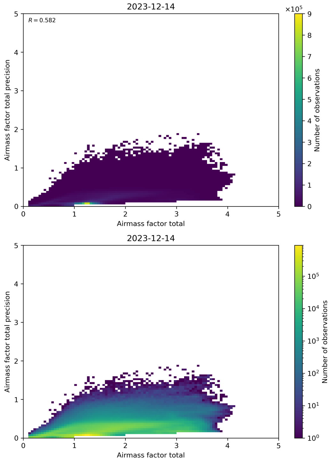
Figure 103: Scatter density plot of “Airmass factor total” against “Airmass factor total precision” for 2023-12-14 to 2023-12-15.
