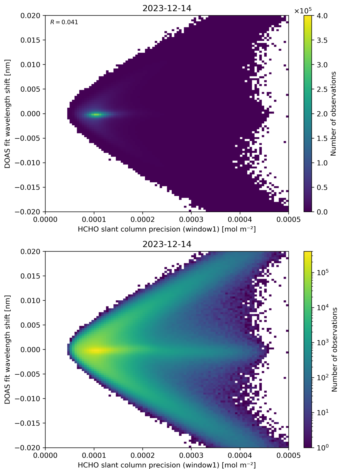
Figure 89: Scatter density plot of “HCHO slant column precision (window1)” against “DOAS fit wavelength shift” for 2023-12-14 to 2023-12-15.
