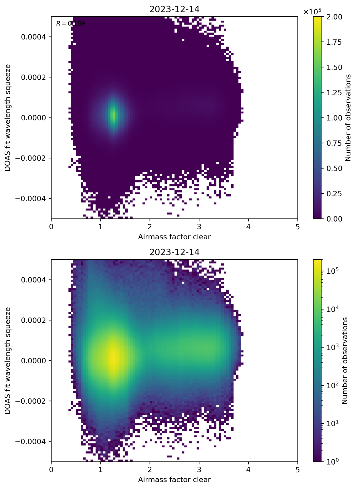
Figure 73: Scatter density plot of “Airmass factor clear” against “DOAS fit wavelength squeeze” for 2023-12-14 to 2023-12-15.
