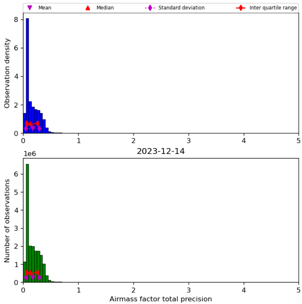
Figure 41: Histogram of “Airmass factor total precision” for 2023-12-14 to 2023-12-15
