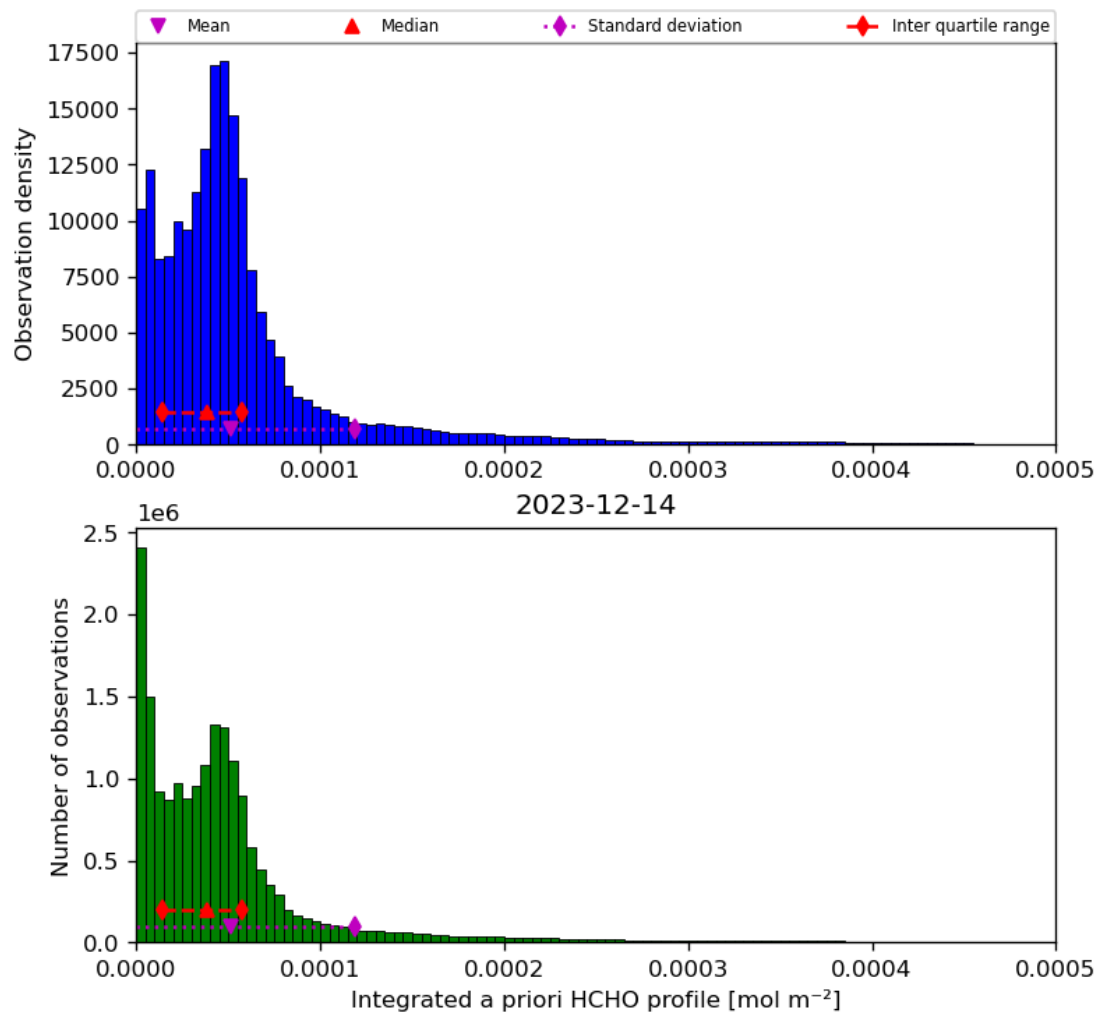
Figure 43: Histogram of “Integrated a priori HCHO profile” for 2023-12-14 to 2023-12-15
