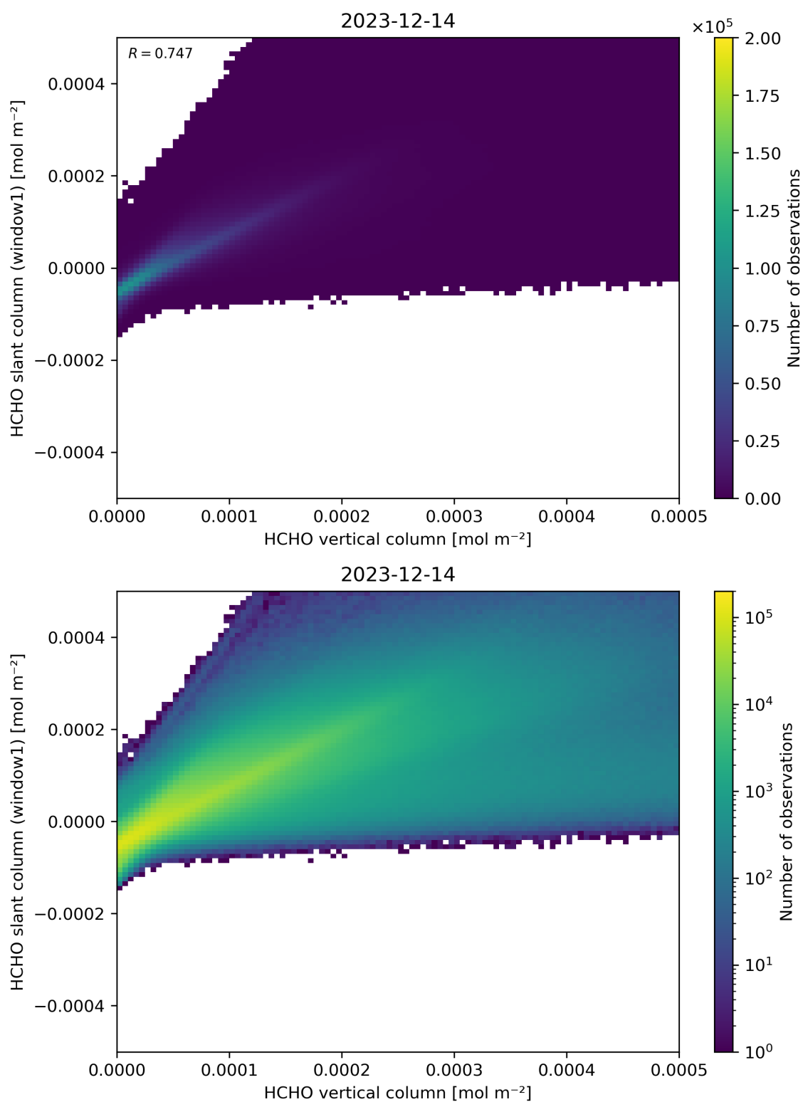
Figure 129: Scatter density plot of “HCHO vertical column” against “HCHO slant column (window1)” for 2023-12-14 to 2023-12-15.
