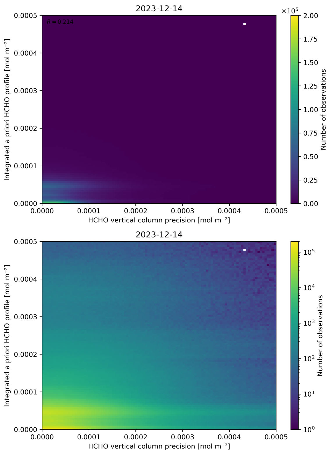
Figure 147: Scatter density plot of “HCHO vertical column precision” against “Integrated a priori HCHO profile” for 2023-12-14 to 2023-12-15.
