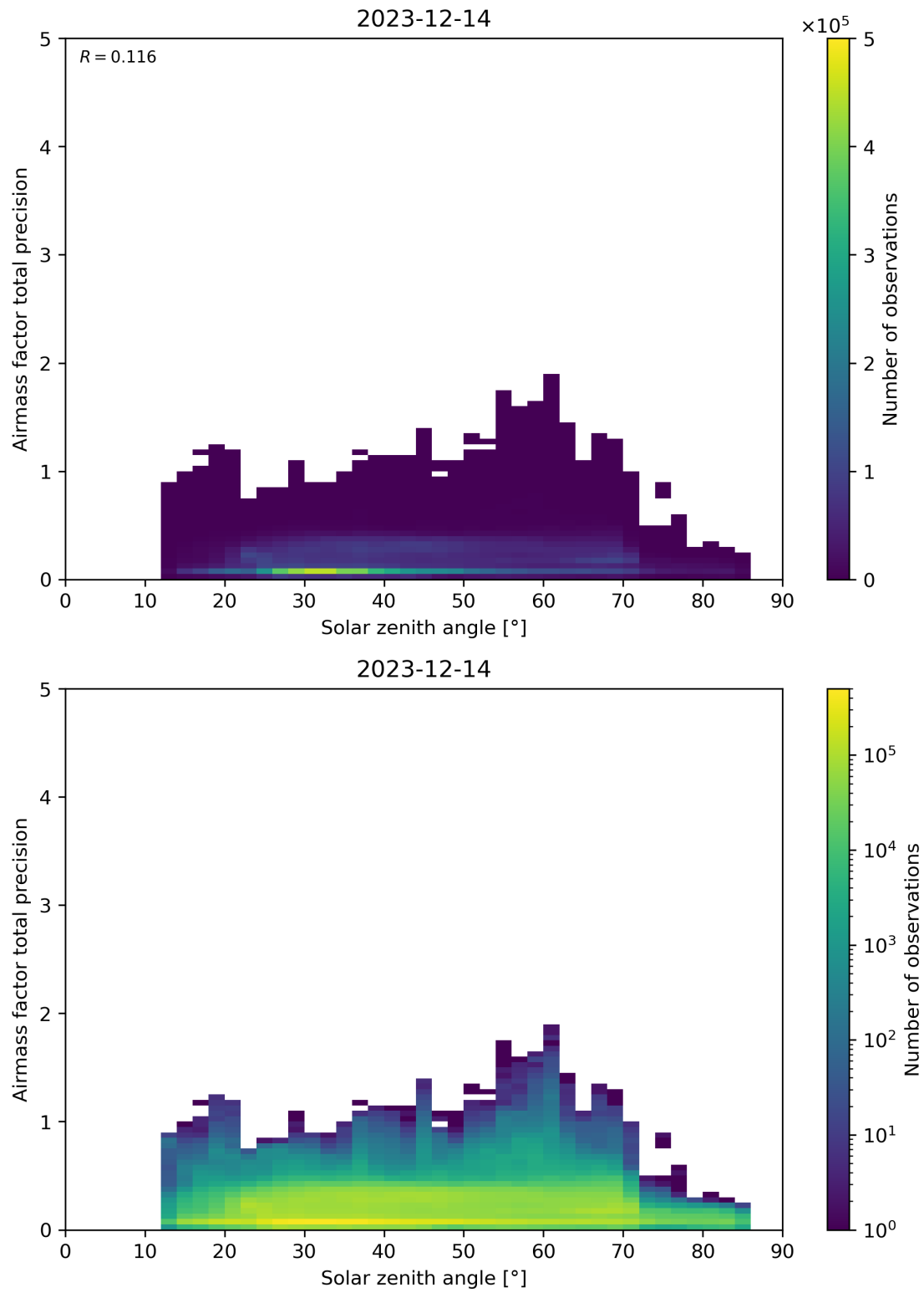
Figure 176: Scatter density plot of “Solar zenith angle” against “Airmass factor total precision” for 2023-12-14 to 2023-12-15.
