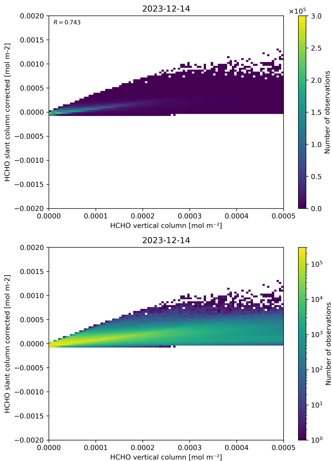
Figure 127: Scatter density plot of “HCHO vertical column” against “HCHO slant column corrected” for 2023-12-14 to 2023-12-15.
