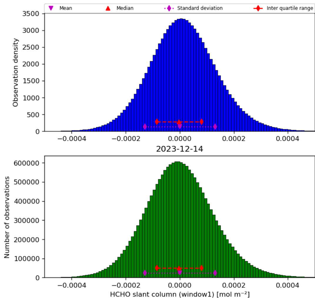
Figure 38: Histogram of “HCHO slant column (window1)” for 2023-12-14 to 2023-12-15
