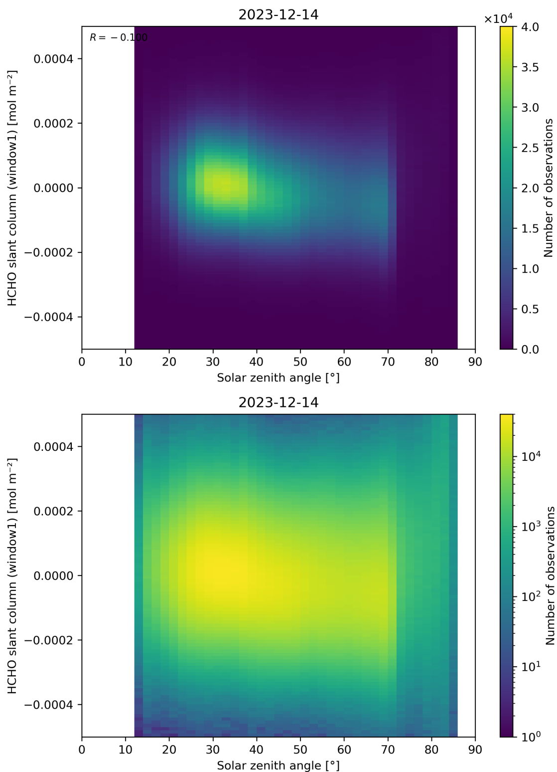
Figure 173: Scatter density plot of “Solar zenith angle” against “HCHO slant column (window1)” for 2023-12-14 to 2023-12-15.
