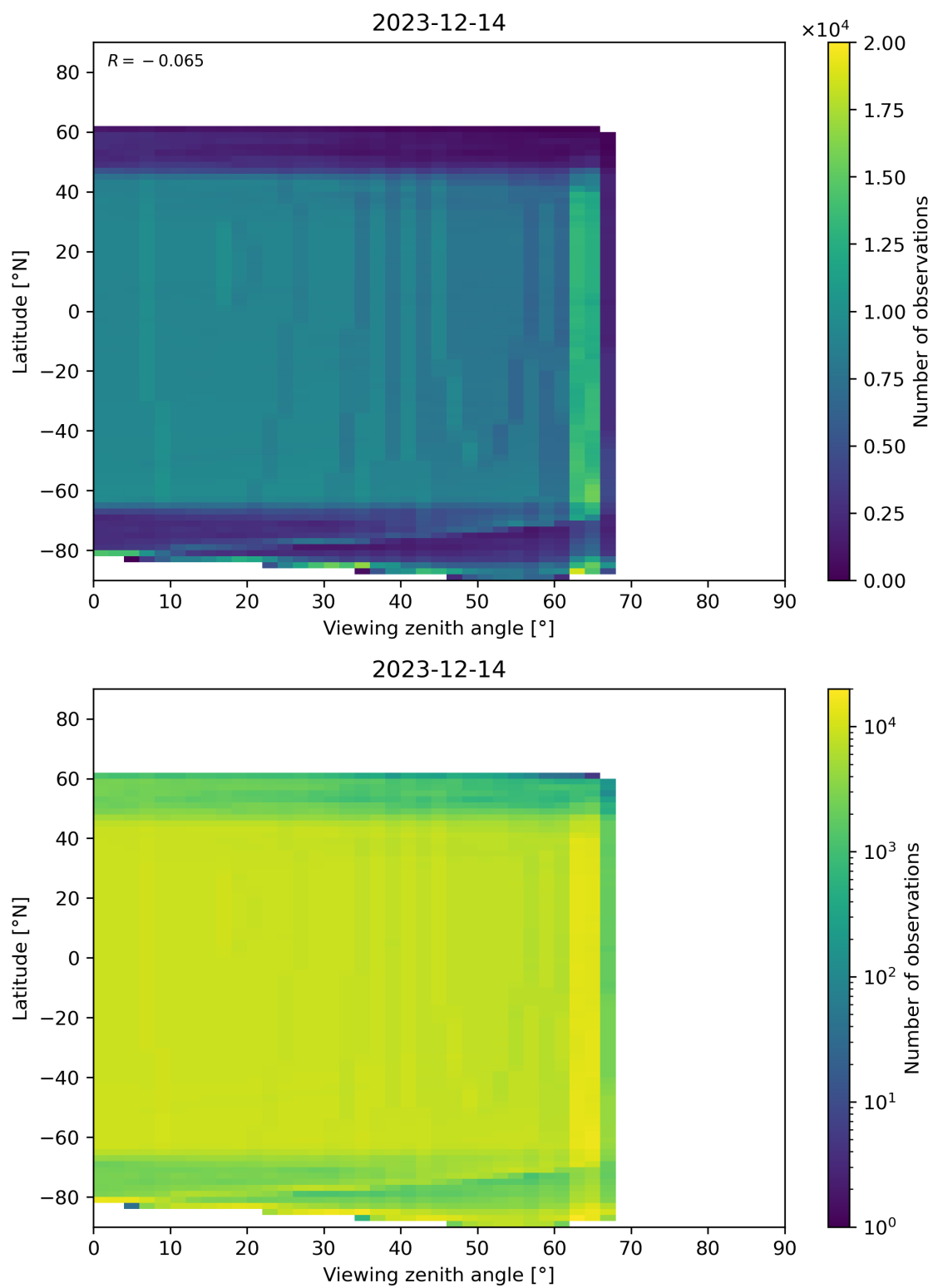
Figure 196: Scatter density plot of “Viewing zenith angle” against “Latitude” for 2023-12-14 to 2023-12-15.
