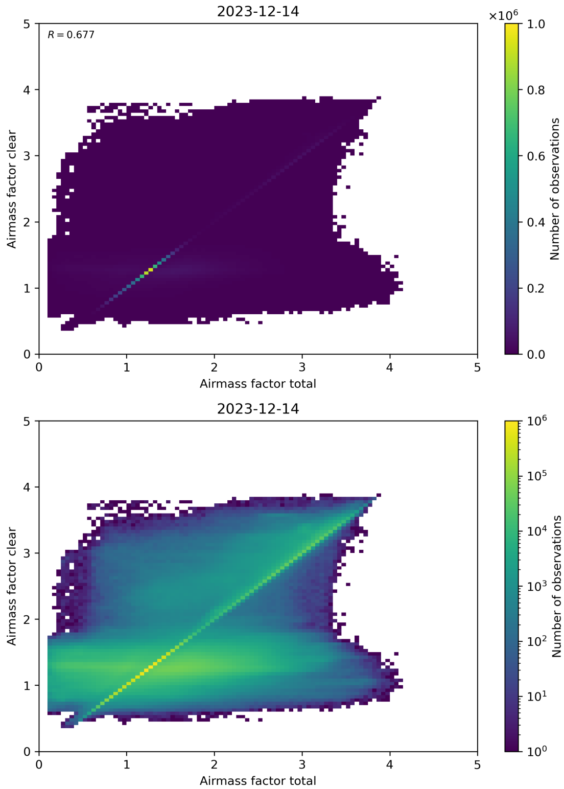
Figure 100: Scatter density plot of “Airmass factor total” against “Airmass factor clear” for 2023-12-14 to 2023-12-15.
