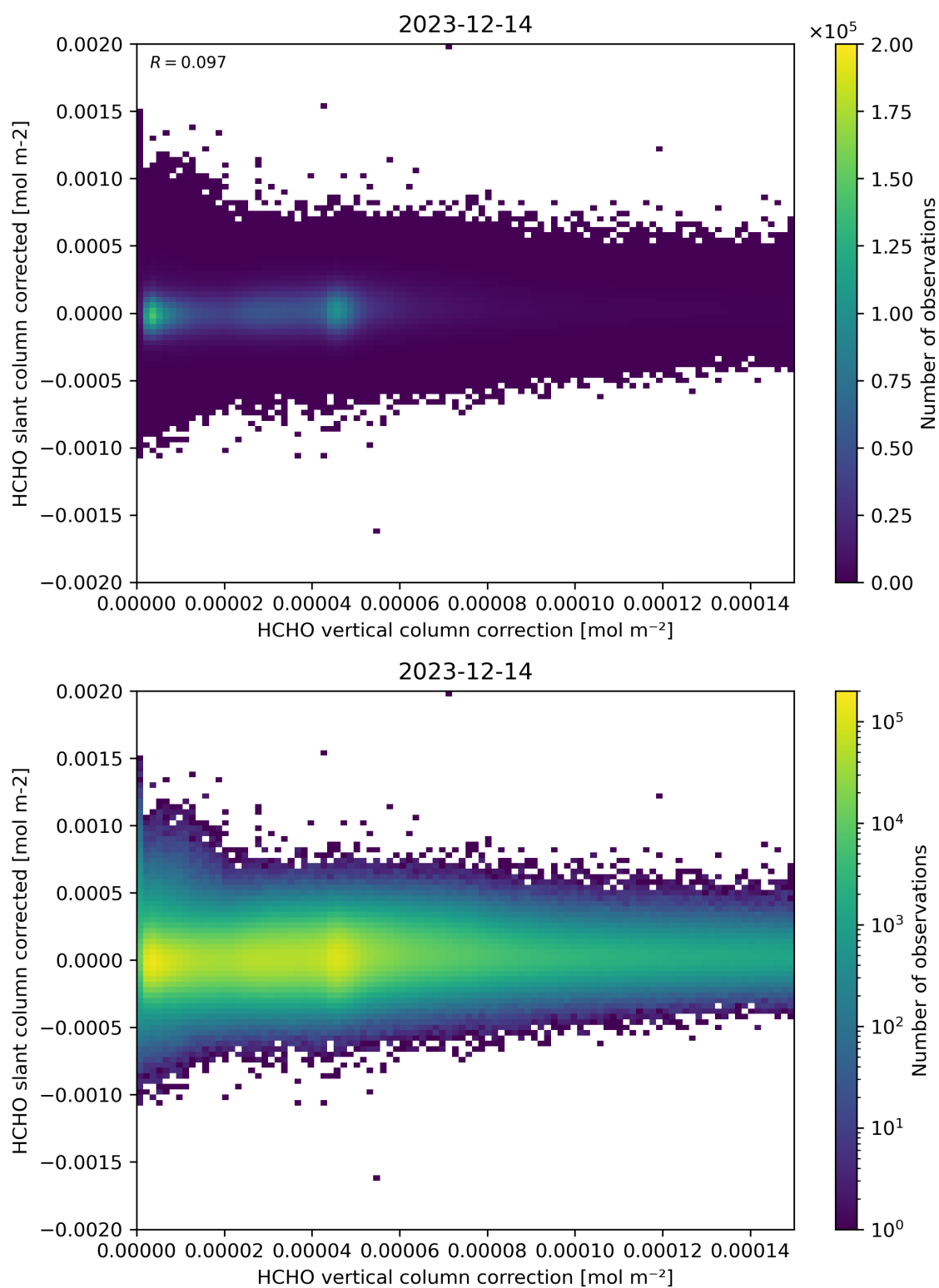
Figure 116: Scatter density plot of “HCHO vertical column correction” against “HCHO slant column corrected” for 2023-12-14 to 2023-12-15.
