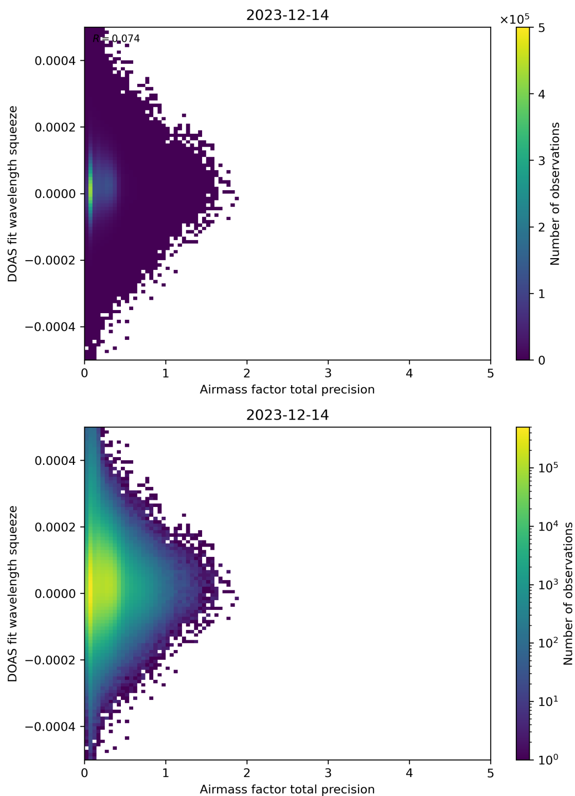
Figure 107: Scatter density plot of “Airmass factor total precision” against “DOAS fit wavelength squeeze” for 2023-12-14 to 2023-12-15.
