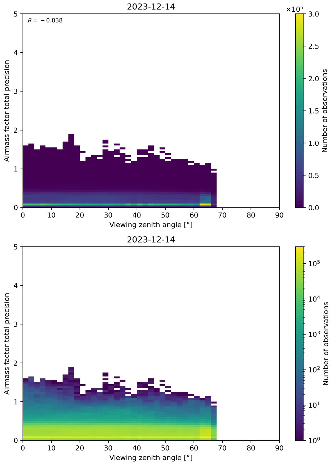
Figure 191: Scatter density plot of “Viewing zenith angle” against “Airmass factor total precision” for 2023-12-14 to 2023-12-15.
