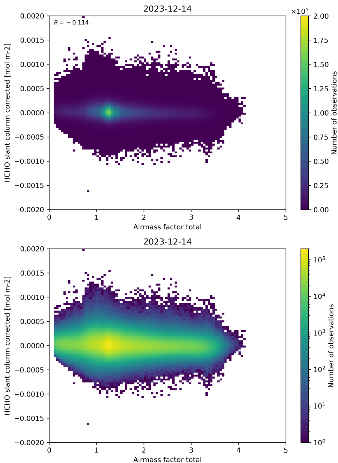
Figure 101: Scatter density plot of “Airmass factor total” against “HCHO slant column corrected” for 2023-12-14 to 2023-12-15.
