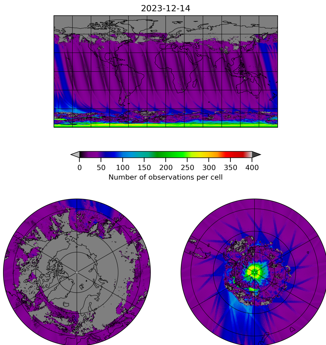
Figure 19: Map of the number of observations for 2023-12-14 to 2023-12-15
