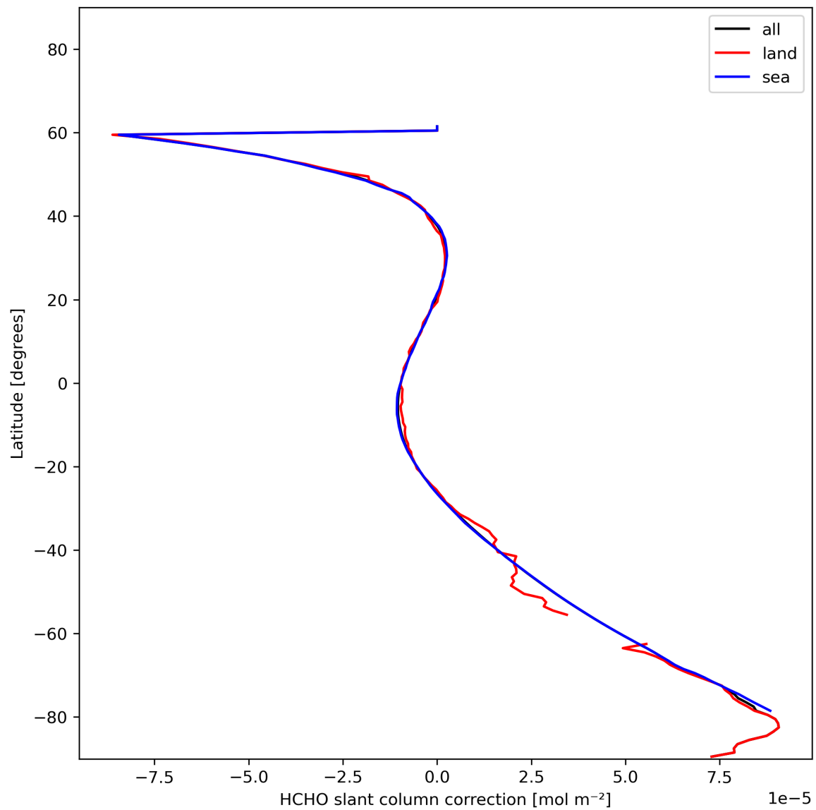
Figure 33: Zonal average of “HCHO slant column correction” for 2023-12-14 to 2023-12-15.
