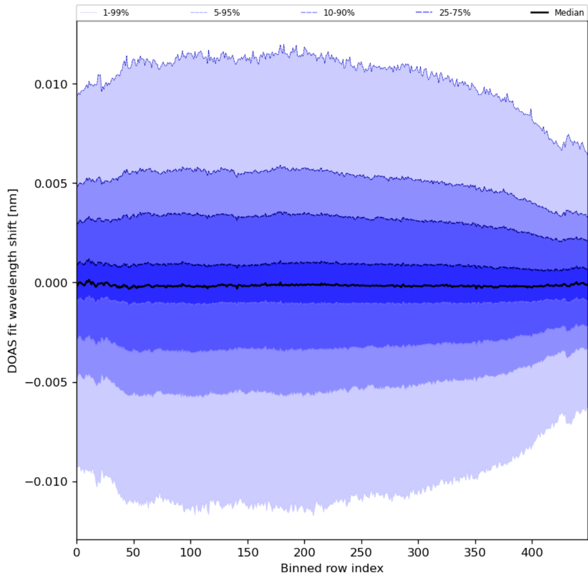
Figure 58: Along track statistics of “DOAS fit wavelength shift” for 2023-12-14 to 2023-12-15
