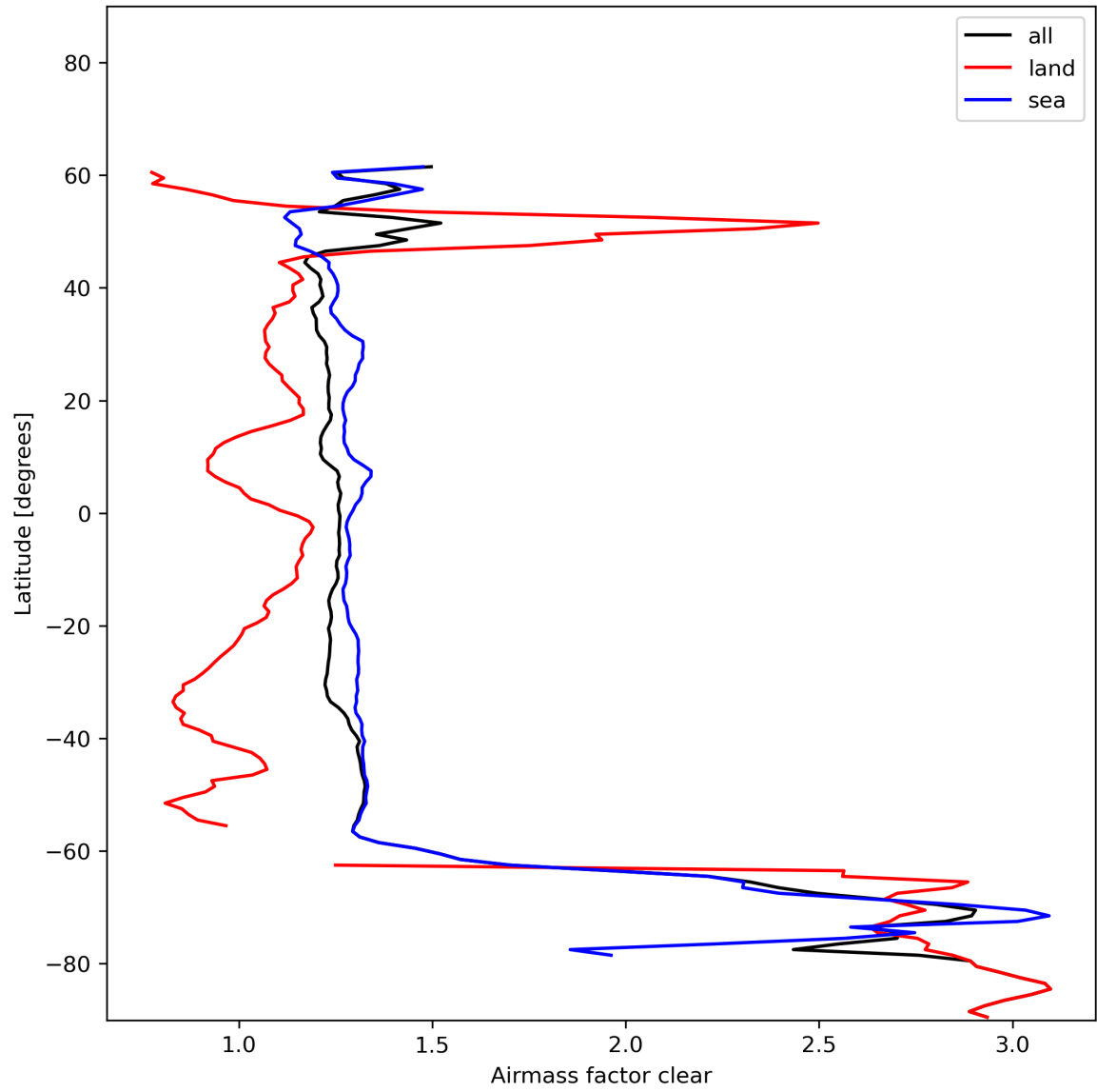
Figure 28: Zonal average of “Airmass factor clear” for 2023-12-14 to 2023-12-15.
