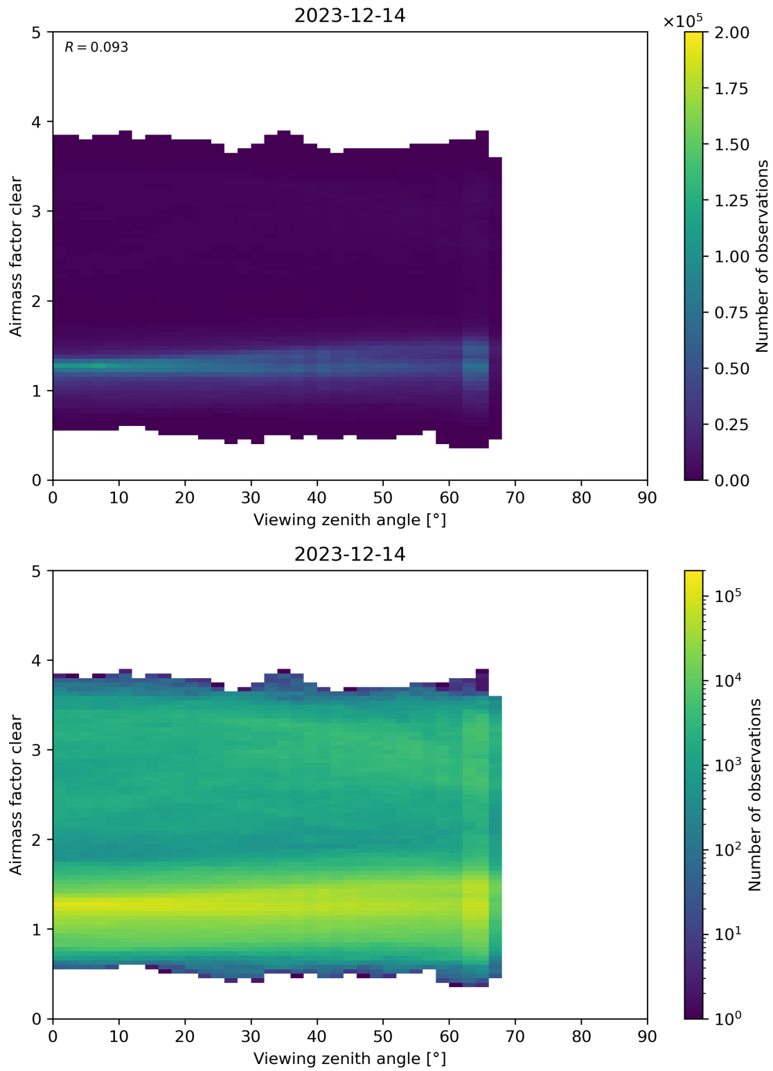
Figure 185: Scatter density plot of “Viewing zenith angle” against “Airmass factor clear” for 2023-12-14 to 2023-12-15.
