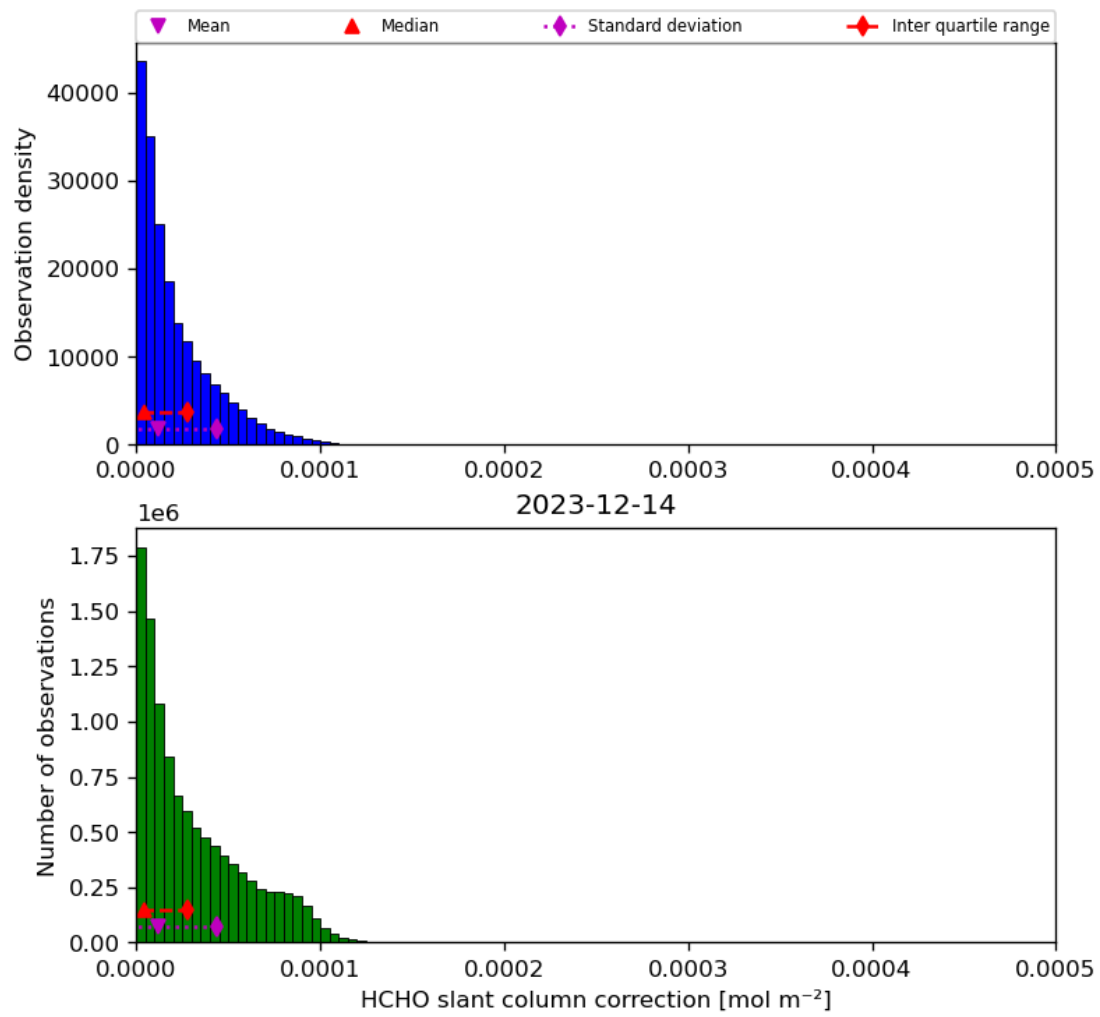
Figure 47: Histogram of “HCHO slant column correction” for 2023-12-14 to 2023-12-15
