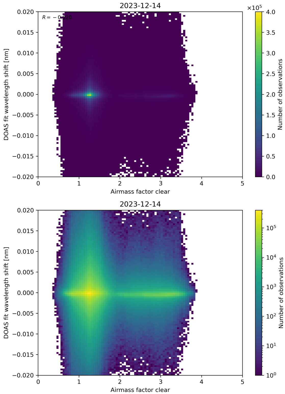
Figure 72: Scatter density plot of “Airmass factor clear” against “DOAS fit wavelength shift” for 2023-12-14 to 2023-12-15.
