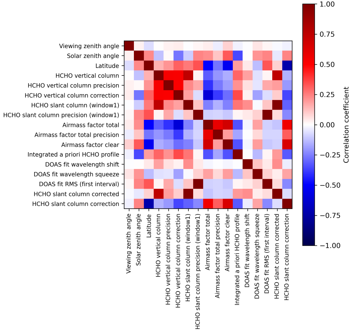
Figure 2: Map of correlation matrix for 2023-12-14 to 2023-12-15.
