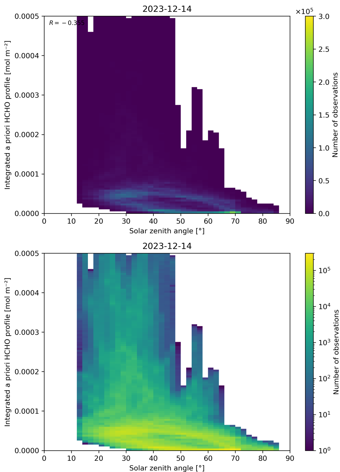
Figure 180: Scatter density plot of “Solar zenith angle” against “Integrated a priori HCHO profile” for 2023-12-14 to 2023-12-15.
