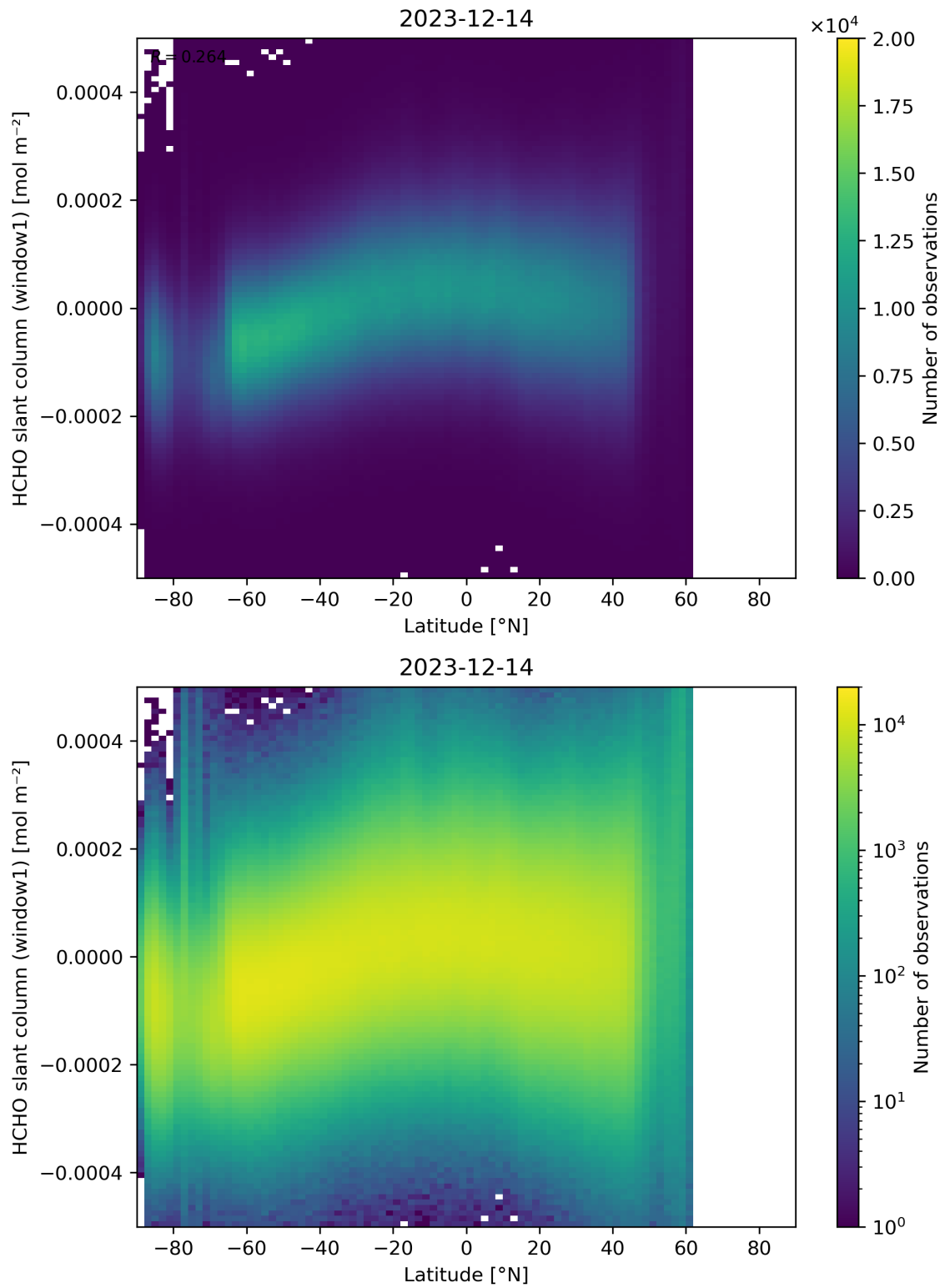
Figure 159: Scatter density plot of “Latitude” against “HCHO slant column (window1)” for 2023-12-14 to 2023-12-15.
