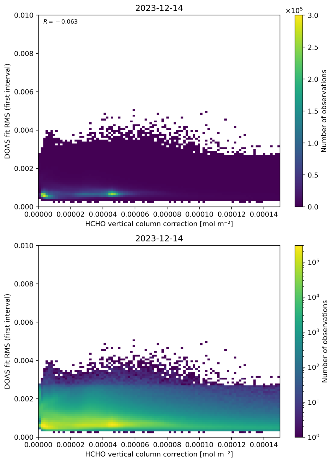
Figure 112: Scatter density plot of “HCHO vertical column correction” against “DOAS fit RMS (first interval)” for 2023-12-14 to 2023-12-15.
