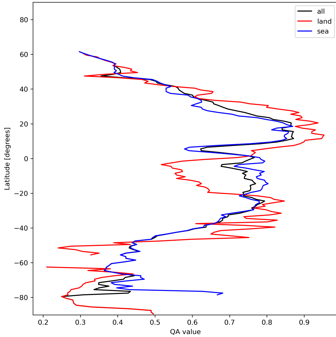
Figure 20: Zonal average of “QA value” for 2023-12-14 to 2023-12-15.
