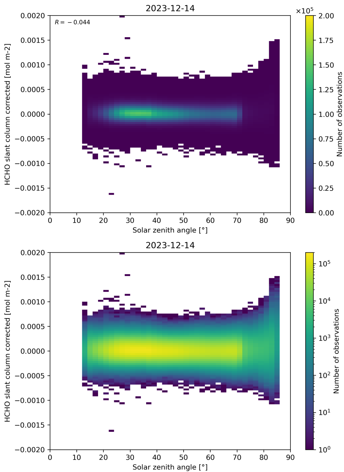
Figure 171: Scatter density plot of “Solar zenith angle” against “HCHO slant column corrected” for 2023-12-14 to 2023-12-15.
