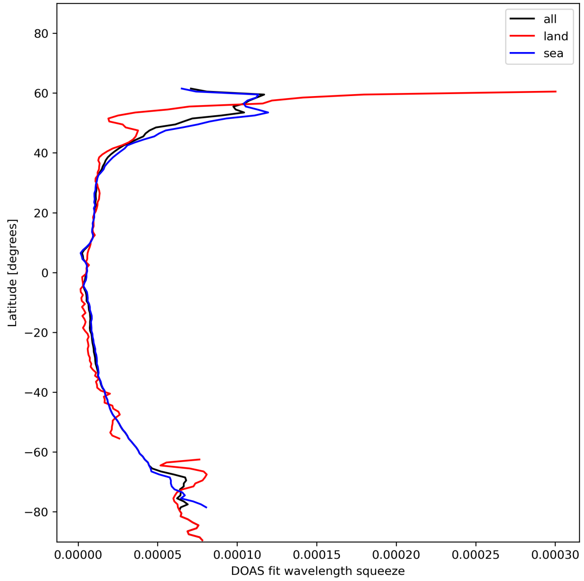
Figure 31: Zonal average of “DOAS fit wavelength squeeze” for 2023-12-14 to 2023-12-15.
