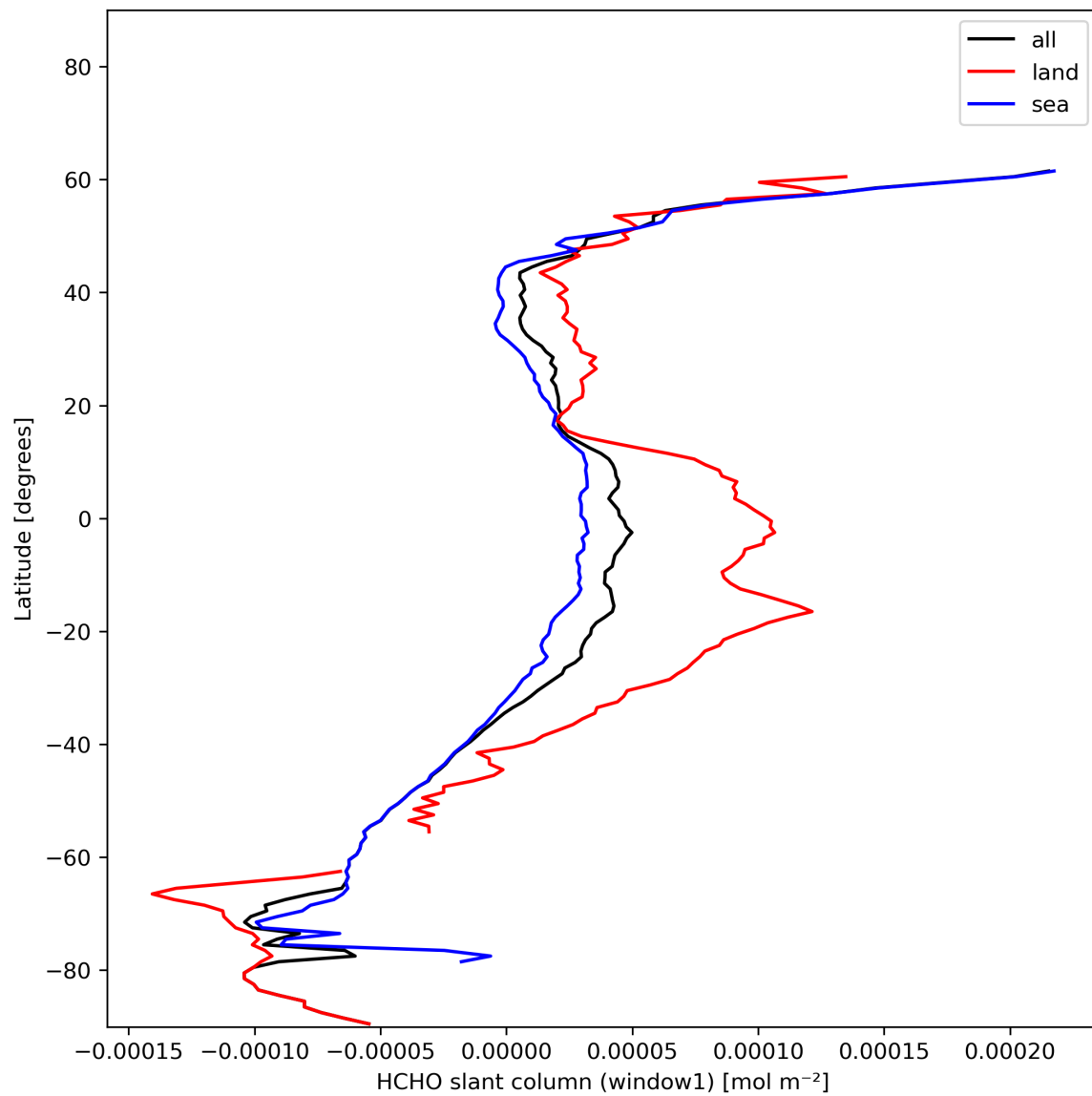
Figure 24: Zonal average of “HCHO slant column (window1)” for 2023-12-14 to 2023-12-15.
