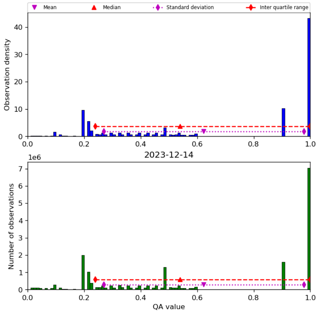
Figure 34: Histogram of “QA value” for 2023-12-14 to 2023-12-15
