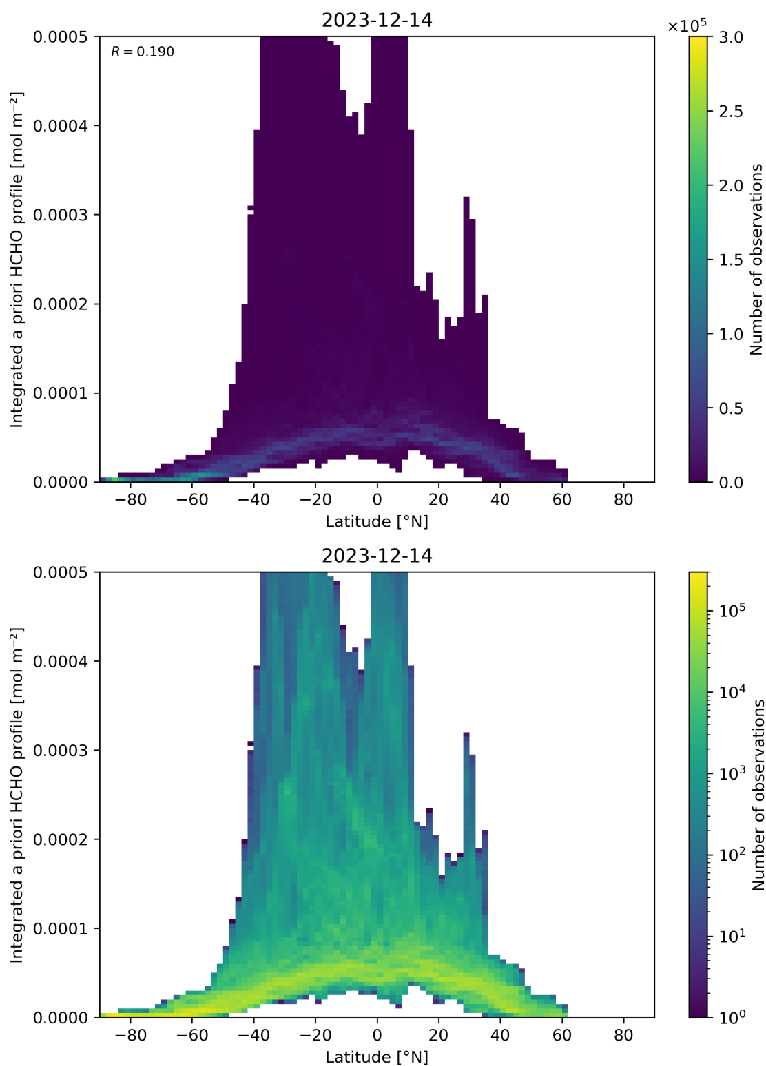
Figure 166: Scatter density plot of “Latitude” against “Integrated a priori HCHO profile” for 2023-12-14 to 2023-12-15.
