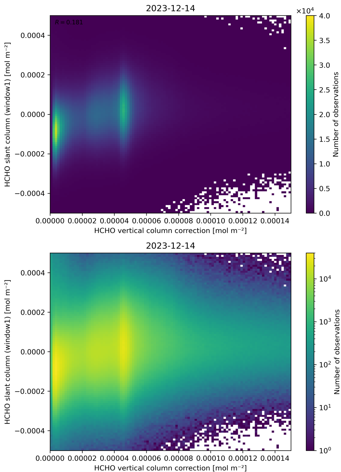
Figure 118: Scatter density plot of “HCHO vertical column correction” against “HCHO slant column (window1)” for 2023-12-14 to 2023-12-15.
