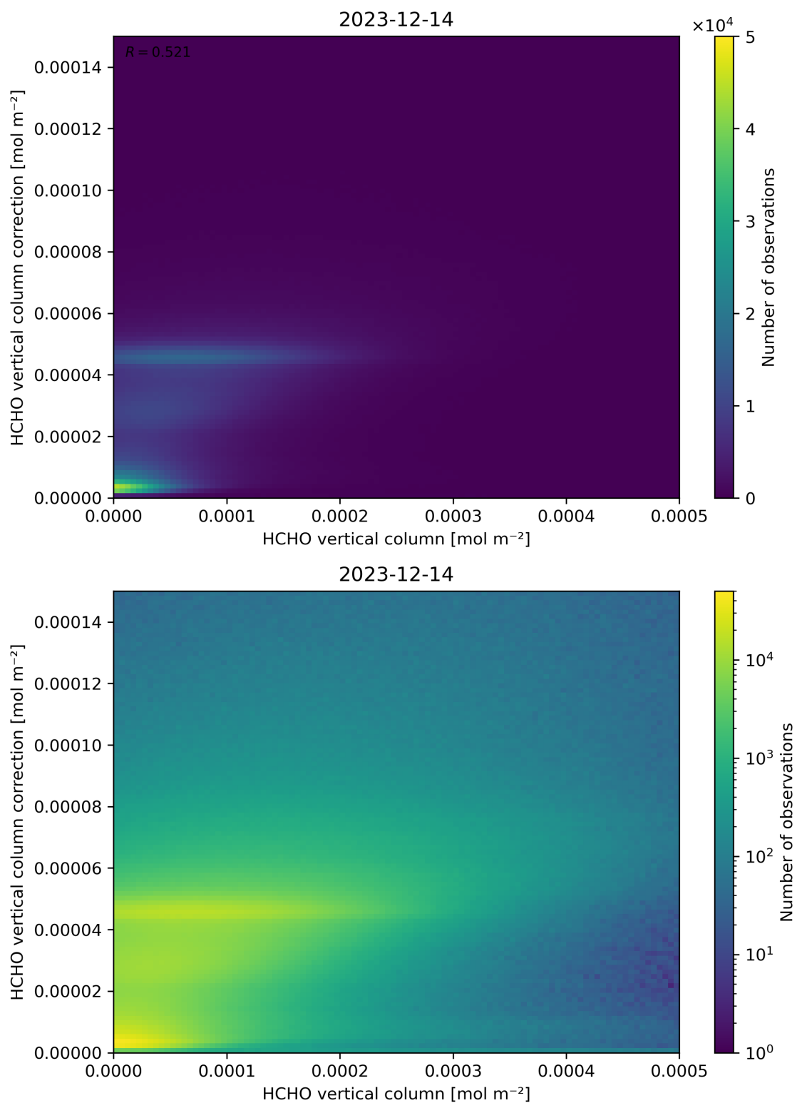
Figure 133: Scatter density plot of “HCHO vertical column” against “HCHO vertical column correction” for 2023-12-14 to 2023-12-15.
