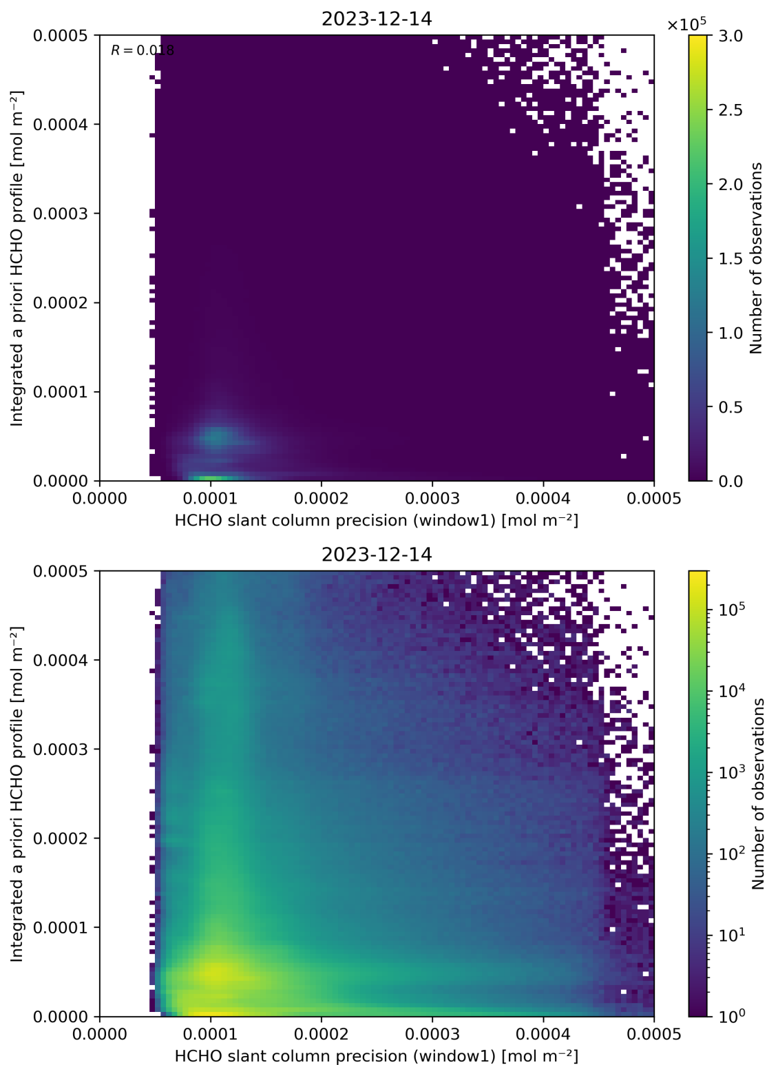
Figure 96: Scatter density plot of “HCHO slant column precision (window1)” against “Integrated a priori HCHO profile” for 2023-12-14 to 2023-12-15.
