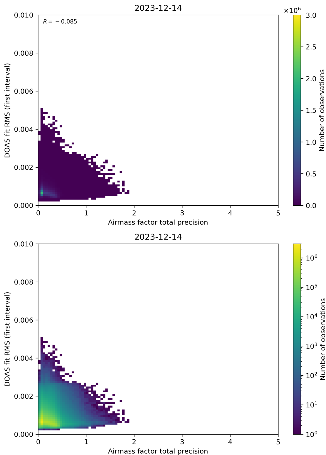
Figure 105: Scatter density plot of “Airmass factor total precision” against “DOAS fit RMS (first interval)” for 2023-12-14 to 2023-12-15.
