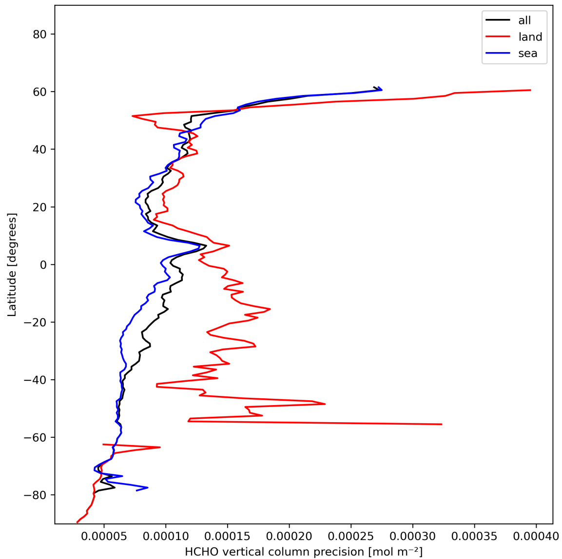
Figure 22: Zonal average of “HCHO vertical column precision” for 2023-12-14 to 2023-12-15.
