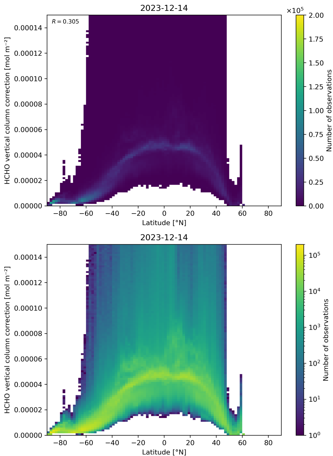
Figure 164: Scatter density plot of “Latitude” against “HCHO vertical column correction” for 2023-12-14 to 2023-12-15.
