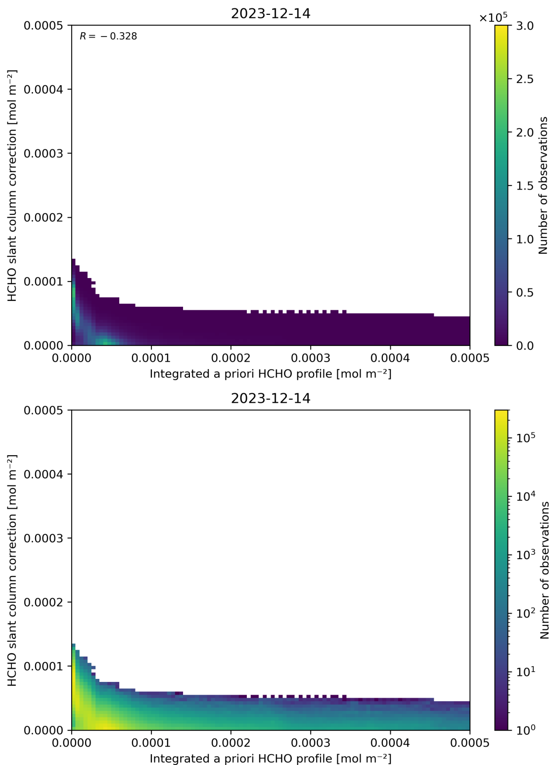
Figure 152: Scatter density plot of “Integrated a priori HCHO profile” against “HCHO slant column correction” for 2023-12-14 to 2023-12-15.
