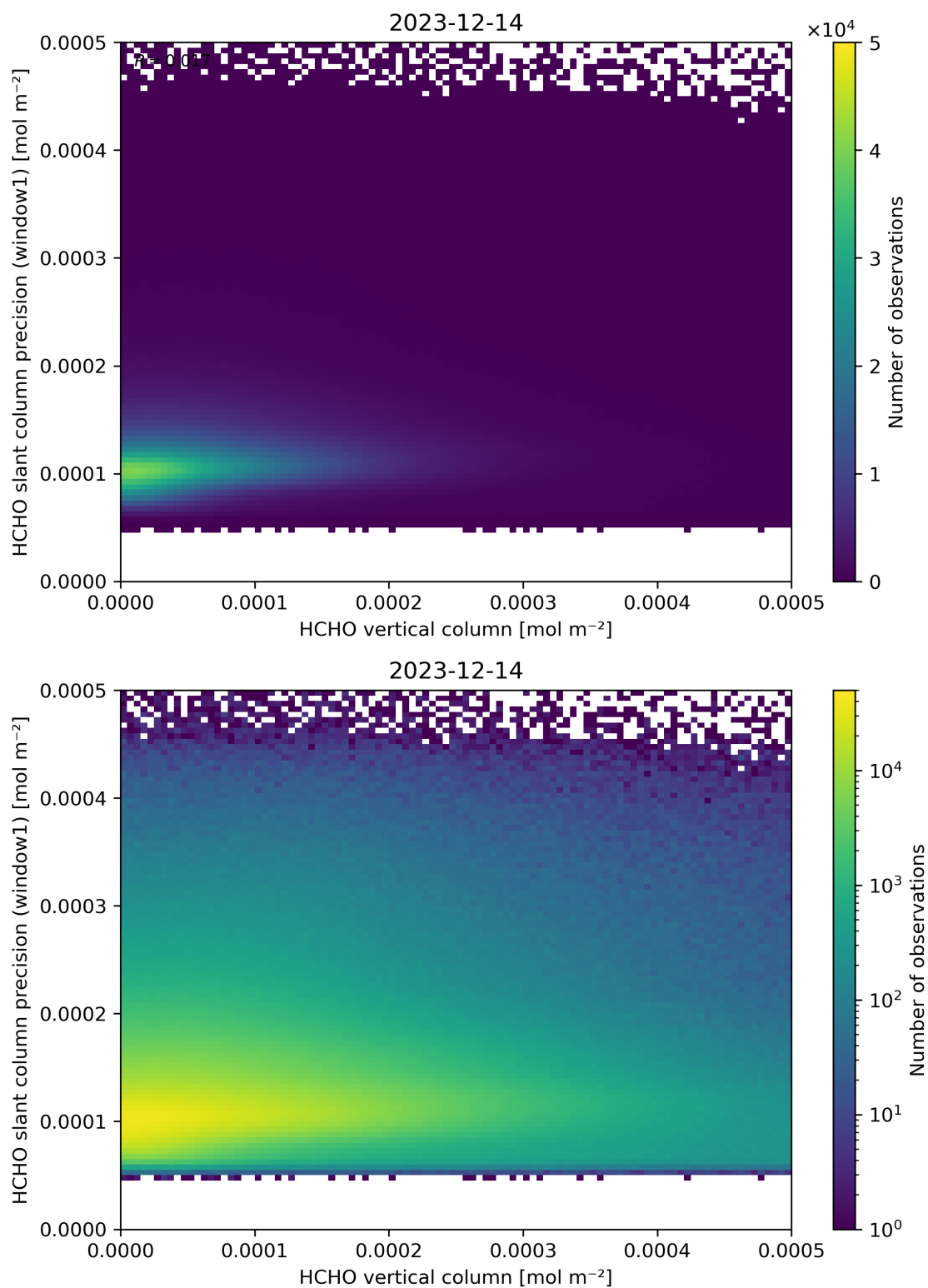
Figure 130: Scatter density plot of “HCHO vertical column” against “HCHO slant column precision (window1)” for 2023-12-14 to 2023-12-15.
