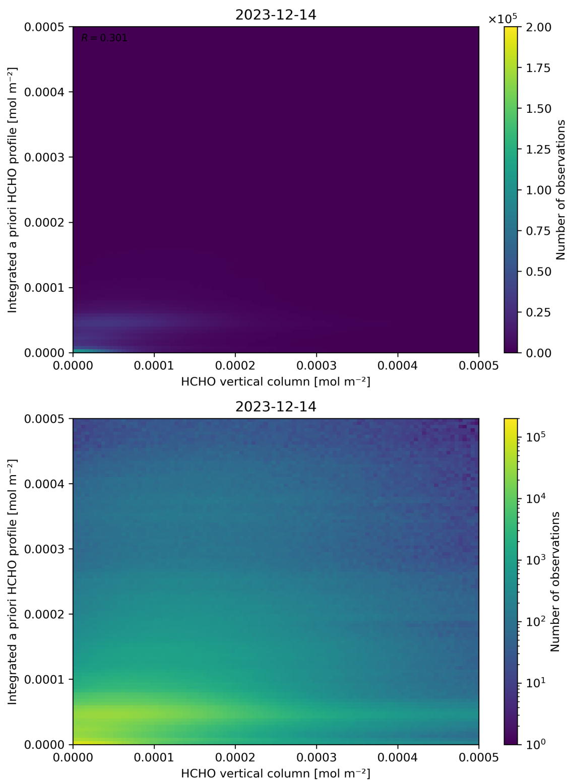
Figure 135: Scatter density plot of “HCHO vertical column” against “Integrated a priori HCHO profile” for 2023-12-14 to 2023-12-15.
