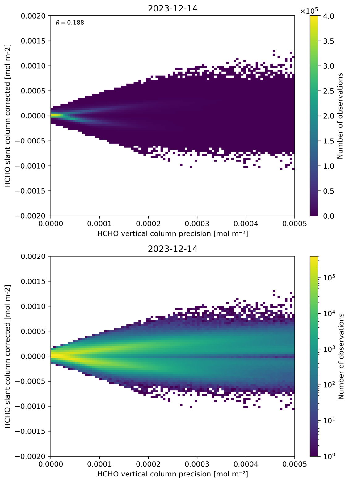
Figure 140: Scatter density plot of “HCHO vertical column precision” against “HCHO slant column corrected” for 2023-12-14 to 2023-12-15.
