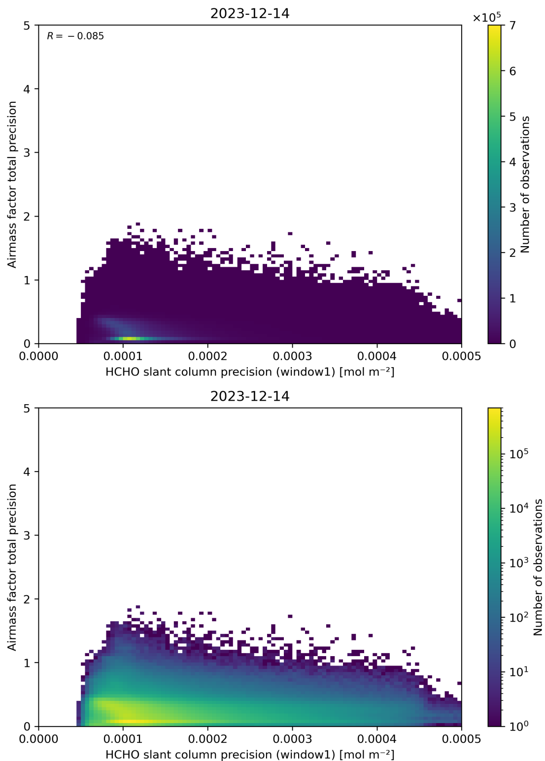
Figure 95: Scatter density plot of “HCHO slant column precision (window1)” against “Airmass factor total precision” for 2023-12-14 to 2023-12-15.
