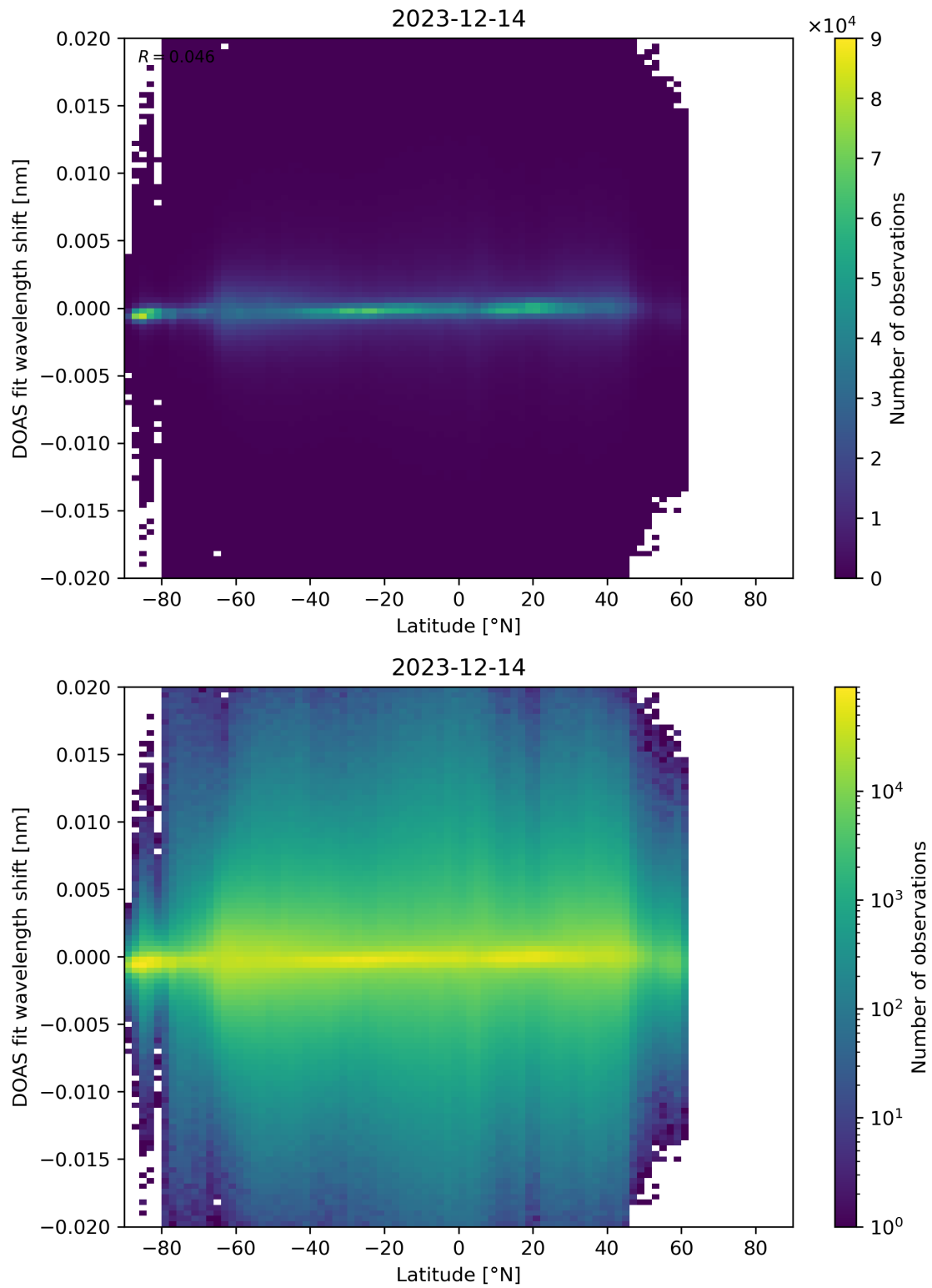
Figure 154: Scatter density plot of “Latitude” against “DOAS fit wavelength shift” for 2023-12-14 to 2023-12-15.
