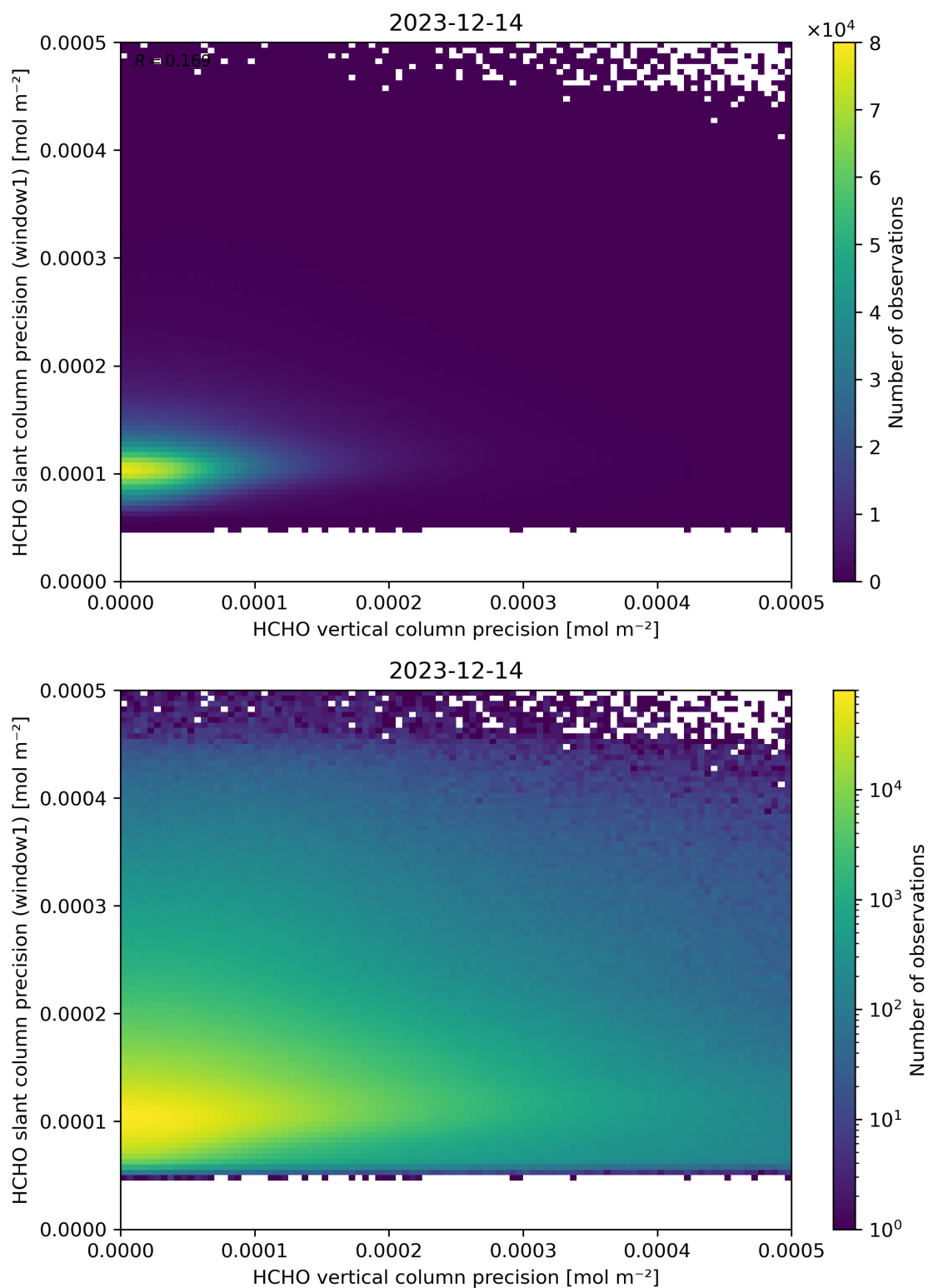
Figure 143: Scatter density plot of “HCHO vertical column precision” against “HCHO slant column precision (window1)” for 2023-12-14 to 2023-12-15.
