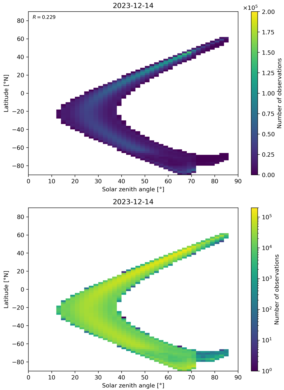
Figure 181: Scatter density plot of “Solar zenith angle” against “Latitude” for 2023-12-14 to 2023-12-15.
