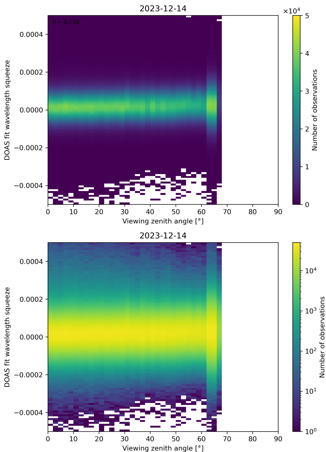
Figure 184: Scatter density plot of “Viewing zenith angle” against “DOAS fit wavelength squeeze” for 2023-12-14 to 2023-12-15.
