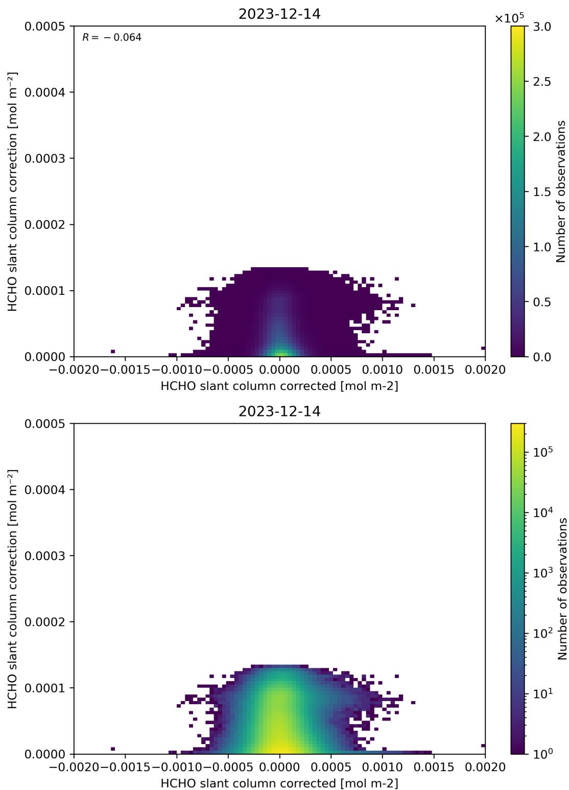
Figure 77: Scatter density plot of “HCHO slant column corrected” against “HCHO slant column correction” for 2023-12-14 to 2023-12-15.
