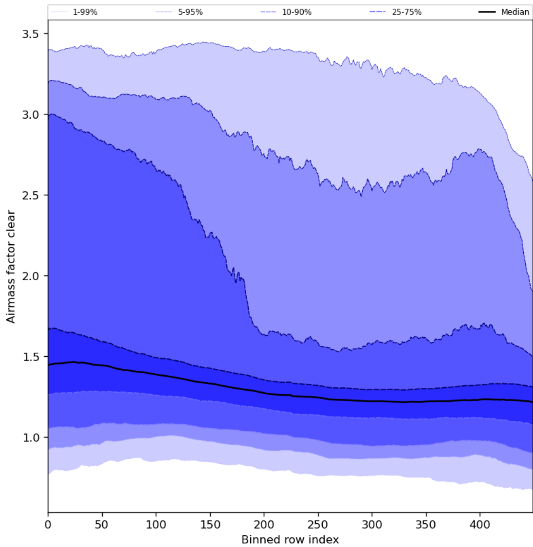
Figure 56: Along track statistics of “Airmass factor clear” for 2023-12-14 to 2023-12-15
