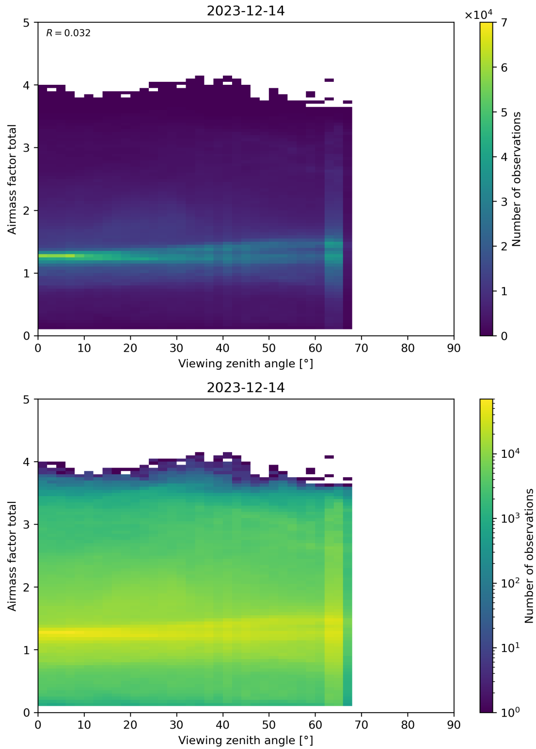
Figure 190: Scatter density plot of “Viewing zenith angle” against “Airmass factor total” for 2023-12-14 to 2023-12-15.
