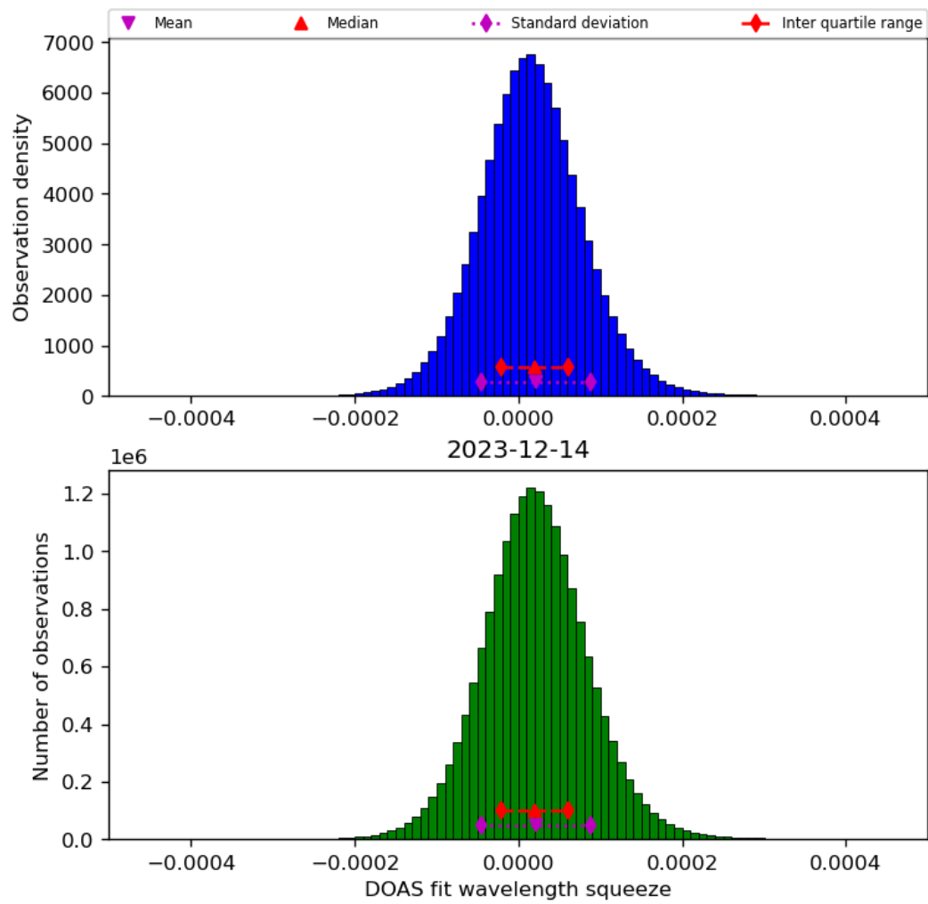
Figure 45: Histogram of “DOAS fit wavelength squeeze” for 2023-12-14 to 2023-12-15
