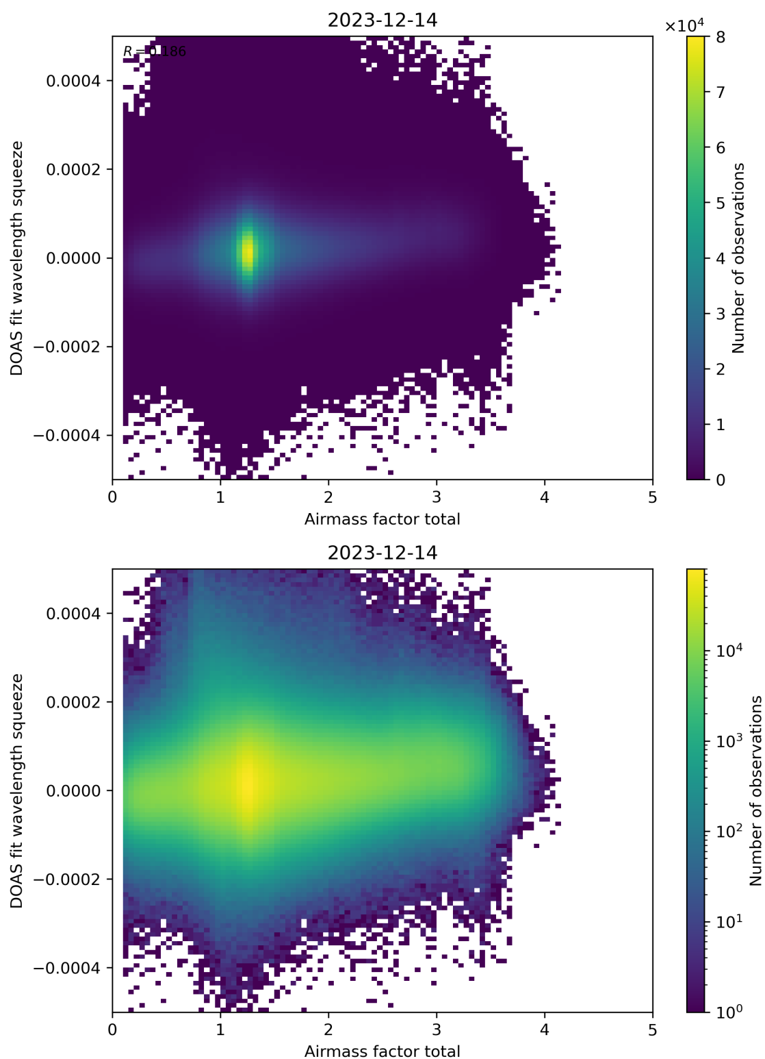
Figure 99: Scatter density plot of “Airmass factor total” against “DOAS fit wavelength squeeze” for 2023-12-14 to 2023-12-15.
