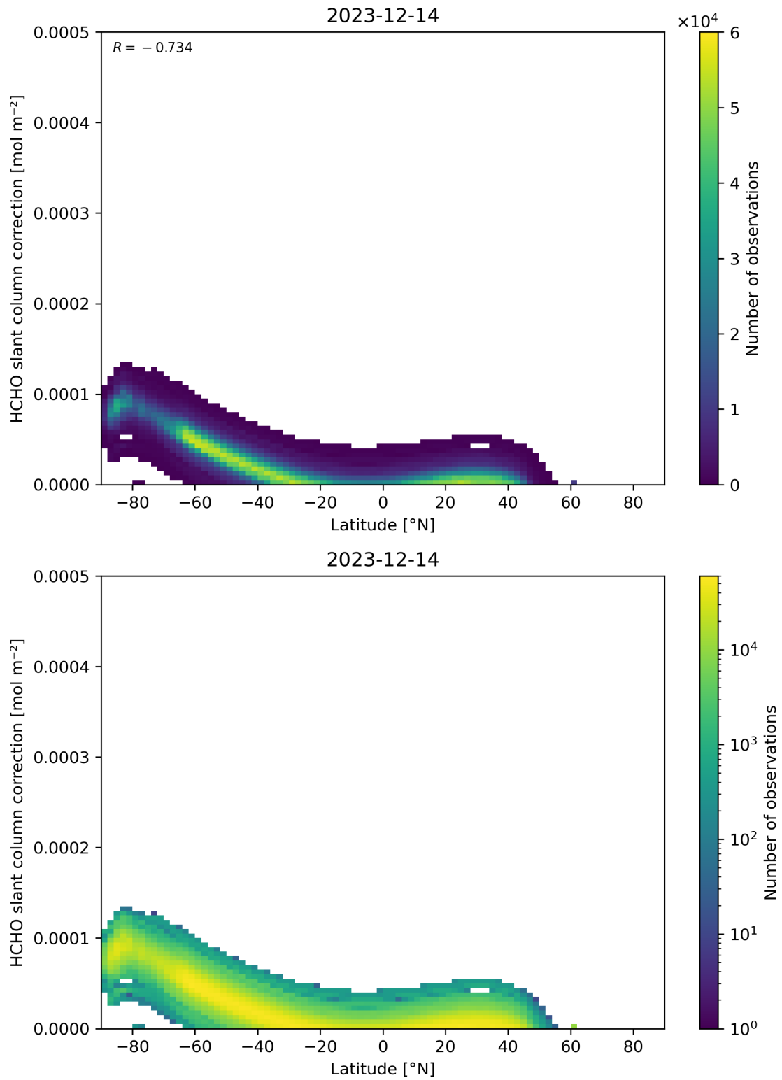
Figure 158: Scatter density plot of “Latitude” against “HCHO slant column correction” for 2023-12-14 to 2023-12-15.
