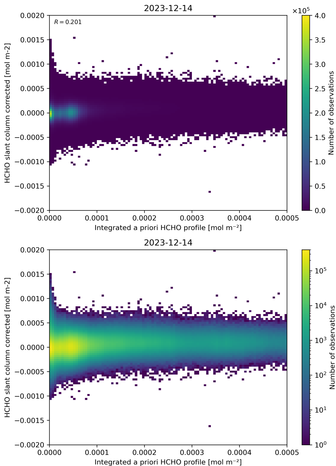
Figure 151: Scatter density plot of “Integrated a priori HCHO profile” against “HCHO slant column corrected” for 2023-12-14 to 2023-12-15.
