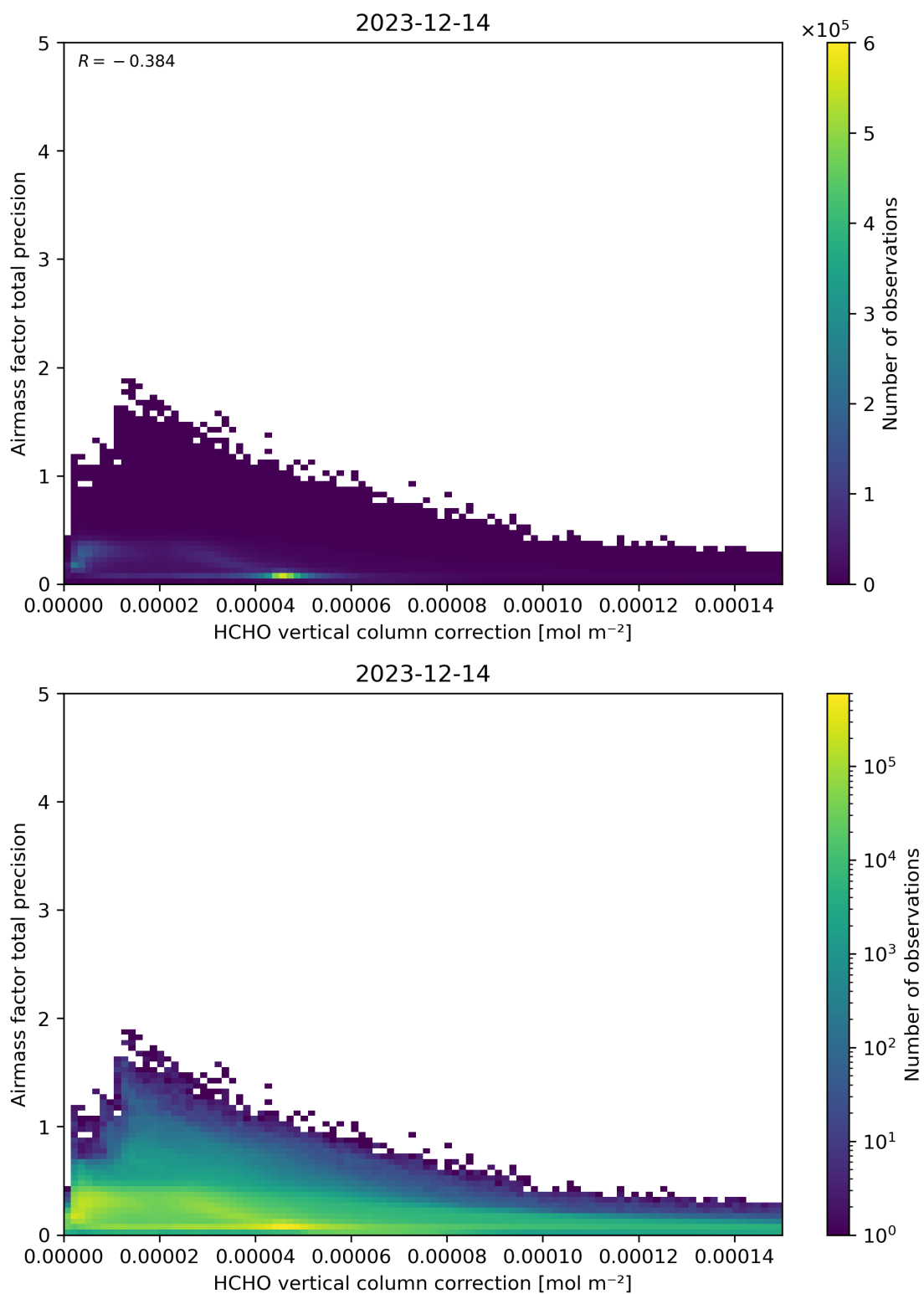
Figure 121: Scatter density plot of “HCHO vertical column correction” against “Airmass factor total precision” for 2023-12-14 to 2023-12-15.
