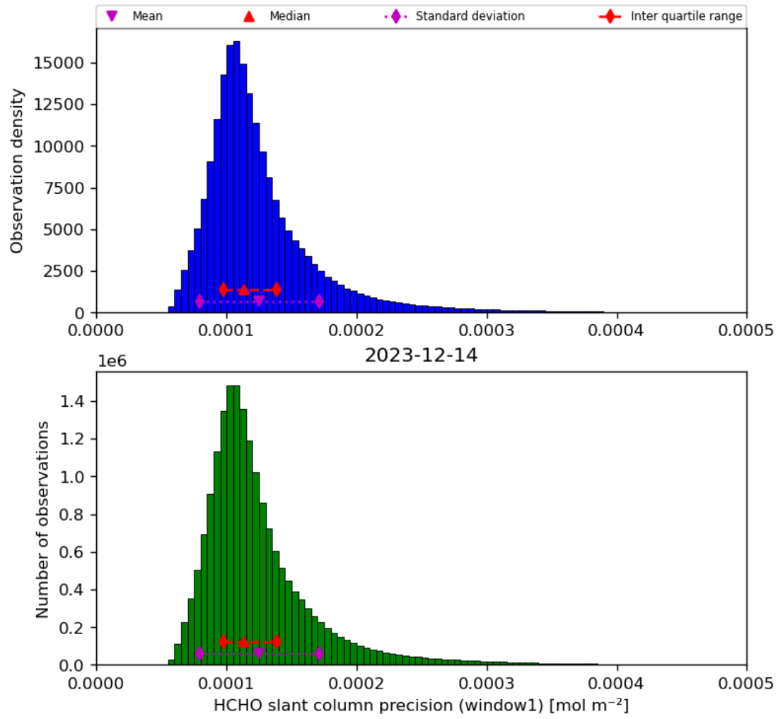
Figure 39: Histogram of “HCHO slant column precision (window1)” for 2023-12-14 to 2023-12-15
