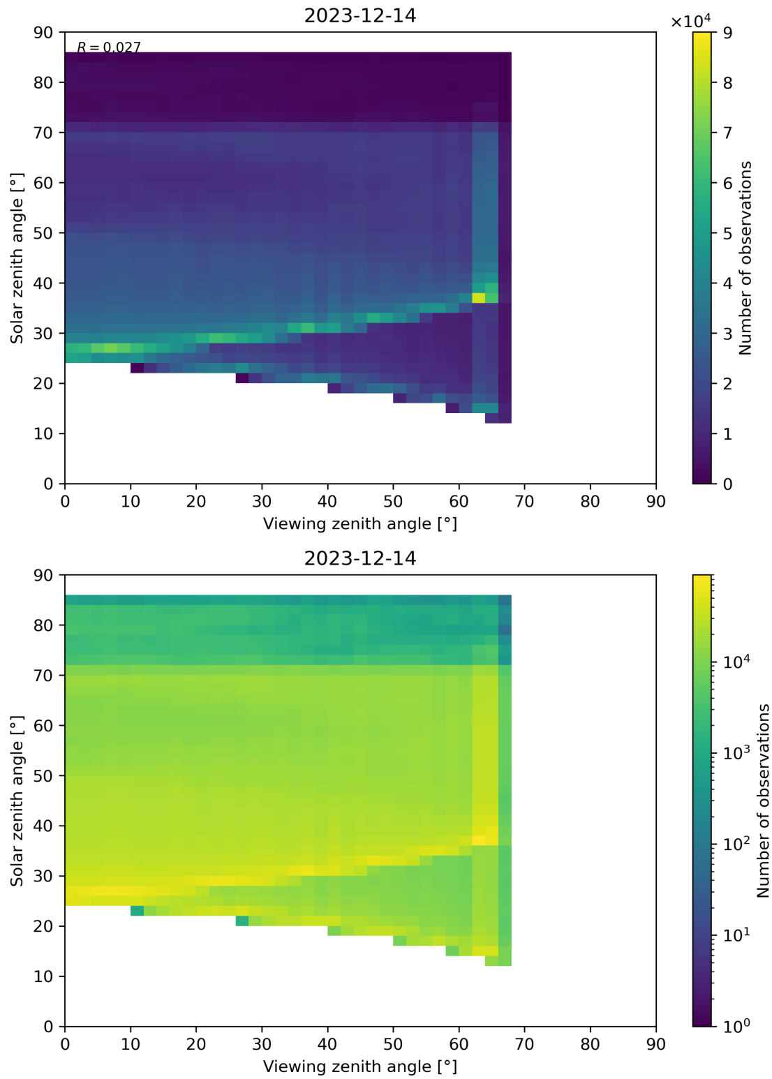
Figure 197: Scatter density plot of “Viewing zenith angle” against “Solar zenith angle” for 2023-12-14 to 2023-12-15.
