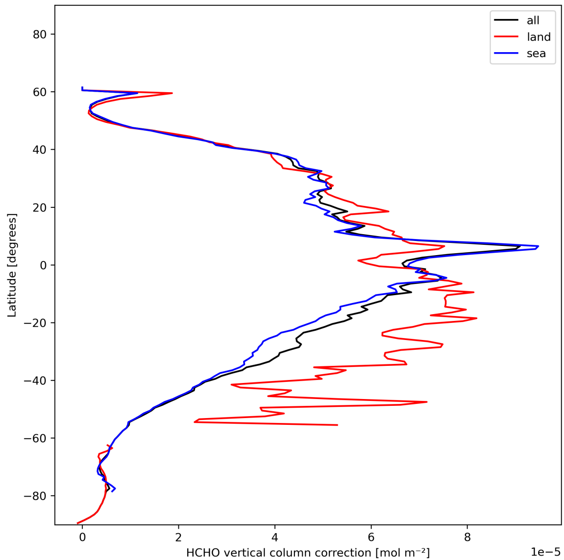
Figure 23: Zonal average of “HCHO vertical column correction” for 2023-12-14 to 2023-12-15.
