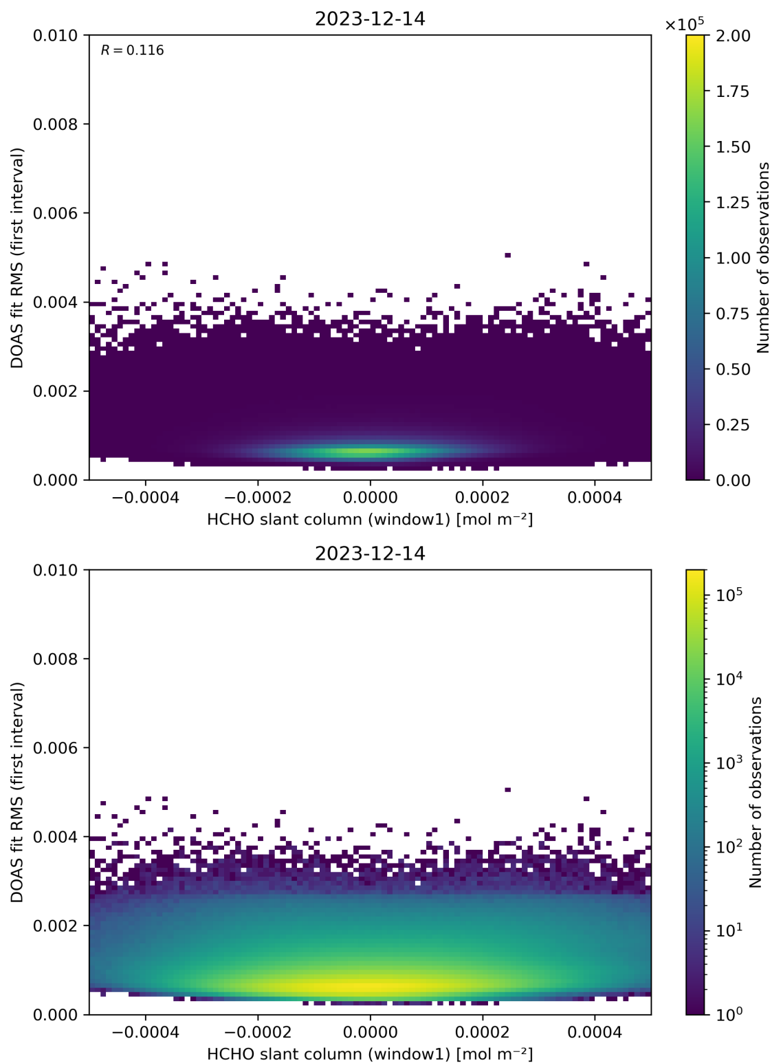
Figure 78: Scatter density plot of “HCHO slant column (window1)” against “DOAS fit RMS (first interval)” for 2023-12-14 to 2023-12-15.
