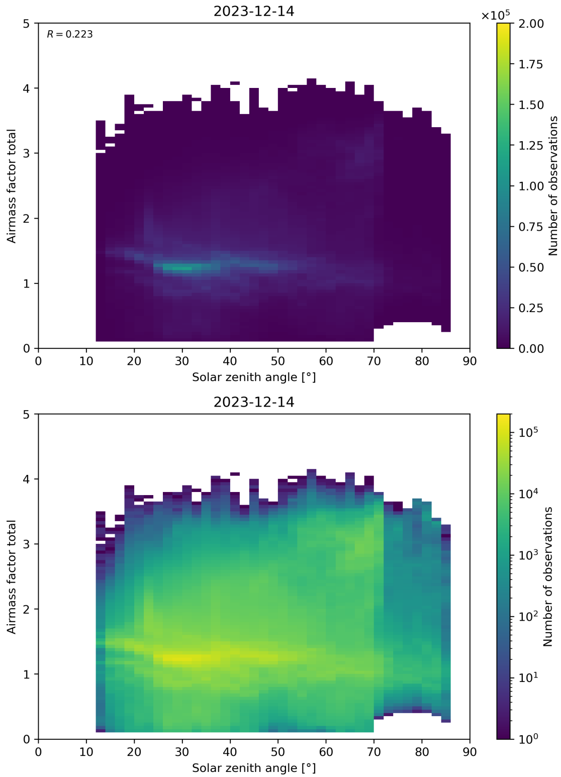
Figure 175: Scatter density plot of “Solar zenith angle” against “Airmass factor total” for 2023-12-14 to 2023-12-15.
