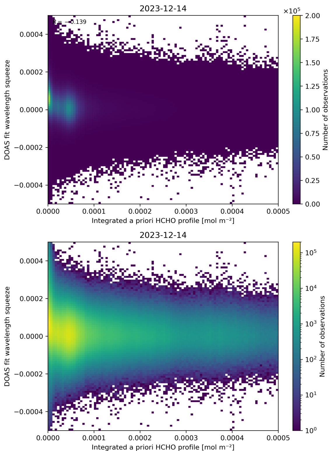
Figure 150: Scatter density plot of “Integrated a priori HCHO profile” against “DOAS fit wavelength squeeze” for 2023-12-14 to 2023-12-15.
