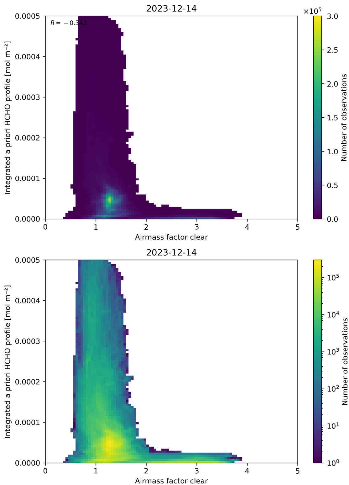
Figure 76: Scatter density plot of “Airmass factor clear” against “Integrated a priori HCHO profile” for 2023-12-14 to 2023-12-15.
