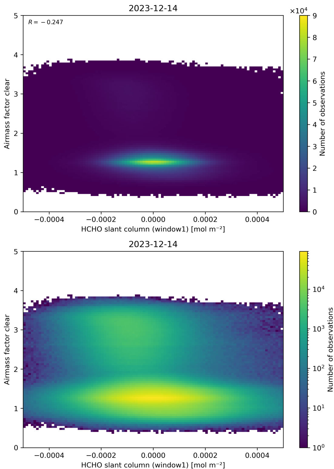
Figure 81: Scatter density plot of “HCHO slant column (window1)” against “Airmass factor clear” for 2023-12-14 to 2023-12-15.
