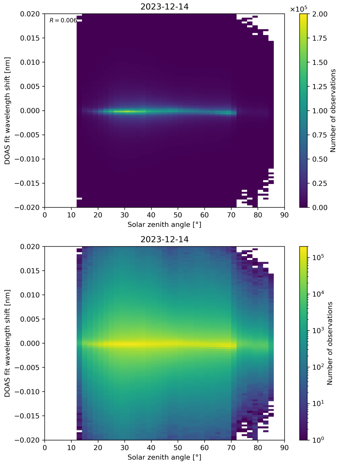
Figure 168: Scatter density plot of “Solar zenith angle” against “DOAS fit wavelength shift” for 2023-12-14 to 2023-12-15.
