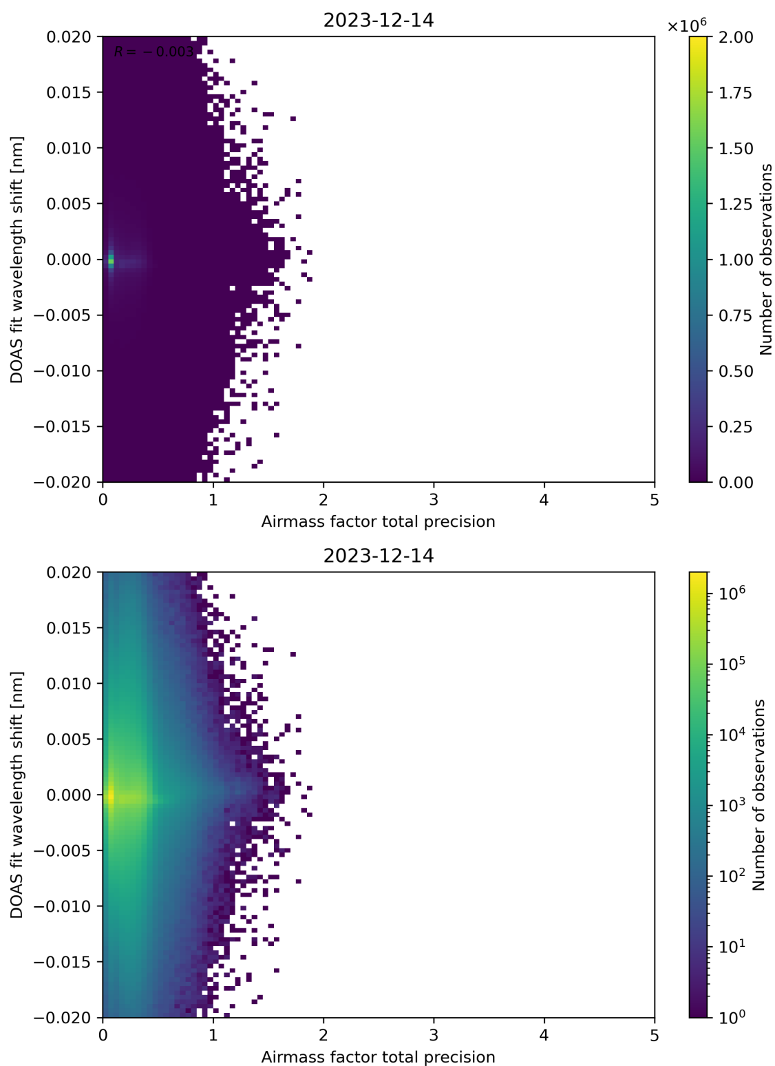
Figure 106: Scatter density plot of “Airmass factor total precision” against “DOAS fit wavelength shift” for 2023-12-14 to 2023-12-15.
