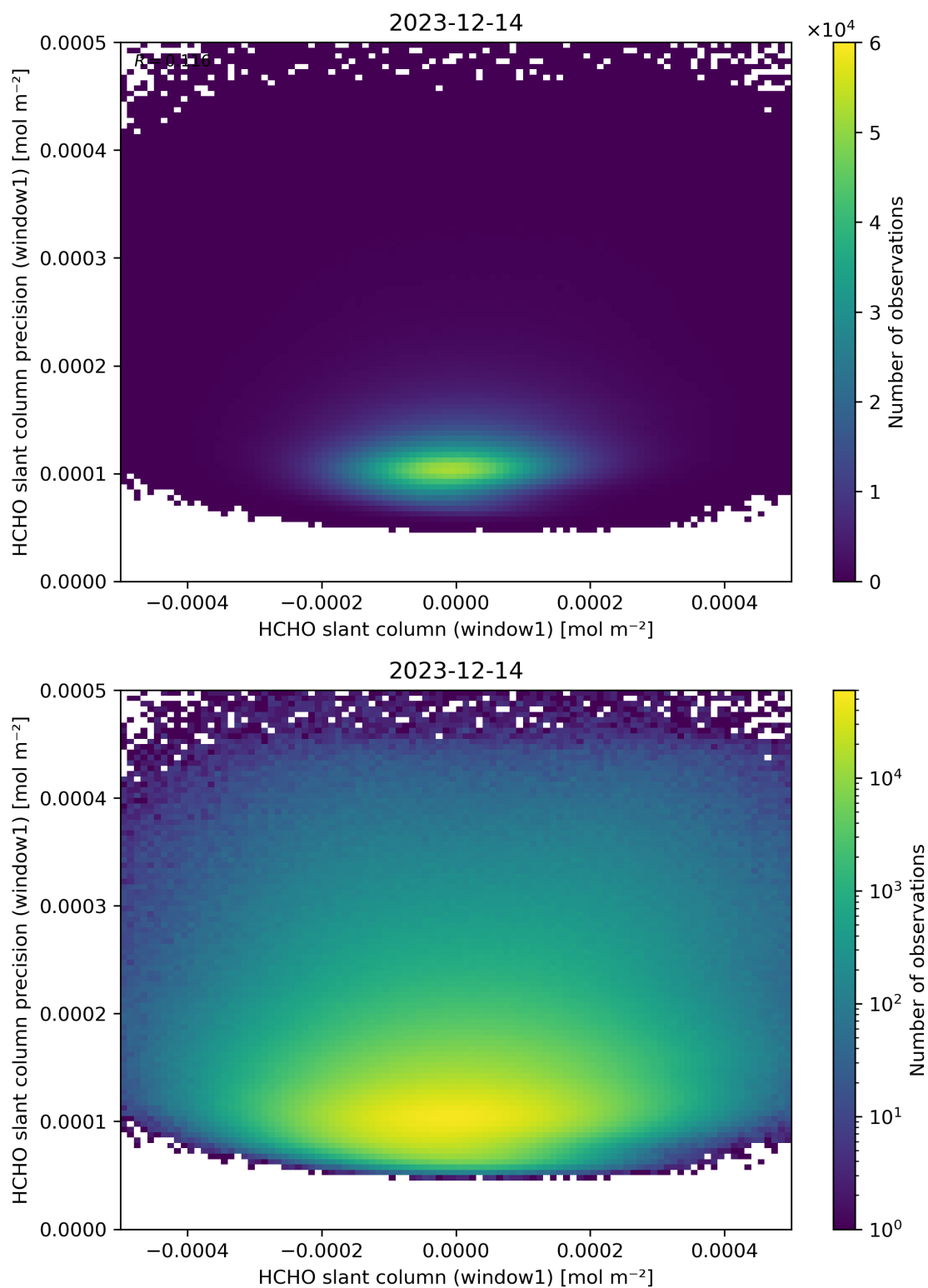
Figure 84: Scatter density plot of “HCHO slant column (window1)” against “HCHO slant column precision (window1)” for 2023-12-14 to 2023-12-15.
