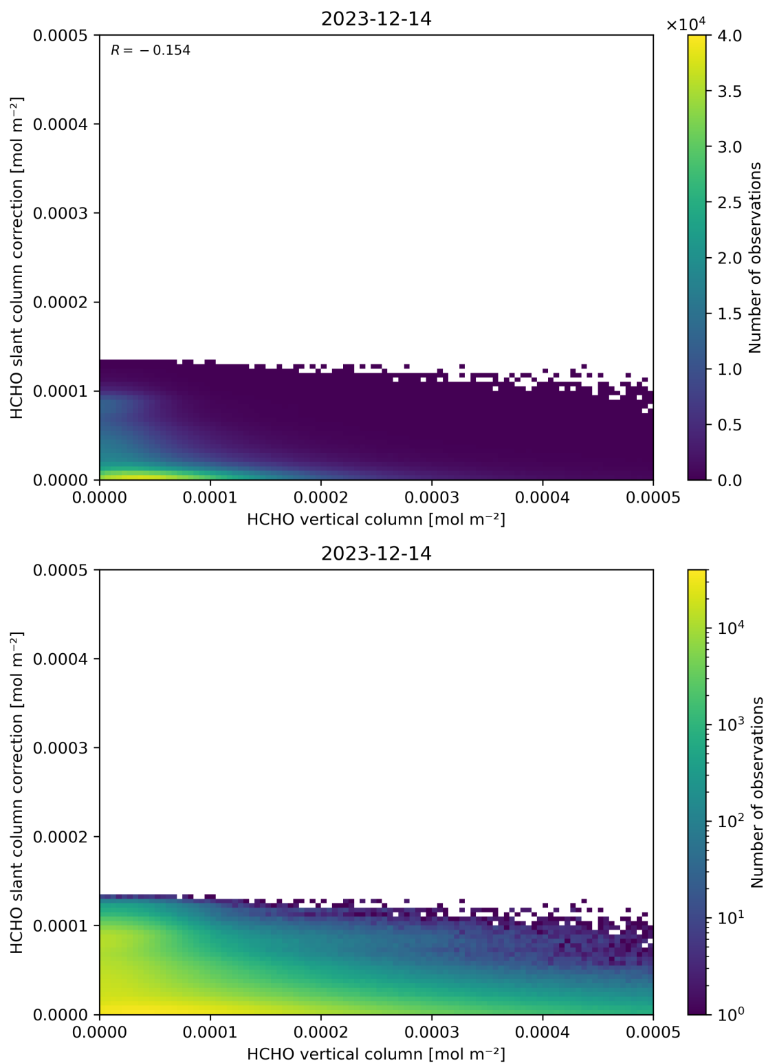
Figure 128: Scatter density plot of “HCHO vertical column” against “HCHO slant column correction” for 2023-12-14 to 2023-12-15.
