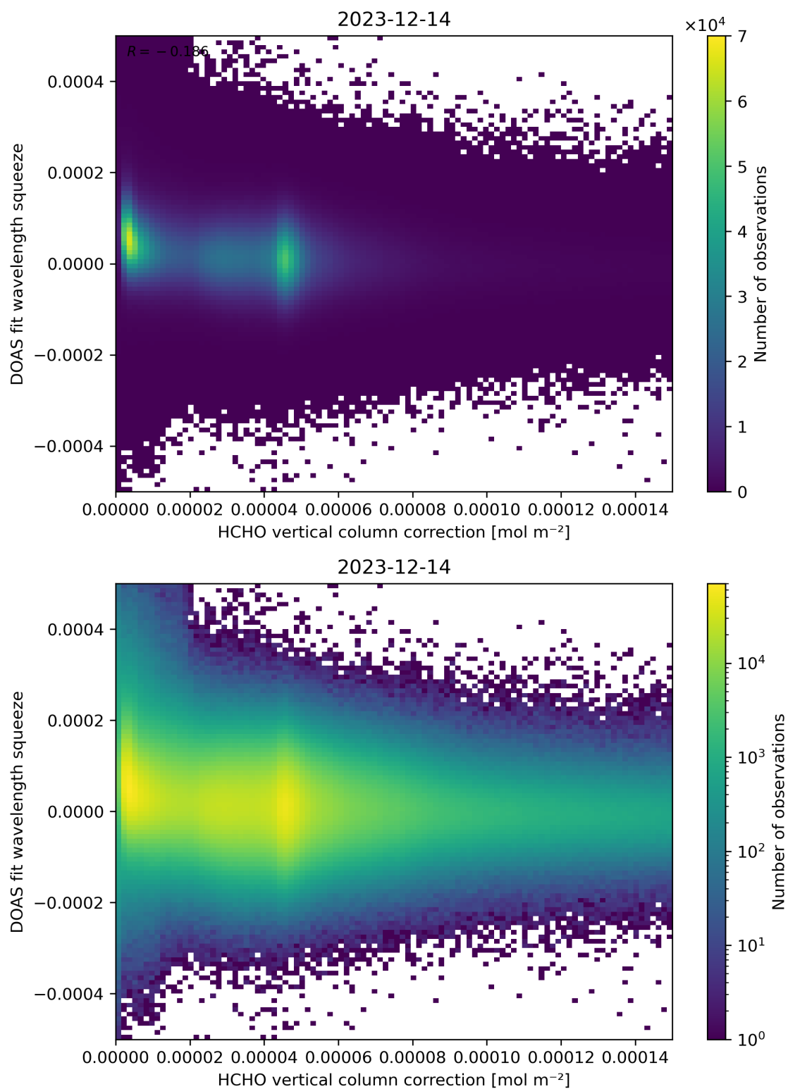
Figure 114: Scatter density plot of “HCHO vertical column correction” against “DOAS fit wavelength squeeze” for 2023-12-14 to 2023-12-15.
