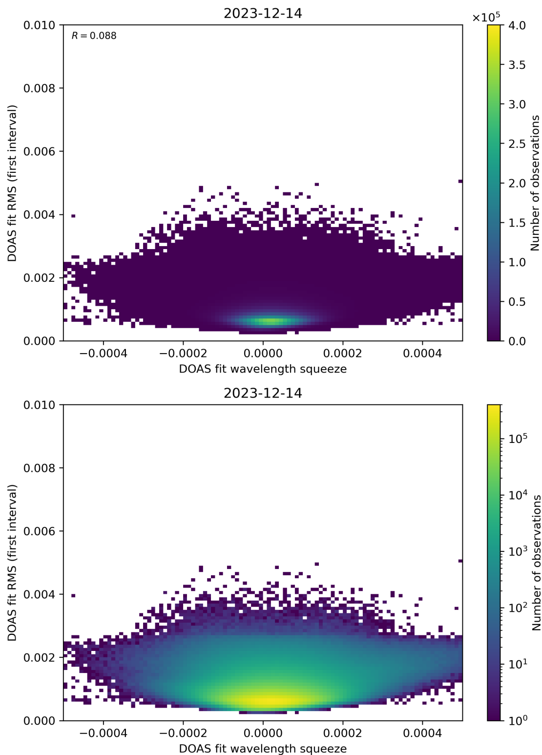
Figure 68: Scatter density plot of “DOAS fit wavelength squeeze” against “DOAS fit RMS (first interval)” for 2023-12-14 to 2023-12-15.
