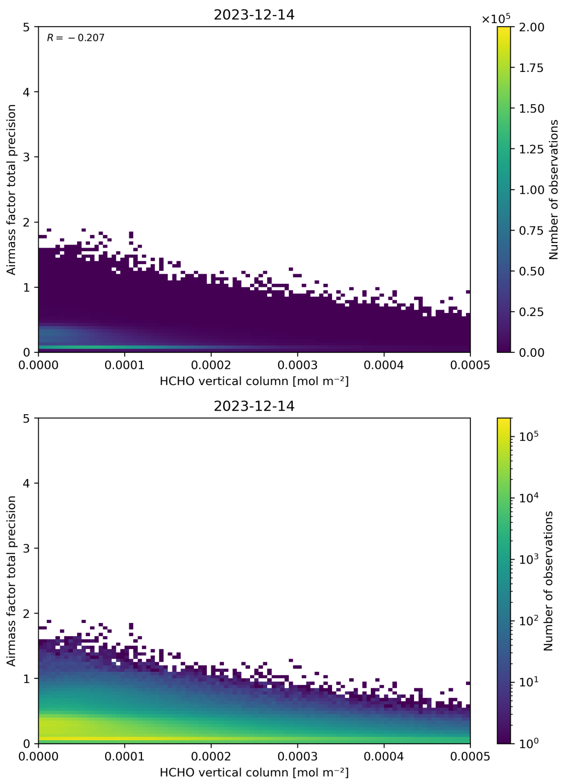
Figure 132: Scatter density plot of “HCHO vertical column” against “Airmass factor total precision” for 2023-12-14 to 2023-12-15.
