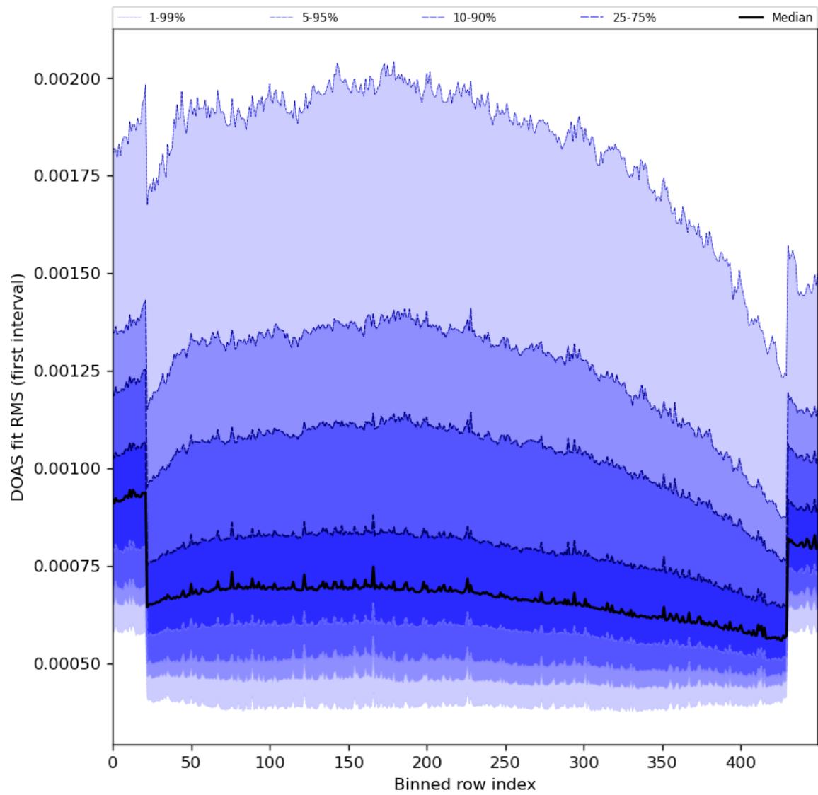
Figure 60: Along track statistics of “DOAS fit RMS (first interval)” for 2023-12-14 to 2023-12-15
