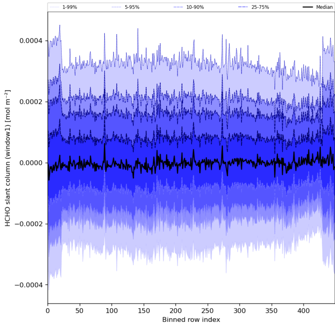
Figure 52: Along track statistics of “HCHO slant column (window1)” for 2023-12-14 to 2023-12-15
