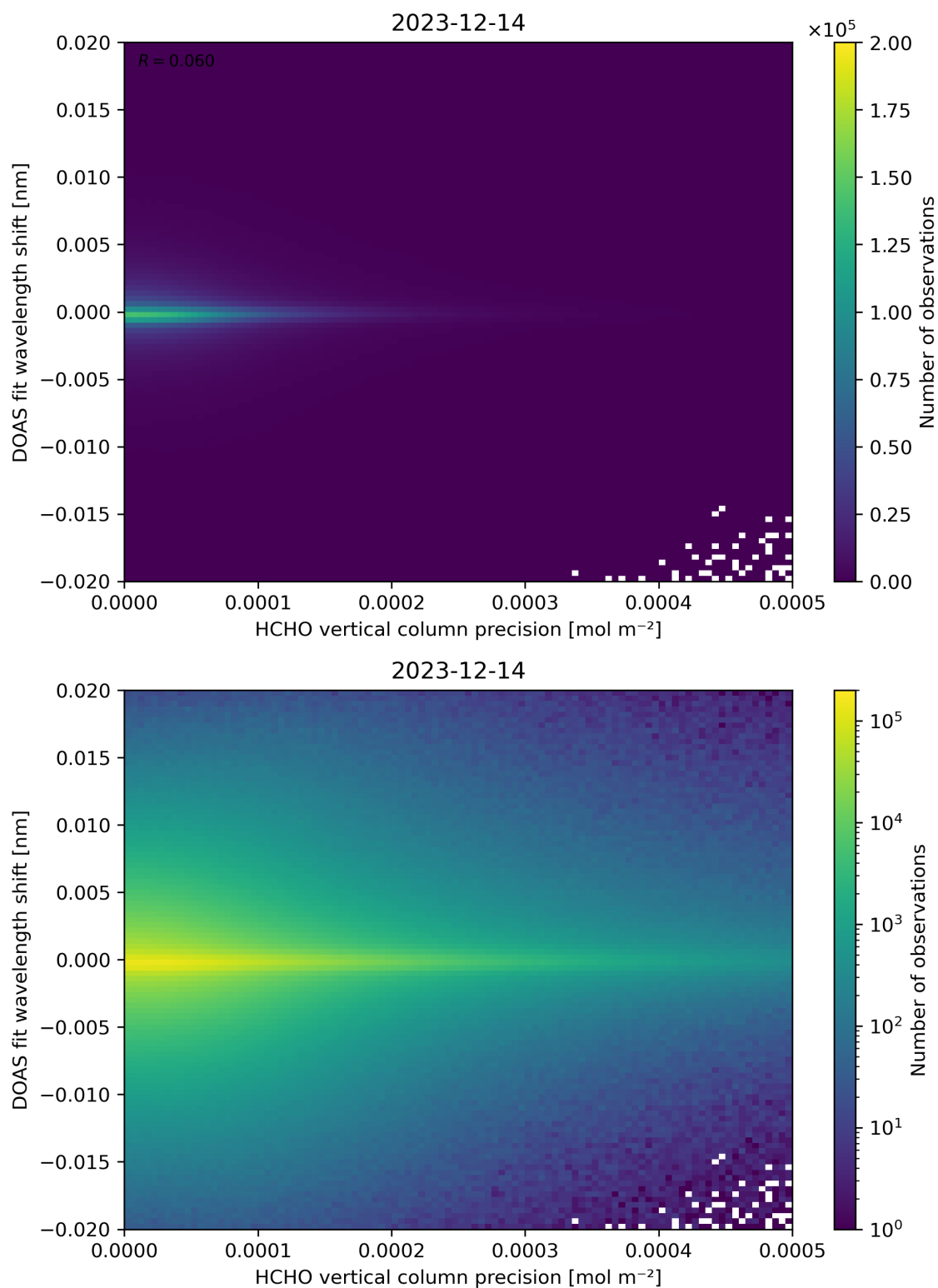
Figure 137: Scatter density plot of “HCHO vertical column precision” against “DOAS fit wavelength shift” for 2023-12-14 to 2023-12-15.
