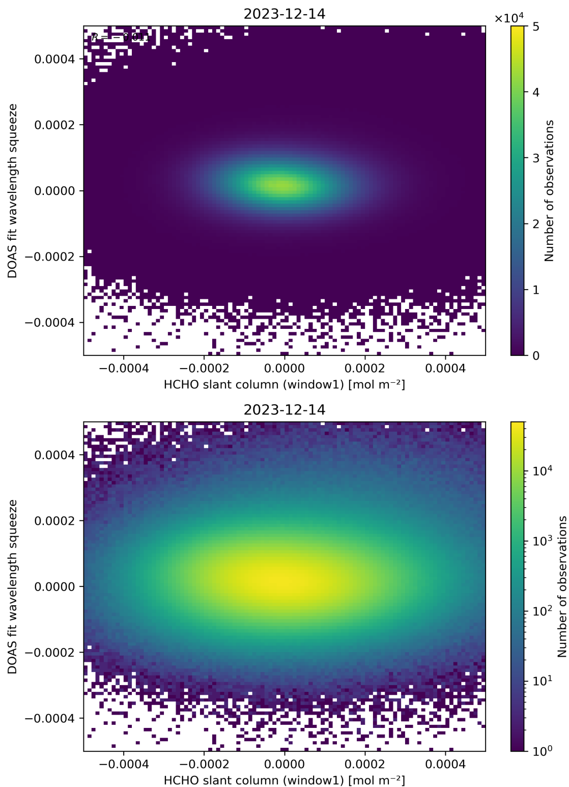
Figure 80: Scatter density plot of “HCHO slant column (window1)” against “DOAS fit wavelength squeeze” for 2023-12-14 to 2023-12-15.
