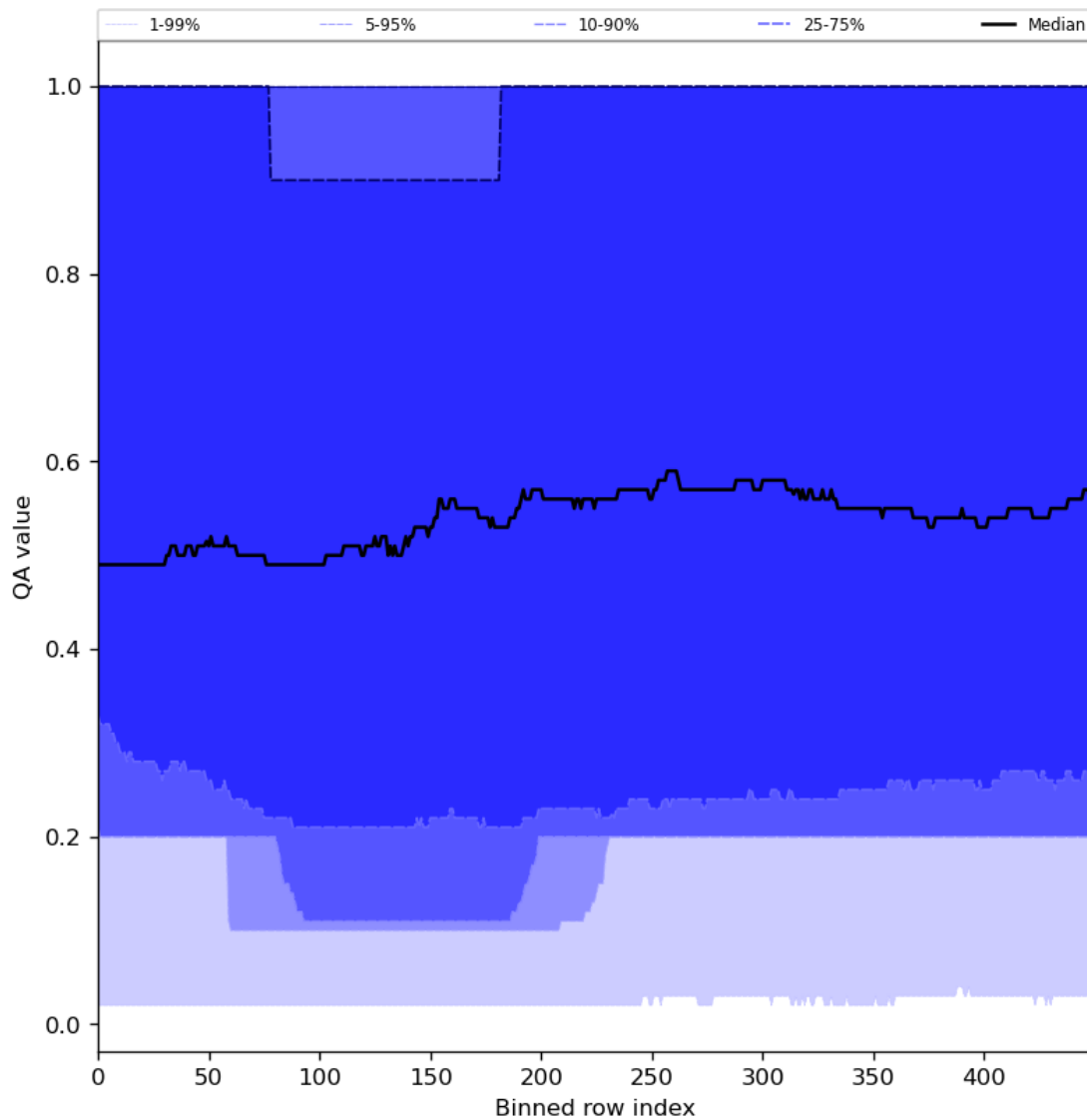
Figure 48: Along track statistics of "QA value" for 2023-12-14 to 2023-12-15
