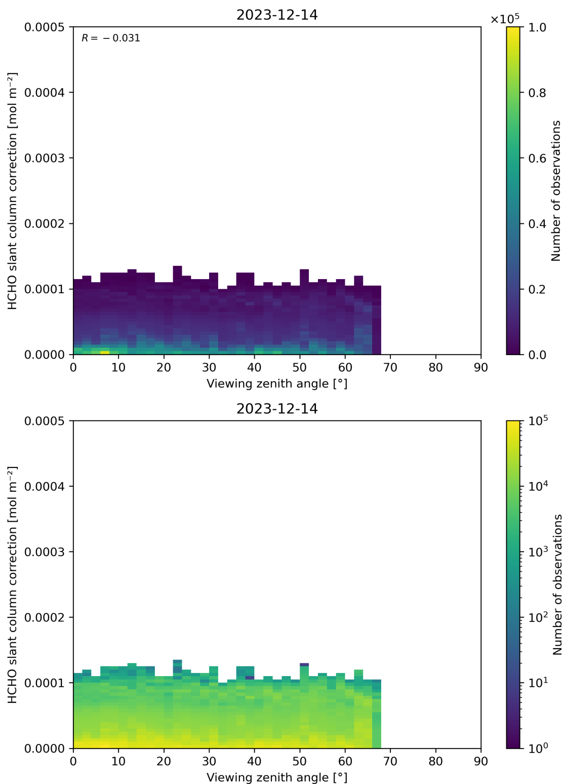
Figure 187: Scatter density plot of “Viewing zenith angle” against “HCHO slant column correction” for 2023-12-14 to 2023-12-15.
