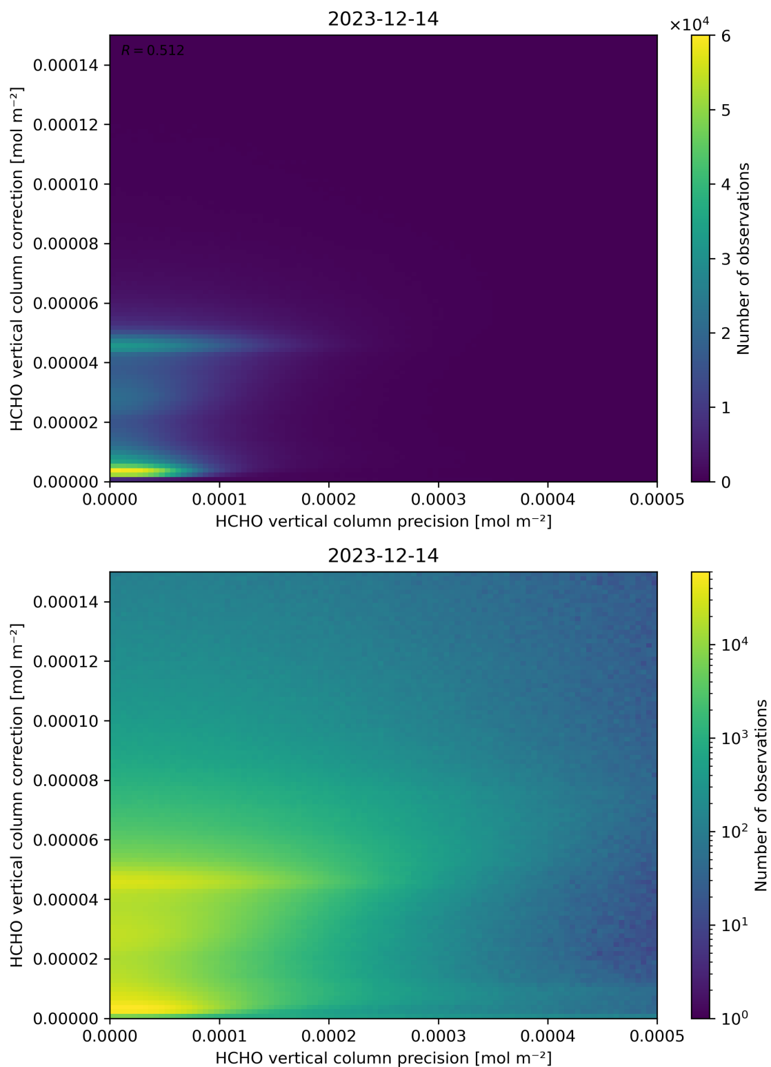
Figure 146: Scatter density plot of “HCHO vertical column precision” against “HCHO vertical column correction” for 2023-12-14 to 2023-12-15.
