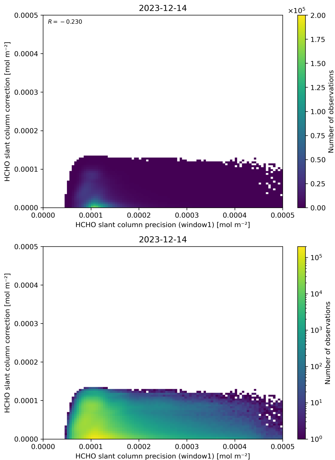
Figure 93: Scatter density plot of “HCHO slant column precision (window1)” against “HCHO slant column correction” for 2023-12-14 to 2023-12-15.
