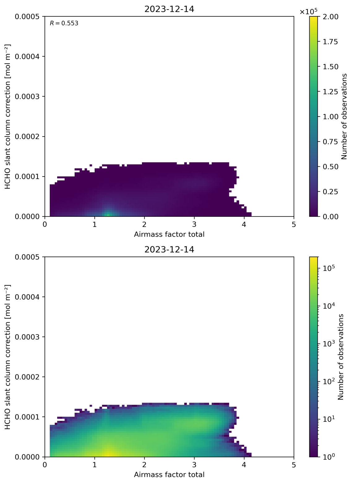
Figure 102: Scatter density plot of “Airmass factor total” against “HCHO slant column correction” for 2023-12-14 to 2023-12-15.
