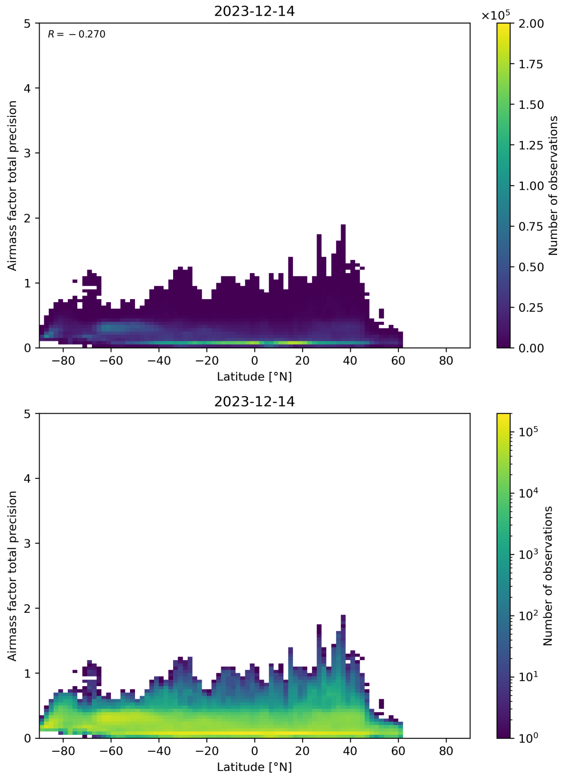
Figure 162: Scatter density plot of “Latitude” against “Airmass factor total precision” for 2023-12-14 to 2023-12-15.
