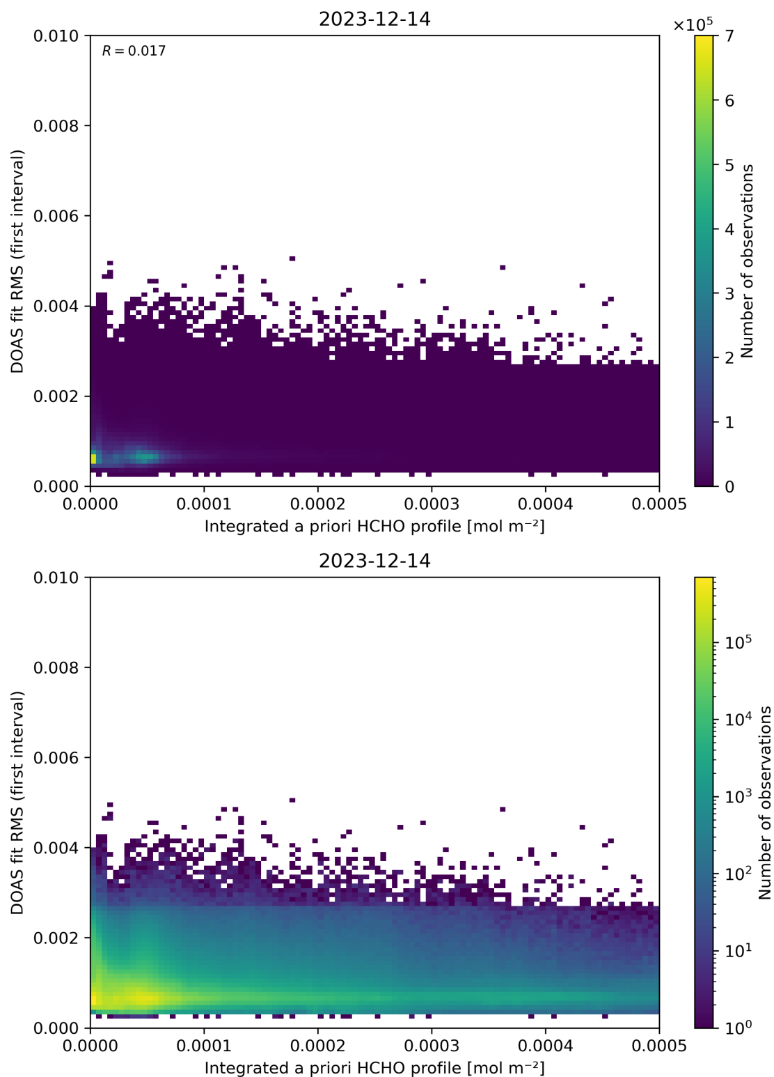
Figure 148: Scatter density plot of “Integrated a priori HCHO profile” against “DOAS fit RMS (first interval)” for 2023-12-14 to 2023-12-15.
