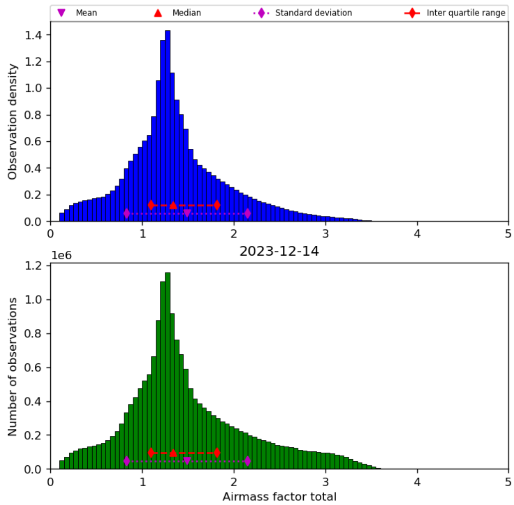
Figure 40: Histogram of “Airmass factor total” for 2023-12-14 to 2023-12-15
