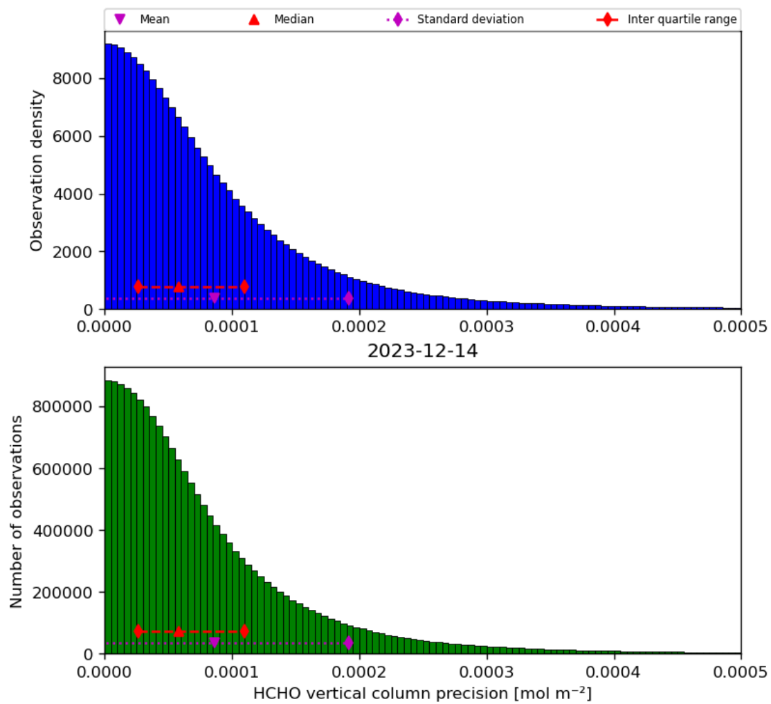
Figure 36: Histogram of “HCHO vertical column precision” for 2023-12-14 to 2023-12-15
