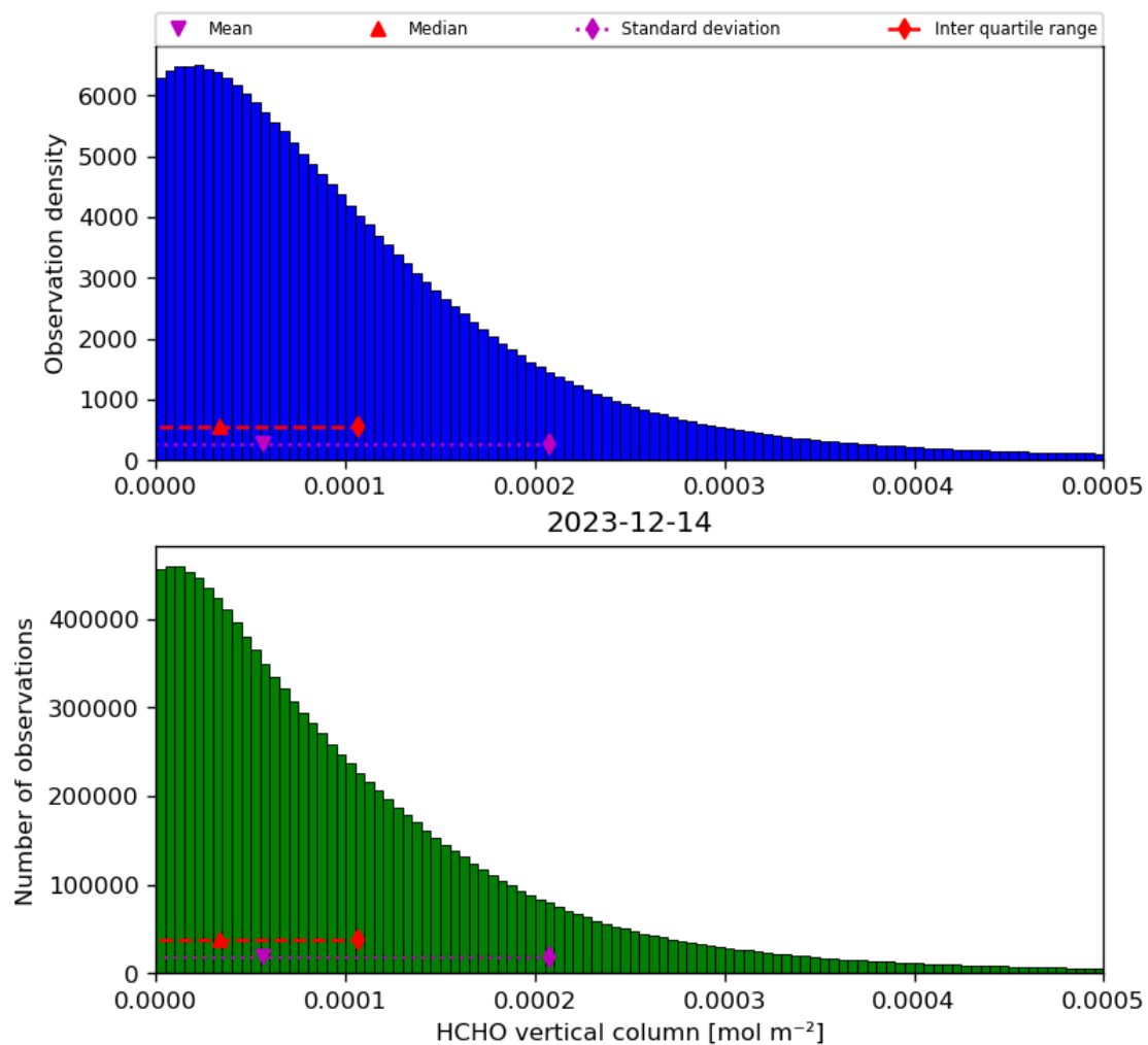
Figure 35: Histogram of “HCHO vertical column” for 2023-12-14 to 2023-12-15
