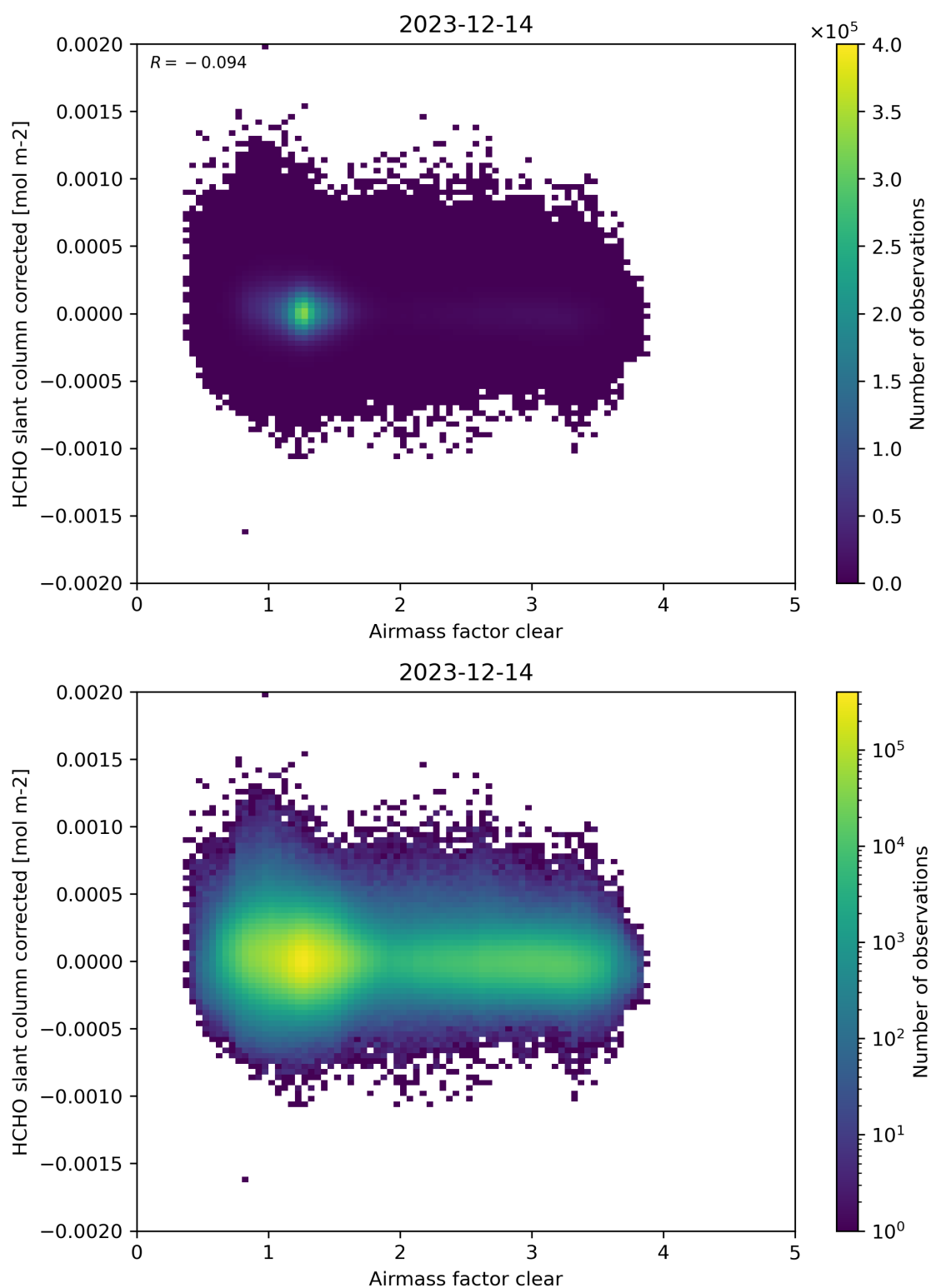
Figure 74: Scatter density plot of “Airmass factor clear” against “HCHO slant column corrected” for 2023-12-14 to 2023-12-15.
