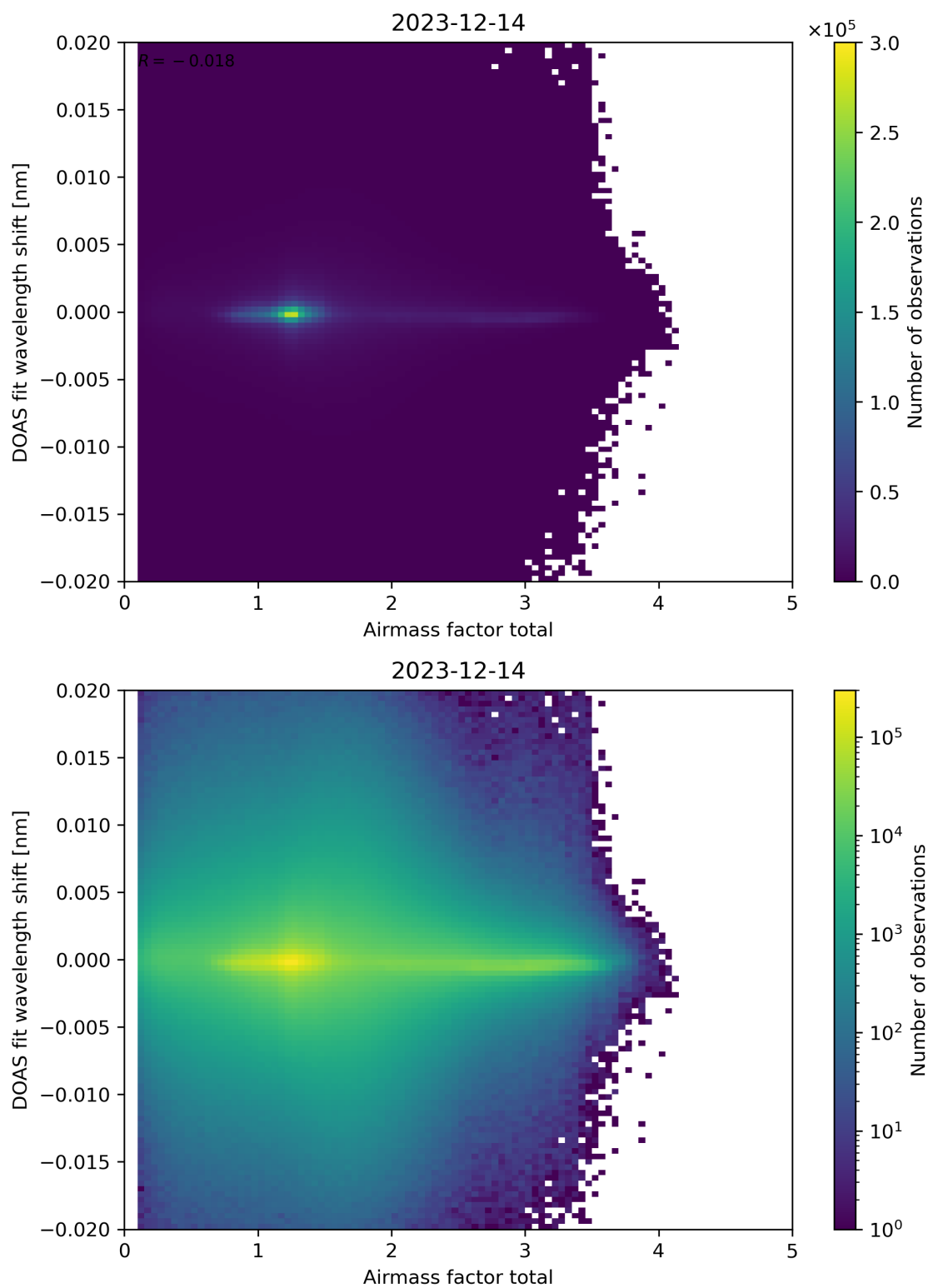
Figure 98: Scatter density plot of “Airmass factor total” against “DOAS fit wavelength shift” for 2023-12-14 to 2023-12-15.
