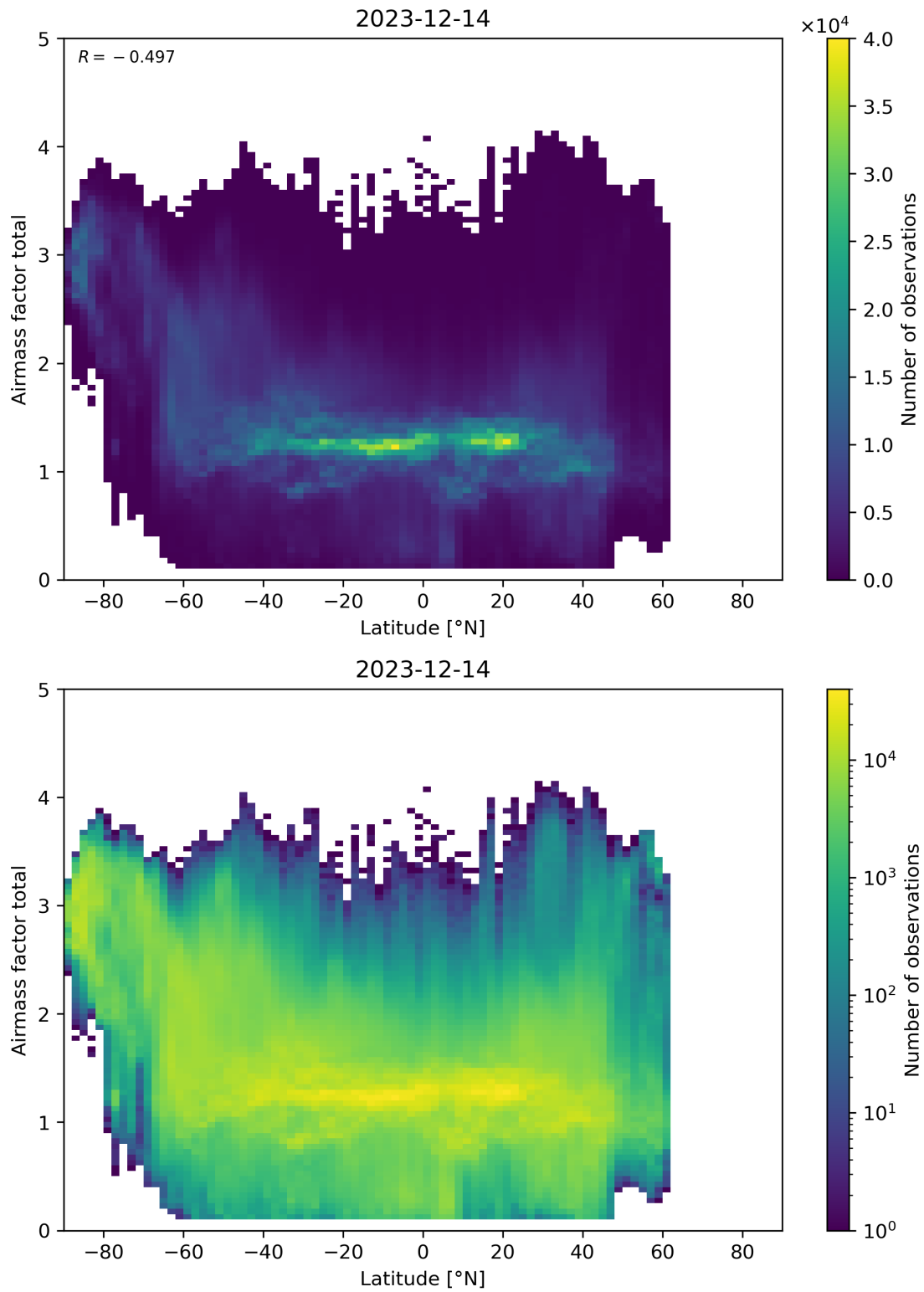
Figure 161: Scatter density plot of “Latitude” against “Airmass factor total” for 2023-12-14 to 2023-12-15.
