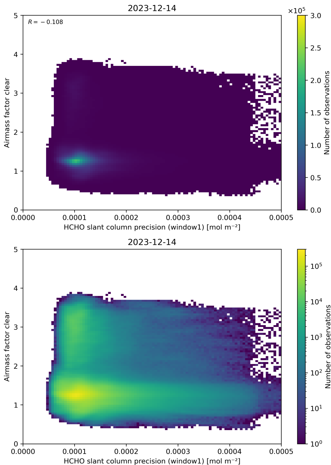
Figure 91: Scatter density plot of “HCHO slant column precision (window1)” against “Airmass factor clear” for 2023-12-14 to 2023-12-15.
