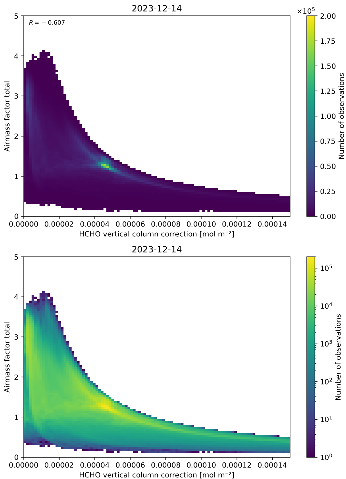
Figure 120: Scatter density plot of “HCHO vertical column correction” against “Airmass factor total” for 2023-12-14 to 2023-12-15.
