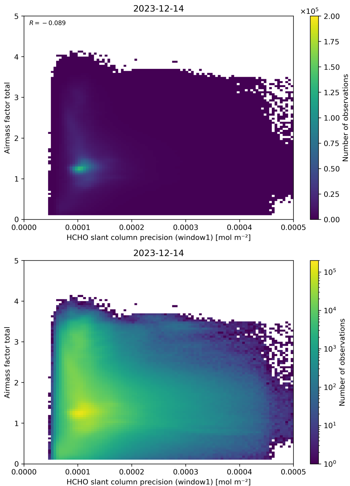
Figure 94: Scatter density plot of “HCHO slant column precision (window1)” against “Airmass factor total” for 2023-12-14 to 2023-12-15.
