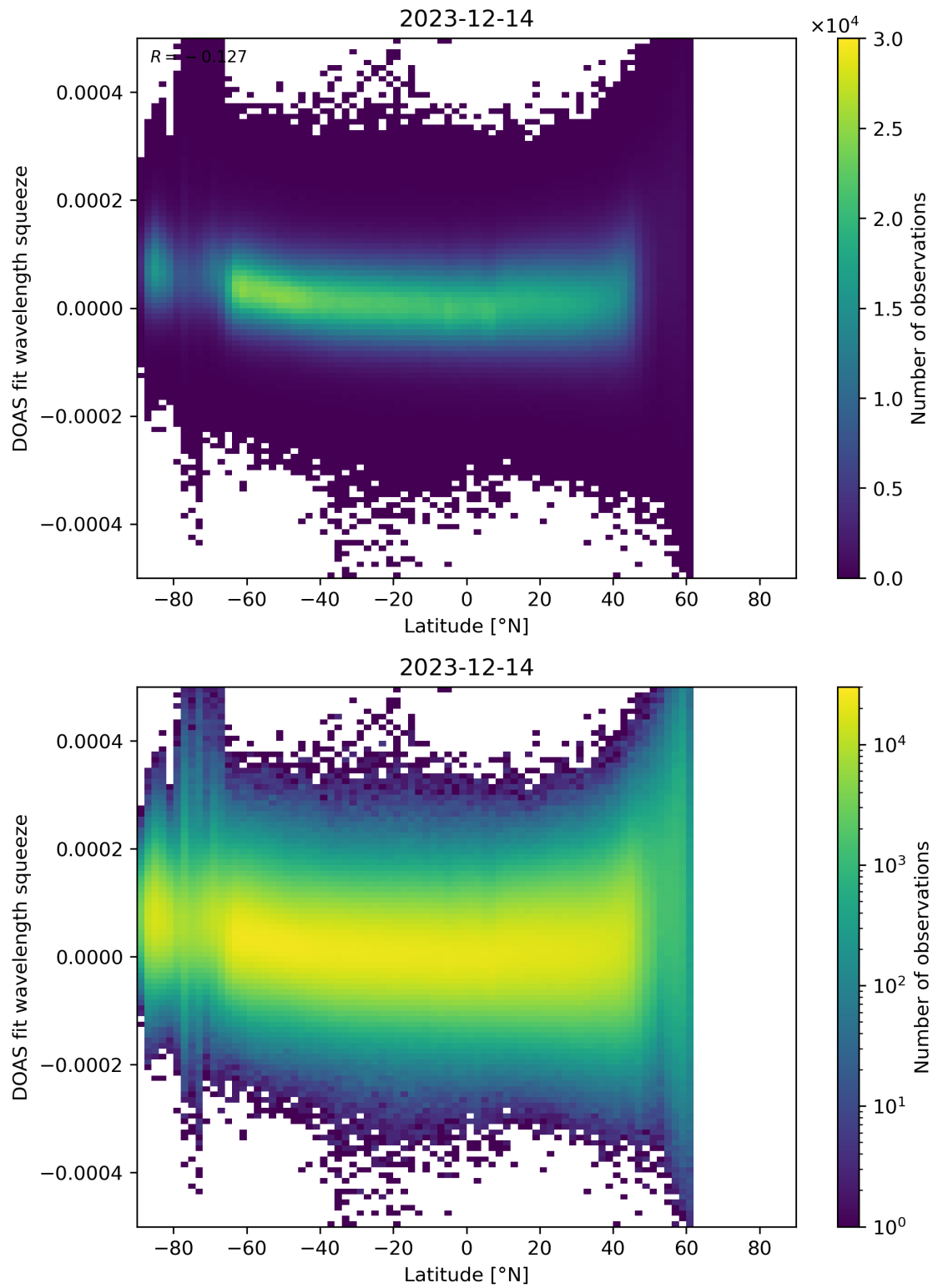
Figure 155: Scatter density plot of “Latitude” against “DOAS fit wavelength squeeze” for 2023-12-14 to 2023-12-15.
