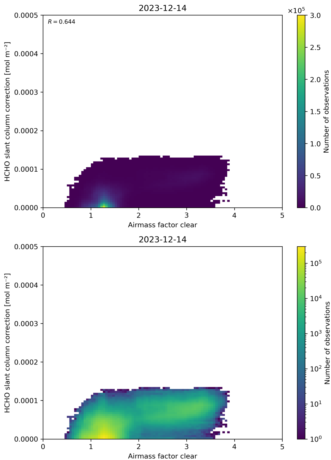
Figure 75: Scatter density plot of “Airmass factor clear” against “HCHO slant column correction” for 2023-12-14 to 2023-12-15.
