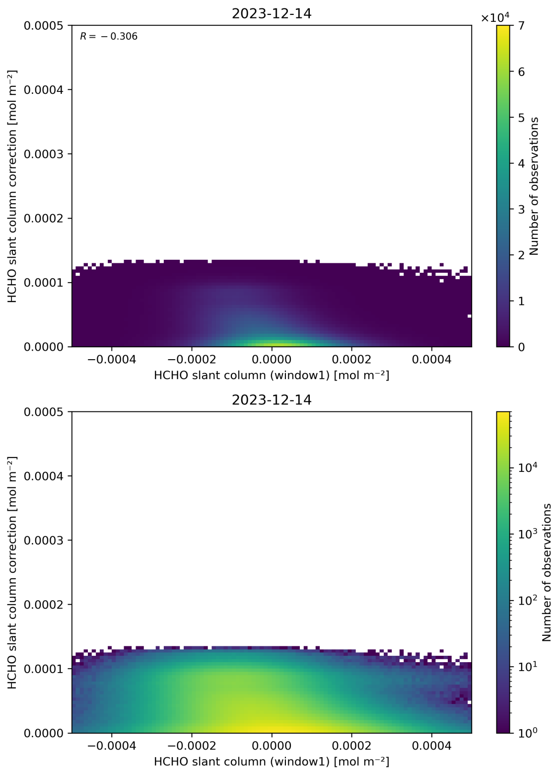
Figure 83: Scatter density plot of “HCHO slant column (window1)” against “HCHO slant column correction” for 2023-12-14 to 2023-12-15.
