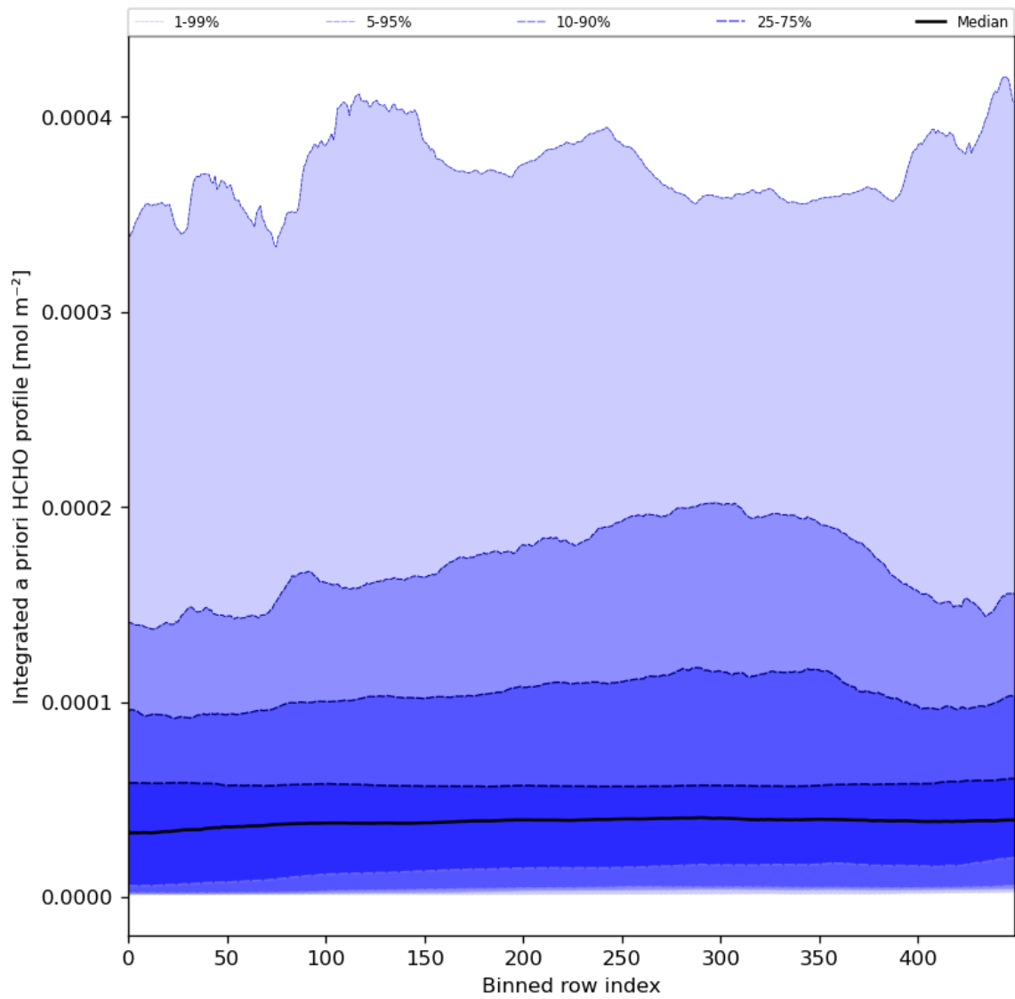
Figure 57: Along track statistics of "Integrated a priori HCHO profile" for 2023-12-14 to 2023-12-15
