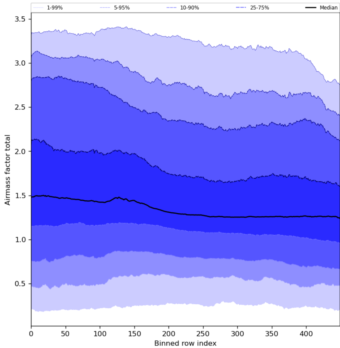
Figure 54: Along track statistics of “Airmass factor total” for 2023-12-14 to 2023-12-15
