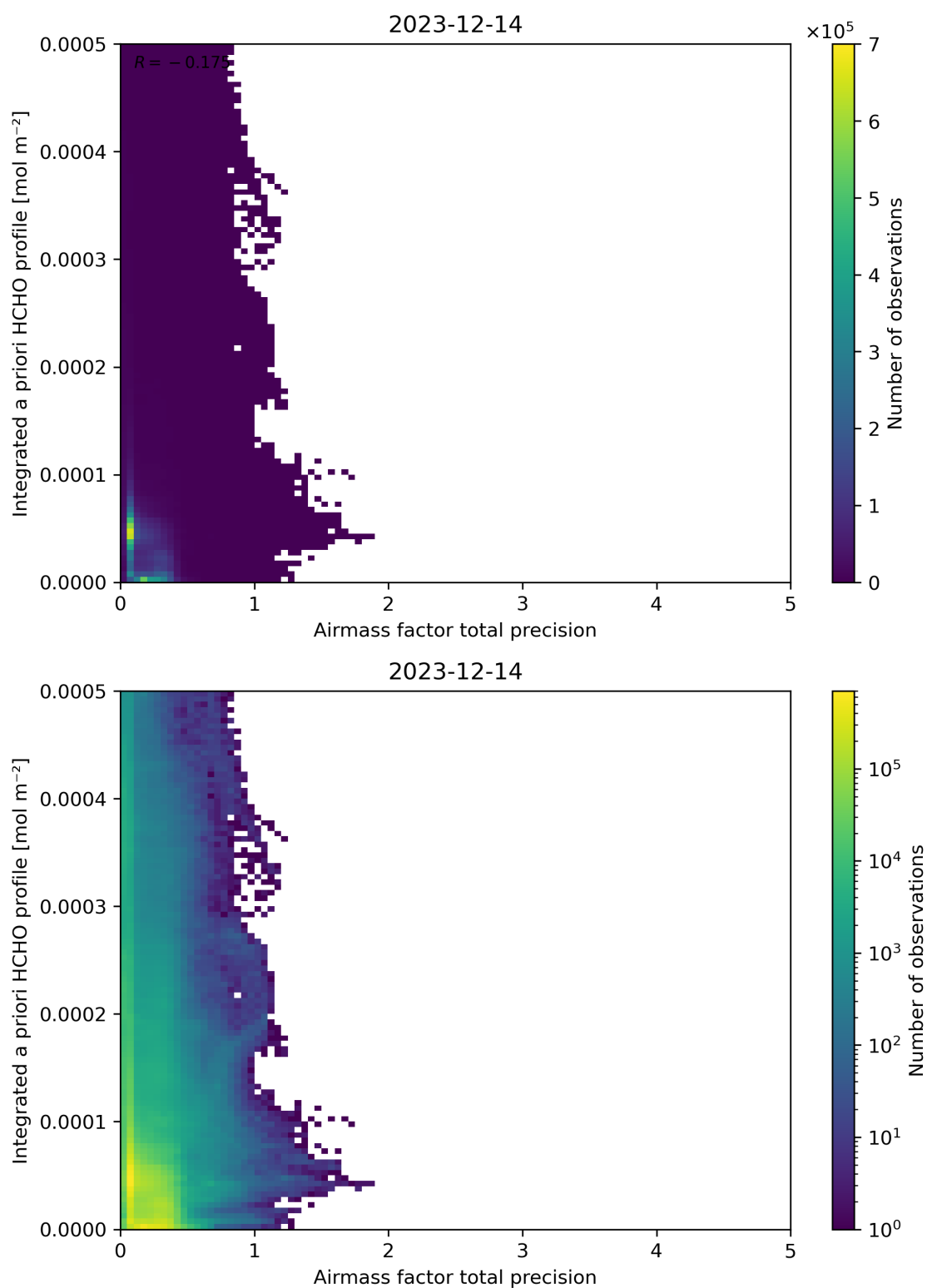
Figure 111: Scatter density plot of “Airmass factor total precision” against “Integrated a priori HCHO profile” for 2023-12-14 to 2023-12-15.
