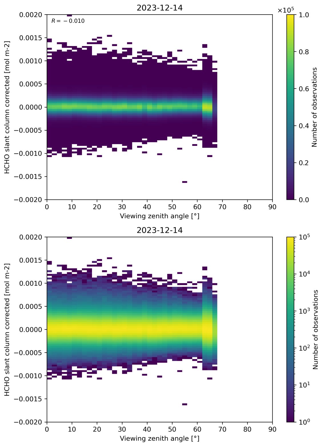
Figure 186: Scatter density plot of “Viewing zenith angle” against “HCHO slant column corrected” for 2023-12-14 to 2023-12-15.
