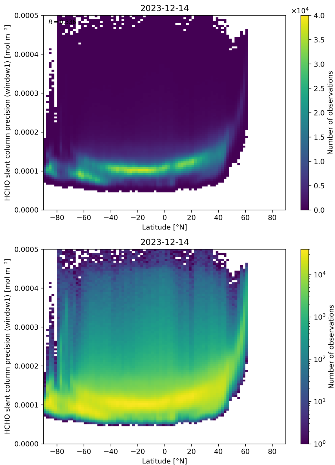
Figure 160: Scatter density plot of “Latitude” against “HCHO slant column precision (window1)” for 2023-12-14 to 2023-12-15.
