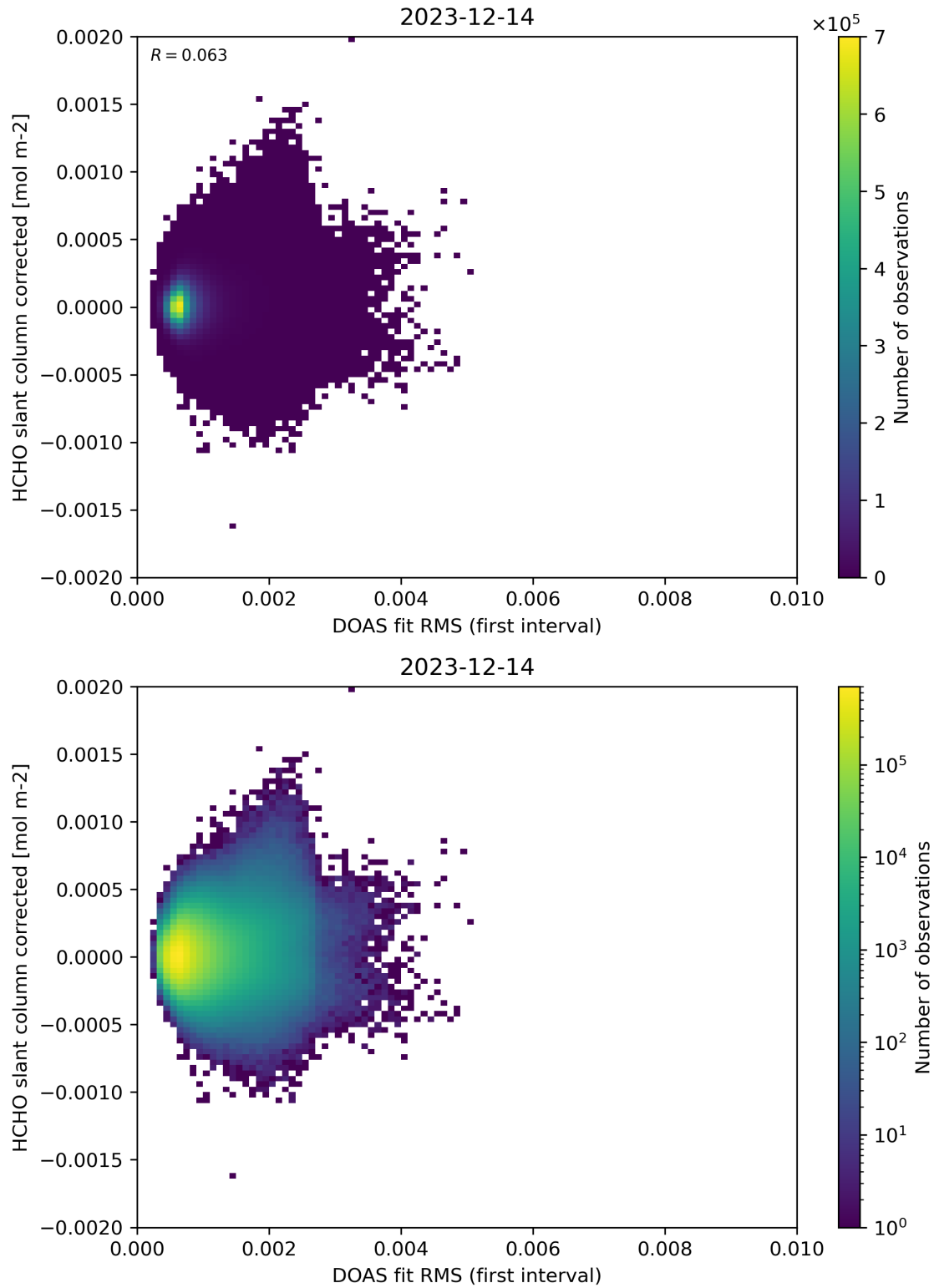
Figure 62: Scatter density plot of “DOAS fit RMS (first interval)” against “HCHO slant column corrected” for 2023-12-14 to 2023-12-15.
