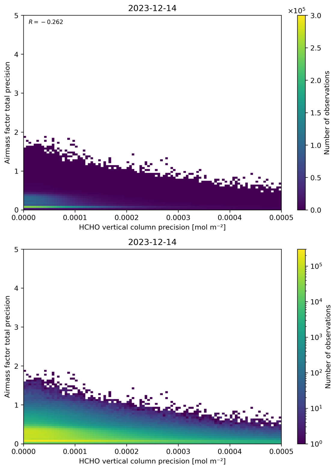
Figure 145: Scatter density plot of “HCHO vertical column precision” against “Airmass factor total precision” for 2023-12-14 to 2023-12-15.
