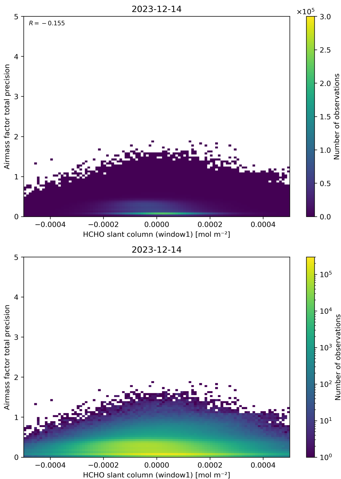
Figure 86: Scatter density plot of “HCHO slant column (window1)” against “Airmass factor total precision” for 2023-12-14 to 2023-12-15.
