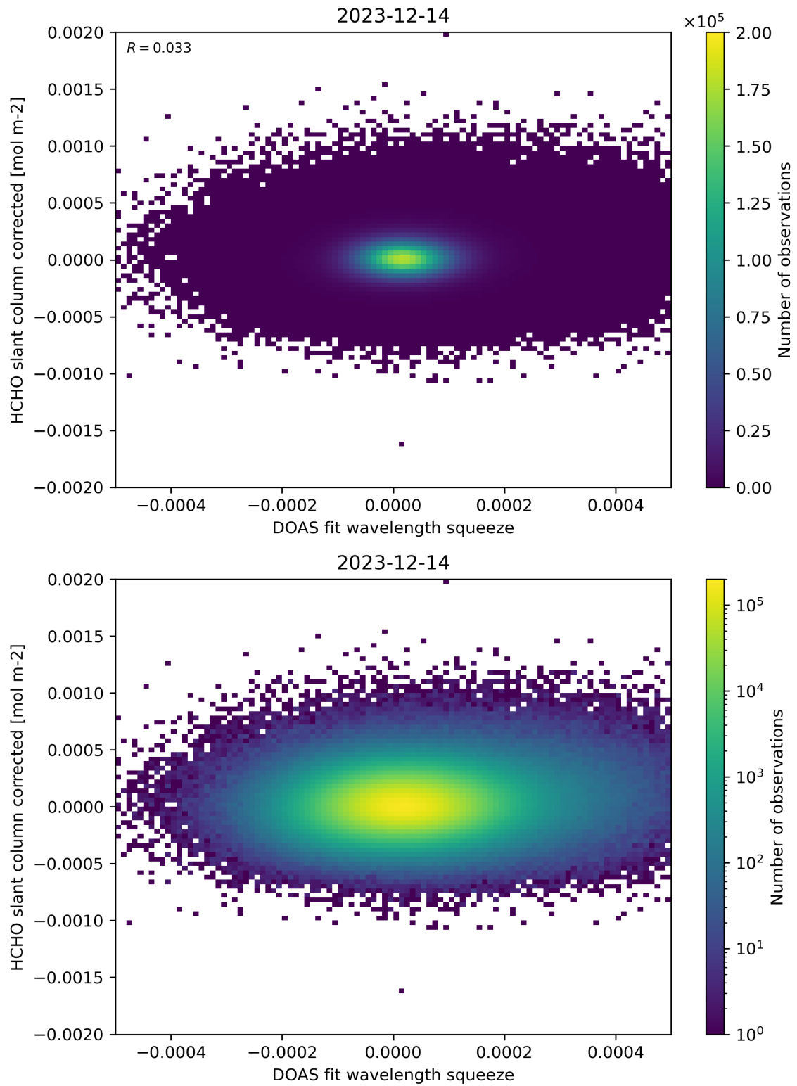
Figure 69: Scatter density plot of “DOAS fit wavelength squeeze” against “HCHO slant column corrected” for 2023-12-14 to 2023-12-15.
