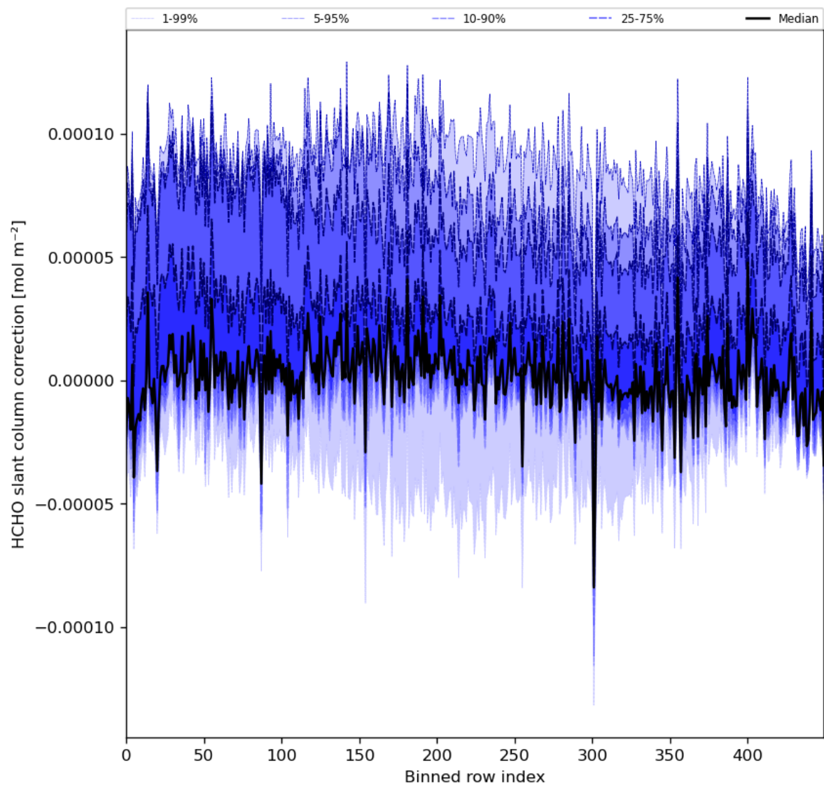
Figure 61: Along track statistics of “HCHO slant column correction” for 2023-12-14 to 2023-12-15
