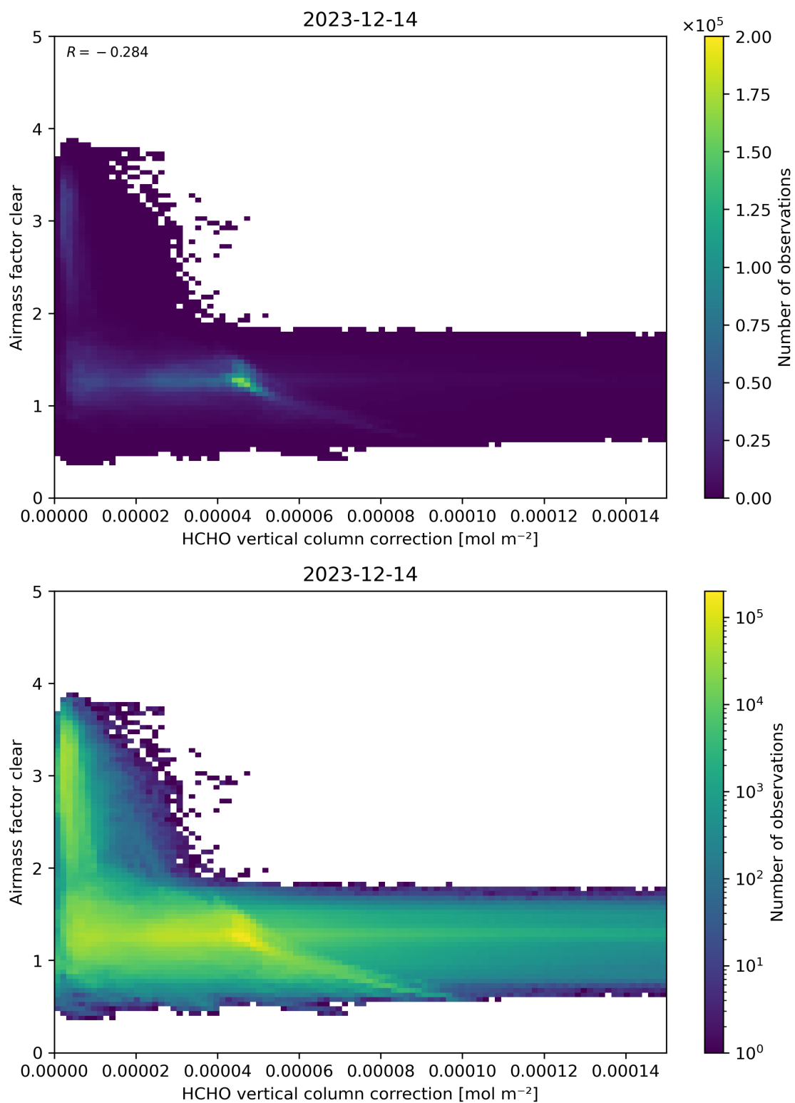
Figure 115: Scatter density plot of “HCHO vertical column correction” against “Airmass factor clear” for 2023-12-14 to 2023-12-15.
