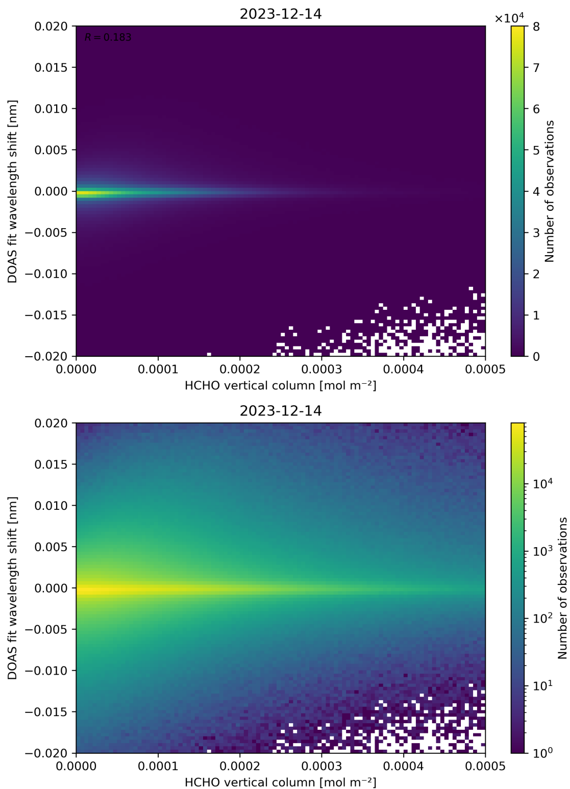
Figure 124: Scatter density plot of “HCHO vertical column” against “DOAS fit wavelength shift” for 2023-12-14 to 2023-12-15.
