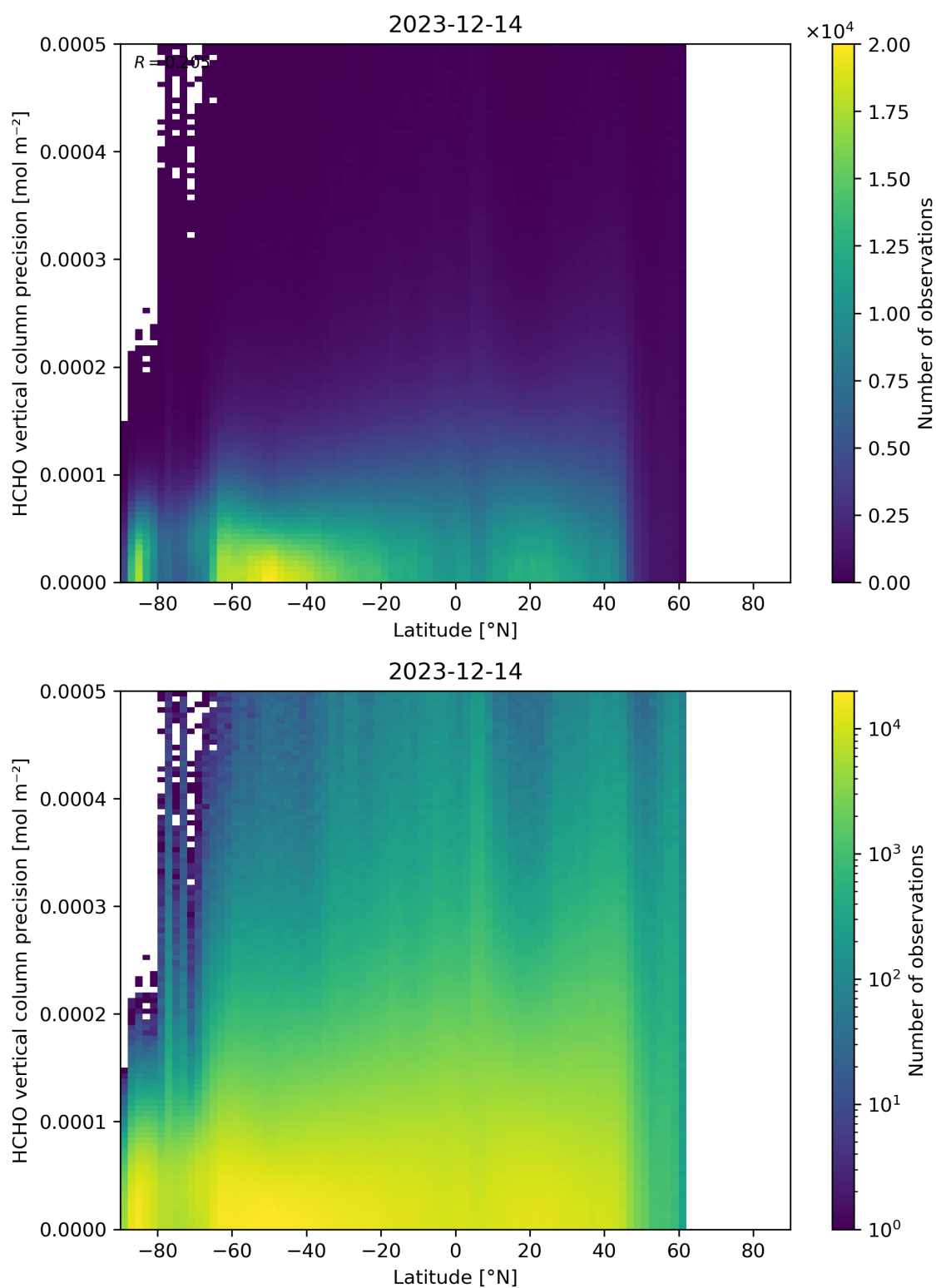
Figure 165: Scatter density plot of “Latitude” against “HCHO vertical column precision” for 2023-12-14 to 2023-12-15.
