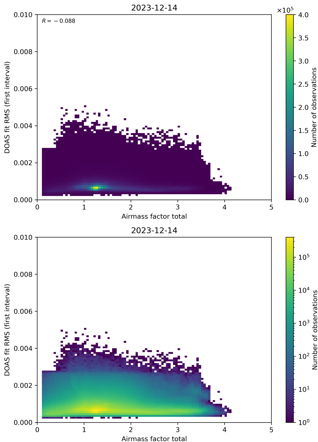
Figure 97: Scatter density plot of “Airmass factor total” against “DOAS fit RMS (first interval)” for 2023-12-14 to 2023-12-15.
