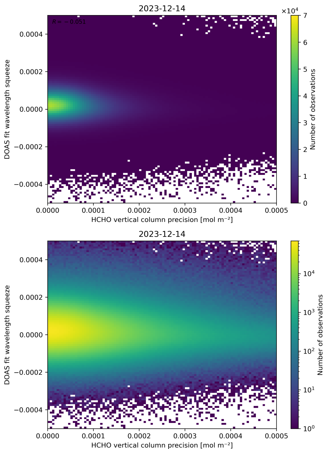
Figure 138: Scatter density plot of “HCHO vertical column precision” against “DOAS fit wavelength squeeze” for 2023-12-14 to 2023-12-15.
