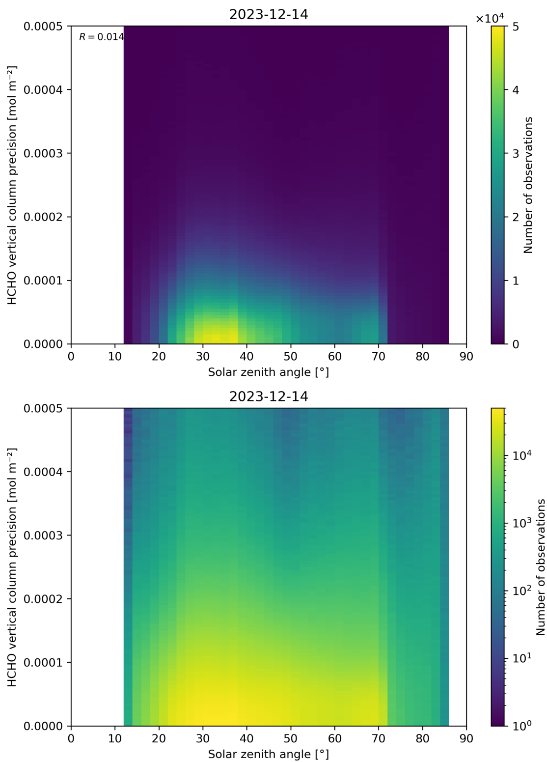
Figure 179: Scatter density plot of “Solar zenith angle” against “HCHO vertical column precision” for 2023-12-14 to 2023-12-15.
