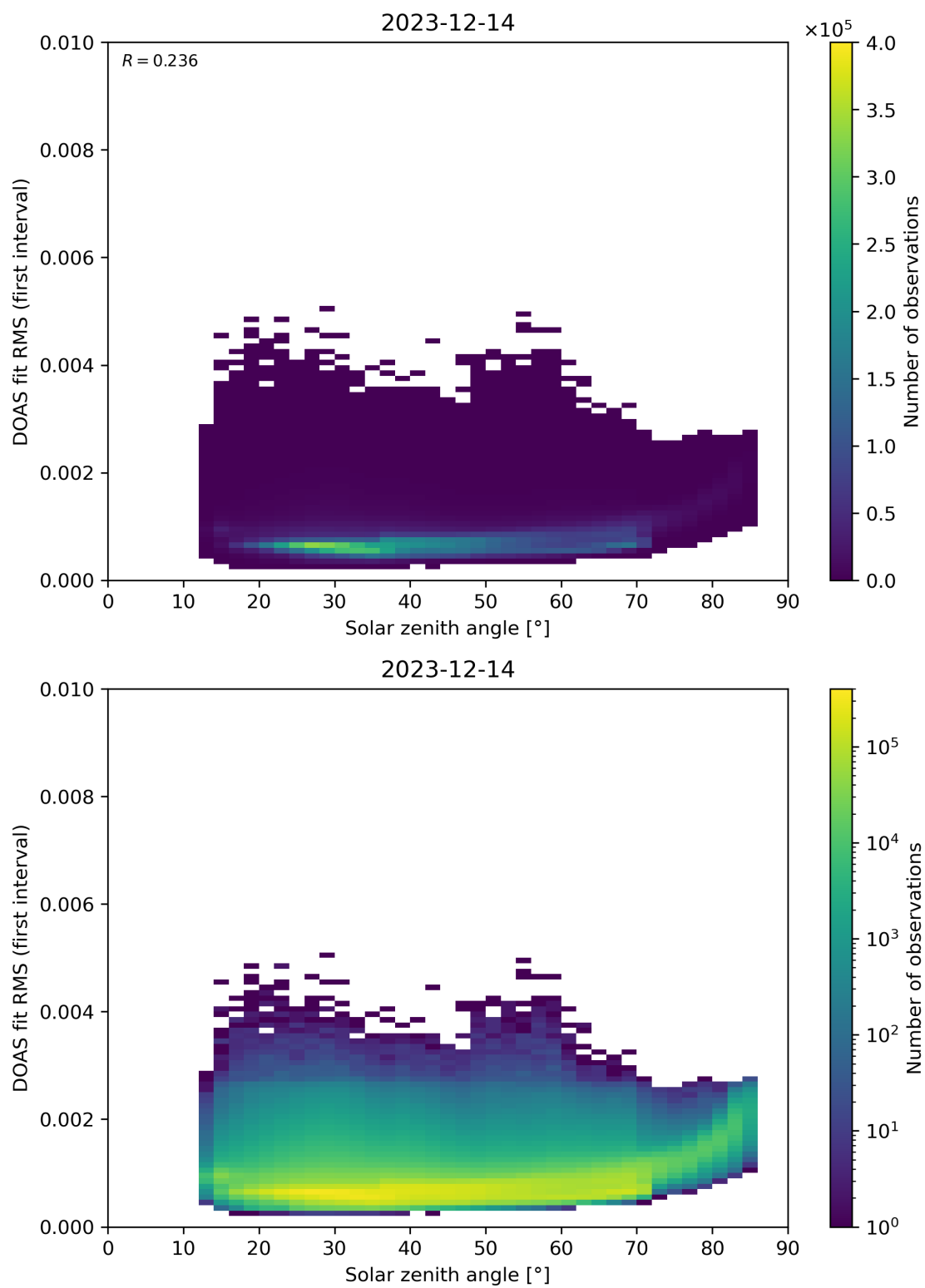
Figure 167: Scatter density plot of “Solar zenith angle” against “DOAS fit RMS (first interval)” for 2023-12-14 to 2023-12-15.
