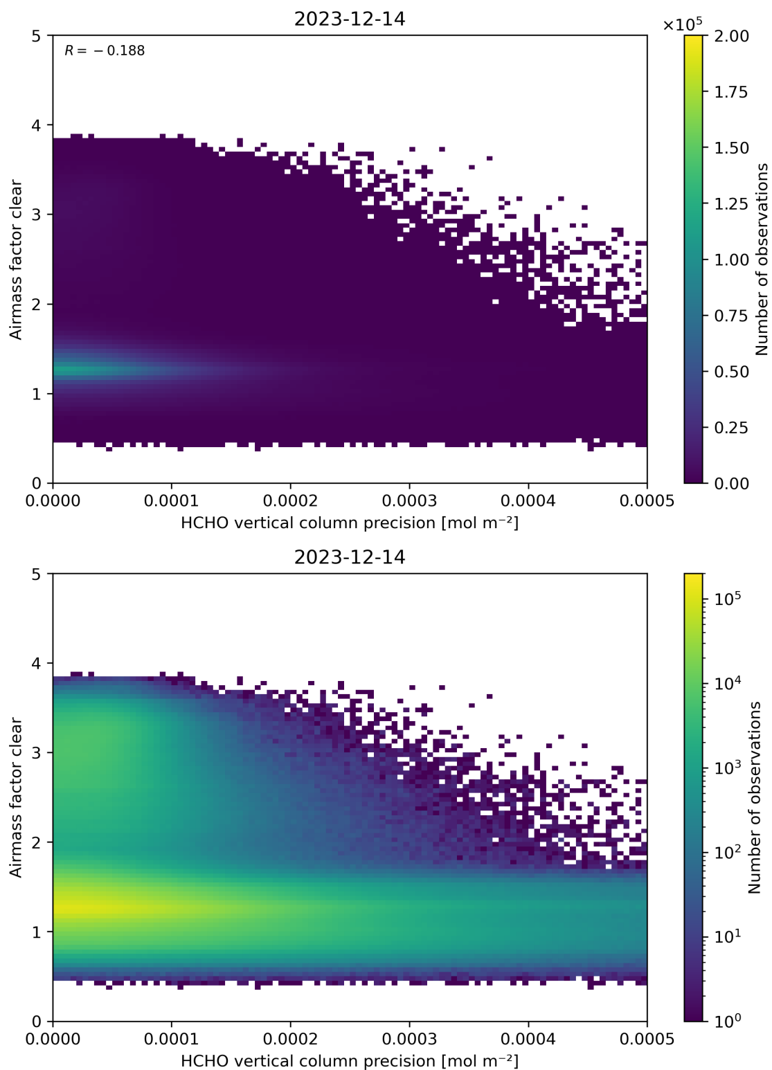
Figure 139: Scatter density plot of “HCHO vertical column precision” against “Airmass factor clear” for 2023-12-14 to 2023-12-15.
