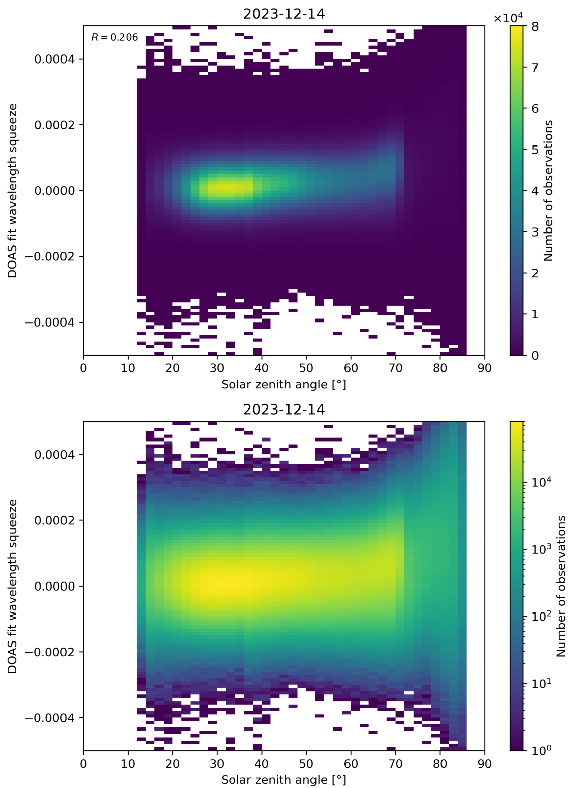
Figure 169: Scatter density plot of “Solar zenith angle” against “DOAS fit wavelength squeeze” for 2023-12-14 to 2023-12-15.
