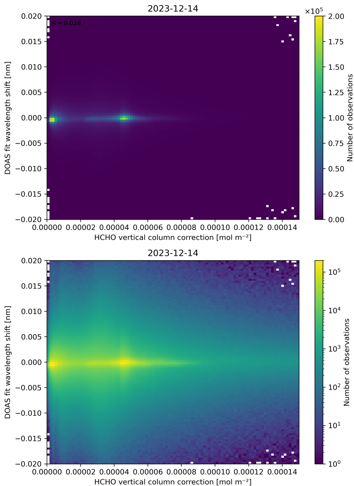
Figure 113: Scatter density plot of “HCHO vertical column correction” against “DOAS fit wavelength shift” for 2023-12-14 to 2023-12-15.
