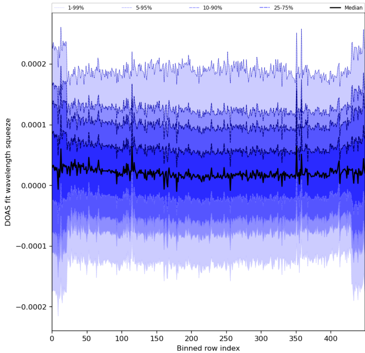
Figure 59: Along track statistics of “DOAS fit wavelength squeeze” for 2023-12-14 to 2023-12-15
