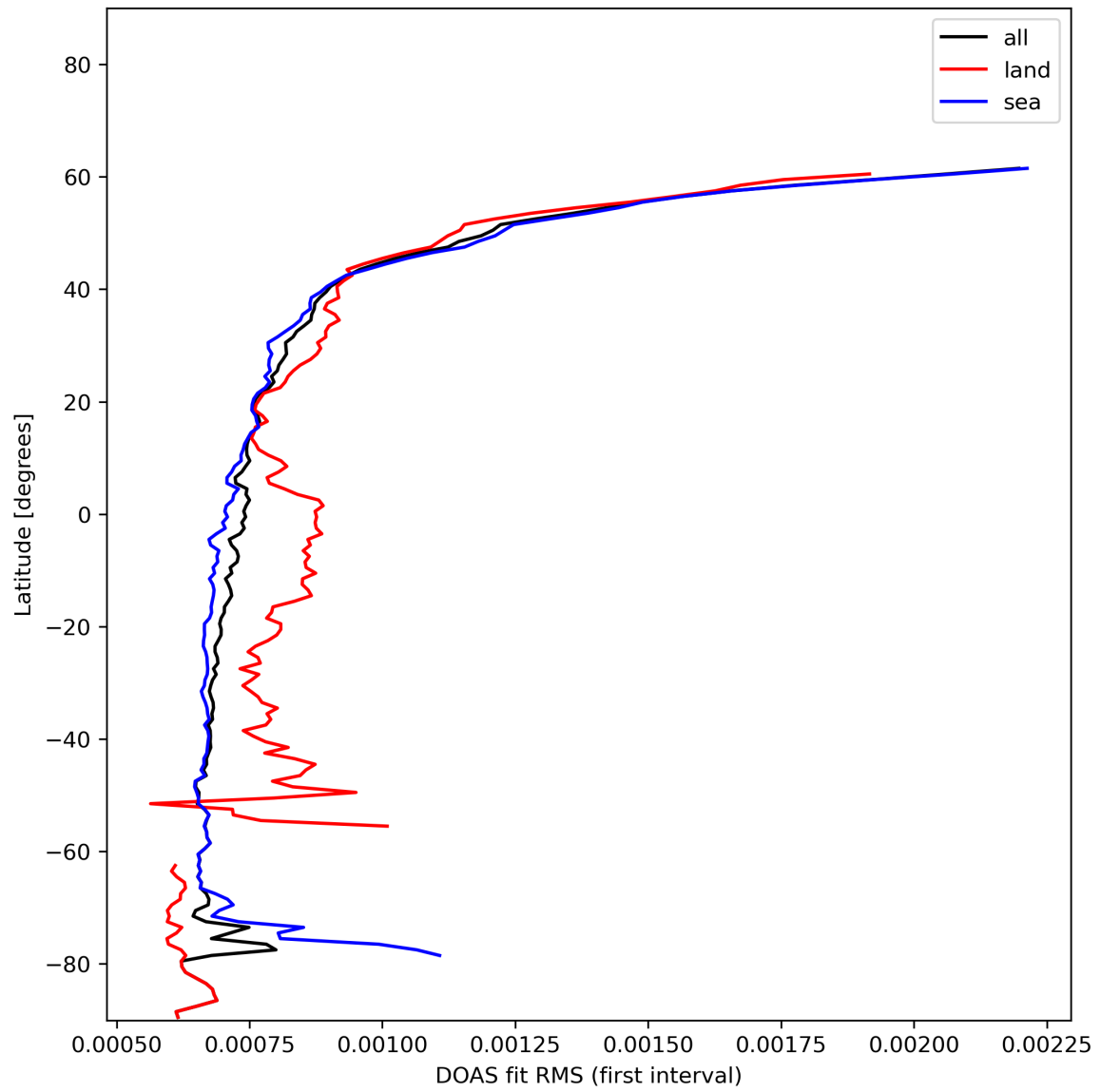
Figure 32: Zonal average of “DOAS fit RMS (first interval)” for 2023-12-14 to 2023-12-15.
