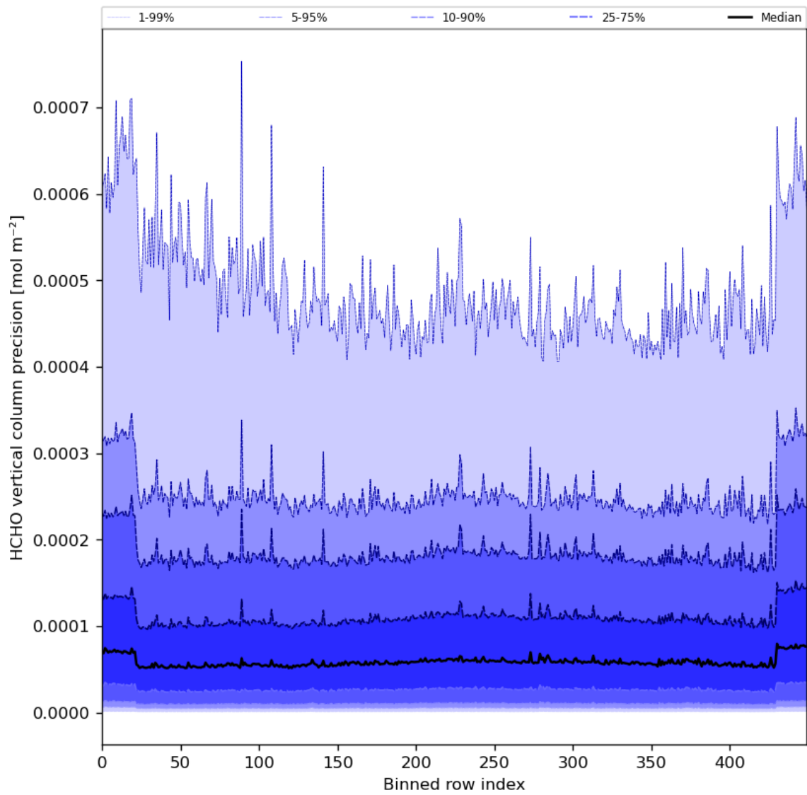
Figure 50: Along track statistics of "HCHO vertical column precision" for 2023-12-14 to 2023-12-15
