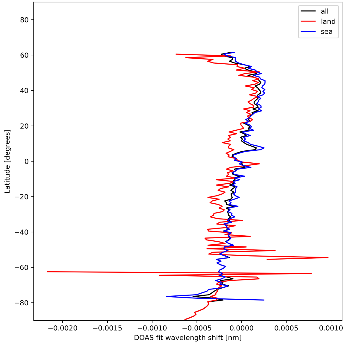
Figure 30: Zonal average of “DOAS fit wavelength shift” for 2023-12-14 to 2023-12-15.
