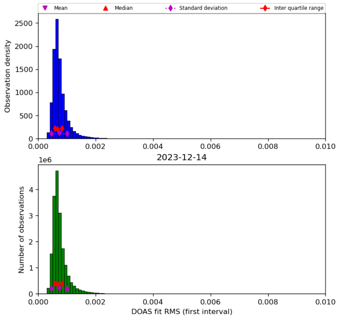
Figure 46: Histogram of “DOAS fit RMS (first interval)” for 2023-12-14 to 2023-12-15
