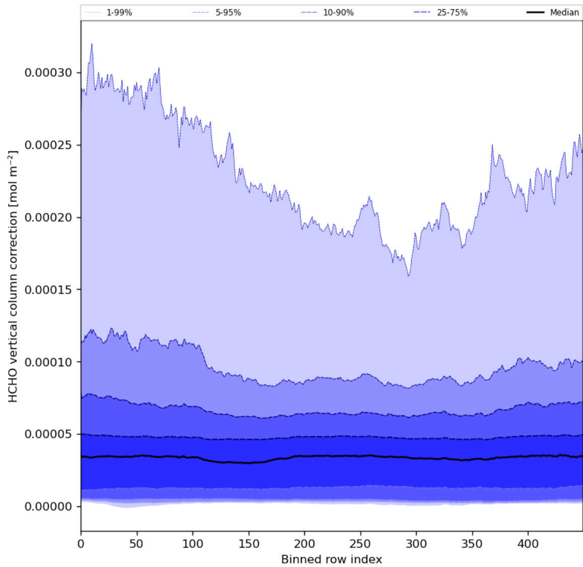
Figure 51: Along track statistics of “HCHO vertical column correction” for 2023-12-14 to 2023-12-15
