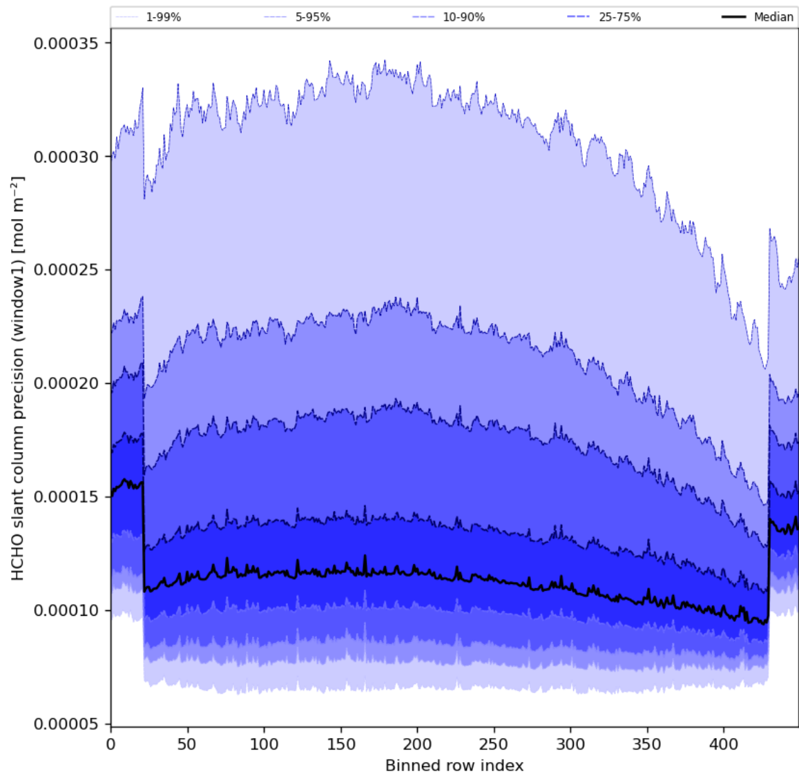
Figure 53: Along track statistics of “HCHO slant column precision (window1)” for 2023-12-14 to 2023-12-15
