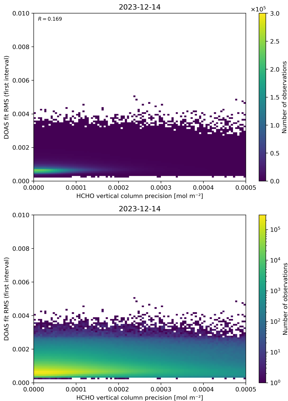
Figure 136: Scatter density plot of “HCHO vertical column precision” against “DOAS fit RMS (first interval)” for 2023-12-14 to 2023-12-15.
