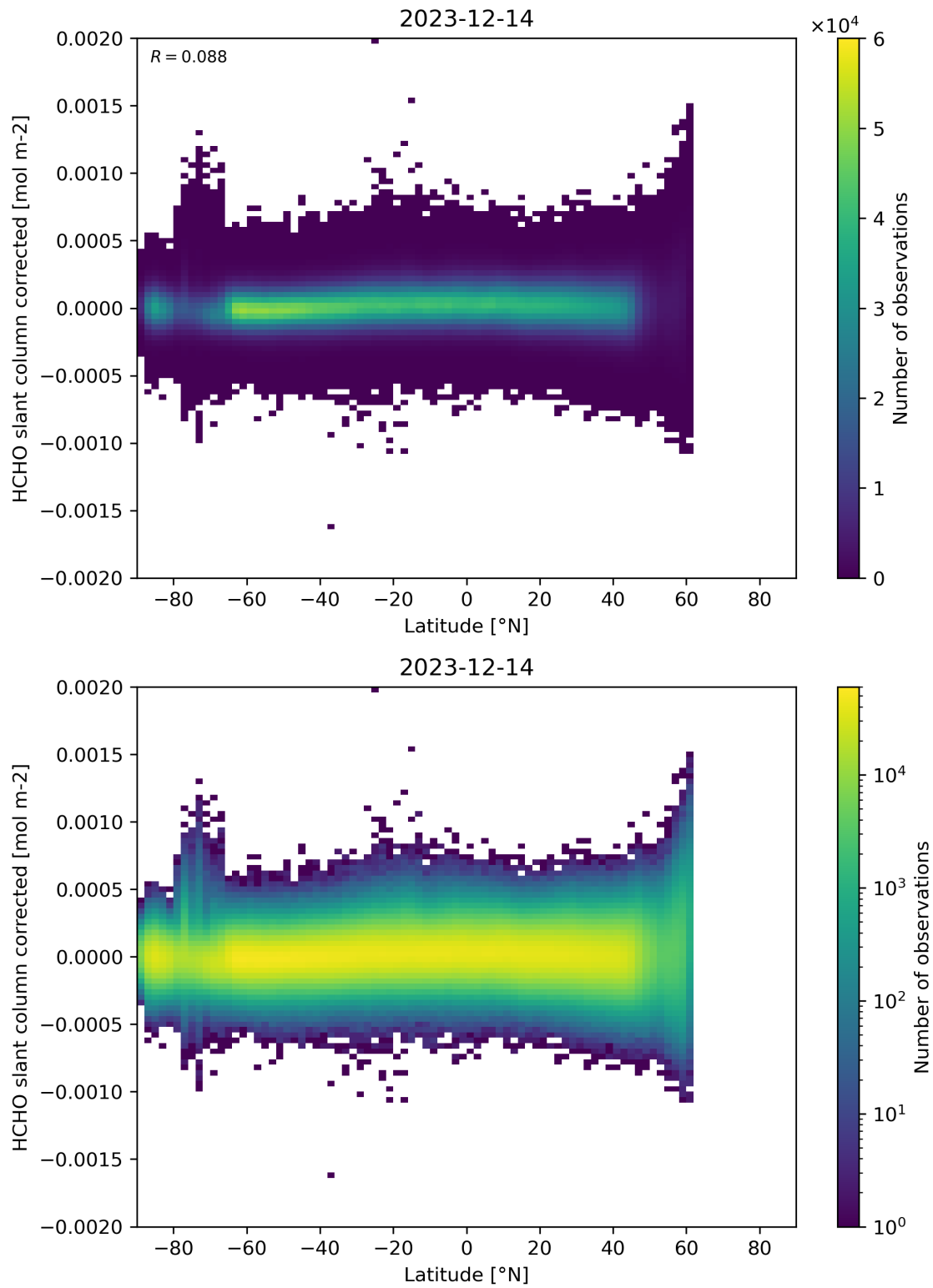
Figure 157: Scatter density plot of “Latitude” against “HCHO slant column corrected” for 2023-12-14 to 2023-12-15.
