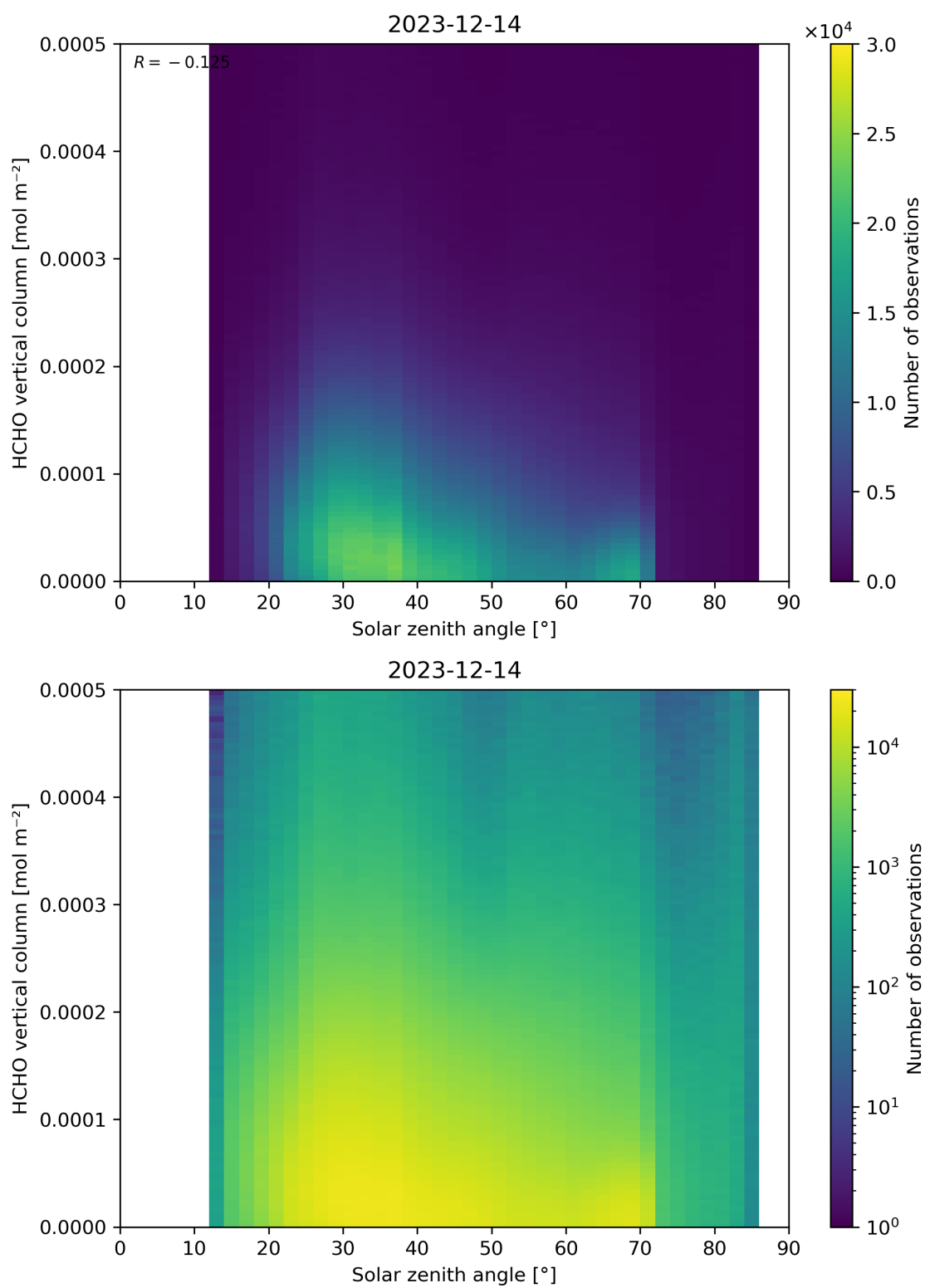
Figure 177: Scatter density plot of “Solar zenith angle” against “HCHO vertical column” for 2023-12-14 to 2023-12-15.
