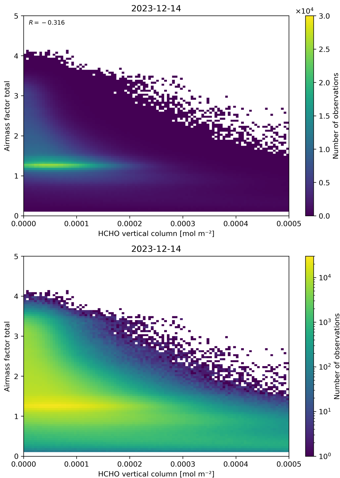
Figure 131: Scatter density plot of “HCHO vertical column” against “Airmass factor total” for 2023-12-14 to 2023-12-15.
