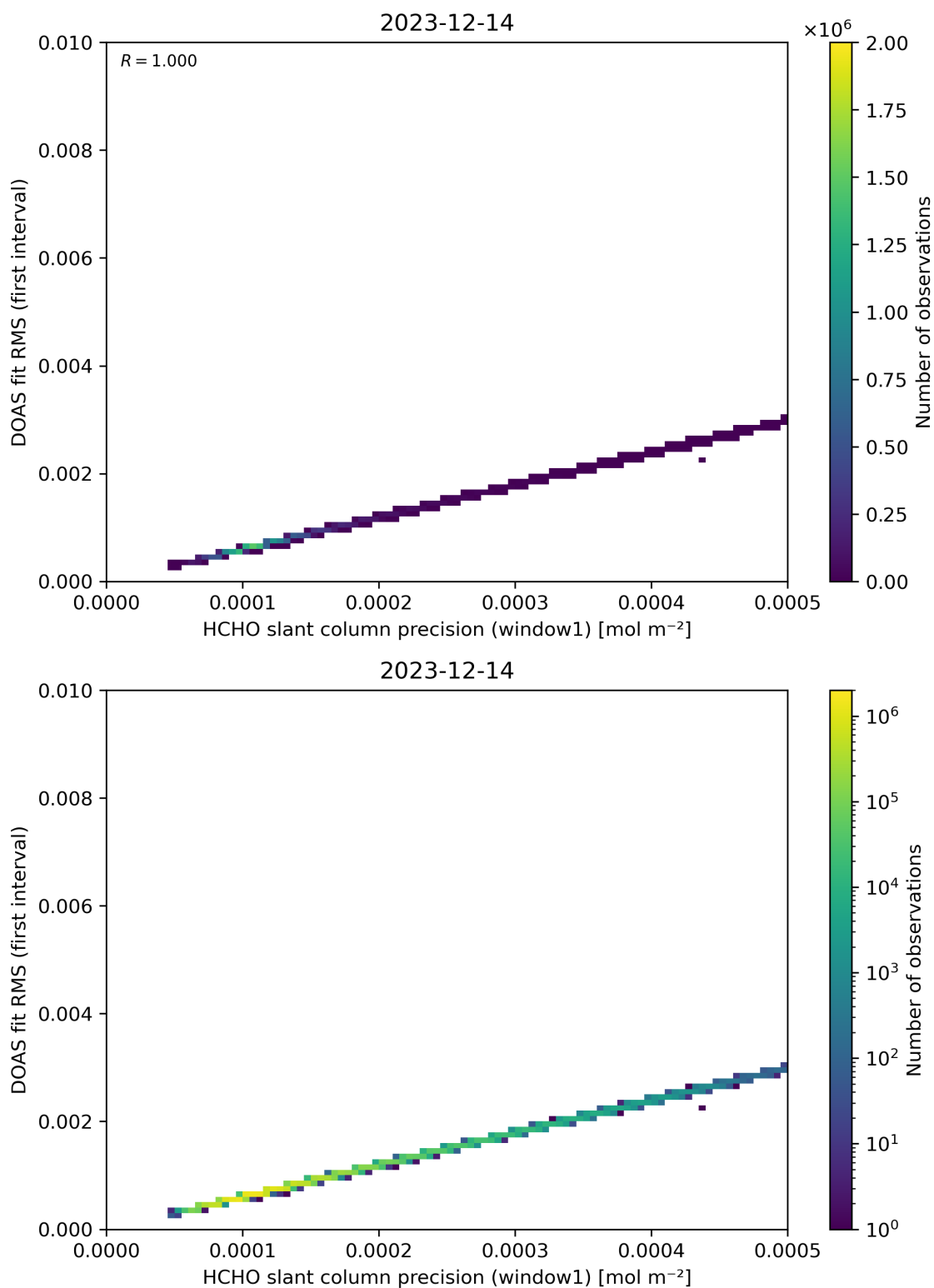
Figure 88: Scatter density plot of “HCHO slant column precision (window1)” against “DOAS fit RMS (first interval)” for 2023-12-14 to 2023-12-15.
