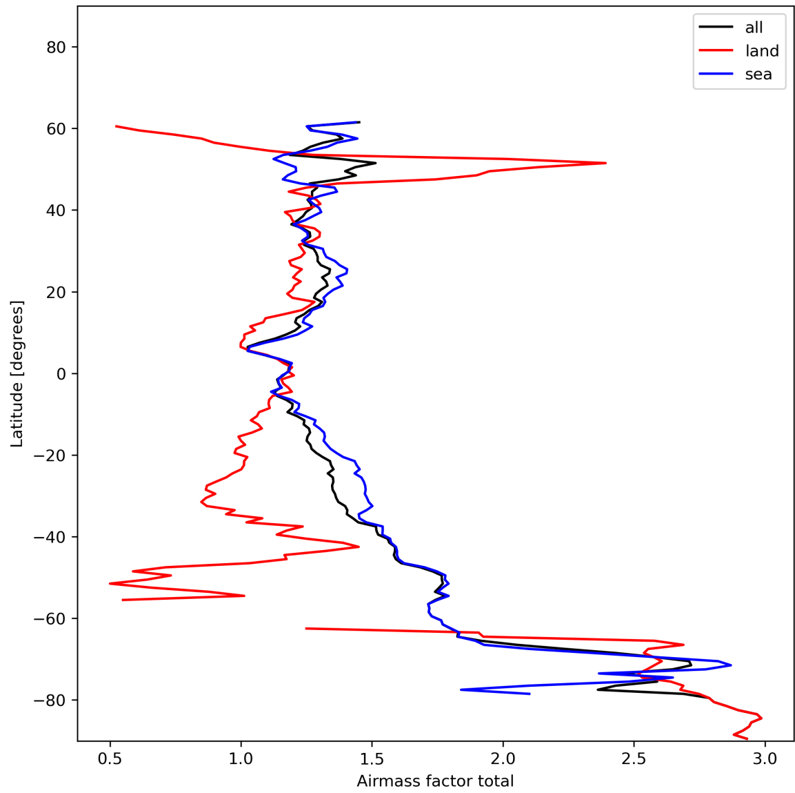
Figure 26: Zonal average of “Airmass factor total” for 2023-12-14 to 2023-12-15.
