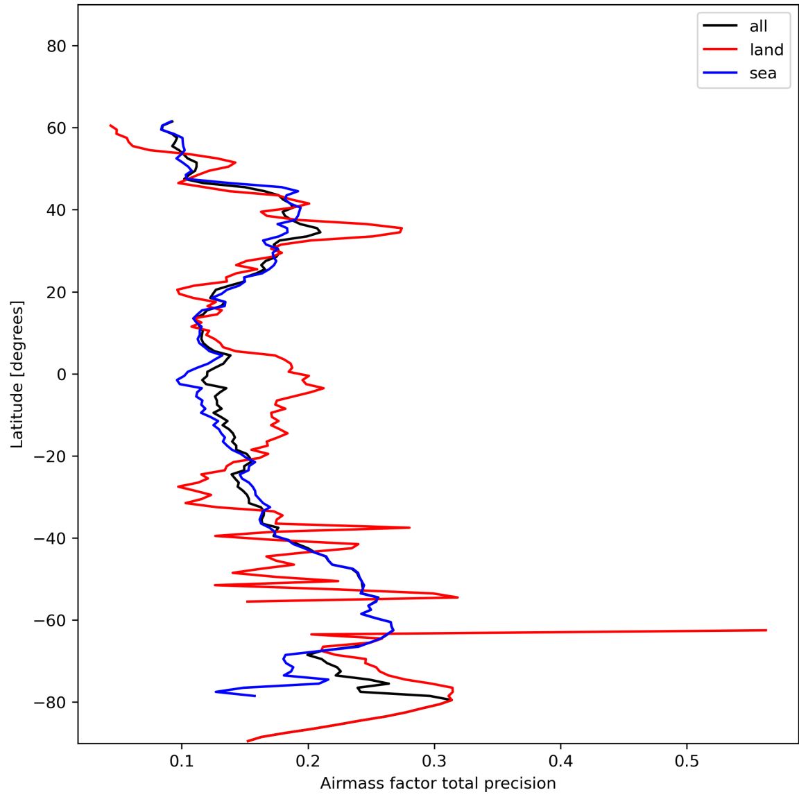
Figure 27: Zonal average of “Airmass factor total precision” for 2023-12-14 to 2023-12-15.
