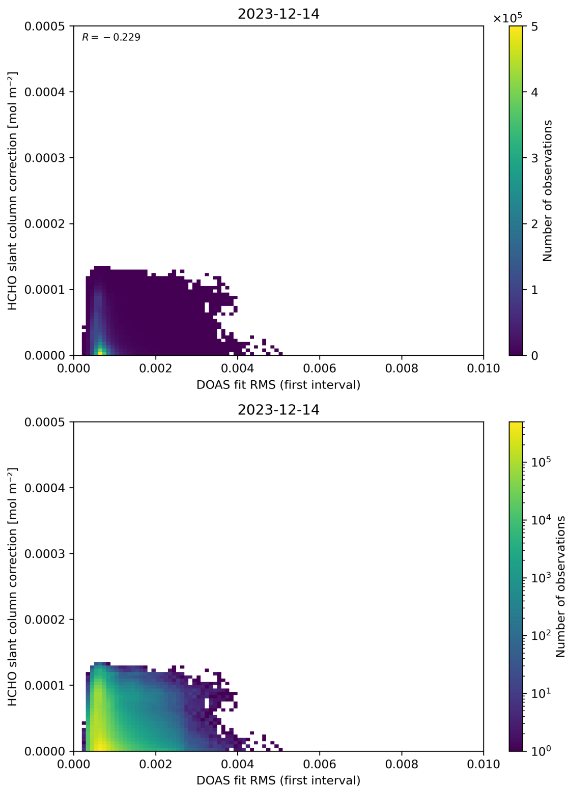
Figure 63: Scatter density plot of “DOAS fit RMS (first interval)” against “HCHO slant column correction” for 2023-12-14 to 2023-12-15.
