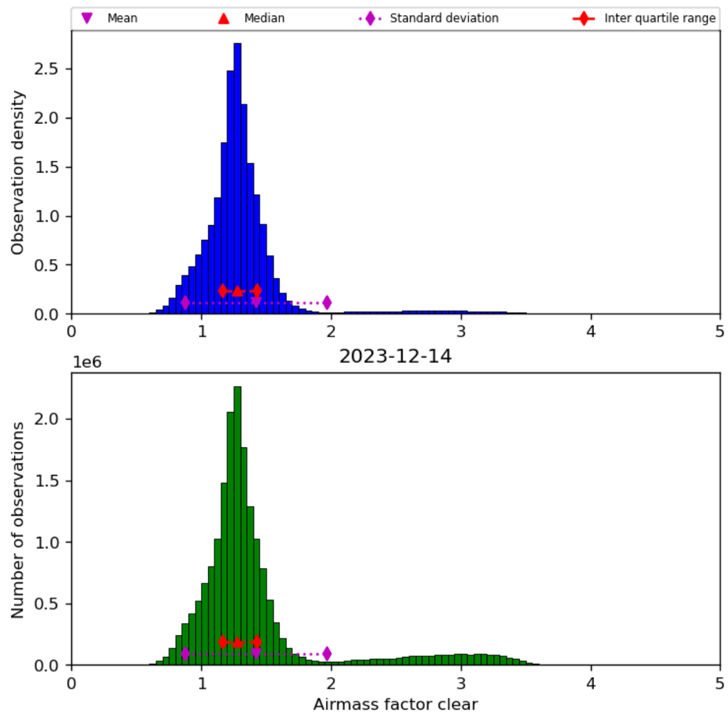
Figure 42: Histogram of “Airmass factor clear” for 2023-12-14 to 2023-12-15
