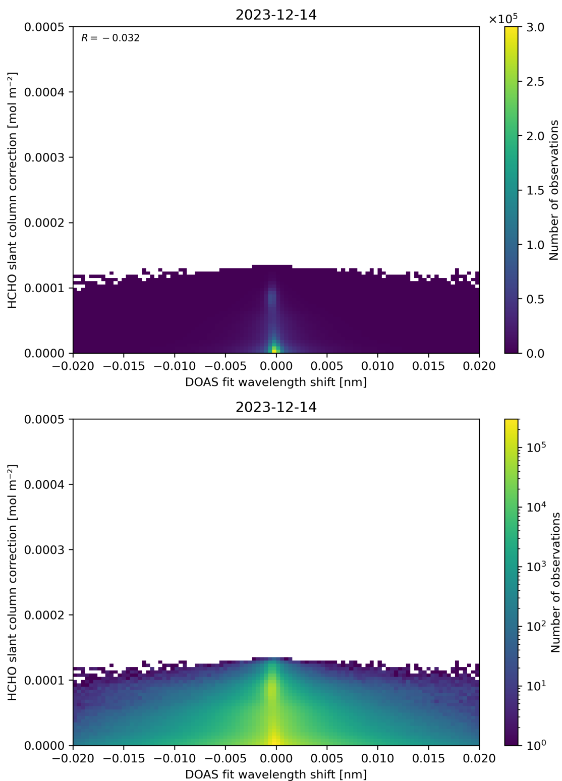
Figure 67: Scatter density plot of “DOAS fit wavelength shift” against “HCHO slant column correction” for 2023-12-14 to 2023-12-15.
