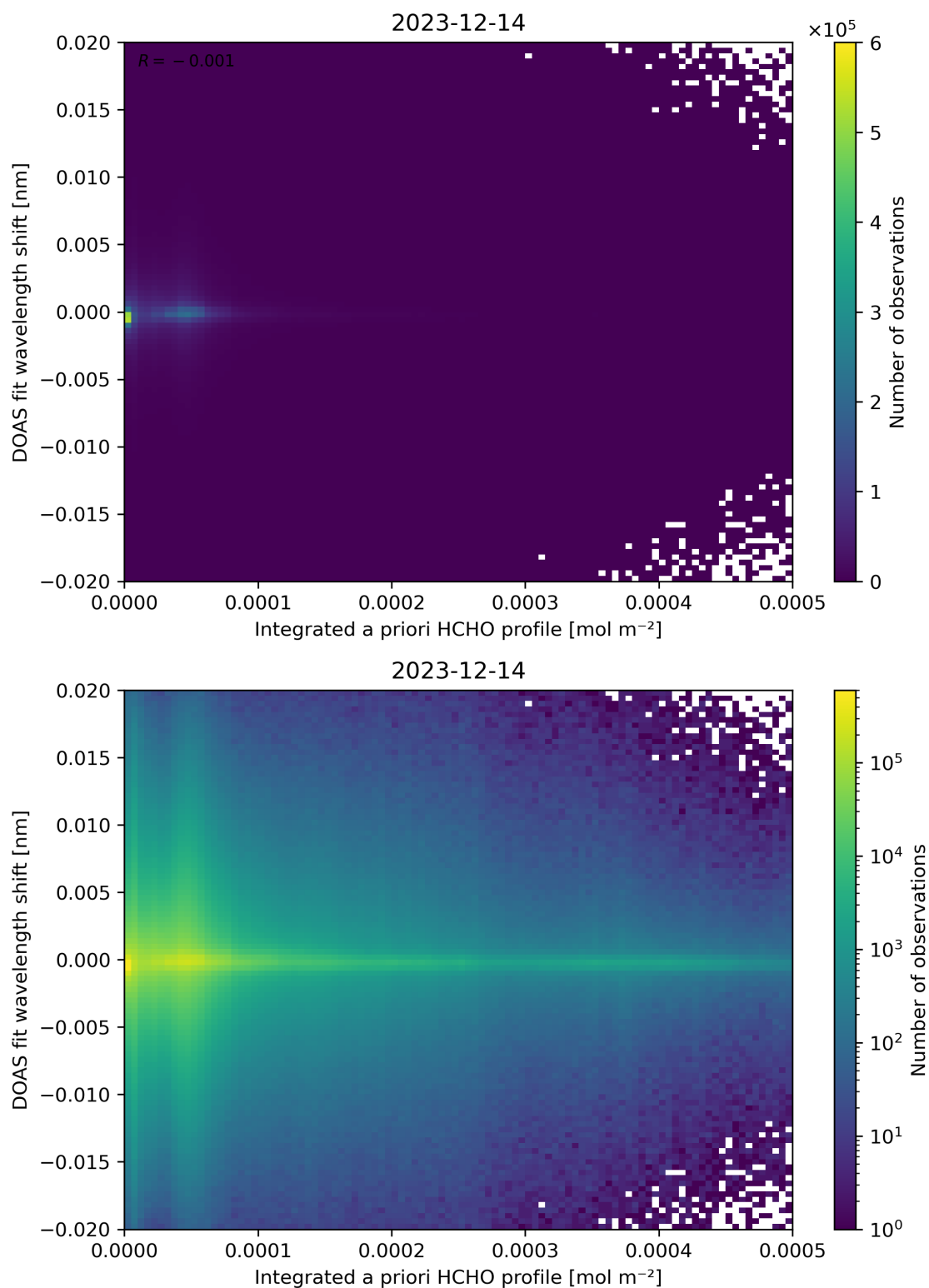
Figure 149: Scatter density plot of “Integrated a priori HCHO profile” against “DOAS fit wavelength shift” for 2023-12-14 to 2023-12-15.
