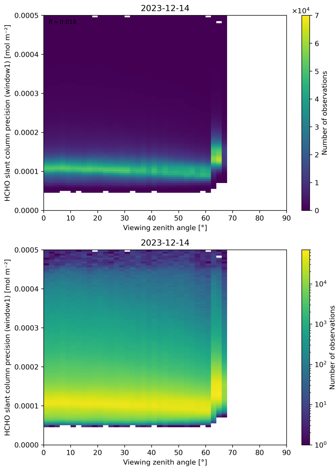
Figure 189: Scatter density plot of “Viewing zenith angle” against “HCHO slant column precision (window1)” for 2023-12-14 to 2023-12-15.
