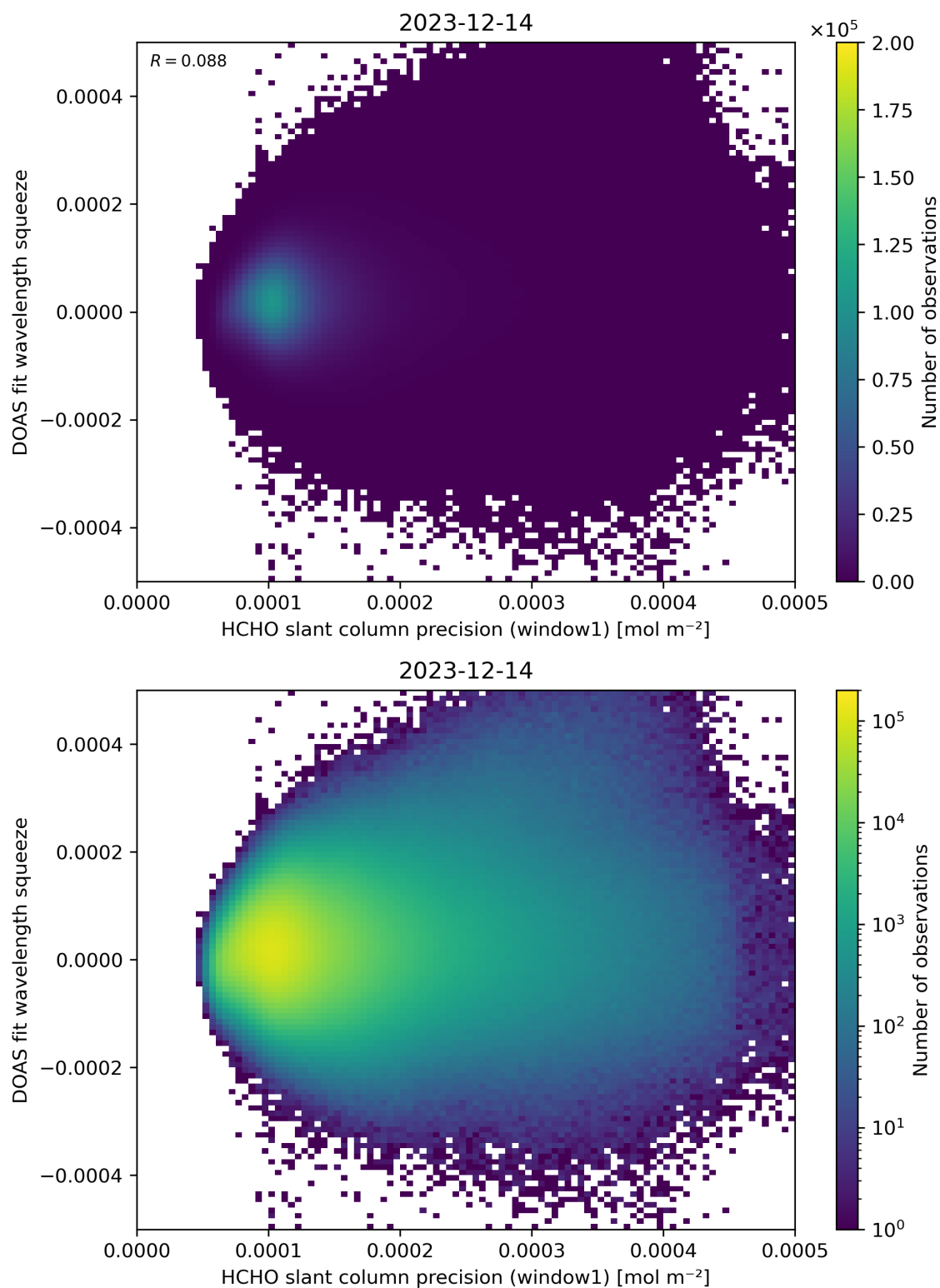
Figure 90: Scatter density plot of “HCHO slant column precision (window1)” against “DOAS fit wavelength squeeze” for 2023-12-14 to 2023-12-15.
