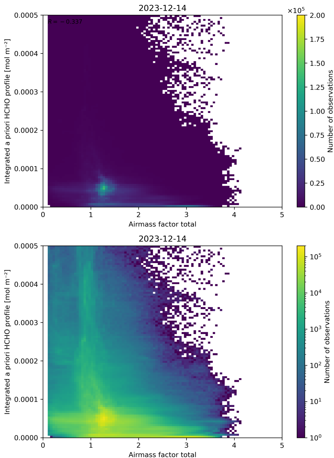
Figure 104: Scatter density plot of “Airmass factor total” against “Integrated a priori HCHO profile” for 2023-12-14 to 2023-12-15.
