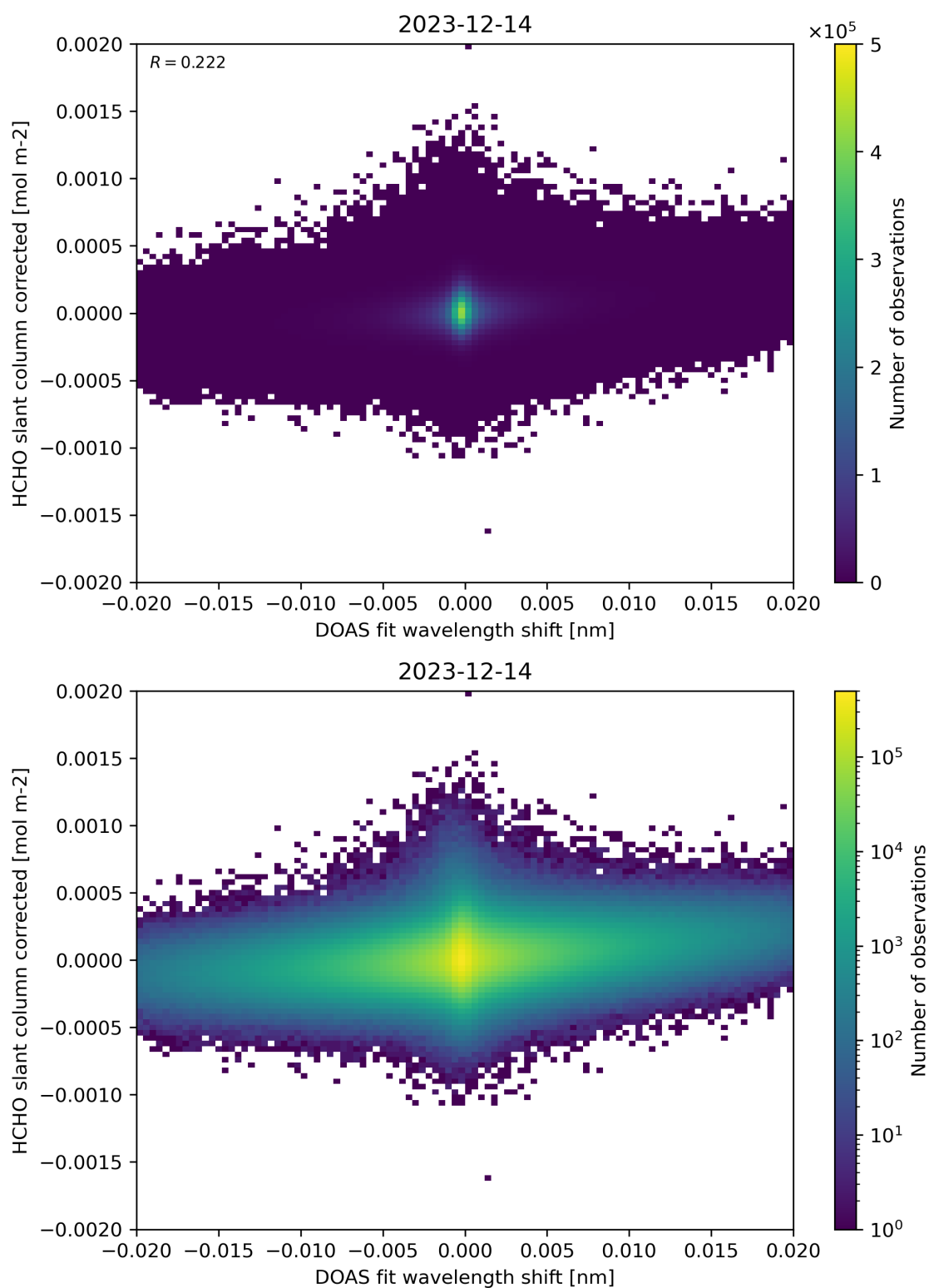
Figure 66: Scatter density plot of “DOAS fit wavelength shift” against “HCHO slant column corrected” for 2023-12-14 to 2023-12-15.
