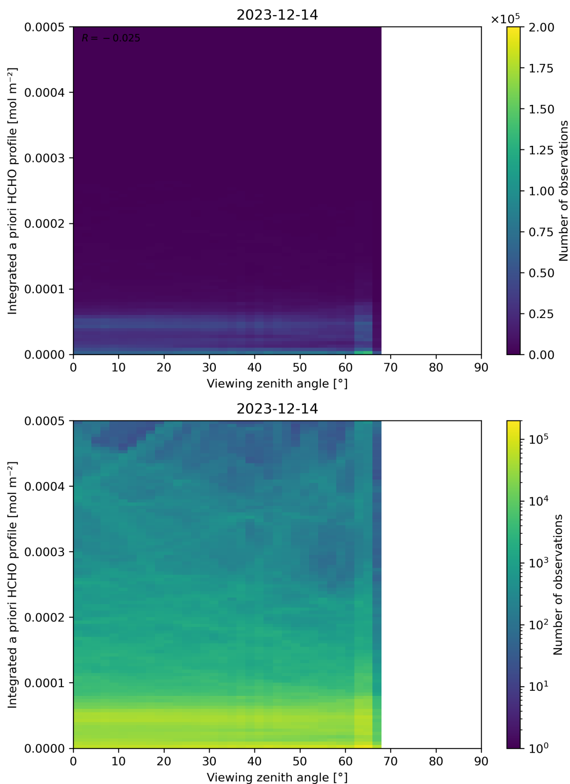
Figure 195: Scatter density plot of “Viewing zenith angle” against “Integrated a priori HCHO profile” for 2023-12-14 to 2023-12-15.
