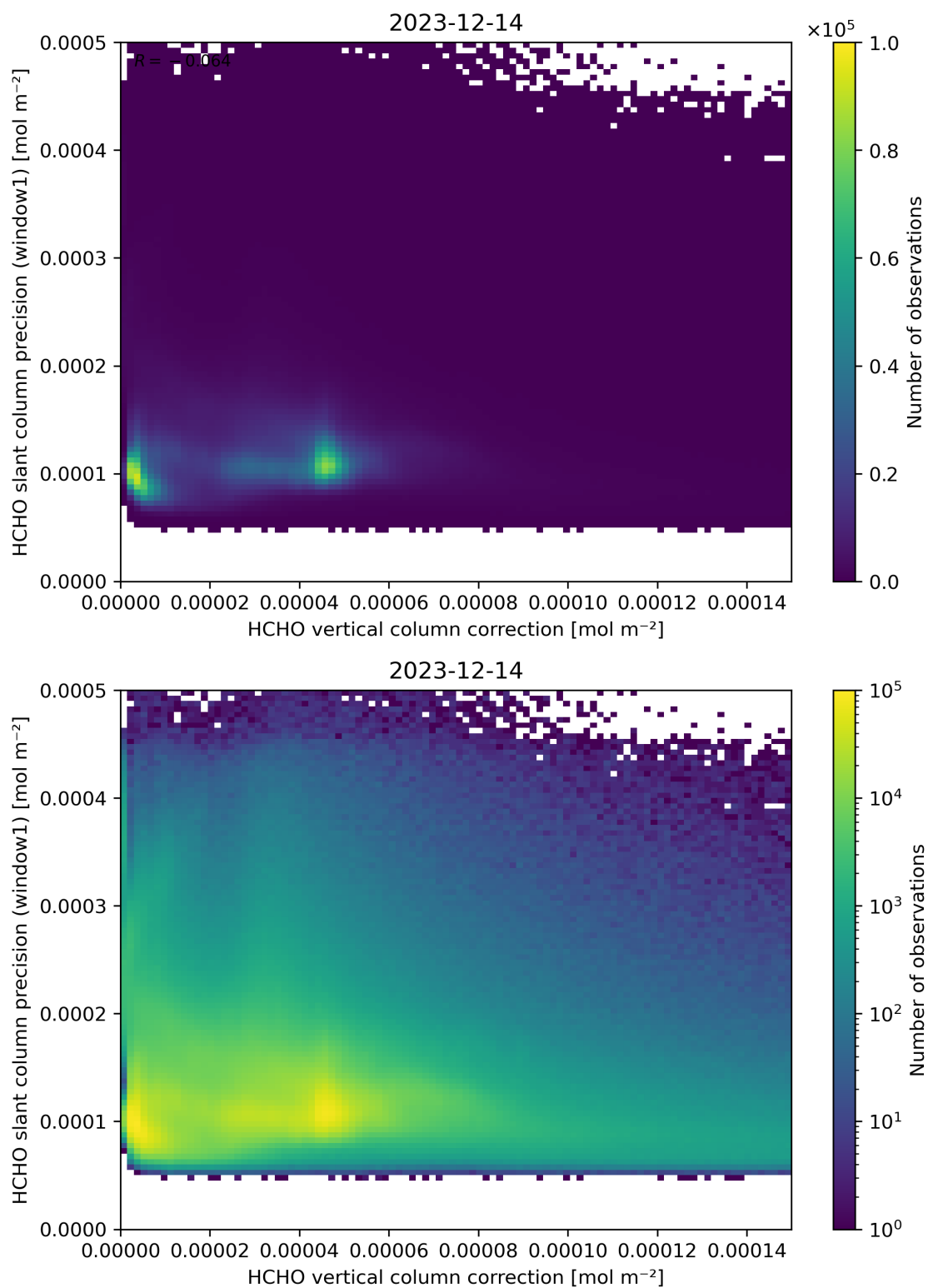
Figure 119: Scatter density plot of “HCHO vertical column correction” against “HCHO slant column precision (window1)” for 2023-12-14 to 2023-12-15.
