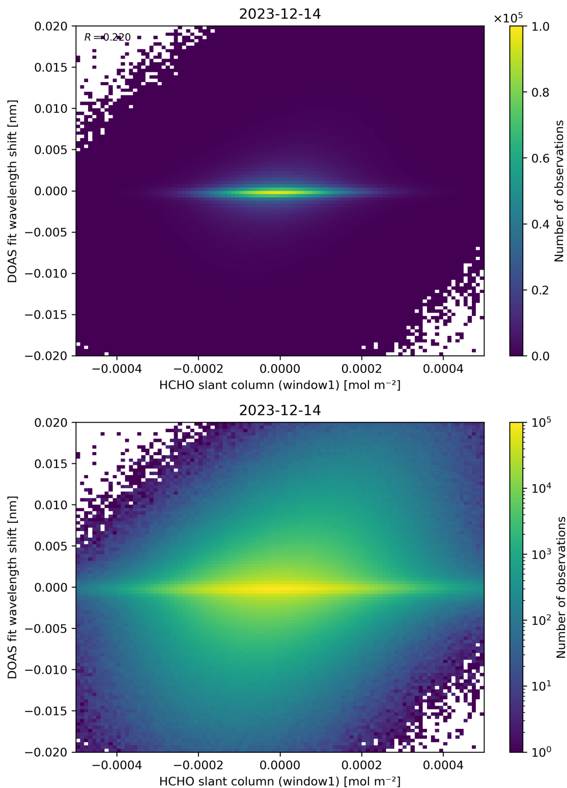
Figure 79: Scatter density plot of “HCHO slant column (window1)” against “DOAS fit wavelength shift” for 2023-12-14 to 2023-12-15.
