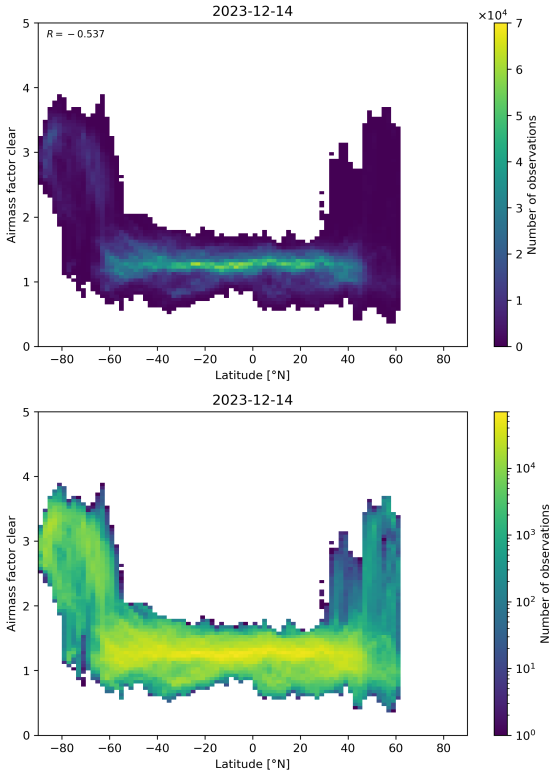
Figure 156: Scatter density plot of “Latitude” against “Airmass factor clear” for 2023-12-14 to 2023-12-15.
