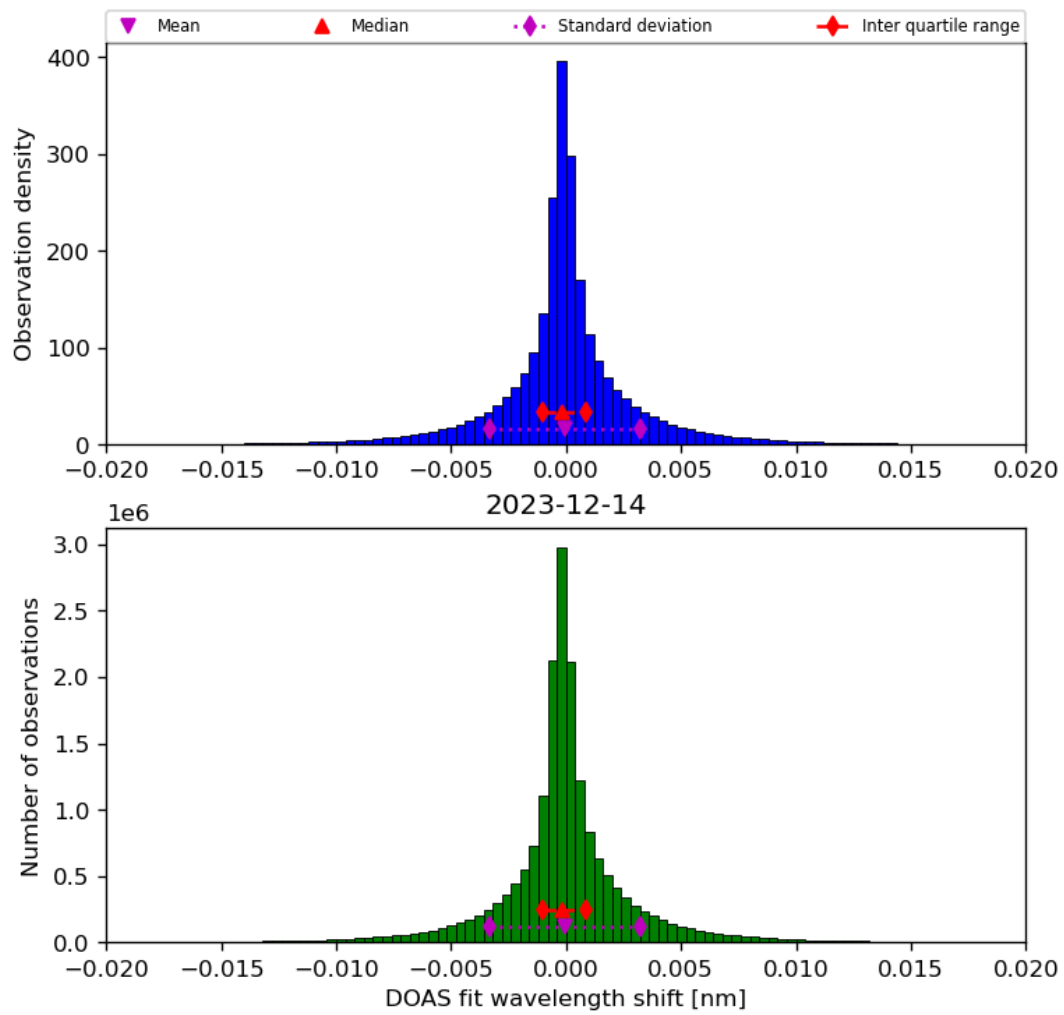
Figure 44: Histogram of “DOAS fit wavelength shift” for 2023-12-14 to 2023-12-15
