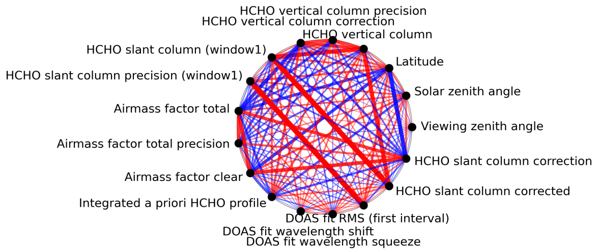
Figure 1: Map of correlation graph for 2023-12-14 to 2023-12-15.
