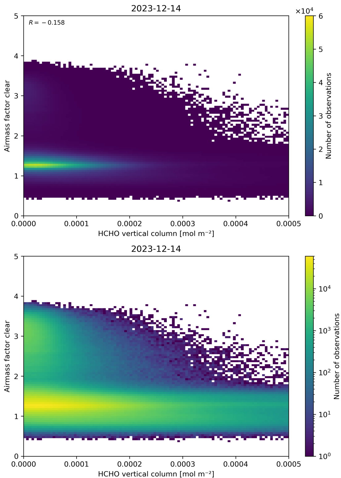
Figure 126: Scatter density plot of “HCHO vertical column” against “Airmass factor clear” for 2023-12-14 to 2023-12-15.
