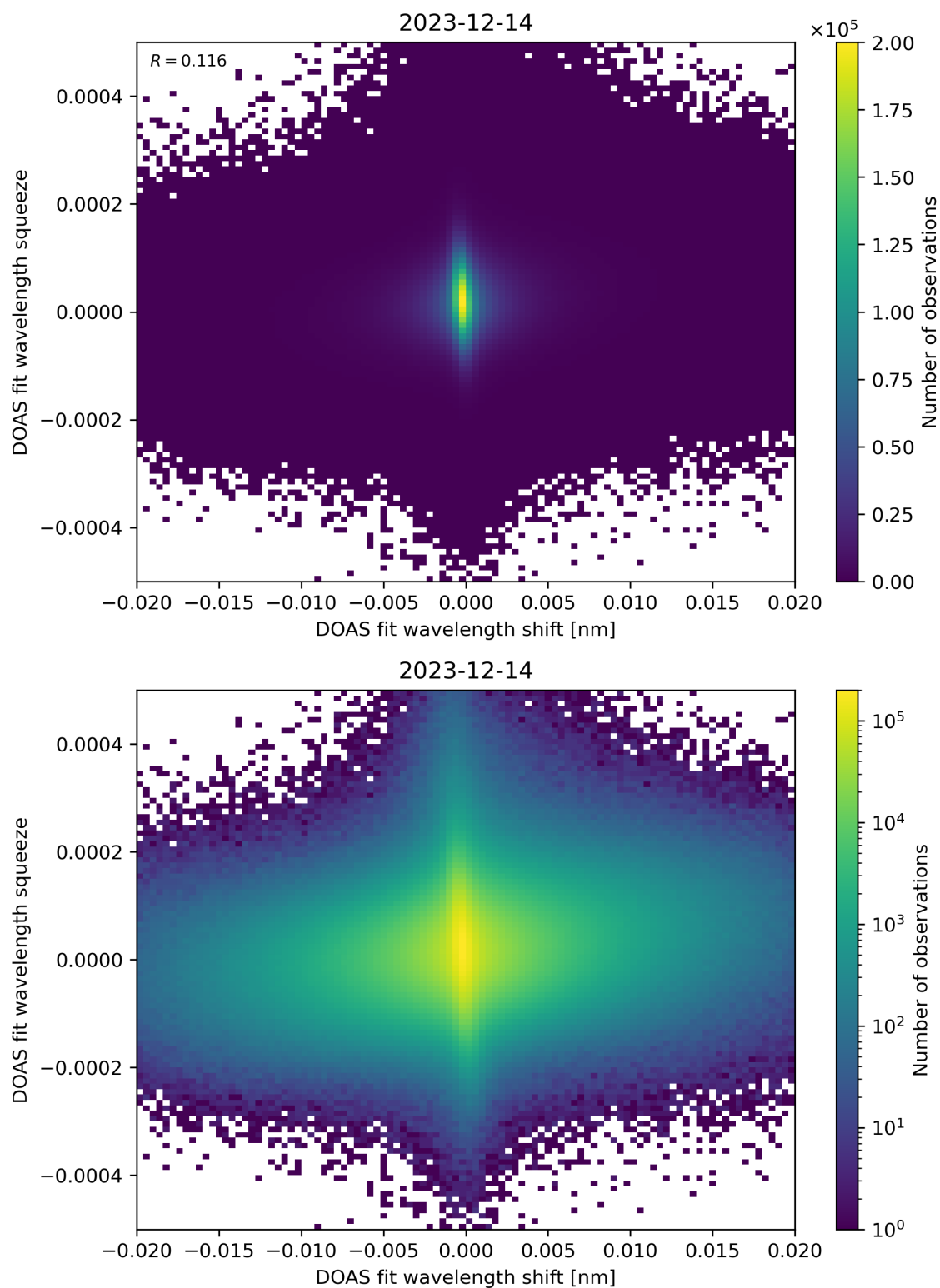
Figure 65: Scatter density plot of “DOAS fit wavelength shift” against “DOAS fit wavelength squeeze” for 2023-12-14 to 2023-12-15.
