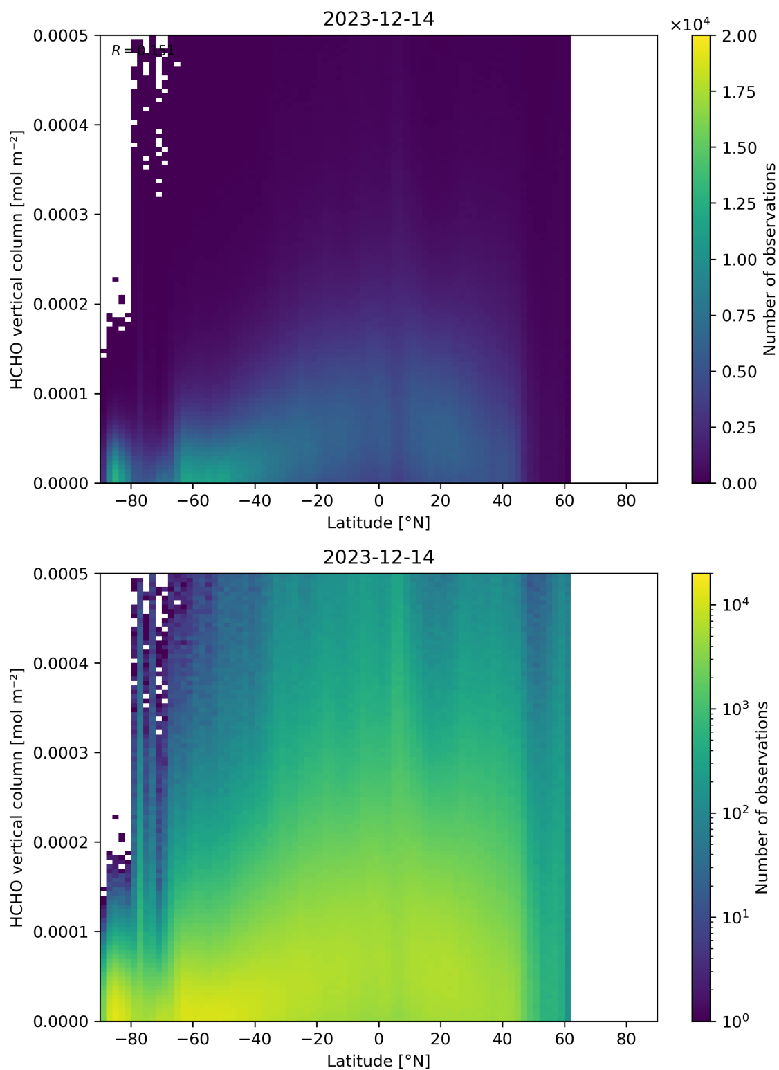
Figure 163: Scatter density plot of “Latitude” against “HCHO vertical column” for 2023-12-14 to 2023-12-15.
