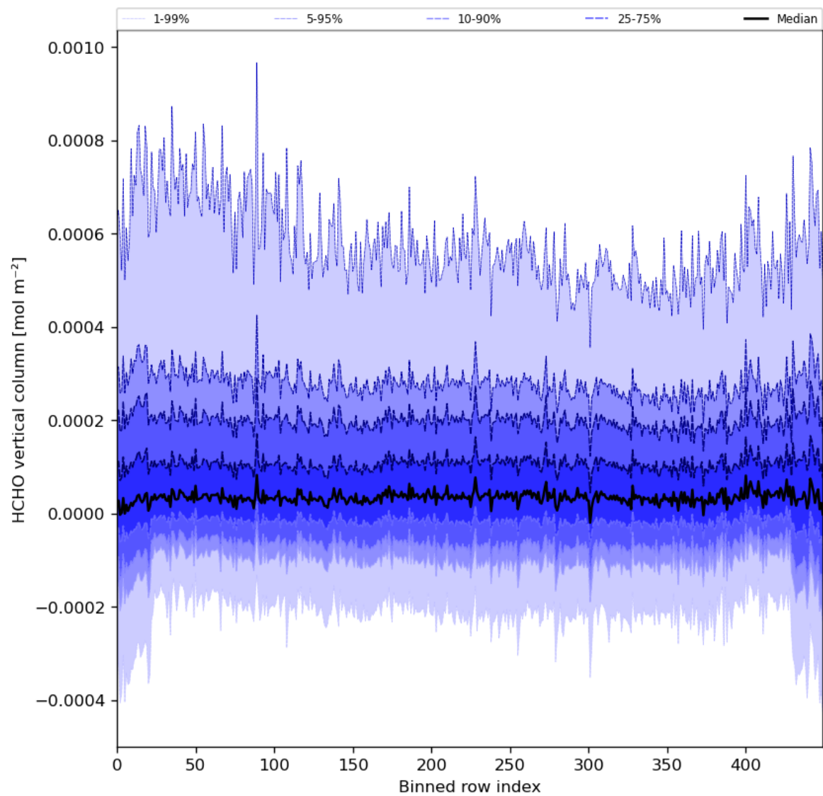
Figure 49: Along track statistics of “HCHO vertical column” for 2023-12-14 to 2023-12-15
