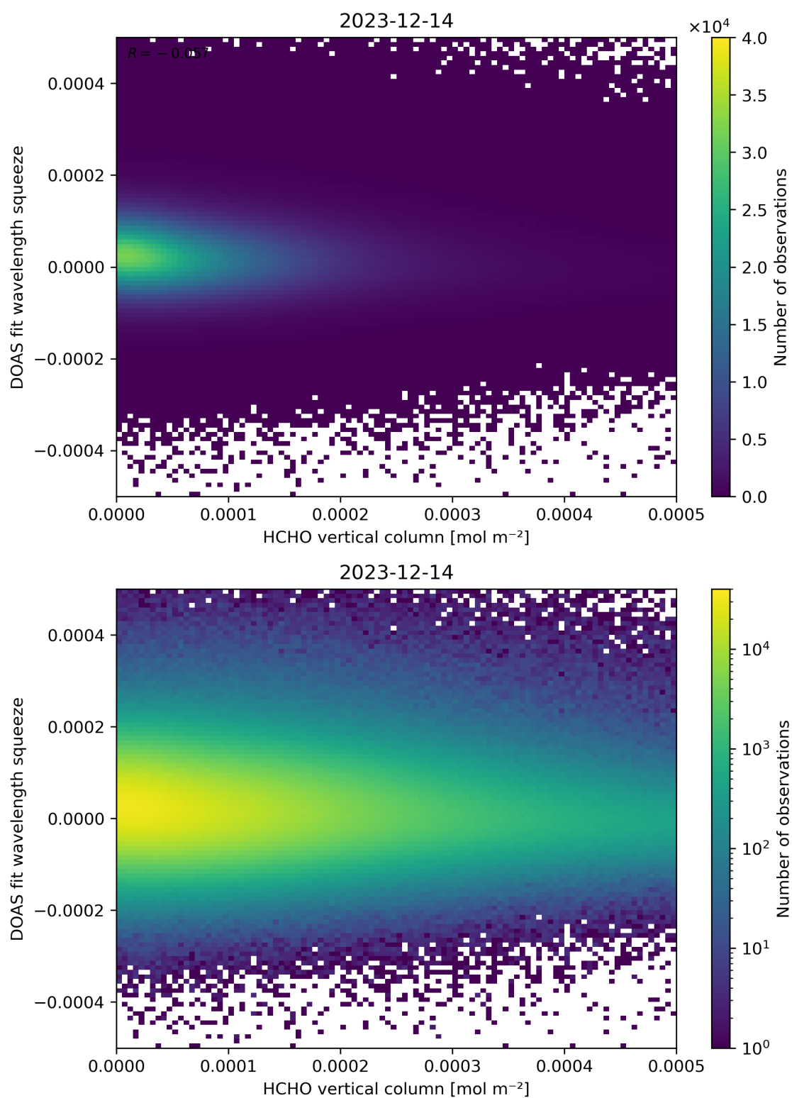
Figure 125: Scatter density plot of “HCHO vertical column” against “DOAS fit wavelength squeeze” for 2023-12-14 to 2023-12-15.
