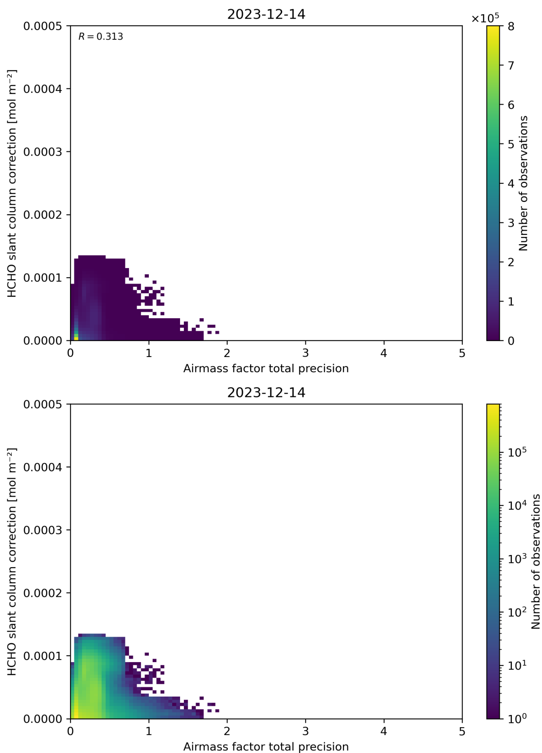
Figure 110: Scatter density plot of “Airmass factor total precision” against “HCHO slant column correction” for 2023-12-14 to 2023-12-15.
