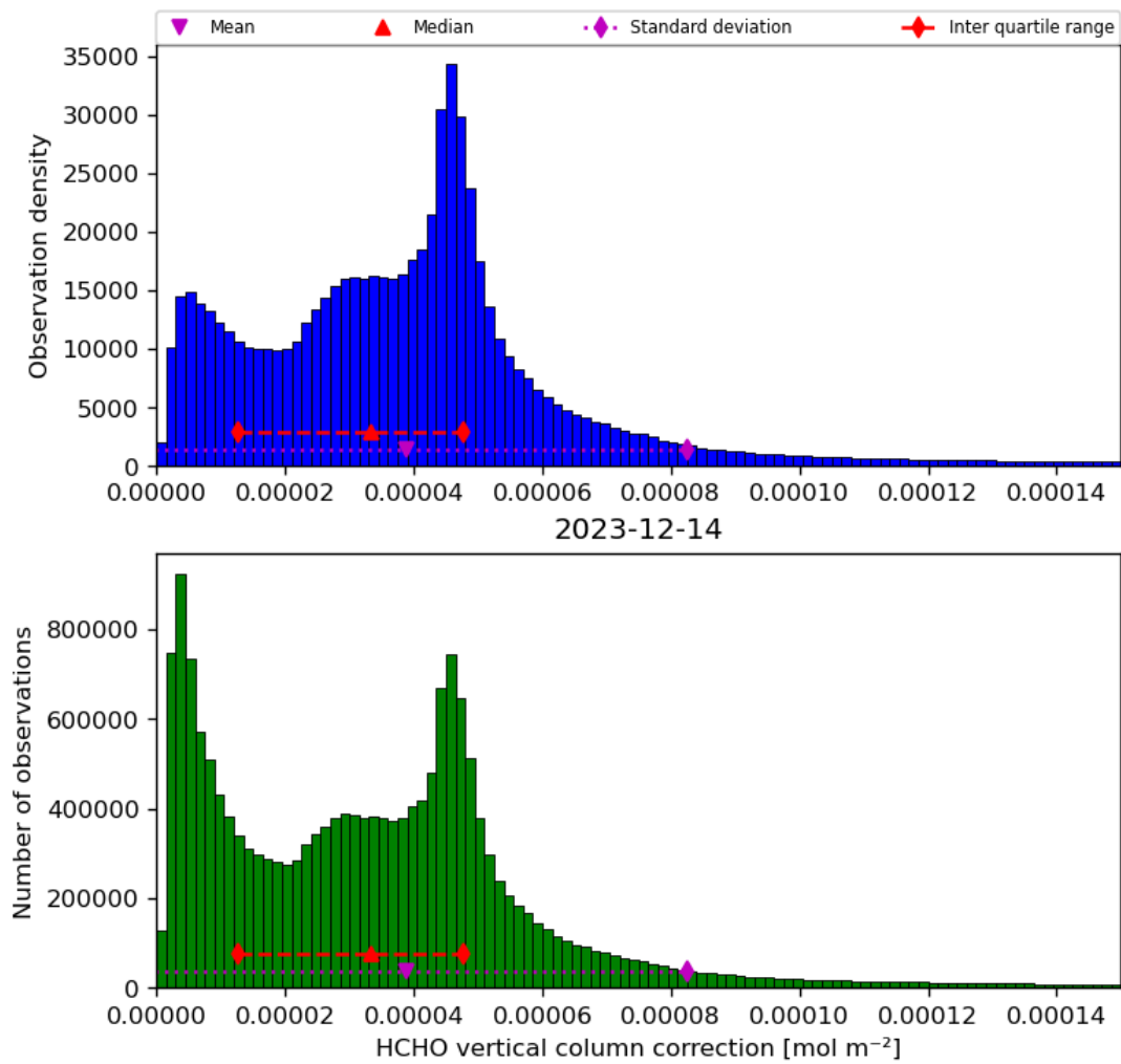
Figure 37: Histogram of “HCHO vertical column correction” for 2023-12-14 to 2023-12-15
