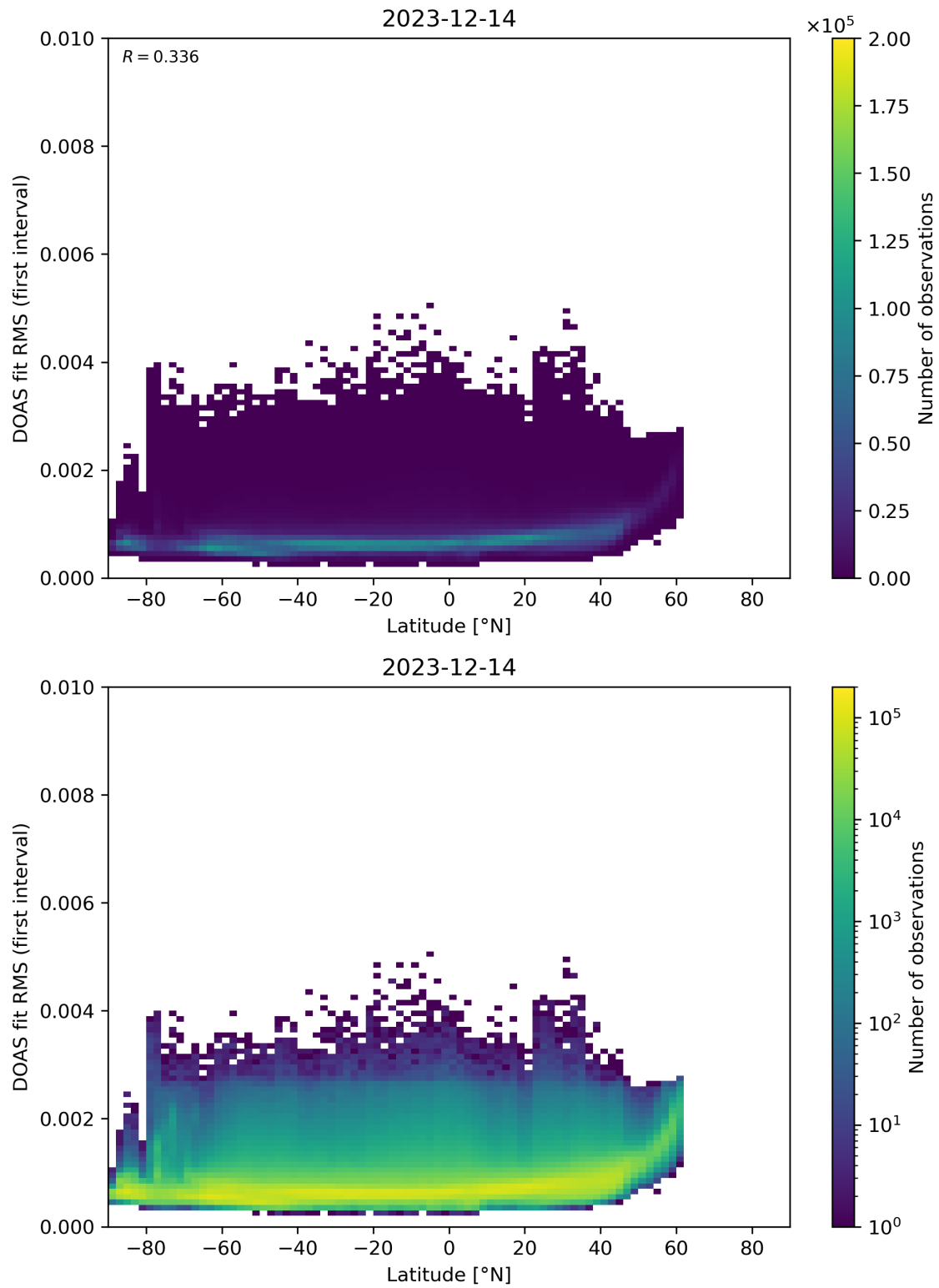
Figure 153: Scatter density plot of “Latitude” against “DOAS fit RMS (first interval)” for 2023-12-14 to 2023-12-15.
