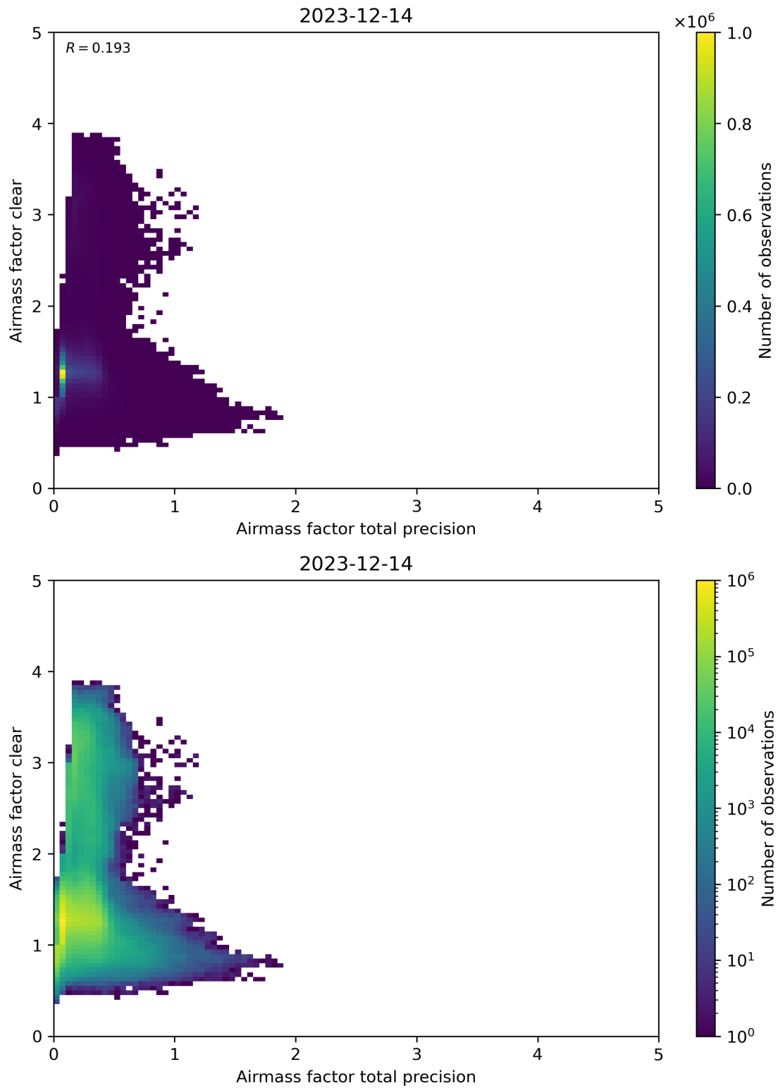
Figure 108: Scatter density plot of “Airmass factor total precision” against “Airmass factor clear” for 2023-12-14 to 2023-12-15.
