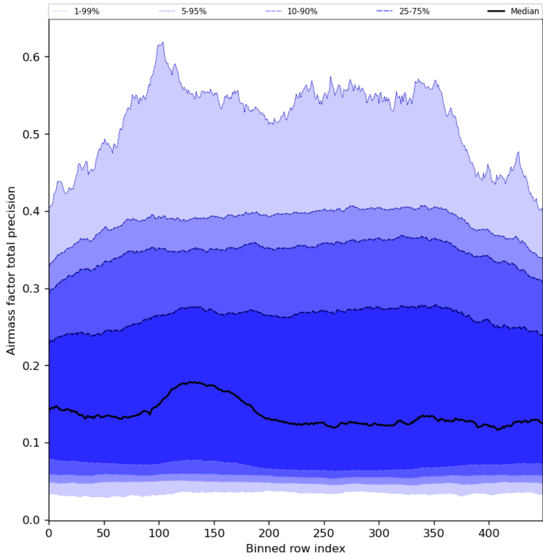
Figure 55: Along track statistics of “Airmass factor total precision” for 2023-12-14 to 2023-12-15
