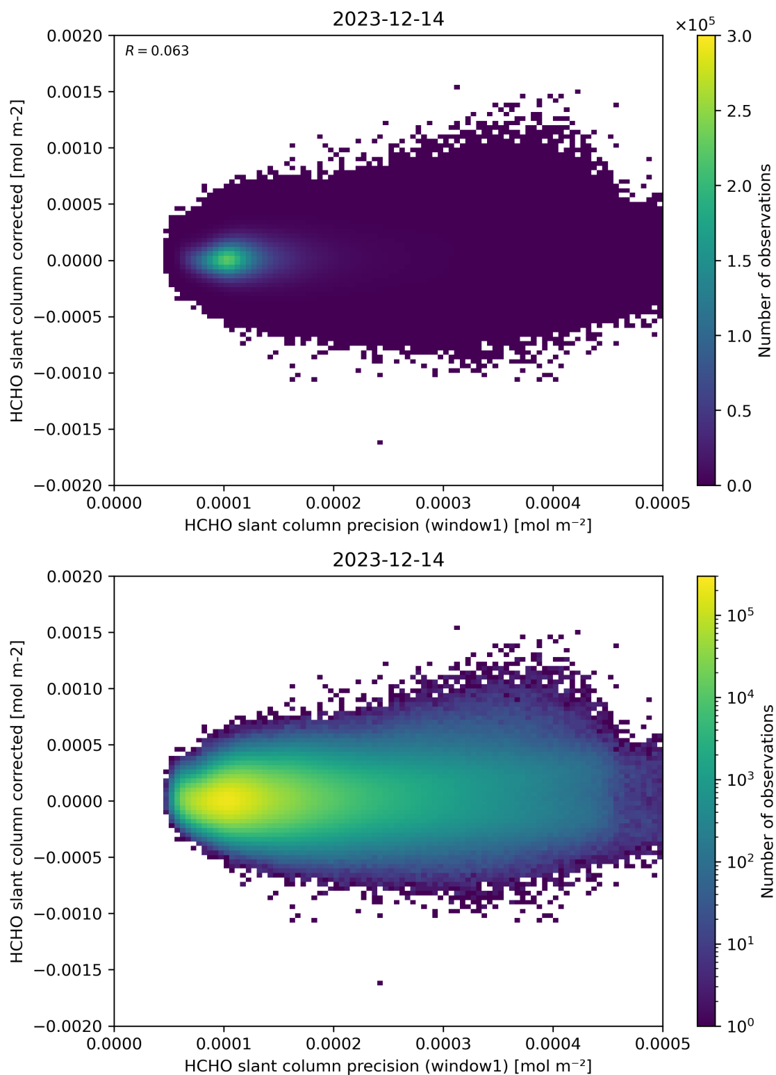
Figure 92: Scatter density plot of “HCHO slant column precision (window1)” against “HCHO slant column corrected” for 2023-12-14 to 2023-12-15.
