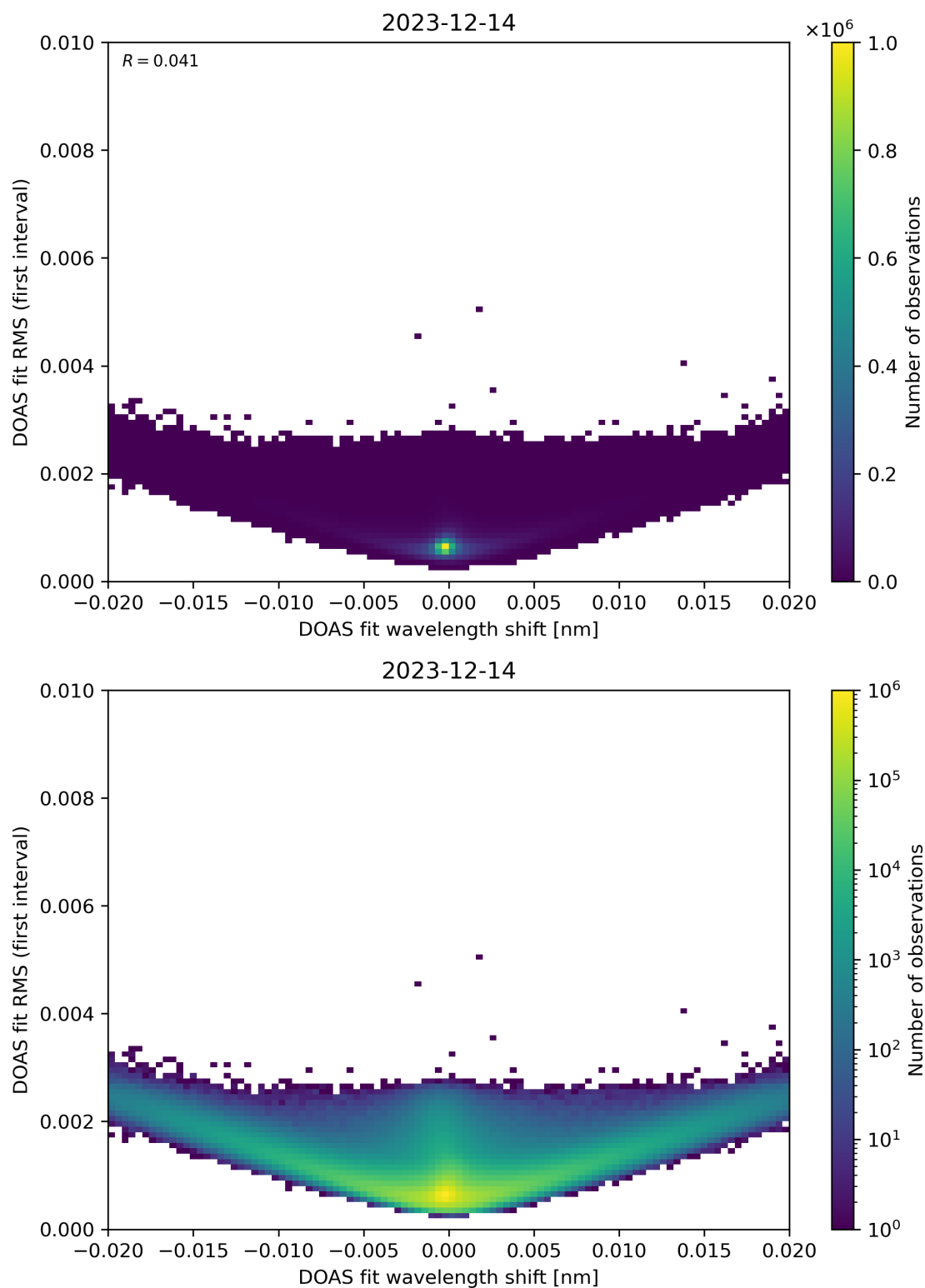
Figure 64: Scatter density plot of “DOAS fit wavelength shift” against “DOAS fit RMS (first interval)” for 2023-12-14 to 2023-12-15.
