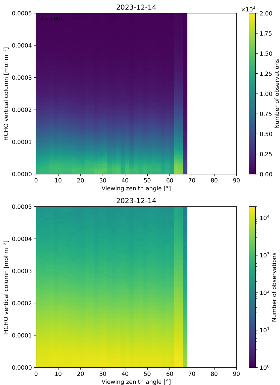
Figure 192: Scatter density plot of “Viewing zenith angle” against “HCHO vertical column” for 2023-12-14 to 2023-12-15.
