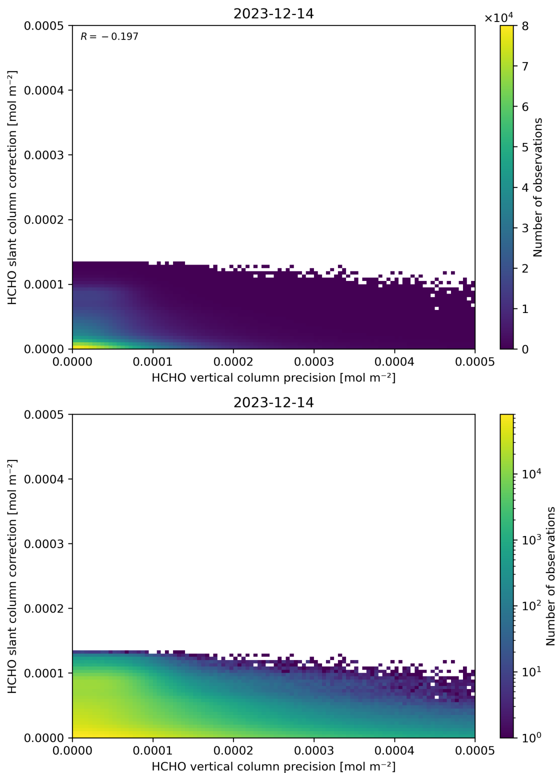
Figure 141: Scatter density plot of “HCHO vertical column precision” against “HCHO slant column correction” for 2023-12-14 to 2023-12-15.
