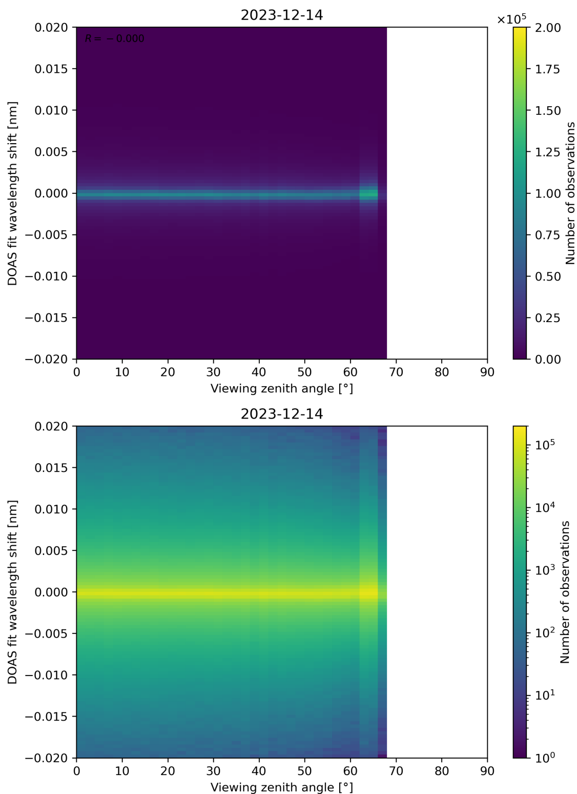
Figure 183: Scatter density plot of “Viewing zenith angle” against “DOAS fit wavelength shift” for 2023-12-14 to 2023-12-15.
