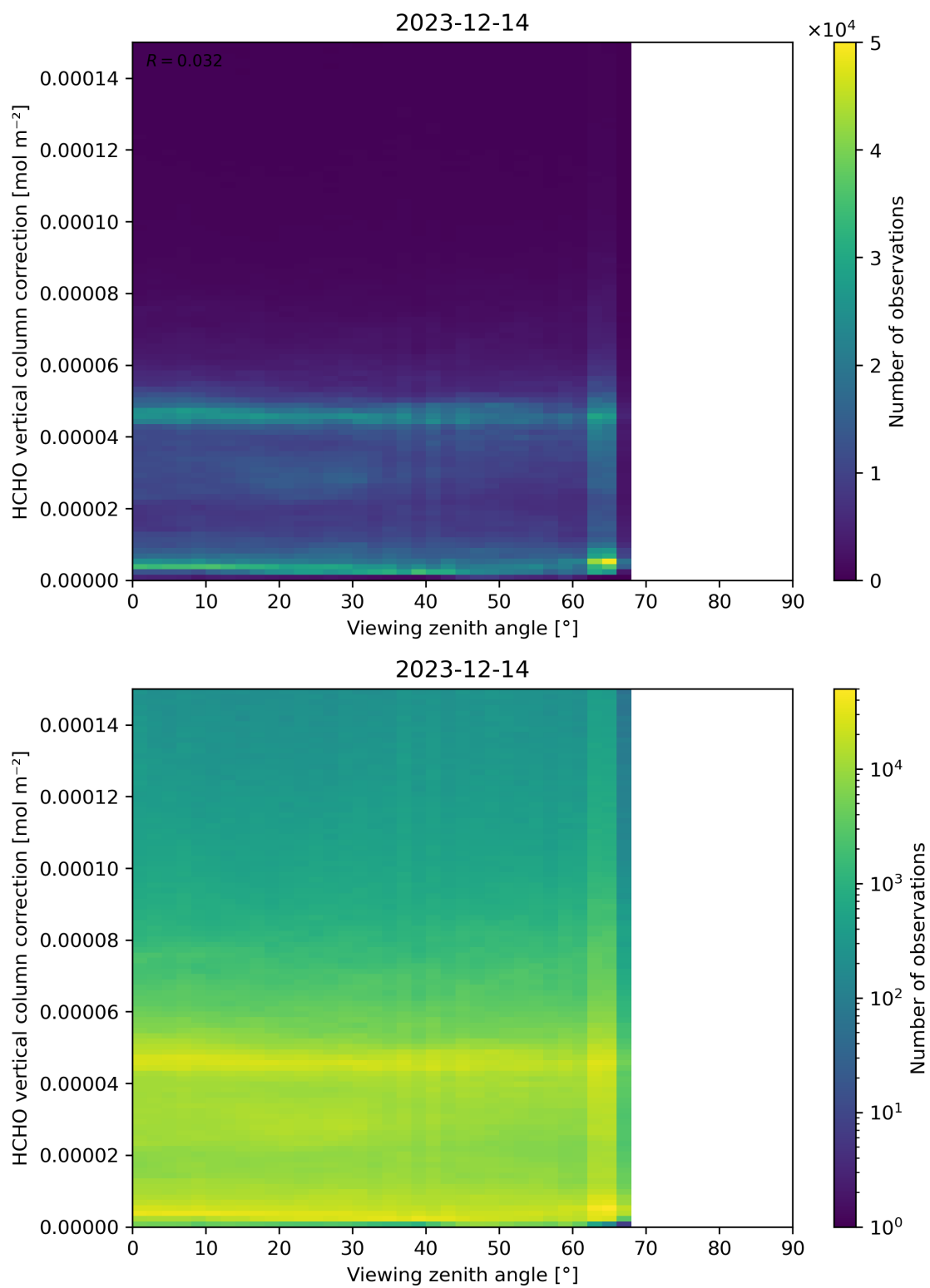
Figure 193: Scatter density plot of “Viewing zenith angle” against “HCHO vertical column correction” for 2023-12-14 to 2023-12-15.
