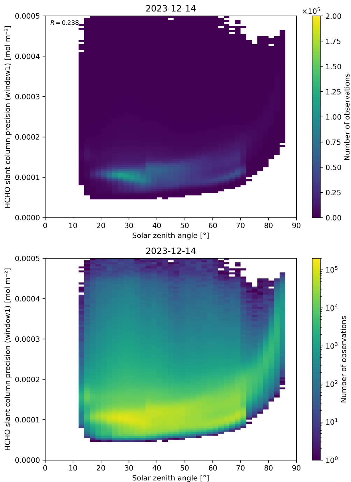
Figure 174: Scatter density plot of “Solar zenith angle” against “HCHO slant column precision (window1)” for 2023-12-14 to 2023-12-15.
