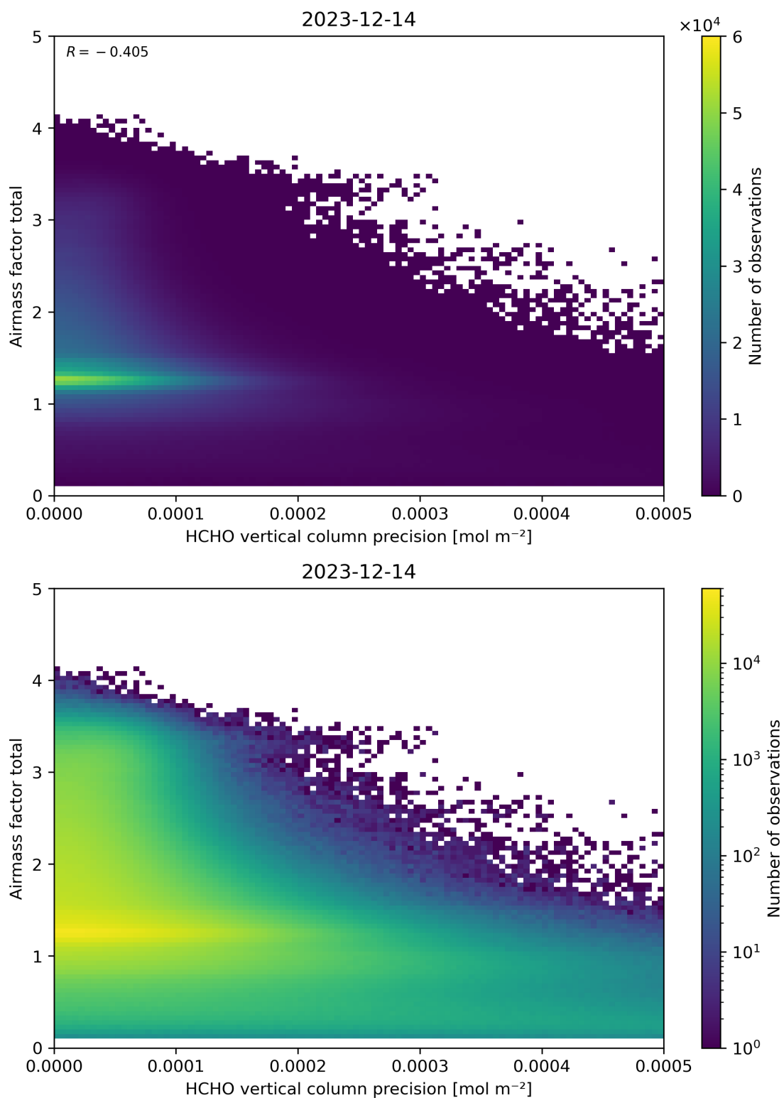
Figure 144: Scatter density plot of “HCHO vertical column precision” against “Airmass factor total” for 2023-12-14 to 2023-12-15.
