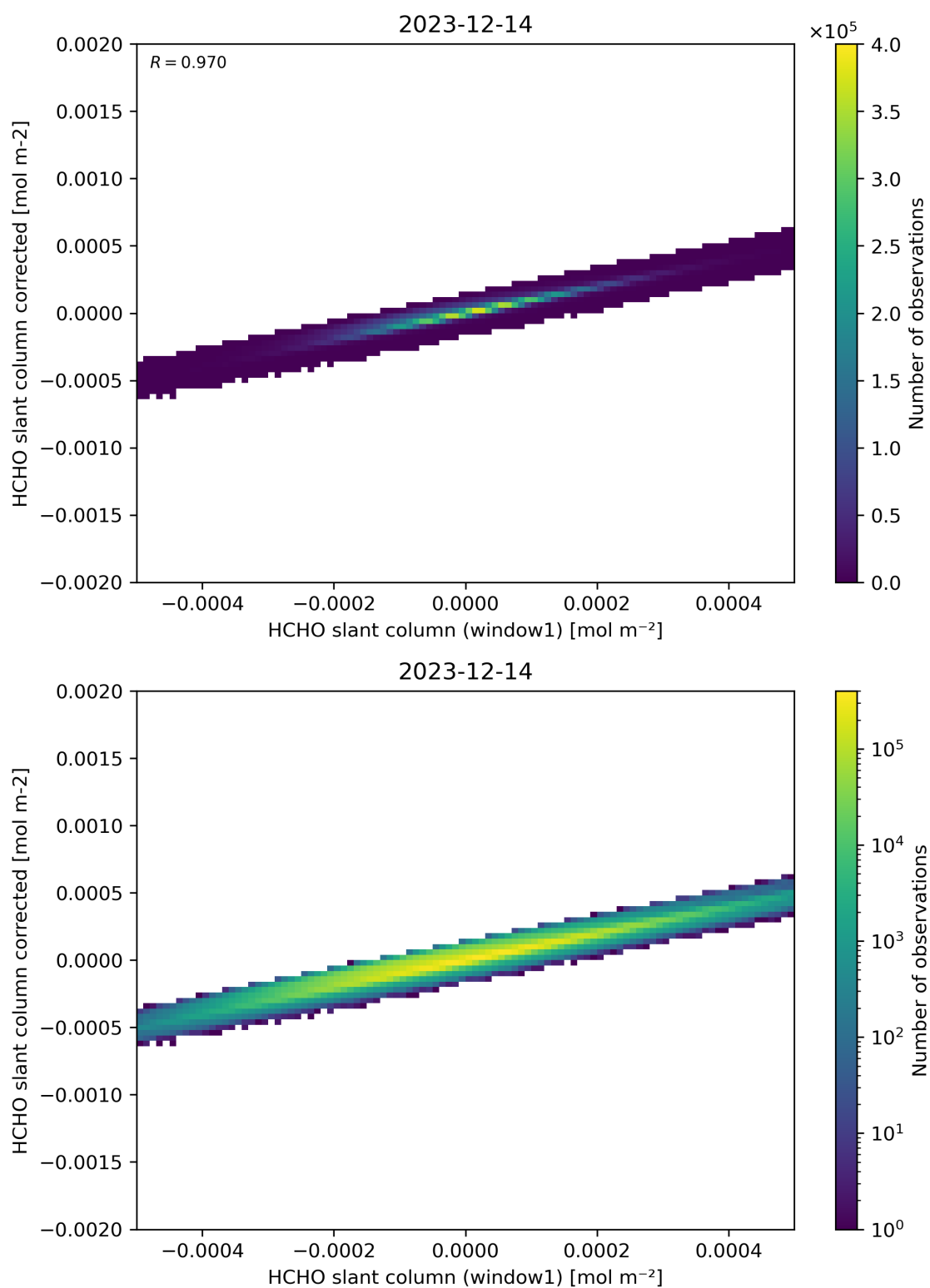
Figure 82: Scatter density plot of “HCHO slant column (window1)” against “HCHO slant column corrected” for 2023-12-14 to 2023-12-15.
