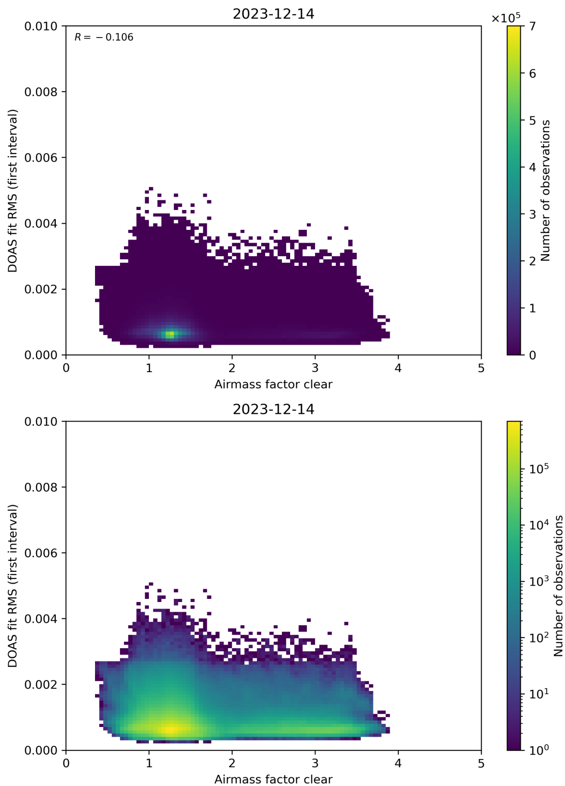
Figure 71: Scatter density plot of “Airmass factor clear” against “DOAS fit RMS (first interval)” for 2023-12-14 to 2023-12-15.
