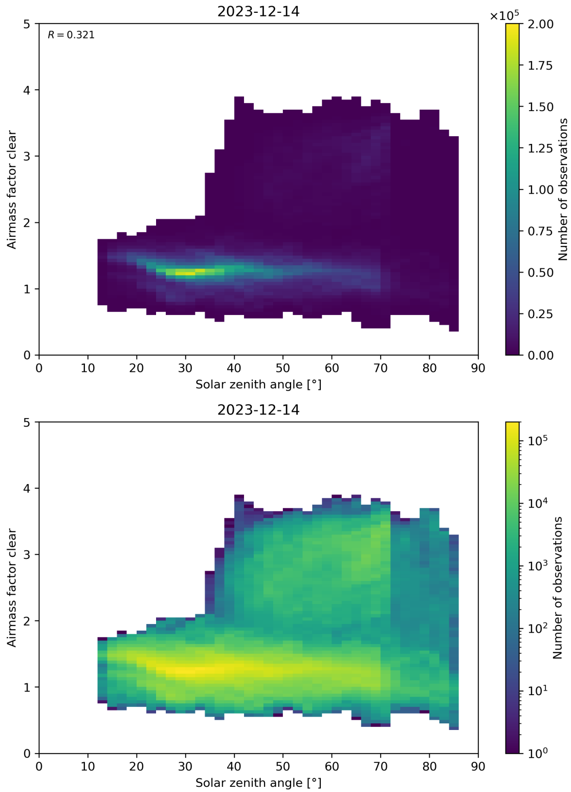
Figure 170: Scatter density plot of “Solar zenith angle” against “Airmass factor clear” for 2023-12-14 to 2023-12-15.
