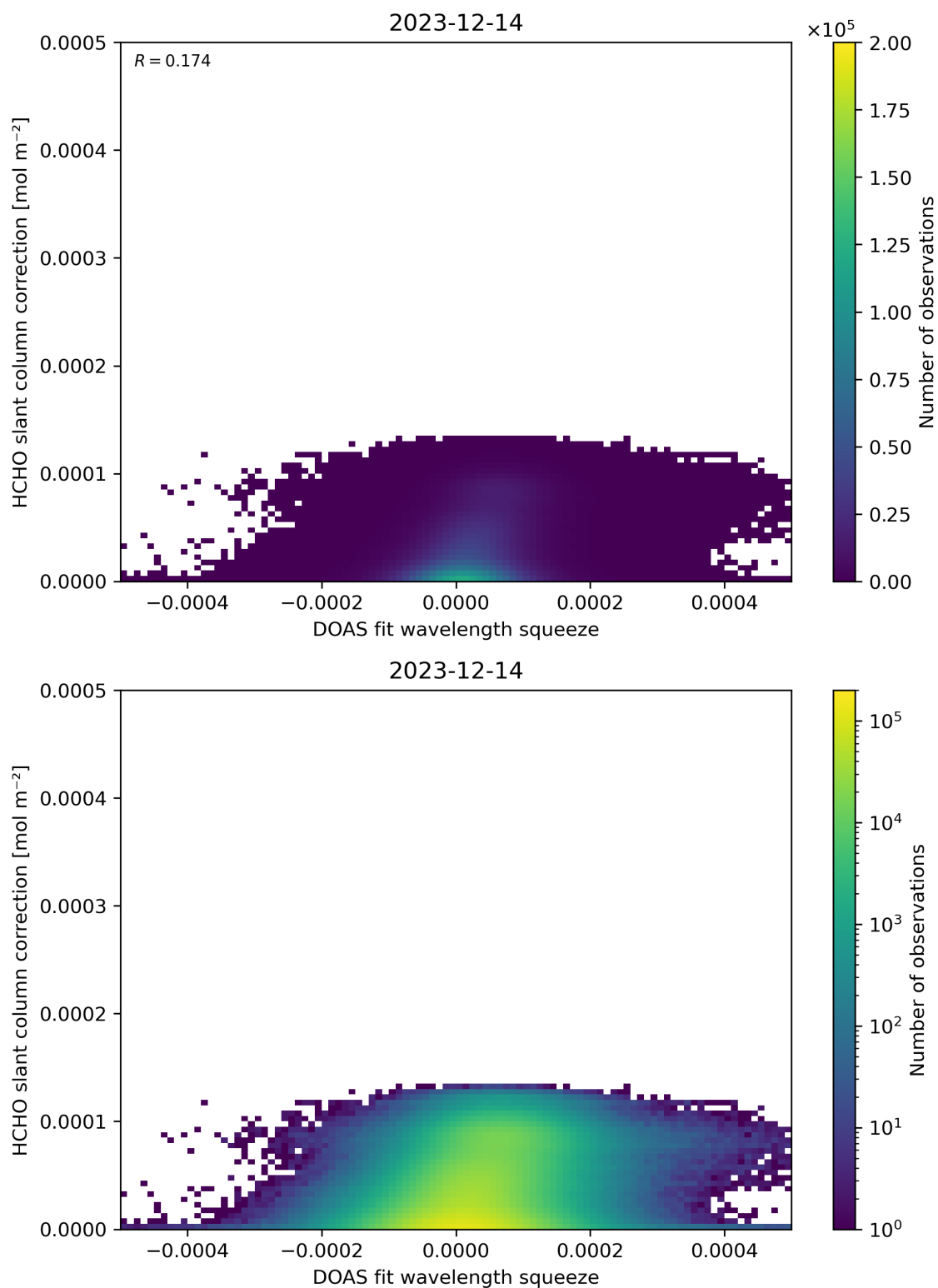
Figure 70: Scatter density plot of “DOAS fit wavelength squeeze” against “HCHO slant column correction” for 2023-12-14 to 2023-12-15.
