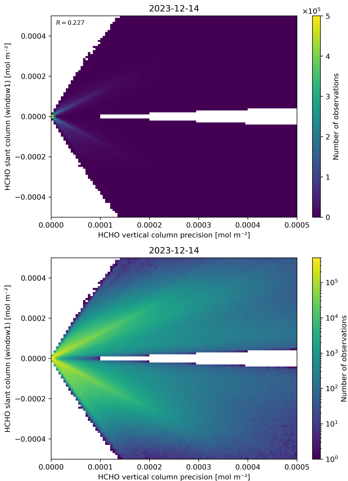
Figure 142: Scatter density plot of “HCHO vertical column precision” against “HCHO slant column (window1)” for 2023-12-14 to 2023-12-15.
