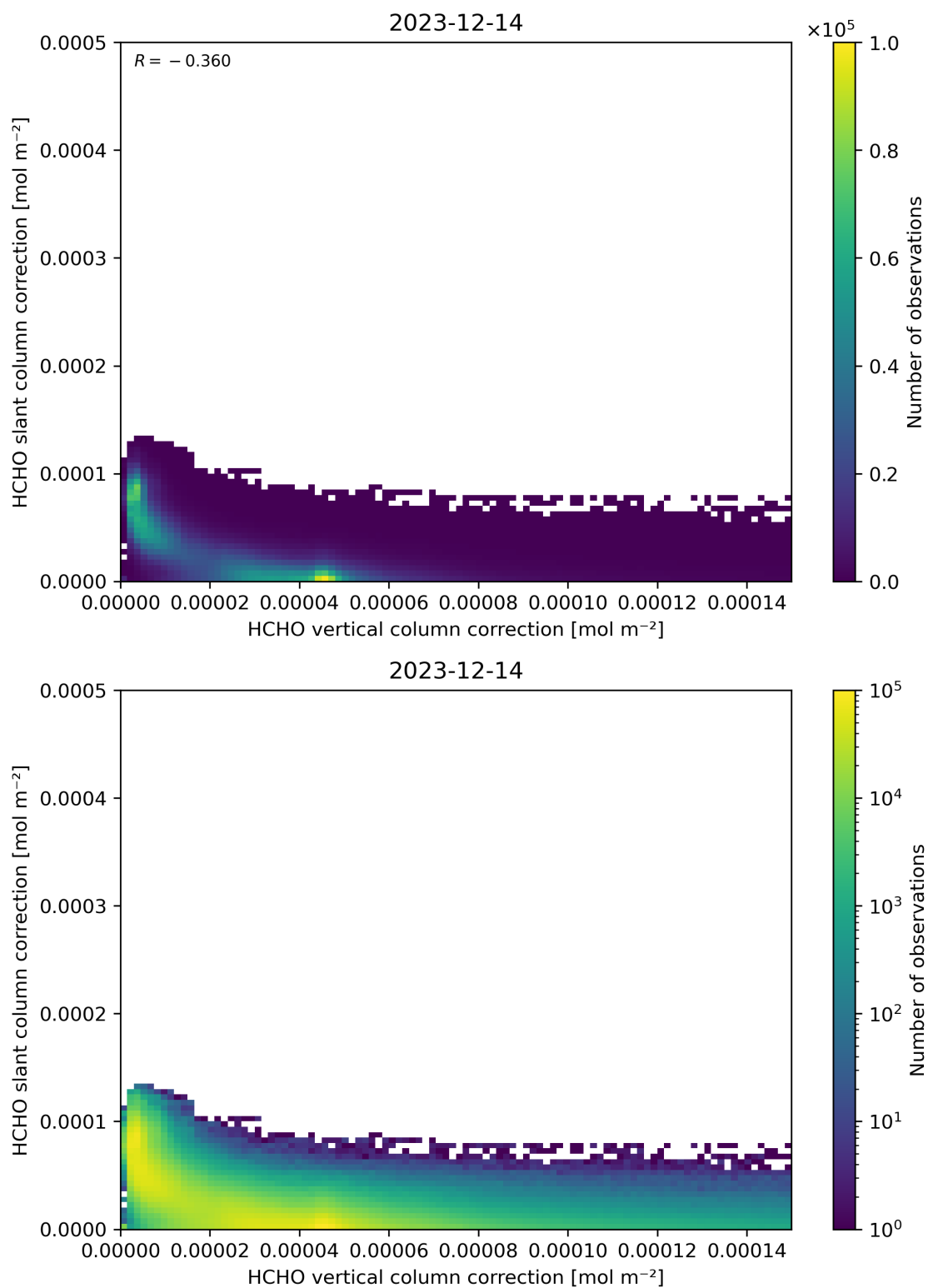
Figure 117: Scatter density plot of “HCHO vertical column correction” against “HCHO slant column correction” for 2023-12-14 to 2023-12-15.
