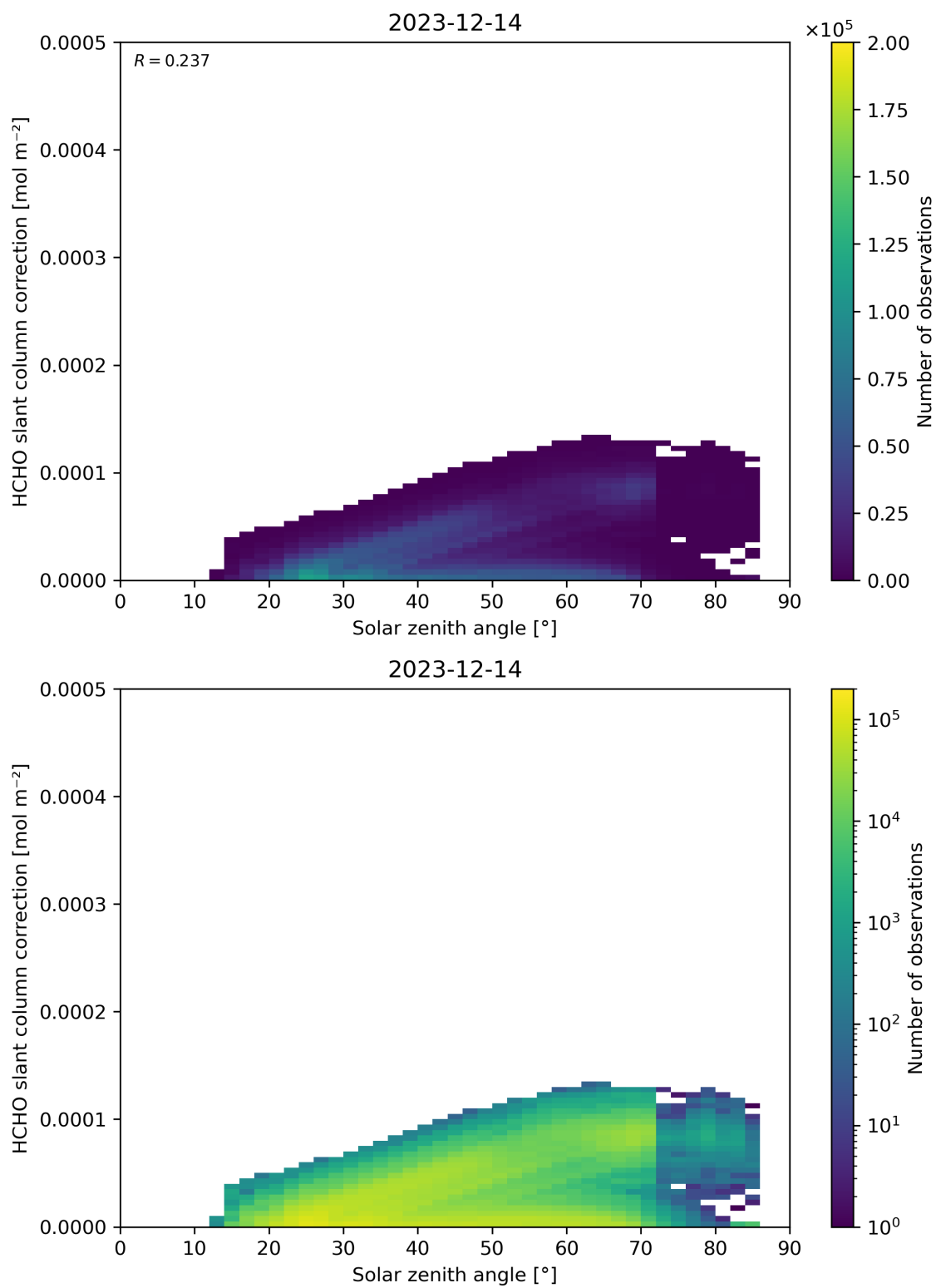
Figure 172: Scatter density plot of “Solar zenith angle” against “HCHO slant column correction” for 2023-12-14 to 2023-12-15.
