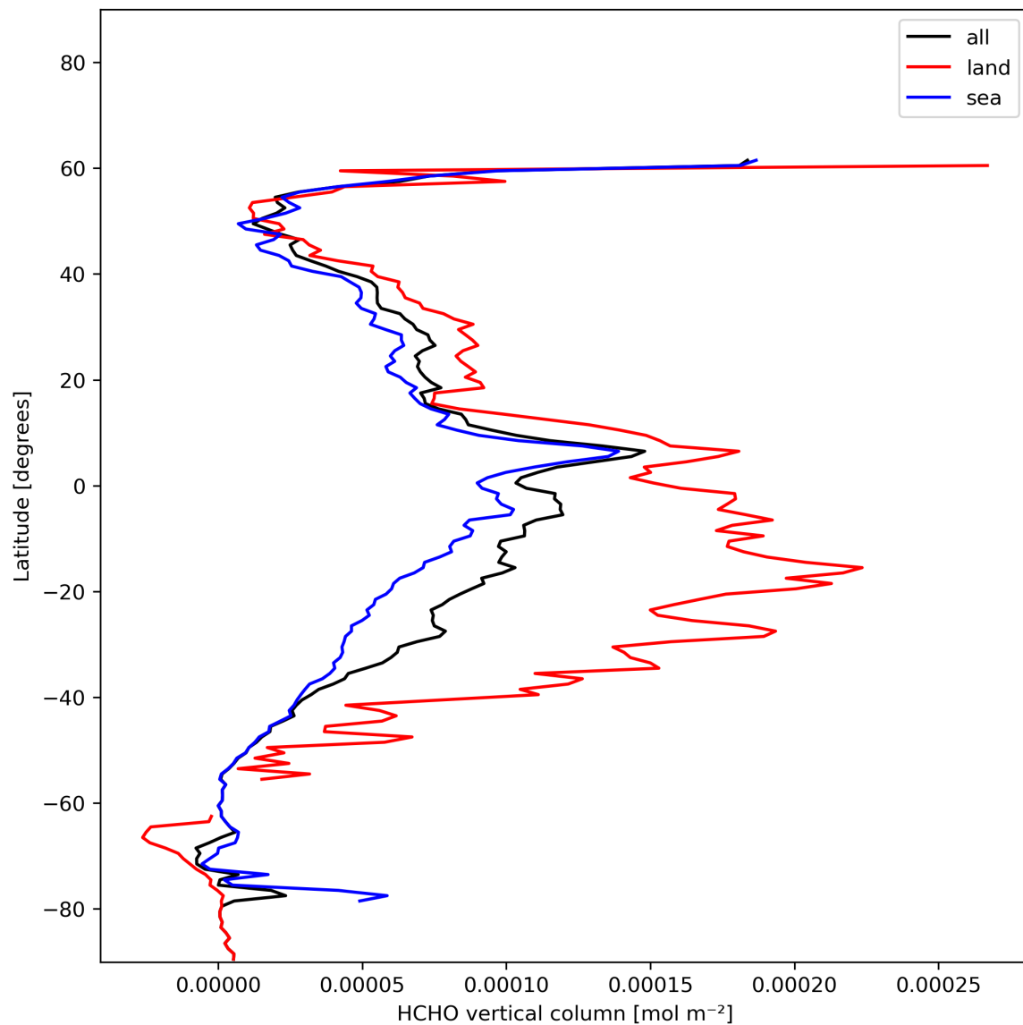
Figure 21: Zonal average of “HCHO vertical column” for 2023-12-14 to 2023-12-15.
