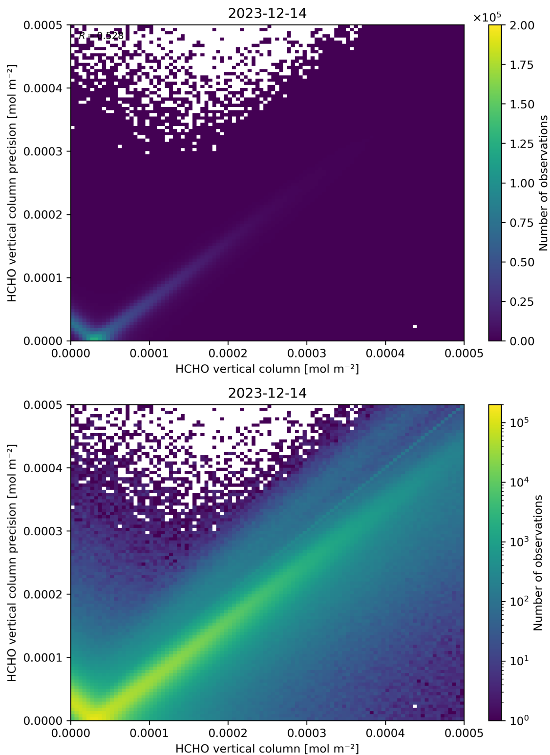
Figure 134: Scatter density plot of “HCHO vertical column” against “HCHO vertical column precision” for 2023-12-14 to 2023-12-15.
