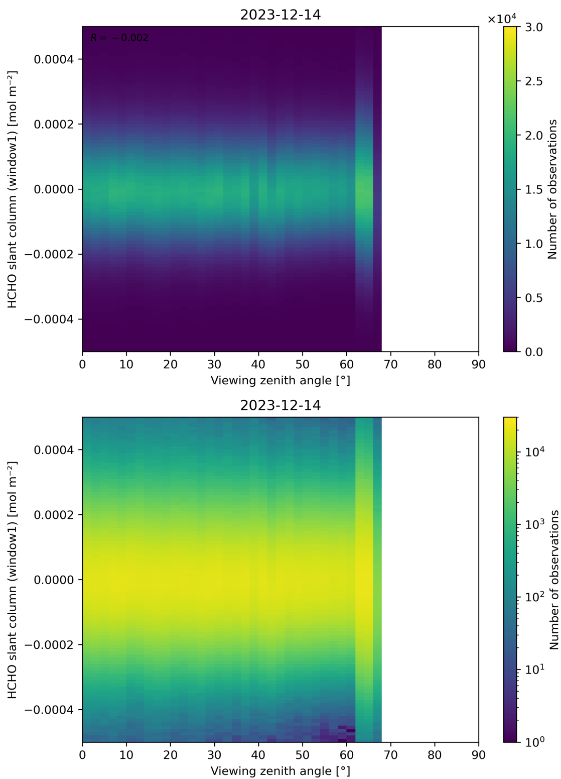
Figure 188: Scatter density plot of “Viewing zenith angle” against “HCHO slant column (window1)” for 2023-12-14 to 2023-12-15.
