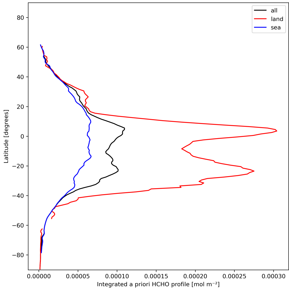
Figure 29: Zonal average of “Integrated a priori HCHO profile” for 2023-12-14 to 2023-12-15.
