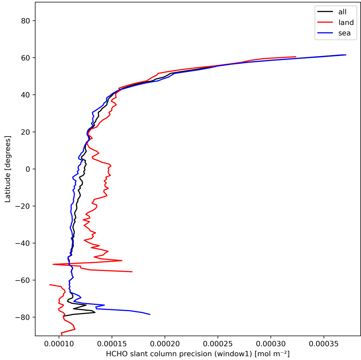
Figure 25: Zonal average of “HCHO slant column precision (window1)” for 2023-12-14 to 2023-12-15.
