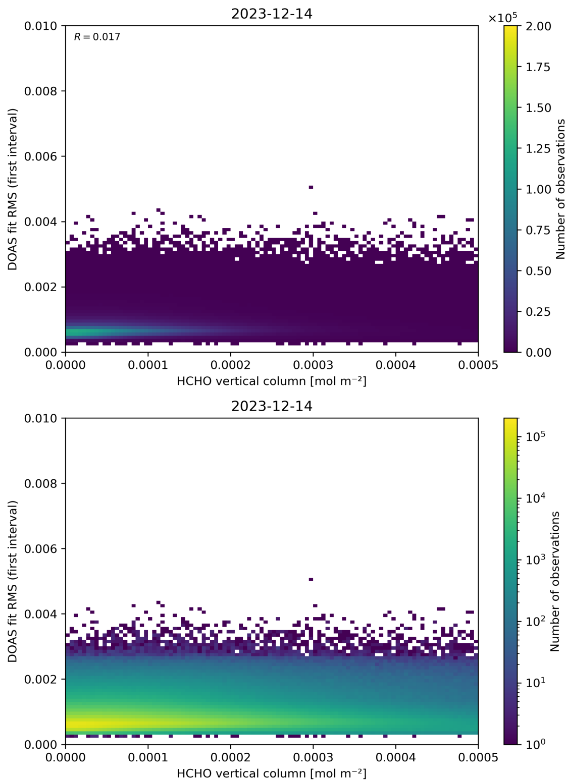
Figure 123: Scatter density plot of “HCHO vertical column” against “DOAS fit RMS (first interval)” for 2023-12-14 to 2023-12-15.
