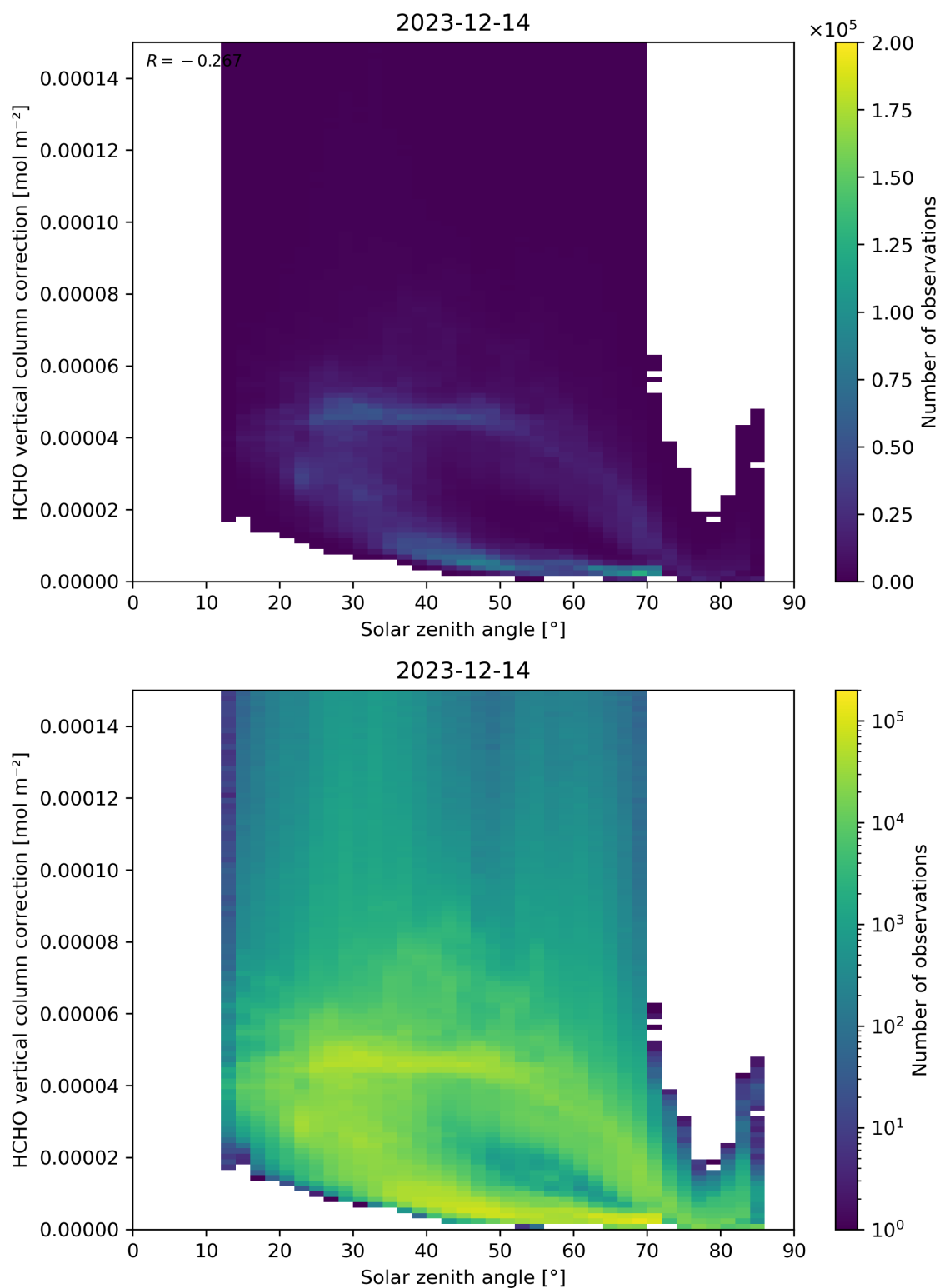
Figure 178: Scatter density plot of “Solar zenith angle” against “HCHO vertical column correction” for 2023-12-14 to 2023-12-15.
