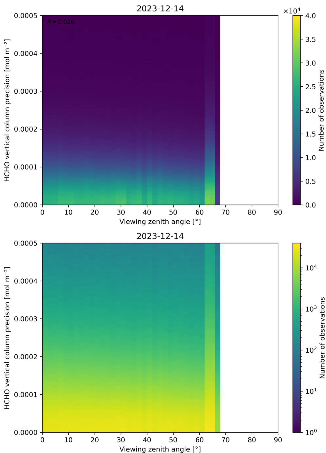
Figure 194: Scatter density plot of “Viewing zenith angle” against “HCHO vertical column precision” for 2023-12-14 to 2023-12-15.
