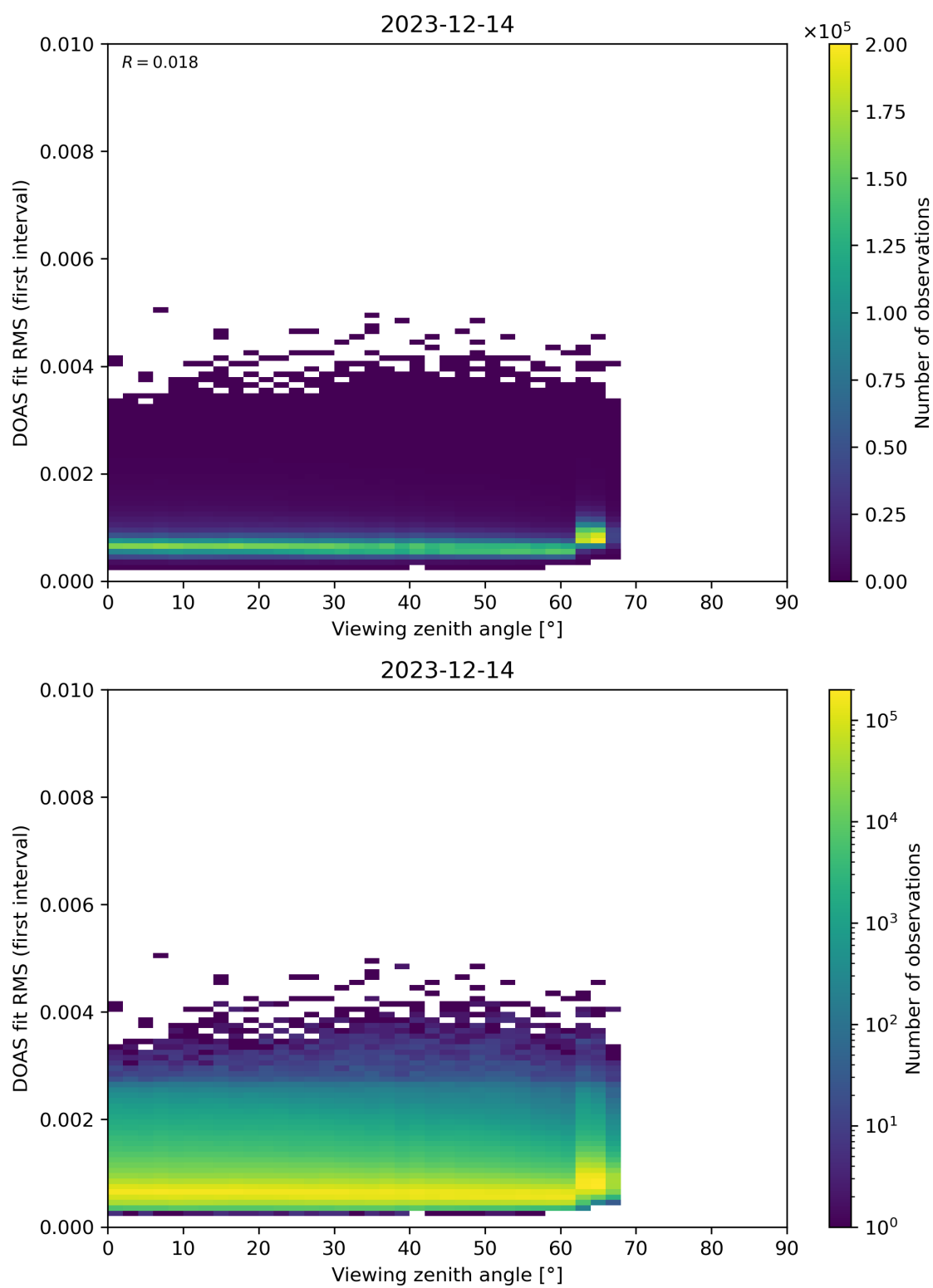
Figure 182: Scatter density plot of “Viewing zenith angle” against “DOAS fit RMS (first interval)” for 2023-12-14 to 2023-12-15.
