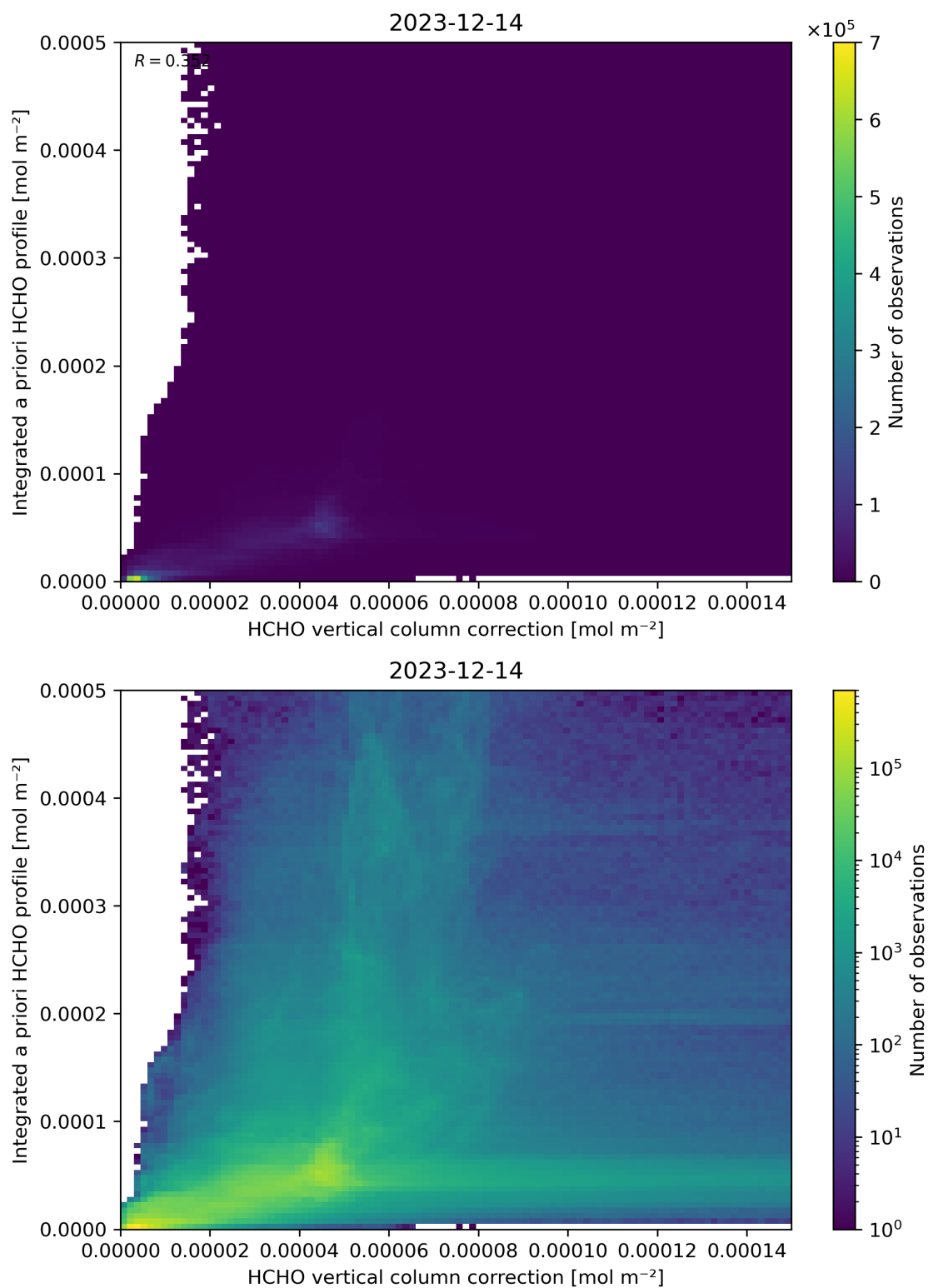
Figure 122: Scatter density plot of “HCHO vertical column correction” against “Integrated a priori HCHO profile” for 2023-12-14 to 2023-12-15.
