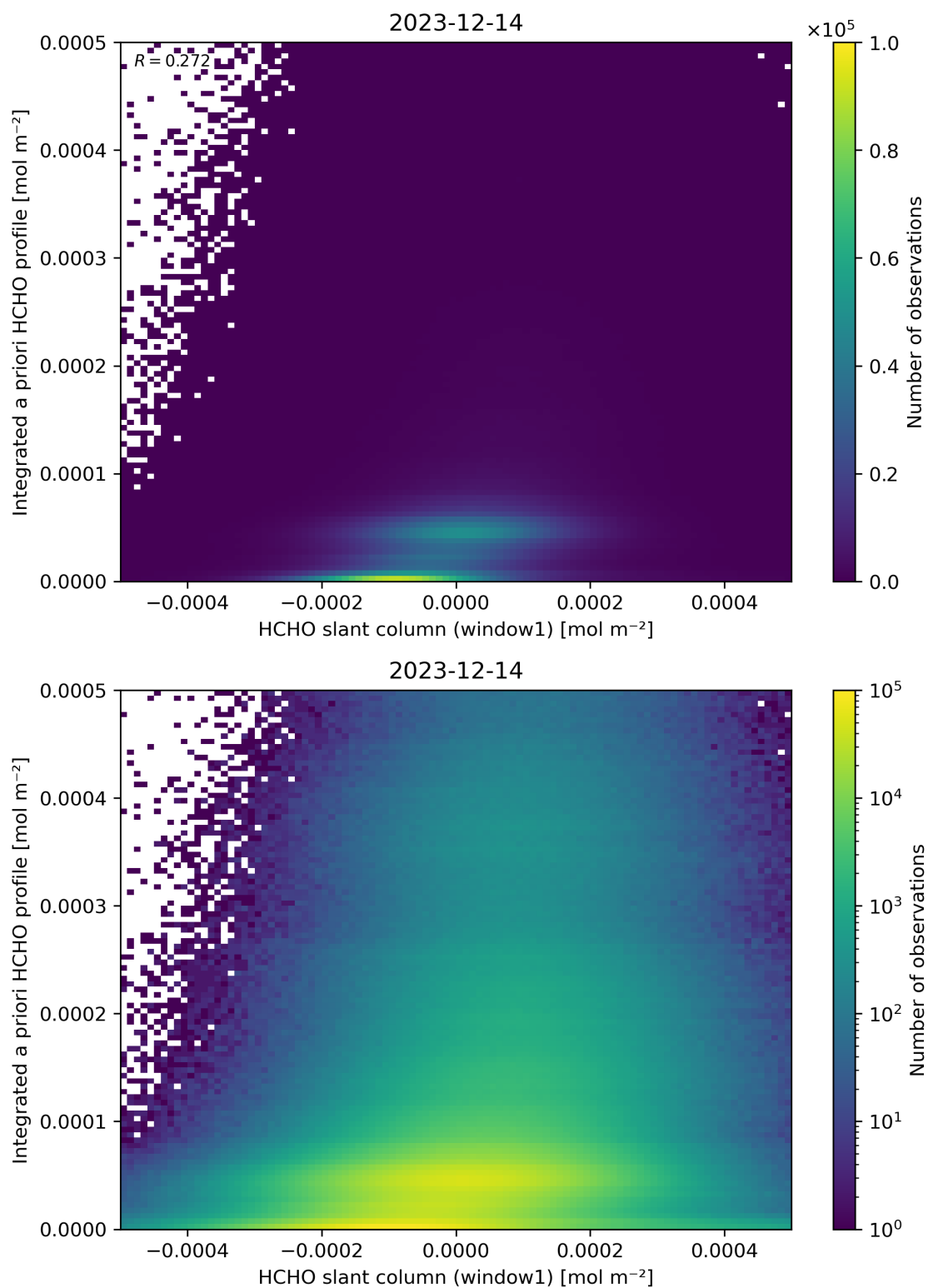
Figure 87: Scatter density plot of “HCHO slant column (window1)” against “Integrated a priori HCHO profile” for 2023-12-14 to 2023-12-15.
