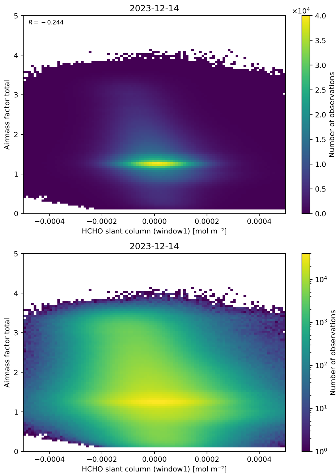
Figure 85: Scatter density plot of “HCHO slant column (window1)” against “Airmass factor total” for 2023-12-14 to 2023-12-15.
