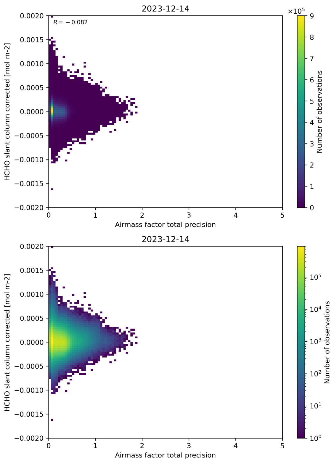
Figure 109: Scatter density plot of “Airmass factor total precision” against “HCHO slant column corrected” for 2023-12-14 to 2023-12-15.
