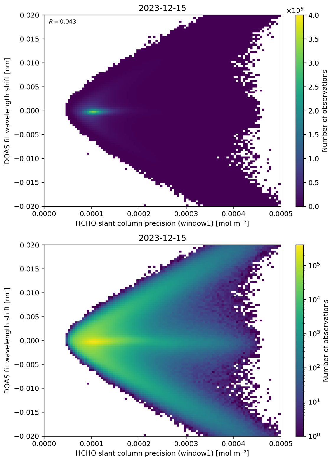
Figure 89: Scatter density plot of “HCHO slant column precision (window1)” against “DOAS fit wavelength shift” for 2023-12-14 to 2023-12-16.
