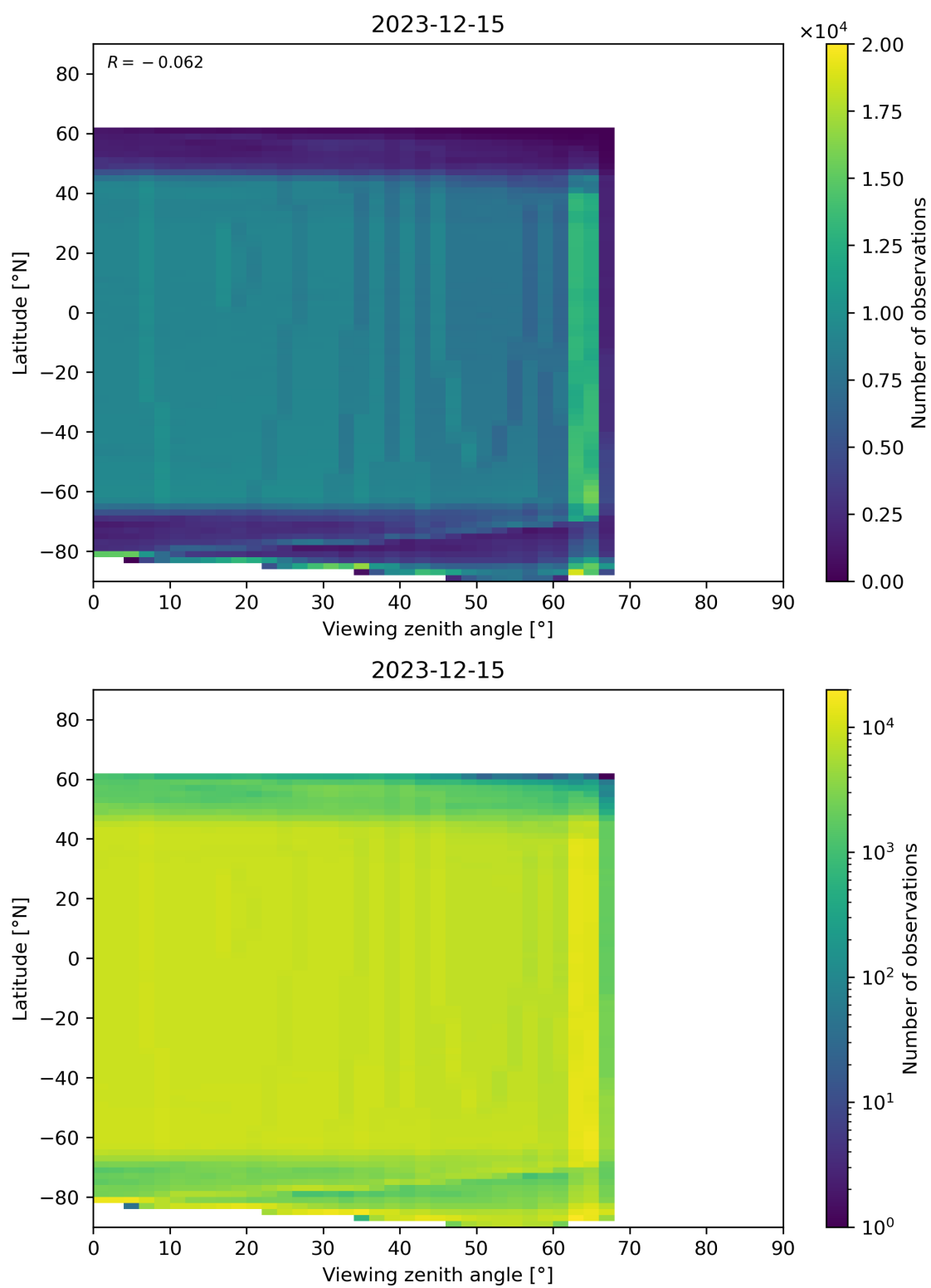
Figure 196: Scatter density plot of “Viewing zenith angle” against “Latitude” for 2023-12-14 to 2023-12-16.
