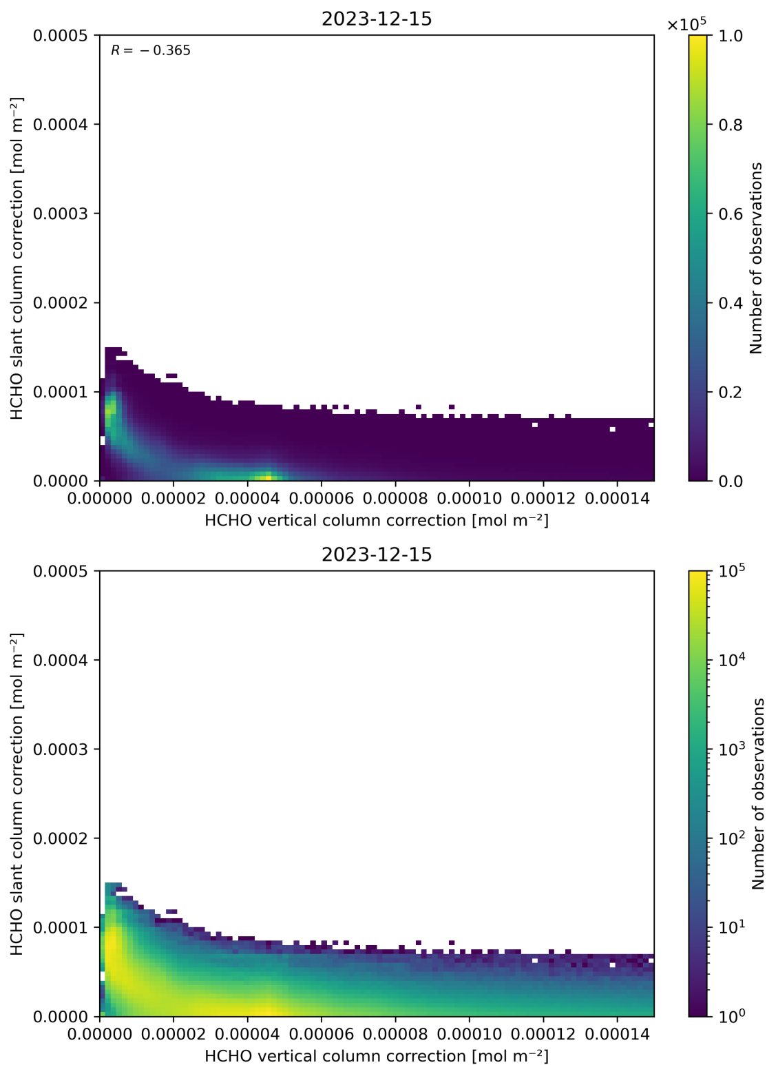
Figure 117: Scatter density plot of “HCHO vertical column correction” against “HCHO slant column correction” for 2023-12-14 to 2023-12-16.
