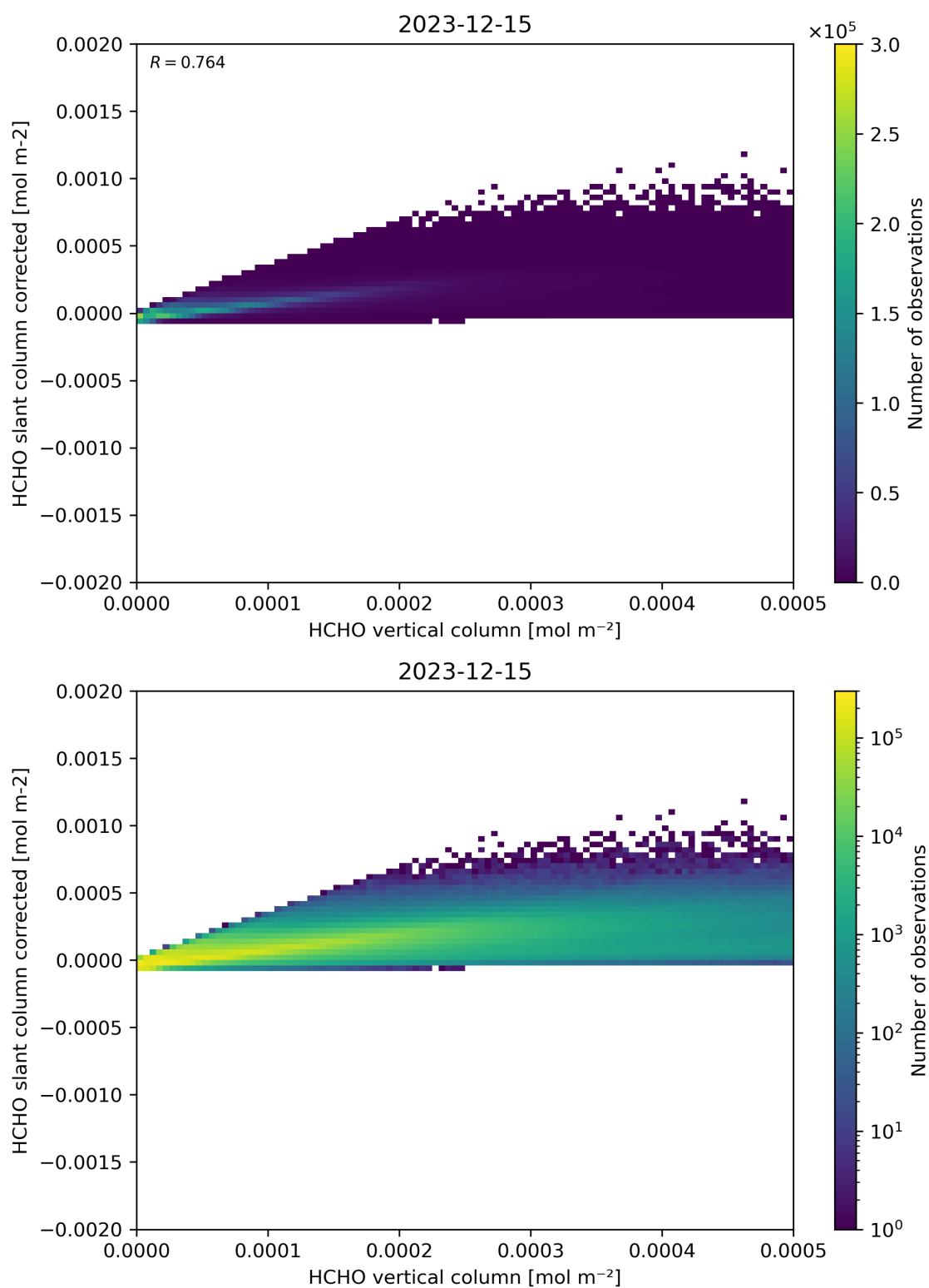
Figure 127: Scatter density plot of “HCHO vertical column” against “HCHO slant column corrected” for 2023-12-14 to 2023-12-16.
