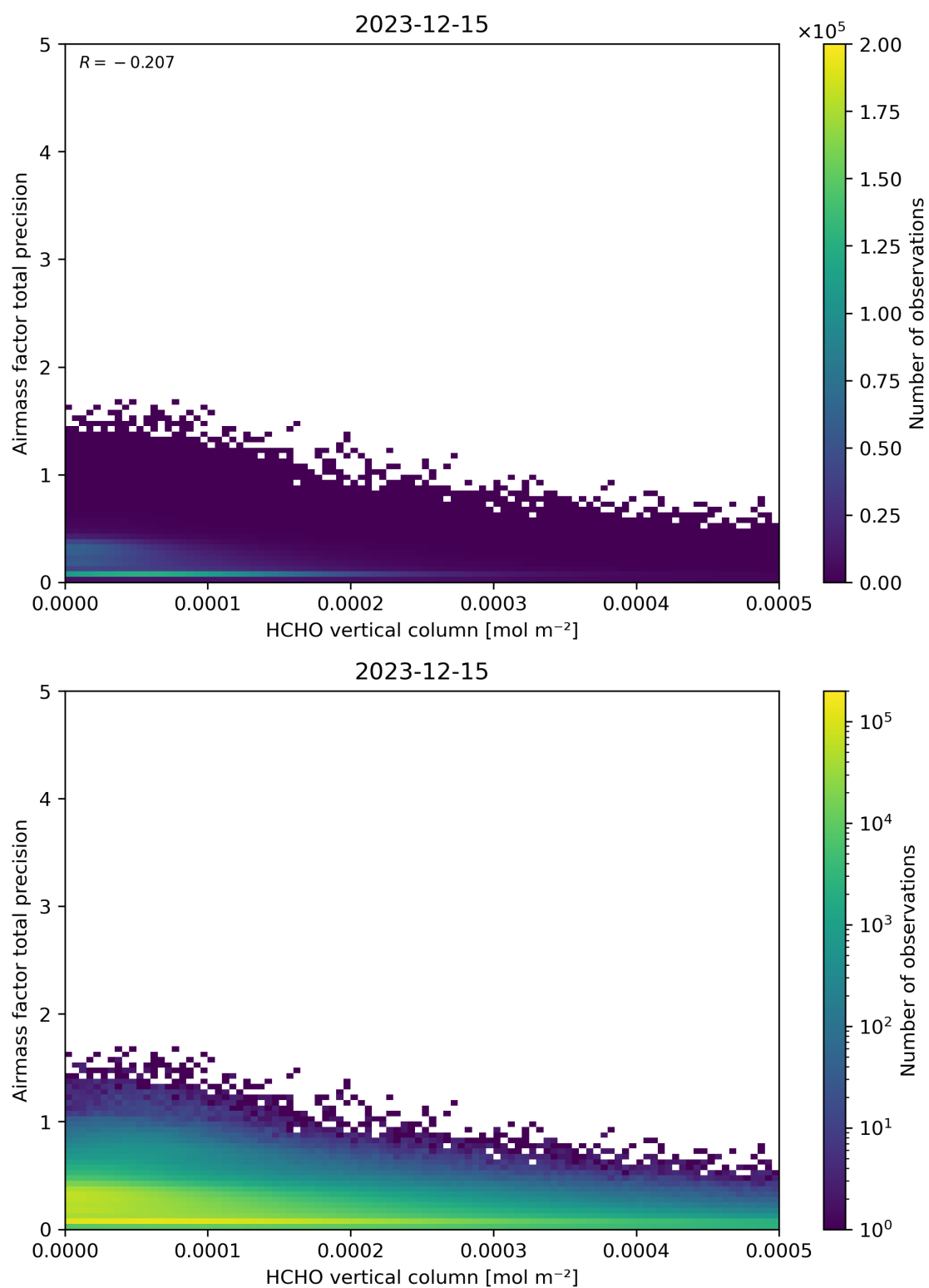
Figure 132: Scatter density plot of “HCHO vertical column” against “Airmass factor total precision” for 2023-12-14 to 2023-12-16.
