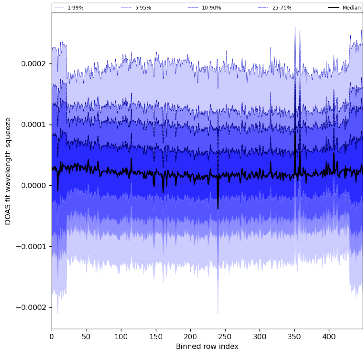
Figure 59: Along track statistics of “DOAS fit wavelength squeeze” for 2023-12-14 to 2023-12-16
