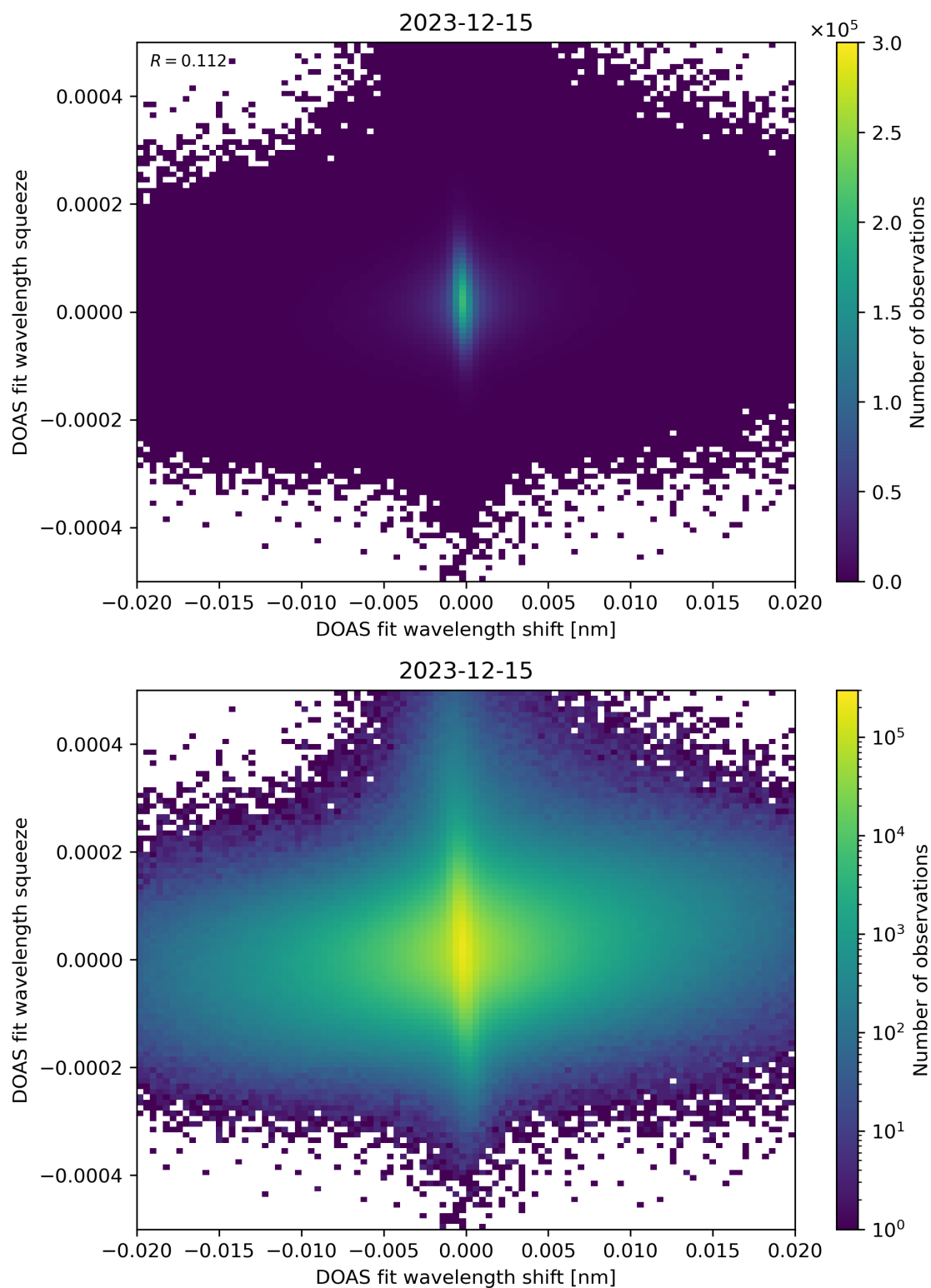
Figure 65: Scatter density plot of “DOAS fit wavelength shift” against “DOAS fit wavelength squeeze” for 2023-12-14 to 2023-12-16.
