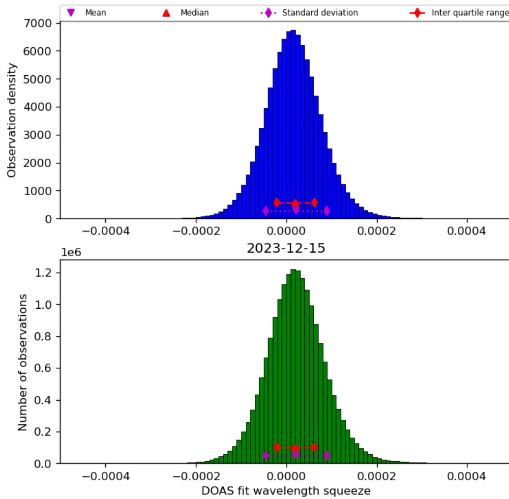
Figure 45: Histogram of “DOAS fit wavelength squeeze” for 2023-12-14 to 2023-12-16
