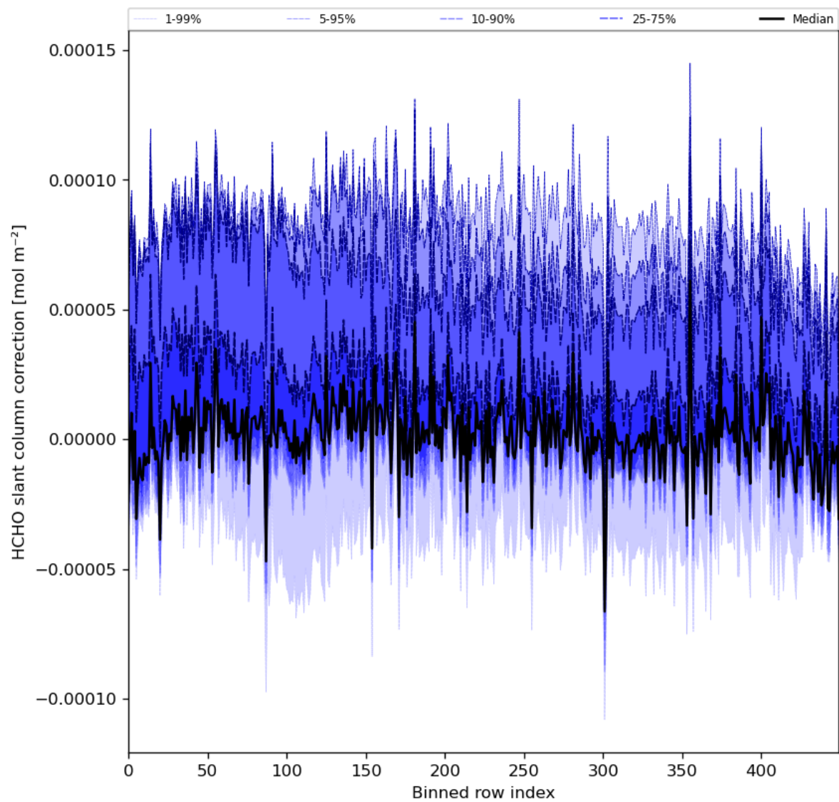
Figure 61: Along track statistics of “HCHO slant column correction” for 2023-12-14 to 2023-12-16
