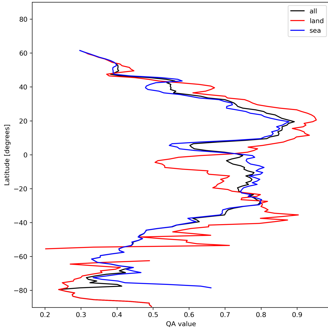
Figure 20: Zonal average of “QA value” for 2023-12-14 to 2023-12-16.
