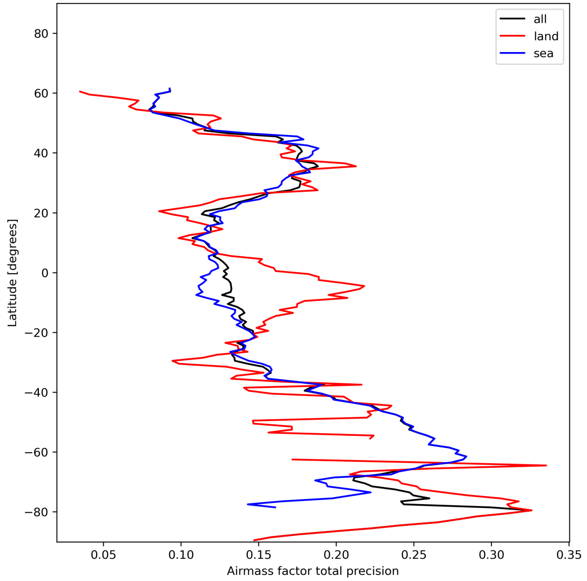
Figure 27: Zonal average of “Airmass factor total precision” for 2023-12-14 to 2023-12-16.
