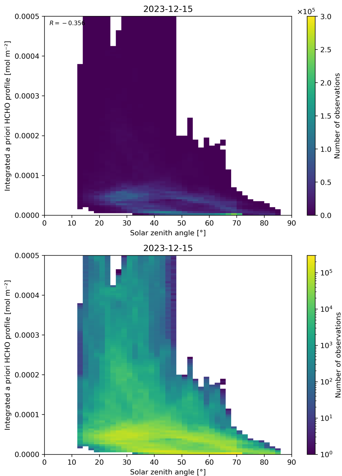
Figure 180: Scatter density plot of “Solar zenith angle” against “Integrated a priori HCHO profile” for 2023-12-14 to 2023-12-16.
