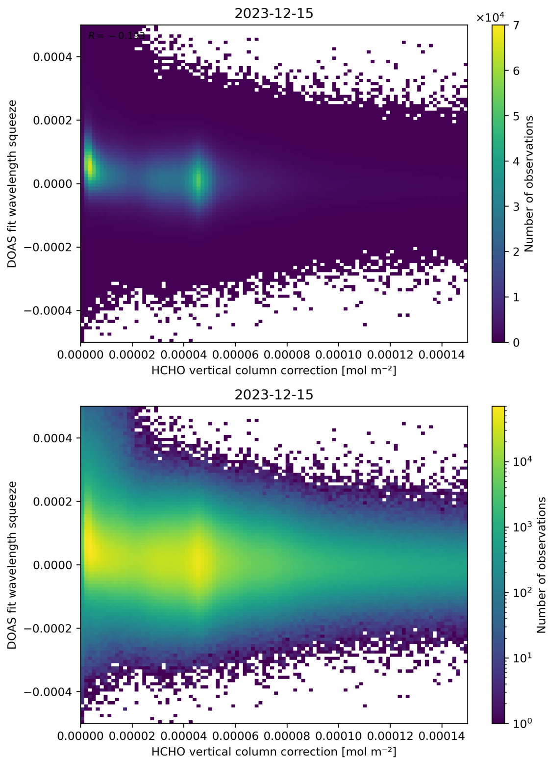
Figure 114: Scatter density plot of “HCHO vertical column correction” against “DOAS fit wavelength squeeze” for 2023-12-14 to 2023-12-16.
