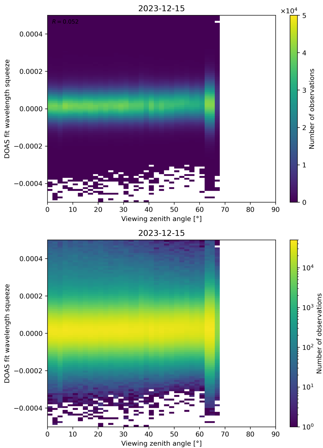
Figure 184: Scatter density plot of “Viewing zenith angle” against “DOAS fit wavelength squeeze” for 2023-12-14 to 2023-12-16.
