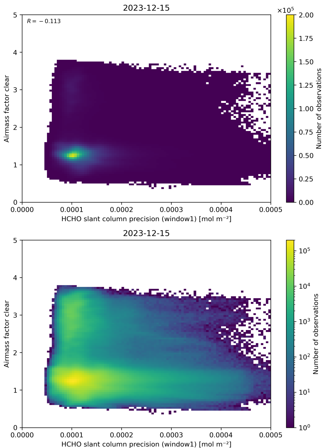
Figure 91: Scatter density plot of “HCHO slant column precision (window1)” against “Airmass factor clear” for 2023-12-14 to 2023-12-16.
