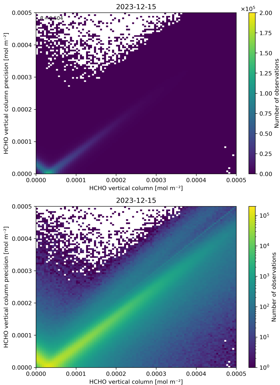
Figure 134: Scatter density plot of “HCHO vertical column” against “HCHO vertical column precision” for 2023-12-14 to 2023-12-16.
