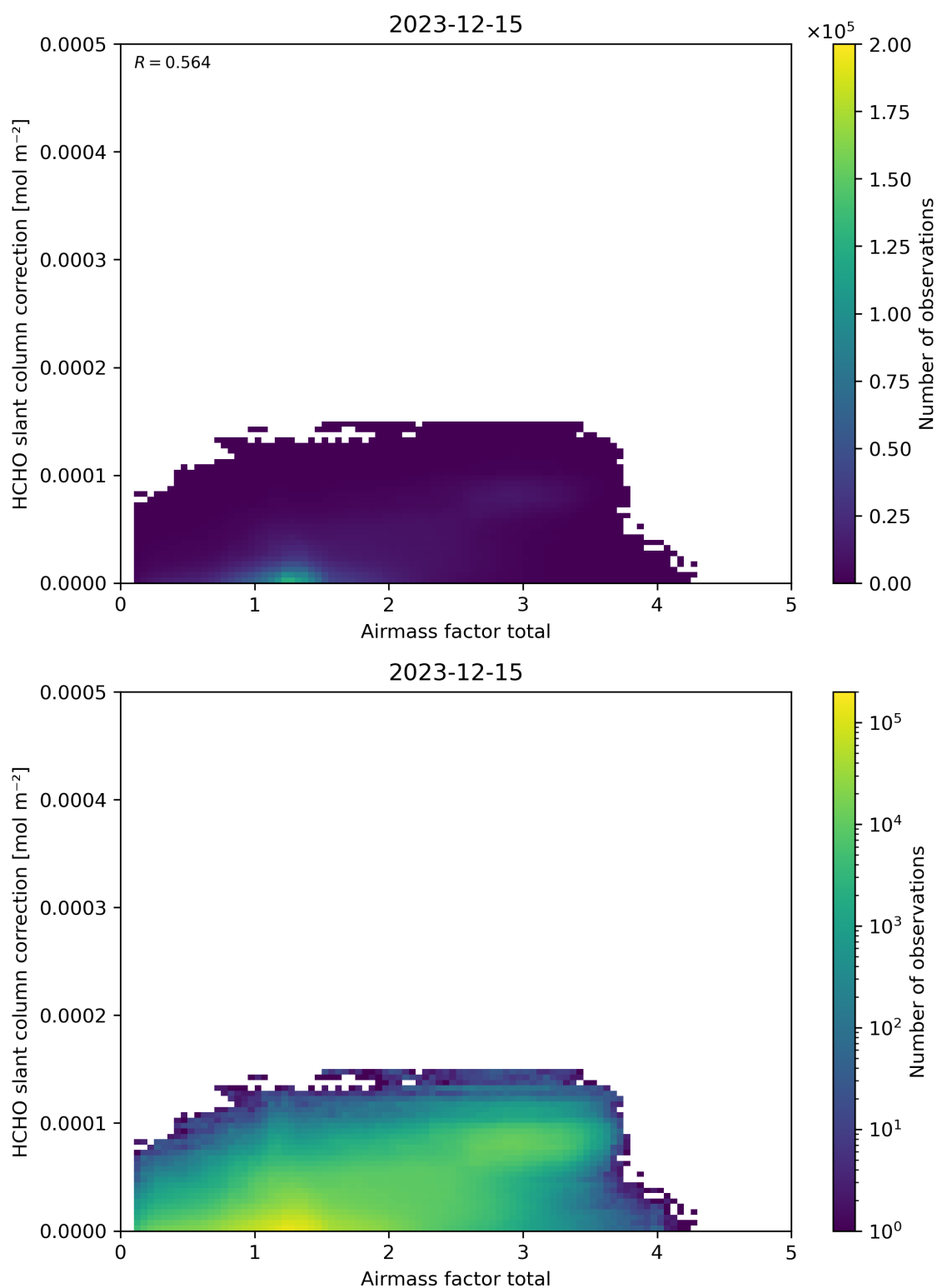
Figure 102: Scatter density plot of “Airmass factor total” against “HCHO slant column correction” for 2023-12-14 to 2023-12-16.
