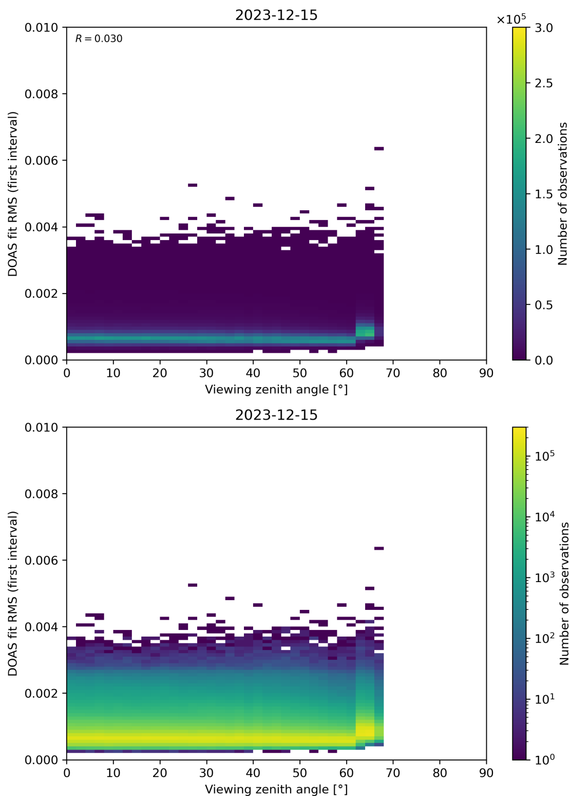
Figure 182: Scatter density plot of “Viewing zenith angle” against “DOAS fit RMS (first interval)” for 2023-12-14 to 2023-12-16.
