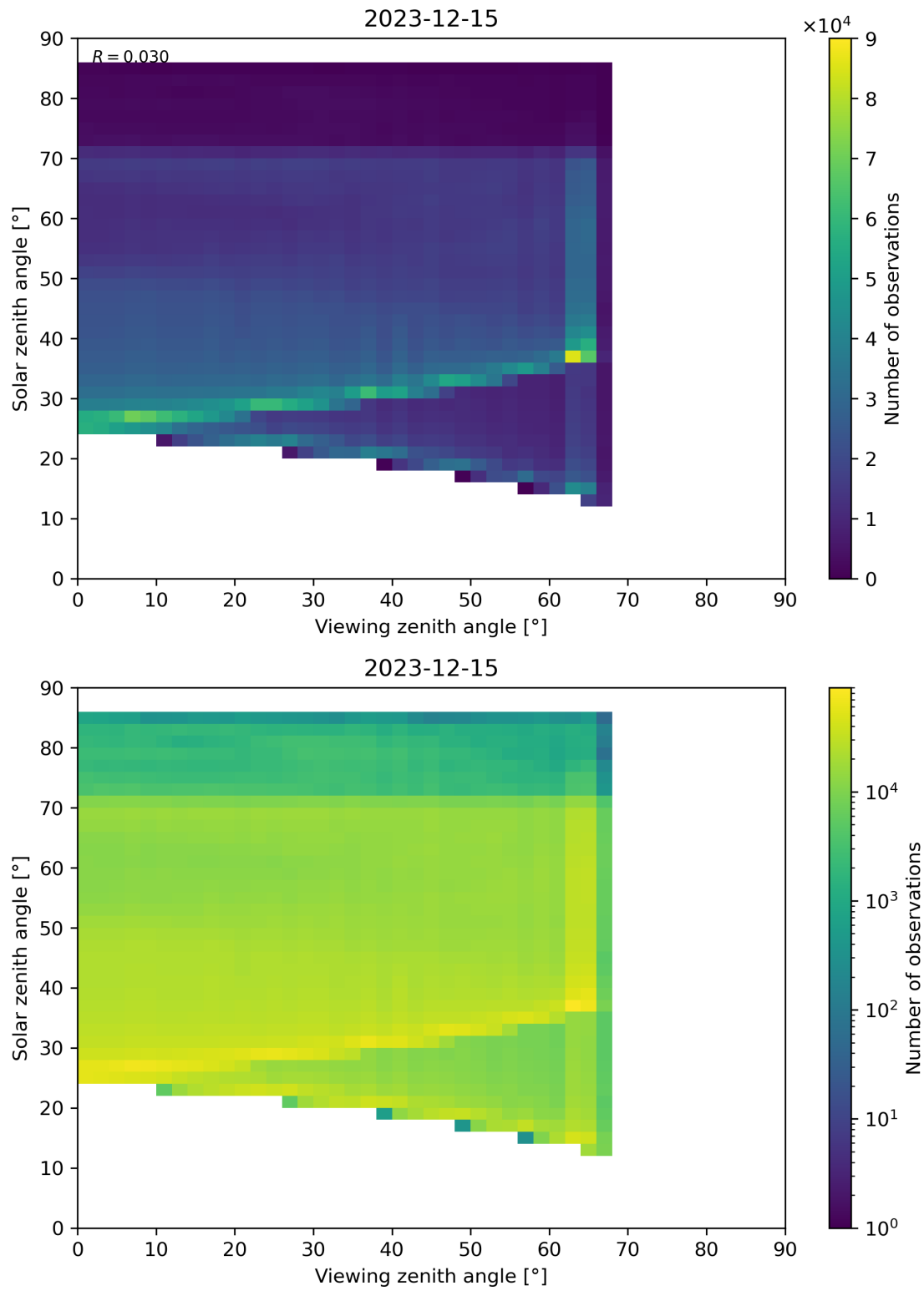
Figure 197: Scatter density plot of “Viewing zenith angle” against “Solar zenith angle” for 2023-12-14 to 2023-12-16.
