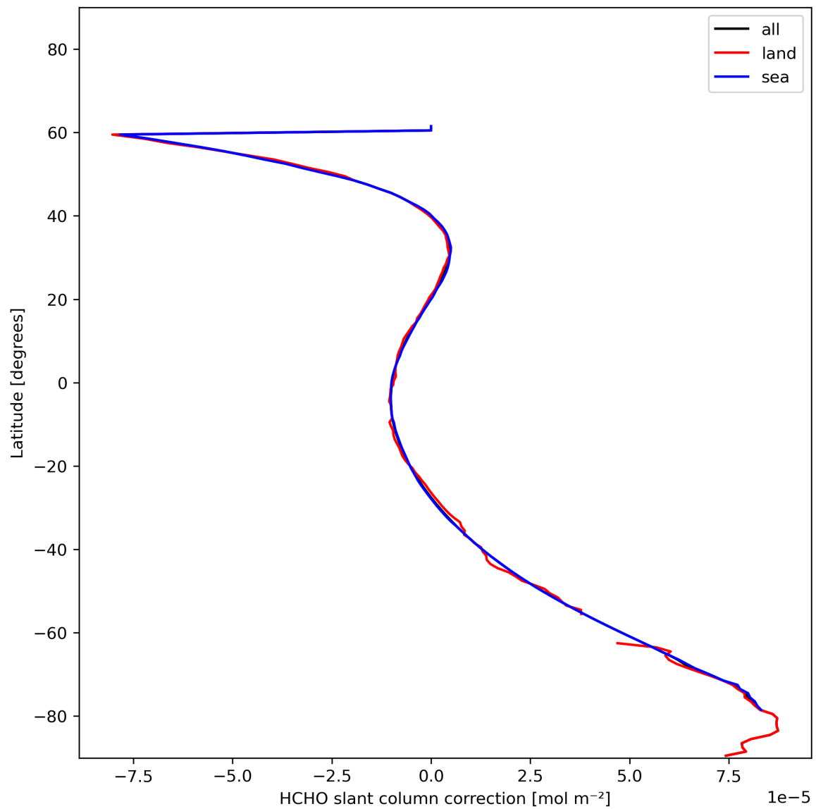
Figure 33: Zonal average of “HCHO slant column correction” for 2023-12-14 to 2023-12-16.
