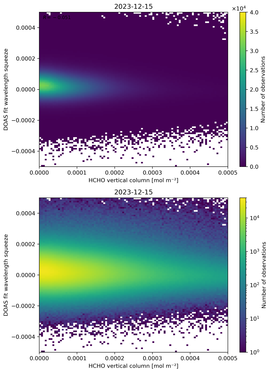
Figure 125: Scatter density plot of “HCHO vertical column” against “DOAS fit wavelength squeeze” for 2023-12-14 to 2023-12-16.
