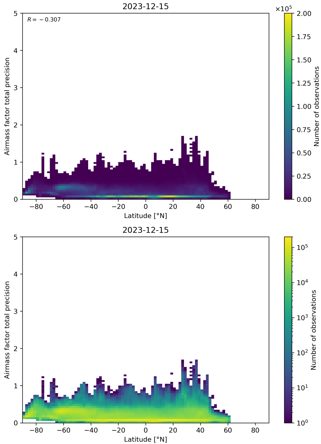
Figure 162: Scatter density plot of “Latitude” against “Airmass factor total precision” for 2023-12-14 to 2023-12-16.
