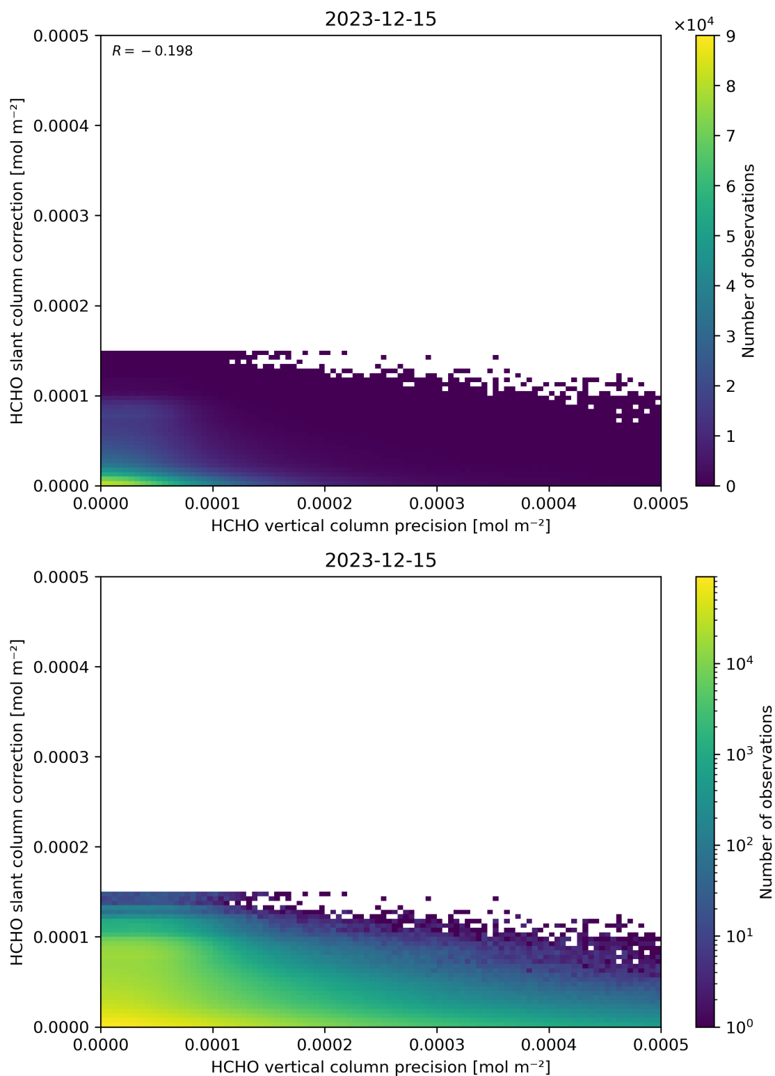
Figure 141: Scatter density plot of “HCHO vertical column precision” against “HCHO slant column correction” for 2023-12-14 to 2023-12-16.
