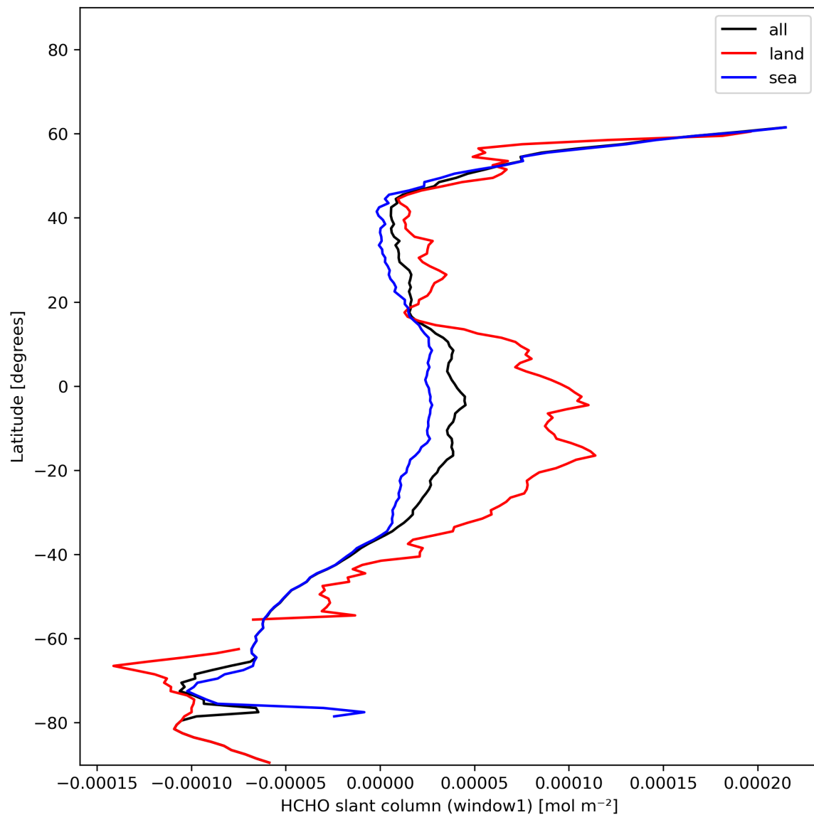
Figure 24: Zonal average of “HCHO slant column (window1)” for 2023-12-14 to 2023-12-16.
