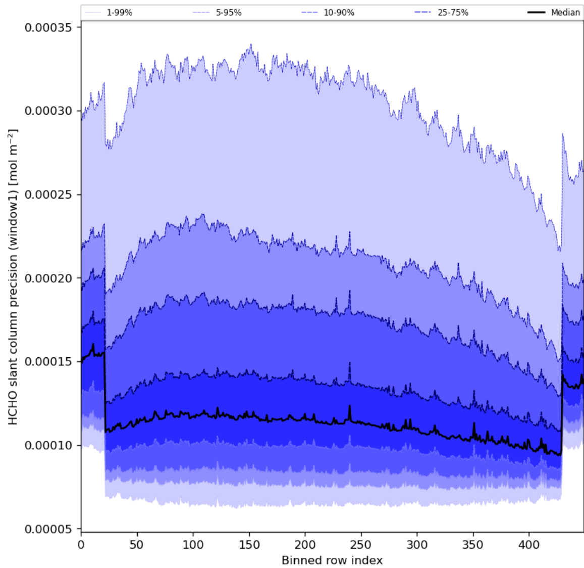
Figure 53: Along track statistics of “HCHO slant column precision (window1)” for 2023-12-14 to 2023-12-16
