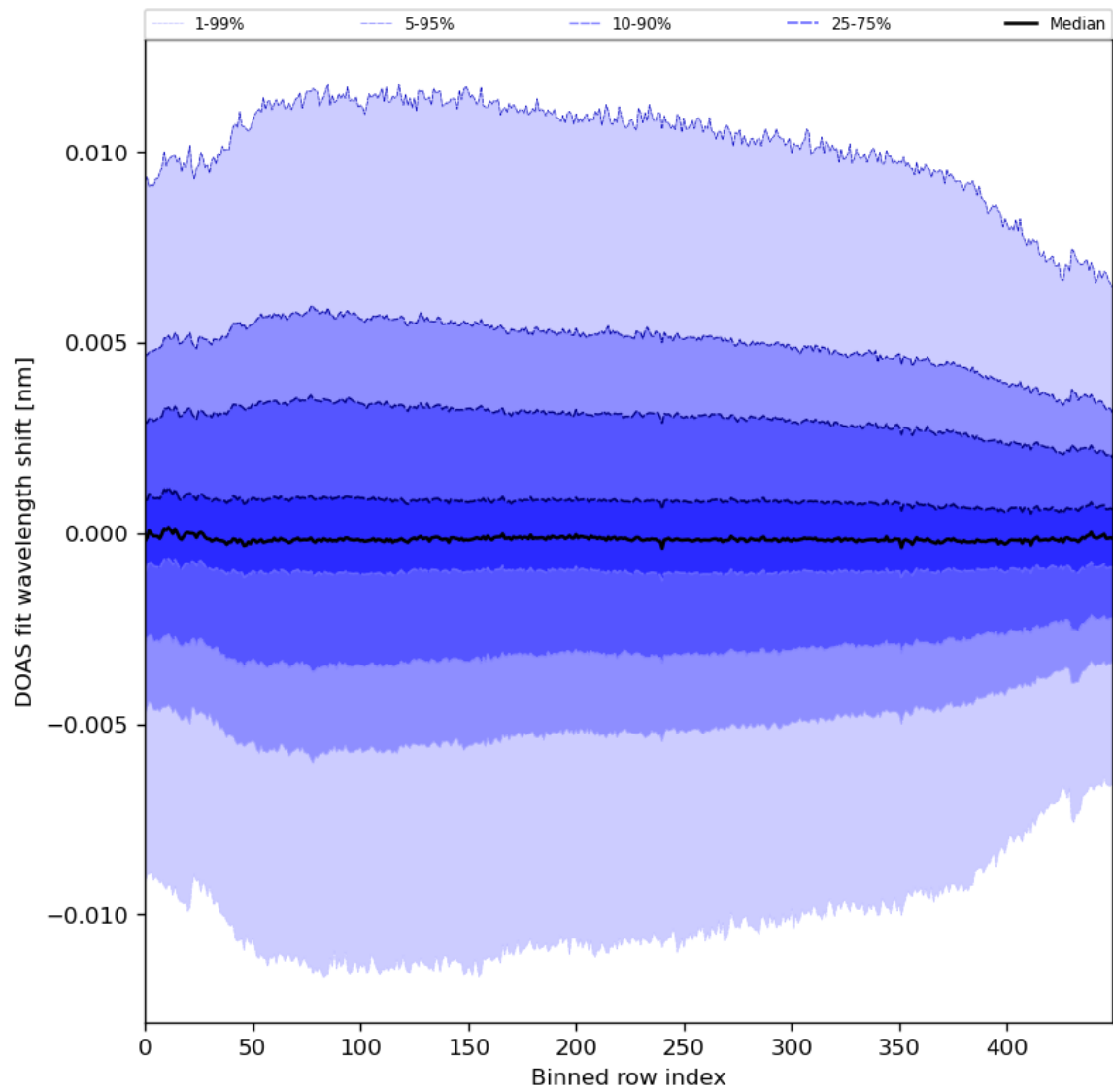
Figure 58: Along track statistics of “DOAS fit wavelength shift” for 2023-12-14 to 2023-12-16
