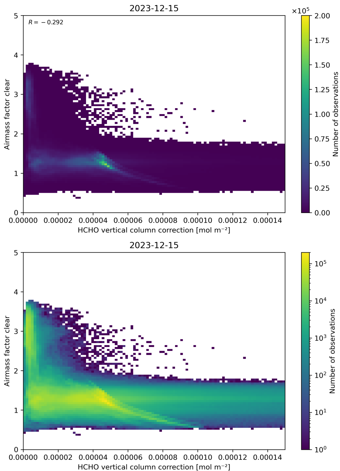
Figure 115: Scatter density plot of “HCHO vertical column correction” against “Airmass factor clear” for 2023-12-14 to 2023-12-16.
