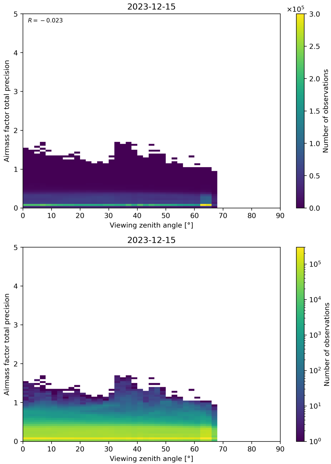
Figure 191: Scatter density plot of “Viewing zenith angle” against “Airmass factor total precision” for 2023-12-14 to 2023-12-16.
