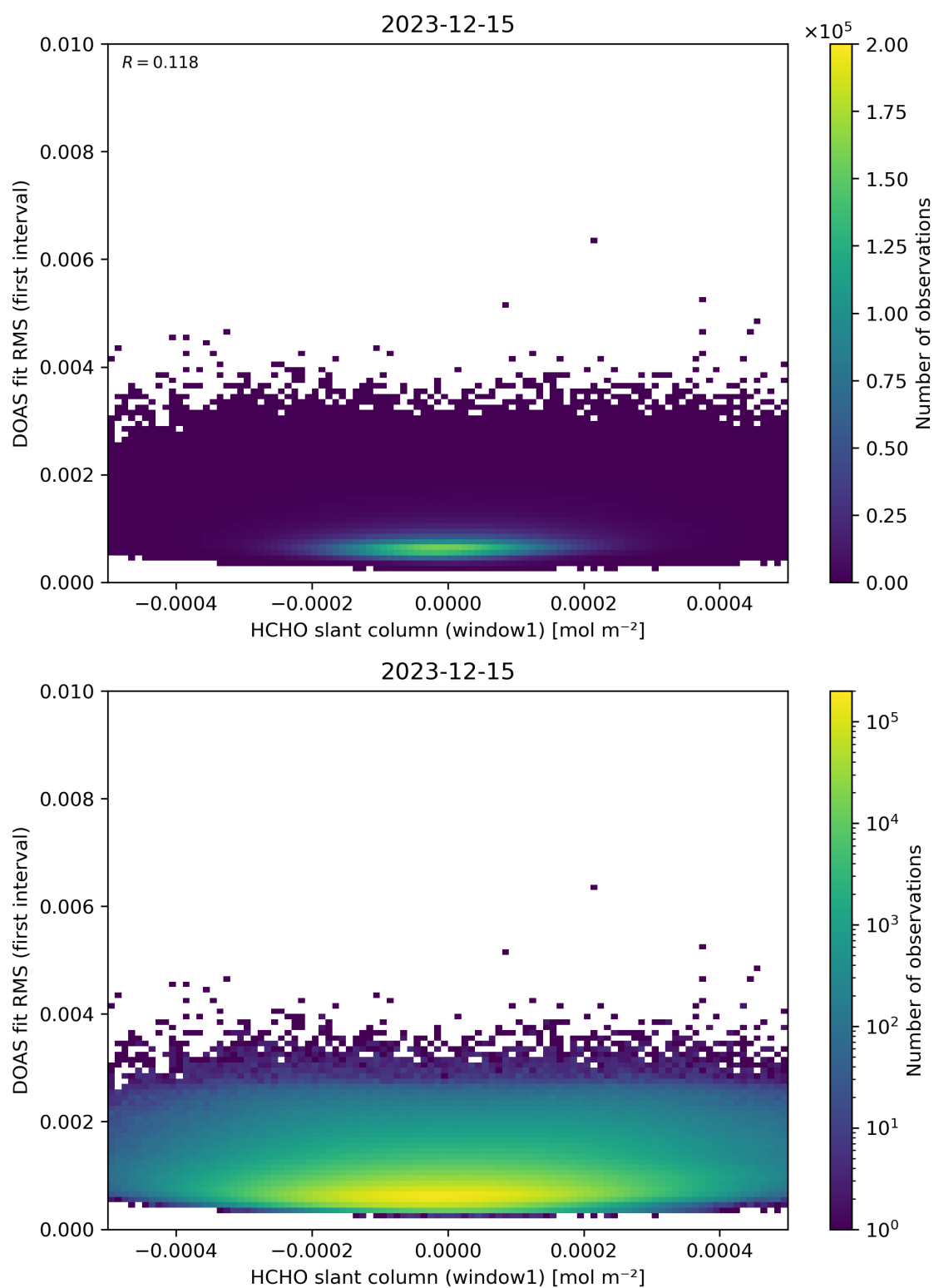
Figure 78: Scatter density plot of “HCHO slant column (window1)” against “DOAS fit RMS (first interval)” for 2023-12-14 to 2023-12-16.
