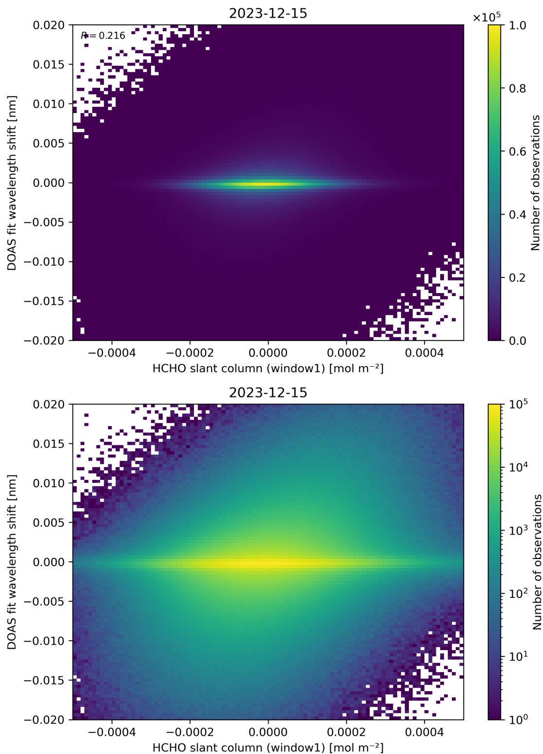
Figure 79: Scatter density plot of “HCHO slant column (window1)” against “DOAS fit wavelength shift” for 2023-12-14 to 2023-12-16.
