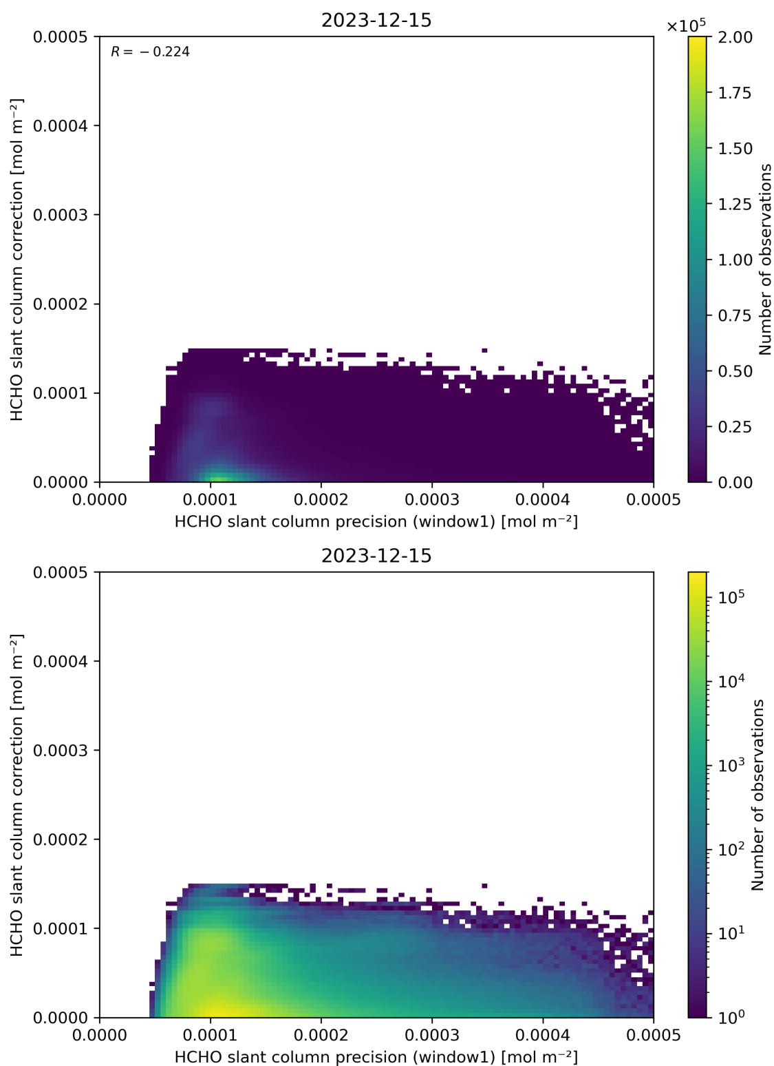
Figure 93: Scatter density plot of “HCHO slant column precision (window1)” against “HCHO slant column correction” for 2023-12-14 to 2023-12-16.
