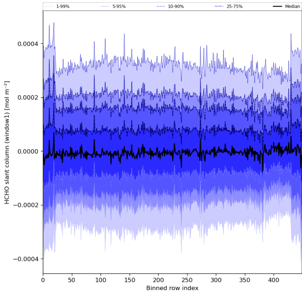
Figure 52: Along track statistics of “HCHO slant column (window1)” for 2023-12-14 to 2023-12-16
