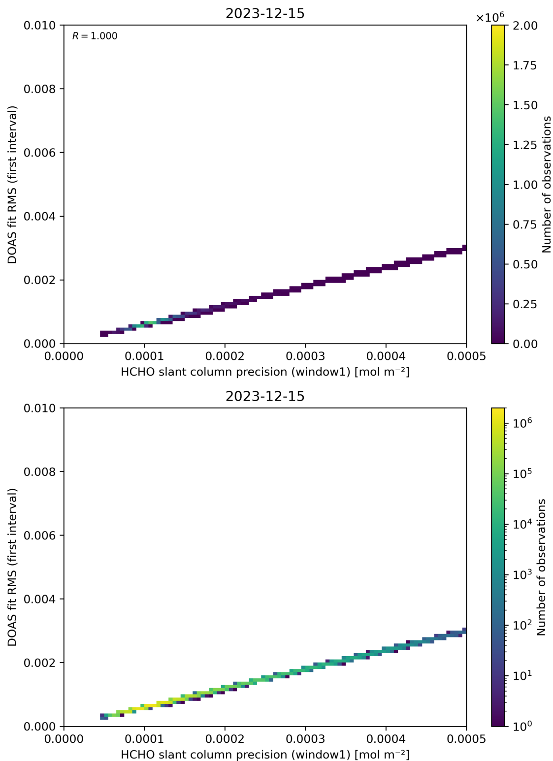
Figure 88: Scatter density plot of “HCHO slant column precision (window1)” against “DOAS fit RMS (first interval)” for 2023-12-14 to 2023-12-16.
