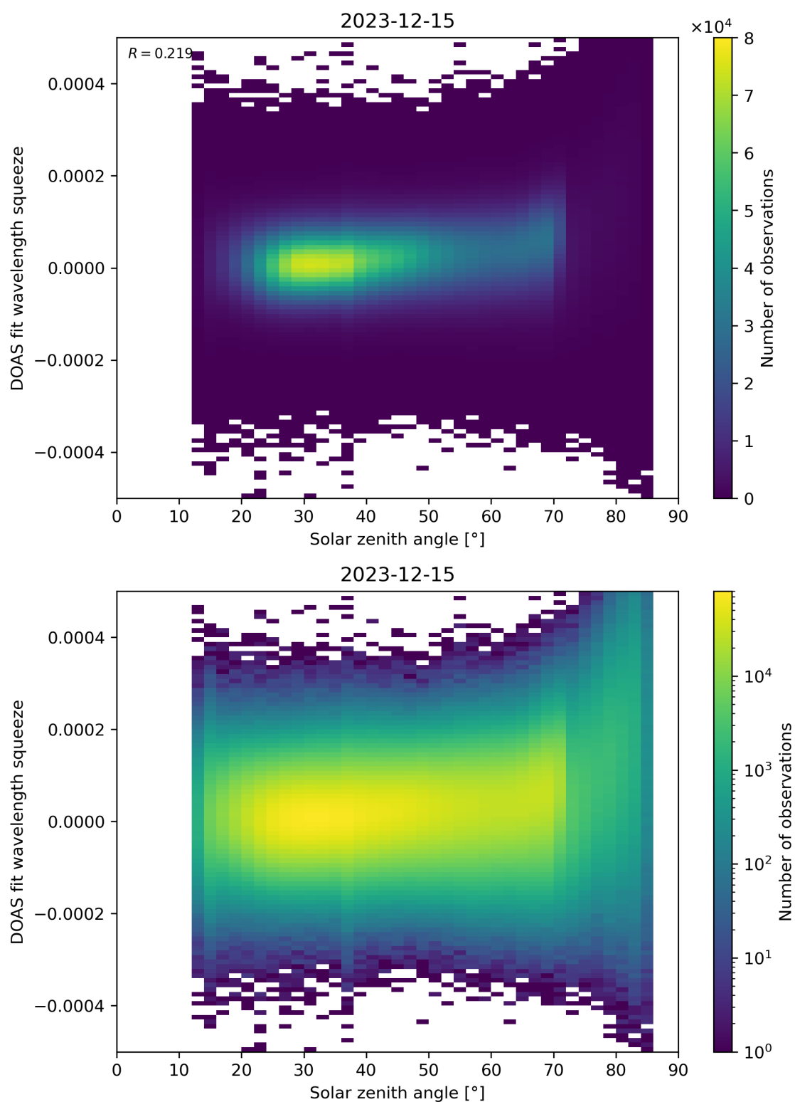
Figure 169: Scatter density plot of “Solar zenith angle” against “DOAS fit wavelength squeeze” for 2023-12-14 to 2023-12-16.
