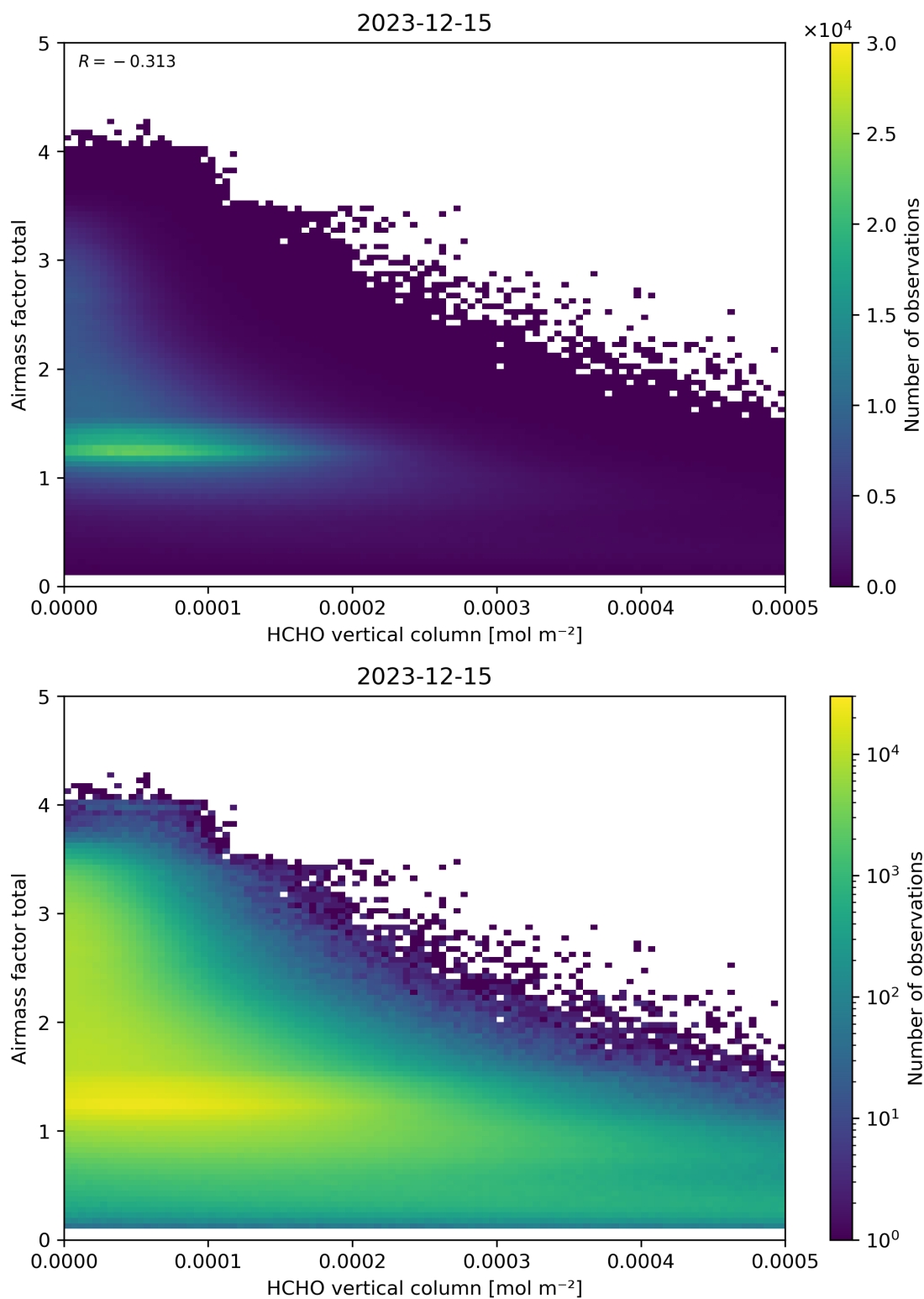
Figure 131: Scatter density plot of “HCHO vertical column” against “Airmass factor total” for 2023-12-14 to 2023-12-16.
