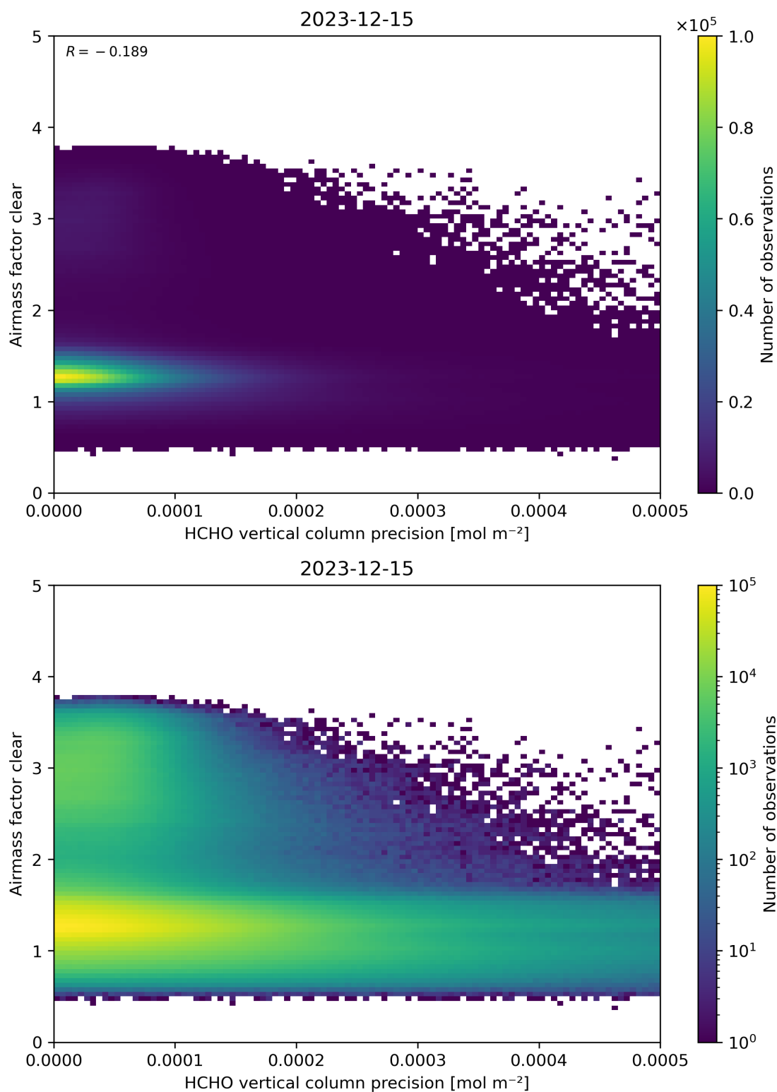
Figure 139: Scatter density plot of “HCHO vertical column precision” against “Airmass factor clear” for 2023-12-14 to 2023-12-16.
