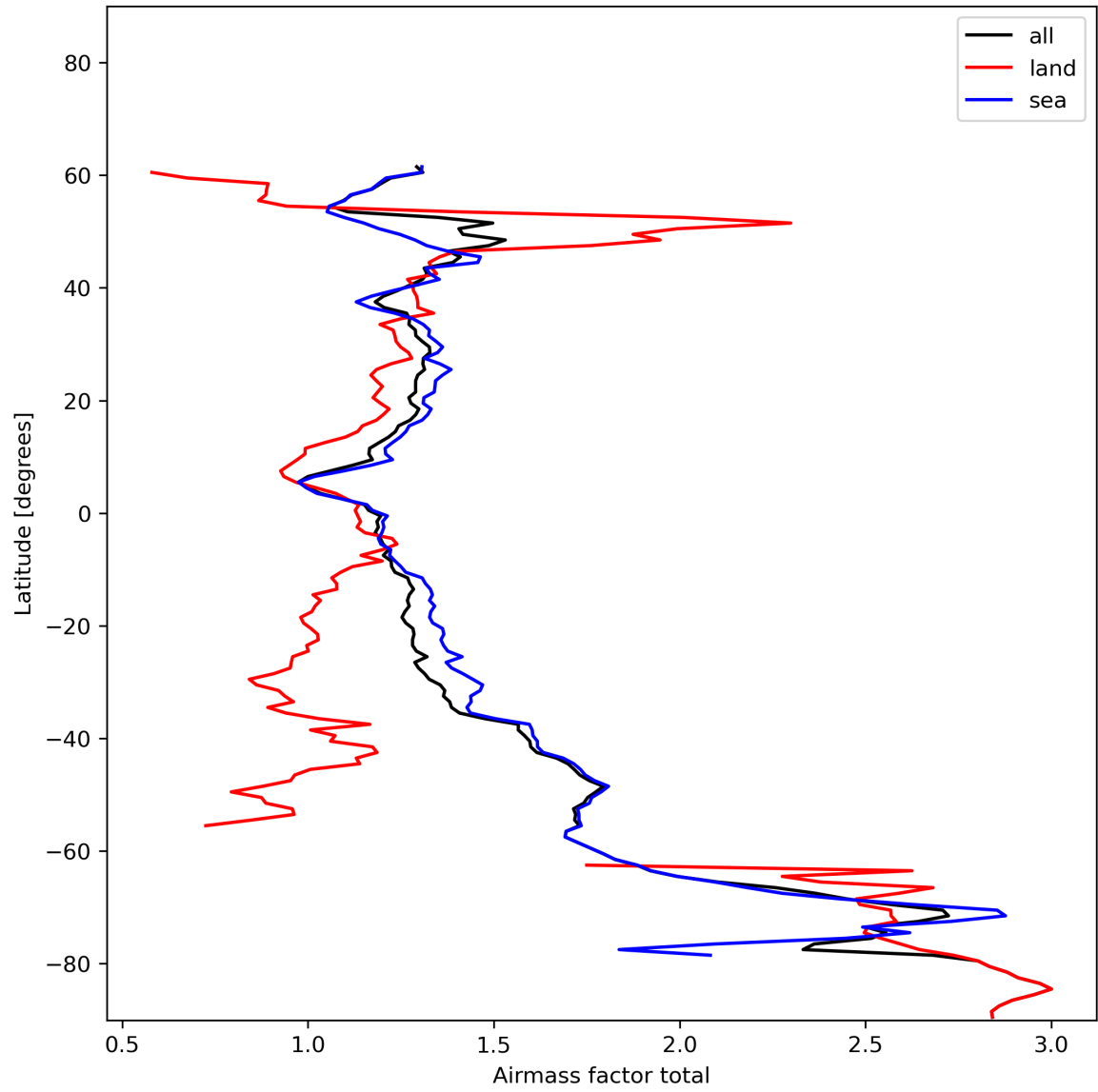
Figure 26: Zonal average of “Airmass factor total” for 2023-12-14 to 2023-12-16.
