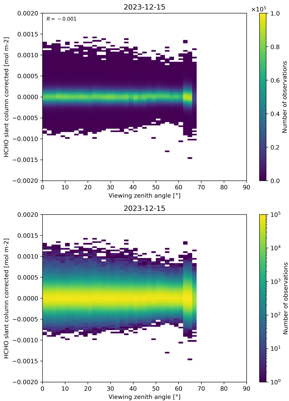
Figure 186: Scatter density plot of “Viewing zenith angle” against “HCHO slant column corrected” for 2023-12-14 to 2023-12-16.
