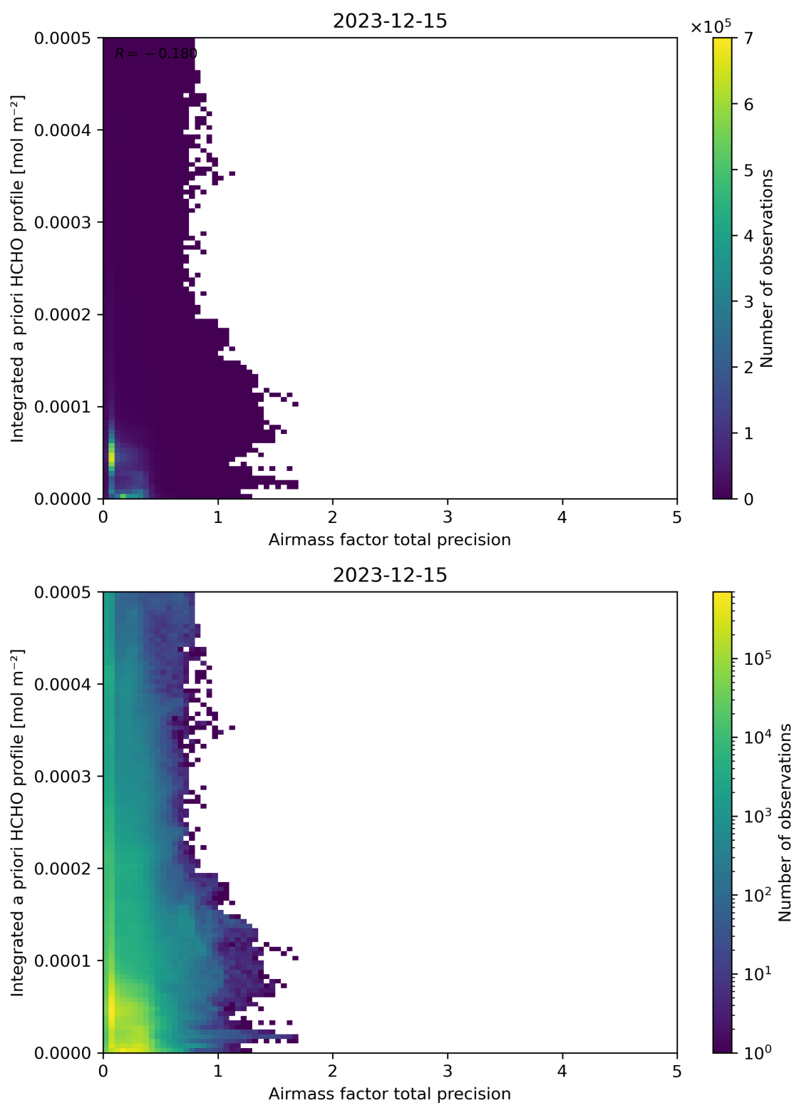
Figure 111: Scatter density plot of “Airmass factor total precision” against “Integrated a priori HCHO profile” for 2023-12-14 to 2023-12-16.
