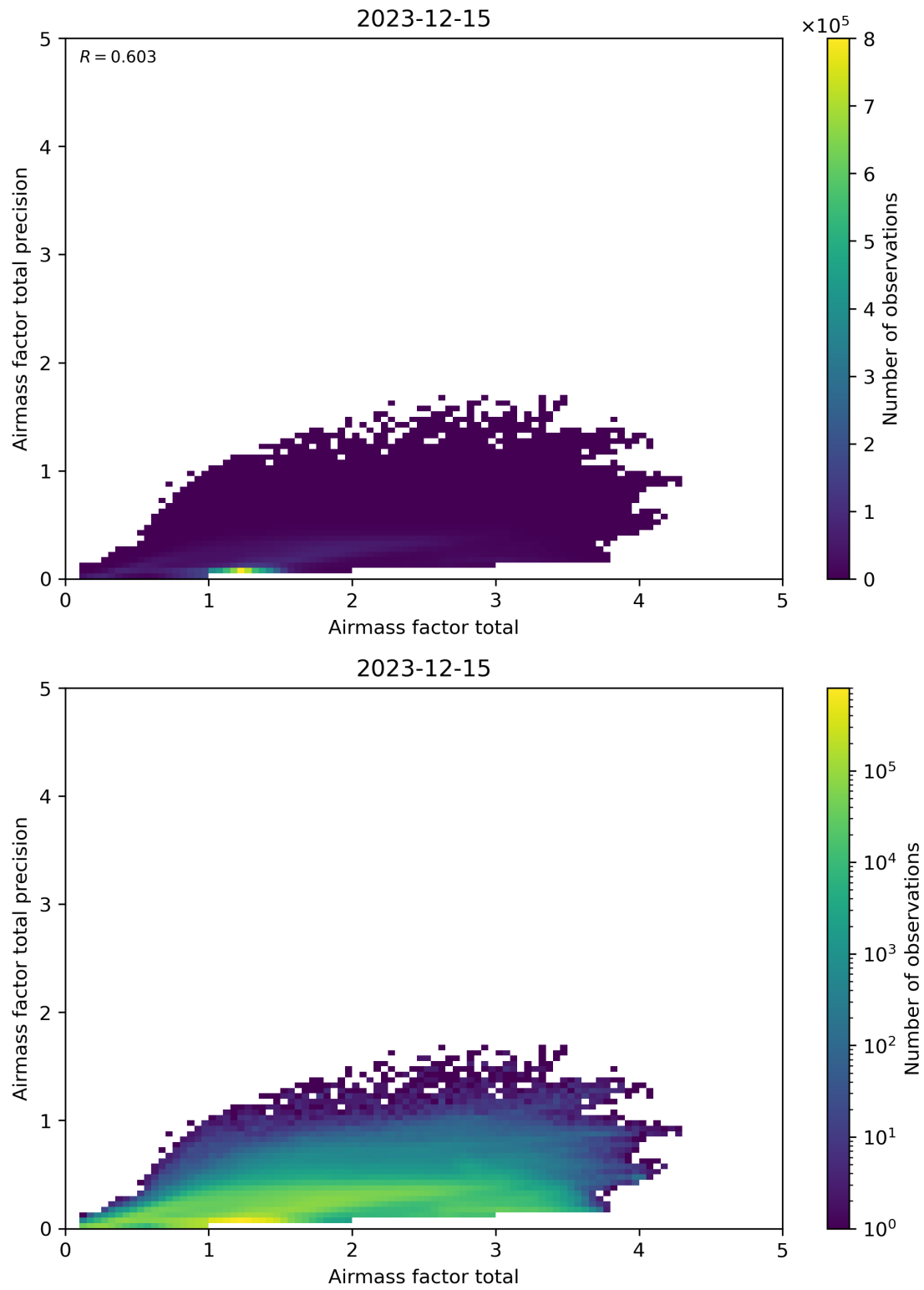
Figure 103: Scatter density plot of “Airmass factor total” against “Airmass factor total precision” for 2023-12-14 to 2023-12-16.
