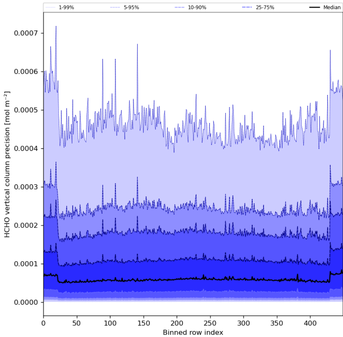
Figure 50: Along track statistics of "HCHO vertical column precision" for 2023-12-14 to 2023-12-16
