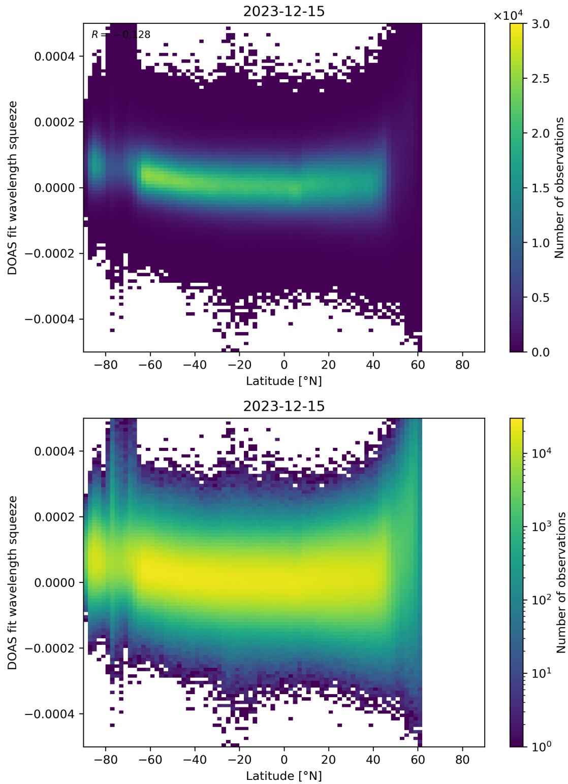
Figure 155: Scatter density plot of “Latitude” against “DOAS fit wavelength squeeze” for 2023-12-14 to 2023-12-16.
