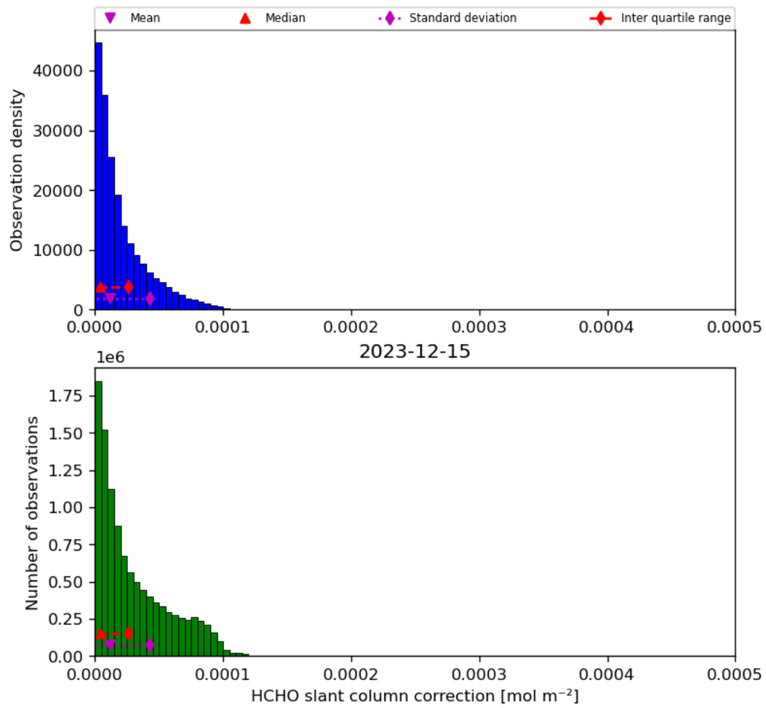
Figure 47: Histogram of “HCHO slant column correction” for 2023-12-14 to 2023-12-16
