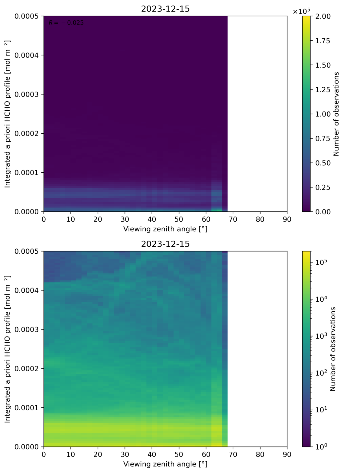
Figure 195: Scatter density plot of “Viewing zenith angle” against “Integrated a priori HCHO profile” for 2023-12-14 to 2023-12-16.
