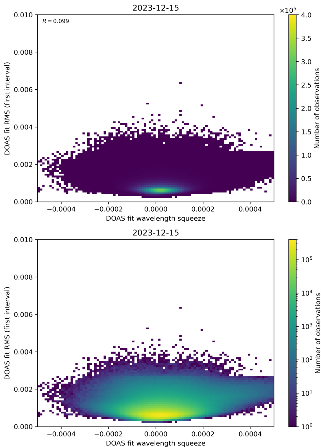
Figure 68: Scatter density plot of “DOAS fit wavelength squeeze” against “DOAS fit RMS (first interval)” for 2023-12-14 to 2023-12-16.
