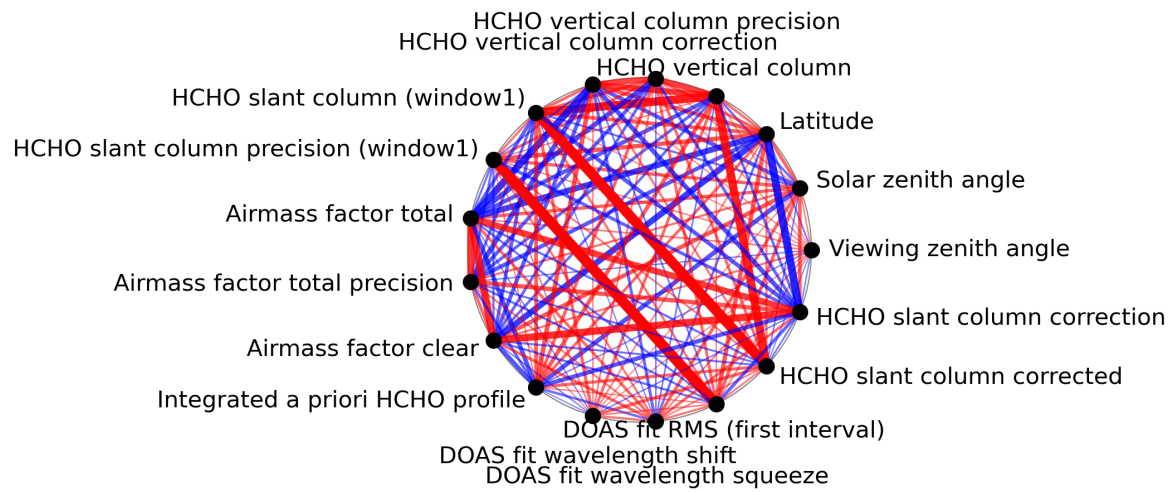
Figure 1: Map of correlation graph for 2023-12-14 to 2023-12-16.
