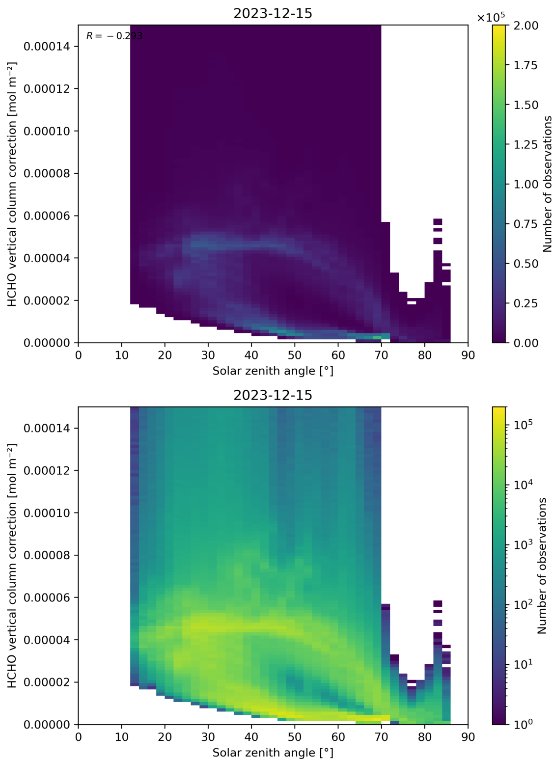
Figure 178: Scatter density plot of “Solar zenith angle” against “HCHO vertical column correction” for 2023-12-14 to 2023-12-16.
