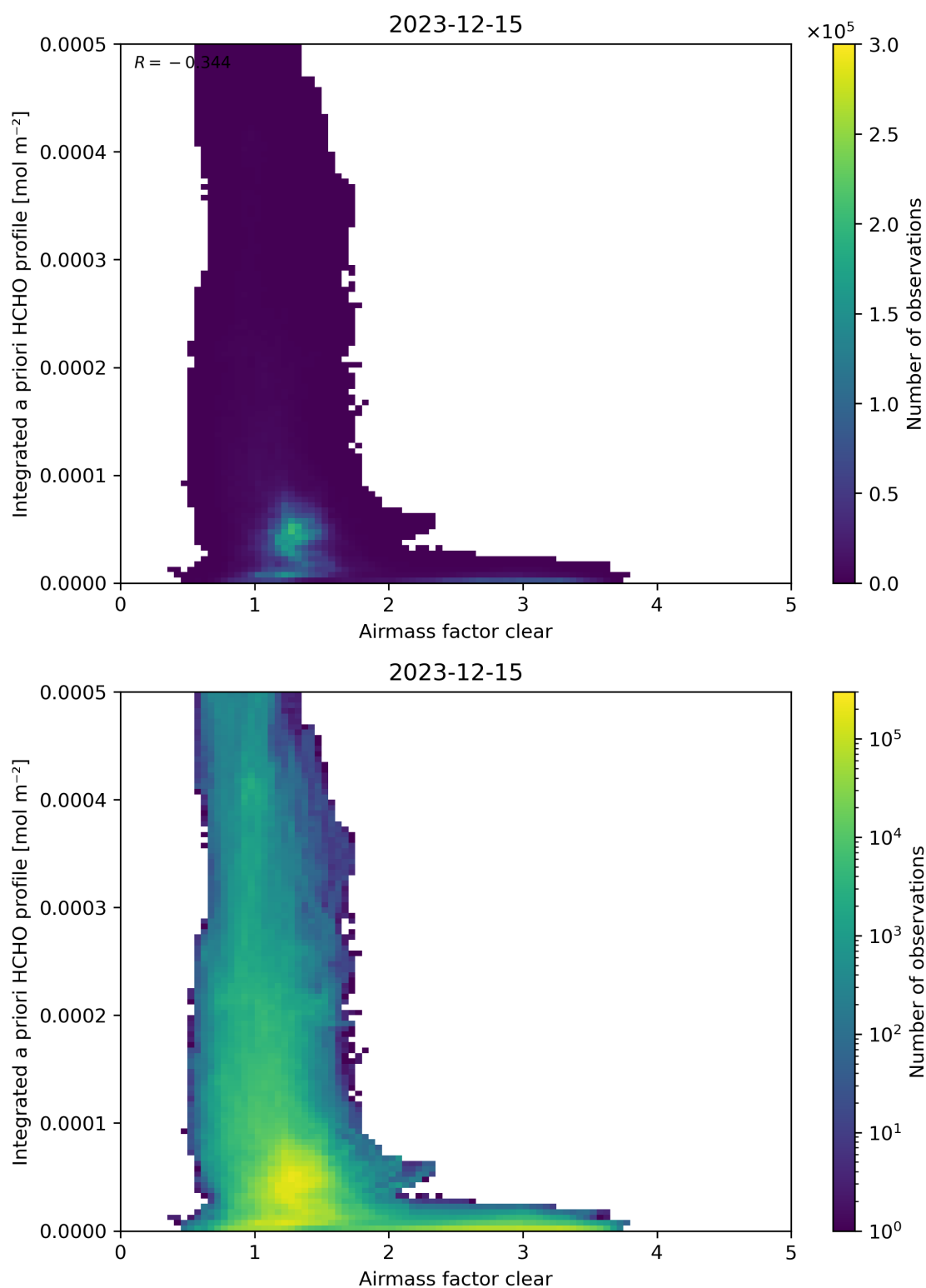
Figure 76: Scatter density plot of “Airmass factor clear” against “Integrated a priori HCHO profile” for 2023-12-14 to 2023-12-16.
