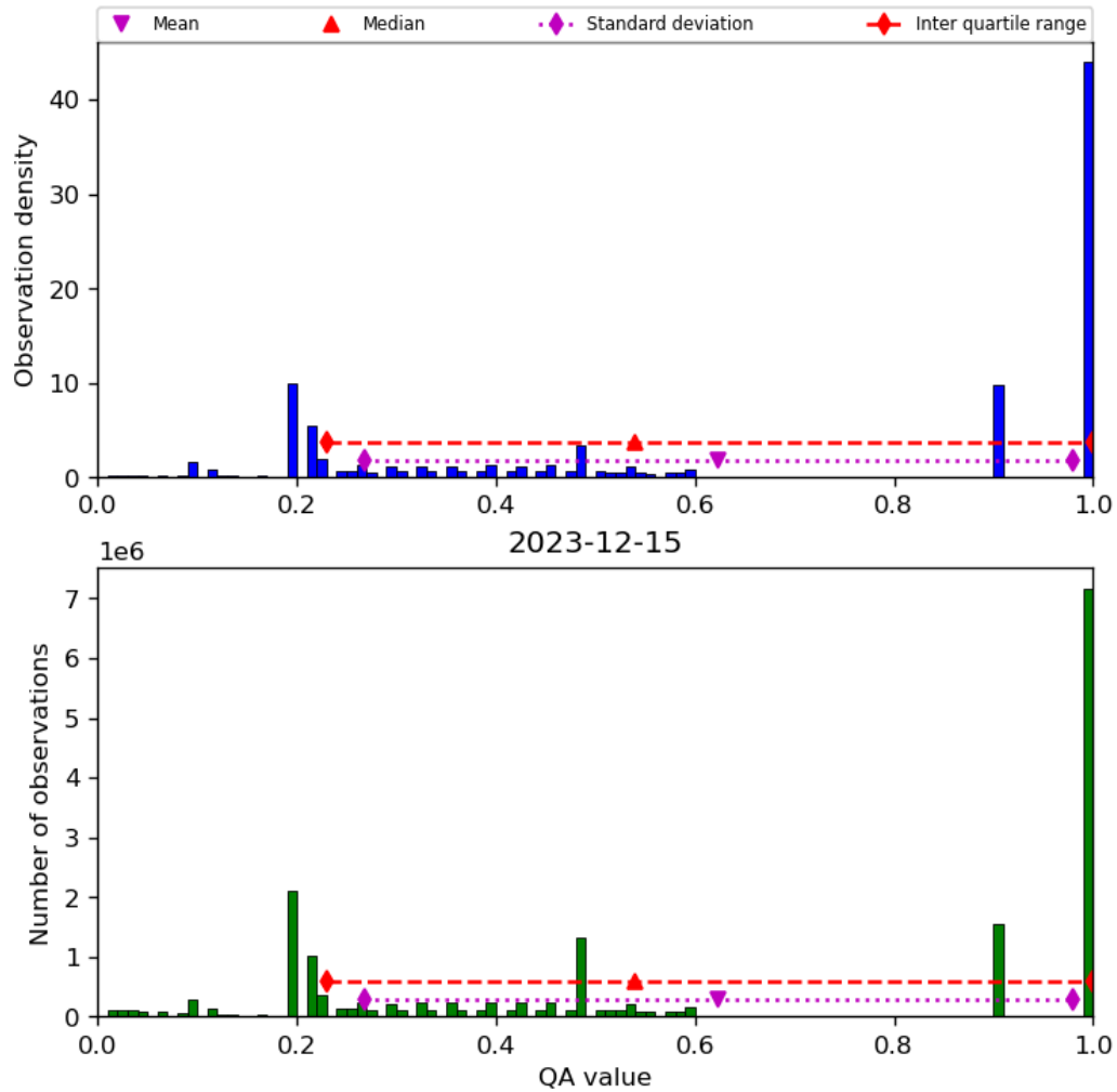
Figure 34: Histogram of “QA value” for 2023-12-14 to 2023-12-16
