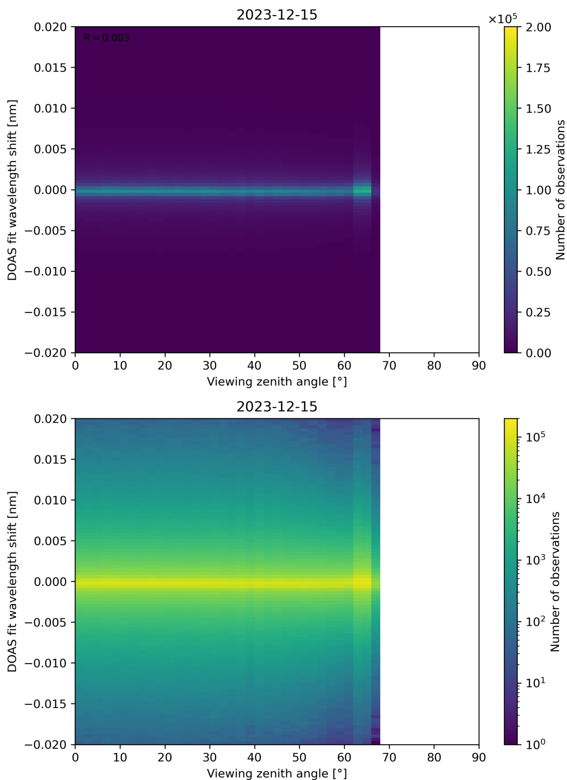
Figure 183: Scatter density plot of “Viewing zenith angle” against “DOAS fit wavelength shift” for 2023-12-14 to 2023-12-16.
