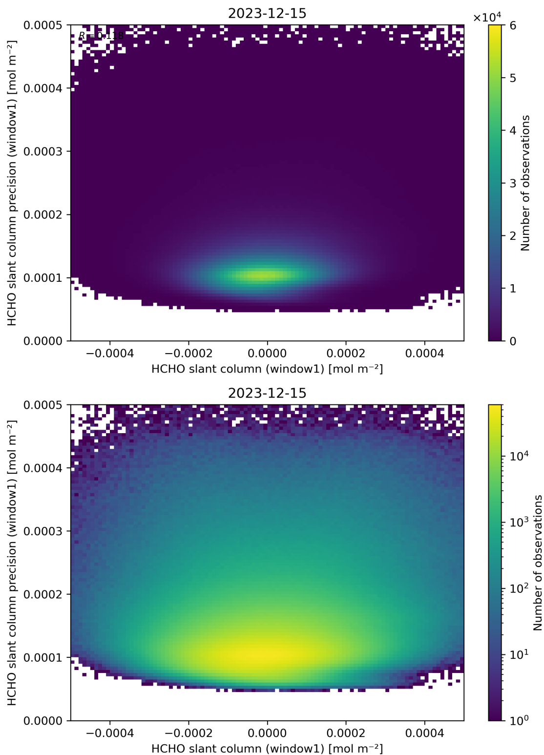
Figure 84: Scatter density plot of “HCHO slant column (window1)” against “HCHO slant column precision (window1)” for 2023-12-14 to 2023-12-16.
