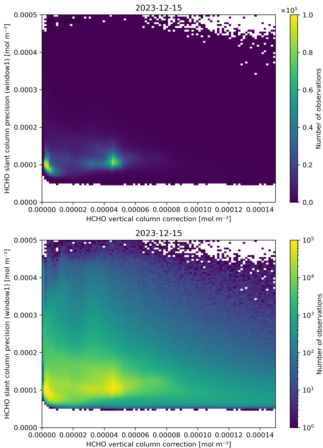
Figure 119: Scatter density plot of “HCHO vertical column correction” against “HCHO slant column precision (window1)” for 2023-12-14 to 2023-12-16.
