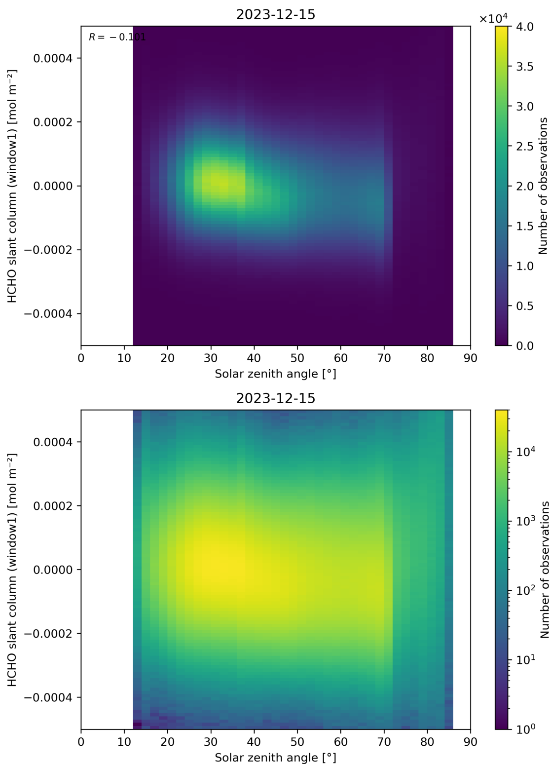
Figure 173: Scatter density plot of “Solar zenith angle” against “HCHO slant column (window1)” for 2023-12-14 to 2023-12-16.
