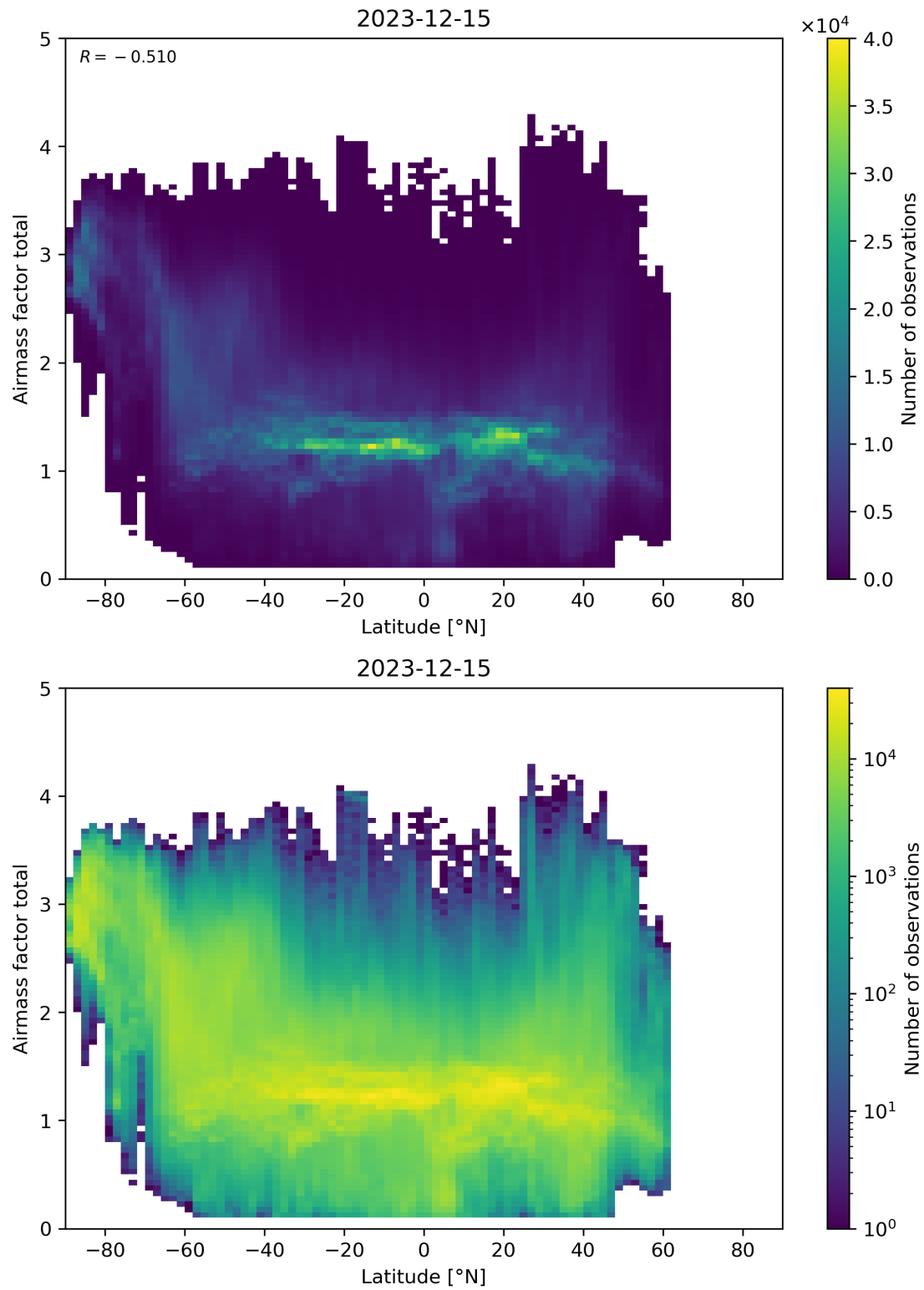
Figure 161: Scatter density plot of “Latitude” against “Airmass factor total” for 2023-12-14 to 2023-12-16.
