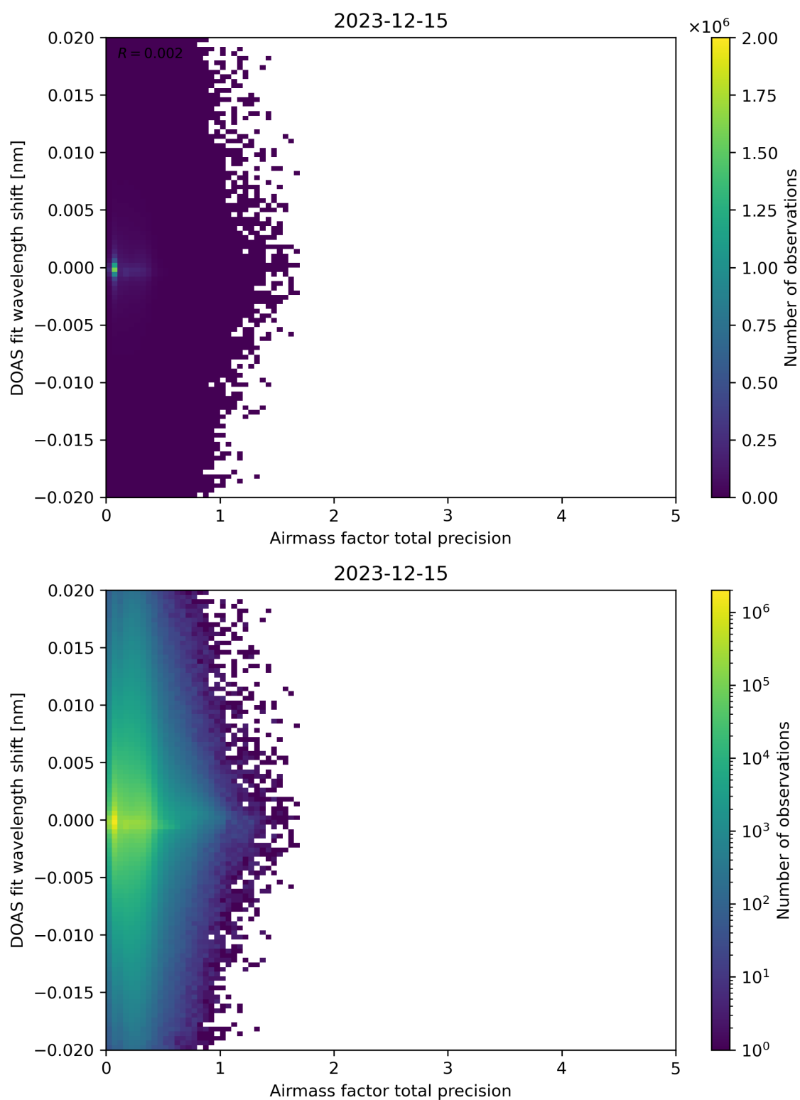
Figure 106: Scatter density plot of “Airmass factor total precision” against “DOAS fit wavelength shift” for 2023-12-14 to 2023-12-16.
