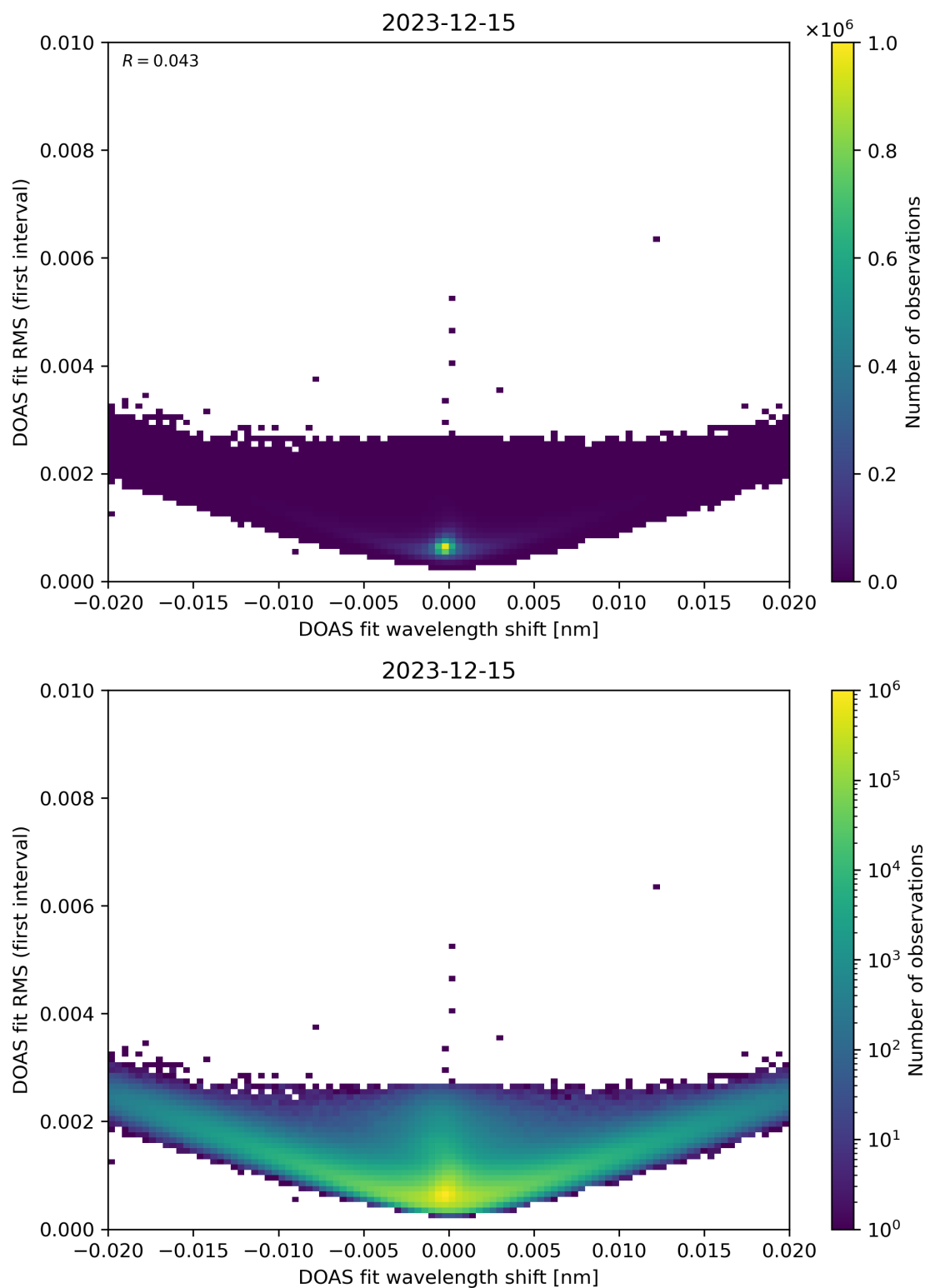
Figure 64: Scatter density plot of “DOAS fit wavelength shift” against “DOAS fit RMS (first interval)” for 2023-12-14 to 2023-12-16.
