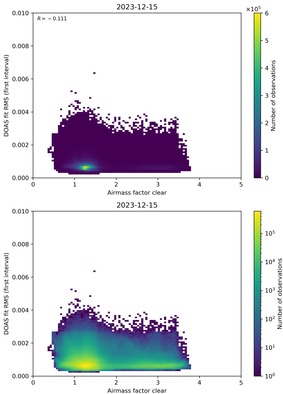
Figure 71: Scatter density plot of “Airmass factor clear” against “DOAS fit RMS (first interval)” for 2023-12-14 to 2023-12-16.
