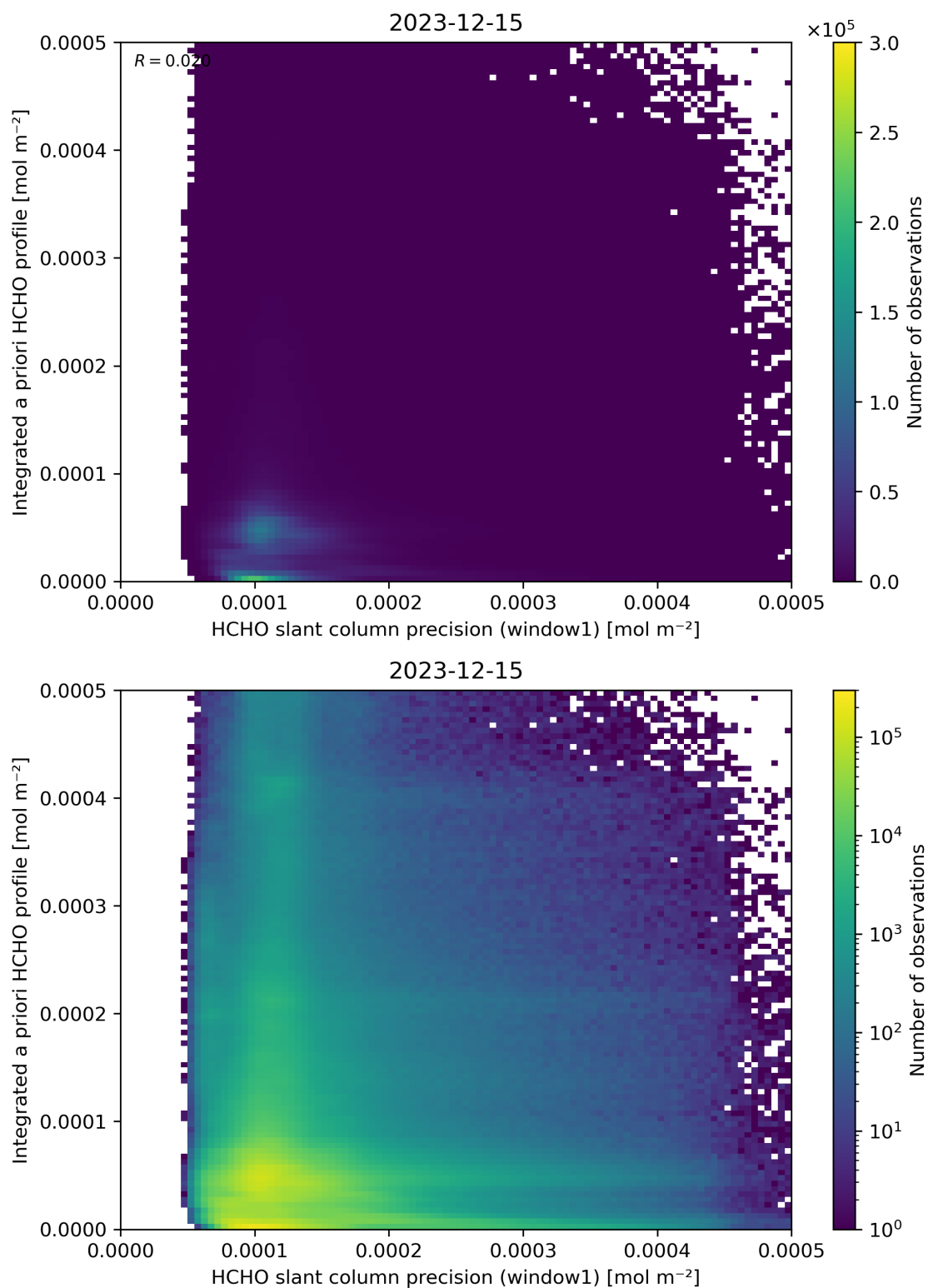
Figure 96: Scatter density plot of “HCHO slant column precision (window1)” against “Integrated a priori HCHO profile” for 2023-12-14 to 2023-12-16.
