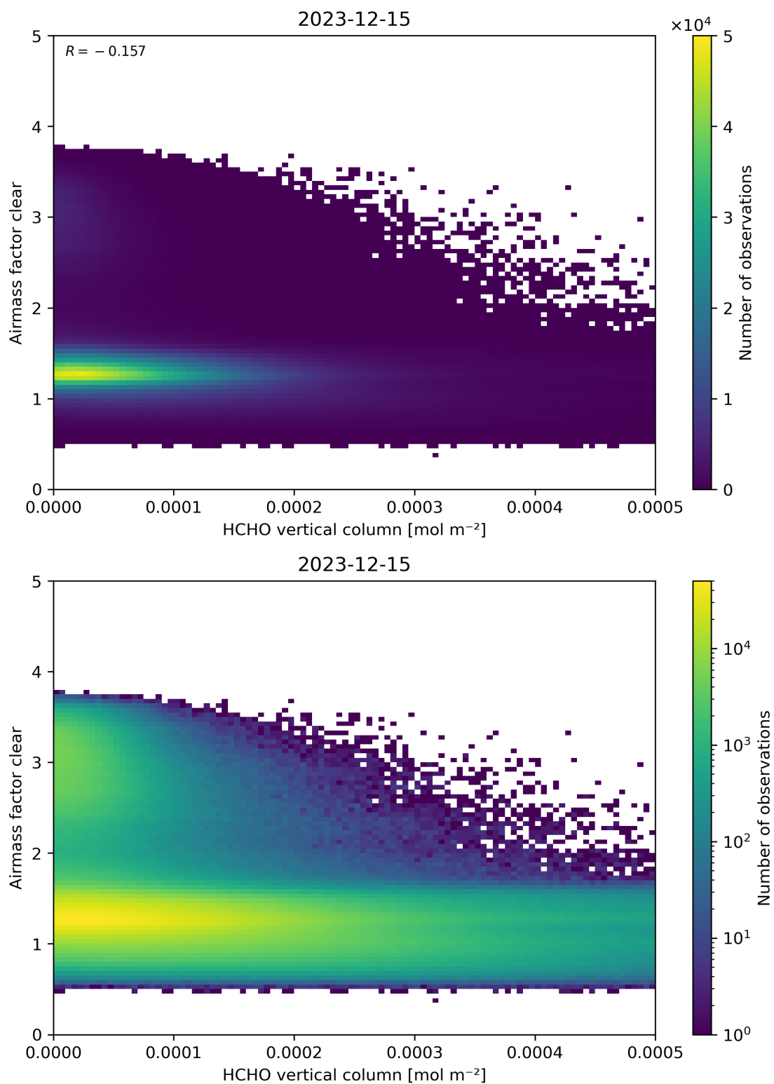
Figure 126: Scatter density plot of “HCHO vertical column” against “Airmass factor clear” for 2023-12-14 to 2023-12-16.
