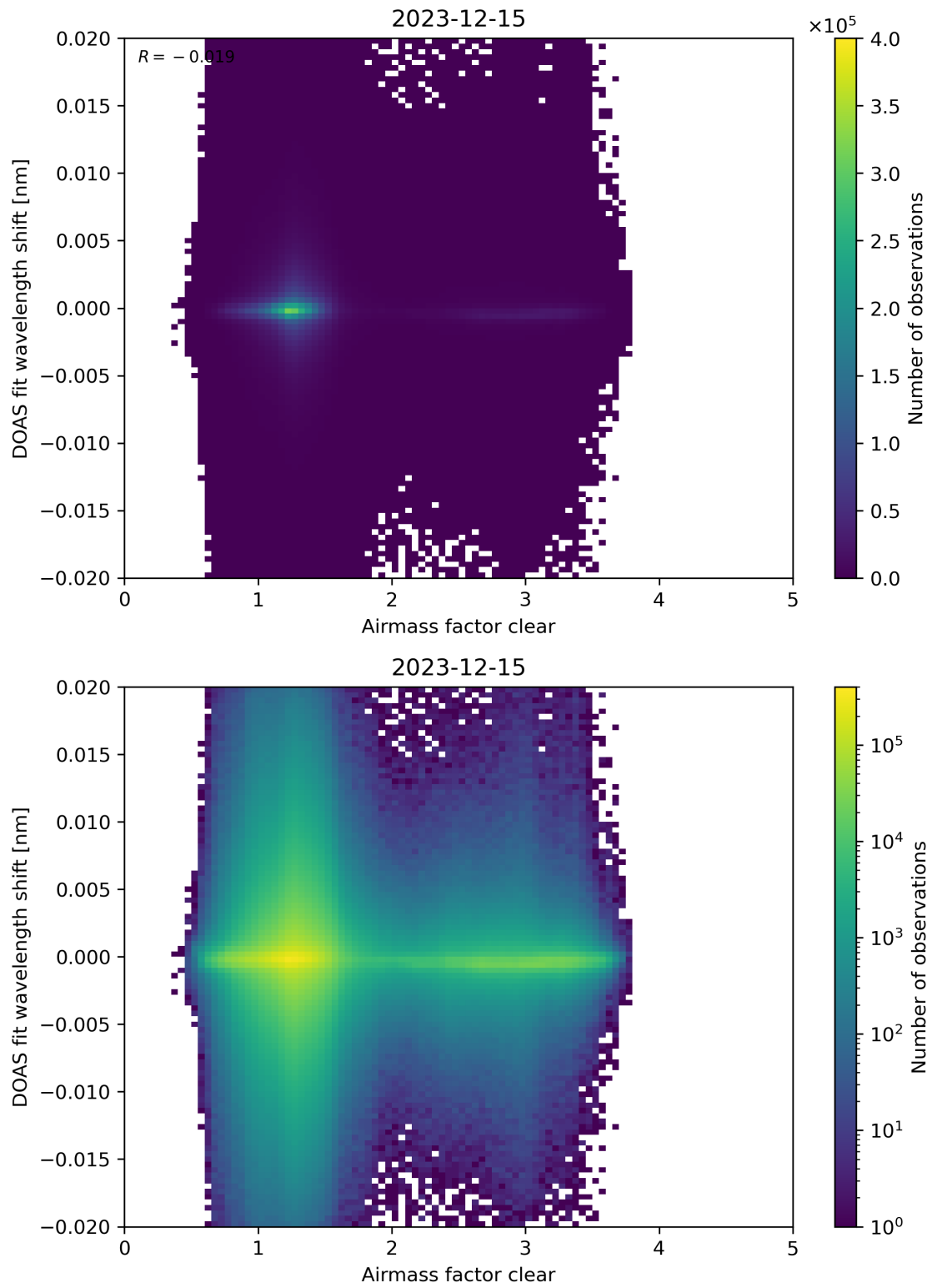
Figure 72: Scatter density plot of “Airmass factor clear” against “DOAS fit wavelength shift” for 2023-12-14 to 2023-12-16.
