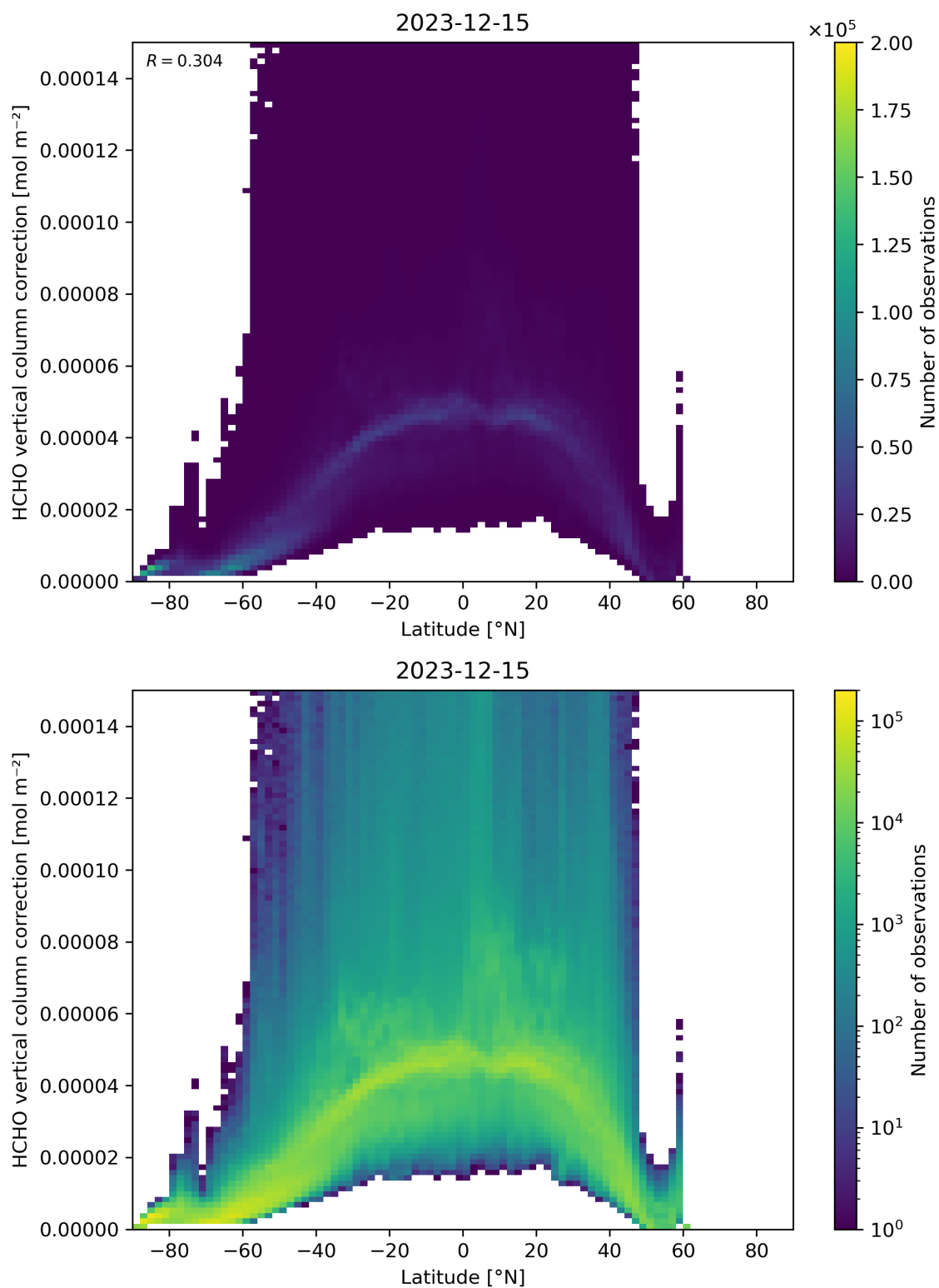
Figure 164: Scatter density plot of “Latitude” against “HCHO vertical column correction” for 2023-12-14 to 2023-12-16.
