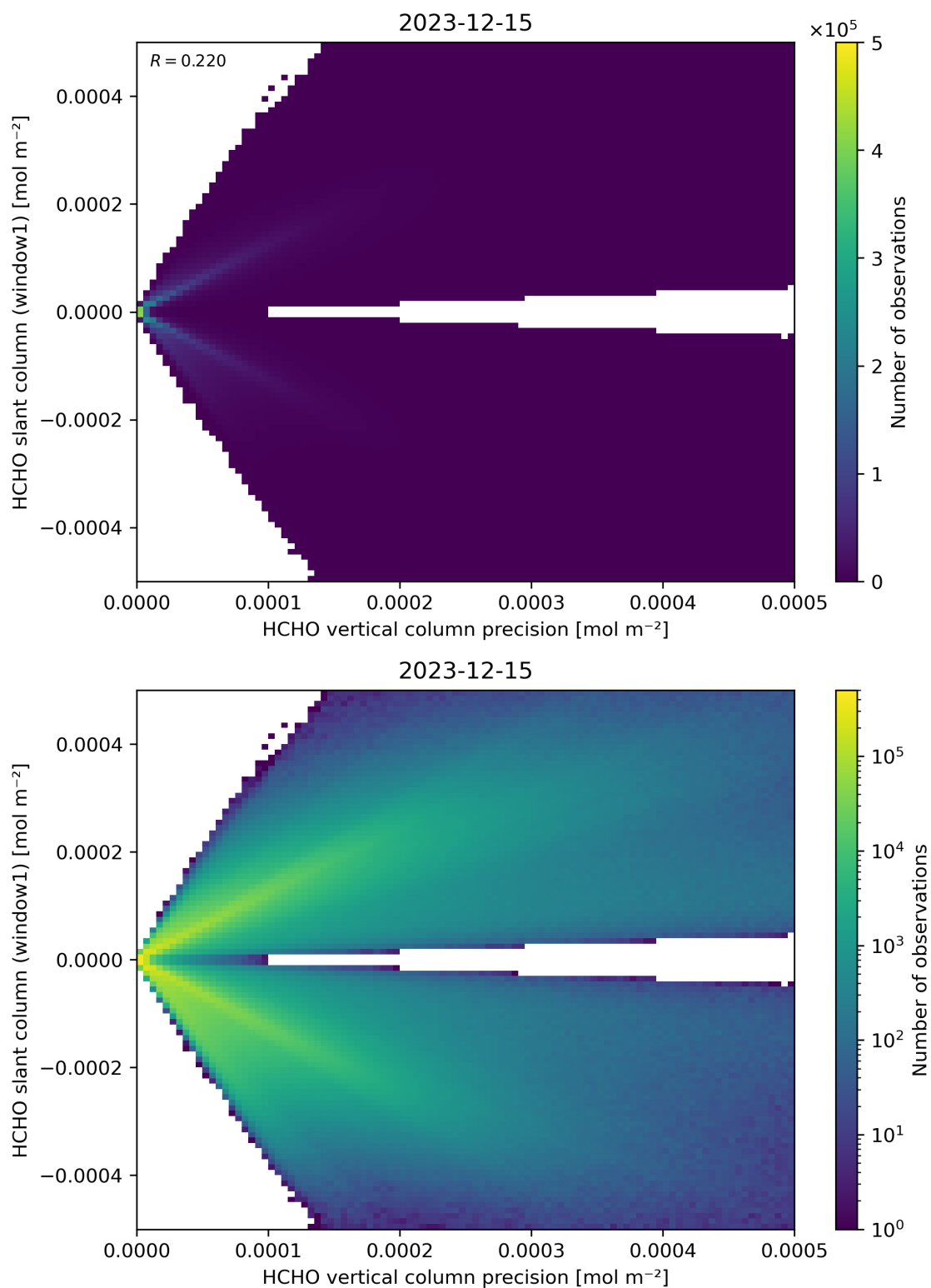
Figure 142: Scatter density plot of “HCHO vertical column precision” against “HCHO slant column (window1)” for 2023-12-14 to 2023-12-16.
