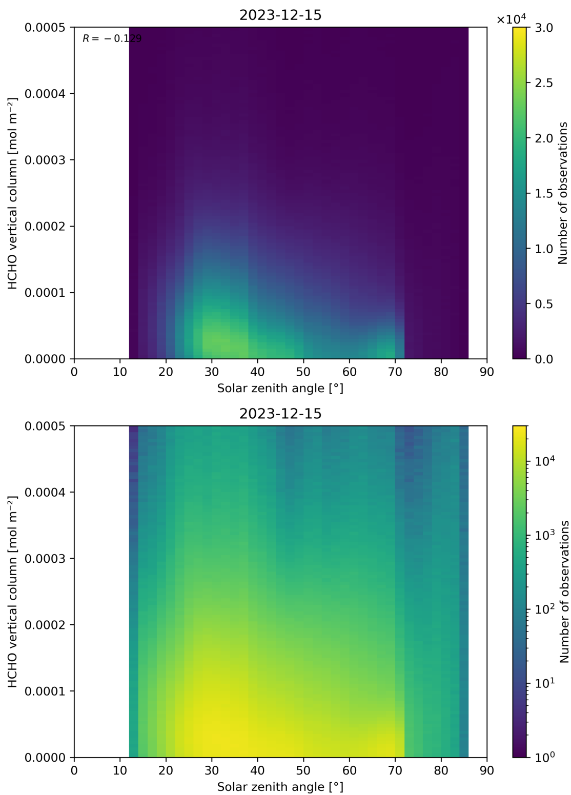
Figure 177: Scatter density plot of “Solar zenith angle” against “HCHO vertical column” for 2023-12-14 to 2023-12-16.
