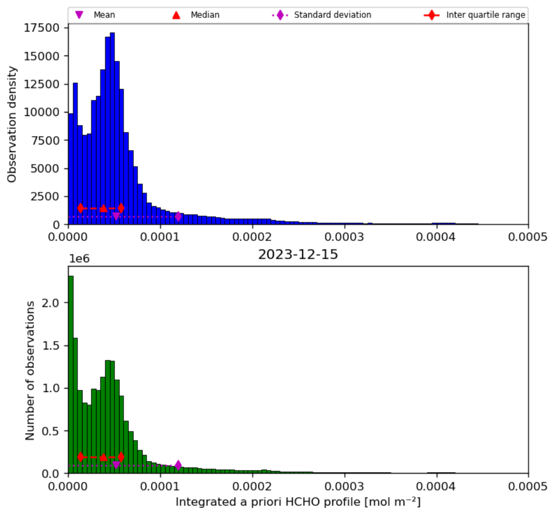
Figure 43: Histogram of “Integrated a priori HCHO profile” for 2023-12-14 to 2023-12-16
