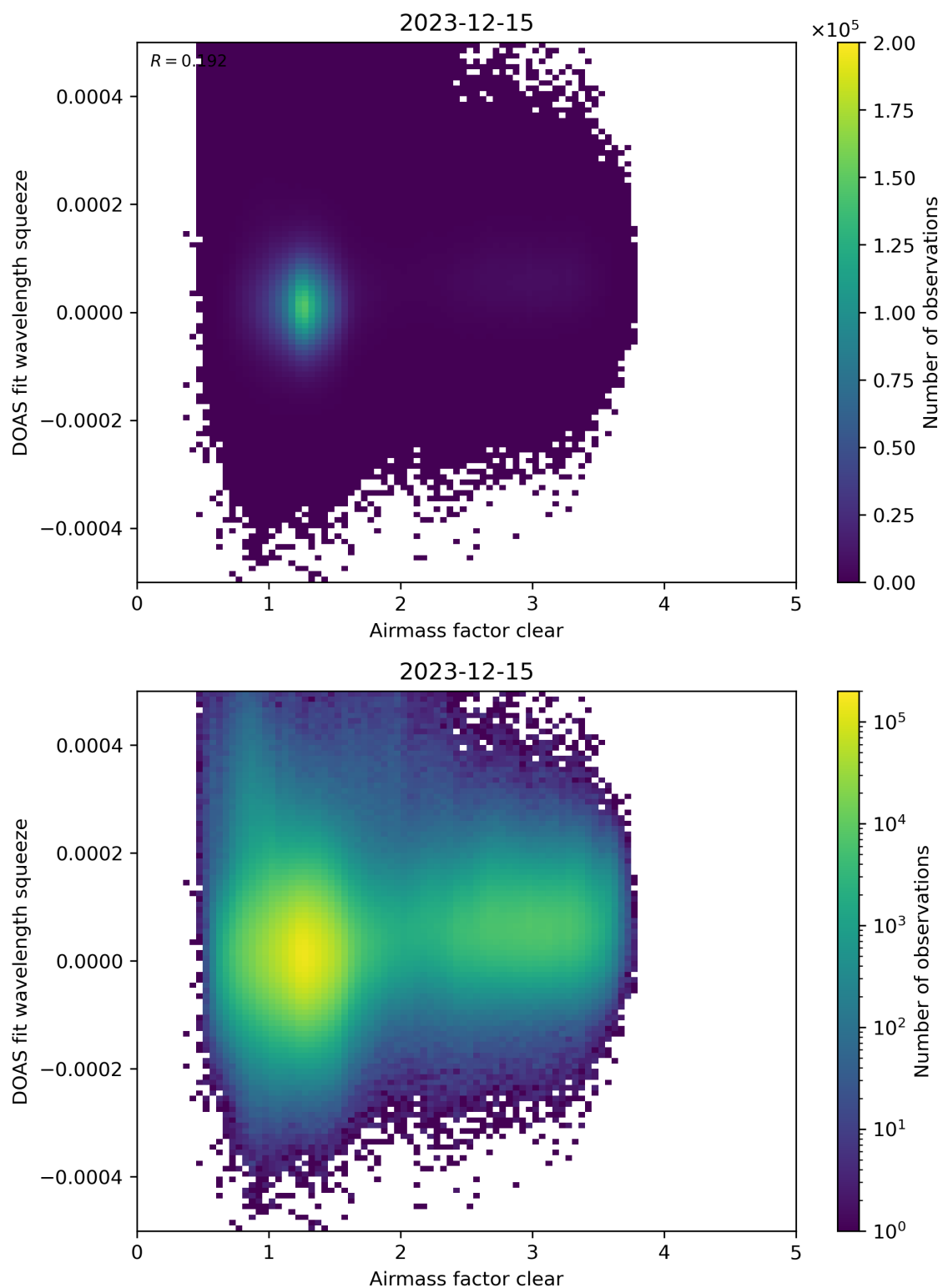
Figure 73: Scatter density plot of “Airmass factor clear” against “DOAS fit wavelength squeeze” for 2023-12-14 to 2023-12-16.
