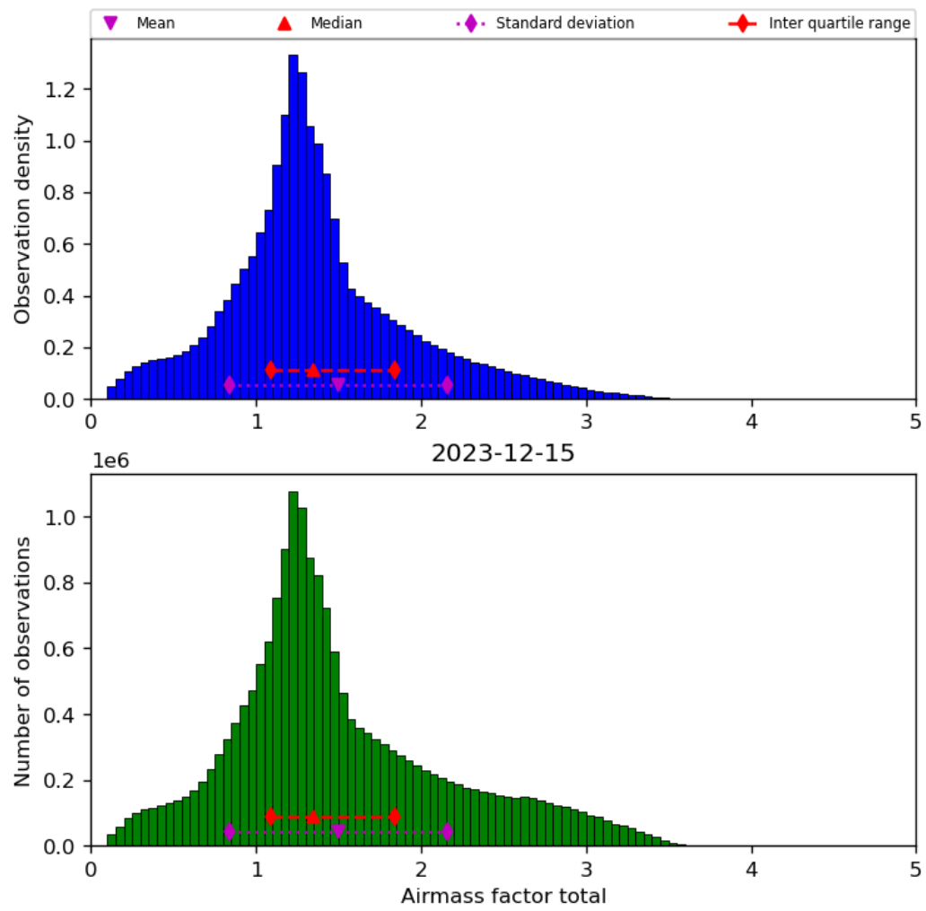
Figure 40: Histogram of “Airmass factor total” for 2023-12-14 to 2023-12-16
