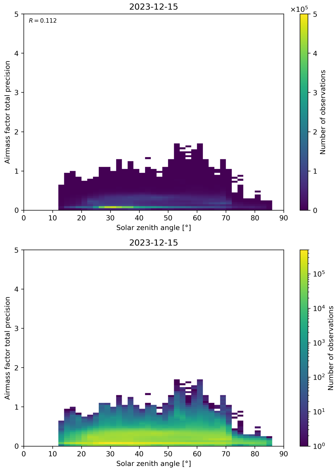
Figure 176: Scatter density plot of “Solar zenith angle” against “Airmass factor total precision” for 2023-12-14 to 2023-12-16.
