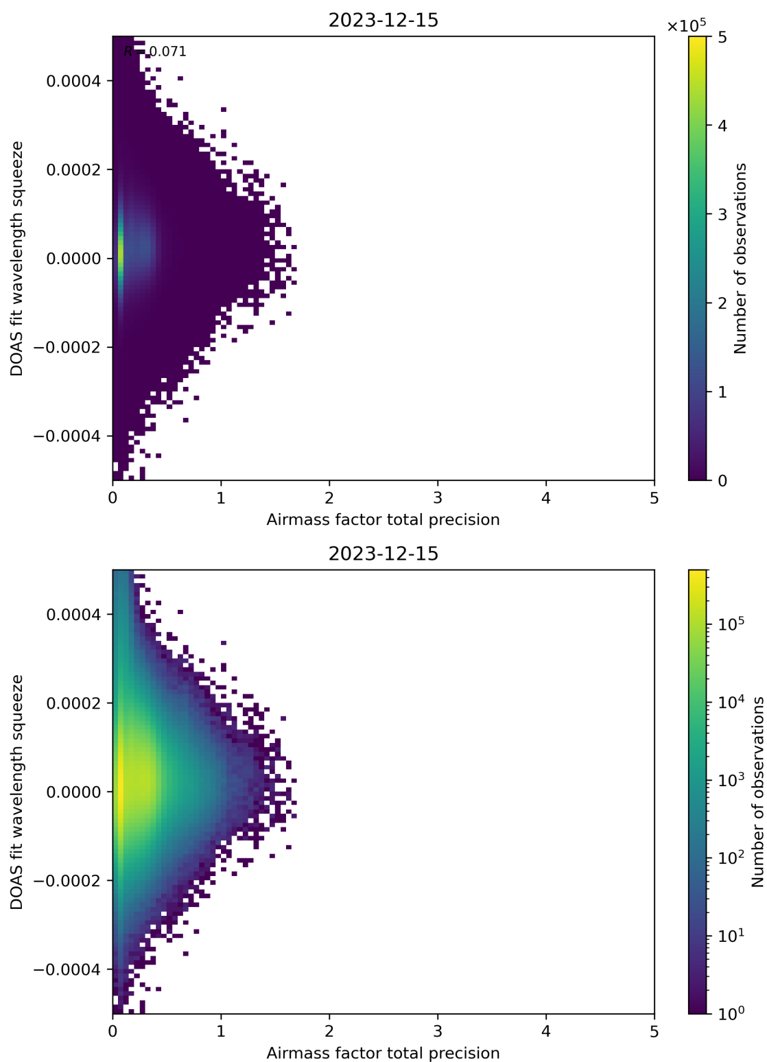
Figure 107: Scatter density plot of “Airmass factor total precision” against “DOAS fit wavelength squeeze” for 2023-12-14 to 2023-12-16.
