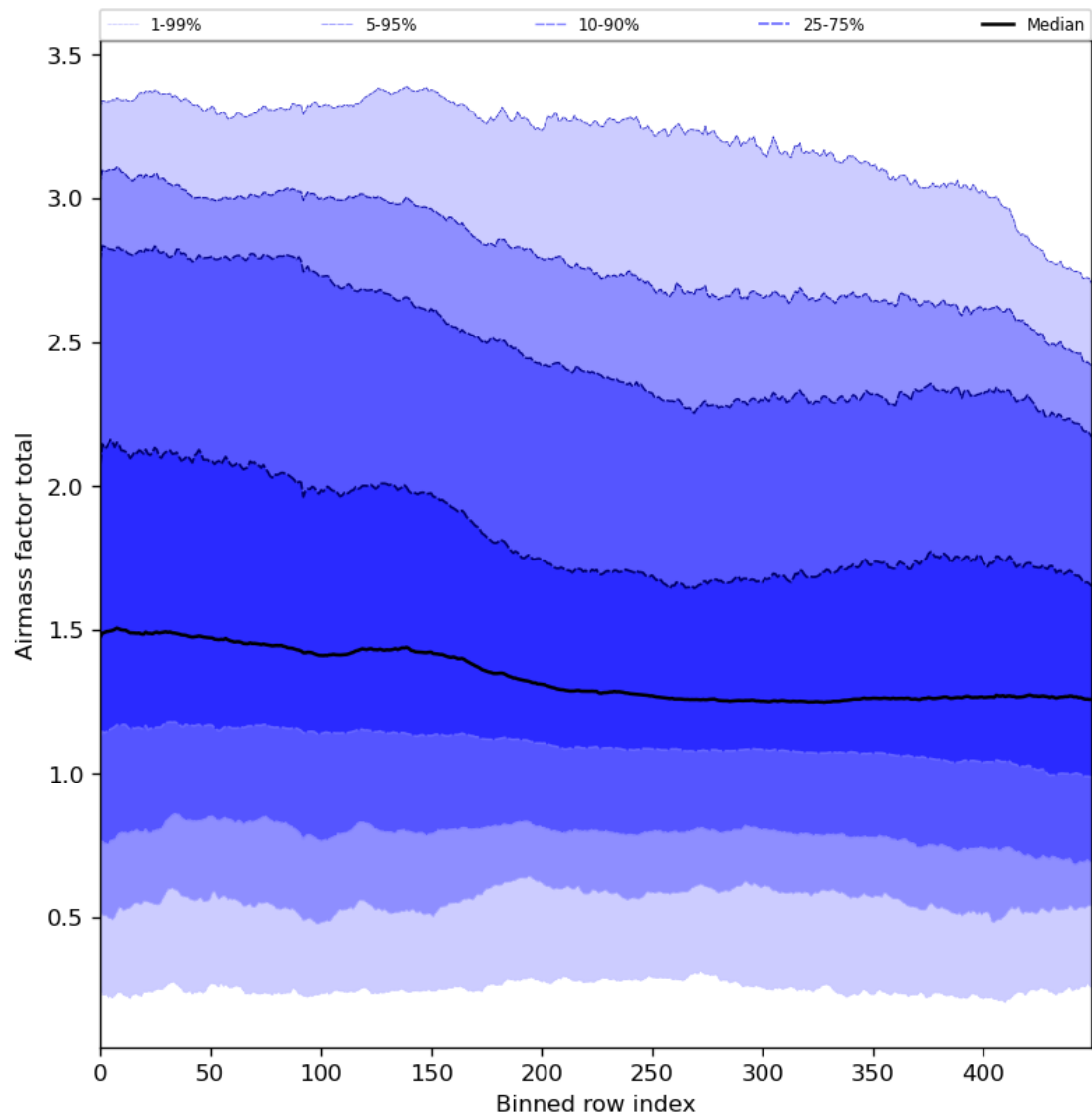
Figure 54: Along track statistics of “Airmass factor total” for 2023-12-14 to 2023-12-16
