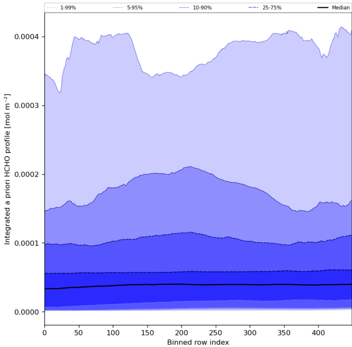
Figure 57: Along track statistics of “Integrated a priori HCHO profile” for 2023-12-14 to 2023-12-16
