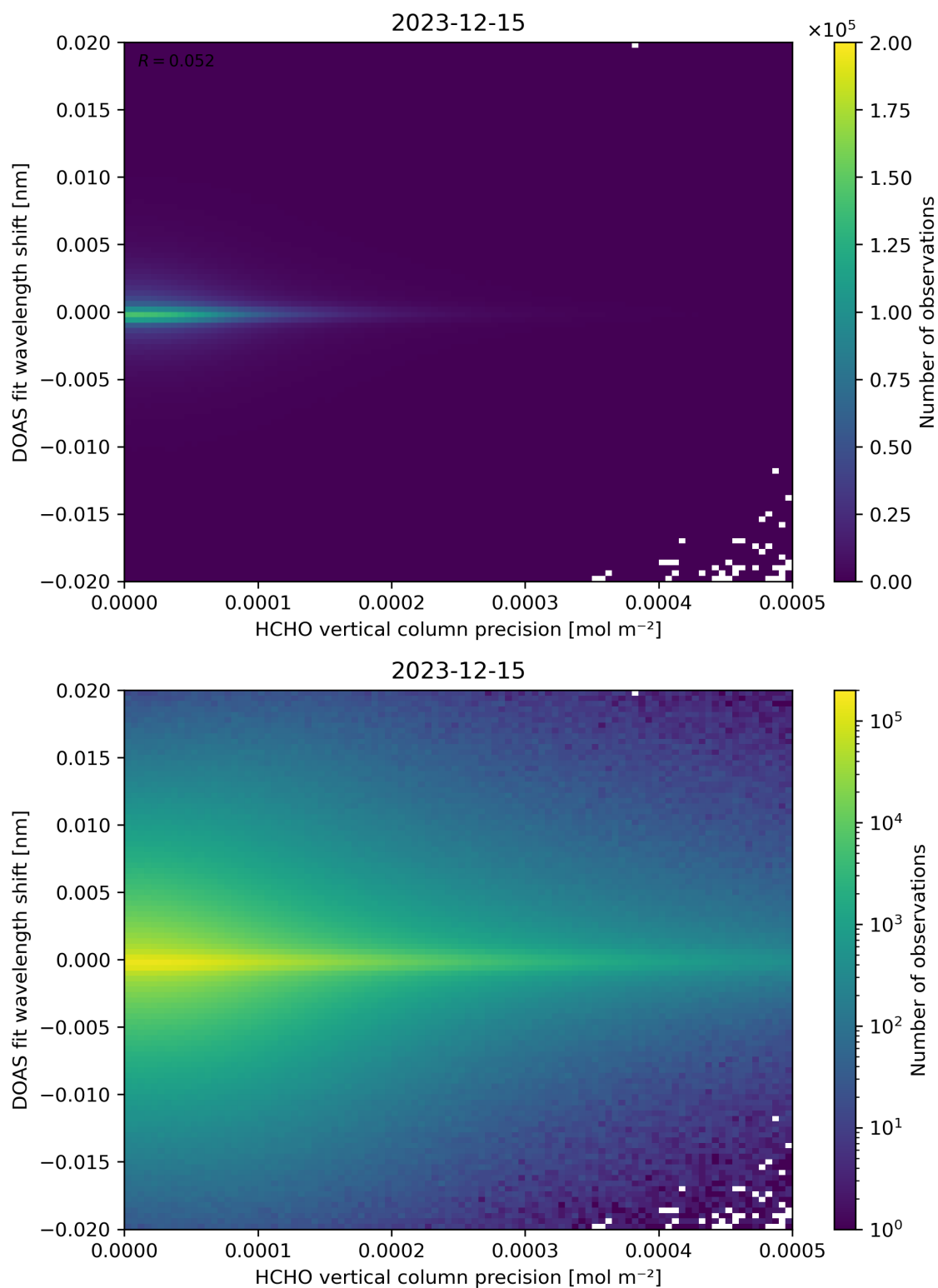
Figure 137: Scatter density plot of “HCHO vertical column precision” against “DOAS fit wavelength shift” for 2023-12-14 to 2023-12-16.
