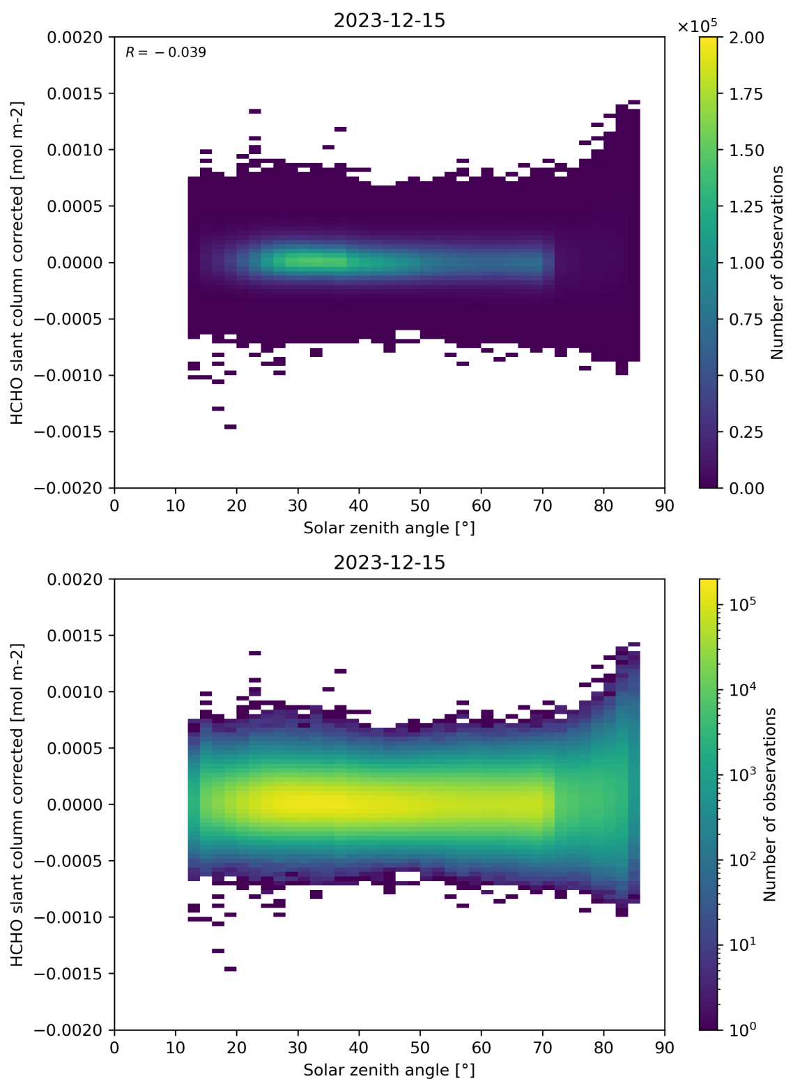
Figure 171: Scatter density plot of “Solar zenith angle” against “HCHO slant column corrected” for 2023-12-14 to 2023-12-16.
