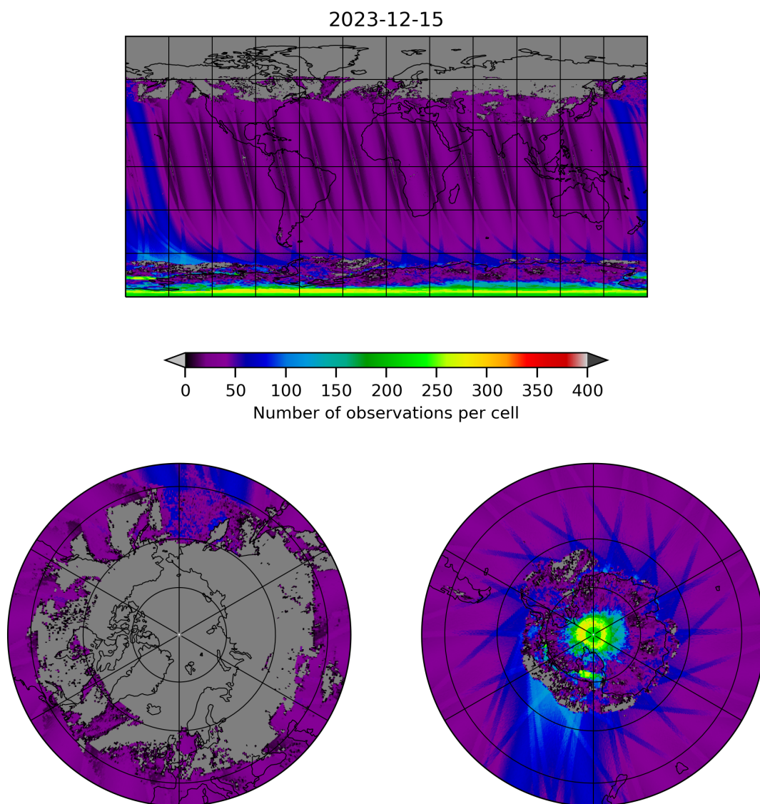
Figure 19: Map of the number of observations for 2023-12-14 to 2023-12-16
