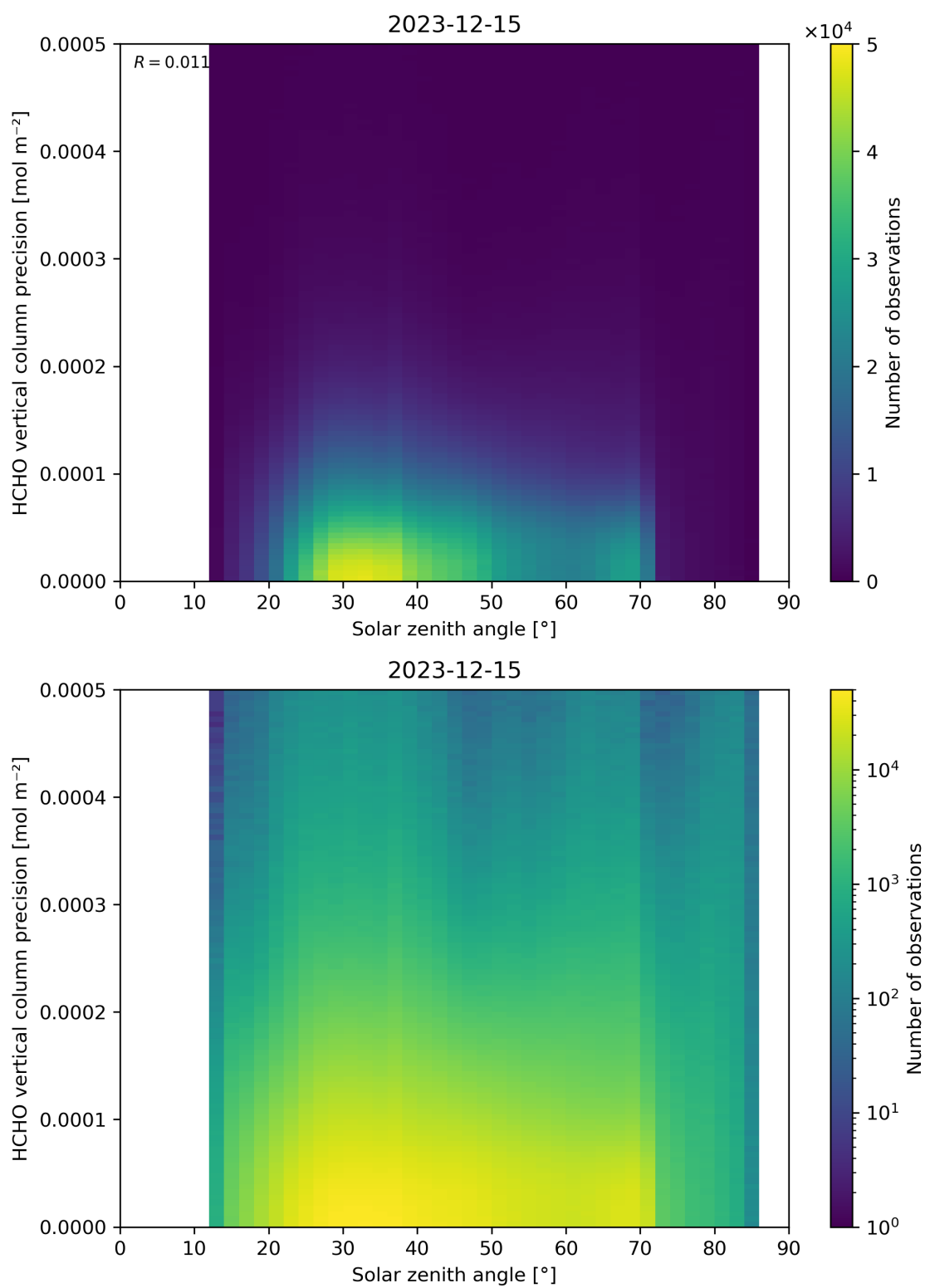
Figure 179: Scatter density plot of “Solar zenith angle” against “HCHO vertical column precision” for 2023-12-14 to 2023-12-16.
