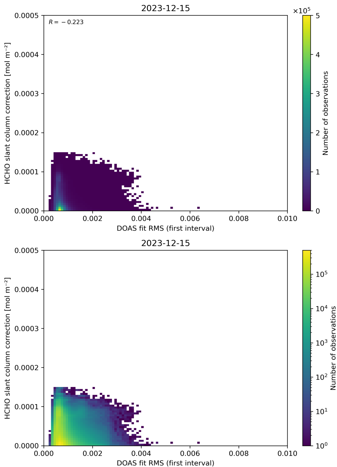
Figure 63: Scatter density plot of “DOAS fit RMS (first interval)” against “HCHO slant column correction” for 2023-12-14 to 2023-12-16.
