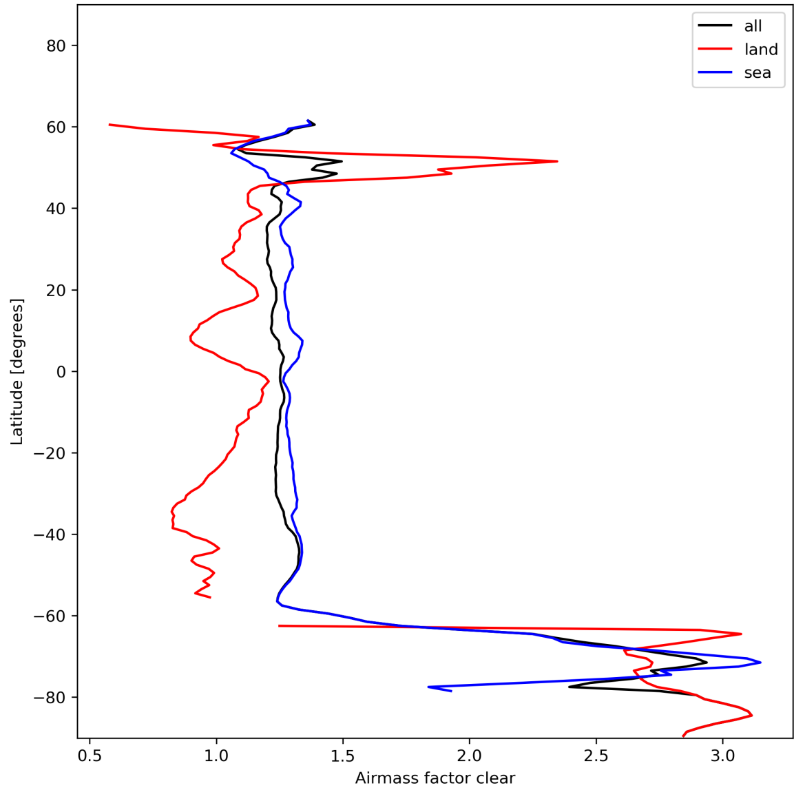
Figure 28: Zonal average of “Airmass factor clear” for 2023-12-14 to 2023-12-16.
