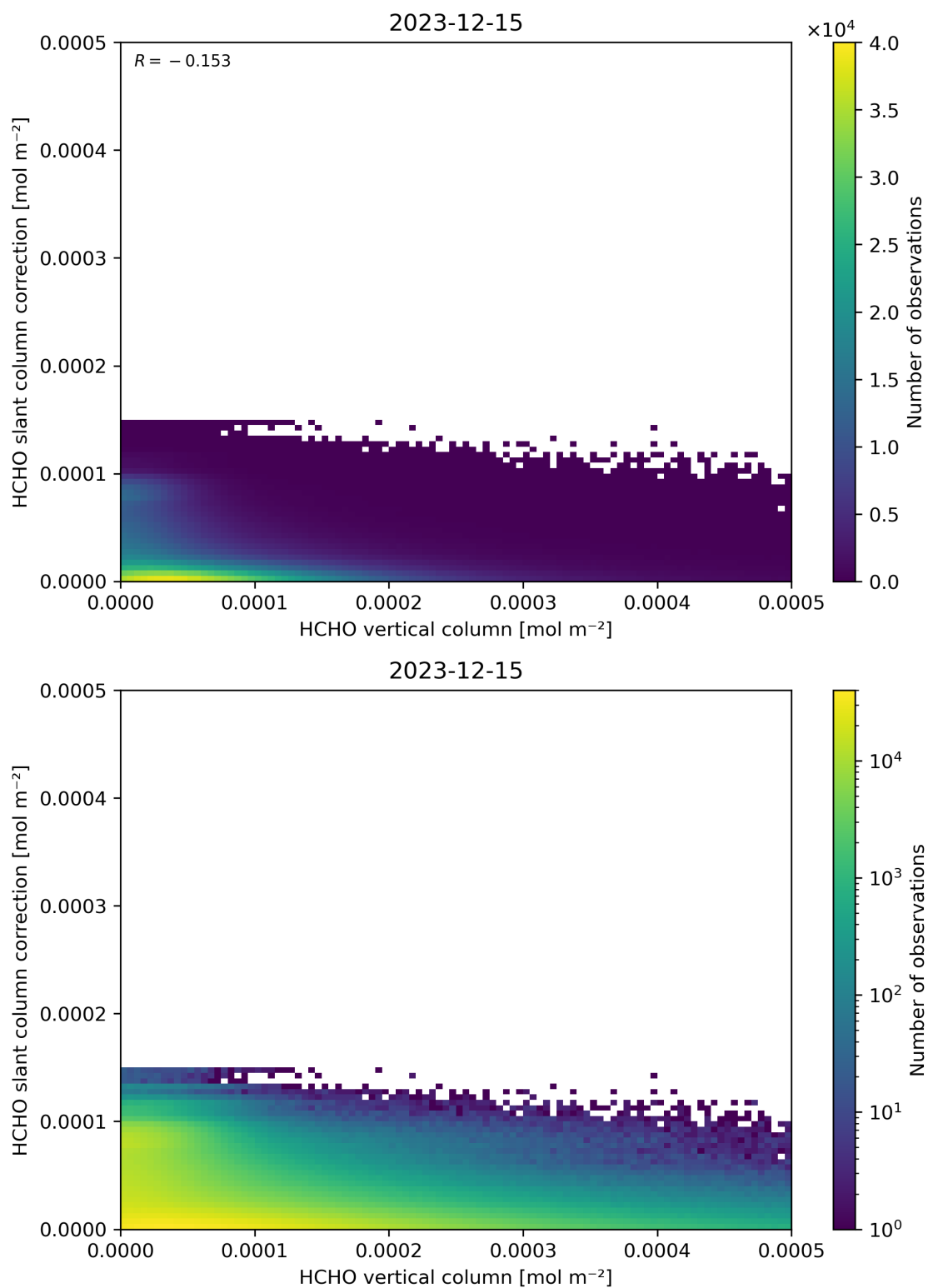
Figure 128: Scatter density plot of “HCHO vertical column” against “HCHO slant column correction” for 2023-12-14 to 2023-12-16.
