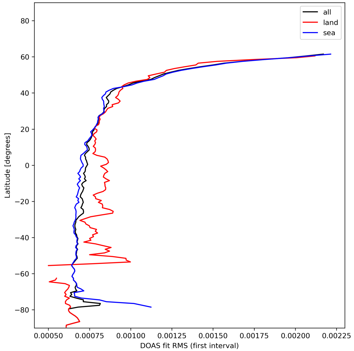
Figure 32: Zonal average of “DOAS fit RMS (first interval)” for 2023-12-14 to 2023-12-16.
