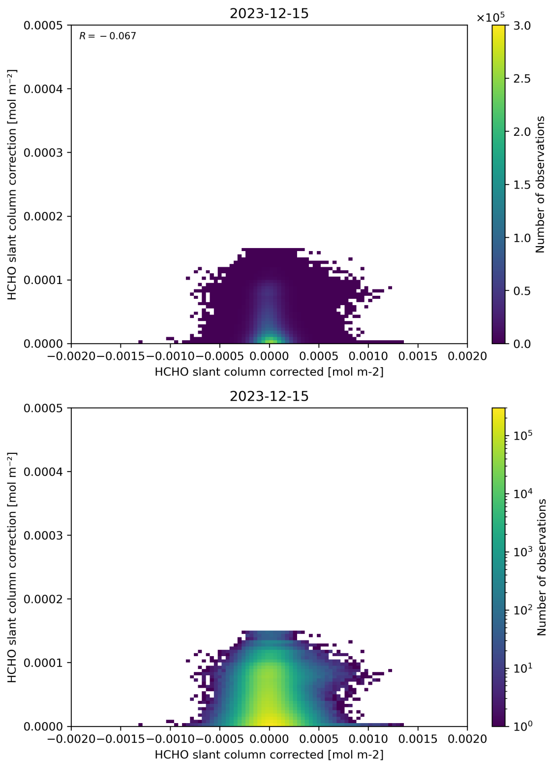
Figure 77: Scatter density plot of “HCHO slant column corrected” against “HCHO slant column correction” for 2023-12-14 to 2023-12-16.
