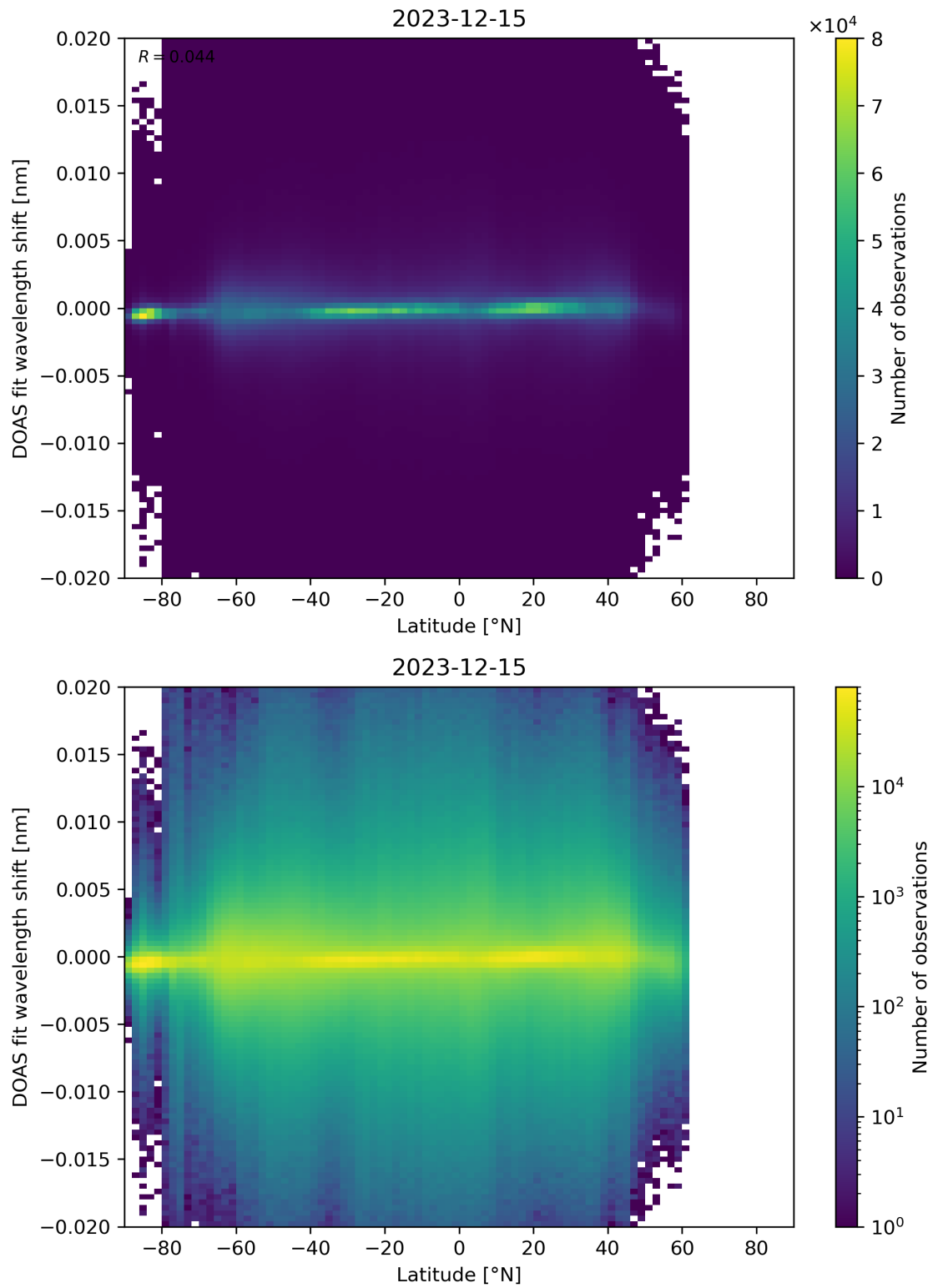
Figure 154: Scatter density plot of “Latitude” against “DOAS fit wavelength shift” for 2023-12-14 to 2023-12-16.
