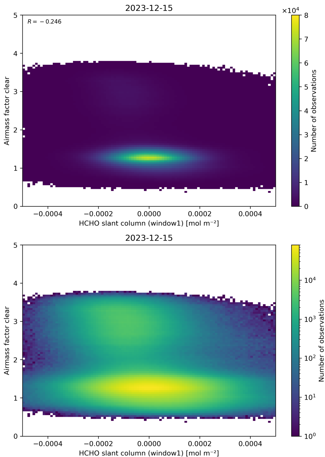
Figure 81: Scatter density plot of “HCHO slant column (window1)” against “Airmass factor clear” for 2023-12-14 to 2023-12-16.
