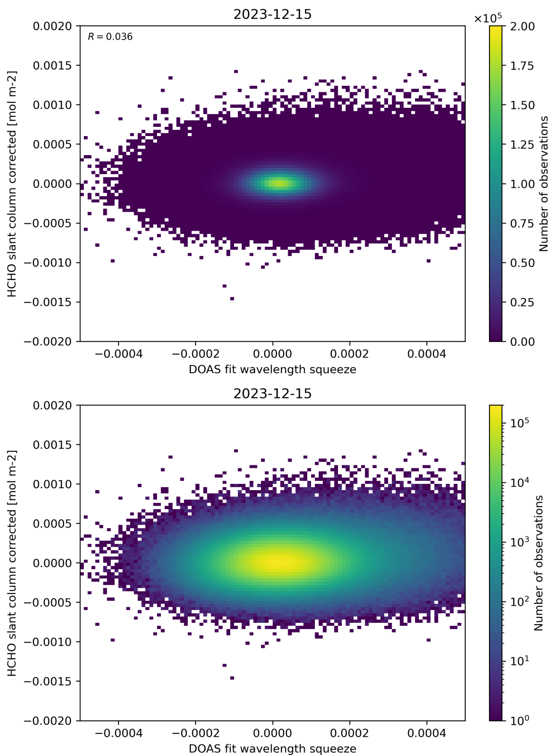
Figure 69: Scatter density plot of “DOAS fit wavelength squeeze” against “HCHO slant column corrected” for 2023-12-14 to 2023-12-16.
