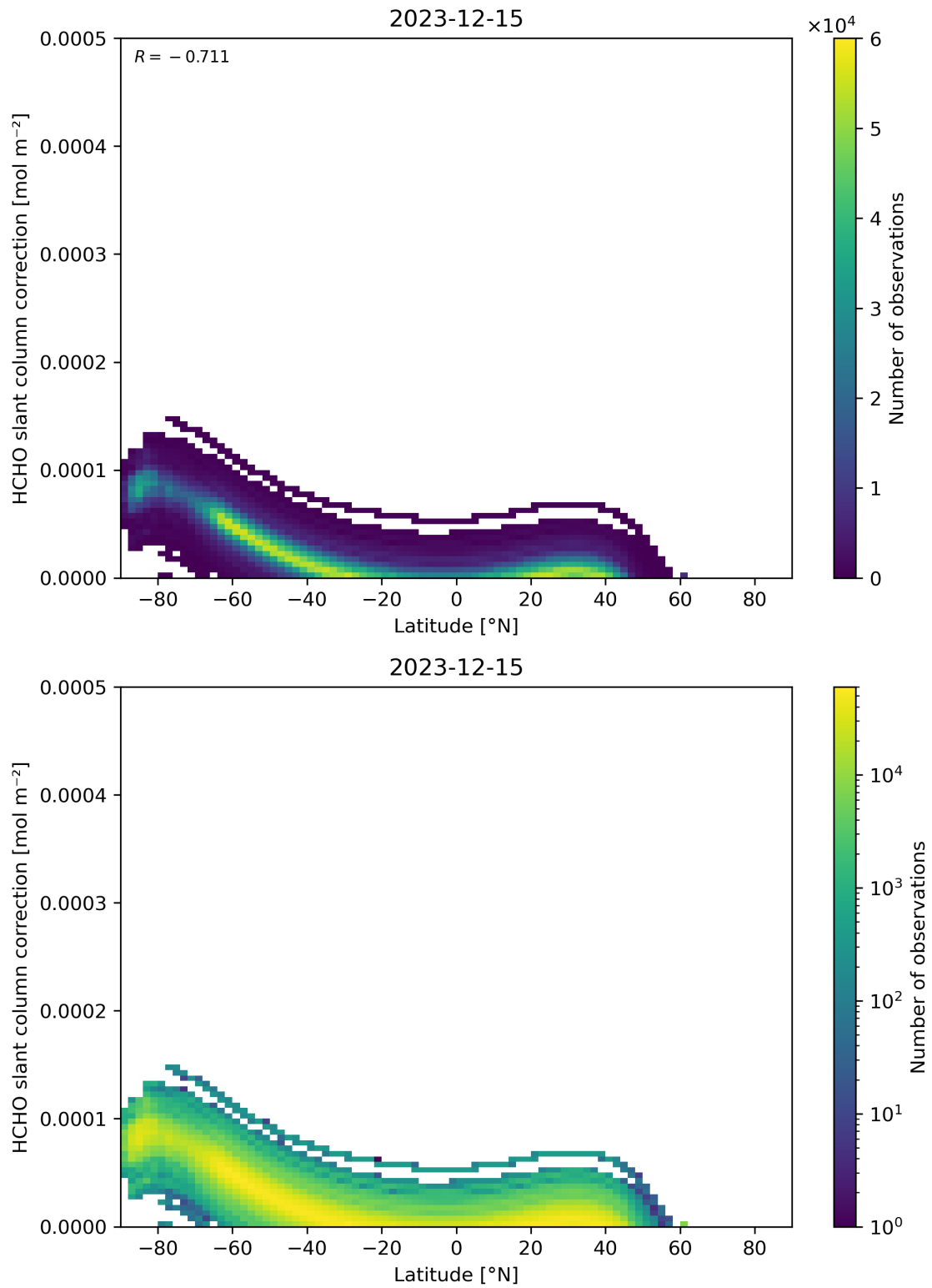
Figure 158: Scatter density plot of “Latitude” against “HCHO slant column correction” for 2023-12-14 to 2023-12-16.
