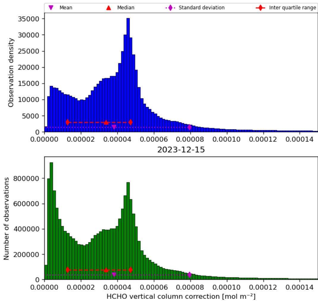
Figure 37: Histogram of “HCHO vertical column correction” for 2023-12-14 to 2023-12-16
