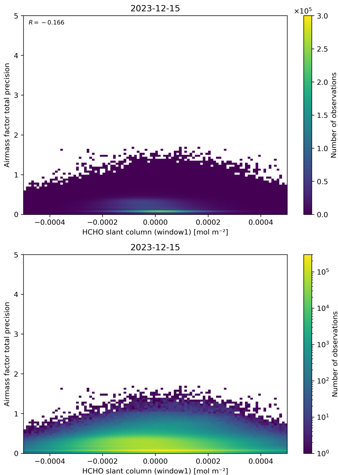
Figure 86: Scatter density plot of “HCHO slant column (window1)” against “Airmass factor total precision” for 2023-12-14 to 2023-12-16.
