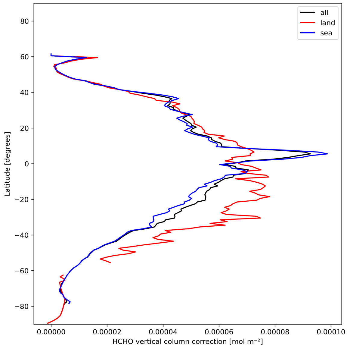
Figure 23: Zonal average of “HCHO vertical column correction” for 2023-12-14 to 2023-12-16.
