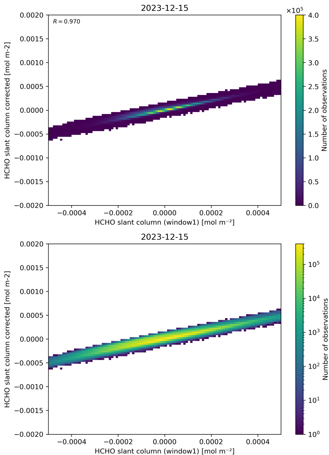
Figure 82: Scatter density plot of “HCHO slant column (window1)” against “HCHO slant column corrected” for 2023-12-14 to 2023-12-16.
