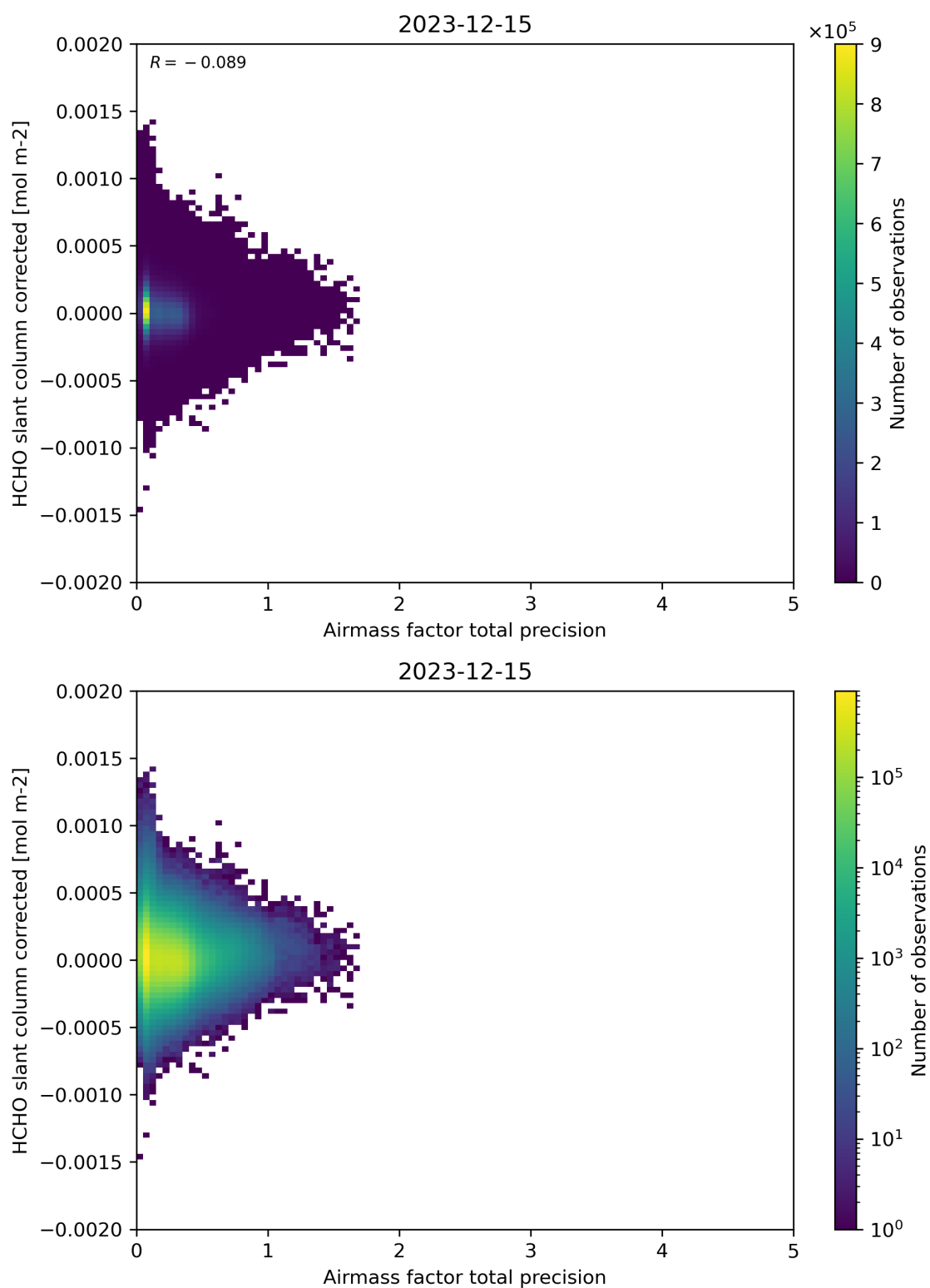
Figure 109: Scatter density plot of “Airmass factor total precision” against “HCHO slant column corrected” for 2023-12-14 to 2023-12-16.
