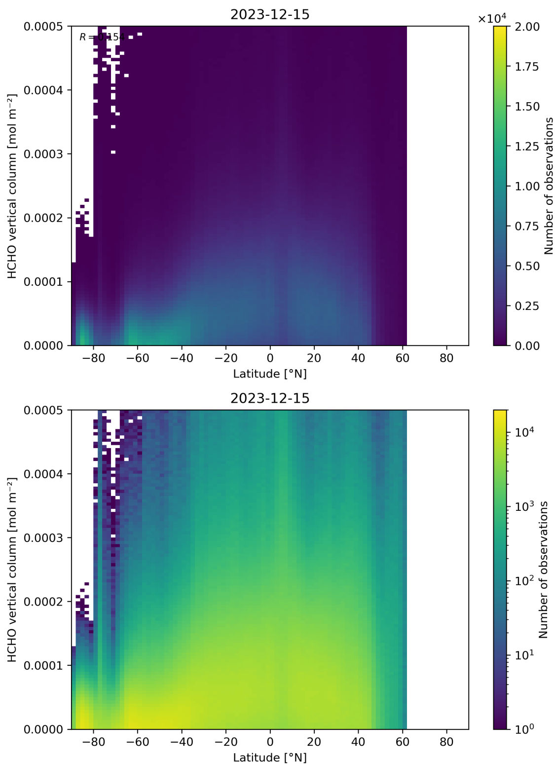
Figure 163: Scatter density plot of “Latitude” against “HCHO vertical column” for 2023-12-14 to 2023-12-16.
