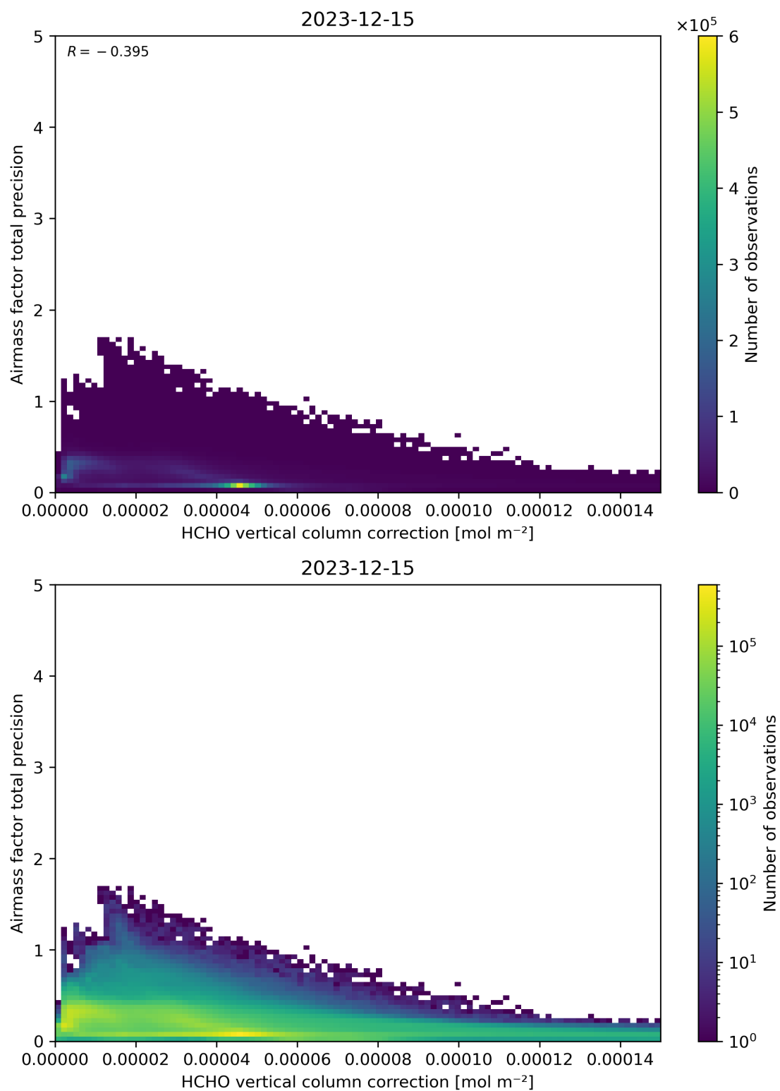
Figure 121: Scatter density plot of “HCHO vertical column correction” against “Airmass factor total precision” for 2023-12-14 to 2023-12-16.
