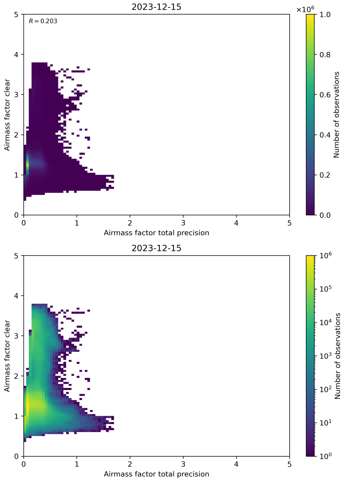
Figure 108: Scatter density plot of “Airmass factor total precision” against “Airmass factor clear” for 2023-12-14 to 2023-12-16.
