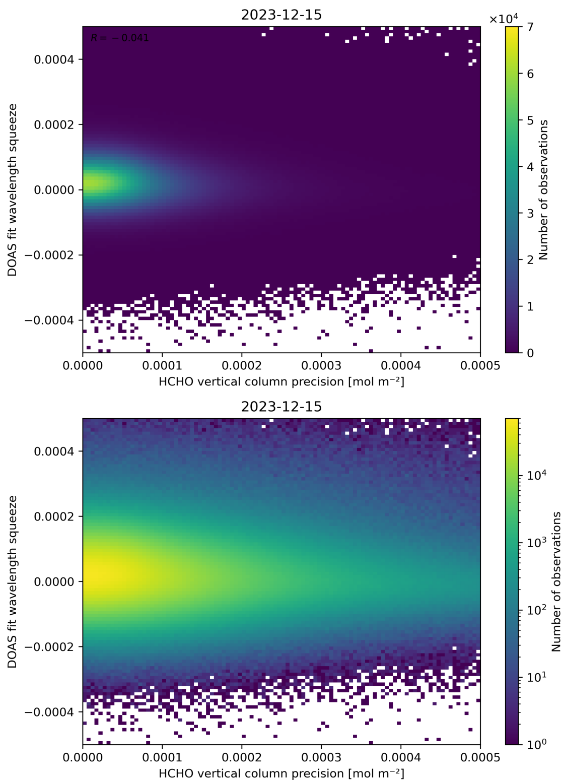
Figure 138: Scatter density plot of “HCHO vertical column precision” against “DOAS fit wavelength squeeze” for 2023-12-14 to 2023-12-16.
