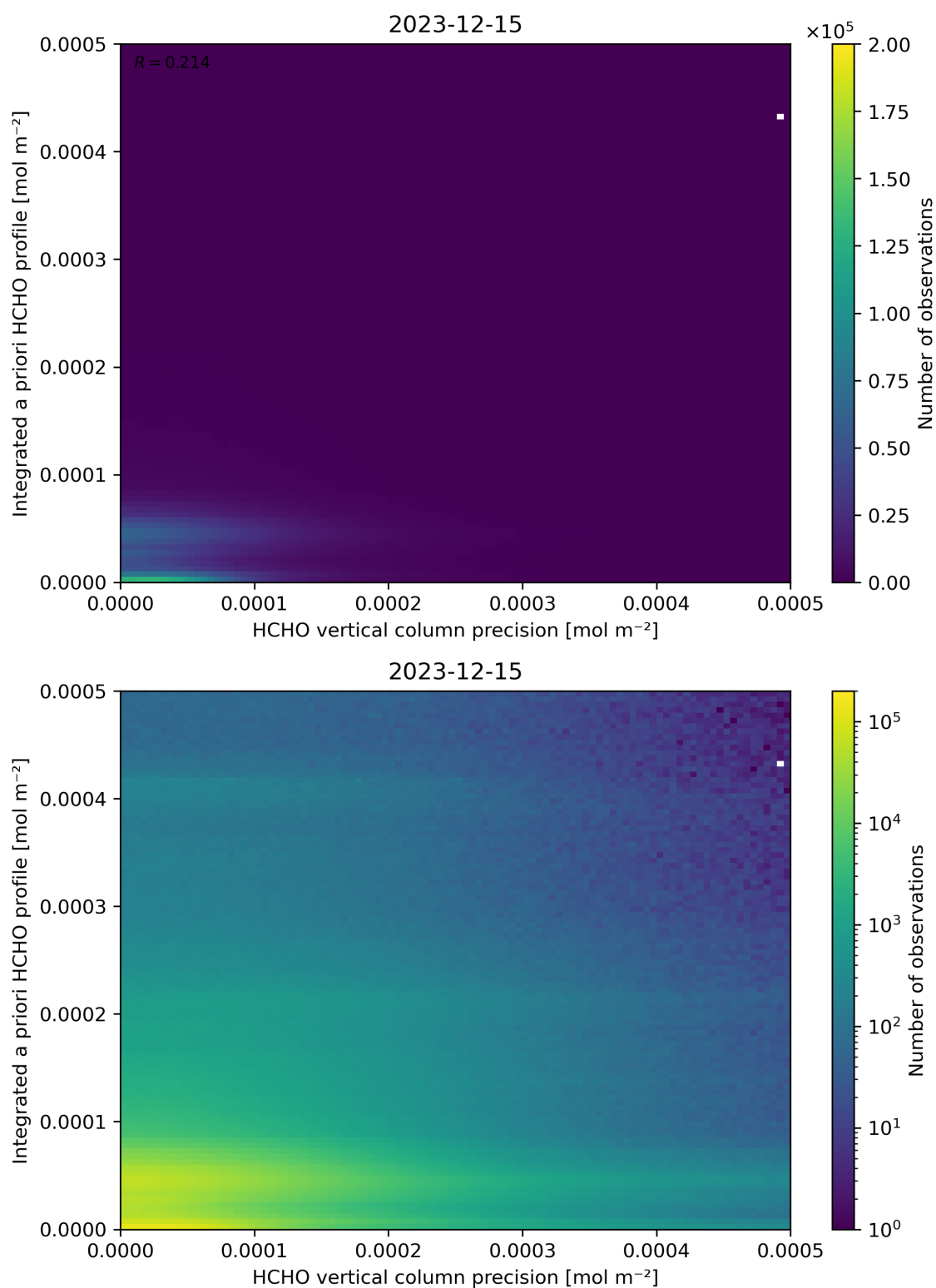
Figure 147: Scatter density plot of “HCHO vertical column precision” against “Integrated a priori HCHO profile” for 2023-12-14 to 2023-12-16.
