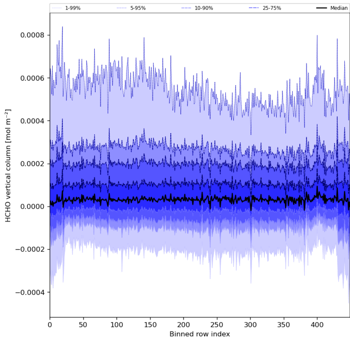
Figure 49: Along track statistics of “HCHO vertical column” for 2023-12-14 to 2023-12-16
