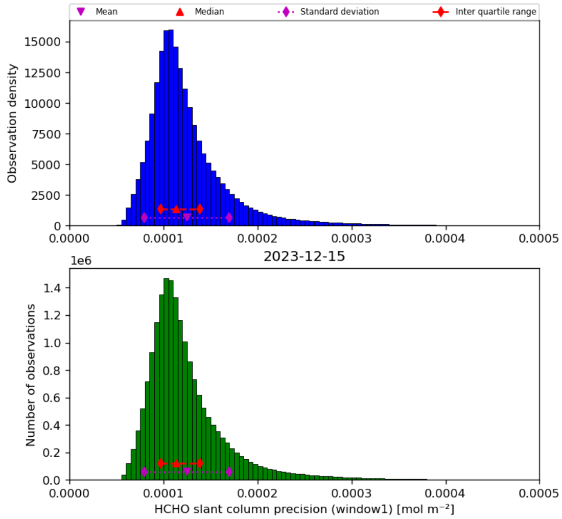
Figure 39: Histogram of “HCHO slant column precision (window1)” for 2023-12-14 to 2023-12-16
