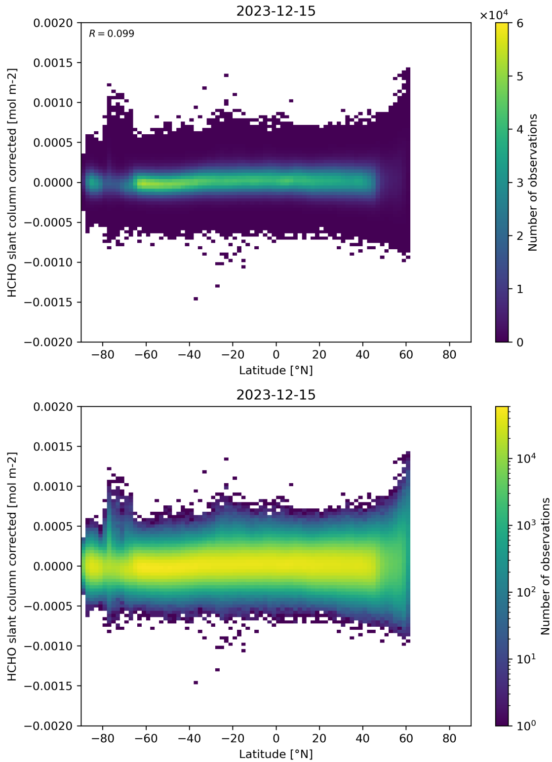
Figure 157: Scatter density plot of “Latitude” against “HCHO slant column corrected” for 2023-12-14 to 2023-12-16.
