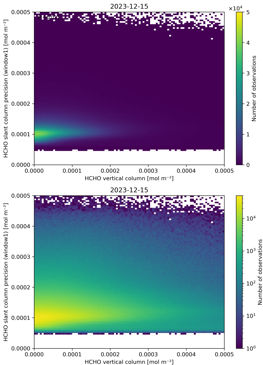
Figure 130: Scatter density plot of “HCHO vertical column” against “HCHO slant column precision (window1)” for 2023-12-14 to 2023-12-16.
