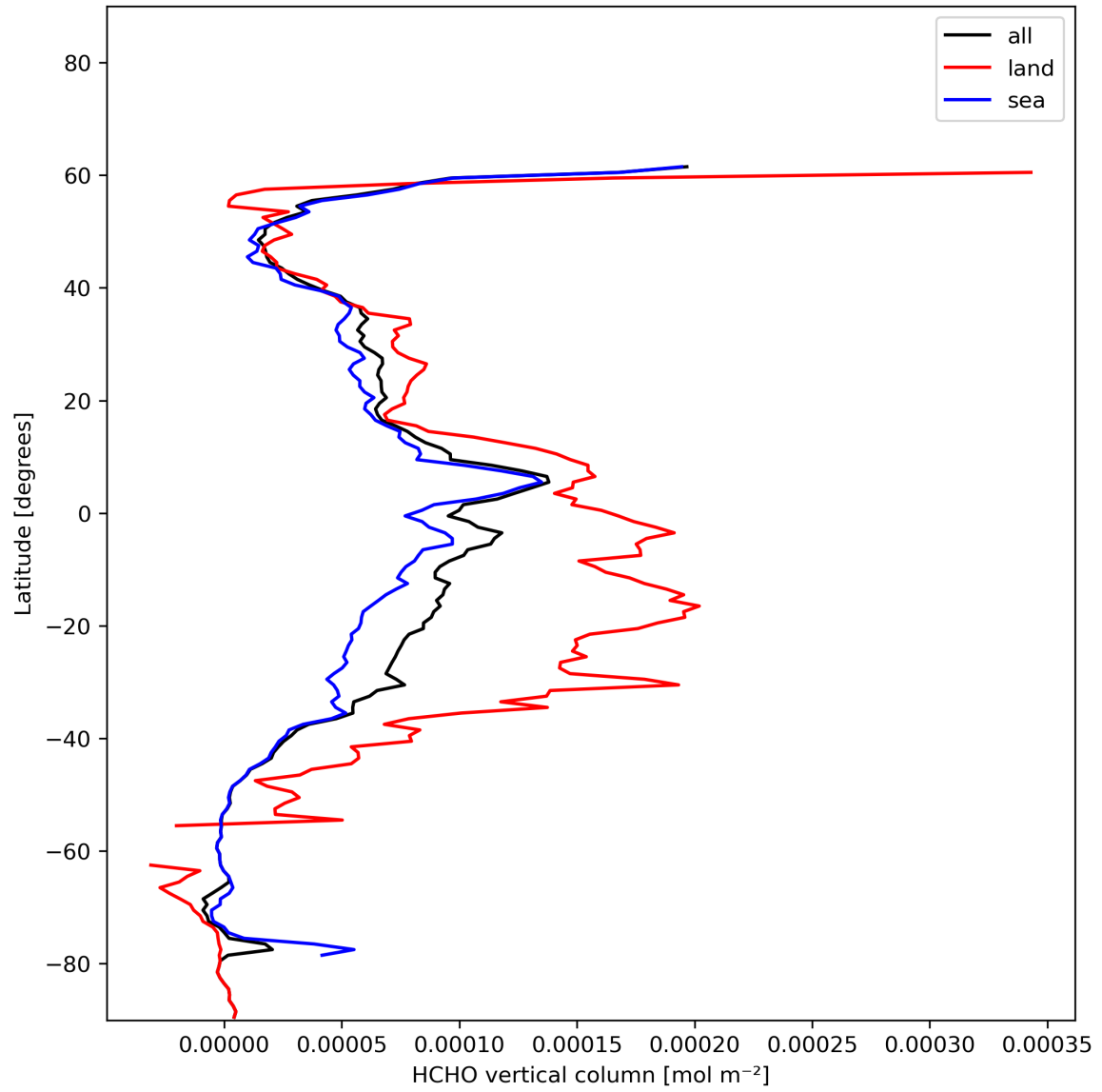
Figure 21: Zonal average of “HCHO vertical column” for 2023-12-14 to 2023-12-16.
