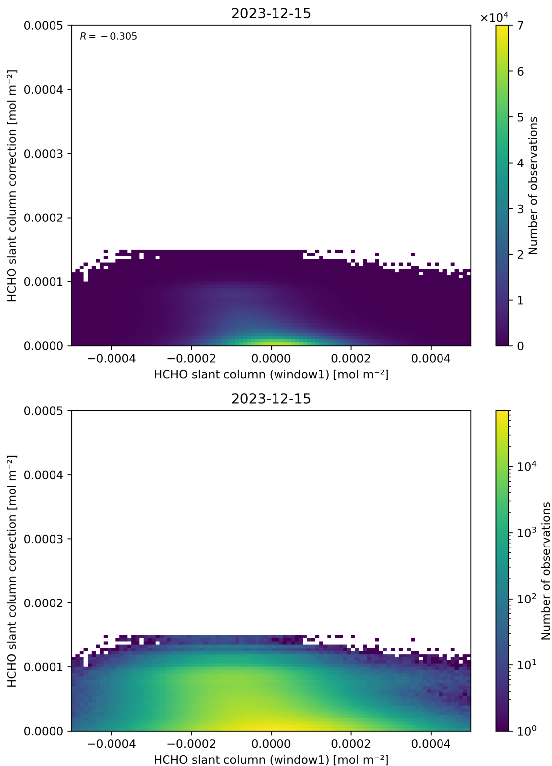
Figure 83: Scatter density plot of “HCHO slant column (window1)” against “HCHO slant column correction” for 2023-12-14 to 2023-12-16.
