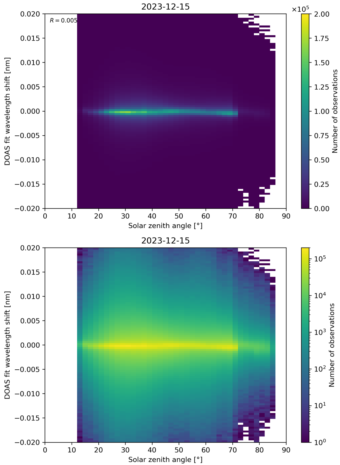
Figure 168: Scatter density plot of “Solar zenith angle” against “DOAS fit wavelength shift” for 2023-12-14 to 2023-12-16.
