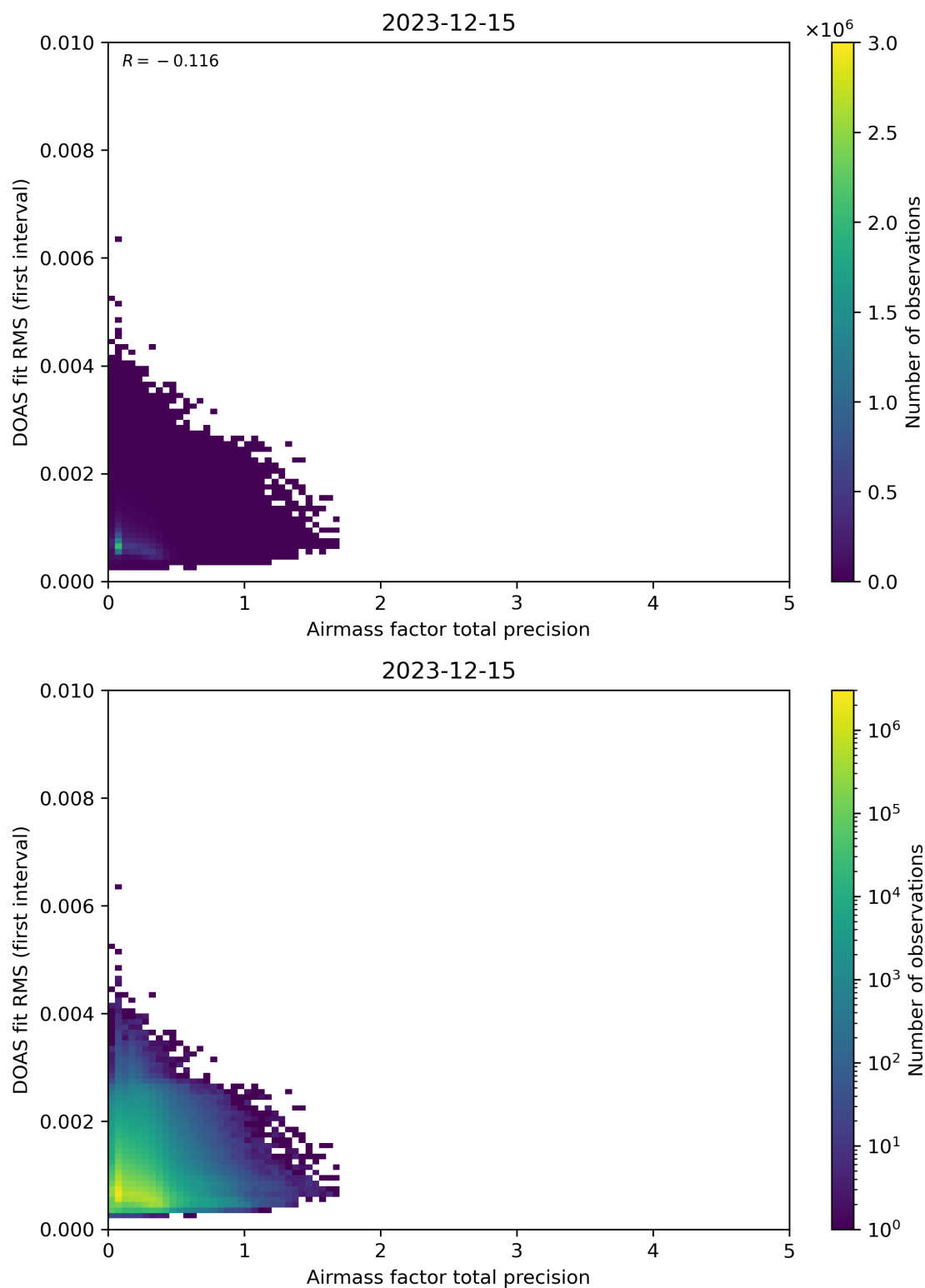
Figure 105: Scatter density plot of “Airmass factor total precision” against “DOAS fit RMS (first interval)” for 2023-12-14 to 2023-12-16.
