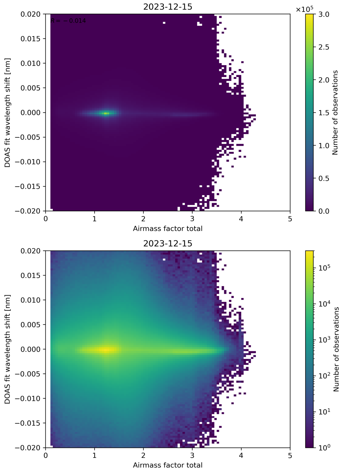
Figure 98: Scatter density plot of “Airmass factor total” against “DOAS fit wavelength shift” for 2023-12-14 to 2023-12-16.
