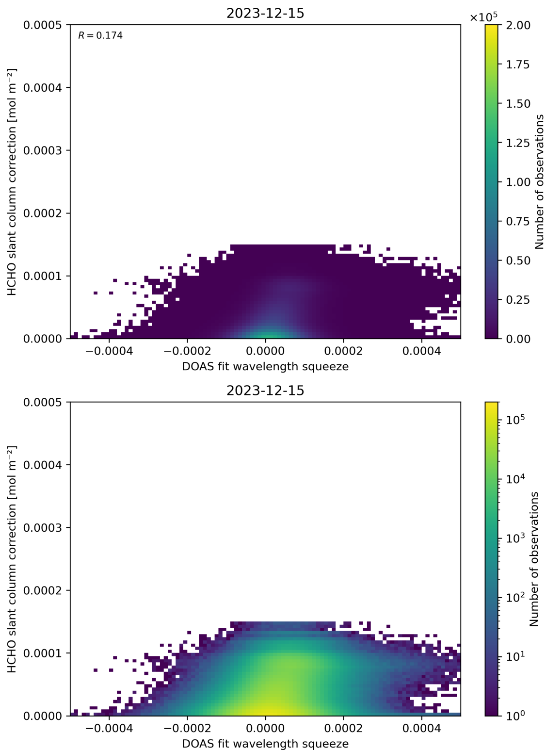
Figure 70: Scatter density plot of “DOAS fit wavelength squeeze” against “HCHO slant column correction” for 2023-12-14 to 2023-12-16.
