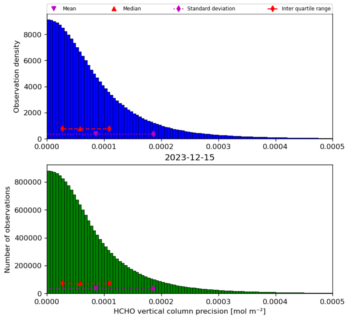
Figure 36: Histogram of “HCHO vertical column precision” for 2023-12-14 to 2023-12-16
