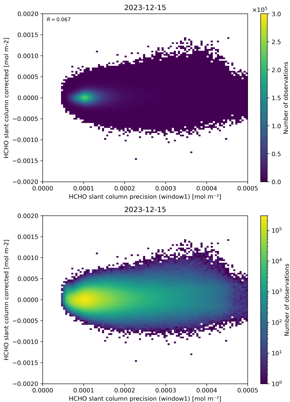
Figure 92: Scatter density plot of “HCHO slant column precision (window1)” against “HCHO slant column corrected” for 2023-12-14 to 2023-12-16.
