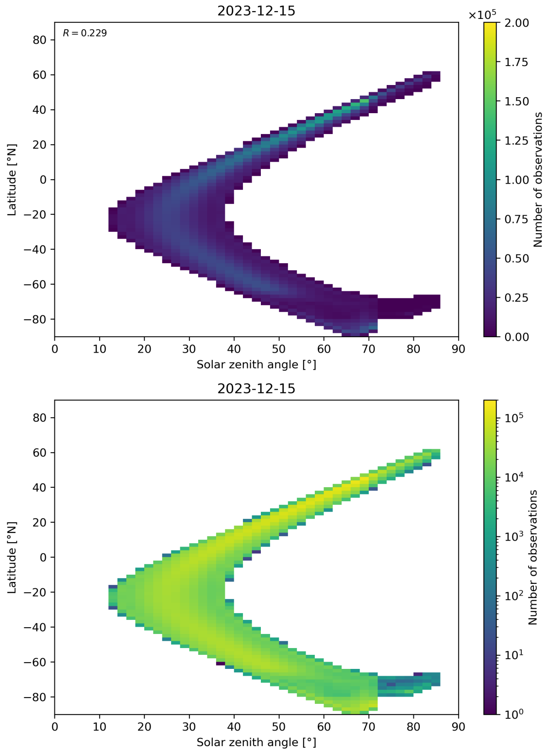
Figure 181: Scatter density plot of “Solar zenith angle” against “Latitude” for 2023-12-14 to 2023-12-16.
