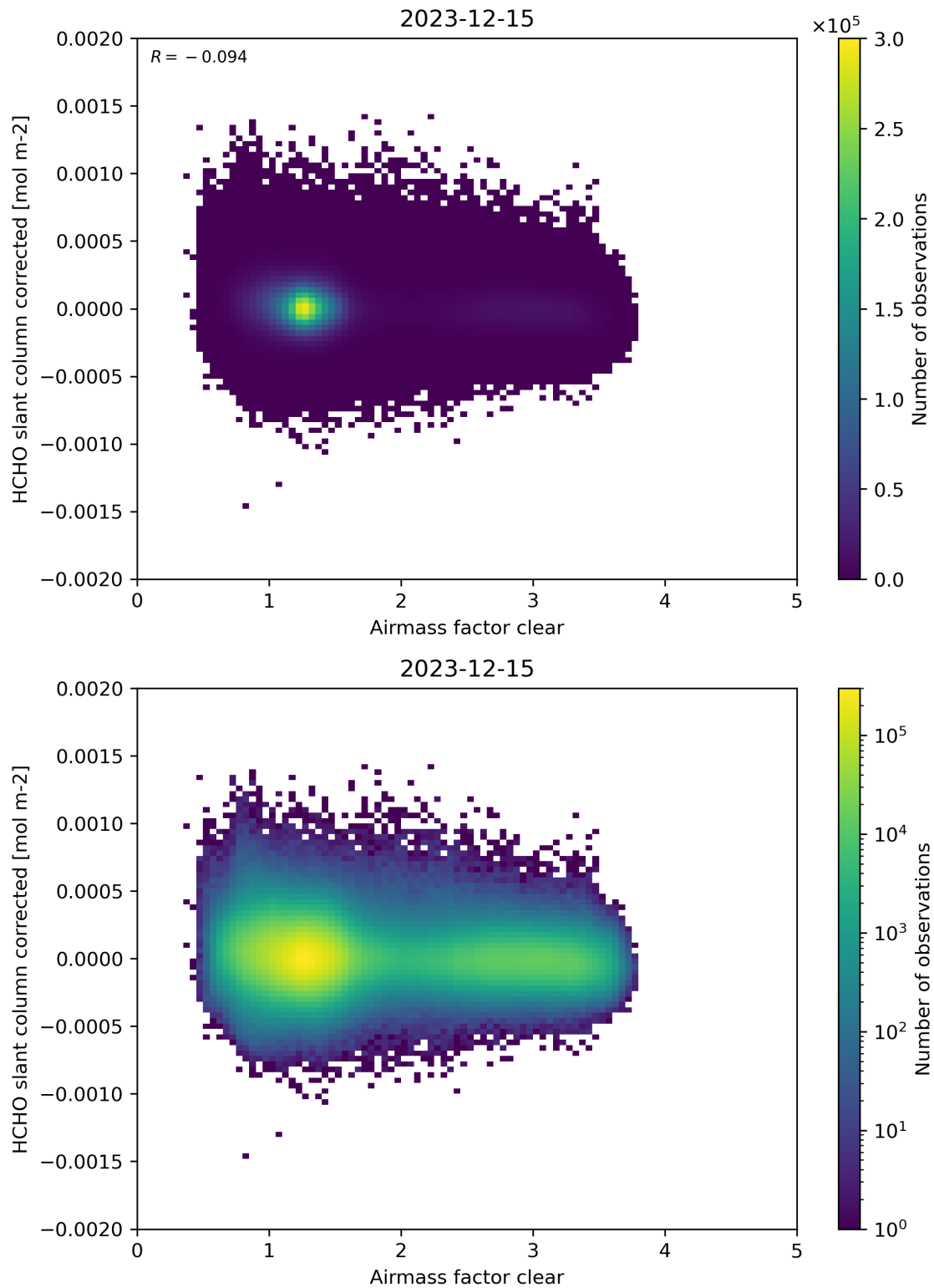
Figure 74: Scatter density plot of “Airmass factor clear” against “HCHO slant column corrected” for 2023-12-14 to 2023-12-16.
