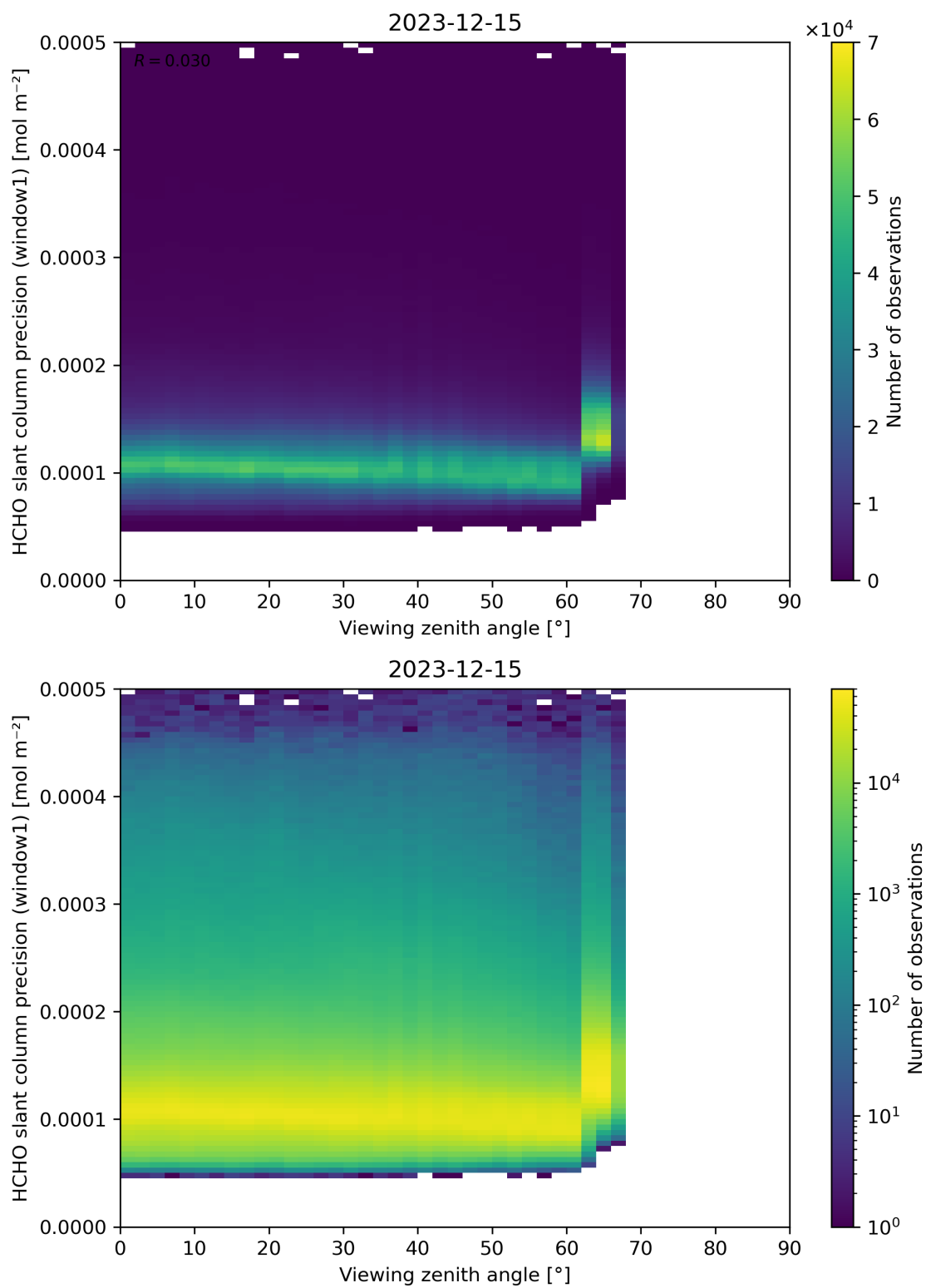
Figure 189: Scatter density plot of “Viewing zenith angle” against “HCHO slant column precision (window1)” for 2023-12-14 to 2023-12-16.
