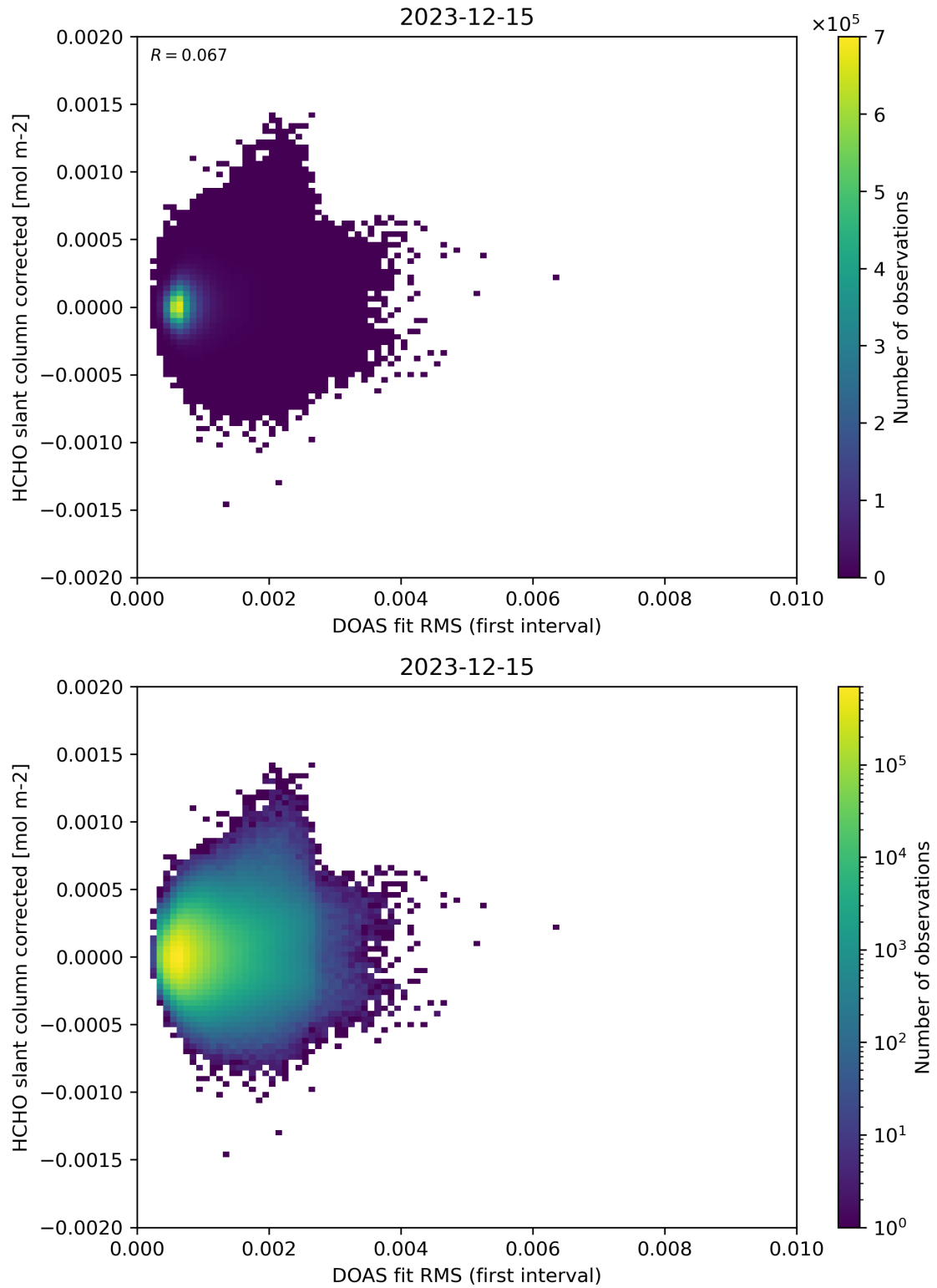
Figure 62: Scatter density plot of “DOAS fit RMS (first interval)” against “HCHO slant column corrected” for 2023-12-14 to 2023-12-16.
