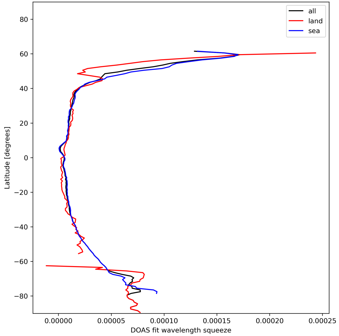
Figure 31: Zonal average of “DOAS fit wavelength squeeze” for 2023-12-14 to 2023-12-16.
