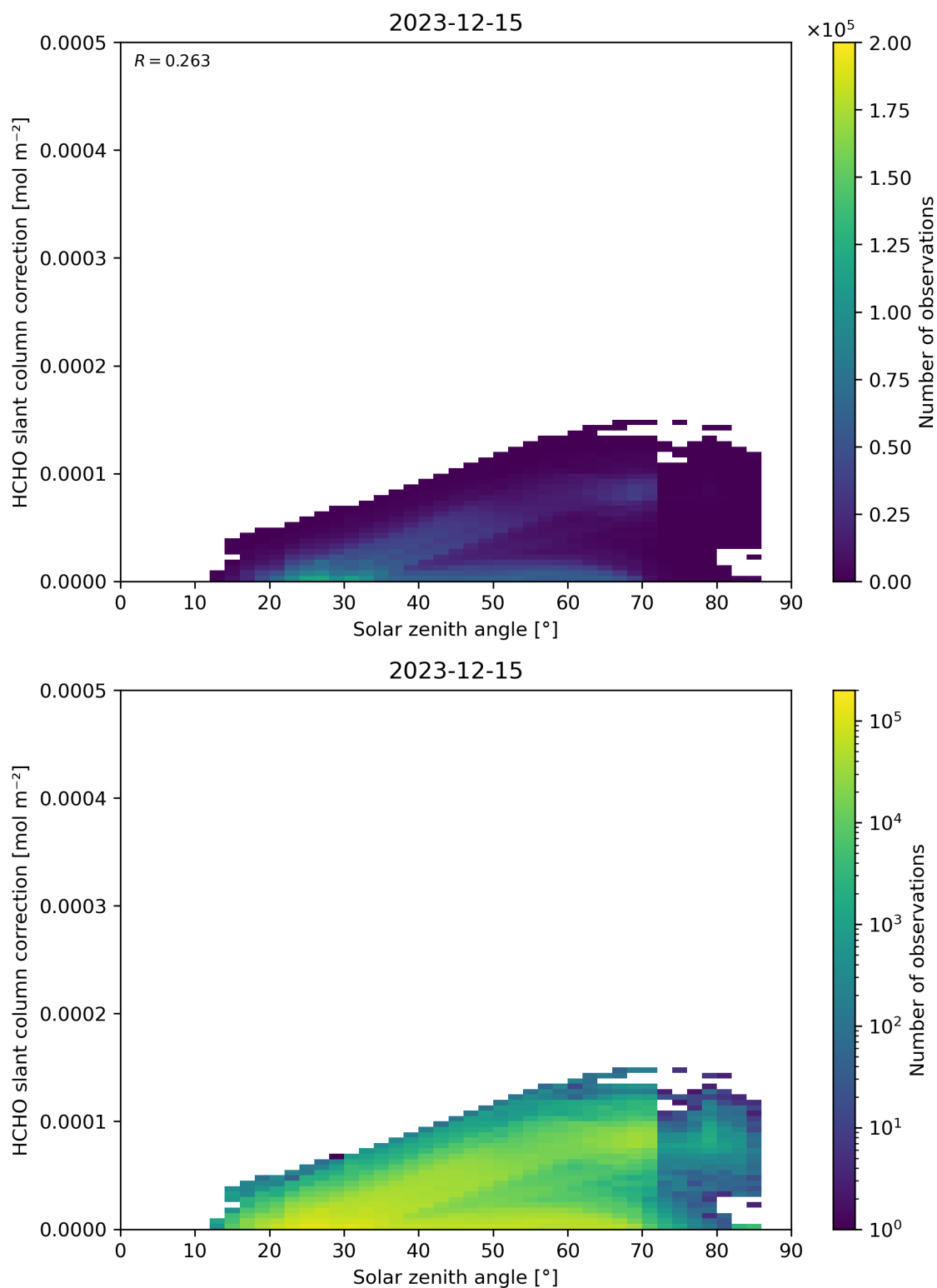
Figure 172: Scatter density plot of “Solar zenith angle” against “HCHO slant column correction” for 2023-12-14 to 2023-12-16.
