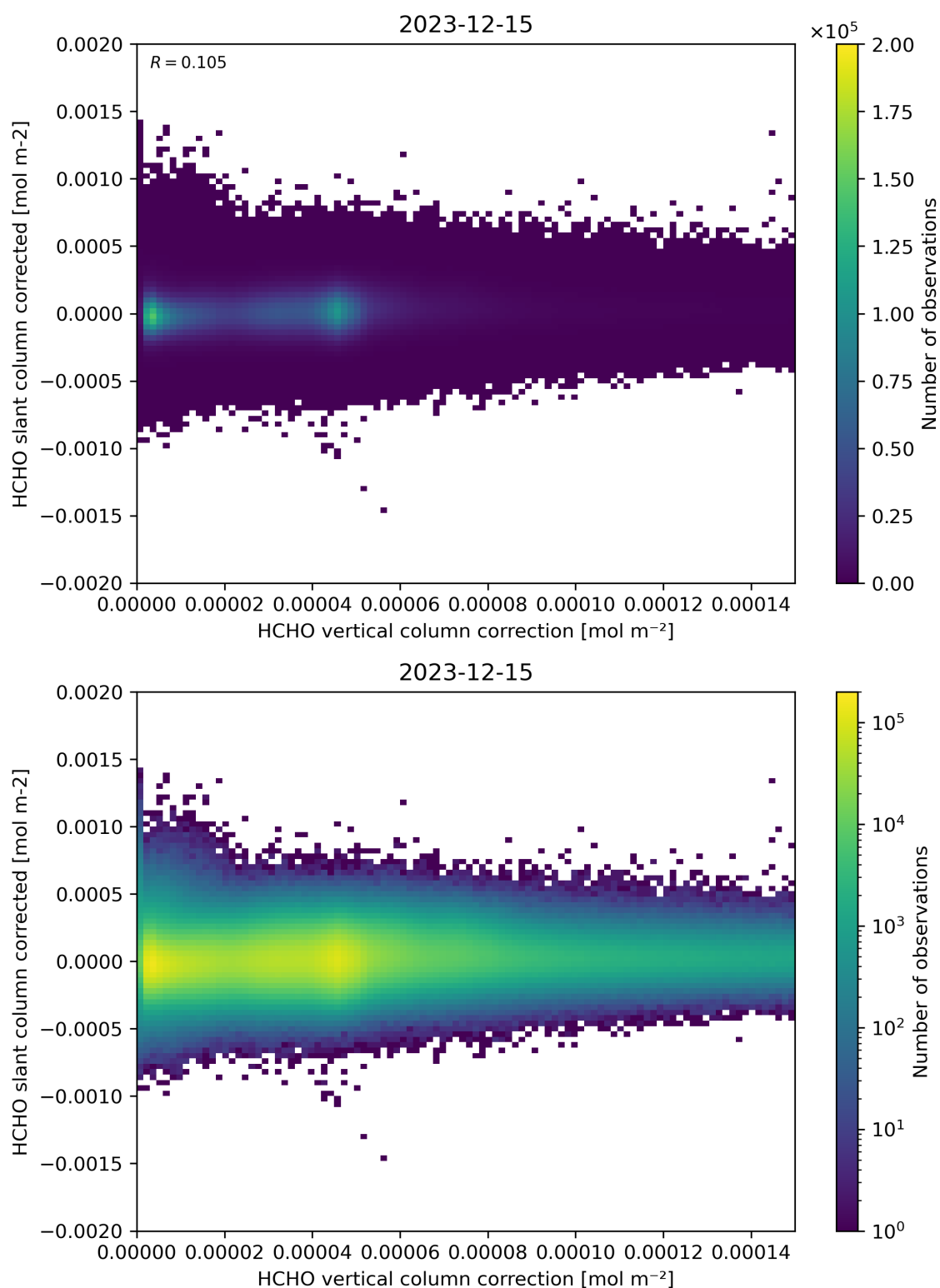
Figure 116: Scatter density plot of “HCHO vertical column correction” against “HCHO slant column corrected” for 2023-12-14 to 2023-12-16.
