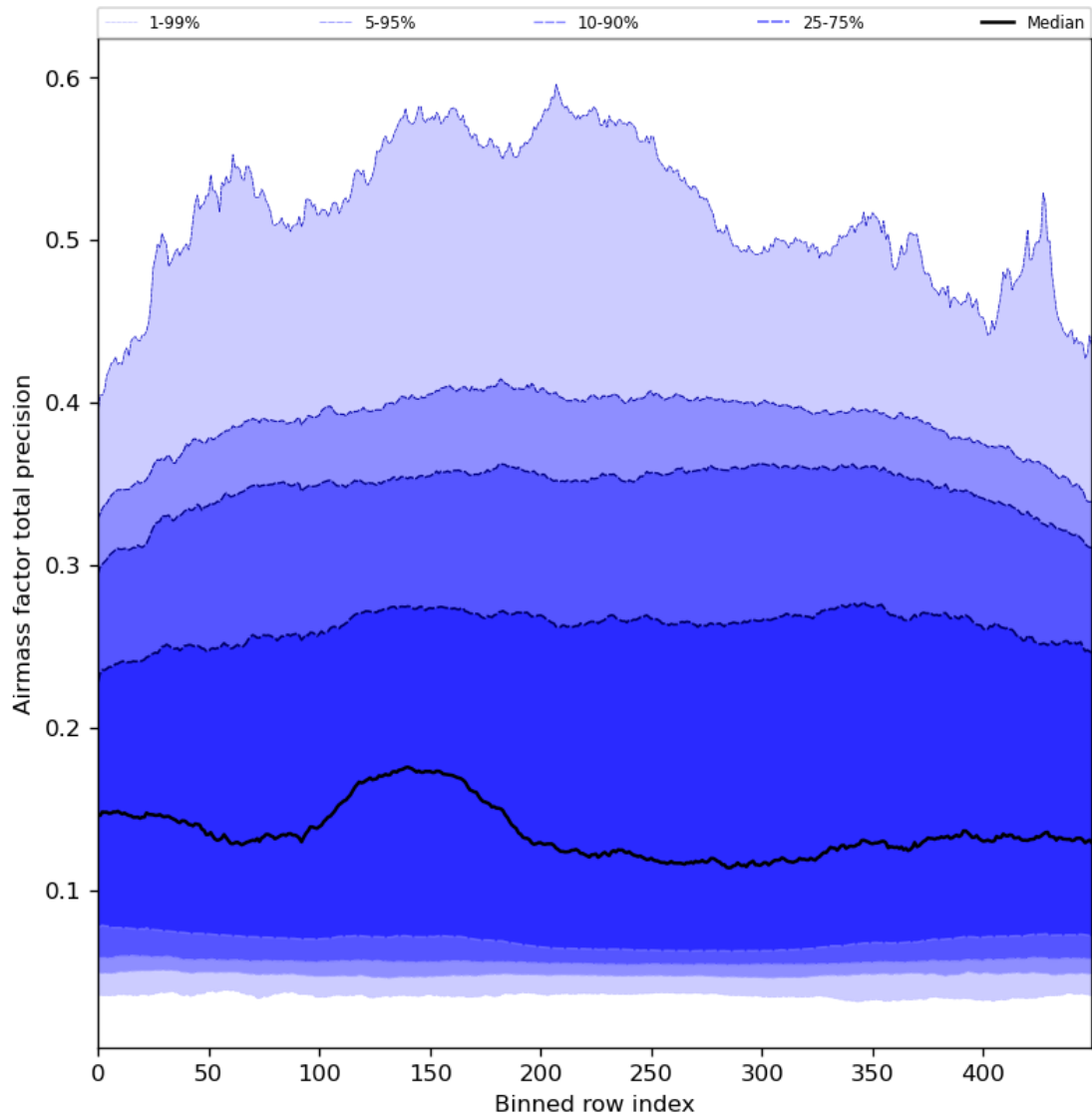
Figure 55: Along track statistics of “Airmass factor total precision” for 2023-12-14 to 2023-12-16
