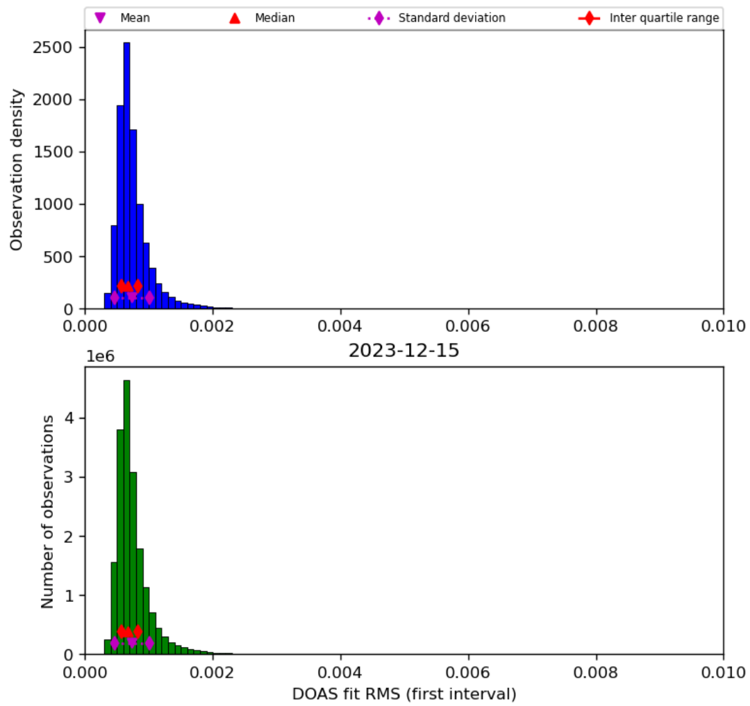
Figure 46: Histogram of “DOAS fit RMS (first interval)” for 2023-12-14 to 2023-12-16
