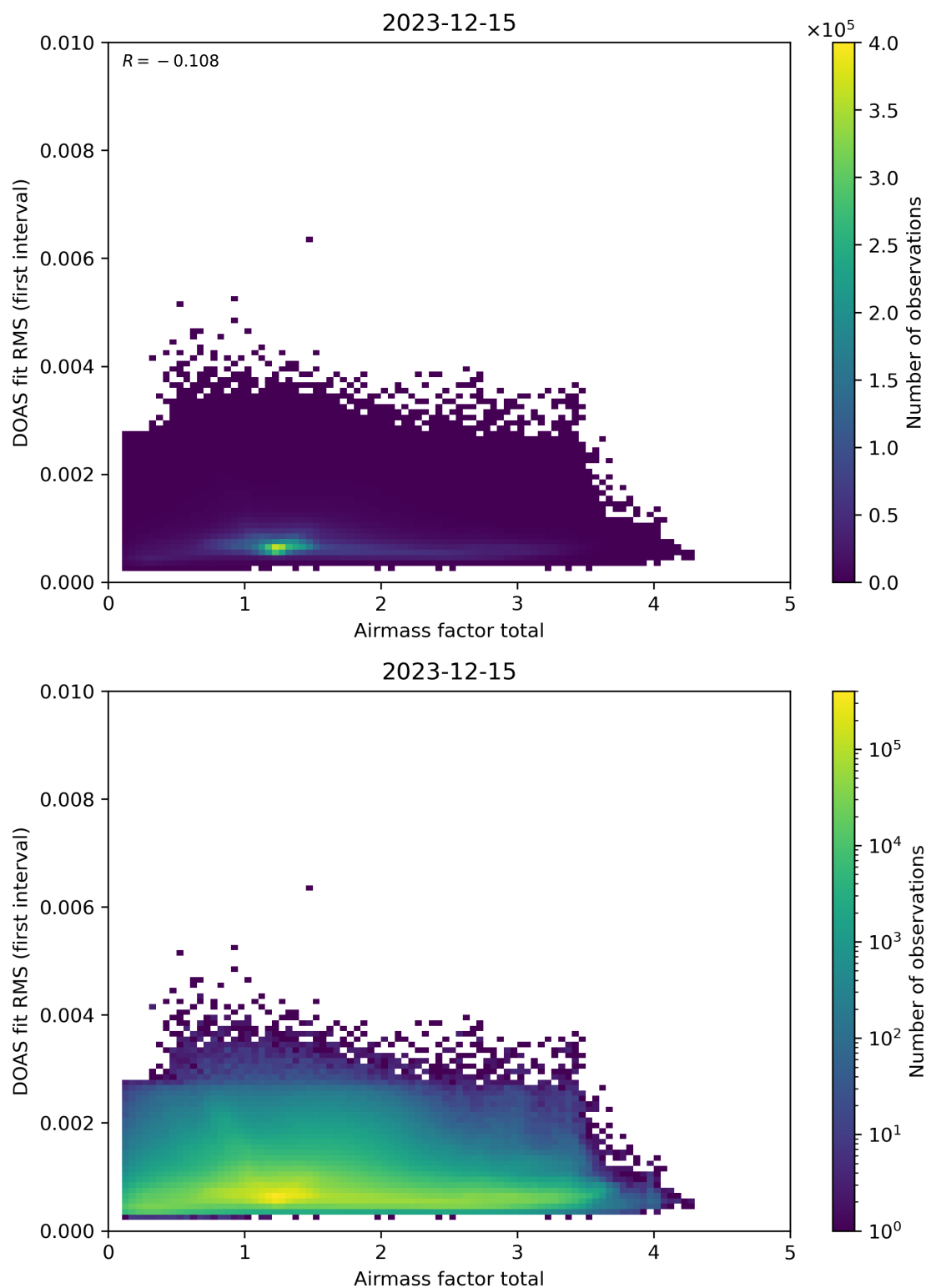
Figure 97: Scatter density plot of “Airmass factor total” against “DOAS fit RMS (first interval)” for 2023-12-14 to 2023-12-16.
