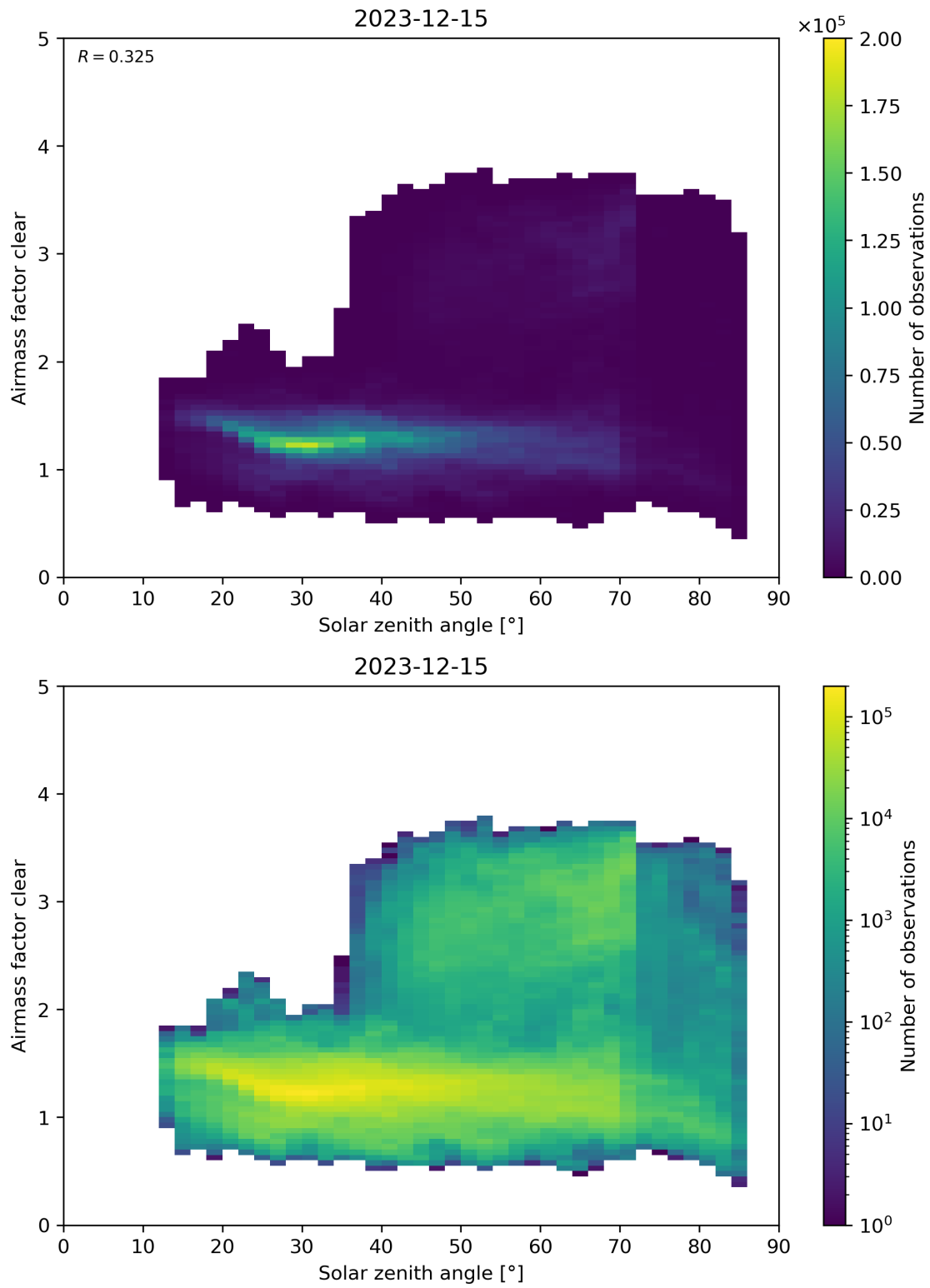
Figure 170: Scatter density plot of “Solar zenith angle” against “Airmass factor clear” for 2023-12-14 to 2023-12-16.
