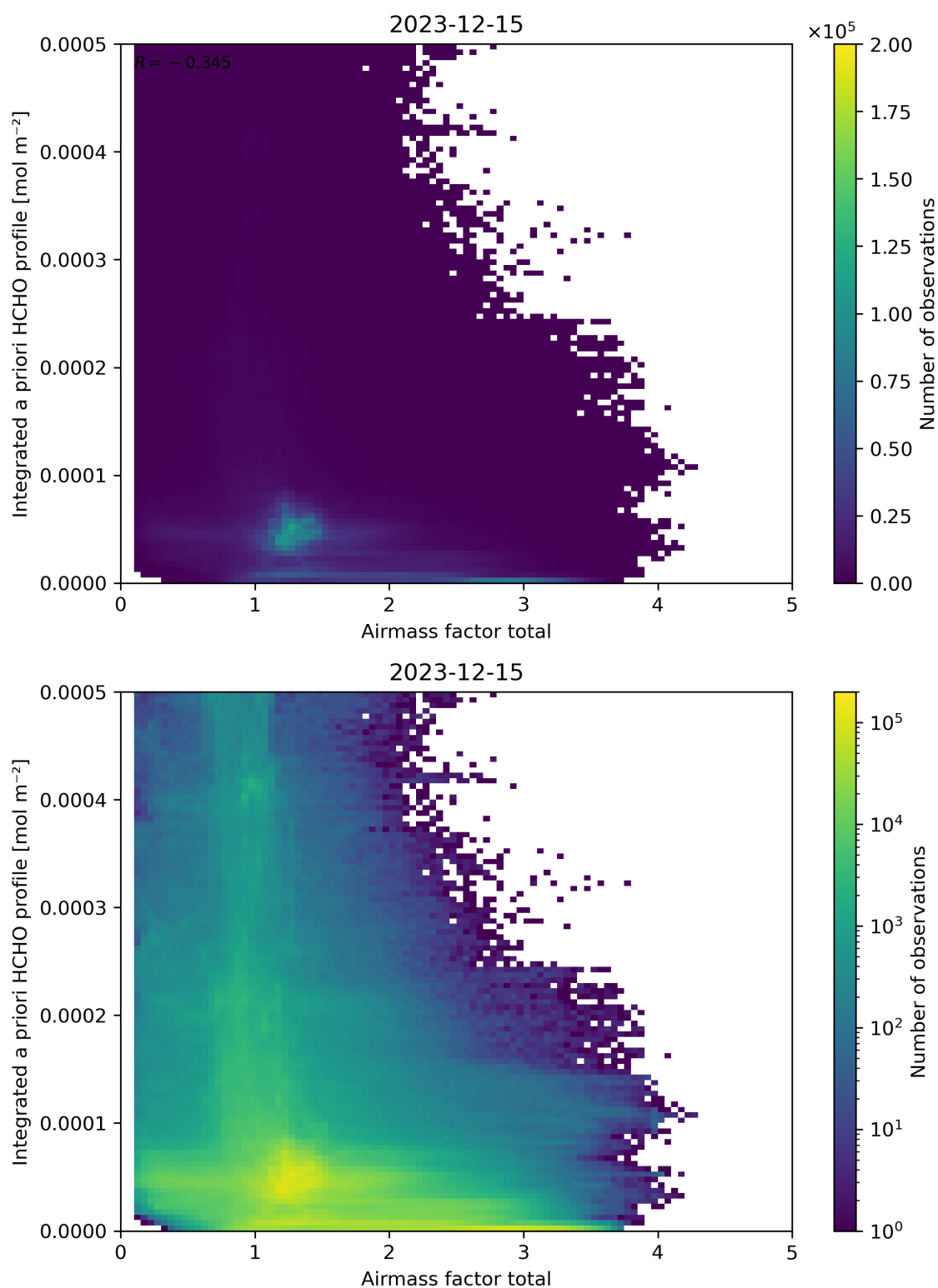
Figure 104: Scatter density plot of “Airmass factor total” against “Integrated a priori HCHO profile” for 2023-12-14 to 2023-12-16.
