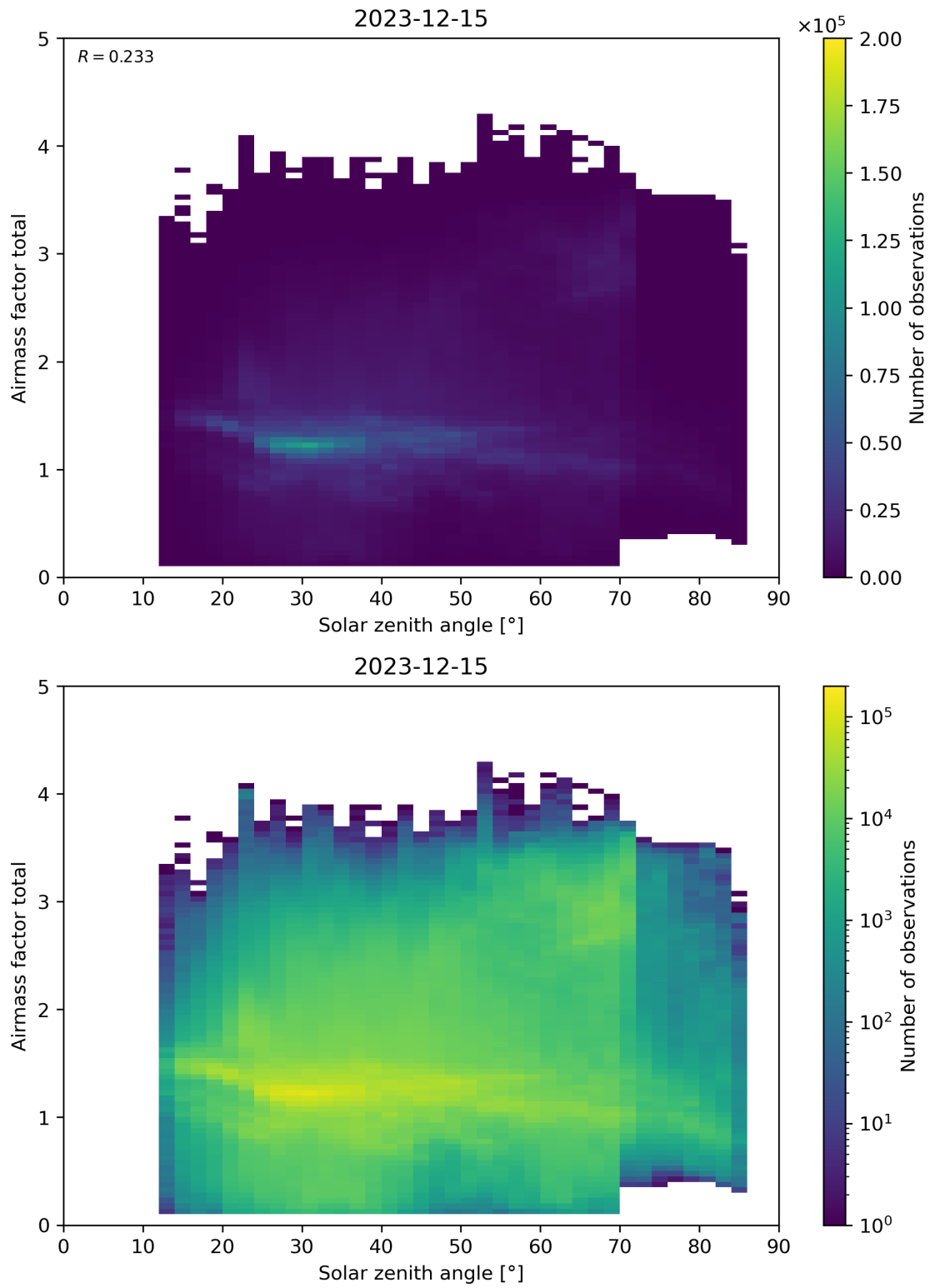
Figure 175: Scatter density plot of “Solar zenith angle” against “Airmass factor total” for 2023-12-14 to 2023-12-16.
