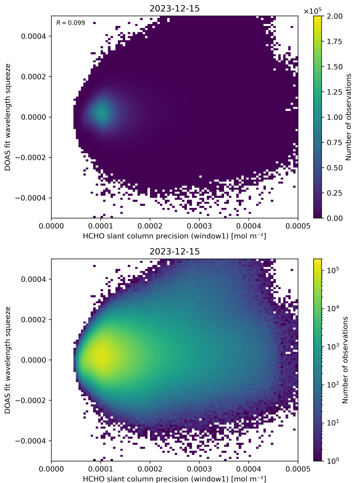
Figure 90: Scatter density plot of “HCHO slant column precision (window1)” against “DOAS fit wavelength squeeze” for 2023-12-14 to 2023-12-16.
