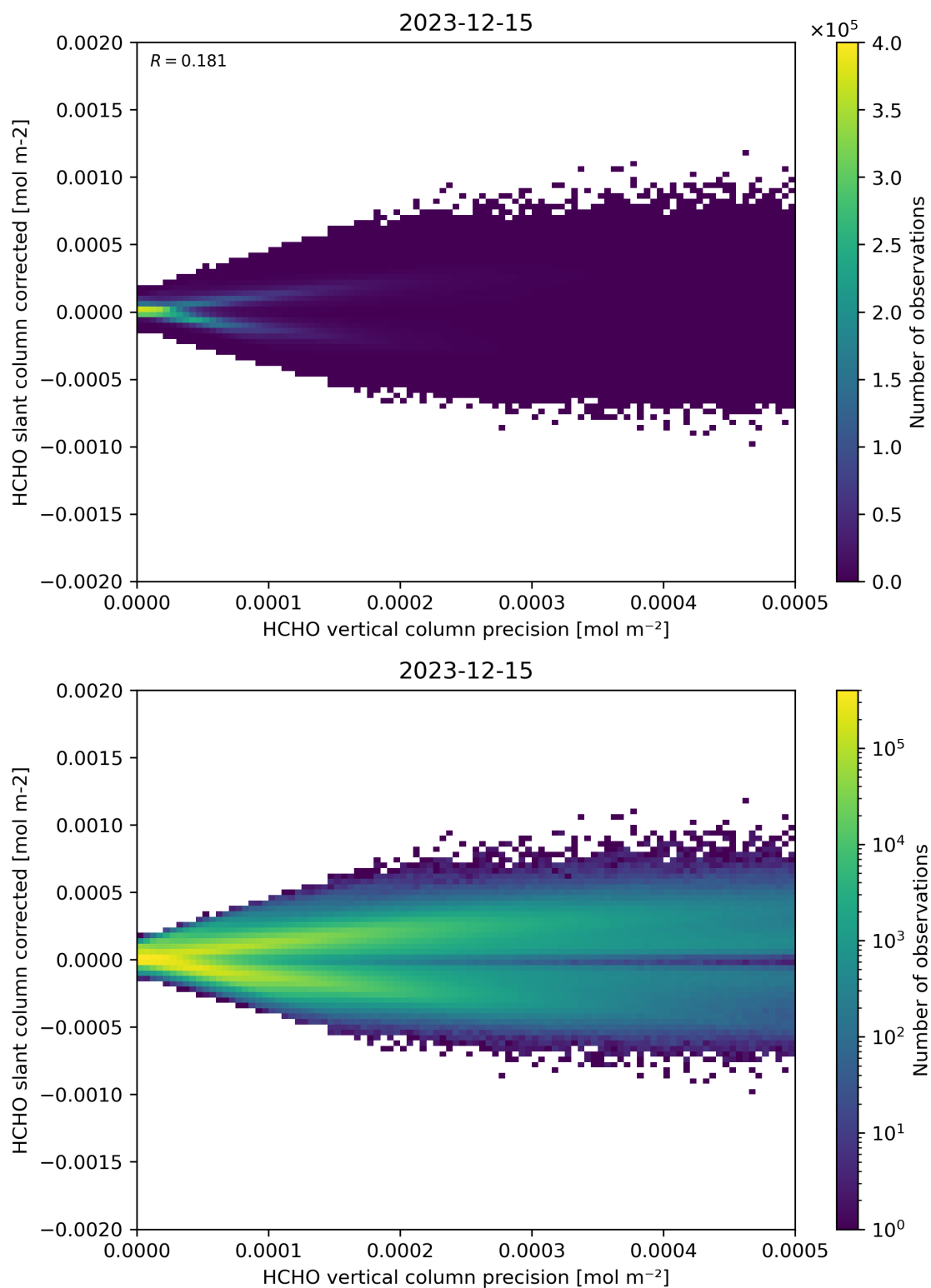
Figure 140: Scatter density plot of “HCHO vertical column precision” against “HCHO slant column corrected” for 2023-12-14 to 2023-12-16.
