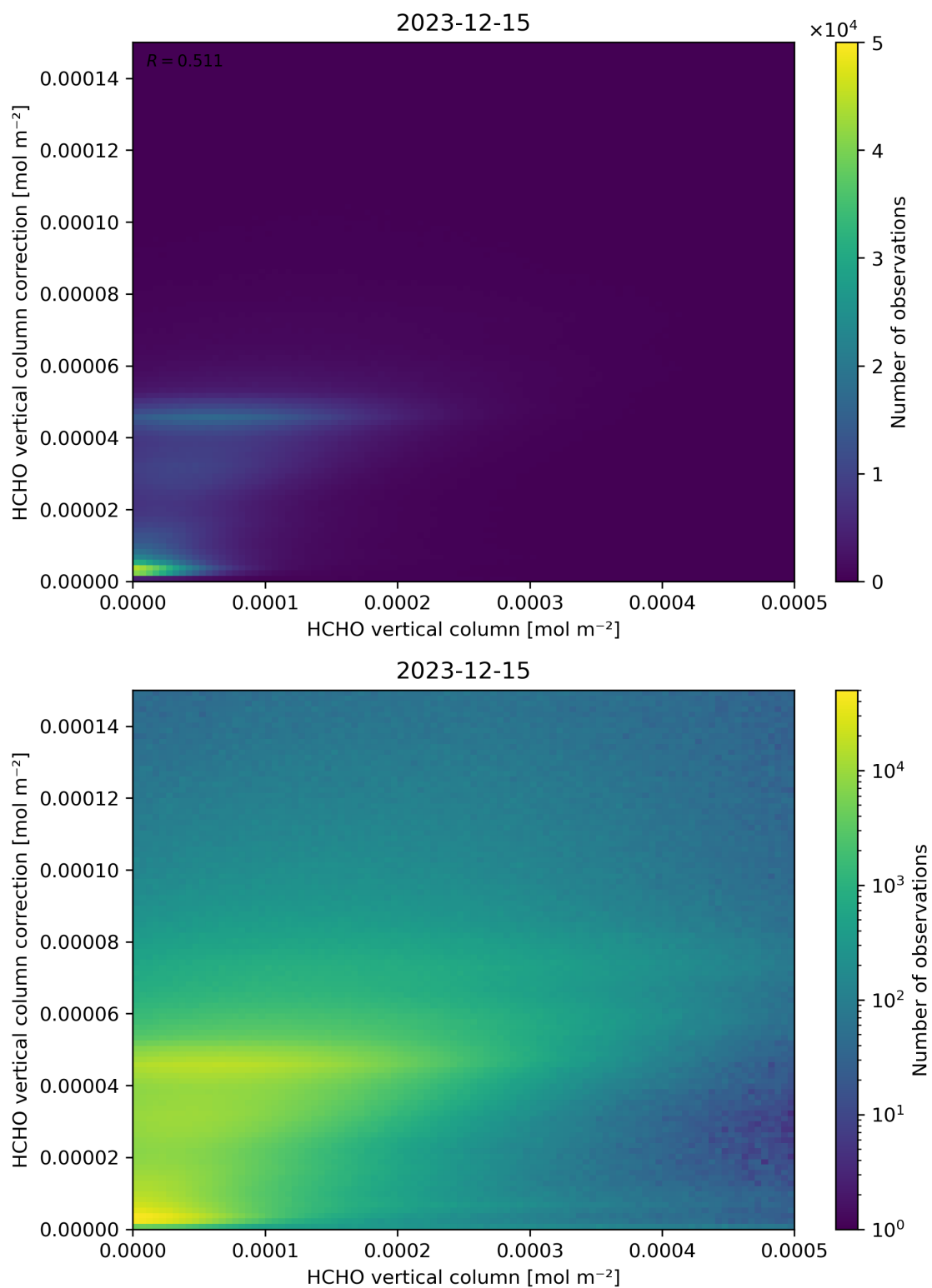
Figure 133: Scatter density plot of “HCHO vertical column” against “HCHO vertical column correction” for 2023-12-14 to 2023-12-16.
