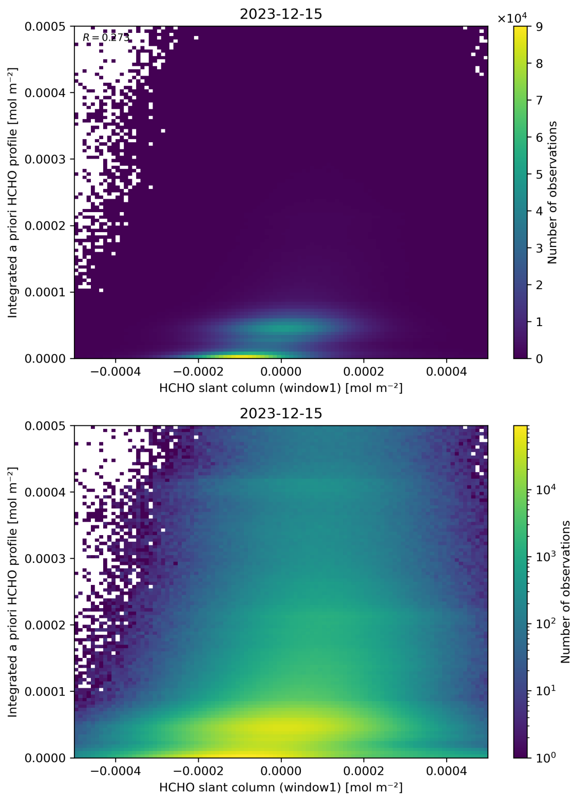
Figure 87: Scatter density plot of “HCHO slant column (window1)” against “Integrated a priori HCHO profile” for 2023-12-14 to 2023-12-16.
