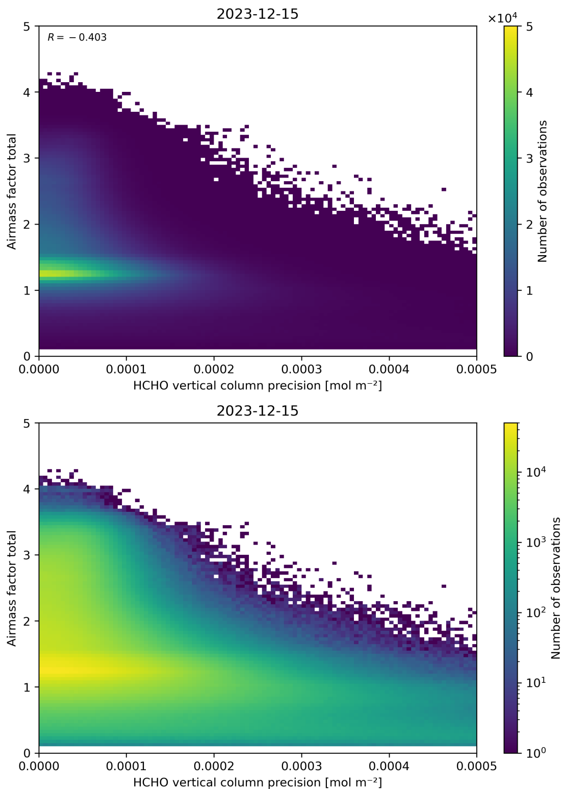
Figure 144: Scatter density plot of “HCHO vertical column precision” against “Airmass factor total” for 2023-12-14 to 2023-12-16.
