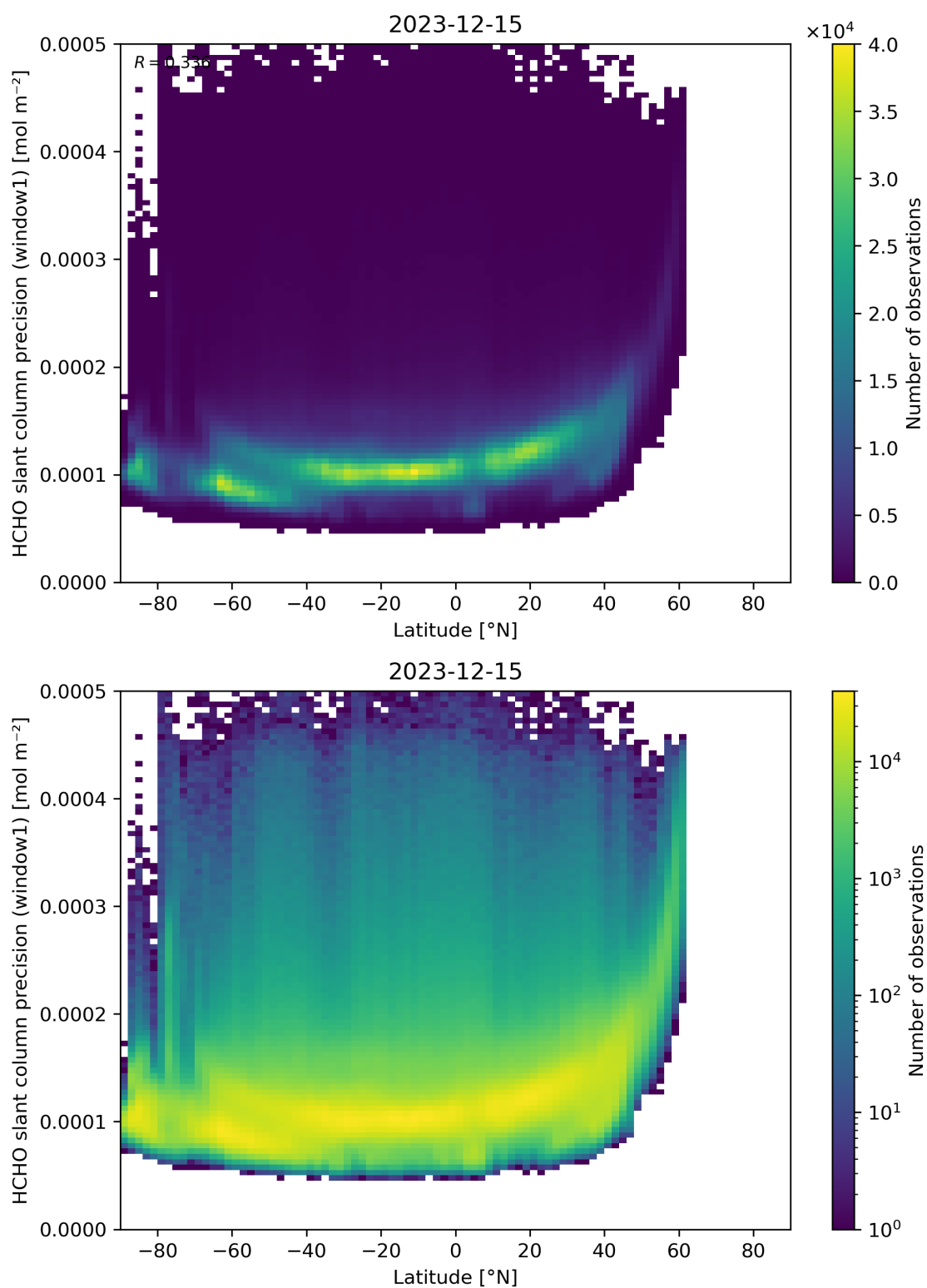
Figure 160: Scatter density plot of “Latitude” against “HCHO slant column precision (window1)” for 2023-12-14 to 2023-12-16.
