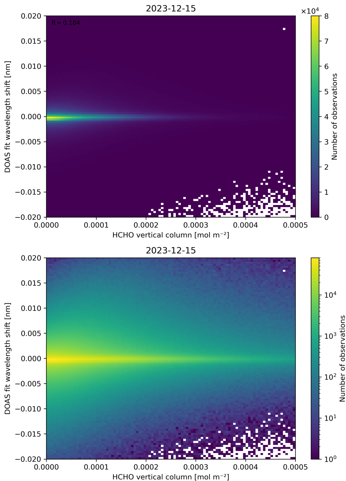
Figure 124: Scatter density plot of “HCHO vertical column” against “DOAS fit wavelength shift” for 2023-12-14 to 2023-12-16.
