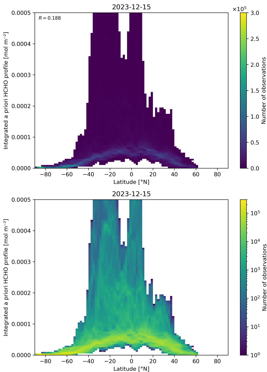
Figure 166: Scatter density plot of “Latitude” against “Integrated a priori HCHO profile” for 2023-12-14 to 2023-12-16.
