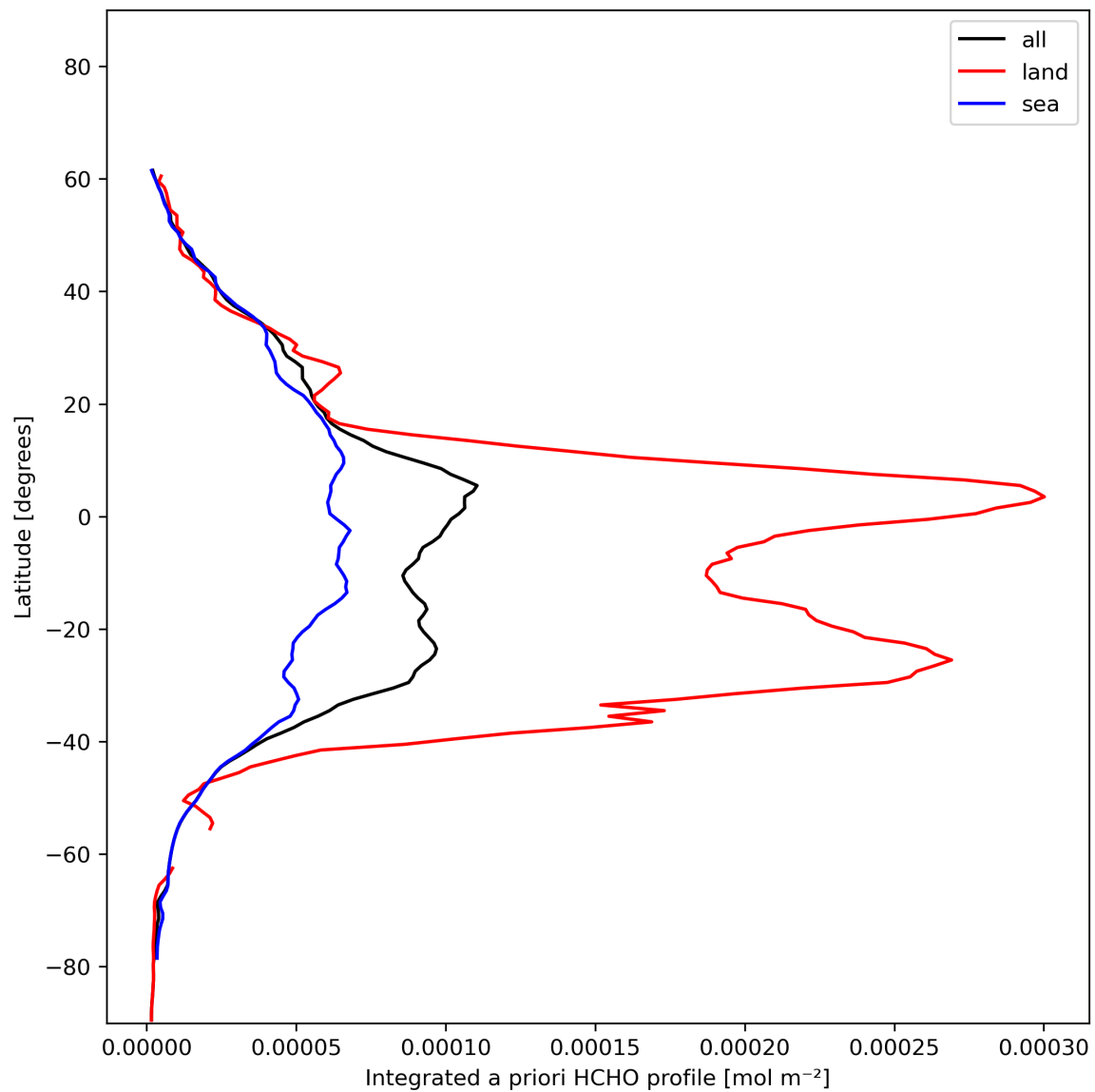
Figure 29: Zonal average of “Integrated a priori HCHO profile” for 2023-12-14 to 2023-12-16.
