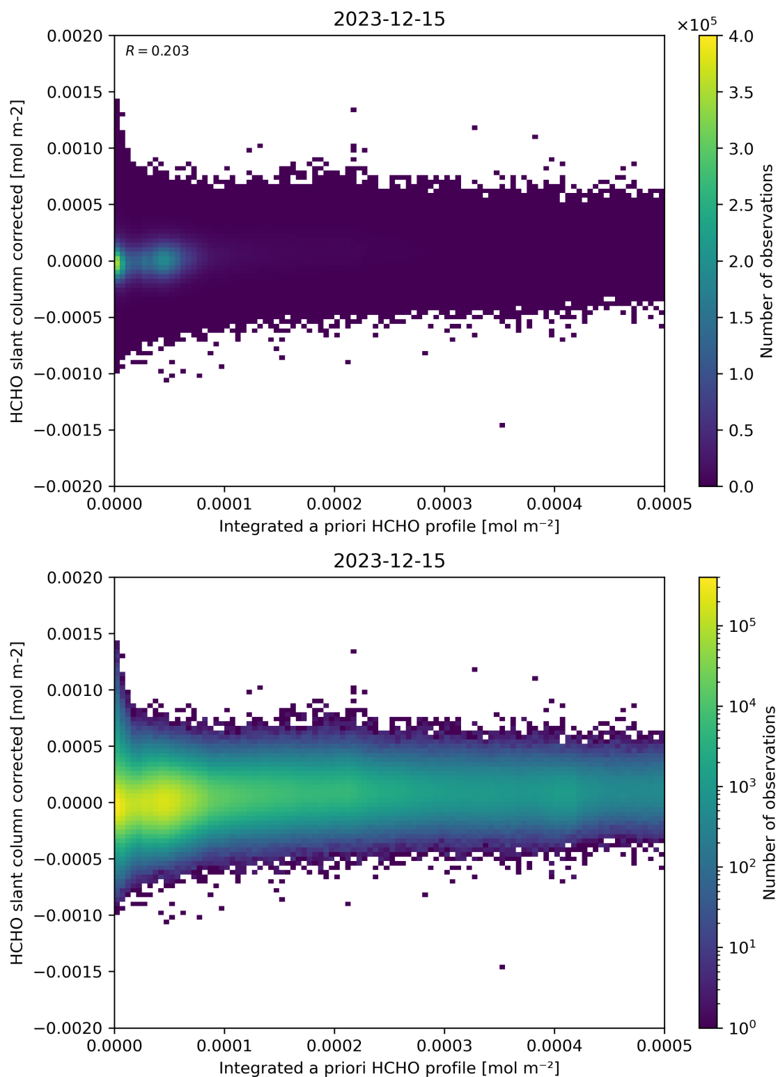
Figure 151: Scatter density plot of “Integrated a priori HCHO profile” against “HCHO slant column corrected” for 2023-12-14 to 2023-12-16.
