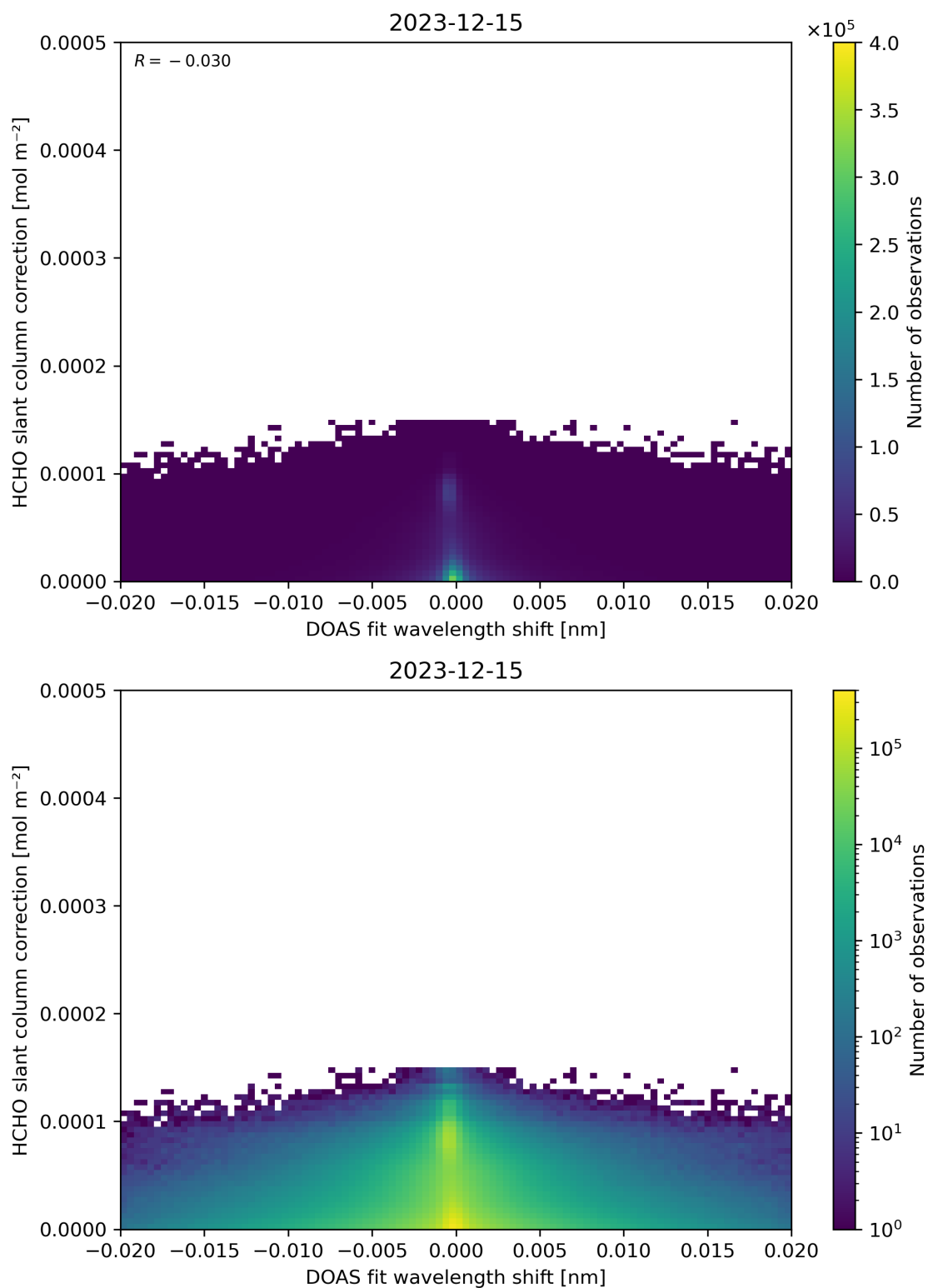
Figure 67: Scatter density plot of “DOAS fit wavelength shift” against “HCHO slant column correction” for 2023-12-14 to 2023-12-16.
