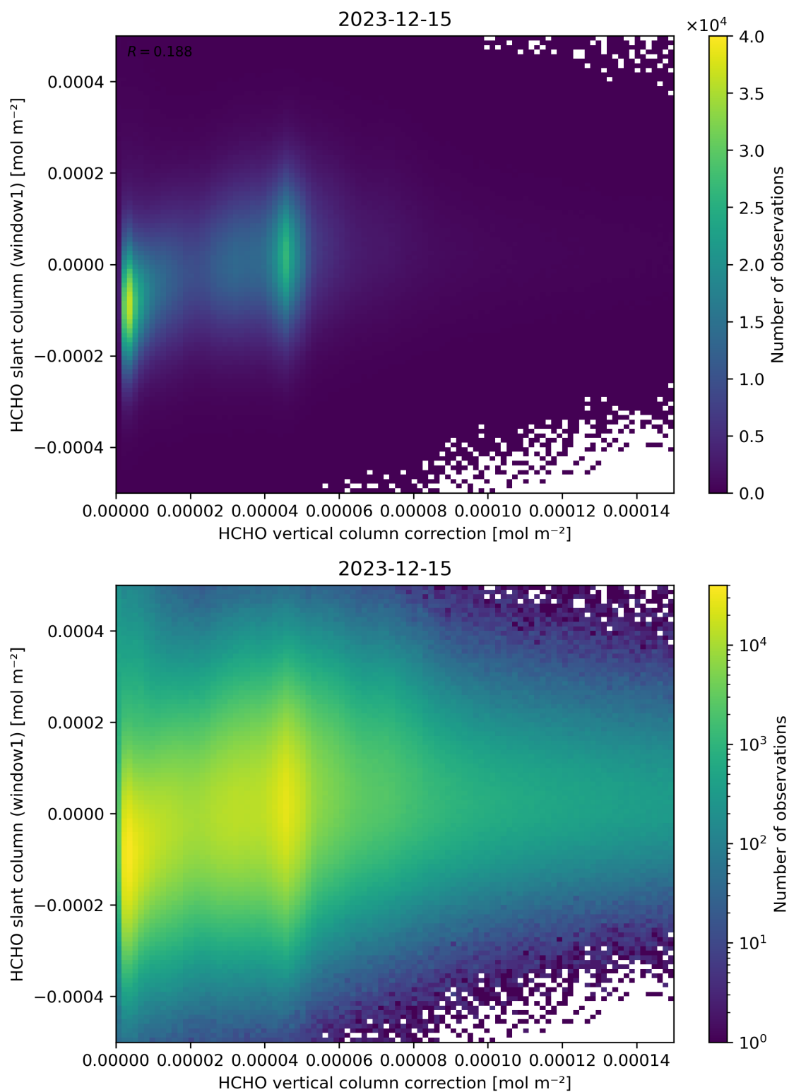
Figure 118: Scatter density plot of “HCHO vertical column correction” against “HCHO slant column (window1)” for 2023-12-14 to 2023-12-16.
