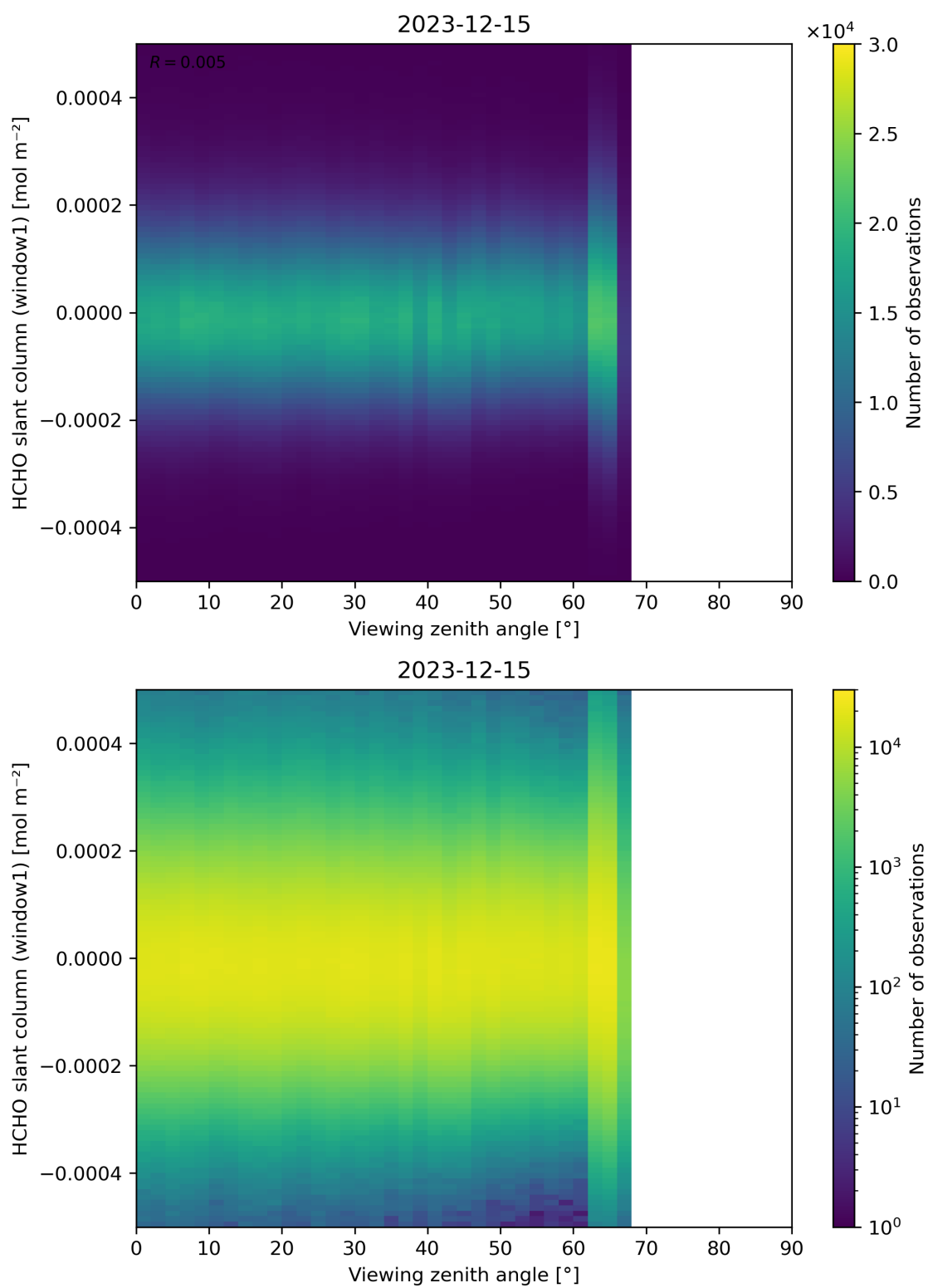
Figure 188: Scatter density plot of “Viewing zenith angle” against “HCHO slant column (window1)” for 2023-12-14 to 2023-12-16.
