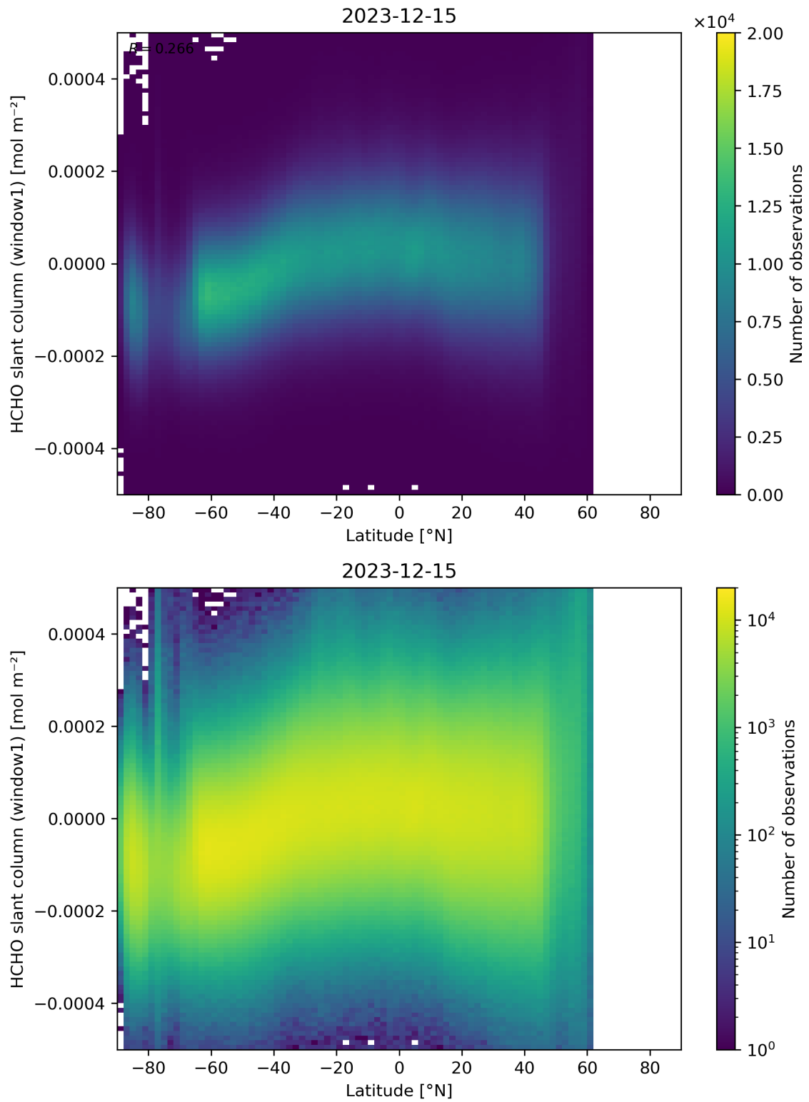
Figure 159: Scatter density plot of “Latitude” against “HCHO slant column (window1)” for 2023-12-14 to 2023-12-16.
