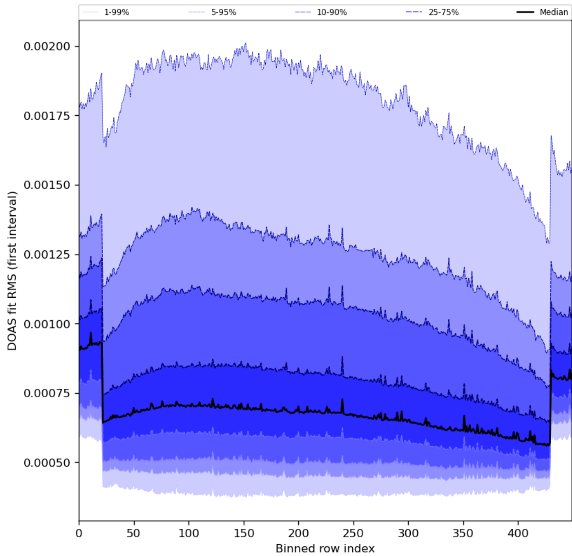
Figure 60: Along track statistics of “DOAS fit RMS (first interval)” for 2023-12-14 to 2023-12-16
