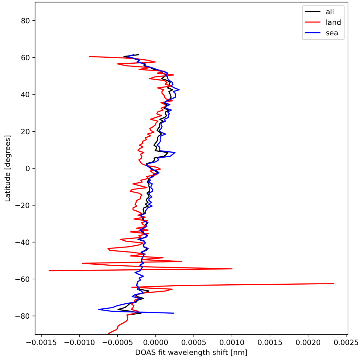
Figure 30: Zonal average of “DOAS fit wavelength shift” for 2023-12-14 to 2023-12-16.
