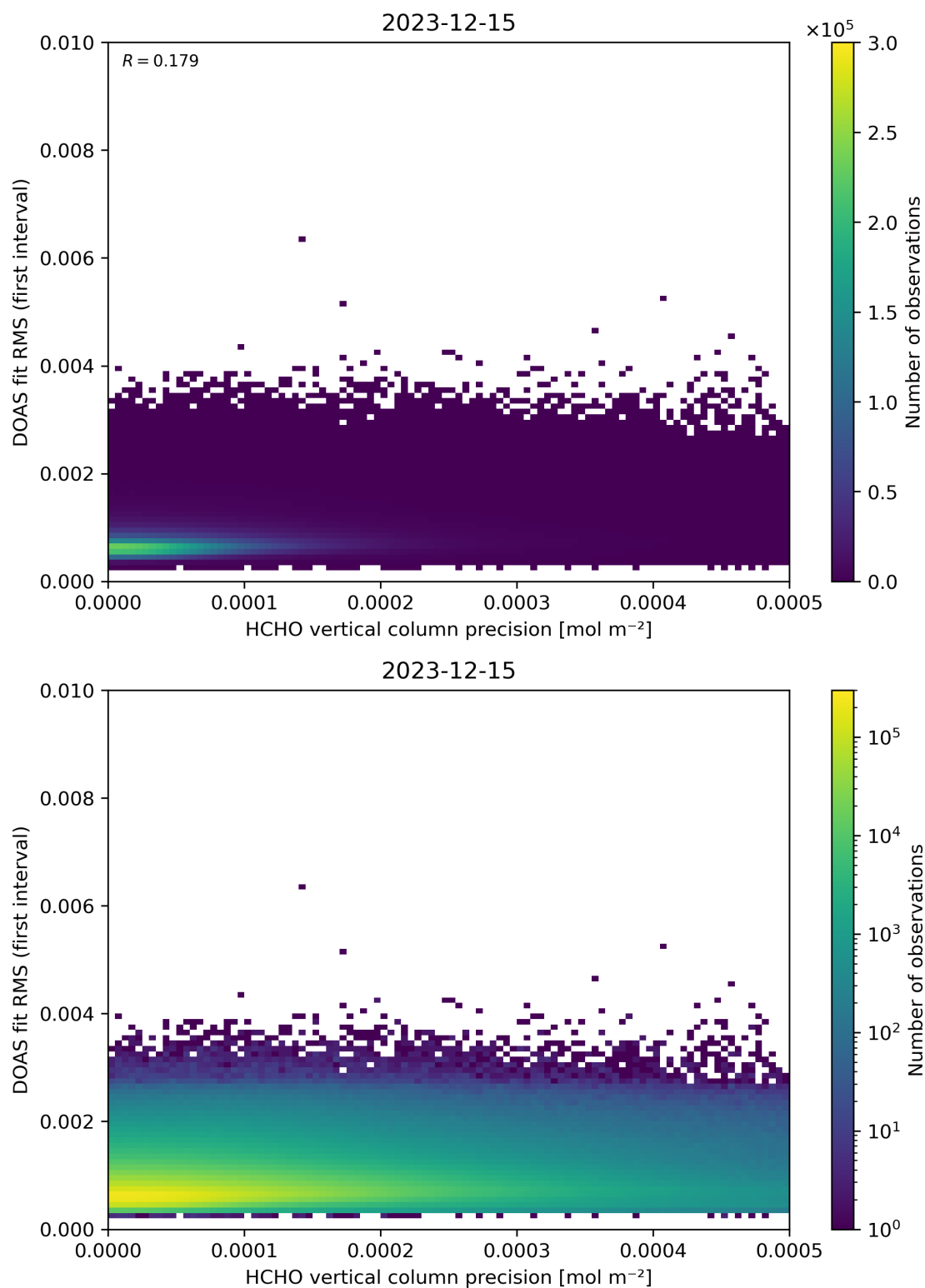
Figure 136: Scatter density plot of “HCHO vertical column precision” against “DOAS fit RMS (first interval)” for 2023-12-14 to 2023-12-16.
