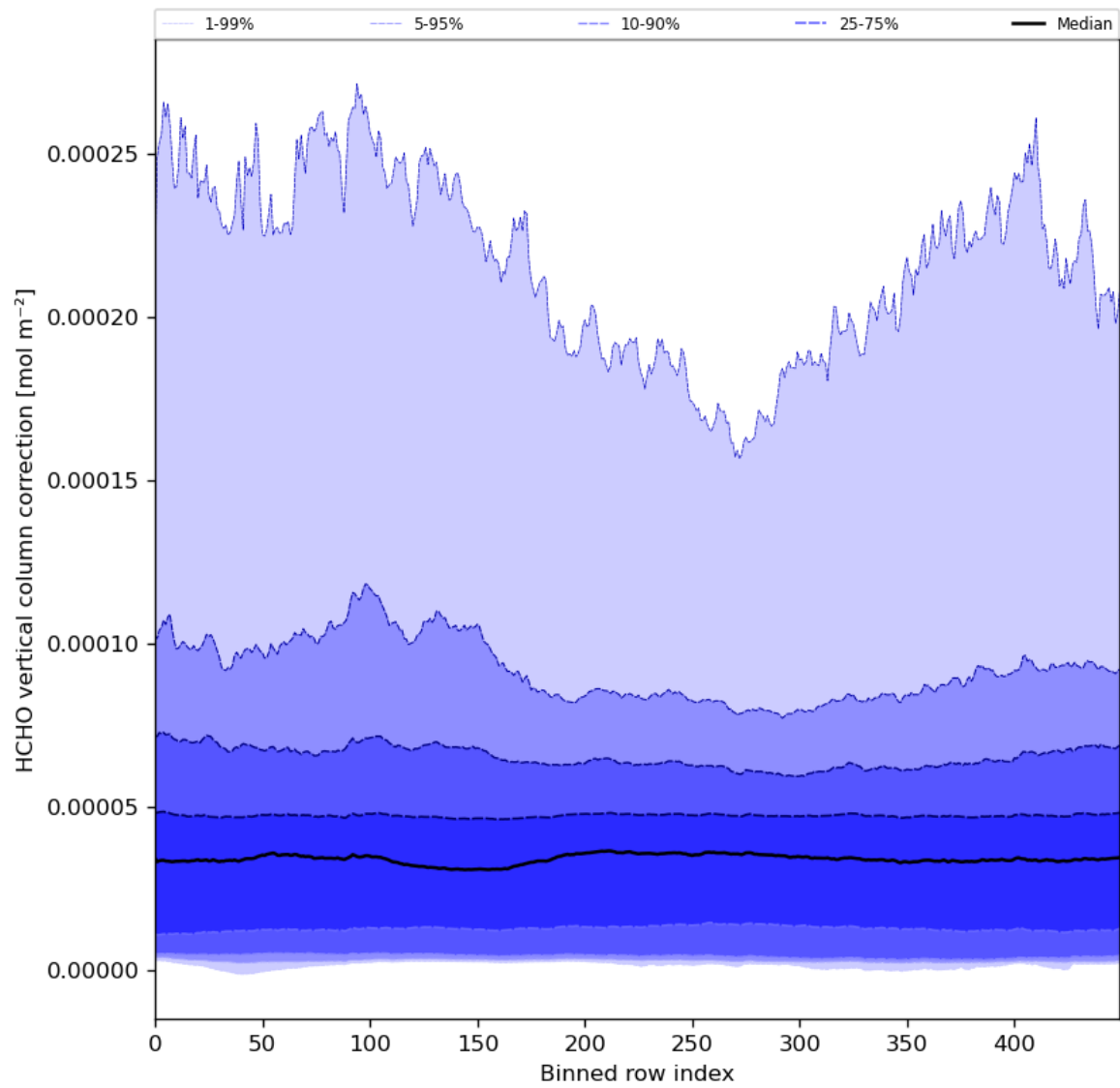
Figure 51: Along track statistics of “HCHO vertical column correction” for 2023-12-14 to 2023-12-16
