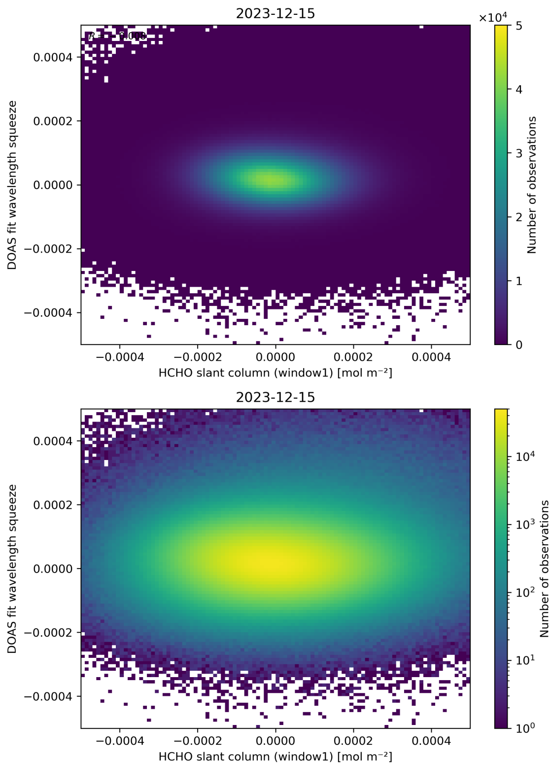
Figure 80: Scatter density plot of “HCHO slant column (window1)” against “DOAS fit wavelength squeeze” for 2023-12-14 to 2023-12-16.
