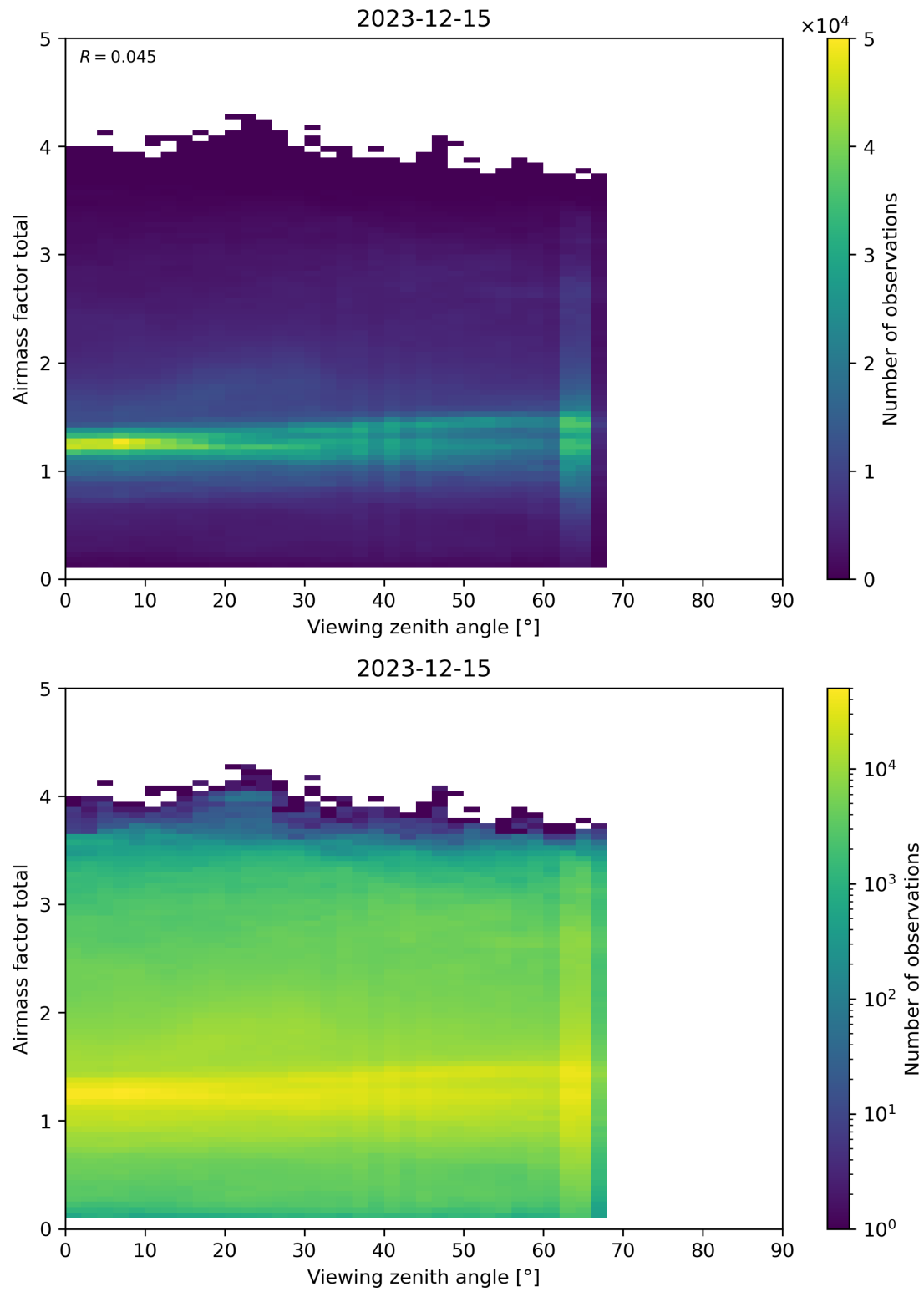
Figure 190: Scatter density plot of “Viewing zenith angle” against “Airmass factor total” for 2023-12-14 to 2023-12-16.
