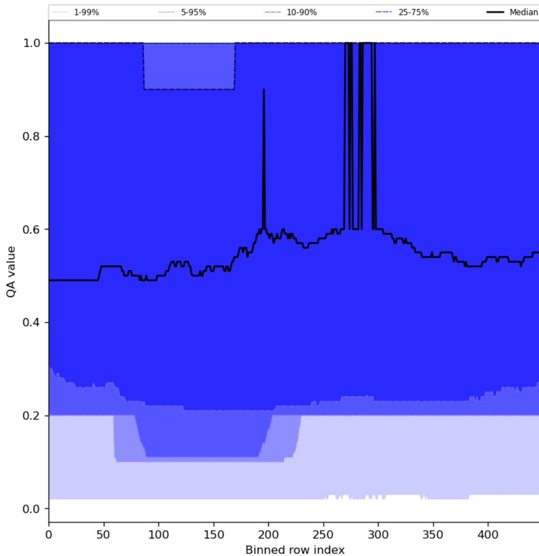
Figure 48: Along track statistics of “QA value” for 2023-12-14 to 2023-12-16
