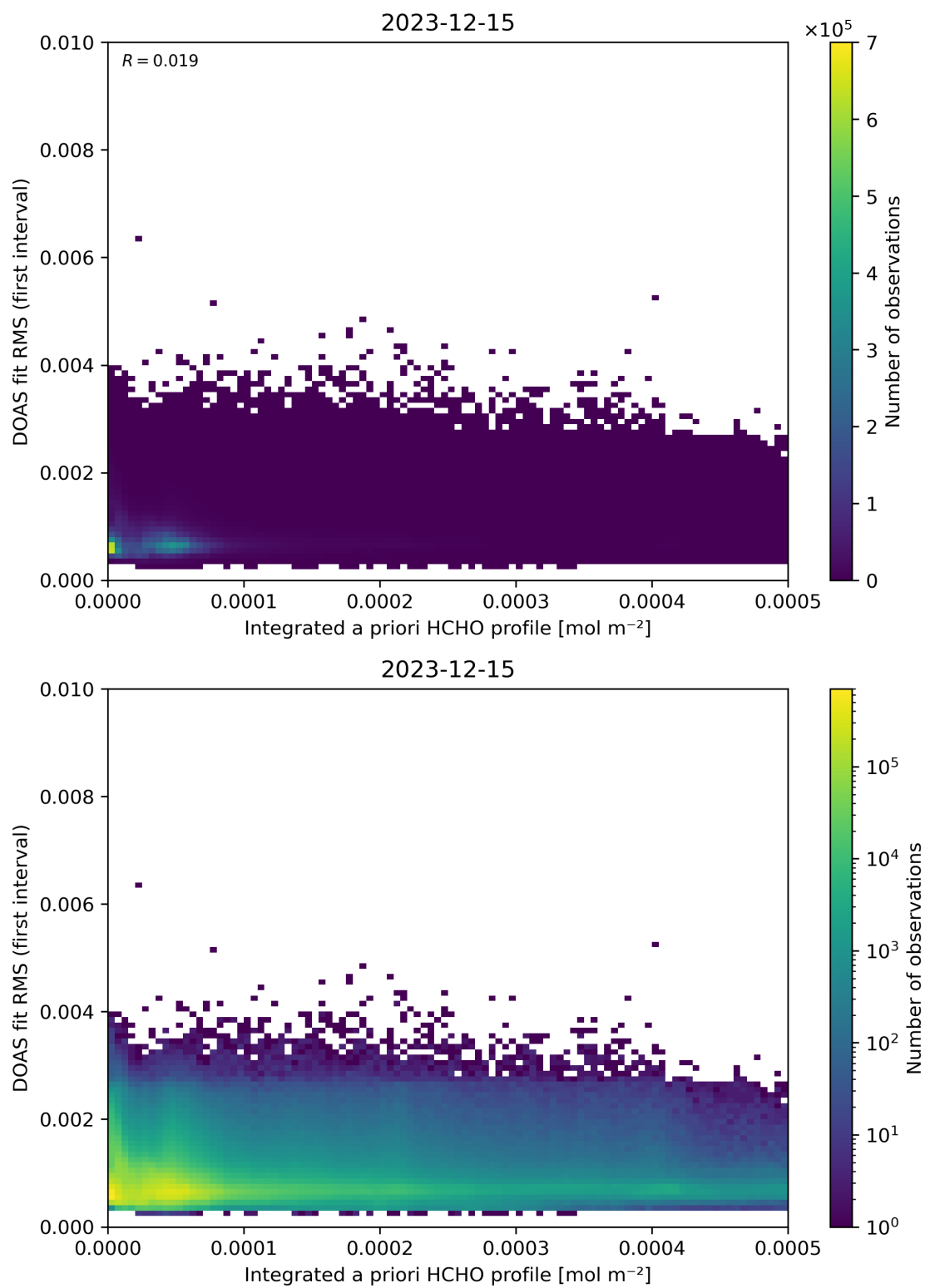
Figure 148: Scatter density plot of “Integrated a priori HCHO profile” against “DOAS fit RMS (first interval)” for 2023-12-14 to 2023-12-16.
