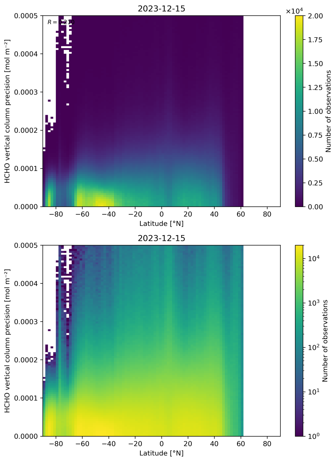
Figure 165: Scatter density plot of “Latitude” against “HCHO vertical column precision” for 2023-12-14 to 2023-12-16.
