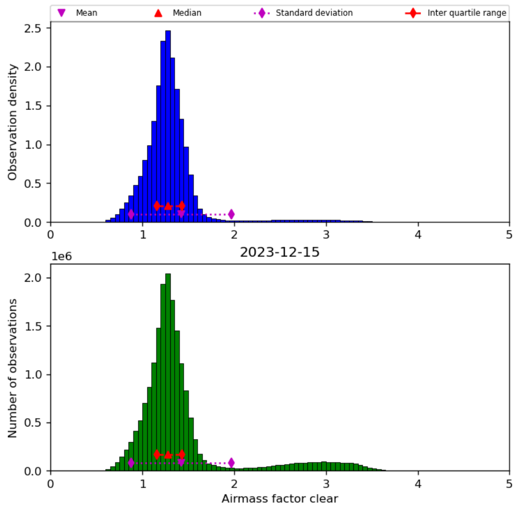
Figure 42: Histogram of “Airmass factor clear” for 2023-12-14 to 2023-12-16
