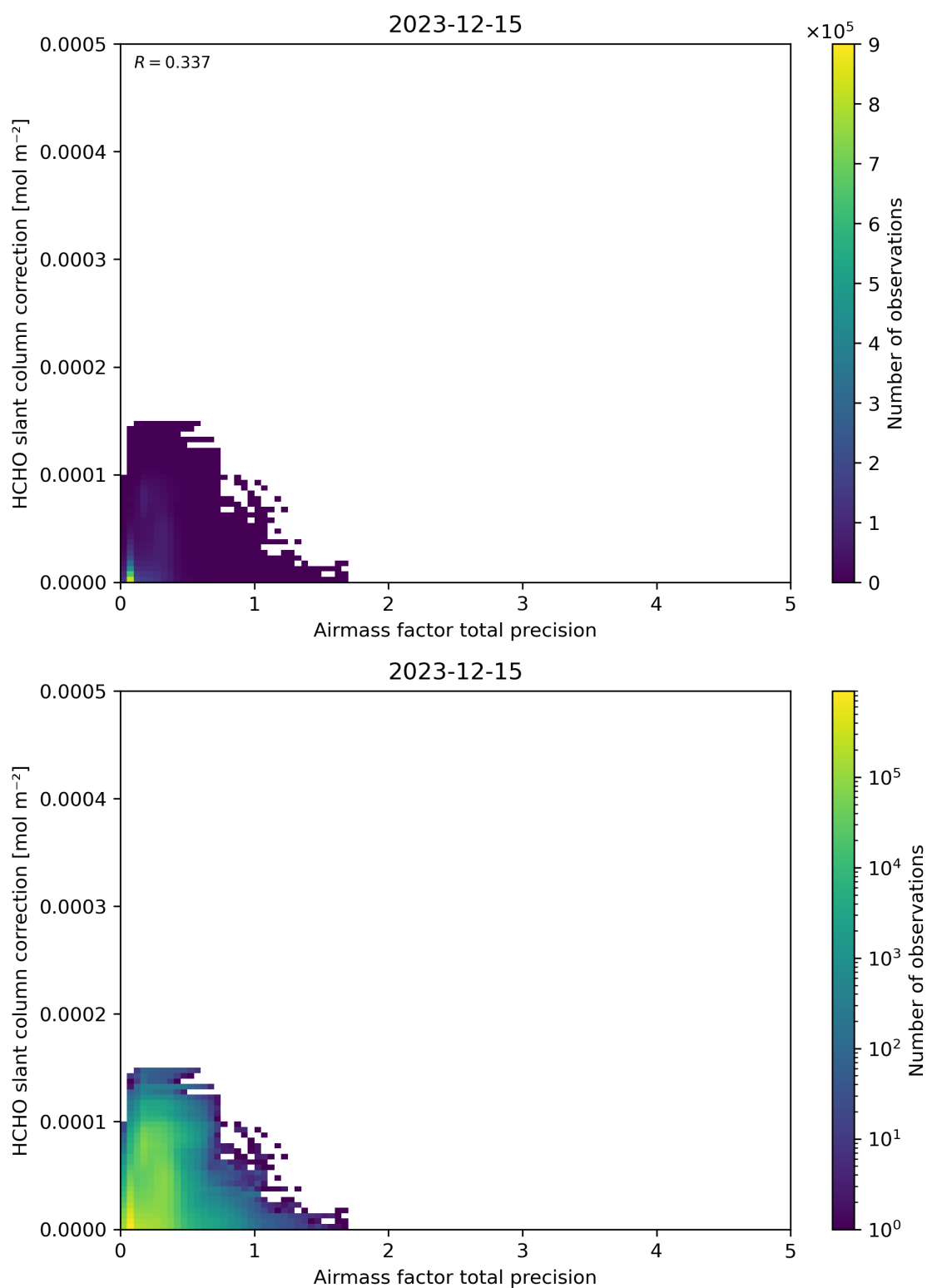
Figure 110: Scatter density plot of “Airmass factor total precision” against “HCHO slant column correction” for 2023-12-14 to 2023-12-16.
