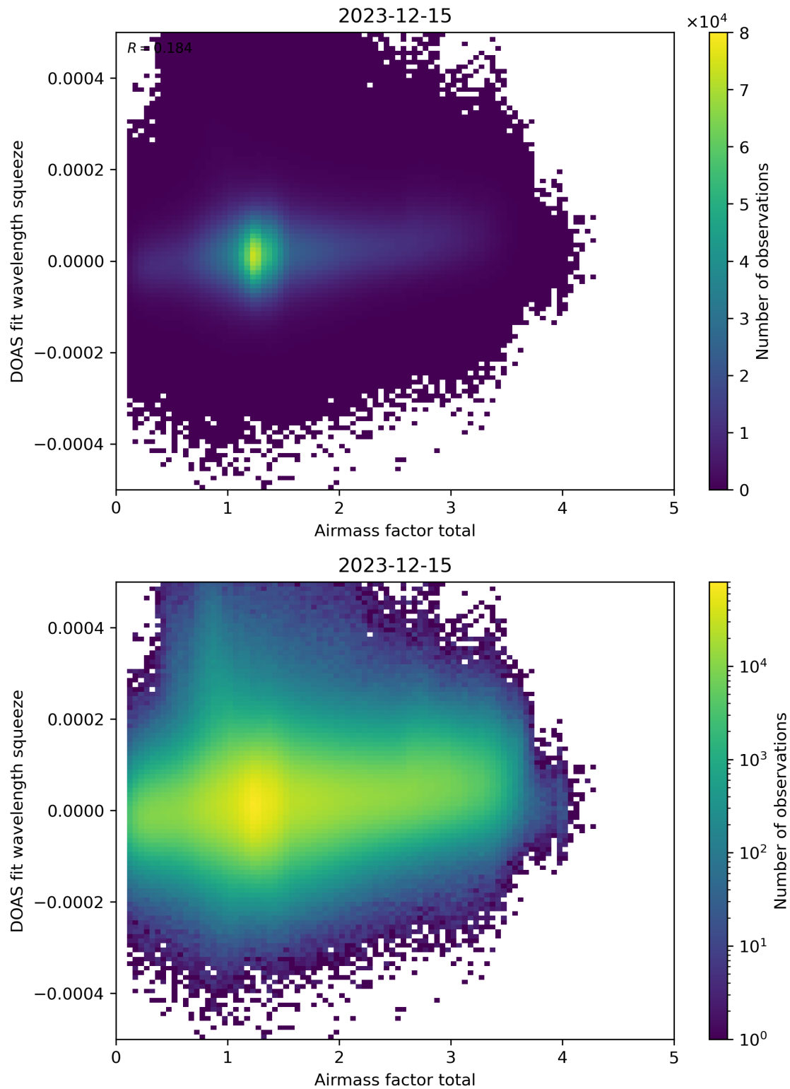
Figure 99: Scatter density plot of “Airmass factor total” against “DOAS fit wavelength squeeze” for 2023-12-14 to 2023-12-16.
