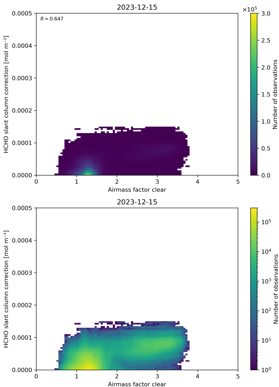
Figure 75: Scatter density plot of “Airmass factor clear” against “HCHO slant column correction” for 2023-12-14 to 2023-12-16.
