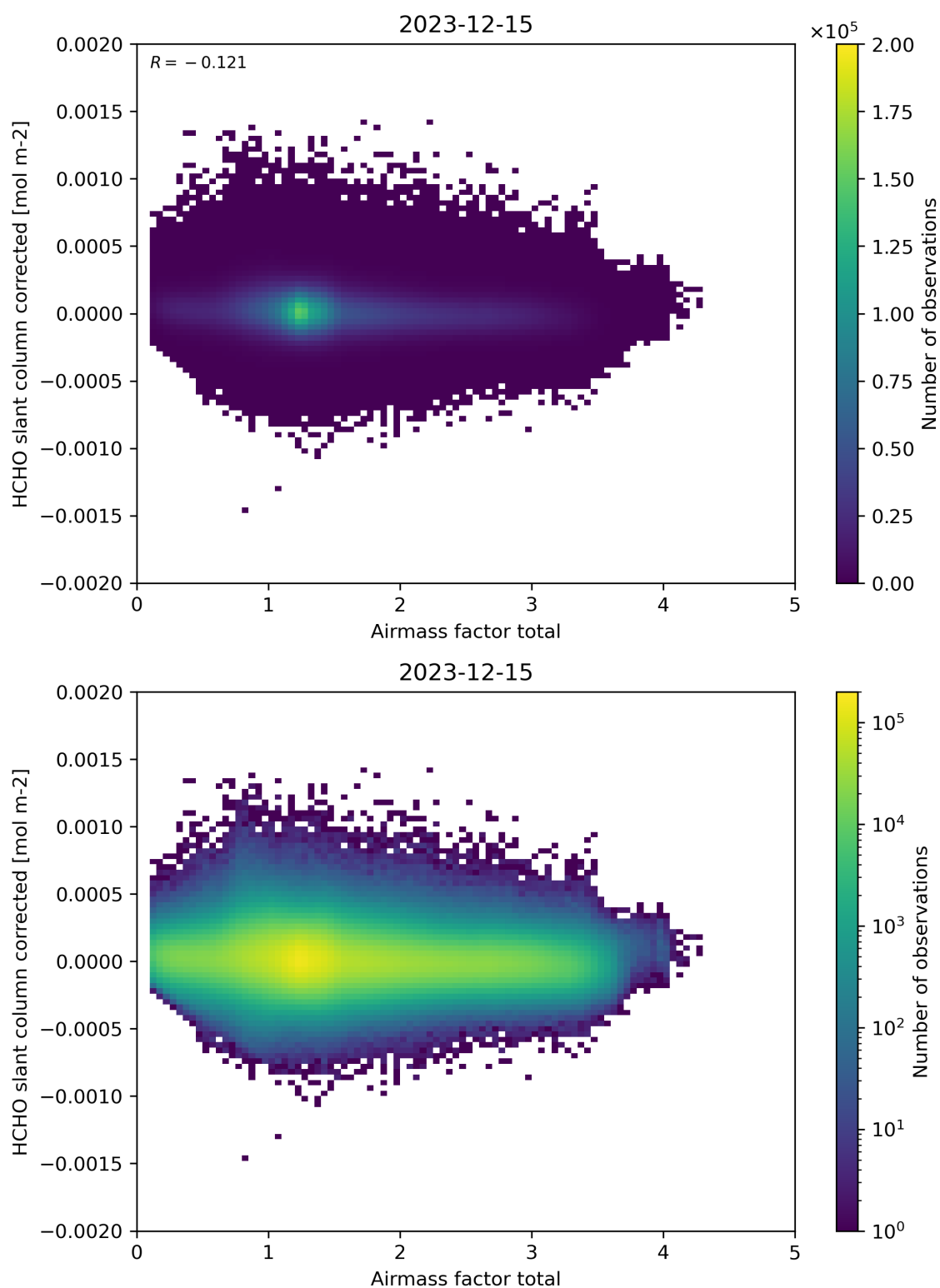
Figure 101: Scatter density plot of “Airmass factor total” against “HCHO slant column corrected” for 2023-12-14 to 2023-12-16.
