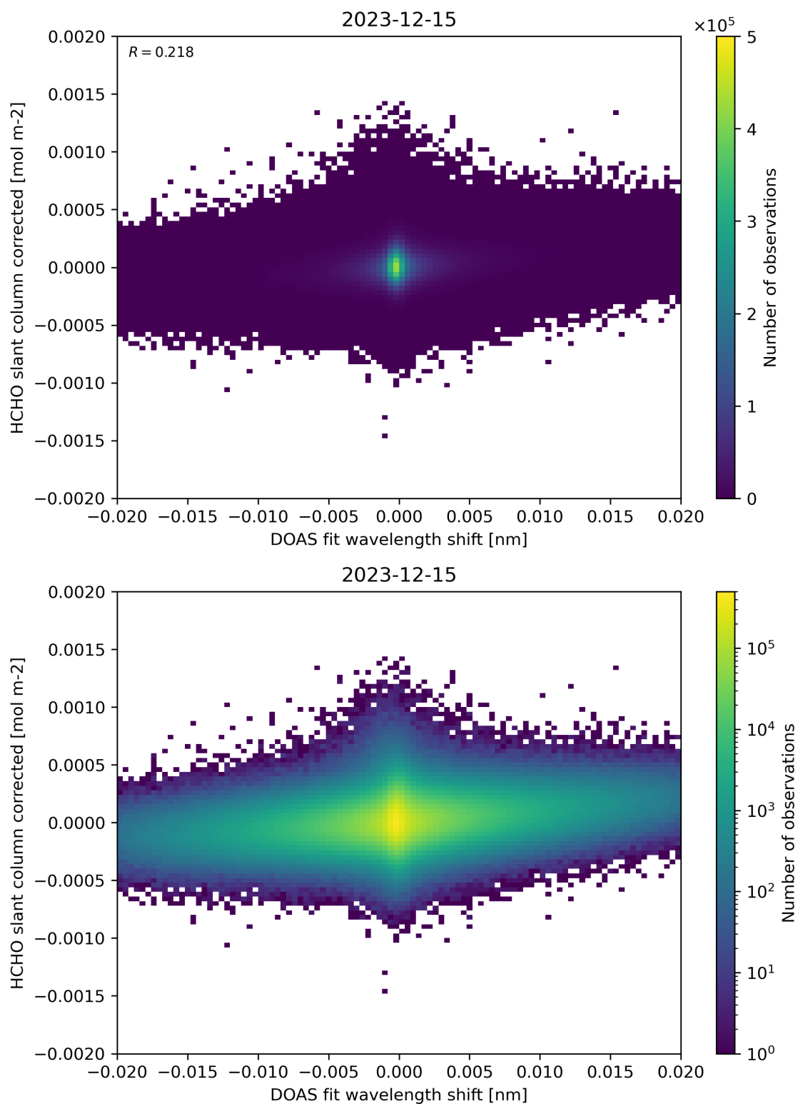
Figure 66: Scatter density plot of “DOAS fit wavelength shift” against “HCHO slant column corrected” for 2023-12-14 to 2023-12-16.
