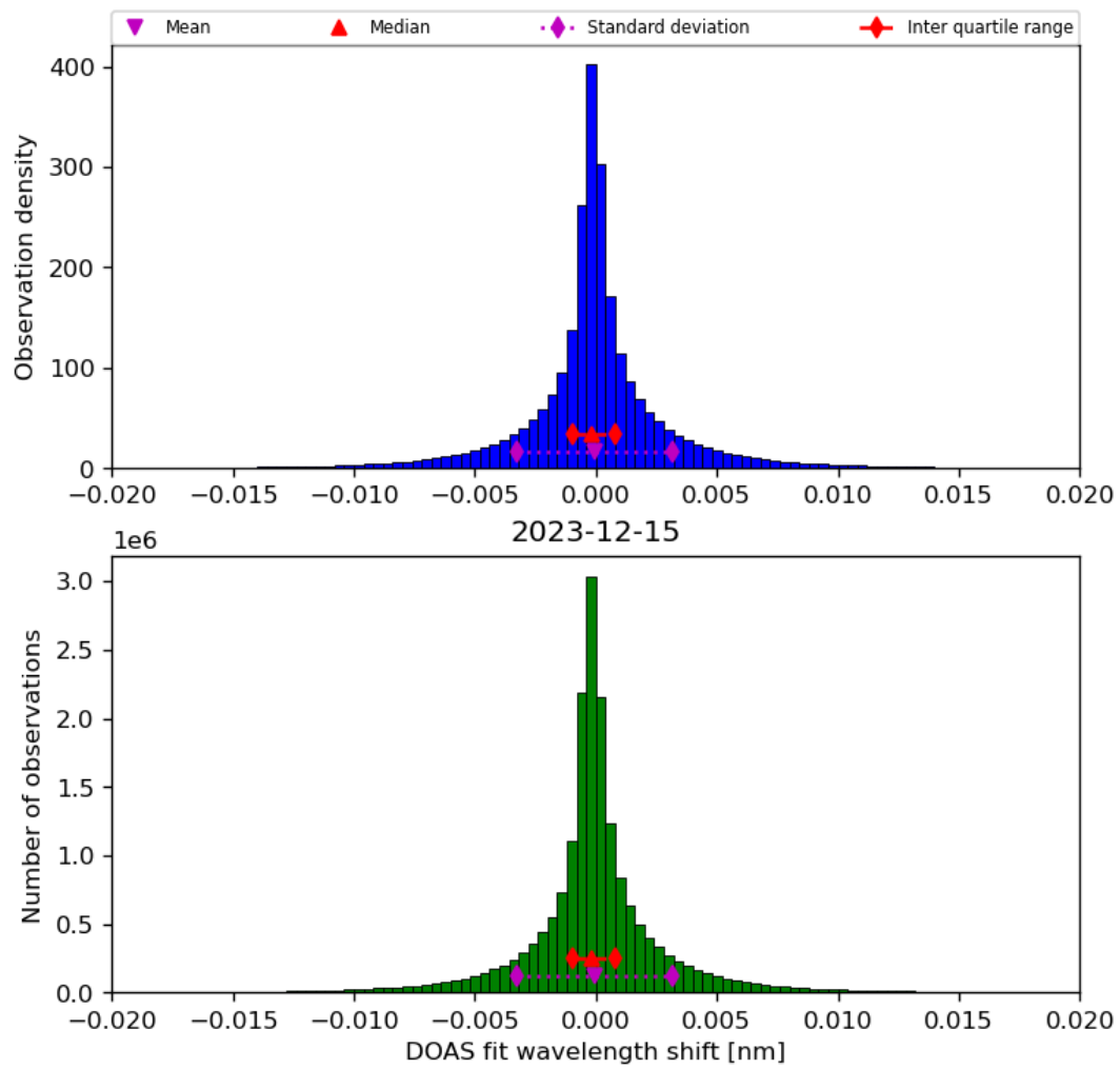
Figure 44: Histogram of “DOAS fit wavelength shift” for 2023-12-14 to 2023-12-16
