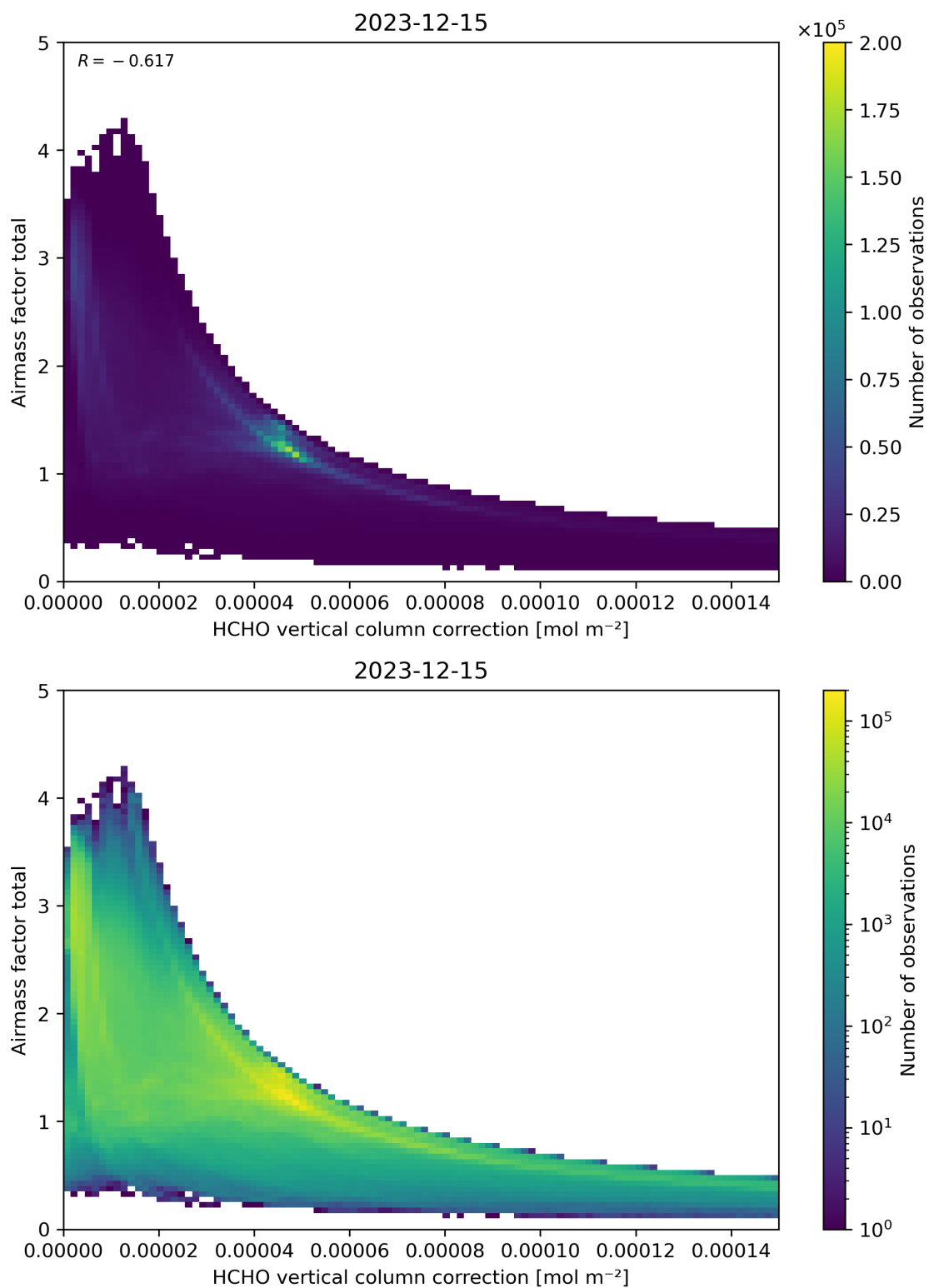
Figure 120: Scatter density plot of “HCHO vertical column correction” against “Airmass factor total” for 2023-12-14 to 2023-12-16.
