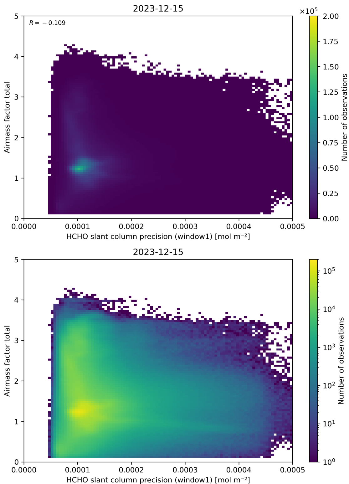
Figure 94: Scatter density plot of “HCHO slant column precision (window1)” against “Airmass factor total” for 2023-12-14 to 2023-12-16.
