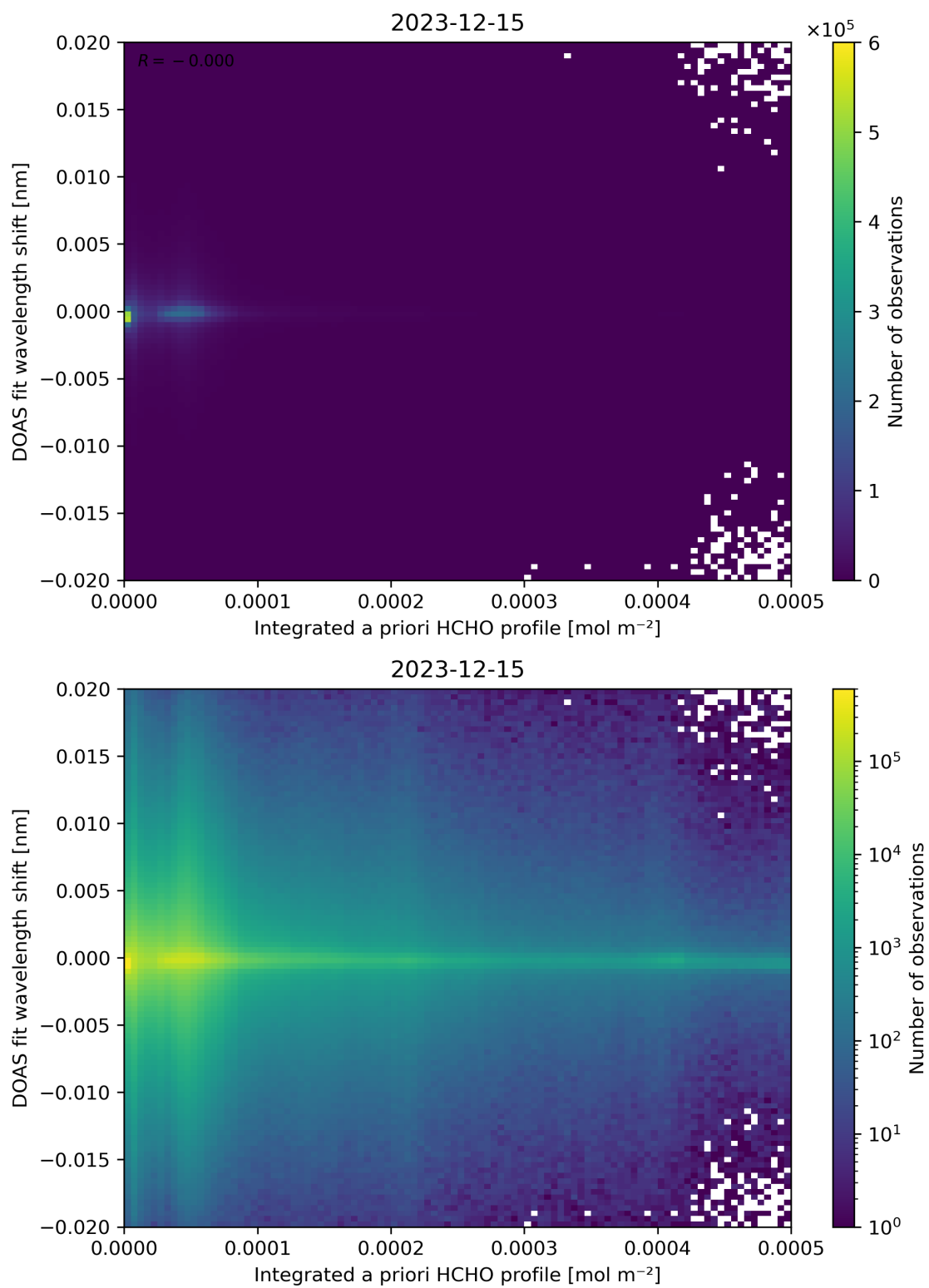
Figure 149: Scatter density plot of “Integrated a priori HCHO profile” against “DOAS fit wavelength shift” for 2023-12-14 to 2023-12-16.
