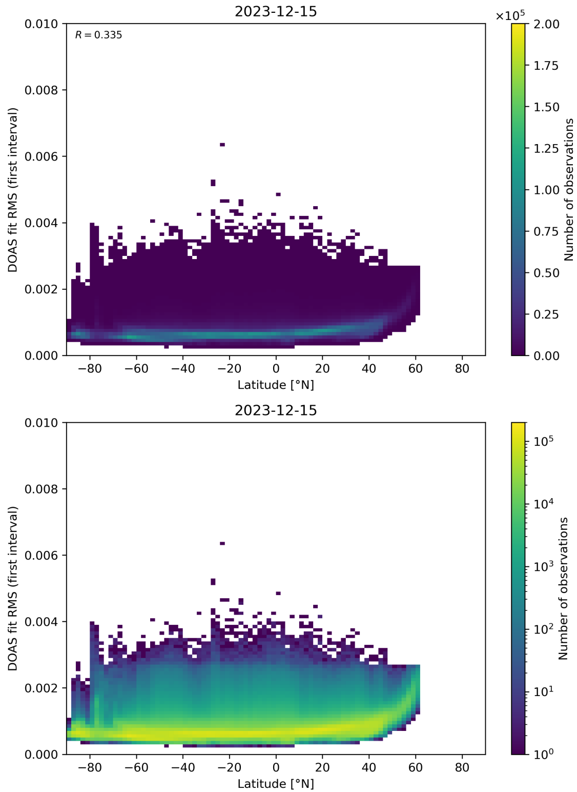
Figure 153: Scatter density plot of “Latitude” against “DOAS fit RMS (first interval)” for 2023-12-14 to 2023-12-16.
