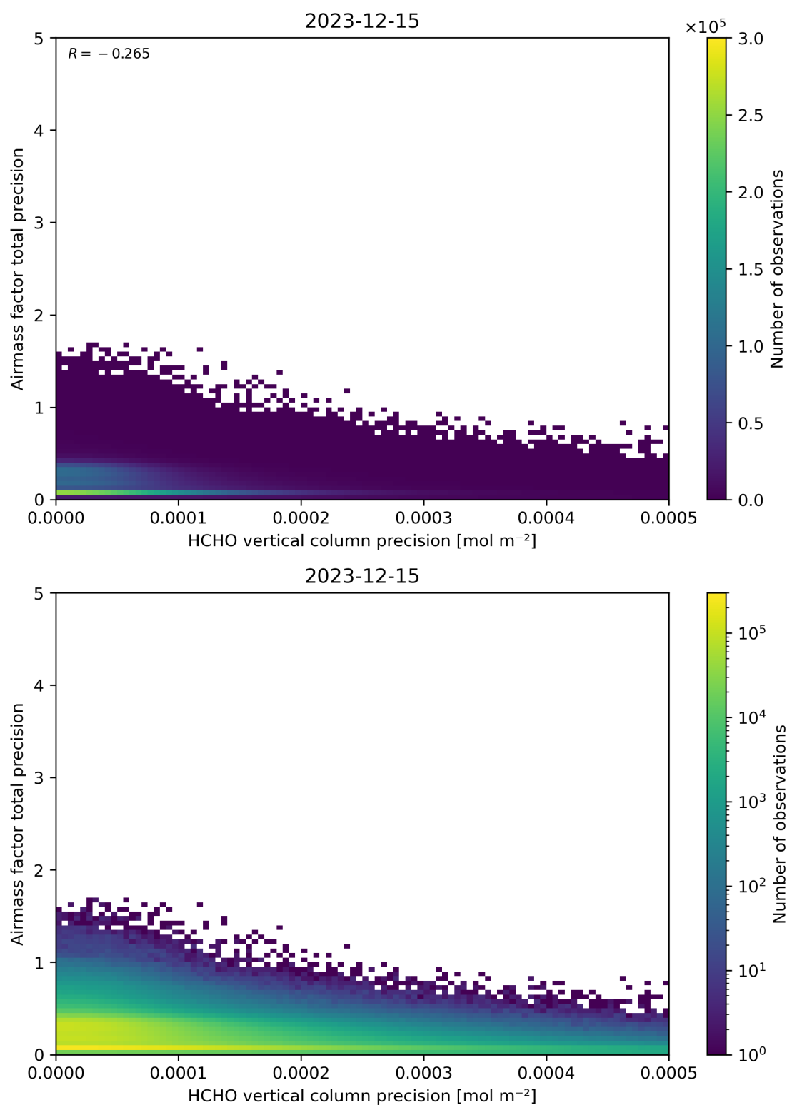
Figure 145: Scatter density plot of “HCHO vertical column precision” against “Airmass factor total precision” for 2023-12-14 to 2023-12-16.
