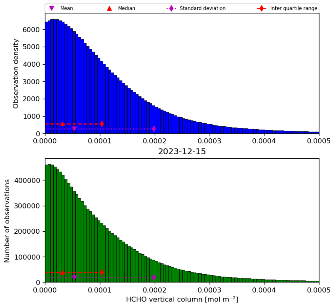
Figure 35: Histogram of “HCHO vertical column” for 2023-12-14 to 2023-12-16
