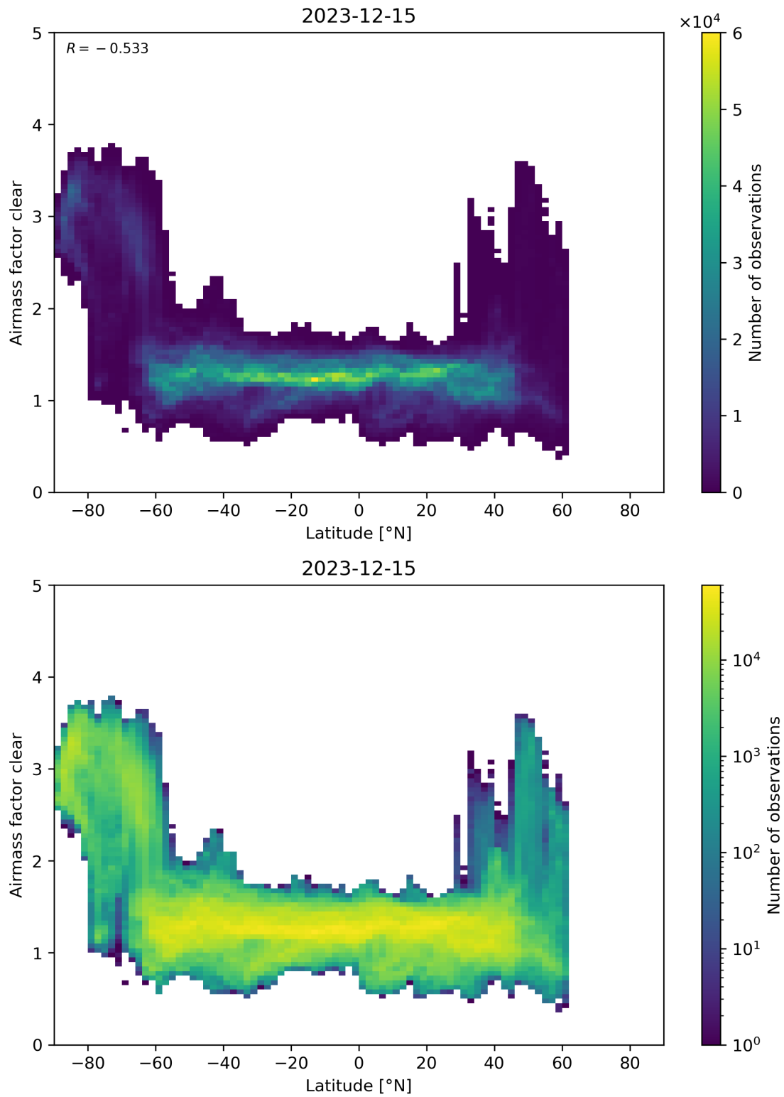
Figure 156: Scatter density plot of “Latitude” against “Airmass factor clear” for 2023-12-14 to 2023-12-16.
