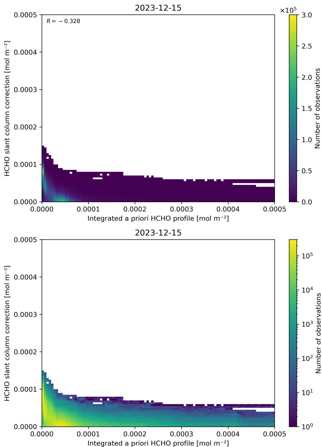
Figure 152: Scatter density plot of “Integrated a priori HCHO profile” against “HCHO slant column correction” for 2023-12-14 to 2023-12-16.
