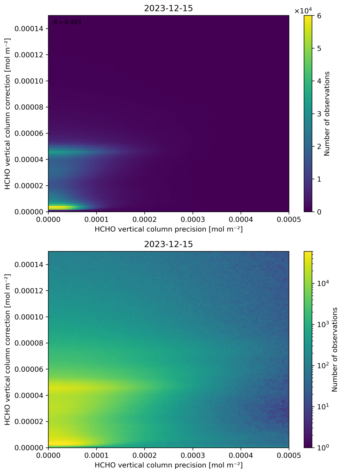
Figure 146: Scatter density plot of “HCHO vertical column precision” against “HCHO vertical column correction” for 2023-12-14 to 2023-12-16.
