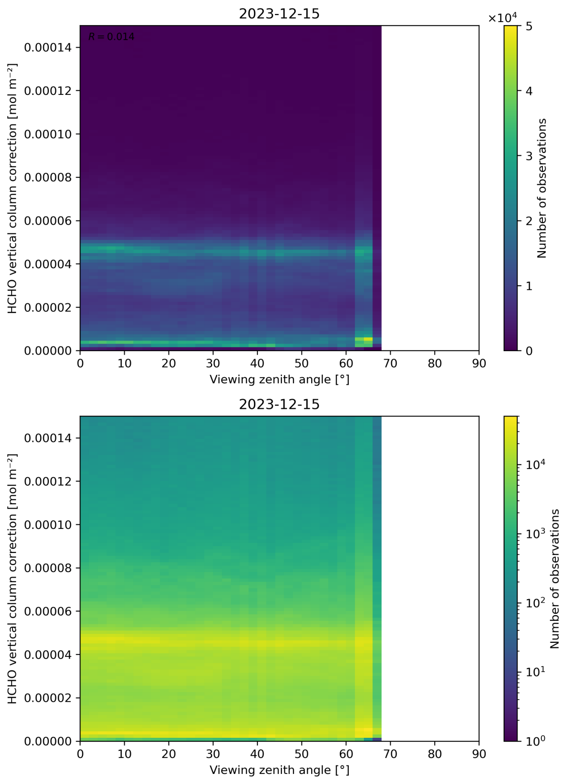
Figure 193: Scatter density plot of “Viewing zenith angle” against “HCHO vertical column correction” for 2023-12-14 to 2023-12-16.
