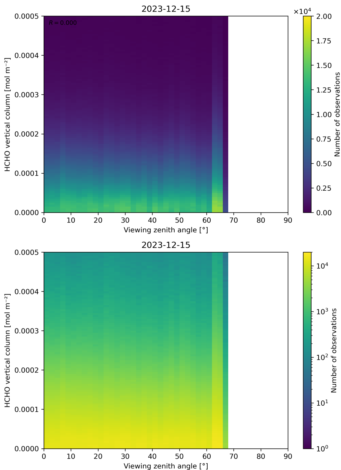
Figure 192: Scatter density plot of “Viewing zenith angle” against “HCHO vertical column” for 2023-12-14 to 2023-12-16.
