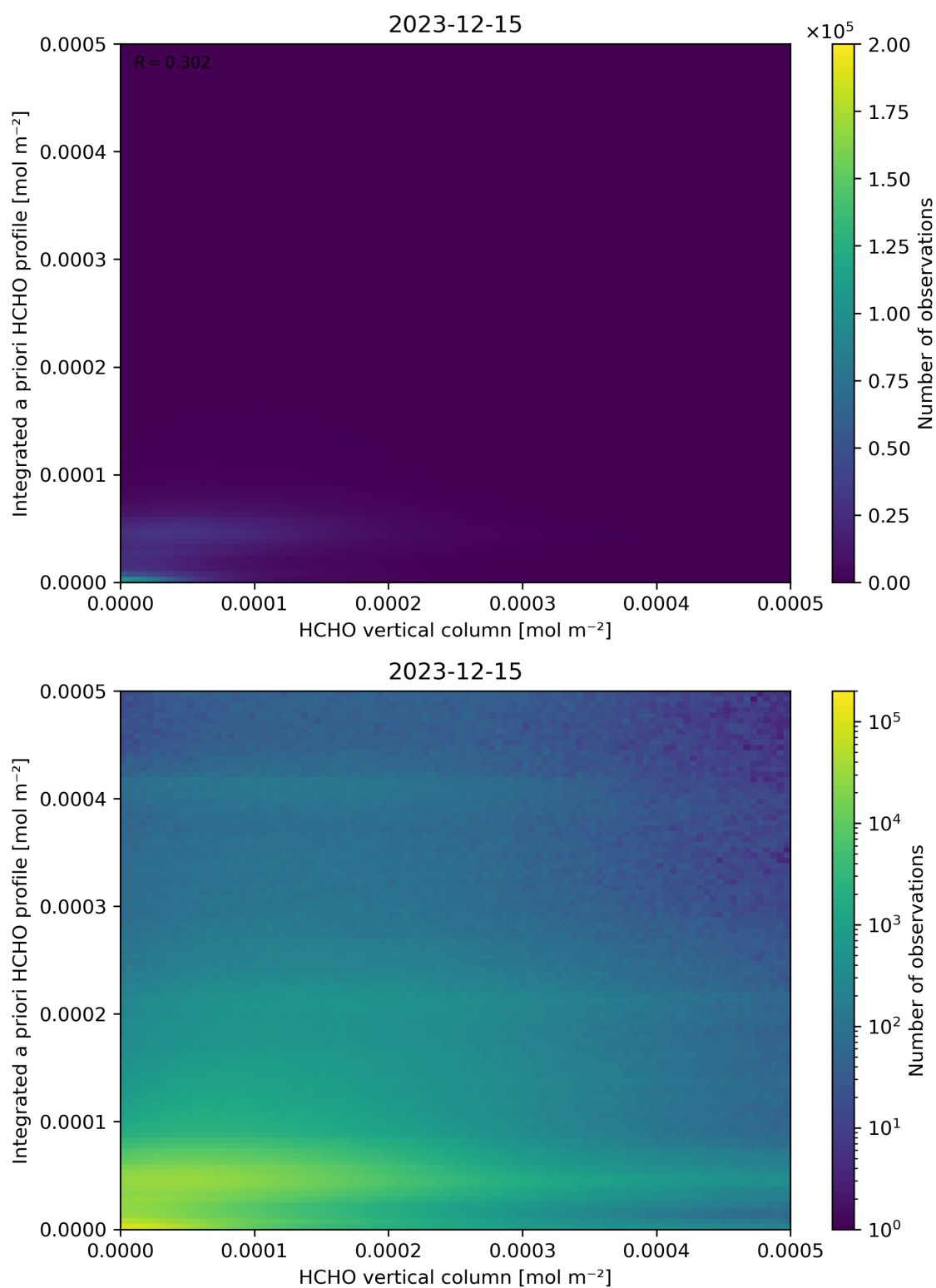
Figure 135: Scatter density plot of “HCHO vertical column” against “Integrated a priori HCHO profile” for 2023-12-14 to 2023-12-16.
