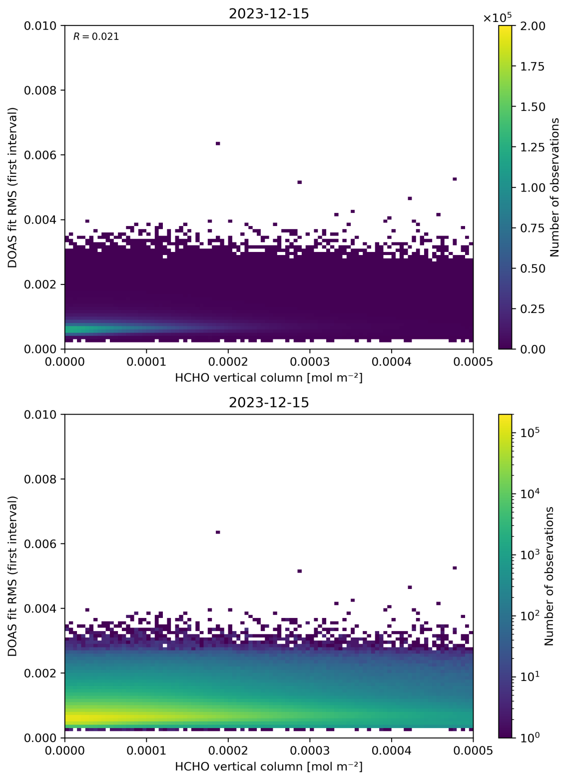
Figure 123: Scatter density plot of “HCHO vertical column” against “DOAS fit RMS (first interval)” for 2023-12-14 to 2023-12-16.
