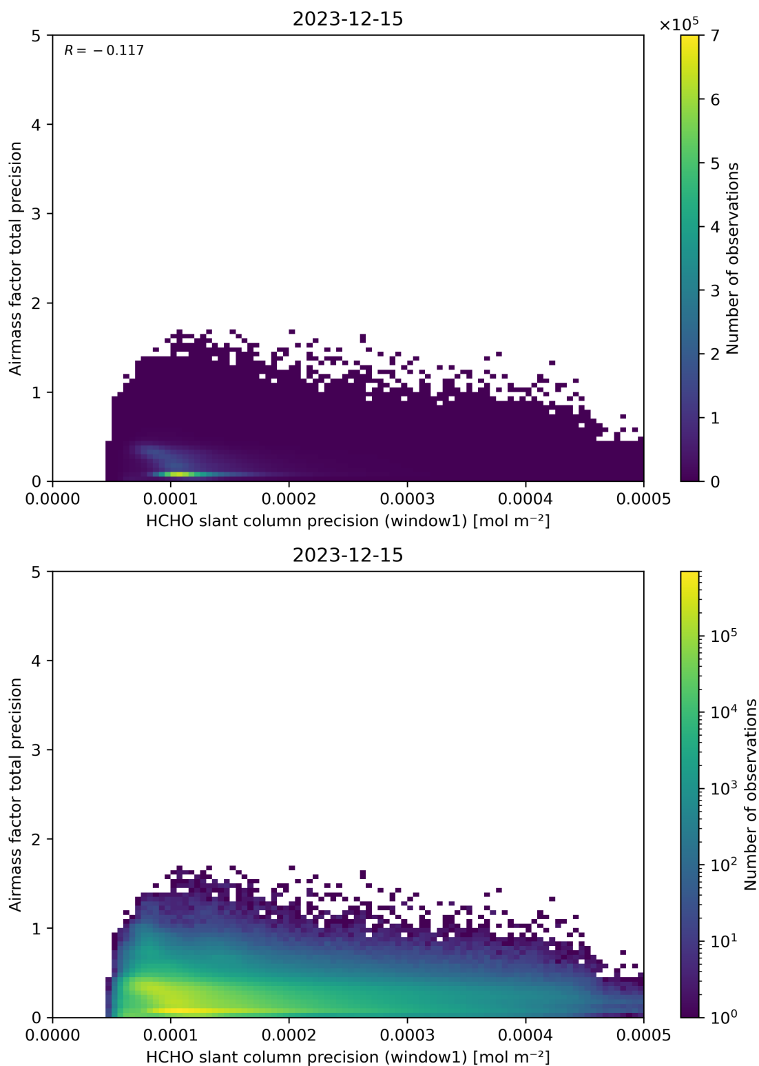
Figure 95: Scatter density plot of “HCHO slant column precision (window1)” against “Airmass factor total precision” for 2023-12-14 to 2023-12-16.
