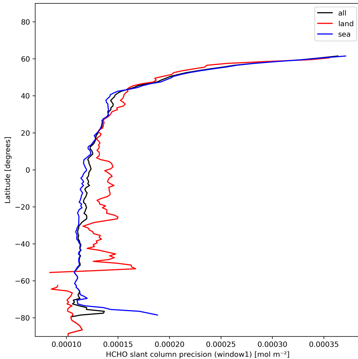
Figure 25: Zonal average of “HCHO slant column precision (window1)” for 2023-12-14 to 2023-12-16.
