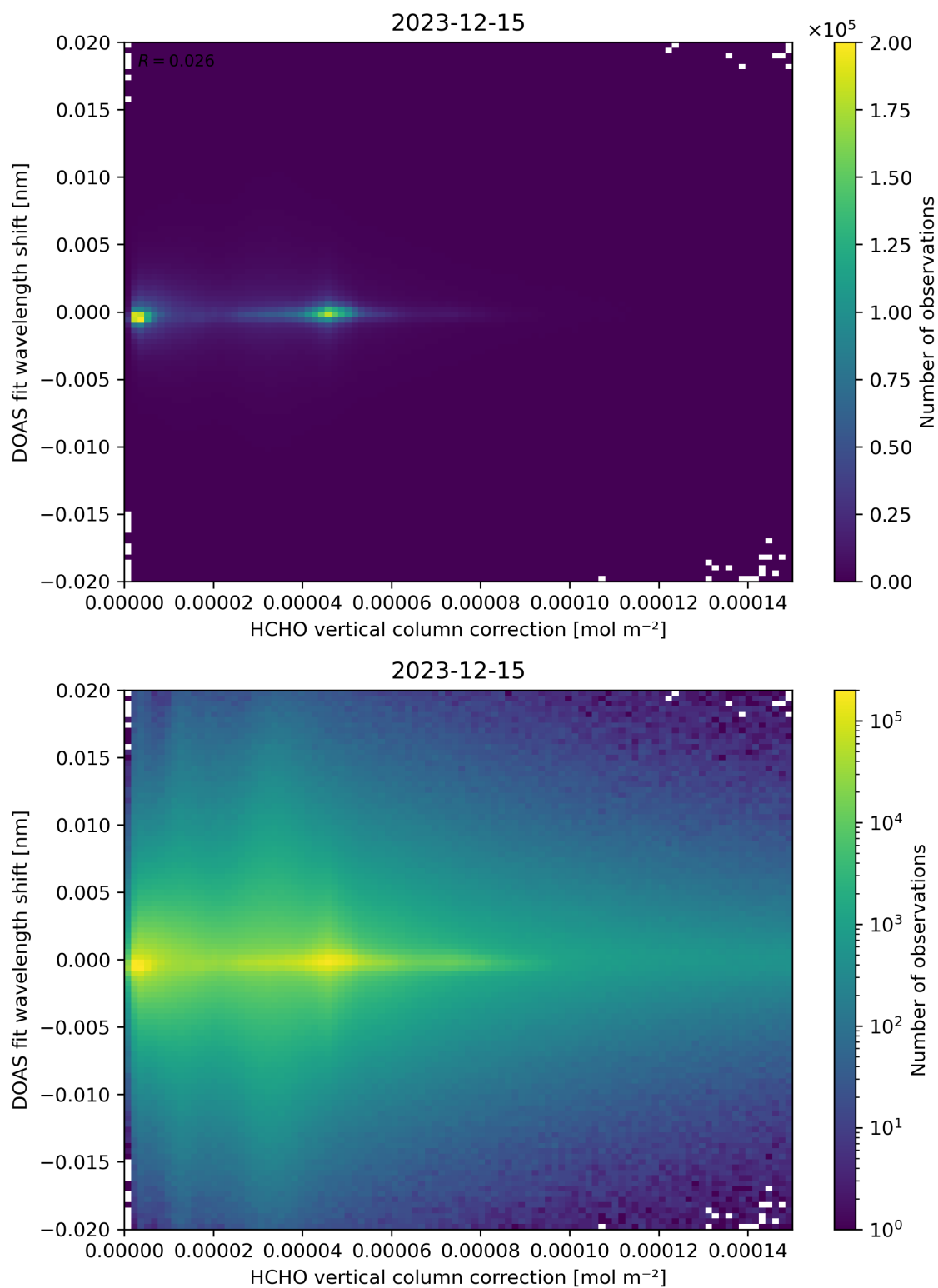
Figure 113: Scatter density plot of “HCHO vertical column correction” against “DOAS fit wavelength shift” for 2023-12-14 to 2023-12-16.
