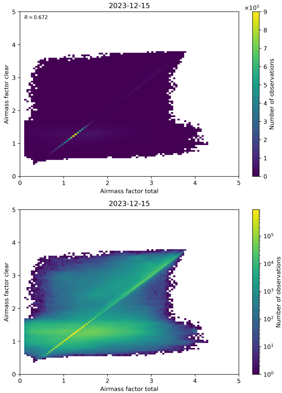
Figure 100: Scatter density plot of “Airmass factor total” against “Airmass factor clear” for 2023-12-14 to 2023-12-16.
