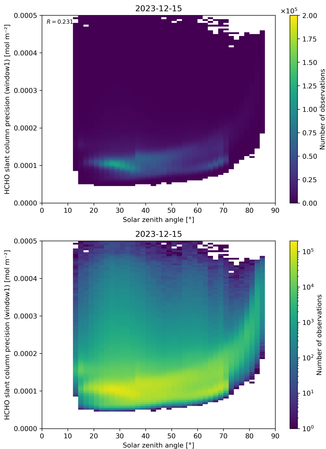
Figure 174: Scatter density plot of “Solar zenith angle” against “HCHO slant column precision (window1)” for 2023-12-14 to 2023-12-16.
