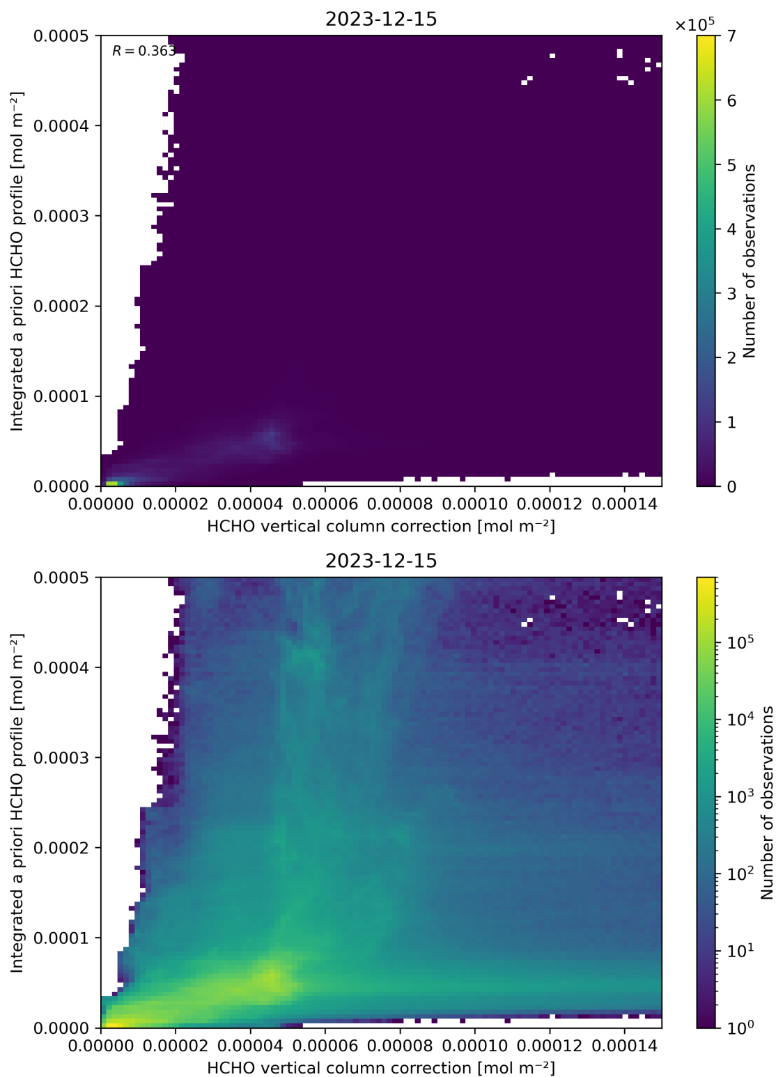
Figure 122: Scatter density plot of “HCHO vertical column correction” against “Integrated a priori HCHO profile” for 2023-12-14 to 2023-12-16.
