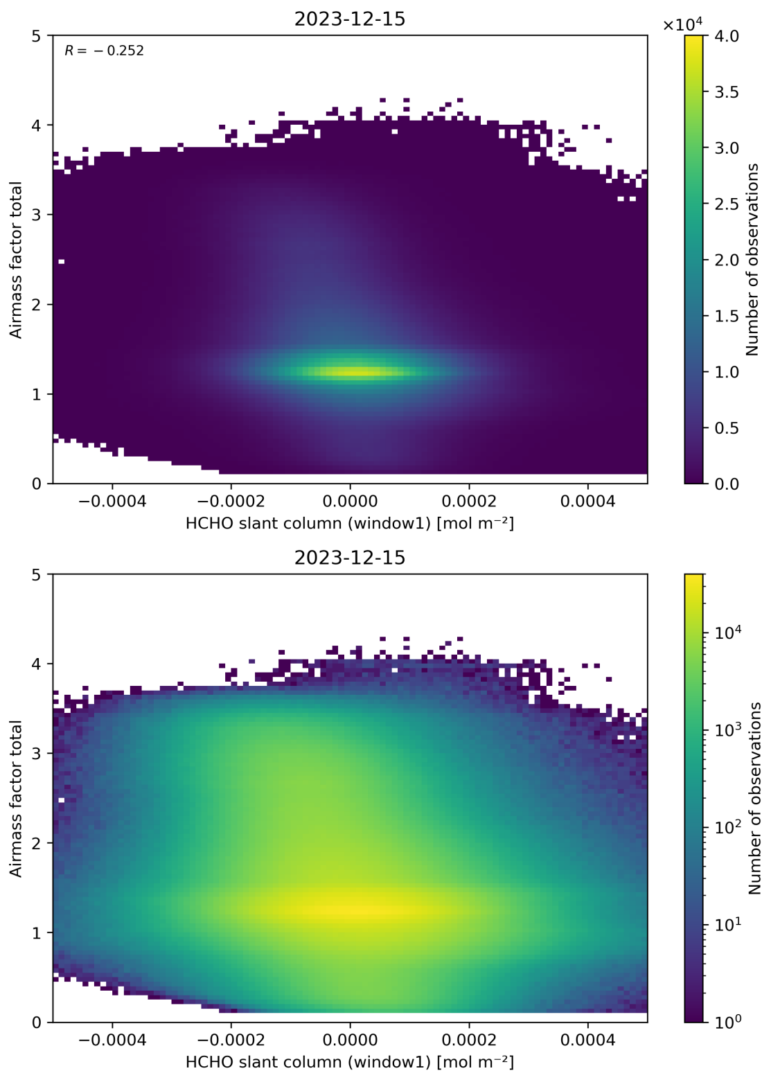
Figure 85: Scatter density plot of “HCHO slant column (window1)” against “Airmass factor total” for 2023-12-14 to 2023-12-16.
