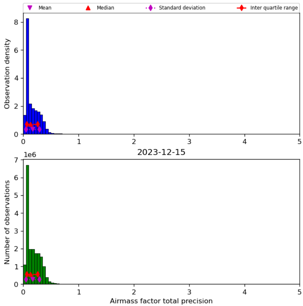
Figure 41: Histogram of “Airmass factor total precision” for 2023-12-14 to 2023-12-16
