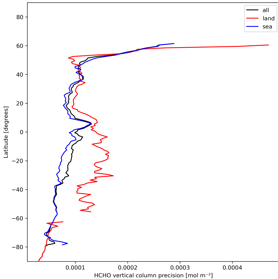
Figure 22: Zonal average of "HCHO vertical column precision" for 2023-12-14 to 2023-12-16.
