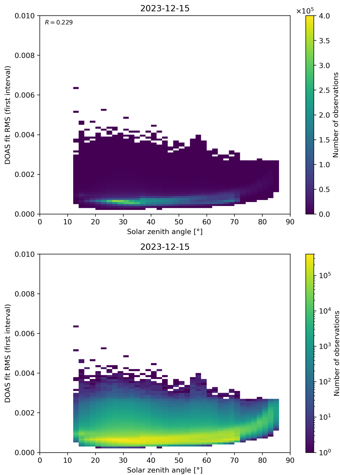
Figure 167: Scatter density plot of “Solar zenith angle” against “DOAS fit RMS (first interval)” for 2023-12-14 to 2023-12-16.
