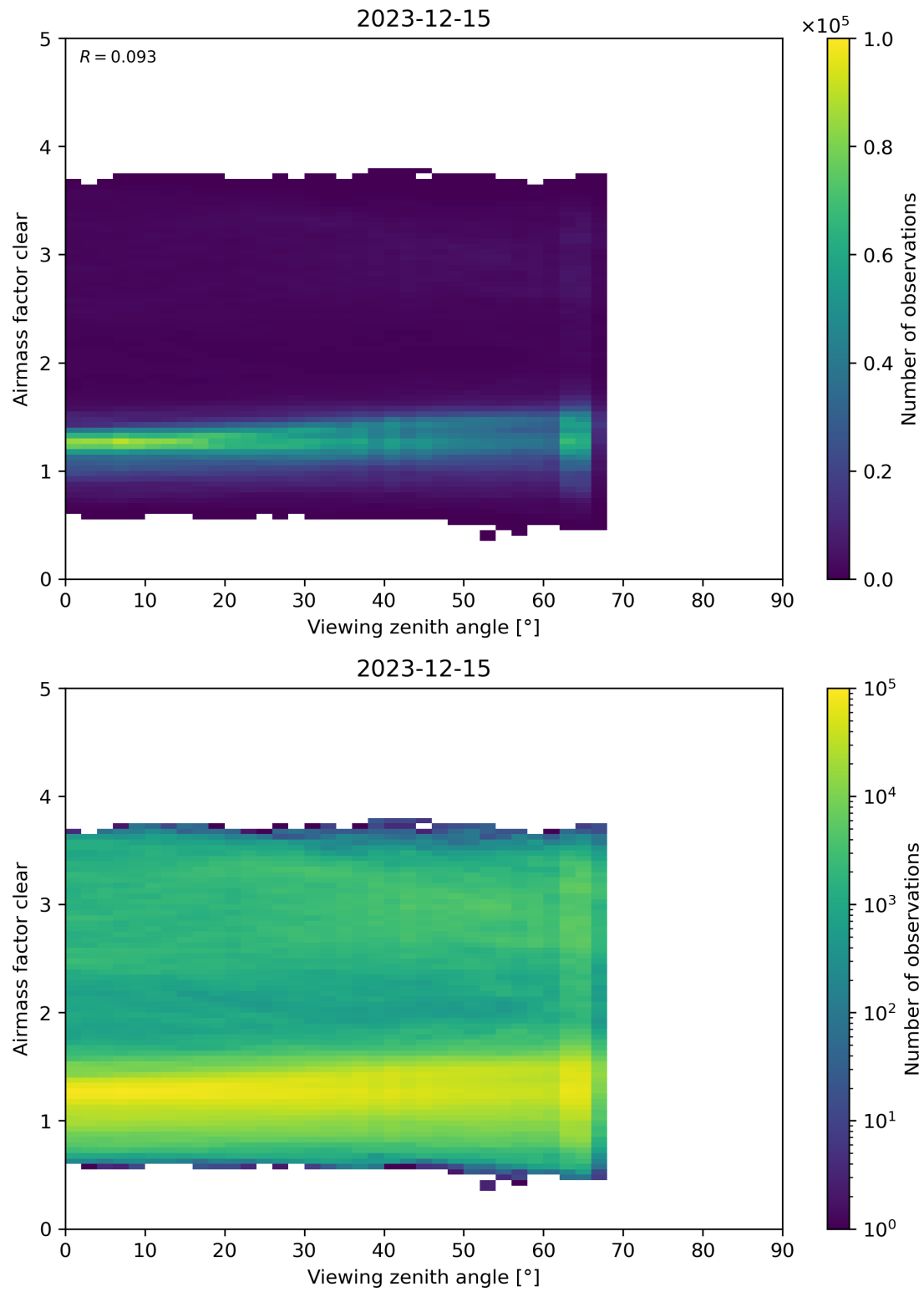
Figure 185: Scatter density plot of “Viewing zenith angle” against “Airmass factor clear” for 2023-12-14 to 2023-12-16.
