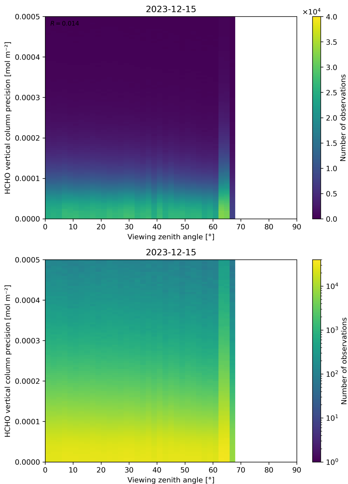
Figure 194: Scatter density plot of “Viewing zenith angle” against “HCHO vertical column precision” for 2023-12-14 to 2023-12-16.
