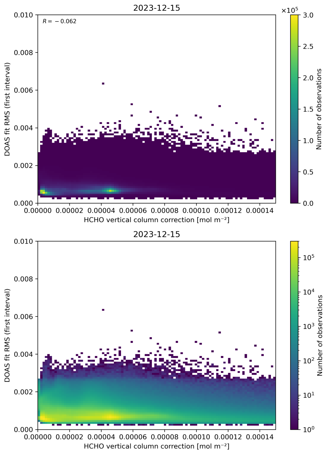
Figure 112: Scatter density plot of “HCHO vertical column correction” against “DOAS fit RMS (first interval)” for 2023-12-14 to 2023-12-16.
