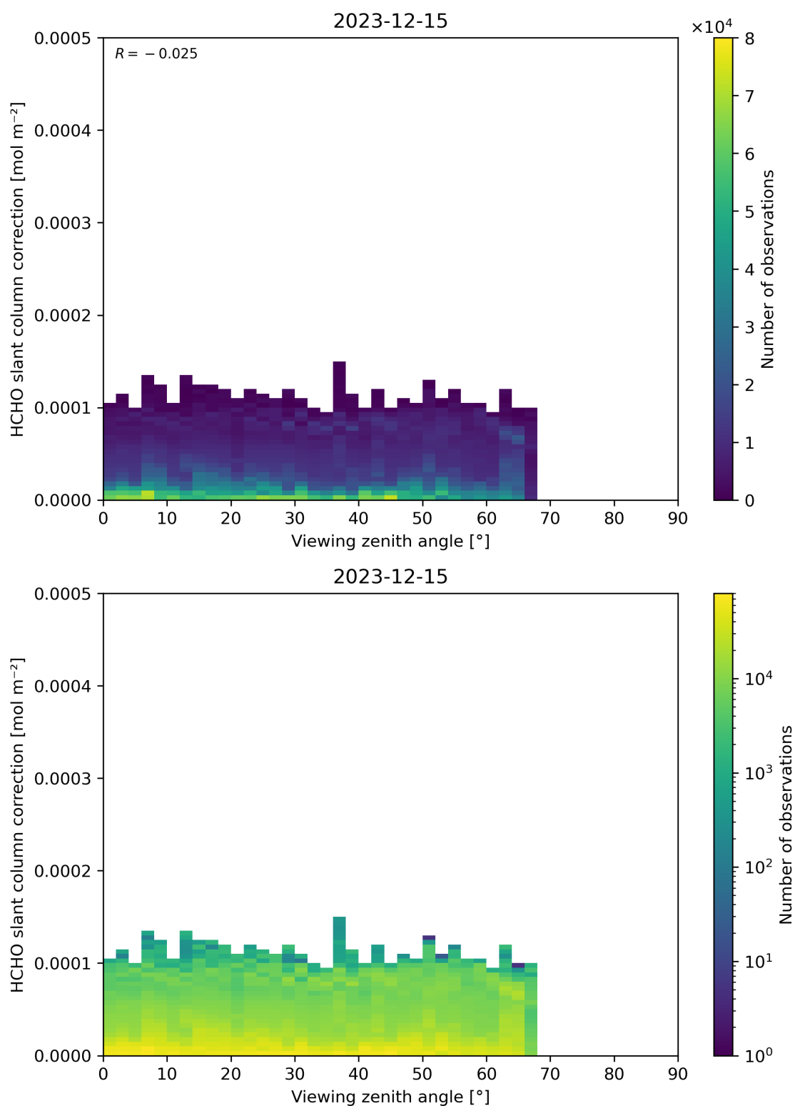
Figure 187: Scatter density plot of “Viewing zenith angle” against “HCHO slant column correction” for 2023-12-14 to 2023-12-16.
