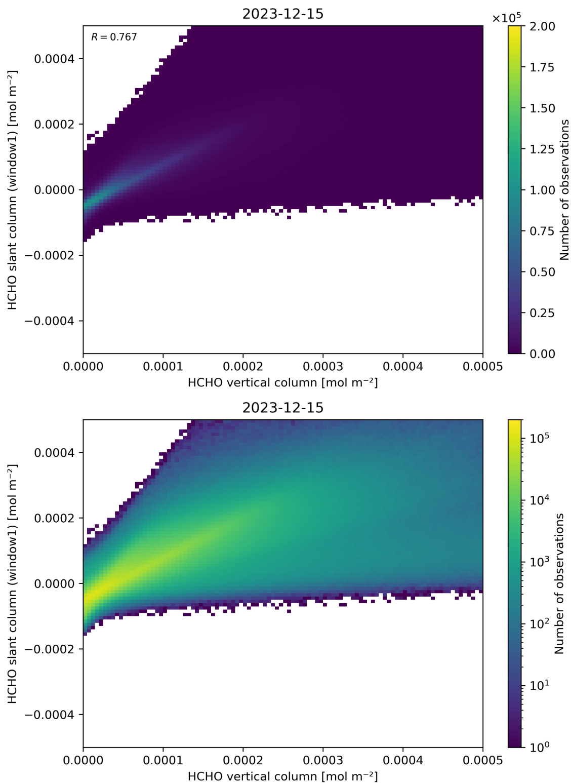
Figure 129: Scatter density plot of “HCHO vertical column” against “HCHO slant column (window1)” for 2023-12-14 to 2023-12-16.
