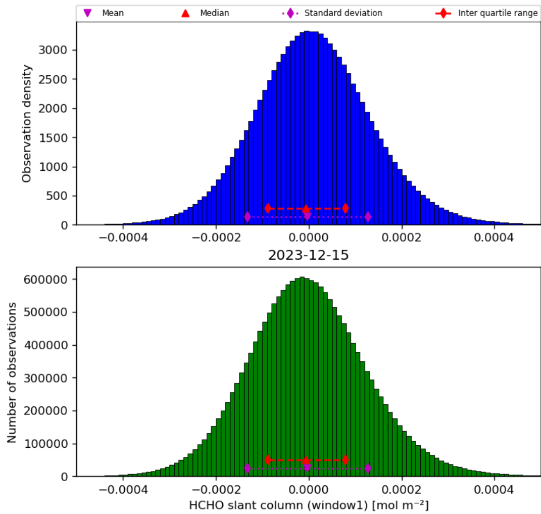
Figure 38: Histogram of “HCHO slant column (window1)” for 2023-12-14 to 2023-12-16
