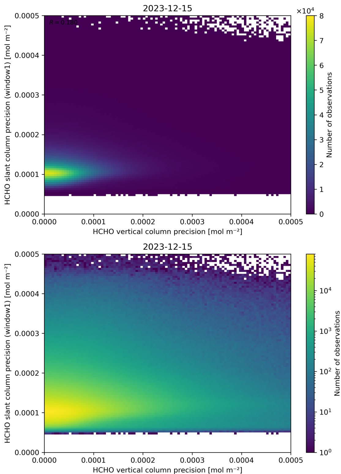
Figure 143: Scatter density plot of “HCHO vertical column precision” against “HCHO slant column precision (window1)” for 2023-12-14 to 2023-12-16.
