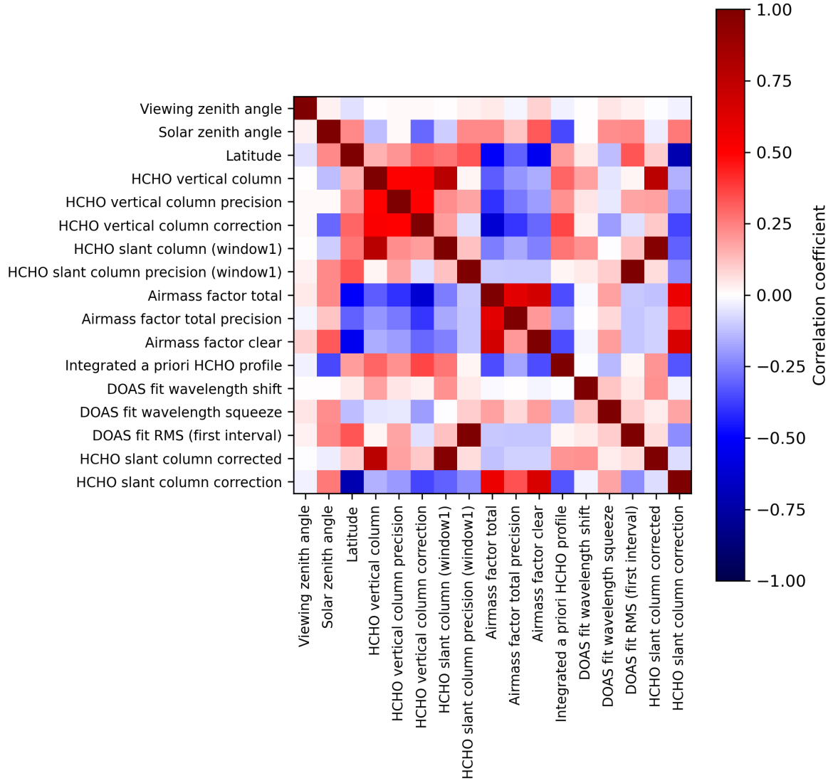
Figure 2: Map of correlation matrix for 2023-12-14 to 2023-12-16.
