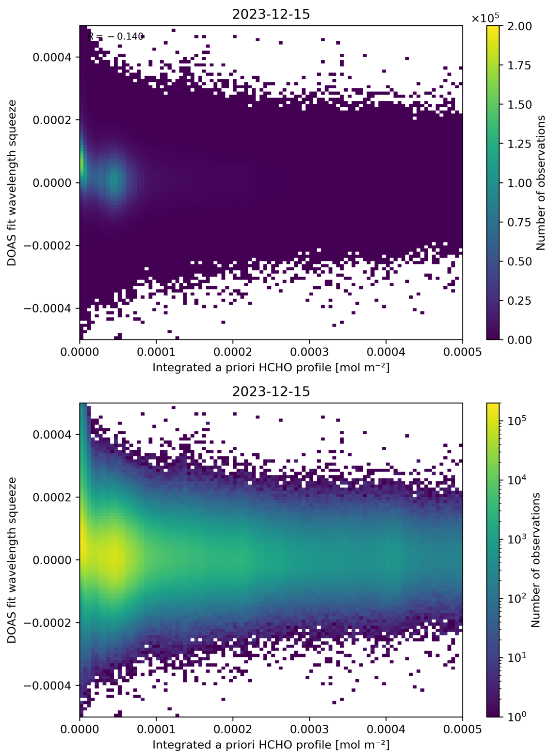
Figure 150: Scatter density plot of “Integrated a priori HCHO profile” against “DOAS fit wavelength squeeze” for 2023-12-14 to 2023-12-16.
