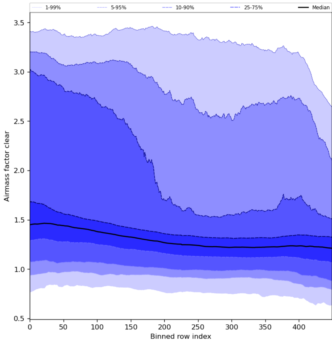
Figure 56: Along track statistics of “Airmass factor clear” for 2023-12-14 to 2023-12-16
