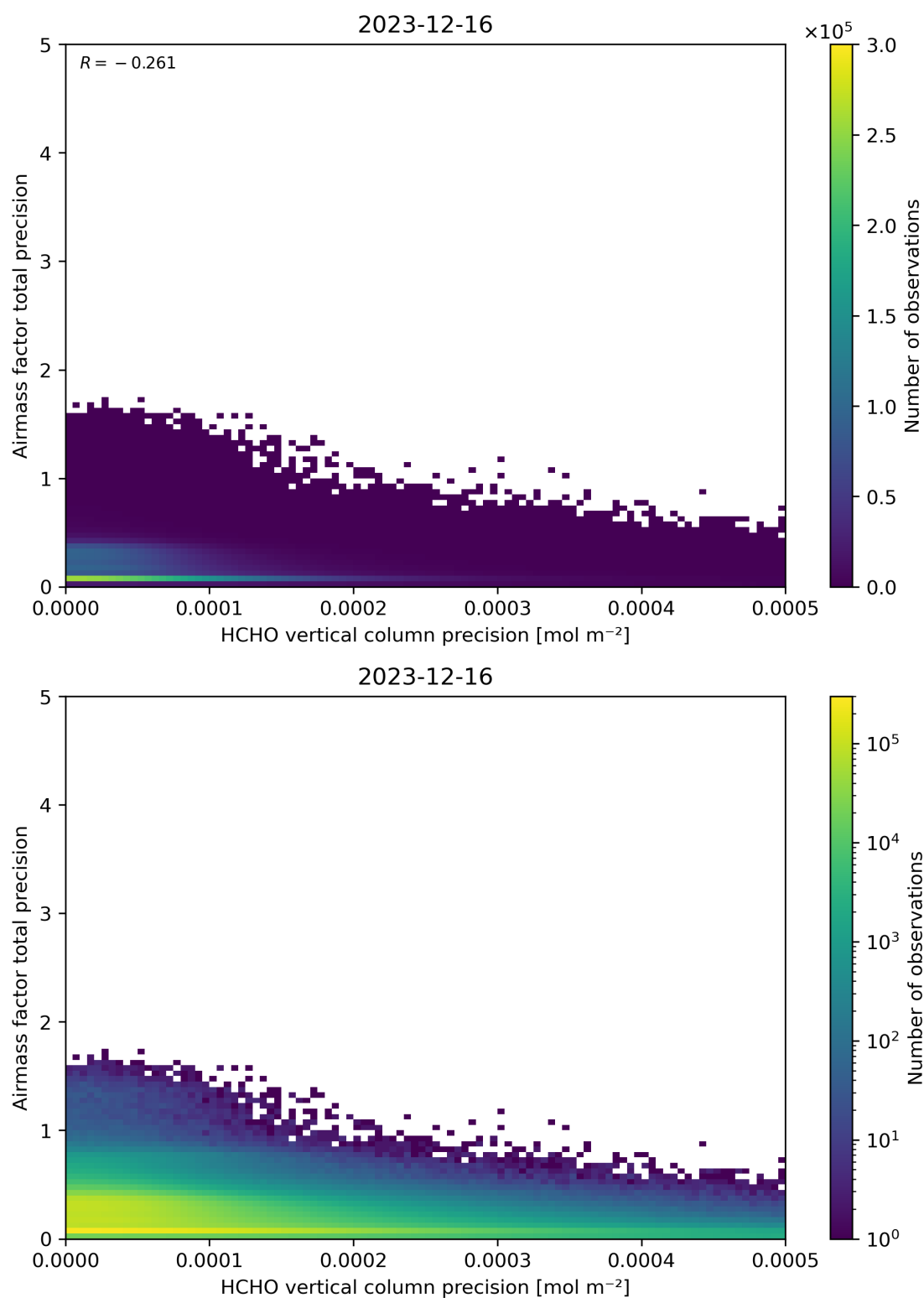
Figure 145: Scatter density plot of “HCHO vertical column precision” against “Airmass factor total precision” for 2023-12-15 to 2023-12-17.
