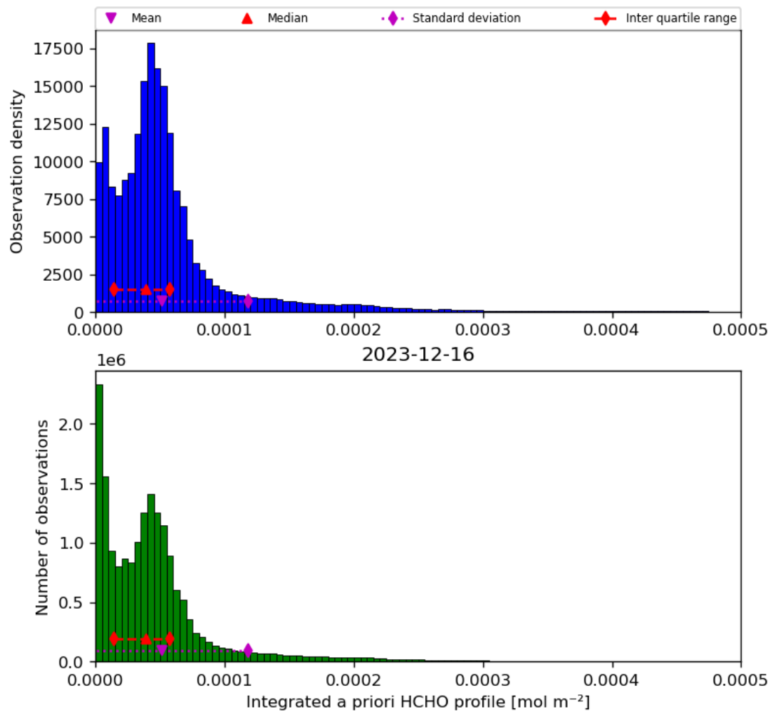
Figure 43: Histogram of “Integrated a priori HCHO profile” for 2023-12-15 to 2023-12-17
