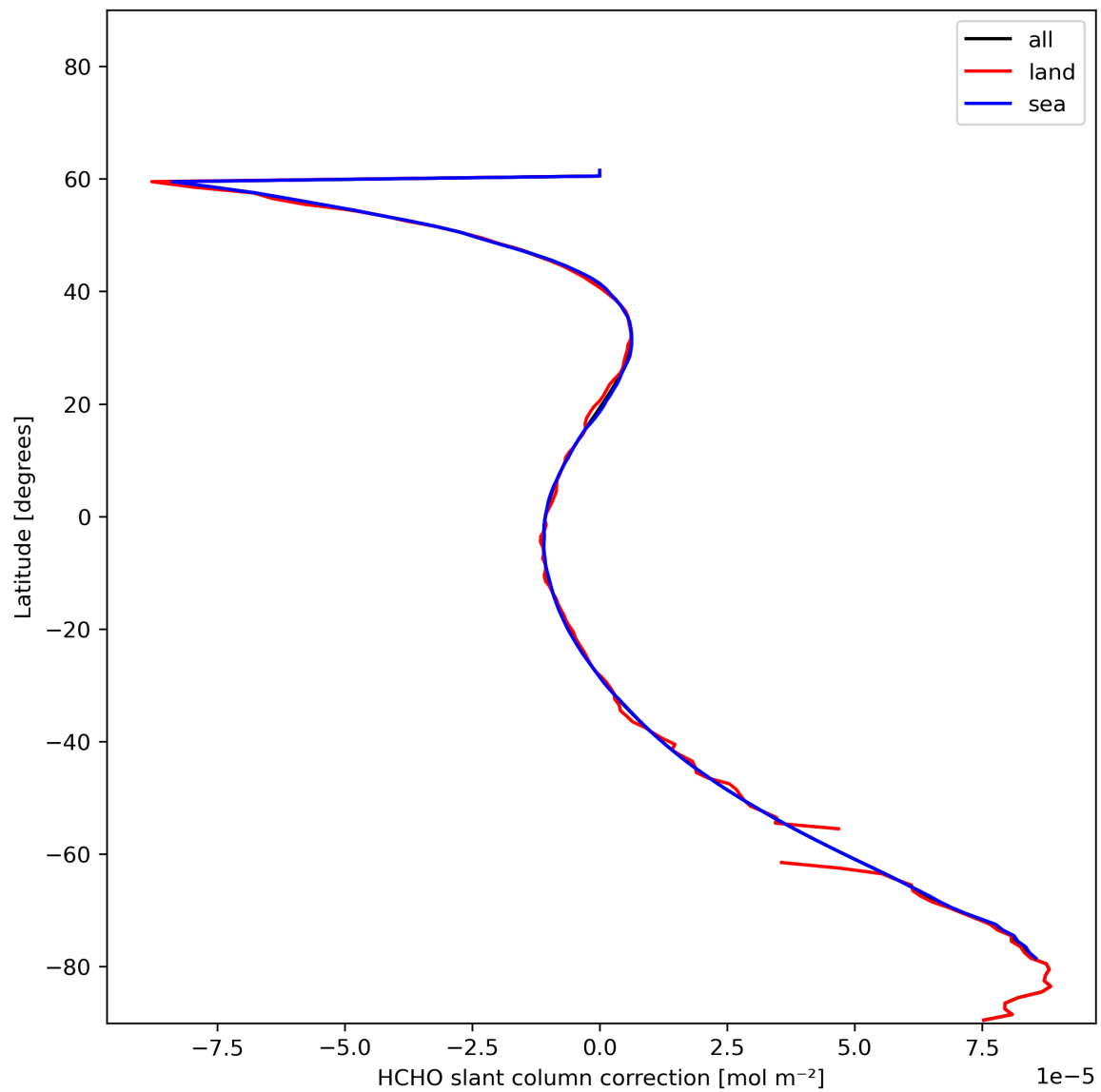
Figure 33: Zonal average of “HCHO slant column correction” for 2023-12-15 to 2023-12-17.
