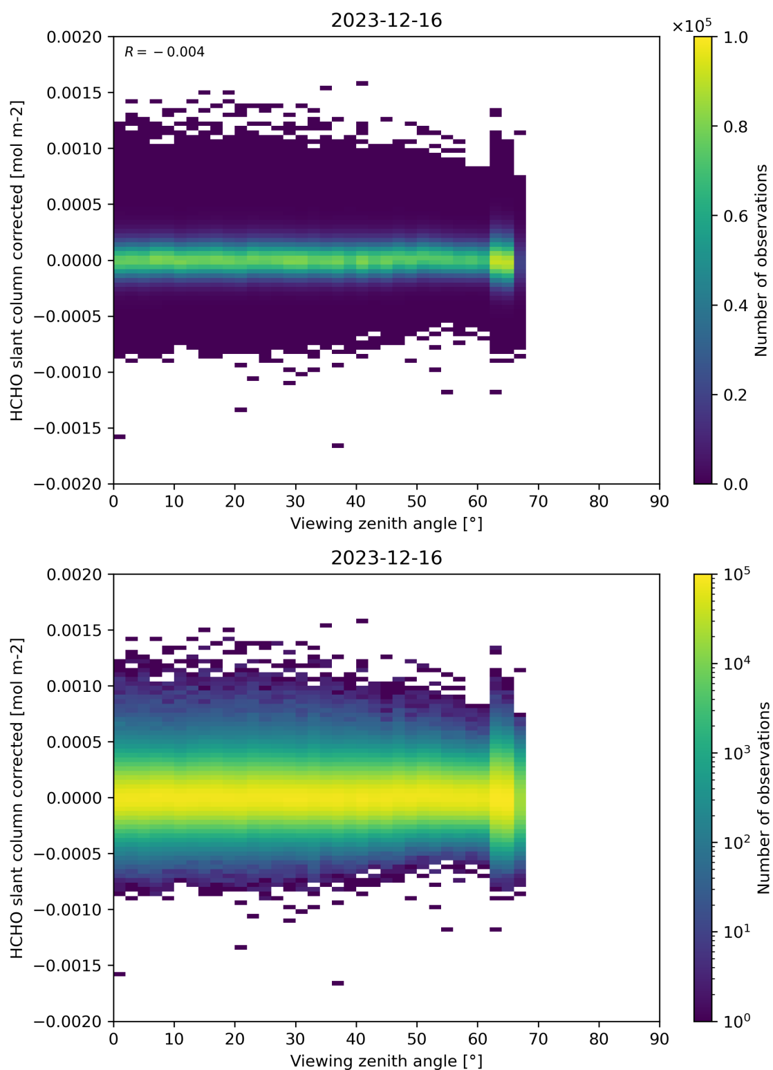
Figure 186: Scatter density plot of “Viewing zenith angle” against “HCHO slant column corrected” for 2023-12-15 to 2023-12-17.
