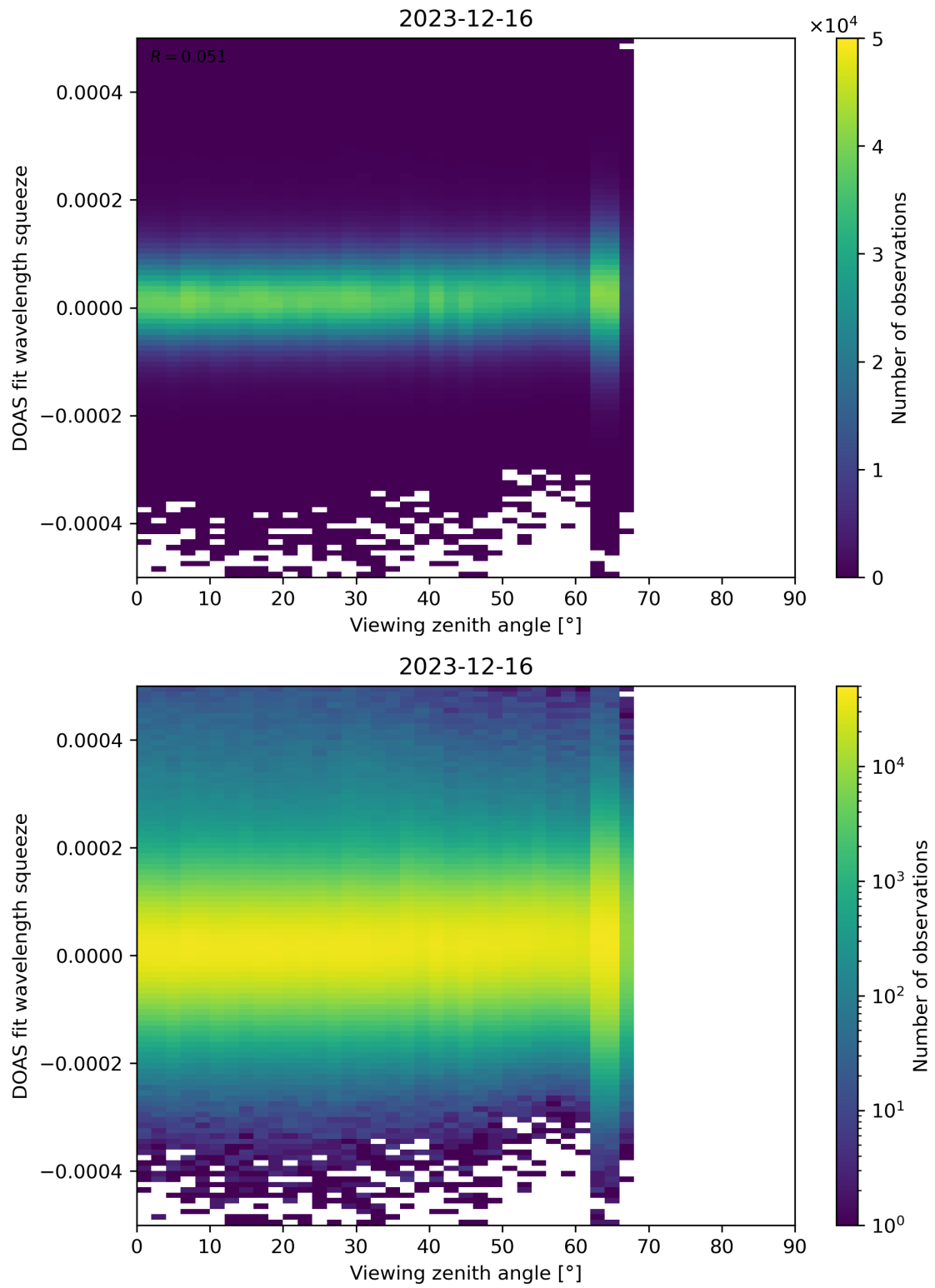
Figure 184: Scatter density plot of “Viewing zenith angle” against “DOAS fit wavelength squeeze” for 2023-12-15 to 2023-12-17.
