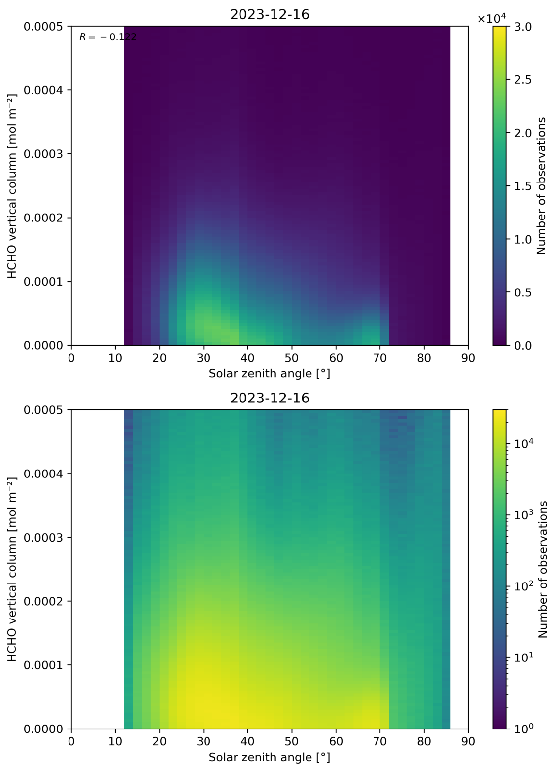
Figure 177: Scatter density plot of “Solar zenith angle” against “HCHO vertical column” for 2023-12-15 to 2023-12-17.
