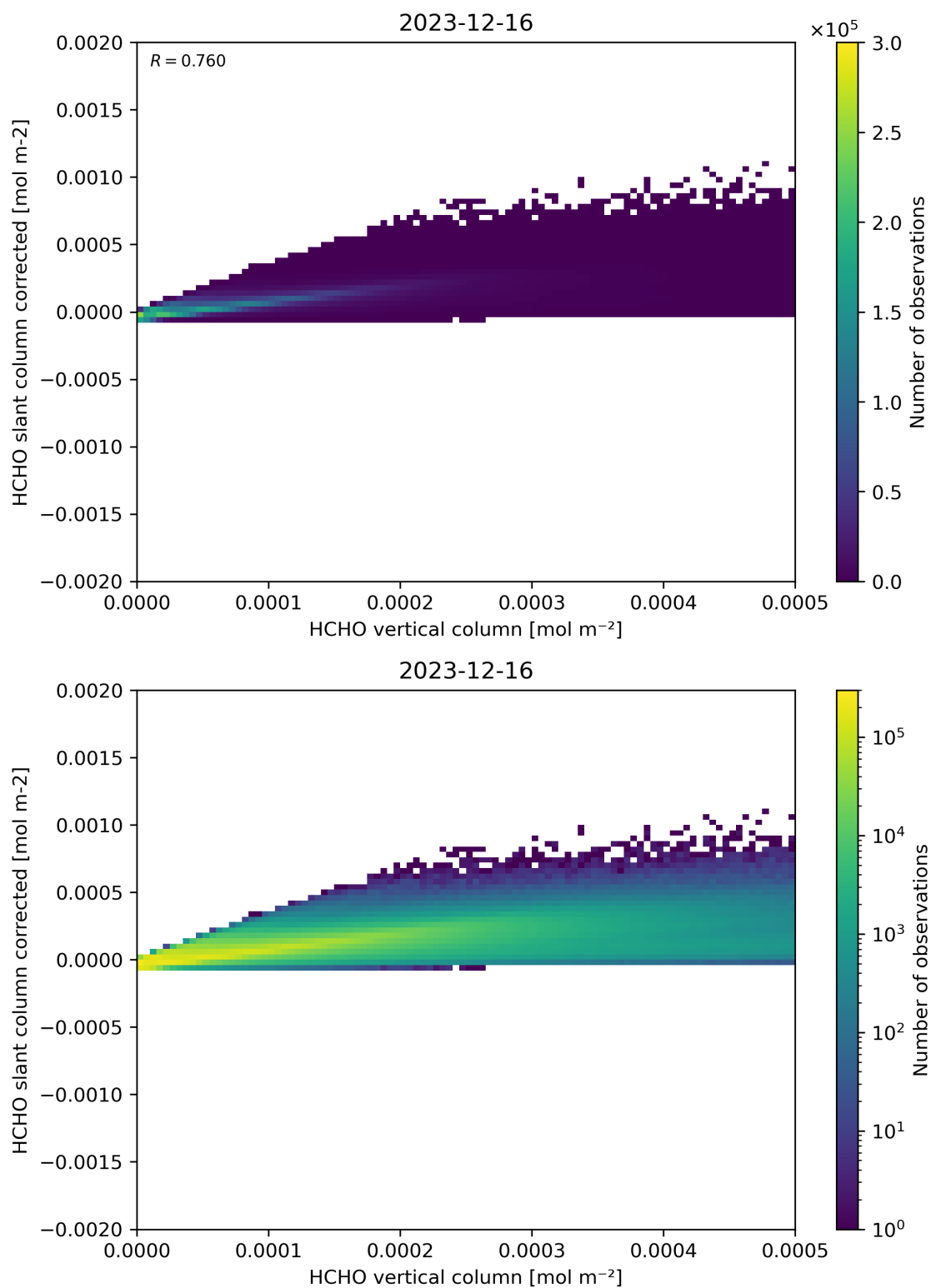
Figure 127: Scatter density plot of “HCHO vertical column” against “HCHO slant column corrected” for 2023-12-15 to 2023-12-17.
