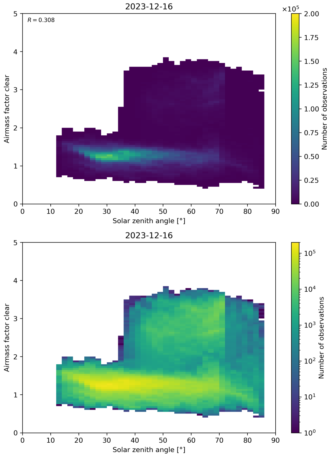
Figure 170: Scatter density plot of “Solar zenith angle” against “Airmass factor clear” for 2023-12-15 to 2023-12-17.
