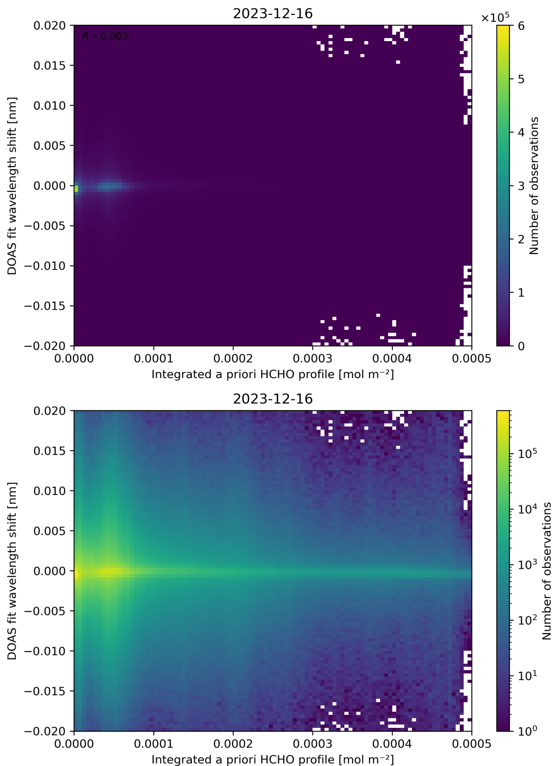
Figure 149: Scatter density plot of “Integrated a priori HCHO profile” against “DOAS fit wavelength shift” for 2023-12-15 to 2023-12-17.
