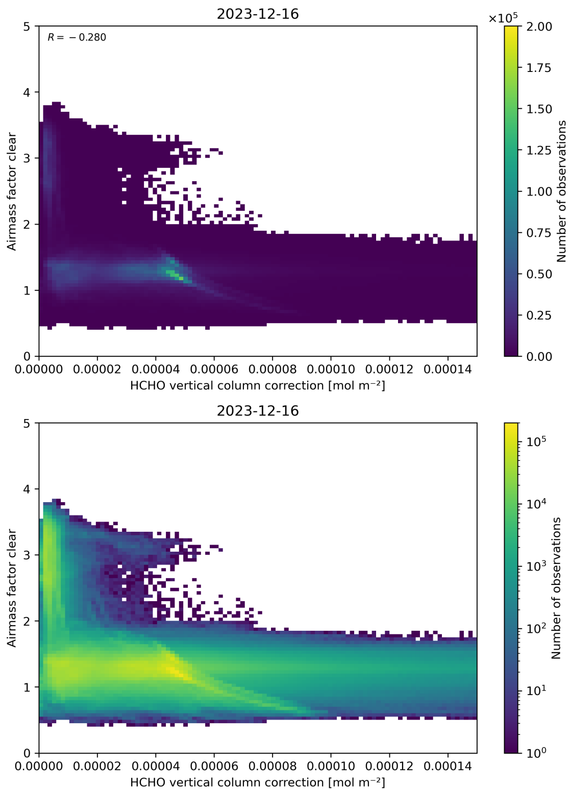
Figure 115: Scatter density plot of “HCHO vertical column correction” against “Airmass factor clear” for 2023-12-15 to 2023-12-17.
