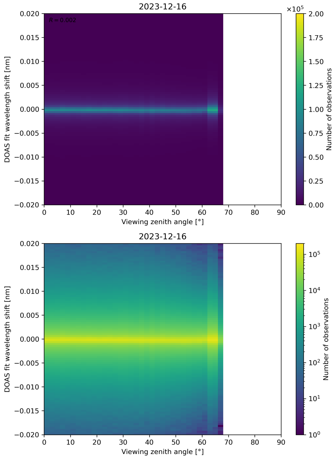
Figure 183: Scatter density plot of “Viewing zenith angle” against “DOAS fit wavelength shift” for 2023-12-15 to 2023-12-17.
