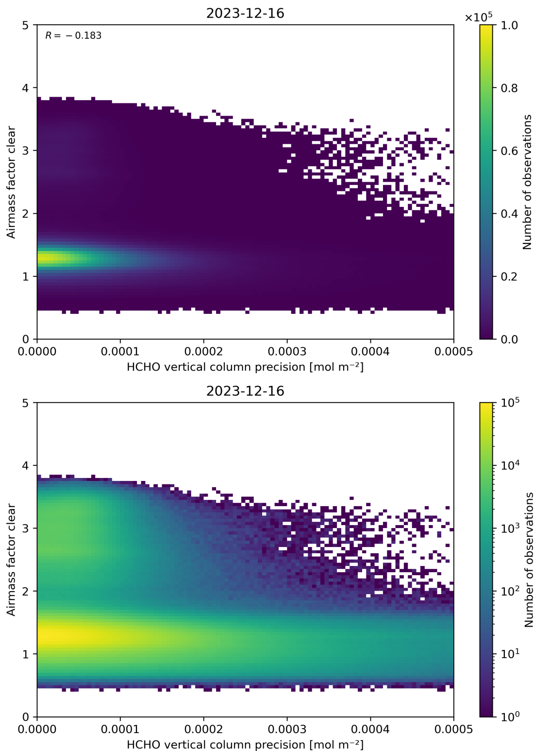
Figure 139: Scatter density plot of “HCHO vertical column precision” against “Airmass factor clear” for 2023-12-15 to 2023-12-17.
