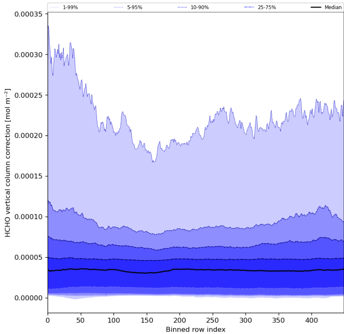
Figure 51: Along track statistics of “HCHO vertical column correction” for 2023-12-15 to 2023-12-17
