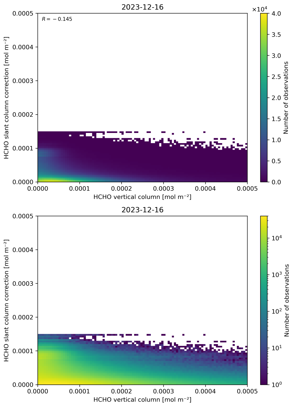
Figure 128: Scatter density plot of “HCHO vertical column” against “HCHO slant column correction” for 2023-12-15 to 2023-12-17.
