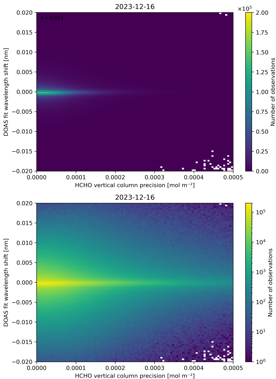
Figure 137: Scatter density plot of “HCHO vertical column precision” against “DOAS fit wavelength shift” for 2023-12-15 to 2023-12-17.
