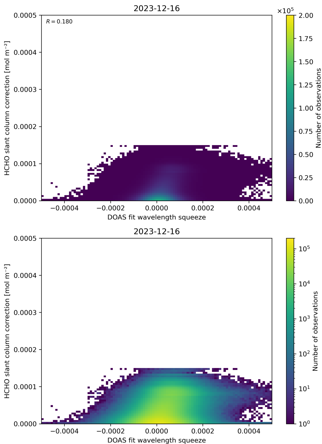
Figure 70: Scatter density plot of “DOAS fit wavelength squeeze” against “HCHO slant column correction” for 2023-12-15 to 2023-12-17.
