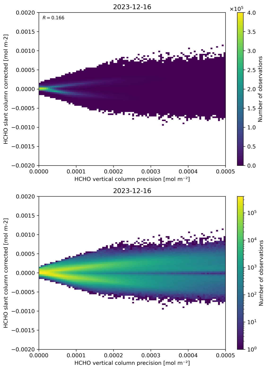
Figure 140: Scatter density plot of “HCHO vertical column precision” against “HCHO slant column corrected” for 2023-12-15 to 2023-12-17.
