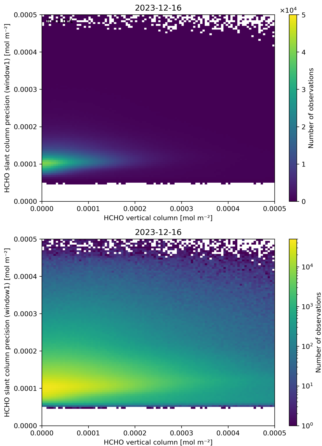
Figure 130: Scatter density plot of “HCHO vertical column” against “HCHO slant column precision (window1)” for 2023-12-15 to 2023-12-17.
