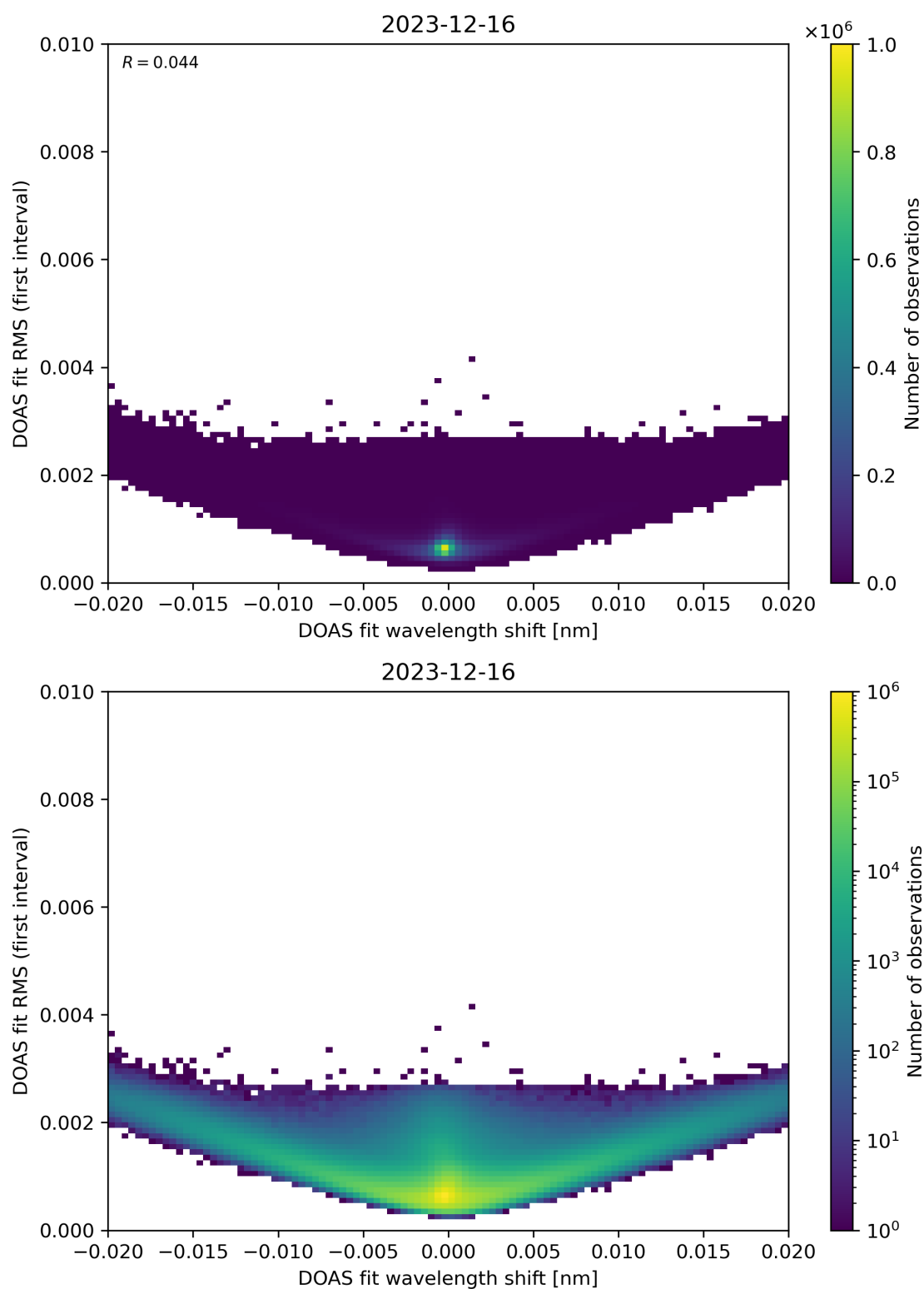
Figure 64: Scatter density plot of “DOAS fit wavelength shift” against “DOAS fit RMS (first interval)” for 2023-12-15 to 2023-12-17.
