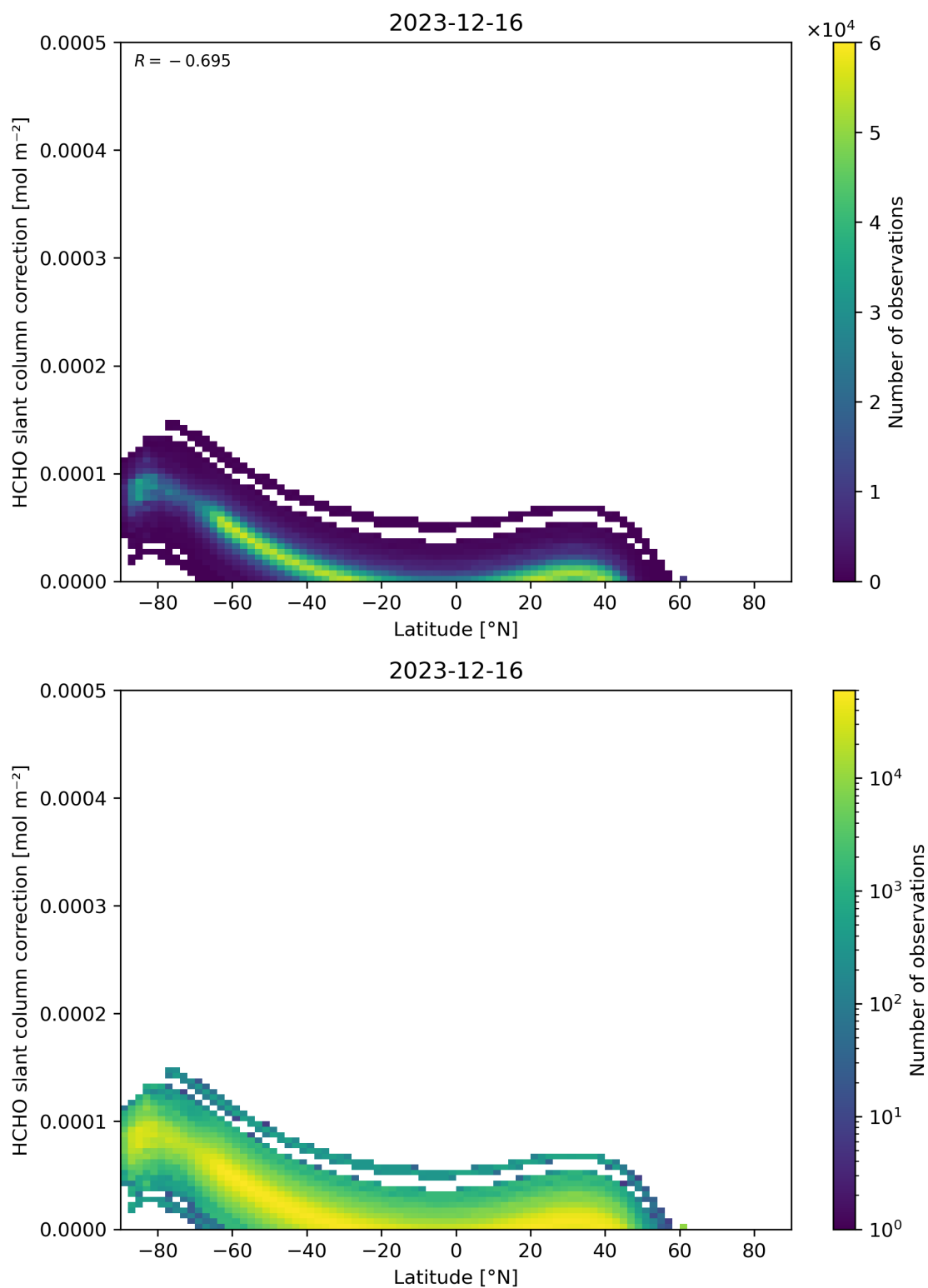
Figure 158: Scatter density plot of “Latitude” against “HCHO slant column correction” for 2023-12-15 to 2023-12-17.
