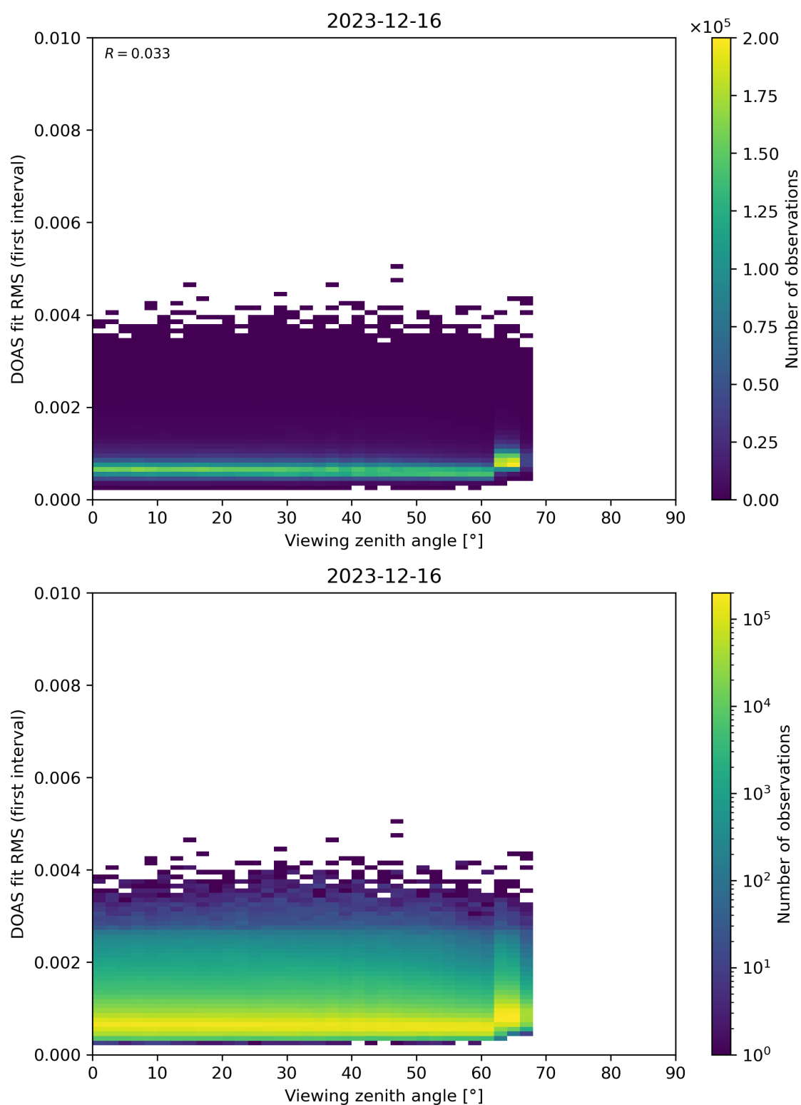
Figure 182: Scatter density plot of “Viewing zenith angle” against “DOAS fit RMS (first interval)” for 2023-12-15 to 2023-12-17.
