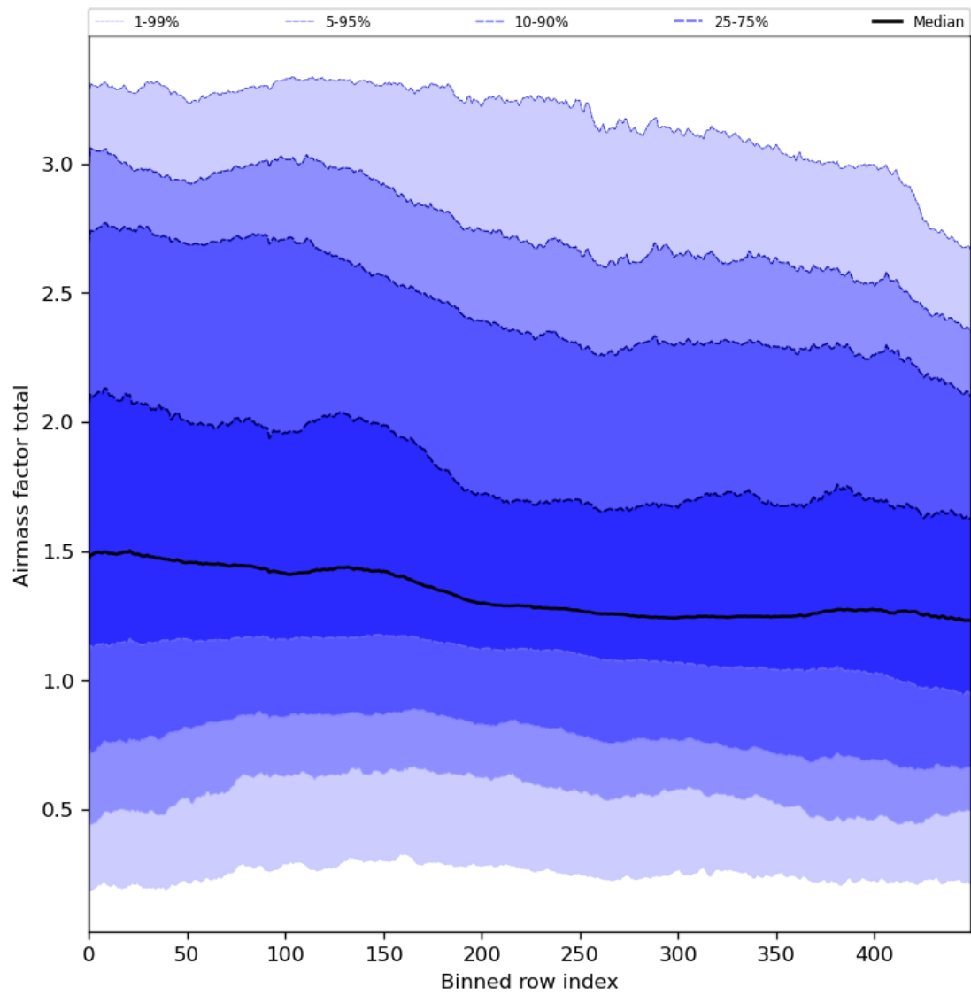
Figure 54: Along track statistics of “Airmass factor total” for 2023-12-15 to 2023-12-17
