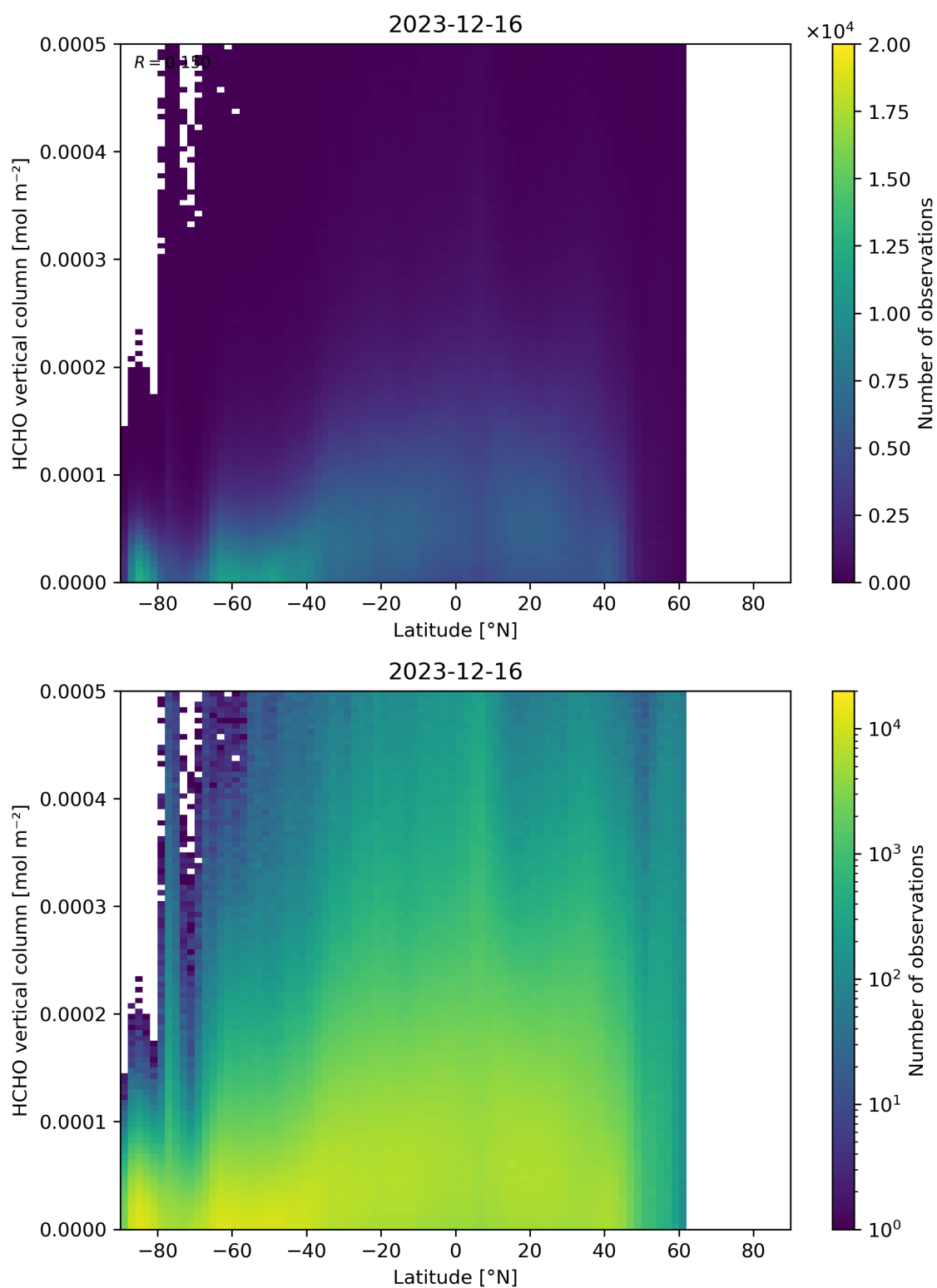
Figure 163: Scatter density plot of “Latitude” against “HCHO vertical column” for 2023-12-15 to 2023-12-17.
