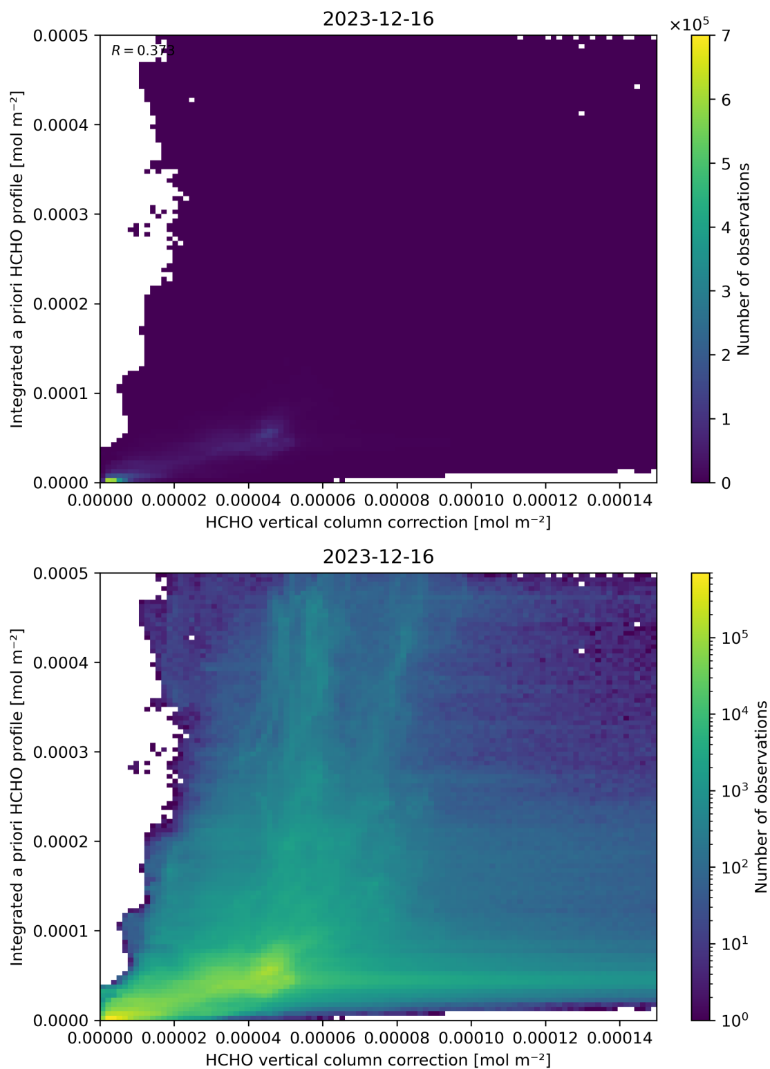
Figure 122: Scatter density plot of “HCHO vertical column correction” against “Integrated a priori HCHO profile” for 2023-12-15 to 2023-12-17.
