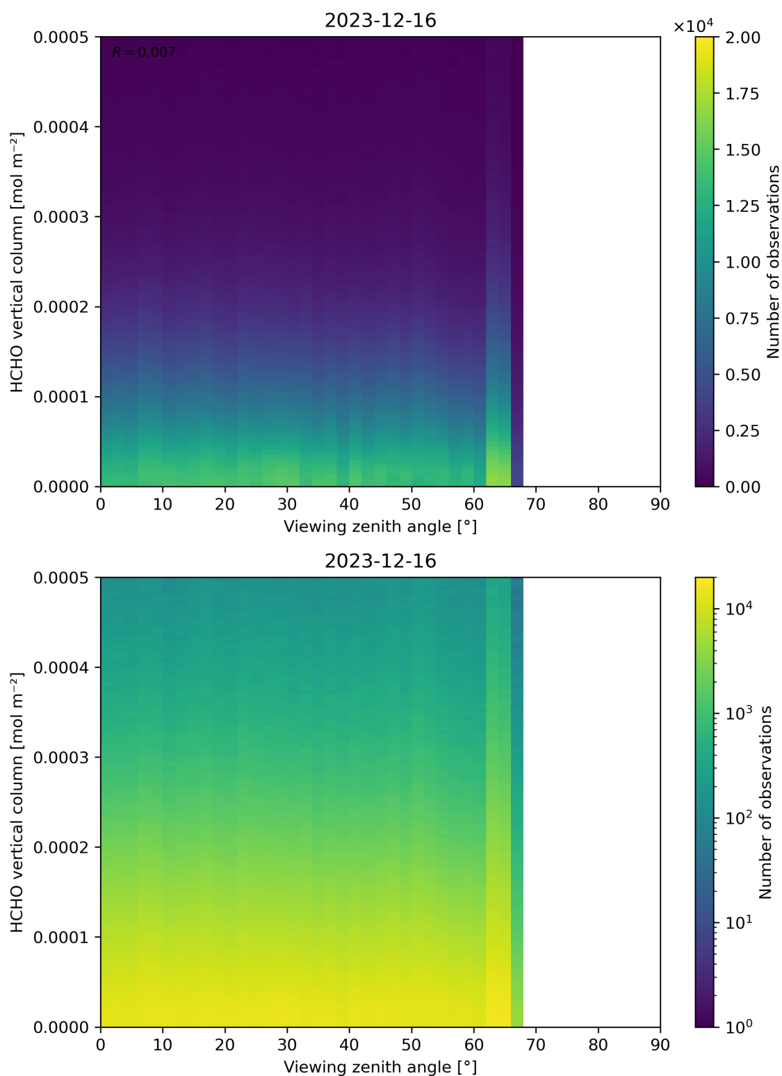
Figure 192: Scatter density plot of “Viewing zenith angle” against “HCHO vertical column” for 2023-12-15 to 2023-12-17.
