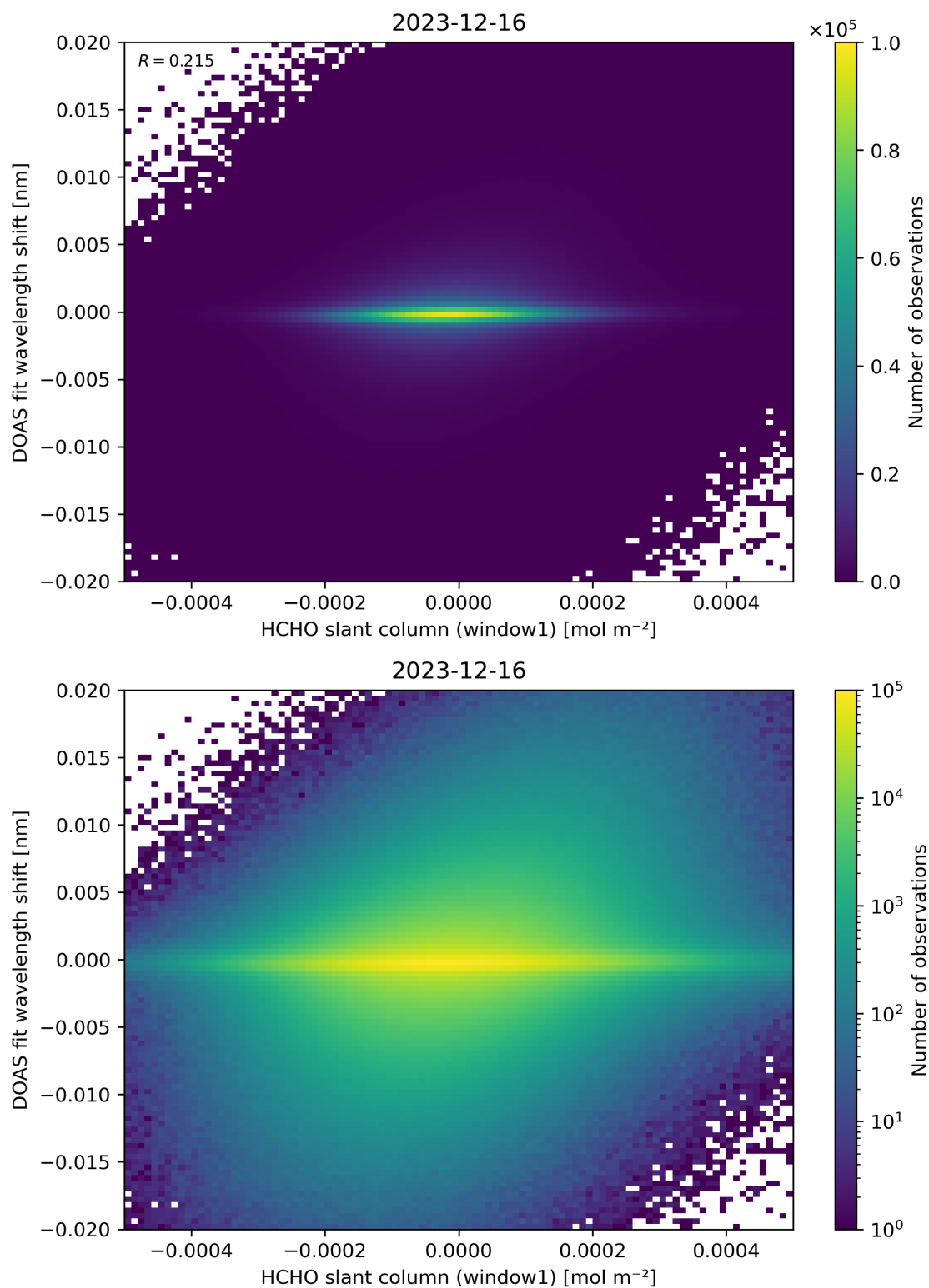
Figure 79: Scatter density plot of “HCHO slant column (window1)” against “DOAS fit wavelength shift” for 2023-12-15 to 2023-12-17.
