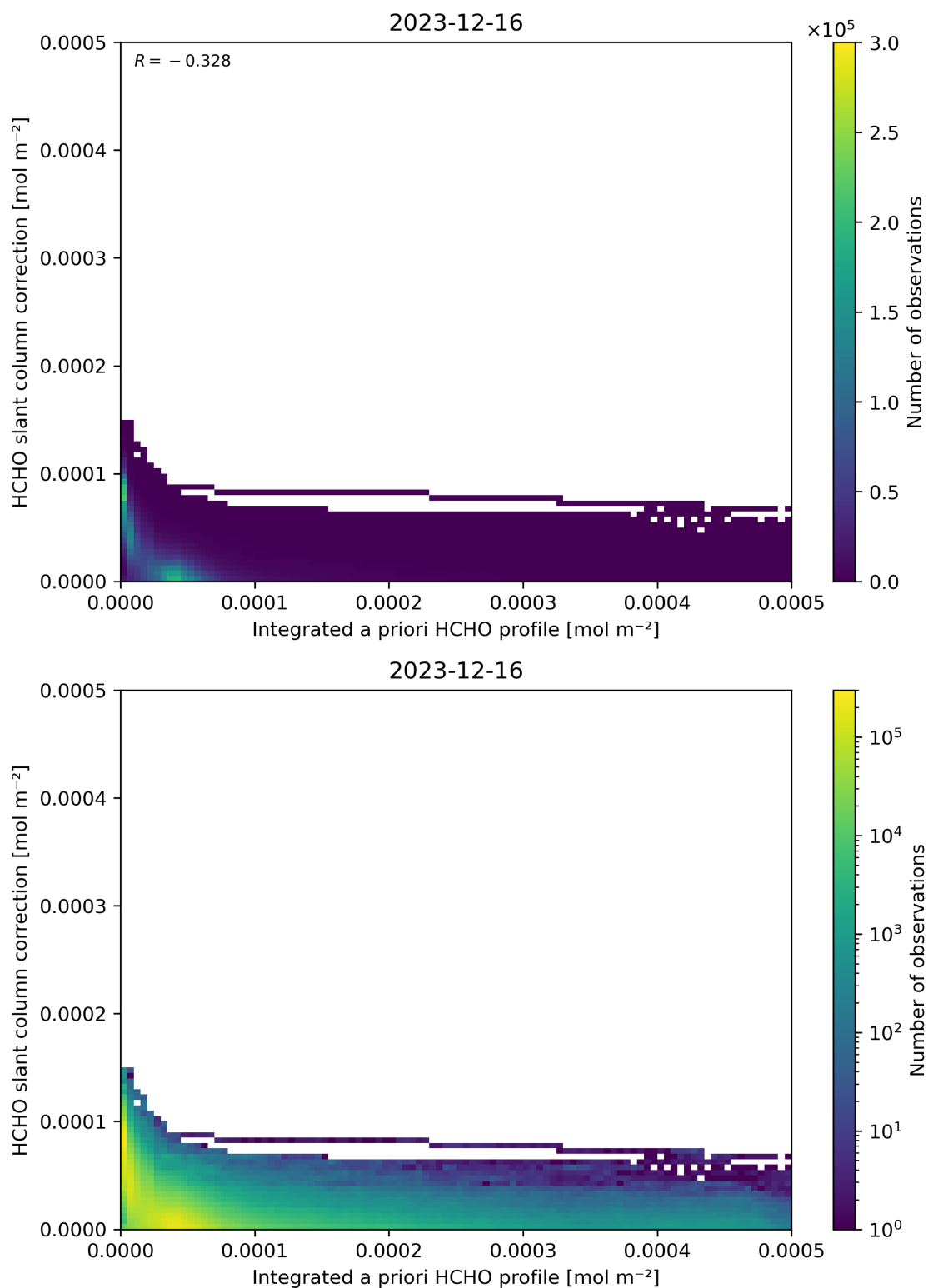
Figure 152: Scatter density plot of “Integrated a priori HCHO profile” against “HCHO slant column correction” for 2023-12-15 to 2023-12-17.
