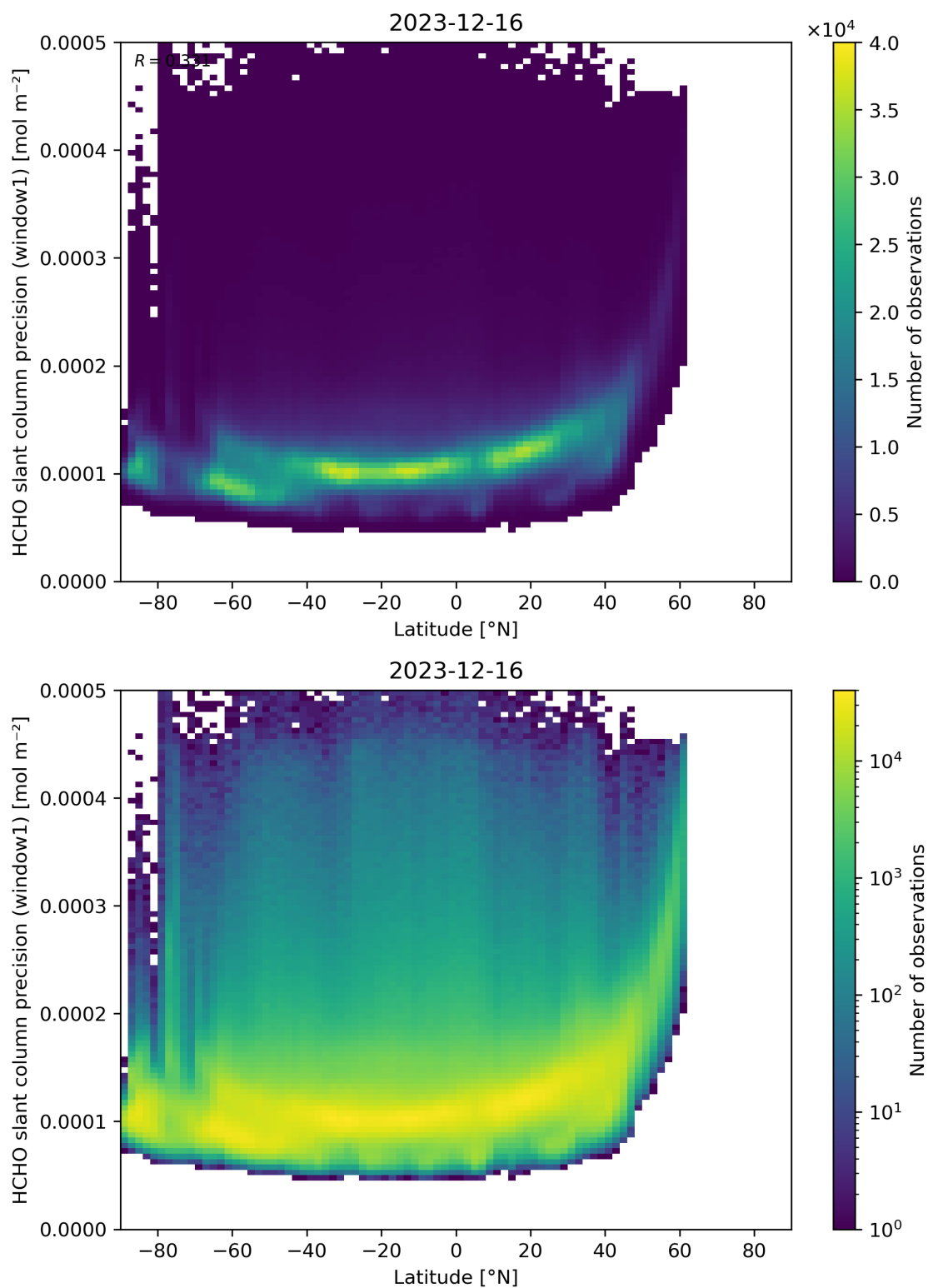
Figure 160: Scatter density plot of “Latitude” against “HCHO slant column precision (window1)” for 2023-12-15 to 2023-12-17.
