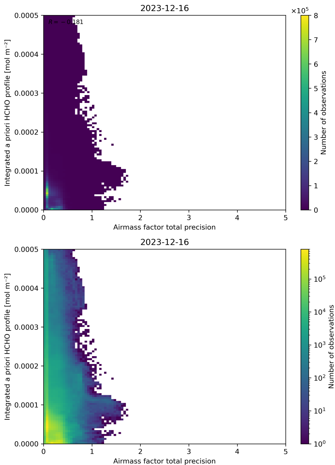
Figure 111: Scatter density plot of “Airmass factor total precision” against “Integrated a priori HCHO profile” for 2023-12-15 to 2023-12-17.
