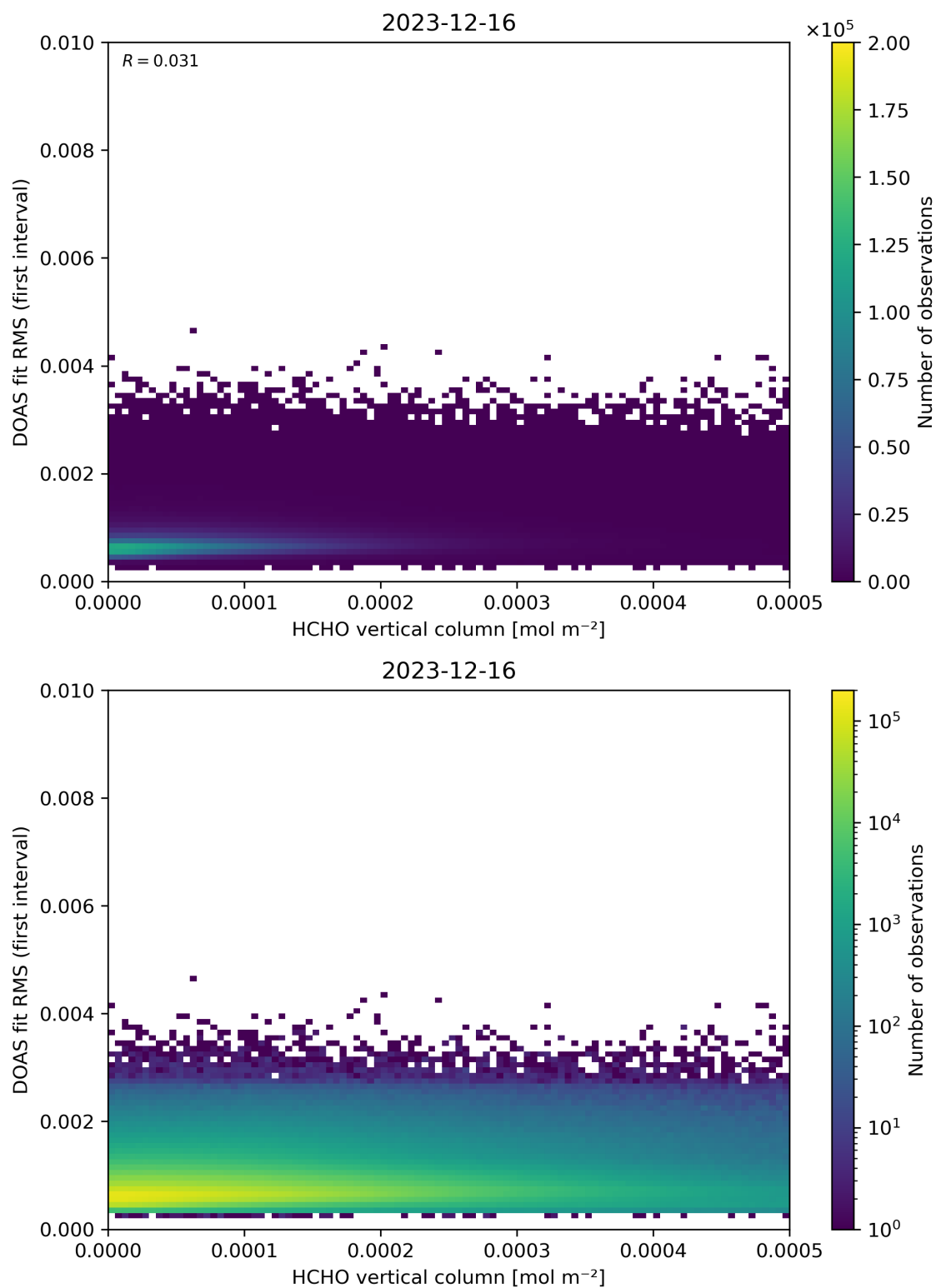
Figure 123: Scatter density plot of “HCHO vertical column” against “DOAS fit RMS (first interval)” for 2023-12-15 to 2023-12-17.
