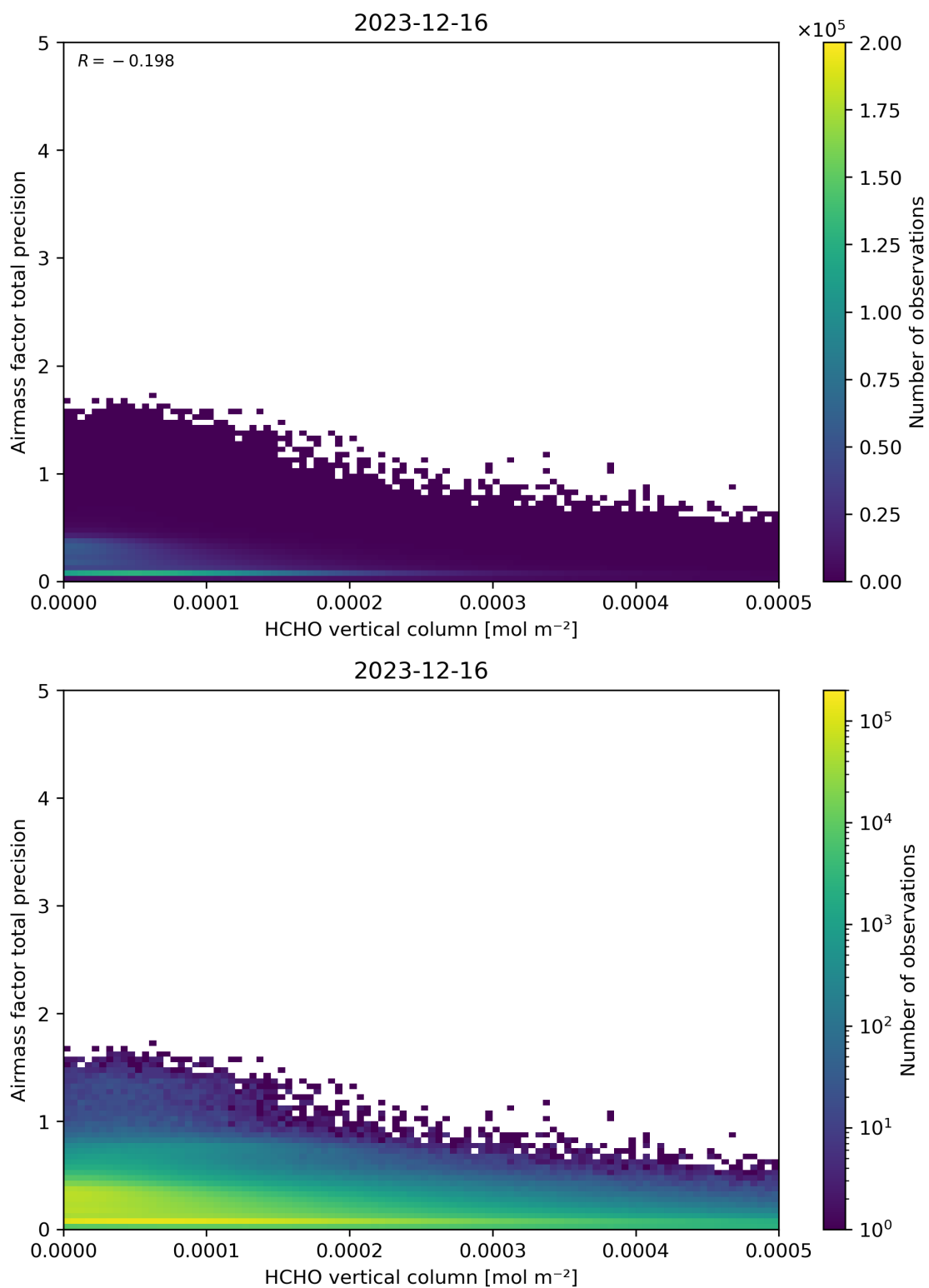
Figure 132: Scatter density plot of “HCHO vertical column” against “Airmass factor total precision” for 2023-12-15 to 2023-12-17.
