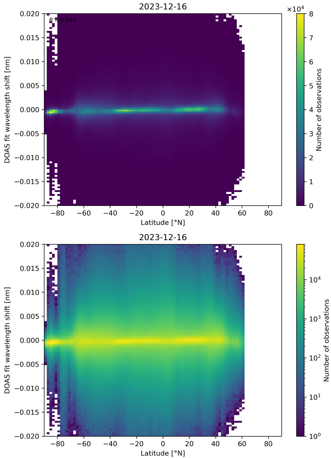
Figure 154: Scatter density plot of “Latitude” against “DOAS fit wavelength shift” for 2023-12-15 to 2023-12-17.
