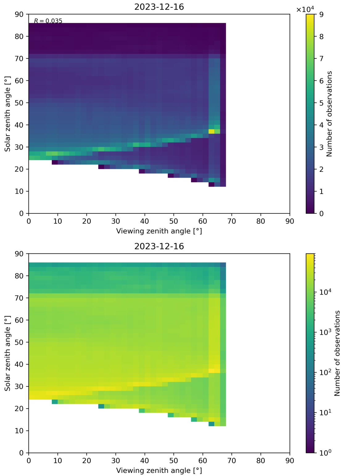
Figure 197: Scatter density plot of “Viewing zenith angle” against “Solar zenith angle” for 2023-12-15 to 2023-12-17.
