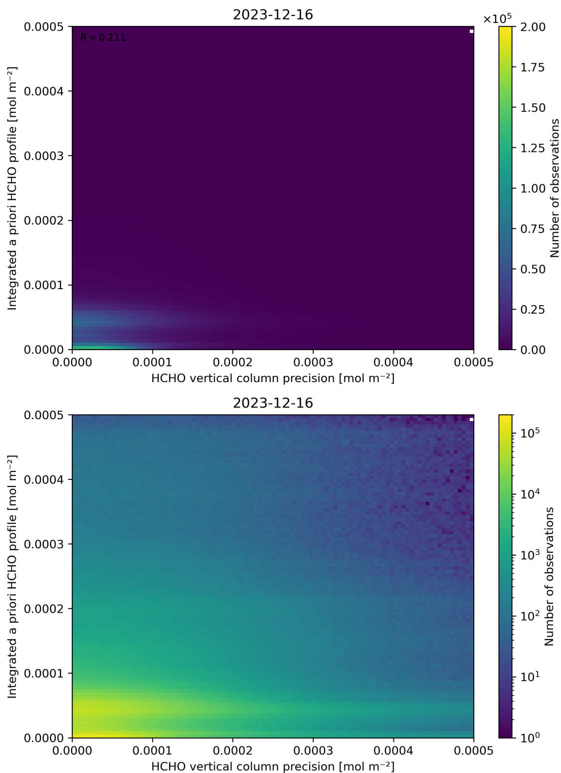
Figure 147: Scatter density plot of “HCHO vertical column precision” against “Integrated a priori HCHO profile” for 2023-12-15 to 2023-12-17.
