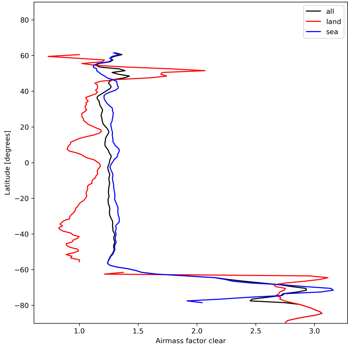
Figure 28: Zonal average of “Airmass factor clear” for 2023-12-15 to 2023-12-17.
