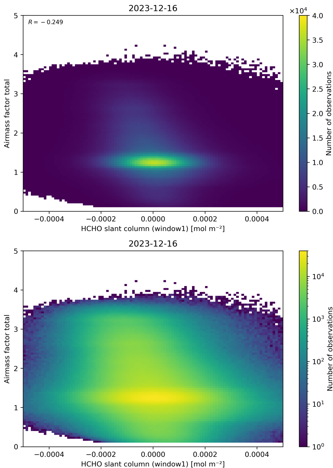
Figure 85: Scatter density plot of “HCHO slant column (window1)” against “Airmass factor total” for 2023-12-15 to 2023-12-17.
