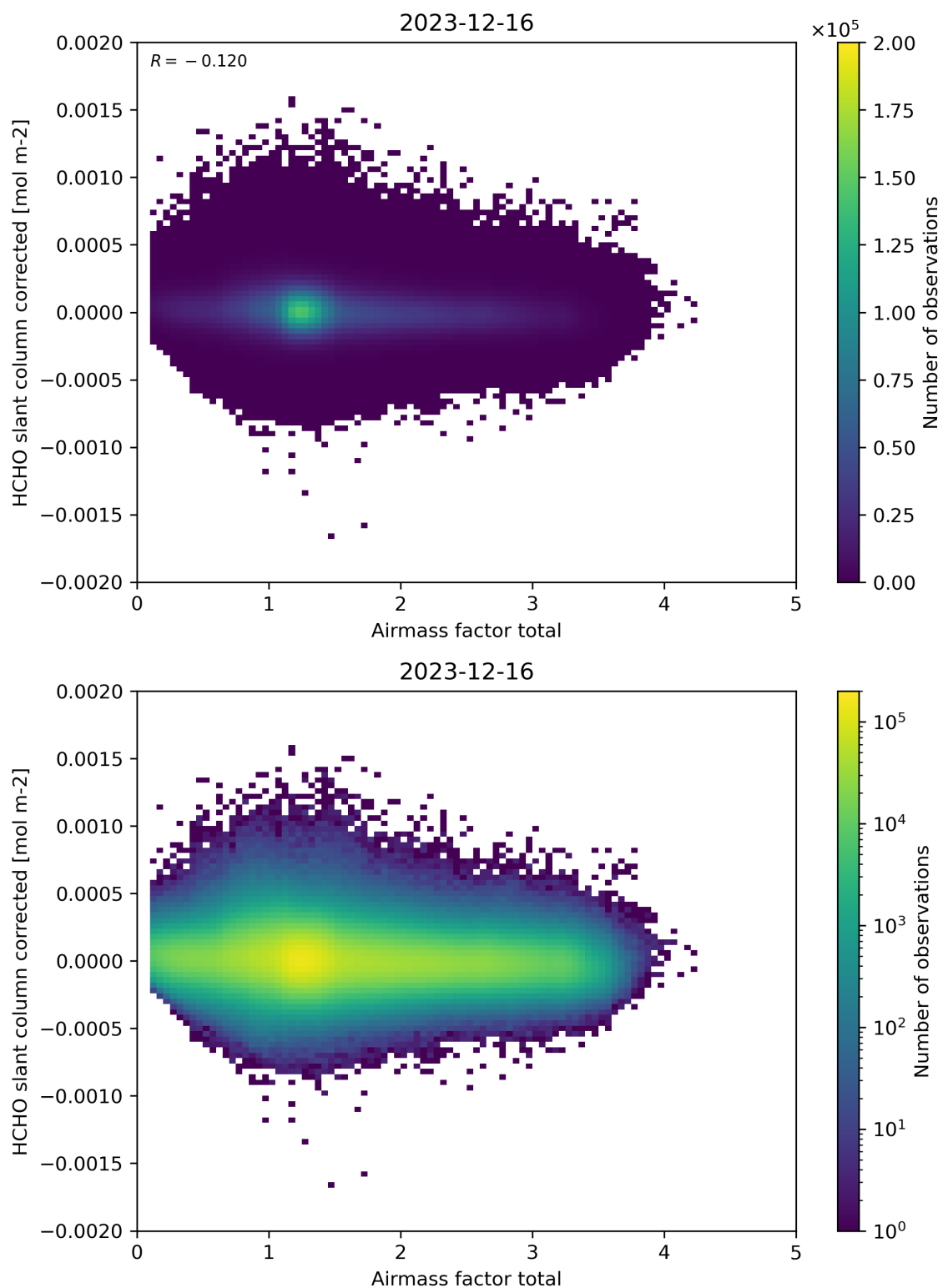
Figure 101: Scatter density plot of “Airmass factor total” against “HCHO slant column corrected” for 2023-12-15 to 2023-12-17.
