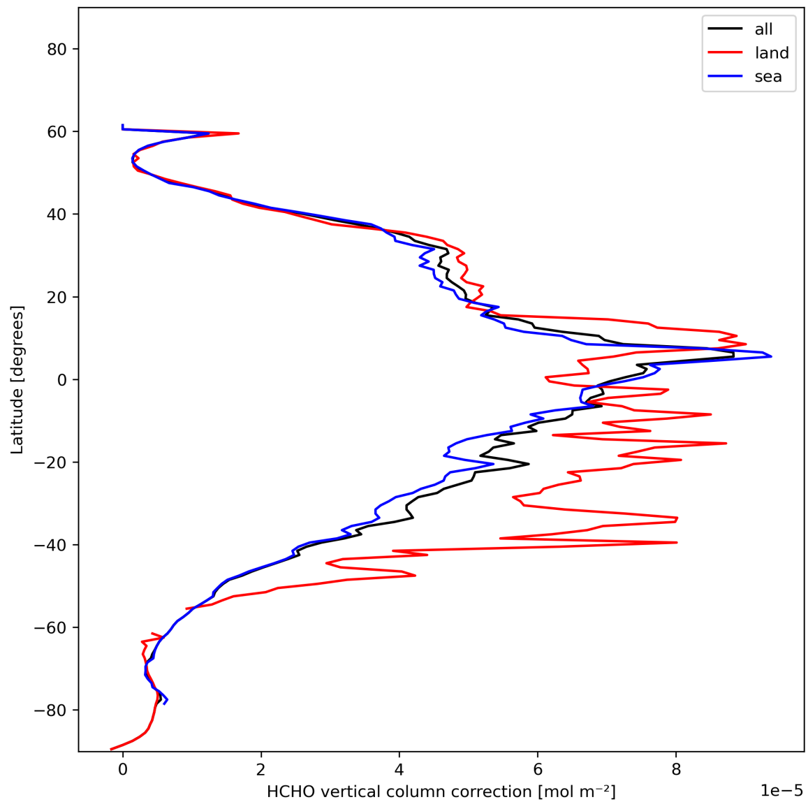
Figure 23: Zonal average of “HCHO vertical column correction” for 2023-12-15 to 2023-12-17.
