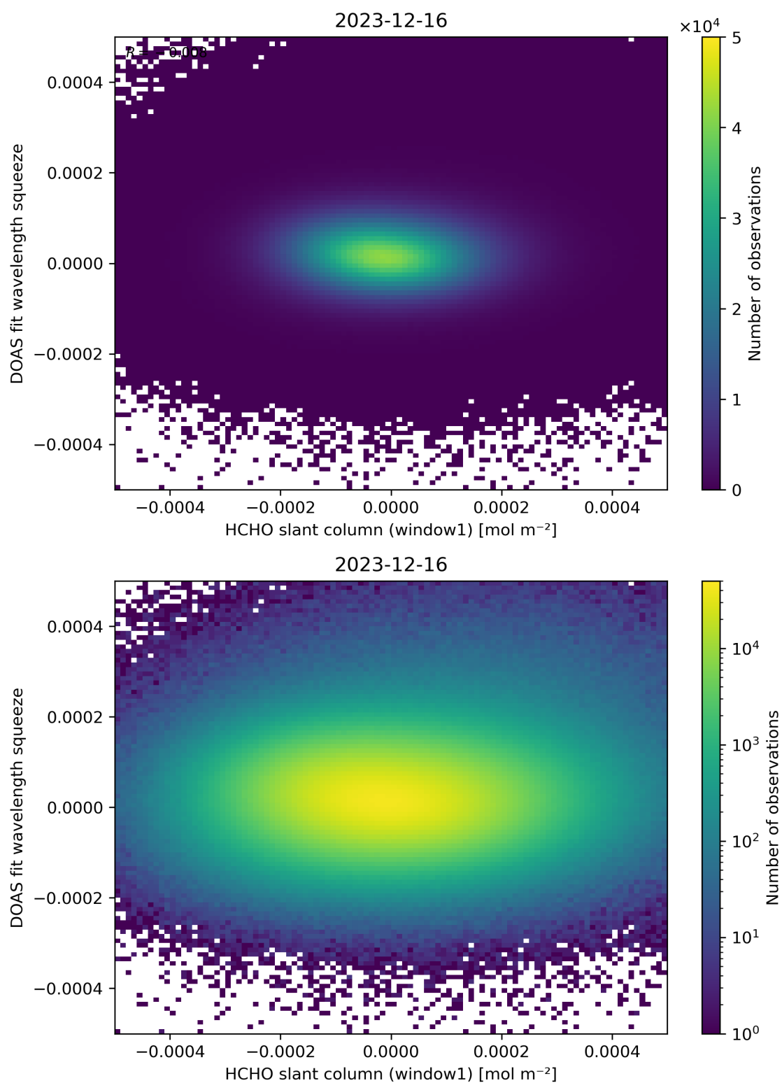
Figure 80: Scatter density plot of “HCHO slant column (window1)” against “DOAS fit wavelength squeeze” for 2023-12-15 to 2023-12-17.
