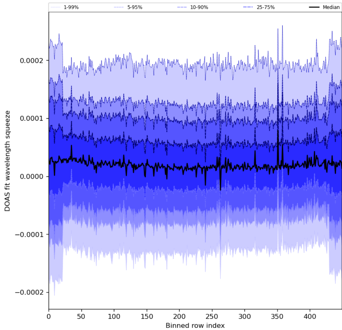
Figure 59: Along track statistics of “DOAS fit wavelength squeeze” for 2023-12-15 to 2023-12-17
