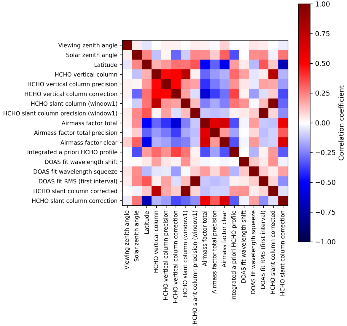
Figure 2: Map of correlation matrix for 2023-12-15 to 2023-12-17.
