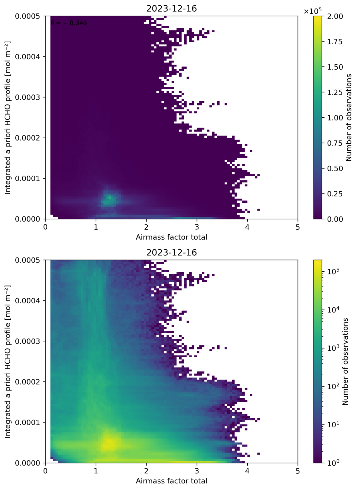
Figure 104: Scatter density plot of “Airmass factor total” against “Integrated a priori HCHO profile” for 2023-12-15 to 2023-12-17.
