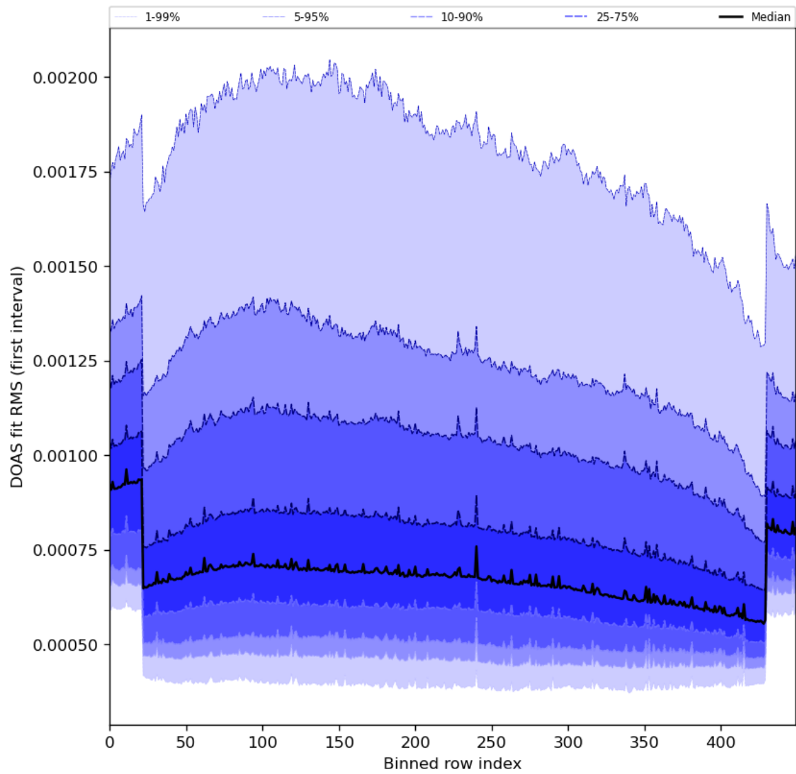
Figure 60: Along track statistics of “DOAS fit RMS (first interval)” for 2023-12-15 to 2023-12-17
