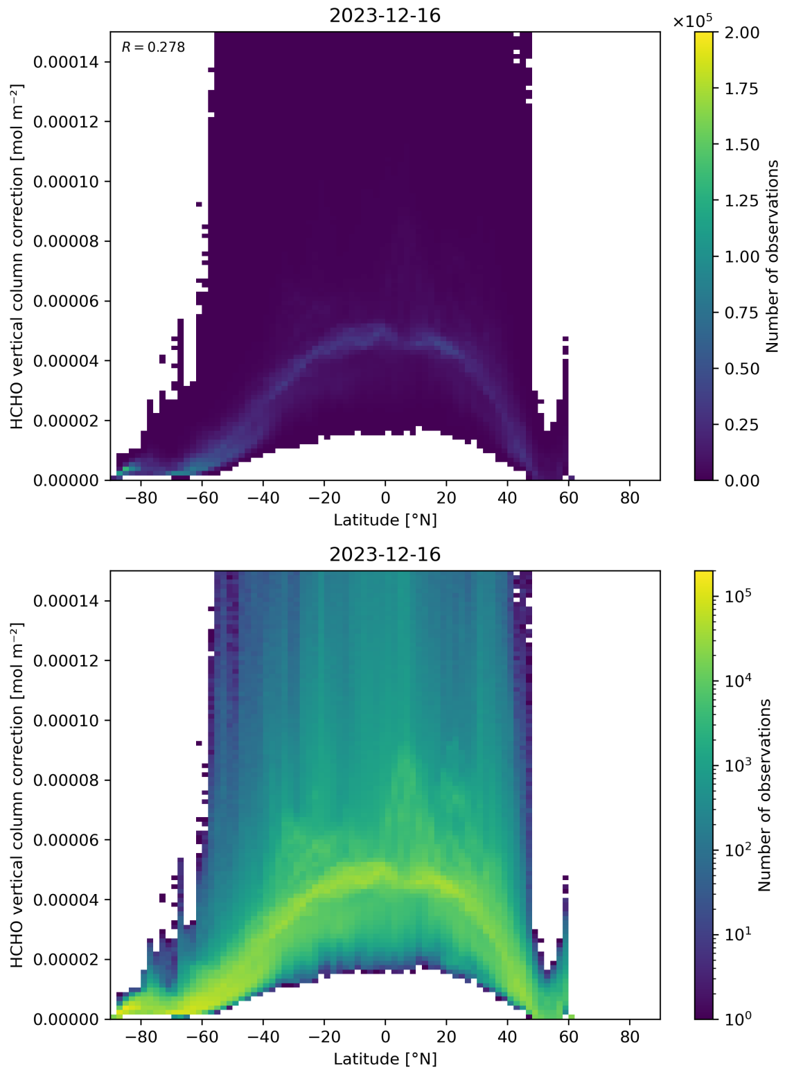
Figure 164: Scatter density plot of “Latitude” against “HCHO vertical column correction” for 2023-12-15 to 2023-12-17.
