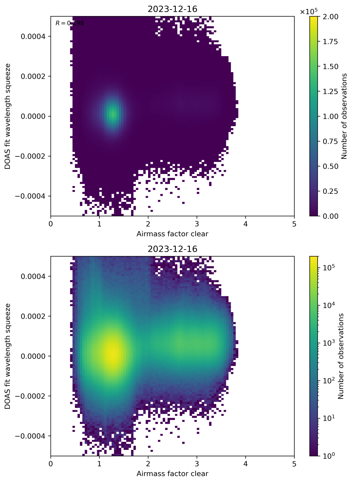
Figure 73: Scatter density plot of “Airmass factor clear” against “DOAS fit wavelength squeeze” for 2023-12-15 to 2023-12-17.
