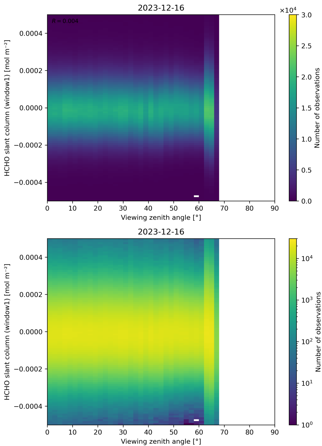
Figure 188: Scatter density plot of “Viewing zenith angle” against “HCHO slant column (window1)” for 2023-12-15 to 2023-12-17.
