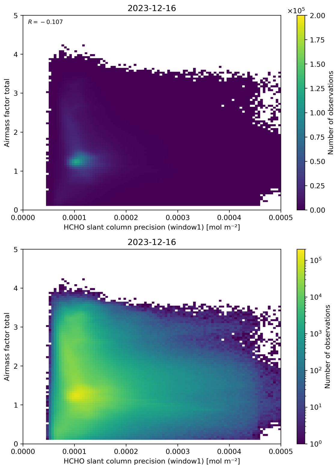
Figure 94: Scatter density plot of “HCHO slant column precision (window1)” against “Airmass factor total” for 2023-12-15 to 2023-12-17.
