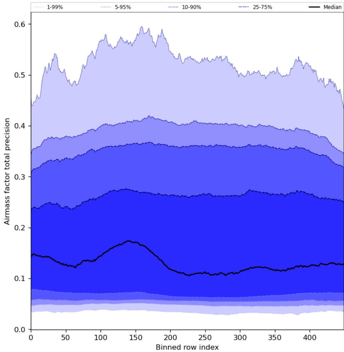
Figure 55: Along track statistics of “Airmass factor total precision” for 2023-12-15 to 2023-12-17
