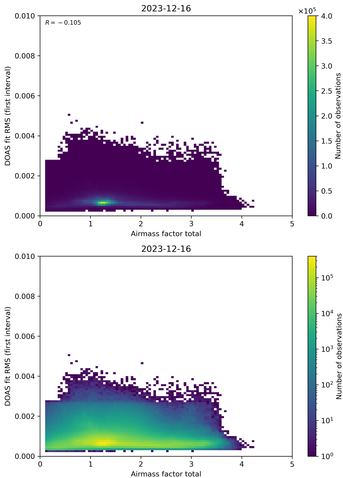
Figure 97: Scatter density plot of “Airmass factor total” against “DOAS fit RMS (first interval)” for 2023-12-15 to 2023-12-17.
