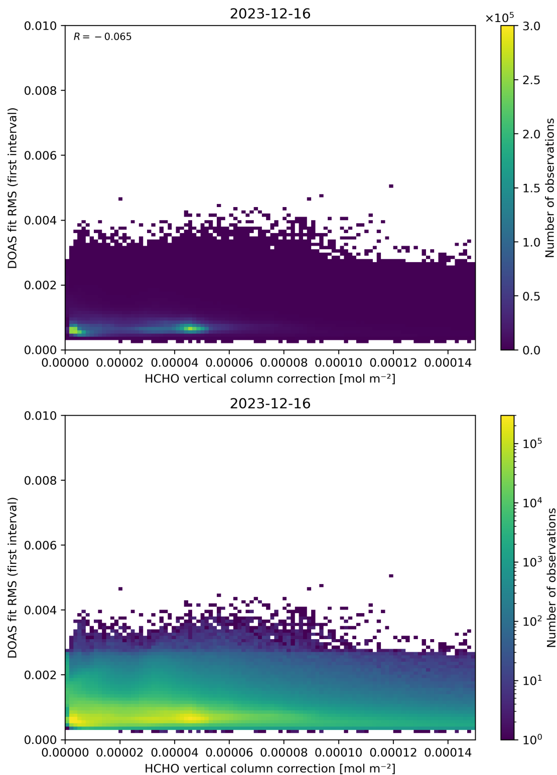
Figure 112: Scatter density plot of “HCHO vertical column correction” against “DOAS fit RMS (first interval)” for 2023-12-15 to 2023-12-17.
