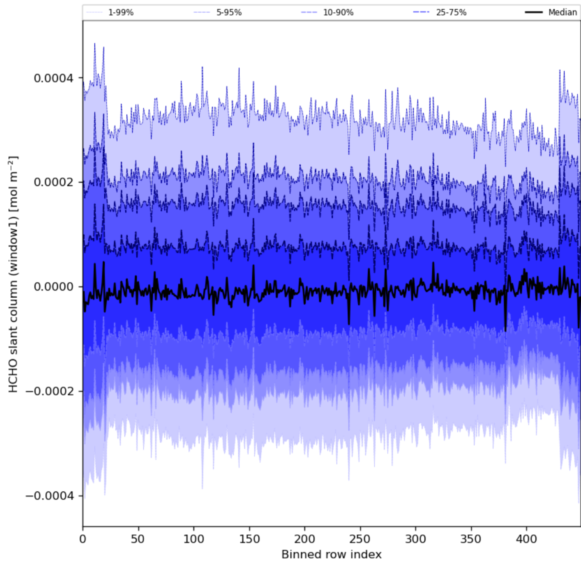
Figure 52: Along track statistics of “HCHO slant column (window1)” for 2023-12-15 to 2023-12-17
