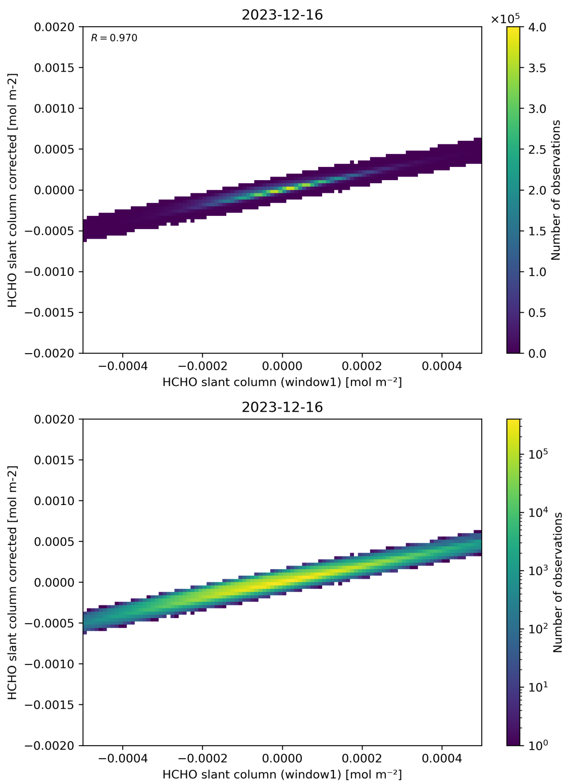
Figure 82: Scatter density plot of “HCHO slant column (window1)” against “HCHO slant column corrected” for 2023-12-15 to 2023-12-17.
