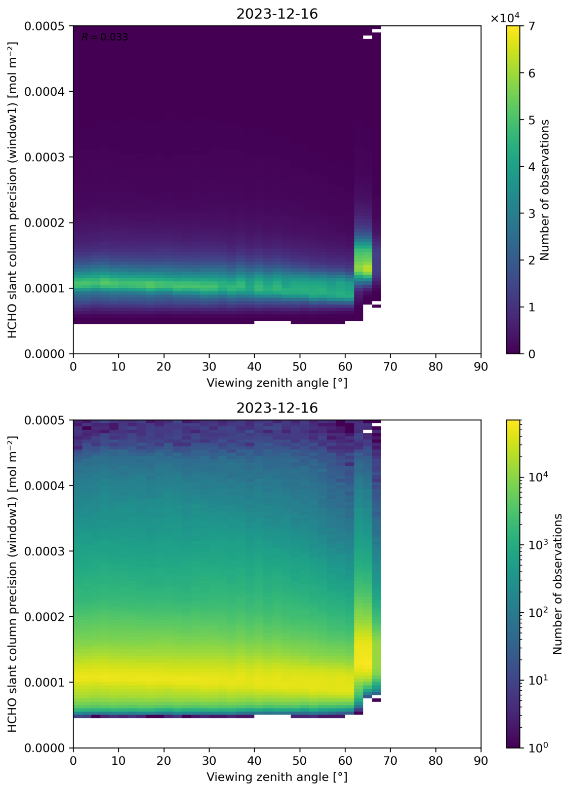
Figure 189: Scatter density plot of “Viewing zenith angle” against “HCHO slant column precision (window1)” for 2023-12-15 to 2023-12-17.
