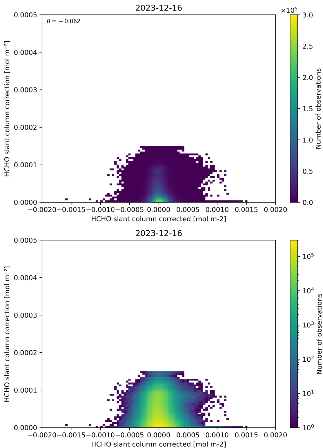
Figure 77: Scatter density plot of “HCHO slant column corrected” against “HCHO slant column correction” for 2023-12-15 to 2023-12-17.
