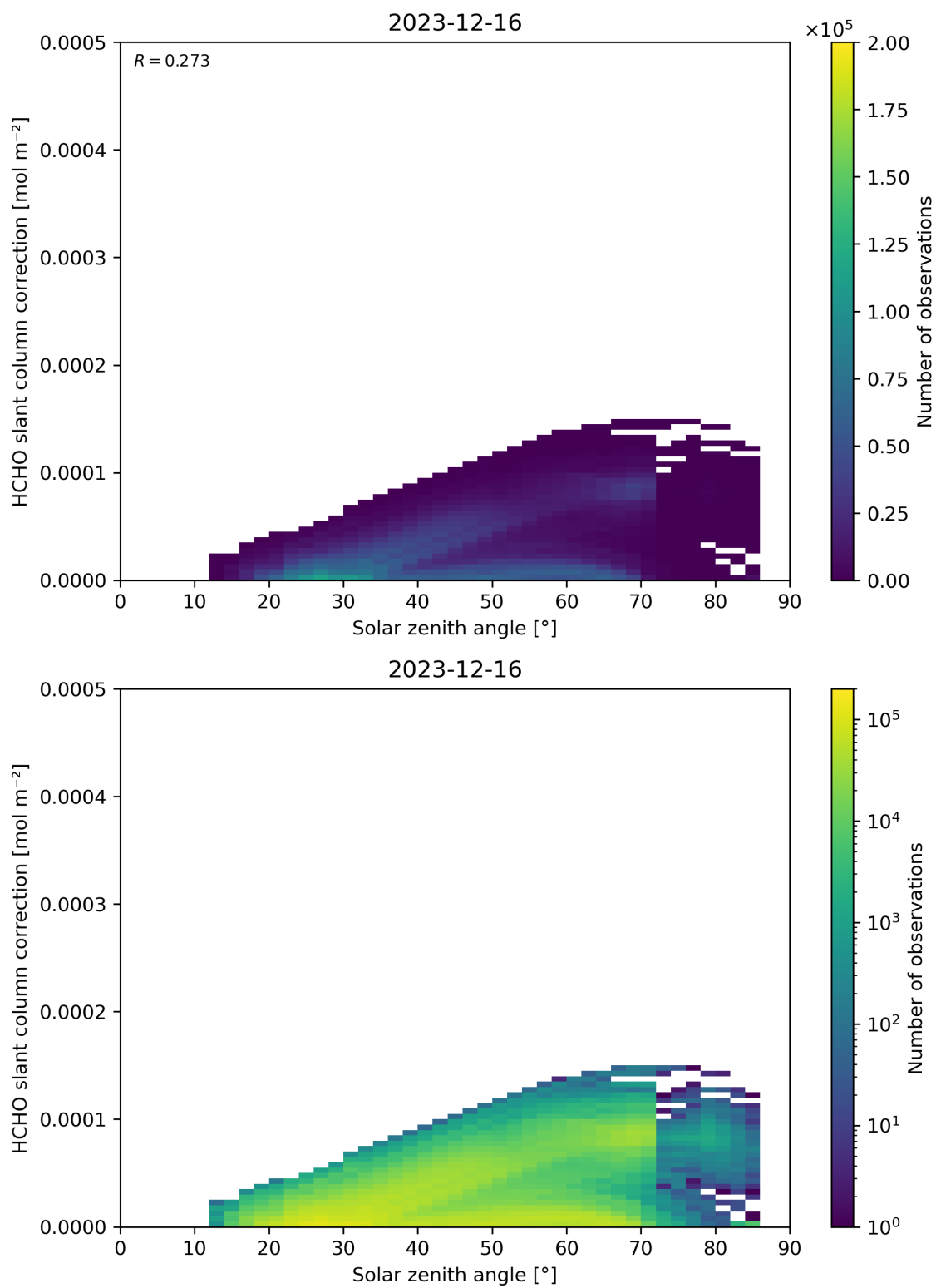
Figure 172: Scatter density plot of “Solar zenith angle” against “HCHO slant column correction” for 2023-12-15 to 2023-12-17.
