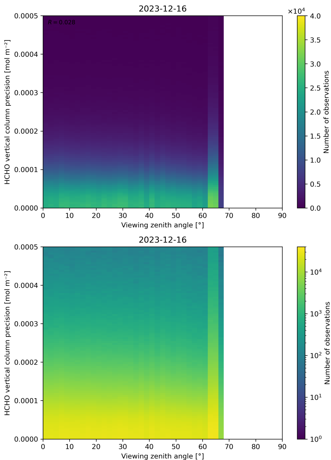
Figure 194: Scatter density plot of “Viewing zenith angle” against “HCHO vertical column precision” for 2023-12-15 to 2023-12-17.
