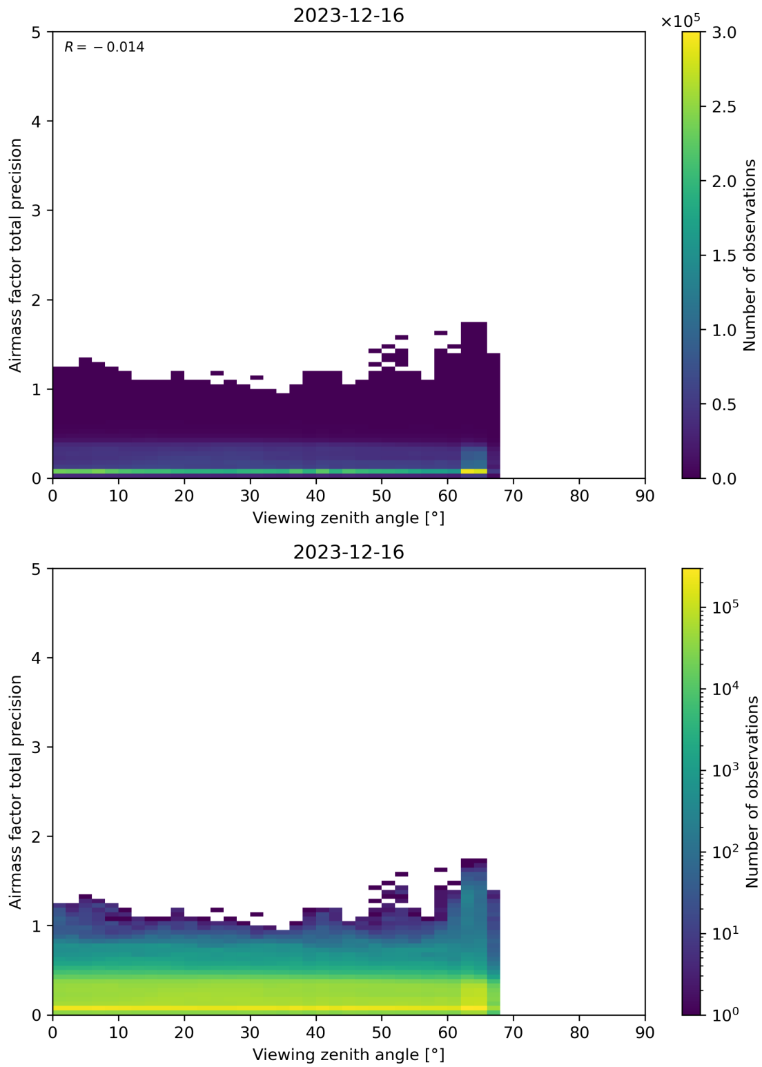
Figure 191: Scatter density plot of “Viewing zenith angle” against “Airmass factor total precision” for 2023-12-15 to 2023-12-17.
