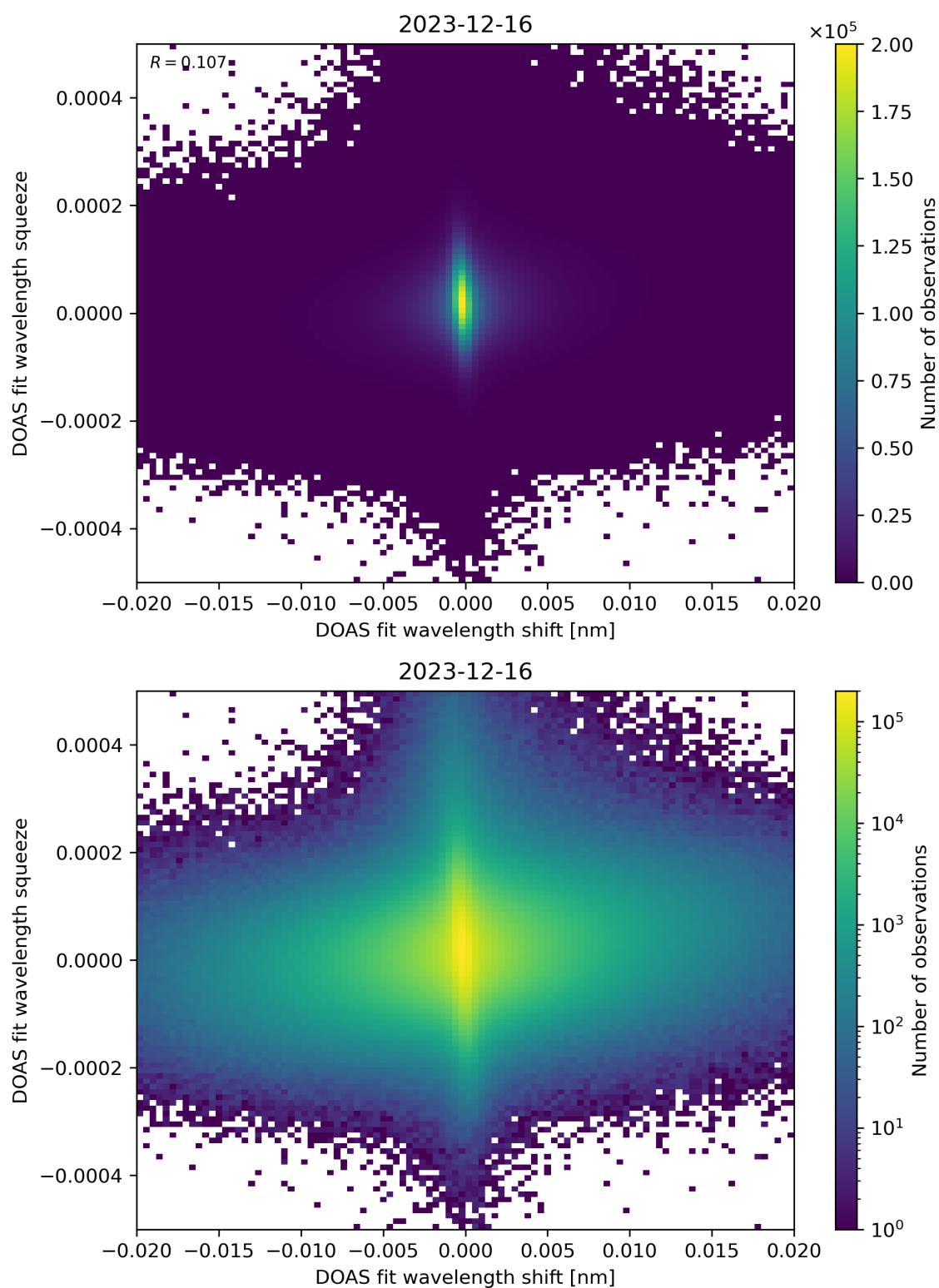
Figure 65: Scatter density plot of “DOAS fit wavelength shift” against “DOAS fit wavelength squeeze” for 2023-12-15 to 2023-12-17.
