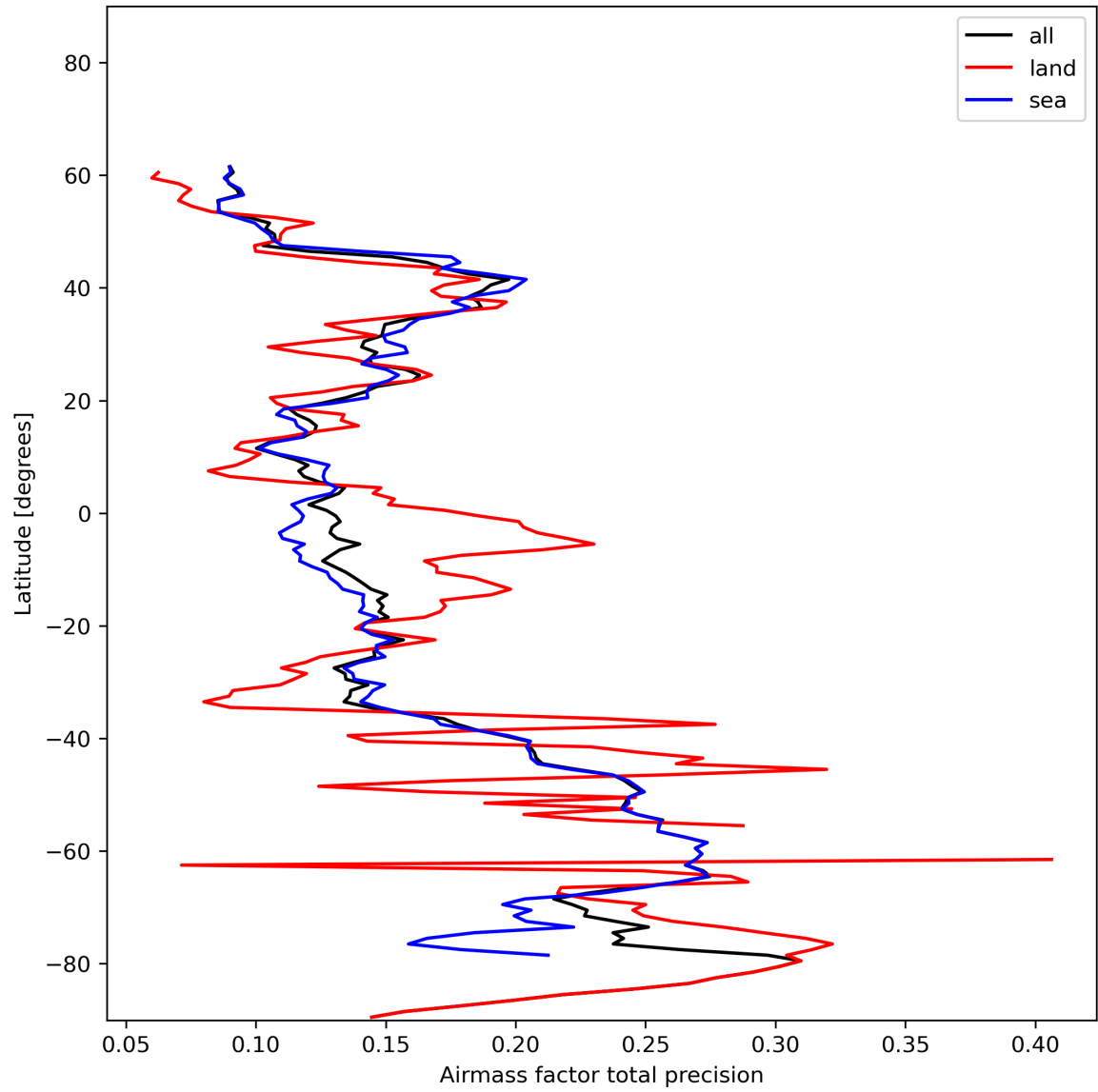
Figure 27: Zonal average of “Airmass factor total precision” for 2023-12-15 to 2023-12-17.
