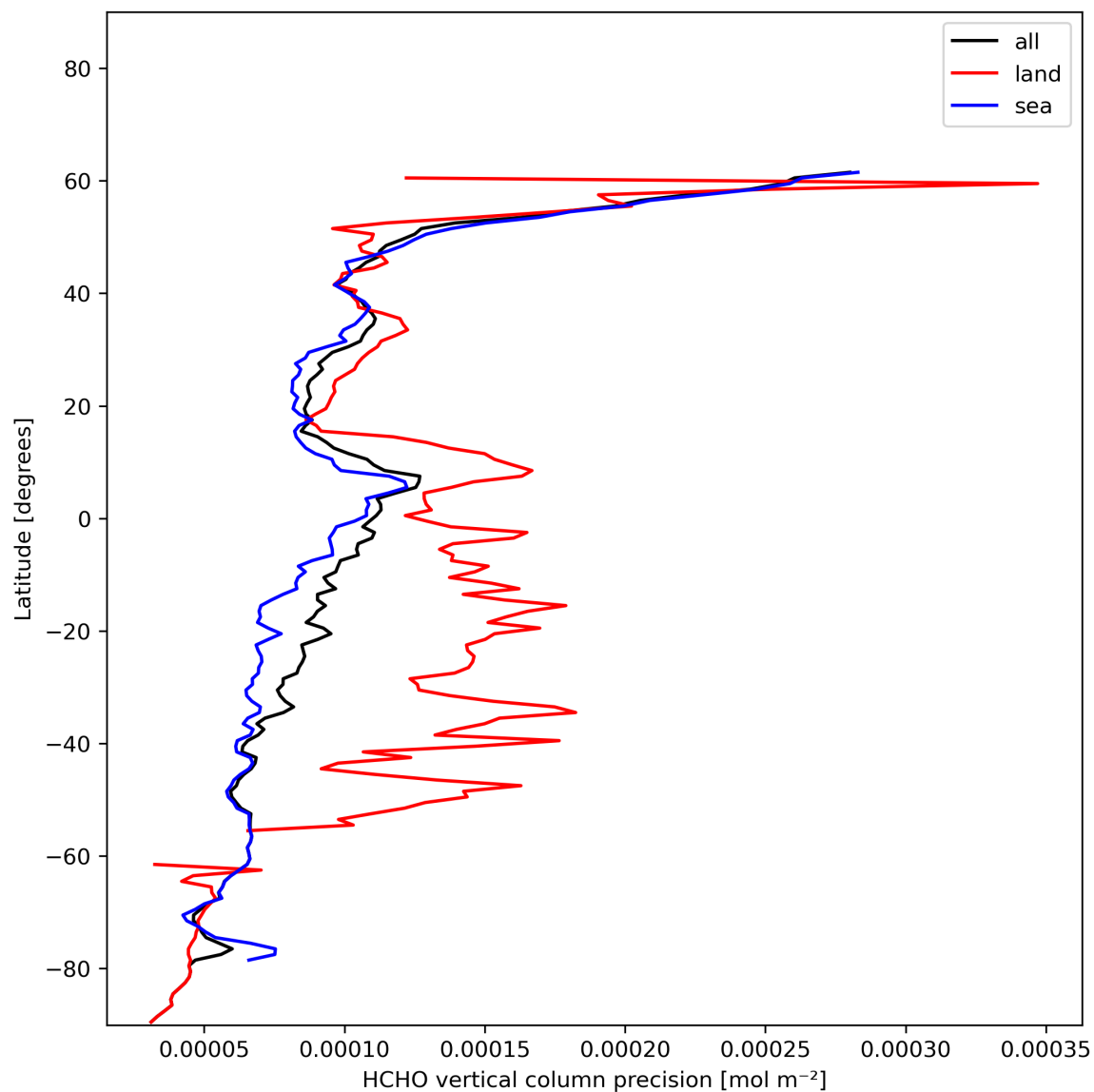
Figure 22: Zonal average of “HCHO vertical column precision” for 2023-12-15 to 2023-12-17.
