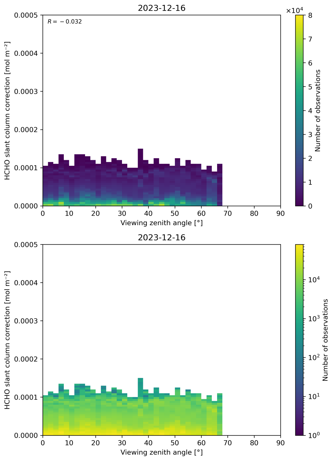
Figure 187: Scatter density plot of “Viewing zenith angle” against “HCHO slant column correction” for 2023-12-15 to 2023-12-17.
