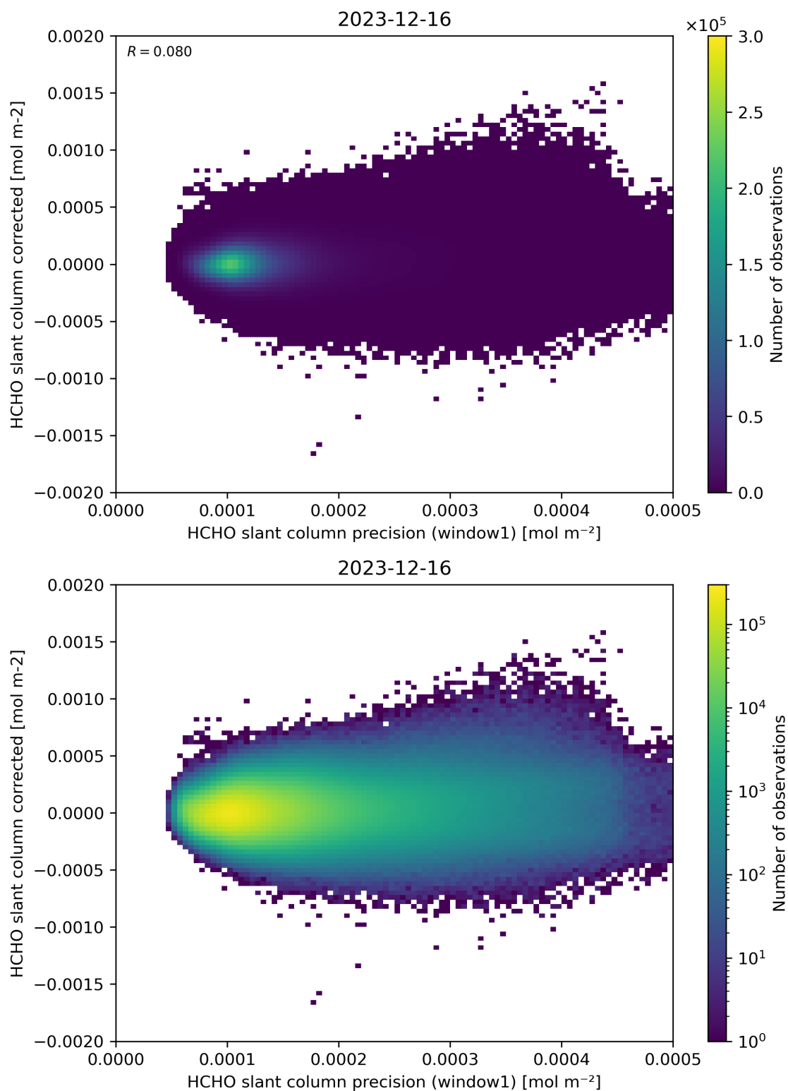
Figure 92: Scatter density plot of “HCHO slant column precision (window1)” against “HCHO slant column corrected” for 2023-12-15 to 2023-12-17.
