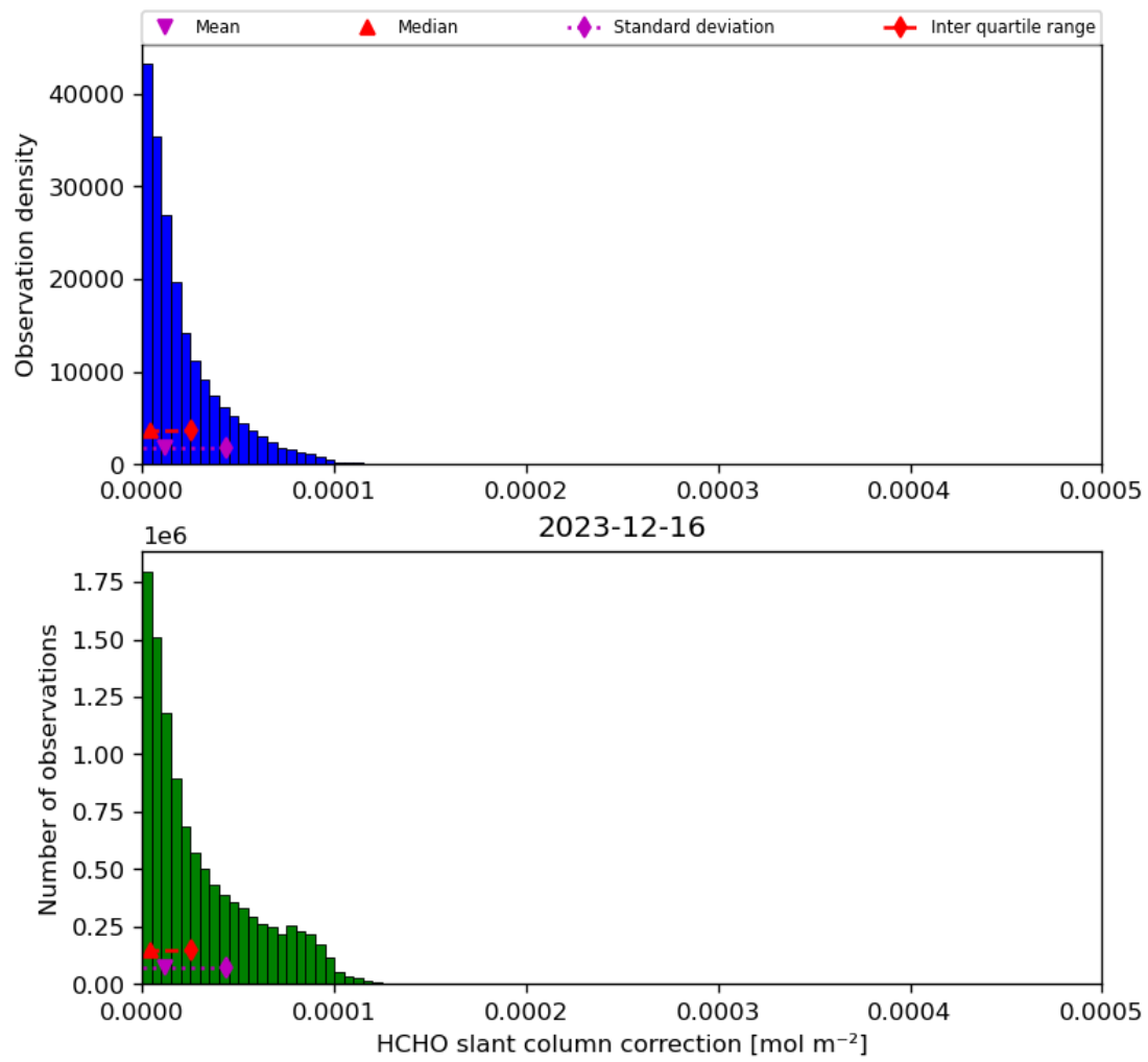
Figure 47: Histogram of “HCHO slant column correction” for 2023-12-15 to 2023-12-17
