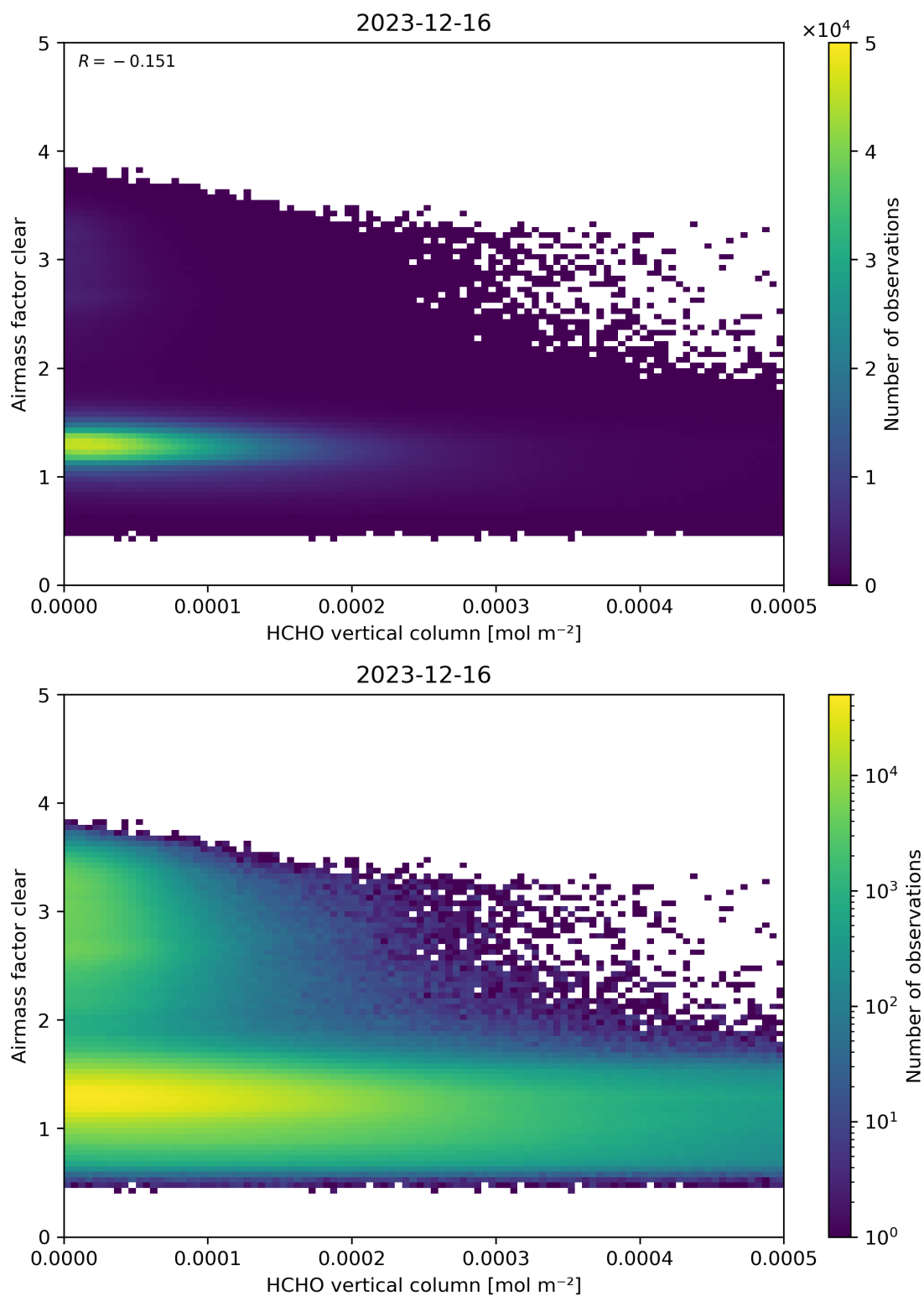
Figure 126: Scatter density plot of “HCHO vertical column” against “Airmass factor clear” for 2023-12-15 to 2023-12-17.
