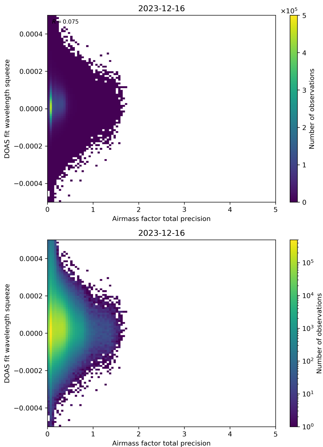
Figure 107: Scatter density plot of “Airmass factor total precision” against “DOAS fit wavelength squeeze” for 2023-12-15 to 2023-12-17.
