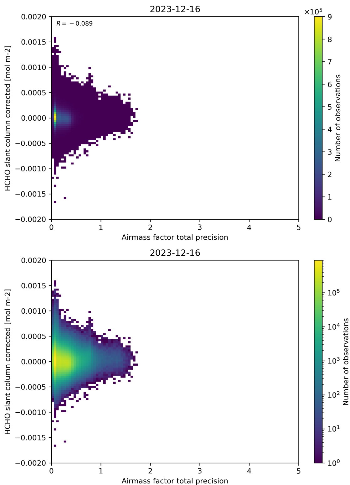
Figure 109: Scatter density plot of “Airmass factor total precision” against “HCHO slant column corrected” for 2023-12-15 to 2023-12-17.
