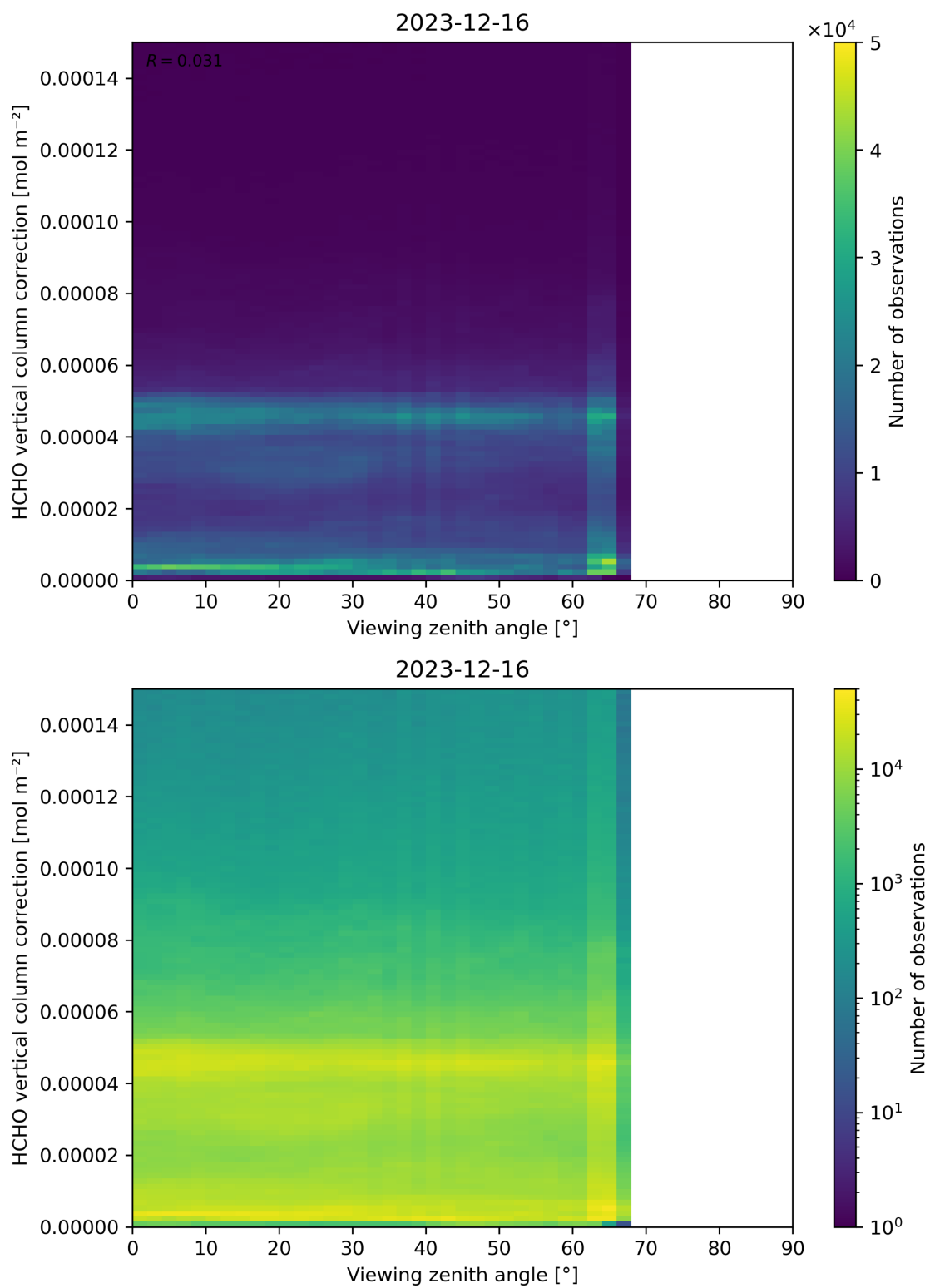
Figure 193: Scatter density plot of “Viewing zenith angle” against “HCHO vertical column correction” for 2023-12-15 to 2023-12-17.
