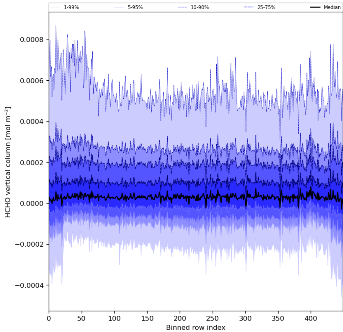
Figure 49: Along track statistics of “HCHO vertical column” for 2023-12-15 to 2023-12-17
