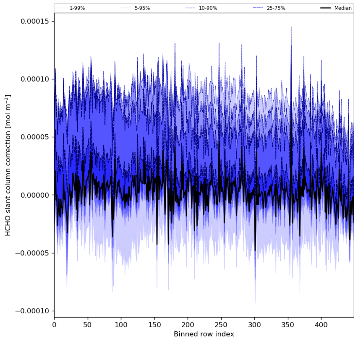
Figure 61: Along track statistics of “HCHO slant column correction” for 2023-12-15 to 2023-12-17
