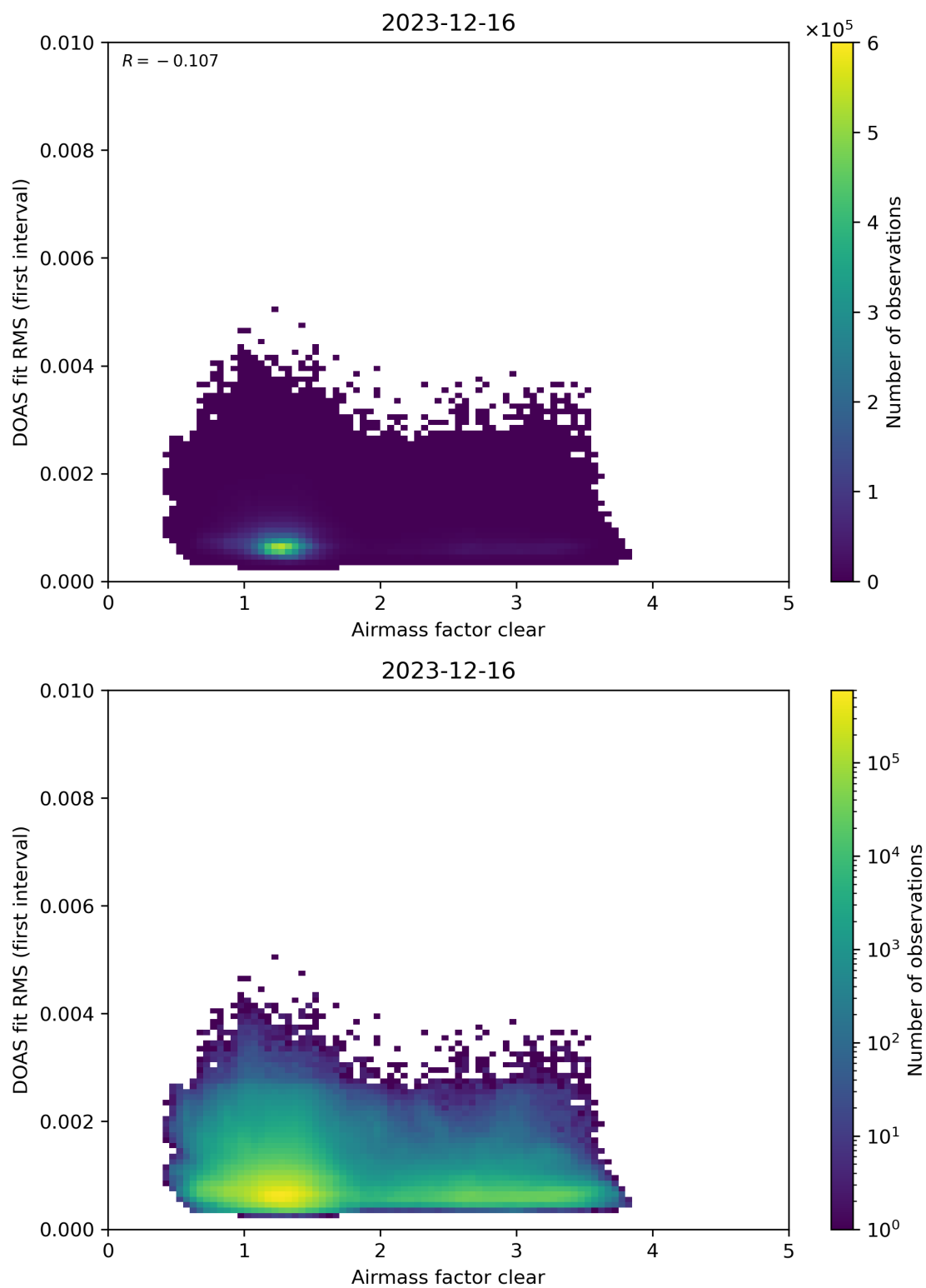
Figure 71: Scatter density plot of “Airmass factor clear” against “DOAS fit RMS (first interval)” for 2023-12-15 to 2023-12-17.
