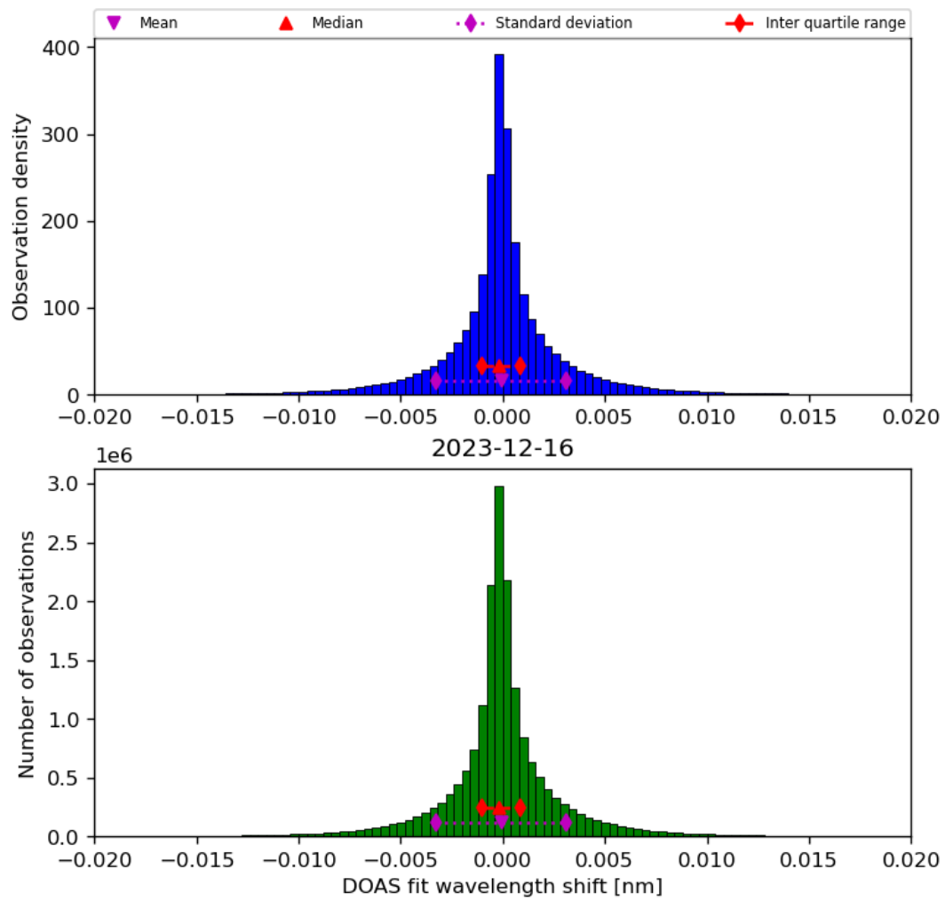
Figure 44: Histogram of “DOAS fit wavelength shift” for 2023-12-15 to 2023-12-17
