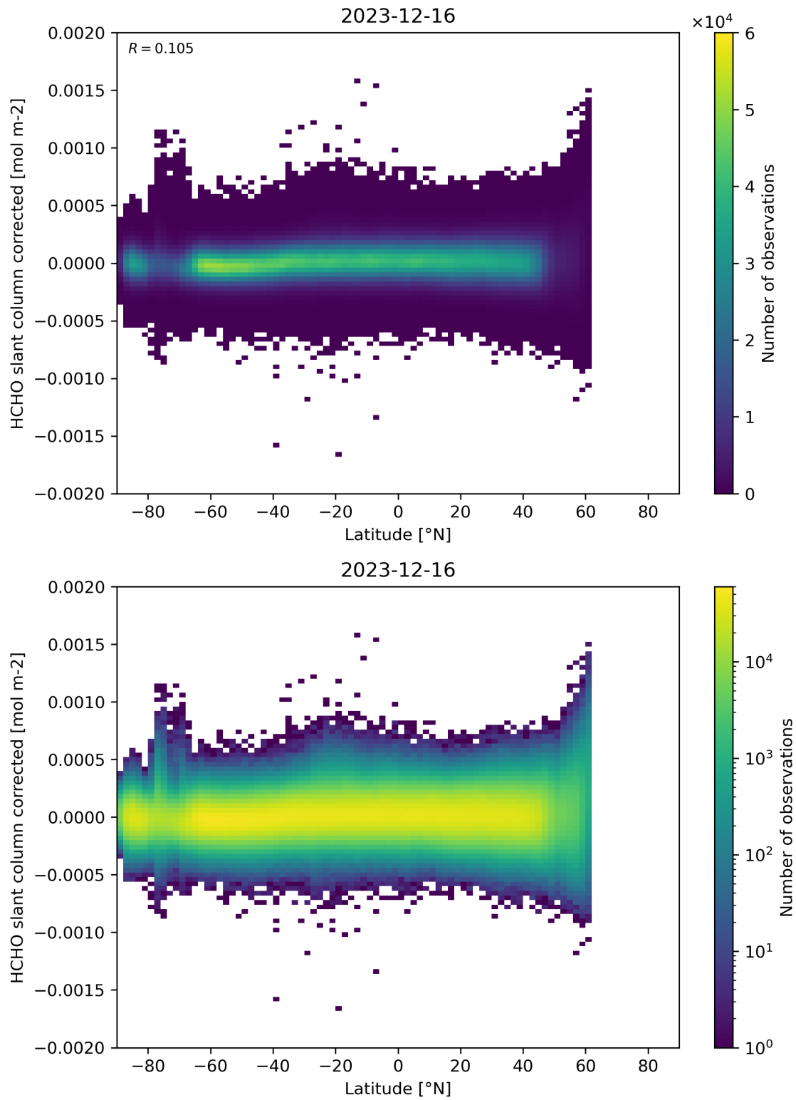
Figure 157: Scatter density plot of “Latitude” against “HCHO slant column corrected” for 2023-12-15 to 2023-12-17.
