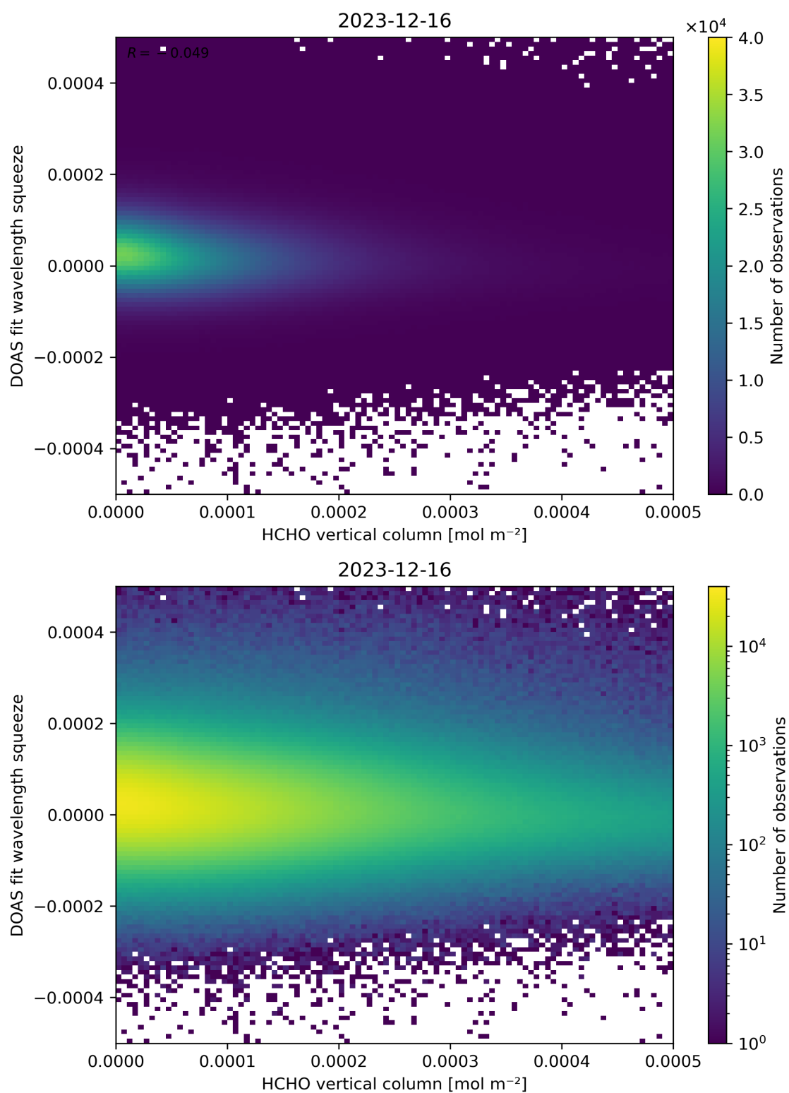
Figure 125: Scatter density plot of “HCHO vertical column” against “DOAS fit wavelength squeeze” for 2023-12-15 to 2023-12-17.
