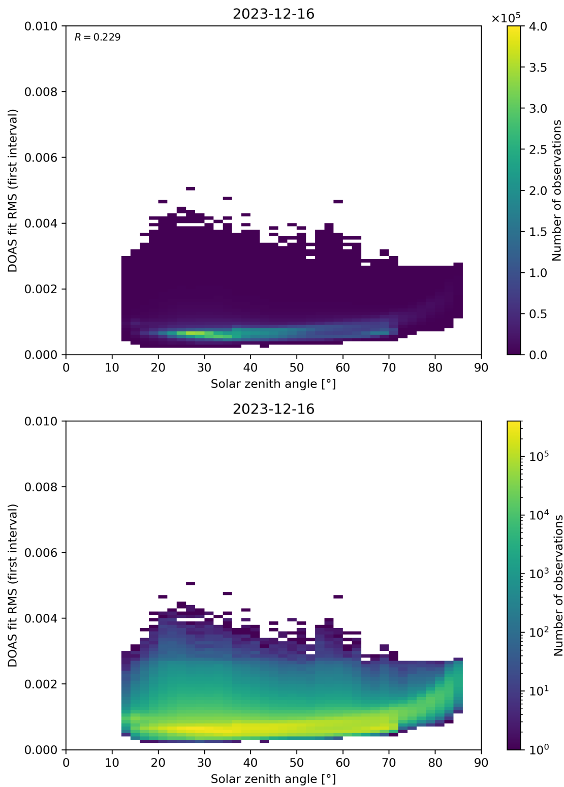
Figure 167: Scatter density plot of “Solar zenith angle” against “DOAS fit RMS (first interval)” for 2023-12-15 to 2023-12-17.
