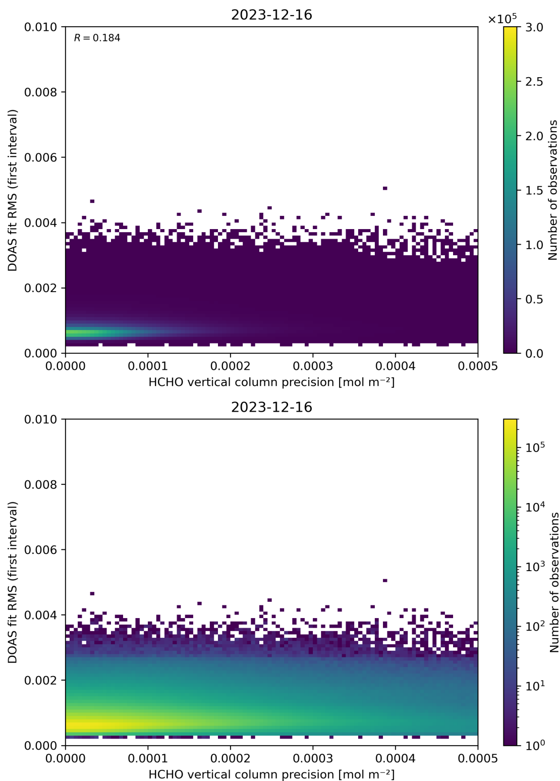
Figure 136: Scatter density plot of “HCHO vertical column precision” against “DOAS fit RMS (first interval)” for 2023-12-15 to 2023-12-17.
