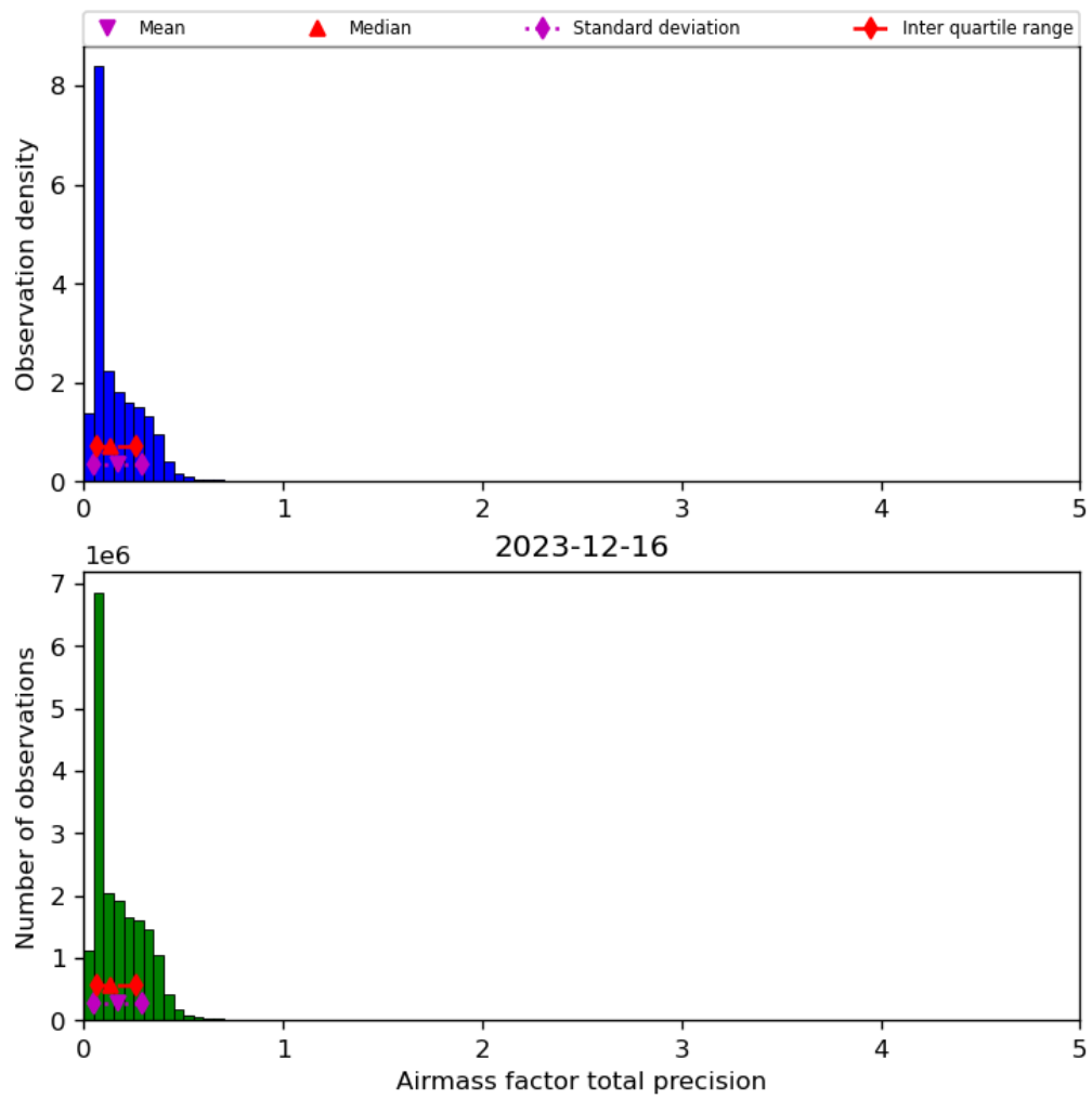
Figure 41: Histogram of “Airmass factor total precision” for 2023-12-15 to 2023-12-17
