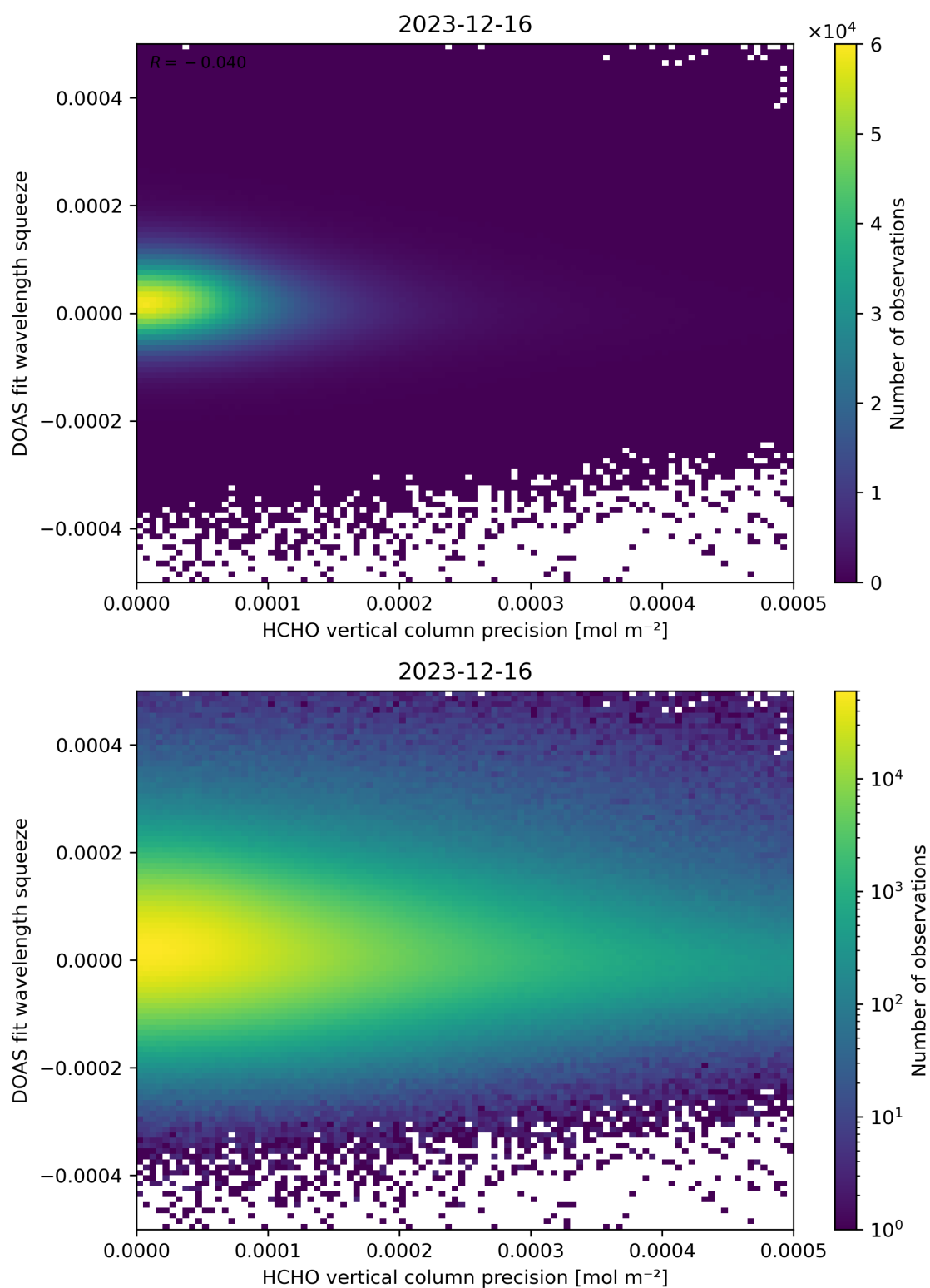
Figure 138: Scatter density plot of “HCHO vertical column precision” against “DOAS fit wavelength squeeze” for 2023-12-15 to 2023-12-17.
