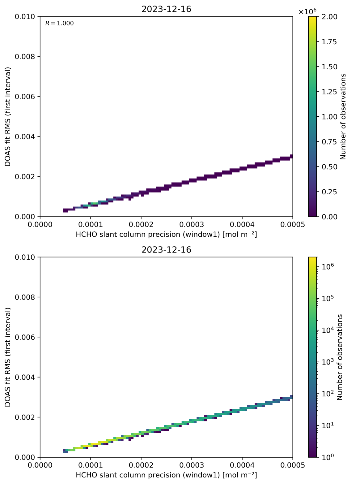
Figure 88: Scatter density plot of “HCHO slant column precision (window1)” against “DOAS fit RMS (first interval)” for 2023-12-15 to 2023-12-17.
