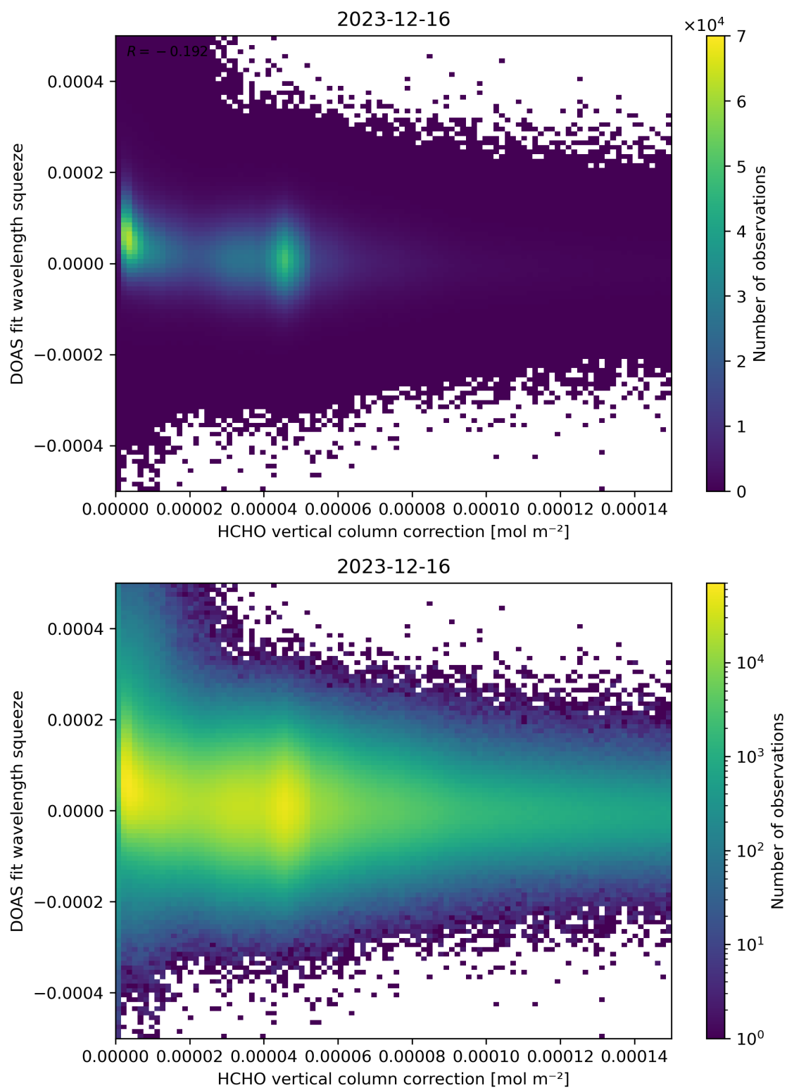
Figure 114: Scatter density plot of “HCHO vertical column correction” against “DOAS fit wavelength squeeze” for 2023-12-15 to 2023-12-17.
