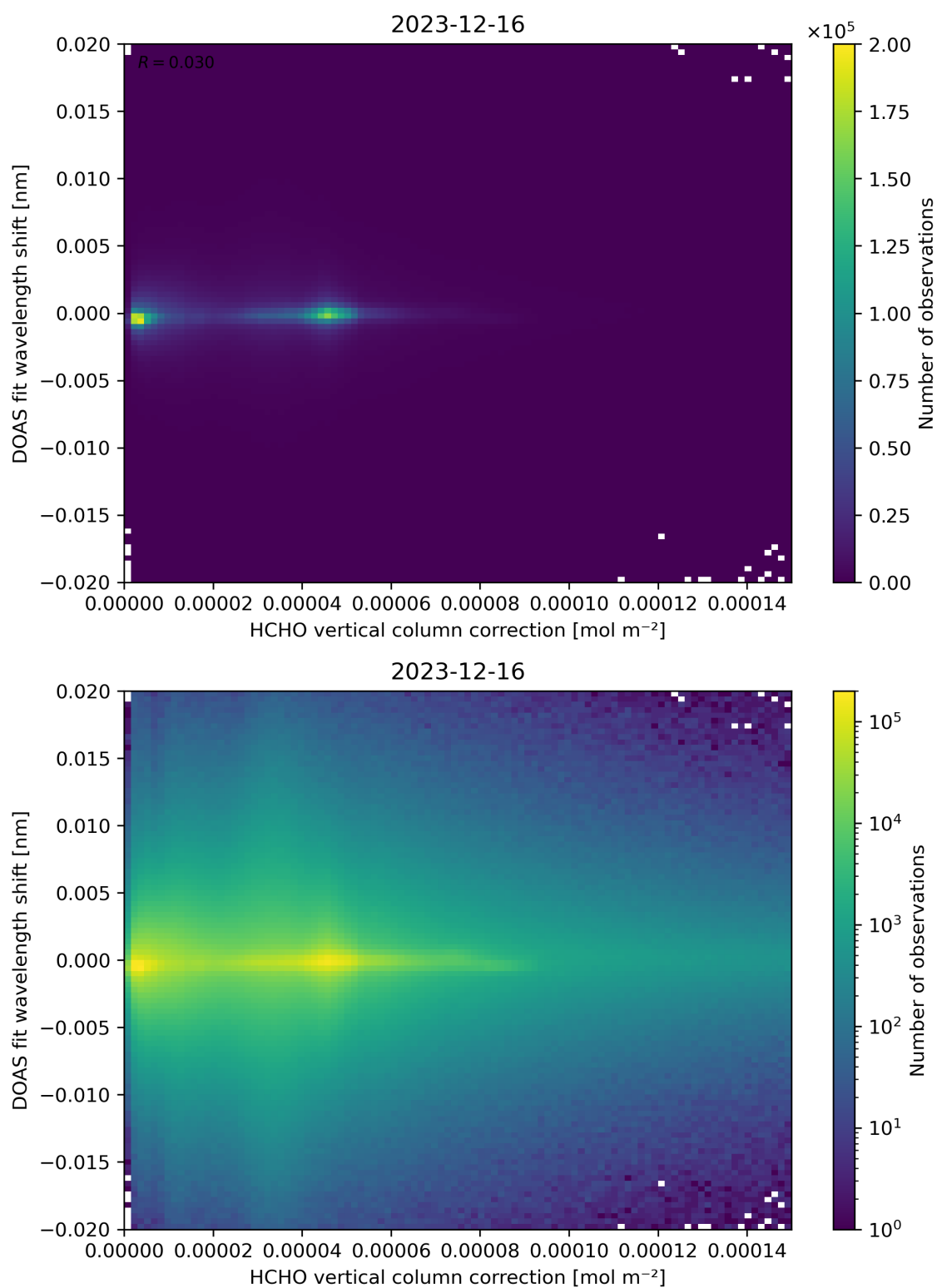
Figure 113: Scatter density plot of “HCHO vertical column correction” against “DOAS fit wavelength shift” for 2023-12-15 to 2023-12-17.
