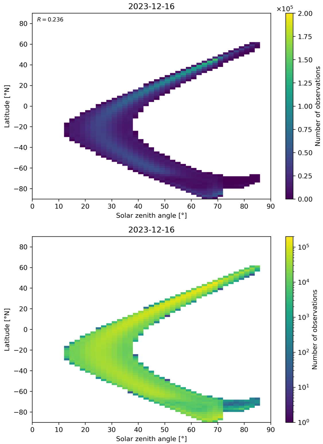
Figure 181: Scatter density plot of “Solar zenith angle” against “Latitude” for 2023-12-15 to 2023-12-17.
