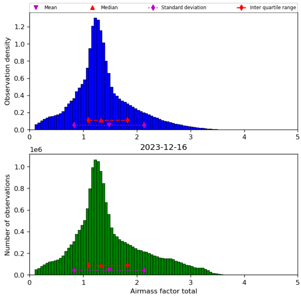
Figure 40: Histogram of “Airmass factor total” for 2023-12-15 to 2023-12-17
