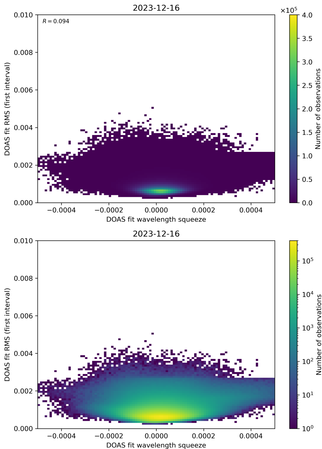
Figure 68: Scatter density plot of “DOAS fit wavelength squeeze” against “DOAS fit RMS (first interval)” for 2023-12-15 to 2023-12-17.
