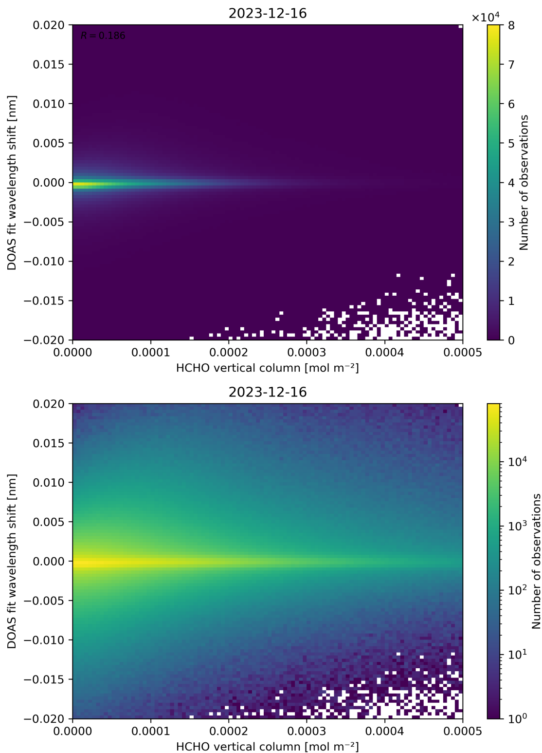
Figure 124: Scatter density plot of “HCHO vertical column” against “DOAS fit wavelength shift” for 2023-12-15 to 2023-12-17.
