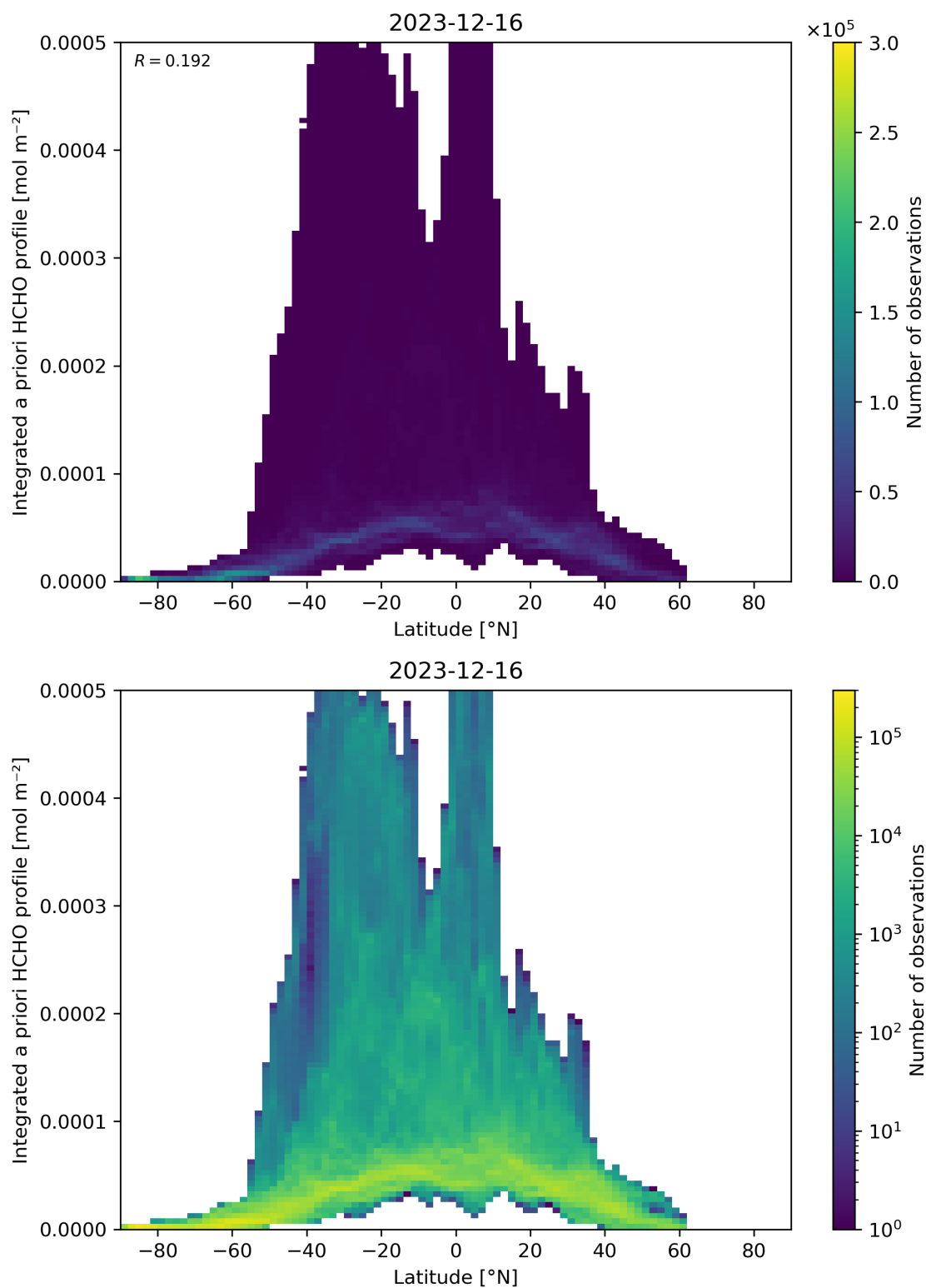
Figure 166: Scatter density plot of “Latitude” against “Integrated a priori HCHO profile” for 2023-12-15 to 2023-12-17.
