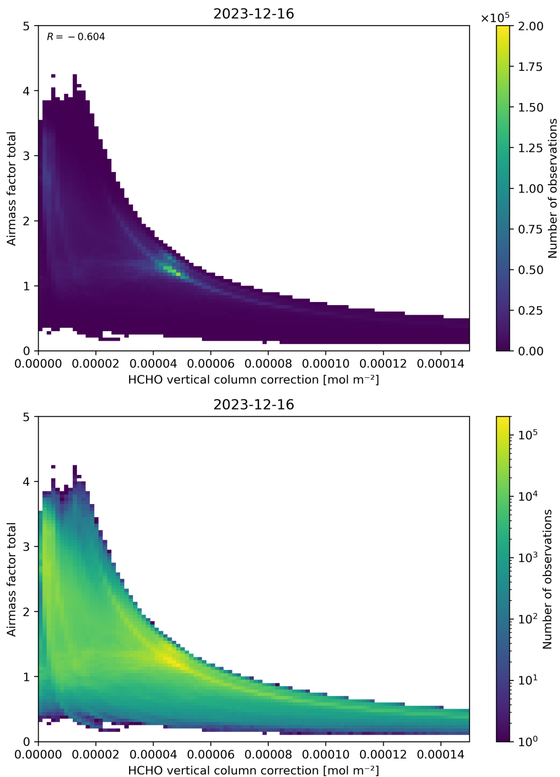
Figure 120: Scatter density plot of “HCHO vertical column correction” against “Airmass factor total” for 2023-12-15 to 2023-12-17.
