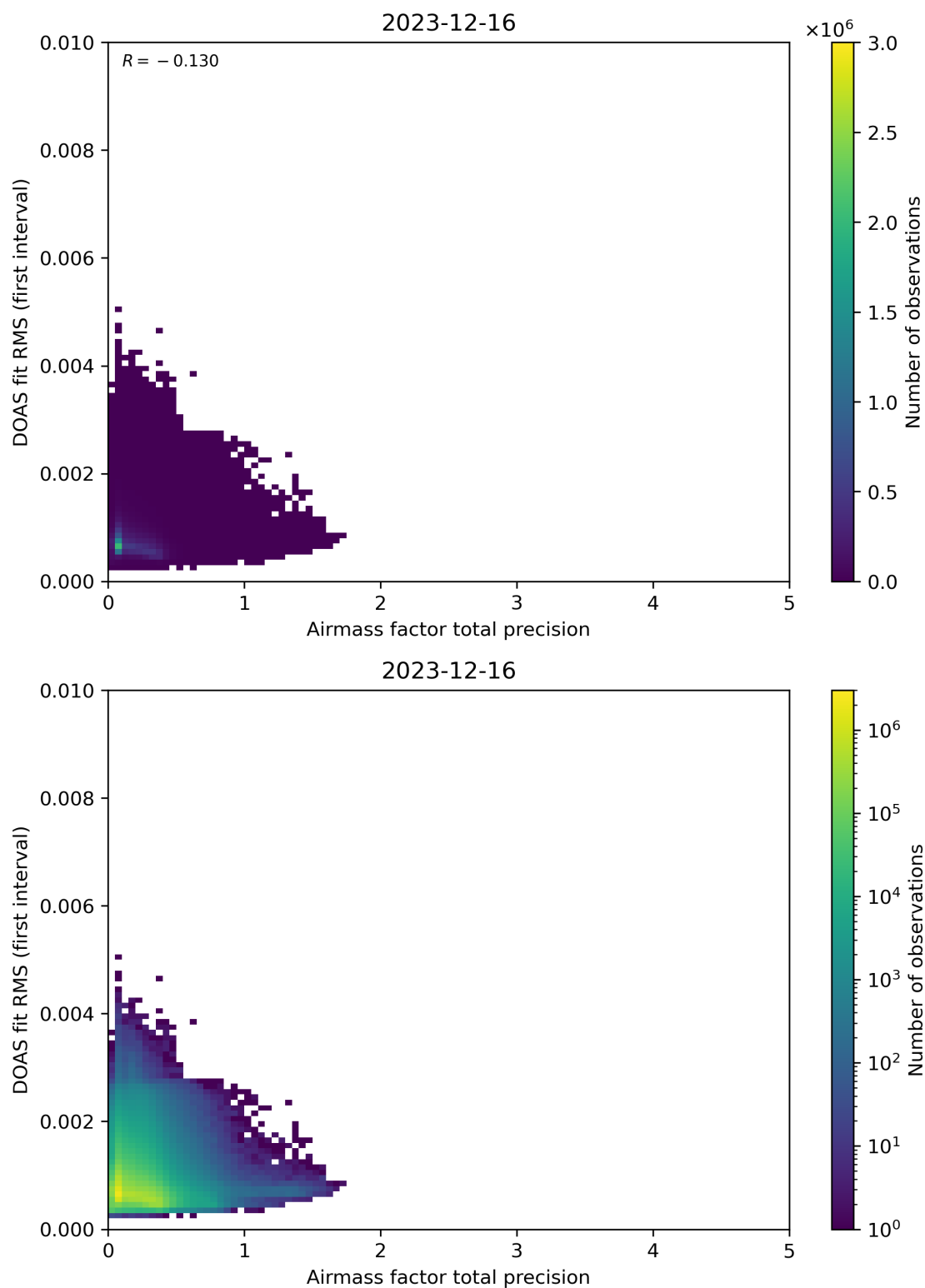
Figure 105: Scatter density plot of “Airmass factor total precision” against “DOAS fit RMS (first interval)” for 2023-12-15 to 2023-12-17.
