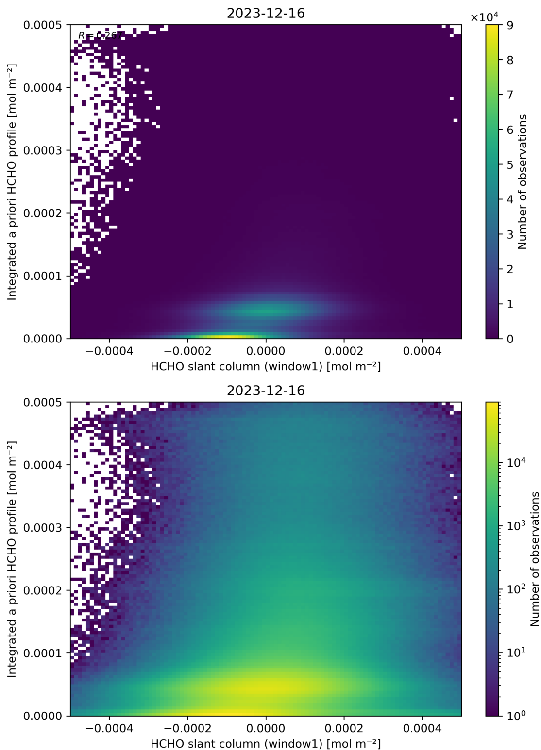
Figure 87: Scatter density plot of “HCHO slant column (window1)” against “Integrated a priori HCHO profile” for 2023-12-15 to 2023-12-17.
