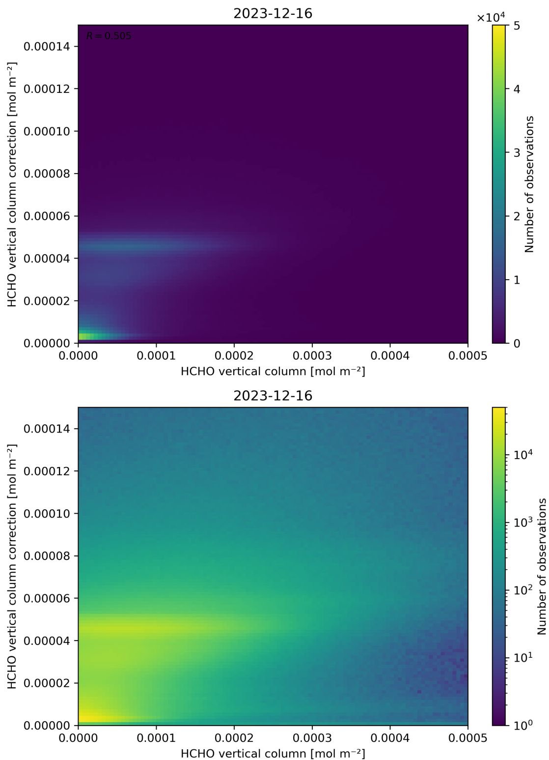
Figure 133: Scatter density plot of “HCHO vertical column” against “HCHO vertical column correction” for 2023-12-15 to 2023-12-17.
