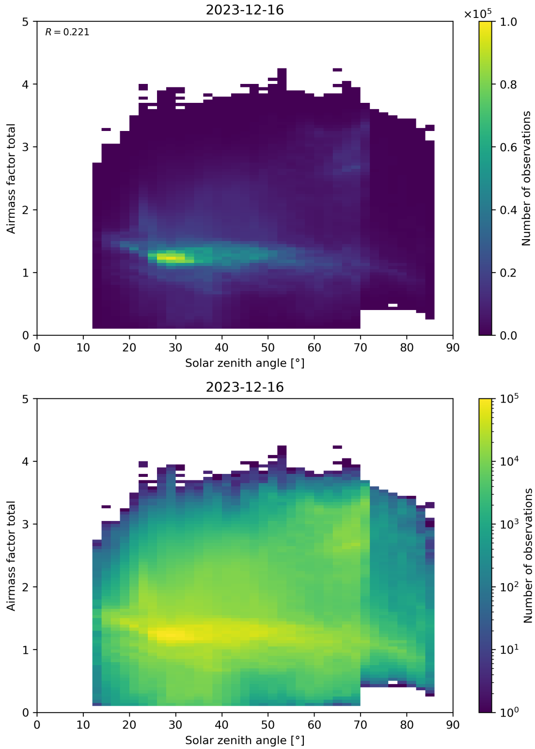
Figure 175: Scatter density plot of “Solar zenith angle” against “Airmass factor total” for 2023-12-15 to 2023-12-17.
