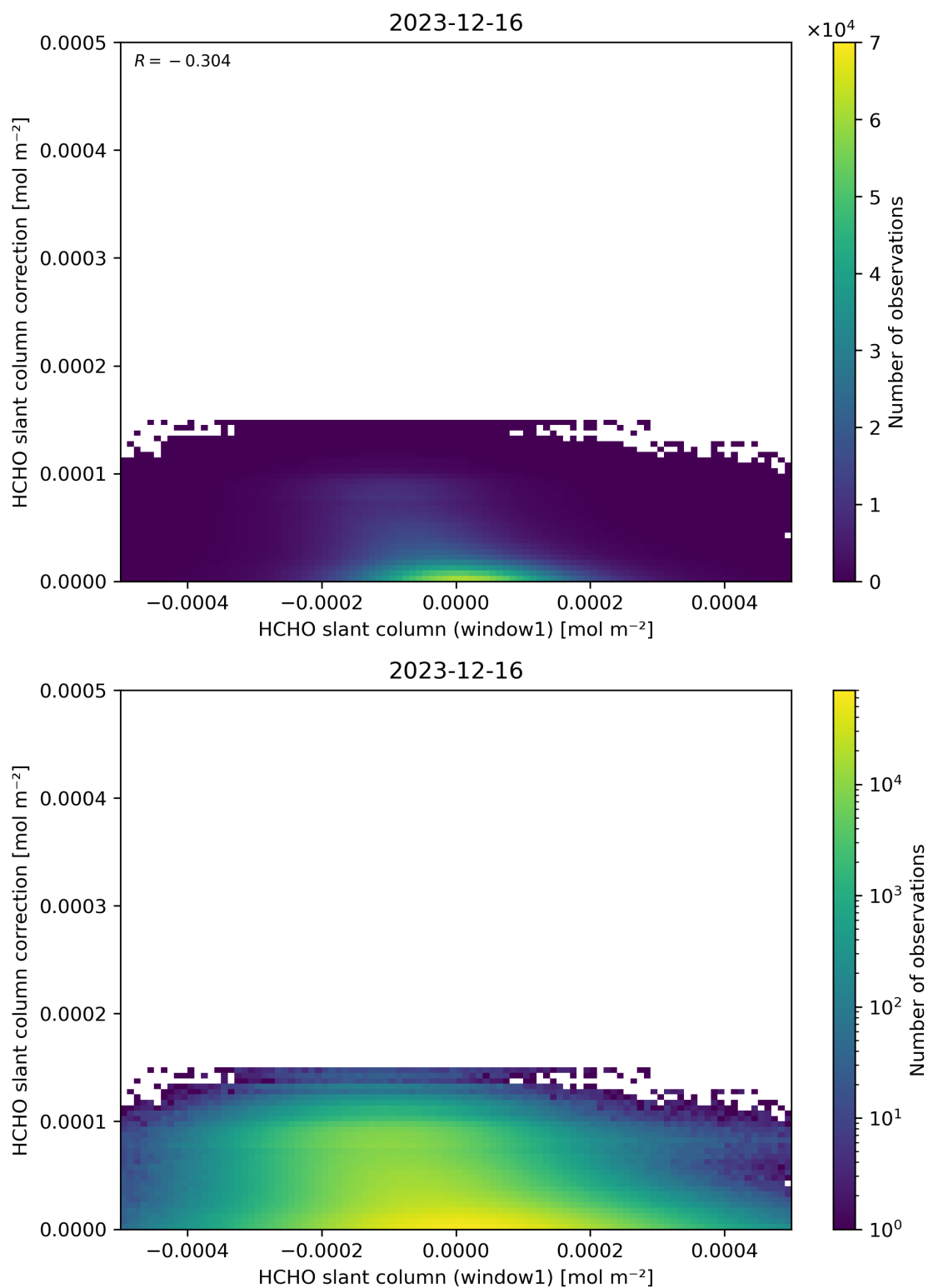
Figure 83: Scatter density plot of “HCHO slant column (window1)” against “HCHO slant column correction” for 2023-12-15 to 2023-12-17.
