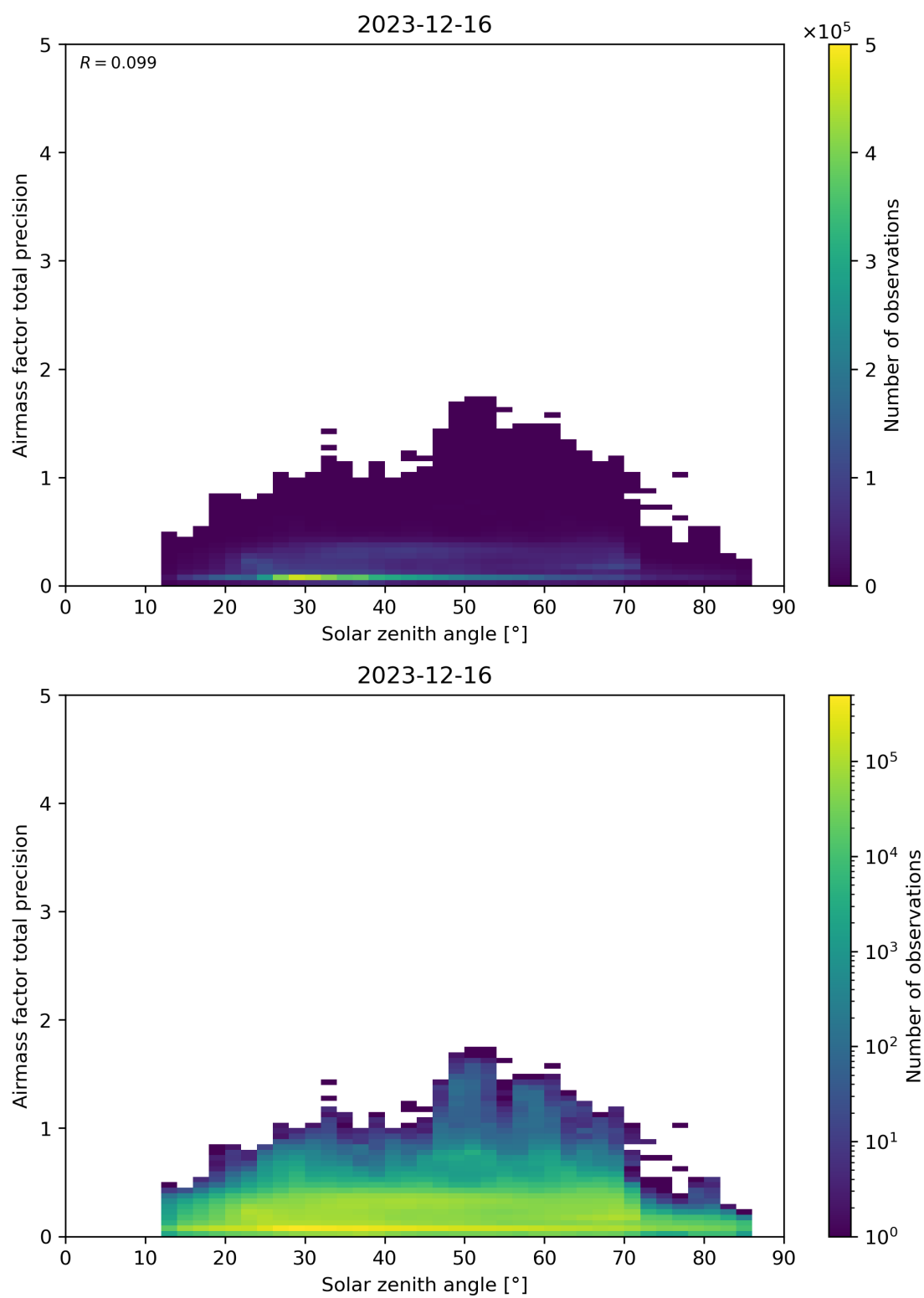
Figure 176: Scatter density plot of “Solar zenith angle” against “Airmass factor total precision” for 2023-12-15 to 2023-12-17.
