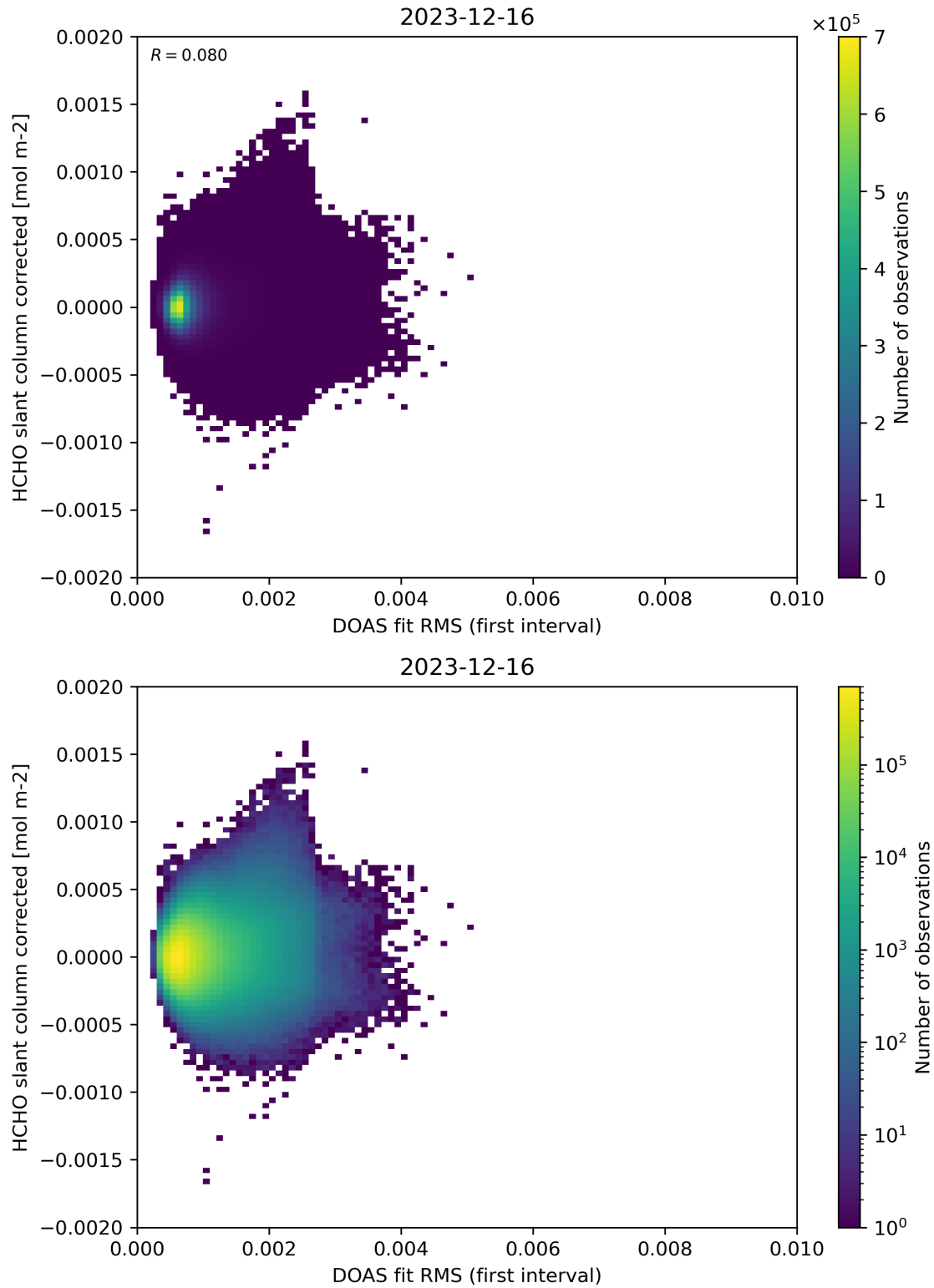
Figure 62: Scatter density plot of “DOAS fit RMS (first interval)” against “HCHO slant column corrected” for 2023-12-15 to 2023-12-17.
