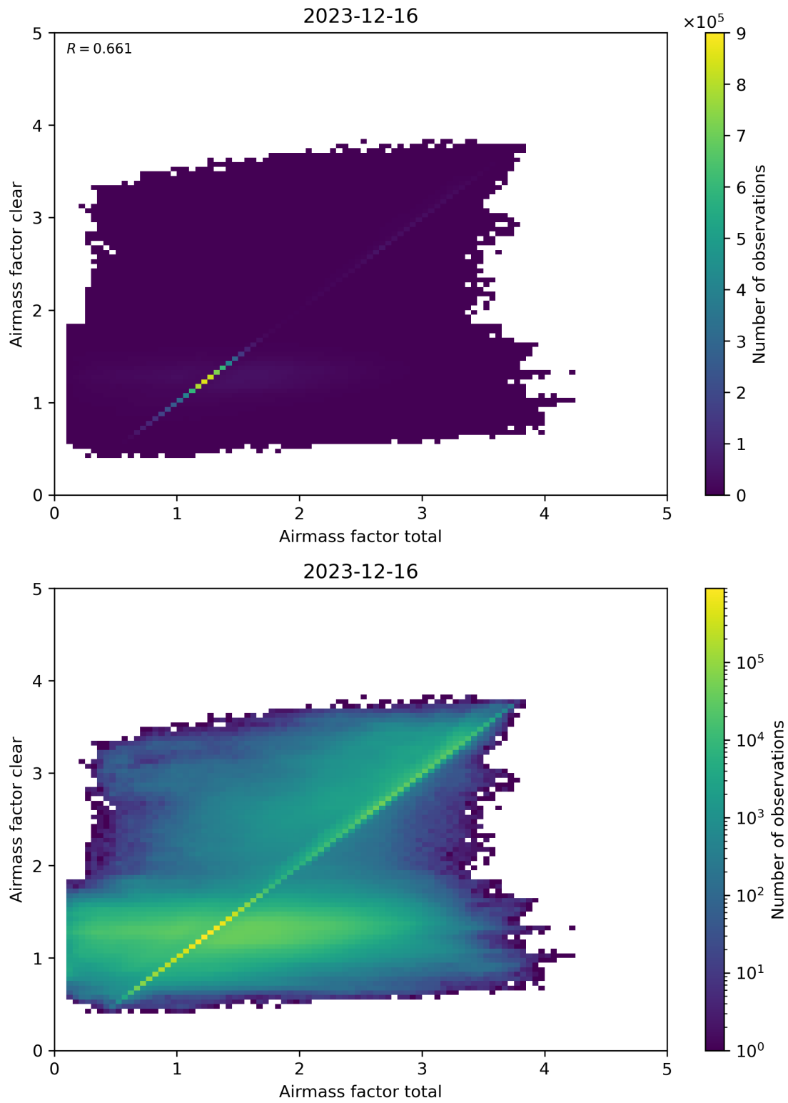
Figure 100: Scatter density plot of “Airmass factor total” against “Airmass factor clear” for 2023-12-15 to 2023-12-17.
