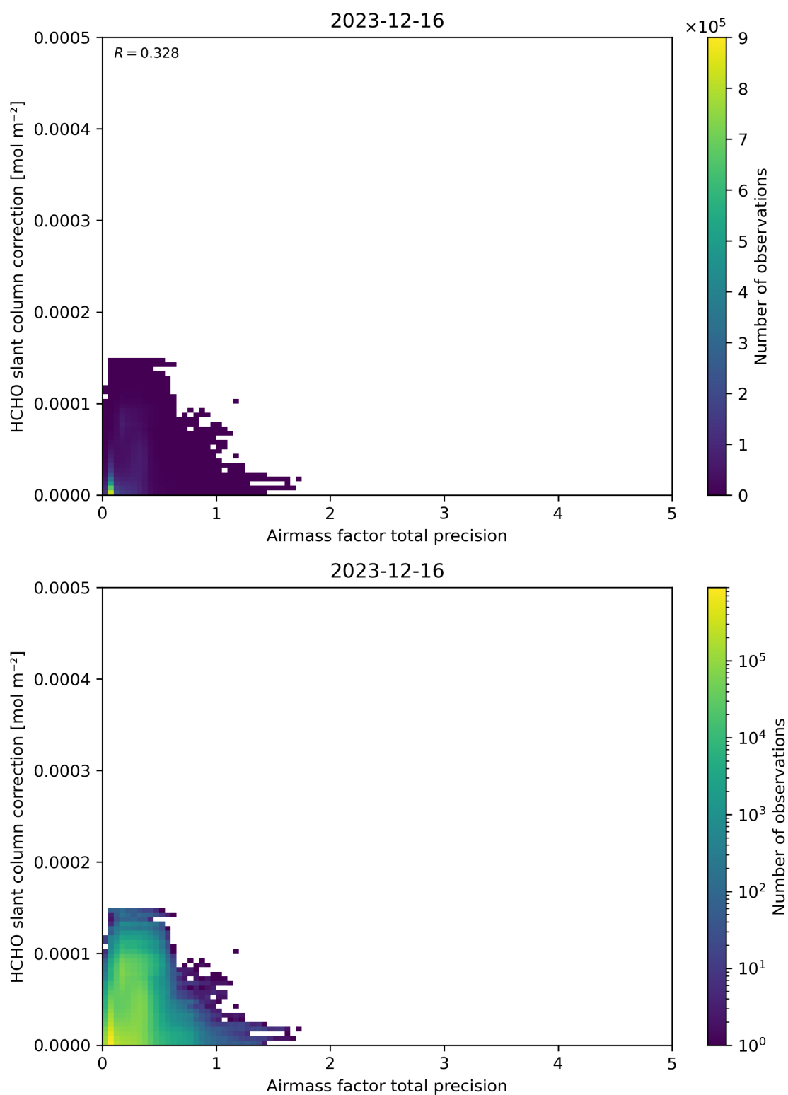
Figure 110: Scatter density plot of “Airmass factor total precision” against “HCHO slant column correction” for 2023-12-15 to 2023-12-17.
