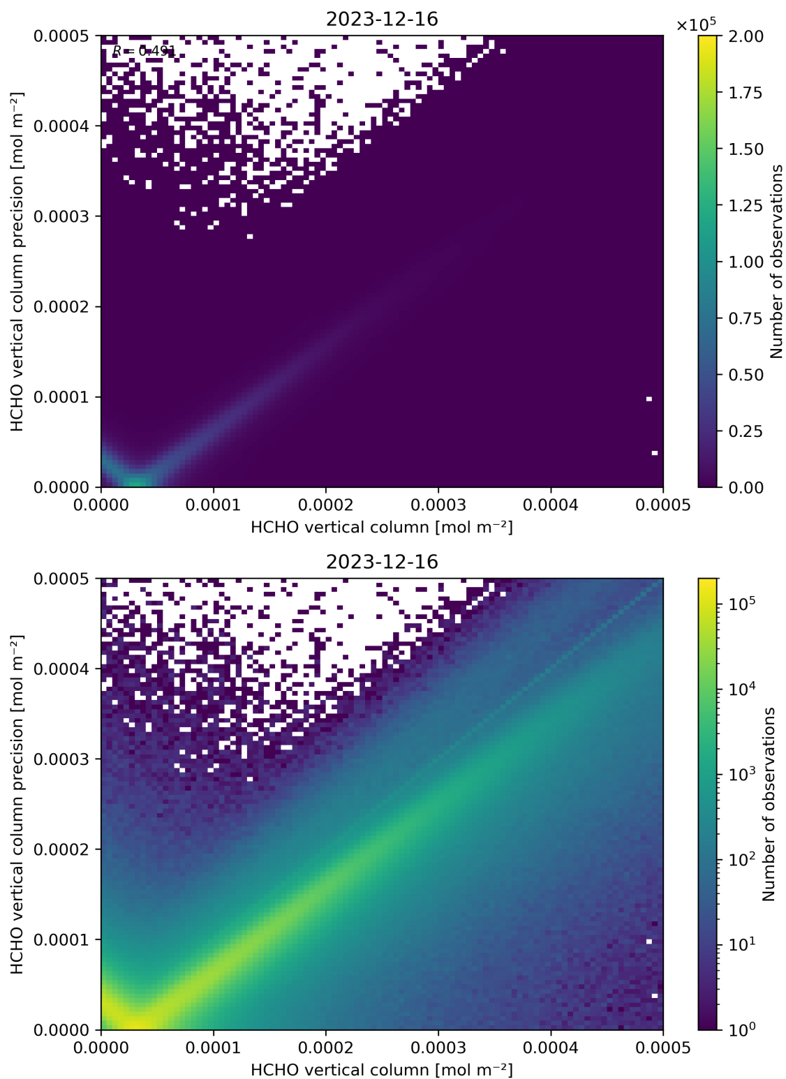
Figure 134: Scatter density plot of “HCHO vertical column” against “HCHO vertical column precision” for 2023-12-15 to 2023-12-17.
