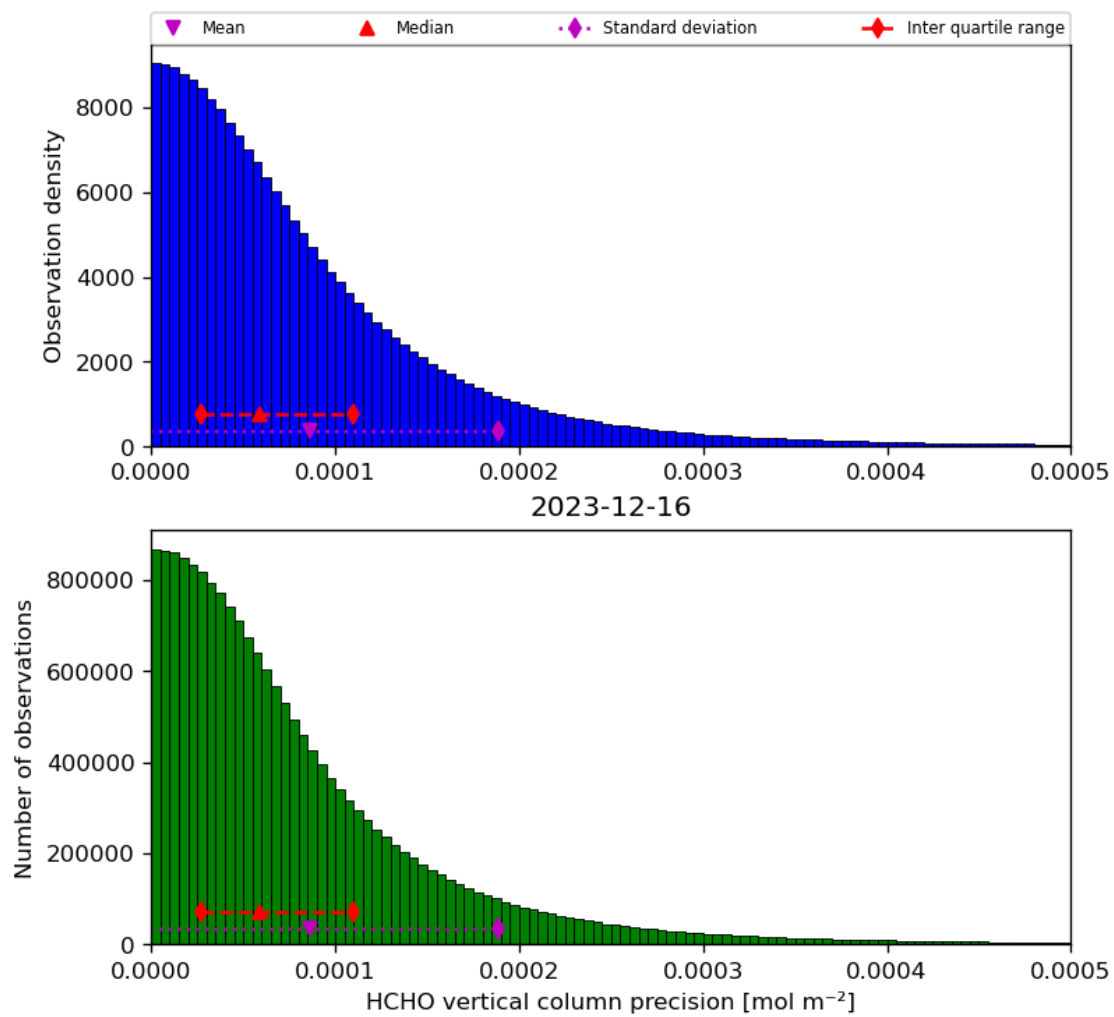
Figure 36: Histogram of “HCHO vertical column precision” for 2023-12-15 to 2023-12-17
