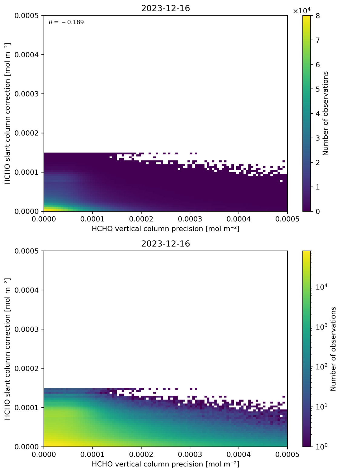
Figure 141: Scatter density plot of “HCHO vertical column precision” against “HCHO slant column correction” for 2023-12-15 to 2023-12-17.
