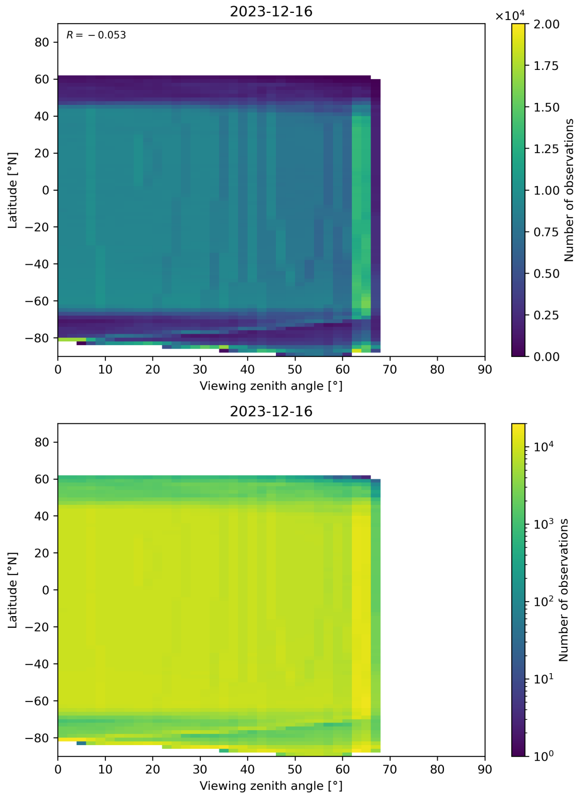
Figure 196: Scatter density plot of “Viewing zenith angle” against “Latitude” for 2023-12-15 to 2023-12-17.
