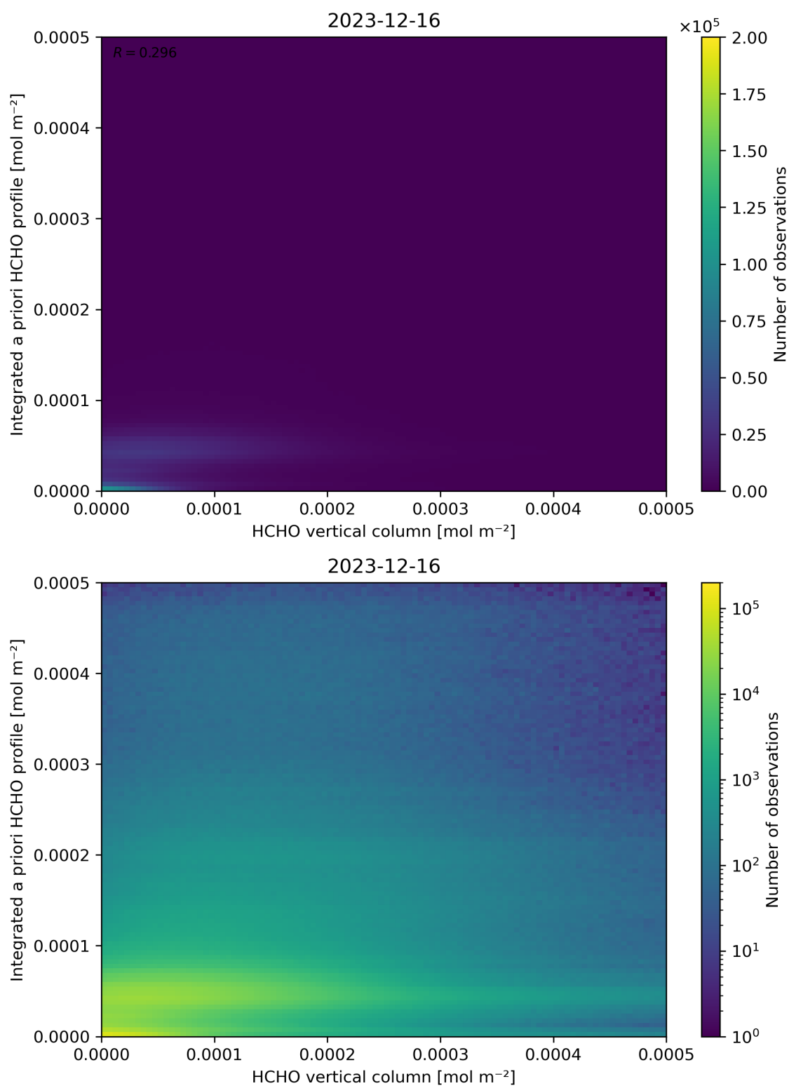
Figure 135: Scatter density plot of “HCHO vertical column” against “Integrated a priori HCHO profile” for 2023-12-15 to 2023-12-17.
