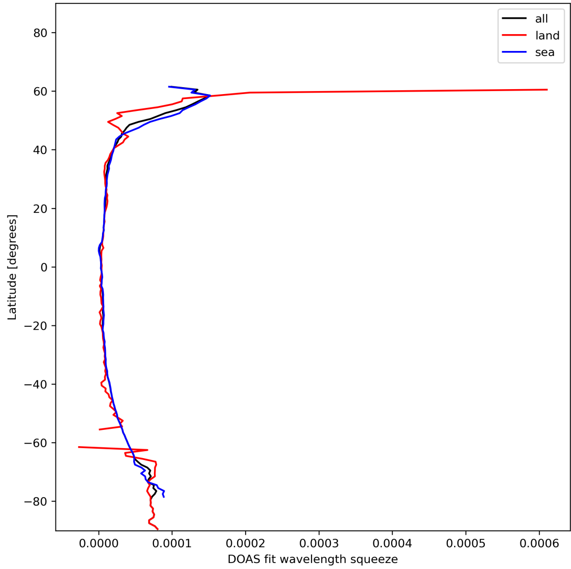
Figure 31: Zonal average of “DOAS fit wavelength squeeze” for 2023-12-15 to 2023-12-17.
