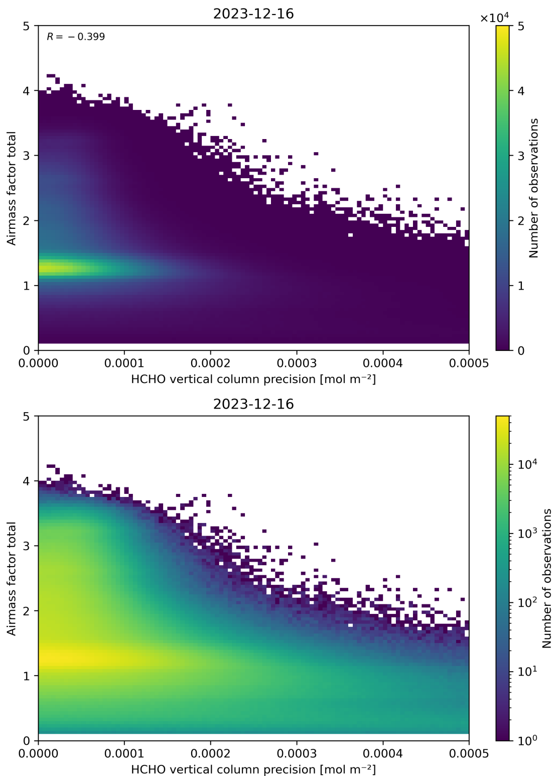
Figure 144: Scatter density plot of “HCHO vertical column precision” against “Airmass factor total” for 2023-12-15 to 2023-12-17.
