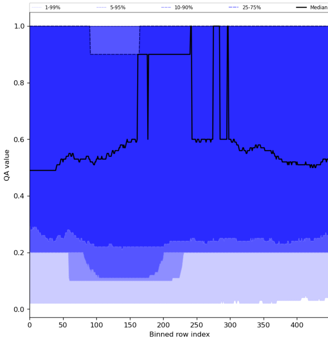
Figure 48: Along track statistics of “QA value” for 2023-12-15 to 2023-12-17
