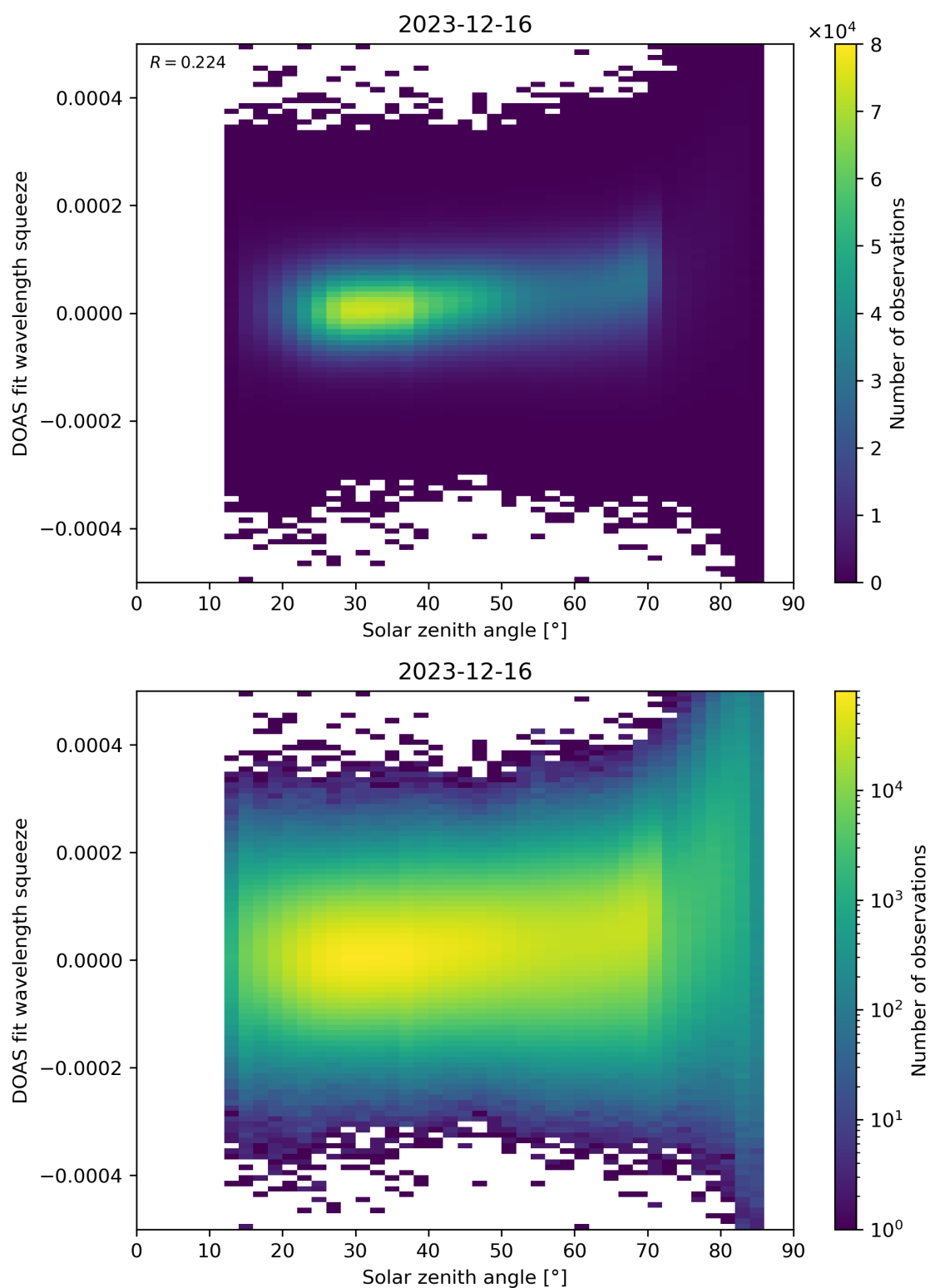
Figure 169: Scatter density plot of “Solar zenith angle” against “DOAS fit wavelength squeeze” for 2023-12-15 to 2023-12-17.
