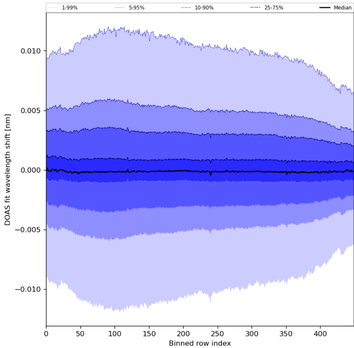
Figure 58: Along track statistics of “DOAS fit wavelength shift” for 2023-12-15 to 2023-12-17
