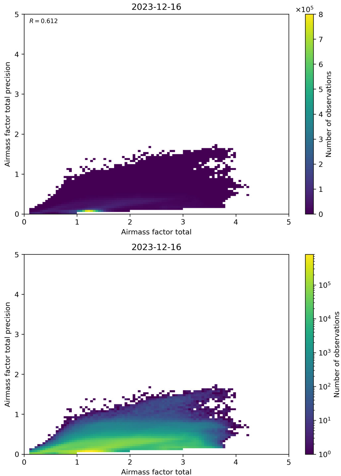
Figure 103: Scatter density plot of “Airmass factor total” against “Airmass factor total precision” for 2023-12-15 to 2023-12-17.
