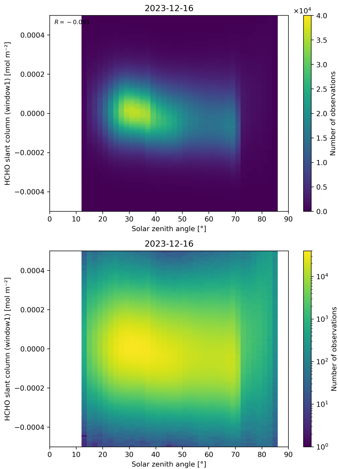
Figure 173: Scatter density plot of “Solar zenith angle” against “HCHO slant column (window1)” for 2023-12-15 to 2023-12-17.
