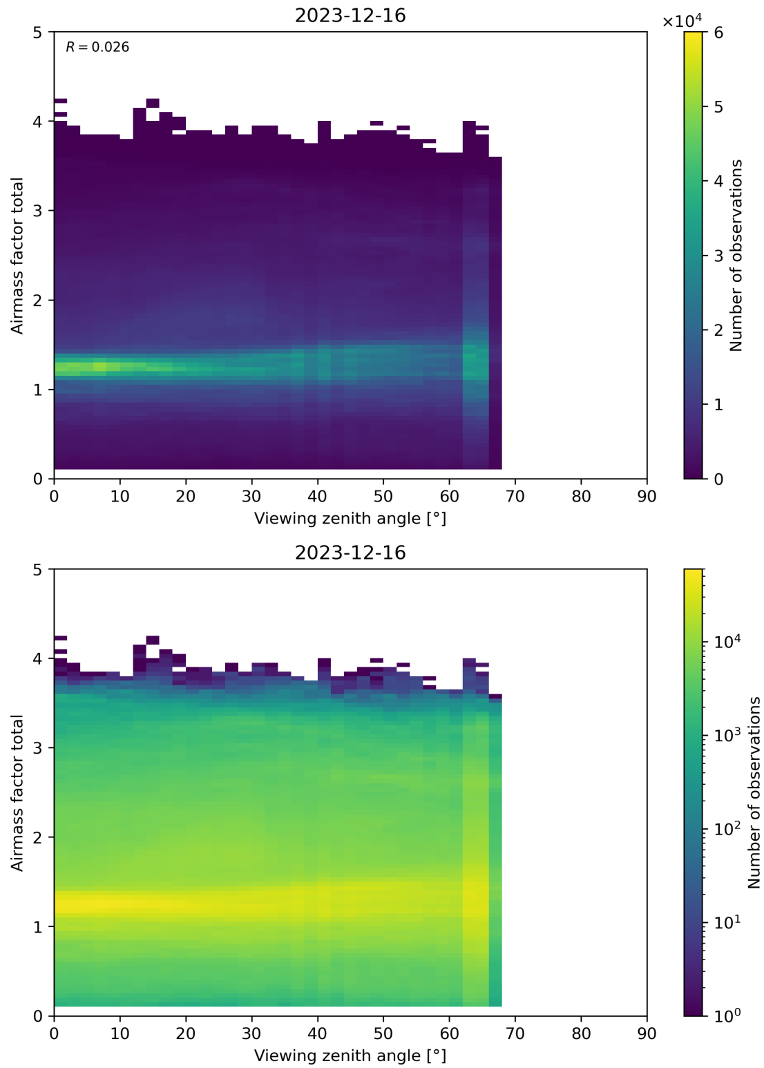
Figure 190: Scatter density plot of “Viewing zenith angle” against “Airmass factor total” for 2023-12-15 to 2023-12-17.
