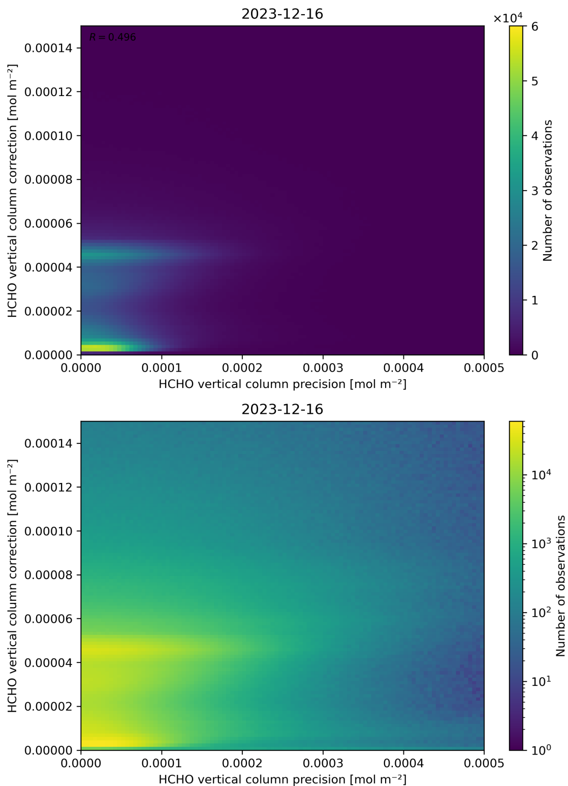
Figure 146: Scatter density plot of “HCHO vertical column precision” against “HCHO vertical column correction” for 2023-12-15 to 2023-12-17.
