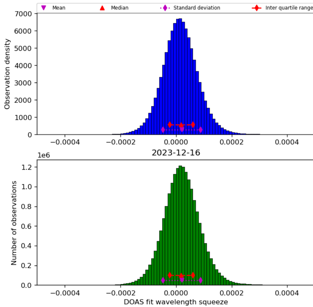
Figure 45: Histogram of “DOAS fit wavelength squeeze” for 2023-12-15 to 2023-12-17
