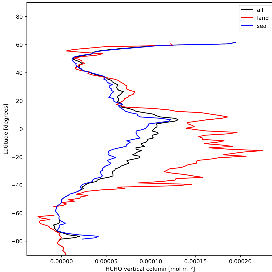
Figure 21: Zonal average of “HCHO vertical column” for 2023-12-15 to 2023-12-17.
