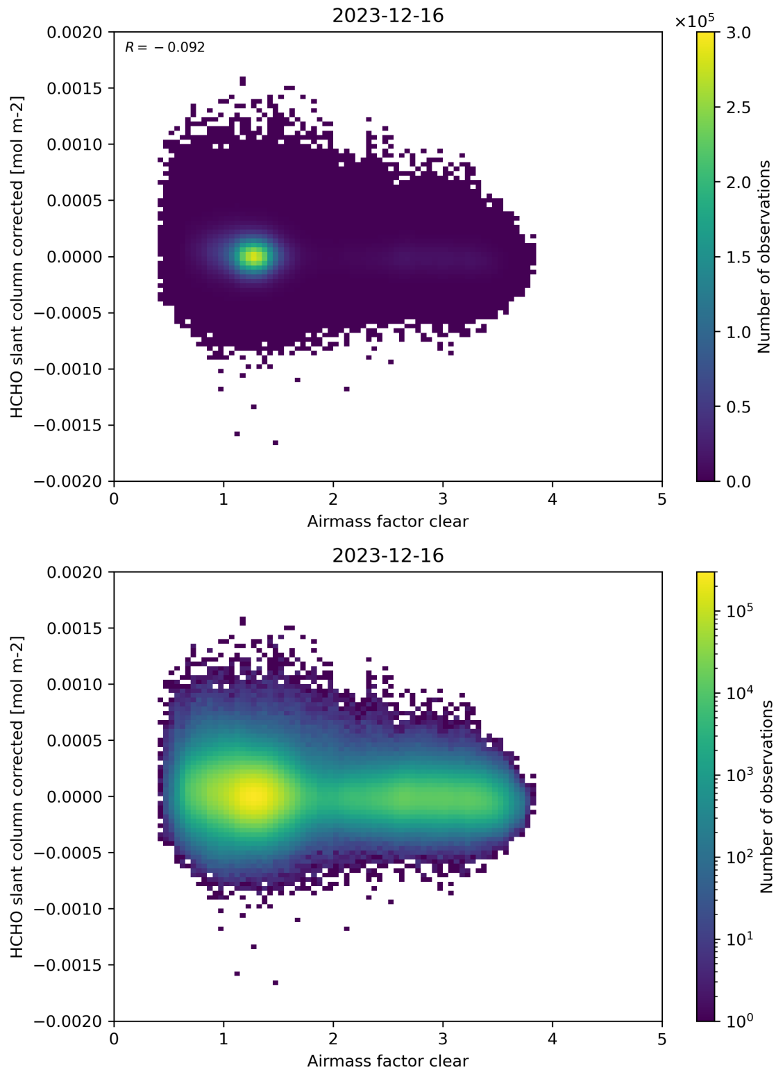
Figure 74: Scatter density plot of “Airmass factor clear” against “HCHO slant column corrected” for 2023-12-15 to 2023-12-17.
