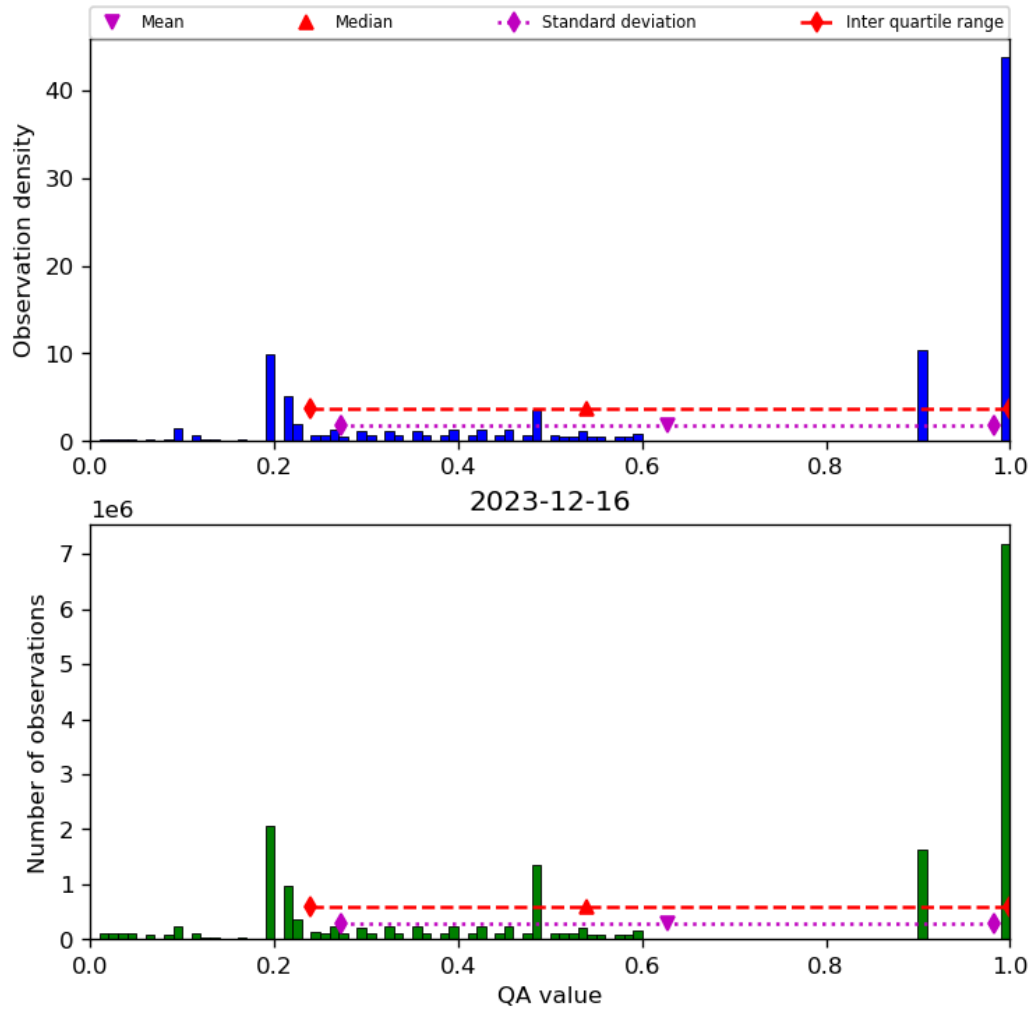
Figure 34: Histogram of “QA value” for 2023-12-15 to 2023-12-17
