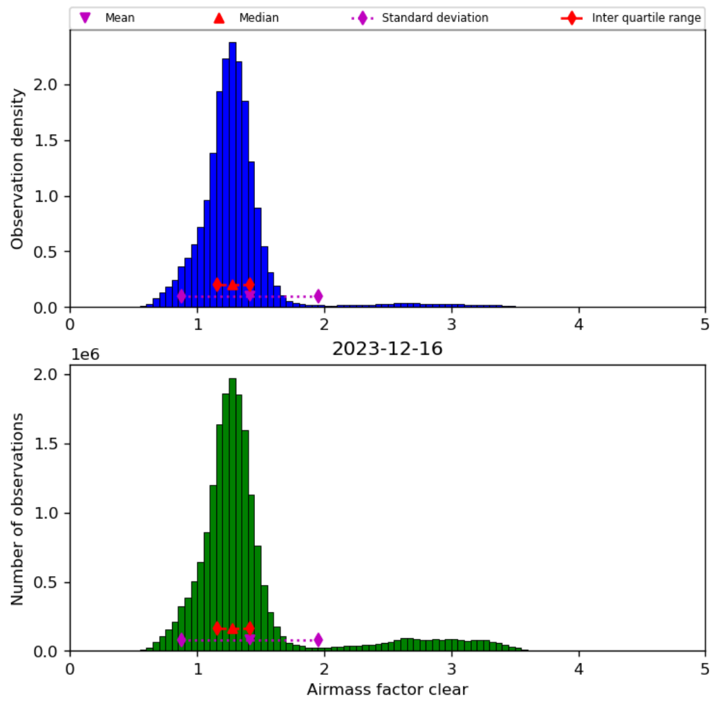
Figure 42: Histogram of “Airmass factor clear” for 2023-12-15 to 2023-12-17
