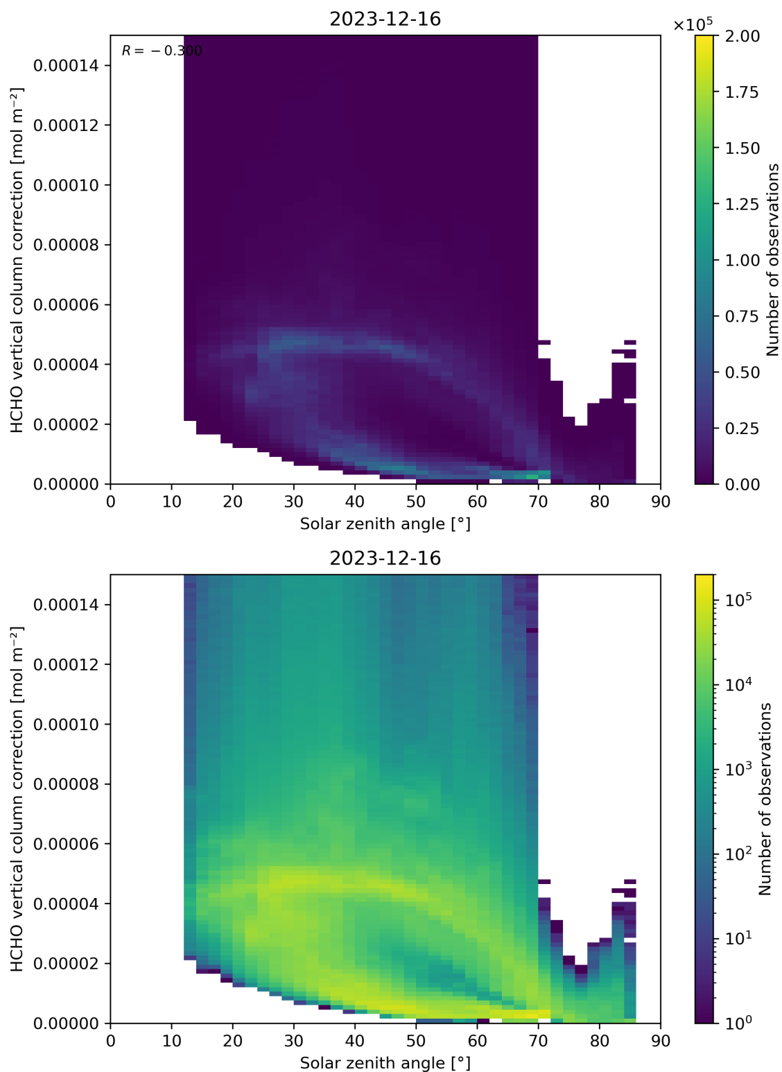
Figure 178: Scatter density plot of “Solar zenith angle” against “HCHO vertical column correction” for 2023-12-15 to 2023-12-17.
