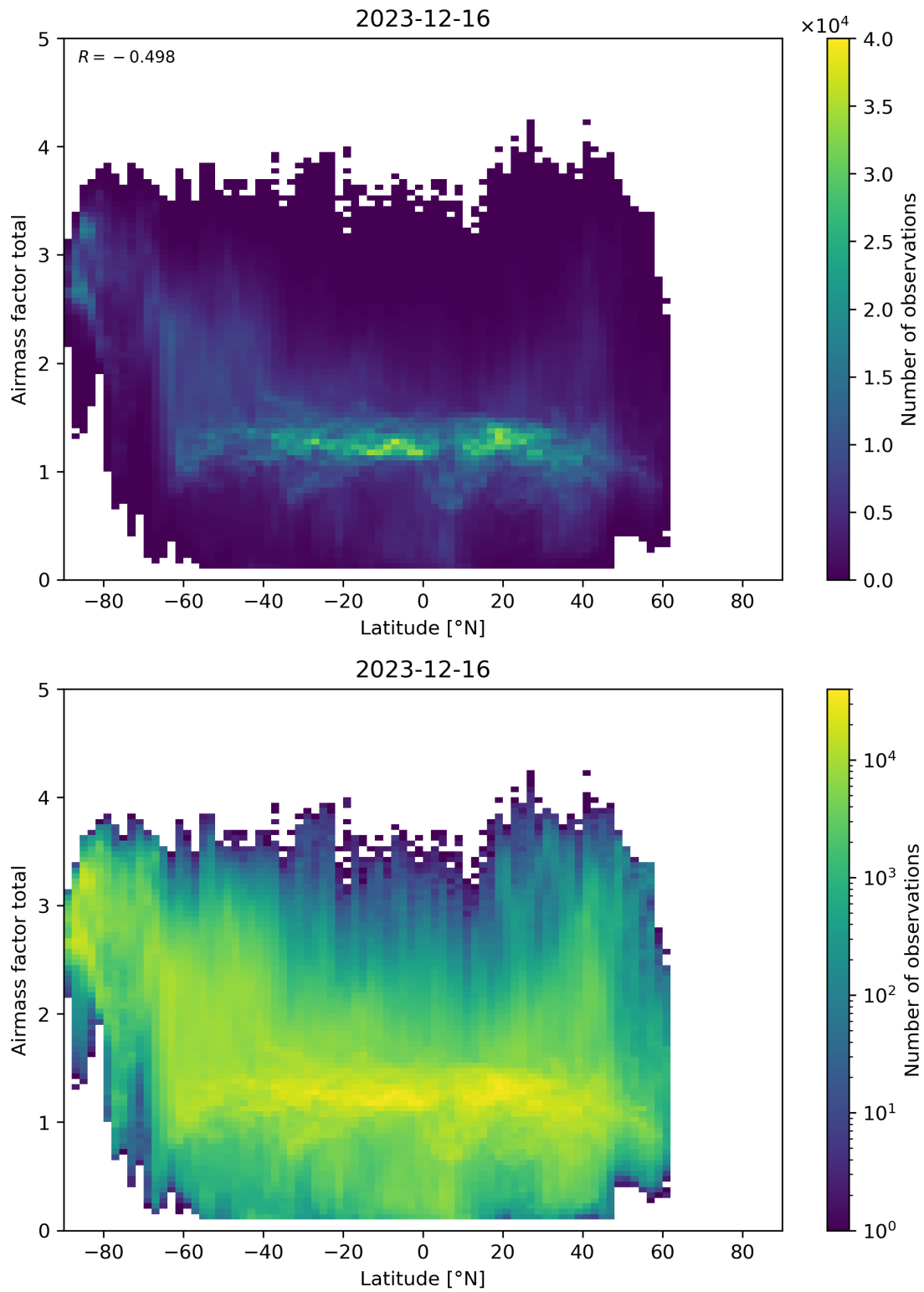
Figure 161: Scatter density plot of “Latitude” against “Airmass factor total” for 2023-12-15 to 2023-12-17.
