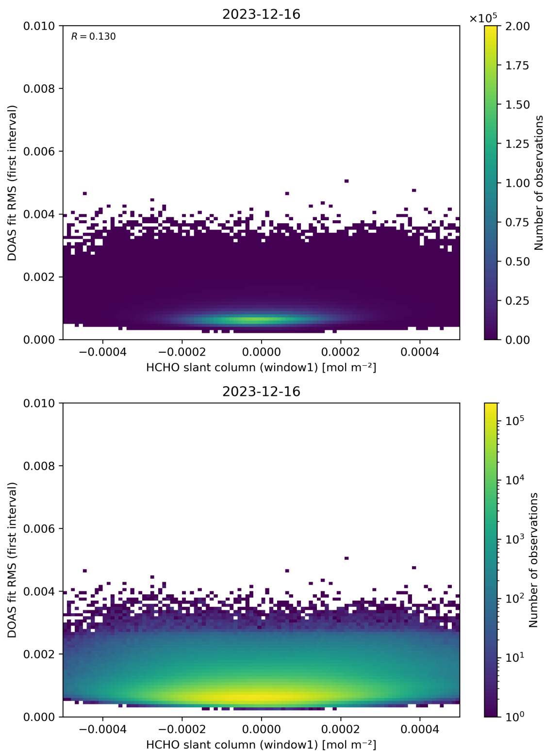
Figure 78: Scatter density plot of “HCHO slant column (window1)” against “DOAS fit RMS (first interval)” for 2023-12-15 to 2023-12-17.
