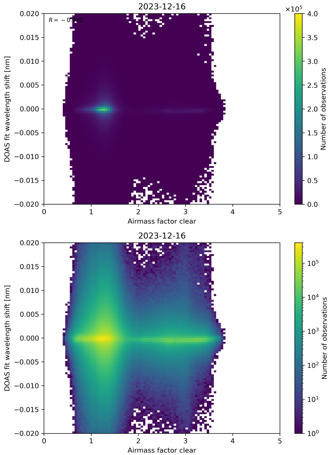
Figure 72: Scatter density plot of “Airmass factor clear” against “DOAS fit wavelength shift” for 2023-12-15 to 2023-12-17.
