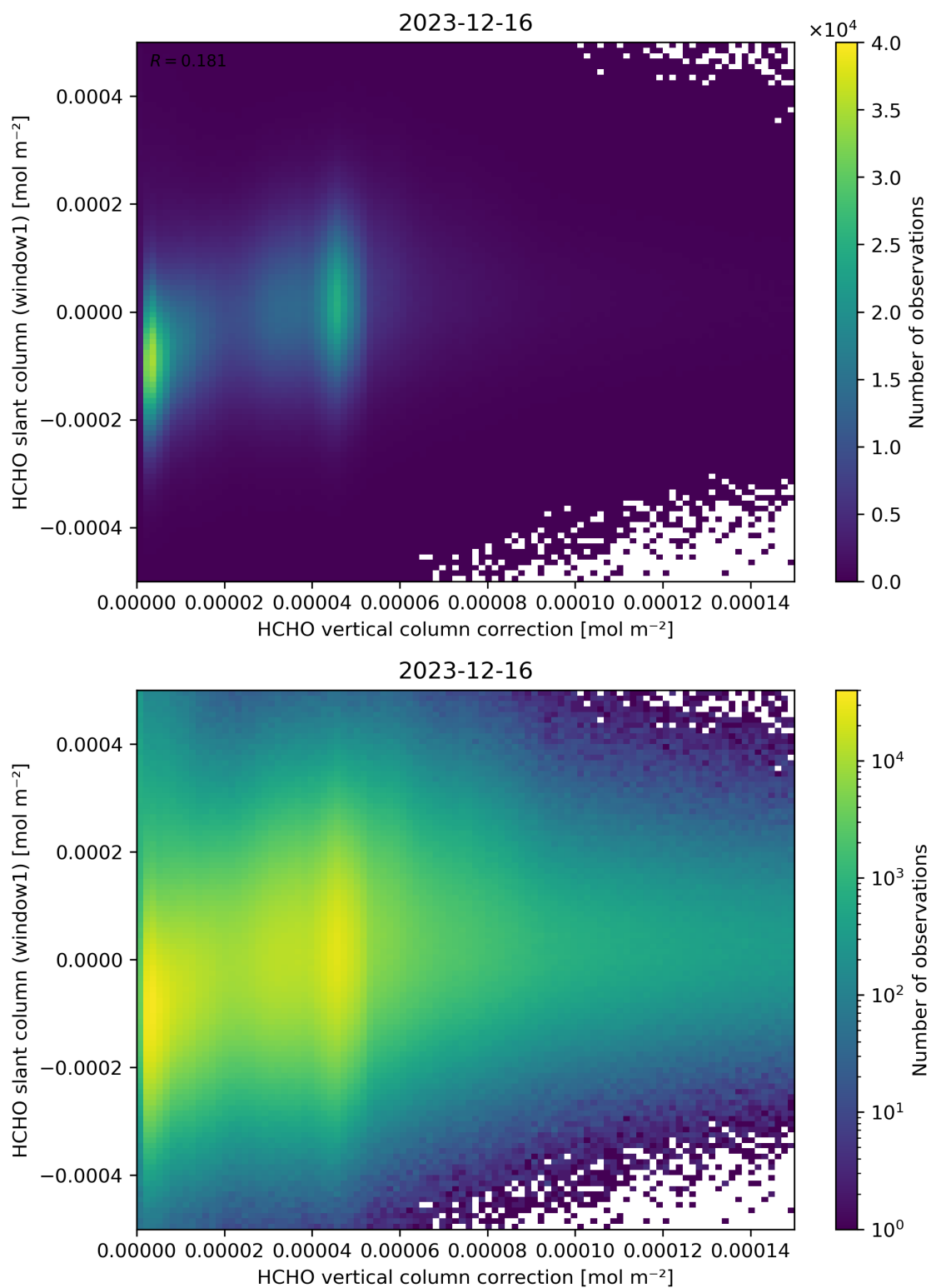
Figure 118: Scatter density plot of “HCHO vertical column correction” against “HCHO slant column (window1)” for 2023-12-15 to 2023-12-17.
