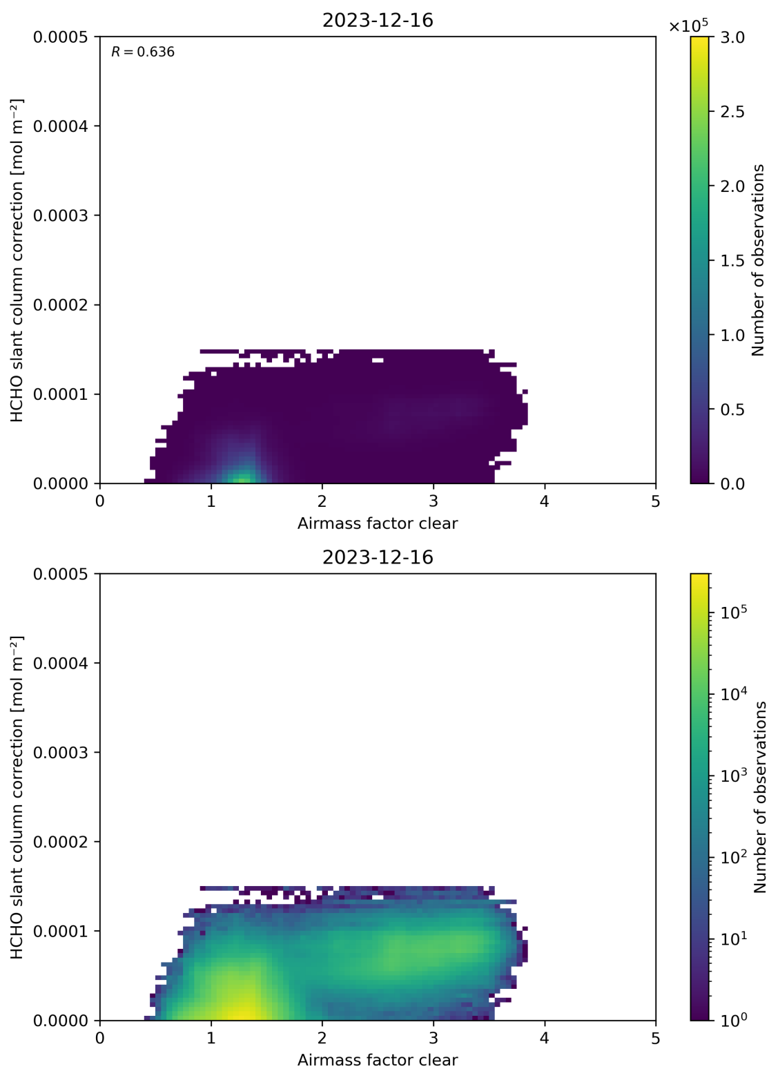
Figure 75: Scatter density plot of “Airmass factor clear” against “HCHO slant column correction” for 2023-12-15 to 2023-12-17.
