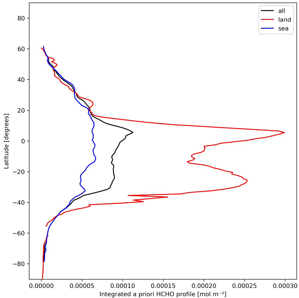
Figure 29: Zonal average of “Integrated a priori HCHO profile” for 2023-12-15 to 2023-12-17.
