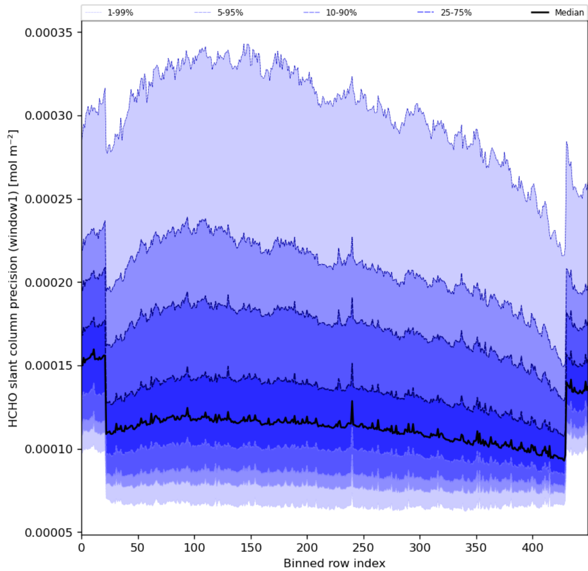
Figure 53: Along track statistics of “HCHO slant column precision (window1)” for 2023-12-15 to 2023-12-17
