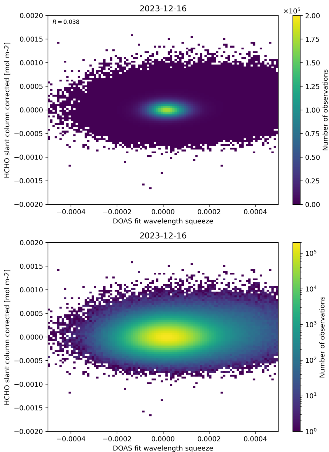
Figure 69: Scatter density plot of “DOAS fit wavelength squeeze” against “HCHO slant column corrected” for 2023-12-15 to 2023-12-17.
