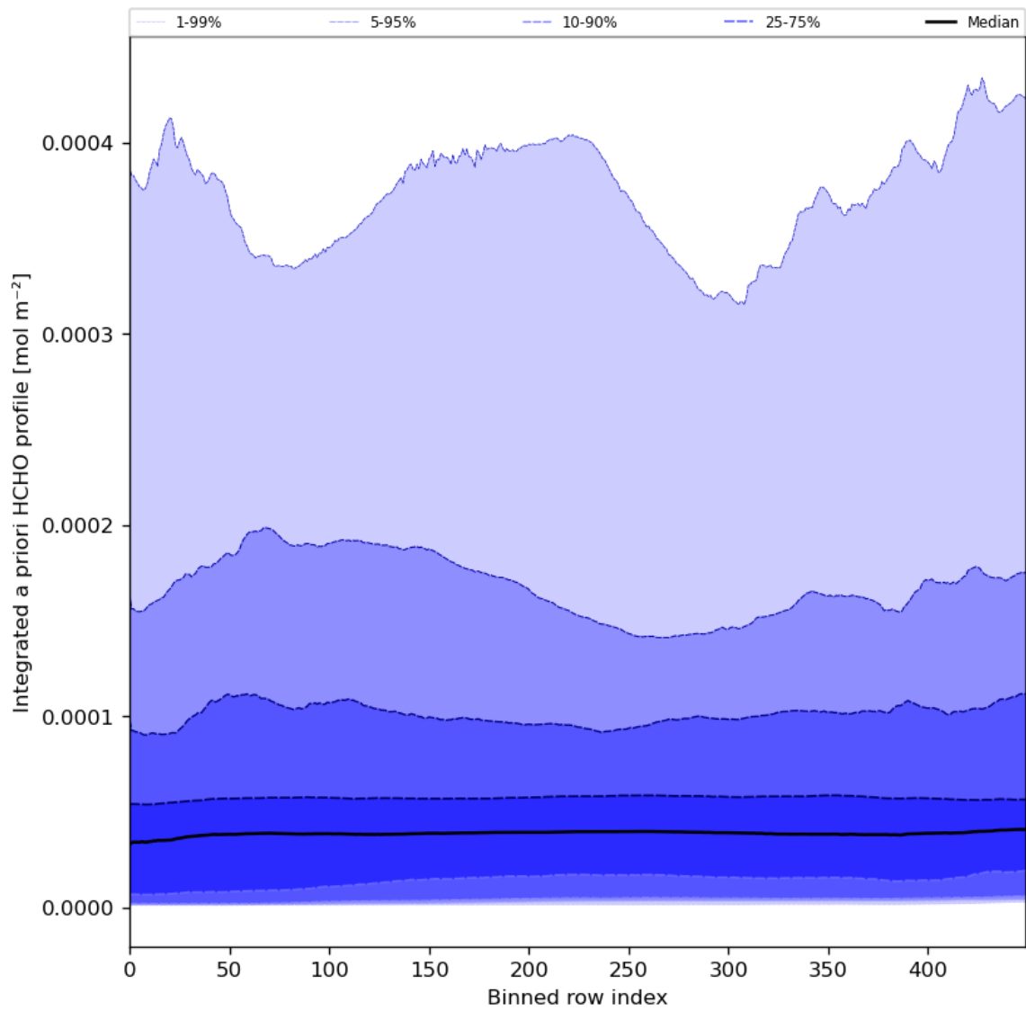
Figure 57: Along track statistics of “Integrated a priori HCHO profile” for 2023-12-15 to 2023-12-17
