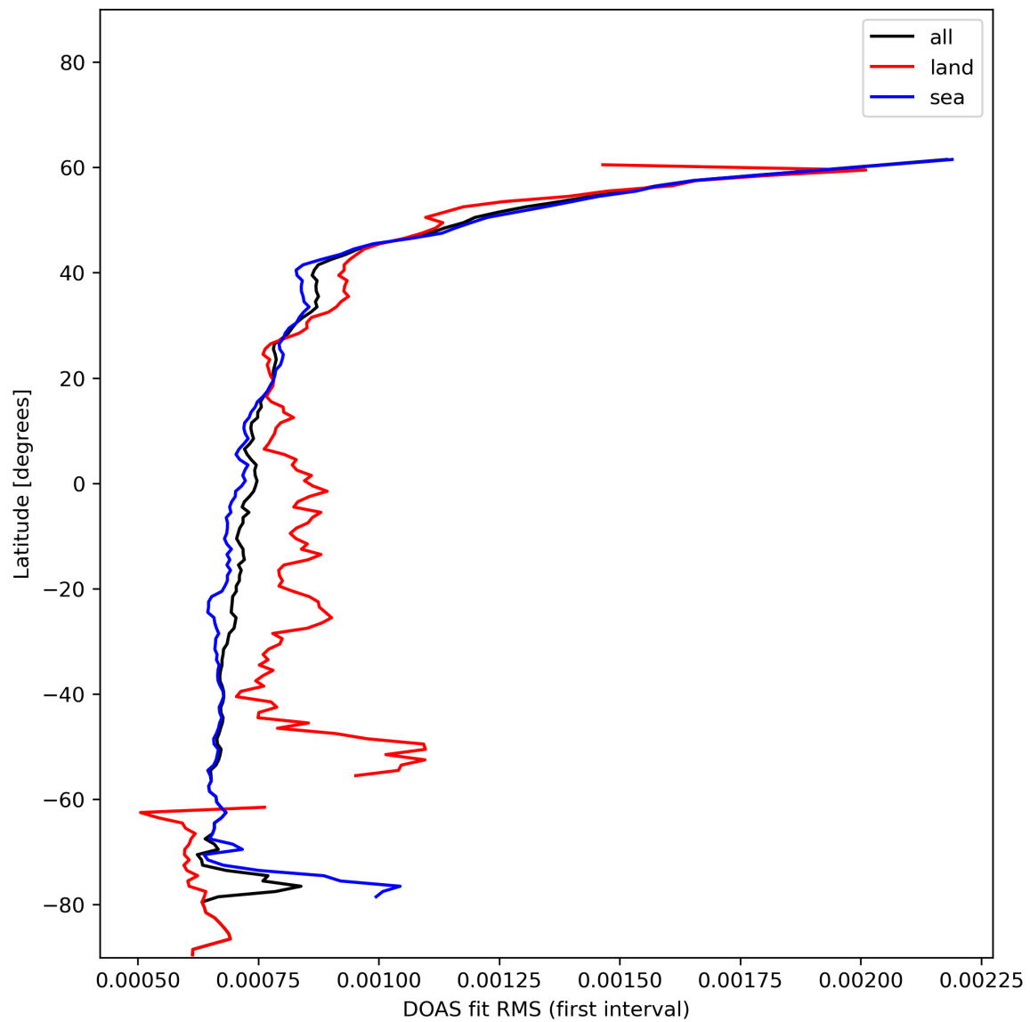
Figure 32: Zonal average of “DOAS fit RMS (first interval)” for 2023-12-15 to 2023-12-17.
