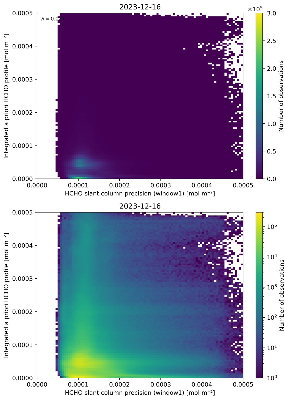
Figure 96: Scatter density plot of “HCHO slant column precision (window1)” against “Integrated a priori HCHO profile” for 2023-12-15 to 2023-12-17.
