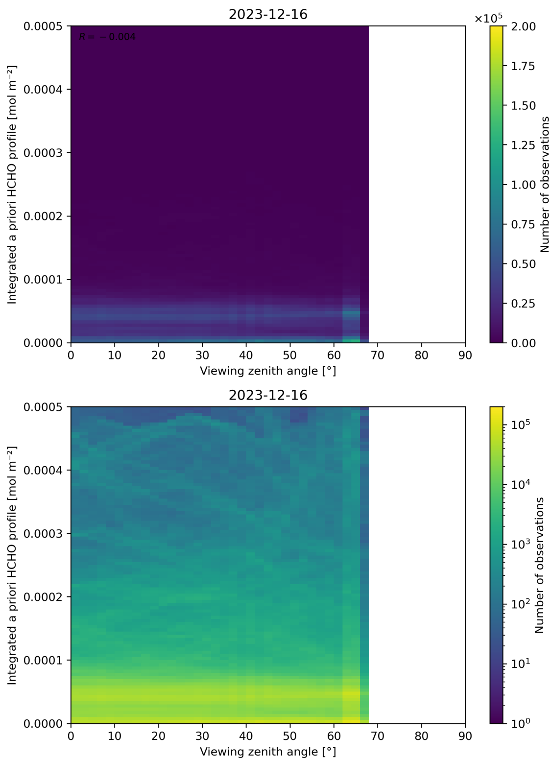
Figure 195: Scatter density plot of “Viewing zenith angle” against “Integrated a priori HCHO profile” for 2023-12-15 to 2023-12-17.
