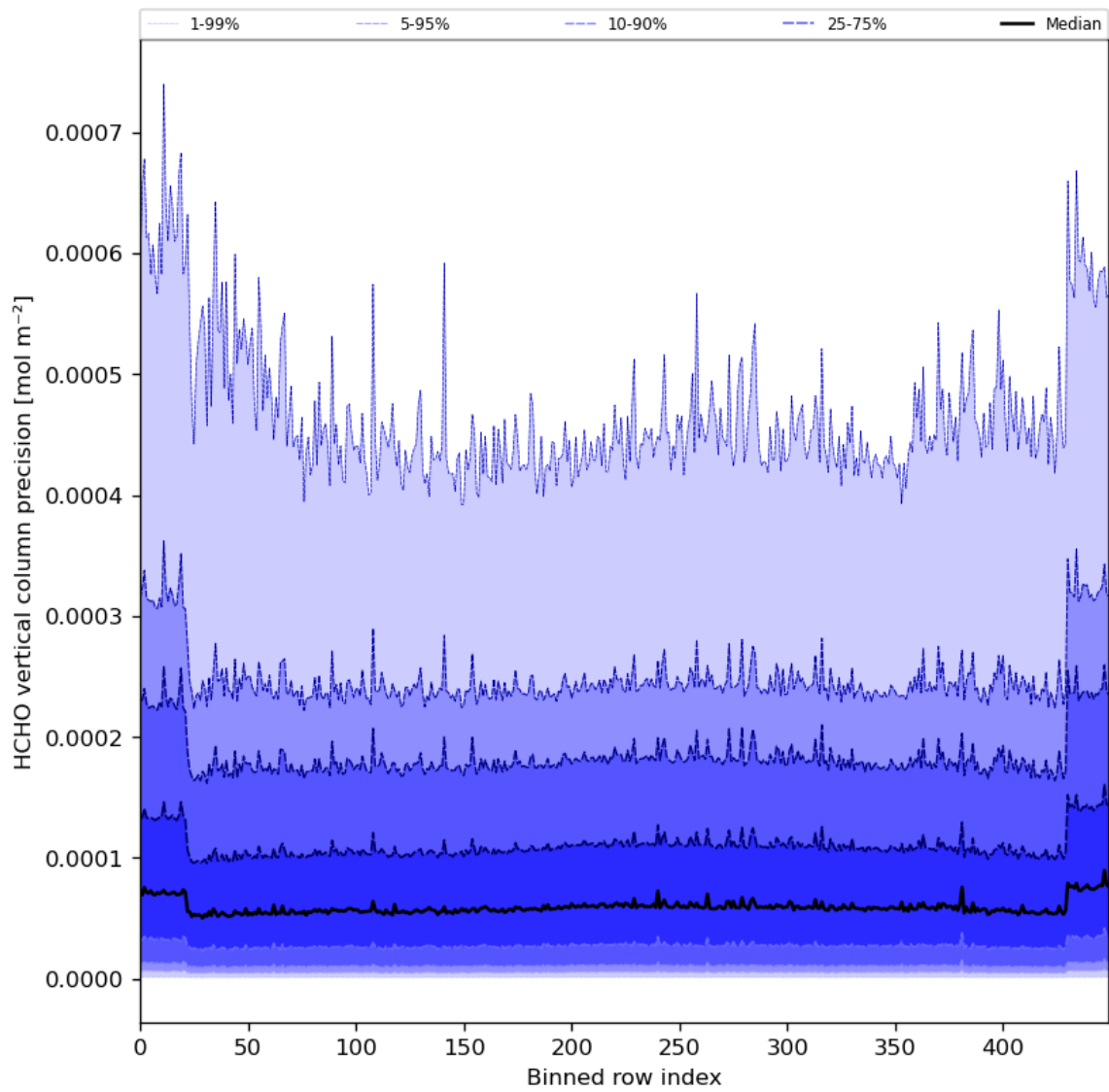
Figure 50: Along track statistics of “HCHO vertical column precision” for 2023-12-15 to 2023-12-17
