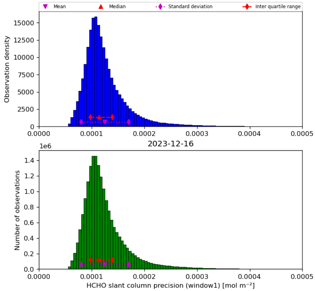
Figure 39: Histogram of “HCHO slant column precision (window1)” for 2023-12-15 to 2023-12-17
