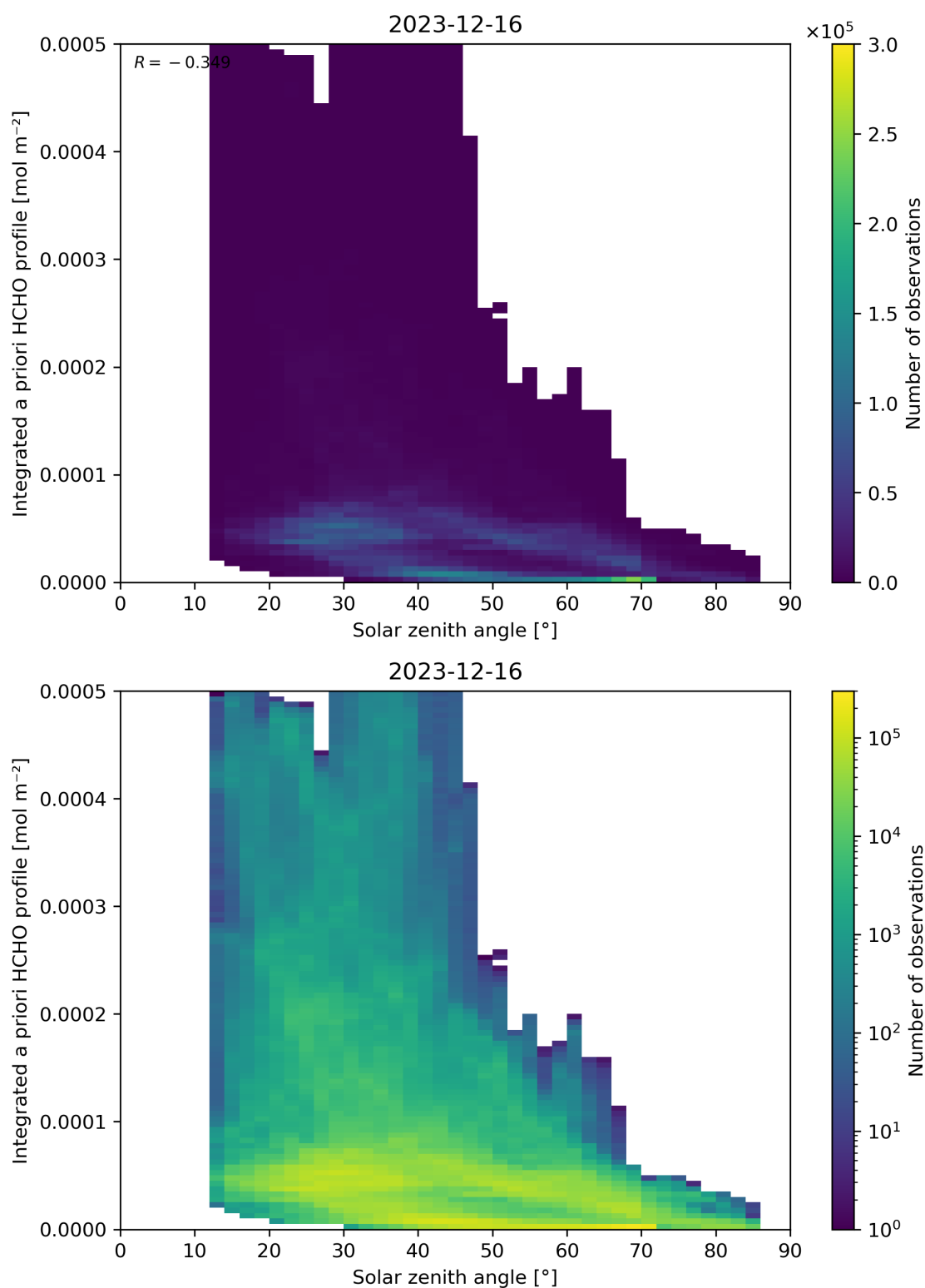
Figure 180: Scatter density plot of “Solar zenith angle” against “Integrated a priori HCHO profile” for 2023-12-15 to 2023-12-17.
