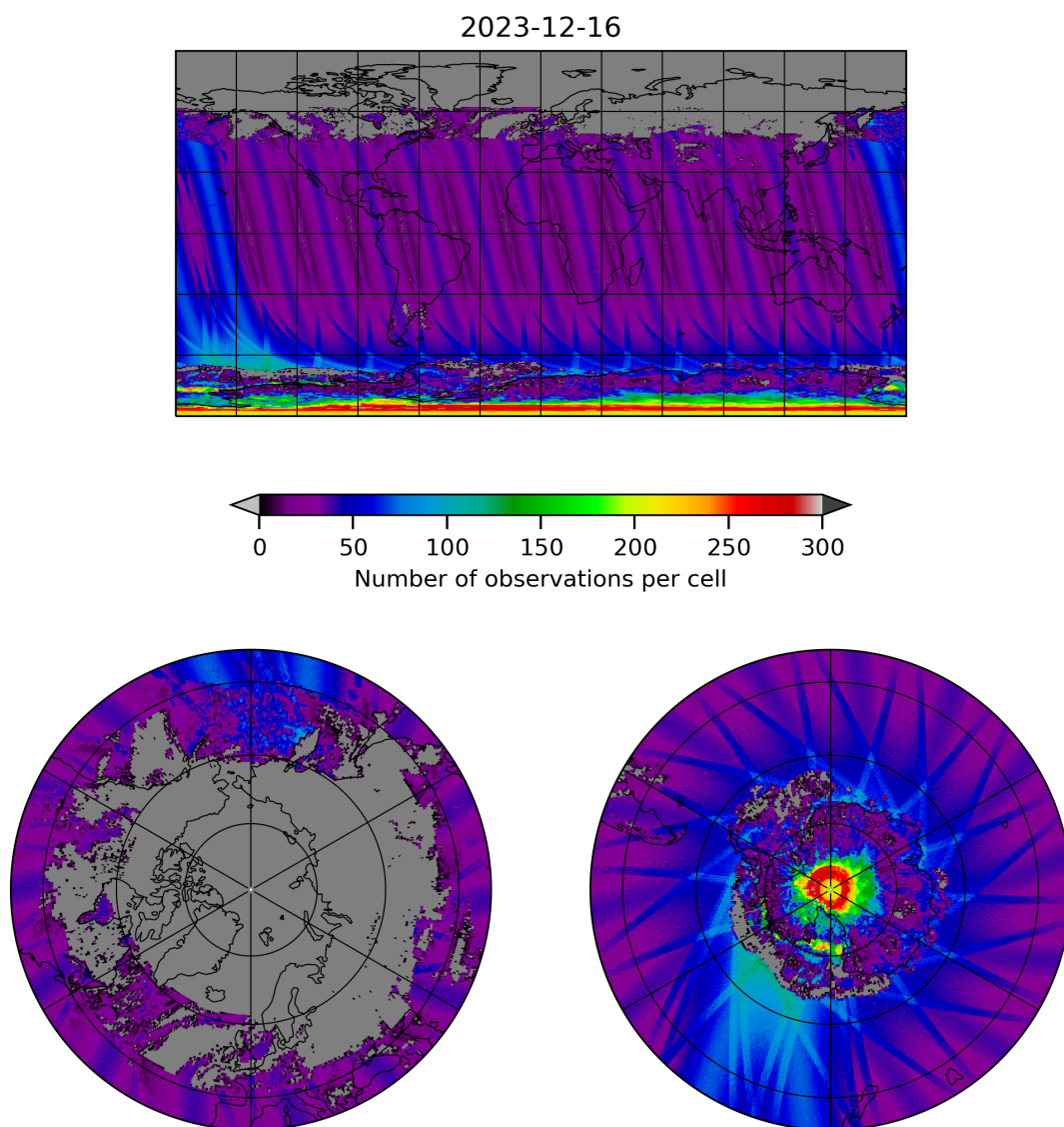
Figure 19: Map of the number of observations for 2023-12-15 to 2023-12-17
