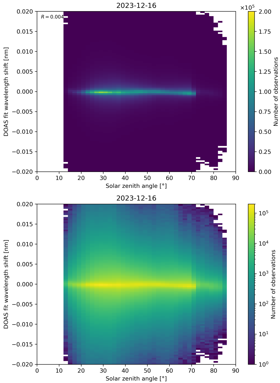
Figure 168: Scatter density plot of “Solar zenith angle” against “DOAS fit wavelength shift” for 2023-12-15 to 2023-12-17.
