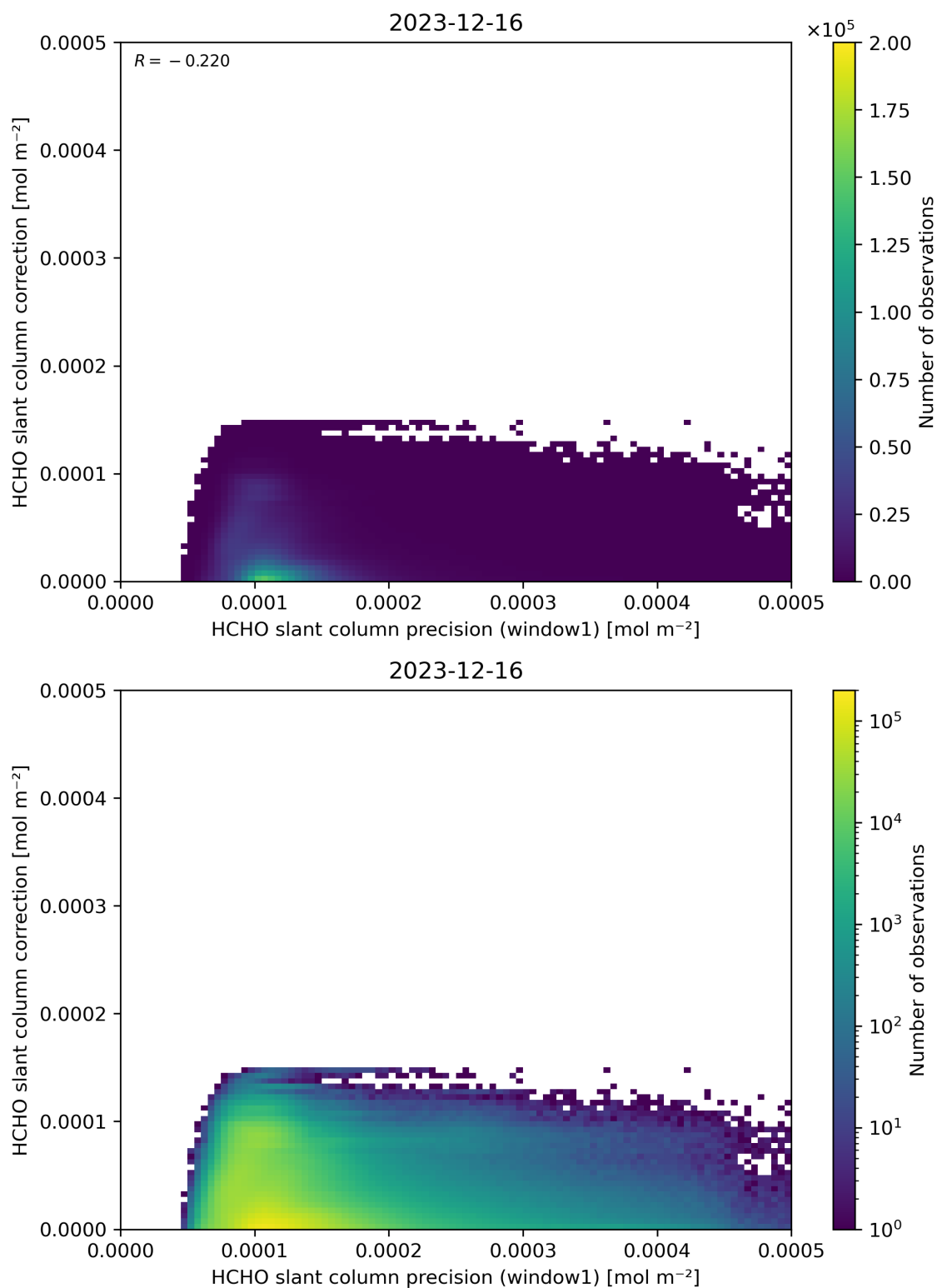
Figure 93: Scatter density plot of “HCHO slant column precision (window1)” against “HCHO slant column correction” for 2023-12-15 to 2023-12-17.
