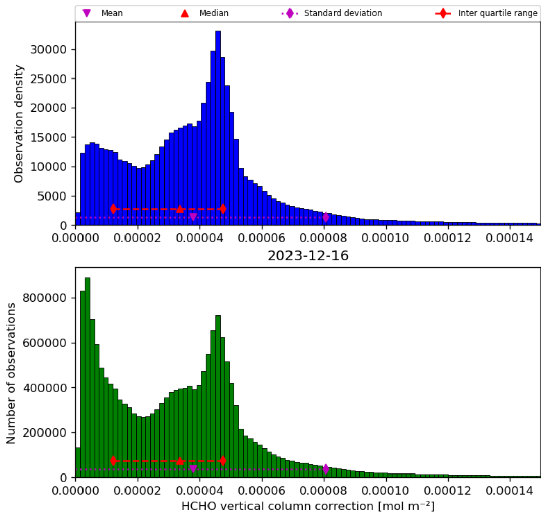
Figure 37: Histogram of “HCHO vertical column correction” for 2023-12-15 to 2023-12-17
