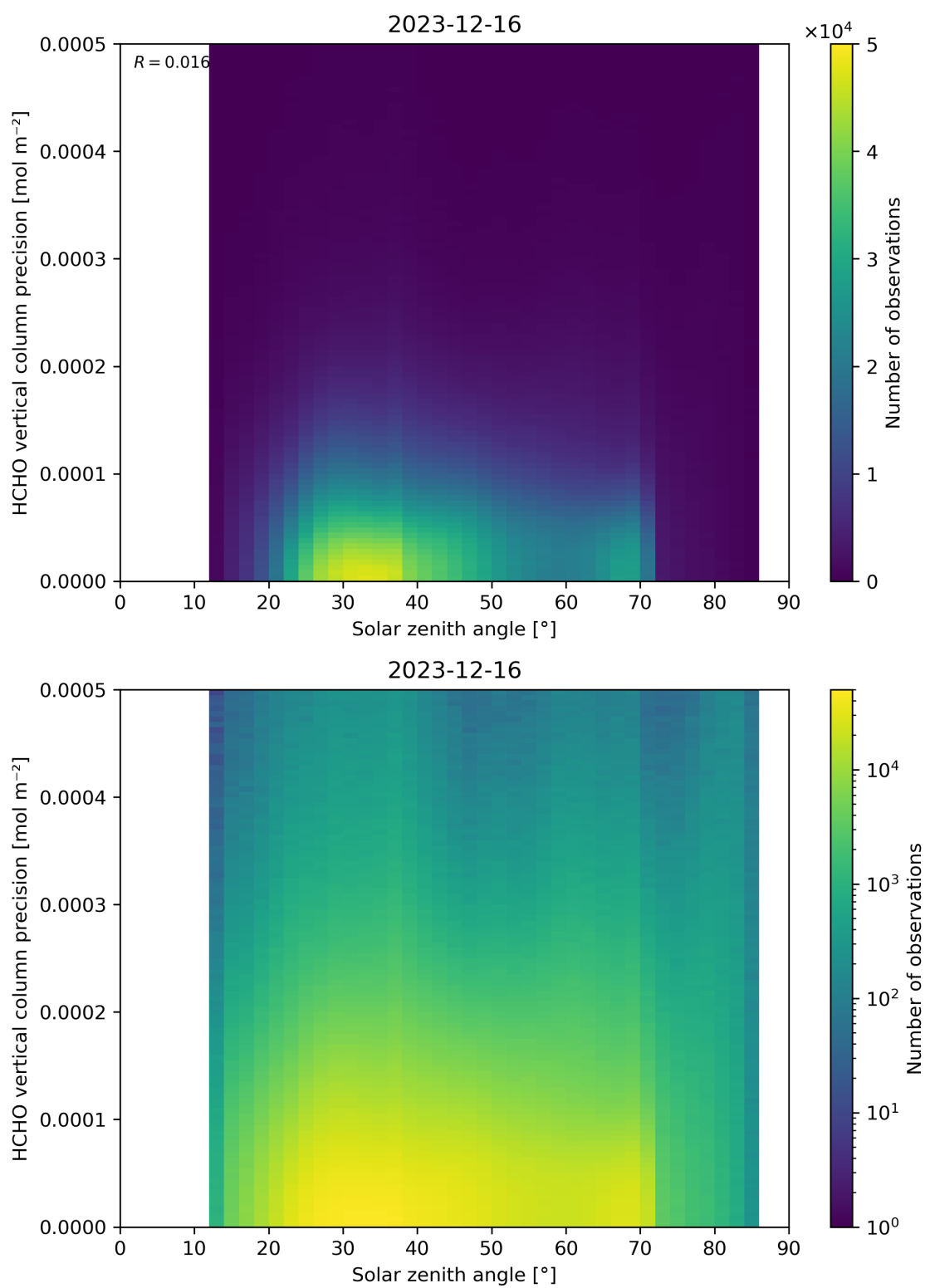
Figure 179: Scatter density plot of “Solar zenith angle” against “HCHO vertical column precision” for 2023-12-15 to 2023-12-17.
