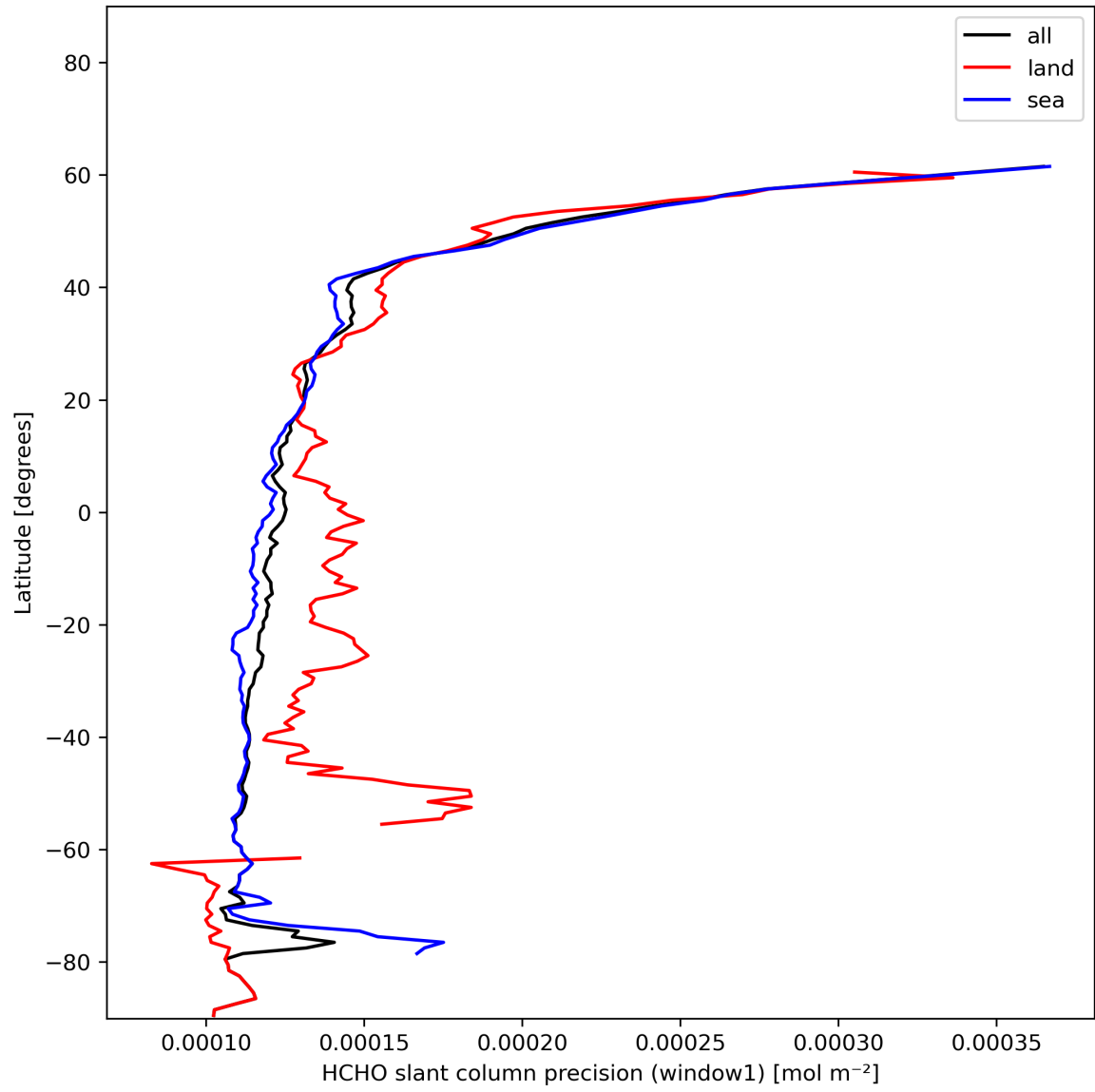
Figure 25: Zonal average of “HCHO slant column precision (window1)” for 2023-12-15 to 2023-12-17.
