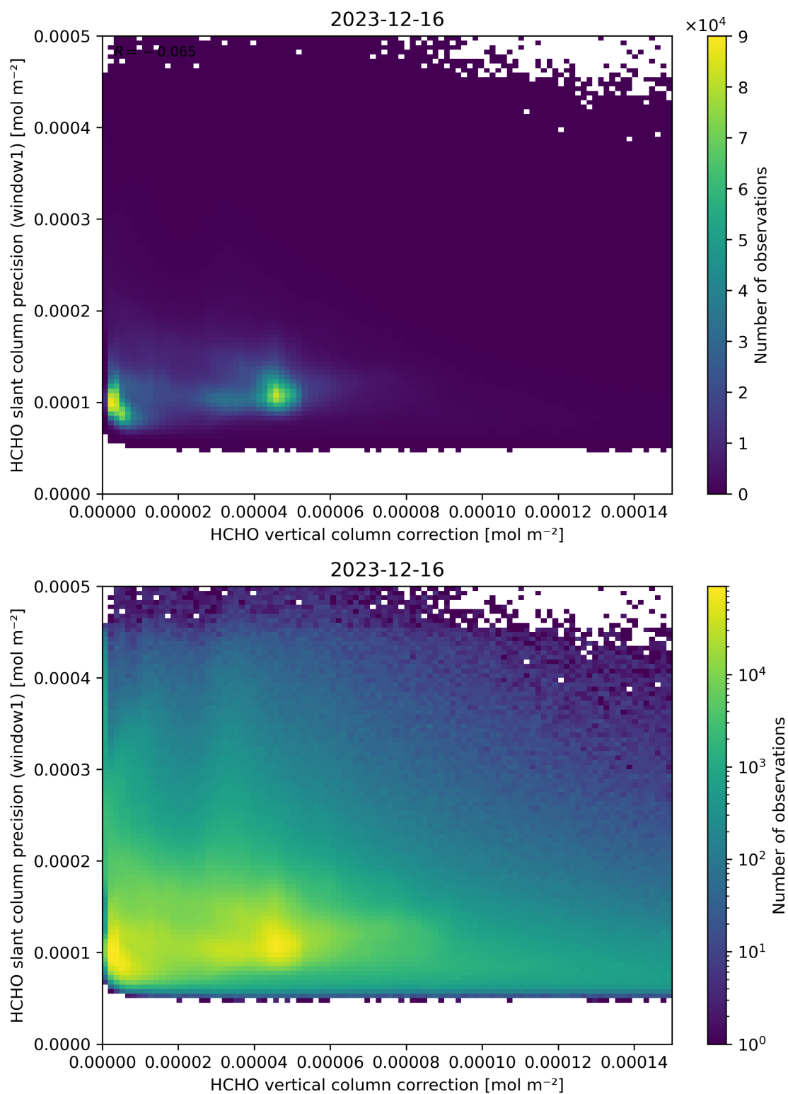
Figure 119: Scatter density plot of “HCHO vertical column correction” against “HCHO slant column precision (window1)” for 2023-12-15 to 2023-12-17.
