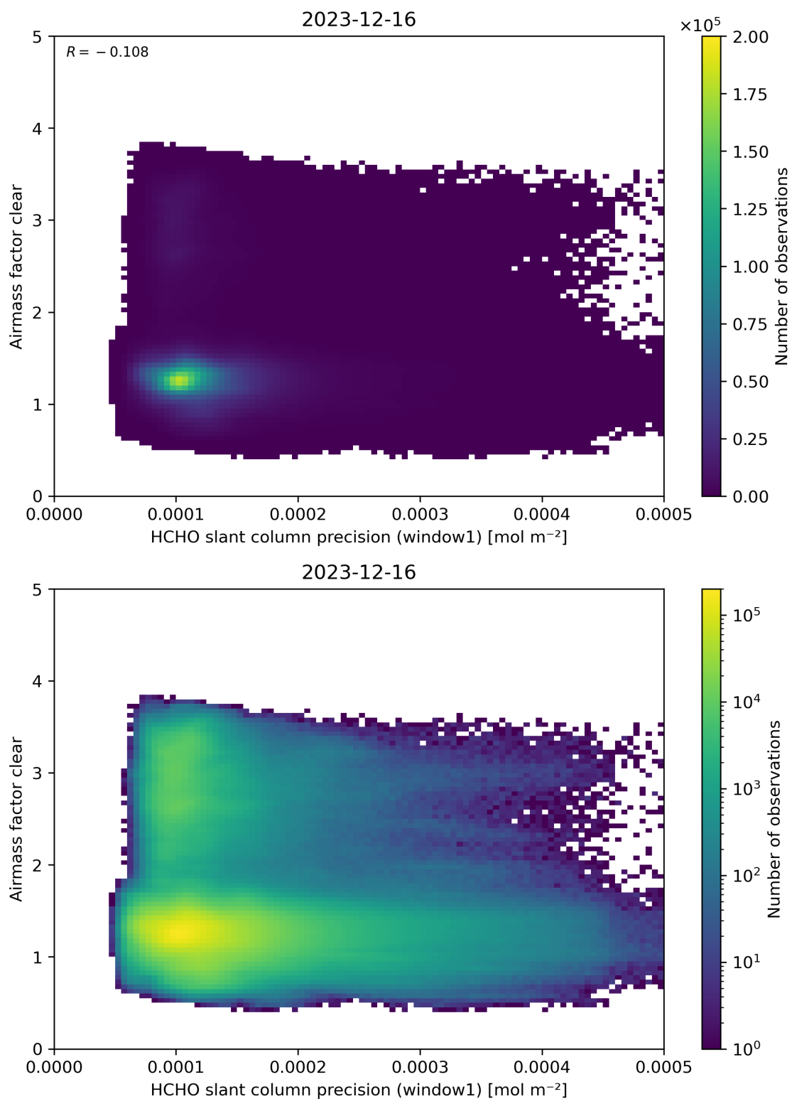
Figure 91: Scatter density plot of “HCHO slant column precision (window1)” against “Airmass factor clear” for 2023-12-15 to 2023-12-17.
