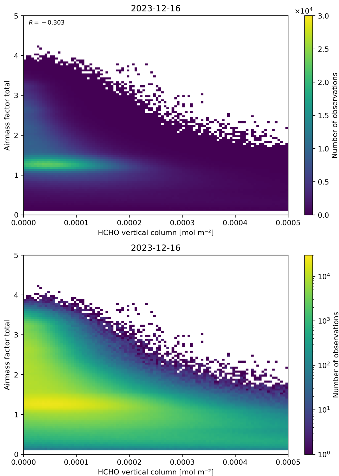
Figure 131: Scatter density plot of “HCHO vertical column” against “Airmass factor total” for 2023-12-15 to 2023-12-17.
