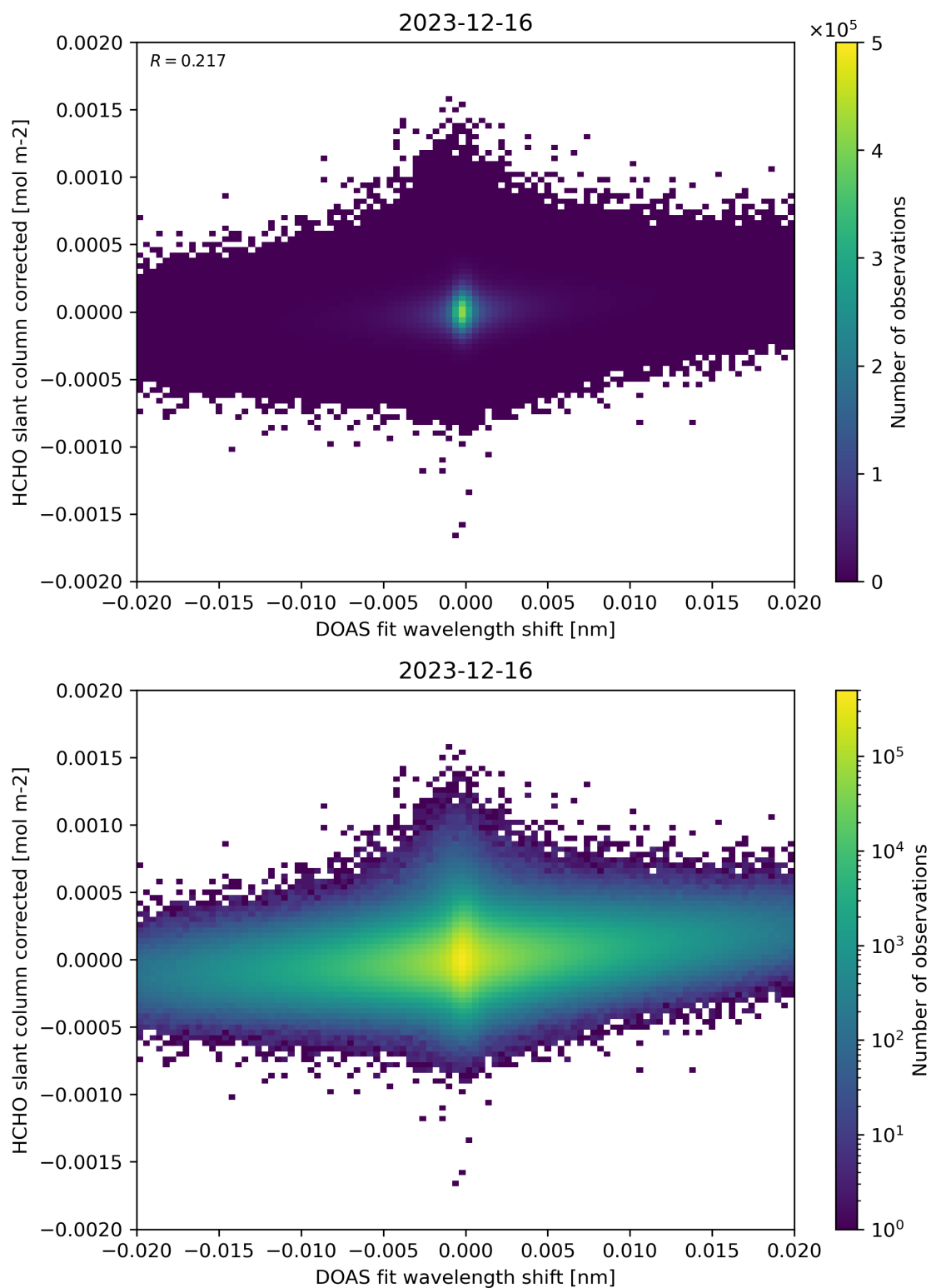
Figure 66: Scatter density plot of “DOAS fit wavelength shift” against “HCHO slant column corrected” for 2023-12-15 to 2023-12-17.
