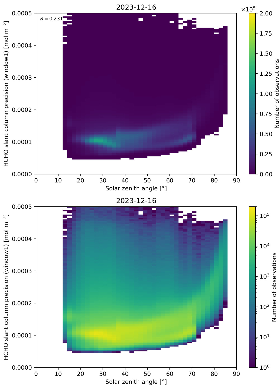
Figure 174: Scatter density plot of “Solar zenith angle” against “HCHO slant column precision (window1)” for 2023-12-15 to 2023-12-17.
