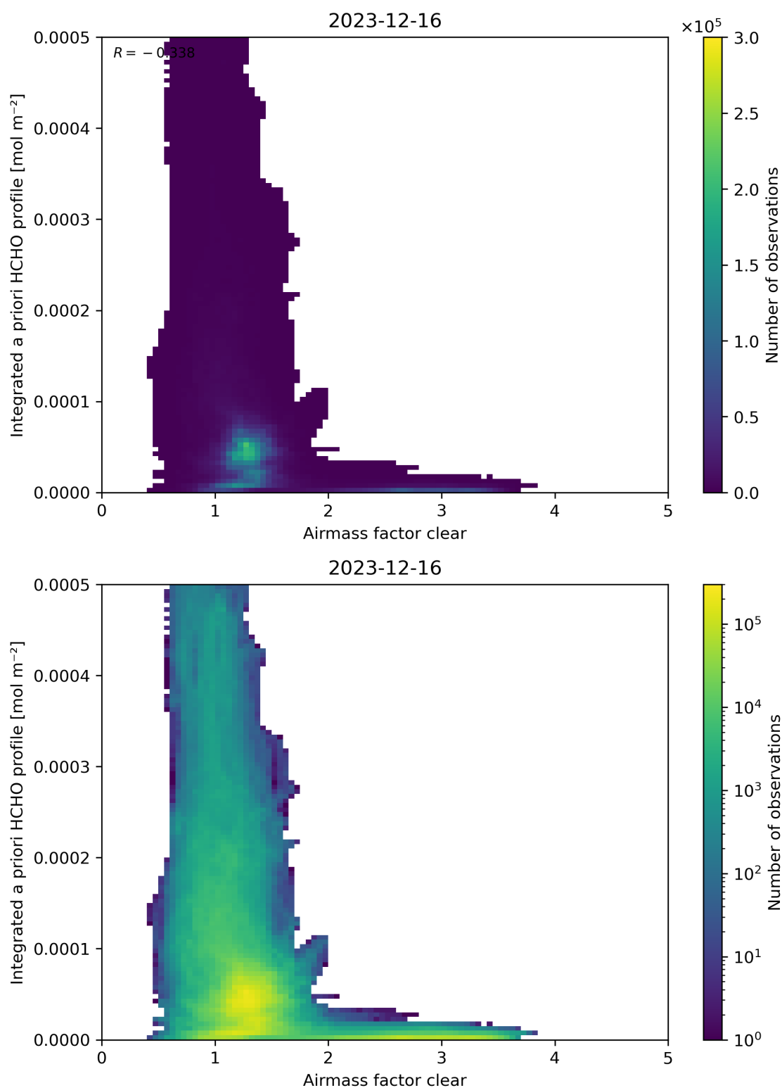
Figure 76: Scatter density plot of “Airmass factor clear” against “Integrated a priori HCHO profile” for 2023-12-15 to 2023-12-17.
