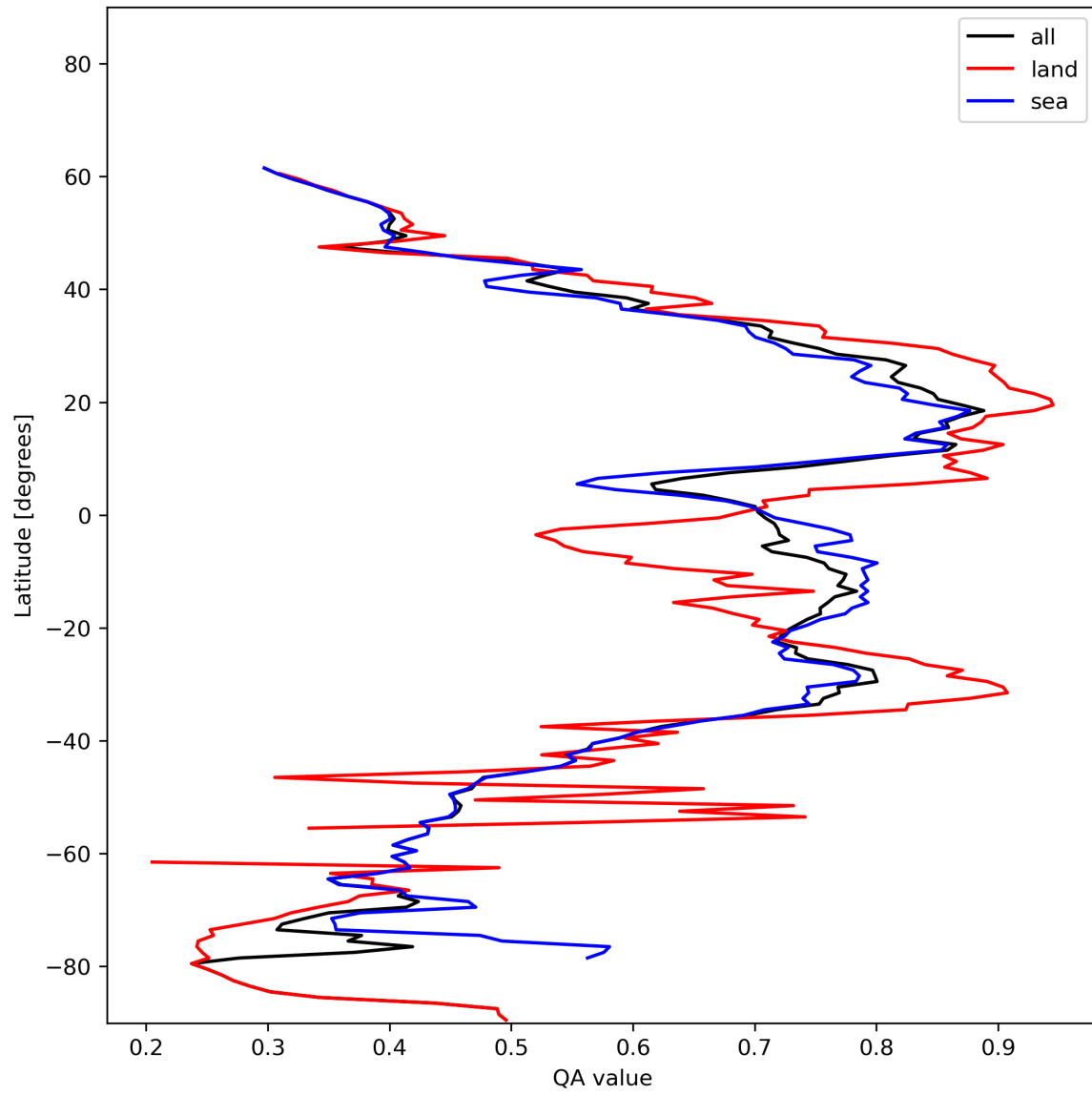
Figure 20: Zonal average of “QA value” for 2023-12-15 to 2023-12-17.
