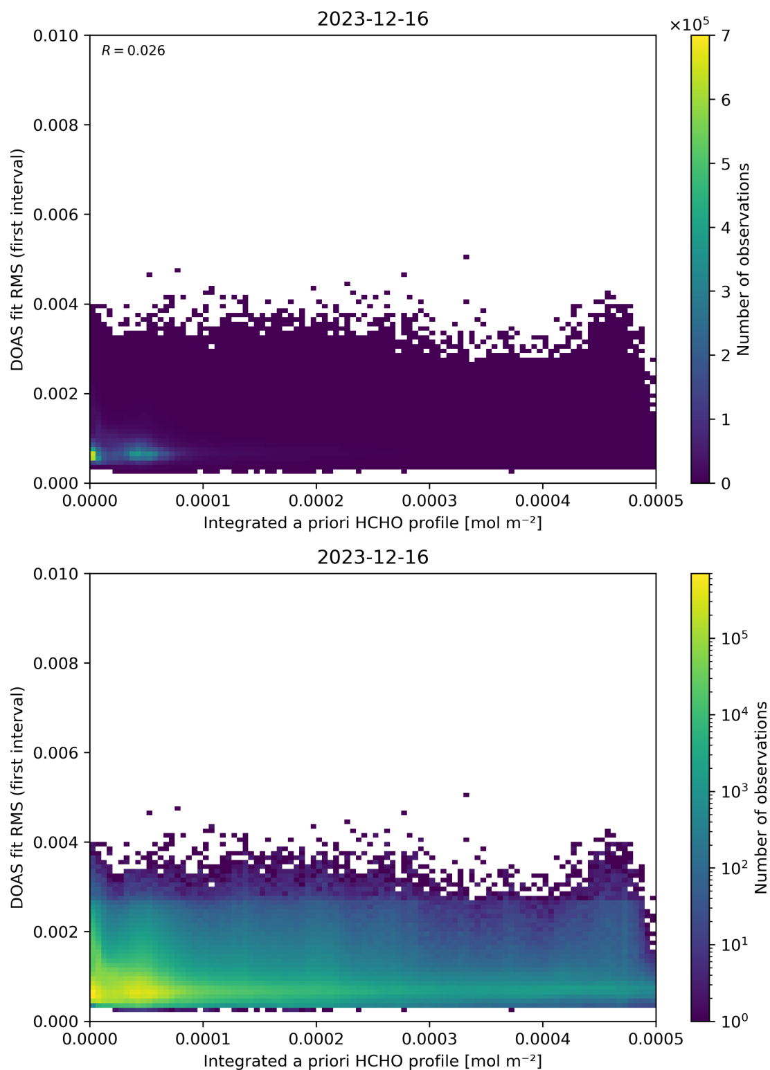
Figure 148: Scatter density plot of “Integrated a priori HCHO profile” against “DOAS fit RMS (first interval)” for 2023-12-15 to 2023-12-17.
