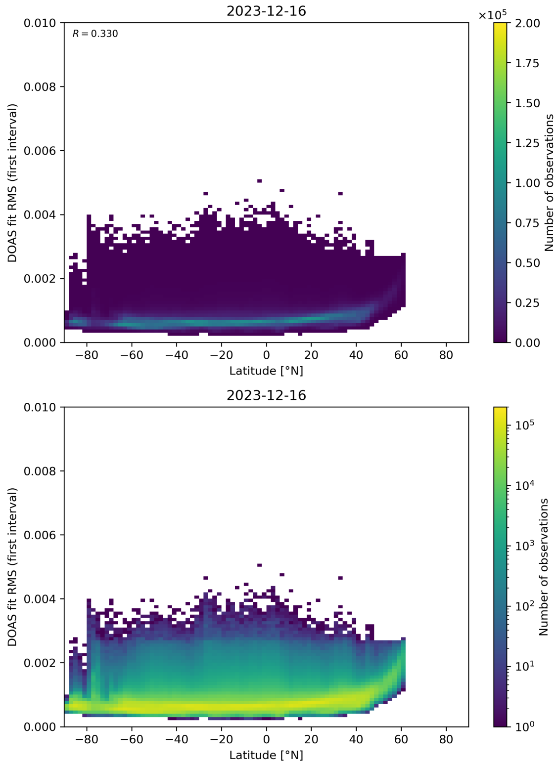
Figure 153: Scatter density plot of “Latitude” against “DOAS fit RMS (first interval)” for 2023-12-15 to 2023-12-17.
