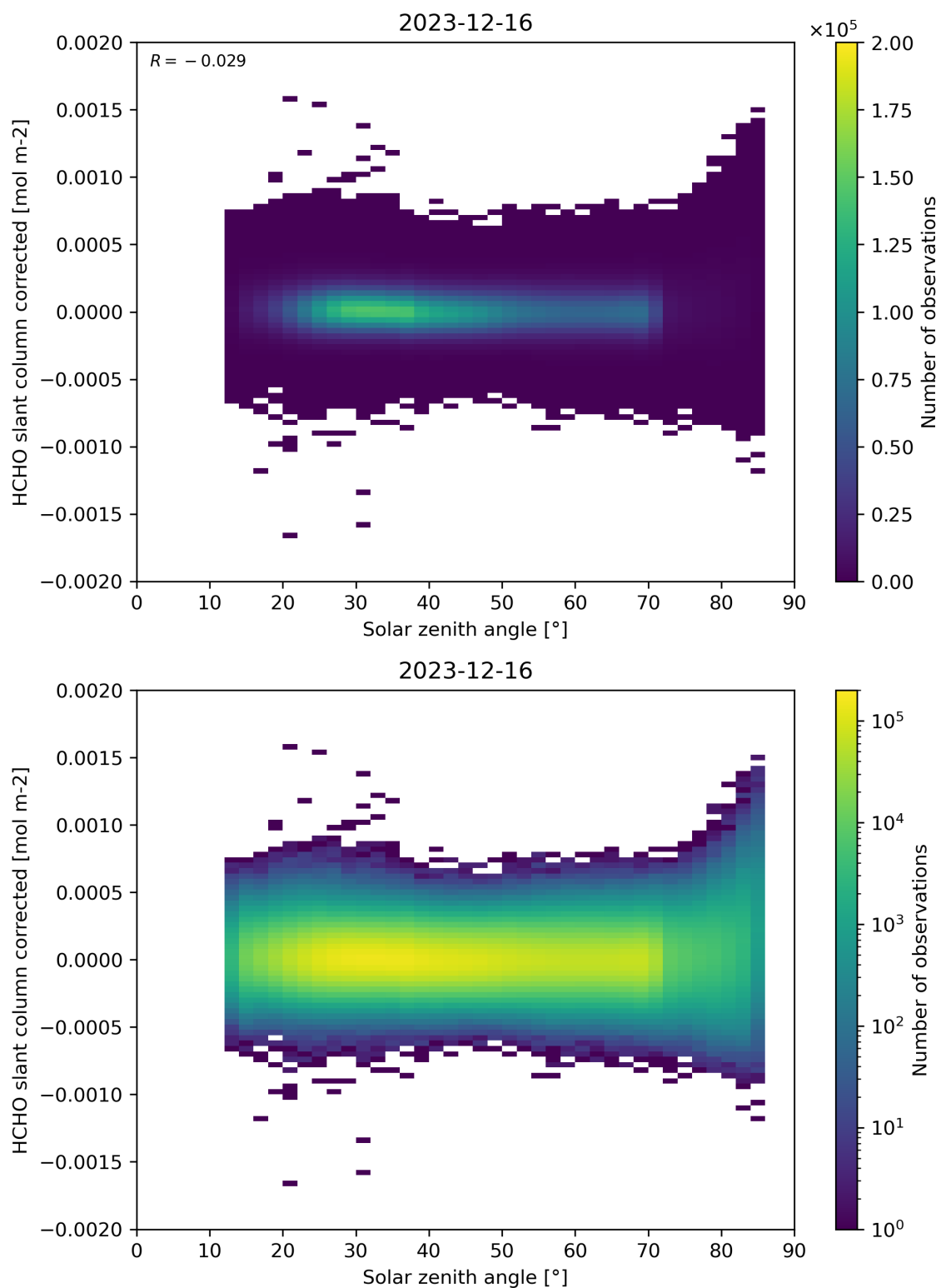
Figure 171: Scatter density plot of “Solar zenith angle” against “HCHO slant column corrected” for 2023-12-15 to 2023-12-17.
