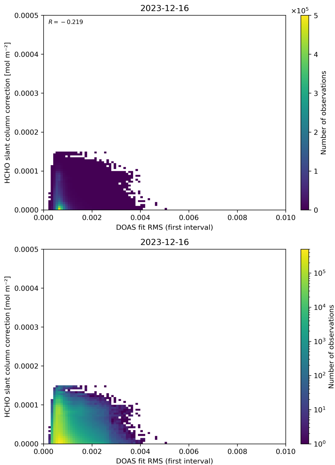
Figure 63: Scatter density plot of “DOAS fit RMS (first interval)” against “HCHO slant column correction” for 2023-12-15 to 2023-12-17.
