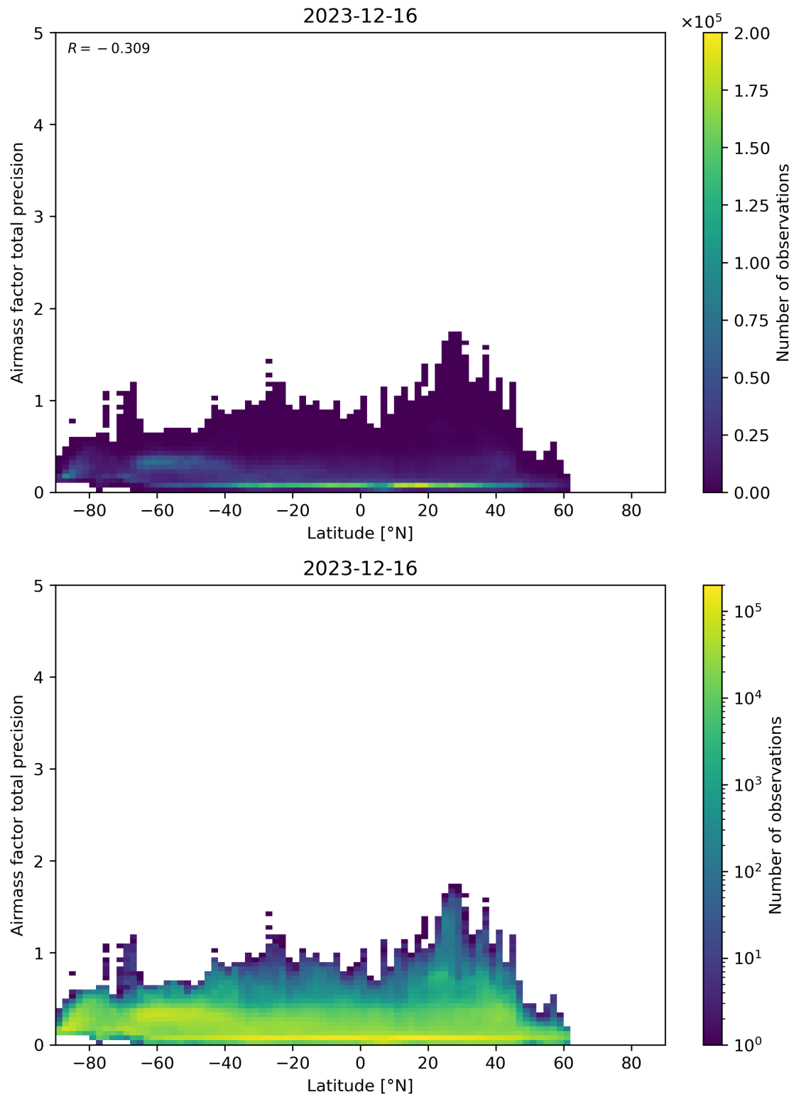
Figure 162: Scatter density plot of “Latitude” against “Airmass factor total precision” for 2023-12-15 to 2023-12-17.
