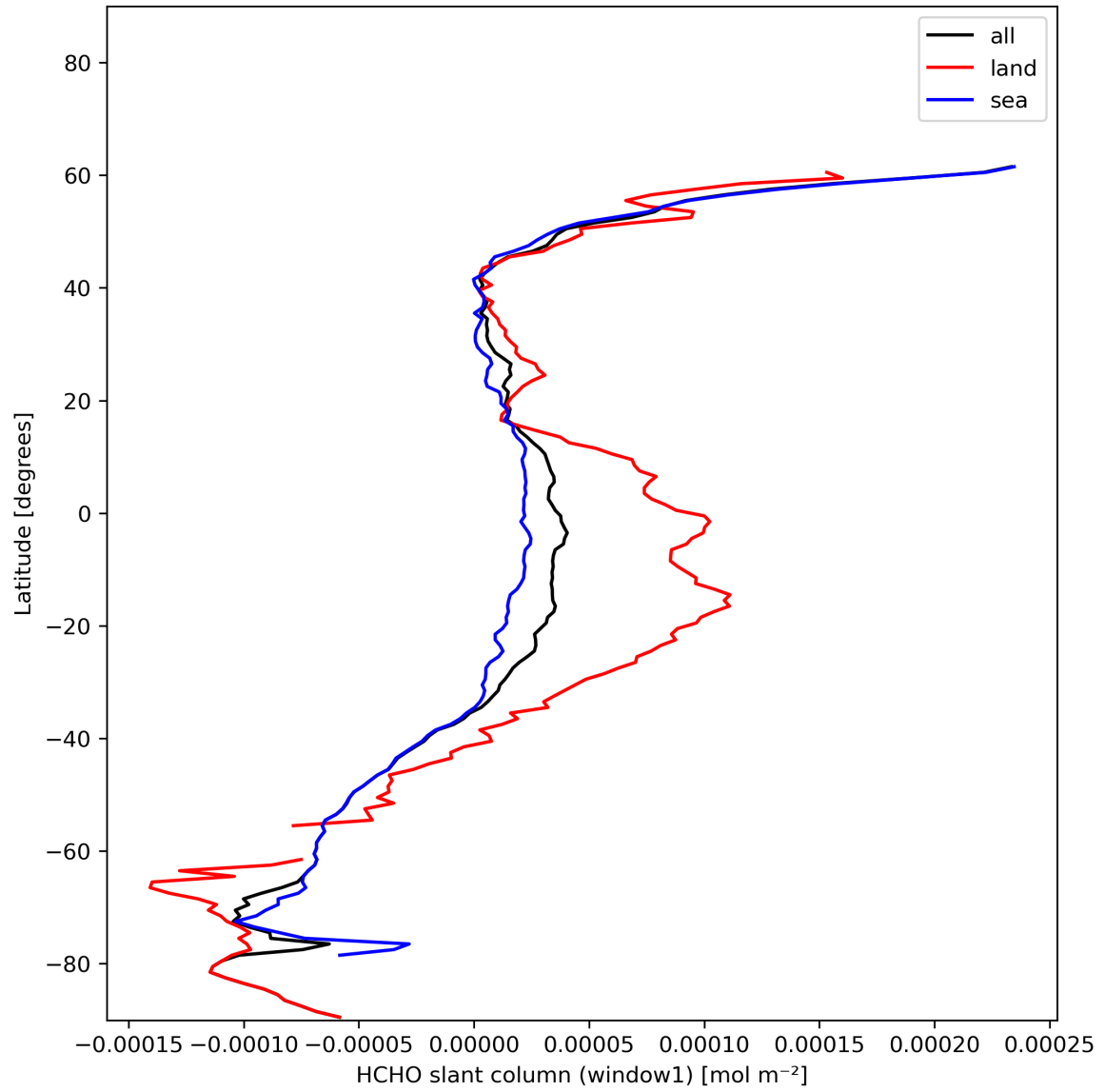
Figure 24: Zonal average of "HCHO slant column (window1)" for 2023-12-15 to 2023-12-17.
