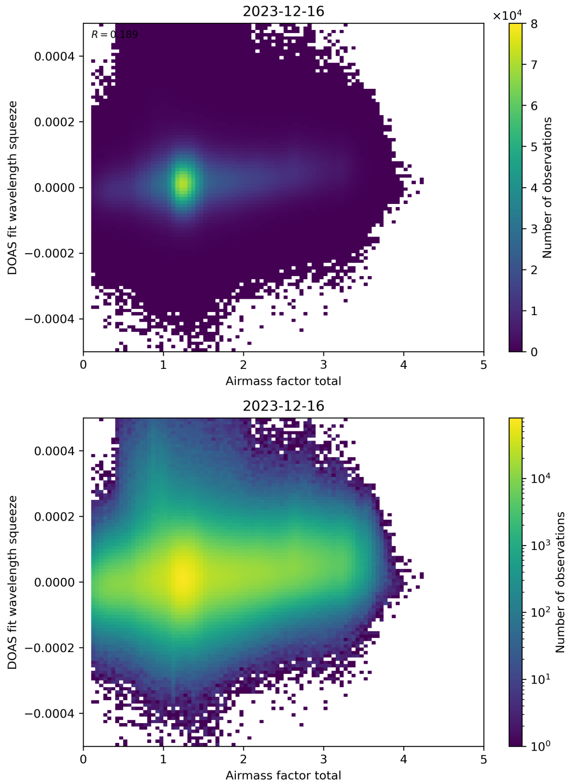
Figure 99: Scatter density plot of “Airmass factor total” against “DOAS fit wavelength squeeze” for 2023-12-15 to 2023-12-17.
