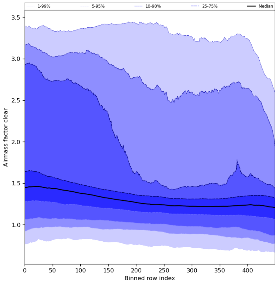
Figure 56: Along track statistics of “Airmass factor clear” for 2023-12-15 to 2023-12-17
