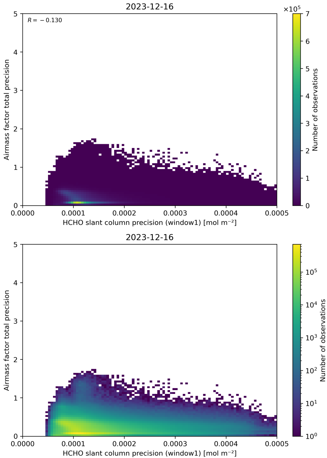
Figure 95: Scatter density plot of “HCHO slant column precision (window1)” against “Airmass factor total precision” for 2023-12-15 to 2023-12-17.
