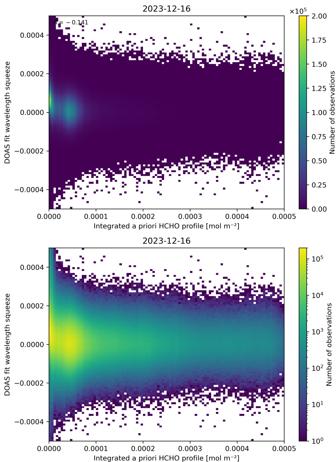
Figure 150: Scatter density plot of “Integrated a priori HCHO profile” against “DOAS fit wavelength squeeze” for 2023-12-15 to 2023-12-17.
