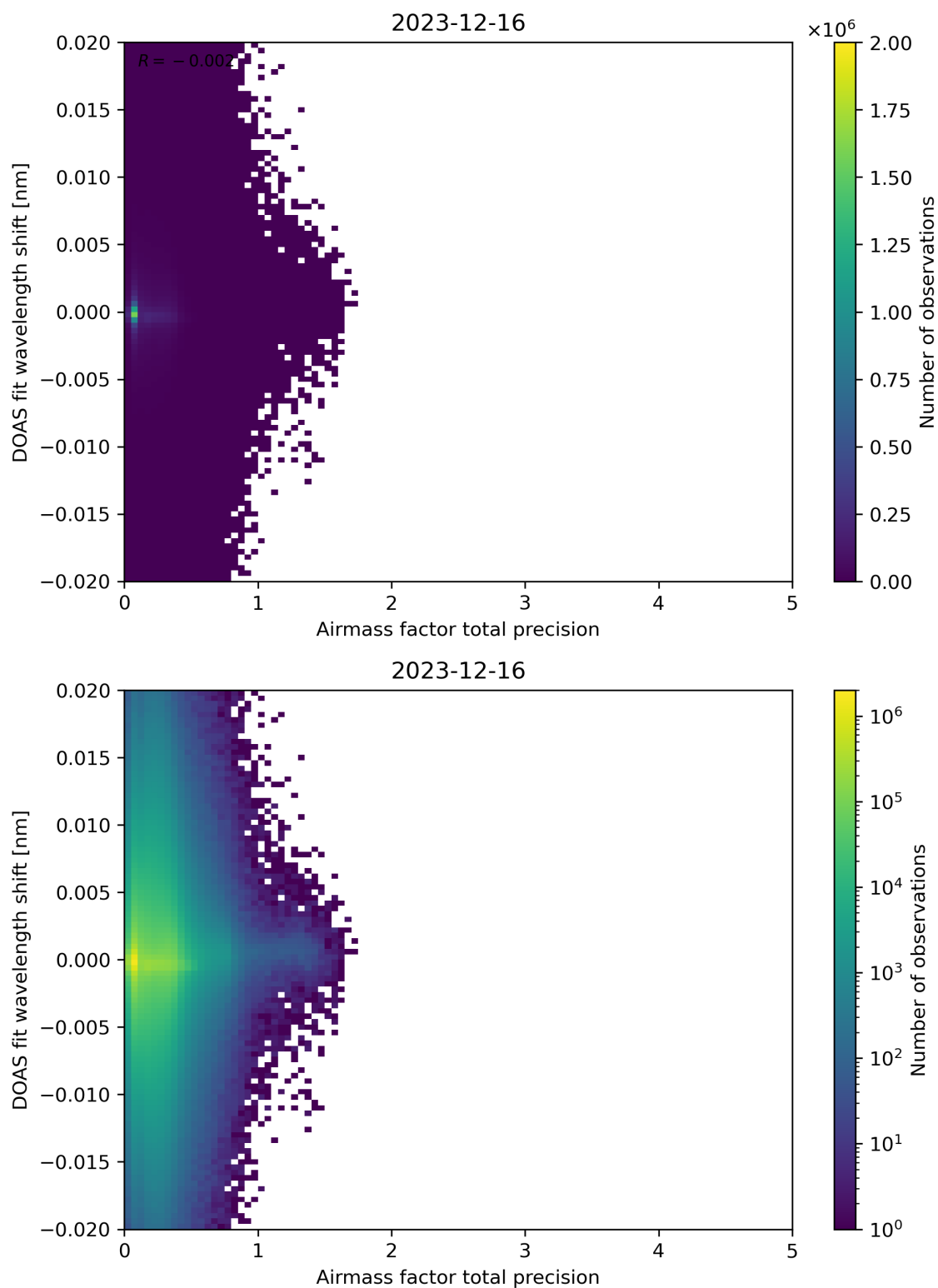
Figure 106: Scatter density plot of “Airmass factor total precision” against “DOAS fit wavelength shift” for 2023-12-15 to 2023-12-17.
