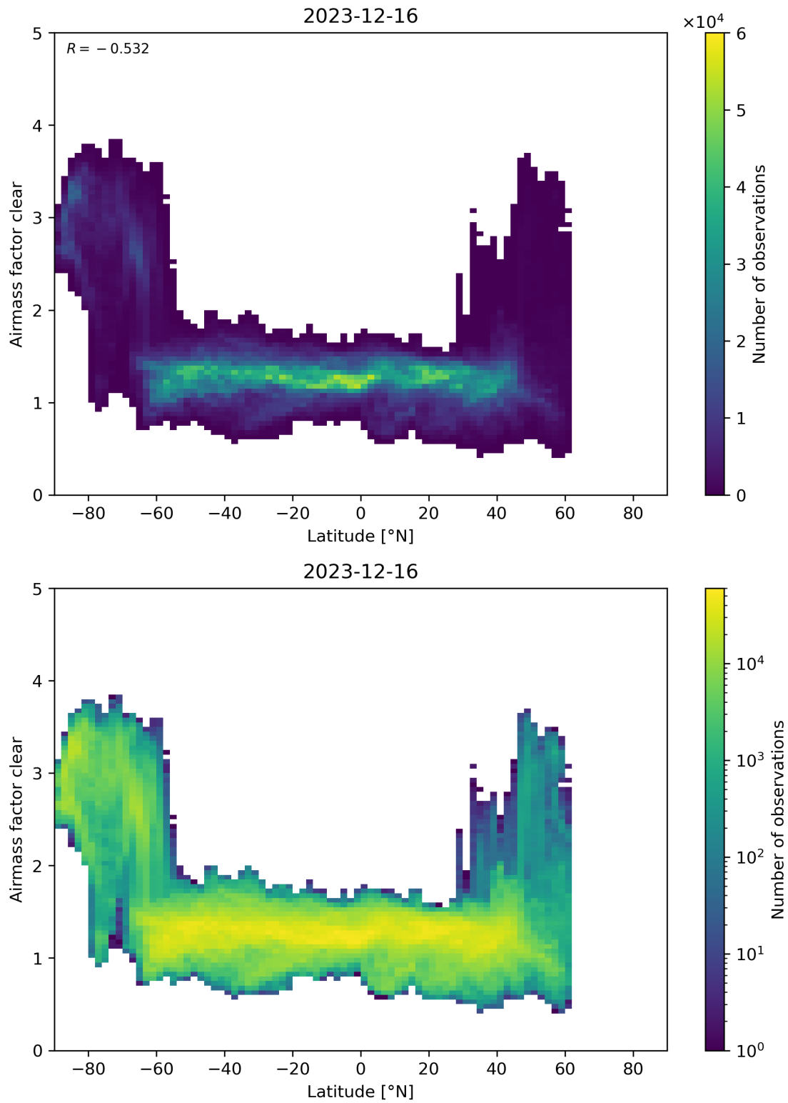
Figure 156: Scatter density plot of “Latitude” against “Airmass factor clear” for 2023-12-15 to 2023-12-17.
