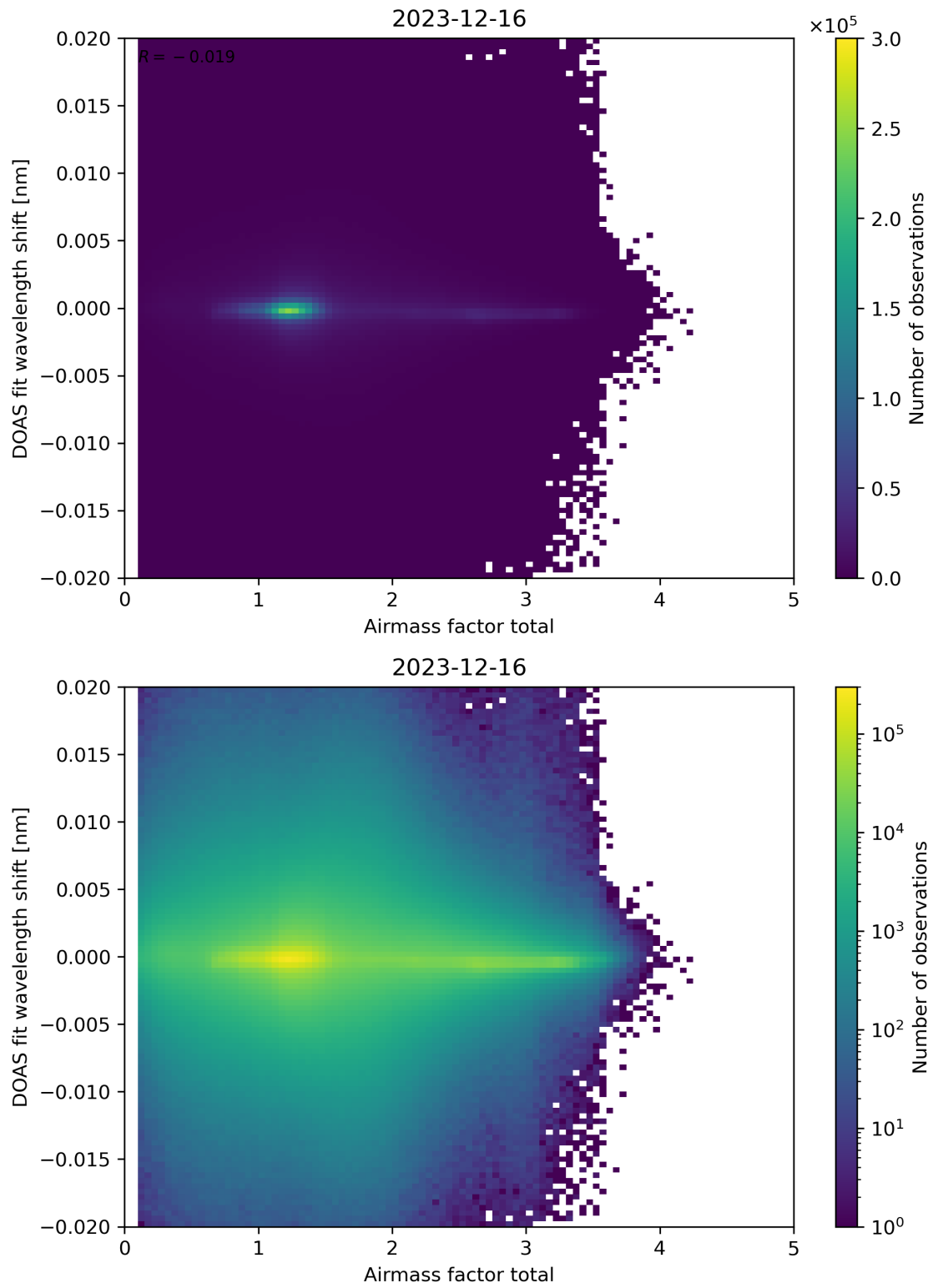
Figure 98: Scatter density plot of “Airmass factor total” against “DOAS fit wavelength shift” for 2023-12-15 to 2023-12-17.
