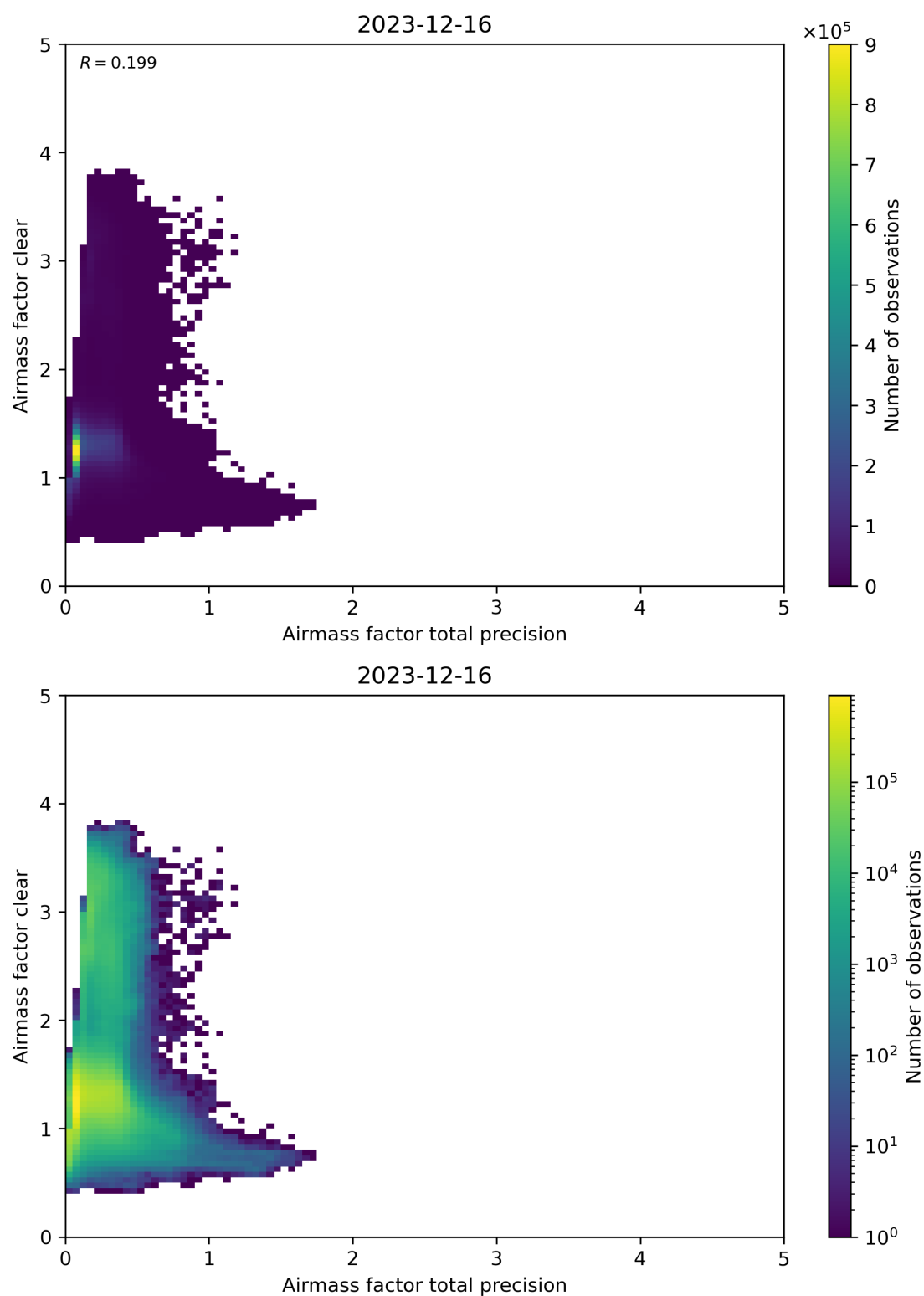
Figure 108: Scatter density plot of “Airmass factor total precision” against “Airmass factor clear” for 2023-12-15 to 2023-12-17.
