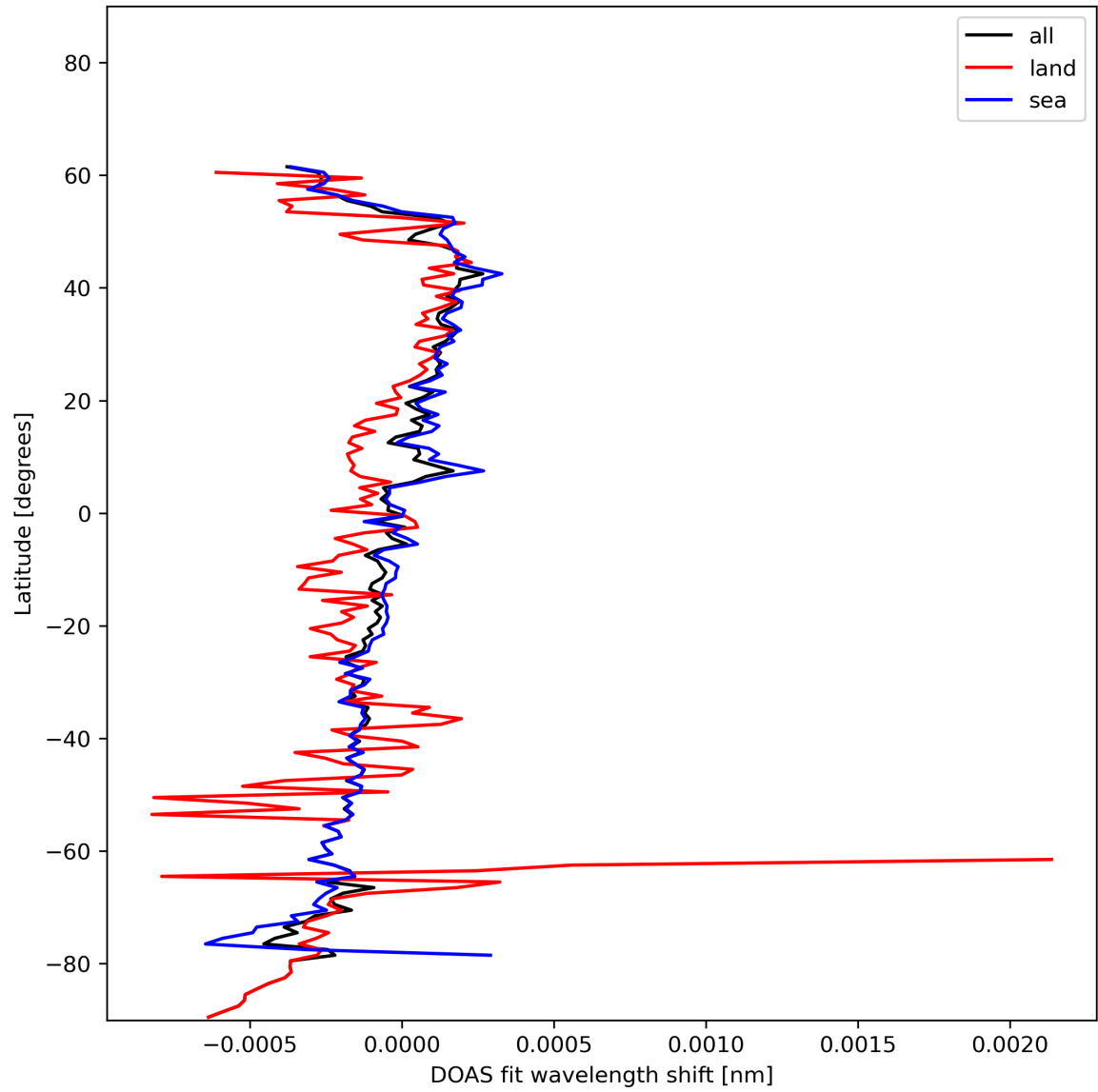
Figure 30: Zonal average of “DOAS fit wavelength shift” for 2023-12-15 to 2023-12-17.
