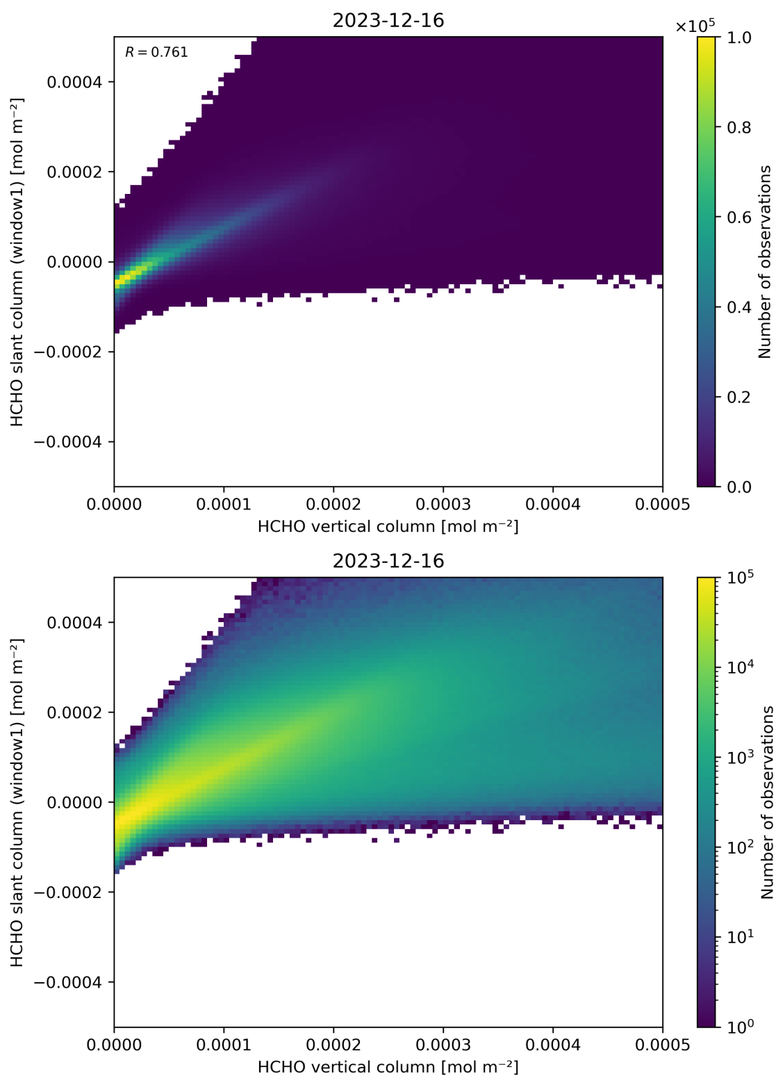
Figure 129: Scatter density plot of “HCHO vertical column” against “HCHO slant column (window1)” for 2023-12-15 to 2023-12-17.
