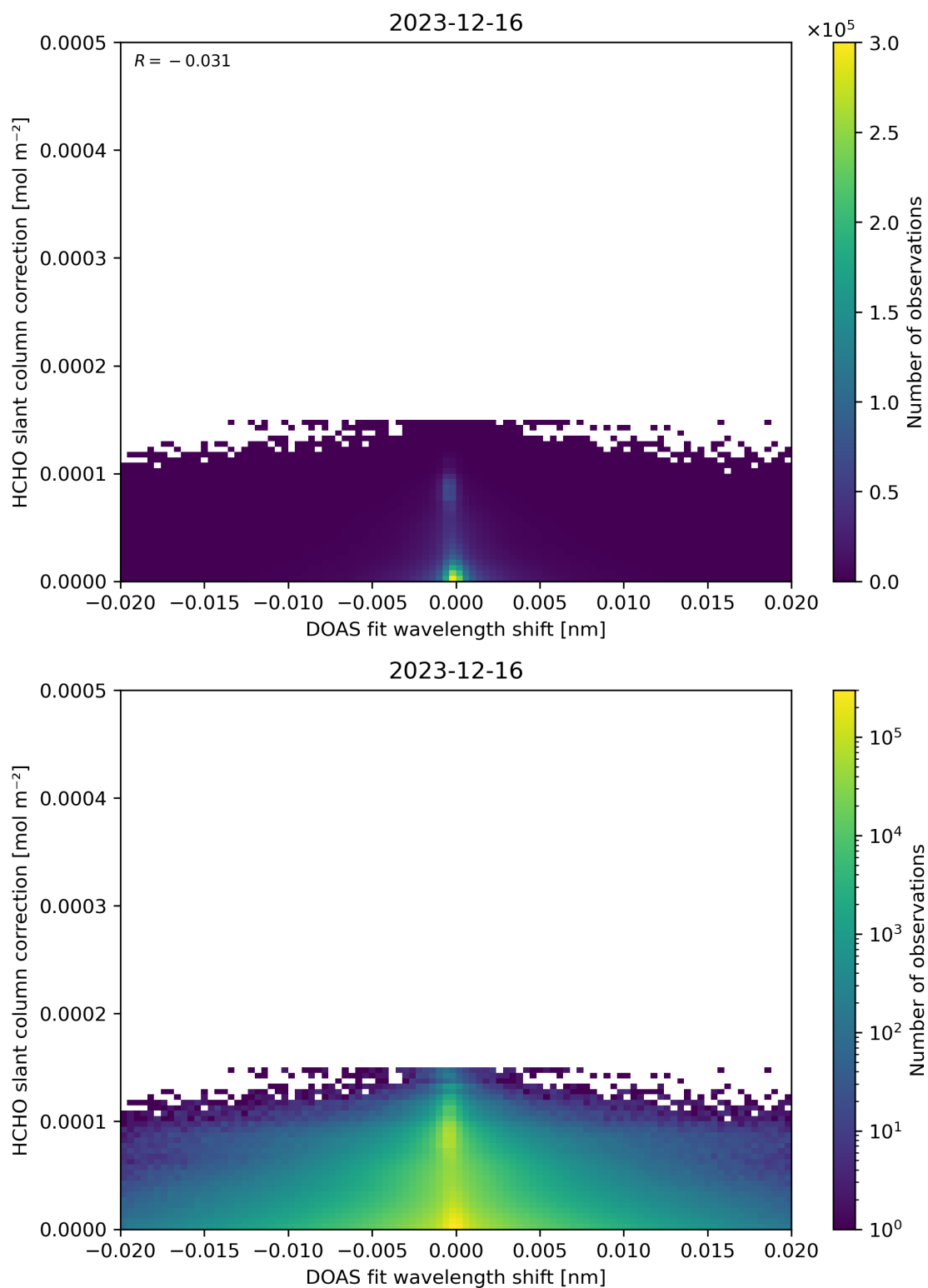
Figure 67: Scatter density plot of “DOAS fit wavelength shift” against “HCHO slant column correction” for 2023-12-15 to 2023-12-17.
