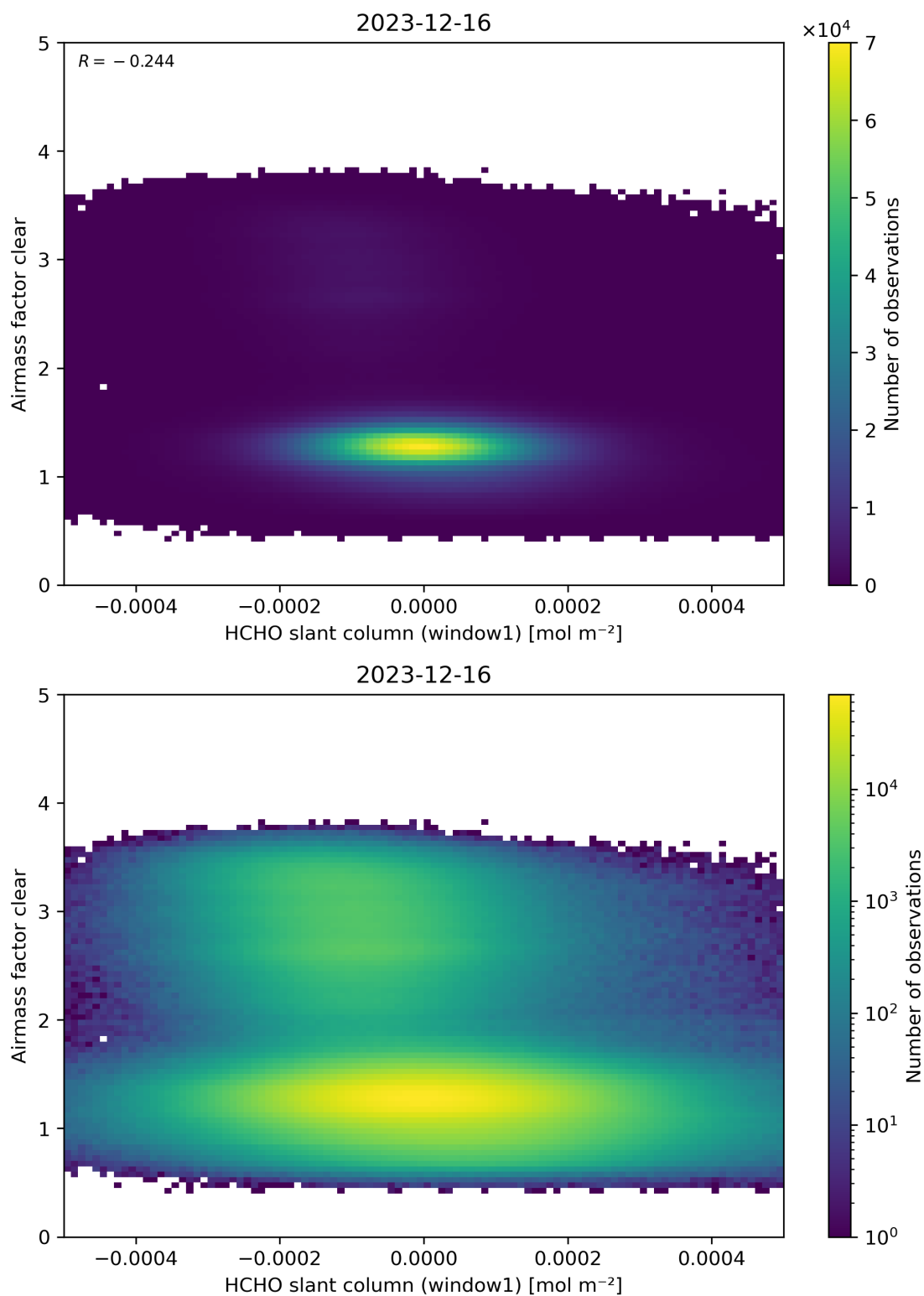
Figure 81: Scatter density plot of “HCHO slant column (window1)” against “Airmass factor clear” for 2023-12-15 to 2023-12-17.
