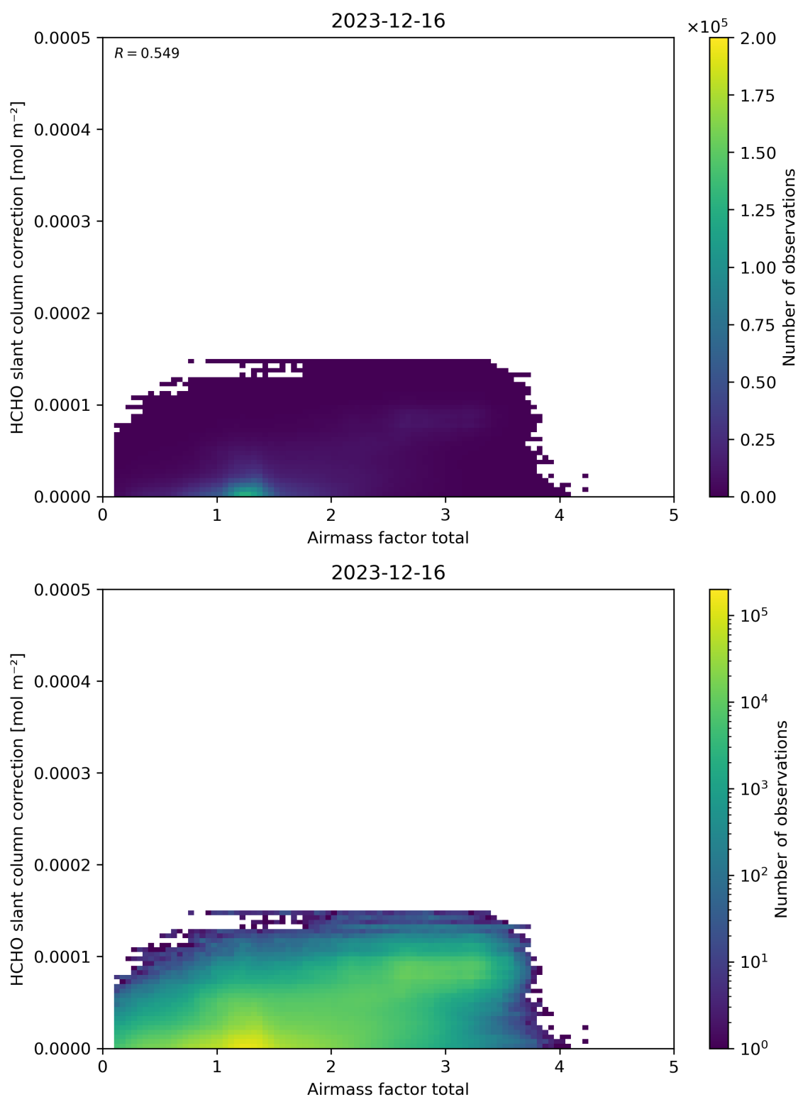
Figure 102: Scatter density plot of “Airmass factor total” against “HCHO slant column correction” for 2023-12-15 to 2023-12-17.
