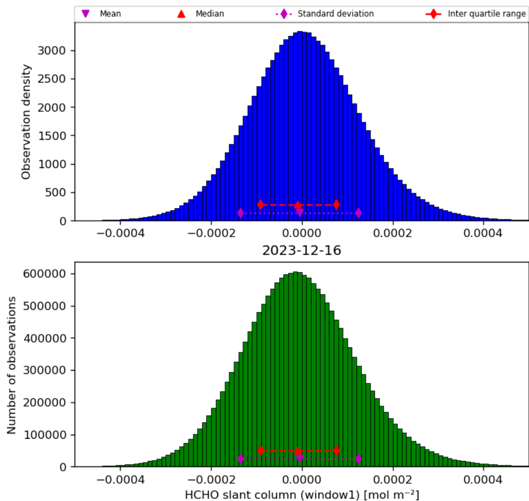
Figure 38: Histogram of “HCHO slant column (window1)” for 2023-12-15 to 2023-12-17
