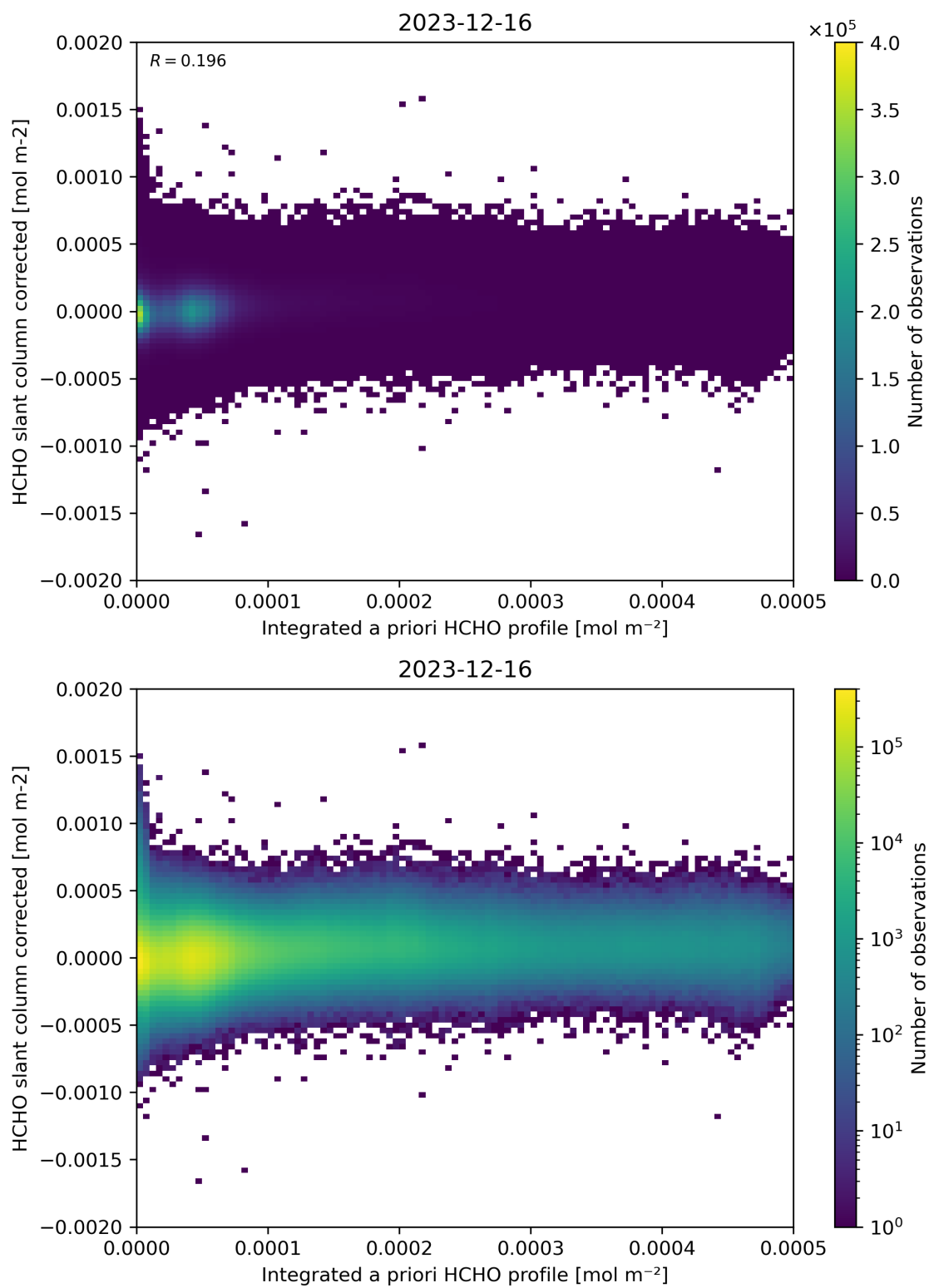
Figure 151: Scatter density plot of “Integrated a priori HCHO profile” against “HCHO slant column corrected” for 2023-12-15 to 2023-12-17.
