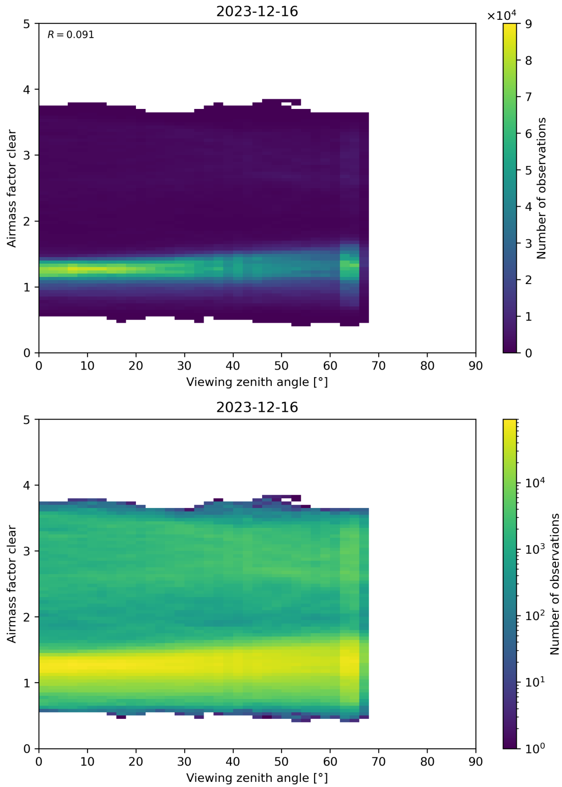
Figure 185: Scatter density plot of “Viewing zenith angle” against “Airmass factor clear” for 2023-12-15 to 2023-12-17.
