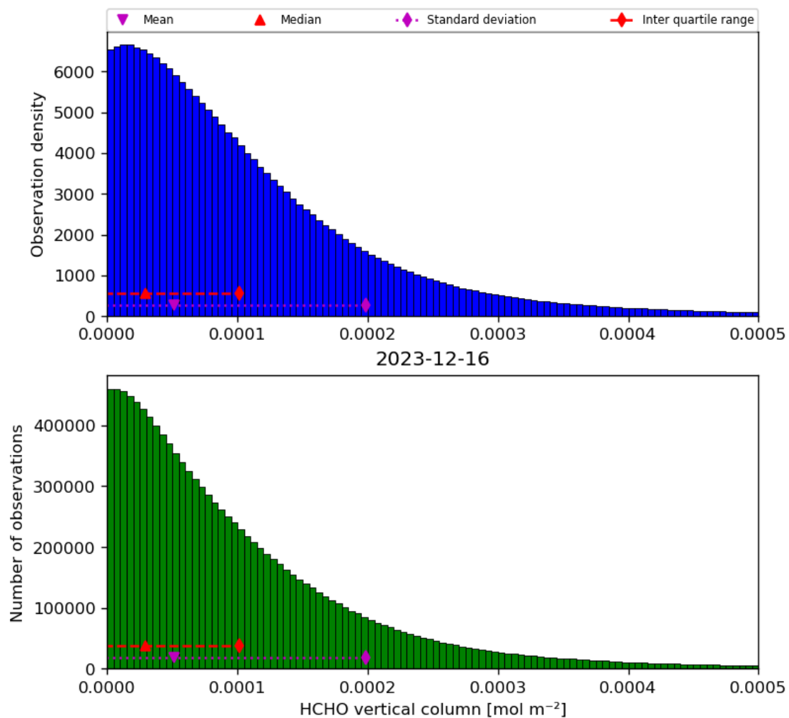
Figure 35: Histogram of “HCHO vertical column” for 2023-12-15 to 2023-12-17
