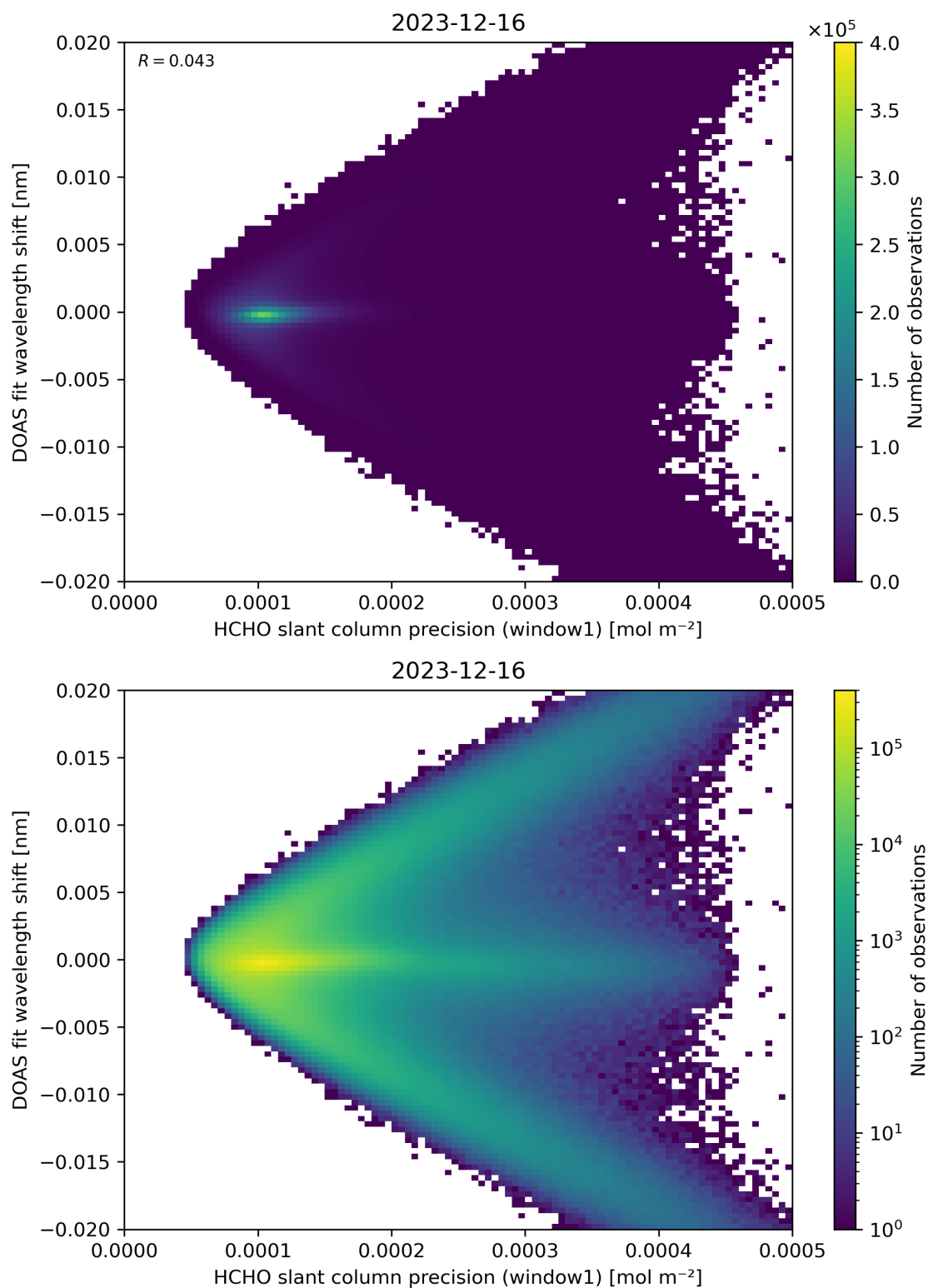
Figure 89: Scatter density plot of “HCHO slant column precision (window1)” against “DOAS fit wavelength shift” for 2023-12-15 to 2023-12-17.
