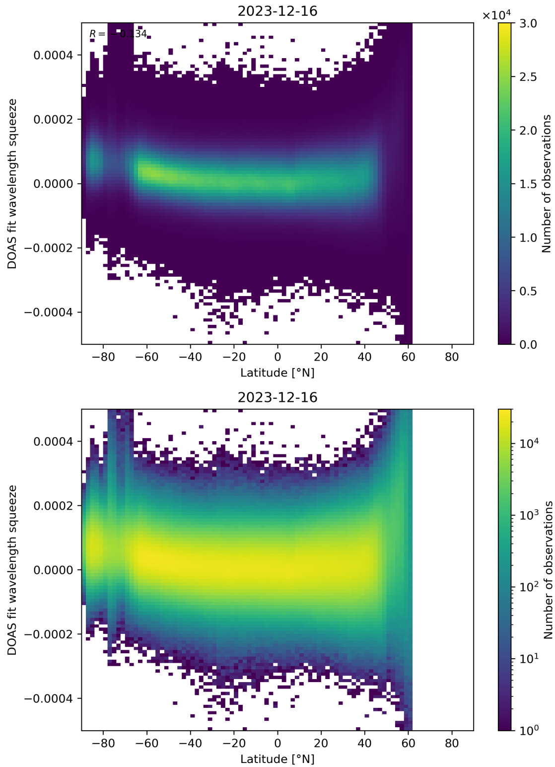
Figure 155: Scatter density plot of “Latitude” against “DOAS fit wavelength squeeze” for 2023-12-15 to 2023-12-17.
