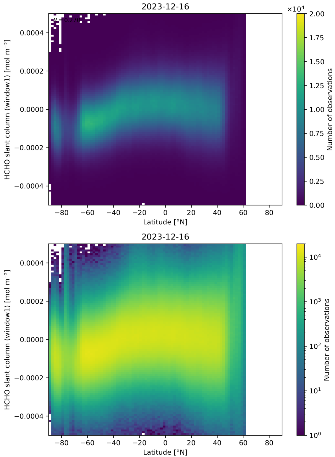
Figure 159: Scatter density plot of “Latitude” against “HCHO slant column (window1)” for 2023-12-15 to 2023-12-17.
