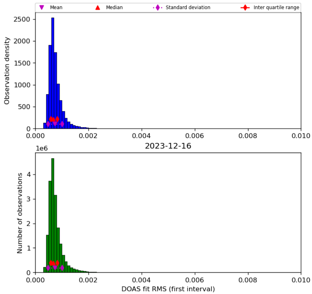
Figure 46: Histogram of “DOAS fit RMS (first interval)” for 2023-12-15 to 2023-12-17
