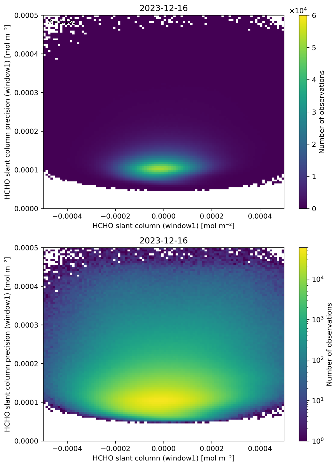
Figure 84: Scatter density plot of “HCHO slant column (window1)” against “HCHO slant column precision (window1)” for 2023-12-15 to 2023-12-17.
