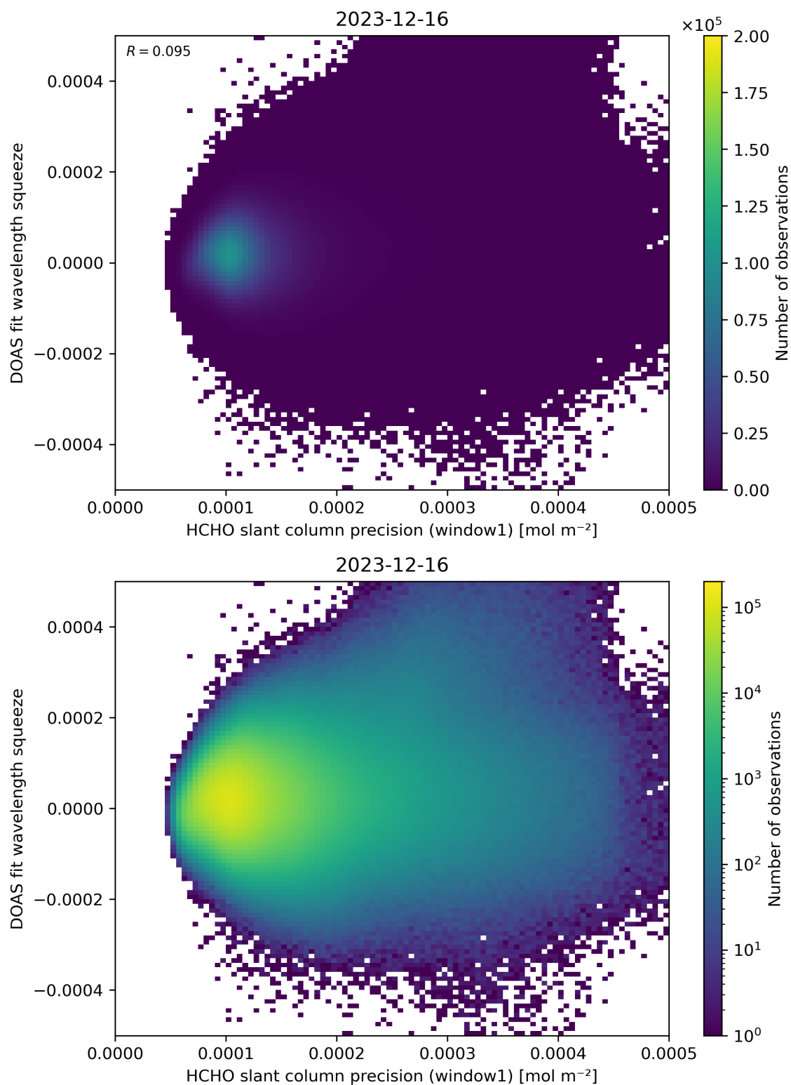
Figure 90: Scatter density plot of “HCHO slant column precision (window1)” against “DOAS fit wavelength squeeze” for 2023-12-15 to 2023-12-17.
