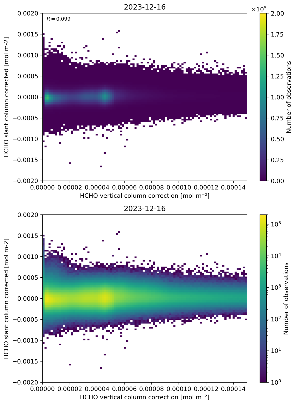
Figure 116: Scatter density plot of “HCHO vertical column correction” against “HCHO slant column corrected” for 2023-12-15 to 2023-12-17.
