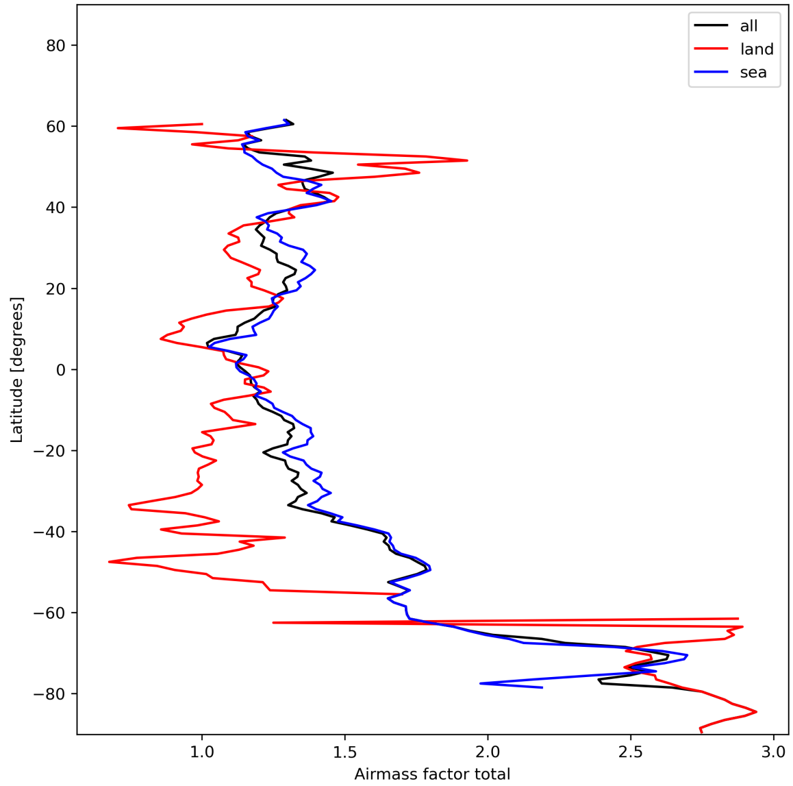
Figure 26: Zonal average of “Airmass factor total” for 2023-12-15 to 2023-12-17.
