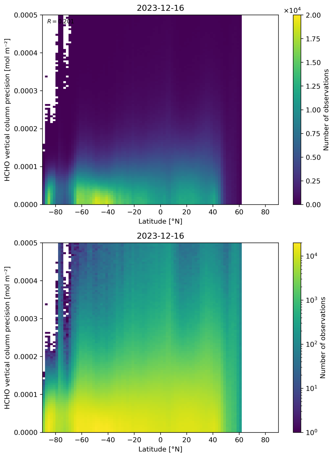
Figure 165: Scatter density plot of “Latitude” against “HCHO vertical column precision” for 2023-12-15 to 2023-12-17.
