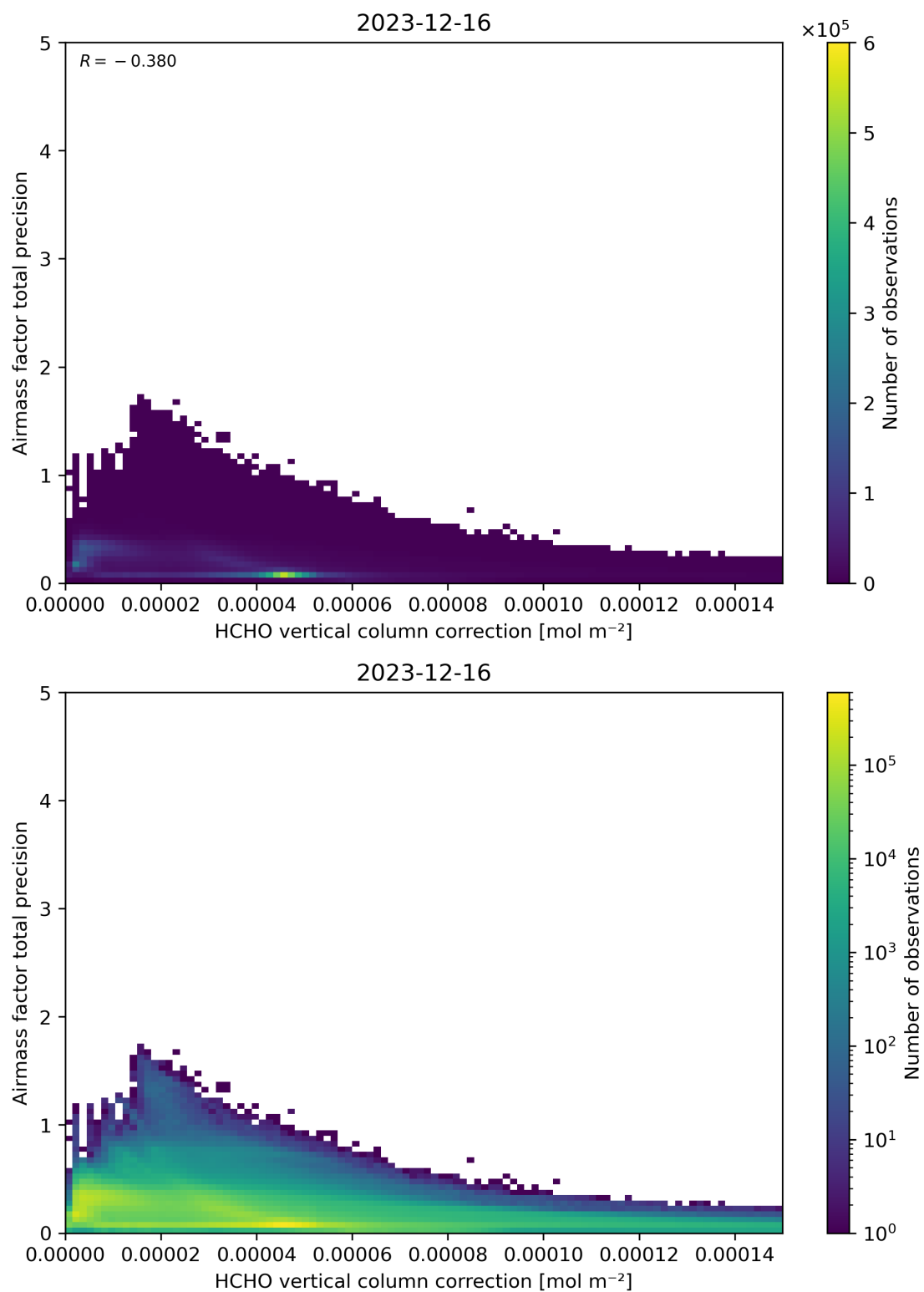
Figure 121: Scatter density plot of “HCHO vertical column correction” against “Airmass factor total precision” for 2023-12-15 to 2023-12-17.
