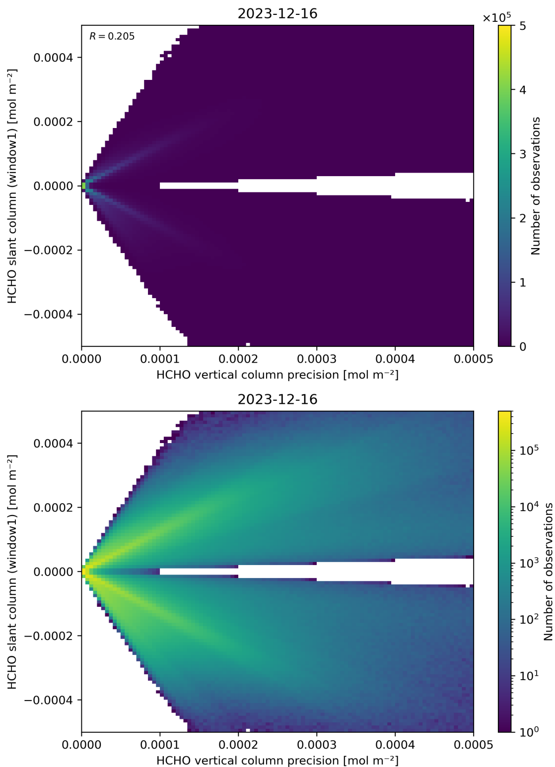
Figure 142: Scatter density plot of “HCHO vertical column precision” against “HCHO slant column (window1)” for 2023-12-15 to 2023-12-17.
