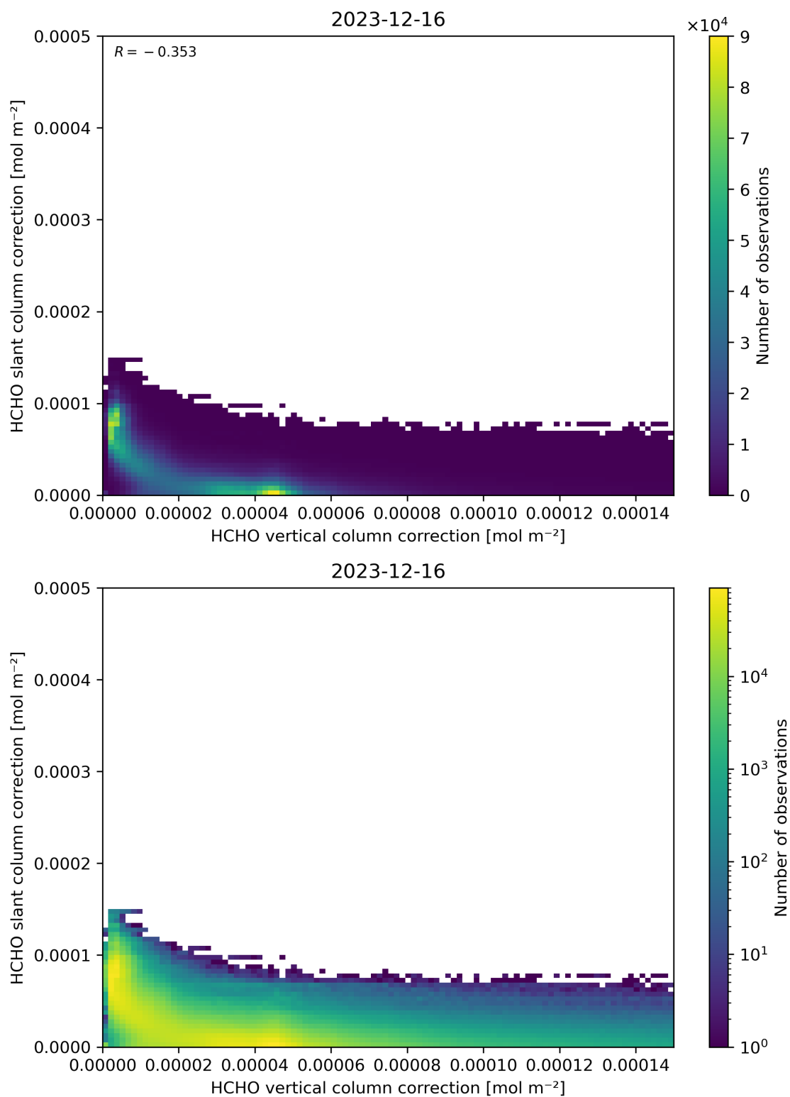
Figure 117: Scatter density plot of “HCHO vertical column correction” against “HCHO slant column correction” for 2023-12-15 to 2023-12-17.
