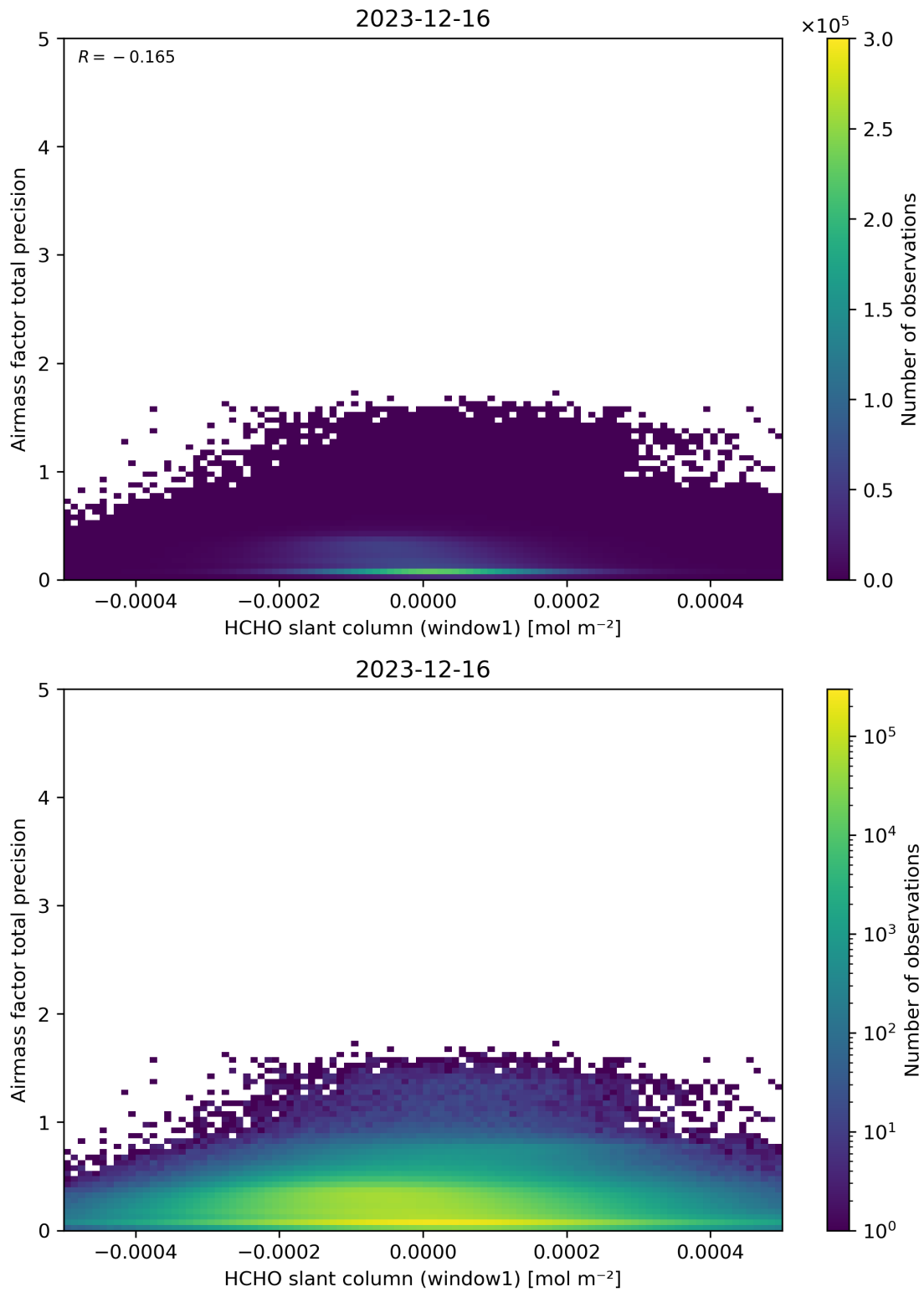
Figure 86: Scatter density plot of “HCHO slant column (window1)” against “Airmass factor total precision” for 2023-12-15 to 2023-12-17.
