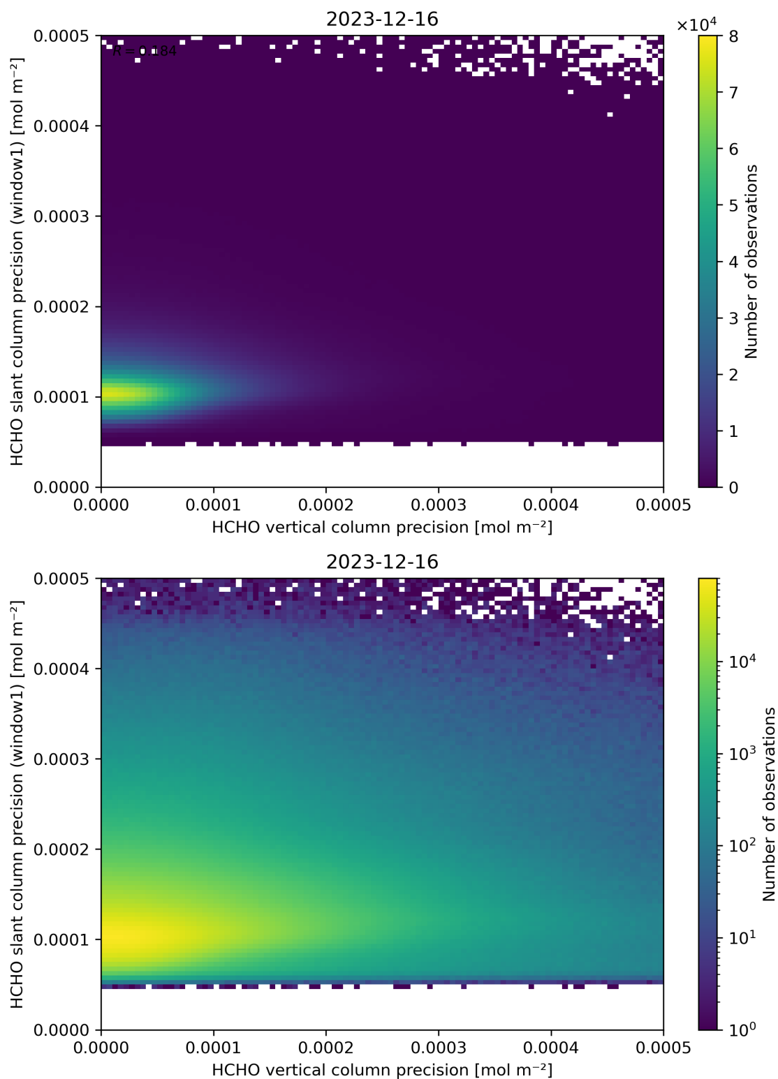
Figure 143: Scatter density plot of “HCHO vertical column precision” against “HCHO slant column precision (window1)” for 2023-12-15 to 2023-12-17.
