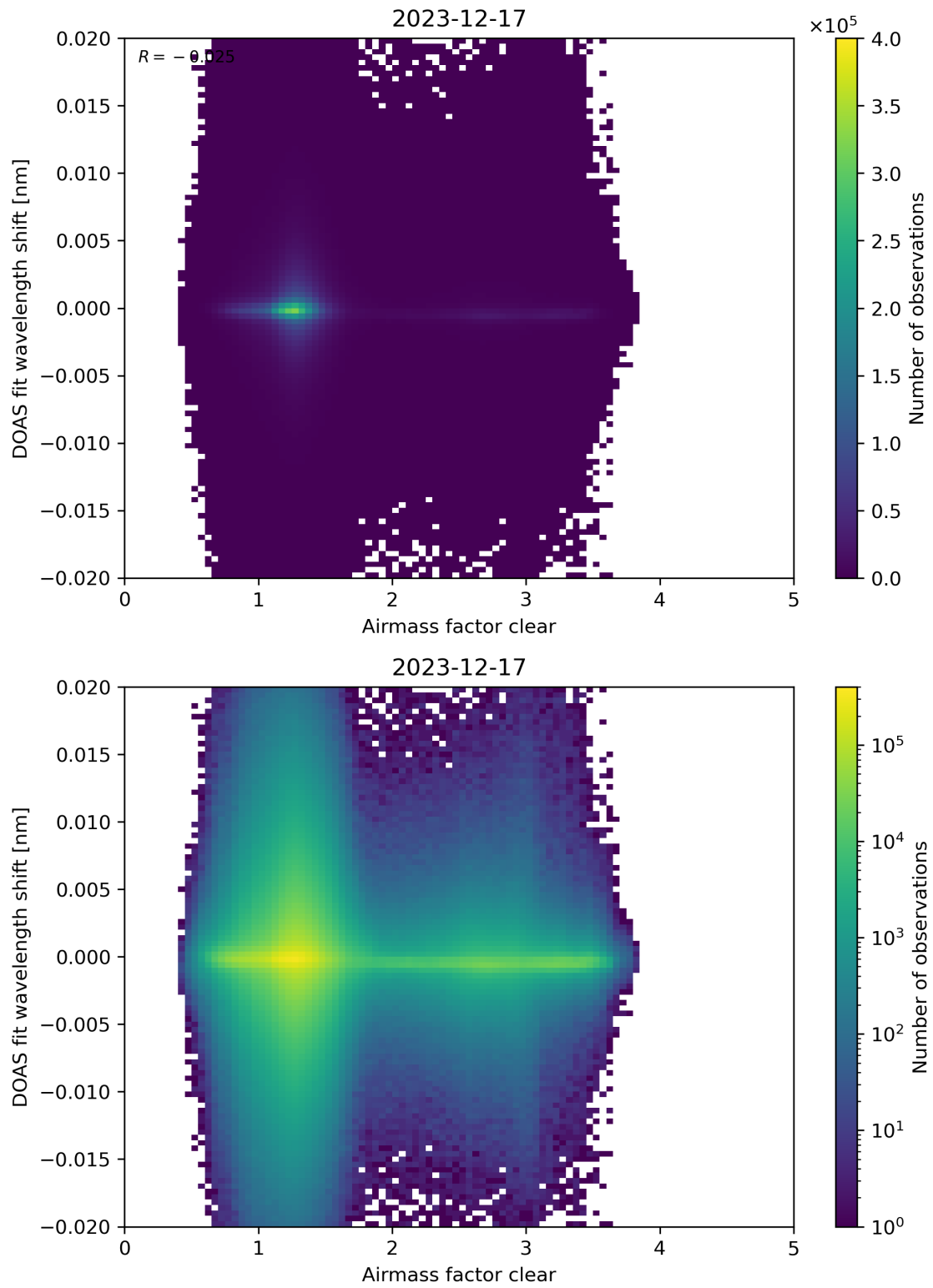
Figure 72: Scatter density plot of “Airmass factor clear” against “DOAS fit wavelength shift” for 2023-12-16 to 2023-12-18.
