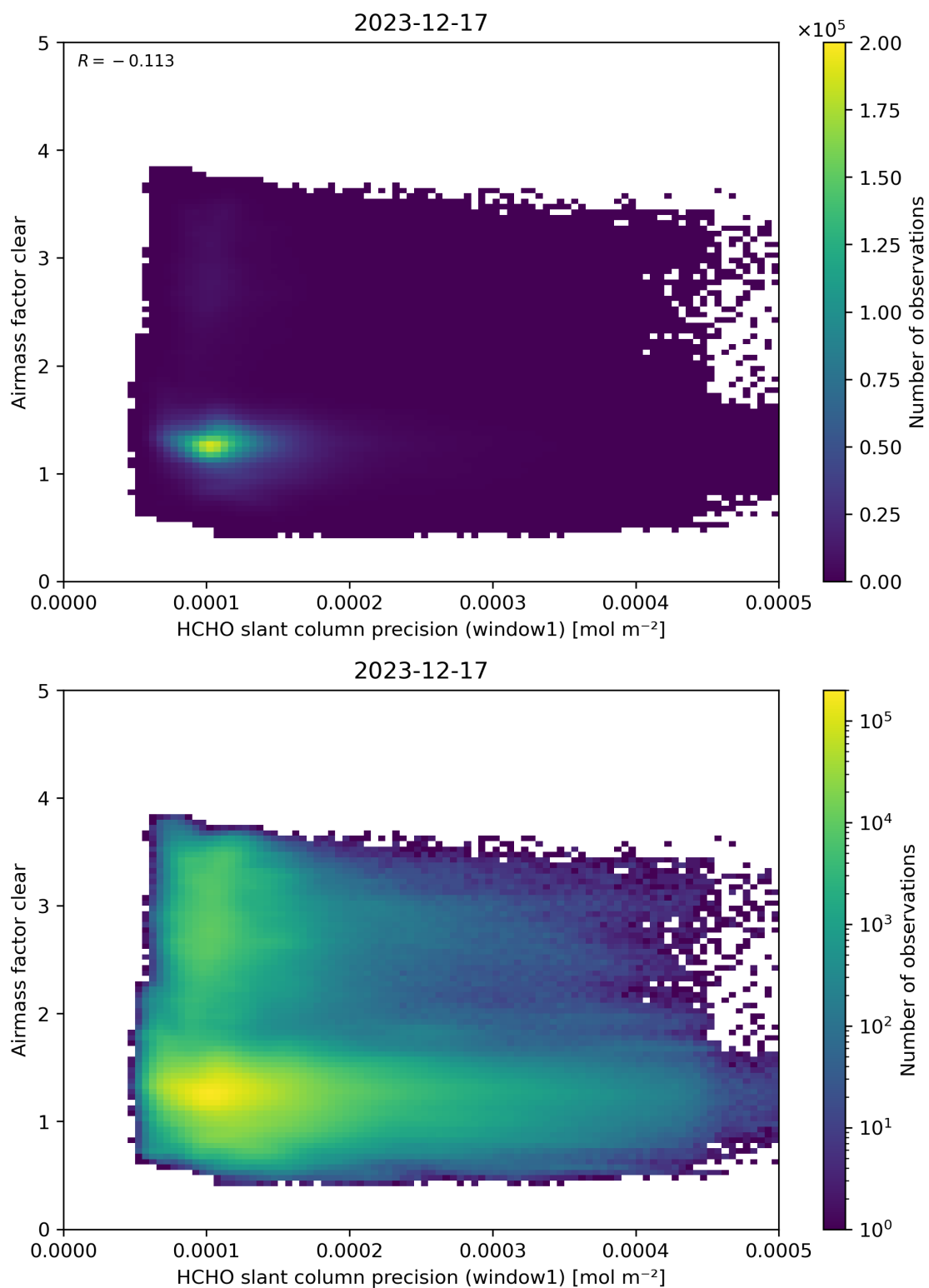
Figure 91: Scatter density plot of “HCHO slant column precision (window1)” against “Airmass factor clear” for 2023-12-16 to 2023-12-18.
