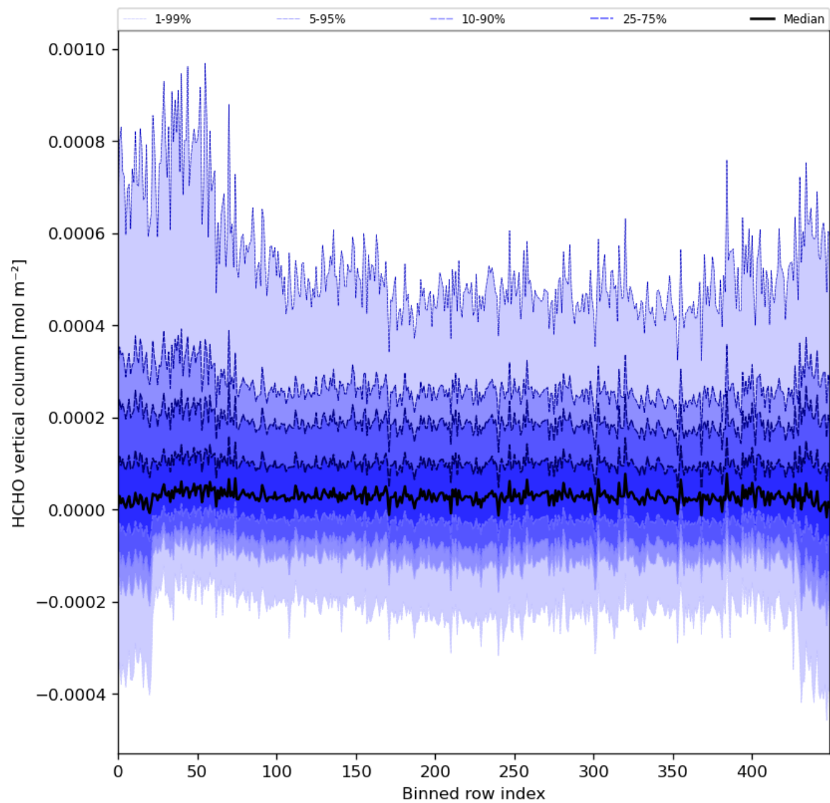
Figure 49: Along track statistics of “HCHO vertical column” for 2023-12-16 to 2023-12-18
