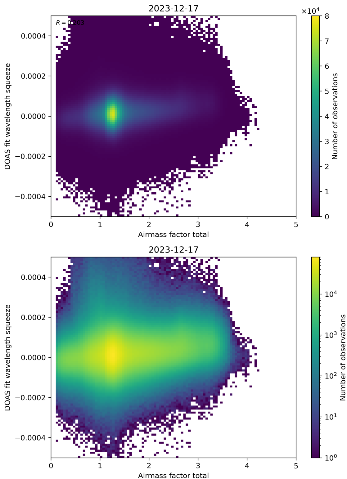
Figure 99: Scatter density plot of “Airmass factor total” against “DOAS fit wavelength squeeze” for 2023-12-16 to 2023-12-18.
