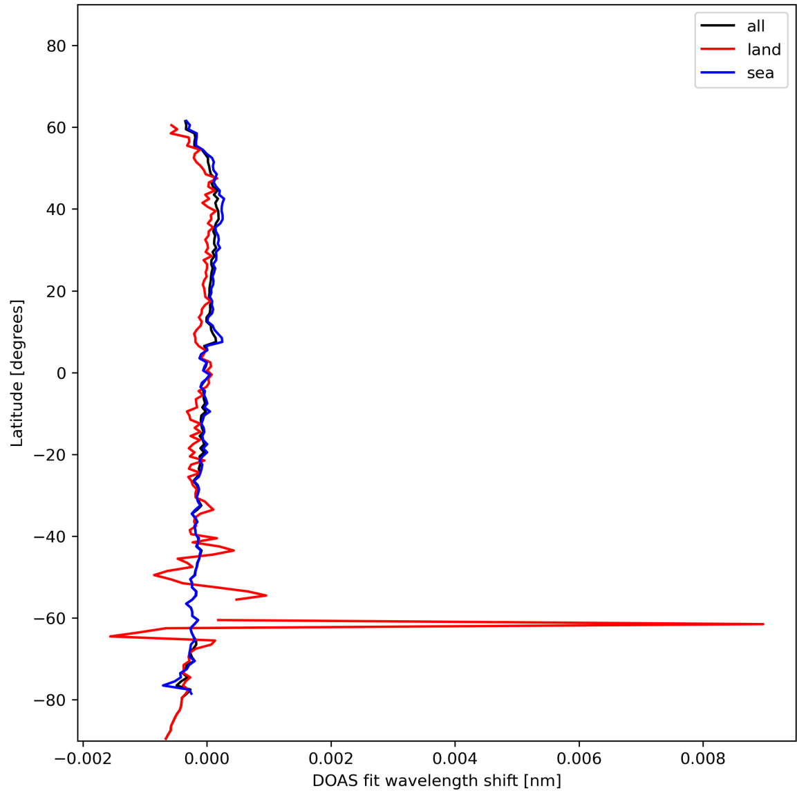
Figure 30: Zonal average of "DOAS fit wavelength shift" for 2023-12-16 to 2023-12-18.
