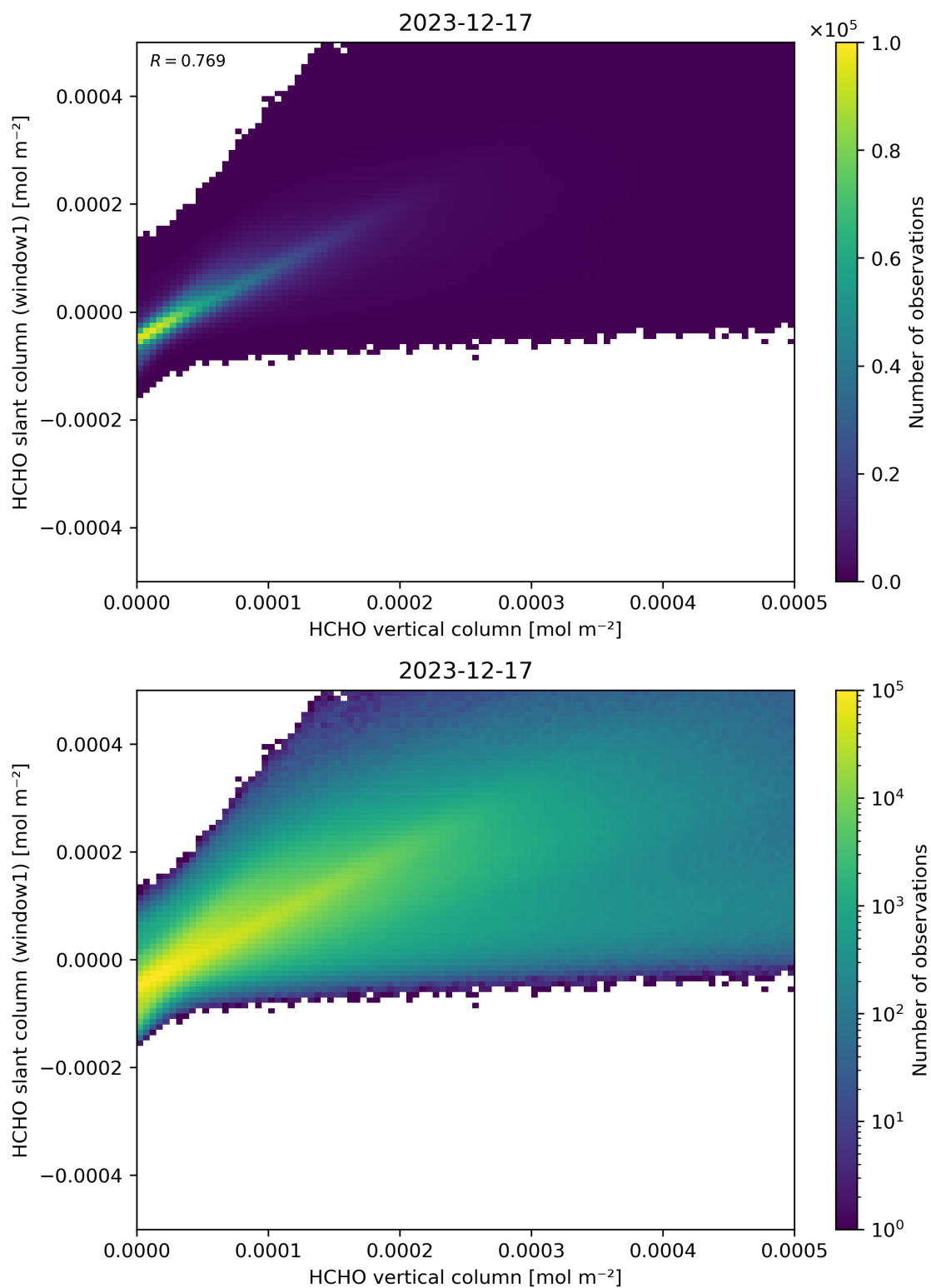
Figure 129: Scatter density plot of “HCHO vertical column” against “HCHO slant column (window1)” for 2023-12-16 to 2023-12-18.
