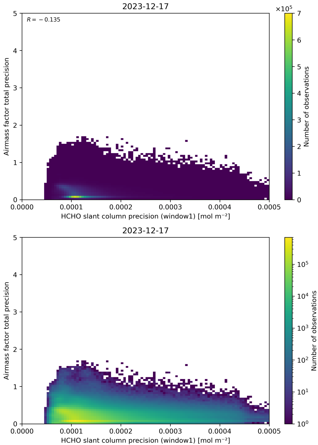
Figure 95: Scatter density plot of “HCHO slant column precision (window1)” against “Airmass factor total precision” for 2023-12-16 to 2023-12-18.
