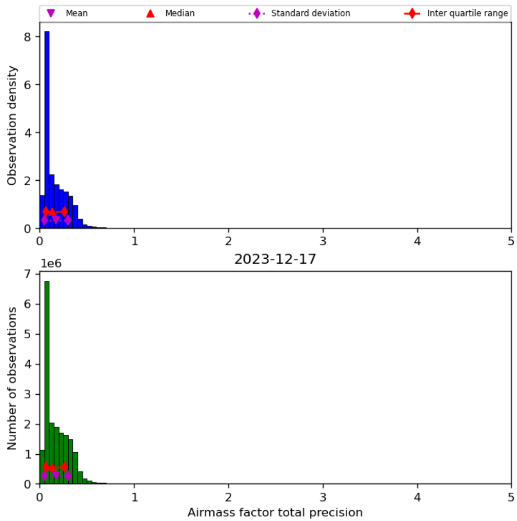
Figure 41: Histogram of “Airmass factor total precision” for 2023-12-16 to 2023-12-18
