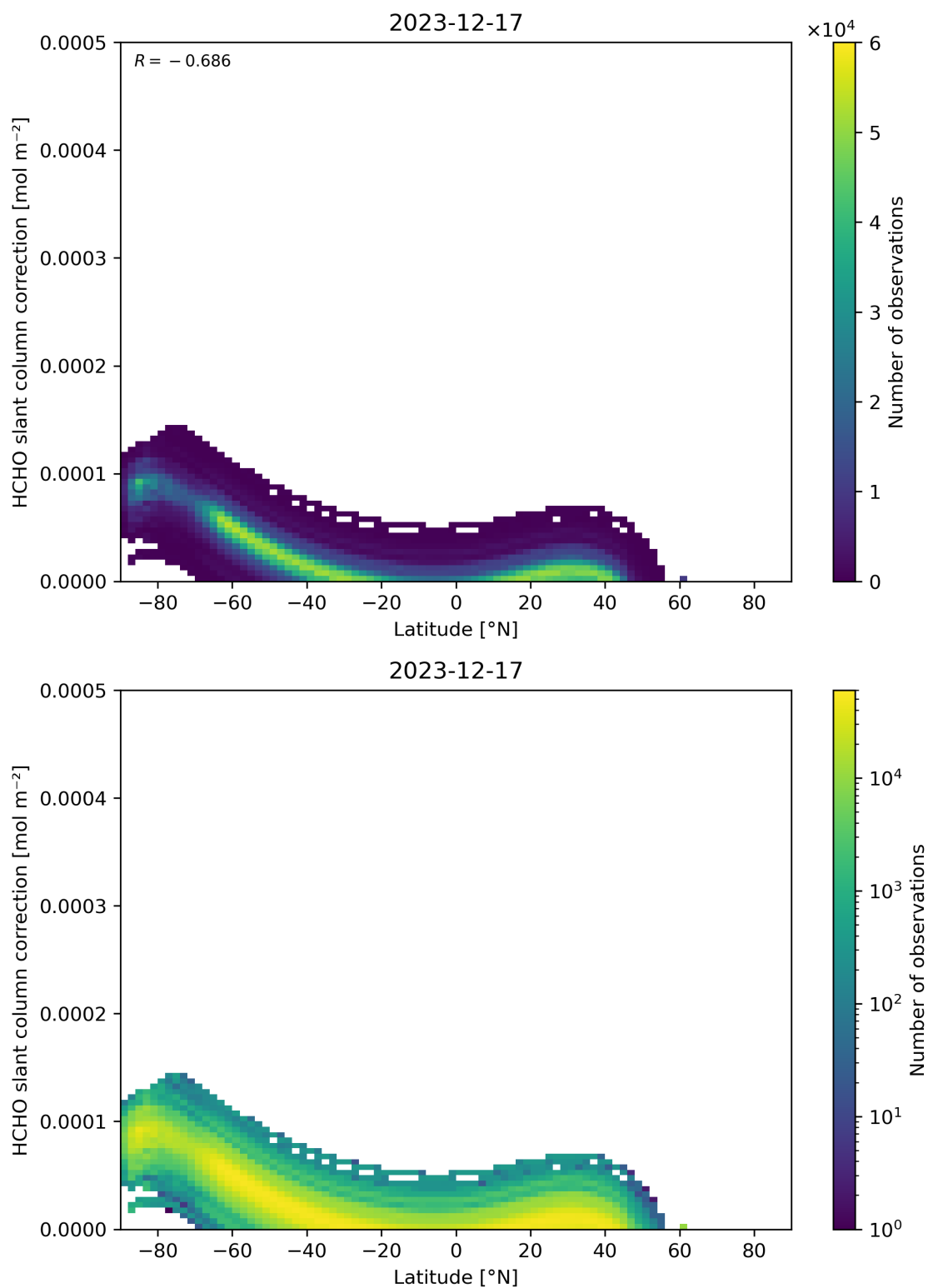
Figure 158: Scatter density plot of “Latitude” against “HCHO slant column correction” for 2023-12-16 to 2023-12-18.
