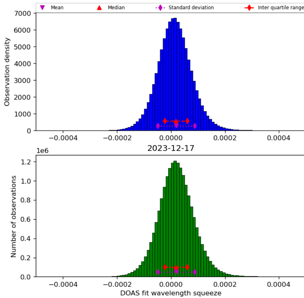
Figure 45: Histogram of “DOAS fit wavelength squeeze” for 2023-12-16 to 2023-12-18
