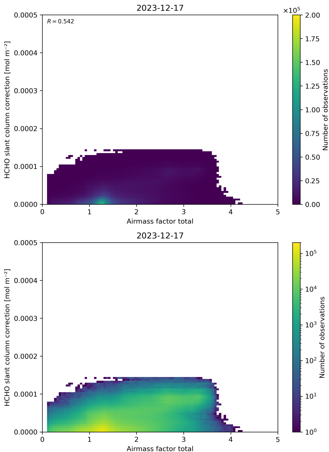
Figure 102: Scatter density plot of “Airmass factor total” against “HCHO slant column correction” for 2023-12-16 to 2023-12-18.
