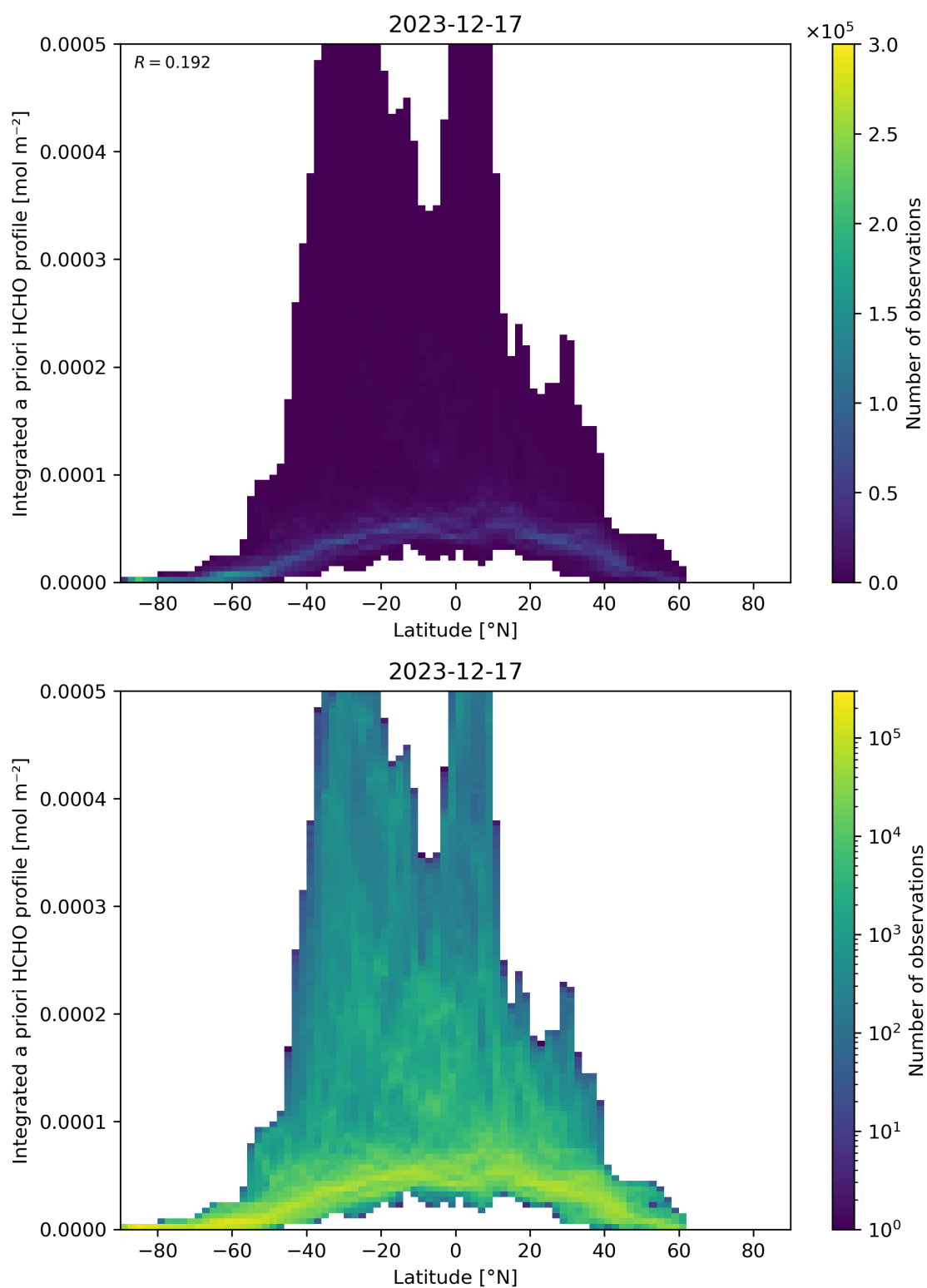
Figure 166: Scatter density plot of “Latitude” against “Integrated a priori HCHO profile” for 2023-12-16 to 2023-12-18.
