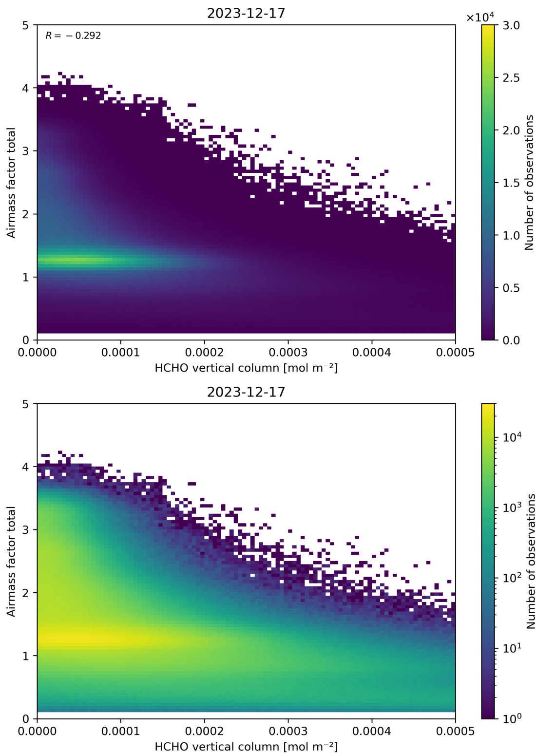
Figure 131: Scatter density plot of “HCHO vertical column” against “Airmass factor total” for 2023-12-16 to 2023-12-18.
