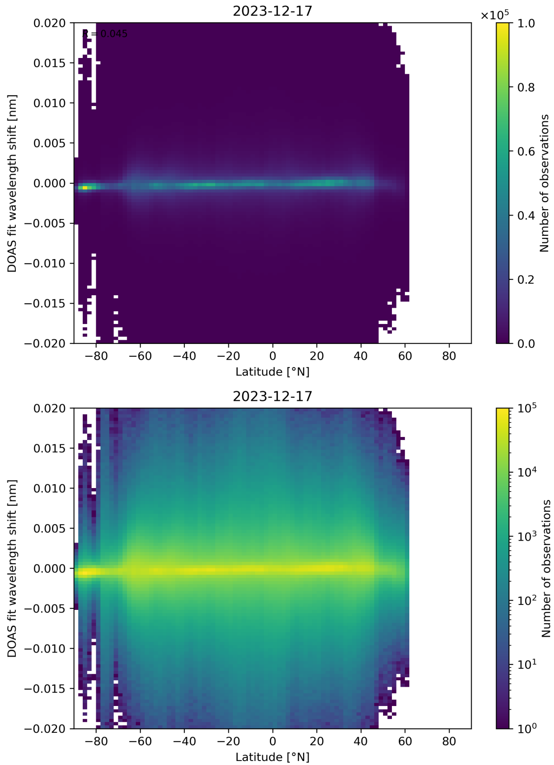
Figure 154: Scatter density plot of “Latitude” against “DOAS fit wavelength shift” for 2023-12-16 to 2023-12-18.
