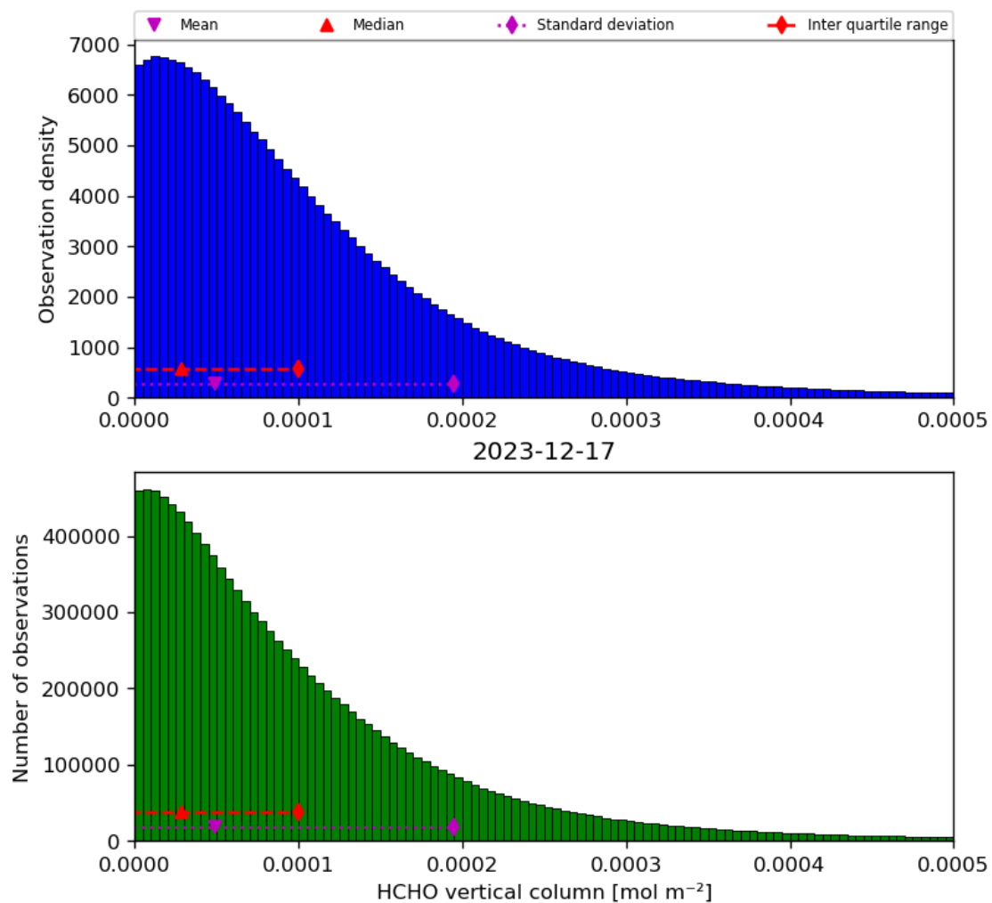
Figure 35: Histogram of “HCHO vertical column” for 2023-12-16 to 2023-12-18
