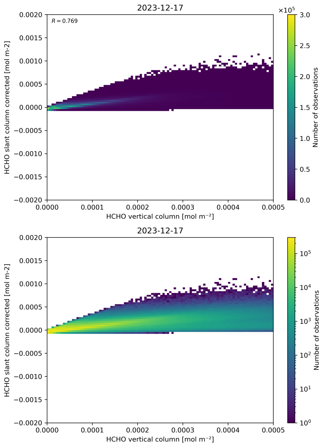
Figure 127: Scatter density plot of “HCHO vertical column” against “HCHO slant column corrected” for 2023-12-16 to 2023-12-18.
