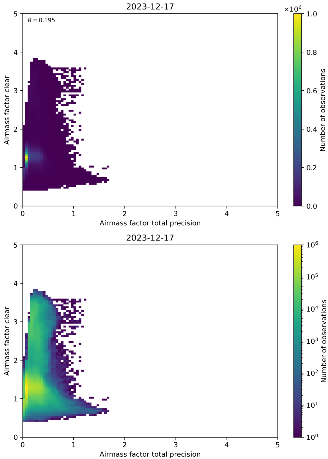
Figure 108: Scatter density plot of “Airmass factor total precision” against “Airmass factor clear” for 2023-12-16 to 2023-12-18.
