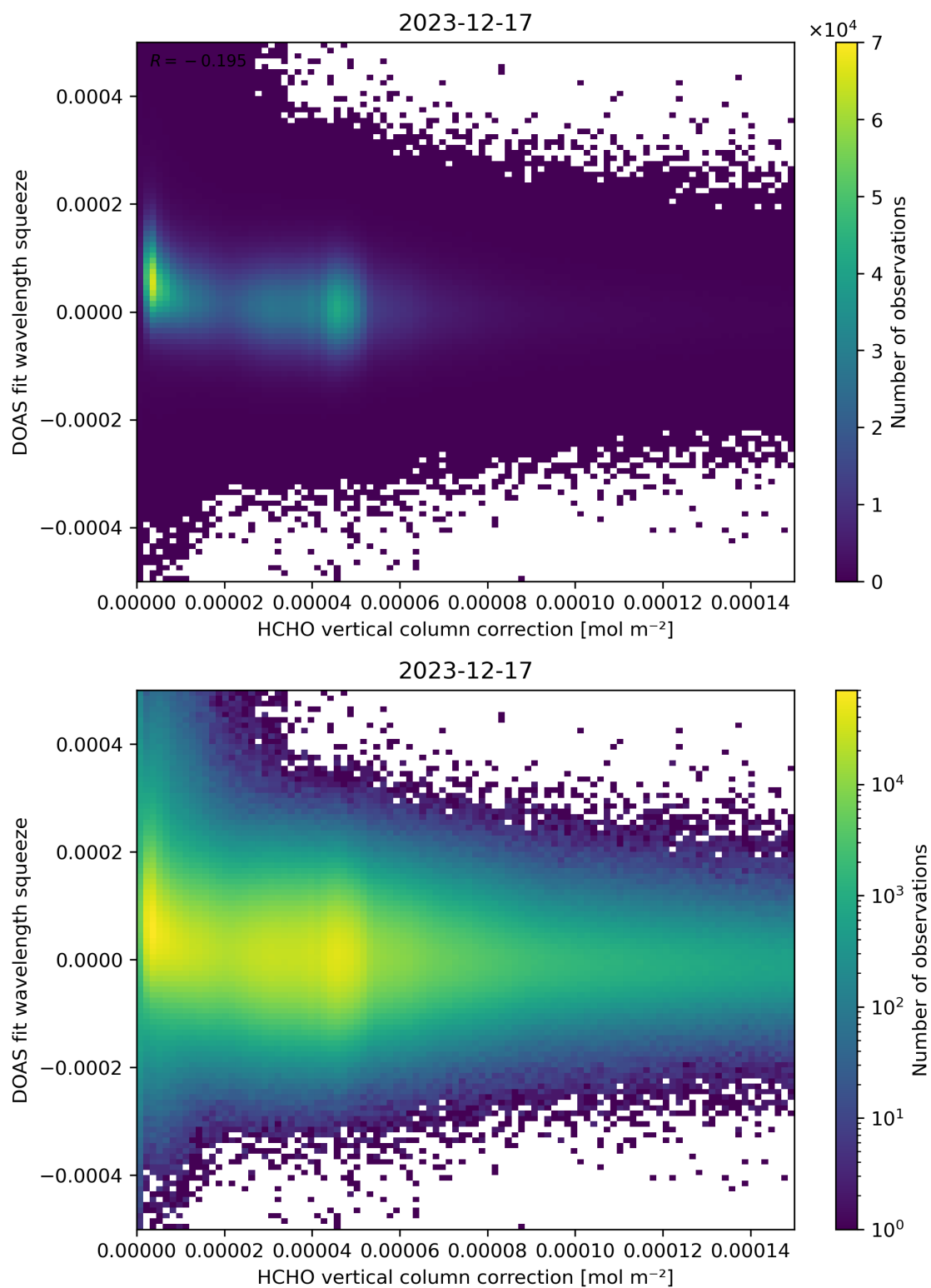
Figure 114: Scatter density plot of “HCHO vertical column correction” against “DOAS fit wavelength squeeze” for 2023-12-16 to 2023-12-18.
