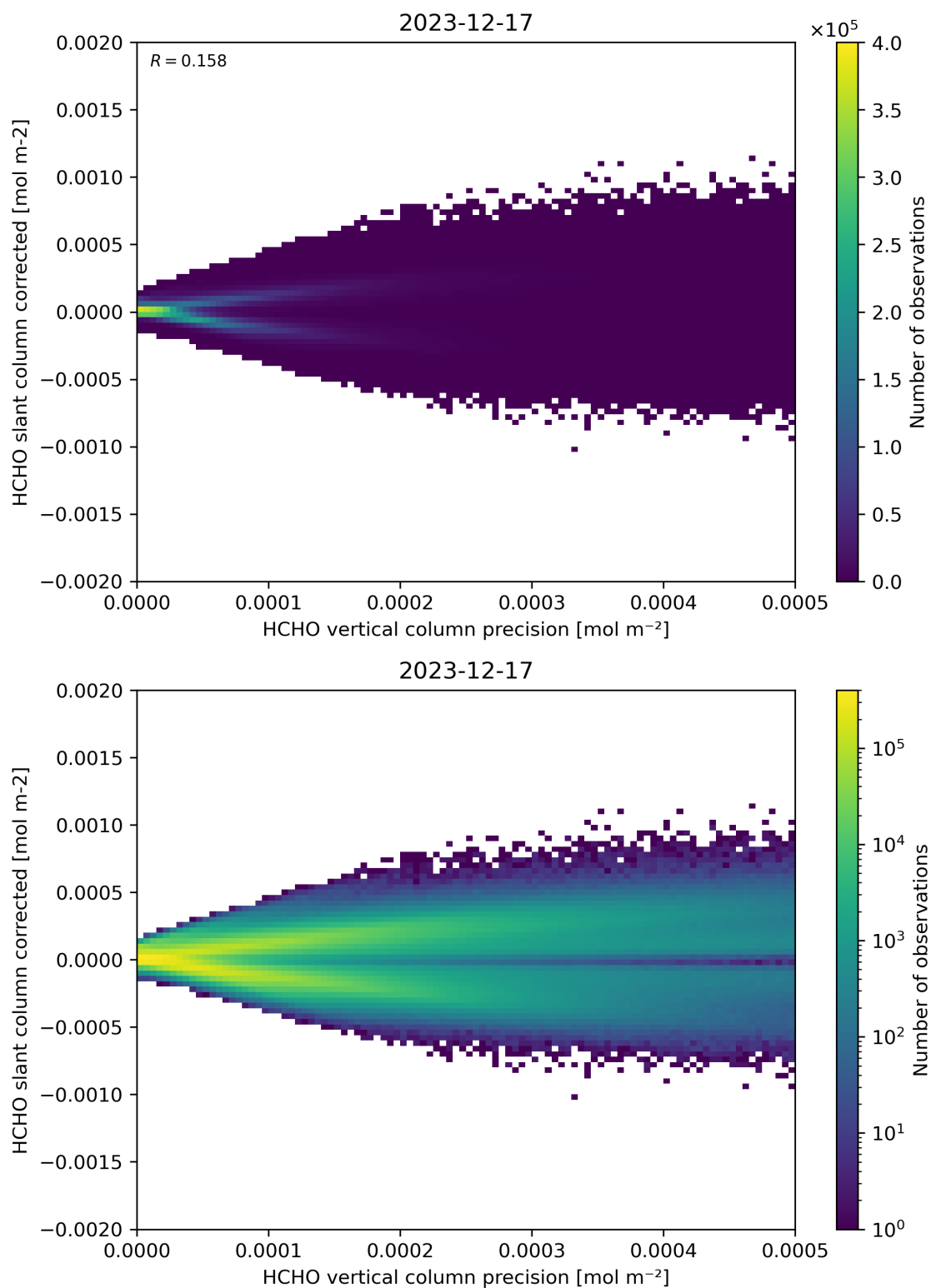
Figure 140: Scatter density plot of “HCHO vertical column precision” against “HCHO slant column corrected” for 2023-12-16 to 2023-12-18.
