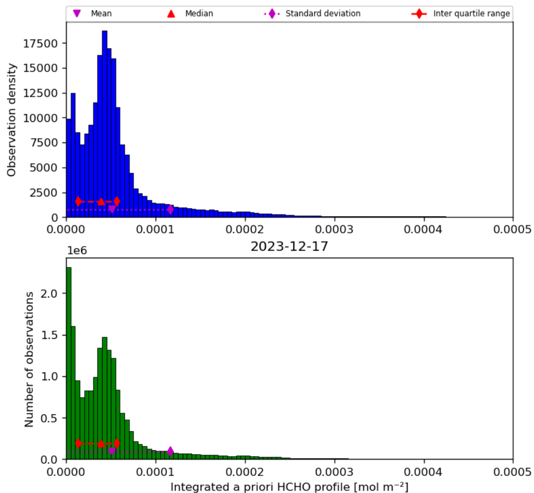
Figure 43: Histogram of “Integrated a priori HCHO profile” for 2023-12-16 to 2023-12-18
