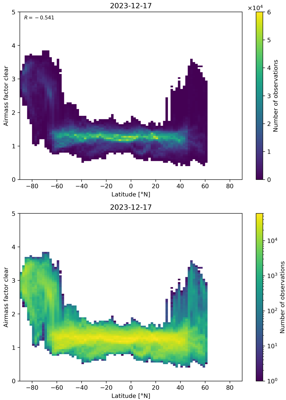
Figure 156: Scatter density plot of “Latitude” against “Airmass factor clear” for 2023-12-16 to 2023-12-18.
