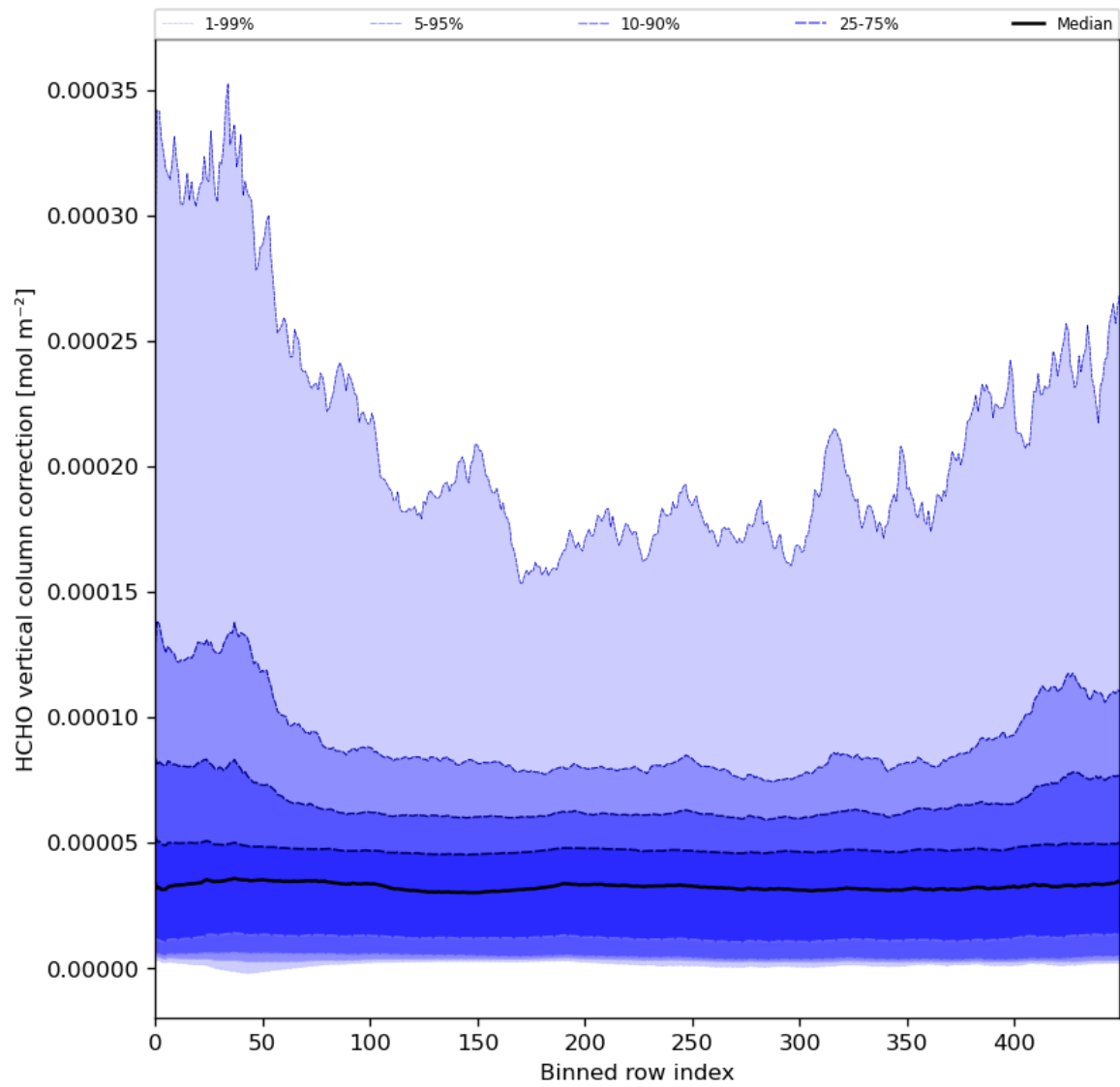
Figure 51: Along track statistics of “HCHO vertical column correction” for 2023-12-16 to 2023-12-18
