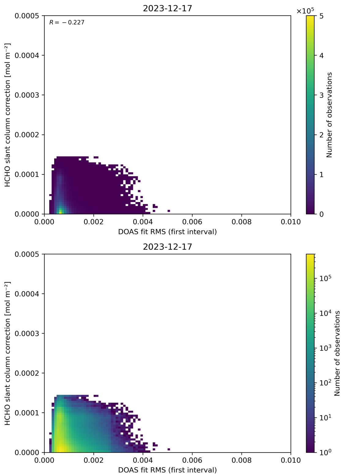
Figure 63: Scatter density plot of “DOAS fit RMS (first interval)” against “HCHO slant column correction” for 2023-12-16 to 2023-12-18.
