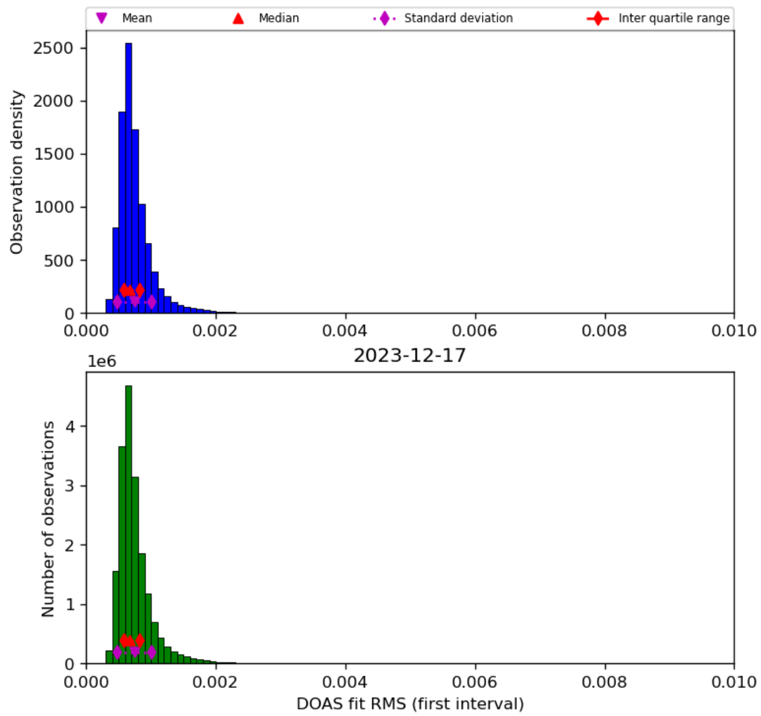
Figure 46: Histogram of “DOAS fit RMS (first interval)” for 2023-12-16 to 2023-12-18
