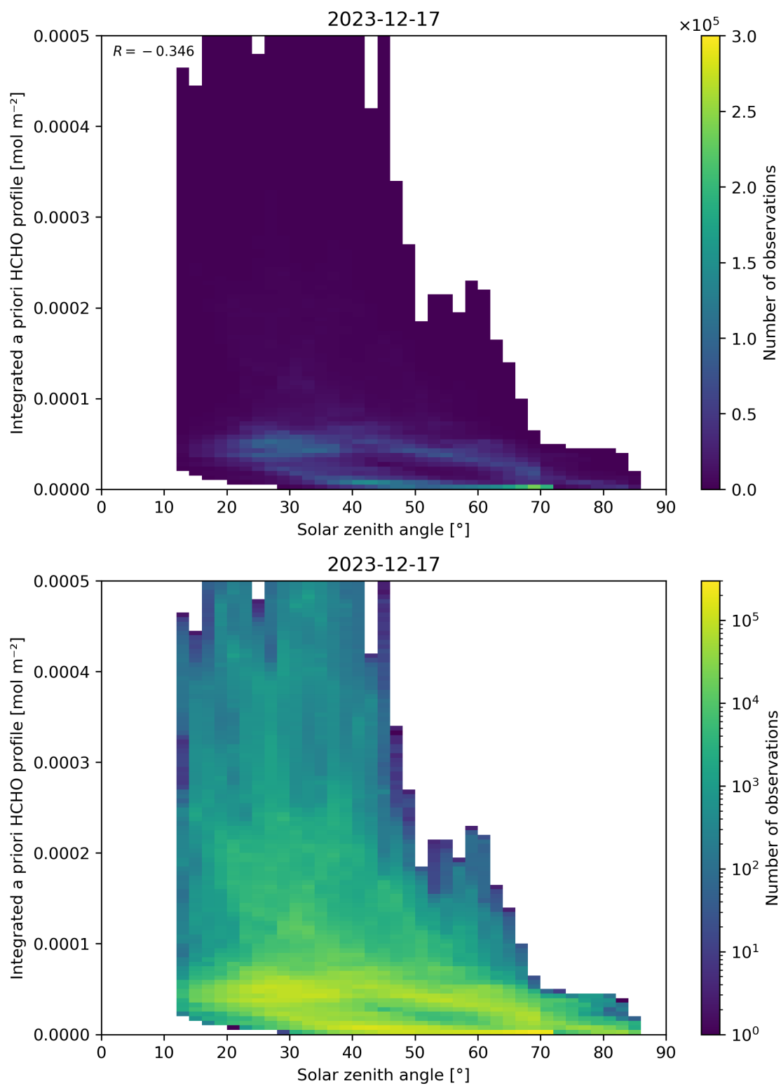
Figure 180: Scatter density plot of “Solar zenith angle” against “Integrated a priori HCHO profile” for 2023-12-16 to 2023-12-18.
