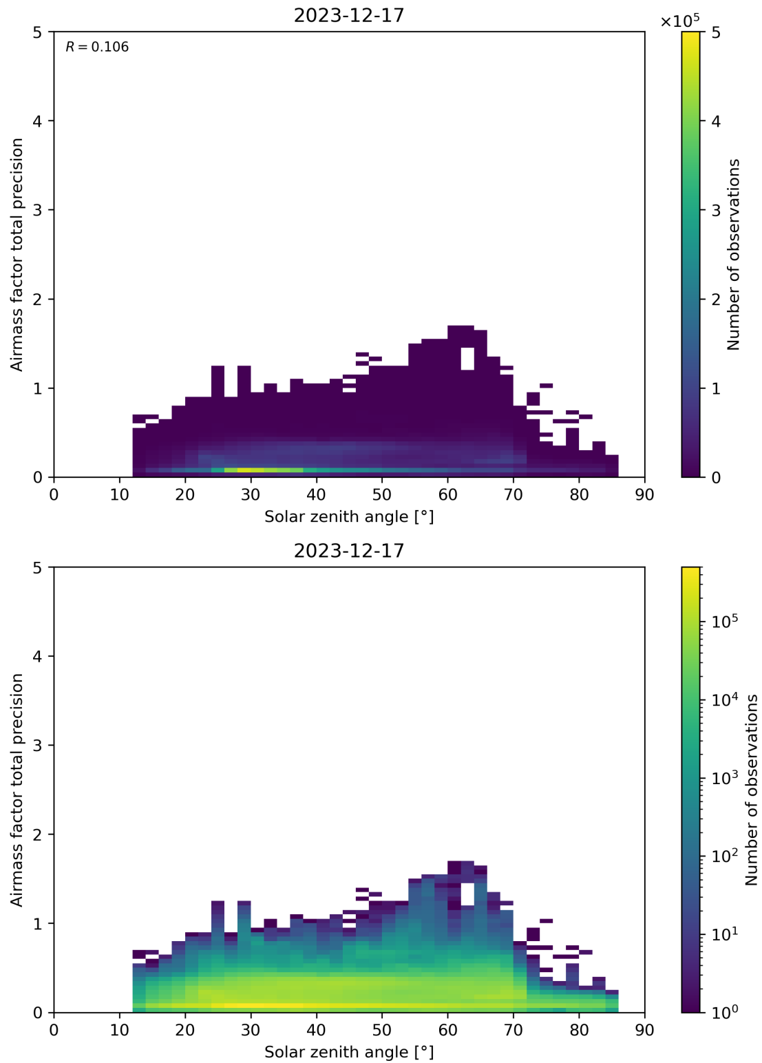
Figure 176: Scatter density plot of “Solar zenith angle” against “Airmass factor total precision” for 2023-12-16 to 2023-12-18.
