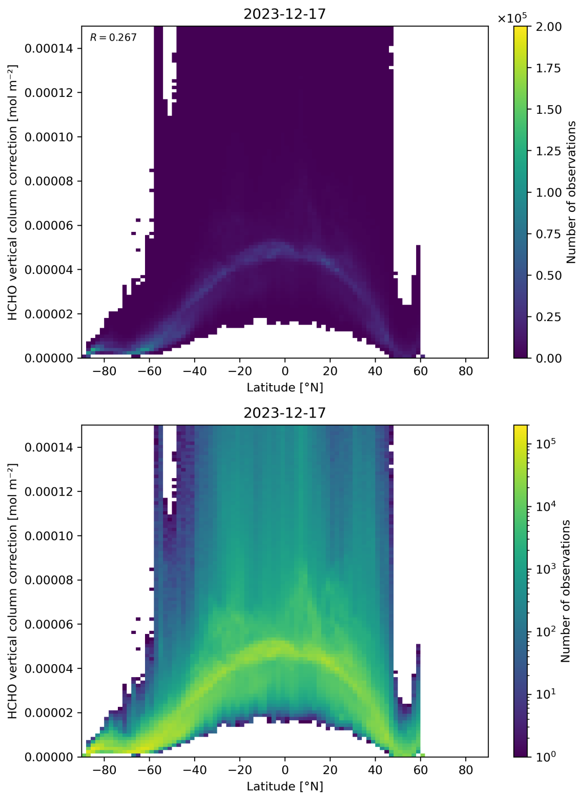
Figure 164: Scatter density plot of “Latitude” against “HCHO vertical column correction” for 2023-12-16 to 2023-12-18.
