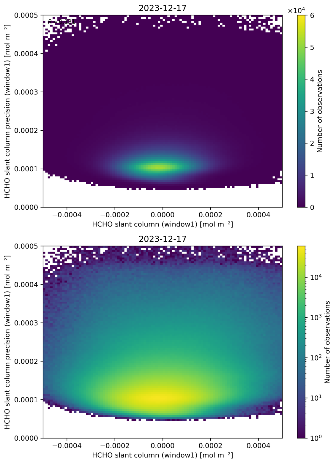
Figure 84: Scatter density plot of “HCHO slant column (window1)” against “HCHO slant column precision (window1)” for 2023-12-16 to 2023-12-18.
