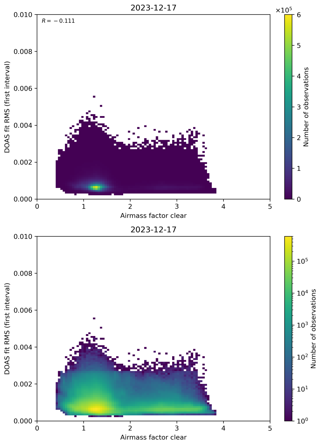
Figure 71: Scatter density plot of “Airmass factor clear” against “DOAS fit RMS (first interval)” for 2023-12-16 to 2023-12-18.
