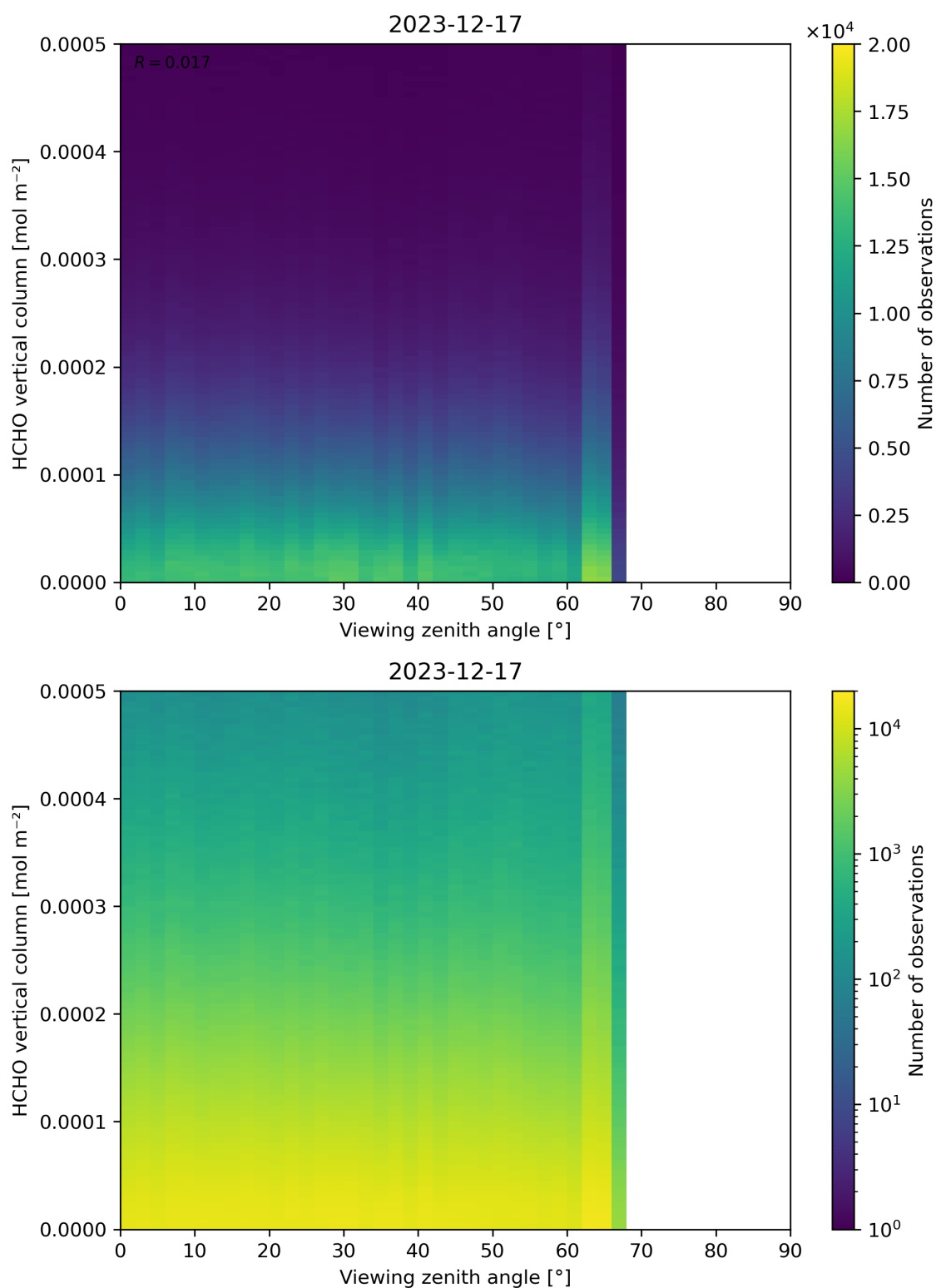
Figure 192: Scatter density plot of “Viewing zenith angle” against “HCHO vertical column” for 2023-12-16 to 2023-12-18.
