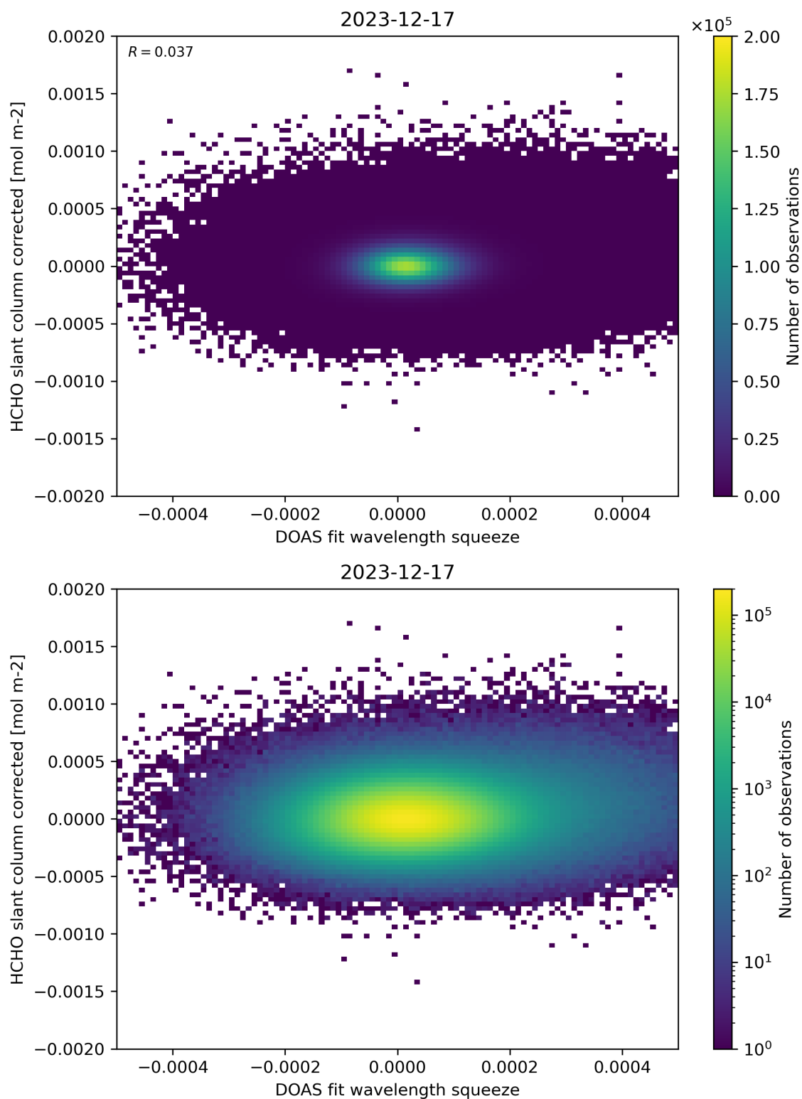
Figure 69: Scatter density plot of “DOAS fit wavelength squeeze” against “HCHO slant column corrected” for 2023-12-16 to 2023-12-18.
