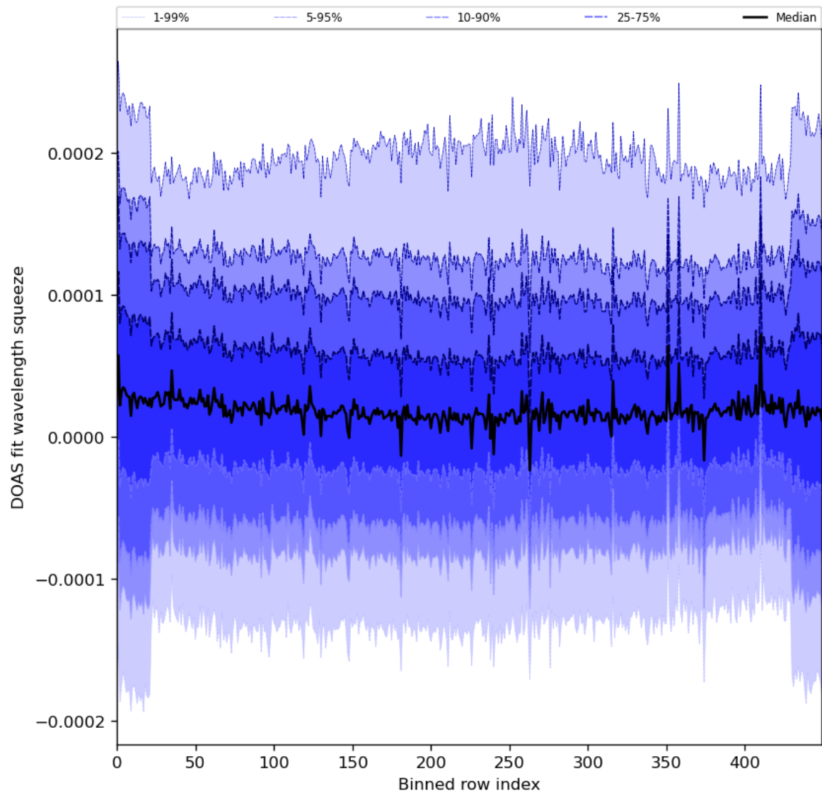
Figure 59: Along track statistics of “DOAS fit wavelength squeeze” for 2023-12-16 to 2023-12-18
