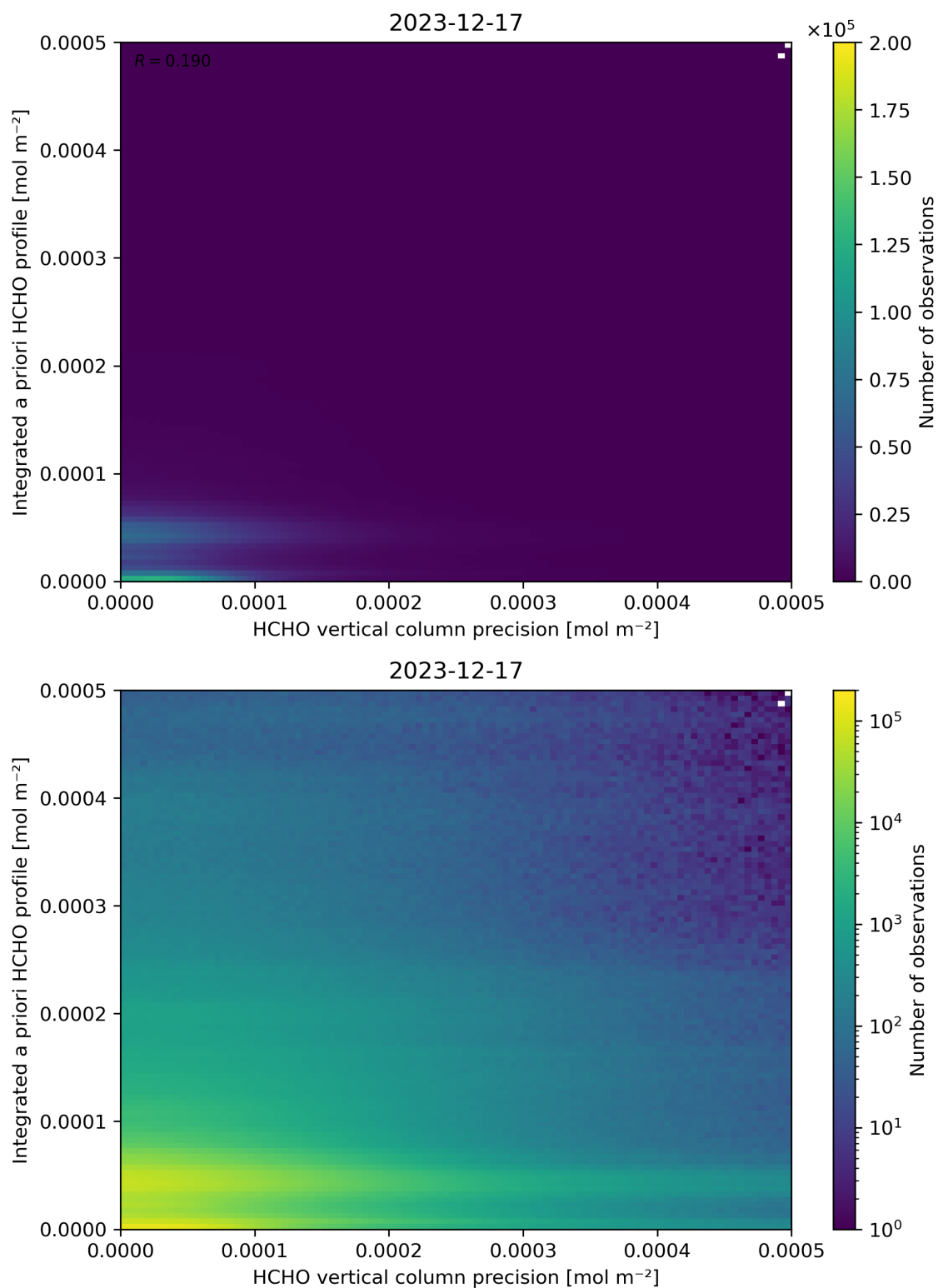
Figure 147: Scatter density plot of “HCHO vertical column precision” against “Integrated a priori HCHO profile” for 2023-12-16 to 2023-12-18.
