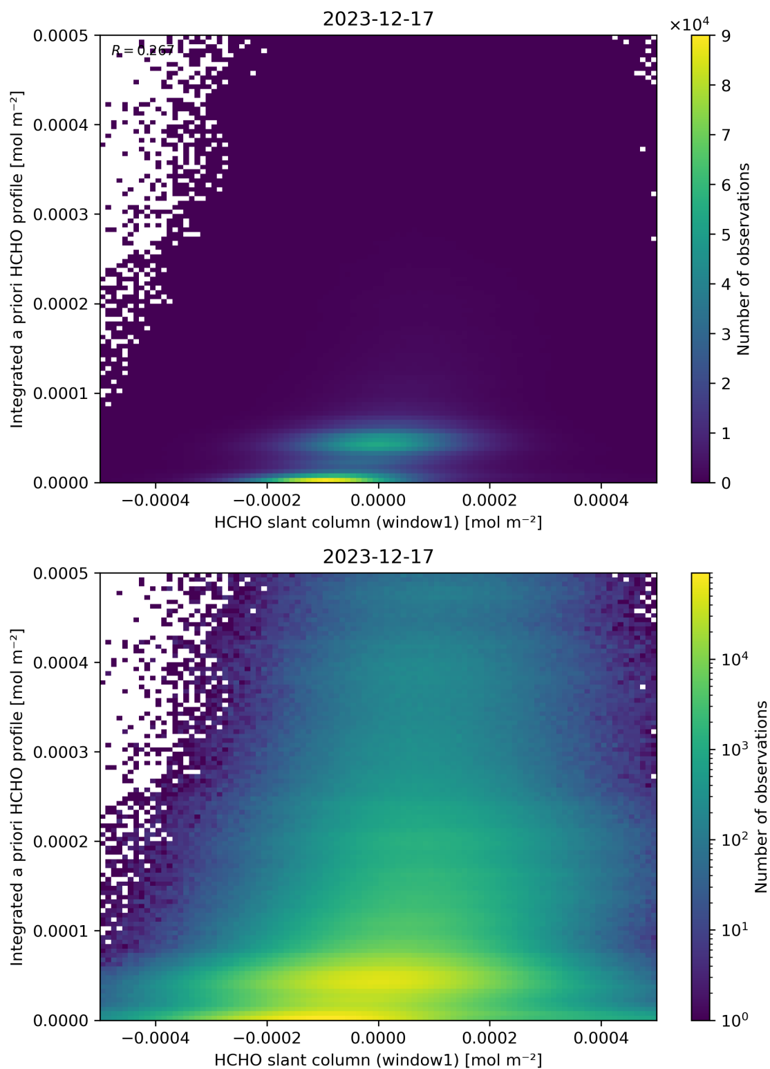
Figure 87: Scatter density plot of “HCHO slant column (window1)” against “Integrated a priori HCHO profile” for 2023-12-16 to 2023-12-18.
