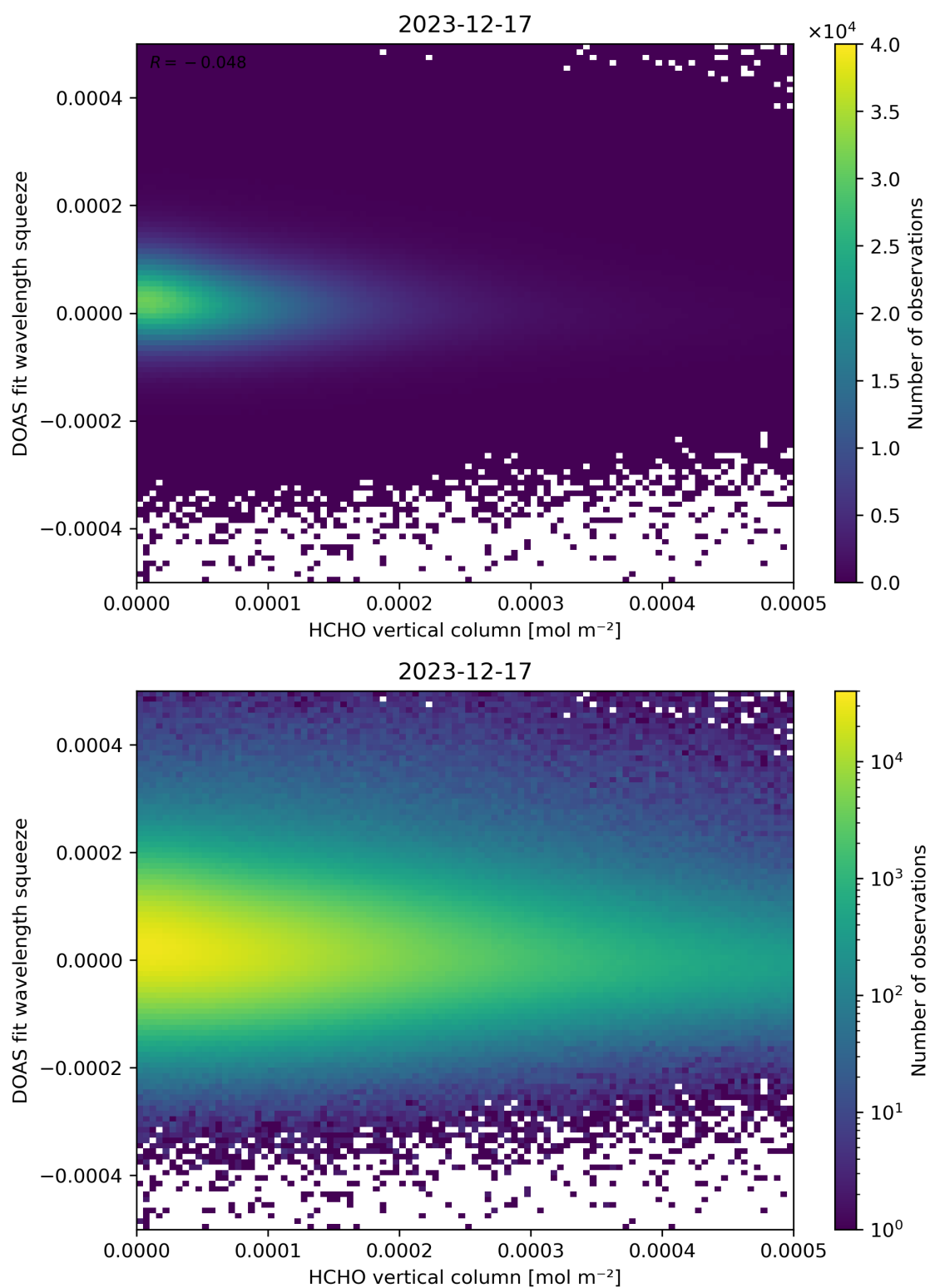
Figure 125: Scatter density plot of “HCHO vertical column” against “DOAS fit wavelength squeeze” for 2023-12-16 to 2023-12-18.
