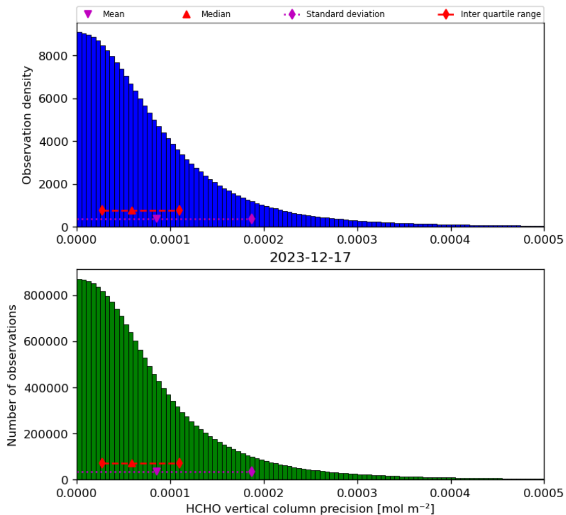
Figure 36: Histogram of “HCHO vertical column precision” for 2023-12-16 to 2023-12-18
