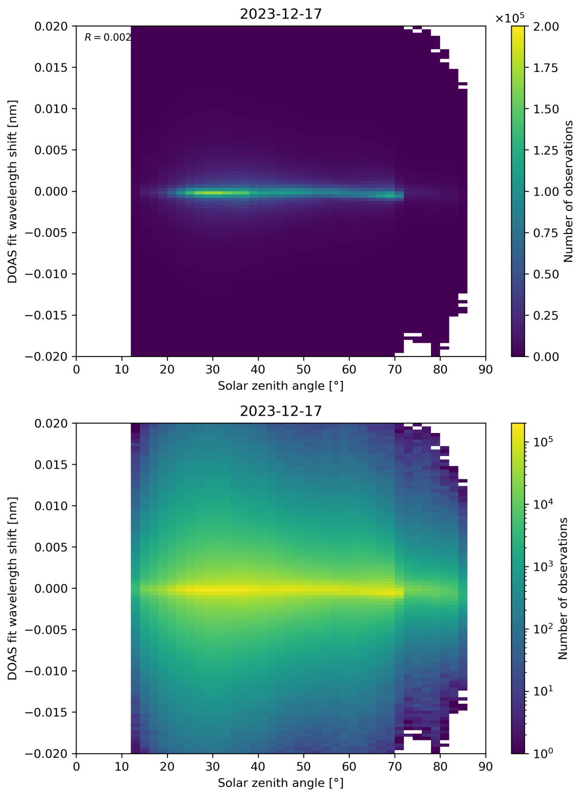
Figure 168: Scatter density plot of “Solar zenith angle” against “DOAS fit wavelength shift” for 2023-12-16 to 2023-12-18.
