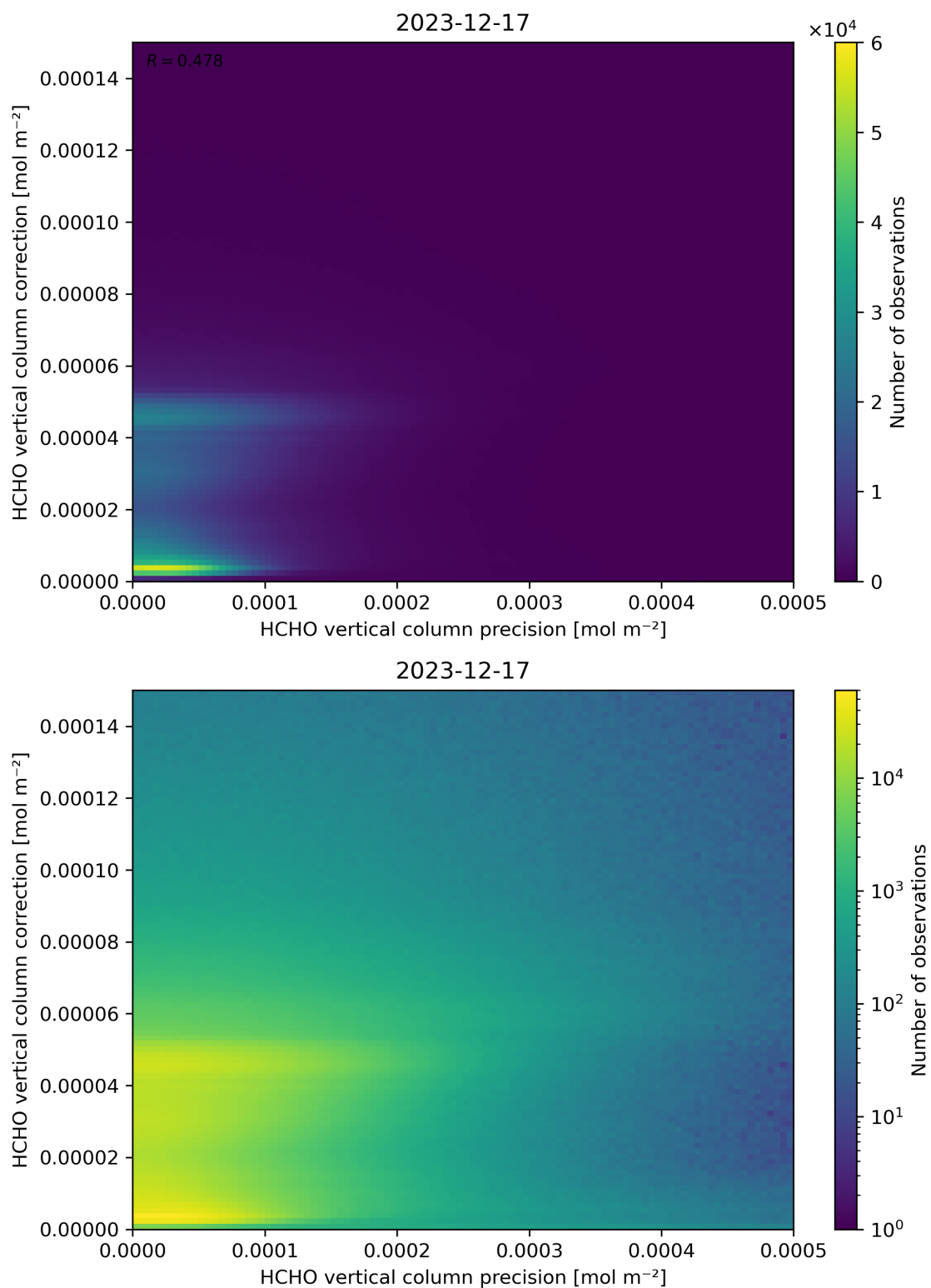
Figure 146: Scatter density plot of “HCHO vertical column precision” against “HCHO vertical column correction” for 2023-12-16 to 2023-12-18.
