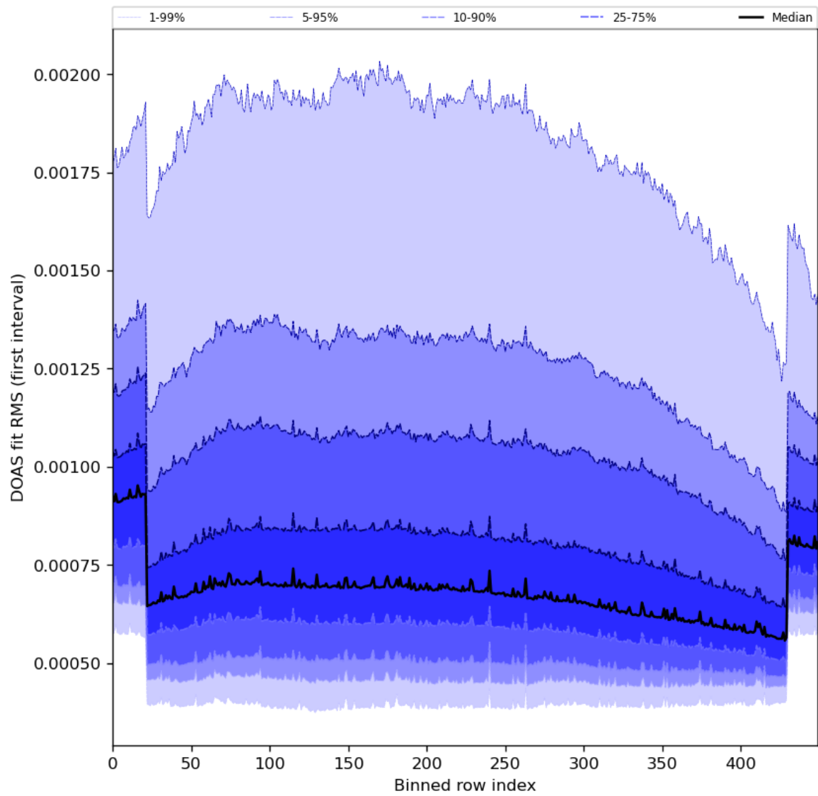
Figure 60: Along track statistics of “DOAS fit RMS (first interval)” for 2023-12-16 to 2023-12-18
