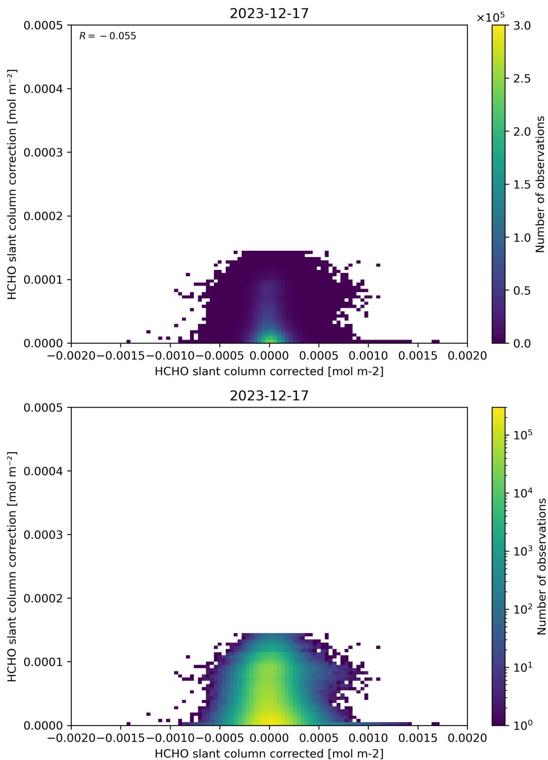
Figure 77: Scatter density plot of “HCHO slant column corrected” against “HCHO slant column correction” for 2023-12-16 to 2023-12-18.
