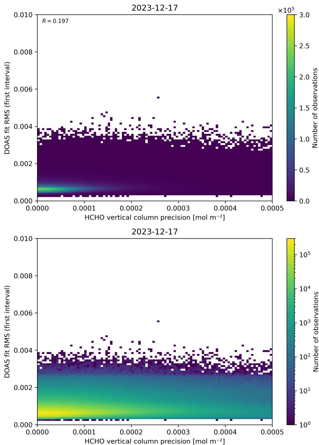
Figure 136: Scatter density plot of “HCHO vertical column precision” against “DOAS fit RMS (first interval)” for 2023-12-16 to 2023-12-18.
