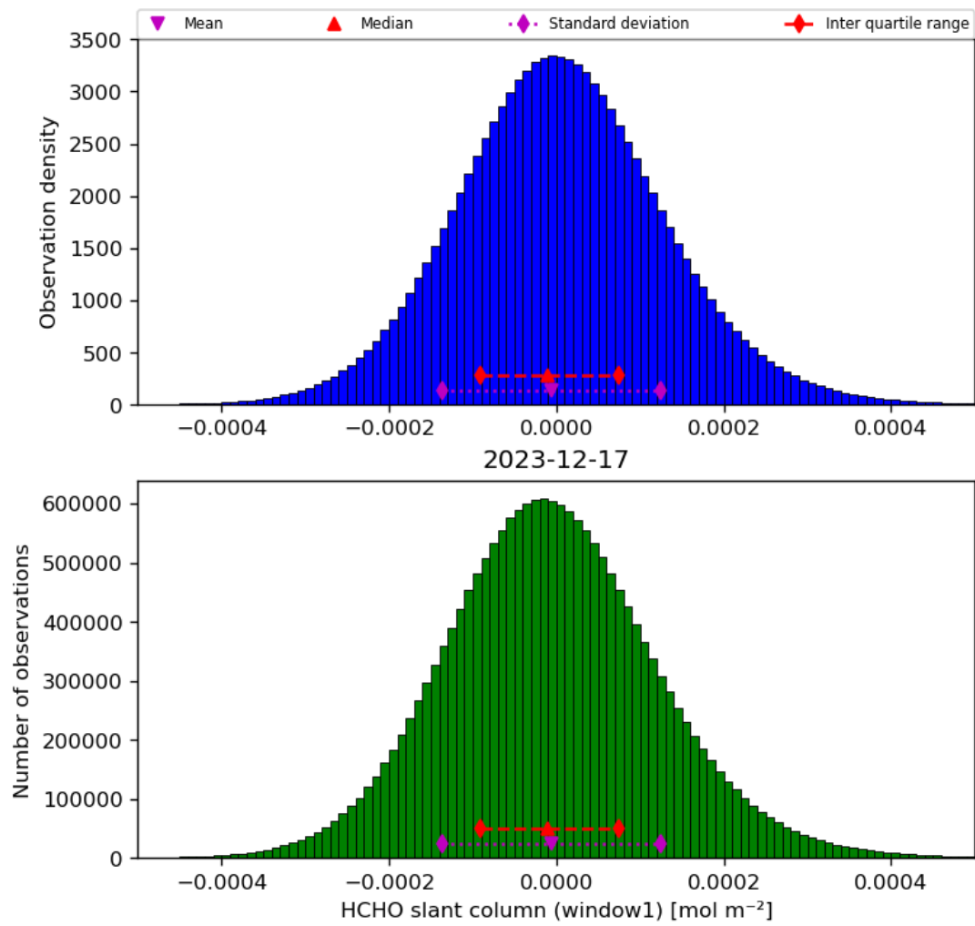
Figure 38: Histogram of “HCHO slant column (window1)” for 2023-12-16 to 2023-12-18
