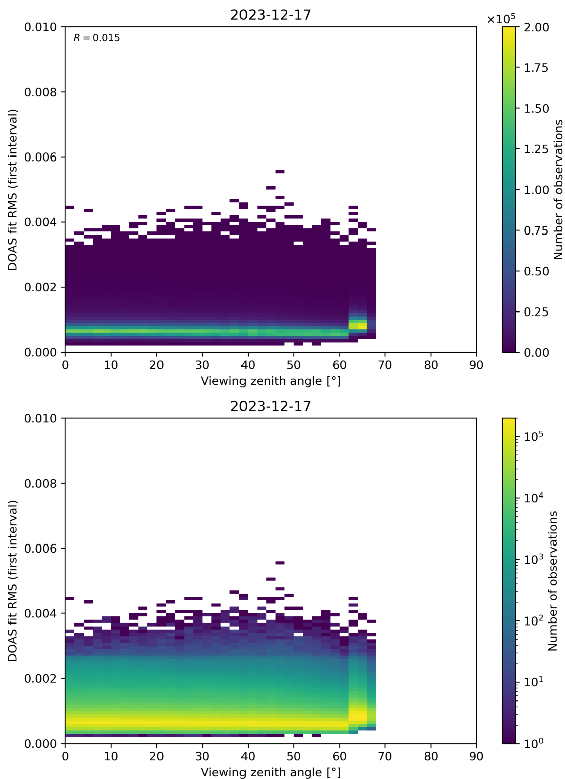
Figure 182: Scatter density plot of “Viewing zenith angle” against “DOAS fit RMS (first interval)” for 2023-12-16 to 2023-12-18.
