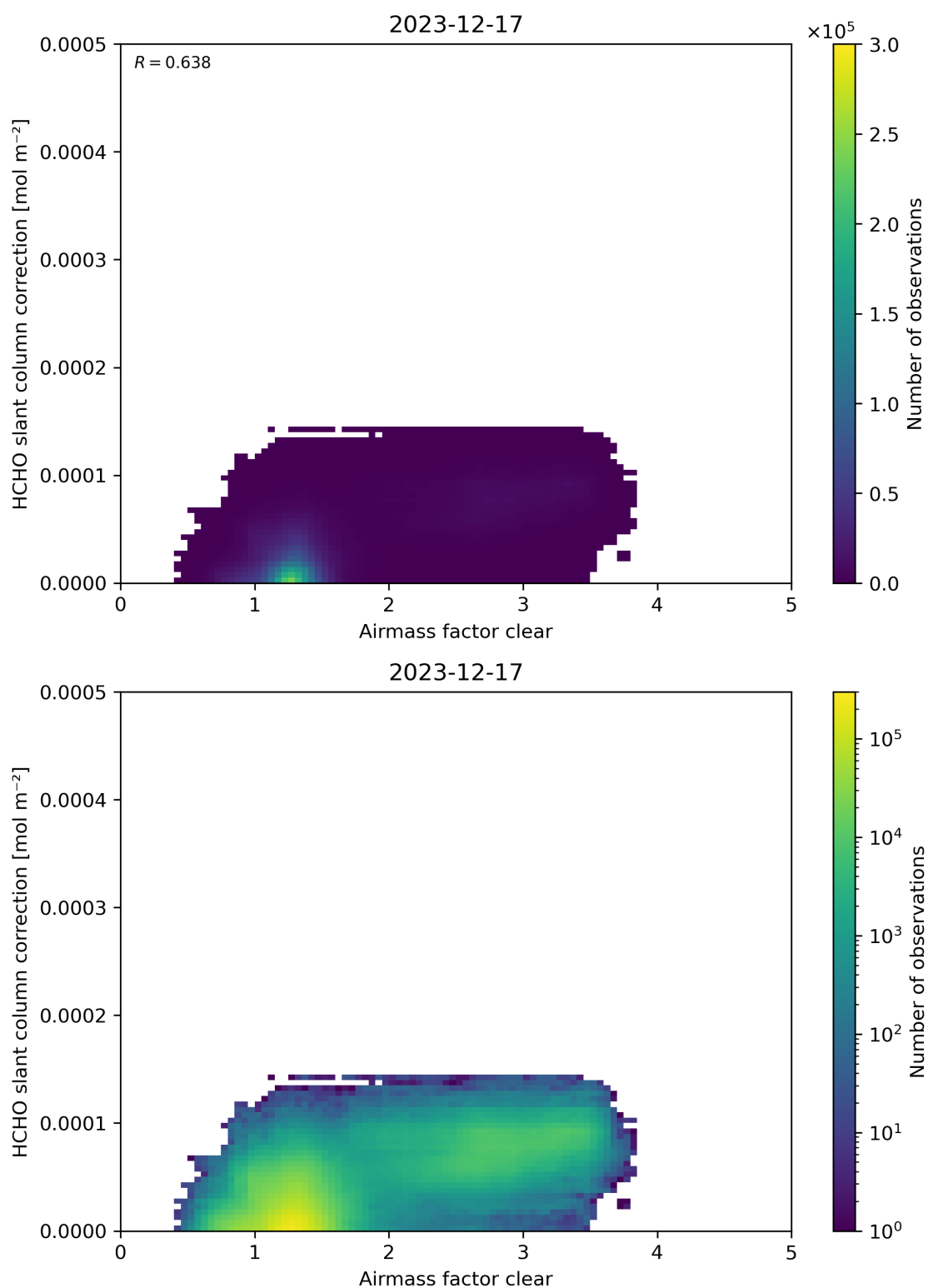
Figure 75: Scatter density plot of “Airmass factor clear” against “HCHO slant column correction” for 2023-12-16 to 2023-12-18.
