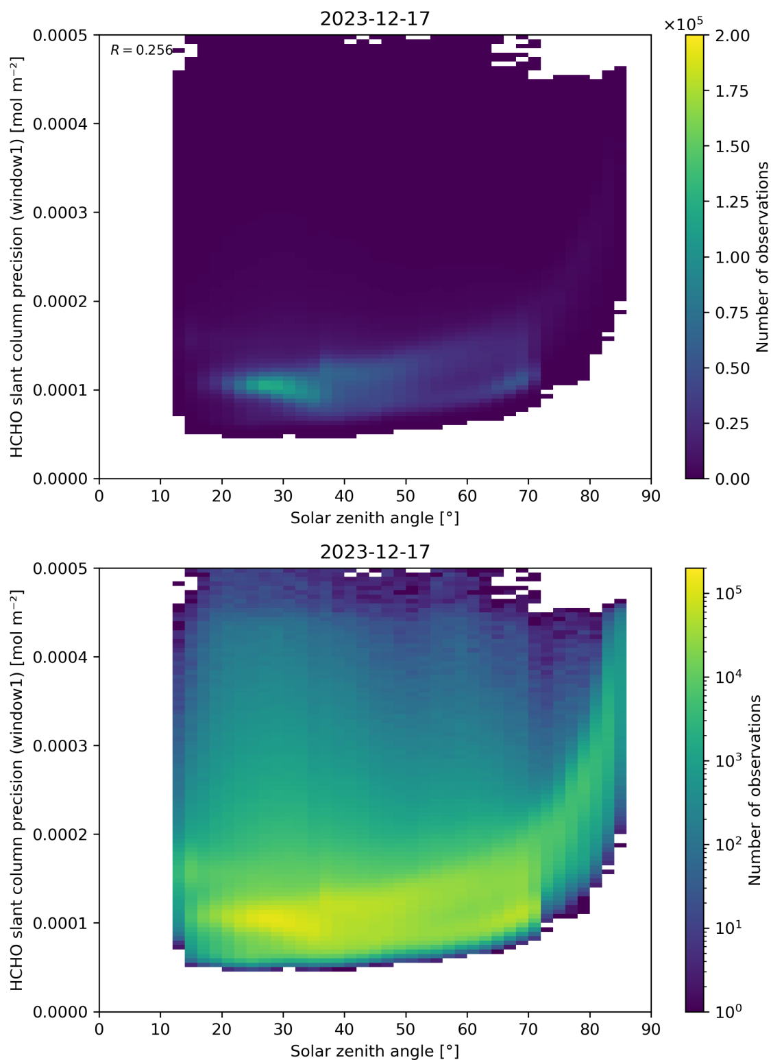
Figure 174: Scatter density plot of “Solar zenith angle” against “HCHO slant column precision (window1)” for 2023-12-16 to 2023-12-18.
