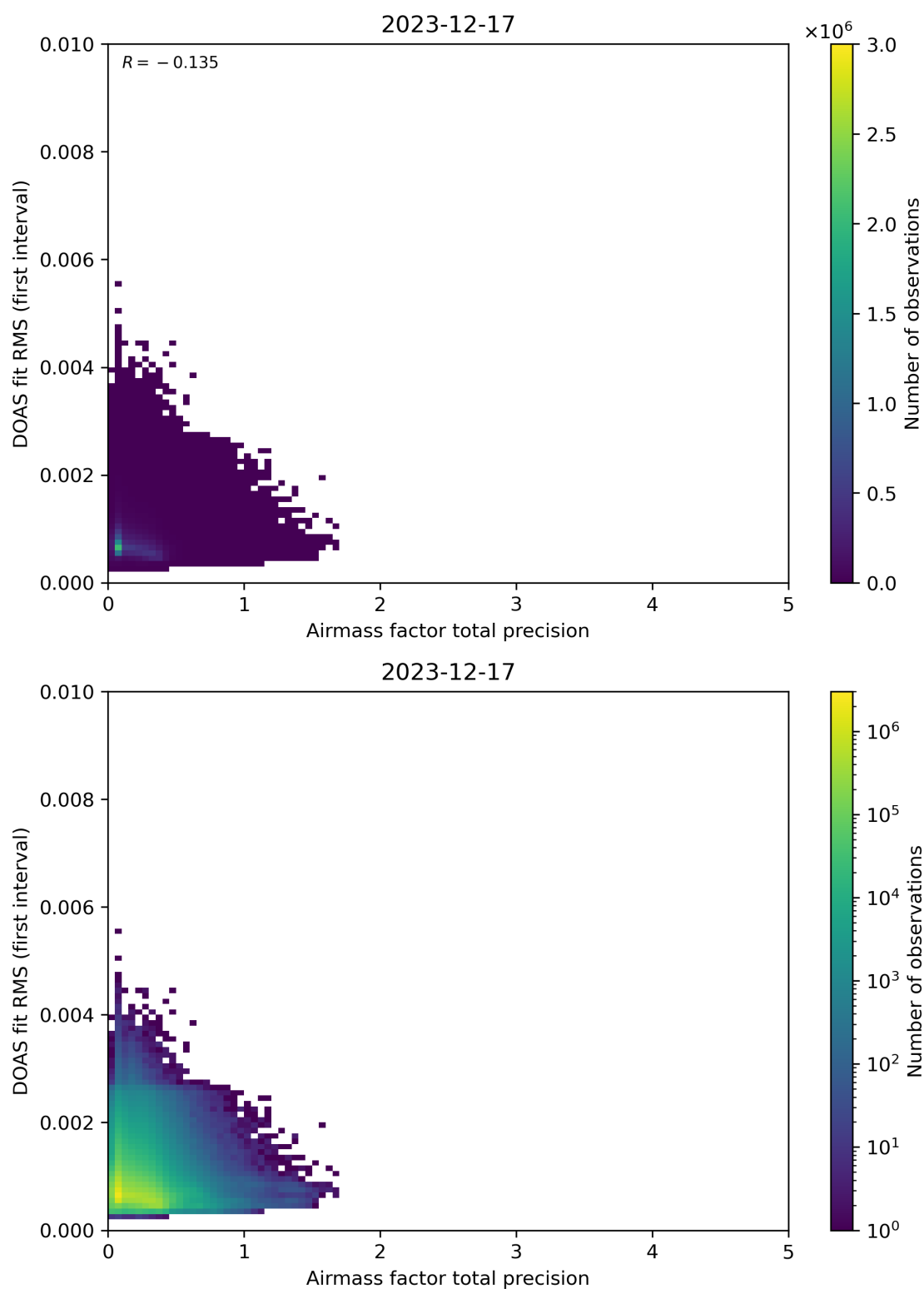
Figure 105: Scatter density plot of “Airmass factor total precision” against “DOAS fit RMS (first interval)” for 2023-12-16 to 2023-12-18.
