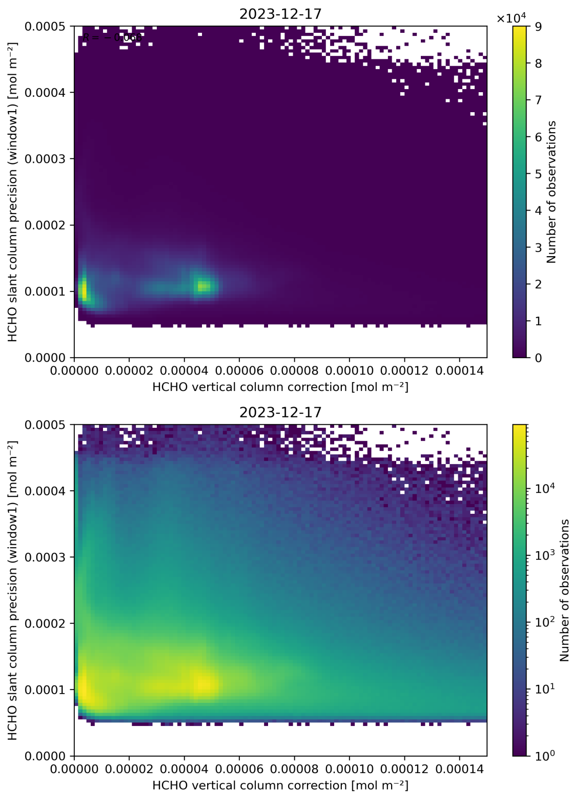
Figure 119: Scatter density plot of “HCHO vertical column correction” against “HCHO slant column precision (window1)” for 2023-12-16 to 2023-12-18.
