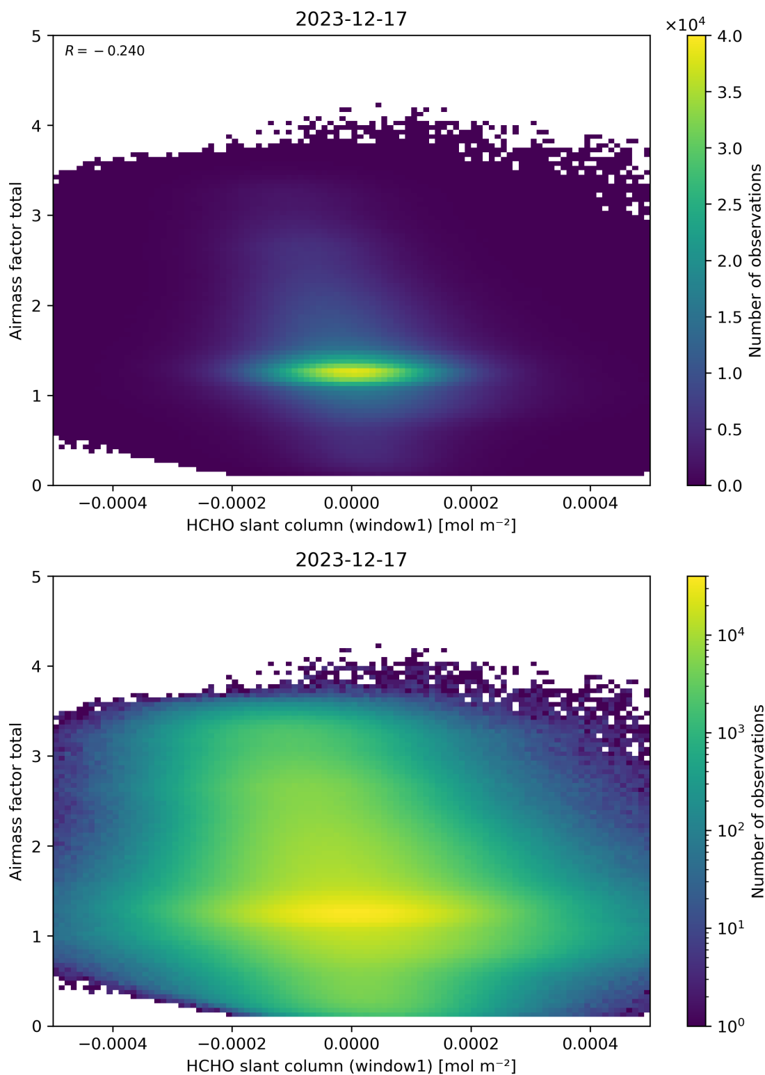
Figure 85: Scatter density plot of “HCHO slant column (window1)” against “Airmass factor total” for 2023-12-16 to 2023-12-18.
