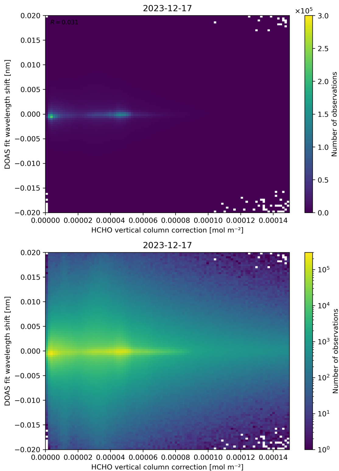
Figure 113: Scatter density plot of “HCHO vertical column correction” against “DOAS fit wavelength shift” for 2023-12-16 to 2023-12-18.
