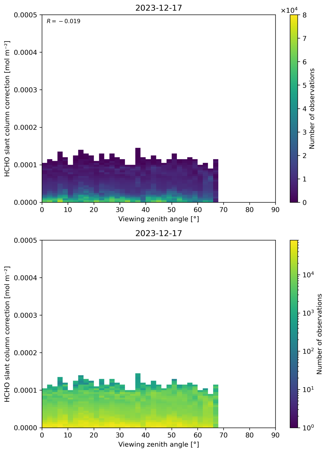
Figure 187: Scatter density plot of “Viewing zenith angle” against “HCHO slant column correction” for 2023-12-16 to 2023-12-18.
