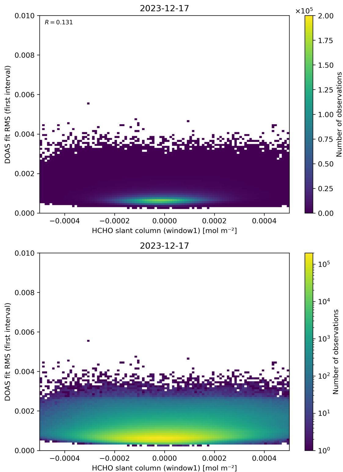
Figure 78: Scatter density plot of “HCHO slant column (window1)” against “DOAS fit RMS (first interval)” for 2023-12-16 to 2023-12-18.
