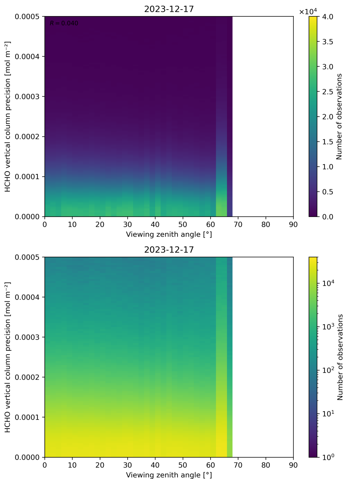
Figure 194: Scatter density plot of “Viewing zenith angle” against “HCHO vertical column precision” for 2023-12-16 to 2023-12-18.
