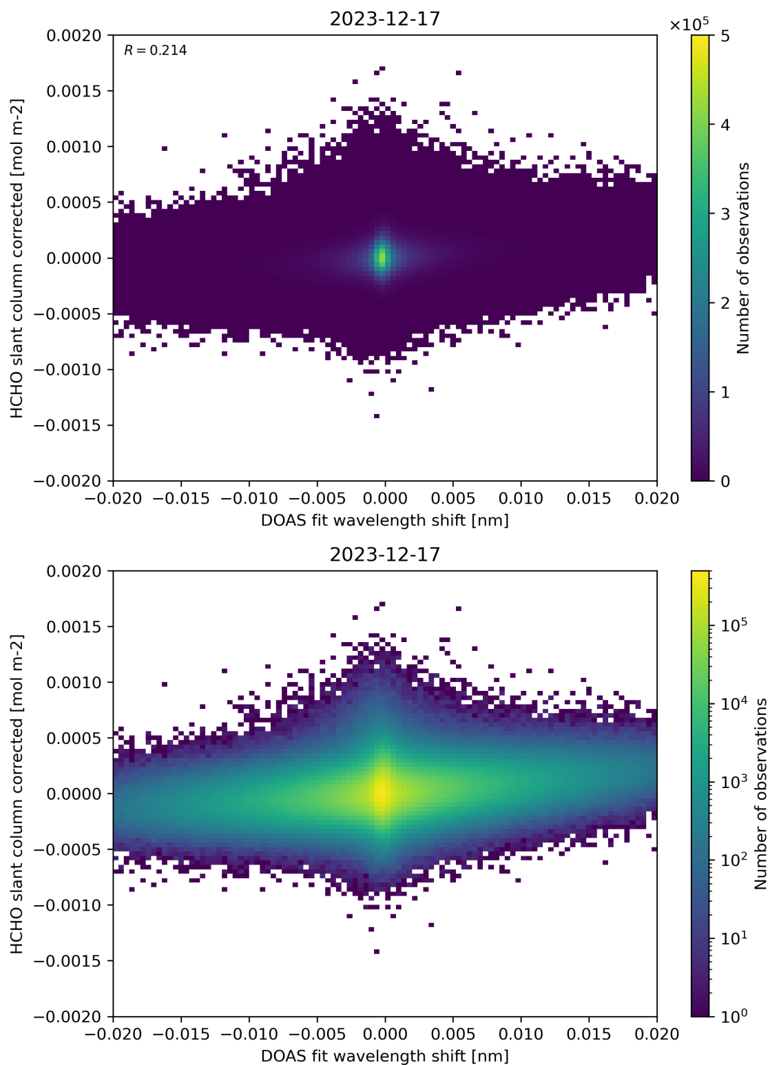
Figure 66: Scatter density plot of “DOAS fit wavelength shift” against “HCHO slant column corrected” for 2023-12-16 to 2023-12-18.
