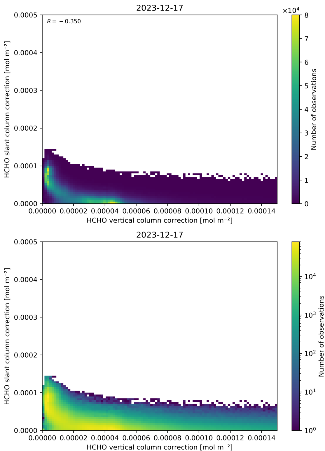
Figure 117: Scatter density plot of “HCHO vertical column correction” against “HCHO slant column correction” for 2023-12-16 to 2023-12-18.
