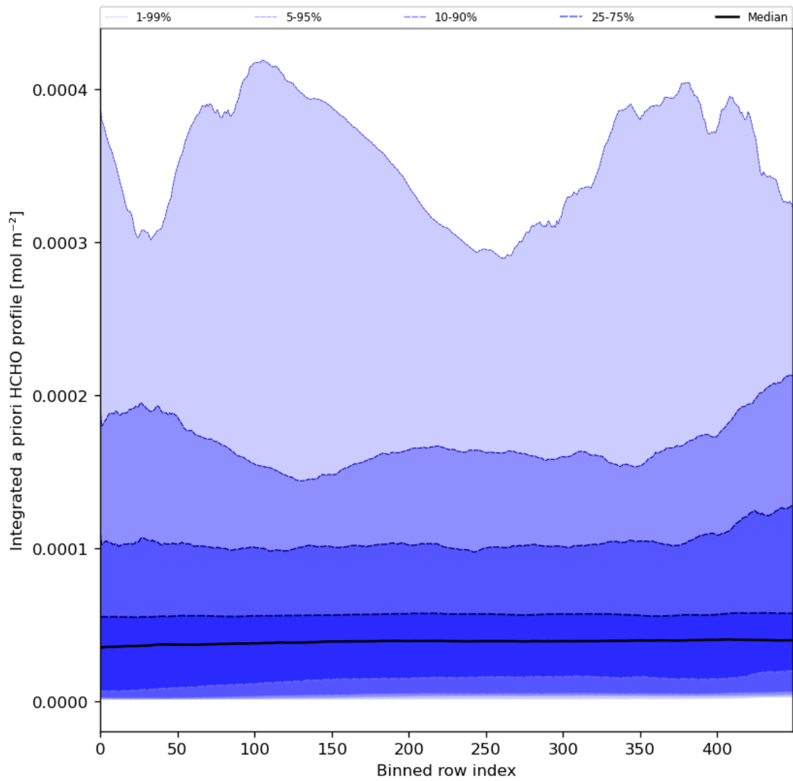
Figure 57: Along track statistics of “Integrated a priori HCHO profile” for 2023-12-16 to 2023-12-18
