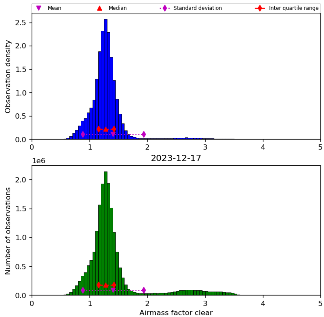
Figure 42: Histogram of “Airmass factor clear” for 2023-12-16 to 2023-12-18
