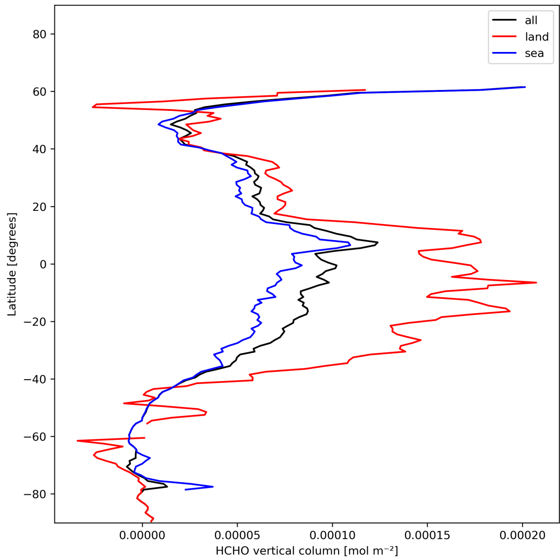
Figure 21: Zonal average of “HCHO vertical column” for 2023-12-16 to 2023-12-18.
