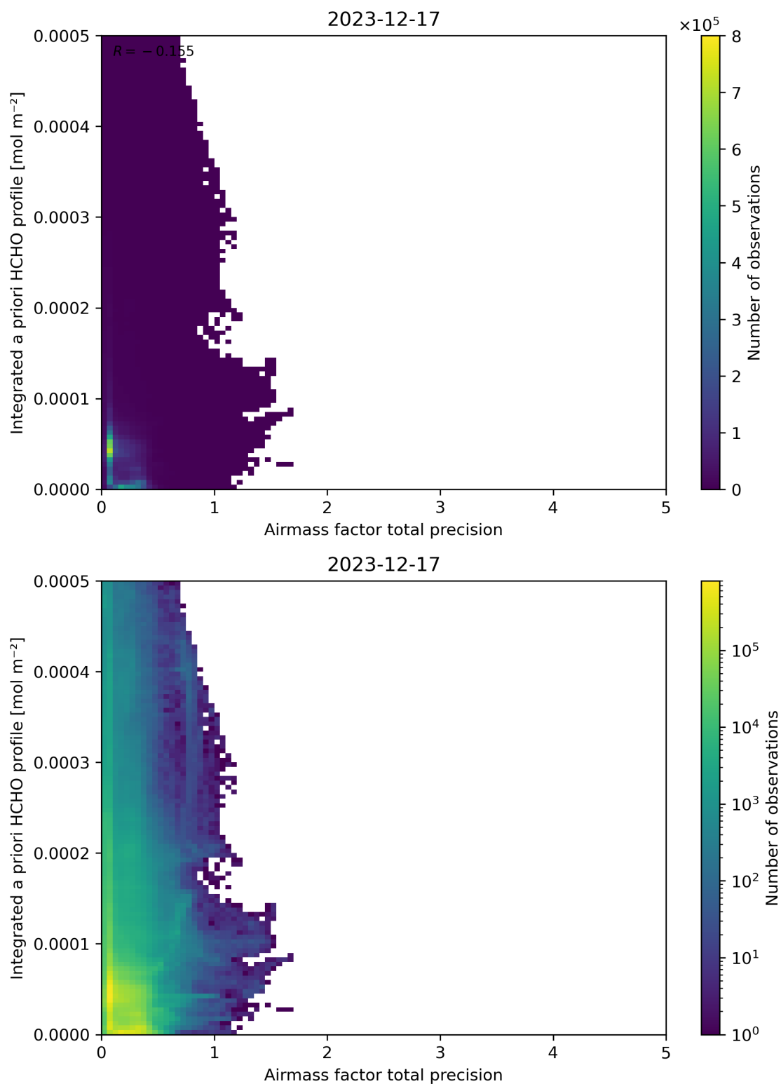
Figure 111: Scatter density plot of “Airmass factor total precision” against “Integrated a priori HCHO profile” for 2023-12-16 to 2023-12-18.
