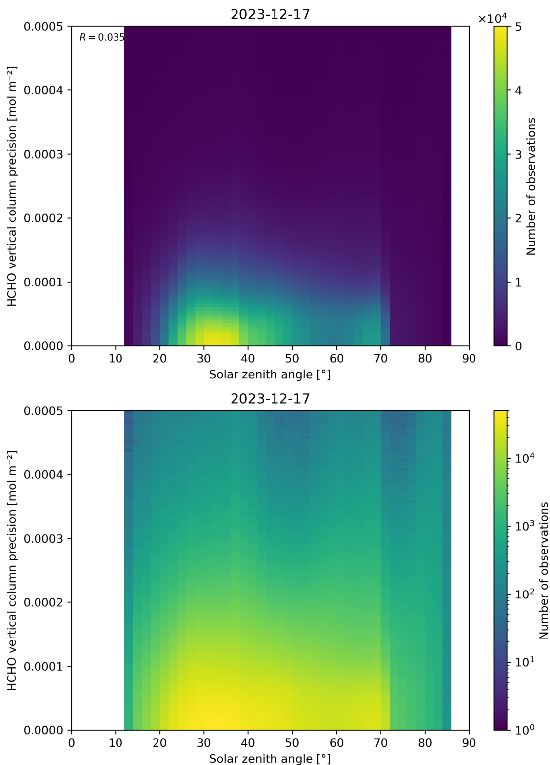
Figure 179: Scatter density plot of “Solar zenith angle” against “HCHO vertical column precision” for 2023-12-16 to 2023-12-18.
