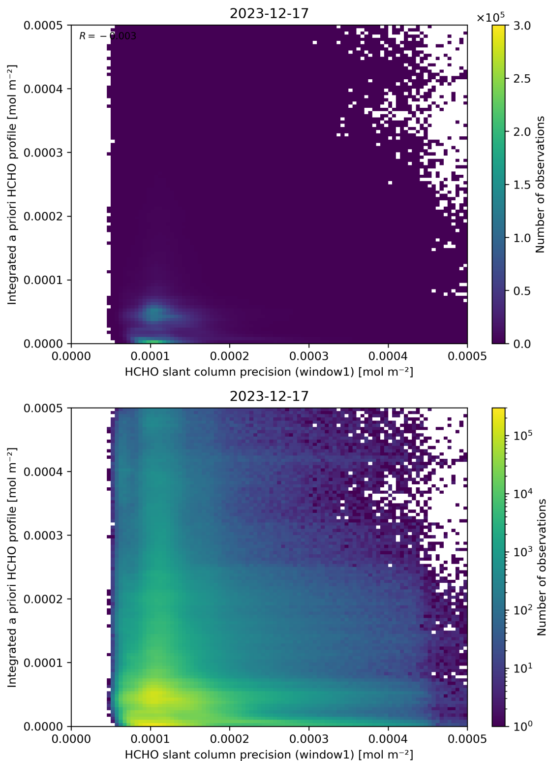
Figure 96: Scatter density plot of “HCHO slant column precision (window1)” against “Integrated a priori HCHO profile” for 2023-12-16 to 2023-12-18.
