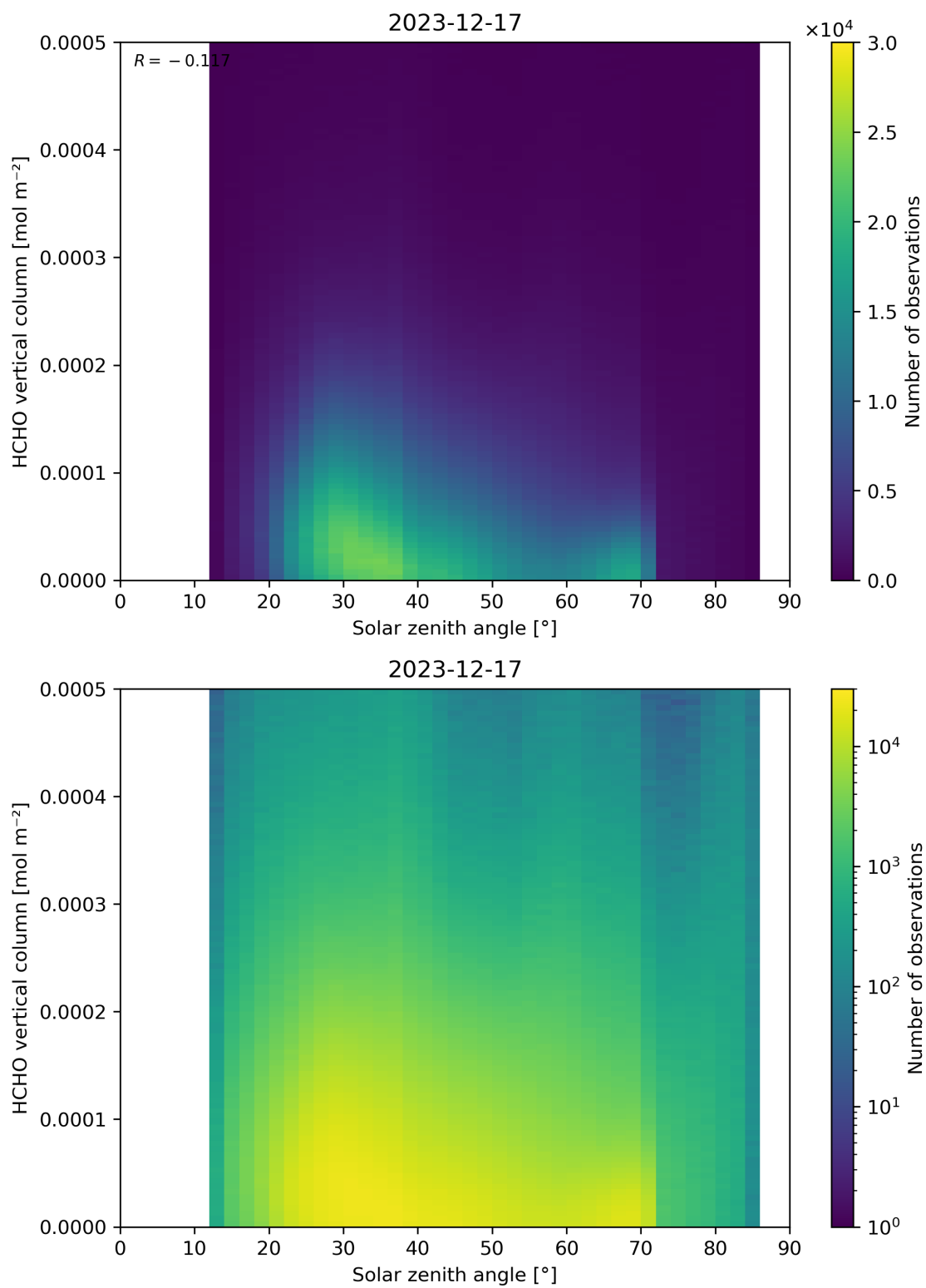
Figure 177: Scatter density plot of “Solar zenith angle” against “HCHO vertical column” for 2023-12-16 to 2023-12-18.
