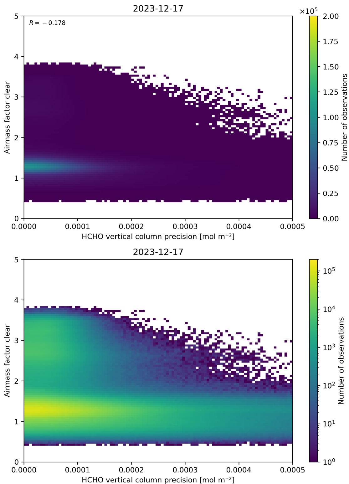
Figure 139: Scatter density plot of “HCHO vertical column precision” against “Airmass factor clear” for 2023-12-16 to 2023-12-18.
