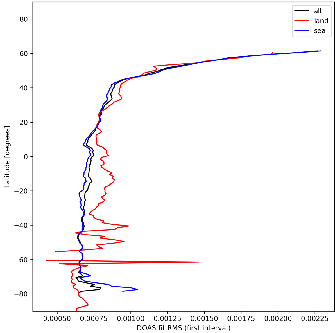
Figure 32: Zonal average of “DOAS fit RMS (first interval)” for 2023-12-16 to 2023-12-18.
