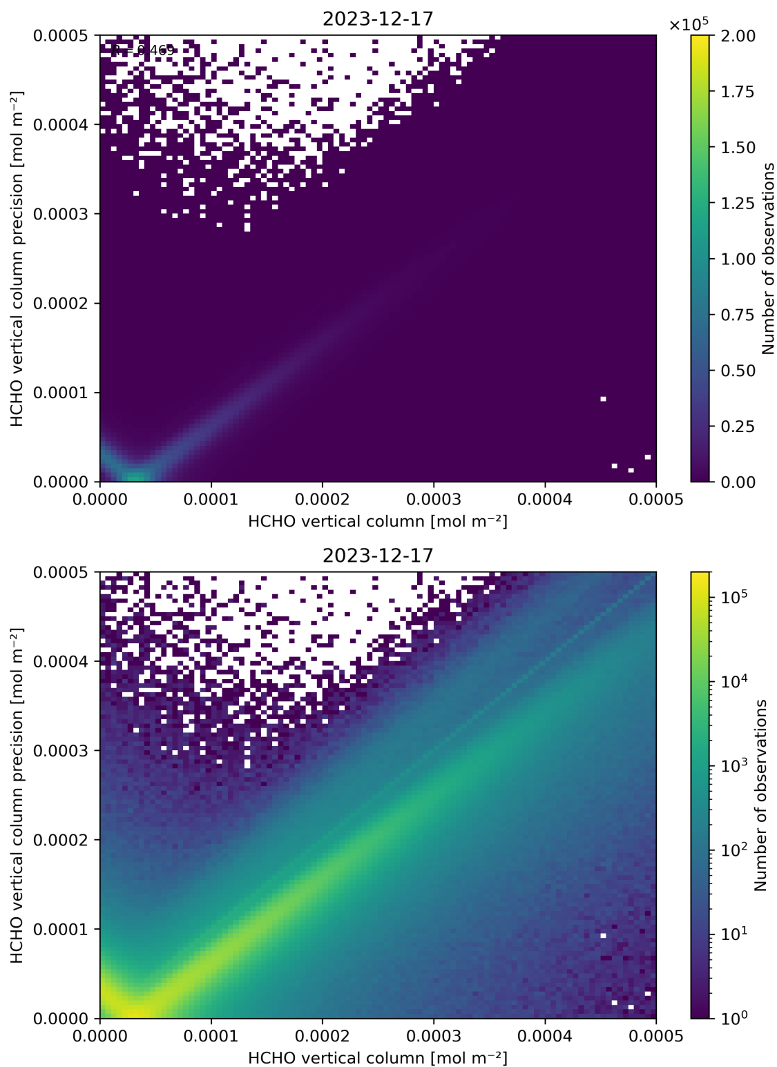
Figure 134: Scatter density plot of “HCHO vertical column” against “HCHO vertical column precision” for 2023-12-16 to 2023-12-18.
