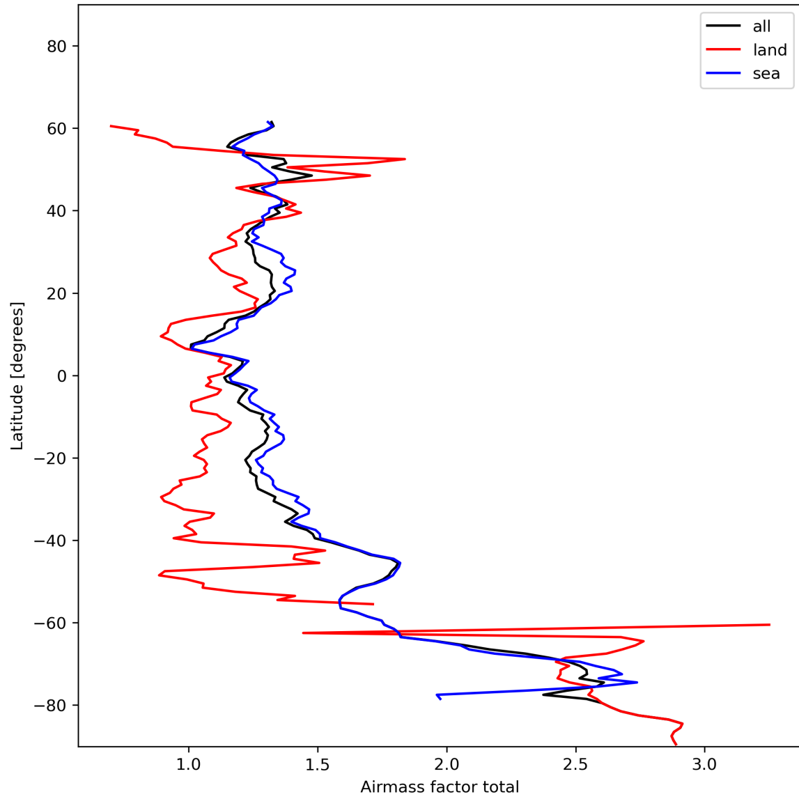
Figure 26: Zonal average of “Airmass factor total” for 2023-12-16 to 2023-12-18.
