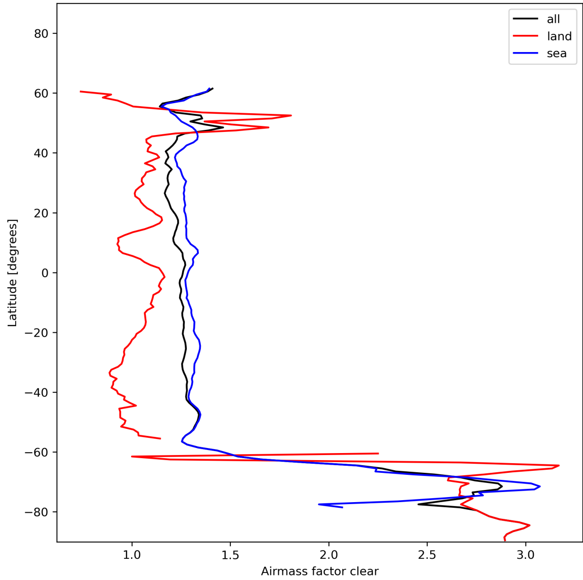
Figure 28: Zonal average of “Airmass factor clear” for 2023-12-16 to 2023-12-18.
