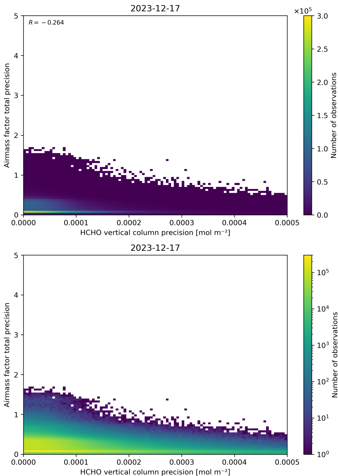
Figure 145: Scatter density plot of “HCHO vertical column precision” against “Airmass factor total precision” for 2023-12-16 to 2023-12-18.
