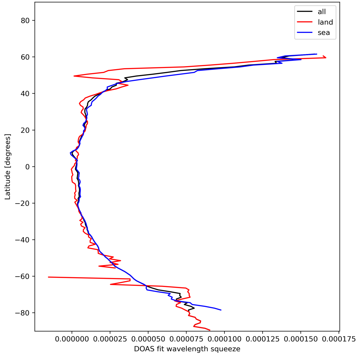
Figure 31: Zonal average of “DOAS fit wavelength squeeze” for 2023-12-16 to 2023-12-18.
