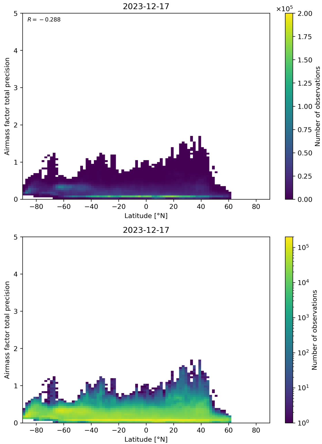
Figure 162: Scatter density plot of “Latitude” against “Airmass factor total precision” for 2023-12-16 to 2023-12-18.
