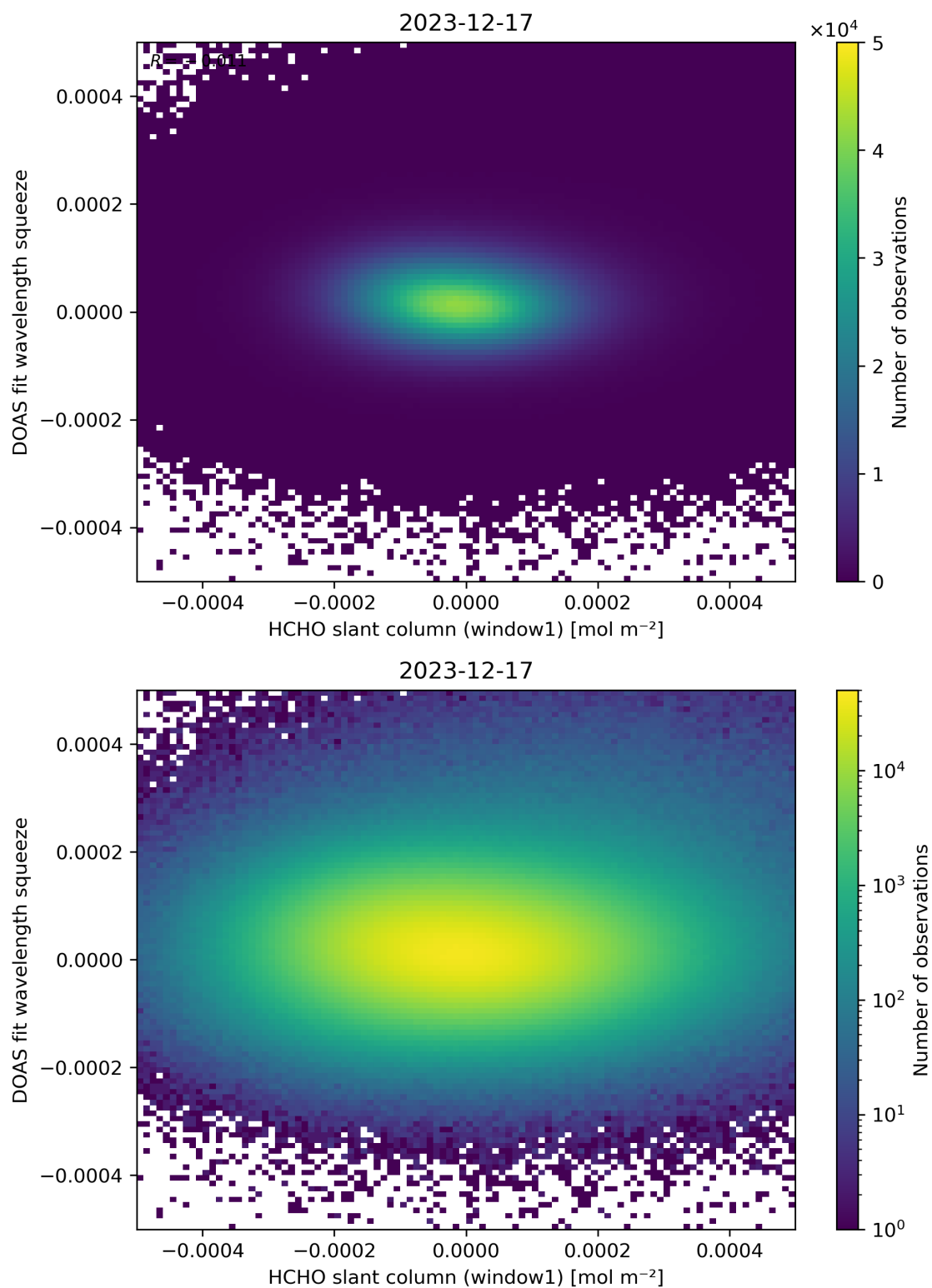
Figure 80: Scatter density plot of “HCHO slant column (window1)” against “DOAS fit wavelength squeeze” for 2023-12-16 to 2023-12-18.
