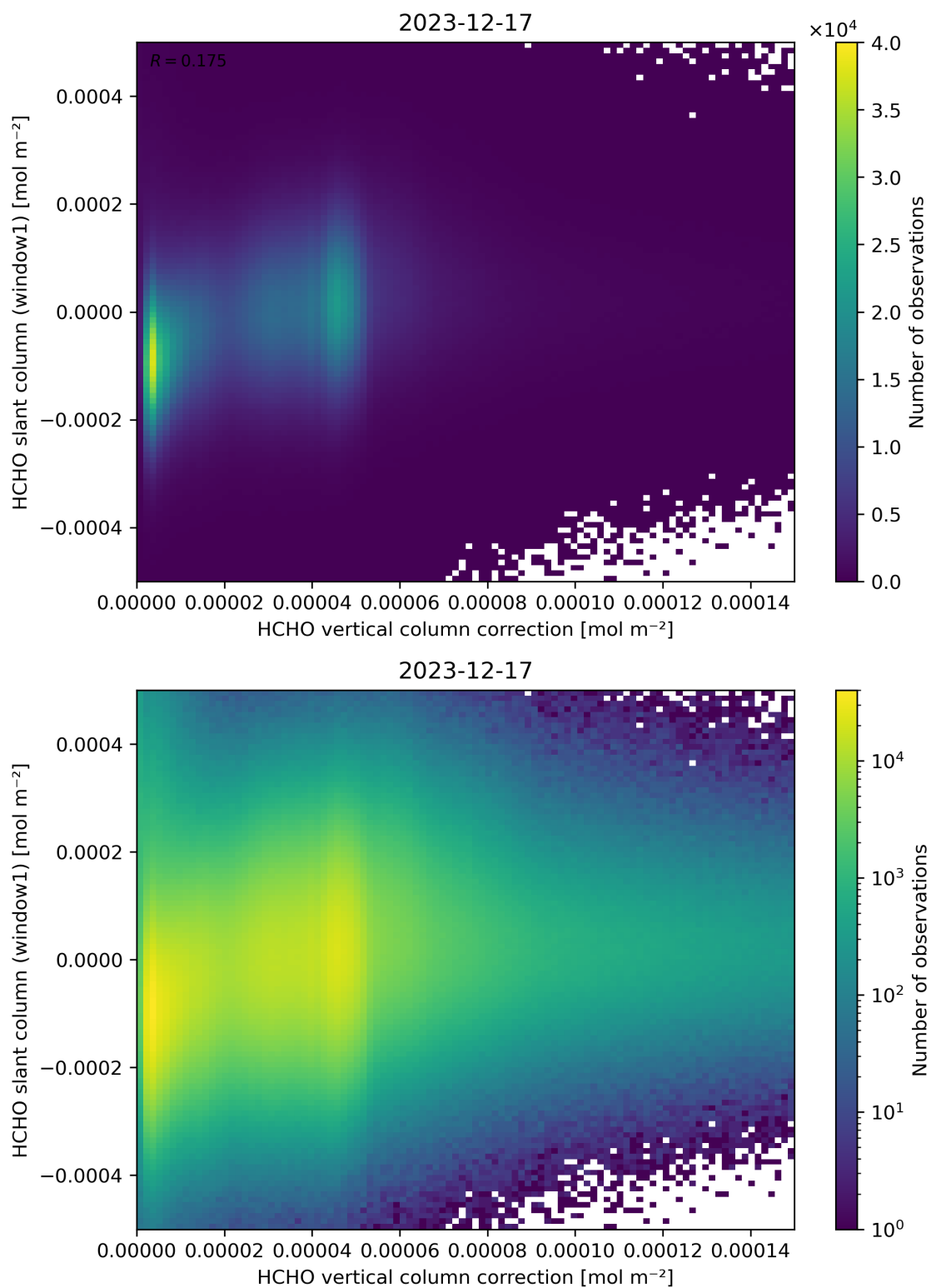
Figure 118: Scatter density plot of “HCHO vertical column correction” against “HCHO slant column (window1)” for 2023-12-16 to 2023-12-18.
