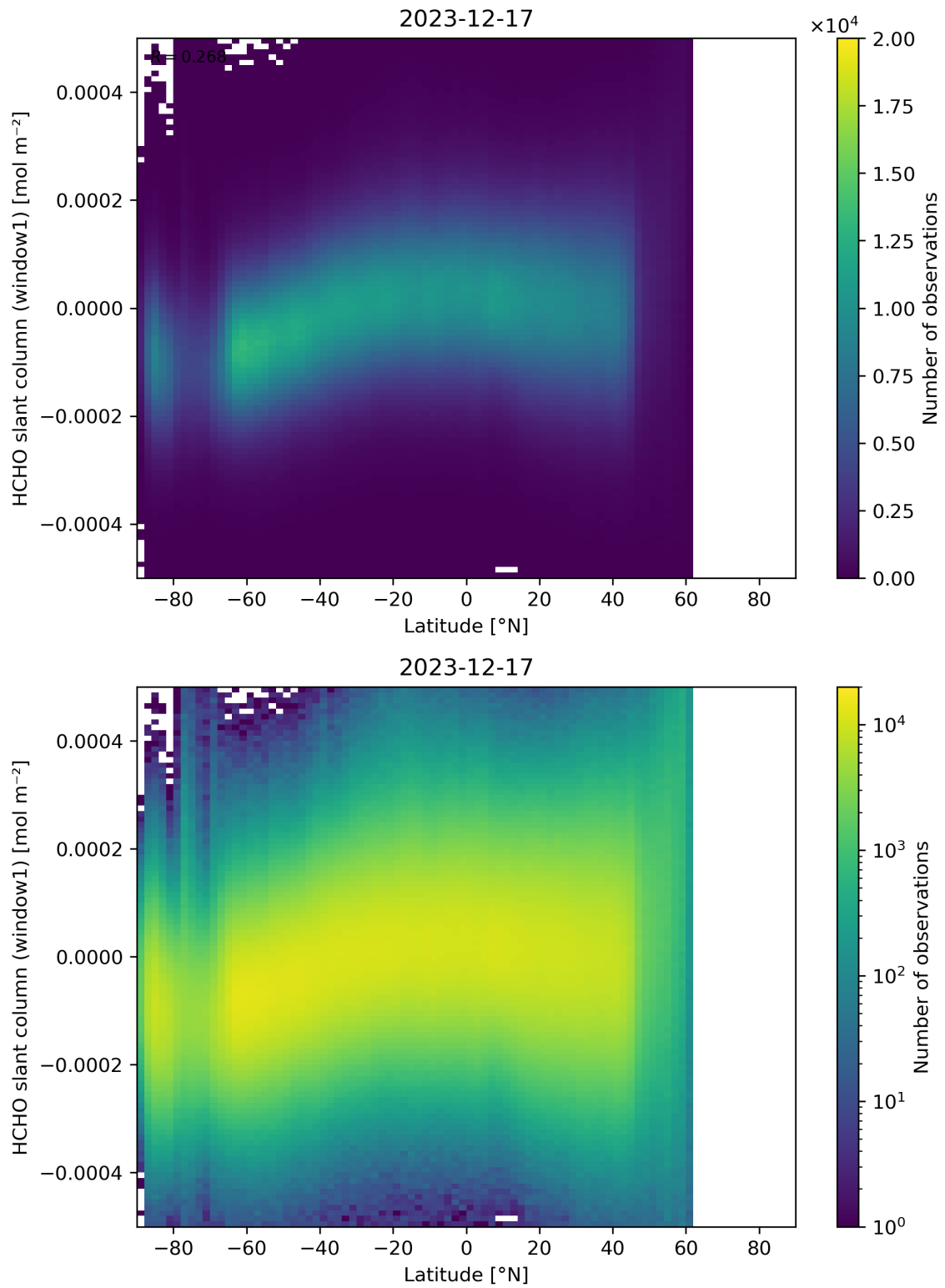
Figure 159: Scatter density plot of “Latitude” against “HCHO slant column (window1)” for 2023-12-16 to 2023-12-18.
