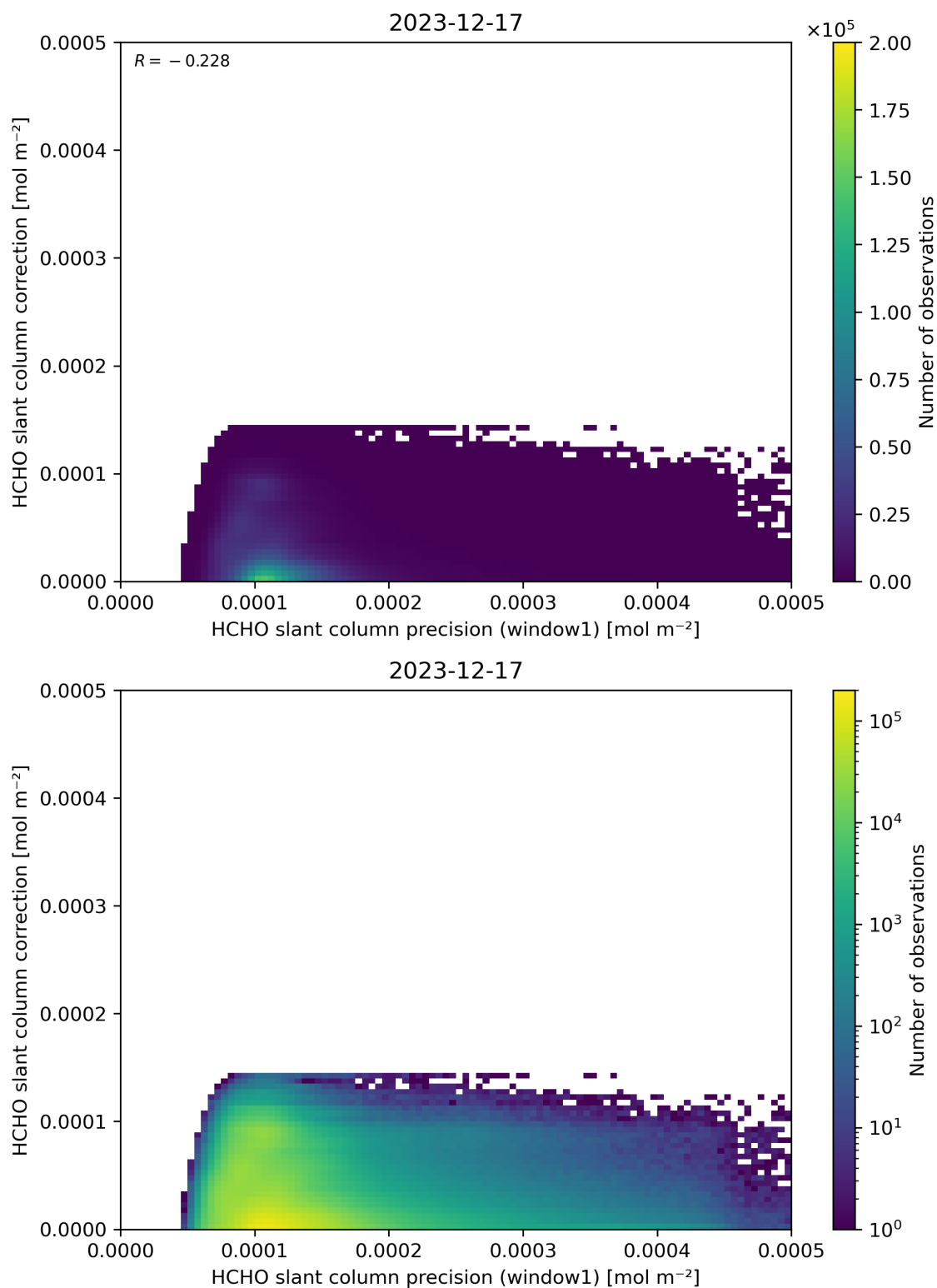
Figure 93: Scatter density plot of “HCHO slant column precision (window1)” against “HCHO slant column correction” for 2023-12-16 to 2023-12-18.
