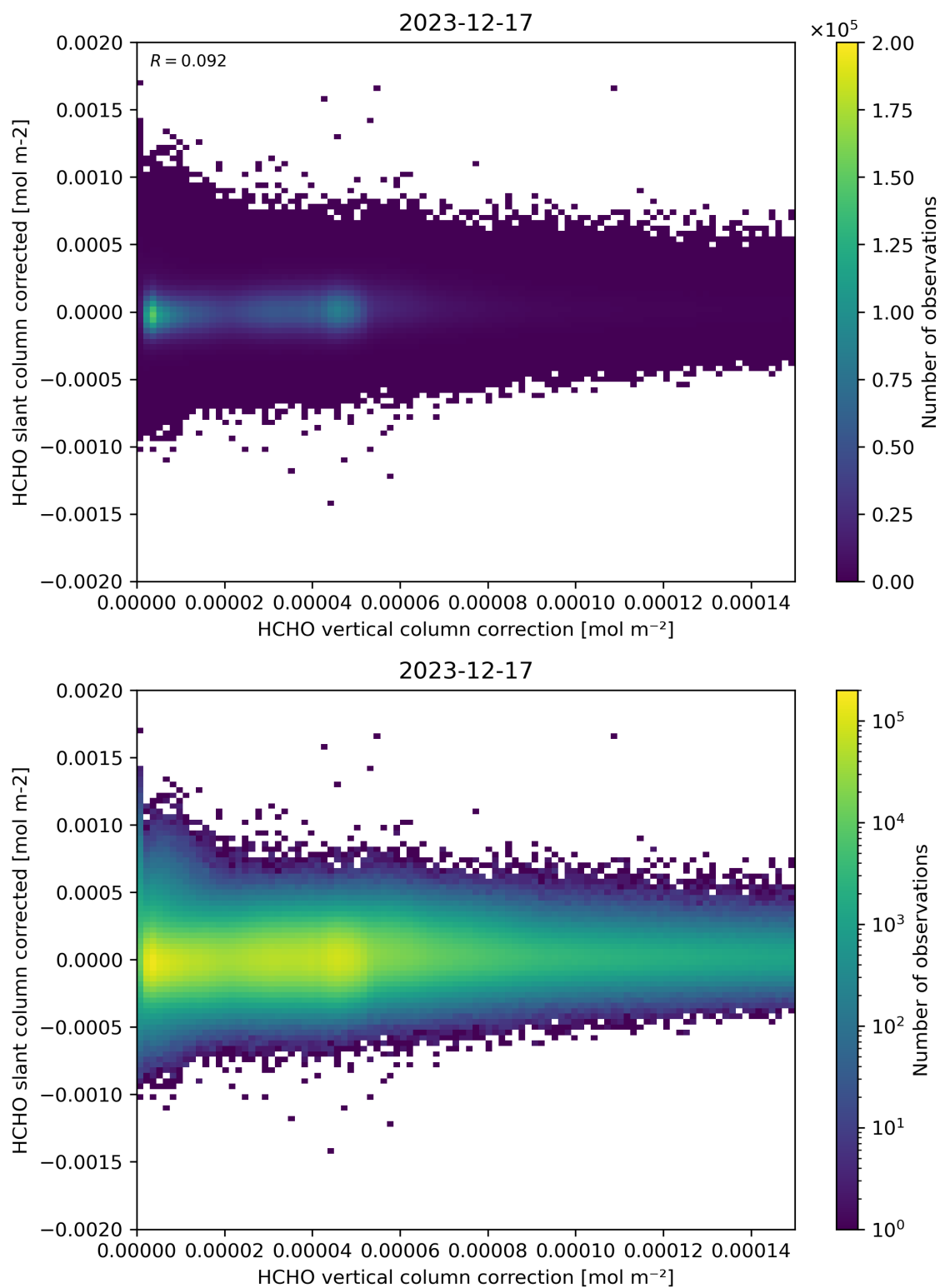
Figure 116: Scatter density plot of “HCHO vertical column correction” against “HCHO slant column corrected” for 2023-12-16 to 2023-12-18.
