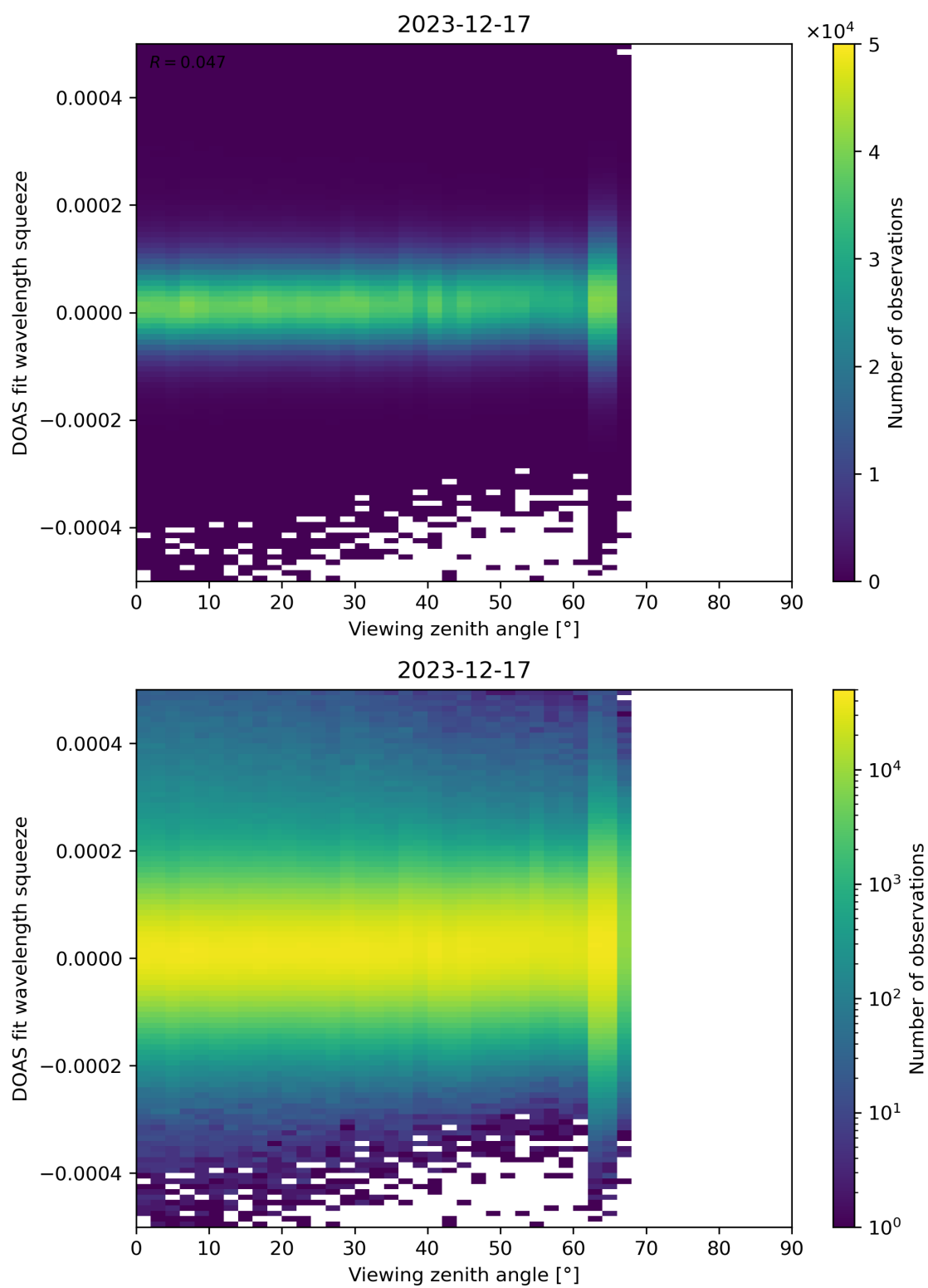
Figure 184: Scatter density plot of “Viewing zenith angle” against “DOAS fit wavelength squeeze” for 2023-12-16 to 2023-12-18.
