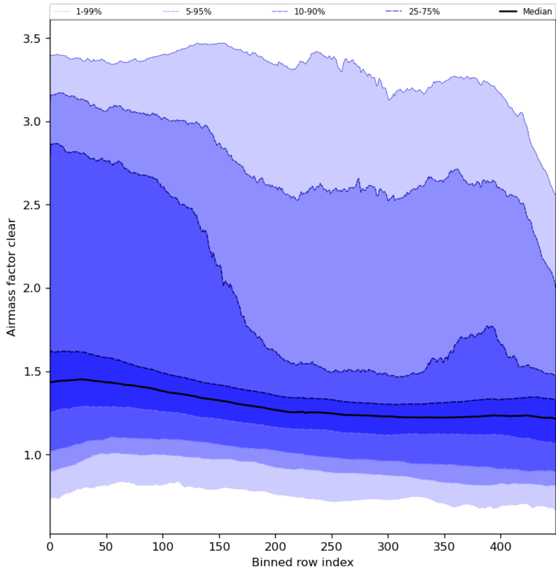
Figure 56: Along track statistics of “Airmass factor clear” for 2023-12-16 to 2023-12-18
