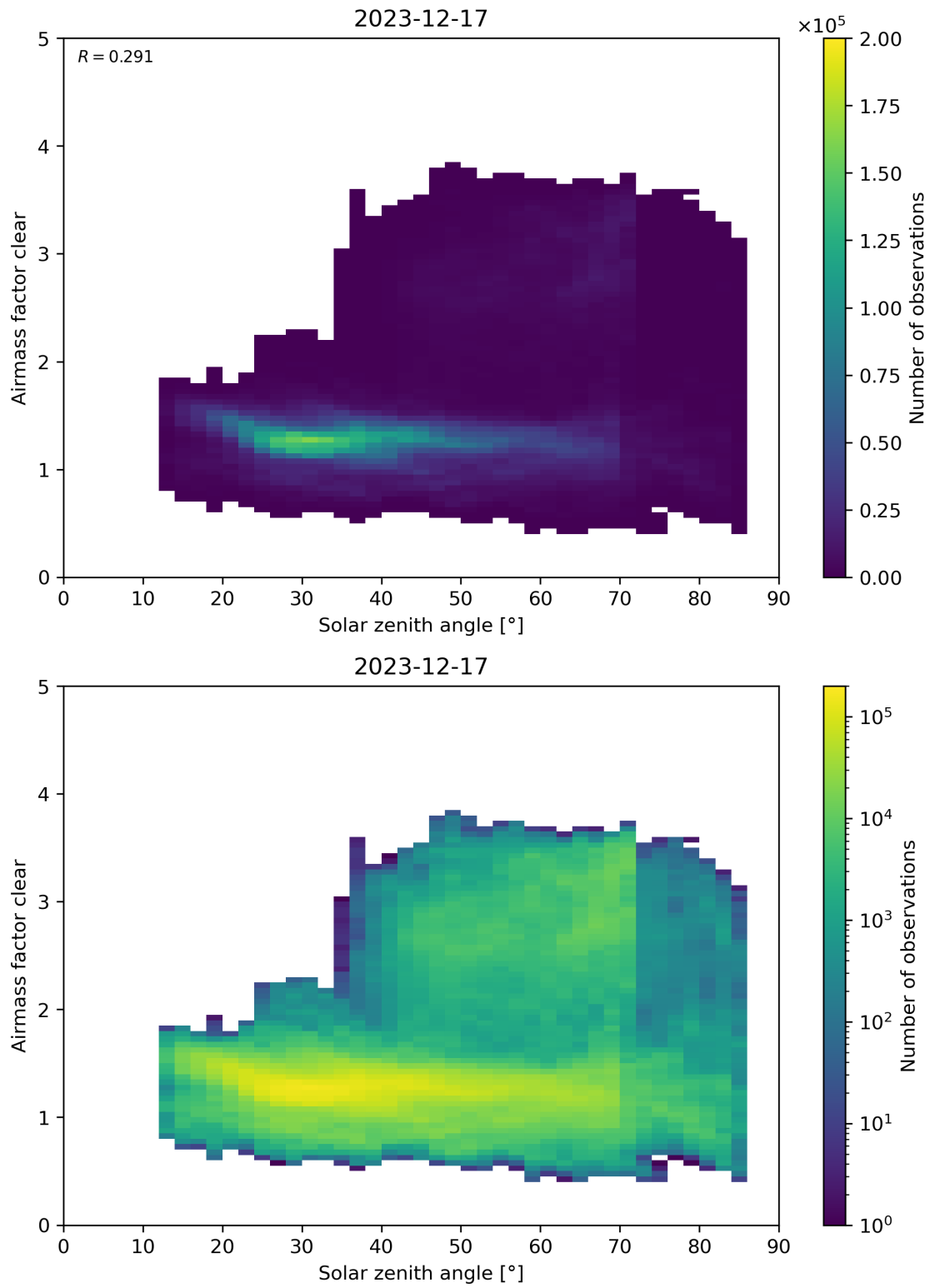
Figure 170: Scatter density plot of “Solar zenith angle” against “Airmass factor clear” for 2023-12-16 to 2023-12-18.
