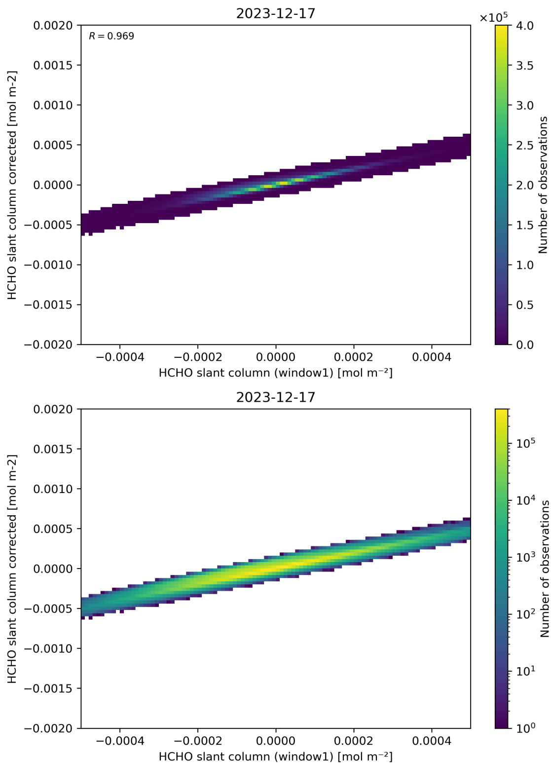
Figure 82: Scatter density plot of “HCHO slant column (window1)” against “HCHO slant column corrected” for 2023-12-16 to 2023-12-18.
