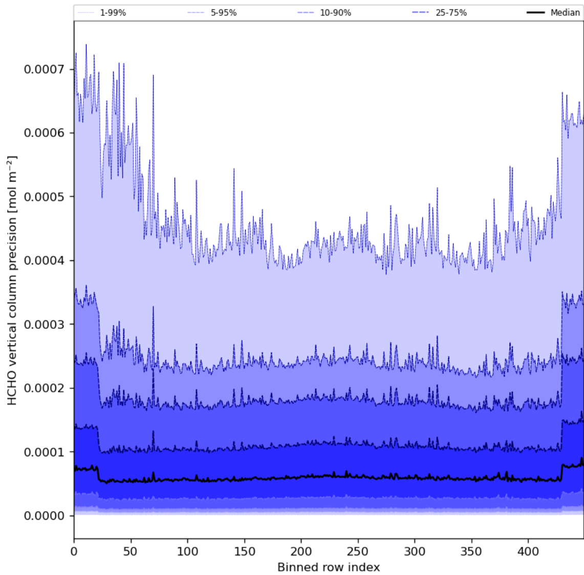
Figure 50: Along track statistics of “HCHO vertical column precision” for 2023-12-16 to 2023-12-18
