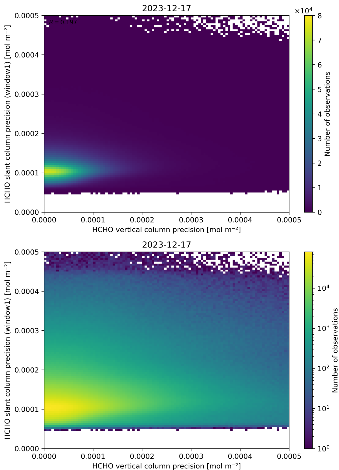
Figure 143: Scatter density plot of “HCHO vertical column precision” against “HCHO slant column precision (window1)” for 2023-12-16 to 2023-12-18.
