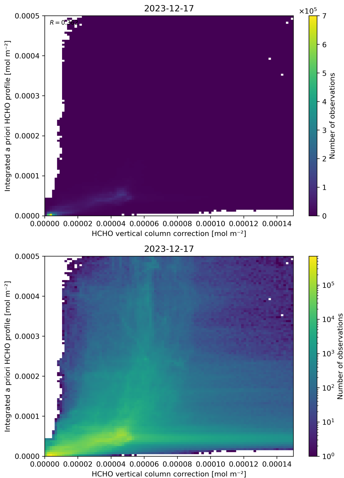
Figure 122: Scatter density plot of “HCHO vertical column correction” against “Integrated a priori HCHO profile” for 2023-12-16 to 2023-12-18.
