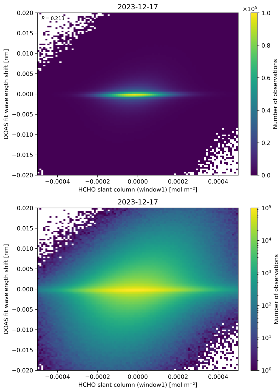
Figure 79: Scatter density plot of “HCHO slant column (window1)” against “DOAS fit wavelength shift” for 2023-12-16 to 2023-12-18.
