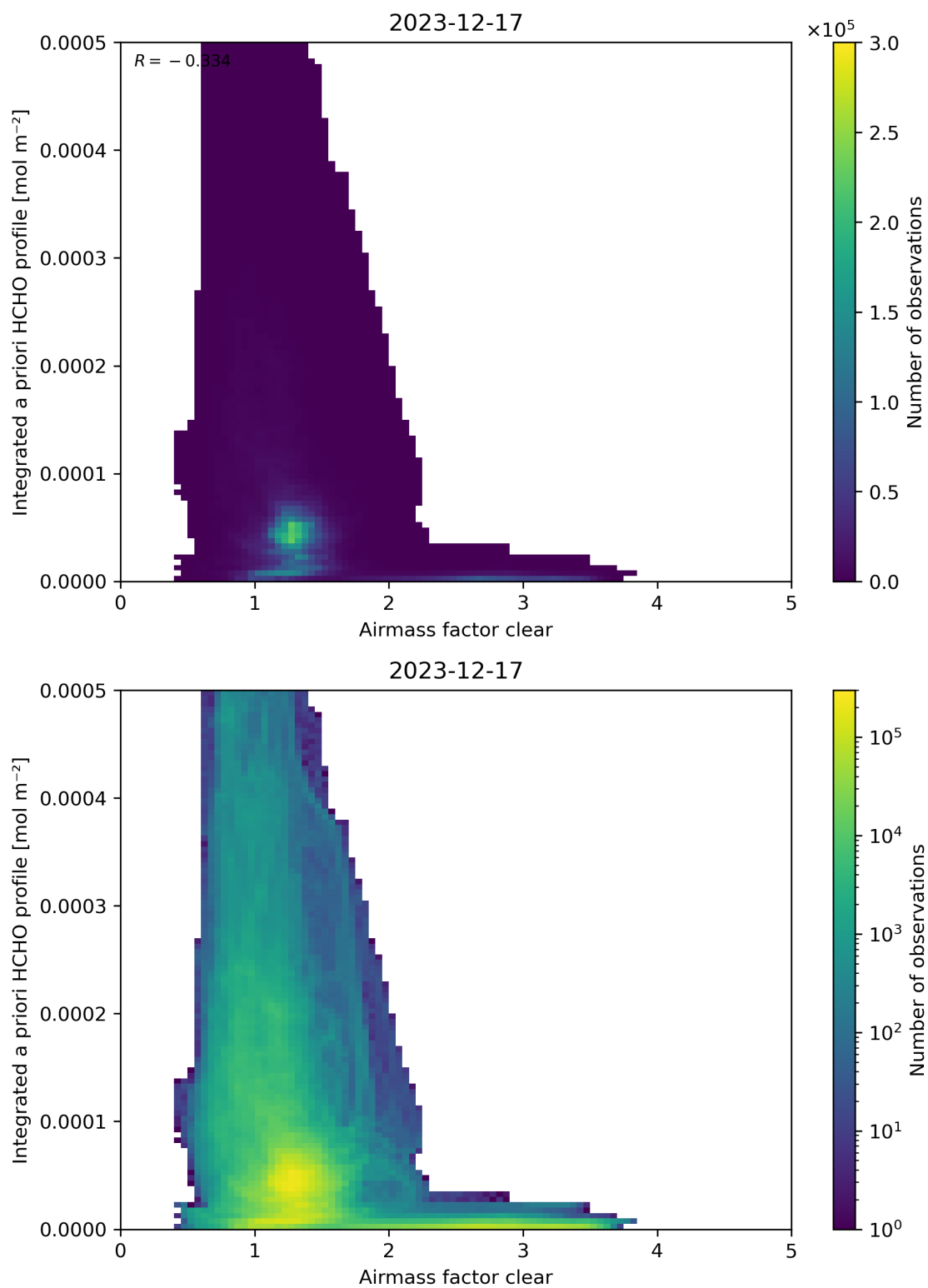
Figure 76: Scatter density plot of “Airmass factor clear” against “Integrated a priori HCHO profile” for 2023-12-16 to 2023-12-18.
