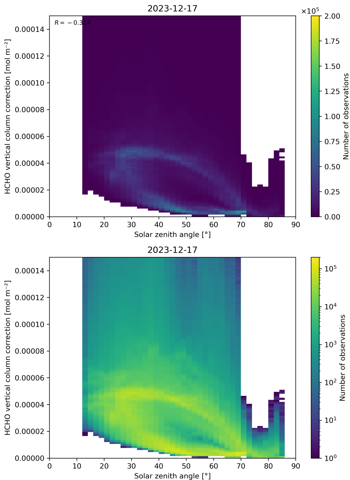
Figure 178: Scatter density plot of “Solar zenith angle” against “HCHO vertical column correction” for 2023-12-16 to 2023-12-18.
