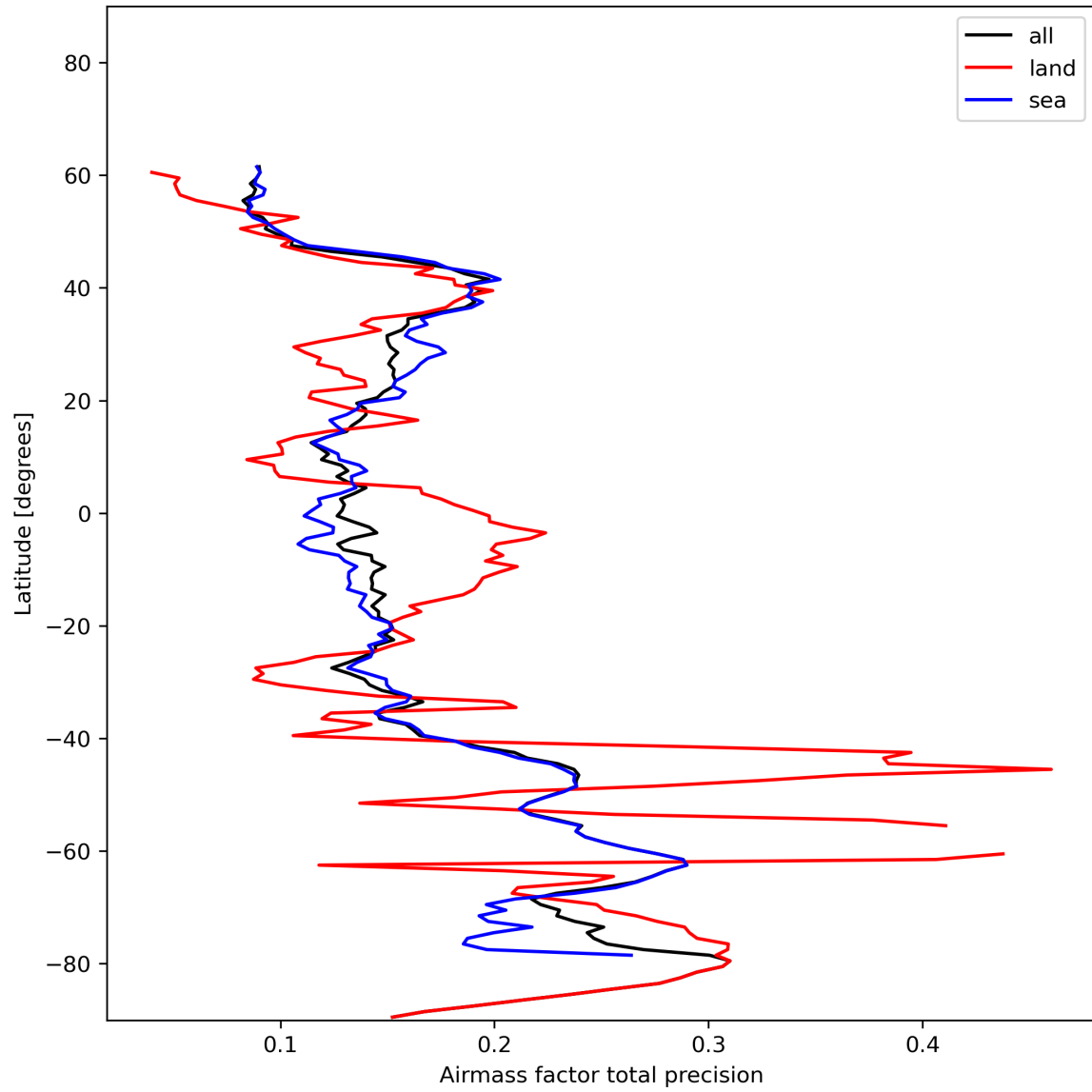
Figure 27: Zonal average of “Airmass factor total precision” for 2023-12-16 to 2023-12-18.
