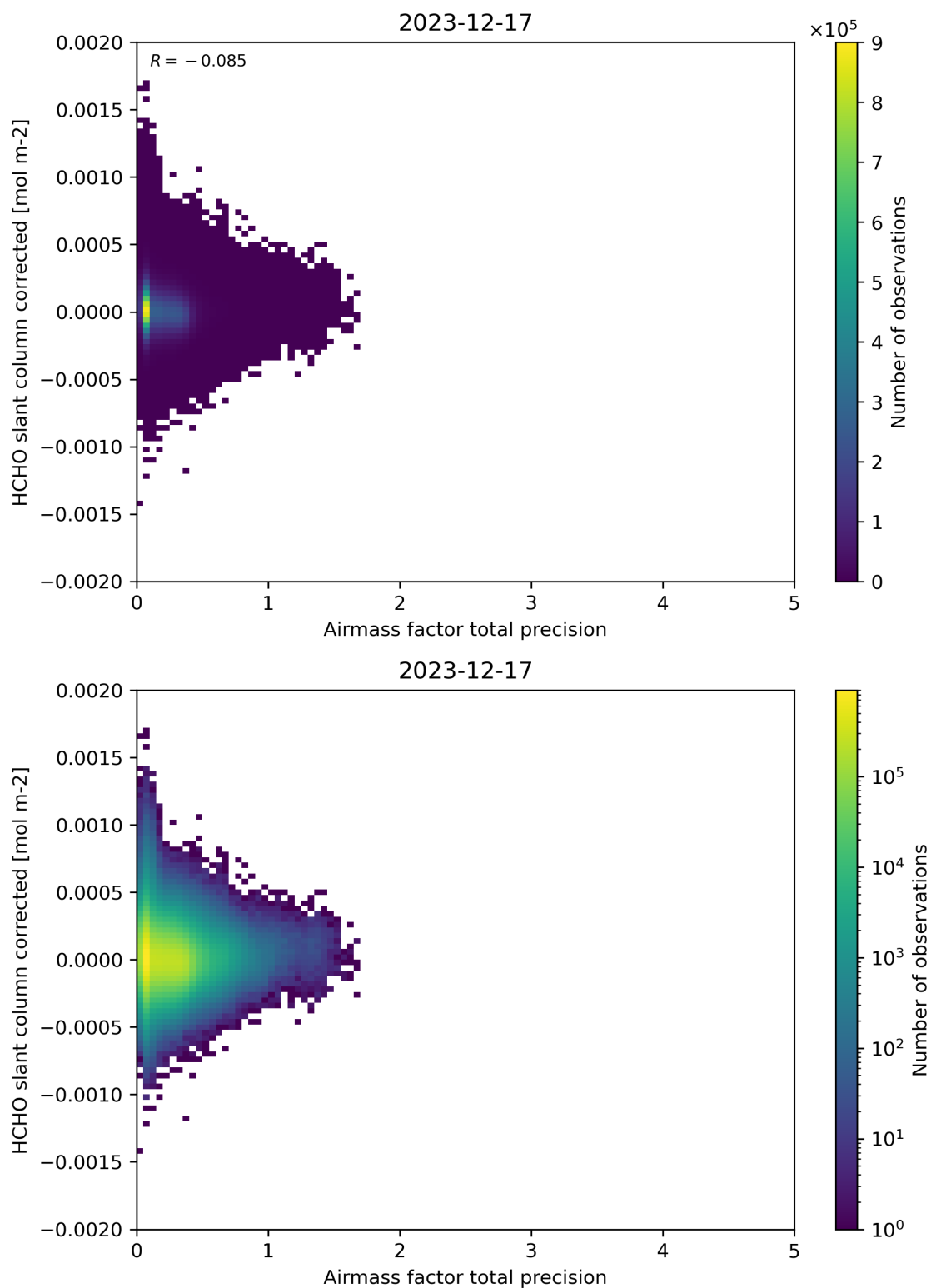
Figure 109: Scatter density plot of “Airmass factor total precision” against “HCHO slant column corrected” for 2023-12-16 to 2023-12-18.
