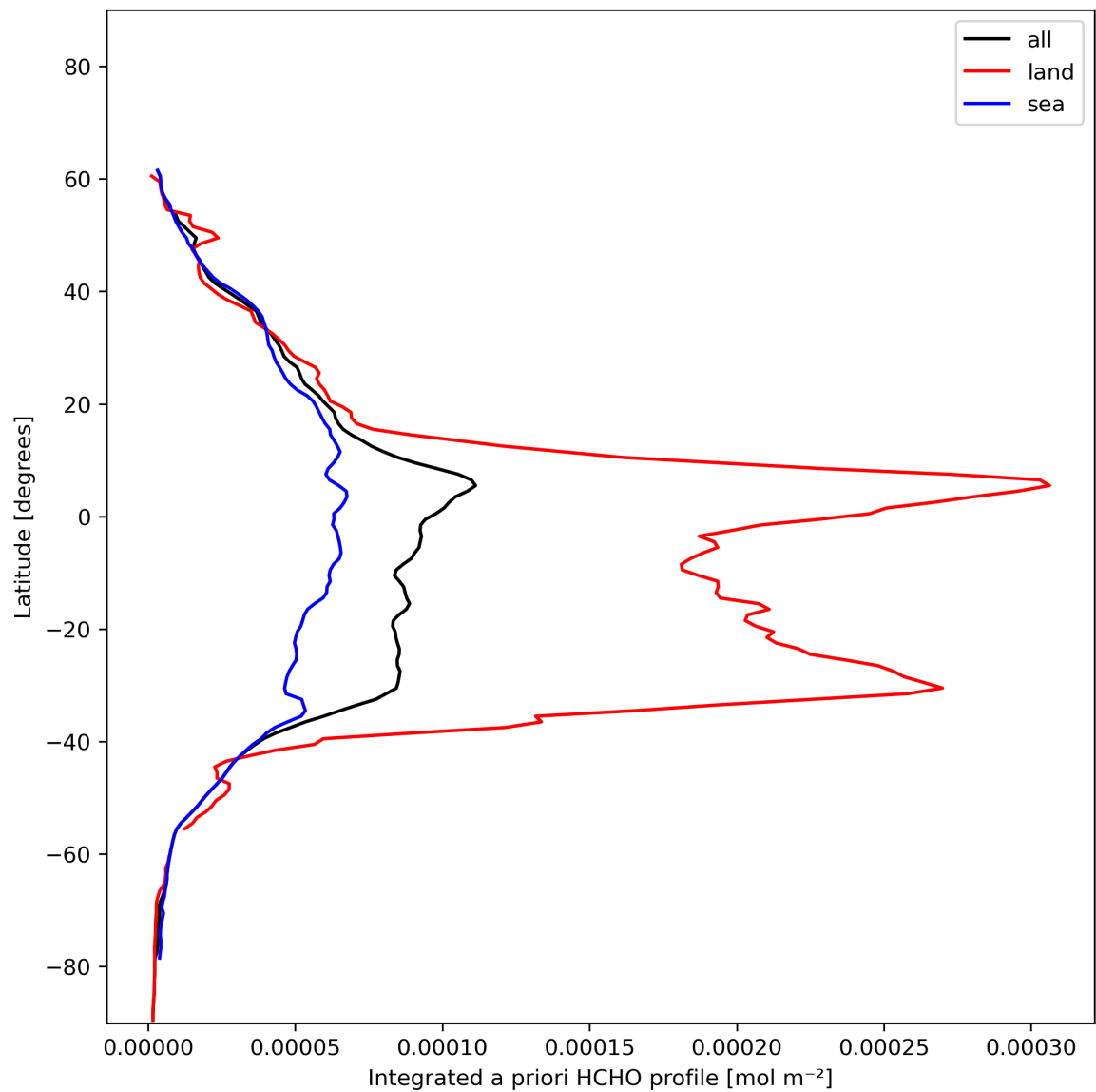
Figure 29: Zonal average of “Integrated a priori HCHO profile” for 2023-12-16 to 2023-12-18.
