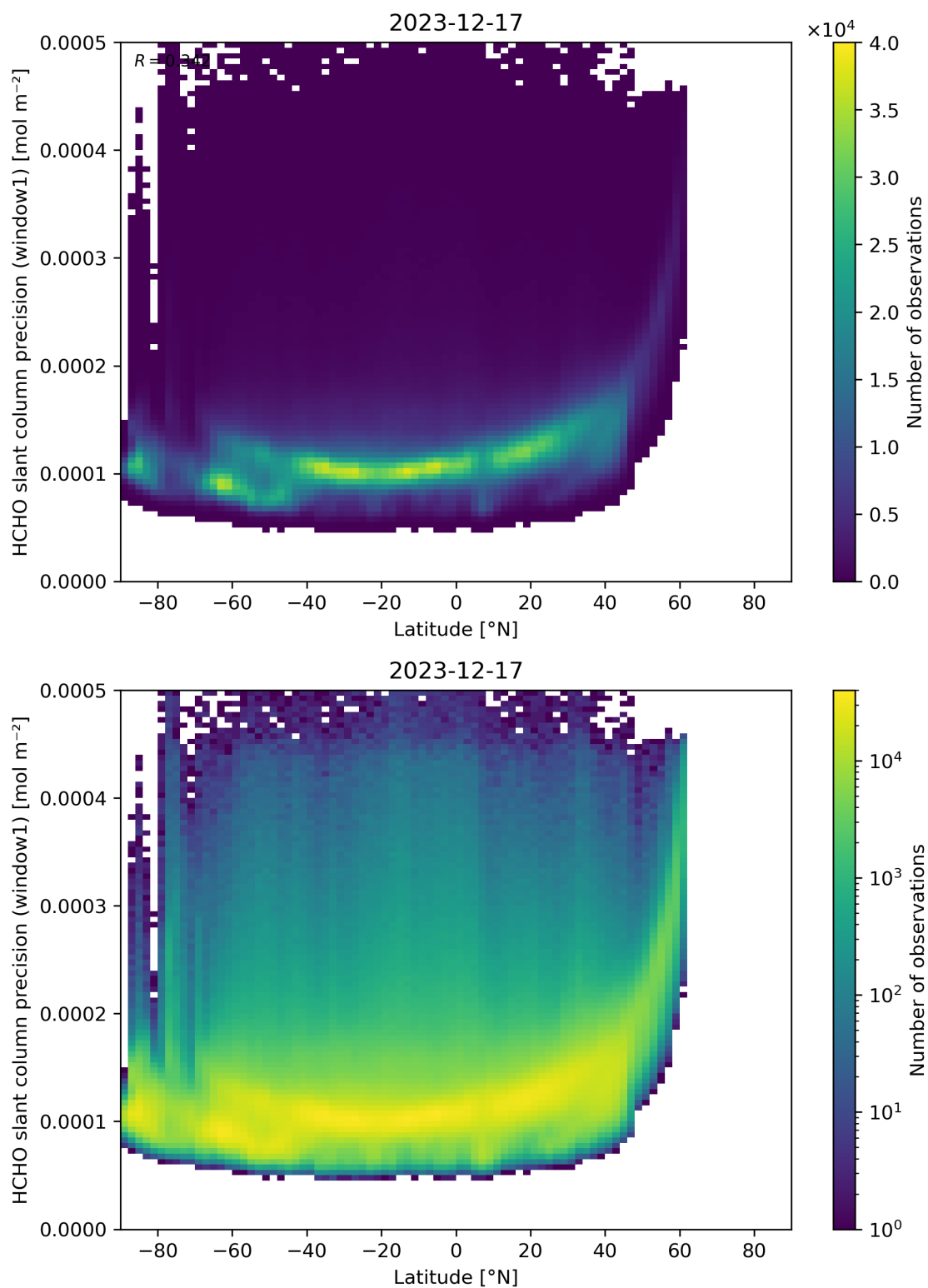
Figure 160: Scatter density plot of “Latitude” against “HCHO slant column precision (window1)” for 2023-12-16 to 2023-12-18.
