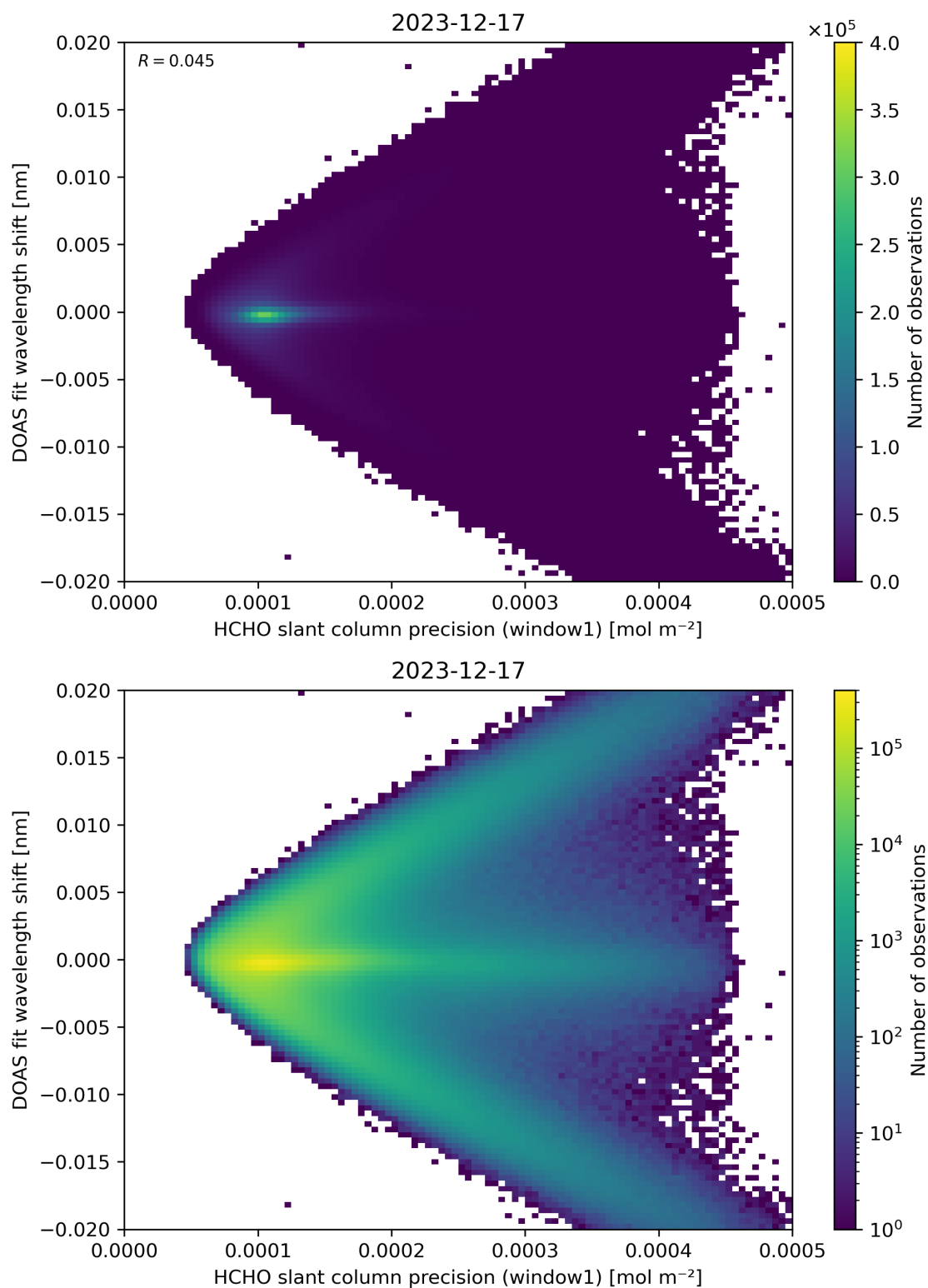
Figure 89: Scatter density plot of “HCHO slant column precision (window1)” against “DOAS fit wavelength shift” for 2023-12-16 to 2023-12-18.
