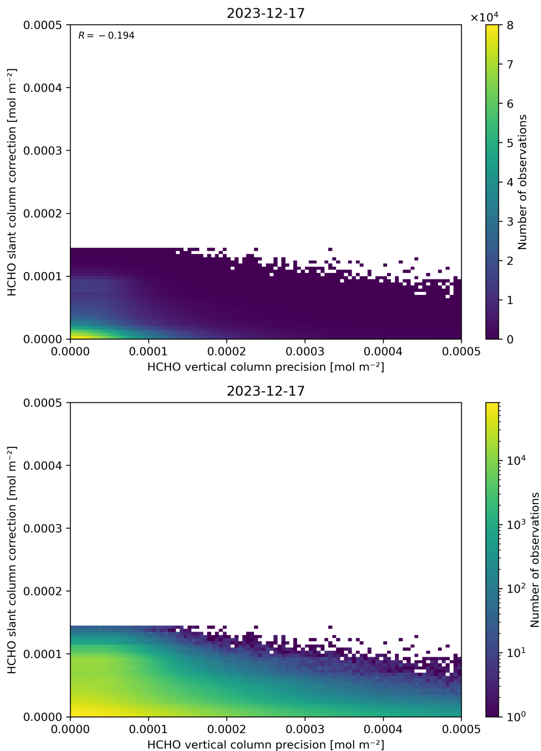
Figure 141: Scatter density plot of “HCHO vertical column precision” against “HCHO slant column correction” for 2023-12-16 to 2023-12-18.
