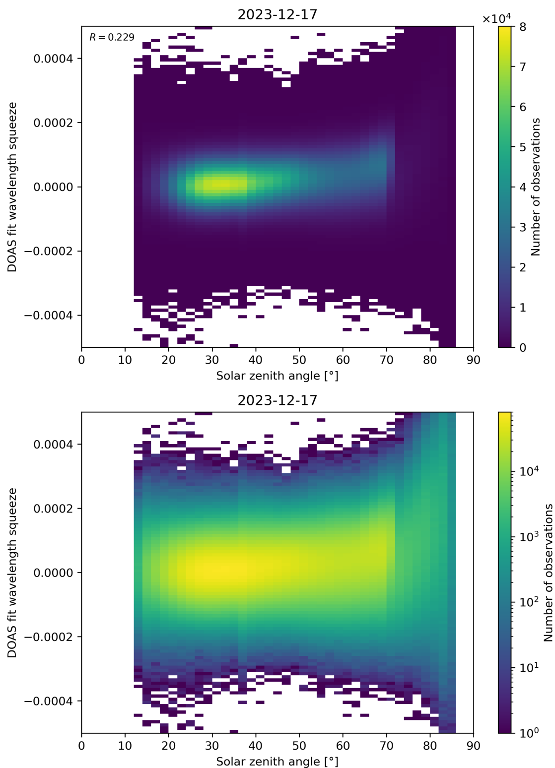
Figure 169: Scatter density plot of “Solar zenith angle” against “DOAS fit wavelength squeeze” for 2023-12-16 to 2023-12-18.
