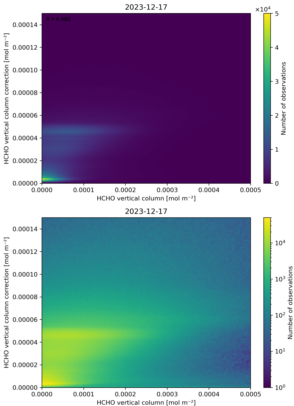
Figure 133: Scatter density plot of “HCHO vertical column” against “HCHO vertical column correction” for 2023-12-16 to 2023-12-18.
