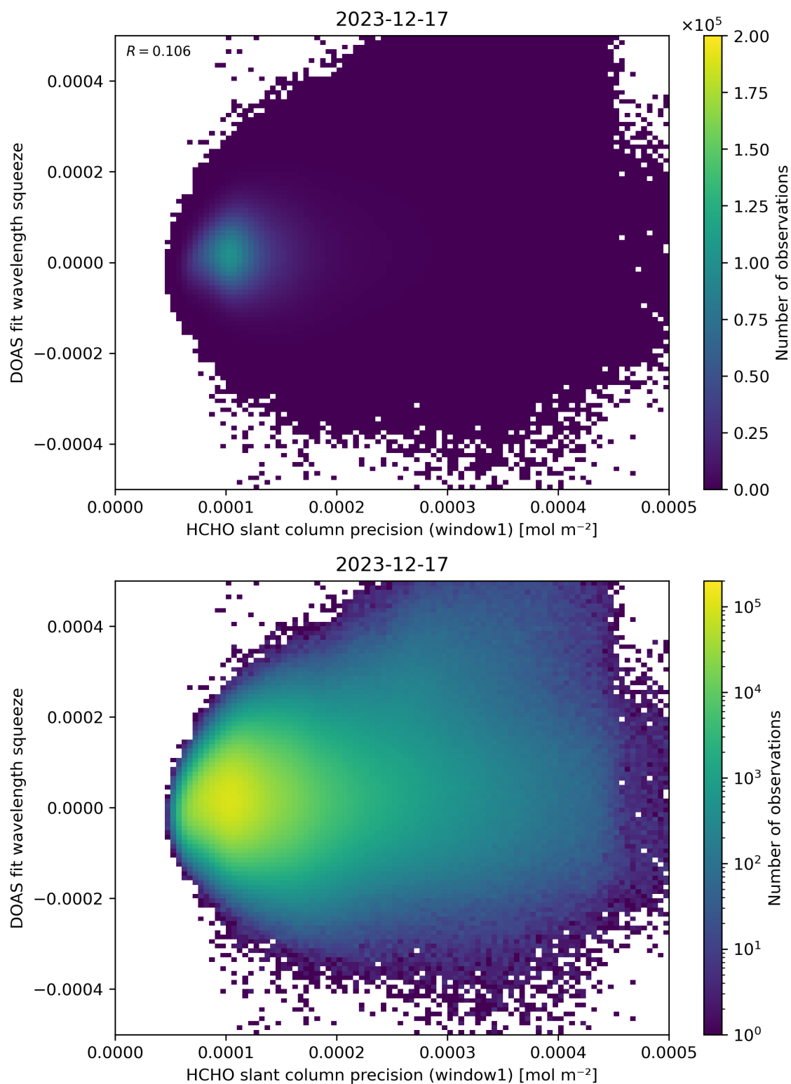
Figure 90: Scatter density plot of “HCHO slant column precision (window1)” against “DOAS fit wavelength squeeze” for 2023-12-16 to 2023-12-18.
