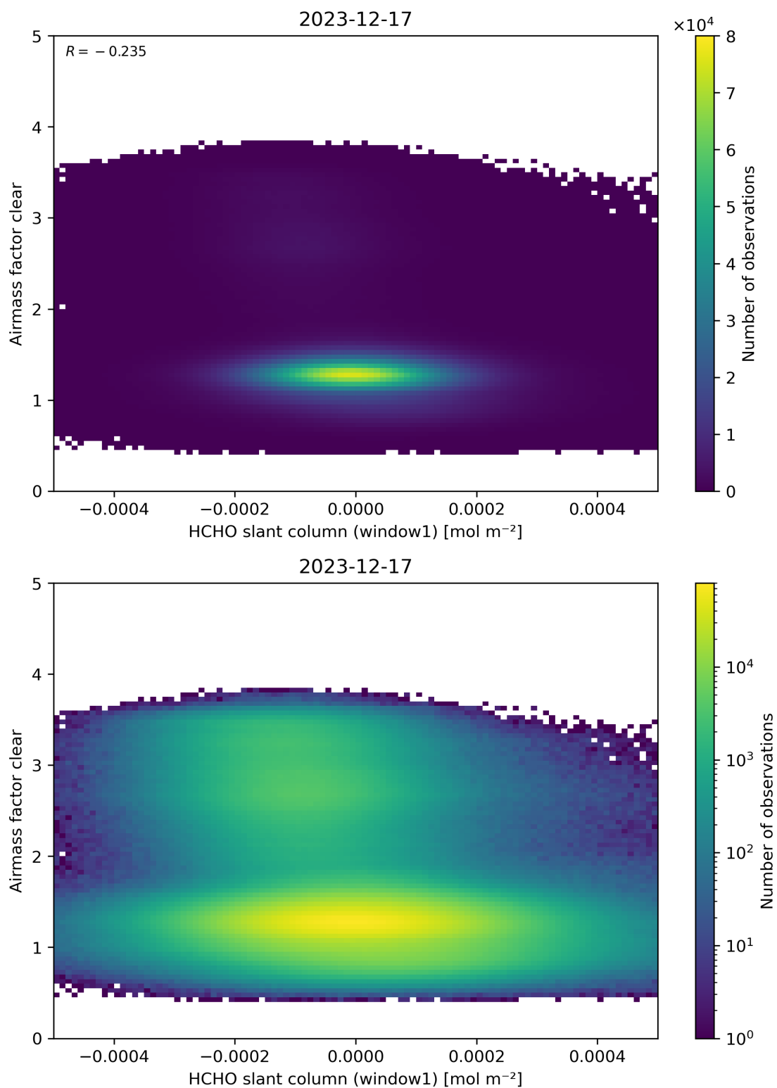
Figure 81: Scatter density plot of “HCHO slant column (window1)” against “Airmass factor clear” for 2023-12-16 to 2023-12-18.
