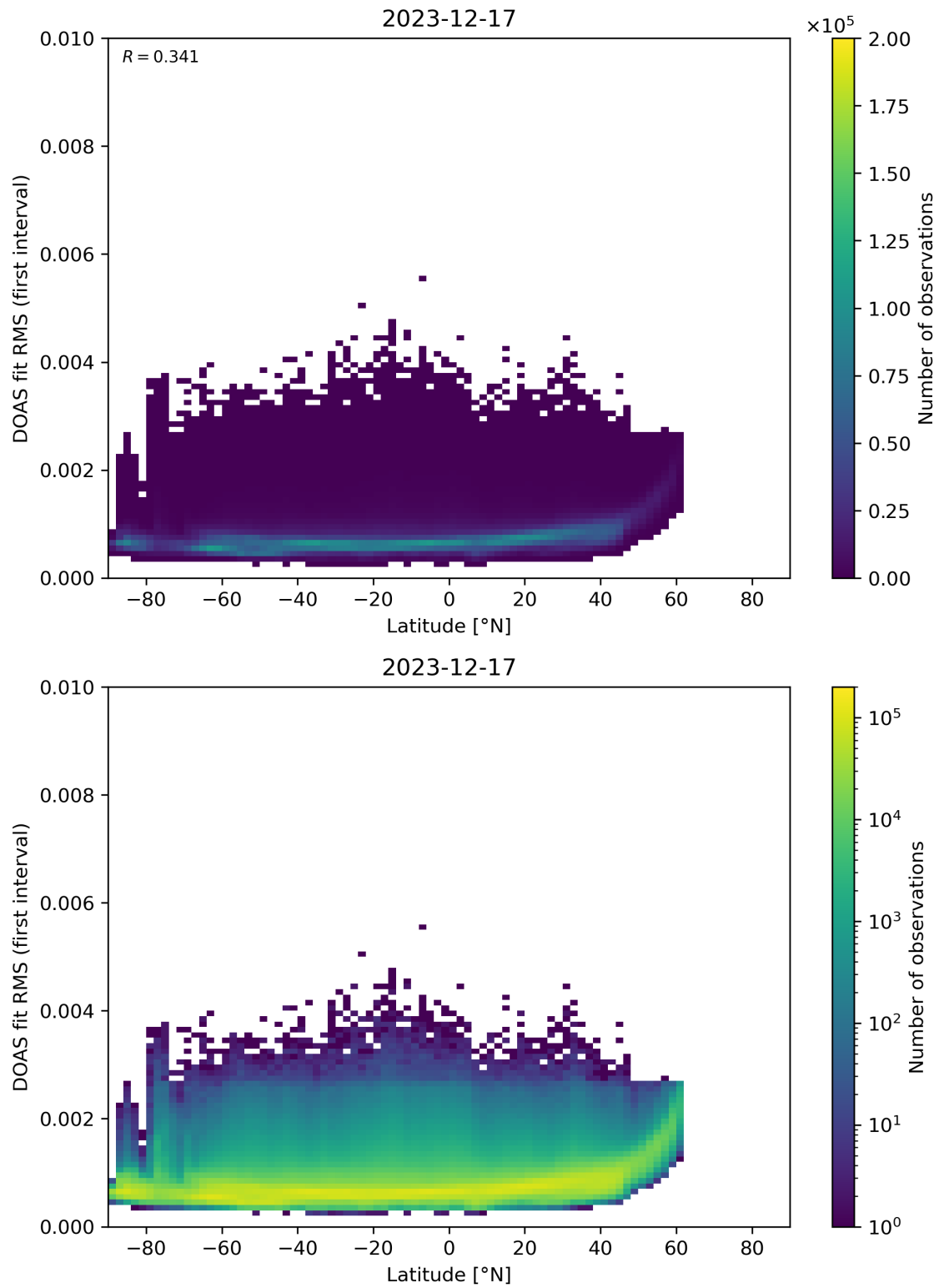
Figure 153: Scatter density plot of “Latitude” against “DOAS fit RMS (first interval)” for 2023-12-16 to 2023-12-18.
