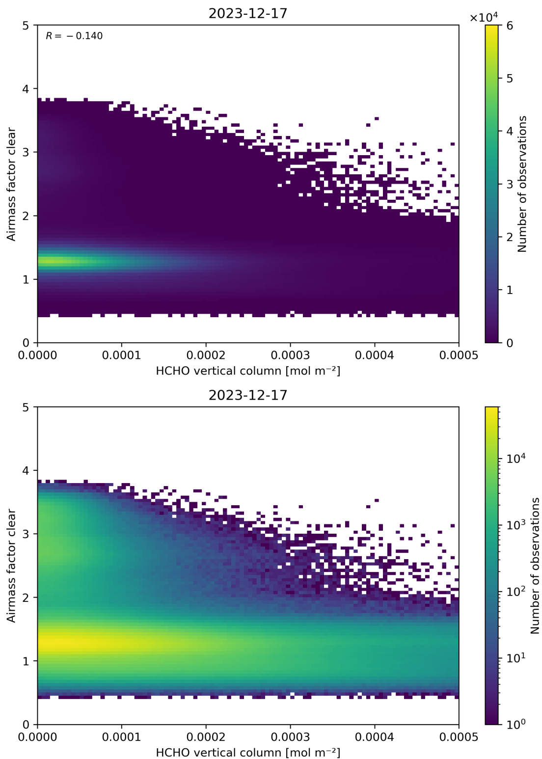
Figure 126: Scatter density plot of “HCHO vertical column” against “Airmass factor clear” for 2023-12-16 to 2023-12-18.
