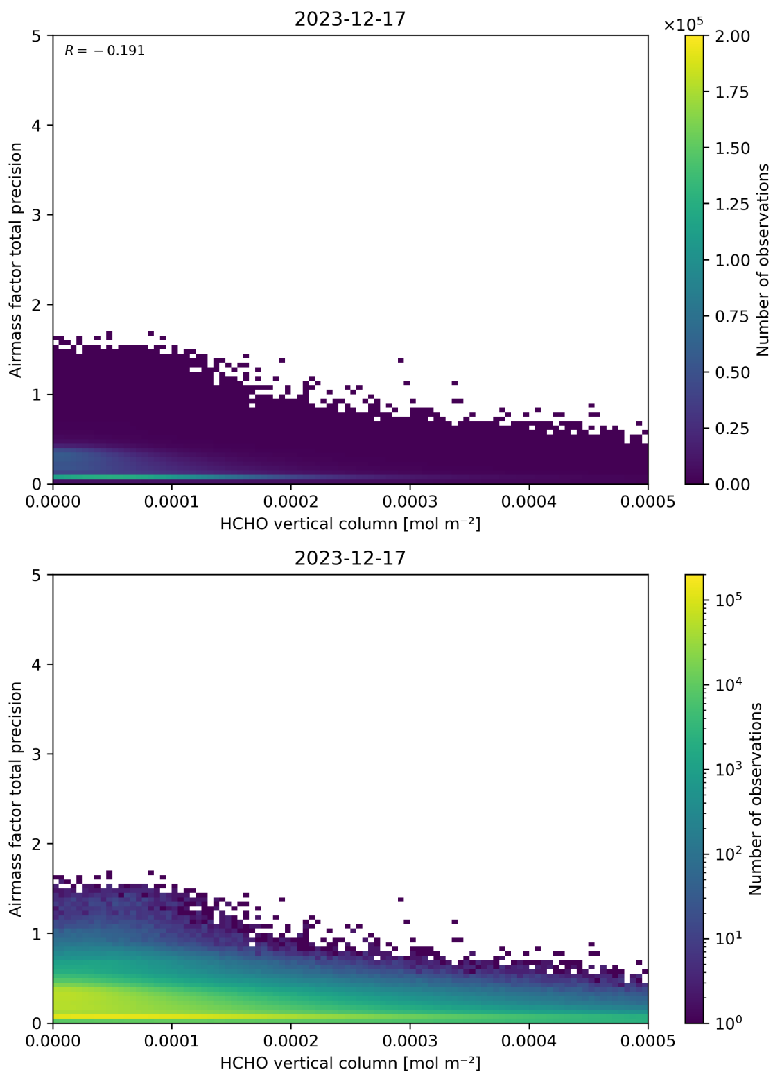
Figure 132: Scatter density plot of “HCHO vertical column” against “Airmass factor total precision” for 2023-12-16 to 2023-12-18.
