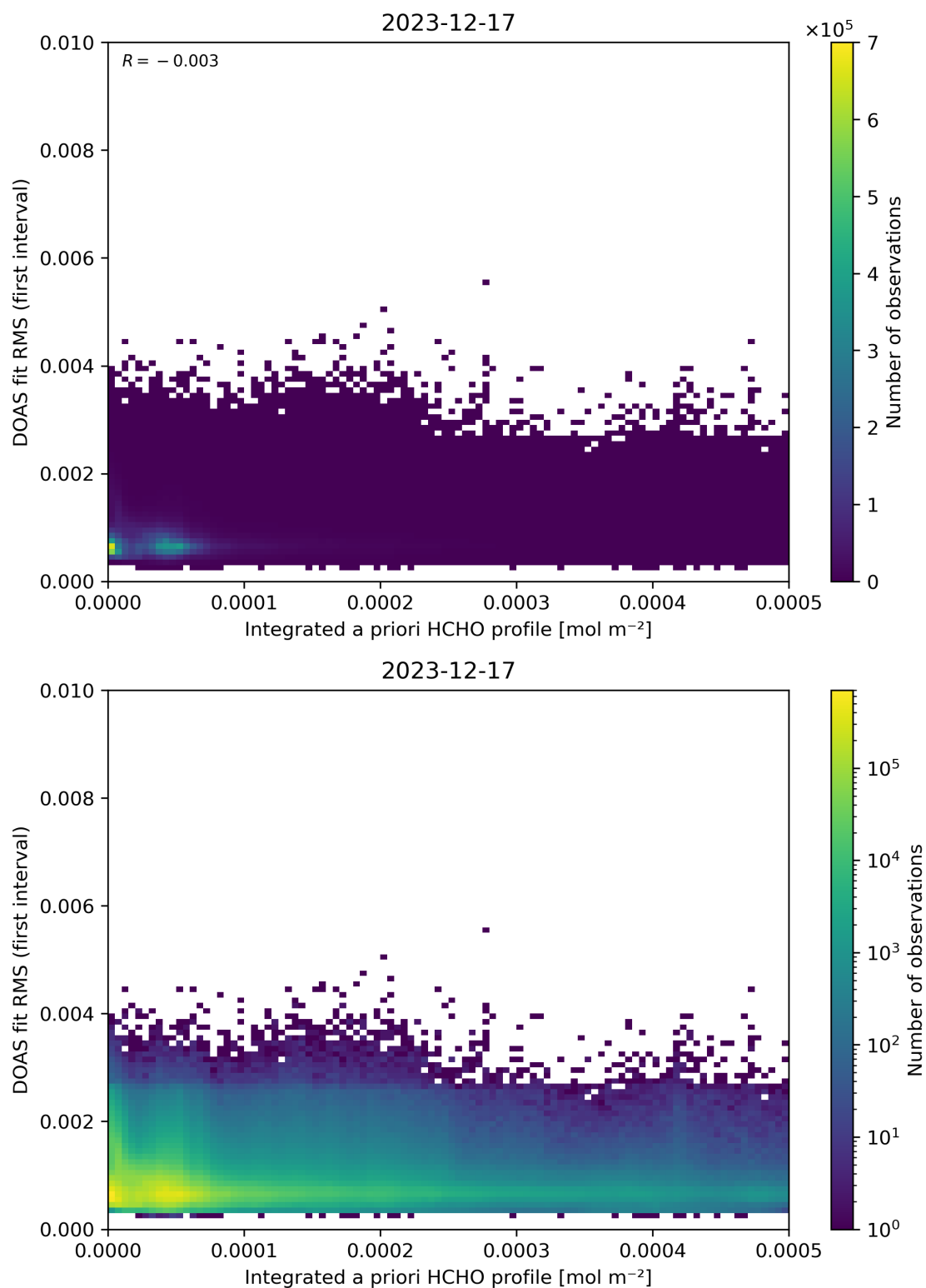
Figure 148: Scatter density plot of “Integrated a priori HCHO profile” against “DOAS fit RMS (first interval)” for 2023-12-16 to 2023-12-18.
