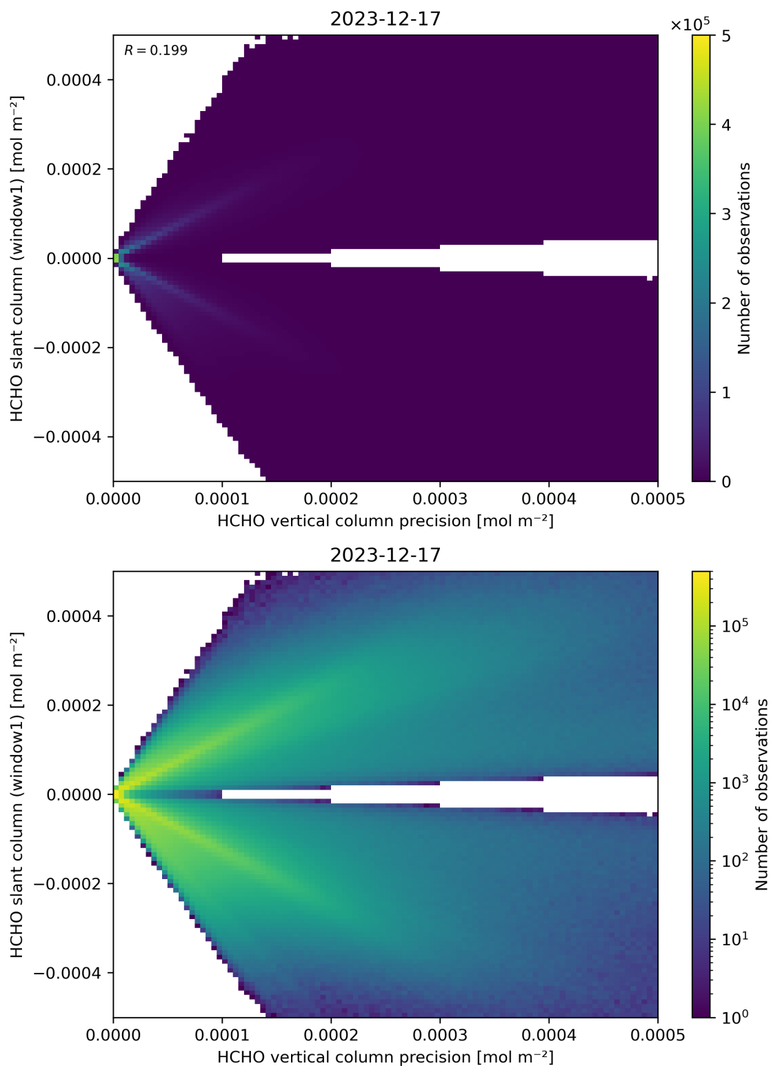
Figure 142: Scatter density plot of “HCHO vertical column precision” against “HCHO slant column (window1)” for 2023-12-16 to 2023-12-18.
