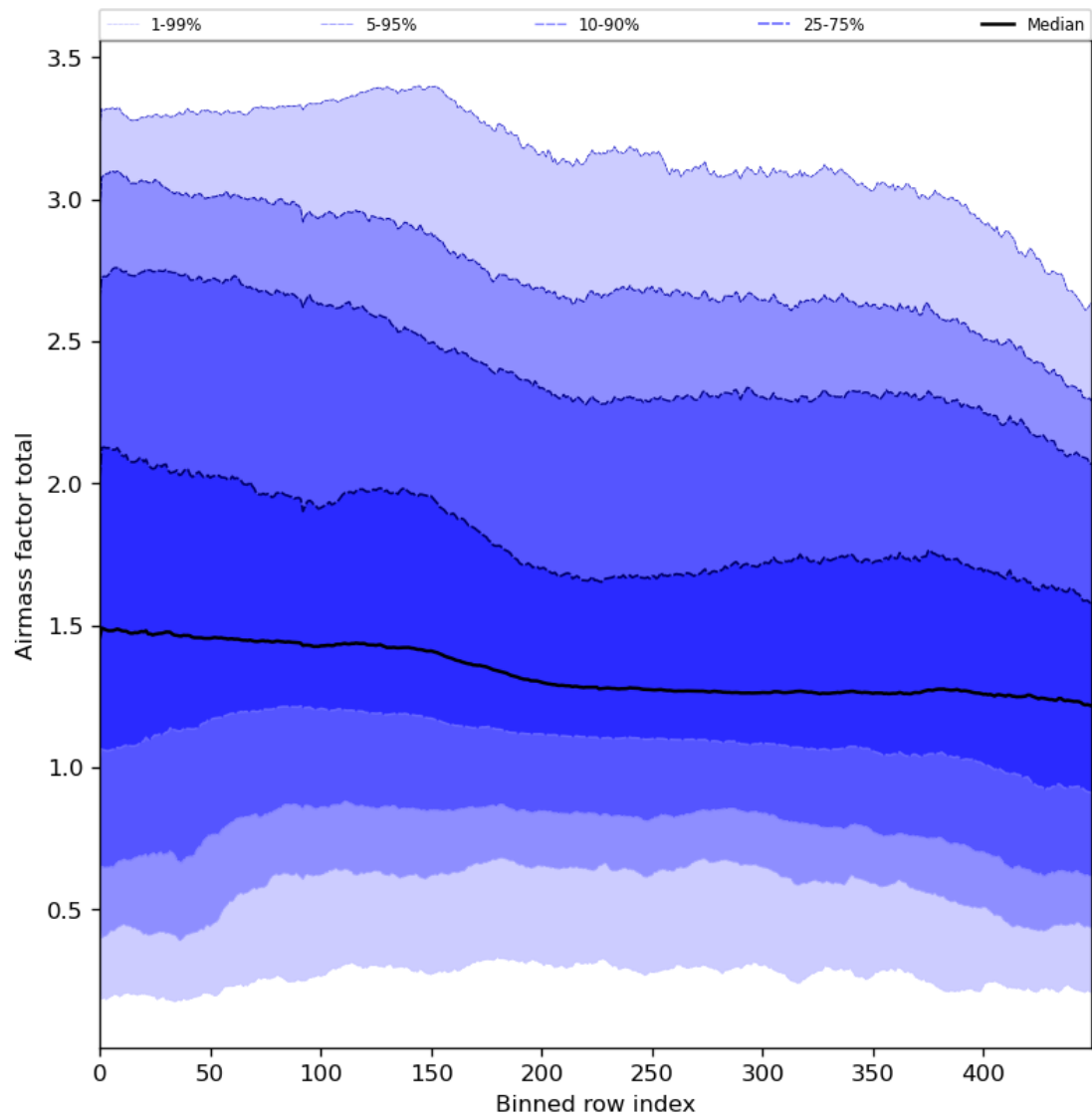
Figure 54: Along track statistics of “Airmass factor total” for 2023-12-16 to 2023-12-18
