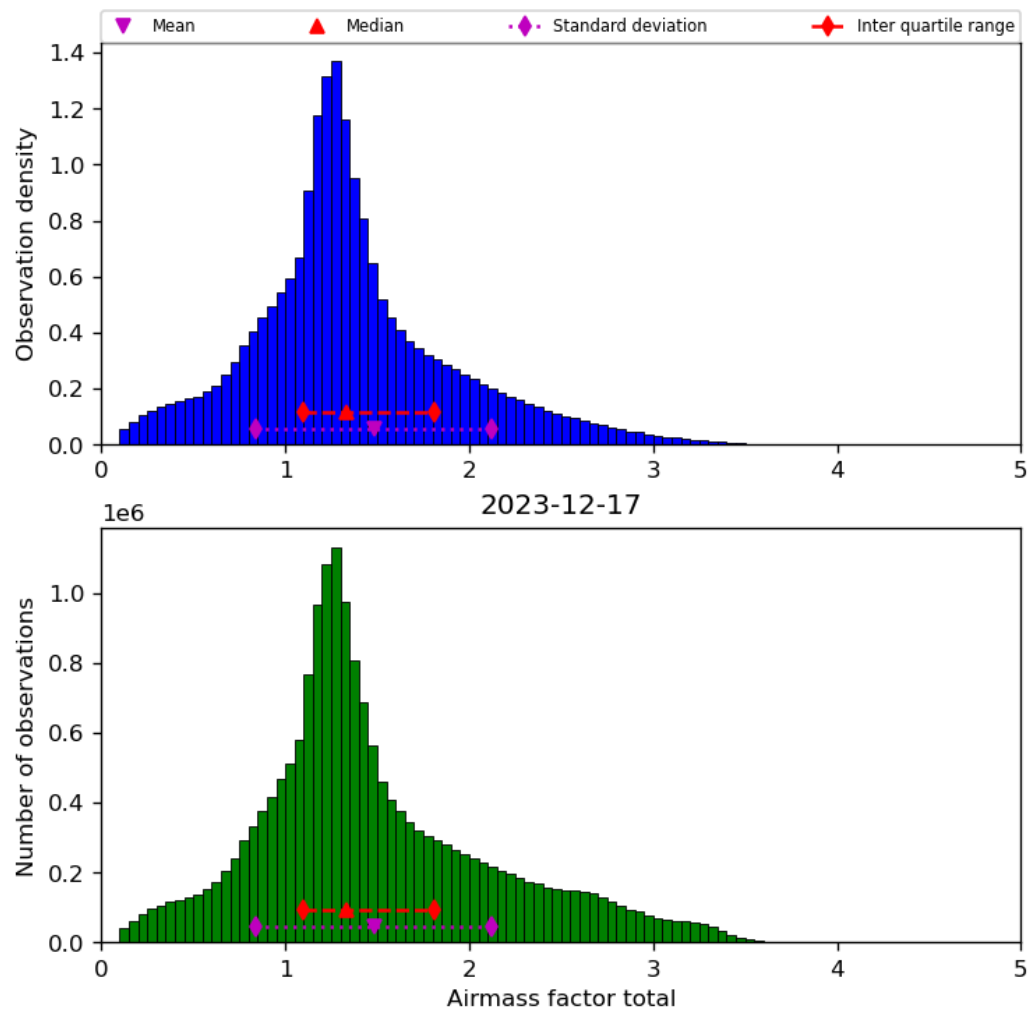
Figure 40: Histogram of “Airmass factor total” for 2023-12-16 to 2023-12-18
