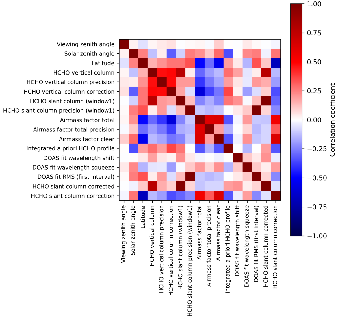
Figure 2: Map of correlation matrix for 2023-12-16 to 2023-12-18.
