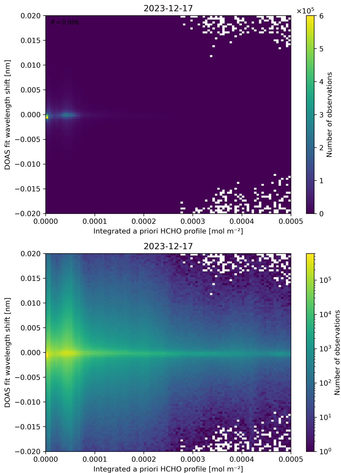
Figure 149: Scatter density plot of “Integrated a priori HCHO profile” against “DOAS fit wavelength shift” for 2023-12-16 to 2023-12-18.
