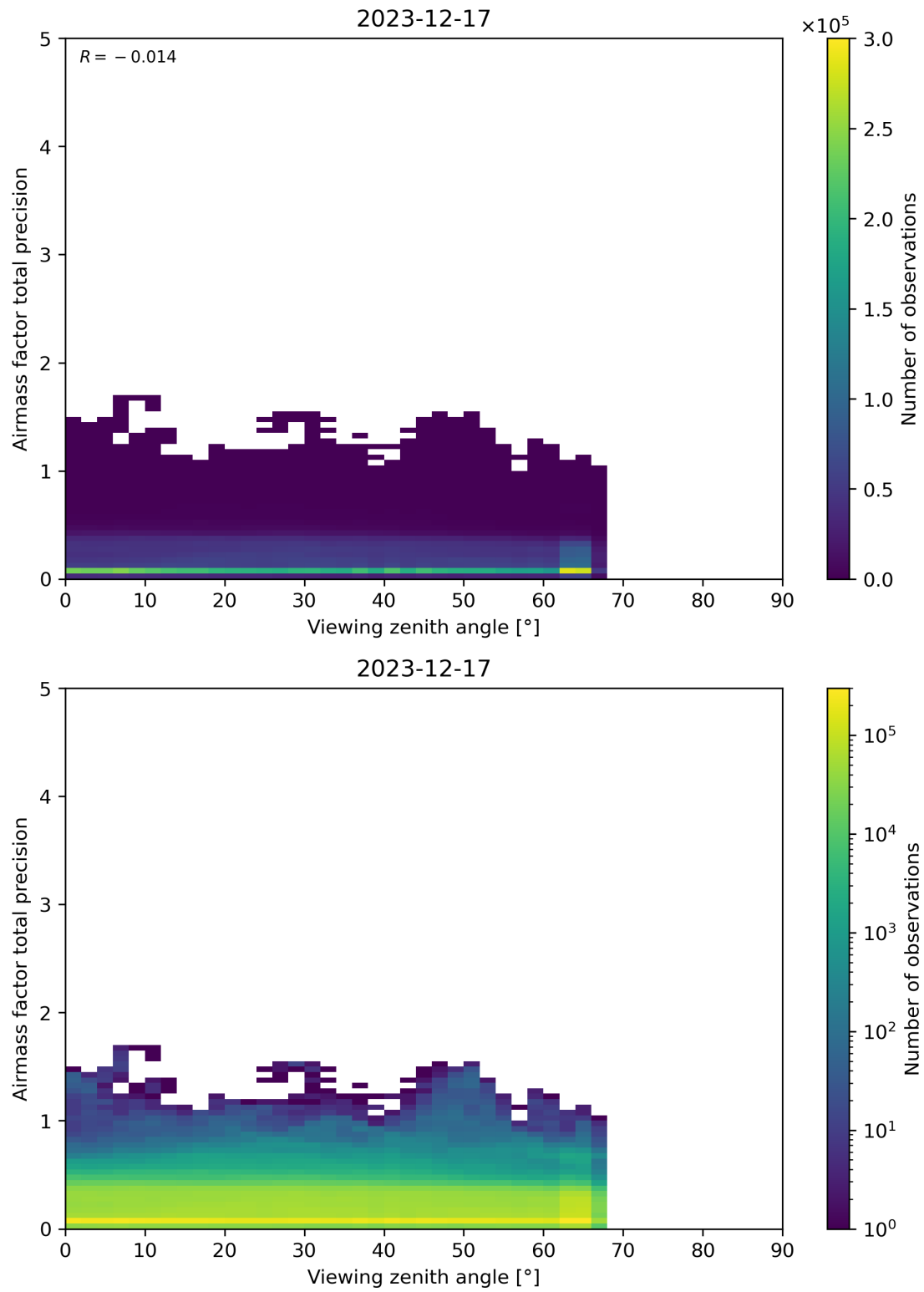
Figure 191: Scatter density plot of “Viewing zenith angle” against “Airmass factor total precision” for 2023-12-16 to 2023-12-18.
