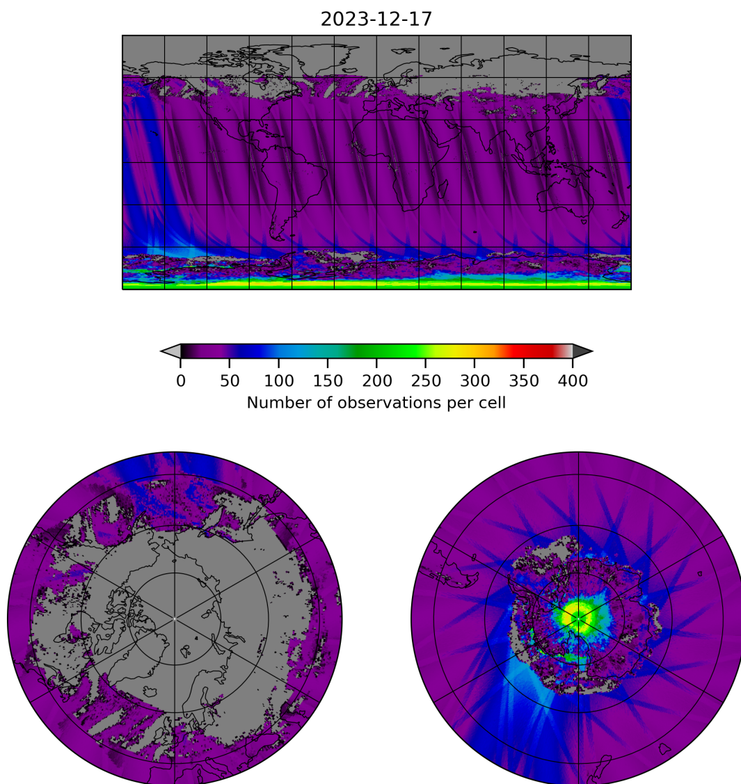
Figure 19: Map of the number of observations for 2023-12-16 to 2023-12-18
