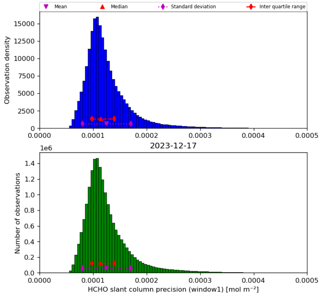
Figure 39: Histogram of “HCHO slant column precision (window1)” for 2023-12-16 to 2023-12-18
