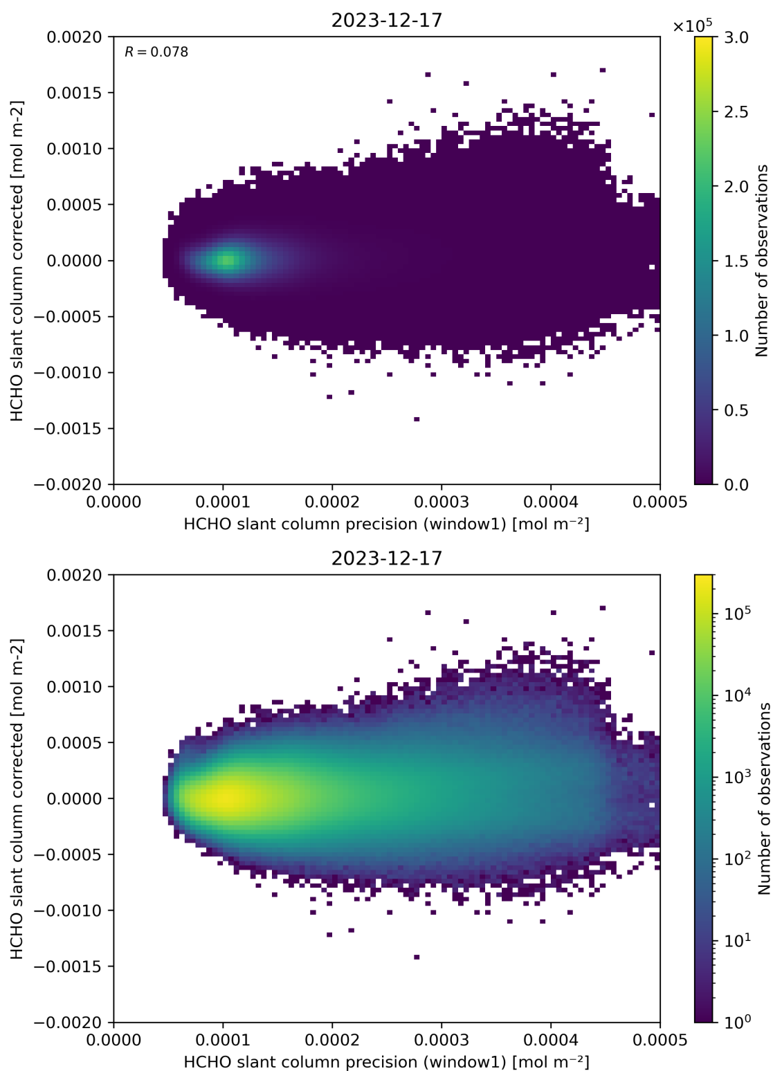
Figure 92: Scatter density plot of “HCHO slant column precision (window1)” against “HCHO slant column corrected” for 2023-12-16 to 2023-12-18.
