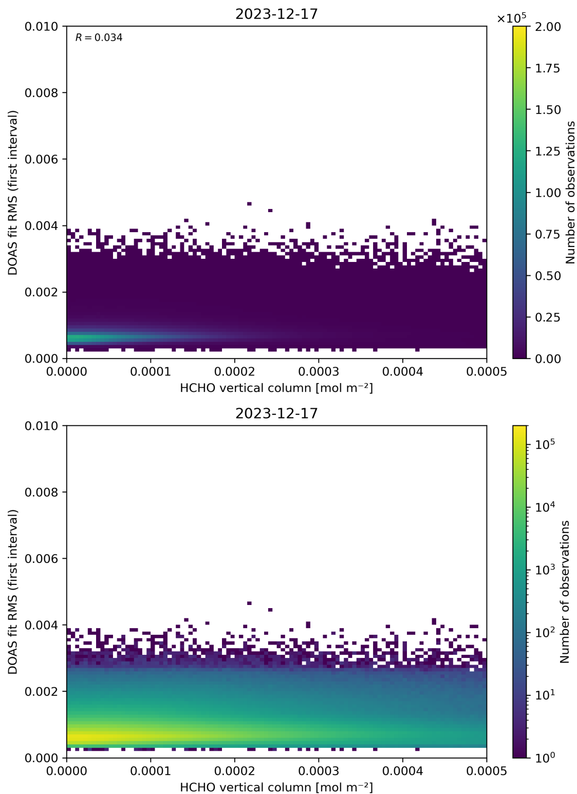
Figure 123: Scatter density plot of “HCHO vertical column” against “DOAS fit RMS (first interval)” for 2023-12-16 to 2023-12-18.
