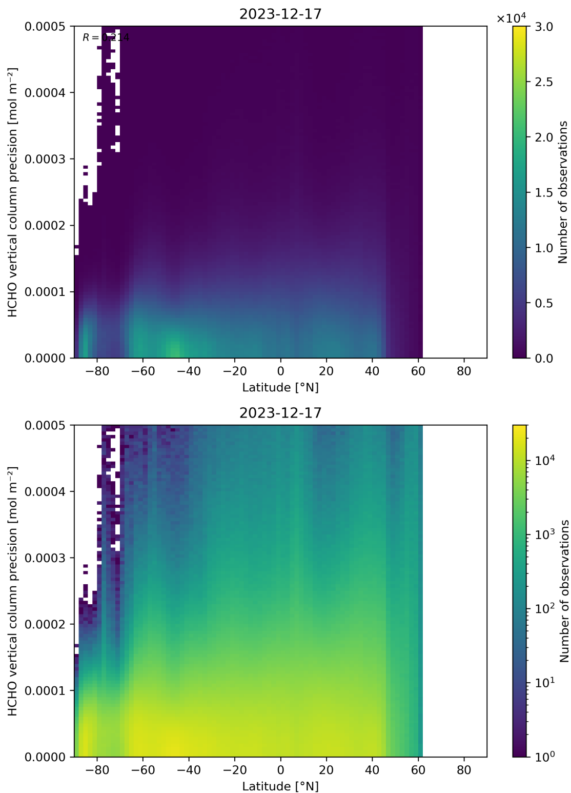
Figure 165: Scatter density plot of “Latitude” against “HCHO vertical column precision” for 2023-12-16 to 2023-12-18.
