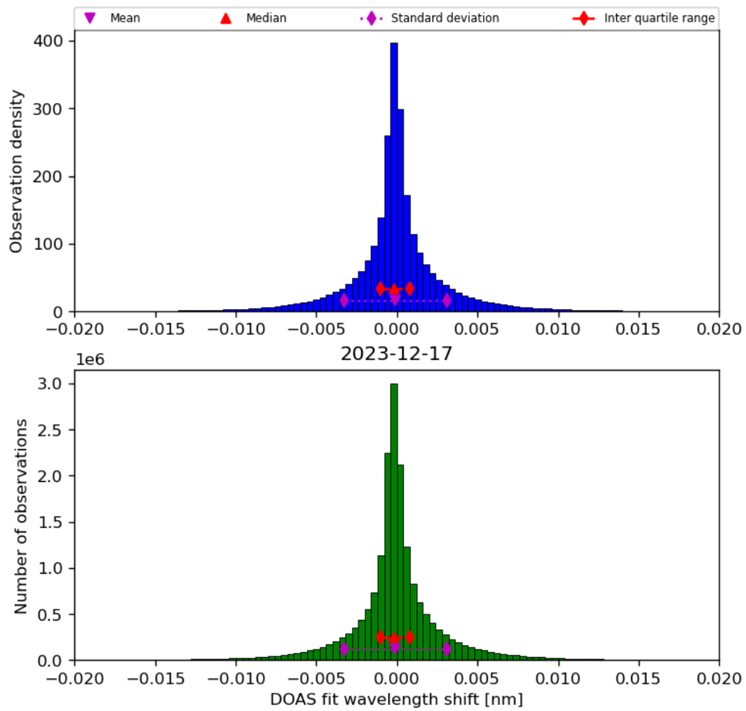
Figure 44: Histogram of “DOAS fit wavelength shift” for 2023-12-16 to 2023-12-18
