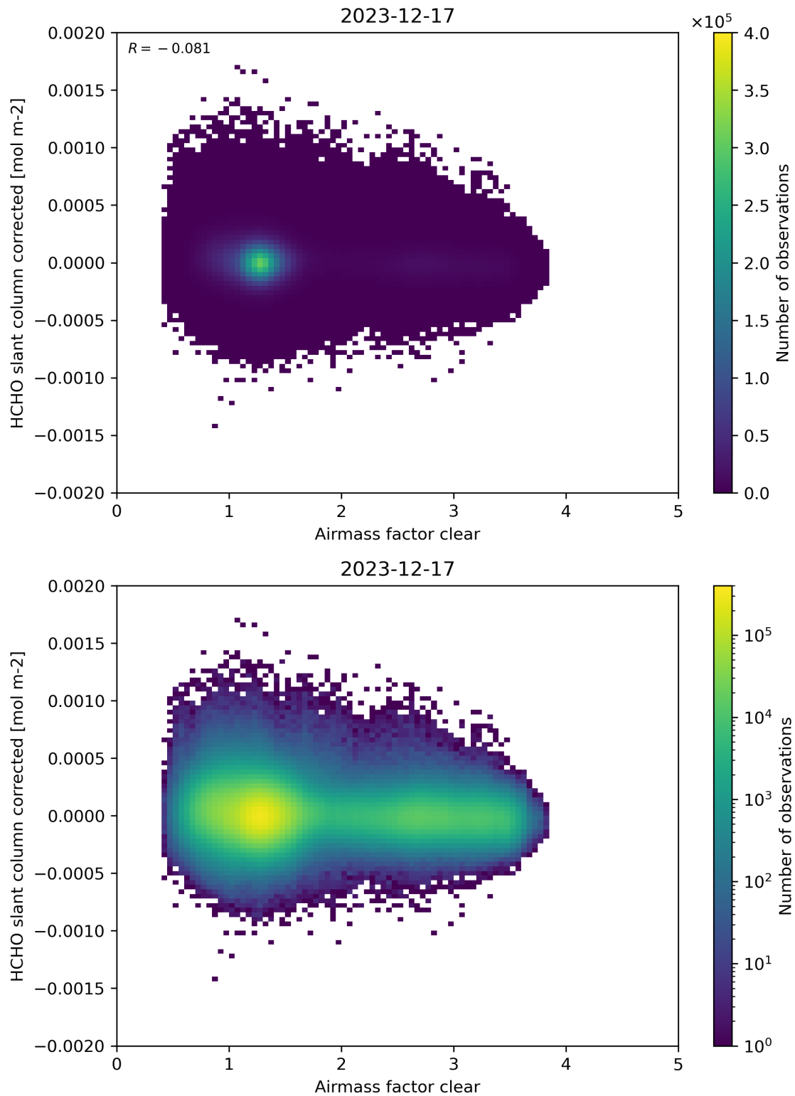
Figure 74: Scatter density plot of “Airmass factor clear” against “HCHO slant column corrected” for 2023-12-16 to 2023-12-18.
