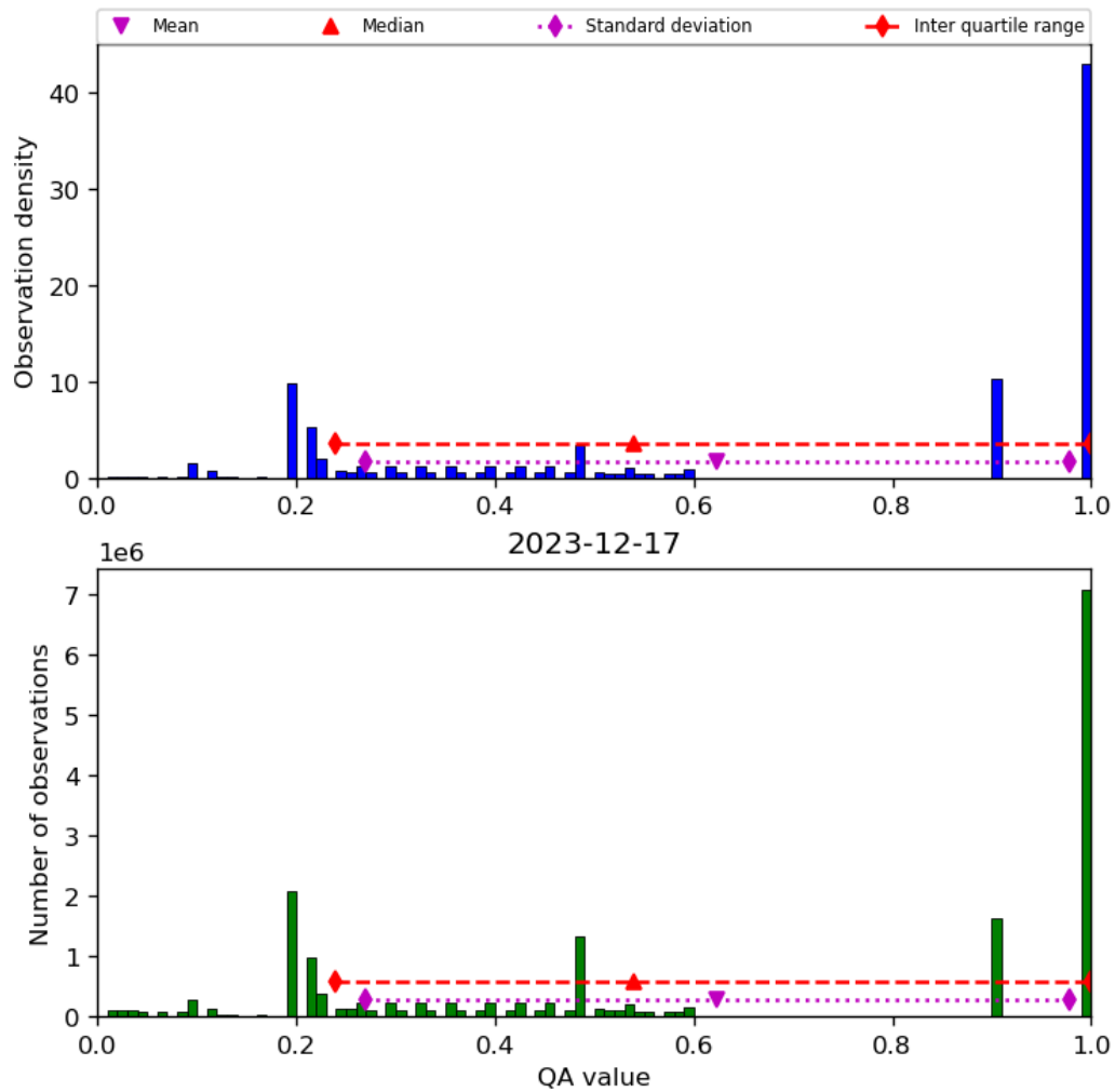
Figure 34: Histogram of “QA value” for 2023-12-16 to 2023-12-18
