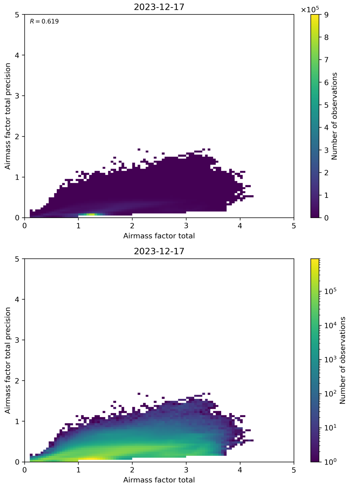
Figure 103: Scatter density plot of “Airmass factor total” against “Airmass factor total precision” for 2023-12-16 to 2023-12-18.
