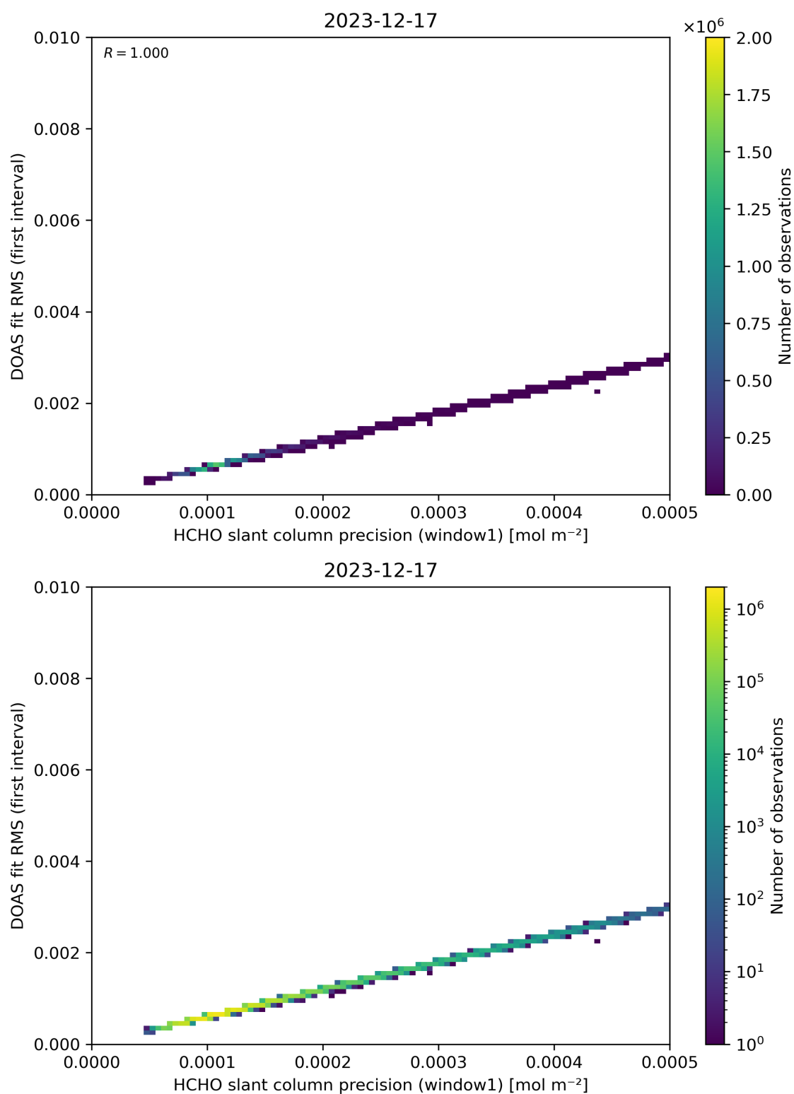
Figure 88: Scatter density plot of “HCHO slant column precision (window1)” against “DOAS fit RMS (first interval)” for 2023-12-16 to 2023-12-18.
