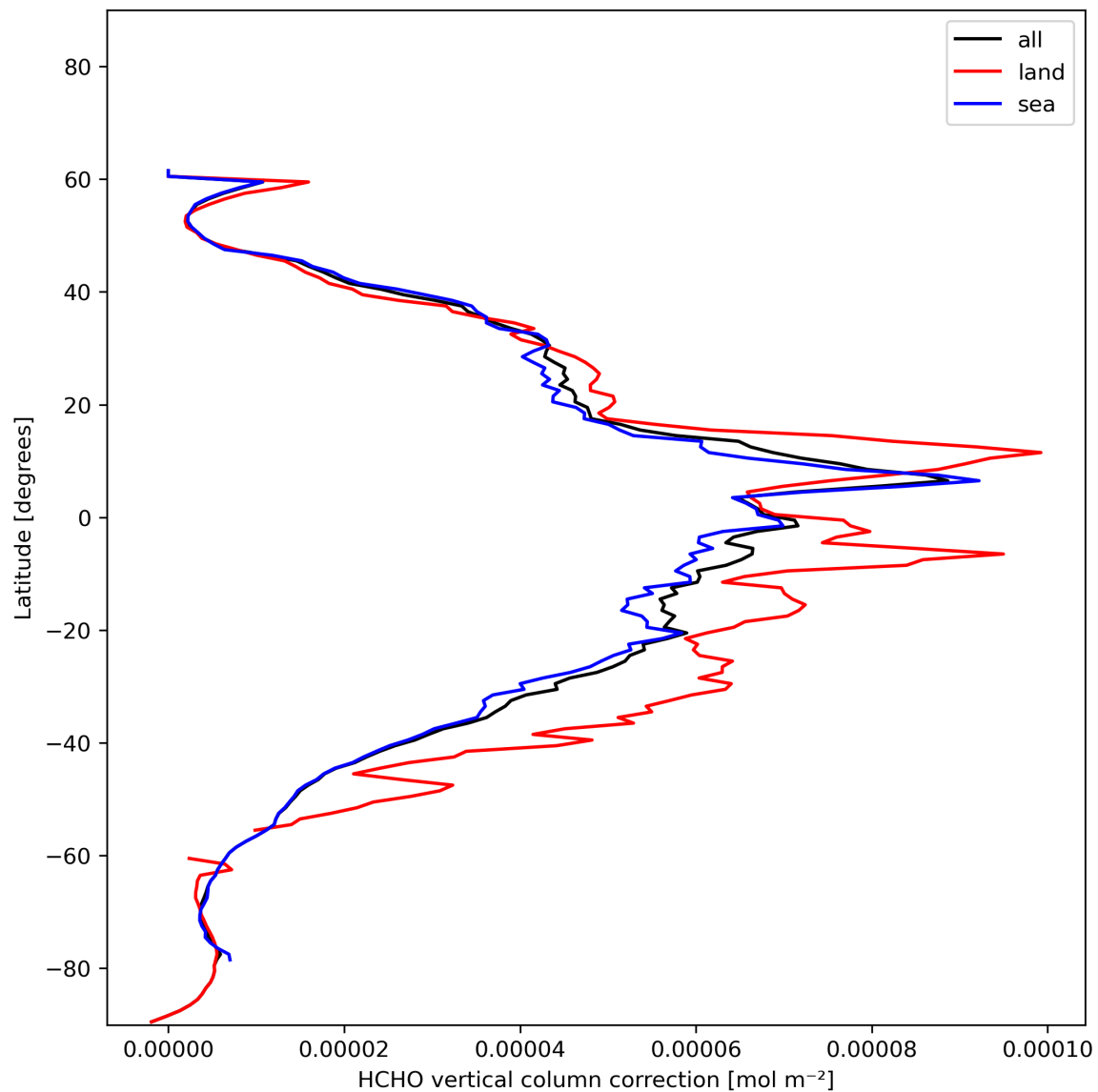
Figure 23: Zonal average of “HCHO vertical column correction” for 2023-12-16 to 2023-12-18.
