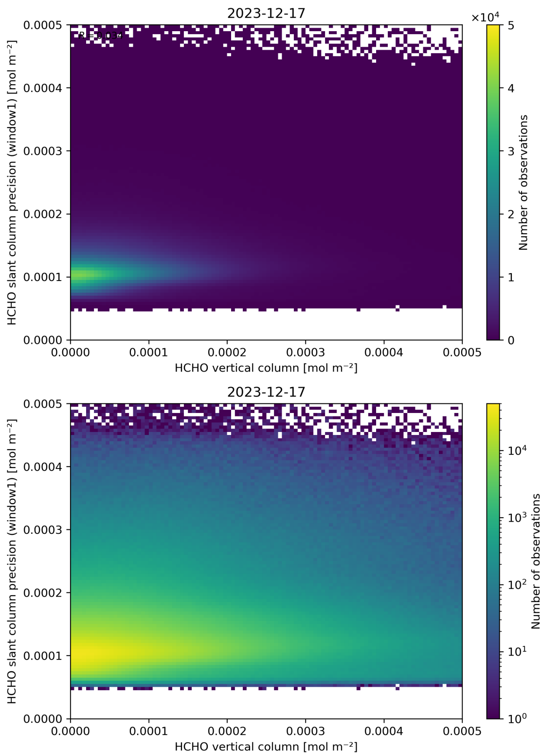
Figure 130: Scatter density plot of “HCHO vertical column” against “HCHO slant column precision (window1)” for 2023-12-16 to 2023-12-18.
