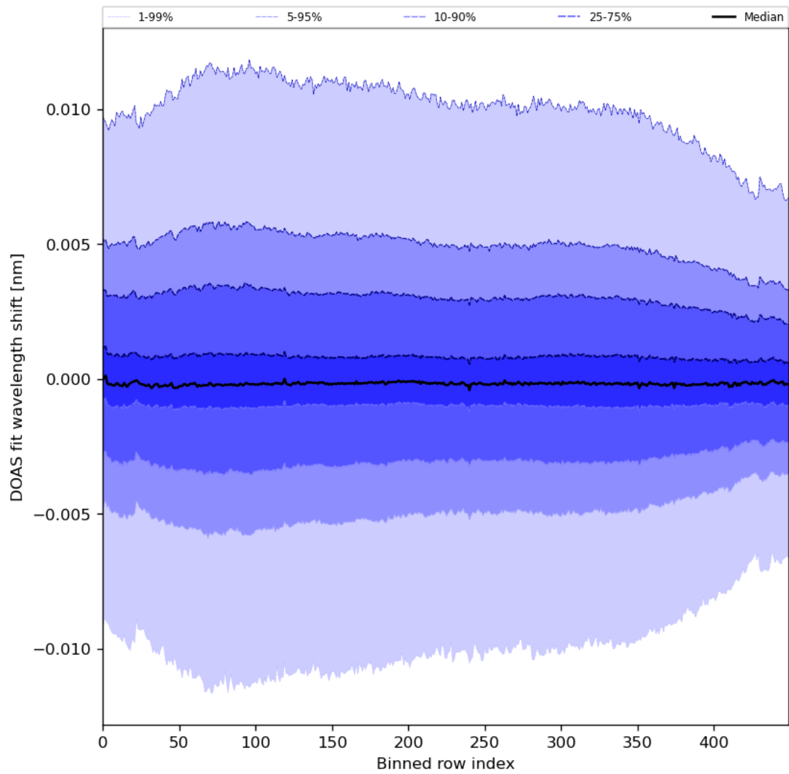
Figure 58: Along track statistics of “DOAS fit wavelength shift” for 2023-12-16 to 2023-12-18
