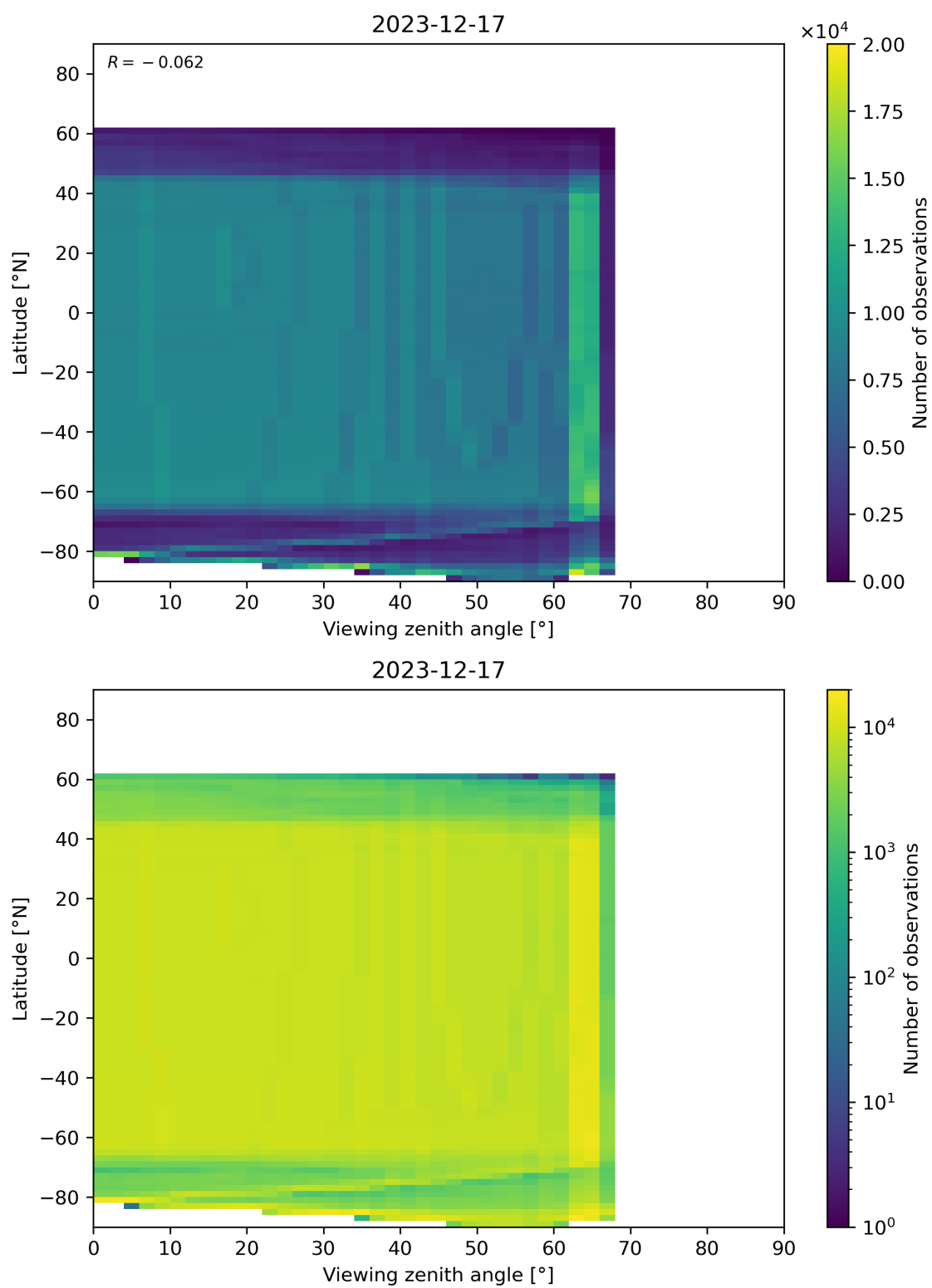
Figure 196: Scatter density plot of “Viewing zenith angle” against “Latitude” for 2023-12-16 to 2023-12-18.
