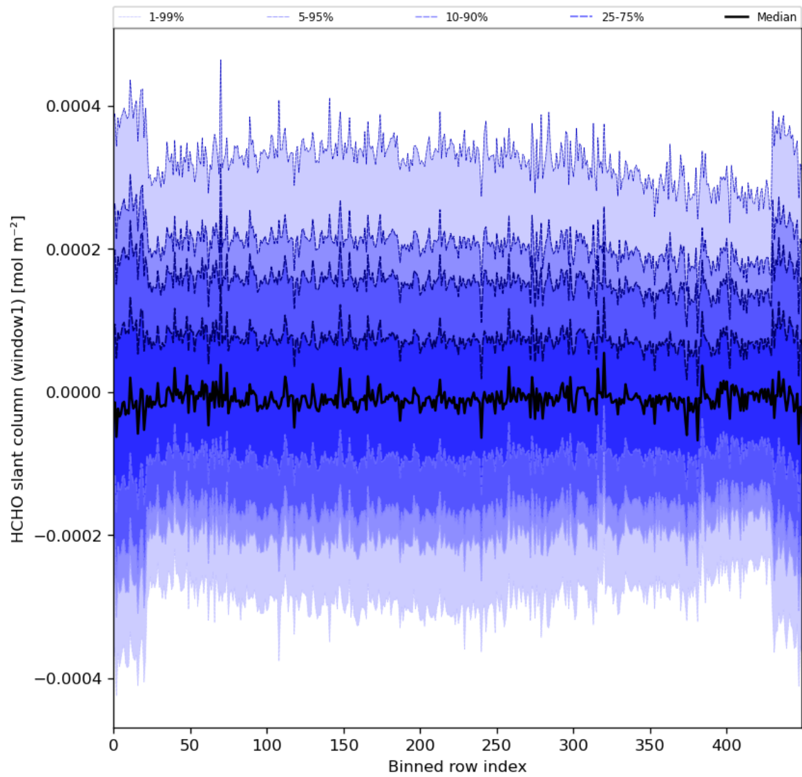
Figure 52: Along track statistics of “HCHO slant column (window1)” for 2023-12-16 to 2023-12-18
