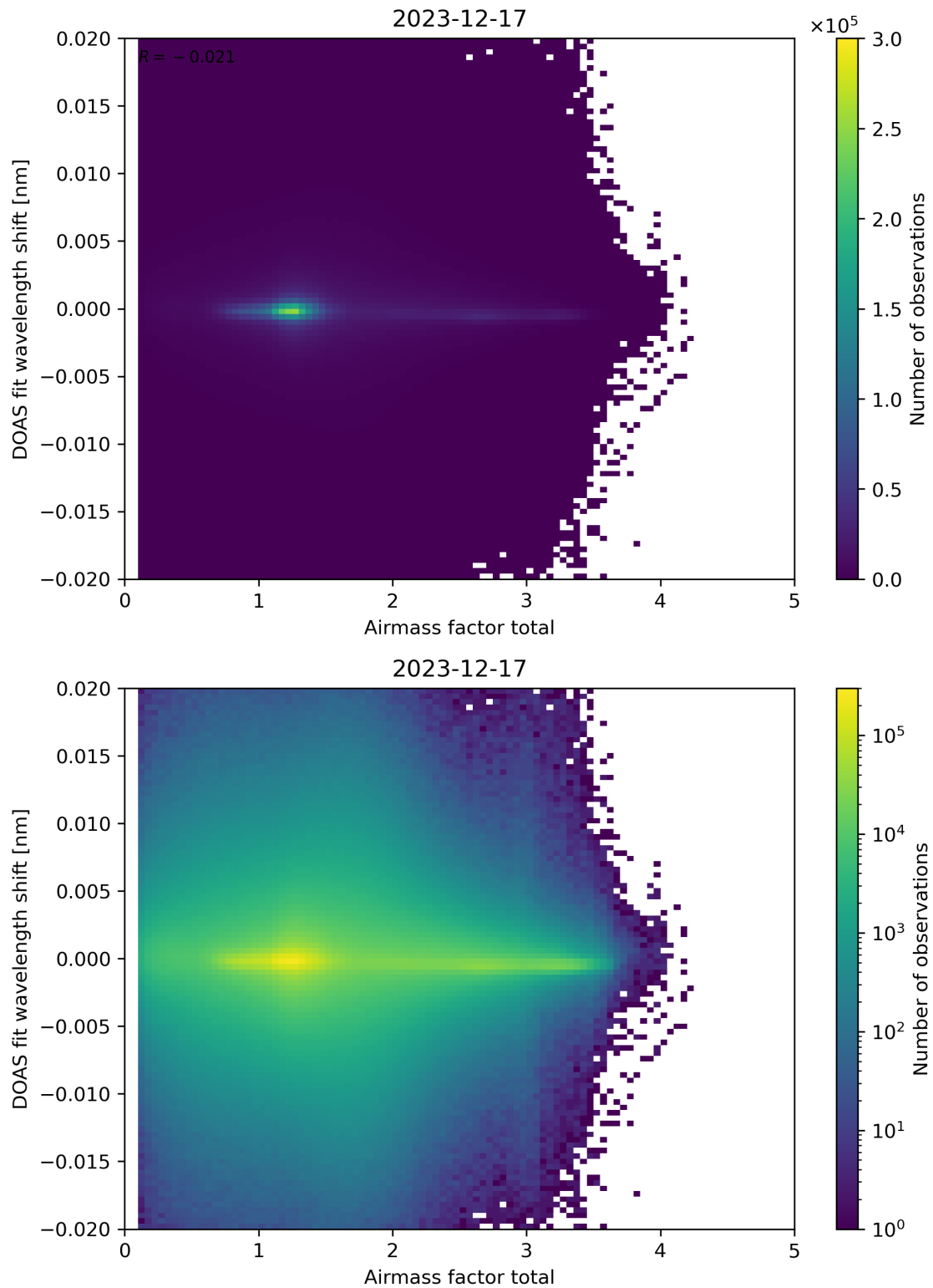
Figure 98: Scatter density plot of “Airmass factor total” against “DOAS fit wavelength shift” for 2023-12-16 to 2023-12-18.
