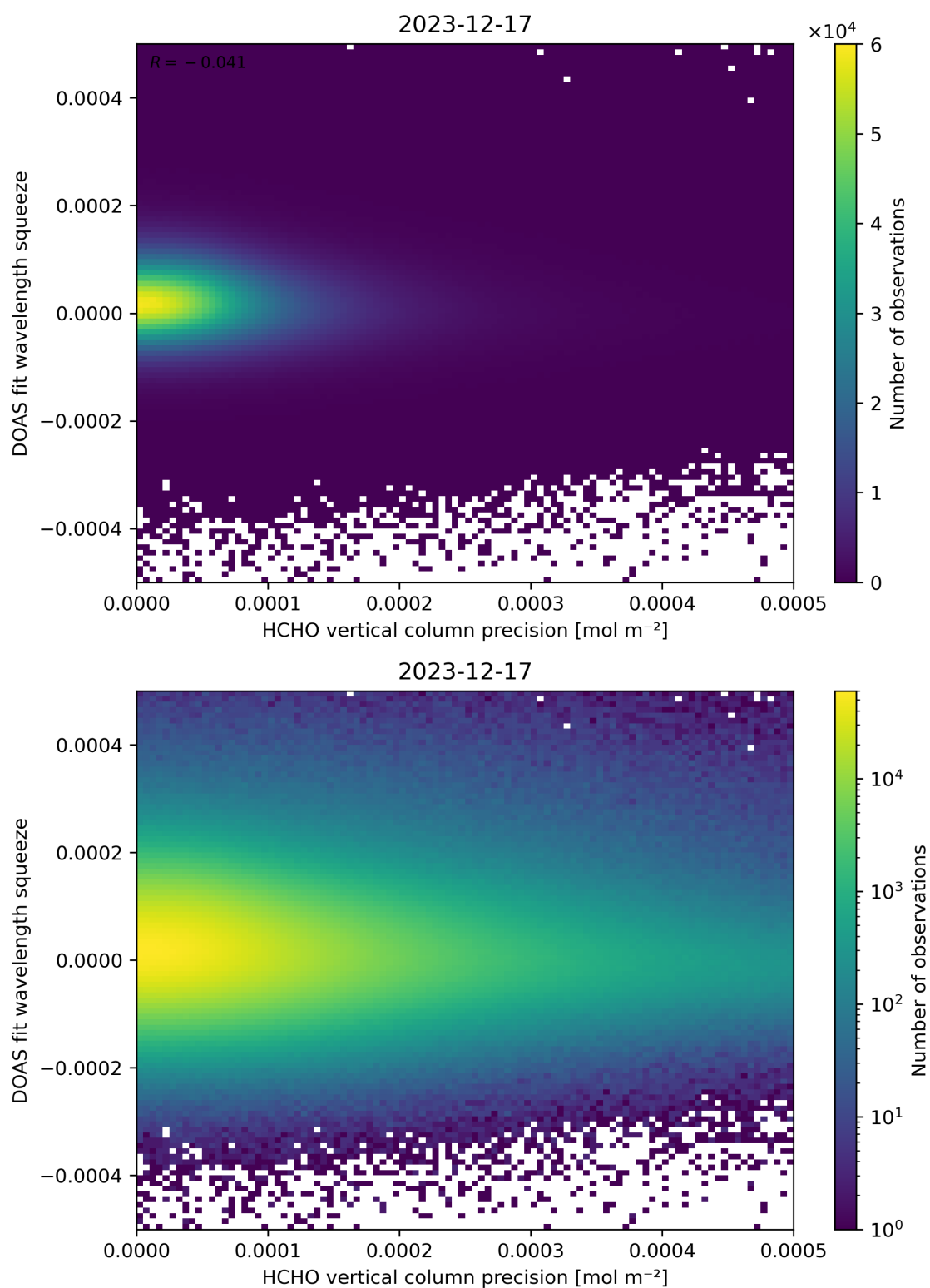
Figure 138: Scatter density plot of “HCHO vertical column precision” against “DOAS fit wavelength squeeze” for 2023-12-16 to 2023-12-18.
