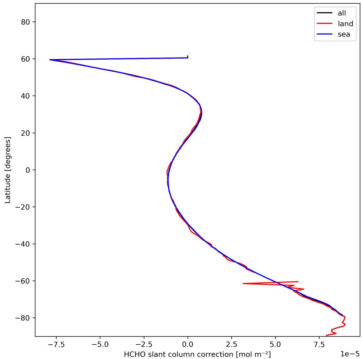
Figure 33: Zonal average of “HCHO slant column correction” for 2023-12-16 to 2023-12-18.
