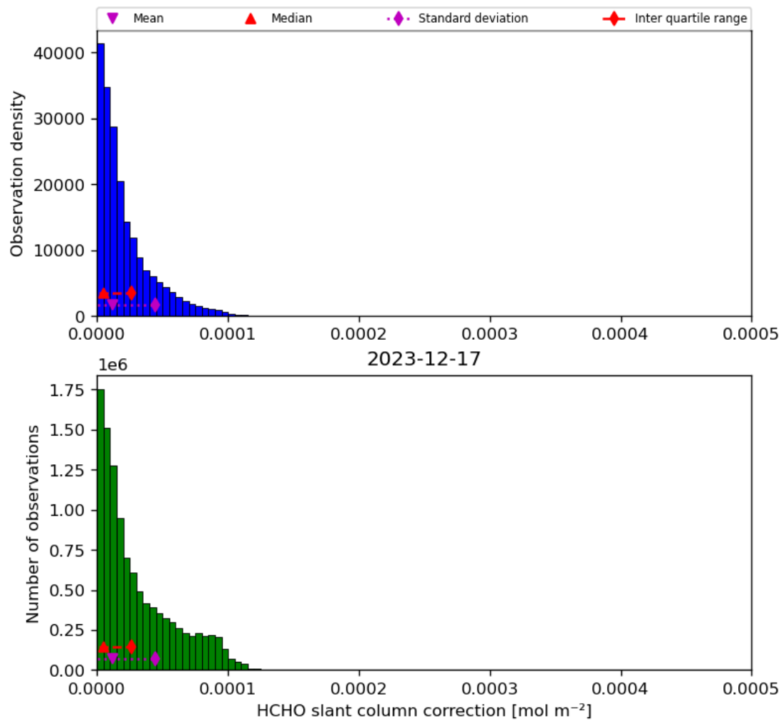
Figure 47: Histogram of “HCHO slant column correction” for 2023-12-16 to 2023-12-18
