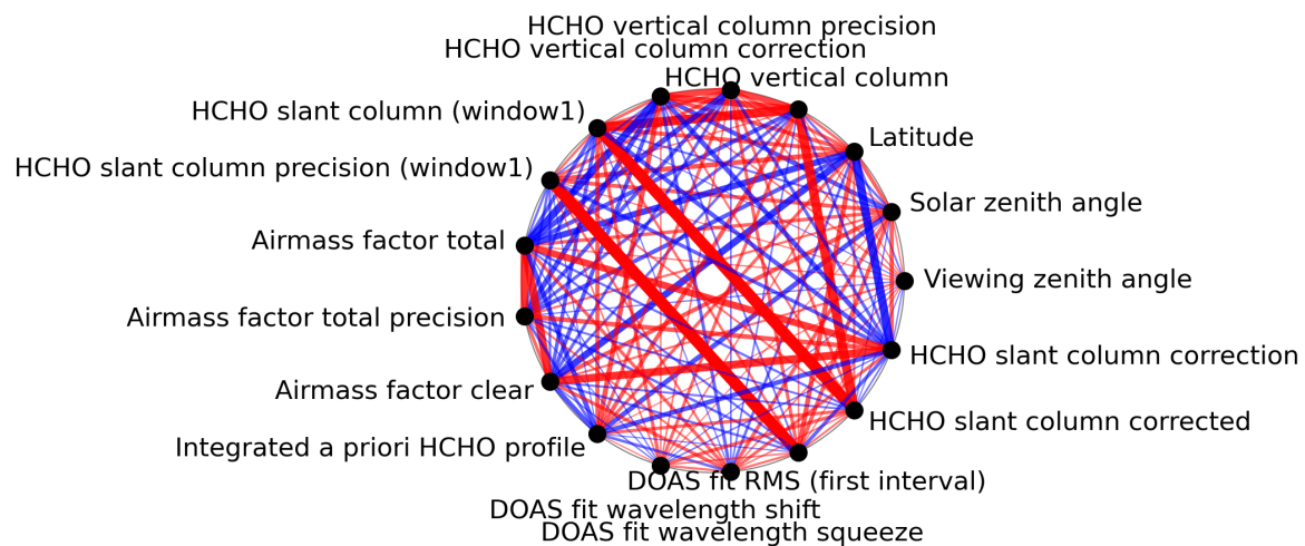
Figure 1: Map of correlation graph for 2023-12-16 to 2023-12-18.
