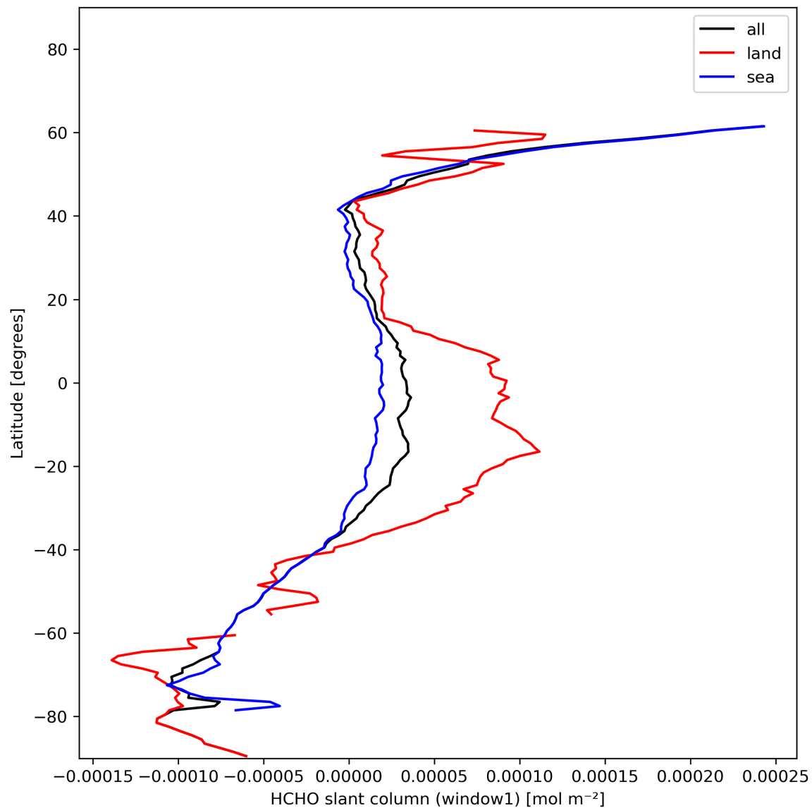
Figure 24: Zonal average of “HCHO slant column (window1)” for 2023-12-16 to 2023-12-18.
