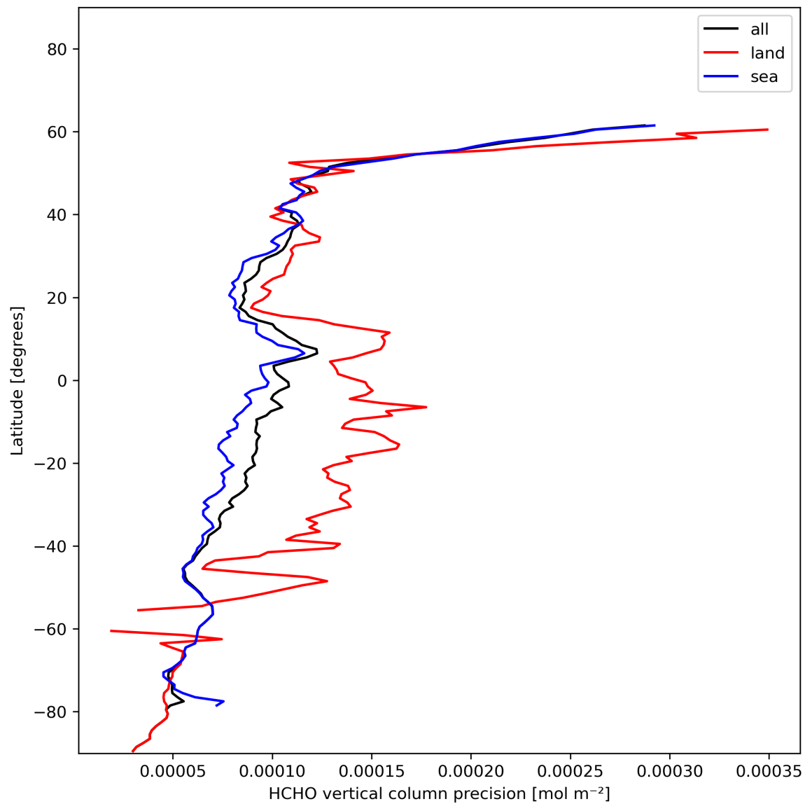
Figure 22: Zonal average of “HCHO vertical column precision” for 2023-12-16 to 2023-12-18.
