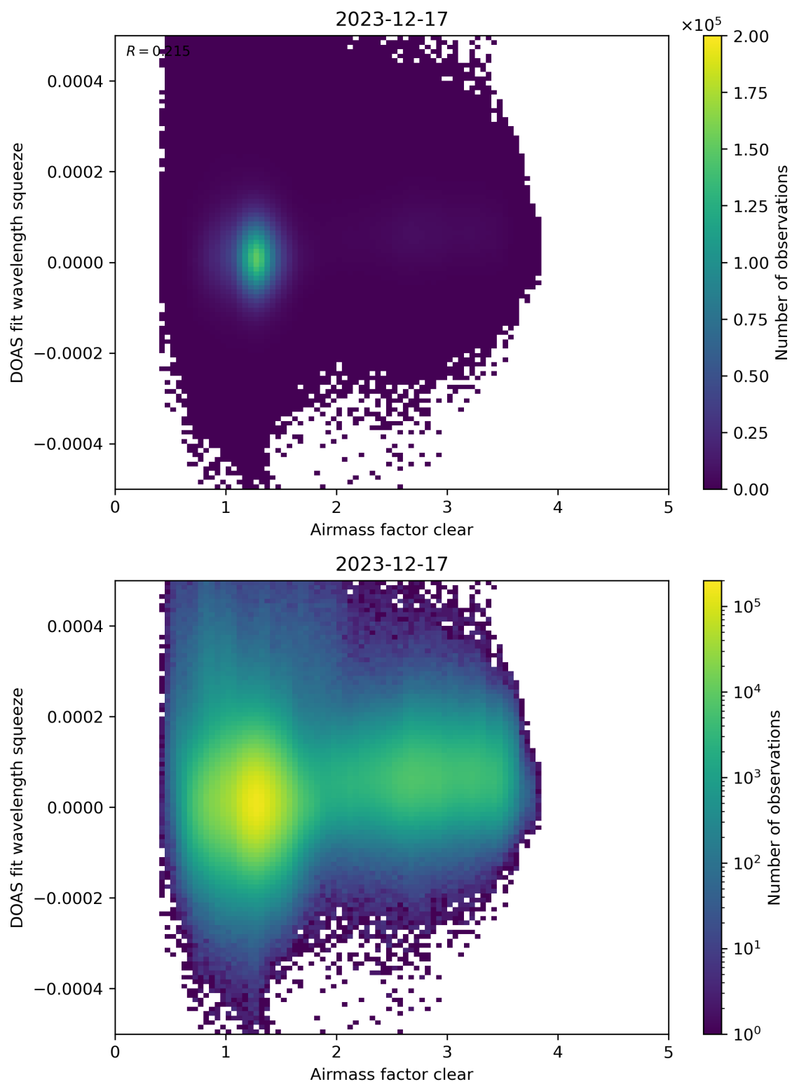
Figure 73: Scatter density plot of “Airmass factor clear” against “DOAS fit wavelength squeeze” for 2023-12-16 to 2023-12-18.
