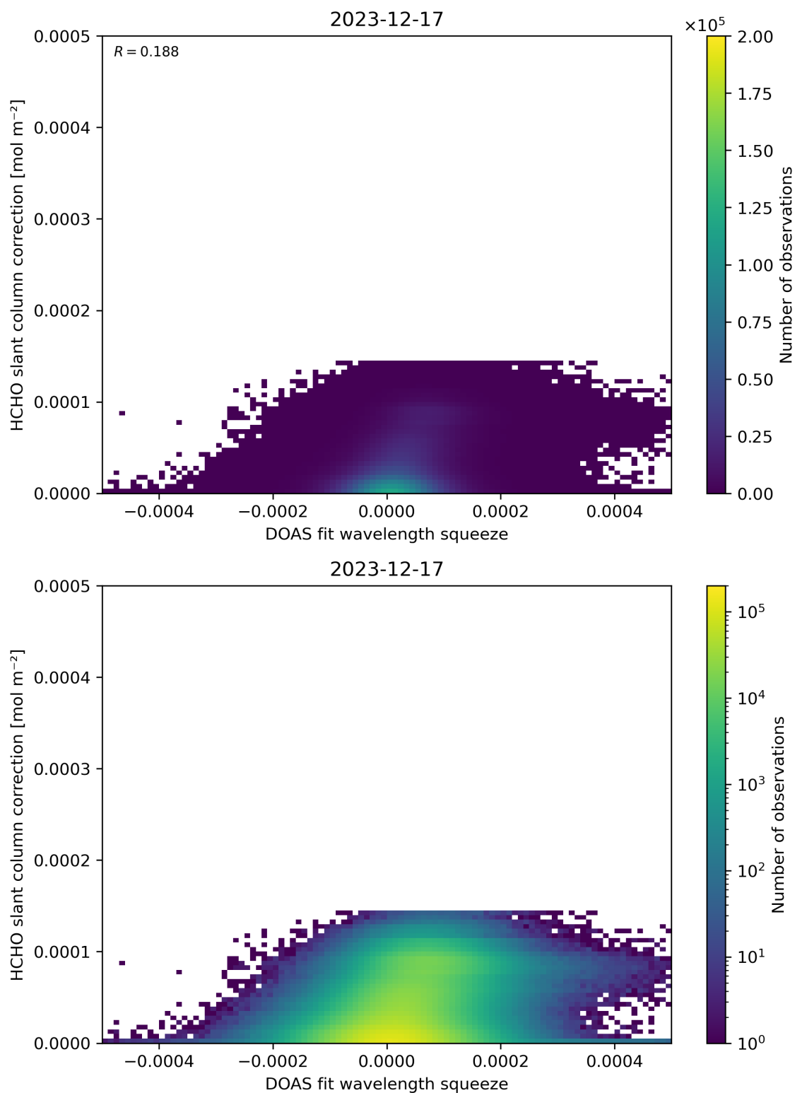
Figure 70: Scatter density plot of “DOAS fit wavelength squeeze” against “HCHO slant column correction” for 2023-12-16 to 2023-12-18.
