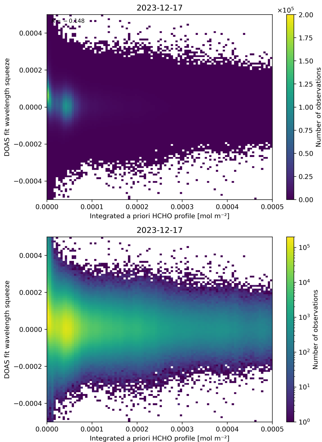
Figure 150: Scatter density plot of “Integrated a priori HCHO profile” against “DOAS fit wavelength squeeze” for 2023-12-16 to 2023-12-18.
