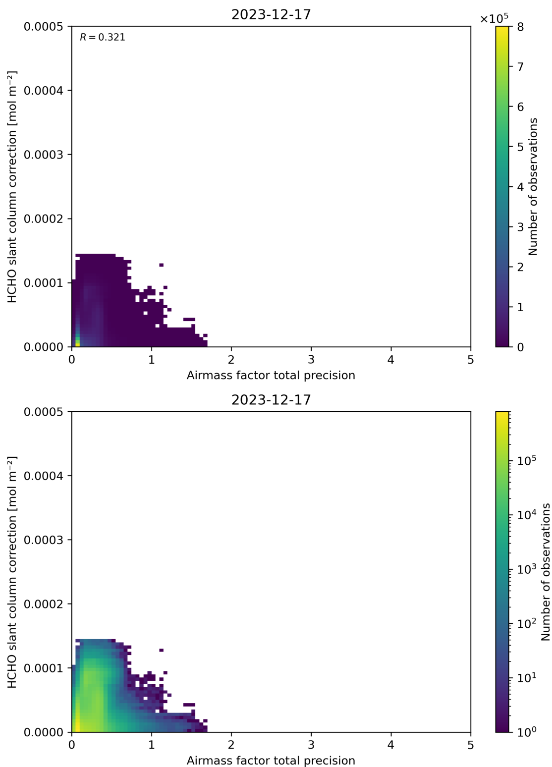
Figure 110: Scatter density plot of “Airmass factor total precision” against “HCHO slant column correction” for 2023-12-16 to 2023-12-18.
