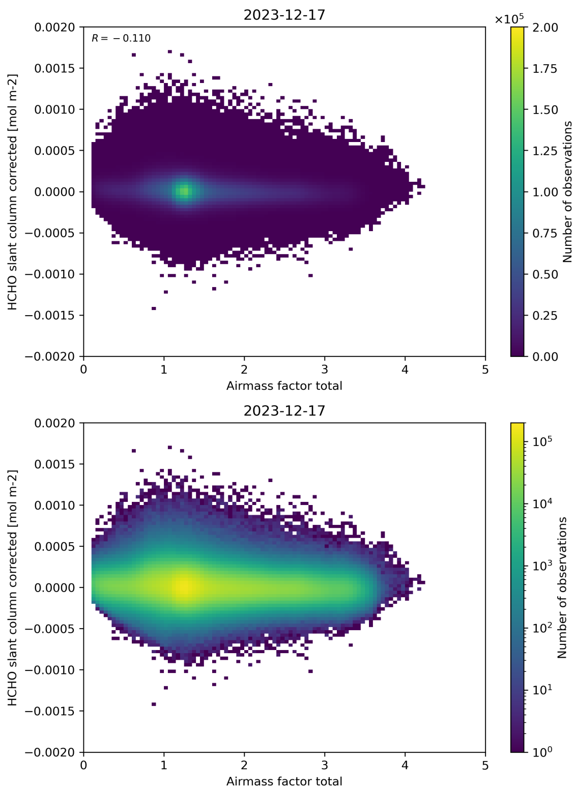
Figure 101: Scatter density plot of “Airmass factor total” against “HCHO slant column corrected” for 2023-12-16 to 2023-12-18.
