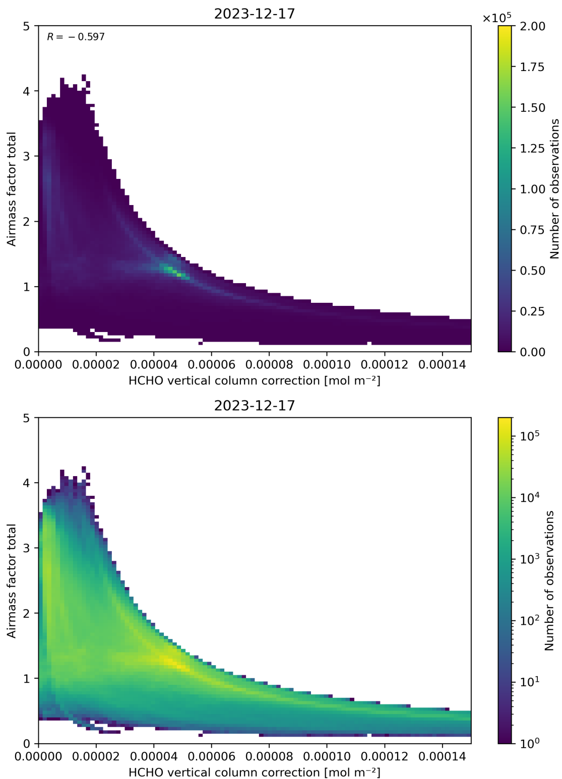
Figure 120: Scatter density plot of “HCHO vertical column correction” against “Airmass factor total” for 2023-12-16 to 2023-12-18.
