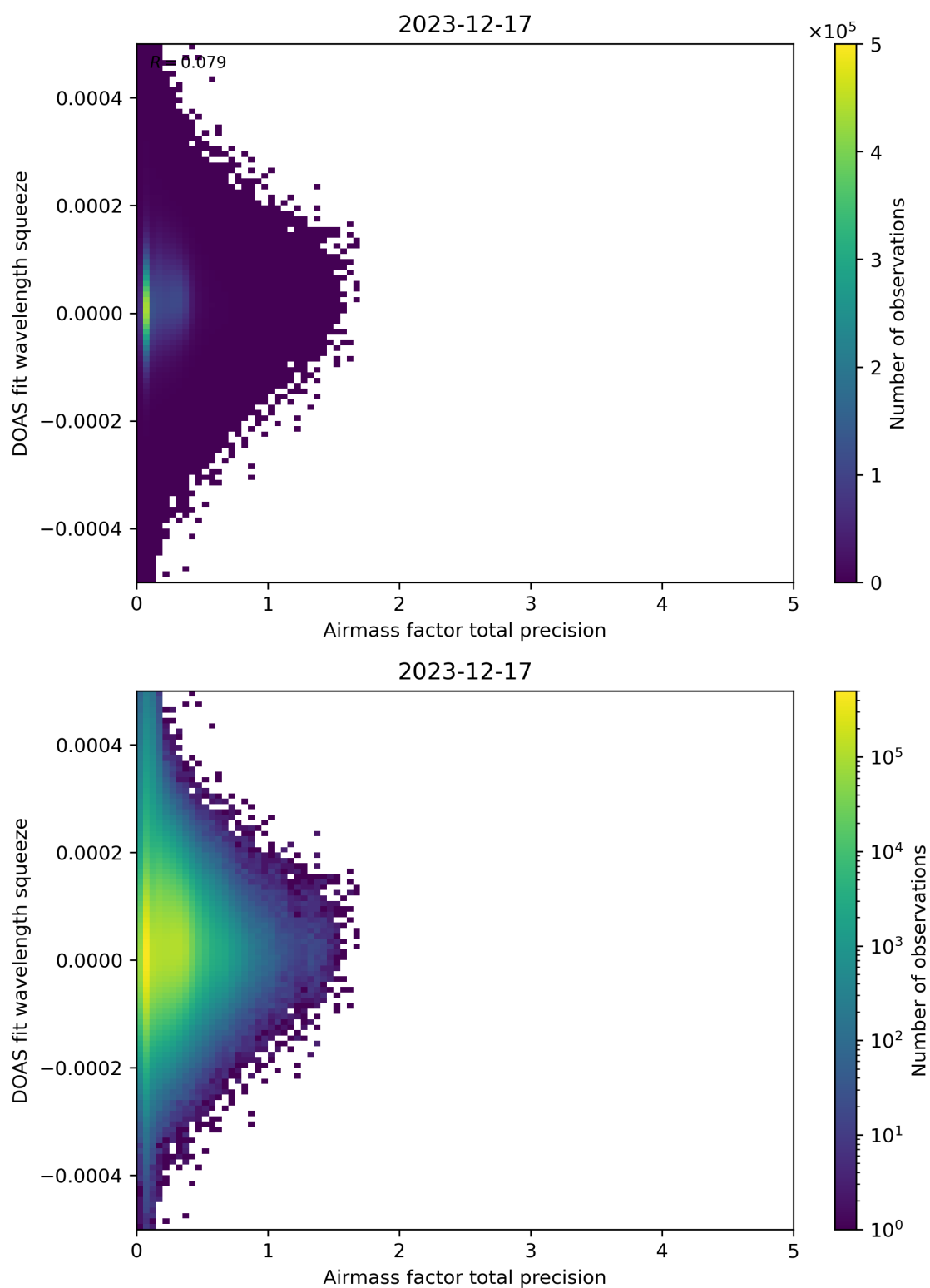
Figure 107: Scatter density plot of “Airmass factor total precision” against “DOAS fit wavelength squeeze” for 2023-12-16 to 2023-12-18.
