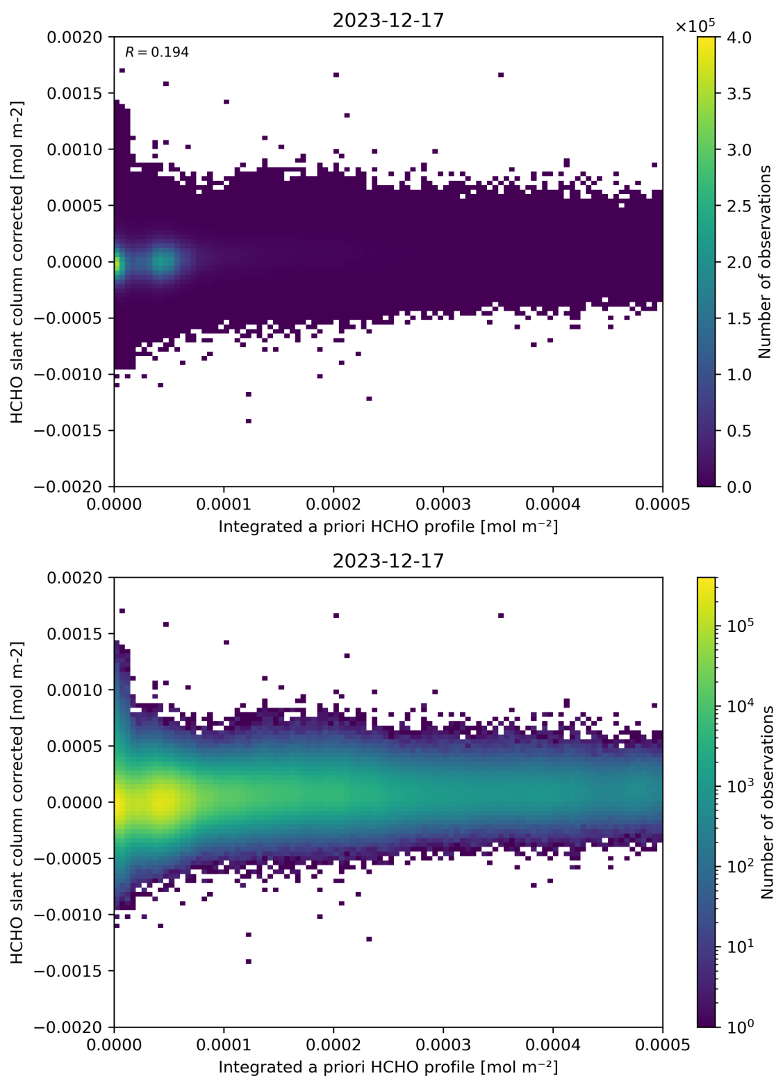
Figure 151: Scatter density plot of “Integrated a priori HCHO profile” against “HCHO slant column corrected” for 2023-12-16 to 2023-12-18.
