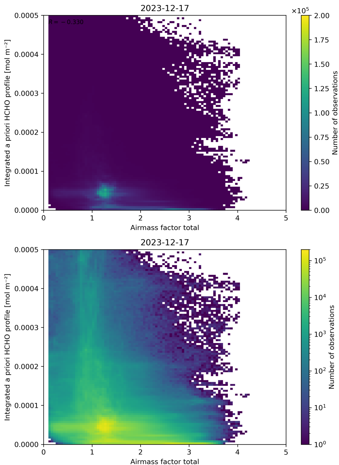
Figure 104: Scatter density plot of “Airmass factor total” against “Integrated a priori HCHO profile” for 2023-12-16 to 2023-12-18.
