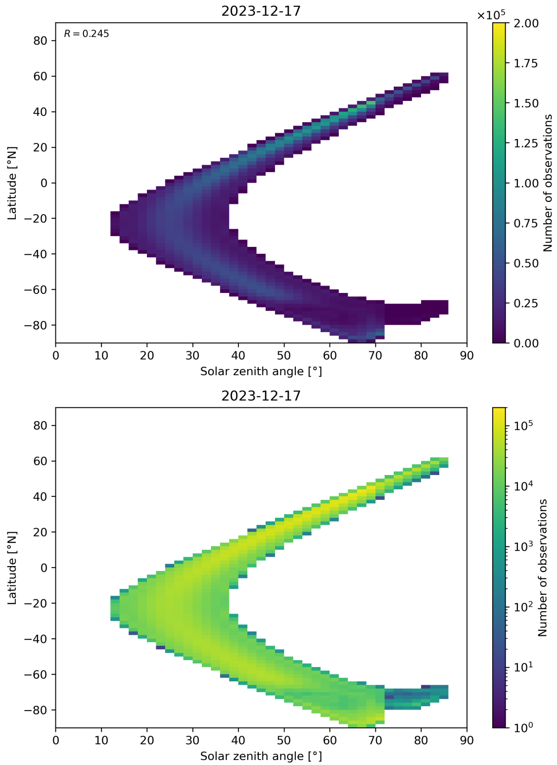
Figure 181: Scatter density plot of “Solar zenith angle” against “Latitude” for 2023-12-16 to 2023-12-18.
