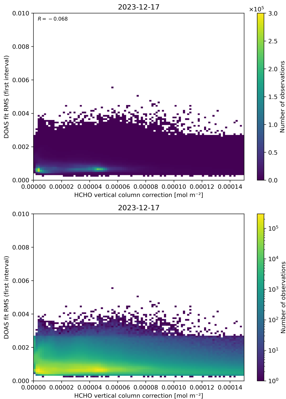
Figure 112: Scatter density plot of “HCHO vertical column correction” against “DOAS fit RMS (first interval)” for 2023-12-16 to 2023-12-18.
