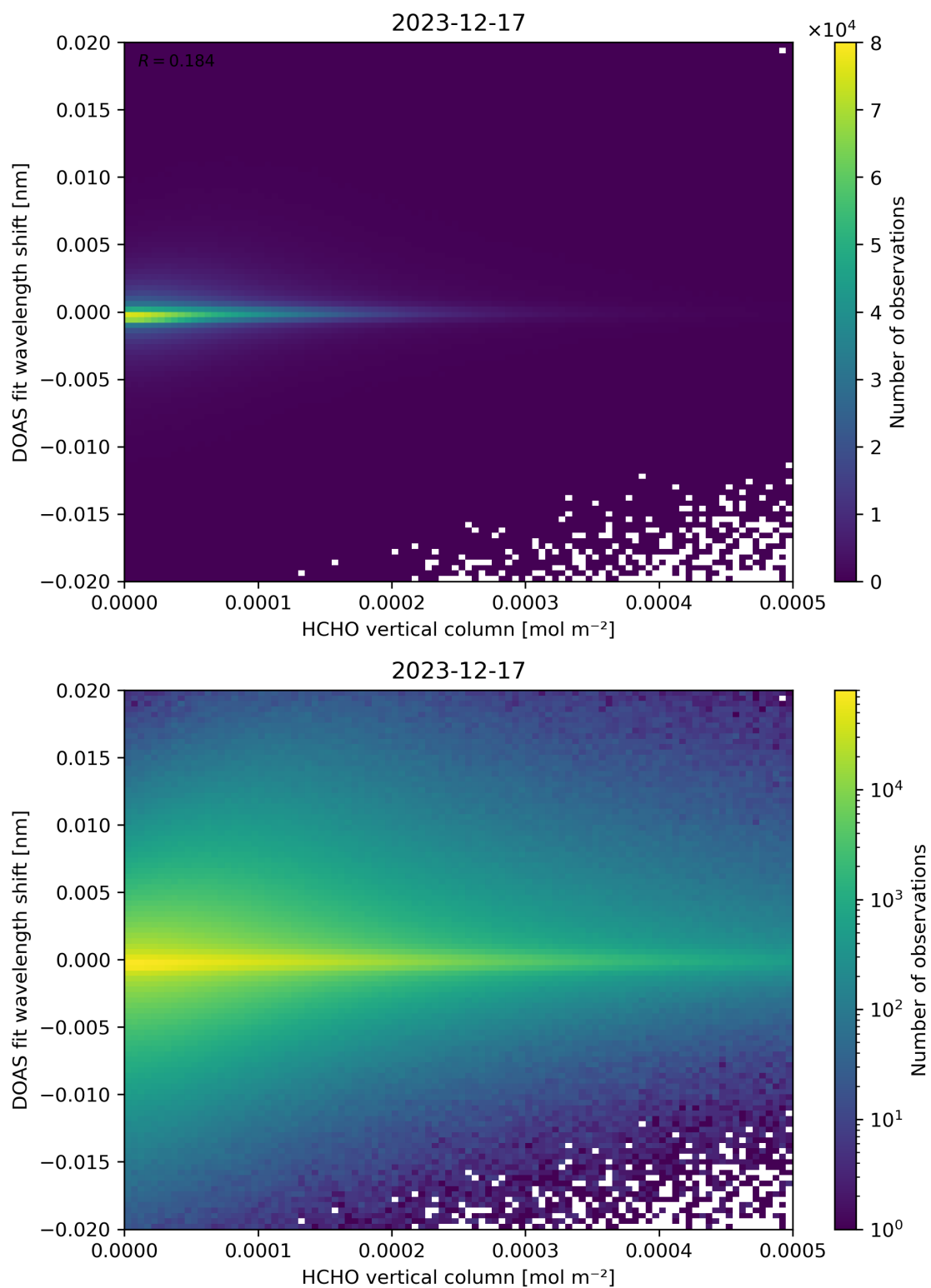
Figure 124: Scatter density plot of “HCHO vertical column” against “DOAS fit wavelength shift” for 2023-12-16 to 2023-12-18.
