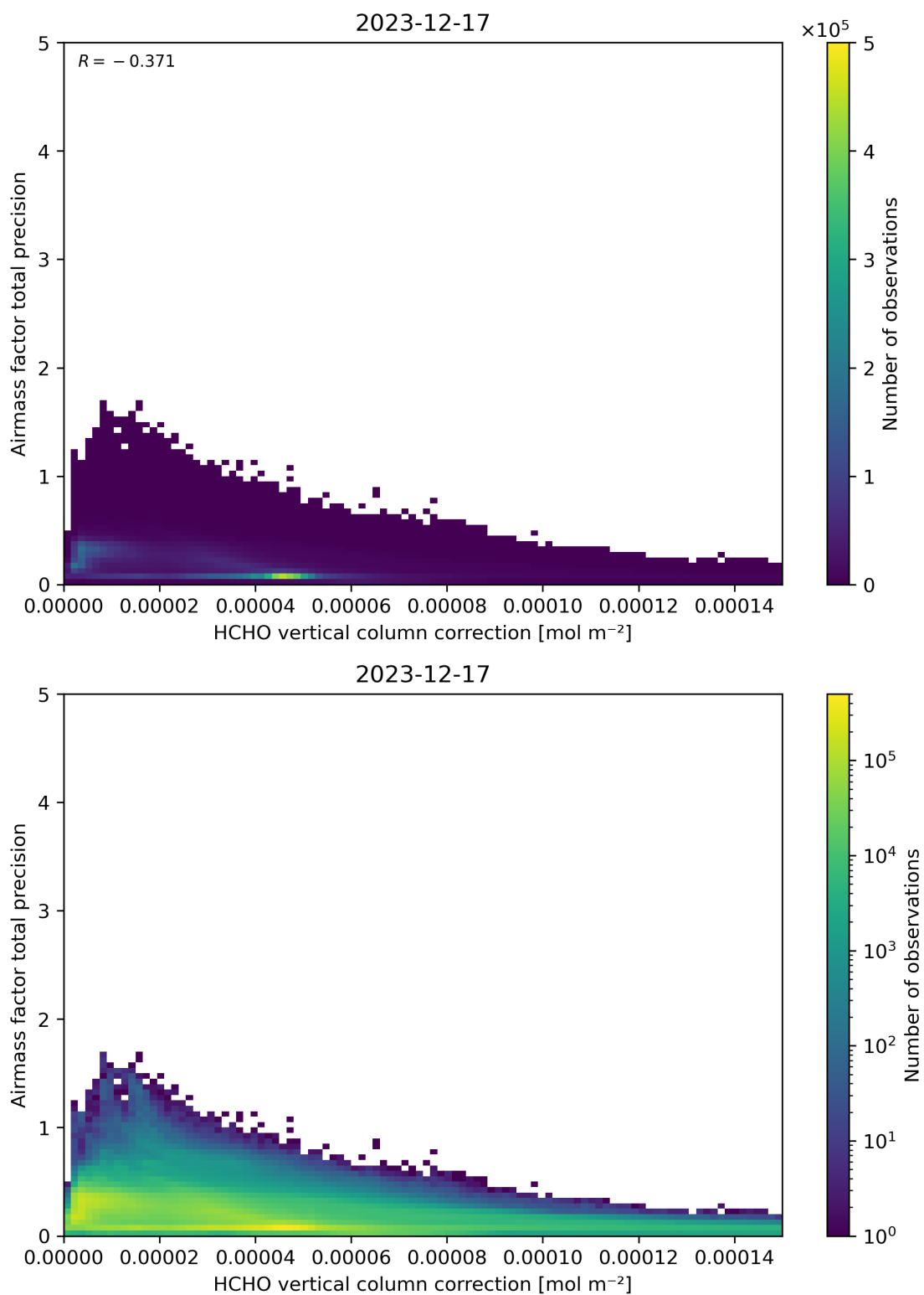
Figure 121: Scatter density plot of “HCHO vertical column correction” against “Airmass factor total precision” for 2023-12-16 to 2023-12-18.
