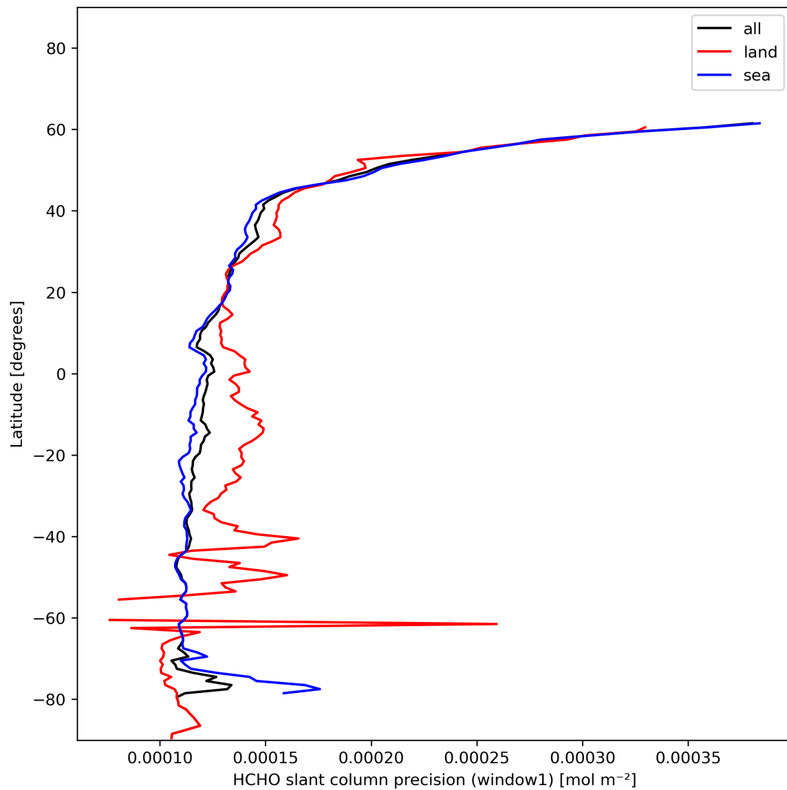
Figure 25: Zonal average of “HCHO slant column precision (window1)” for 2023-12-16 to 2023-12-18.
