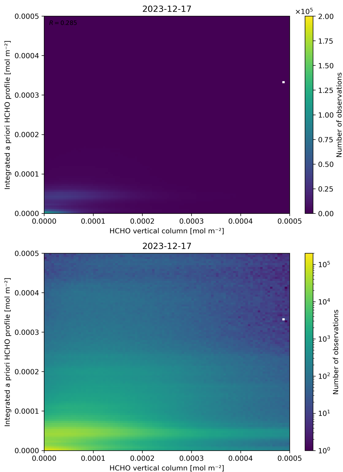
Figure 135: Scatter density plot of “HCHO vertical column” against “Integrated a priori HCHO profile” for 2023-12-16 to 2023-12-18.
