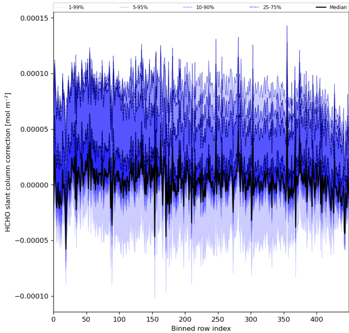
Figure 61: Along track statistics of “HCHO slant column correction” for 2023-12-16 to 2023-12-18
