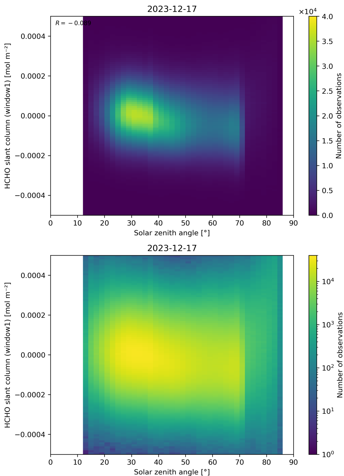
Figure 173: Scatter density plot of “Solar zenith angle” against “HCHO slant column (window1)” for 2023-12-16 to 2023-12-18.
