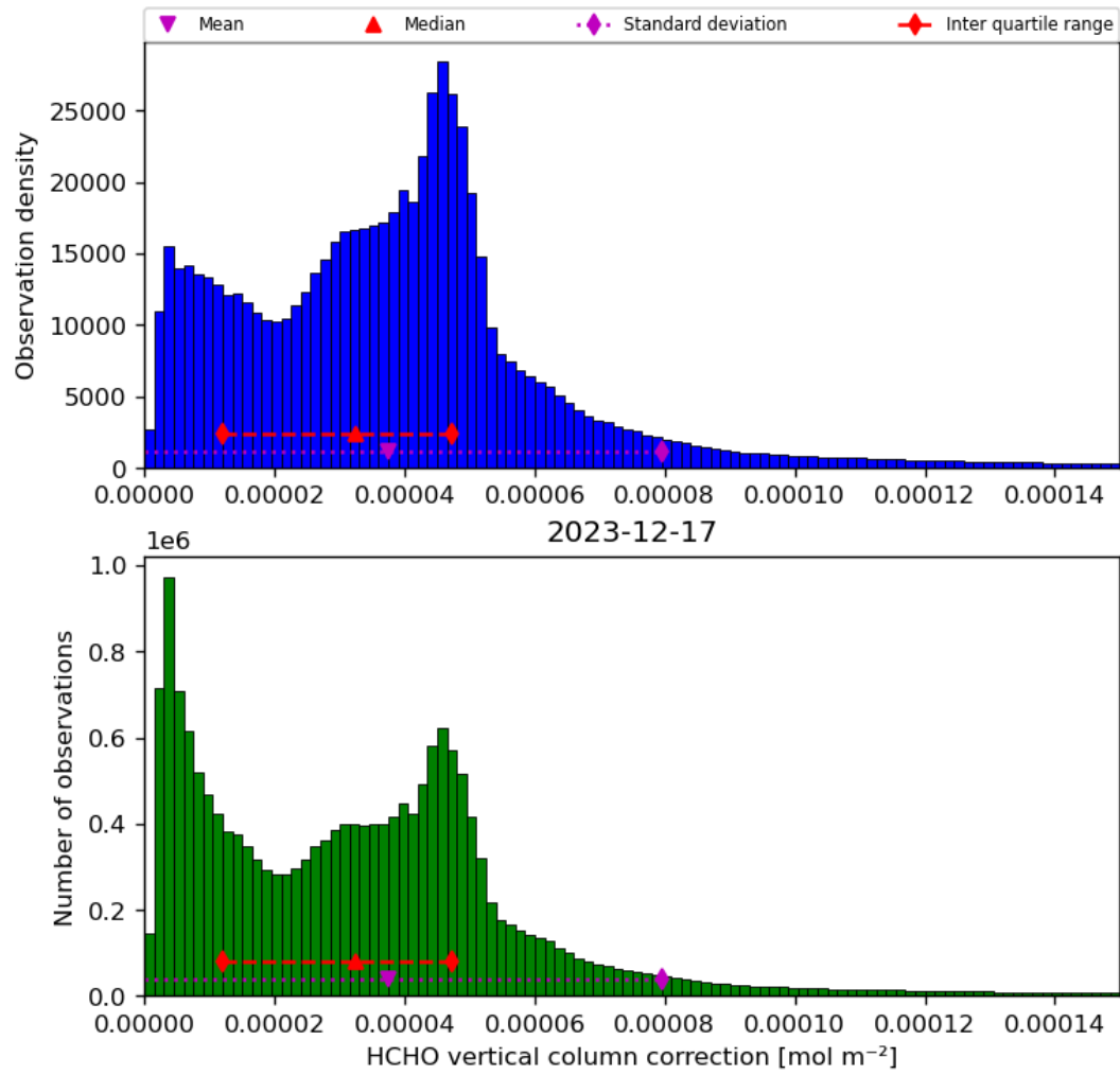
Figure 37: Histogram of “HCHO vertical column correction” for 2023-12-16 to 2023-12-18
