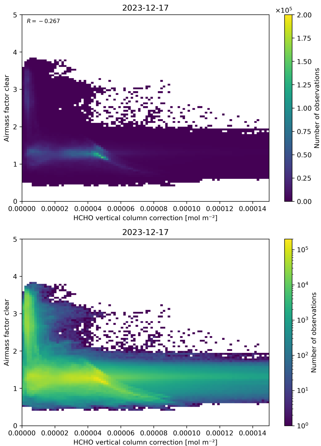
Figure 115: Scatter density plot of “HCHO vertical column correction” against “Airmass factor clear” for 2023-12-16 to 2023-12-18.
