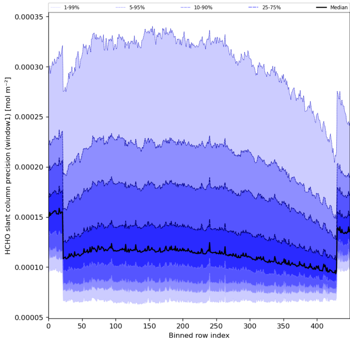
Figure 53: Along track statistics of “HCHO slant column precision (window1)” for 2023-12-16 to 2023-12-18
