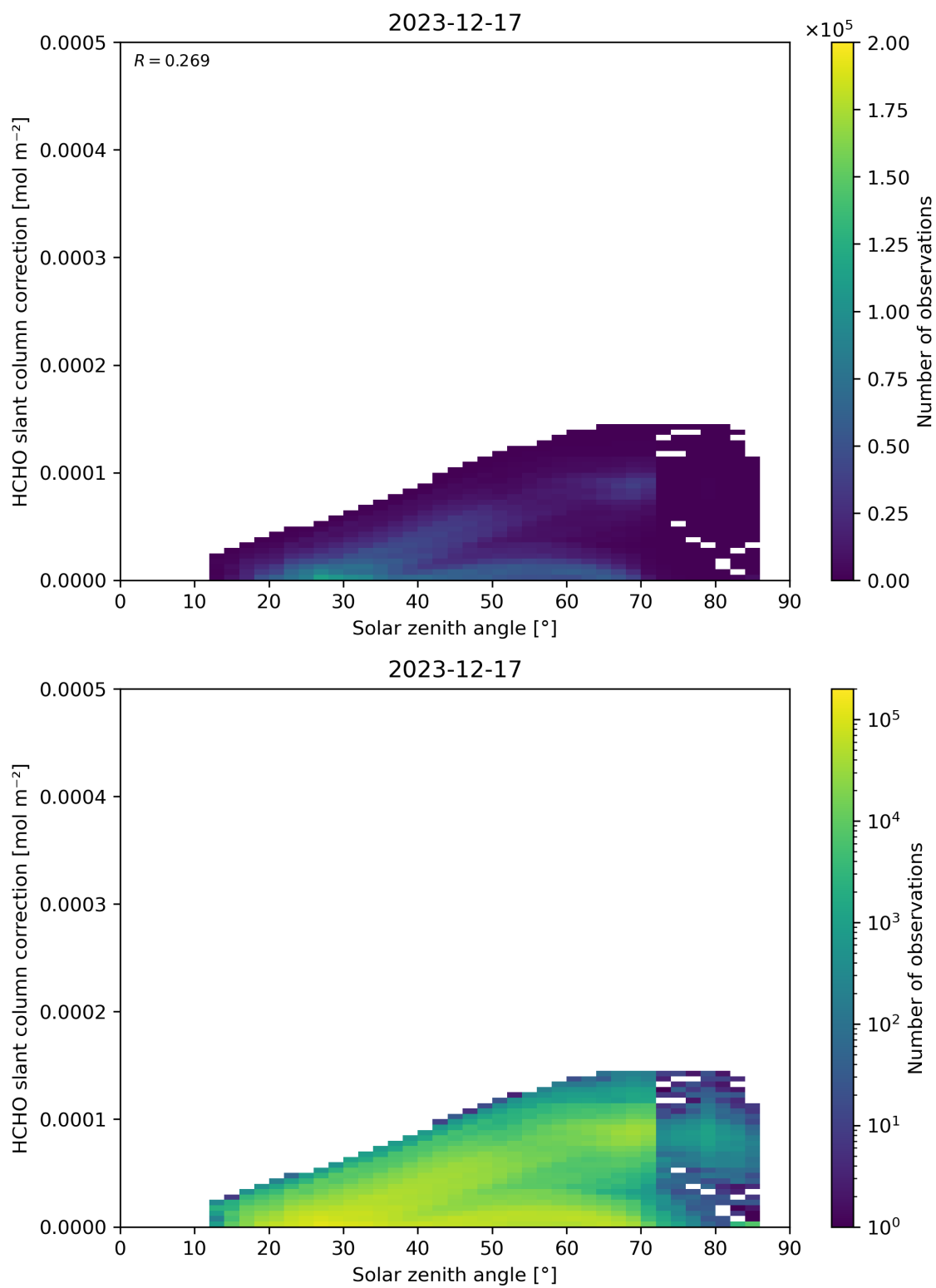
Figure 172: Scatter density plot of “Solar zenith angle” against “HCHO slant column correction” for 2023-12-16 to 2023-12-18.
