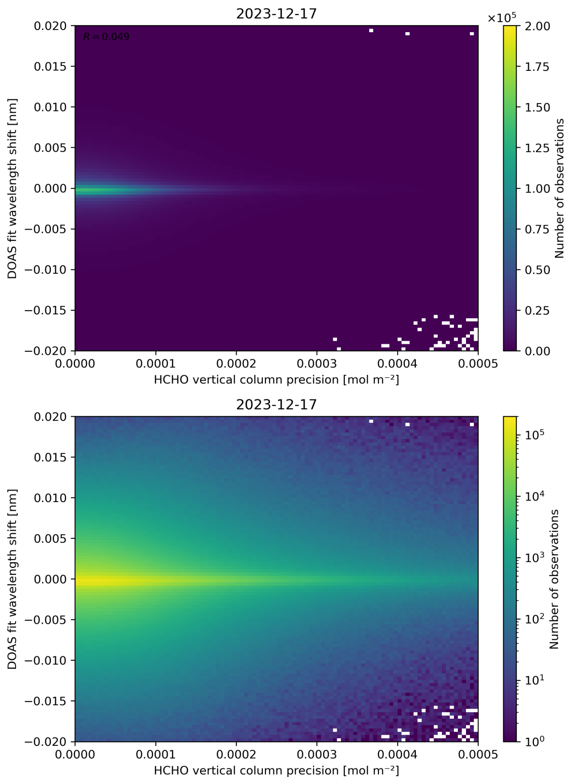
Figure 137: Scatter density plot of “HCHO vertical column precision” against “DOAS fit wavelength shift” for 2023-12-16 to 2023-12-18.
