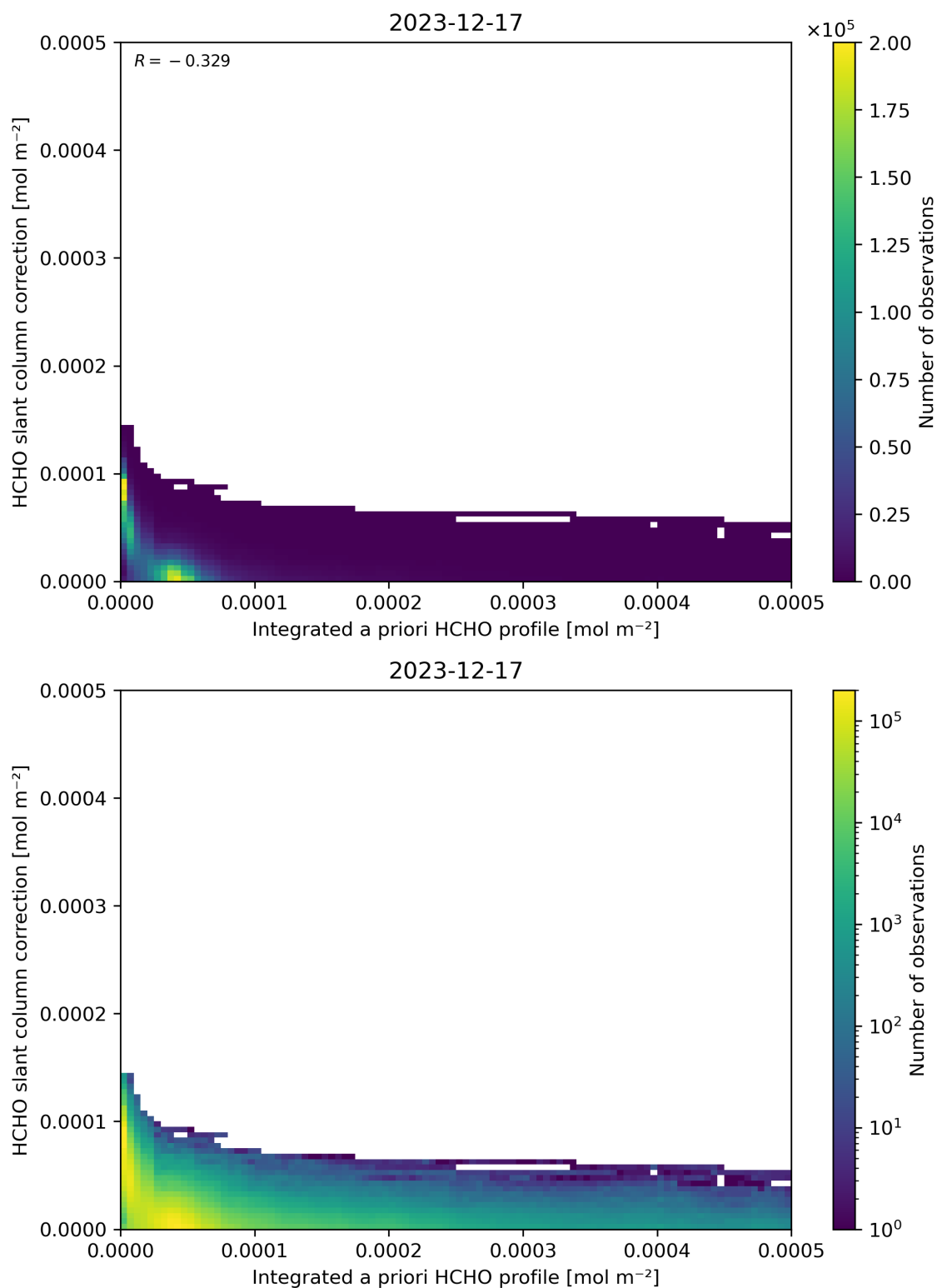
Figure 152: Scatter density plot of “Integrated a priori HCHO profile” against “HCHO slant column correction” for 2023-12-16 to 2023-12-18.
