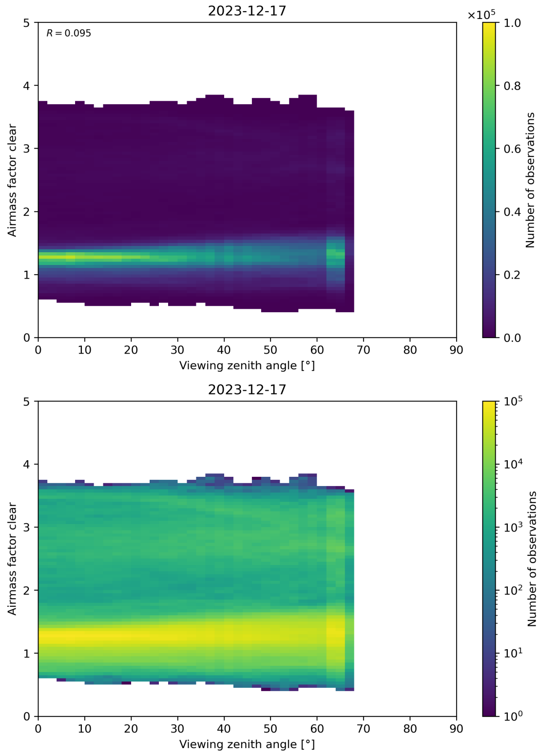
Figure 185: Scatter density plot of “Viewing zenith angle” against “Airmass factor clear” for 2023-12-16 to 2023-12-18.
