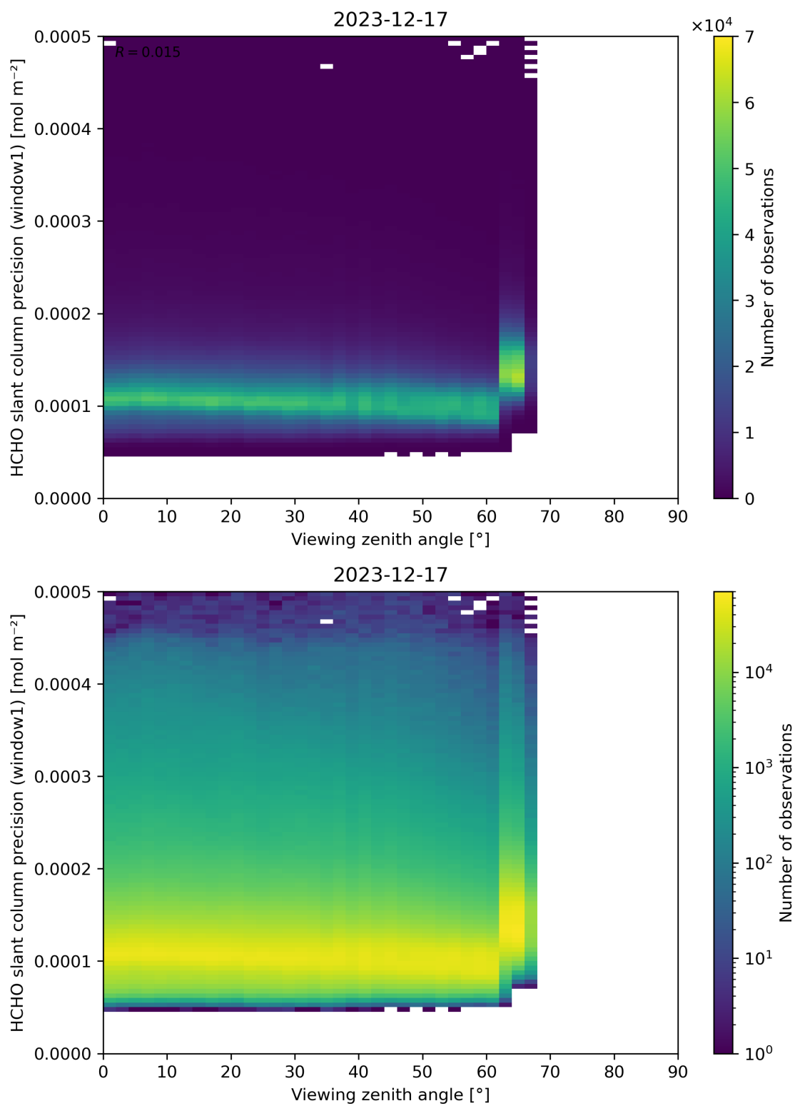
Figure 189: Scatter density plot of “Viewing zenith angle” against “HCHO slant column precision (window1)” for 2023-12-16 to 2023-12-18.
