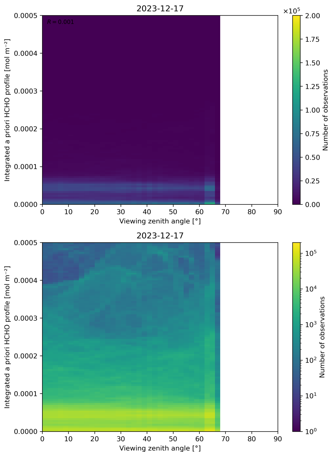
Figure 195: Scatter density plot of “Viewing zenith angle” against “Integrated a priori HCHO profile” for 2023-12-16 to 2023-12-18.
