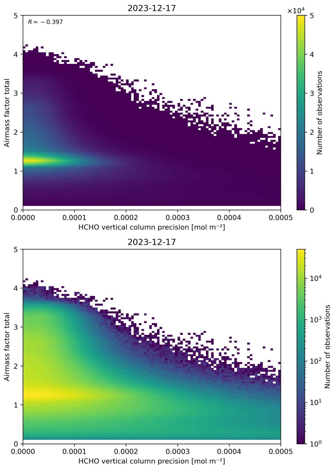
Figure 144: Scatter density plot of “HCHO vertical column precision” against “Airmass factor total” for 2023-12-16 to 2023-12-18.
