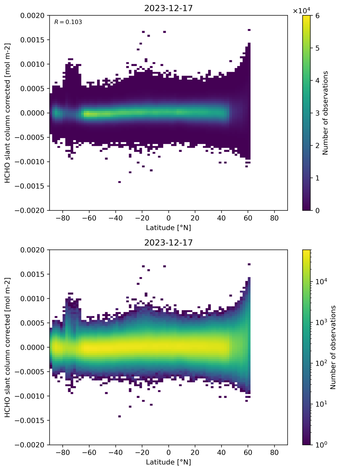
Figure 157: Scatter density plot of “Latitude” against “HCHO slant column corrected” for 2023-12-16 to 2023-12-18.
