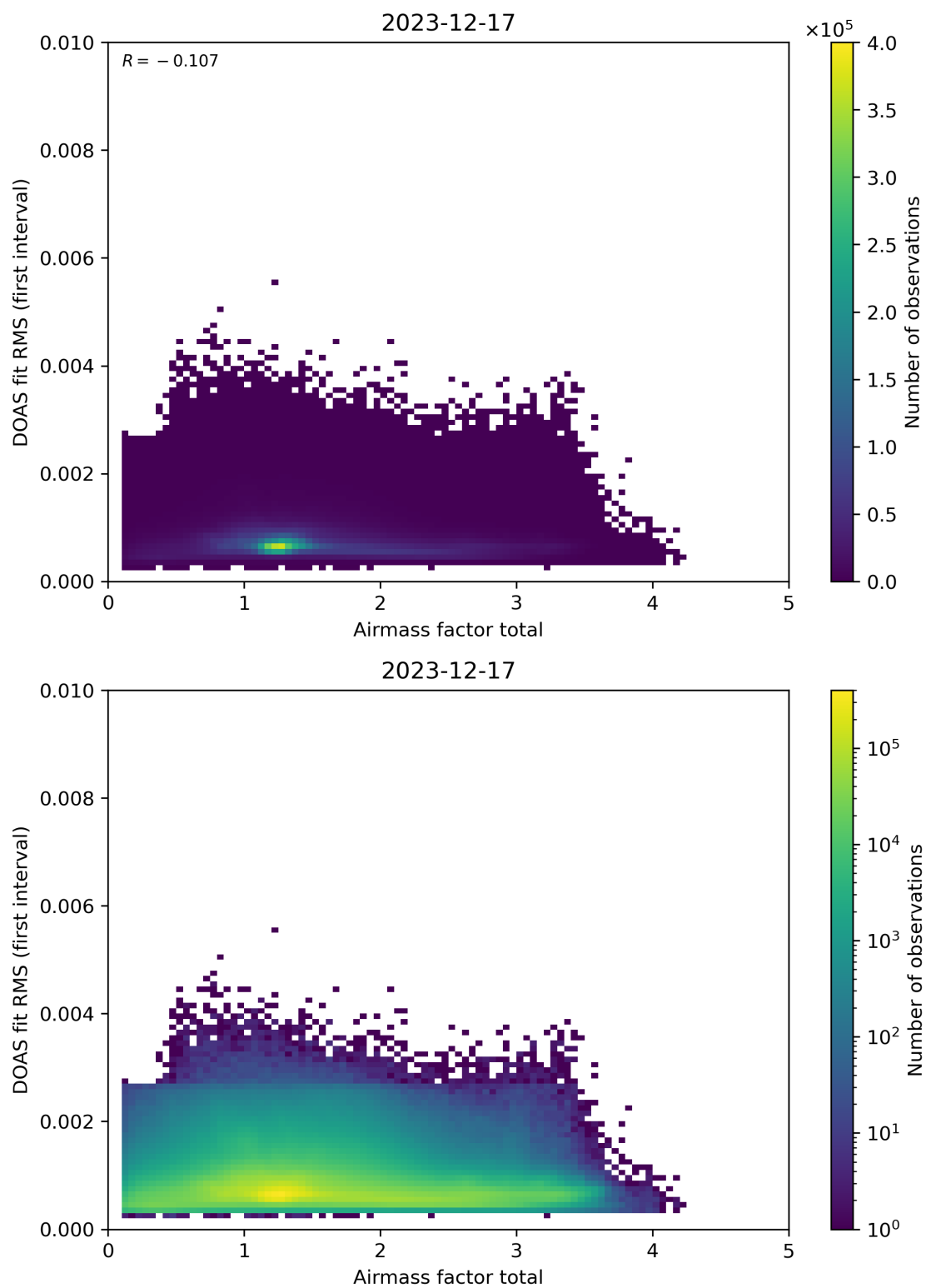
Figure 97: Scatter density plot of “Airmass factor total” against “DOAS fit RMS (first interval)” for 2023-12-16 to 2023-12-18.
