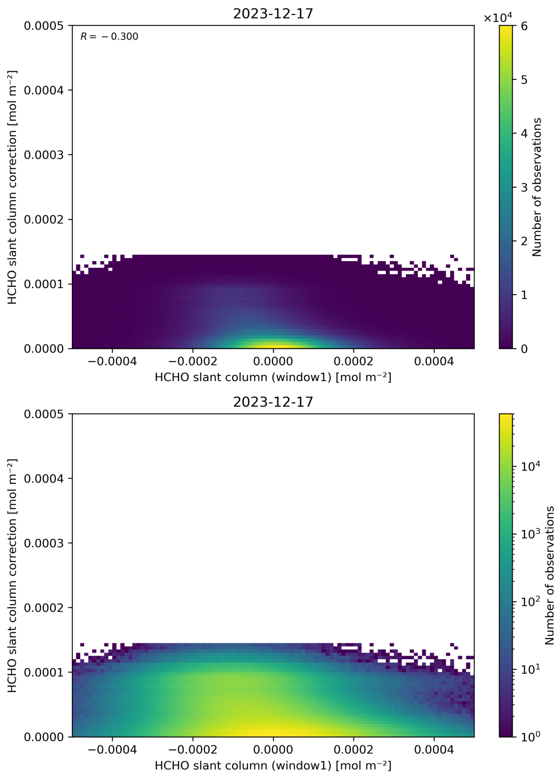
Figure 83: Scatter density plot of “HCHO slant column (window1)” against “HCHO slant column correction” for 2023-12-16 to 2023-12-18.
