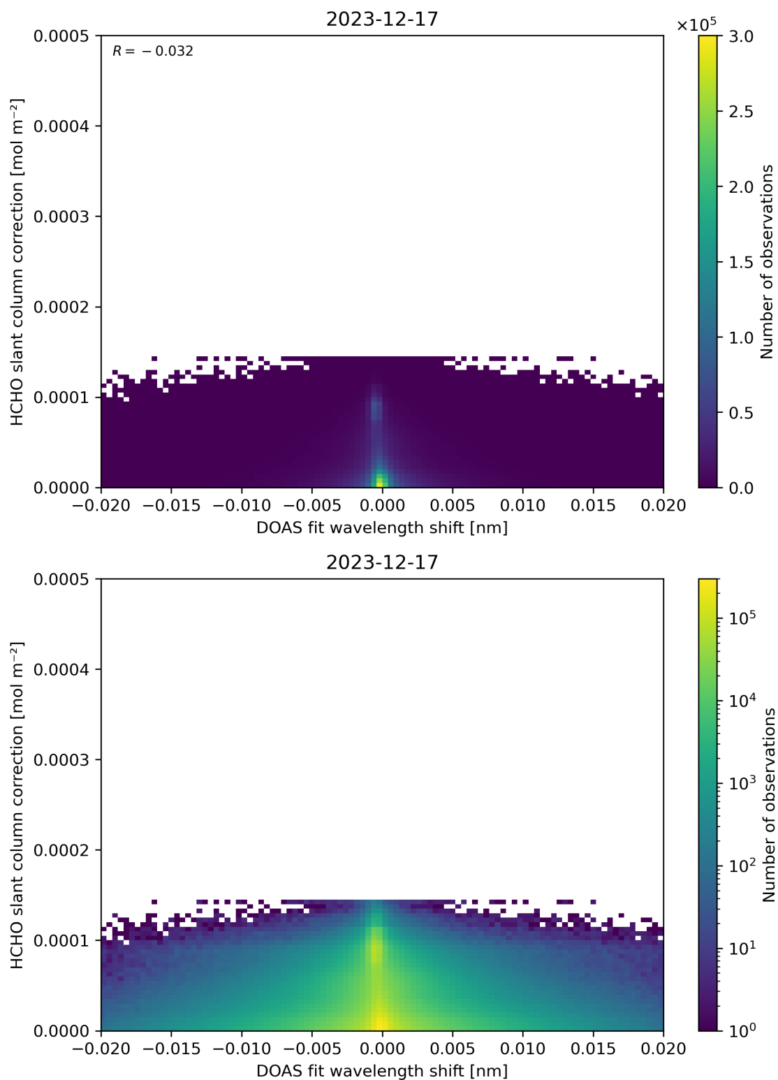
Figure 67: Scatter density plot of “DOAS fit wavelength shift” against “HCHO slant column correction” for 2023-12-16 to 2023-12-18.
