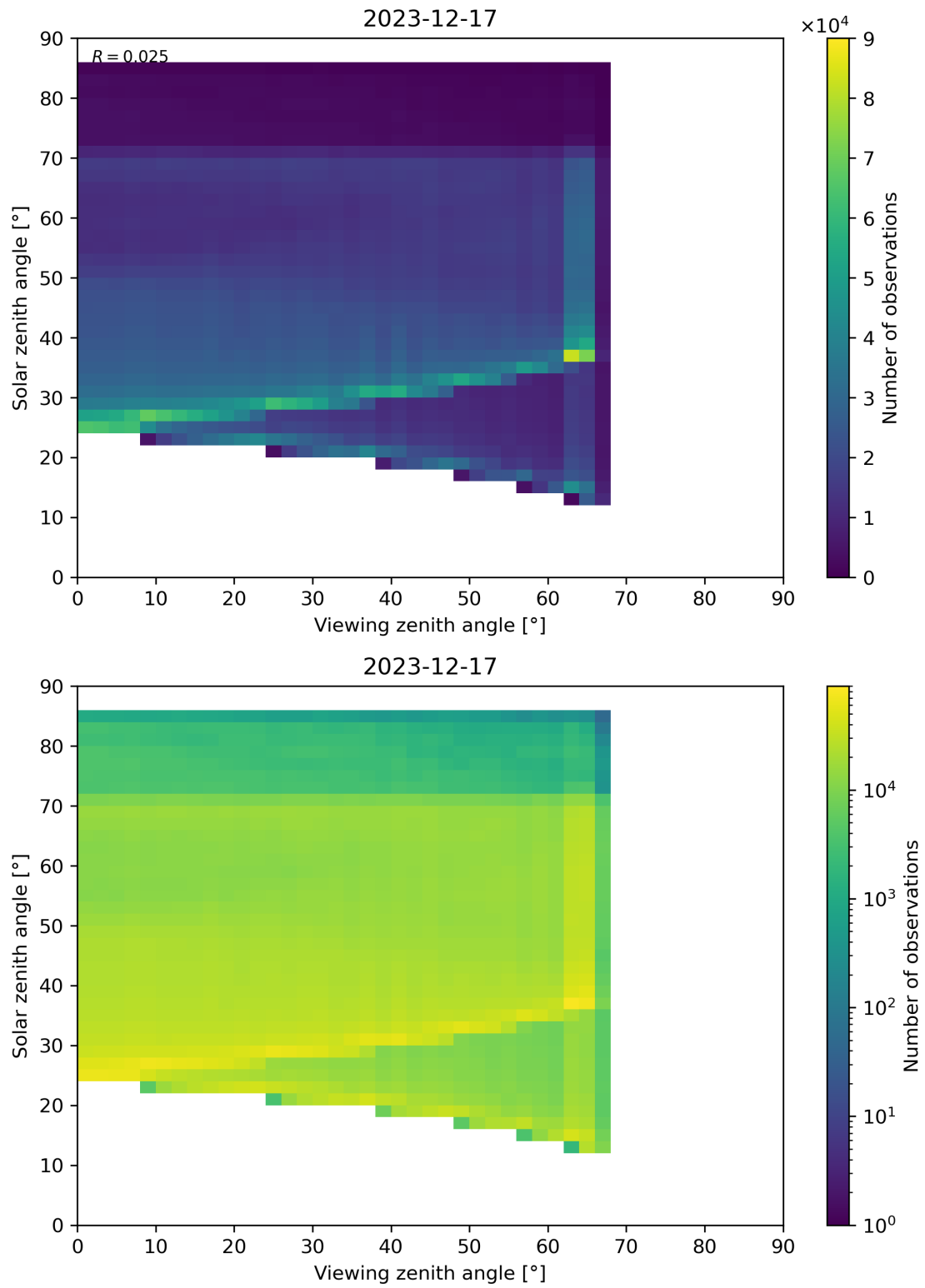
Figure 197: Scatter density plot of “Viewing zenith angle” against “Solar zenith angle” for 2023-12-16 to 2023-12-18.
