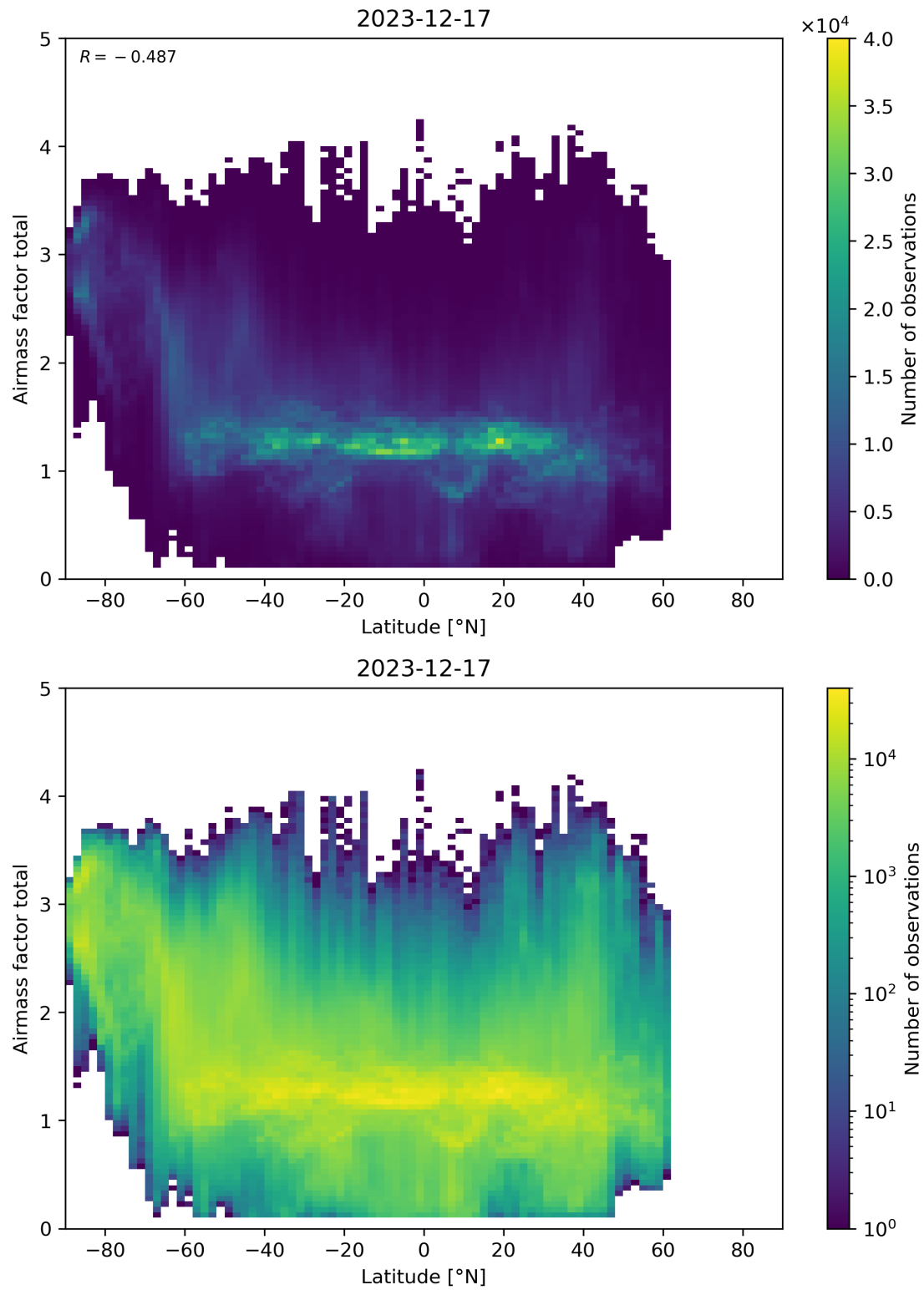
Figure 161: Scatter density plot of “Latitude” against “Airmass factor total” for 2023-12-16 to 2023-12-18.
