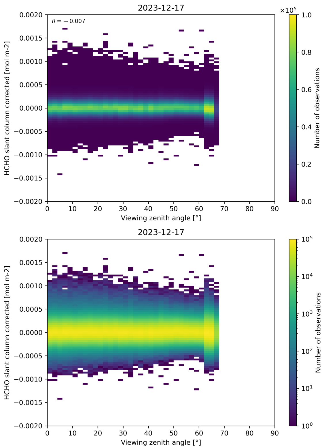
Figure 186: Scatter density plot of “Viewing zenith angle” against “HCHO slant column corrected” for 2023-12-16 to 2023-12-18.
