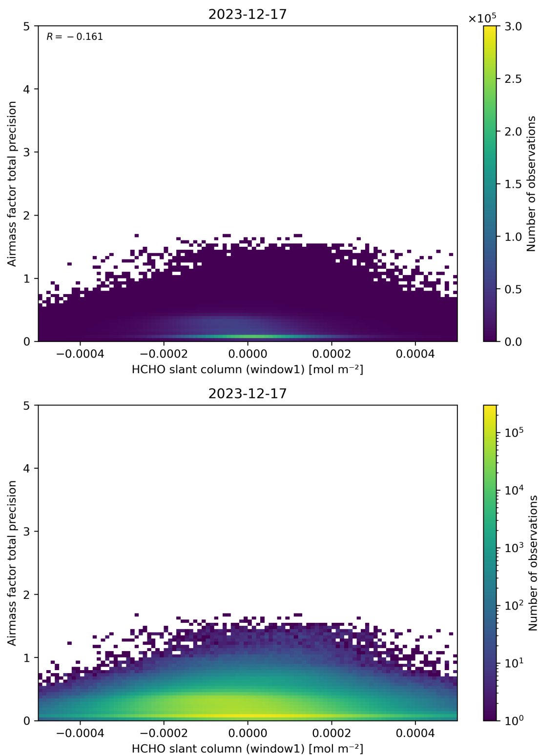
Figure 86: Scatter density plot of “HCHO slant column (window1)” against “Airmass factor total precision” for 2023-12-16 to 2023-12-18.
