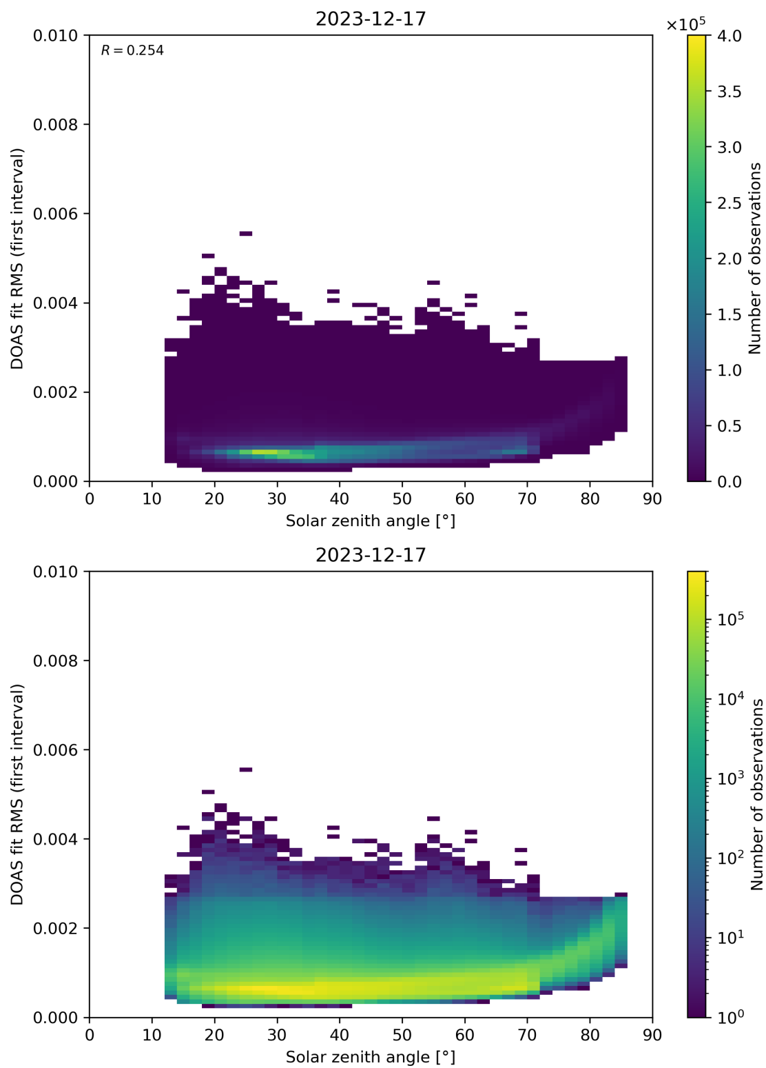
Figure 167: Scatter density plot of “Solar zenith angle” against “DOAS fit RMS (first interval)” for 2023-12-16 to 2023-12-18.
