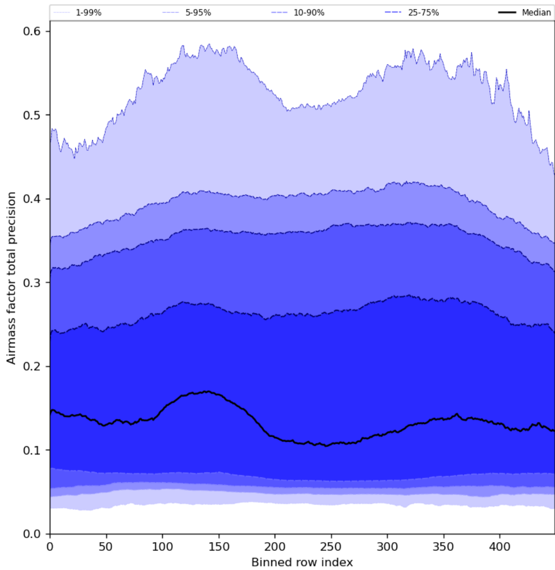
Figure 55: Along track statistics of “Airmass factor total precision” for 2023-12-16 to 2023-12-18
