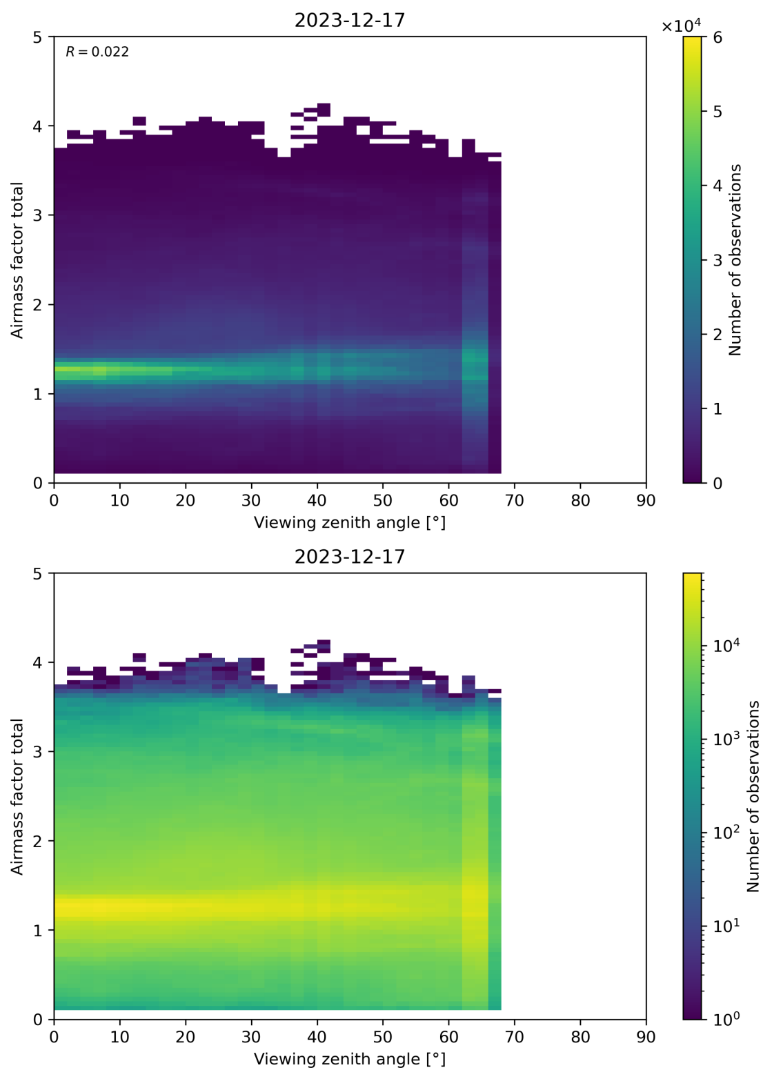
Figure 190: Scatter density plot of “Viewing zenith angle” against “Airmass factor total” for 2023-12-16 to 2023-12-18.
