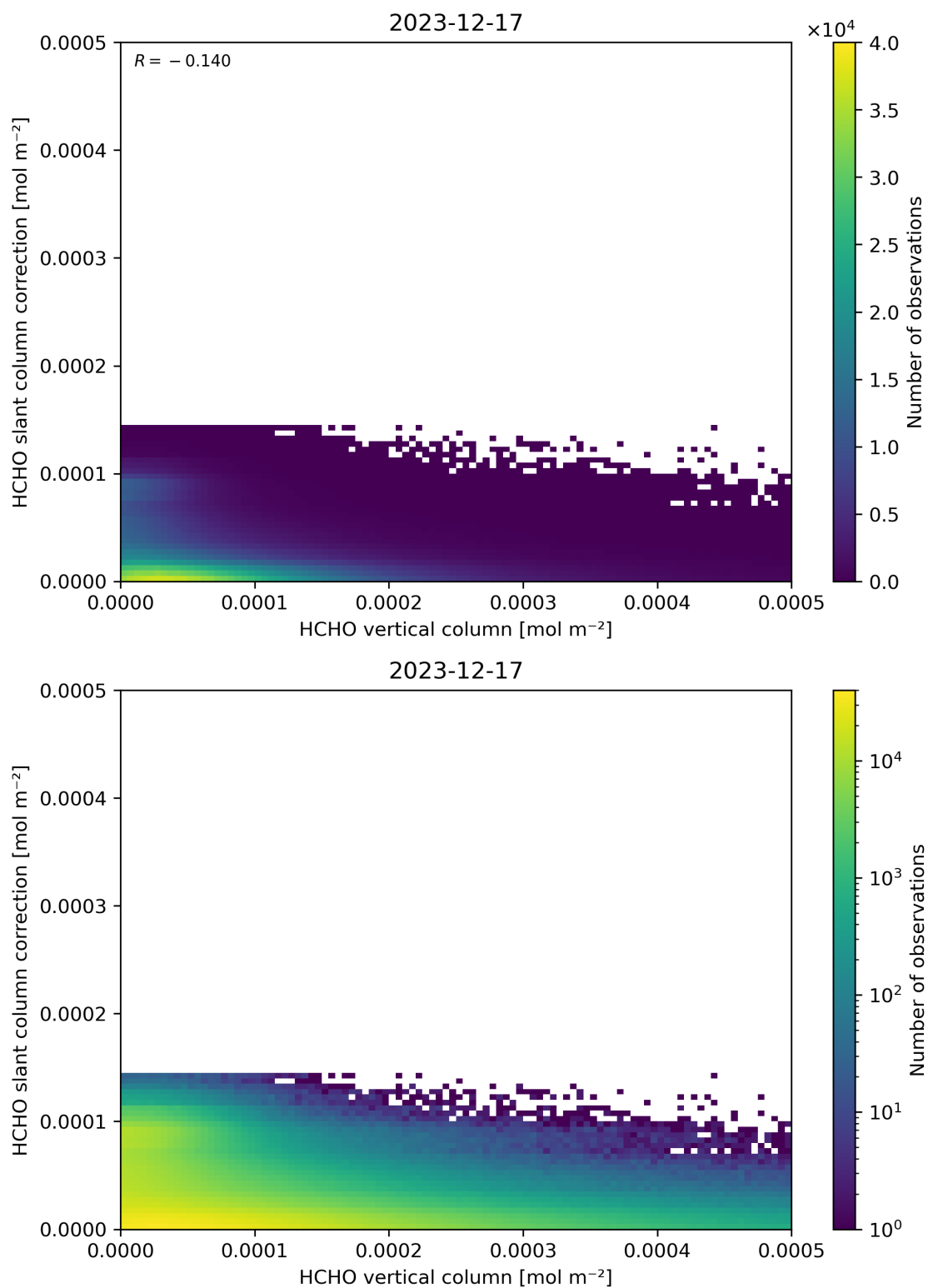
Figure 128: Scatter density plot of “HCHO vertical column” against “HCHO slant column correction” for 2023-12-16 to 2023-12-18.
