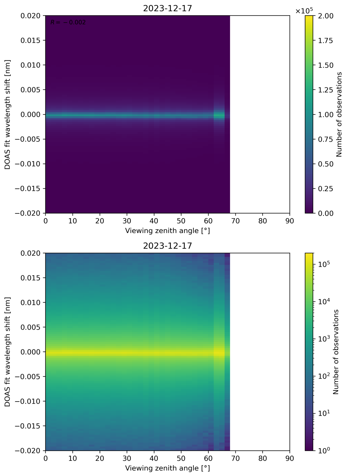
Figure 183: Scatter density plot of “Viewing zenith angle” against “DOAS fit wavelength shift” for 2023-12-16 to 2023-12-18.
