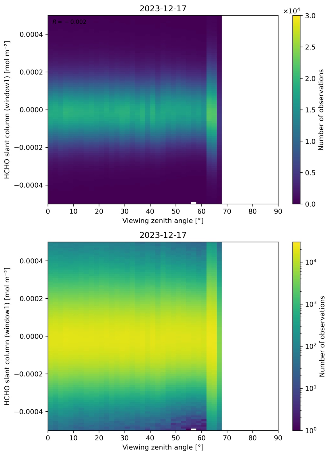
Figure 188: Scatter density plot of “Viewing zenith angle” against “HCHO slant column (window1)” for 2023-12-16 to 2023-12-18.
