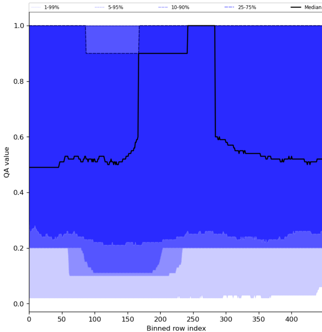
Figure 48: Along track statistics of "QA value" for 2023-12-16 to 2023-12-18
