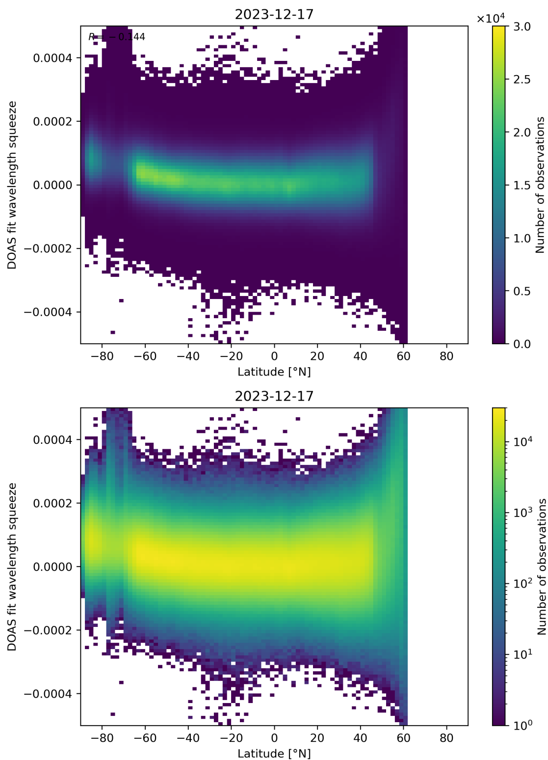
Figure 155: Scatter density plot of “Latitude” against “DOAS fit wavelength squeeze” for 2023-12-16 to 2023-12-18.
