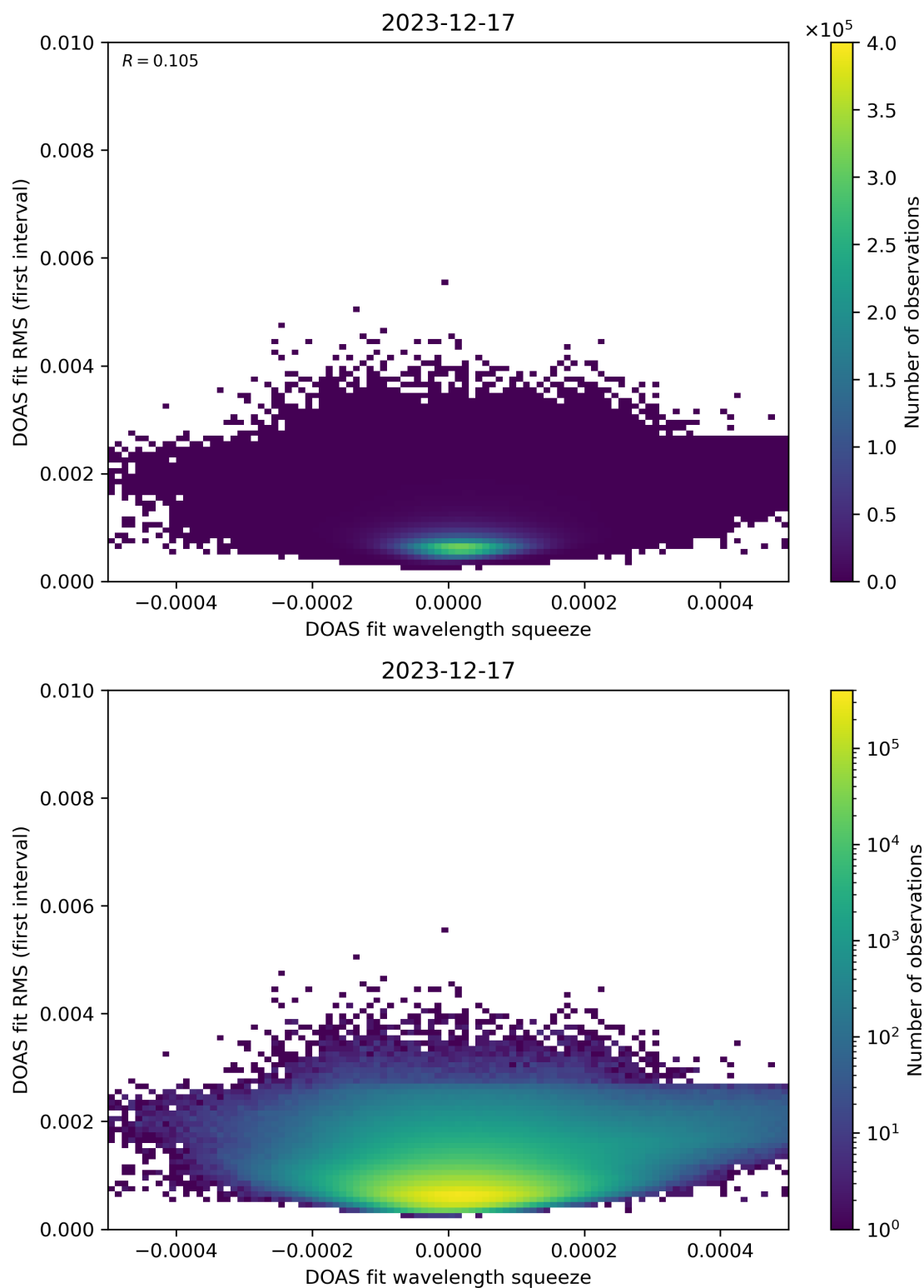
Figure 68: Scatter density plot of “DOAS fit wavelength squeeze” against “DOAS fit RMS (first interval)” for 2023-12-16 to 2023-12-18.
