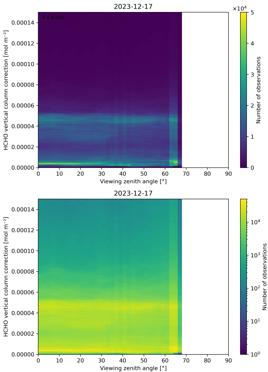
Figure 193: Scatter density plot of “Viewing zenith angle” against “HCHO vertical column correction” for 2023-12-16 to 2023-12-18.
