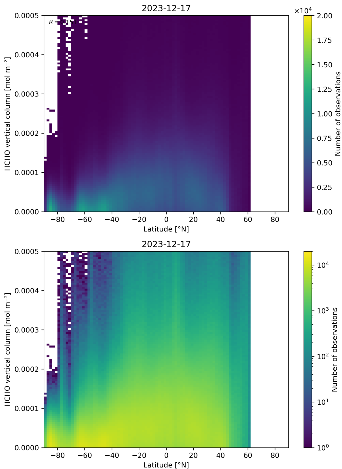
Figure 163: Scatter density plot of “Latitude” against “HCHO vertical column” for 2023-12-16 to 2023-12-18.
