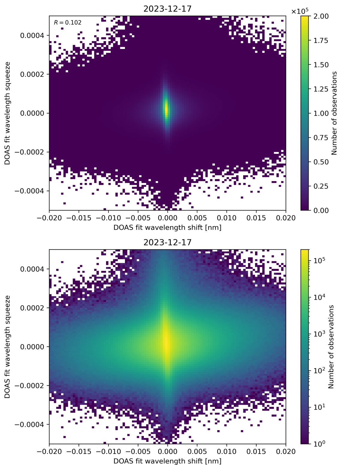
Figure 65: Scatter density plot of “DOAS fit wavelength shift” against “DOAS fit wavelength squeeze” for 2023-12-16 to 2023-12-18.
