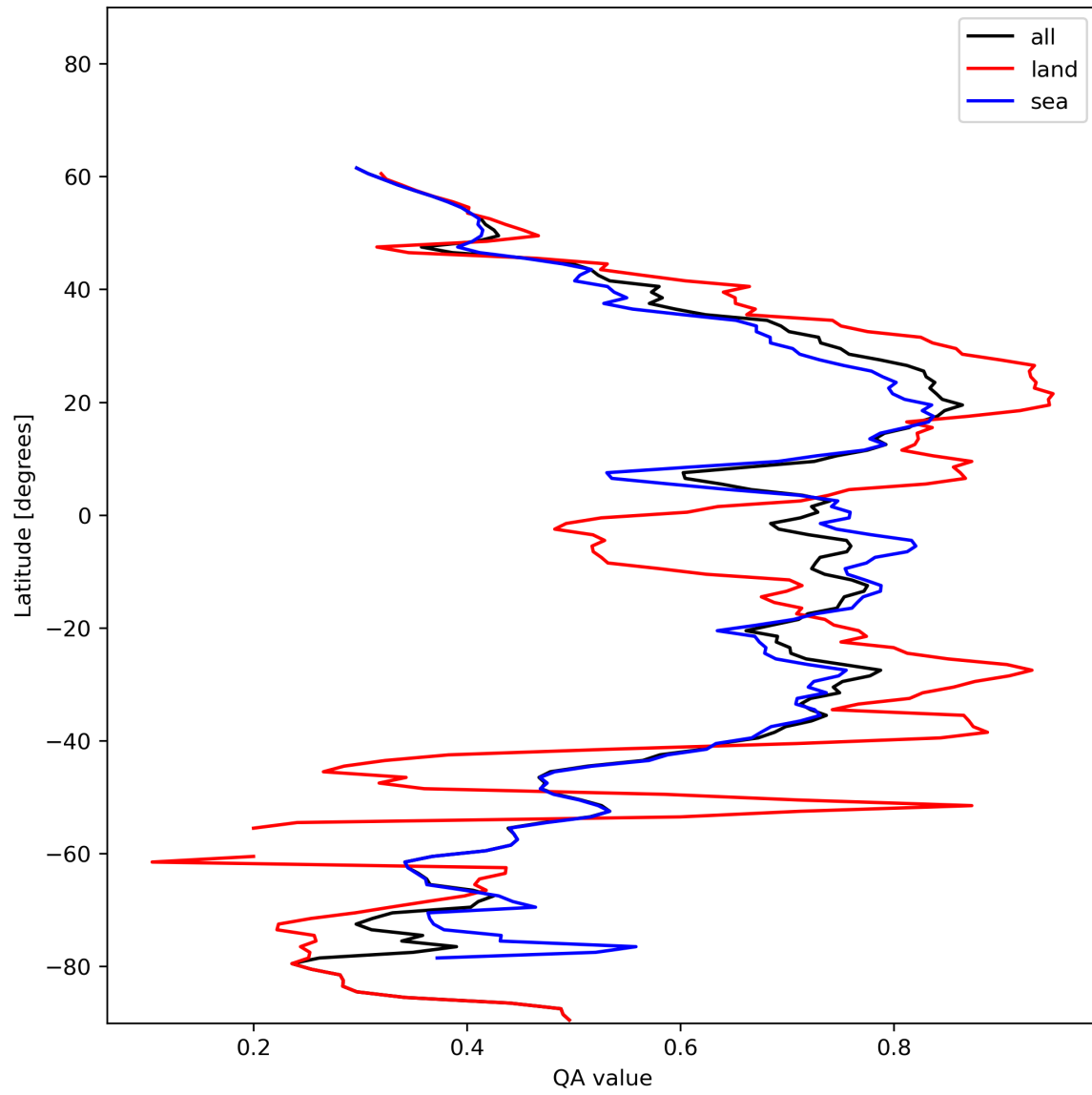
Figure 20: Zonal average of “QA value” for 2023-12-16 to 2023-12-18.
