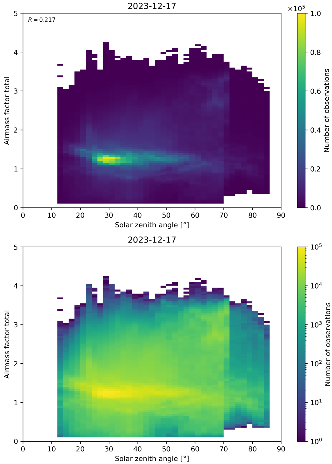
Figure 175: Scatter density plot of “Solar zenith angle” against “Airmass factor total” for 2023-12-16 to 2023-12-18.
