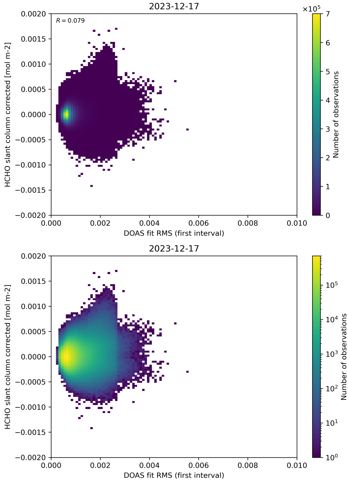
Figure 62: Scatter density plot of “DOAS fit RMS (first interval)” against “HCHO slant column corrected” for 2023-12-16 to 2023-12-18.
