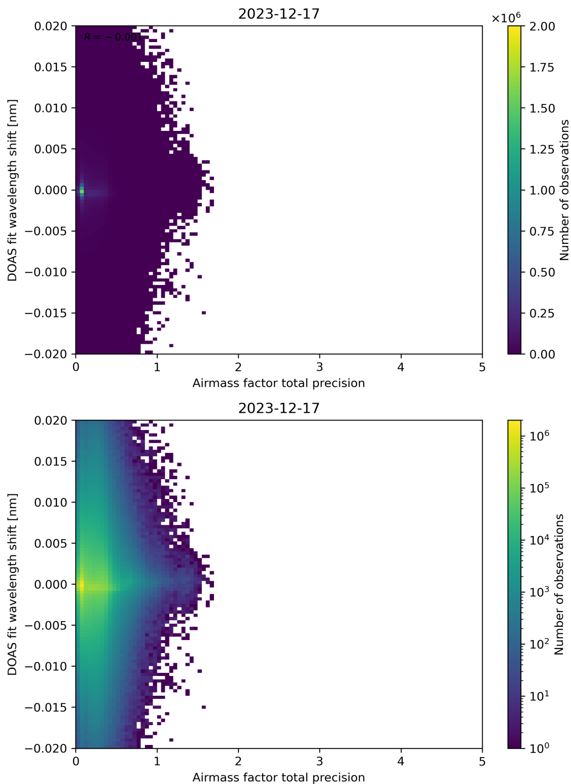
Figure 106: Scatter density plot of “Airmass factor total precision” against “DOAS fit wavelength shift” for 2023-12-16 to 2023-12-18.
