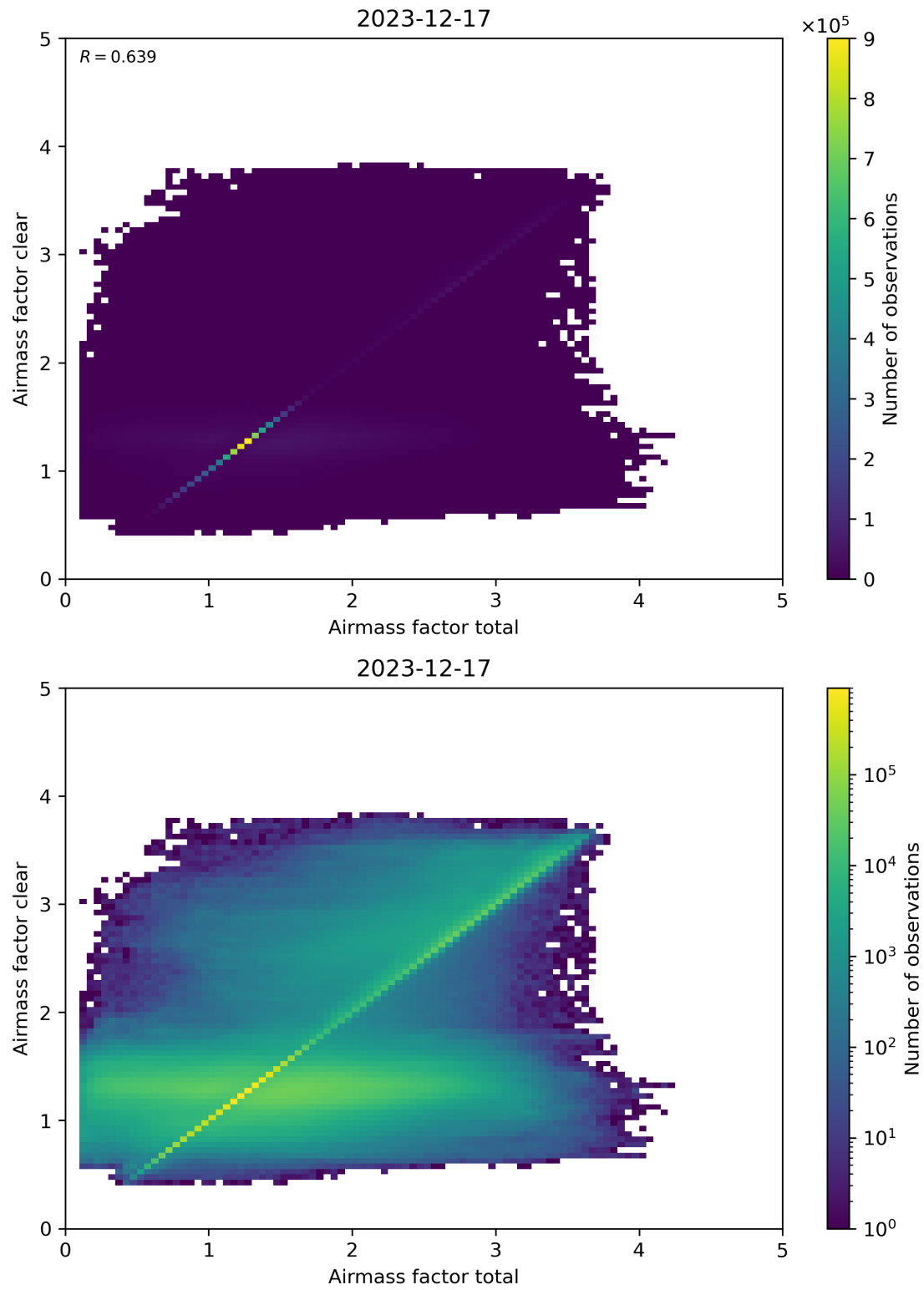
Figure 100: Scatter density plot of “Airmass factor total” against “Airmass factor clear” for 2023-12-16 to 2023-12-18.
