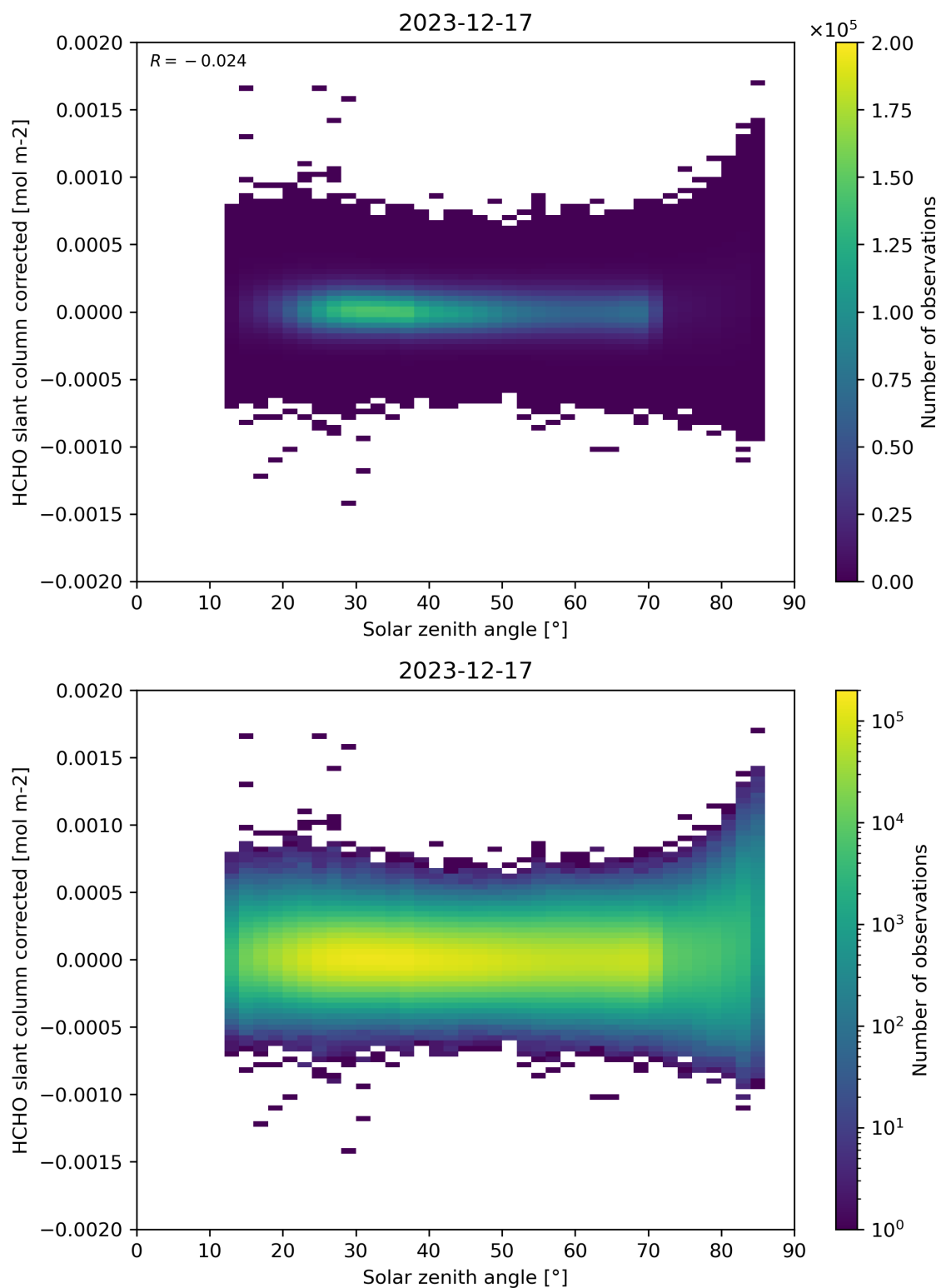
Figure 171: Scatter density plot of “Solar zenith angle” against “HCHO slant column corrected” for 2023-12-16 to 2023-12-18.
