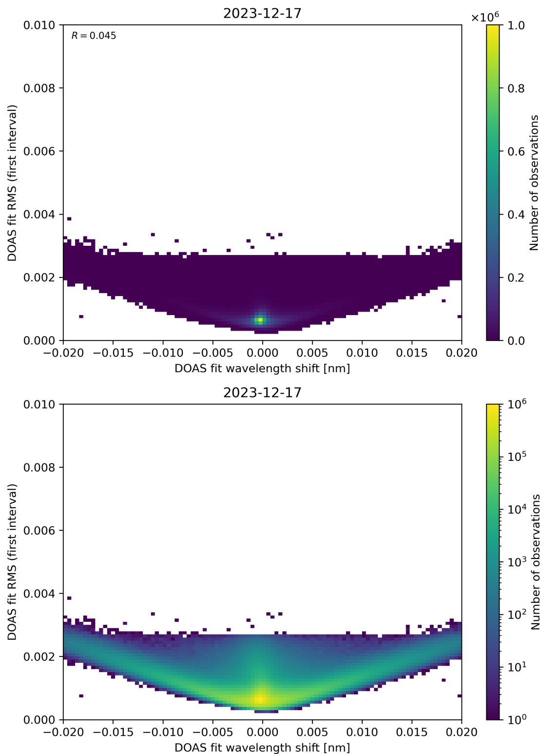
Figure 64: Scatter density plot of “DOAS fit wavelength shift” against “DOAS fit RMS (first interval)” for 2023-12-16 to 2023-12-18.
