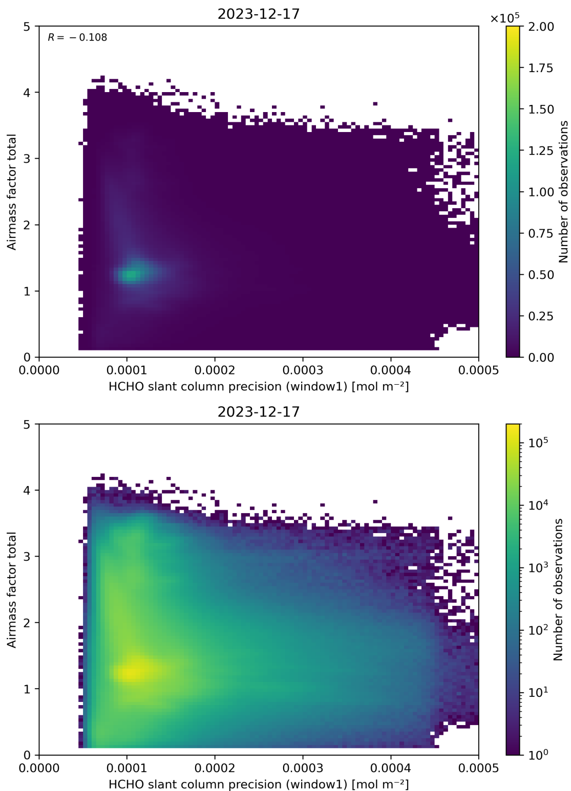
Figure 94: Scatter density plot of “HCHO slant column precision (window1)” against “Airmass factor total” for 2023-12-16 to 2023-12-18.
