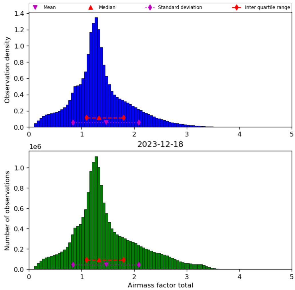
Figure 40: Histogram of “Airmass factor total” for 2023-12-17 to 2023-12-19
