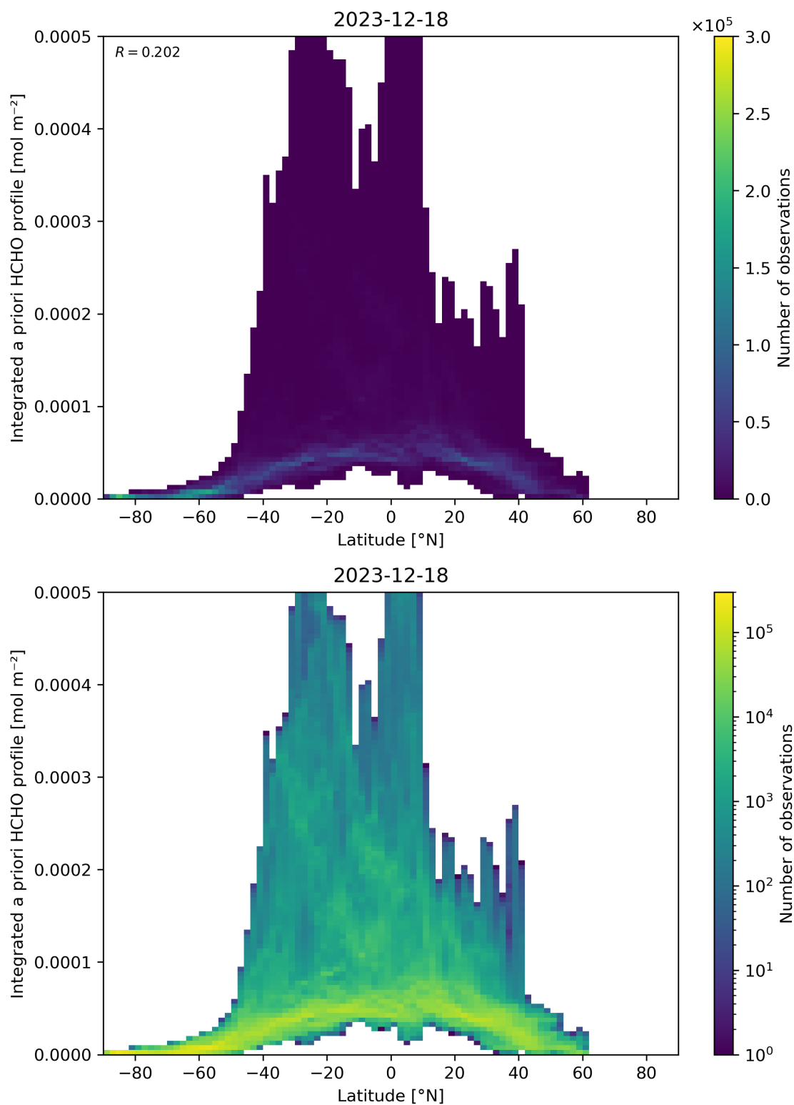
Figure 166: Scatter density plot of “Latitude” against “Integrated a priori HCHO profile” for 2023-12-17 to 2023-12-19.
