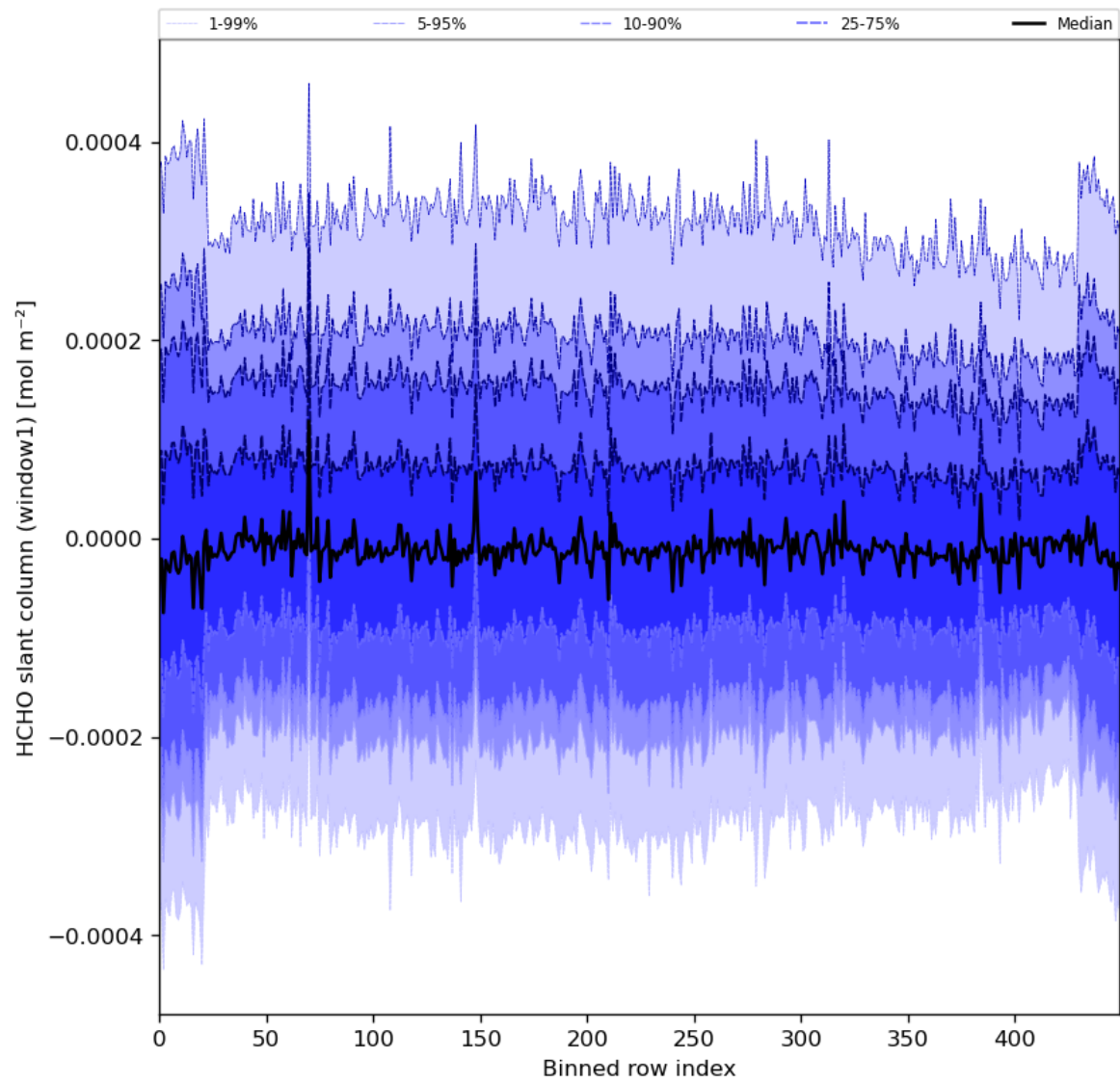
Figure 52: Along track statistics of “HCHO slant column (window1)” for 2023-12-17 to 2023-12-19
