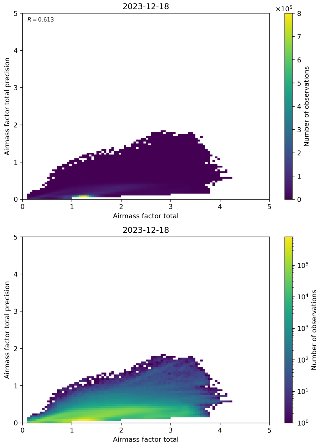
Figure 103: Scatter density plot of “Airmass factor total” against “Airmass factor total precision” for 2023-12-17 to 2023-12-19.
