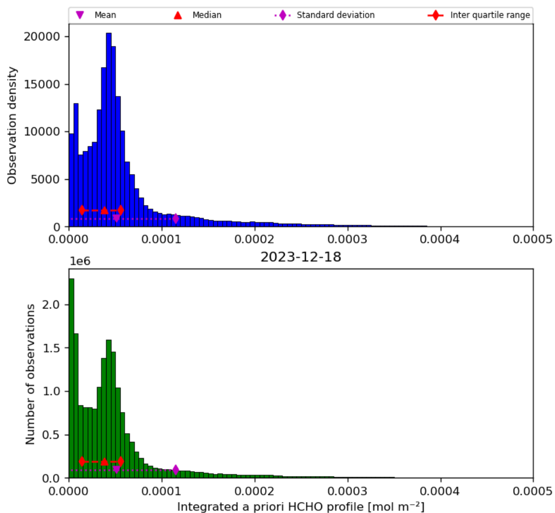
Figure 43: Histogram of “Integrated a priori HCHO profile” for 2023-12-17 to 2023-12-19
