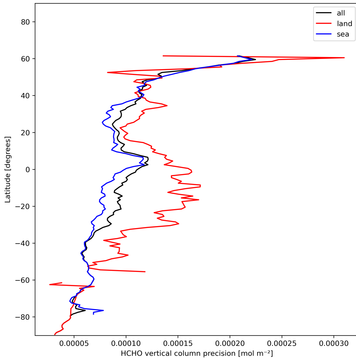
Figure 22: Zonal average of “HCHO vertical column precision” for 2023-12-17 to 2023-12-19.
