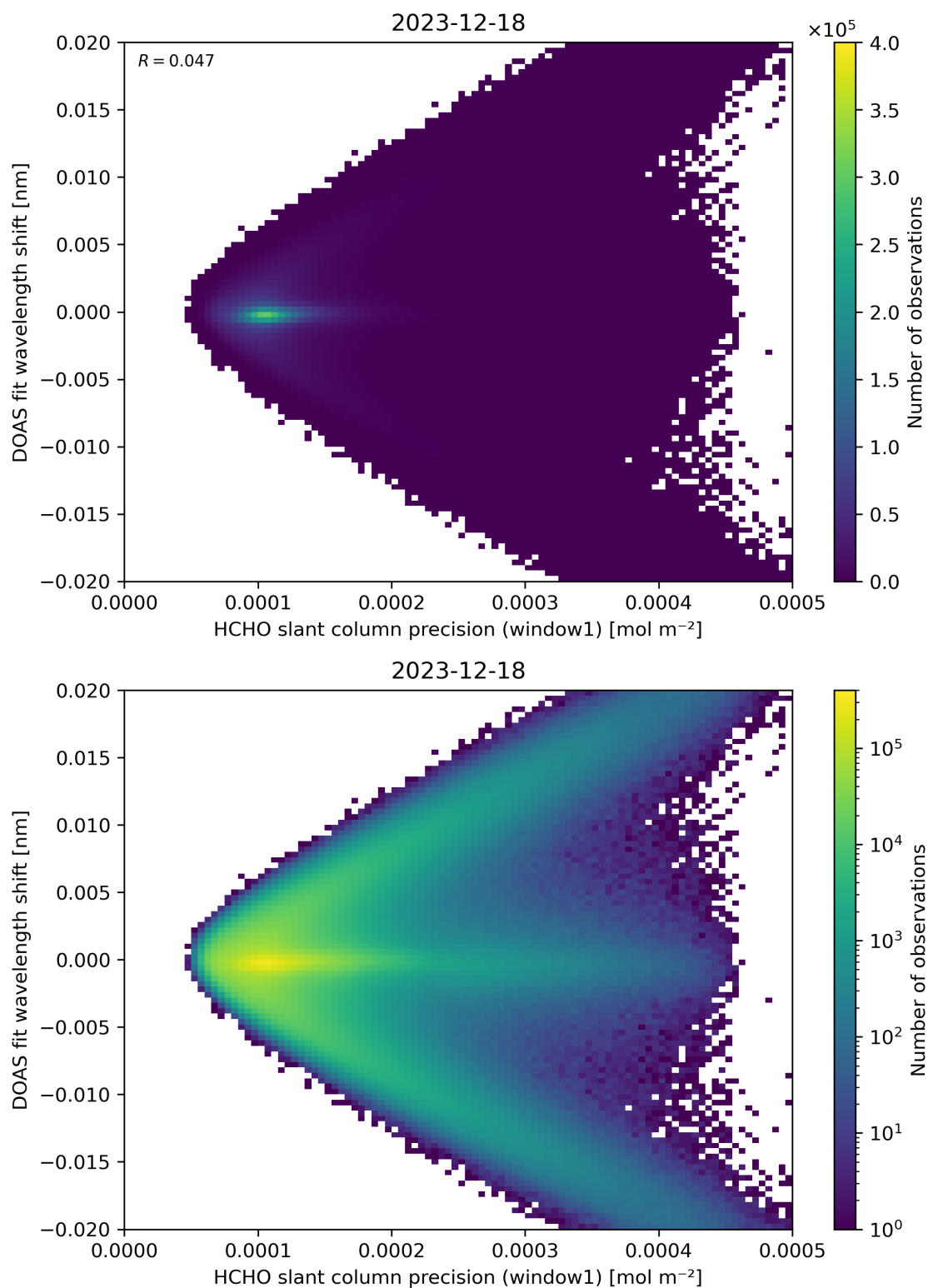
Figure 89: Scatter density plot of “HCHO slant column precision (window1)” against “DOAS fit wavelength shift” for 2023-12-17 to 2023-12-19.
