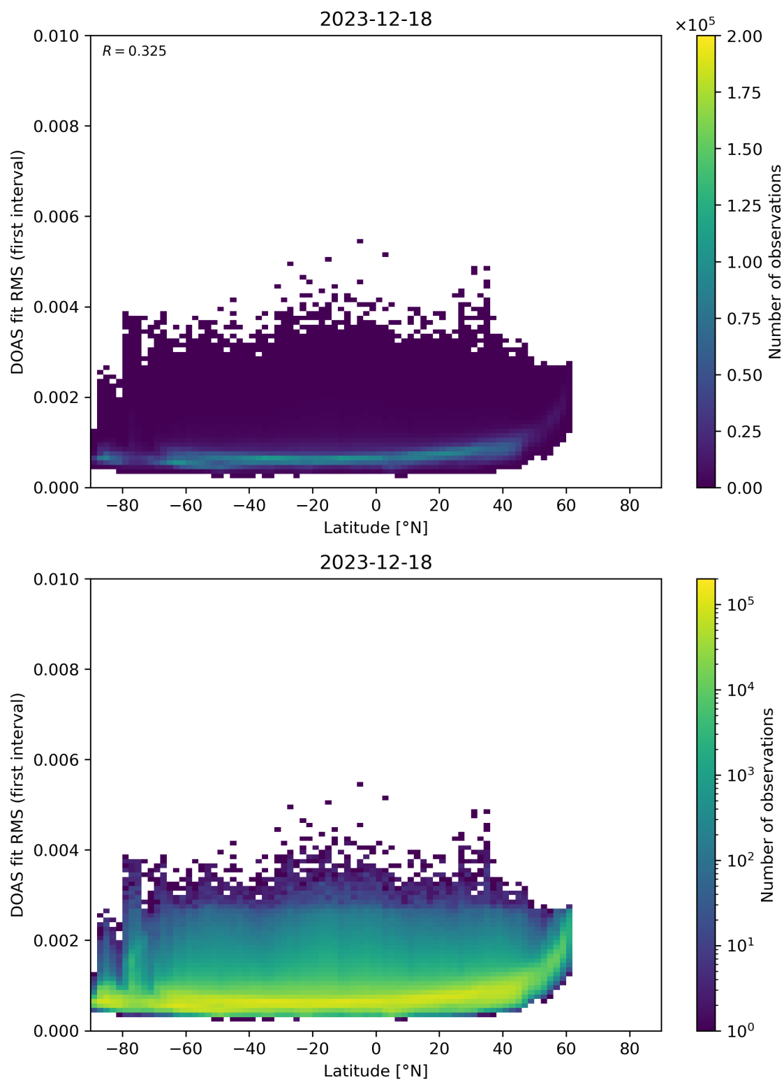
Figure 153: Scatter density plot of “Latitude” against “DOAS fit RMS (first interval)” for 2023-12-17 to 2023-12-19.
