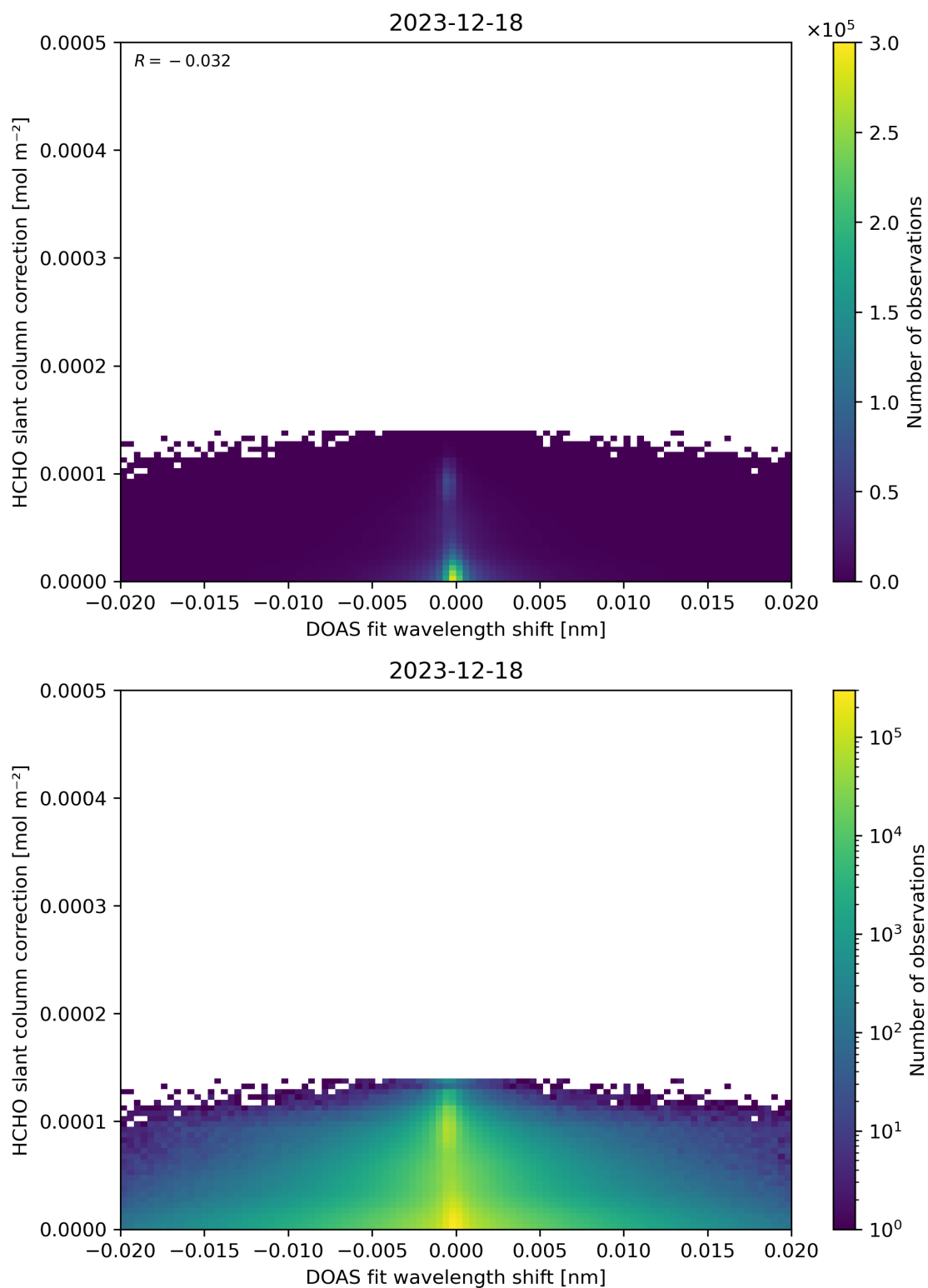
Figure 67: Scatter density plot of “DOAS fit wavelength shift” against “HCHO slant column correction” for 2023-12-17 to 2023-12-19.
