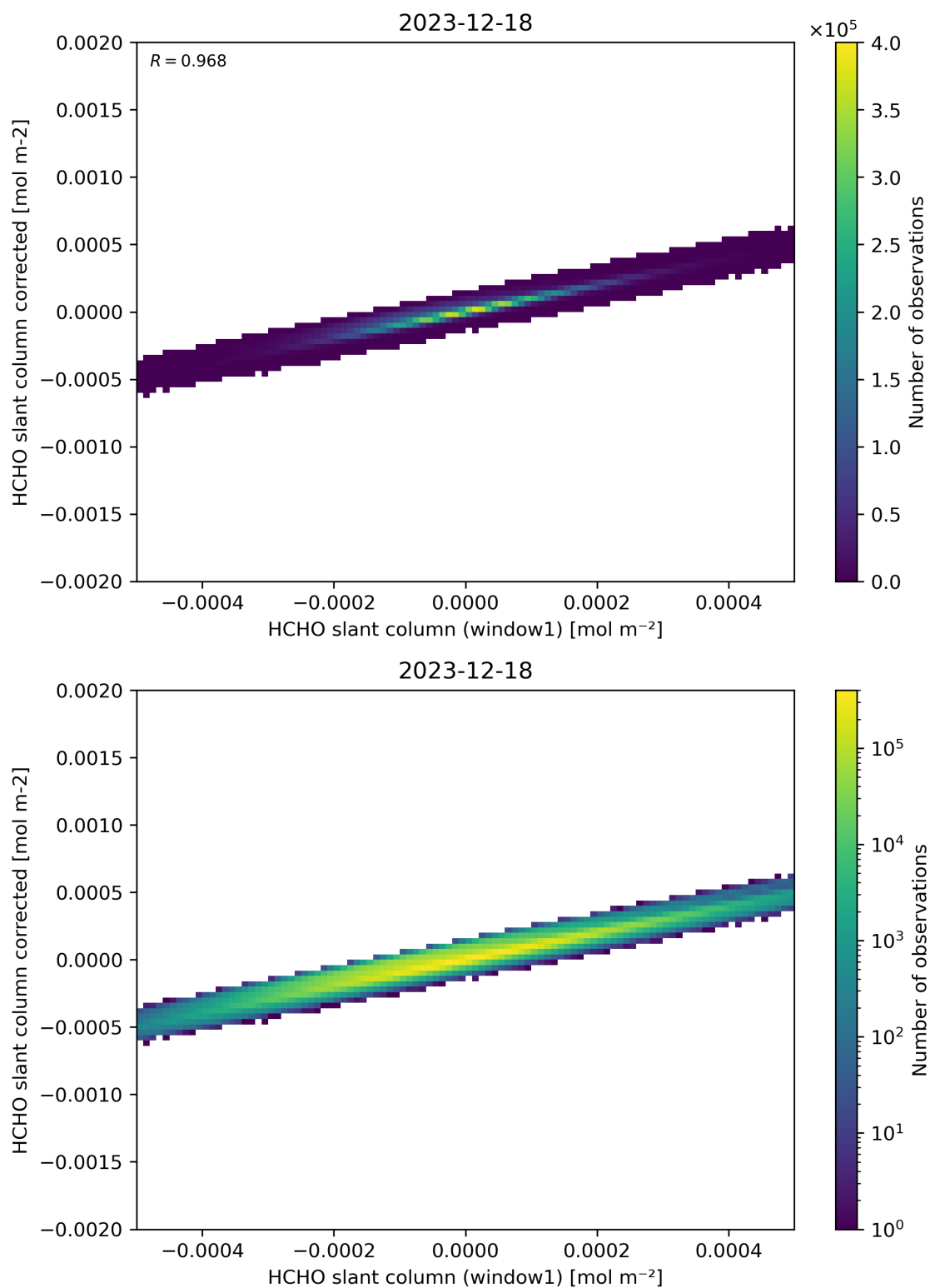
Figure 82: Scatter density plot of “HCHO slant column (window1)” against “HCHO slant column corrected” for 2023-12-17 to 2023-12-19.
