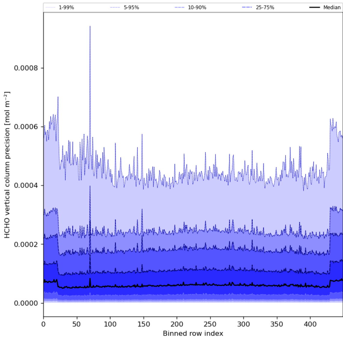
Figure 50: Along track statistics of “HCHO vertical column precision” for 2023-12-17 to 2023-12-19
