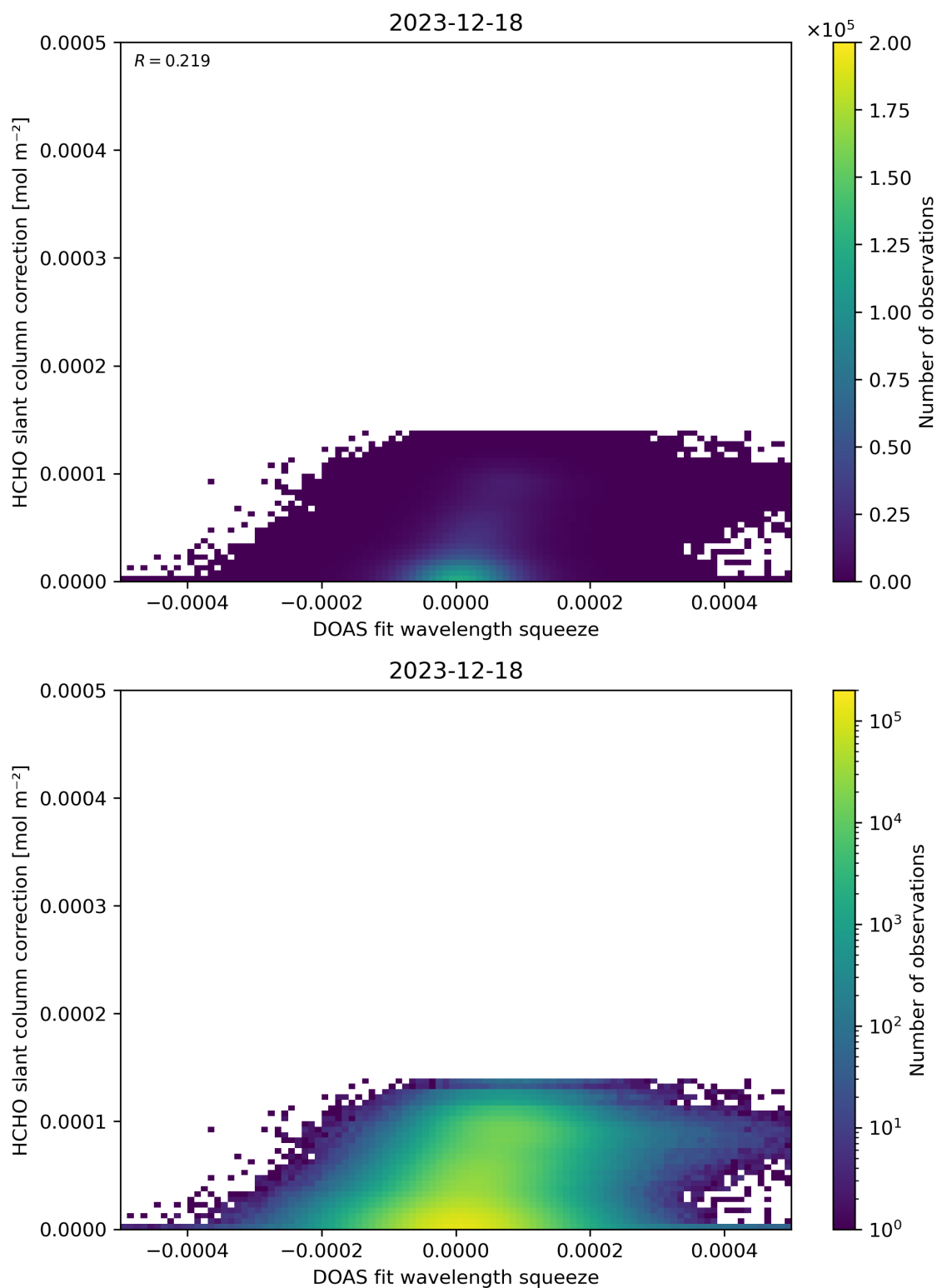
Figure 70: Scatter density plot of “DOAS fit wavelength squeeze” against “HCHO slant column correction” for 2023-12-17 to 2023-12-19.
