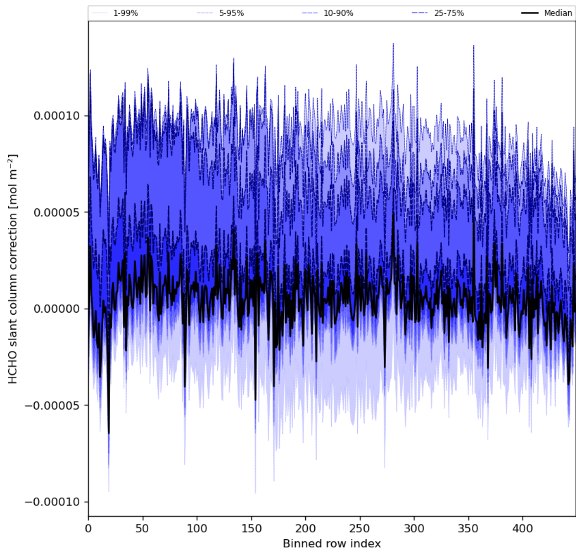
Figure 61: Along track statistics of “HCHO slant column correction” for 2023-12-17 to 2023-12-19
