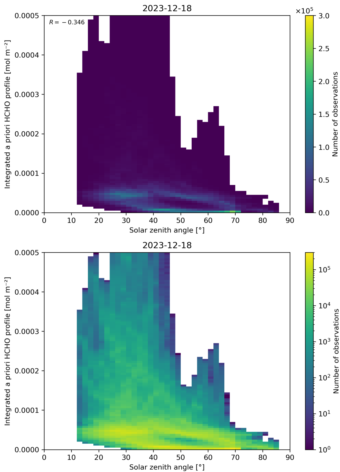
Figure 180: Scatter density plot of “Solar zenith angle” against “Integrated a priori HCHO profile” for 2023-12-17 to 2023-12-19.
