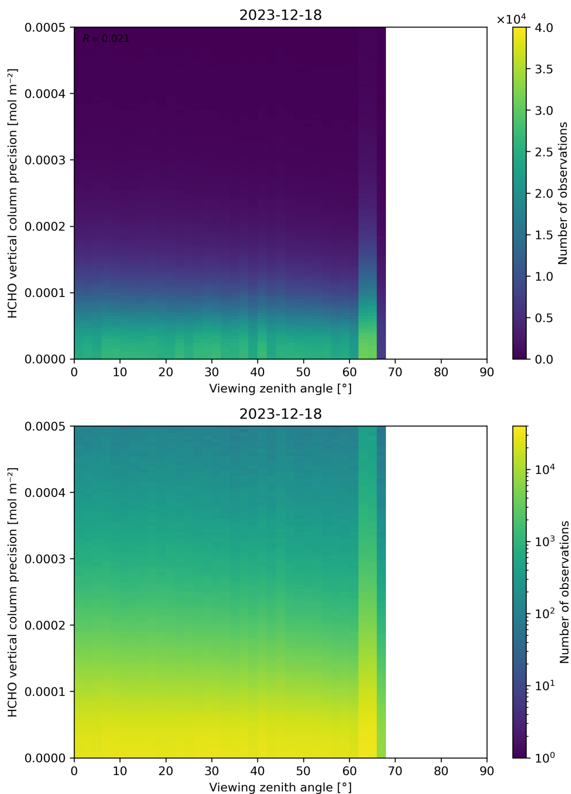
Figure 194: Scatter density plot of “Viewing zenith angle” against “HCHO vertical column precision” for 2023-12-17 to 2023-12-19.
