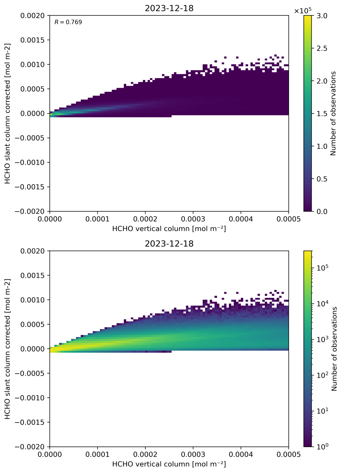
Figure 127: Scatter density plot of “HCHO vertical column” against “HCHO slant column corrected” for 2023-12-17 to 2023-12-19.
