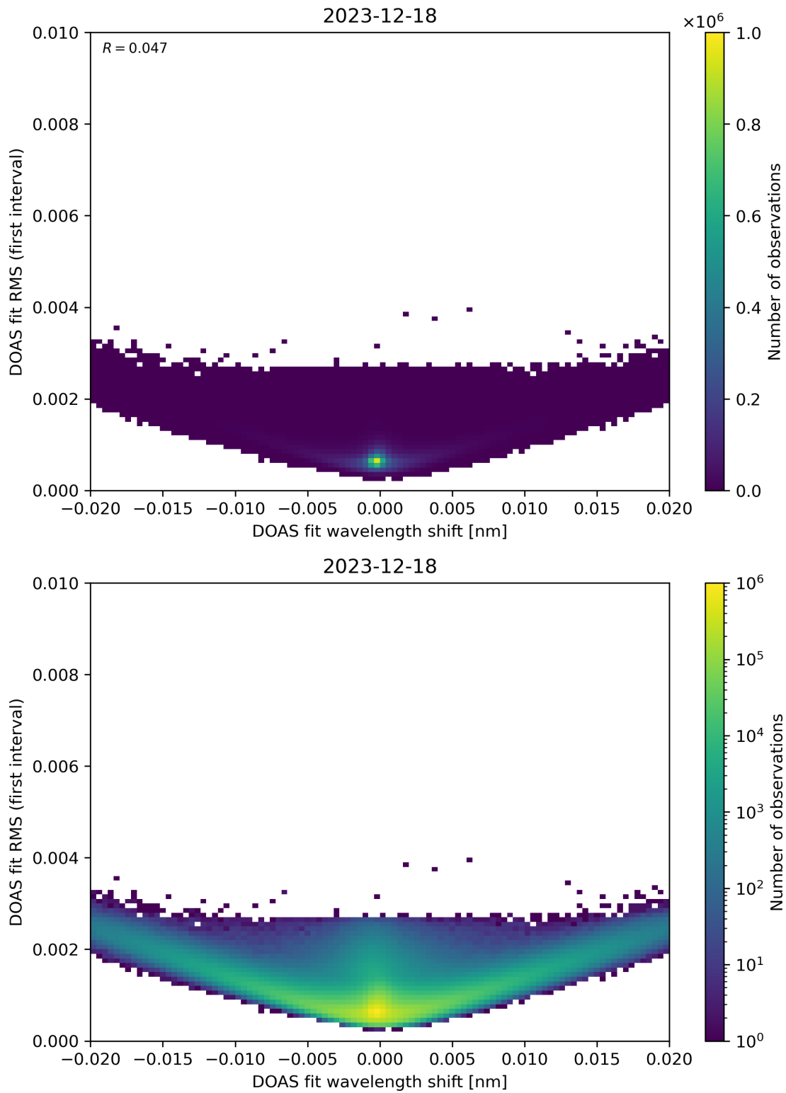
Figure 64: Scatter density plot of “DOAS fit wavelength shift” against “DOAS fit RMS (first interval)” for 2023-12-17 to 2023-12-19.
