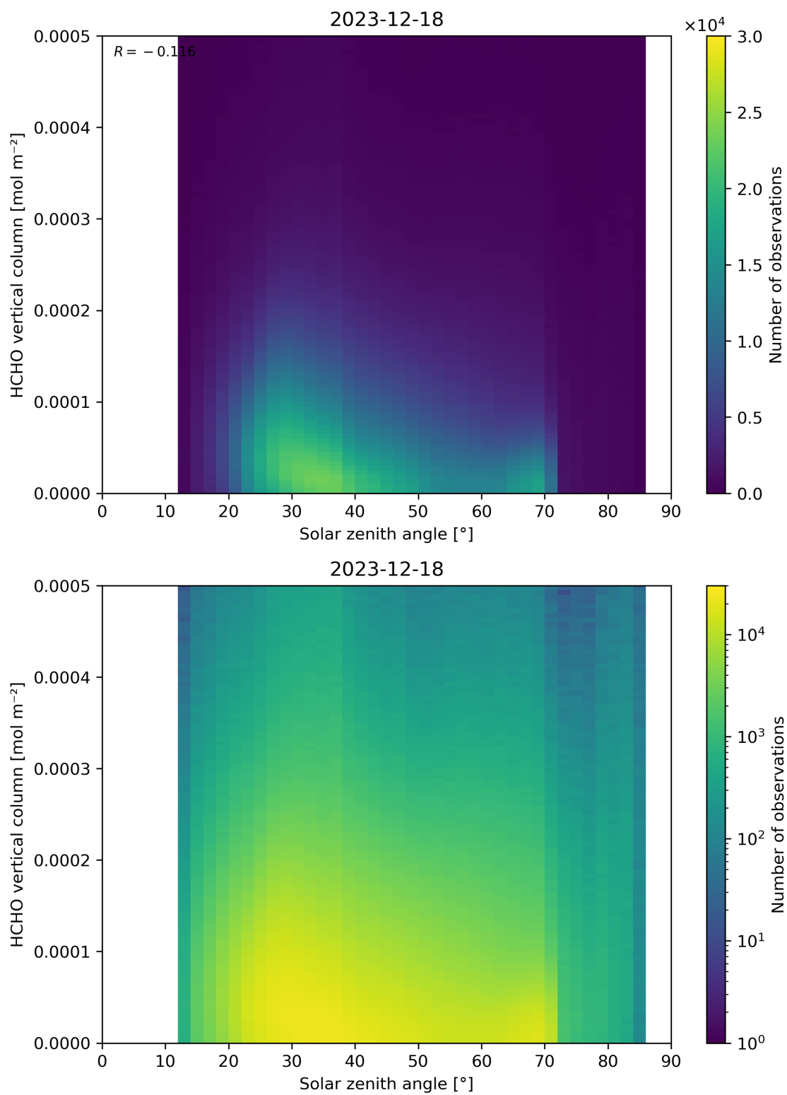
Figure 177: Scatter density plot of “Solar zenith angle” against “HCHO vertical column” for 2023-12-17 to 2023-12-19.
