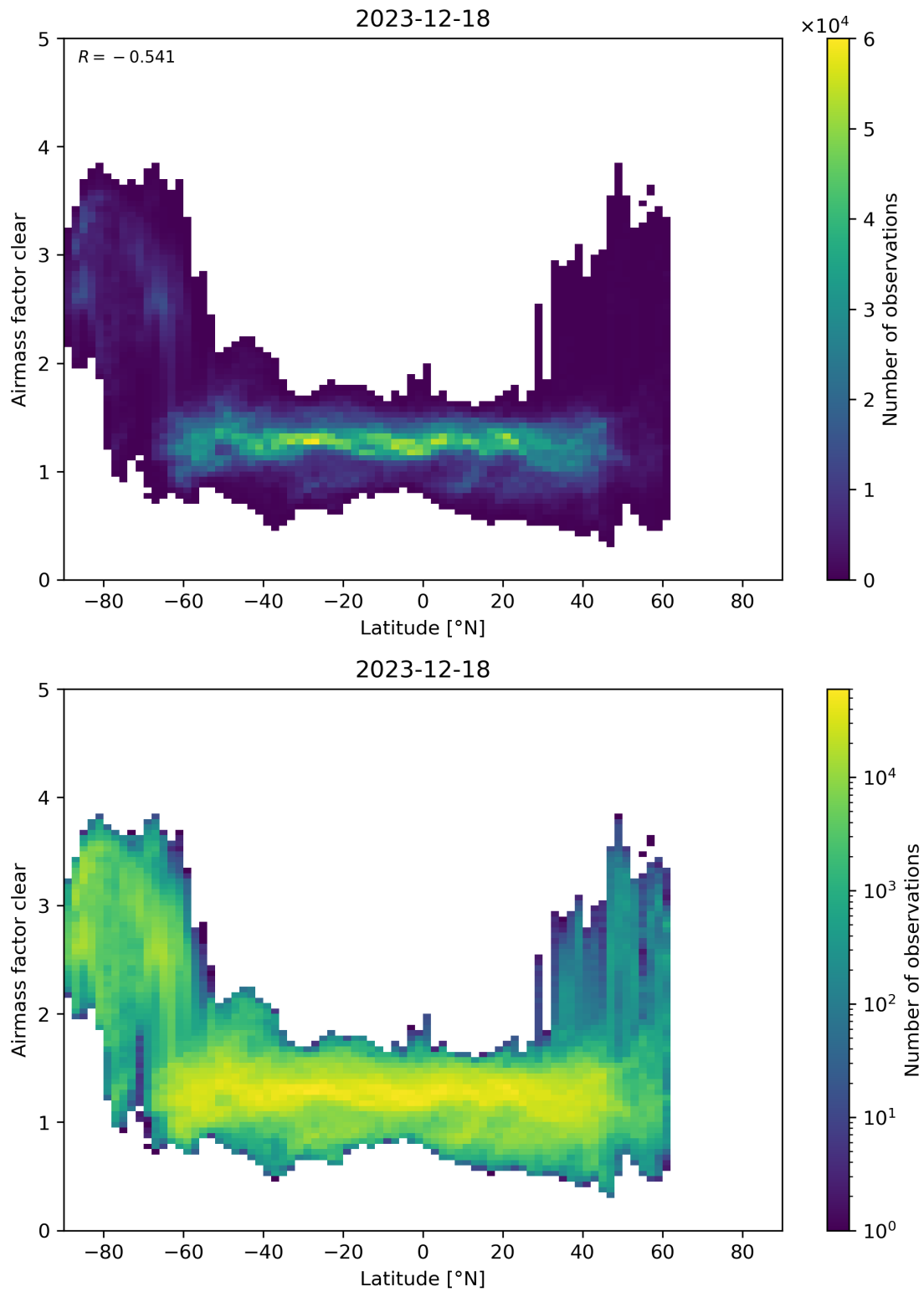
Figure 156: Scatter density plot of “Latitude” against “Airmass factor clear” for 2023-12-17 to 2023-12-19.
