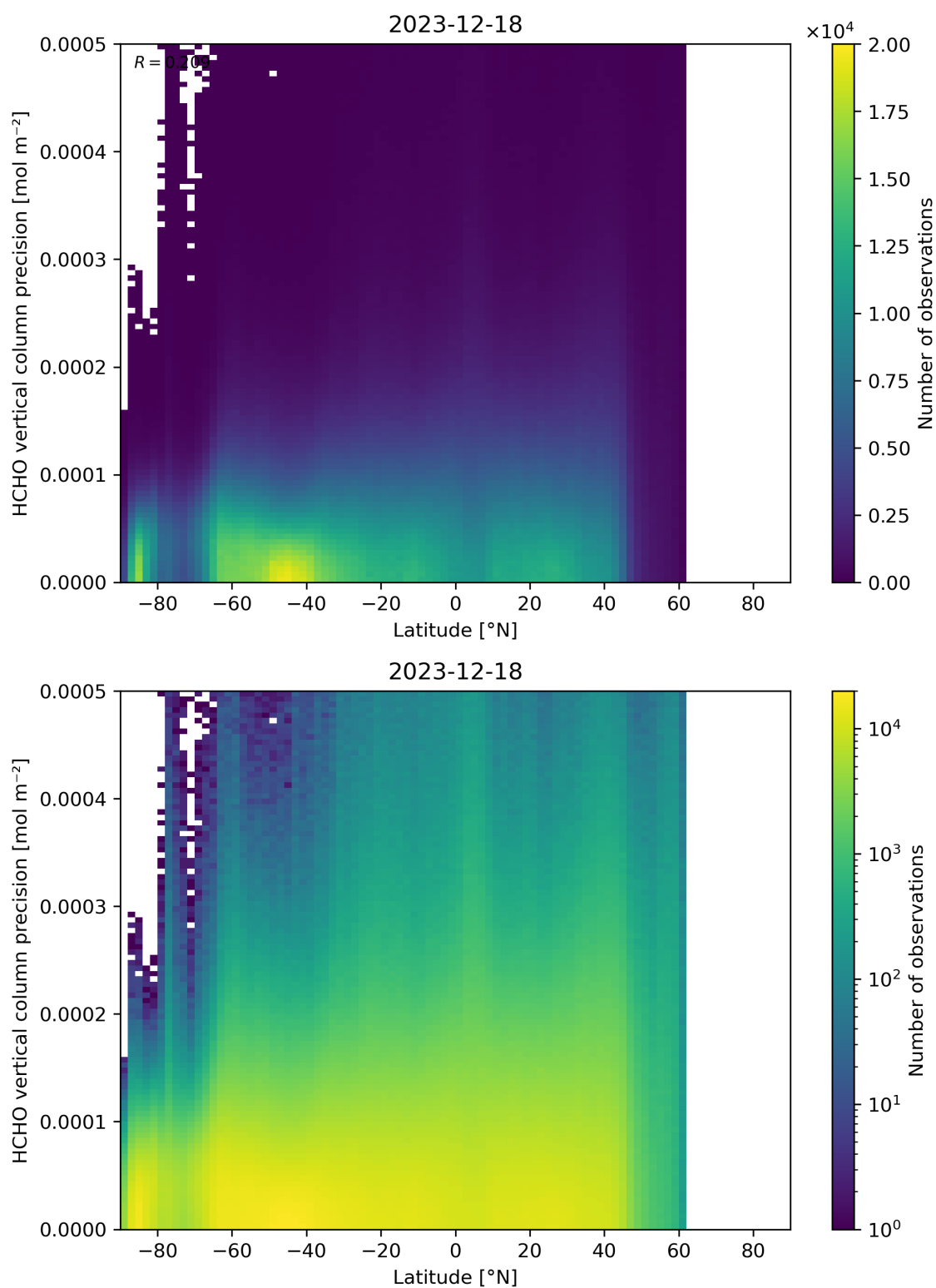
Figure 165: Scatter density plot of “Latitude” against “HCHO vertical column precision” for 2023-12-17 to 2023-12-19.
