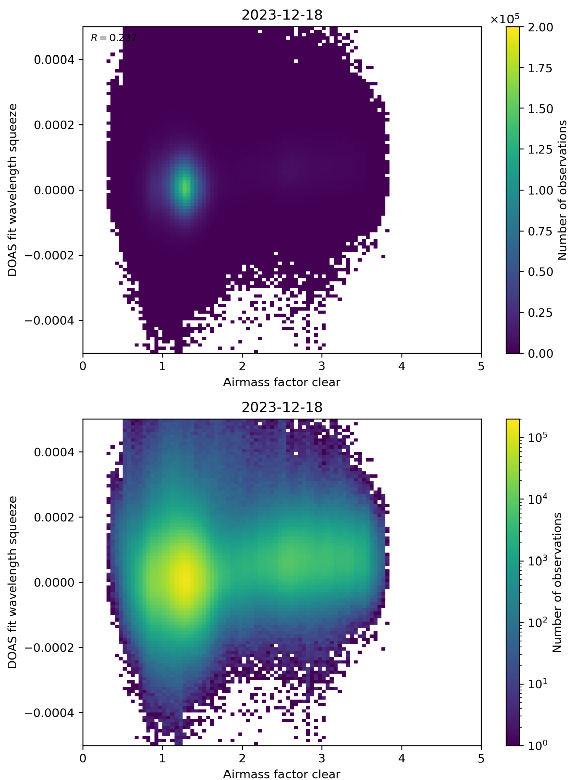
Figure 73: Scatter density plot of “Airmass factor clear” against “DOAS fit wavelength squeeze” for 2023-12-17 to 2023-12-19.
