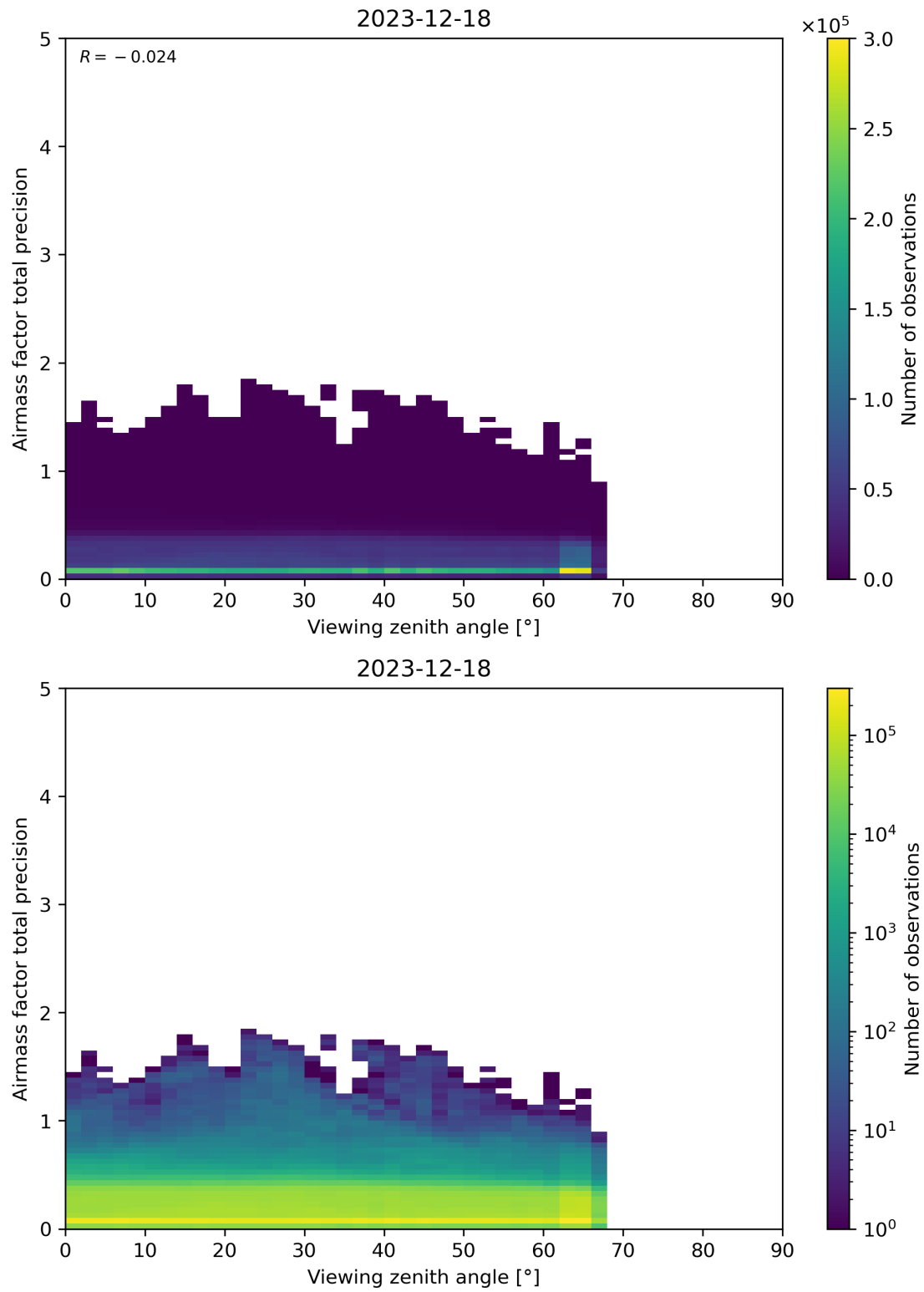
Figure 191: Scatter density plot of “Viewing zenith angle” against “Airmass factor total precision” for 2023-12-17 to 2023-12-19.
