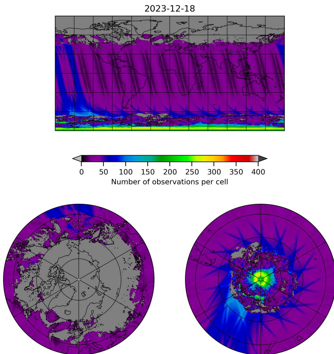
Figure 19: Map of the number of observations for 2023-12-17 to 2023-12-19
