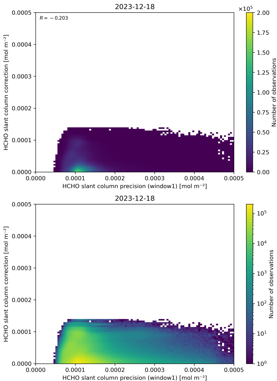
Figure 93: Scatter density plot of “HCHO slant column precision (window1)” against “HCHO slant column correction” for 2023-12-17 to 2023-12-19.
