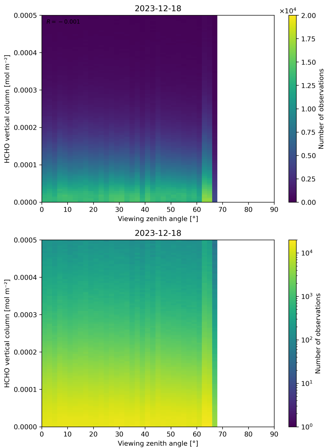
Figure 192: Scatter density plot of “Viewing zenith angle” against “HCHO vertical column” for 2023-12-17 to 2023-12-19.
