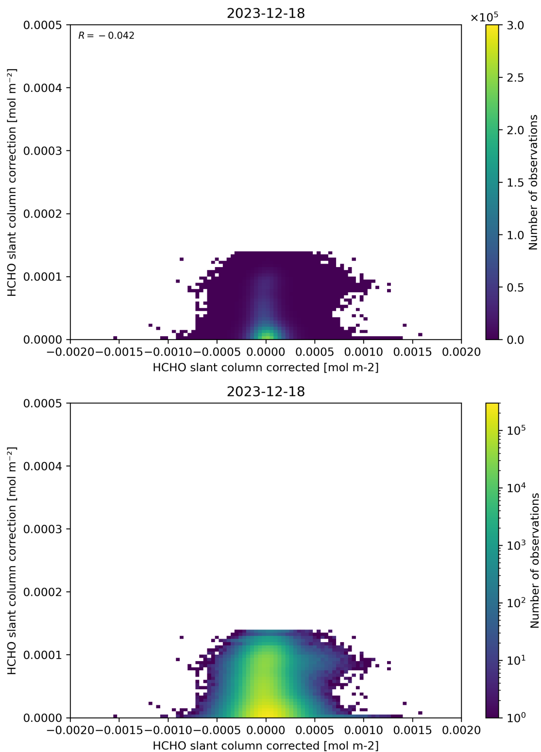
Figure 77: Scatter density plot of “HCHO slant column corrected” against “HCHO slant column correction” for 2023-12-17 to 2023-12-19.
