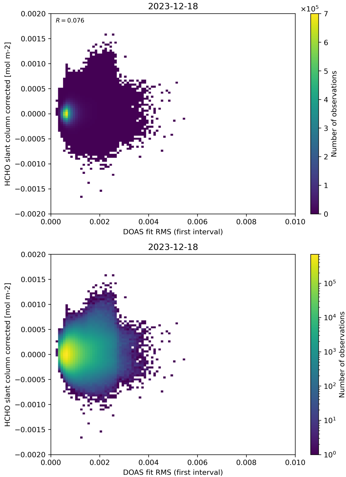
Figure 62: Scatter density plot of “DOAS fit RMS (first interval)” against “HCHO slant column corrected” for 2023-12-17 to 2023-12-19.
