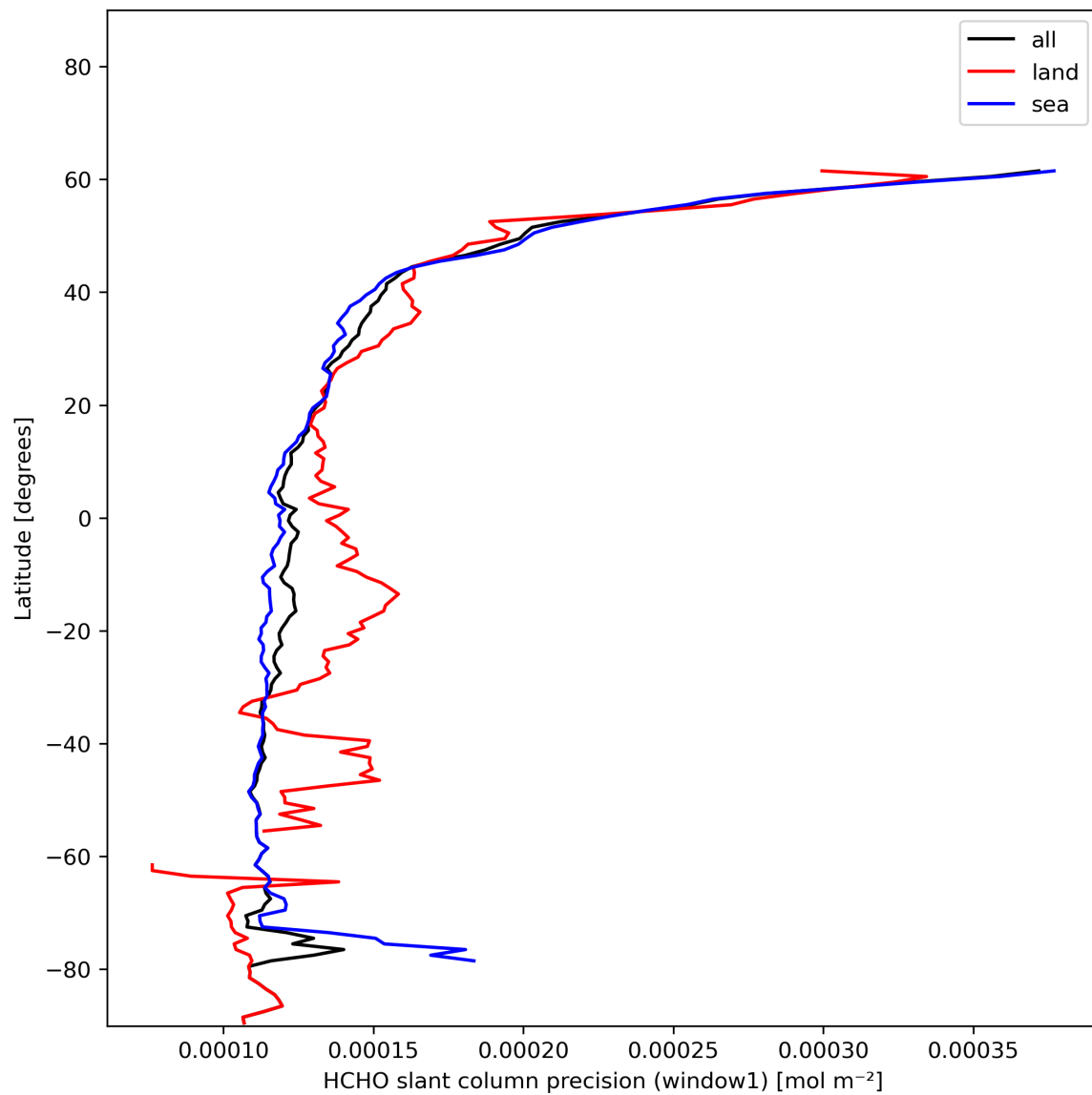
Figure 25: Zonal average of “HCHO slant column precision (window1)” for 2023-12-17 to 2023-12-19.
