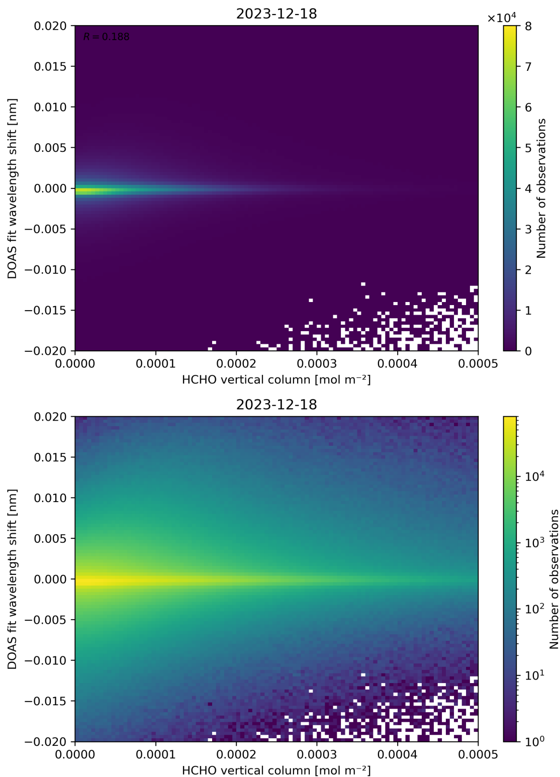
Figure 124: Scatter density plot of “HCHO vertical column” against “DOAS fit wavelength shift” for 2023-12-17 to 2023-12-19.
