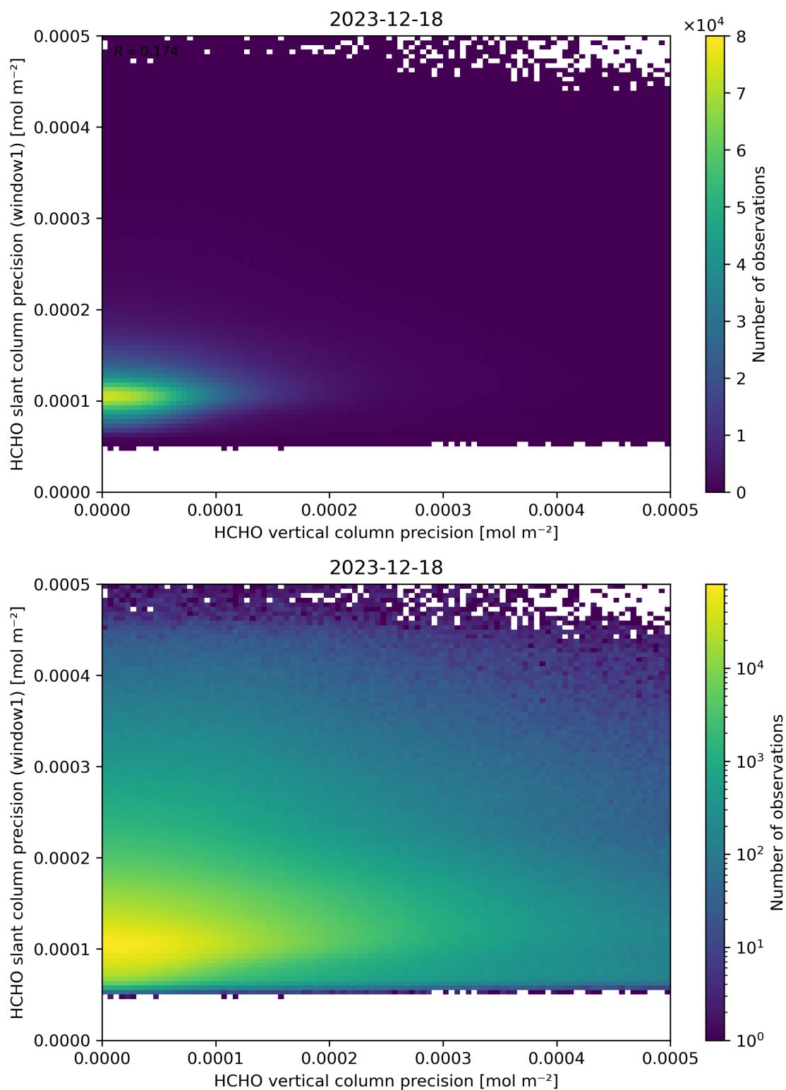
Figure 143: Scatter density plot of “HCHO vertical column precision” against “HCHO slant column precision (window1)” for 2023-12-17 to 2023-12-19.
