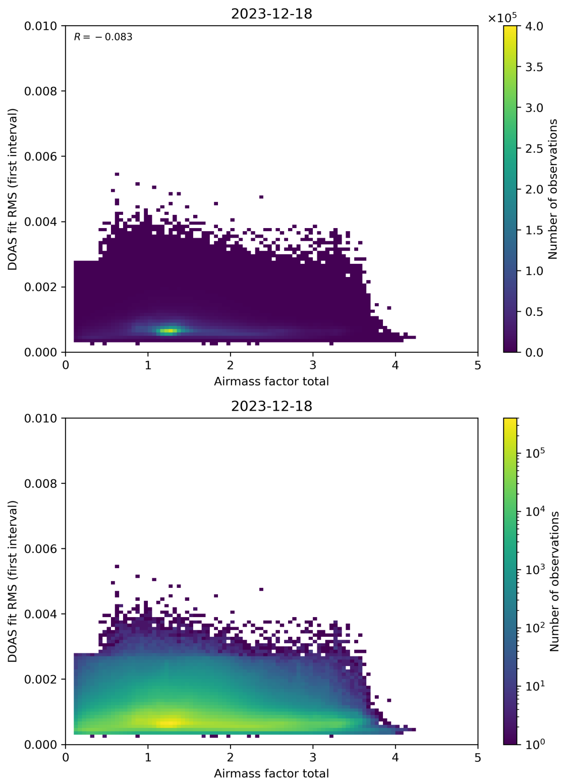
Figure 97: Scatter density plot of “Airmass factor total” against “DOAS fit RMS (first interval)” for 2023-12-17 to 2023-12-19.
