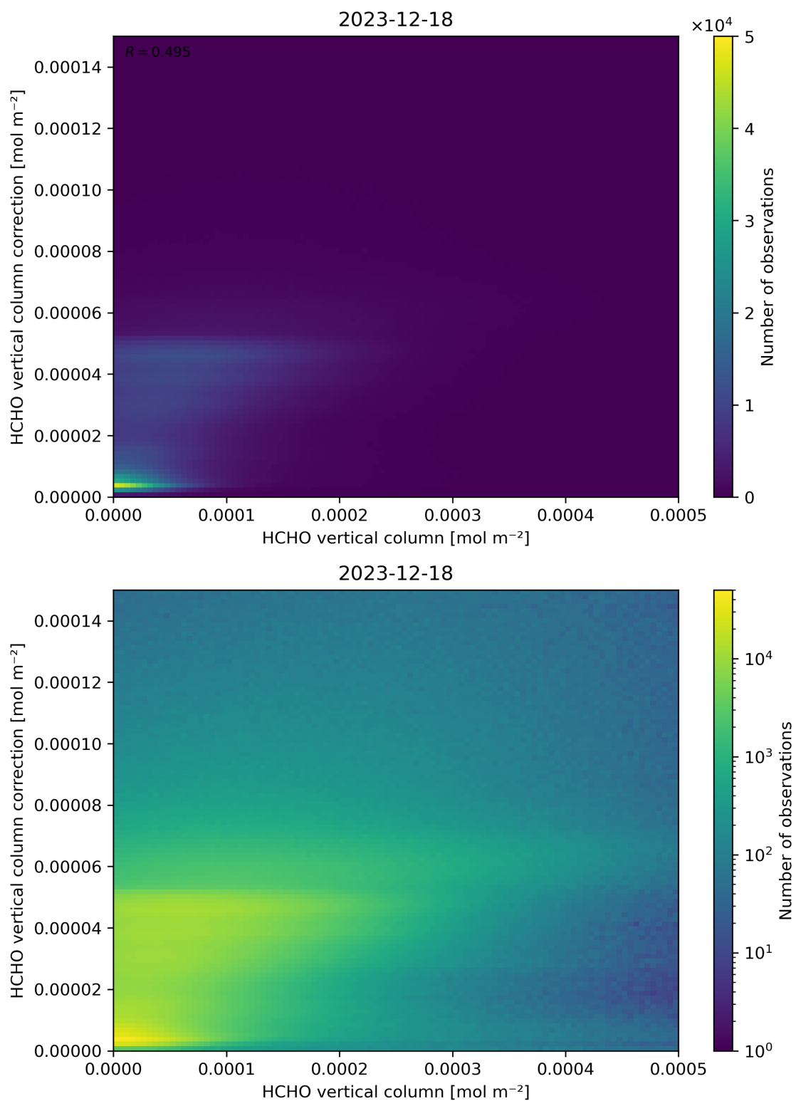
Figure 133: Scatter density plot of “HCHO vertical column” against “HCHO vertical column correction” for 2023-12-17 to 2023-12-19.
