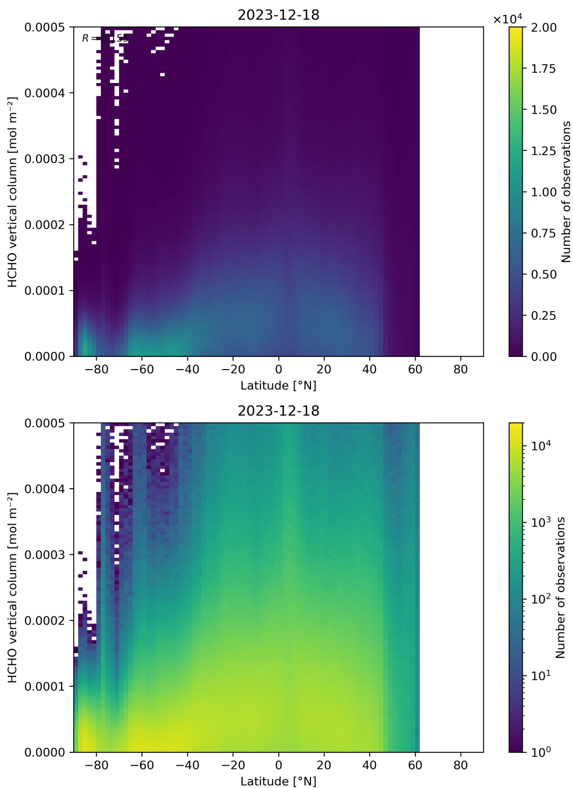
Figure 163: Scatter density plot of “Latitude” against “HCHO vertical column” for 2023-12-17 to 2023-12-19.
