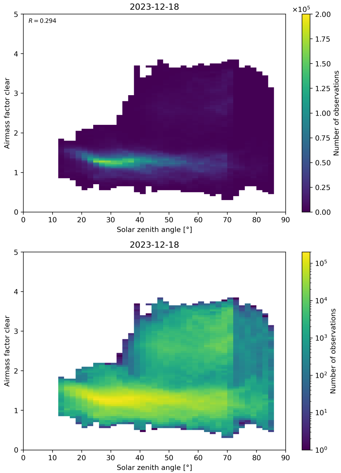
Figure 170: Scatter density plot of “Solar zenith angle” against “Airmass factor clear” for 2023-12-17 to 2023-12-19.
