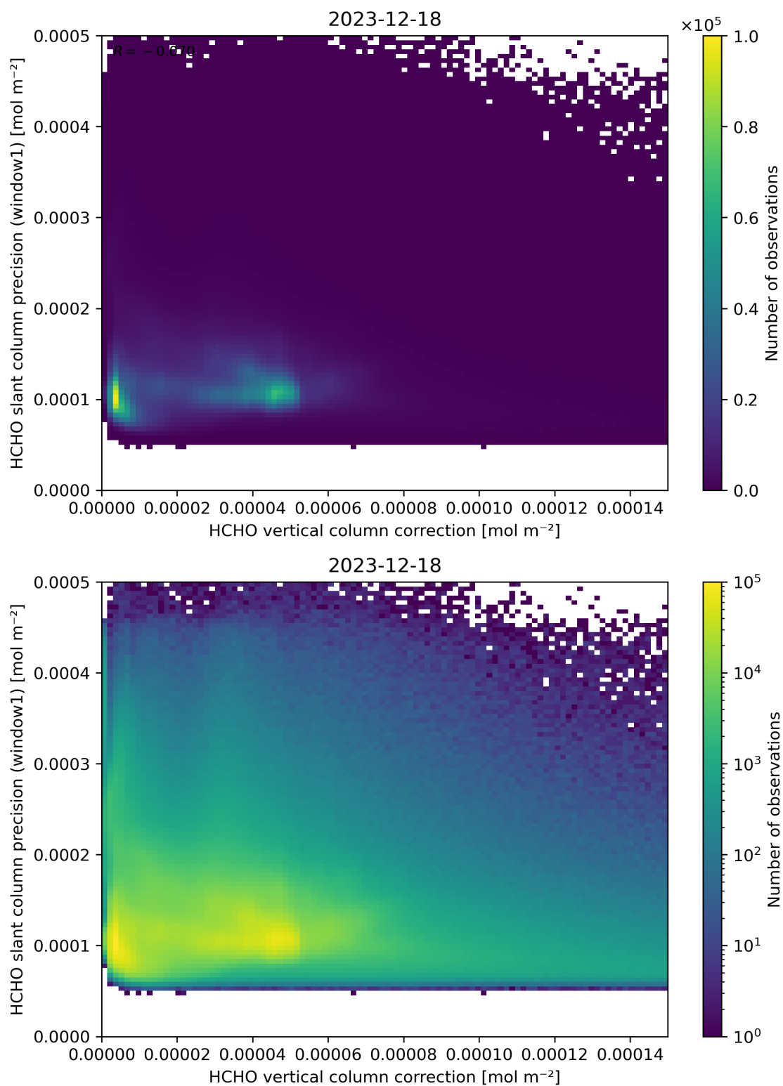
Figure 119: Scatter density plot of “HCHO vertical column correction” against “HCHO slant column precision (window1)” for 2023-12-17 to 2023-12-19.
