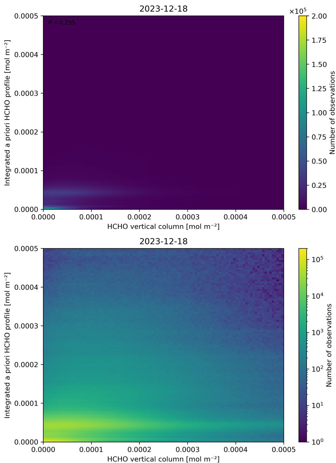
Figure 135: Scatter density plot of “HCHO vertical column” against “Integrated a priori HCHO profile” for 2023-12-17 to 2023-12-19.
