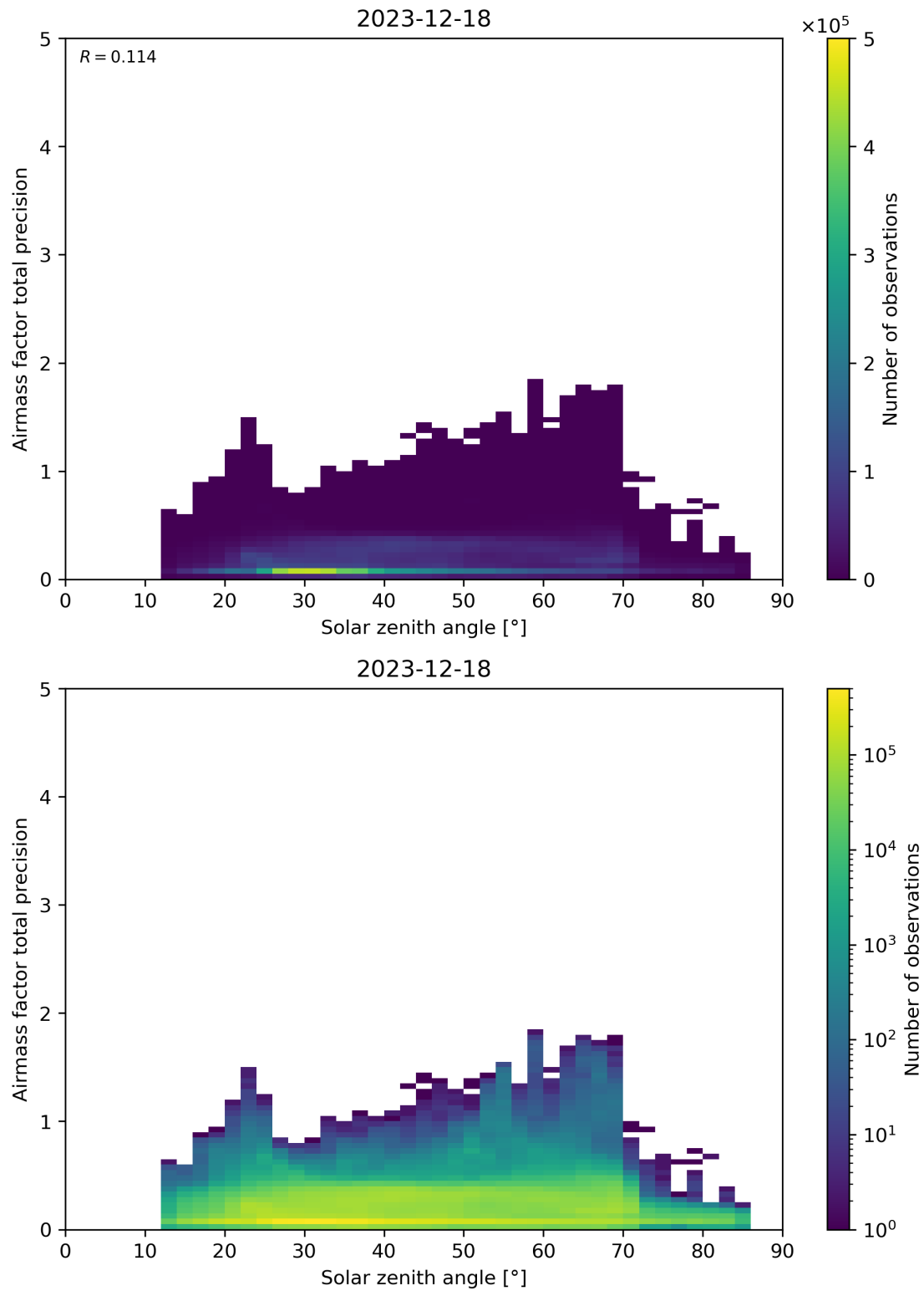
Figure 176: Scatter density plot of “Solar zenith angle” against “Airmass factor total precision” for 2023-12-17 to 2023-12-19.
