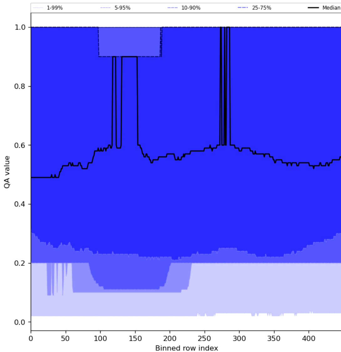
Figure 48: Along track statistics of “QA value” for 2023-12-17 to 2023-12-19
