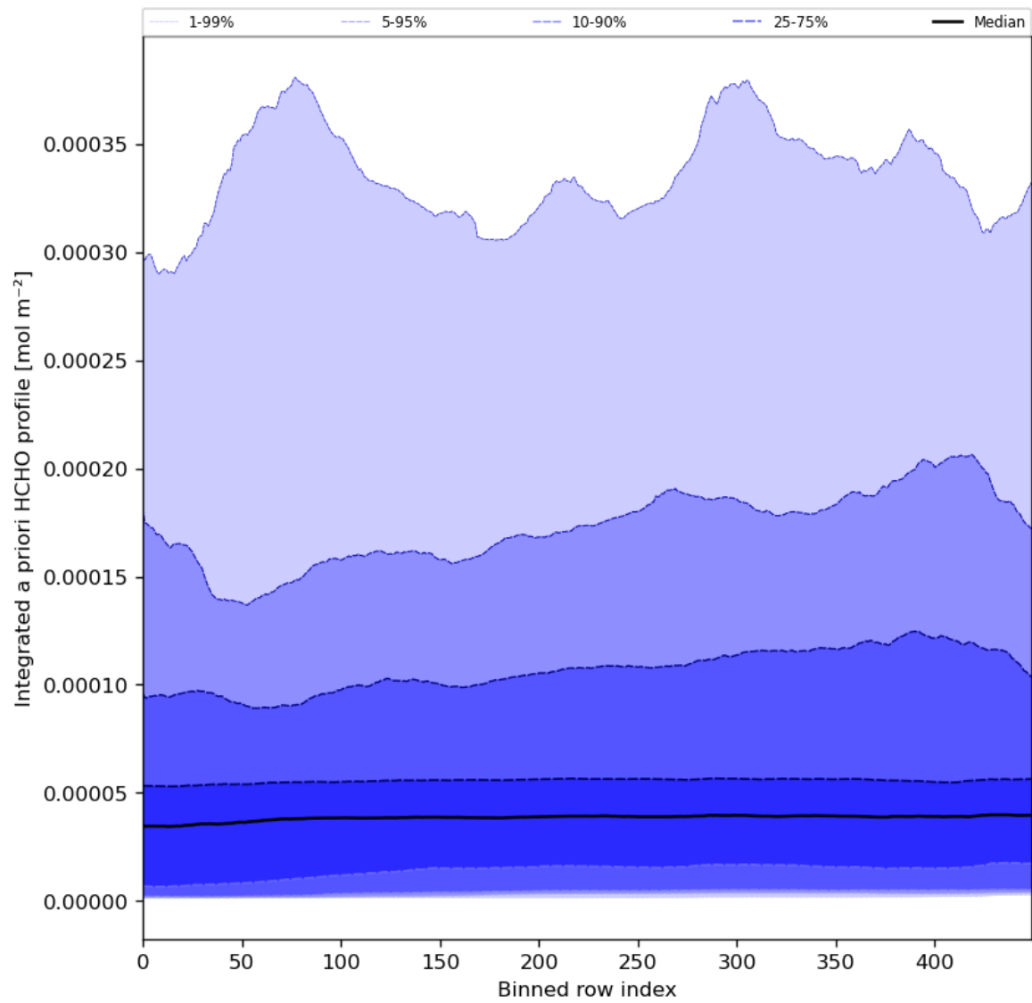
Figure 57: Along track statistics of “Integrated a priori HCHO profile” for 2023-12-17 to 2023-12-19
