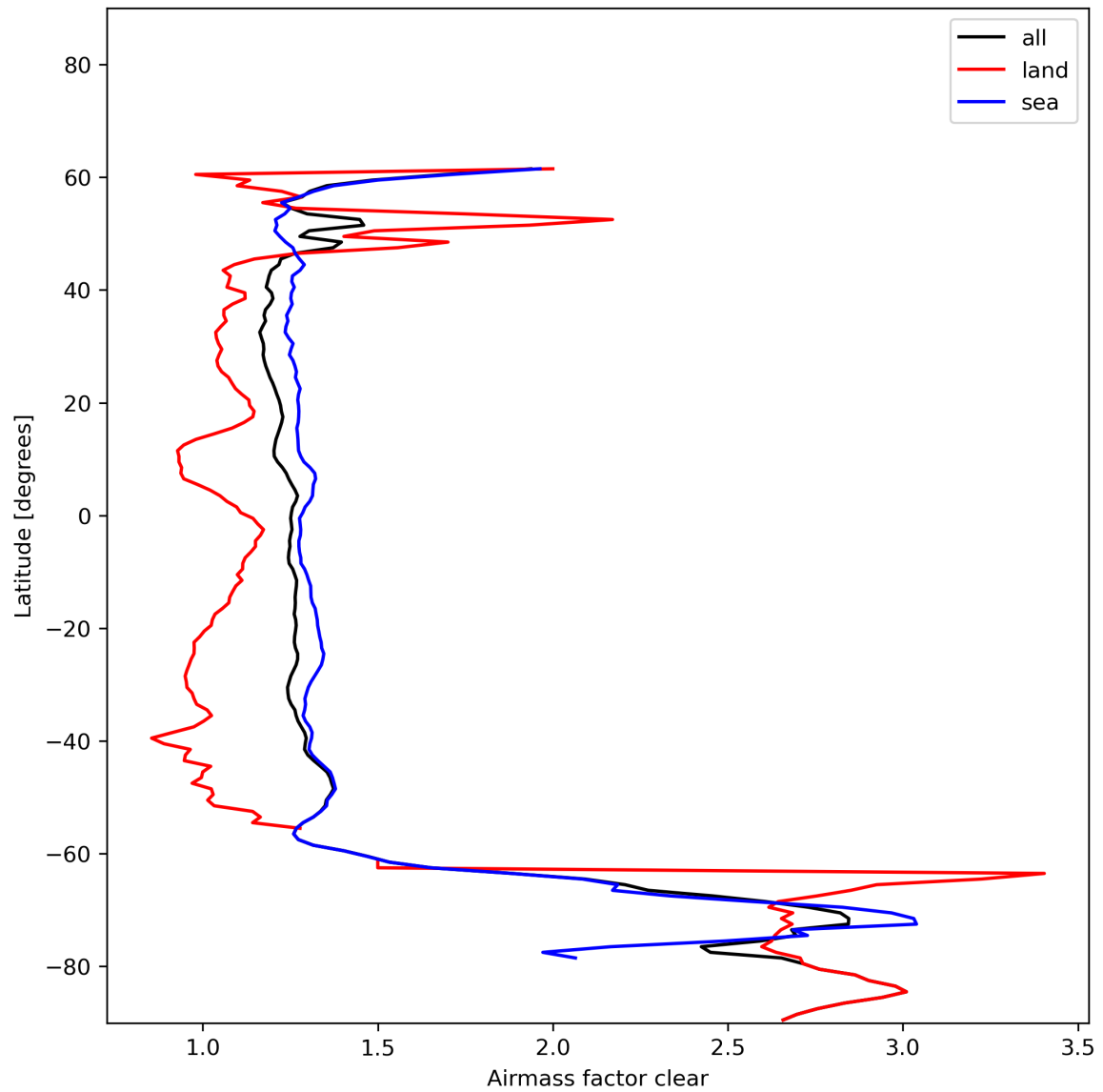
Figure 28: Zonal average of “Airmass factor clear” for 2023-12-17 to 2023-12-19.
