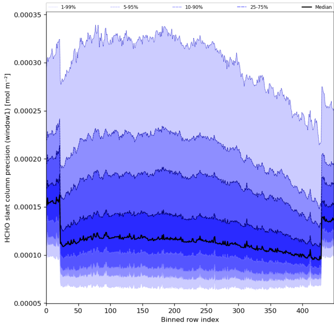
Figure 53: Along track statistics of “HCHO slant column precision (window1)” for 2023-12-17 to 2023-12-19
