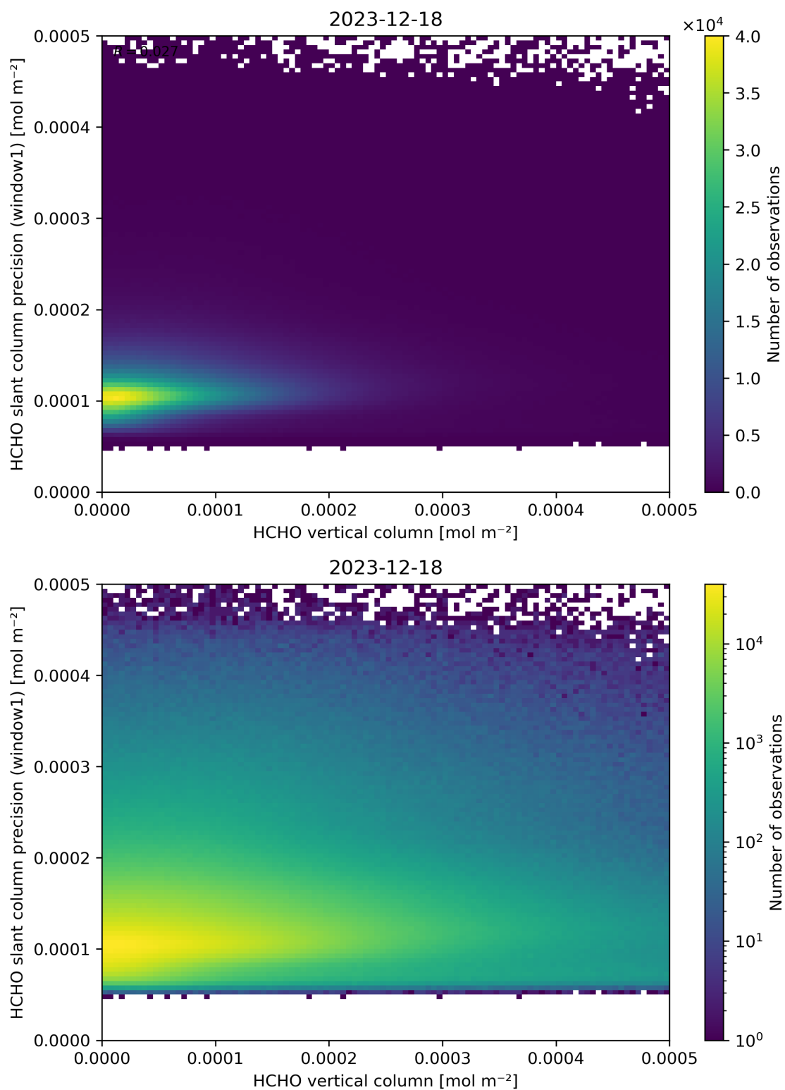
Figure 130: Scatter density plot of “HCHO vertical column” against “HCHO slant column precision (window1)” for 2023-12-17 to 2023-12-19.
