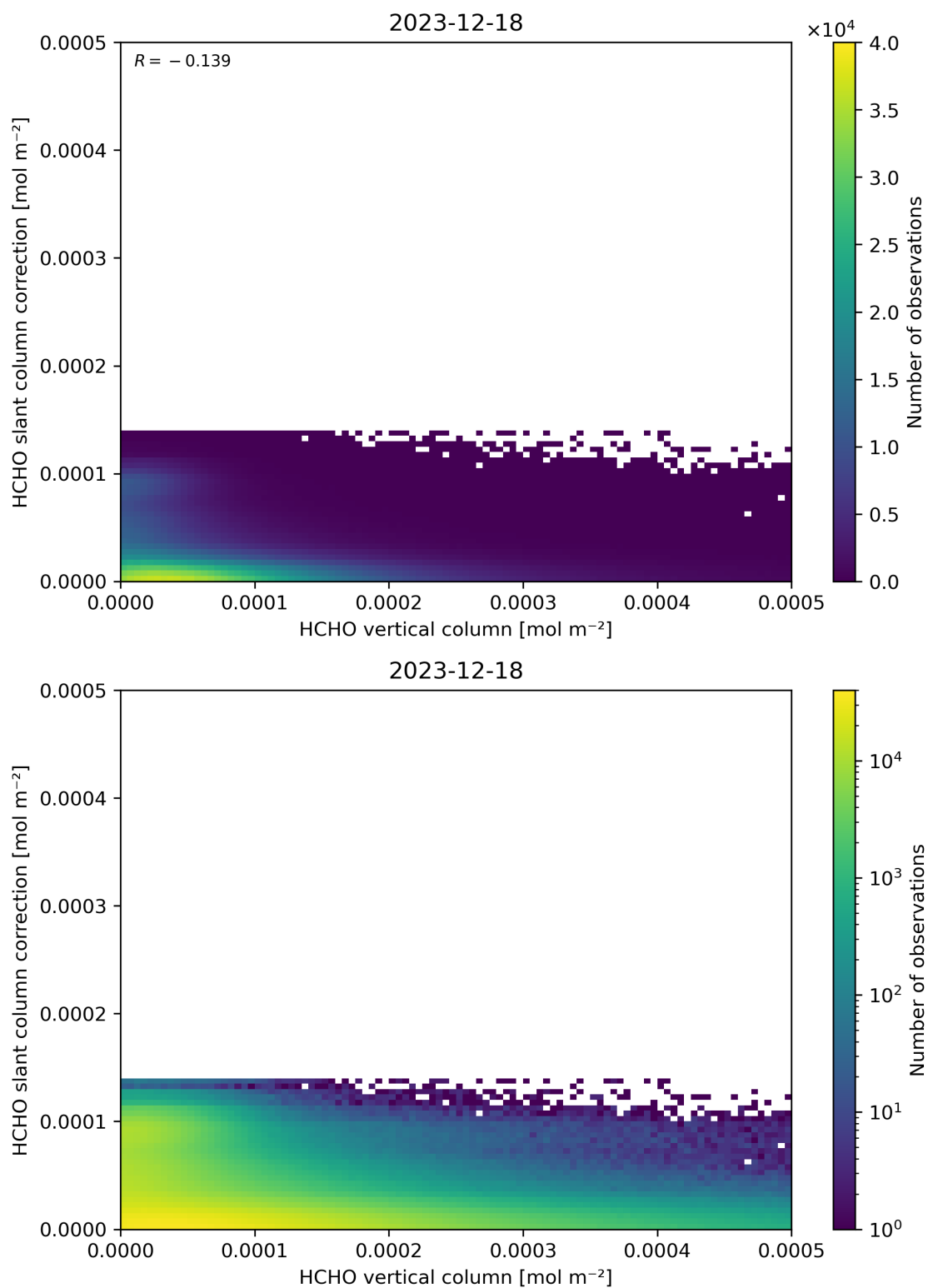
Figure 128: Scatter density plot of “HCHO vertical column” against “HCHO slant column correction” for 2023-12-17 to 2023-12-19.
