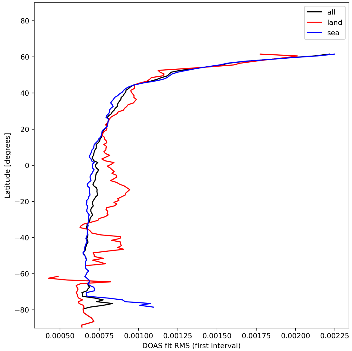
Figure 32: Zonal average of “DOAS fit RMS (first interval)” for 2023-12-17 to 2023-12-19.
