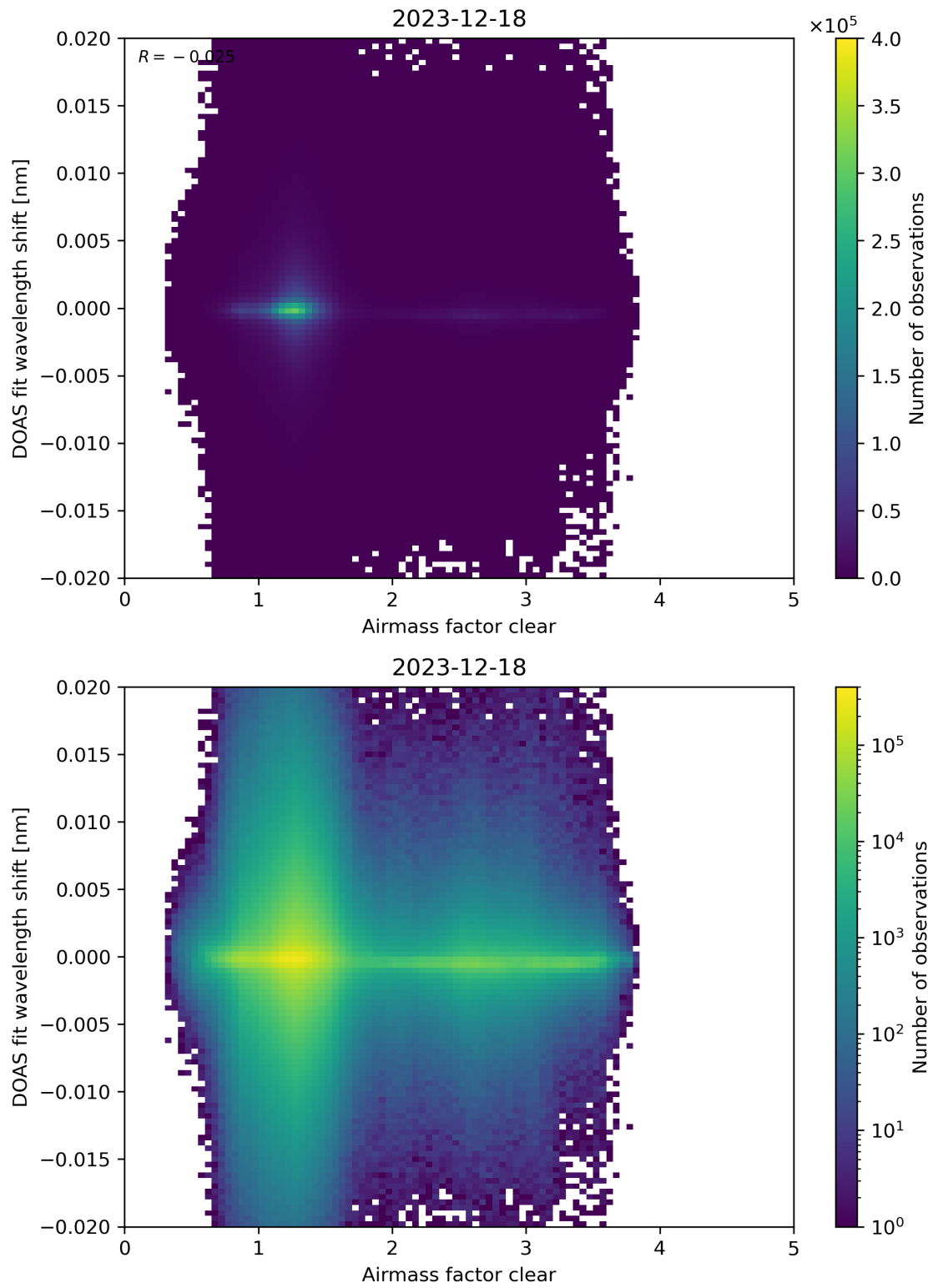
Figure 72: Scatter density plot of “Airmass factor clear” against “DOAS fit wavelength shift” for 2023-12-17 to 2023-12-19.
