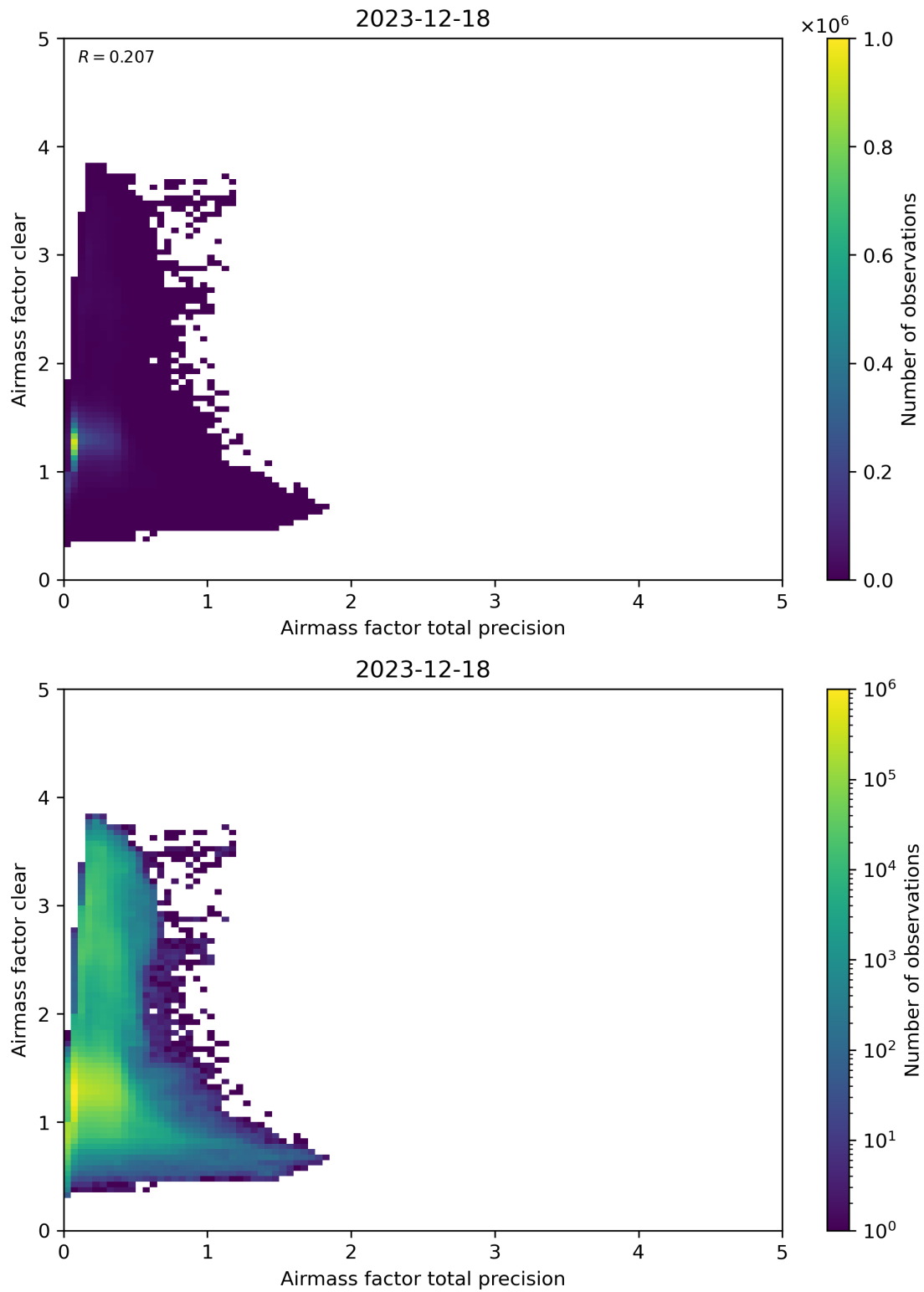
Figure 108: Scatter density plot of “Airmass factor total precision” against “Airmass factor clear” for 2023-12-17 to 2023-12-19.
