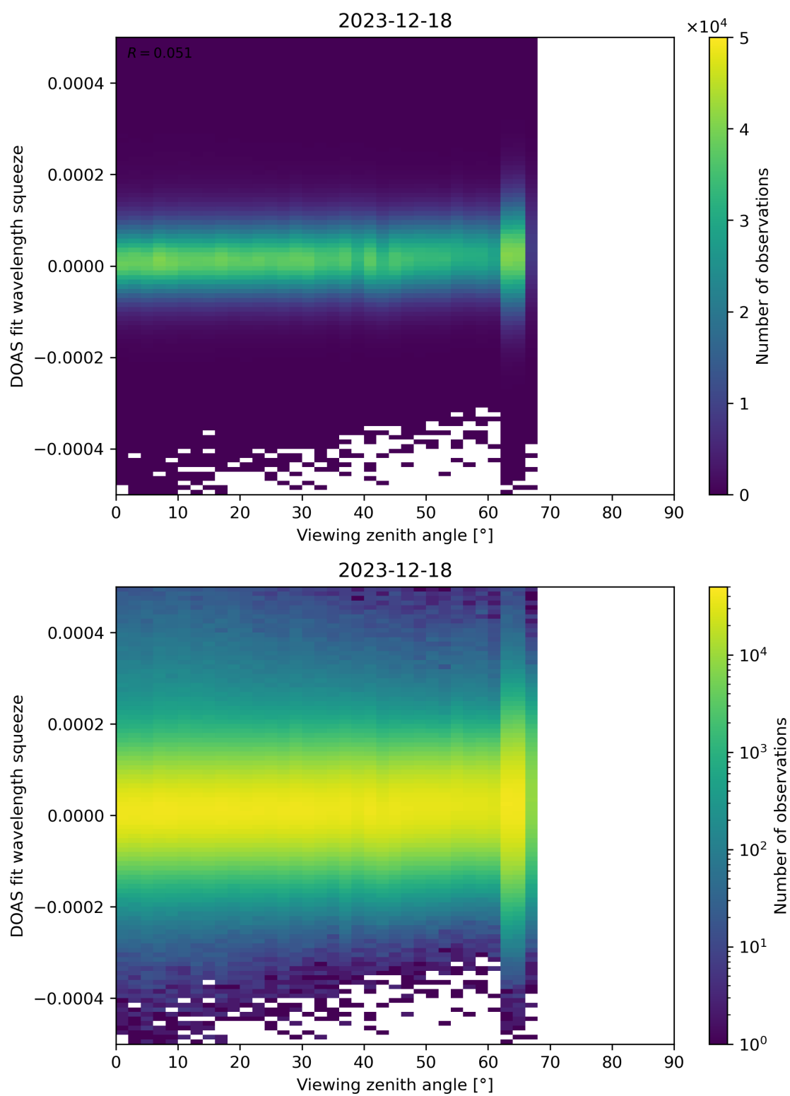
Figure 184: Scatter density plot of “Viewing zenith angle” against “DOAS fit wavelength squeeze” for 2023-12-17 to 2023-12-19.
