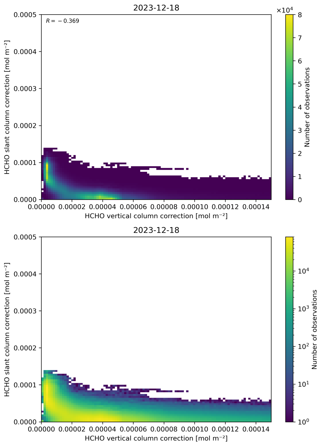
Figure 117: Scatter density plot of “HCHO vertical column correction” against “HCHO slant column correction” for 2023-12-17 to 2023-12-19.
