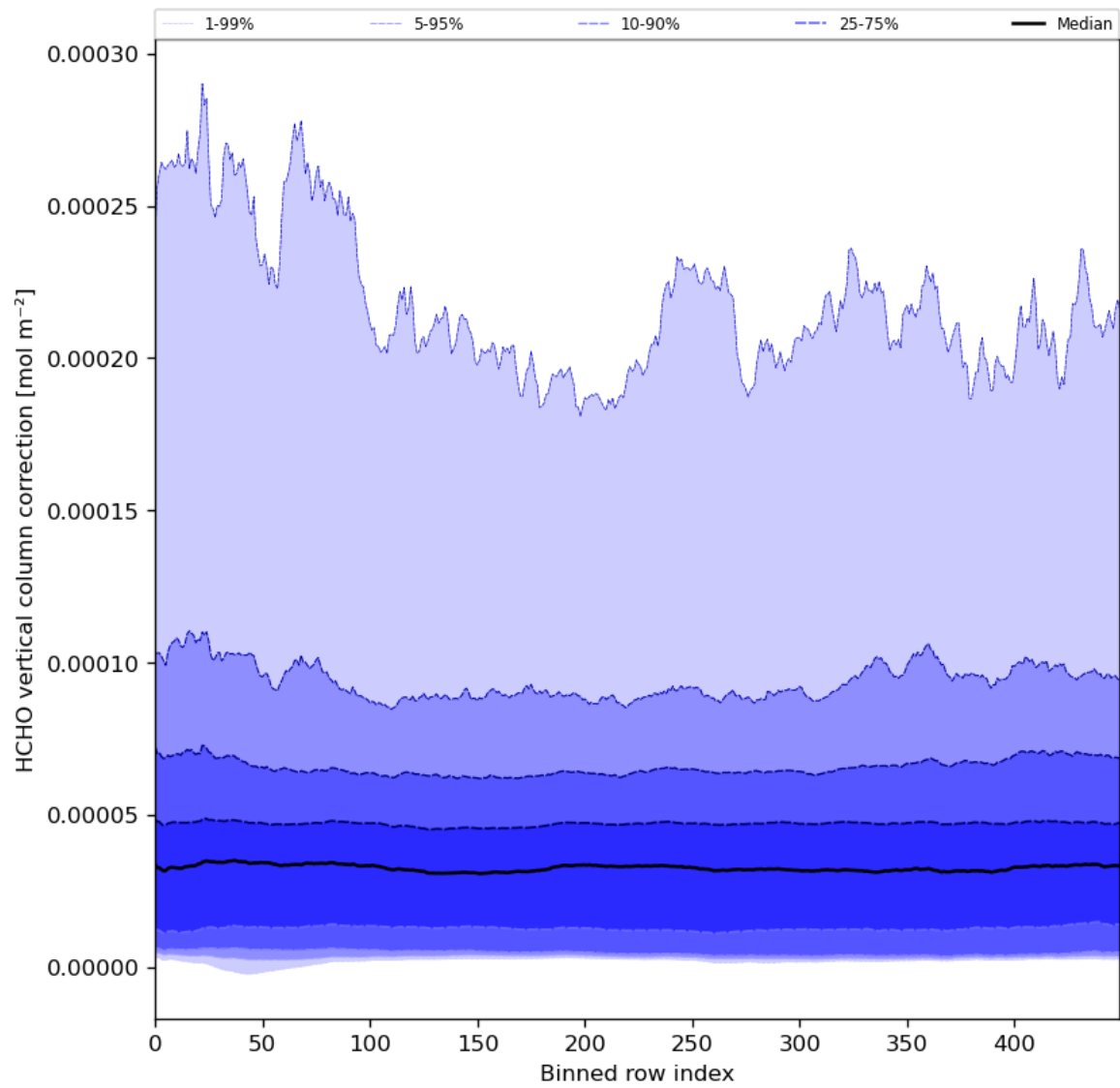
Figure 51: Along track statistics of “HCHO vertical column correction” for 2023-12-17 to 2023-12-19
