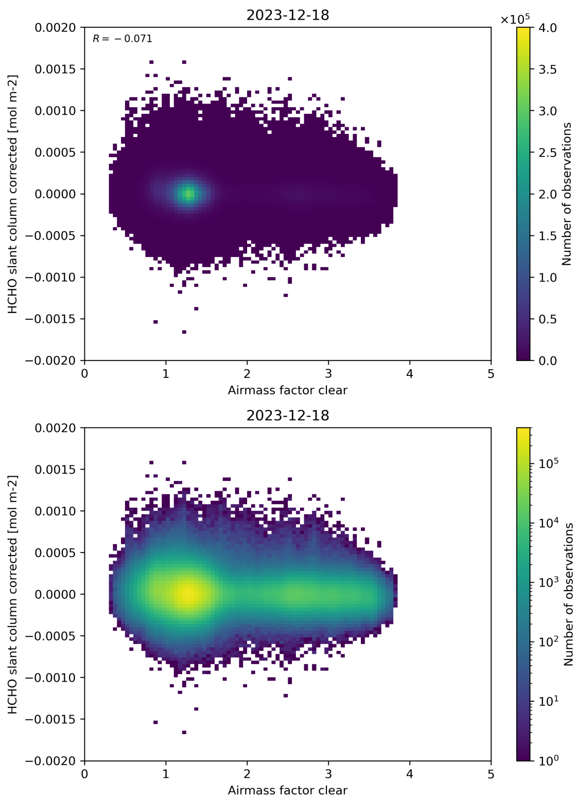
Figure 74: Scatter density plot of “Airmass factor clear” against “HCHO slant column corrected” for 2023-12-17 to 2023-12-19.
