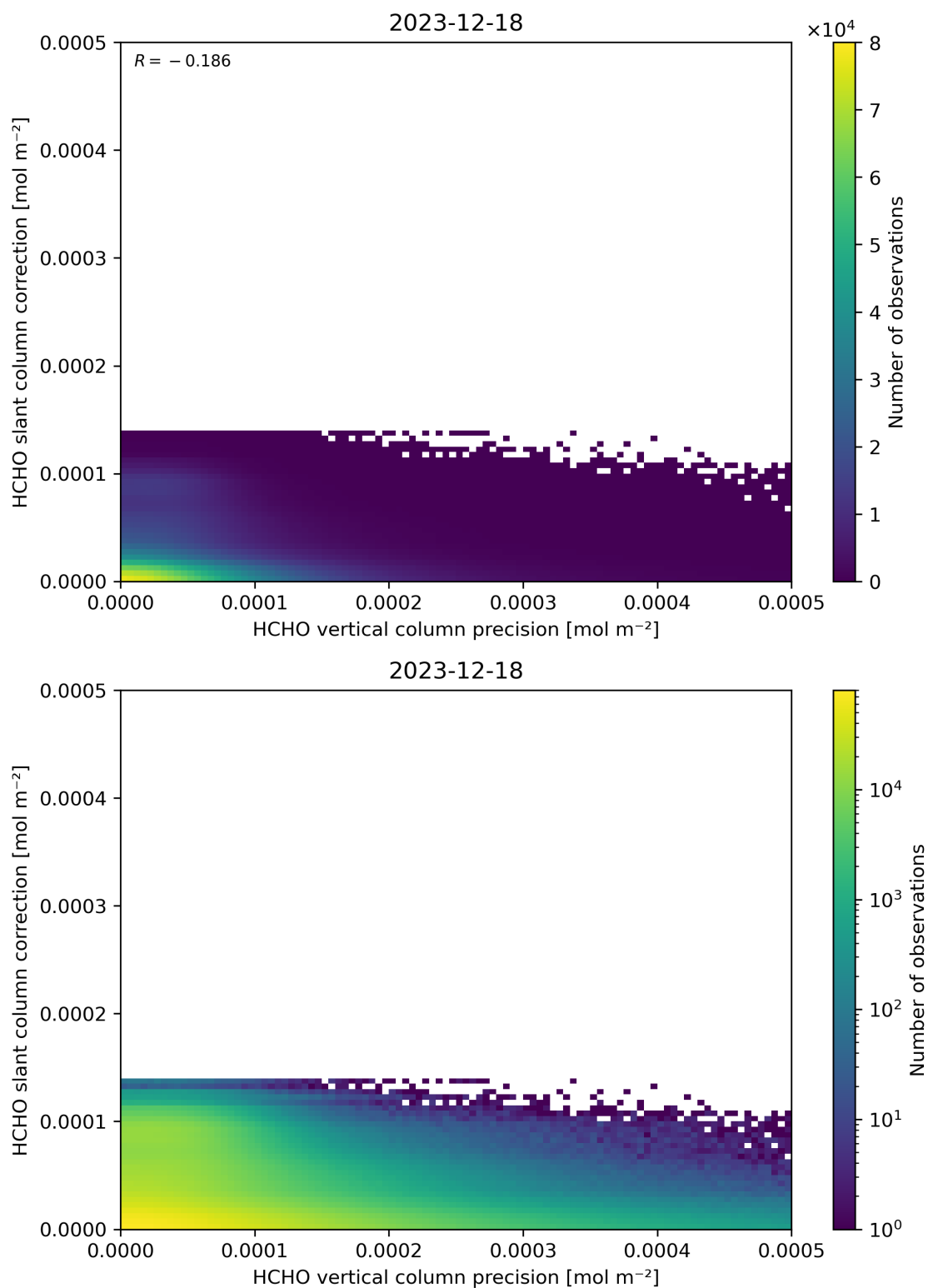
Figure 141: Scatter density plot of “HCHO vertical column precision” against “HCHO slant column correction” for 2023-12-17 to 2023-12-19.
