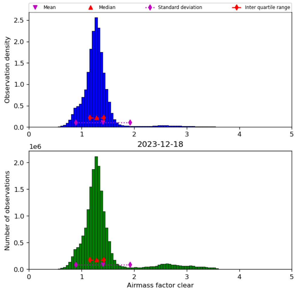
Figure 42: Histogram of “Airmass factor clear” for 2023-12-17 to 2023-12-19
