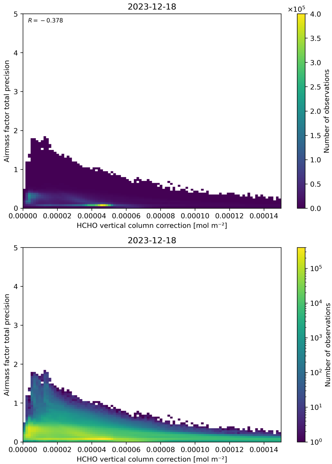
Figure 121: Scatter density plot of “HCHO vertical column correction” against “Airmass factor total precision” for 2023-12-17 to 2023-12-19.
