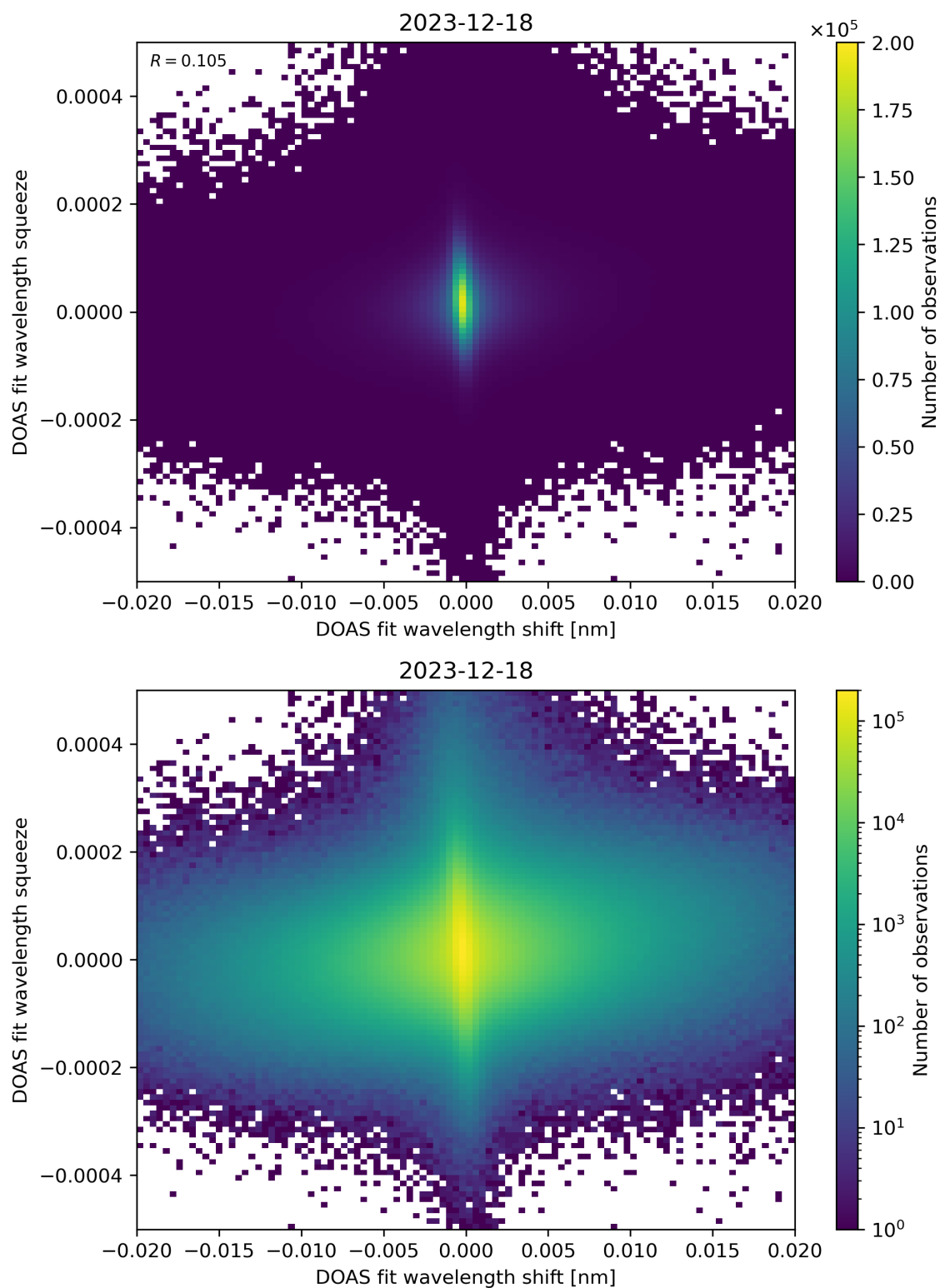
Figure 65: Scatter density plot of “DOAS fit wavelength shift” against “DOAS fit wavelength squeeze” for 2023-12-17 to 2023-12-19.
