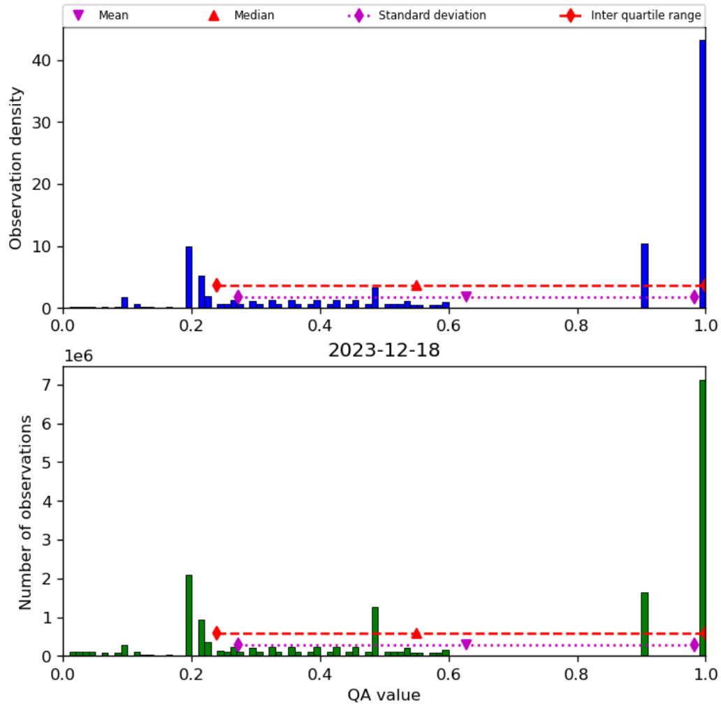
Figure 34: Histogram of “QA value” for 2023-12-17 to 2023-12-19
