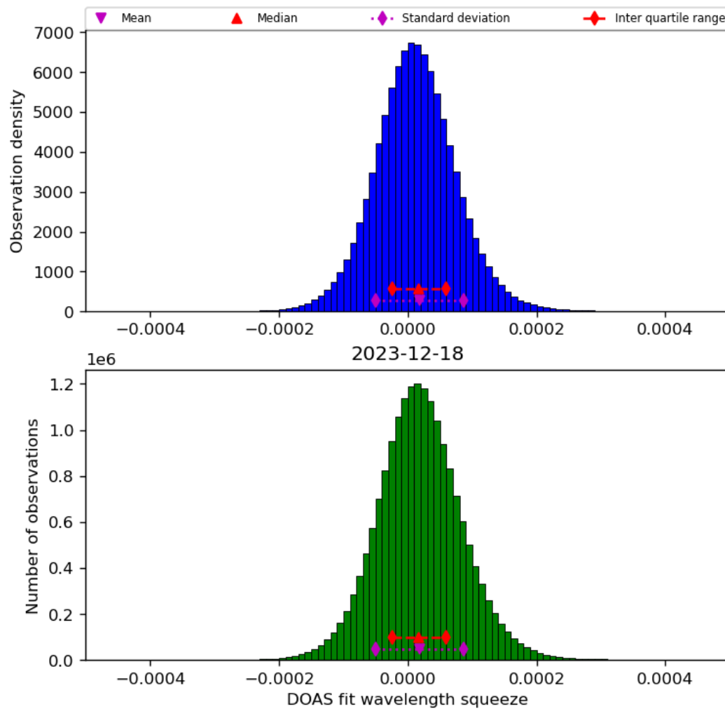
Figure 45: Histogram of “DOAS fit wavelength squeeze” for 2023-12-17 to 2023-12-19
