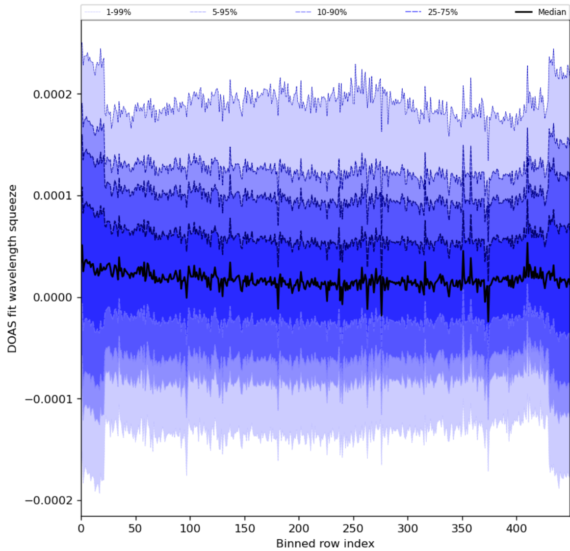
Figure 59: Along track statistics of “DOAS fit wavelength squeeze” for 2023-12-17 to 2023-12-19
