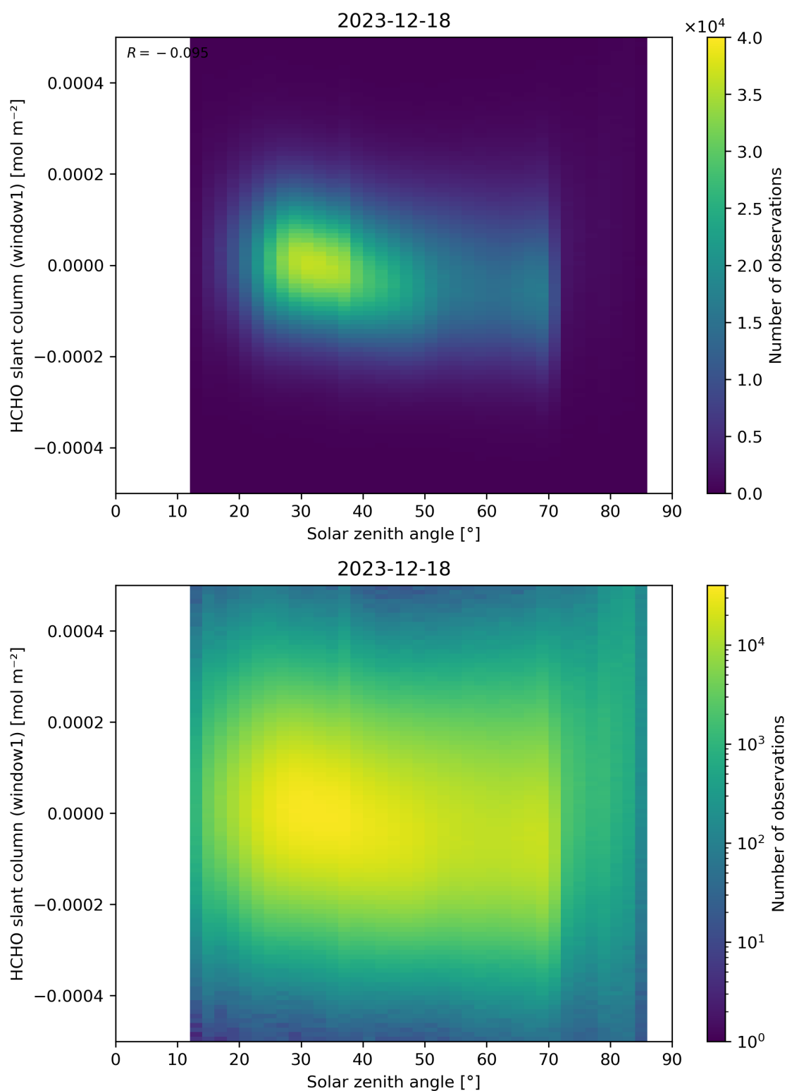
Figure 173: Scatter density plot of “Solar zenith angle” against “HCHO slant column (window1)” for 2023-12-17 to 2023-12-19.
