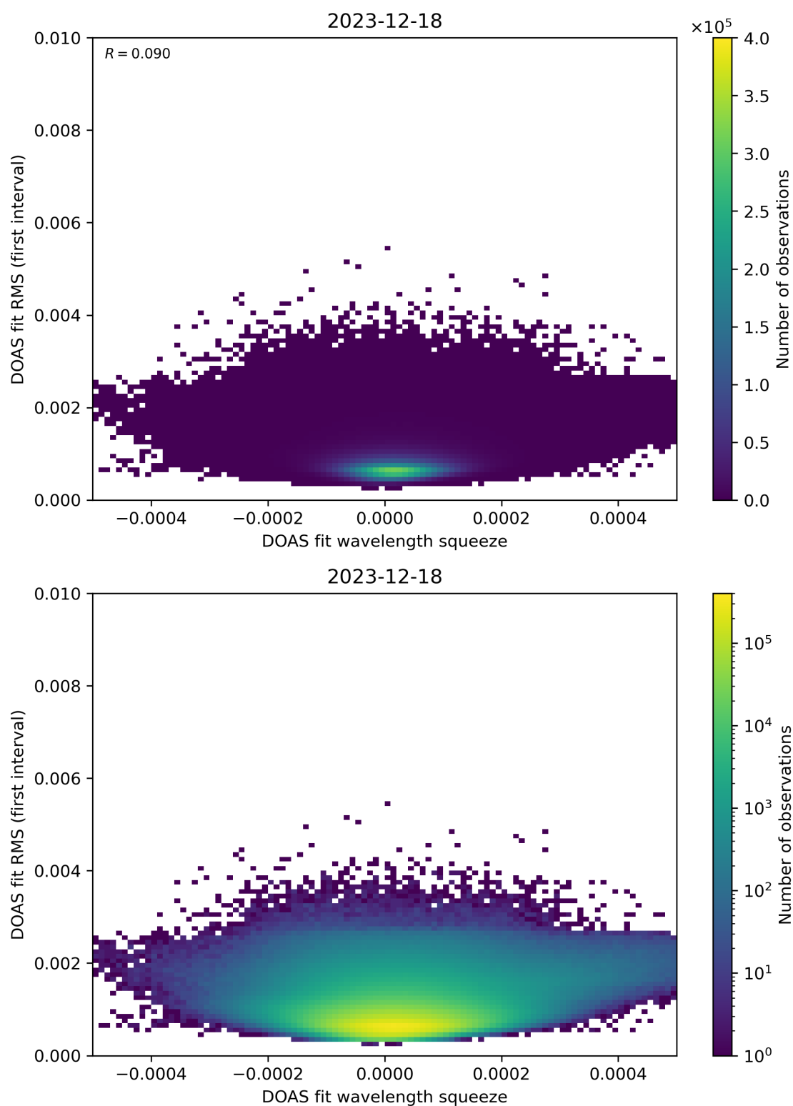
Figure 68: Scatter density plot of “DOAS fit wavelength squeeze” against “DOAS fit RMS (first interval)” for 2023-12-17 to 2023-12-19.
