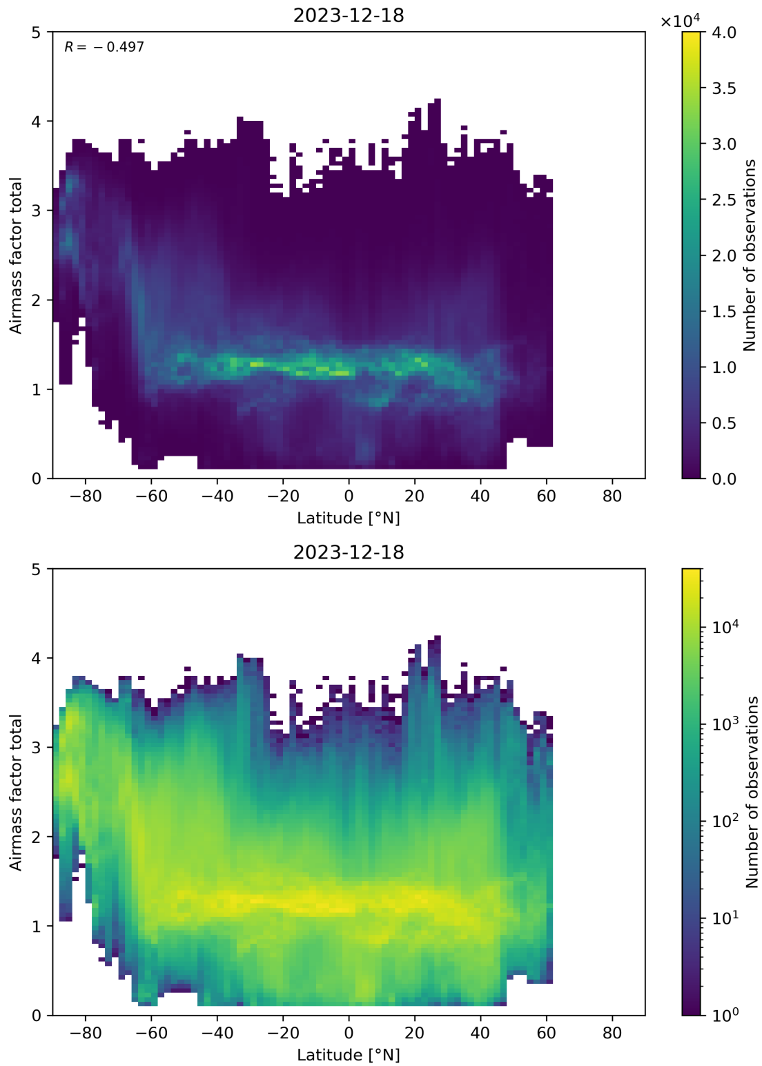
Figure 161: Scatter density plot of “Latitude” against “Airmass factor total” for 2023-12-17 to 2023-12-19.
