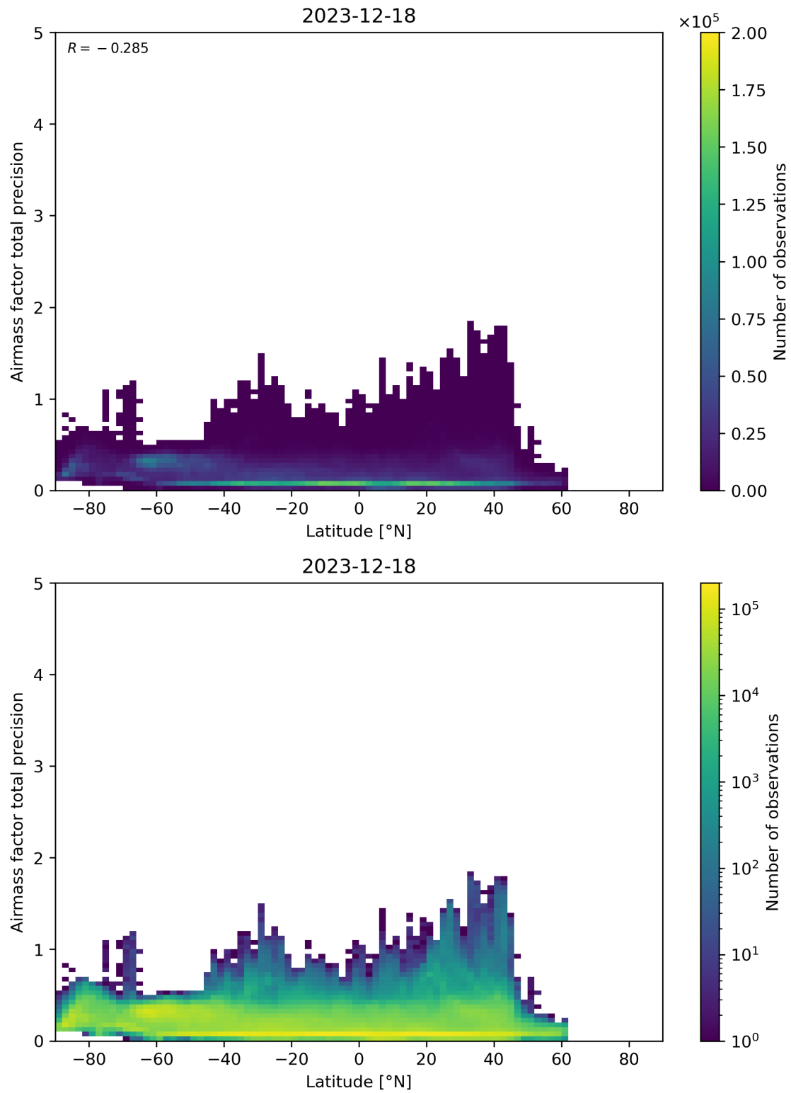
Figure 162: Scatter density plot of “Latitude” against “Airmass factor total precision” for 2023-12-17 to 2023-12-19.
