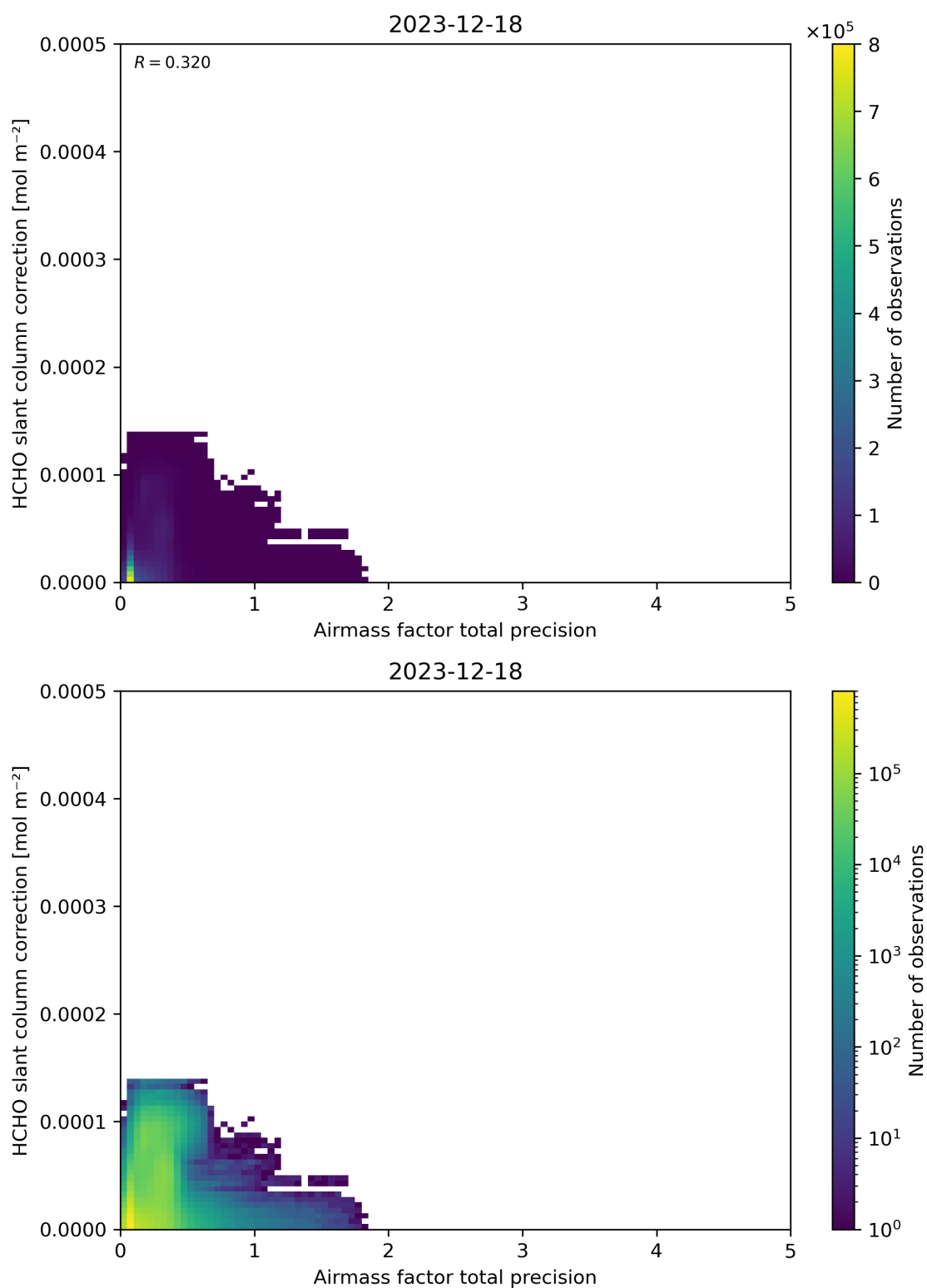
Figure 110: Scatter density plot of “Airmass factor total precision” against “HCHO slant column correction” for 2023-12-17 to 2023-12-19.
