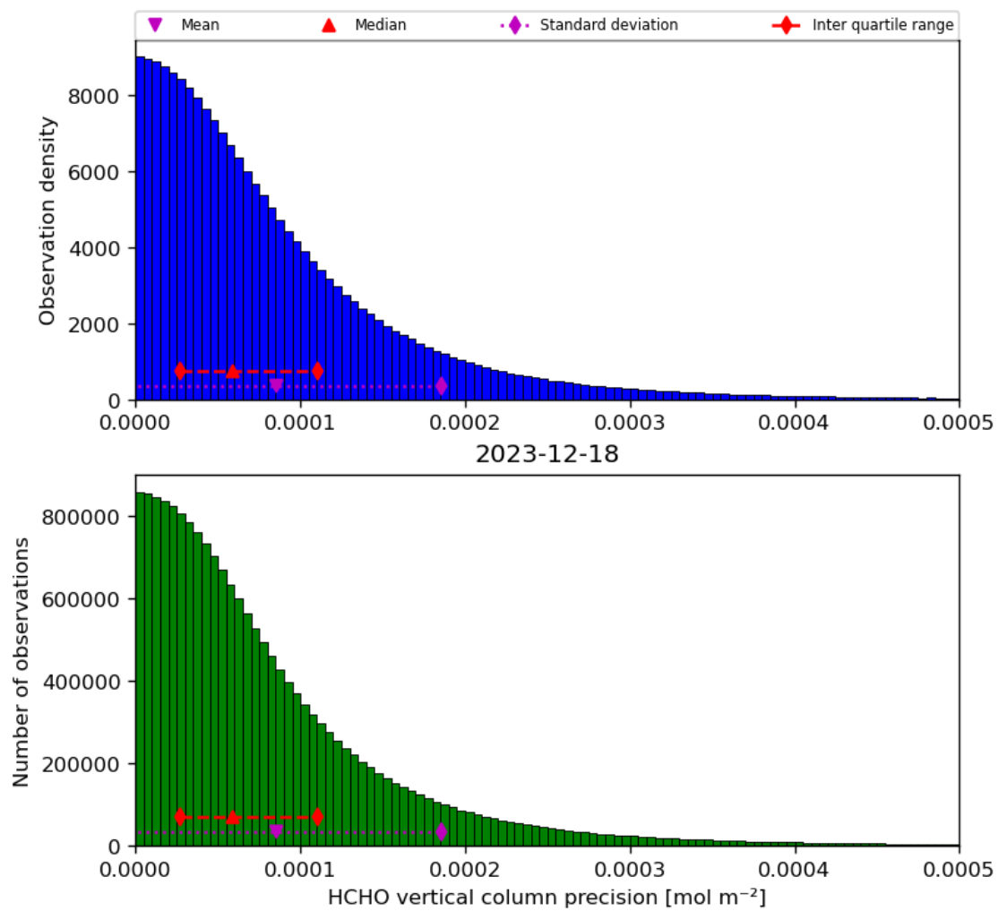
Figure 36: Histogram of “HCHO vertical column precision” for 2023-12-17 to 2023-12-19
