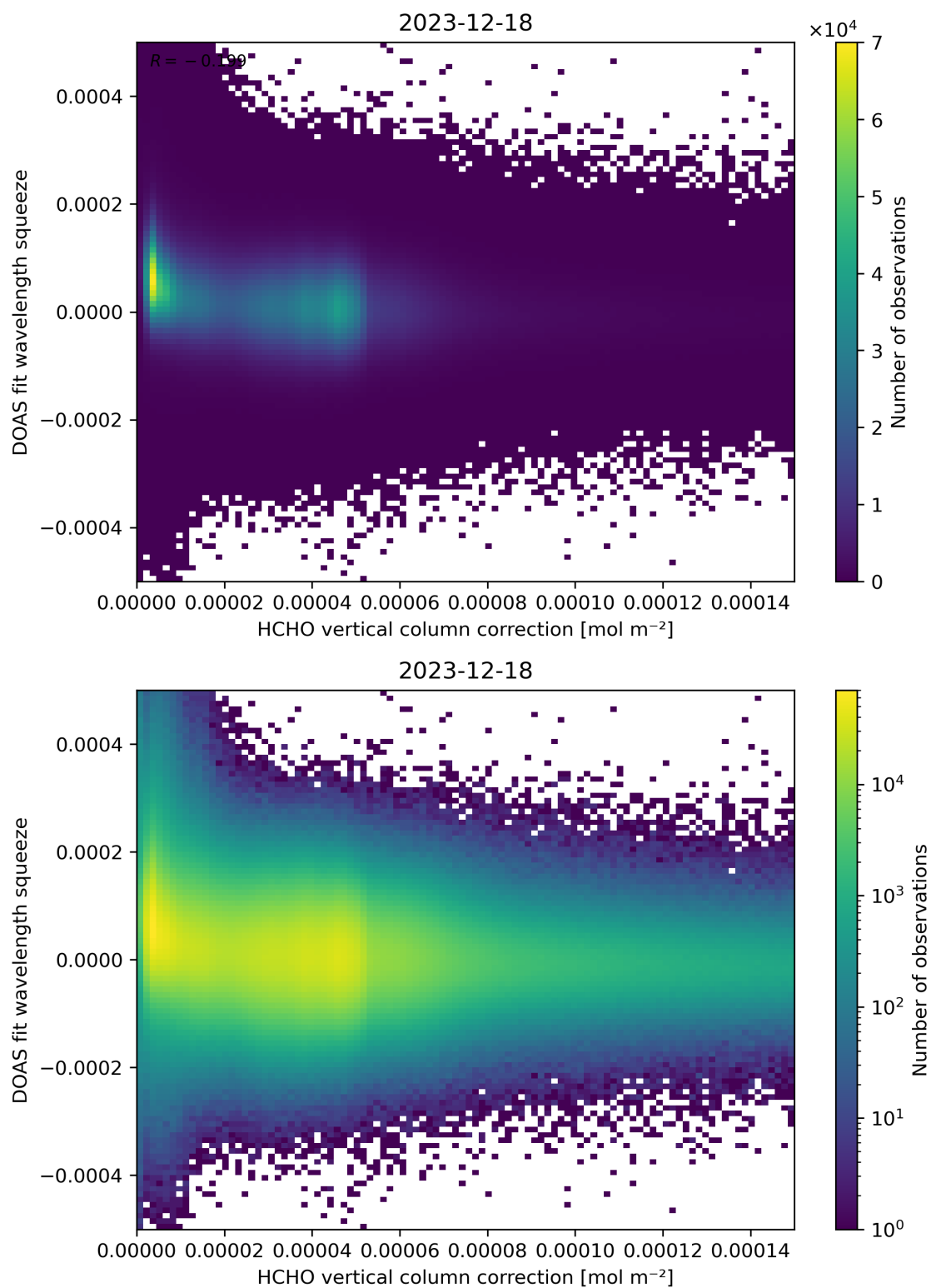
Figure 114: Scatter density plot of “HCHO vertical column correction” against “DOAS fit wavelength squeeze” for 2023-12-17 to 2023-12-19.
