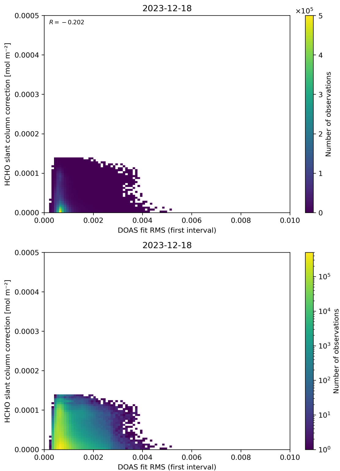
Figure 63: Scatter density plot of “DOAS fit RMS (first interval)” against “HCHO slant column correction” for 2023-12-17 to 2023-12-19.
