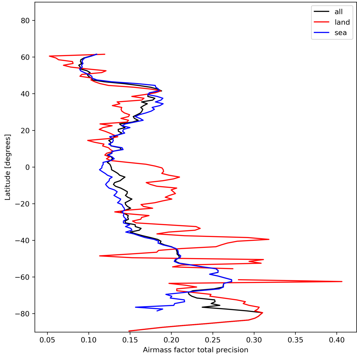
Figure 27: Zonal average of “Airmass factor total precision” for 2023-12-17 to 2023-12-19.
