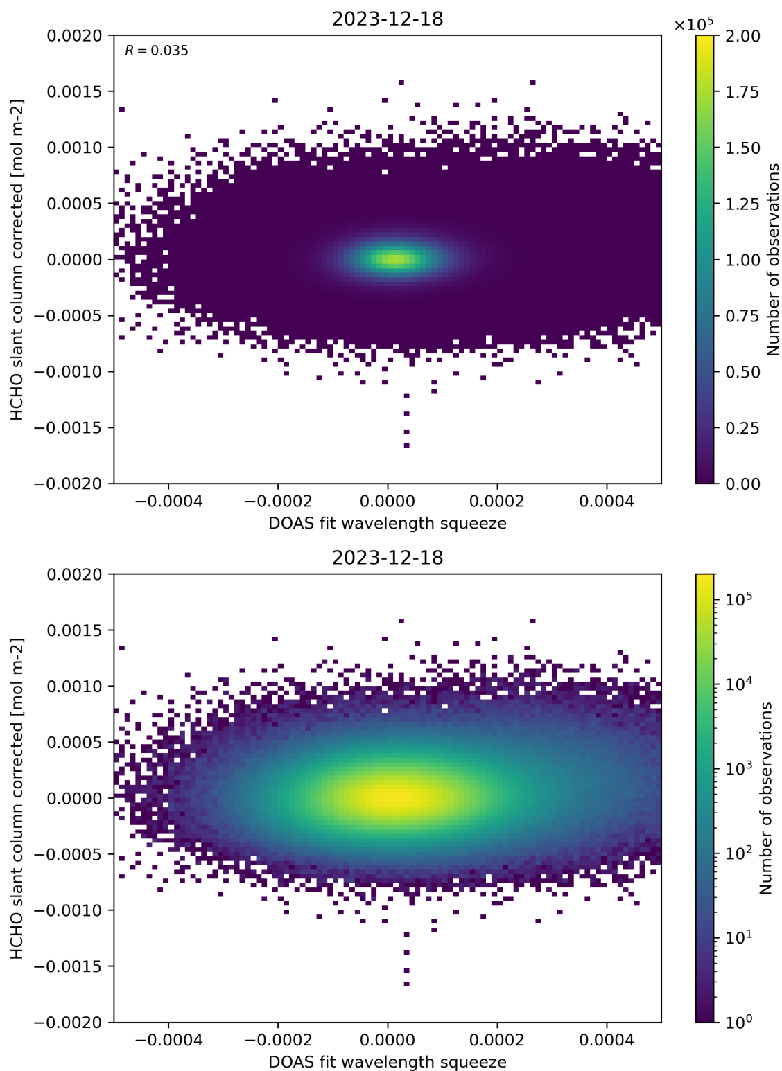
Figure 69: Scatter density plot of “DOAS fit wavelength squeeze” against “HCHO slant column corrected” for 2023-12-17 to 2023-12-19.
