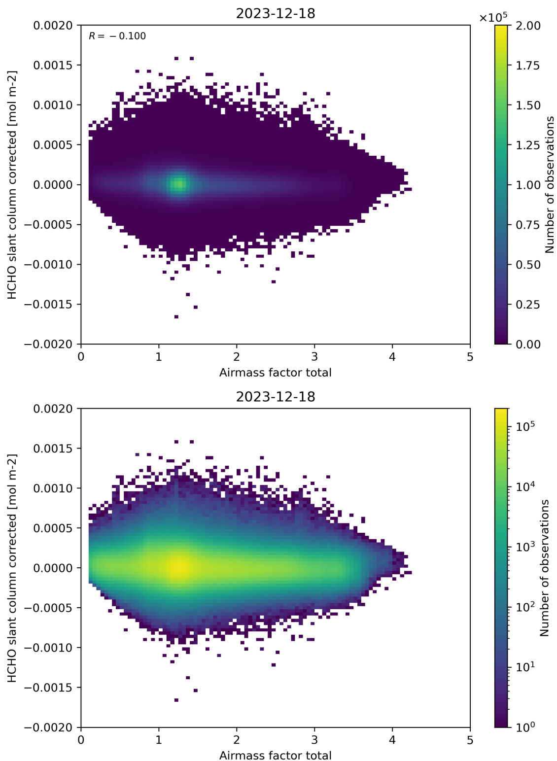
Figure 101: Scatter density plot of “Airmass factor total” against “HCHO slant column corrected” for 2023-12-17 to 2023-12-19.
