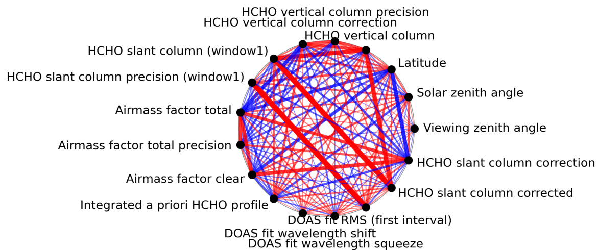
Figure 1: Map of correlation graph for 2023-12-17 to 2023-12-19.
