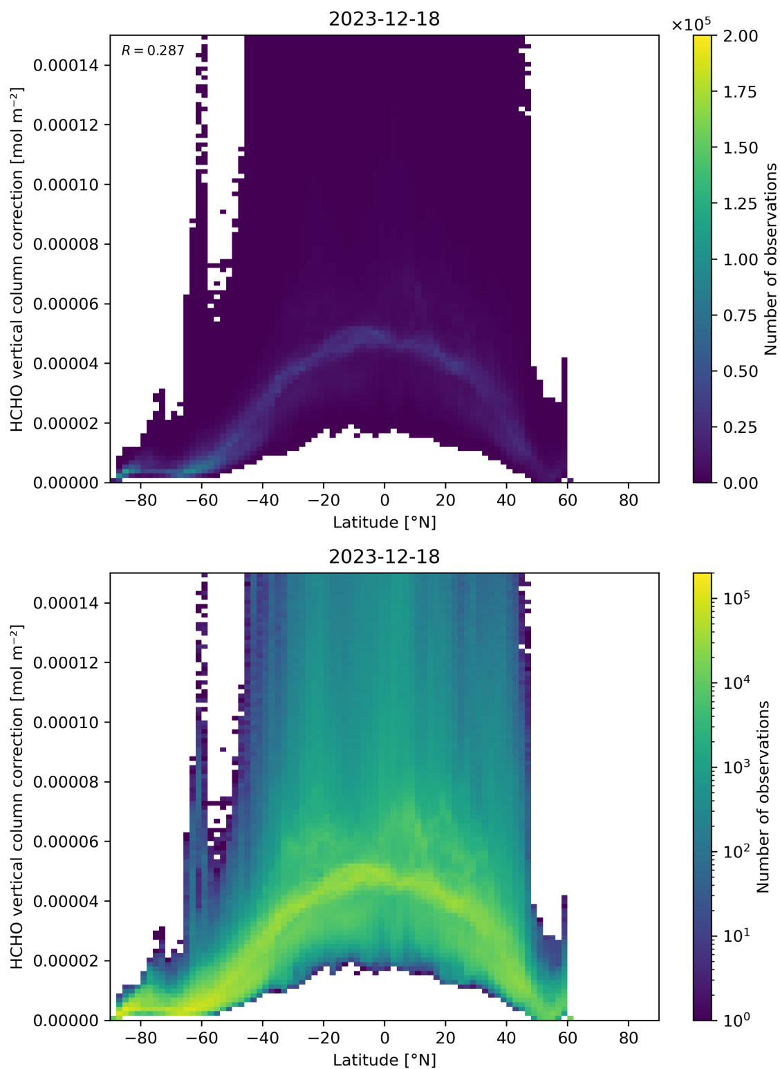
Figure 164: Scatter density plot of “Latitude” against “HCHO vertical column correction” for 2023-12-17 to 2023-12-19.
