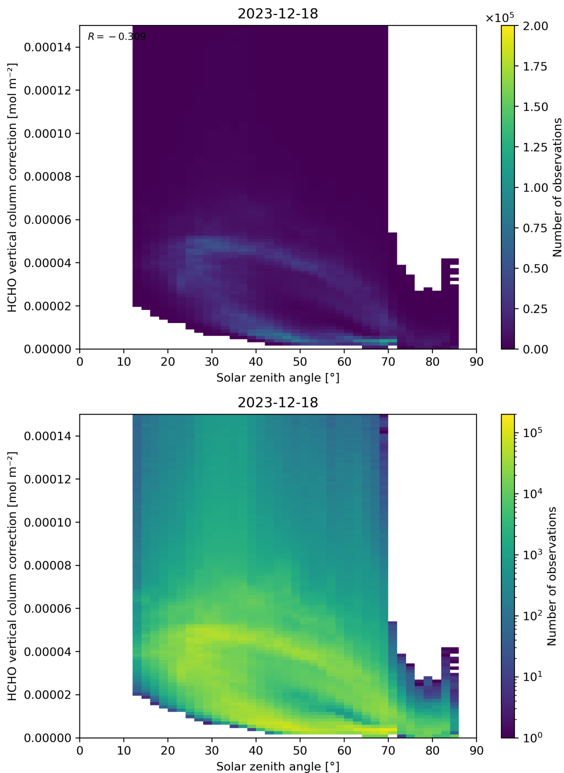
Figure 178: Scatter density plot of “Solar zenith angle” against “HCHO vertical column correction” for 2023-12-17 to 2023-12-19.
