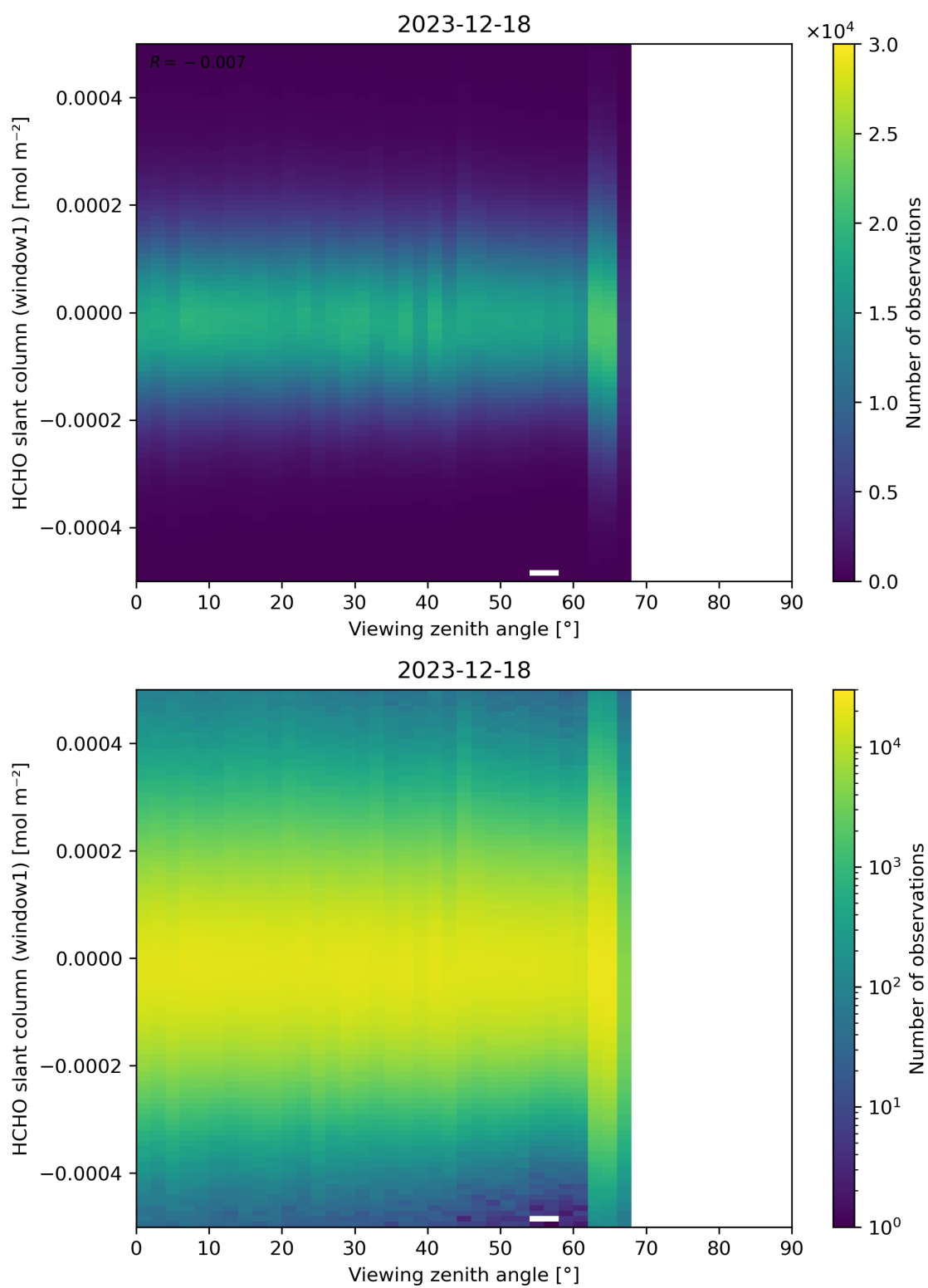
Figure 188: Scatter density plot of “Viewing zenith angle” against “HCHO slant column (window1)” for 2023-12-17 to 2023-12-19.
