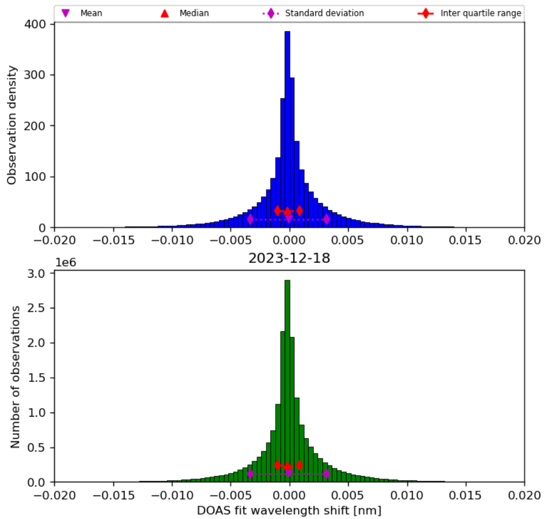
Figure 44: Histogram of “DOAS fit wavelength shift” for 2023-12-17 to 2023-12-19
