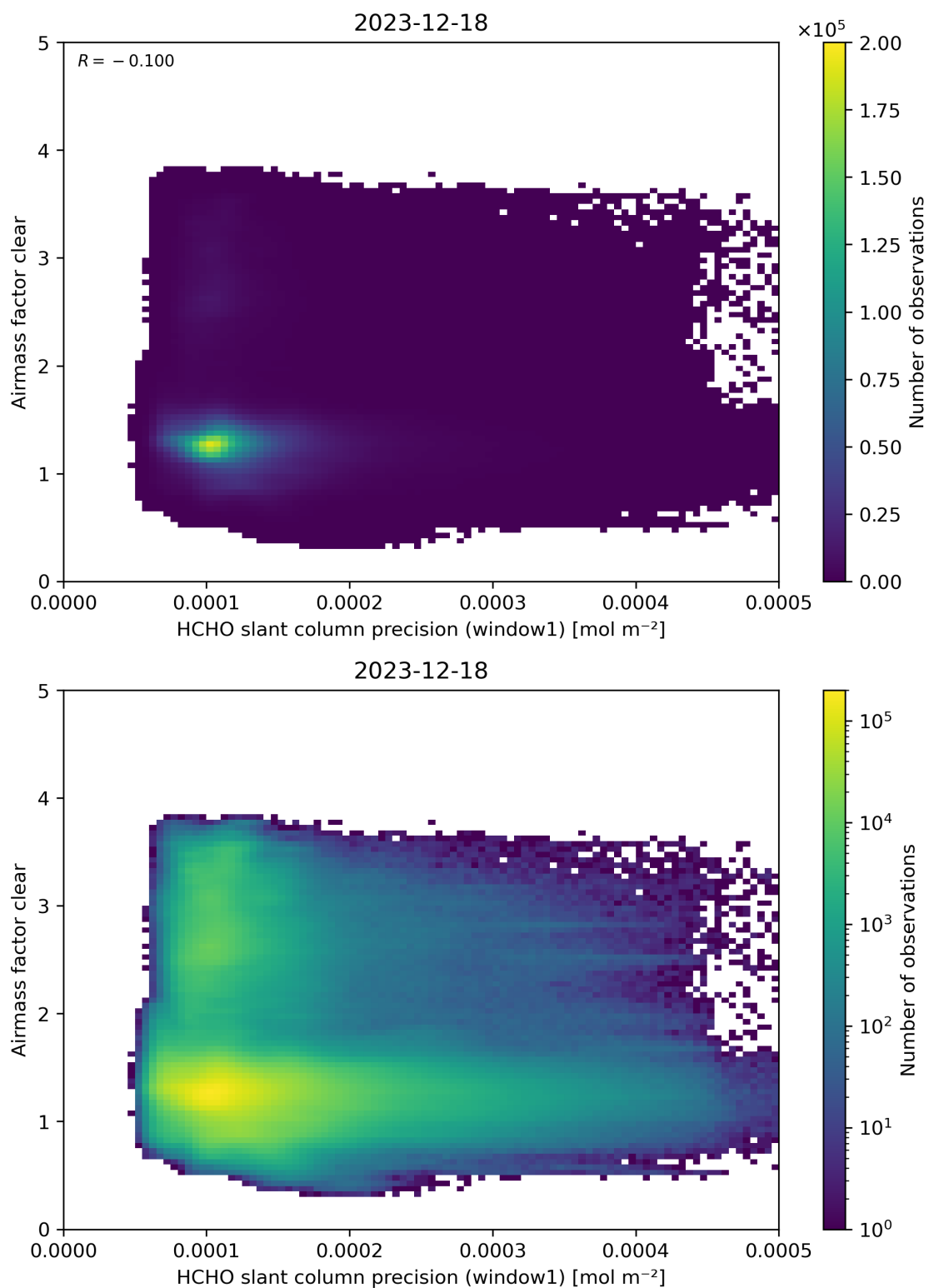
Figure 91: Scatter density plot of “HCHO slant column precision (window1)” against “Airmass factor clear” for 2023-12-17 to 2023-12-19.
