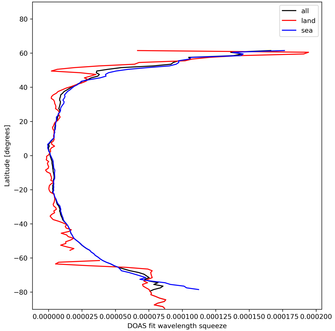
Figure 31: Zonal average of “DOAS fit wavelength squeeze” for 2023-12-17 to 2023-12-19.
