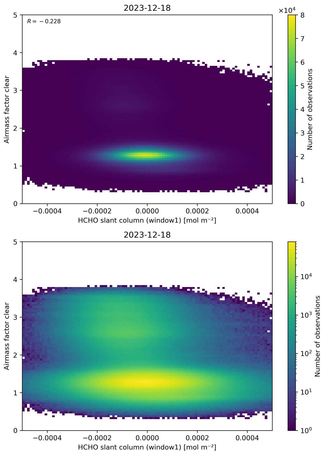
Figure 81: Scatter density plot of “HCHO slant column (window1)” against “Airmass factor clear” for 2023-12-17 to 2023-12-19.
