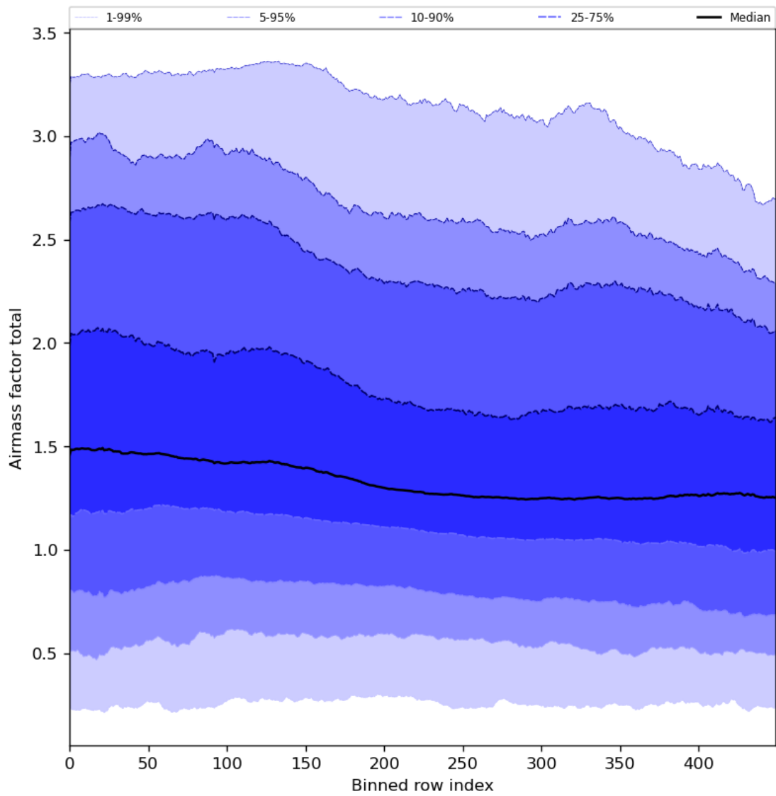
Figure 54: Along track statistics of “Airmass factor total” for 2023-12-17 to 2023-12-19
