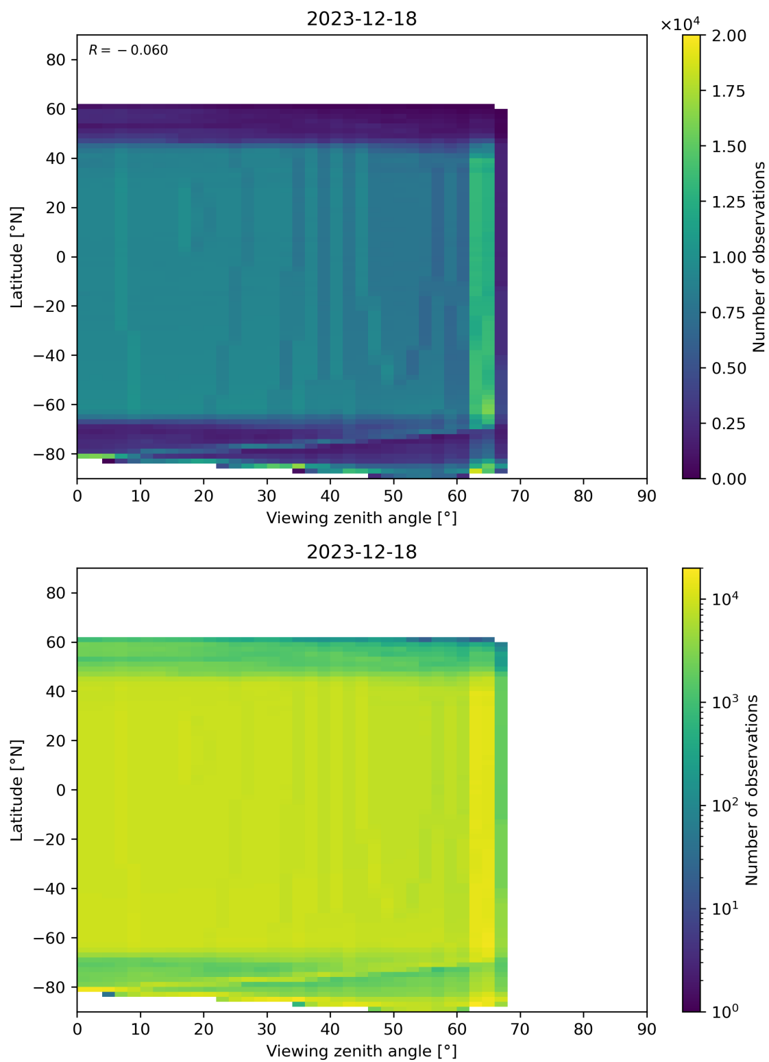
Figure 196: Scatter density plot of “Viewing zenith angle” against “Latitude” for 2023-12-17 to 2023-12-19.
