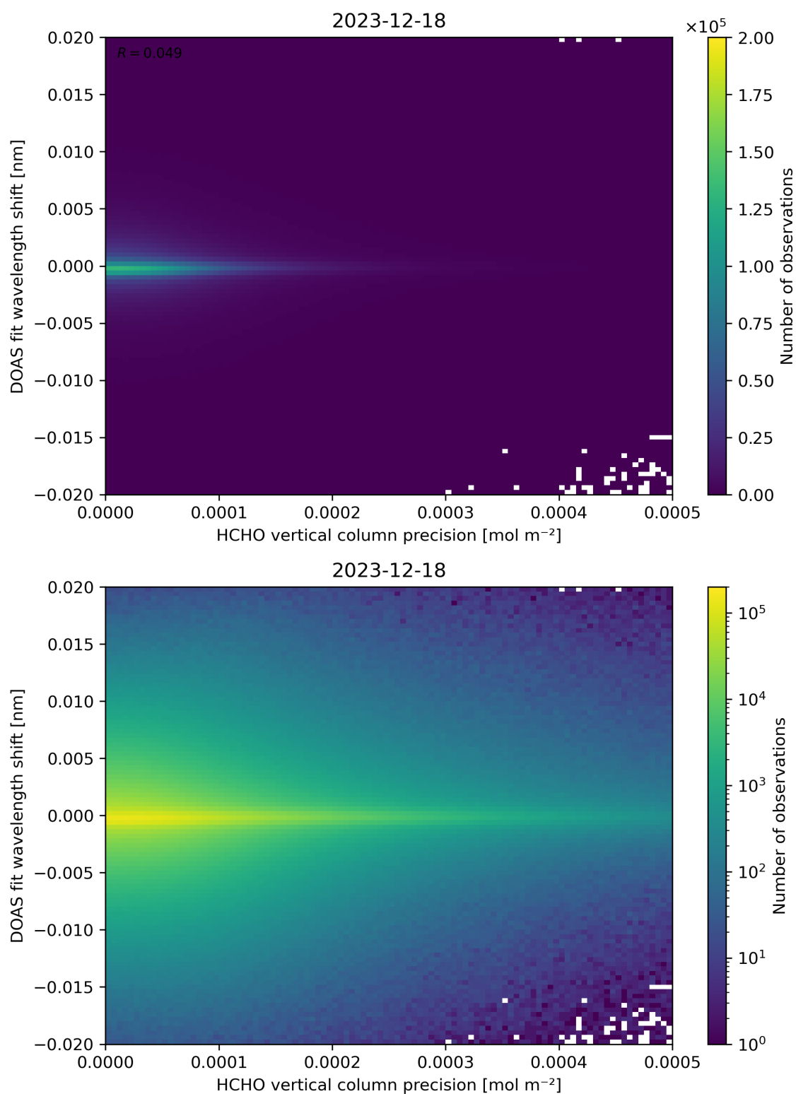
Figure 137: Scatter density plot of “HCHO vertical column precision” against “DOAS fit wavelength shift” for 2023-12-17 to 2023-12-19.
