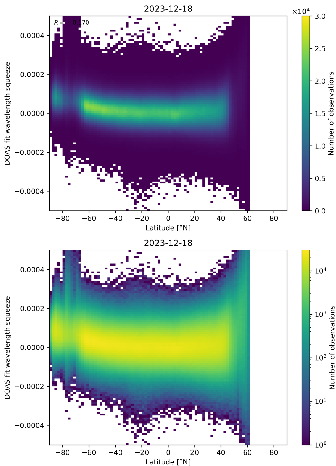
Figure 155: Scatter density plot of “Latitude” against “DOAS fit wavelength squeeze” for 2023-12-17 to 2023-12-19.
