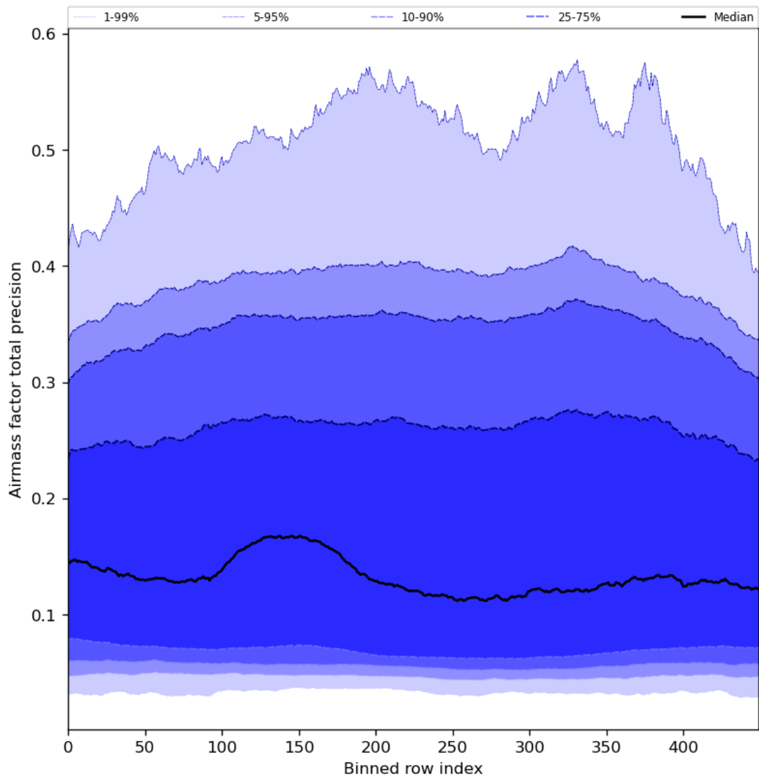
Figure 55: Along track statistics of “Airmass factor total precision” for 2023-12-17 to 2023-12-19
