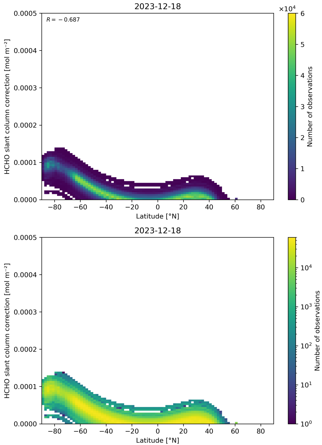
Figure 158: Scatter density plot of “Latitude” against “HCHO slant column correction” for 2023-12-17 to 2023-12-19.
