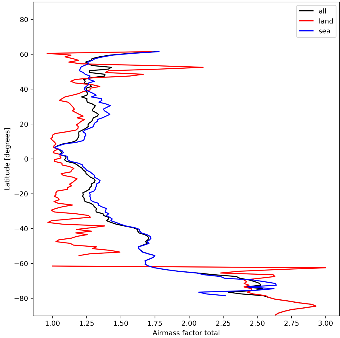
Figure 26: Zonal average of “Airmass factor total” for 2023-12-17 to 2023-12-19.
