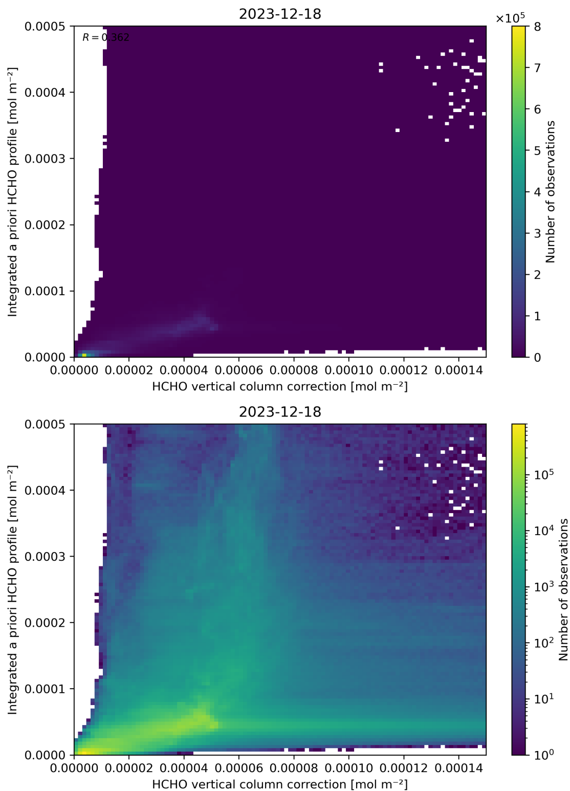
Figure 122: Scatter density plot of “HCHO vertical column correction” against “Integrated a priori HCHO profile” for 2023-12-17 to 2023-12-19.
