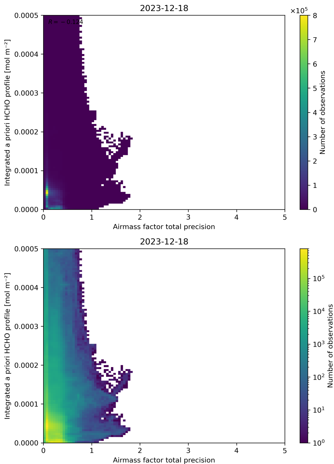
Figure 111: Scatter density plot of “Airmass factor total precision” against “Integrated a priori HCHO profile” for 2023-12-17 to 2023-12-19.
