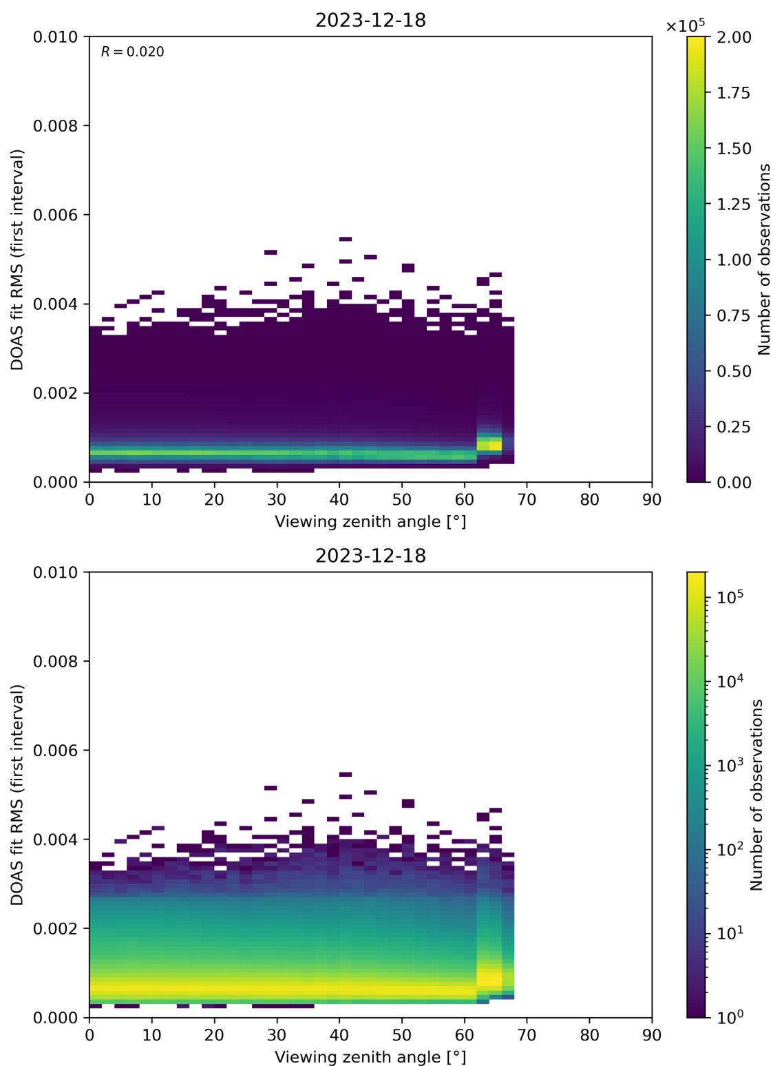
Figure 182: Scatter density plot of “Viewing zenith angle” against “DOAS fit RMS (first interval)” for 2023-12-17 to 2023-12-19.
