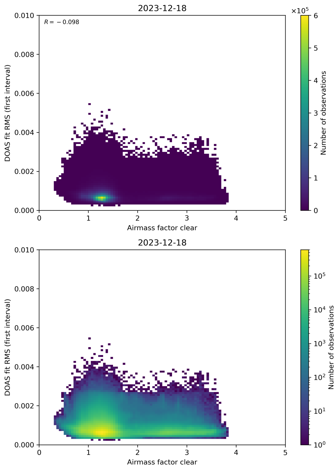
Figure 71: Scatter density plot of “Airmass factor clear” against “DOAS fit RMS (first interval)” for 2023-12-17 to 2023-12-19.
