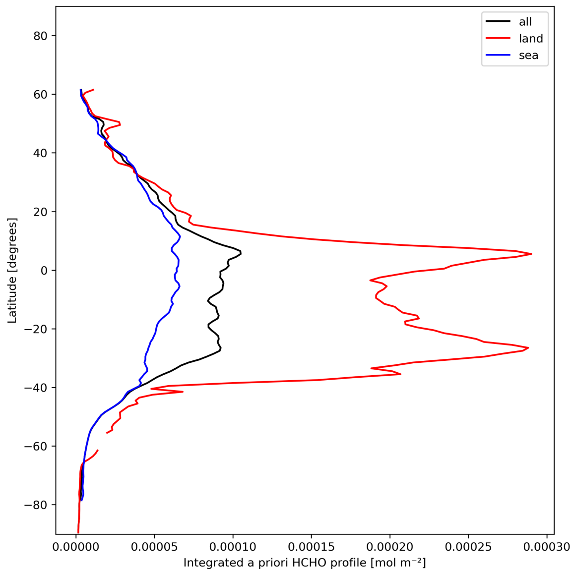
Figure 29: Zonal average of “Integrated a priori HCHO profile” for 2023-12-17 to 2023-12-19.
