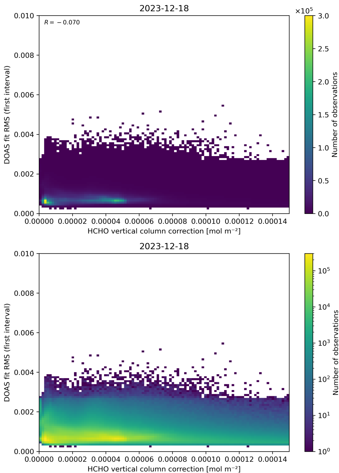
Figure 112: Scatter density plot of “HCHO vertical column correction” against “DOAS fit RMS (first interval)” for 2023-12-17 to 2023-12-19.
