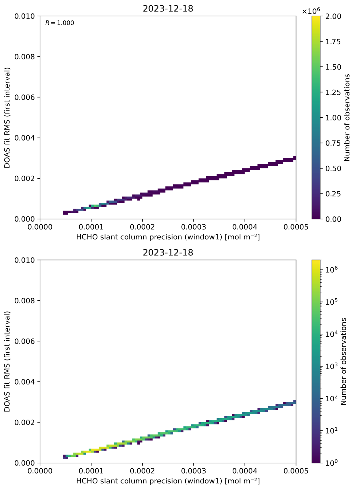
Figure 88: Scatter density plot of “HCHO slant column precision (window1)” against “DOAS fit RMS (first interval)” for 2023-12-17 to 2023-12-19.
