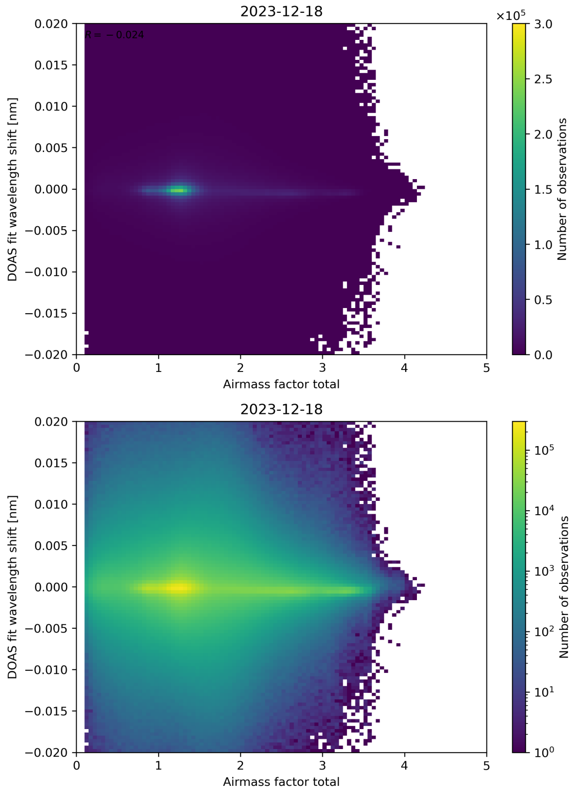
Figure 98: Scatter density plot of “Airmass factor total” against “DOAS fit wavelength shift” for 2023-12-17 to 2023-12-19.
