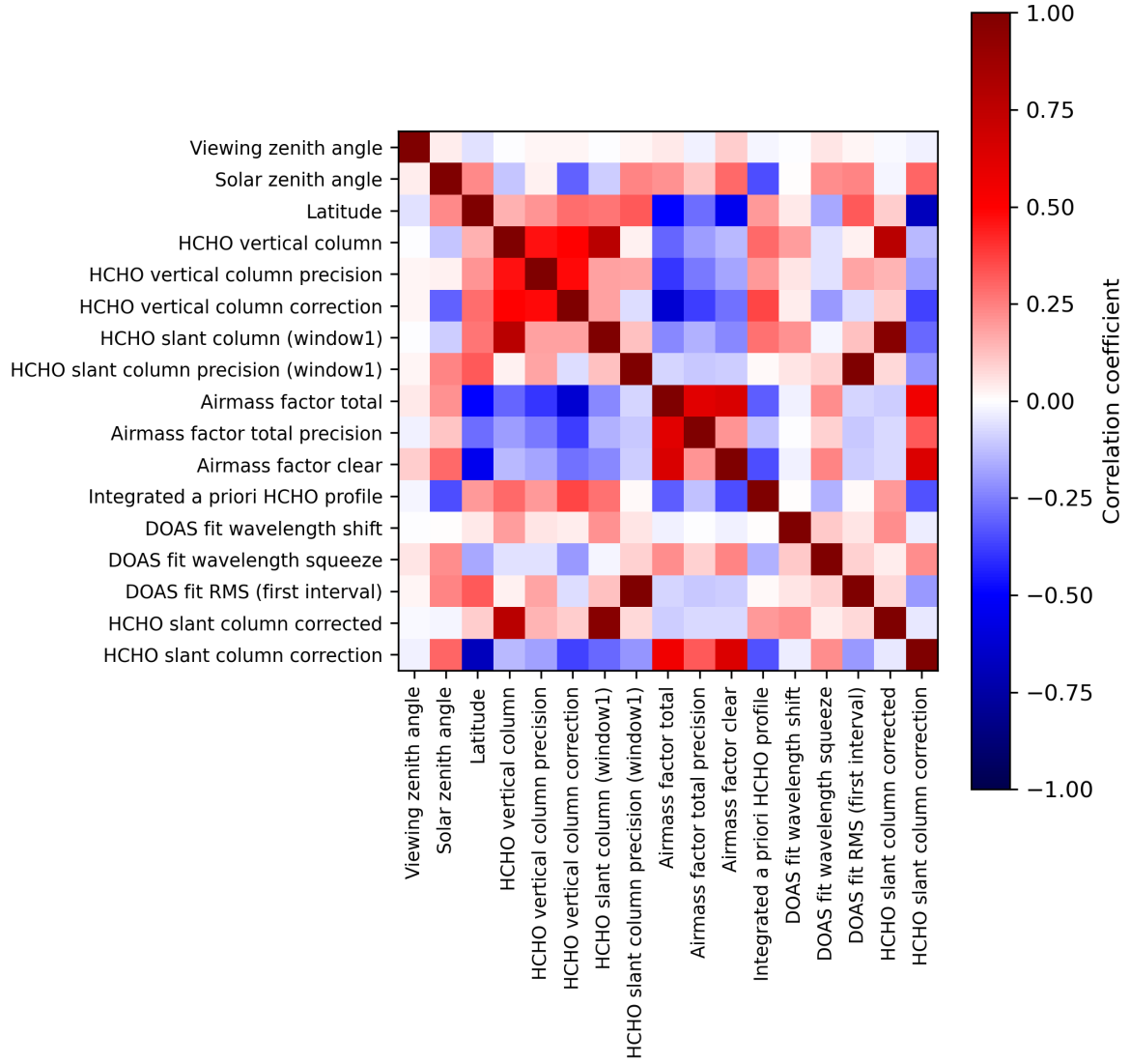
Figure 2: Map of correlation matrix for 2023-12-17 to 2023-12-19.
