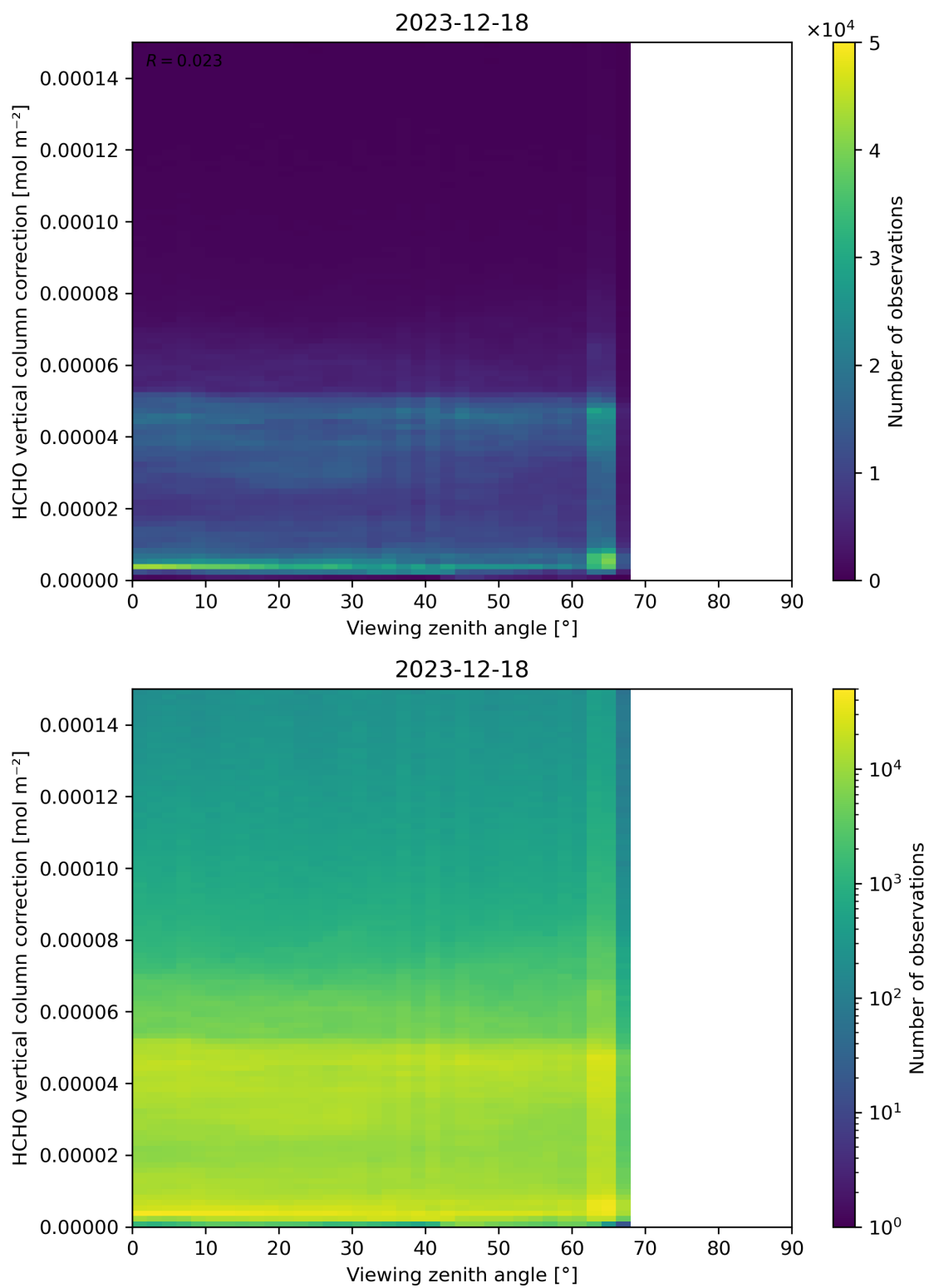
Figure 193: Scatter density plot of “Viewing zenith angle” against “HCHO vertical column correction” for 2023-12-17 to 2023-12-19.
