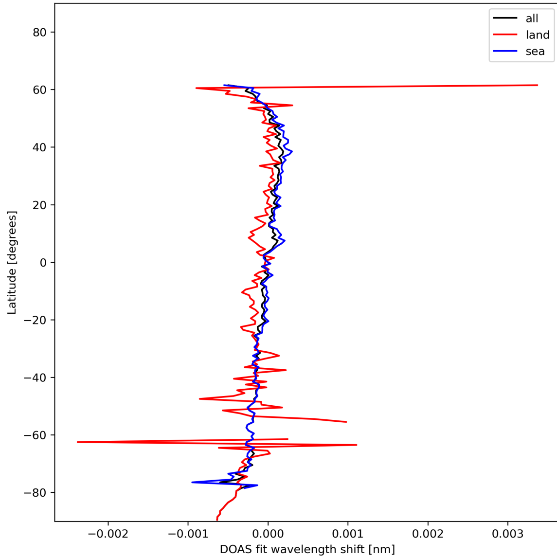
Figure 30: Zonal average of “DOAS fit wavelength shift” for 2023-12-17 to 2023-12-19.
