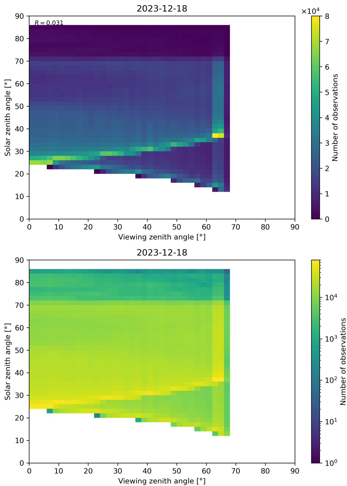
Figure 197: Scatter density plot of “Viewing zenith angle” against “Solar zenith angle” for 2023-12-17 to 2023-12-19.
