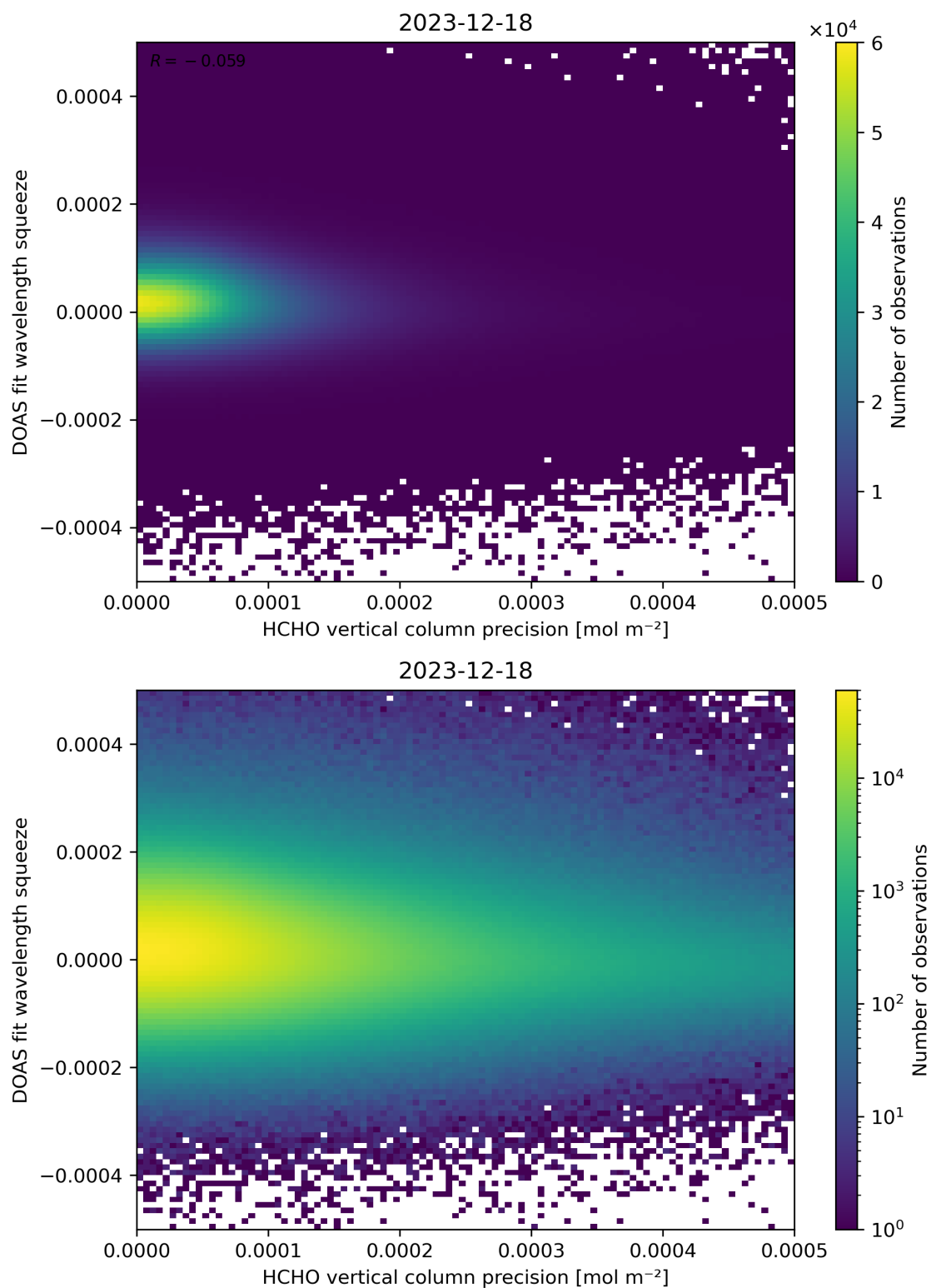
Figure 138: Scatter density plot of “HCHO vertical column precision” against “DOAS fit wavelength squeeze” for 2023-12-17 to 2023-12-19.
