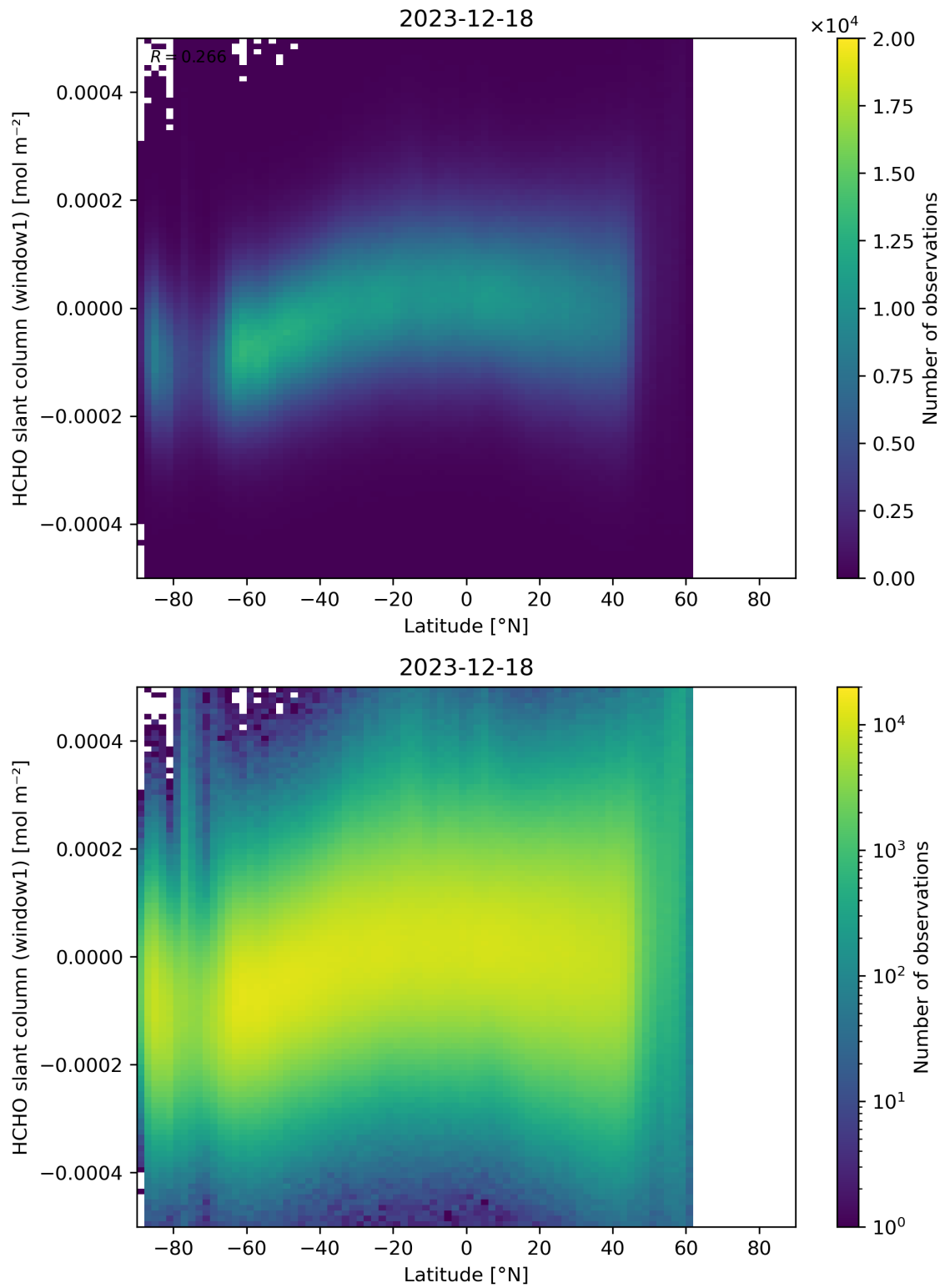
Figure 159: Scatter density plot of “Latitude” against “HCHO slant column (window1)” for 2023-12-17 to 2023-12-19.
