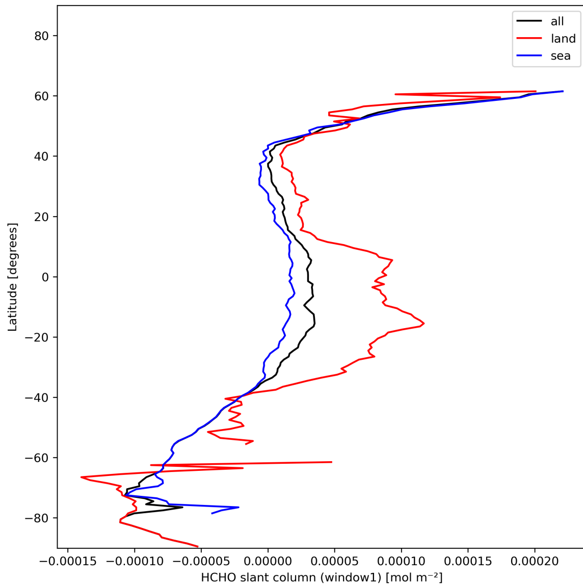
Figure 24: Zonal average of “HCHO slant column (window1)” for 2023-12-17 to 2023-12-19.
