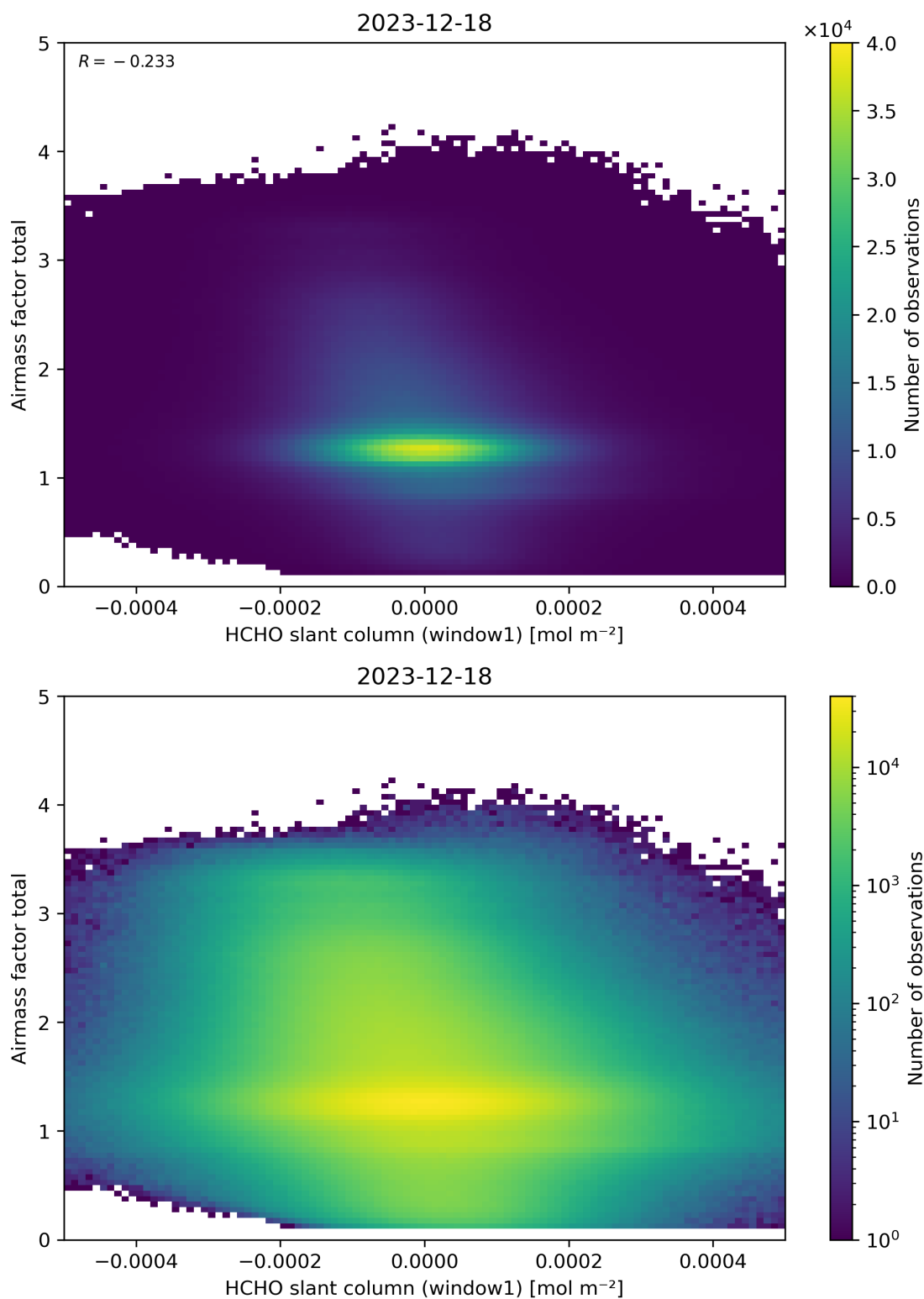
Figure 85: Scatter density plot of “HCHO slant column (window1)” against “Airmass factor total” for 2023-12-17 to 2023-12-19.
