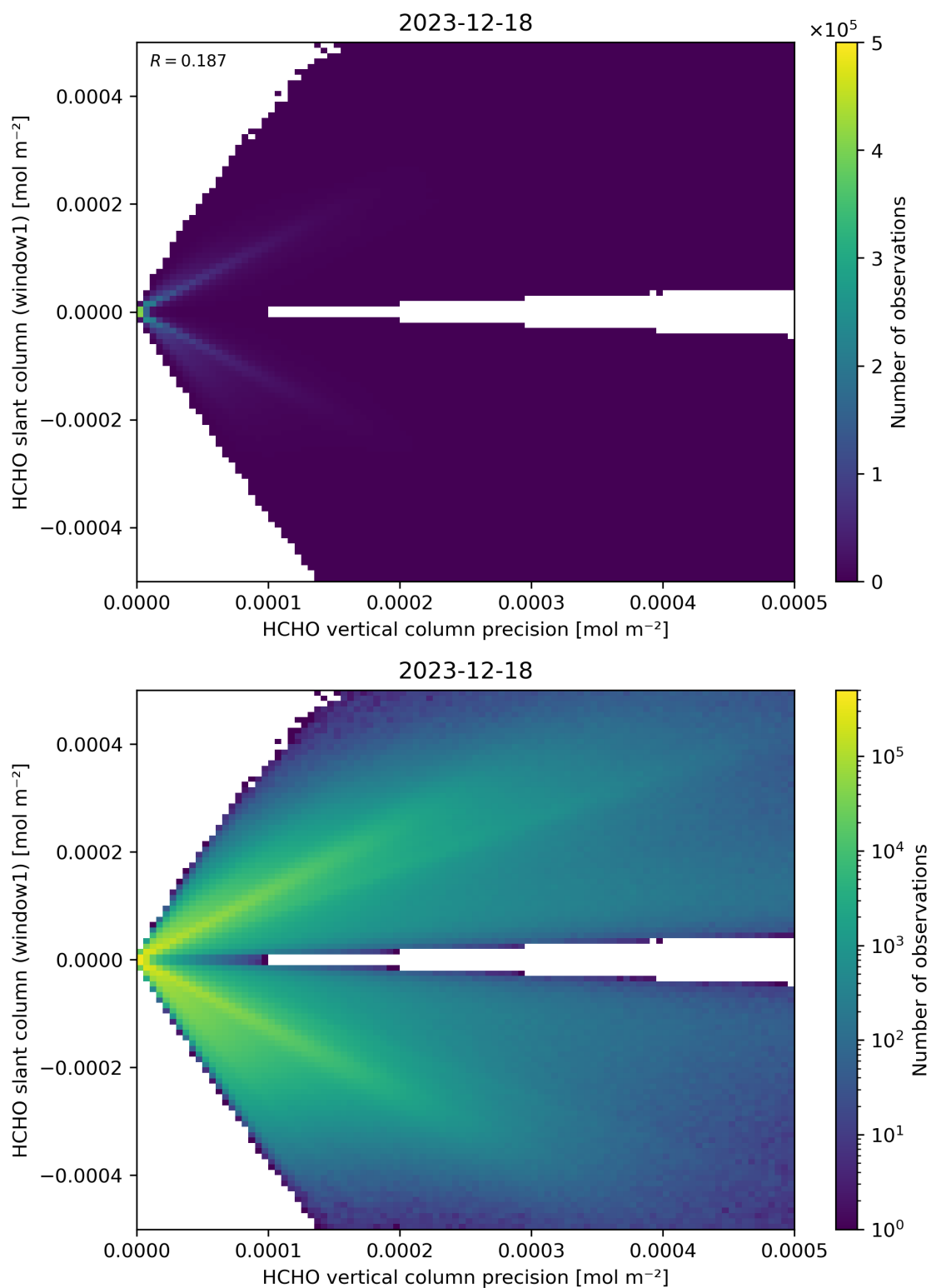
Figure 142: Scatter density plot of “HCHO vertical column precision” against “HCHO slant column (window1)” for 2023-12-17 to 2023-12-19.
