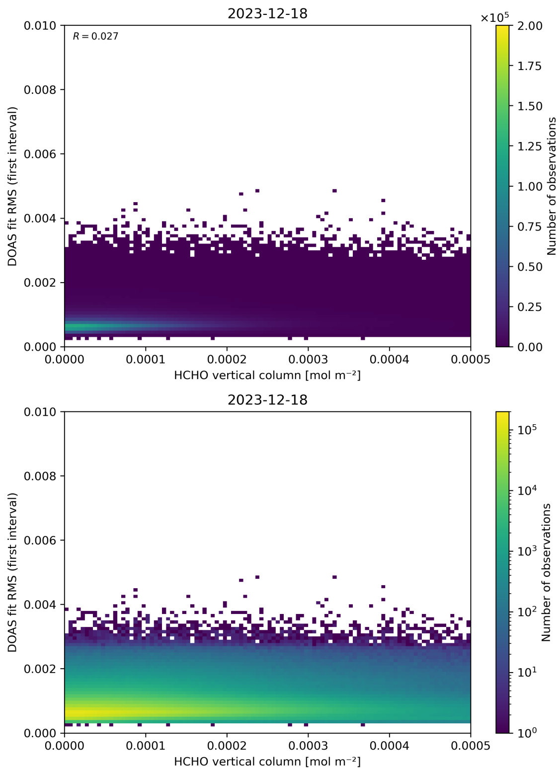
Figure 123: Scatter density plot of “HCHO vertical column” against “DOAS fit RMS (first interval)” for 2023-12-17 to 2023-12-19.
