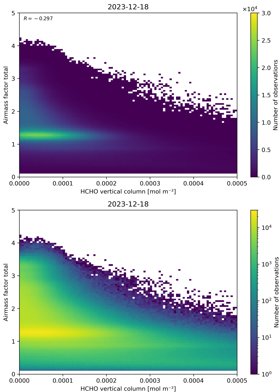
Figure 131: Scatter density plot of “HCHO vertical column” against “Airmass factor total” for 2023-12-17 to 2023-12-19.
