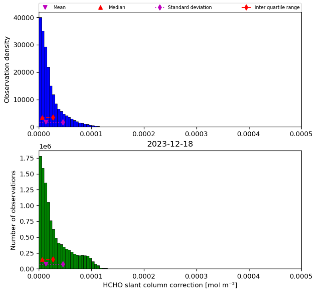
Figure 47: Histogram of “HCHO slant column correction” for 2023-12-17 to 2023-12-19
