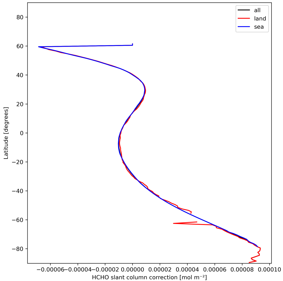
Figure 33: Zonal average of “HCHO slant column correction” for 2023-12-17 to 2023-12-19.
