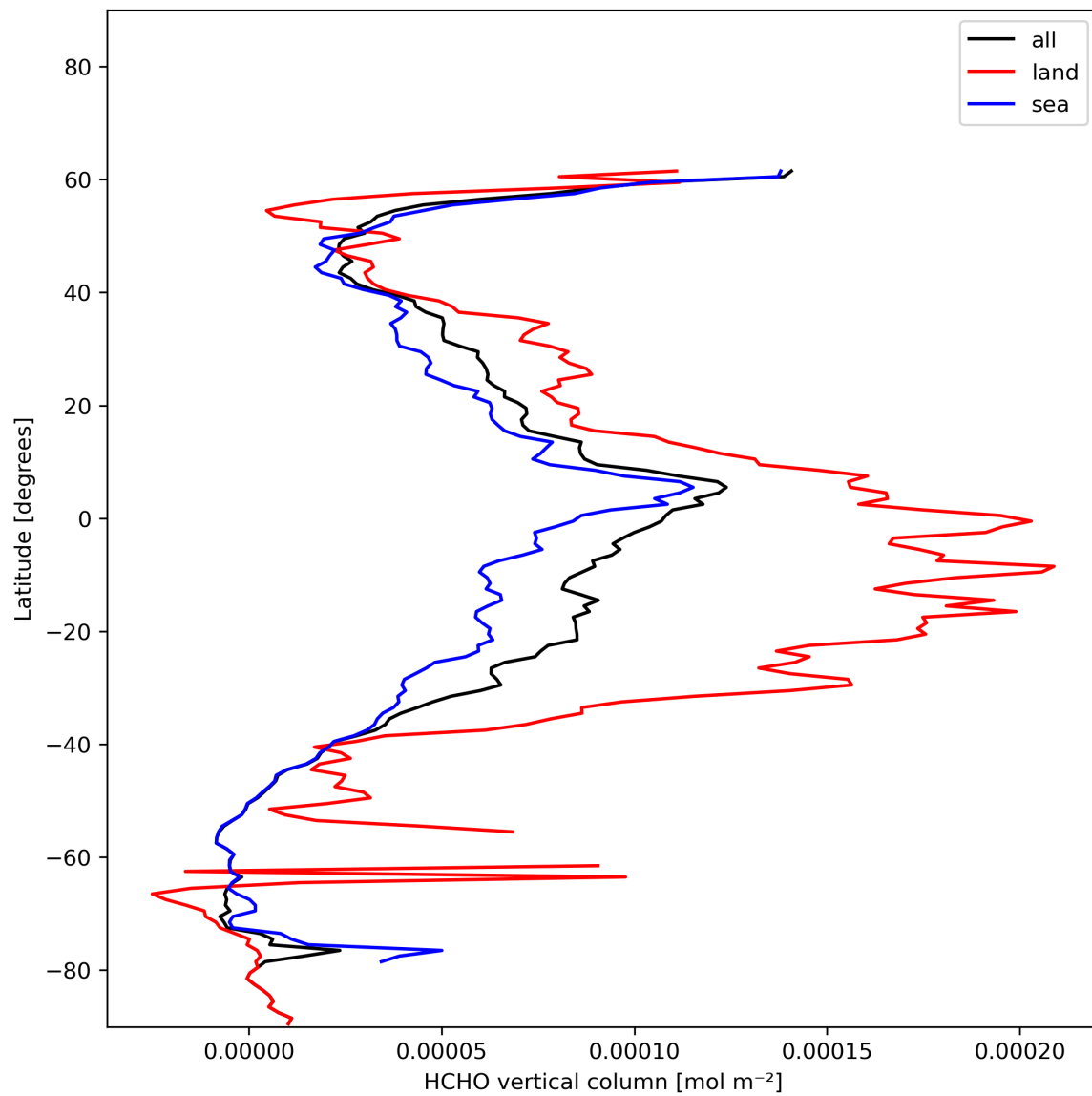
Figure 21: Zonal average of “HCHO vertical column” for 2023-12-17 to 2023-12-19.
