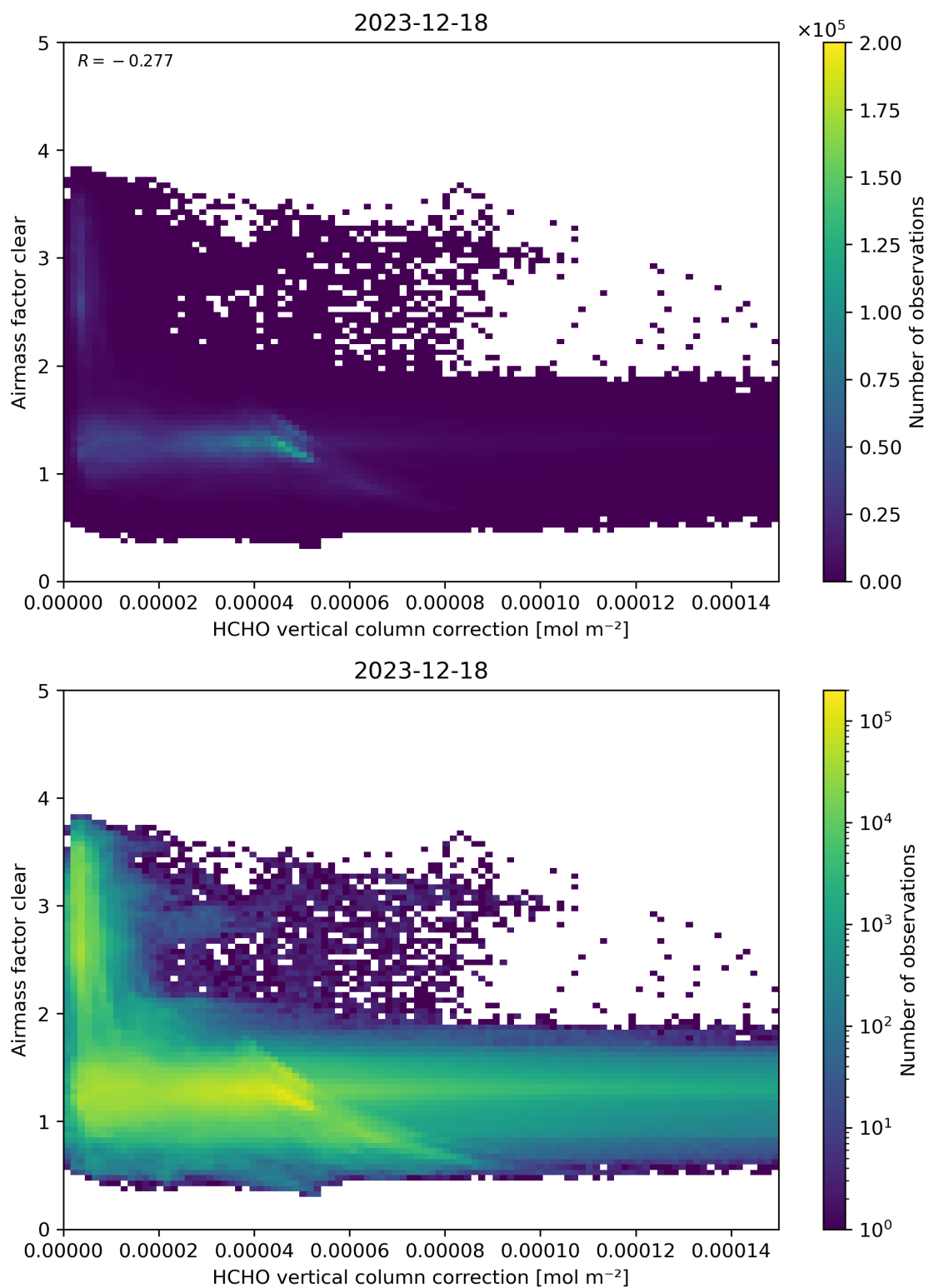
Figure 115: Scatter density plot of “HCHO vertical column correction” against “Airmass factor clear” for 2023-12-17 to 2023-12-19.
