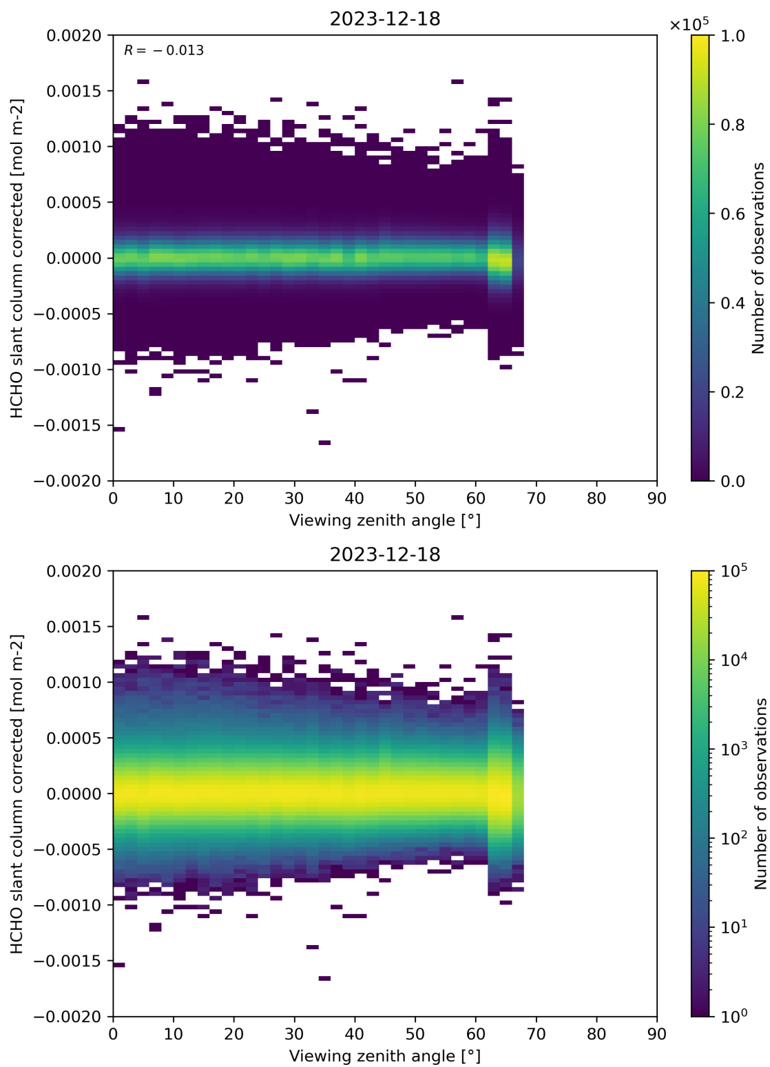
Figure 186: Scatter density plot of “Viewing zenith angle” against “HCHO slant column corrected” for 2023-12-17 to 2023-12-19.
