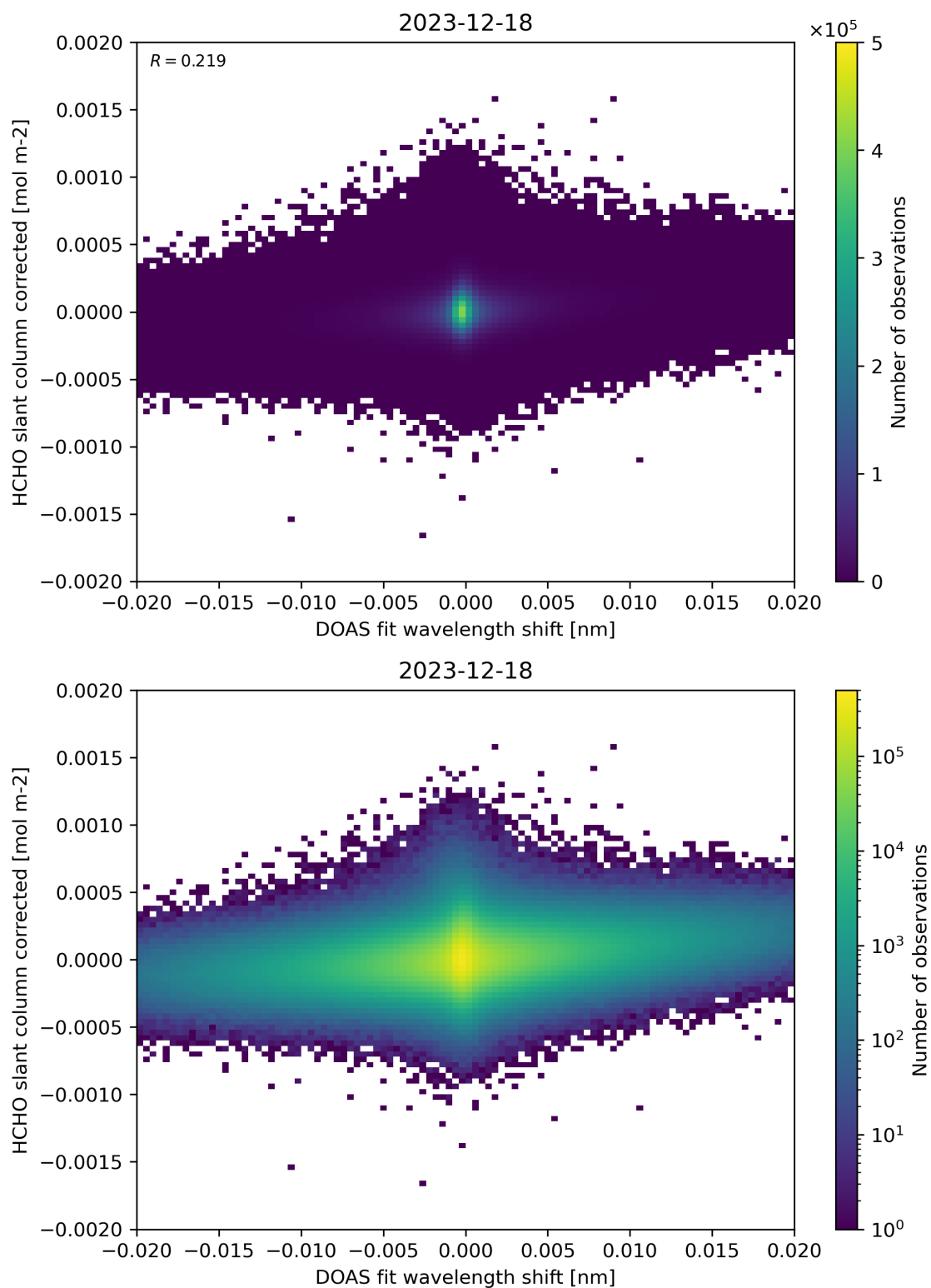
Figure 66: Scatter density plot of “DOAS fit wavelength shift” against “HCHO slant column corrected” for 2023-12-17 to 2023-12-19.
