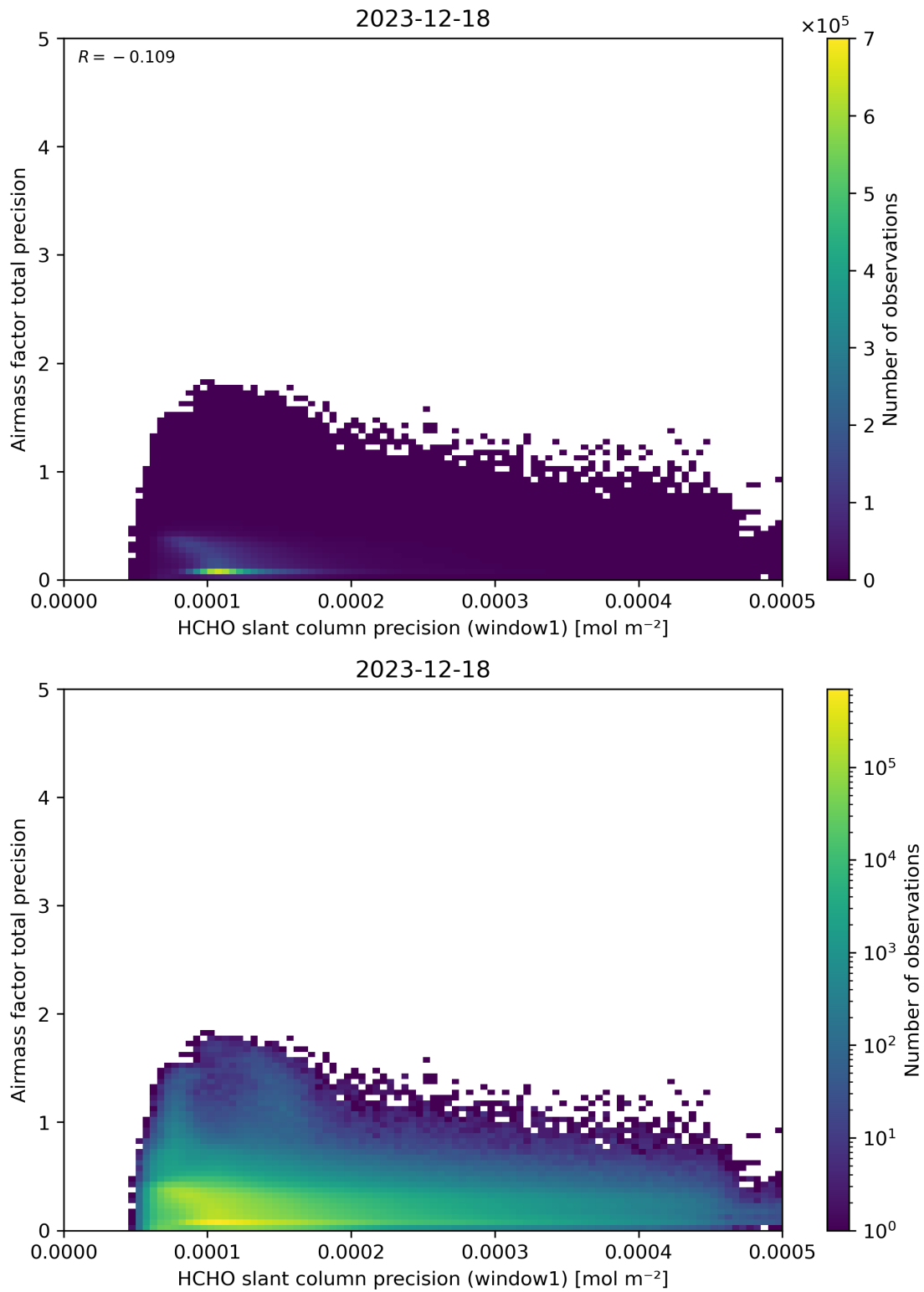
Figure 95: Scatter density plot of “HCHO slant column precision (window1)” against “Airmass factor total precision” for 2023-12-17 to 2023-12-19.
