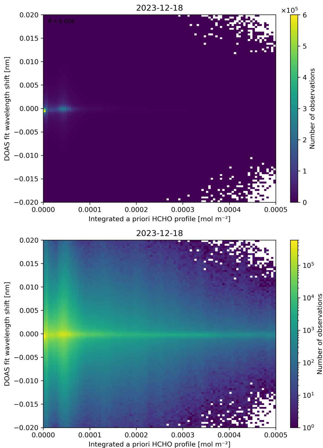
Figure 149: Scatter density plot of “Integrated a priori HCHO profile” against “DOAS fit wavelength shift” for 2023-12-17 to 2023-12-19.
