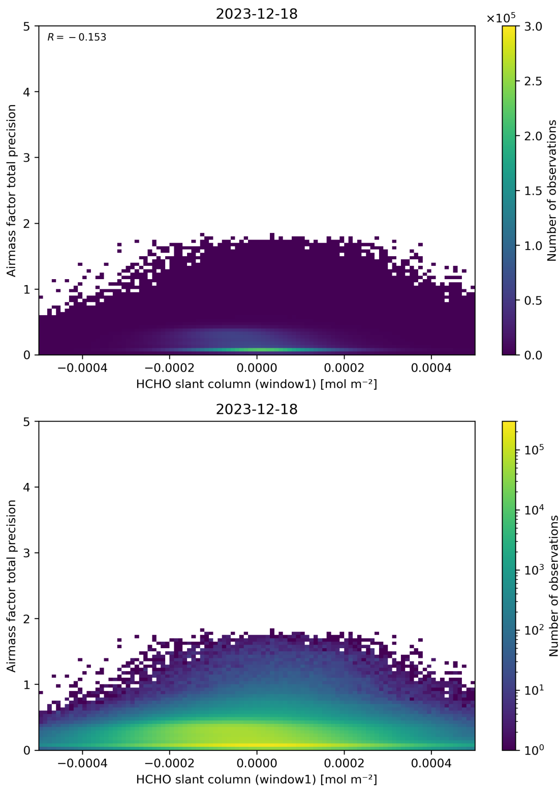
Figure 86: Scatter density plot of “HCHO slant column (window1)” against “Airmass factor total precision” for 2023-12-17 to 2023-12-19.
