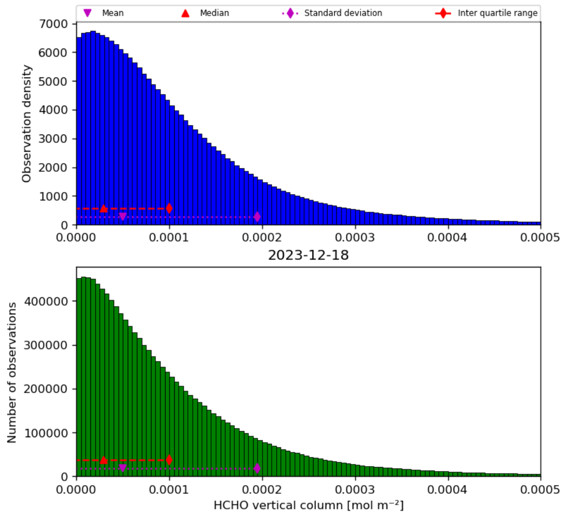
Figure 35: Histogram of “HCHO vertical column” for 2023-12-17 to 2023-12-19
