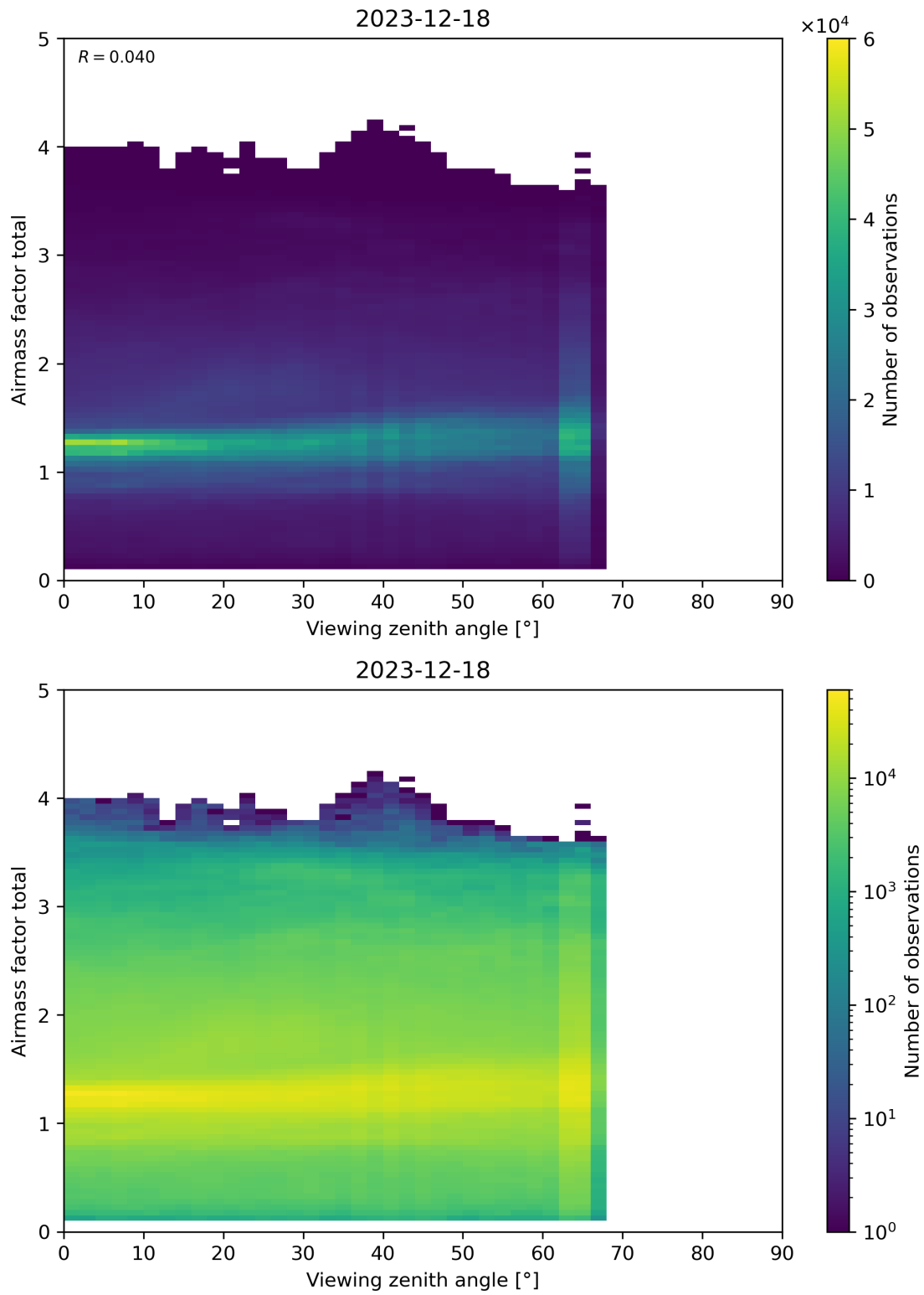
Figure 190: Scatter density plot of “Viewing zenith angle” against “Airmass factor total” for 2023-12-17 to 2023-12-19.
