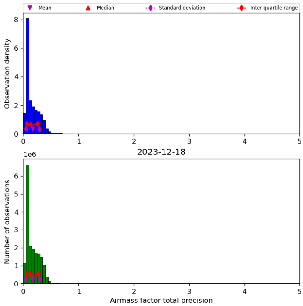
Figure 41: Histogram of “Airmass factor total precision” for 2023-12-17 to 2023-12-19
