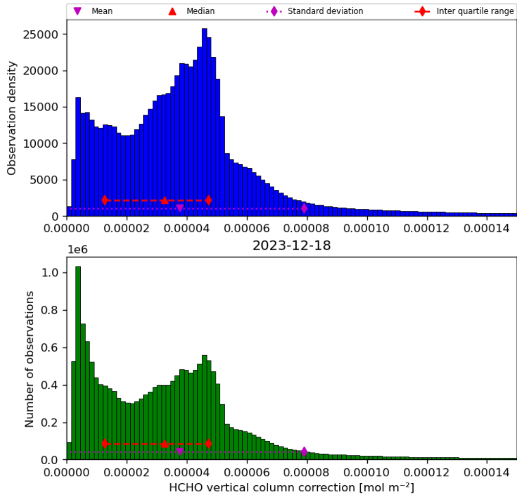
Figure 37: Histogram of “HCHO vertical column correction” for 2023-12-17 to 2023-12-19
