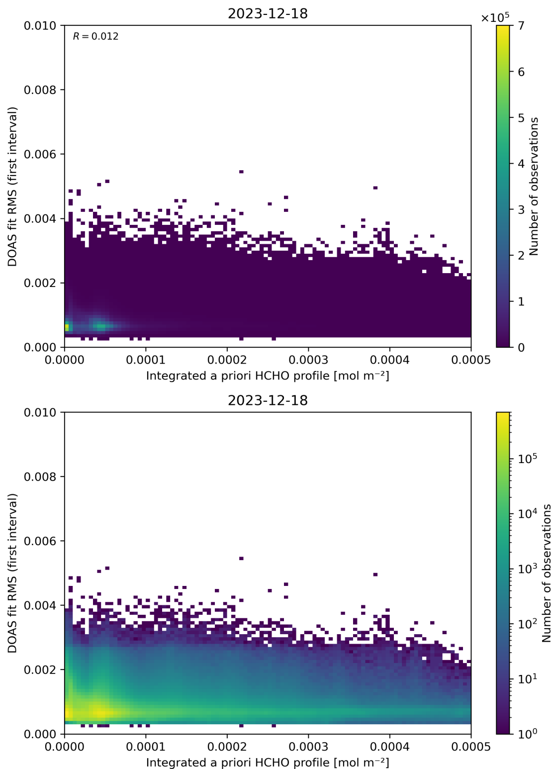
Figure 148: Scatter density plot of “Integrated a priori HCHO profile” against “DOAS fit RMS (first interval)” for 2023-12-17 to 2023-12-19.
