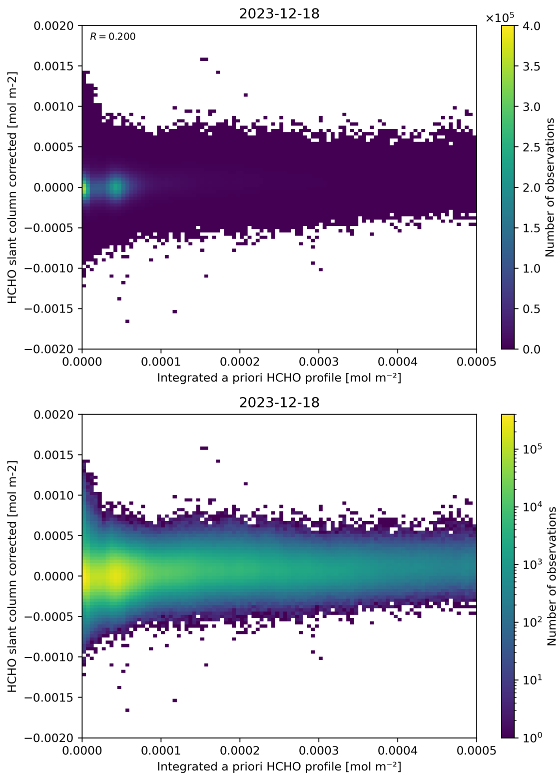
Figure 151: Scatter density plot of “Integrated a priori HCHO profile” against “HCHO slant column corrected” for 2023-12-17 to 2023-12-19.
