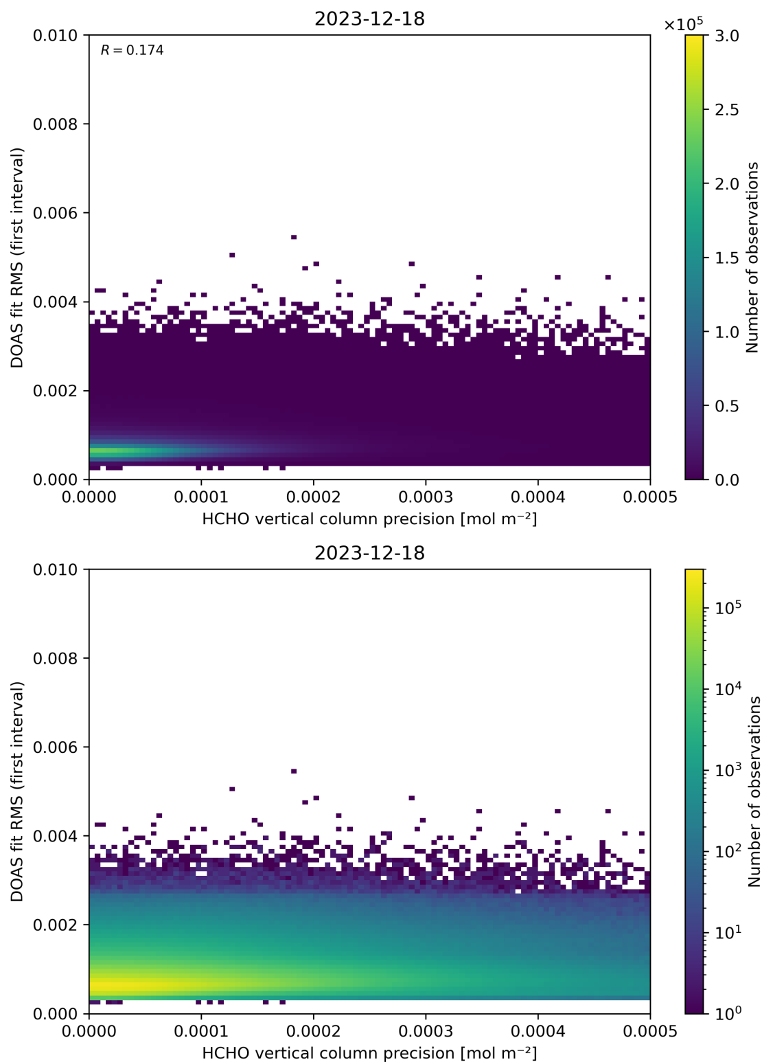
Figure 136: Scatter density plot of “HCHO vertical column precision” against “DOAS fit RMS (first interval)” for 2023-12-17 to 2023-12-19.
