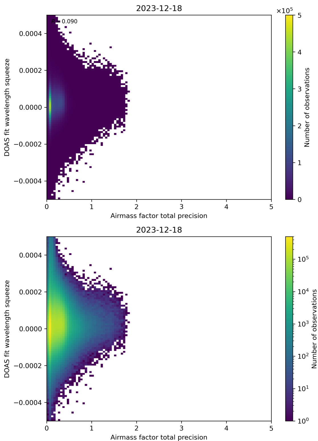
Figure 107: Scatter density plot of “Airmass factor total precision” against “DOAS fit wavelength squeeze” for 2023-12-17 to 2023-12-19.
