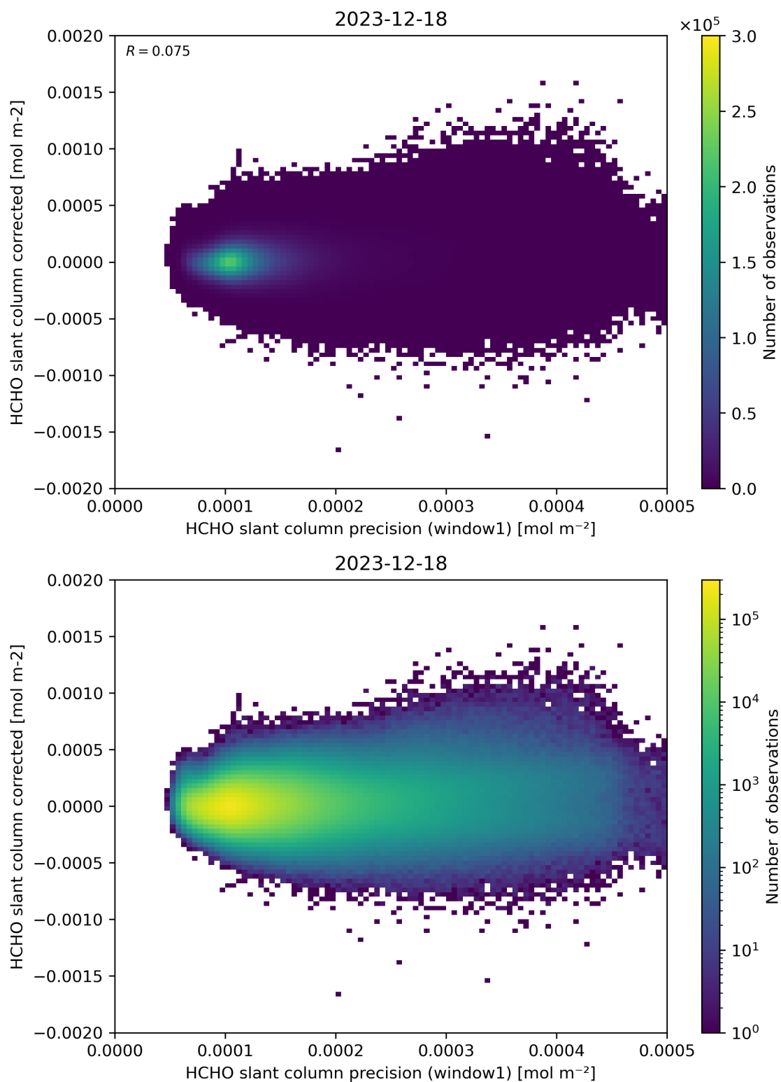
Figure 92: Scatter density plot of “HCHO slant column precision (window1)” against “HCHO slant column corrected” for 2023-12-17 to 2023-12-19.
