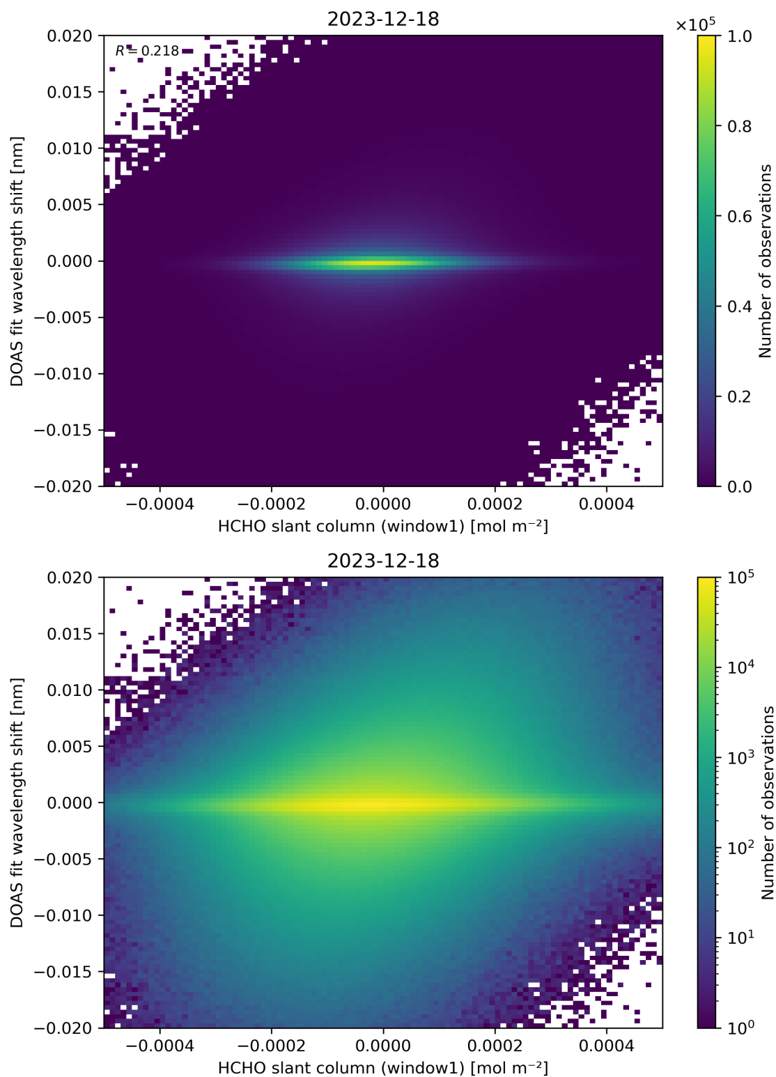
Figure 79: Scatter density plot of “HCHO slant column (window1)” against “DOAS fit wavelength shift” for 2023-12-17 to 2023-12-19.
