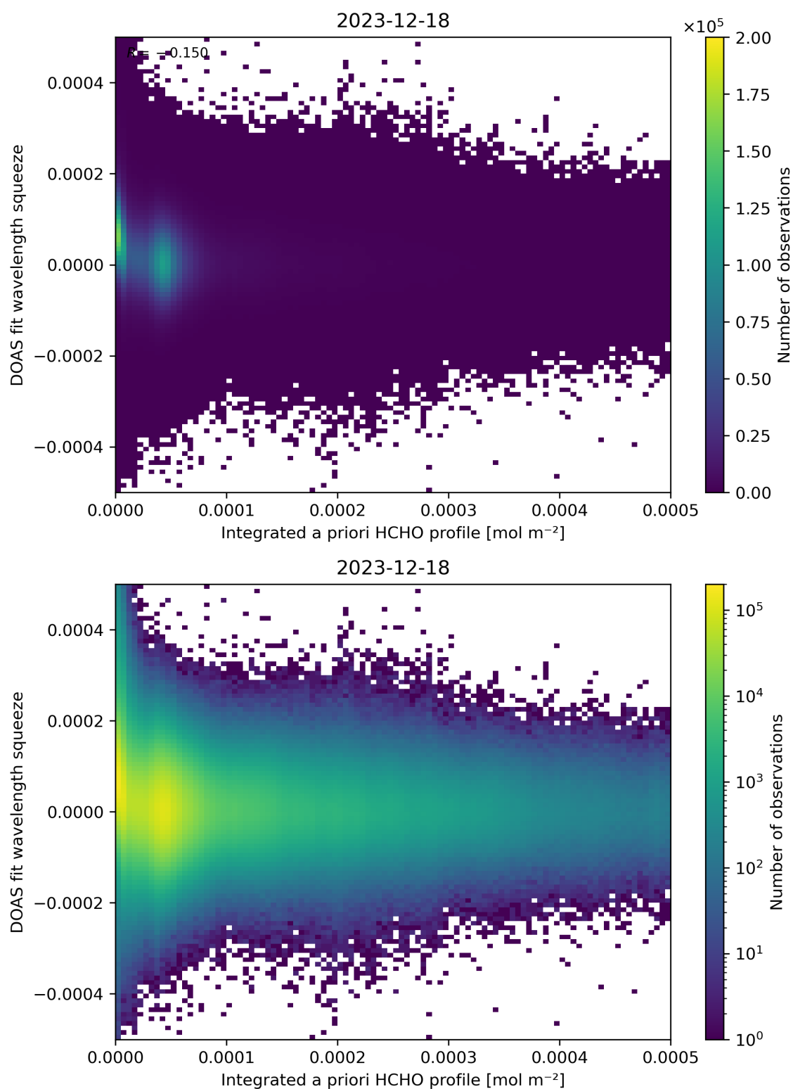
Figure 150: Scatter density plot of “Integrated a priori HCHO profile” against “DOAS fit wavelength squeeze” for 2023-12-17 to 2023-12-19.
