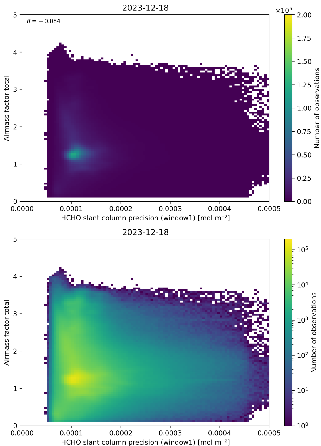
Figure 94: Scatter density plot of “HCHO slant column precision (window1)” against “Airmass factor total” for 2023-12-17 to 2023-12-19.
