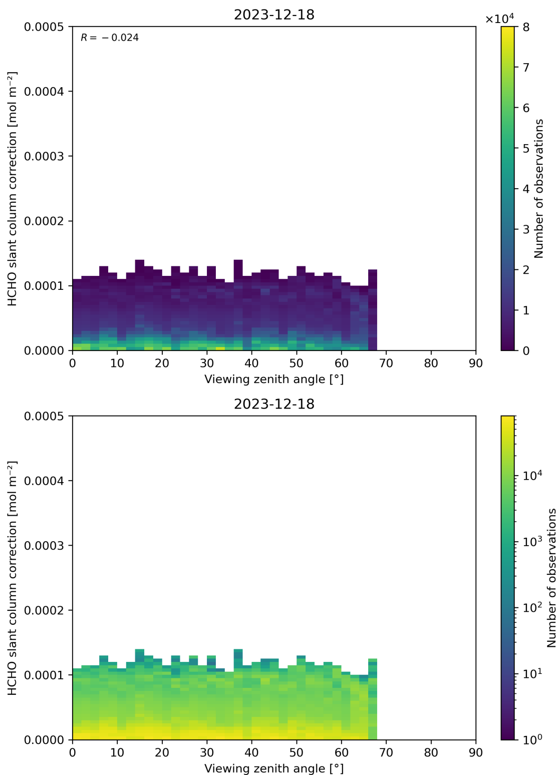
Figure 187: Scatter density plot of “Viewing zenith angle” against “HCHO slant column correction” for 2023-12-17 to 2023-12-19.
