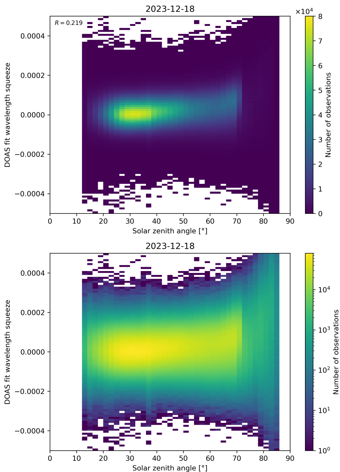
Figure 169: Scatter density plot of “Solar zenith angle” against “DOAS fit wavelength squeeze” for 2023-12-17 to 2023-12-19.
