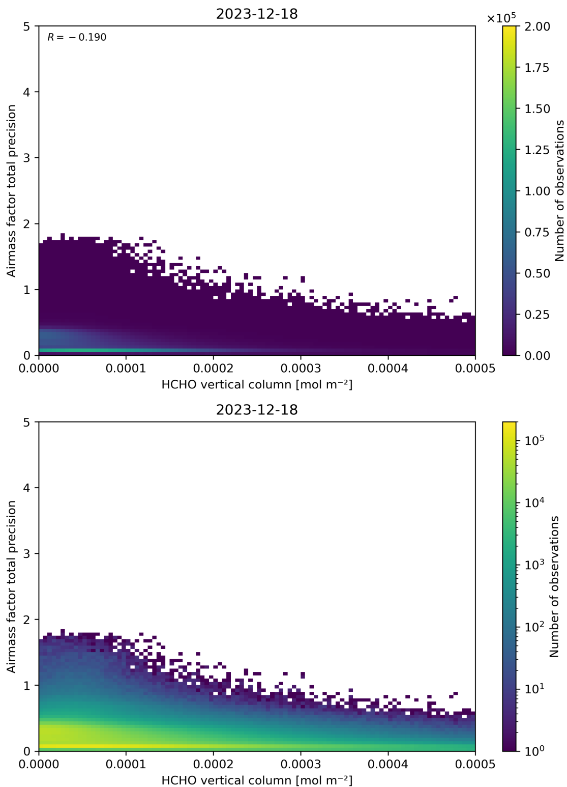
Figure 132: Scatter density plot of “HCHO vertical column” against “Airmass factor total precision” for 2023-12-17 to 2023-12-19.
