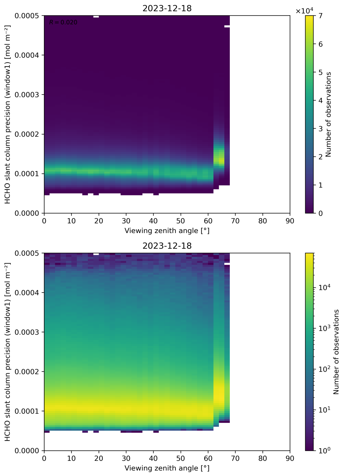
Figure 189: Scatter density plot of “Viewing zenith angle” against “HCHO slant column precision (window1)” for 2023-12-17 to 2023-12-19.
