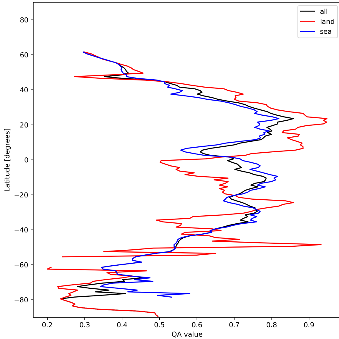
Figure 20: Zonal average of “QA value” for 2023-12-17 to 2023-12-19.
