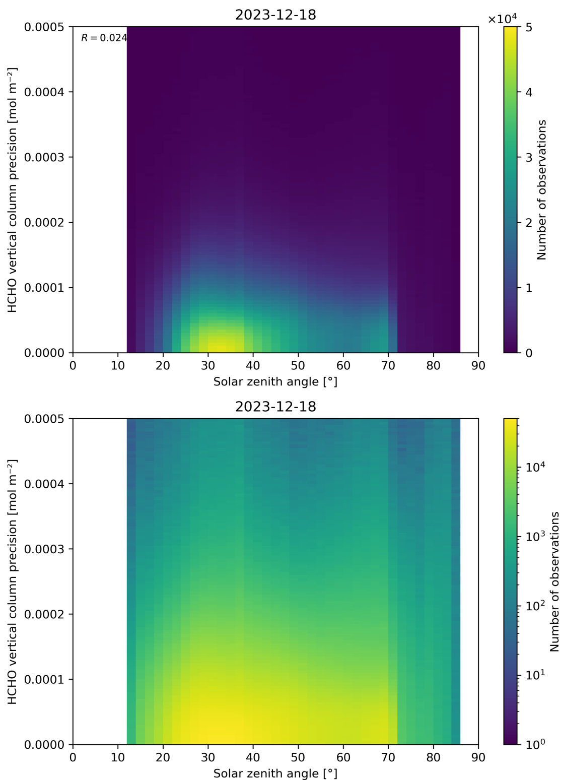
Figure 179: Scatter density plot of “Solar zenith angle” against “HCHO vertical column precision” for 2023-12-17 to 2023-12-19.
