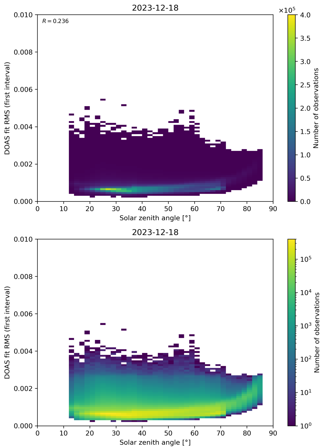
Figure 167: Scatter density plot of “Solar zenith angle” against “DOAS fit RMS (first interval)” for 2023-12-17 to 2023-12-19.
