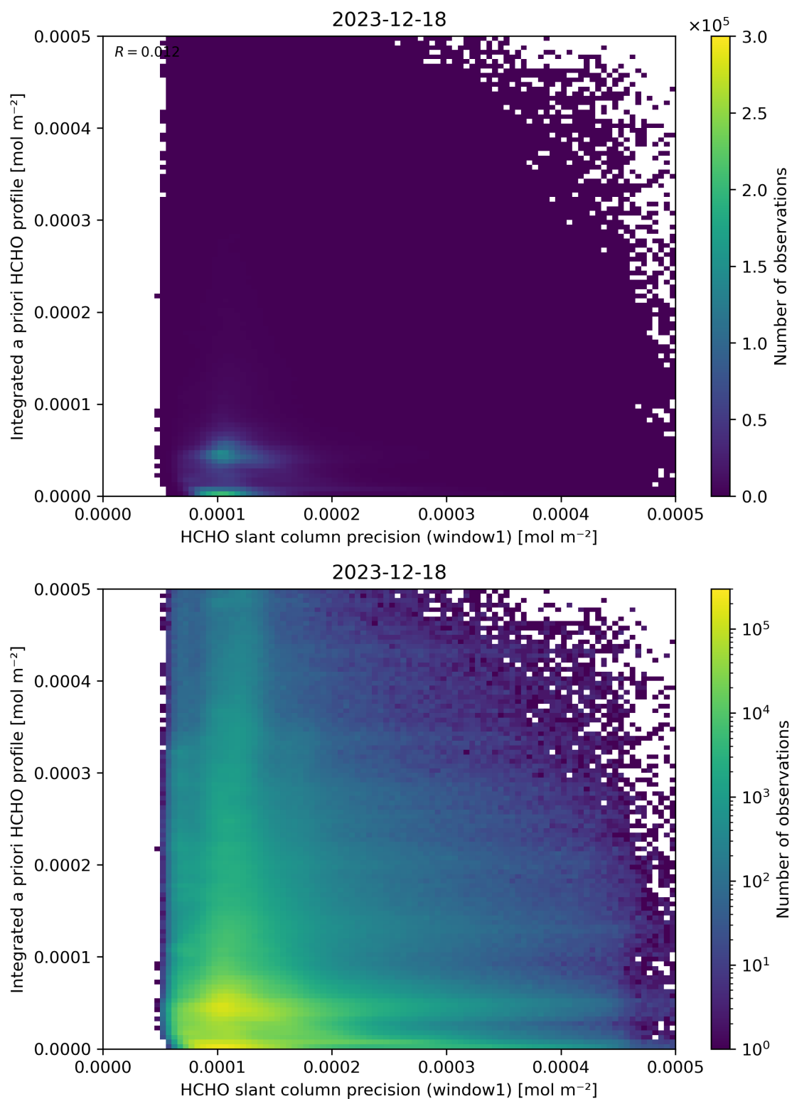
Figure 96: Scatter density plot of “HCHO slant column precision (window1)” against “Integrated a priori HCHO profile” for 2023-12-17 to 2023-12-19.
