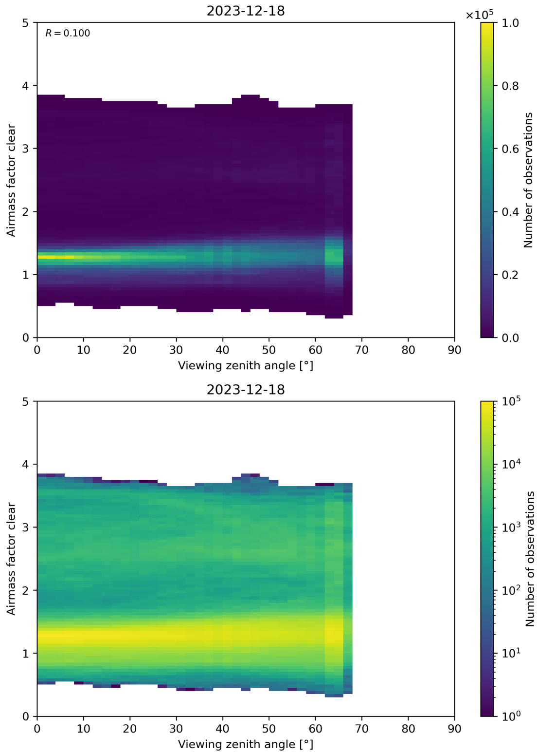
Figure 185: Scatter density plot of “Viewing zenith angle” against “Airmass factor clear” for 2023-12-17 to 2023-12-19.
