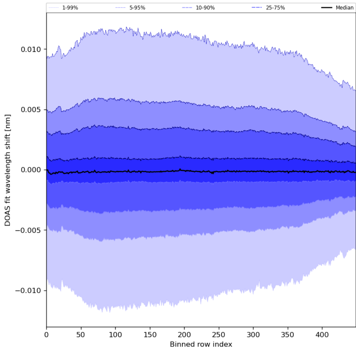
Figure 58: Along track statistics of “DOAS fit wavelength shift” for 2023-12-17 to 2023-12-19
