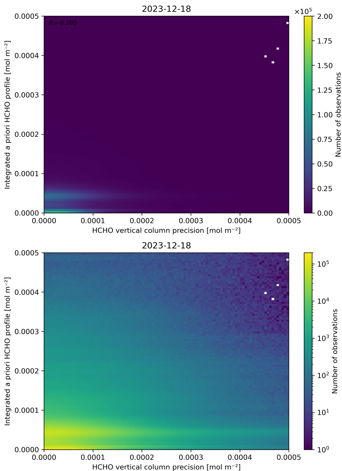
Figure 147: Scatter density plot of “HCHO vertical column precision” against “Integrated a priori HCHO profile” for 2023-12-17 to 2023-12-19.
