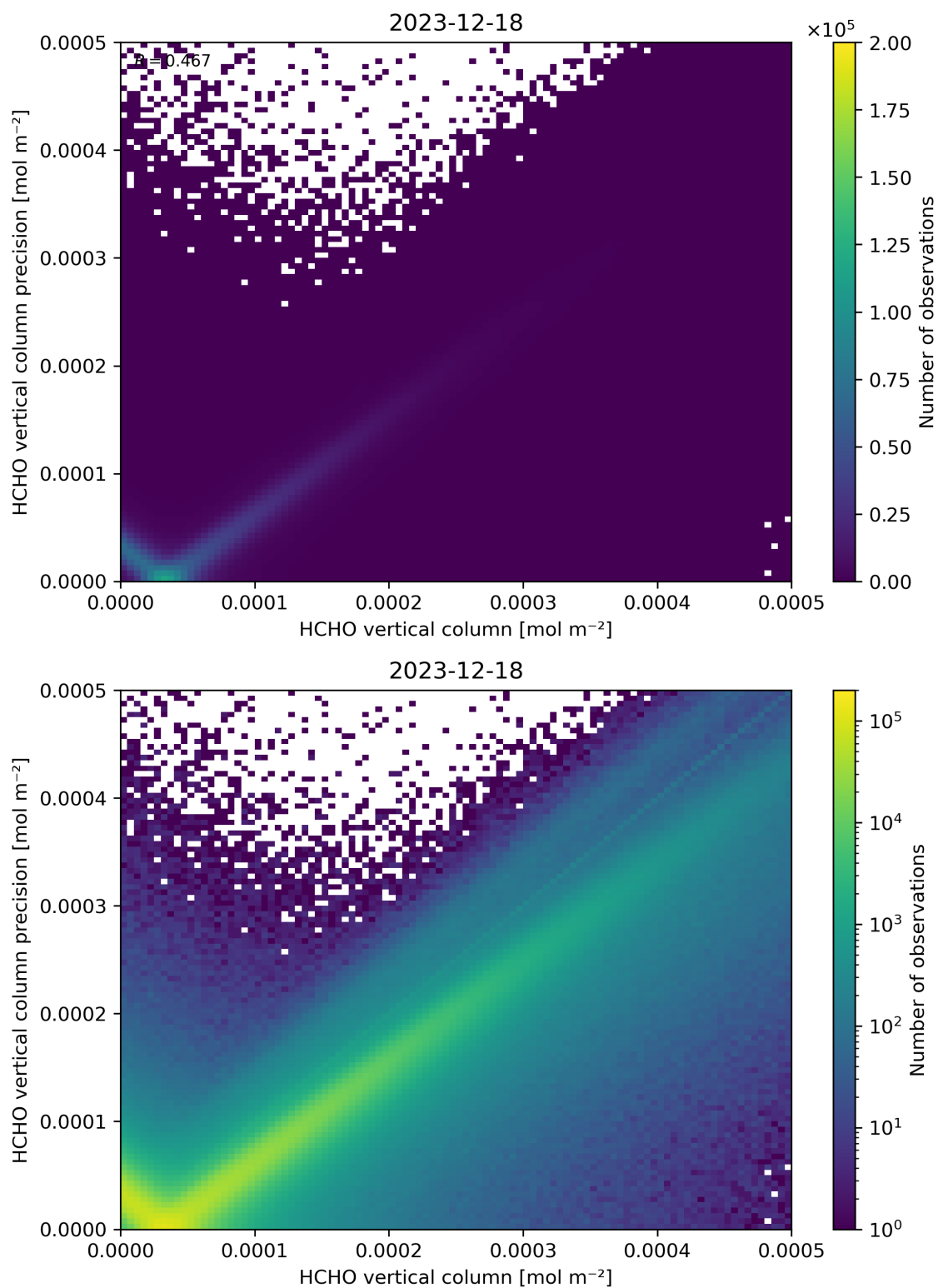
Figure 134: Scatter density plot of “HCHO vertical column” against “HCHO vertical column precision” for 2023-12-17 to 2023-12-19.
