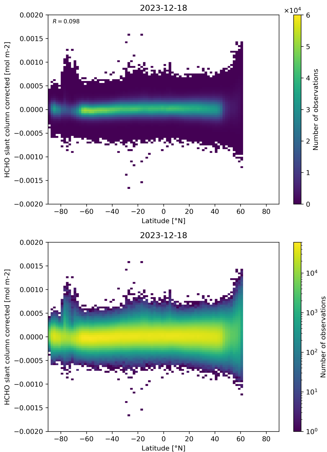
Figure 157: Scatter density plot of “Latitude” against “HCHO slant column corrected” for 2023-12-17 to 2023-12-19.
