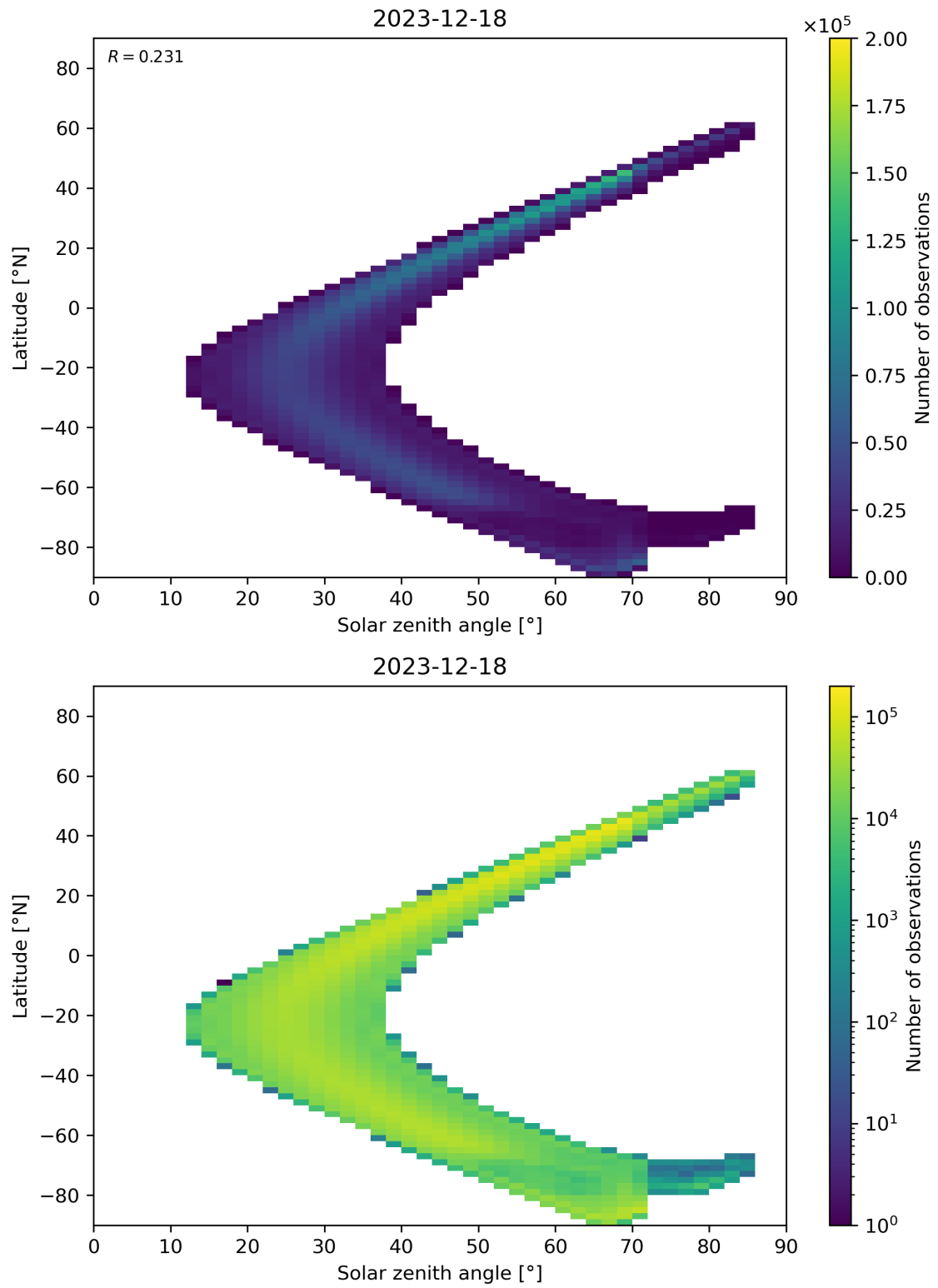
Figure 181: Scatter density plot of “Solar zenith angle” against “Latitude” for 2023-12-17 to 2023-12-19.
