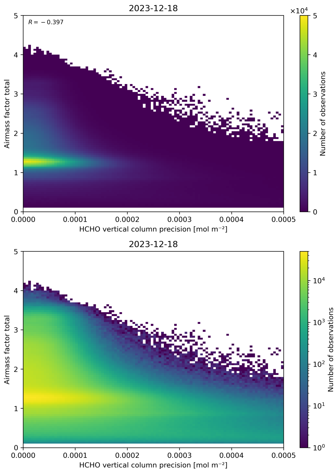
Figure 144: Scatter density plot of “HCHO vertical column precision” against “Airmass factor total” for 2023-12-17 to 2023-12-19.
