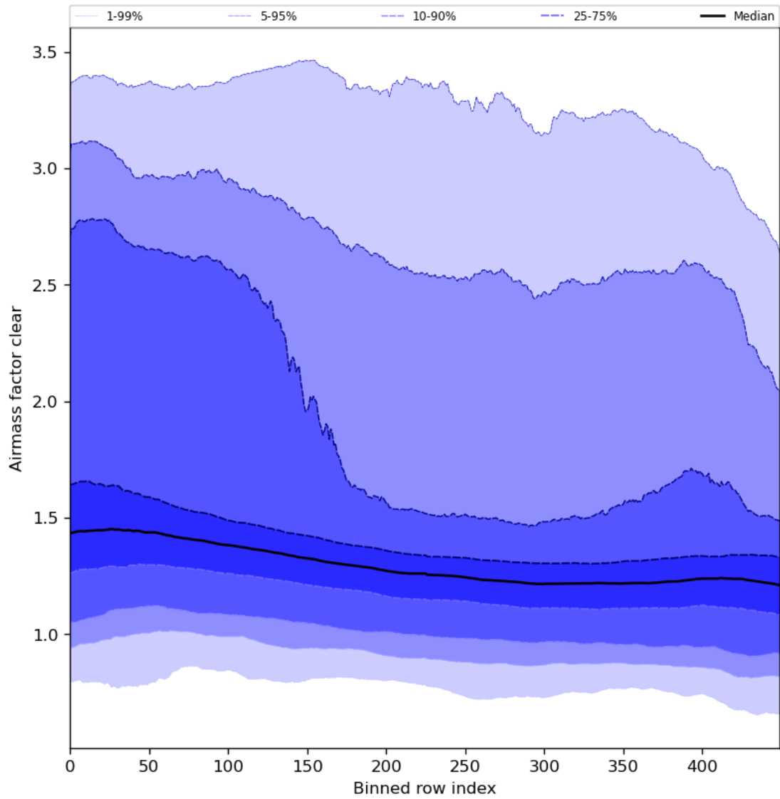
Figure 56: Along track statistics of “Airmass factor clear” for 2023-12-17 to 2023-12-19
