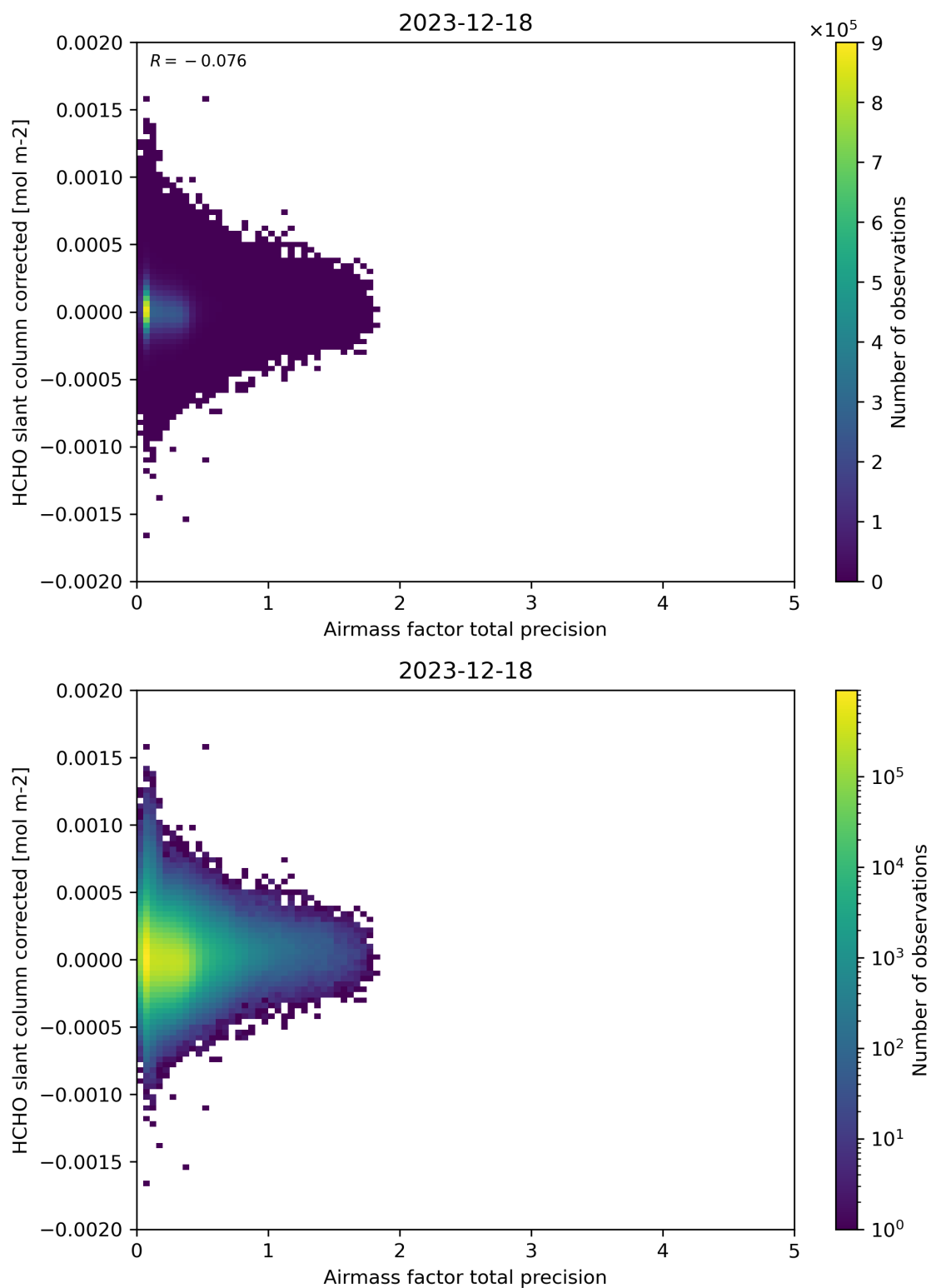
Figure 109: Scatter density plot of “Airmass factor total precision” against “HCHO slant column corrected” for 2023-12-17 to 2023-12-19.
