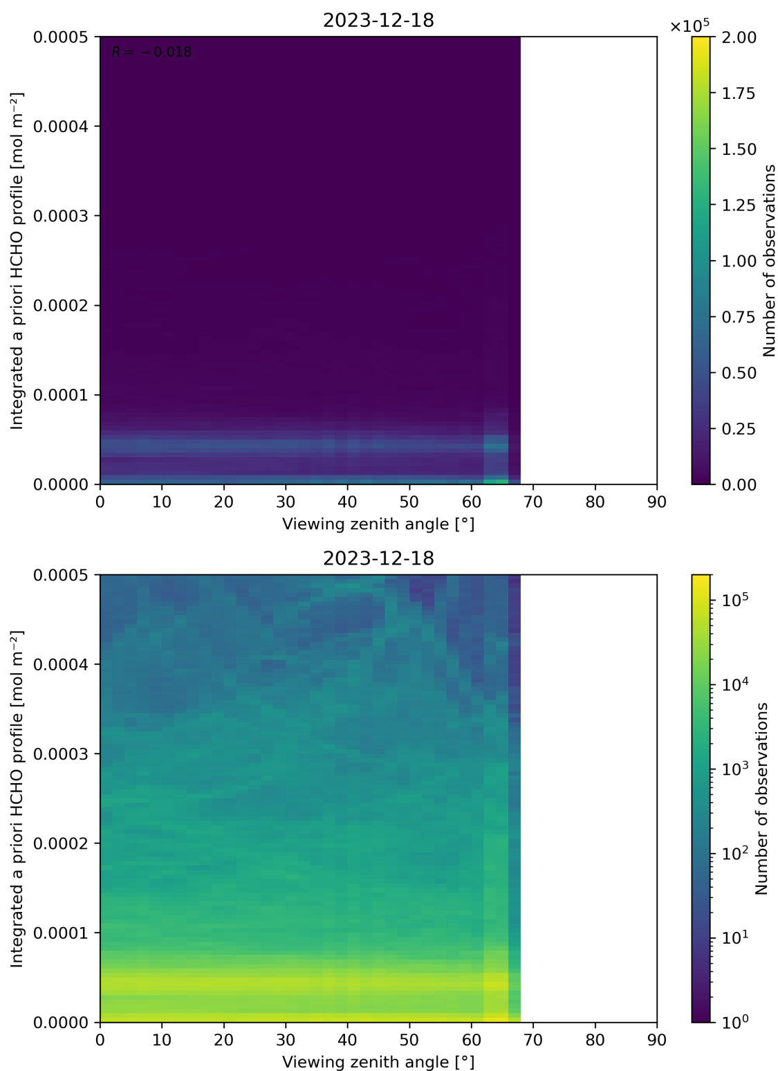
Figure 195: Scatter density plot of “Viewing zenith angle” against “Integrated a priori HCHO profile” for 2023-12-17 to 2023-12-19.
