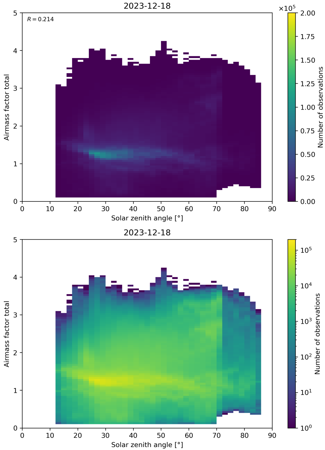
Figure 175: Scatter density plot of “Solar zenith angle” against “Airmass factor total” for 2023-12-17 to 2023-12-19.
