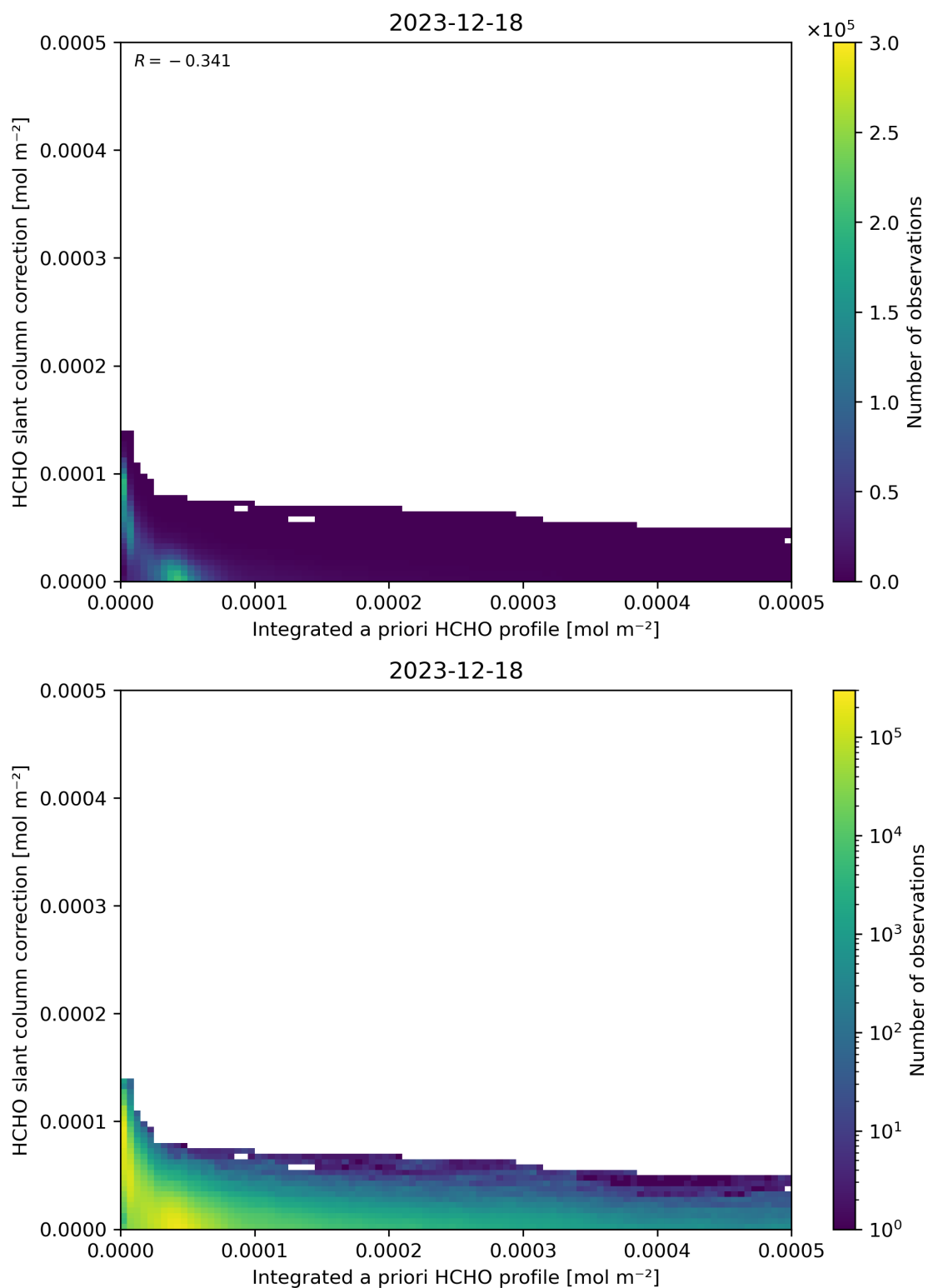
Figure 152: Scatter density plot of “Integrated a priori HCHO profile” against “HCHO slant column correction” for 2023-12-17 to 2023-12-19.
