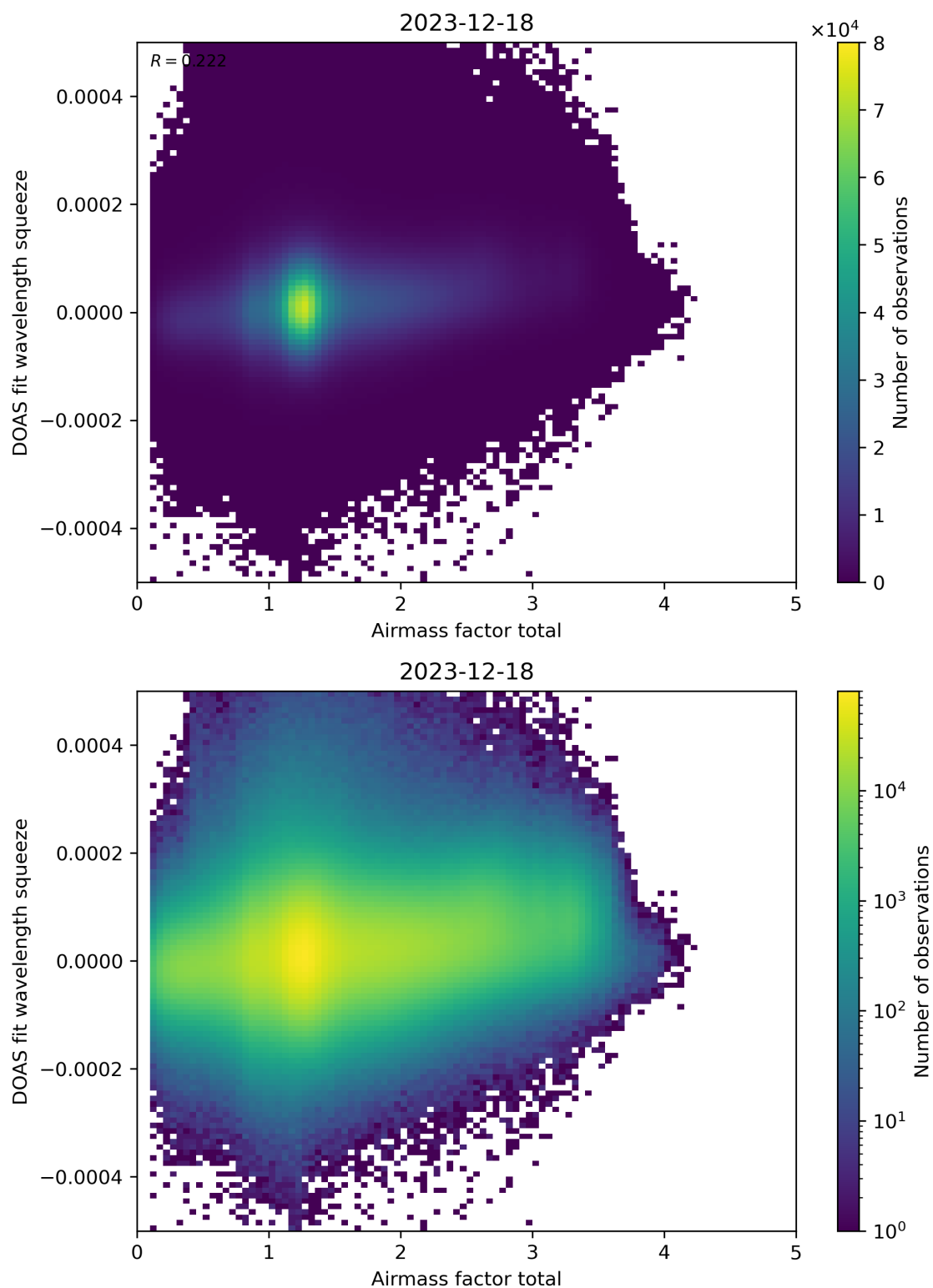
Figure 99: Scatter density plot of “Airmass factor total” against “DOAS fit wavelength squeeze” for 2023-12-17 to 2023-12-19.
