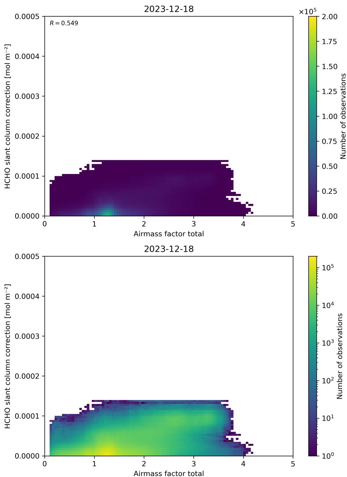
Figure 102: Scatter density plot of “Airmass factor total” against “HCHO slant column correction” for 2023-12-17 to 2023-12-19.
