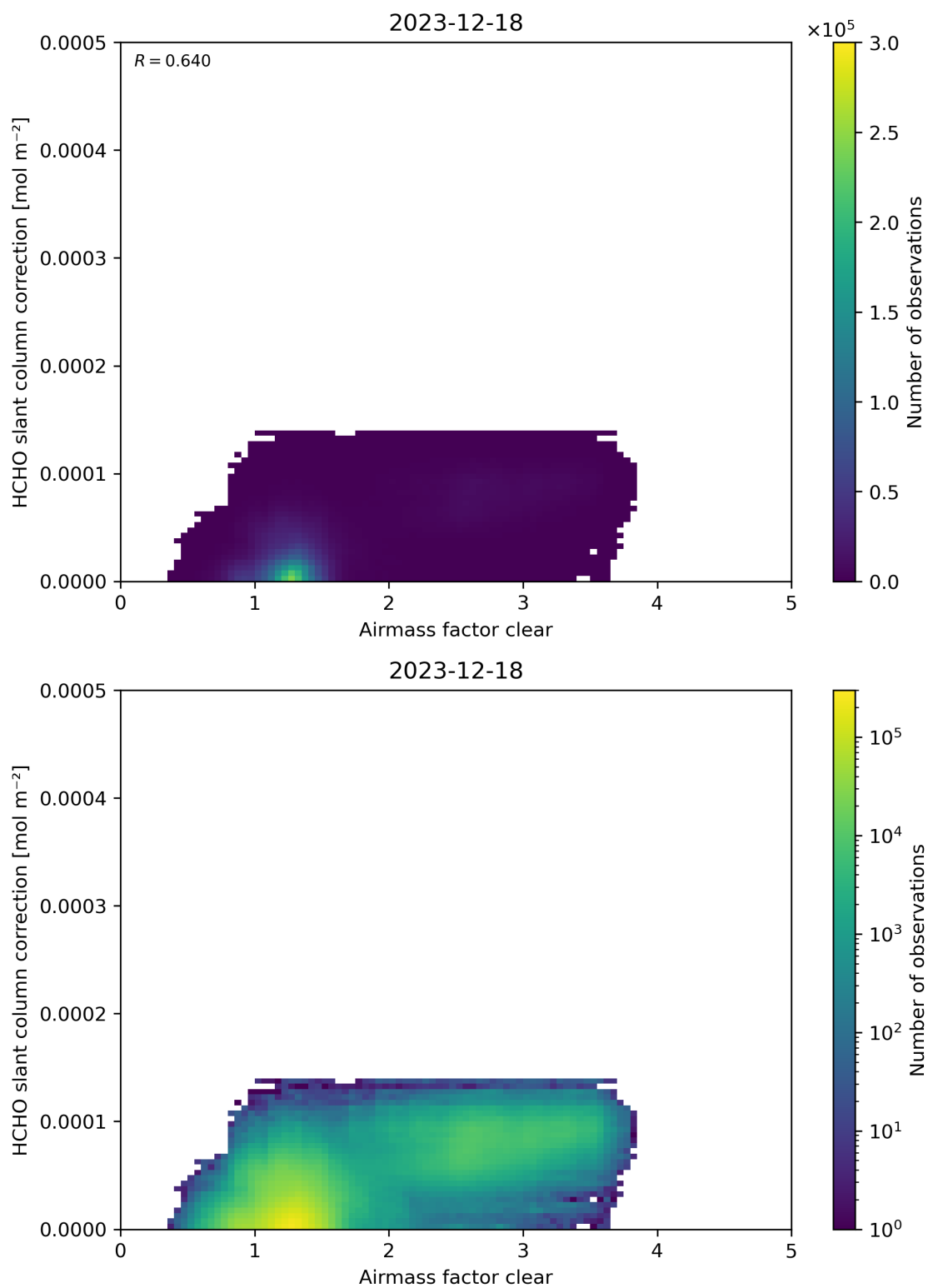
Figure 75: Scatter density plot of “Airmass factor clear” against “HCHO slant column correction” for 2023-12-17 to 2023-12-19.
