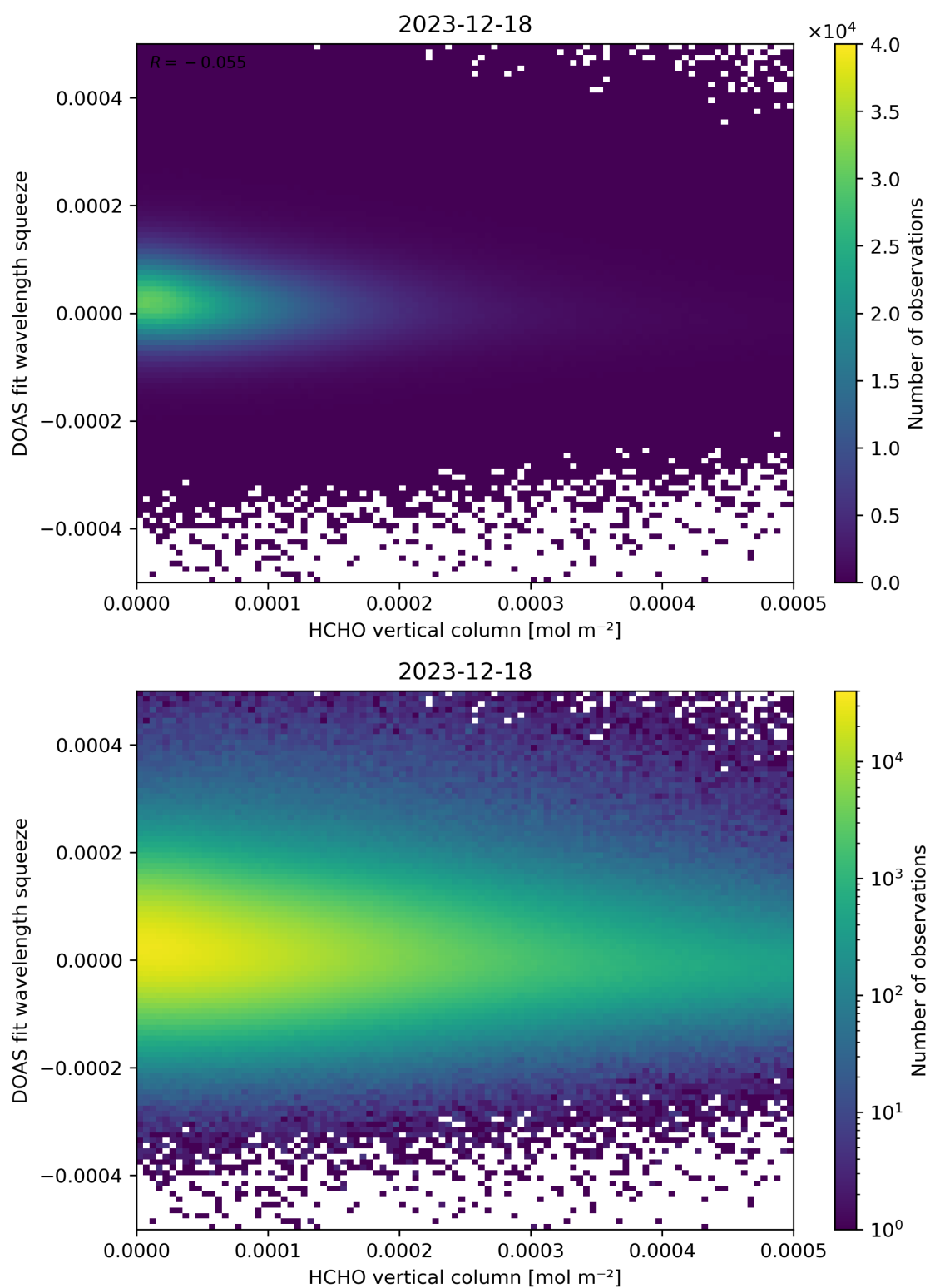
Figure 125: Scatter density plot of “HCHO vertical column” against “DOAS fit wavelength squeeze” for 2023-12-17 to 2023-12-19.
