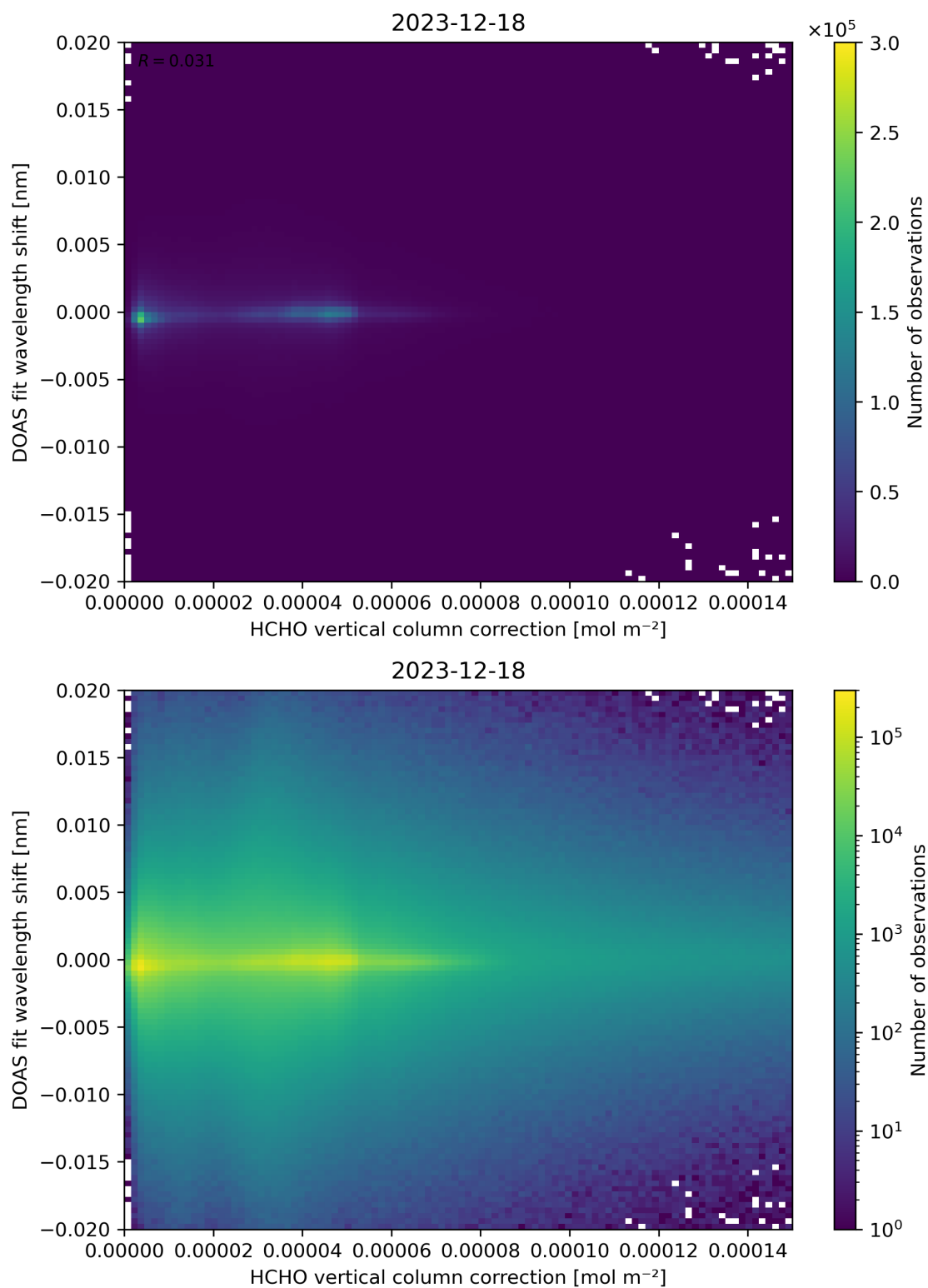
Figure 113: Scatter density plot of “HCHO vertical column correction” against “DOAS fit wavelength shift” for 2023-12-17 to 2023-12-19.
