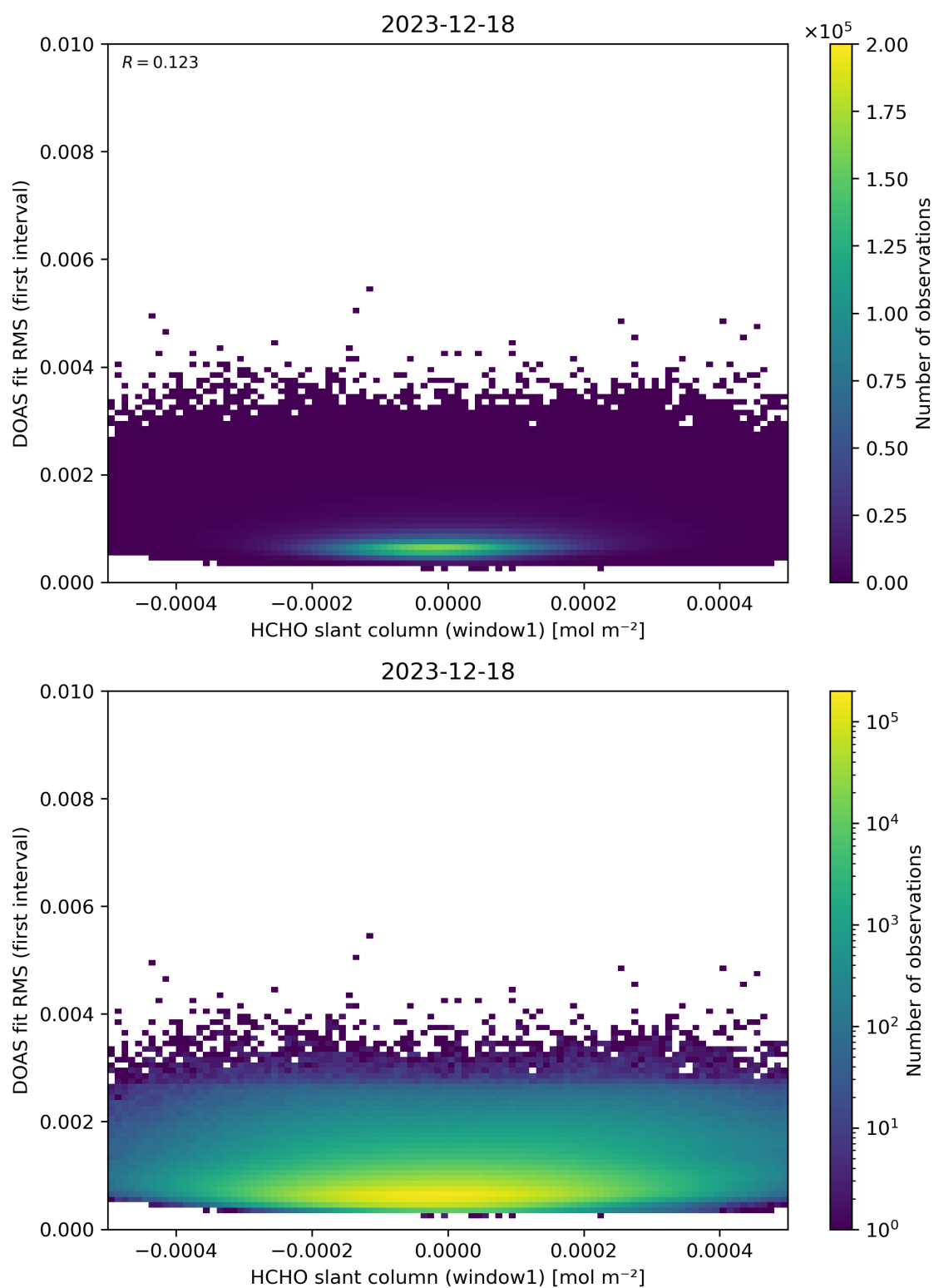
Figure 78: Scatter density plot of “HCHO slant column (window1)” against “DOAS fit RMS (first interval)” for 2023-12-17 to 2023-12-19.
