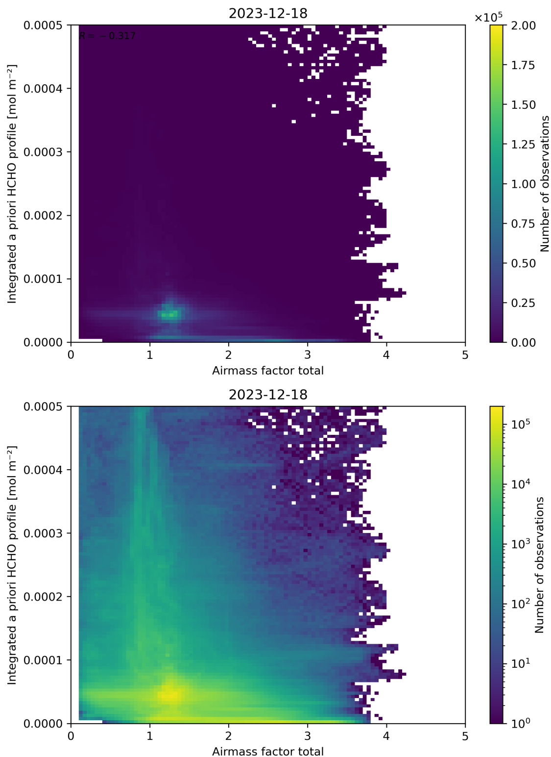
Figure 104: Scatter density plot of “Airmass factor total” against “Integrated a priori HCHO profile” for 2023-12-17 to 2023-12-19.
