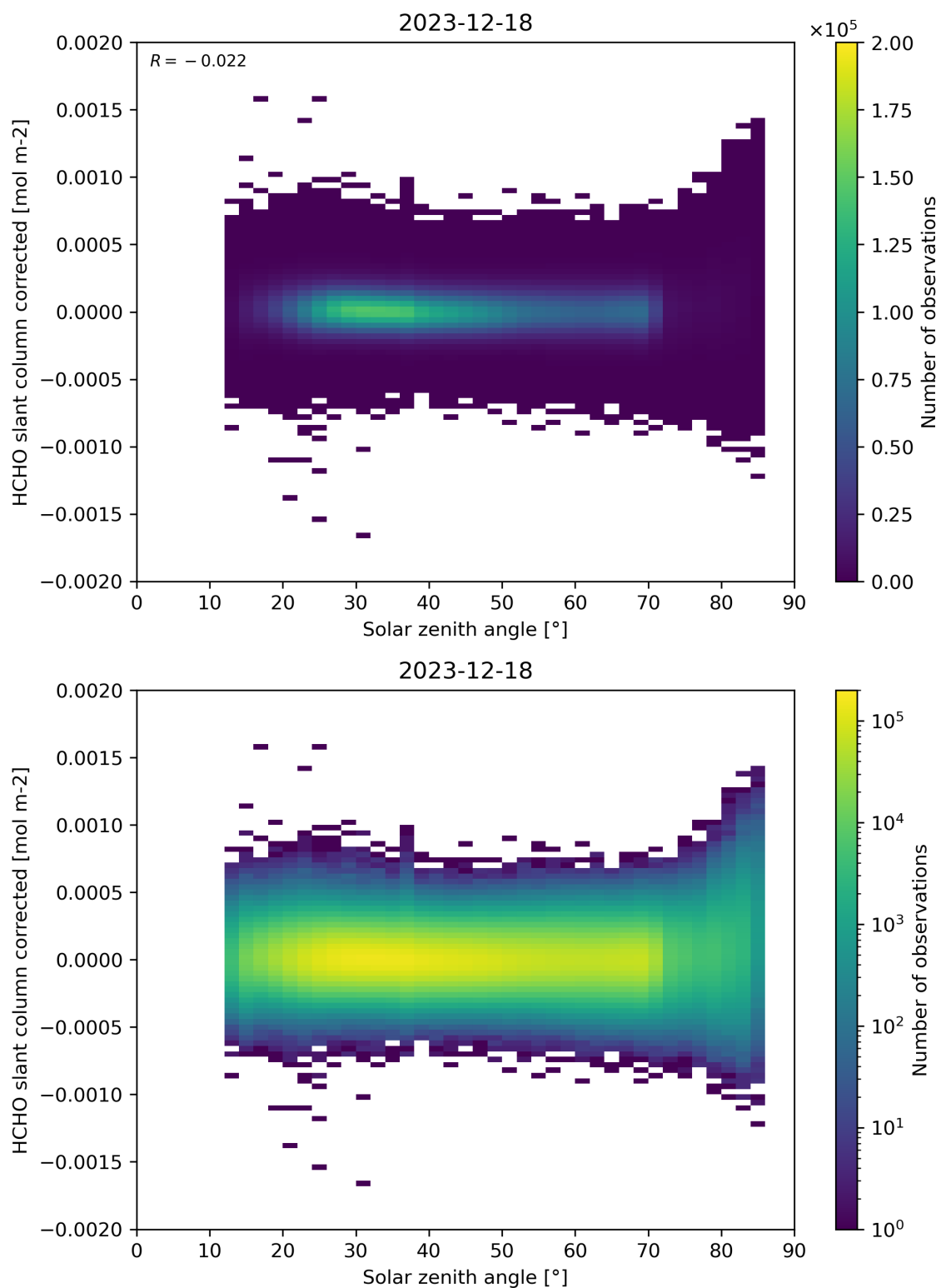
Figure 171: Scatter density plot of “Solar zenith angle” against “HCHO slant column corrected” for 2023-12-17 to 2023-12-19.
