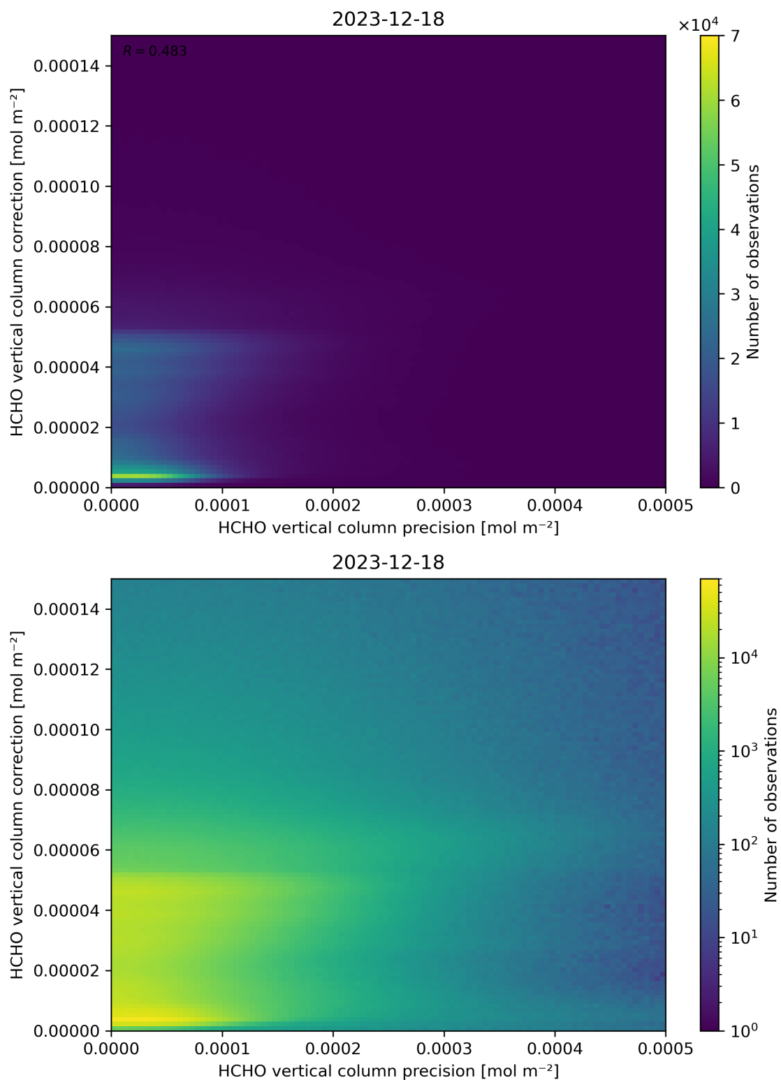
Figure 146: Scatter density plot of “HCHO vertical column precision” against “HCHO vertical column correction” for 2023-12-17 to 2023-12-19.
