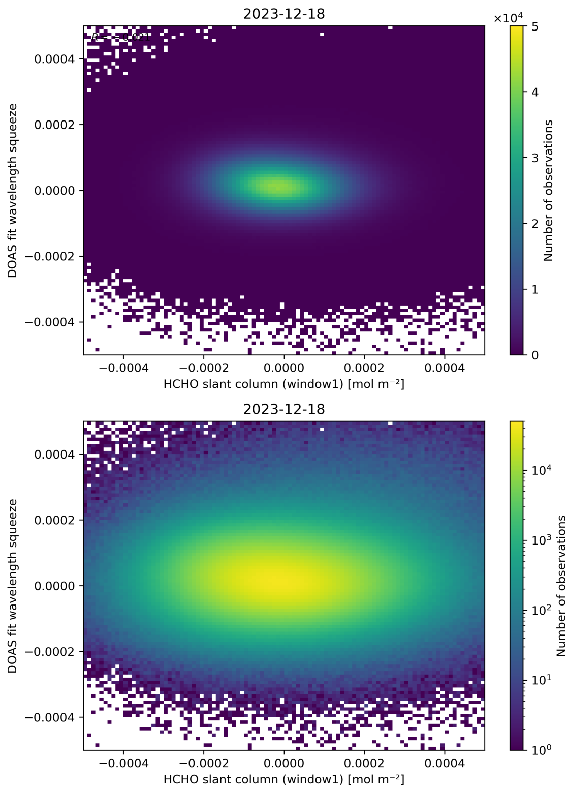
Figure 80: Scatter density plot of “HCHO slant column (window1)” against “DOAS fit wavelength squeeze” for 2023-12-17 to 2023-12-19.
