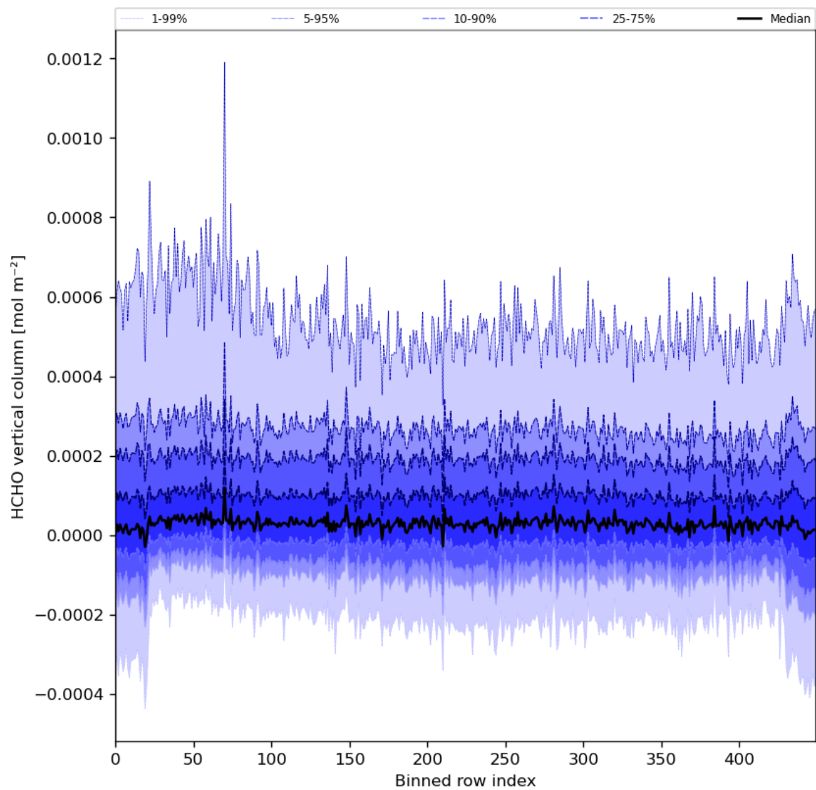
Figure 49: Along track statistics of “HCHO vertical column” for 2023-12-17 to 2023-12-19
