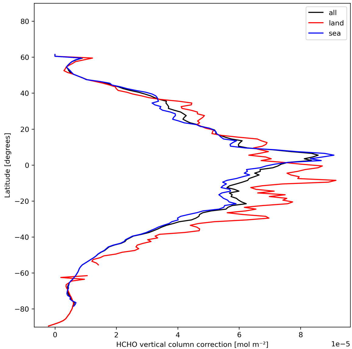
Figure 23: Zonal average of “HCHO vertical column correction” for 2023-12-17 to 2023-12-19.
