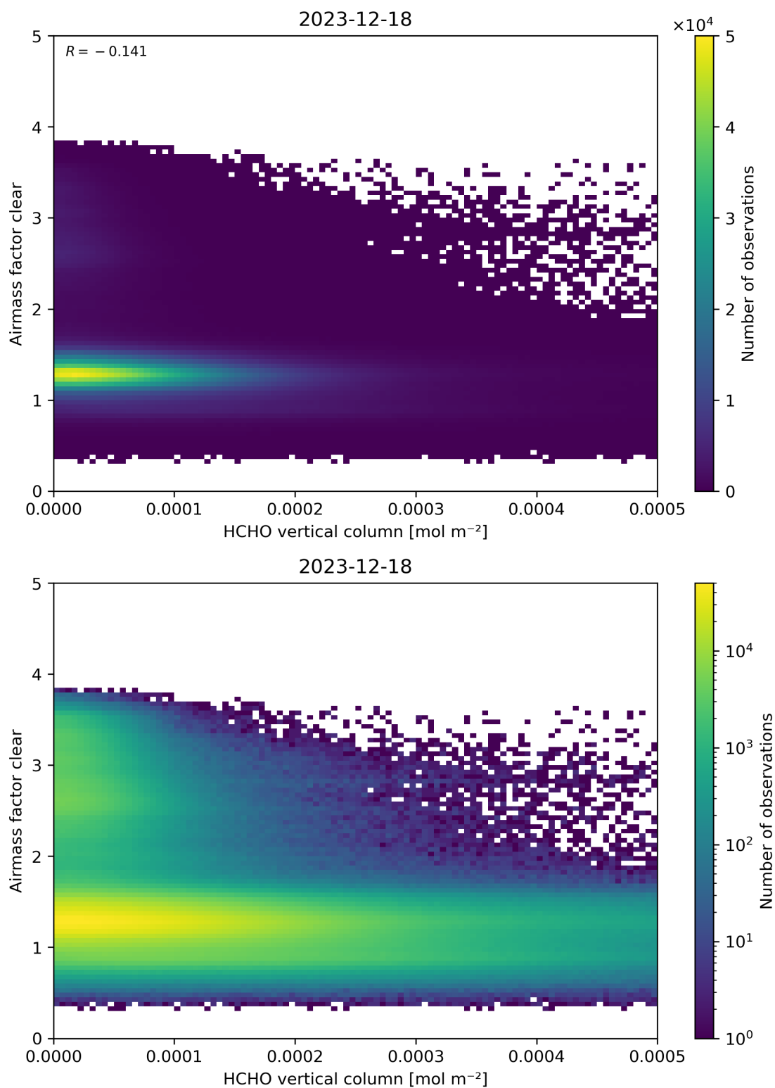
Figure 126: Scatter density plot of “HCHO vertical column” against “Airmass factor clear” for 2023-12-17 to 2023-12-19.
