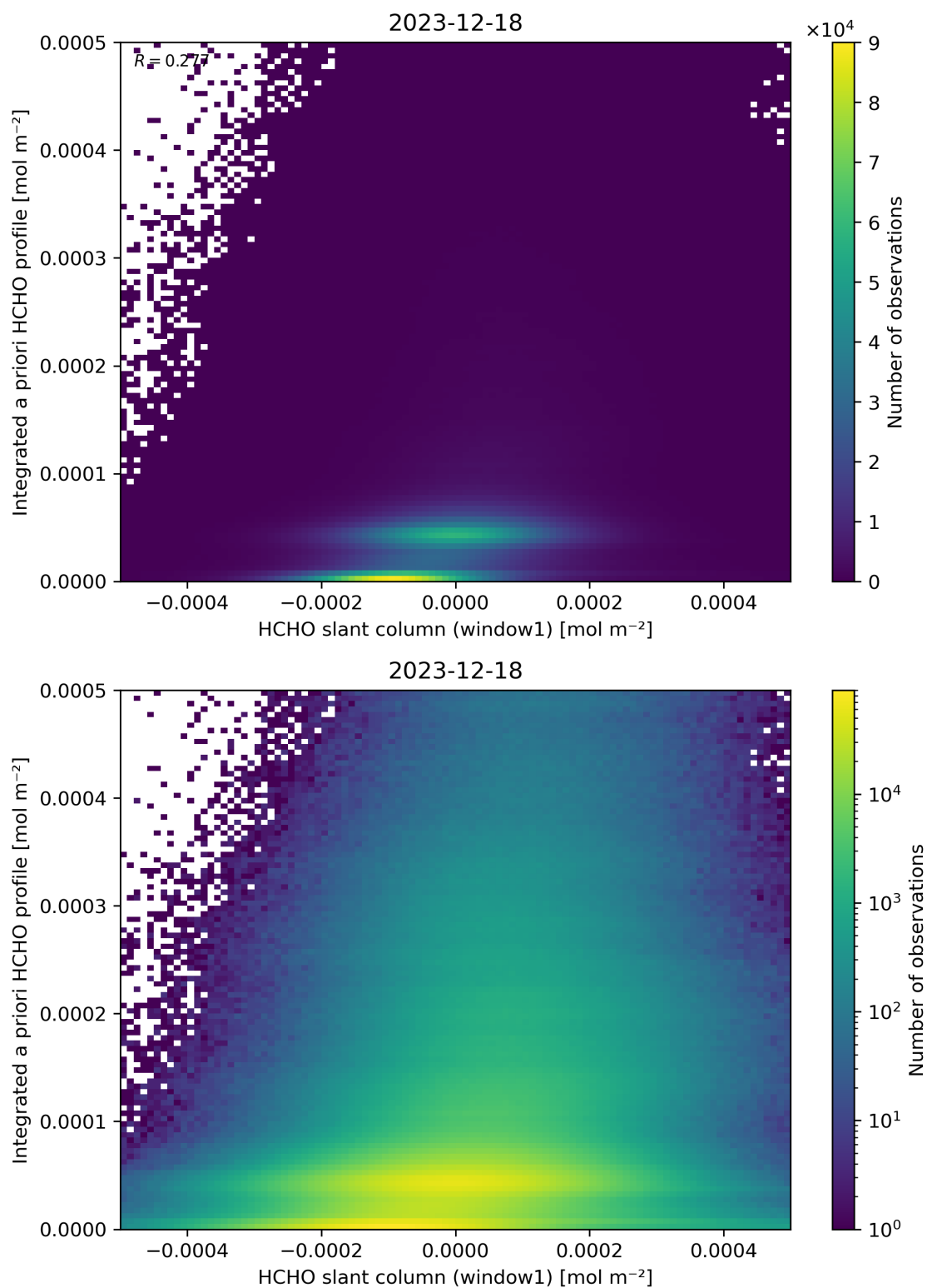
Figure 87: Scatter density plot of “HCHO slant column (window1)” against “Integrated a priori HCHO profile” for 2023-12-17 to 2023-12-19.
