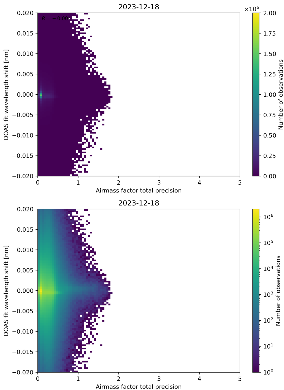
Figure 106: Scatter density plot of “Airmass factor total precision” against “DOAS fit wavelength shift” for 2023-12-17 to 2023-12-19.
