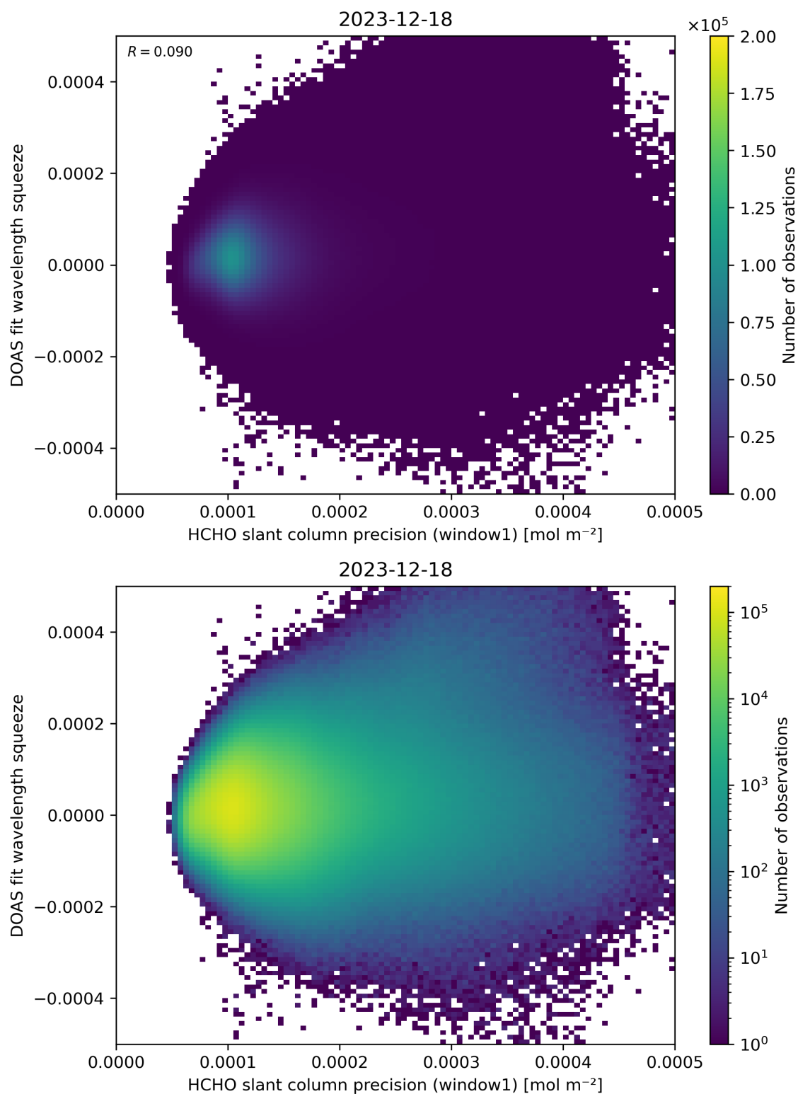
Figure 90: Scatter density plot of “HCHO slant column precision (window1)” against “DOAS fit wavelength squeeze” for 2023-12-17 to 2023-12-19.
