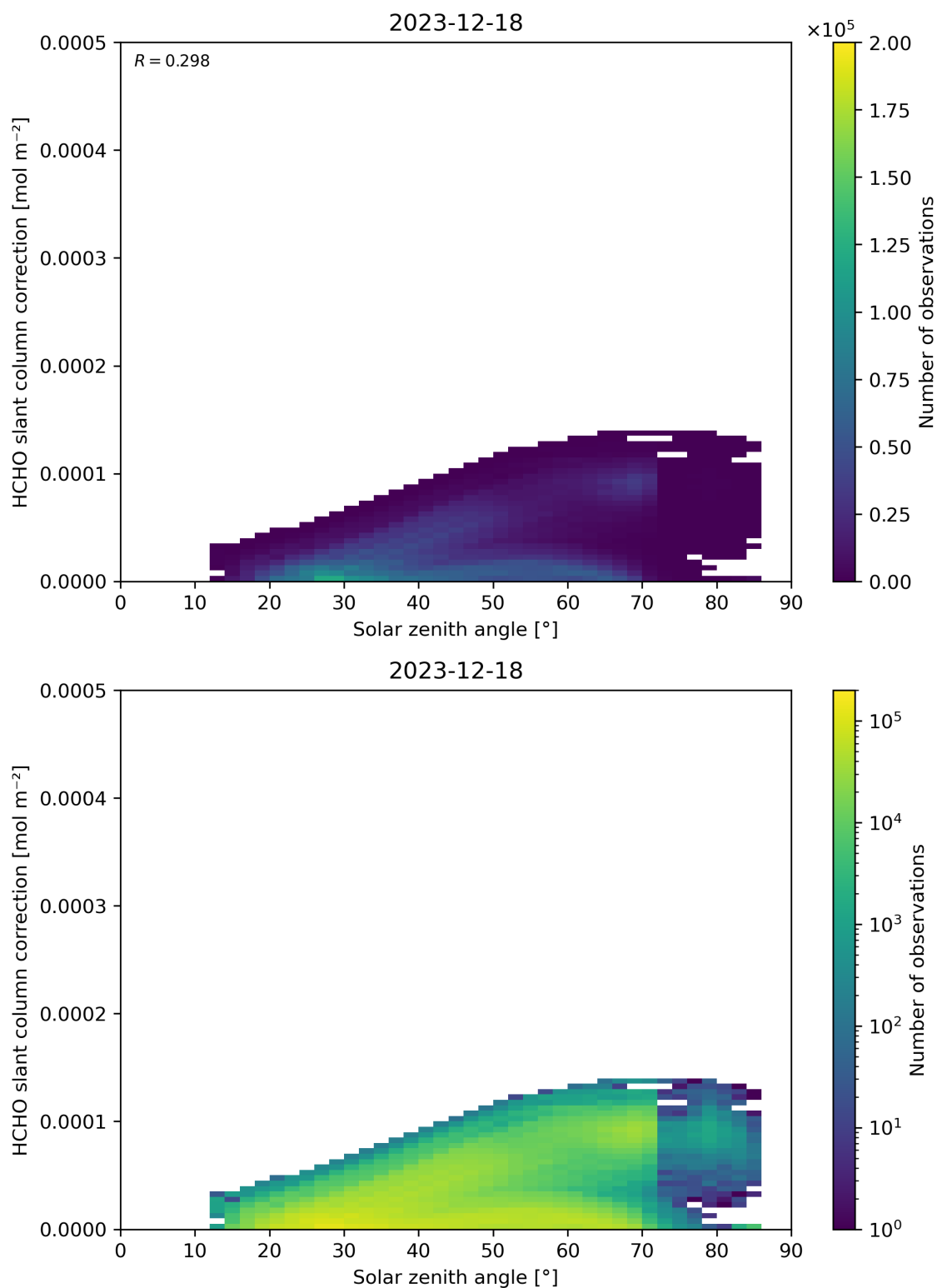
Figure 172: Scatter density plot of “Solar zenith angle” against “HCHO slant column correction” for 2023-12-17 to 2023-12-19.
