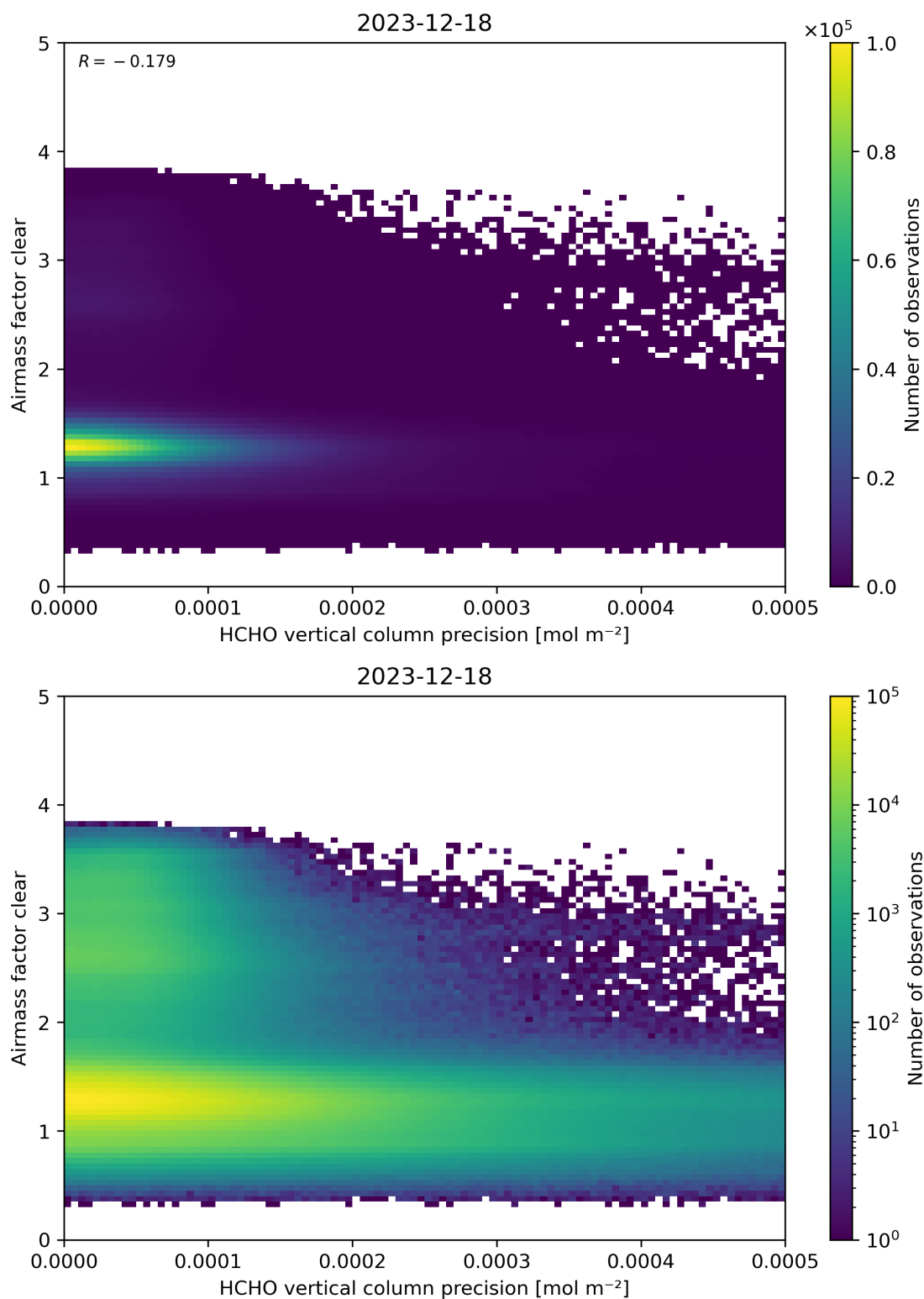
Figure 139: Scatter density plot of “HCHO vertical column precision” against “Airmass factor clear” for 2023-12-17 to 2023-12-19.
