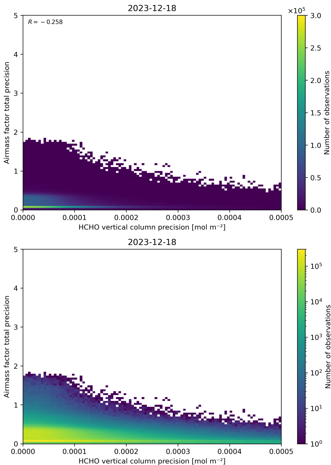
Figure 145: Scatter density plot of “HCHO vertical column precision” against “Airmass factor total precision” for 2023-12-17 to 2023-12-19.
