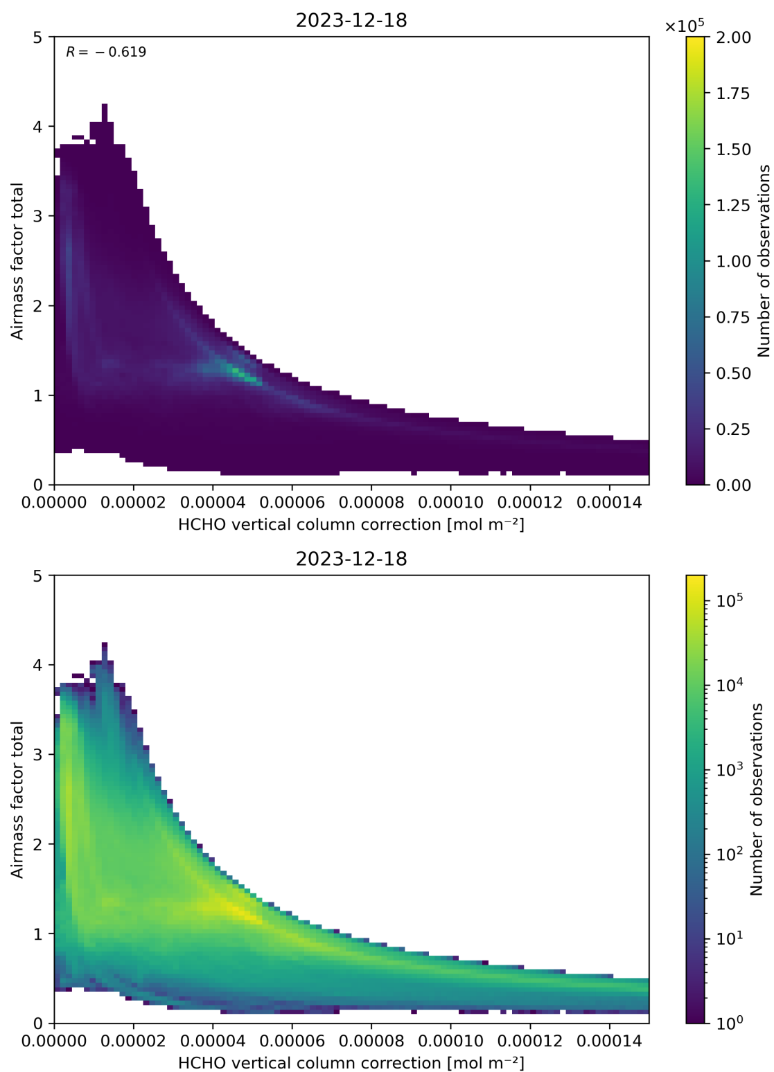
Figure 120: Scatter density plot of “HCHO vertical column correction” against “Airmass factor total” for 2023-12-17 to 2023-12-19.
