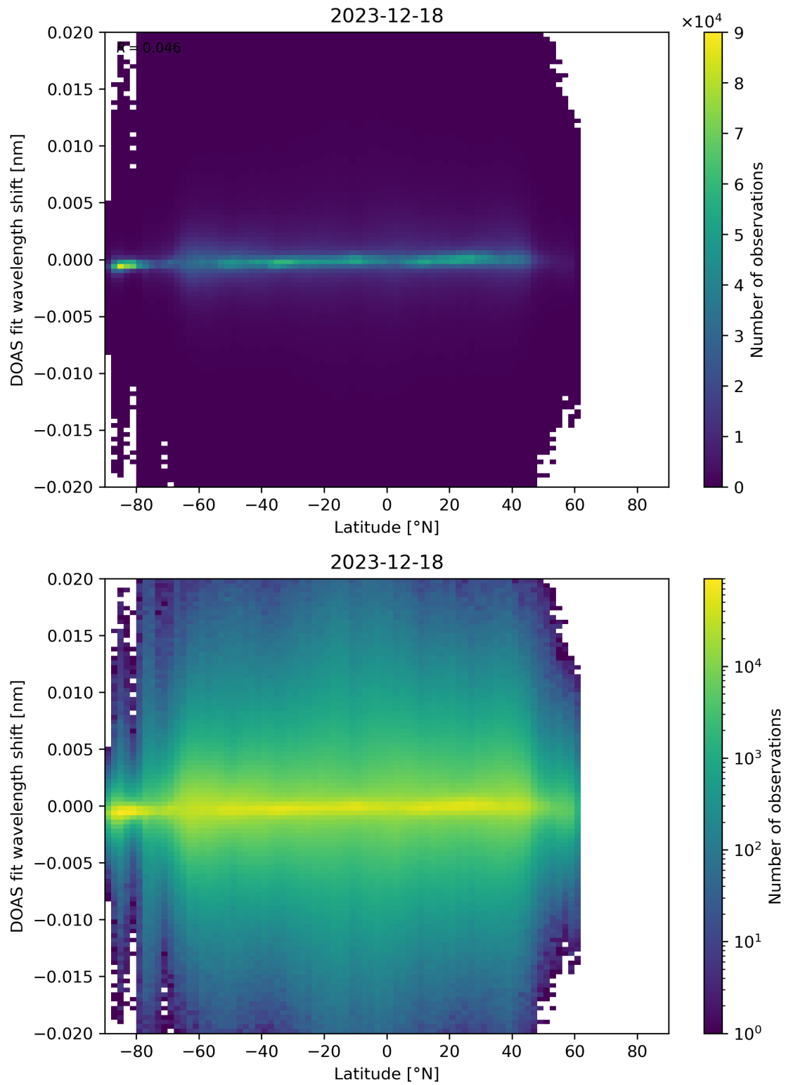
Figure 154: Scatter density plot of “Latitude” against “DOAS fit wavelength shift” for 2023-12-17 to 2023-12-19.
