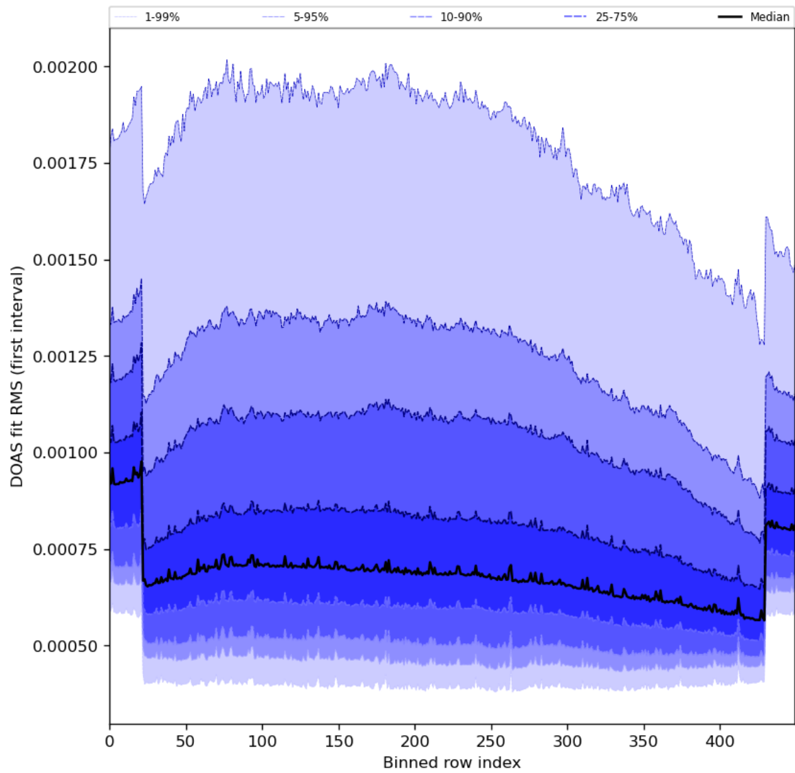
Figure 60: Along track statistics of “DOAS fit RMS (first interval)” for 2023-12-17 to 2023-12-19
