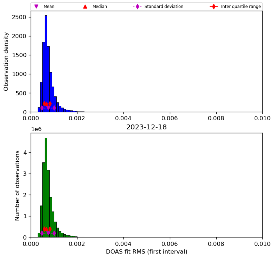
Figure 46: Histogram of “DOAS fit RMS (first interval)” for 2023-12-17 to 2023-12-19
