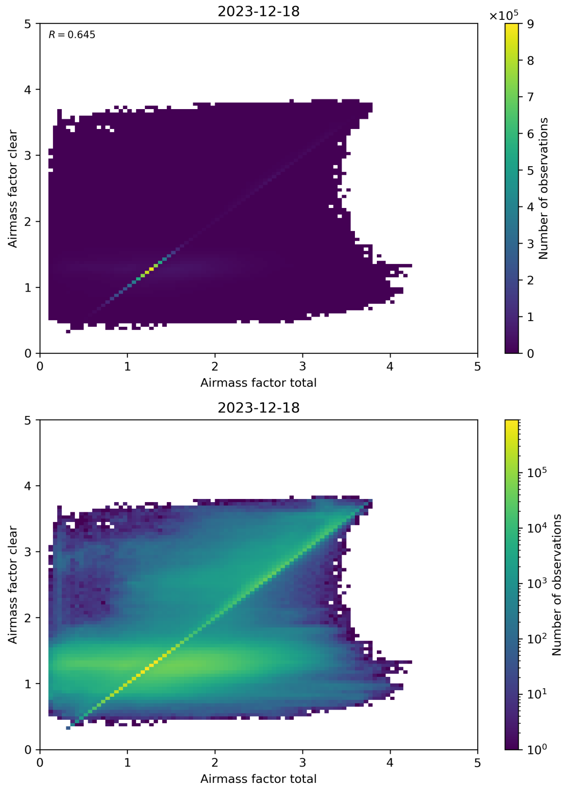
Figure 100: Scatter density plot of “Airmass factor total” against “Airmass factor clear” for 2023-12-17 to 2023-12-19.
