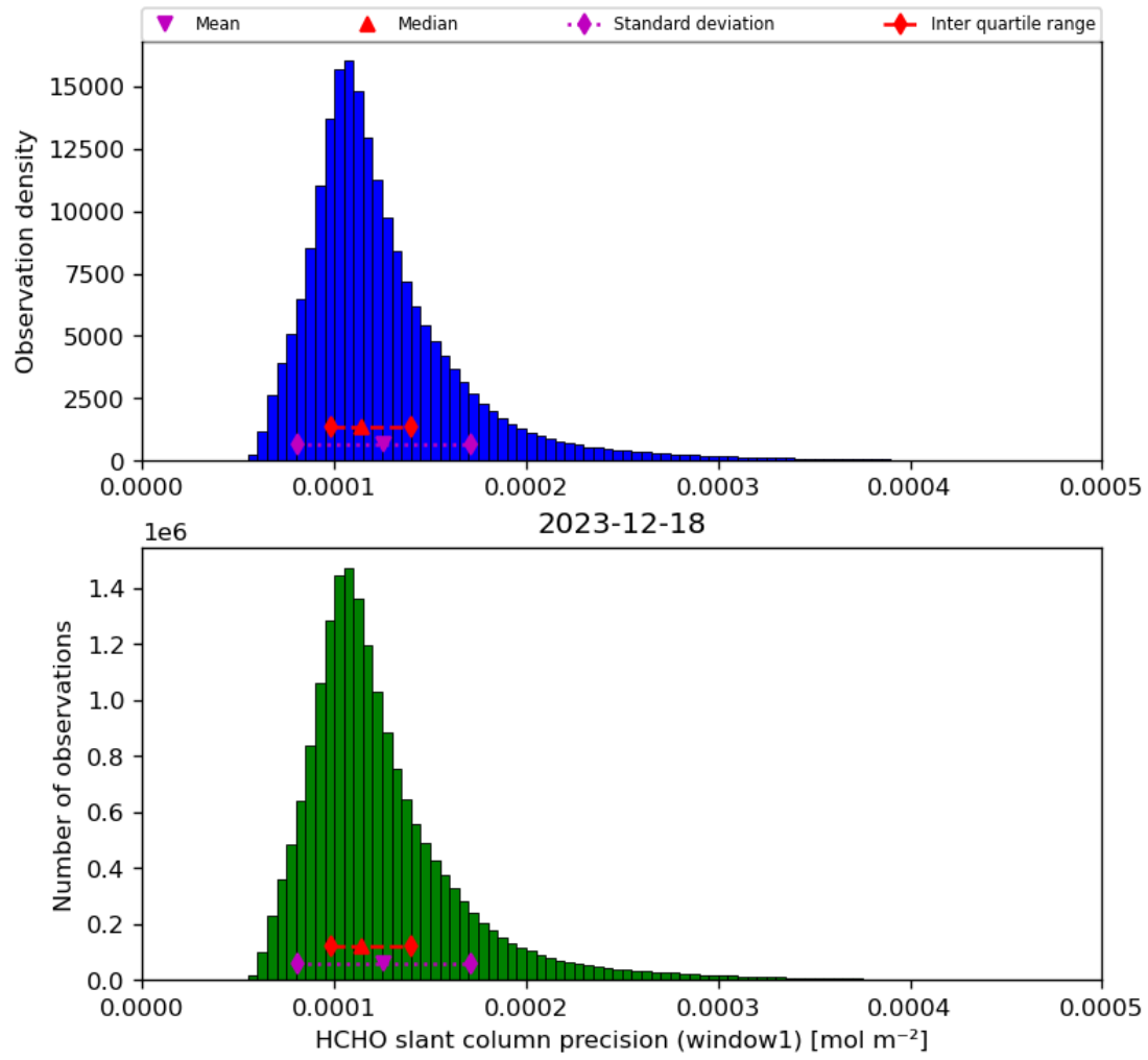
Figure 39: Histogram of “HCHO slant column precision (window1)” for 2023-12-17 to 2023-12-19
