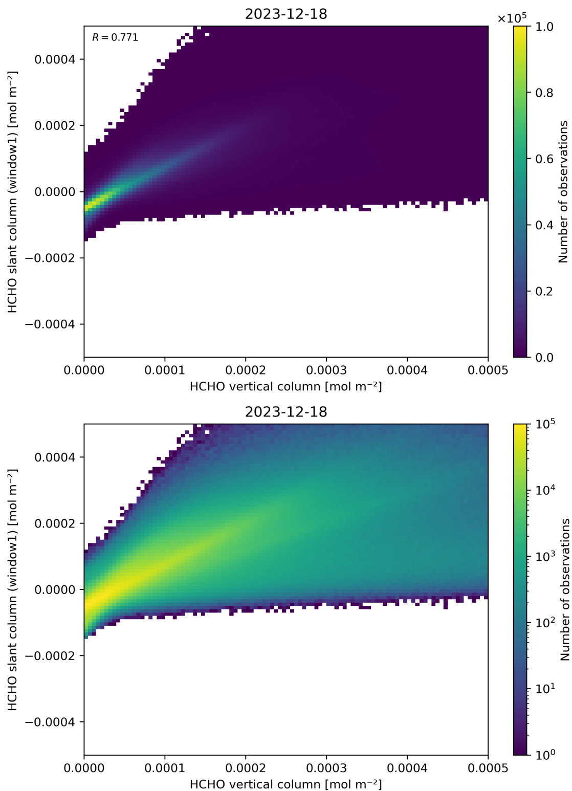
Figure 129: Scatter density plot of “HCHO vertical column” against “HCHO slant column (window1)” for 2023-12-17 to 2023-12-19.
