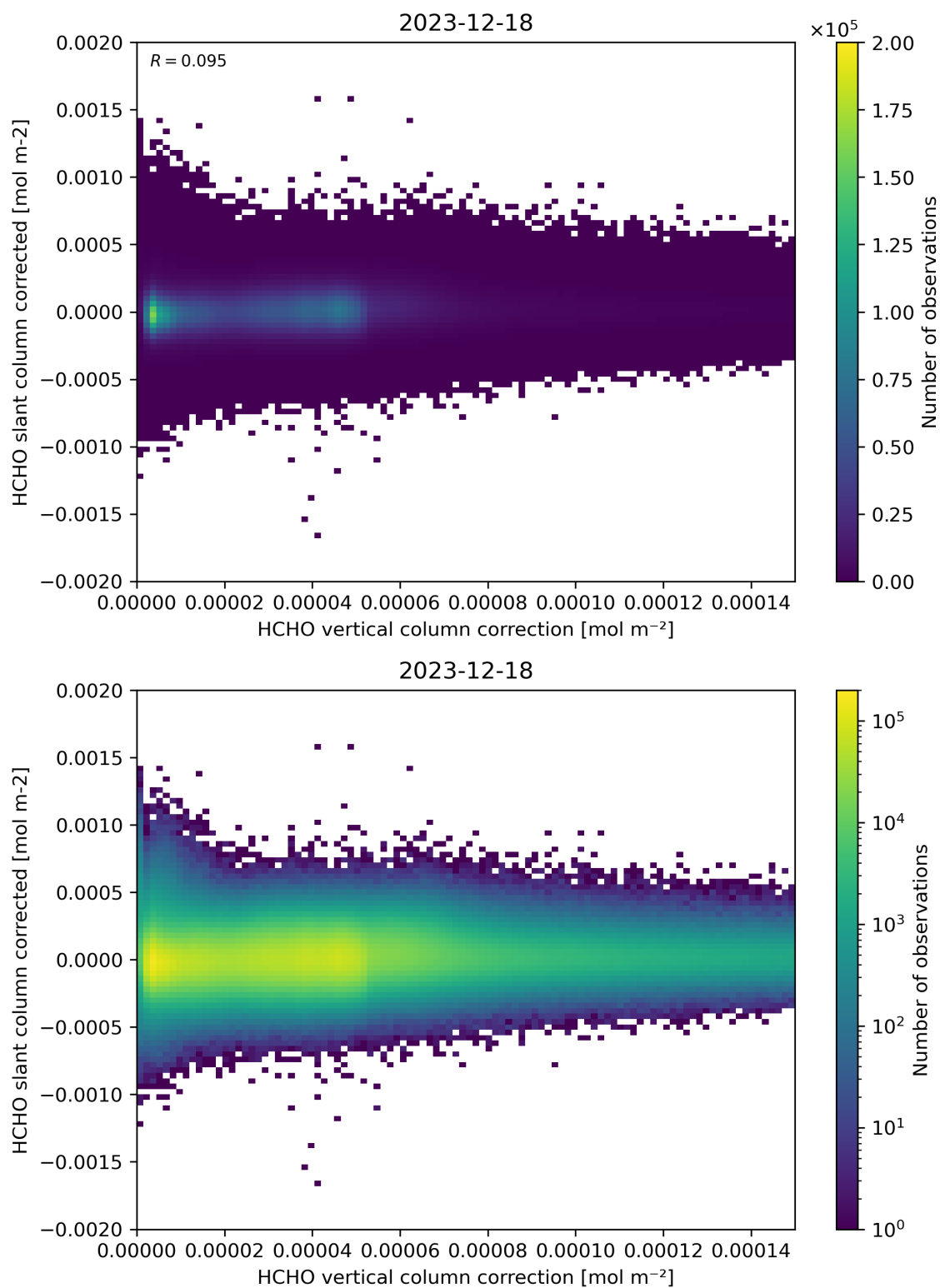
Figure 116: Scatter density plot of “HCHO vertical column correction” against “HCHO slant column corrected” for 2023-12-17 to 2023-12-19.
