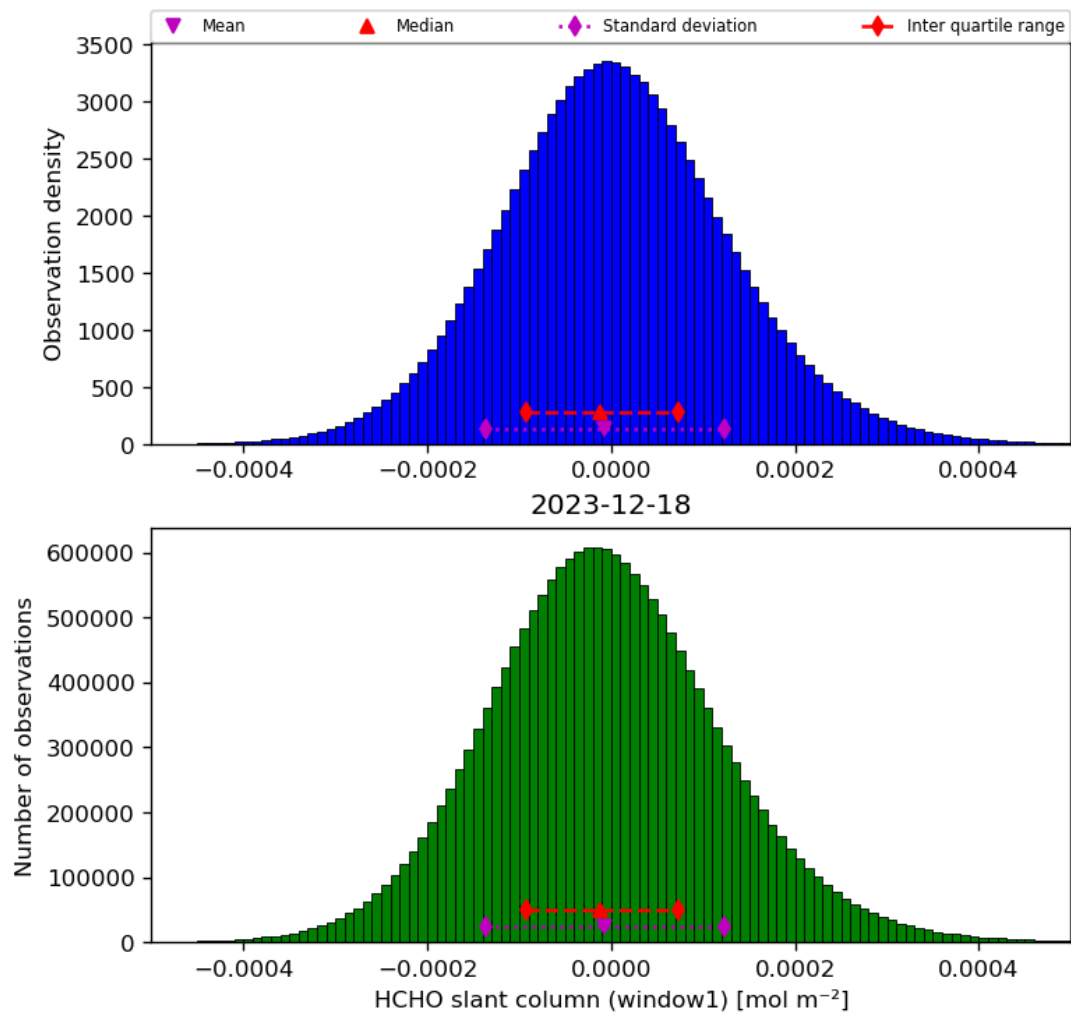
Figure 38: Histogram of “HCHO slant column (window1)” for 2023-12-17 to 2023-12-19
