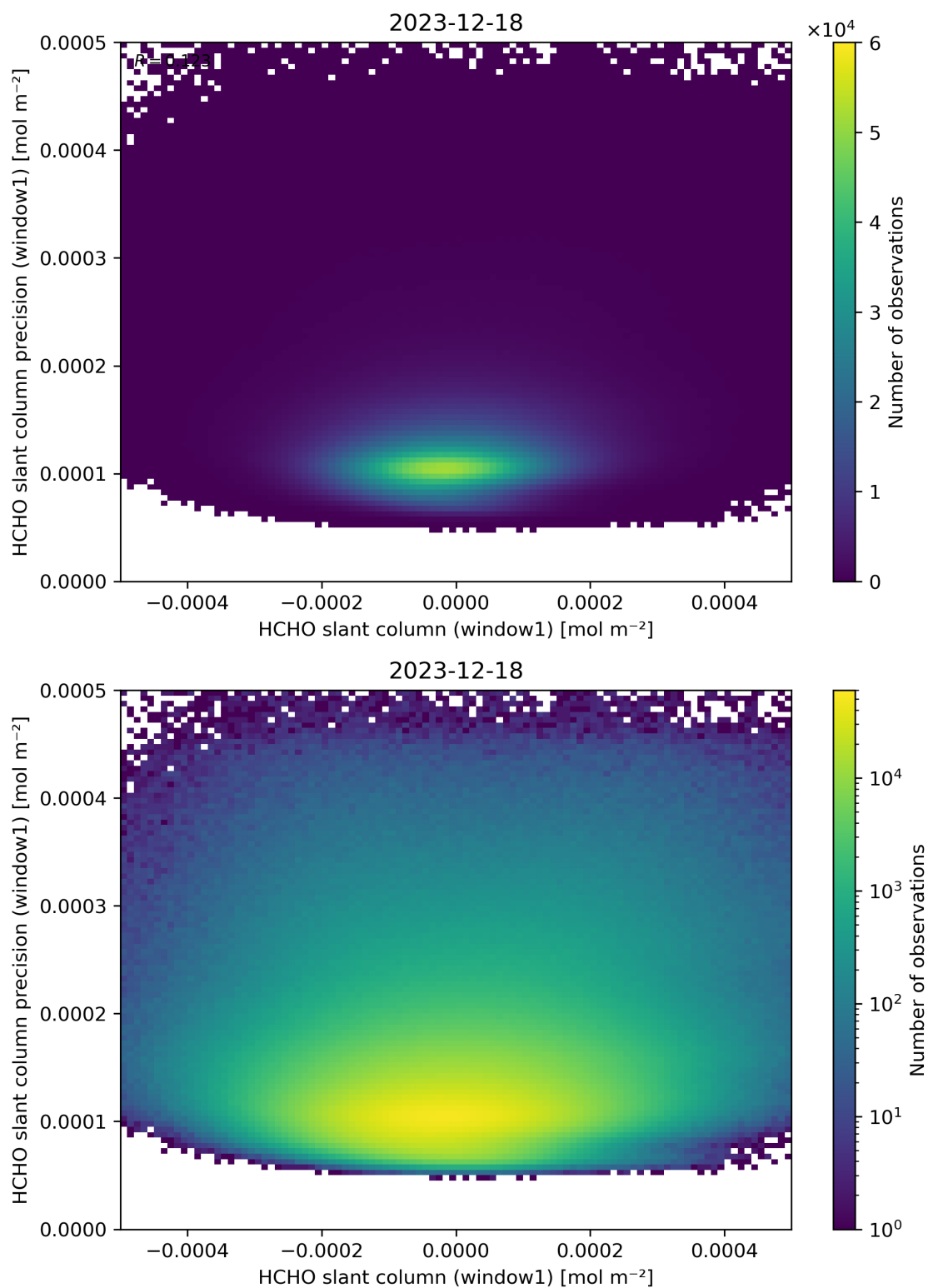
Figure 84: Scatter density plot of “HCHO slant column (window1)” against “HCHO slant column precision (window1)” for 2023-12-17 to 2023-12-19.
