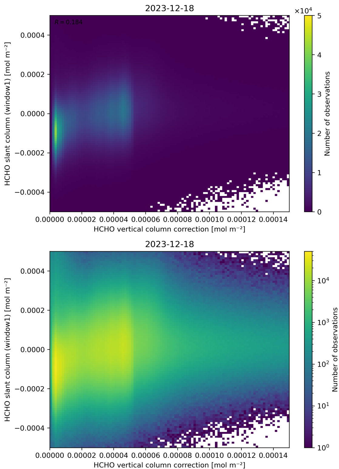
Figure 118: Scatter density plot of “HCHO vertical column correction” against “HCHO slant column (window1)” for 2023-12-17 to 2023-12-19.
