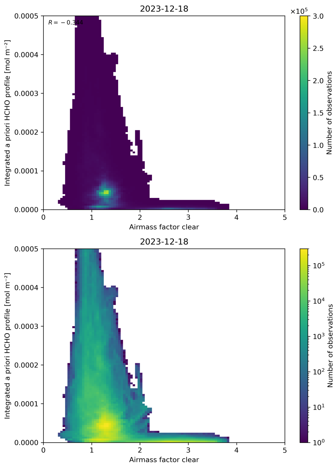
Figure 76: Scatter density plot of “Airmass factor clear” against “Integrated a priori HCHO profile” for 2023-12-17 to 2023-12-19.
