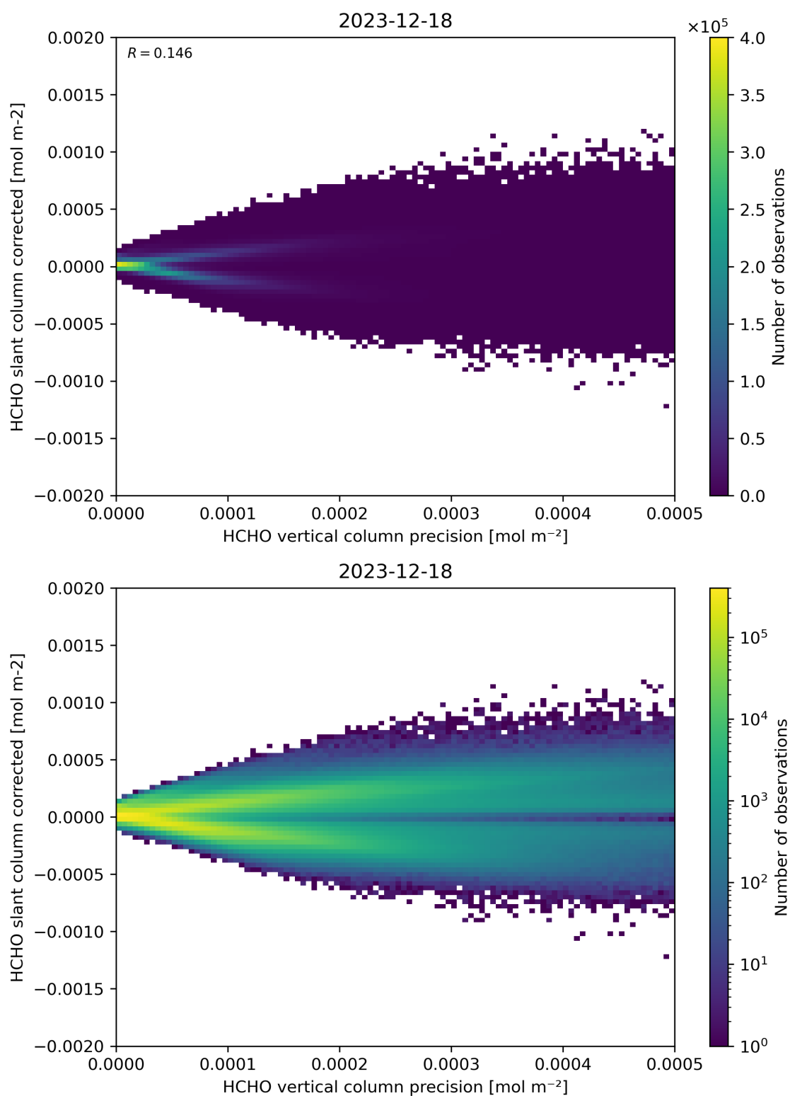
Figure 140: Scatter density plot of “HCHO vertical column precision” against “HCHO slant column corrected” for 2023-12-17 to 2023-12-19.
