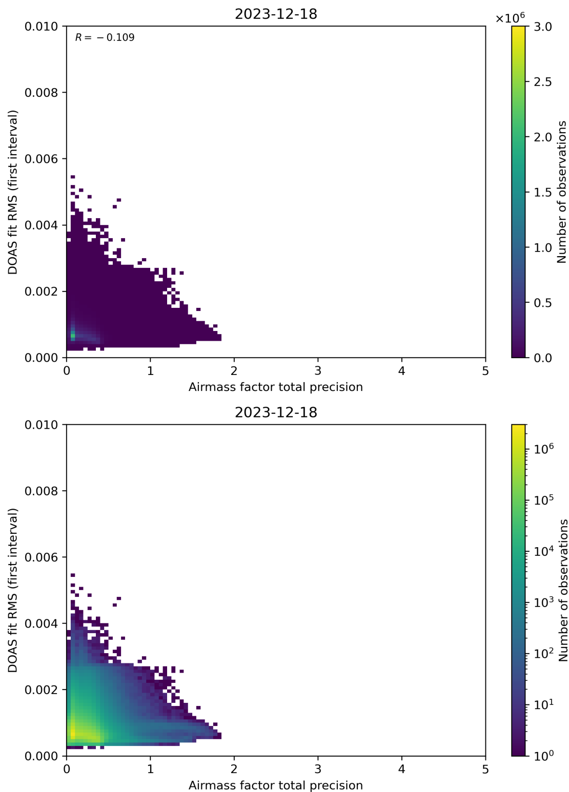
Figure 105: Scatter density plot of “Airmass factor total precision” against “DOAS fit RMS (first interval)” for 2023-12-17 to 2023-12-19.
