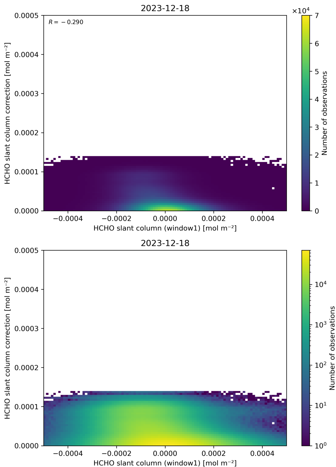
Figure 83: Scatter density plot of “HCHO slant column (window1)” against “HCHO slant column correction” for 2023-12-17 to 2023-12-19.
