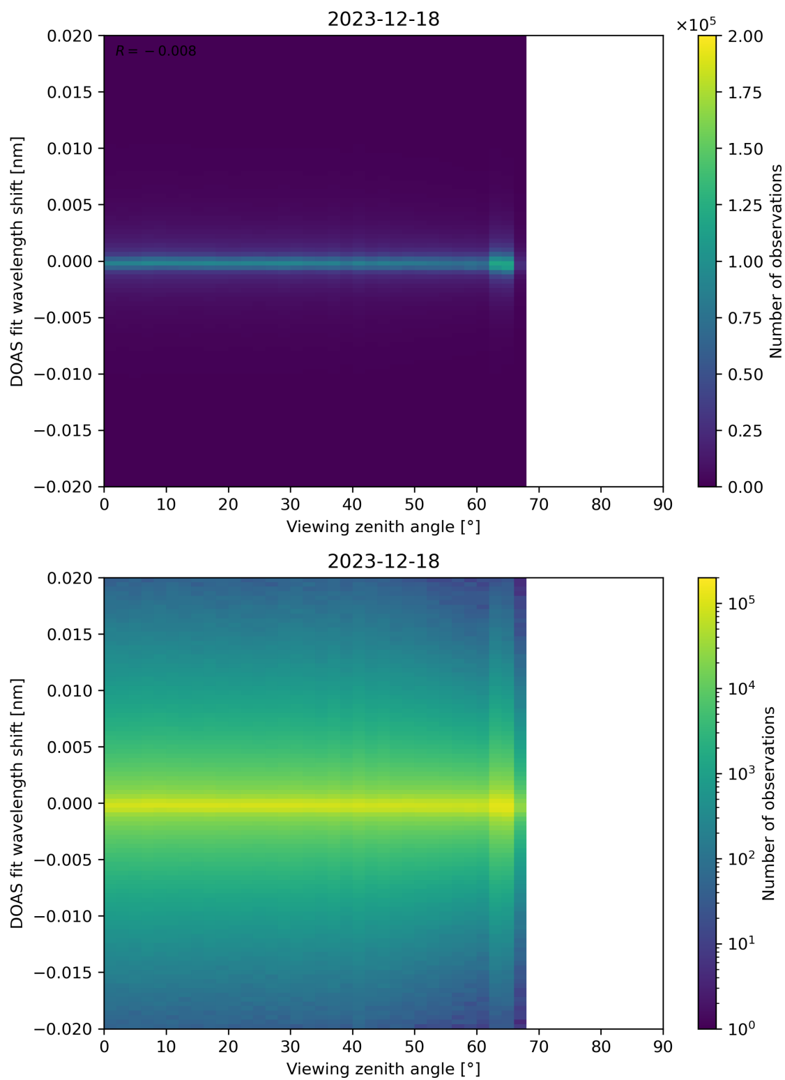
Figure 183: Scatter density plot of “Viewing zenith angle” against “DOAS fit wavelength shift” for 2023-12-17 to 2023-12-19.
