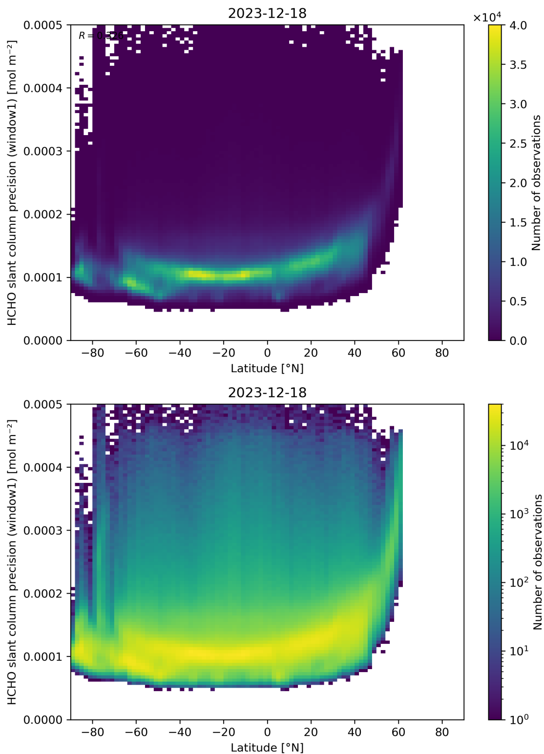
Figure 160: Scatter density plot of “Latitude” against “HCHO slant column precision (window1)” for 2023-12-17 to 2023-12-19.
