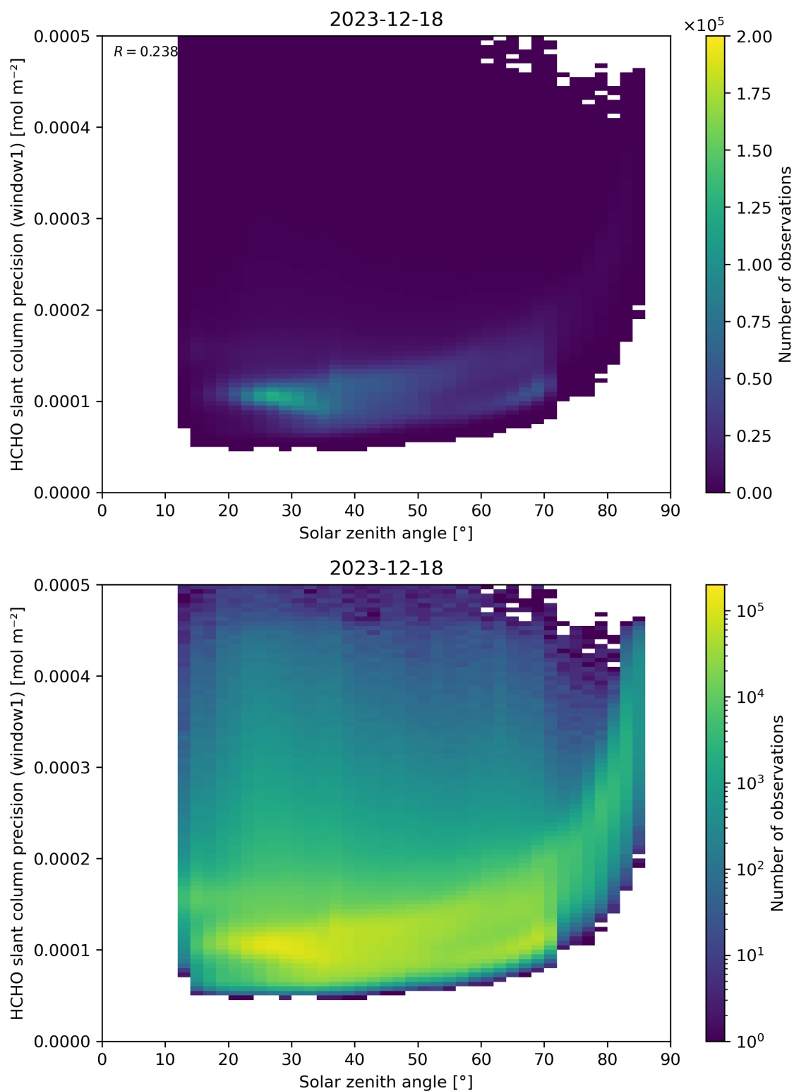
Figure 174: Scatter density plot of “Solar zenith angle” against “HCHO slant column precision (window1)” for 2023-12-17 to 2023-12-19.
