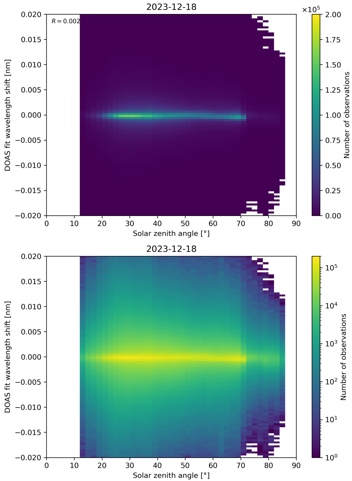
Figure 168: Scatter density plot of “Solar zenith angle” against “DOAS fit wavelength shift” for 2023-12-17 to 2023-12-19.
