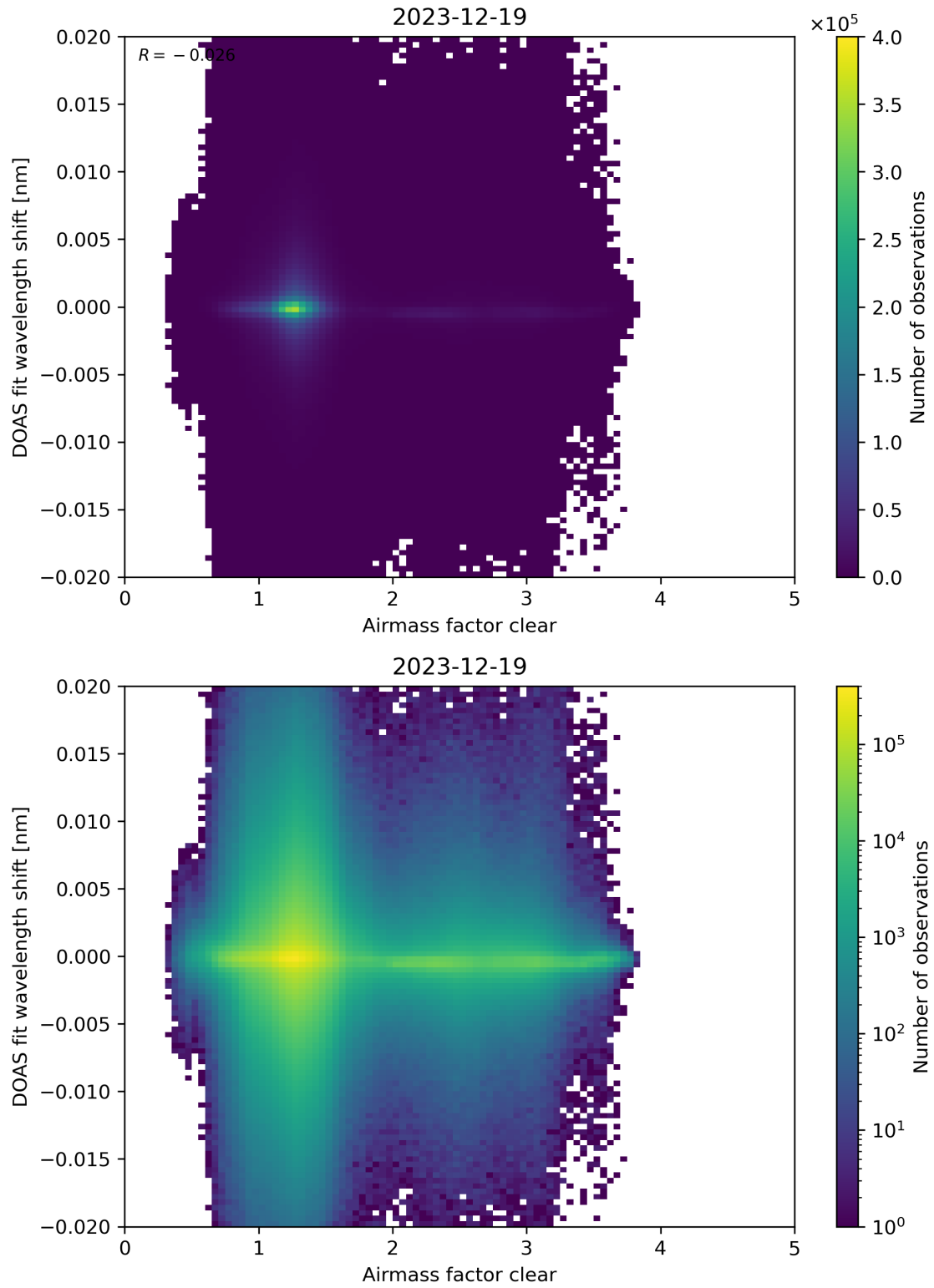
Figure 72: Scatter density plot of “Airmass factor clear” against “DOAS fit wavelength shift” for 2023-12-18 to 2023-12-20.
