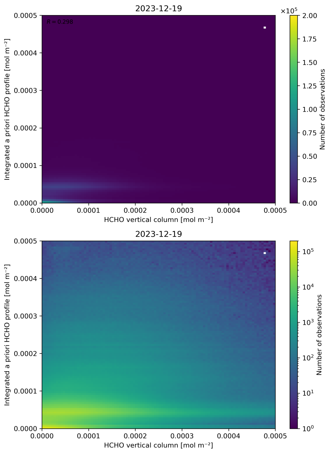
Figure 135: Scatter density plot of “HCHO vertical column” against “Integrated a priori HCHO profile” for 2023-12-18 to 2023-12-20.
