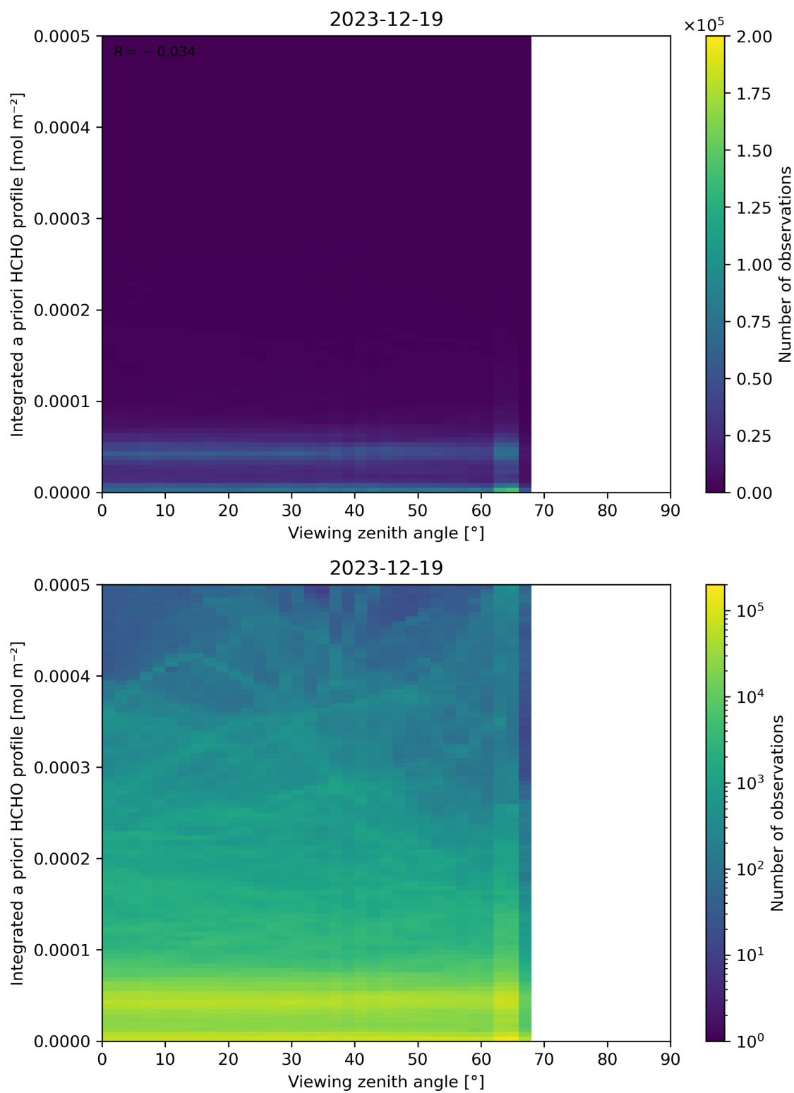
Figure 195: Scatter density plot of “Viewing zenith angle” against “Integrated a priori HCHO profile” for 2023-12-18 to 2023-12-20.
