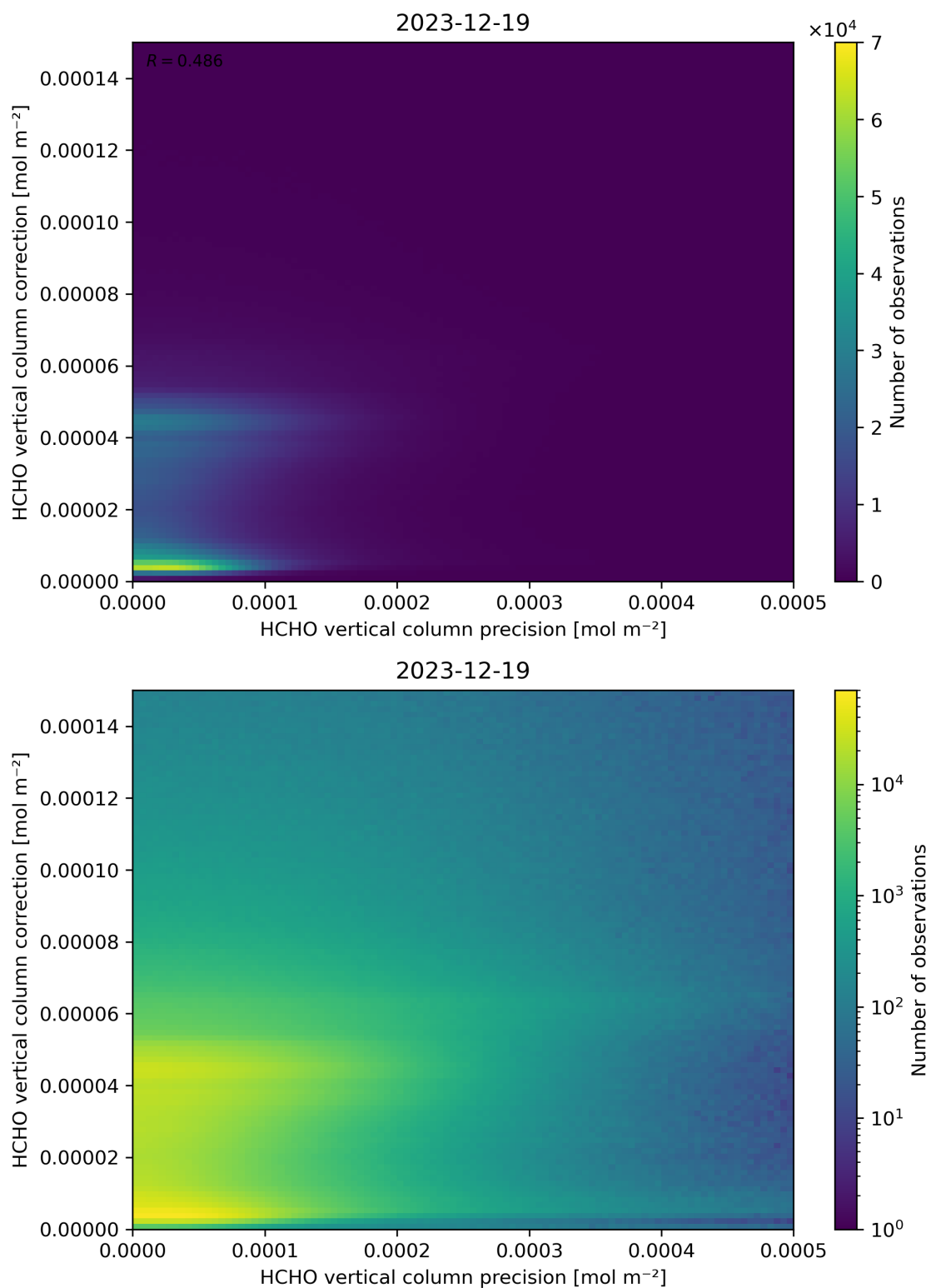
Figure 146: Scatter density plot of “HCHO vertical column precision” against “HCHO vertical column correction” for 2023-12-18 to 2023-12-20.
