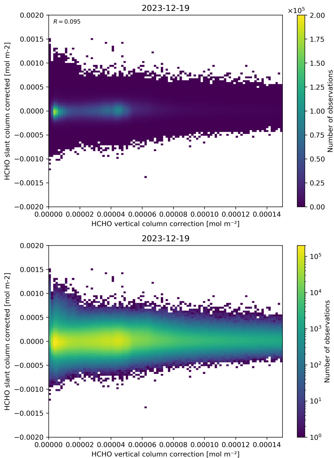
Figure 116: Scatter density plot of “HCHO vertical column correction” against “HCHO slant column corrected” for 2023-12-18 to 2023-12-20.
