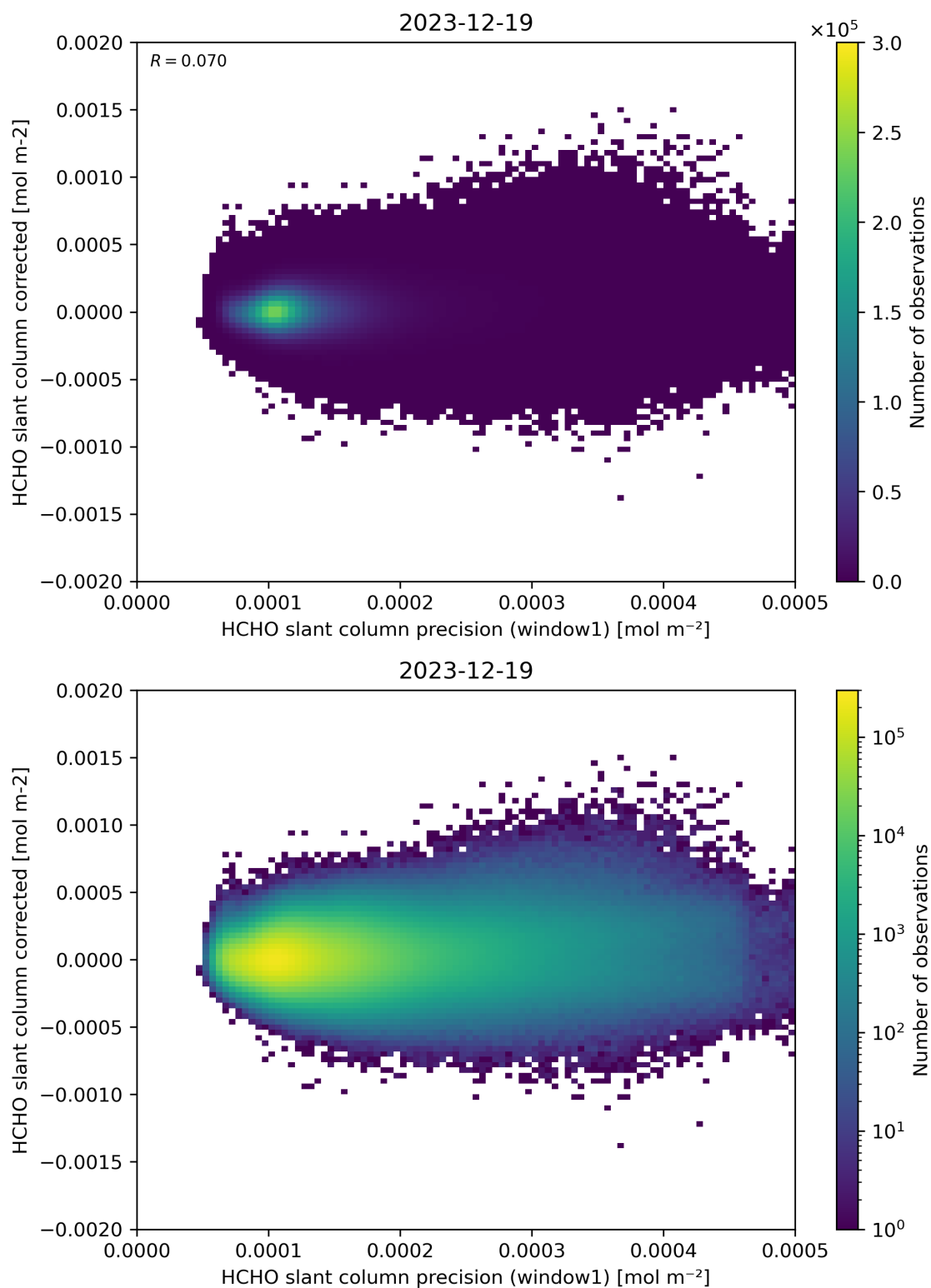
Figure 92: Scatter density plot of “HCHO slant column precision (window1)” against “HCHO slant column corrected” for 2023-12-18 to 2023-12-20.
