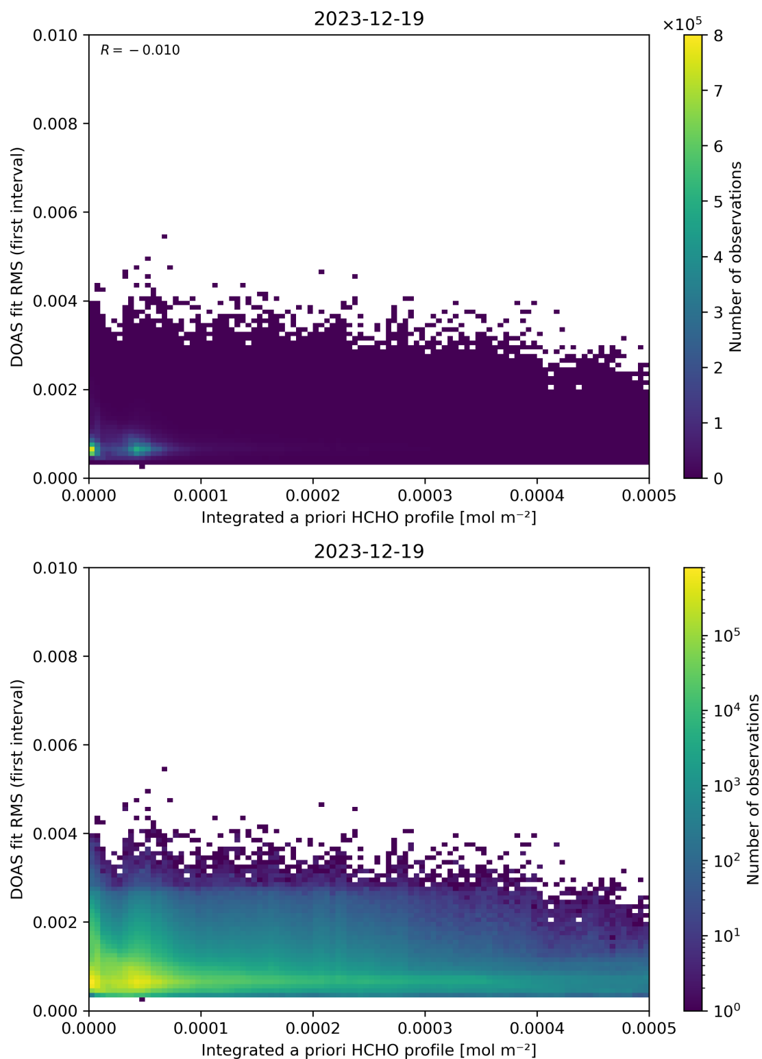
Figure 148: Scatter density plot of “Integrated a priori HCHO profile” against “DOAS fit RMS (first interval)” for 2023-12-18 to 2023-12-20.
