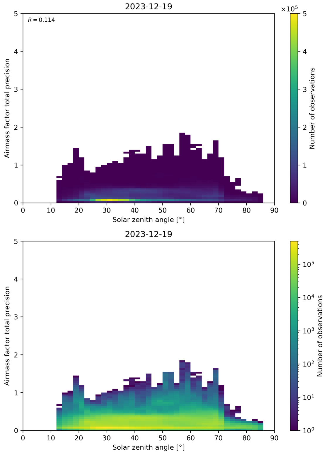
Figure 176: Scatter density plot of “Solar zenith angle” against “Airmass factor total precision” for 2023-12-18 to 2023-12-20.
