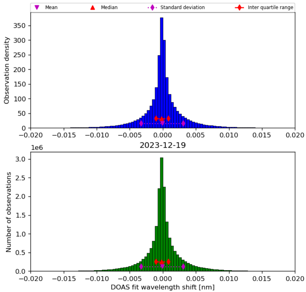
Figure 44: Histogram of “DOAS fit wavelength shift” for 2023-12-18 to 2023-12-20
