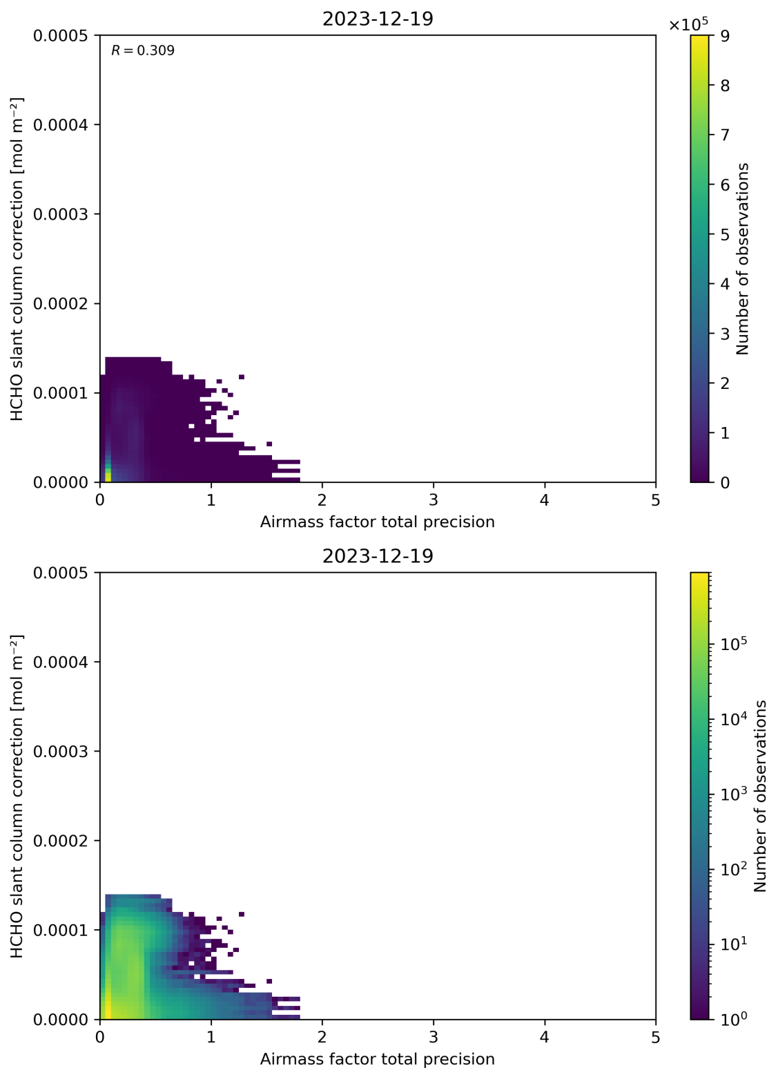
Figure 110: Scatter density plot of “Airmass factor total precision” against “HCHO slant column correction” for 2023-12-18 to 2023-12-20.
