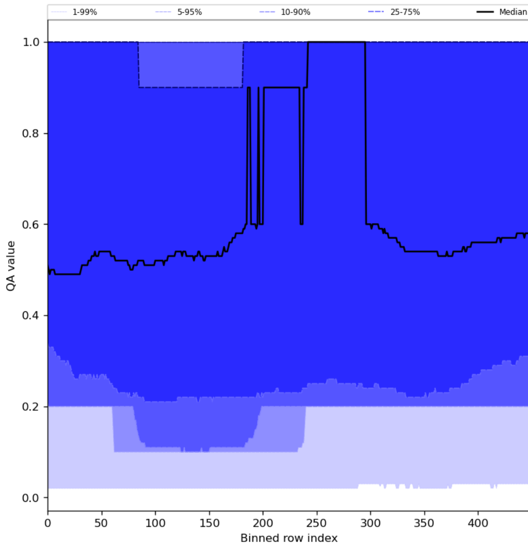
Figure 48: Along track statistics of “QA value” for 2023-12-18 to 2023-12-20
