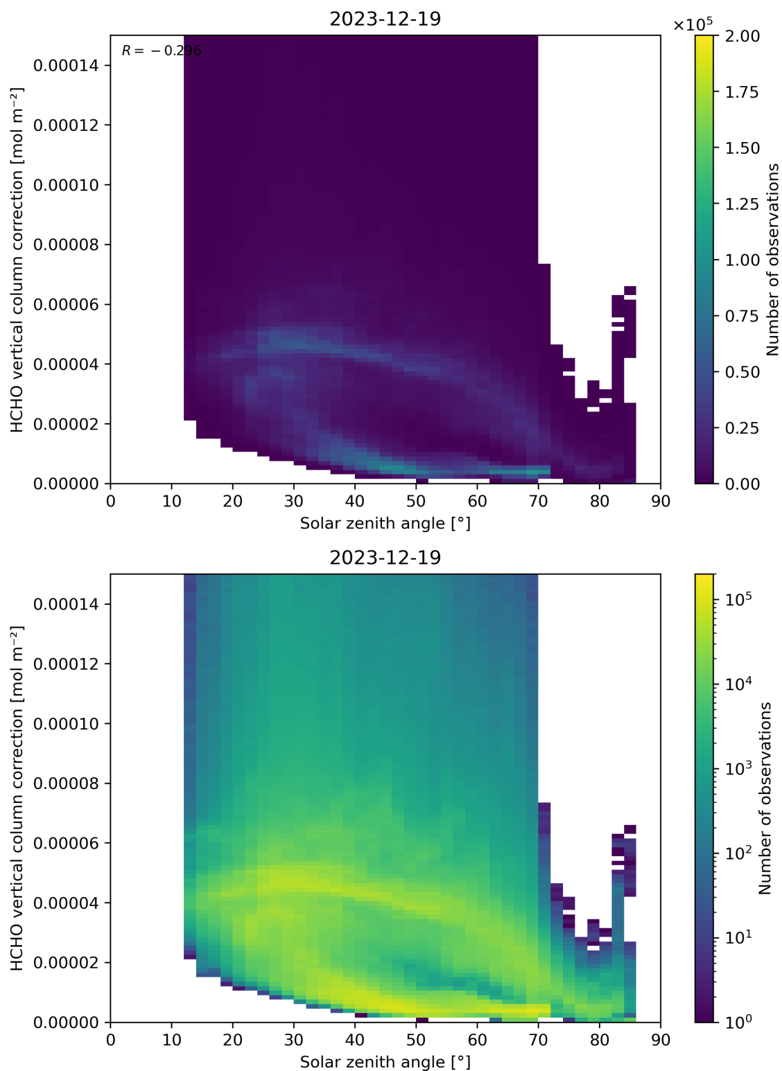
Figure 178: Scatter density plot of “Solar zenith angle” against “HCHO vertical column correction” for 2023-12-18 to 2023-12-20.
