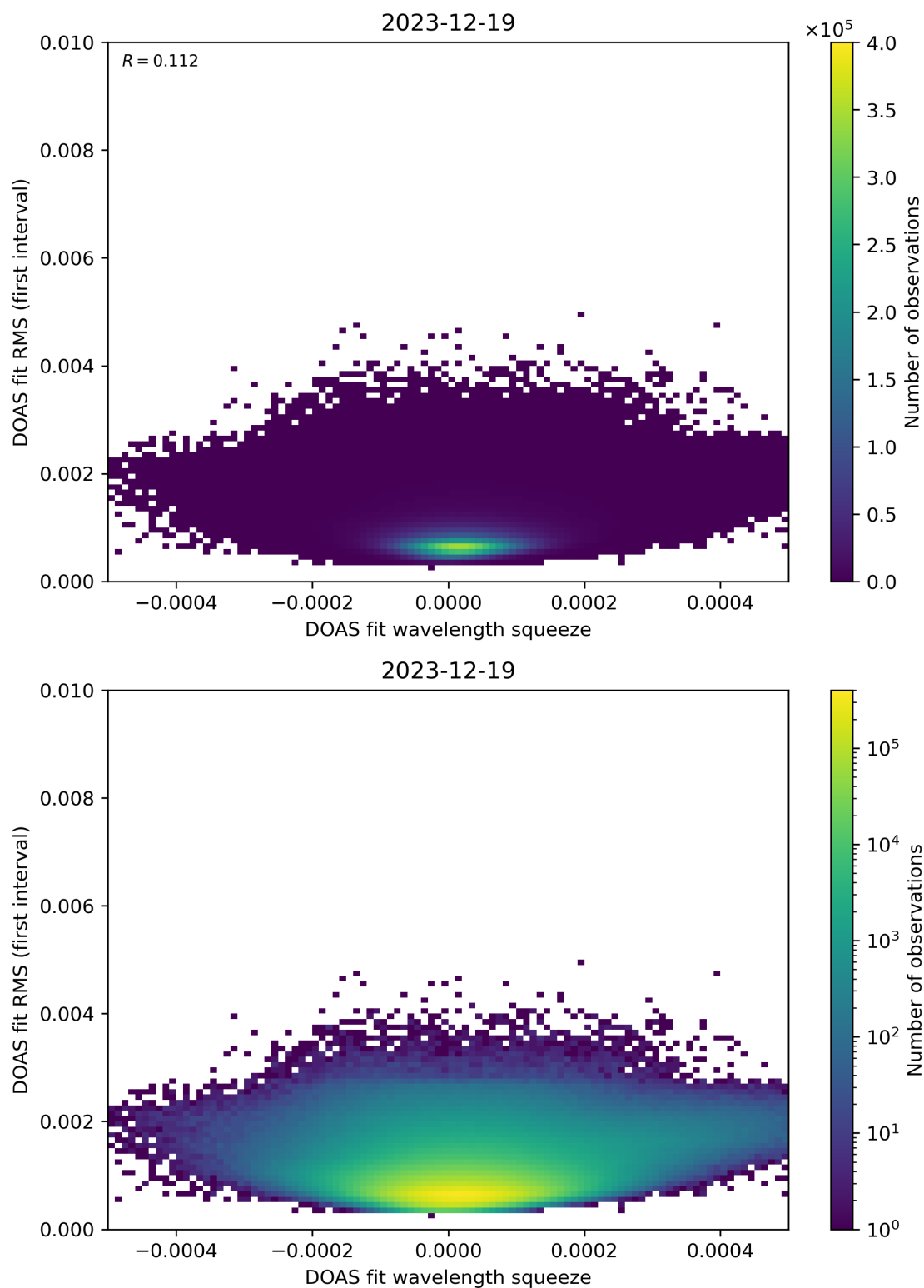
Figure 68: Scatter density plot of “DOAS fit wavelength squeeze” against “DOAS fit RMS (first interval)” for 2023-12-18 to 2023-12-20.
