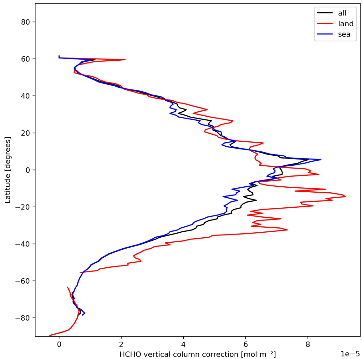
Figure 23: Zonal average of “HCHO vertical column correction” for 2023-12-18 to 2023-12-20.
