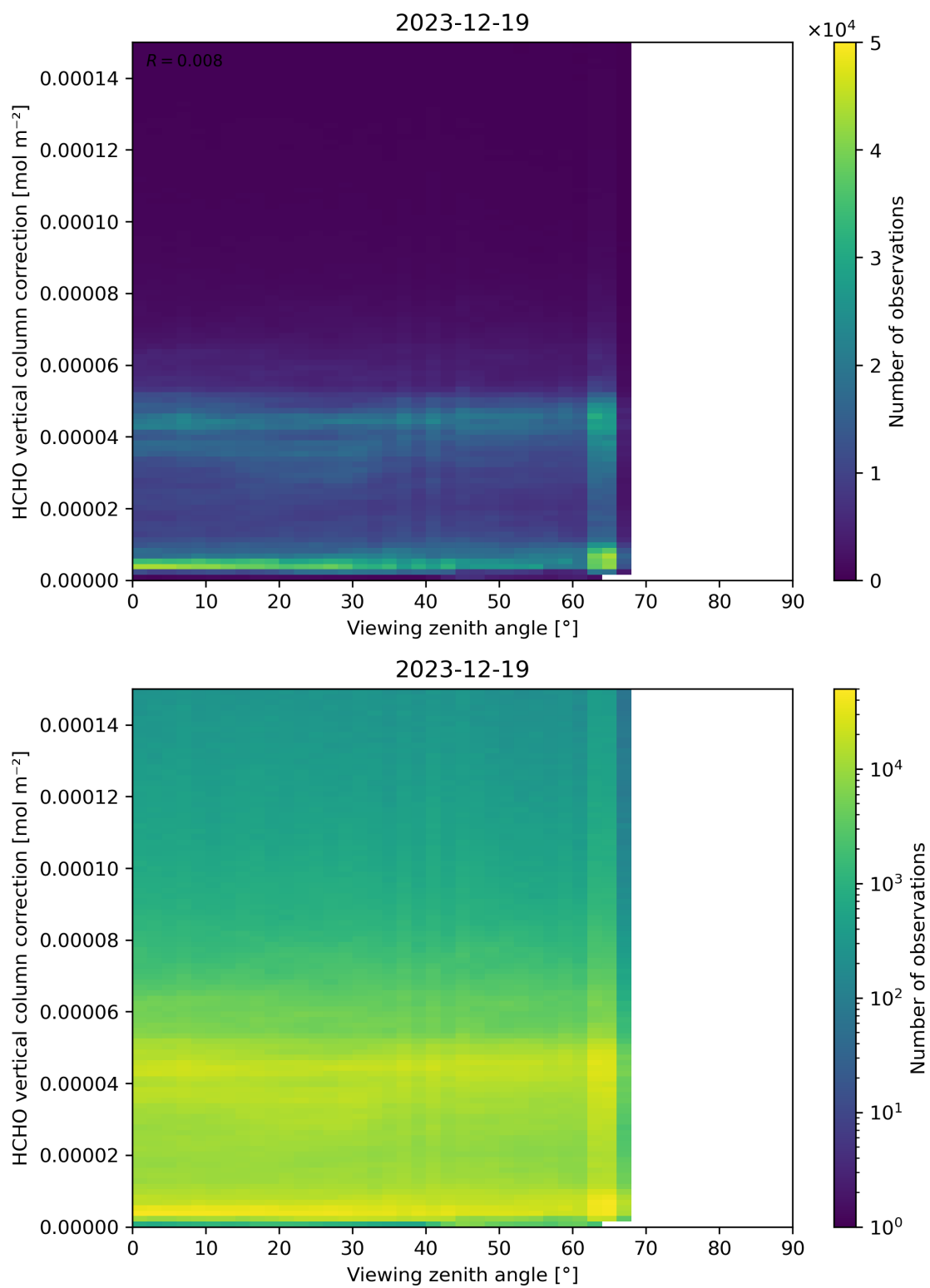
Figure 193: Scatter density plot of “Viewing zenith angle” against “HCHO vertical column correction” for 2023-12-18 to 2023-12-20.
