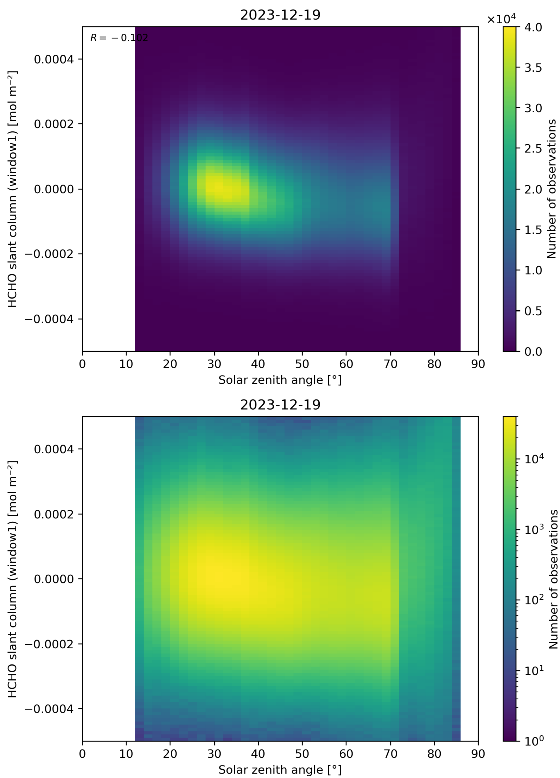
Figure 173: Scatter density plot of “Solar zenith angle” against “HCHO slant column (window1)” for 2023-12-18 to 2023-12-20.
