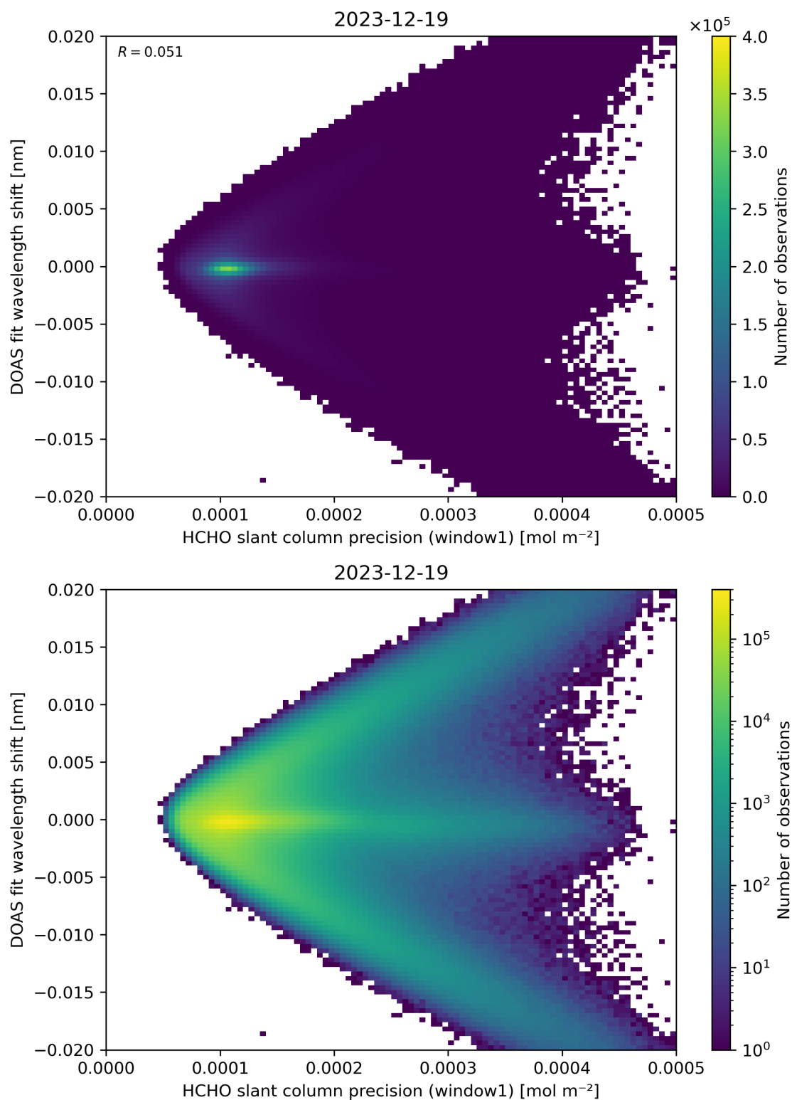
Figure 89: Scatter density plot of “HCHO slant column precision (window1)” against “DOAS fit wavelength shift” for 2023-12-18 to 2023-12-20.
