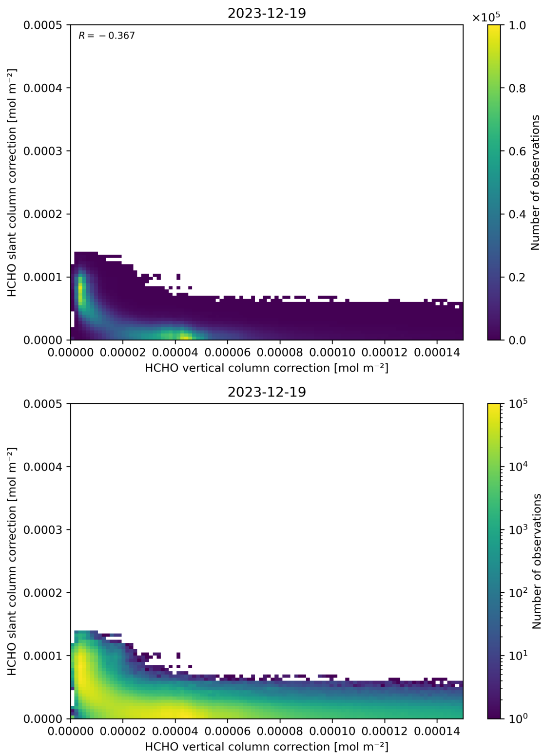
Figure 117: Scatter density plot of “HCHO vertical column correction” against “HCHO slant column correction” for 2023-12-18 to 2023-12-20.
