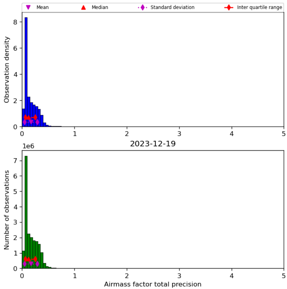
Figure 41: Histogram of “Airmass factor total precision” for 2023-12-18 to 2023-12-20
