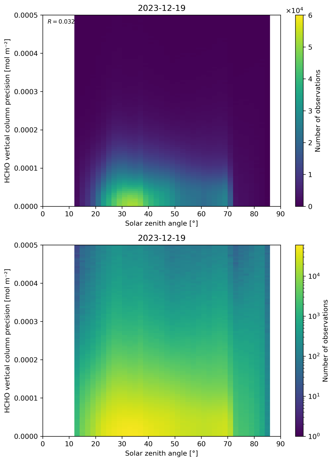
Figure 179: Scatter density plot of “Solar zenith angle” against “HCHO vertical column precision” for 2023-12-18 to 2023-12-20.
