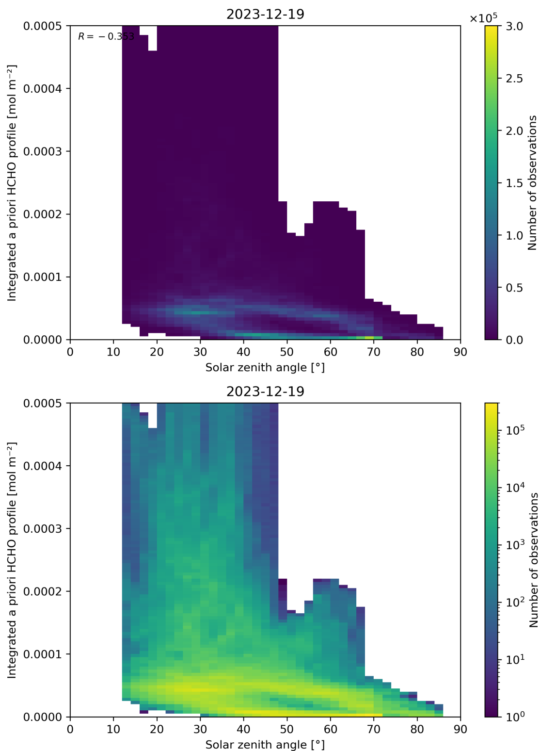
Figure 180: Scatter density plot of “Solar zenith angle” against “Integrated a priori HCHO profile” for 2023-12-18 to 2023-12-20.
