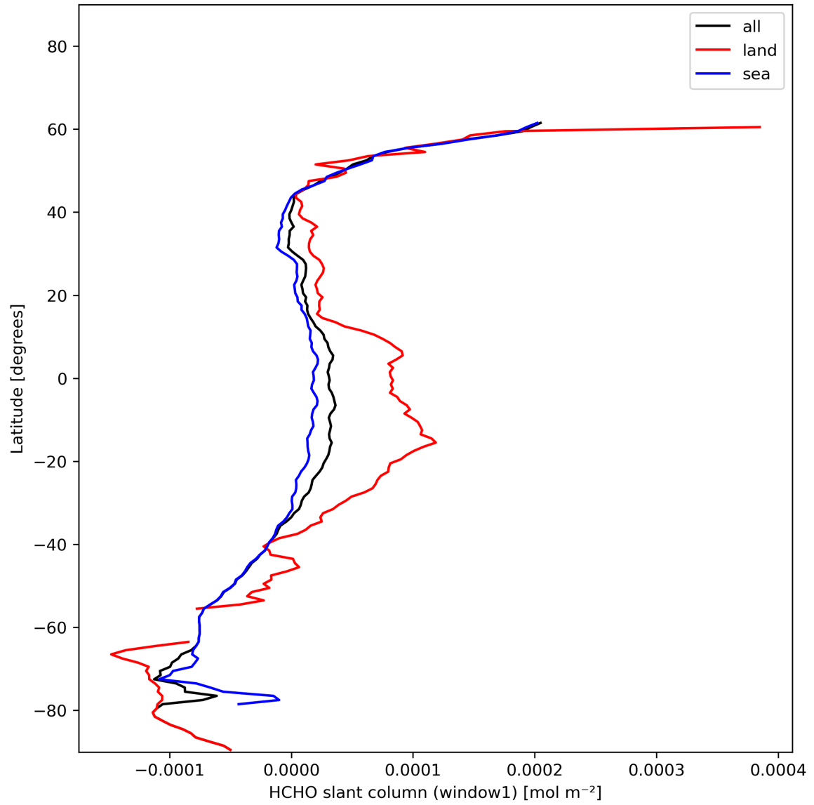
Figure 24: Zonal average of “HCHO slant column (window1)” for 2023-12-18 to 2023-12-20.
