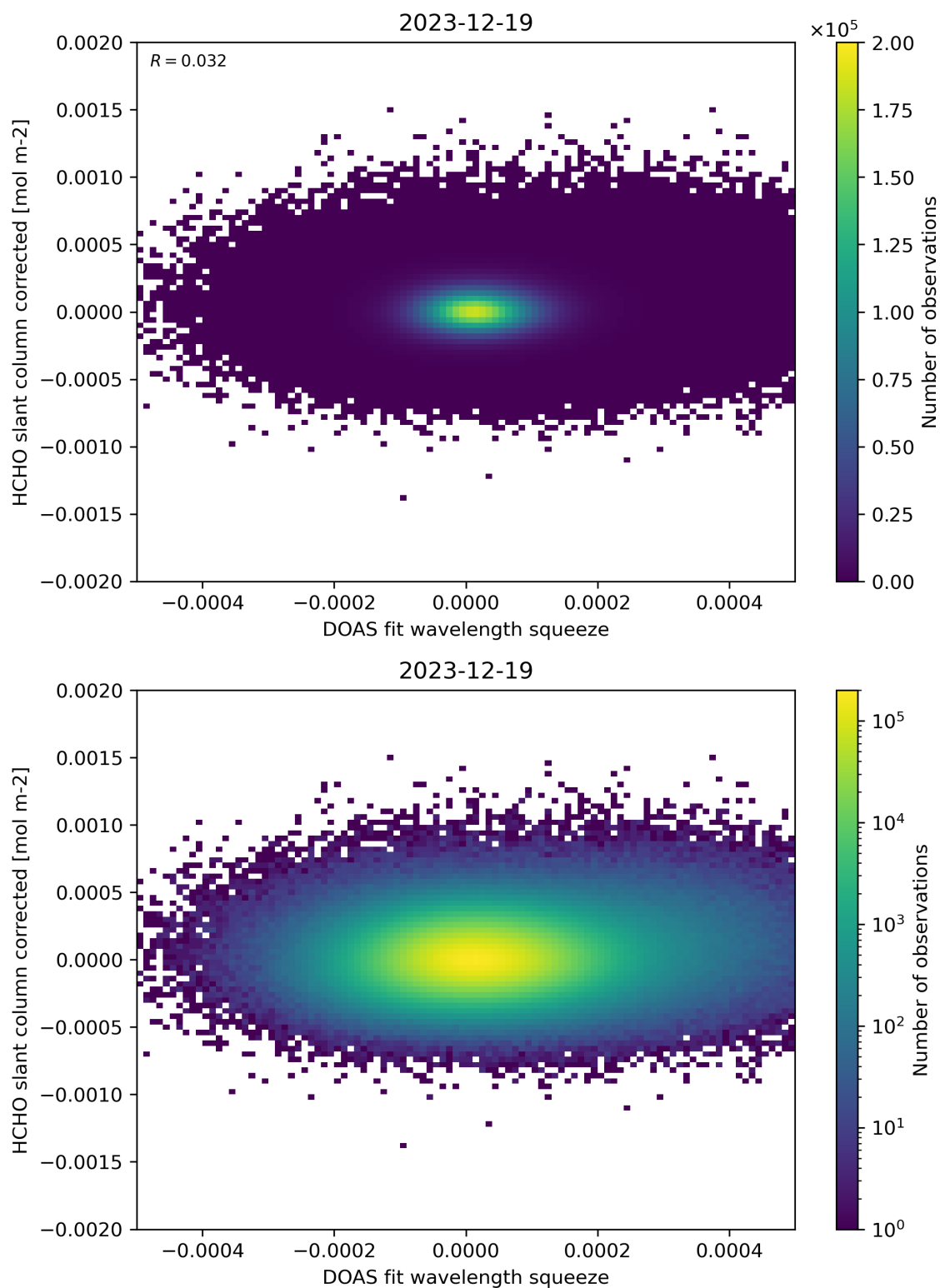
Figure 69: Scatter density plot of “DOAS fit wavelength squeeze” against “HCHO slant column corrected” for 2023-12-18 to 2023-12-20.
