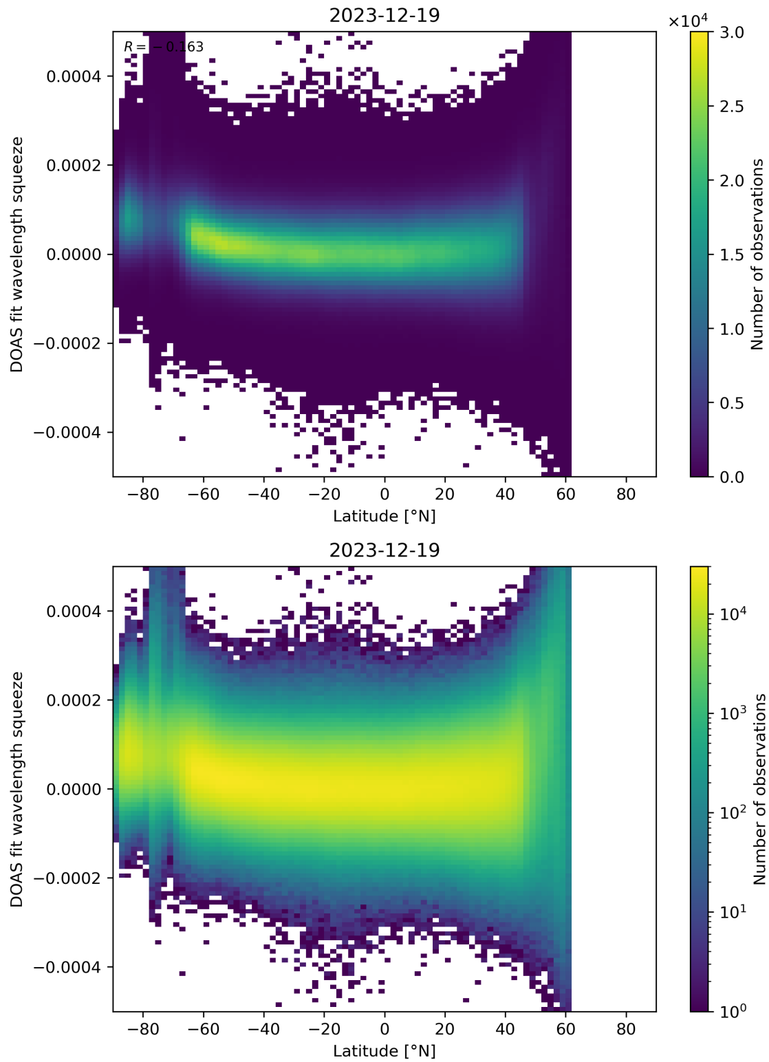
Figure 155: Scatter density plot of “Latitude” against “DOAS fit wavelength squeeze” for 2023-12-18 to 2023-12-20.
