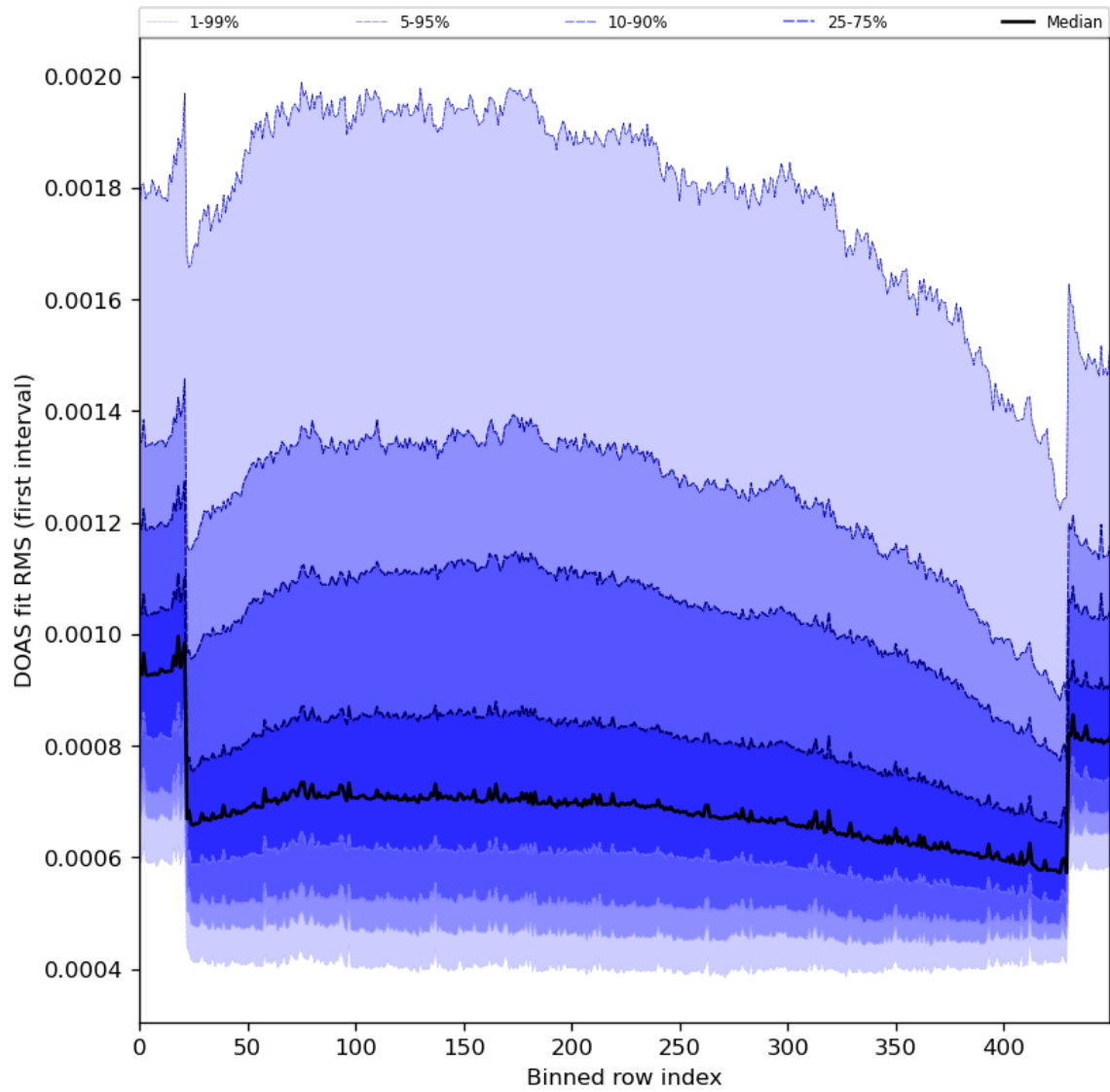
Figure 60: Along track statistics of “DOAS fit RMS (first interval)” for 2023-12-18 to 2023-12-20
