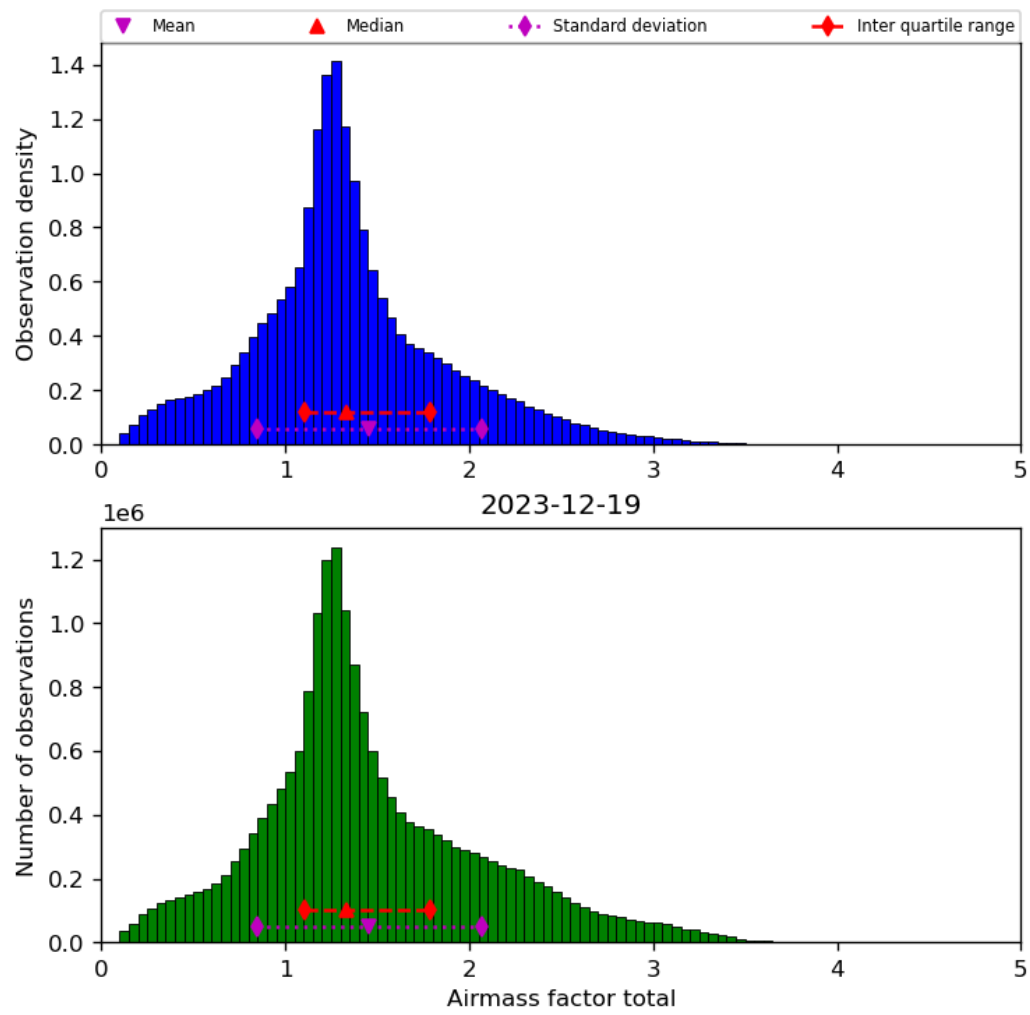
Figure 40: Histogram of “Airmass factor total” for 2023-12-18 to 2023-12-20
