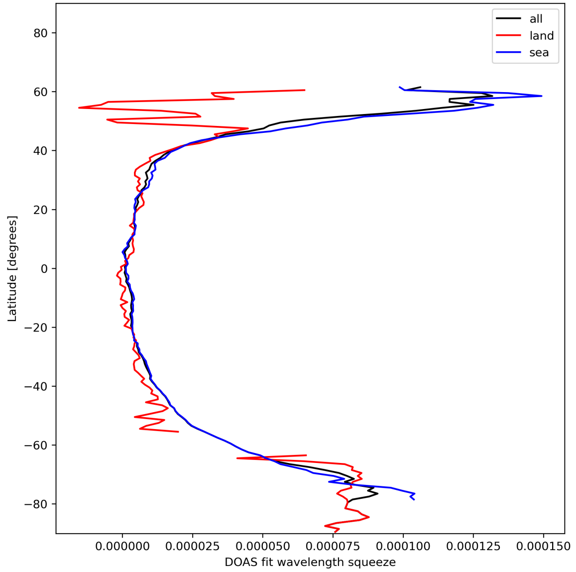
Figure 31: Zonal average of “DOAS fit wavelength squeeze” for 2023-12-18 to 2023-12-20.
