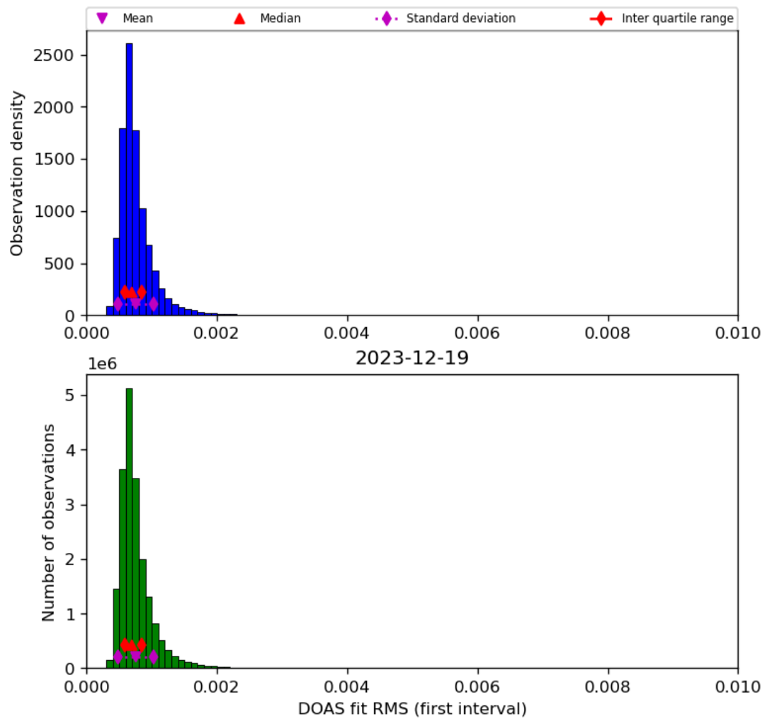
Figure 46: Histogram of “DOAS fit RMS (first interval)” for 2023-12-18 to 2023-12-20
