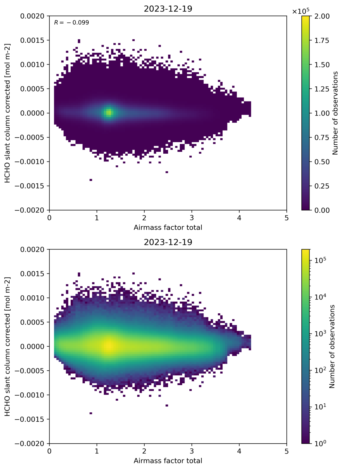
Figure 101: Scatter density plot of “Airmass factor total” against “HCHO slant column corrected” for 2023-12-18 to 2023-12-20.
