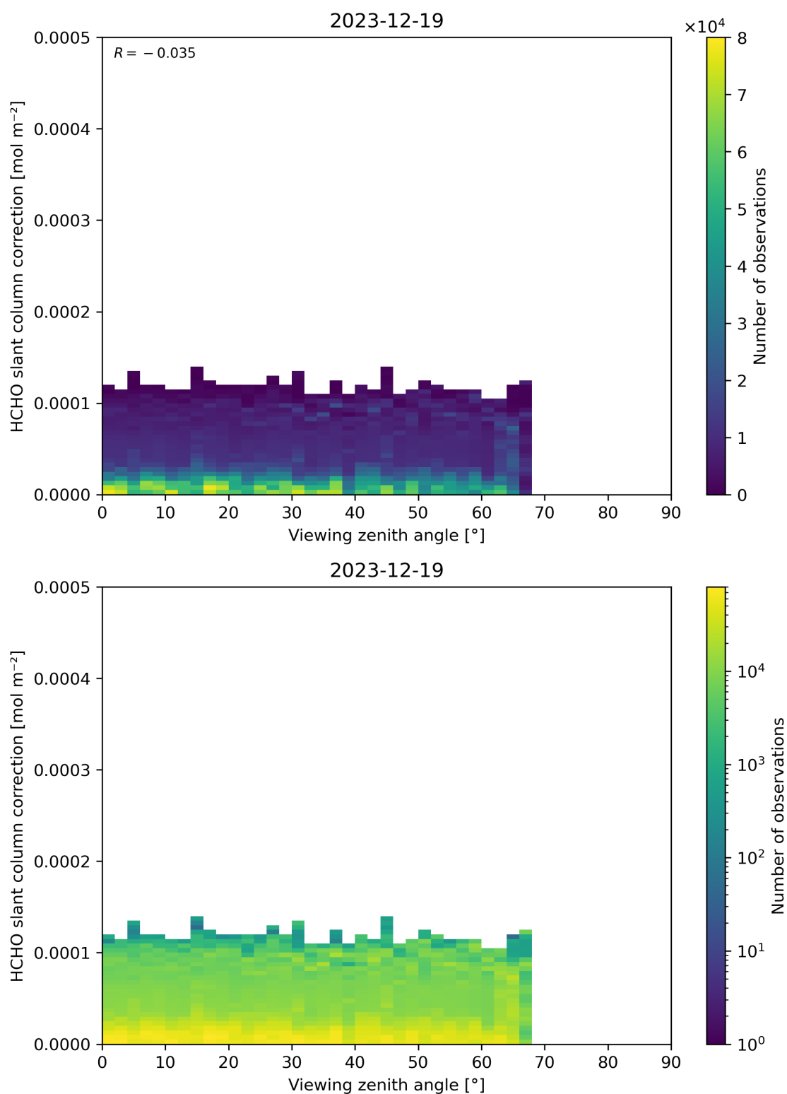
Figure 187: Scatter density plot of “Viewing zenith angle” against “HCHO slant column correction” for 2023-12-18 to 2023-12-20.
