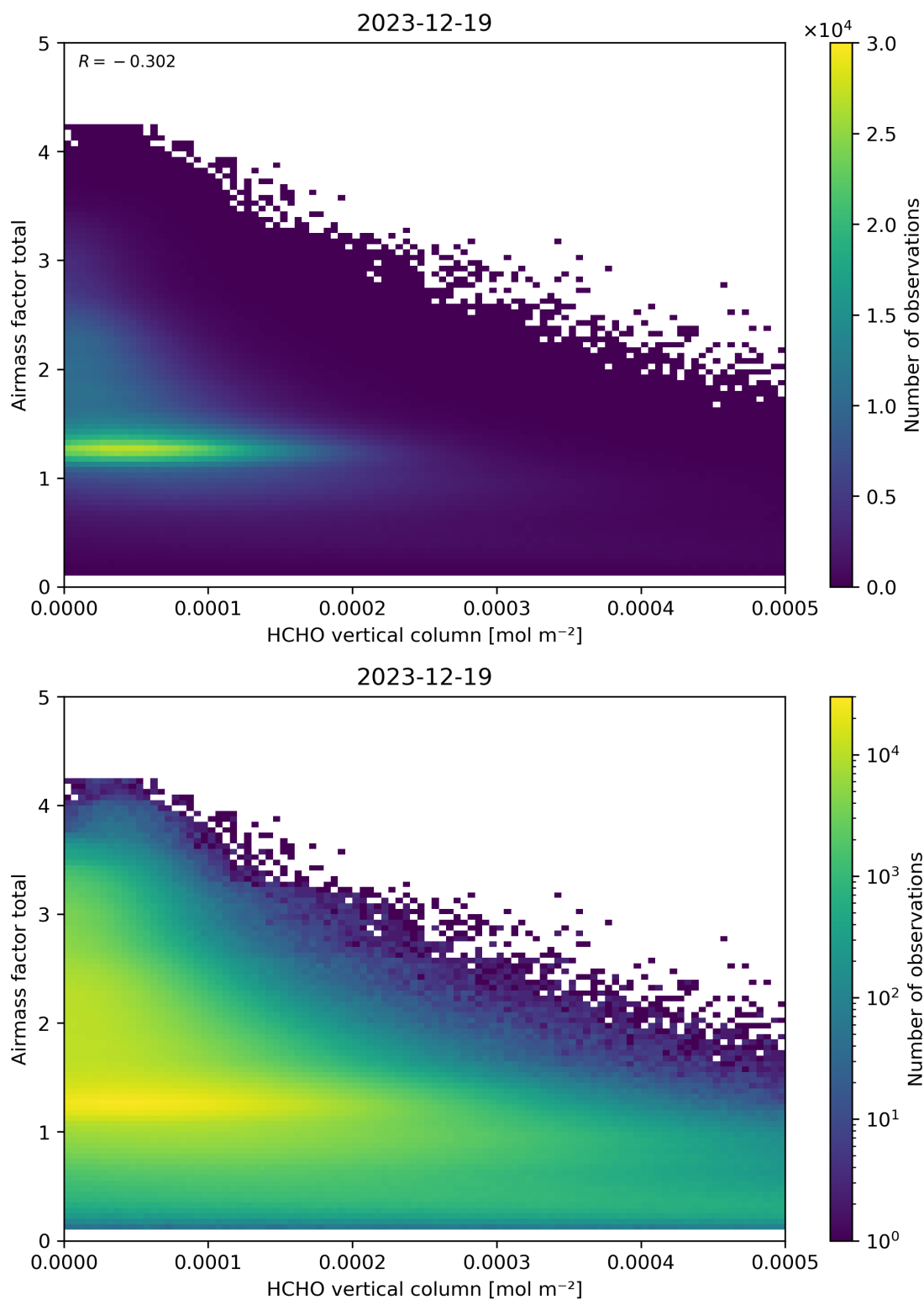
Figure 131: Scatter density plot of “HCHO vertical column” against “Airmass factor total” for 2023-12-18 to 2023-12-20.
