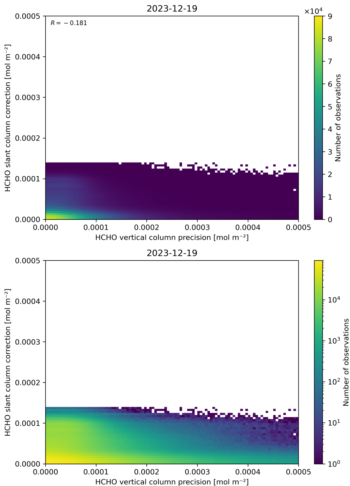
Figure 141: Scatter density plot of “HCHO vertical column precision” against “HCHO slant column correction” for 2023-12-18 to 2023-12-20.
