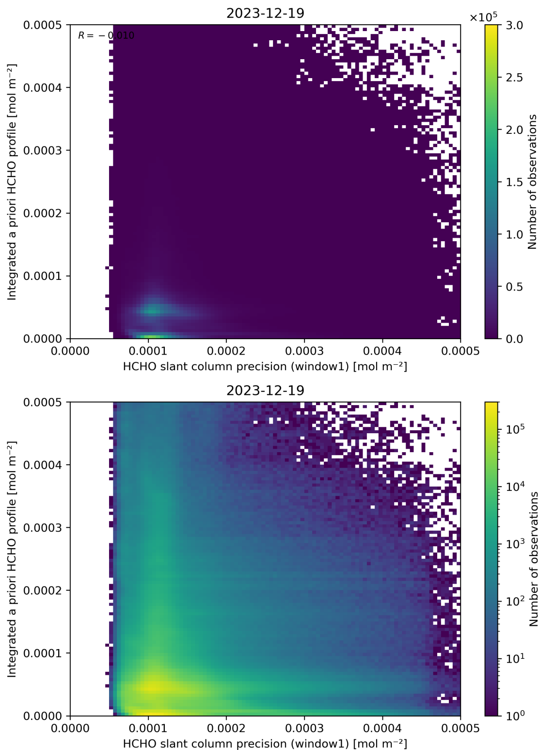
Figure 96: Scatter density plot of “HCHO slant column precision (window1)” against “Integrated a priori HCHO profile” for 2023-12-18 to 2023-12-20.
