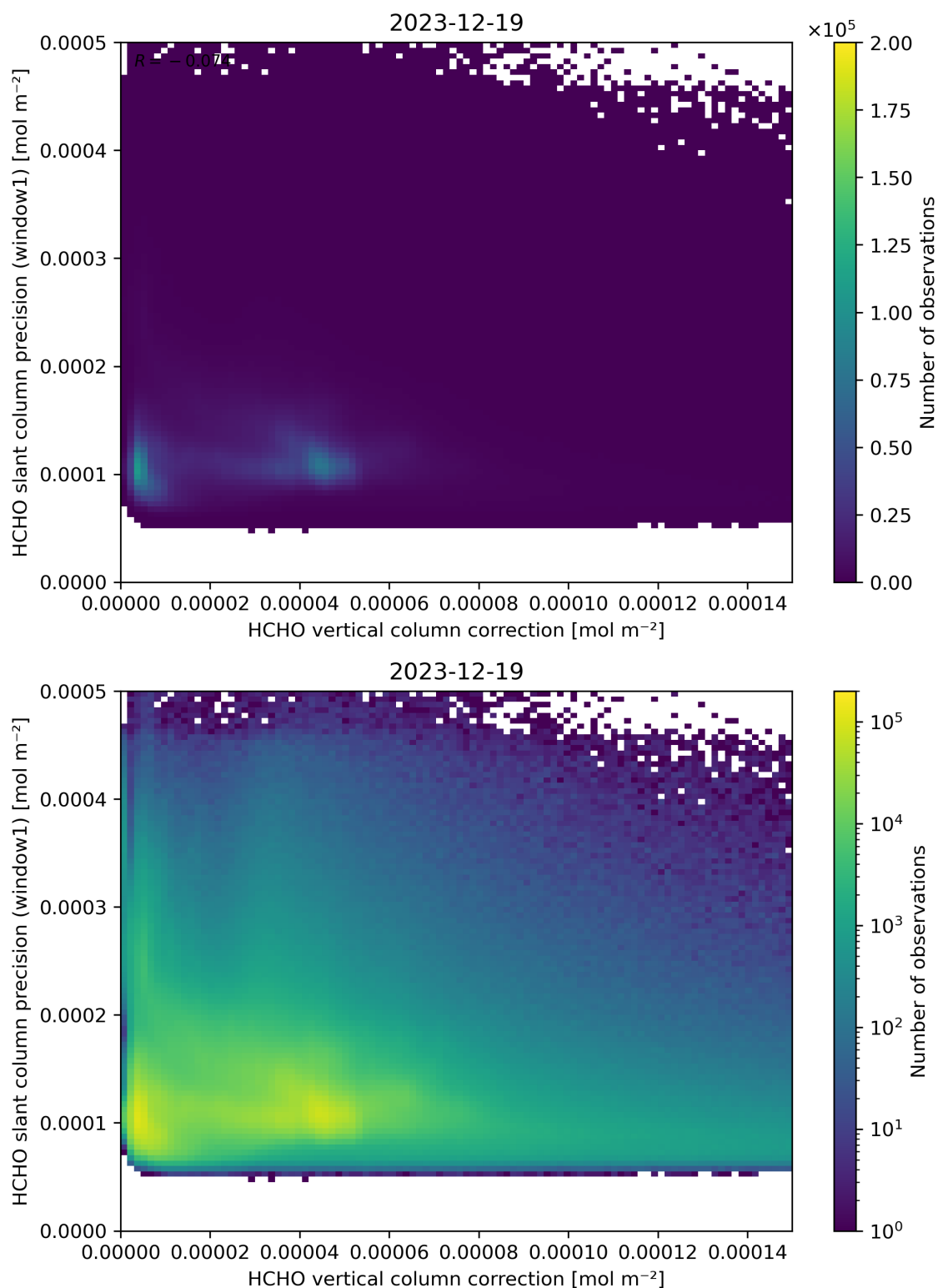
Figure 119: Scatter density plot of “HCHO vertical column correction” against “HCHO slant column precision (window1)” for 2023-12-18 to 2023-12-20.
