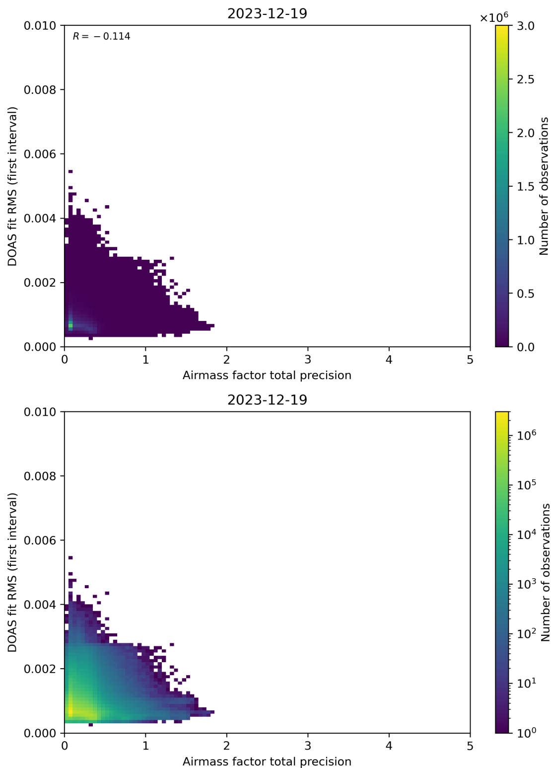
Figure 105: Scatter density plot of “Airmass factor total precision” against “DOAS fit RMS (first interval)” for 2023-12-18 to 2023-12-20.
