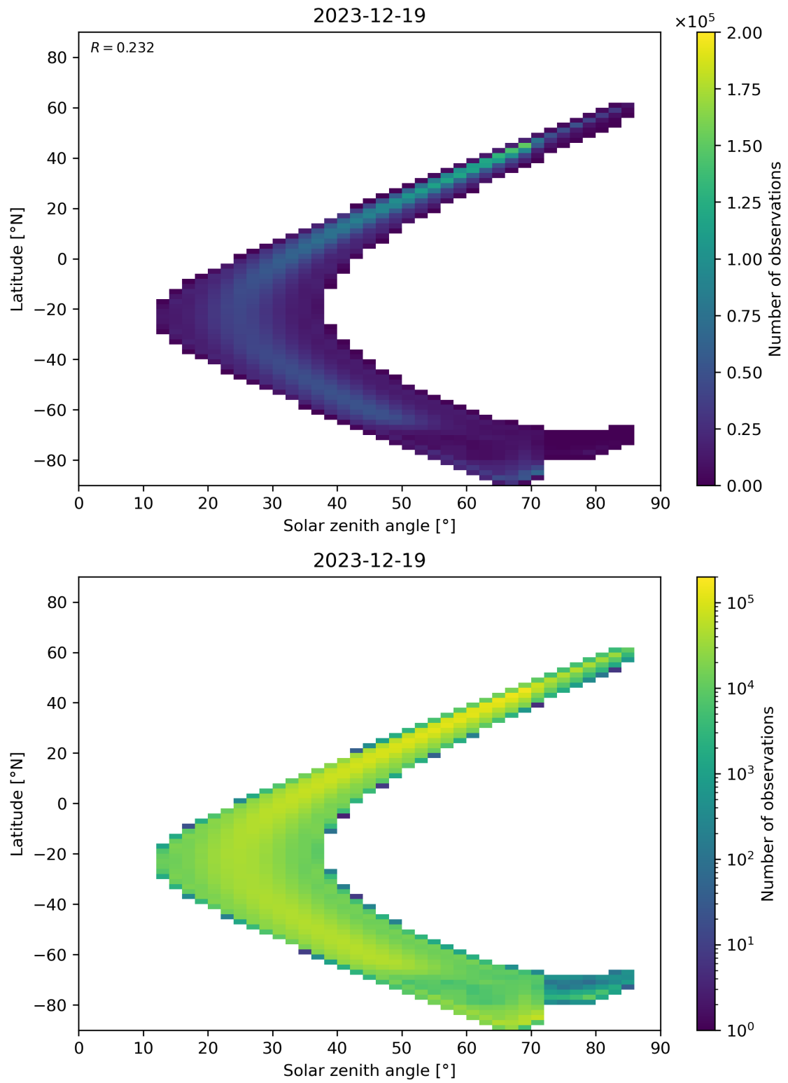
Figure 181: Scatter density plot of “Solar zenith angle” against “Latitude” for 2023-12-18 to 2023-12-20.
