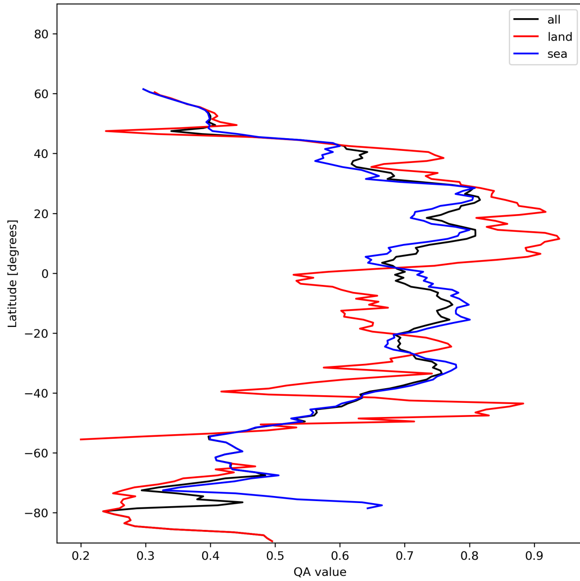
Figure 20: Zonal average of “QA value” for 2023-12-18 to 2023-12-20.
