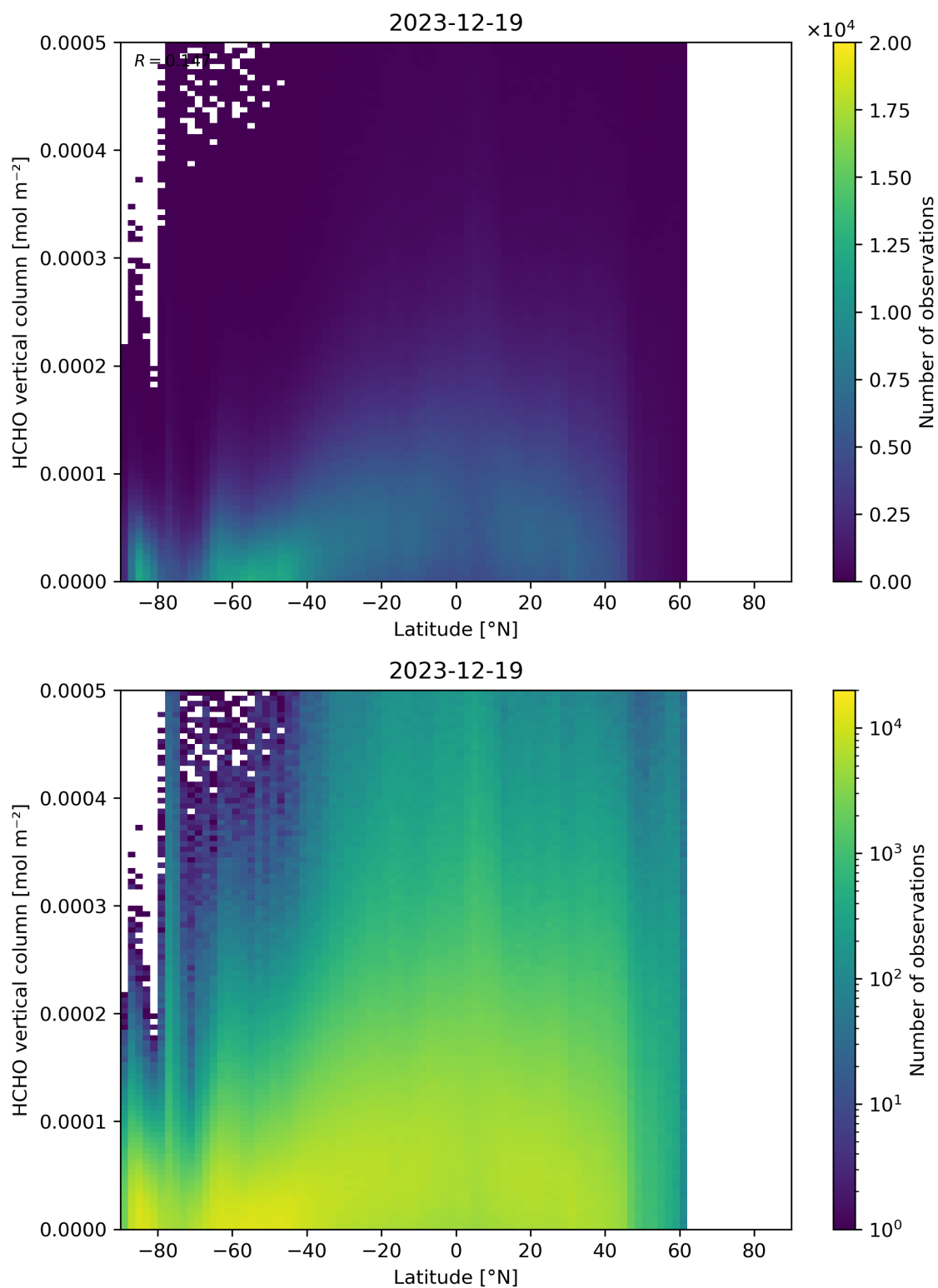
Figure 163: Scatter density plot of “Latitude” against “HCHO vertical column” for 2023-12-18 to 2023-12-20.
