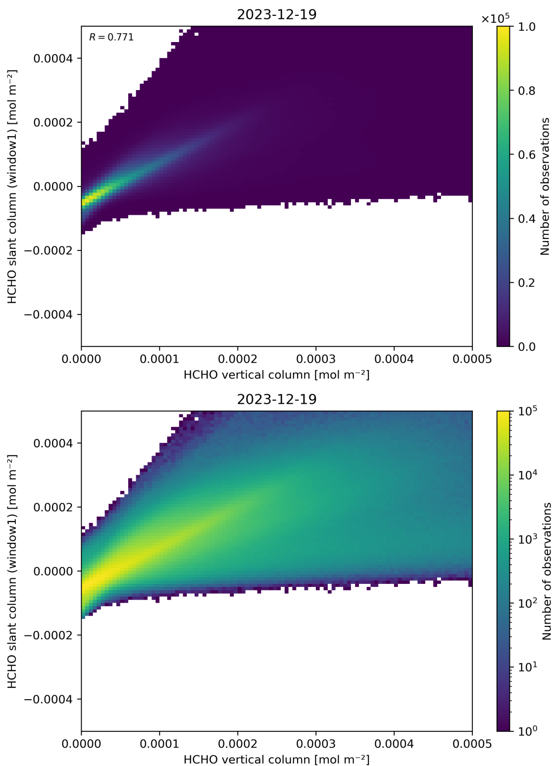
Figure 129: Scatter density plot of “HCHO vertical column” against “HCHO slant column (window1)” for 2023-12-18 to 2023-12-20.
