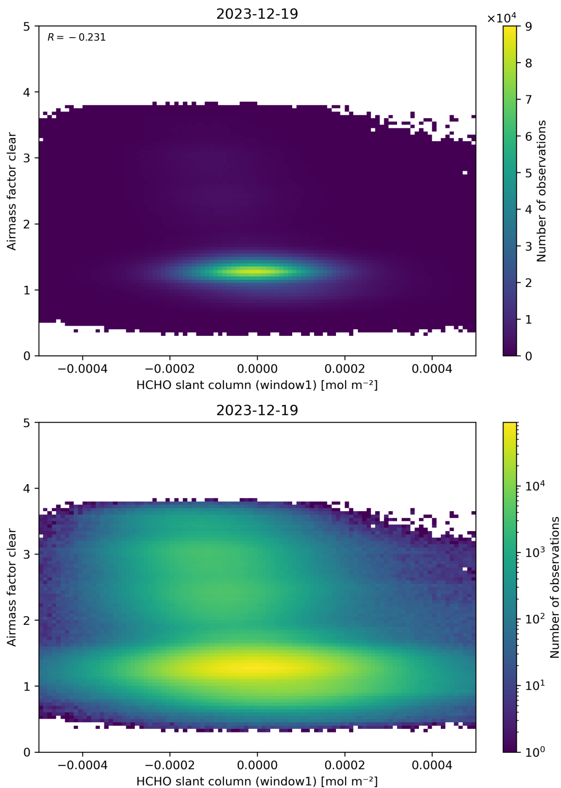
Figure 81: Scatter density plot of “HCHO slant column (window1)” against “Airmass factor clear” for 2023-12-18 to 2023-12-20.
