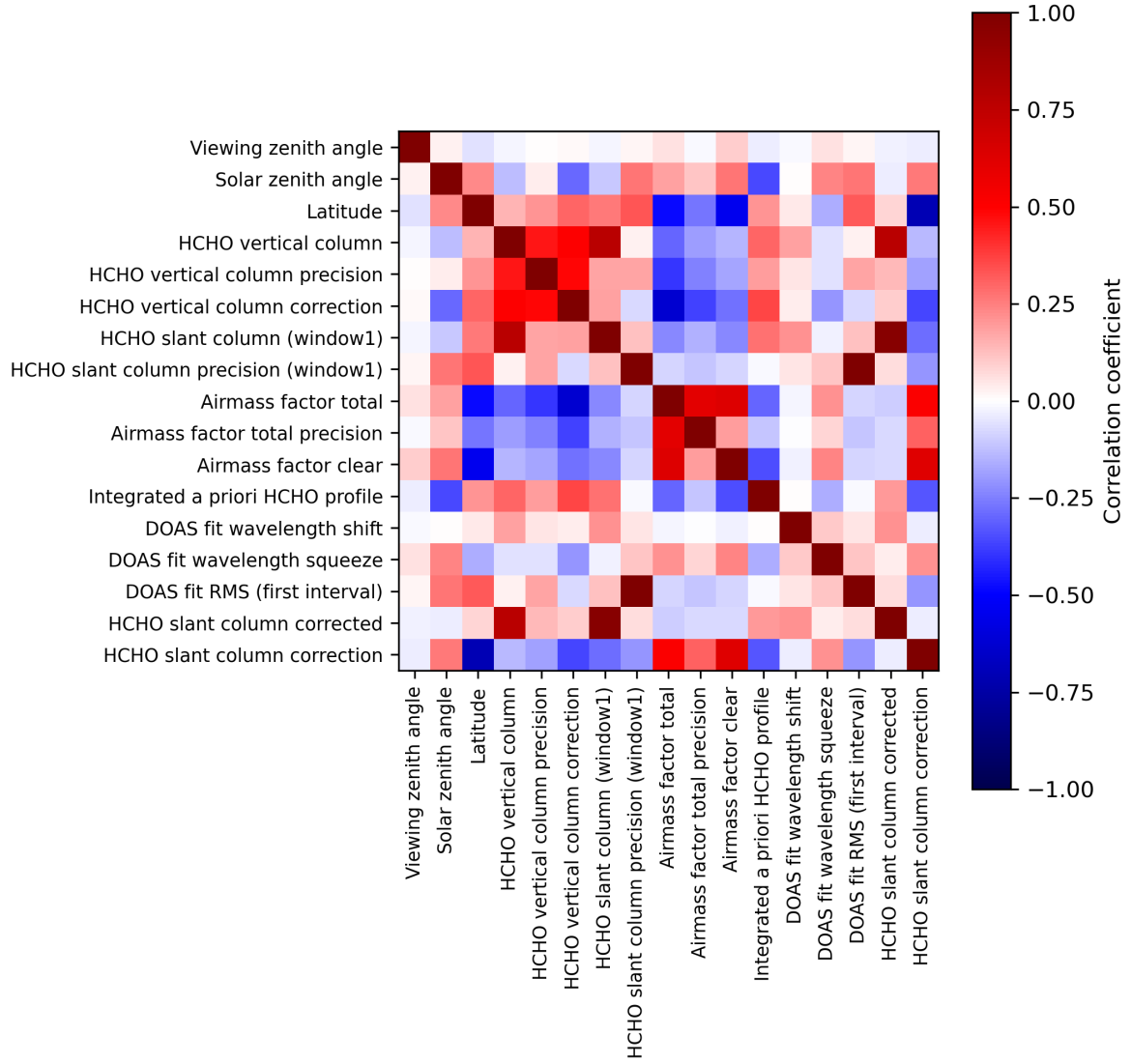
Figure 2: Map of correlation matrix for 2023-12-18 to 2023-12-20.
