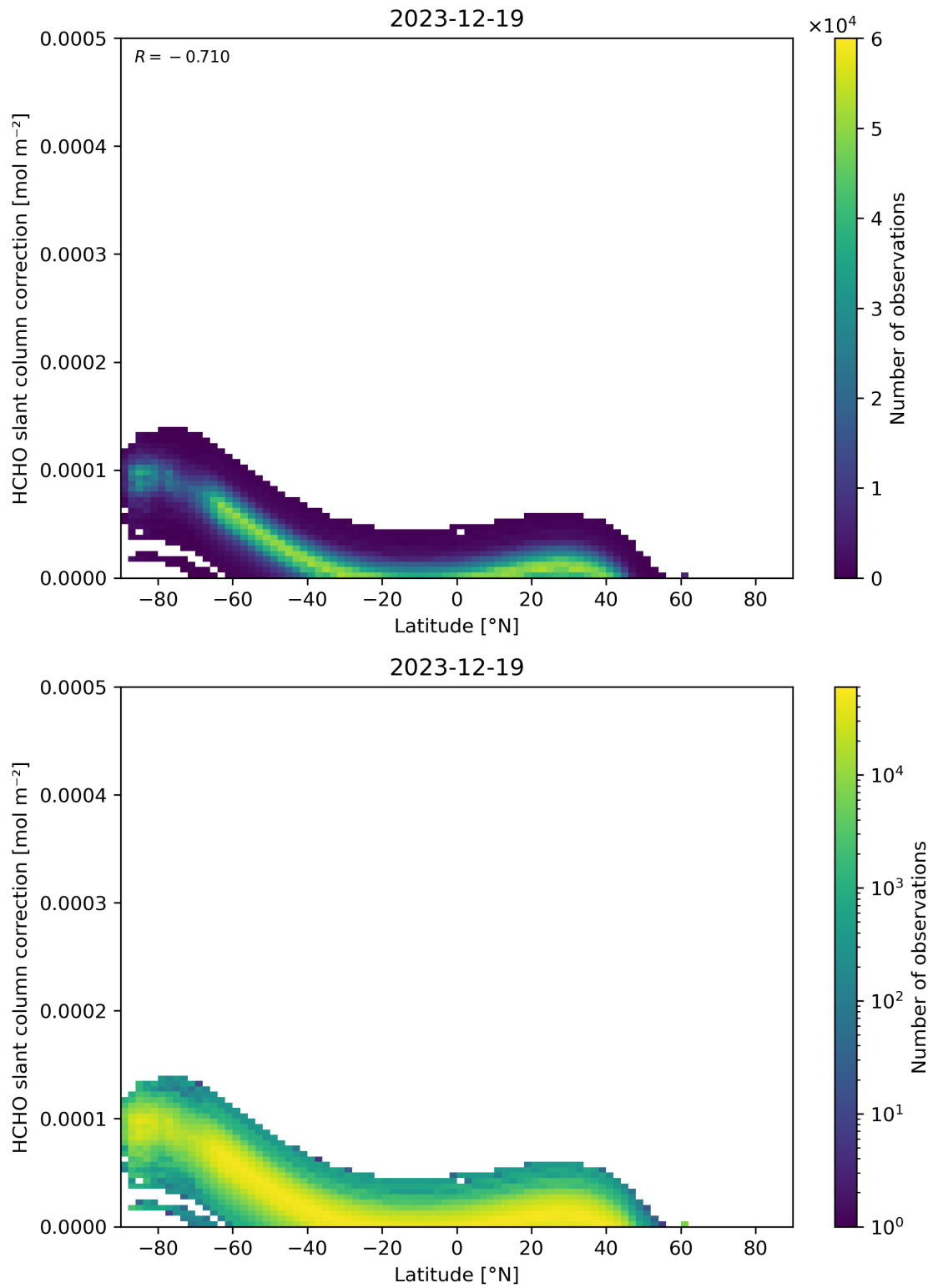
Figure 158: Scatter density plot of “Latitude” against “HCHO slant column correction” for 2023-12-18 to 2023-12-20.
