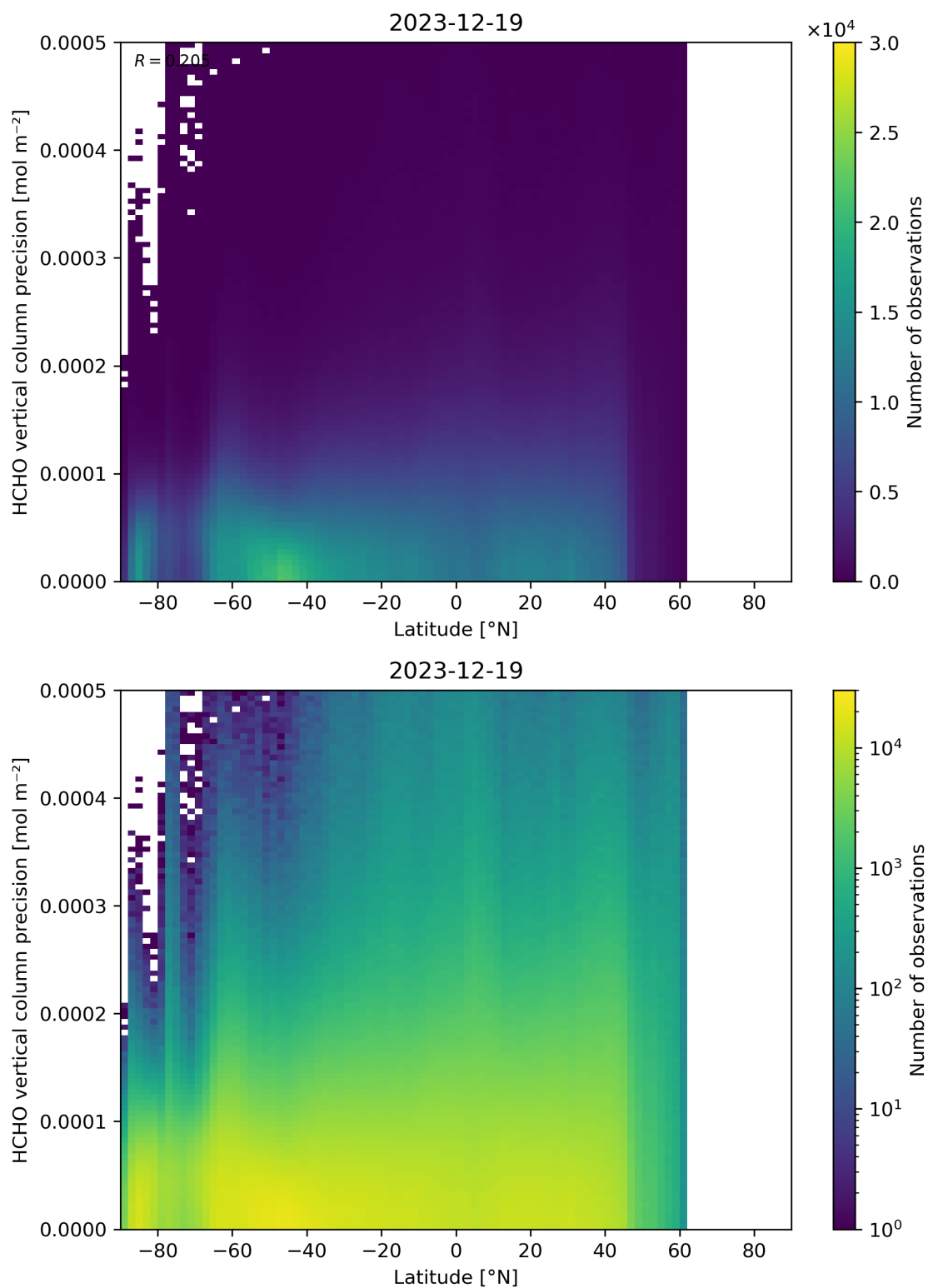
Figure 165: Scatter density plot of “Latitude” against “HCHO vertical column precision” for 2023-12-18 to 2023-12-20.
