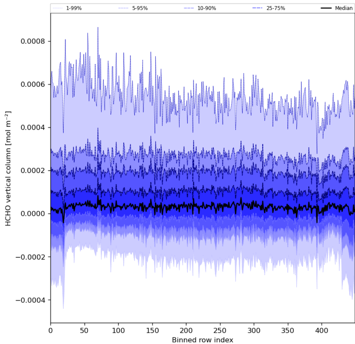
Figure 49: Along track statistics of "HCHO vertical column" for 2023-12-18 to 2023-12-20
