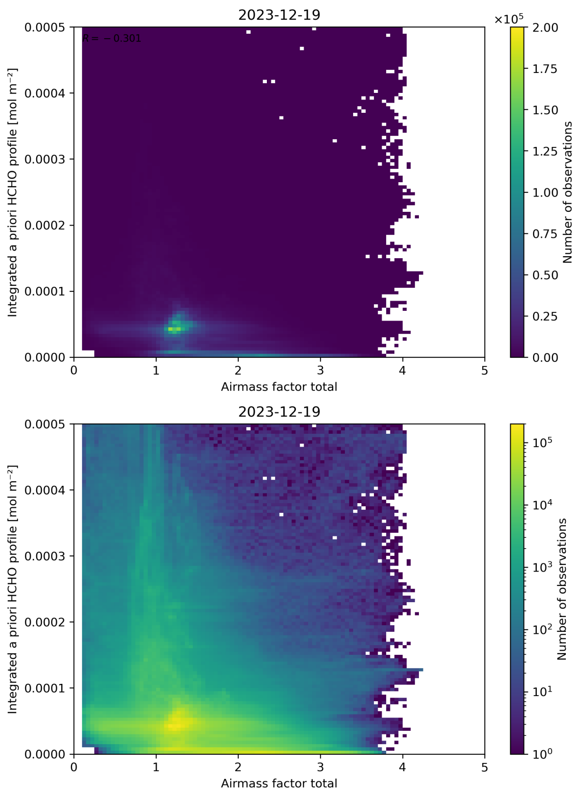
Figure 104: Scatter density plot of “Airmass factor total” against “Integrated a priori HCHO profile” for 2023-12-18 to 2023-12-20.
