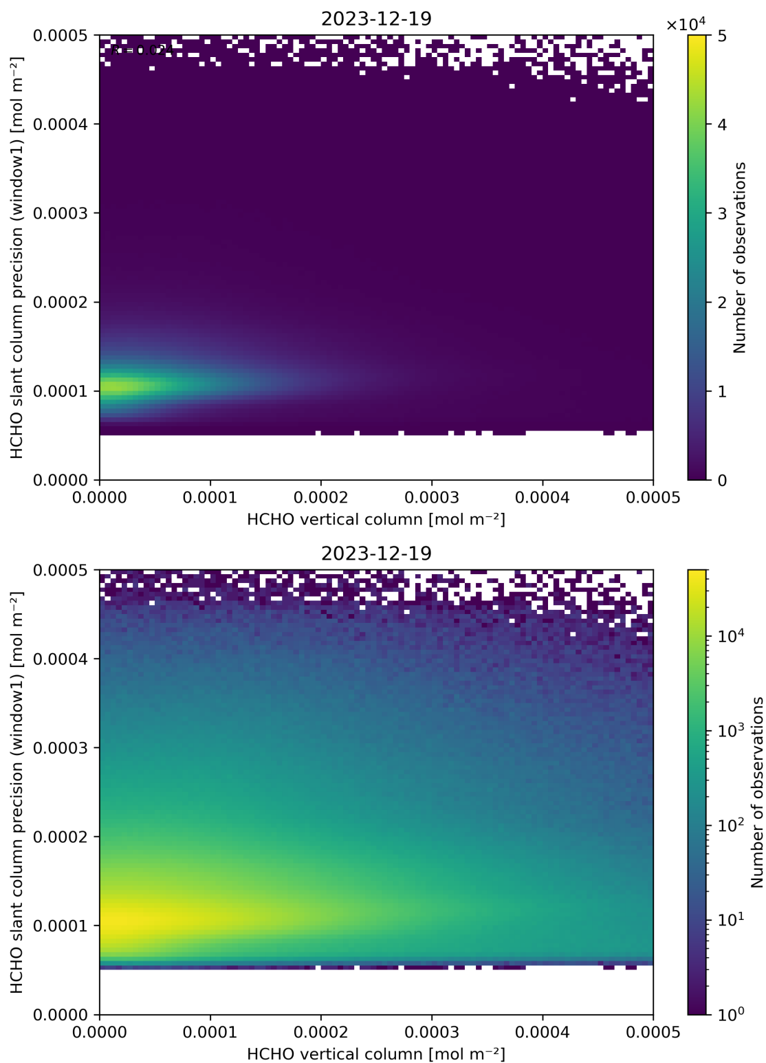
Figure 130: Scatter density plot of “HCHO vertical column” against “HCHO slant column precision (window1)” for 2023-12-18 to 2023-12-20.
