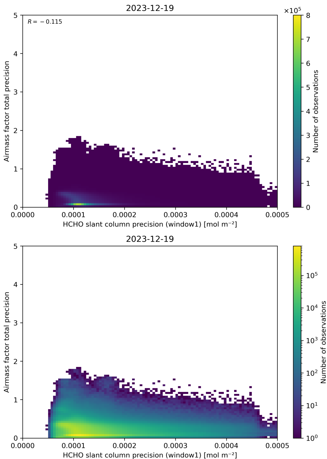
Figure 95: Scatter density plot of “HCHO slant column precision (window1)” against “Airmass factor total precision” for 2023-12-18 to 2023-12-20.
