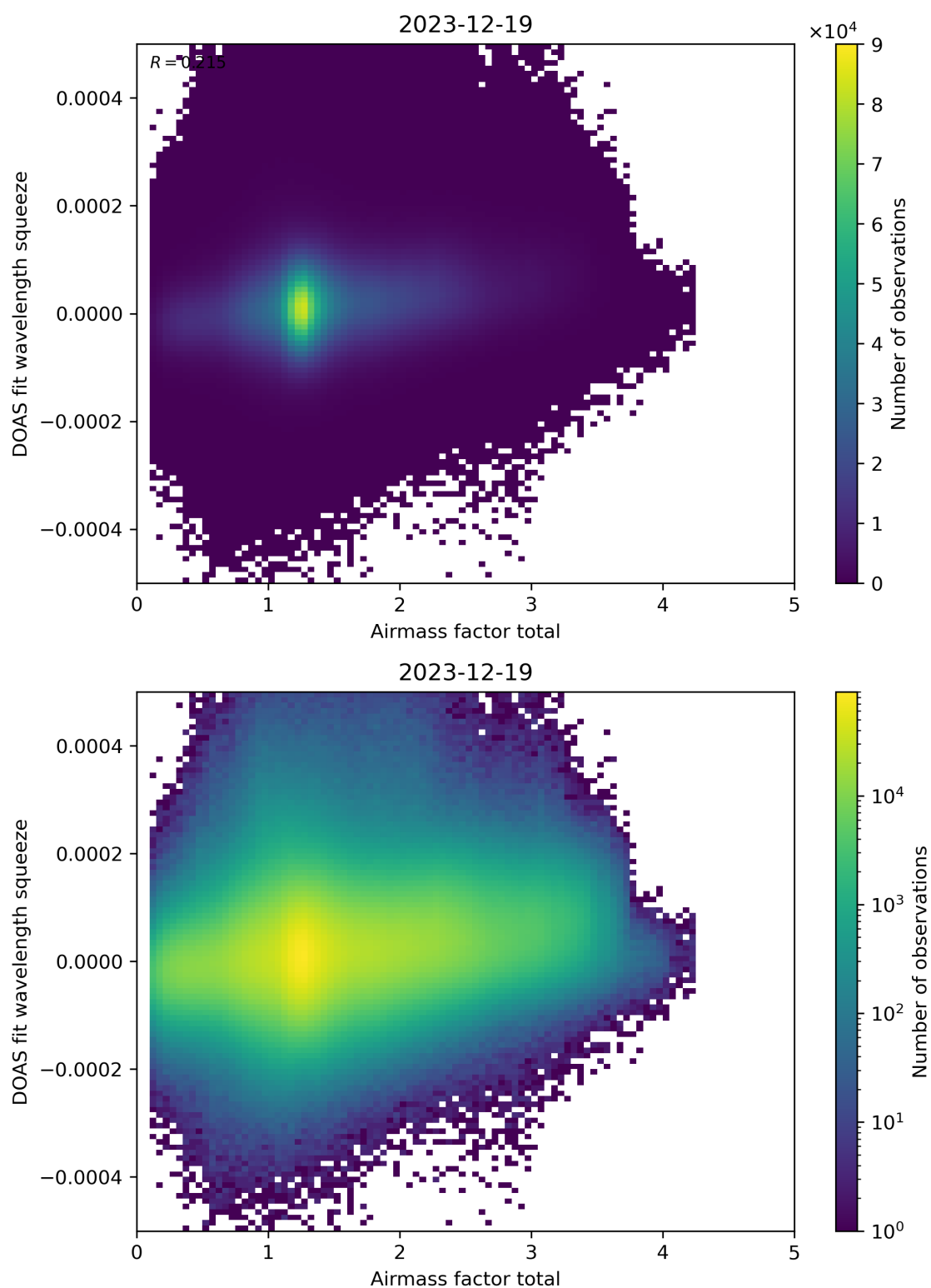
Figure 99: Scatter density plot of “Airmass factor total” against “DOAS fit wavelength squeeze” for 2023-12-18 to 2023-12-20.
