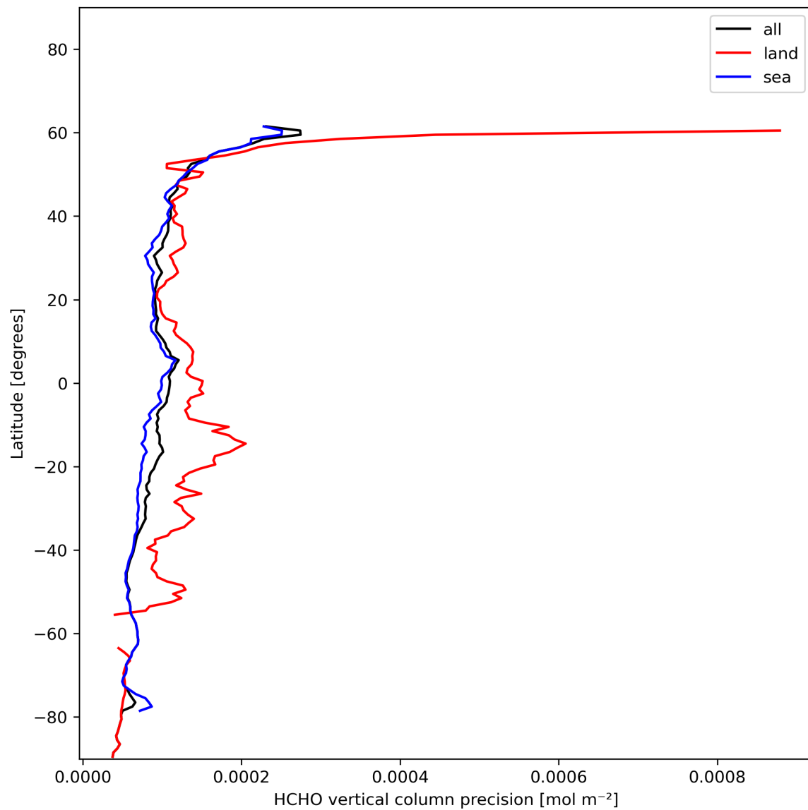
Figure 22: Zonal average of “HCHO vertical column precision” for 2023-12-18 to 2023-12-20.
