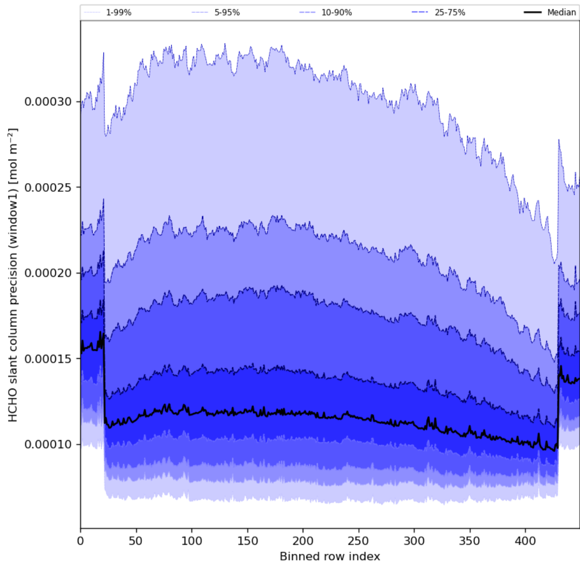
Figure 53: Along track statistics of “HCHO slant column precision (window1)” for 2023-12-18 to 2023-12-20
