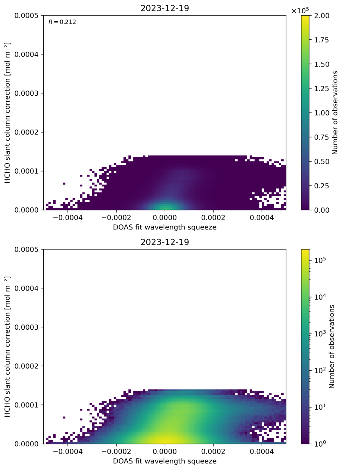
Figure 70: Scatter density plot of “DOAS fit wavelength squeeze” against “HCHO slant column correction” for 2023-12-18 to 2023-12-20.
