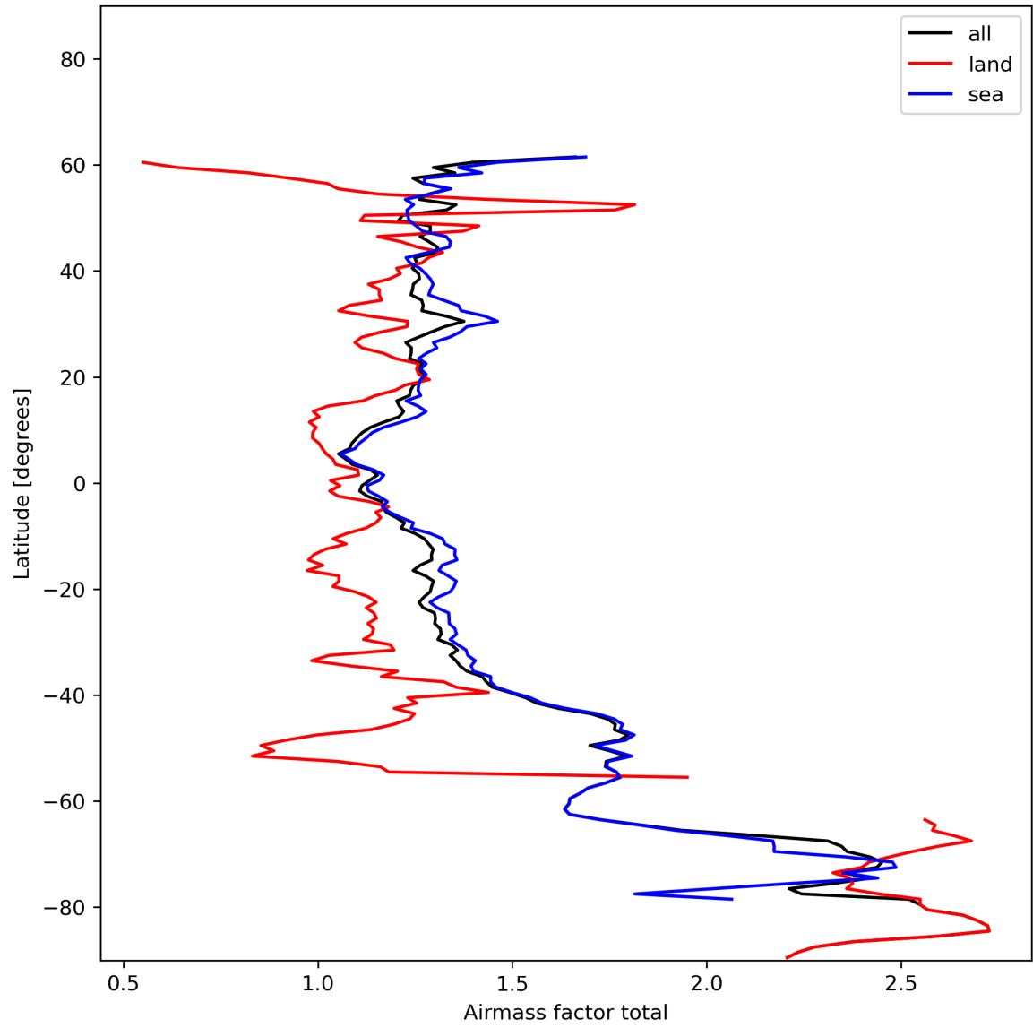
Figure 26: Zonal average of “Airmass factor total” for 2023-12-18 to 2023-12-20.
