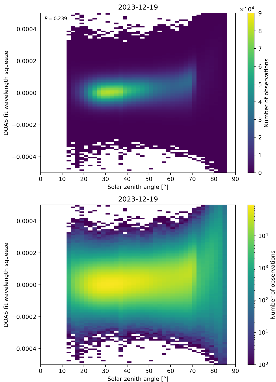
Figure 169: Scatter density plot of “Solar zenith angle” against “DOAS fit wavelength squeeze” for 2023-12-18 to 2023-12-20.
