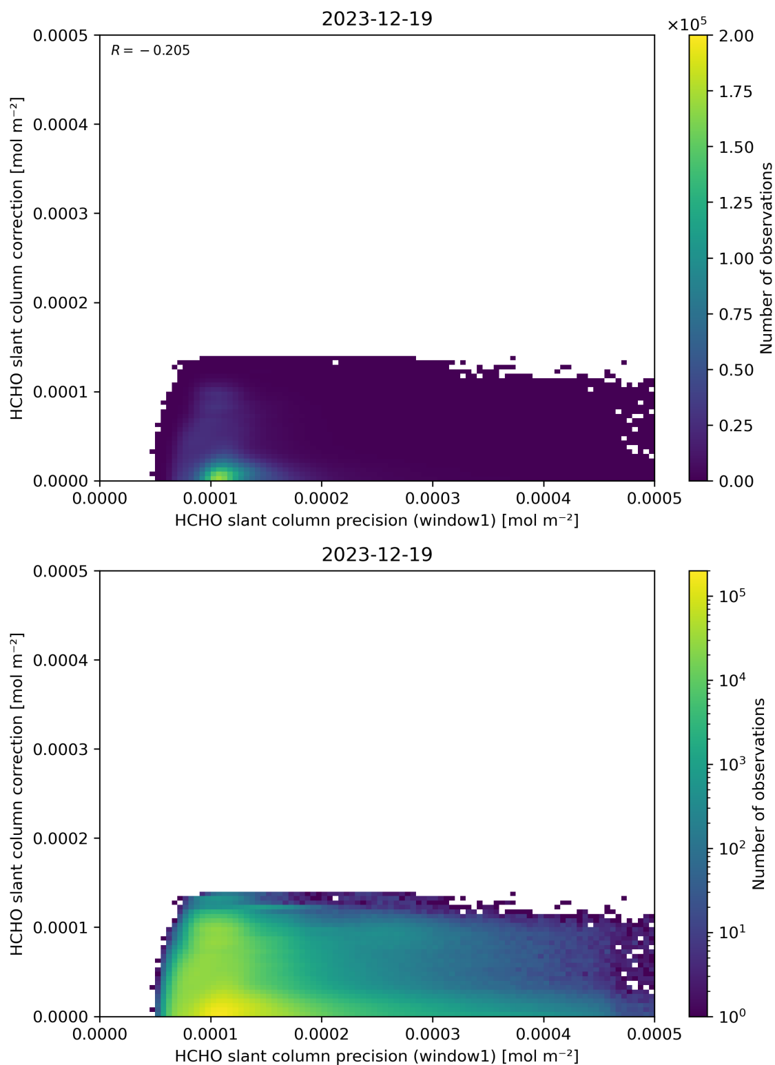
Figure 93: Scatter density plot of “HCHO slant column precision (window1)” against “HCHO slant column correction” for 2023-12-18 to 2023-12-20.
