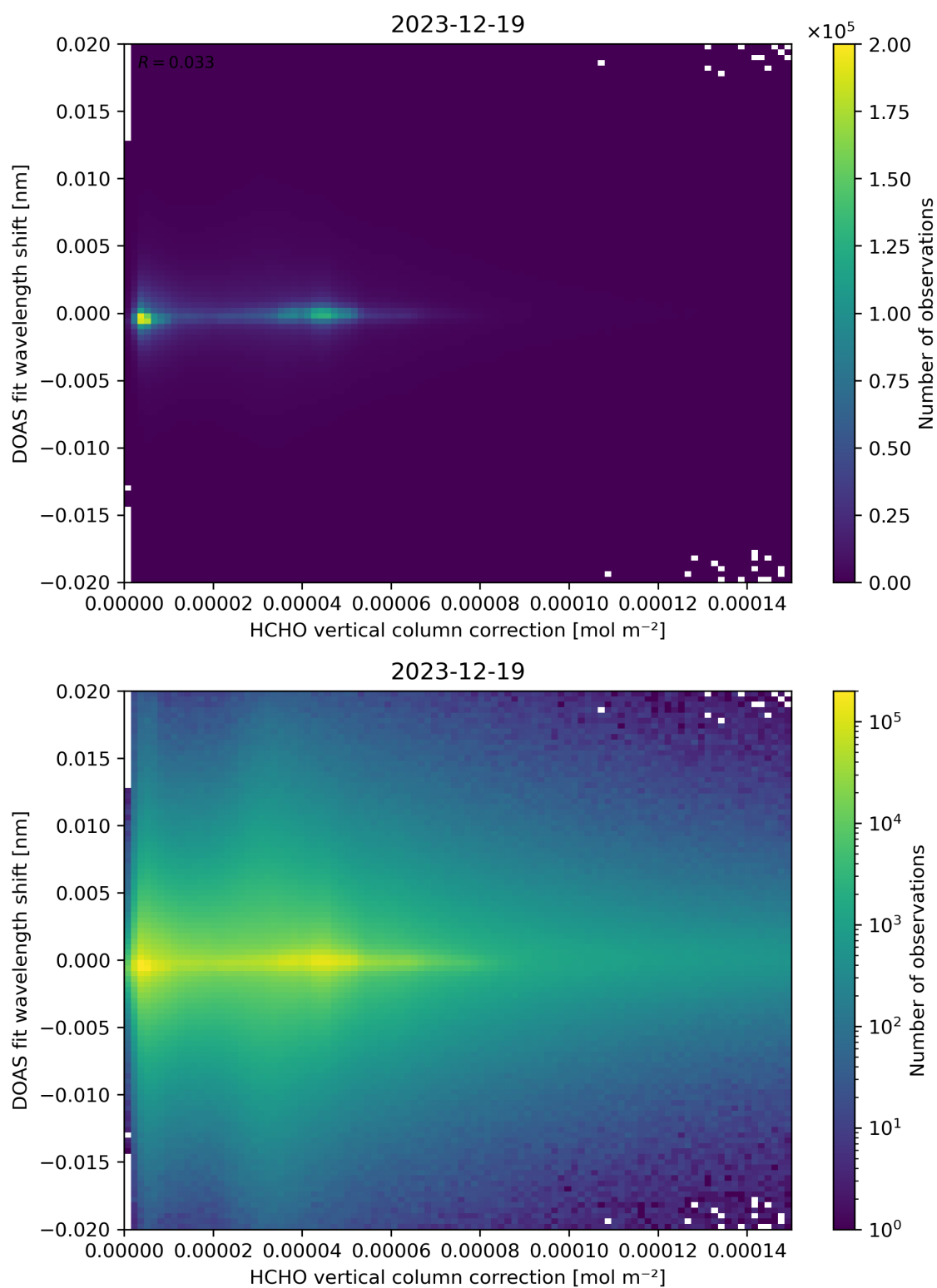
Figure 113: Scatter density plot of “HCHO vertical column correction” against “DOAS fit wavelength shift” for 2023-12-18 to 2023-12-20.
