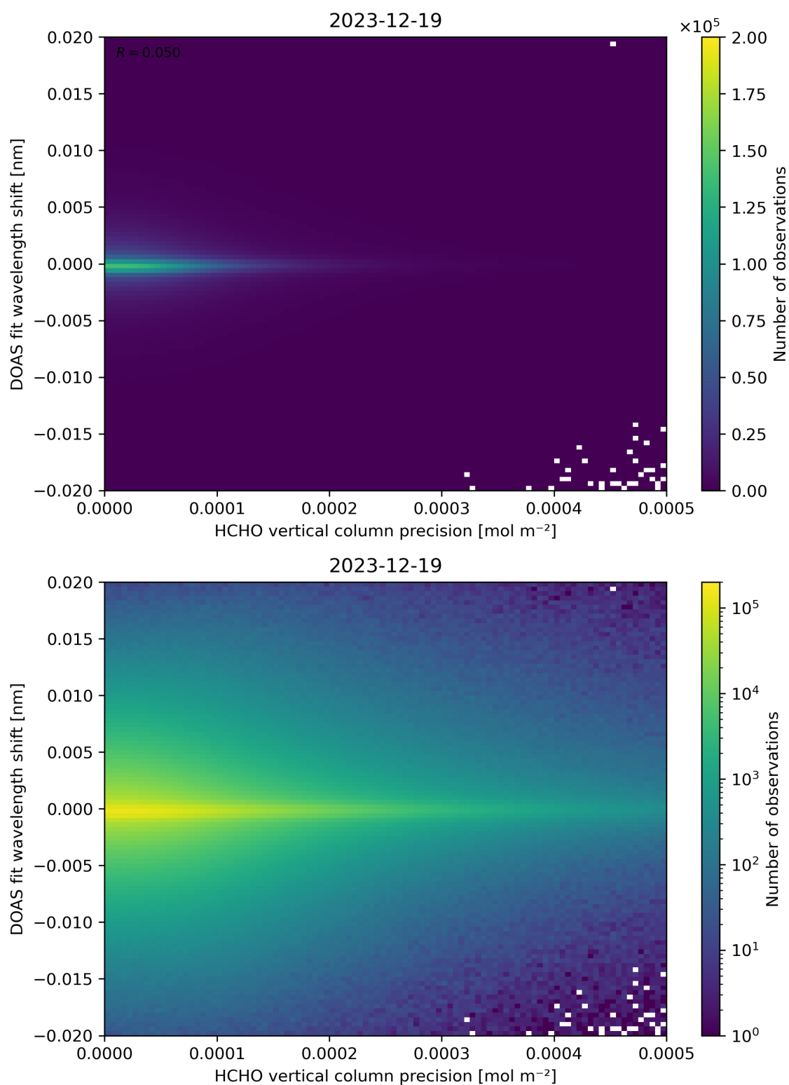
Figure 137: Scatter density plot of “HCHO vertical column precision” against “DOAS fit wavelength shift” for 2023-12-18 to 2023-12-20.
