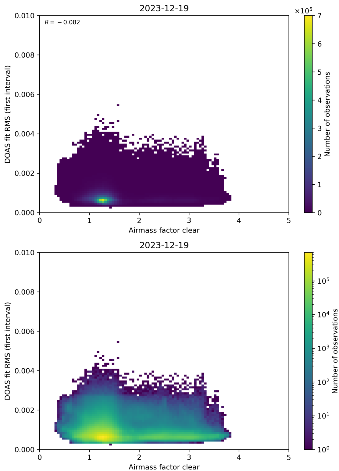
Figure 71: Scatter density plot of “Airmass factor clear” against “DOAS fit RMS (first interval)” for 2023-12-18 to 2023-12-20.
