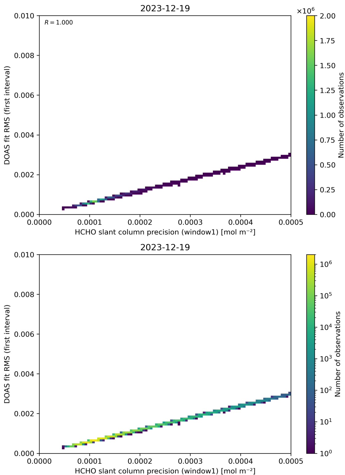
Figure 88: Scatter density plot of “HCHO slant column precision (window1)” against “DOAS fit RMS (first interval)” for 2023-12-18 to 2023-12-20.
