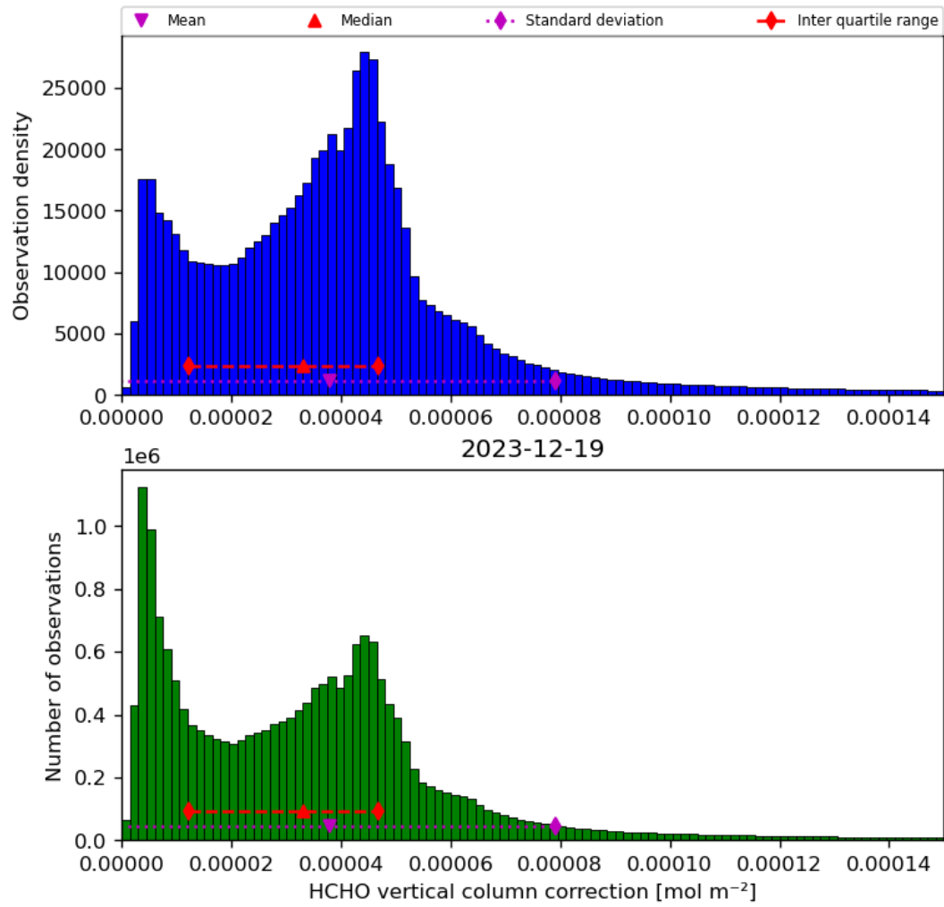
Figure 37: Histogram of “HCHO vertical column correction” for 2023-12-18 to 2023-12-20
