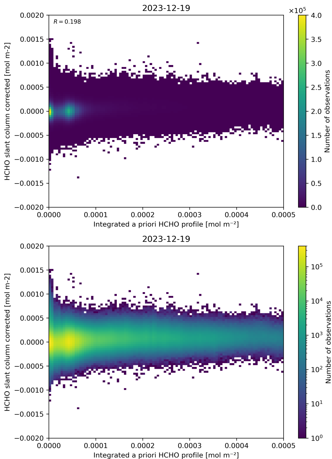
Figure 151: Scatter density plot of “Integrated a priori HCHO profile” against “HCHO slant column corrected” for 2023-12-18 to 2023-12-20.
