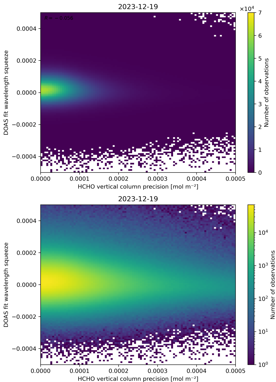
Figure 138: Scatter density plot of “HCHO vertical column precision” against “DOAS fit wavelength squeeze” for 2023-12-18 to 2023-12-20.
