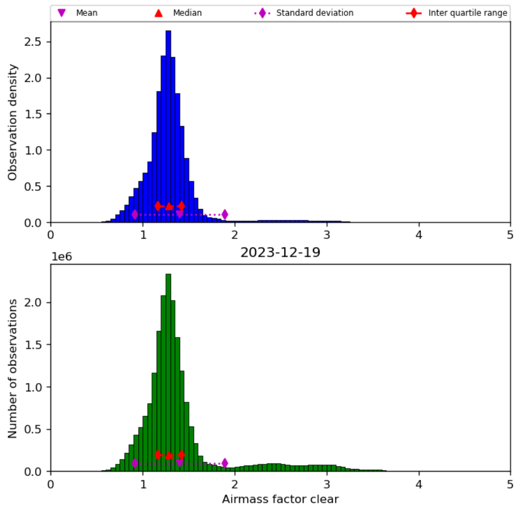
Figure 42: Histogram of “Airmass factor clear” for 2023-12-18 to 2023-12-20
