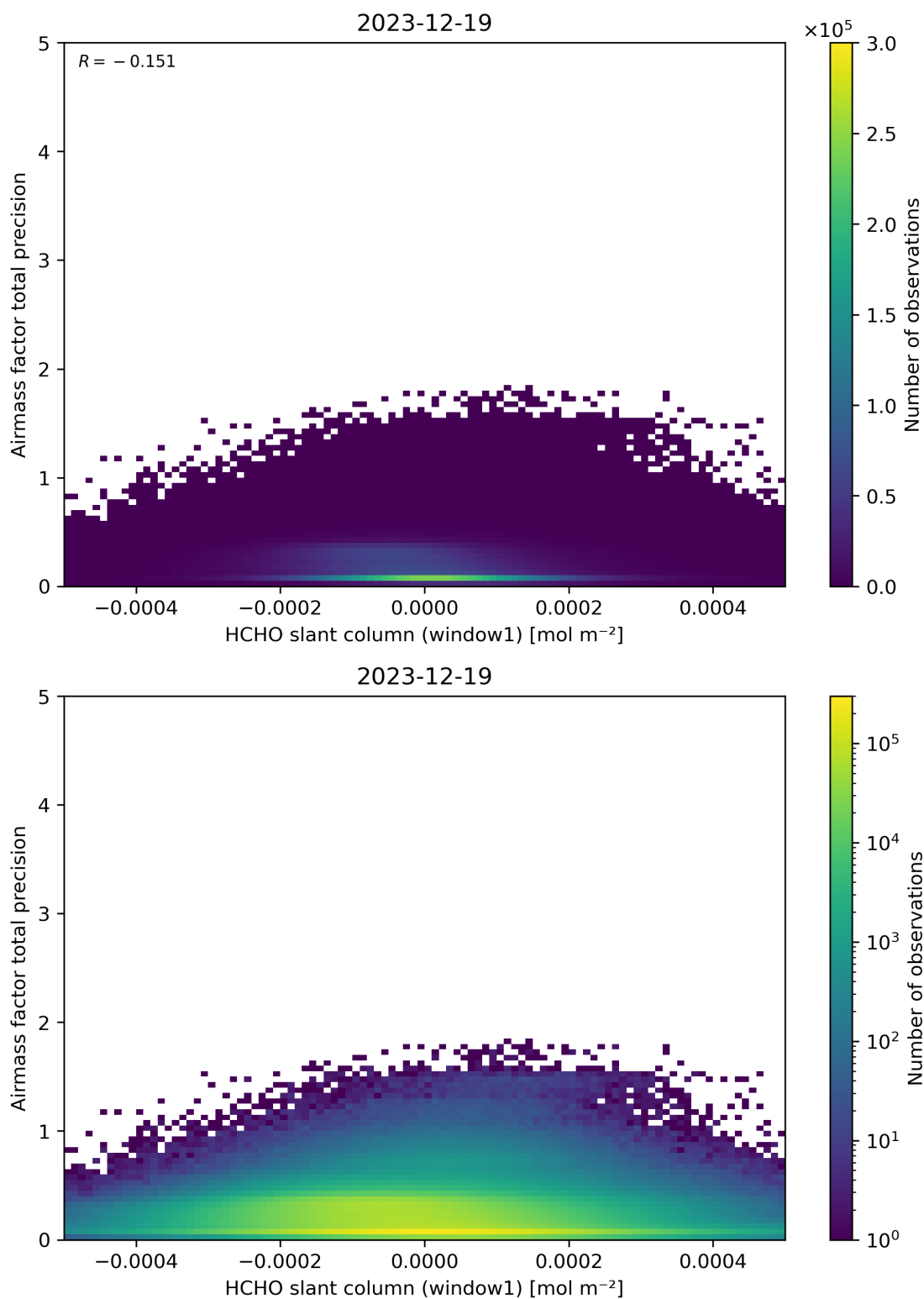
Figure 86: Scatter density plot of “HCHO slant column (window1)” against “Airmass factor total precision” for 2023-12-18 to 2023-12-20.
