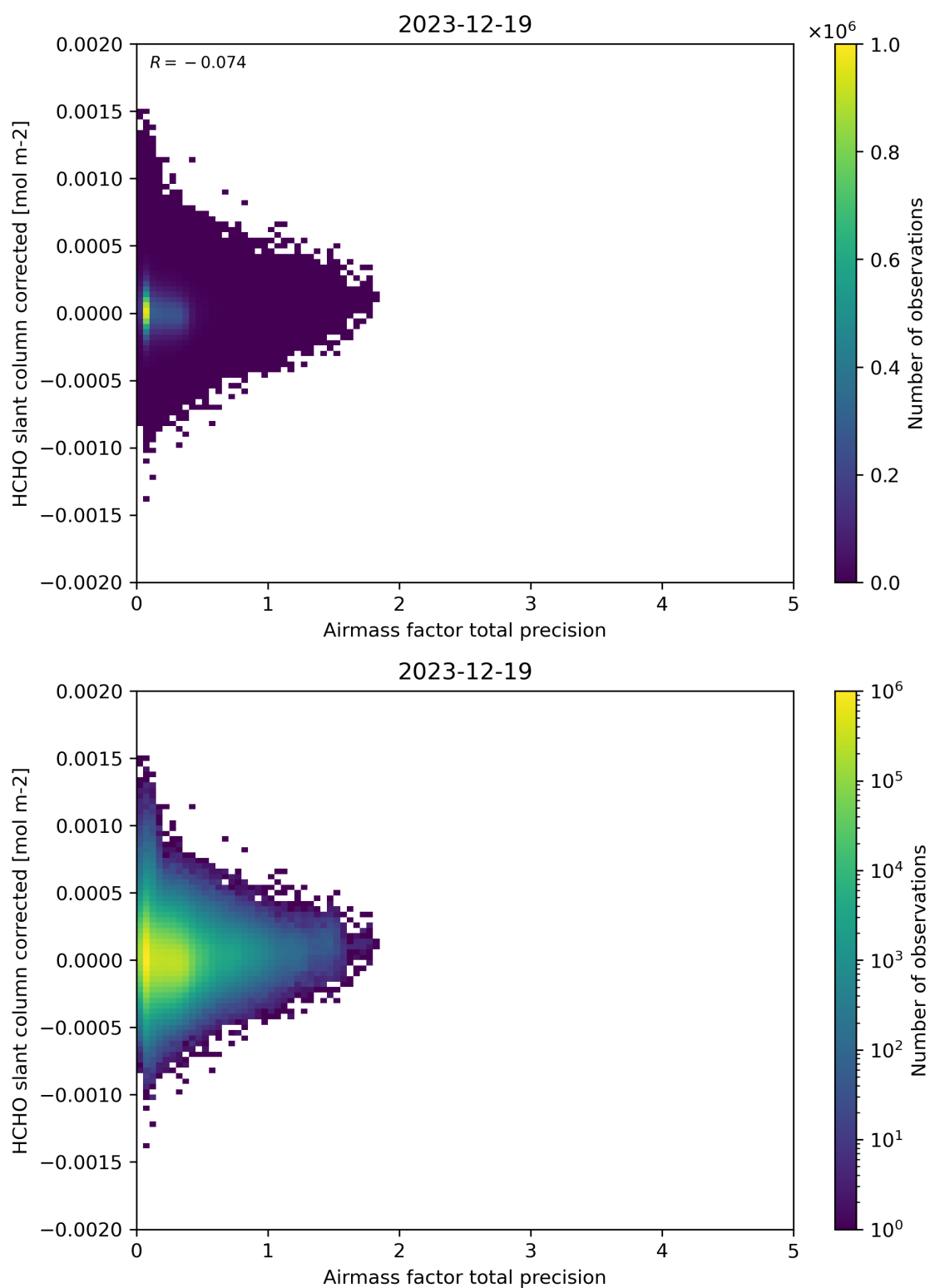
Figure 109: Scatter density plot of “Airmass factor total precision” against “HCHO slant column corrected” for 2023-12-18 to 2023-12-20.
