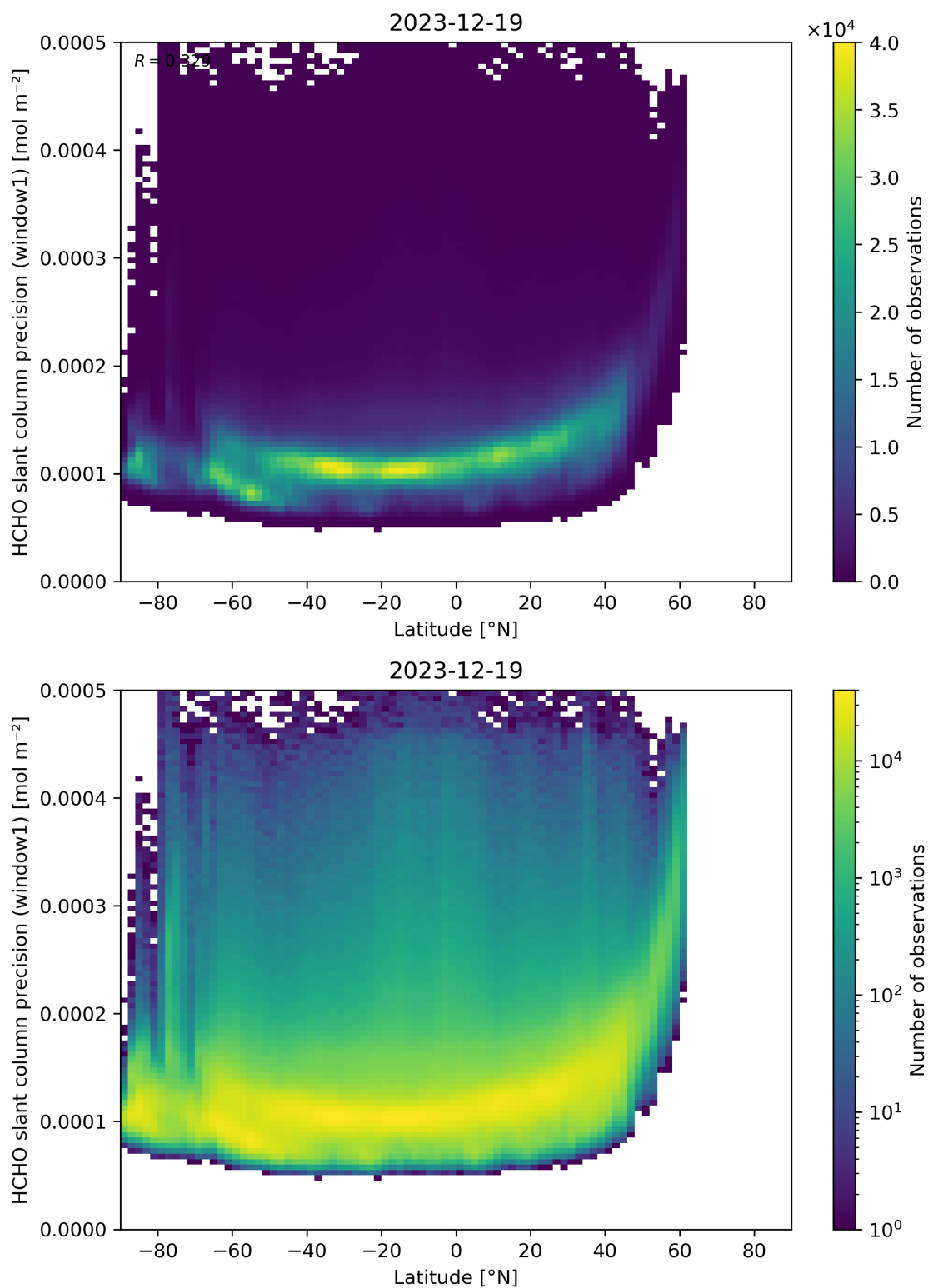
Figure 160: Scatter density plot of “Latitude” against “HCHO slant column precision (window1)” for 2023-12-18 to 2023-12-20.
