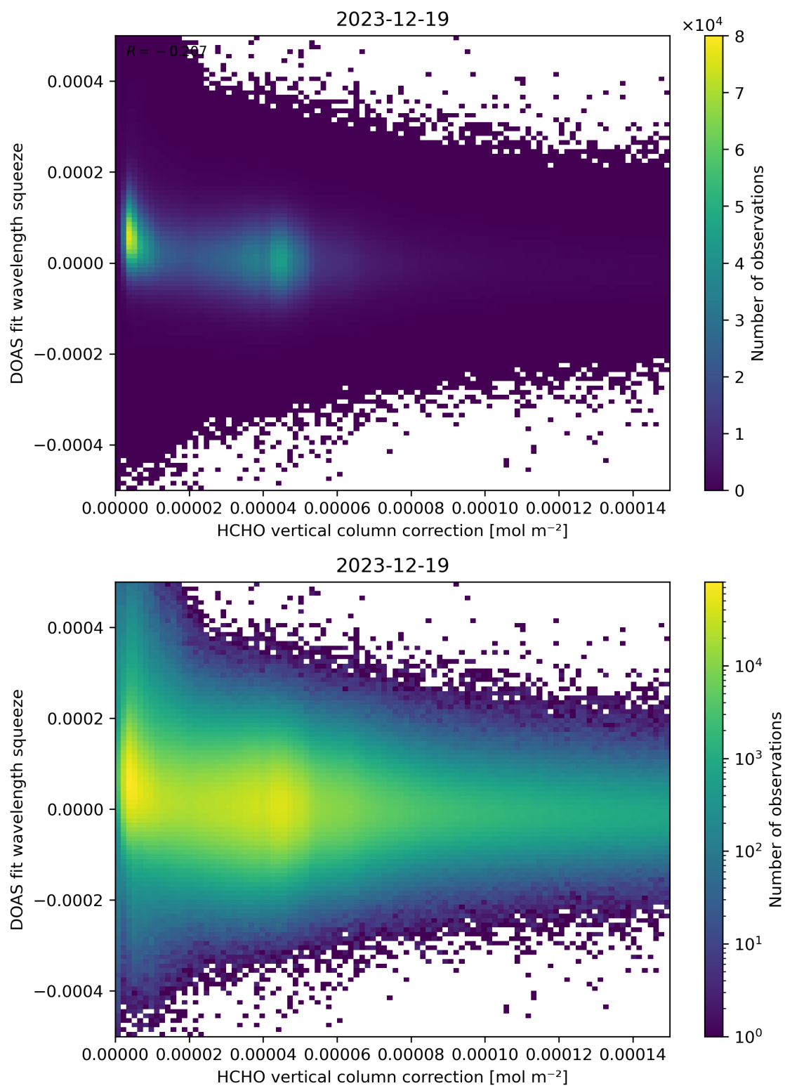
Figure 114: Scatter density plot of “HCHO vertical column correction” against “DOAS fit wavelength squeeze” for 2023-12-18 to 2023-12-20.
