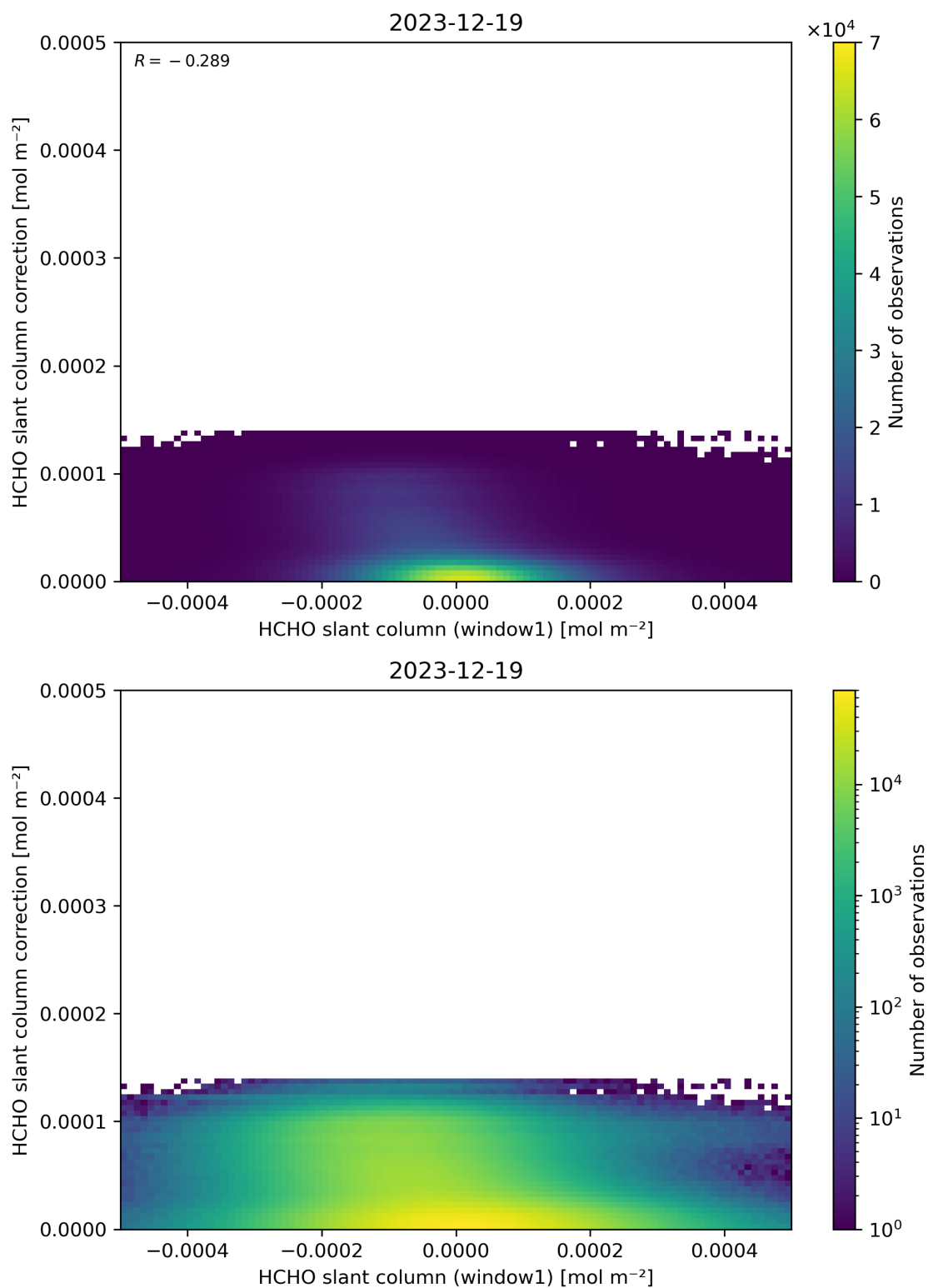
Figure 83: Scatter density plot of “HCHO slant column (window1)” against “HCHO slant column correction” for 2023-12-18 to 2023-12-20.
