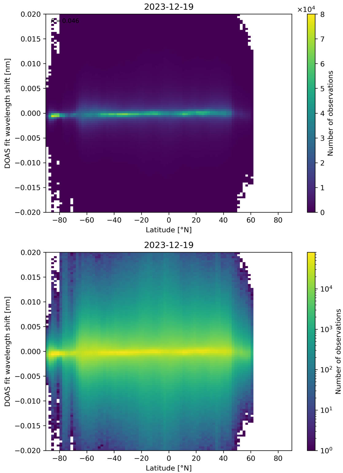
Figure 154: Scatter density plot of “Latitude” against “DOAS fit wavelength shift” for 2023-12-18 to 2023-12-20.
