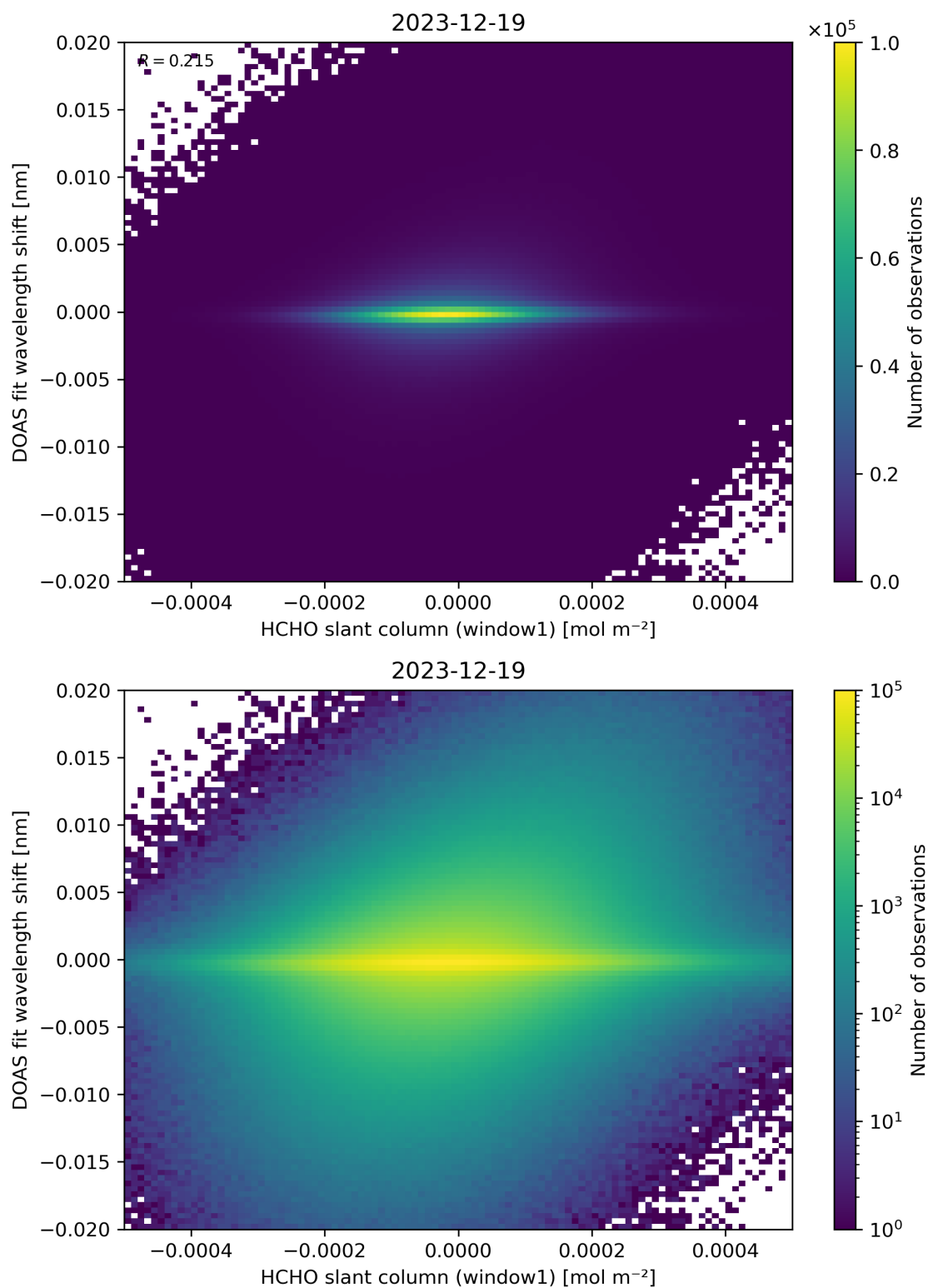
Figure 79: Scatter density plot of “HCHO slant column (window1)” against “DOAS fit wavelength shift” for 2023-12-18 to 2023-12-20.
