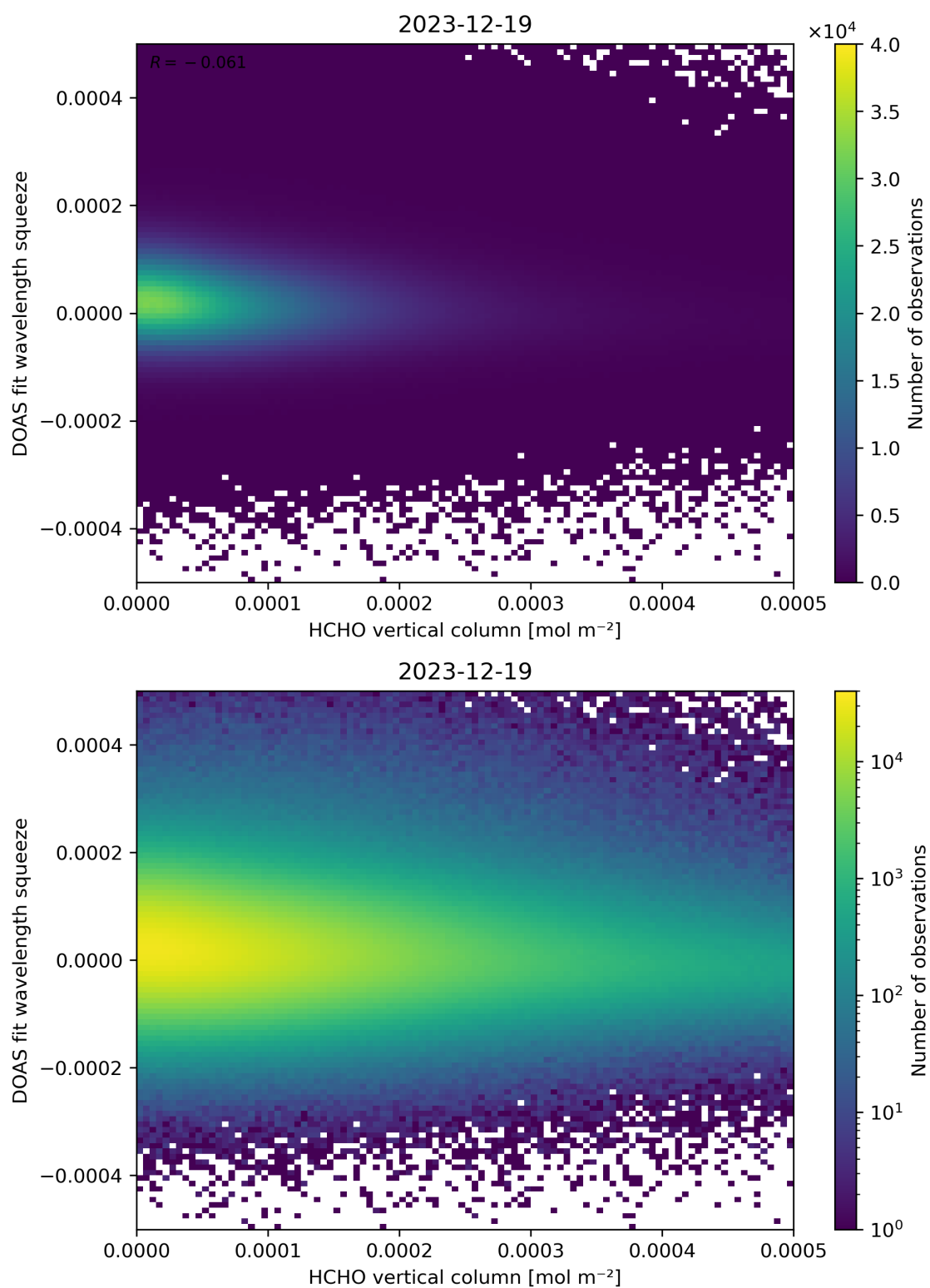
Figure 125: Scatter density plot of “HCHO vertical column” against “DOAS fit wavelength squeeze” for 2023-12-18 to 2023-12-20.
