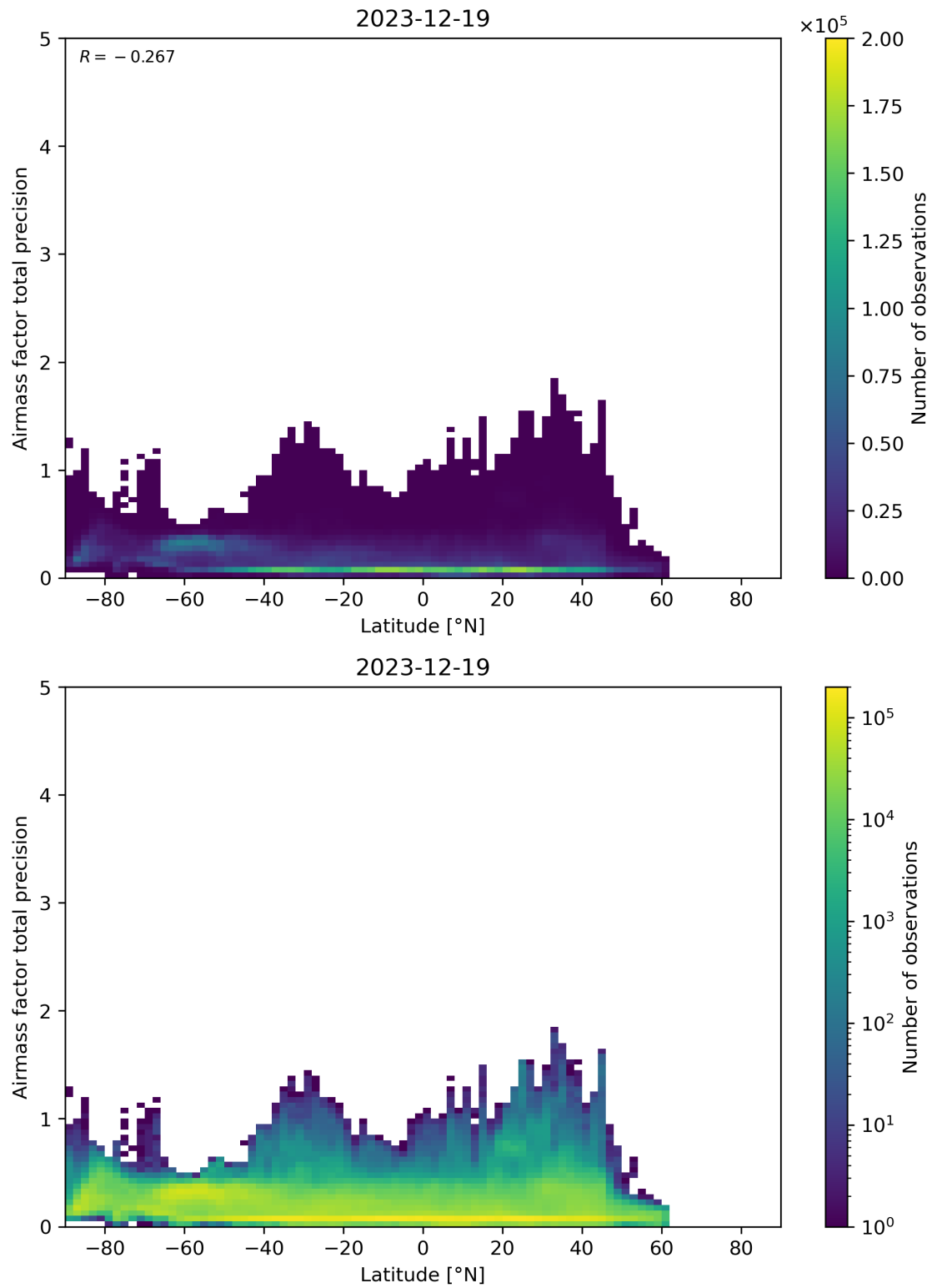
Figure 162: Scatter density plot of “Latitude” against “Airmass factor total precision” for 2023-12-18 to 2023-12-20.
