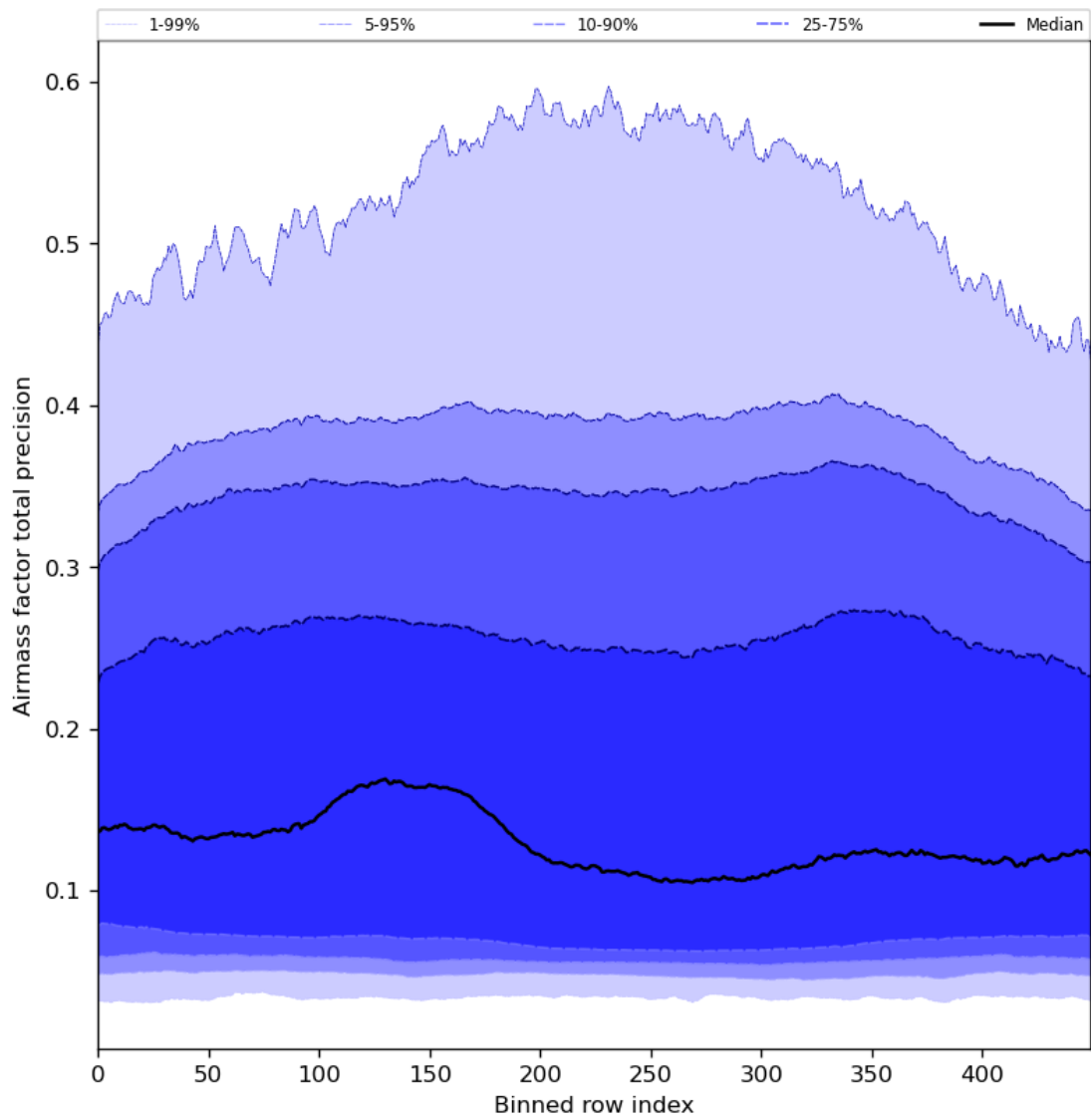
Figure 55: Along track statistics of “Airmass factor total precision” for 2023-12-18 to 2023-12-20
