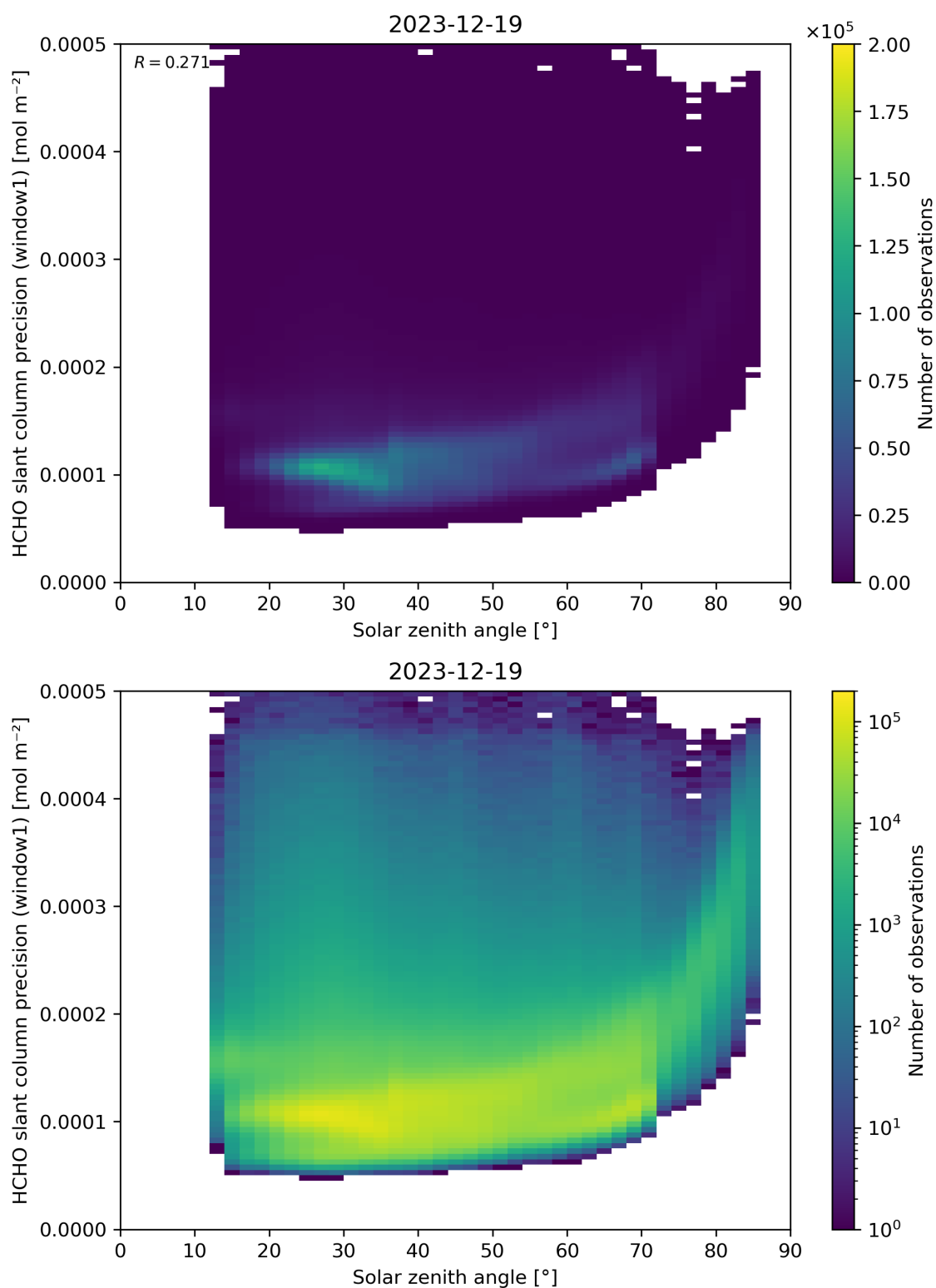
Figure 174: Scatter density plot of “Solar zenith angle” against “HCHO slant column precision (window1)” for 2023-12-18 to 2023-12-20.
