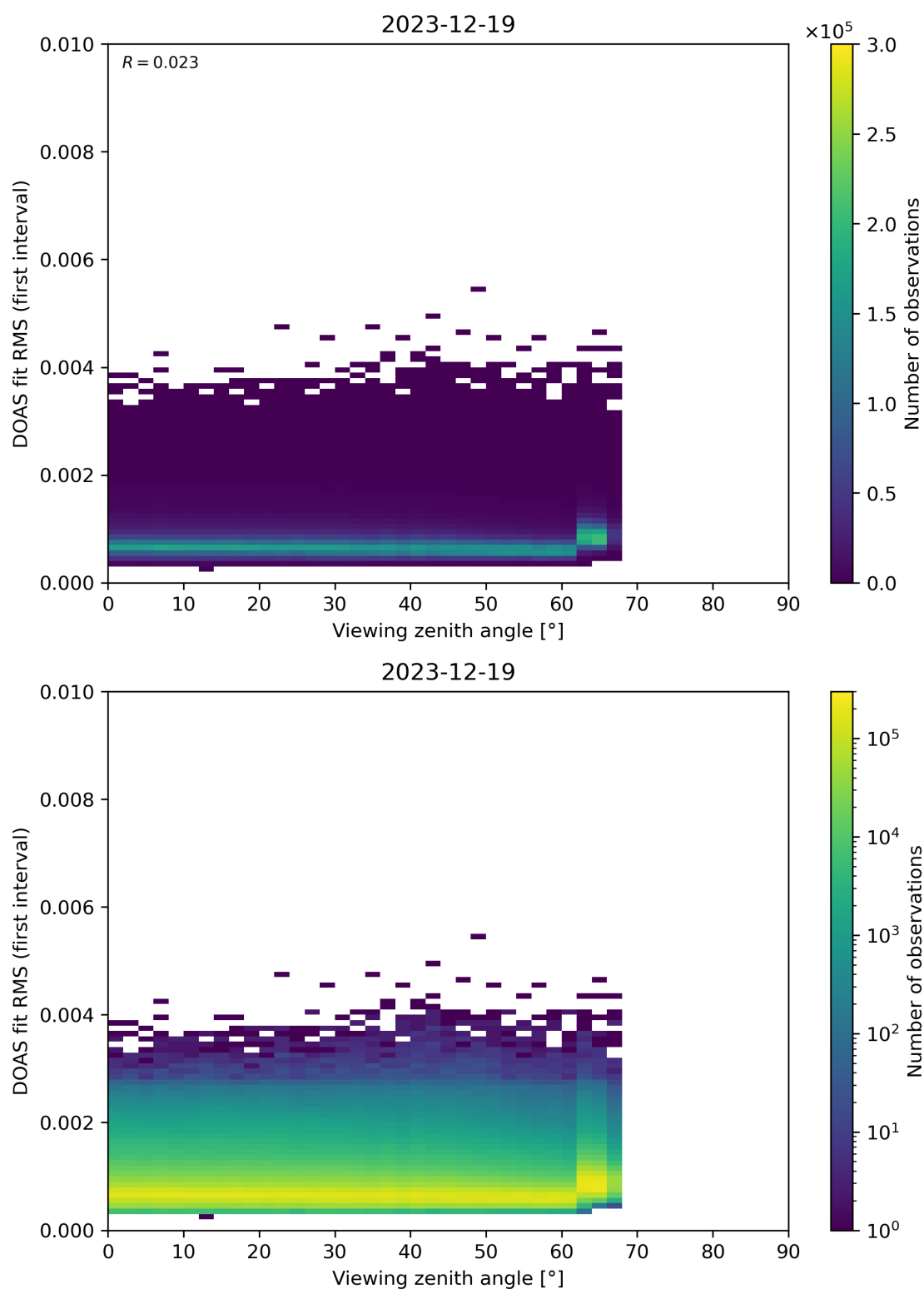
Figure 182: Scatter density plot of “Viewing zenith angle” against “DOAS fit RMS (first interval)” for 2023-12-18 to 2023-12-20.
