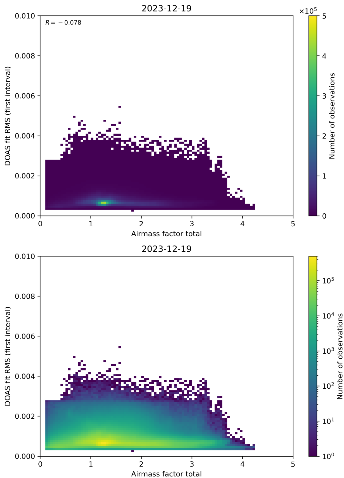
Figure 97: Scatter density plot of “Airmass factor total” against “DOAS fit RMS (first interval)” for 2023-12-18 to 2023-12-20.
