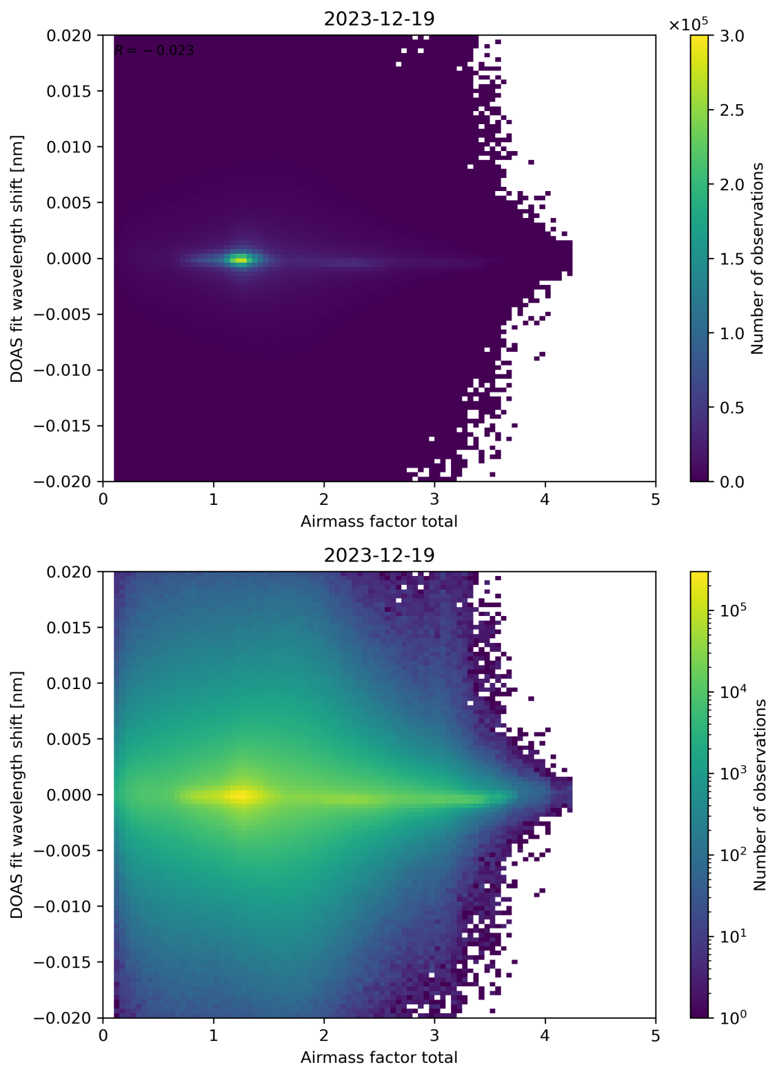
Figure 98: Scatter density plot of “Airmass factor total” against “DOAS fit wavelength shift” for 2023-12-18 to 2023-12-20.
