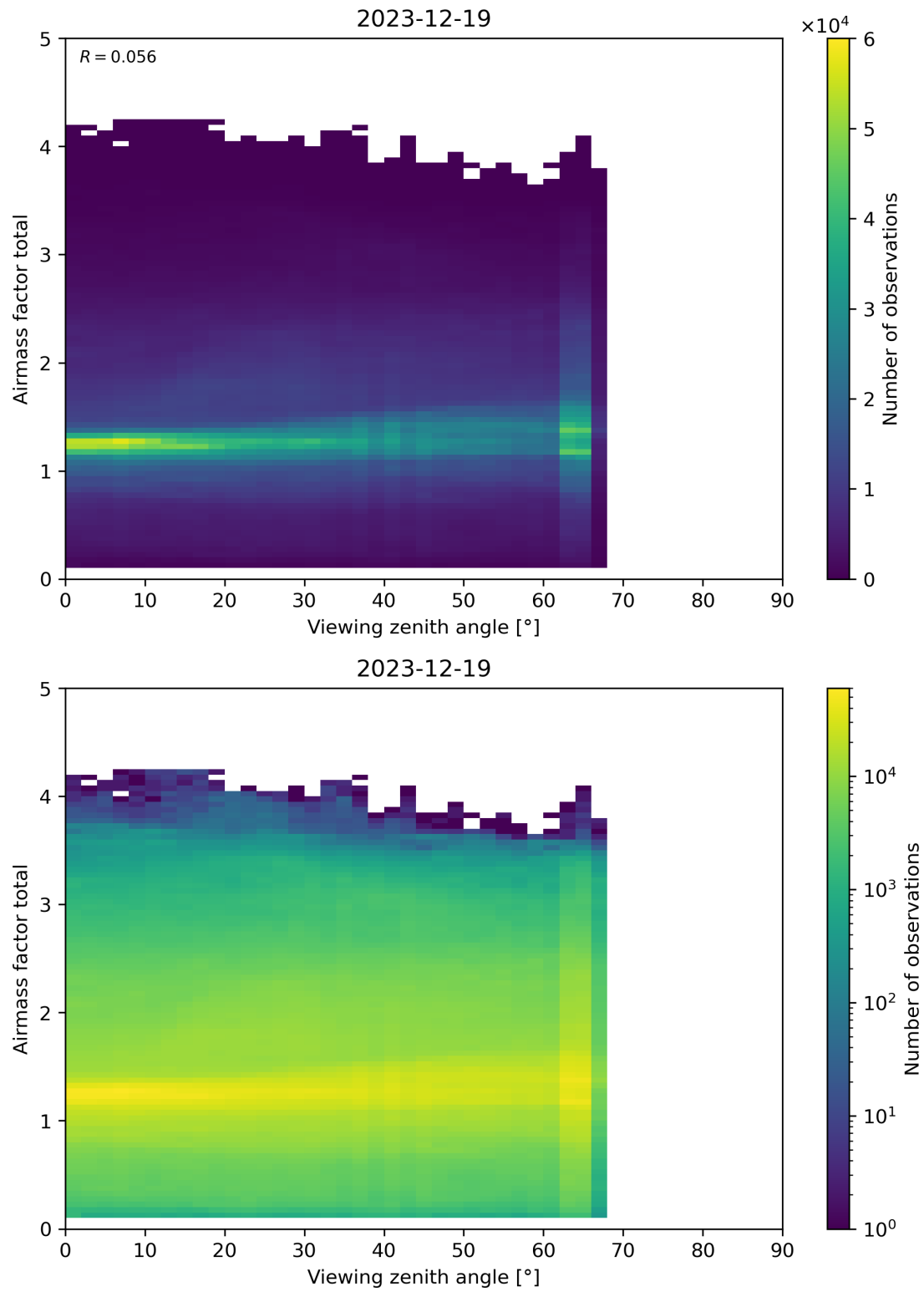
Figure 190: Scatter density plot of “Viewing zenith angle” against “Airmass factor total” for 2023-12-18 to 2023-12-20.
