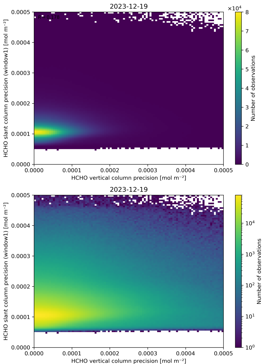
Figure 143: Scatter density plot of “HCHO vertical column precision” against “HCHO slant column precision (window1)” for 2023-12-18 to 2023-12-20.
