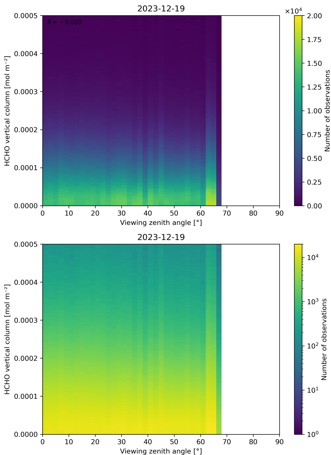
Figure 192: Scatter density plot of “Viewing zenith angle” against “HCHO vertical column” for 2023-12-18 to 2023-12-20.
