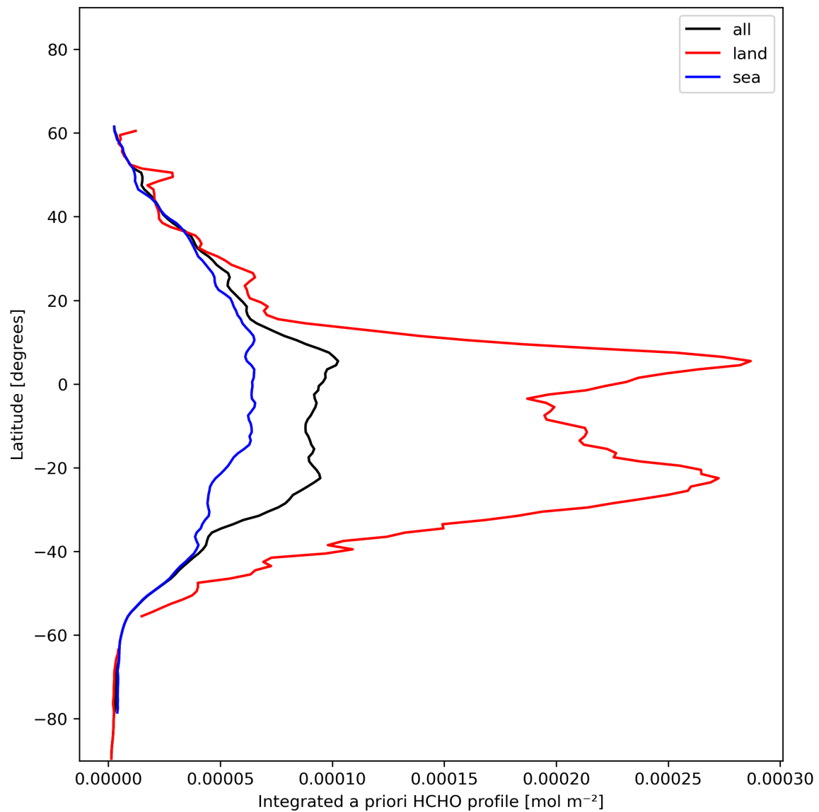
Figure 29: Zonal average of “Integrated a priori HCHO profile” for 2023-12-18 to 2023-12-20.
