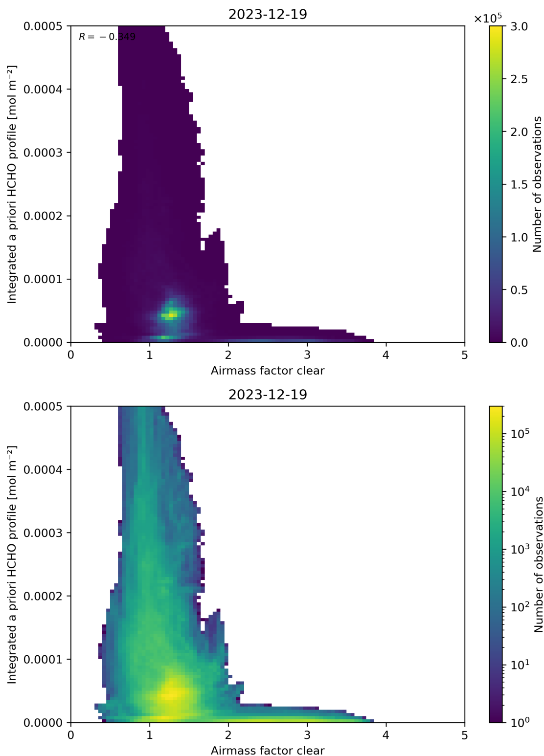
Figure 76: Scatter density plot of “Airmass factor clear” against “Integrated a priori HCHO profile” for 2023-12-18 to 2023-12-20.
