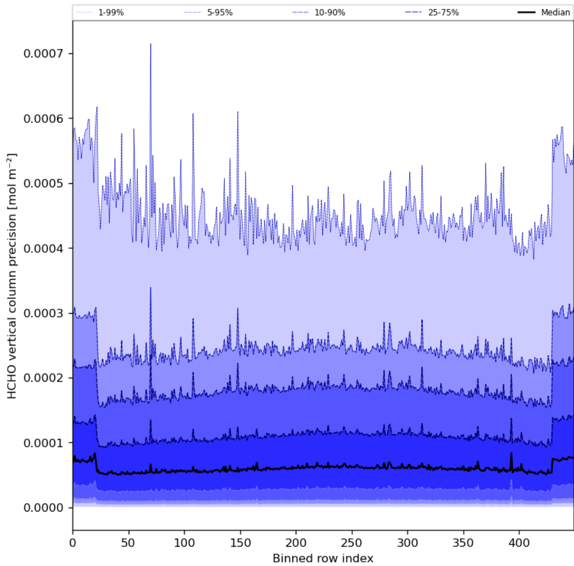
Figure 50: Along track statistics of “HCHO vertical column precision” for 2023-12-18 to 2023-12-20
