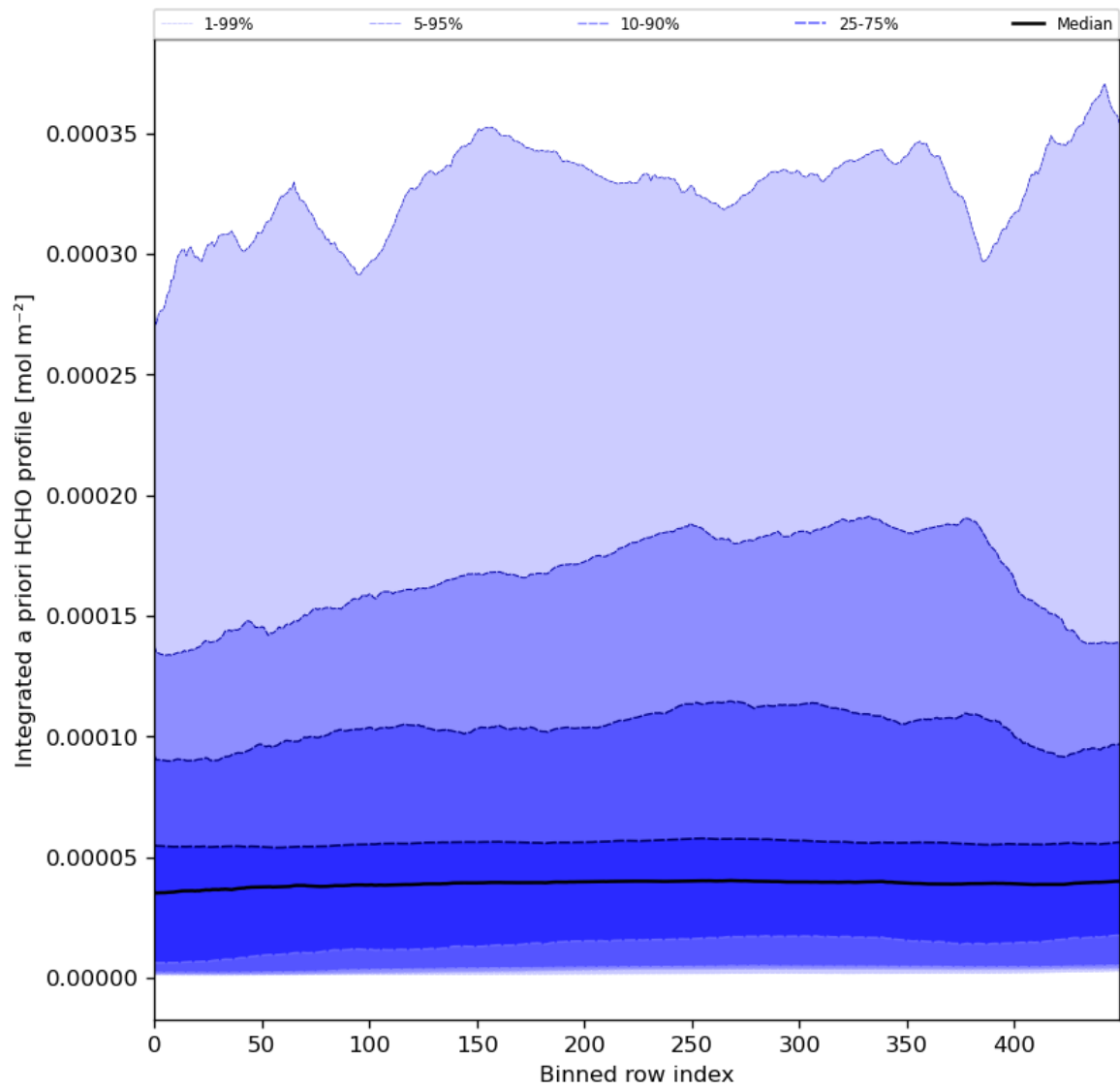
Figure 57: Along track statistics of “Integrated a priori HCHO profile” for 2023-12-18 to 2023-12-20
