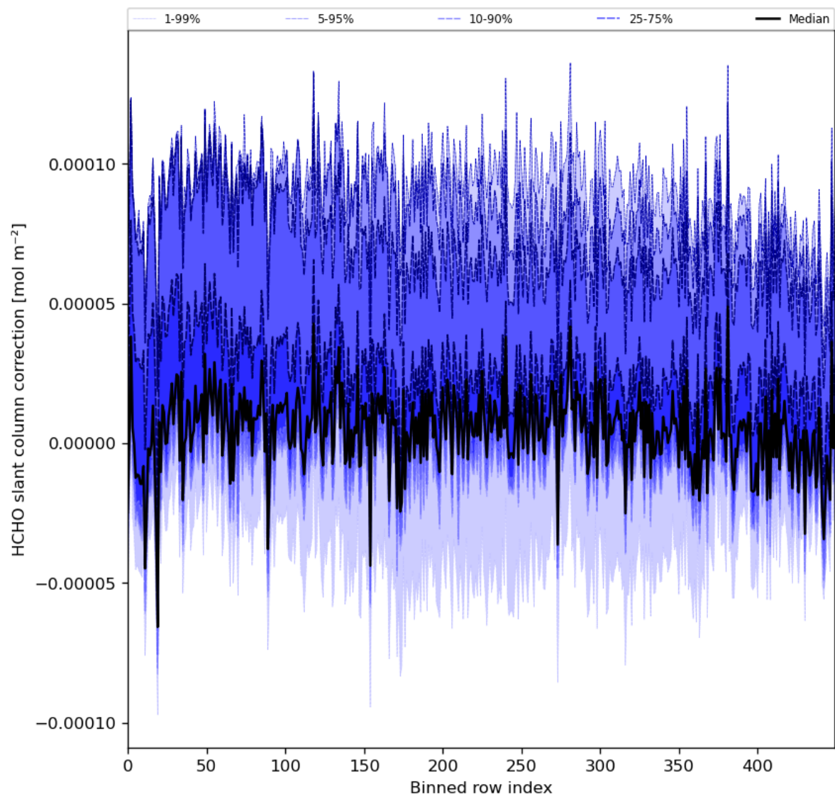
Figure 61: Along track statistics of “HCHO slant column correction” for 2023-12-18 to 2023-12-20
