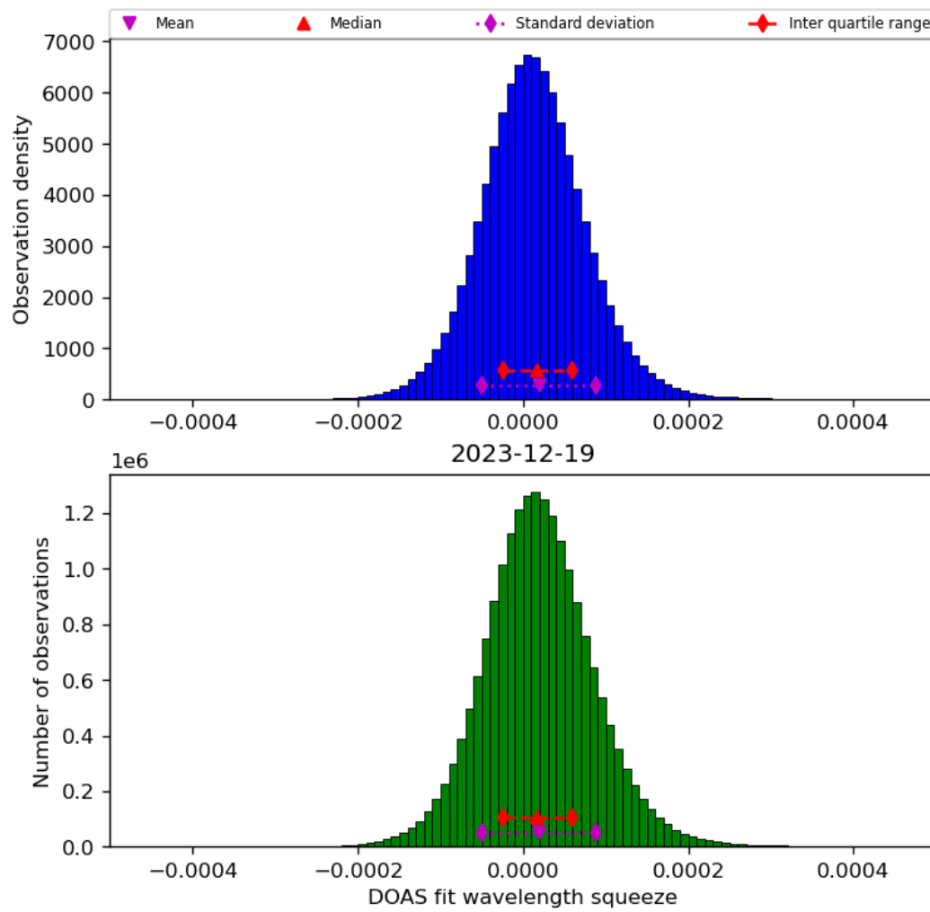
Figure 45: Histogram of “DOAS fit wavelength squeeze” for 2023-12-18 to 2023-12-20
