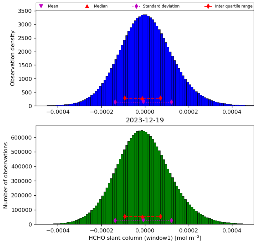
Figure 38: Histogram of “HCHO slant column (window1)” for 2023-12-18 to 2023-12-20
