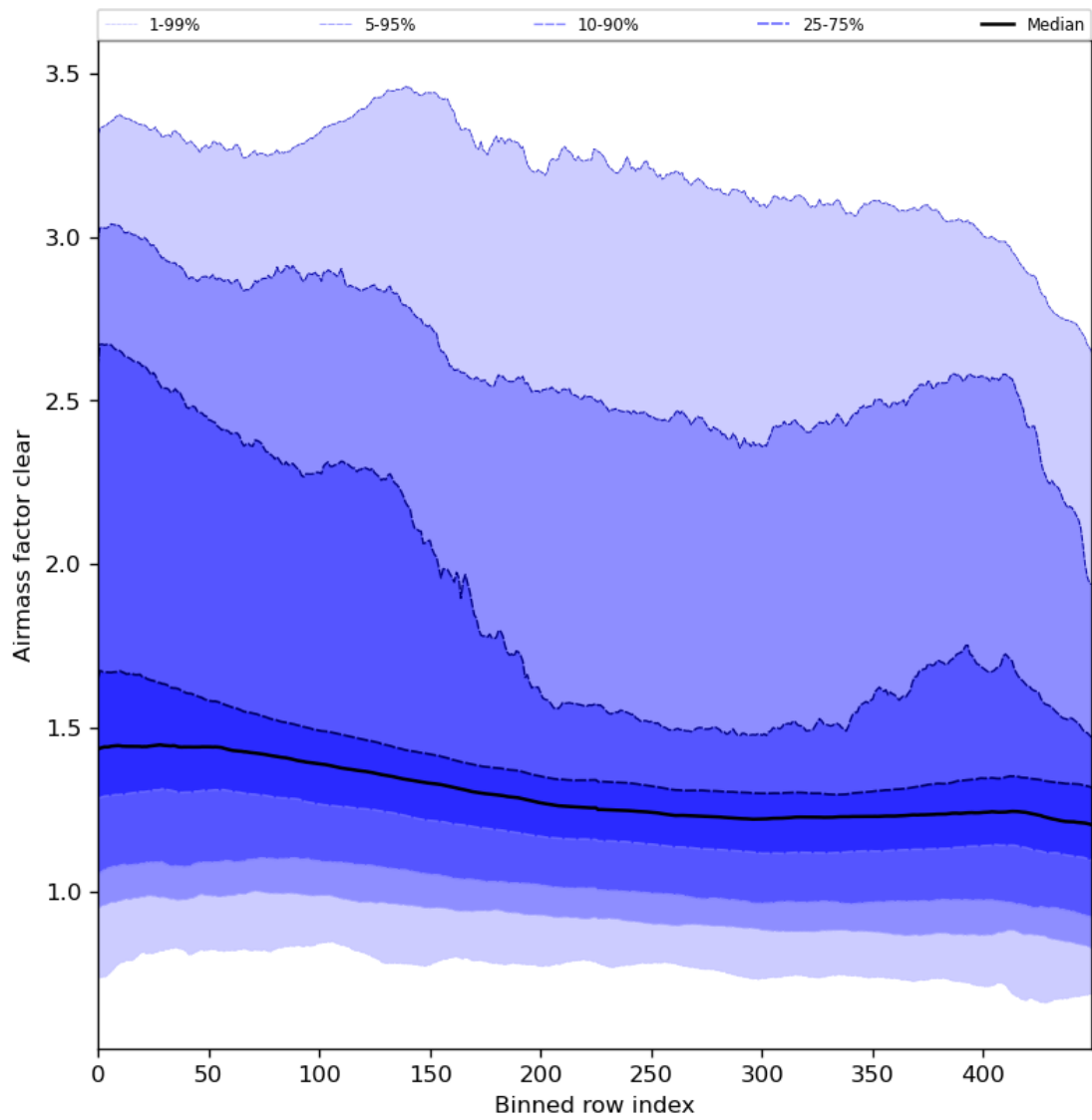
Figure 56: Along track statistics of “Airmass factor clear” for 2023-12-18 to 2023-12-20
