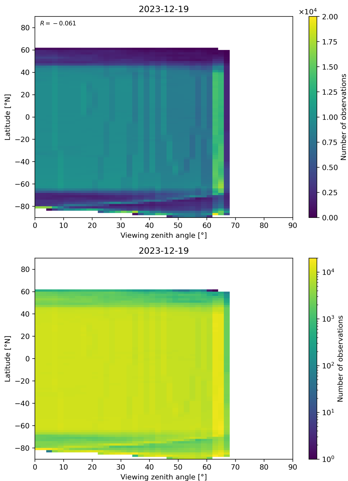
Figure 196: Scatter density plot of “Viewing zenith angle” against “Latitude” for 2023-12-18 to 2023-12-20.
