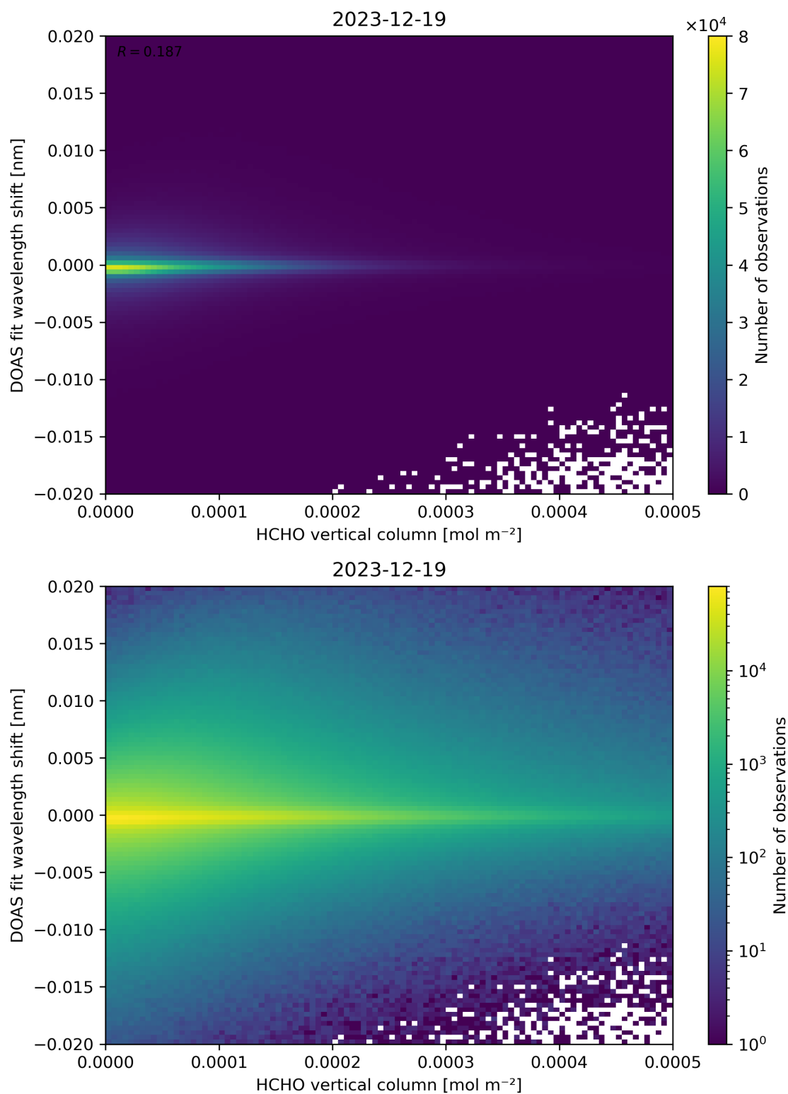
Figure 124: Scatter density plot of “HCHO vertical column” against “DOAS fit wavelength shift” for 2023-12-18 to 2023-12-20.
