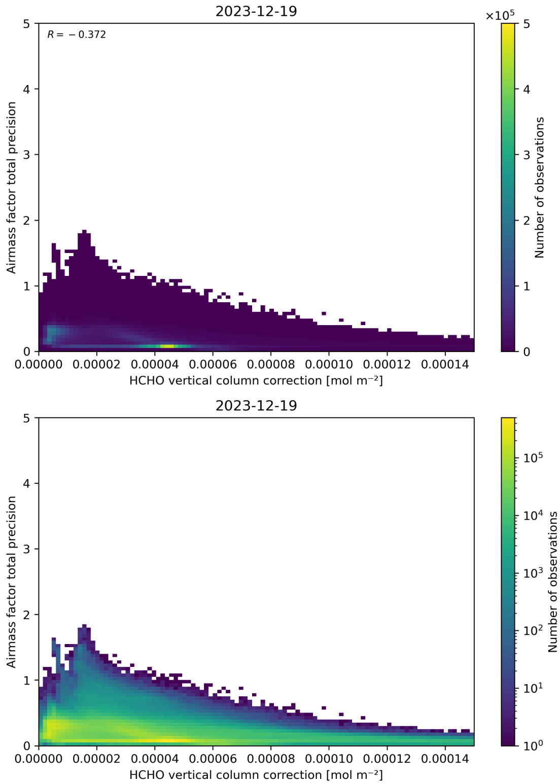
Figure 121: Scatter density plot of “HCHO vertical column correction” against “Airmass factor total precision” for 2023-12-18 to 2023-12-20.
