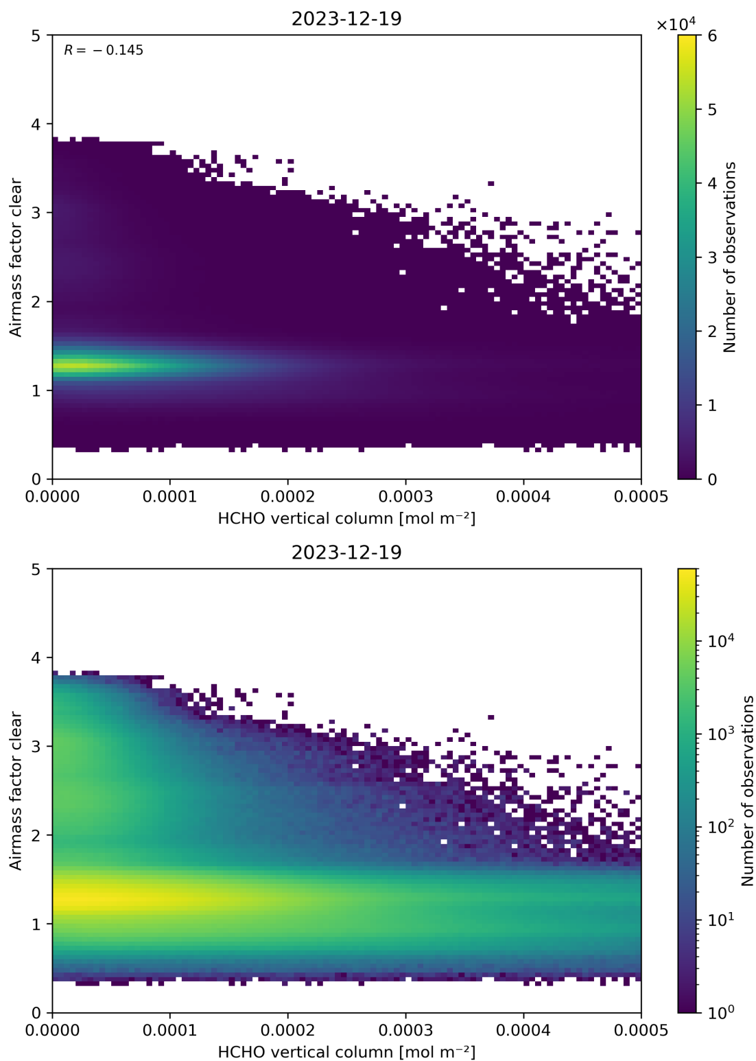
Figure 126: Scatter density plot of “HCHO vertical column” against “Airmass factor clear” for 2023-12-18 to 2023-12-20.
