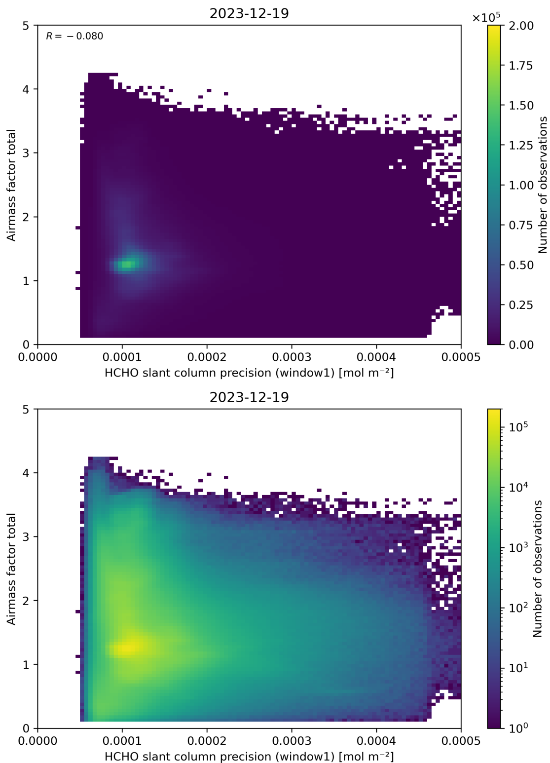
Figure 94: Scatter density plot of “HCHO slant column precision (window1)” against “Airmass factor total” for 2023-12-18 to 2023-12-20.
