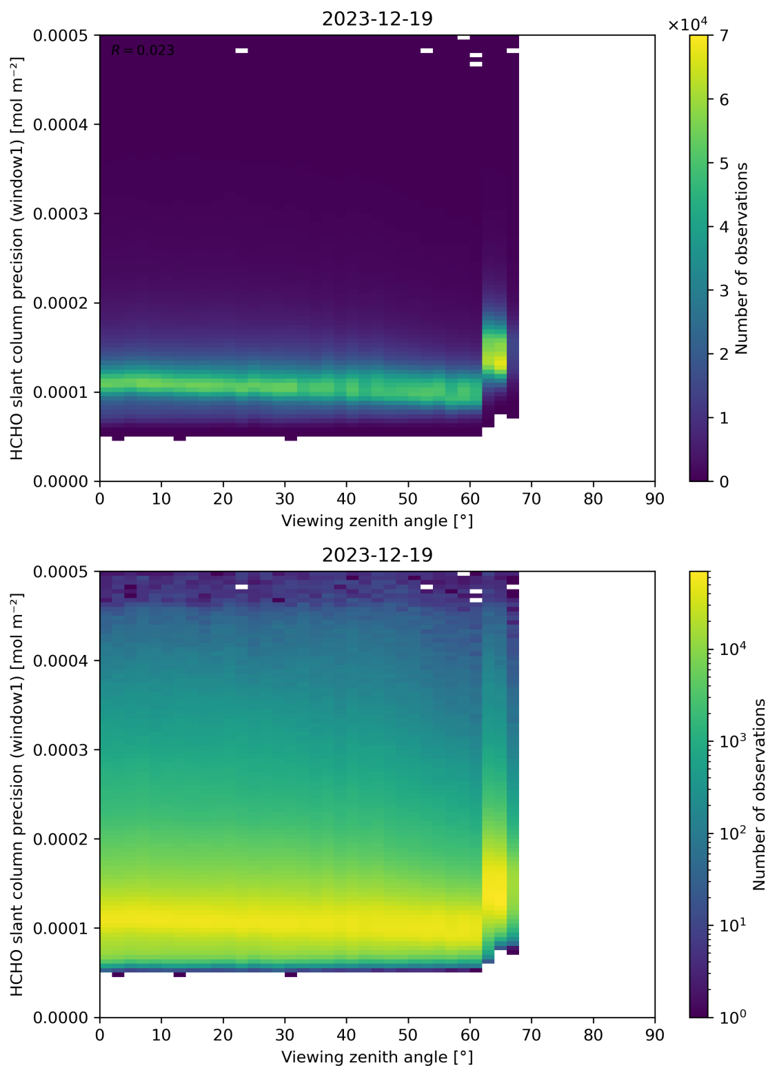
Figure 189: Scatter density plot of “Viewing zenith angle” against “HCHO slant column precision (window1)” for 2023-12-18 to 2023-12-20.
