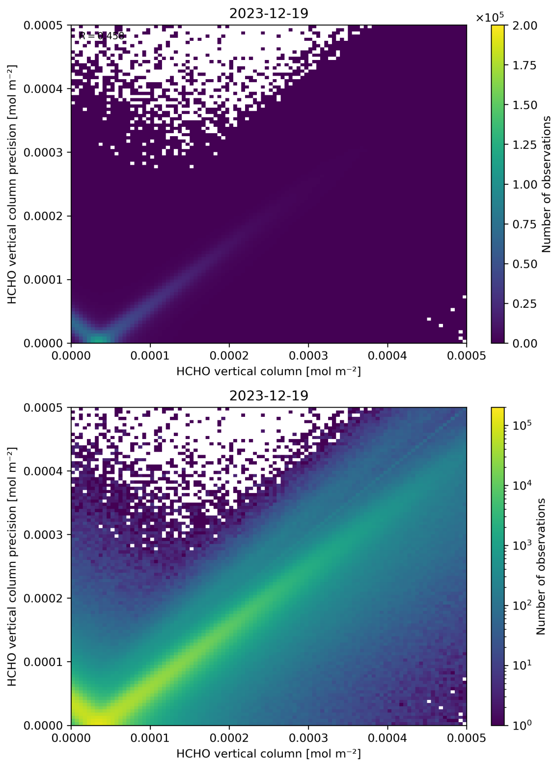
Figure 134: Scatter density plot of “HCHO vertical column” against “HCHO vertical column precision” for 2023-12-18 to 2023-12-20.
