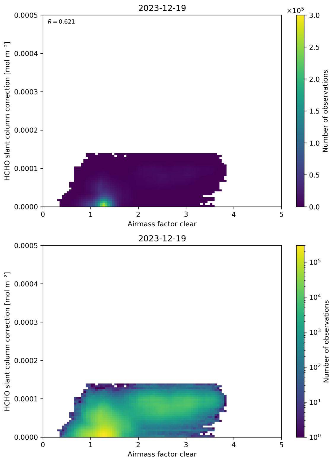
Figure 75: Scatter density plot of “Airmass factor clear” against “HCHO slant column correction” for 2023-12-18 to 2023-12-20.
