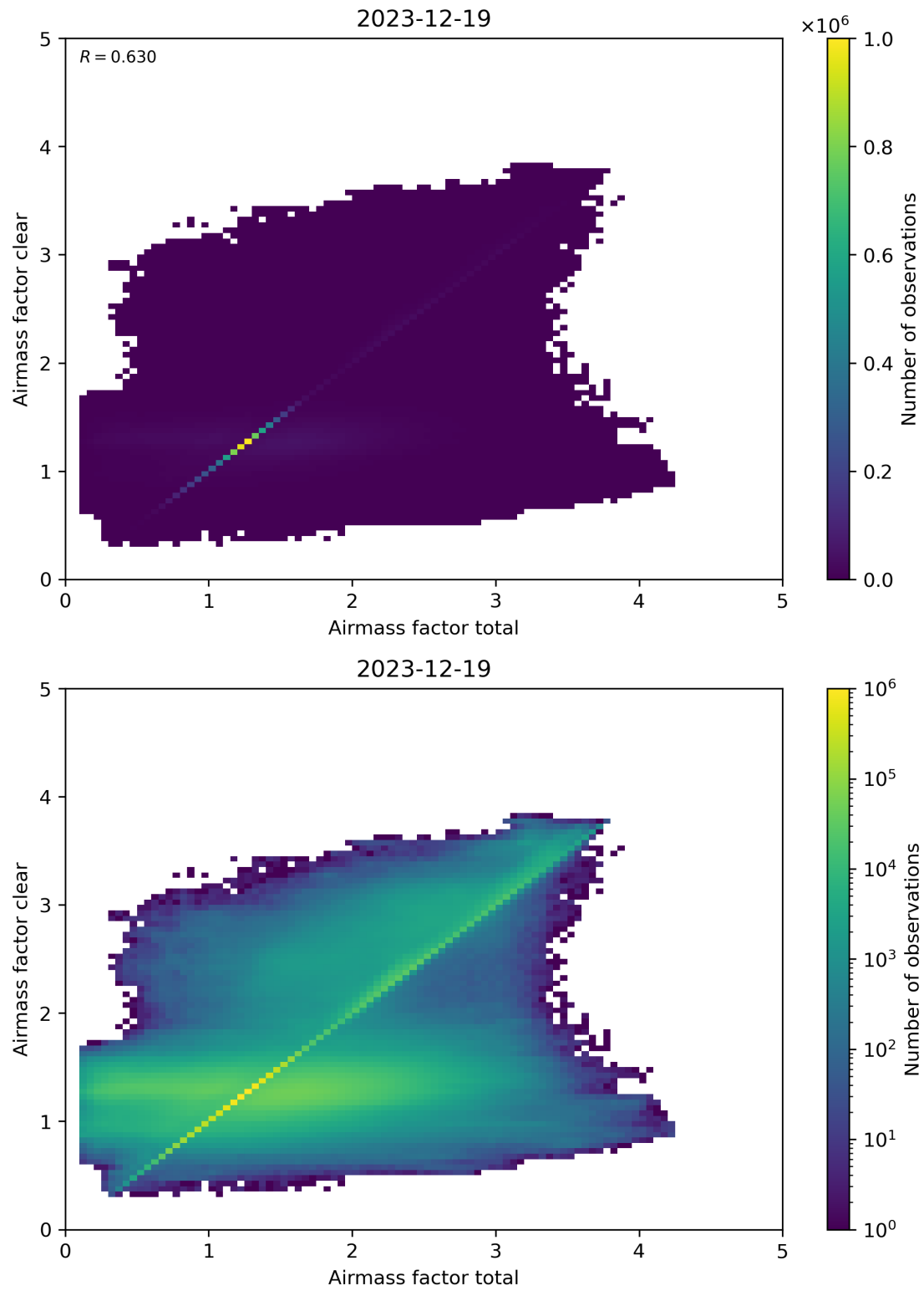
Figure 100: Scatter density plot of “Airmass factor total” against “Airmass factor clear” for 2023-12-18 to 2023-12-20.
