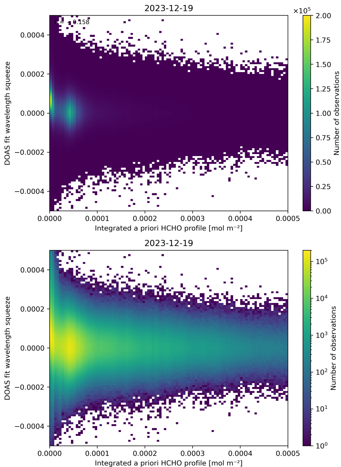
Figure 150: Scatter density plot of “Integrated a priori HCHO profile” against “DOAS fit wavelength squeeze” for 2023-12-18 to 2023-12-20.
