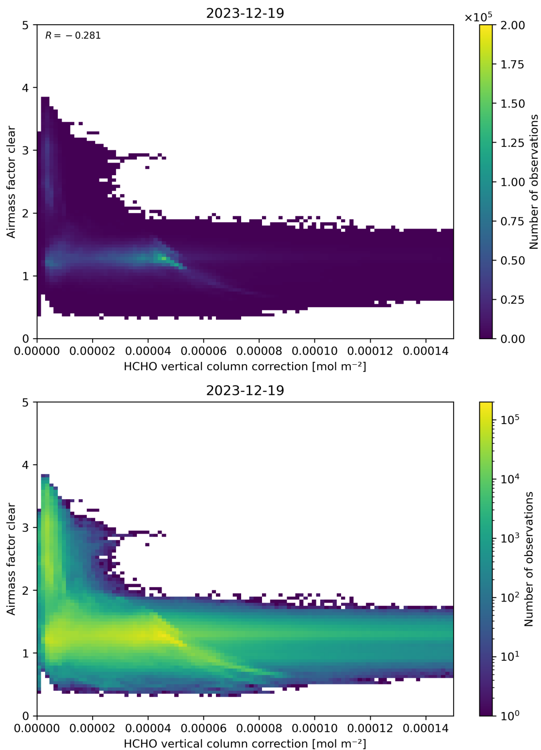
Figure 115: Scatter density plot of “HCHO vertical column correction” against “Airmass factor clear” for 2023-12-18 to 2023-12-20.
