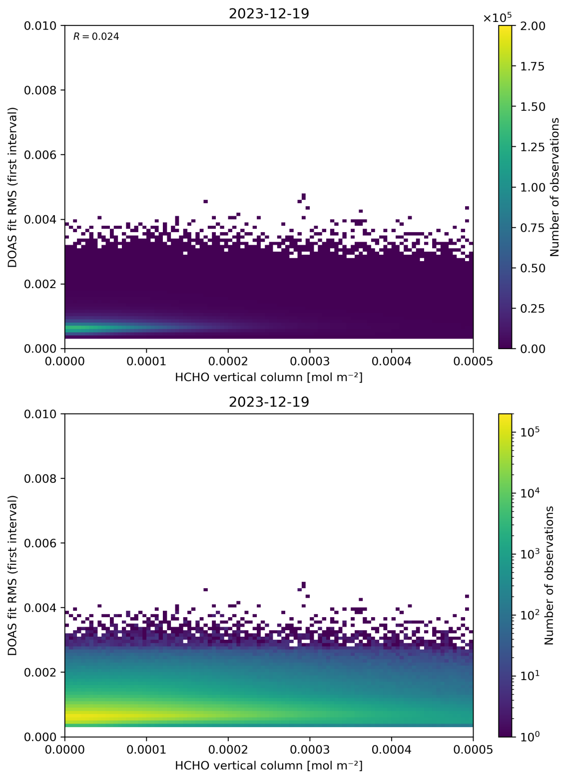
Figure 123: Scatter density plot of “HCHO vertical column” against “DOAS fit RMS (first interval)” for 2023-12-18 to 2023-12-20.
