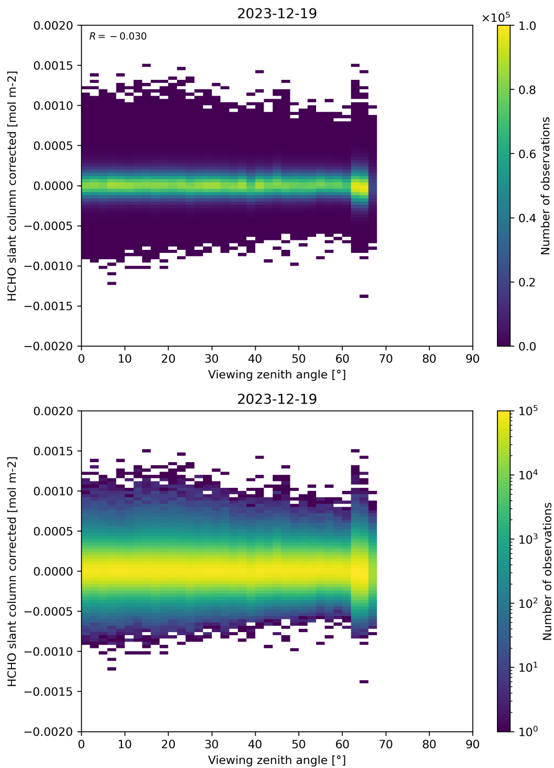
Figure 186: Scatter density plot of “Viewing zenith angle” against “HCHO slant column corrected” for 2023-12-18 to 2023-12-20.
