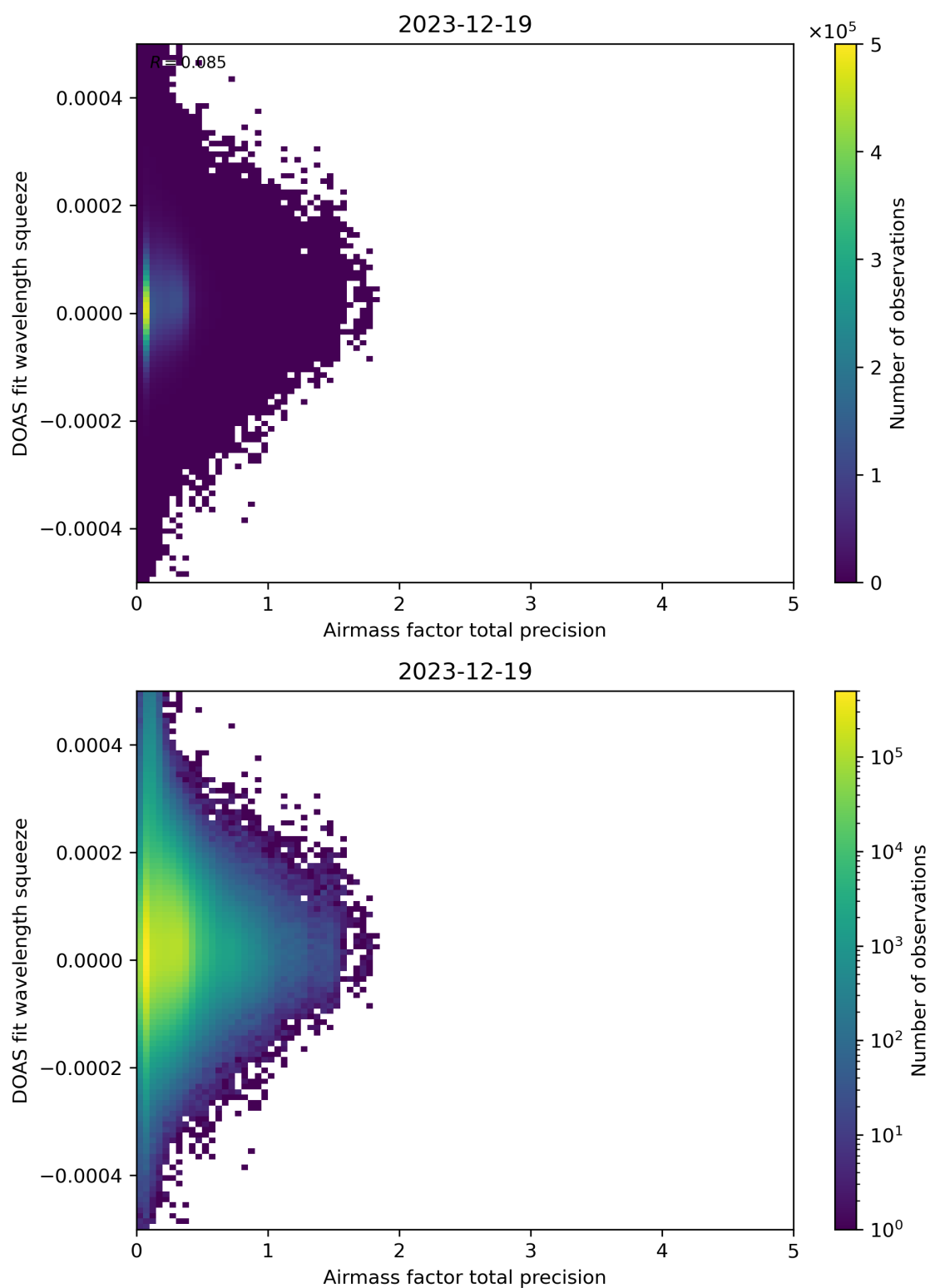
Figure 107: Scatter density plot of “Airmass factor total precision” against “DOAS fit wavelength squeeze” for 2023-12-18 to 2023-12-20.
