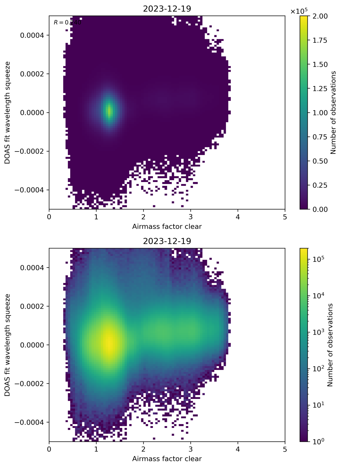
Figure 73: Scatter density plot of “Airmass factor clear” against “DOAS fit wavelength squeeze” for 2023-12-18 to 2023-12-20.
