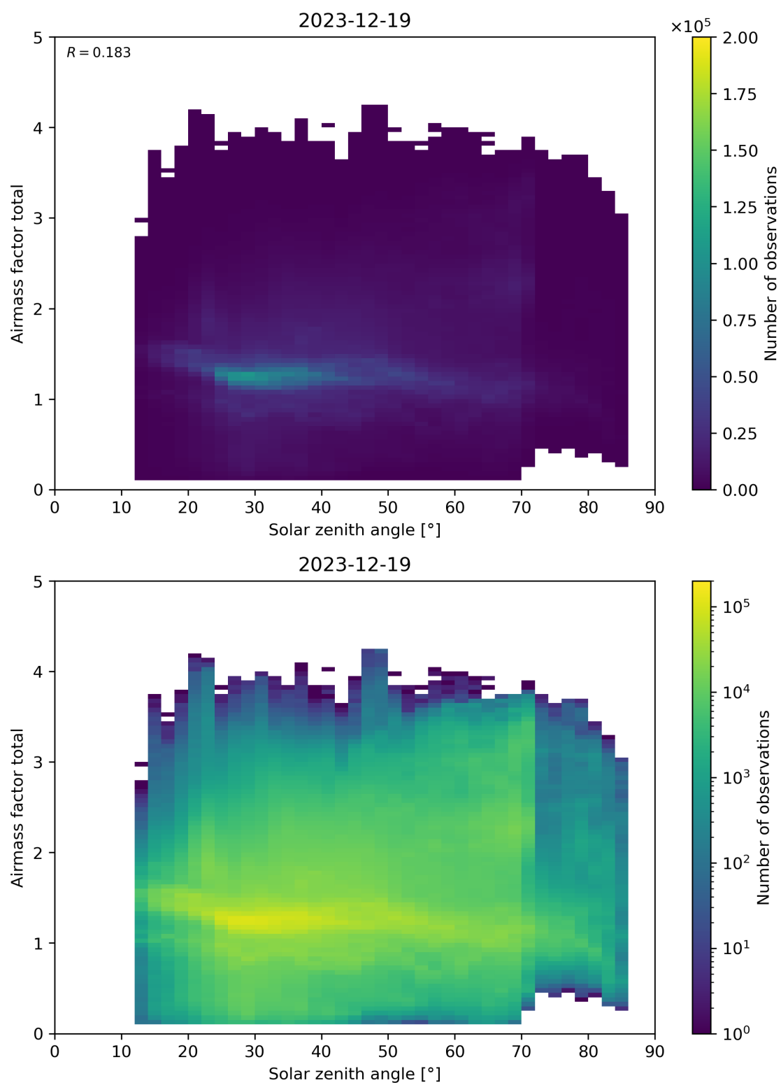
Figure 175: Scatter density plot of “Solar zenith angle” against “Airmass factor total” for 2023-12-18 to 2023-12-20.
