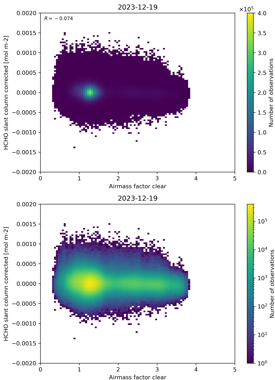
Figure 74: Scatter density plot of “Airmass factor clear” against “HCHO slant column corrected” for 2023-12-18 to 2023-12-20.
