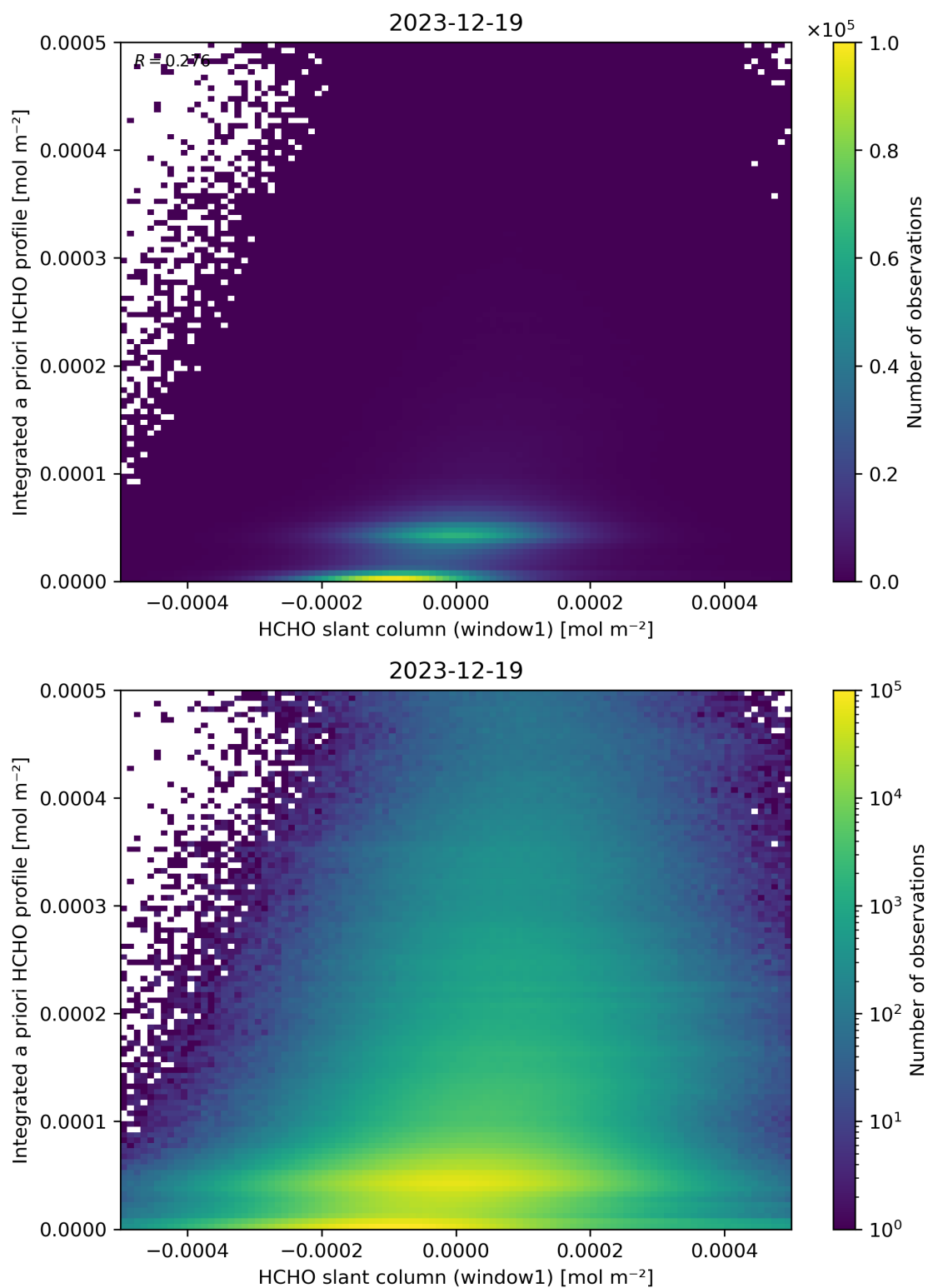
Figure 87: Scatter density plot of “HCHO slant column (window1)” against “Integrated a priori HCHO profile” for 2023-12-18 to 2023-12-20.
