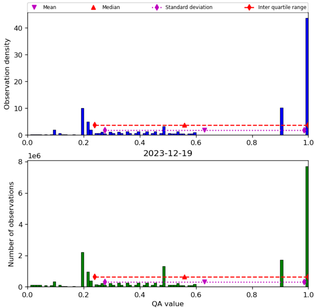
Figure 34: Histogram of “QA value” for 2023-12-18 to 2023-12-20
