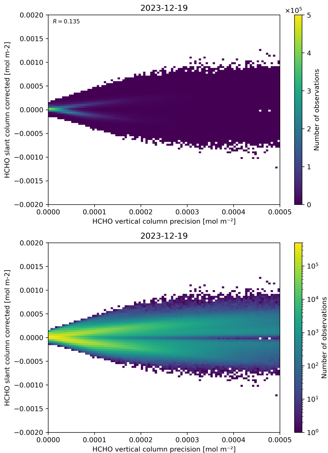
Figure 140: Scatter density plot of “HCHO vertical column precision” against “HCHO slant column corrected” for 2023-12-18 to 2023-12-20.
