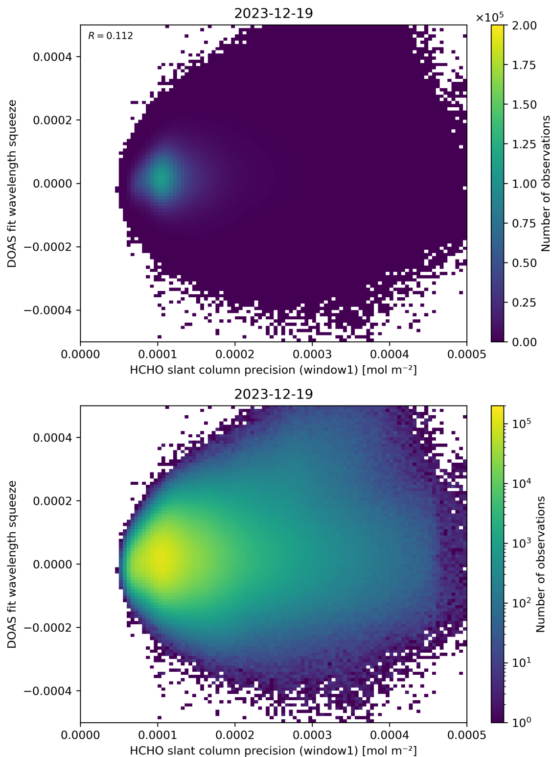
Figure 90: Scatter density plot of “HCHO slant column precision (window1)” against “DOAS fit wavelength squeeze” for 2023-12-18 to 2023-12-20.
