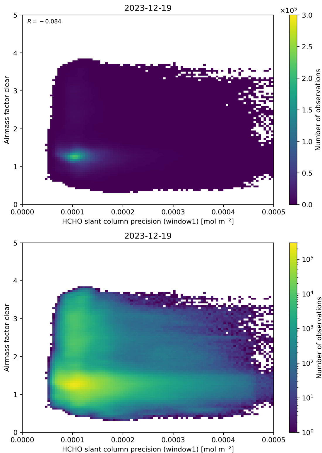
Figure 91: Scatter density plot of “HCHO slant column precision (window1)” against “Airmass factor clear” for 2023-12-18 to 2023-12-20.
