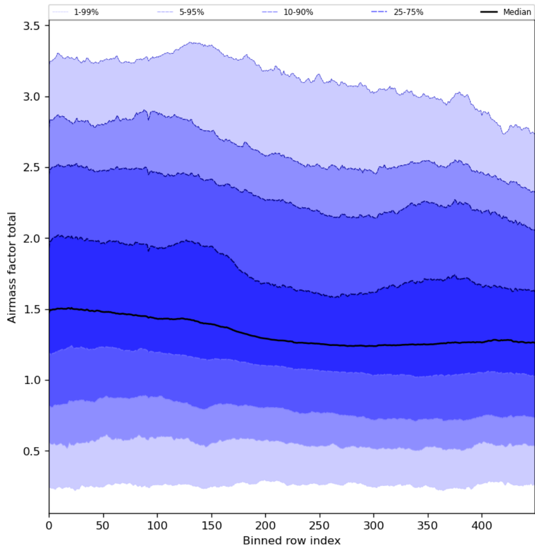
Figure 54: Along track statistics of “Airmass factor total” for 2023-12-18 to 2023-12-20
