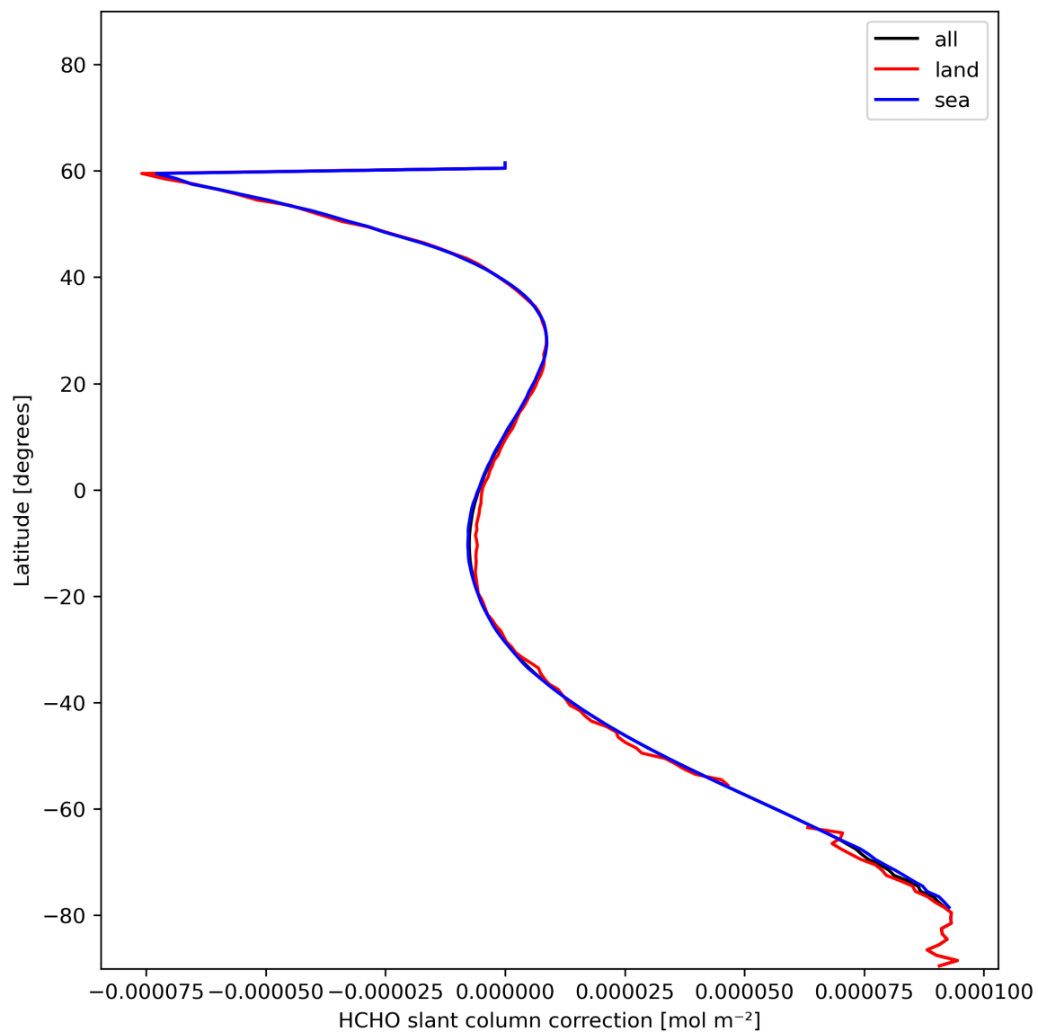
Figure 33: Zonal average of “HCHO slant column correction” for 2023-12-18 to 2023-12-20.
