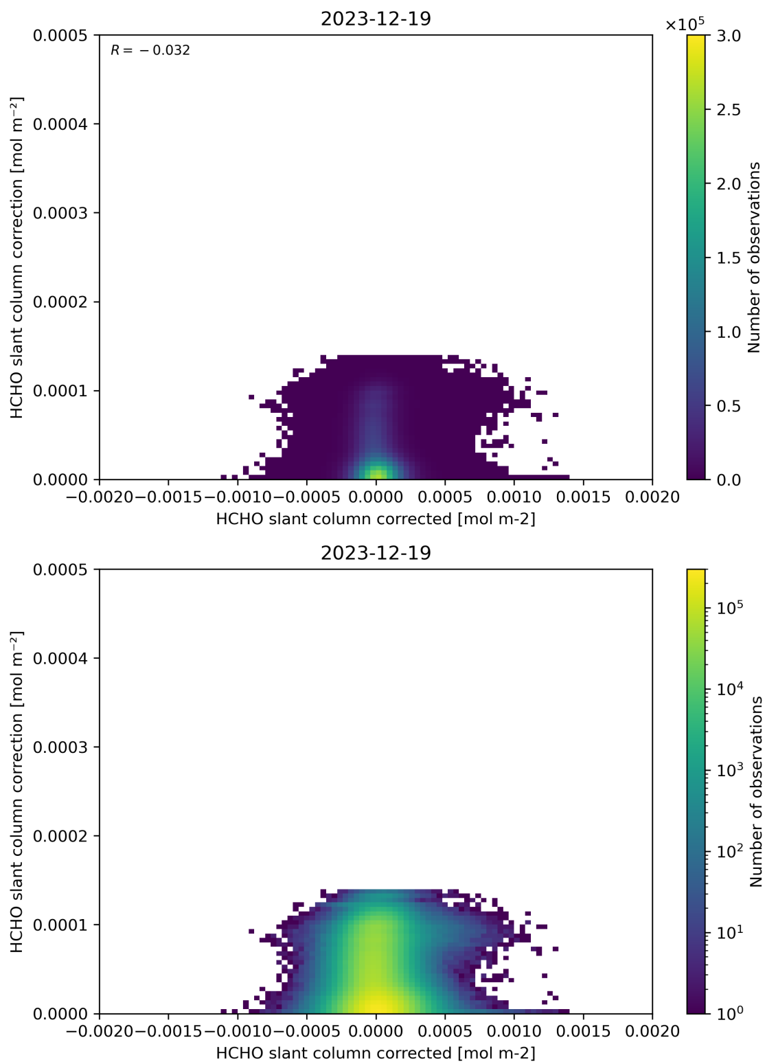
Figure 77: Scatter density plot of “HCHO slant column corrected” against “HCHO slant column correction” for 2023-12-18 to 2023-12-20.
