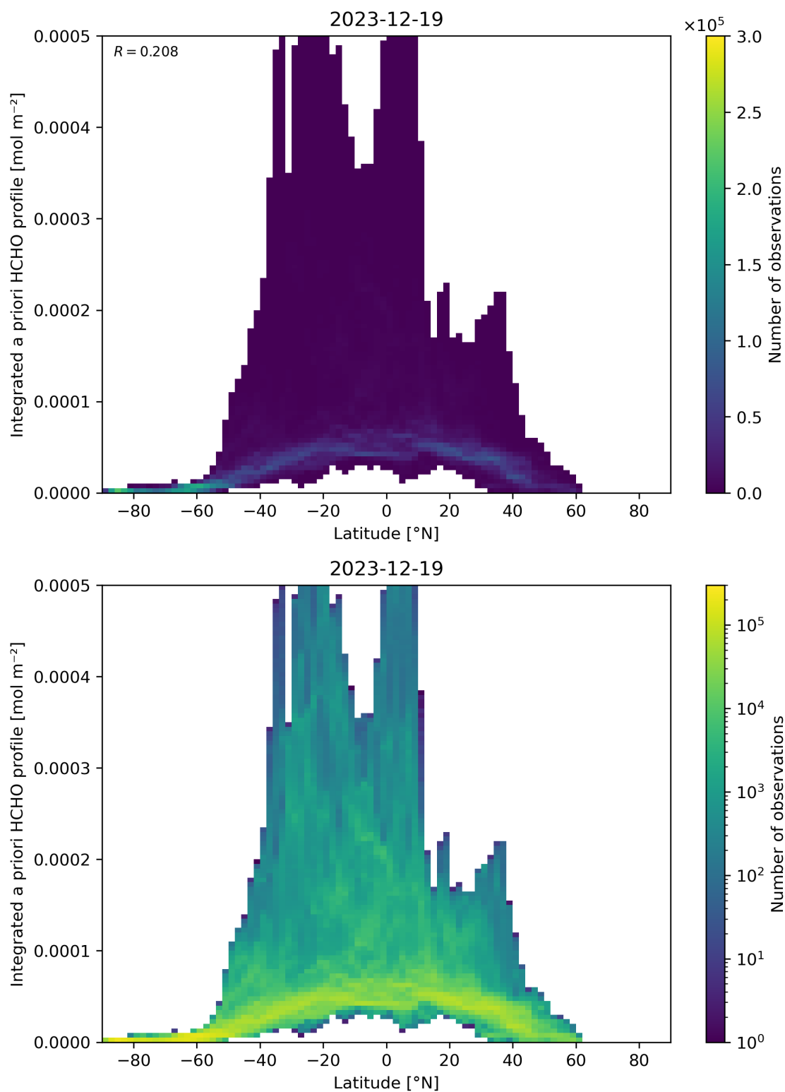
Figure 166: Scatter density plot of “Latitude” against “Integrated a priori HCHO profile” for 2023-12-18 to 2023-12-20.
