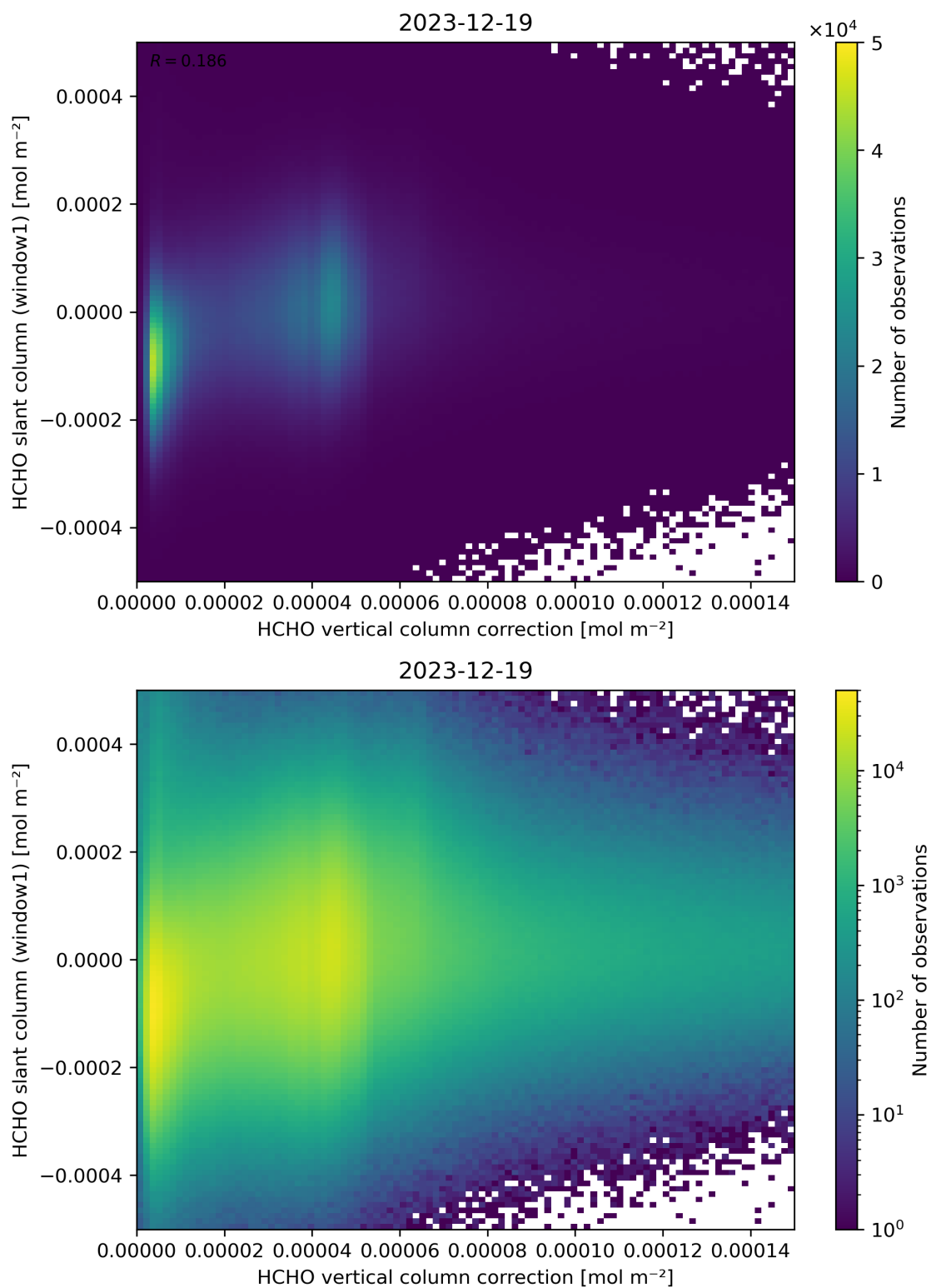
Figure 118: Scatter density plot of “HCHO vertical column correction” against “HCHO slant column (window1)” for 2023-12-18 to 2023-12-20.
