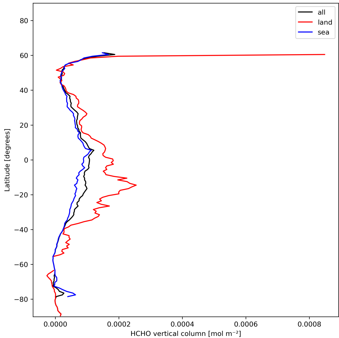
Figure 21: Zonal average of “HCHO vertical column” for 2023-12-18 to 2023-12-20.
