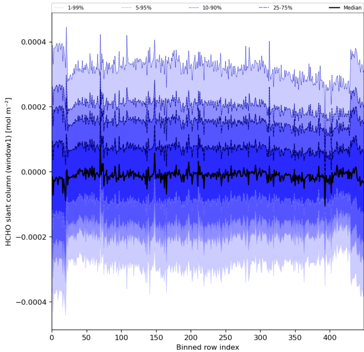
Figure 52: Along track statistics of “HCHO slant column (window1)” for 2023-12-18 to 2023-12-20
