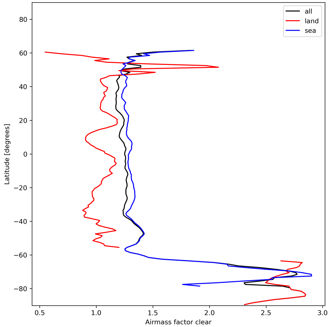
Figure 28: Zonal average of “Airmass factor clear” for 2023-12-18 to 2023-12-20.
