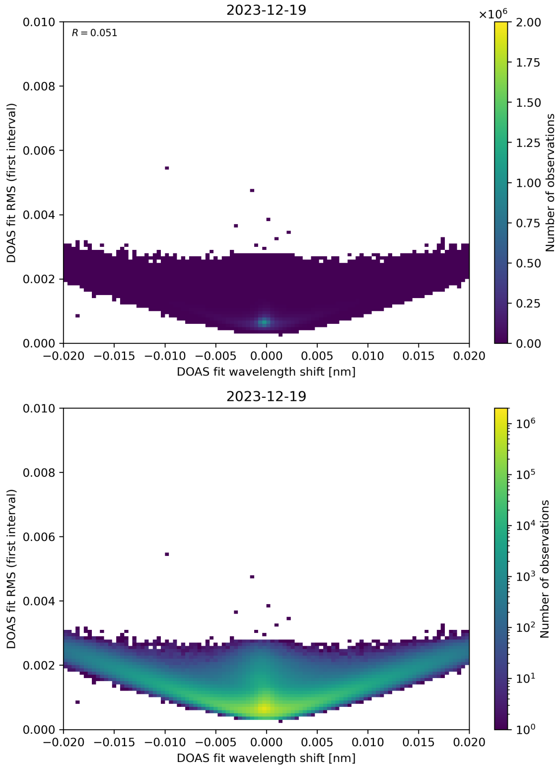
Figure 64: Scatter density plot of “DOAS fit wavelength shift” against “DOAS fit RMS (first interval)” for 2023-12-18 to 2023-12-20.
