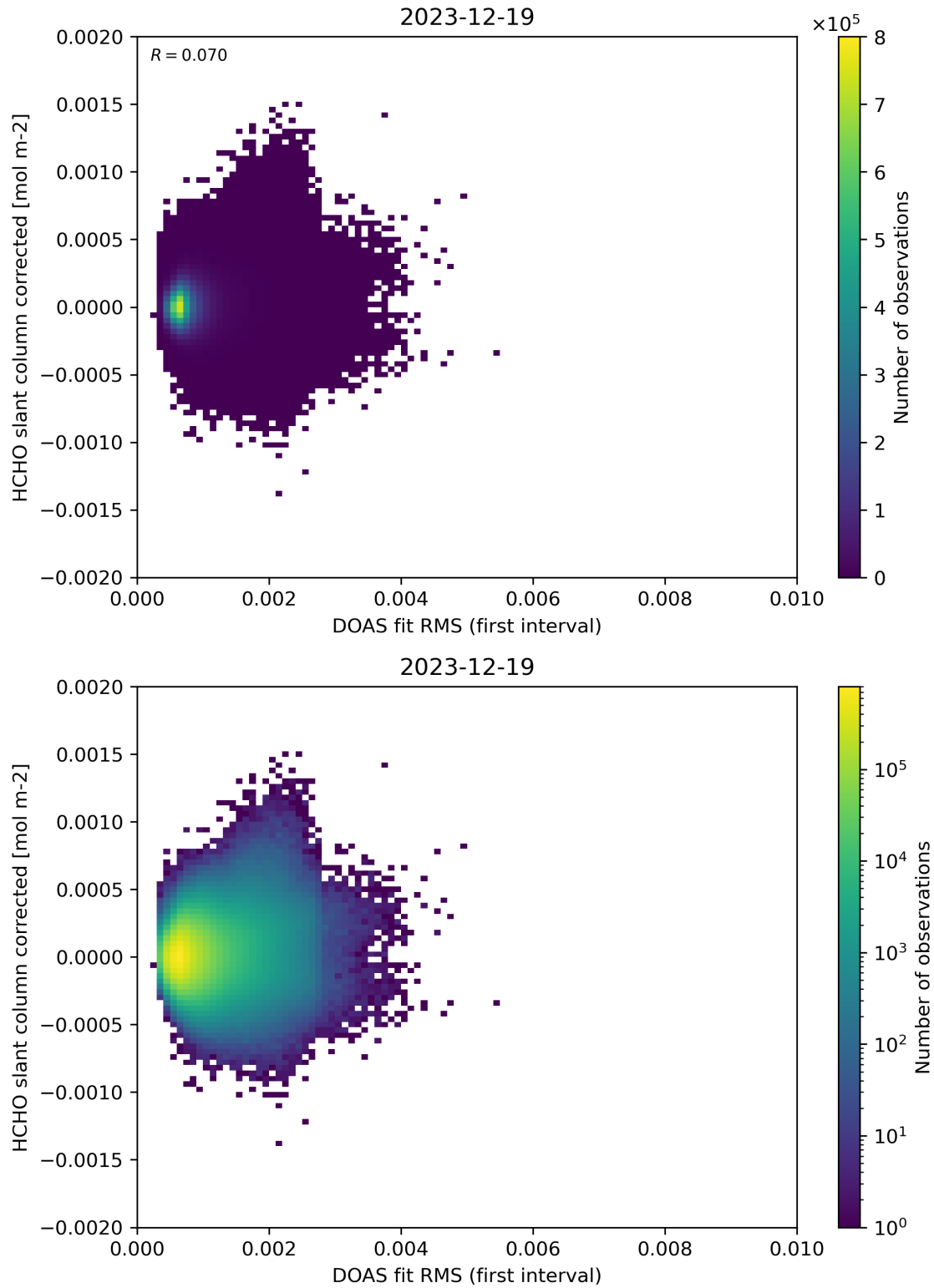
Figure 62: Scatter density plot of “DOAS fit RMS (first interval)” against “HCHO slant column corrected” for 2023-12-18 to 2023-12-20.
