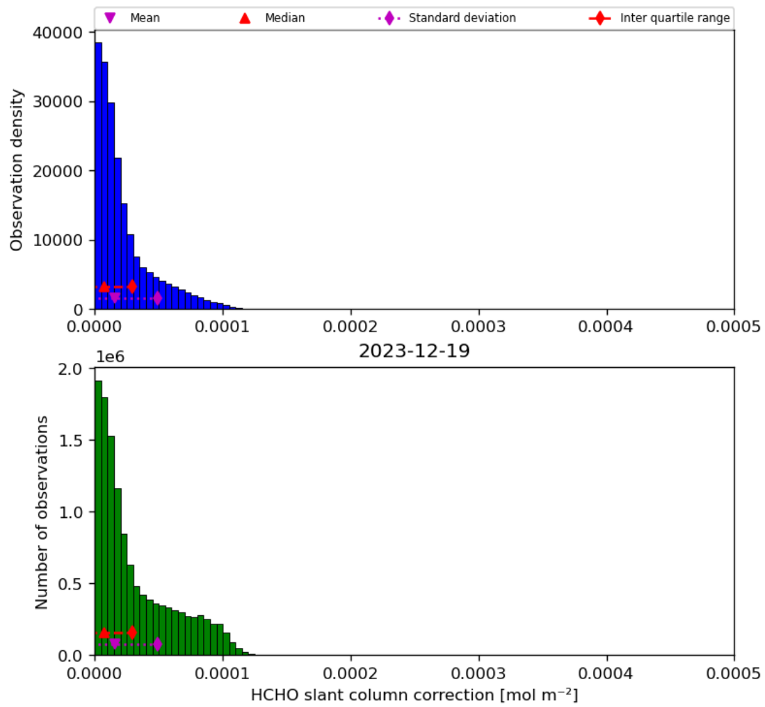
Figure 47: Histogram of “HCHO slant column correction” for 2023-12-18 to 2023-12-20
