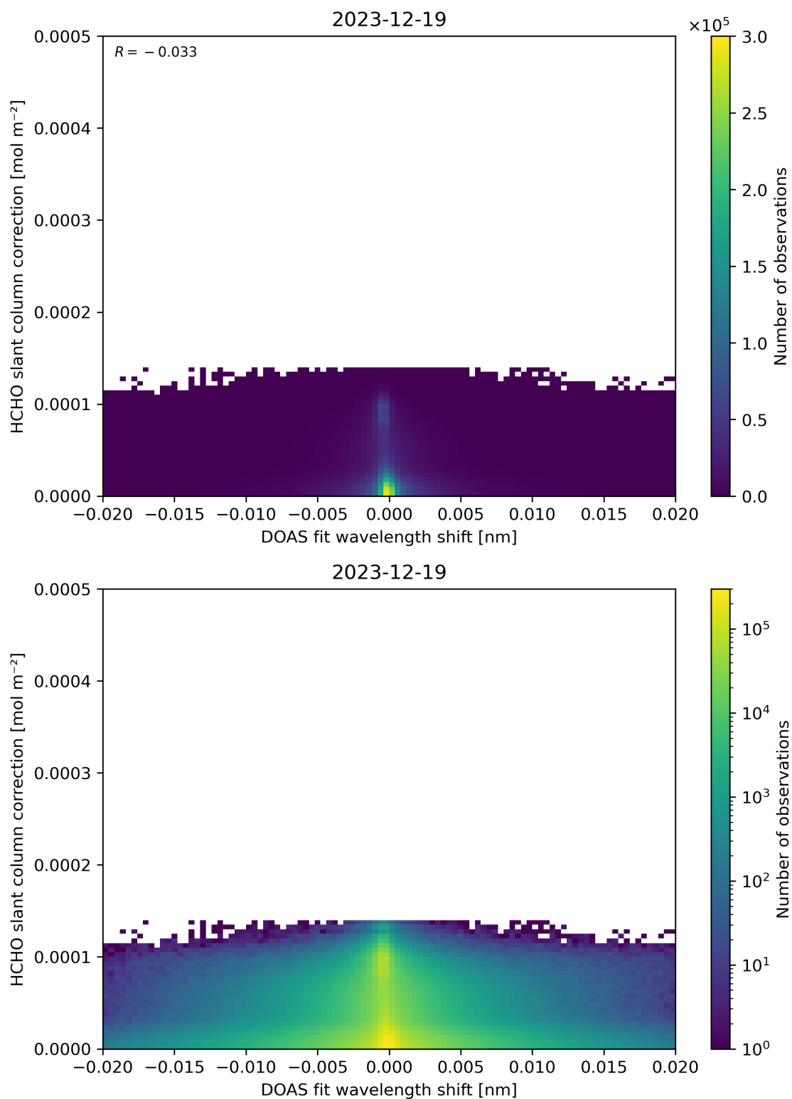
Figure 67: Scatter density plot of “DOAS fit wavelength shift” against “HCHO slant column correction” for 2023-12-18 to 2023-12-20.
