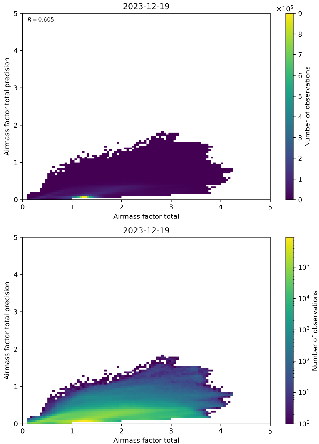
Figure 103: Scatter density plot of “Airmass factor total” against “Airmass factor total precision” for 2023-12-18 to 2023-12-20.
