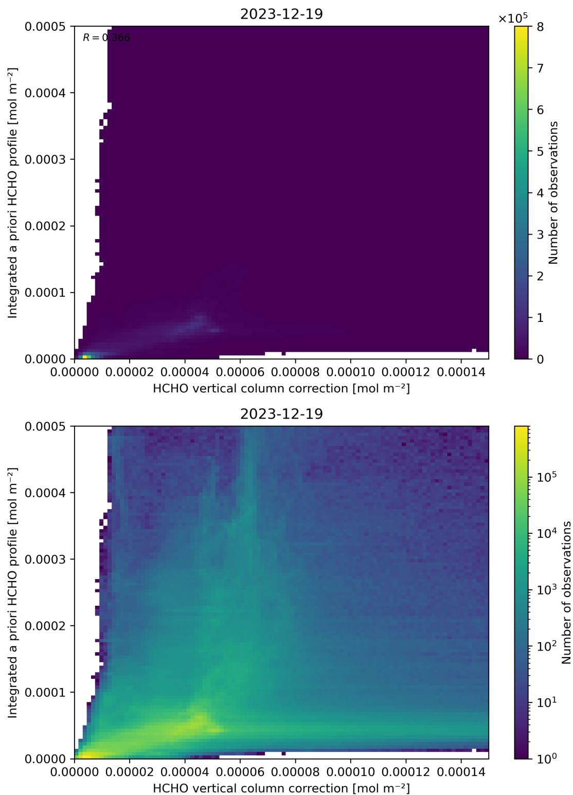
Figure 122: Scatter density plot of “HCHO vertical column correction” against “Integrated a priori HCHO profile” for 2023-12-18 to 2023-12-20.
