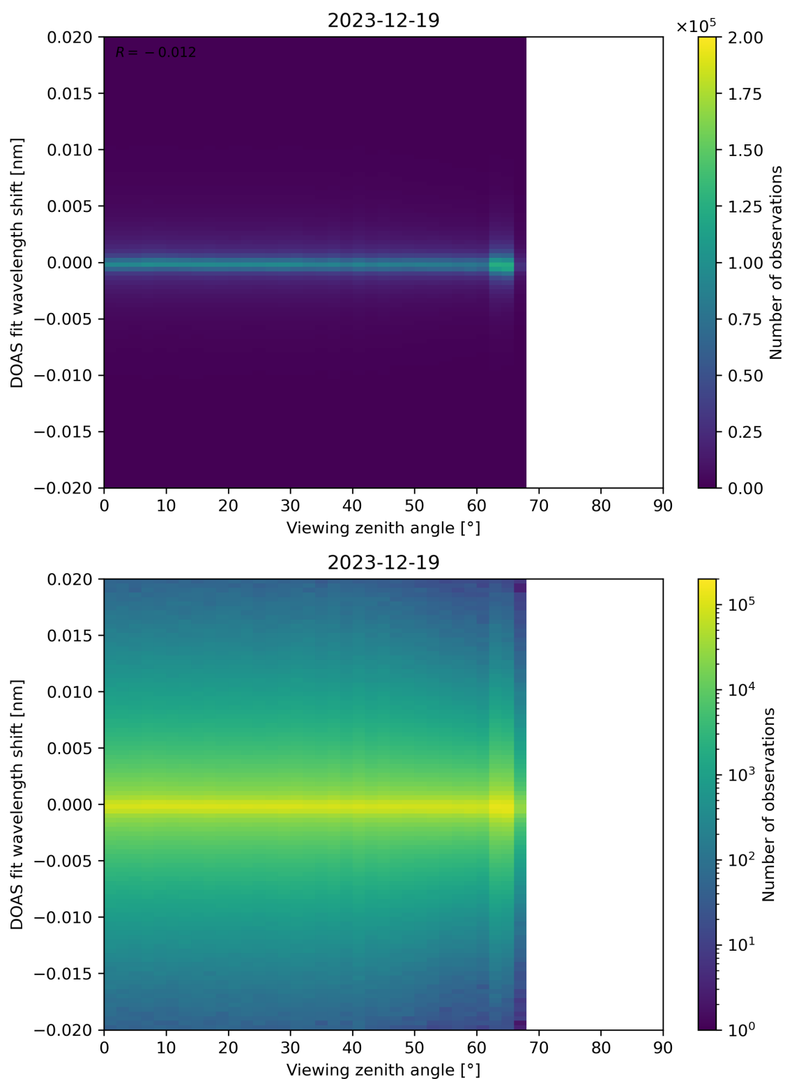
Figure 183: Scatter density plot of “Viewing zenith angle” against “DOAS fit wavelength shift” for 2023-12-18 to 2023-12-20.
