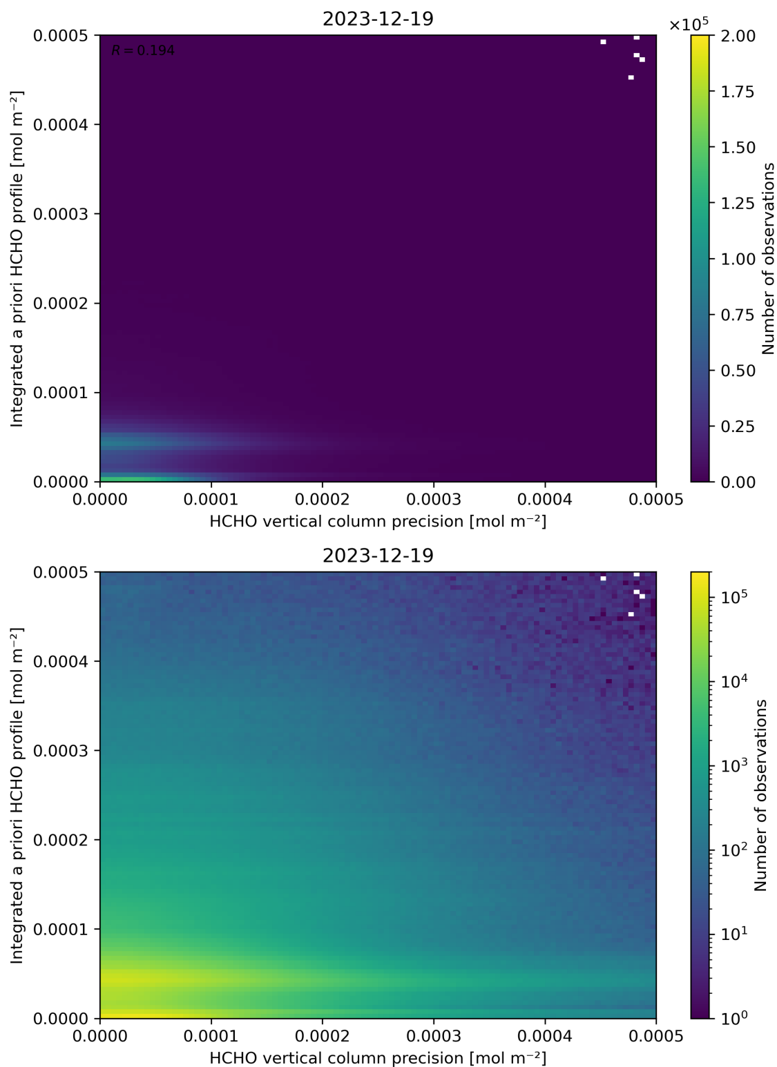
Figure 147: Scatter density plot of “HCHO vertical column precision” against “Integrated a priori HCHO profile” for 2023-12-18 to 2023-12-20.
