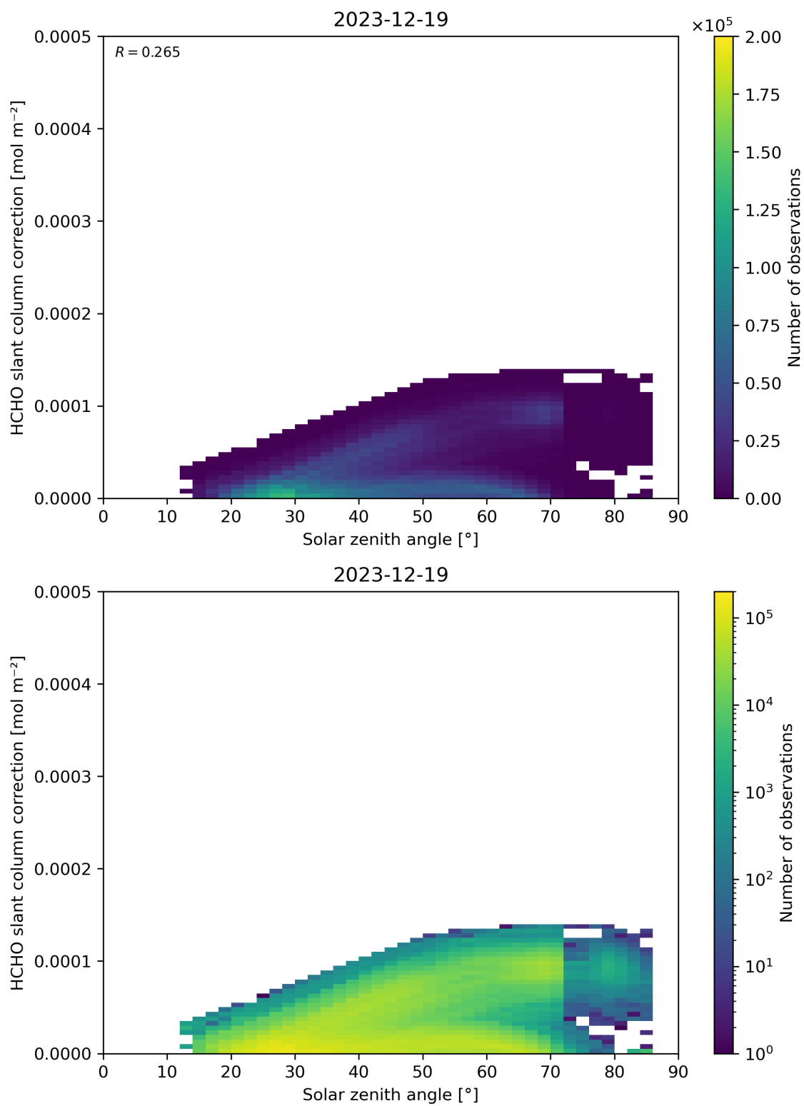
Figure 172: Scatter density plot of “Solar zenith angle” against “HCHO slant column correction” for 2023-12-18 to 2023-12-20.
