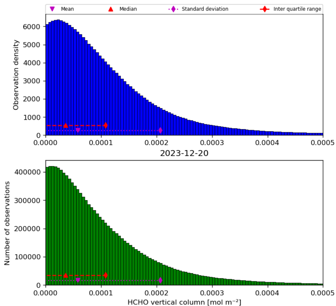
Figure 35: Histogram of “HCHO vertical column” for 2023-12-20 to 2023-12-21
