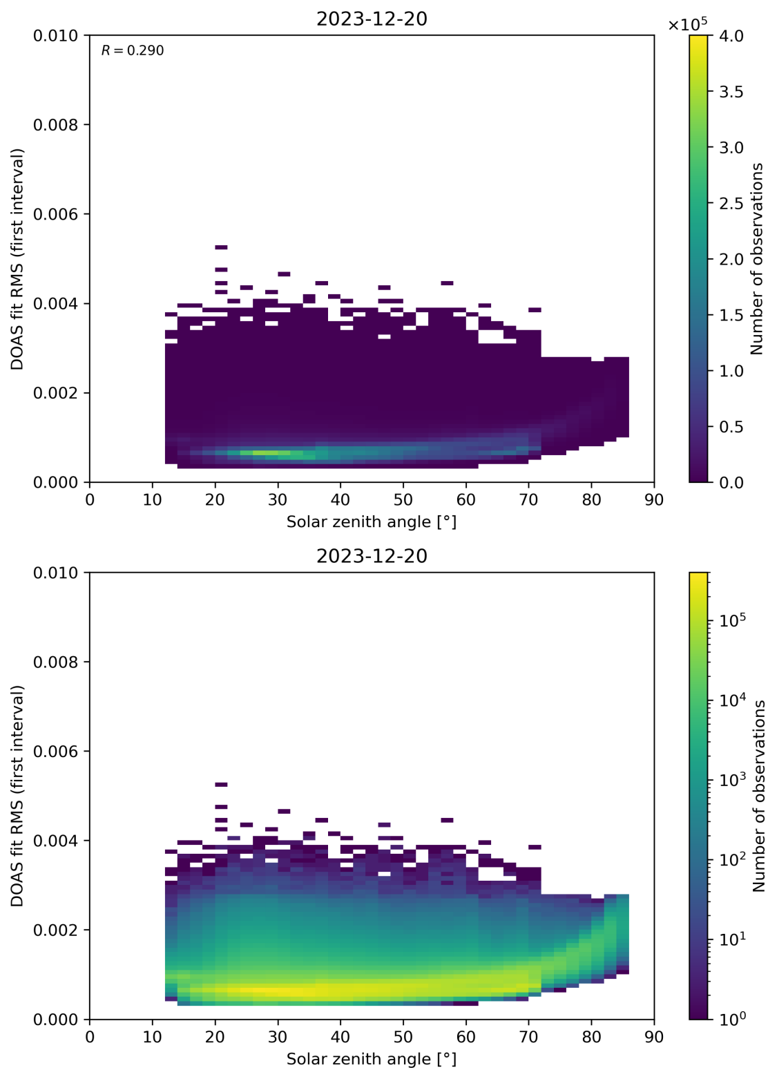
Figure 167: Scatter density plot of “Solar zenith angle” against “DOAS fit RMS (first interval)” for 2023-12-20 to 2023-12-21.
