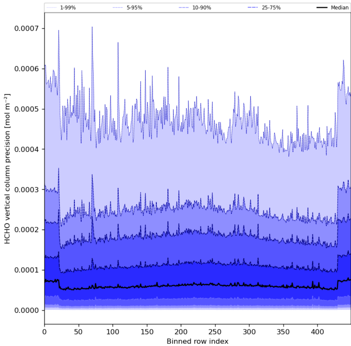
Figure 50: Along track statistics of “HCHO vertical column precision” for 2023-12-20 to 2023-12-21
