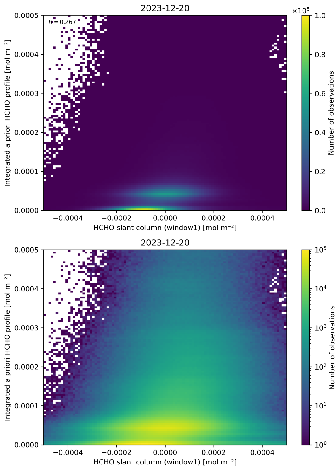
Figure 87: Scatter density plot of “HCHO slant column (window1)” against “Integrated a priori HCHO profile” for 2023-12-20 to 2023-12-21.
