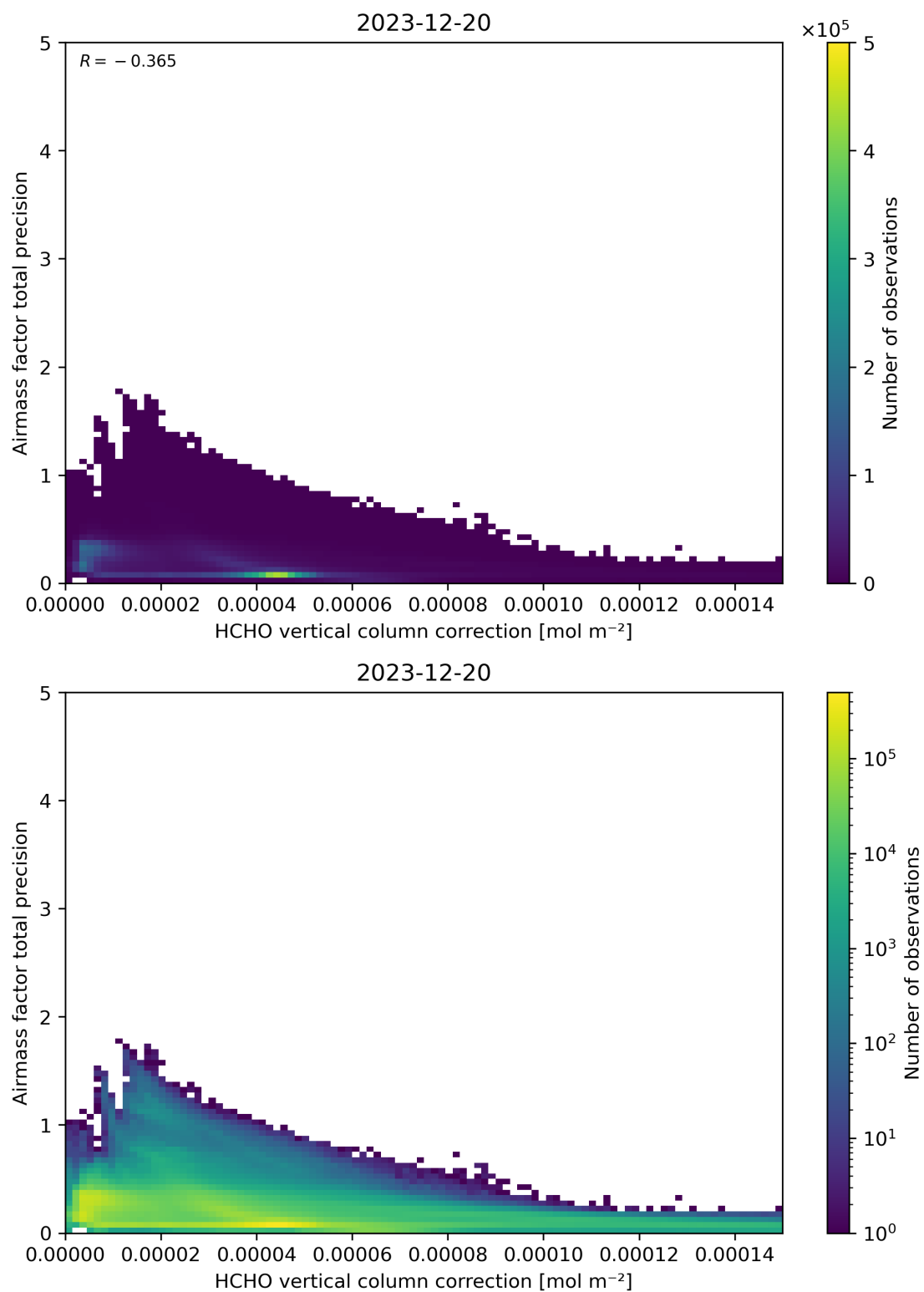
Figure 121: Scatter density plot of “HCHO vertical column correction” against “Airmass factor total precision” for 2023-12-20 to 2023-12-21.
