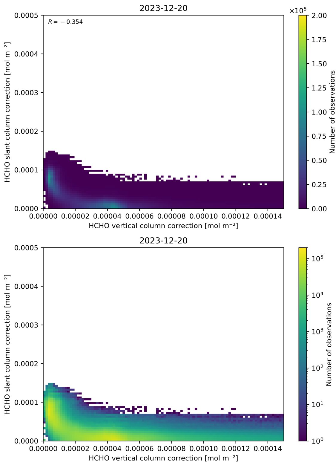
Figure 117: Scatter density plot of “HCHO vertical column correction” against “HCHO slant column correction” for 2023-12-20 to 2023-12-21.
