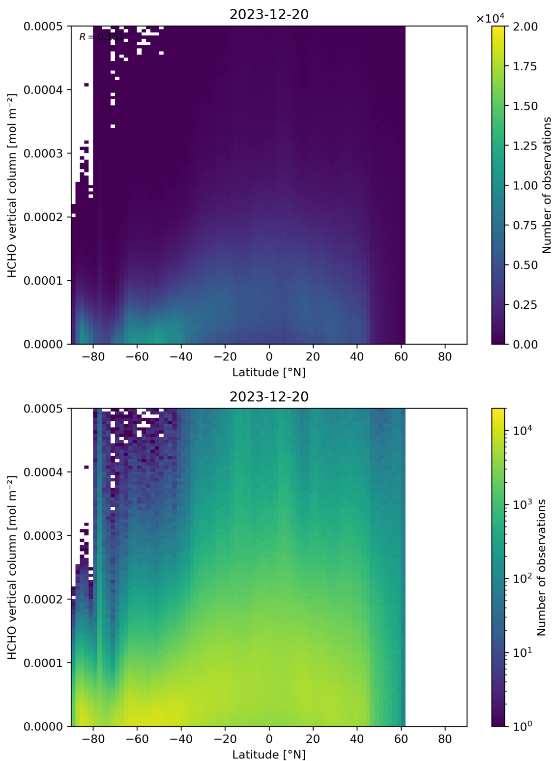
Figure 163: Scatter density plot of “Latitude” against “HCHO vertical column” for 2023-12-20 to 2023-12-21.
