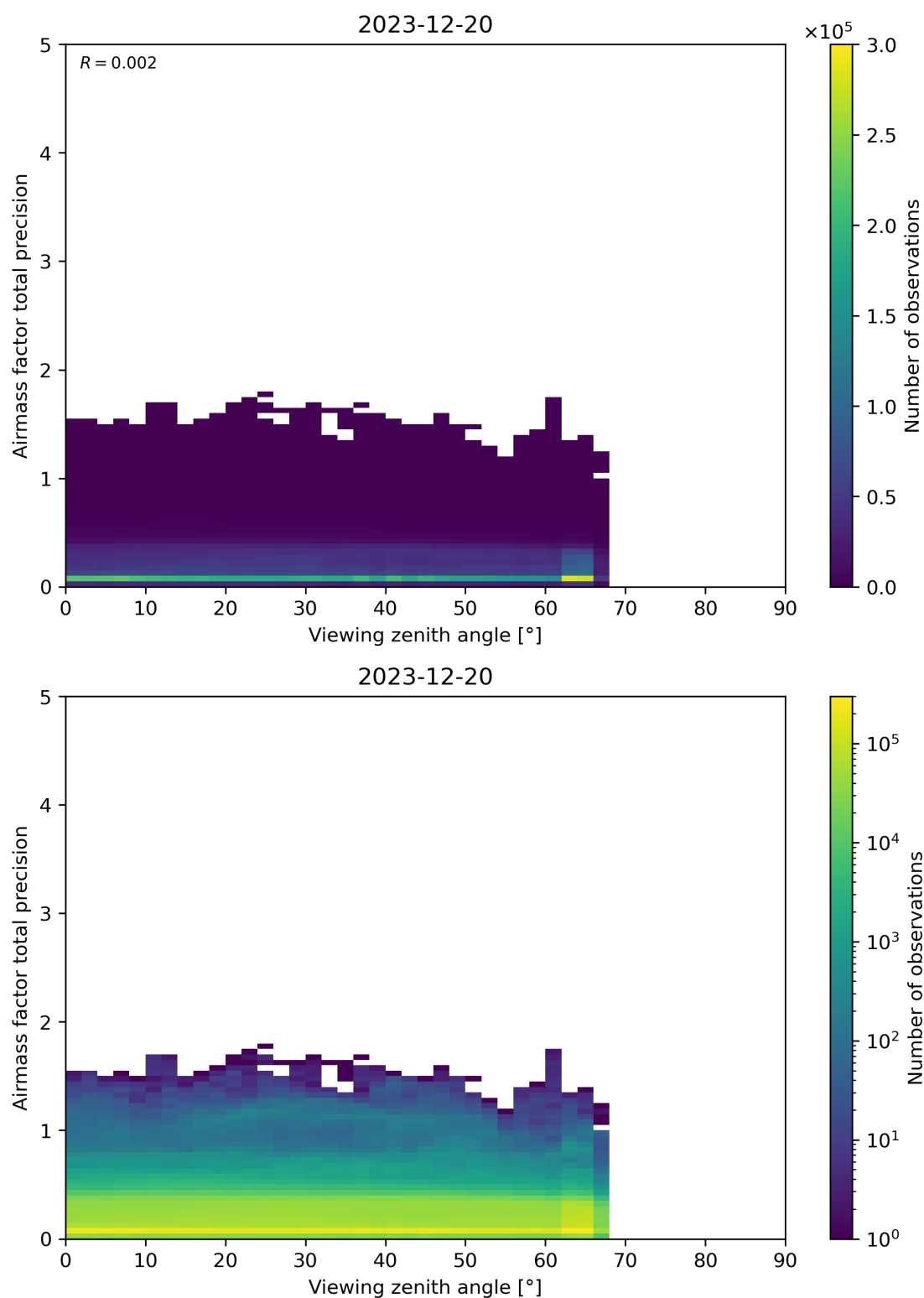
Figure 191: Scatter density plot of “Viewing zenith angle” against “Airmass factor total precision” for 2023-12-20 to 2023-12-21.
