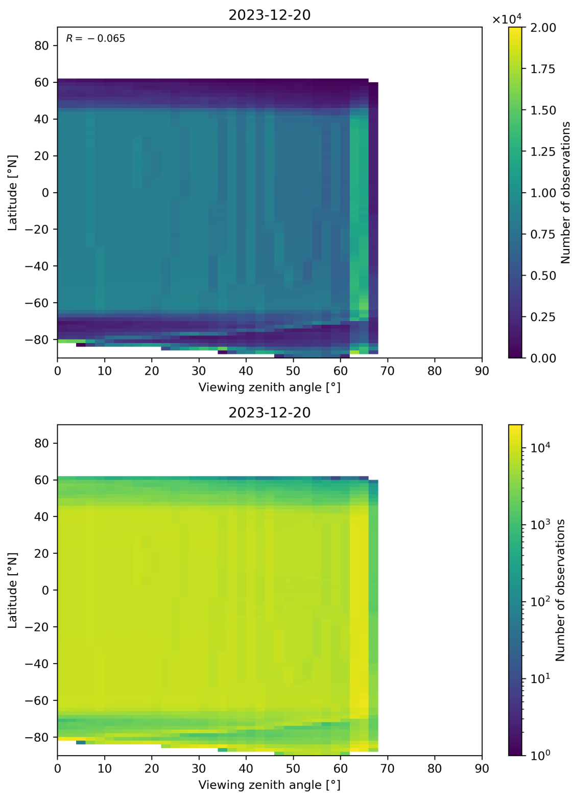
Figure 196: Scatter density plot of “Viewing zenith angle” against “Latitude” for 2023-12-20 to 2023-12-21.
