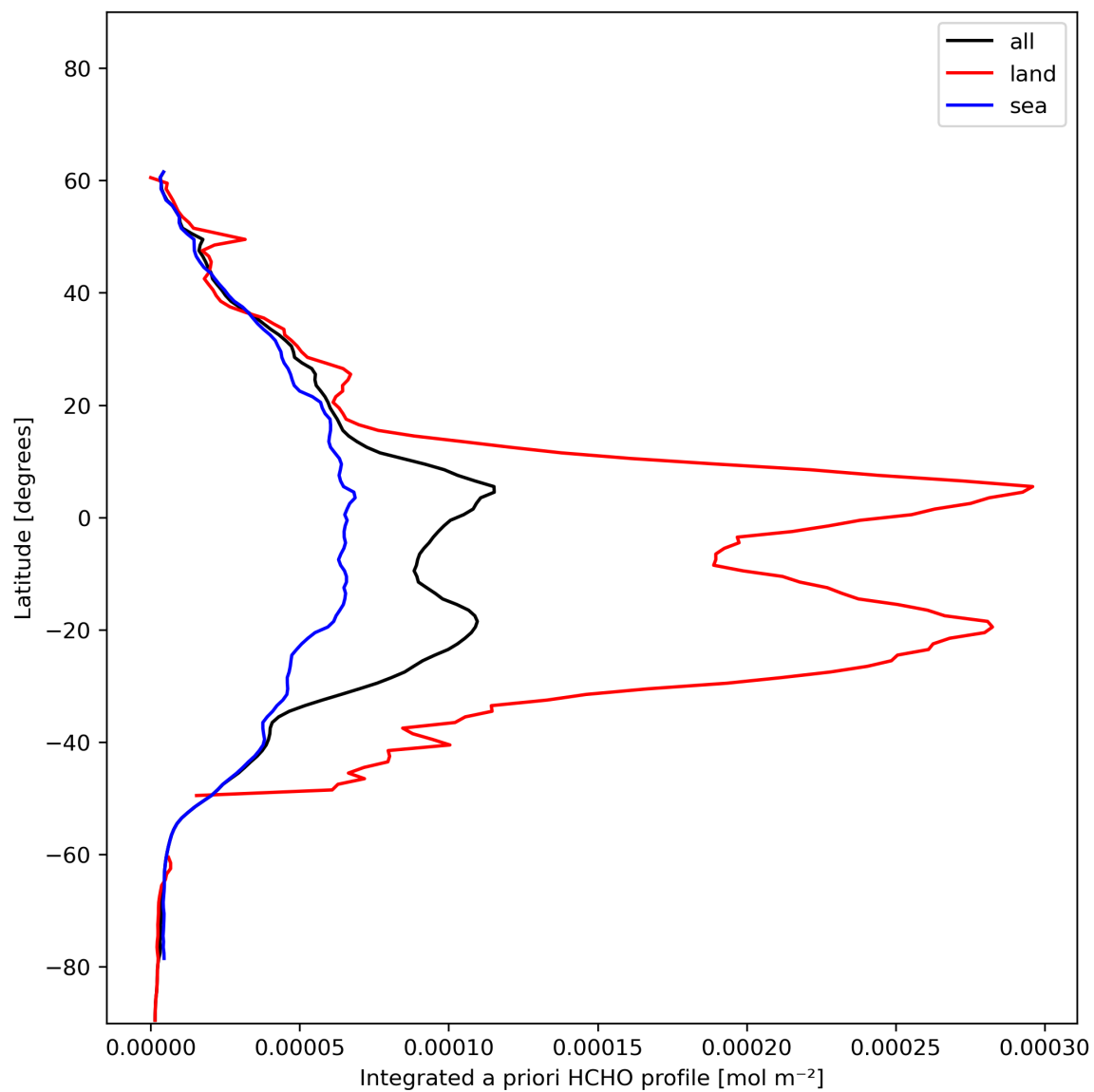
Figure 29: Zonal average of “Integrated a priori HCHO profile” for 2023-12-20 to 2023-12-21.
