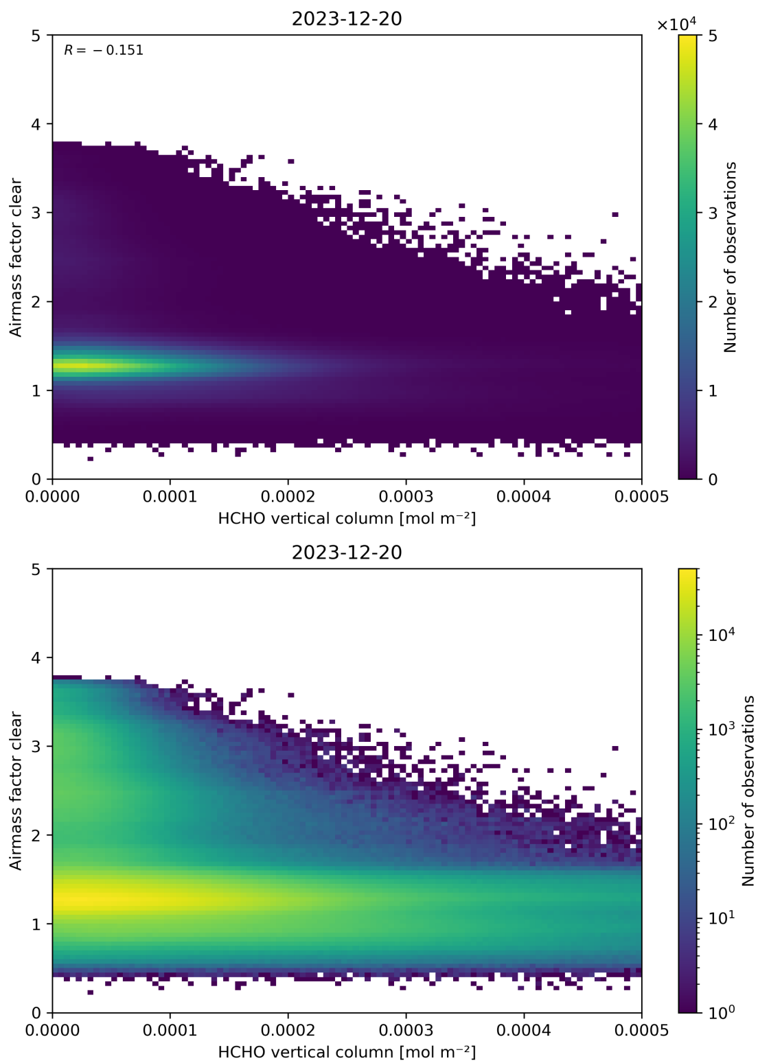
Figure 126: Scatter density plot of “HCHO vertical column” against “Airmass factor clear” for 2023-12-20 to 2023-12-21.
