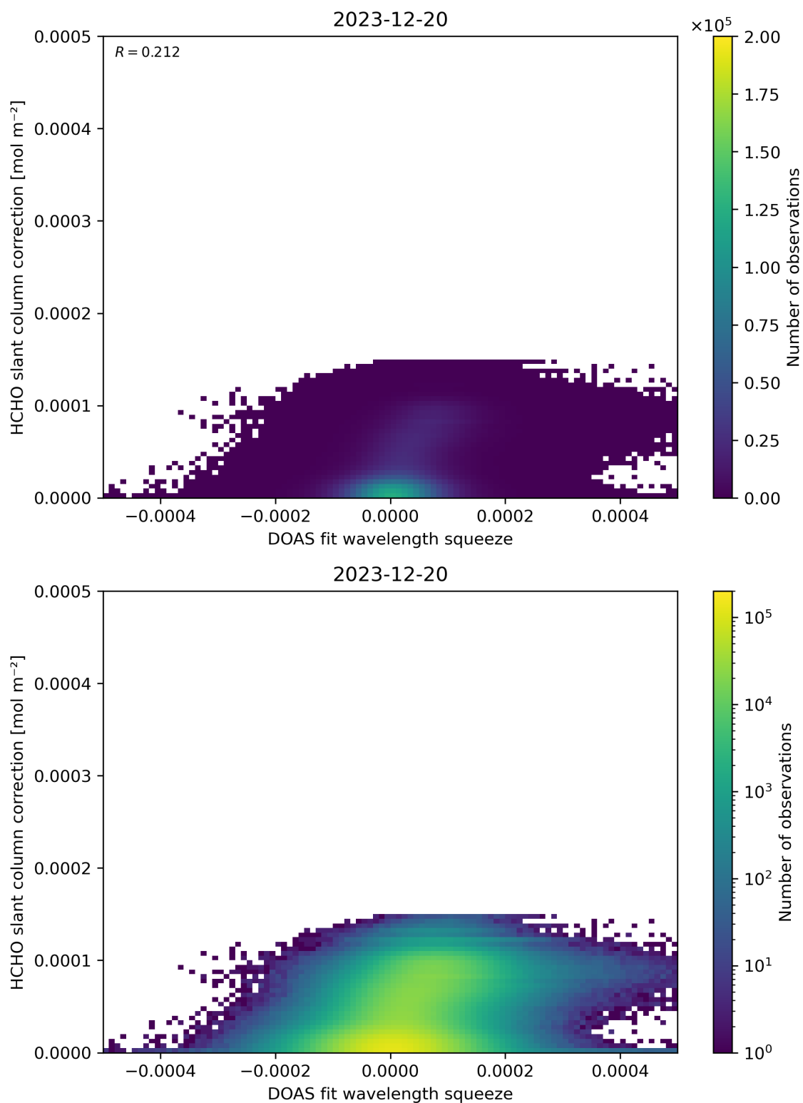
Figure 70: Scatter density plot of “DOAS fit wavelength squeeze” against “HCHO slant column correction” for 2023-12-20 to 2023-12-21.
