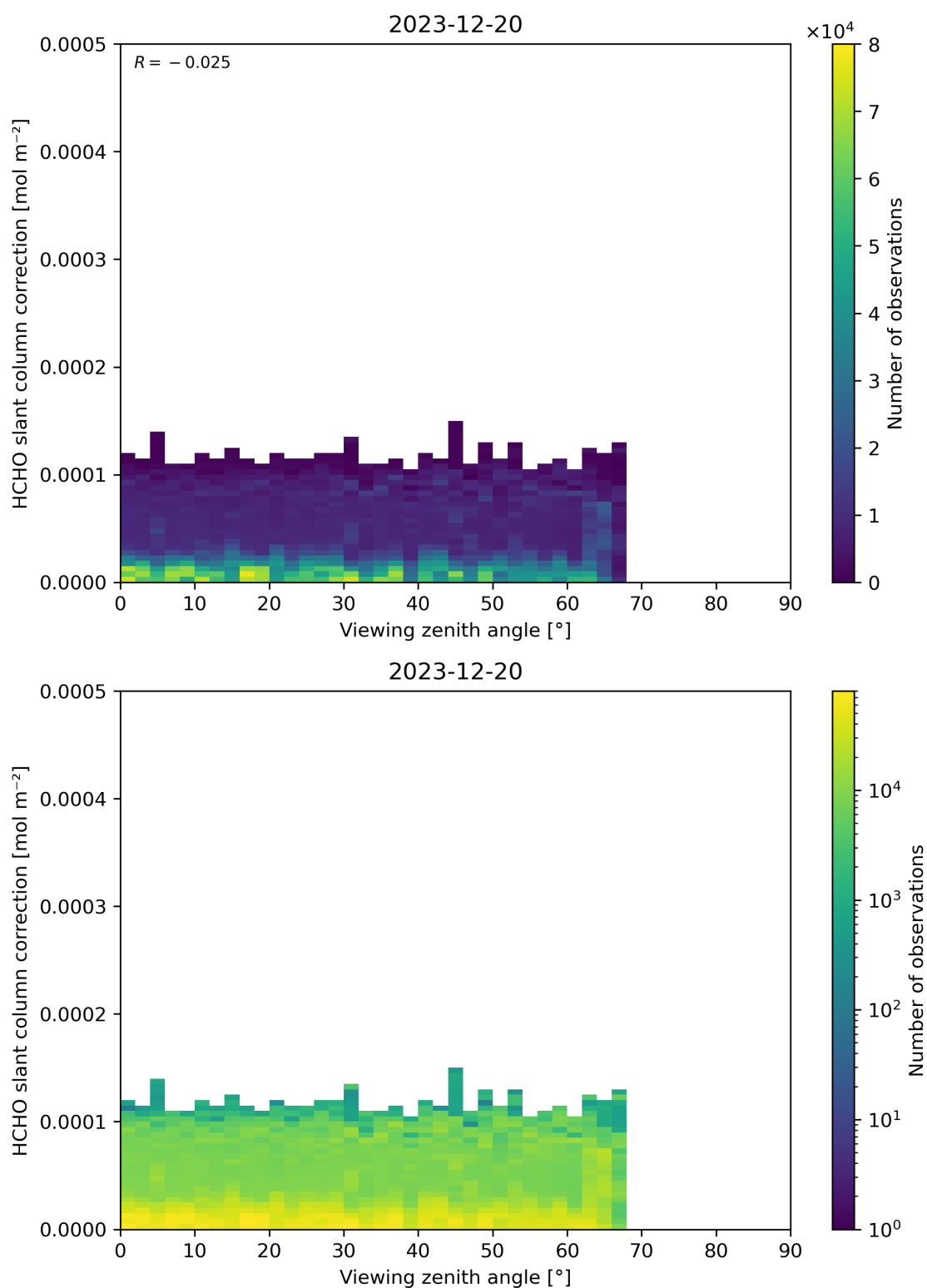
Figure 187: Scatter density plot of “Viewing zenith angle” against “HCHO slant column correction” for 2023-12-20 to 2023-12-21.
