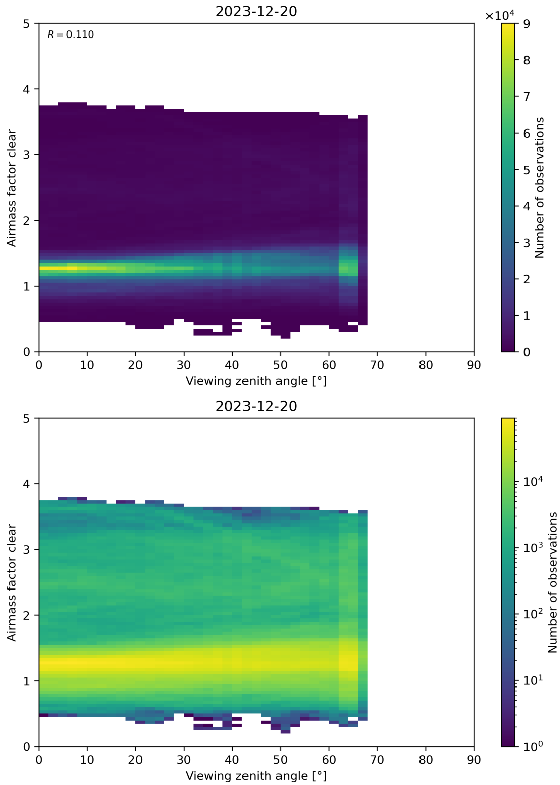
Figure 185: Scatter density plot of “Viewing zenith angle” against “Airmass factor clear” for 2023-12-20 to 2023-12-21.
