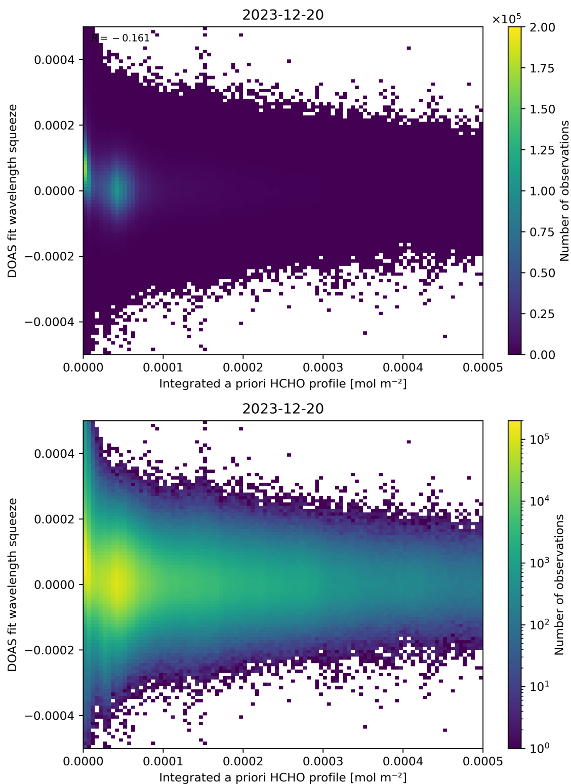
Figure 150: Scatter density plot of “Integrated a priori HCHO profile” against “DOAS fit wavelength squeeze” for 2023-12-20 to 2023-12-21.
