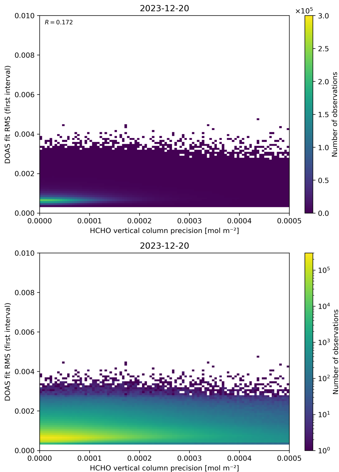
Figure 136: Scatter density plot of “HCHO vertical column precision” against “DOAS fit RMS (first interval)” for 2023-12-20 to 2023-12-21.
