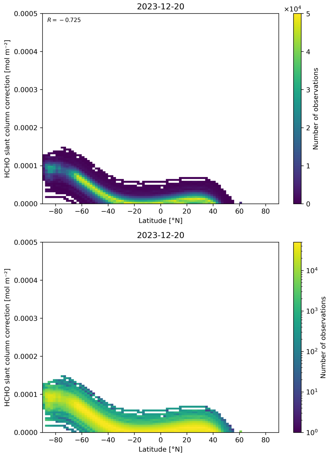
Figure 158: Scatter density plot of “Latitude” against “HCHO slant column correction” for 2023-12-20 to 2023-12-21.
