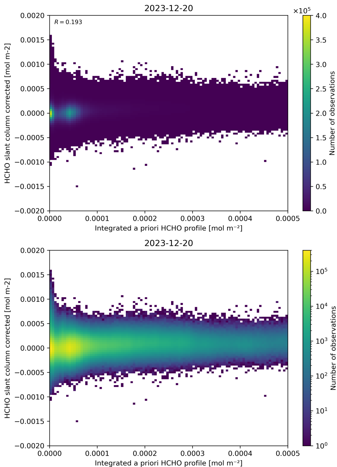
Figure 151: Scatter density plot of “Integrated a priori HCHO profile” against “HCHO slant column corrected” for 2023-12-20 to 2023-12-21.
