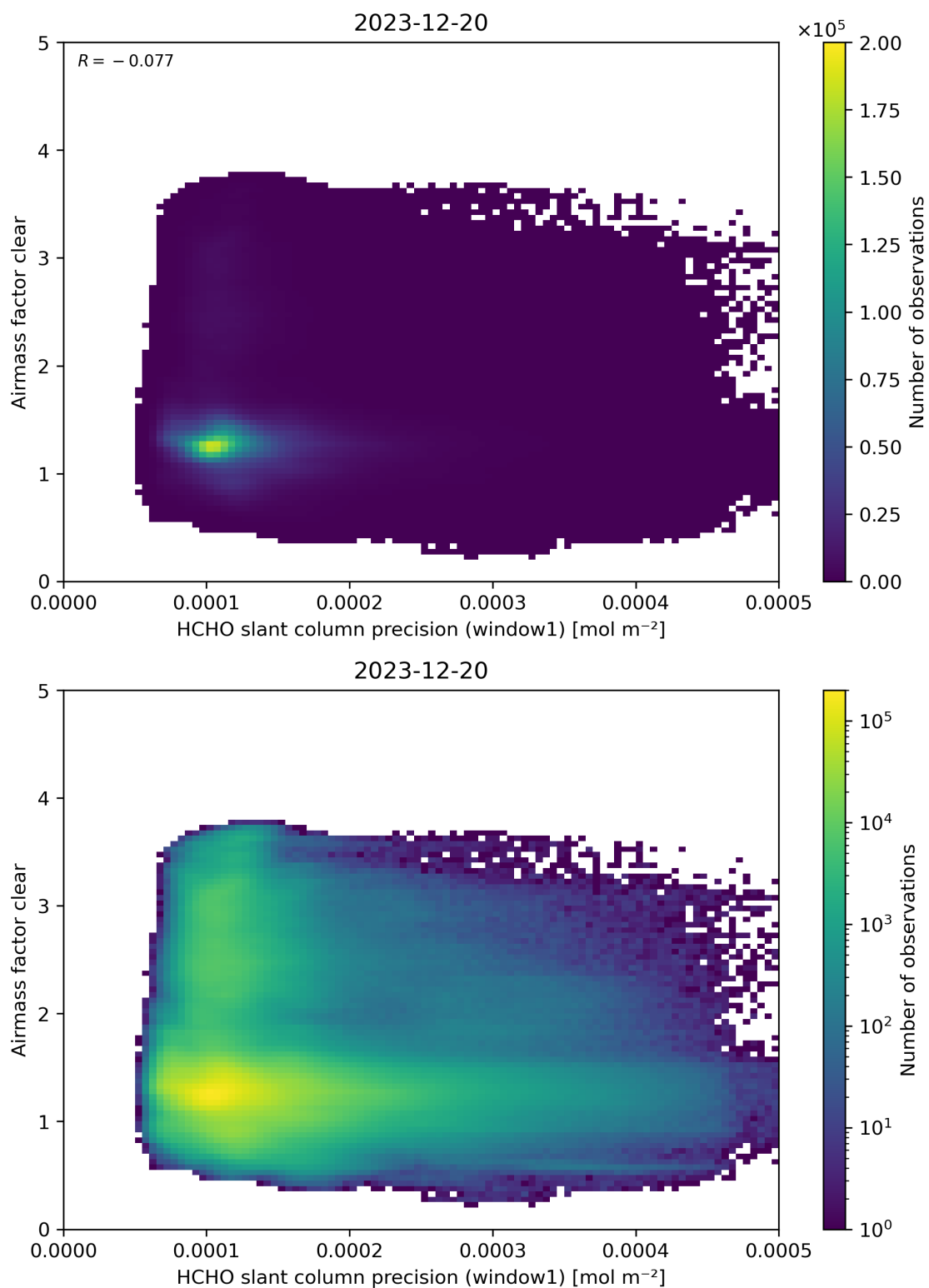
Figure 91: Scatter density plot of “HCHO slant column precision (window1)” against “Airmass factor clear” for 2023-12-20 to 2023-12-21.
