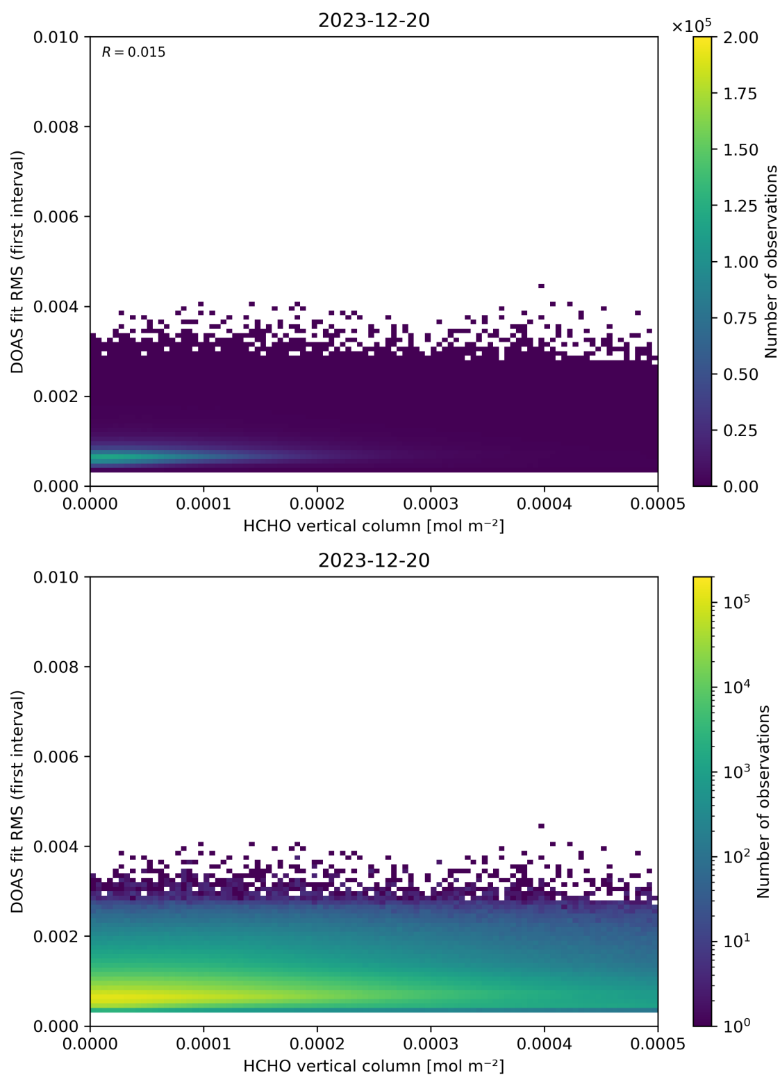
Figure 123: Scatter density plot of “HCHO vertical column” against “DOAS fit RMS (first interval)” for 2023-12-20 to 2023-12-21.
