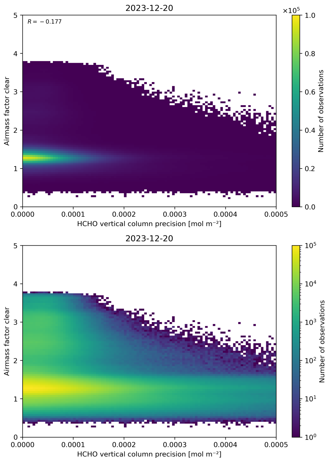
Figure 139: Scatter density plot of “HCHO vertical column precision” against “Airmass factor clear” for 2023-12-20 to 2023-12-21.
