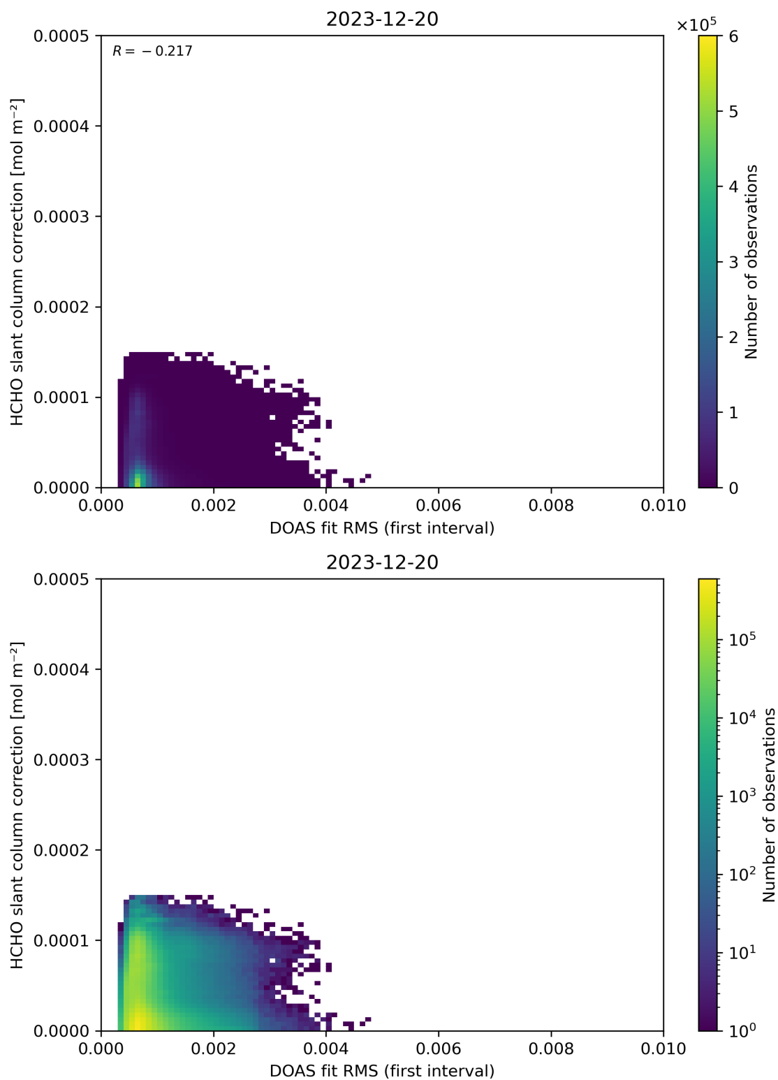
Figure 63: Scatter density plot of “DOAS fit RMS (first interval)” against “HCHO slant column correction” for 2023-12-20 to 2023-12-21.
