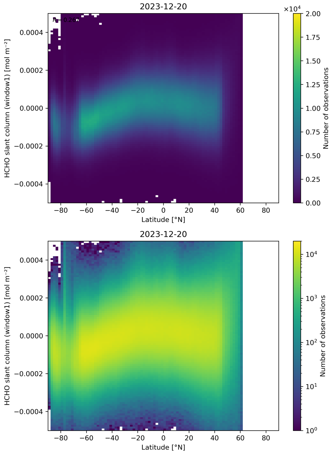
Figure 159: Scatter density plot of “Latitude” against “HCHO slant column (window1)” for 2023-12-20 to 2023-12-21.
