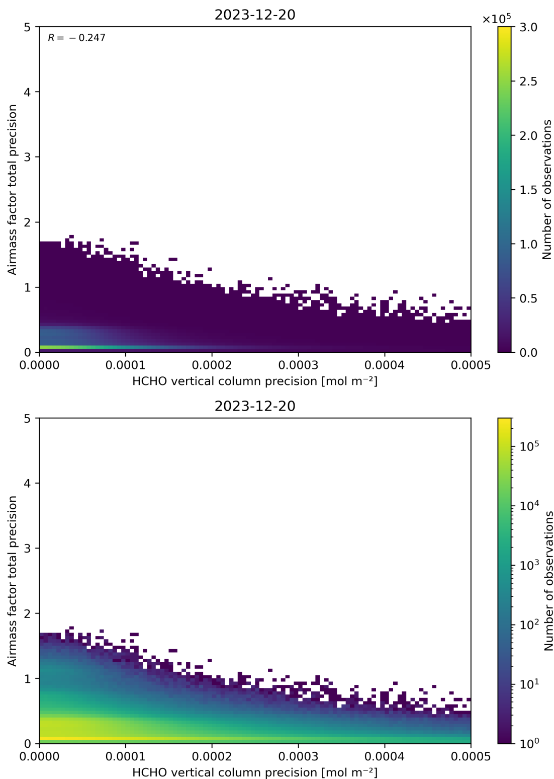
Figure 145: Scatter density plot of “HCHO vertical column precision” against “Airmass factor total precision” for 2023-12-20 to 2023-12-21.
