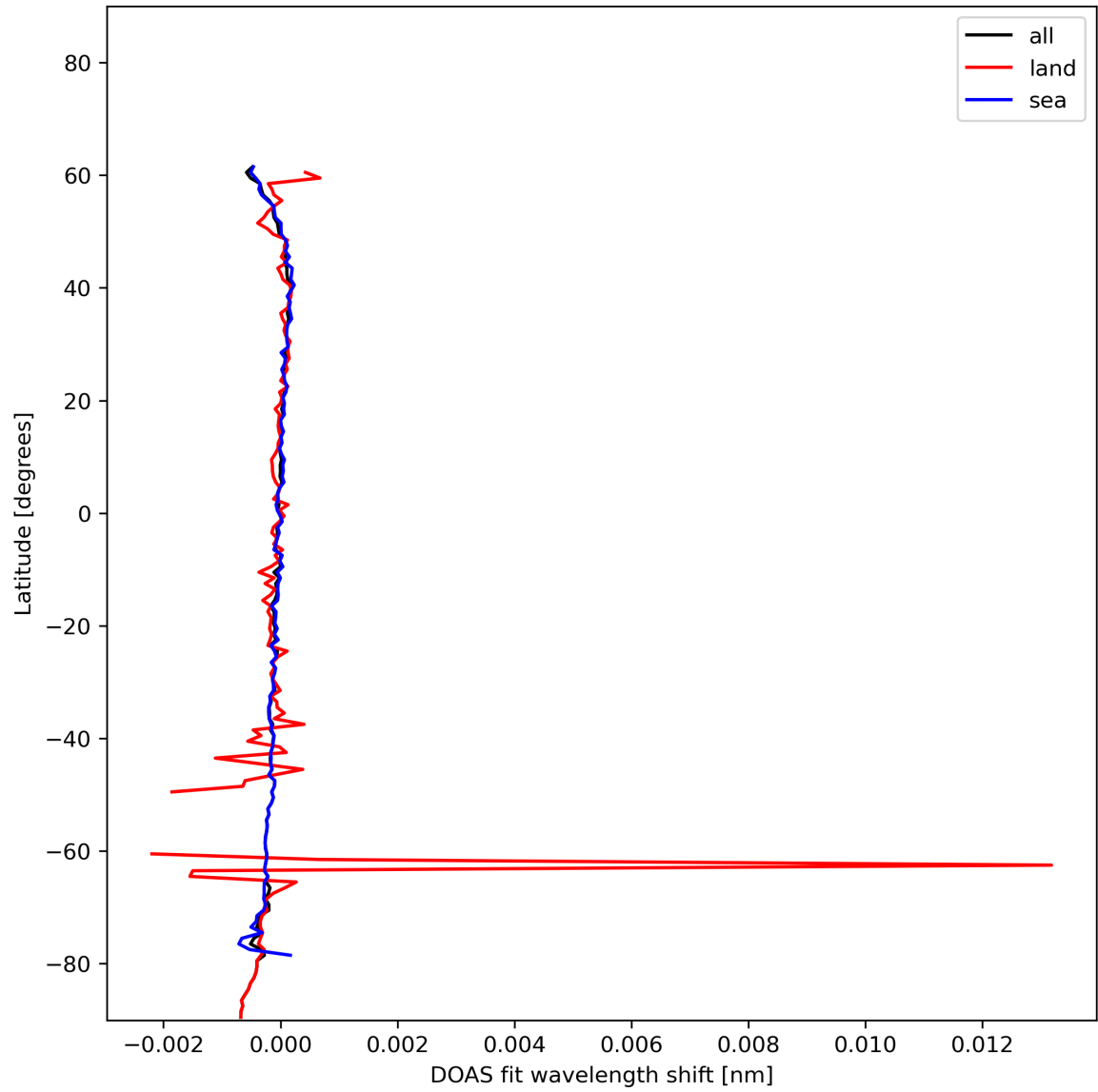
Figure 30: Zonal average of “DOAS fit wavelength shift” for 2023-12-20 to 2023-12-21.
