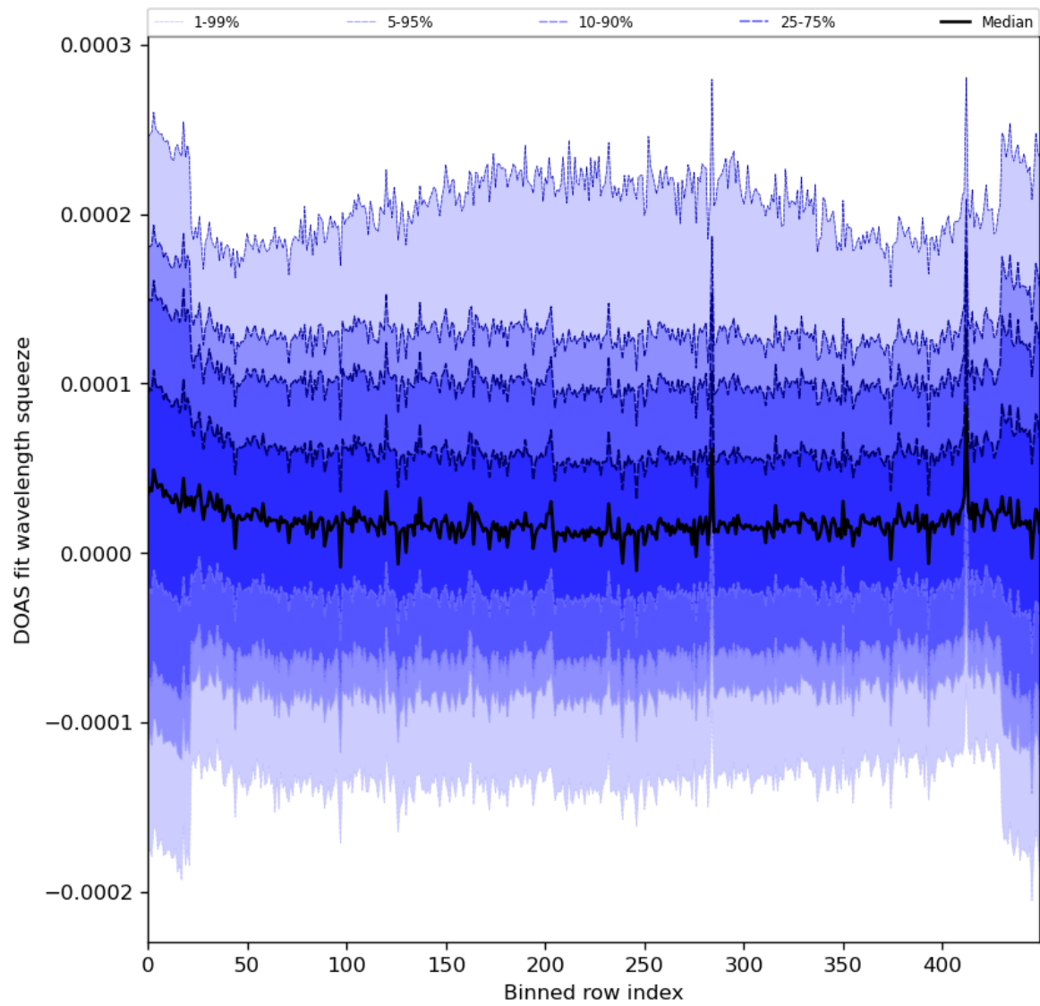
Figure 59: Along track statistics of “DOAS fit wavelength squeeze” for 2023-12-20 to 2023-12-21
