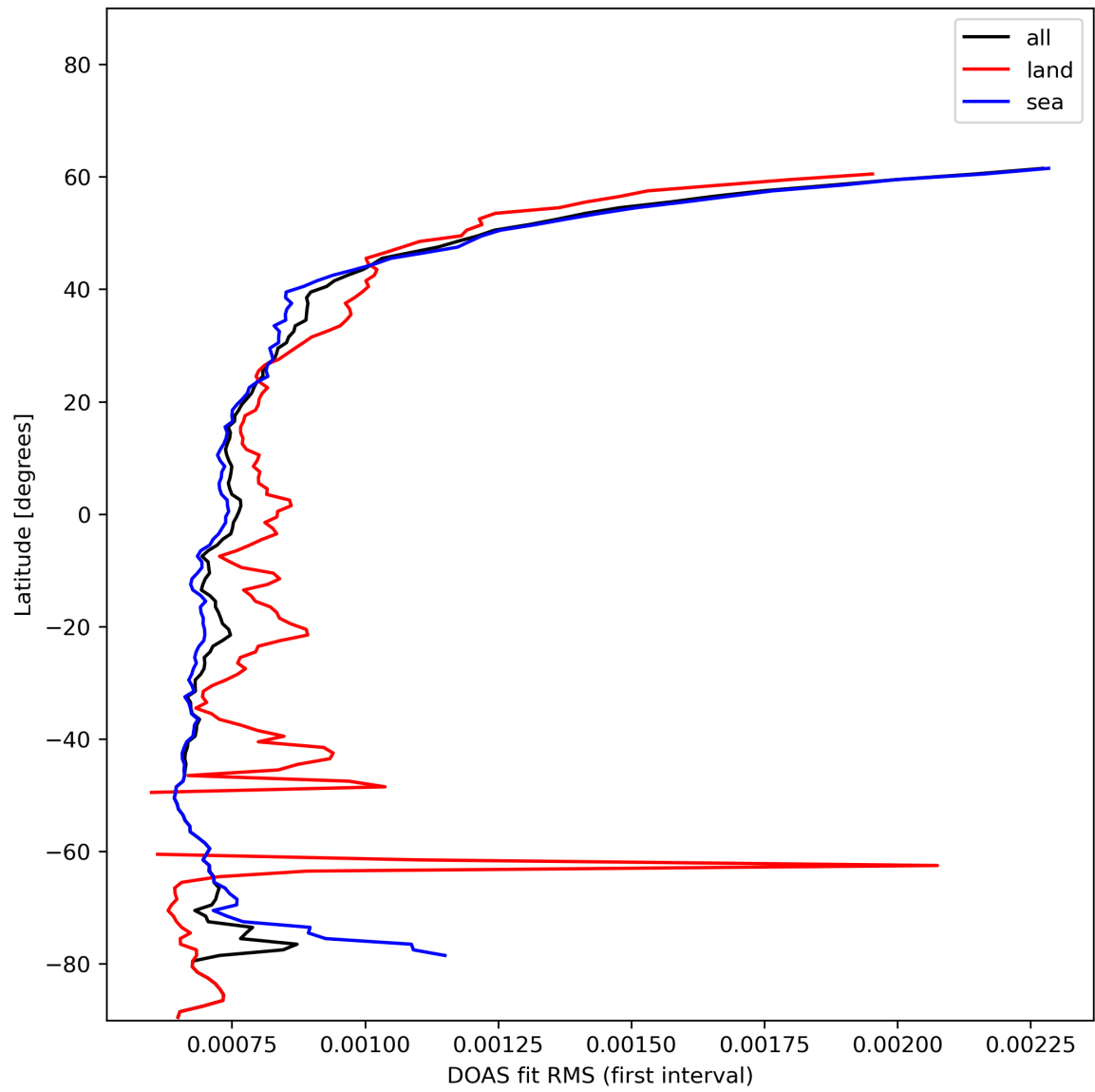
Figure 32: Zonal average of “DOAS fit RMS (first interval)” for 2023-12-20 to 2023-12-21.
