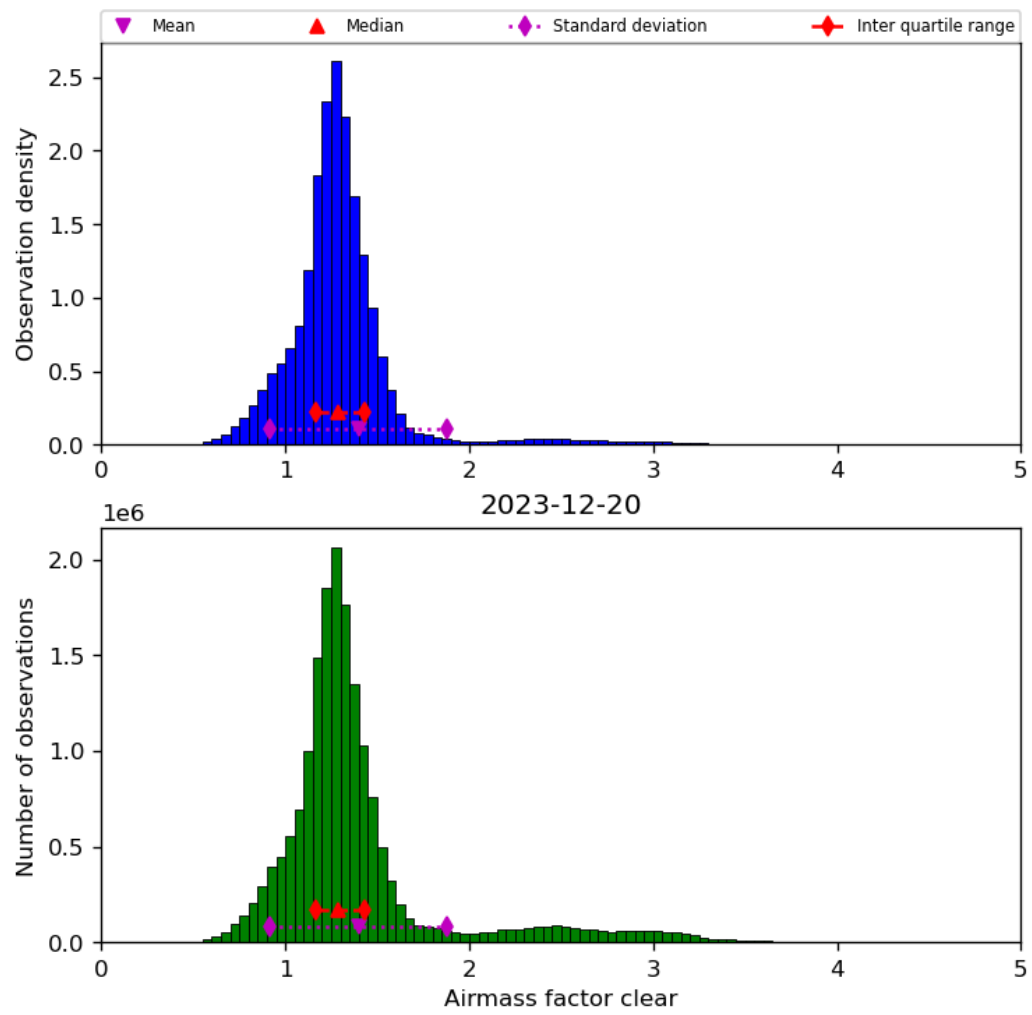
Figure 42: Histogram of “Airmass factor clear” for 2023-12-20 to 2023-12-21
