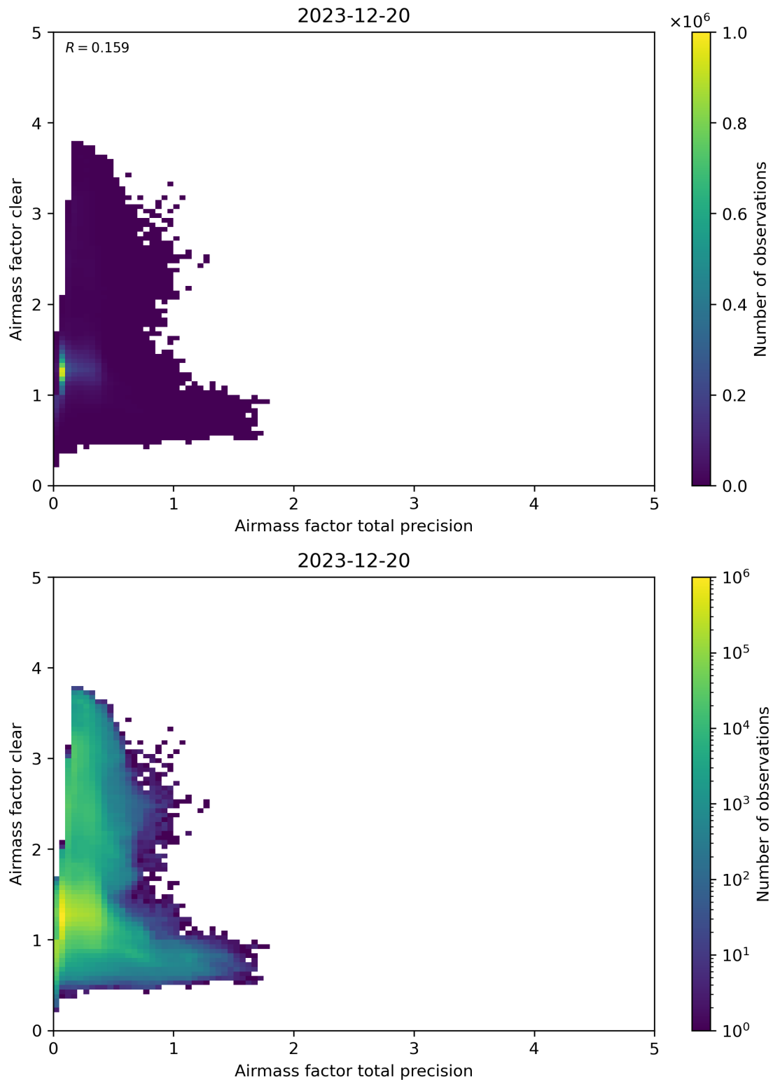
Figure 108: Scatter density plot of “Airmass factor total precision” against “Airmass factor clear” for 2023-12-20 to 2023-12-21.
