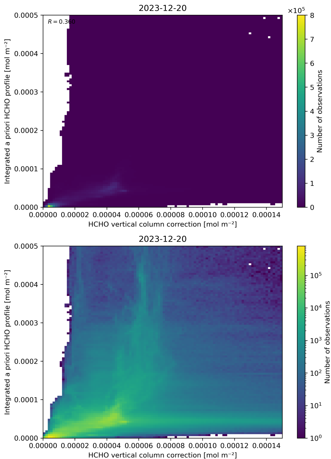
Figure 122: Scatter density plot of “HCHO vertical column correction” against “Integrated a priori HCHO profile” for 2023-12-20 to 2023-12-21.
