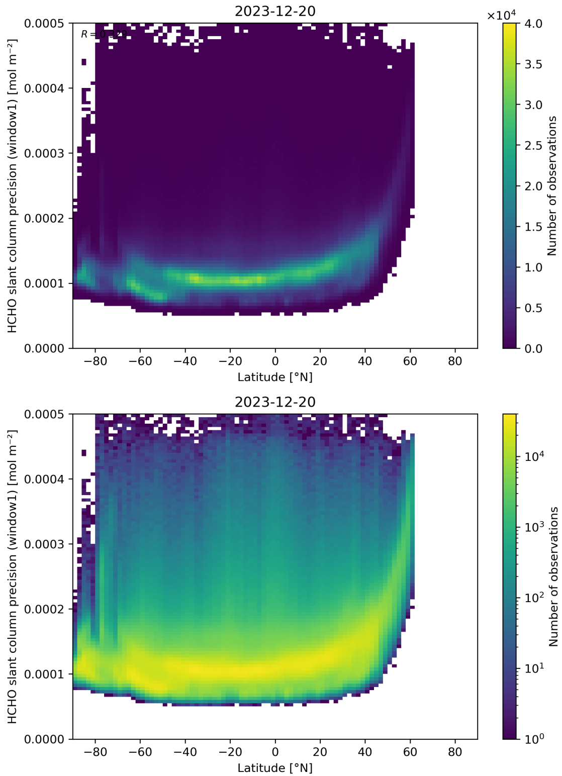
Figure 160: Scatter density plot of “Latitude” against “HCHO slant column precision (window1)” for 2023-12-20 to 2023-12-21.
