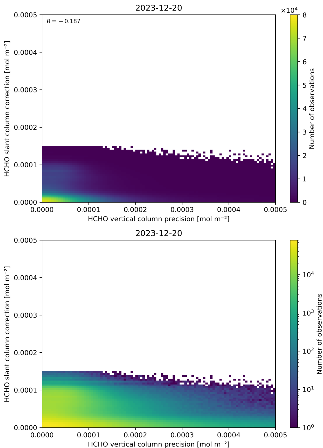
Figure 141: Scatter density plot of “HCHO vertical column precision” against “HCHO slant column correction” for 2023-12-20 to 2023-12-21.
