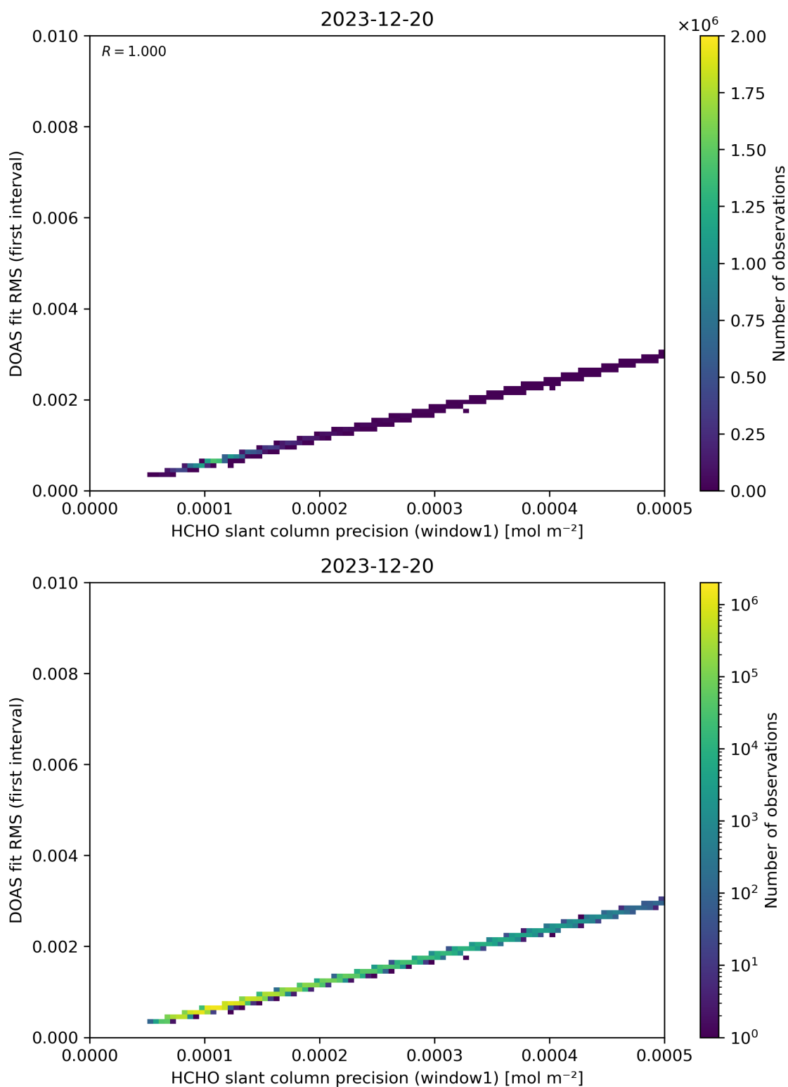
Figure 88: Scatter density plot of “HCHO slant column precision (window1)” against “DOAS fit RMS (first interval)” for 2023-12-20 to 2023-12-21.
