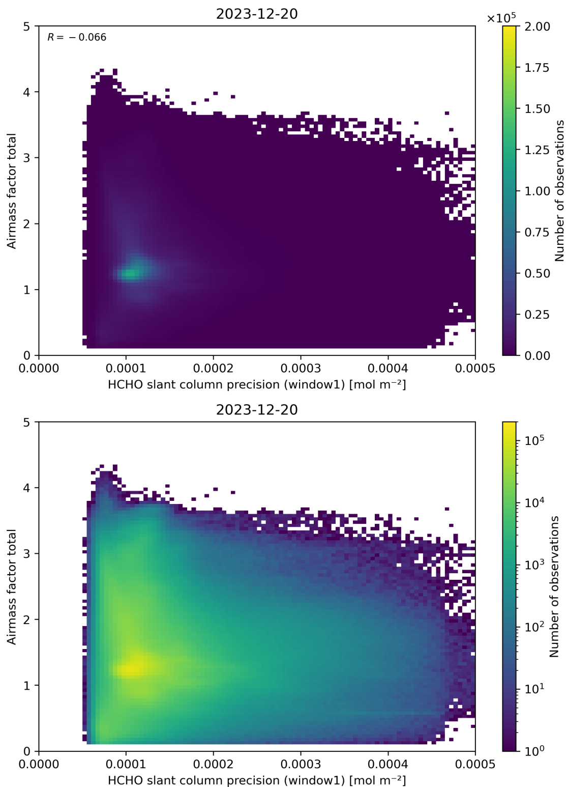
Figure 94: Scatter density plot of “HCHO slant column precision (window1)” against “Airmass factor total” for 2023-12-20 to 2023-12-21.
