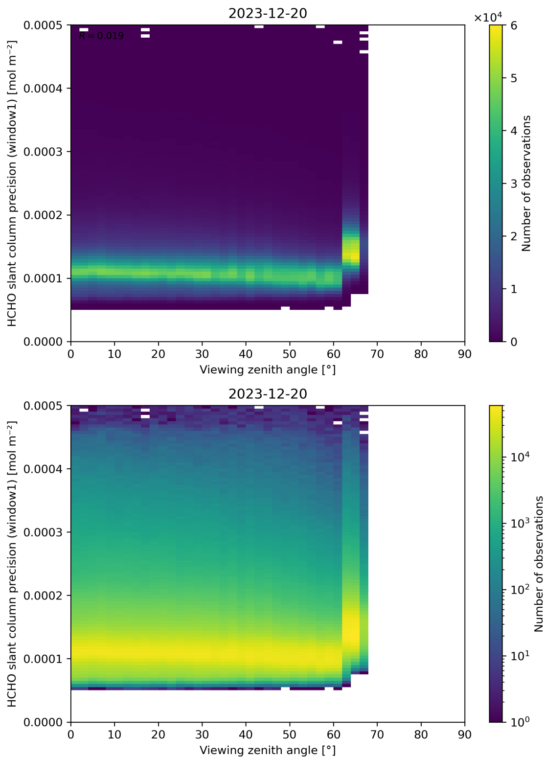
Figure 189: Scatter density plot of “Viewing zenith angle” against “HCHO slant column precision (window1)” for 2023-12-20 to 2023-12-21.
