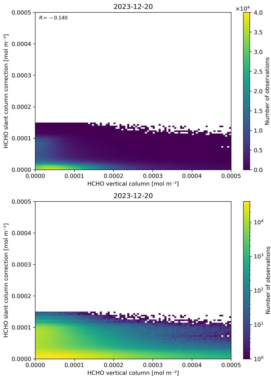
Figure 128: Scatter density plot of “HCHO vertical column” against “HCHO slant column correction” for 2023-12-20 to 2023-12-21.
