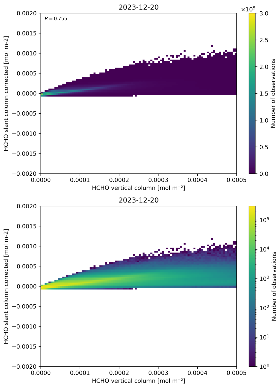
Figure 127: Scatter density plot of “HCHO vertical column” against “HCHO slant column corrected” for 2023-12-20 to 2023-12-21.
