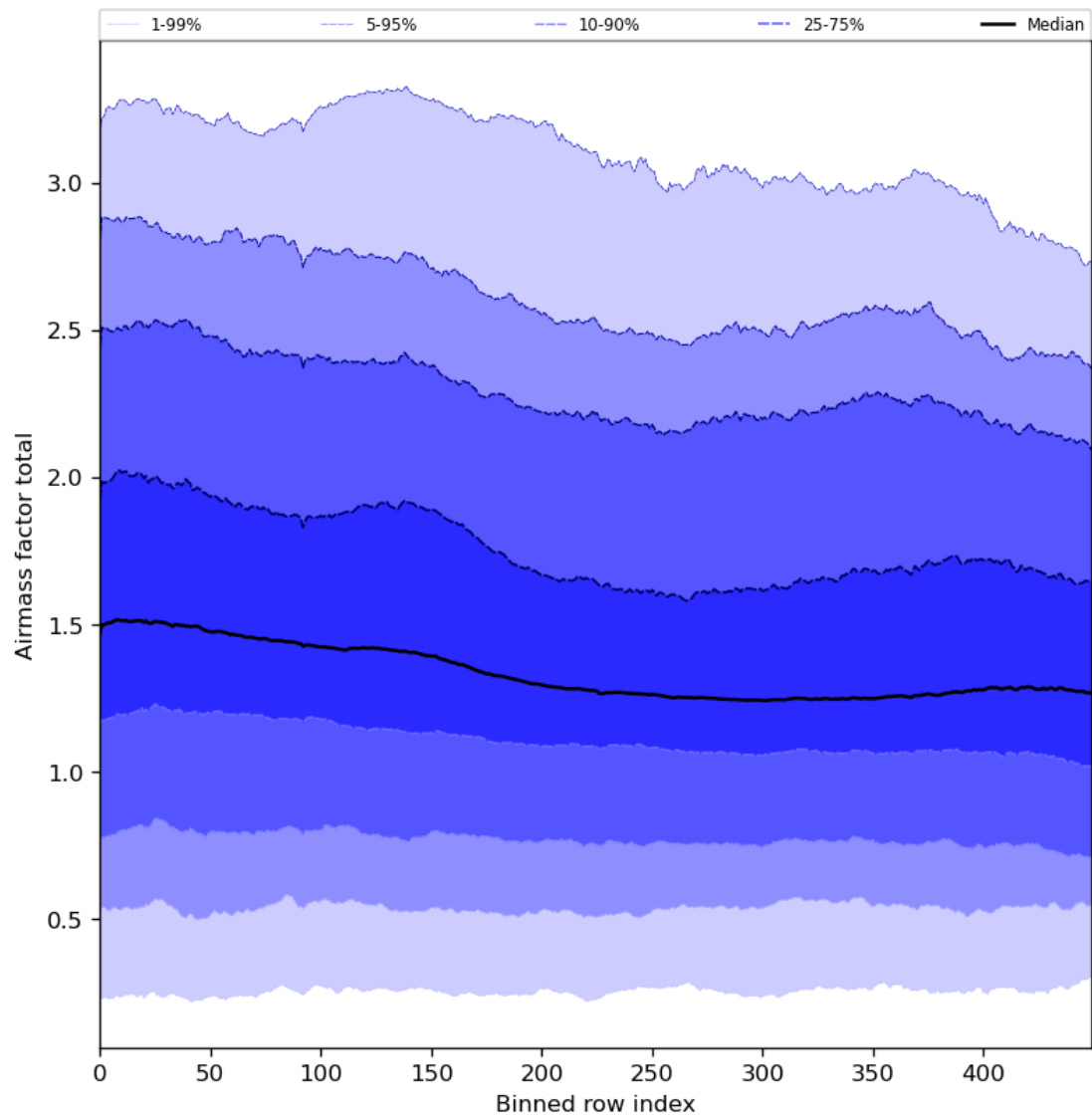
Figure 54: Along track statistics of “Airmass factor total” for 2023-12-20 to 2023-12-21
