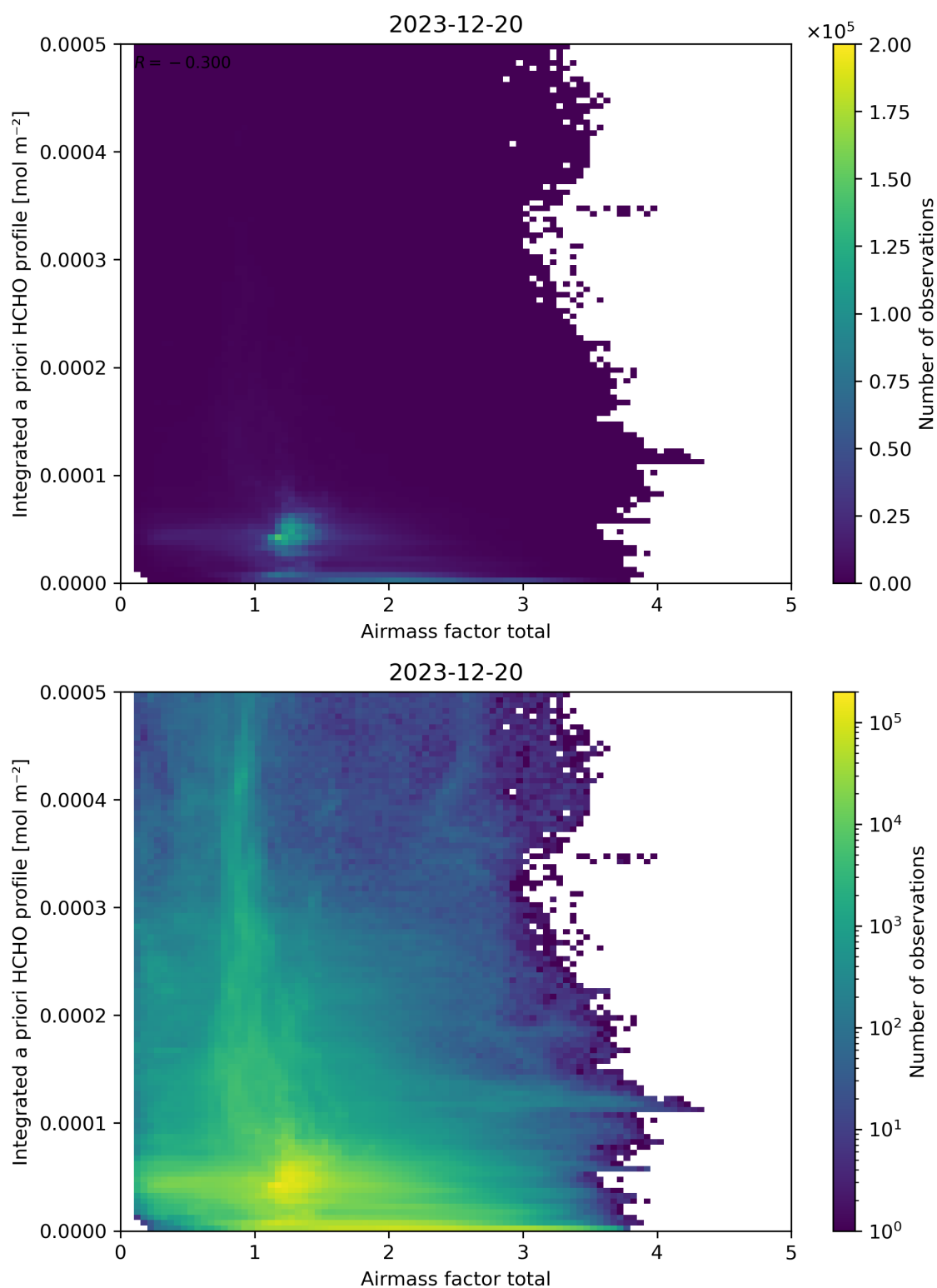
Figure 104: Scatter density plot of “Airmass factor total” against “Integrated a priori HCHO profile” for 2023-12-20 to 2023-12-21.
