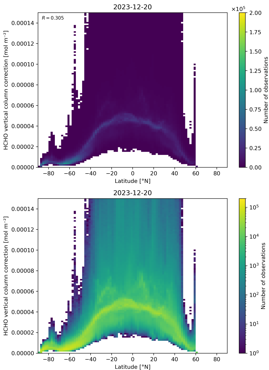
Figure 164: Scatter density plot of “Latitude” against “HCHO vertical column correction” for 2023-12-20 to 2023-12-21.
