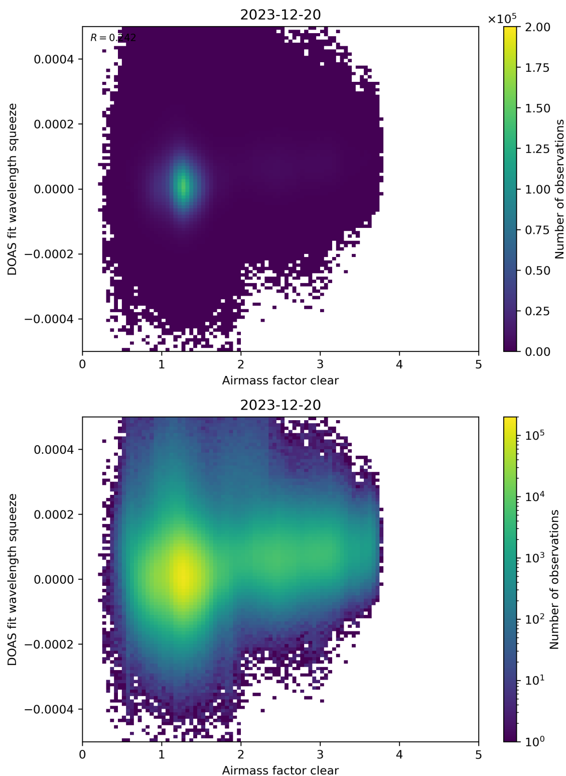
Figure 73: Scatter density plot of “Airmass factor clear” against “DOAS fit wavelength squeeze” for 2023-12-20 to 2023-12-21.
