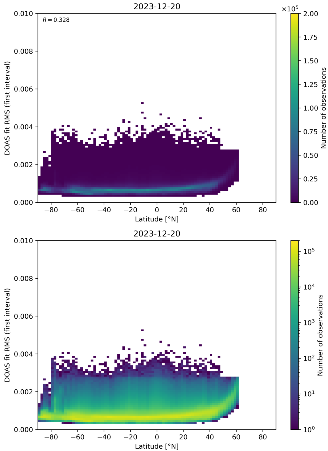
Figure 153: Scatter density plot of “Latitude” against “DOAS fit RMS (first interval)” for 2023-12-20 to 2023-12-21.
