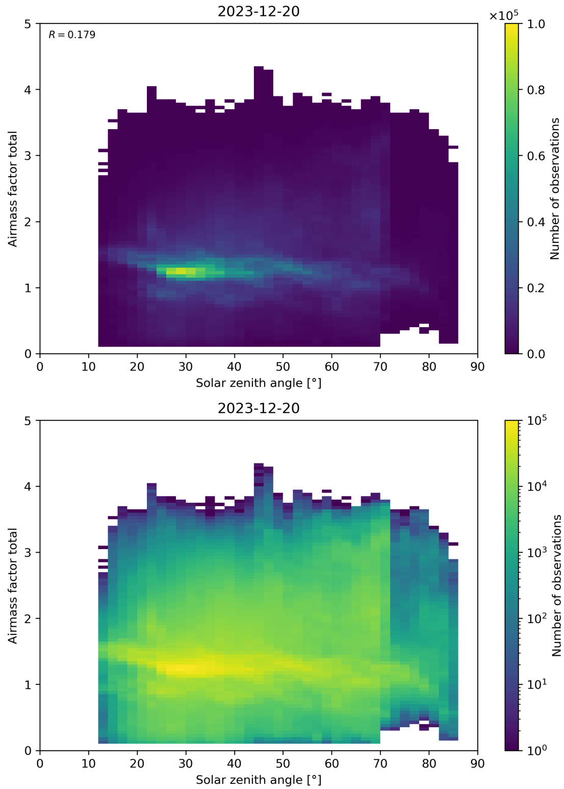
Figure 175: Scatter density plot of “Solar zenith angle” against “Airmass factor total” for 2023-12-20 to 2023-12-21.
