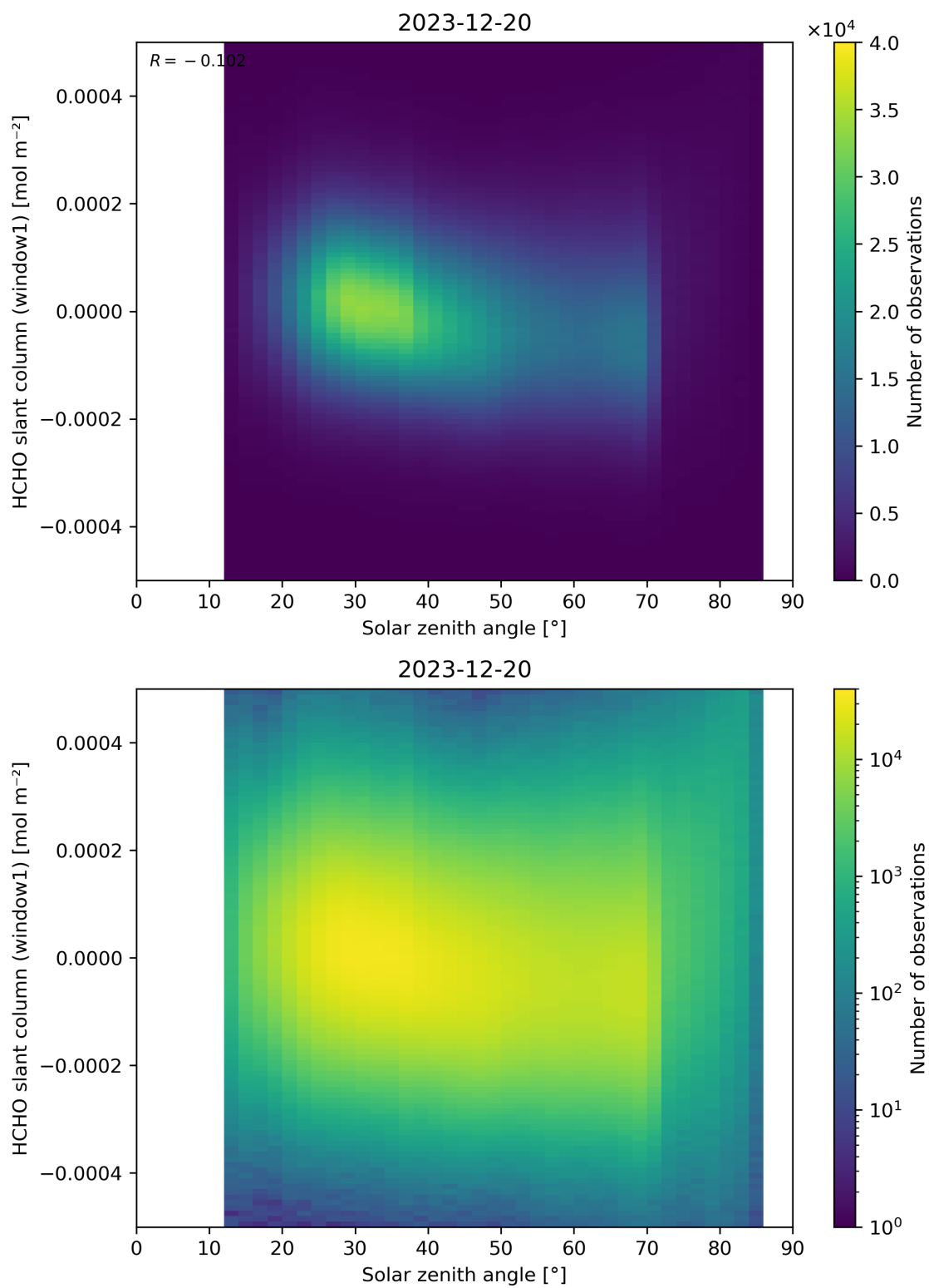
Figure 173: Scatter density plot of “Solar zenith angle” against “HCHO slant column (window1)” for 2023-12-20 to 2023-12-21.
