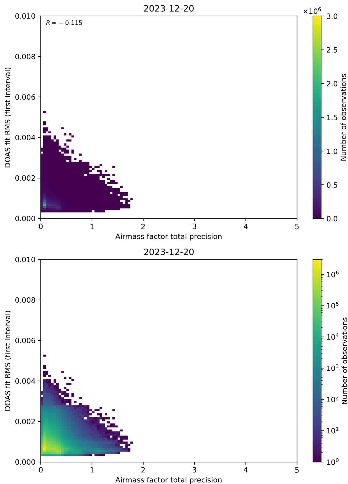
Figure 105: Scatter density plot of “Airmass factor total precision” against “DOAS fit RMS (first interval)” for 2023-12-20 to 2023-12-21.
