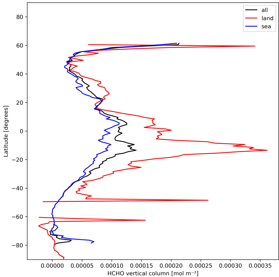
Figure 21: Zonal average of “HCHO vertical column” for 2023-12-20 to 2023-12-21.
