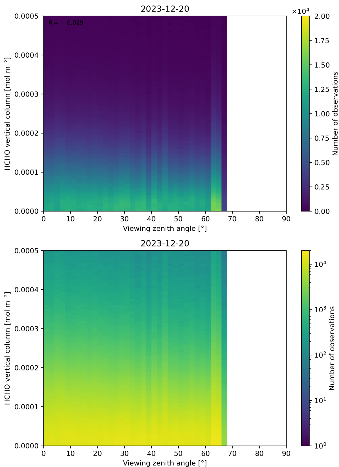
Figure 192: Scatter density plot of “Viewing zenith angle” against “HCHO vertical column” for 2023-12-20 to 2023-12-21.
