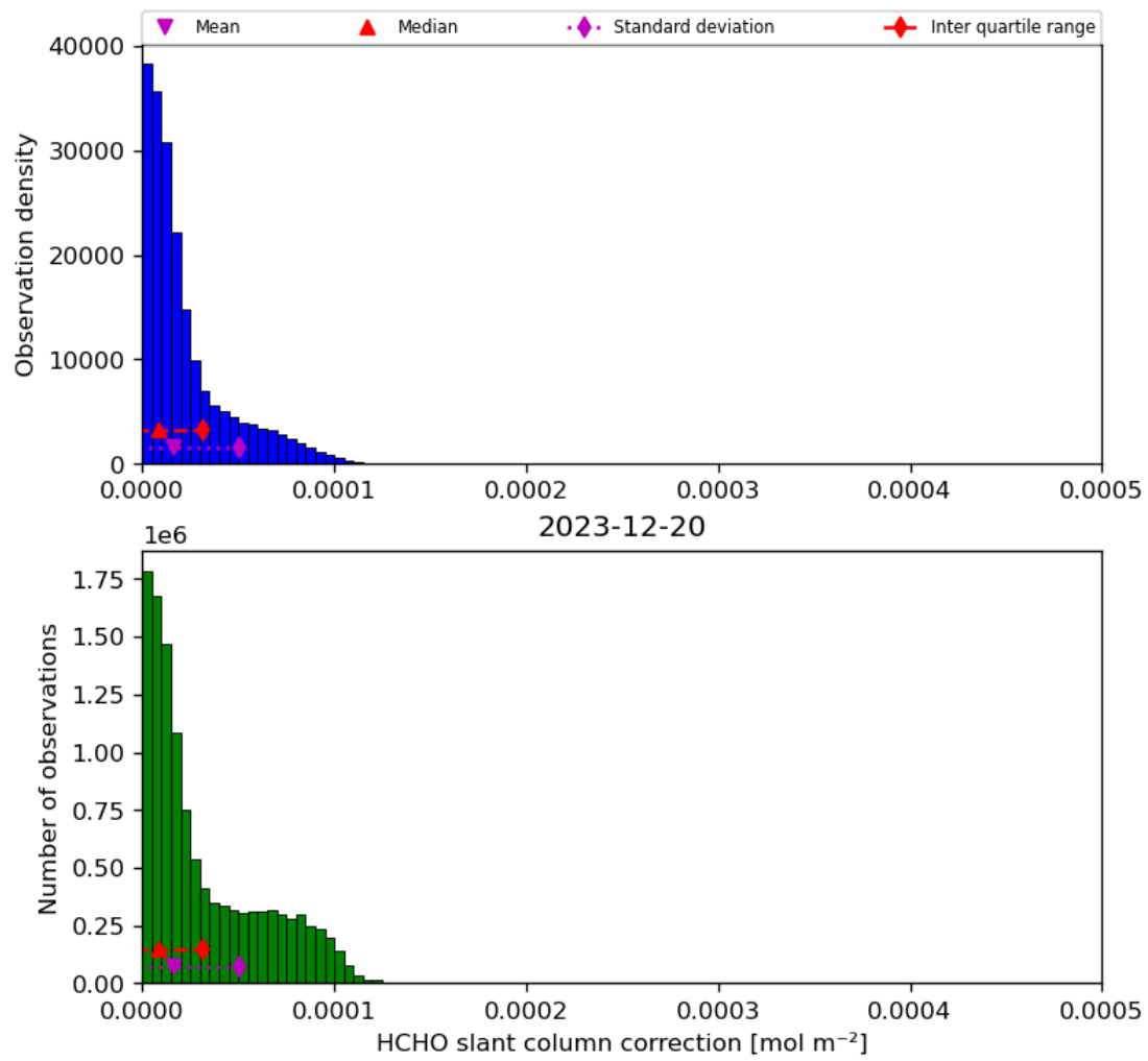
Figure 47: Histogram of “HCHO slant column correction” for 2023-12-20 to 2023-12-21
