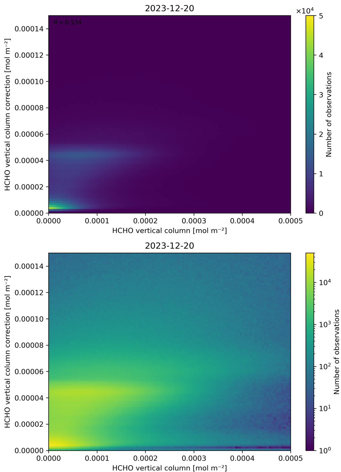
Figure 133: Scatter density plot of “HCHO vertical column” against “HCHO vertical column correction” for 2023-12-20 to 2023-12-21.
