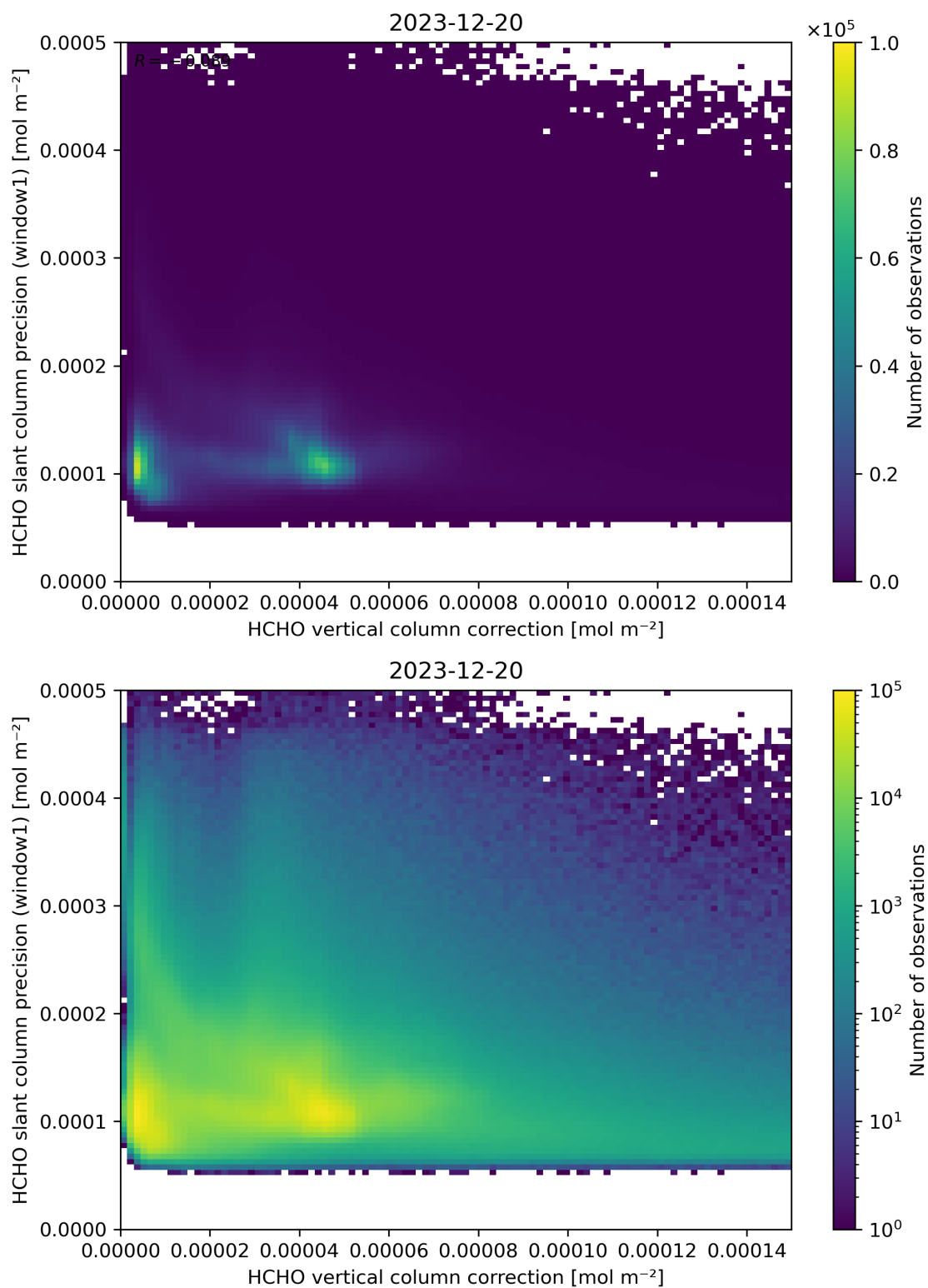
Figure 119: Scatter density plot of “HCHO vertical column correction” against “HCHO slant column precision (window1)” for 2023-12-20 to 2023-12-21.
