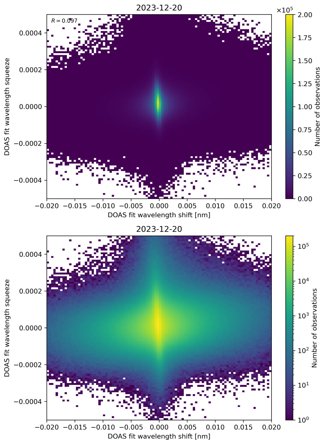
Figure 65: Scatter density plot of “DOAS fit wavelength shift” against “DOAS fit wavelength squeeze” for 2023-12-20 to 2023-12-21.
