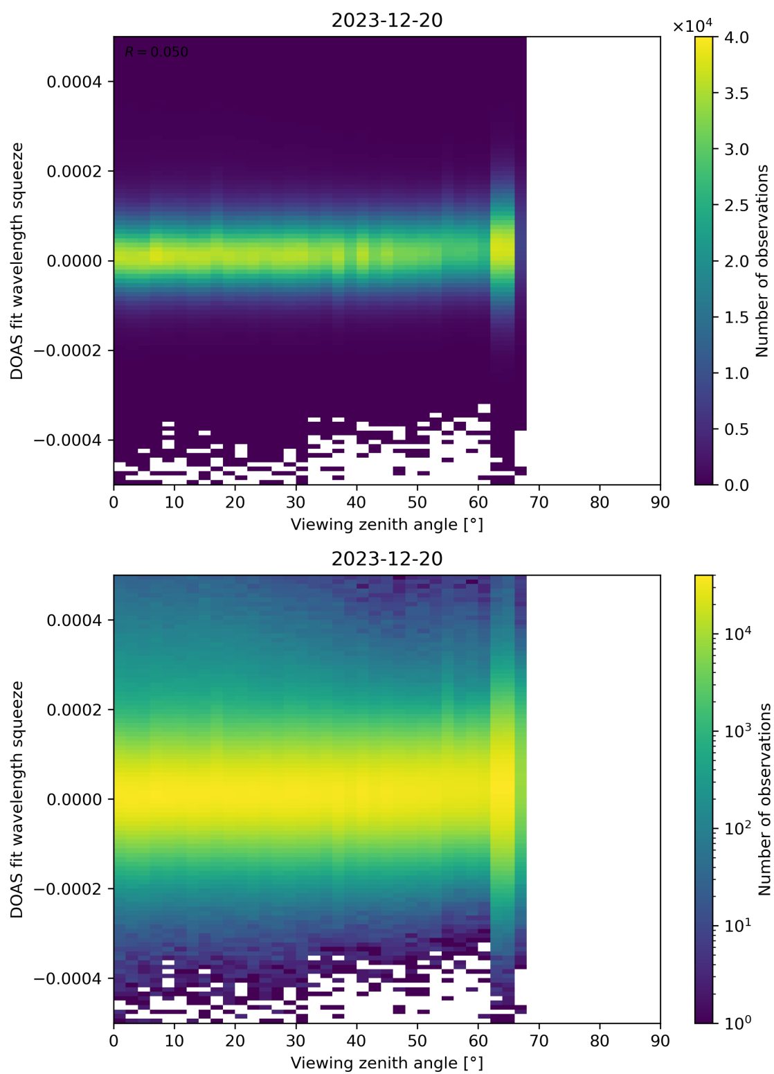
Figure 184: Scatter density plot of “Viewing zenith angle” against “DOAS fit wavelength squeeze” for 2023-12-20 to 2023-12-21.
