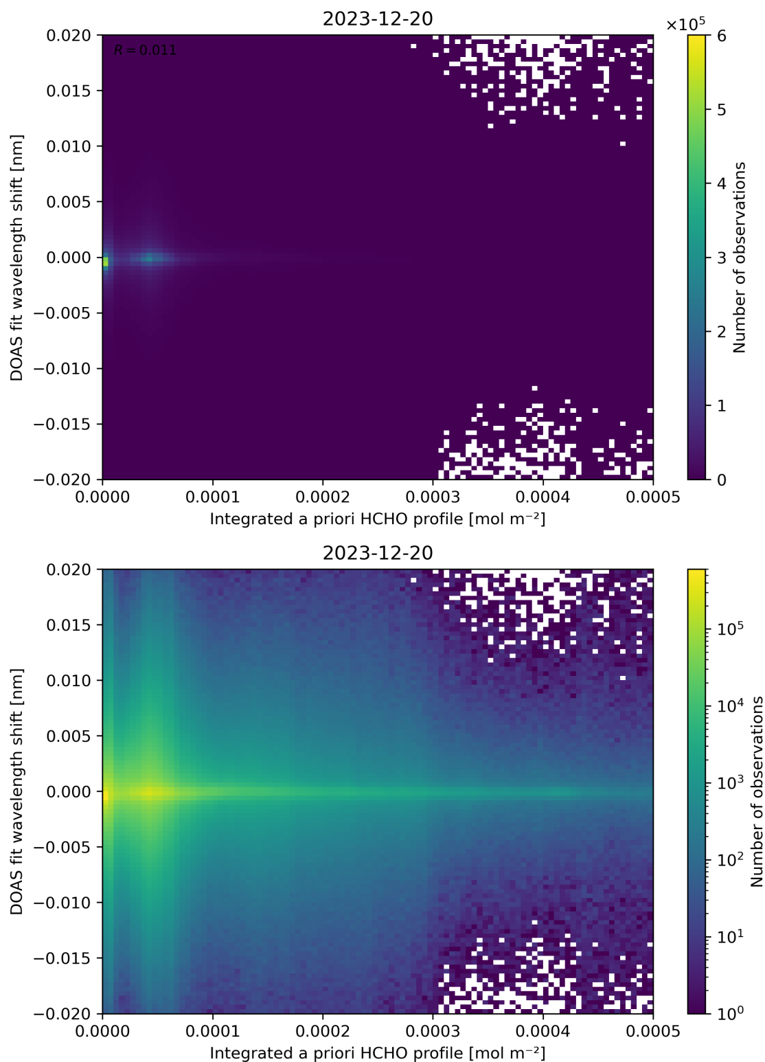
Figure 149: Scatter density plot of “Integrated a priori HCHO profile” against “DOAS fit wavelength shift” for 2023-12-20 to 2023-12-21.
