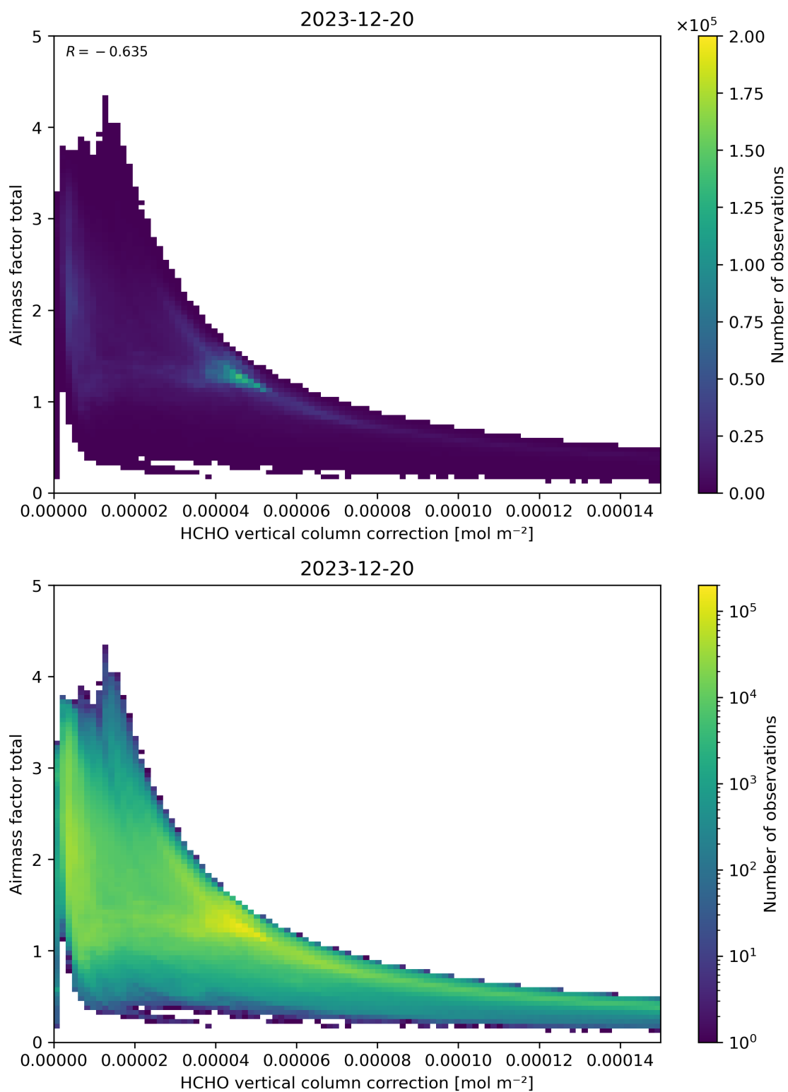
Figure 120: Scatter density plot of “HCHO vertical column correction” against “Airmass factor total” for 2023-12-20 to 2023-12-21.
