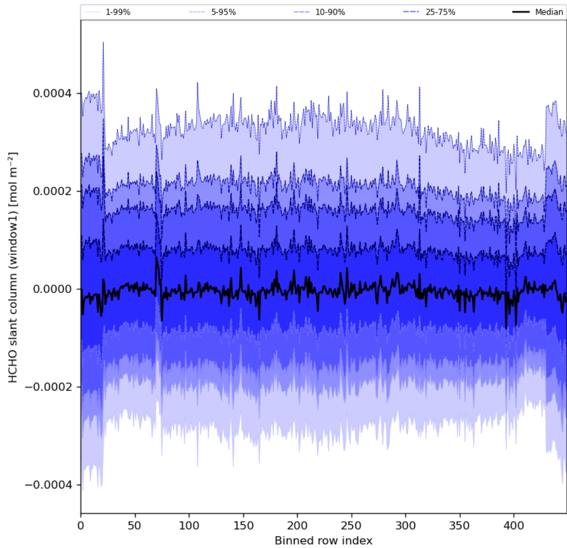
Figure 52: Along track statistics of “HCHO slant column (window1)” for 2023-12-20 to 2023-12-21
