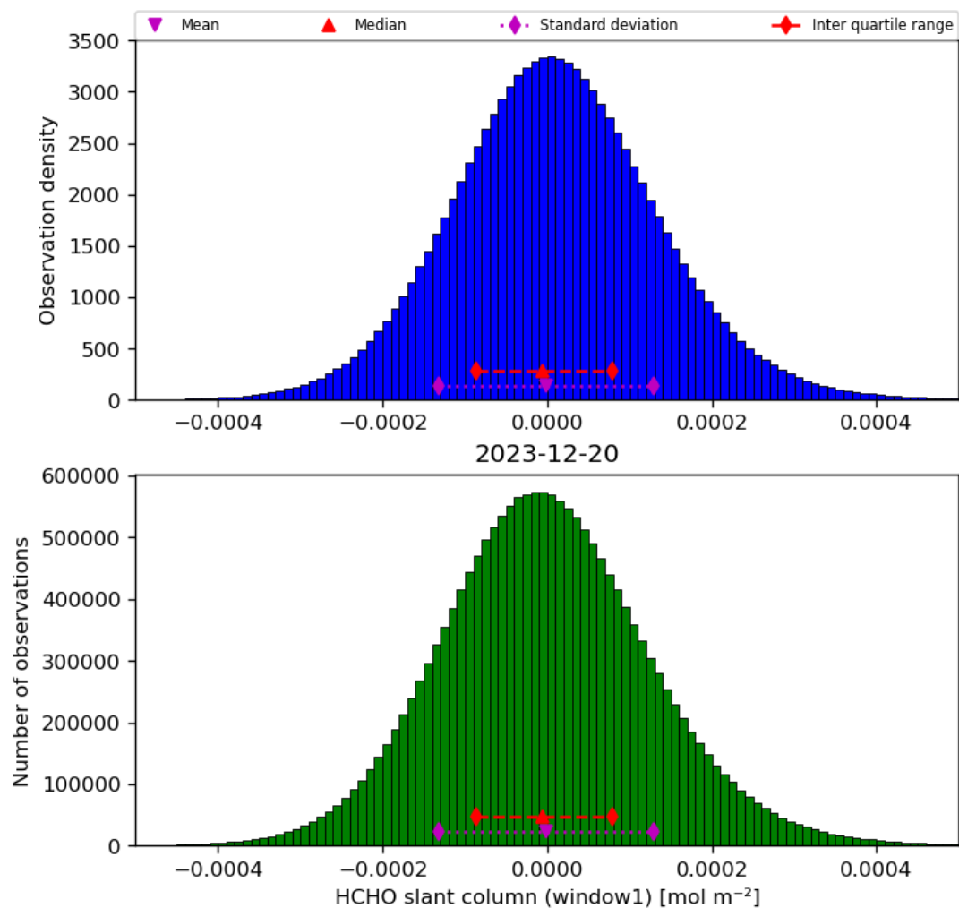
Figure 38: Histogram of “HCHO slant column (window1)” for 2023-12-20 to 2023-12-21
