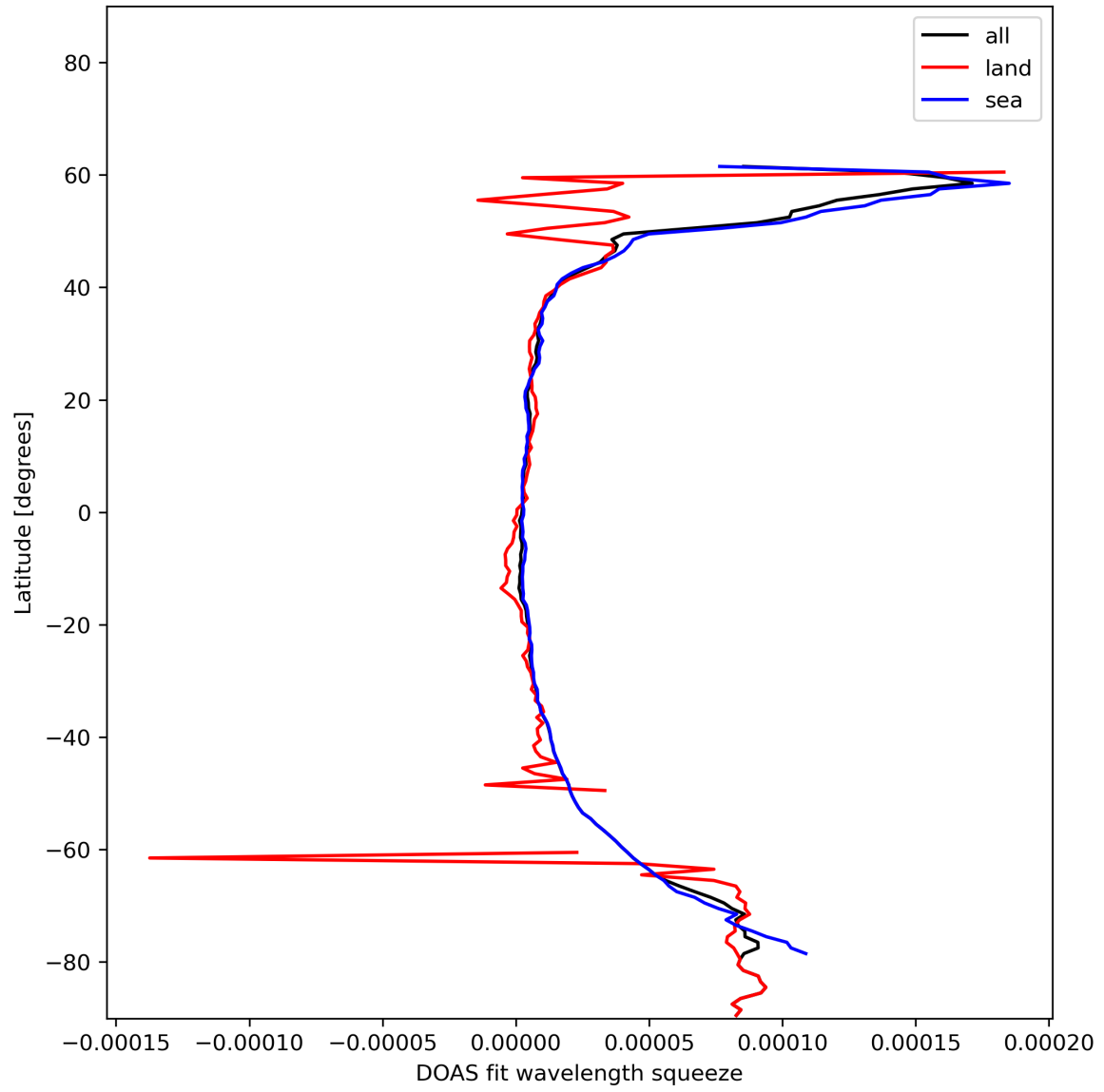
Figure 31: Zonal average of “DOAS fit wavelength squeeze” for 2023-12-20 to 2023-12-21.
