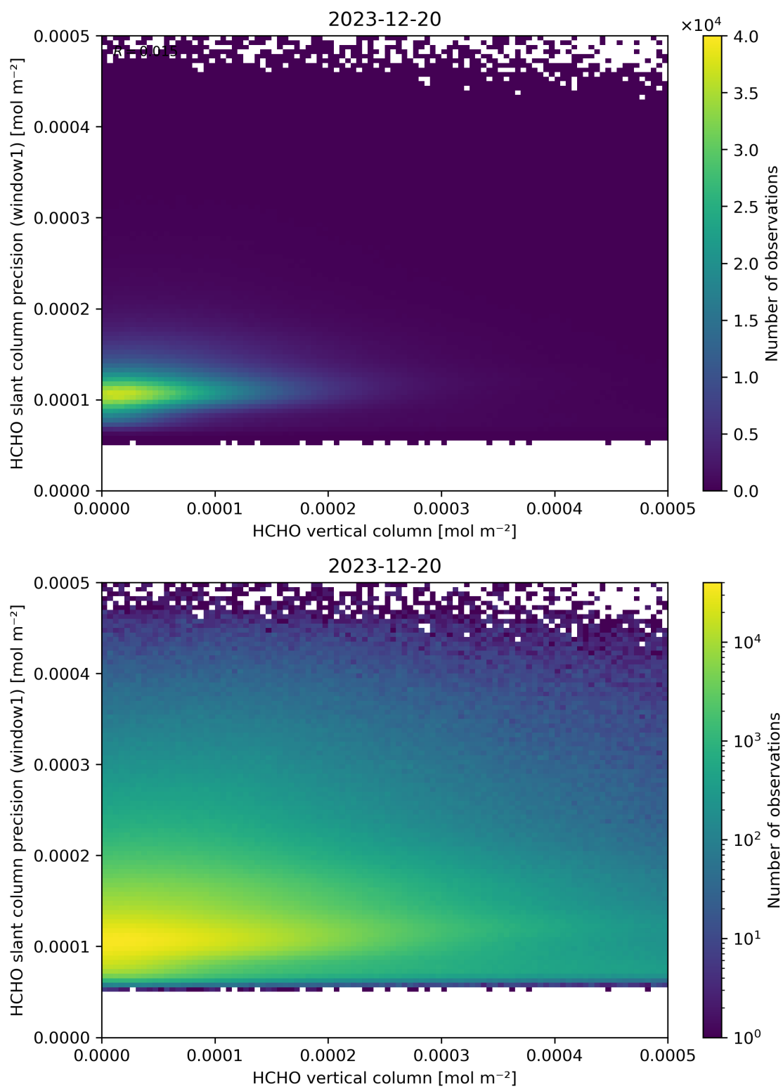
Figure 130: Scatter density plot of “HCHO vertical column” against “HCHO slant column precision (window1)” for 2023-12-20 to 2023-12-21.
