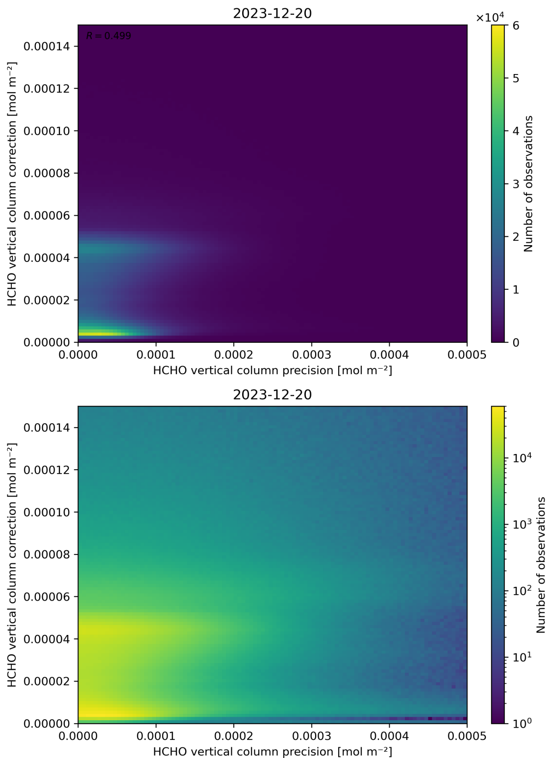
Figure 146: Scatter density plot of “HCHO vertical column precision” against “HCHO vertical column correction” for 2023-12-20 to 2023-12-21.
