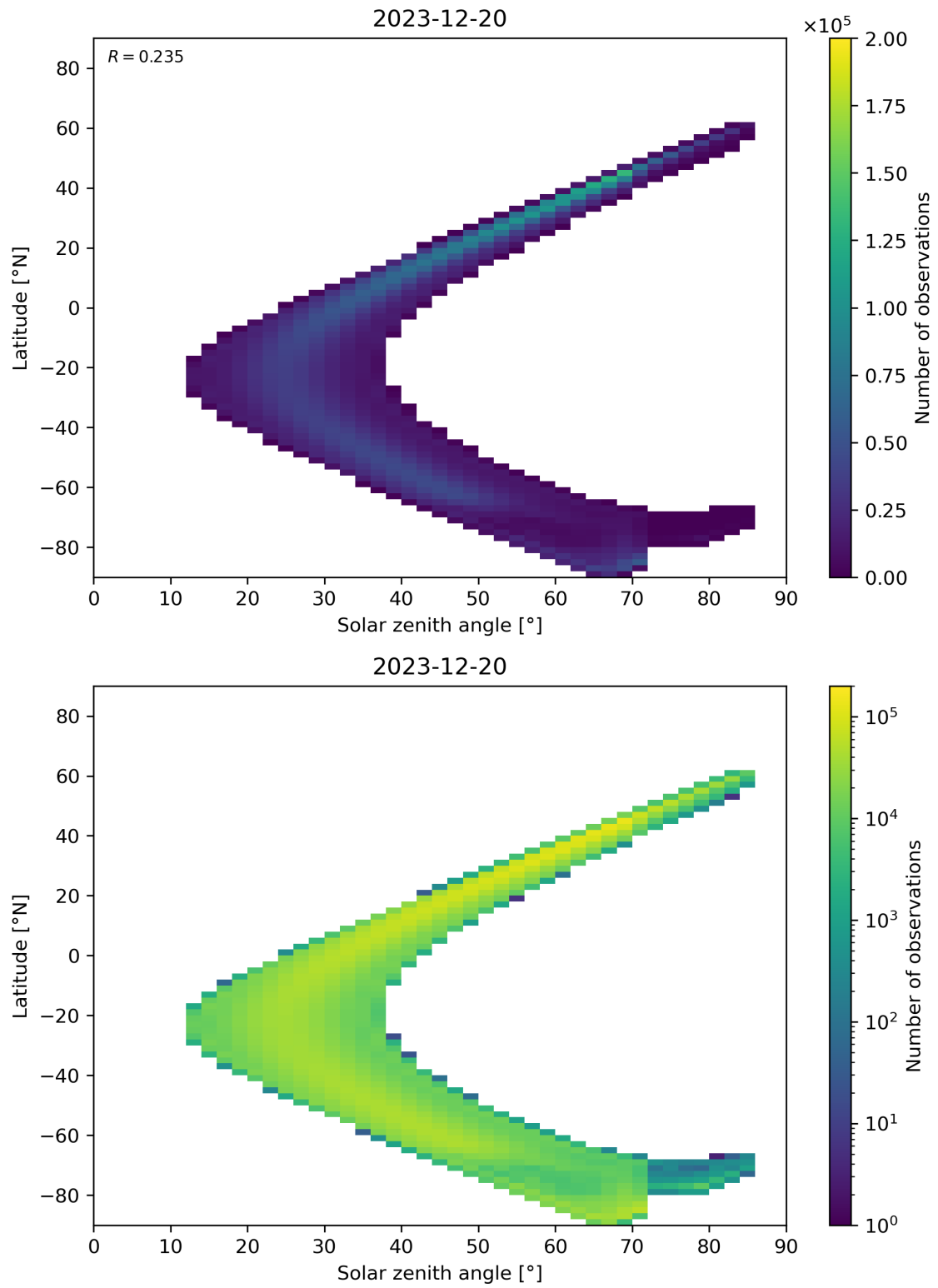
Figure 181: Scatter density plot of “Solar zenith angle” against “Latitude” for 2023-12-20 to 2023-12-21.
