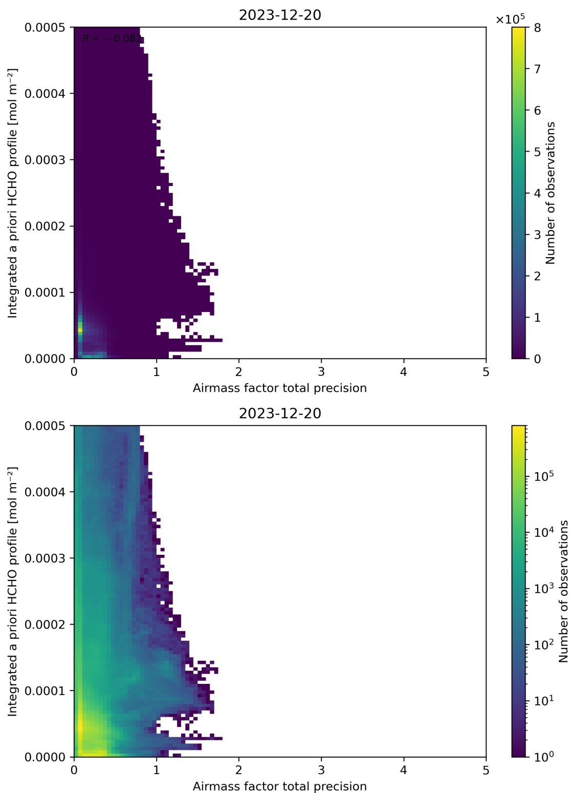
Figure 111: Scatter density plot of “Airmass factor total precision” against “Integrated a priori HCHO profile” for 2023-12-20 to 2023-12-21.
