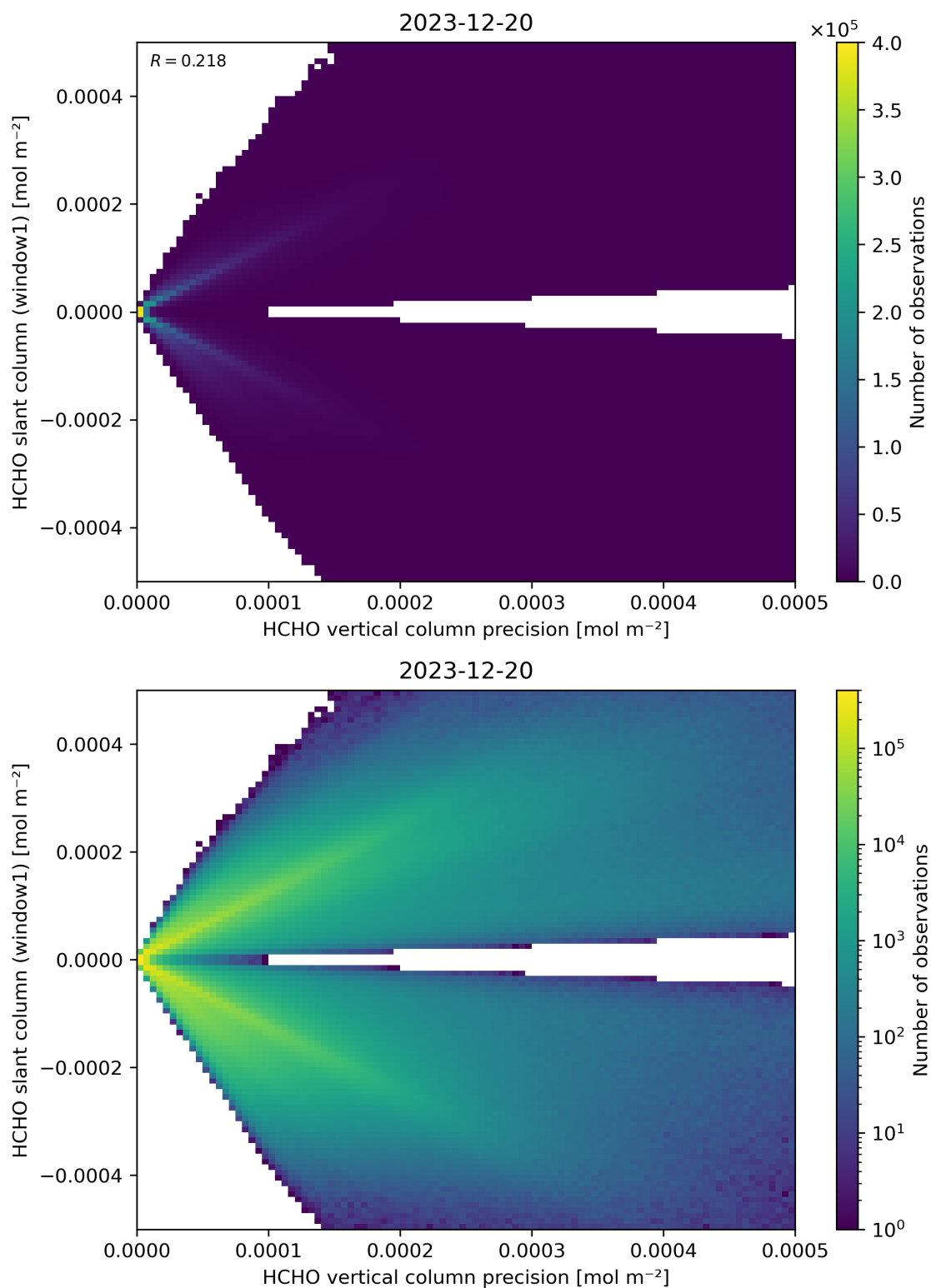
Figure 142: Scatter density plot of “HCHO vertical column precision” against “HCHO slant column (window1)” for 2023-12-20 to 2023-12-21.
