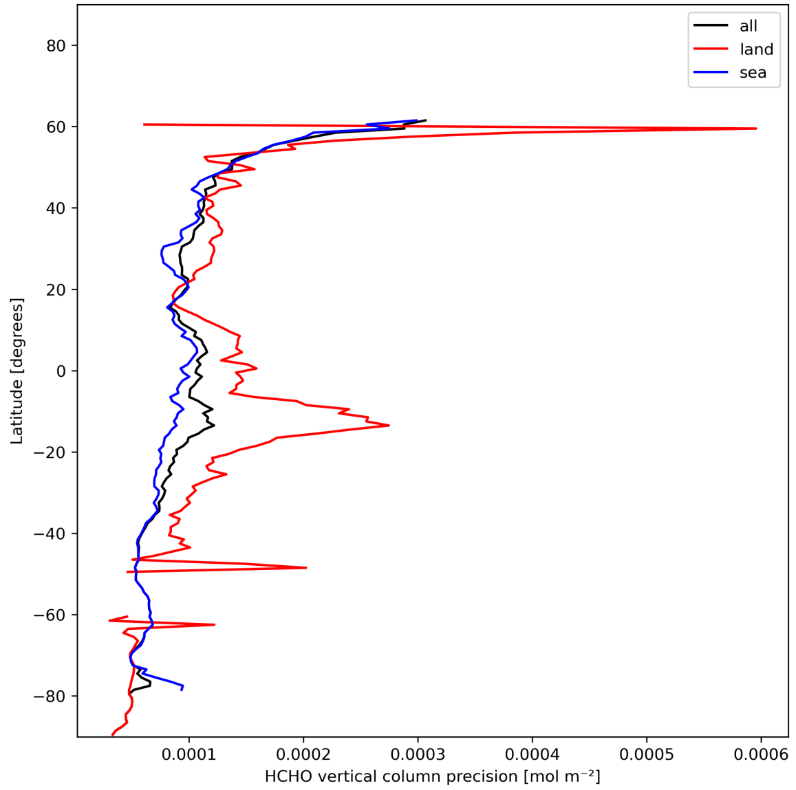
Figure 22: Zonal average of “HCHO vertical column precision” for 2023-12-20 to 2023-12-21.
