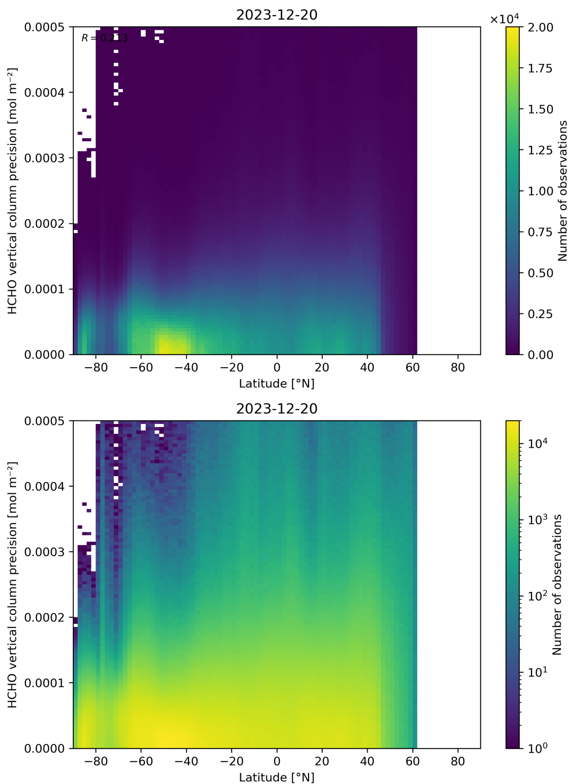
Figure 165: Scatter density plot of “Latitude” against “HCHO vertical column precision” for 2023-12-20 to 2023-12-21.
