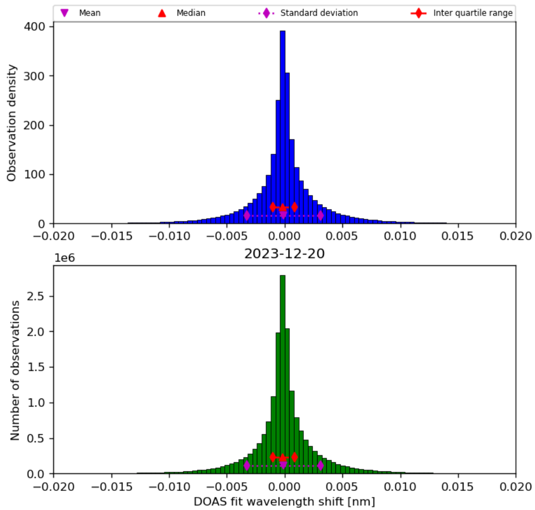
Figure 44: Histogram of “DOAS fit wavelength shift” for 2023-12-20 to 2023-12-21
