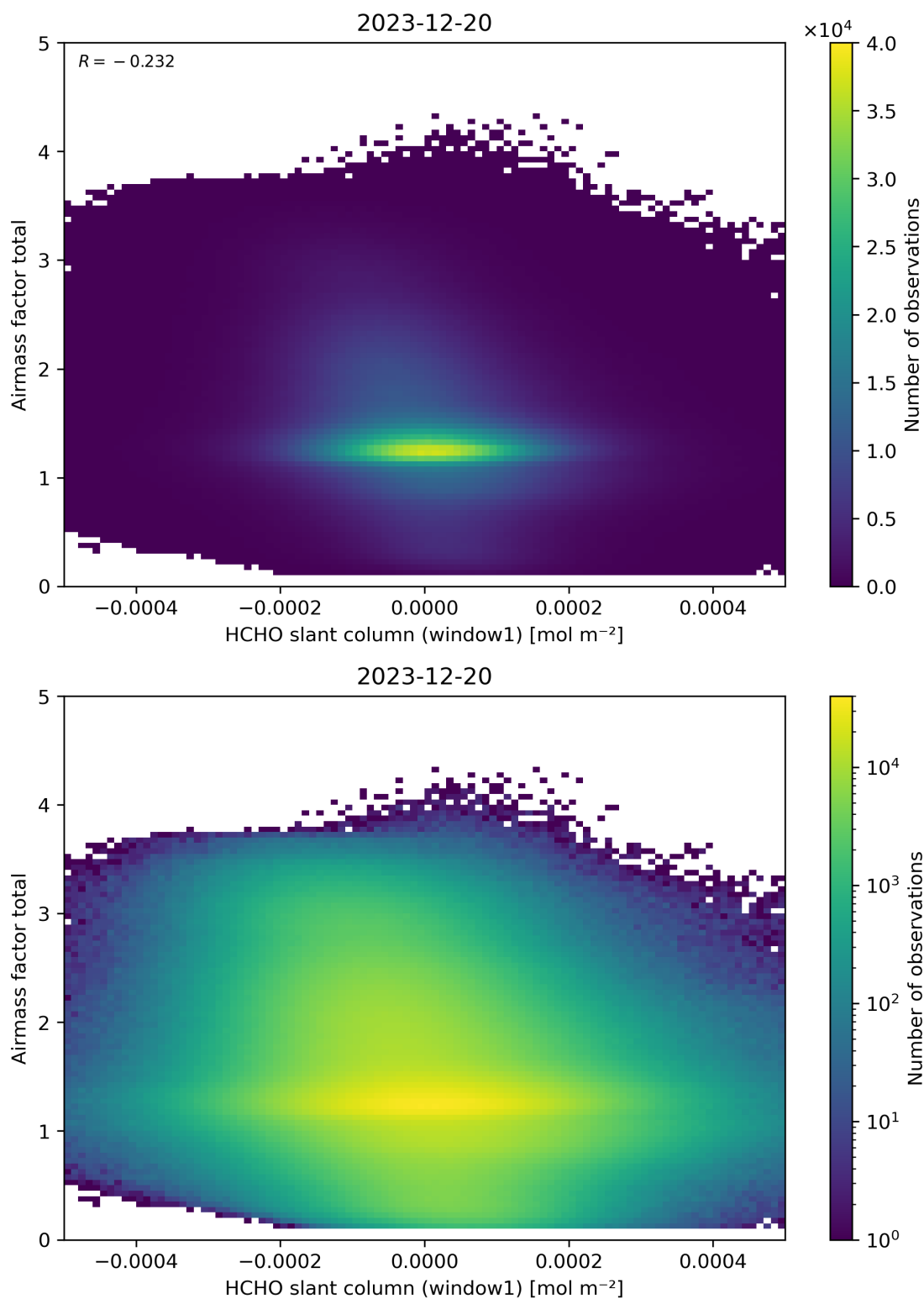
Figure 85: Scatter density plot of “HCHO slant column (window1)” against “Airmass factor total” for 2023-12-20 to 2023-12-21.
