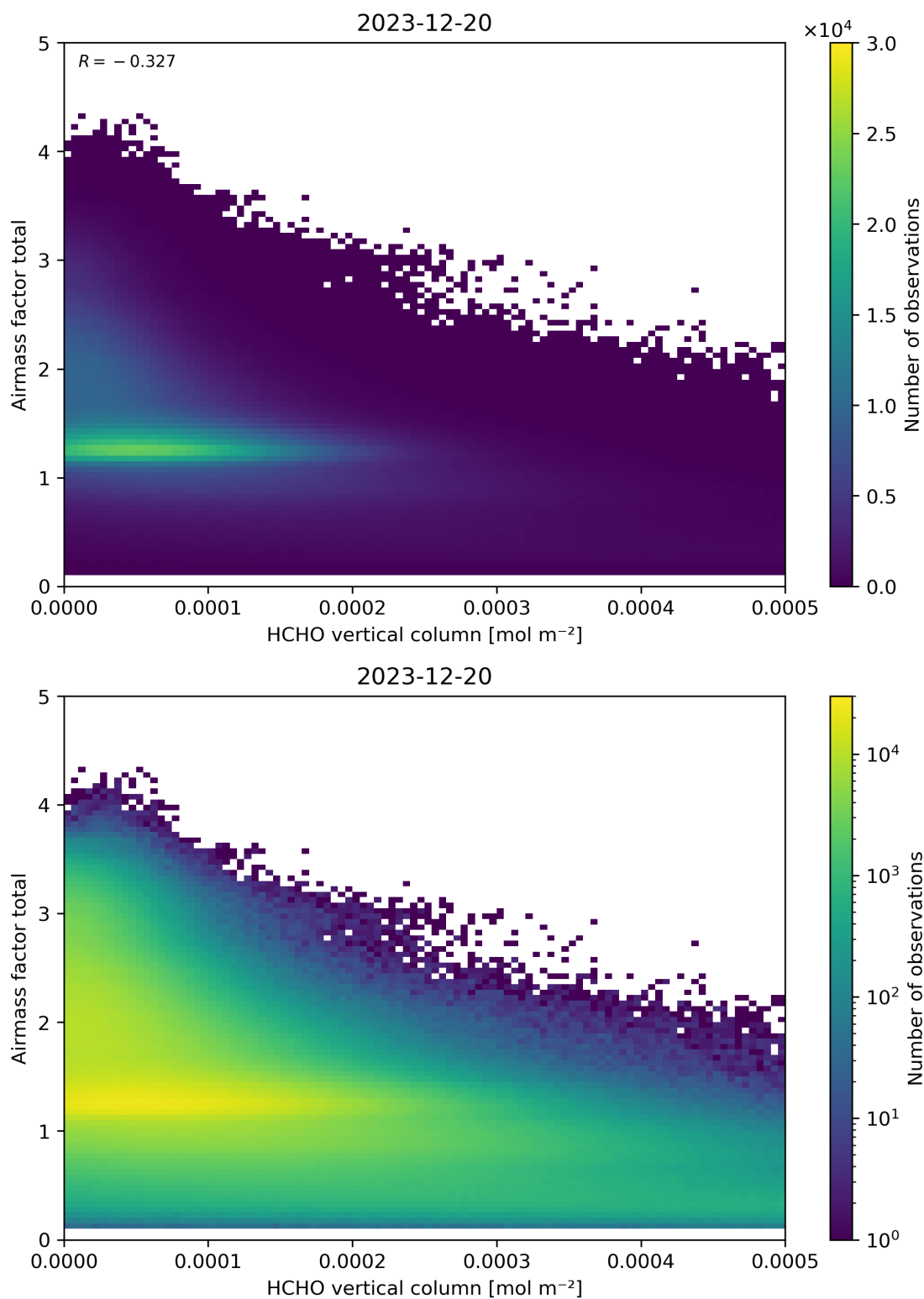
Figure 131: Scatter density plot of “HCHO vertical column” against “Airmass factor total” for 2023-12-20 to 2023-12-21.
