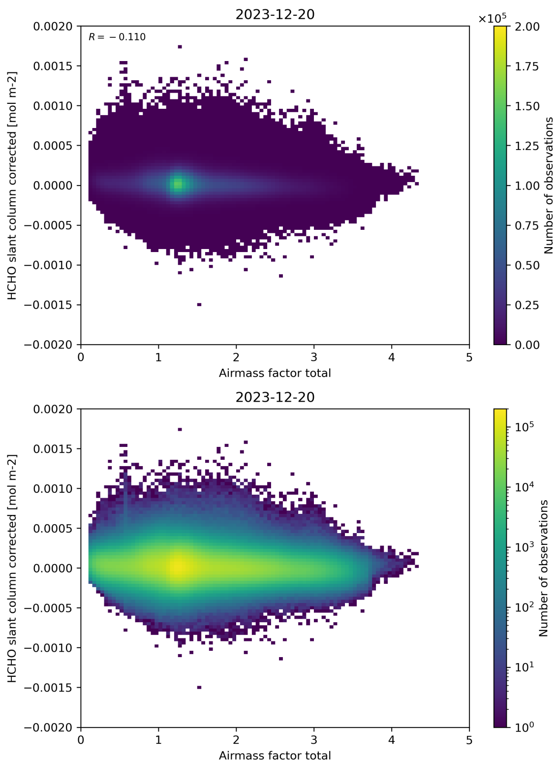
Figure 101: Scatter density plot of “Airmass factor total” against “HCHO slant column corrected” for 2023-12-20 to 2023-12-21.
