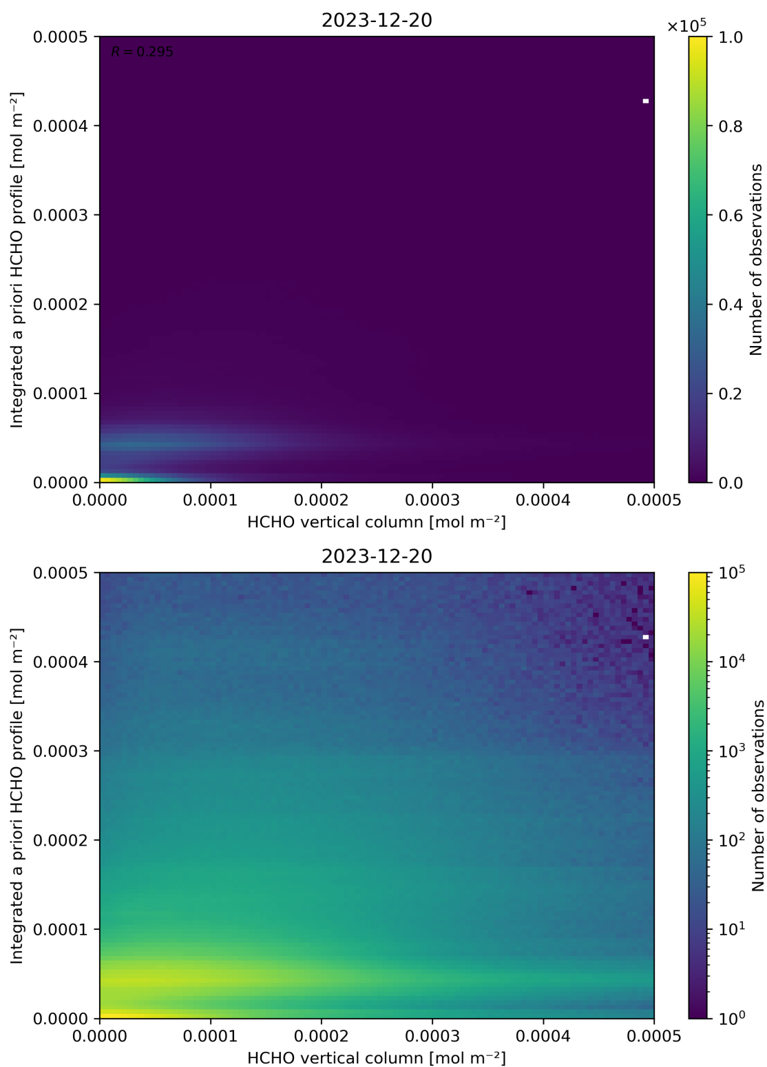
Figure 135: Scatter density plot of “HCHO vertical column” against “Integrated a priori HCHO profile” for 2023-12-20 to 2023-12-21.
