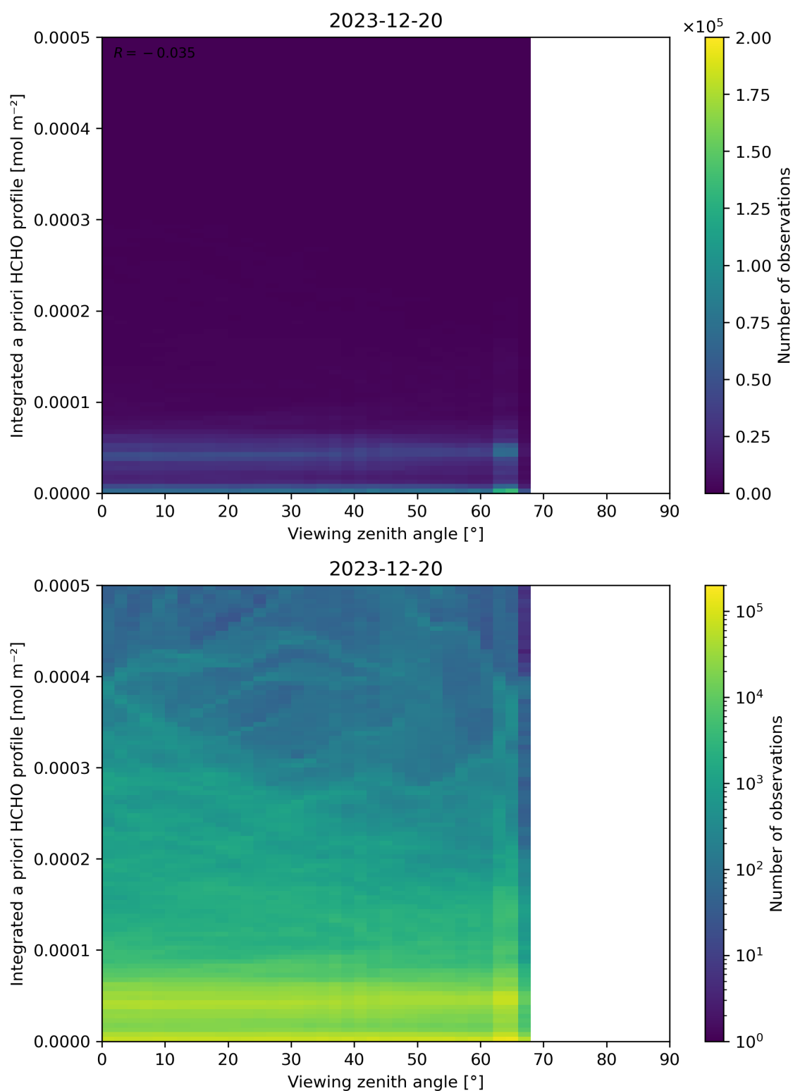
Figure 195: Scatter density plot of “Viewing zenith angle” against “Integrated a priori HCHO profile” for 2023-12-20 to 2023-12-21.
