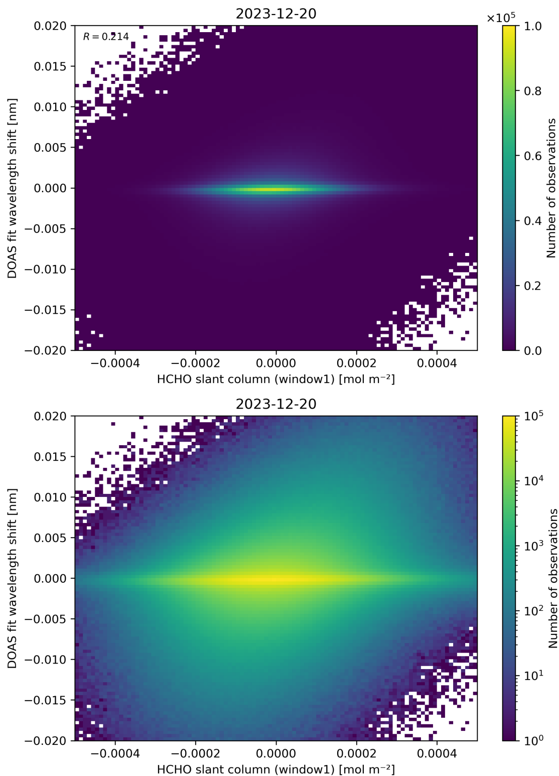
Figure 79: Scatter density plot of “HCHO slant column (window1)” against “DOAS fit wavelength shift” for 2023-12-20 to 2023-12-21.
