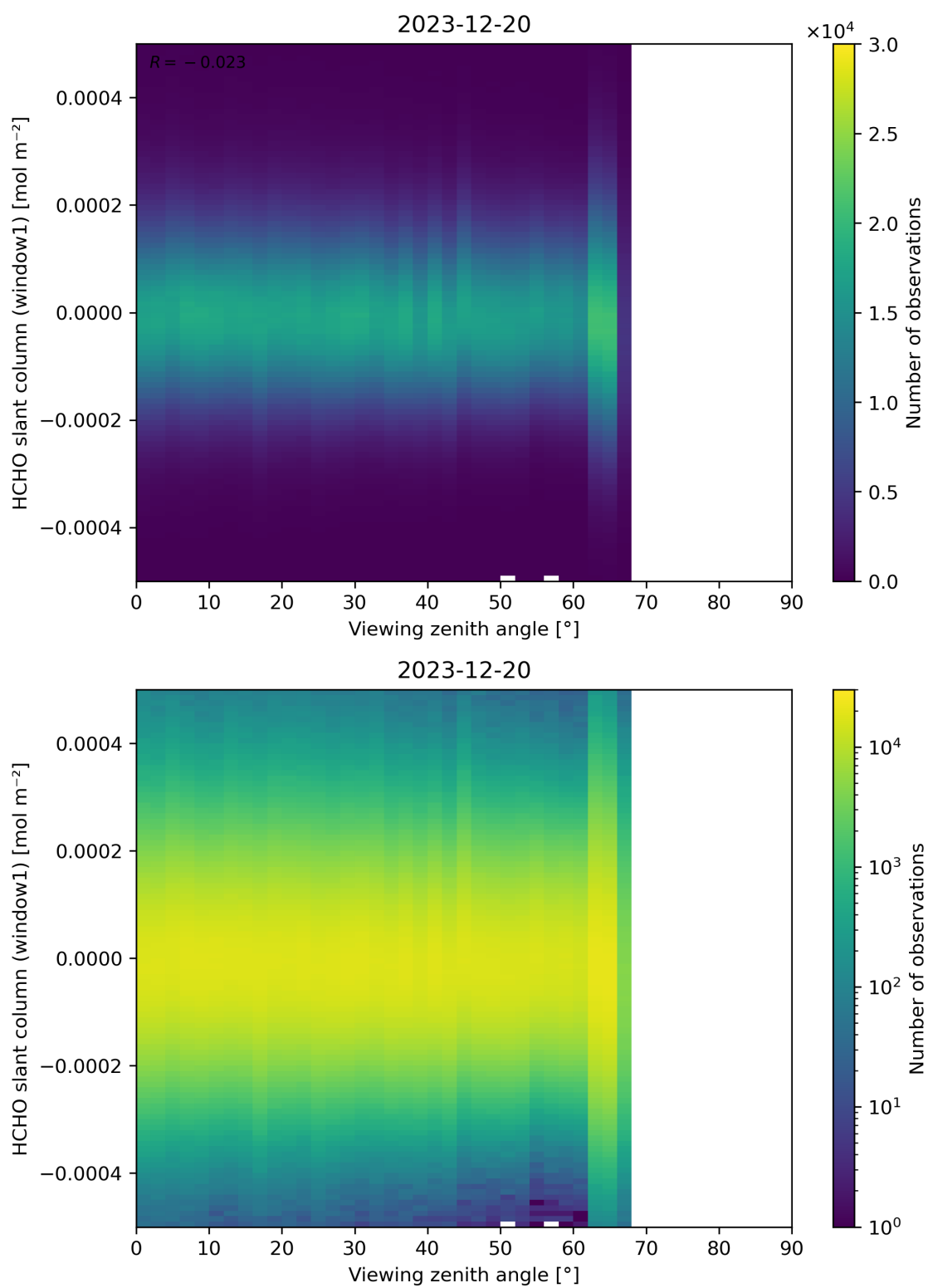
Figure 188: Scatter density plot of “Viewing zenith angle” against “HCHO slant column (window1)” for 2023-12-20 to 2023-12-21.
