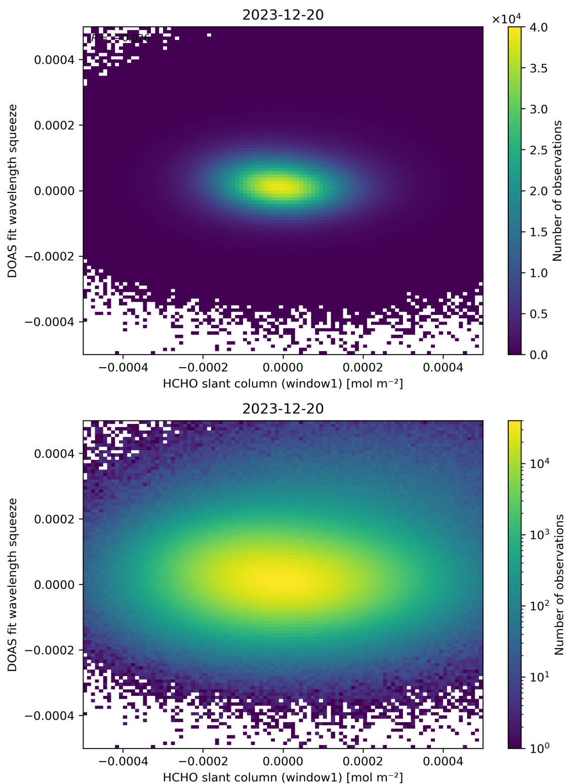
Figure 80: Scatter density plot of “HCHO slant column (window1)” against “DOAS fit wavelength squeeze” for 2023-12-20 to 2023-12-21.
