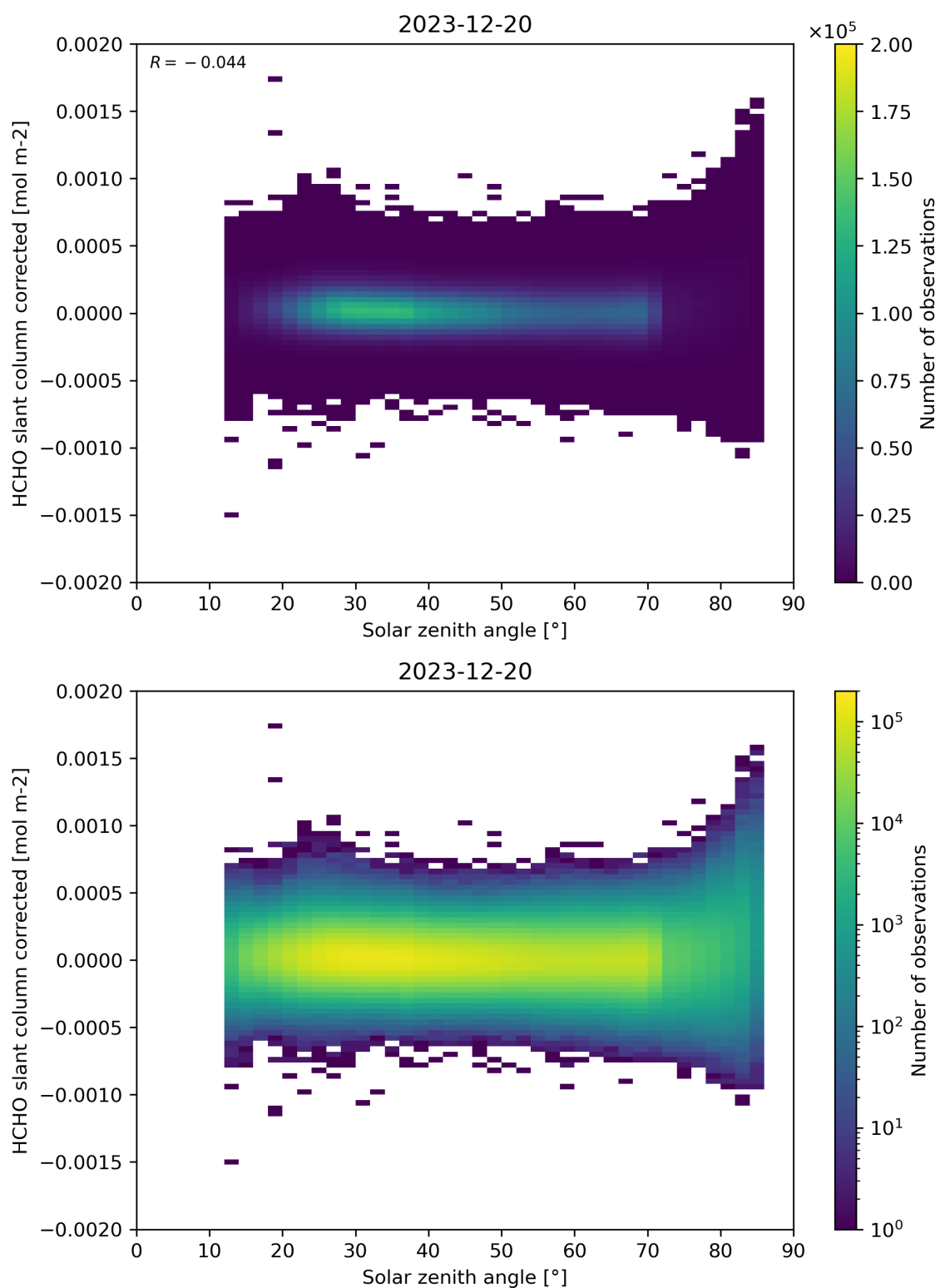
Figure 171: Scatter density plot of “Solar zenith angle” against “HCHO slant column corrected” for 2023-12-20 to 2023-12-21.
