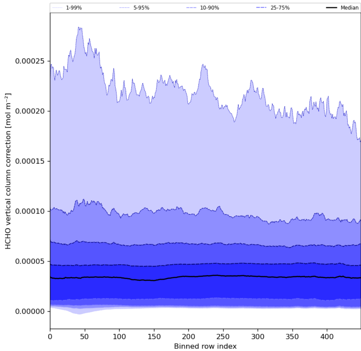
Figure 51: Along track statistics of “HCHO vertical column correction” for 2023-12-20 to 2023-12-21
