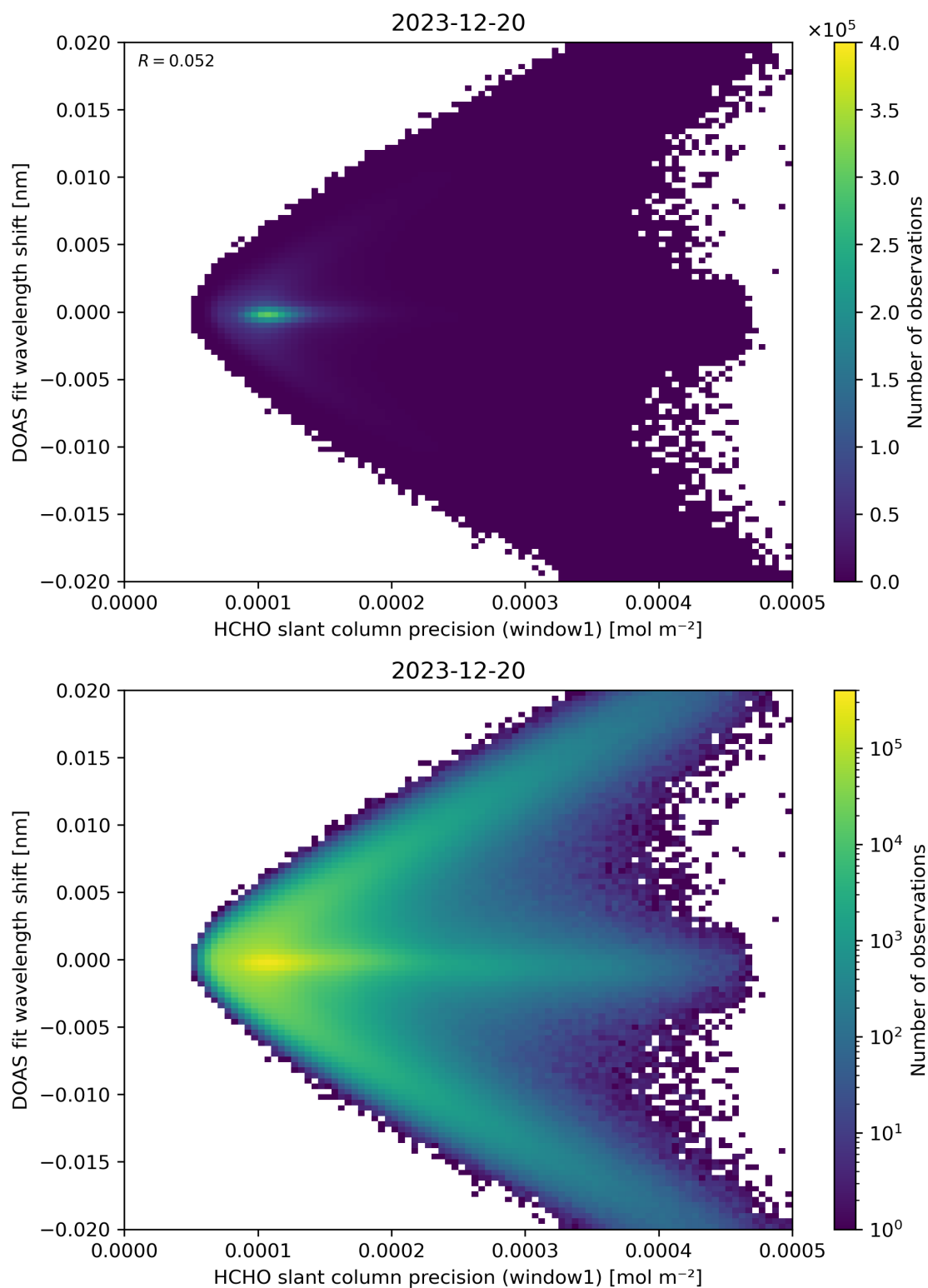
Figure 89: Scatter density plot of “HCHO slant column precision (window1)” against “DOAS fit wavelength shift” for 2023-12-20 to 2023-12-21.
