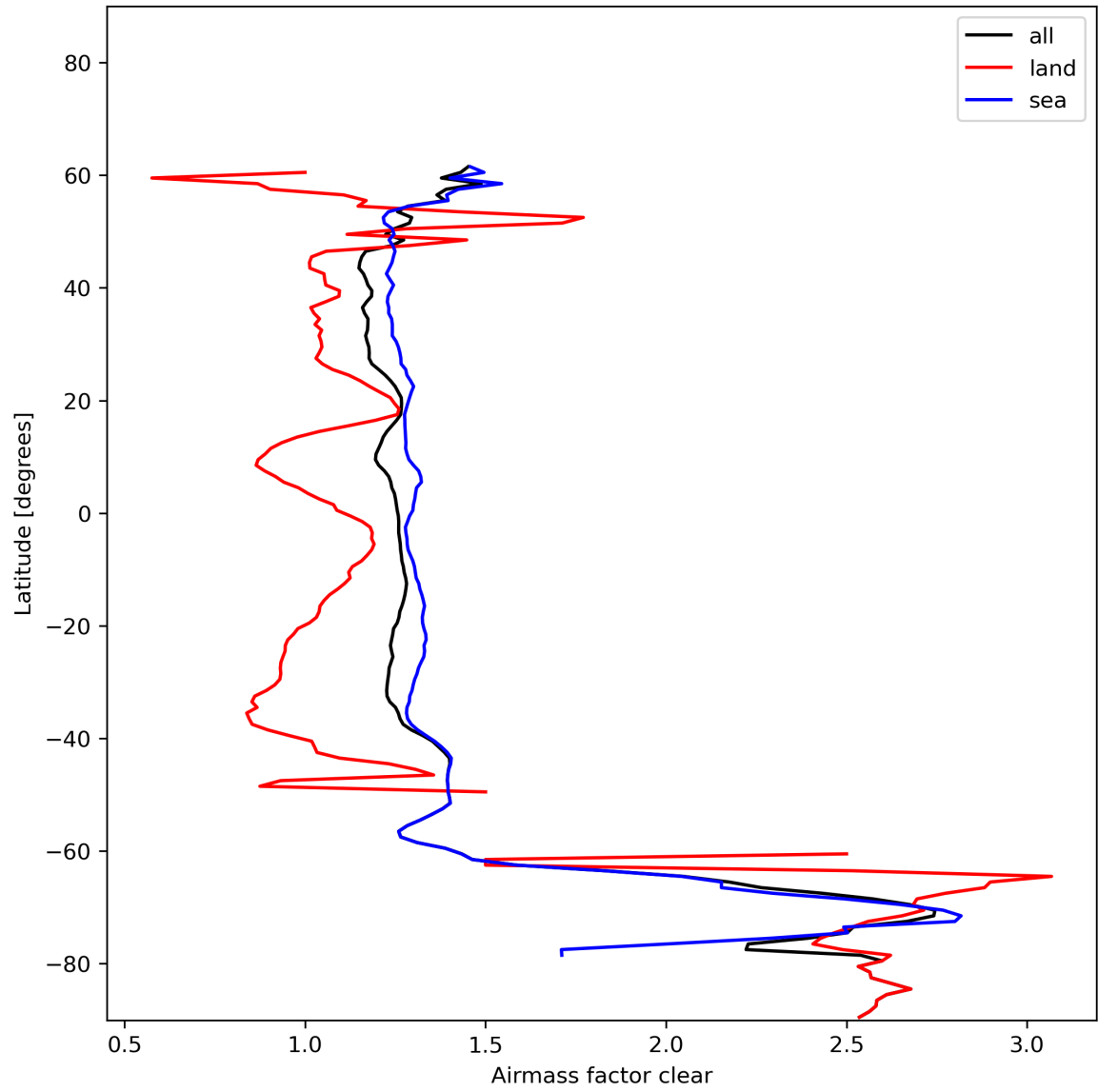
Figure 28: Zonal average of “Airmass factor clear” for 2023-12-20 to 2023-12-21.
