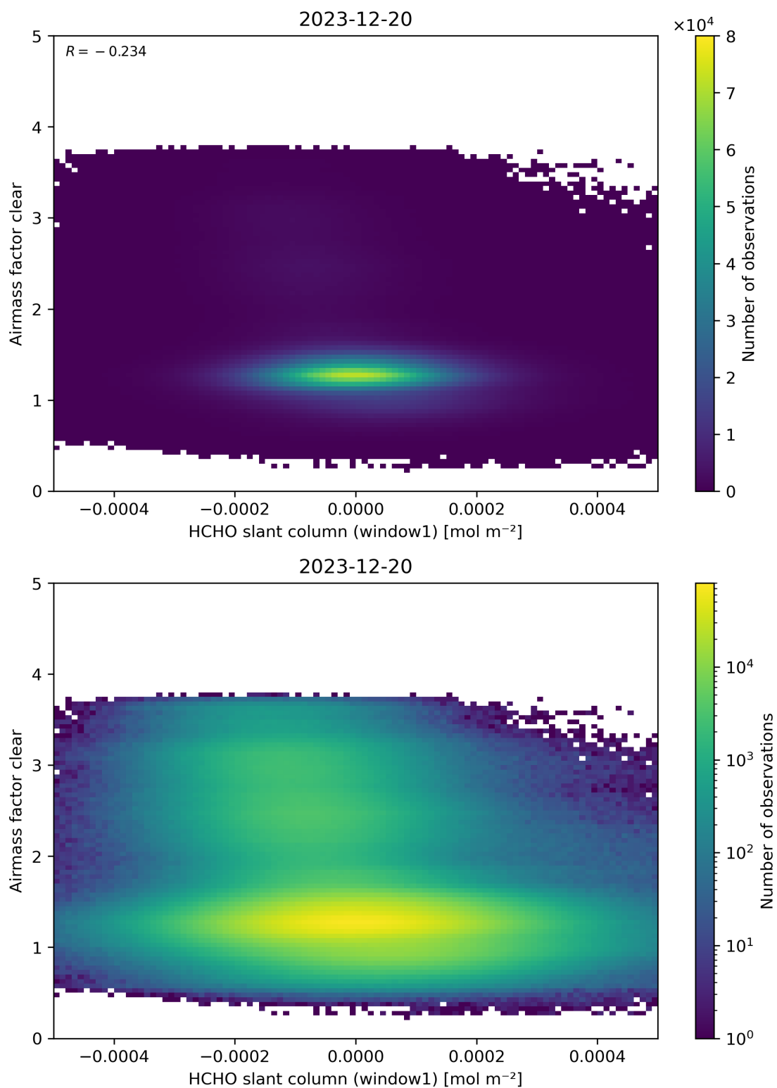
Figure 81: Scatter density plot of “HCHO slant column (window1)” against “Airmass factor clear” for 2023-12-20 to 2023-12-21.
