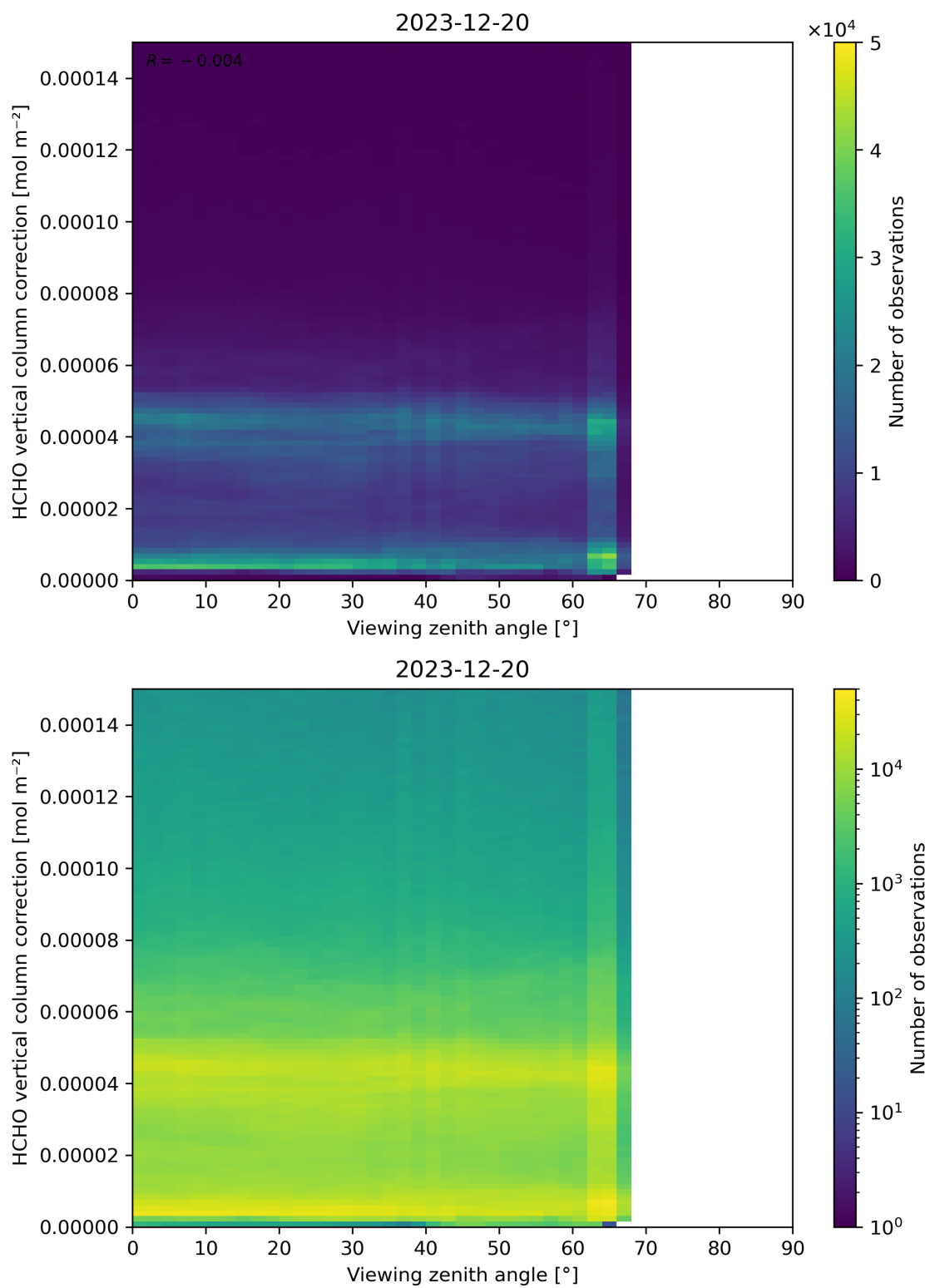
Figure 193: Scatter density plot of “Viewing zenith angle” against “HCHO vertical column correction” for 2023-12-20 to 2023-12-21.
