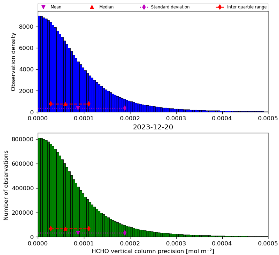
Figure 36: Histogram of “HCHO vertical column precision” for 2023-12-20 to 2023-12-21
