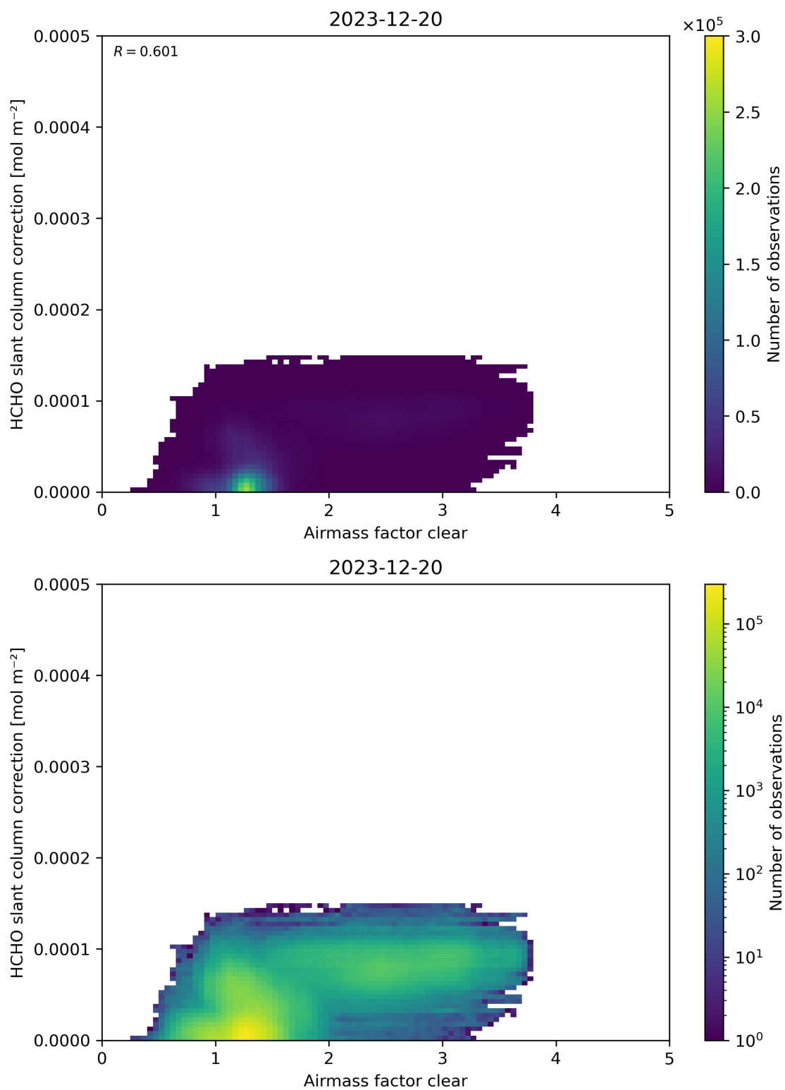
Figure 75: Scatter density plot of “Airmass factor clear” against “HCHO slant column correction” for 2023-12-20 to 2023-12-21.
