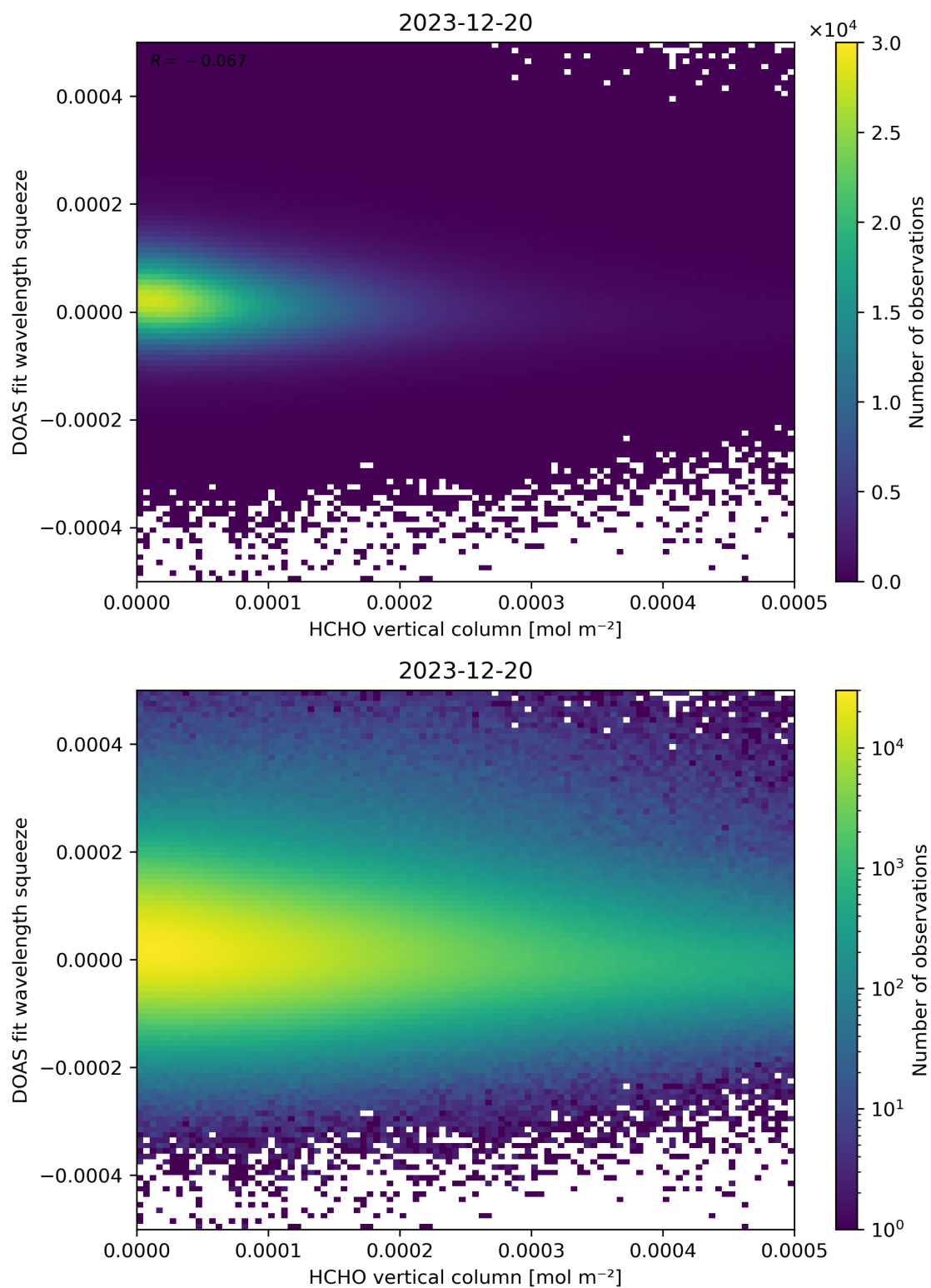
Figure 125: Scatter density plot of “HCHO vertical column” against “DOAS fit wavelength squeeze” for 2023-12-20 to 2023-12-21.
