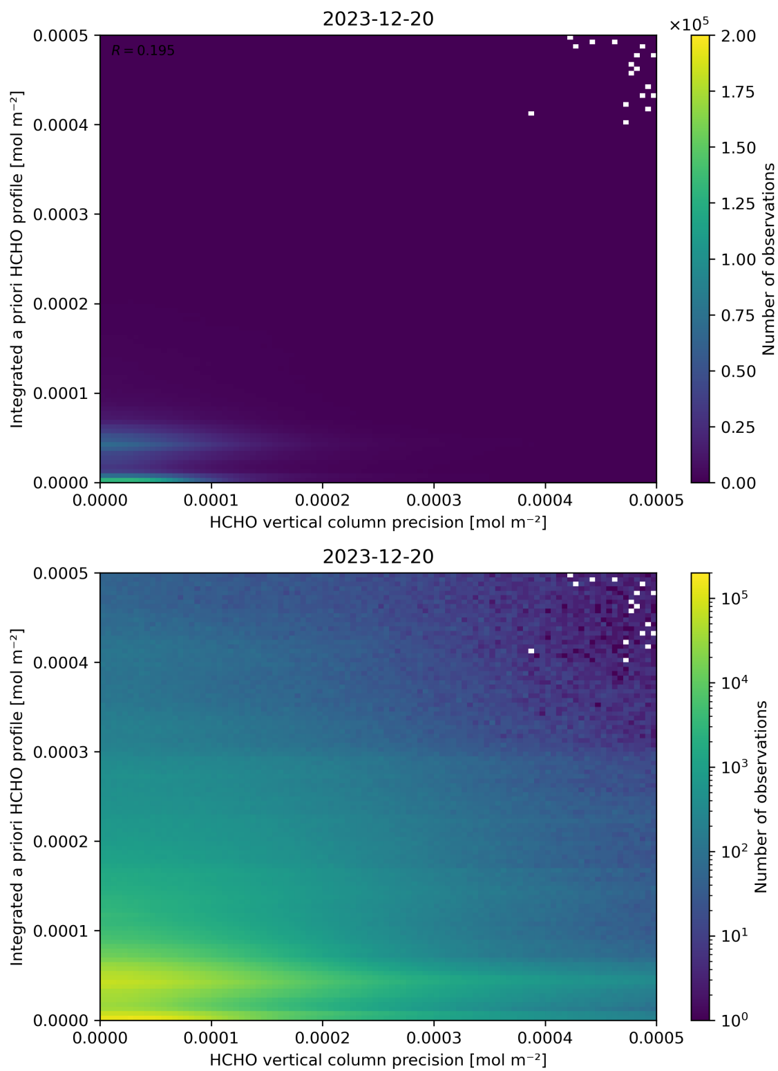
Figure 147: Scatter density plot of “HCHO vertical column precision” against “Integrated a priori HCHO profile” for 2023-12-20 to 2023-12-21.
