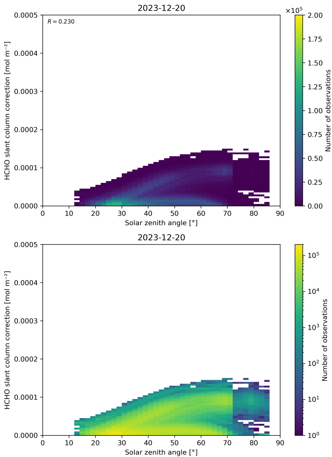
Figure 172: Scatter density plot of “Solar zenith angle” against “HCHO slant column correction” for 2023-12-20 to 2023-12-21.
