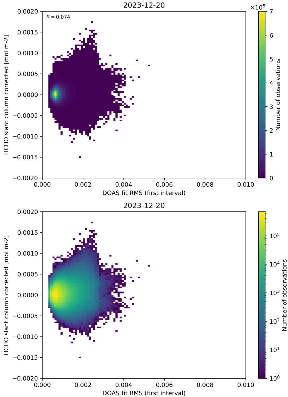
Figure 62: Scatter density plot of “DOAS fit RMS (first interval)” against “HCHO slant column corrected” for 2023-12-20 to 2023-12-21.
