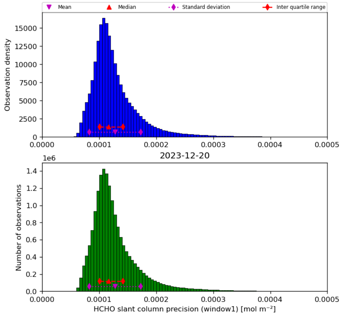
Figure 39: Histogram of “HCHO slant column precision (window1)” for 2023-12-20 to 2023-12-21
