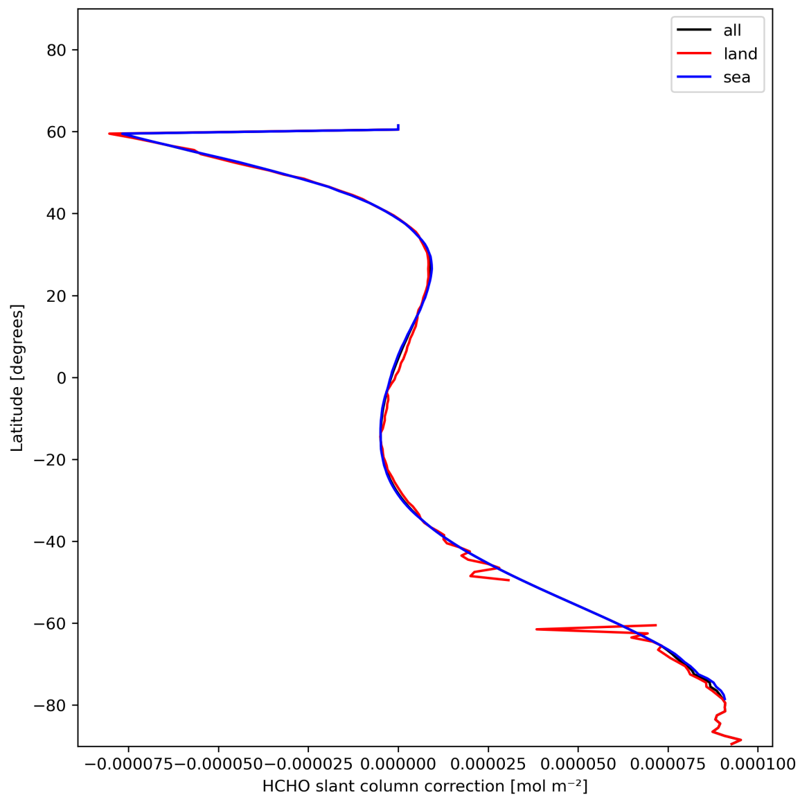
Figure 33: Zonal average of “HCHO slant column correction” for 2023-12-20 to 2023-12-21.
