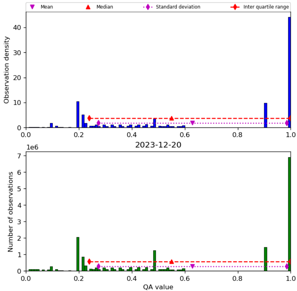
Figure 34: Histogram of “QA value” for 2023-12-20 to 2023-12-21
