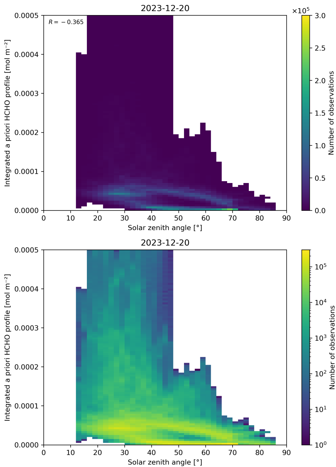
Figure 180: Scatter density plot of “Solar zenith angle” against “Integrated a priori HCHO profile” for 2023-12-20 to 2023-12-21.
