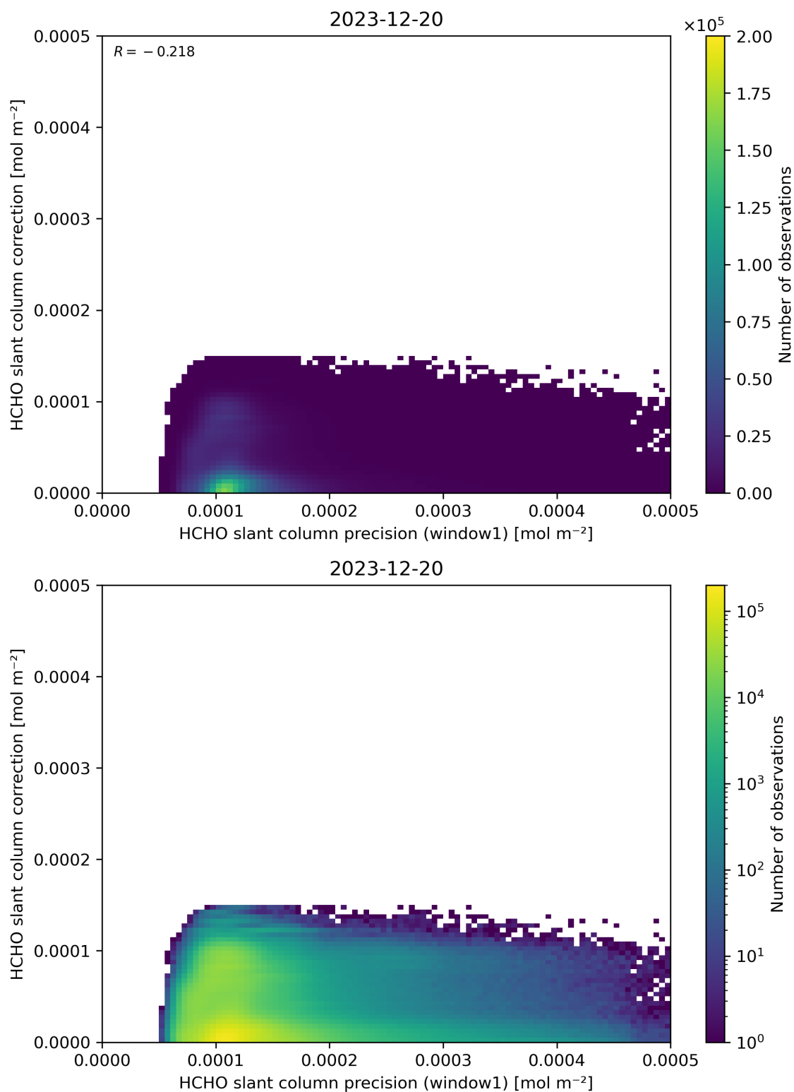
Figure 93: Scatter density plot of “HCHO slant column precision (window1)” against “HCHO slant column correction” for 2023-12-20 to 2023-12-21.
