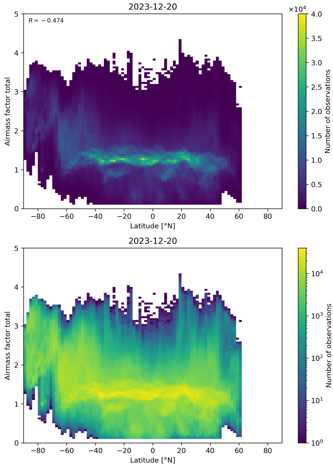
Figure 161: Scatter density plot of “Latitude” against “Airmass factor total” for 2023-12-20 to 2023-12-21.
