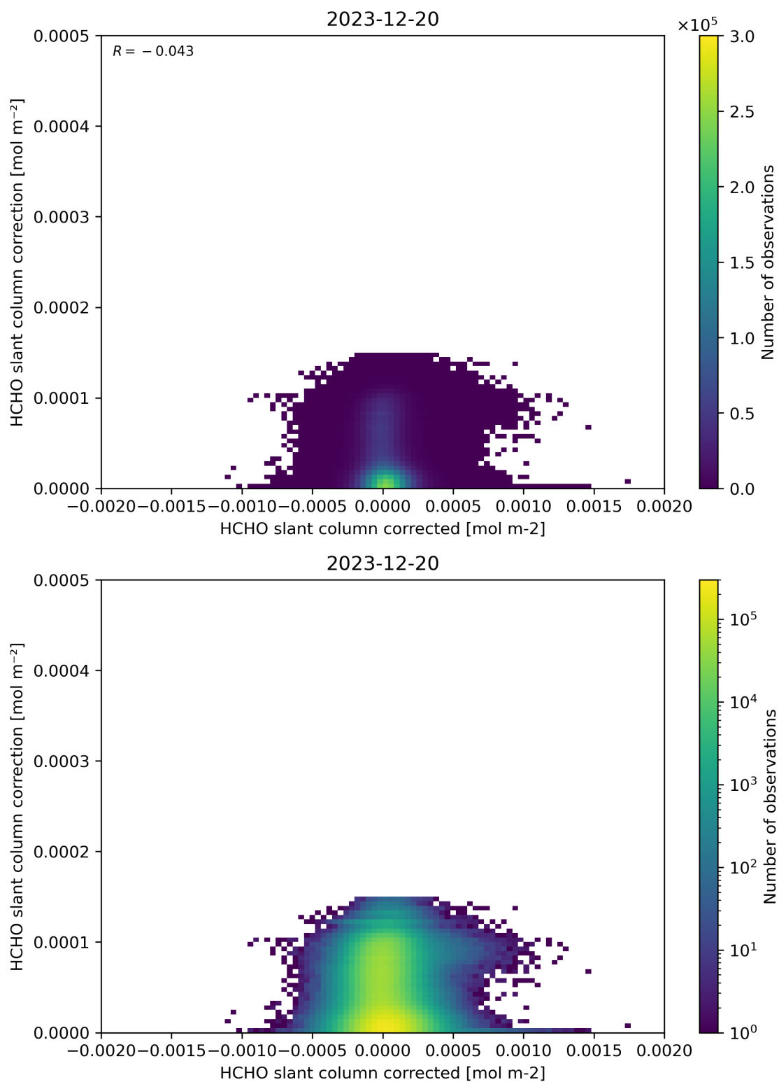
Figure 77: Scatter density plot of “HCHO slant column corrected” against “HCHO slant column correction” for 2023-12-20 to 2023-12-21.
