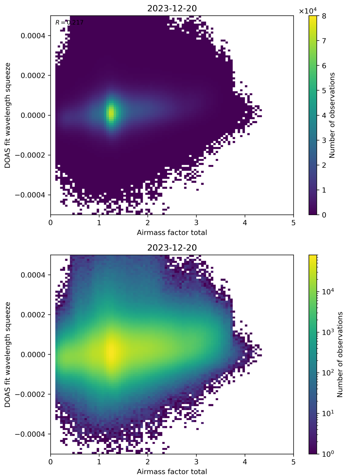
Figure 99: Scatter density plot of “Airmass factor total” against “DOAS fit wavelength squeeze” for 2023-12-20 to 2023-12-21.
