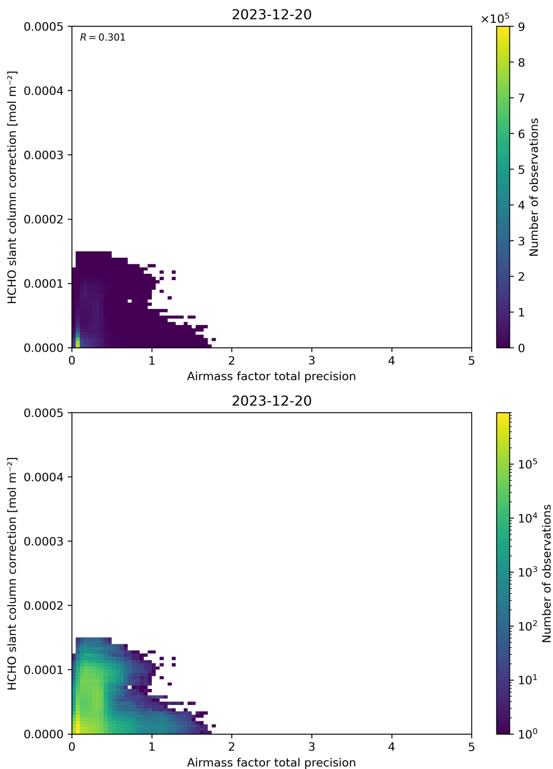
Figure 110: Scatter density plot of “Airmass factor total precision” against “HCHO slant column correction” for 2023-12-20 to 2023-12-21.
