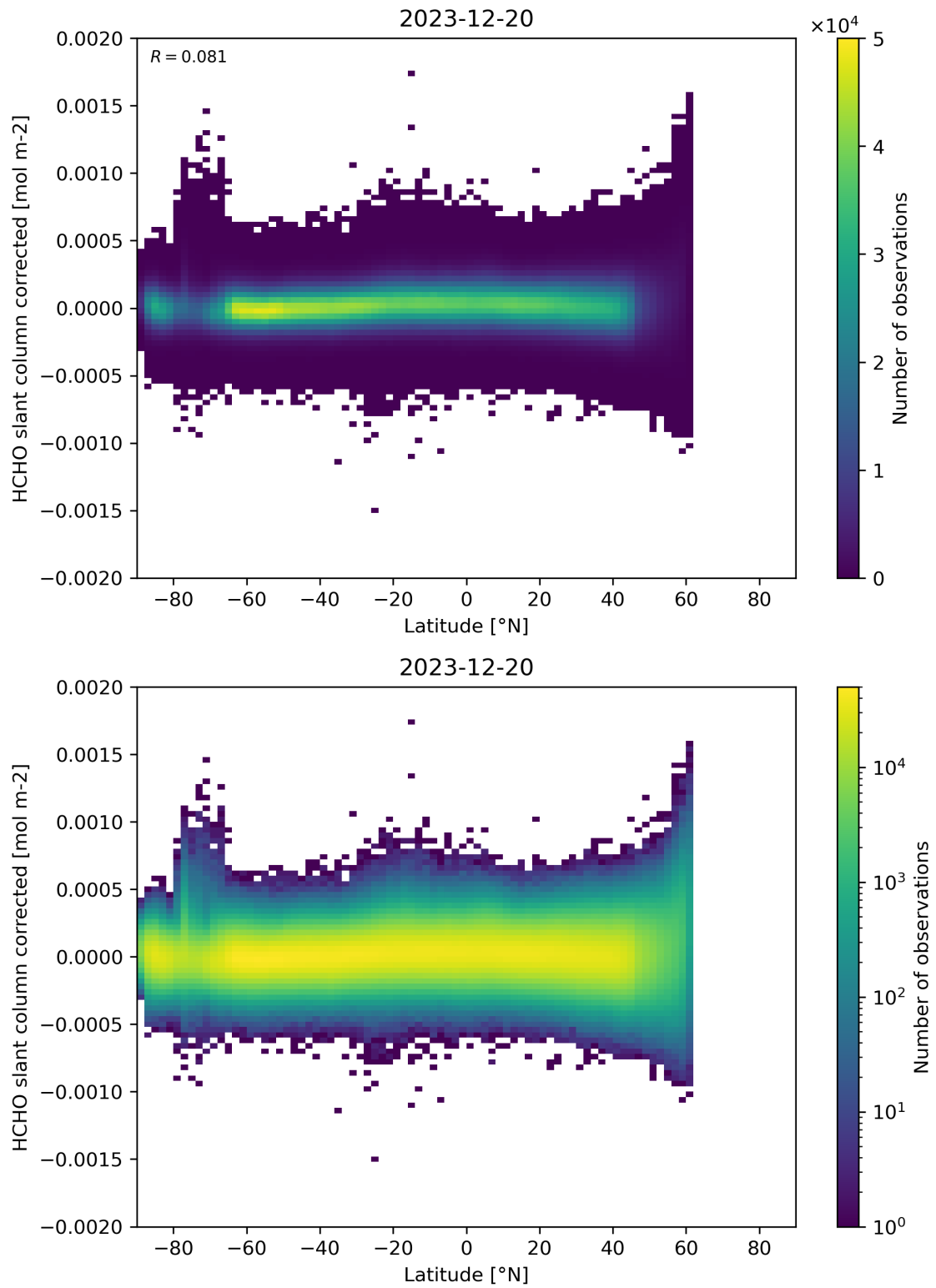
Figure 157: Scatter density plot of “Latitude” against “HCHO slant column corrected” for 2023-12-20 to 2023-12-21.
