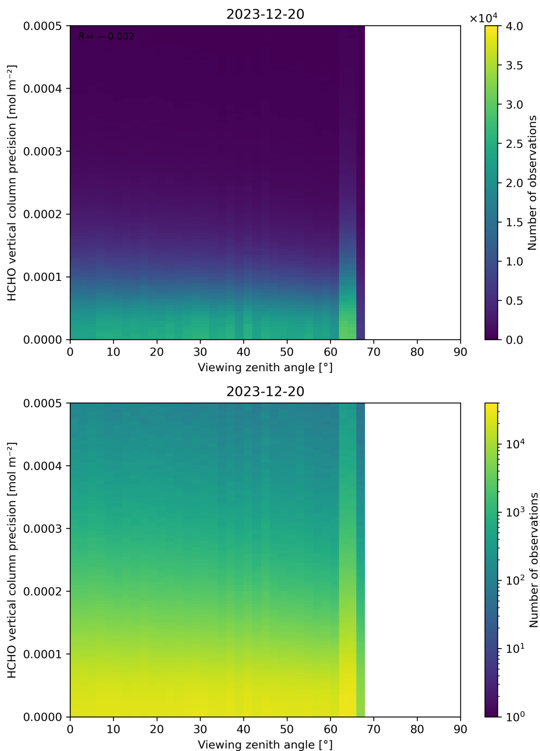
Figure 194: Scatter density plot of “Viewing zenith angle” against “HCHO vertical column precision” for 2023-12-20 to 2023-12-21.
