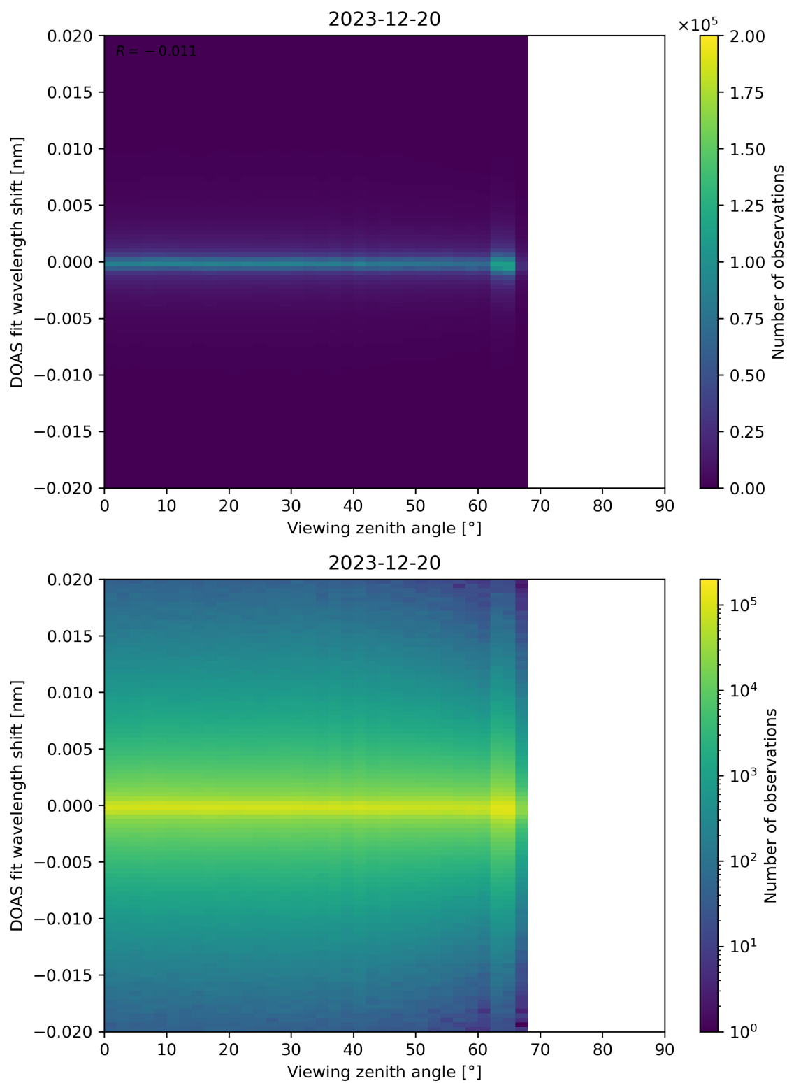
Figure 183: Scatter density plot of “Viewing zenith angle” against “DOAS fit wavelength shift” for 2023-12-20 to 2023-12-21.
