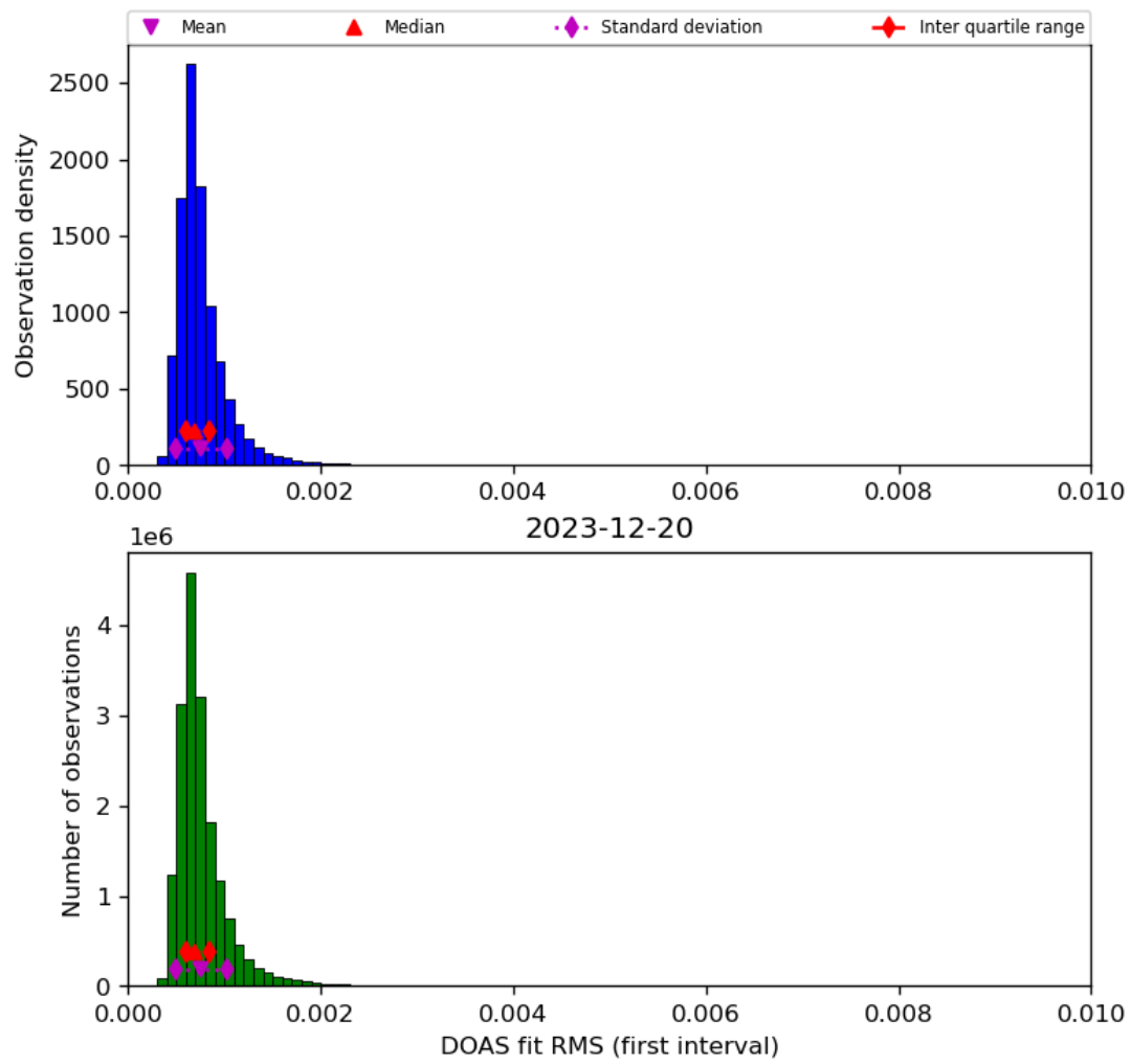
Figure 46: Histogram of “DOAS fit RMS (first interval)” for 2023-12-20 to 2023-12-21
