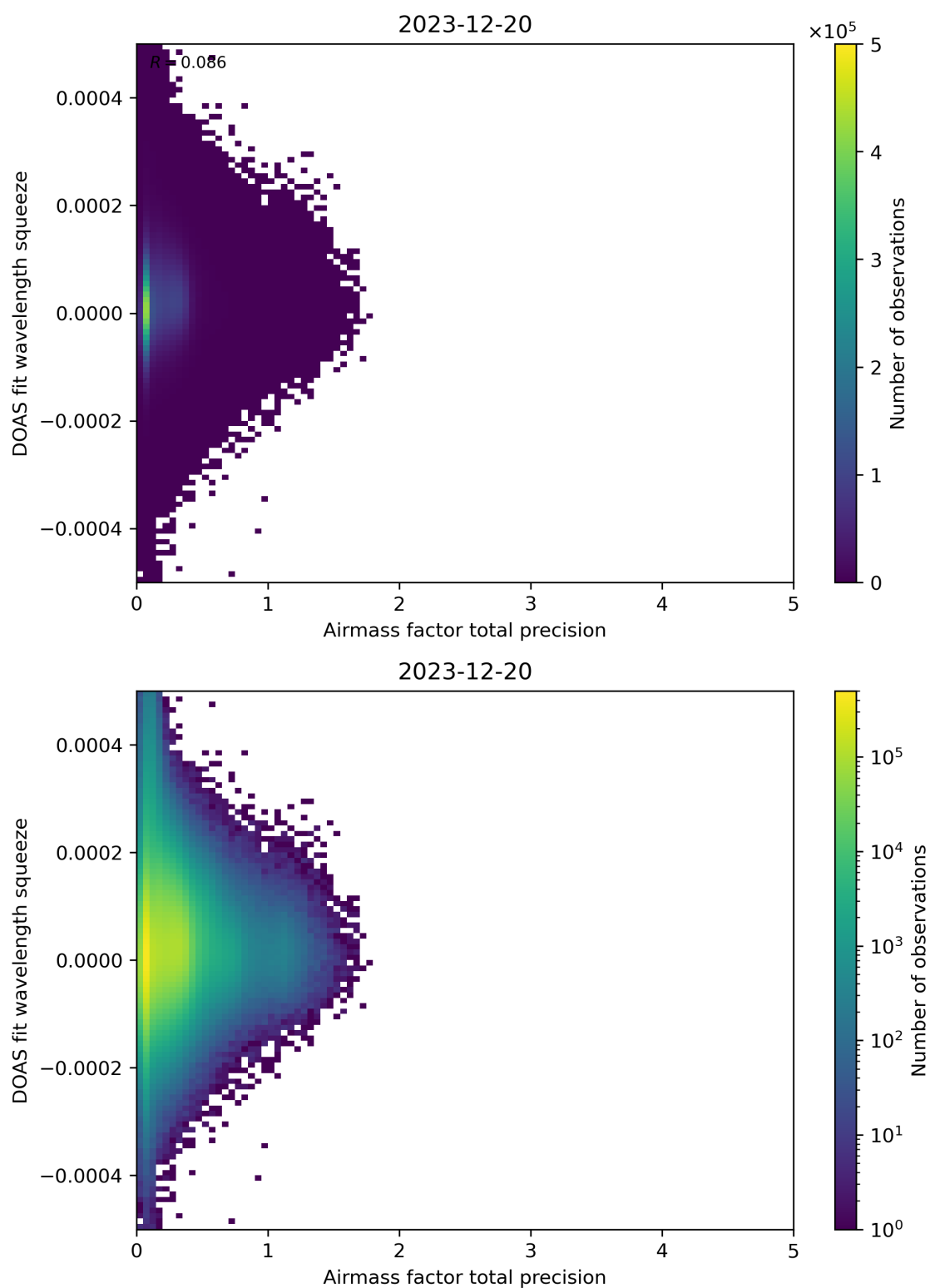
Figure 107: Scatter density plot of “Airmass factor total precision” against “DOAS fit wavelength squeeze” for 2023-12-20 to 2023-12-21.
