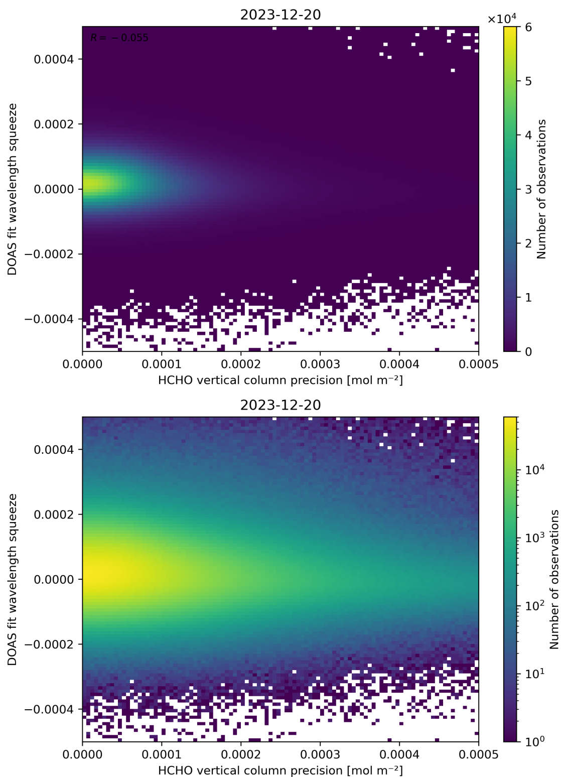
Figure 138: Scatter density plot of “HCHO vertical column precision” against “DOAS fit wavelength squeeze” for 2023-12-20 to 2023-12-21.
