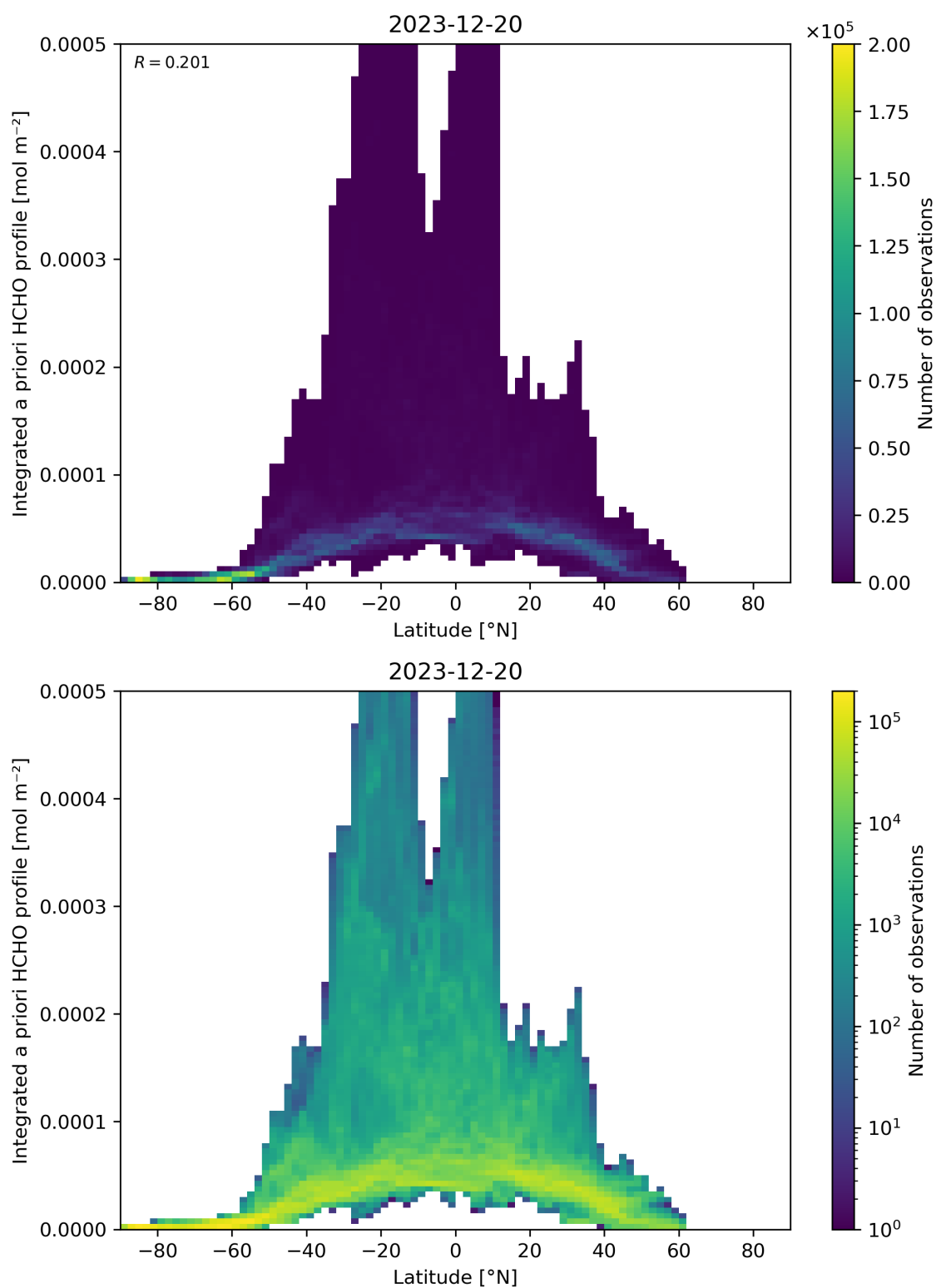
Figure 166: Scatter density plot of “Latitude” against “Integrated a priori HCHO profile” for 2023-12-20 to 2023-12-21.
