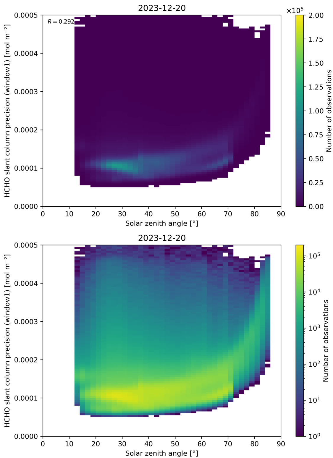
Figure 174: Scatter density plot of “Solar zenith angle” against “HCHO slant column precision (window1)” for 2023-12-20 to 2023-12-21.
