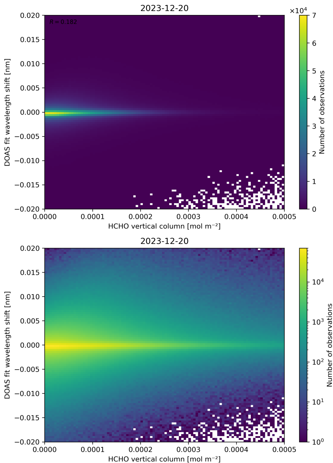
Figure 124: Scatter density plot of “HCHO vertical column” against “DOAS fit wavelength shift” for 2023-12-20 to 2023-12-21.
