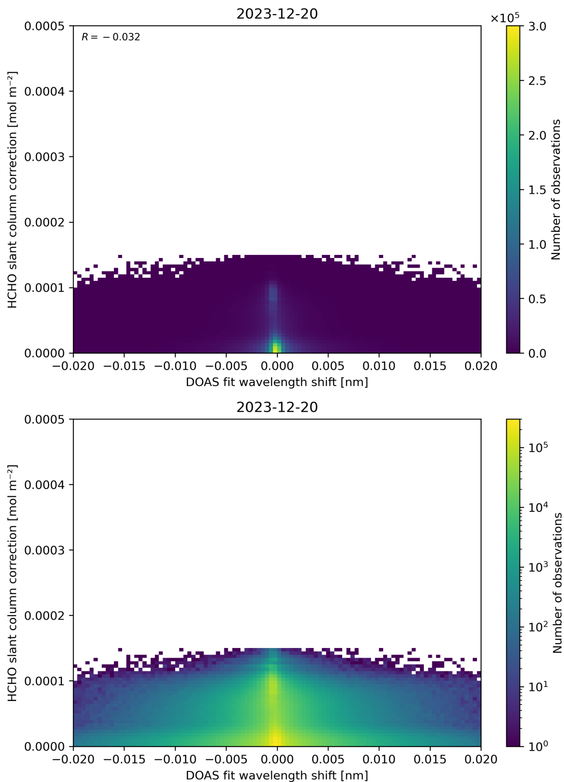
Figure 67: Scatter density plot of “DOAS fit wavelength shift” against “HCHO slant column correction” for 2023-12-20 to 2023-12-21.
