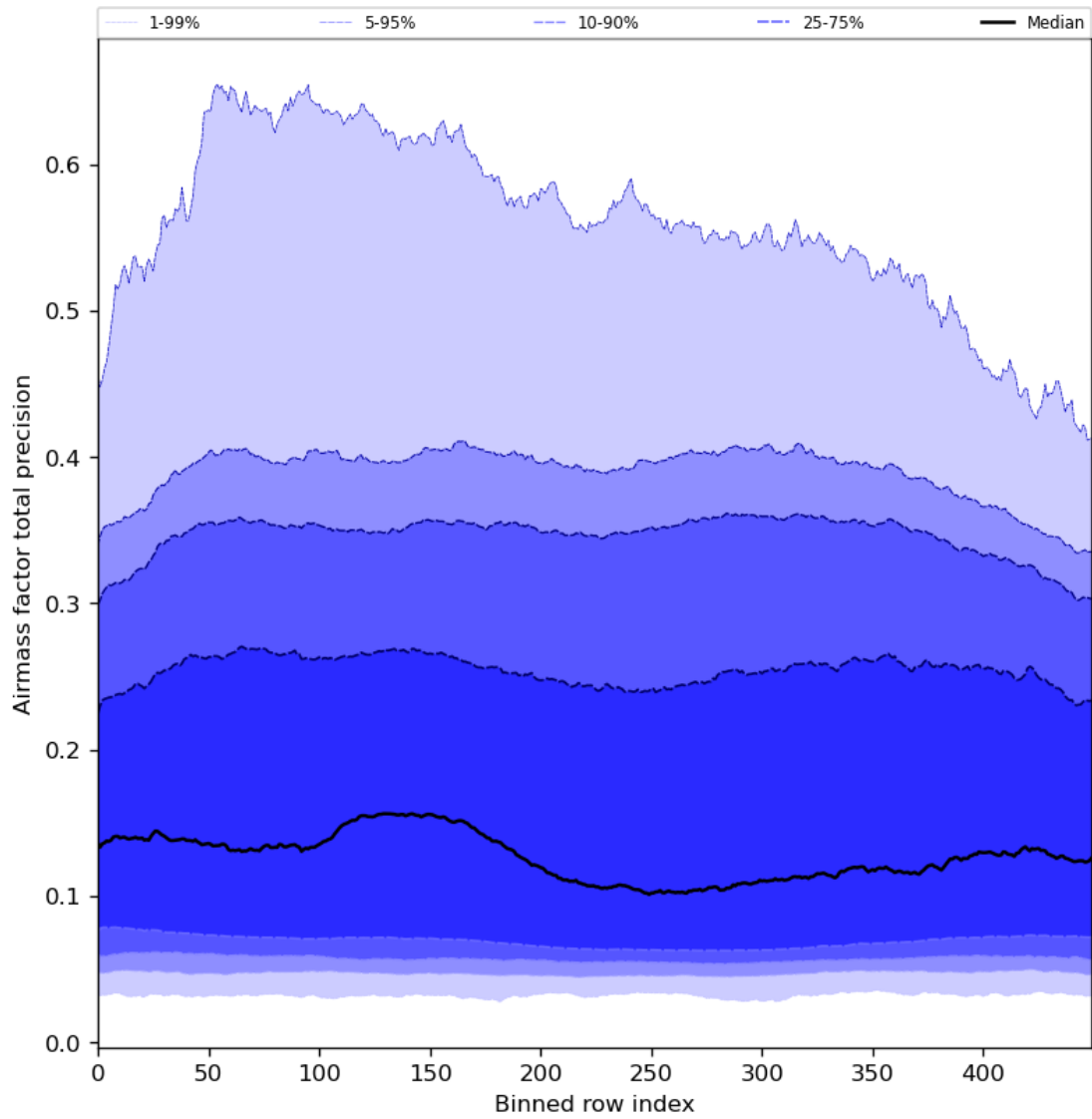
Figure 55: Along track statistics of “Airmass factor total precision” for 2023-12-20 to 2023-12-21
