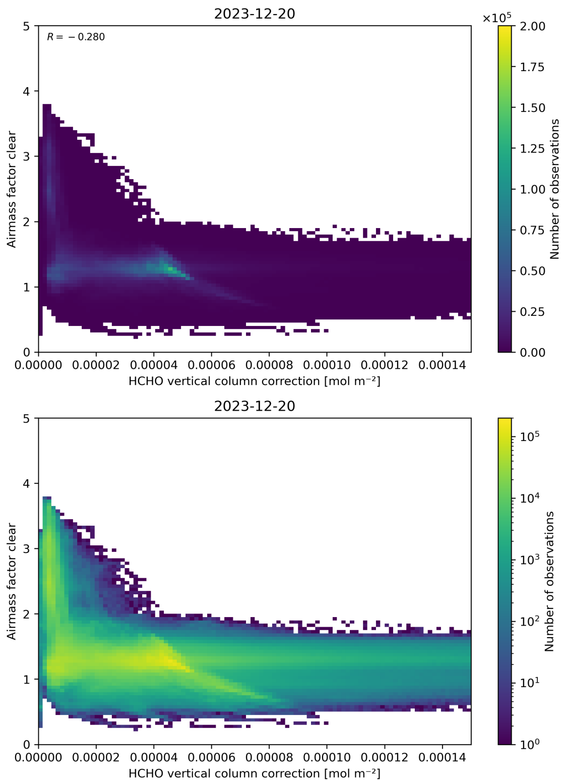
Figure 115: Scatter density plot of “HCHO vertical column correction” against “Airmass factor clear” for 2023-12-20 to 2023-12-21.
