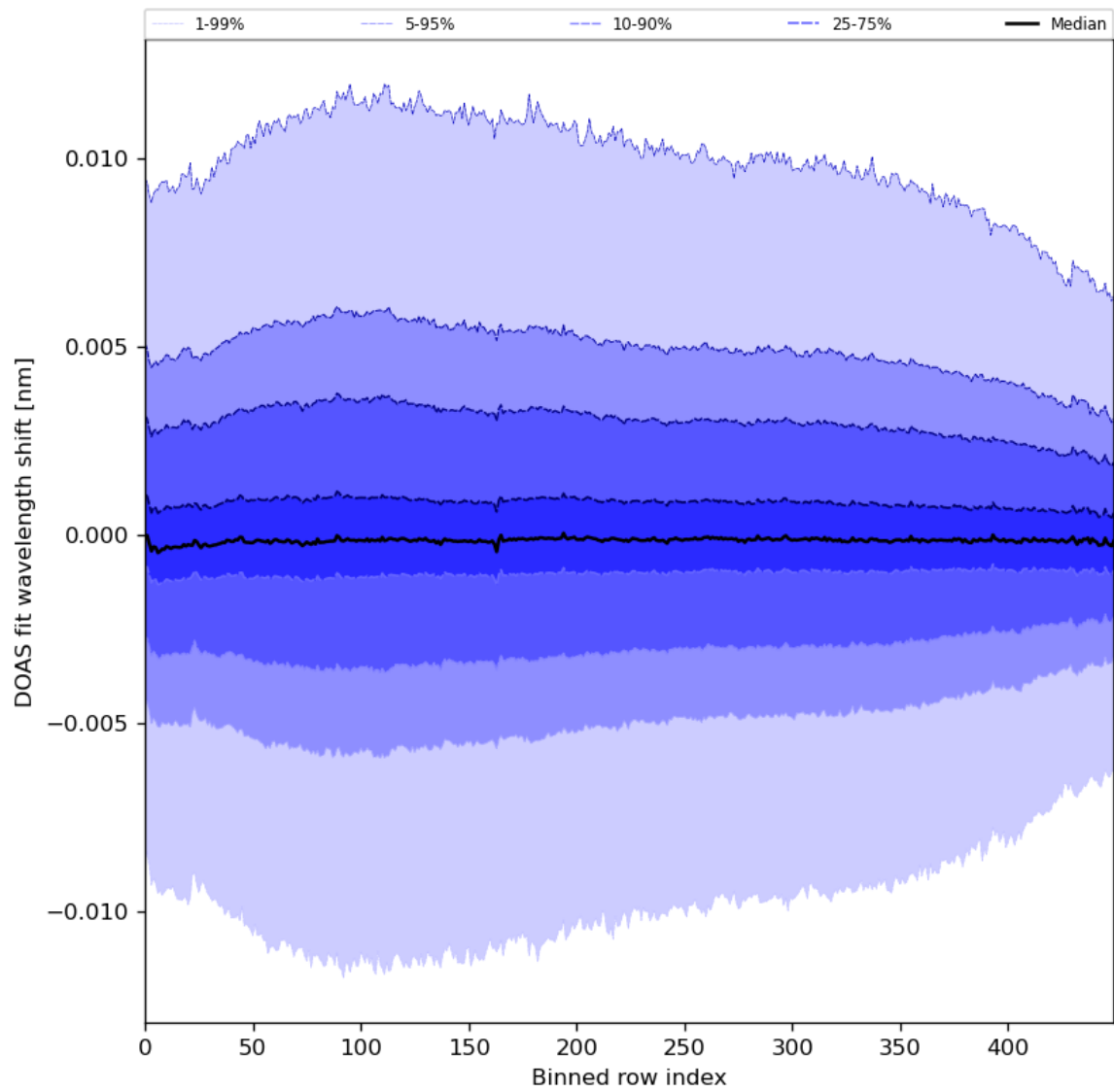
Figure 58: Along track statistics of “DOAS fit wavelength shift” for 2023-12-20 to 2023-12-21
