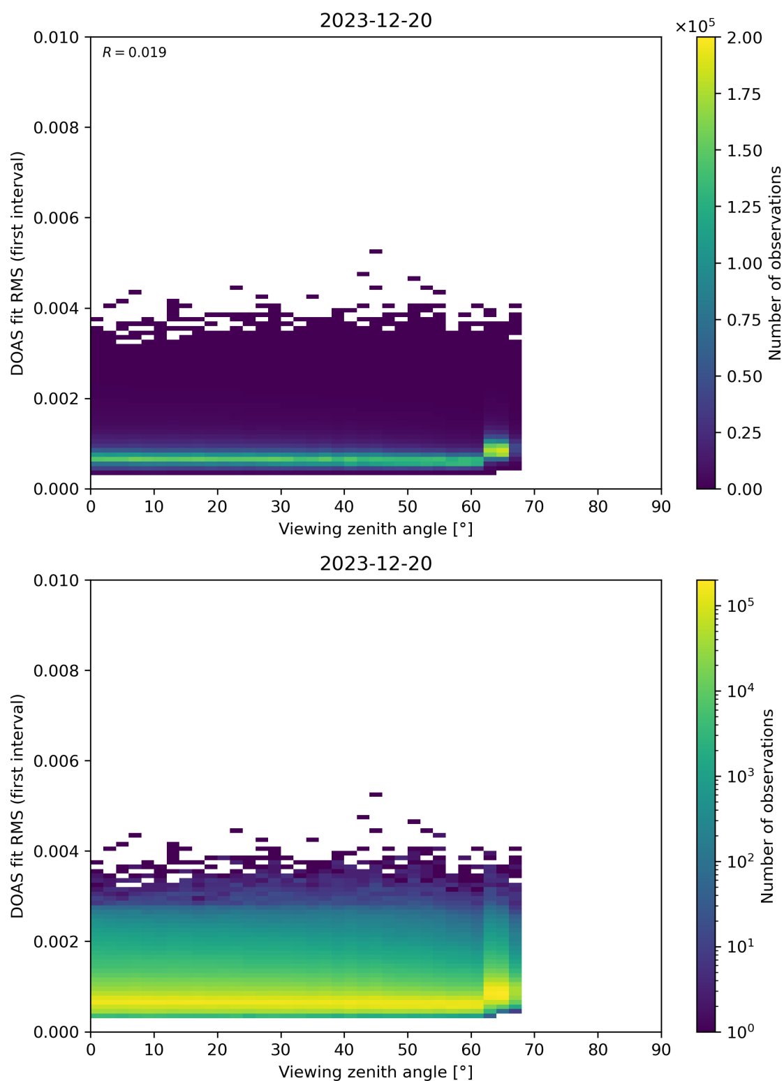
Figure 182: Scatter density plot of “Viewing zenith angle” against “DOAS fit RMS (first interval)” for 2023-12-20 to 2023-12-21.
