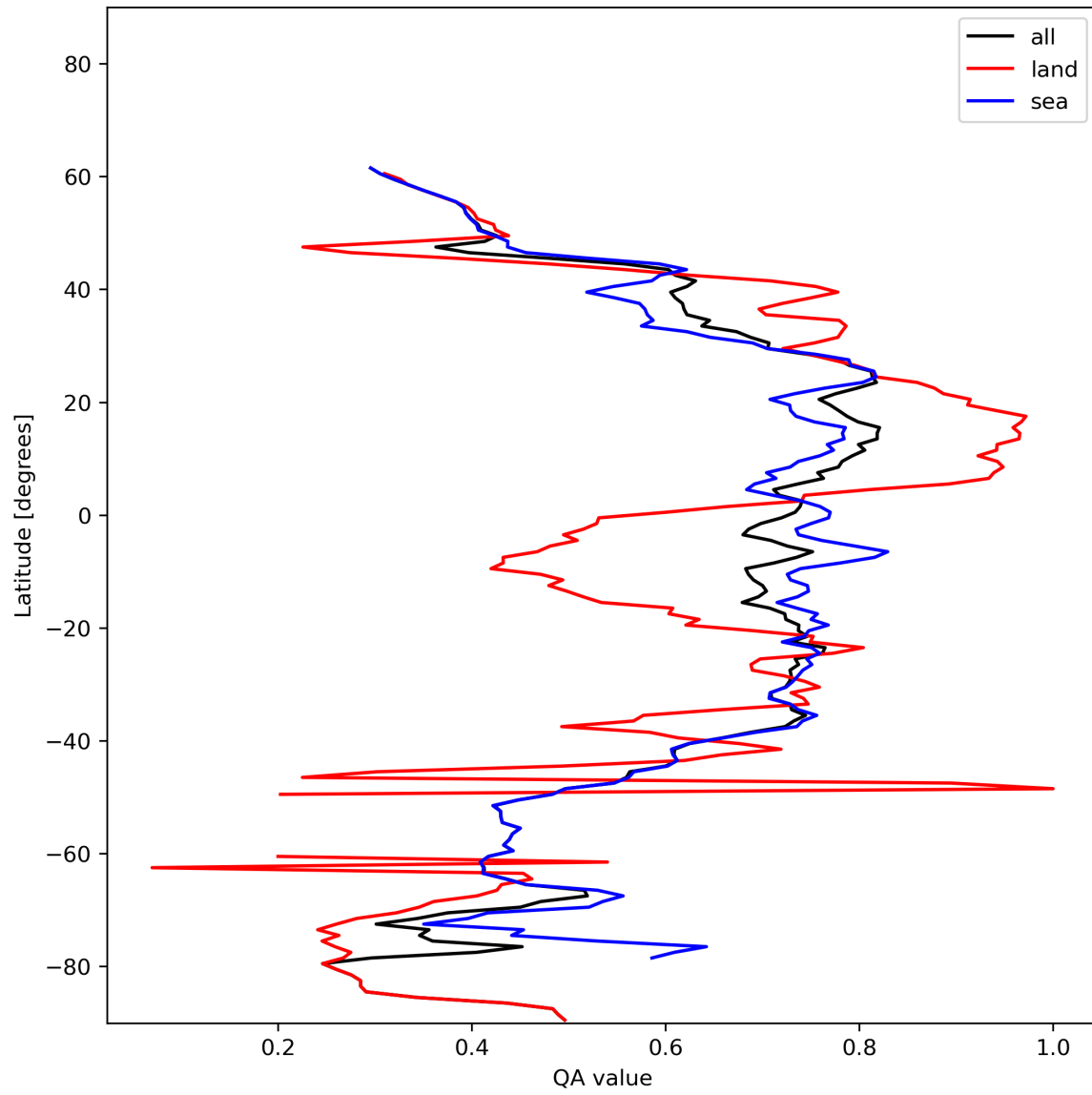
Figure 20: Zonal average of “QA value” for 2023-12-20 to 2023-12-21.
