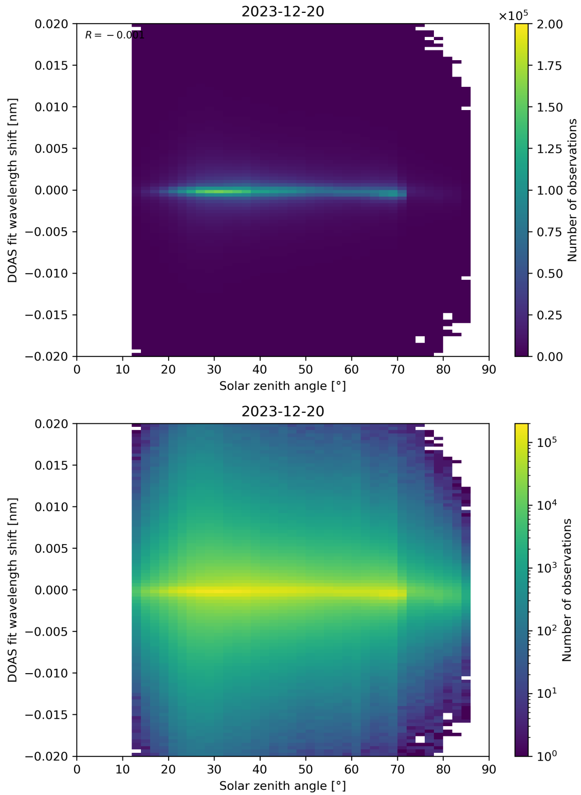
Figure 168: Scatter density plot of “Solar zenith angle” against “DOAS fit wavelength shift” for 2023-12-20 to 2023-12-21.
