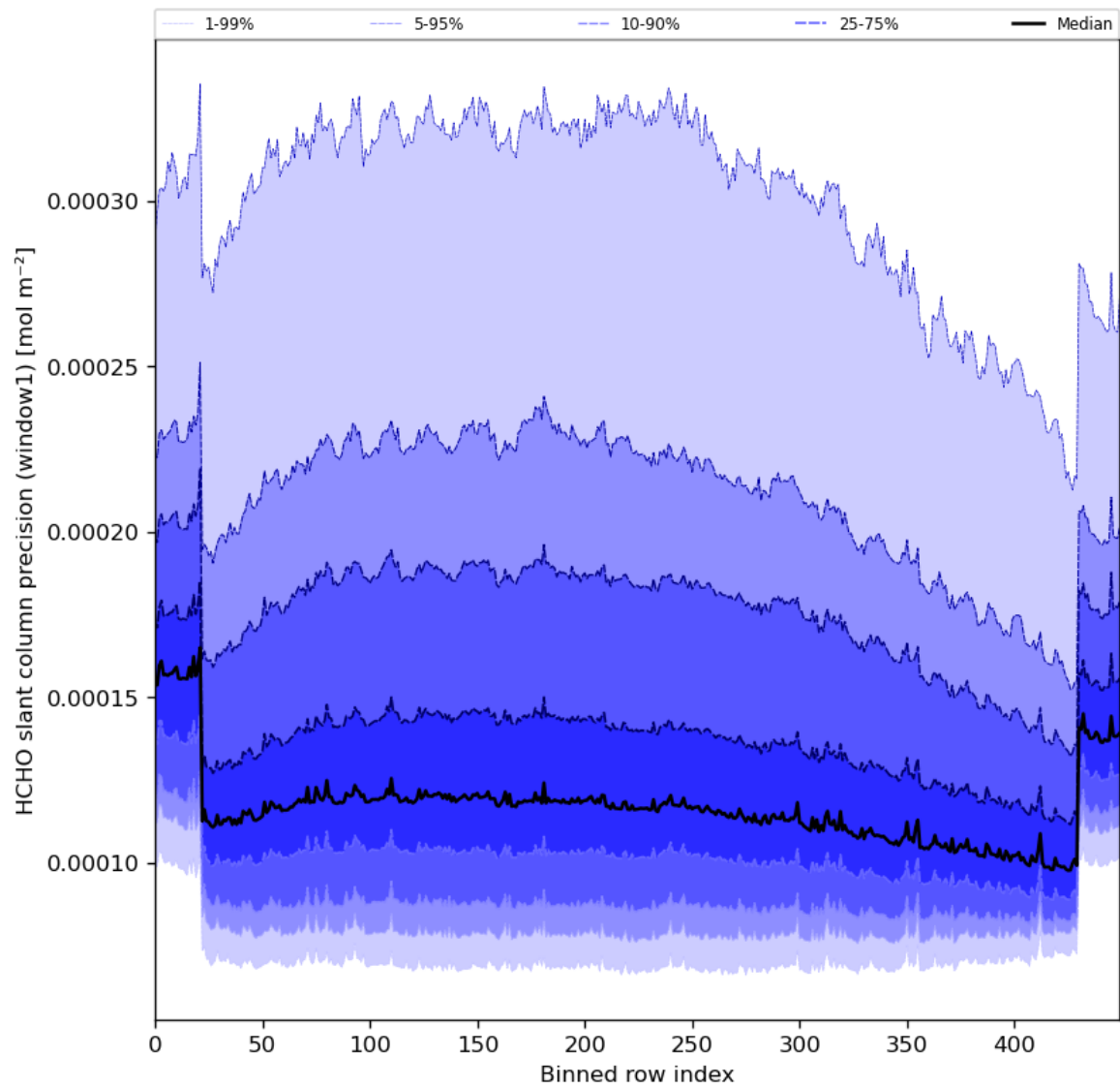
Figure 53: Along track statistics of “HCHO slant column precision (window1)” for 2023-12-20 to 2023-12-21
