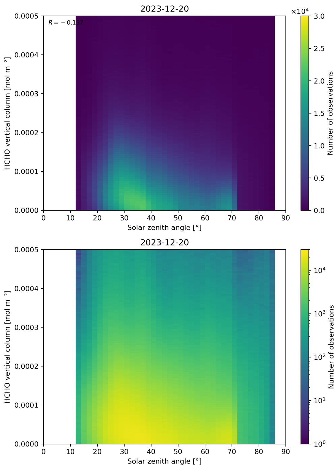
Figure 177: Scatter density plot of “Solar zenith angle” against “HCHO vertical column” for 2023-12-20 to 2023-12-21.
