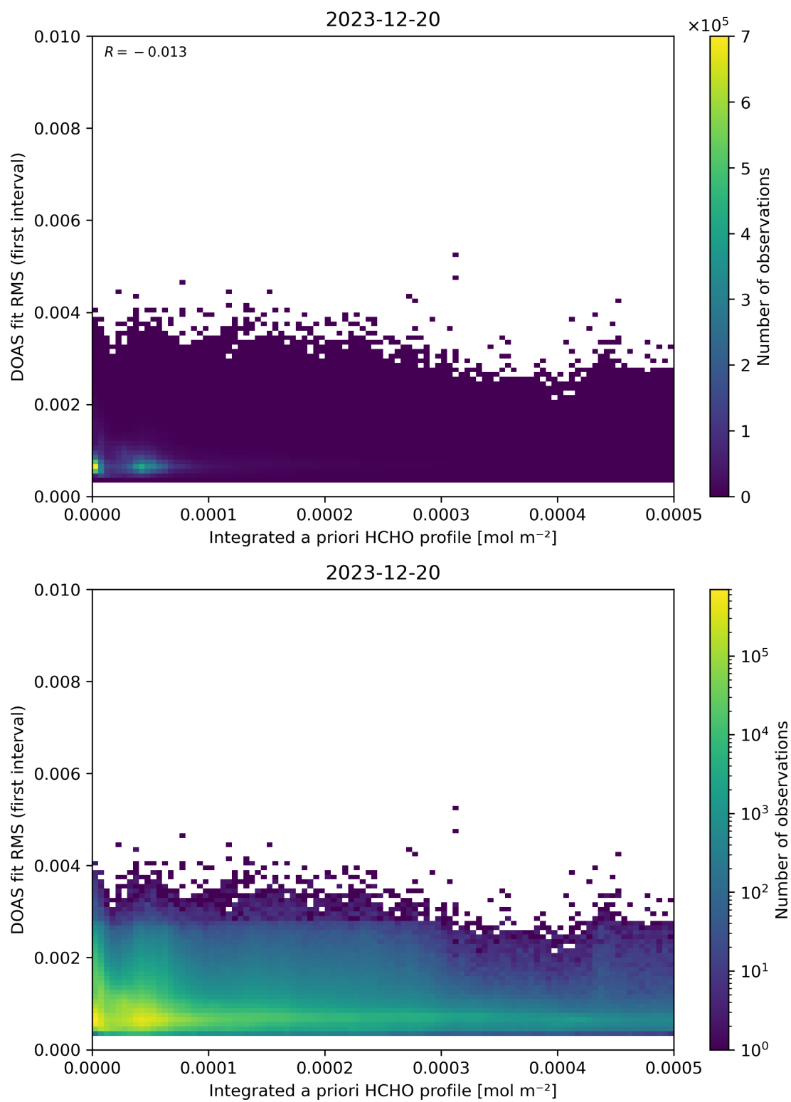
Figure 148: Scatter density plot of “Integrated a priori HCHO profile” against “DOAS fit RMS (first interval)” for 2023-12-20 to 2023-12-21.
