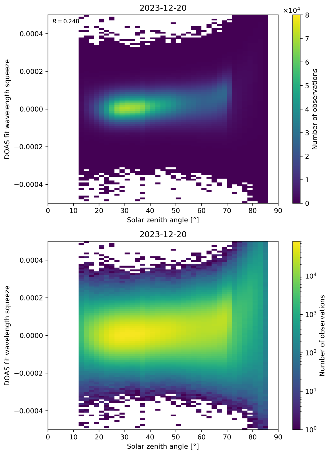
Figure 169: Scatter density plot of “Solar zenith angle” against “DOAS fit wavelength squeeze” for 2023-12-20 to 2023-12-21.
