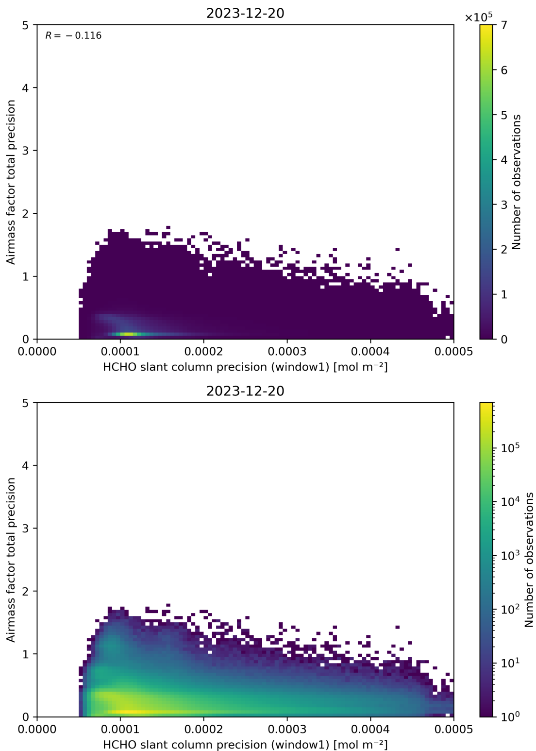
Figure 95: Scatter density plot of “HCHO slant column precision (window1)” against “Airmass factor total precision” for 2023-12-20 to 2023-12-21.
