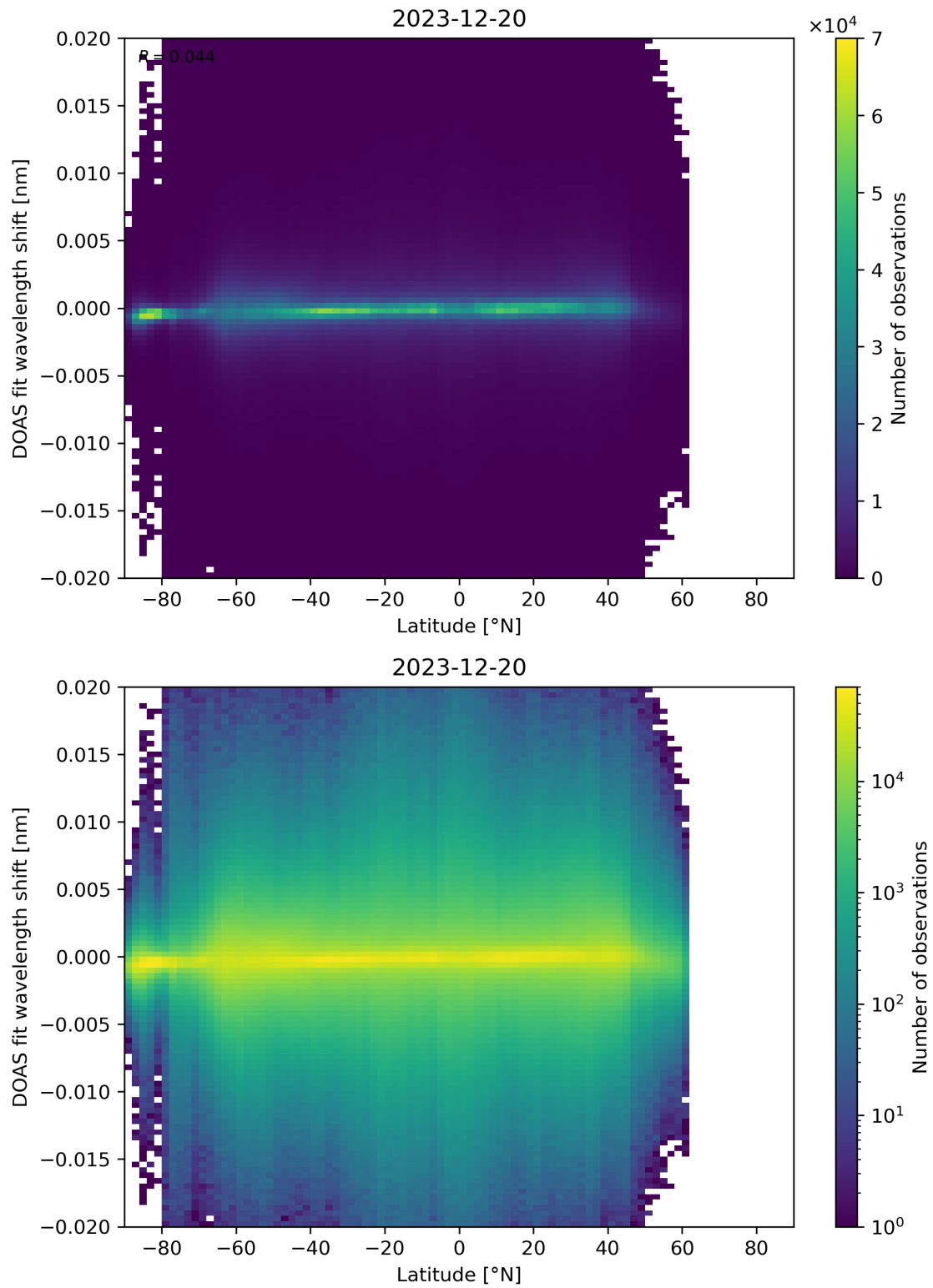
Figure 154: Scatter density plot of “Latitude” against “DOAS fit wavelength shift” for 2023-12-20 to 2023-12-21.
