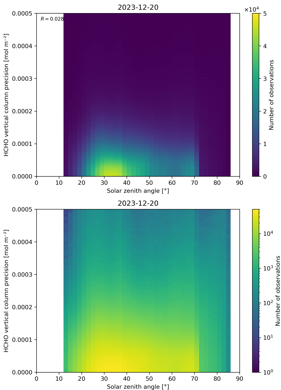
Figure 179: Scatter density plot of “Solar zenith angle” against “HCHO vertical column precision” for 2023-12-20 to 2023-12-21.
