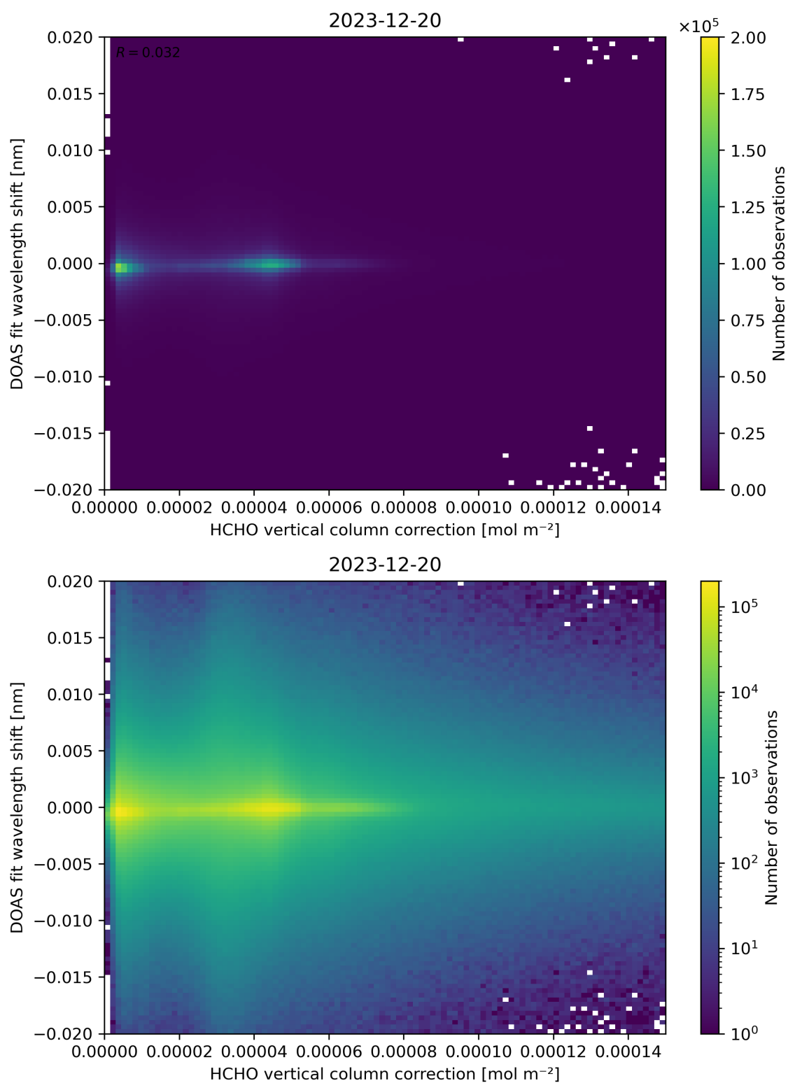
Figure 113: Scatter density plot of “HCHO vertical column correction” against “DOAS fit wavelength shift” for 2023-12-20 to 2023-12-21.
