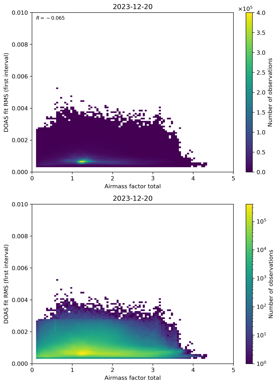
Figure 97: Scatter density plot of “Airmass factor total” against “DOAS fit RMS (first interval)” for 2023-12-20 to 2023-12-21.
