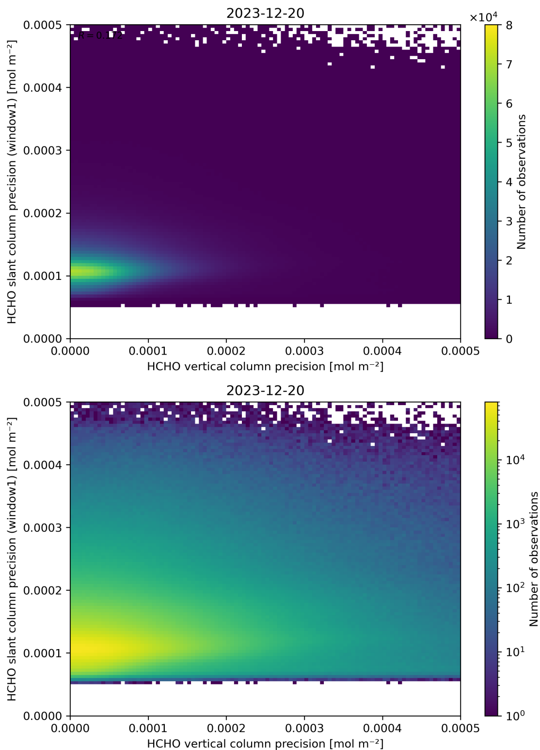
Figure 143: Scatter density plot of “HCHO vertical column precision” against “HCHO slant column precision (window1)” for 2023-12-20 to 2023-12-21.
