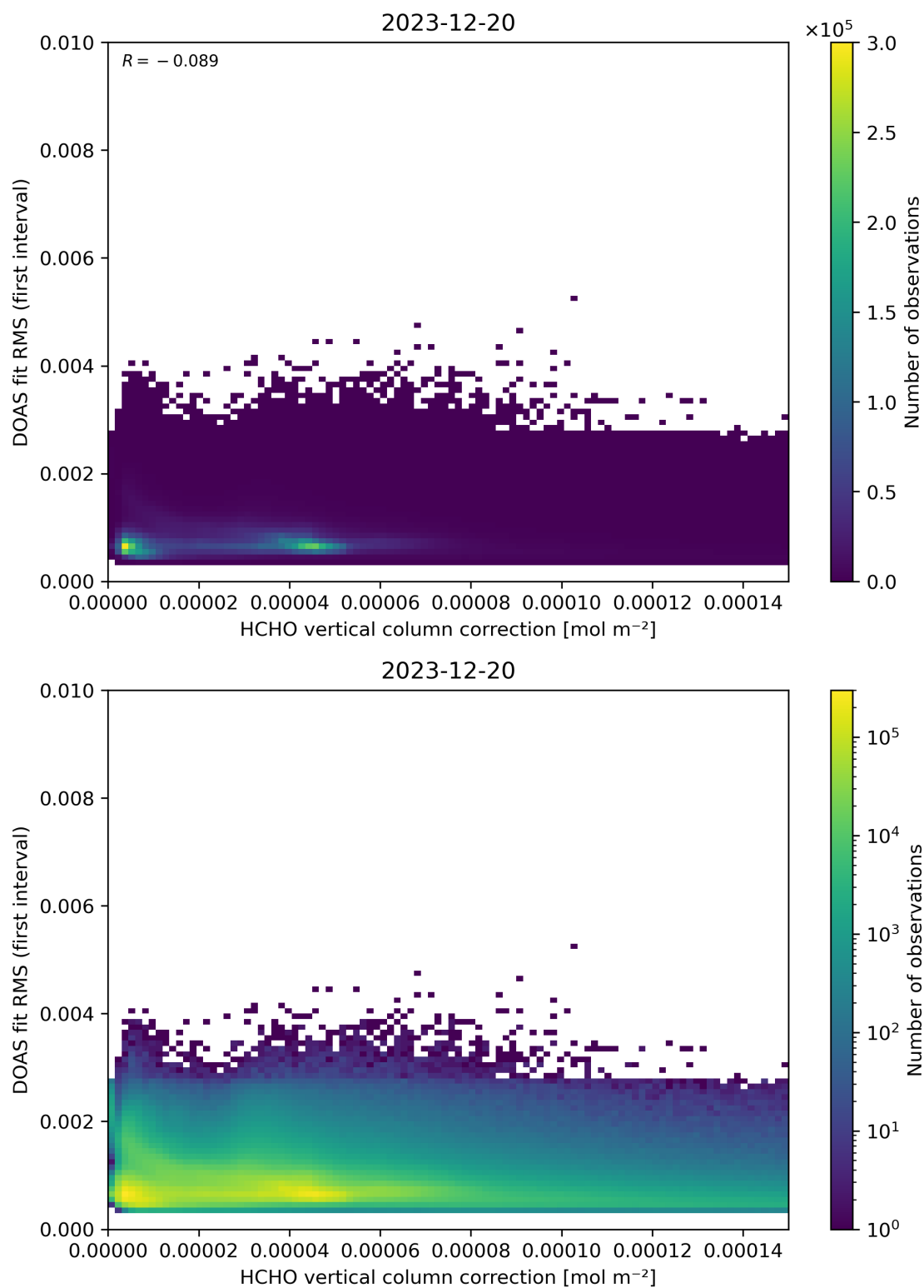
Figure 112: Scatter density plot of “HCHO vertical column correction” against “DOAS fit RMS (first interval)” for 2023-12-20 to 2023-12-21.
