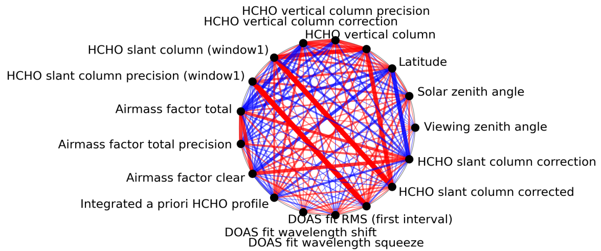
Figure 1: Map of correlation graph for 2023-12-20 to 2023-12-21.
