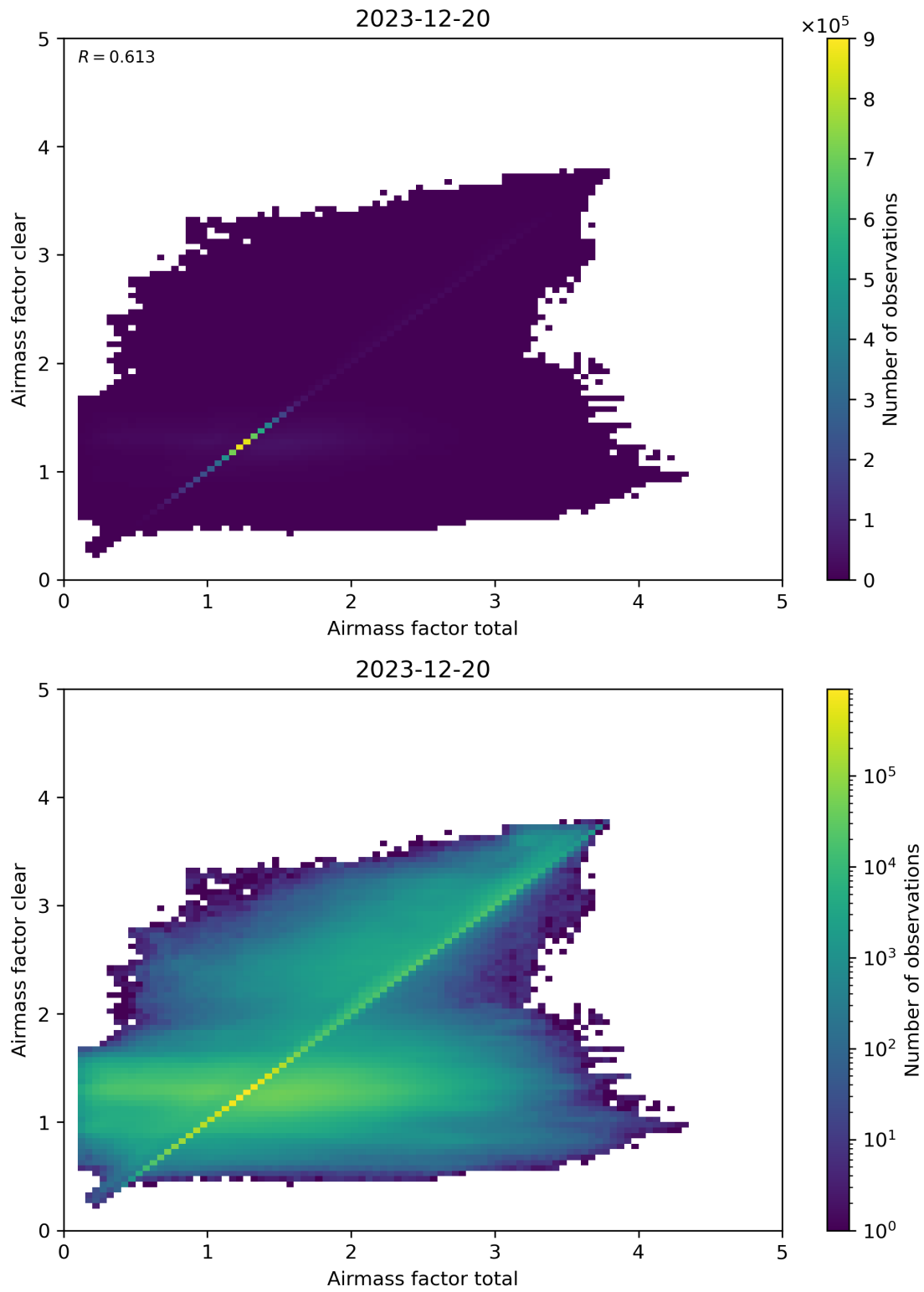
Figure 100: Scatter density plot of “Airmass factor total” against “Airmass factor clear” for 2023-12-20 to 2023-12-21.
