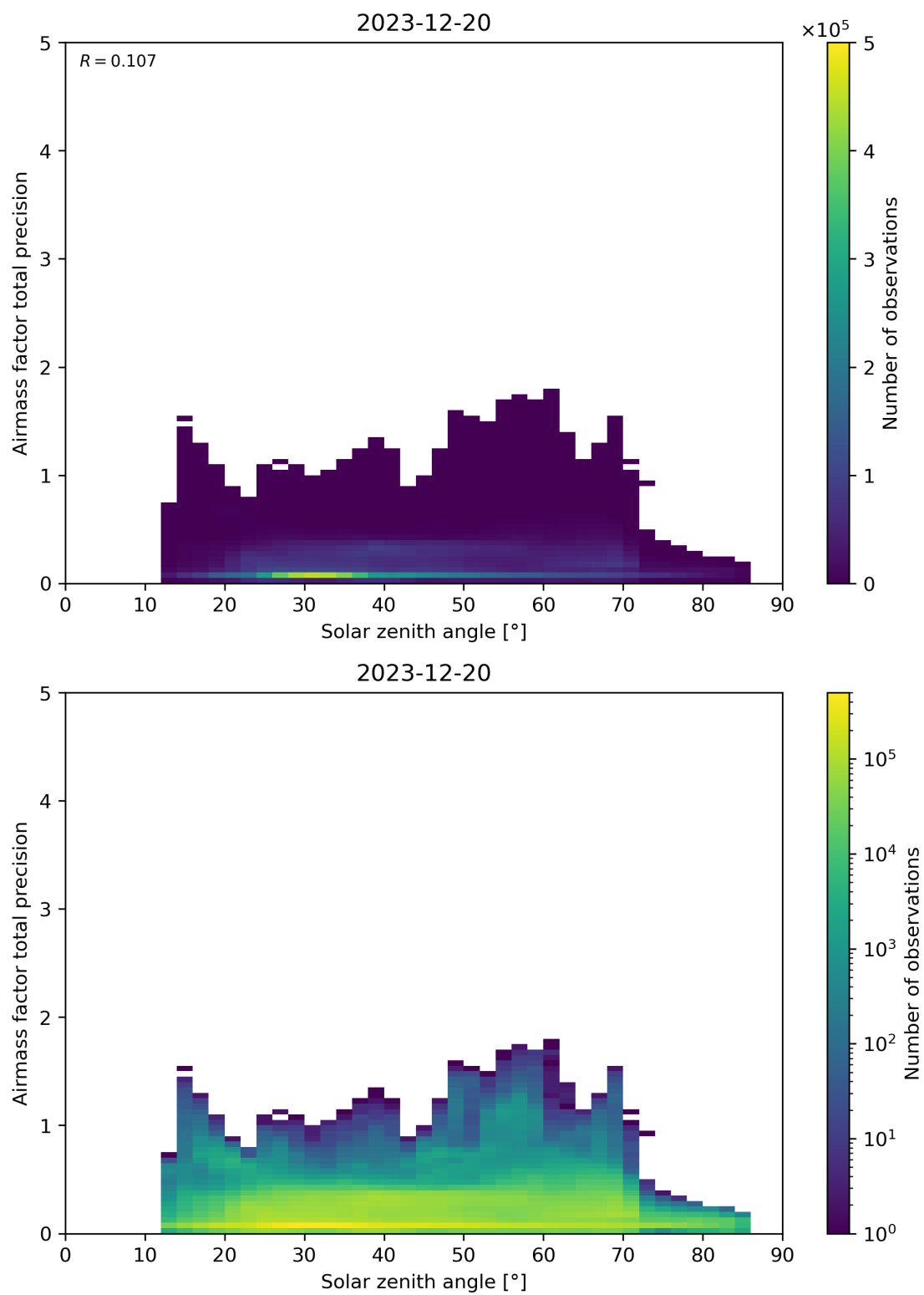
Figure 176: Scatter density plot of “Solar zenith angle” against “Airmass factor total precision” for 2023-12-20 to 2023-12-21.
