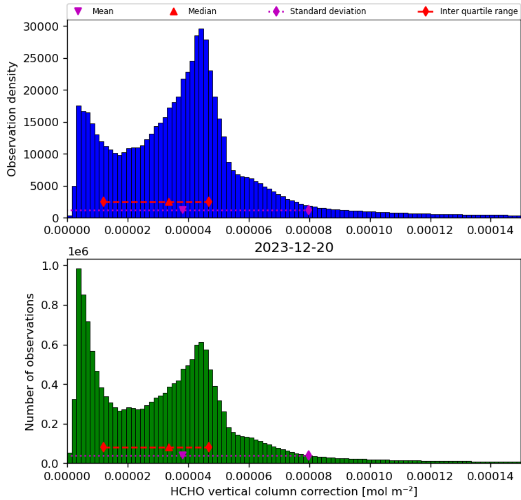
Figure 37: Histogram of “HCHO vertical column correction” for 2023-12-20 to 2023-12-21
