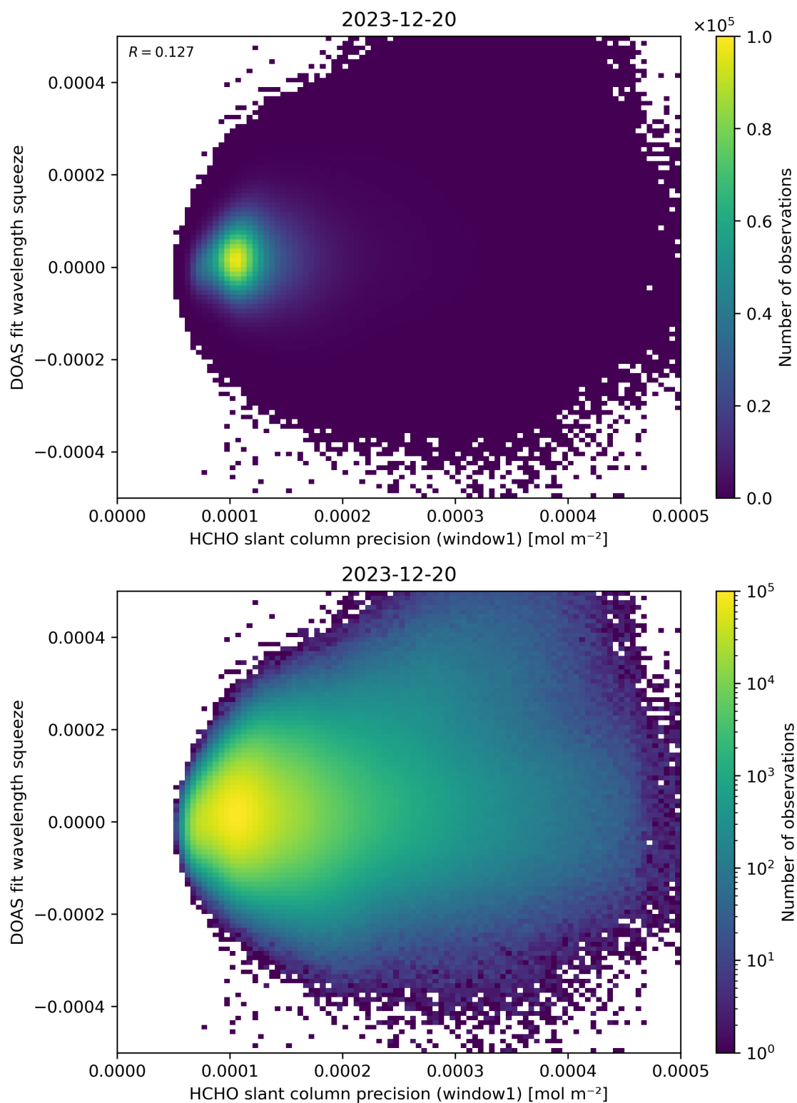
Figure 90: Scatter density plot of “HCHO slant column precision (window1)” against “DOAS fit wavelength squeeze” for 2023-12-20 to 2023-12-21.
