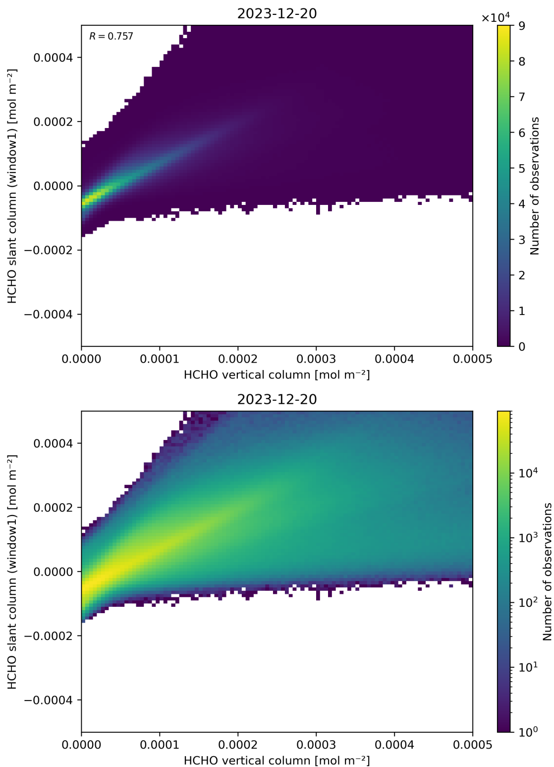
Figure 129: Scatter density plot of “HCHO vertical column” against “HCHO slant column (window1)” for 2023-12-20 to 2023-12-21.
