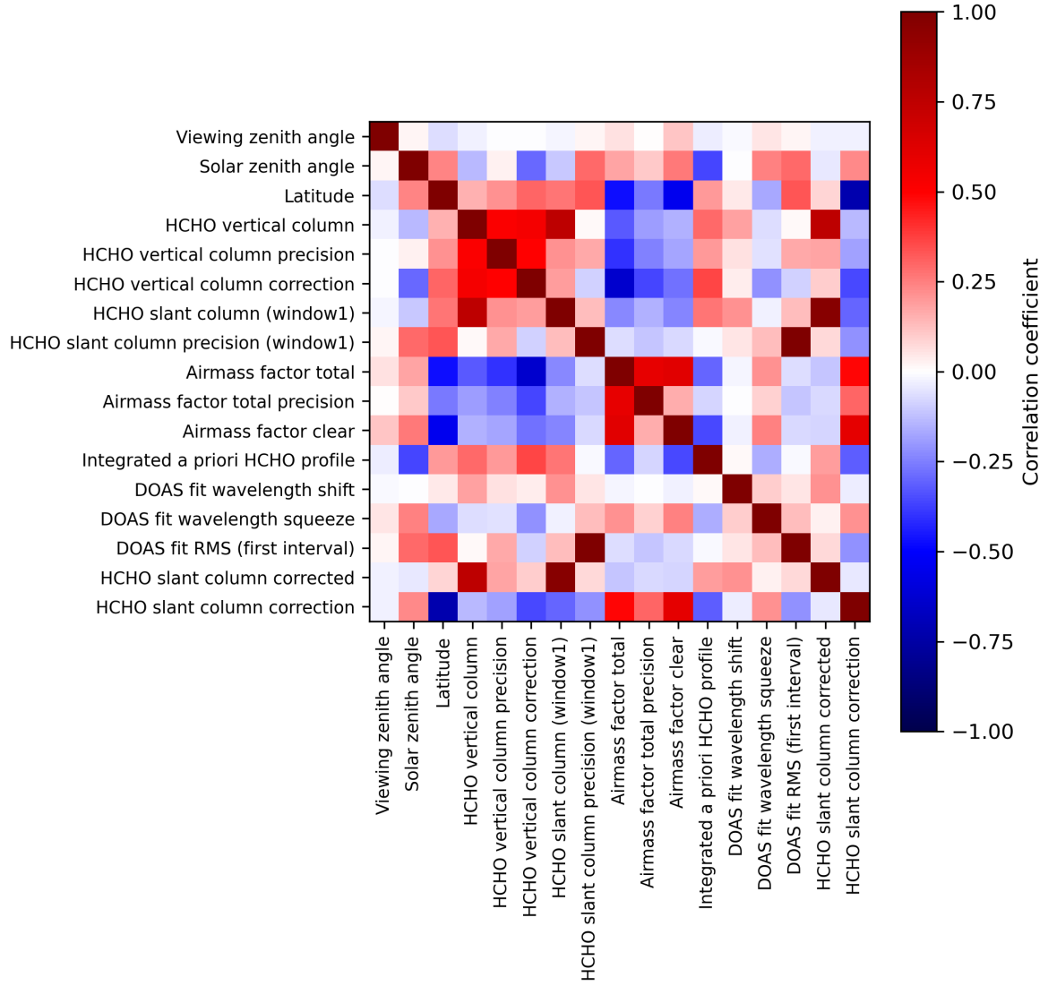
Figure 2: Map of correlation matrix for 2023-12-20 to 2023-12-21.
