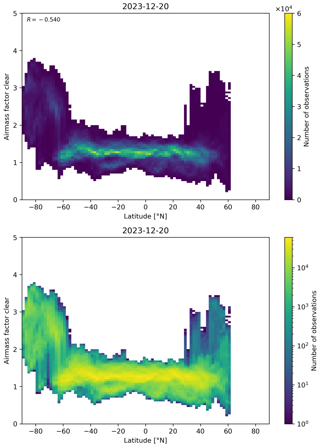
Figure 156: Scatter density plot of “Latitude” against “Airmass factor clear” for 2023-12-20 to 2023-12-21.
