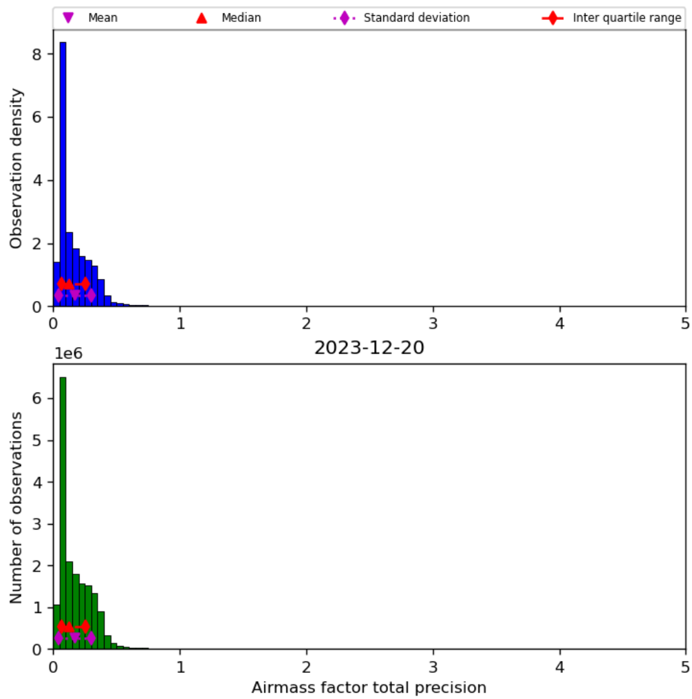
Figure 41: Histogram of “Airmass factor total precision” for 2023-12-20 to 2023-12-21
