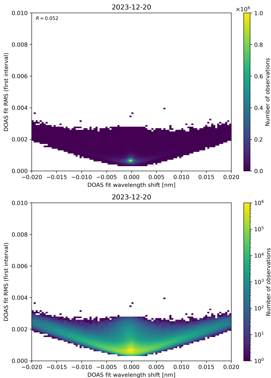
Figure 64: Scatter density plot of “DOAS fit wavelength shift” against “DOAS fit RMS (first interval)” for 2023-12-20 to 2023-12-21.
