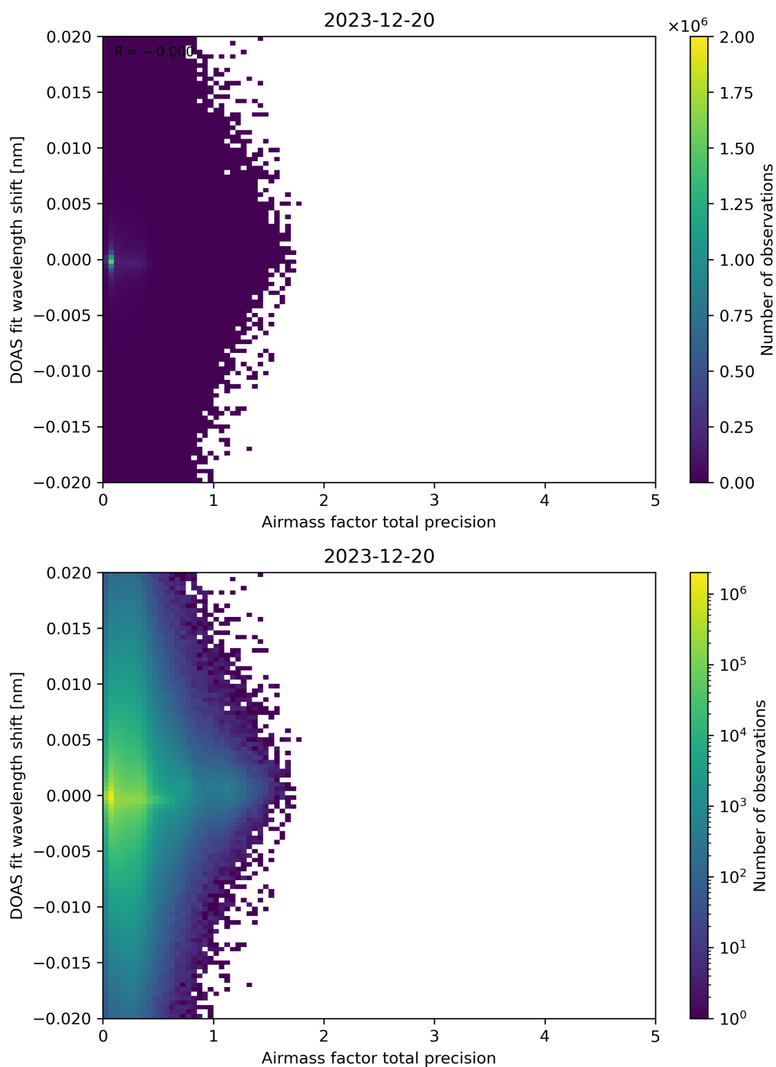
Figure 106: Scatter density plot of “Airmass factor total precision” against “DOAS fit wavelength shift” for 2023-12-20 to 2023-12-21.
