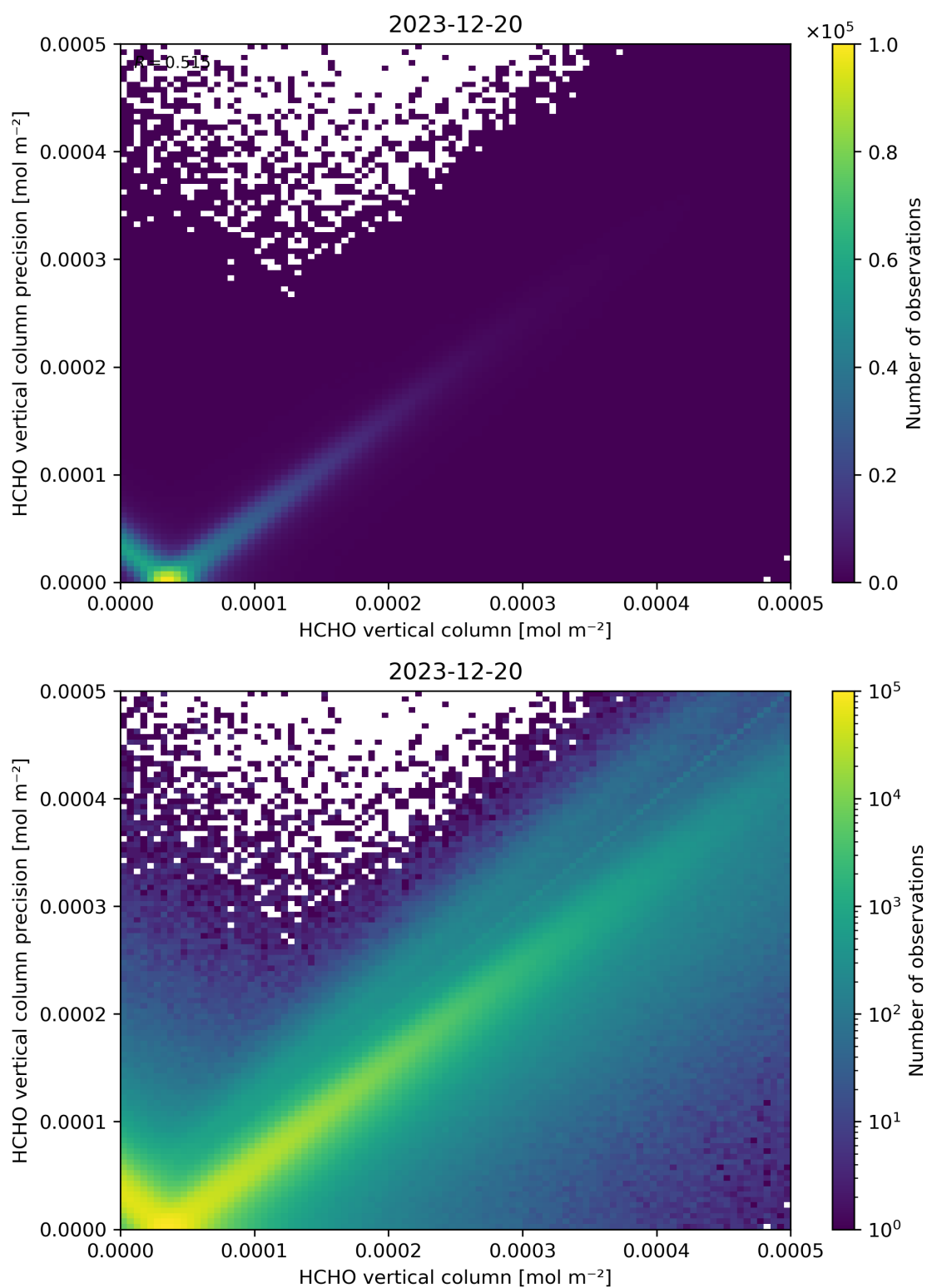
Figure 134: Scatter density plot of “HCHO vertical column” against “HCHO vertical column precision” for 2023-12-20 to 2023-12-21.
