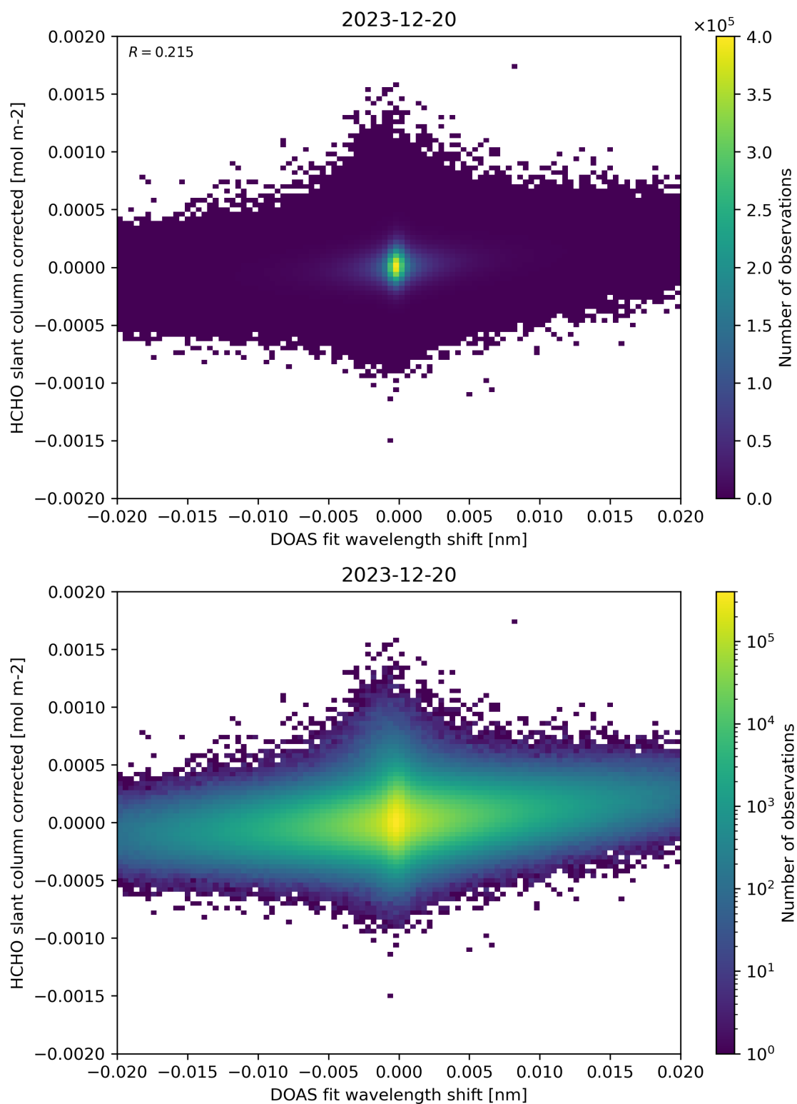
Figure 66: Scatter density plot of “DOAS fit wavelength shift” against “HCHO slant column corrected” for 2023-12-20 to 2023-12-21.
