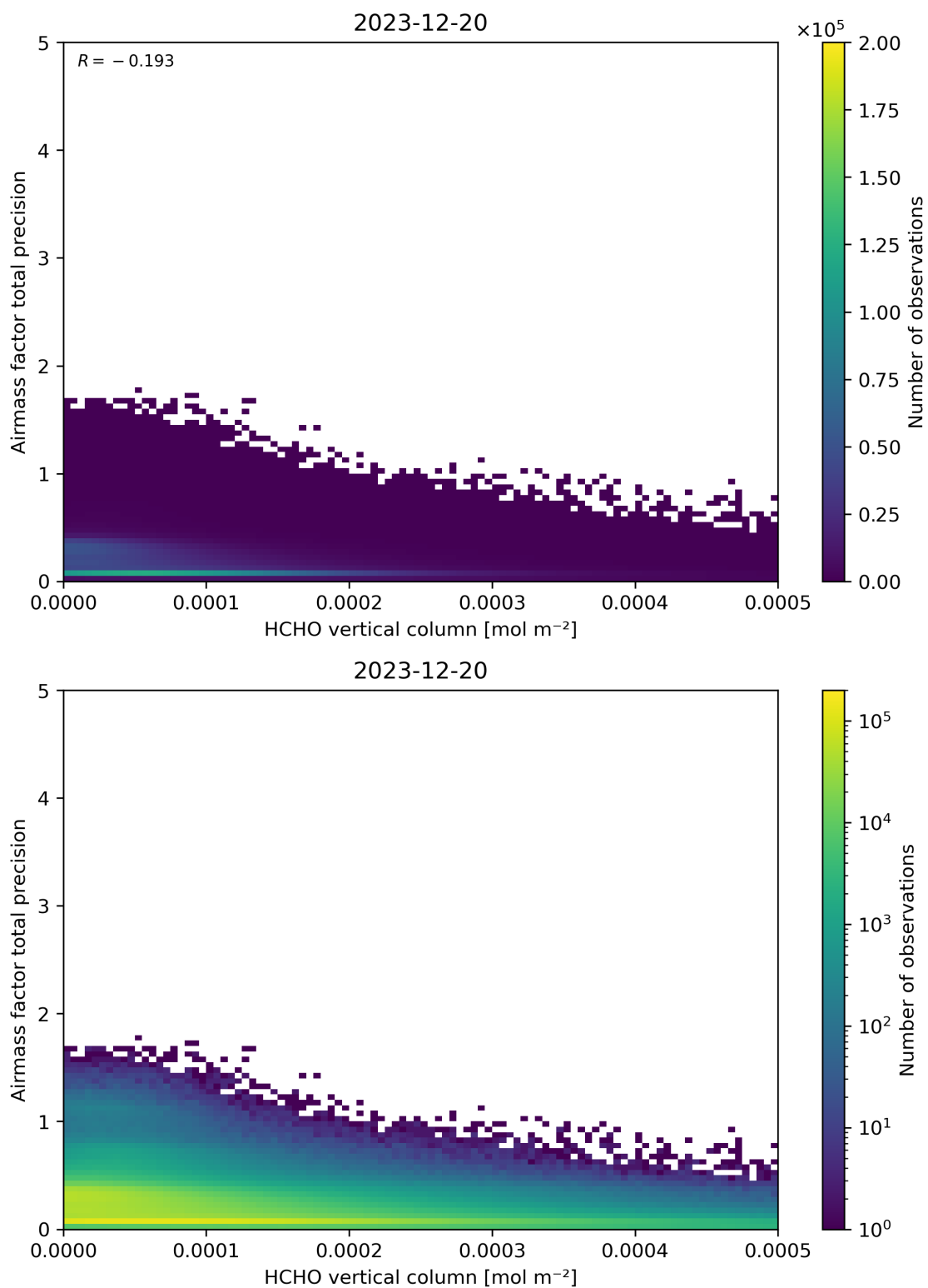
Figure 132: Scatter density plot of “HCHO vertical column” against “Airmass factor total precision” for 2023-12-20 to 2023-12-21.
