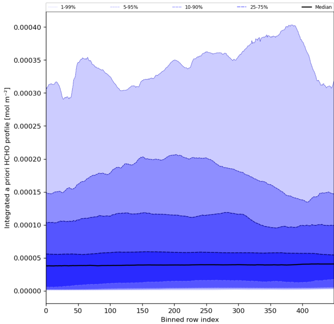
Figure 57: Along track statistics of "Integrated a priori HCHO profile" for 2023-12-20 to 2023-12-21
