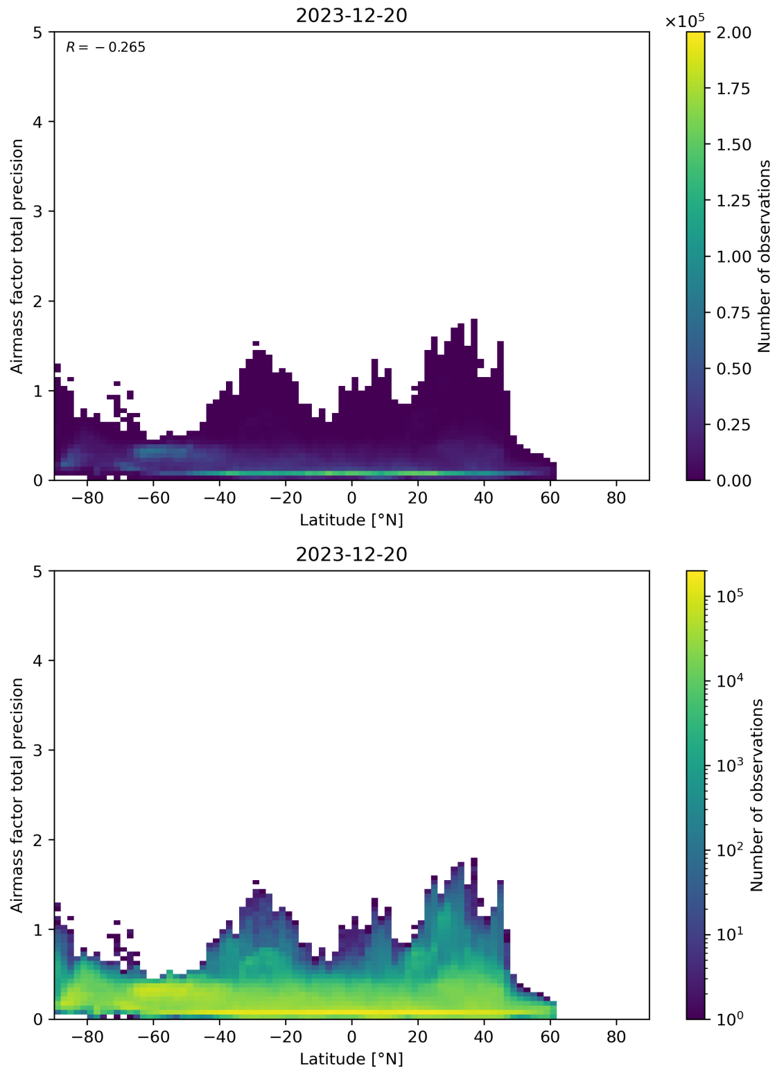
Figure 162: Scatter density plot of “Latitude” against “Airmass factor total precision” for 2023-12-20 to 2023-12-21.
