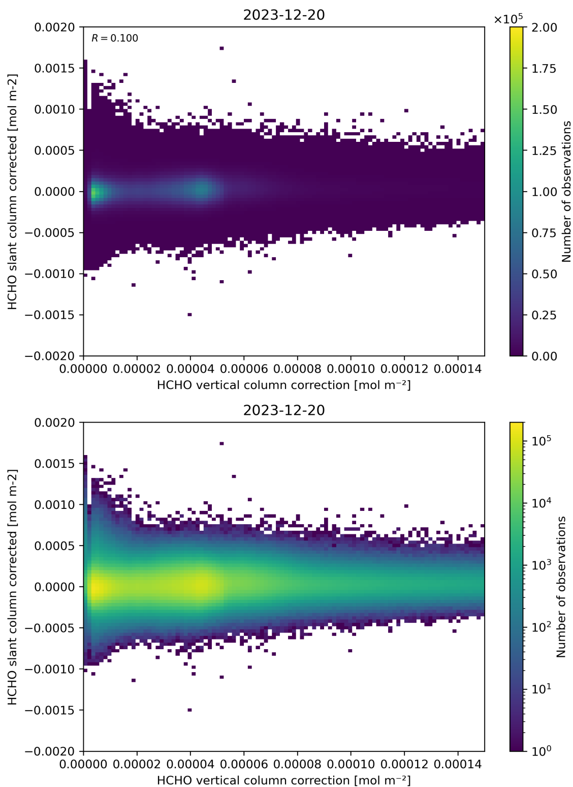
Figure 116: Scatter density plot of “HCHO vertical column correction” against “HCHO slant column corrected” for 2023-12-20 to 2023-12-21.
