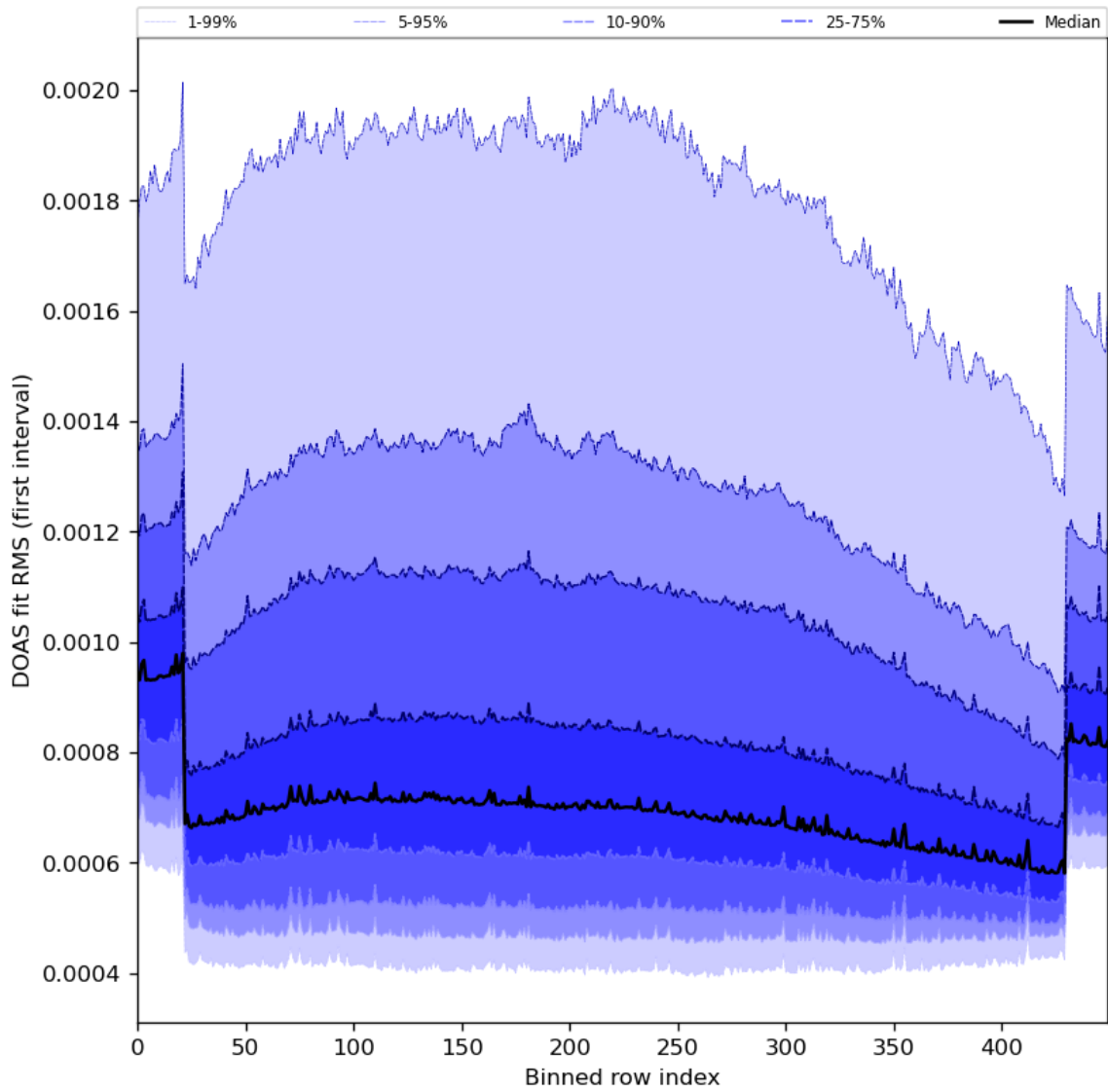
Figure 60: Along track statistics of “DOAS fit RMS (first interval)” for 2023-12-20 to 2023-12-21
