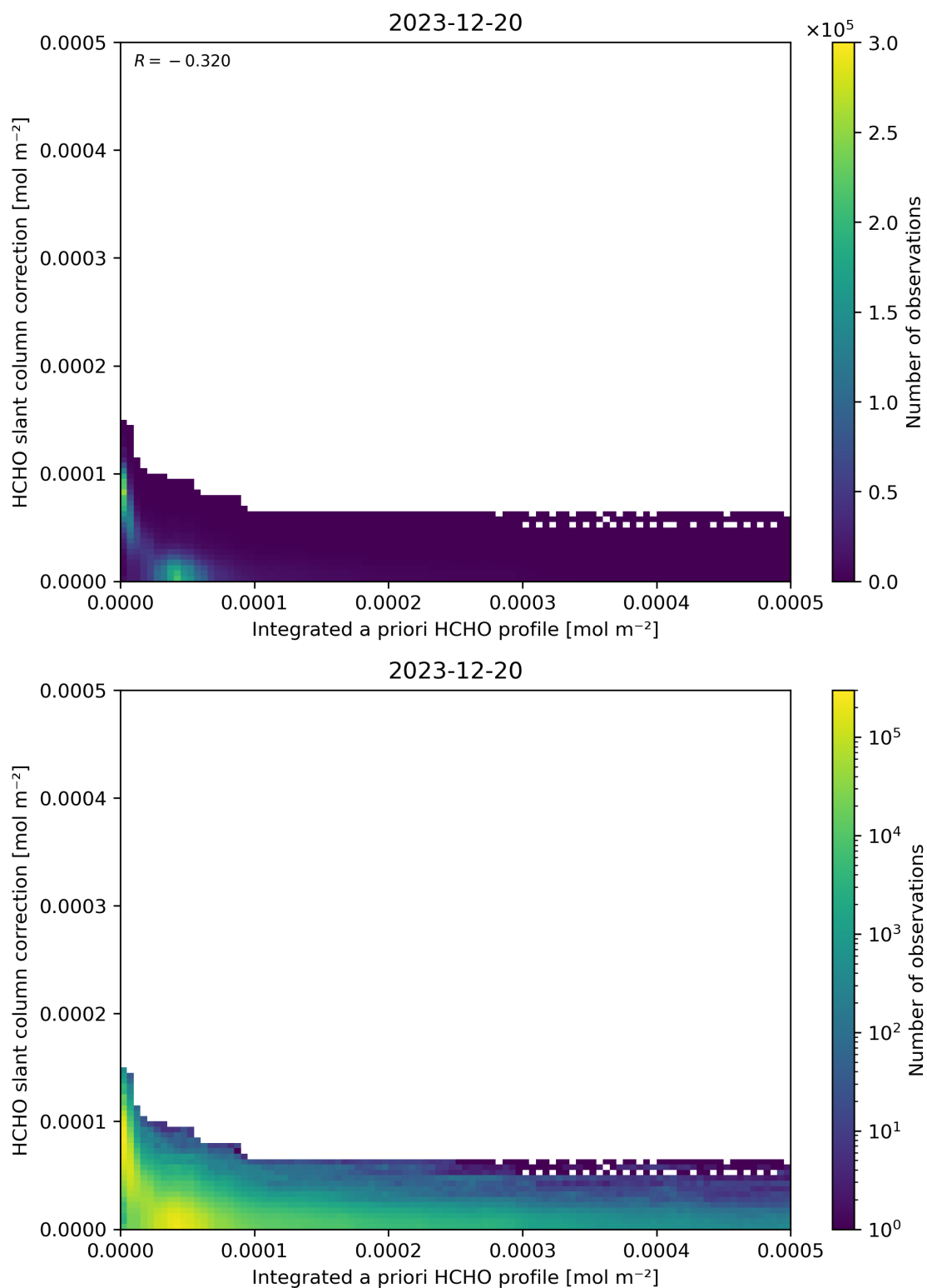
Figure 152: Scatter density plot of “Integrated a priori HCHO profile” against “HCHO slant column correction” for 2023-12-20 to 2023-12-21.
