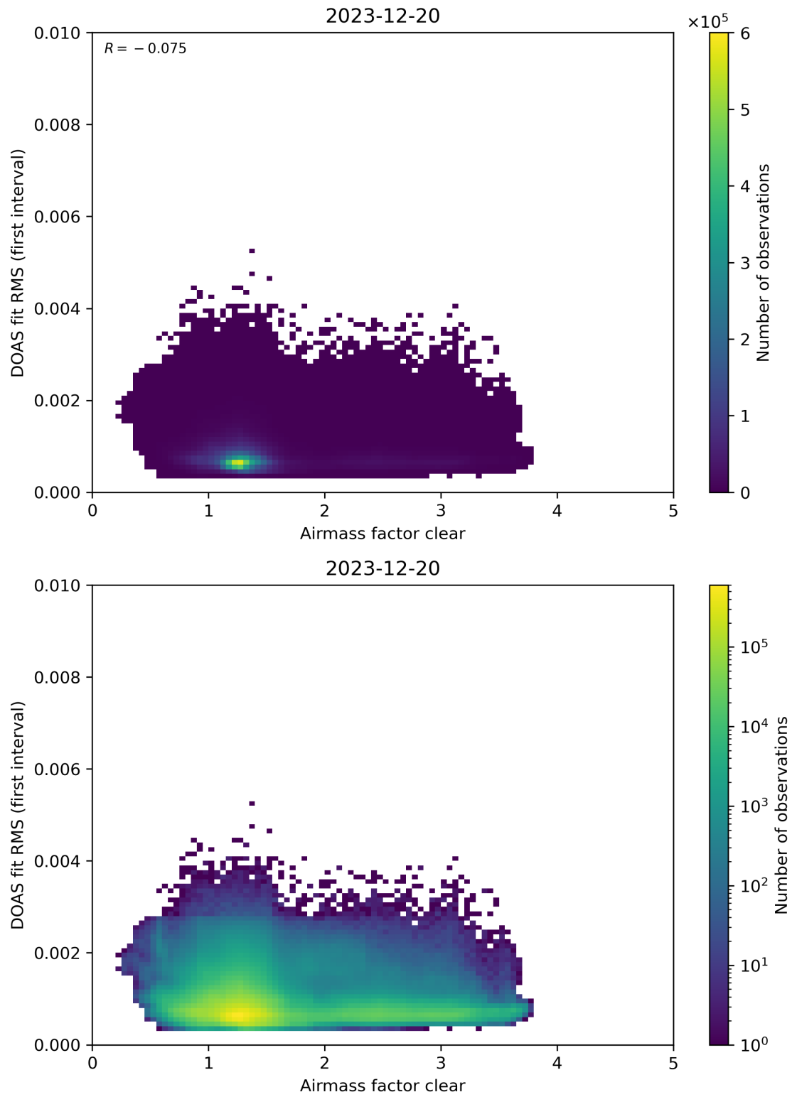
Figure 71: Scatter density plot of “Airmass factor clear” against “DOAS fit RMS (first interval)” for 2023-12-20 to 2023-12-21.
