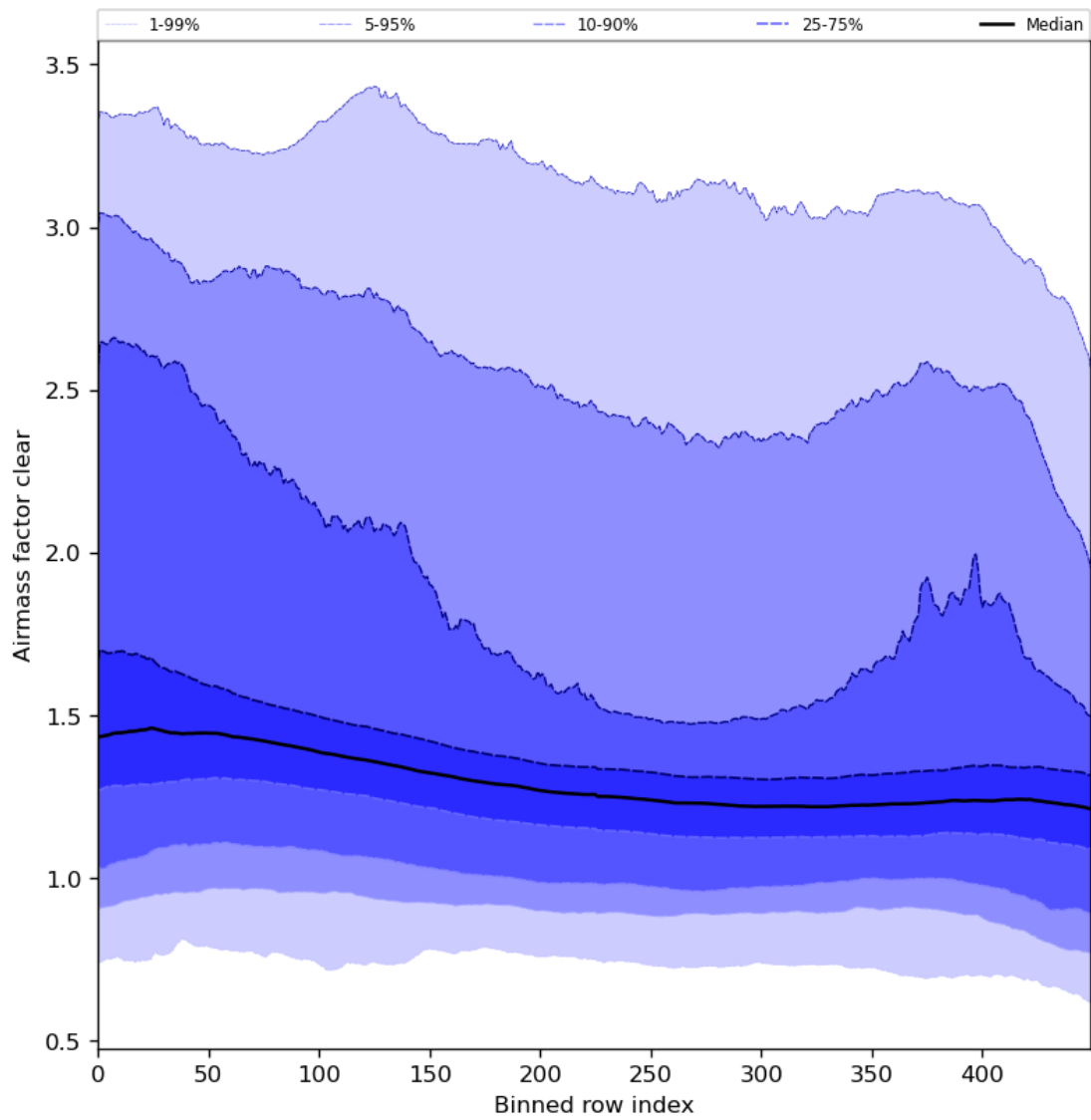
Figure 56: Along track statistics of “Airmass factor clear” for 2023-12-20 to 2023-12-21
