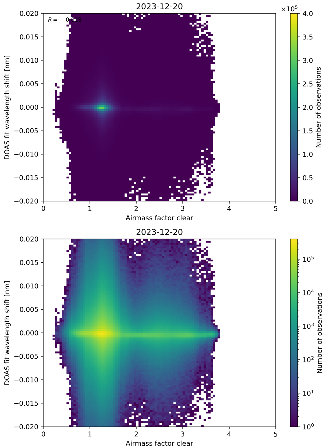
Figure 72: Scatter density plot of “Airmass factor clear” against “DOAS fit wavelength shift” for 2023-12-20 to 2023-12-21.
