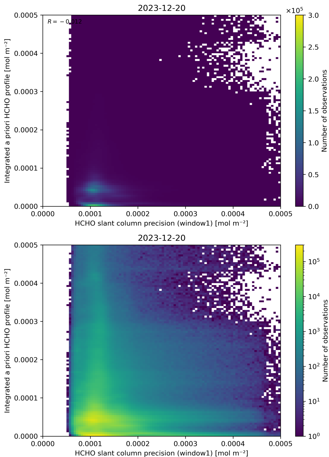
Figure 96: Scatter density plot of “HCHO slant column precision (window1)” against “Integrated a priori HCHO profile” for 2023-12-20 to 2023-12-21.
