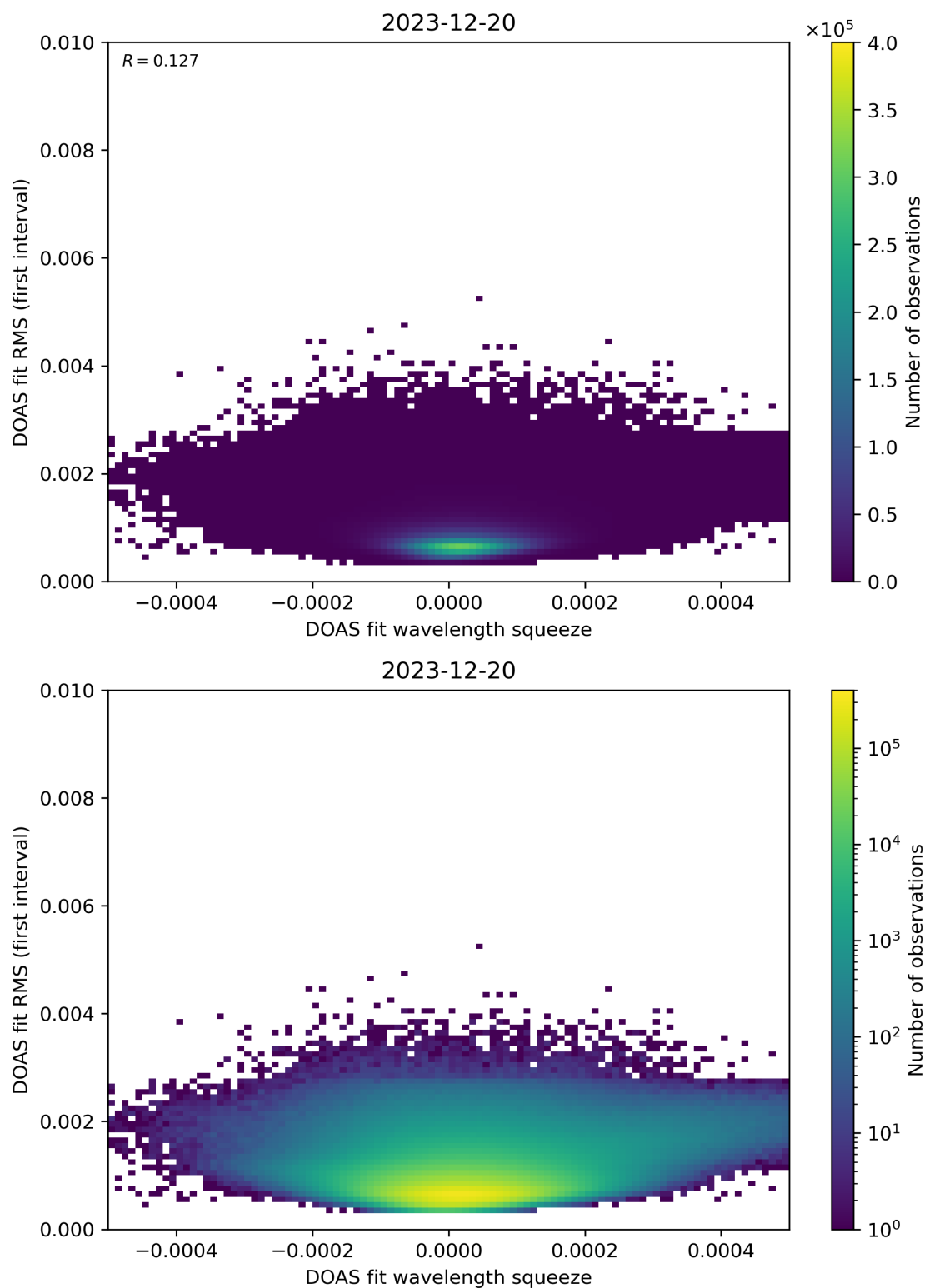
Figure 68: Scatter density plot of “DOAS fit wavelength squeeze” against “DOAS fit RMS (first interval)” for 2023-12-20 to 2023-12-21.
