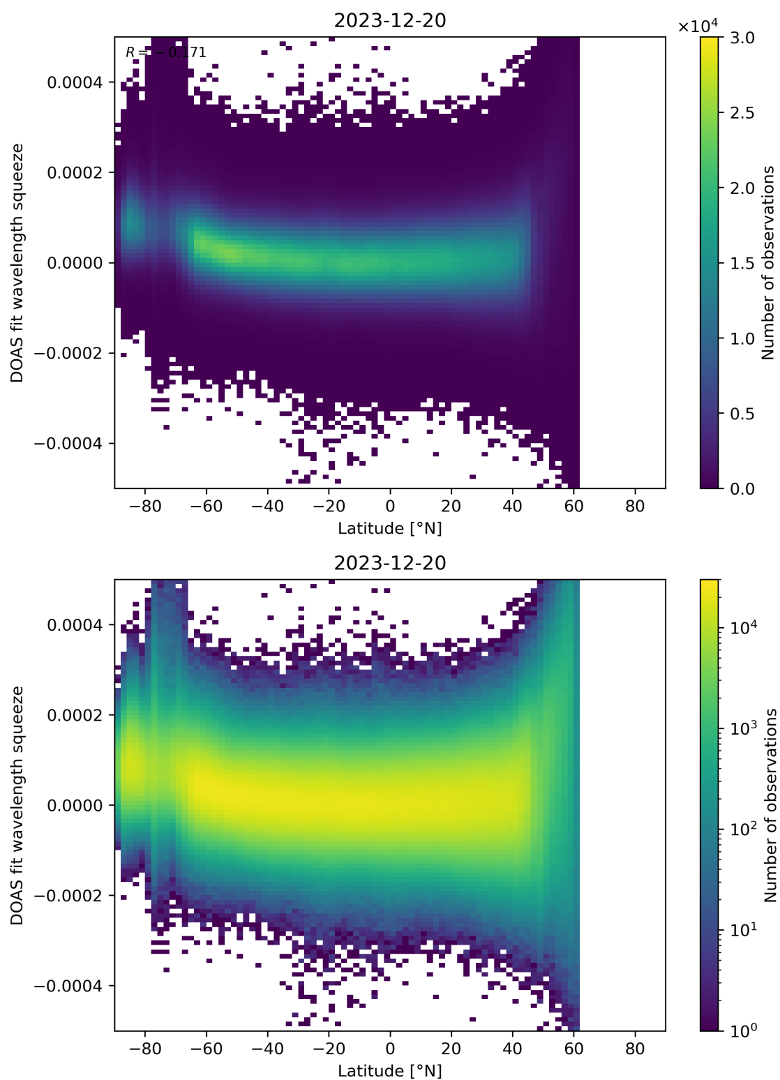
Figure 155: Scatter density plot of “Latitude” against “DOAS fit wavelength squeeze” for 2023-12-20 to 2023-12-21.
