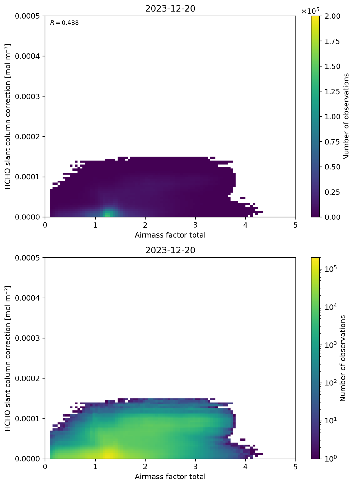
Figure 102: Scatter density plot of “Airmass factor total” against “HCHO slant column correction” for 2023-12-20 to 2023-12-21.
