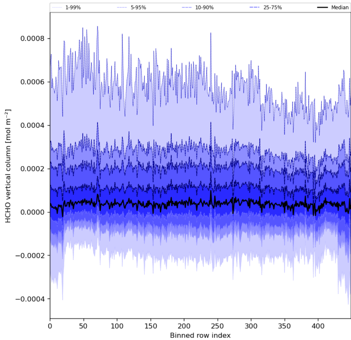
Figure 49: Along track statistics of “HCHO vertical column” for 2023-12-20 to 2023-12-21
