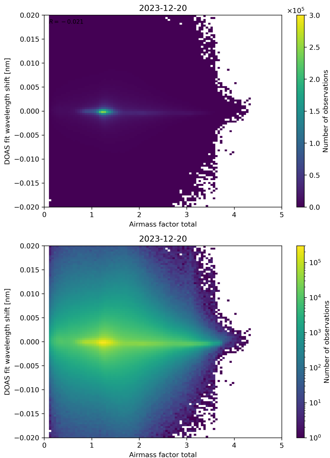
Figure 98: Scatter density plot of “Airmass factor total” against “DOAS fit wavelength shift” for 2023-12-20 to 2023-12-21.
