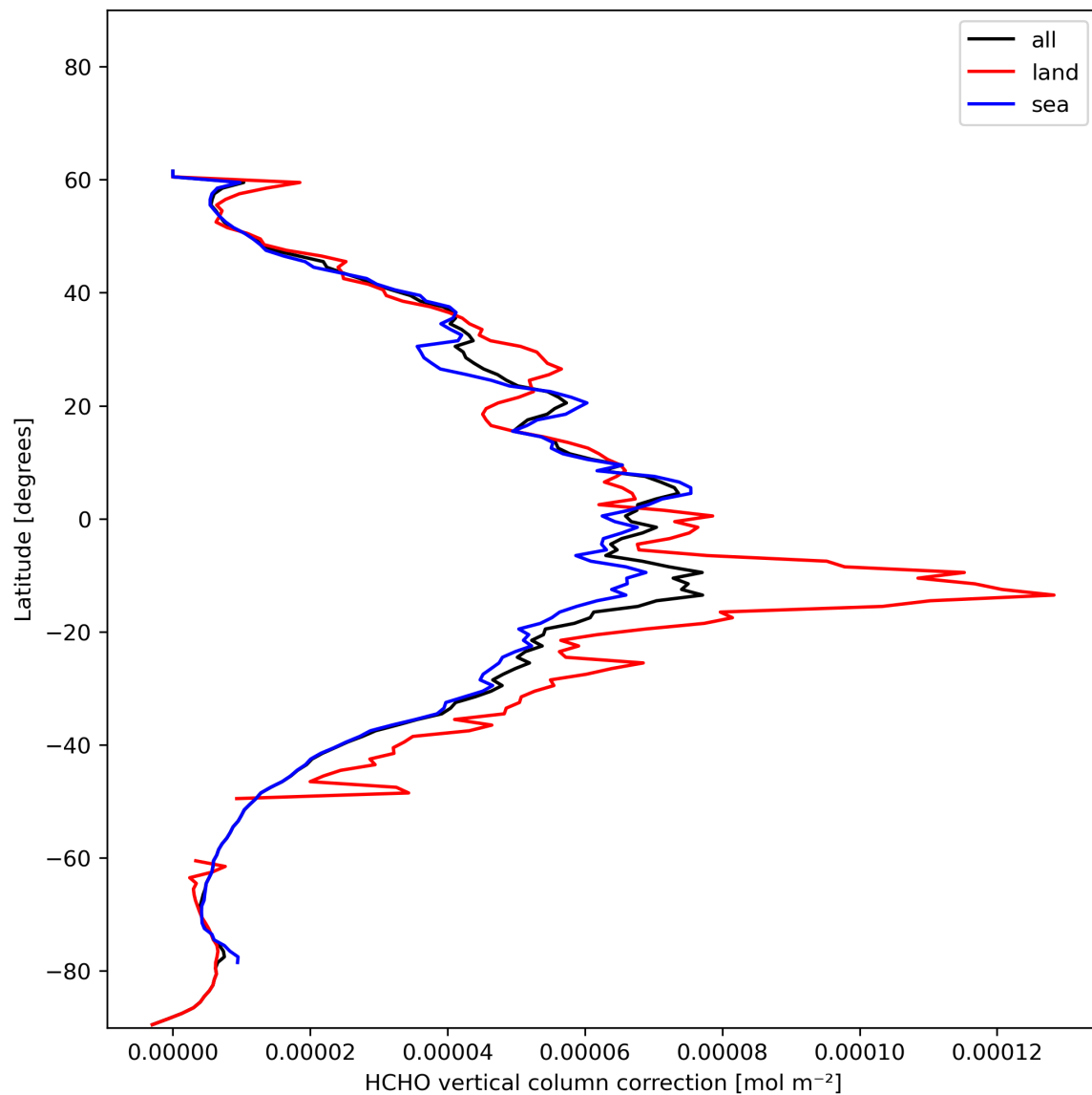
Figure 23: Zonal average of “HCHO vertical column correction” for 2023-12-20 to 2023-12-21.
