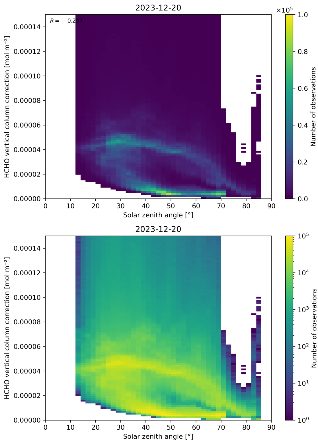
Figure 178: Scatter density plot of “Solar zenith angle” against “HCHO vertical column correction” for 2023-12-20 to 2023-12-21.
