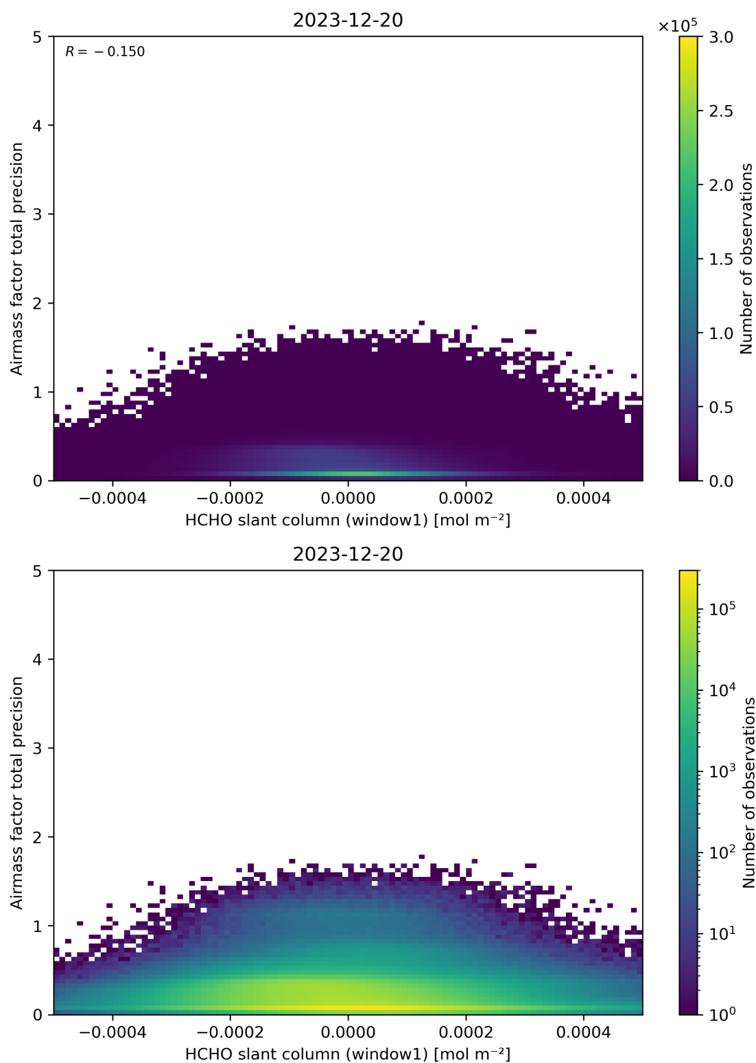
Figure 86: Scatter density plot of “HCHO slant column (window1)” against “Airmass factor total precision” for 2023-12-20 to 2023-12-21.
