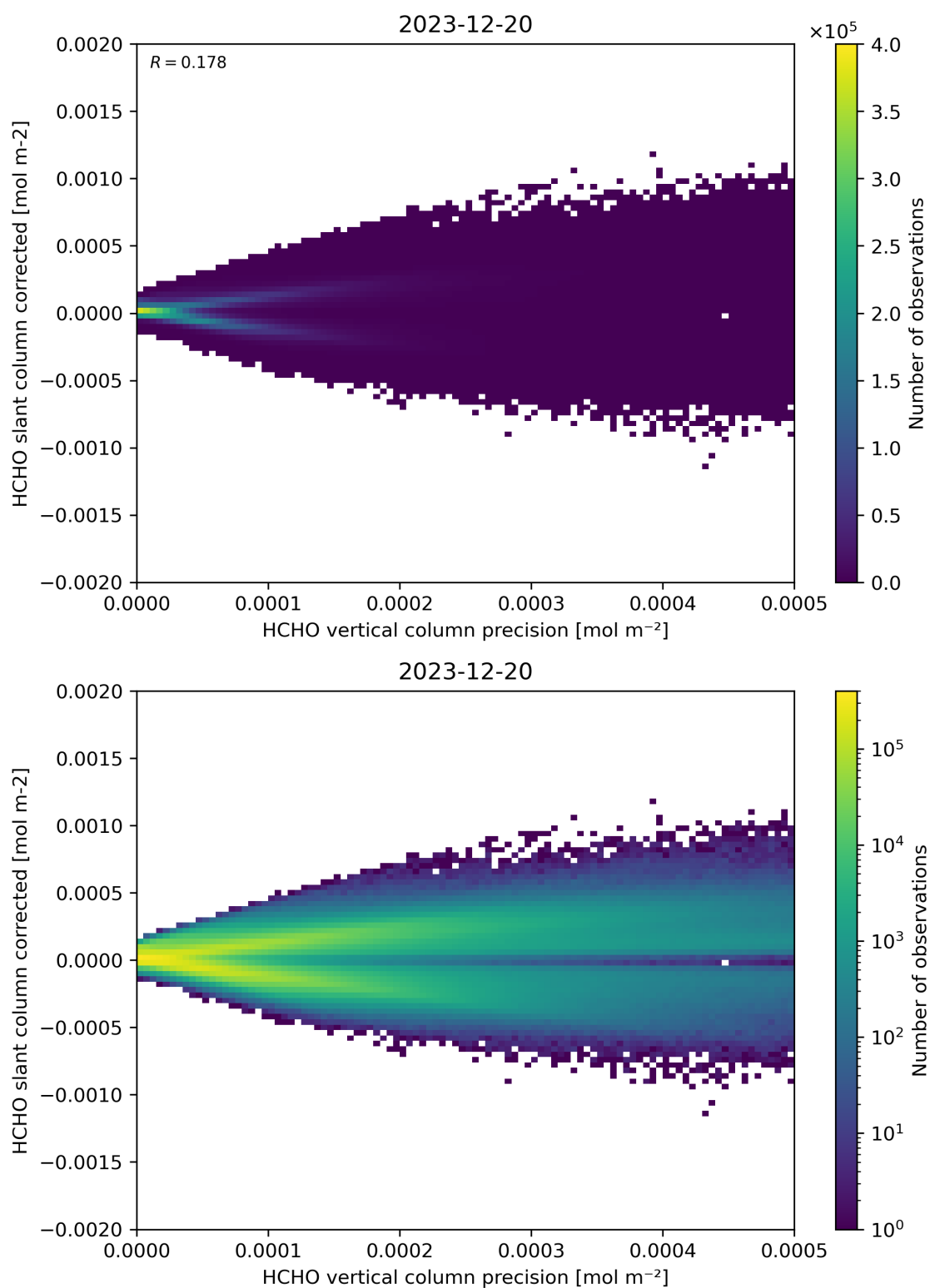
Figure 140: Scatter density plot of “HCHO vertical column precision” against “HCHO slant column corrected” for 2023-12-20 to 2023-12-21.
