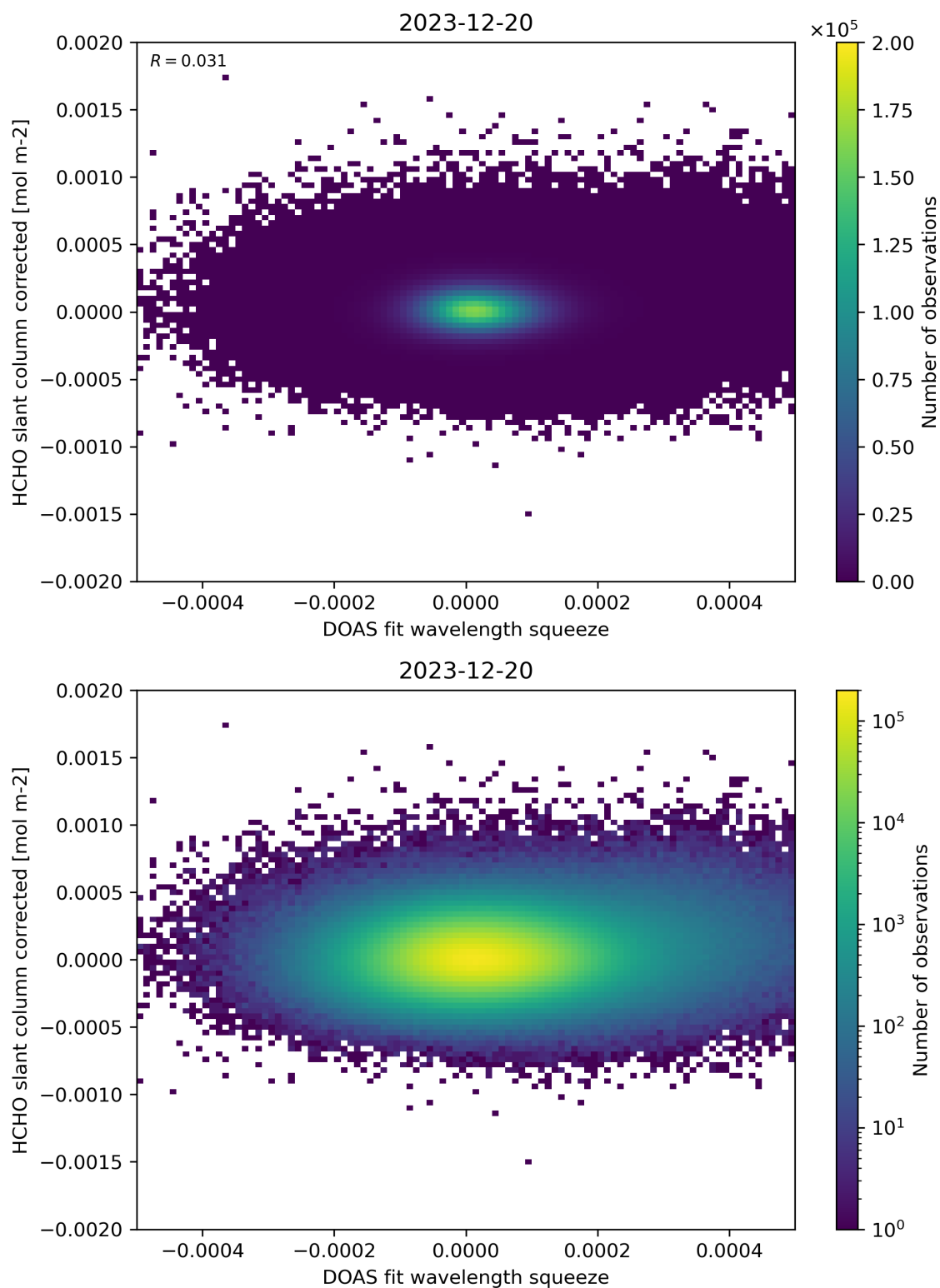
Figure 69: Scatter density plot of “DOAS fit wavelength squeeze” against “HCHO slant column corrected” for 2023-12-20 to 2023-12-21.
