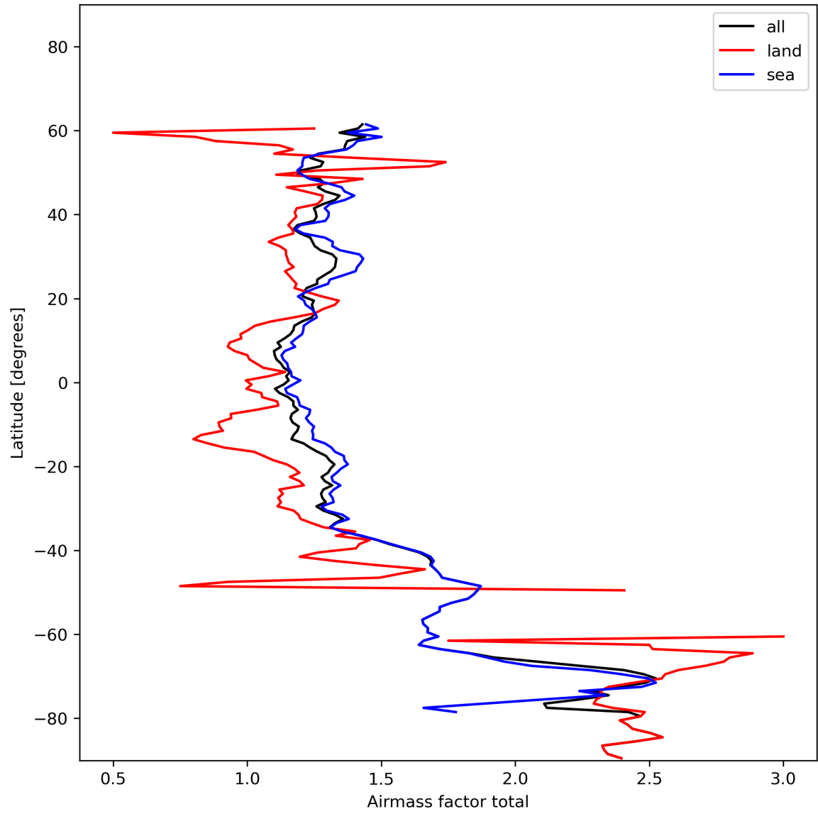
Figure 26: Zonal average of “Airmass factor total” for 2023-12-20 to 2023-12-21.
