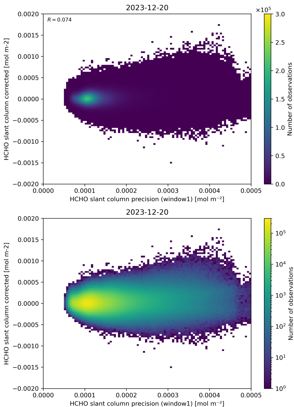
Figure 92: Scatter density plot of “HCHO slant column precision (window1)” against “HCHO slant column corrected” for 2023-12-20 to 2023-12-21.
