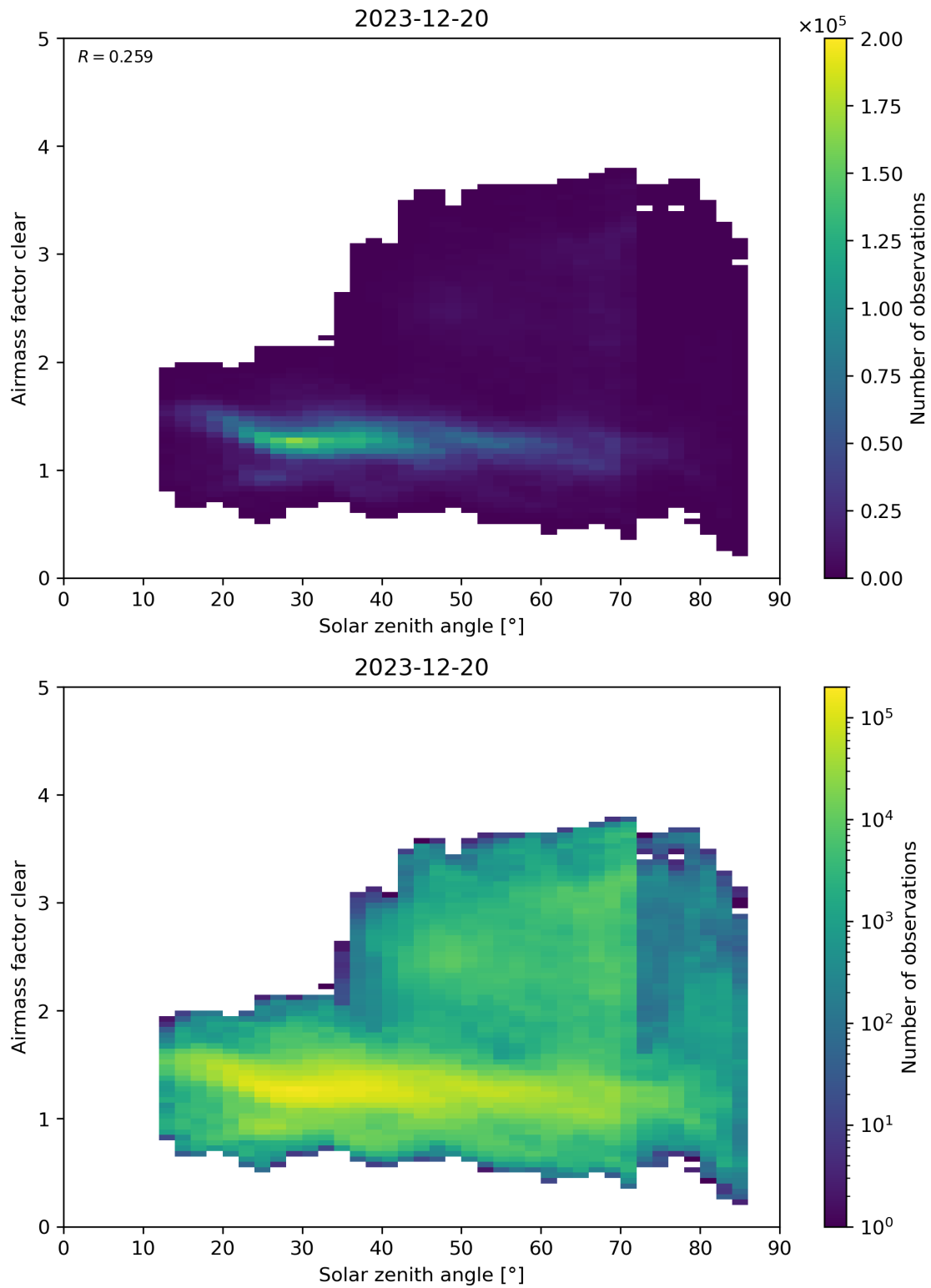
Figure 170: Scatter density plot of “Solar zenith angle” against “Airmass factor clear” for 2023-12-20 to 2023-12-21.
