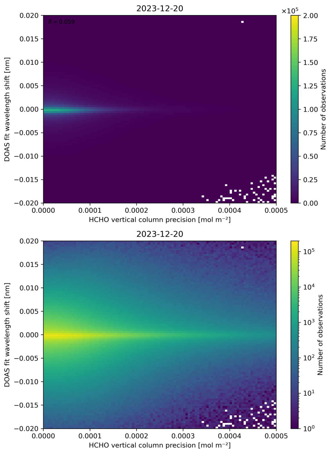
Figure 137: Scatter density plot of “HCHO vertical column precision” against “DOAS fit wavelength shift” for 2023-12-20 to 2023-12-21.
