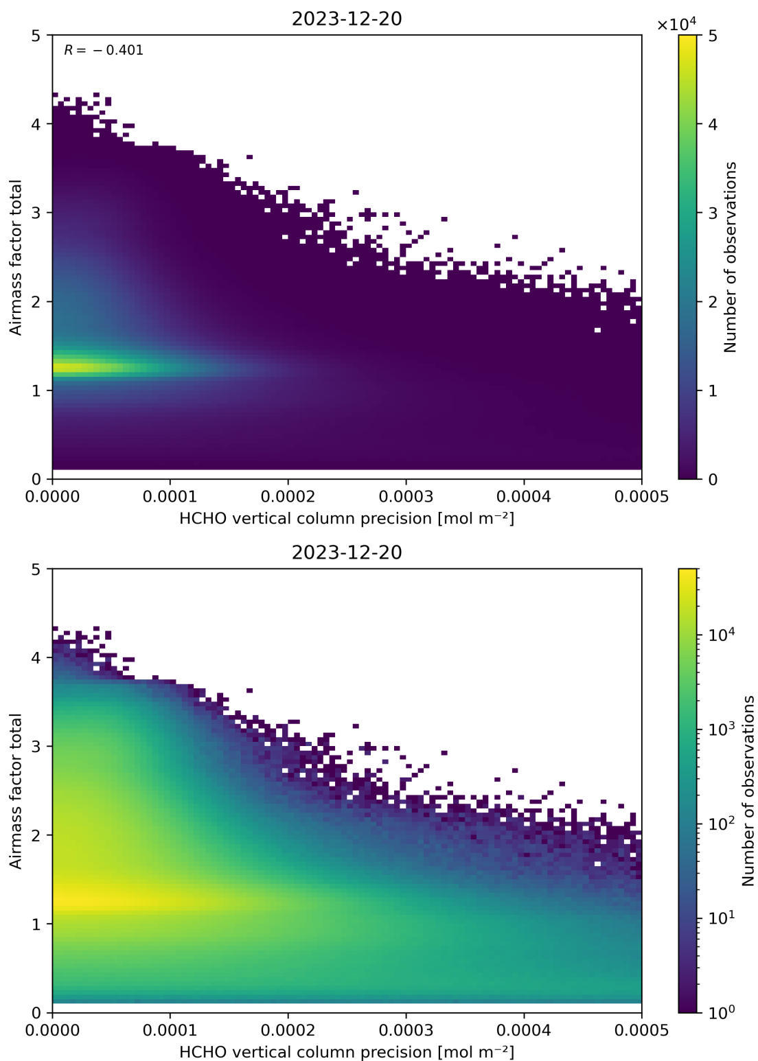
Figure 144: Scatter density plot of “HCHO vertical column precision” against “Airmass factor total” for 2023-12-20 to 2023-12-21.
