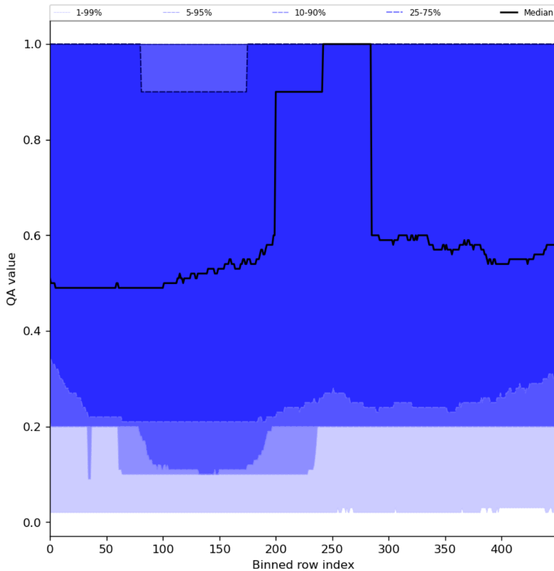
Figure 48: Along track statistics of “QA value” for 2023-12-20 to 2023-12-21
