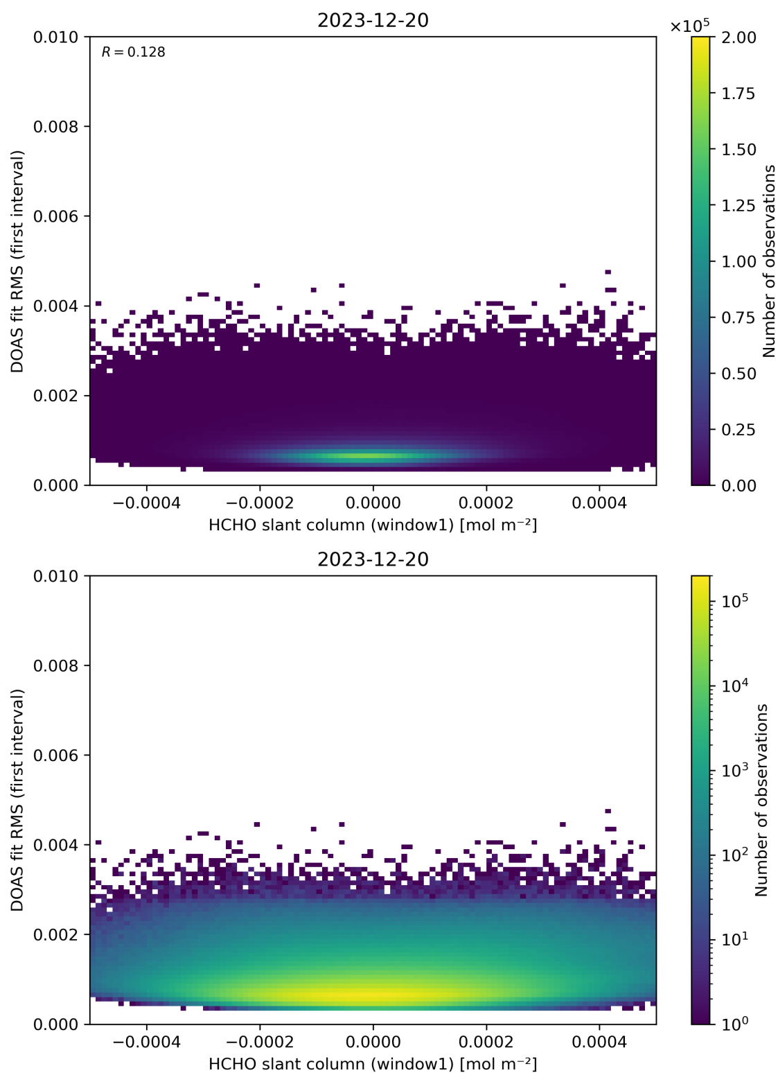
Figure 78: Scatter density plot of “HCHO slant column (window1)” against “DOAS fit RMS (first interval)” for 2023-12-20 to 2023-12-21.
