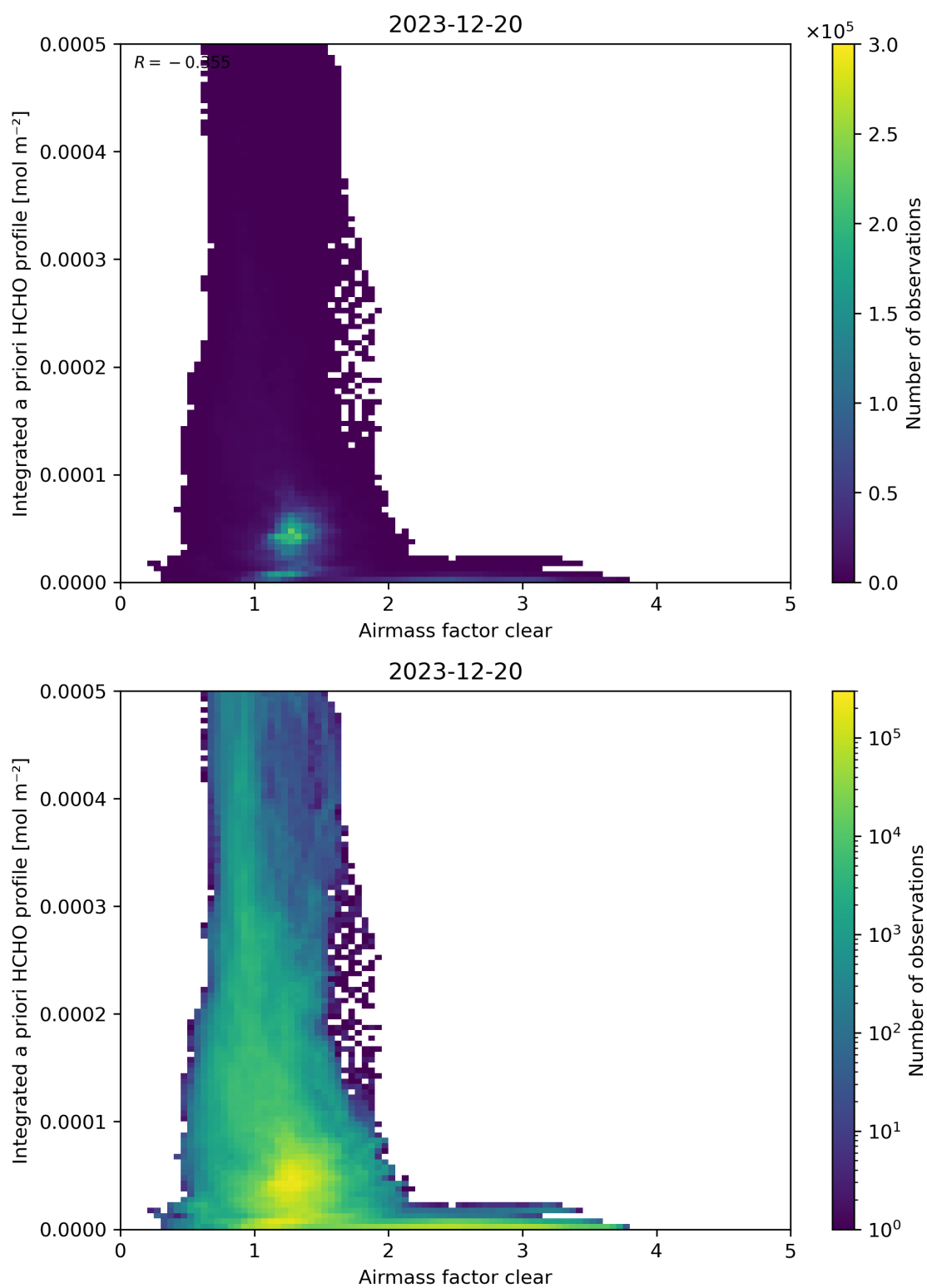
Figure 76: Scatter density plot of “Airmass factor clear” against “Integrated a priori HCHO profile” for 2023-12-20 to 2023-12-21.
