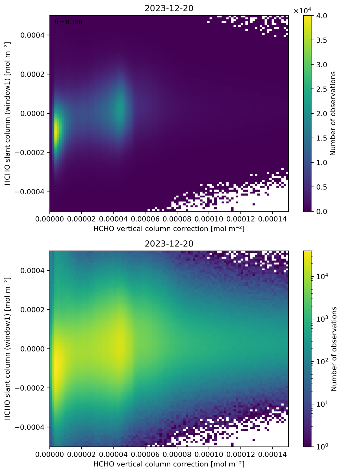
Figure 118: Scatter density plot of “HCHO vertical column correction” against “HCHO slant column (window1)” for 2023-12-20 to 2023-12-21.
