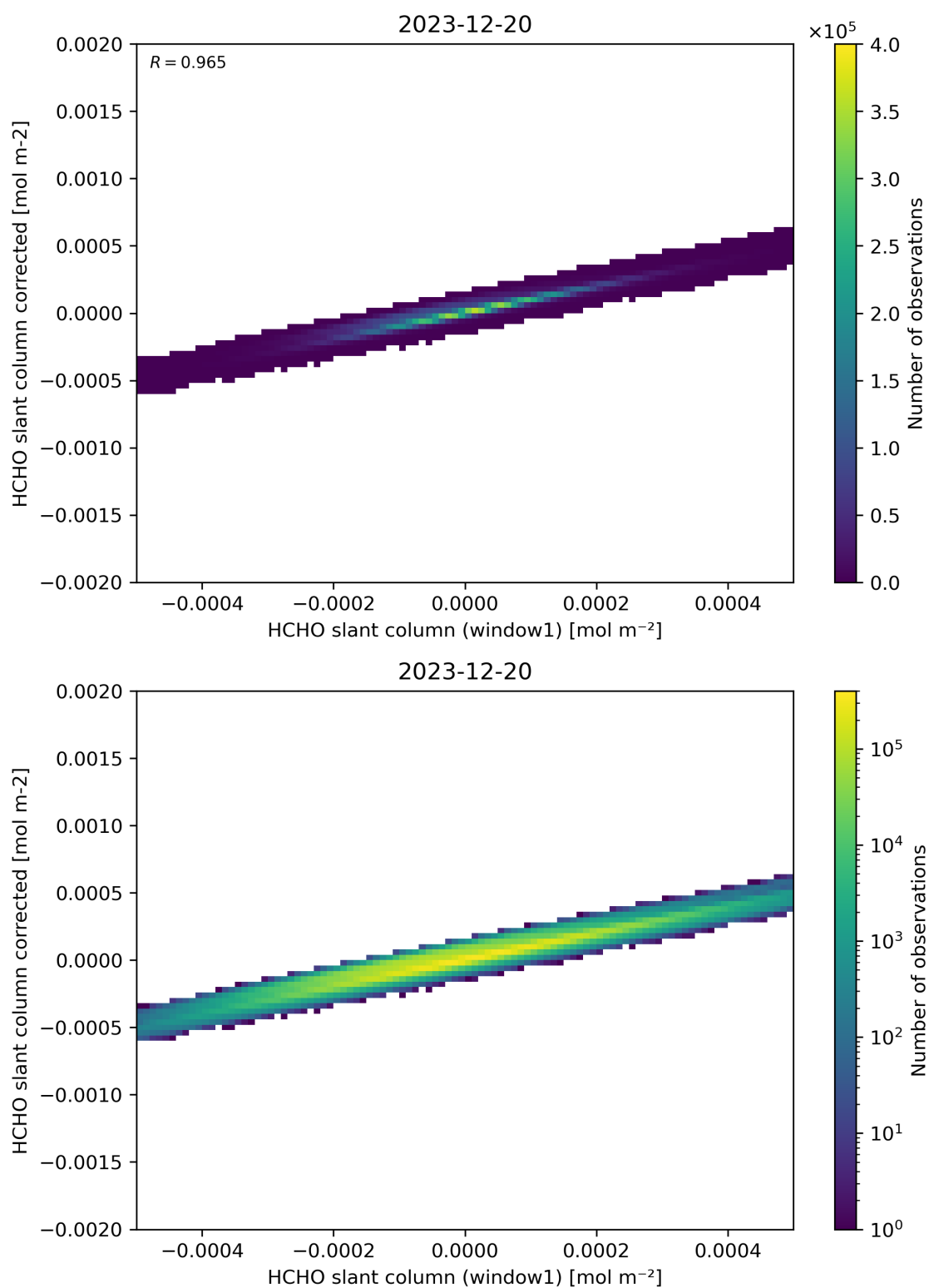
Figure 82: Scatter density plot of “HCHO slant column (window1)” against “HCHO slant column corrected” for 2023-12-20 to 2023-12-21.
