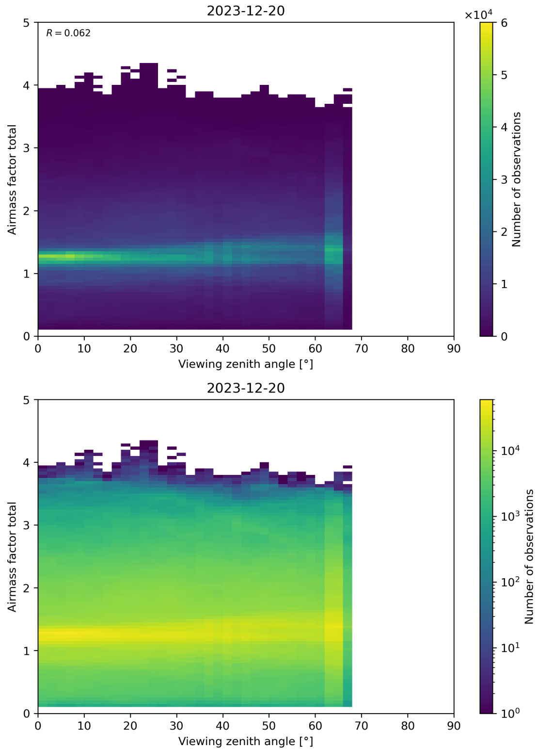
Figure 190: Scatter density plot of “Viewing zenith angle” against “Airmass factor total” for 2023-12-20 to 2023-12-21.
