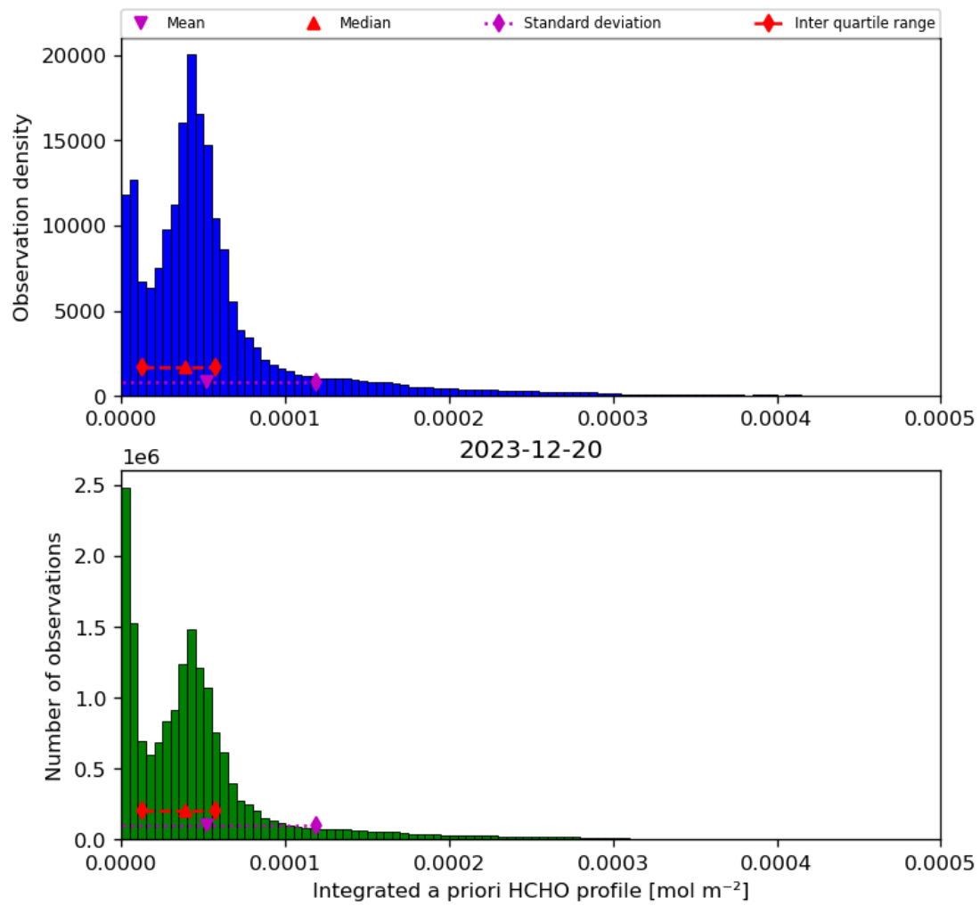
Figure 43: Histogram of “Integrated a priori HCHO profile” for 2023-12-20 to 2023-12-21
