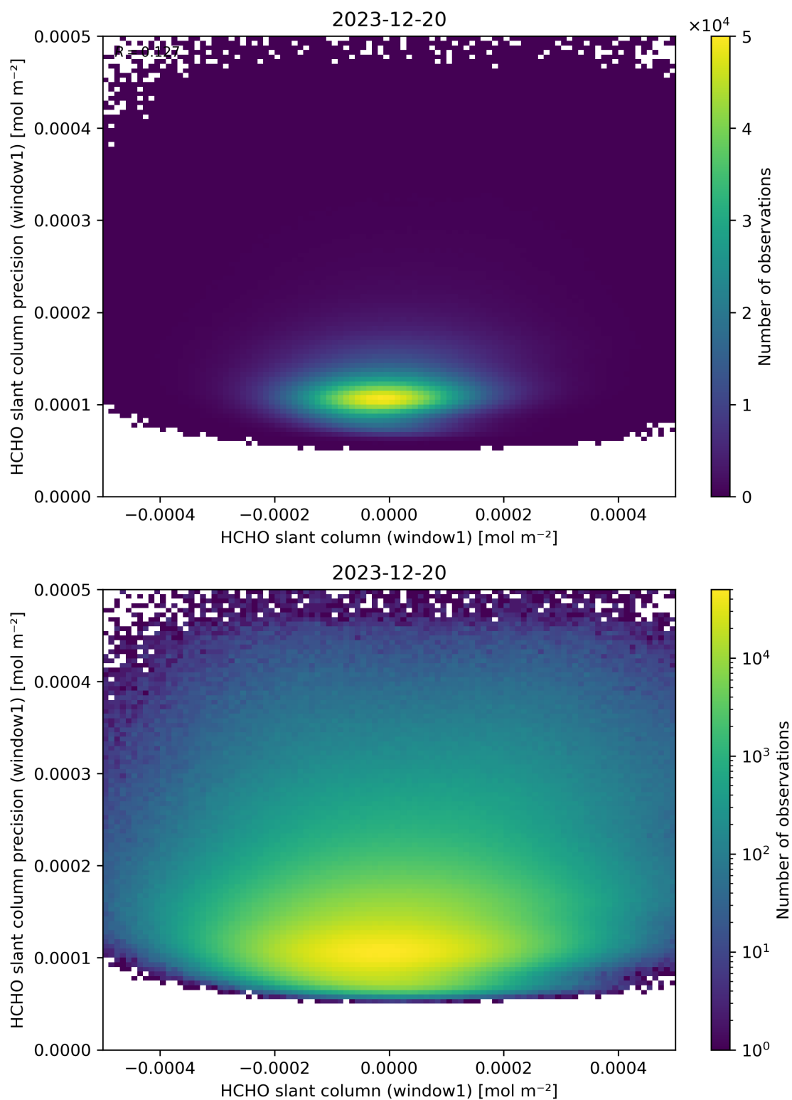
Figure 84: Scatter density plot of “HCHO slant column (window1)” against “HCHO slant column precision (window1)” for 2023-12-20 to 2023-12-21.
