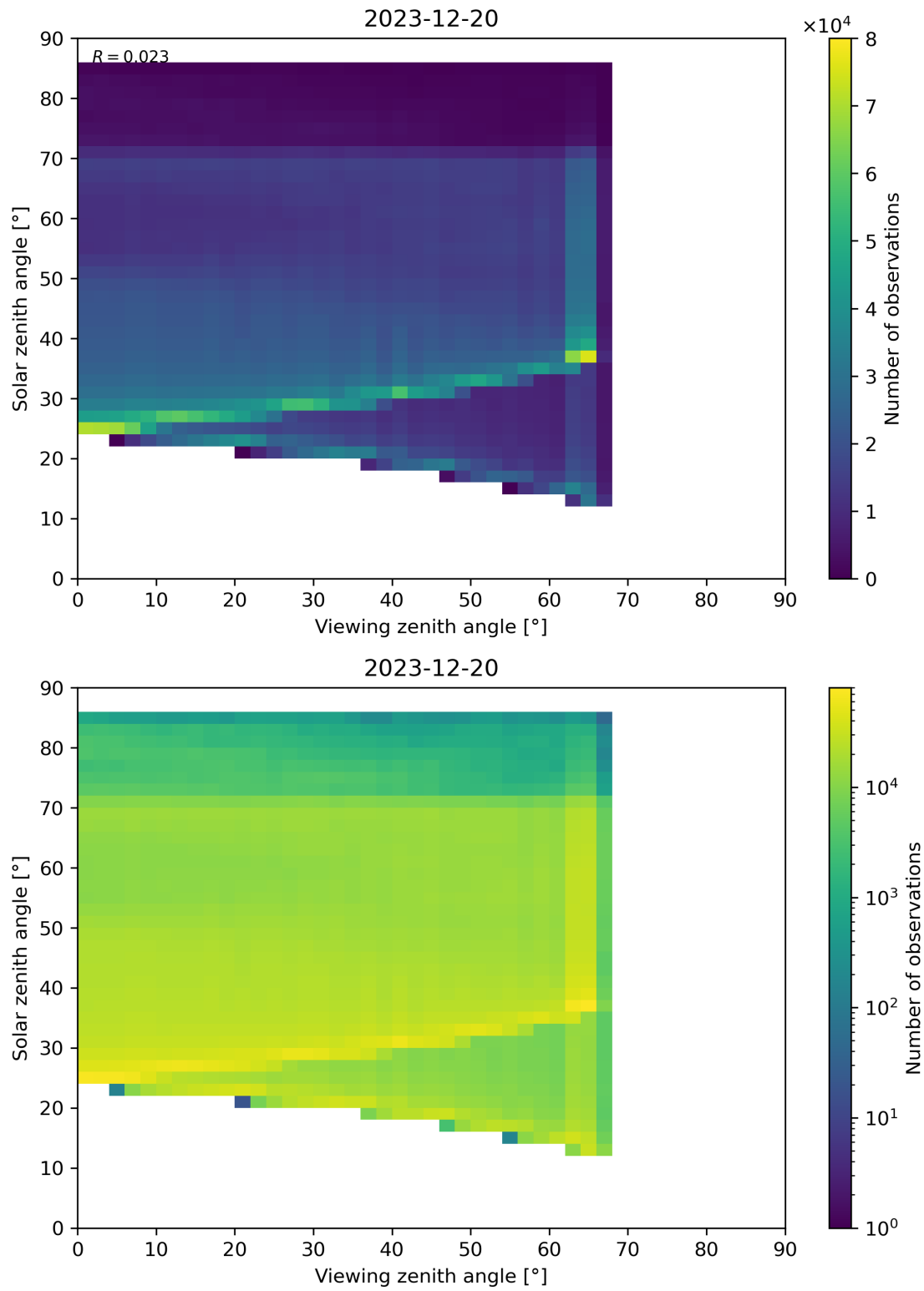
Figure 197: Scatter density plot of “Viewing zenith angle” against “Solar zenith angle” for 2023-12-20 to 2023-12-21.
