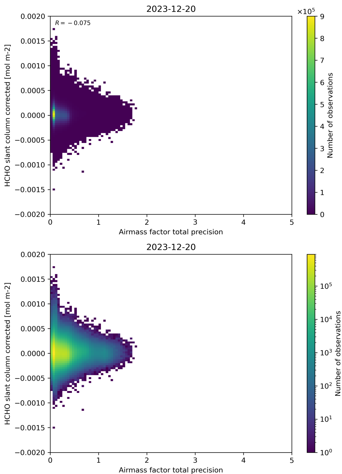
Figure 109: Scatter density plot of “Airmass factor total precision” against “HCHO slant column corrected” for 2023-12-20 to 2023-12-21.
