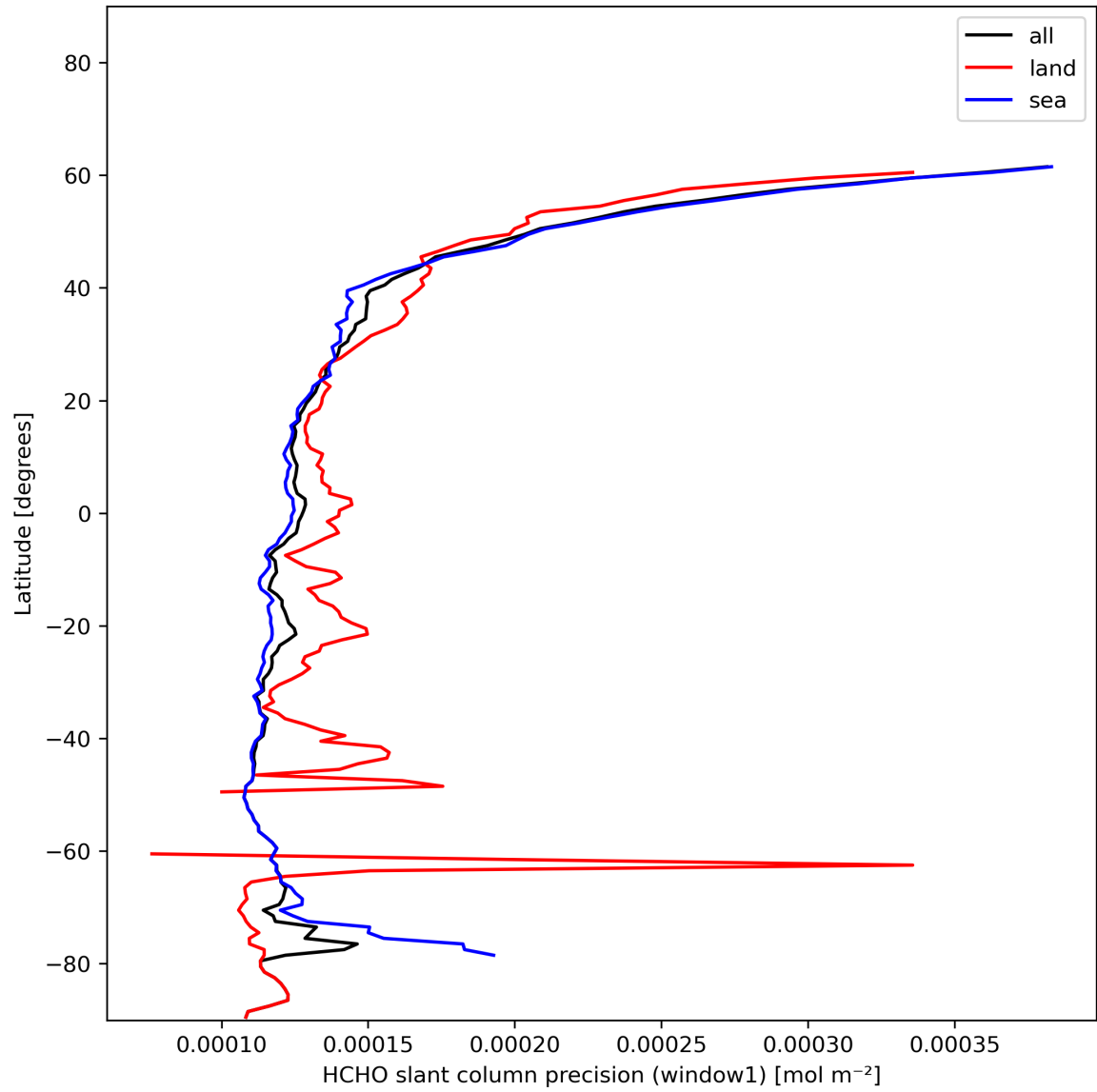
Figure 25: Zonal average of “HCHO slant column precision (window1)” for 2023-12-20 to 2023-12-21.
