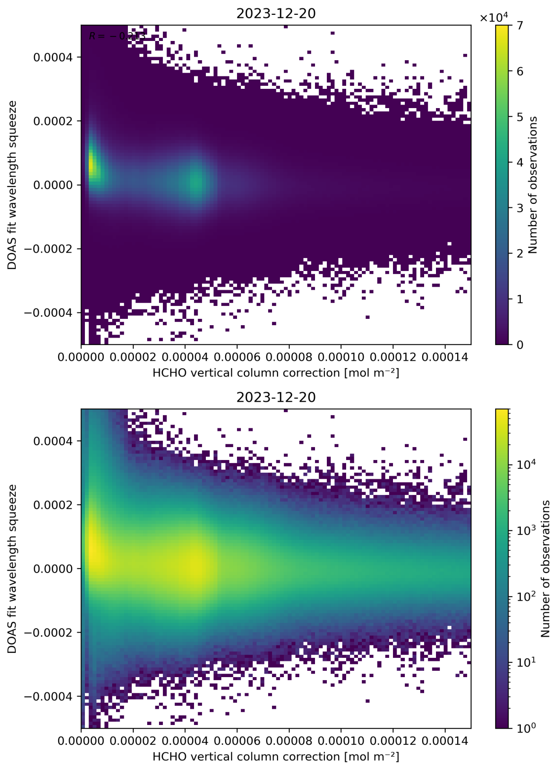
Figure 114: Scatter density plot of “HCHO vertical column correction” against “DOAS fit wavelength squeeze” for 2023-12-20 to 2023-12-21.
