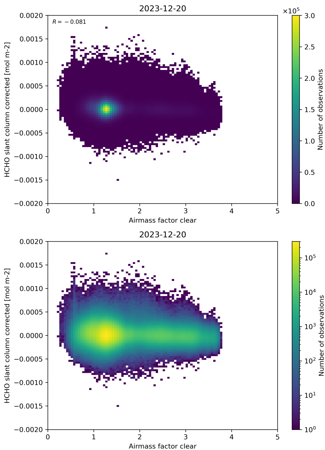
Figure 74: Scatter density plot of “Airmass factor clear” against “HCHO slant column corrected” for 2023-12-20 to 2023-12-21.
