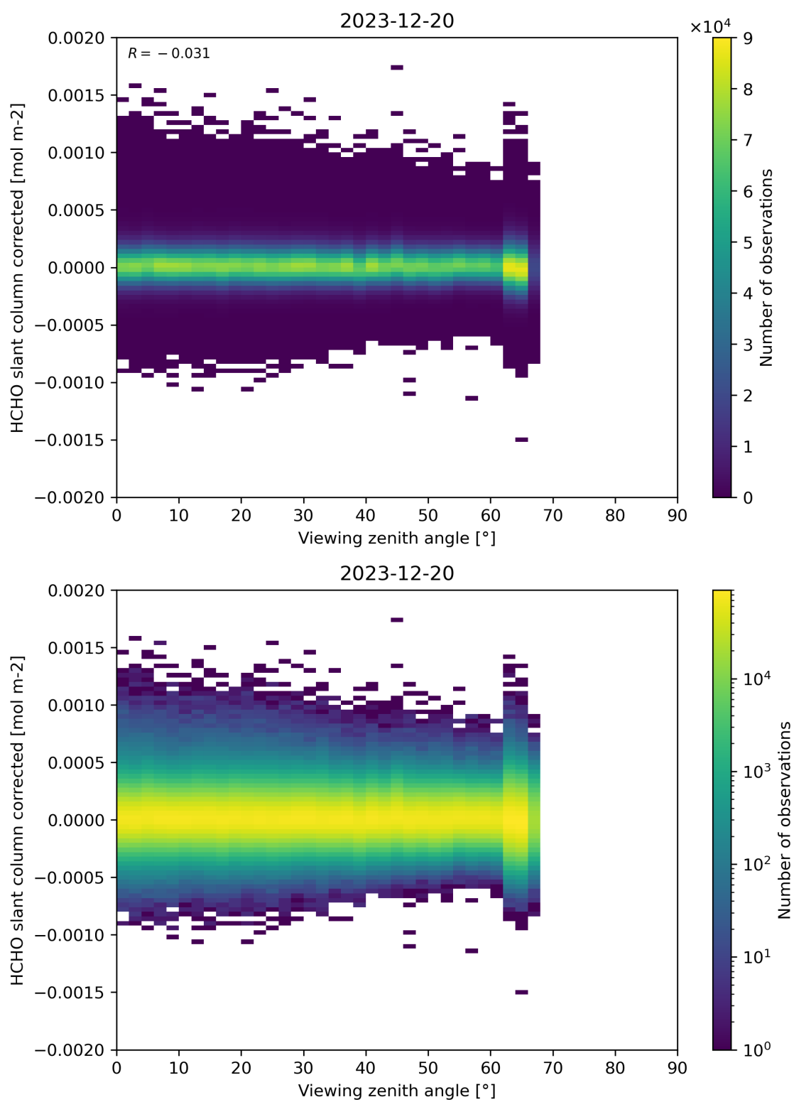
Figure 186: Scatter density plot of “Viewing zenith angle” against “HCHO slant column corrected” for 2023-12-20 to 2023-12-21.
