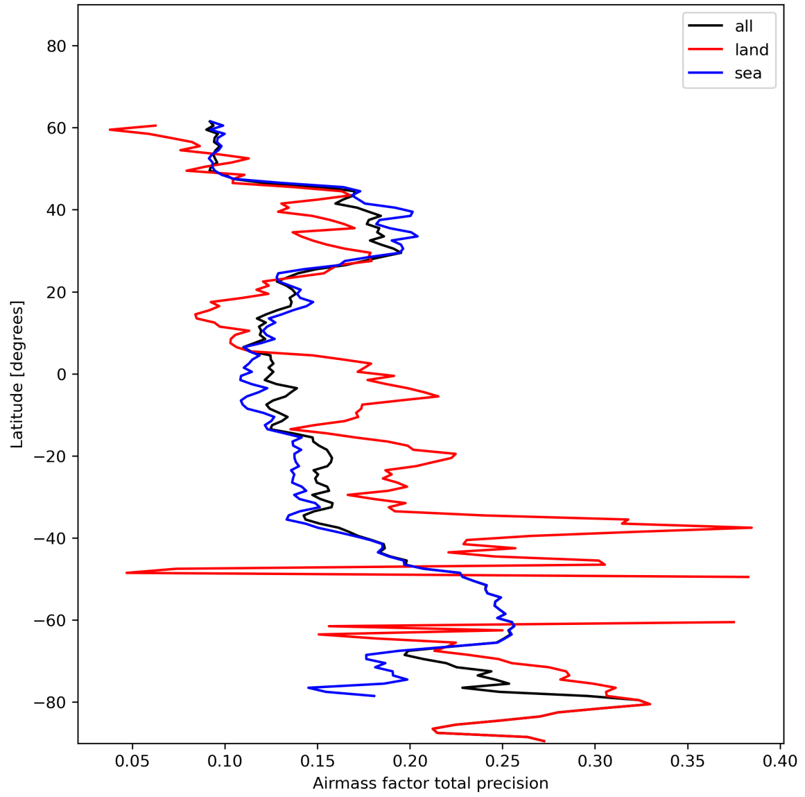
Figure 27: Zonal average of “Airmass factor total precision” for 2023-12-20 to 2023-12-21.
