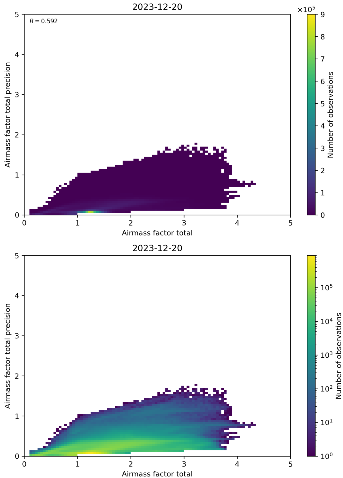
Figure 103: Scatter density plot of “Airmass factor total” against “Airmass factor total precision” for 2023-12-20 to 2023-12-21.
