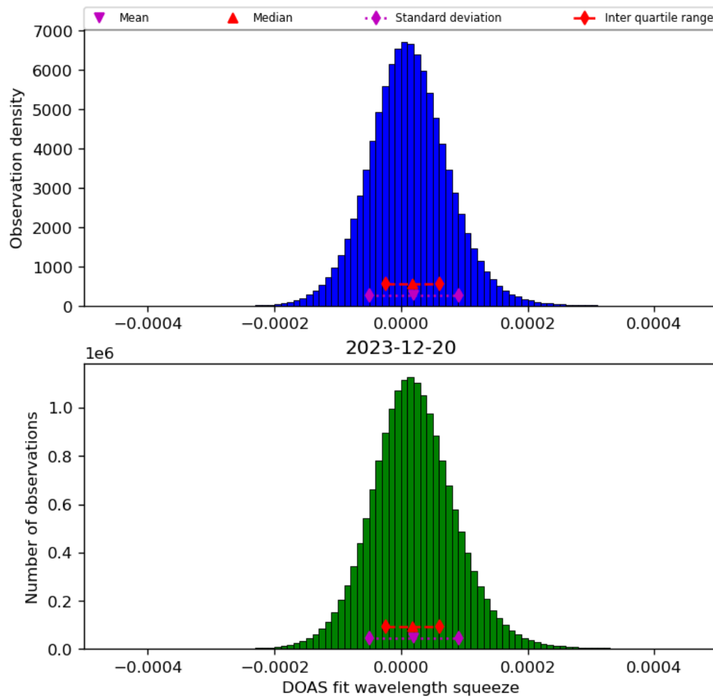
Figure 45: Histogram of “DOAS fit wavelength squeeze” for 2023-12-20 to 2023-12-21
