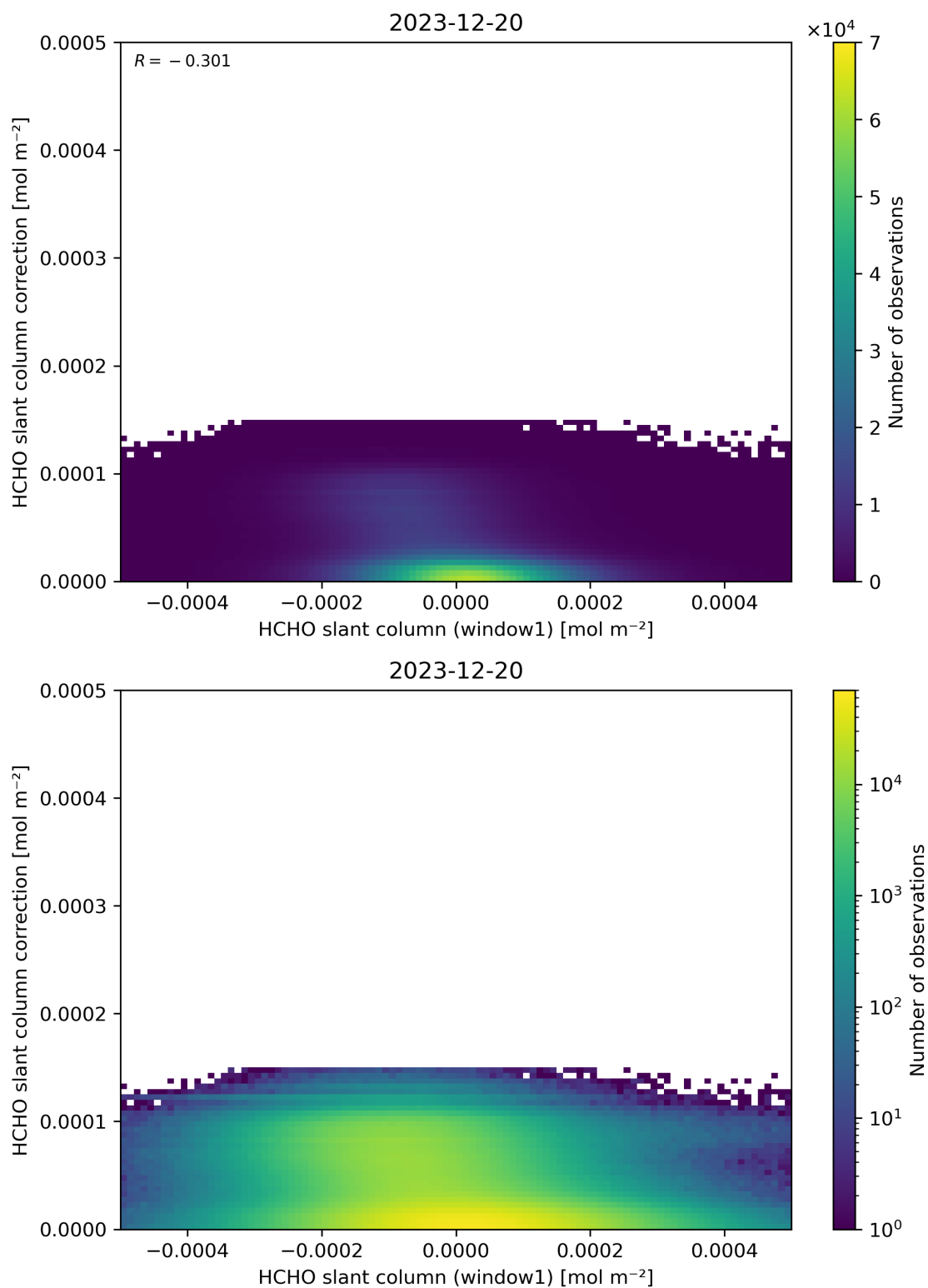
Figure 83: Scatter density plot of “HCHO slant column (window1)” against “HCHO slant column correction” for 2023-12-20 to 2023-12-21.
