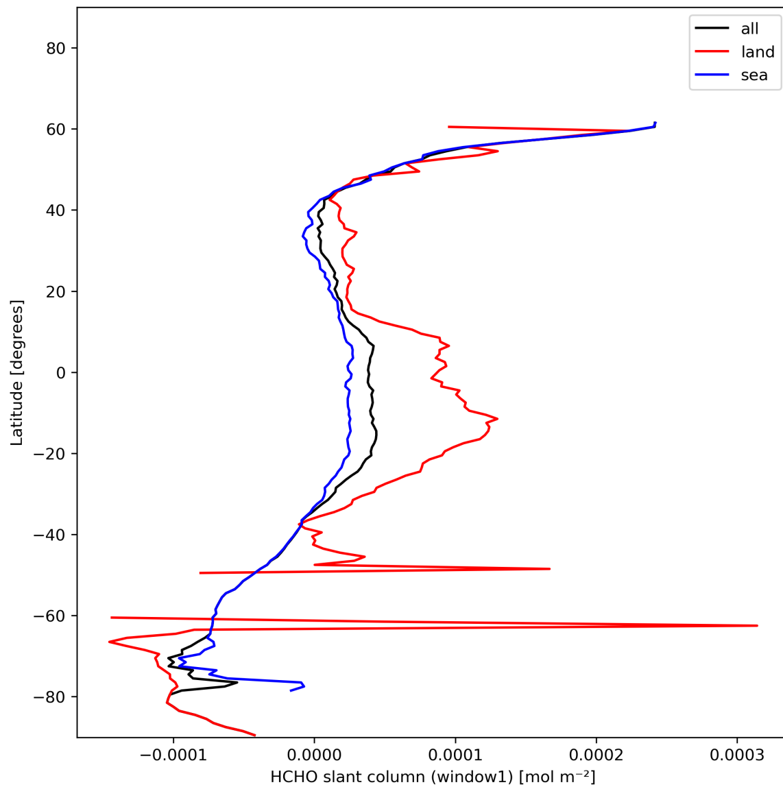
Figure 24: Zonal average of “HCHO slant column (window1)” for 2023-12-20 to 2023-12-21.
