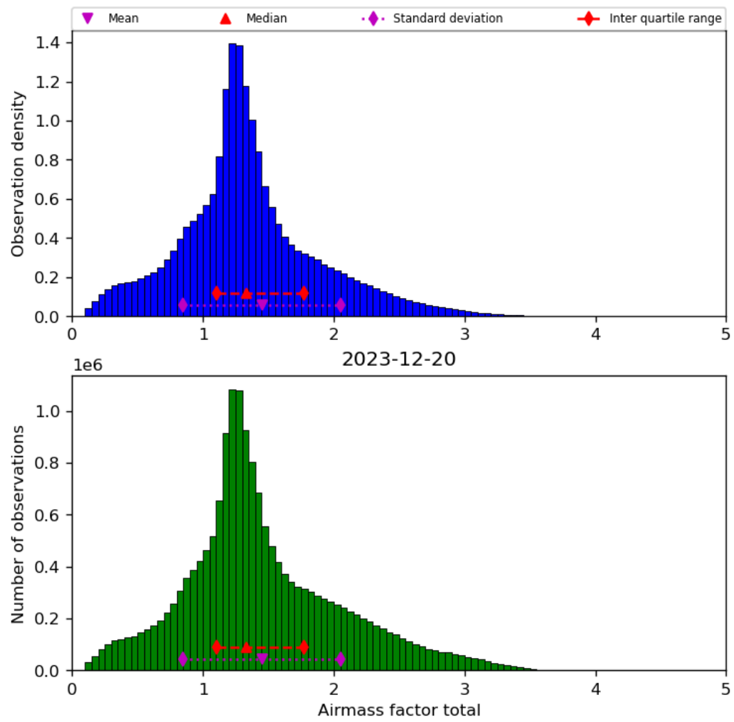
Figure 40: Histogram of “Airmass factor total” for 2023-12-20 to 2023-12-21
