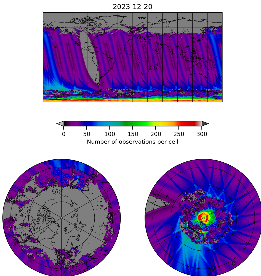
Figure 19: Map of the number of observations for 2023-12-20 to 2023-12-21
