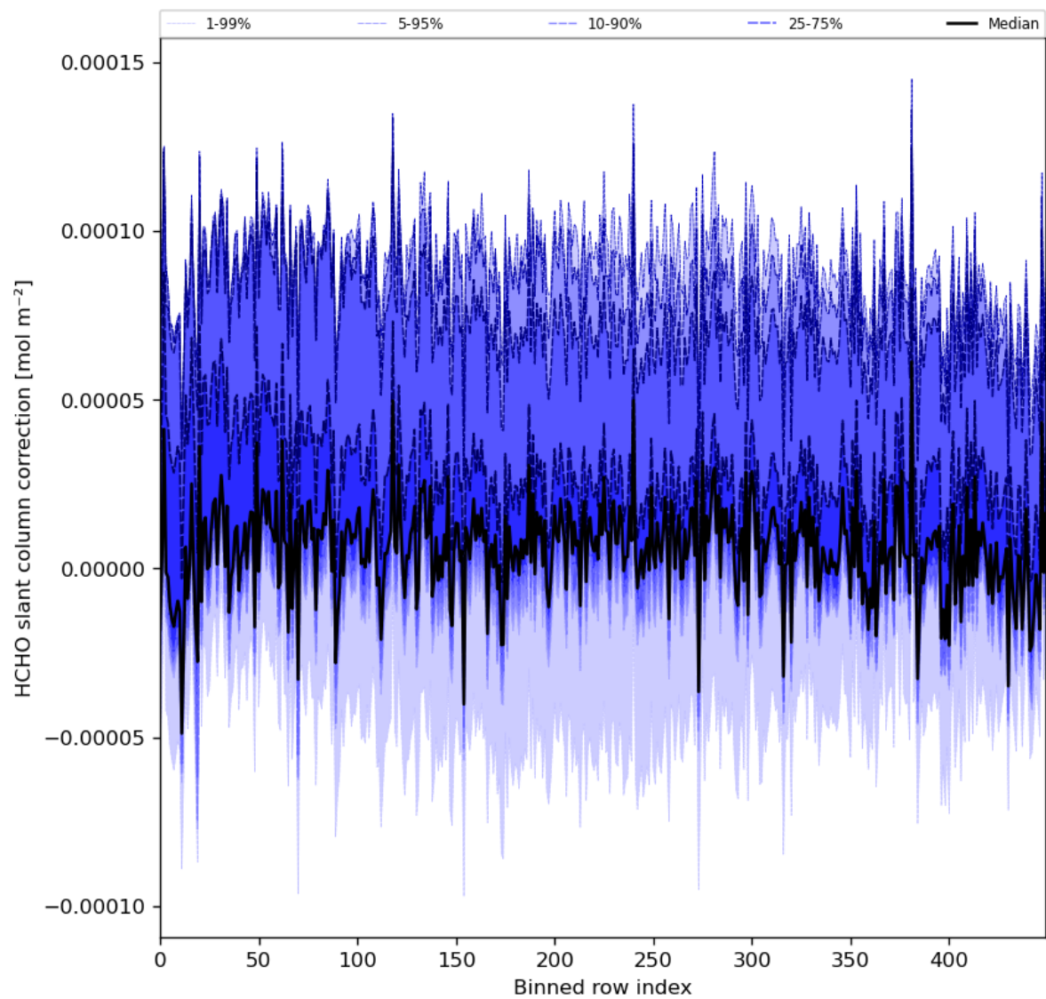
Figure 61: Along track statistics of “HCHO slant column correction” for 2023-12-20 to 2023-12-21
