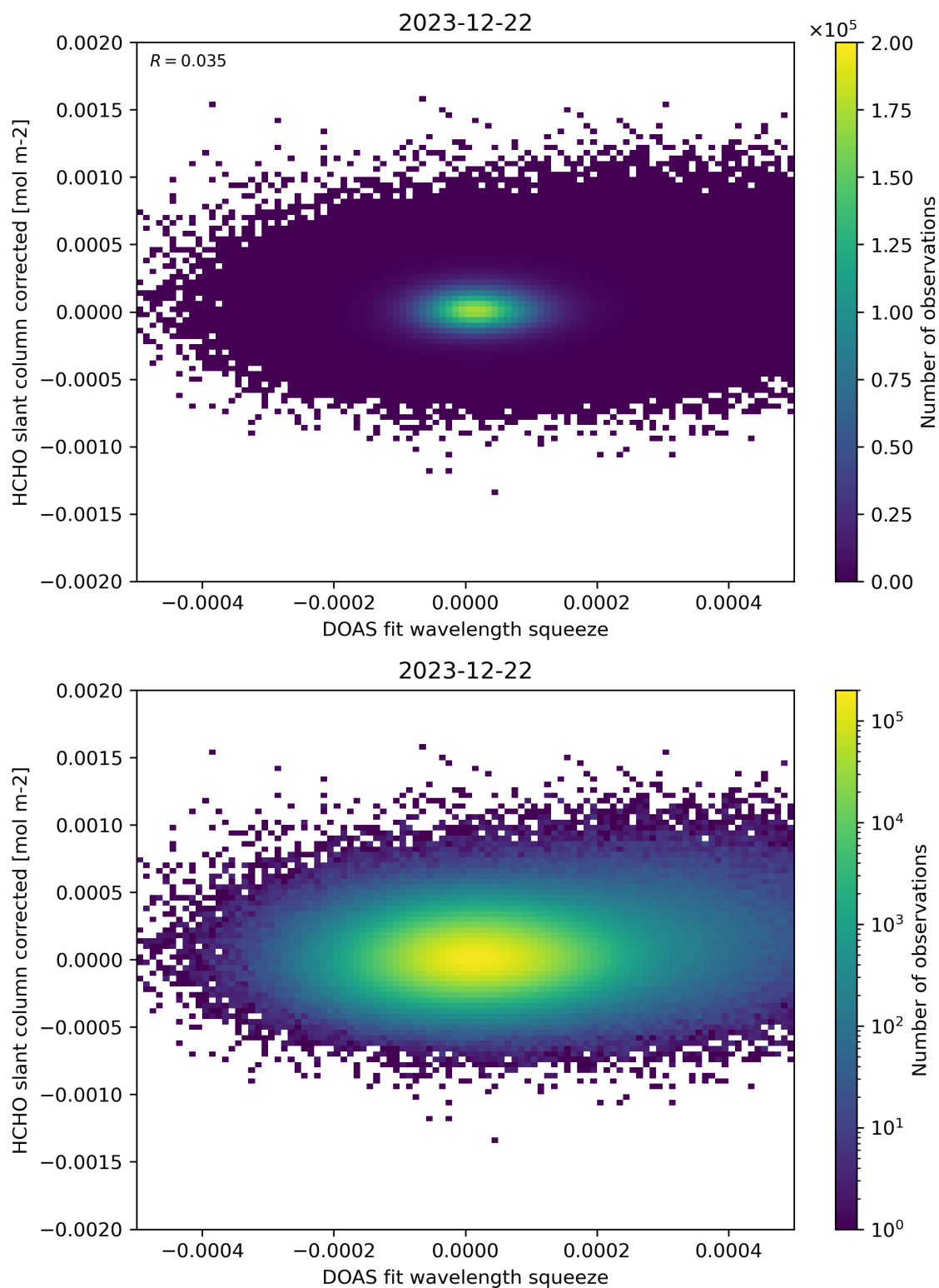
Figure 69: Scatter density plot of “DOAS fit wavelength squeeze” against “HCHO slant column corrected” for 2023-12-21 to 2023-12-23.
