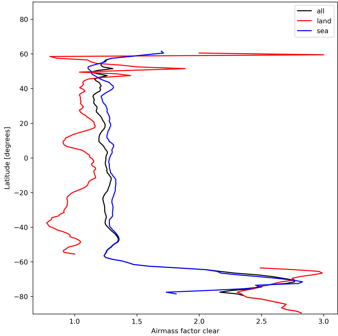
Figure 28: Zonal average of “Airmass factor clear” for 2023-12-21 to 2023-12-23.
