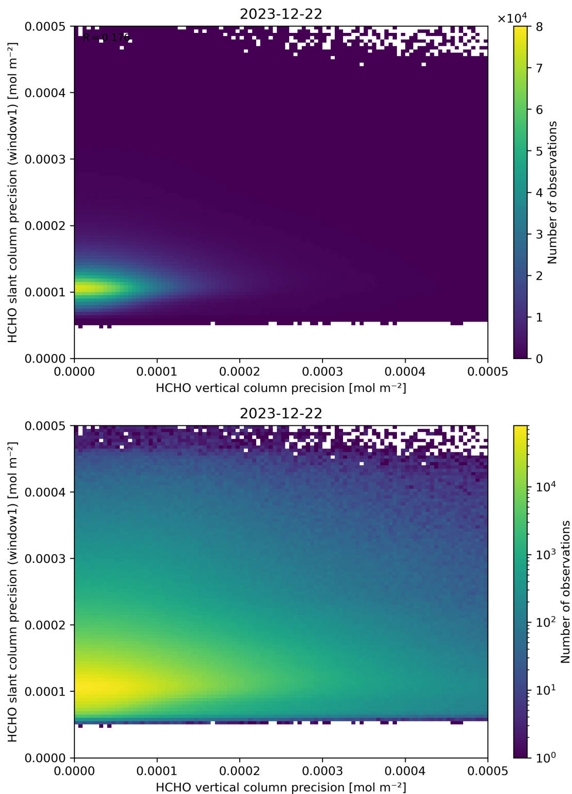
Figure 143: Scatter density plot of “HCHO vertical column precision” against “HCHO slant column precision (window1)” for 2023-12-21 to 2023-12-23.
