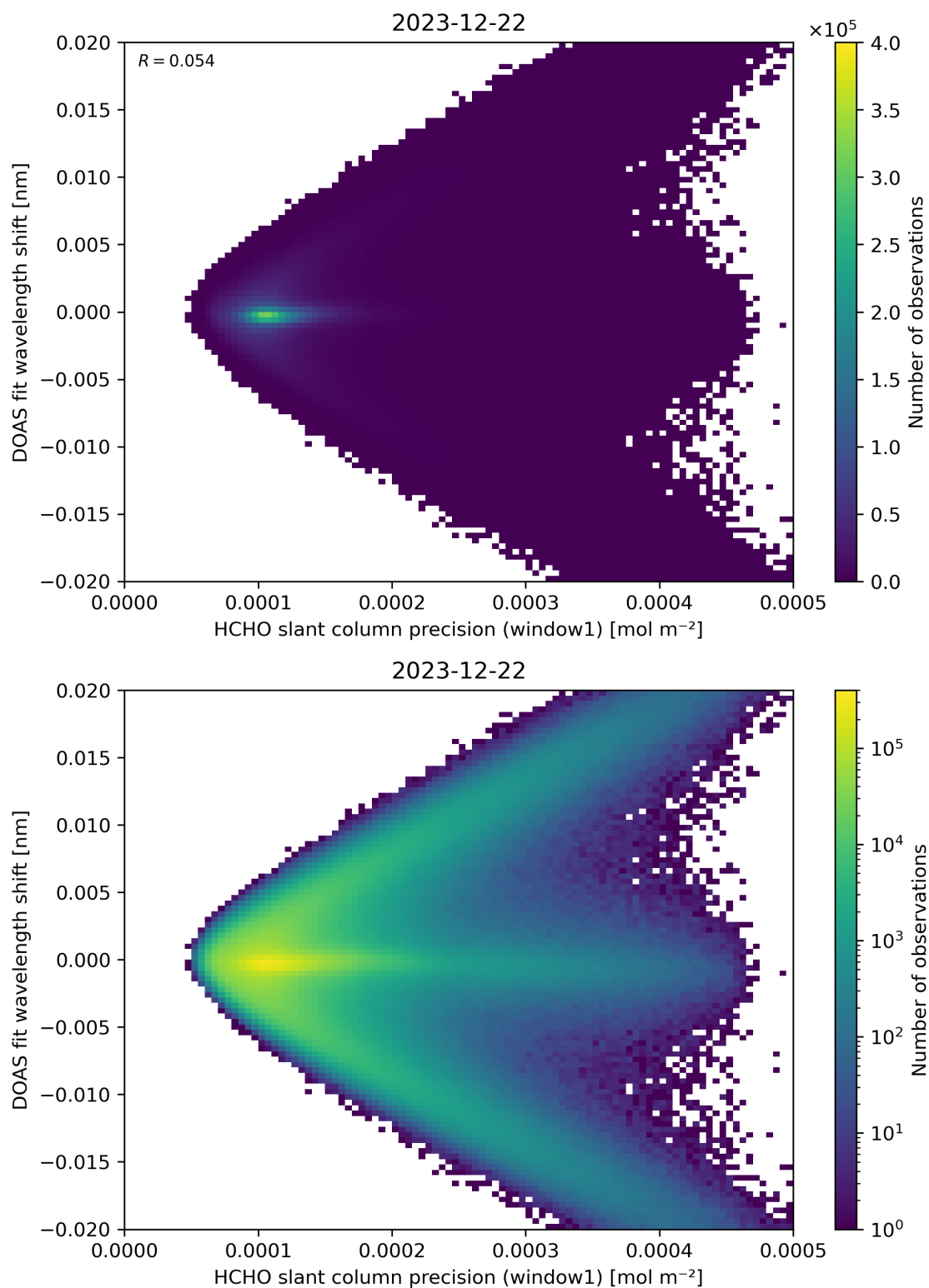
Figure 89: Scatter density plot of “HCHO slant column precision (window1)” against “DOAS fit wavelength shift” for 2023-12-21 to 2023-12-23.
