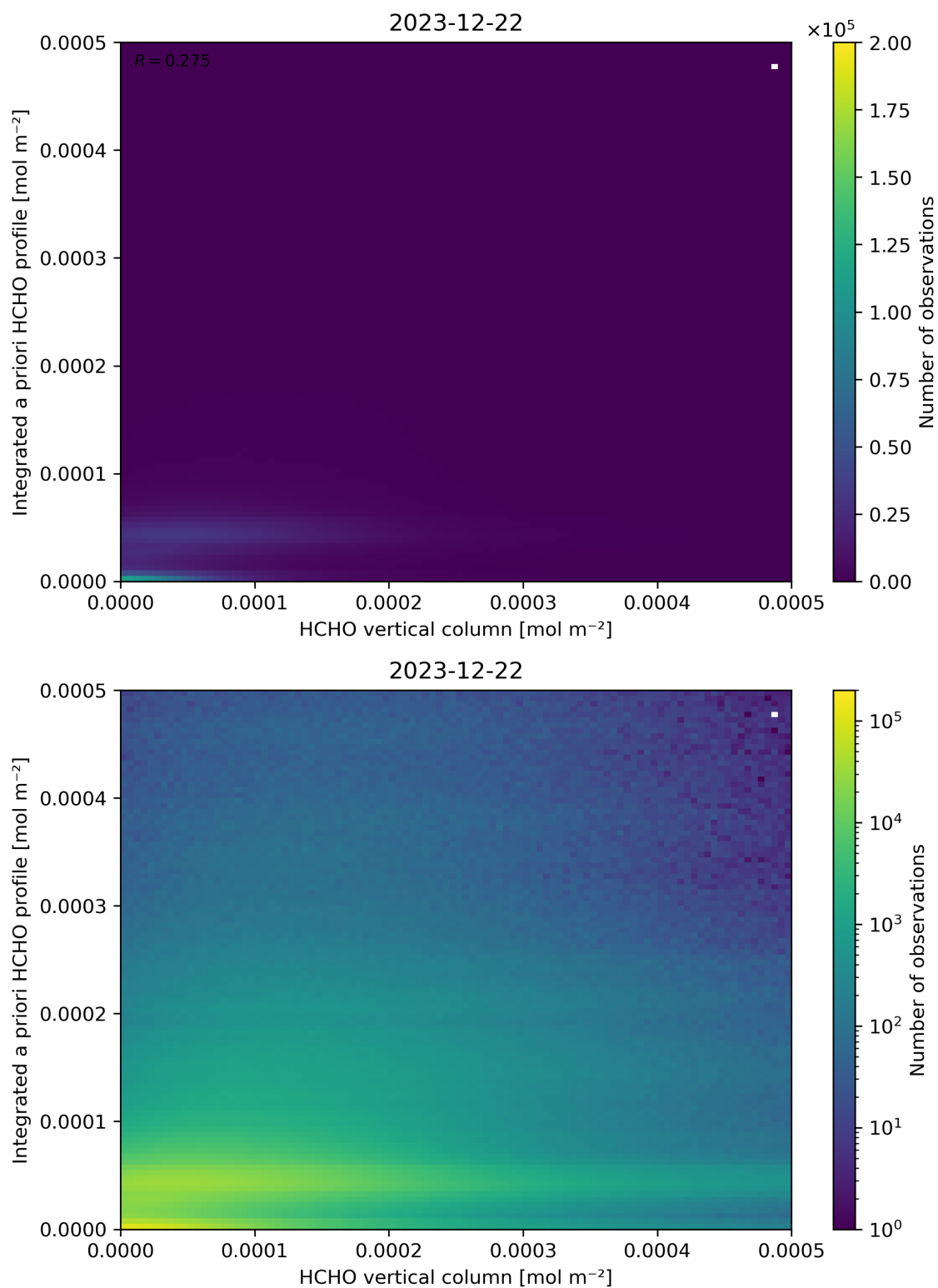
Figure 135: Scatter density plot of “HCHO vertical column” against “Integrated a priori HCHO profile” for 2023-12-21 to 2023-12-23.
