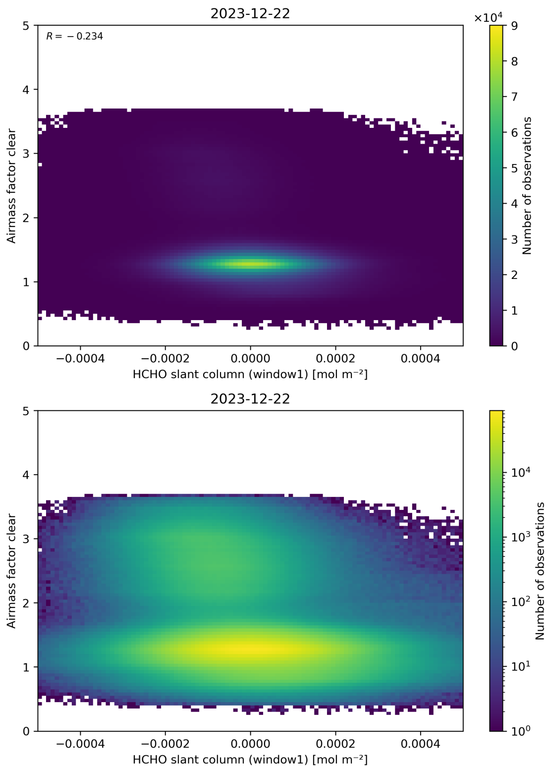
Figure 81: Scatter density plot of “HCHO slant column (window1)” against “Airmass factor clear” for 2023-12-21 to 2023-12-23.
