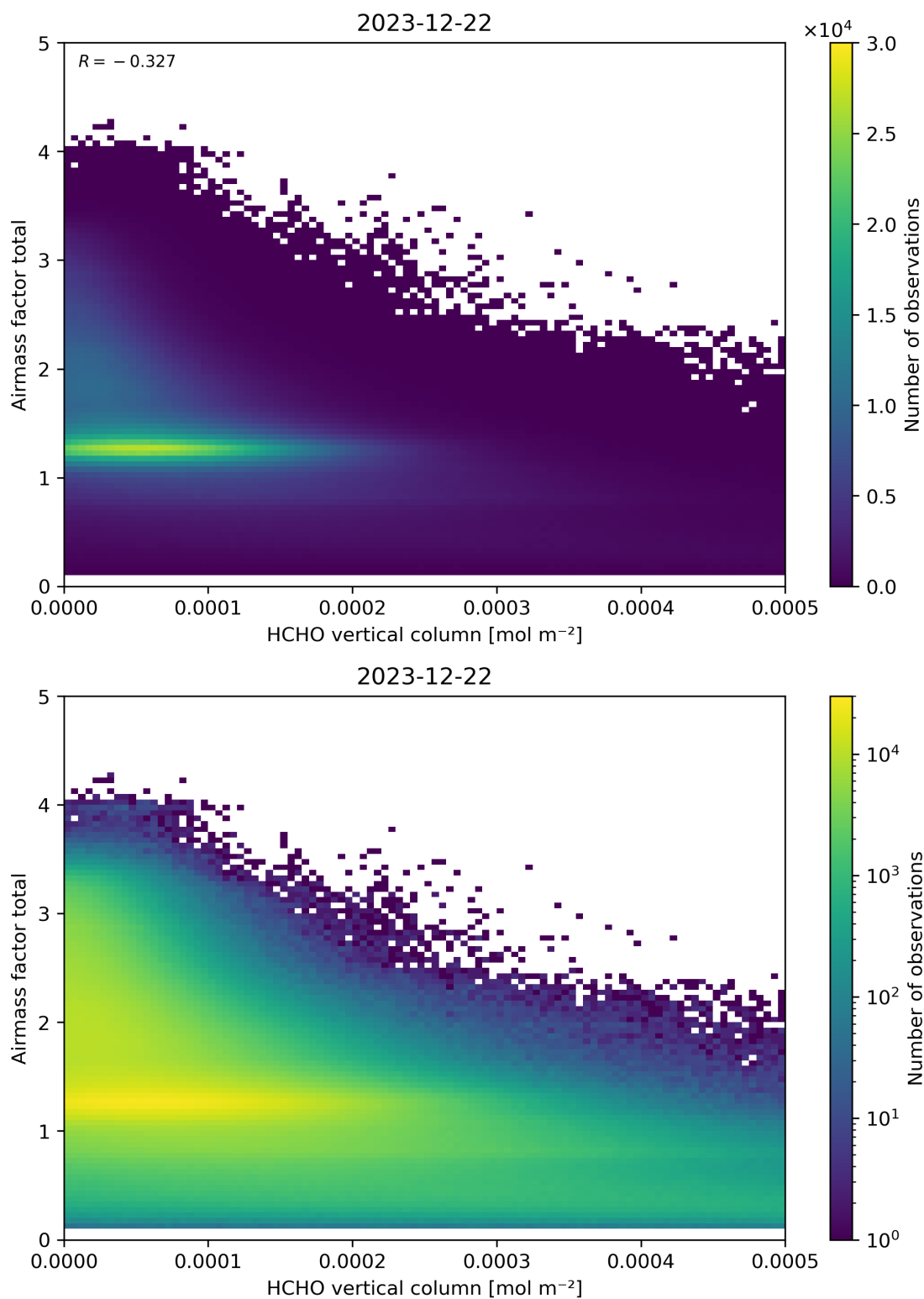
Figure 131: Scatter density plot of “HCHO vertical column” against “Airmass factor total” for 2023-12-21 to 2023-12-23.
