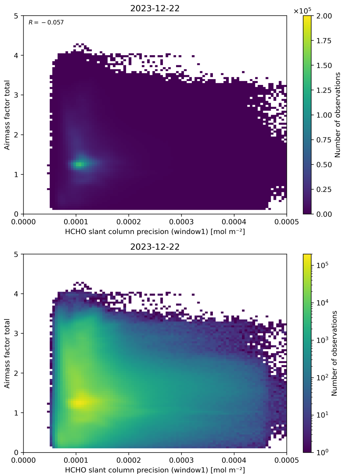
Figure 94: Scatter density plot of “HCHO slant column precision (window1)” against “Airmass factor total” for 2023-12-21 to 2023-12-23.
