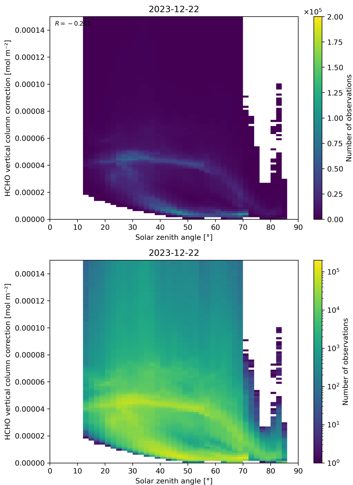
Figure 178: Scatter density plot of “Solar zenith angle” against “HCHO vertical column correction” for 2023-12-21 to 2023-12-23.
