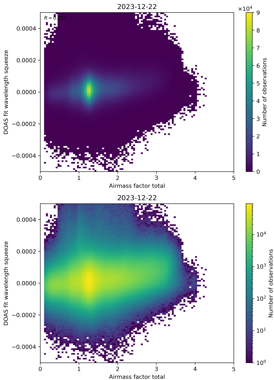
Figure 99: Scatter density plot of “Airmass factor total” against “DOAS fit wavelength squeeze” for 2023-12-21 to 2023-12-23.
