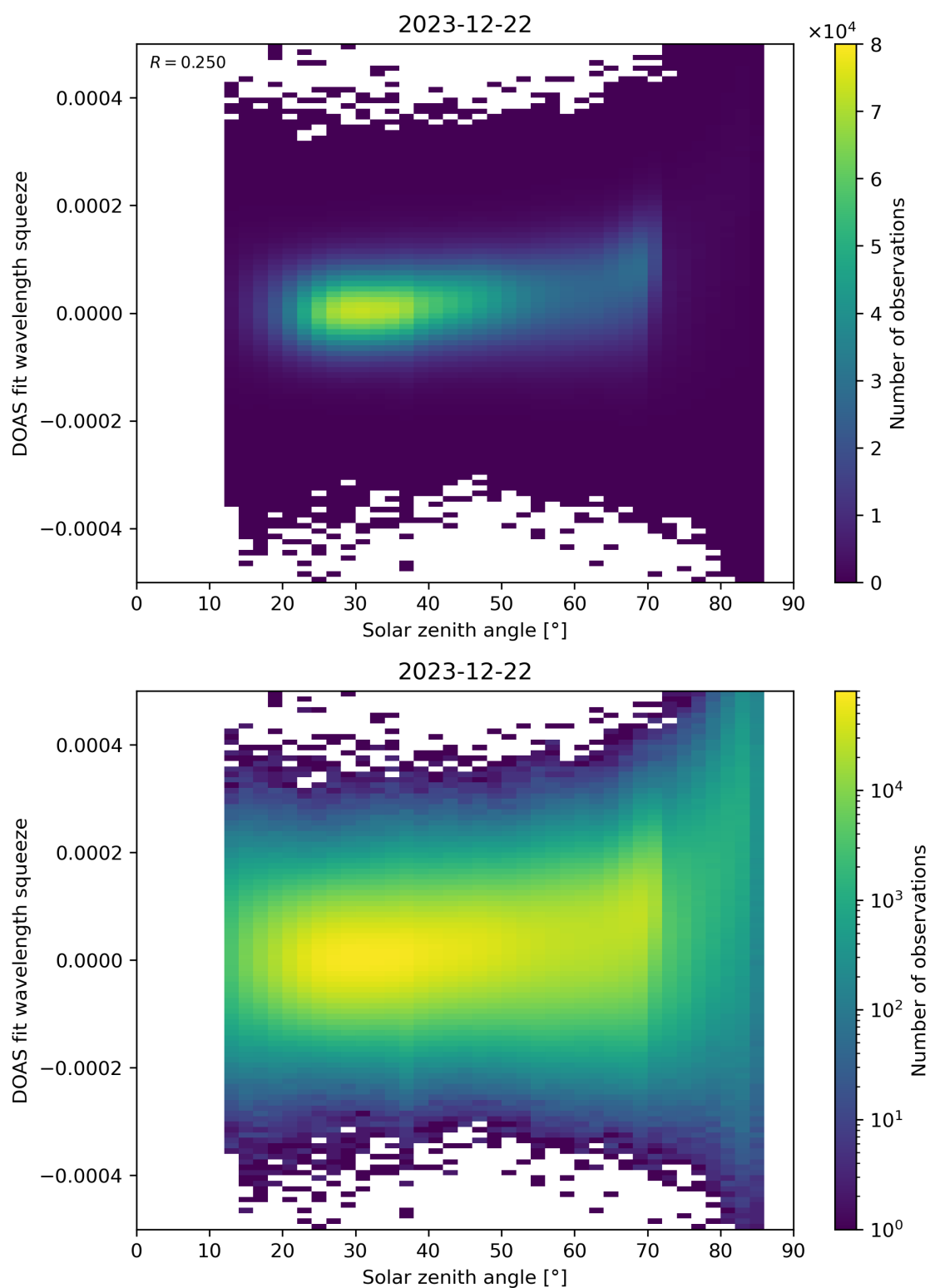
Figure 169: Scatter density plot of “Solar zenith angle” against “DOAS fit wavelength squeeze” for 2023-12-21 to 2023-12-23.
