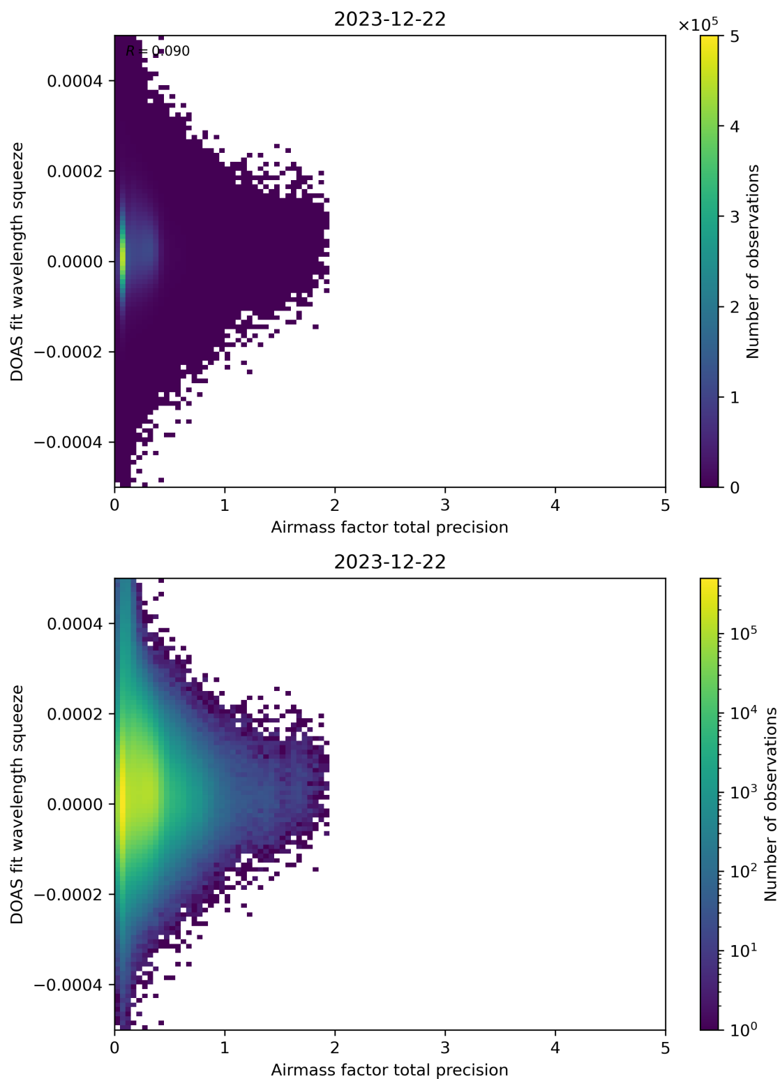
Figure 107: Scatter density plot of “Airmass factor total precision” against “DOAS fit wavelength squeeze” for 2023-12-21 to 2023-12-23.
