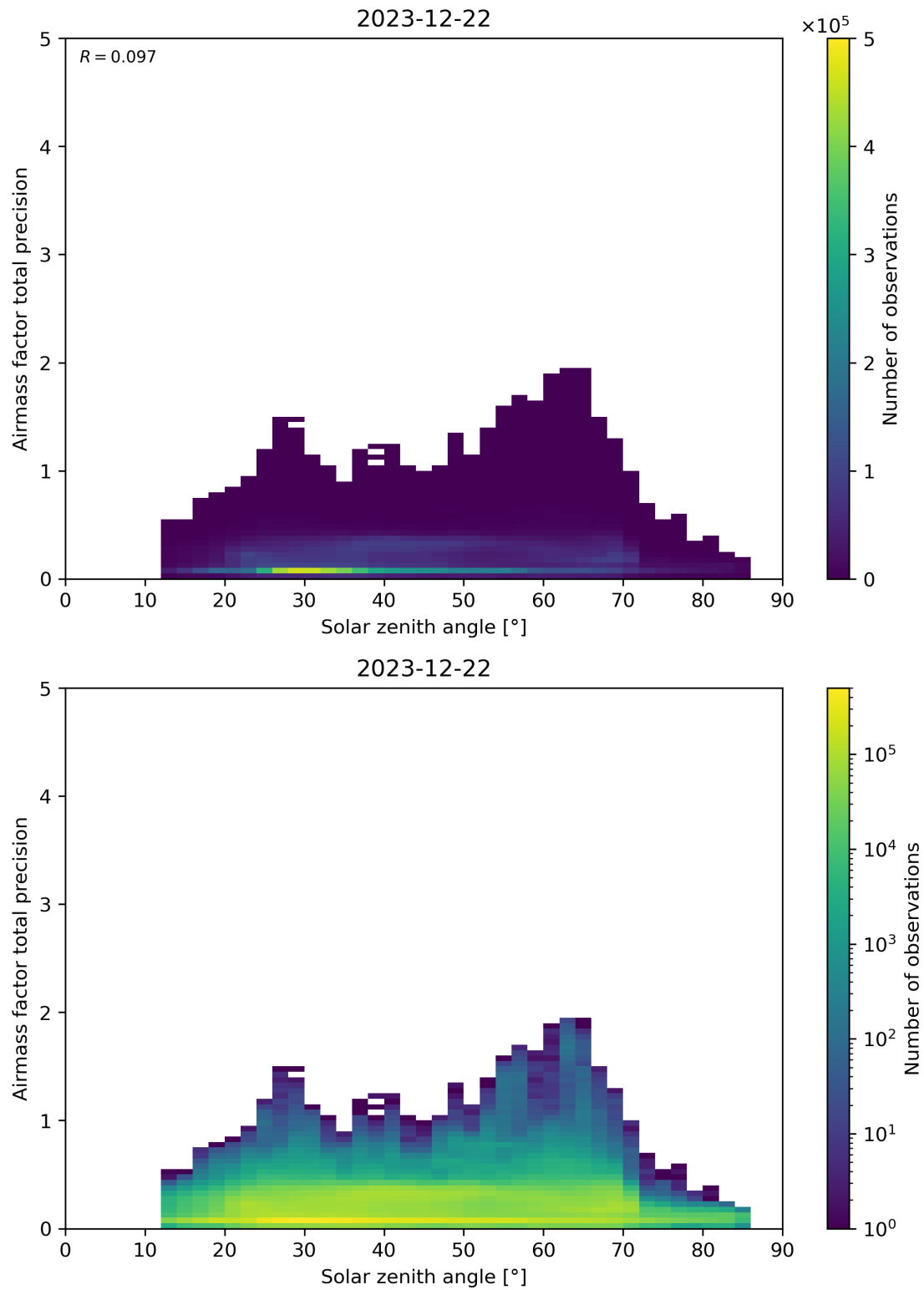
Figure 176: Scatter density plot of “Solar zenith angle” against “Airmass factor total precision” for 2023-12-21 to 2023-12-23.
