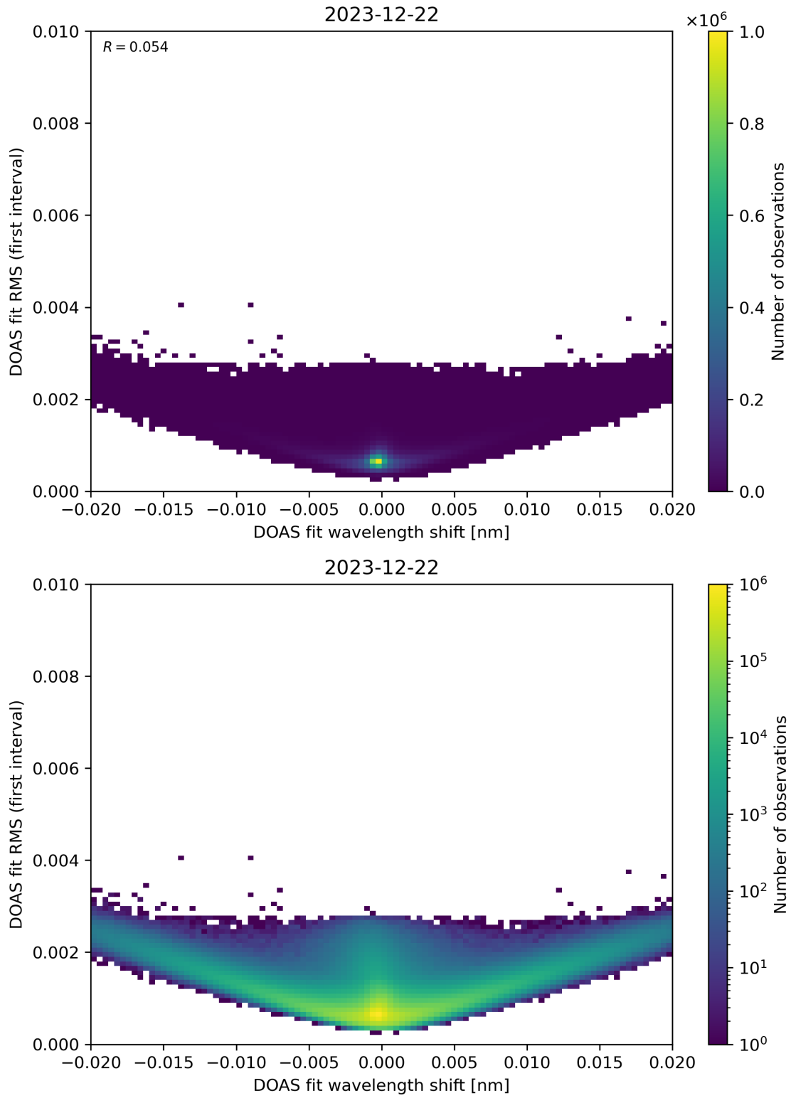
Figure 64: Scatter density plot of “DOAS fit wavelength shift” against “DOAS fit RMS (first interval)” for 2023-12-21 to 2023-12-23.
