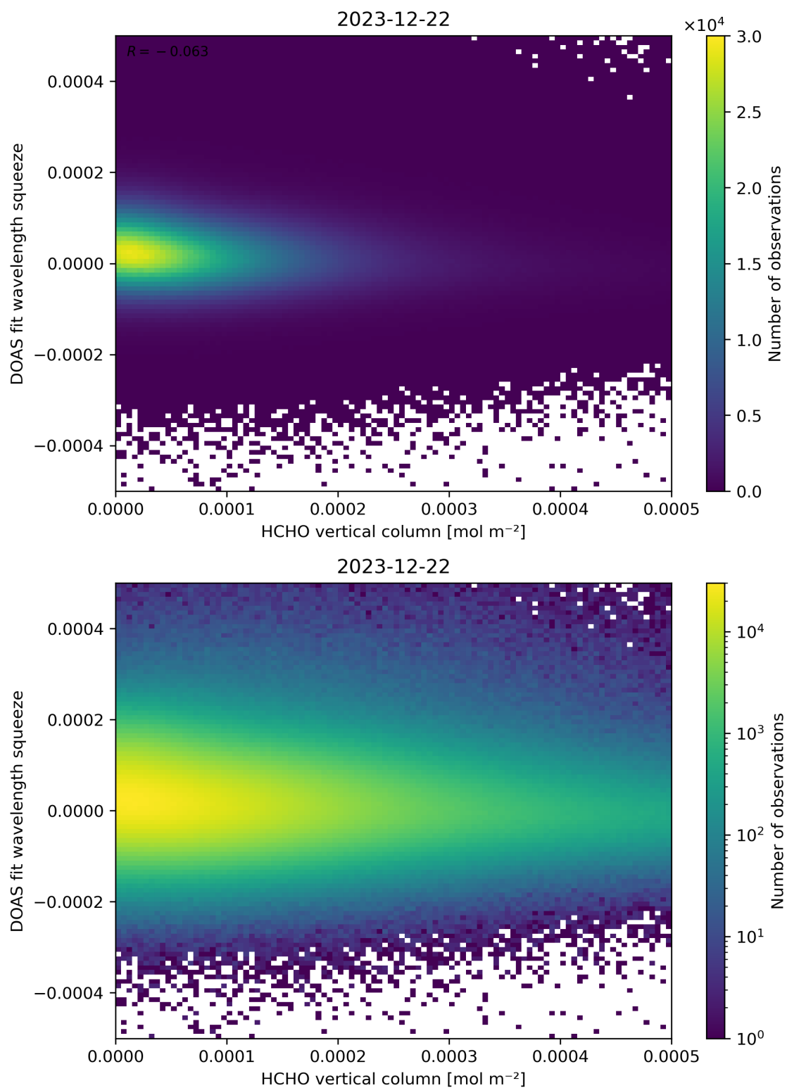
Figure 125: Scatter density plot of “HCHO vertical column” against “DOAS fit wavelength squeeze” for 2023-12-21 to 2023-12-23.
