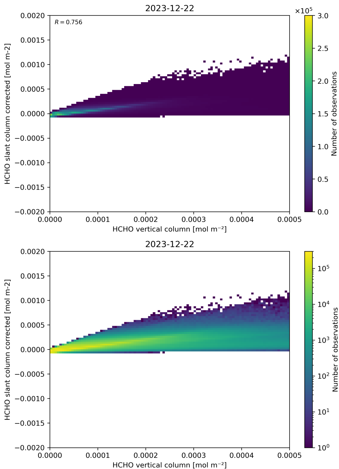
Figure 127: Scatter density plot of “HCHO vertical column” against “HCHO slant column corrected” for 2023-12-21 to 2023-12-23.
