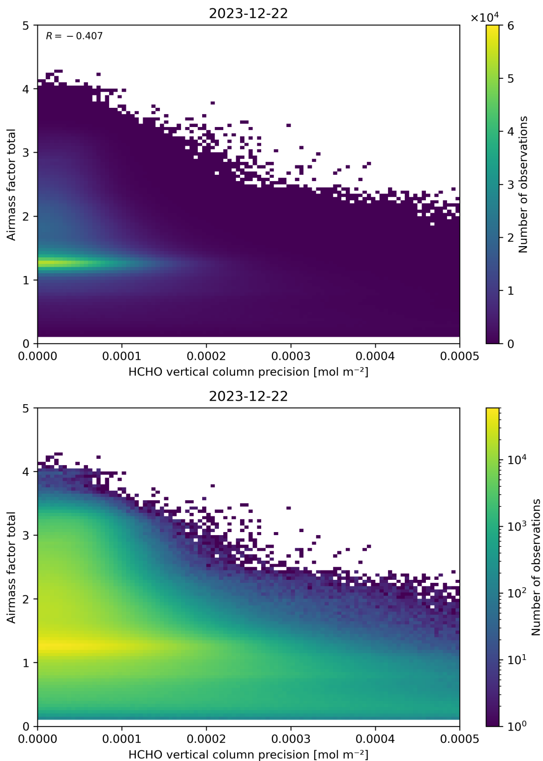
Figure 144: Scatter density plot of “HCHO vertical column precision” against “Airmass factor total” for 2023-12-21 to 2023-12-23.
