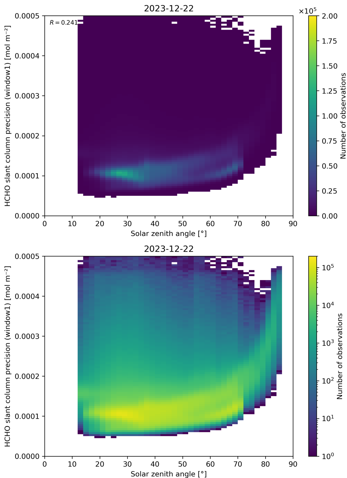
Figure 174: Scatter density plot of “Solar zenith angle” against “HCHO slant column precision (window1)” for 2023-12-21 to 2023-12-23.
