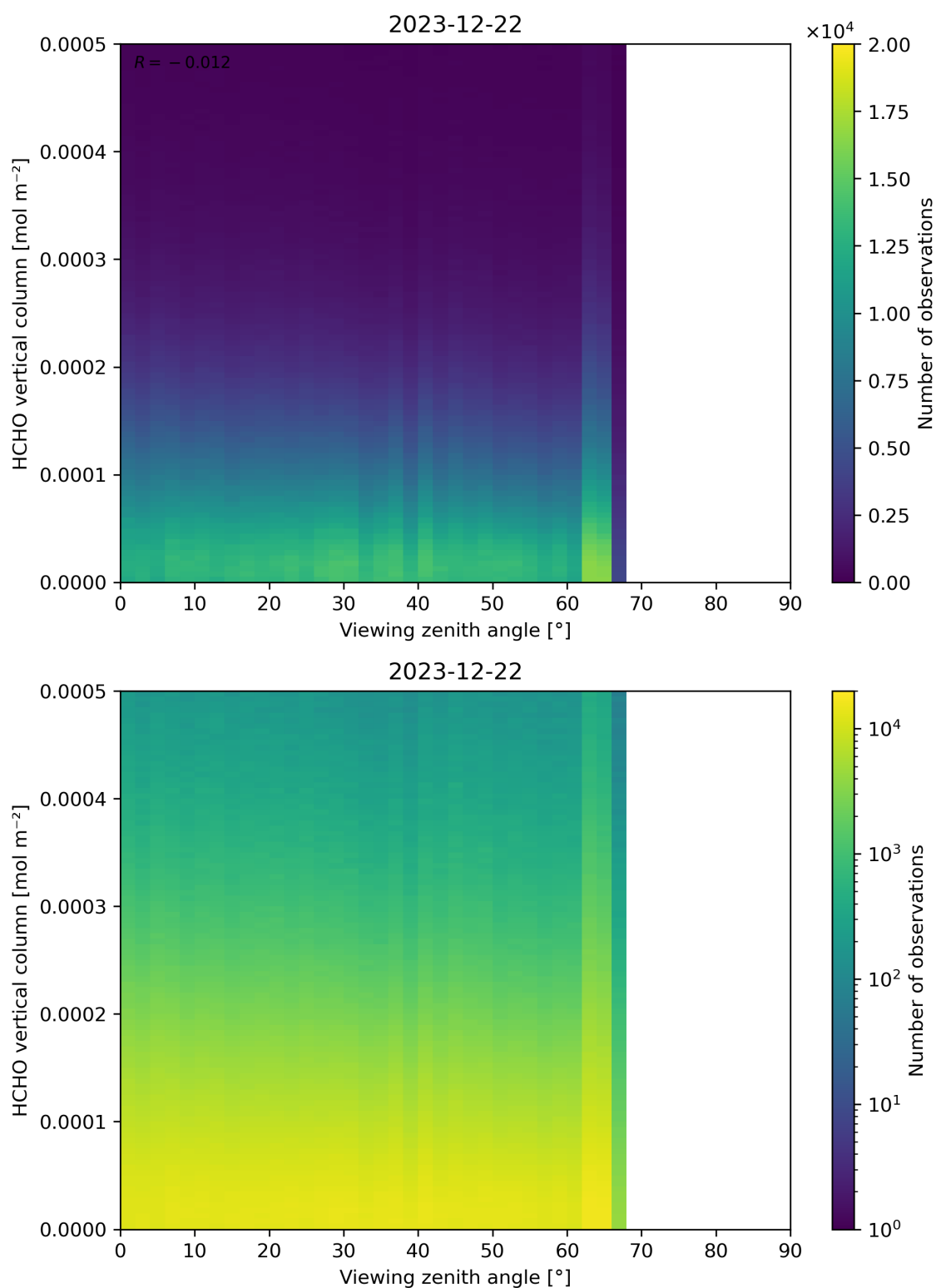
Figure 192: Scatter density plot of “Viewing zenith angle” against “HCHO vertical column” for 2023-12-21 to 2023-12-23.
