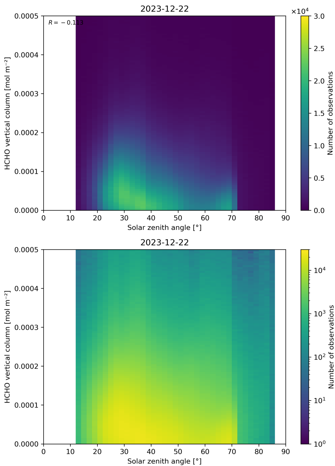
Figure 177: Scatter density plot of “Solar zenith angle” against “HCHO vertical column” for 2023-12-21 to 2023-12-23.
