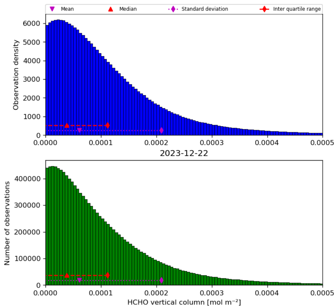
Figure 35: Histogram of “HCHO vertical column” for 2023-12-21 to 2023-12-23
