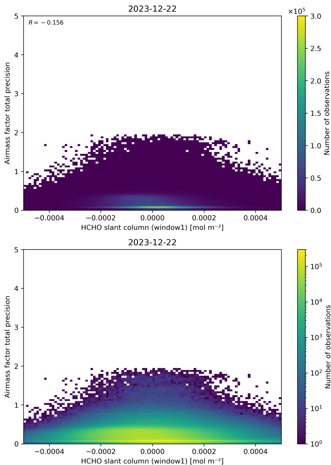
Figure 86: Scatter density plot of “HCHO slant column (window1)” against “Airmass factor total precision” for 2023-12-21 to 2023-12-23.
