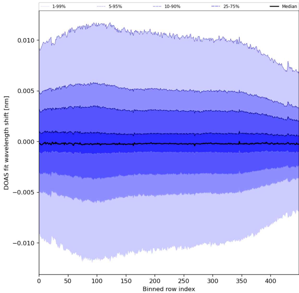
Figure 58: Along track statistics of “DOAS fit wavelength shift” for 2023-12-21 to 2023-12-23
