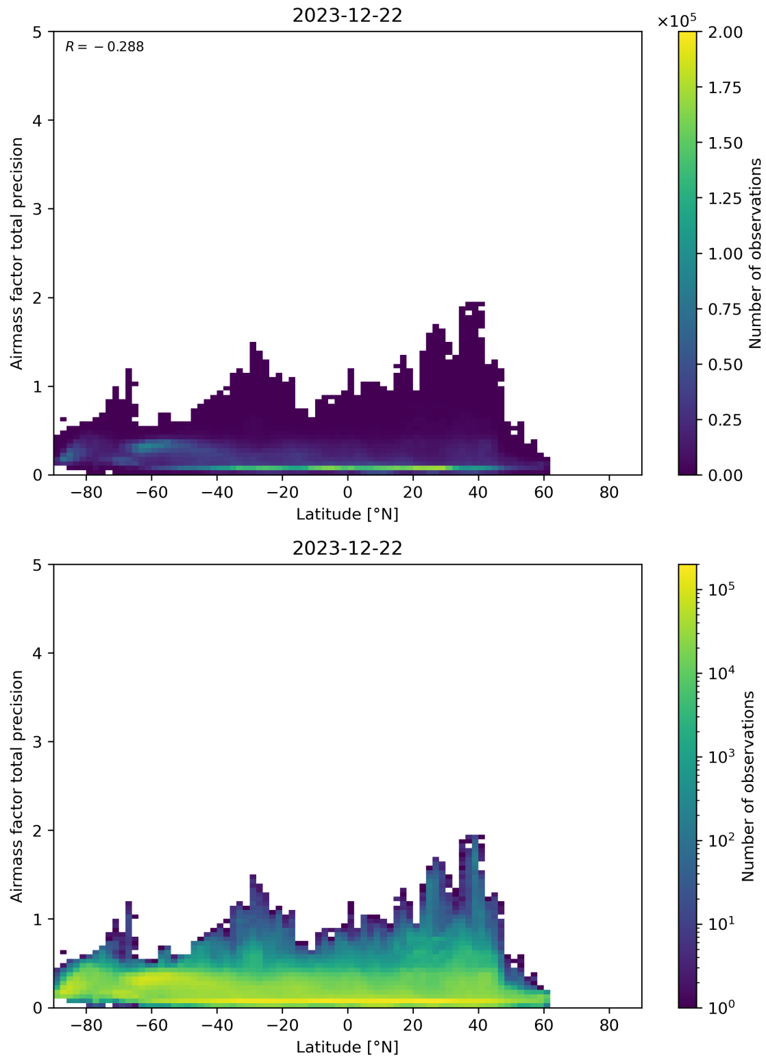
Figure 162: Scatter density plot of “Latitude” against “Airmass factor total precision” for 2023-12-21 to 2023-12-23.
