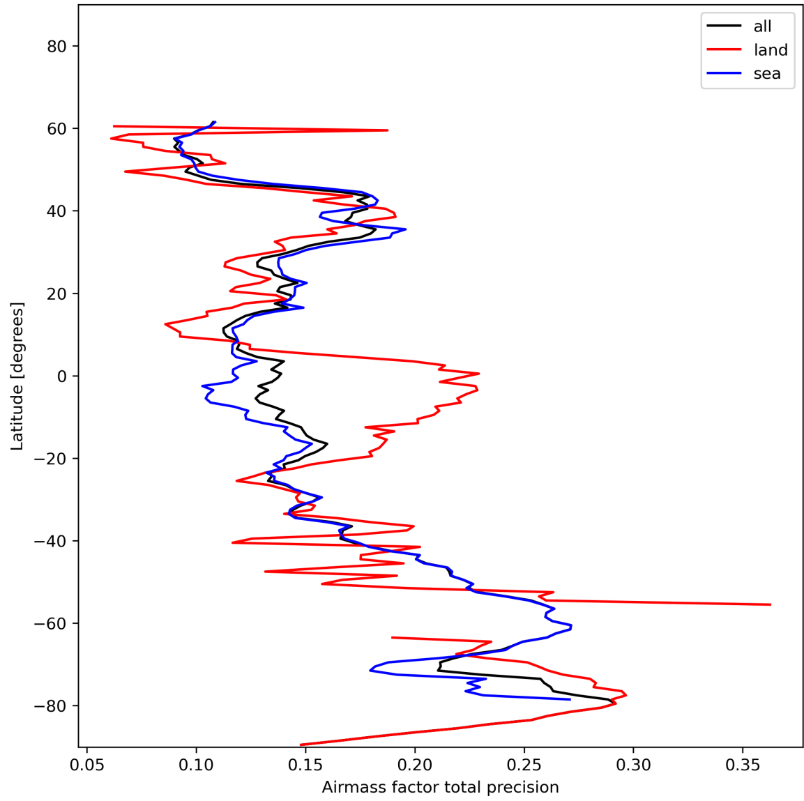
Figure 27: Zonal average of “Airmass factor total precision” for 2023-12-21 to 2023-12-23.
