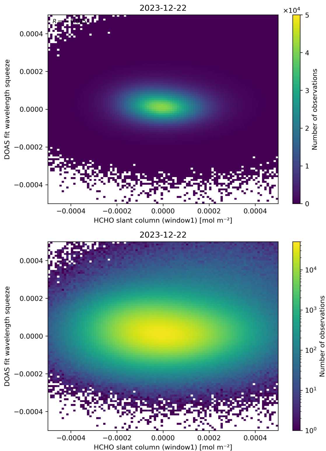
Figure 80: Scatter density plot of “HCHO slant column (window1)” against “DOAS fit wavelength squeeze” for 2023-12-21 to 2023-12-23.
