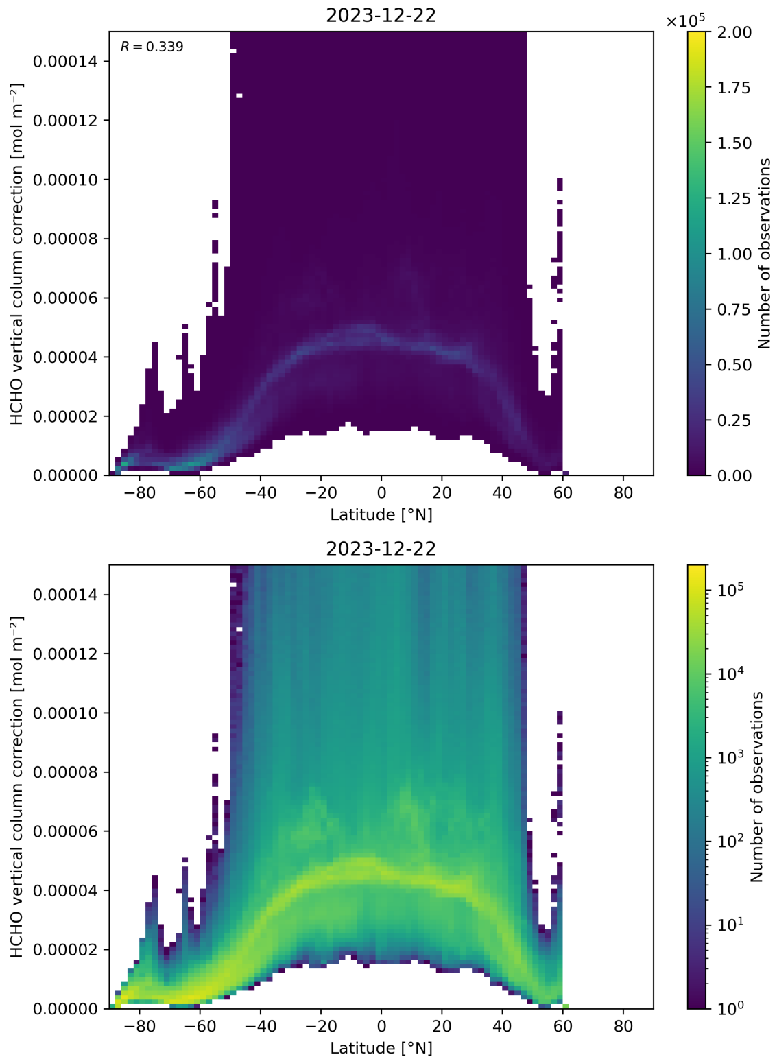
Figure 164: Scatter density plot of “Latitude” against “HCHO vertical column correction” for 2023-12-21 to 2023-12-23.
