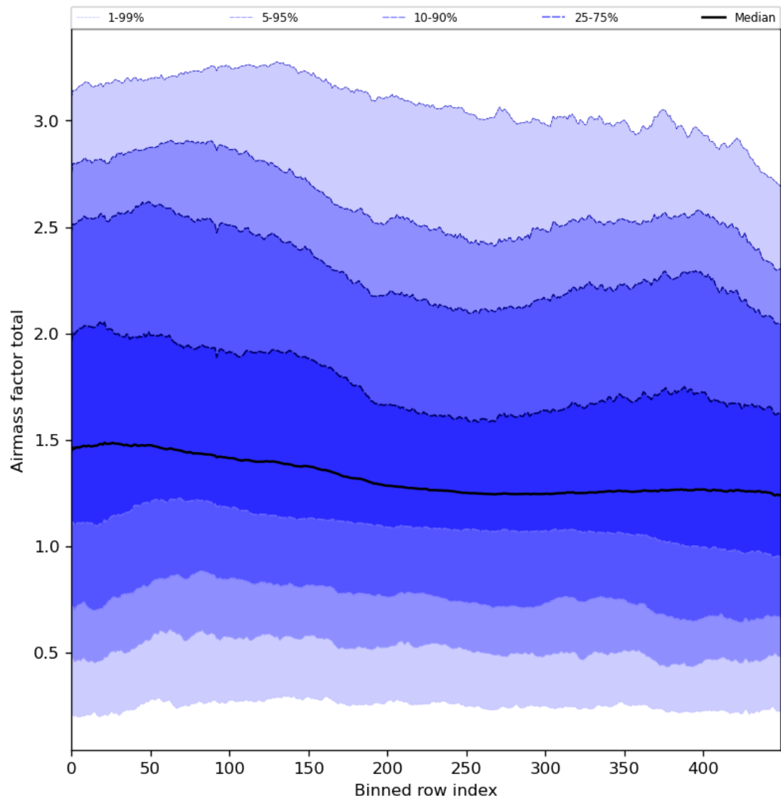
Figure 54: Along track statistics of “Airmass factor total” for 2023-12-21 to 2023-12-23
