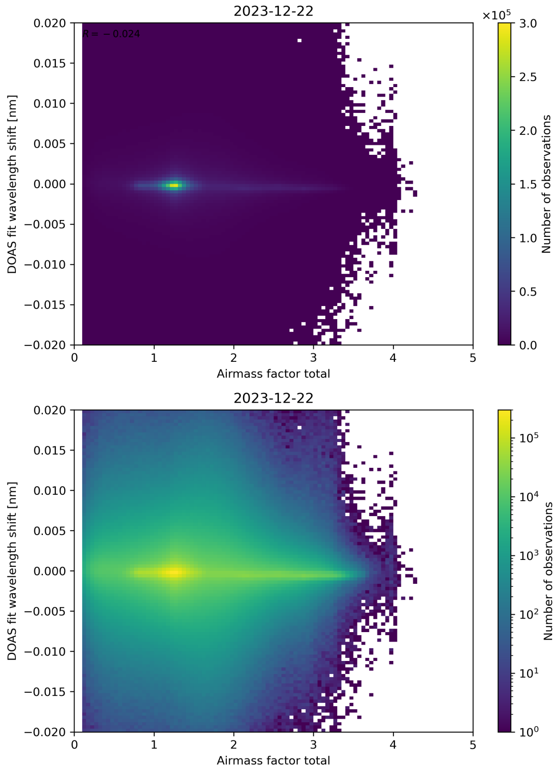
Figure 98: Scatter density plot of “Airmass factor total” against “DOAS fit wavelength shift” for 2023-12-21 to 2023-12-23.
