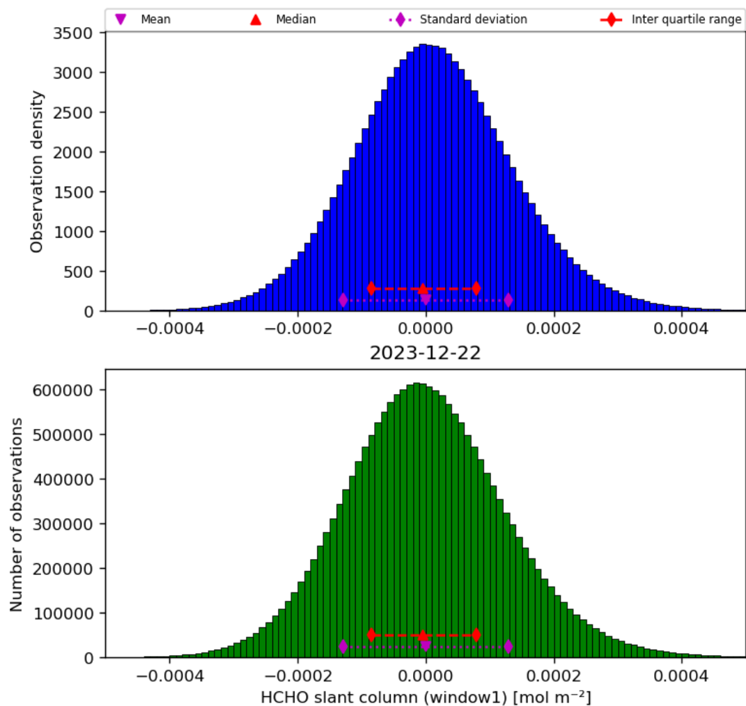
Figure 38: Histogram of “HCHO slant column (window1)” for 2023-12-21 to 2023-12-23
