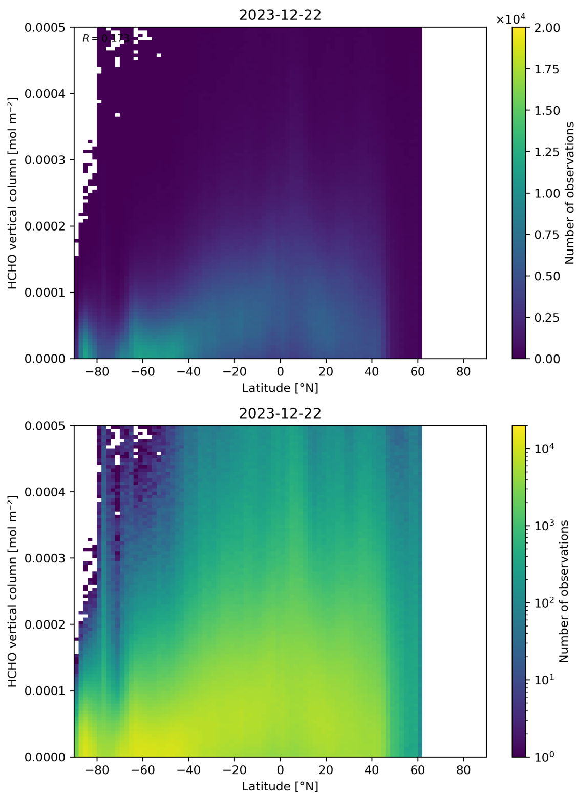
Figure 163: Scatter density plot of “Latitude” against “HCHO vertical column” for 2023-12-21 to 2023-12-23.
