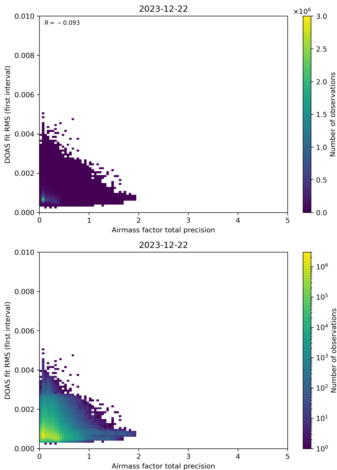
Figure 105: Scatter density plot of “Airmass factor total precision” against “DOAS fit RMS (first interval)” for 2023-12-21 to 2023-12-23.
