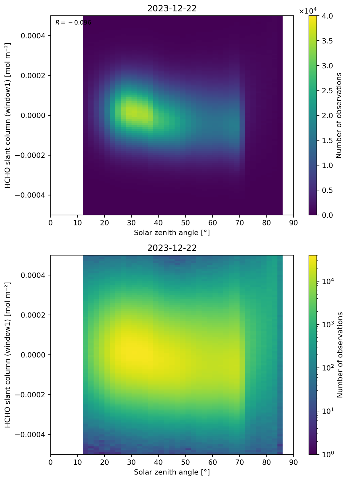
Figure 173: Scatter density plot of “Solar zenith angle” against “HCHO slant column (window1)” for 2023-12-21 to 2023-12-23.
