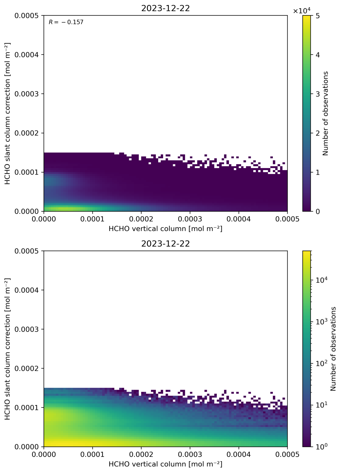
Figure 128: Scatter density plot of “HCHO vertical column” against “HCHO slant column correction” for 2023-12-21 to 2023-12-23.
