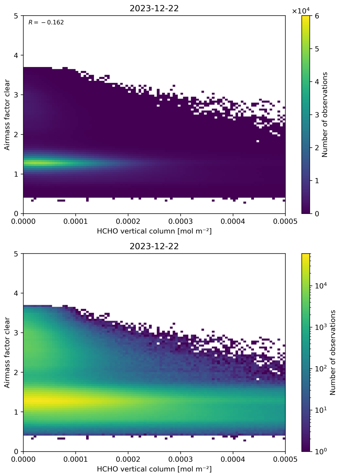
Figure 126: Scatter density plot of “HCHO vertical column” against “Airmass factor clear” for 2023-12-21 to 2023-12-23.
