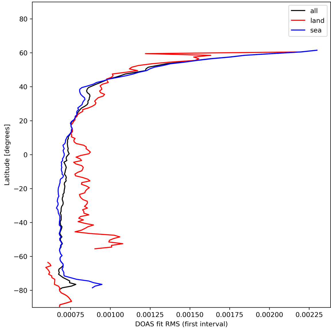
Figure 32: Zonal average of “DOAS fit RMS (first interval)” for 2023-12-21 to 2023-12-23.
