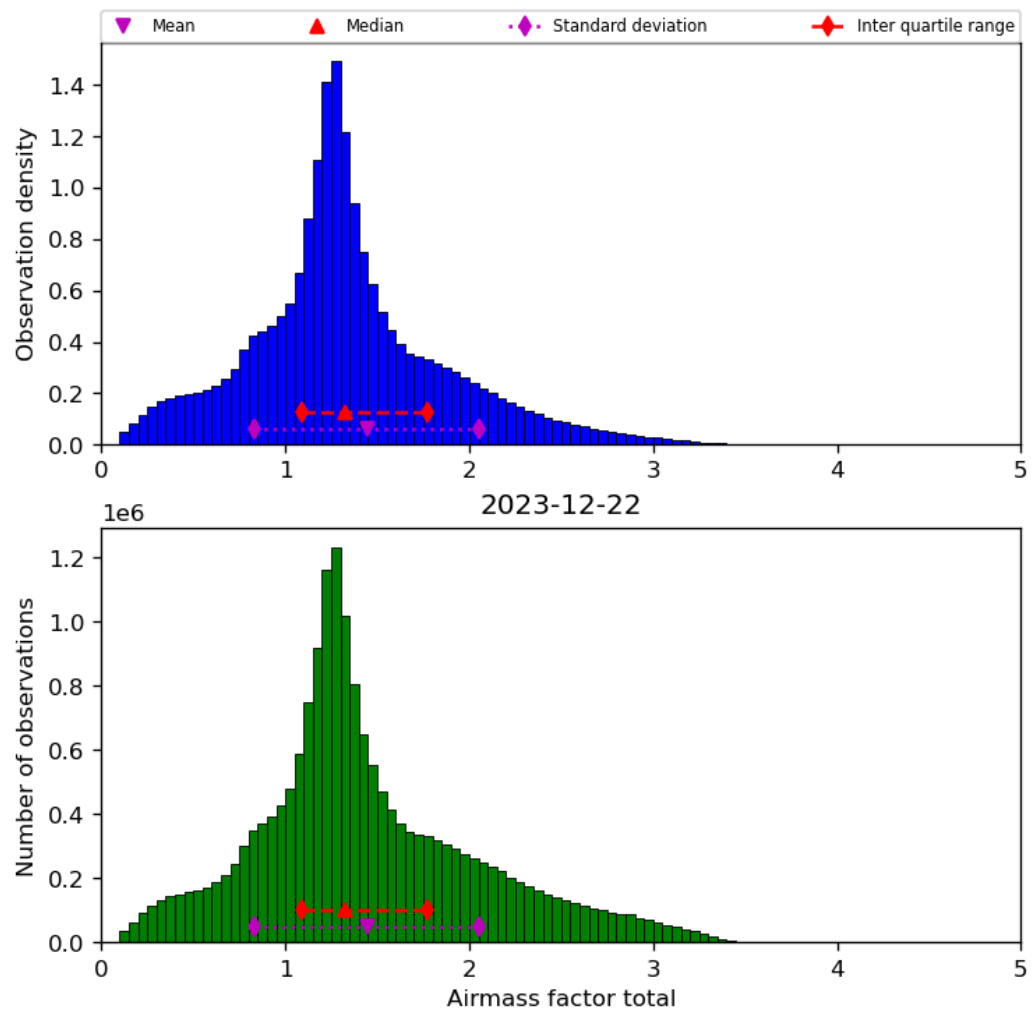
Figure 40: Histogram of “Airmass factor total” for 2023-12-21 to 2023-12-23
