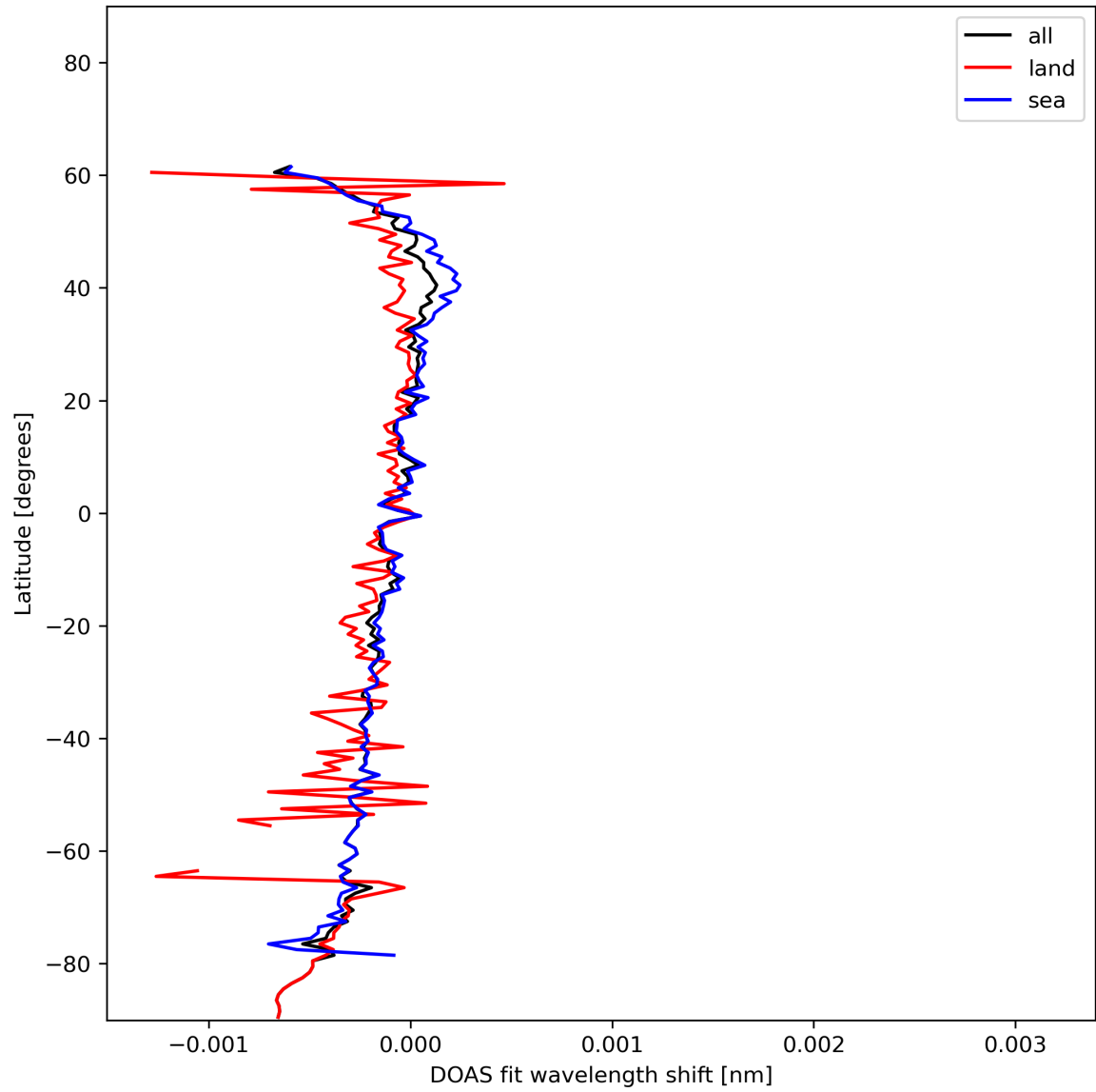
Figure 30: Zonal average of "DOAS fit wavelength shift" for 2023-12-21 to 2023-12-23.
