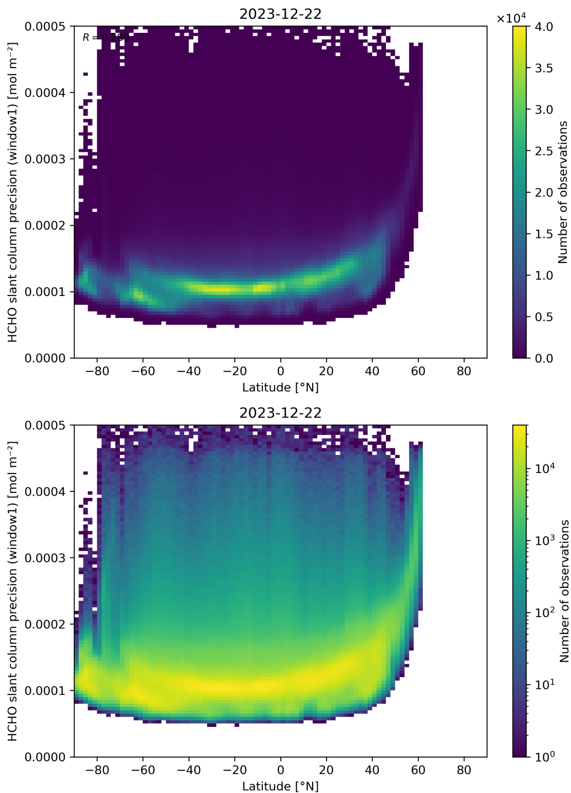
Figure 160: Scatter density plot of “Latitude” against “HCHO slant column precision (window1)” for 2023-12-21 to 2023-12-23.
