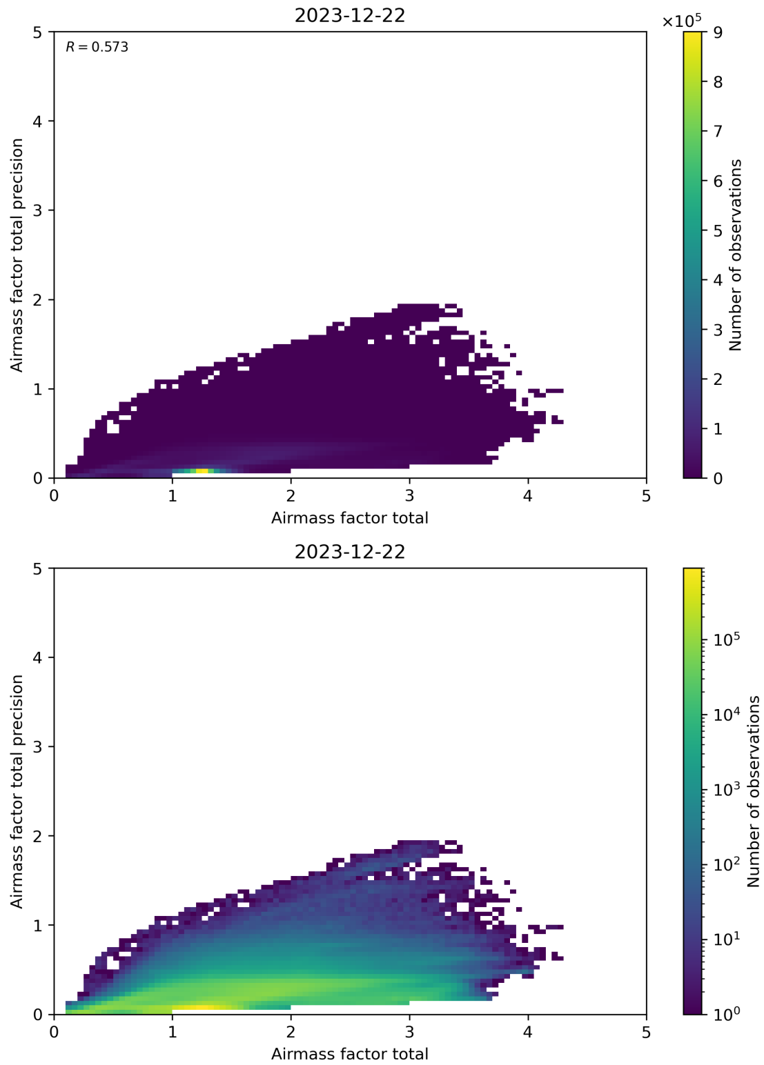
Figure 103: Scatter density plot of “Airmass factor total” against “Airmass factor total precision” for 2023-12-21 to 2023-12-23.
