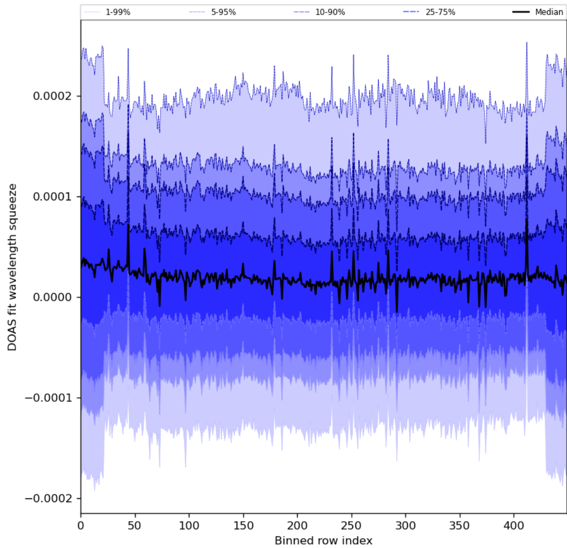
Figure 59: Along track statistics of “DOAS fit wavelength squeeze” for 2023-12-21 to 2023-12-23
