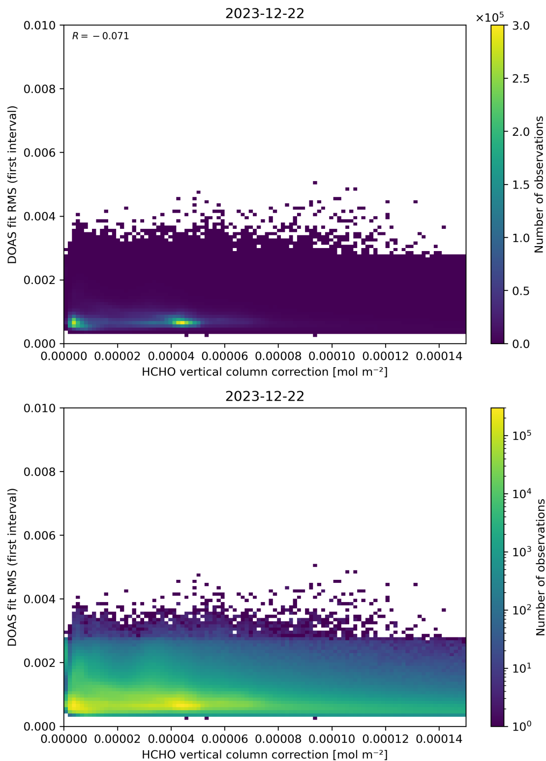
Figure 112: Scatter density plot of “HCHO vertical column correction” against “DOAS fit RMS (first interval)” for 2023-12-21 to 2023-12-23.
