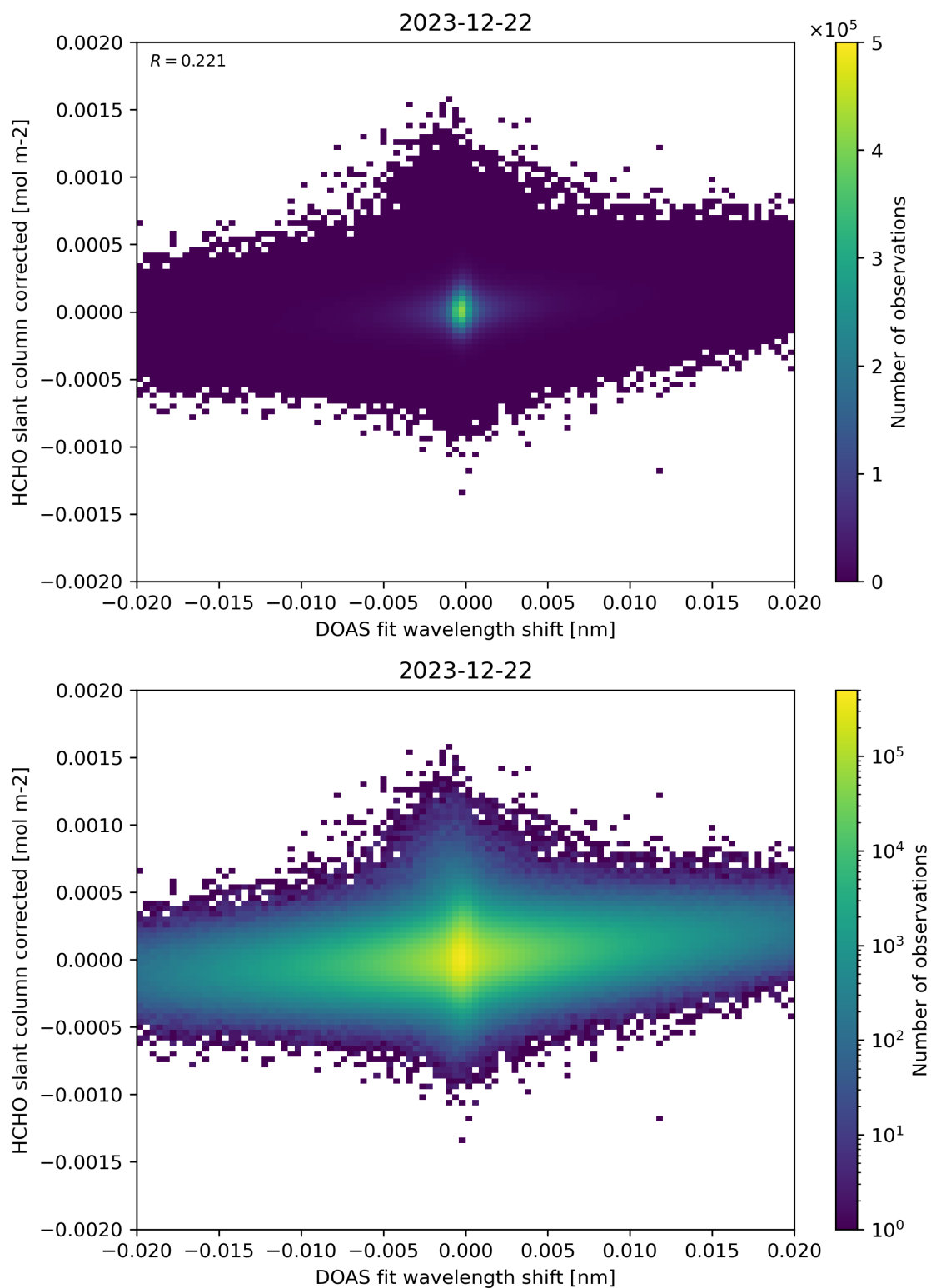
Figure 66: Scatter density plot of “DOAS fit wavelength shift” against “HCHO slant column corrected” for 2023-12-21 to 2023-12-23.
