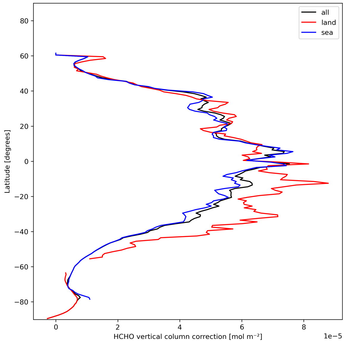
Figure 23: Zonal average of “HCHO vertical column correction” for 2023-12-21 to 2023-12-23.
