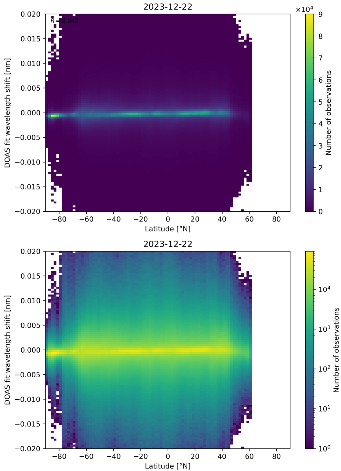
Figure 154: Scatter density plot of “Latitude” against “DOAS fit wavelength shift” for 2023-12-21 to 2023-12-23.
