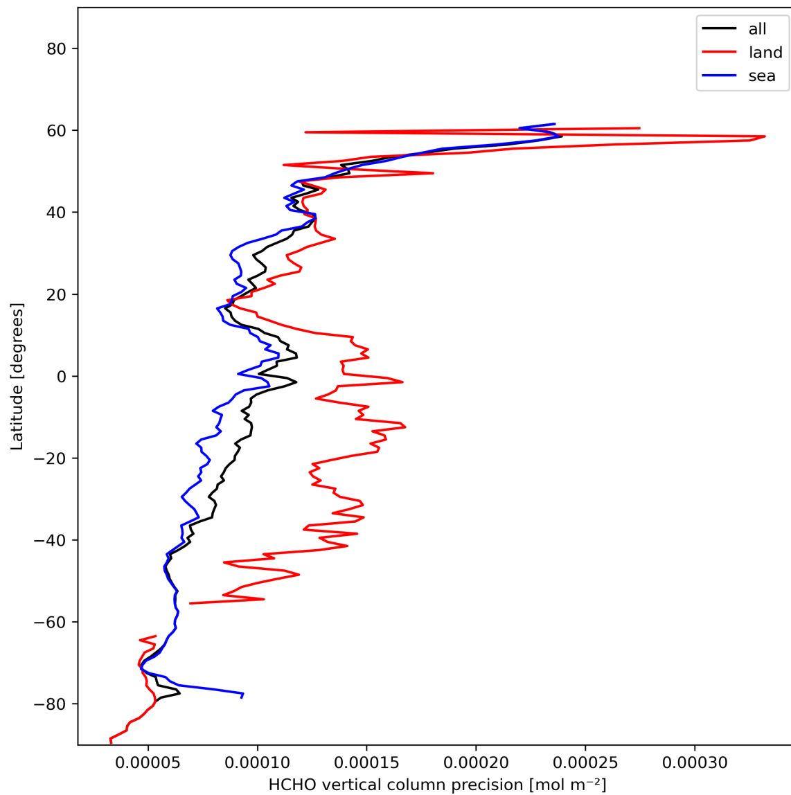
Figure 22: Zonal average of “HCHO vertical column precision” for 2023-12-21 to 2023-12-23.
