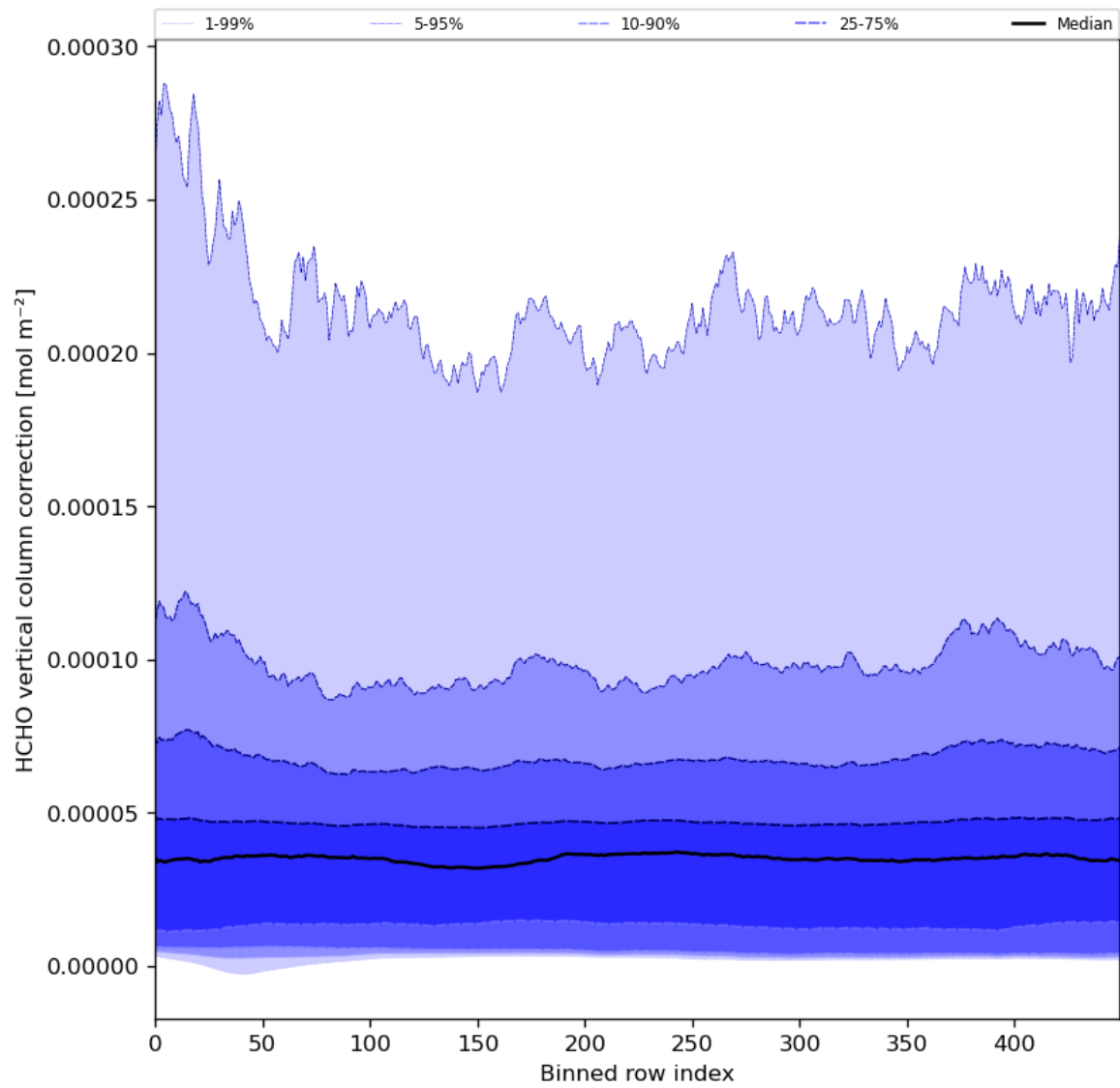
Figure 51: Along track statistics of “HCHO vertical column correction” for 2023-12-21 to 2023-12-23
