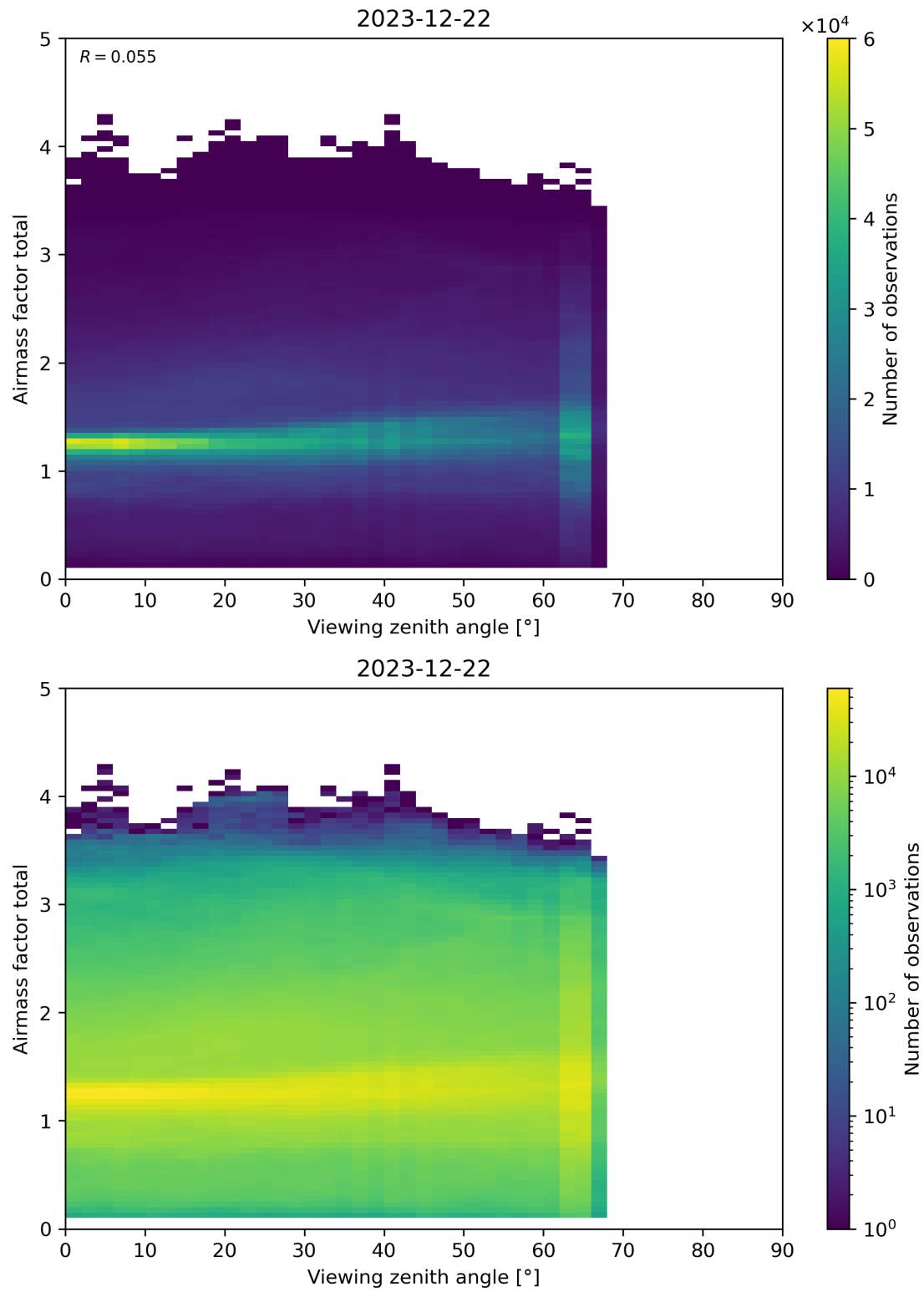
Figure 190: Scatter density plot of “Viewing zenith angle” against “Airmass factor total” for 2023-12-21 to 2023-12-23.
