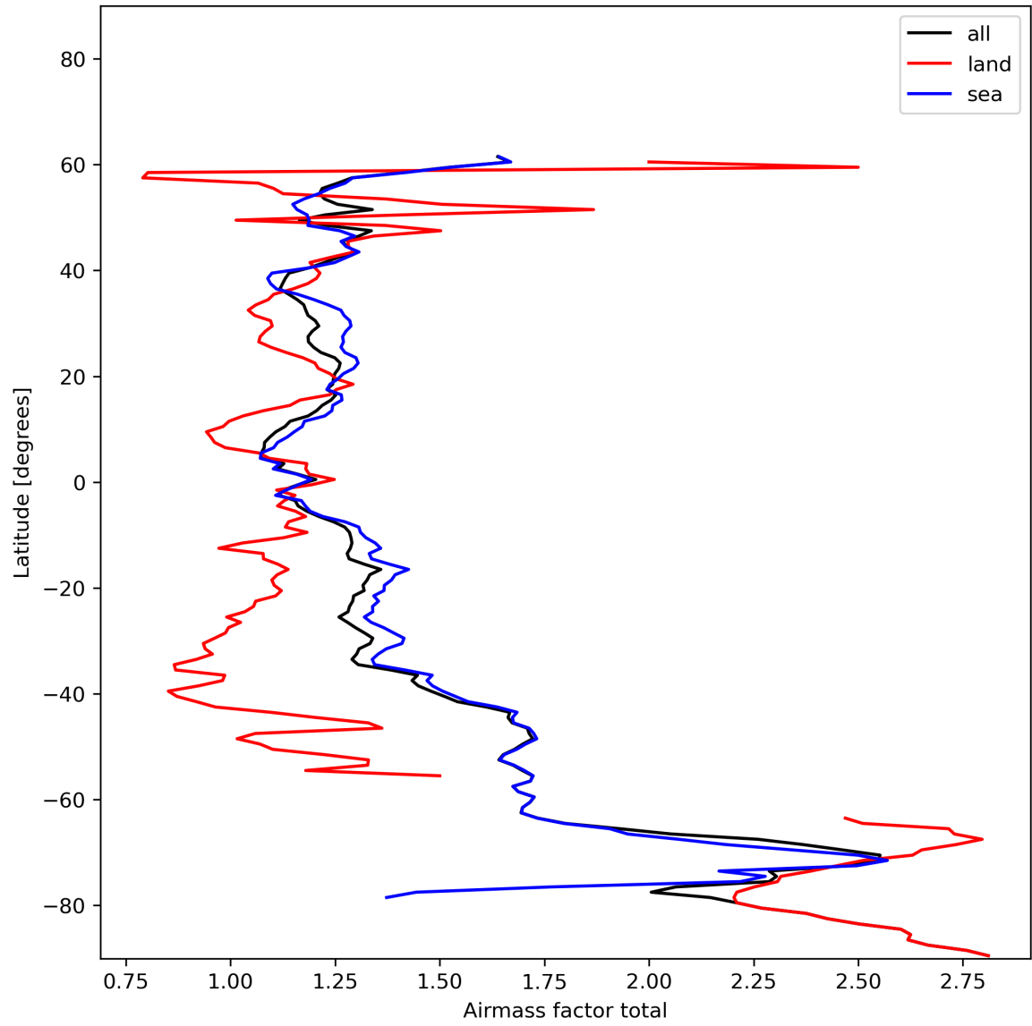
Figure 26: Zonal average of “Airmass factor total” for 2023-12-21 to 2023-12-23.
