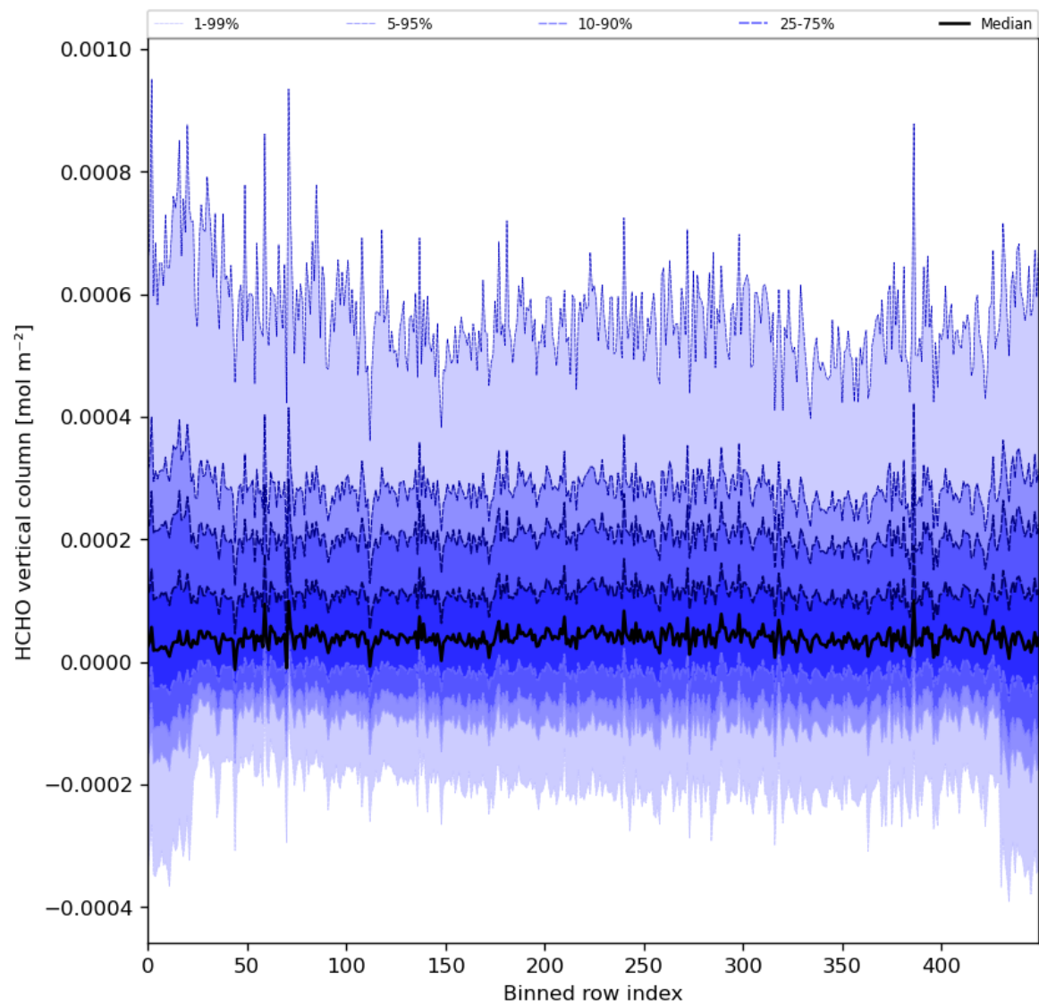
Figure 49: Along track statistics of “HCHO vertical column” for 2023-12-21 to 2023-12-23
