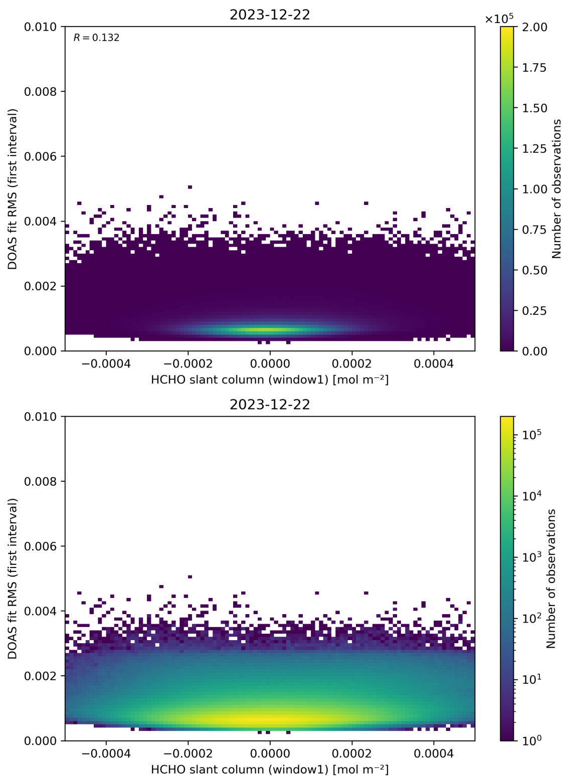
Figure 78: Scatter density plot of “HCHO slant column (window1)” against “DOAS fit RMS (first interval)” for 2023-12-21 to 2023-12-23.
