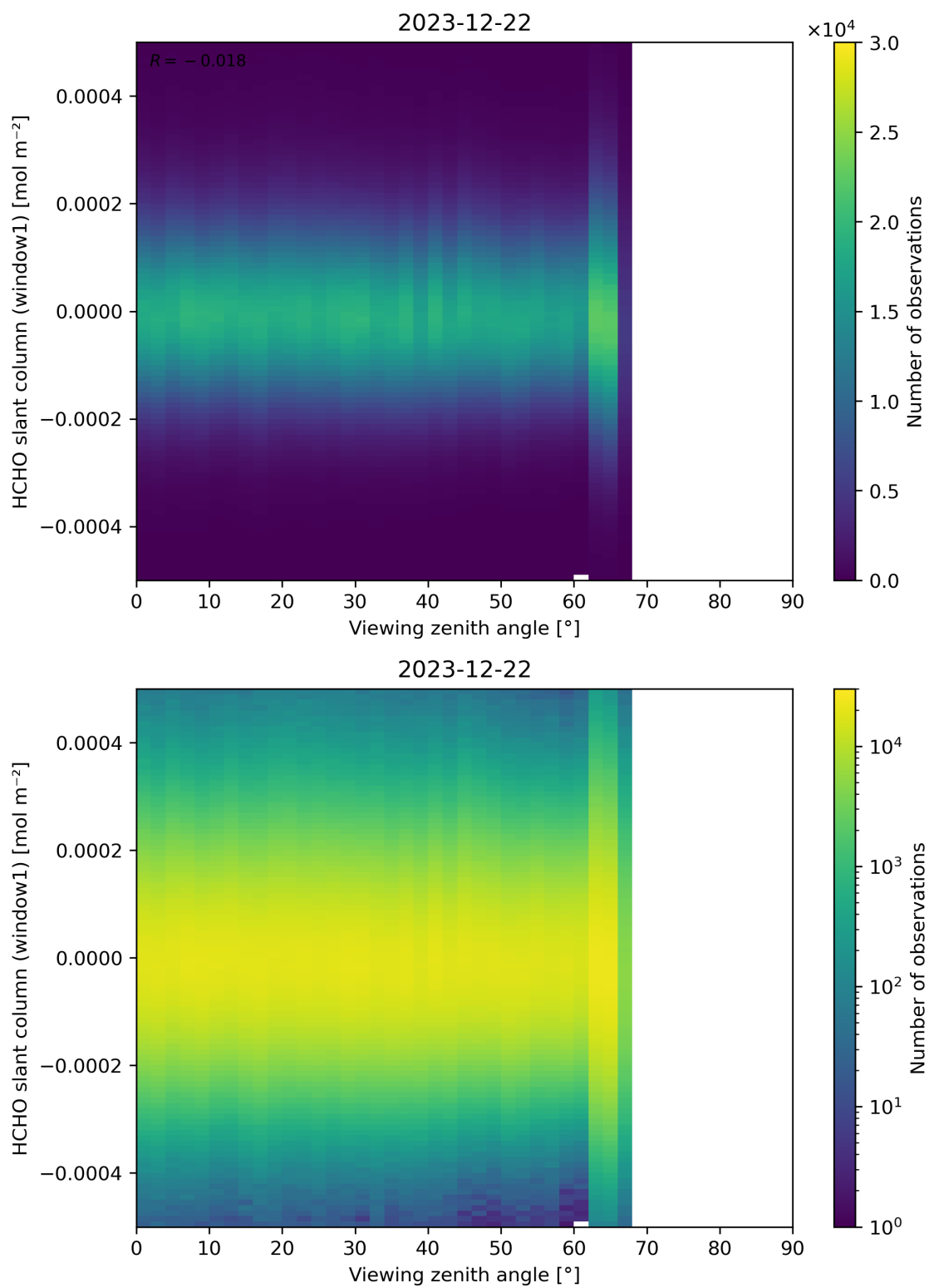
Figure 188: Scatter density plot of “Viewing zenith angle” against “HCHO slant column (window1)” for 2023-12-21 to 2023-12-23.
