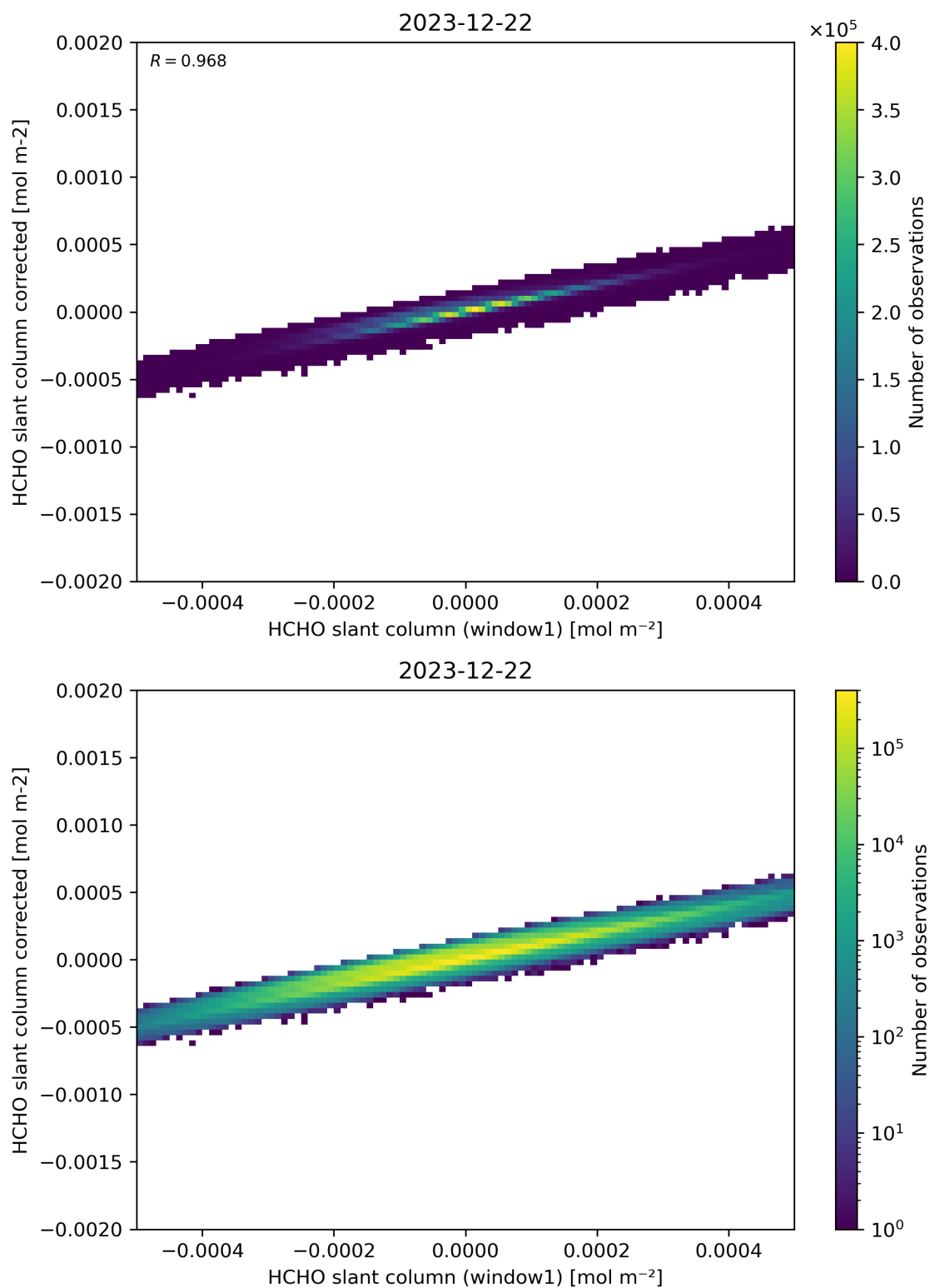
Figure 82: Scatter density plot of “HCHO slant column (window1)” against “HCHO slant column corrected” for 2023-12-21 to 2023-12-23.
