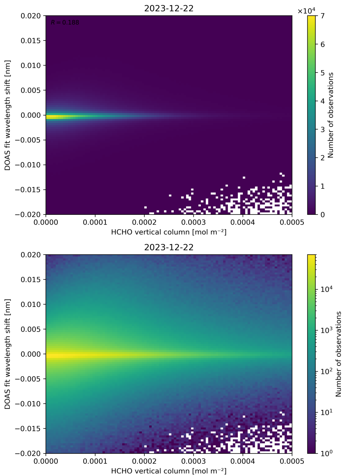
Figure 124: Scatter density plot of “HCHO vertical column” against “DOAS fit wavelength shift” for 2023-12-21 to 2023-12-23.
