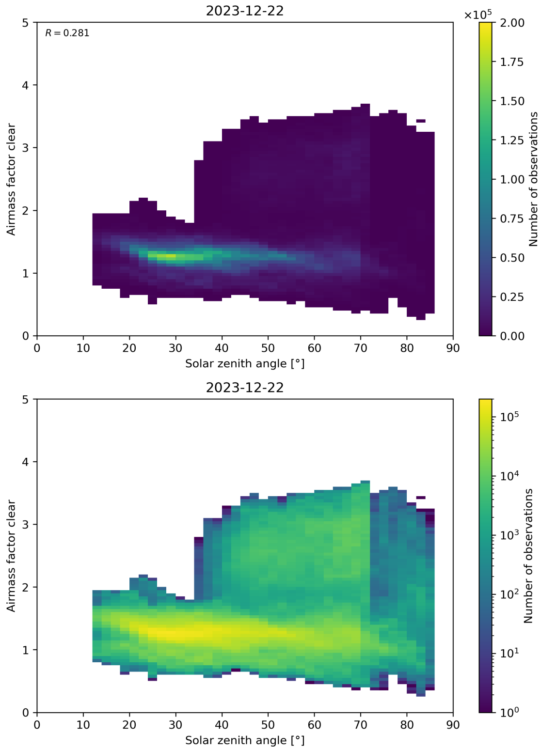
Figure 170: Scatter density plot of “Solar zenith angle” against “Airmass factor clear” for 2023-12-21 to 2023-12-23.
