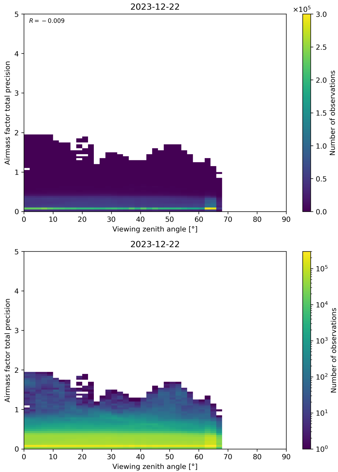
Figure 191: Scatter density plot of “Viewing zenith angle” against “Airmass factor total precision” for 2023-12-21 to 2023-12-23.
