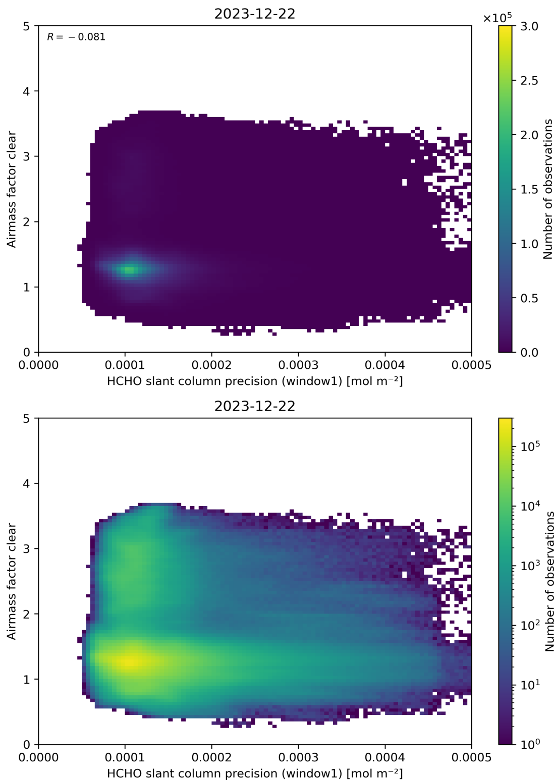
Figure 91: Scatter density plot of “HCHO slant column precision (window1)” against “Airmass factor clear” for 2023-12-21 to 2023-12-23.
