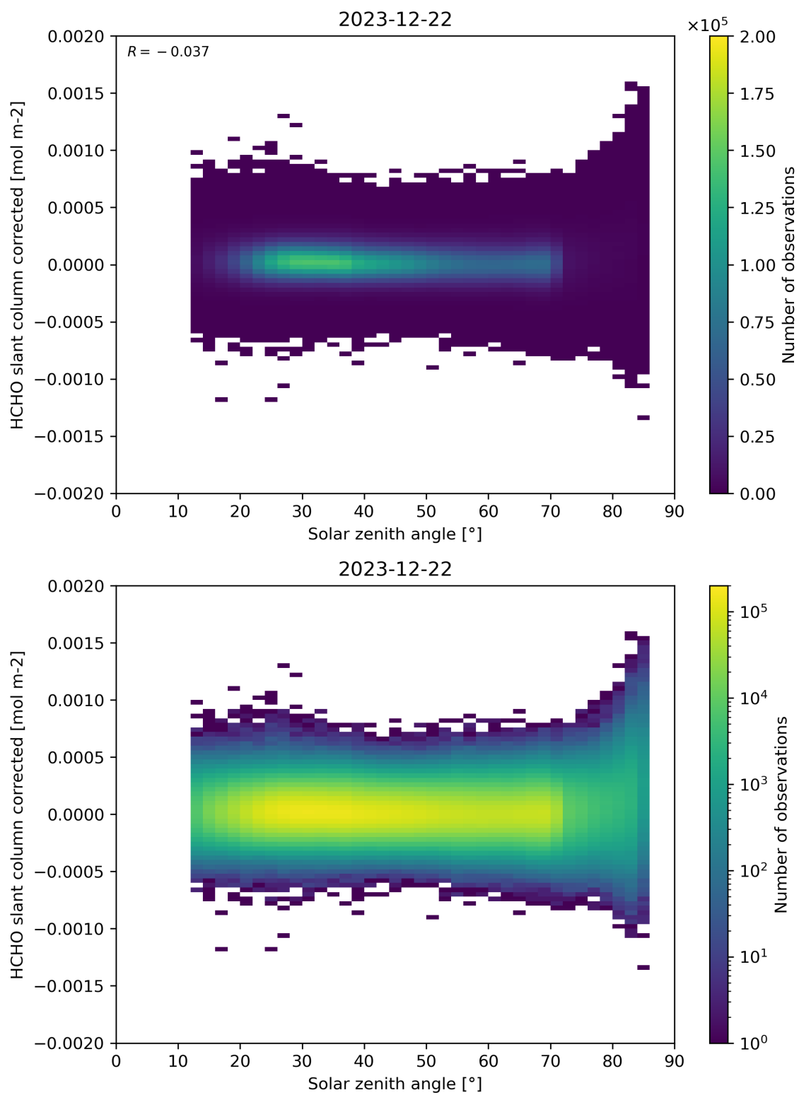
Figure 171: Scatter density plot of “Solar zenith angle” against “HCHO slant column corrected” for 2023-12-21 to 2023-12-23.
