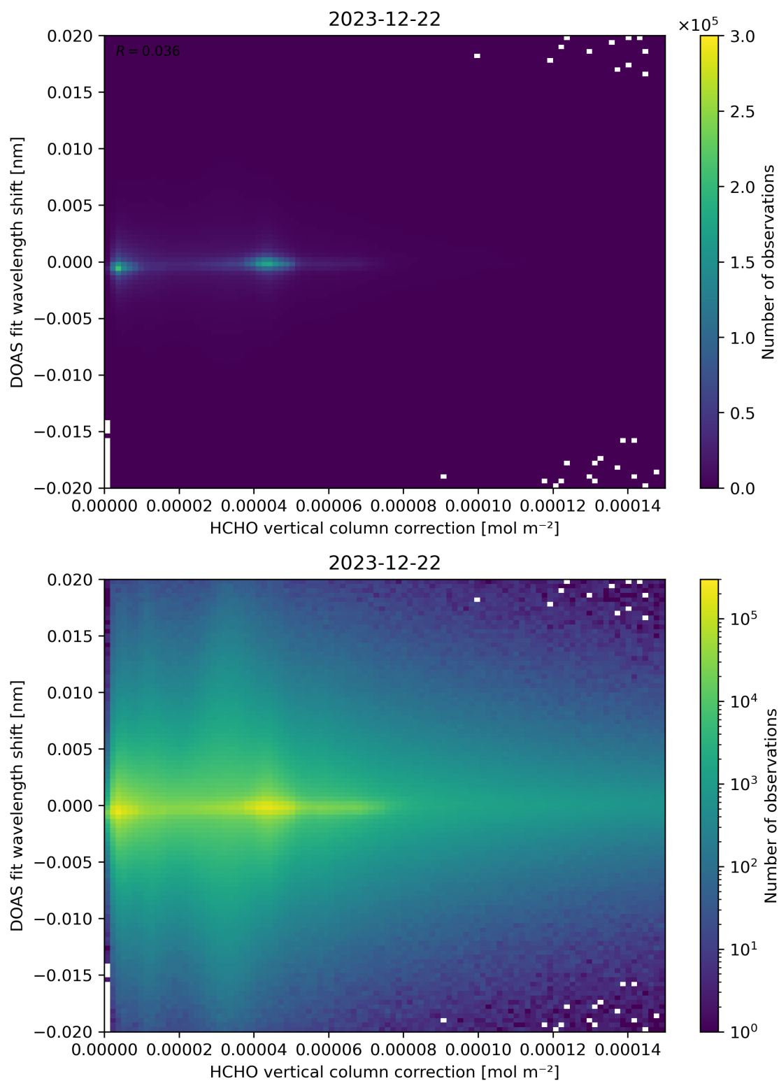
Figure 113: Scatter density plot of “HCHO vertical column correction” against “DOAS fit wavelength shift” for 2023-12-21 to 2023-12-23.
