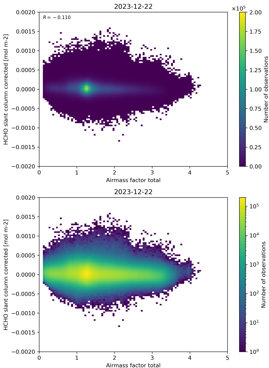
Figure 101: Scatter density plot of “Airmass factor total” against “HCHO slant column corrected” for 2023-12-21 to 2023-12-23.
