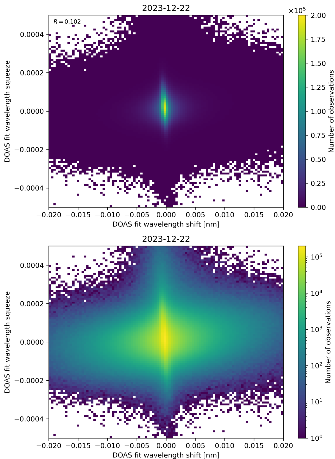
Figure 65: Scatter density plot of “DOAS fit wavelength shift” against “DOAS fit wavelength squeeze” for 2023-12-21 to 2023-12-23.
