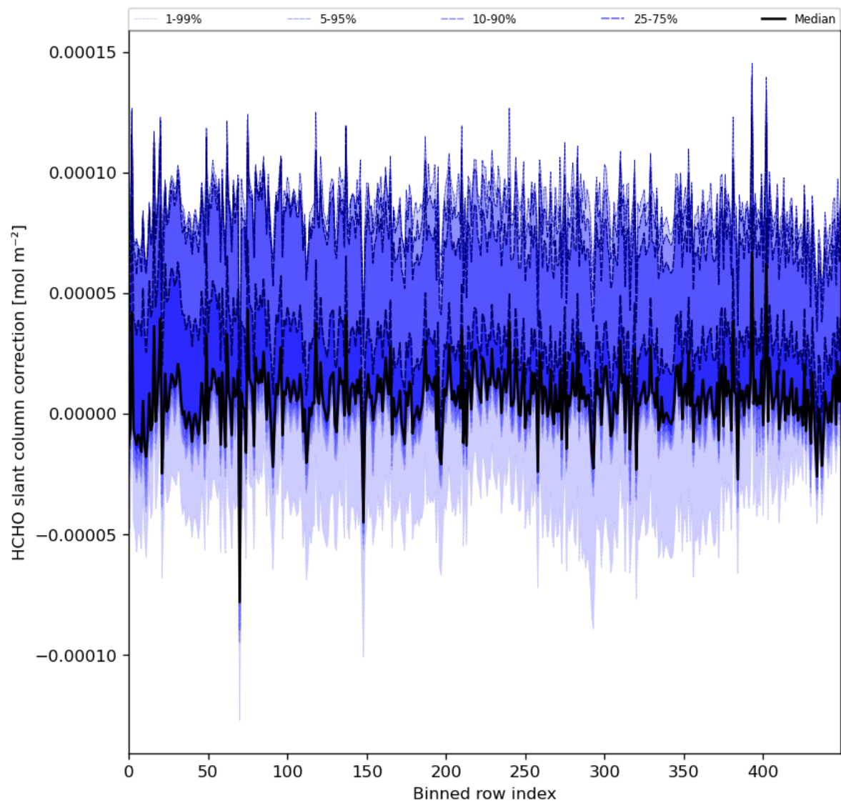
Figure 61: Along track statistics of “HCHO slant column correction” for 2023-12-21 to 2023-12-23
