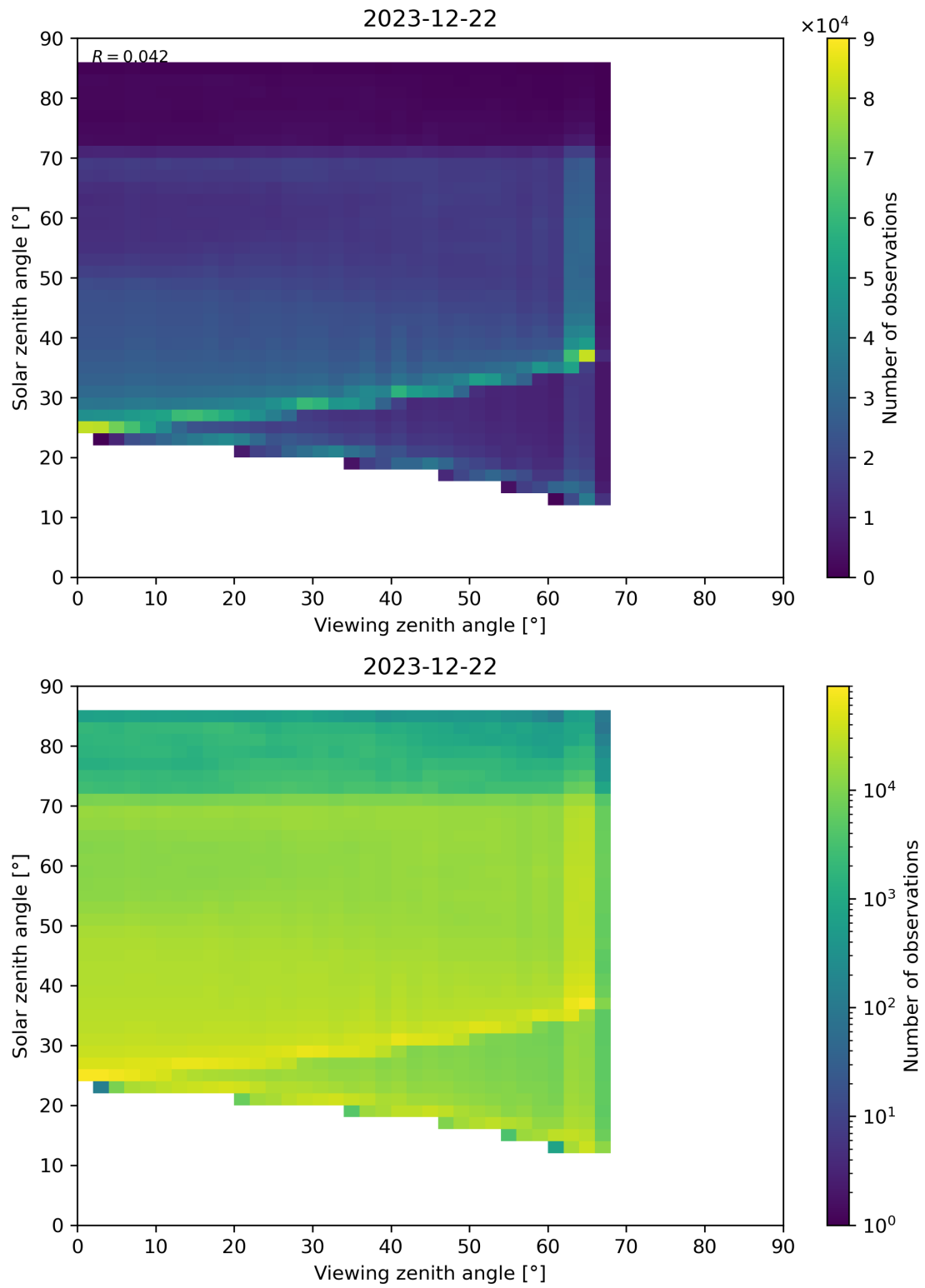
Figure 197: Scatter density plot of “Viewing zenith angle” against “Solar zenith angle” for 2023-12-21 to 2023-12-23.
