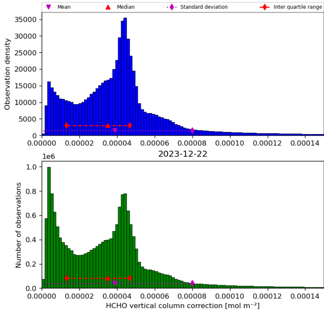
Figure 37: Histogram of “HCHO vertical column correction” for 2023-12-21 to 2023-12-23
