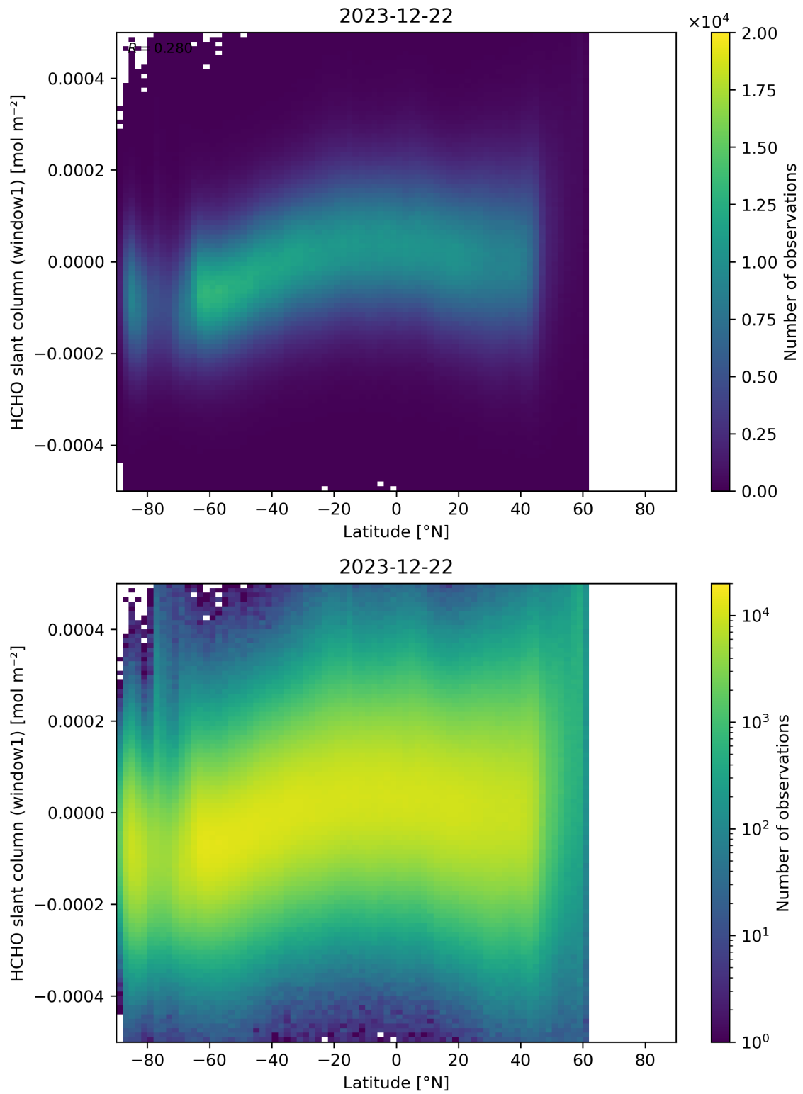
Figure 159: Scatter density plot of “Latitude” against “HCHO slant column (window1)” for 2023-12-21 to 2023-12-23.
