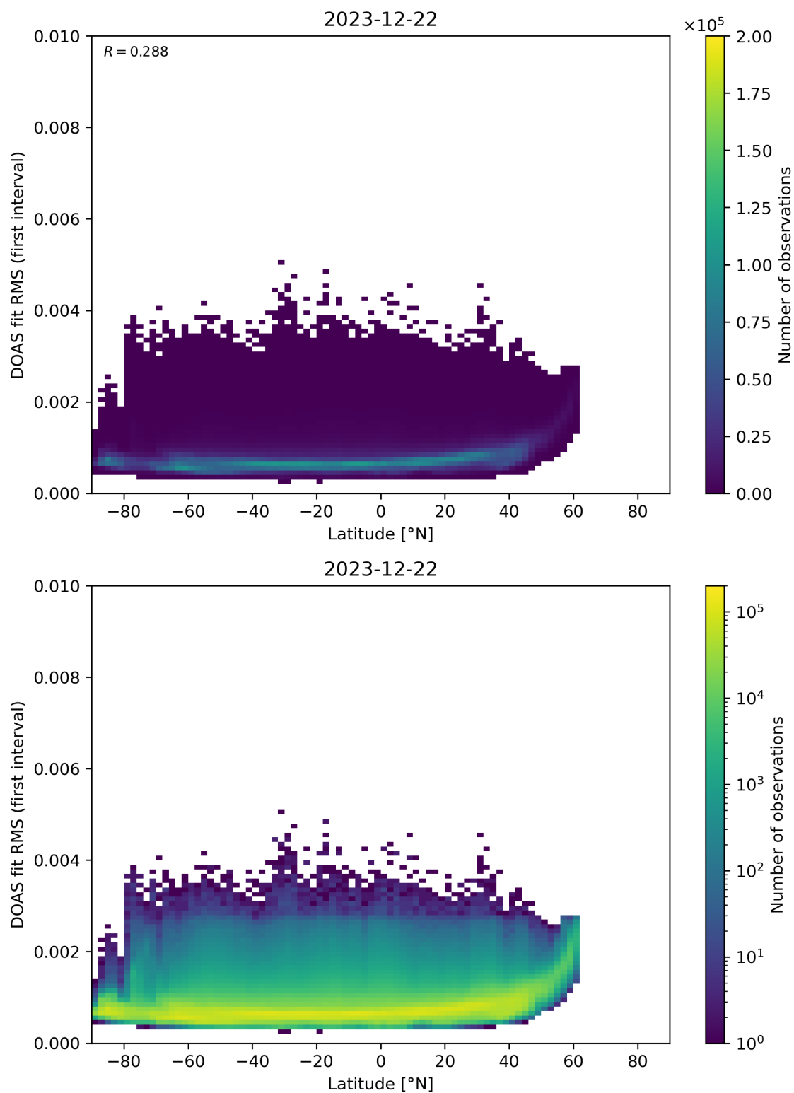
Figure 153: Scatter density plot of “Latitude” against “DOAS fit RMS (first interval)” for 2023-12-21 to 2023-12-23.
