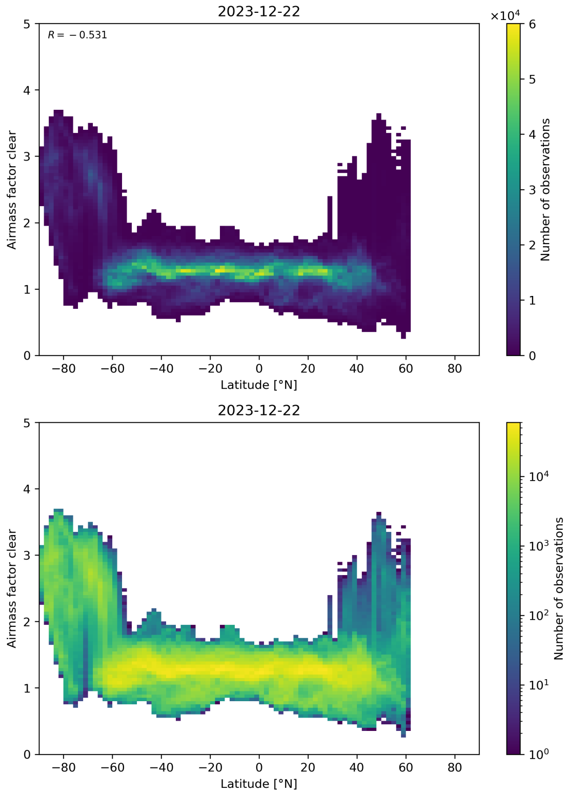
Figure 156: Scatter density plot of “Latitude” against “Airmass factor clear” for 2023-12-21 to 2023-12-23.
