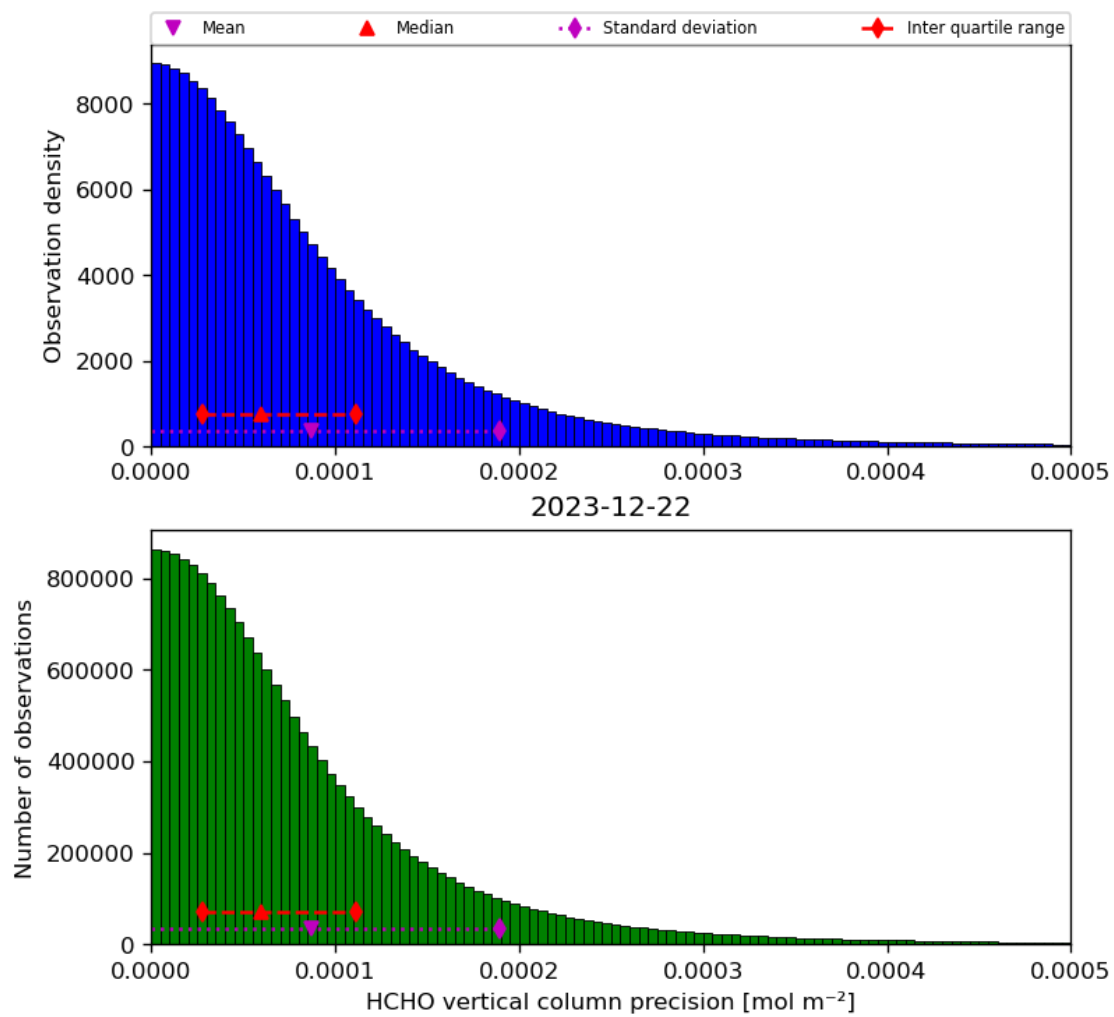
Figure 36: Histogram of “HCHO vertical column precision” for 2023-12-21 to 2023-12-23
