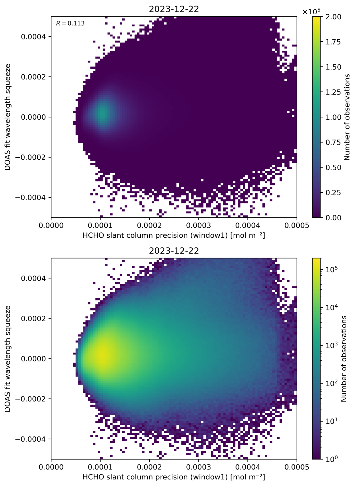
Figure 90: Scatter density plot of “HCHO slant column precision (window1)” against “DOAS fit wavelength squeeze” for 2023-12-21 to 2023-12-23.
