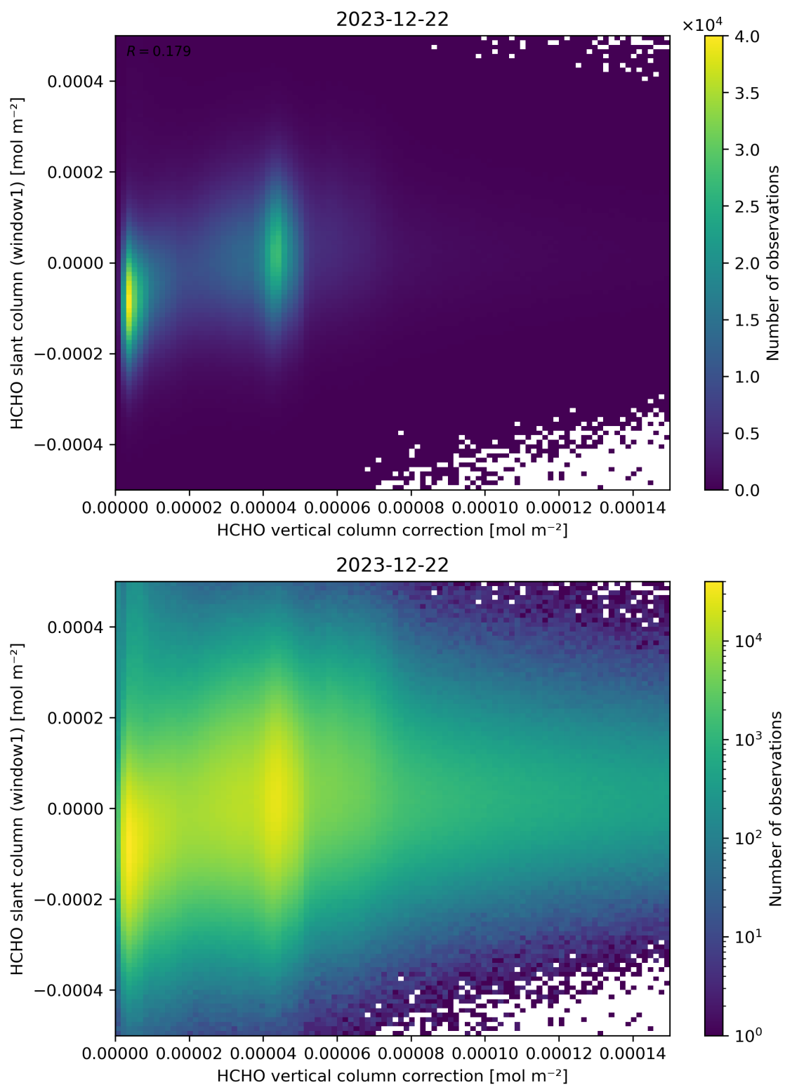
Figure 118: Scatter density plot of “HCHO vertical column correction” against “HCHO slant column (window1)” for 2023-12-21 to 2023-12-23.
