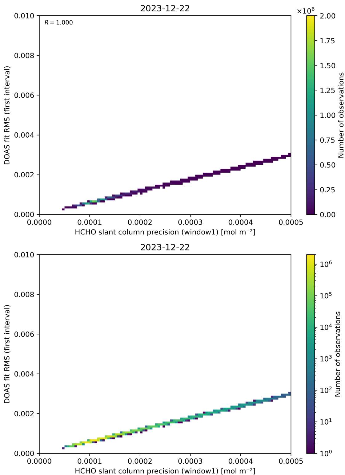
Figure 88: Scatter density plot of “HCHO slant column precision (window1)” against “DOAS fit RMS (first interval)” for 2023-12-21 to 2023-12-23.
