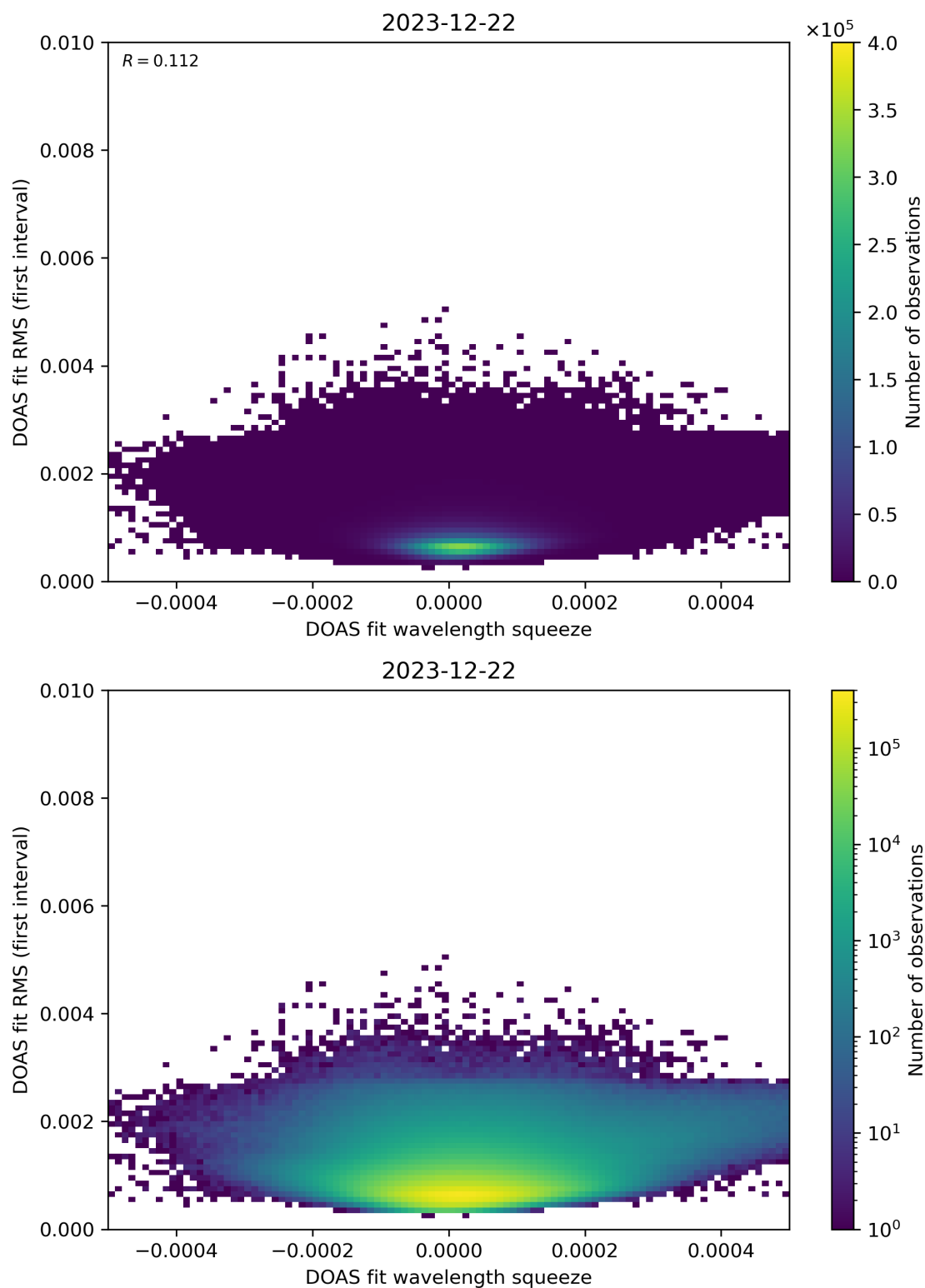
Figure 68: Scatter density plot of “DOAS fit wavelength squeeze” against “DOAS fit RMS (first interval)” for 2023-12-21 to 2023-12-23.
