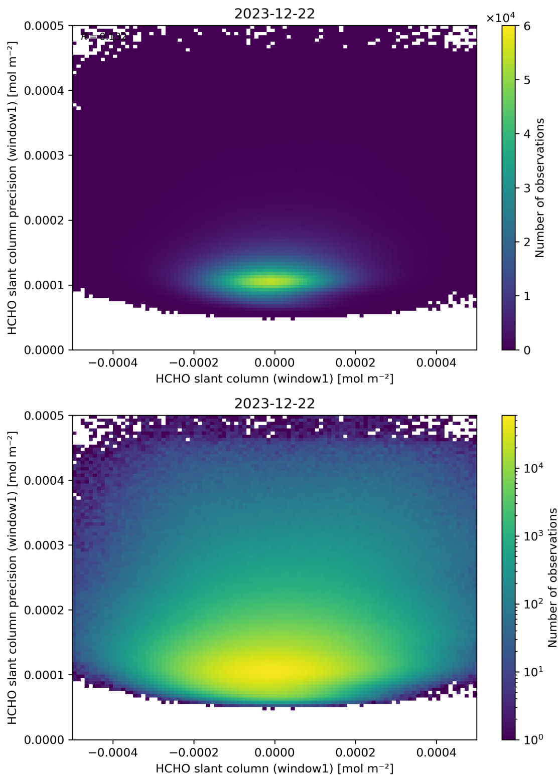
Figure 84: Scatter density plot of “HCHO slant column (window1)” against “HCHO slant column precision (window1)” for 2023-12-21 to 2023-12-23.
