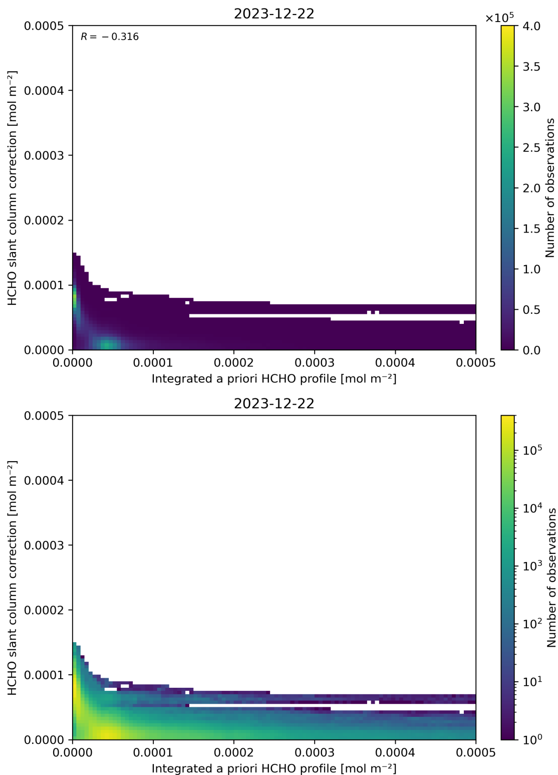
Figure 152: Scatter density plot of “Integrated a priori HCHO profile” against “HCHO slant column correction” for 2023-12-21 to 2023-12-23.
