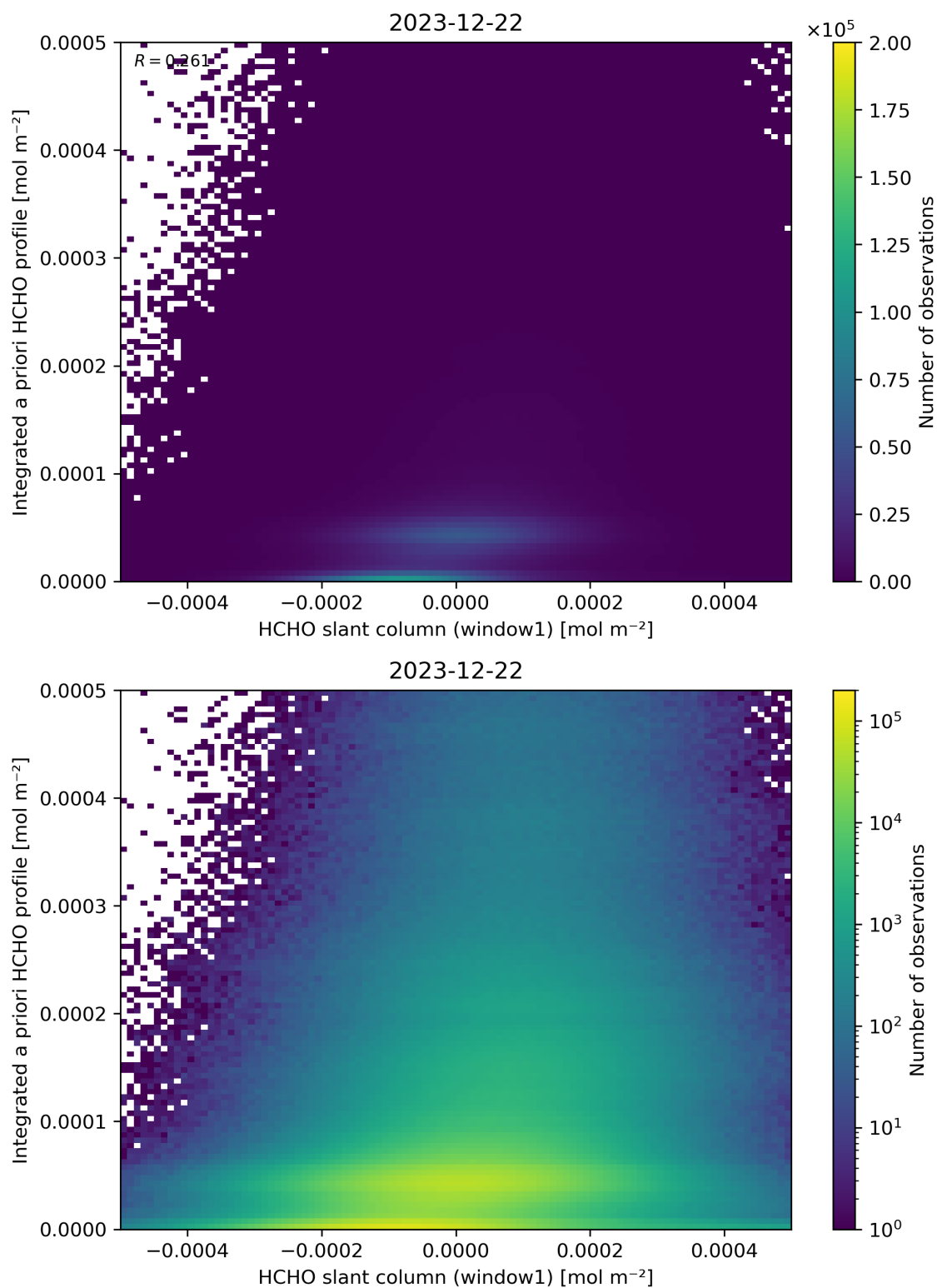
Figure 87: Scatter density plot of “HCHO slant column (window1)” against “Integrated a priori HCHO profile” for 2023-12-21 to 2023-12-23.
