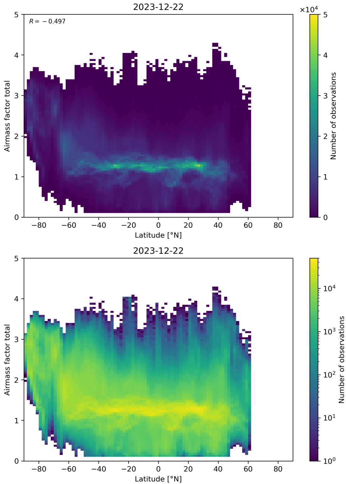
Figure 161: Scatter density plot of “Latitude” against “Airmass factor total” for 2023-12-21 to 2023-12-23.
