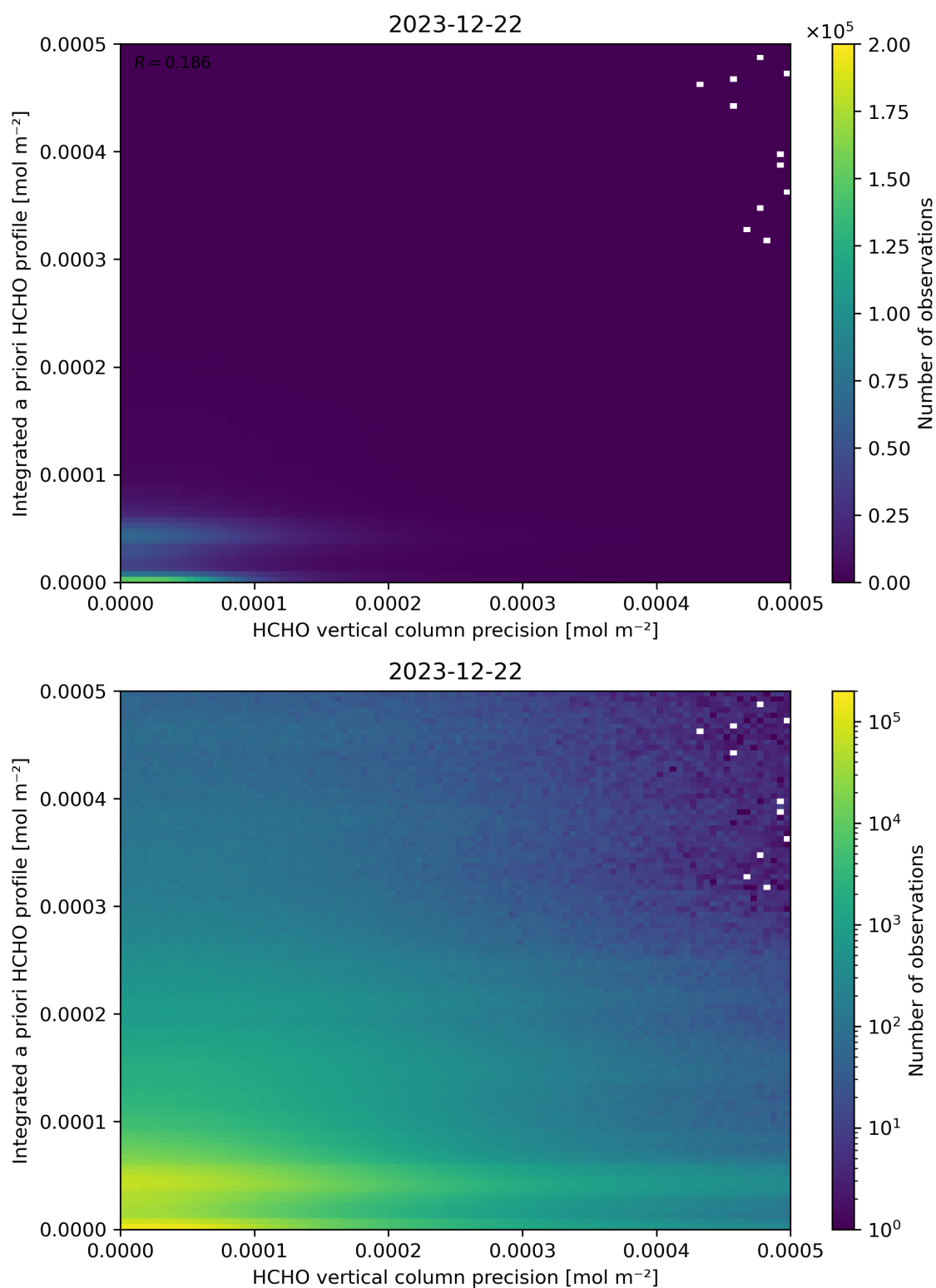
Figure 147: Scatter density plot of “HCHO vertical column precision” against “Integrated a priori HCHO profile” for 2023-12-21 to 2023-12-23.
