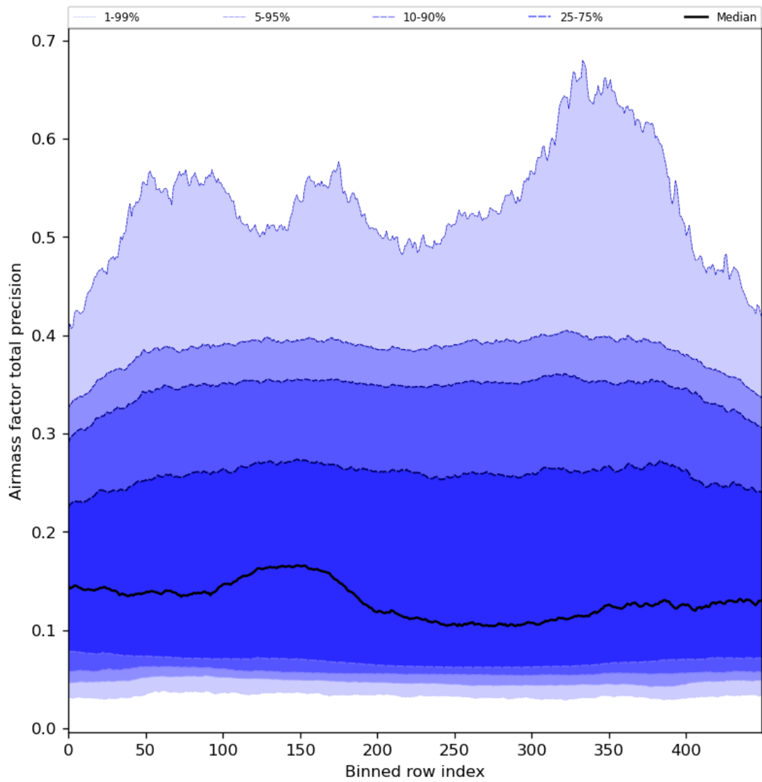
Figure 55: Along track statistics of “Airmass factor total precision” for 2023-12-21 to 2023-12-23
