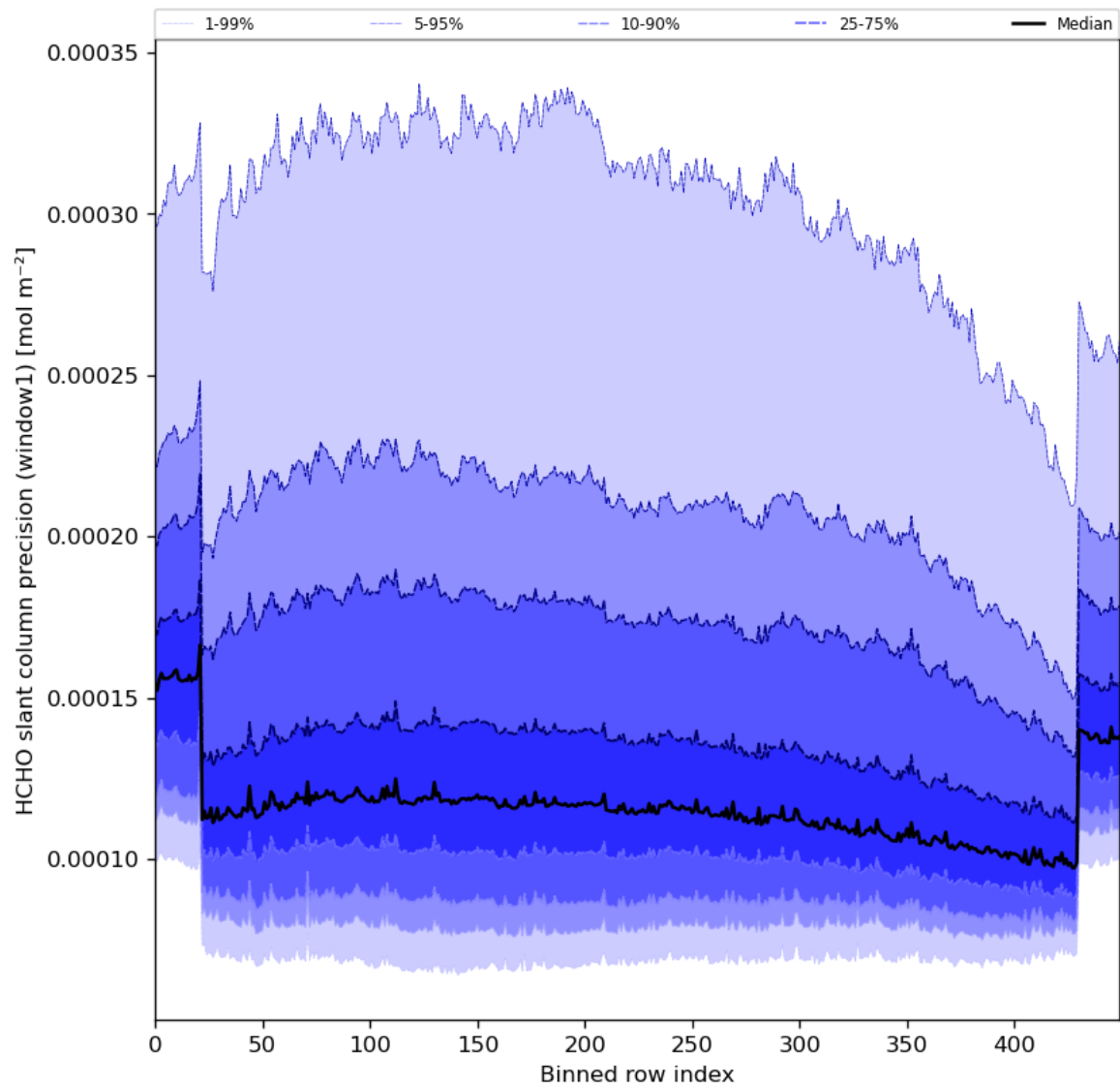
Figure 53: Along track statistics of “HCHO slant column precision (window1)” for 2023-12-21 to 2023-12-23
