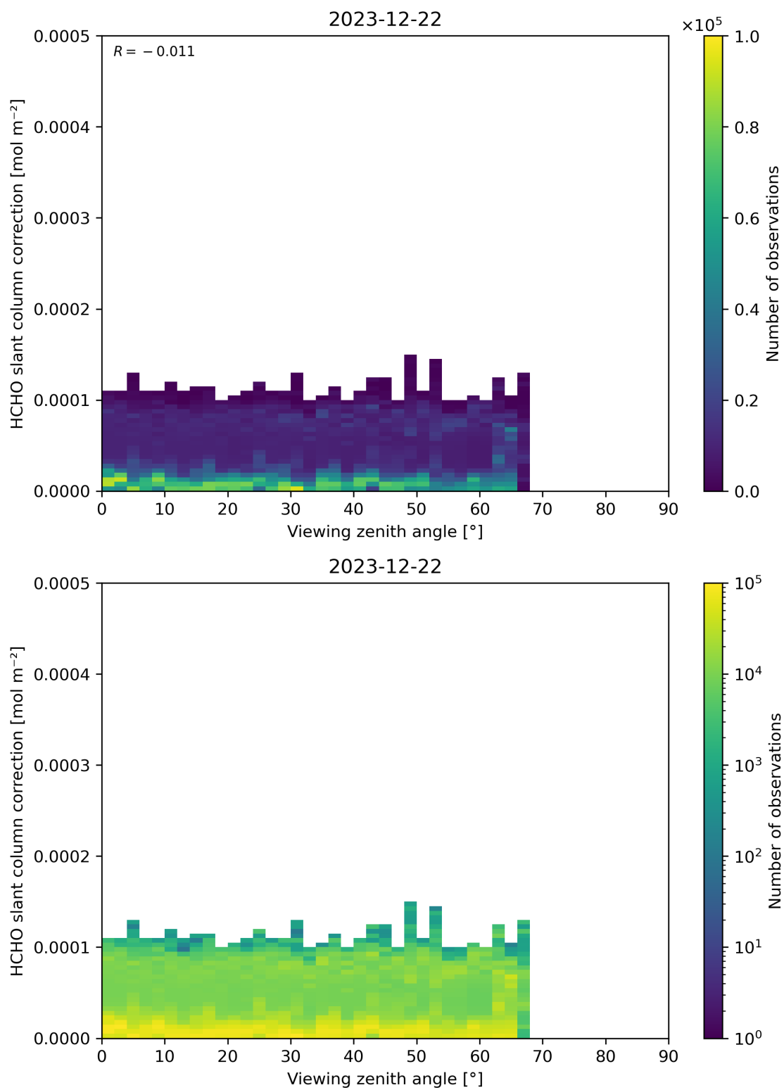
Figure 187: Scatter density plot of “Viewing zenith angle” against “HCHO slant column correction” for 2023-12-21 to 2023-12-23.
