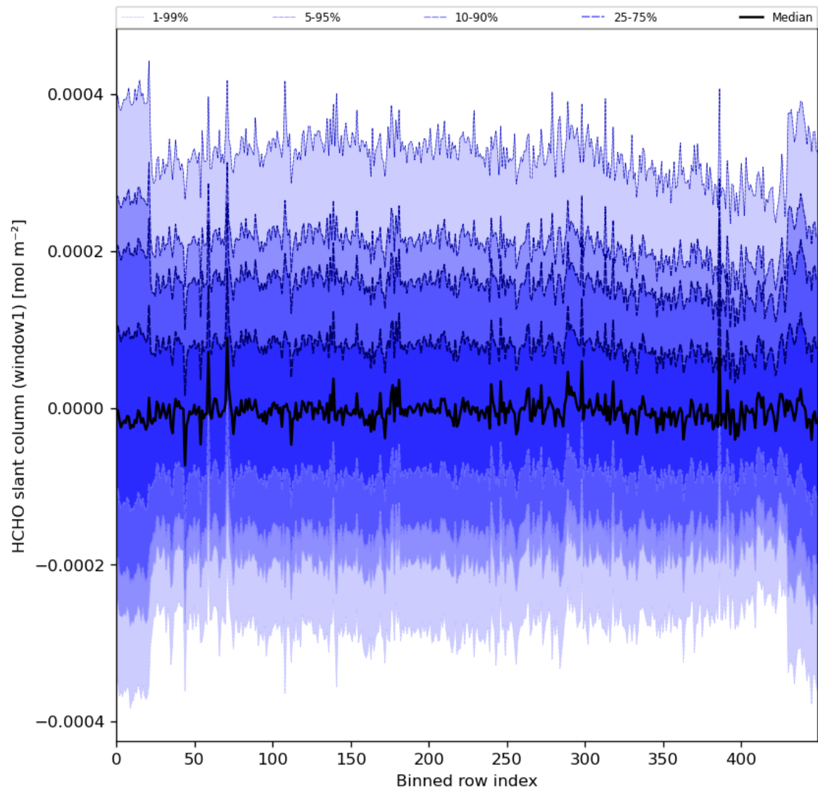
Figure 52: Along track statistics of “HCHO slant column (window1)” for 2023-12-21 to 2023-12-23
