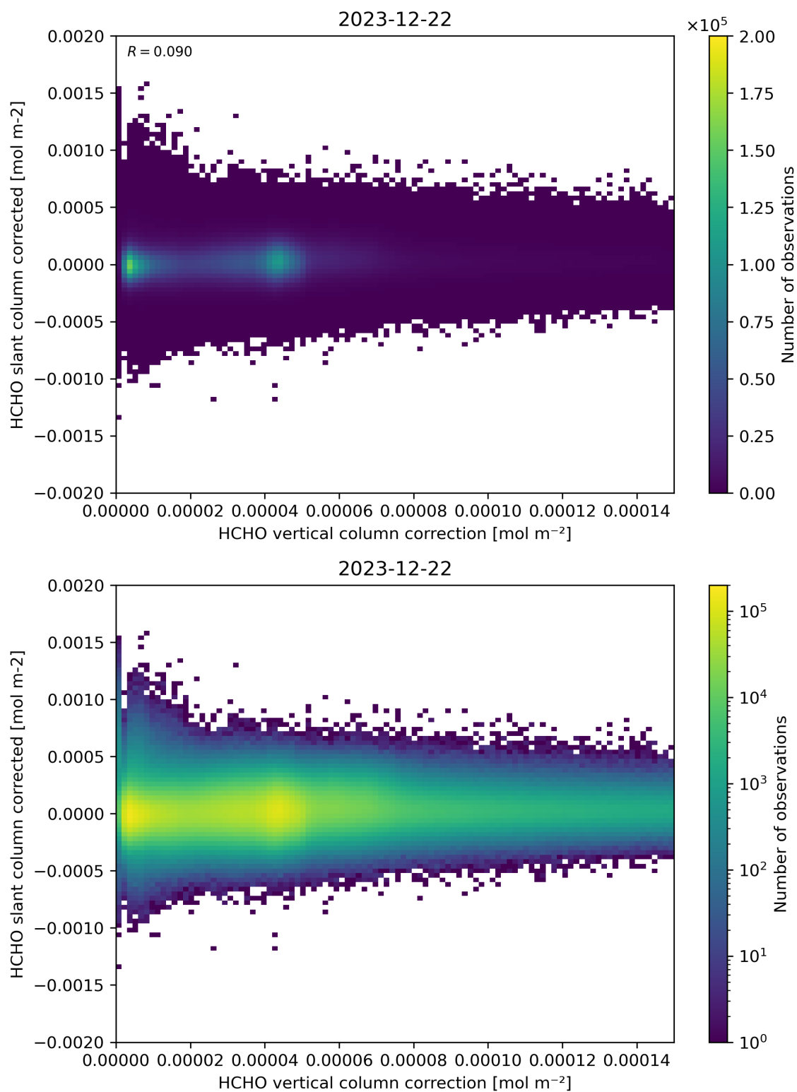
Figure 116: Scatter density plot of “HCHO vertical column correction” against “HCHO slant column corrected” for 2023-12-21 to 2023-12-23.
