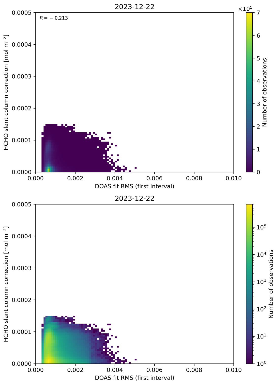
Figure 63: Scatter density plot of “DOAS fit RMS (first interval)” against “HCHO slant column correction” for 2023-12-21 to 2023-12-23.
