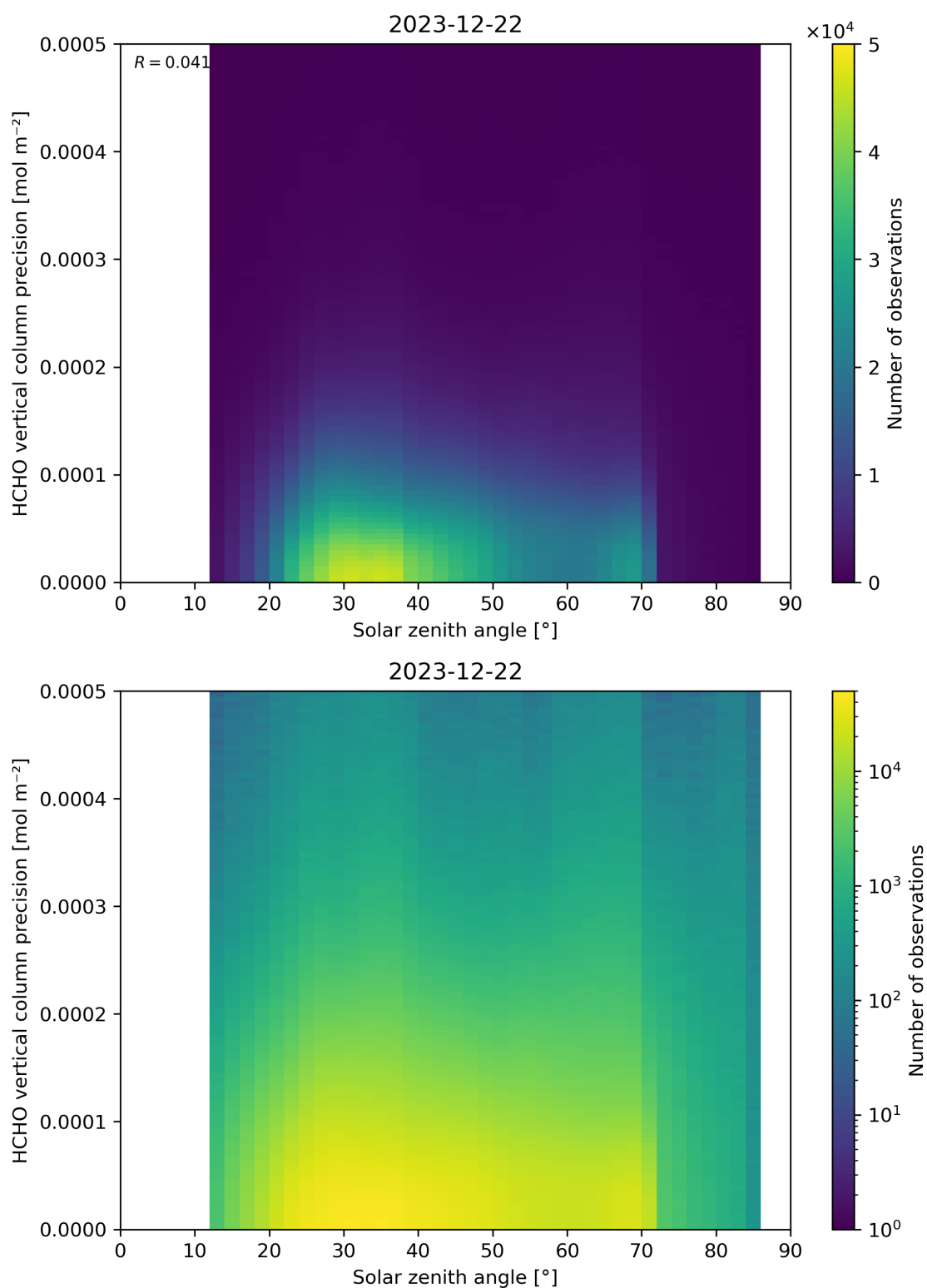
Figure 179: Scatter density plot of “Solar zenith angle” against “HCHO vertical column precision” for 2023-12-21 to 2023-12-23.
