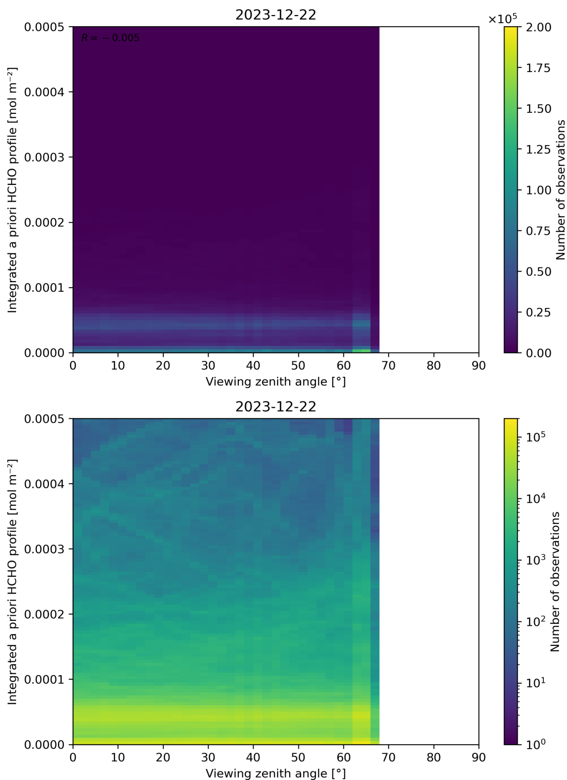
Figure 195: Scatter density plot of “Viewing zenith angle” against “Integrated a priori HCHO profile” for 2023-12-21 to 2023-12-23.
