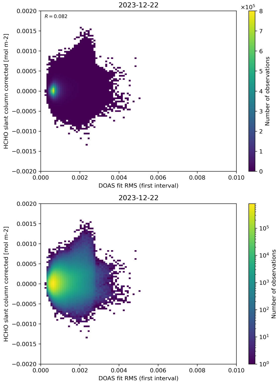
Figure 62: Scatter density plot of “DOAS fit RMS (first interval)” against “HCHO slant column corrected” for 2023-12-21 to 2023-12-23.
