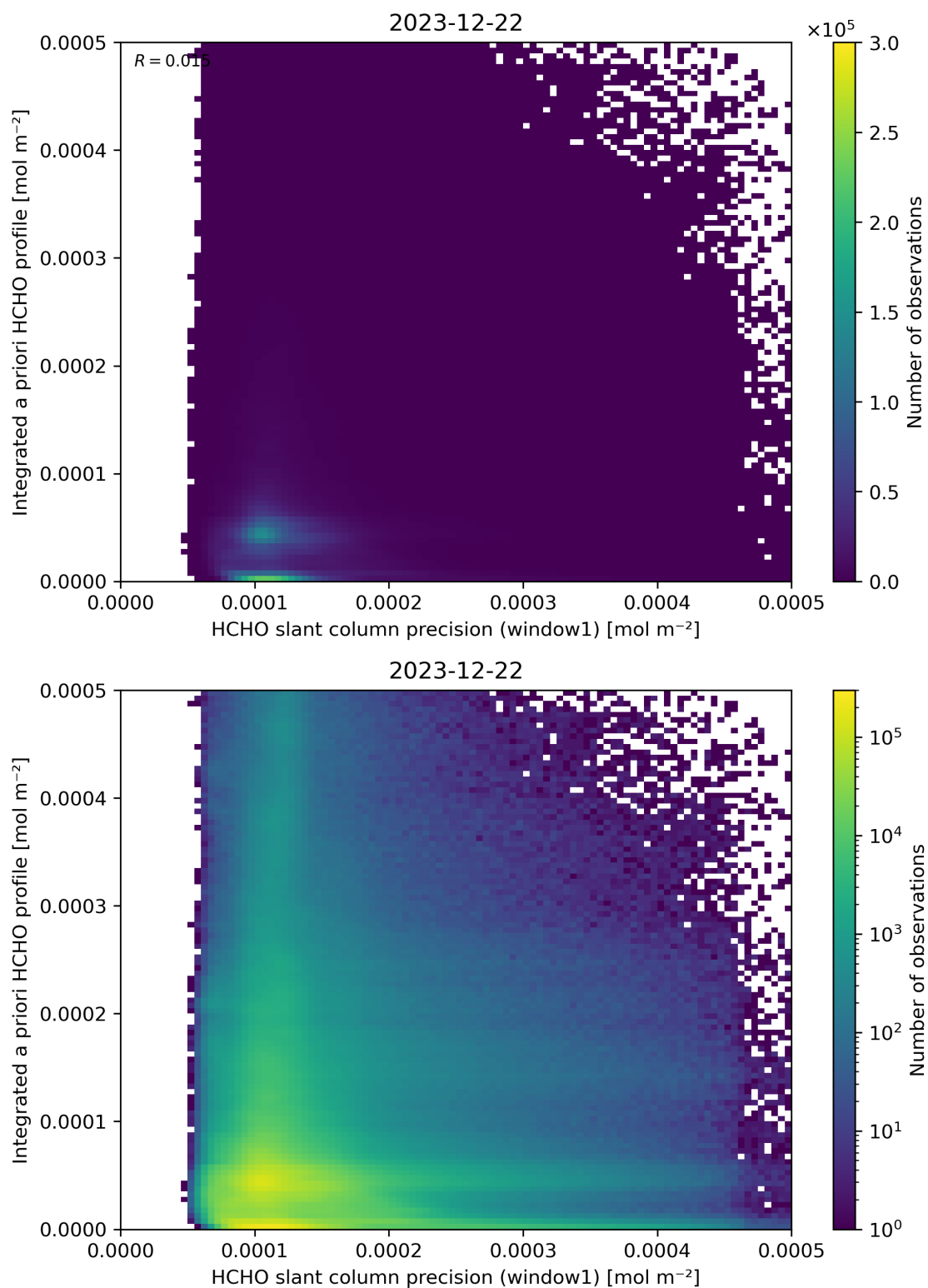
Figure 96: Scatter density plot of “HCHO slant column precision (window1)” against “Integrated a priori HCHO profile” for 2023-12-21 to 2023-12-23.
