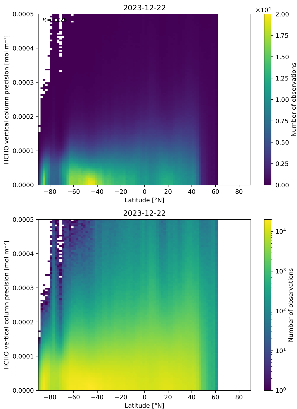
Figure 165: Scatter density plot of “Latitude” against “HCHO vertical column precision” for 2023-12-21 to 2023-12-23.
