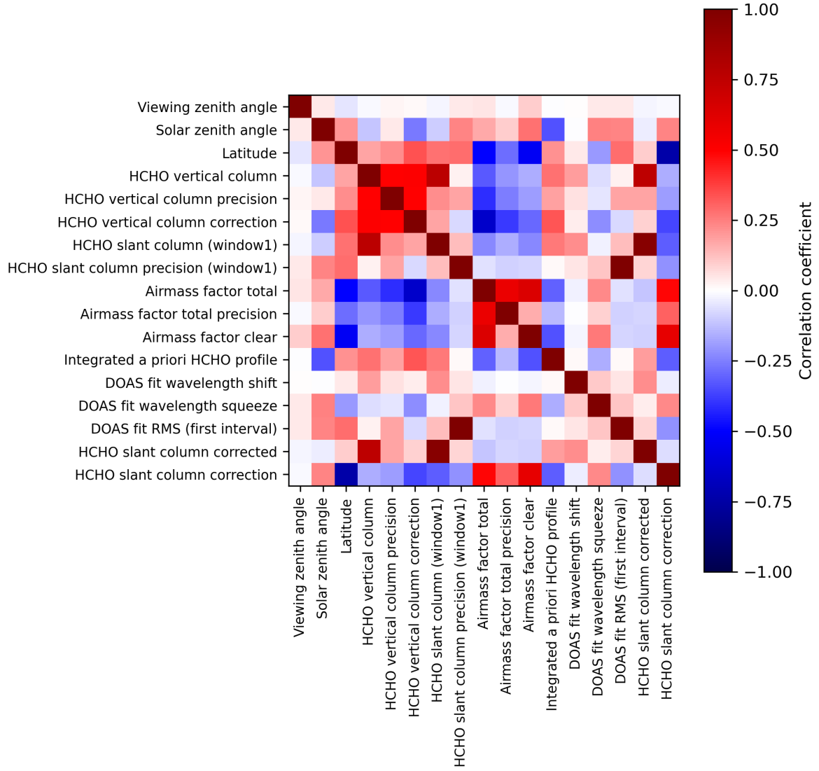
Figure 2: Map of correlation matrix for 2023-12-21 to 2023-12-23.
