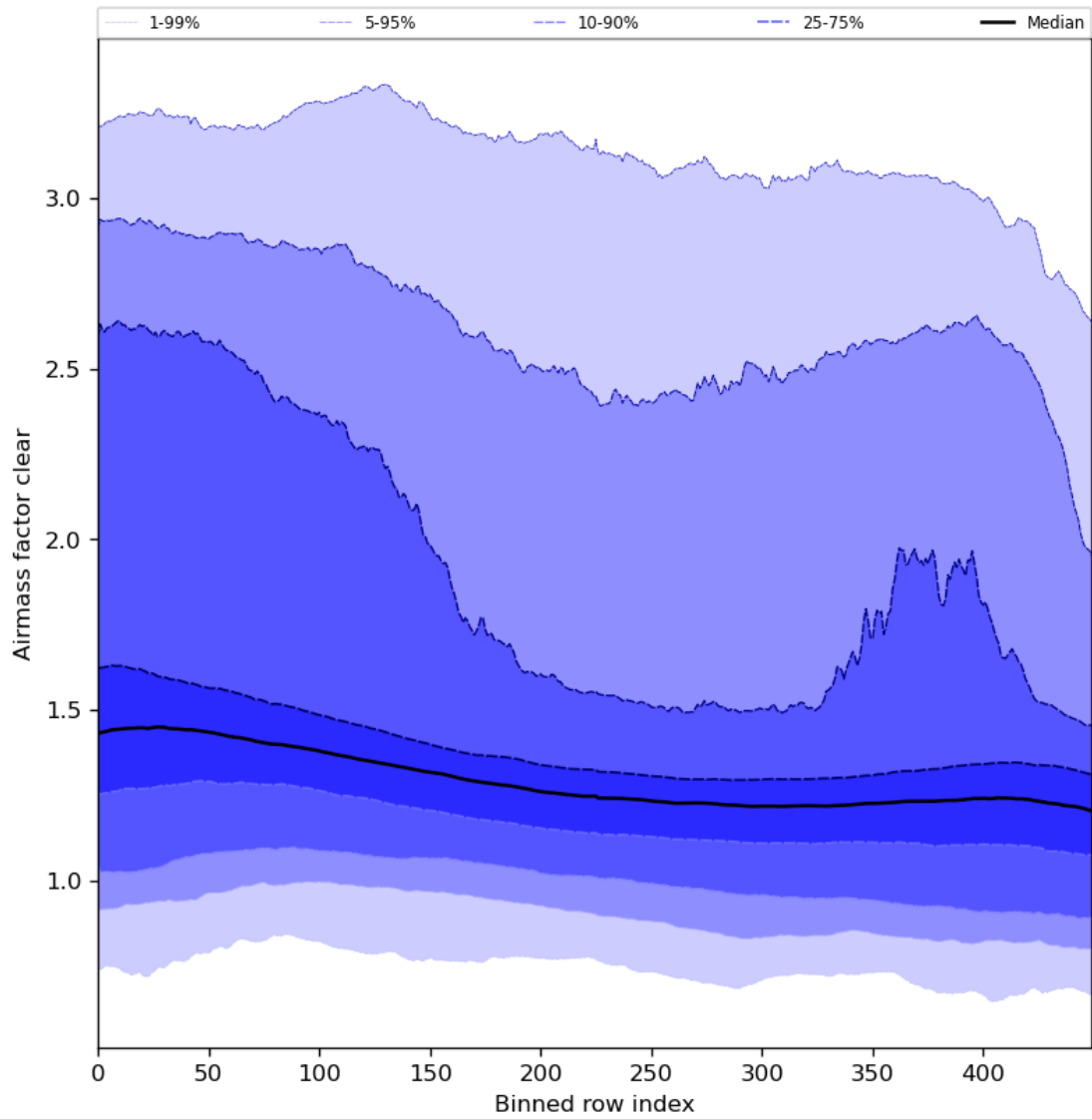
Figure 56: Along track statistics of “Airmass factor clear” for 2023-12-21 to 2023-12-23
