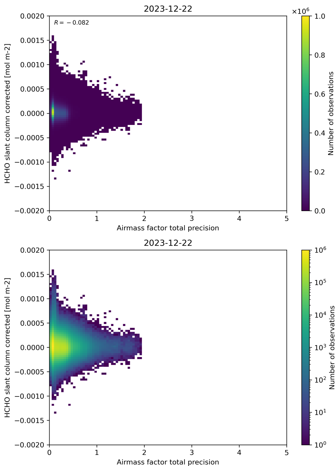
Figure 109: Scatter density plot of “Airmass factor total precision” against “HCHO slant column corrected” for 2023-12-21 to 2023-12-23.
