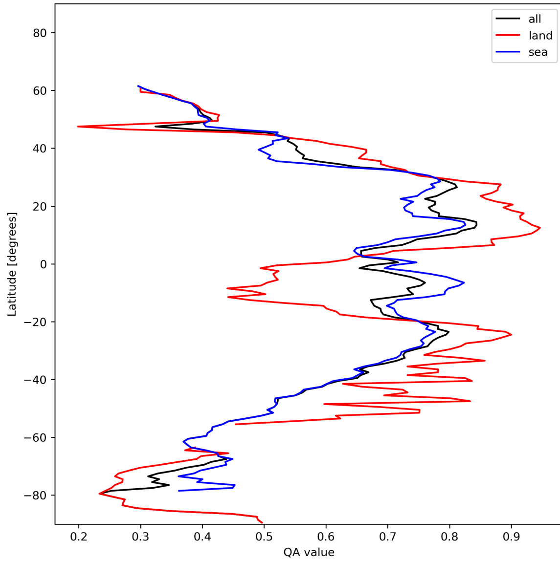
Figure 20: Zonal average of “QA value” for 2023-12-21 to 2023-12-23.
