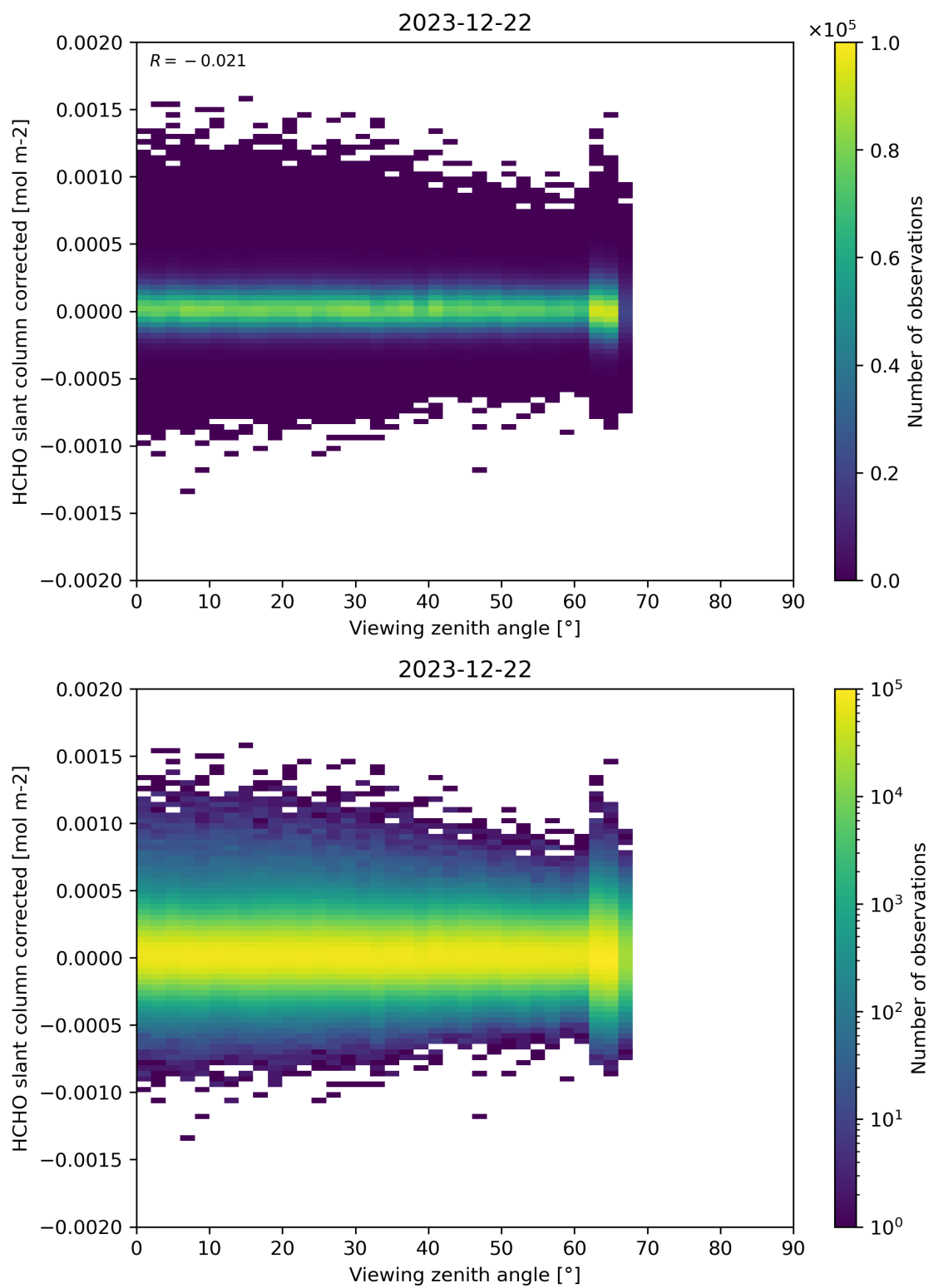
Figure 186: Scatter density plot of “Viewing zenith angle” against “HCHO slant column corrected” for 2023-12-21 to 2023-12-23.
