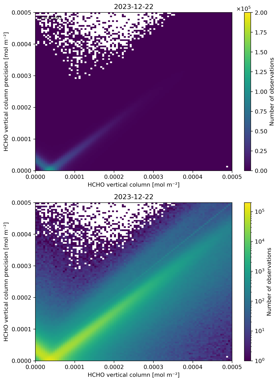
Figure 134: Scatter density plot of “HCHO vertical column” against “HCHO vertical column precision” for 2023-12-21 to 2023-12-23.
