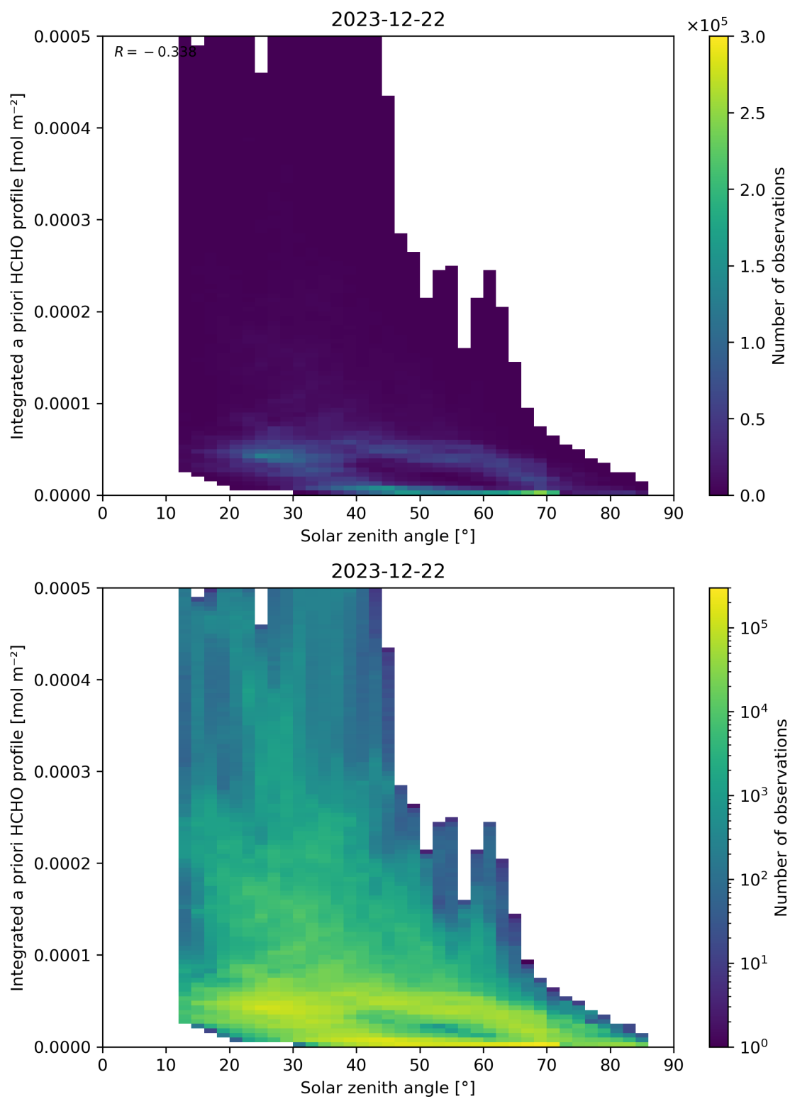
Figure 180: Scatter density plot of “Solar zenith angle” against “Integrated a priori HCHO profile” for 2023-12-21 to 2023-12-23.
