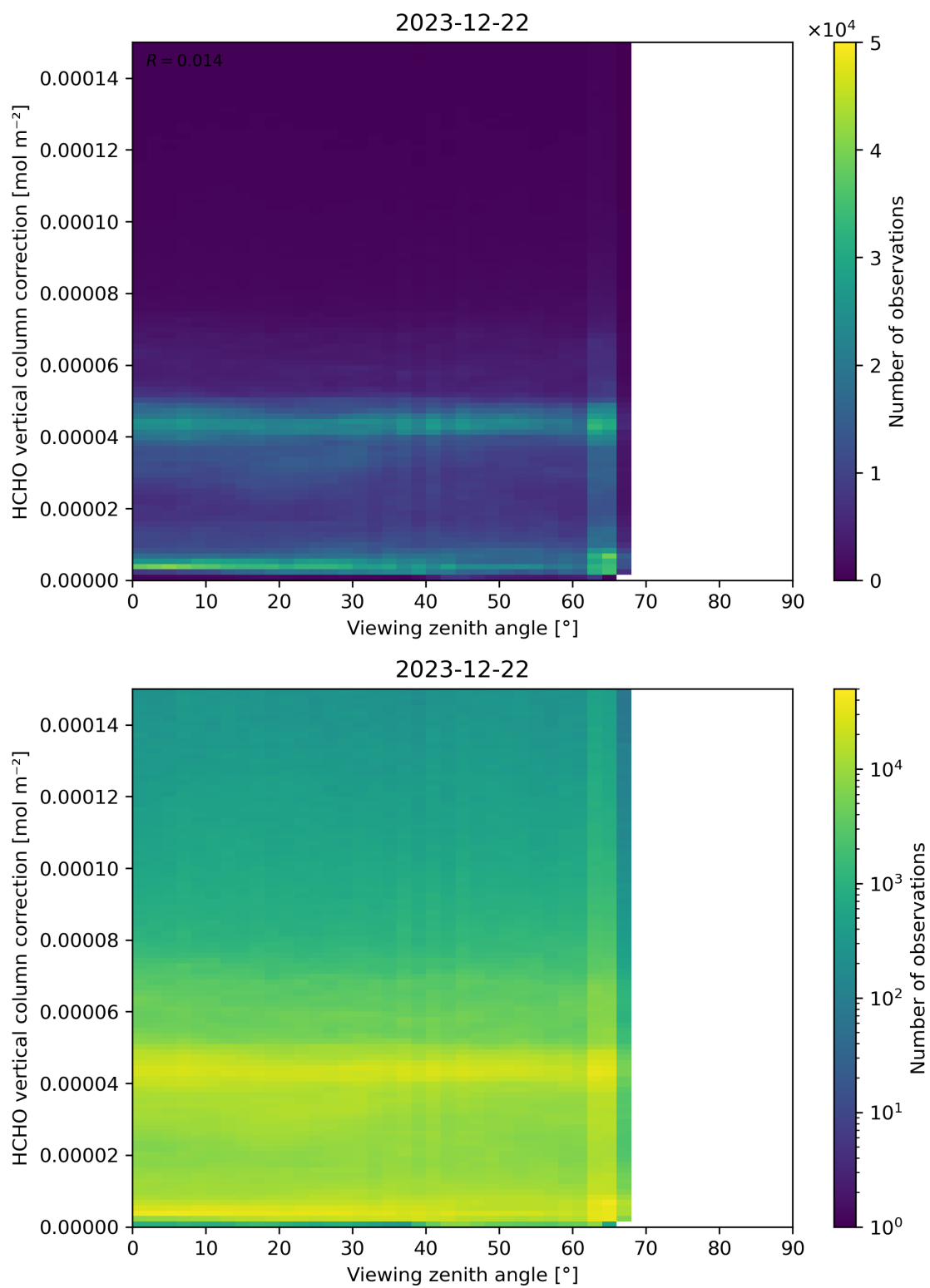
Figure 193: Scatter density plot of “Viewing zenith angle” against “HCHO vertical column correction” for 2023-12-21 to 2023-12-23.
