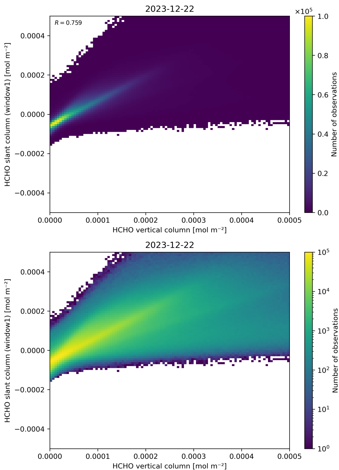
Figure 129: Scatter density plot of “HCHO vertical column” against “HCHO slant column (window1)” for 2023-12-21 to 2023-12-23.
