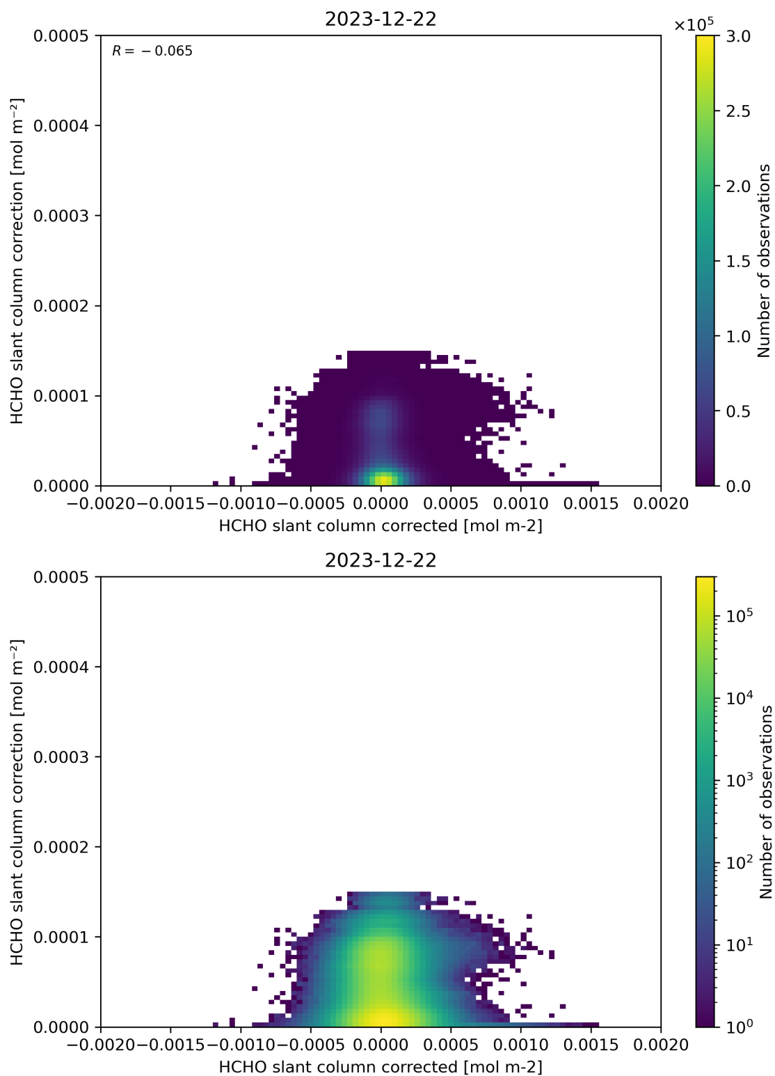
Figure 77: Scatter density plot of “HCHO slant column corrected” against “HCHO slant column correction” for 2023-12-21 to 2023-12-23.
