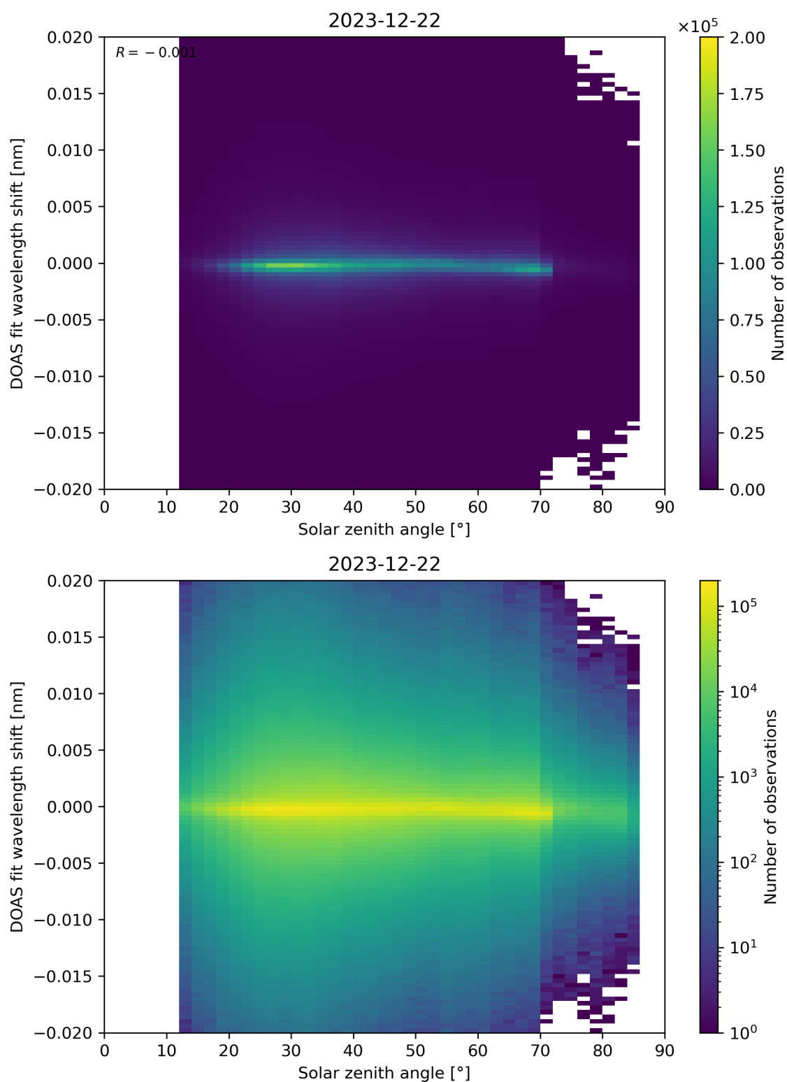
Figure 168: Scatter density plot of “Solar zenith angle” against “DOAS fit wavelength shift” for 2023-12-21 to 2023-12-23.
