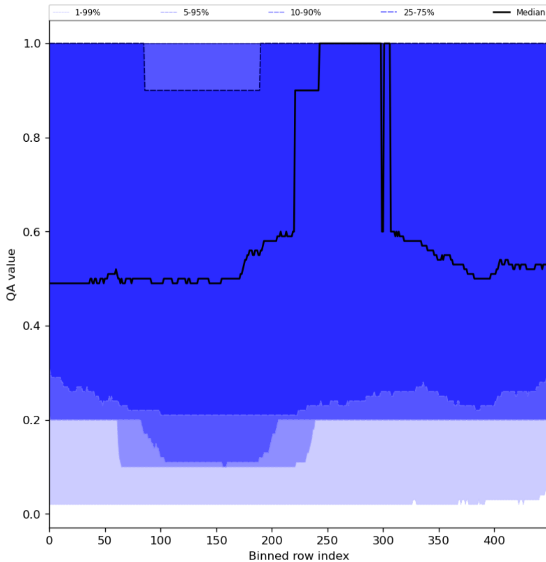
Figure 48: Along track statistics of "QA value" for 2023-12-21 to 2023-12-23
