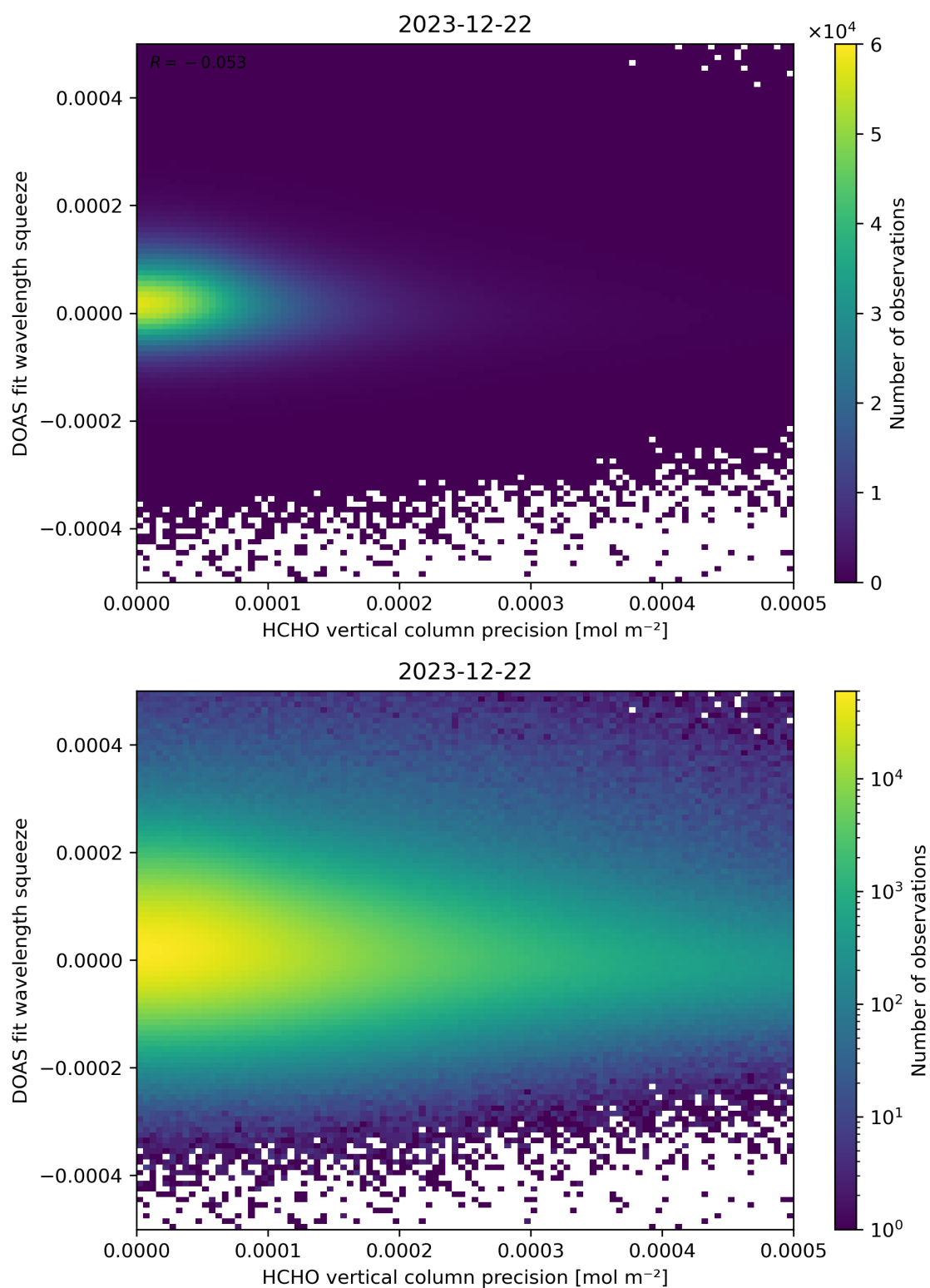
Figure 138: Scatter density plot of “HCHO vertical column precision” against “DOAS fit wavelength squeeze” for 2023-12-21 to 2023-12-23.
