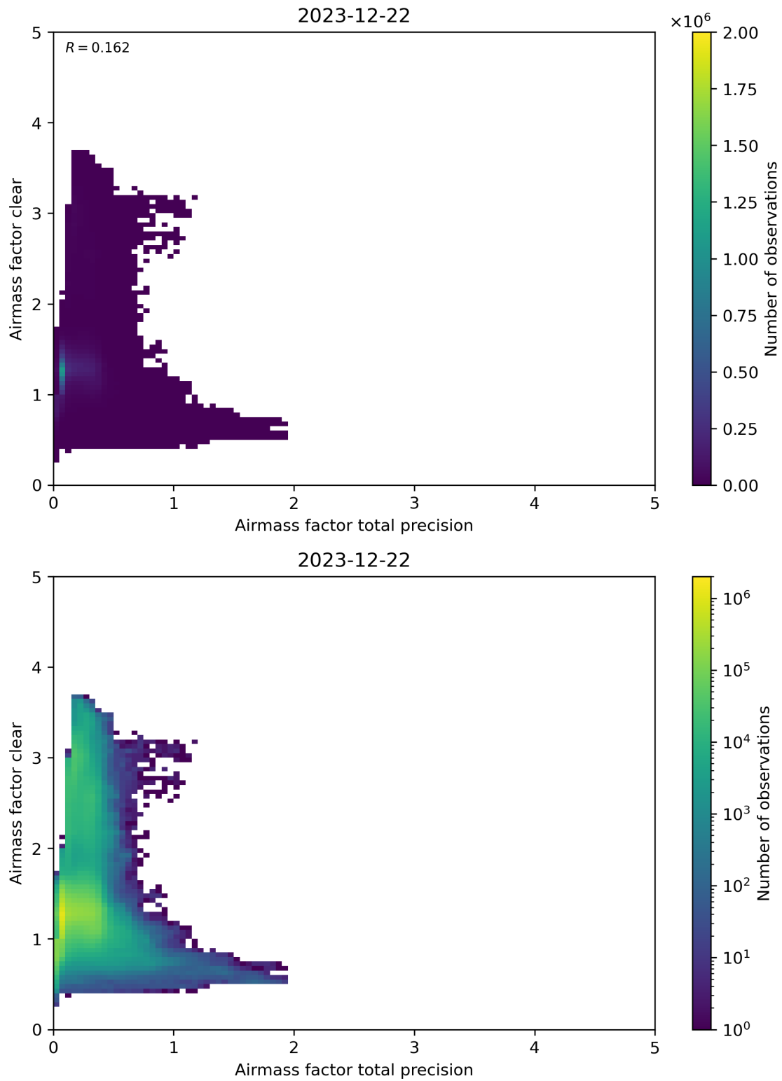
Figure 108: Scatter density plot of “Airmass factor total precision” against “Airmass factor clear” for 2023-12-21 to 2023-12-23.
