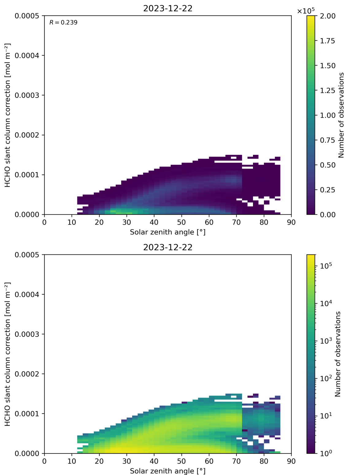
Figure 172: Scatter density plot of “Solar zenith angle” against “HCHO slant column correction” for 2023-12-21 to 2023-12-23.
