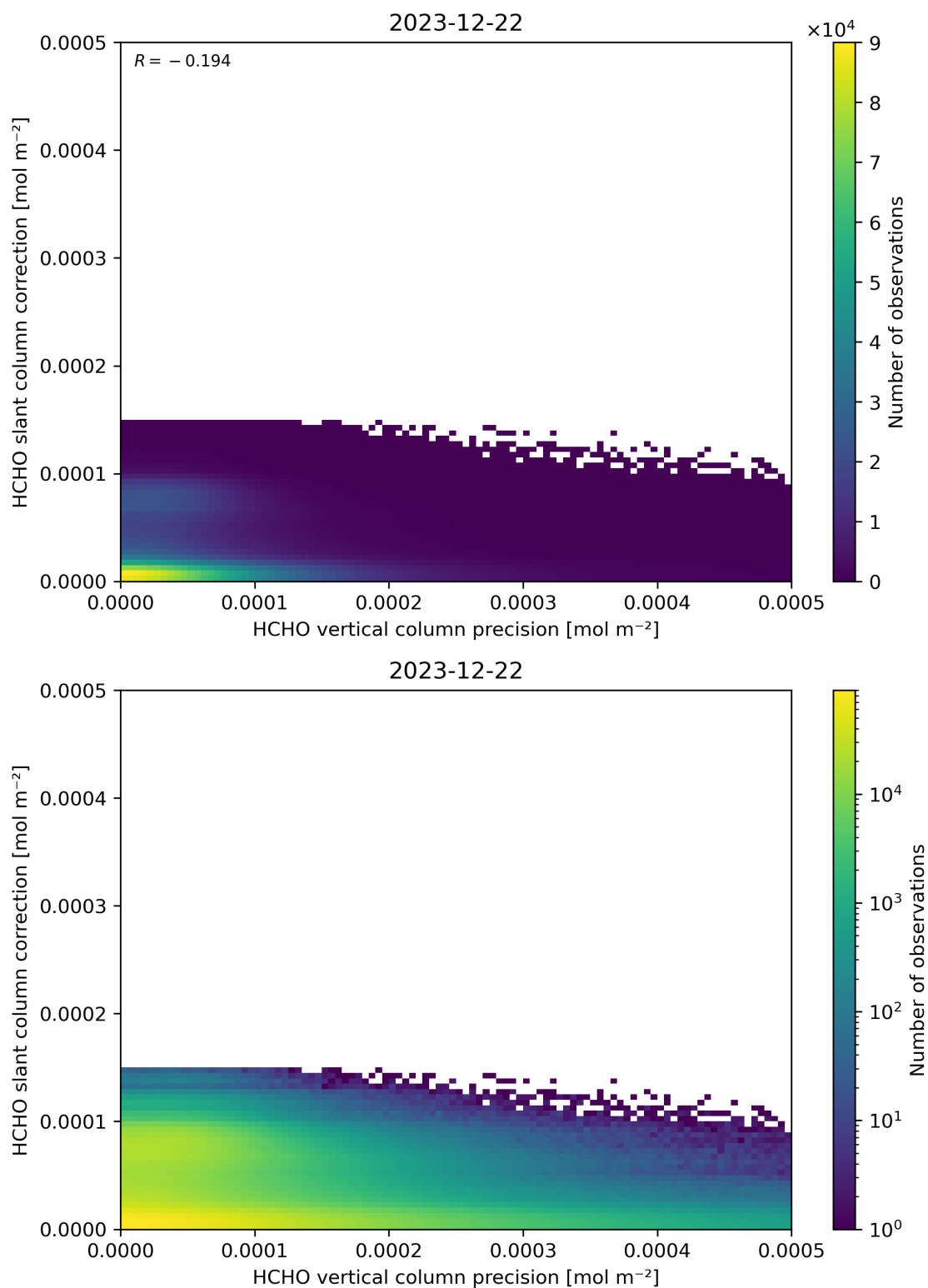
Figure 141: Scatter density plot of “HCHO vertical column precision” against “HCHO slant column correction” for 2023-12-21 to 2023-12-23.
