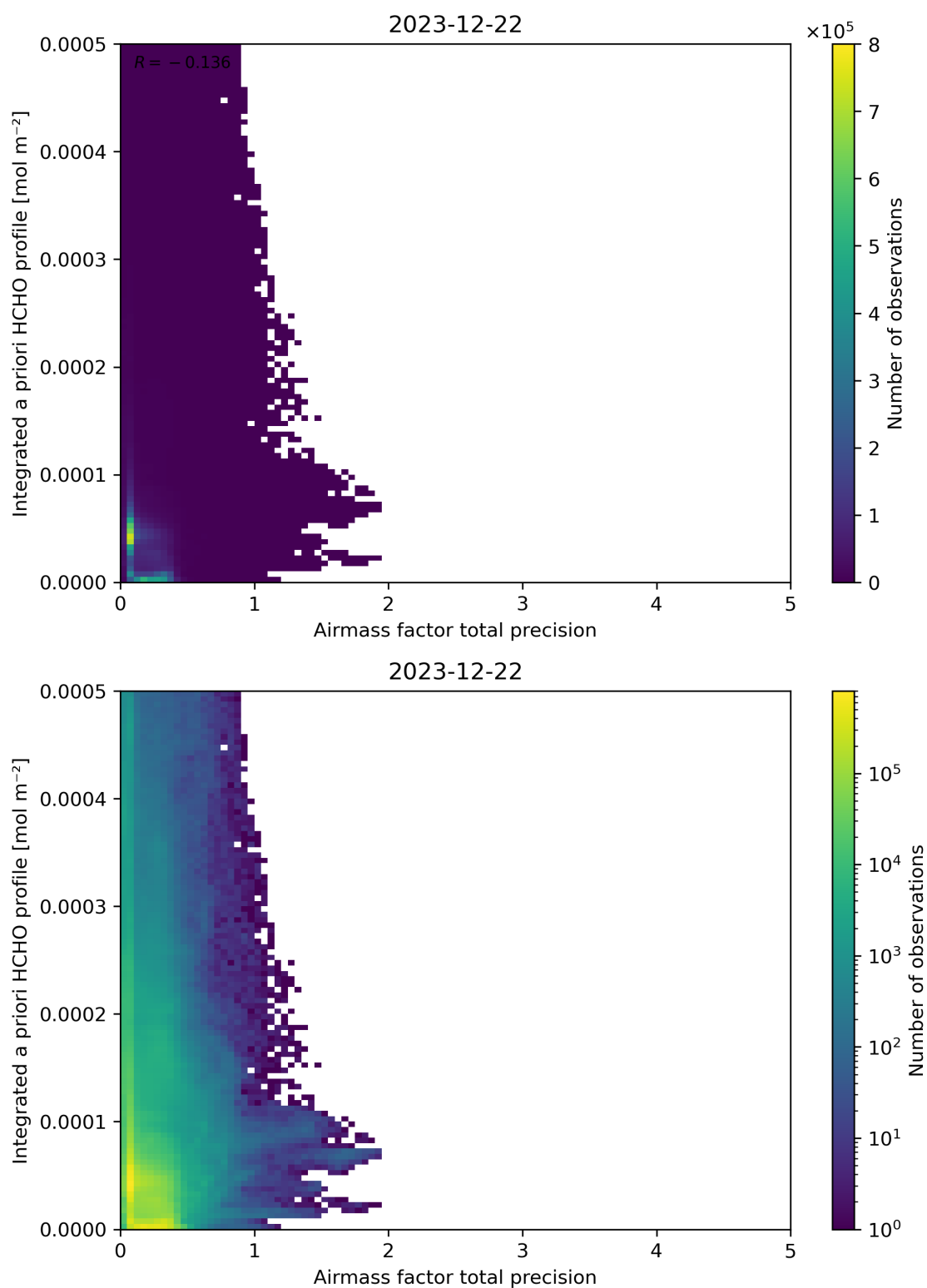
Figure 111: Scatter density plot of “Airmass factor total precision” against “Integrated a priori HCHO profile” for 2023-12-21 to 2023-12-23.
