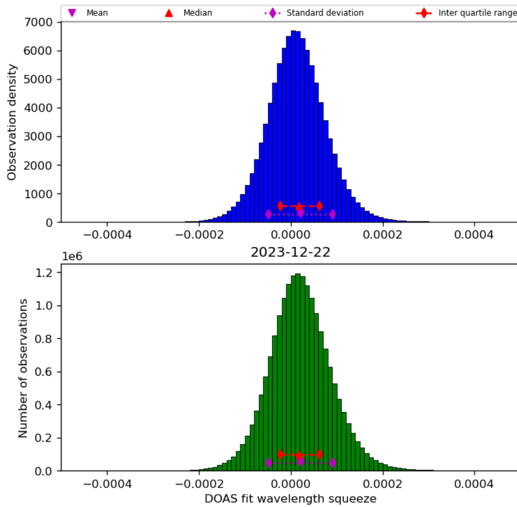
Figure 45: Histogram of “DOAS fit wavelength squeeze” for 2023-12-21 to 2023-12-23
