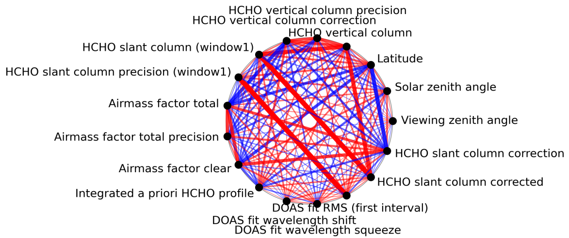
Figure 1: Map of correlation graph for 2023-12-21 to 2023-12-23.
