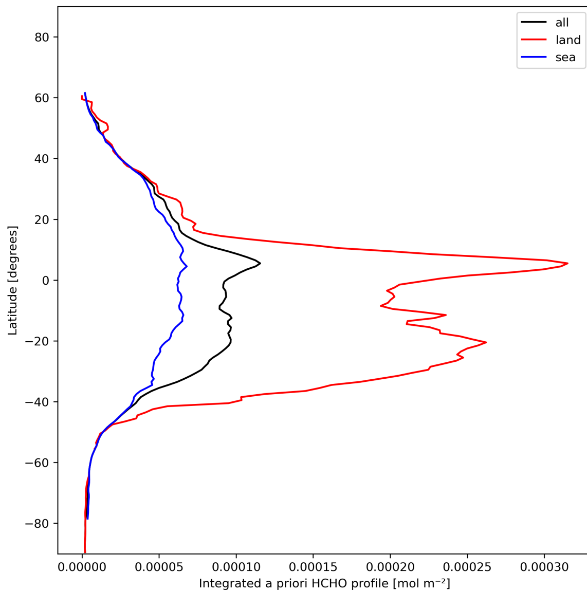
Figure 29: Zonal average of “Integrated a priori HCHO profile” for 2023-12-21 to 2023-12-23.
