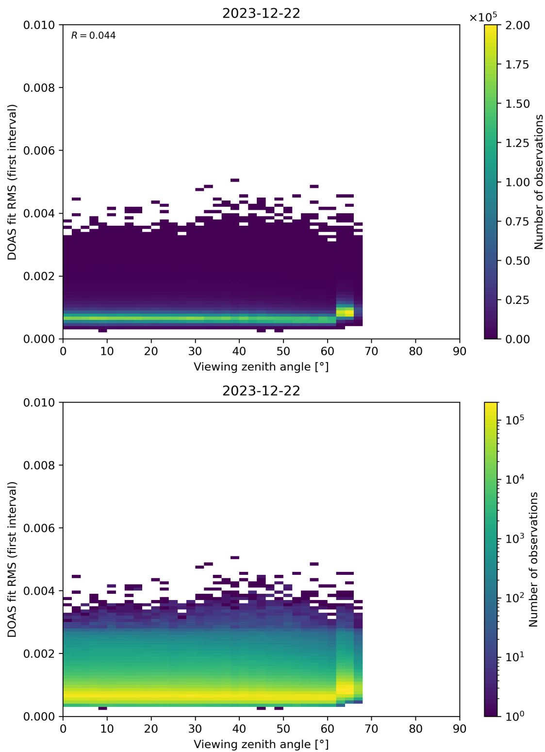
Figure 182: Scatter density plot of “Viewing zenith angle” against “DOAS fit RMS (first interval)” for 2023-12-21 to 2023-12-23.
