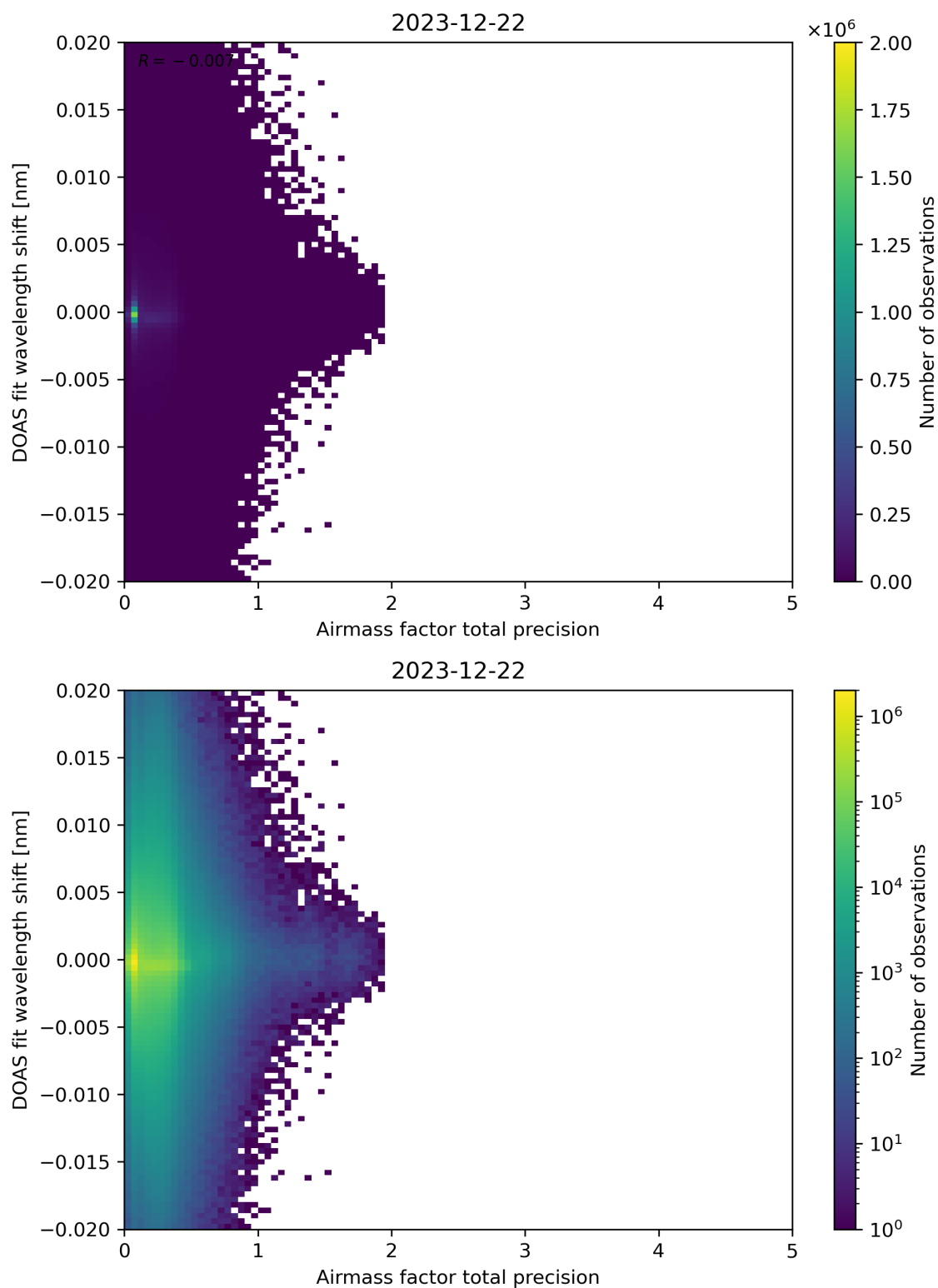
Figure 106: Scatter density plot of “Airmass factor total precision” against “DOAS fit wavelength shift” for 2023-12-21 to 2023-12-23.
