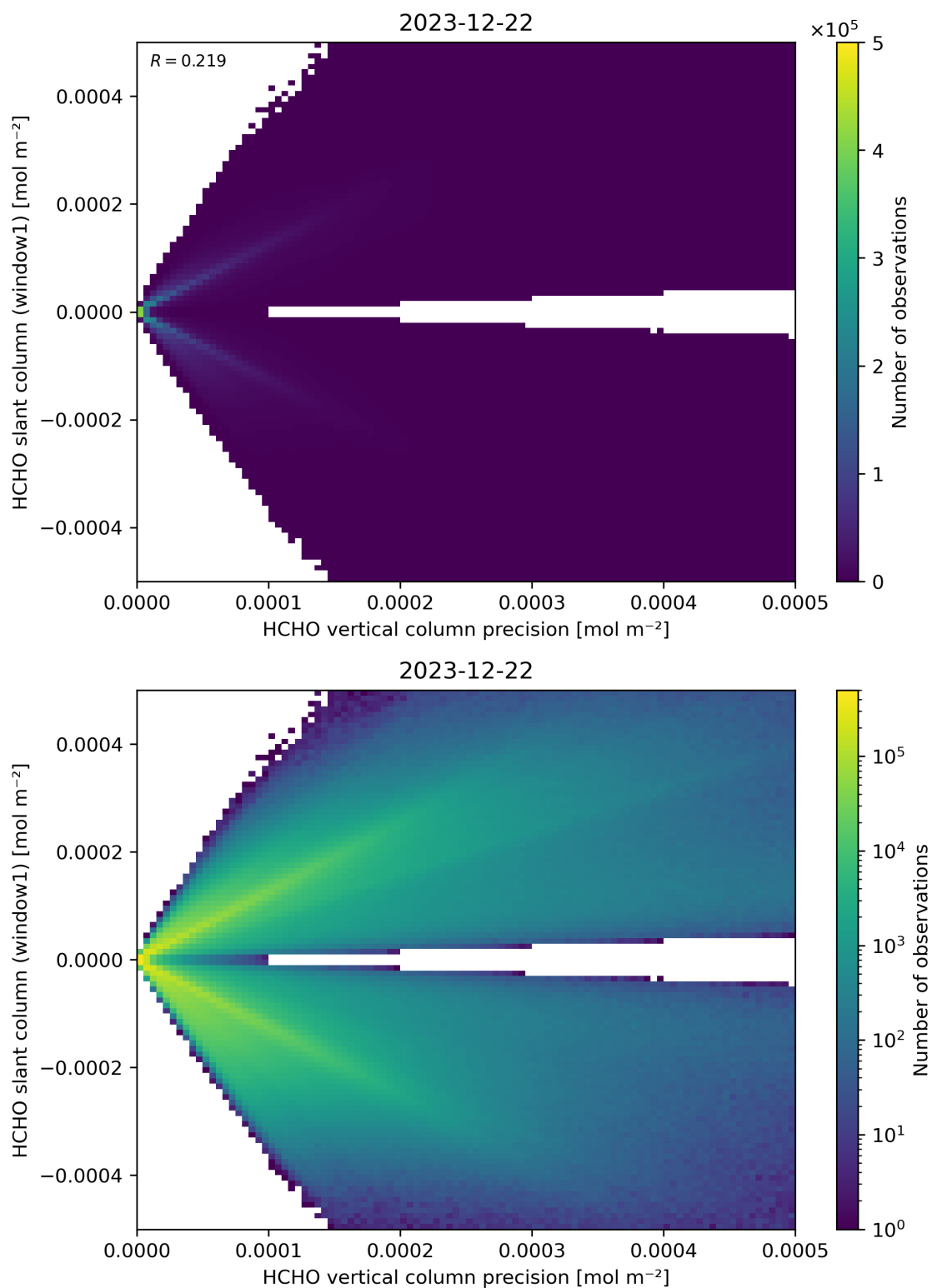
Figure 142: Scatter density plot of “HCHO vertical column precision” against “HCHO slant column (window1)” for 2023-12-21 to 2023-12-23.
