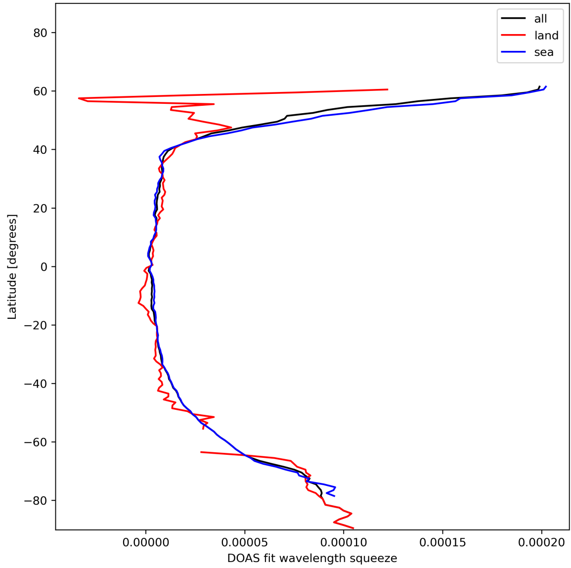
Figure 31: Zonal average of “DOAS fit wavelength squeeze” for 2023-12-21 to 2023-12-23.
