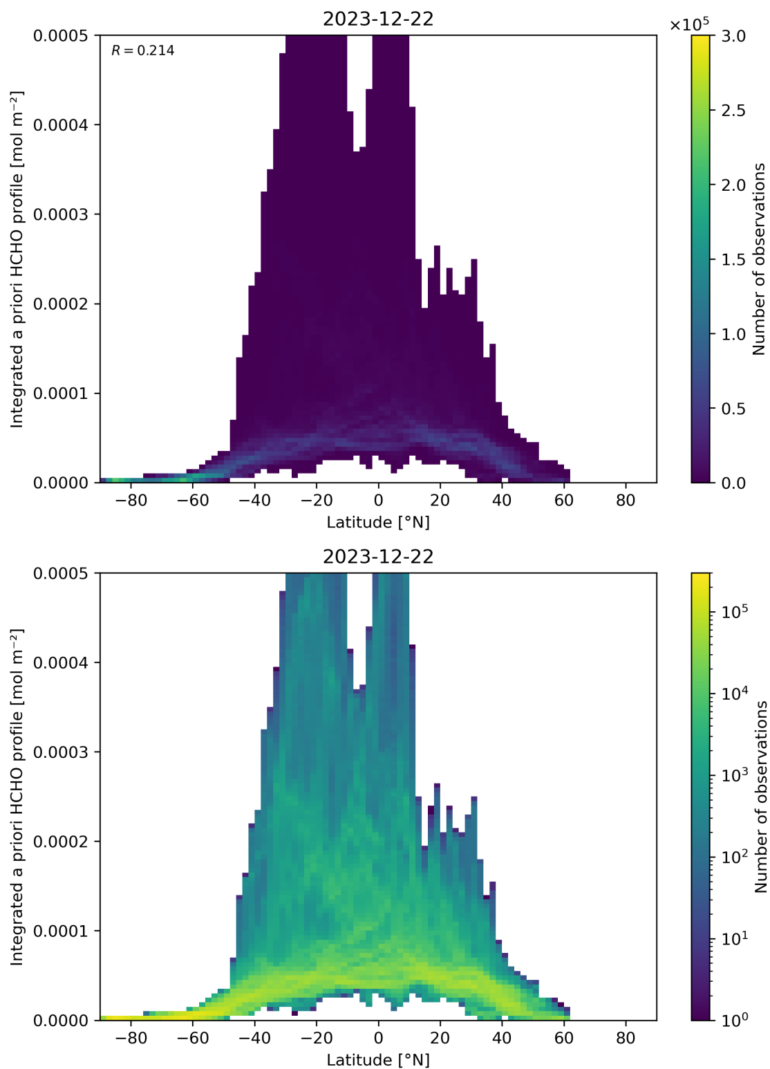
Figure 166: Scatter density plot of “Latitude” against “Integrated a priori HCHO profile” for 2023-12-21 to 2023-12-23.
