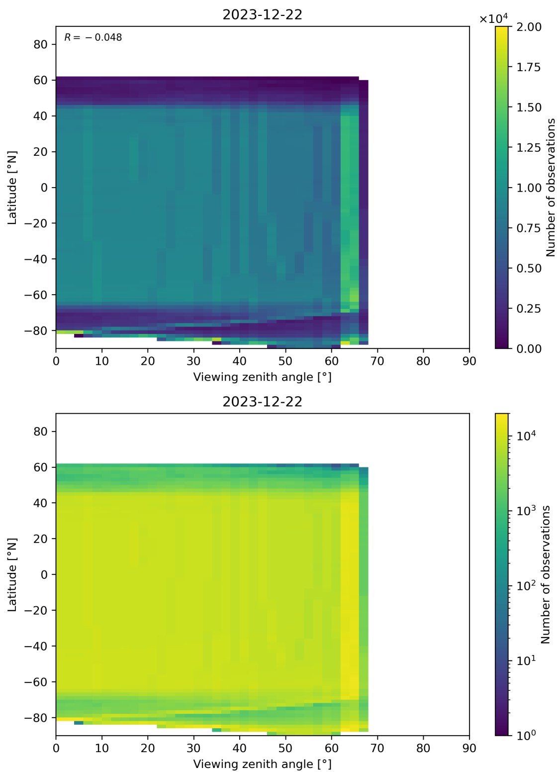
Figure 196: Scatter density plot of “Viewing zenith angle” against “Latitude” for 2023-12-21 to 2023-12-23.
