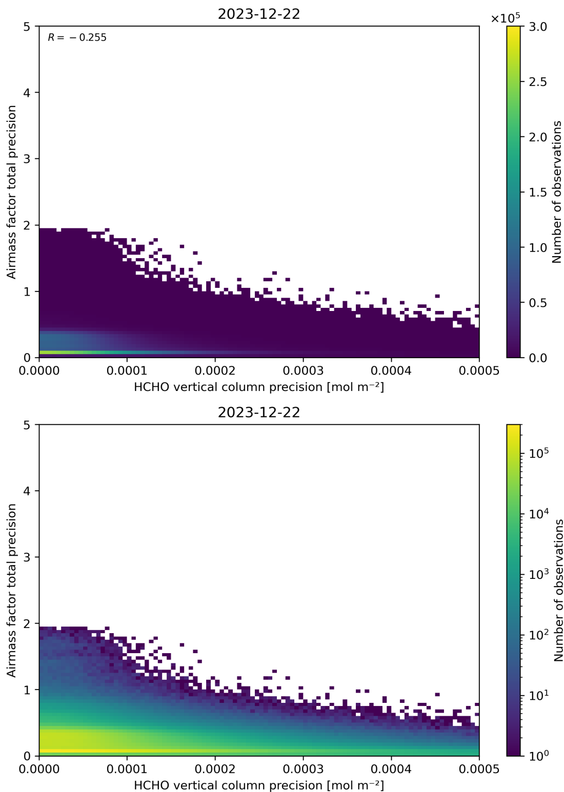
Figure 145: Scatter density plot of “HCHO vertical column precision” against “Airmass factor total precision” for 2023-12-21 to 2023-12-23.
