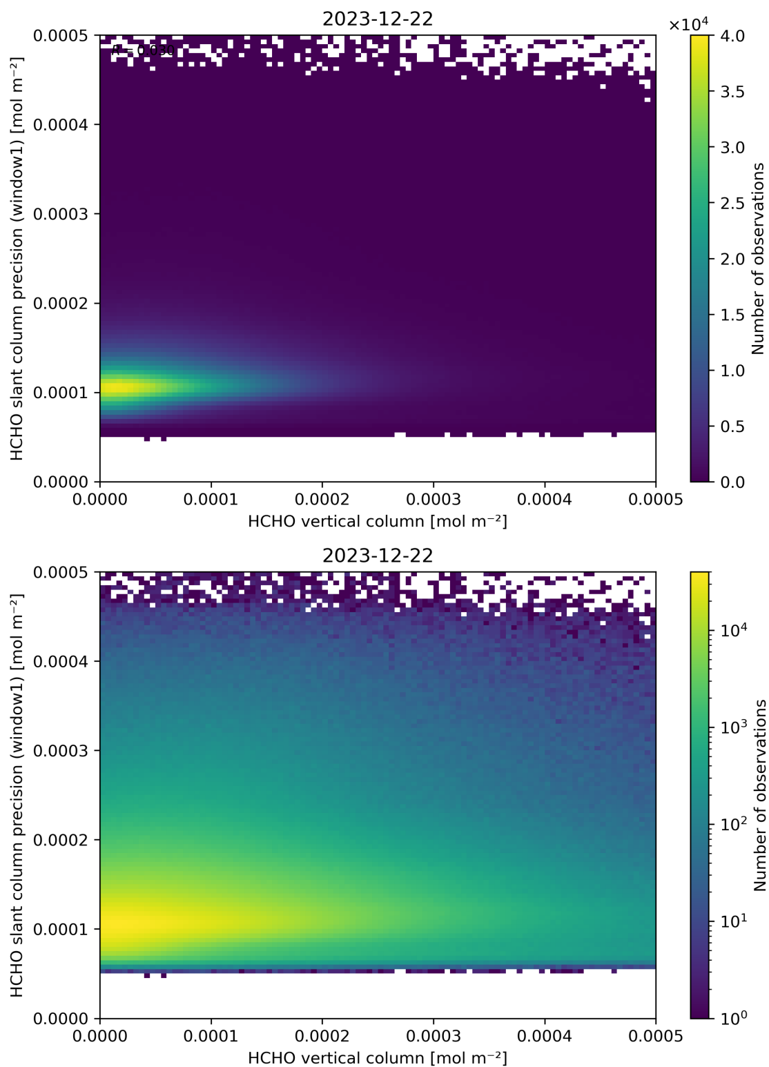
Figure 130: Scatter density plot of “HCHO vertical column” against “HCHO slant column precision (window1)” for 2023-12-21 to 2023-12-23.
