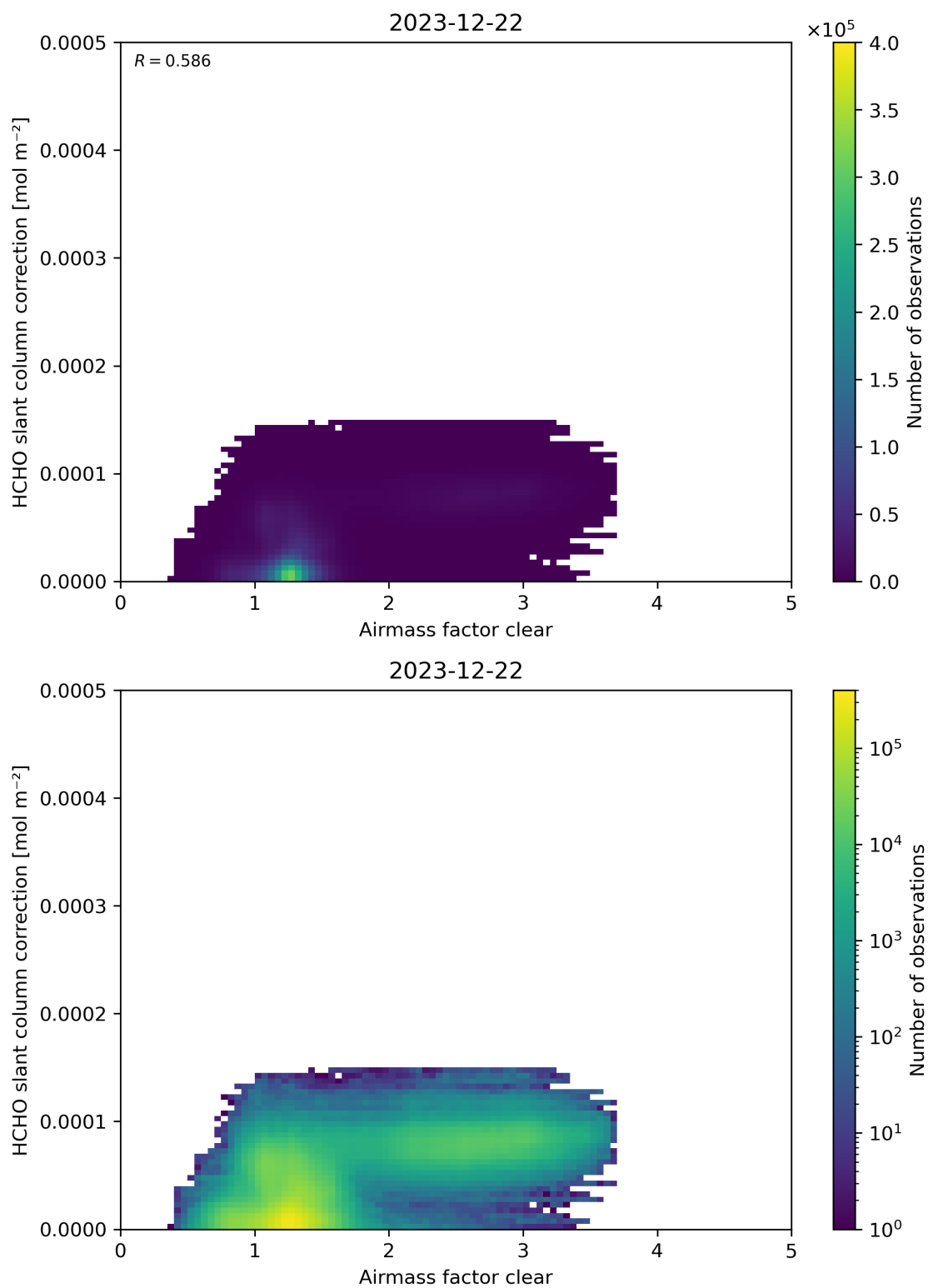
Figure 75: Scatter density plot of “Airmass factor clear” against “HCHO slant column correction” for 2023-12-21 to 2023-12-23.
