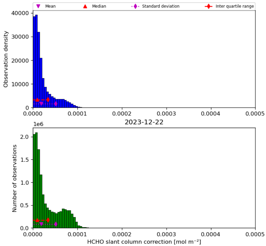
Figure 47: Histogram of “HCHO slant column correction” for 2023-12-21 to 2023-12-23
