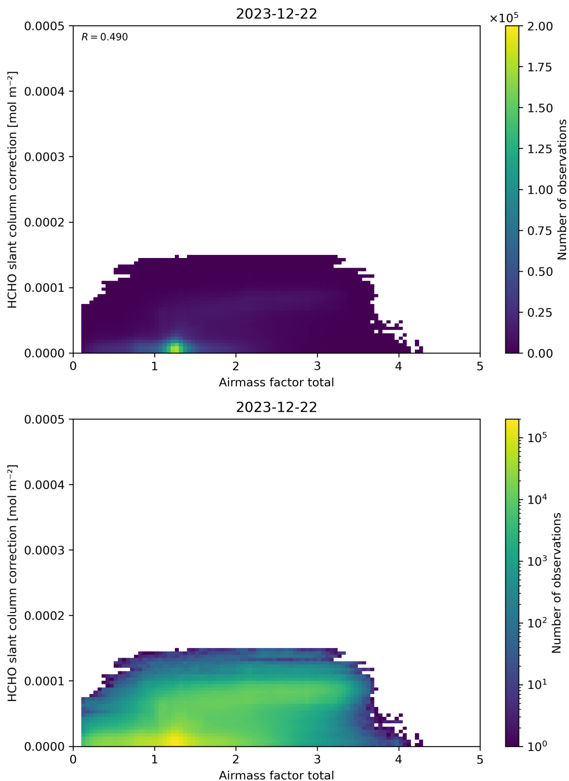
Figure 102: Scatter density plot of “Airmass factor total” against “HCHO slant column correction” for 2023-12-21 to 2023-12-23.
