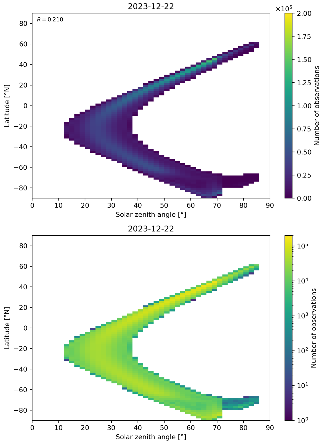
Figure 181: Scatter density plot of “Solar zenith angle” against “Latitude” for 2023-12-21 to 2023-12-23.
