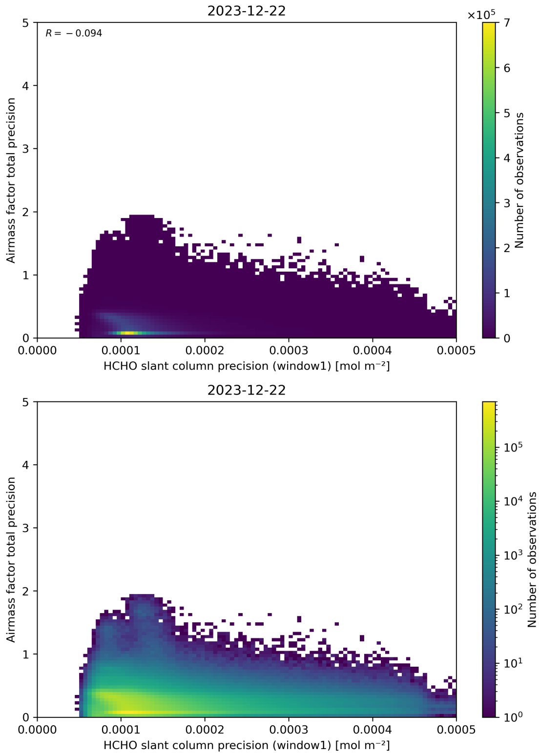
Figure 95: Scatter density plot of “HCHO slant column precision (window1)” against “Airmass factor total precision” for 2023-12-21 to 2023-12-23.
