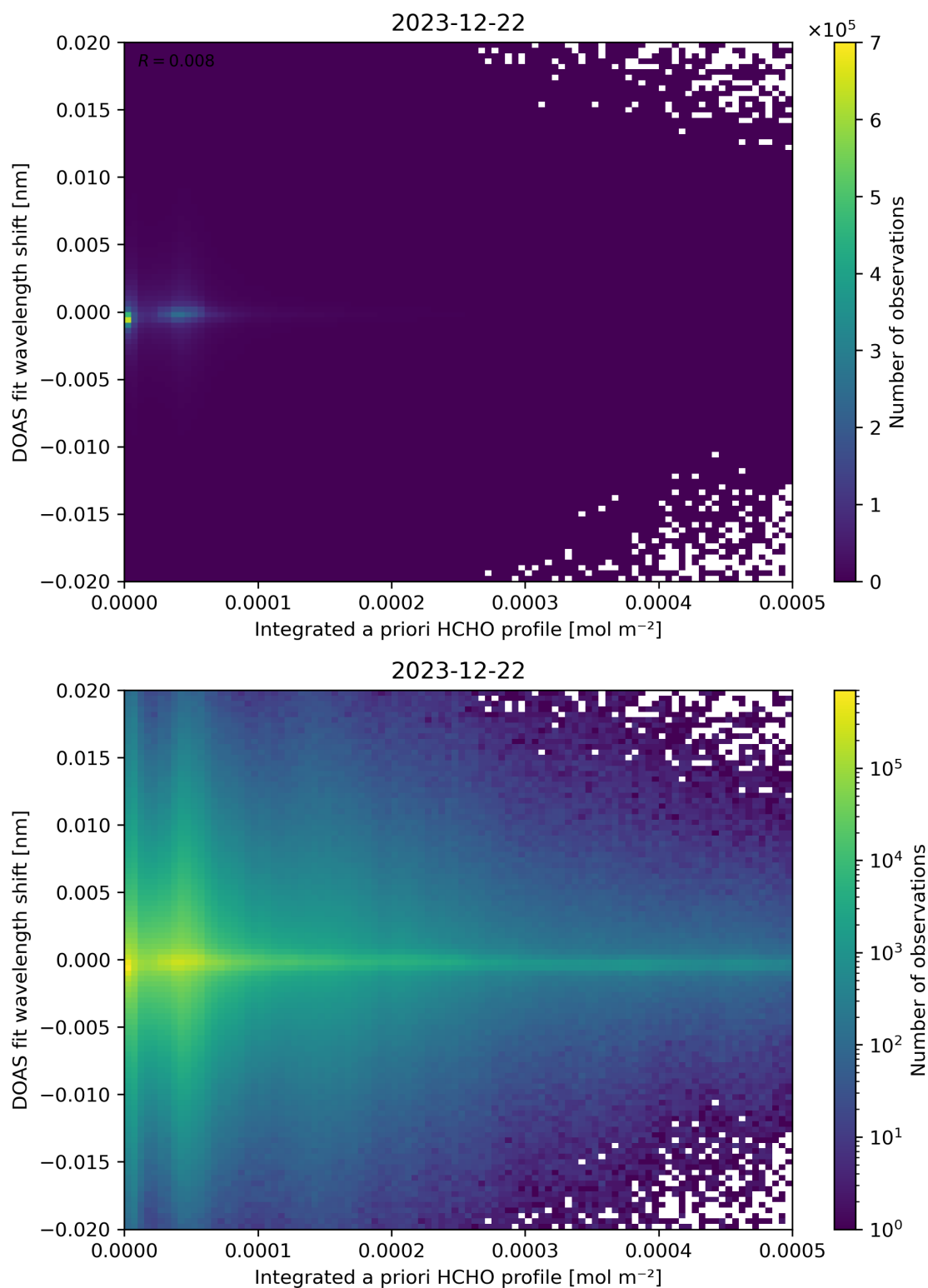
Figure 149: Scatter density plot of “Integrated a priori HCHO profile” against “DOAS fit wavelength shift” for 2023-12-21 to 2023-12-23.
