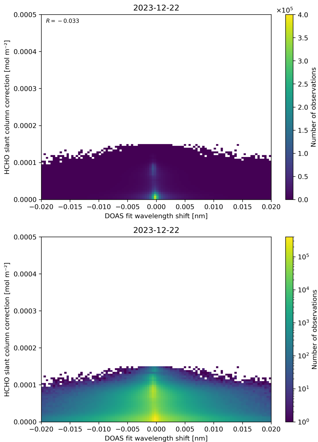
Figure 67: Scatter density plot of “DOAS fit wavelength shift” against “HCHO slant column correction” for 2023-12-21 to 2023-12-23.
