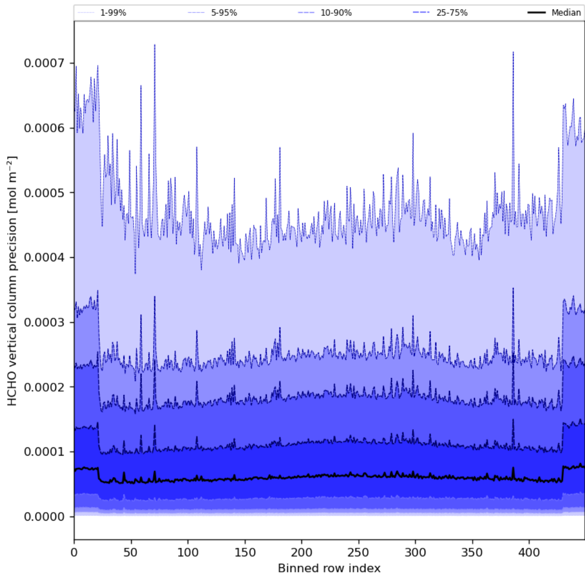
Figure 50: Along track statistics of “HCHO vertical column precision” for 2023-12-21 to 2023-12-23
