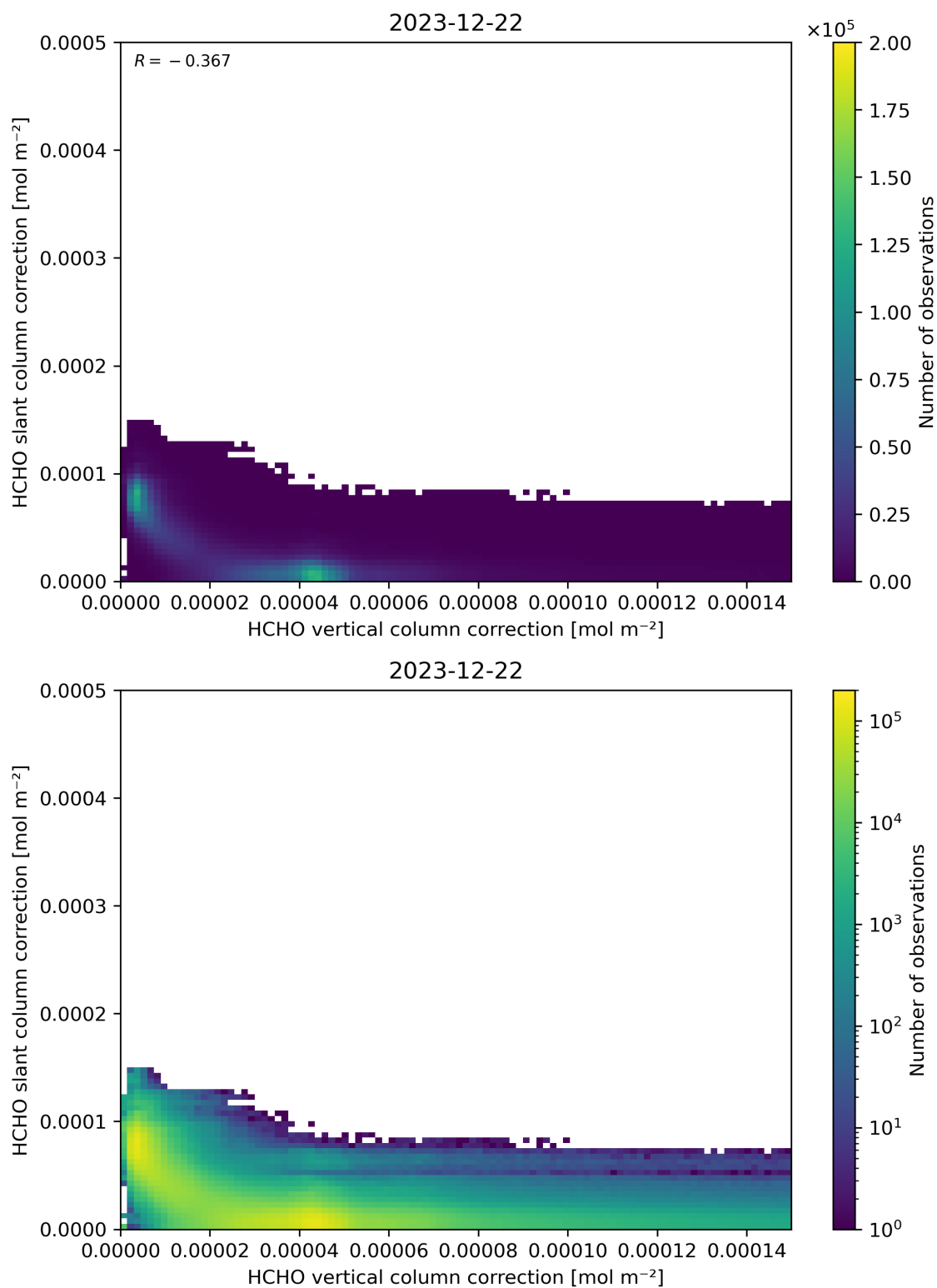
Figure 117: Scatter density plot of “HCHO vertical column correction” against “HCHO slant column correction” for 2023-12-21 to 2023-12-23.
