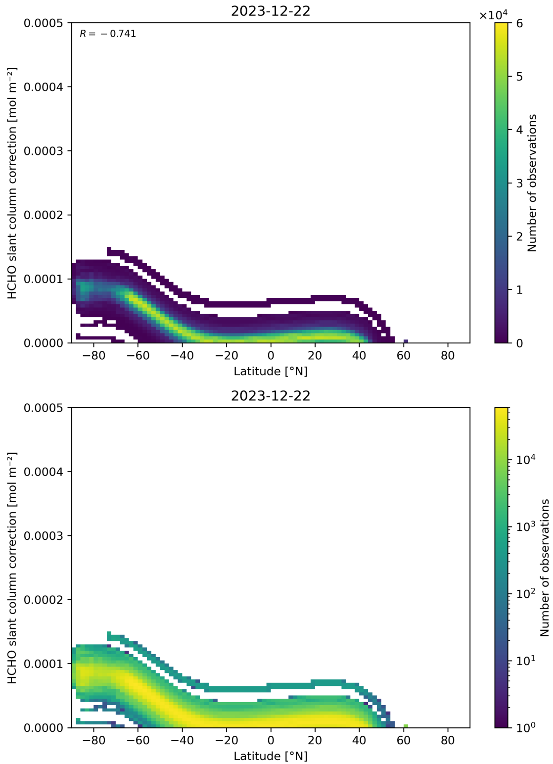
Figure 158: Scatter density plot of “Latitude” against “HCHO slant column correction” for 2023-12-21 to 2023-12-23.
