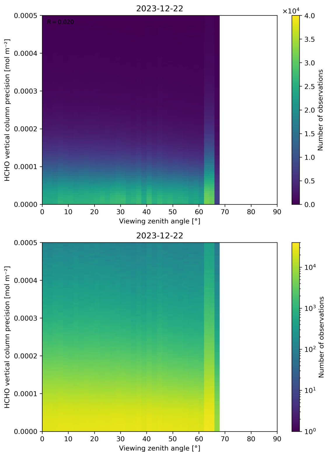
Figure 194: Scatter density plot of “Viewing zenith angle” against “HCHO vertical column precision” for 2023-12-21 to 2023-12-23.
