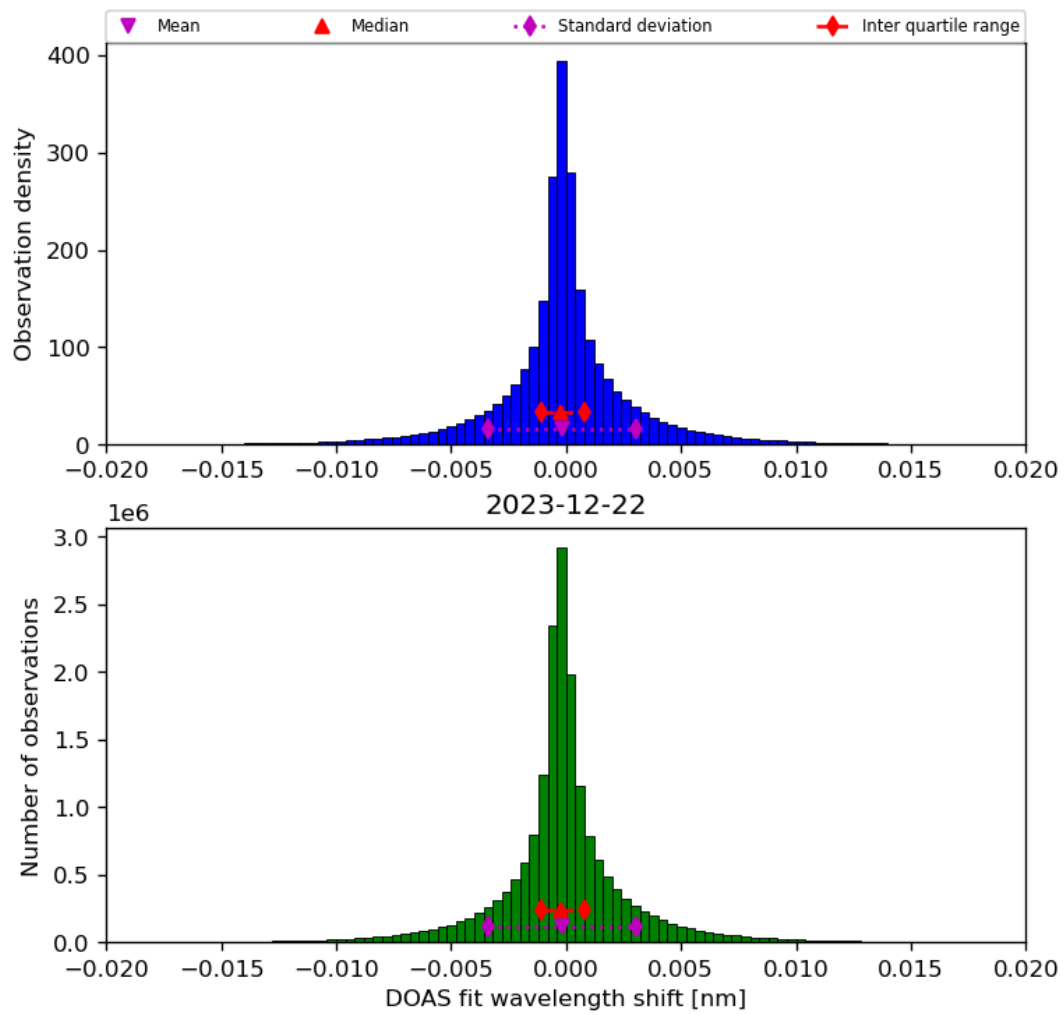
Figure 44: Histogram of “DOAS fit wavelength shift” for 2023-12-21 to 2023-12-23
