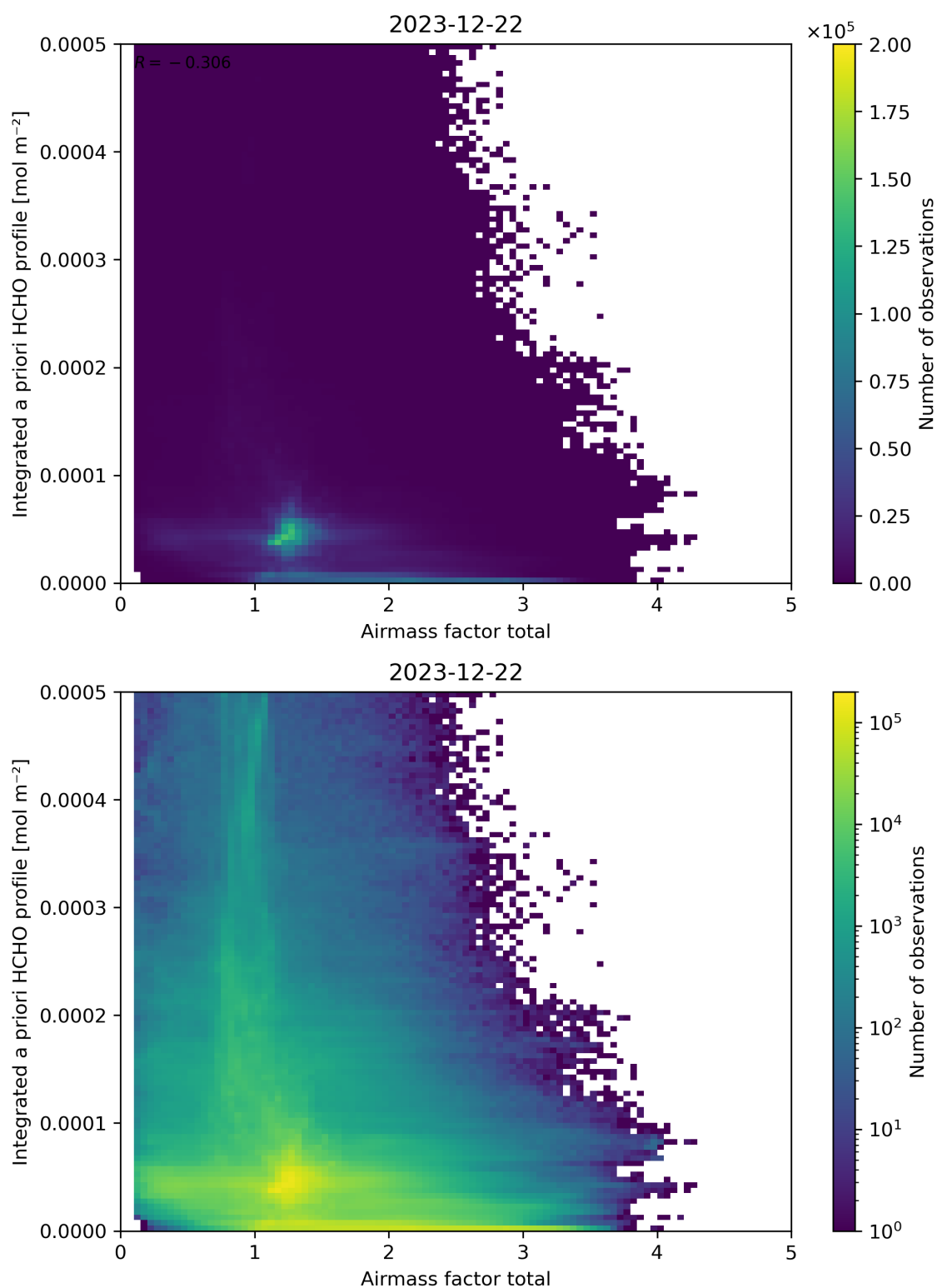
Figure 104: Scatter density plot of “Airmass factor total” against “Integrated a priori HCHO profile” for 2023-12-21 to 2023-12-23.
