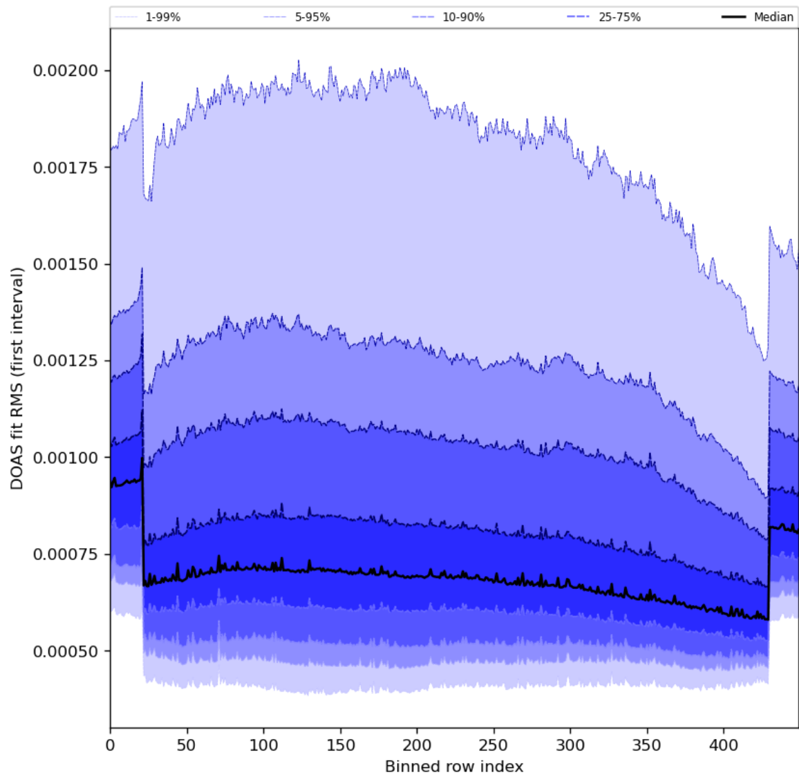
Figure 60: Along track statistics of “DOAS fit RMS (first interval)” for 2023-12-21 to 2023-12-23
