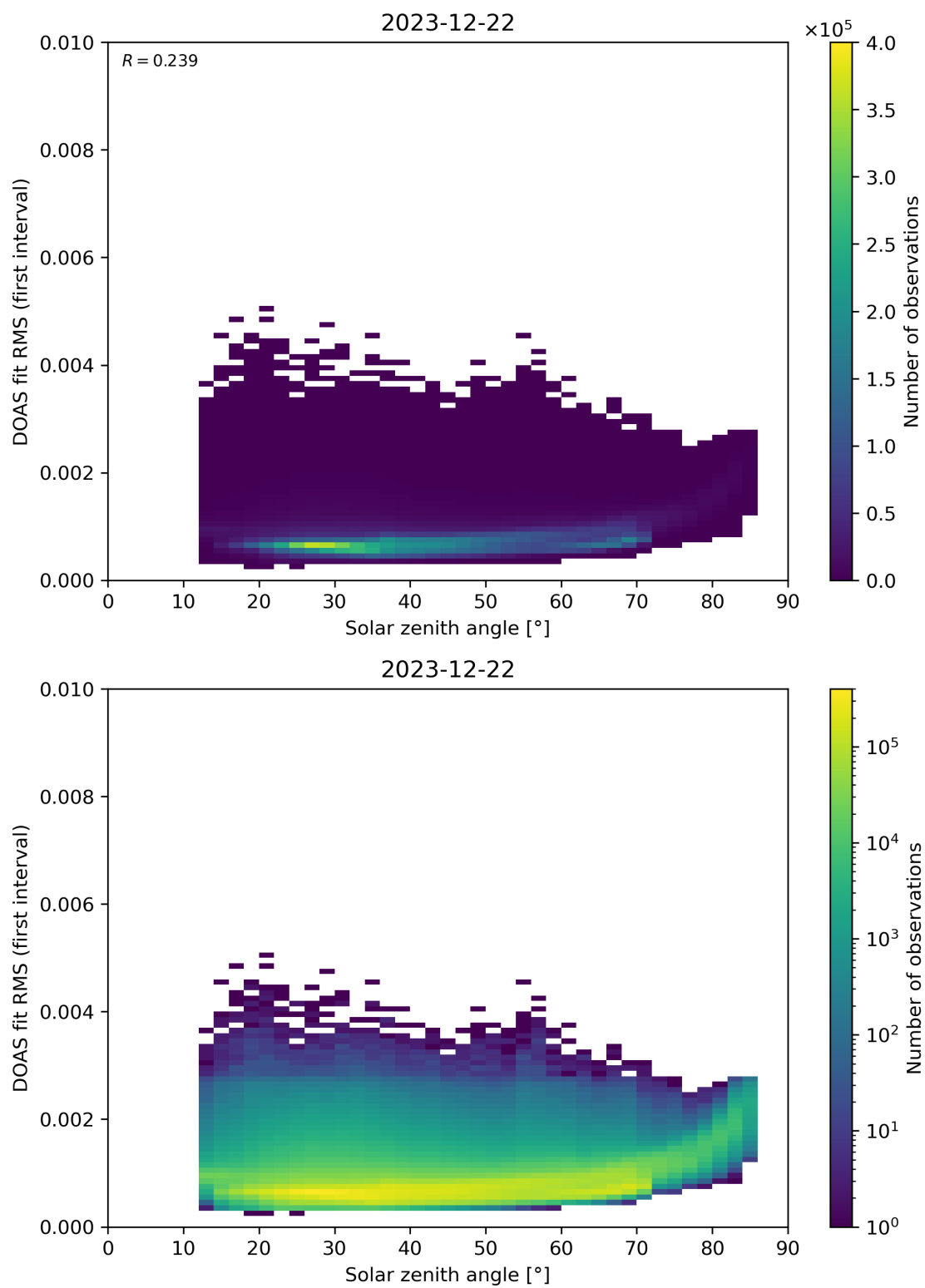
Figure 167: Scatter density plot of “Solar zenith angle” against “DOAS fit RMS (first interval)” for 2023-12-21 to 2023-12-23.
