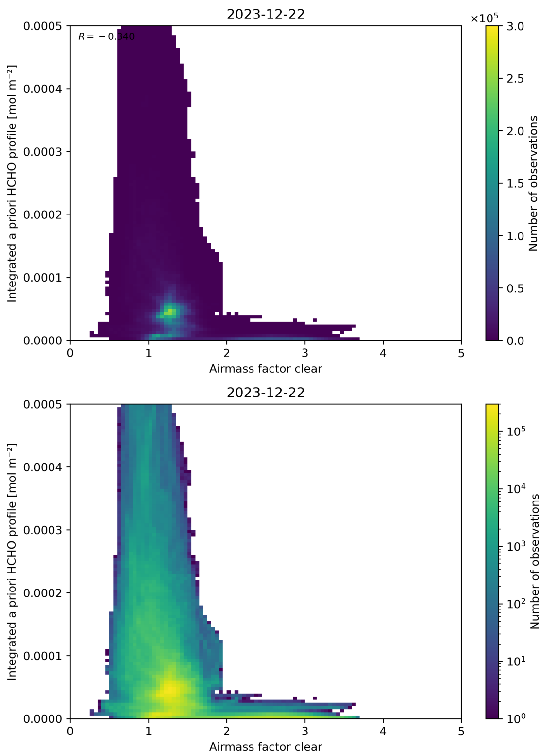
Figure 76: Scatter density plot of “Airmass factor clear” against “Integrated a priori HCHO profile” for 2023-12-21 to 2023-12-23.
