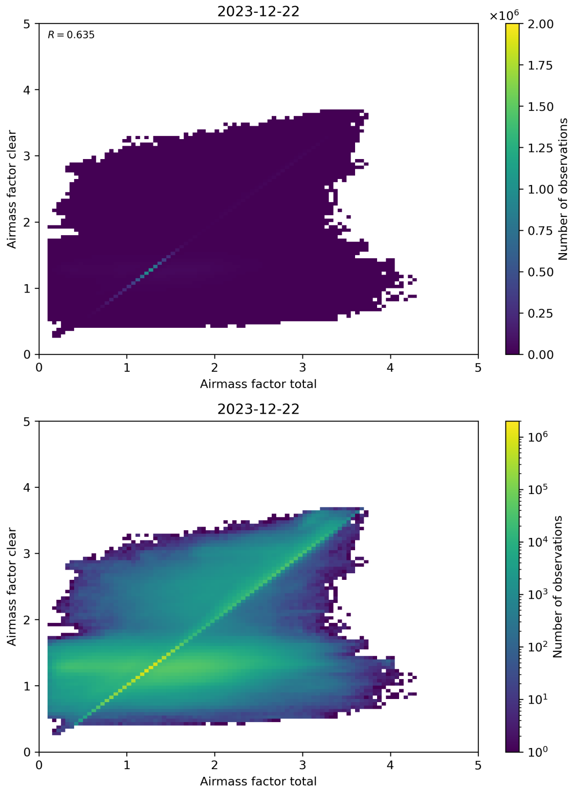
Figure 100: Scatter density plot of “Airmass factor total” against “Airmass factor clear” for 2023-12-21 to 2023-12-23.
