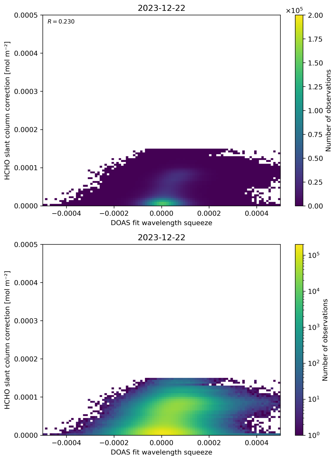
Figure 70: Scatter density plot of “DOAS fit wavelength squeeze” against “HCHO slant column correction” for 2023-12-21 to 2023-12-23.
