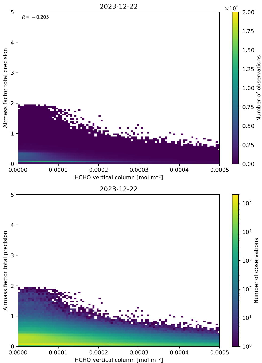
Figure 132: Scatter density plot of “HCHO vertical column” against “Airmass factor total precision” for 2023-12-21 to 2023-12-23.
