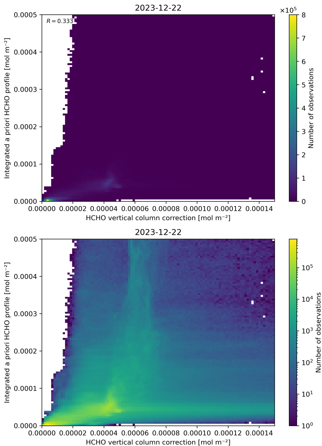
Figure 122: Scatter density plot of “HCHO vertical column correction” against “Integrated a priori HCHO profile” for 2023-12-21 to 2023-12-23.
