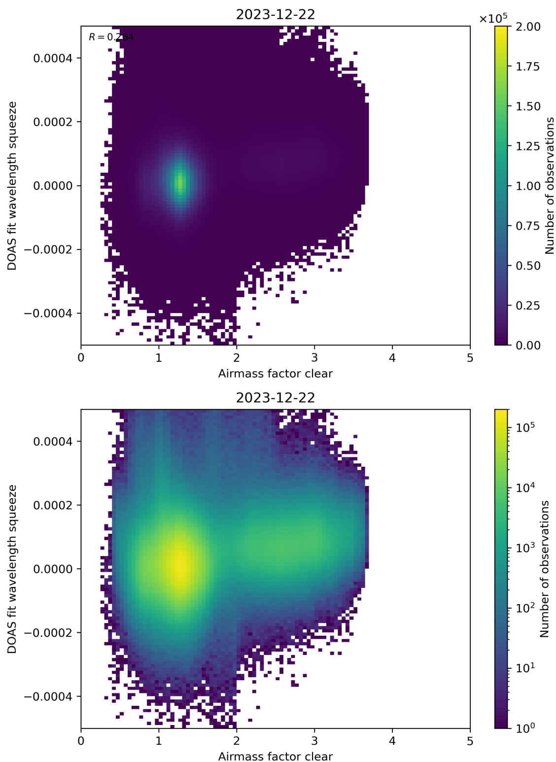
Figure 73: Scatter density plot of “Airmass factor clear” against “DOAS fit wavelength squeeze” for 2023-12-21 to 2023-12-23.
