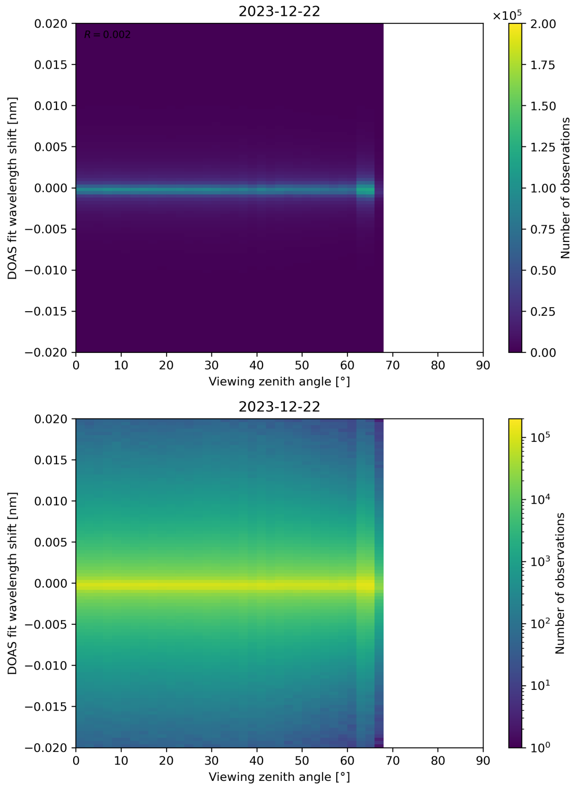
Figure 183: Scatter density plot of “Viewing zenith angle” against “DOAS fit wavelength shift” for 2023-12-21 to 2023-12-23.
