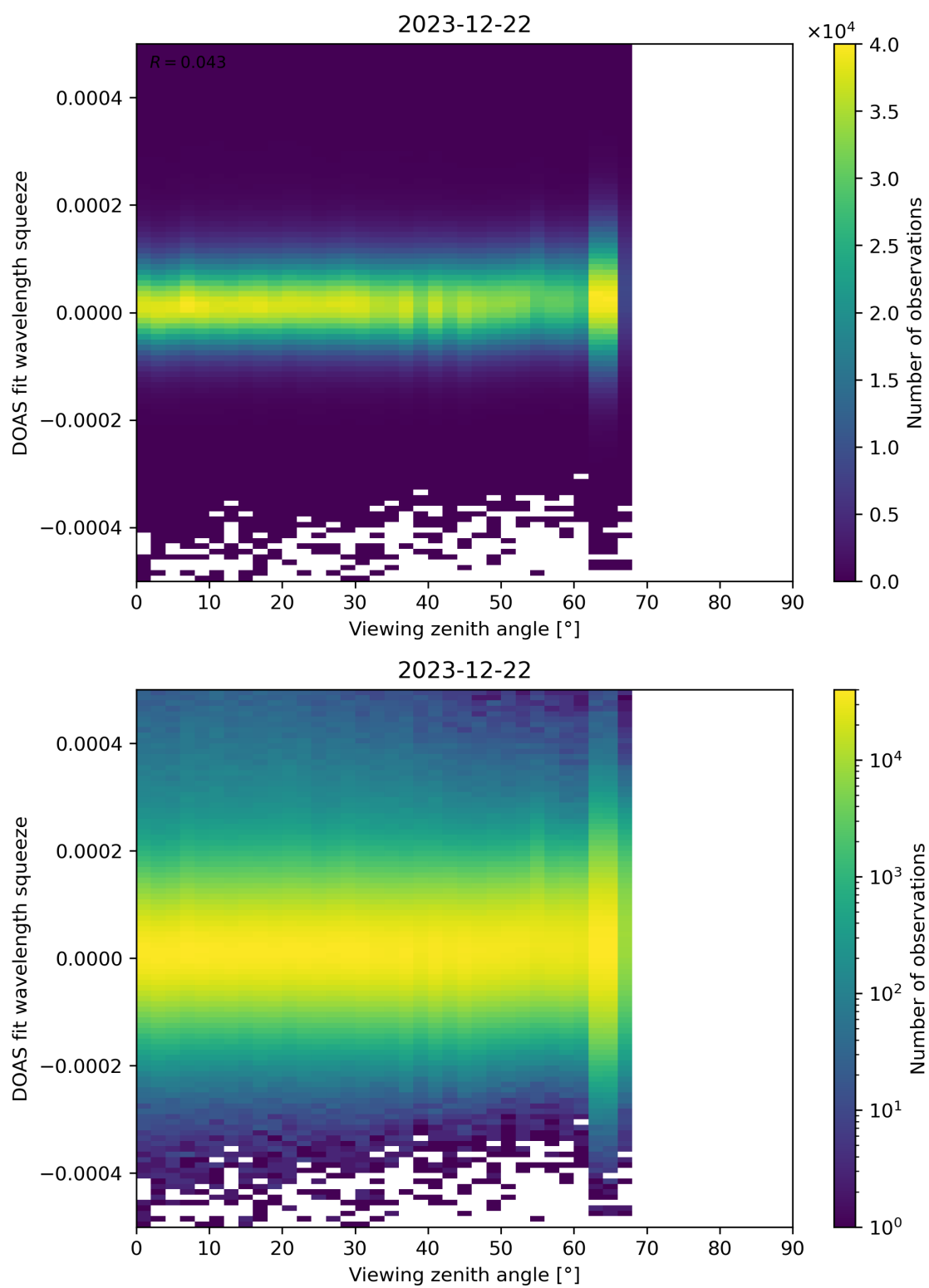
Figure 184: Scatter density plot of “Viewing zenith angle” against “DOAS fit wavelength squeeze” for 2023-12-21 to 2023-12-23.
