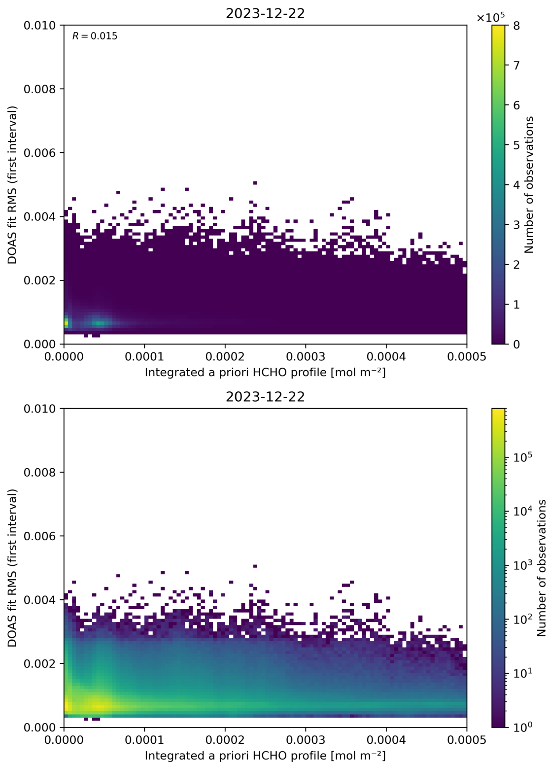
Figure 148: Scatter density plot of “Integrated a priori HCHO profile” against “DOAS fit RMS (first interval)” for 2023-12-21 to 2023-12-23.
