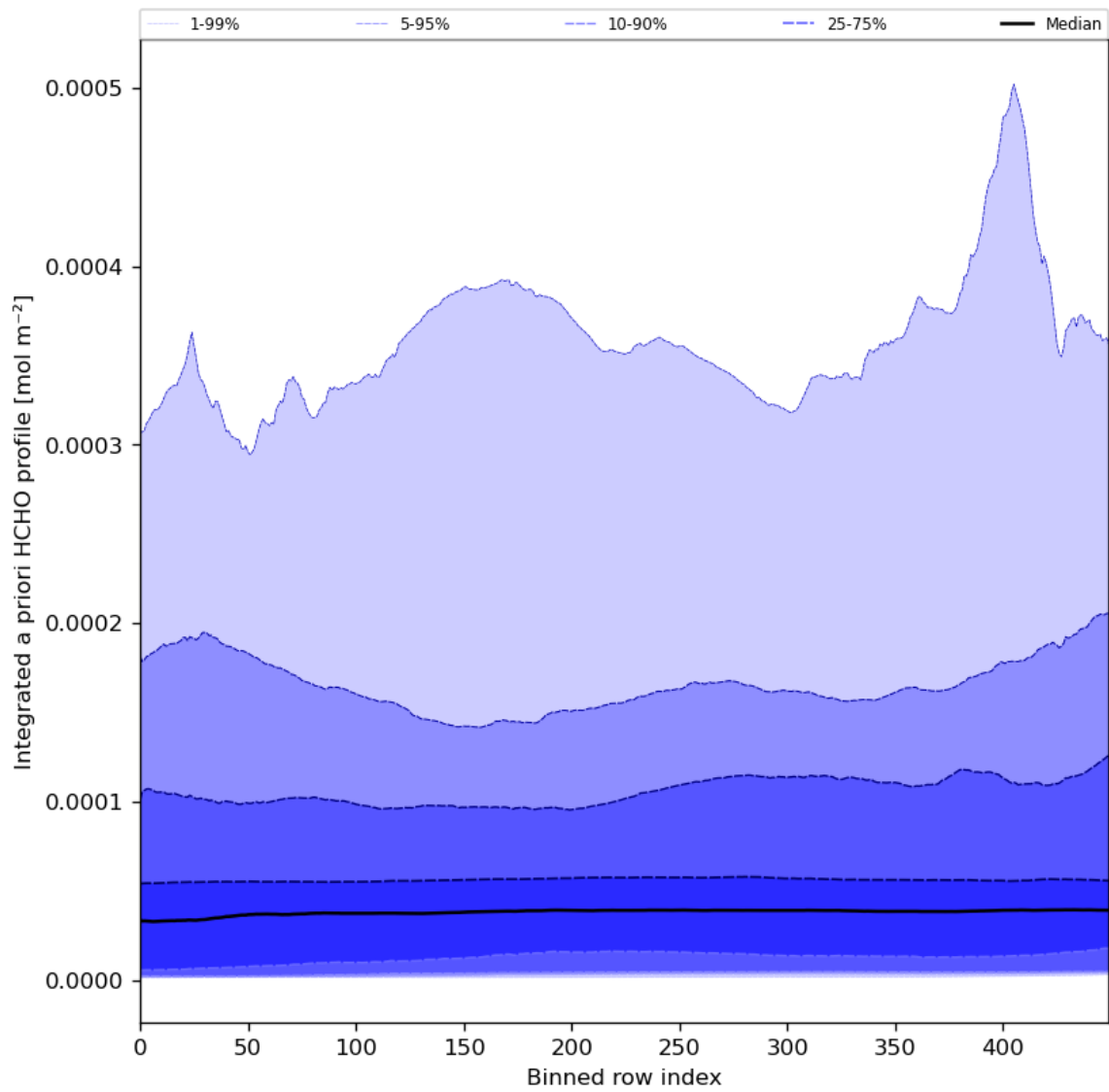
Figure 57: Along track statistics of “Integrated a priori HCHO profile” for 2023-12-21 to 2023-12-23
