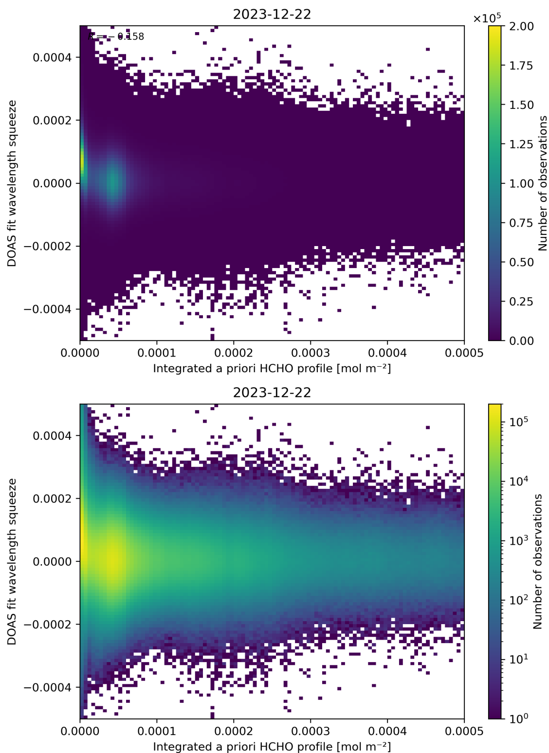
Figure 150: Scatter density plot of “Integrated a priori HCHO profile” against “DOAS fit wavelength squeeze” for 2023-12-21 to 2023-12-23.
