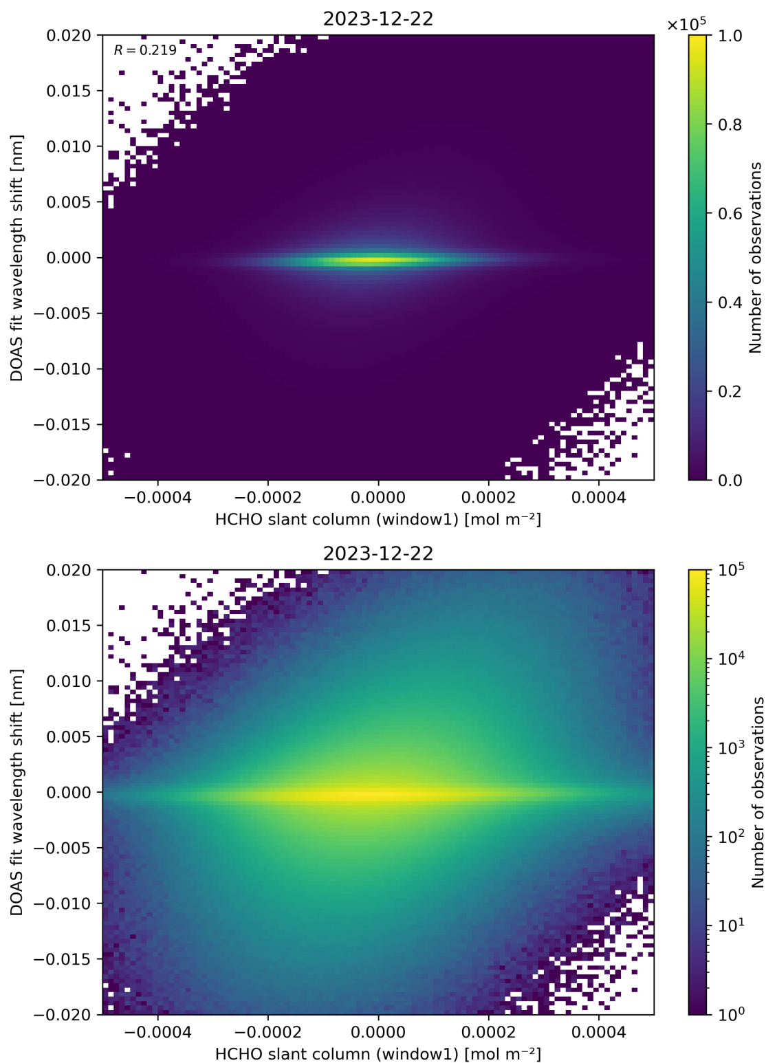
Figure 79: Scatter density plot of “HCHO slant column (window1)” against “DOAS fit wavelength shift” for 2023-12-21 to 2023-12-23.
