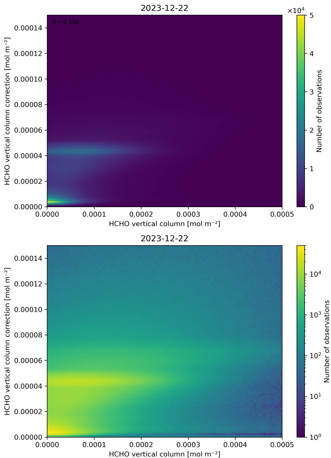
Figure 133: Scatter density plot of “HCHO vertical column” against “HCHO vertical column correction” for 2023-12-21 to 2023-12-23.
