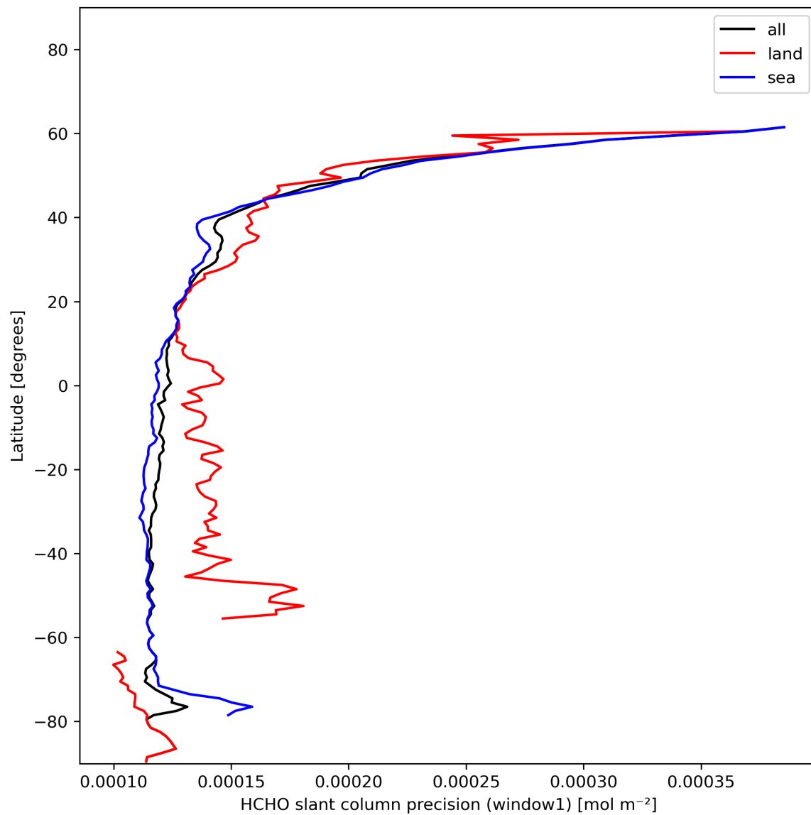
Figure 25: Zonal average of “HCHO slant column precision (window1)” for 2023-12-21 to 2023-12-23.
