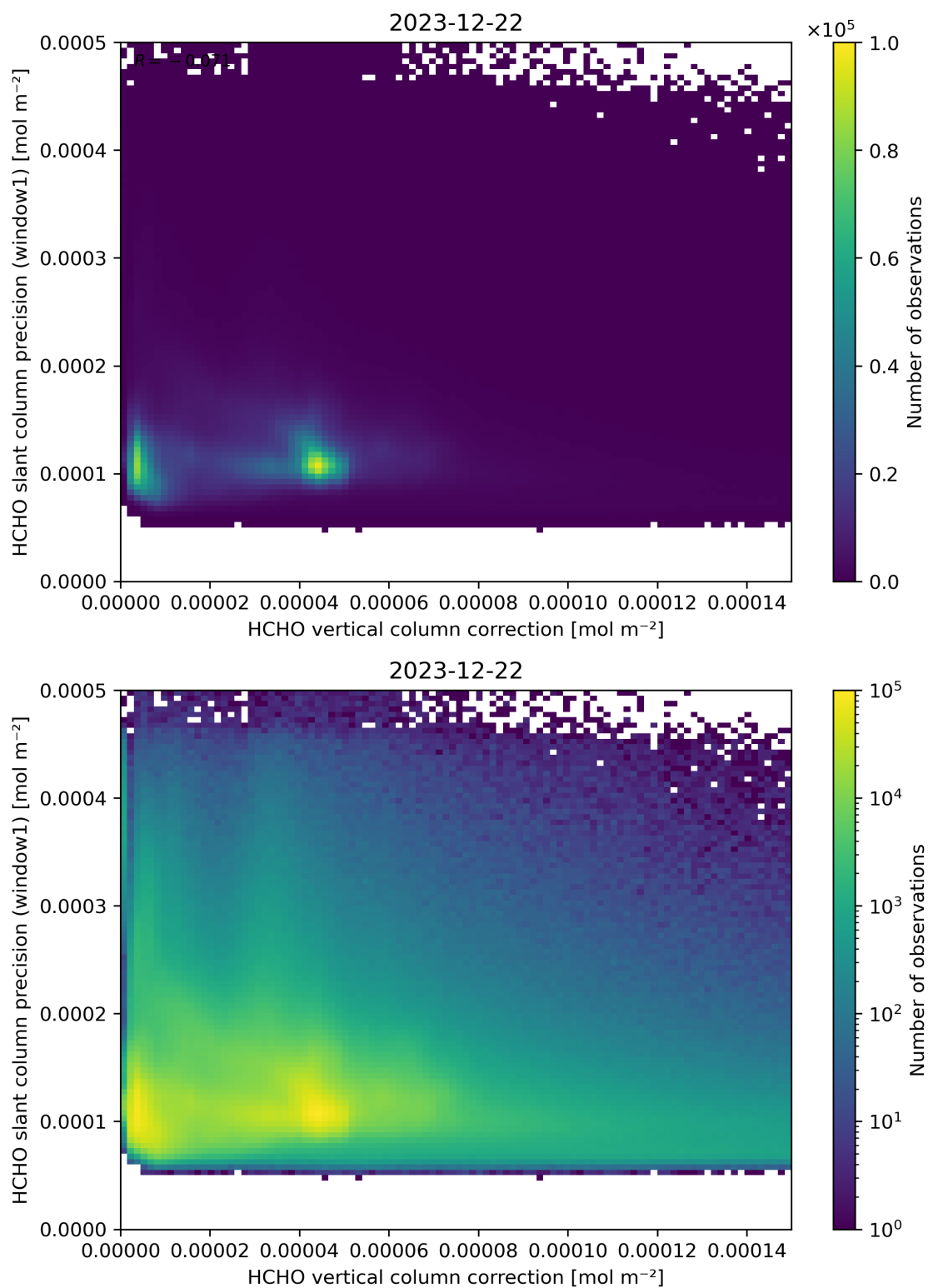
Figure 119: Scatter density plot of “HCHO vertical column correction” against “HCHO slant column precision (window1)” for 2023-12-21 to 2023-12-23.
