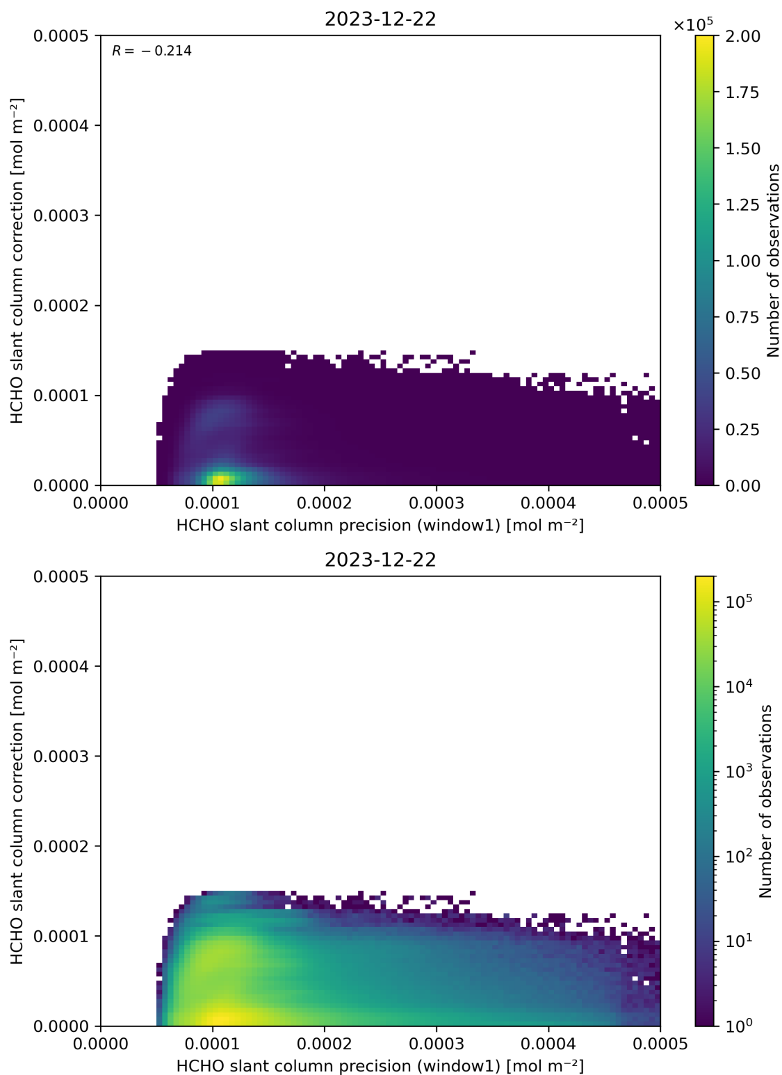
Figure 93: Scatter density plot of “HCHO slant column precision (window1)” against “HCHO slant column correction” for 2023-12-21 to 2023-12-23.
