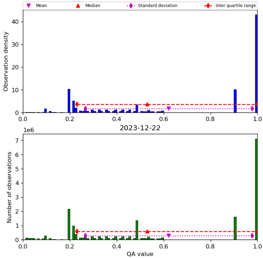
Figure 34: Histogram of “QA value” for 2023-12-21 to 2023-12-23
