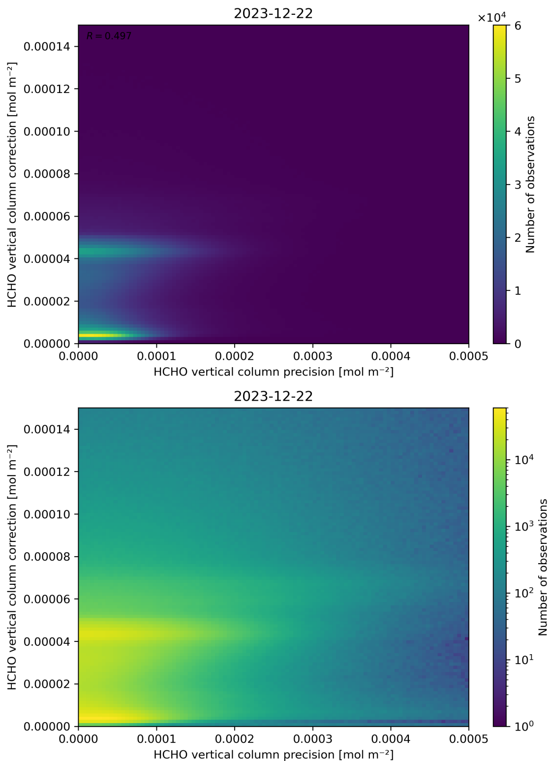
Figure 146: Scatter density plot of “HCHO vertical column precision” against “HCHO vertical column correction” for 2023-12-21 to 2023-12-23.
