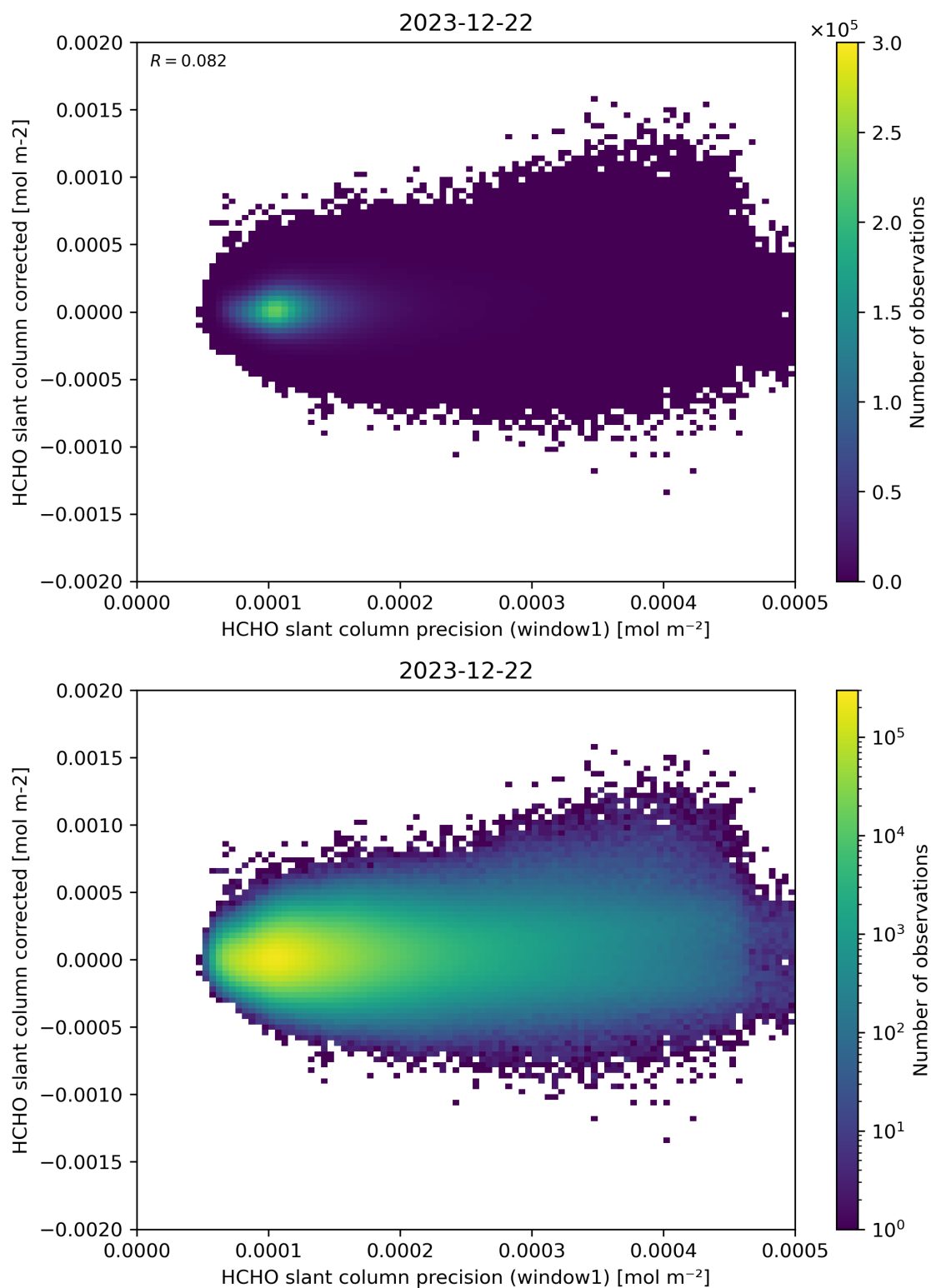
Figure 92: Scatter density plot of “HCHO slant column precision (window1)” against “HCHO slant column corrected” for 2023-12-21 to 2023-12-23.
