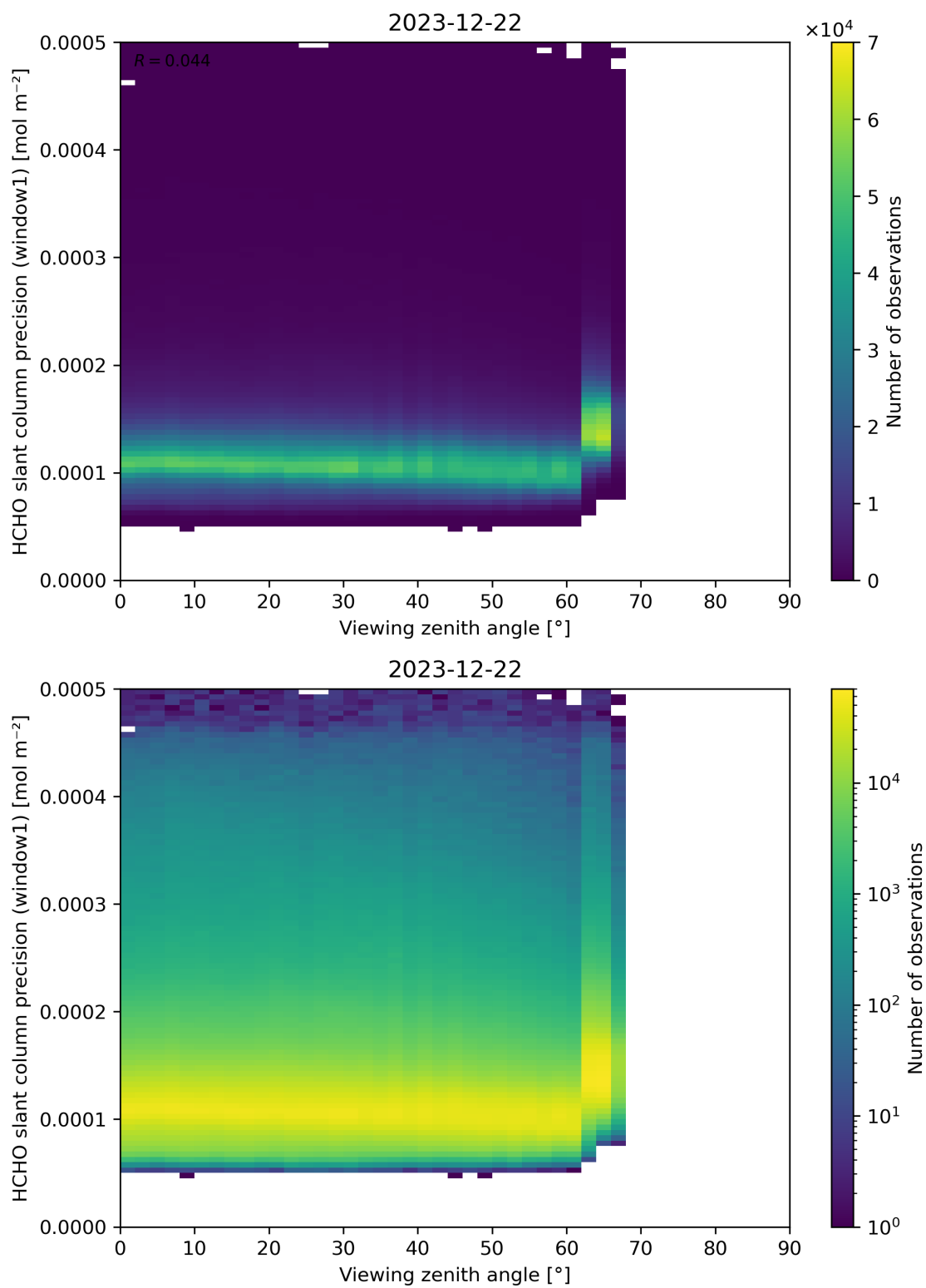
Figure 189: Scatter density plot of “Viewing zenith angle” against “HCHO slant column precision (window1)” for 2023-12-21 to 2023-12-23.
