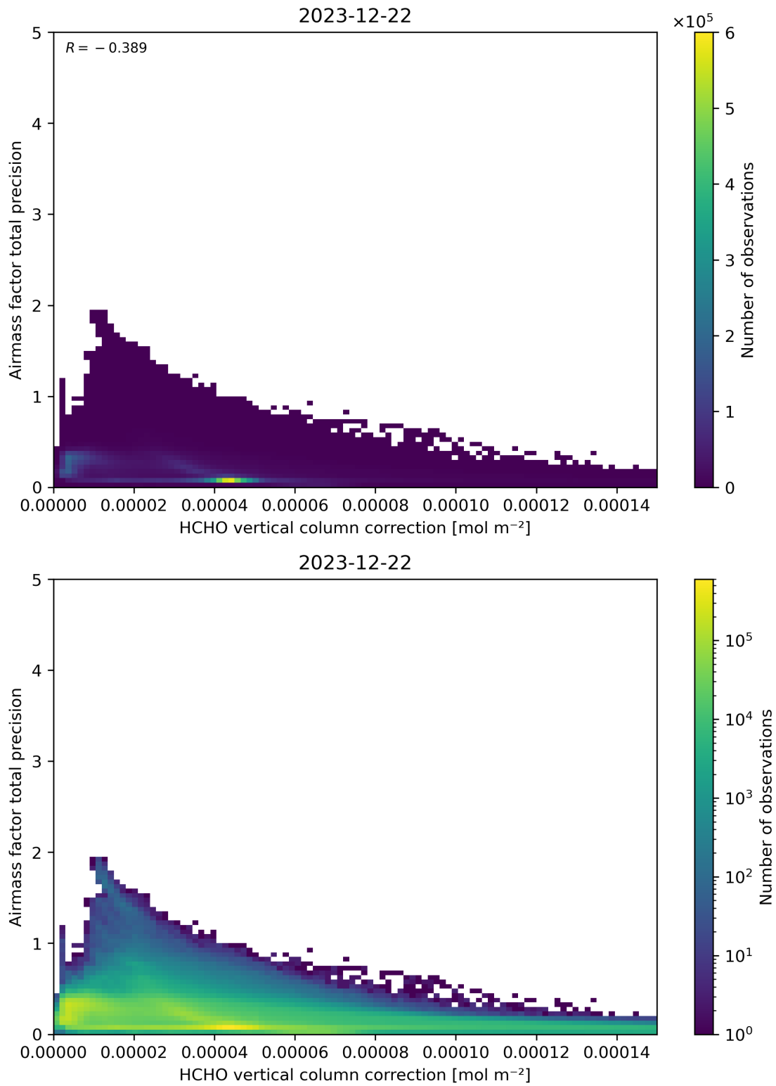
Figure 121: Scatter density plot of “HCHO vertical column correction” against “Airmass factor total precision” for 2023-12-21 to 2023-12-23.
