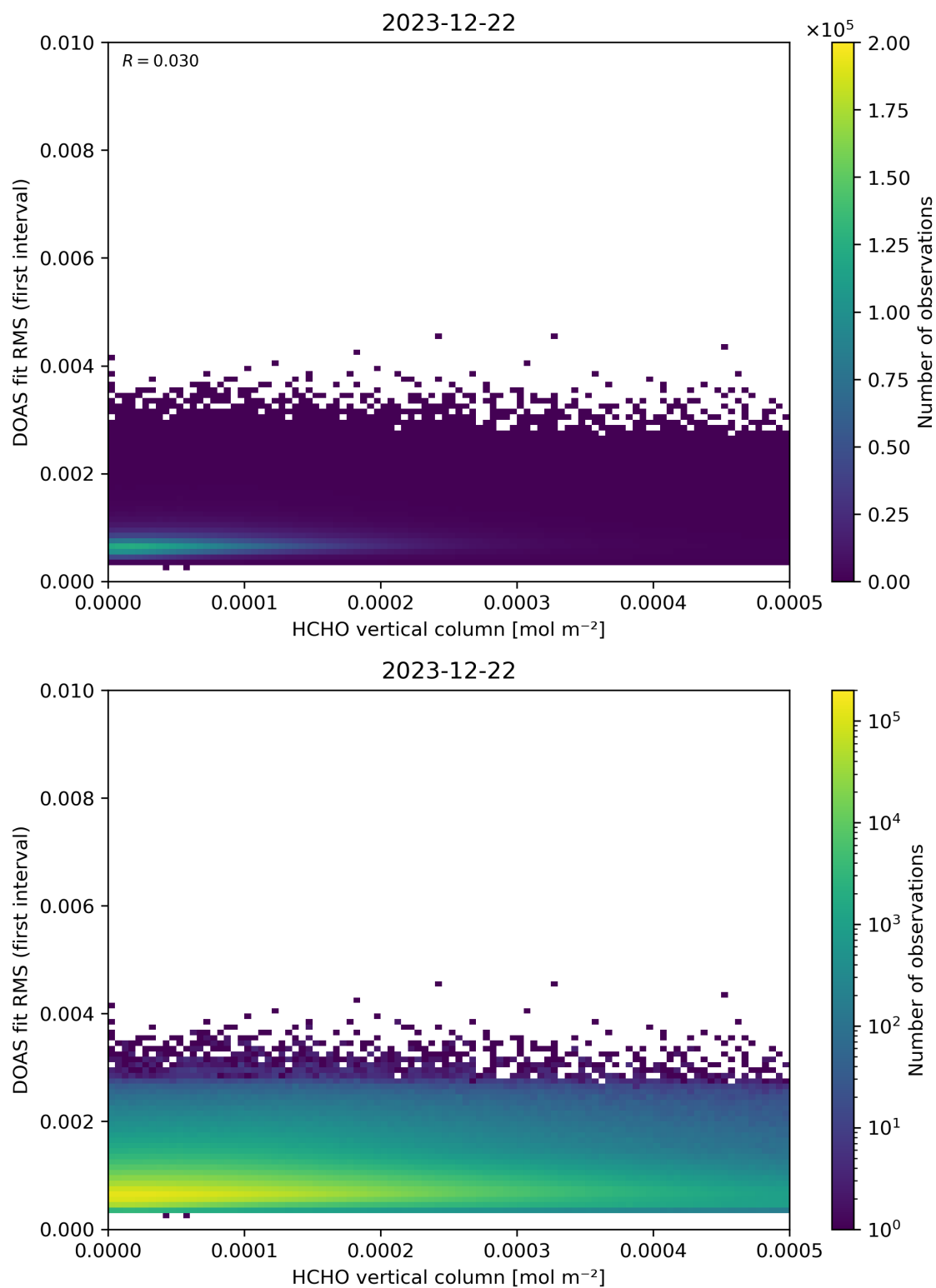
Figure 123: Scatter density plot of “HCHO vertical column” against “DOAS fit RMS (first interval)” for 2023-12-21 to 2023-12-23.
