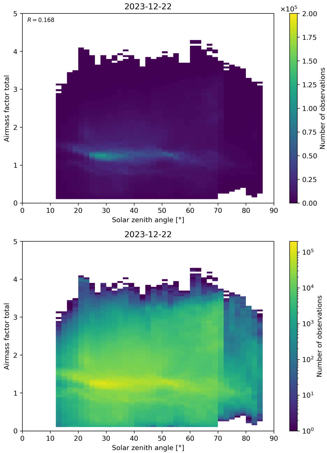
Figure 175: Scatter density plot of “Solar zenith angle” against “Airmass factor total” for 2023-12-21 to 2023-12-23.
