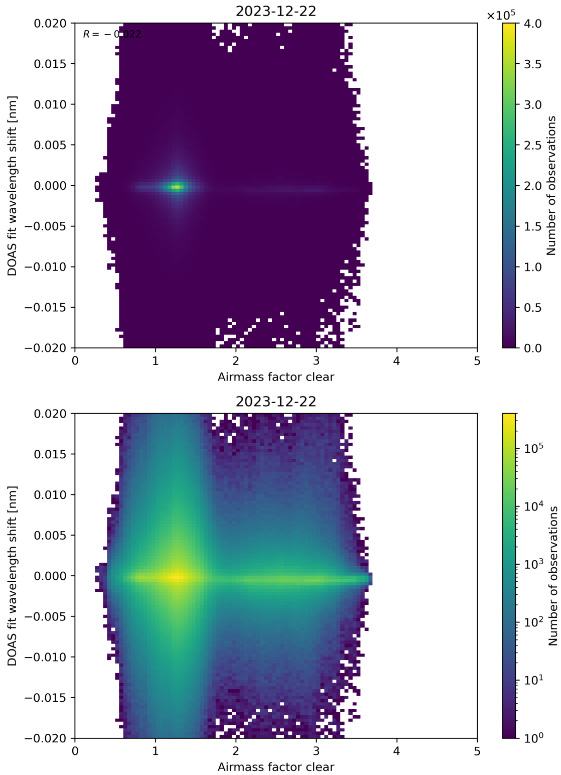
Figure 72: Scatter density plot of “Airmass factor clear” against “DOAS fit wavelength shift” for 2023-12-21 to 2023-12-23.
