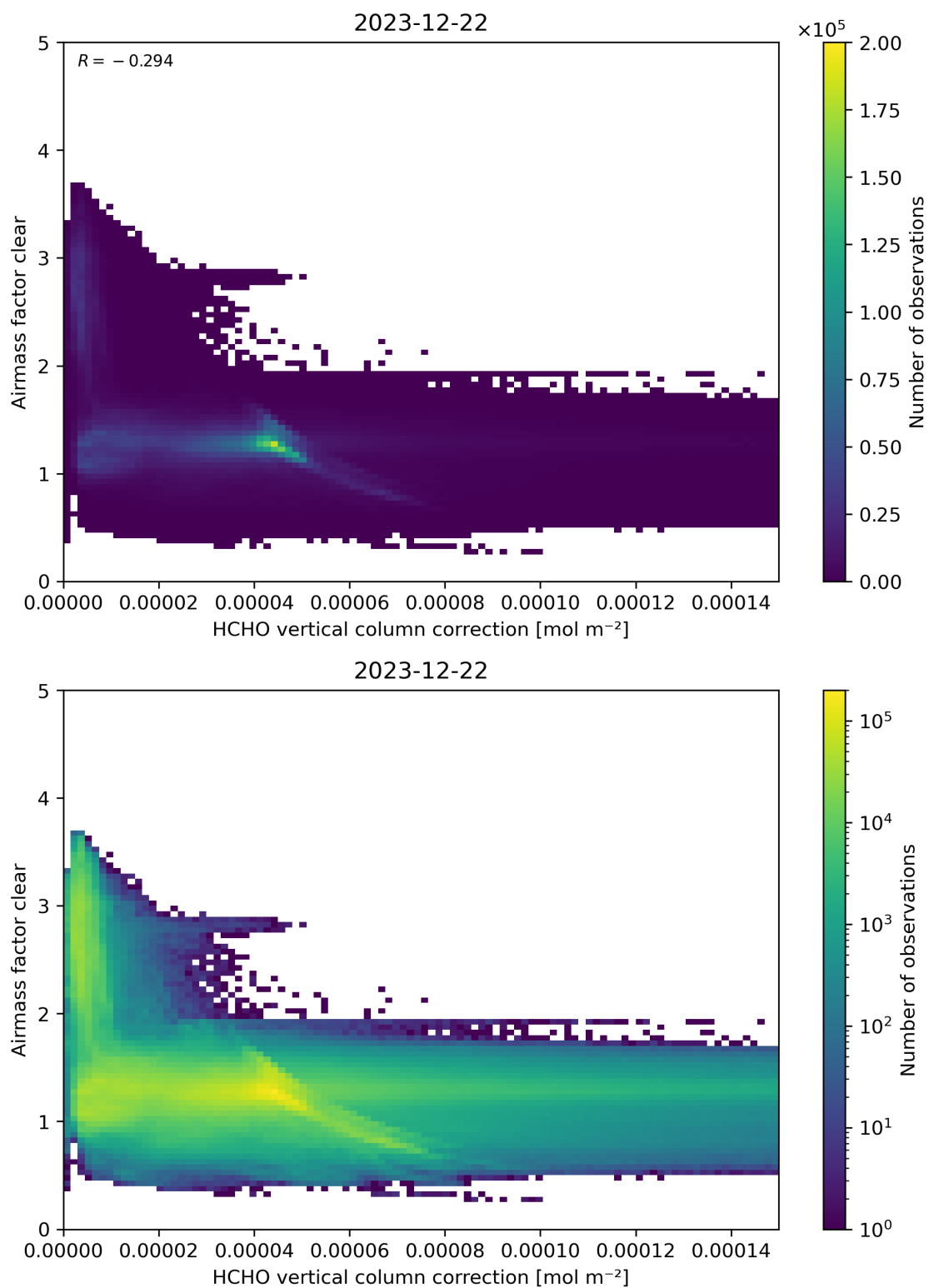
Figure 115: Scatter density plot of “HCHO vertical column correction” against “Airmass factor clear” for 2023-12-21 to 2023-12-23.
