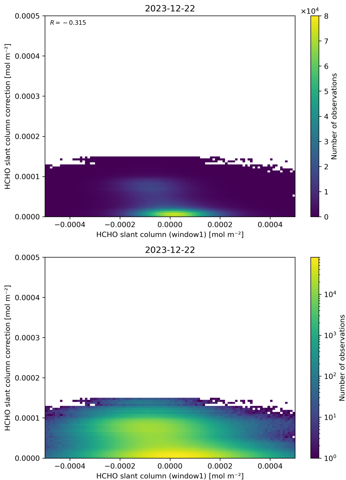
Figure 83: Scatter density plot of “HCHO slant column (window1)” against “HCHO slant column correction” for 2023-12-21 to 2023-12-23.
