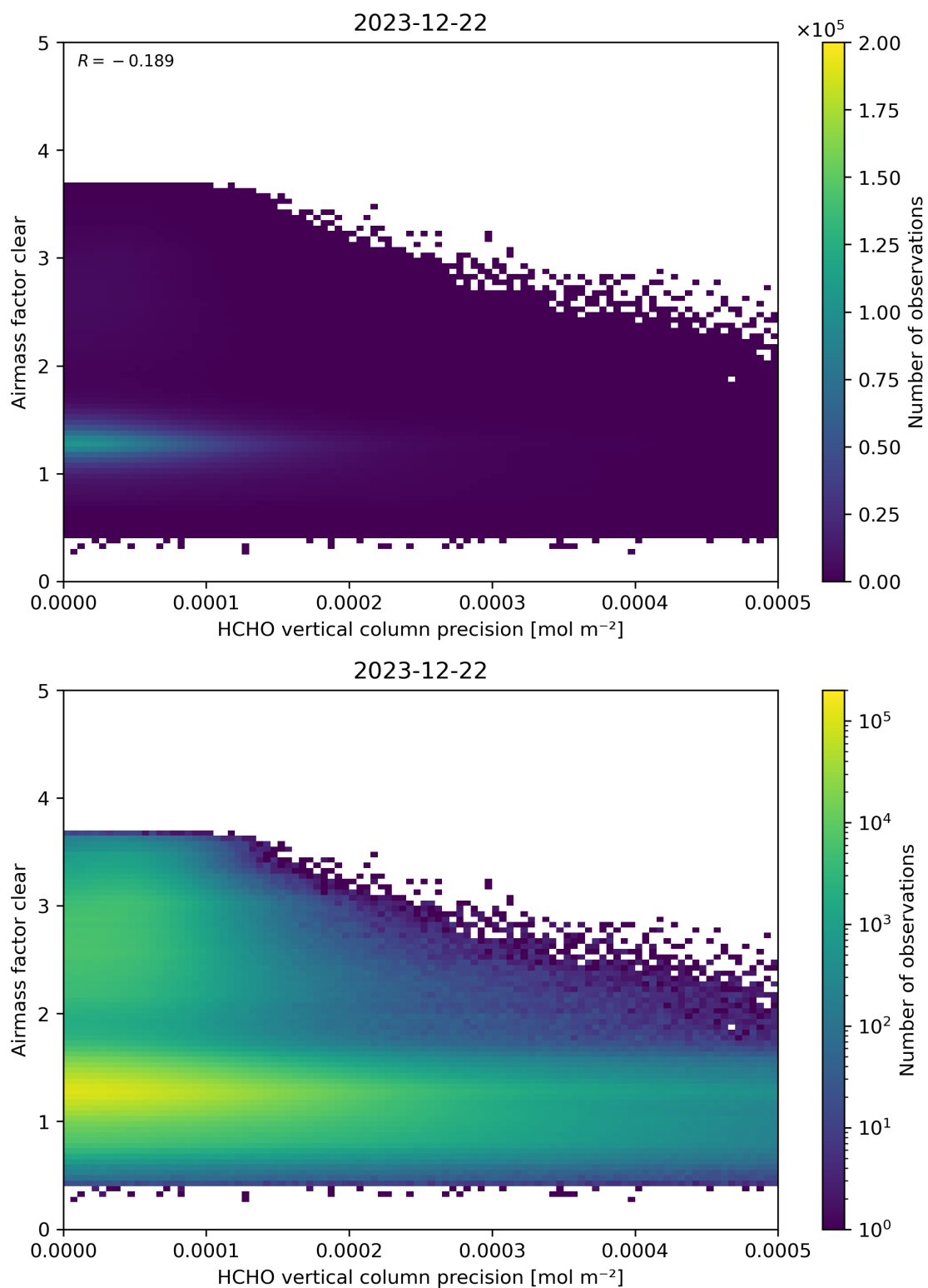
Figure 139: Scatter density plot of “HCHO vertical column precision” against “Airmass factor clear” for 2023-12-21 to 2023-12-23.
