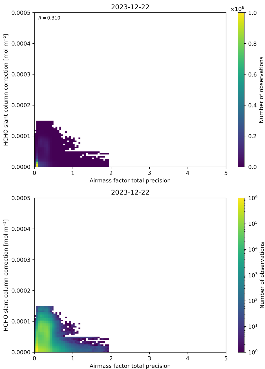
Figure 110: Scatter density plot of “Airmass factor total precision” against “HCHO slant column correction” for 2023-12-21 to 2023-12-23.
