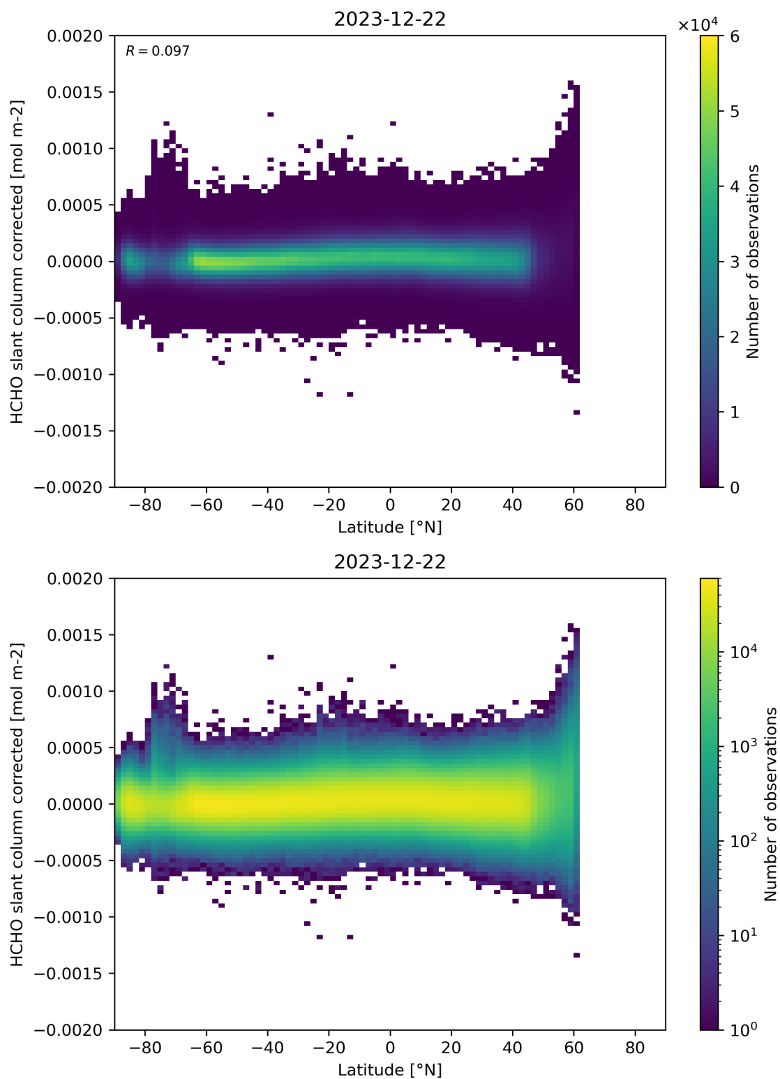
Figure 157: Scatter density plot of “Latitude” against “HCHO slant column corrected” for 2023-12-21 to 2023-12-23.
