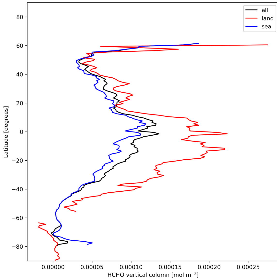
Figure 21: Zonal average of “HCHO vertical column” for 2023-12-21 to 2023-12-23.
