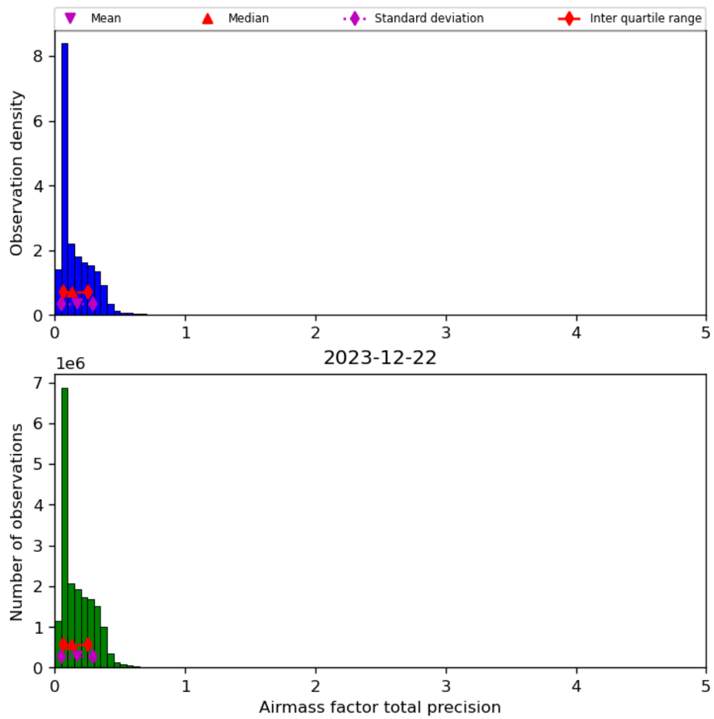
Figure 41: Histogram of “Airmass factor total precision” for 2023-12-21 to 2023-12-23
