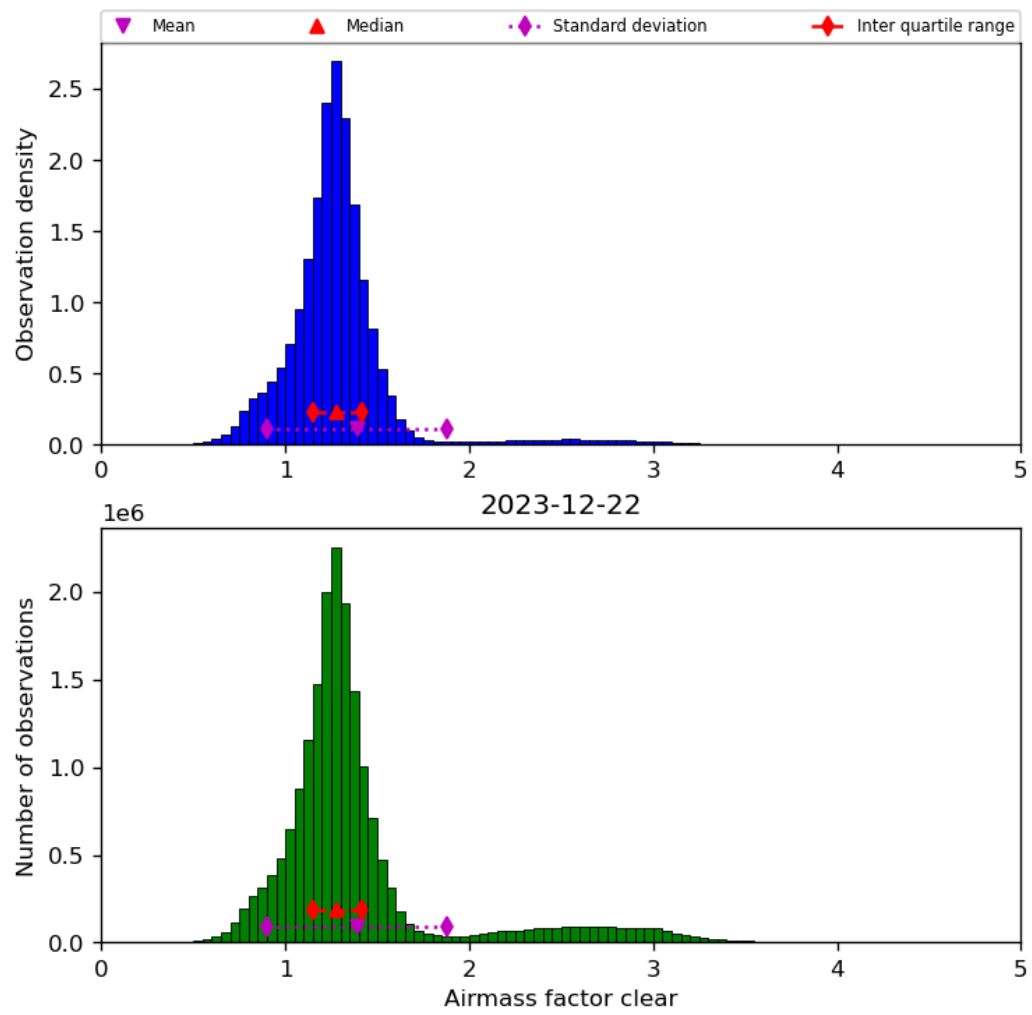
Figure 42: Histogram of “Airmass factor clear” for 2023-12-21 to 2023-12-23
