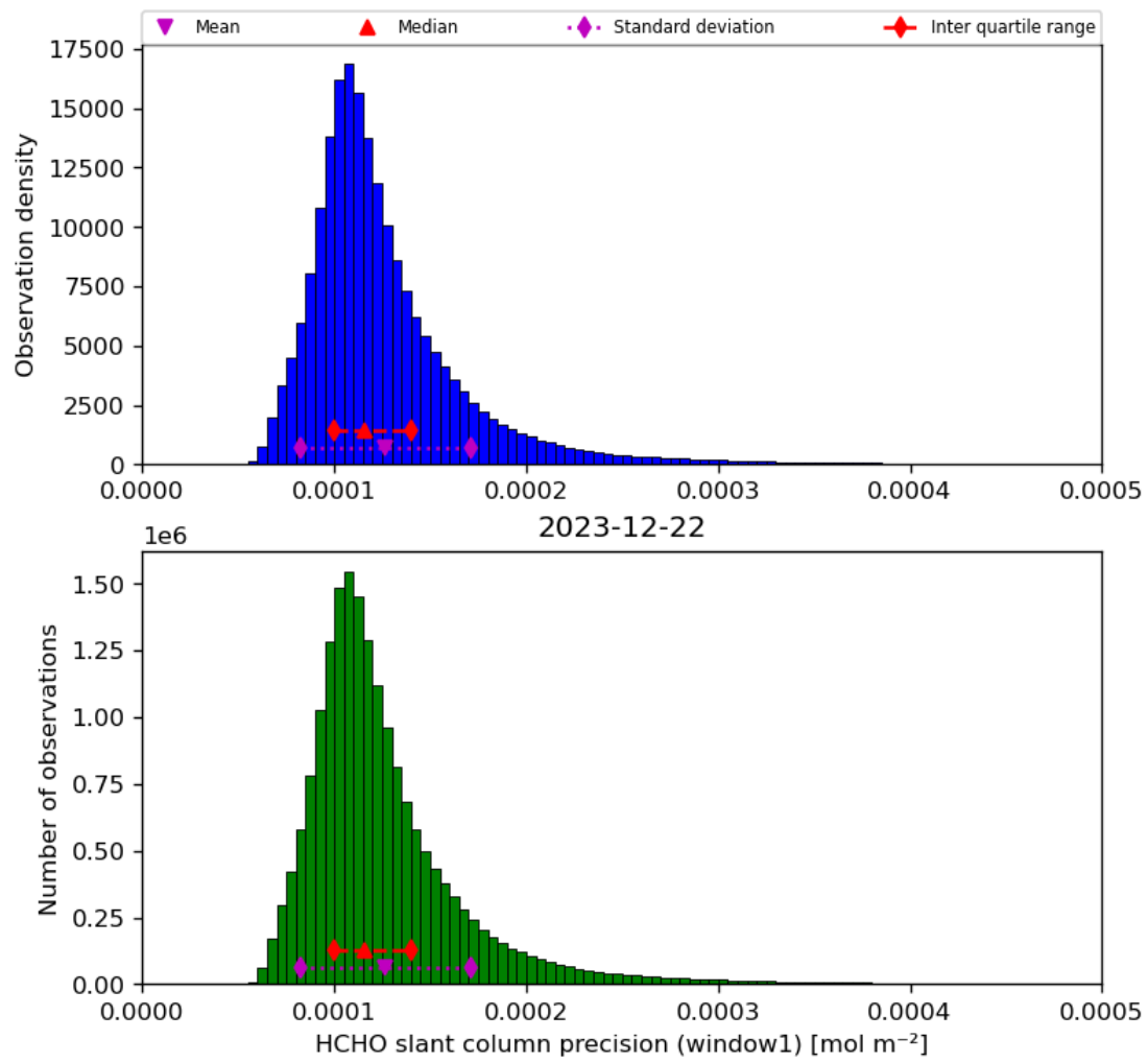
Figure 39: Histogram of “HCHO slant column precision (window1)” for 2023-12-21 to 2023-12-23
