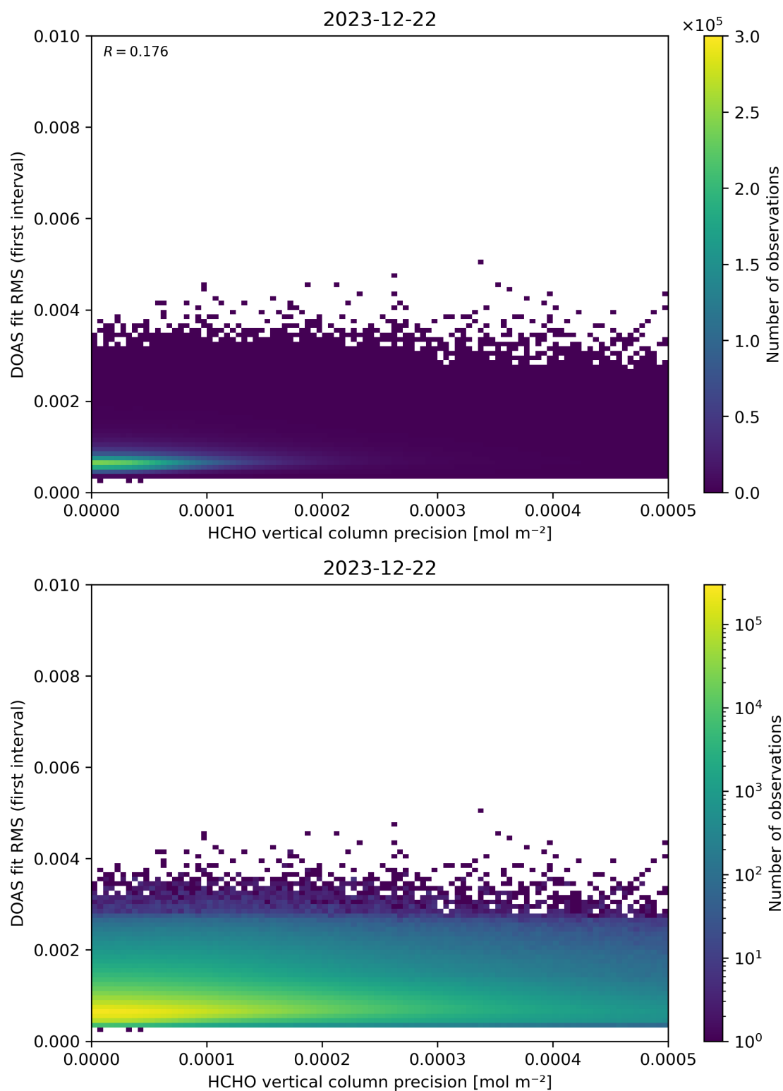
Figure 136: Scatter density plot of “HCHO vertical column precision” against “DOAS fit RMS (first interval)” for 2023-12-21 to 2023-12-23.
