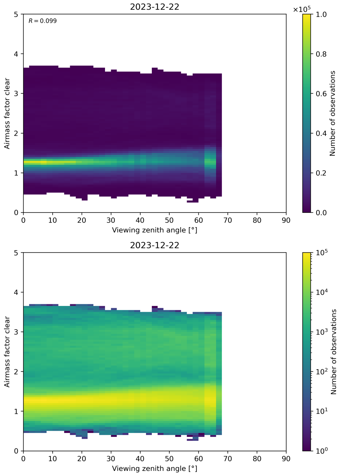
Figure 185: Scatter density plot of “Viewing zenith angle” against “Airmass factor clear” for 2023-12-21 to 2023-12-23.
