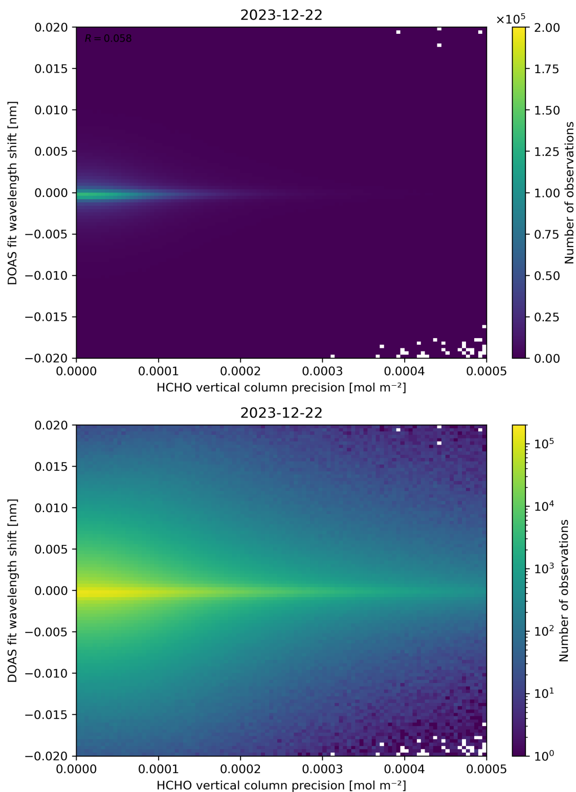
Figure 137: Scatter density plot of “HCHO vertical column precision” against “DOAS fit wavelength shift” for 2023-12-21 to 2023-12-23.
