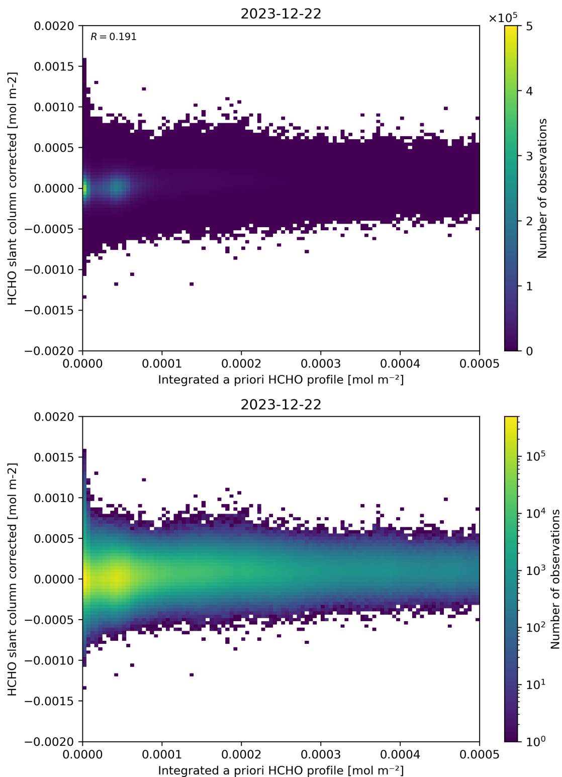
Figure 151: Scatter density plot of “Integrated a priori HCHO profile” against “HCHO slant column corrected” for 2023-12-21 to 2023-12-23.
