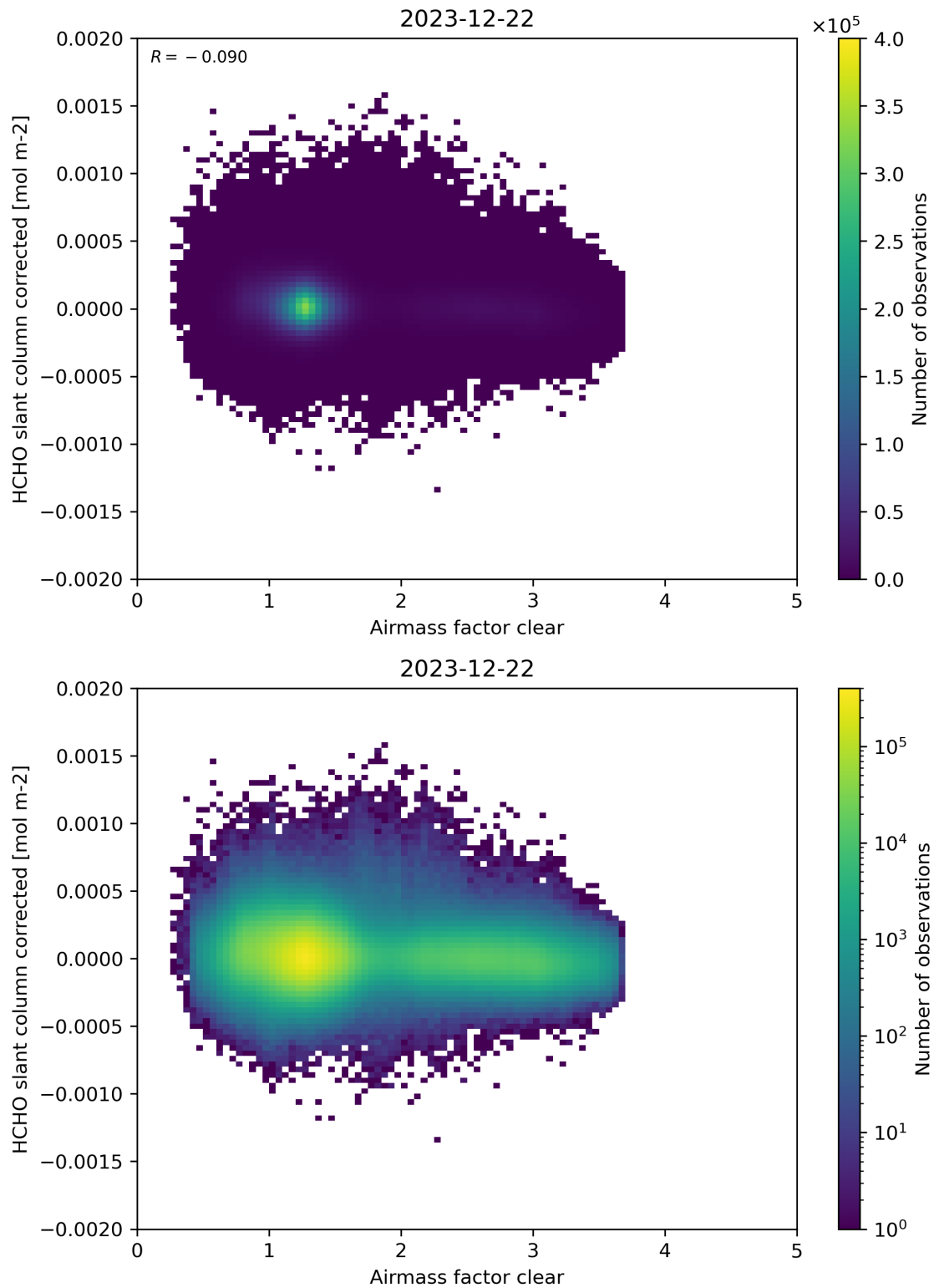
Figure 74: Scatter density plot of “Airmass factor clear” against “HCHO slant column corrected” for 2023-12-21 to 2023-12-23.
