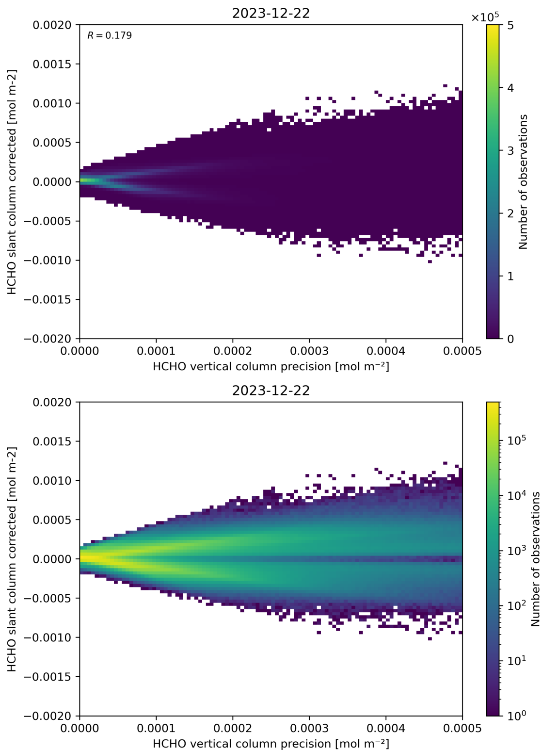
Figure 140: Scatter density plot of “HCHO vertical column precision” against “HCHO slant column corrected” for 2023-12-21 to 2023-12-23.
