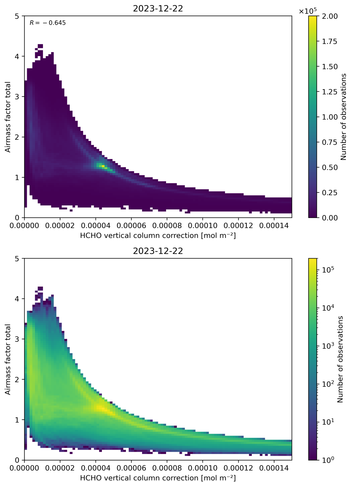
Figure 120: Scatter density plot of “HCHO vertical column correction” against “Airmass factor total” for 2023-12-21 to 2023-12-23.
