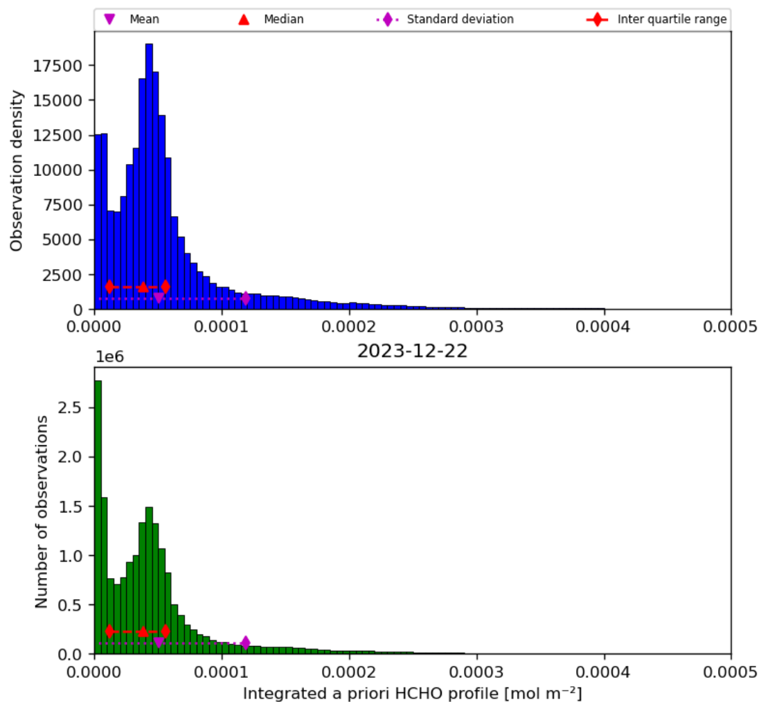
Figure 43: Histogram of “Integrated a priori HCHO profile” for 2023-12-21 to 2023-12-23
