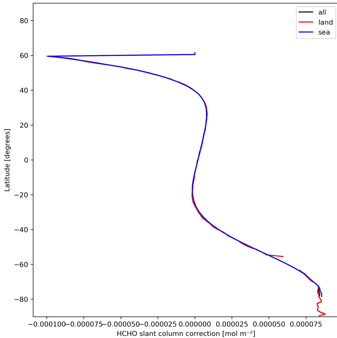
Figure 33: Zonal average of “HCHO slant column correction” for 2023-12-21 to 2023-12-23.
