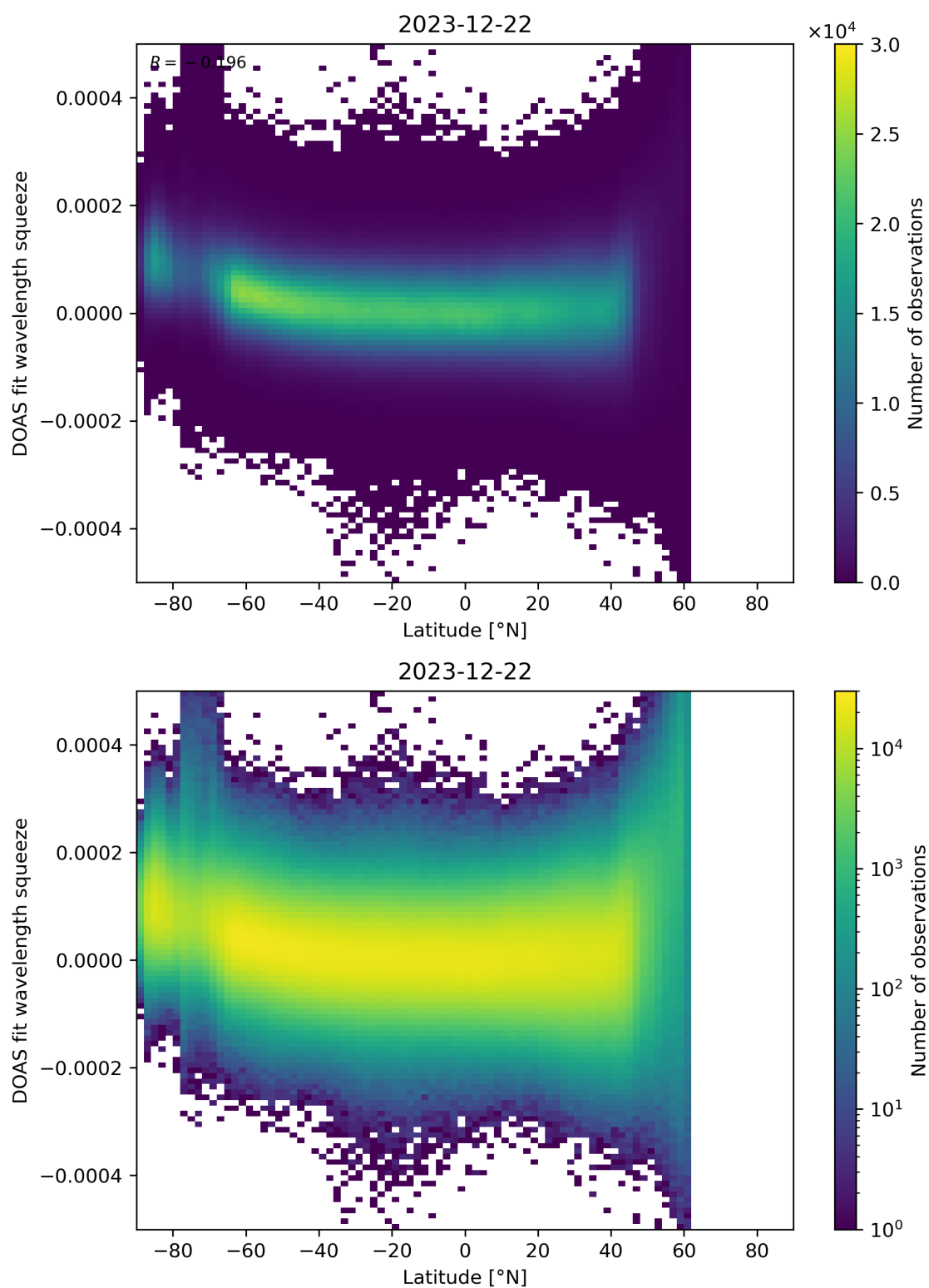
Figure 155: Scatter density plot of “Latitude” against “DOAS fit wavelength squeeze” for 2023-12-21 to 2023-12-23.
