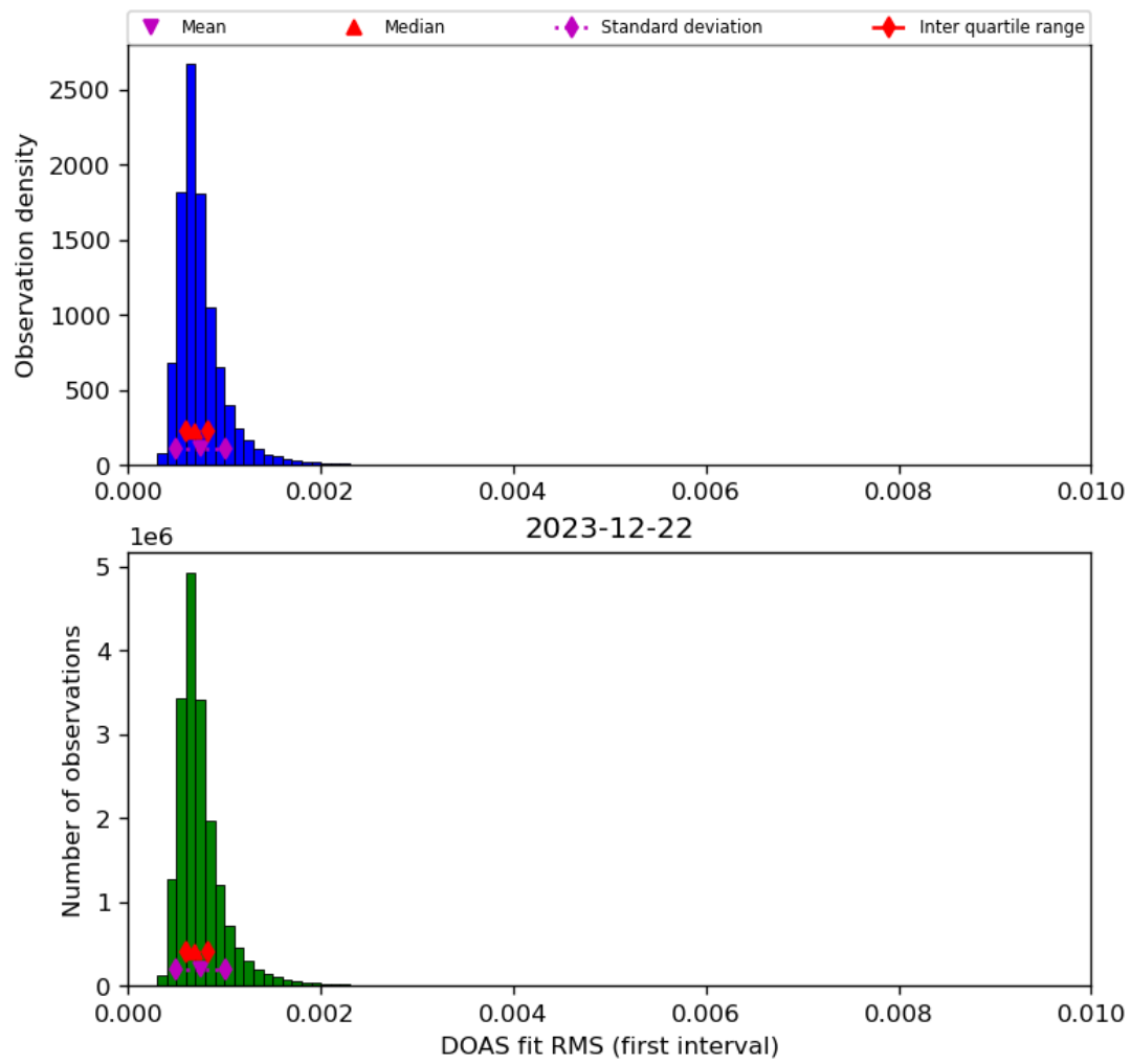
Figure 46: Histogram of “DOAS fit RMS (first interval)” for 2023-12-21 to 2023-12-23
