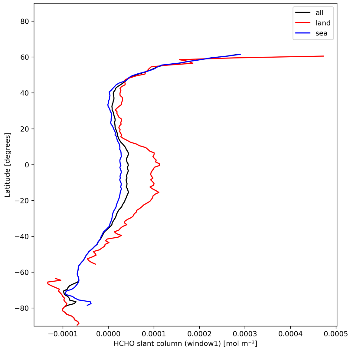
Figure 24: Zonal average of “HCHO slant column (window1)” for 2023-12-21 to 2023-12-23.
