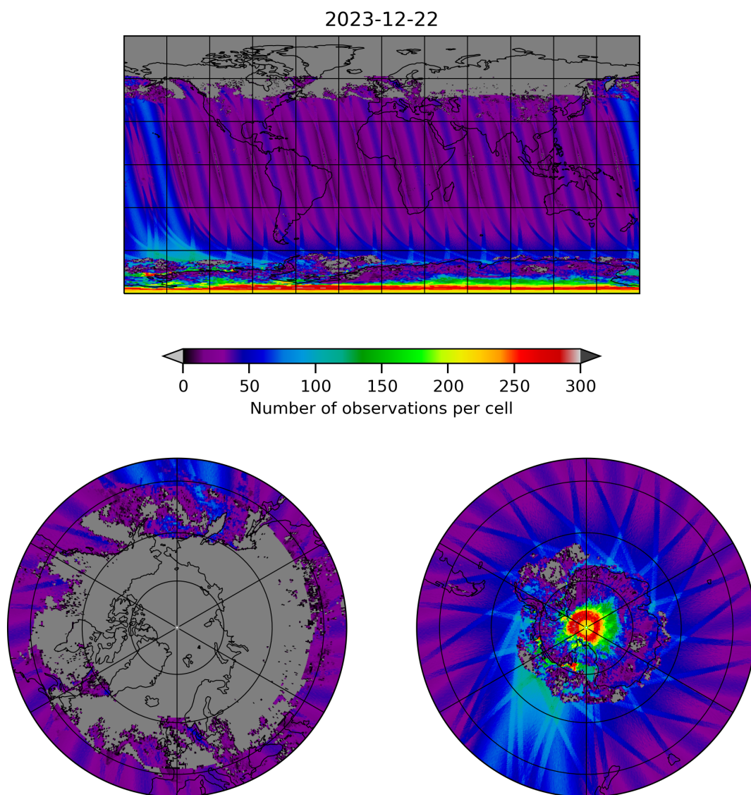
Figure 19: Map of the number of observations for 2023-12-21 to 2023-12-23
