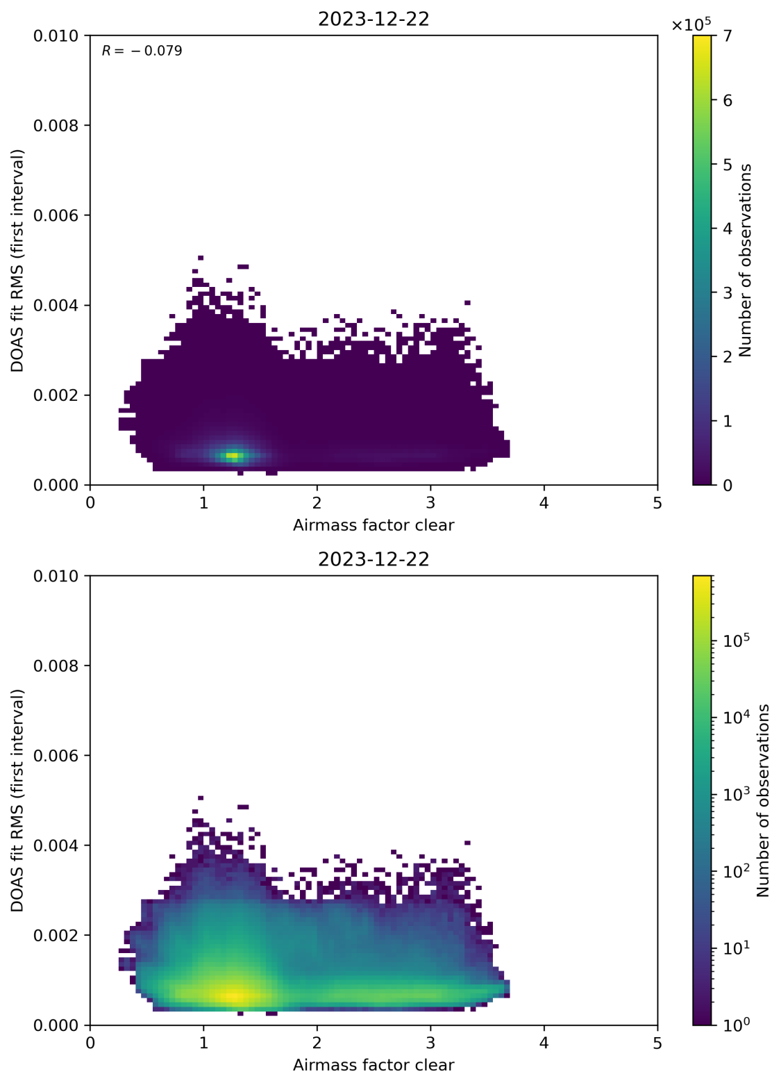
Figure 71: Scatter density plot of “Airmass factor clear” against “DOAS fit RMS (first interval)” for 2023-12-21 to 2023-12-23.
