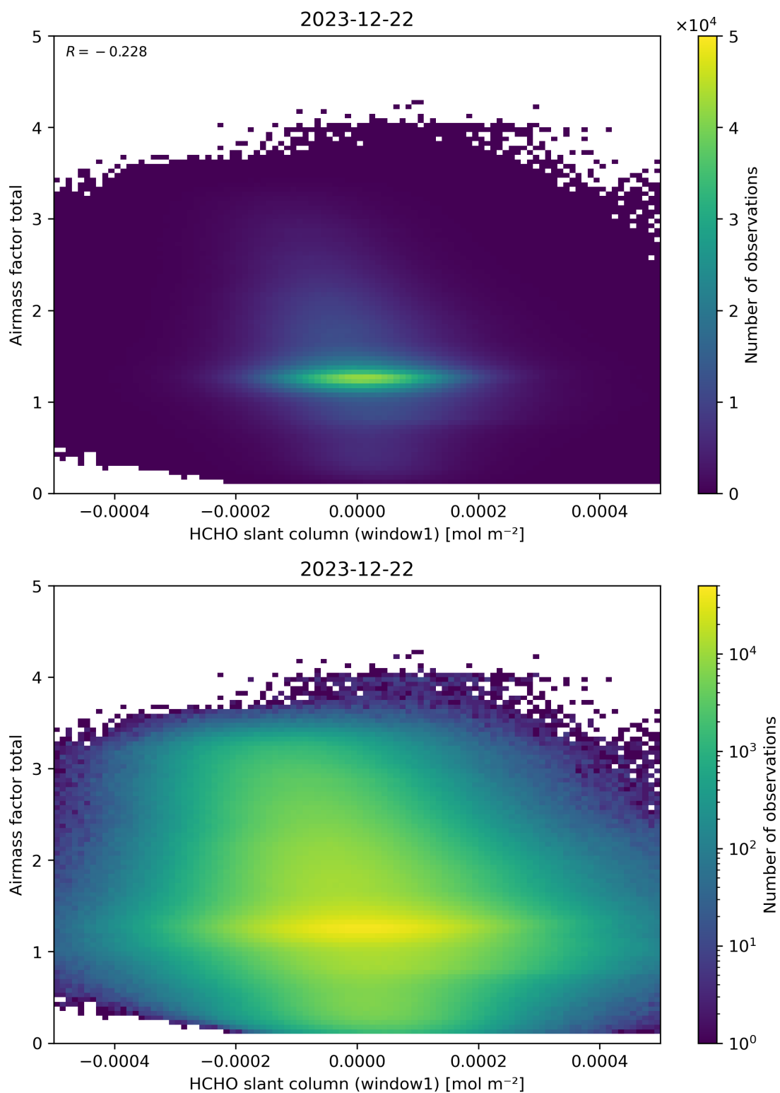
Figure 85: Scatter density plot of “HCHO slant column (window1)” against “Airmass factor total” for 2023-12-21 to 2023-12-23.
