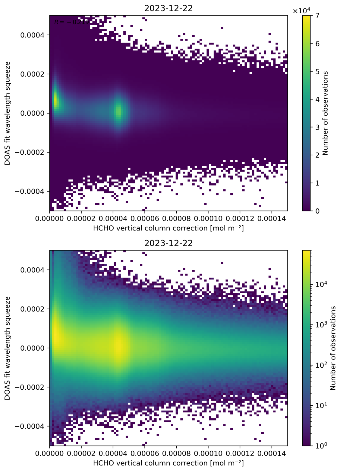
Figure 114: Scatter density plot of “HCHO vertical column correction” against “DOAS fit wavelength squeeze” for 2023-12-21 to 2023-12-23.
