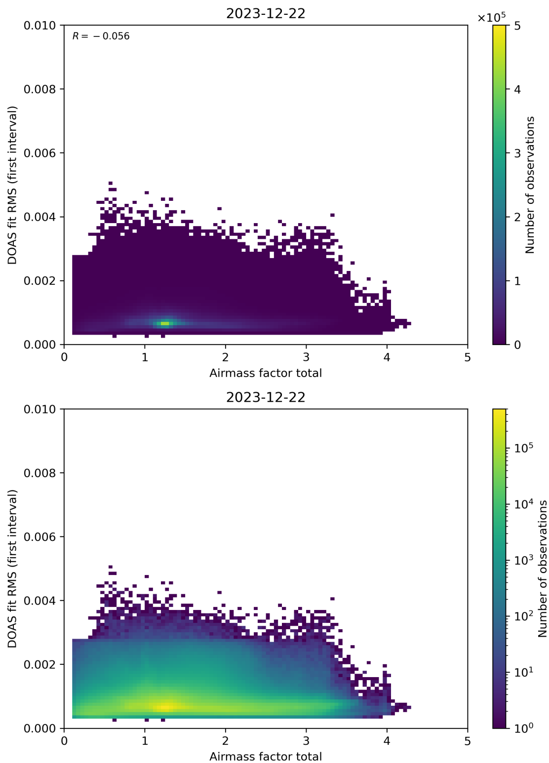
Figure 97: Scatter density plot of “Airmass factor total” against “DOAS fit RMS (first interval)” for 2023-12-21 to 2023-12-23.
