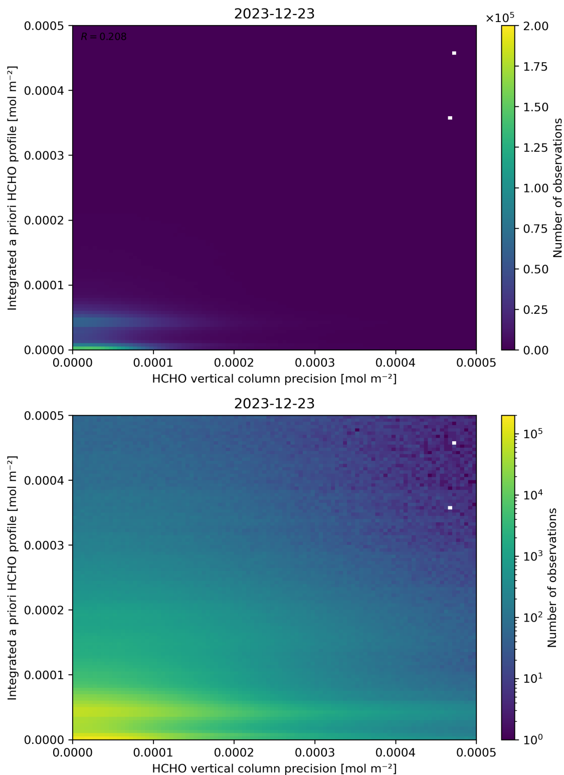
Figure 147: Scatter density plot of “HCHO vertical column precision” against “Integrated a priori HCHO profile” for 2023-12-22 to 2023-12-24.
