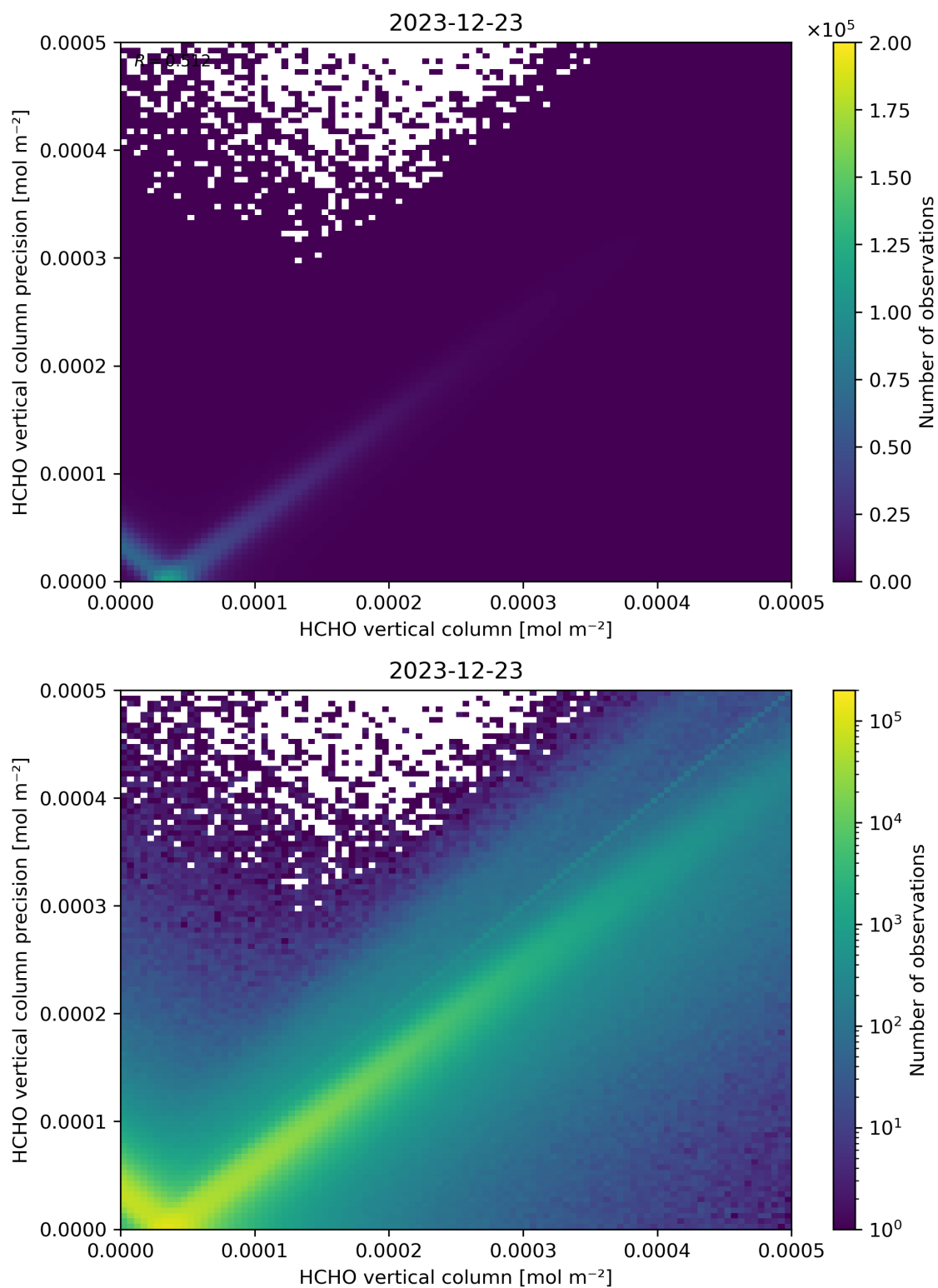
Figure 134: Scatter density plot of “HCHO vertical column” against “HCHO vertical column precision” for 2023-12-22 to 2023-12-24.
