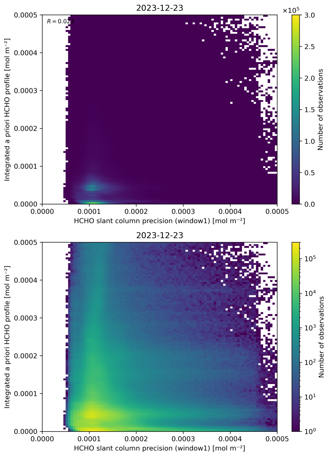
Figure 96: Scatter density plot of “HCHO slant column precision (window1)” against “Integrated a priori HCHO profile” for 2023-12-22 to 2023-12-24.
