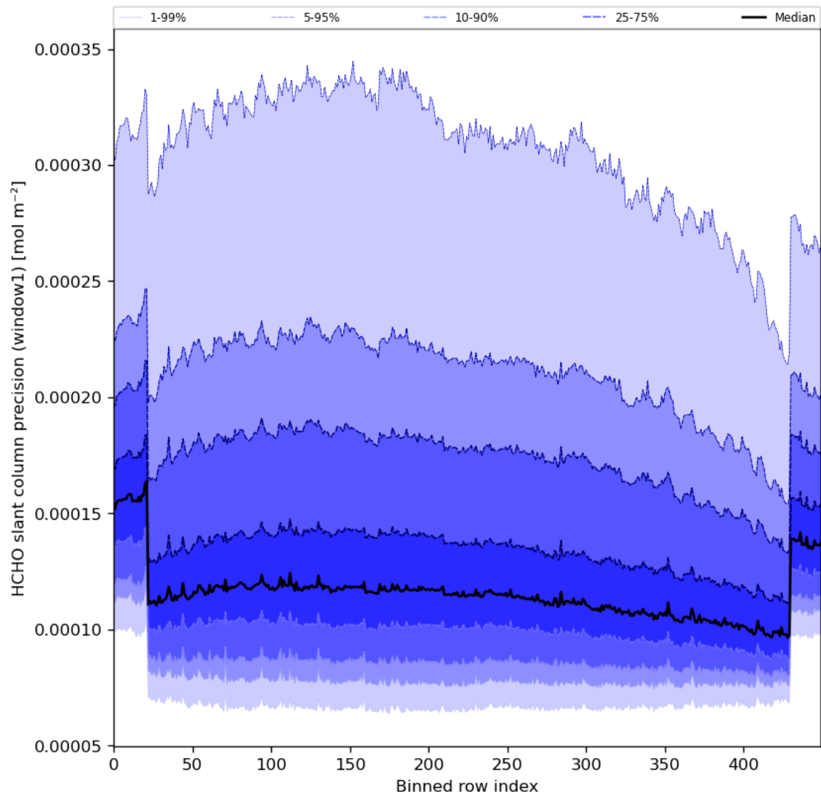
Figure 53: Along track statistics of “HCHO slant column precision (window1)” for 2023-12-22 to 2023-12-24
