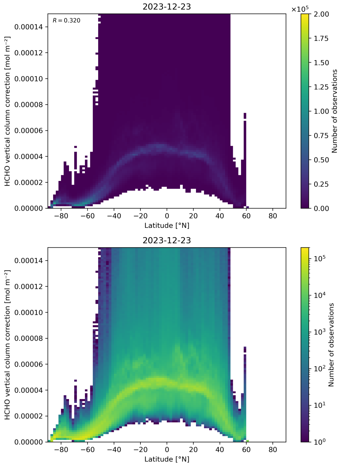
Figure 164: Scatter density plot of “Latitude” against “HCHO vertical column correction” for 2023-12-22 to 2023-12-24.
