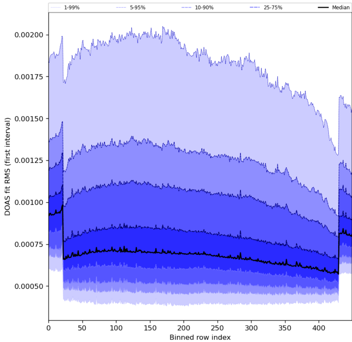
Figure 60: Along track statistics of “DOAS fit RMS (first interval)” for 2023-12-22 to 2023-12-24
