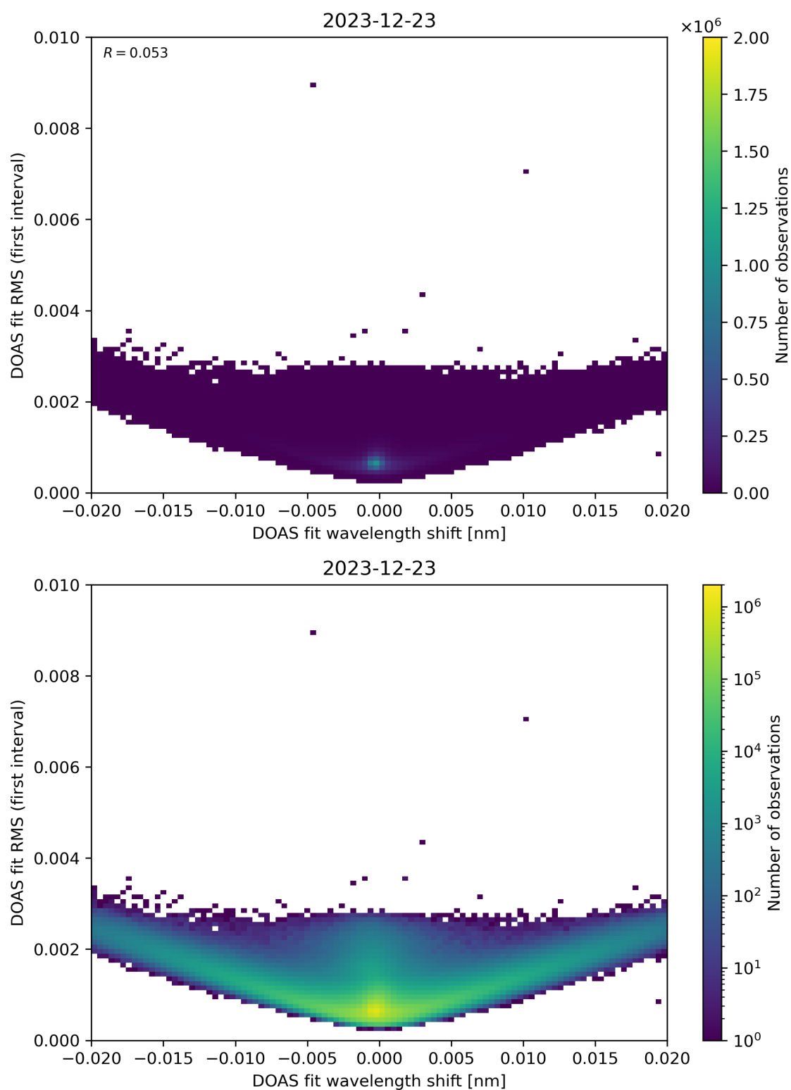
Figure 64: Scatter density plot of “DOAS fit wavelength shift” against “DOAS fit RMS (first interval)” for 2023-12-22 to 2023-12-24.
