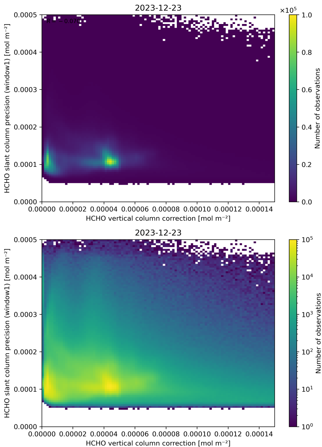
Figure 119: Scatter density plot of “HCHO vertical column correction” against “HCHO slant column precision (window1)” for 2023-12-22 to 2023-12-24.
