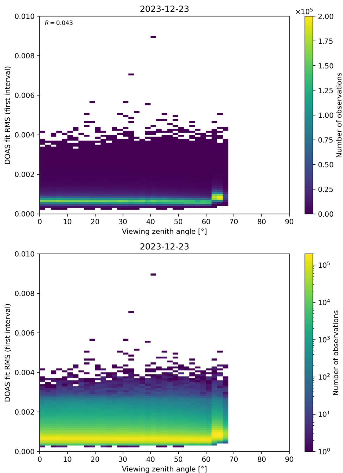
Figure 182: Scatter density plot of “Viewing zenith angle” against “DOAS fit RMS (first interval)” for 2023-12-22 to 2023-12-24.
