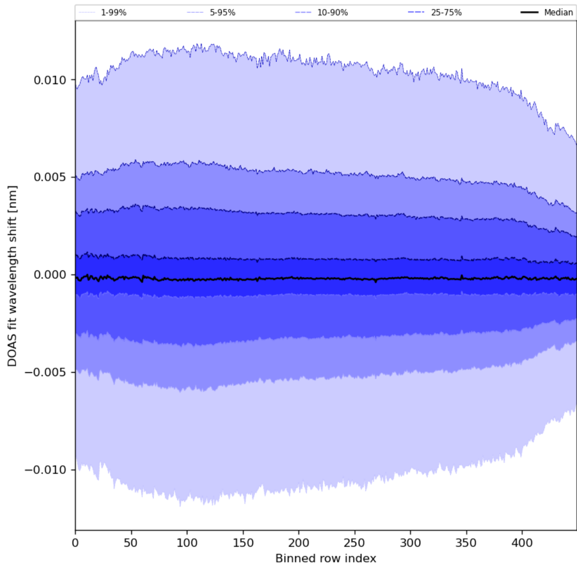
Figure 58: Along track statistics of “DOAS fit wavelength shift” for 2023-12-22 to 2023-12-24
