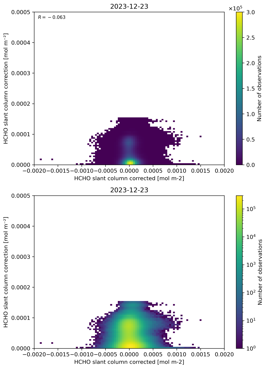
Figure 77: Scatter density plot of “HCHO slant column corrected” against “HCHO slant column correction” for 2023-12-22 to 2023-12-24.
