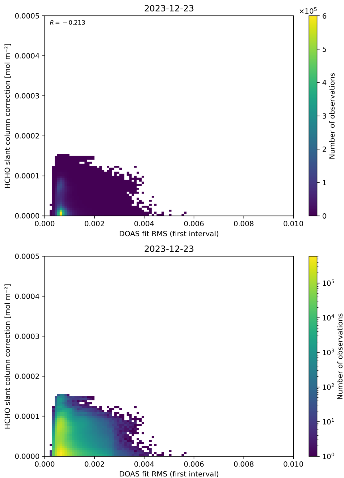
Figure 63: Scatter density plot of “DOAS fit RMS (first interval)” against “HCHO slant column correction” for 2023-12-22 to 2023-12-24.
