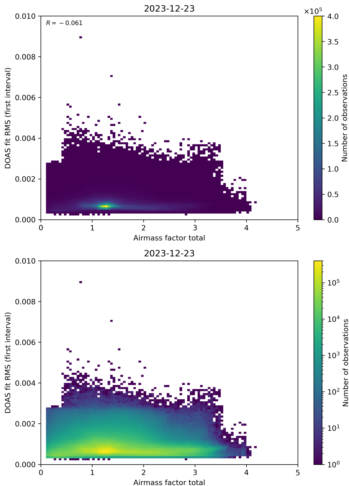
Figure 97: Scatter density plot of “Airmass factor total” against “DOAS fit RMS (first interval)” for 2023-12-22 to 2023-12-24.
