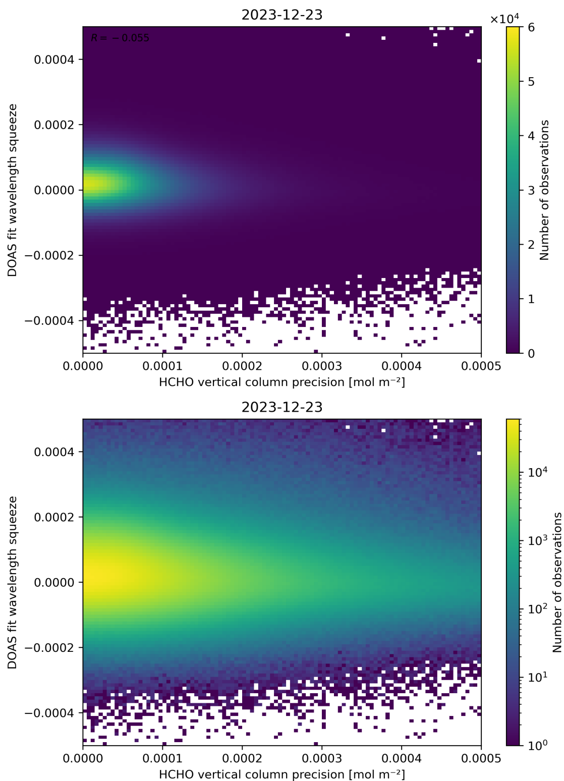
Figure 138: Scatter density plot of “HCHO vertical column precision” against “DOAS fit wavelength squeeze” for 2023-12-22 to 2023-12-24.
