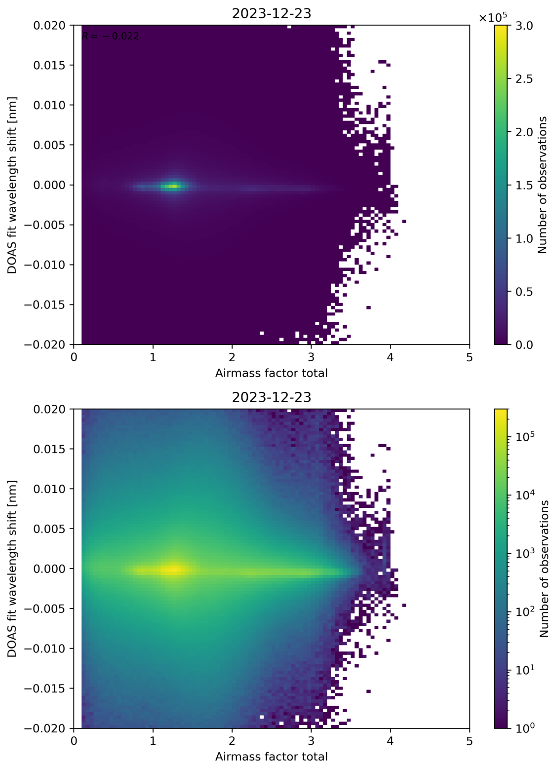
Figure 98: Scatter density plot of “Airmass factor total” against “DOAS fit wavelength shift” for 2023-12-22 to 2023-12-24.
