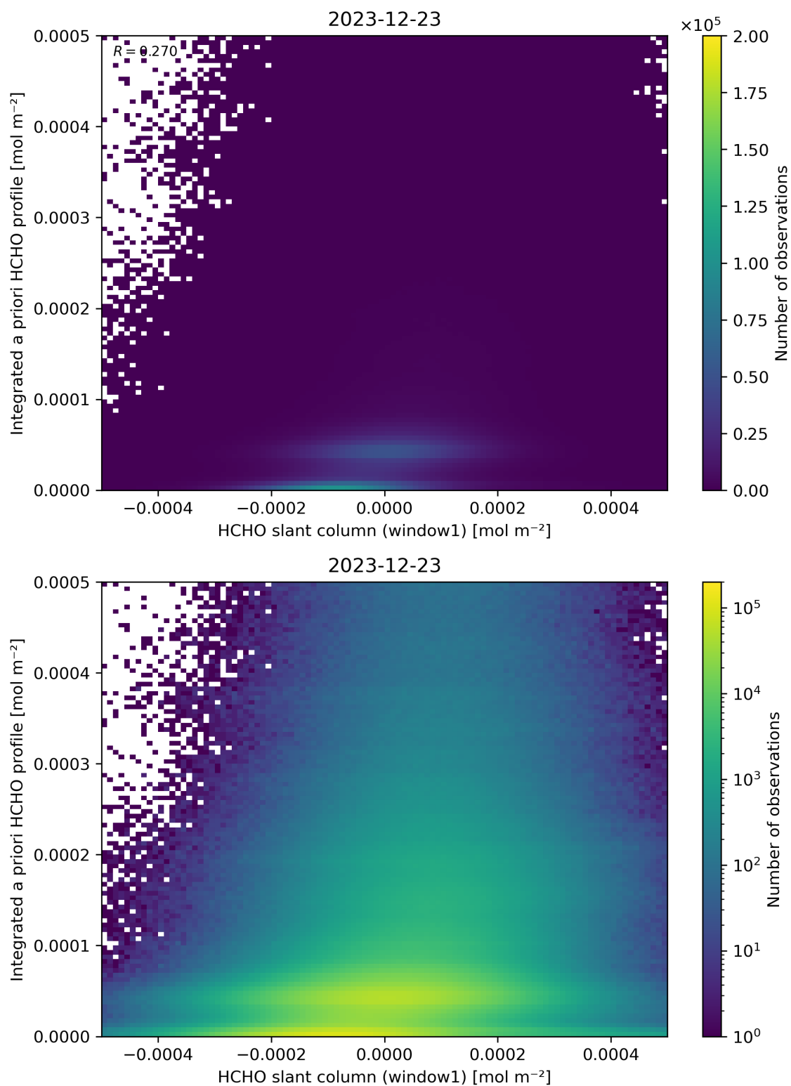
Figure 87: Scatter density plot of “HCHO slant column (window1)” against “Integrated a priori HCHO profile” for 2023-12-22 to 2023-12-24.
