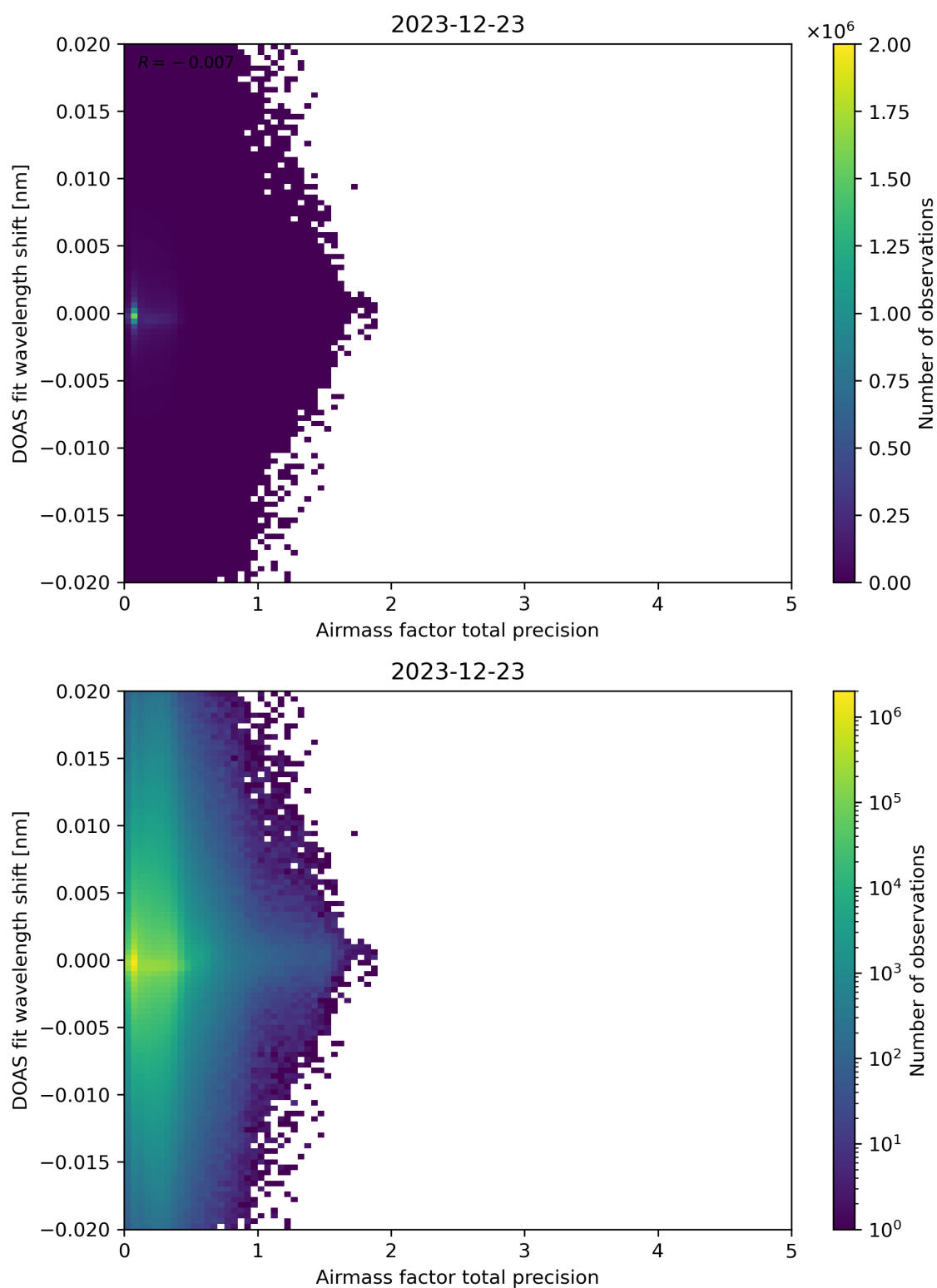
Figure 106: Scatter density plot of “Airmass factor total precision” against “DOAS fit wavelength shift” for 2023-12-22 to 2023-12-24.
