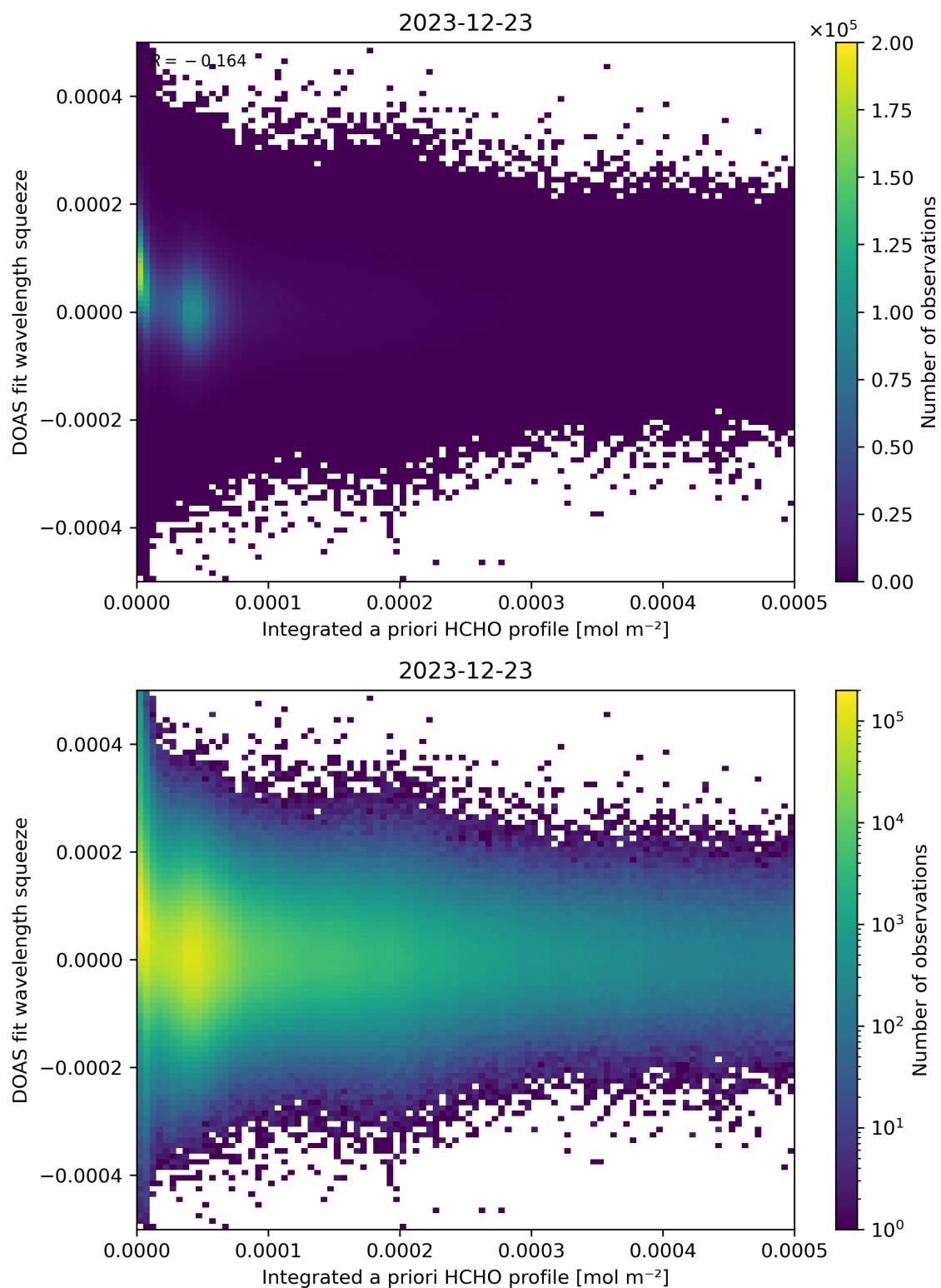
Figure 150: Scatter density plot of “Integrated a priori HCHO profile” against “DOAS fit wavelength squeeze” for 2023-12-22 to 2023-12-24.
