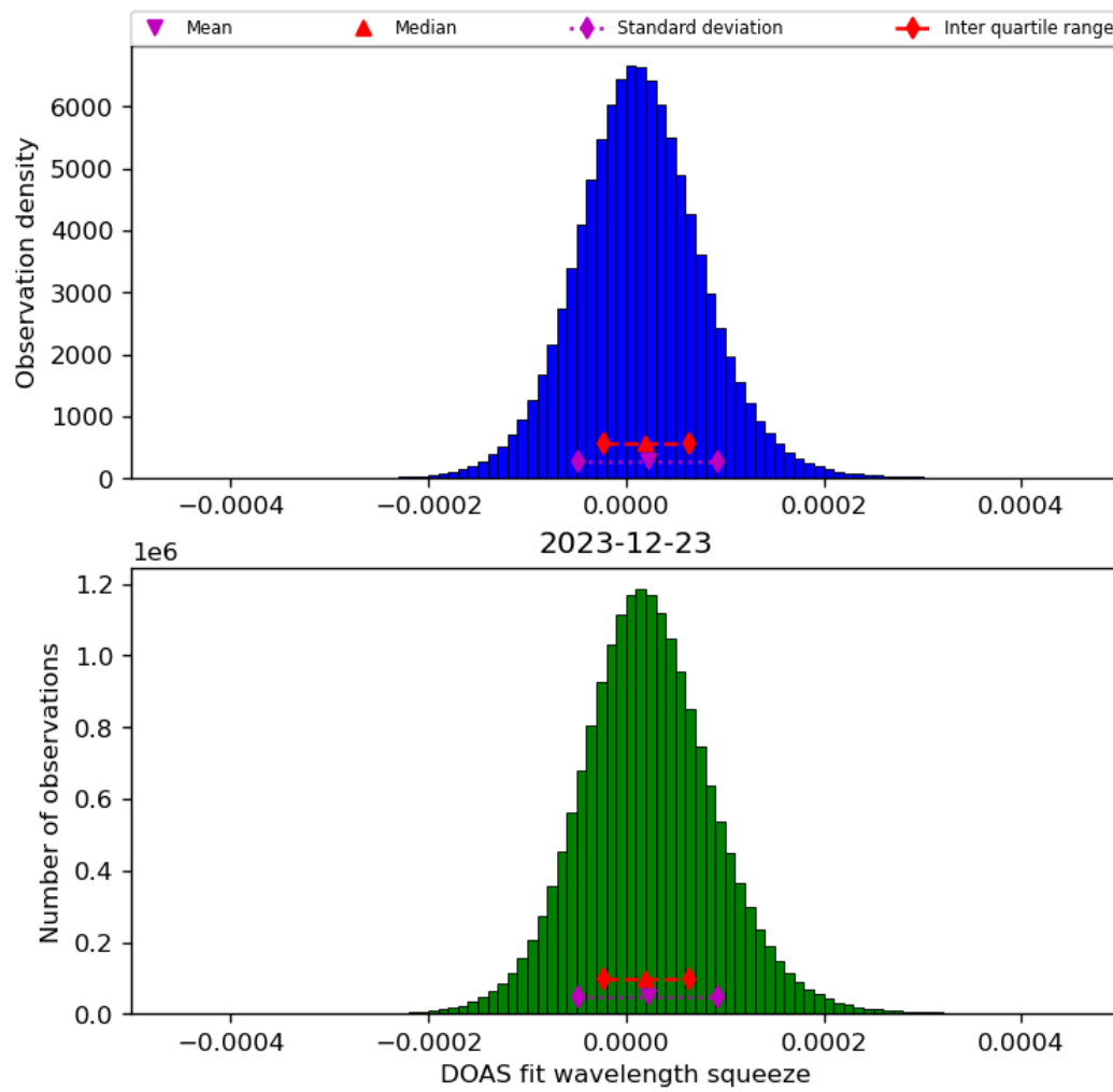
Figure 45: Histogram of “DOAS fit wavelength squeeze” for 2023-12-22 to 2023-12-24
