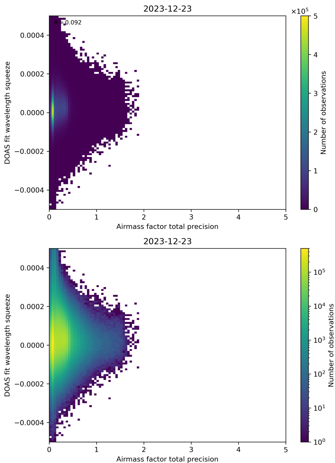
Figure 107: Scatter density plot of “Airmass factor total precision” against “DOAS fit wavelength squeeze” for 2023-12-22 to 2023-12-24.
