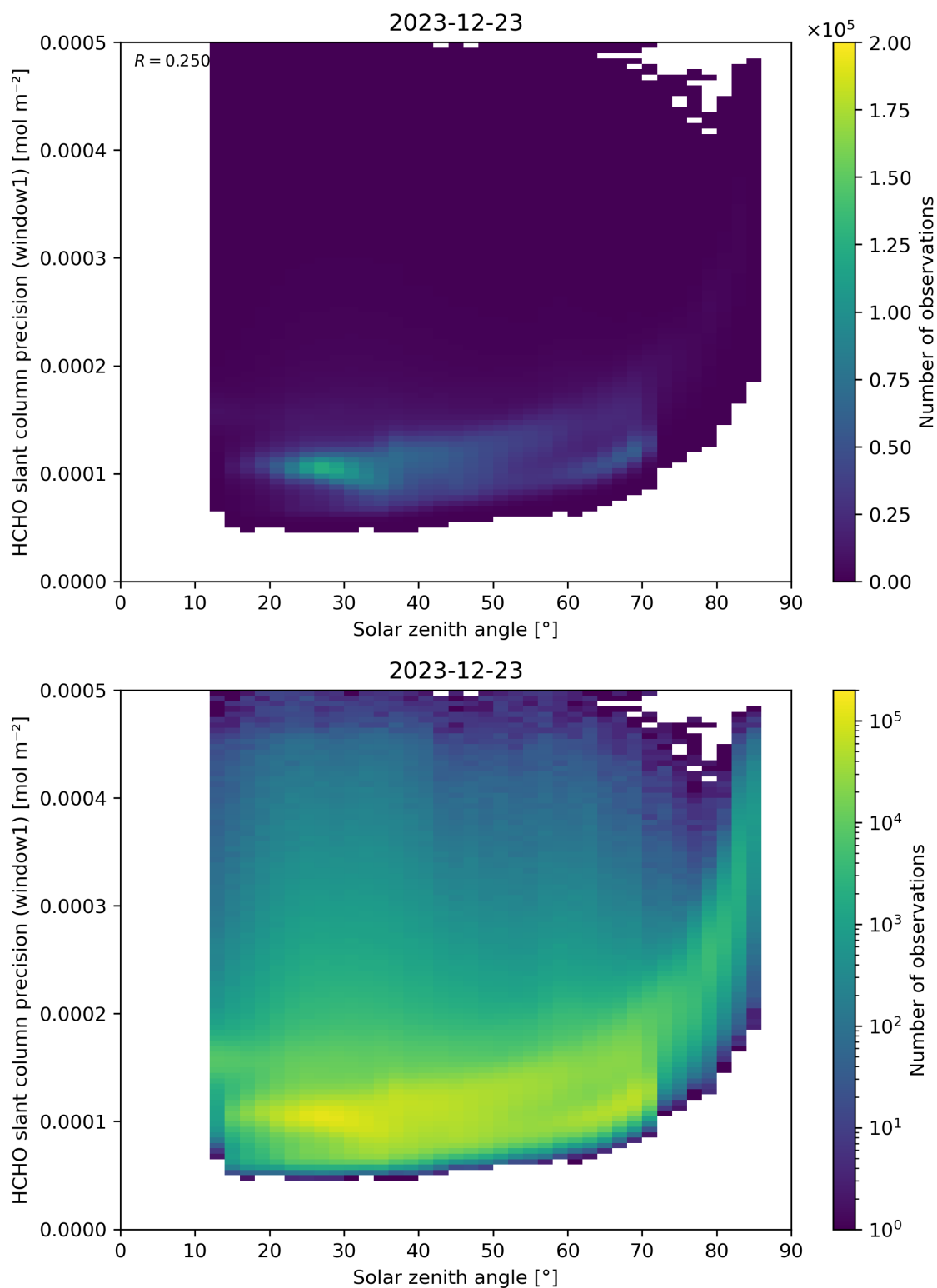
Figure 174: Scatter density plot of “Solar zenith angle” against “HCHO slant column precision (window1)” for 2023-12-22 to 2023-12-24.
