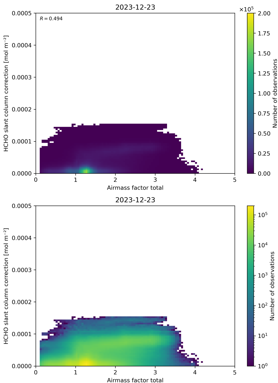
Figure 102: Scatter density plot of “Airmass factor total” against “HCHO slant column correction” for 2023-12-22 to 2023-12-24.
