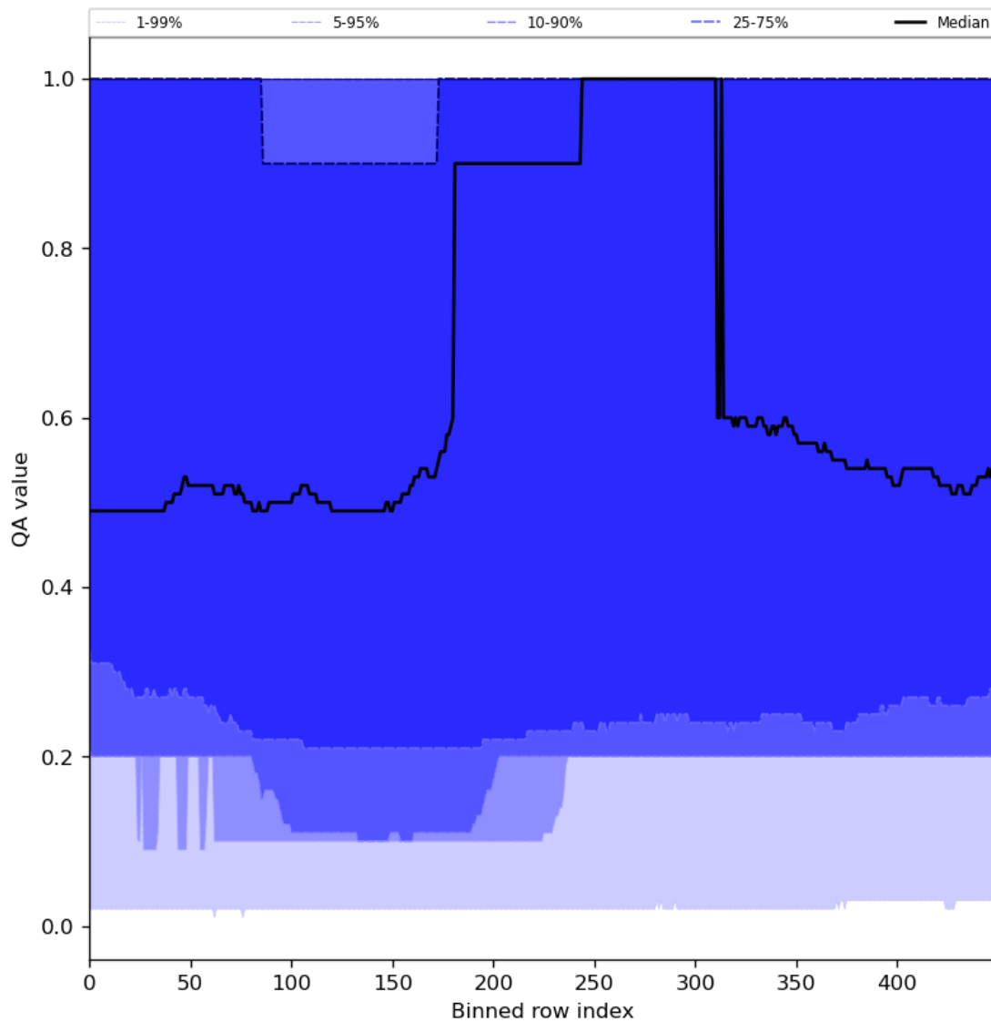
Figure 48: Along track statistics of “QA value” for 2023-12-22 to 2023-12-24
