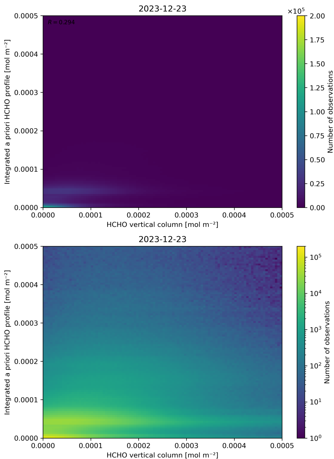
Figure 135: Scatter density plot of “HCHO vertical column” against “Integrated a priori HCHO profile” for 2023-12-22 to 2023-12-24.
