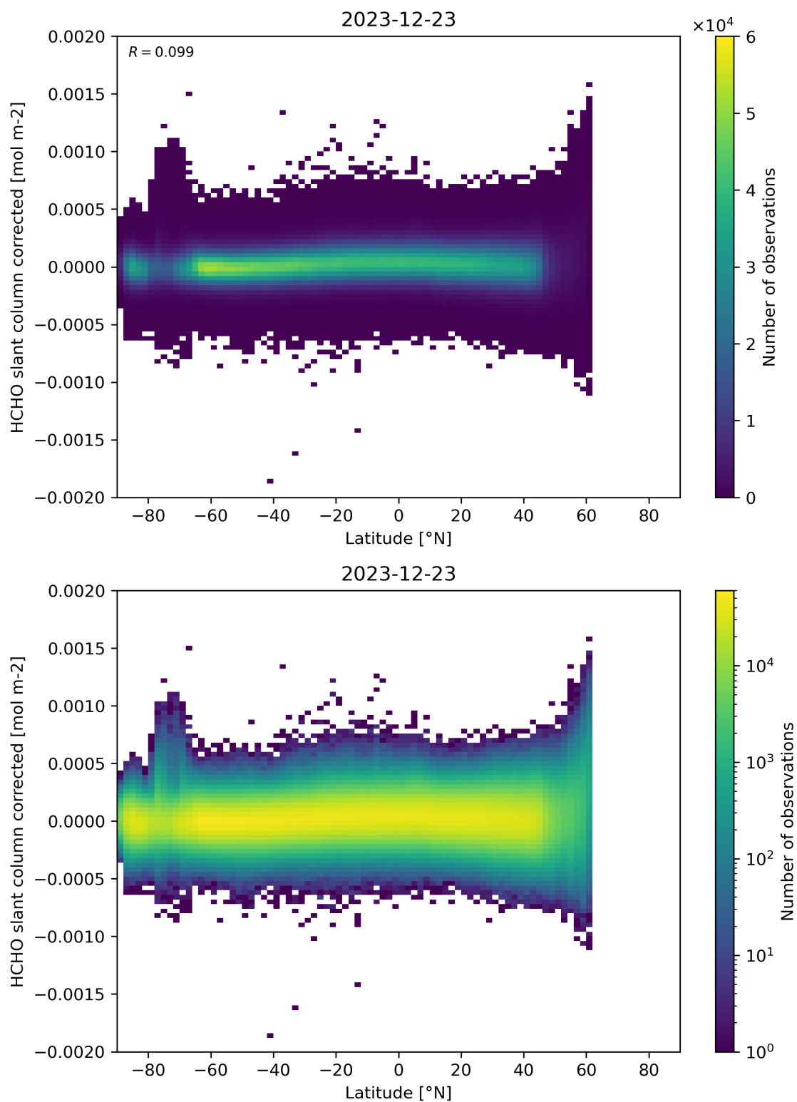
Figure 157: Scatter density plot of “Latitude” against “HCHO slant column corrected” for 2023-12-22 to 2023-12-24.
