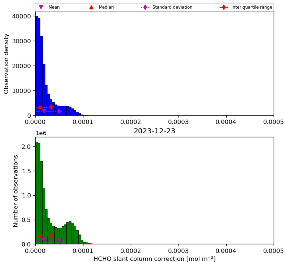
Figure 47: Histogram of “HCHO slant column correction” for 2023-12-22 to 2023-12-24
