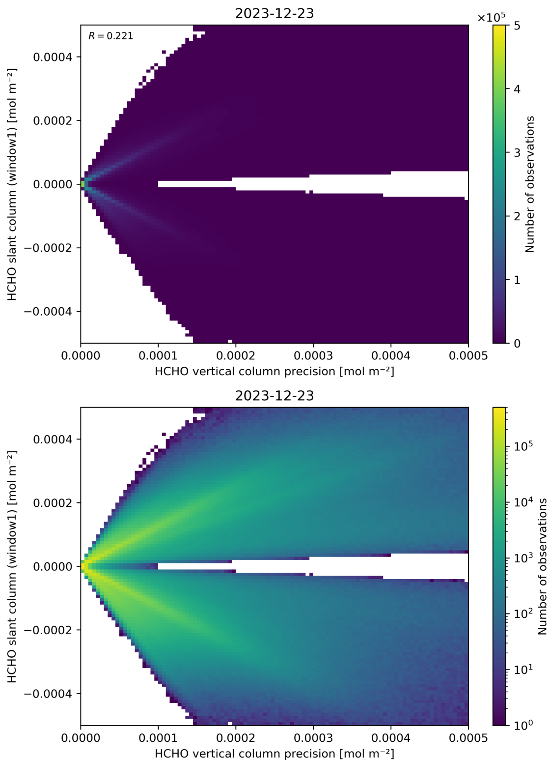
Figure 142: Scatter density plot of “HCHO vertical column precision” against “HCHO slant column (window1)” for 2023-12-22 to 2023-12-24.
