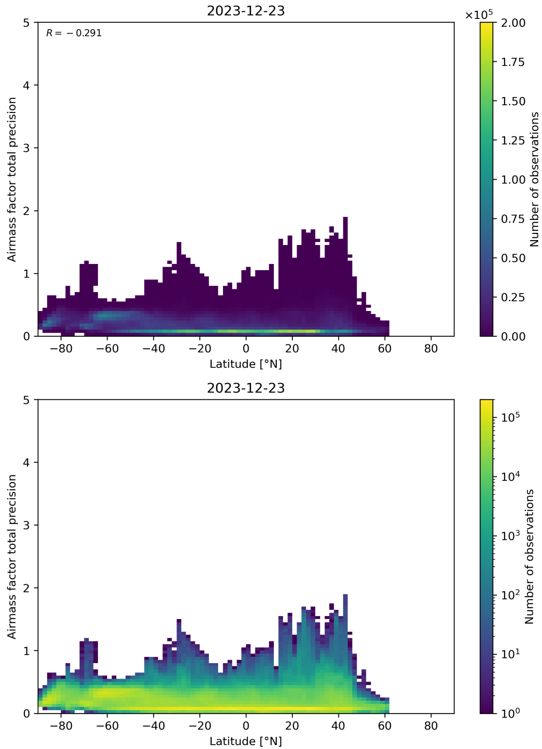
Figure 162: Scatter density plot of “Latitude” against “Airmass factor total precision” for 2023-12-22 to 2023-12-24.
