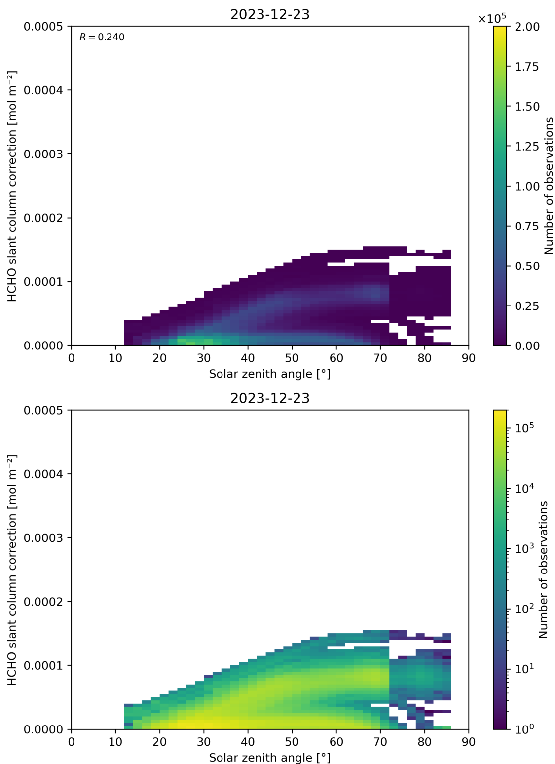
Figure 172: Scatter density plot of “Solar zenith angle” against “HCHO slant column correction” for 2023-12-22 to 2023-12-24.
