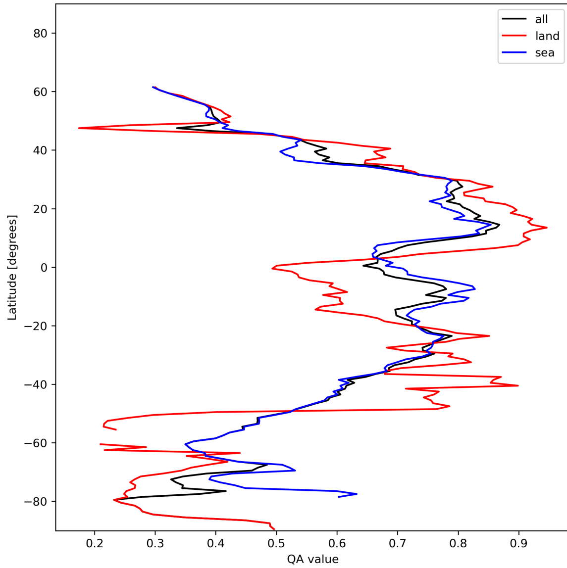
Figure 20: Zonal average of “QA value” for 2023-12-22 to 2023-12-24.
