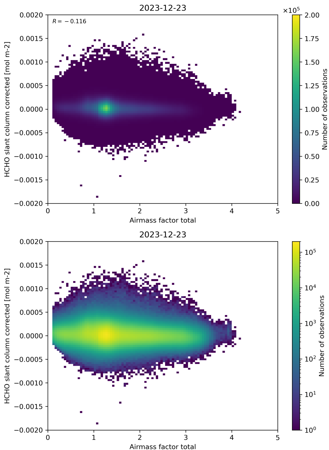
Figure 101: Scatter density plot of “Airmass factor total” against “HCHO slant column corrected” for 2023-12-22 to 2023-12-24.
