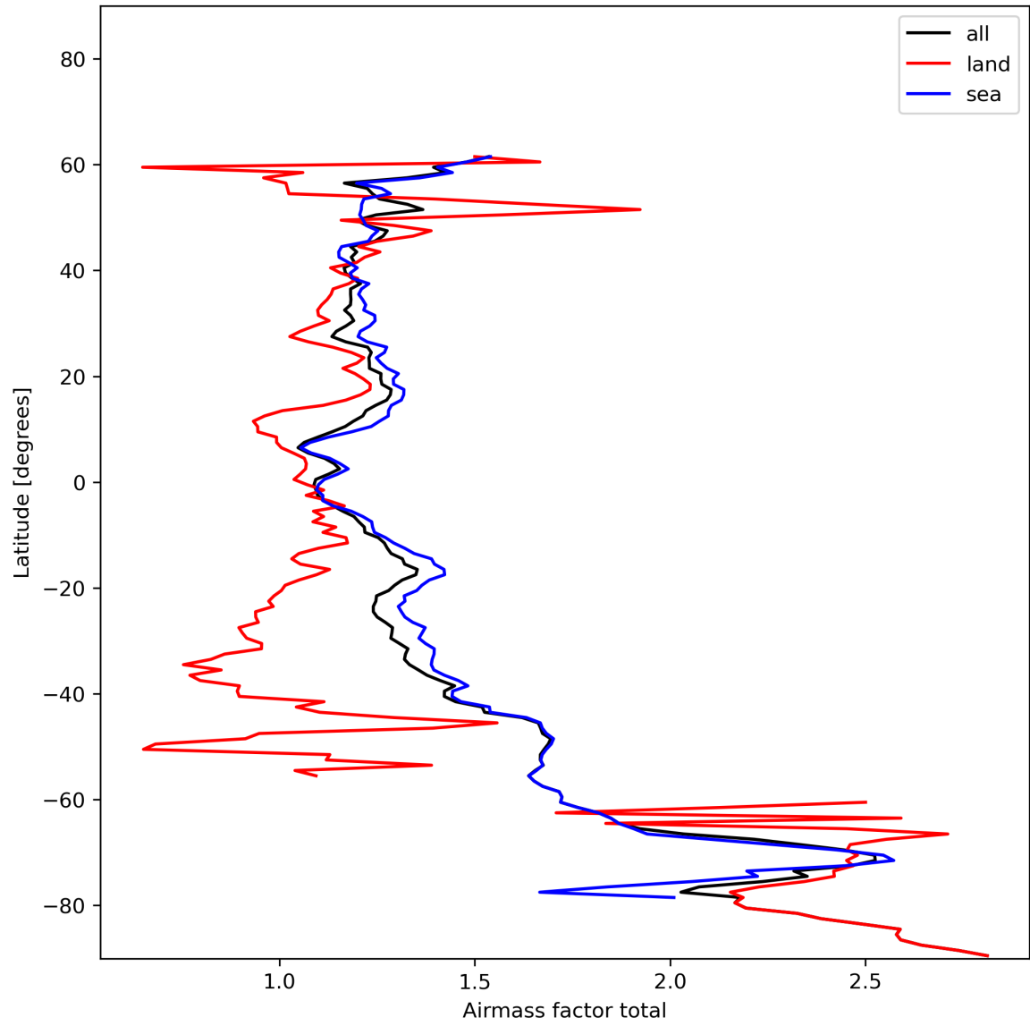
Figure 26: Zonal average of “Airmass factor total” for 2023-12-22 to 2023-12-24.
