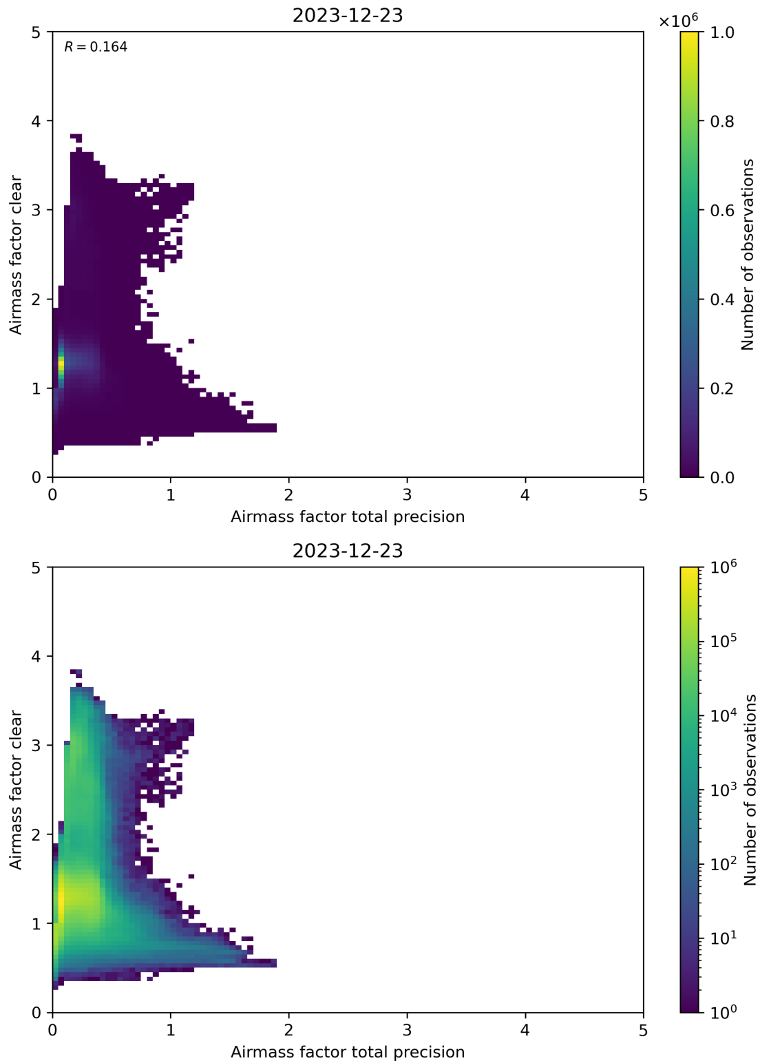
Figure 108: Scatter density plot of “Airmass factor total precision” against “Airmass factor clear” for 2023-12-22 to 2023-12-24.
