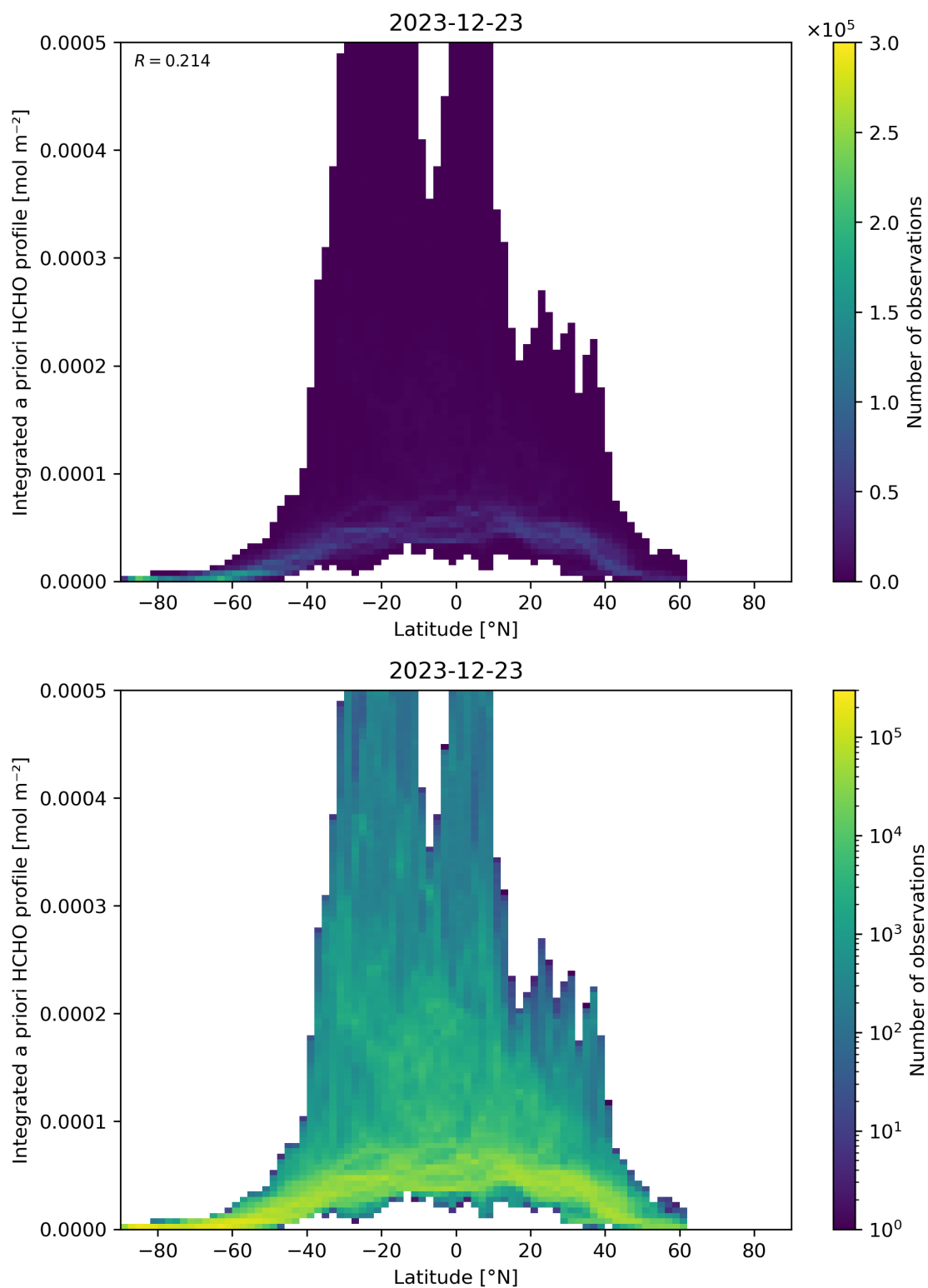
Figure 166: Scatter density plot of “Latitude” against “Integrated a priori HCHO profile” for 2023-12-22 to 2023-12-24.
