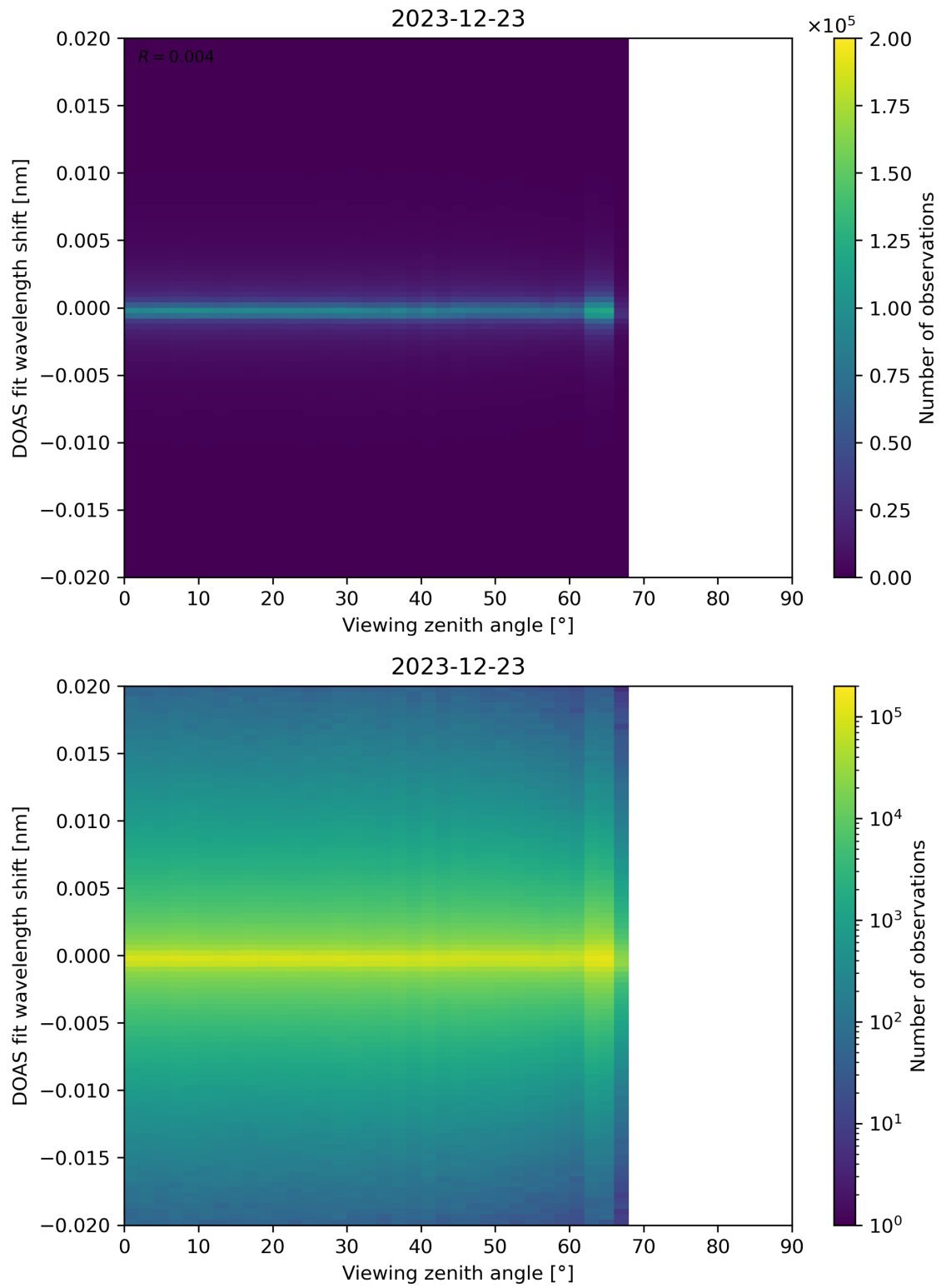
Figure 183: Scatter density plot of “Viewing zenith angle” against “DOAS fit wavelength shift” for 2023-12-22 to 2023-12-24.
