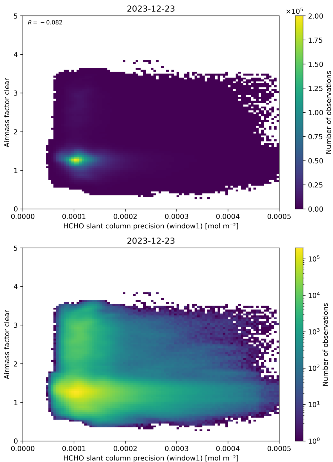
Figure 91: Scatter density plot of “HCHO slant column precision (window1)” against “Airmass factor clear” for 2023-12-22 to 2023-12-24.
