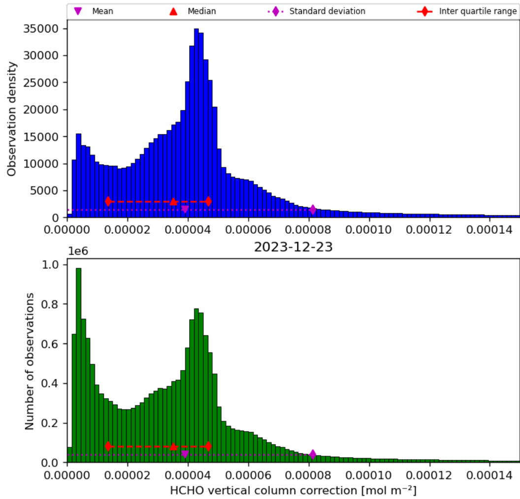
Figure 37: Histogram of “HCHO vertical column correction” for 2023-12-22 to 2023-12-24
