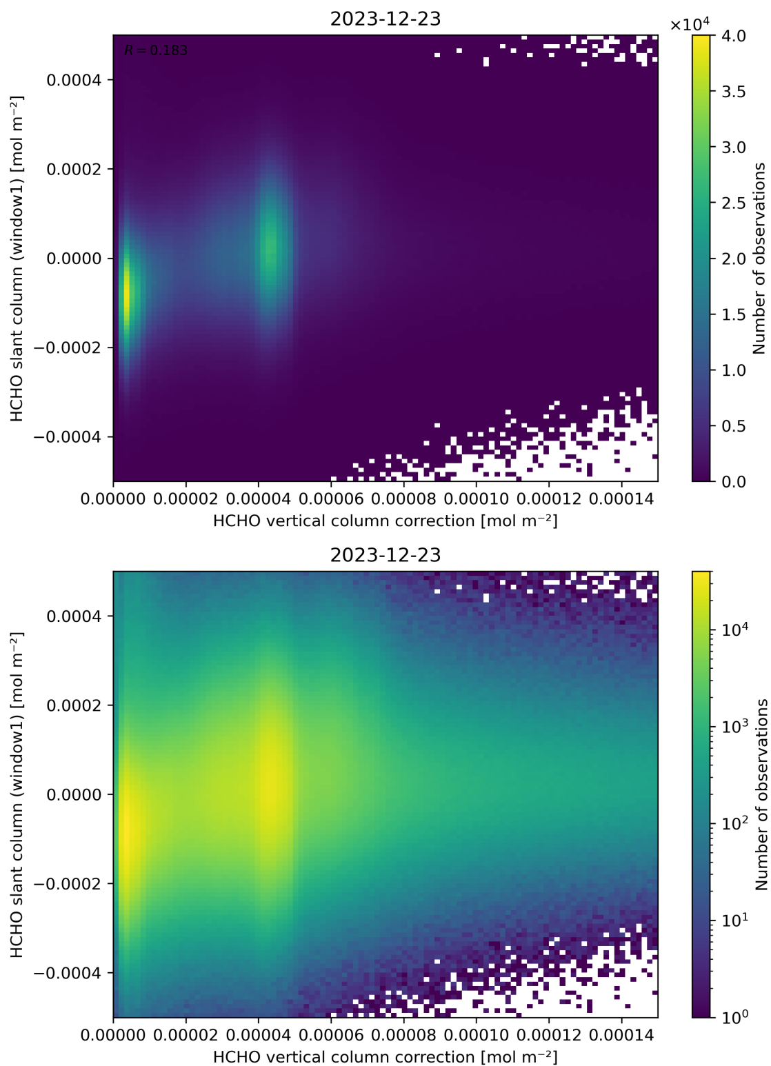
Figure 118: Scatter density plot of “HCHO vertical column correction” against “HCHO slant column (window1)” for 2023-12-22 to 2023-12-24.
