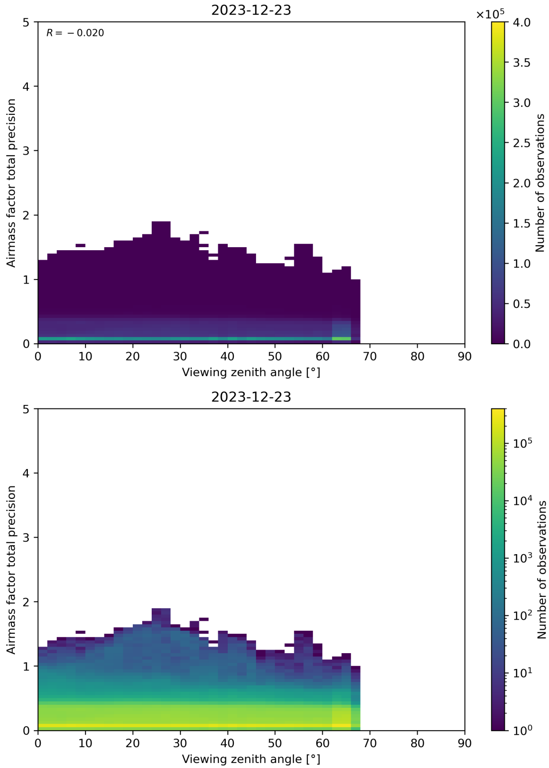
Figure 191: Scatter density plot of “Viewing zenith angle” against “Airmass factor total precision” for 2023-12-22 to 2023-12-24.
