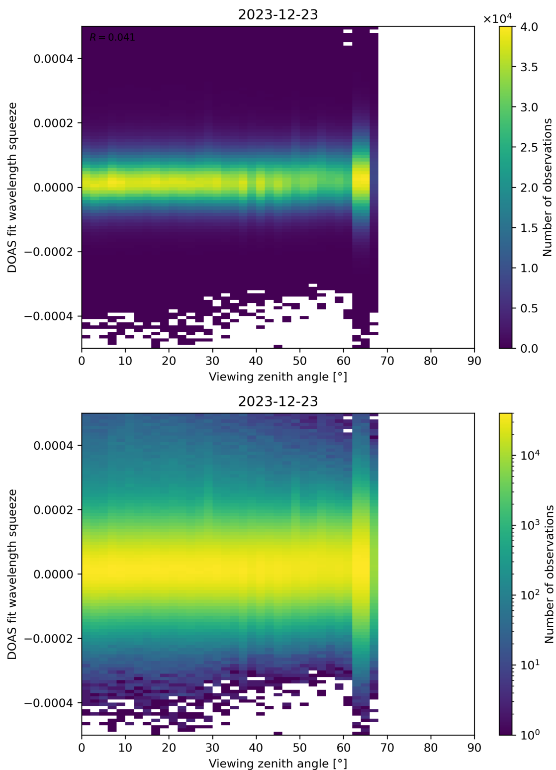
Figure 184: Scatter density plot of “Viewing zenith angle” against “DOAS fit wavelength squeeze” for 2023-12-22 to 2023-12-24.
