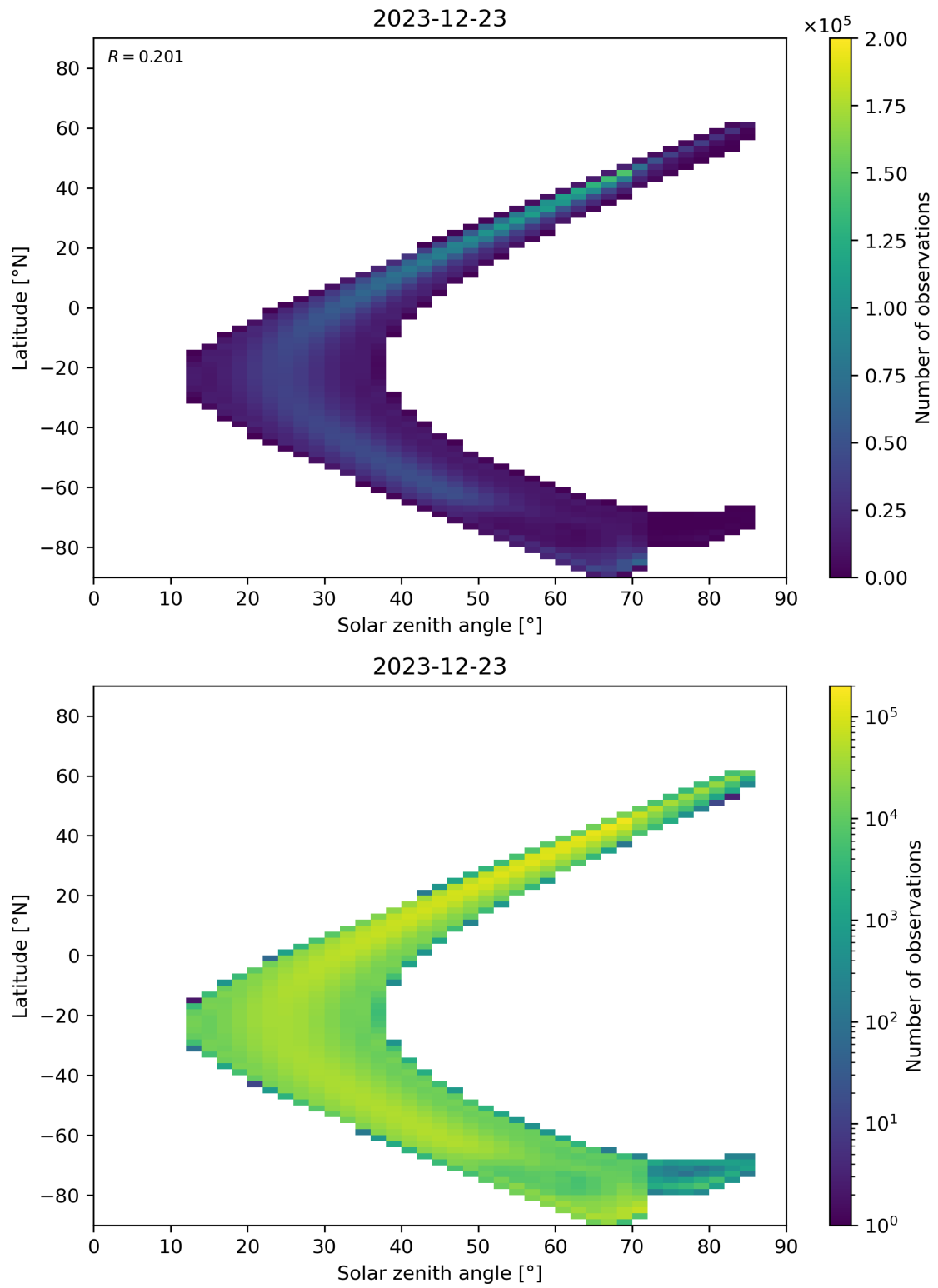
Figure 181: Scatter density plot of “Solar zenith angle” against “Latitude” for 2023-12-22 to 2023-12-24.
