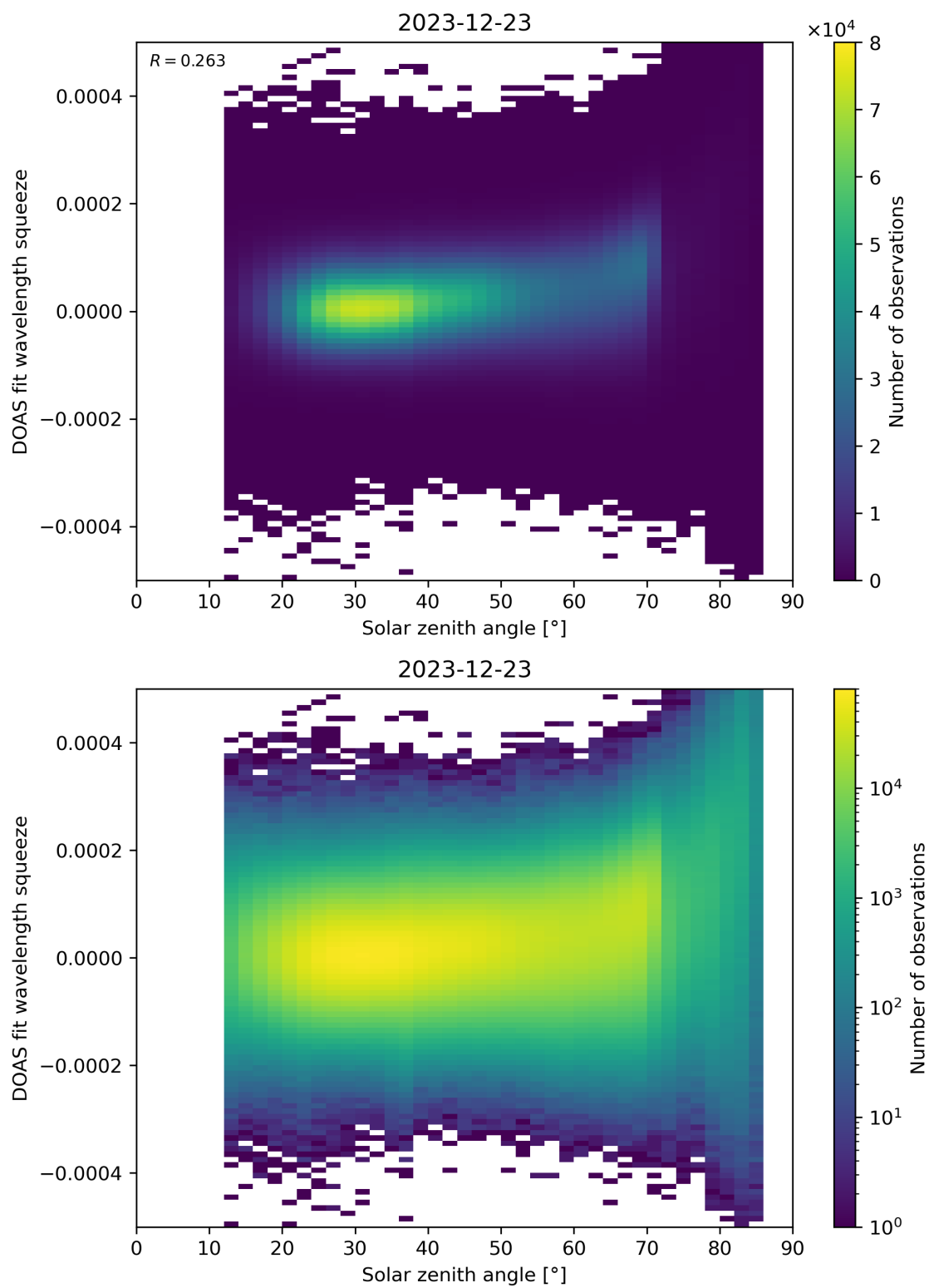
Figure 169: Scatter density plot of “Solar zenith angle” against “DOAS fit wavelength squeeze” for 2023-12-22 to 2023-12-24.
