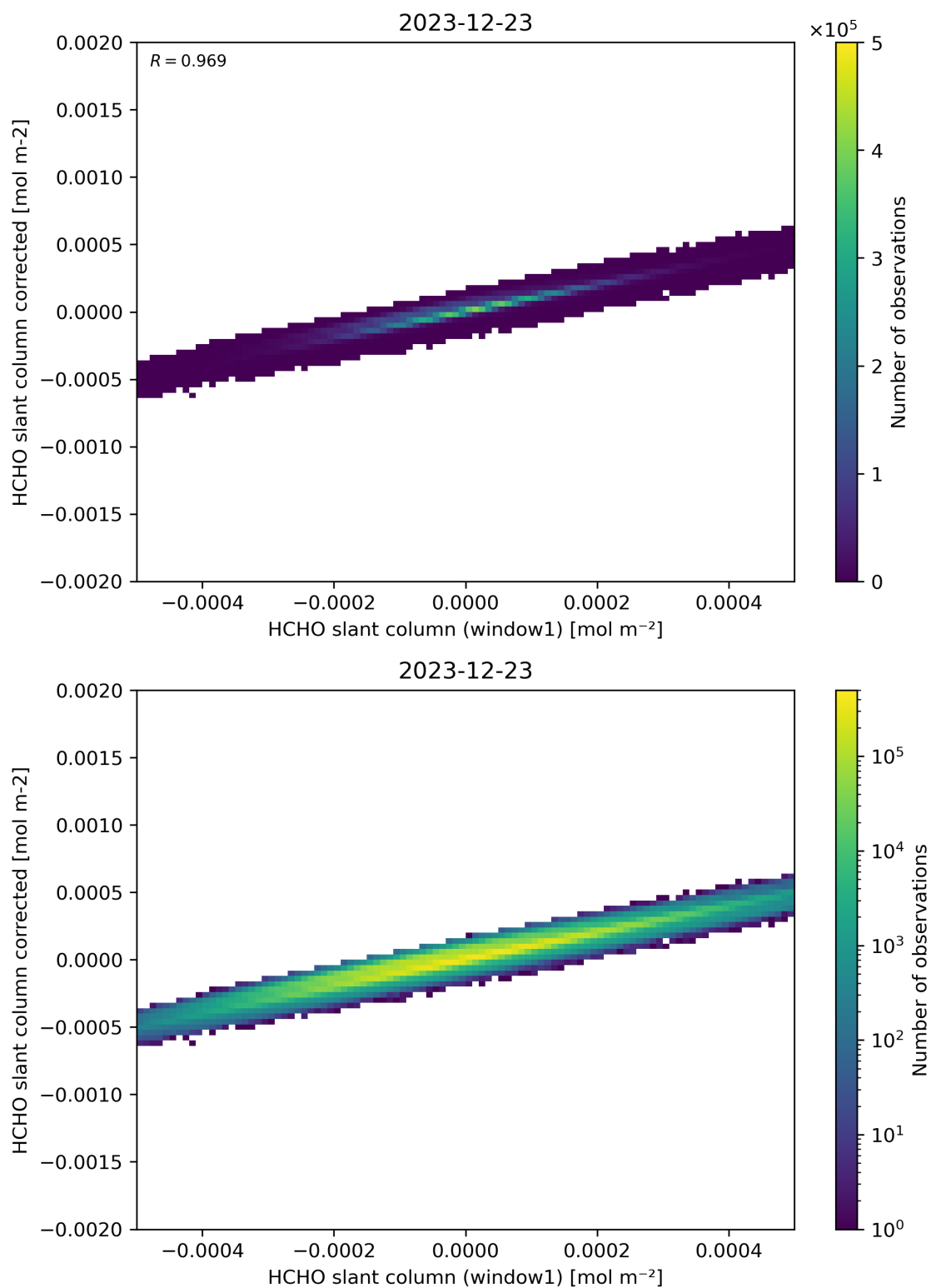
Figure 82: Scatter density plot of “HCHO slant column (window1)” against “HCHO slant column corrected” for 2023-12-22 to 2023-12-24.
