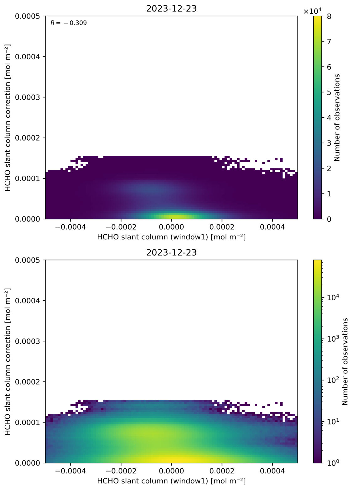
Figure 83: Scatter density plot of “HCHO slant column (window1)” against “HCHO slant column correction” for 2023-12-22 to 2023-12-24.
