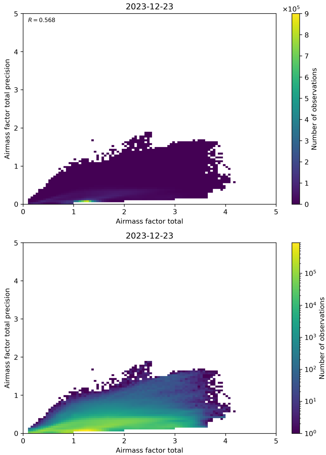
Figure 103: Scatter density plot of “Airmass factor total” against “Airmass factor total precision” for 2023-12-22 to 2023-12-24.
