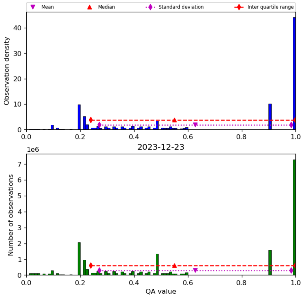
Figure 34: Histogram of “QA value” for 2023-12-22 to 2023-12-24
