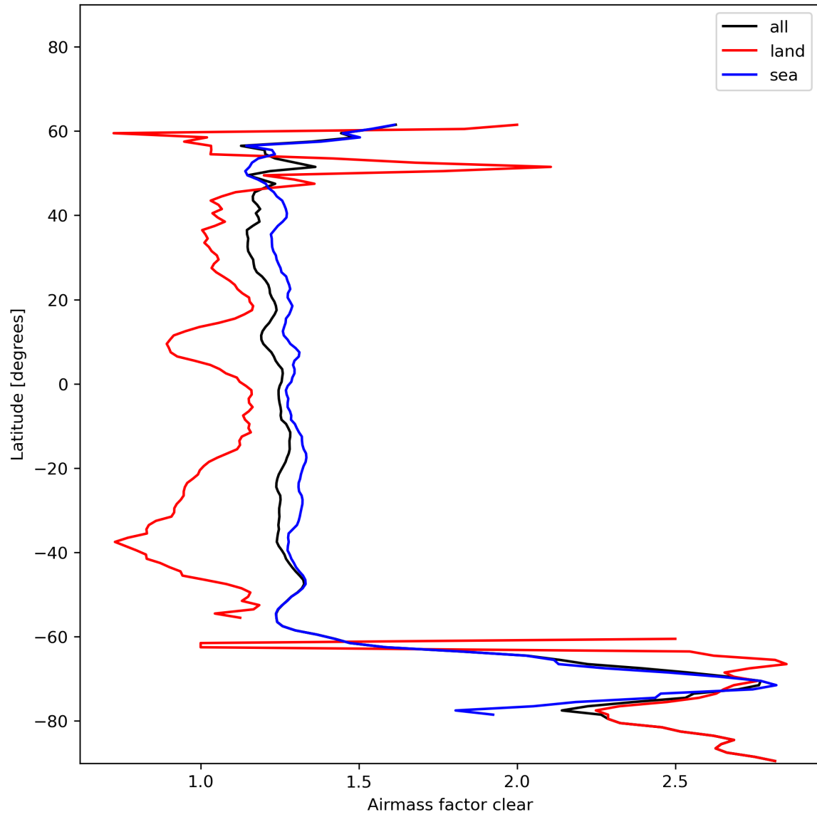
Figure 28: Zonal average of “Airmass factor clear” for 2023-12-22 to 2023-12-24.
