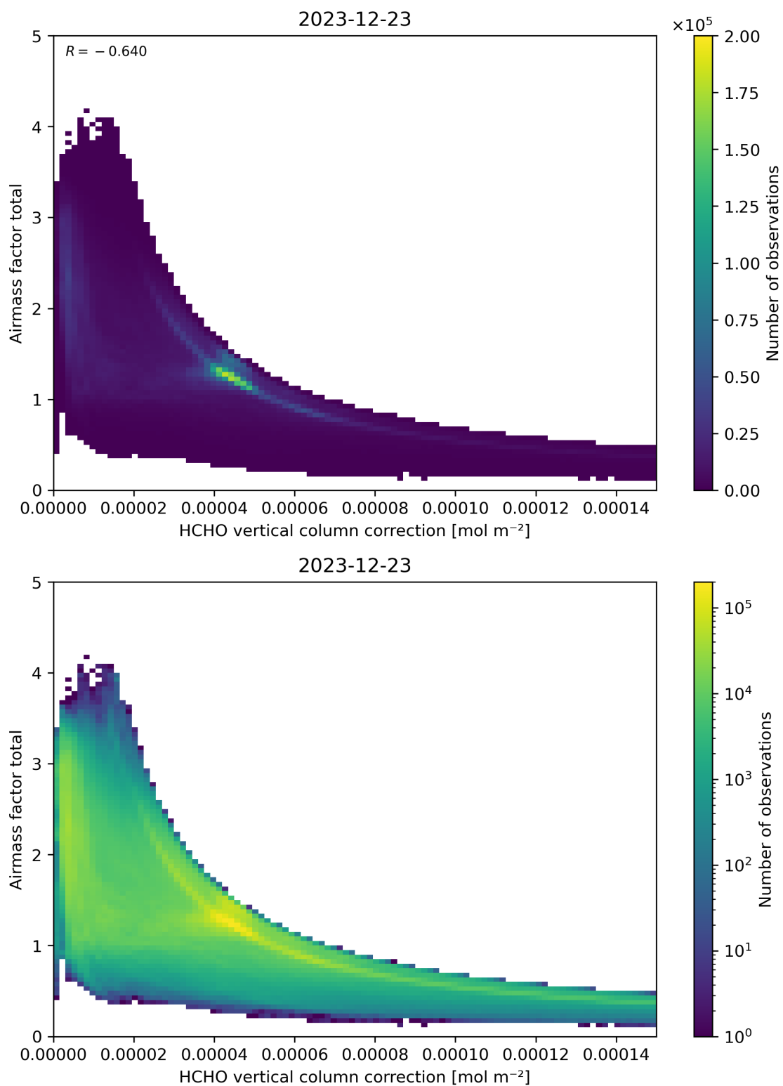
Figure 120: Scatter density plot of “HCHO vertical column correction” against “Airmass factor total” for 2023-12-22 to 2023-12-24.
