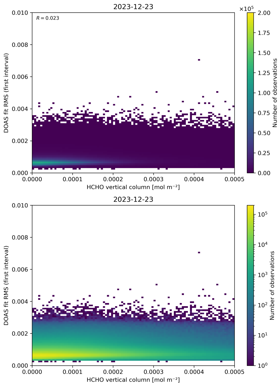
Figure 123: Scatter density plot of “HCHO vertical column” against “DOAS fit RMS (first interval)” for 2023-12-22 to 2023-12-24.
