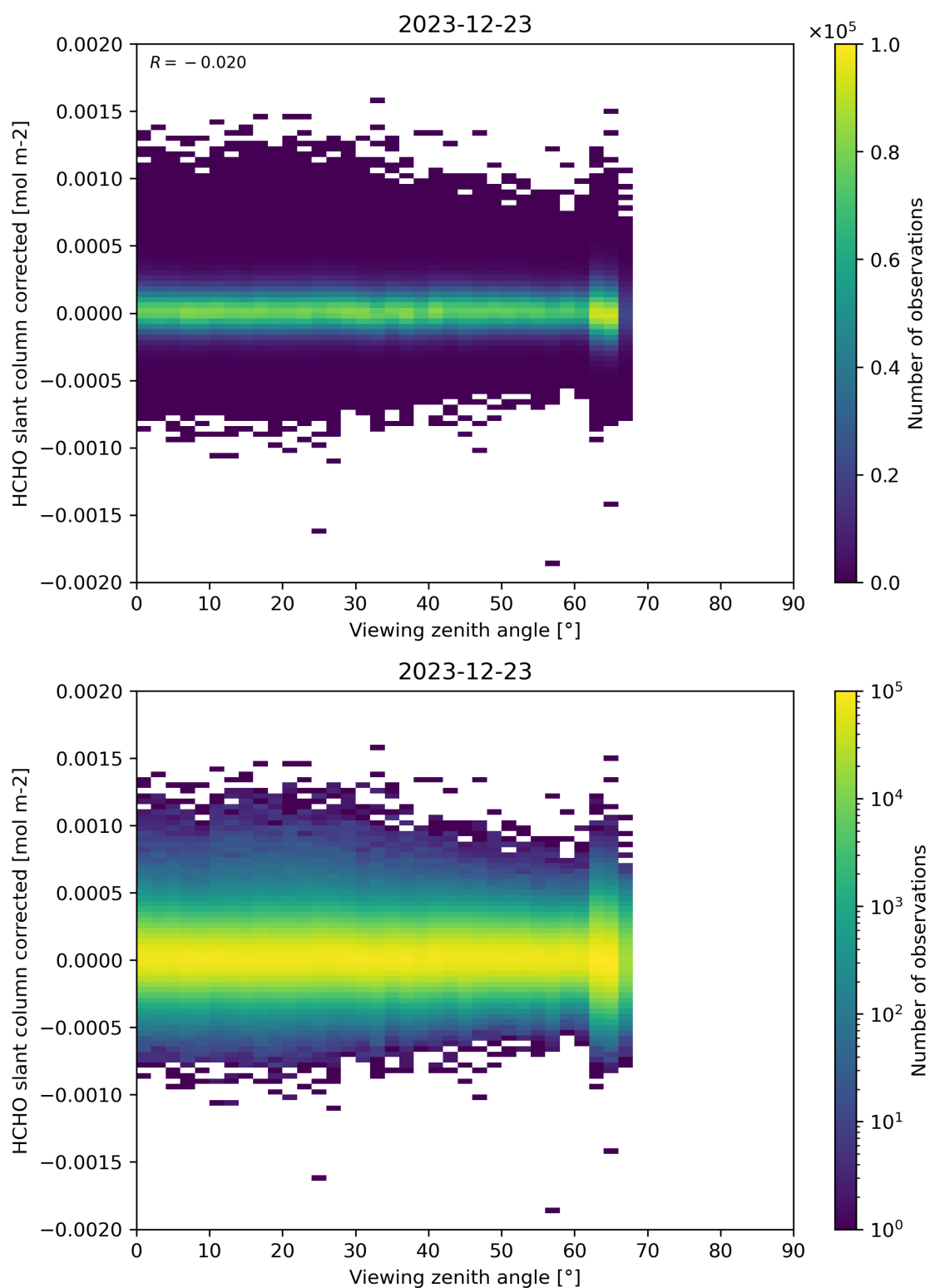
Figure 186: Scatter density plot of “Viewing zenith angle” against “HCHO slant column corrected” for 2023-12-22 to 2023-12-24.
