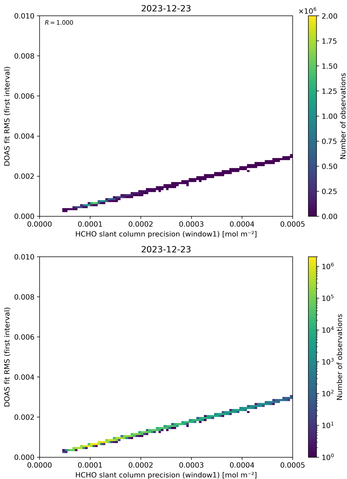
Figure 88: Scatter density plot of “HCHO slant column precision (window1)” against “DOAS fit RMS (first interval)” for 2023-12-22 to 2023-12-24.
