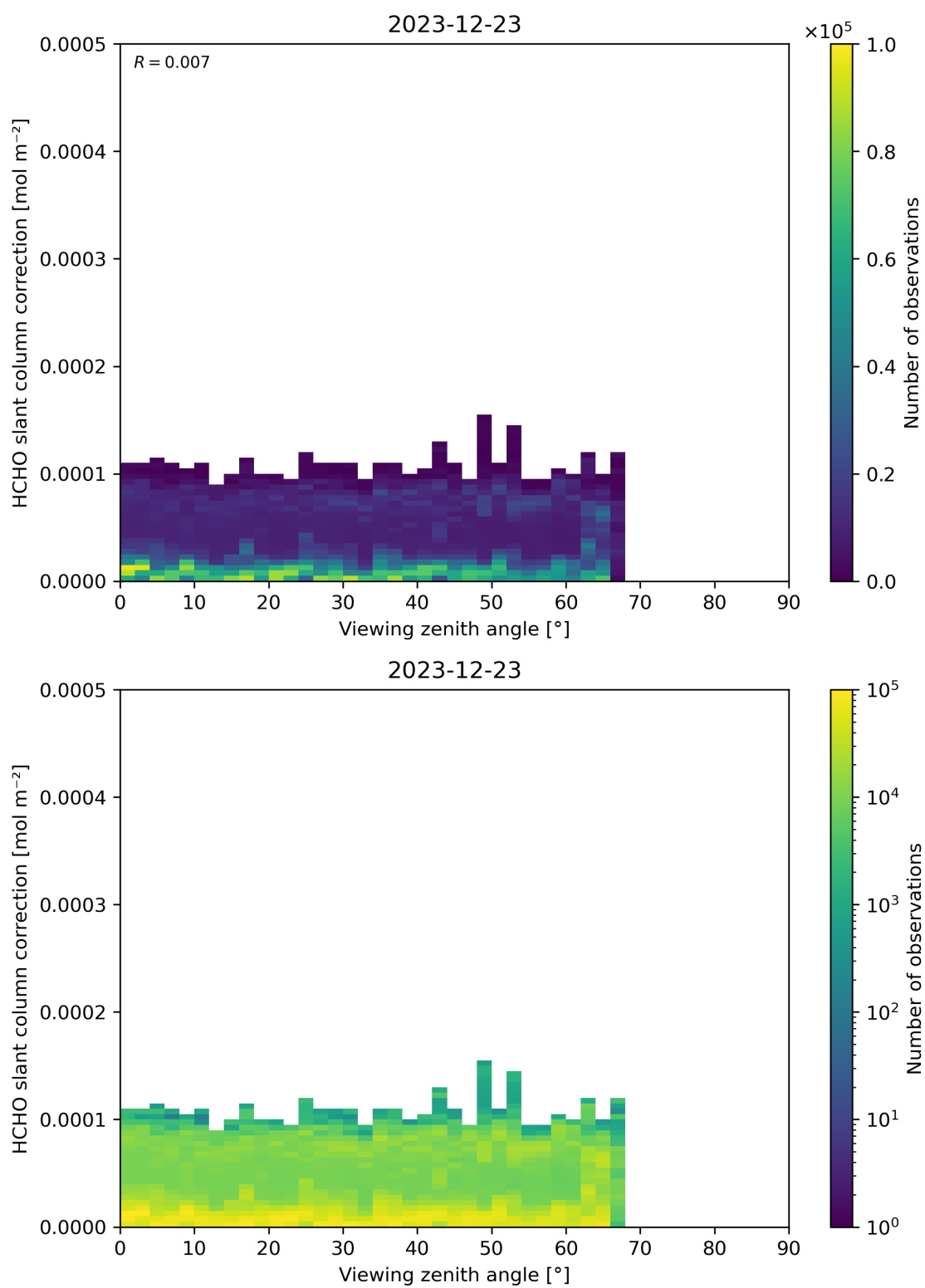
Figure 187: Scatter density plot of “Viewing zenith angle” against “HCHO slant column correction” for 2023-12-22 to 2023-12-24.
