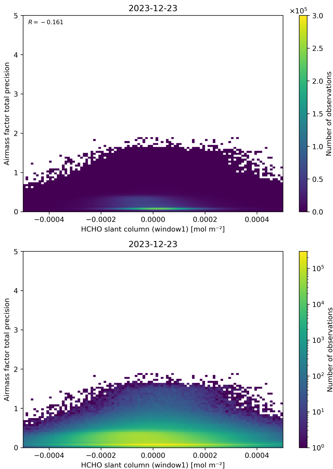
Figure 86: Scatter density plot of “HCHO slant column (window1)” against “Airmass factor total precision” for 2023-12-22 to 2023-12-24.
