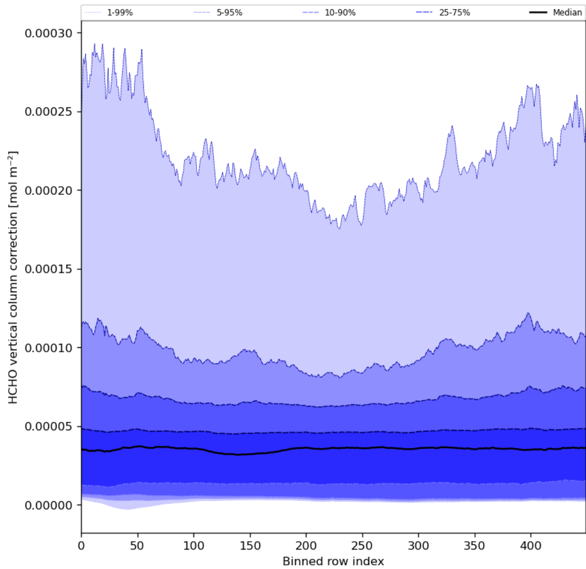
Figure 51: Along track statistics of “HCHO vertical column correction” for 2023-12-22 to 2023-12-24
