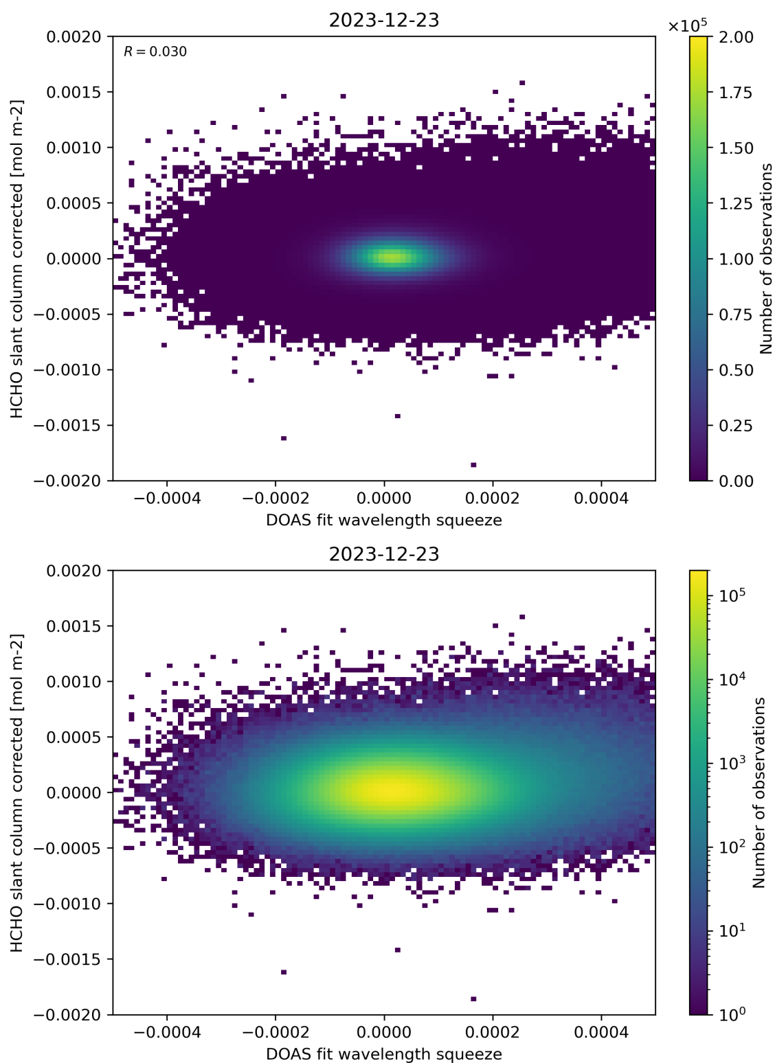
Figure 69: Scatter density plot of “DOAS fit wavelength squeeze” against “HCHO slant column corrected” for 2023-12-22 to 2023-12-24.
