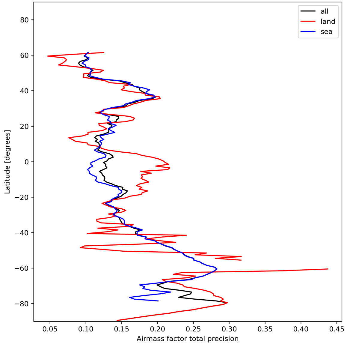
Figure 27: Zonal average of “Airmass factor total precision” for 2023-12-22 to 2023-12-24.
