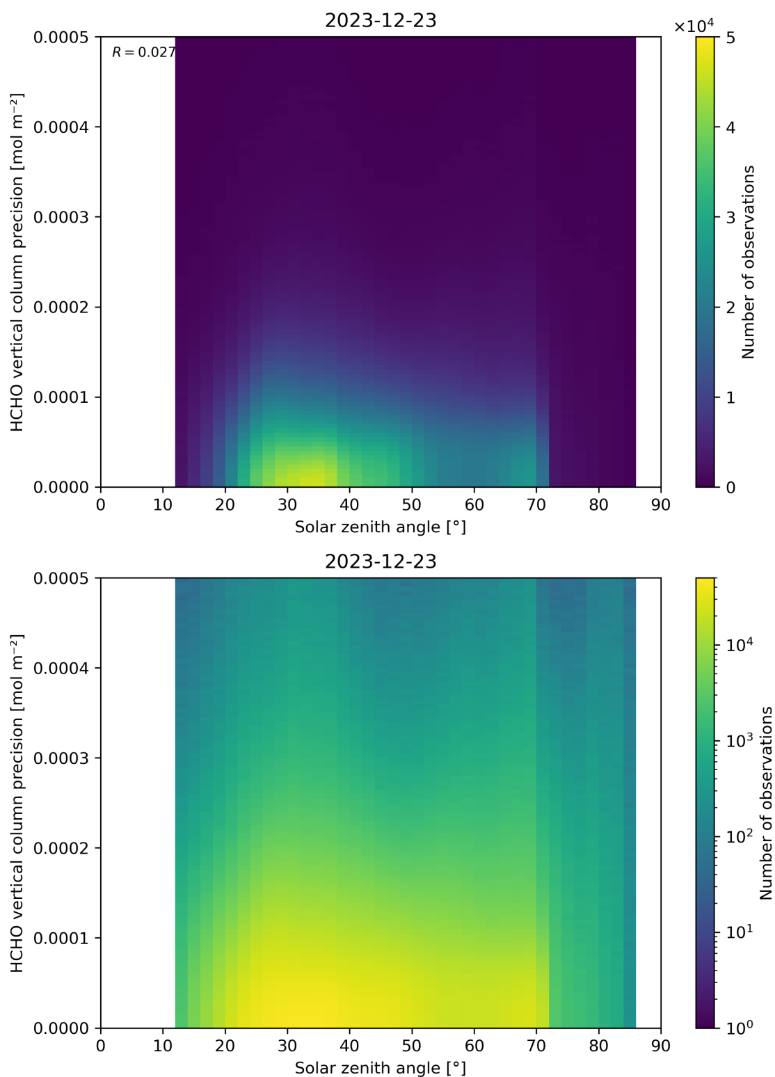
Figure 179: Scatter density plot of “Solar zenith angle” against “HCHO vertical column precision” for 2023-12-22 to 2023-12-24.
