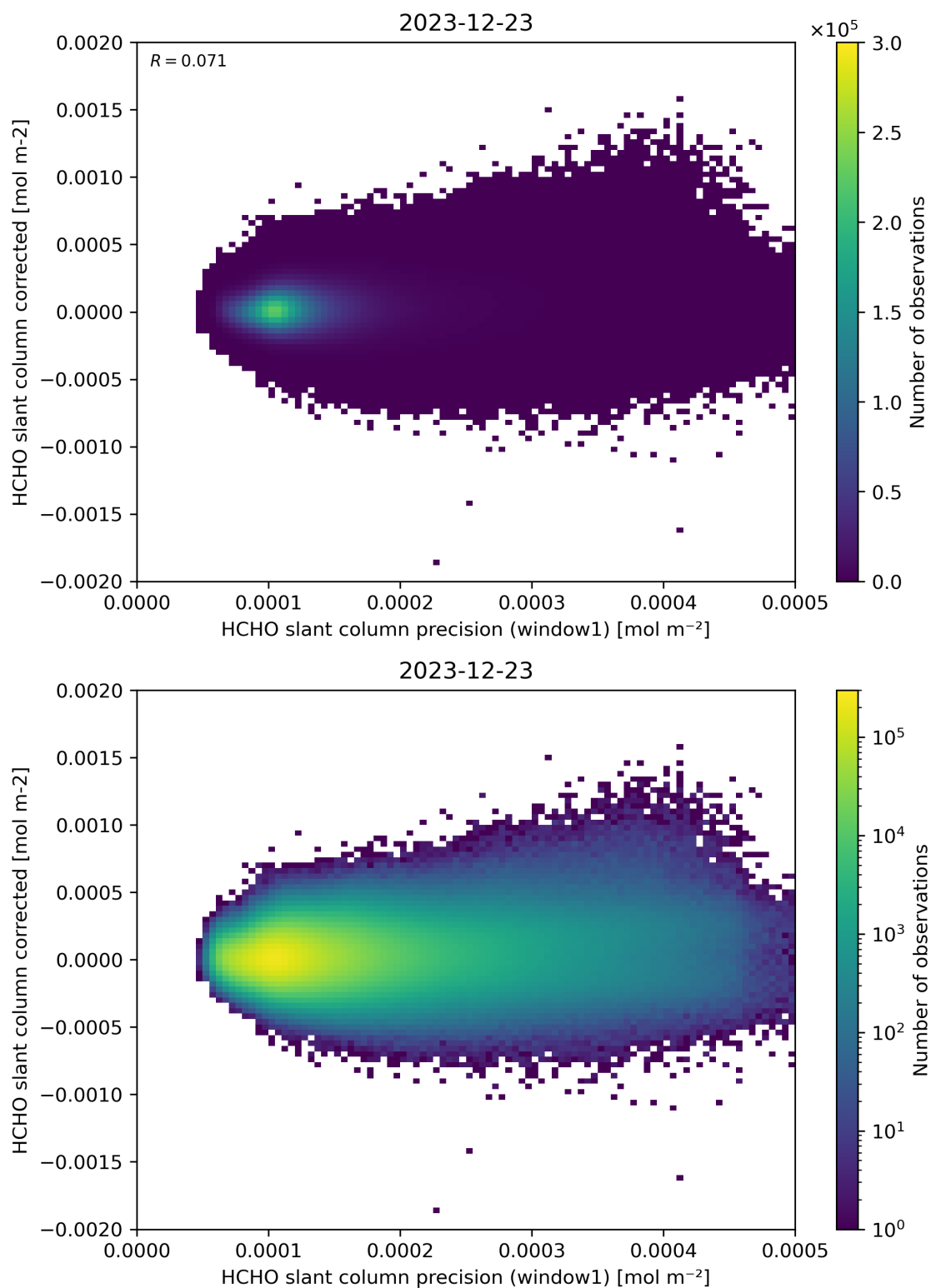
Figure 92: Scatter density plot of “HCHO slant column precision (window1)” against “HCHO slant column corrected” for 2023-12-22 to 2023-12-24.
