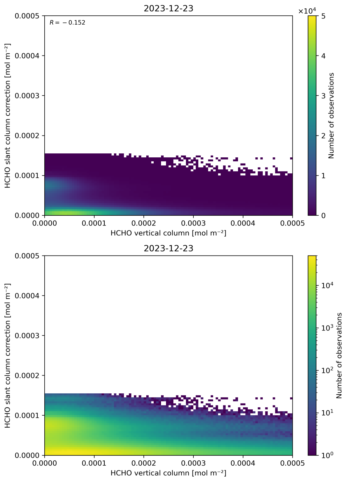
Figure 128: Scatter density plot of “HCHO vertical column” against “HCHO slant column correction” for 2023-12-22 to 2023-12-24.
