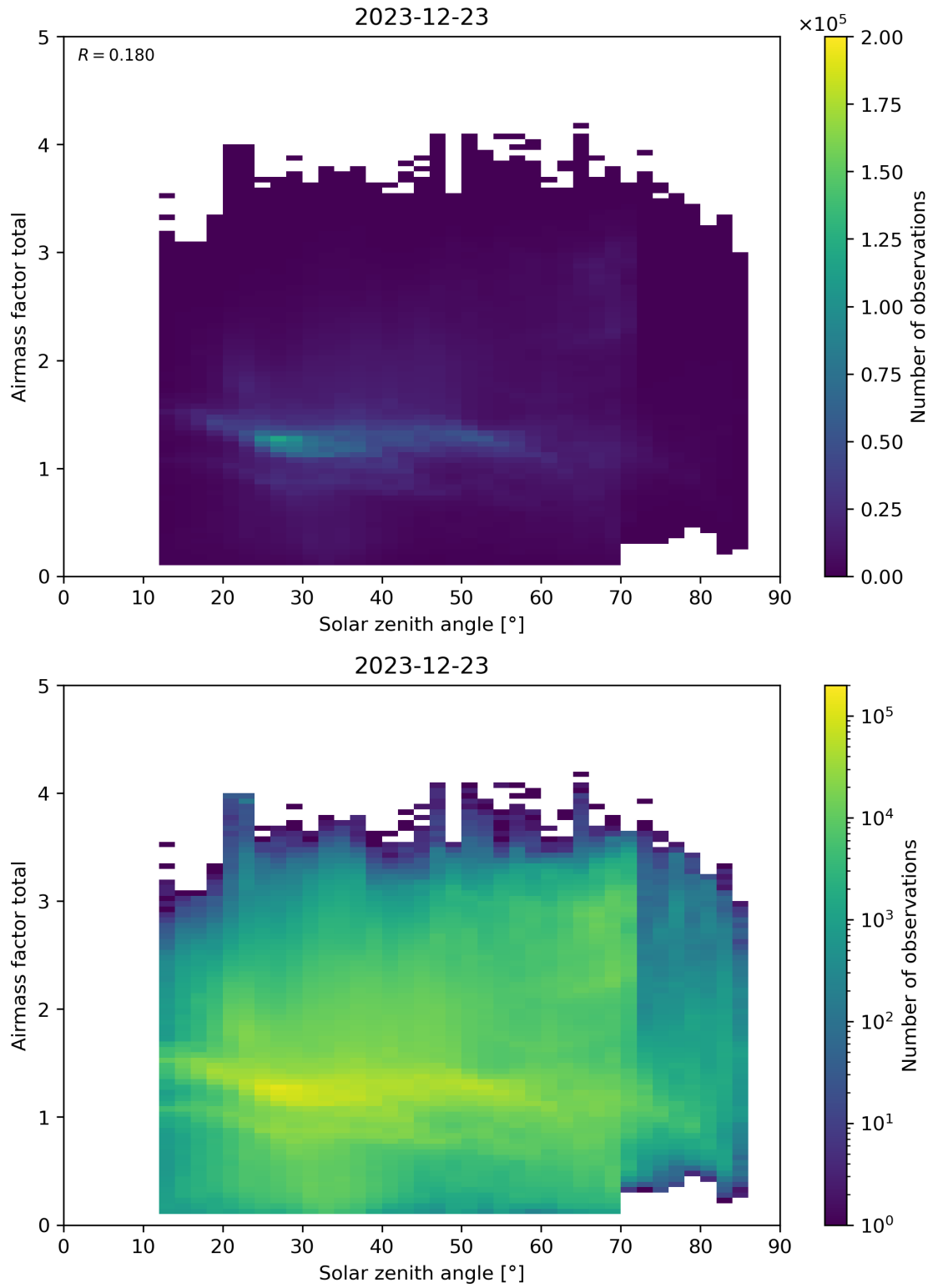
Figure 175: Scatter density plot of “Solar zenith angle” against “Airmass factor total” for 2023-12-22 to 2023-12-24.
