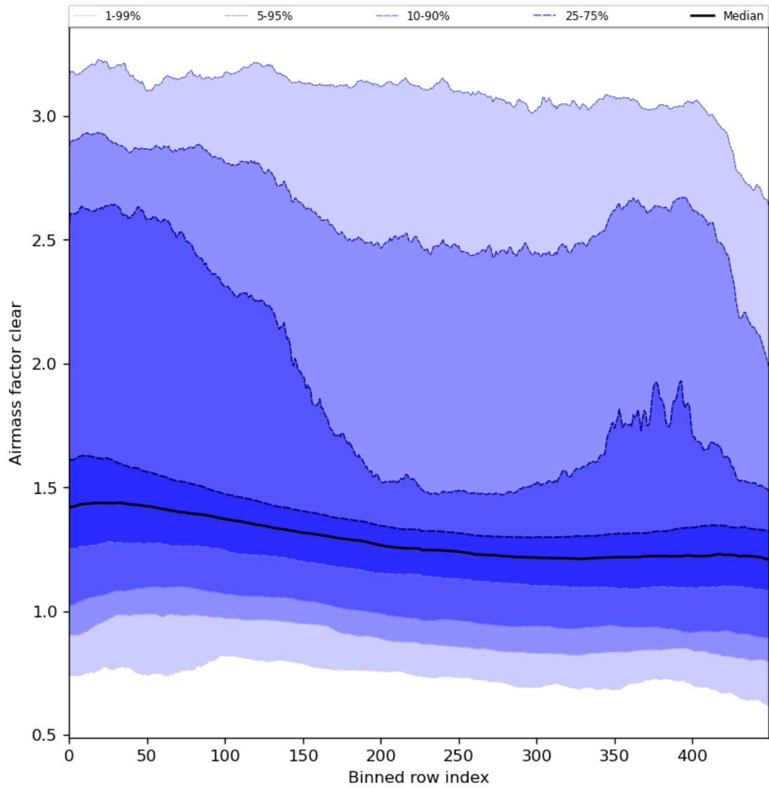
Figure 56: Along track statistics of “Airmass factor clear” for 2023-12-22 to 2023-12-24
