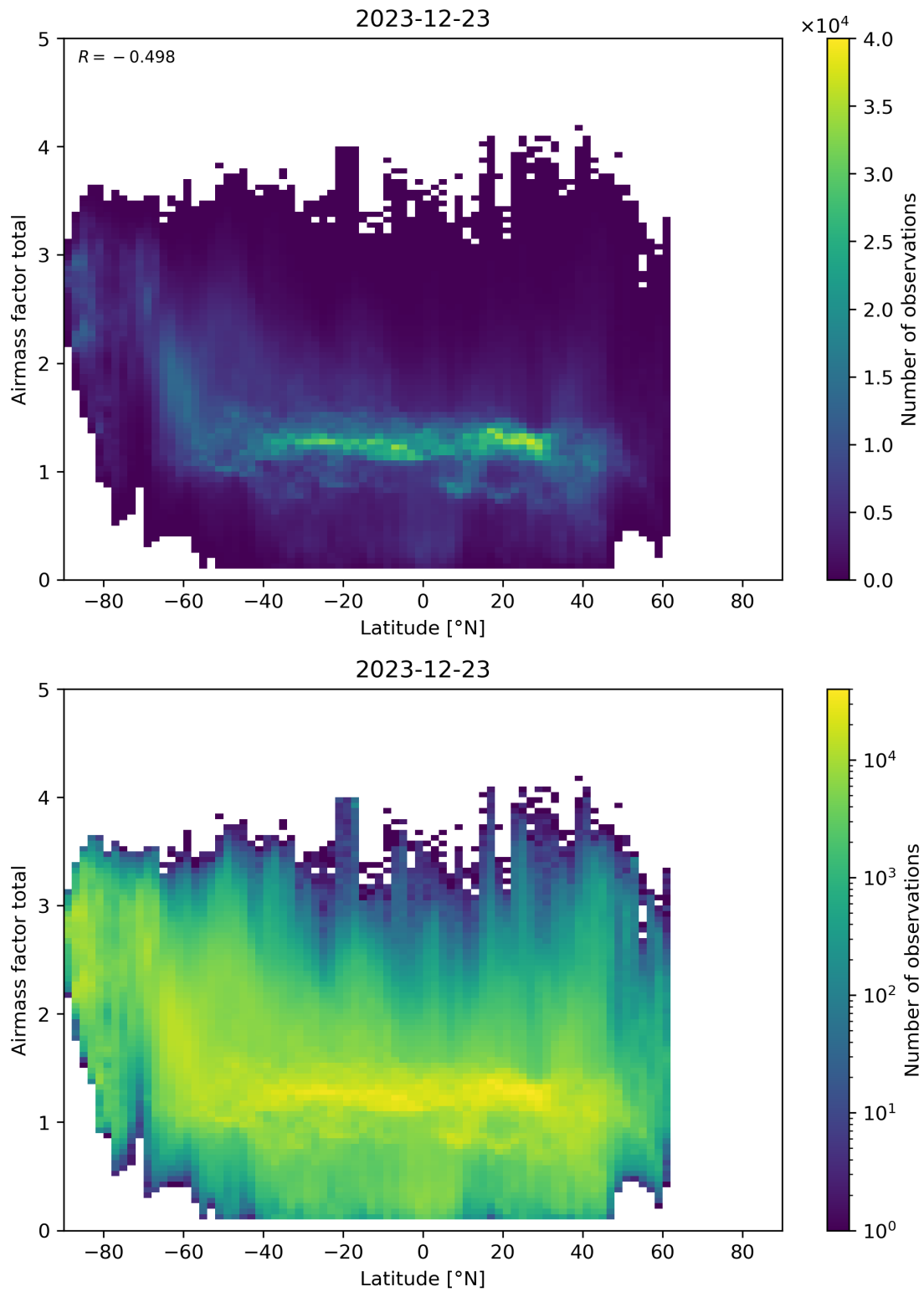
Figure 161: Scatter density plot of “Latitude” against “Airmass factor total” for 2023-12-22 to 2023-12-24.
