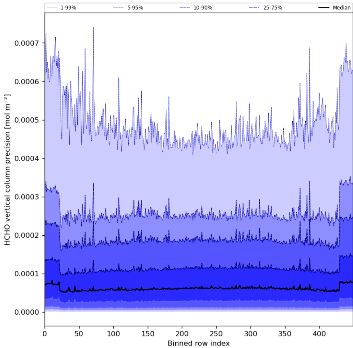
Figure 50: Along track statistics of “HCHO vertical column precision” for 2023-12-22 to 2023-12-24
