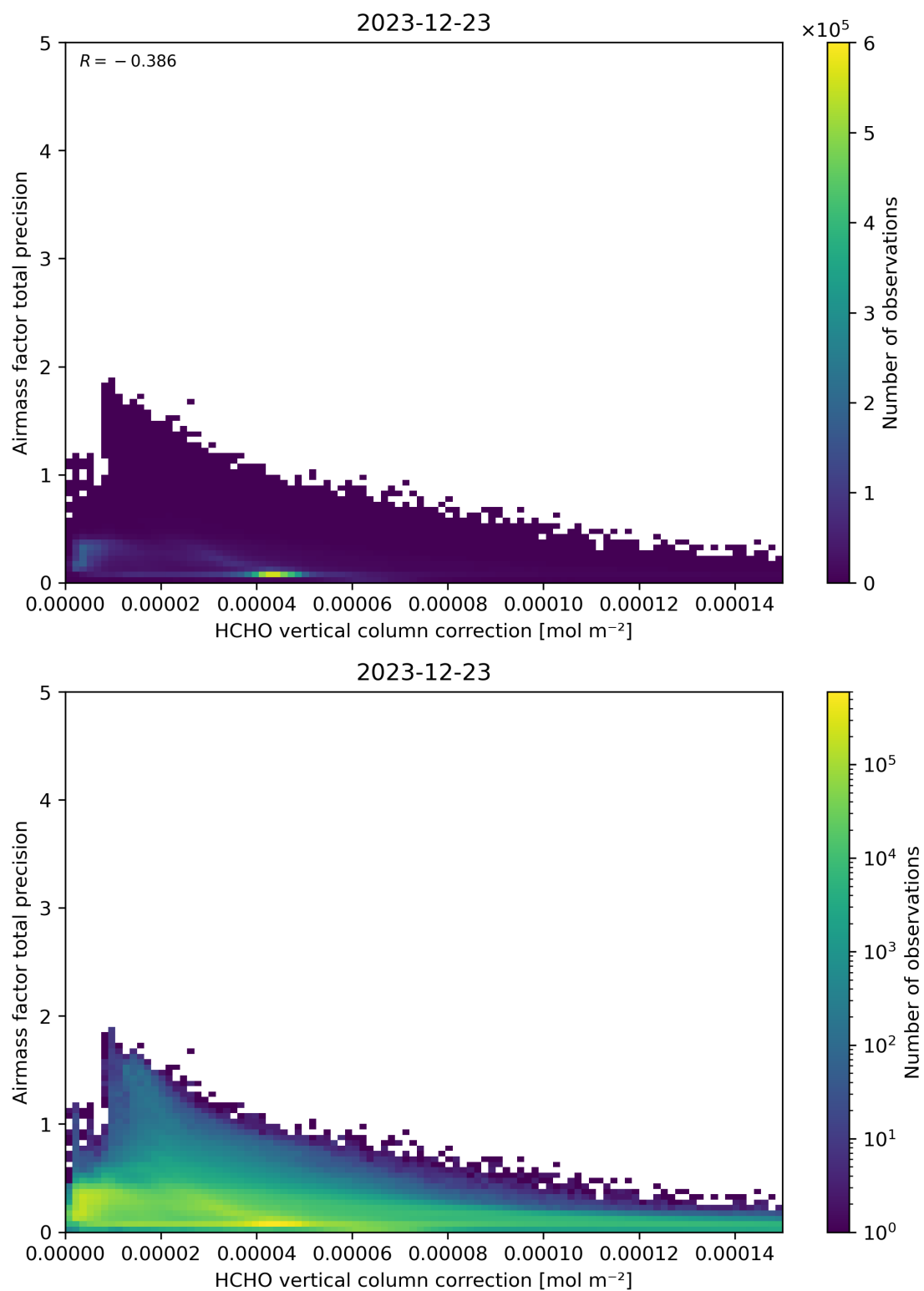
Figure 121: Scatter density plot of “HCHO vertical column correction” against “Airmass factor total precision” for 2023-12-22 to 2023-12-24.
