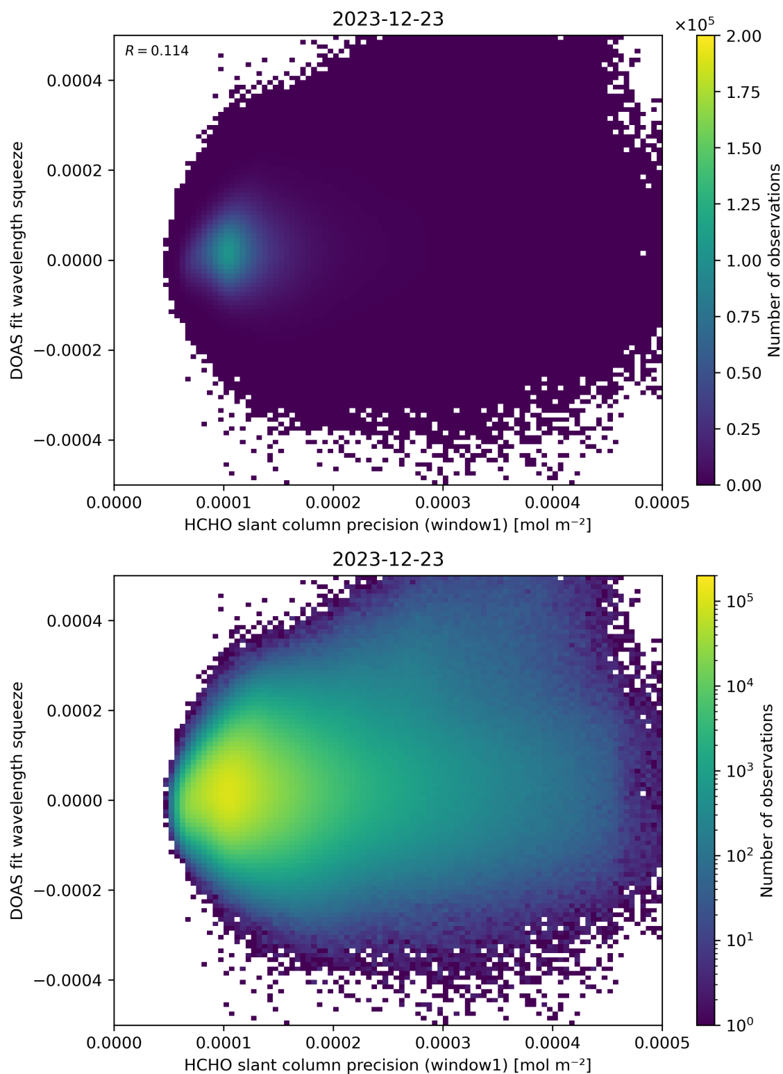
Figure 90: Scatter density plot of “HCHO slant column precision (window1)” against “DOAS fit wavelength squeeze” for 2023-12-22 to 2023-12-24.
