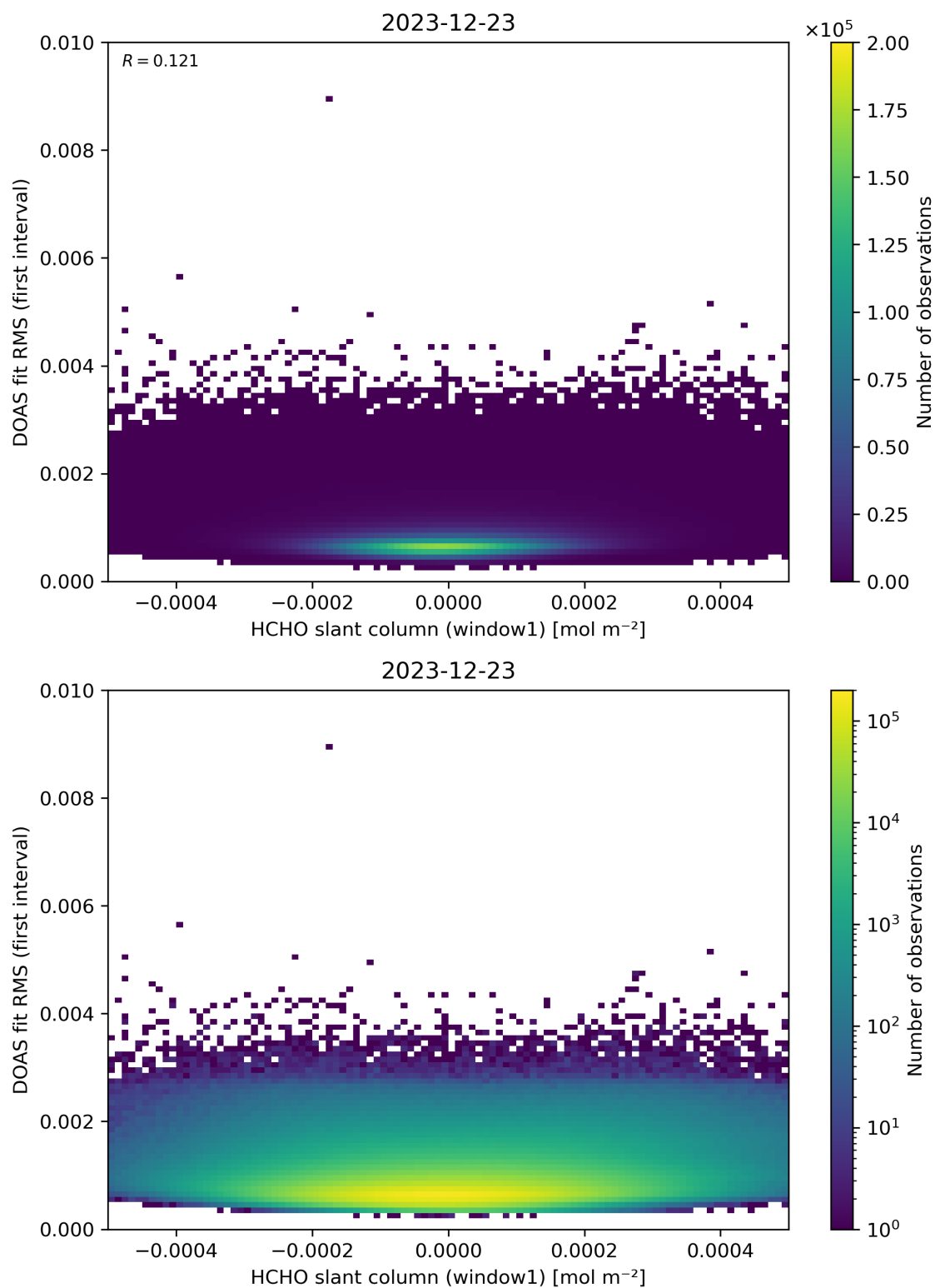
Figure 78: Scatter density plot of “HCHO slant column (window1)” against “DOAS fit RMS (first interval)” for 2023-12-22 to 2023-12-24.
