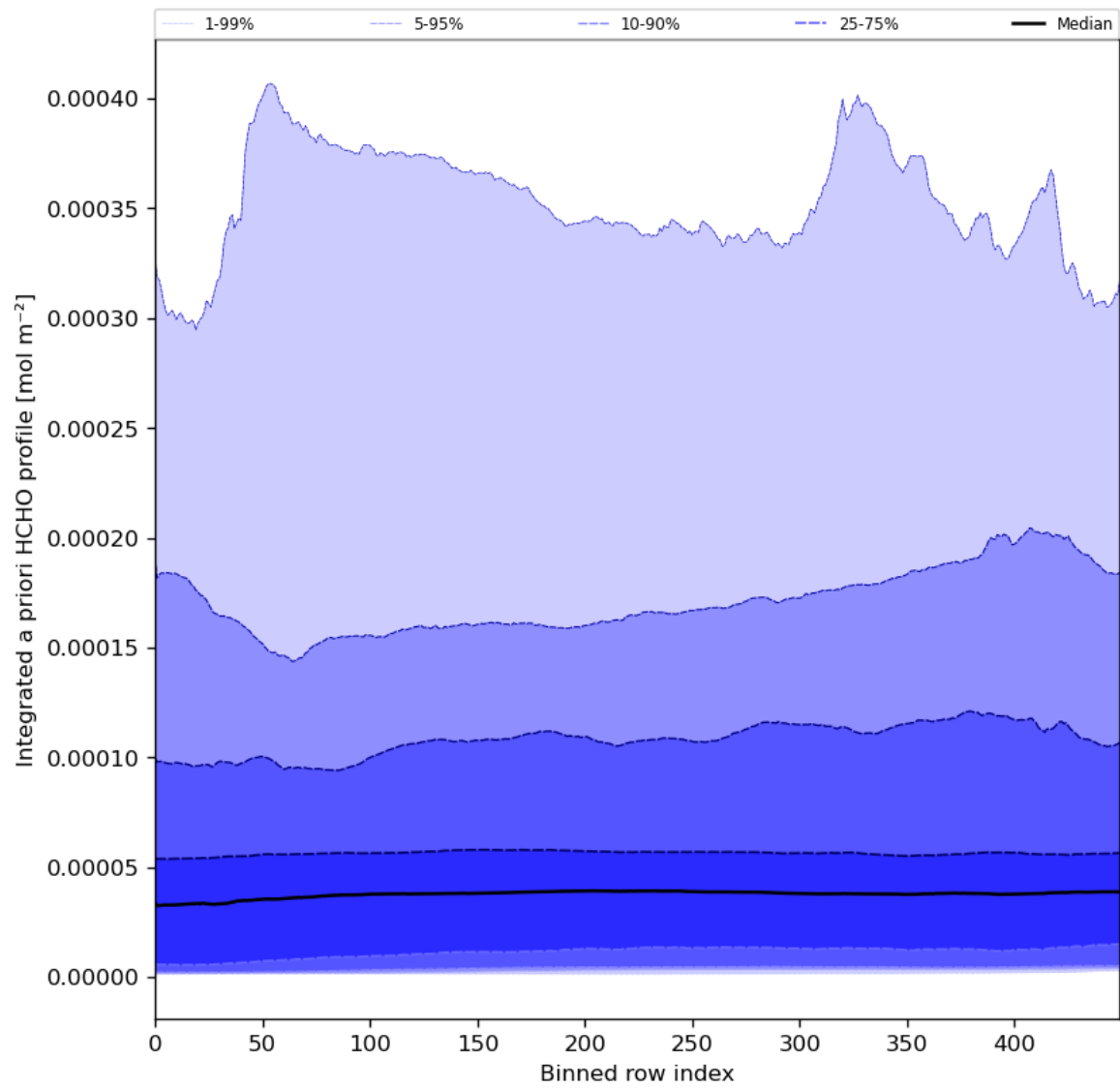
Figure 57: Along track statistics of “Integrated a priori HCHO profile” for 2023-12-22 to 2023-12-24
