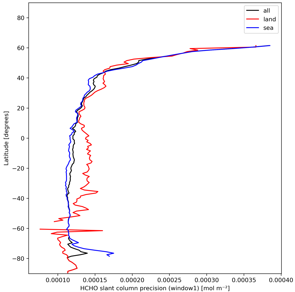
Figure 25: Zonal average of “HCHO slant column precision (window1)” for 2023-12-22 to 2023-12-24.
