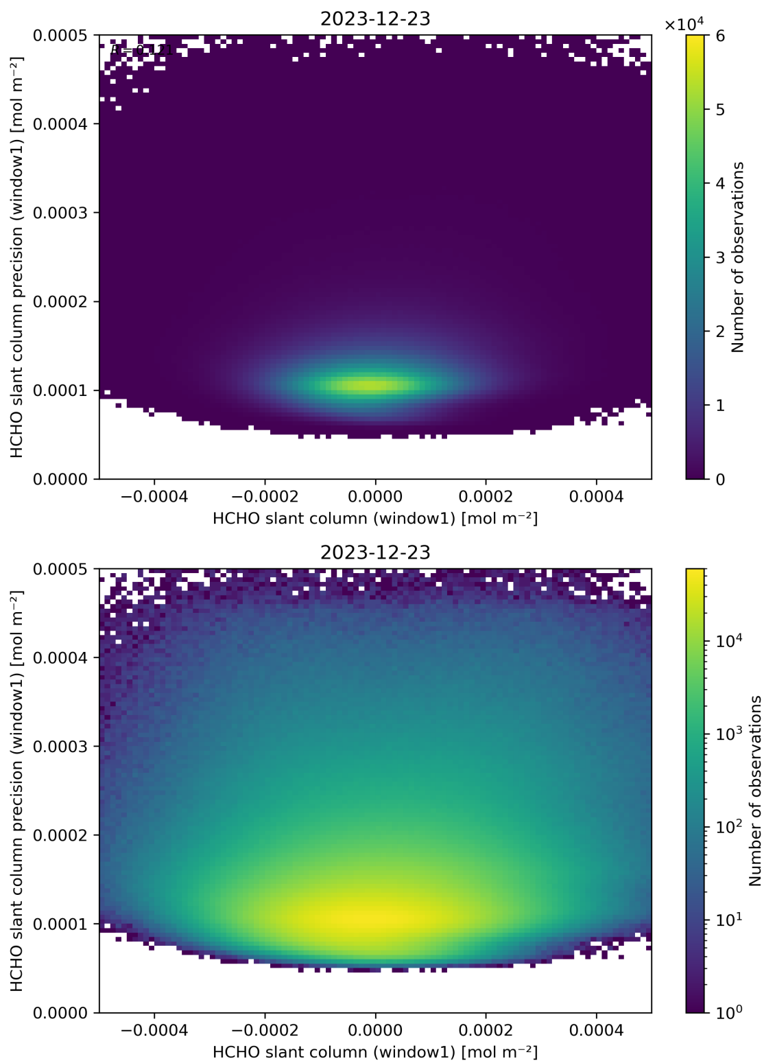
Figure 84: Scatter density plot of “HCHO slant column (window1)” against “HCHO slant column precision (window1)” for 2023-12-22 to 2023-12-24.
