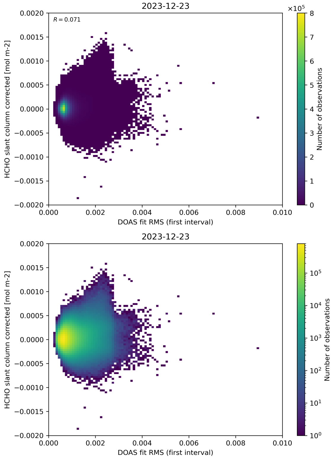
Figure 62: Scatter density plot of “DOAS fit RMS (first interval)” against “HCHO slant column corrected” for 2023-12-22 to 2023-12-24.
