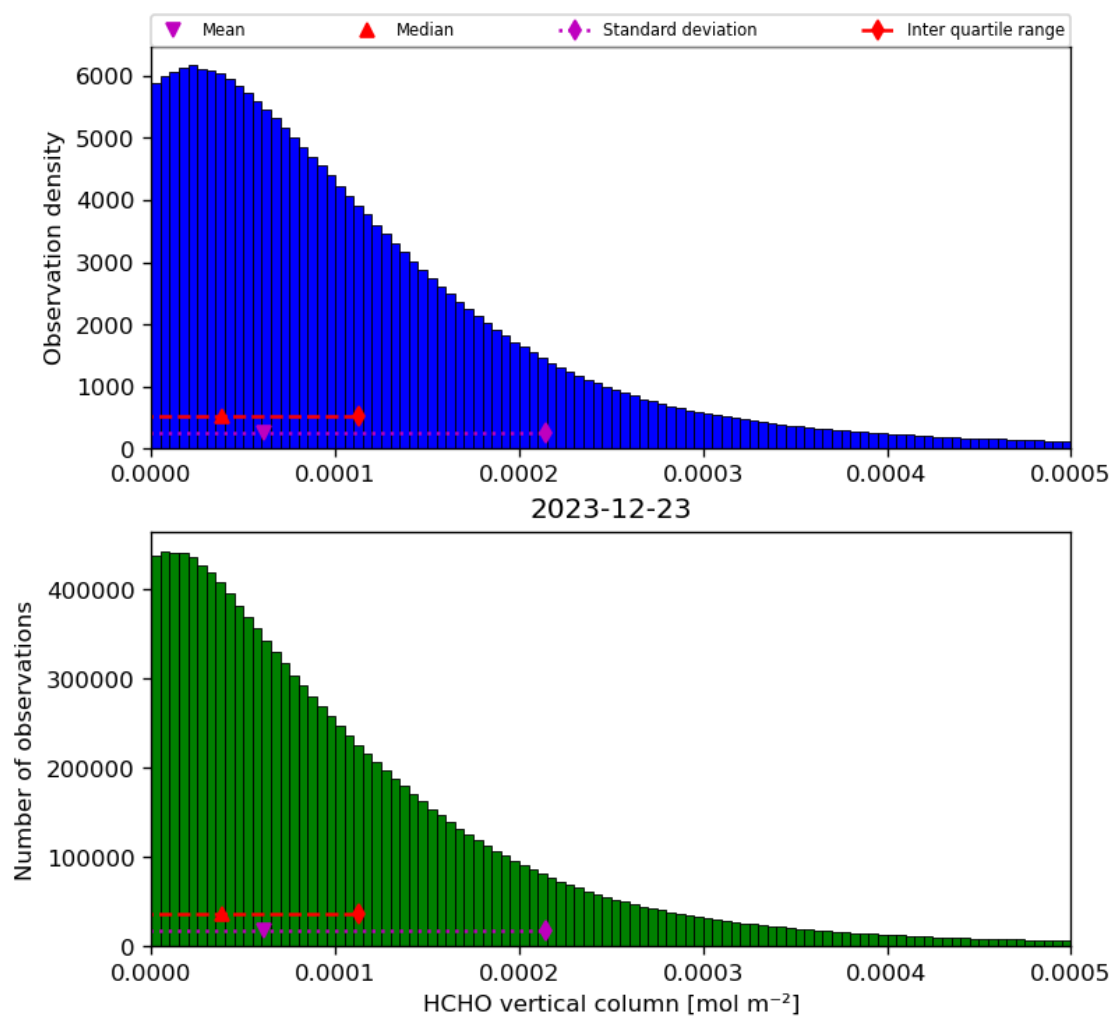
Figure 35: Histogram of “HCHO vertical column” for 2023-12-22 to 2023-12-24
