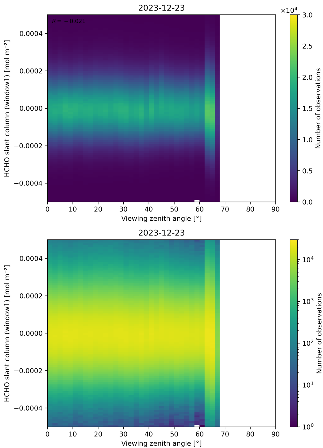
Figure 188: Scatter density plot of “Viewing zenith angle” against “HCHO slant column (window1)” for 2023-12-22 to 2023-12-24.
