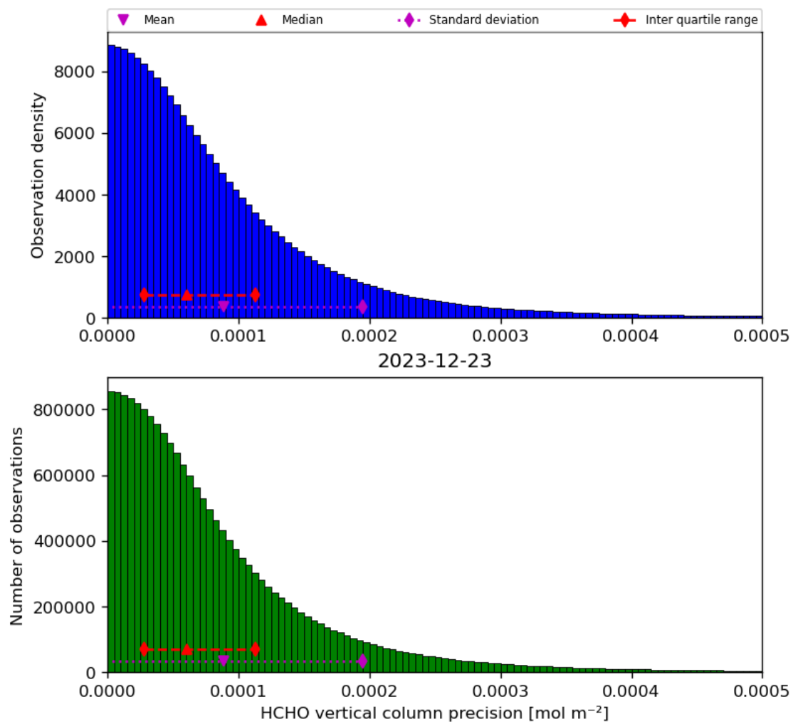
Figure 36: Histogram of “HCHO vertical column precision” for 2023-12-22 to 2023-12-24
