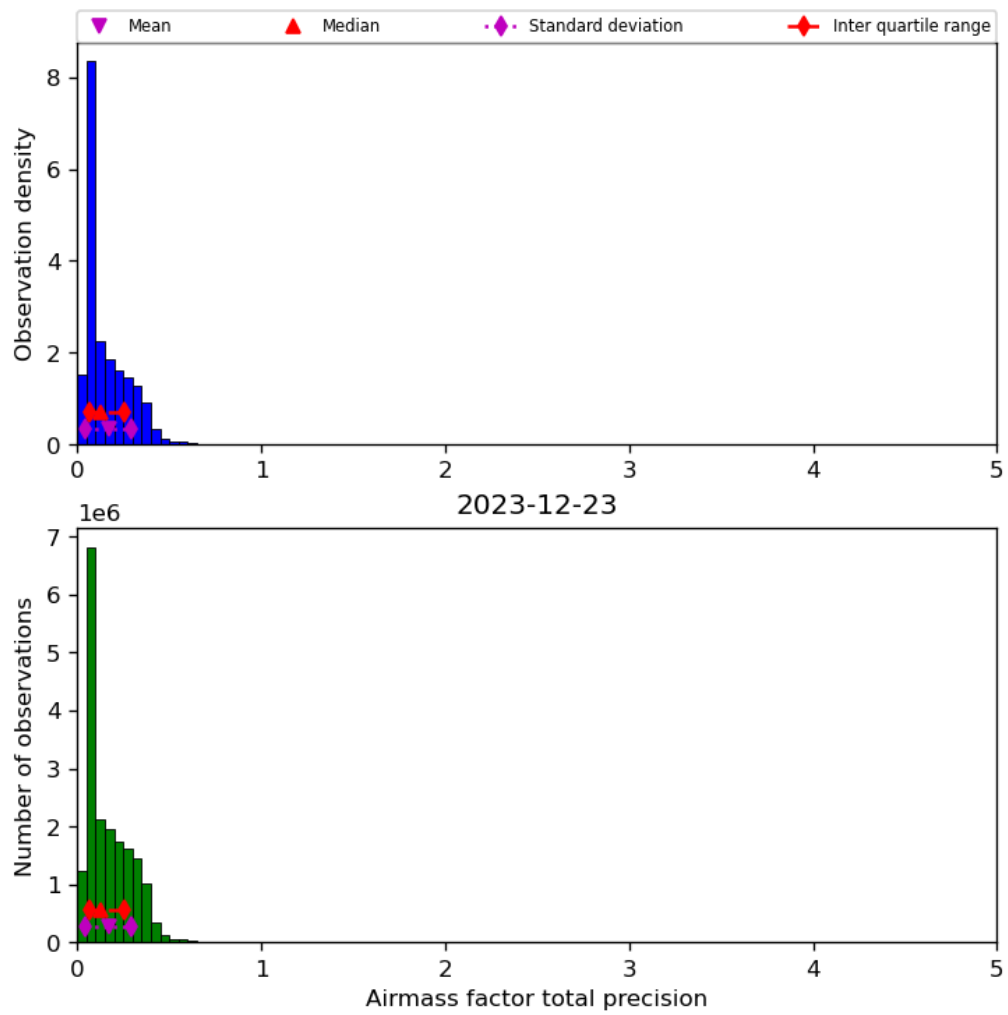
Figure 41: Histogram of “Airmass factor total precision” for 2023-12-22 to 2023-12-24
