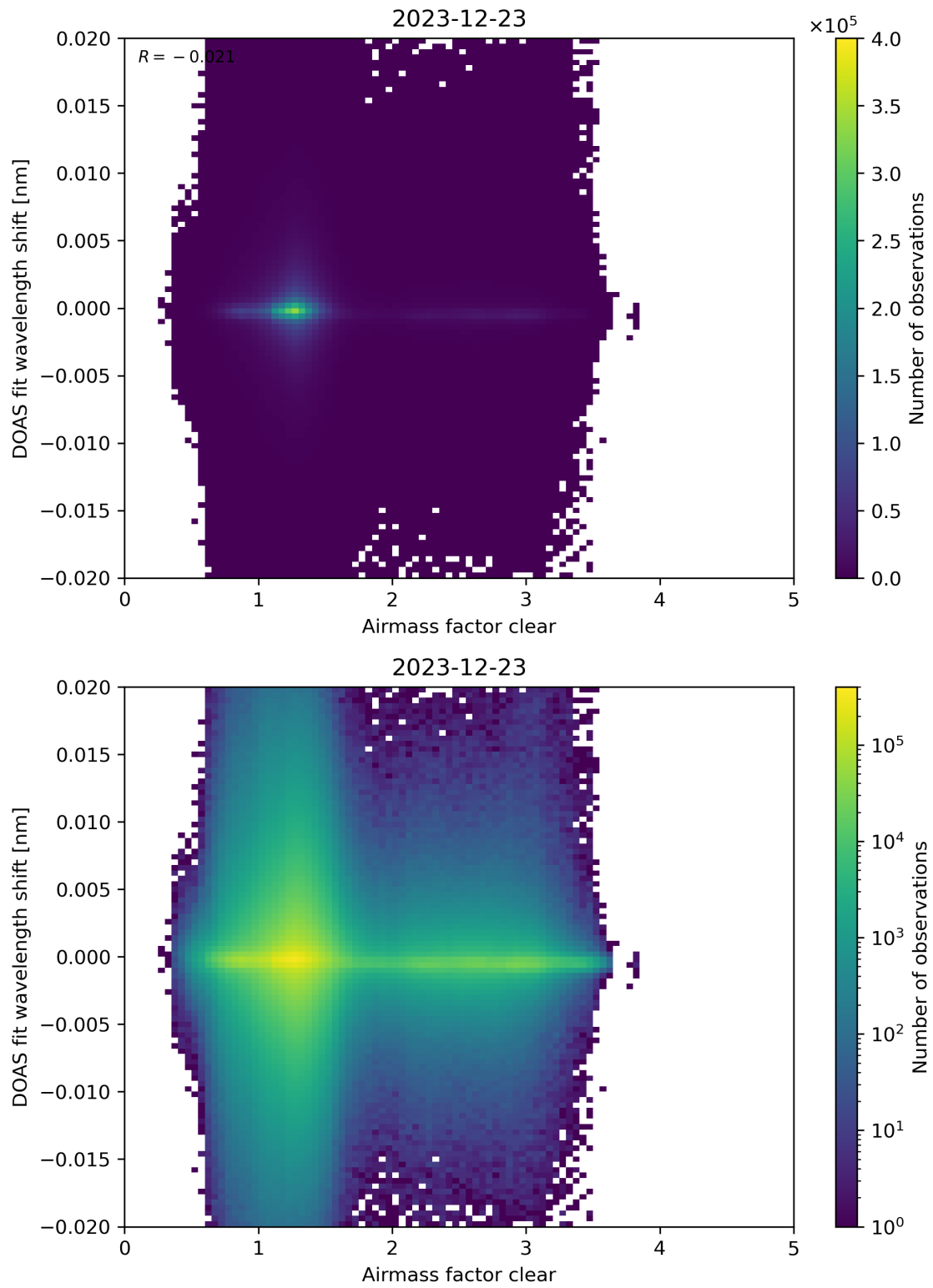
Figure 72: Scatter density plot of “Airmass factor clear” against “DOAS fit wavelength shift” for 2023-12-22 to 2023-12-24.
