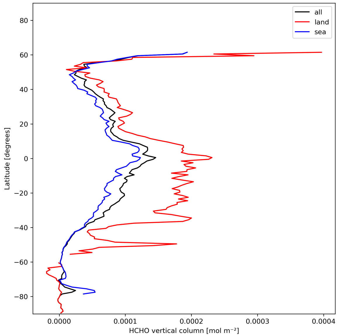
Figure 21: Zonal average of “HCHO vertical column” for 2023-12-22 to 2023-12-24.
