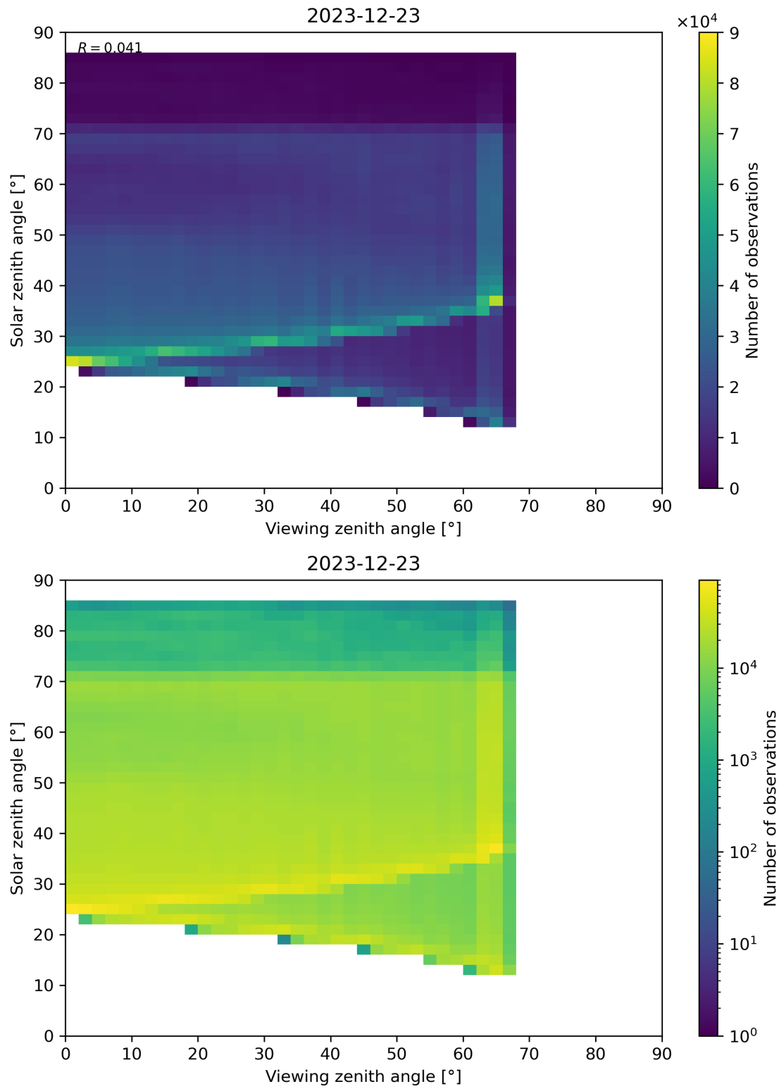
Figure 197: Scatter density plot of “Viewing zenith angle” against “Solar zenith angle” for 2023-12-22 to 2023-12-24.
