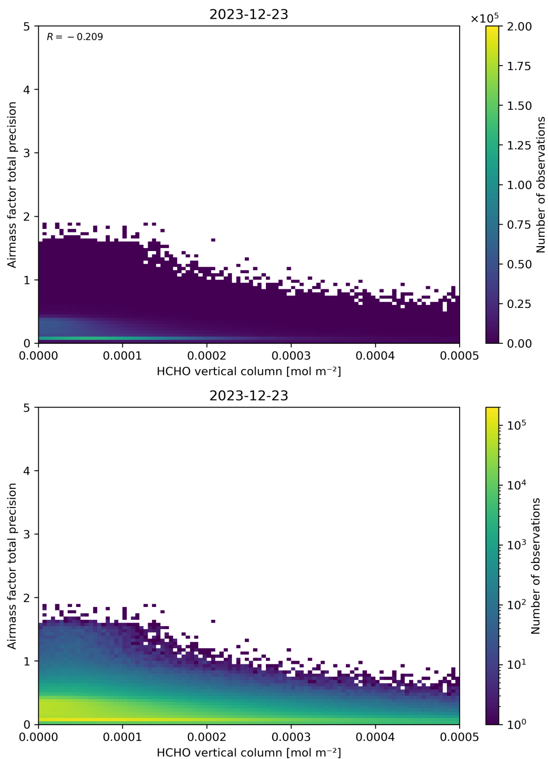
Figure 132: Scatter density plot of “HCHO vertical column” against “Airmass factor total precision” for 2023-12-22 to 2023-12-24.
