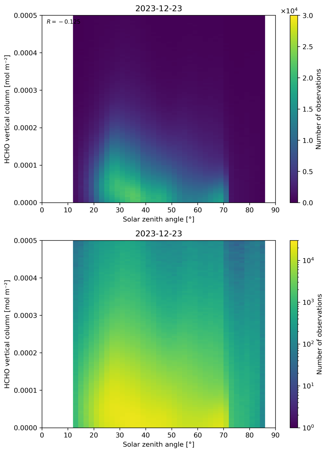
Figure 177: Scatter density plot of “Solar zenith angle” against “HCHO vertical column” for 2023-12-22 to 2023-12-24.
