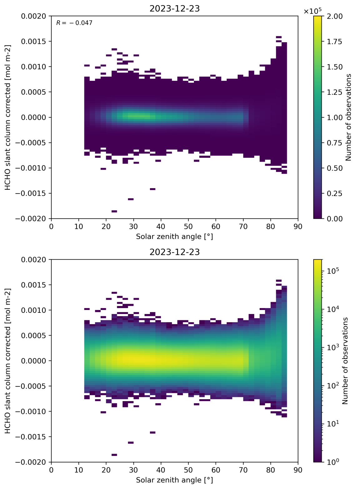
Figure 171: Scatter density plot of “Solar zenith angle” against “HCHO slant column corrected” for 2023-12-22 to 2023-12-24.
