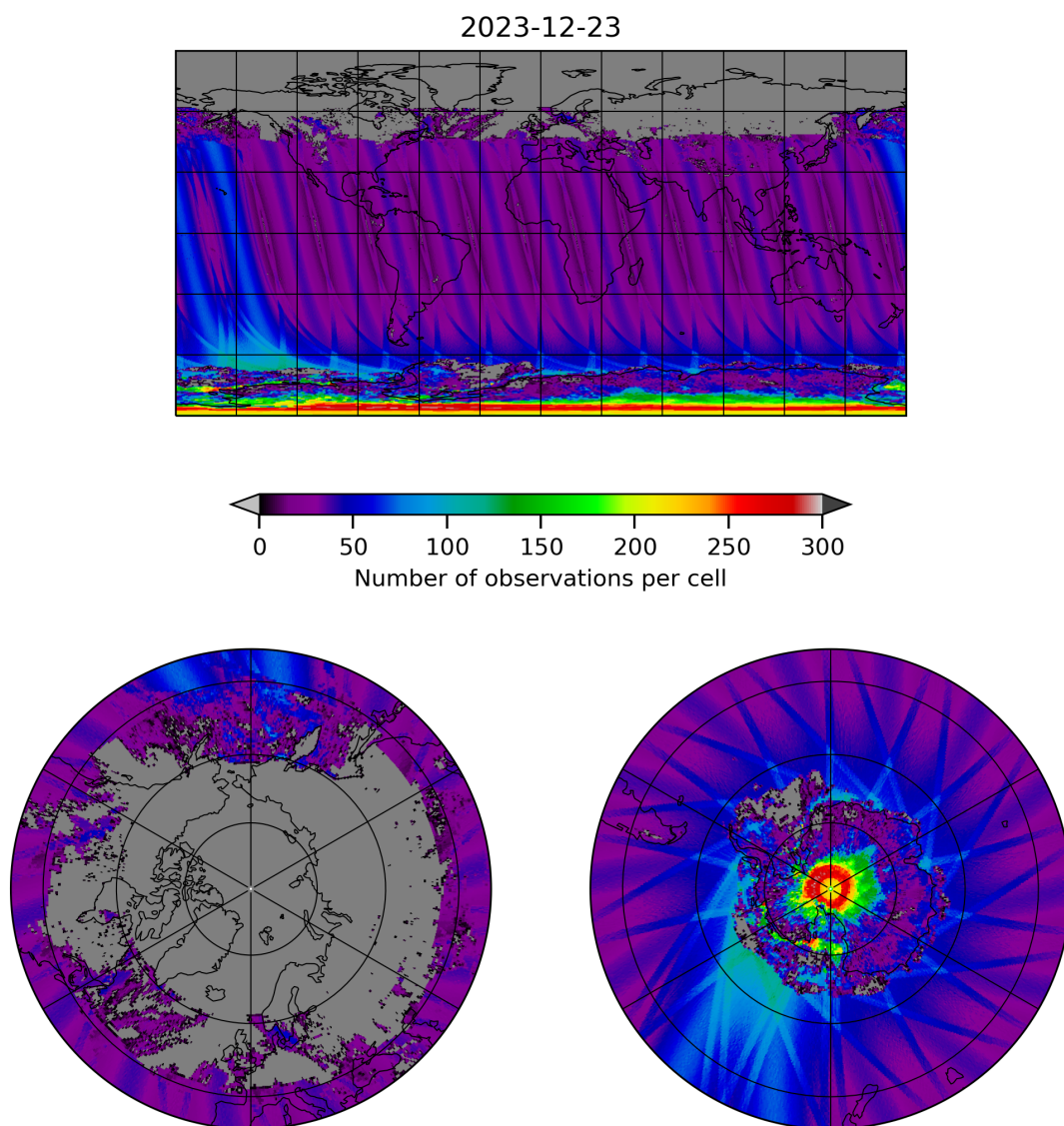
Figure 19: Map of the number of observations for 2023-12-22 to 2023-12-24
