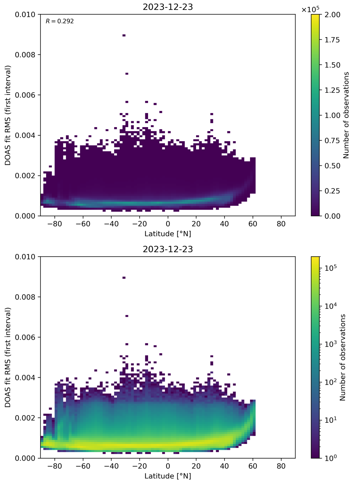
Figure 153: Scatter density plot of “Latitude” against “DOAS fit RMS (first interval)” for 2023-12-22 to 2023-12-24.
