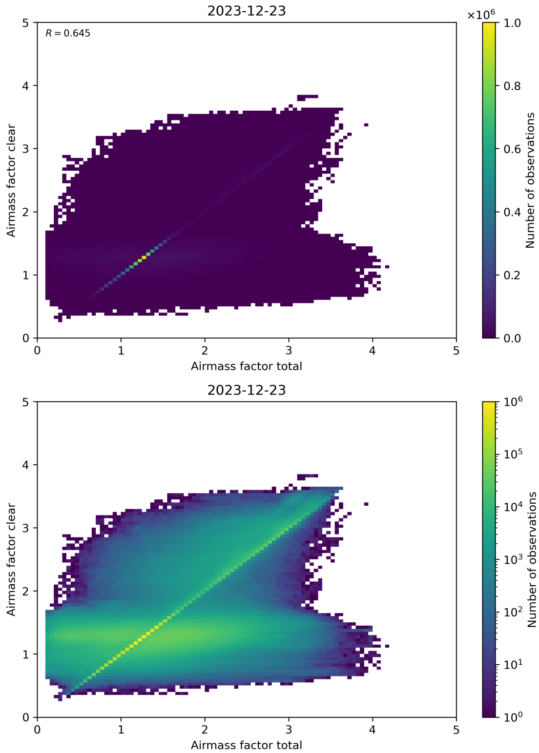
Figure 100: Scatter density plot of “Airmass factor total” against “Airmass factor clear” for 2023-12-22 to 2023-12-24.
