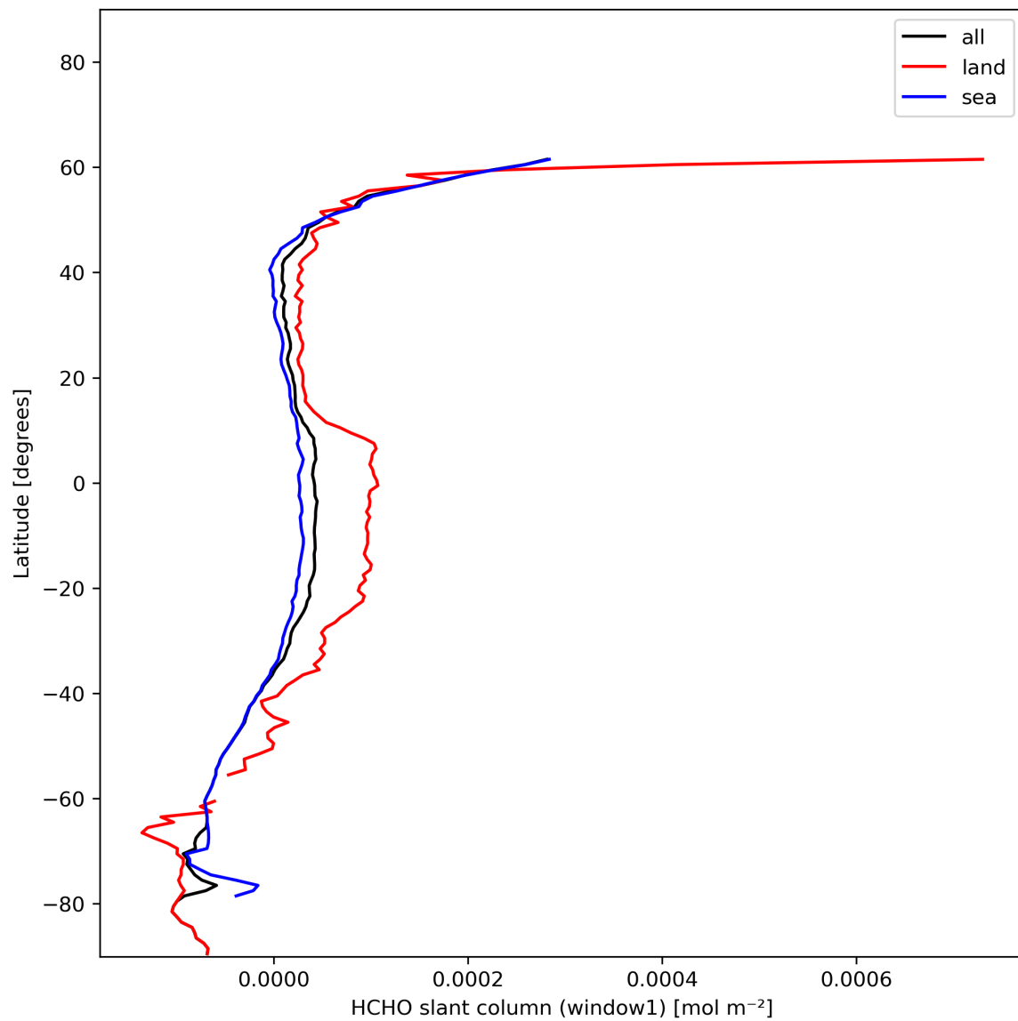
Figure 24: Zonal average of “HCHO slant column (window1)” for 2023-12-22 to 2023-12-24.
