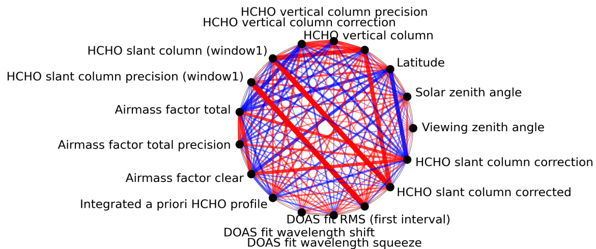
Figure 1: Map of correlation graph for 2023-12-22 to 2023-12-24.
