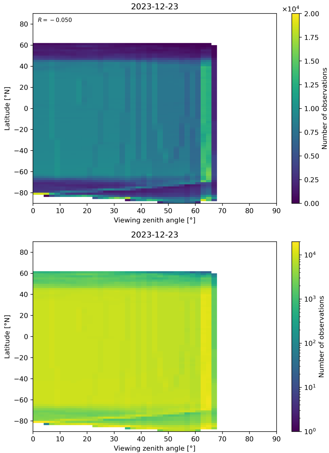
Figure 196: Scatter density plot of “Viewing zenith angle” against “Latitude” for 2023-12-22 to 2023-12-24.
