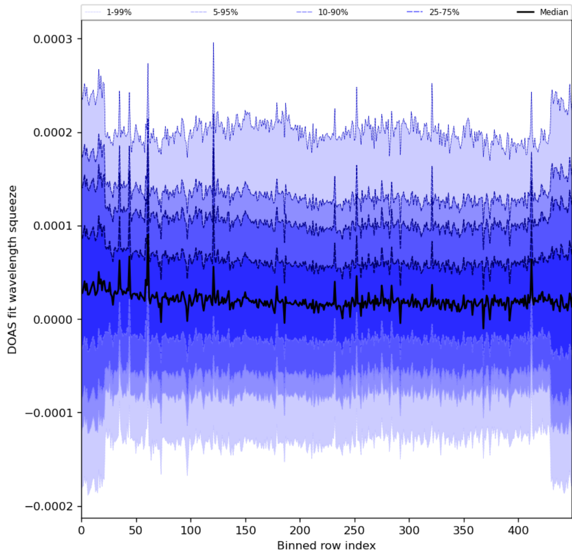
Figure 59: Along track statistics of “DOAS fit wavelength squeeze” for 2023-12-22 to 2023-12-24
