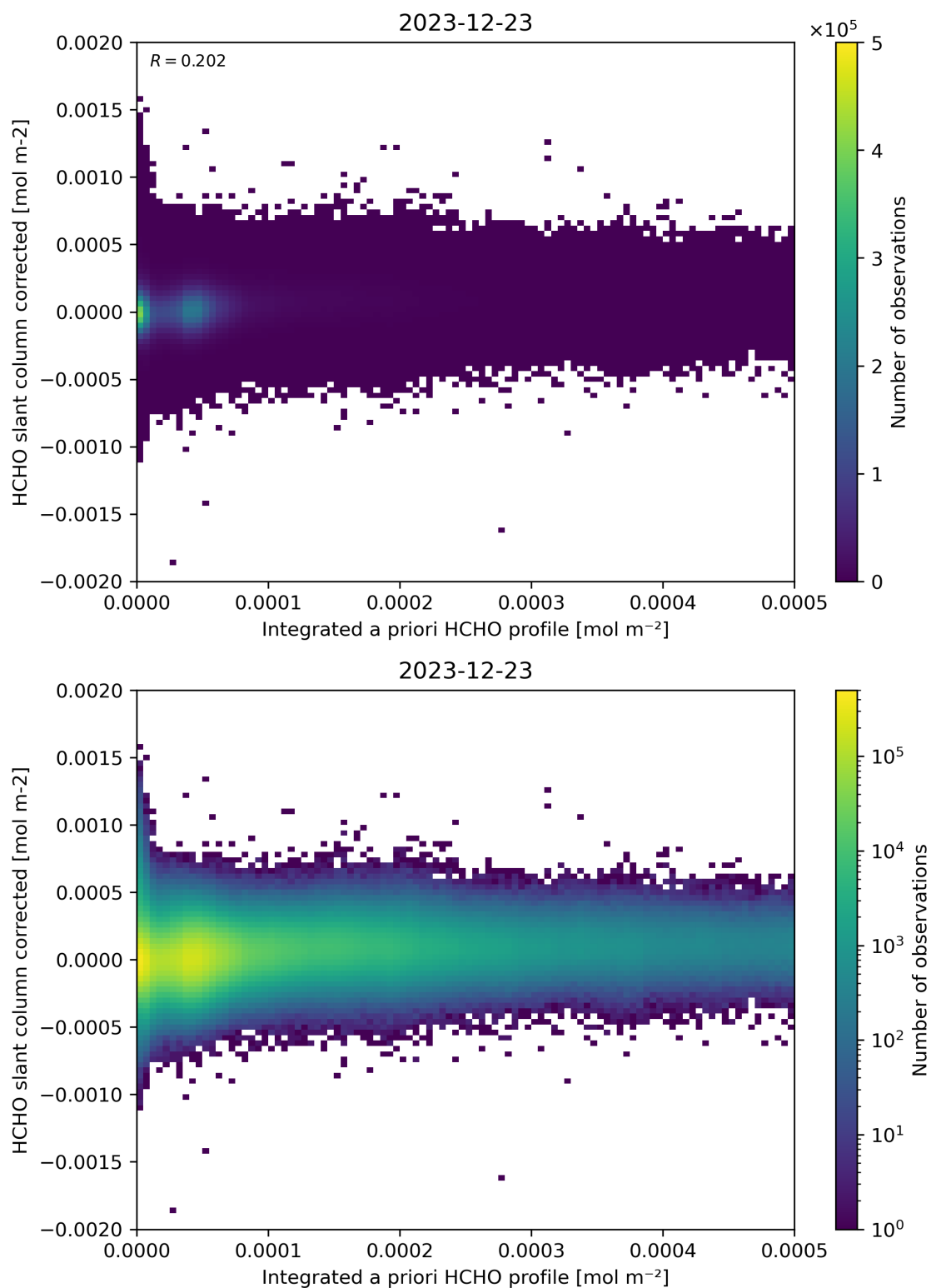
Figure 151: Scatter density plot of “Integrated a priori HCHO profile” against “HCHO slant column corrected” for 2023-12-22 to 2023-12-24.
