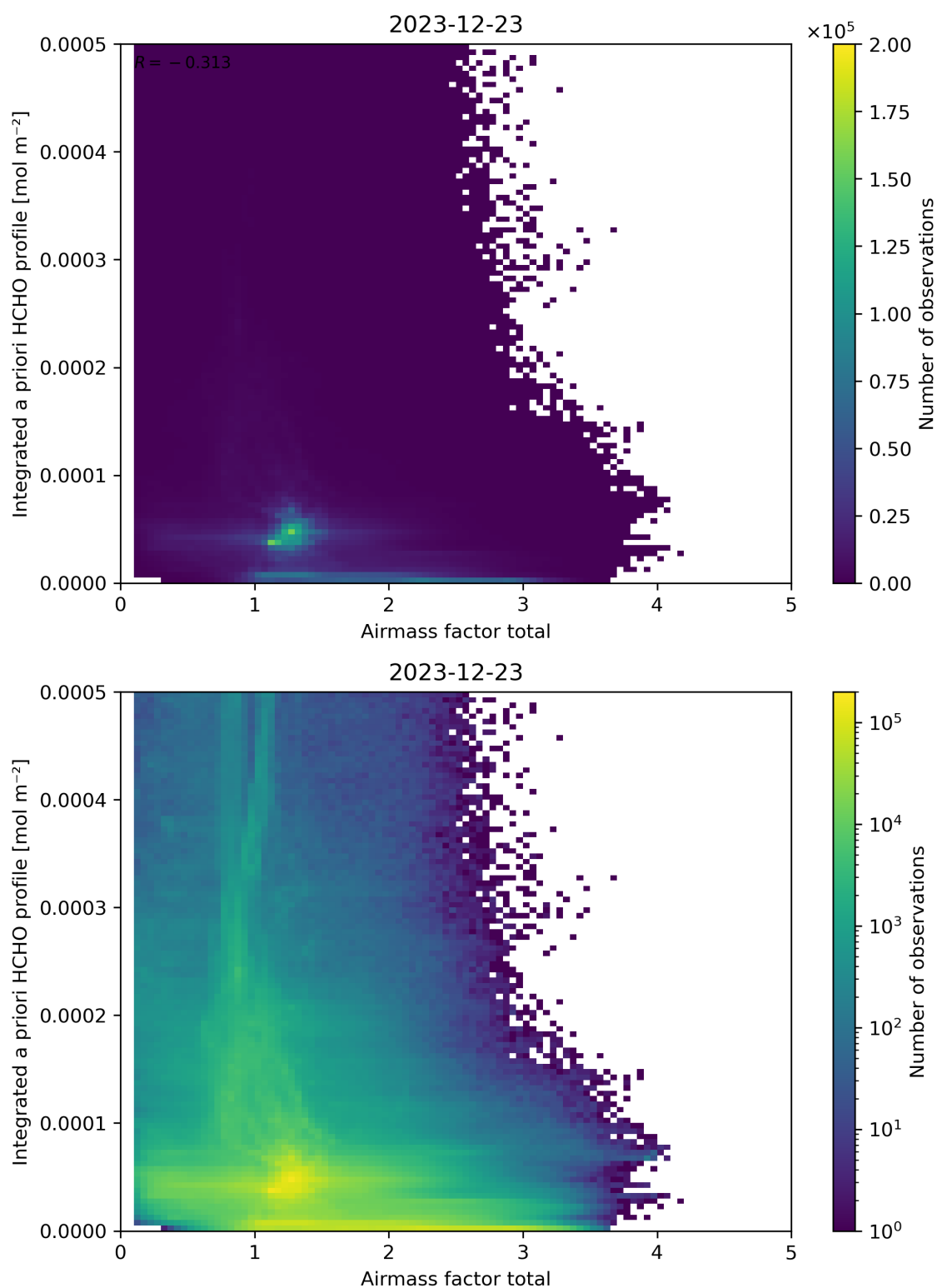
Figure 104: Scatter density plot of “Airmass factor total” against “Integrated a priori HCHO profile” for 2023-12-22 to 2023-12-24.
