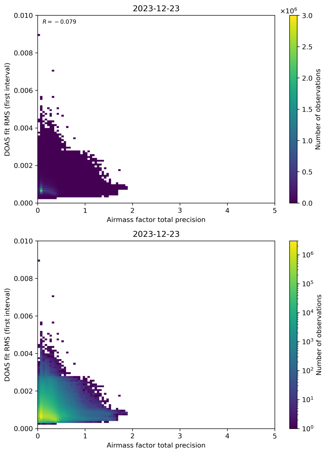
Figure 105: Scatter density plot of “Airmass factor total precision” against “DOAS fit RMS (first interval)” for 2023-12-22 to 2023-12-24.
