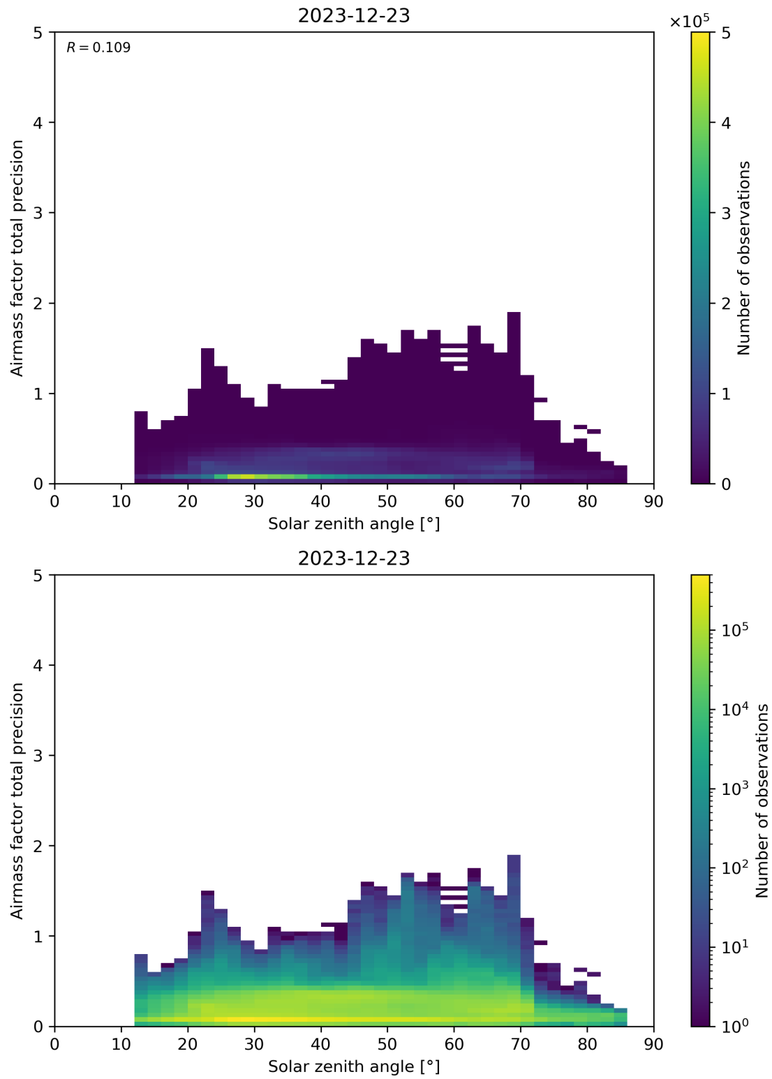
Figure 176: Scatter density plot of “Solar zenith angle” against “Airmass factor total precision” for 2023-12-22 to 2023-12-24.
