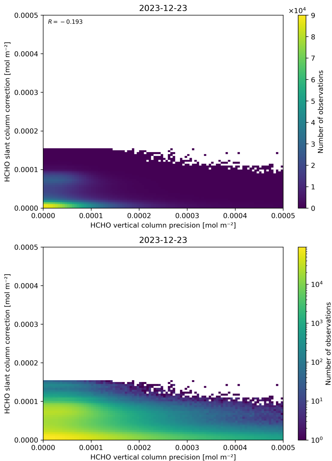
Figure 141: Scatter density plot of “HCHO vertical column precision” against “HCHO slant column correction” for 2023-12-22 to 2023-12-24.
