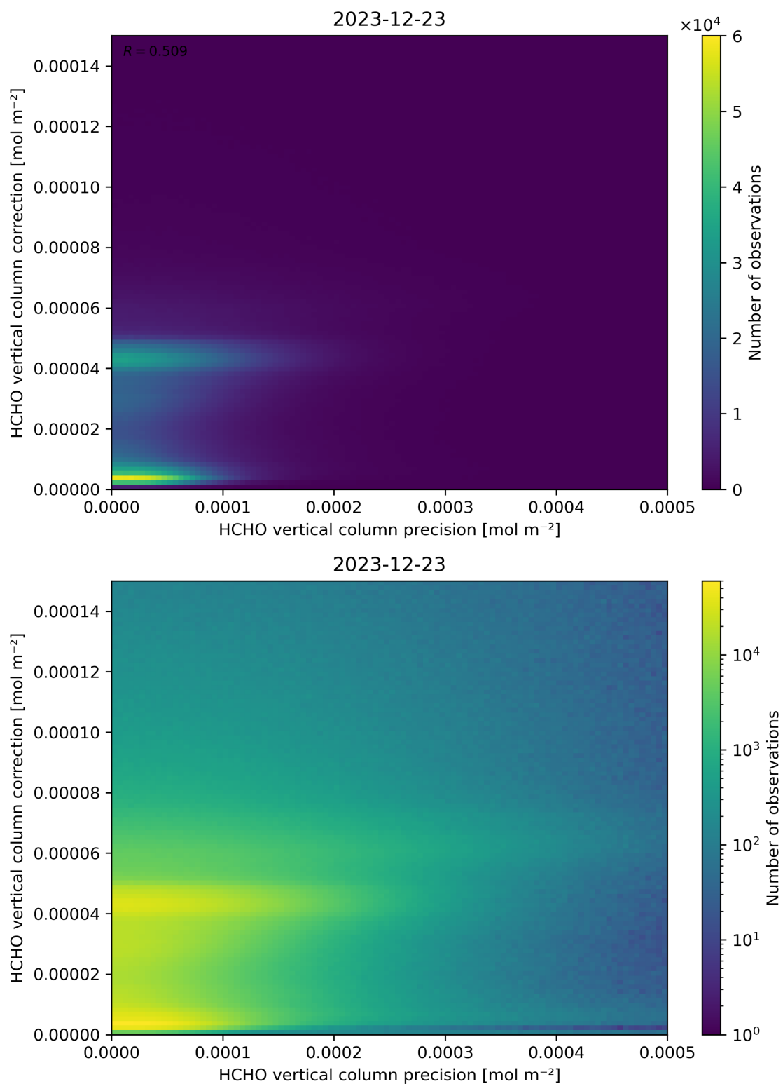
Figure 146: Scatter density plot of “HCHO vertical column precision” against “HCHO vertical column correction” for 2023-12-22 to 2023-12-24.
