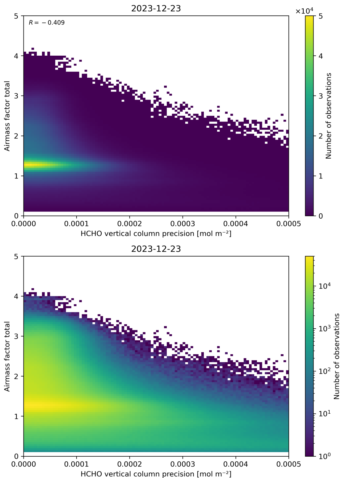
Figure 144: Scatter density plot of “HCHO vertical column precision” against “Airmass factor total” for 2023-12-22 to 2023-12-24.
