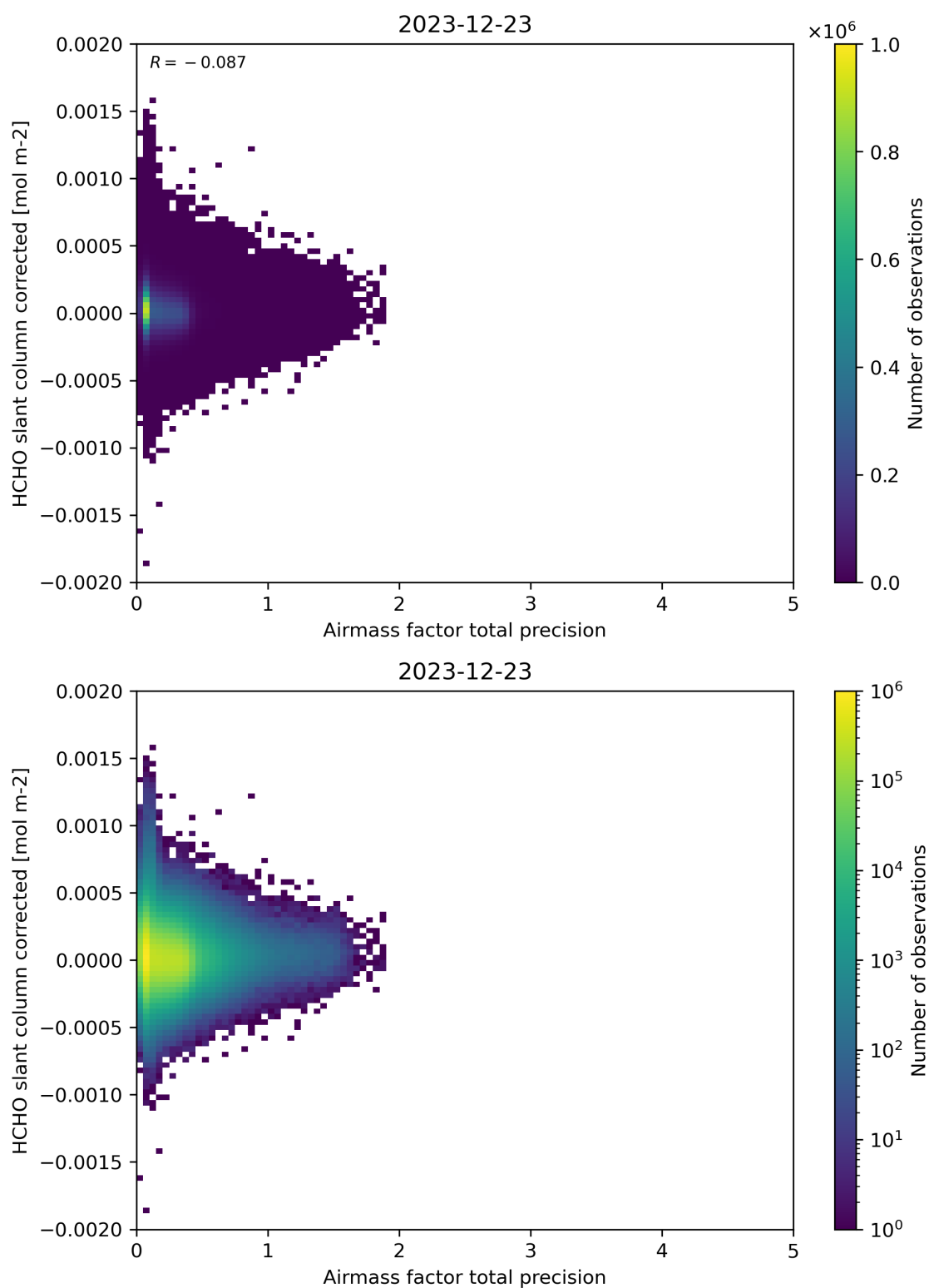
Figure 109: Scatter density plot of “Airmass factor total precision” against “HCHO slant column corrected” for 2023-12-22 to 2023-12-24.
