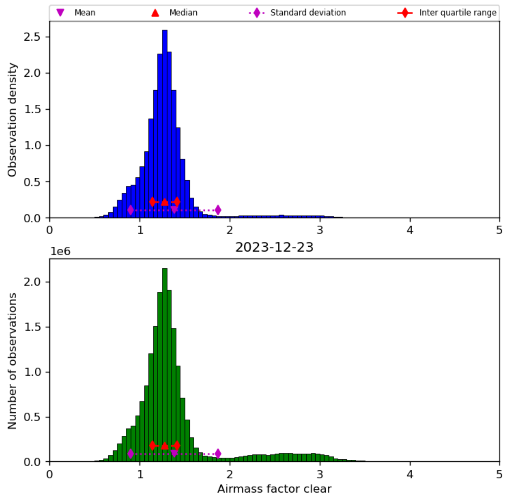
Figure 42: Histogram of “Airmass factor clear” for 2023-12-22 to 2023-12-24
