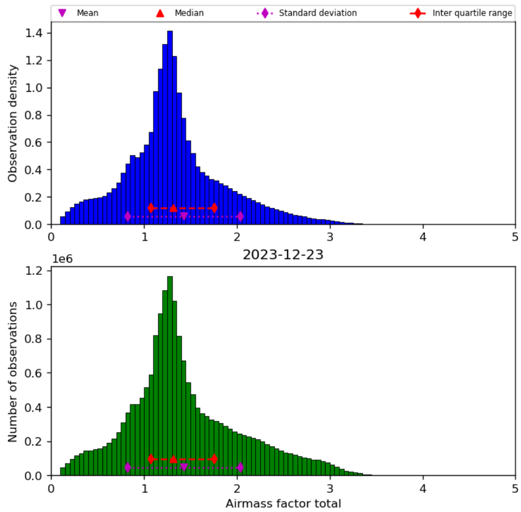
Figure 40: Histogram of “Airmass factor total” for 2023-12-22 to 2023-12-24
