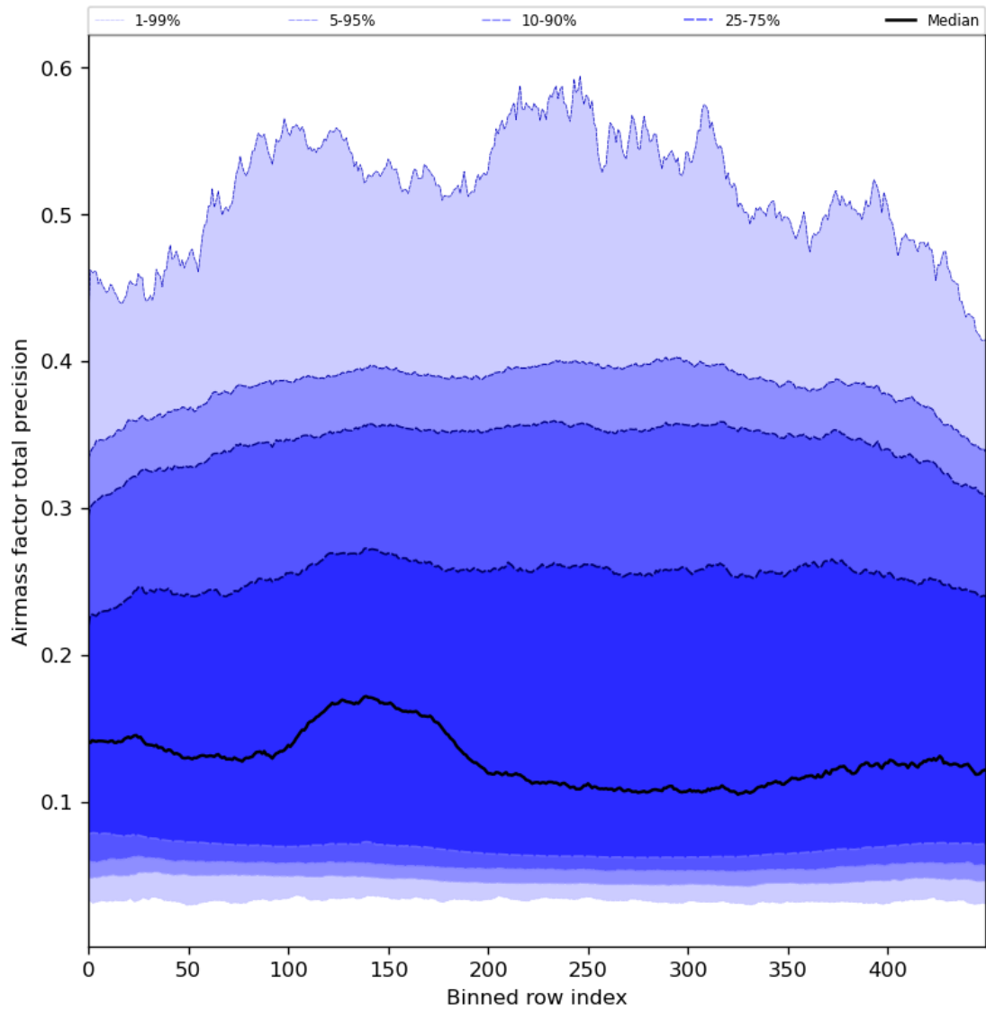
Figure 55: Along track statistics of “Airmass factor total precision” for 2023-12-22 to 2023-12-24
