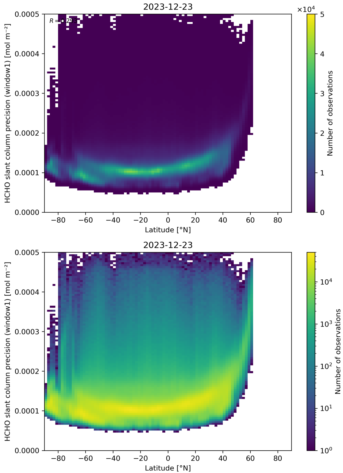
Figure 160: Scatter density plot of “Latitude” against “HCHO slant column precision (window1)” for 2023-12-22 to 2023-12-24.
