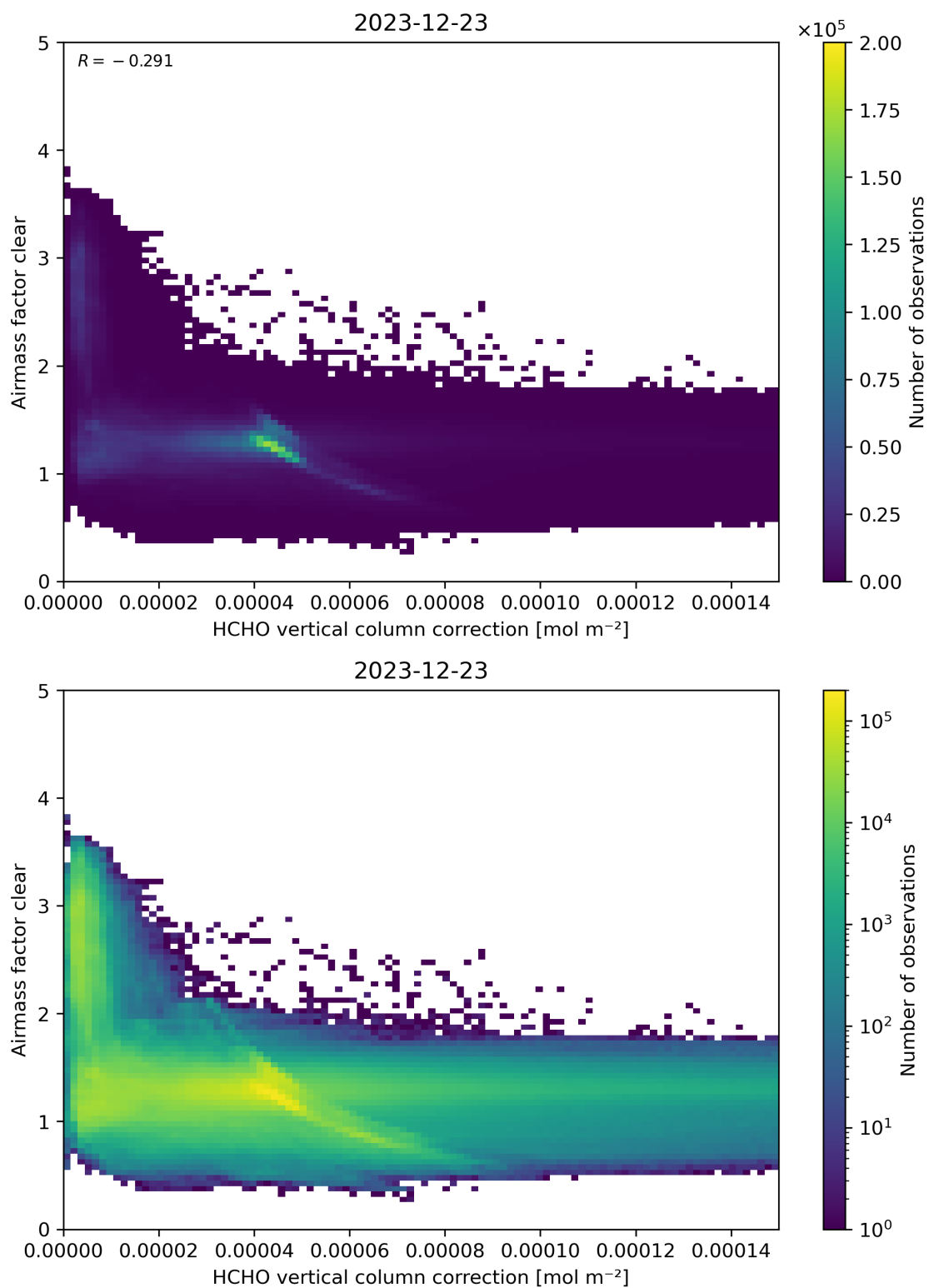
Figure 115: Scatter density plot of “HCHO vertical column correction” against “Airmass factor clear” for 2023-12-22 to 2023-12-24.
