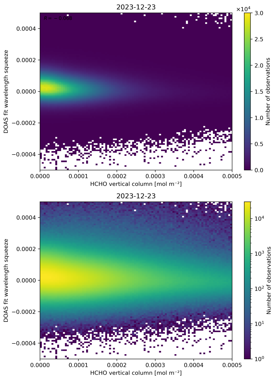
Figure 125: Scatter density plot of “HCHO vertical column” against “DOAS fit wavelength squeeze” for 2023-12-22 to 2023-12-24.
