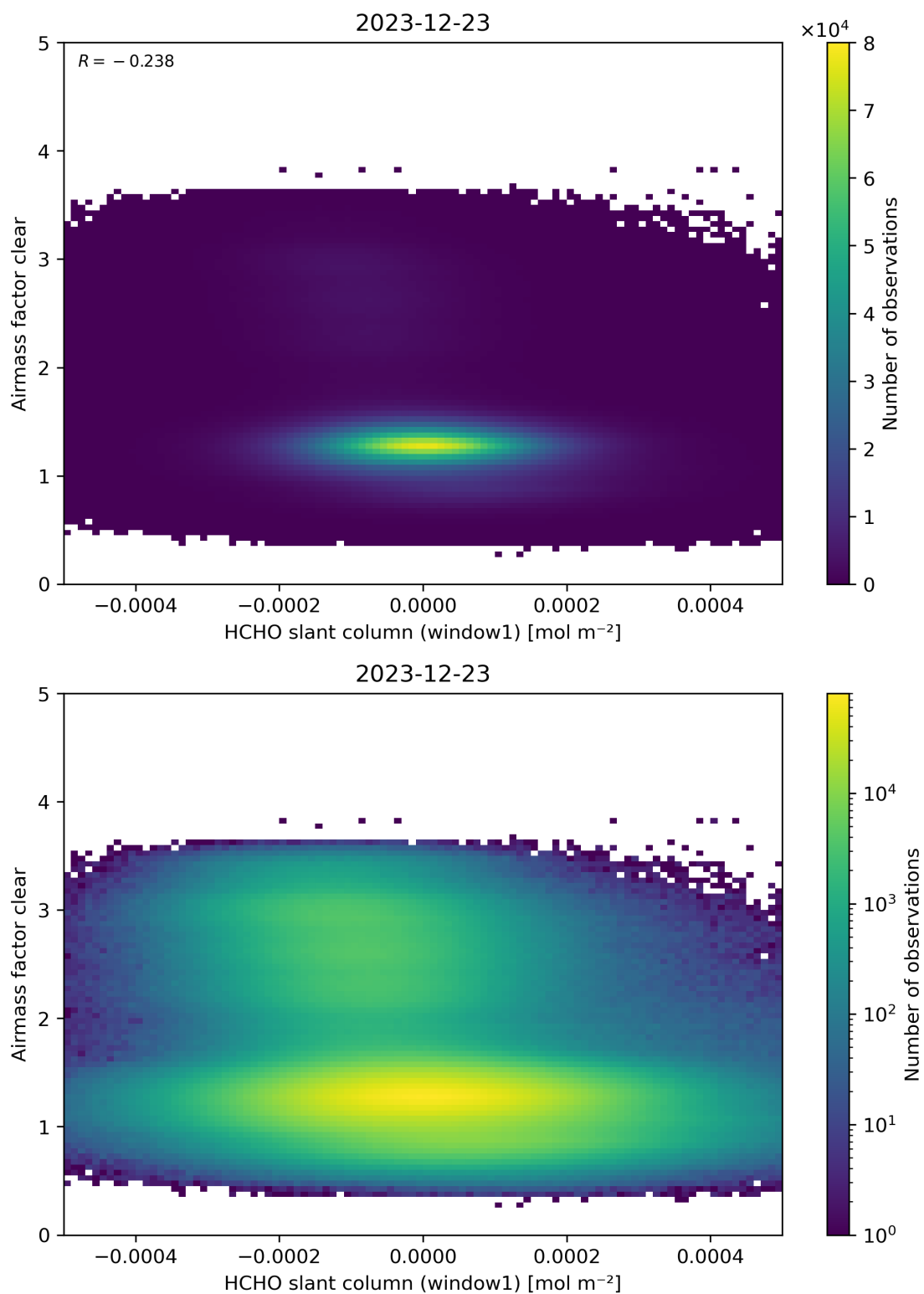
Figure 81: Scatter density plot of “HCHO slant column (window1)” against “Airmass factor clear” for 2023-12-22 to 2023-12-24.
