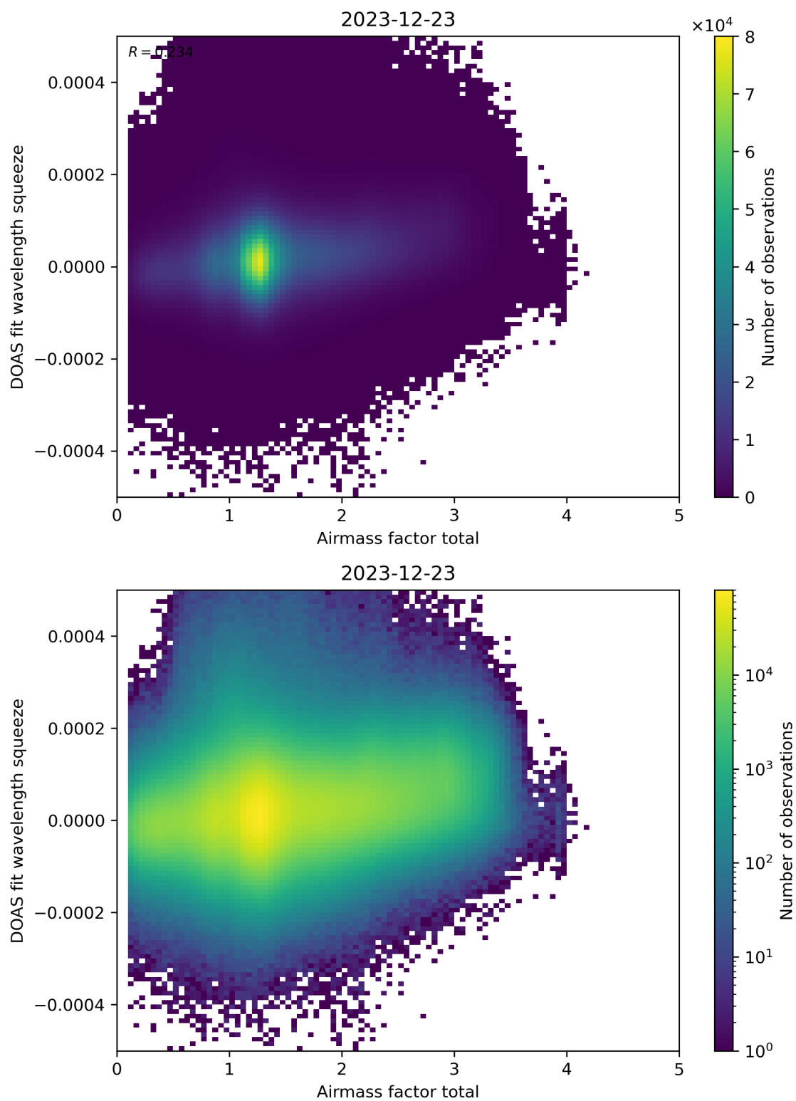
Figure 99: Scatter density plot of “Airmass factor total” against “DOAS fit wavelength squeeze” for 2023-12-22 to 2023-12-24.
