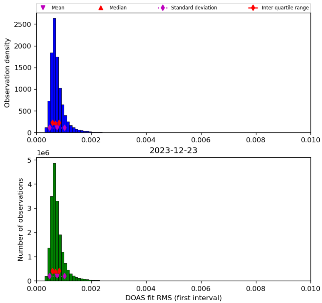
Figure 46: Histogram of “DOAS fit RMS (first interval)” for 2023-12-22 to 2023-12-24
