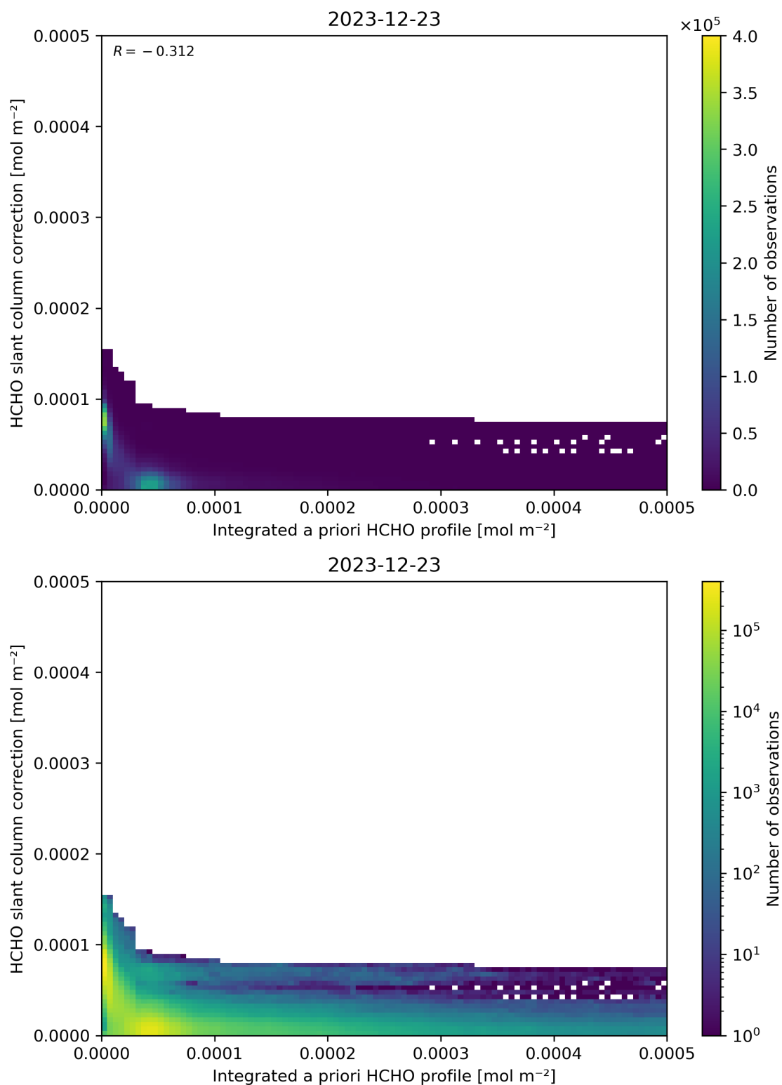
Figure 152: Scatter density plot of “Integrated a priori HCHO profile” against “HCHO slant column correction” for 2023-12-22 to 2023-12-24.
