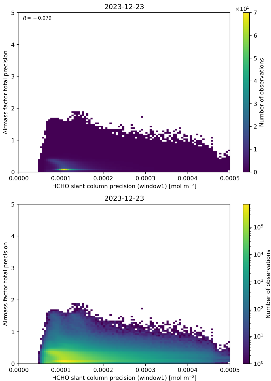
Figure 95: Scatter density plot of “HCHO slant column precision (window1)” against “Airmass factor total precision” for 2023-12-22 to 2023-12-24.
