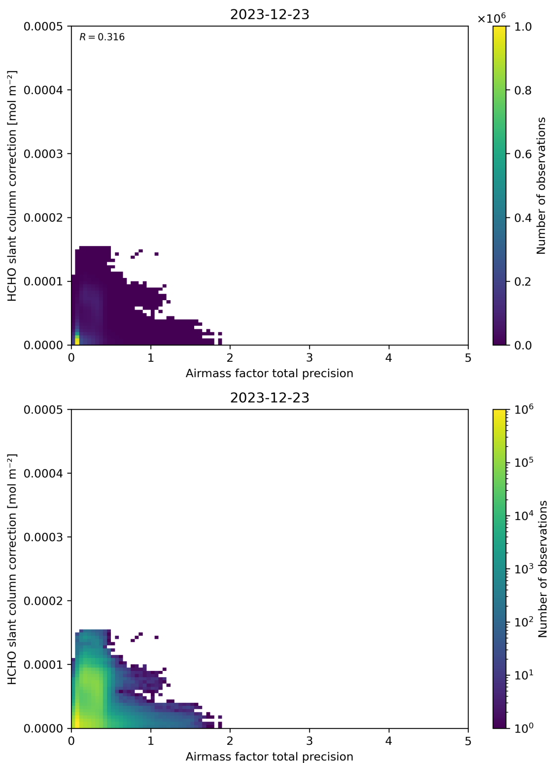
Figure 110: Scatter density plot of “Airmass factor total precision” against “HCHO slant column correction” for 2023-12-22 to 2023-12-24.
