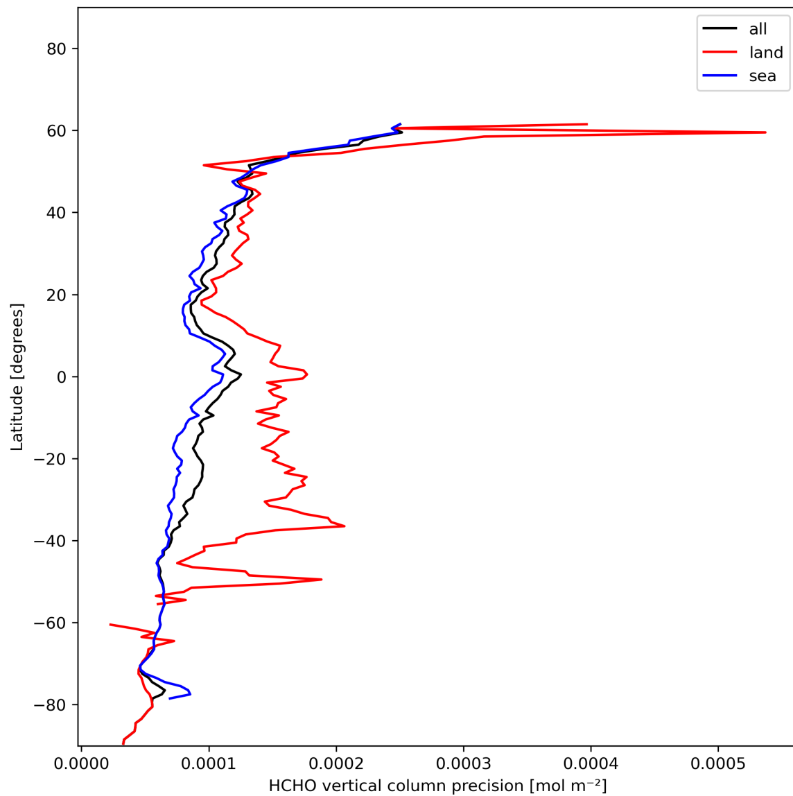
Figure 22: Zonal average of “HCHO vertical column precision” for 2023-12-22 to 2023-12-24.
