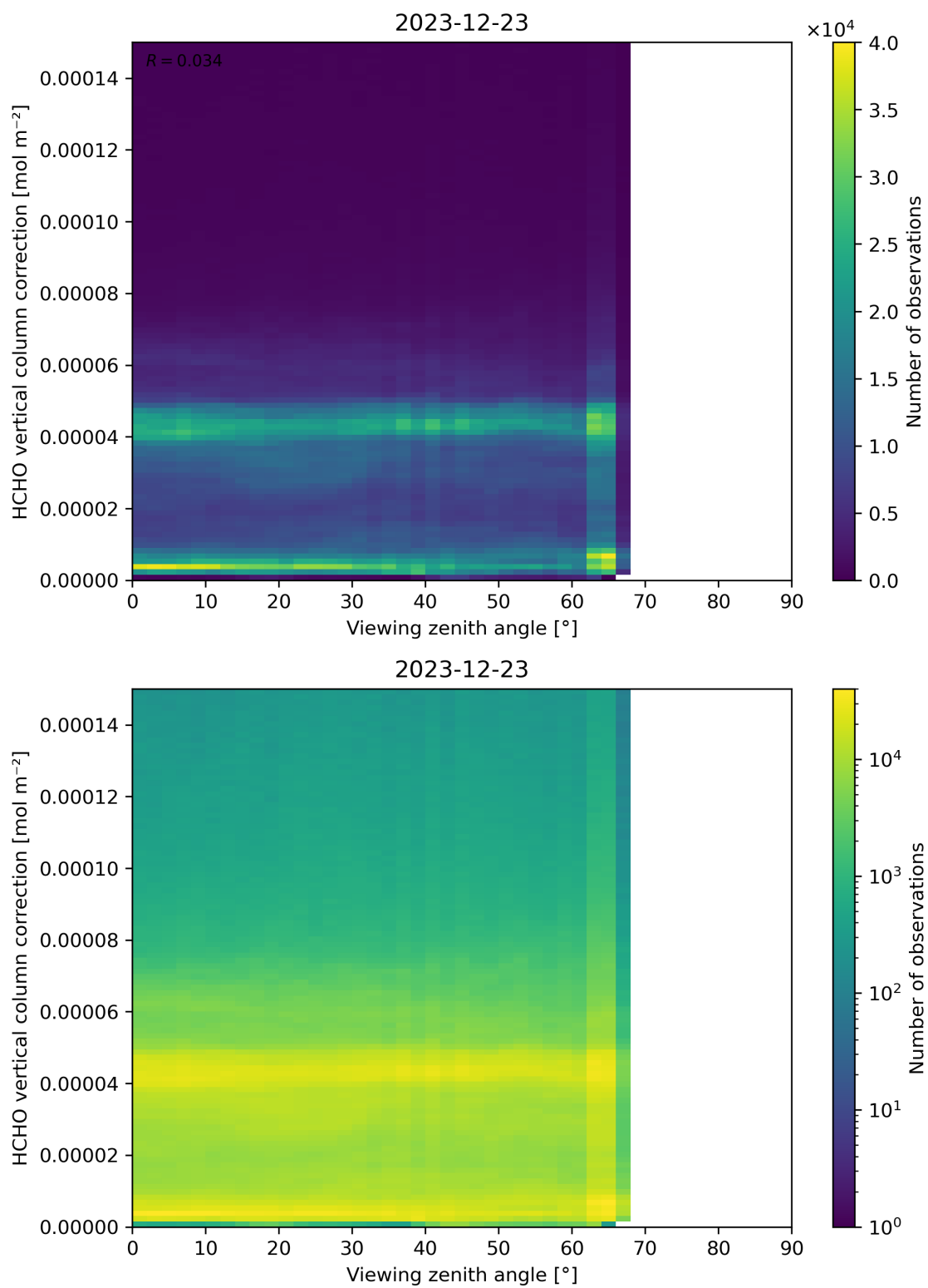
Figure 193: Scatter density plot of “Viewing zenith angle” against “HCHO vertical column correction” for 2023-12-22 to 2023-12-24.
