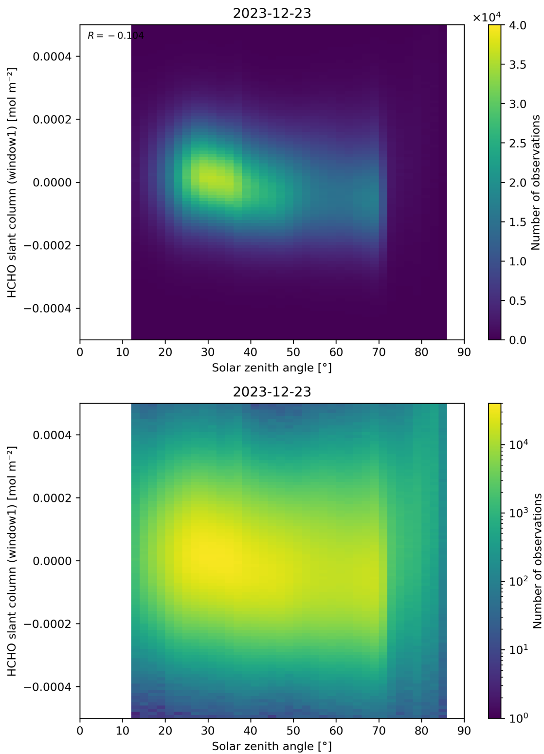
Figure 173: Scatter density plot of “Solar zenith angle” against “HCHO slant column (window1)” for 2023-12-22 to 2023-12-24.
