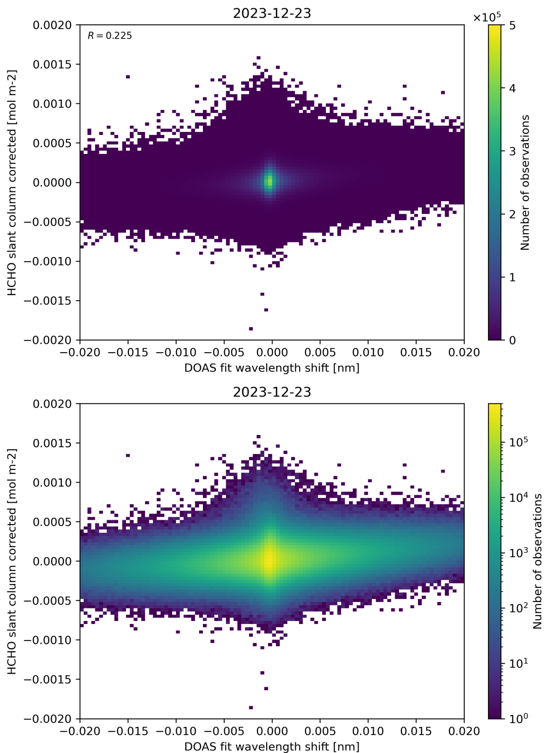
Figure 66: Scatter density plot of “DOAS fit wavelength shift” against “HCHO slant column corrected” for 2023-12-22 to 2023-12-24.
