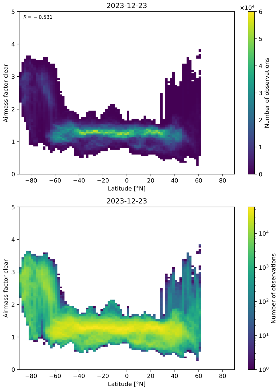
Figure 156: Scatter density plot of “Latitude” against “Airmass factor clear” for 2023-12-22 to 2023-12-24.
