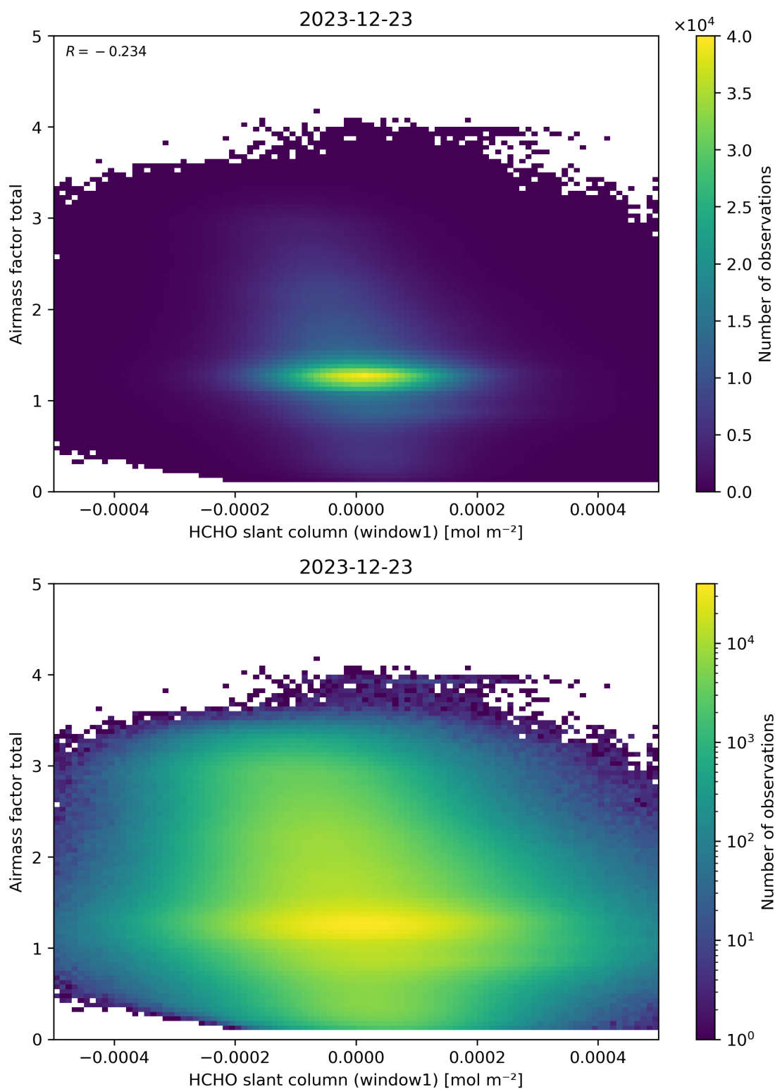
Figure 85: Scatter density plot of “HCHO slant column (window1)” against “Airmass factor total” for 2023-12-22 to 2023-12-24.
