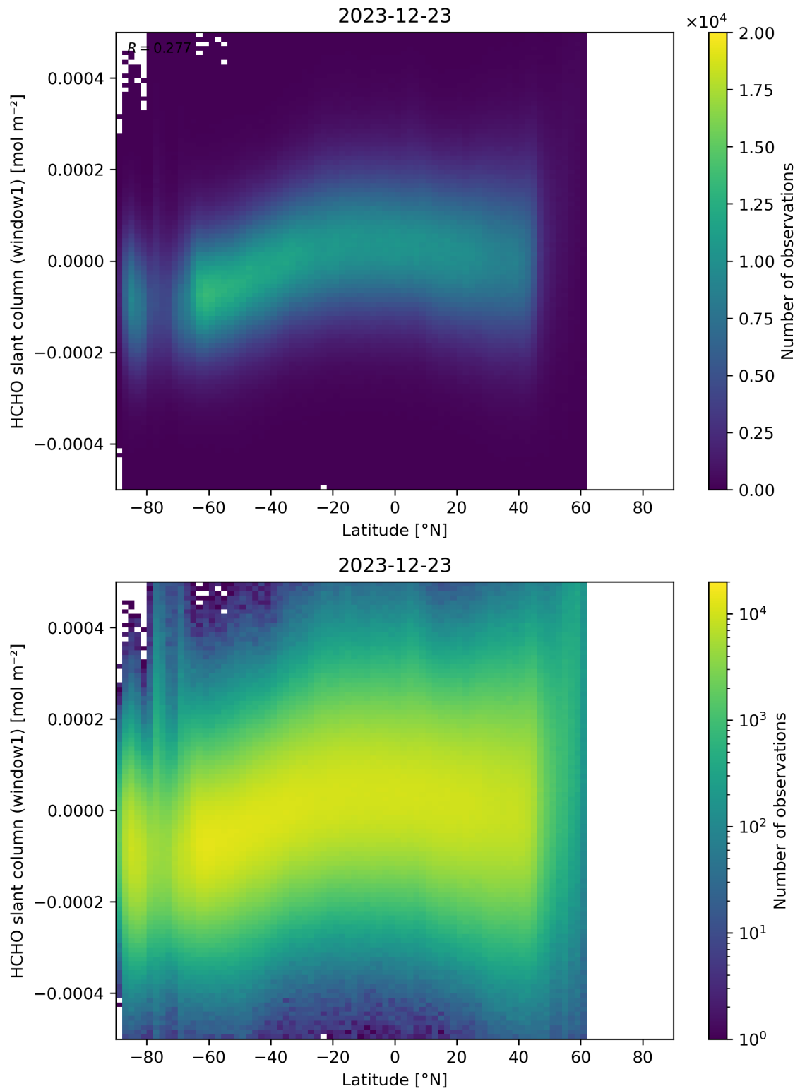
Figure 159: Scatter density plot of “Latitude” against “HCHO slant column (window1)” for 2023-12-22 to 2023-12-24.
