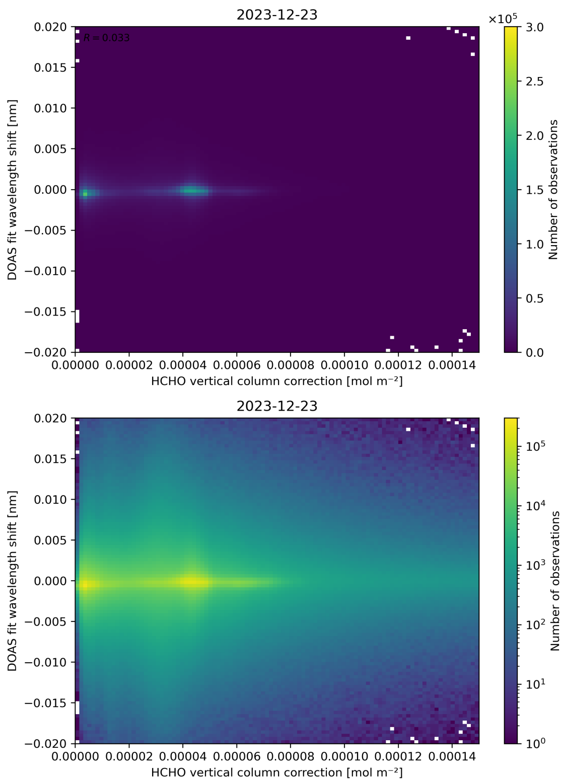
Figure 113: Scatter density plot of “HCHO vertical column correction” against “DOAS fit wavelength shift” for 2023-12-22 to 2023-12-24.
