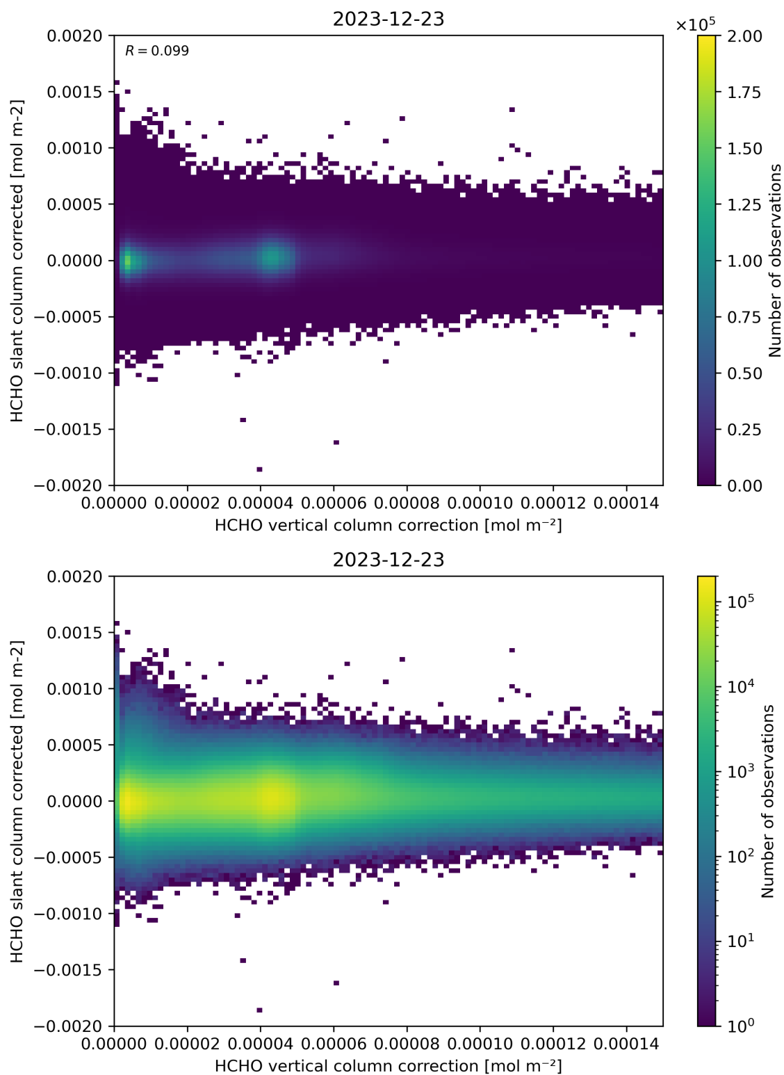
Figure 116: Scatter density plot of “HCHO vertical column correction” against “HCHO slant column corrected” for 2023-12-22 to 2023-12-24.
