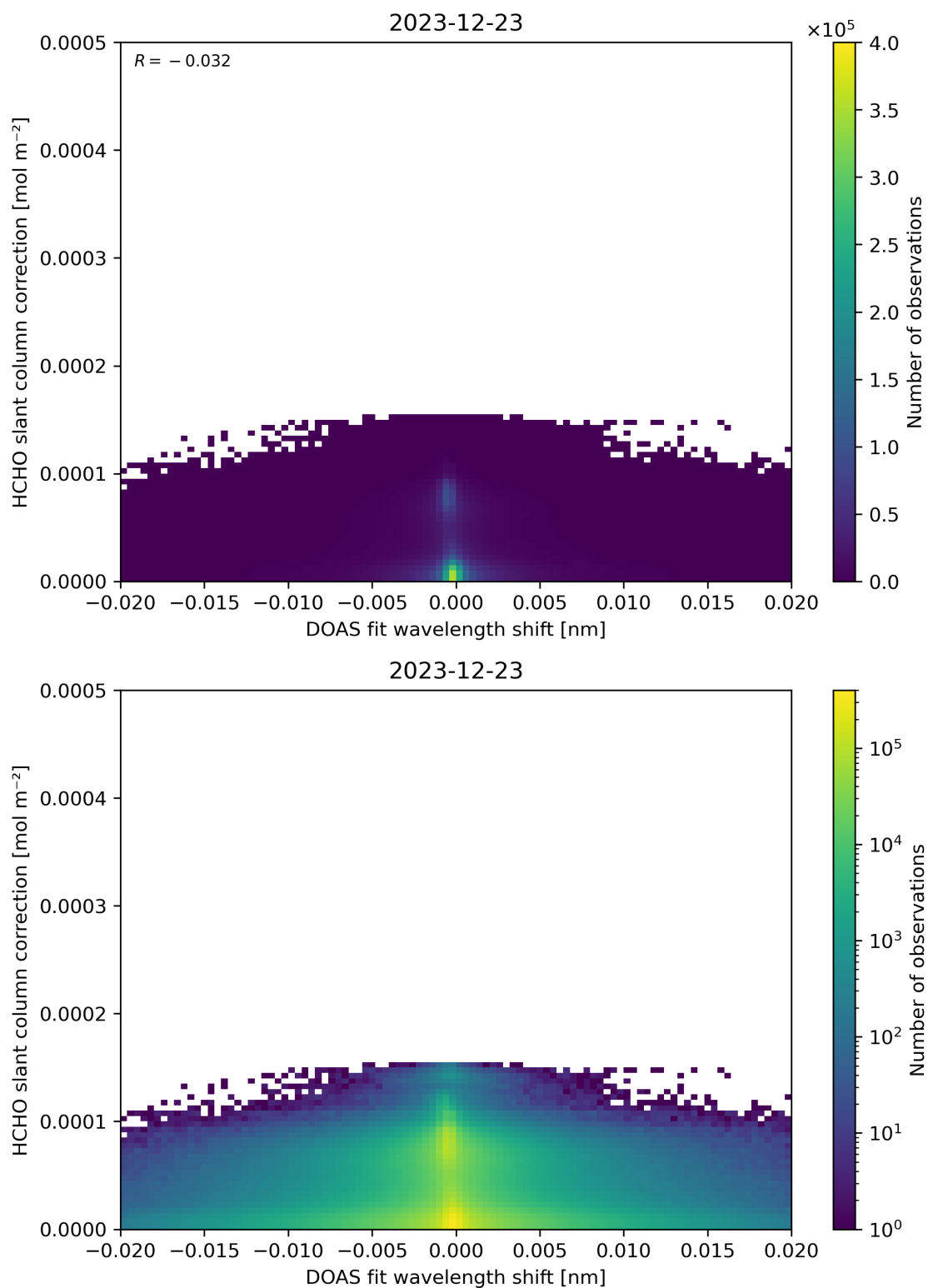
Figure 67: Scatter density plot of “DOAS fit wavelength shift” against “HCHO slant column correction” for 2023-12-22 to 2023-12-24.
