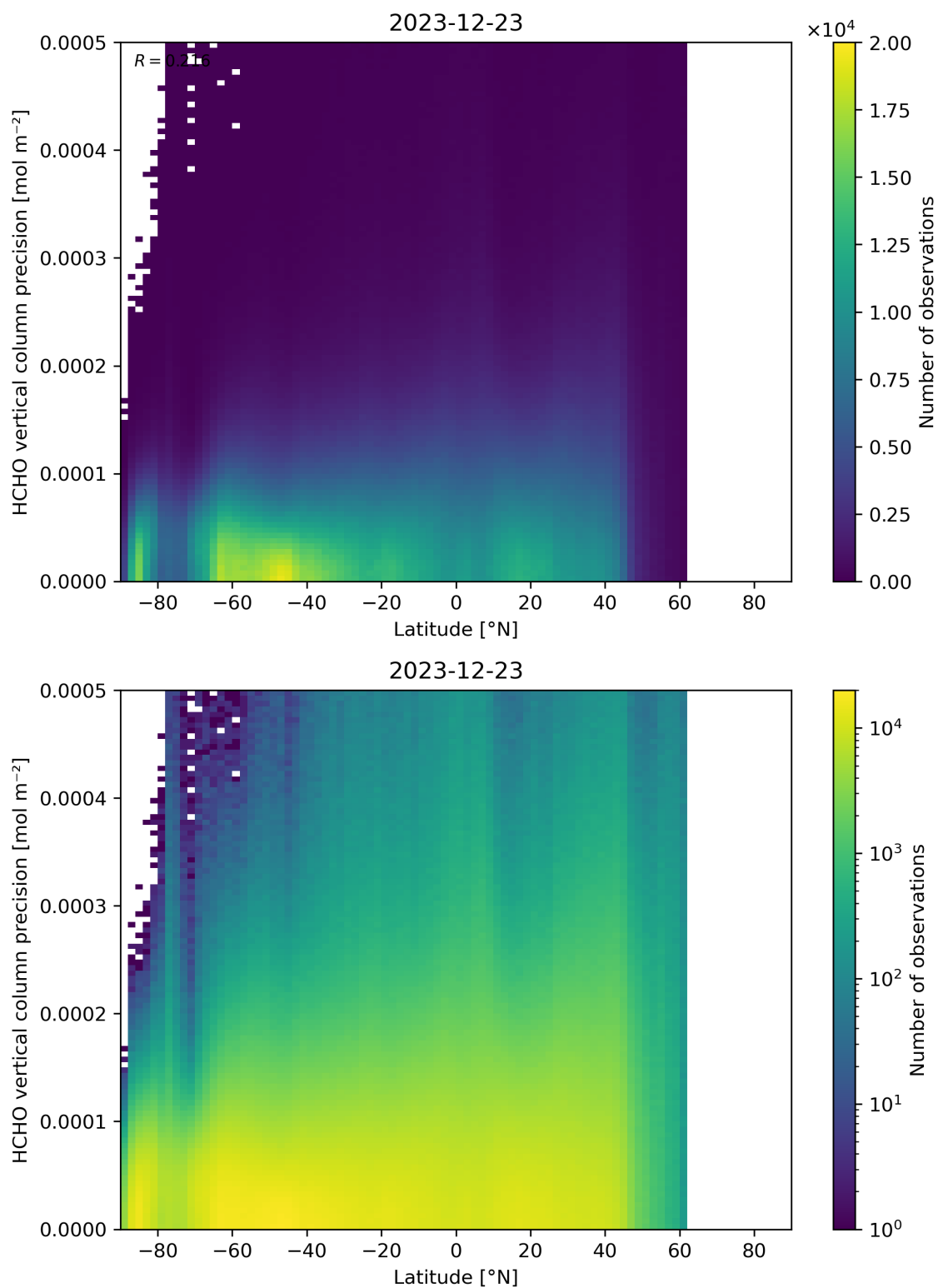
Figure 165: Scatter density plot of “Latitude” against “HCHO vertical column precision” for 2023-12-22 to 2023-12-24.
