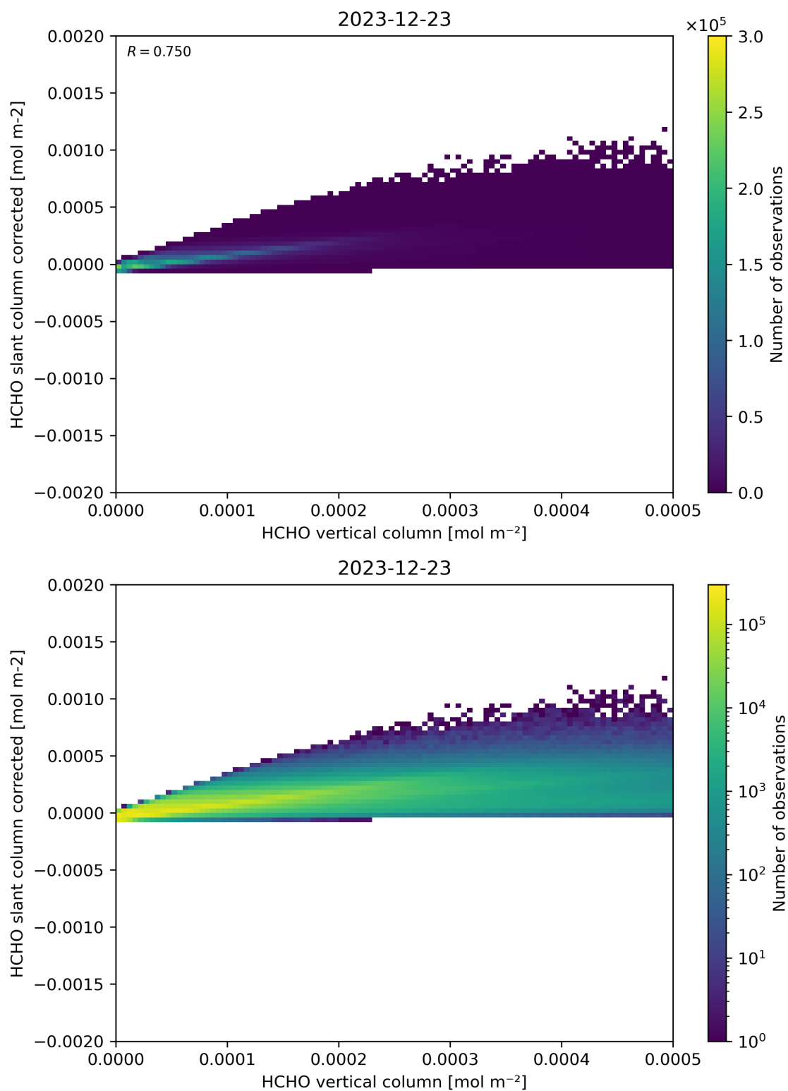
Figure 127: Scatter density plot of “HCHO vertical column” against “HCHO slant column corrected” for 2023-12-22 to 2023-12-24.
