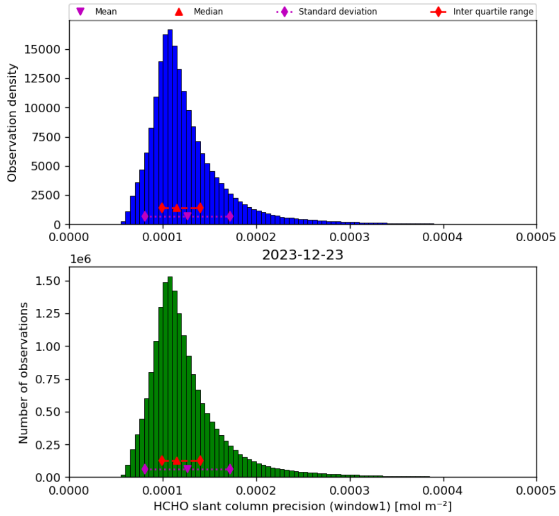
Figure 39: Histogram of “HCHO slant column precision (window1)” for 2023-12-22 to 2023-12-24
