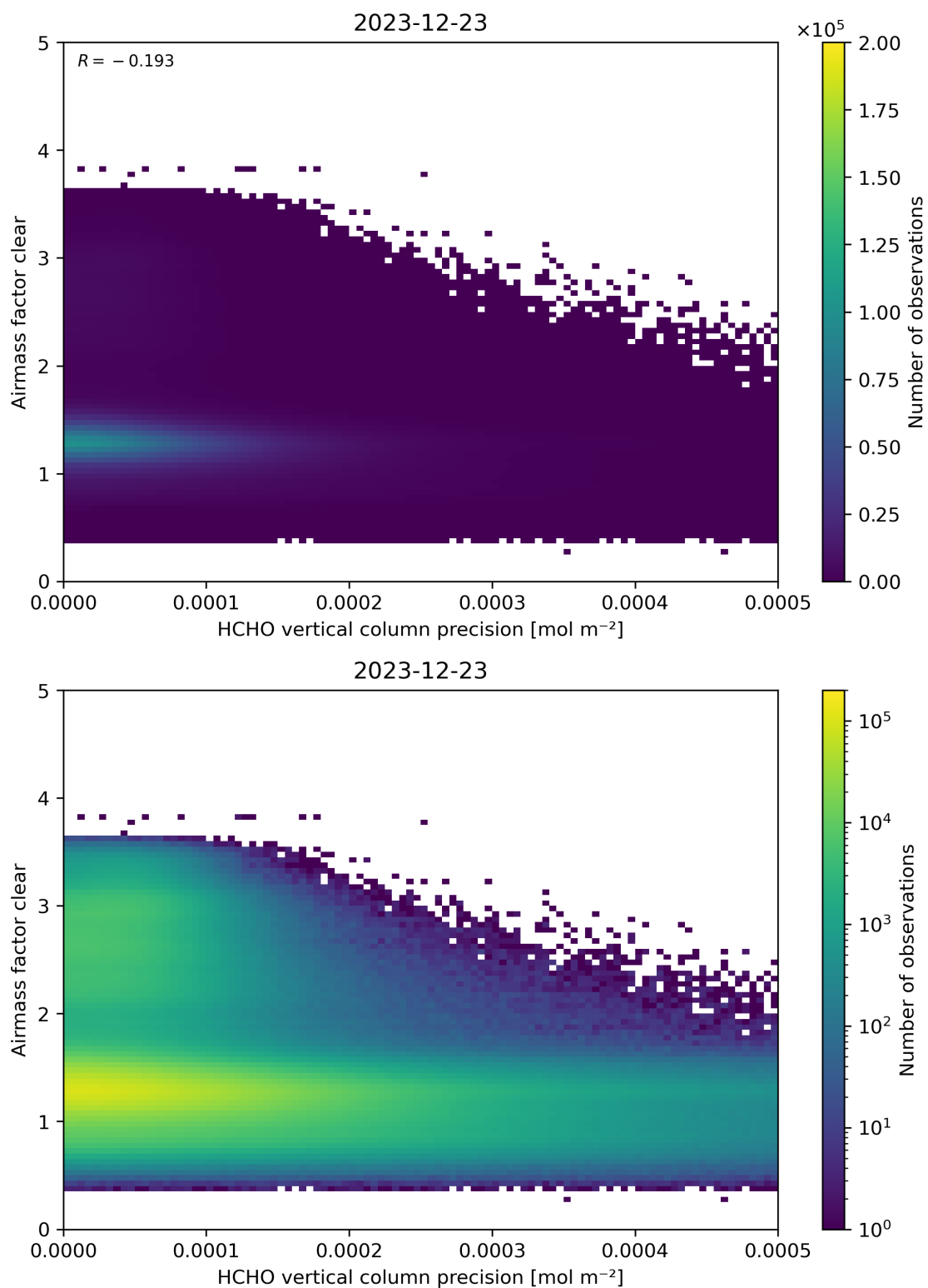
Figure 139: Scatter density plot of “HCHO vertical column precision” against “Airmass factor clear” for 2023-12-22 to 2023-12-24.
