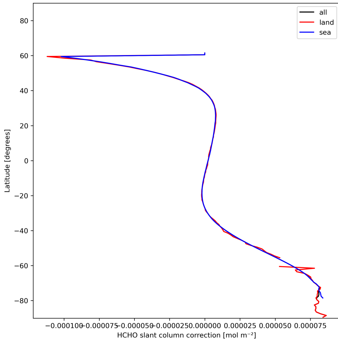
Figure 33: Zonal average of “HCHO slant column correction” for 2023-12-22 to 2023-12-24.
