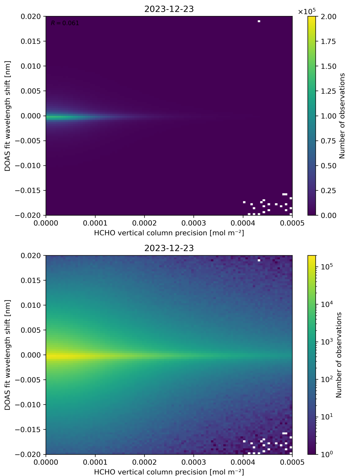
Figure 137: Scatter density plot of “HCHO vertical column precision” against “DOAS fit wavelength shift” for 2023-12-22 to 2023-12-24.
