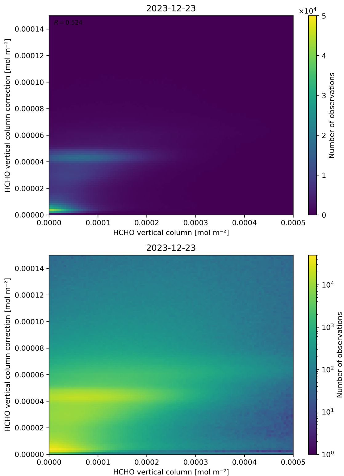
Figure 133: Scatter density plot of “HCHO vertical column” against “HCHO vertical column correction” for 2023-12-22 to 2023-12-24.
