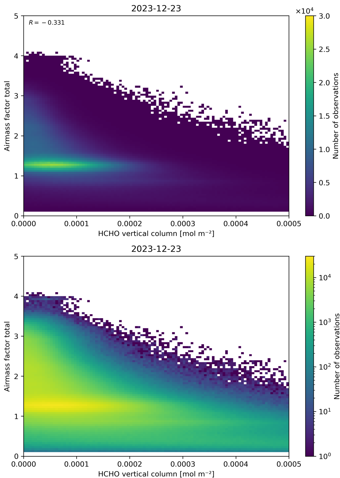
Figure 131: Scatter density plot of “HCHO vertical column” against “Airmass factor total” for 2023-12-22 to 2023-12-24.
