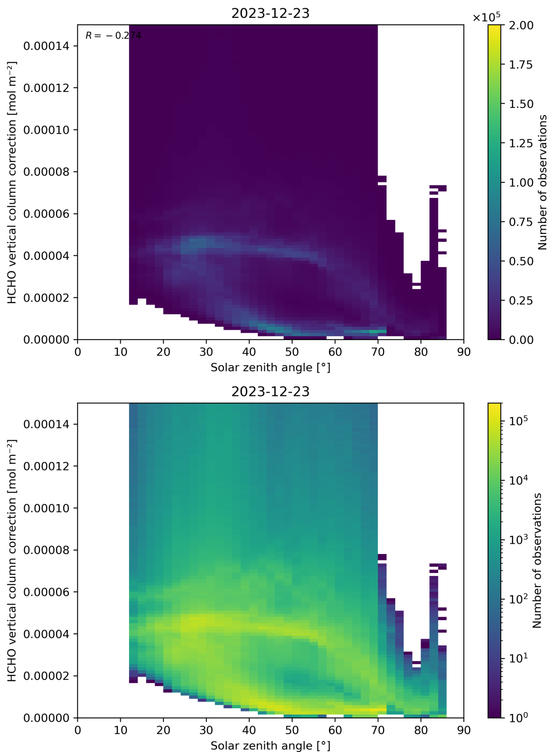
Figure 178: Scatter density plot of “Solar zenith angle” against “HCHO vertical column correction” for 2023-12-22 to 2023-12-24.
