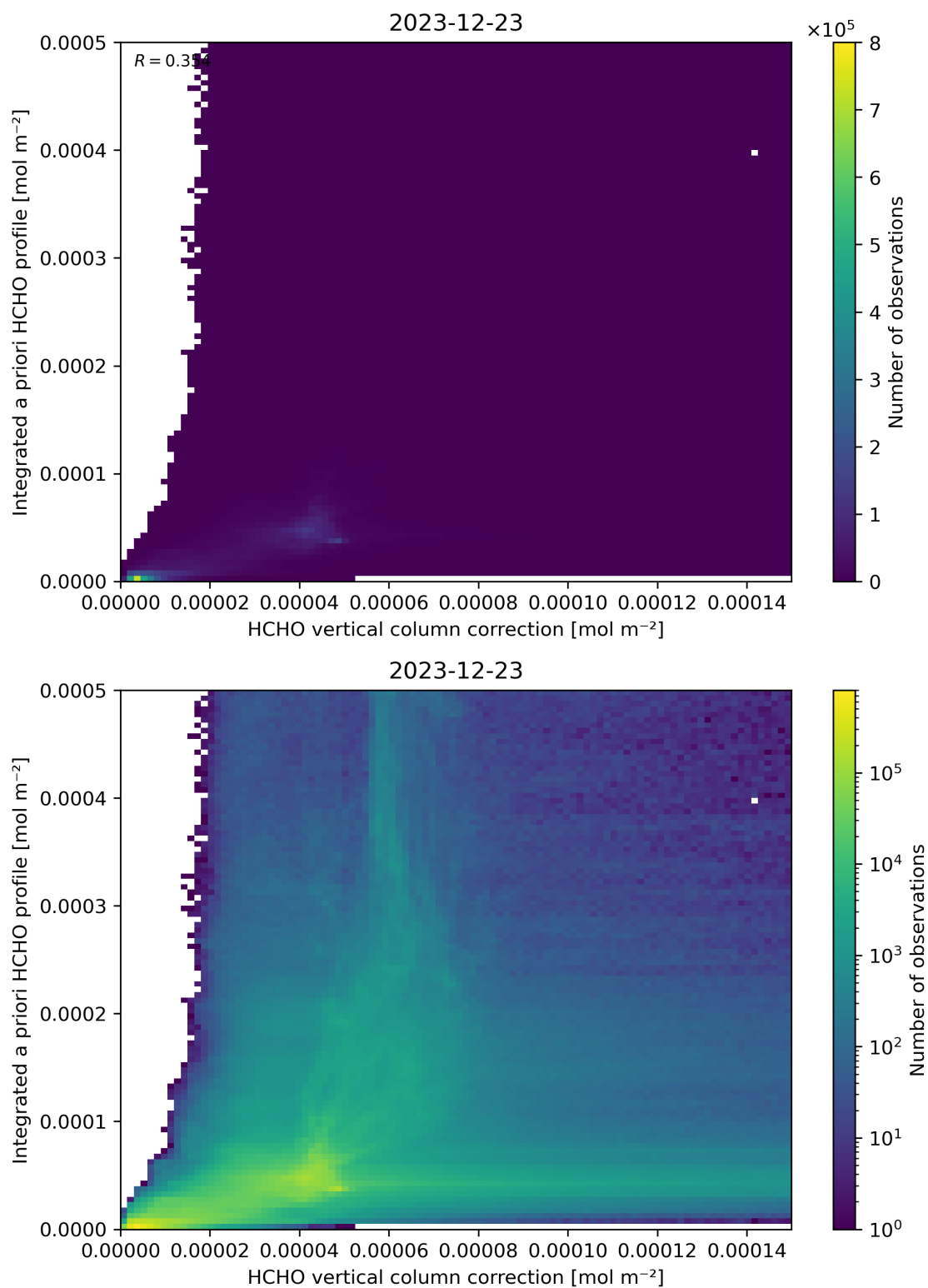
Figure 122: Scatter density plot of “HCHO vertical column correction” against “Integrated a priori HCHO profile” for 2023-12-22 to 2023-12-24.
