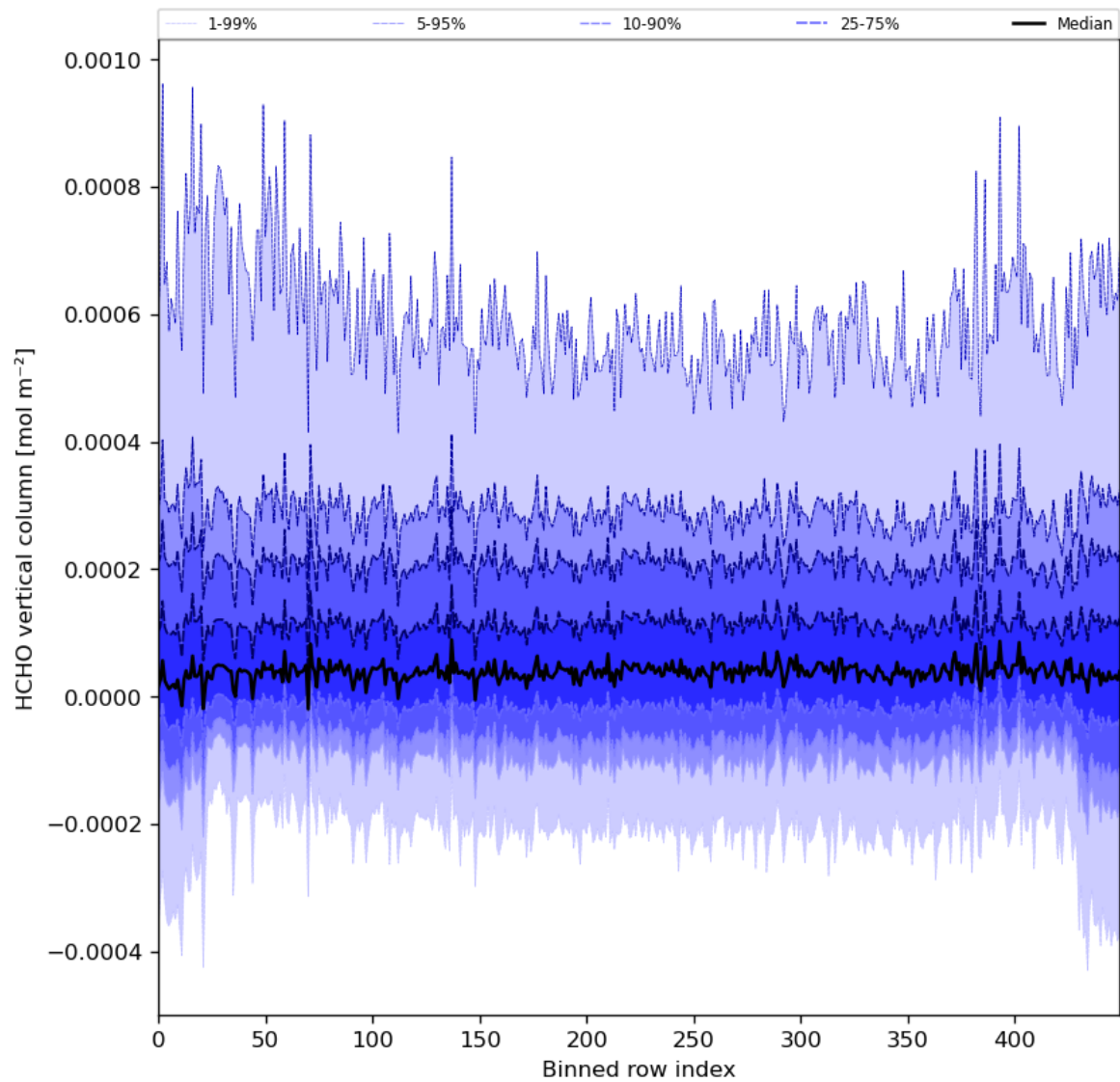
Figure 49: Along track statistics of “HCHO vertical column” for 2023-12-22 to 2023-12-24
