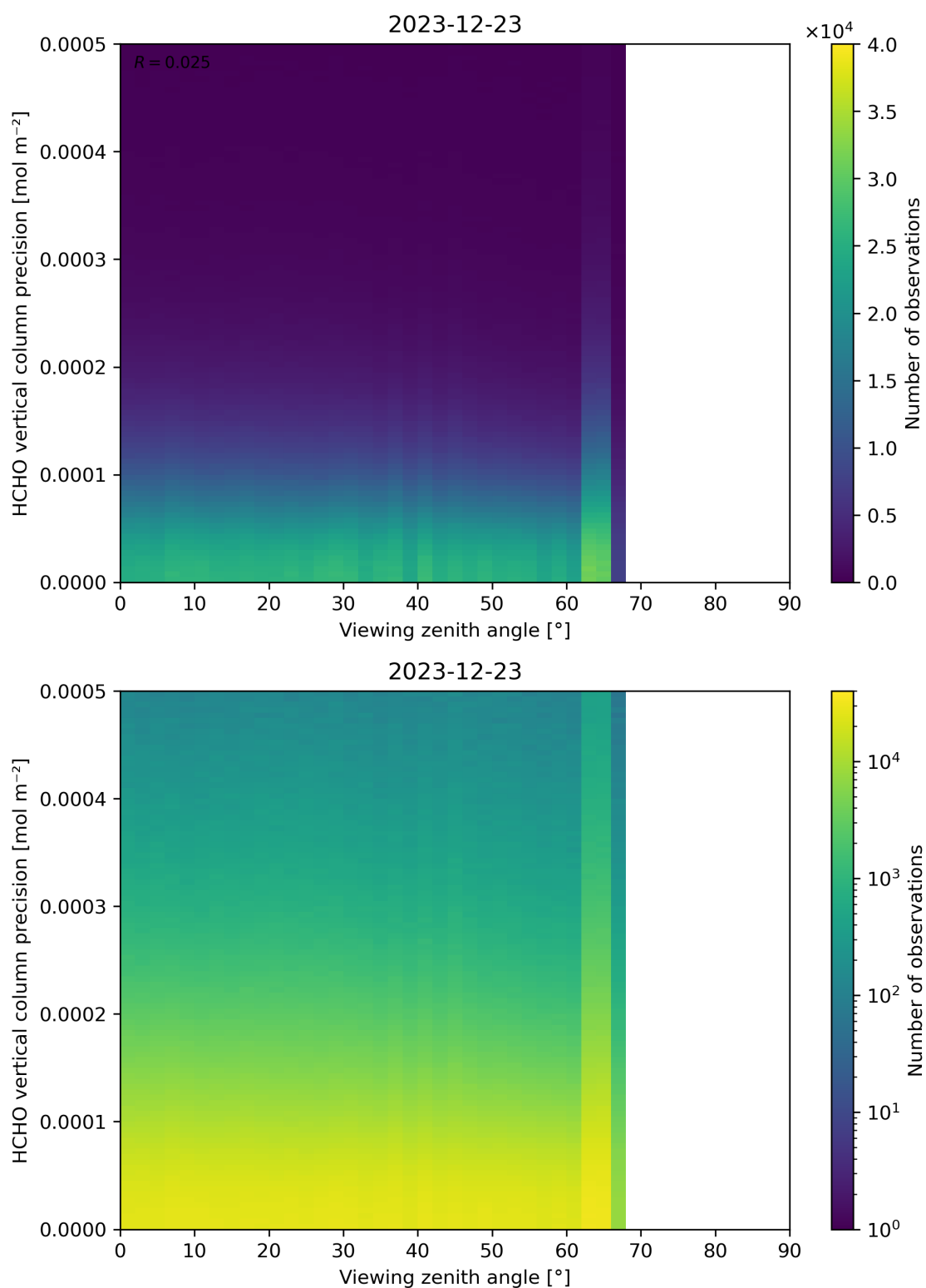
Figure 194: Scatter density plot of “Viewing zenith angle” against “HCHO vertical column precision” for 2023-12-22 to 2023-12-24.
