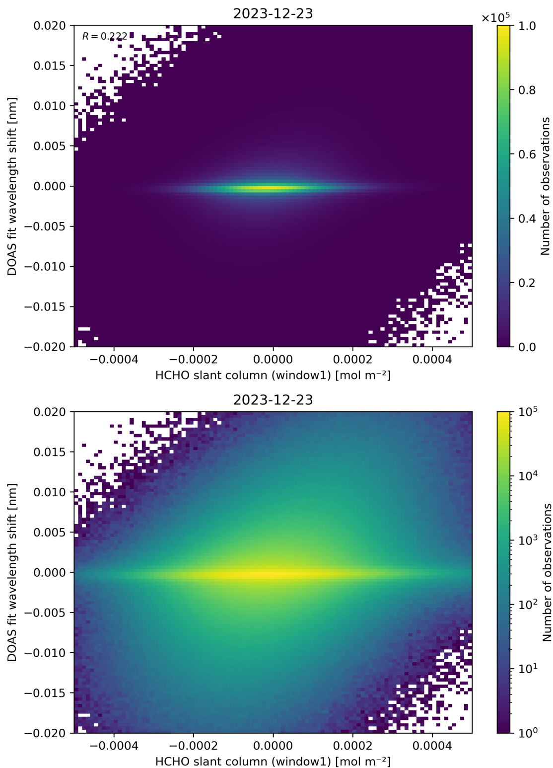
Figure 79: Scatter density plot of “HCHO slant column (window1)” against “DOAS fit wavelength shift” for 2023-12-22 to 2023-12-24.
