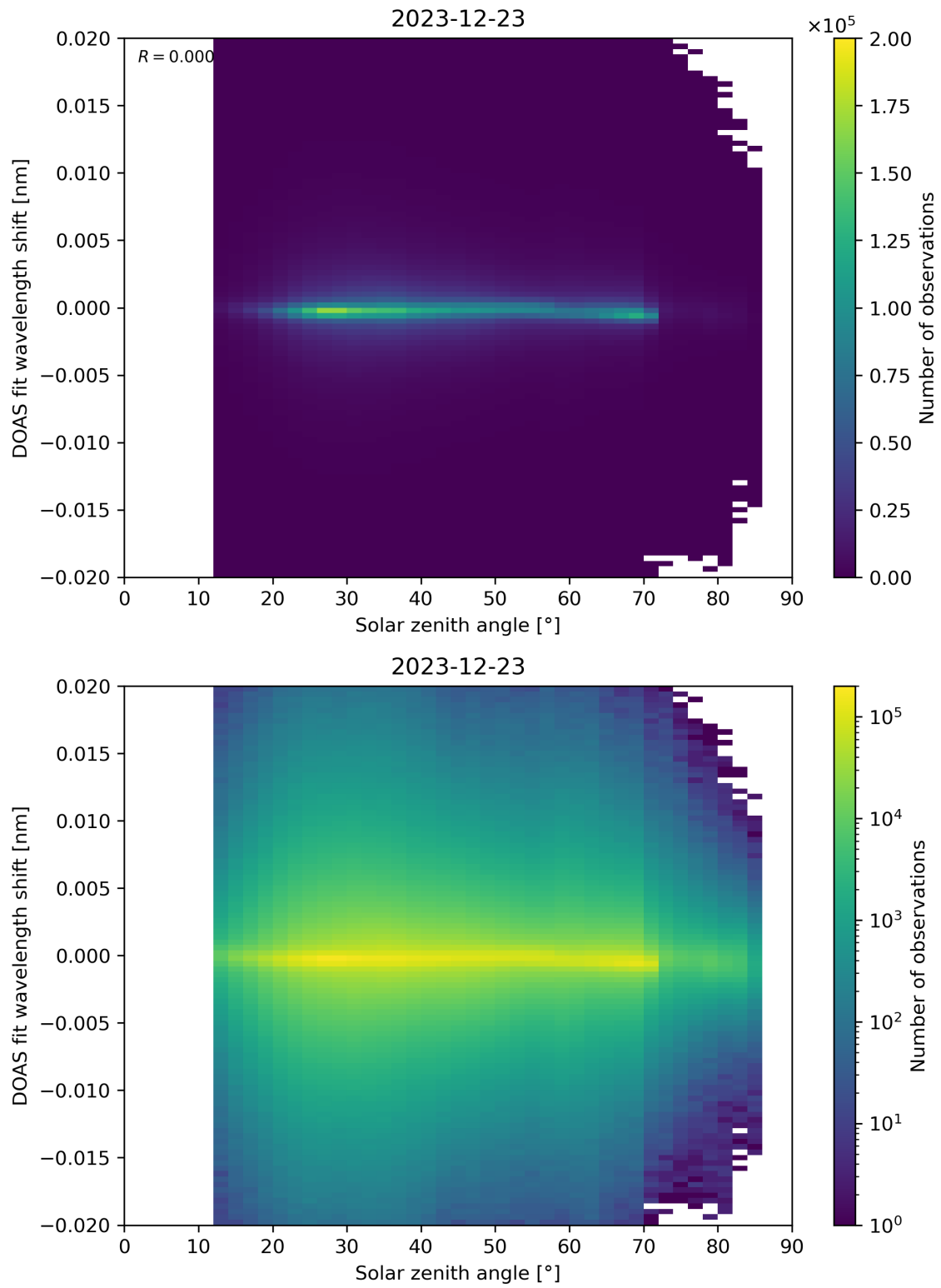
Figure 168: Scatter density plot of “Solar zenith angle” against “DOAS fit wavelength shift” for 2023-12-22 to 2023-12-24.
