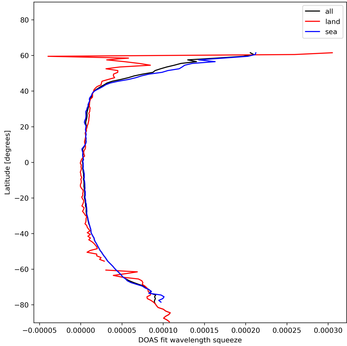
Figure 31: Zonal average of “DOAS fit wavelength squeeze” for 2023-12-22 to 2023-12-24.
