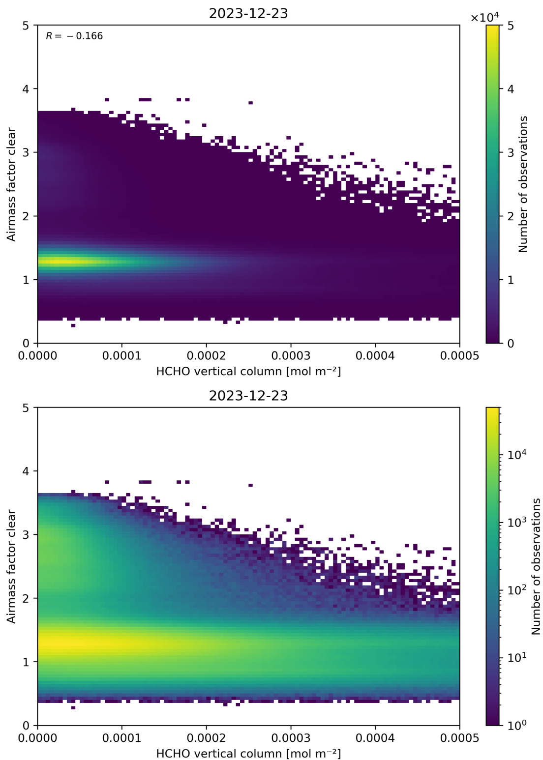
Figure 126: Scatter density plot of “HCHO vertical column” against “Airmass factor clear” for 2023-12-22 to 2023-12-24.
