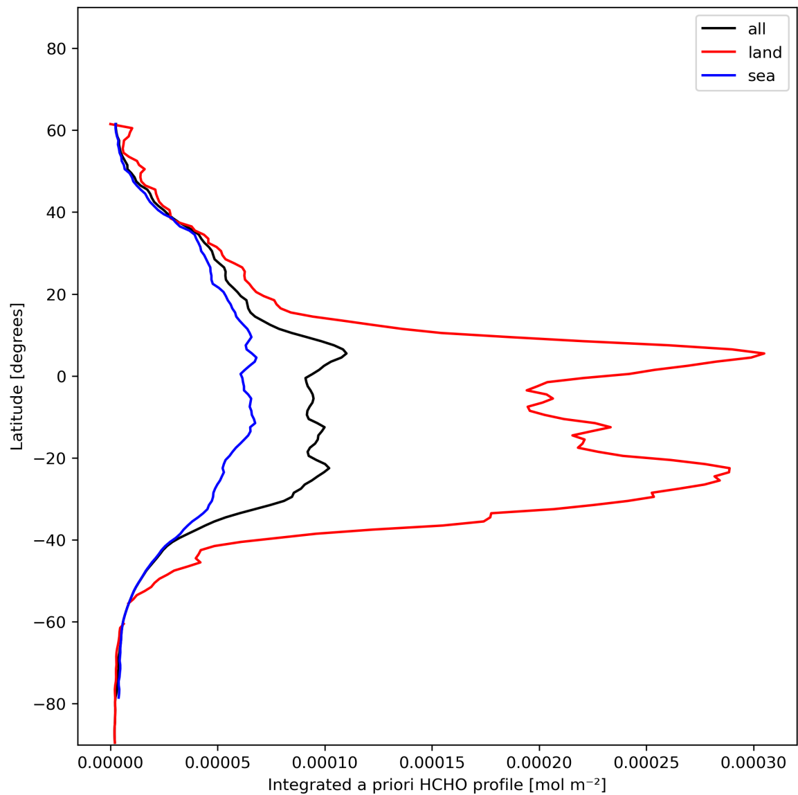
Figure 29: Zonal average of “Integrated a priori HCHO profile” for 2023-12-22 to 2023-12-24.
