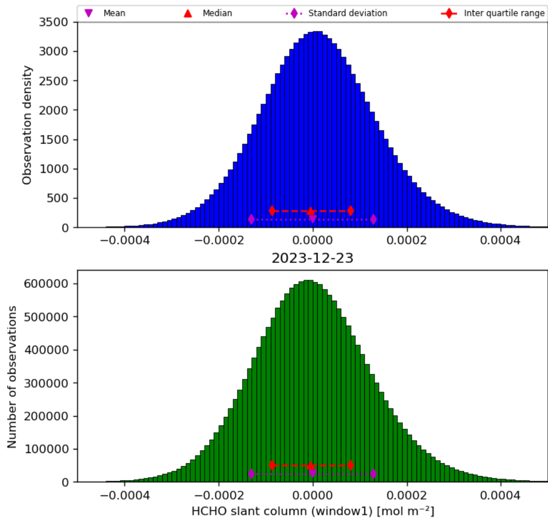
Figure 38: Histogram of “HCHO slant column (window1)” for 2023-12-22 to 2023-12-24
