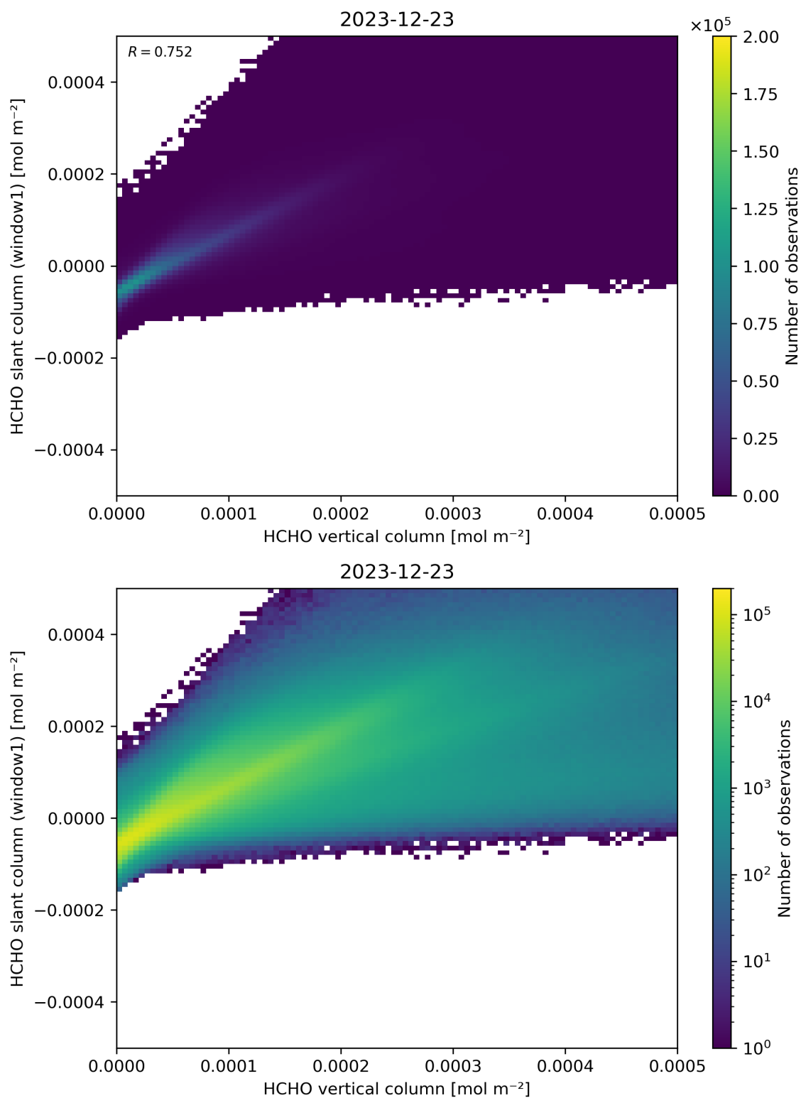
Figure 129: Scatter density plot of “HCHO vertical column” against “HCHO slant column (window1)” for 2023-12-22 to 2023-12-24.
