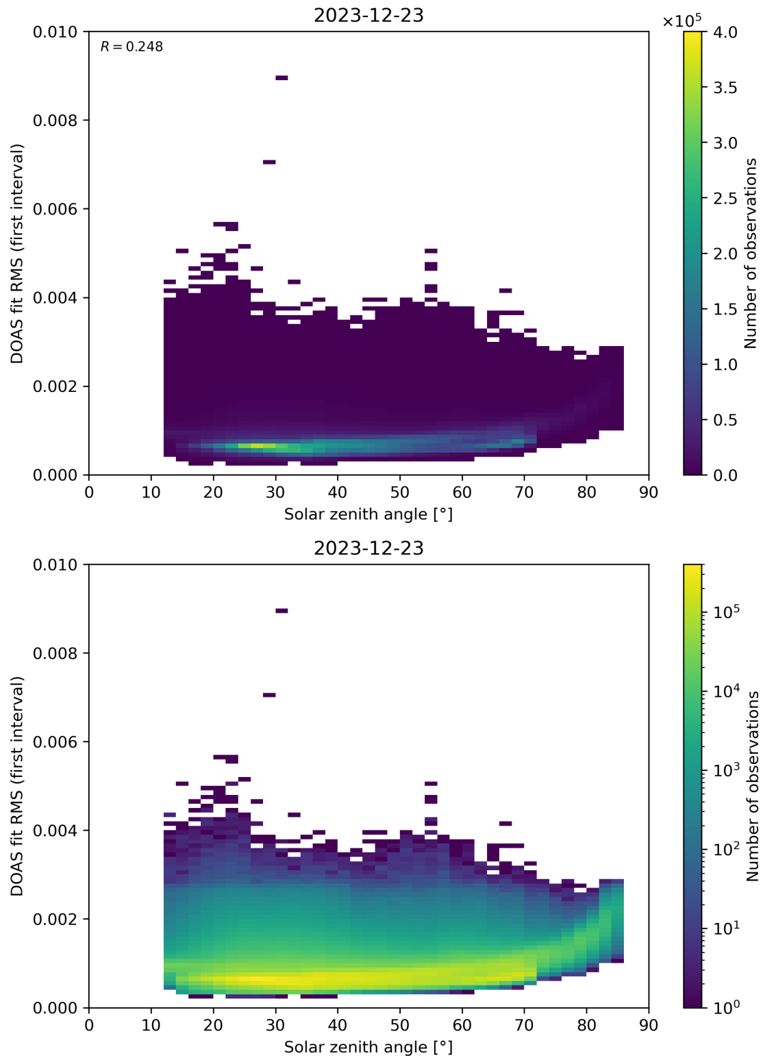
Figure 167: Scatter density plot of “Solar zenith angle” against “DOAS fit RMS (first interval)” for 2023-12-22 to 2023-12-24.
