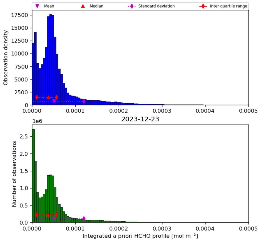
Figure 43: Histogram of “Integrated a priori HCHO profile” for 2023-12-22 to 2023-12-24
