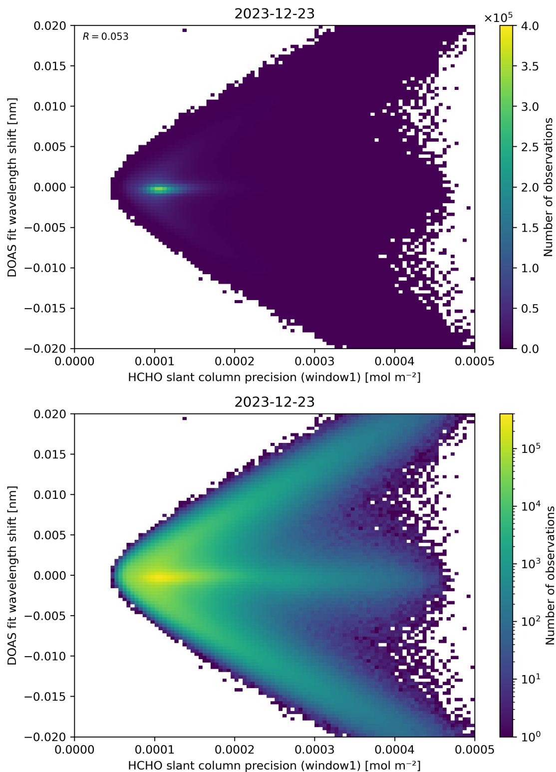
Figure 89: Scatter density plot of “HCHO slant column precision (window1)” against “DOAS fit wavelength shift” for 2023-12-22 to 2023-12-24.
