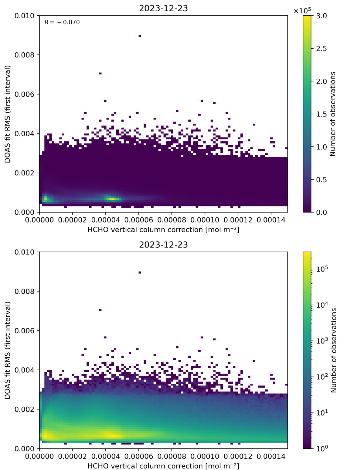
Figure 112: Scatter density plot of “HCHO vertical column correction” against “DOAS fit RMS (first interval)” for 2023-12-22 to 2023-12-24.
