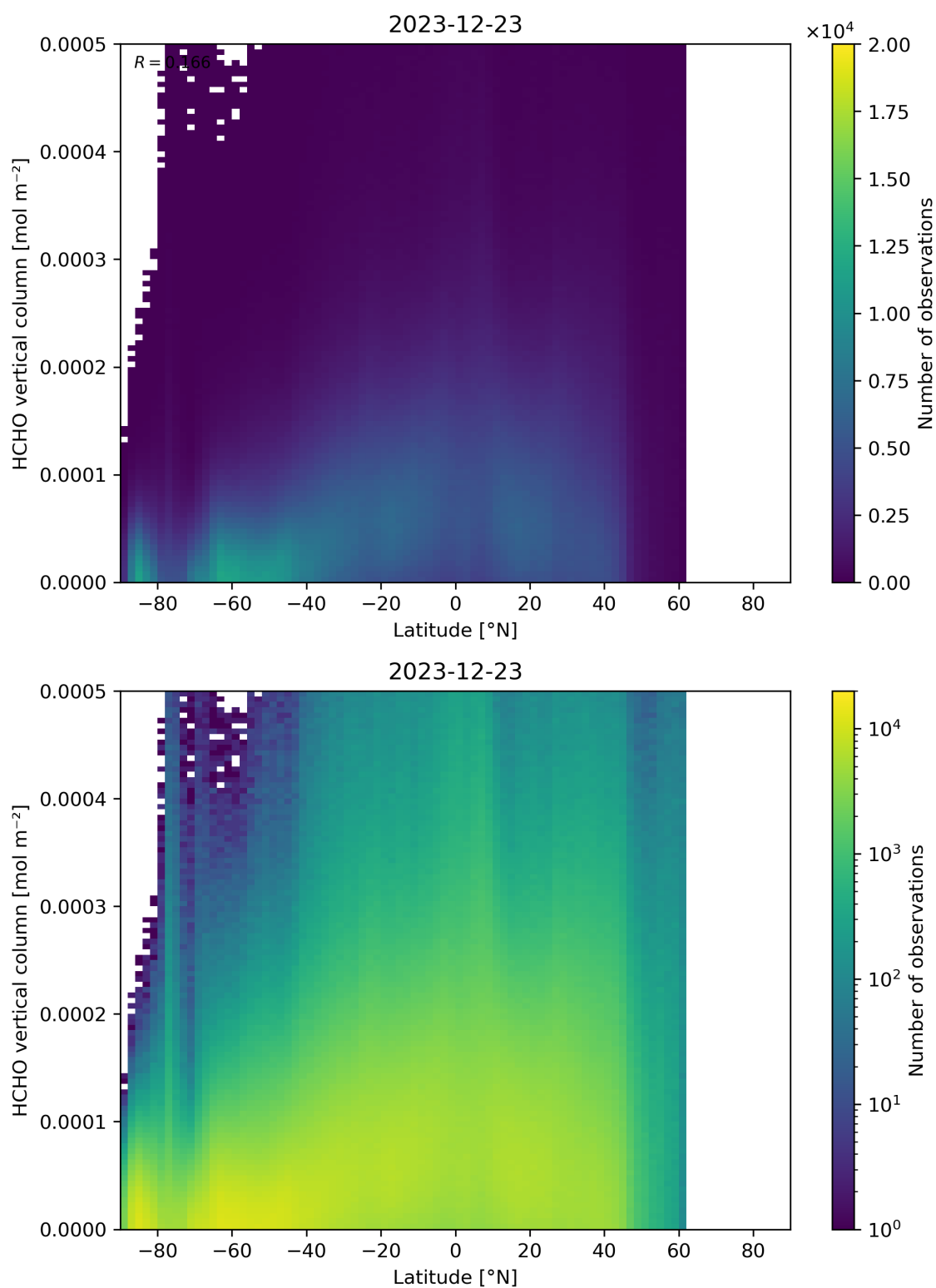
Figure 163: Scatter density plot of “Latitude” against “HCHO vertical column” for 2023-12-22 to 2023-12-24.
