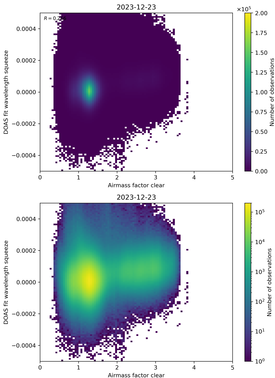
Figure 73: Scatter density plot of “Airmass factor clear” against “DOAS fit wavelength squeeze” for 2023-12-22 to 2023-12-24.
