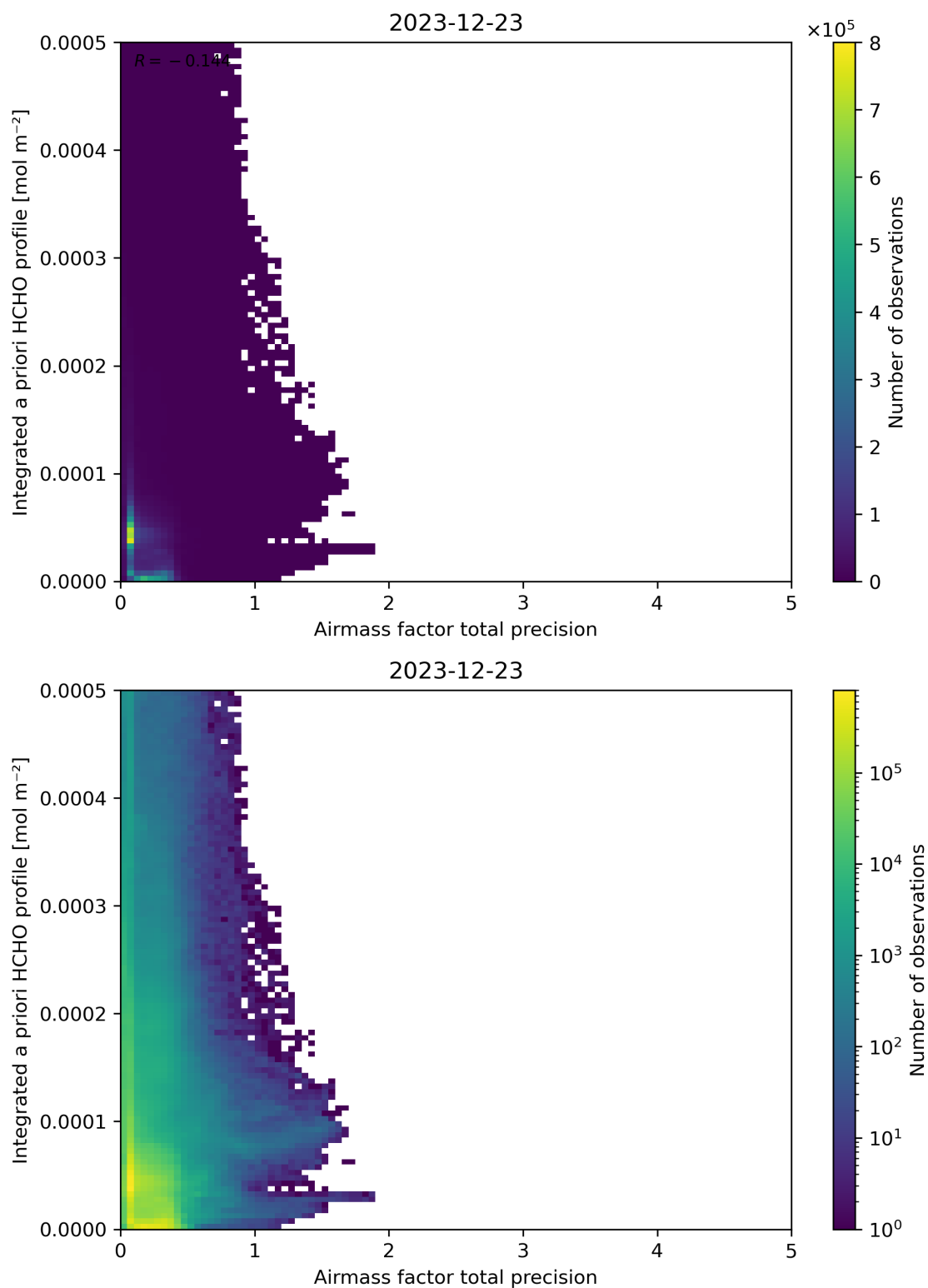
Figure 111: Scatter density plot of “Airmass factor total precision” against “Integrated a priori HCHO profile” for 2023-12-22 to 2023-12-24.
