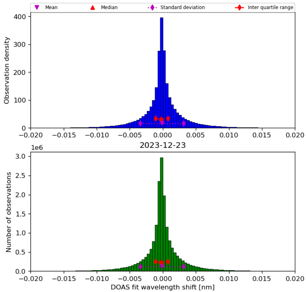
Figure 44: Histogram of “DOAS fit wavelength shift” for 2023-12-22 to 2023-12-24
