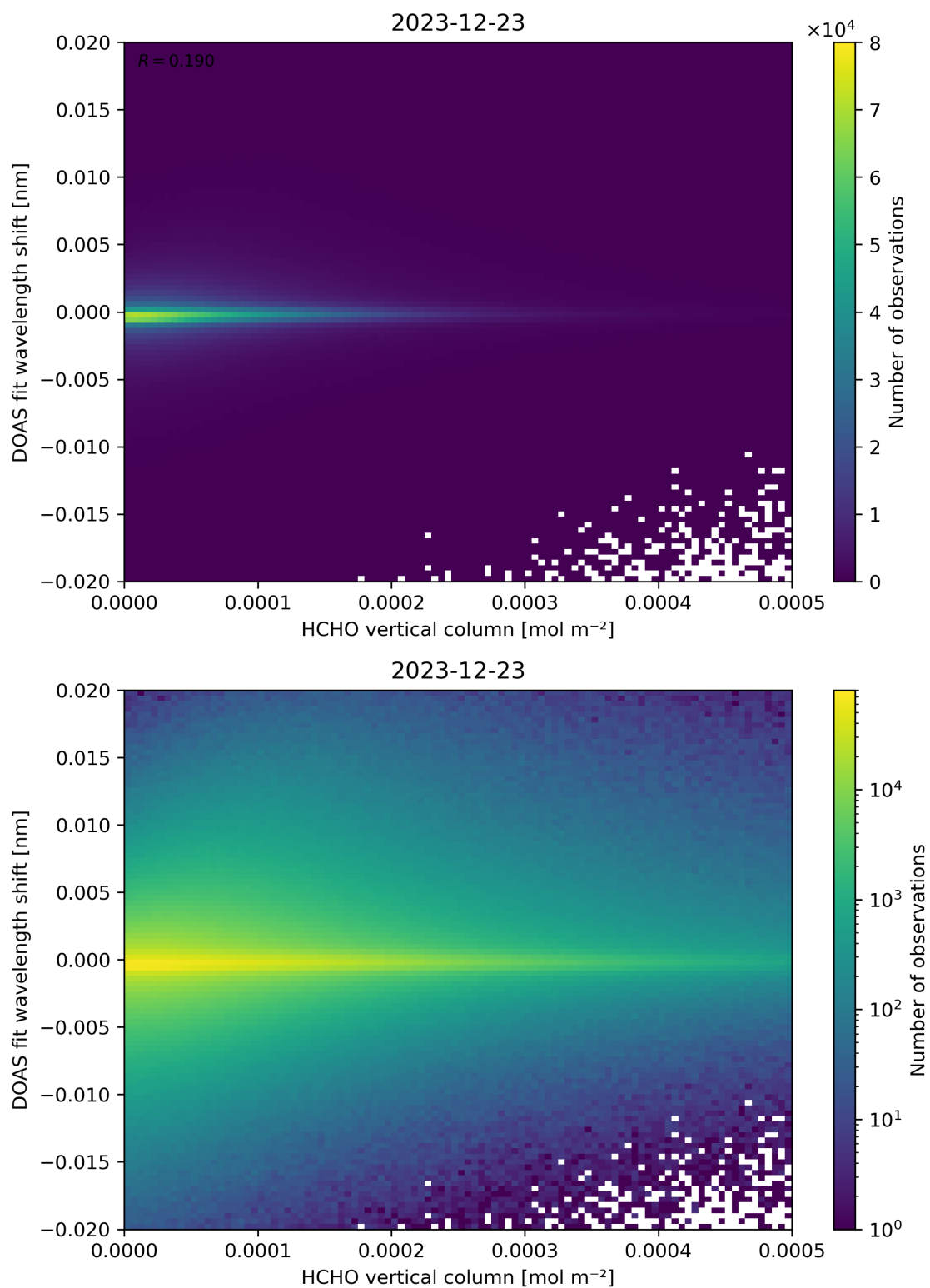
Figure 124: Scatter density plot of “HCHO vertical column” against “DOAS fit wavelength shift” for 2023-12-22 to 2023-12-24.
