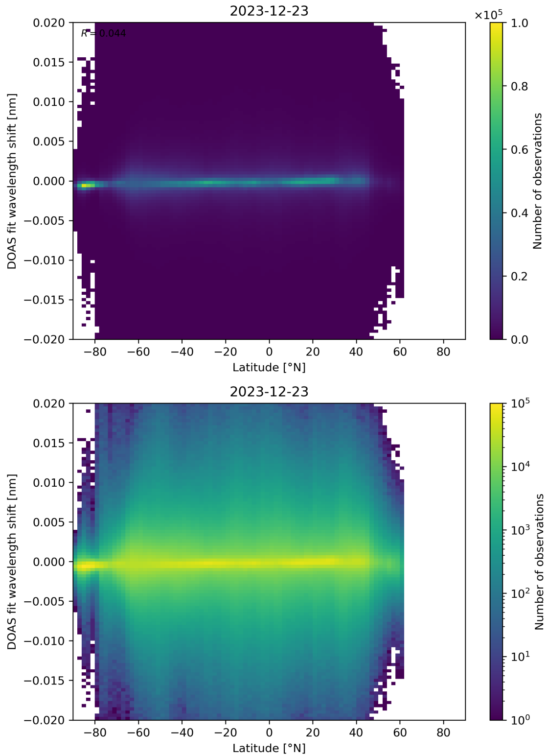
Figure 154: Scatter density plot of “Latitude” against “DOAS fit wavelength shift” for 2023-12-22 to 2023-12-24.
