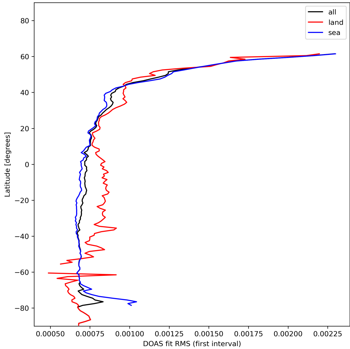
Figure 32: Zonal average of “DOAS fit RMS (first interval)” for 2023-12-22 to 2023-12-24.
