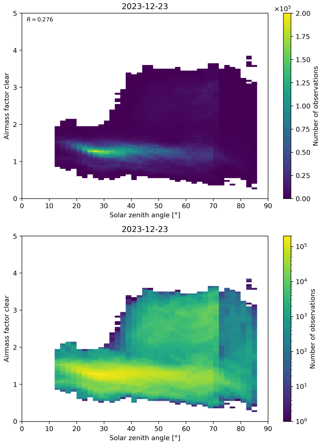
Figure 170: Scatter density plot of “Solar zenith angle” against “Airmass factor clear” for 2023-12-22 to 2023-12-24.
