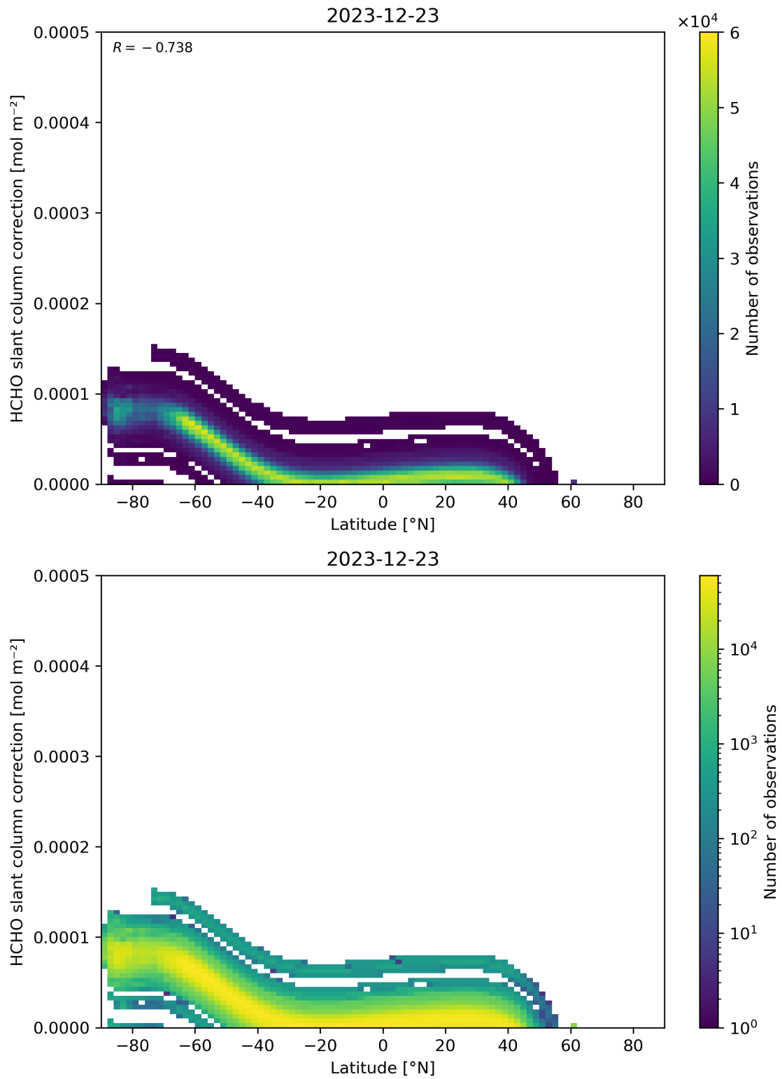
Figure 158: Scatter density plot of “Latitude” against “HCHO slant column correction” for 2023-12-22 to 2023-12-24.
