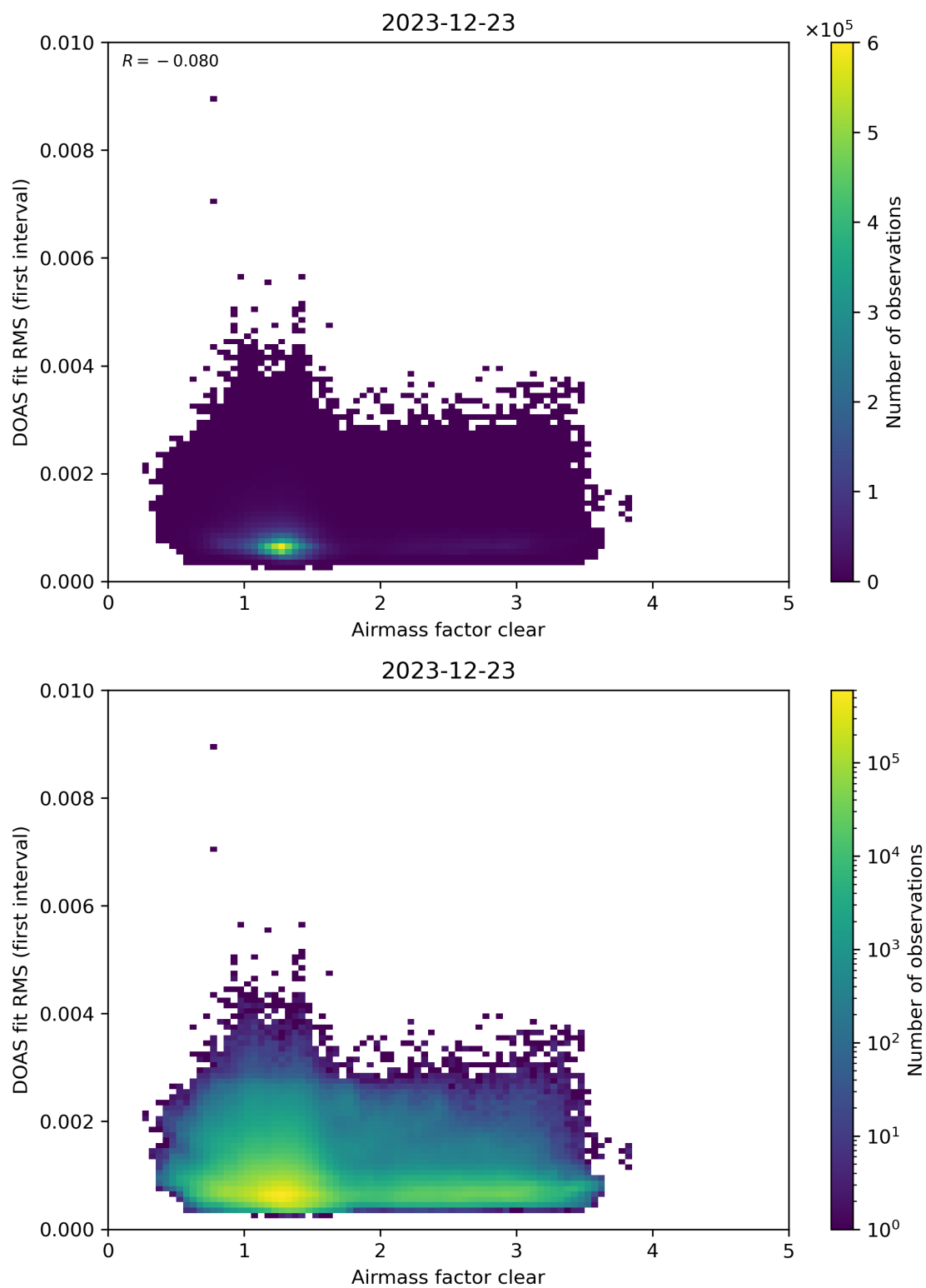
Figure 71: Scatter density plot of “Airmass factor clear” against “DOAS fit RMS (first interval)” for 2023-12-22 to 2023-12-24.
