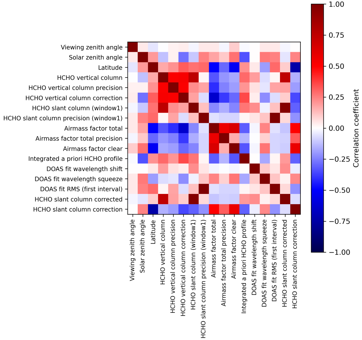
Figure 2: Map of correlation matrix for 2023-12-22 to 2023-12-24.
