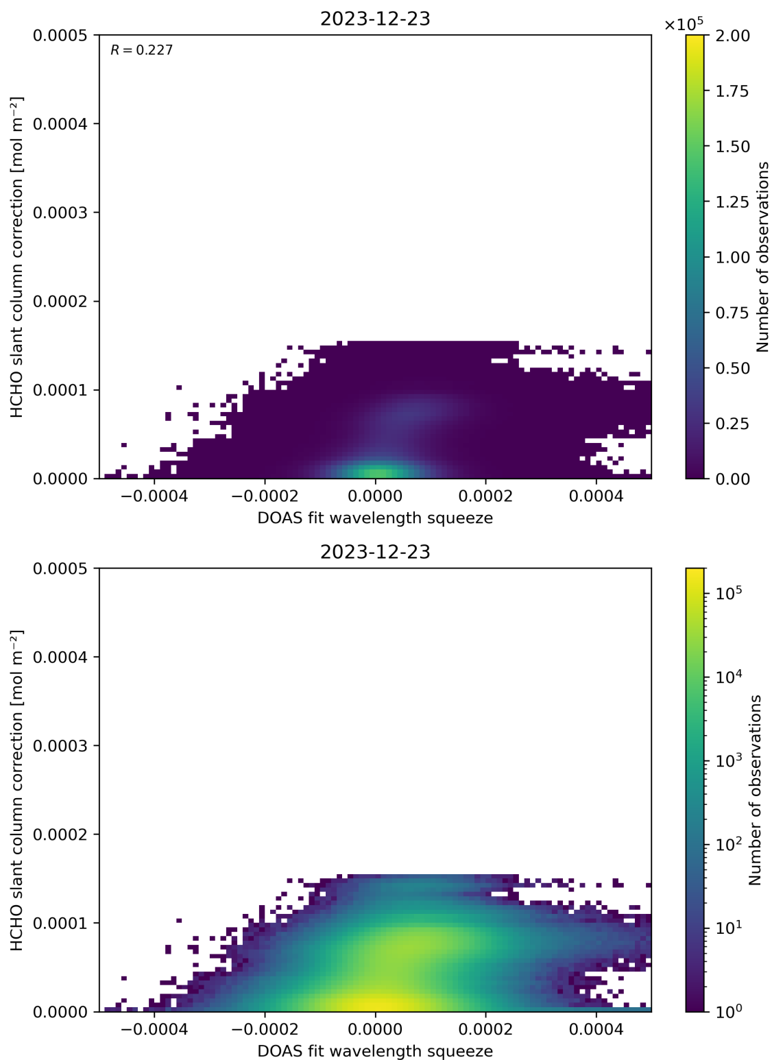
Figure 70: Scatter density plot of “DOAS fit wavelength squeeze” against “HCHO slant column correction” for 2023-12-22 to 2023-12-24.
