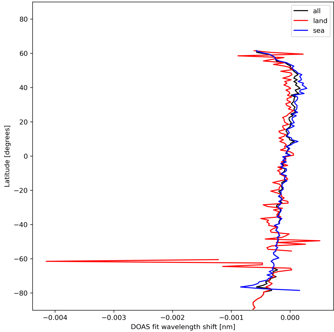
Figure 30: Zonal average of "DOAS fit wavelength shift" for 2023-12-22 to 2023-12-24.
