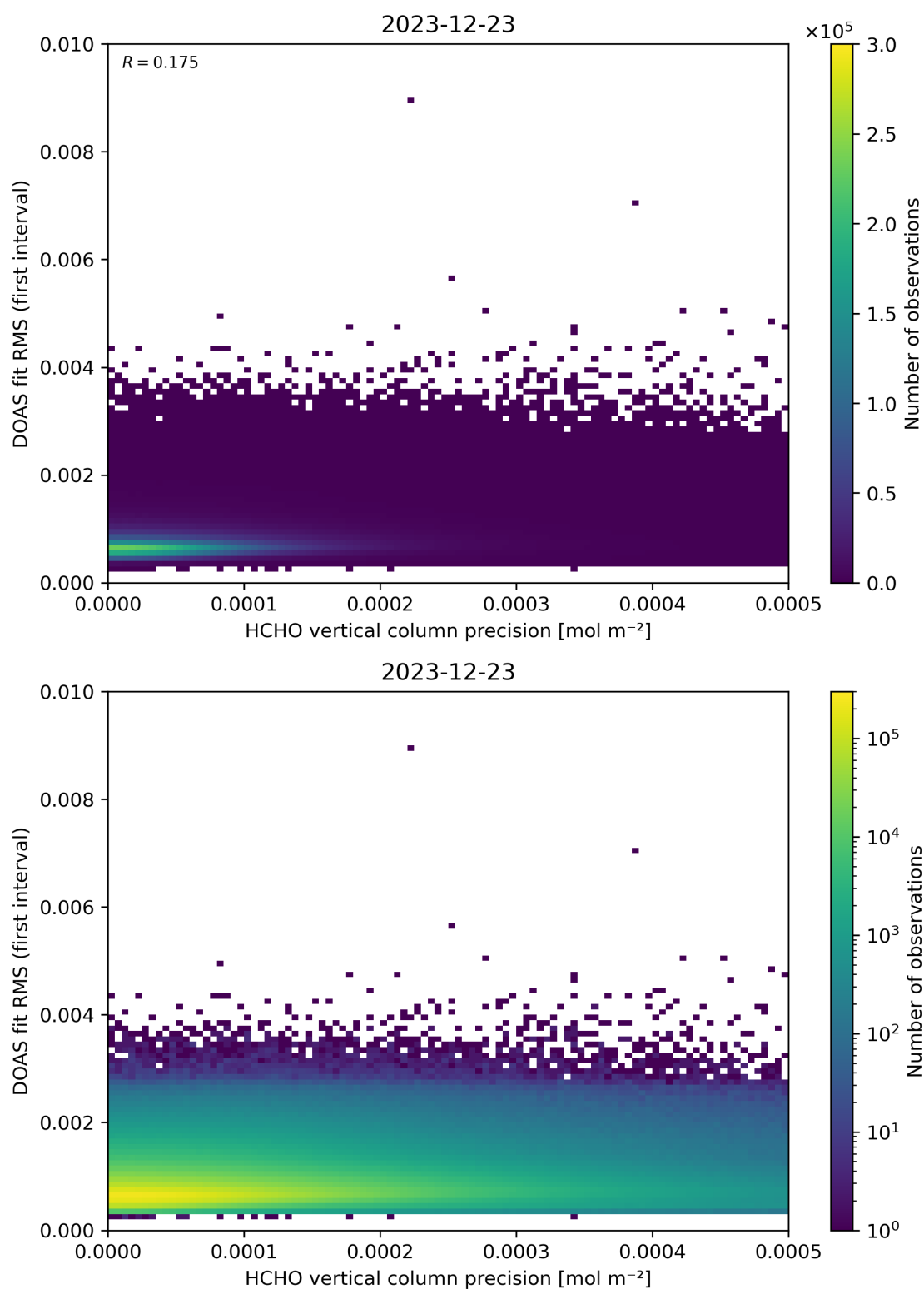
Figure 136: Scatter density plot of “HCHO vertical column precision” against “DOAS fit RMS (first interval)” for 2023-12-22 to 2023-12-24.
