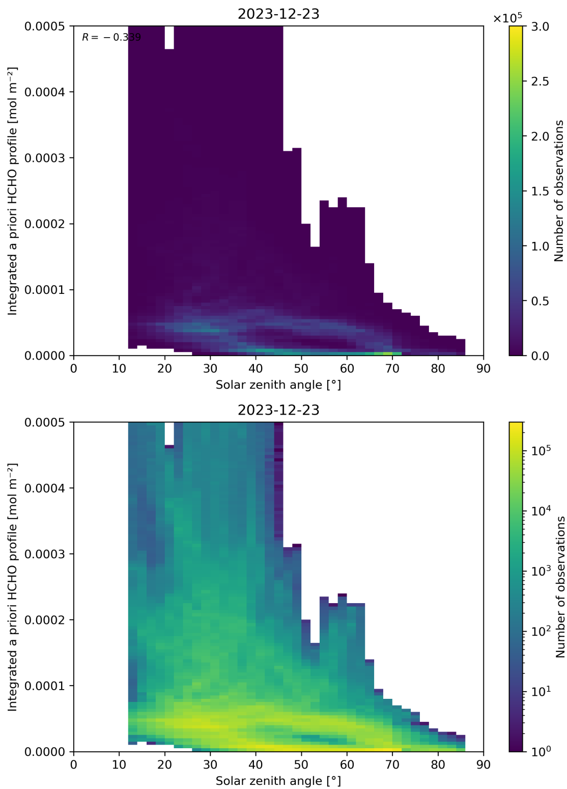
Figure 180: Scatter density plot of “Solar zenith angle” against “Integrated a priori HCHO profile” for 2023-12-22 to 2023-12-24.
