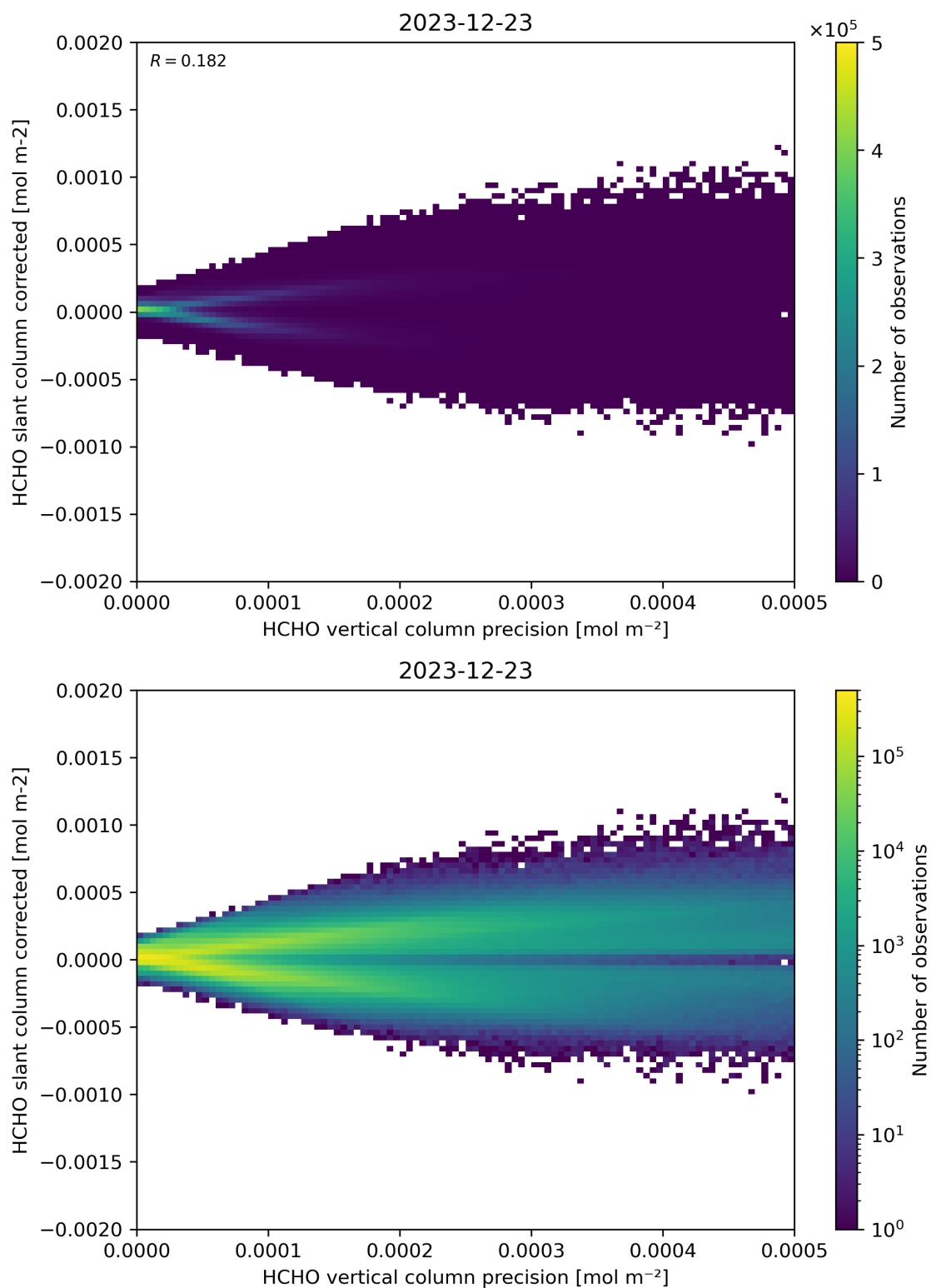
Figure 140: Scatter density plot of “HCHO vertical column precision” against “HCHO slant column corrected” for 2023-12-22 to 2023-12-24.
