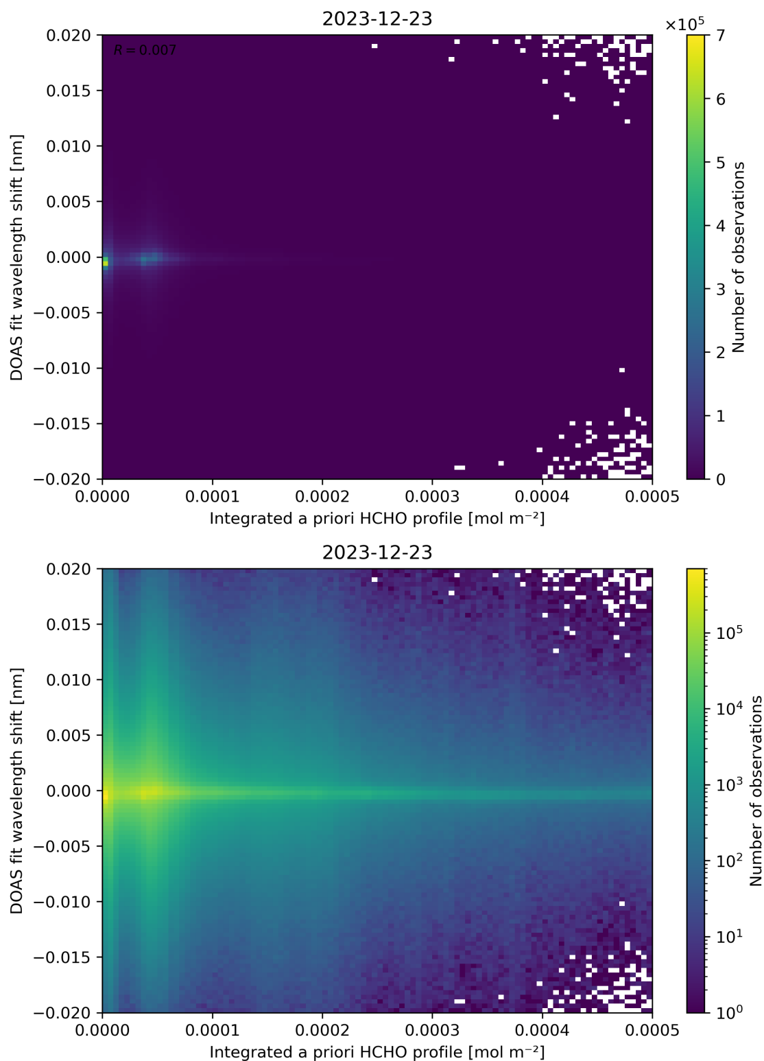
Figure 149: Scatter density plot of “Integrated a priori HCHO profile” against “DOAS fit wavelength shift” for 2023-12-22 to 2023-12-24.
