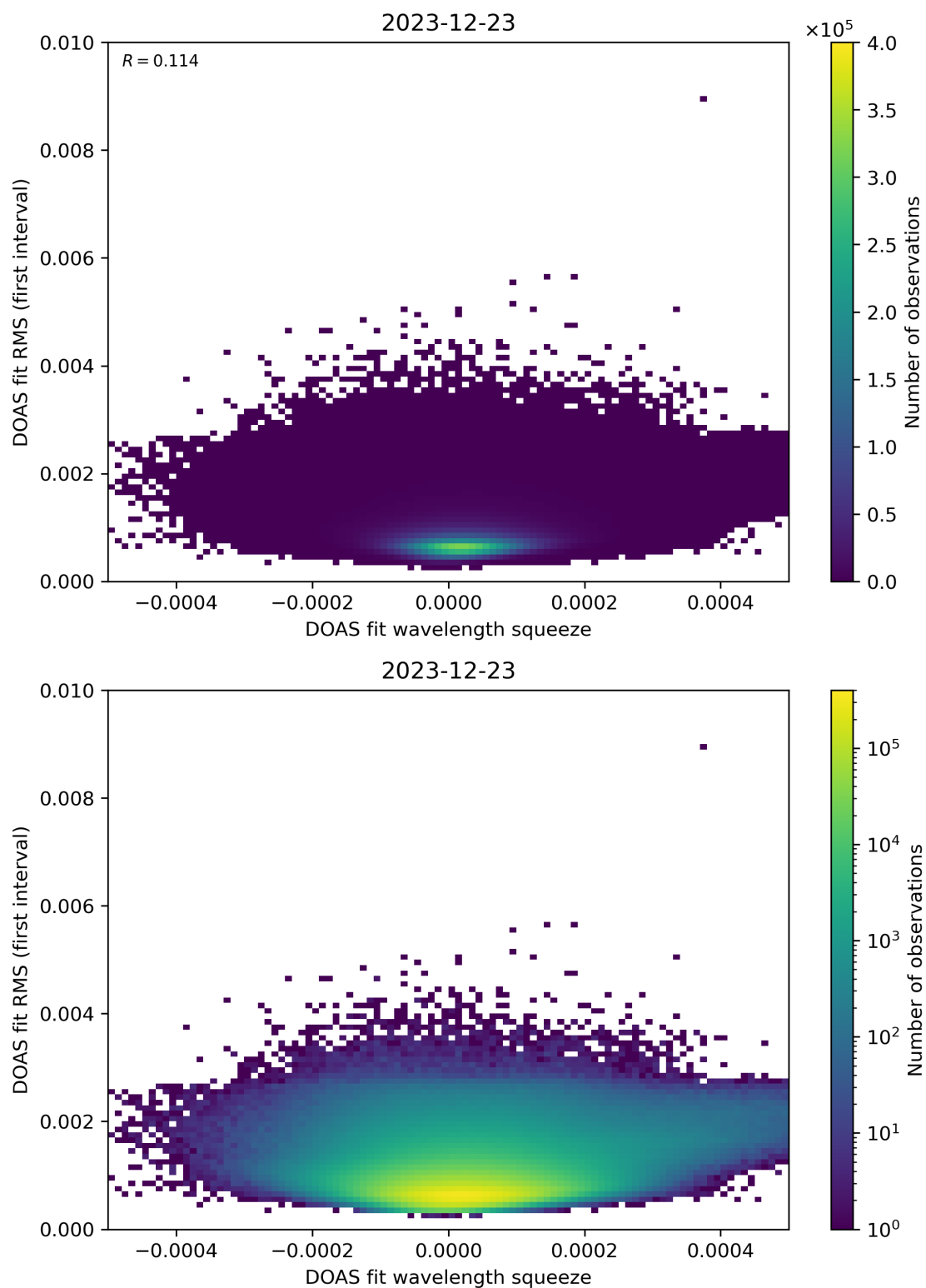
Figure 68: Scatter density plot of “DOAS fit wavelength squeeze” against “DOAS fit RMS (first interval)” for 2023-12-22 to 2023-12-24.
