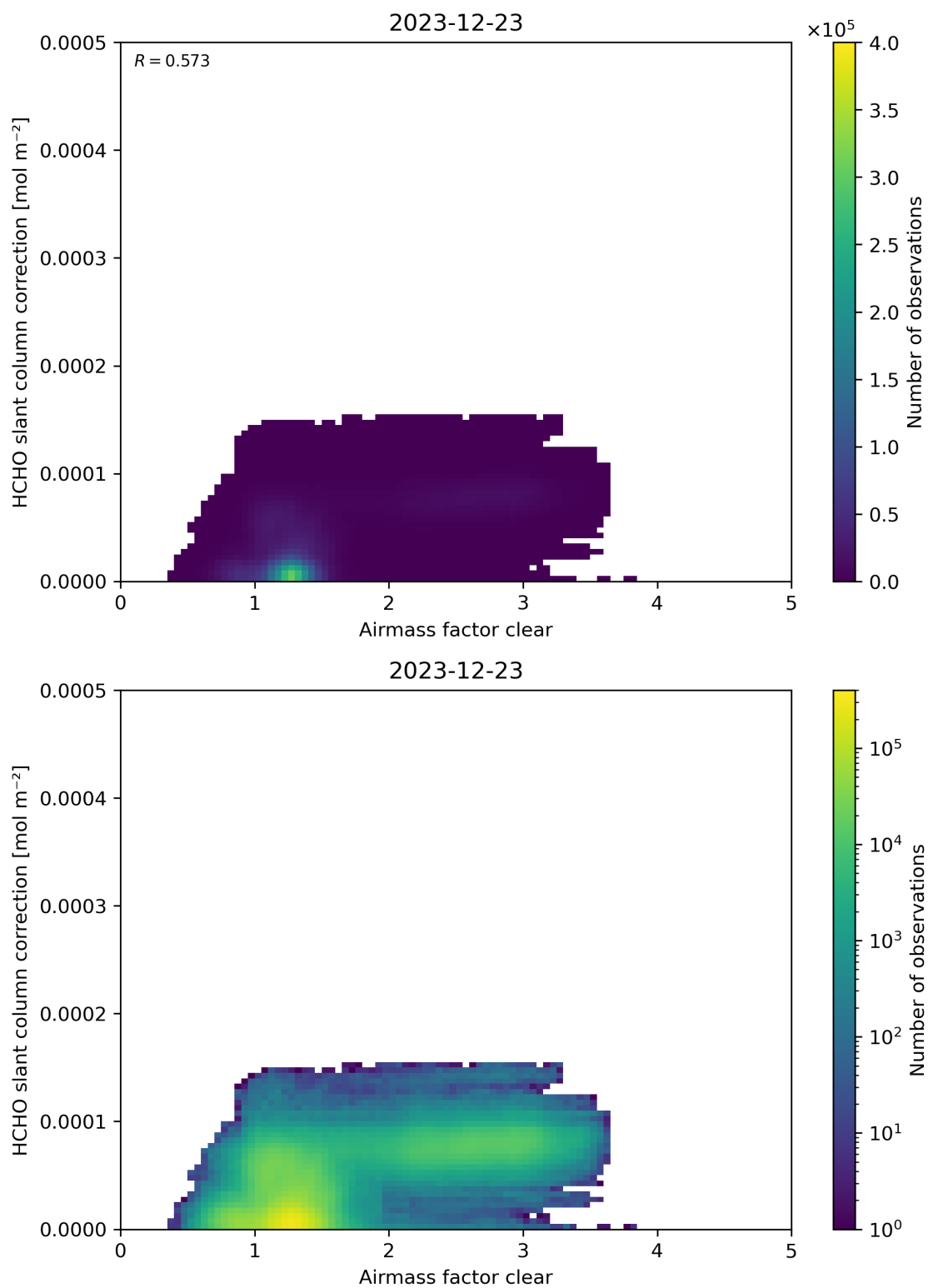
Figure 75: Scatter density plot of “Airmass factor clear” against “HCHO slant column correction” for 2023-12-22 to 2023-12-24.
