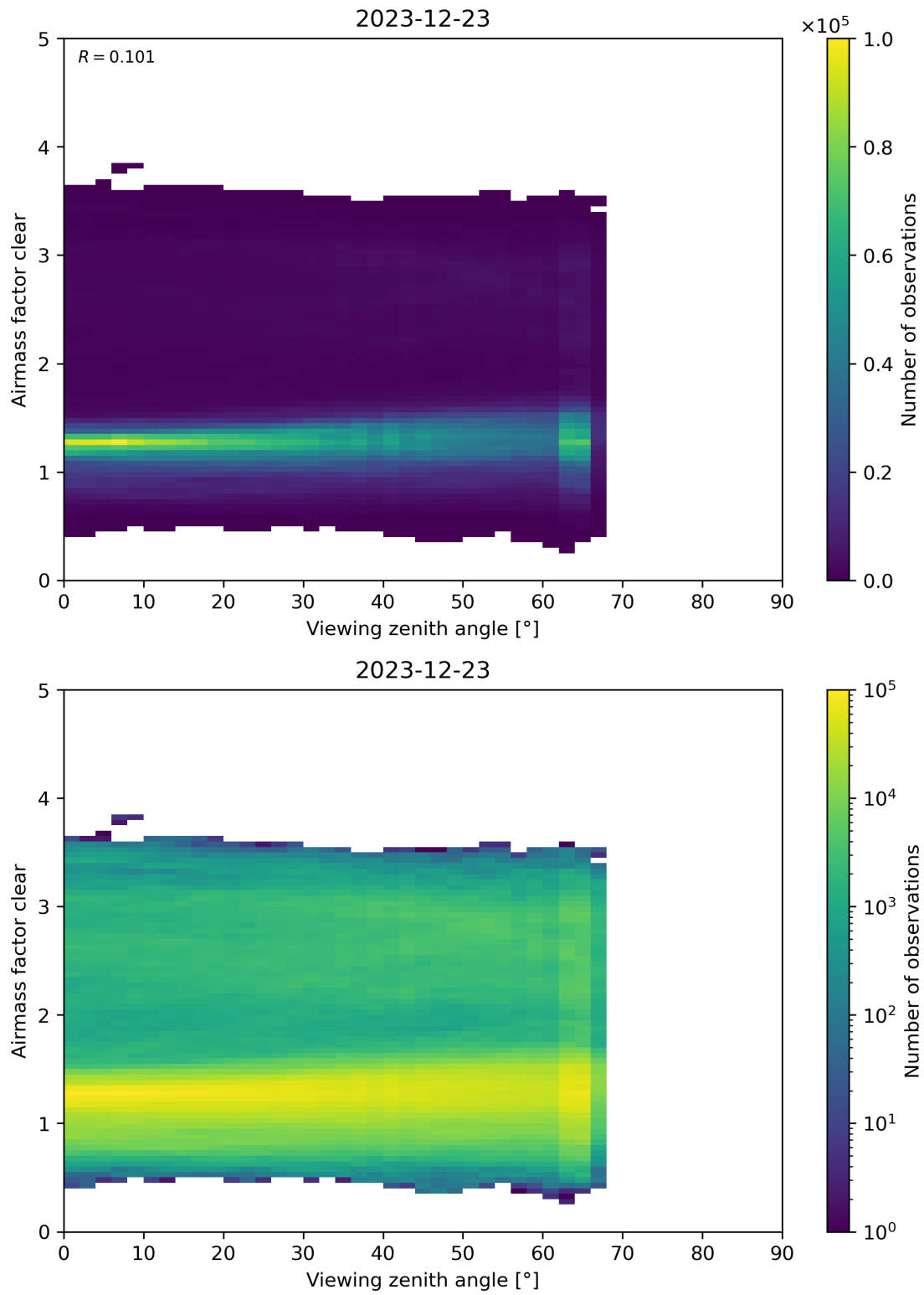
Figure 185: Scatter density plot of “Viewing zenith angle” against “Airmass factor clear” for 2023-12-22 to 2023-12-24.
