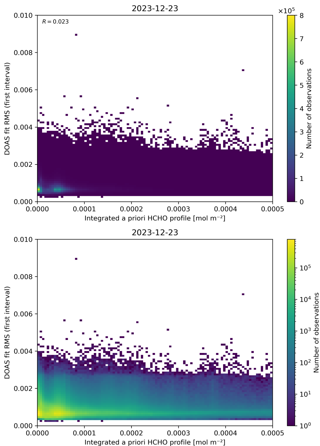
Figure 148: Scatter density plot of “Integrated a priori HCHO profile” against “DOAS fit RMS (first interval)” for 2023-12-22 to 2023-12-24.
