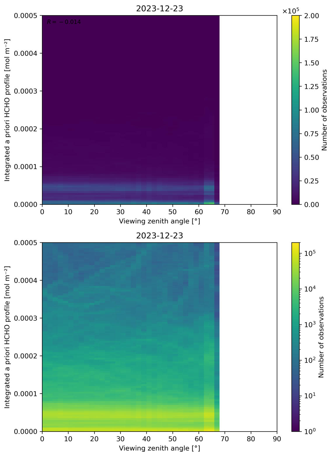
Figure 195: Scatter density plot of “Viewing zenith angle” against “Integrated a priori HCHO profile” for 2023-12-22 to 2023-12-24.
