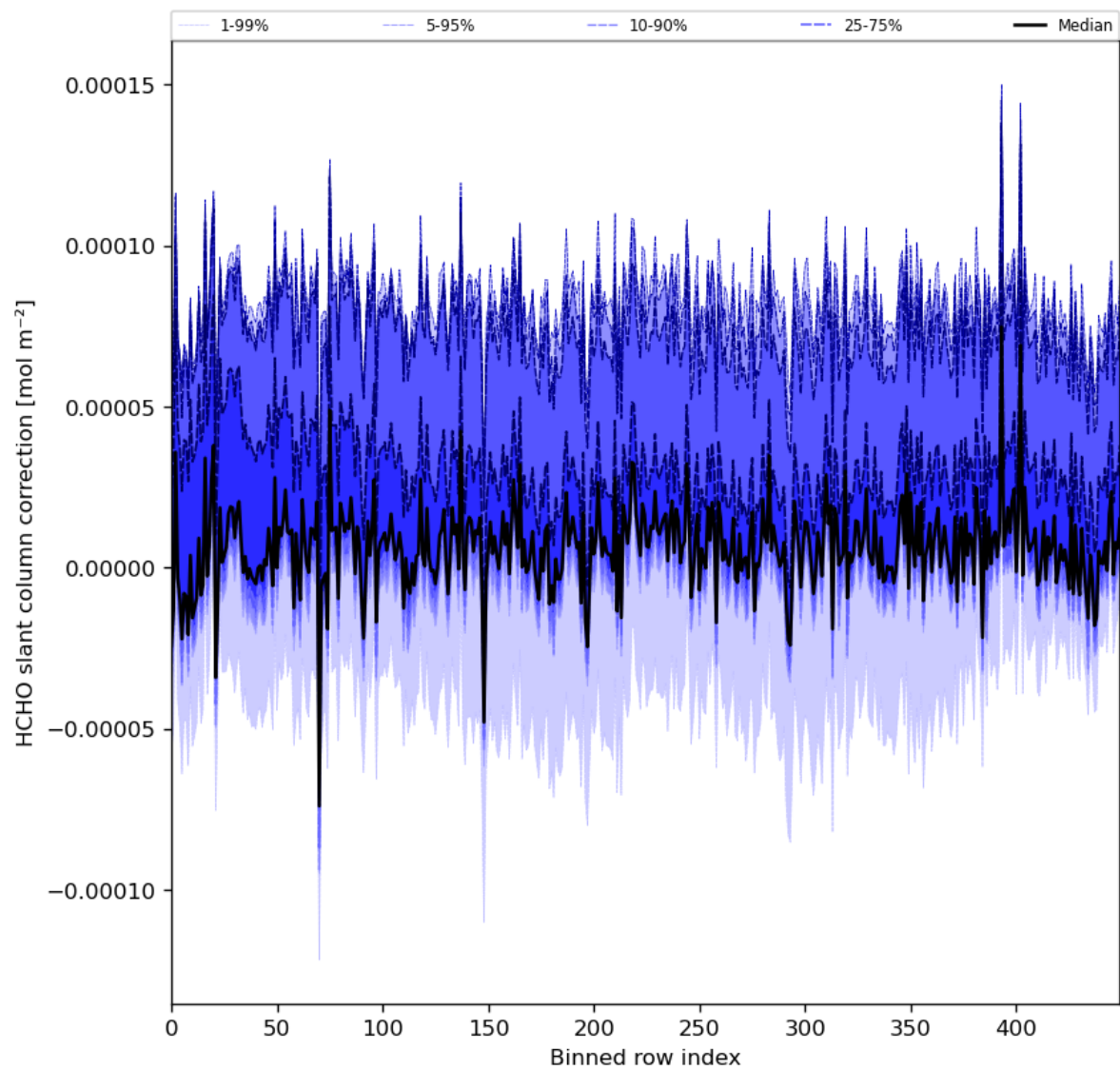
Figure 61: Along track statistics of “HCHO slant column correction” for 2023-12-22 to 2023-12-24
