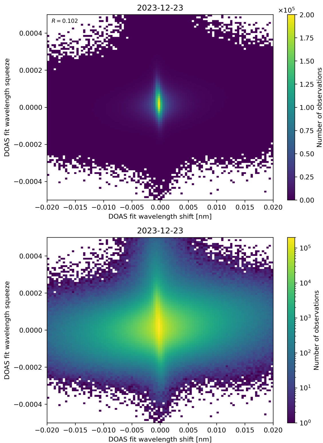
Figure 65: Scatter density plot of “DOAS fit wavelength shift” against “DOAS fit wavelength squeeze” for 2023-12-22 to 2023-12-24.
