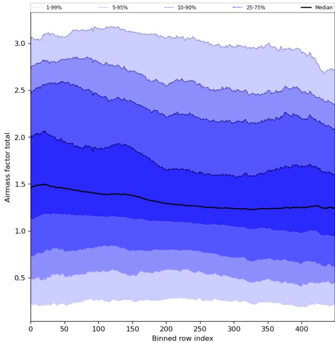
Figure 54: Along track statistics of “Airmass factor total” for 2023-12-22 to 2023-12-24
