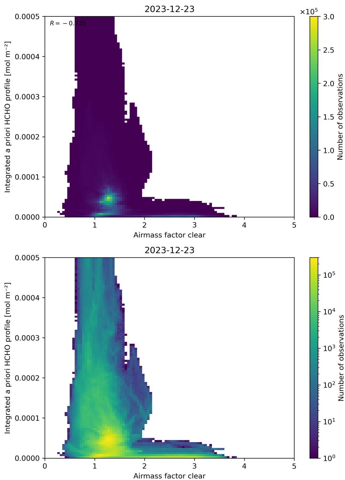
Figure 76: Scatter density plot of “Airmass factor clear” against “Integrated a priori HCHO profile” for 2023-12-22 to 2023-12-24.
