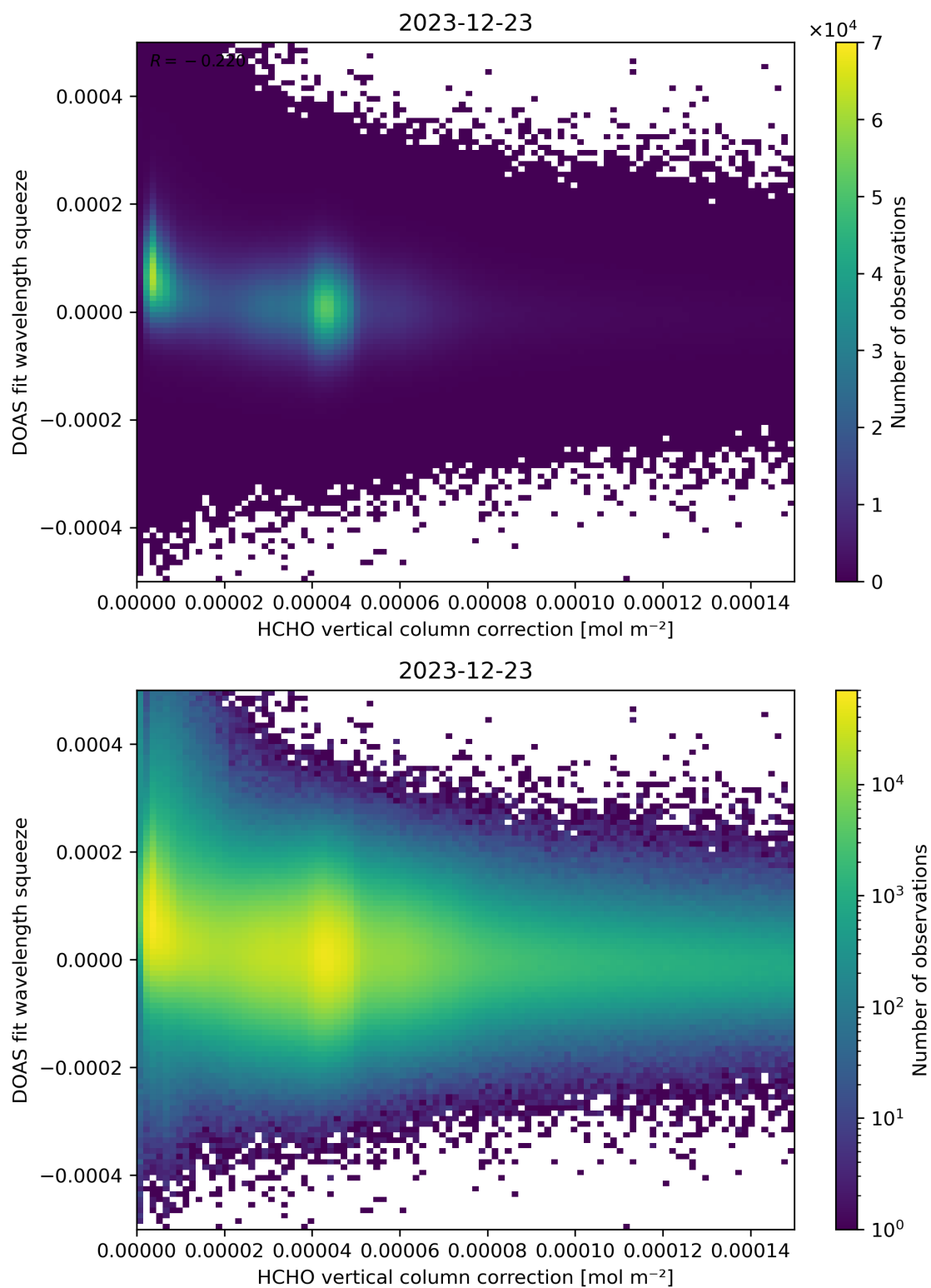
Figure 114: Scatter density plot of “HCHO vertical column correction” against “DOAS fit wavelength squeeze” for 2023-12-22 to 2023-12-24.
