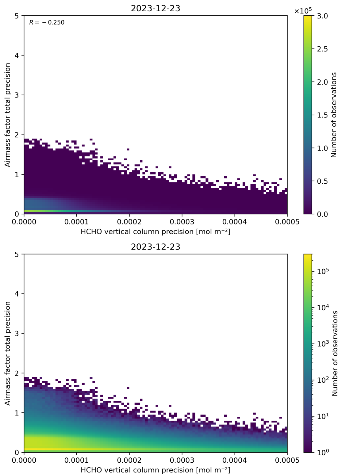
Figure 145: Scatter density plot of “HCHO vertical column precision” against “Airmass factor total precision” for 2023-12-22 to 2023-12-24.
