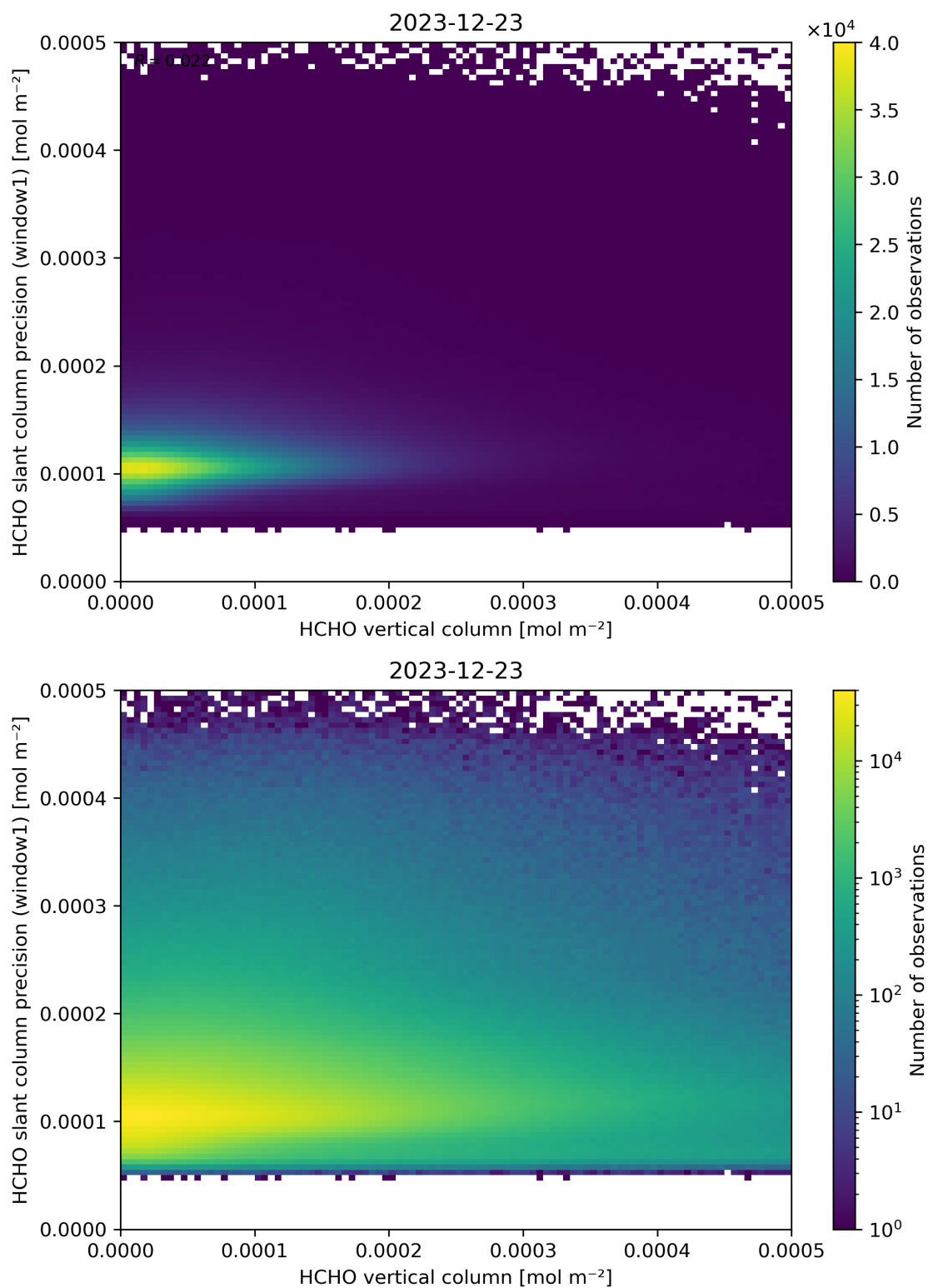
Figure 130: Scatter density plot of “HCHO vertical column” against “HCHO slant column precision (window1)” for 2023-12-22 to 2023-12-24.
