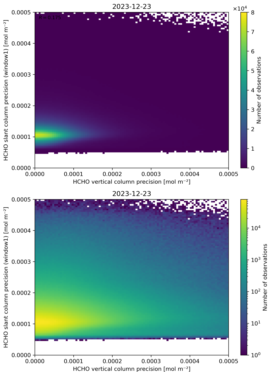
Figure 143: Scatter density plot of “HCHO vertical column precision” against “HCHO slant column precision (window1)” for 2023-12-22 to 2023-12-24.
