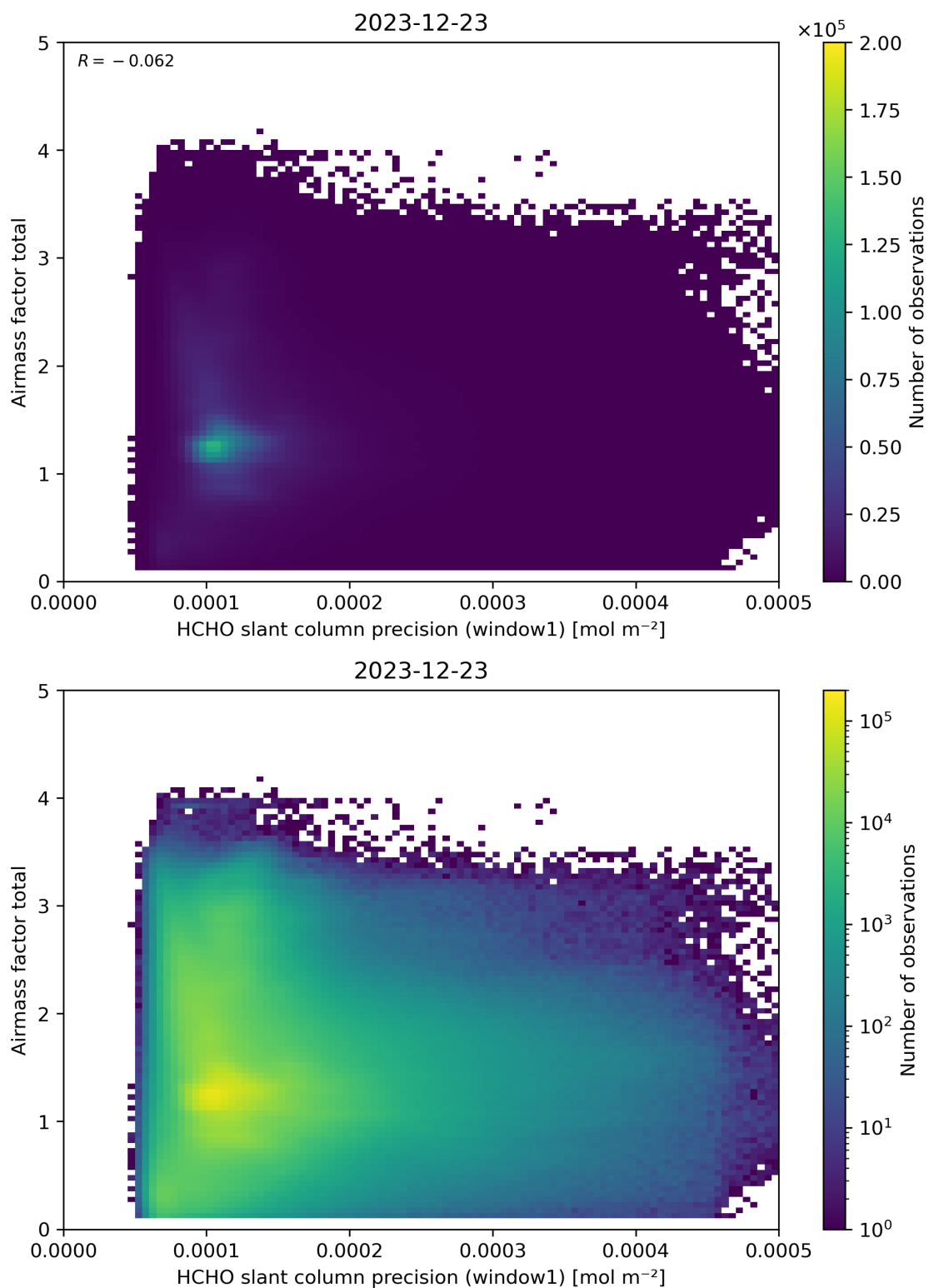
Figure 94: Scatter density plot of “HCHO slant column precision (window1)” against “Airmass factor total” for 2023-12-22 to 2023-12-24.
