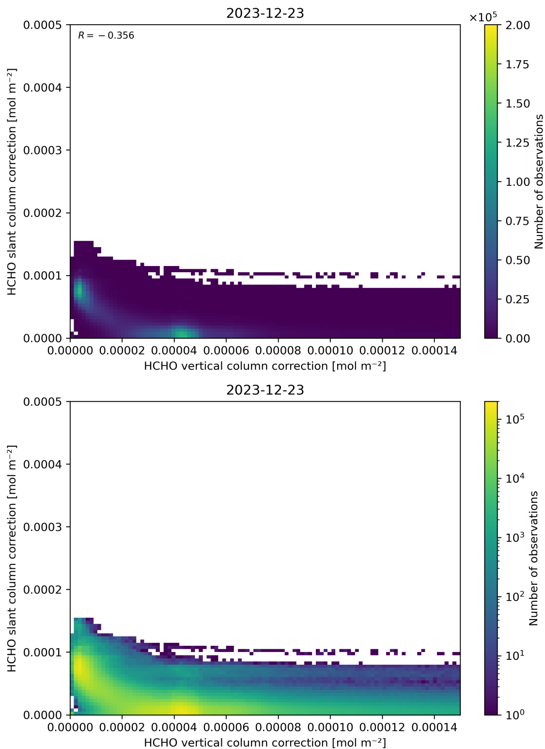
Figure 117: Scatter density plot of “HCHO vertical column correction” against “HCHO slant column correction” for 2023-12-22 to 2023-12-24.
