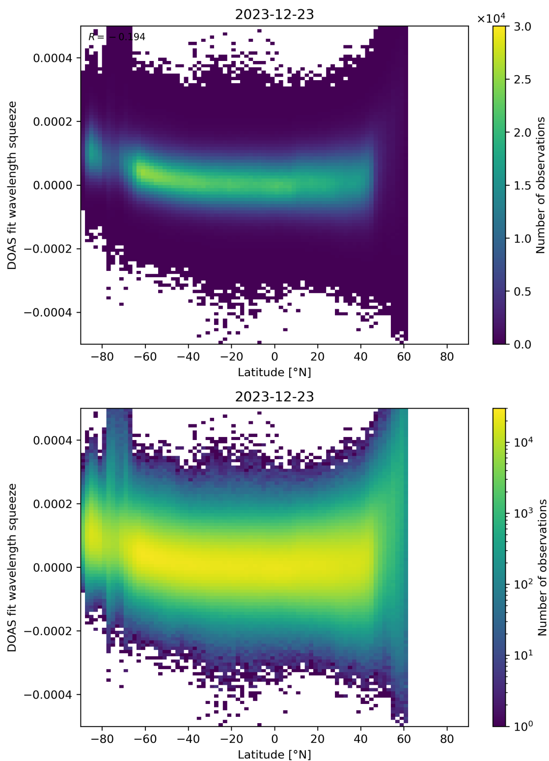
Figure 155: Scatter density plot of “Latitude” against “DOAS fit wavelength squeeze” for 2023-12-22 to 2023-12-24.
