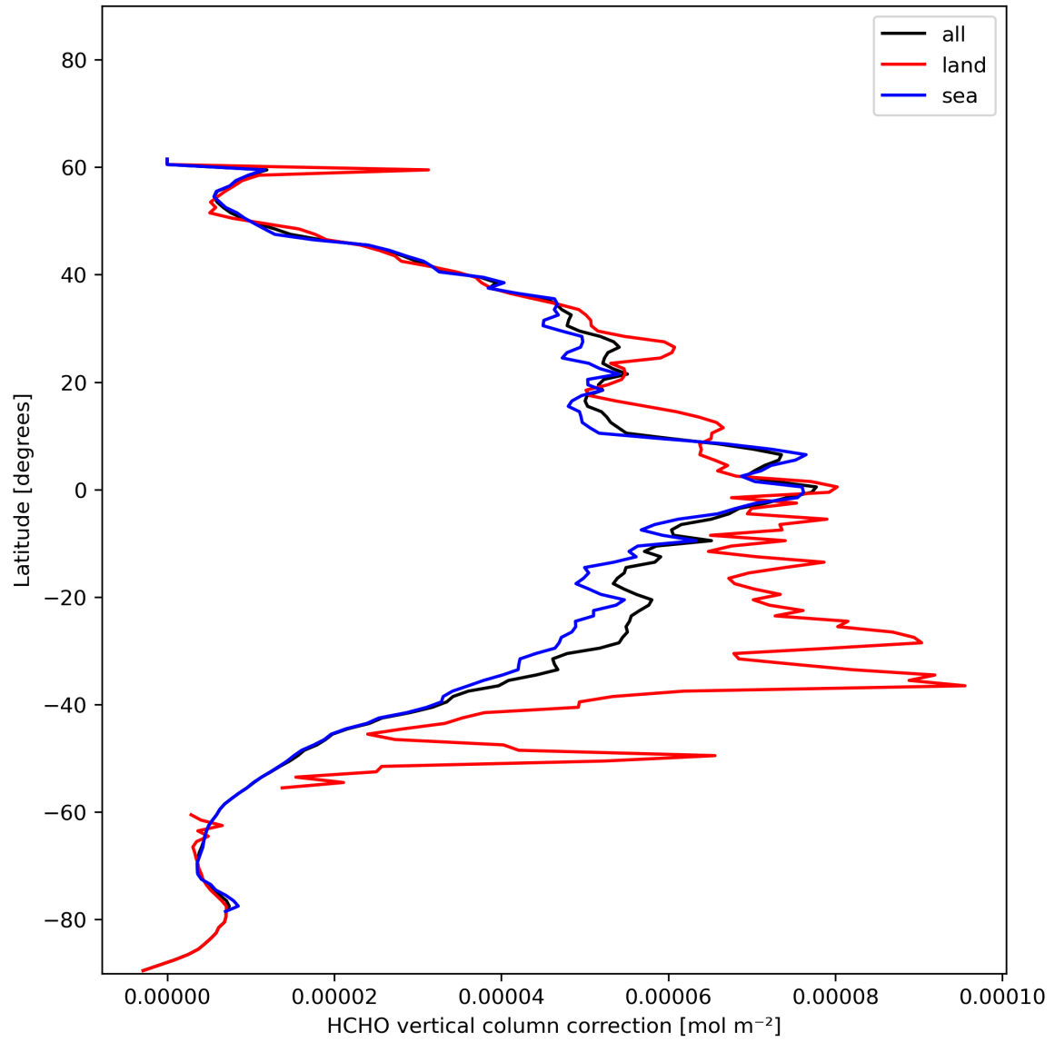
Figure 23: Zonal average of “HCHO vertical column correction” for 2023-12-22 to 2023-12-24.
