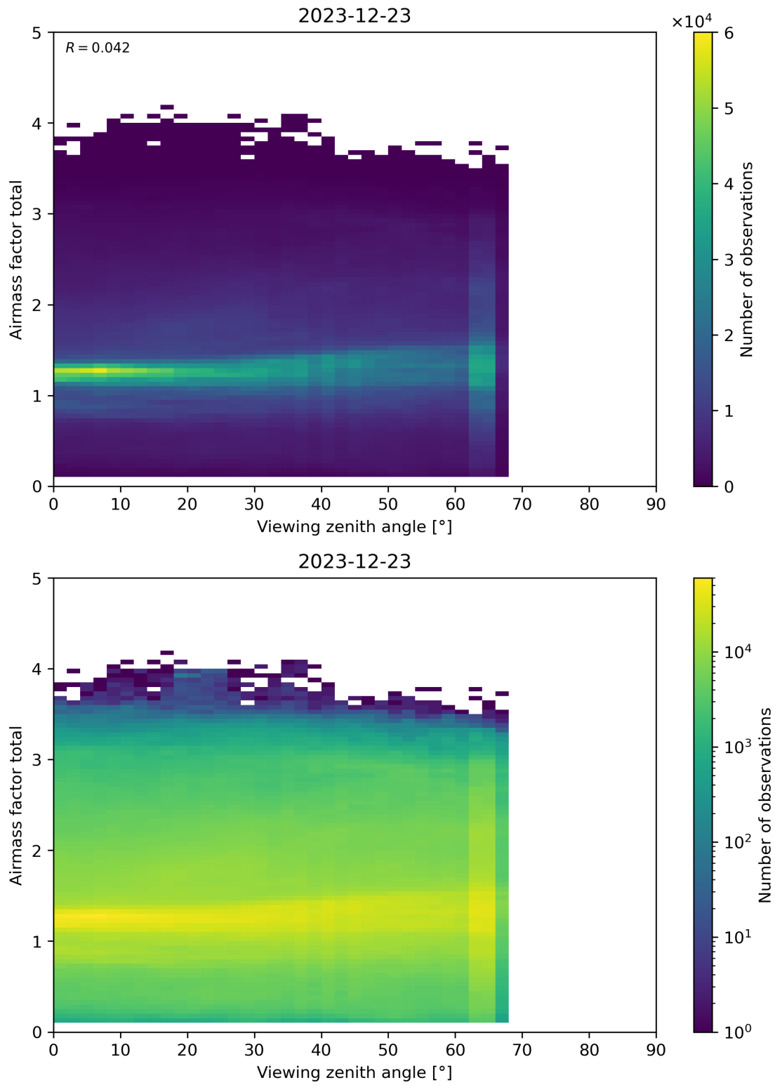
Figure 190: Scatter density plot of “Viewing zenith angle” against “Airmass factor total” for 2023-12-22 to 2023-12-24.
