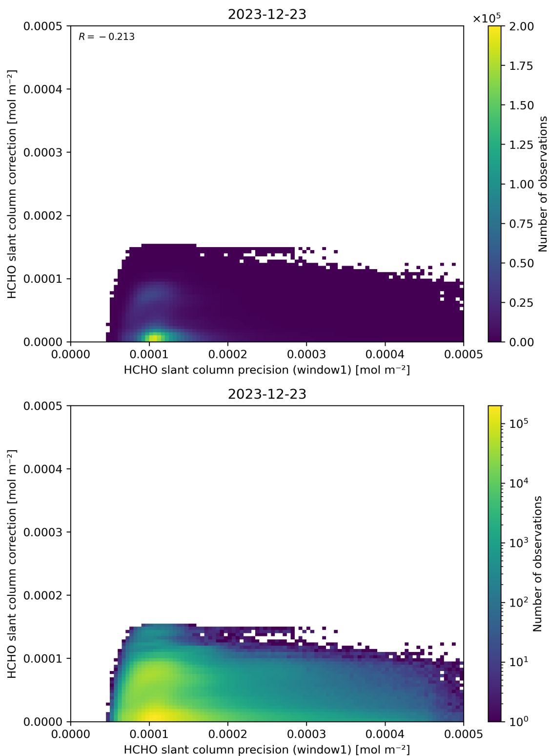
Figure 93: Scatter density plot of “HCHO slant column precision (window1)” against “HCHO slant column correction” for 2023-12-22 to 2023-12-24.
