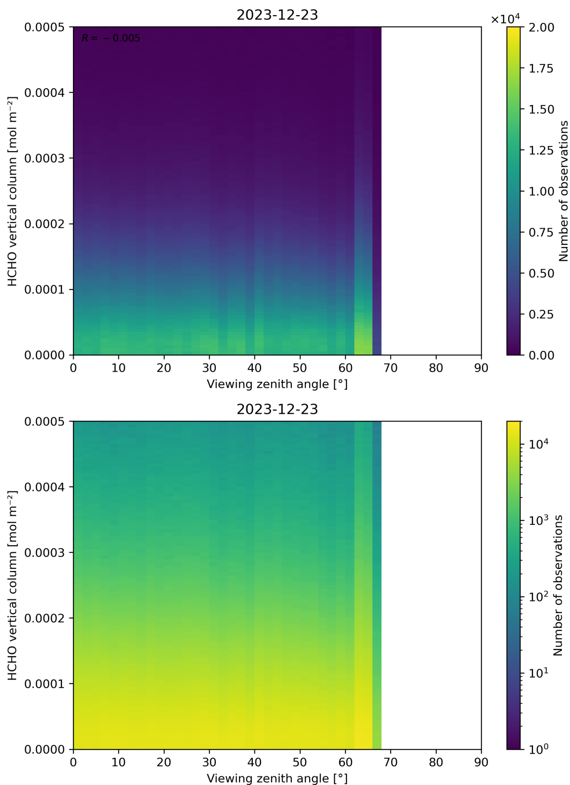
Figure 192: Scatter density plot of “Viewing zenith angle” against “HCHO vertical column” for 2023-12-22 to 2023-12-24.
