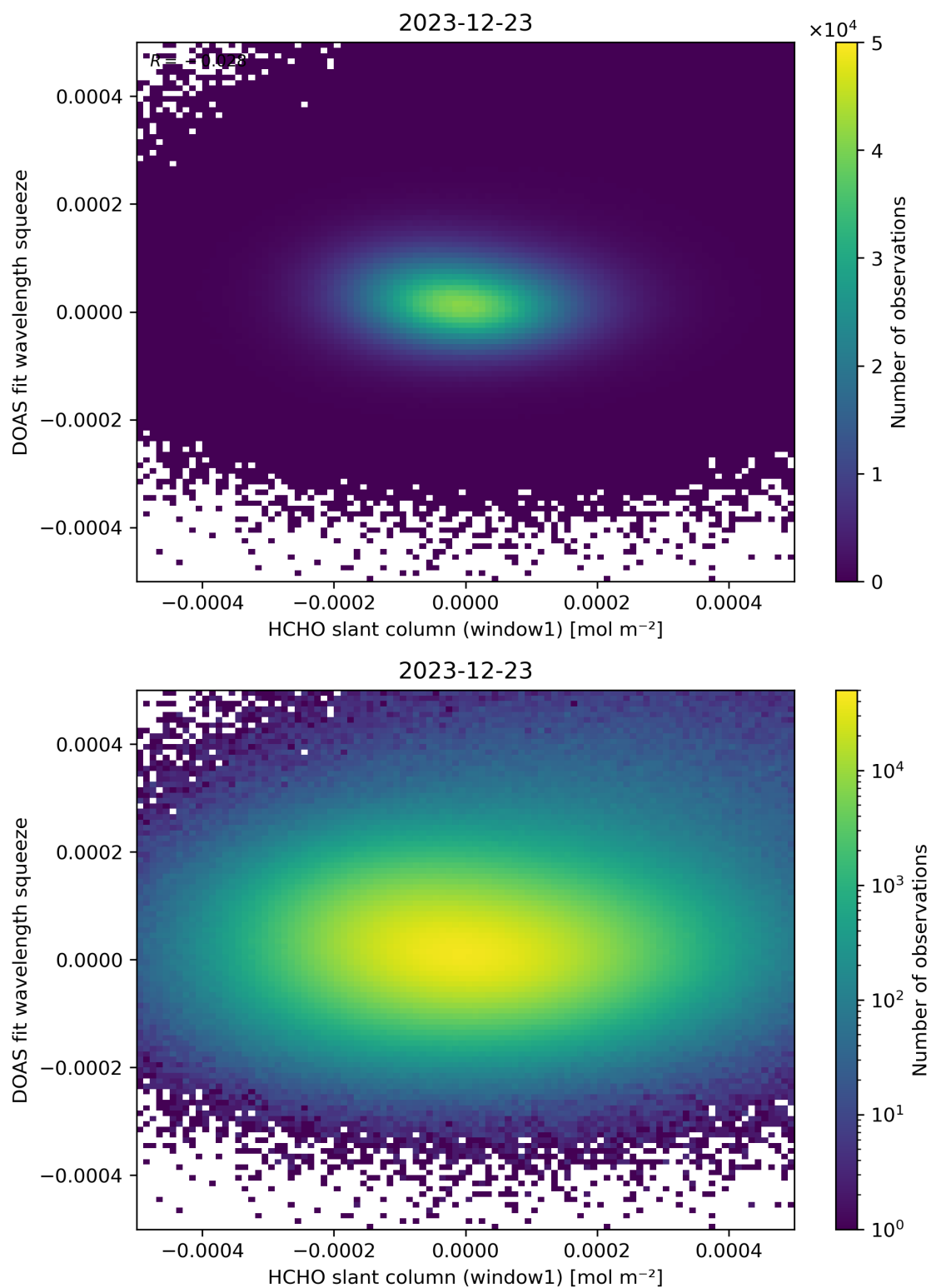
Figure 80: Scatter density plot of “HCHO slant column (window1)” against “DOAS fit wavelength squeeze” for 2023-12-22 to 2023-12-24.
