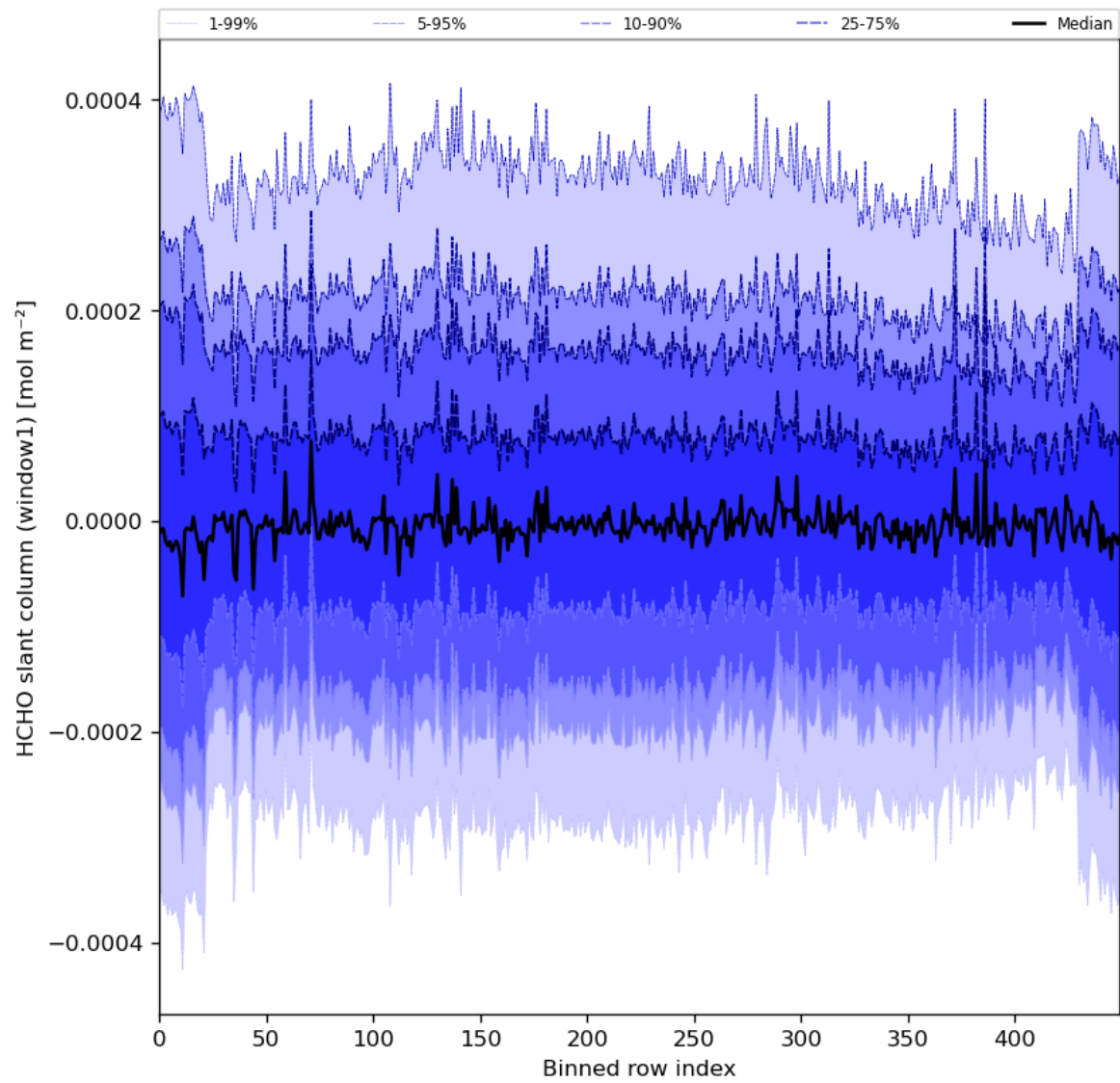
Figure 52: Along track statistics of “HCHO slant column (window1)” for 2023-12-22 to 2023-12-24
