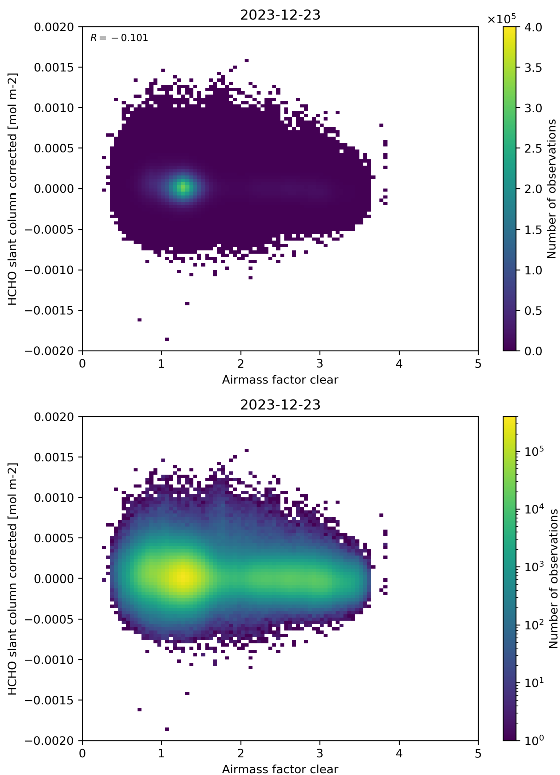
Figure 74: Scatter density plot of “Airmass factor clear” against “HCHO slant column corrected” for 2023-12-22 to 2023-12-24.
