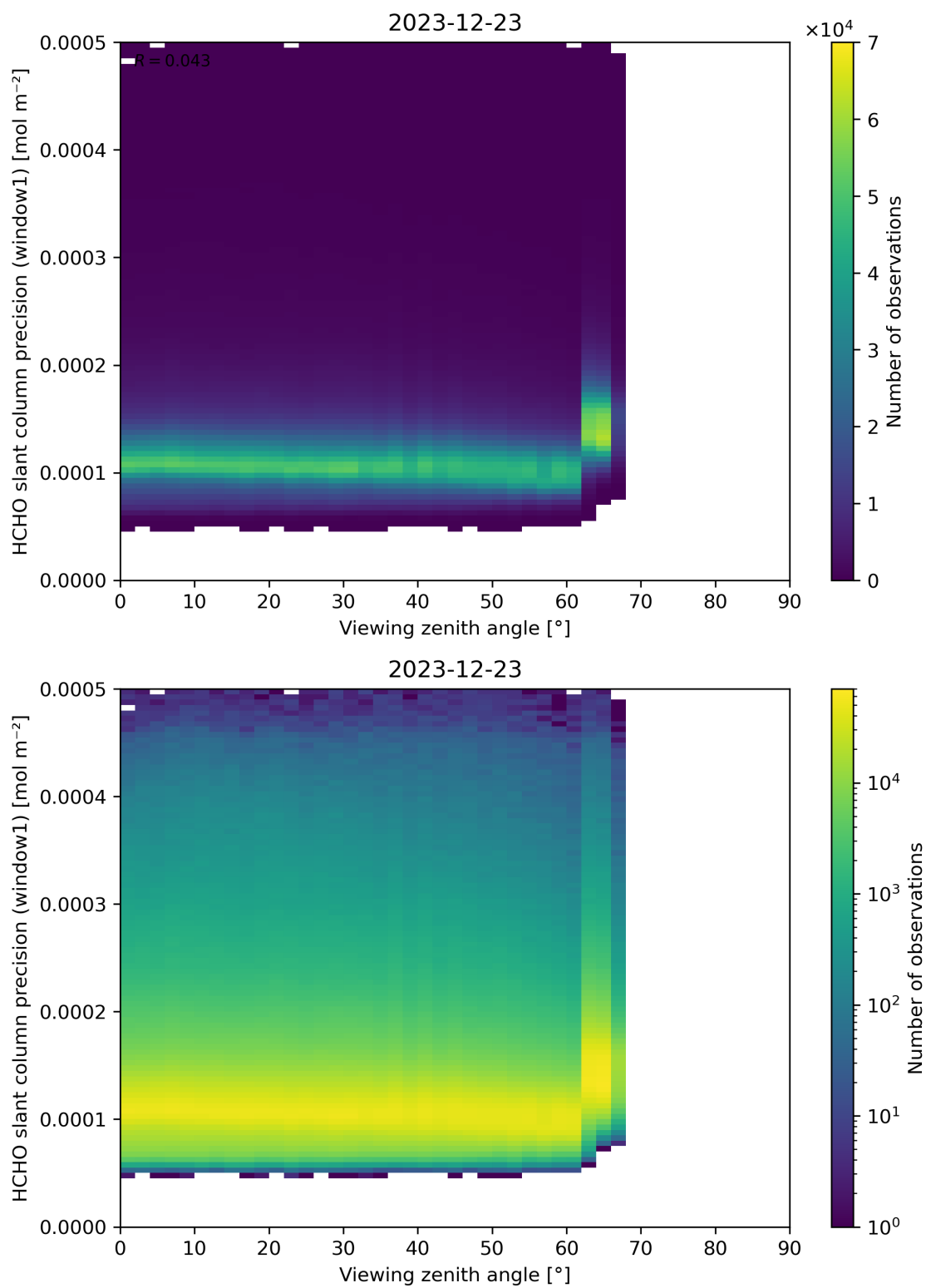
Figure 189: Scatter density plot of “Viewing zenith angle” against “HCHO slant column precision (window1)” for 2023-12-22 to 2023-12-24.
