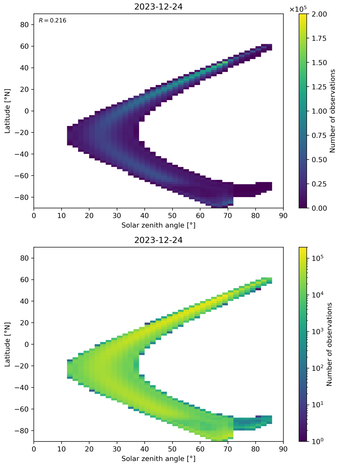
Figure 181: Scatter density plot of “Solar zenith angle” against “Latitude” for 2023-12-23 to 2023-12-25.
