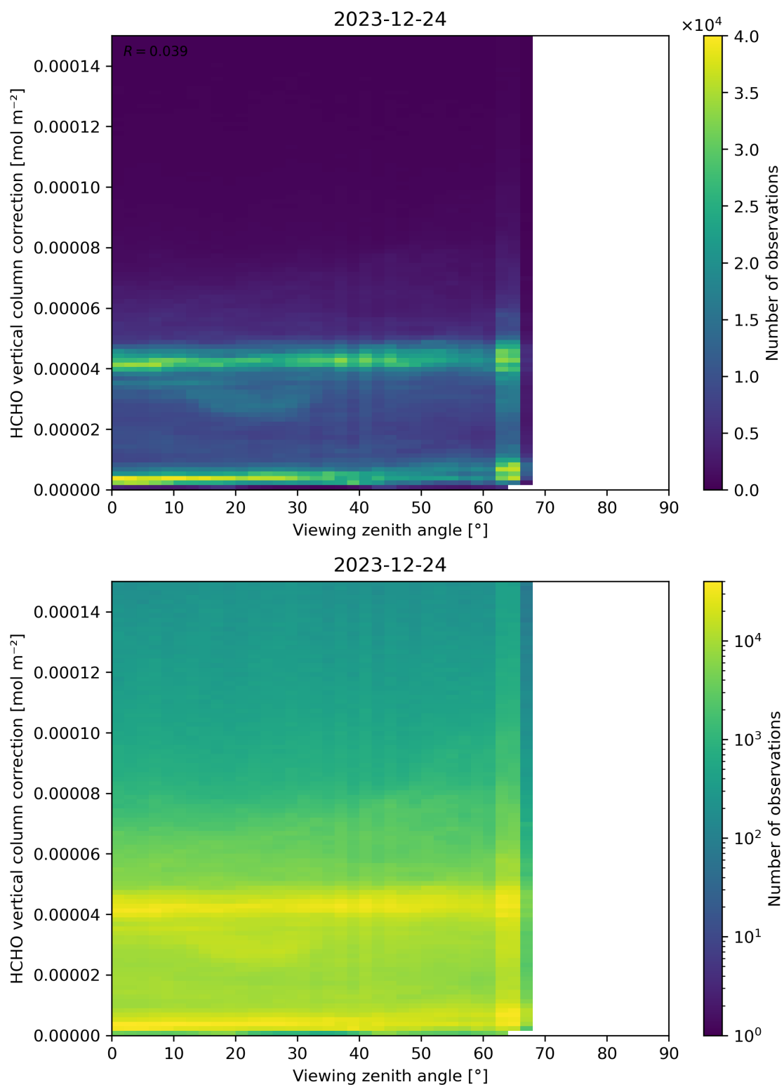
Figure 193: Scatter density plot of “Viewing zenith angle” against “HCHO vertical column correction” for 2023-12-23 to 2023-12-25.
