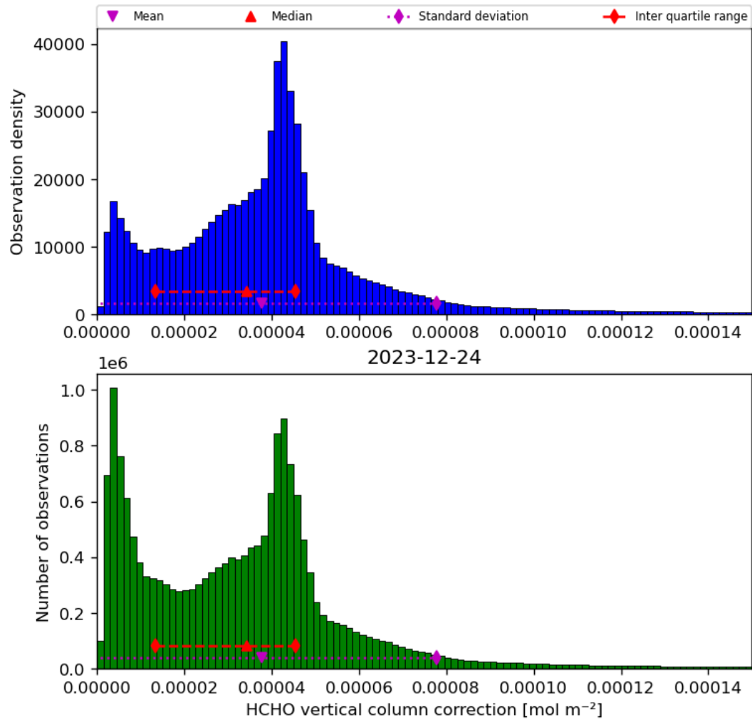
Figure 37: Histogram of “HCHO vertical column correction” for 2023-12-23 to 2023-12-25
