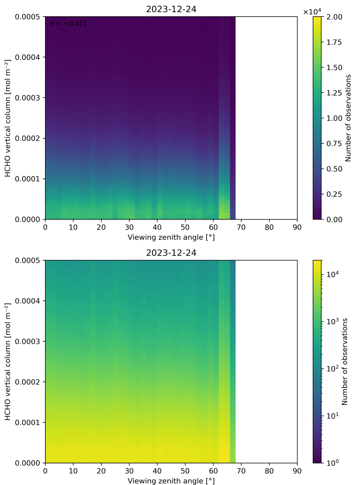
Figure 192: Scatter density plot of “Viewing zenith angle” against “HCHO vertical column” for 2023-12-23 to 2023-12-25.
