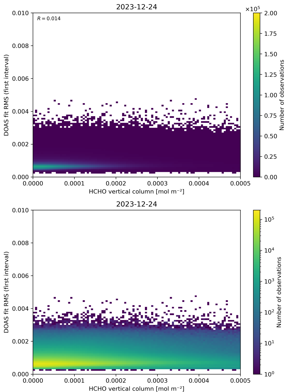
Figure 123: Scatter density plot of “HCHO vertical column” against “DOAS fit RMS (first interval)” for 2023-12-23 to 2023-12-25.
