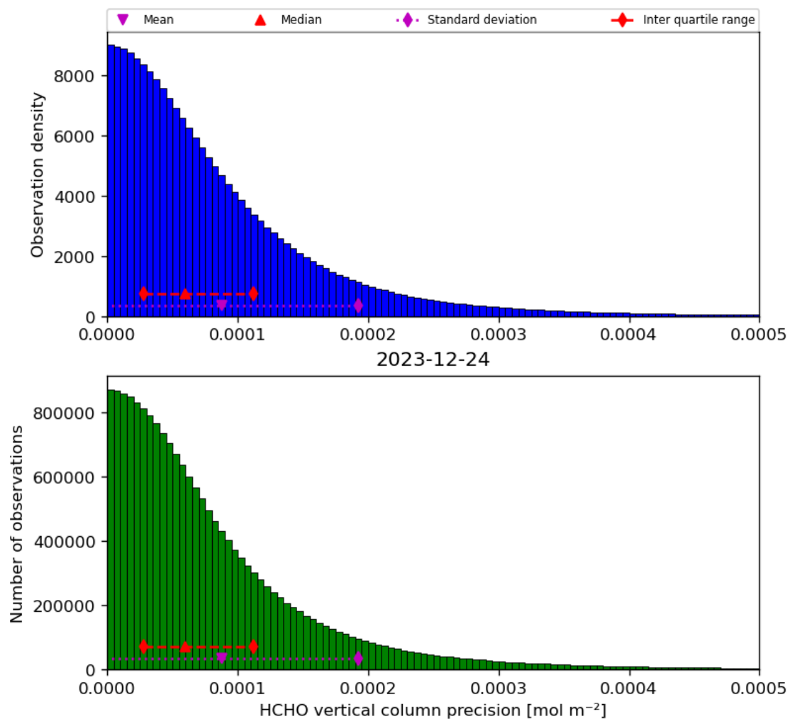
Figure 36: Histogram of “HCHO vertical column precision” for 2023-12-23 to 2023-12-25
