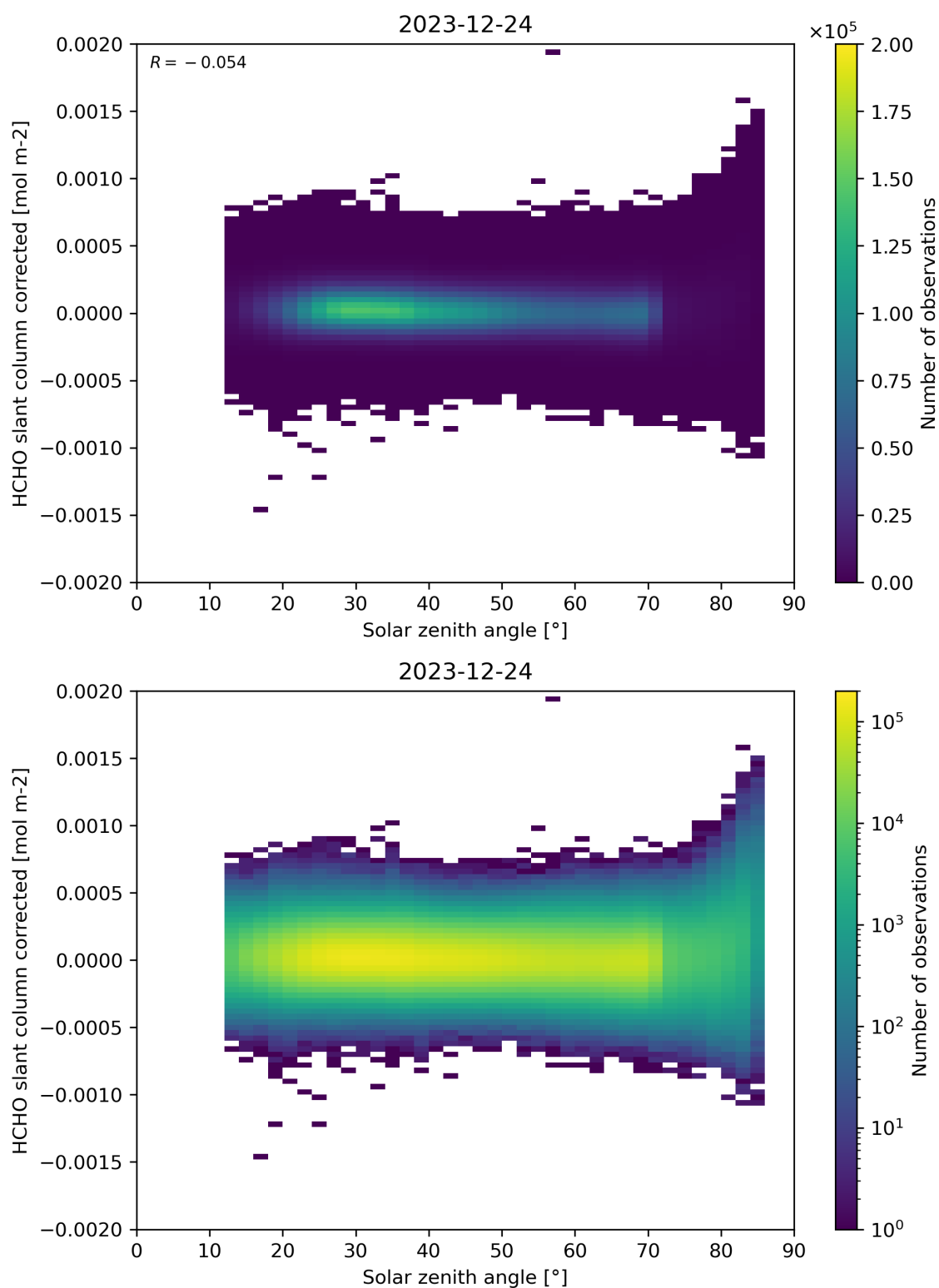
Figure 171: Scatter density plot of “Solar zenith angle” against “HCHO slant column corrected” for 2023-12-23 to 2023-12-25.
