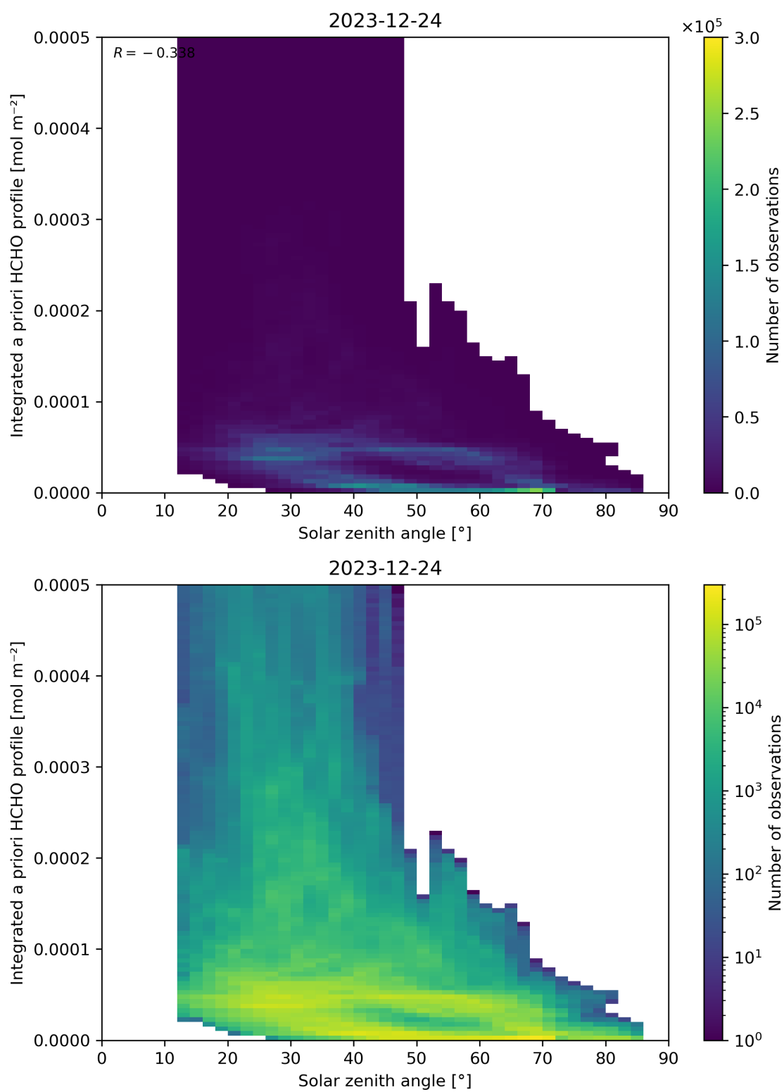
Figure 180: Scatter density plot of “Solar zenith angle” against “Integrated a priori HCHO profile” for 2023-12-23 to 2023-12-25.
