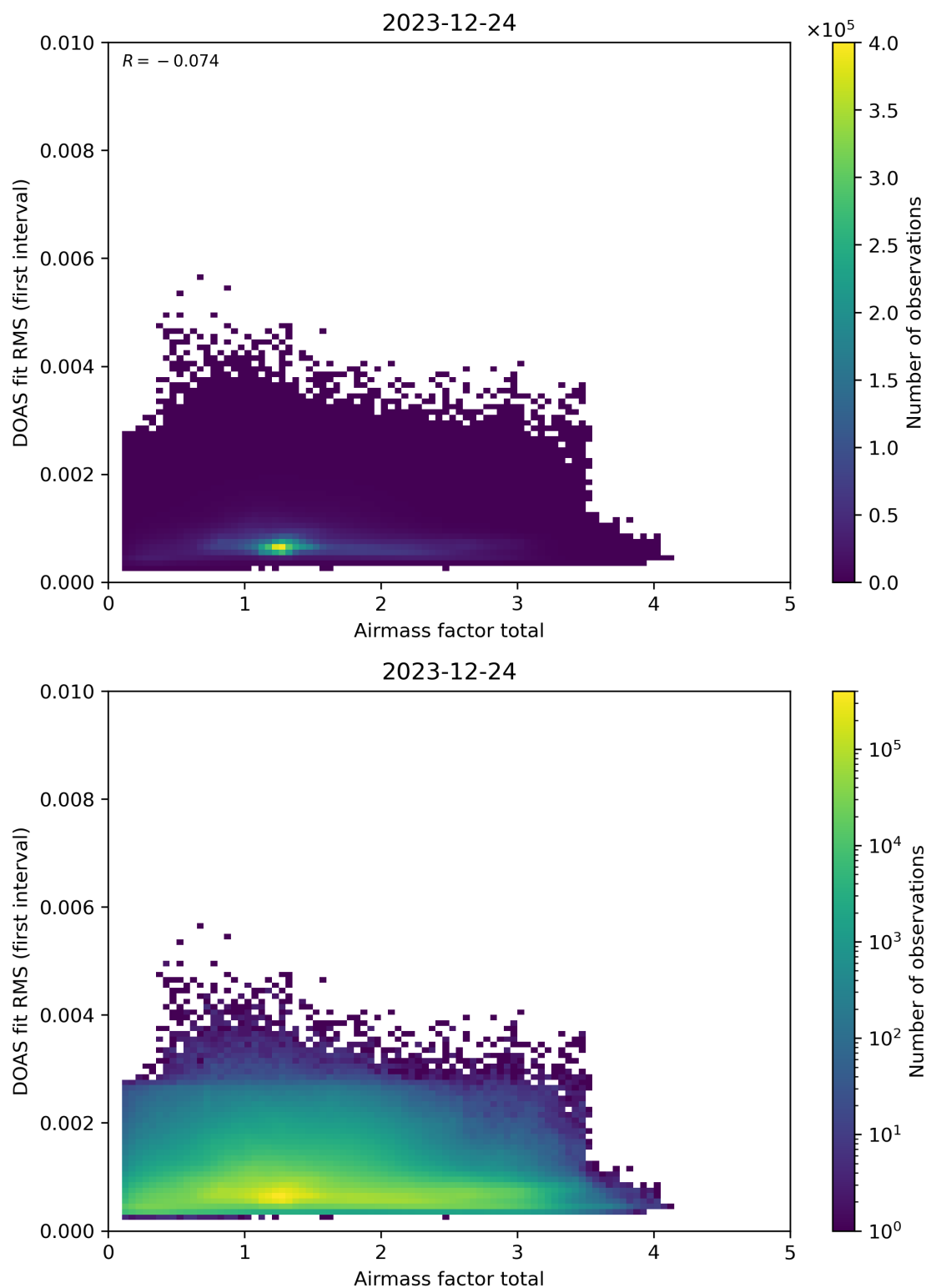
Figure 97: Scatter density plot of “Airmass factor total” against “DOAS fit RMS (first interval)” for 2023-12-23 to 2023-12-25.
