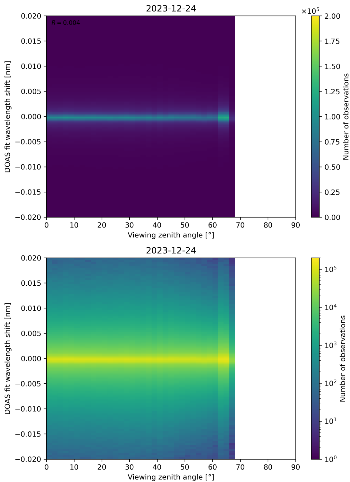
Figure 183: Scatter density plot of “Viewing zenith angle” against “DOAS fit wavelength shift” for 2023-12-23 to 2023-12-25.
