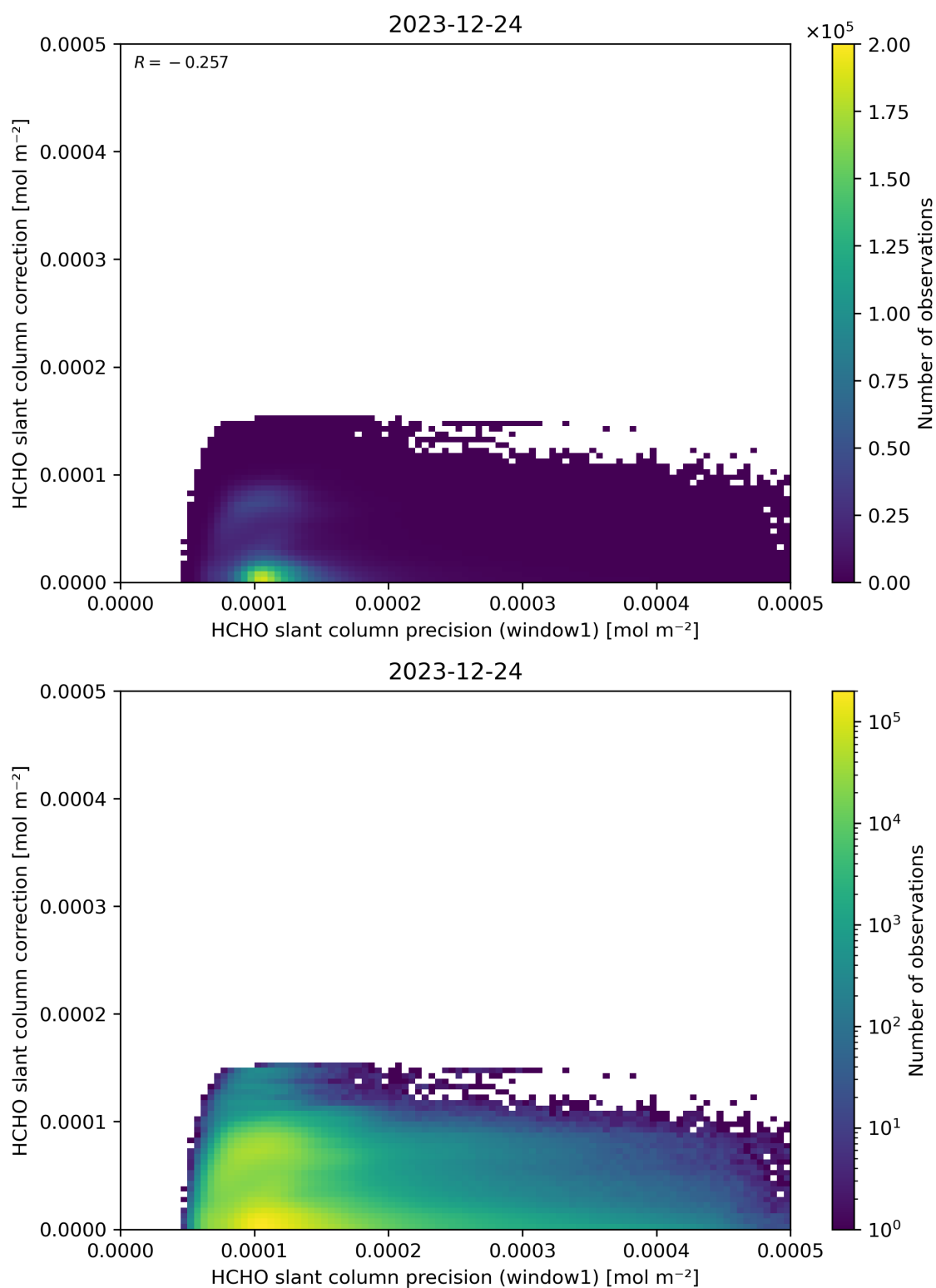
Figure 93: Scatter density plot of “HCHO slant column precision (window1)” against “HCHO slant column correction” for 2023-12-23 to 2023-12-25.
