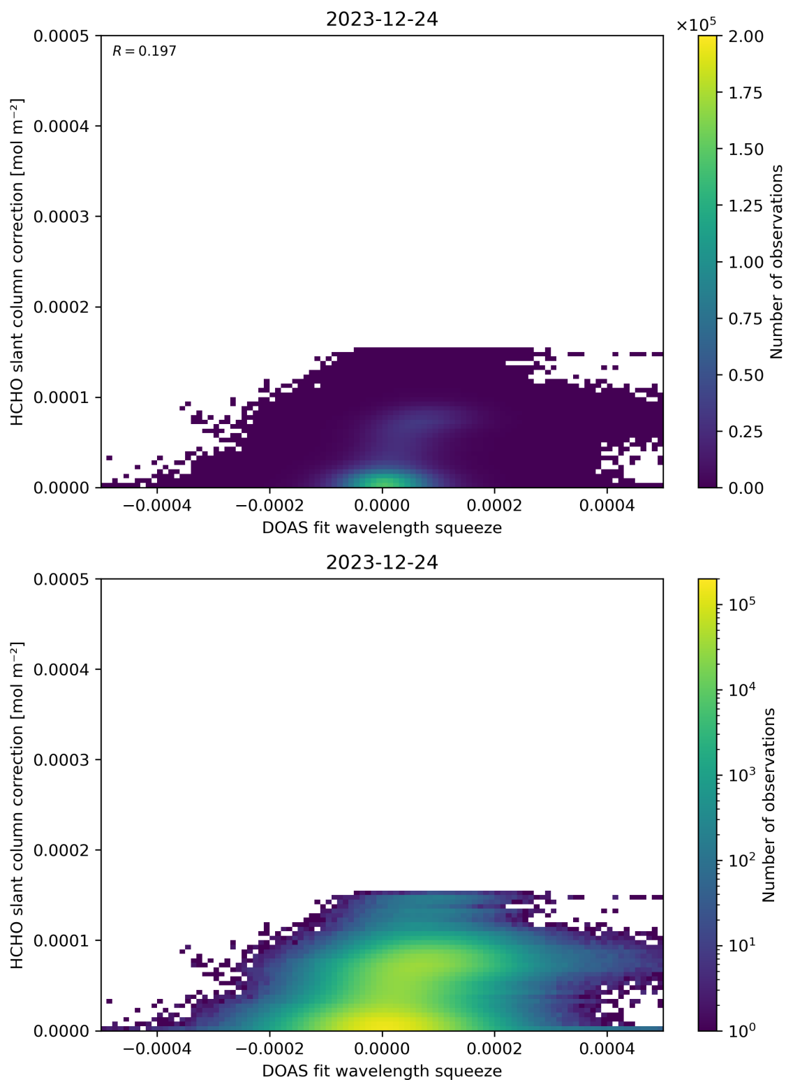
Figure 70: Scatter density plot of “DOAS fit wavelength squeeze” against “HCHO slant column correction” for 2023-12-23 to 2023-12-25.
