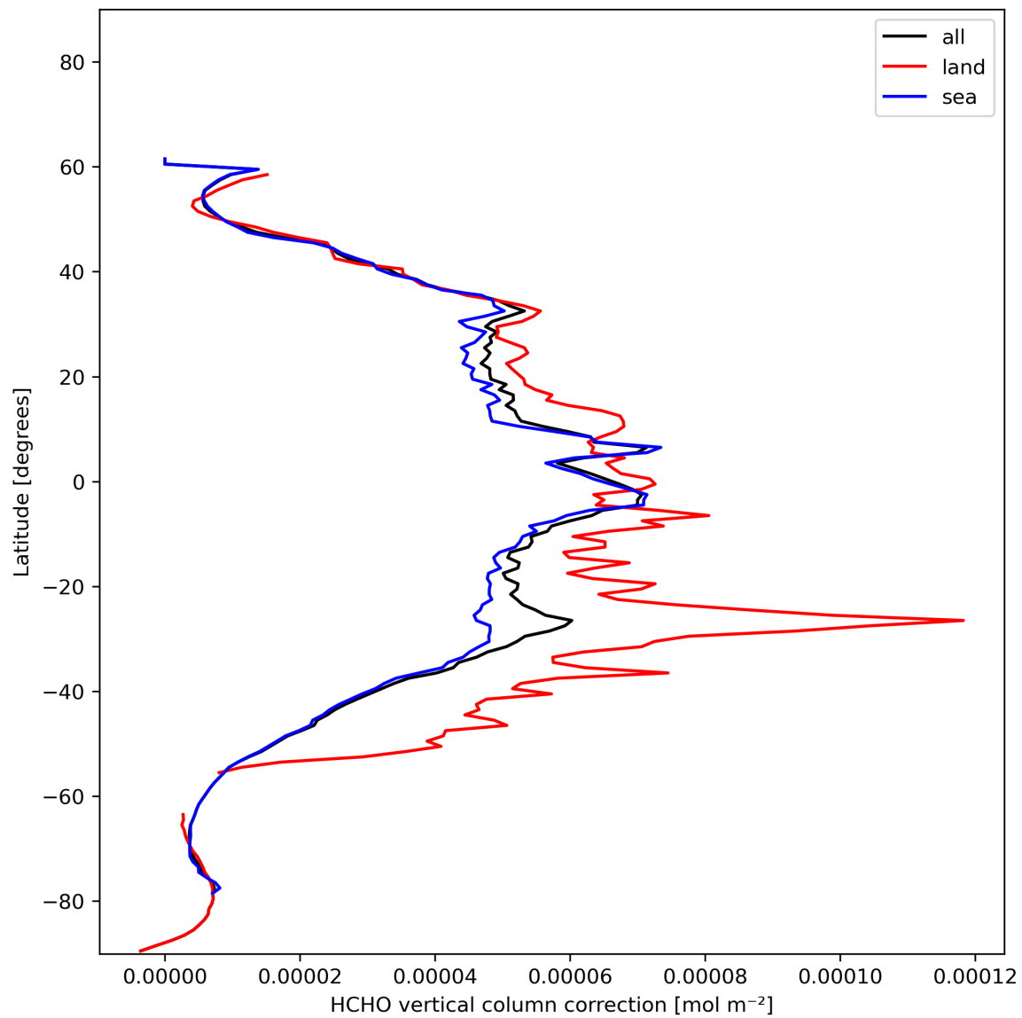
Figure 23: Zonal average of “HCHO vertical column correction” for 2023-12-23 to 2023-12-25.
