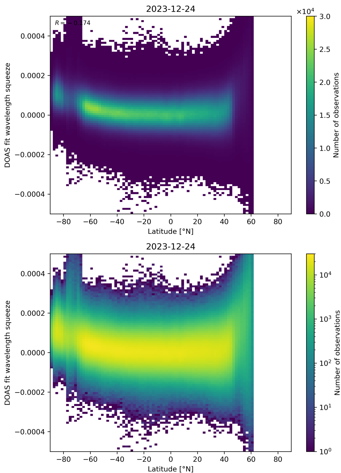
Figure 155: Scatter density plot of “Latitude” against “DOAS fit wavelength squeeze” for 2023-12-23 to 2023-12-25.
