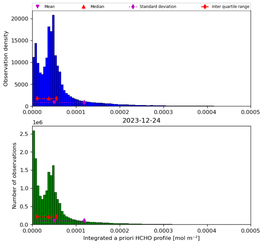
Figure 43: Histogram of “Integrated a priori HCHO profile” for 2023-12-23 to 2023-12-25
