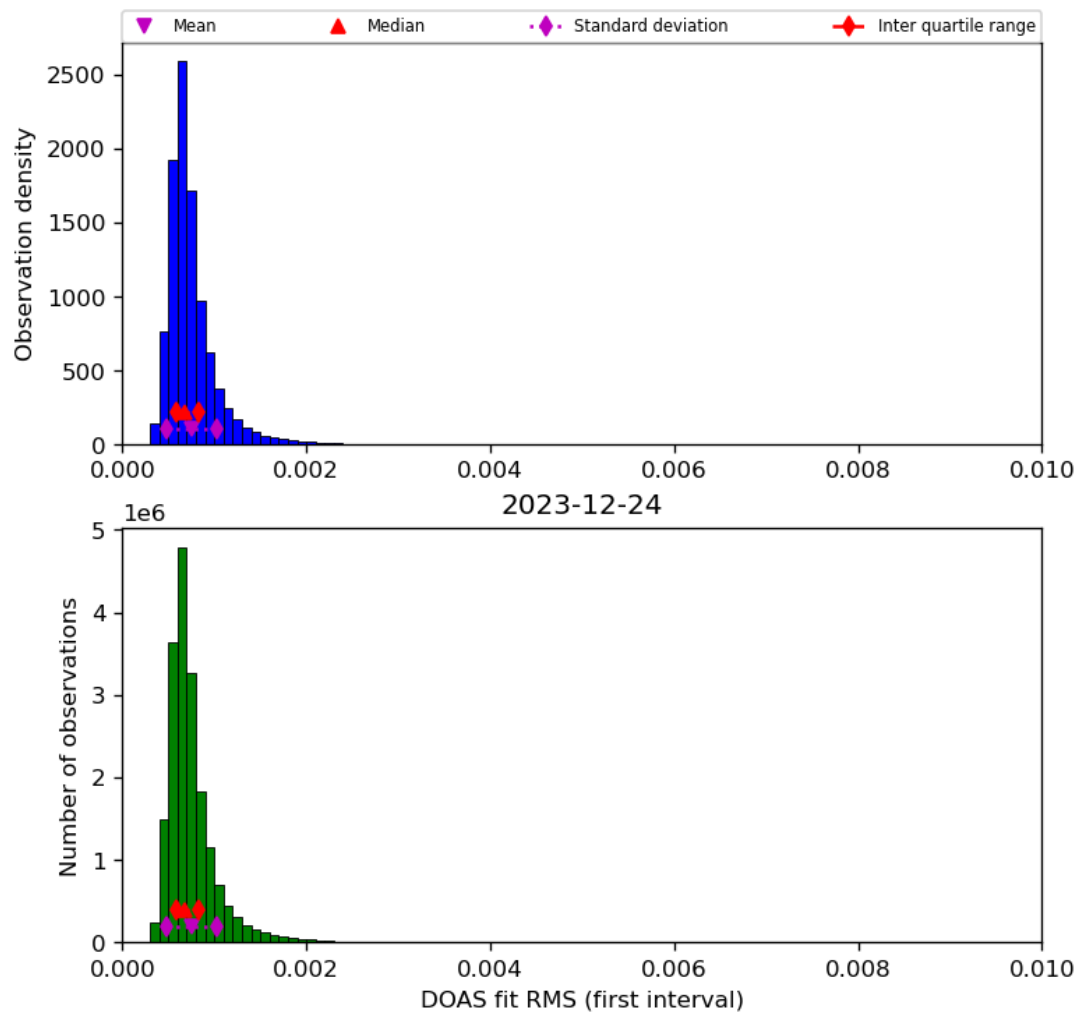
Figure 46: Histogram of “DOAS fit RMS (first interval)” for 2023-12-23 to 2023-12-25
