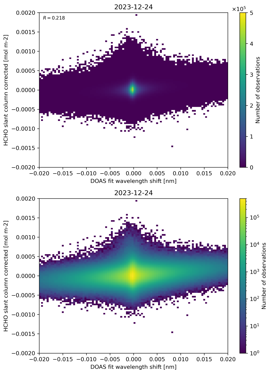
Figure 66: Scatter density plot of “DOAS fit wavelength shift” against “HCHO slant column corrected” for 2023-12-23 to 2023-12-25.
