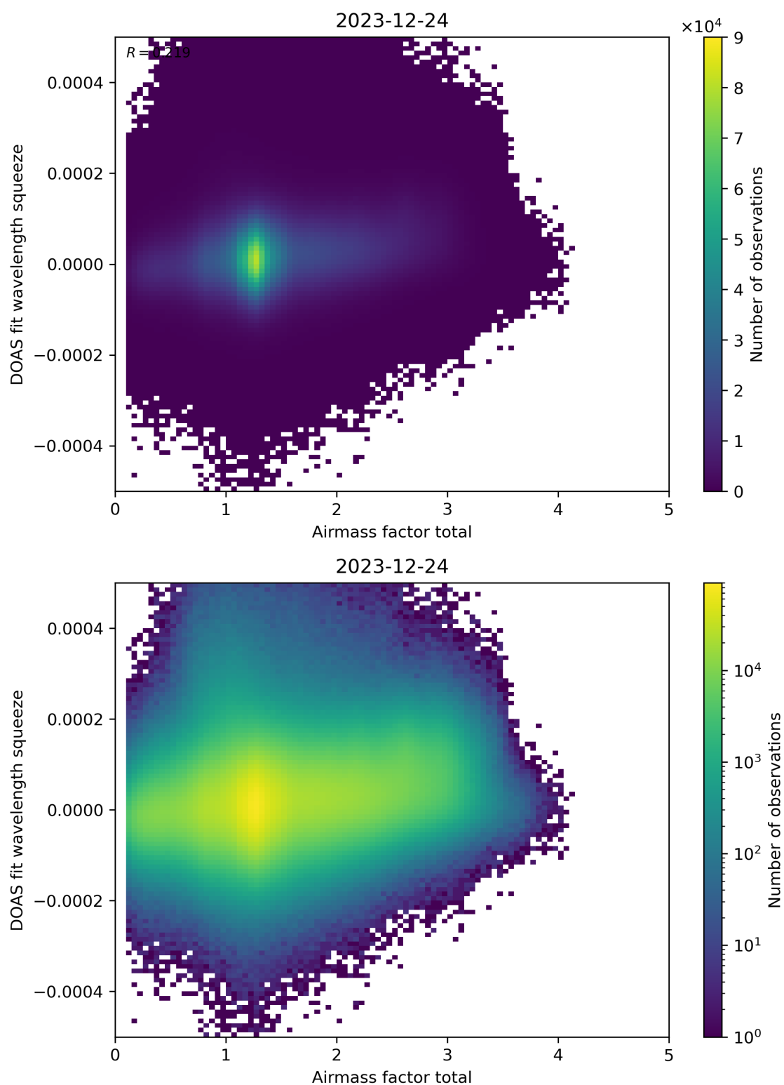
Figure 99: Scatter density plot of “Airmass factor total” against “DOAS fit wavelength squeeze” for 2023-12-23 to 2023-12-25.
