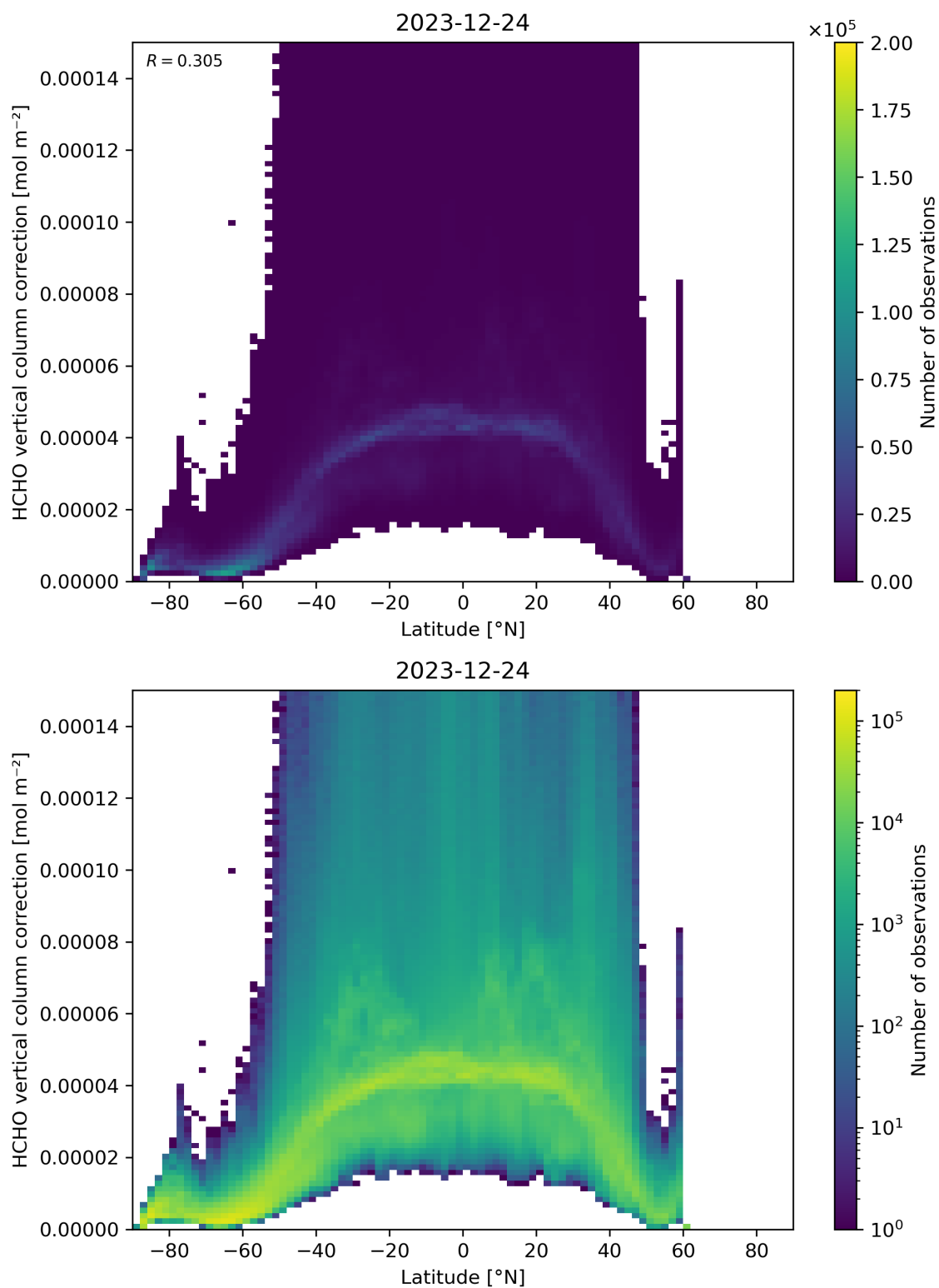
Figure 164: Scatter density plot of “Latitude” against “HCHO vertical column correction” for 2023-12-23 to 2023-12-25.
