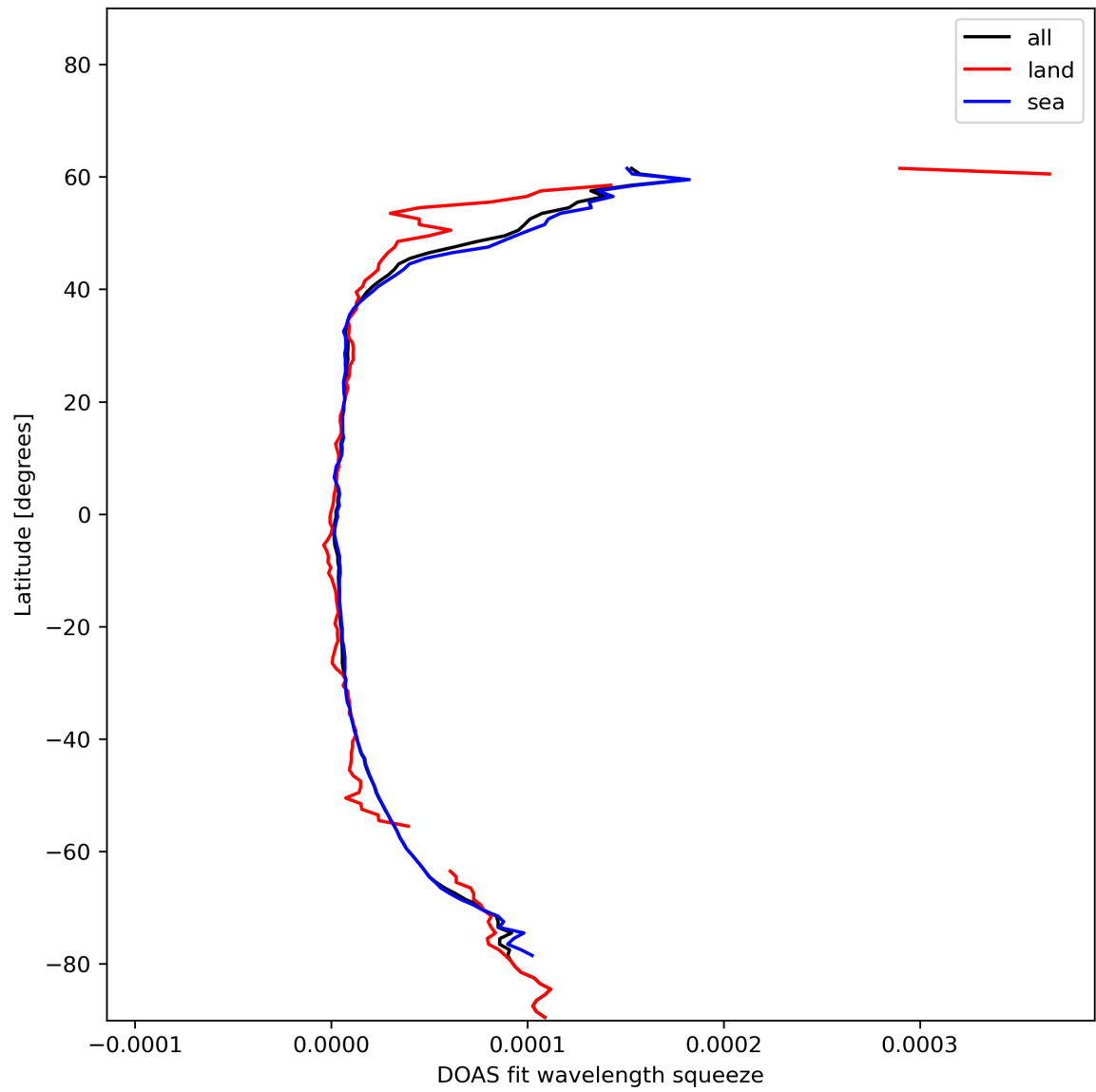
Figure 31: Zonal average of “DOAS fit wavelength squeeze” for 2023-12-23 to 2023-12-25.
