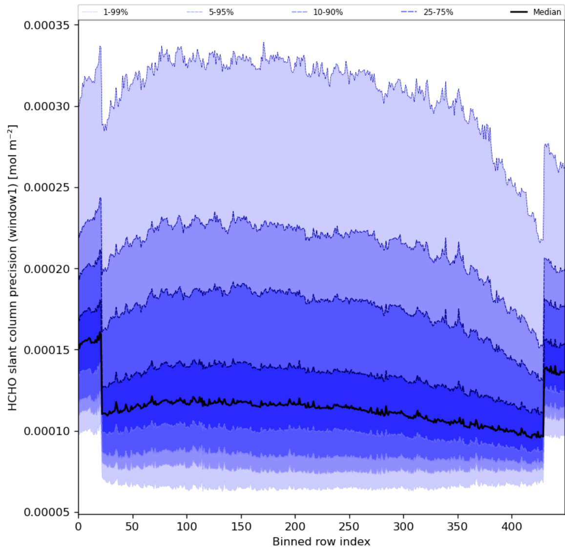
Figure 53: Along track statistics of “HCHO slant column precision (window1)” for 2023-12-23 to 2023-12-25
