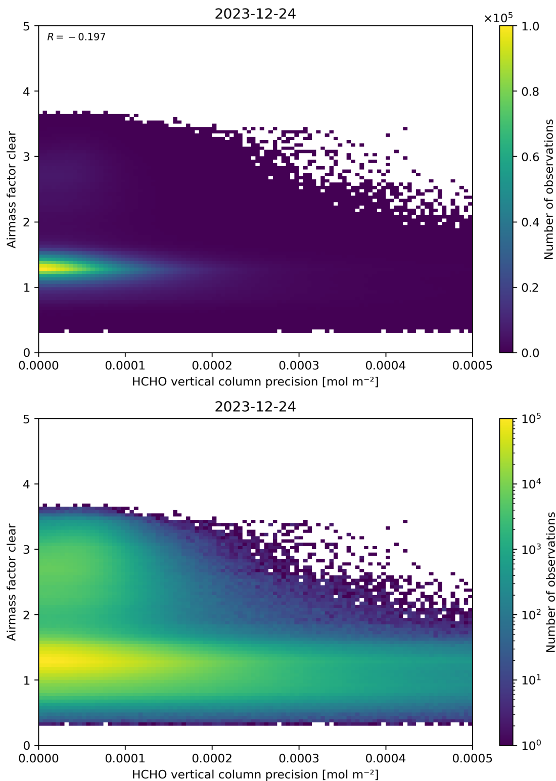
Figure 139: Scatter density plot of “HCHO vertical column precision” against “Airmass factor clear” for 2023-12-23 to 2023-12-25.
