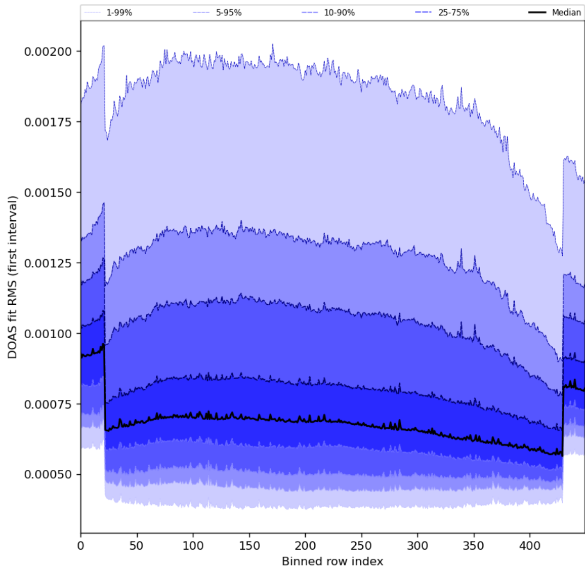
Figure 60: Along track statistics of “DOAS fit RMS (first interval)” for 2023-12-23 to 2023-12-25
