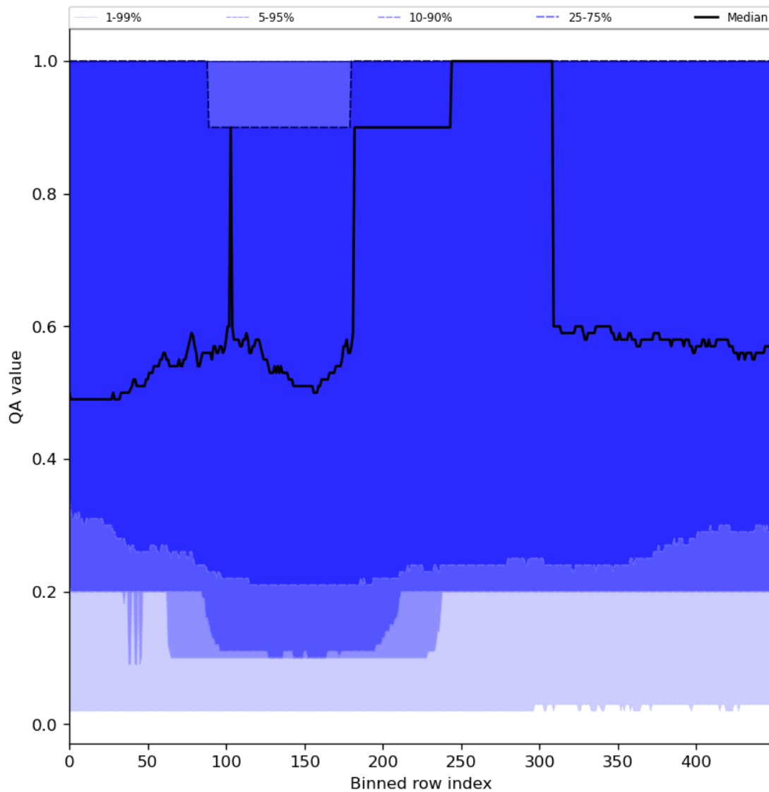
Figure 48: Along track statistics of "QA value" for 2023-12-23 to 2023-12-25
