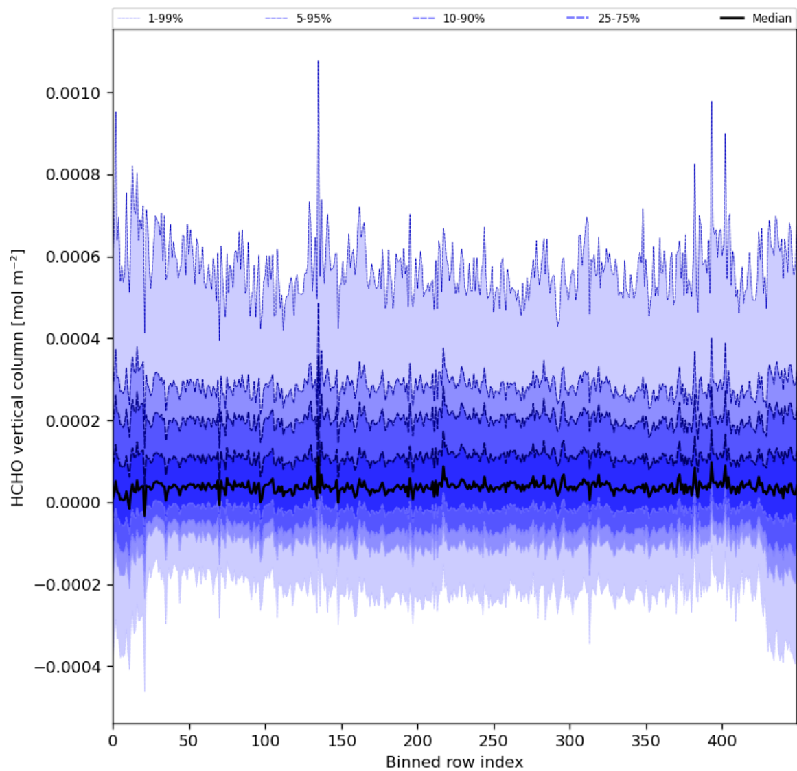
Figure 49: Along track statistics of “HCHO vertical column” for 2023-12-23 to 2023-12-25
