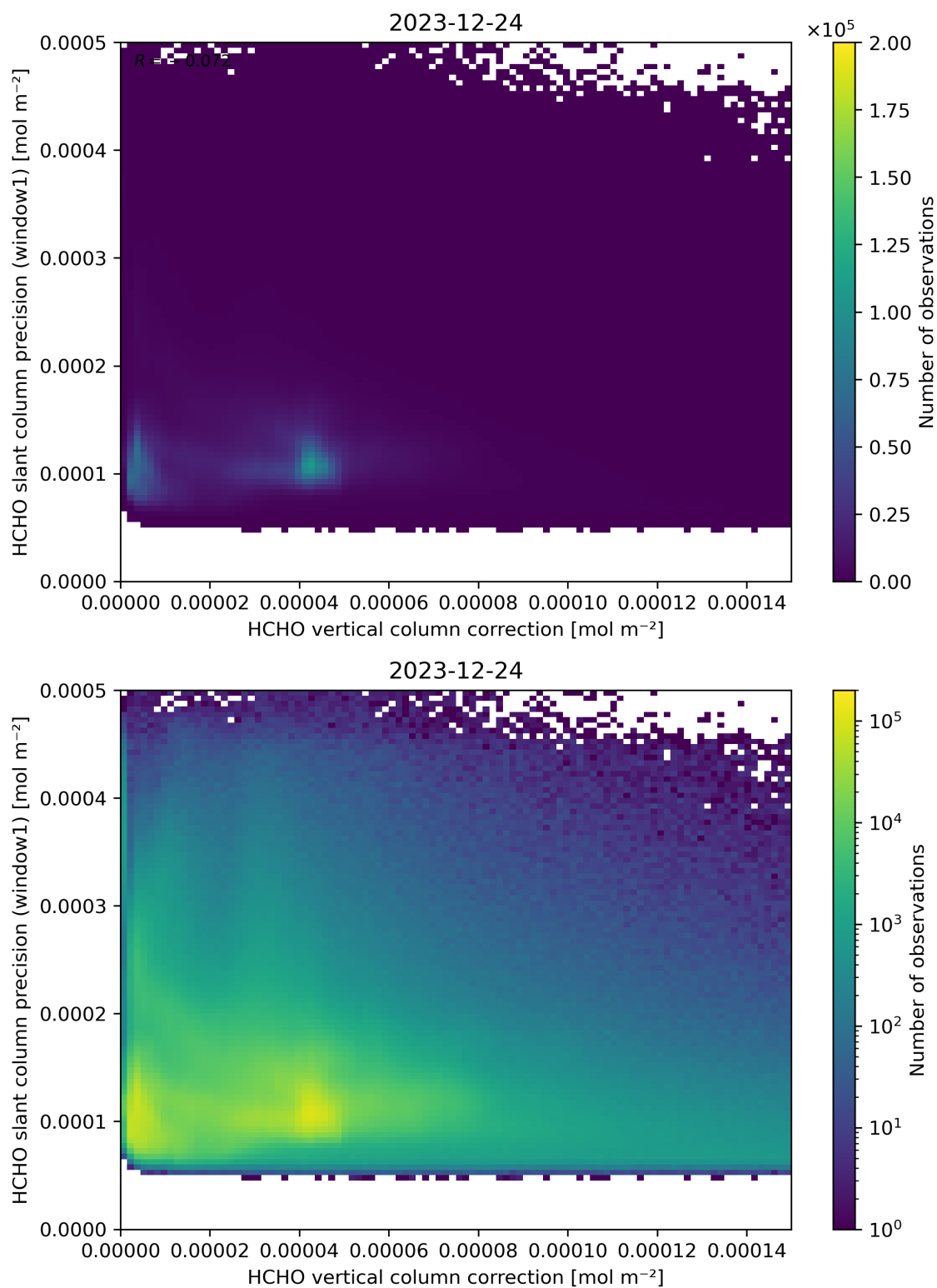
Figure 119: Scatter density plot of “HCHO vertical column correction” against “HCHO slant column precision (window1)” for 2023-12-23 to 2023-12-25.
