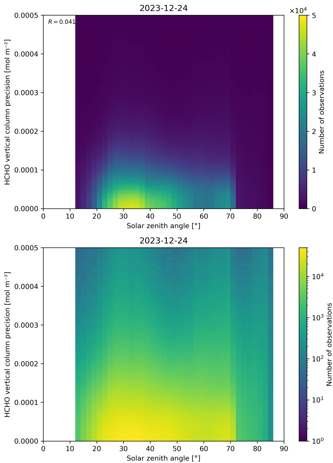
Figure 179: Scatter density plot of “Solar zenith angle” against “HCHO vertical column precision” for 2023-12-23 to 2023-12-25.
