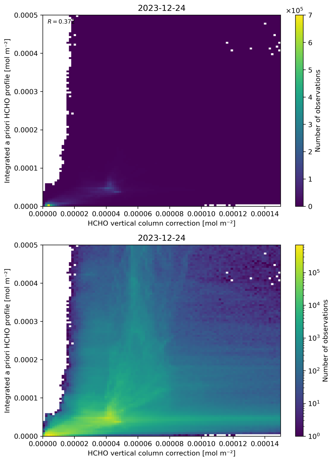
Figure 122: Scatter density plot of “HCHO vertical column correction” against “Integrated a priori HCHO profile” for 2023-12-23 to 2023-12-25.
