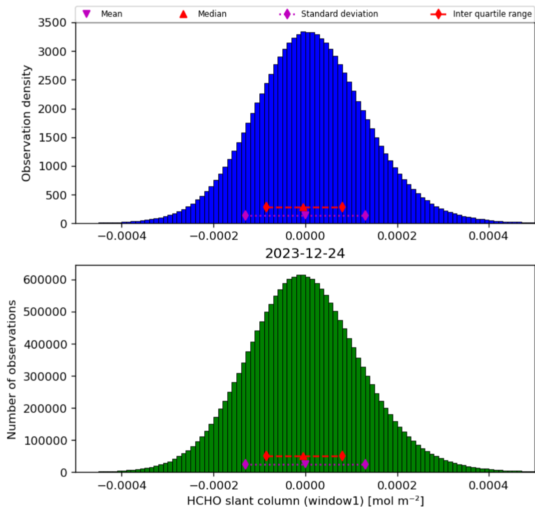
Figure 38: Histogram of “HCHO slant column (window1)” for 2023-12-23 to 2023-12-25
