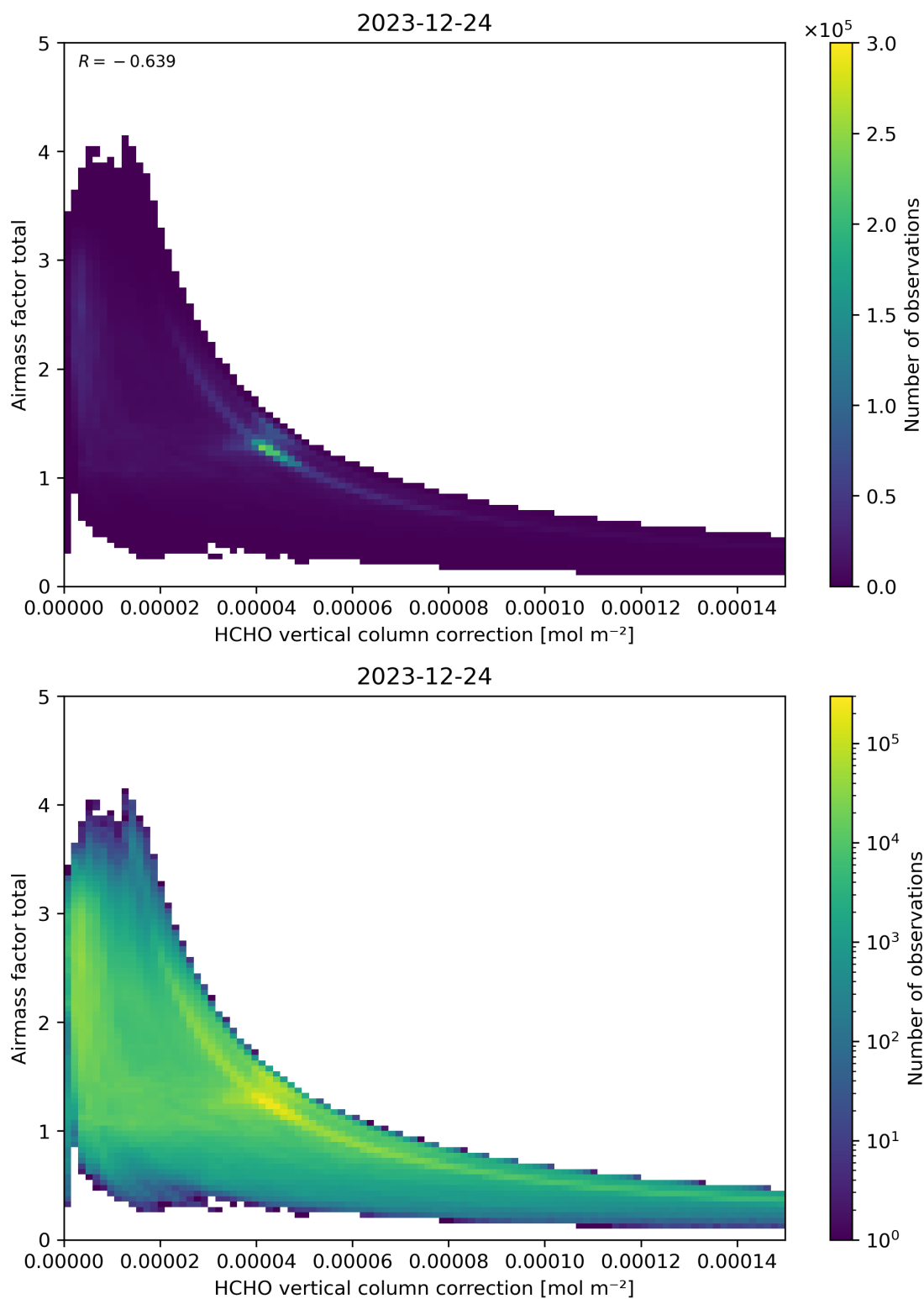
Figure 120: Scatter density plot of “HCHO vertical column correction” against “Airmass factor total” for 2023-12-23 to 2023-12-25.
