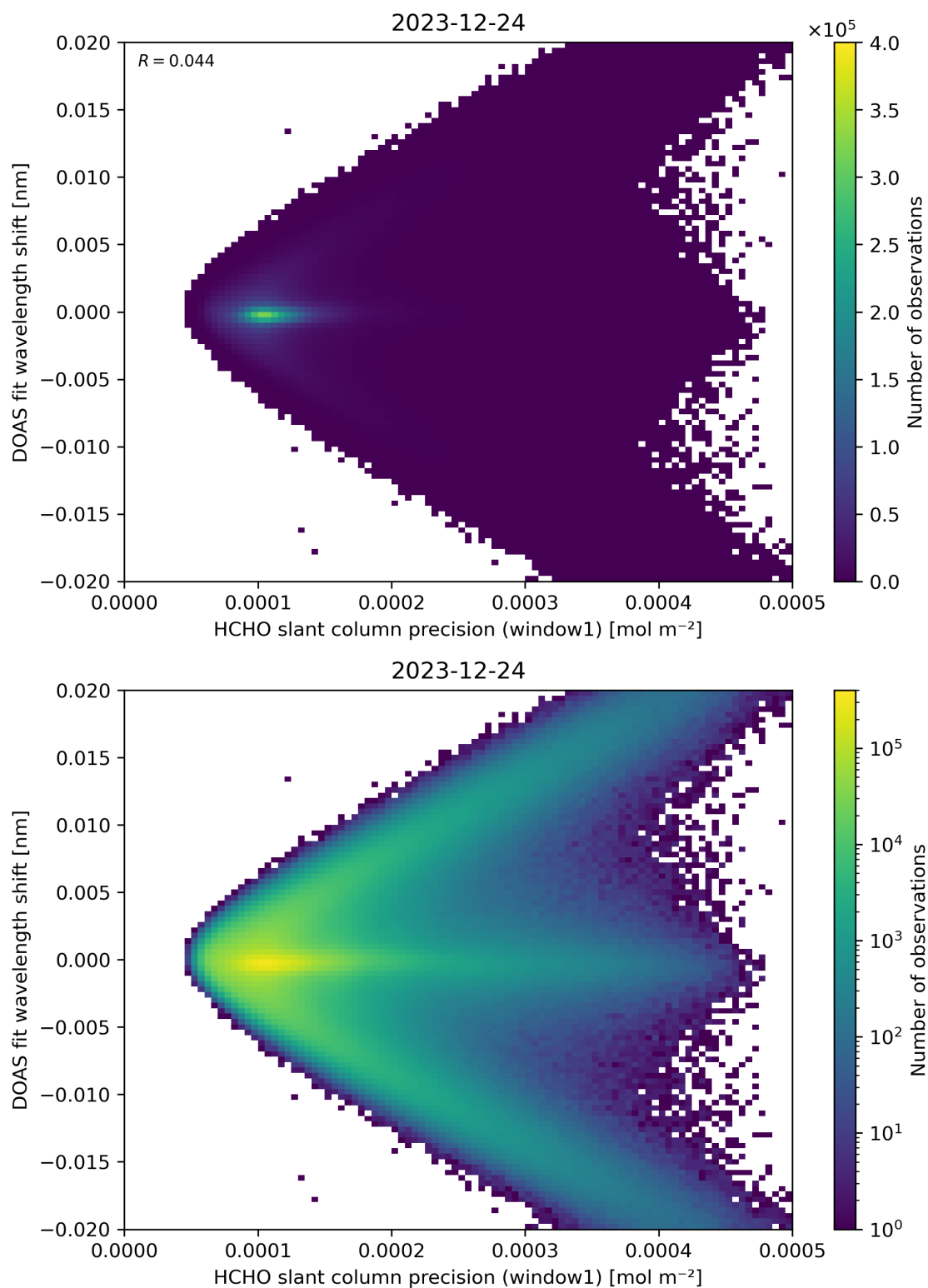
Figure 89: Scatter density plot of “HCHO slant column precision (window1)” against “DOAS fit wavelength shift” for 2023-12-23 to 2023-12-25.
