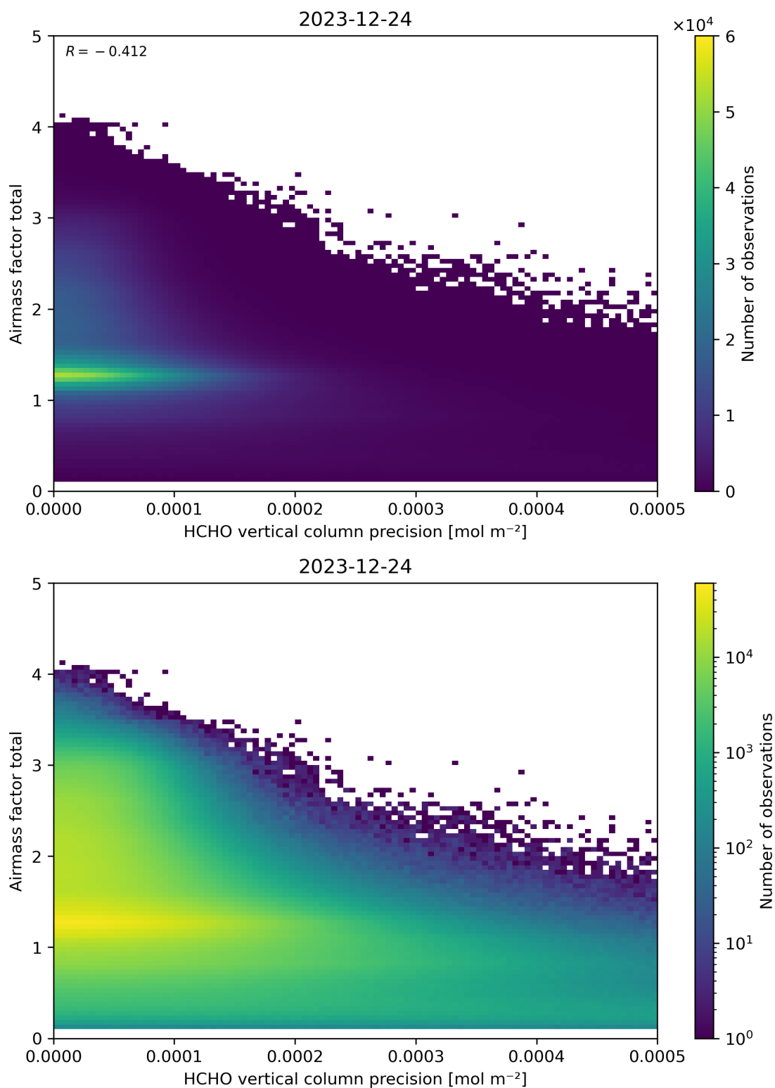
Figure 144: Scatter density plot of “HCHO vertical column precision” against “Airmass factor total” for 2023-12-23 to 2023-12-25.
