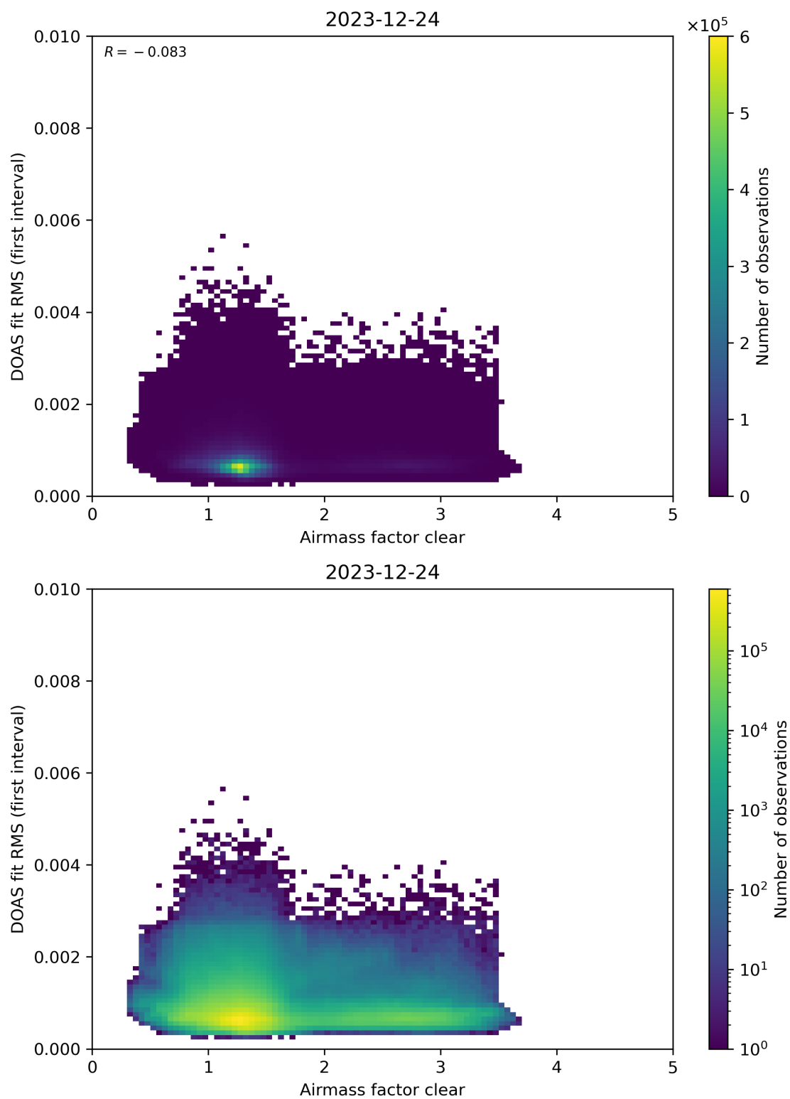
Figure 71: Scatter density plot of “Airmass factor clear” against “DOAS fit RMS (first interval)” for 2023-12-23 to 2023-12-25.
