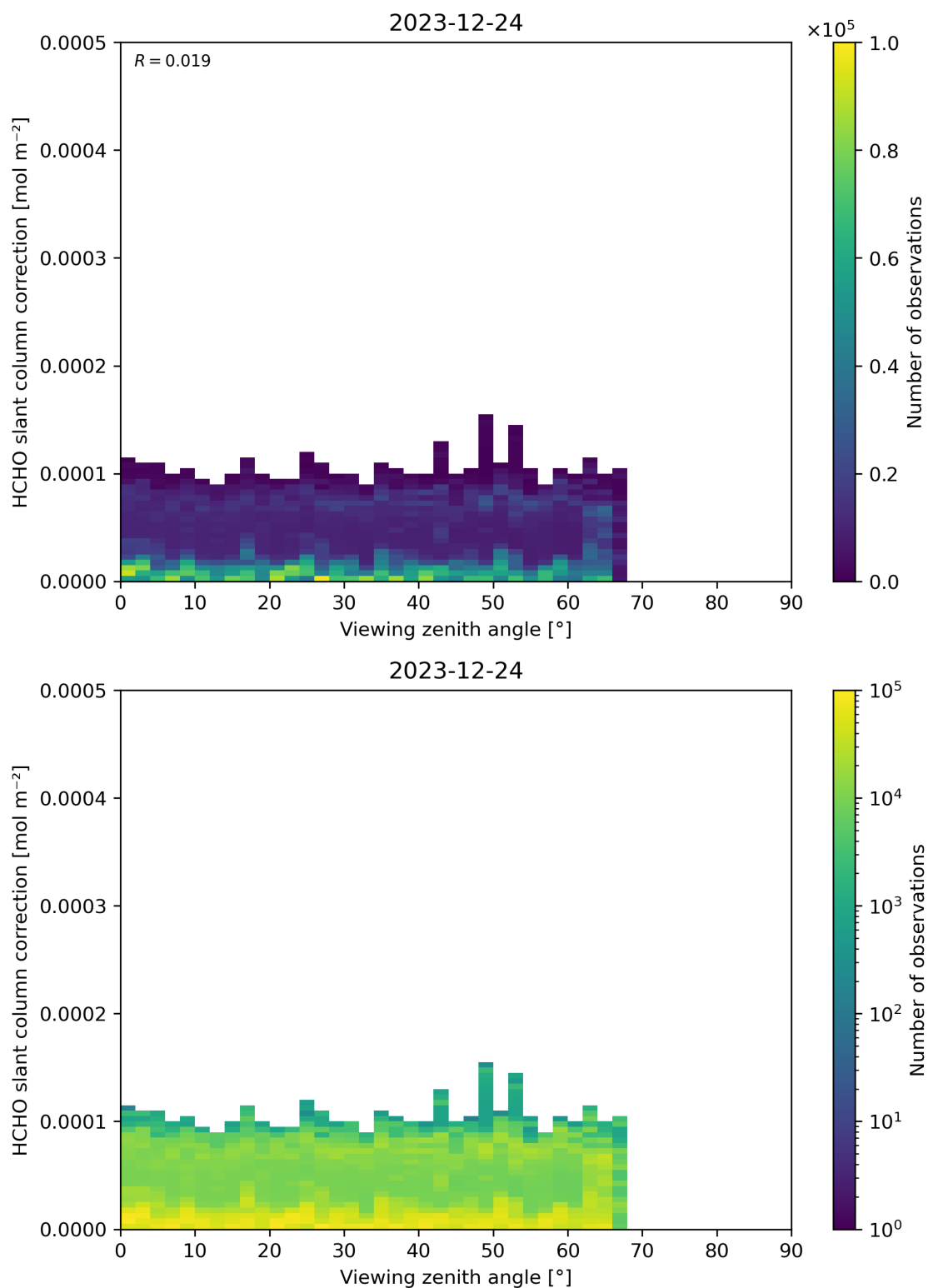
Figure 187: Scatter density plot of “Viewing zenith angle” against “HCHO slant column correction” for 2023-12-23 to 2023-12-25.
