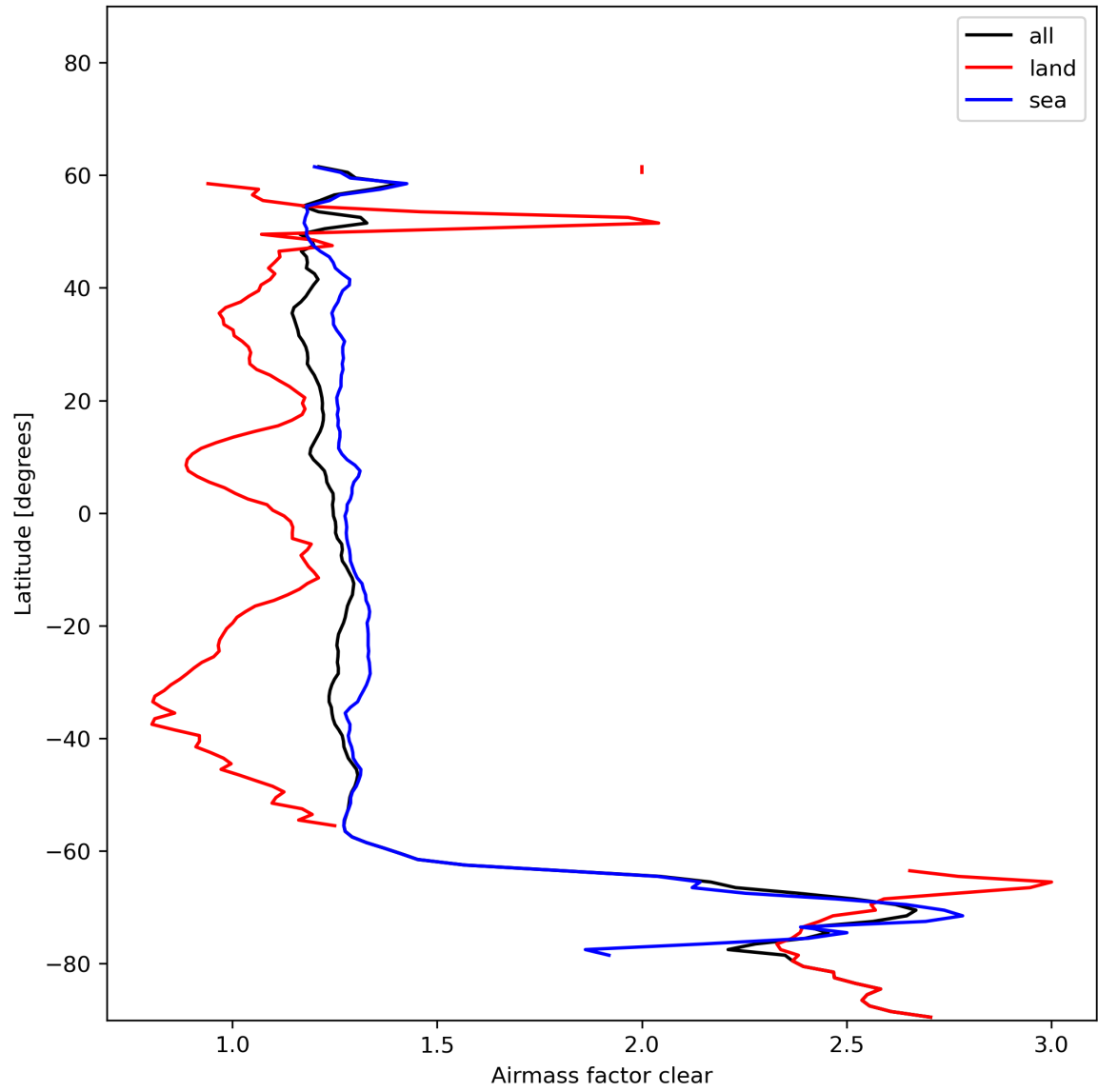
Figure 28: Zonal average of “Airmass factor clear” for 2023-12-23 to 2023-12-25.
