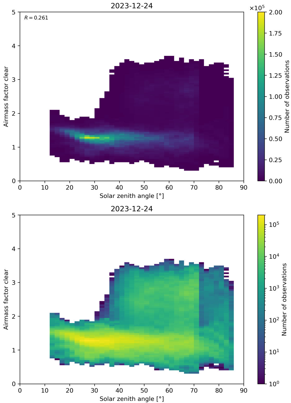
Figure 170: Scatter density plot of “Solar zenith angle” against “Airmass factor clear” for 2023-12-23 to 2023-12-25.
