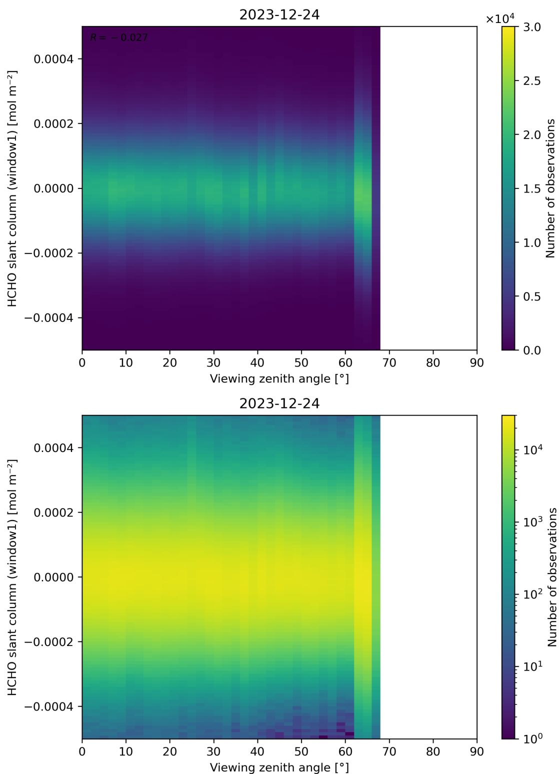
Figure 188: Scatter density plot of “Viewing zenith angle” against “HCHO slant column (window1)” for 2023-12-23 to 2023-12-25.
