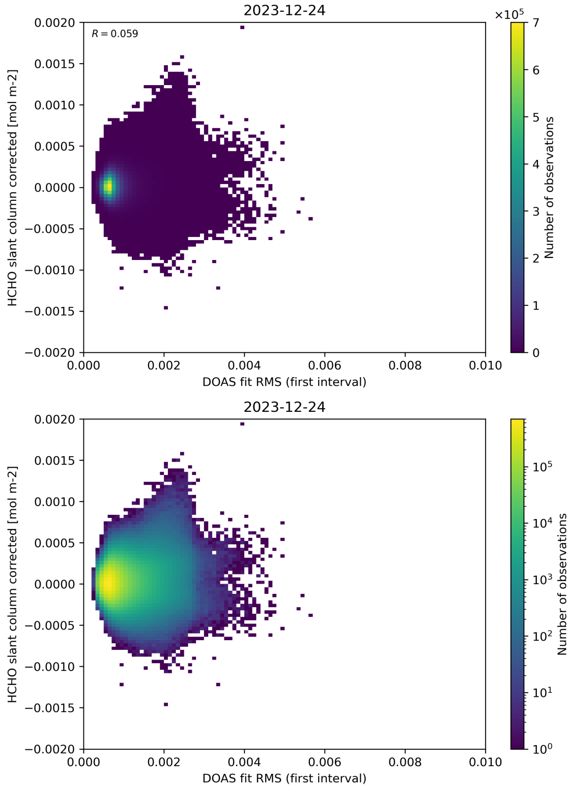
Figure 62: Scatter density plot of “DOAS fit RMS (first interval)” against “HCHO slant column corrected” for 2023-12-23 to 2023-12-25.
