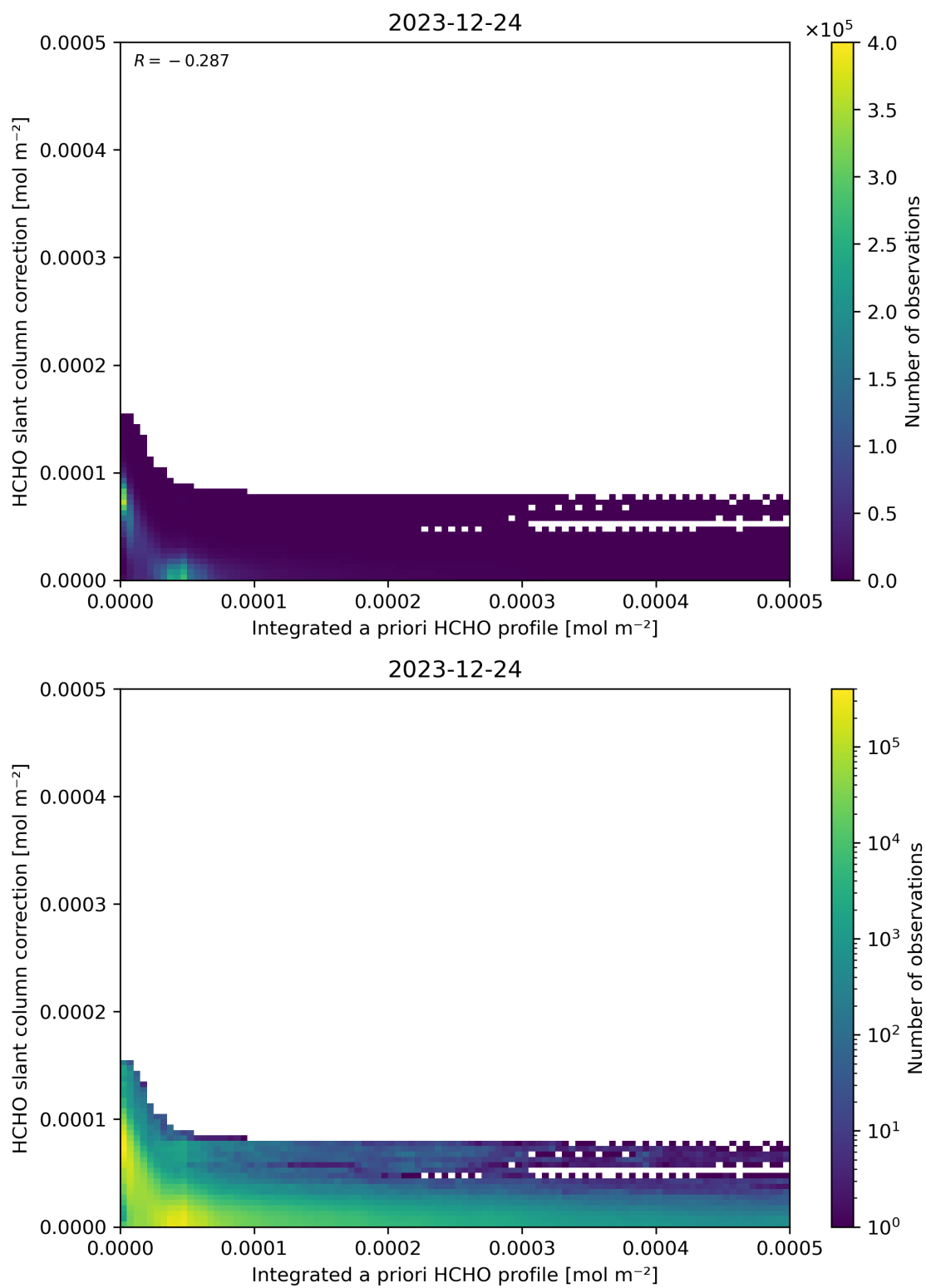
Figure 152: Scatter density plot of “Integrated a priori HCHO profile” against “HCHO slant column correction” for 2023-12-23 to 2023-12-25.
