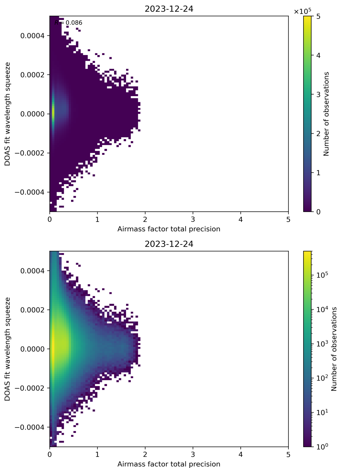
Figure 107: Scatter density plot of “Airmass factor total precision” against “DOAS fit wavelength squeeze” for 2023-12-23 to 2023-12-25.
