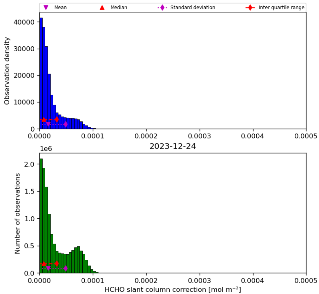
Figure 47: Histogram of “HCHO slant column correction” for 2023-12-23 to 2023-12-25
