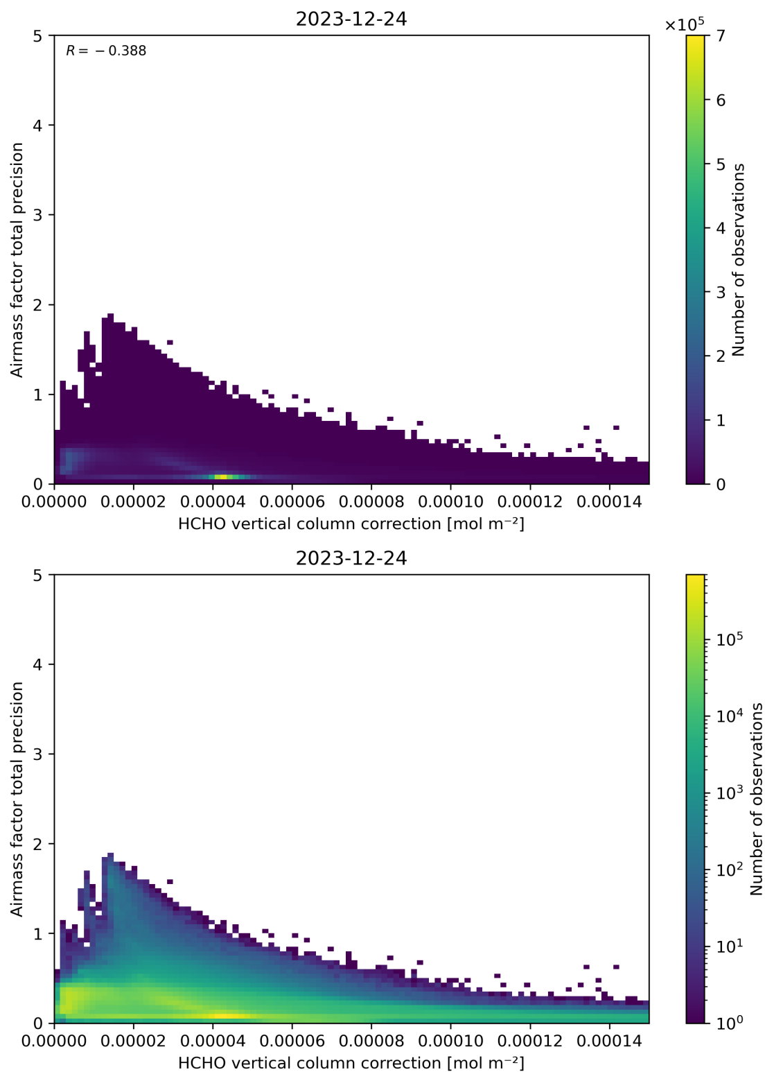
Figure 121: Scatter density plot of “HCHO vertical column correction” against “Airmass factor total precision” for 2023-12-23 to 2023-12-25.
