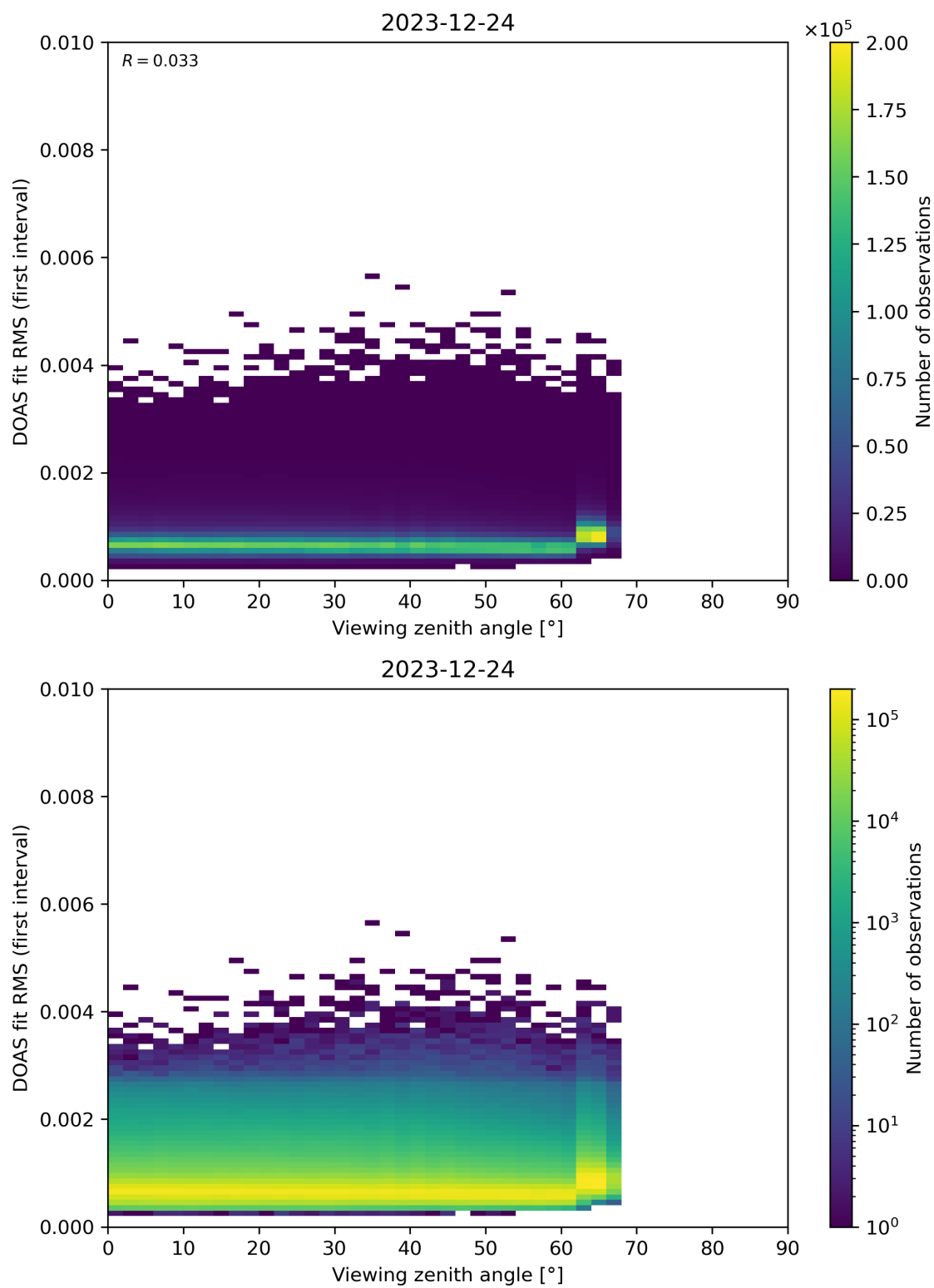
Figure 182: Scatter density plot of “Viewing zenith angle” against “DOAS fit RMS (first interval)” for 2023-12-23 to 2023-12-25.
