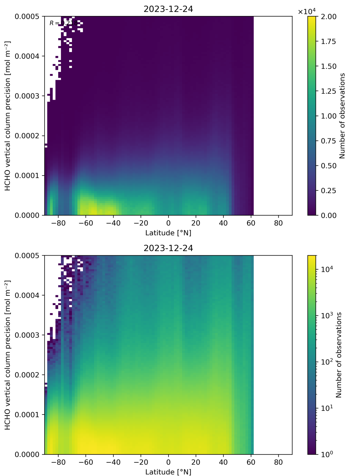
Figure 165: Scatter density plot of “Latitude” against “HCHO vertical column precision” for 2023-12-23 to 2023-12-25.
