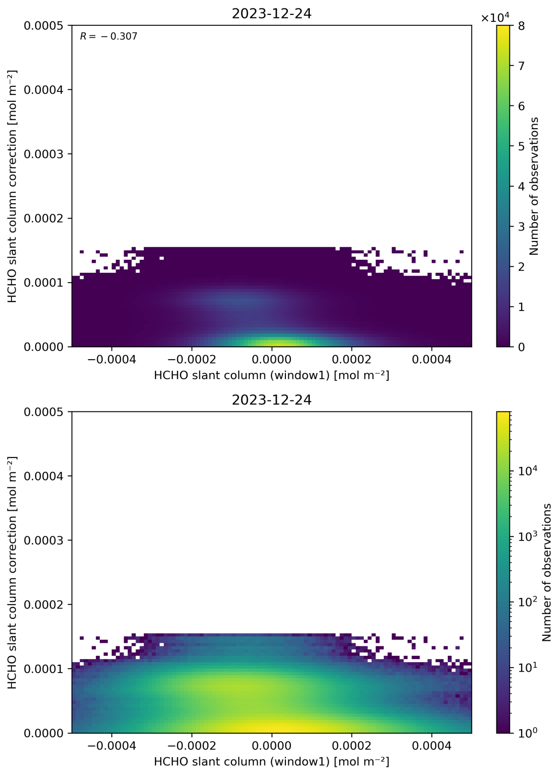
Figure 83: Scatter density plot of “HCHO slant column (window1)” against “HCHO slant column correction” for 2023-12-23 to 2023-12-25.
