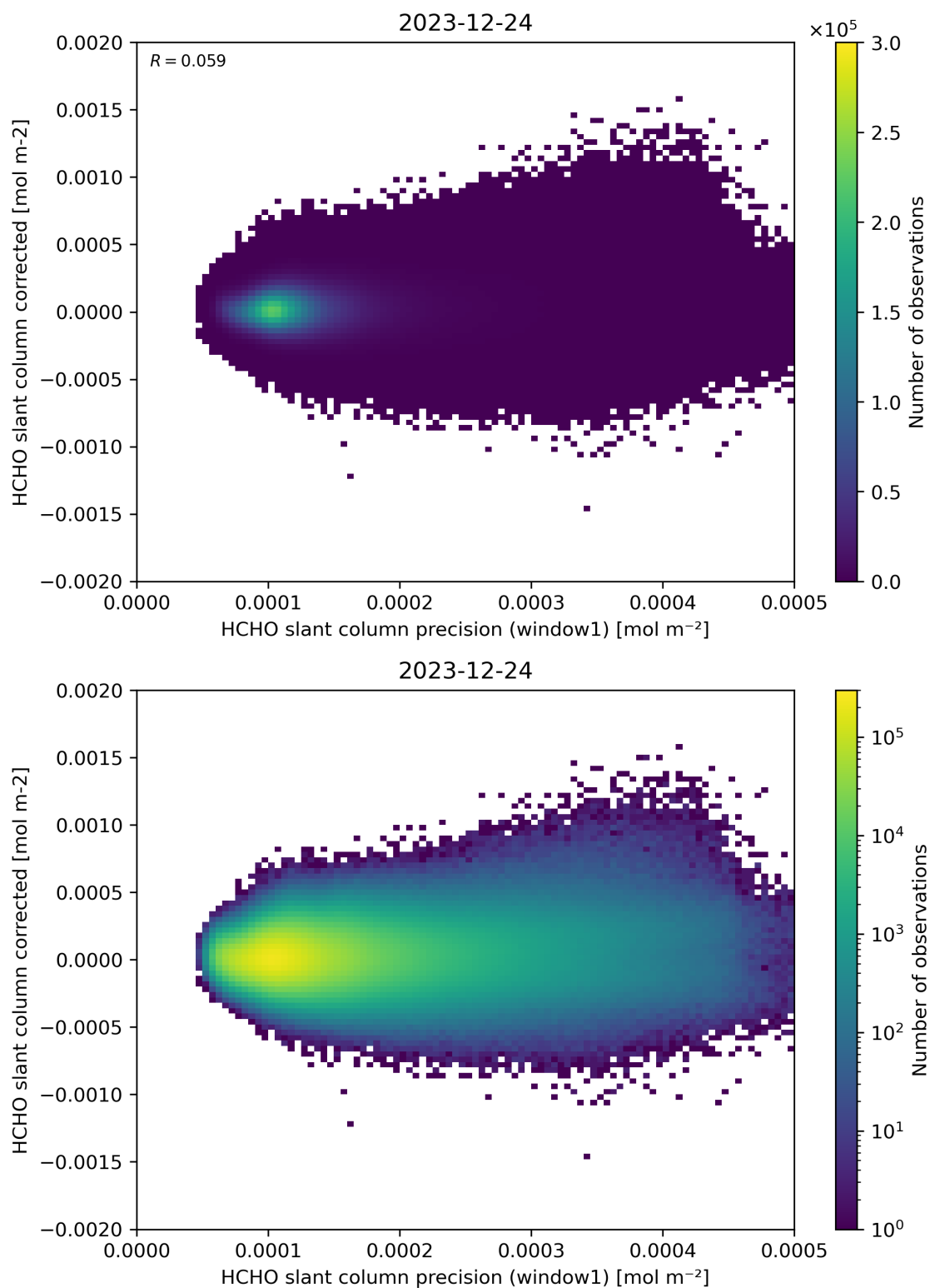
Figure 92: Scatter density plot of “HCHO slant column precision (window1)” against “HCHO slant column corrected” for 2023-12-23 to 2023-12-25.
