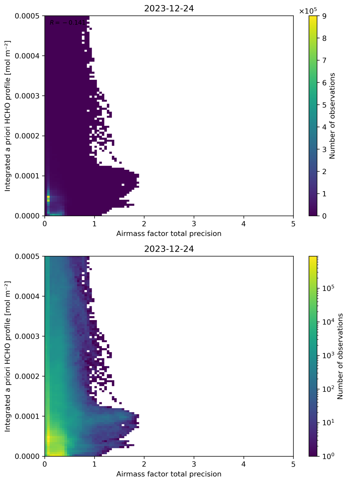
Figure 111: Scatter density plot of “Airmass factor total precision” against “Integrated a priori HCHO profile” for 2023-12-23 to 2023-12-25.
