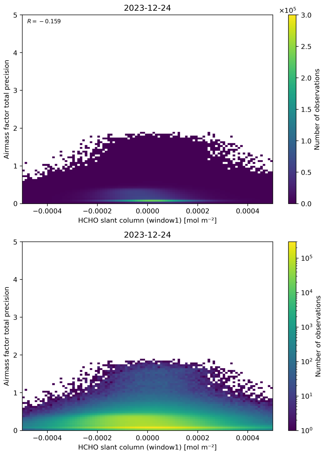
Figure 86: Scatter density plot of “HCHO slant column (window1)” against “Airmass factor total precision” for 2023-12-23 to 2023-12-25.
