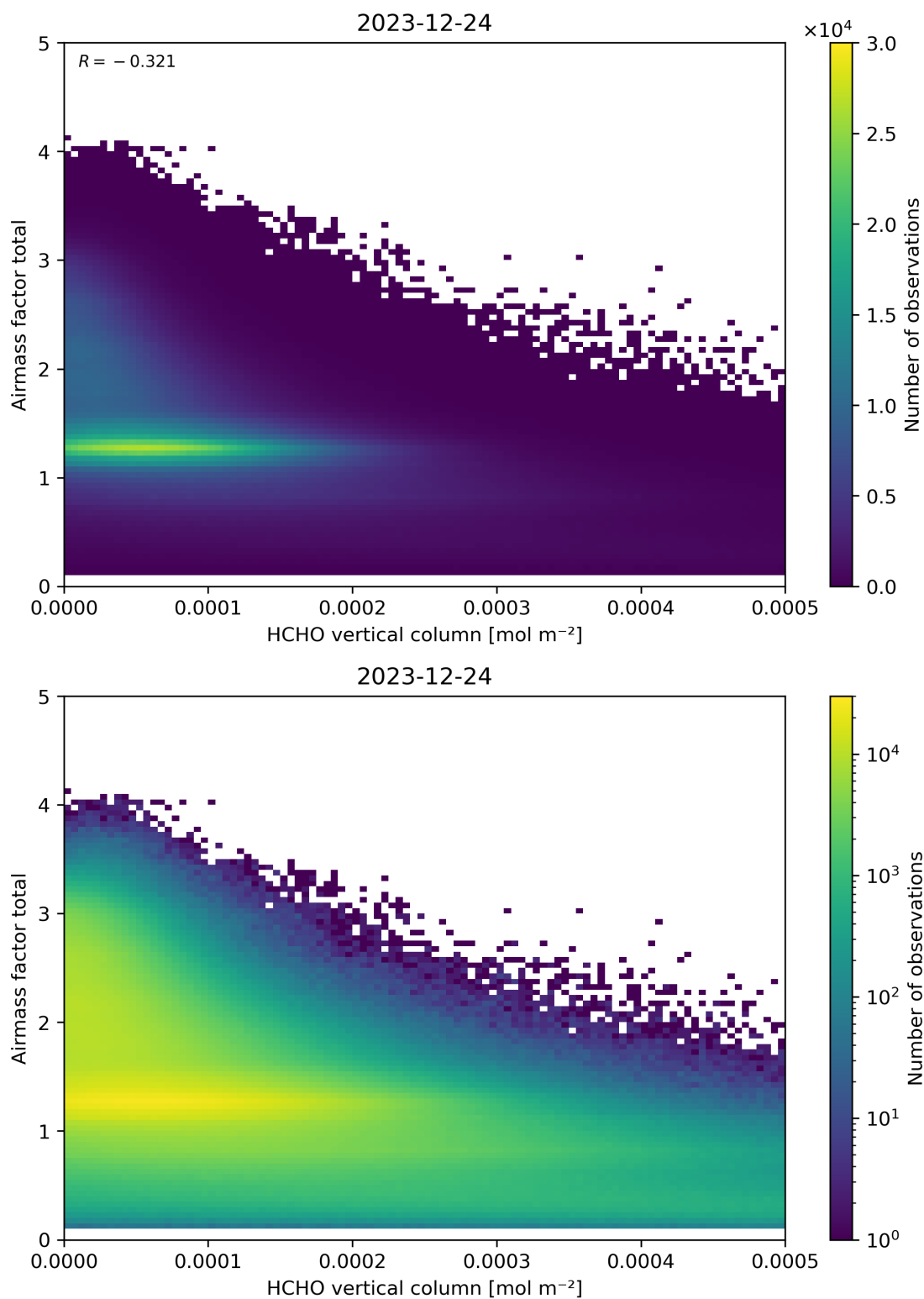
Figure 131: Scatter density plot of “HCHO vertical column” against “Airmass factor total” for 2023-12-23 to 2023-12-25.
