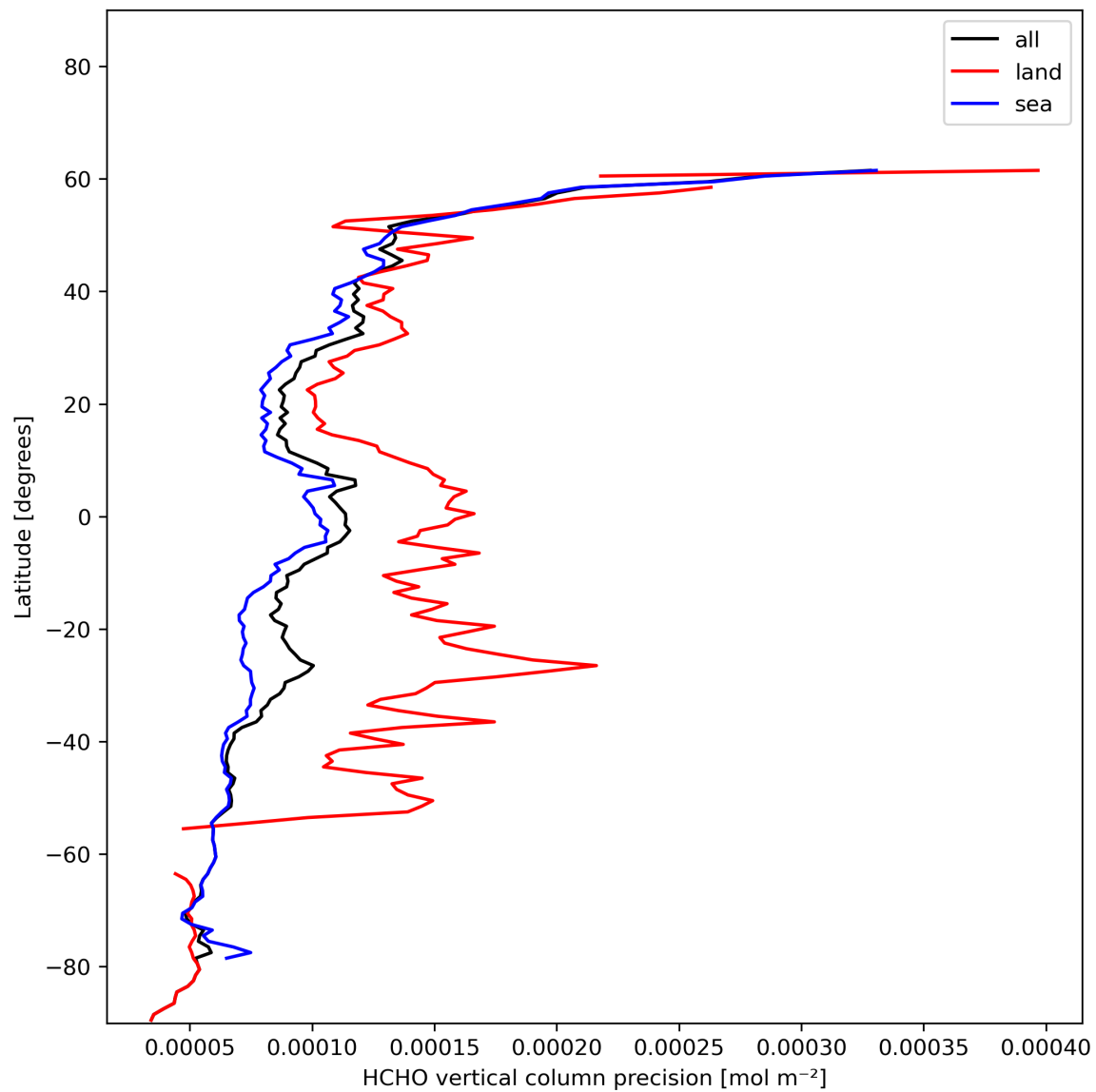
Figure 22: Zonal average of “HCHO vertical column precision” for 2023-12-23 to 2023-12-25.
