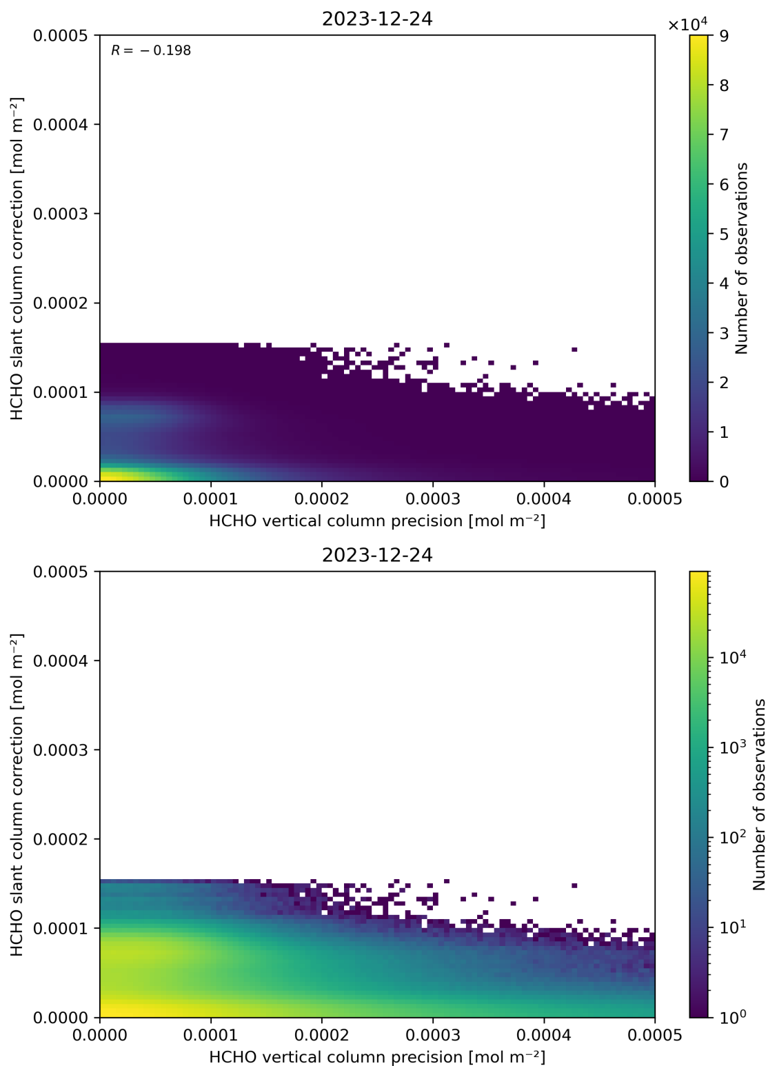
Figure 141: Scatter density plot of “HCHO vertical column precision” against “HCHO slant column correction” for 2023-12-23 to 2023-12-25.
