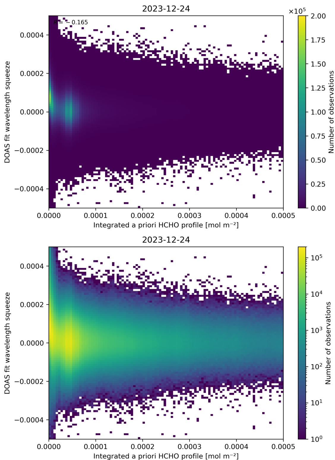
Figure 150: Scatter density plot of “Integrated a priori HCHO profile” against “DOAS fit wavelength squeeze” for 2023-12-23 to 2023-12-25.
