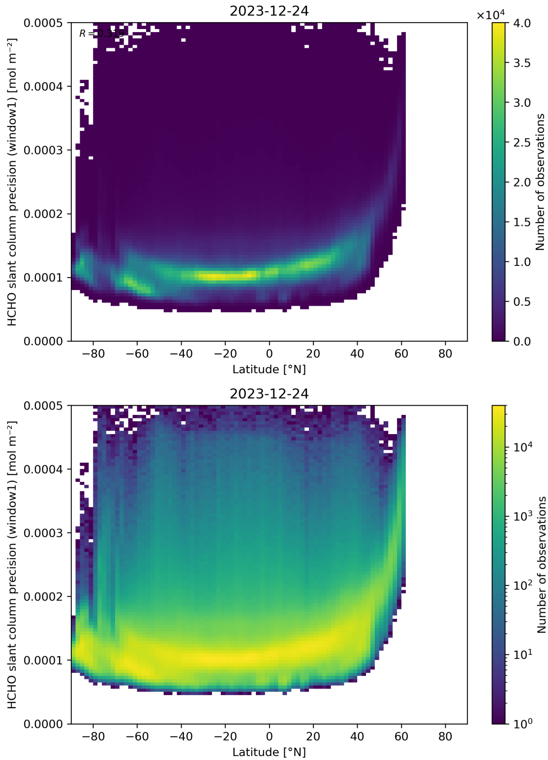
Figure 160: Scatter density plot of “Latitude” against “HCHO slant column precision (window1)” for 2023-12-23 to 2023-12-25.
