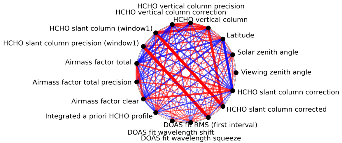
Figure 1: Map of correlation graph for 2023-12-23 to 2023-12-25.
