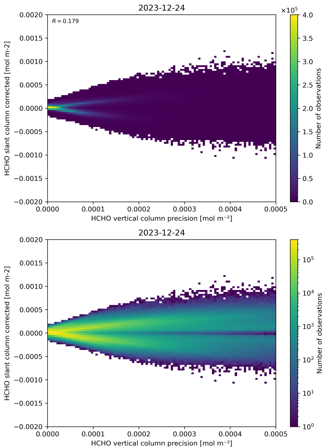
Figure 140: Scatter density plot of “HCHO vertical column precision” against “HCHO slant column corrected” for 2023-12-23 to 2023-12-25.
