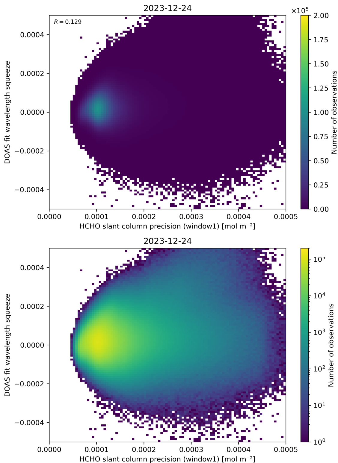
Figure 90: Scatter density plot of “HCHO slant column precision (window1)” against “DOAS fit wavelength squeeze” for 2023-12-23 to 2023-12-25.
