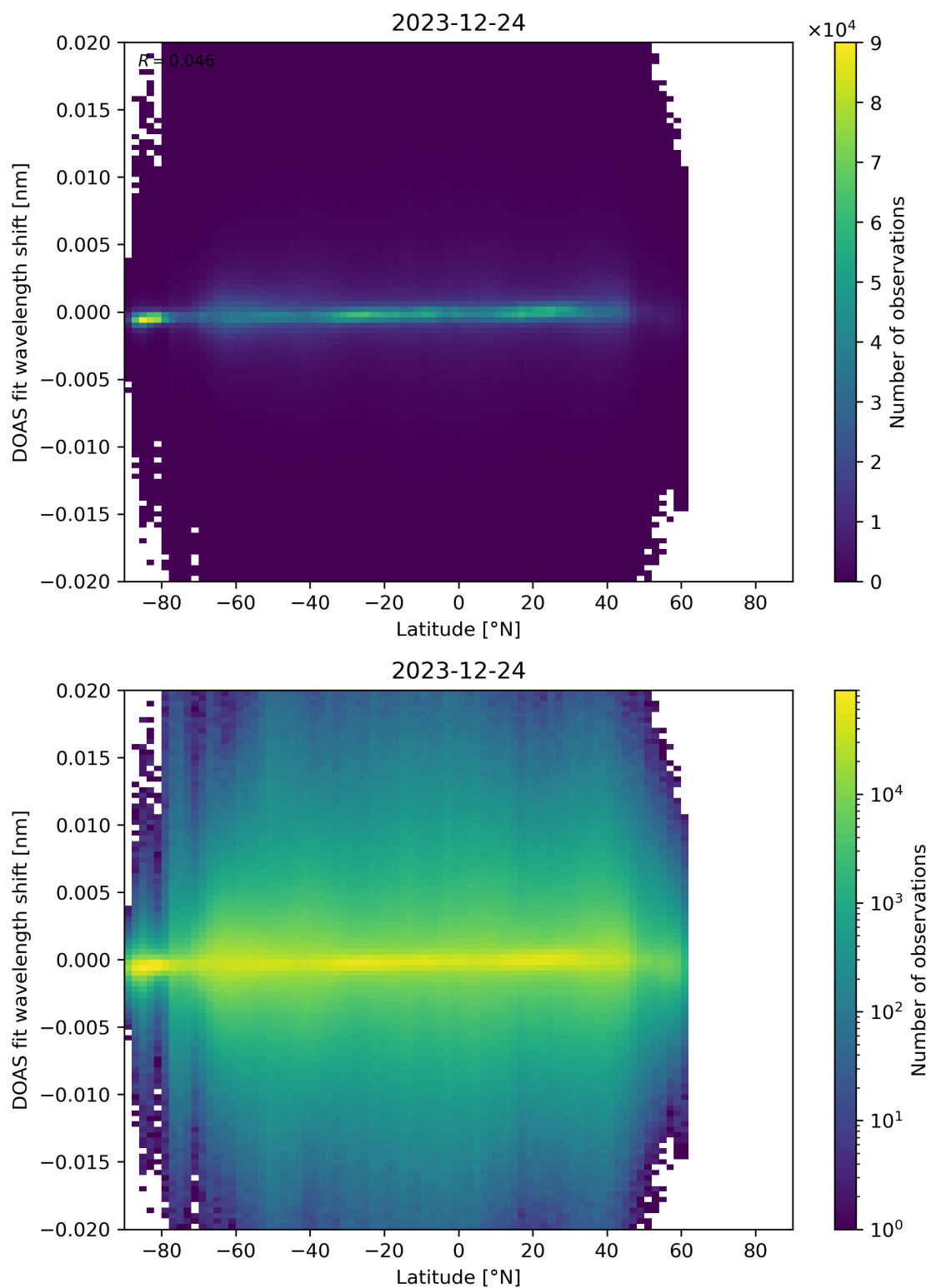
Figure 154: Scatter density plot of “Latitude” against “DOAS fit wavelength shift” for 2023-12-23 to 2023-12-25.
