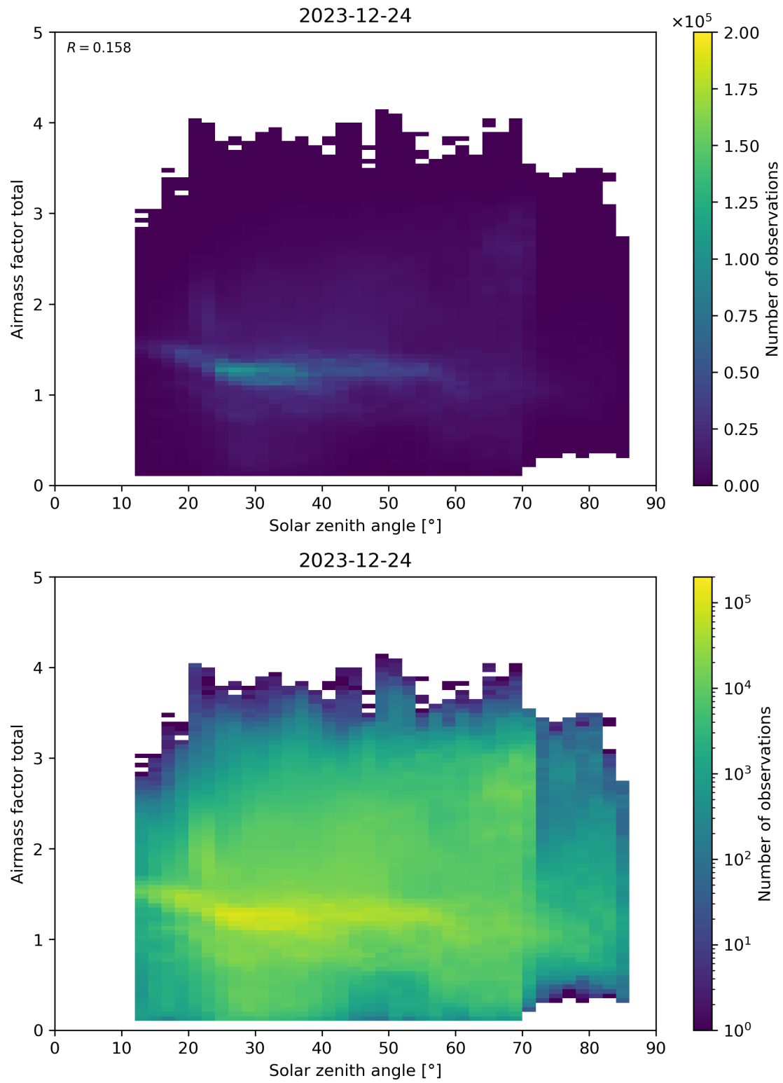
Figure 175: Scatter density plot of “Solar zenith angle” against “Airmass factor total” for 2023-12-23 to 2023-12-25.
