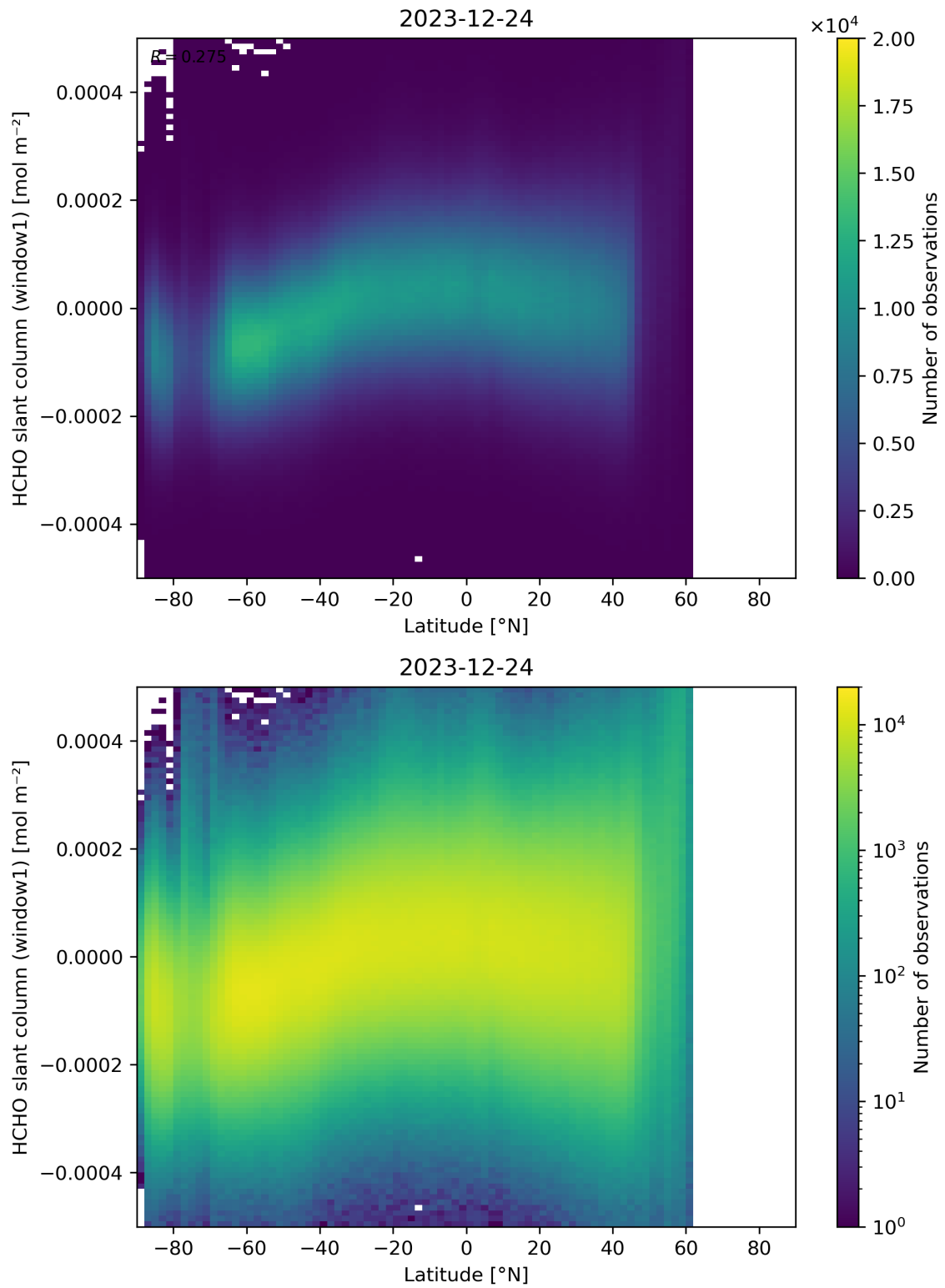
Figure 159: Scatter density plot of “Latitude” against “HCHO slant column (window1)” for 2023-12-23 to 2023-12-25.
