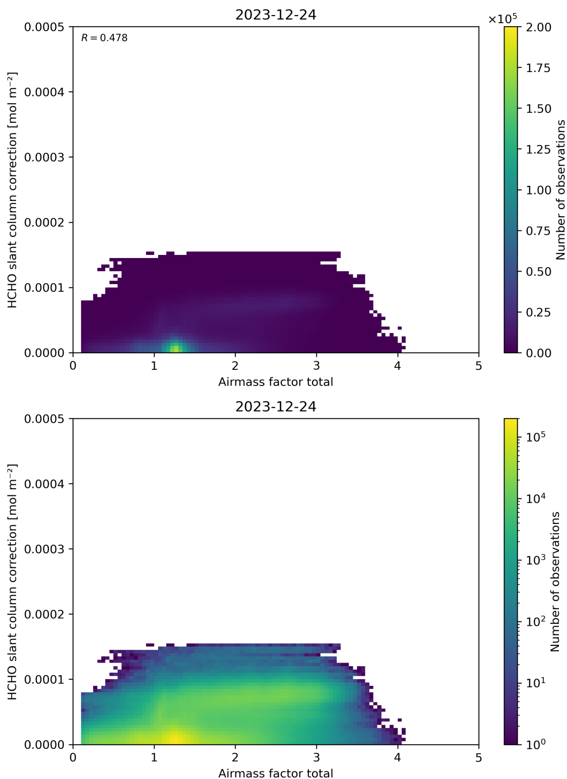
Figure 102: Scatter density plot of “Airmass factor total” against “HCHO slant column correction” for 2023-12-23 to 2023-12-25.
