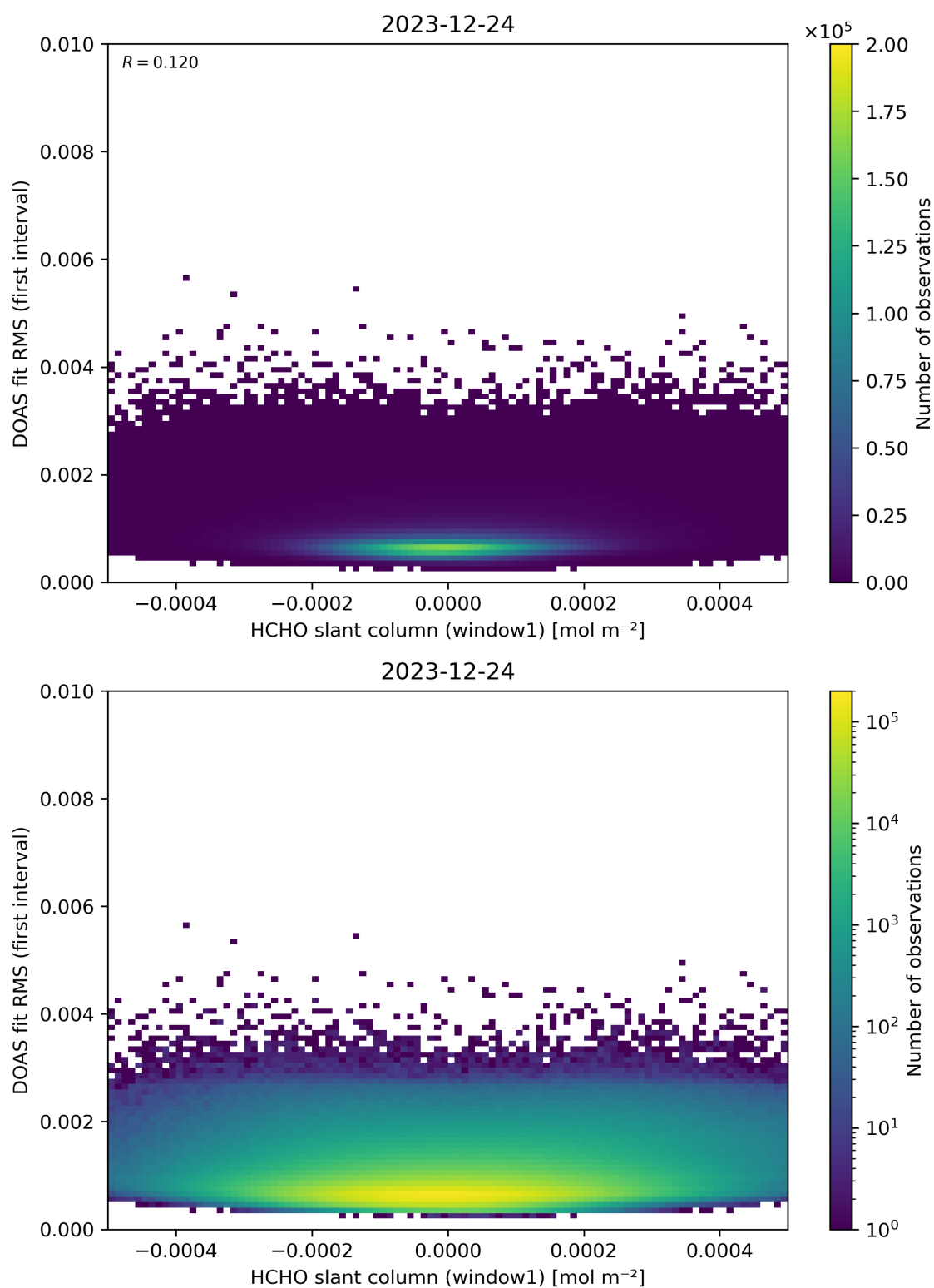
Figure 78: Scatter density plot of “HCHO slant column (window1)” against “DOAS fit RMS (first interval)” for 2023-12-23 to 2023-12-25.
