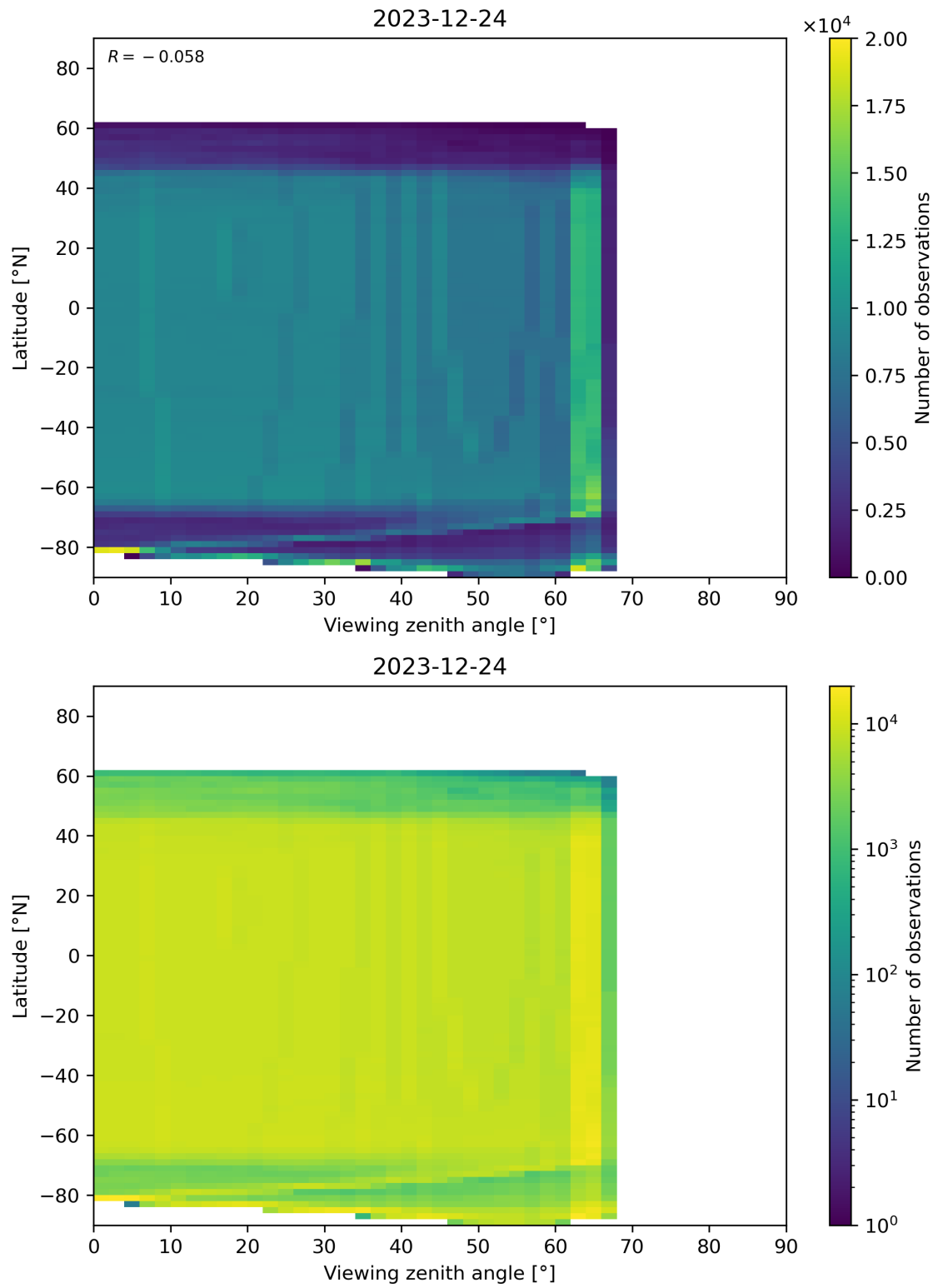
Figure 196: Scatter density plot of “Viewing zenith angle” against “Latitude” for 2023-12-23 to 2023-12-25.
