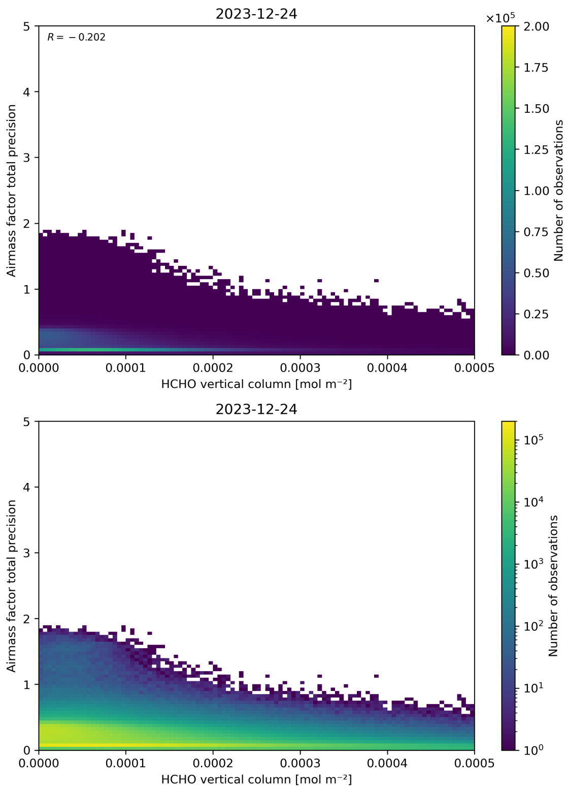
Figure 132: Scatter density plot of “HCHO vertical column” against “Airmass factor total precision” for 2023-12-23 to 2023-12-25.
