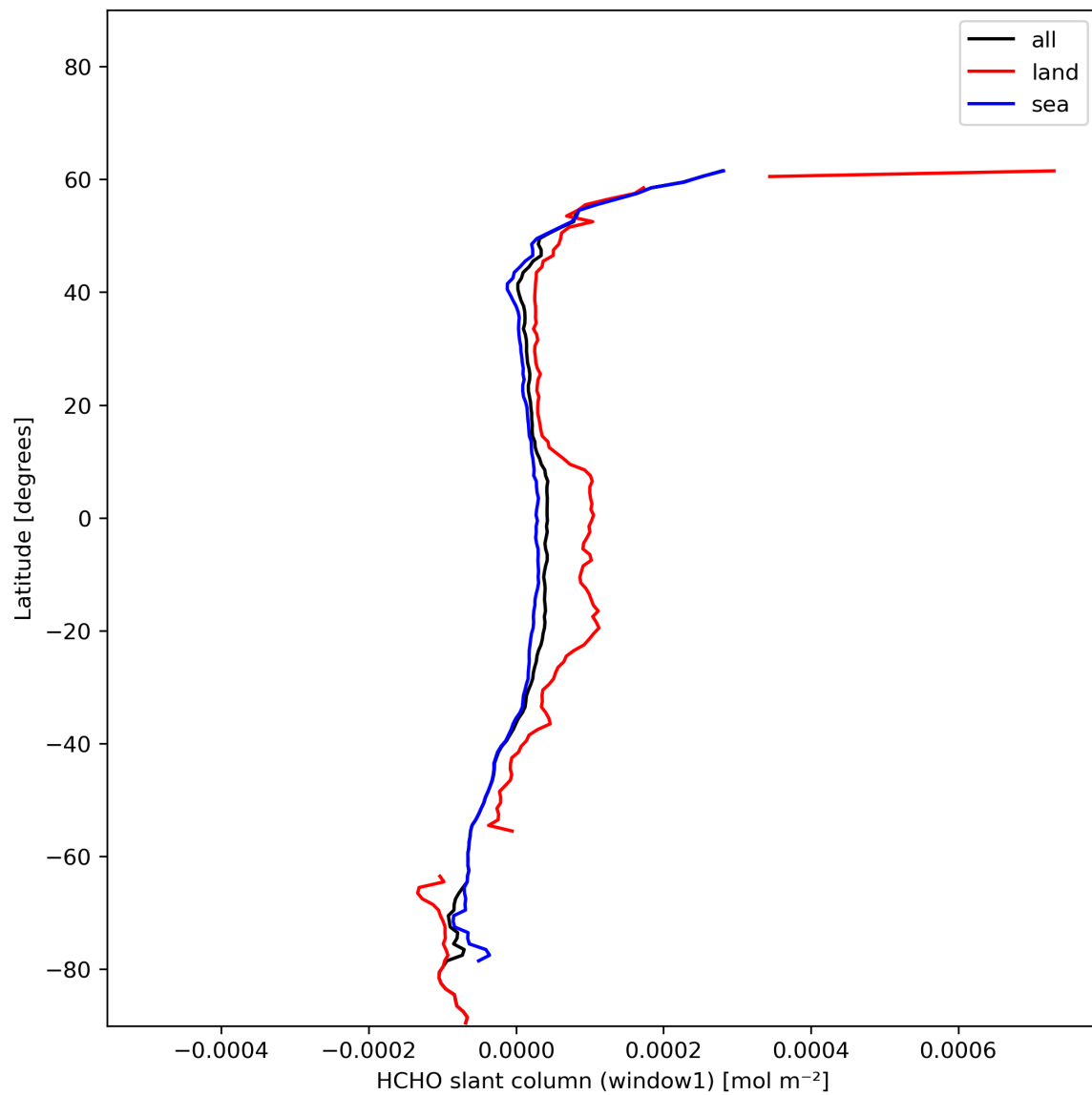
Figure 24: Zonal average of “HCHO slant column (window1)” for 2023-12-23 to 2023-12-25.
