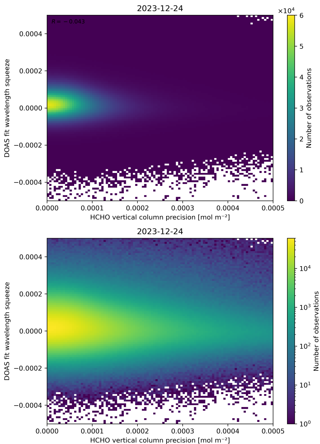
Figure 138: Scatter density plot of “HCHO vertical column precision” against “DOAS fit wavelength squeeze” for 2023-12-23 to 2023-12-25.
