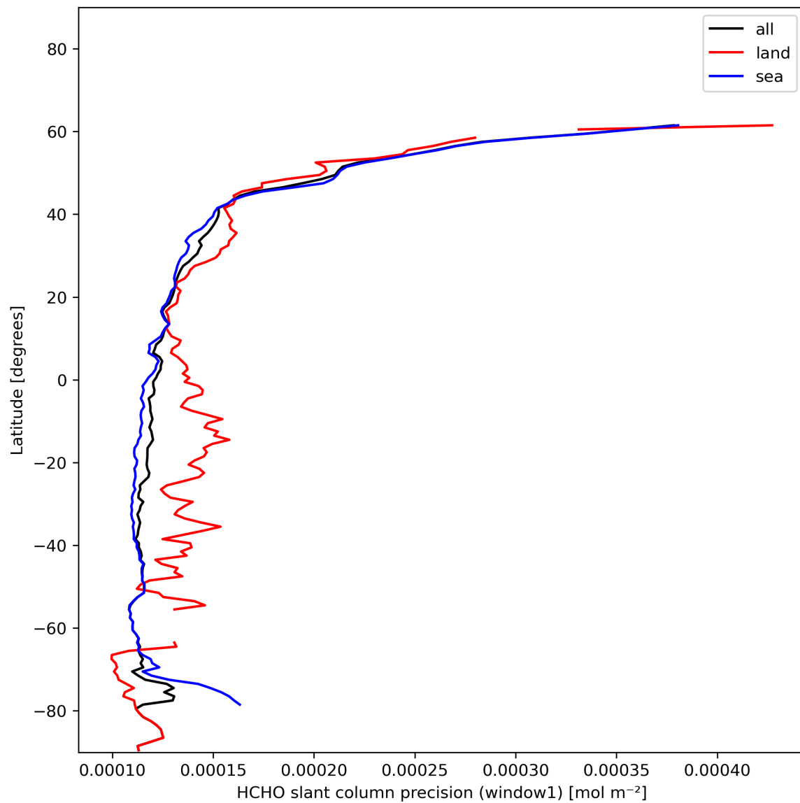
Figure 25: Zonal average of "HCHO slant column precision (window1)" for 2023-12-23 to 2023-12-25.
