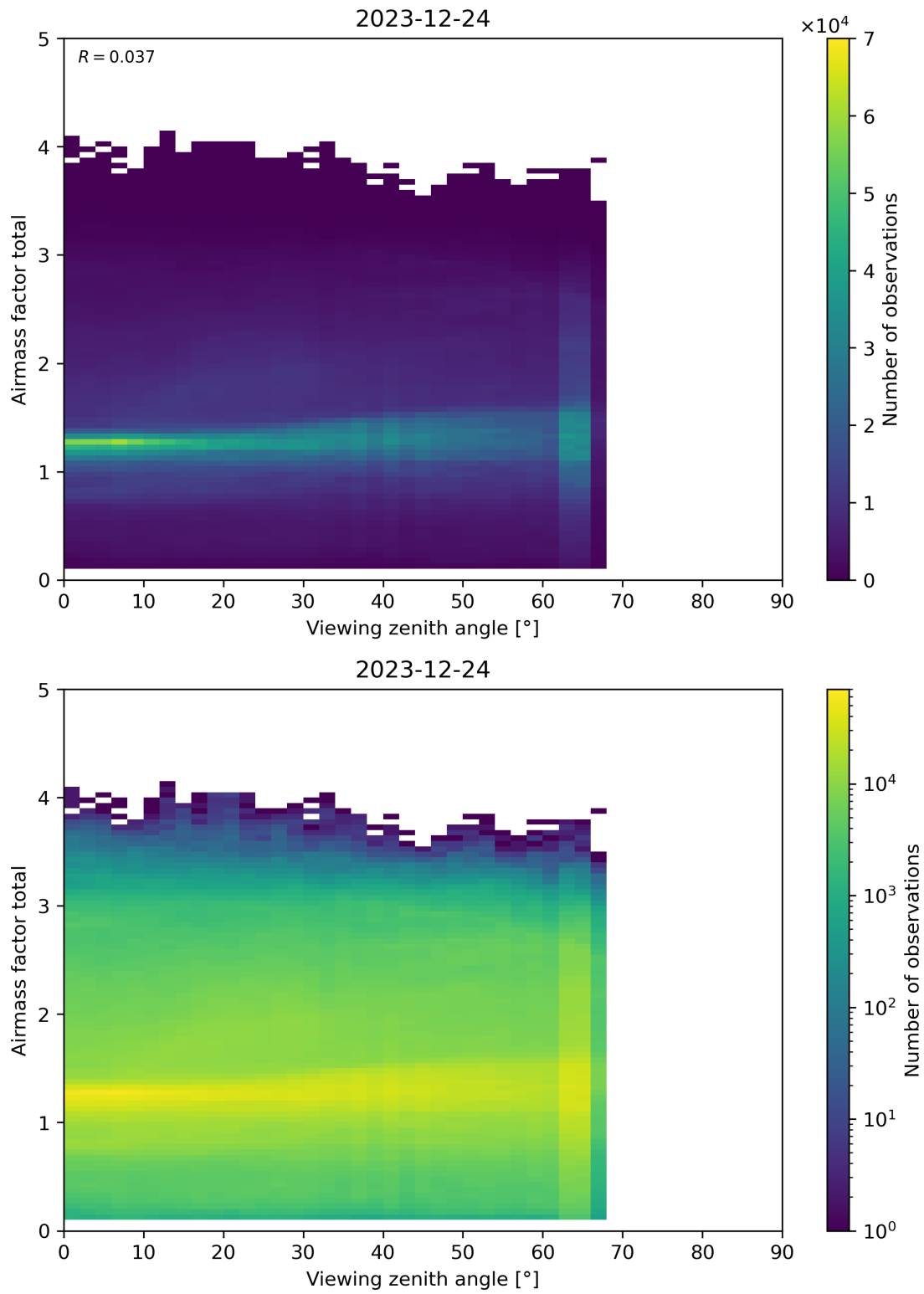
Figure 190: Scatter density plot of “Viewing zenith angle” against “Airmass factor total” for 2023-12-23 to 2023-12-25.
