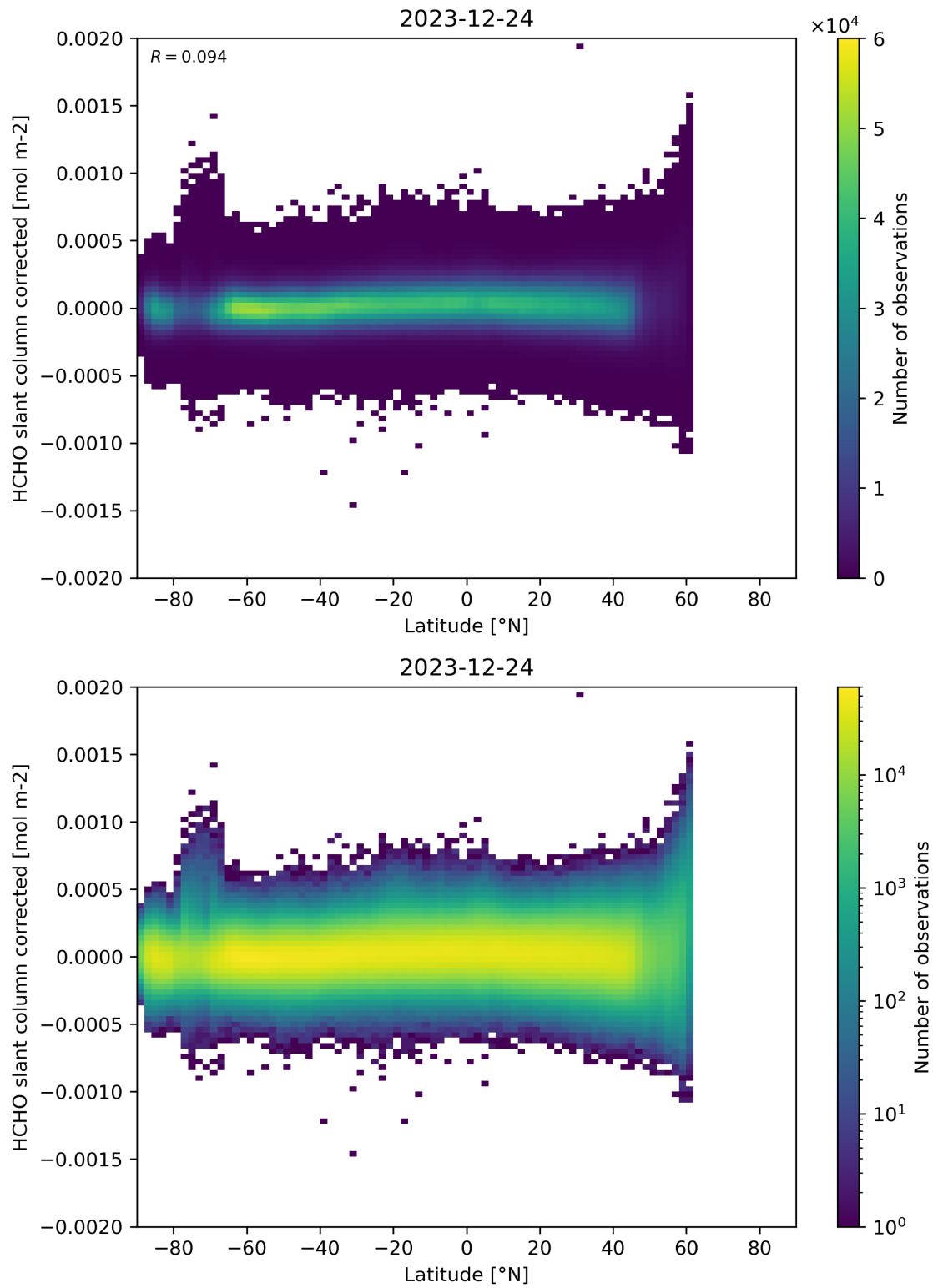
Figure 157: Scatter density plot of “Latitude” against “HCHO slant column corrected” for 2023-12-23 to 2023-12-25.
