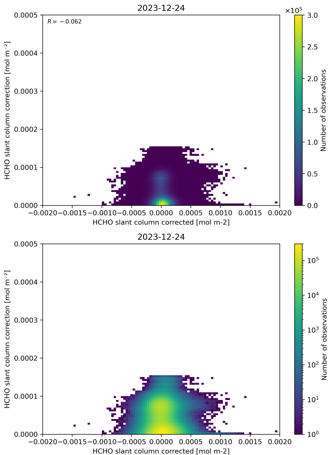
Figure 77: Scatter density plot of “HCHO slant column corrected” against “HCHO slant column correction” for 2023-12-23 to 2023-12-25.
