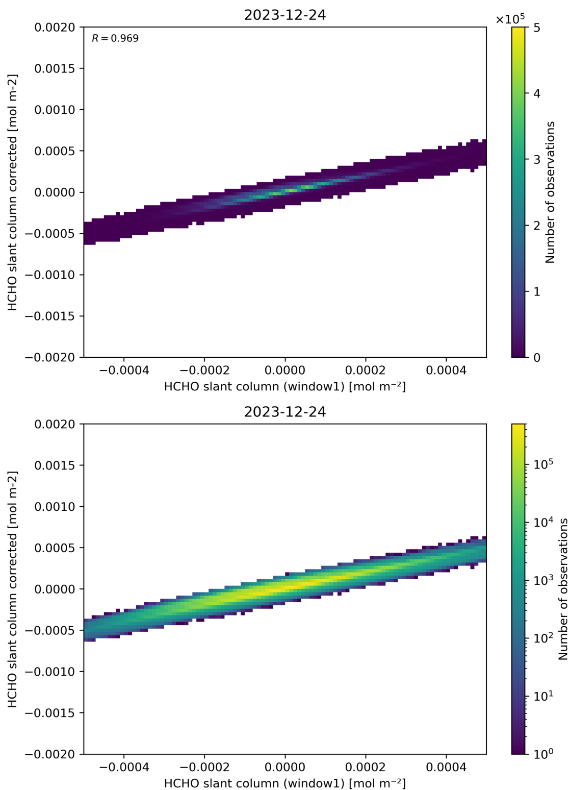
Figure 82: Scatter density plot of “HCHO slant column (window1)” against “HCHO slant column corrected” for 2023-12-23 to 2023-12-25.
