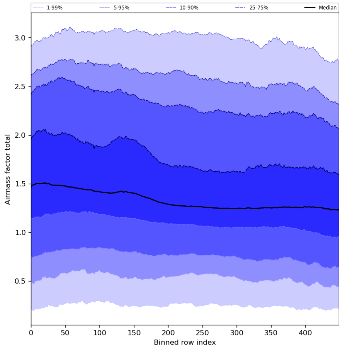
Figure 54: Along track statistics of “Airmass factor total” for 2023-12-23 to 2023-12-25
