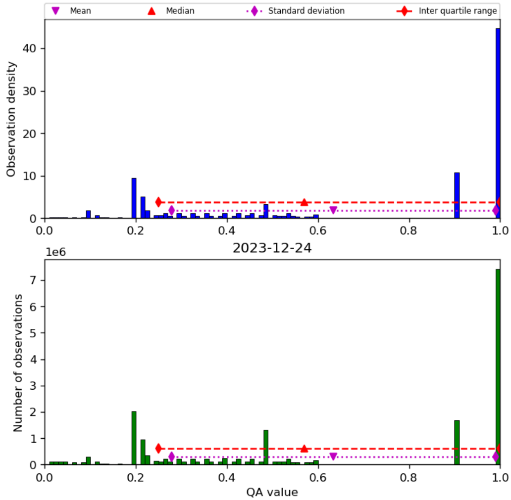
Figure 34: Histogram of “QA value” for 2023-12-23 to 2023-12-25
