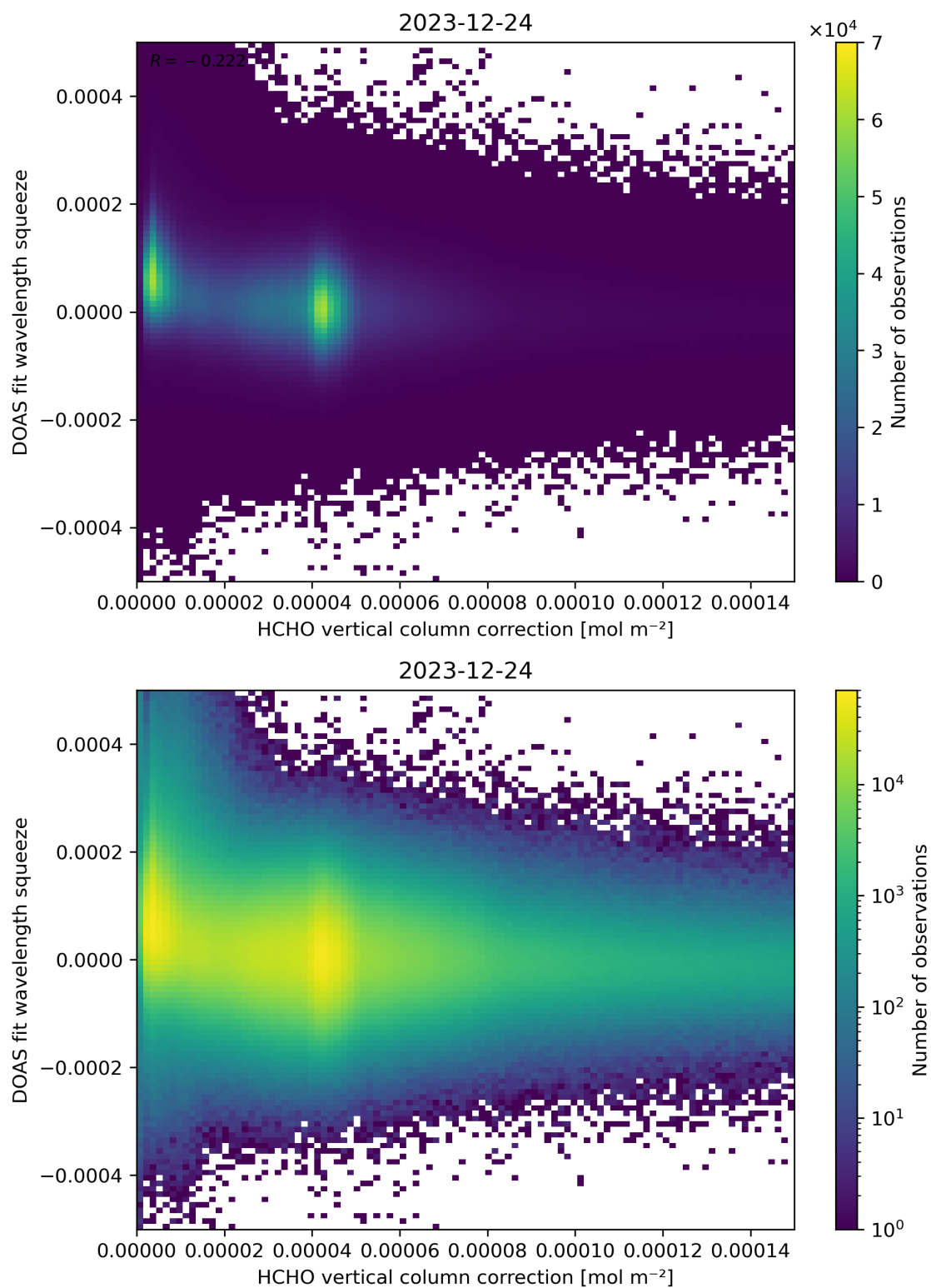
Figure 114: Scatter density plot of “HCHO vertical column correction” against “DOAS fit wavelength squeeze” for 2023-12-23 to 2023-12-25.
