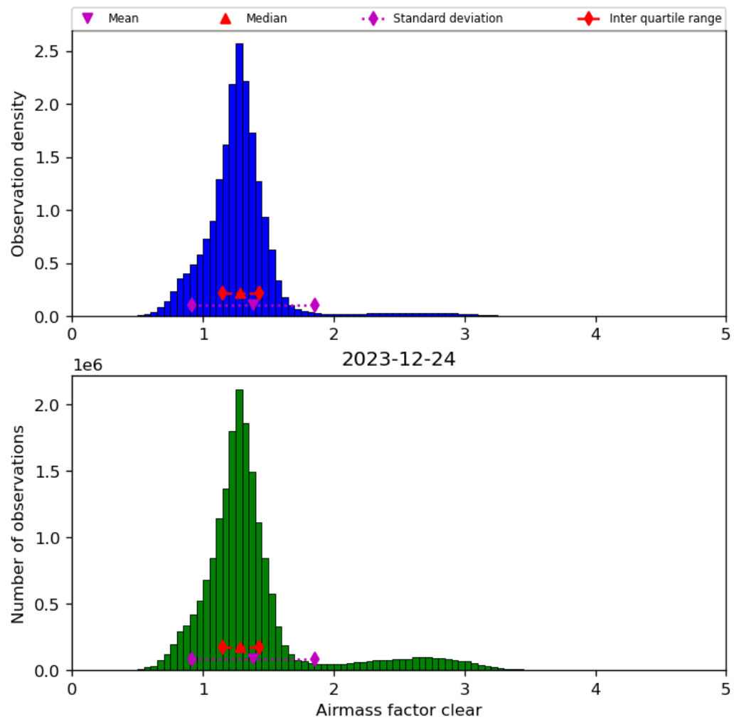
Figure 42: Histogram of “Airmass factor clear” for 2023-12-23 to 2023-12-25
