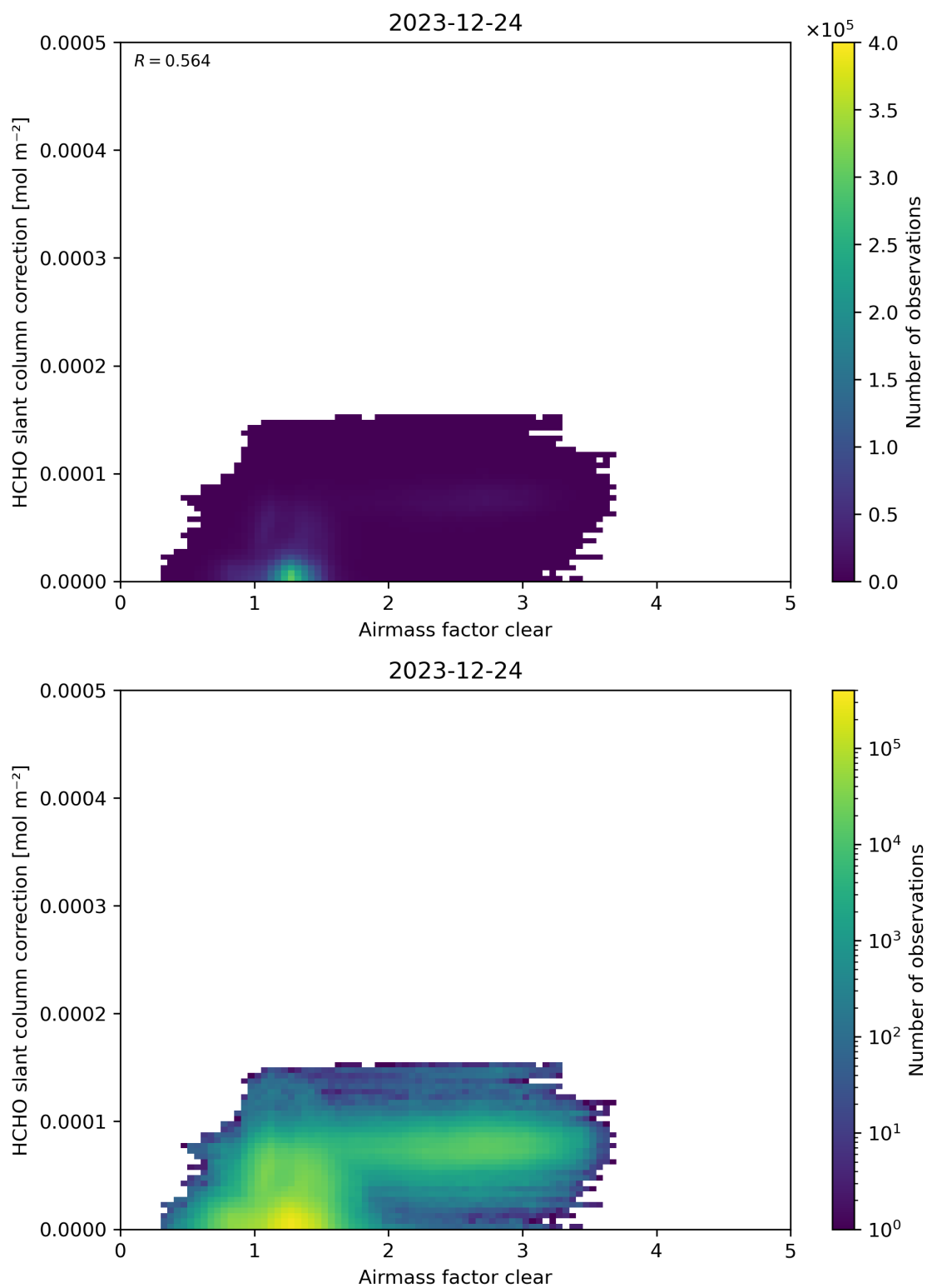
Figure 75: Scatter density plot of “Airmass factor clear” against “HCHO slant column correction” for 2023-12-23 to 2023-12-25.
