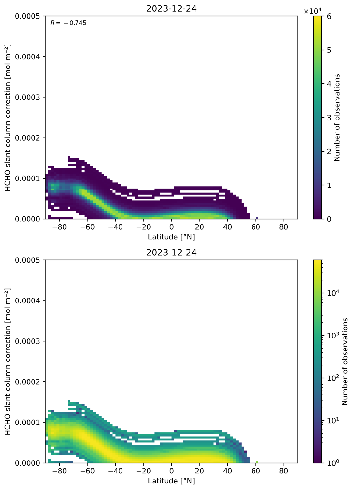
Figure 158: Scatter density plot of “Latitude” against “HCHO slant column correction” for 2023-12-23 to 2023-12-25.
