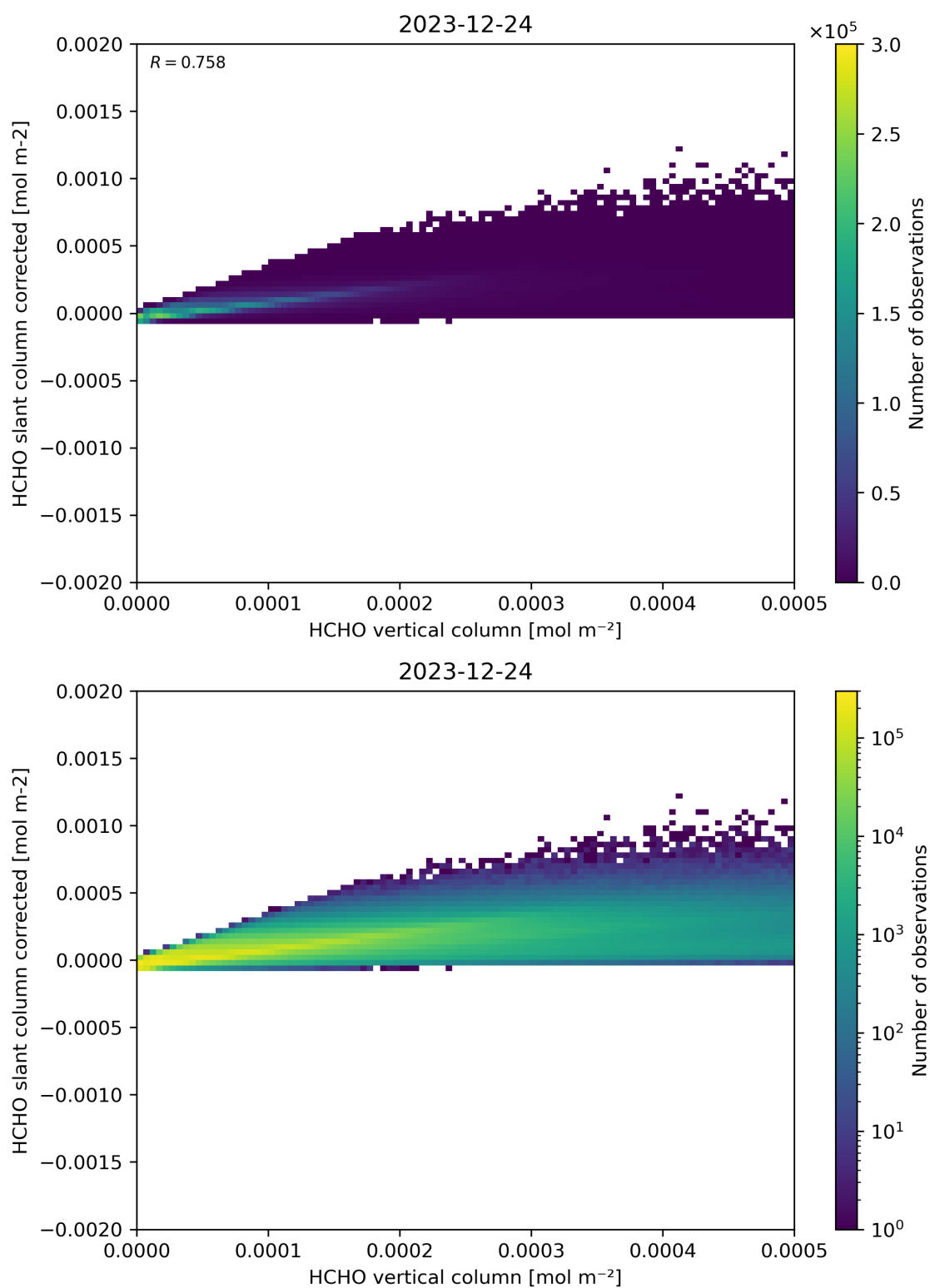
Figure 127: Scatter density plot of “HCHO vertical column” against “HCHO slant column corrected” for 2023-12-23 to 2023-12-25.
