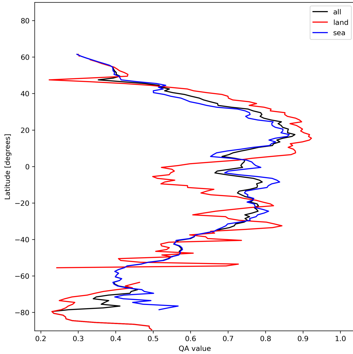
Figure 20: Zonal average of “QA value” for 2023-12-23 to 2023-12-25.
