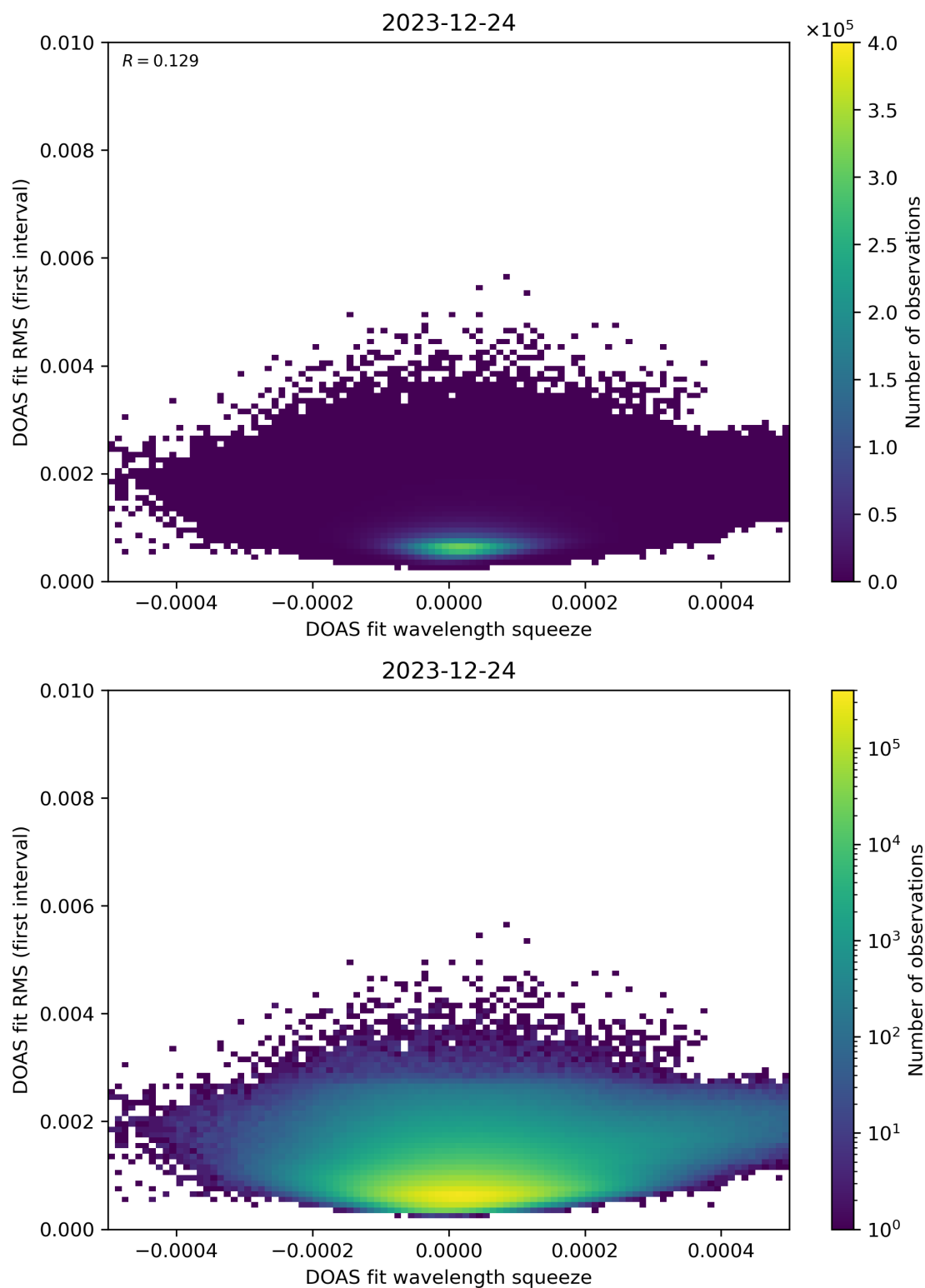
Figure 68: Scatter density plot of “DOAS fit wavelength squeeze” against “DOAS fit RMS (first interval)” for 2023-12-23 to 2023-12-25.
