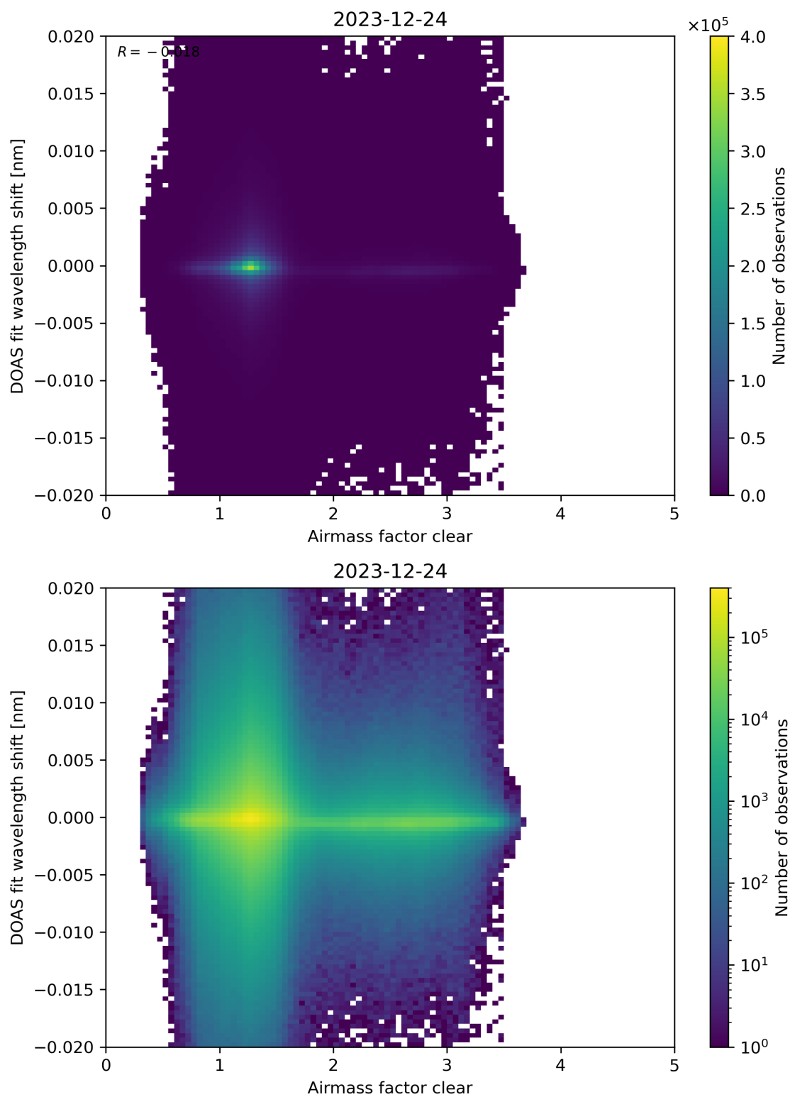
Figure 72: Scatter density plot of “Airmass factor clear” against “DOAS fit wavelength shift” for 2023-12-23 to 2023-12-25.
