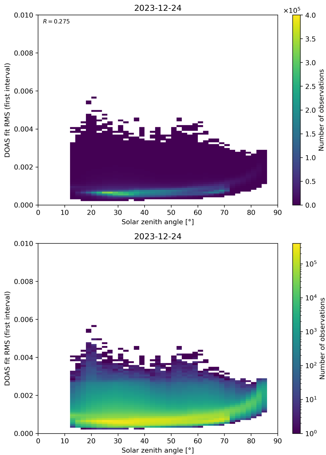
Figure 167: Scatter density plot of “Solar zenith angle” against “DOAS fit RMS (first interval)” for 2023-12-23 to 2023-12-25.
