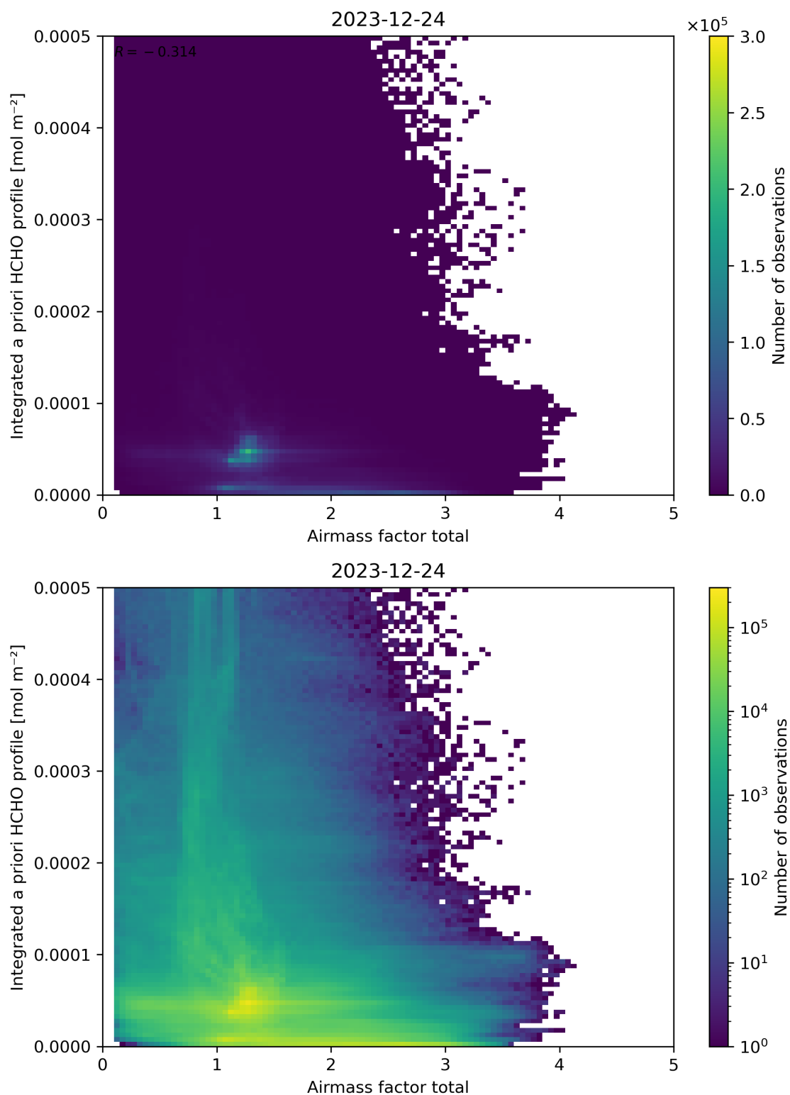
Figure 104: Scatter density plot of “Airmass factor total” against “Integrated a priori HCHO profile” for 2023-12-23 to 2023-12-25.
