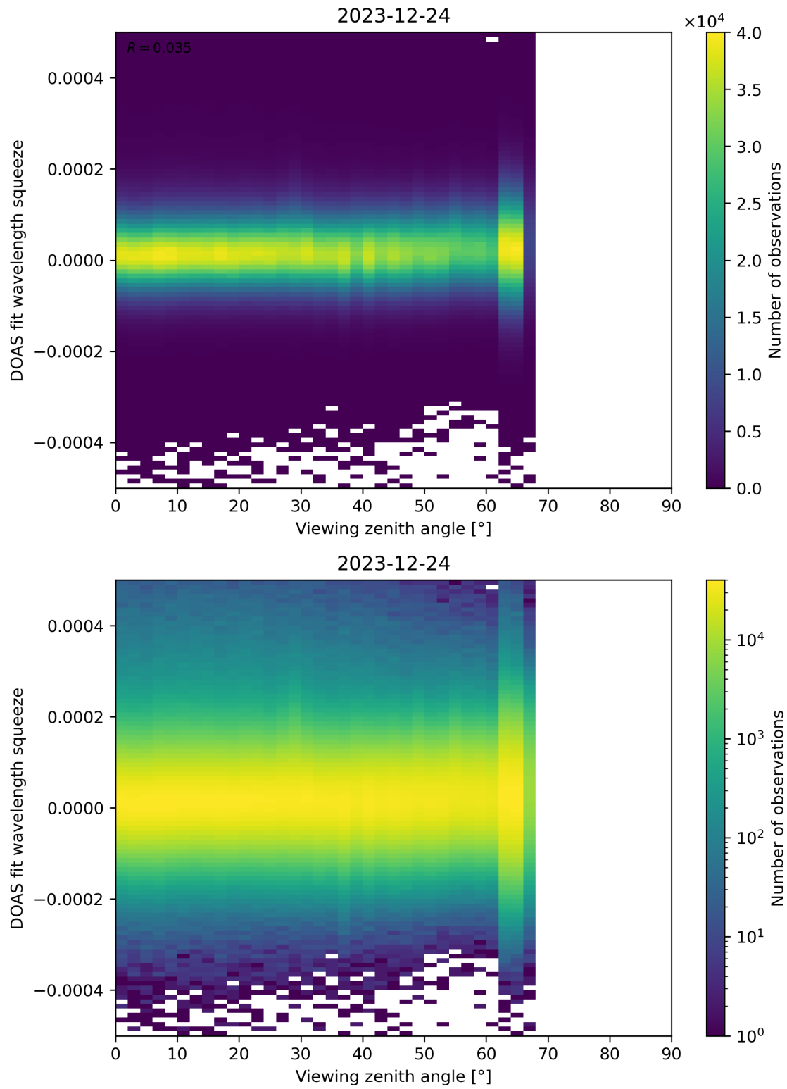
Figure 184: Scatter density plot of “Viewing zenith angle” against “DOAS fit wavelength squeeze” for 2023-12-23 to 2023-12-25.
