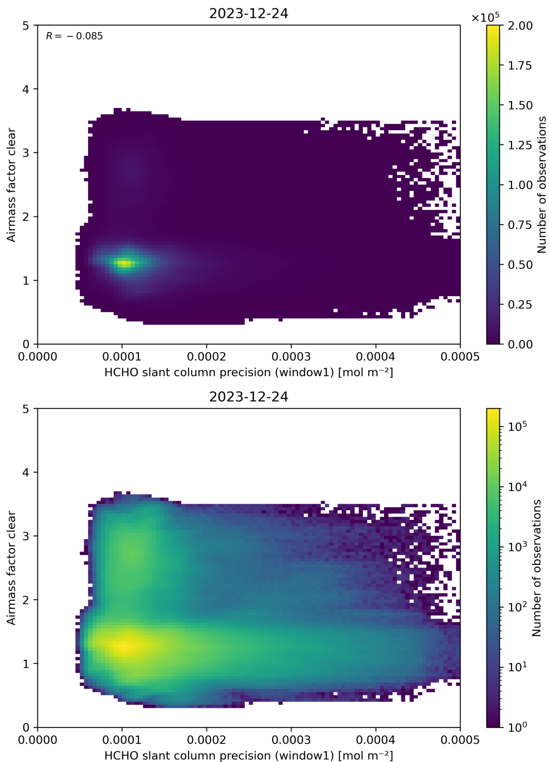
Figure 91: Scatter density plot of “HCHO slant column precision (window1)” against “Airmass factor clear” for 2023-12-23 to 2023-12-25.
