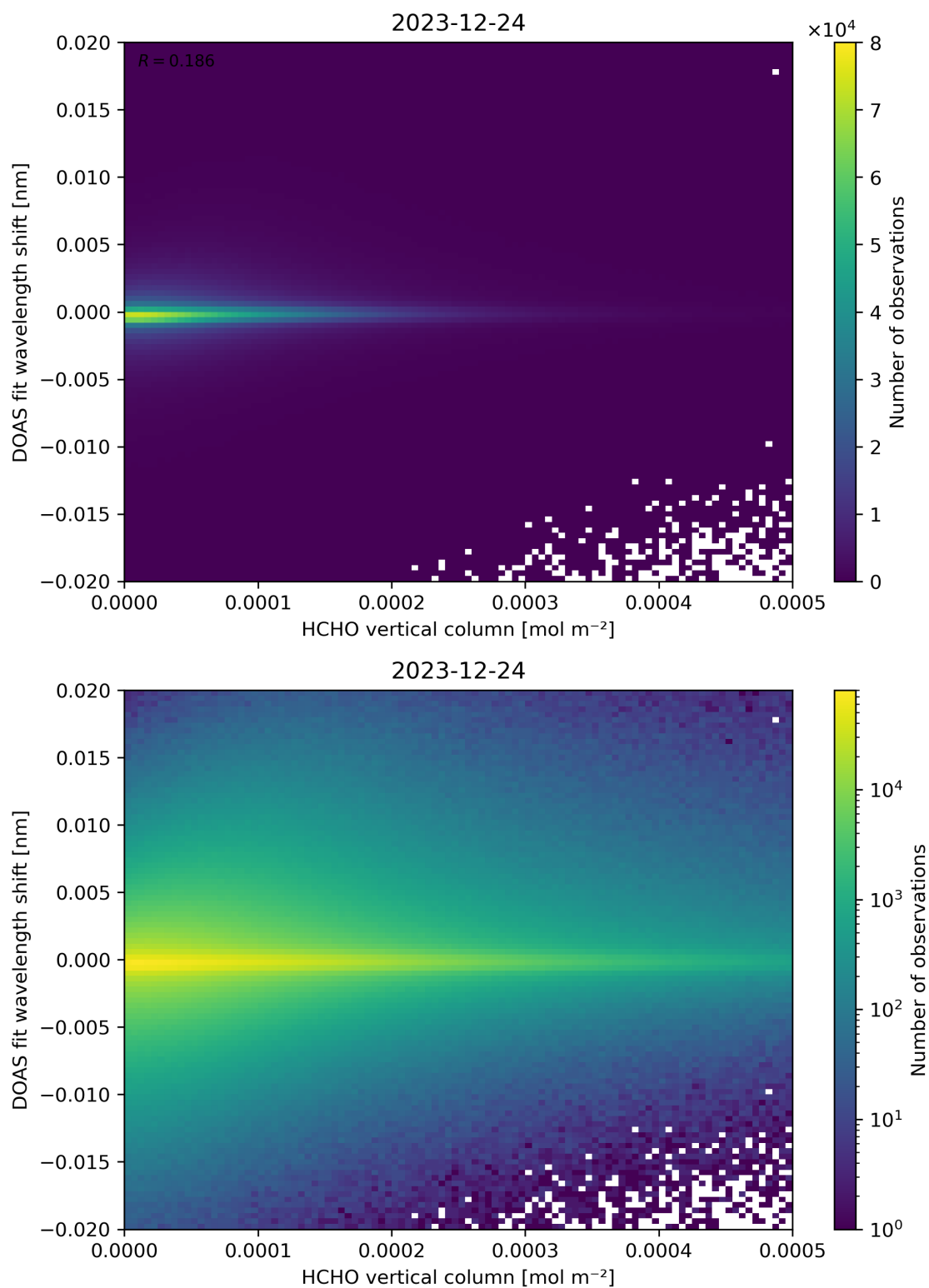
Figure 124: Scatter density plot of “HCHO vertical column” against “DOAS fit wavelength shift” for 2023-12-23 to 2023-12-25.
