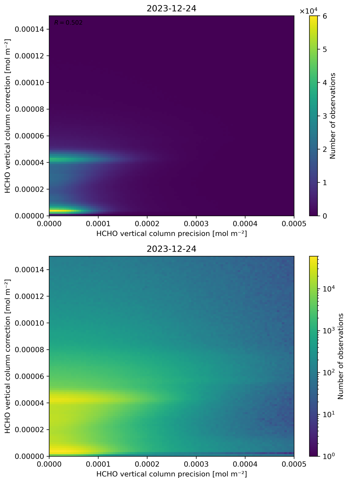
Figure 146: Scatter density plot of “HCHO vertical column precision” against “HCHO vertical column correction” for 2023-12-23 to 2023-12-25.
