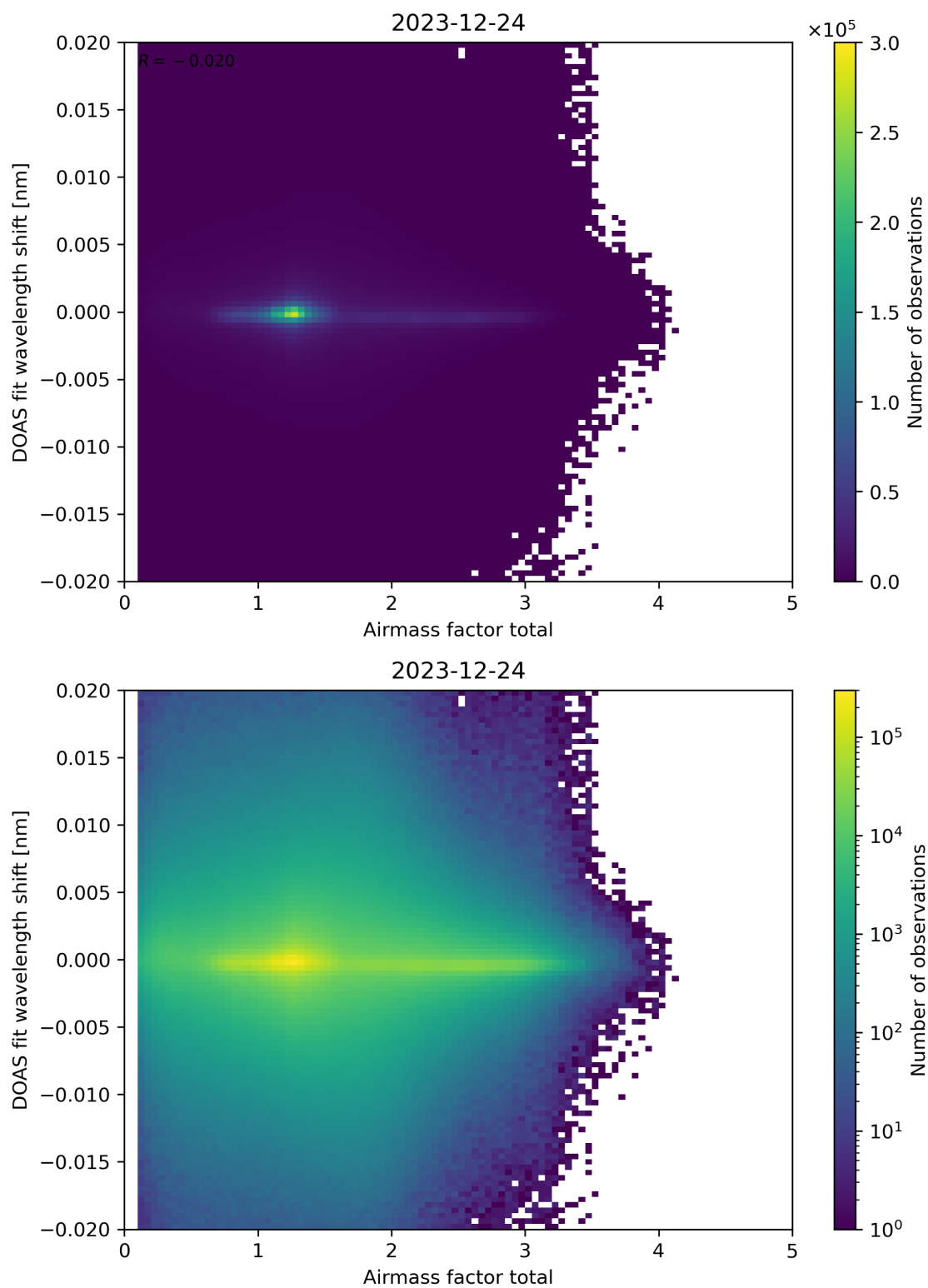
Figure 98: Scatter density plot of “Airmass factor total” against “DOAS fit wavelength shift” for 2023-12-23 to 2023-12-25.
