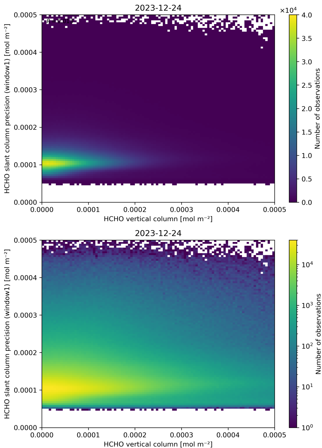
Figure 130: Scatter density plot of “HCHO vertical column” against “HCHO slant column precision (window1)” for 2023-12-23 to 2023-12-25.
