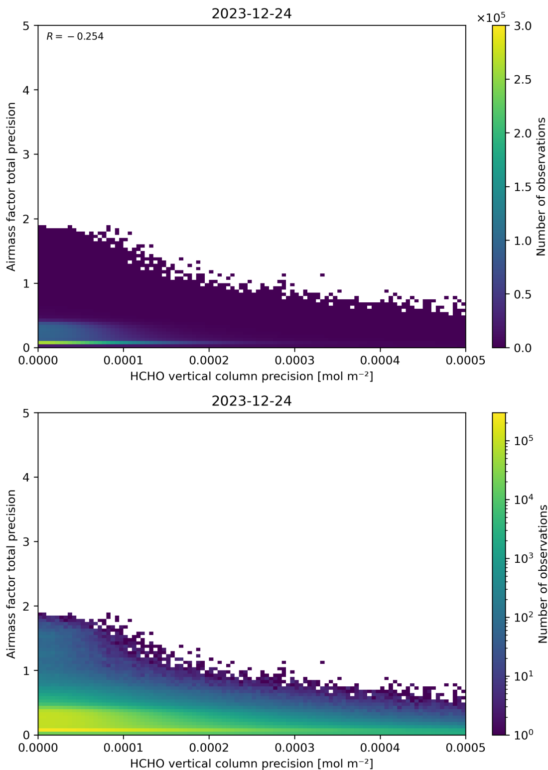
Figure 145: Scatter density plot of “HCHO vertical column precision” against “Airmass factor total precision” for 2023-12-23 to 2023-12-25.
