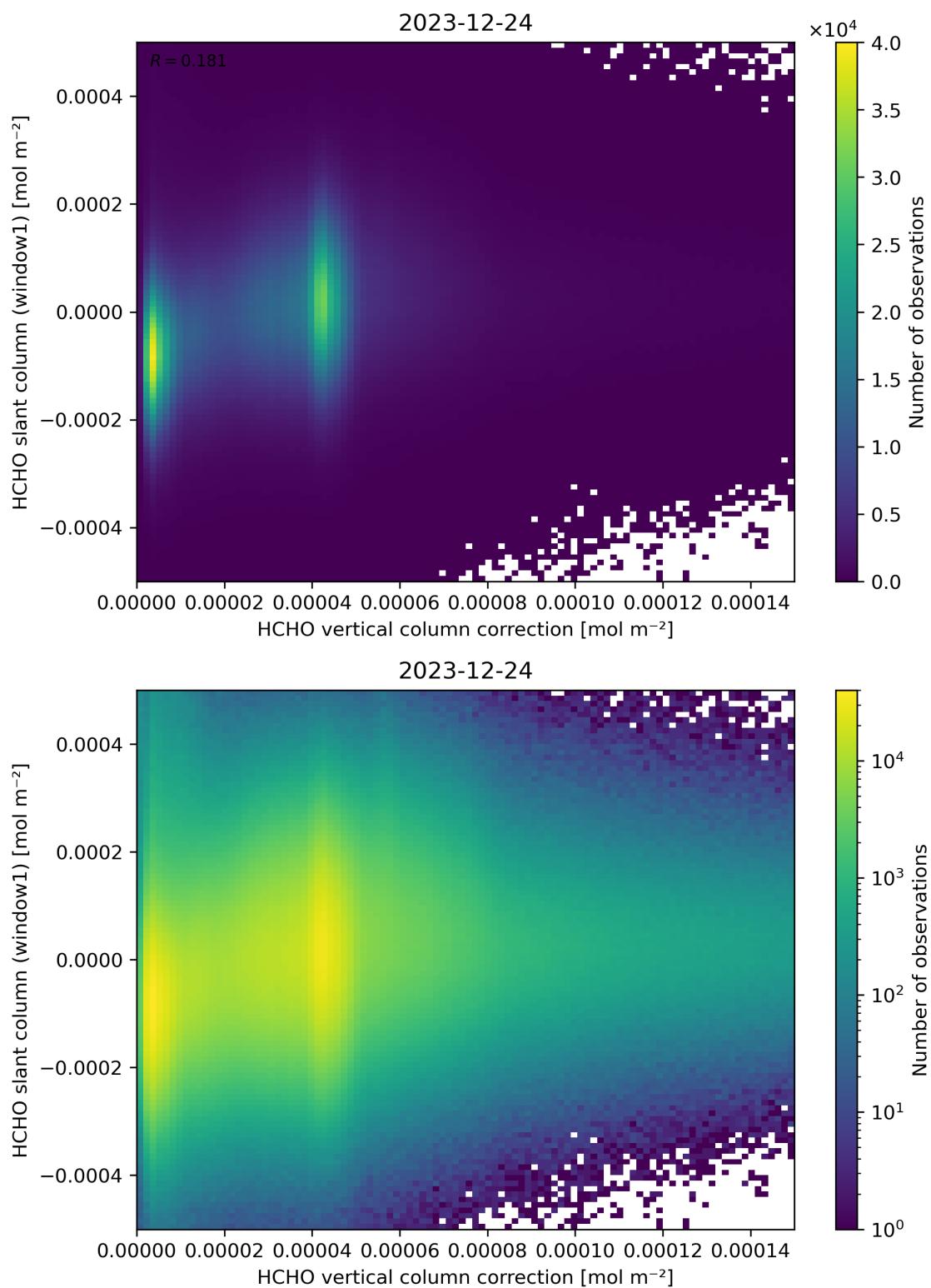
Figure 118: Scatter density plot of “HCHO vertical column correction” against “HCHO slant column (window1)” for 2023-12-23 to 2023-12-25.
