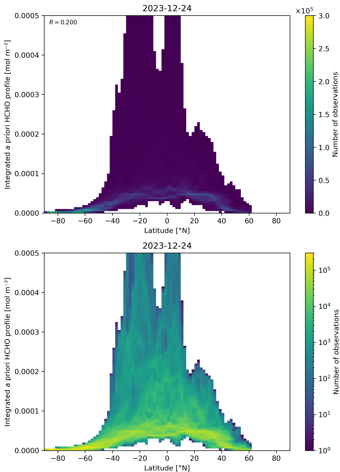
Figure 166: Scatter density plot of “Latitude” against “Integrated a priori HCHO profile” for 2023-12-23 to 2023-12-25.
