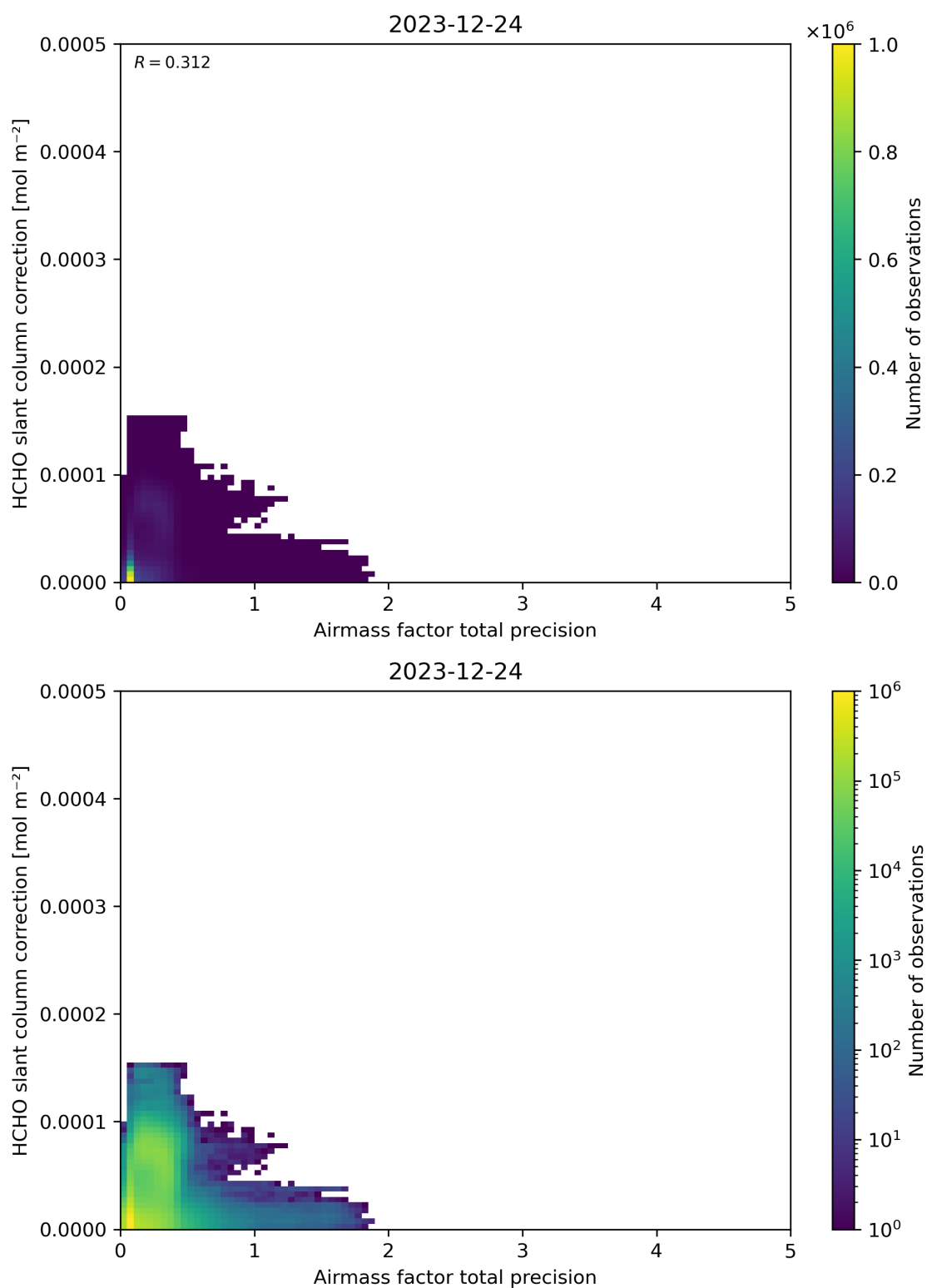
Figure 110: Scatter density plot of “Airmass factor total precision” against “HCHO slant column correction” for 2023-12-23 to 2023-12-25.
