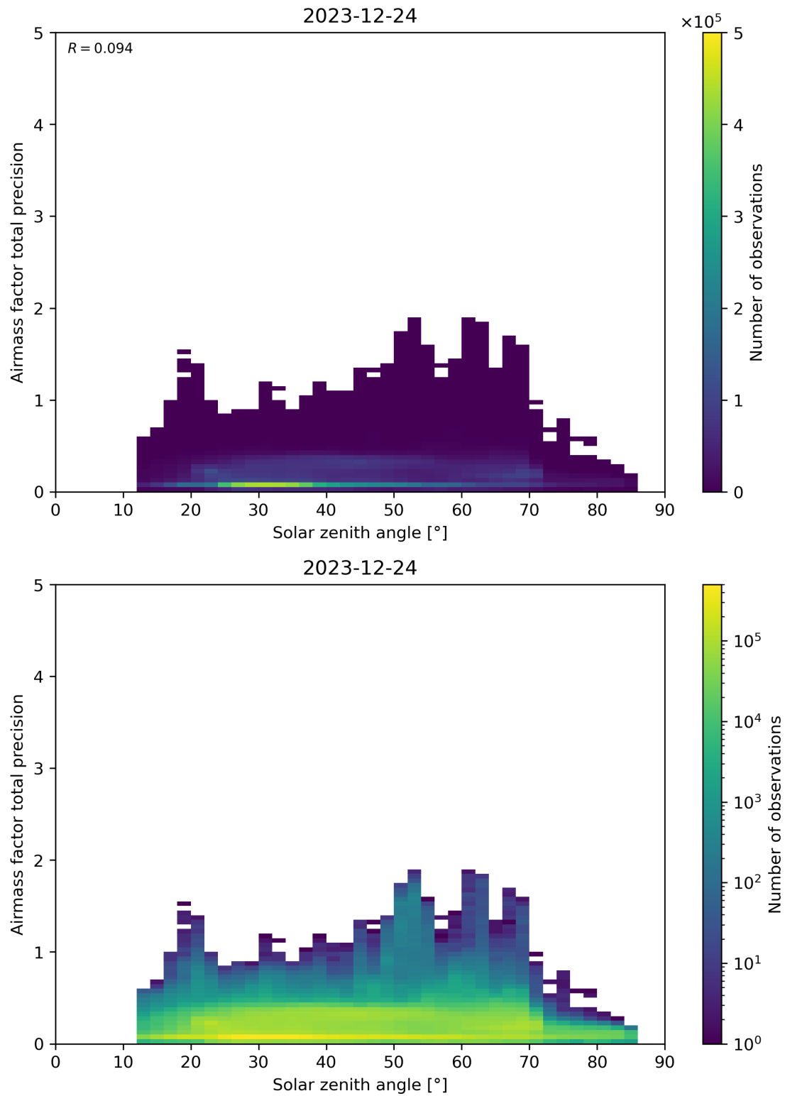
Figure 176: Scatter density plot of “Solar zenith angle” against “Airmass factor total precision” for 2023-12-23 to 2023-12-25.
