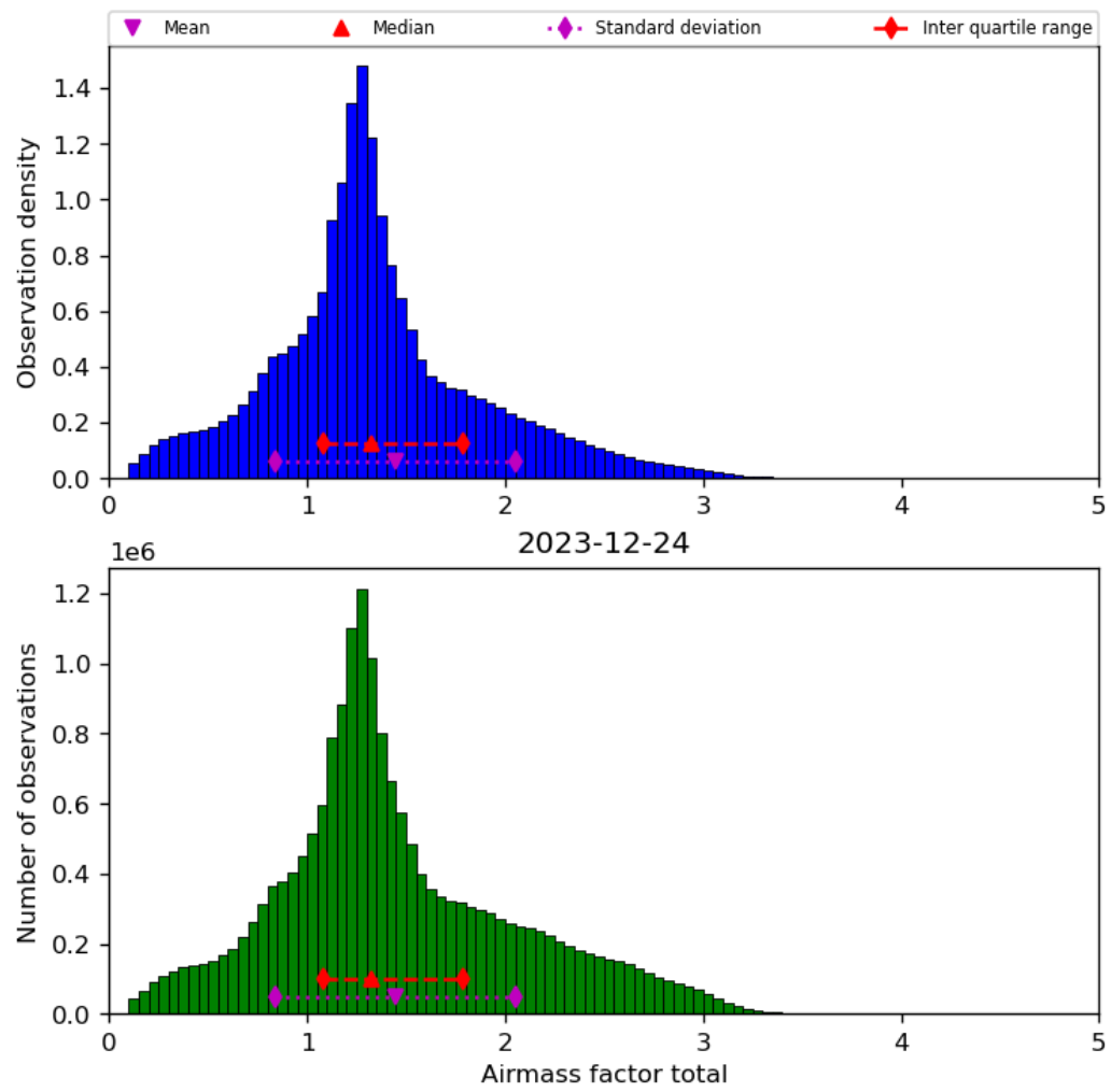
Figure 40: Histogram of “Airmass factor total” for 2023-12-23 to 2023-12-25
