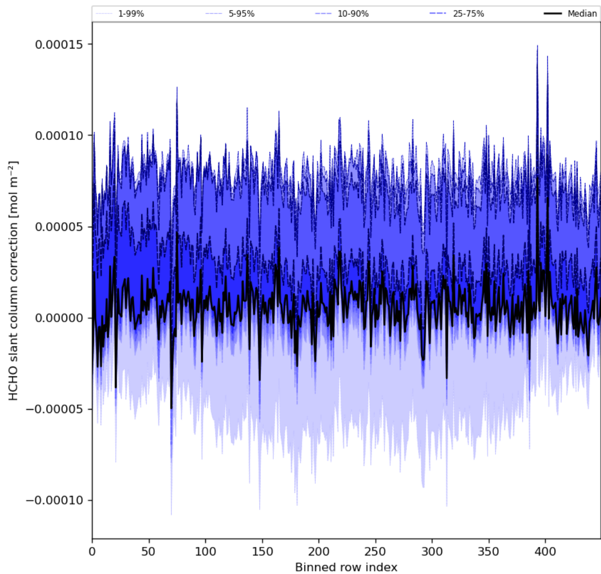
Figure 61: Along track statistics of “HCHO slant column correction” for 2023-12-23 to 2023-12-25
