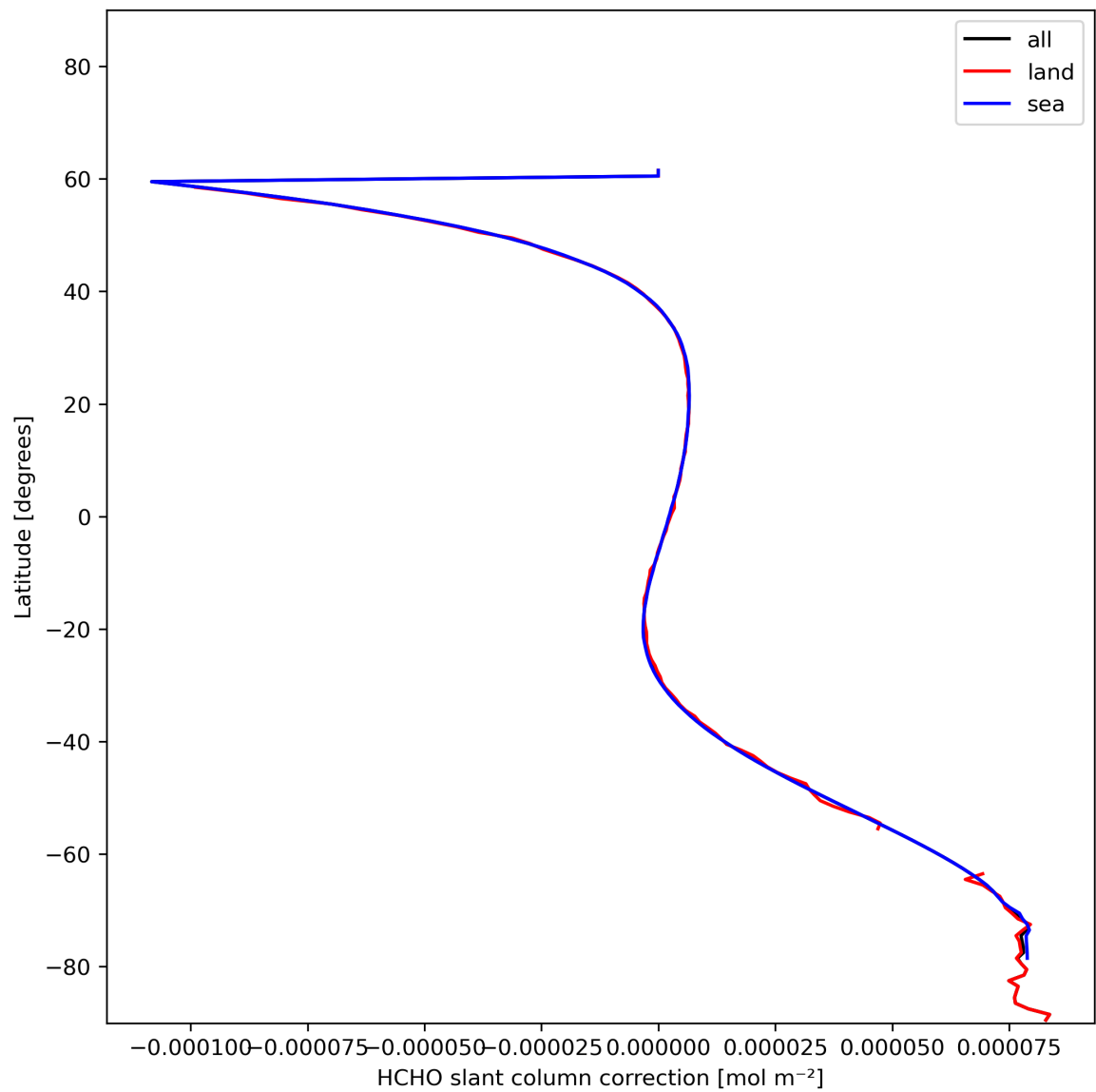
Figure 33: Zonal average of “HCHO slant column correction” for 2023-12-23 to 2023-12-25.
