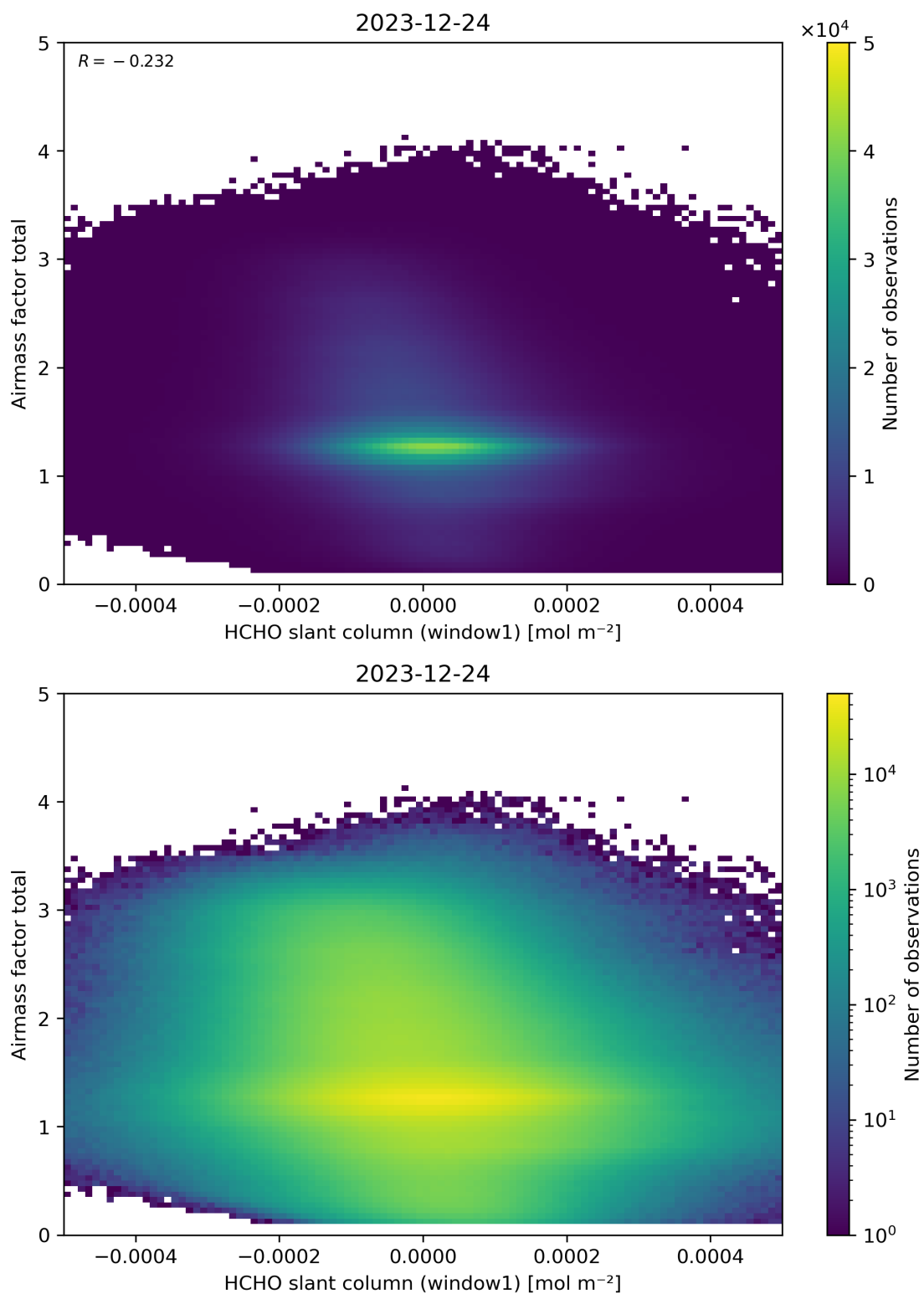
Figure 85: Scatter density plot of “HCHO slant column (window1)” against “Airmass factor total” for 2023-12-23 to 2023-12-25.
