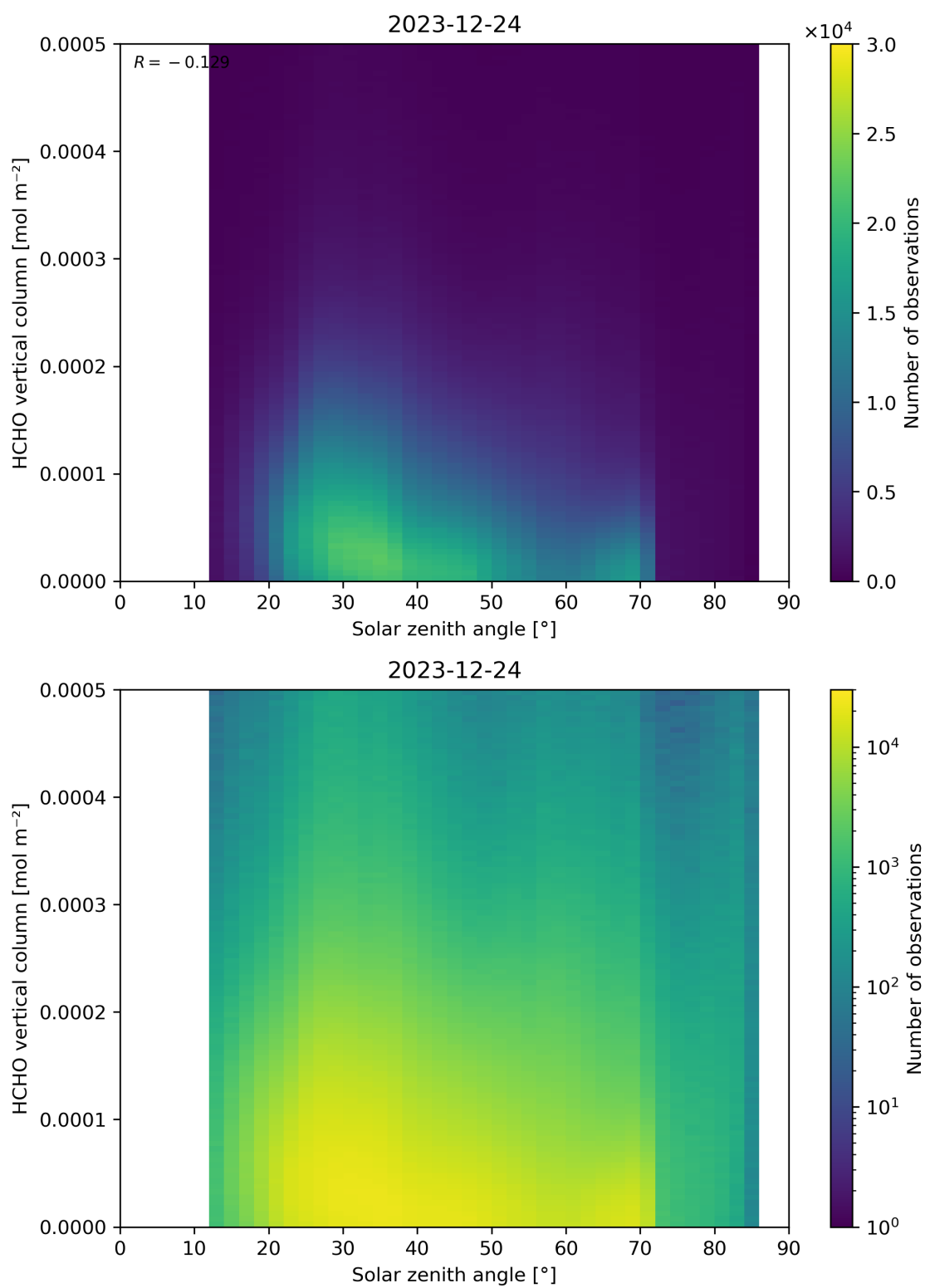
Figure 177: Scatter density plot of “Solar zenith angle” against “HCHO vertical column” for 2023-12-23 to 2023-12-25.
