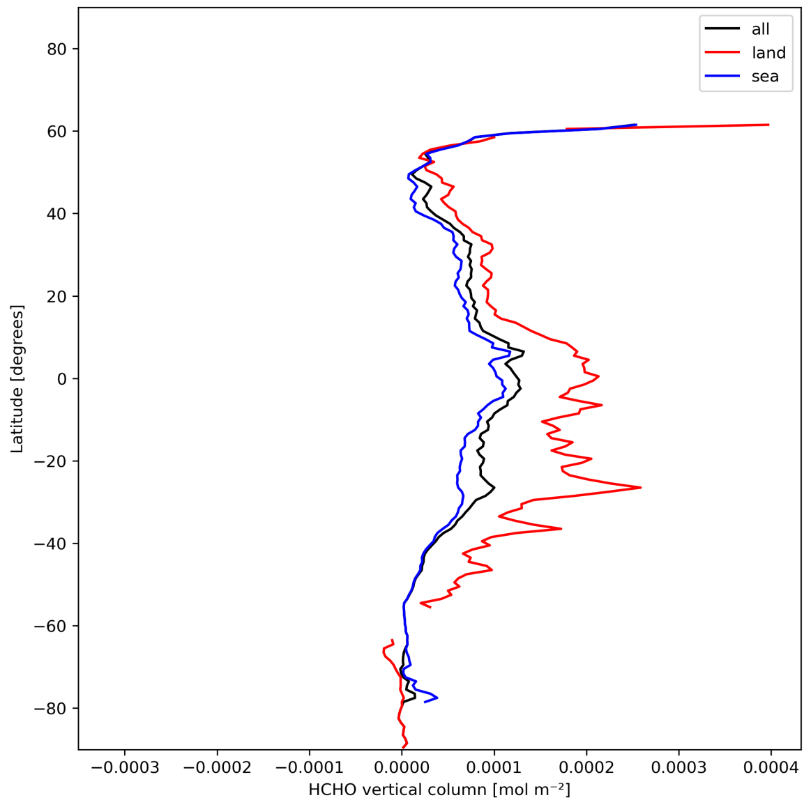
Figure 21: Zonal average of “HCHO vertical column” for 2023-12-23 to 2023-12-25.
