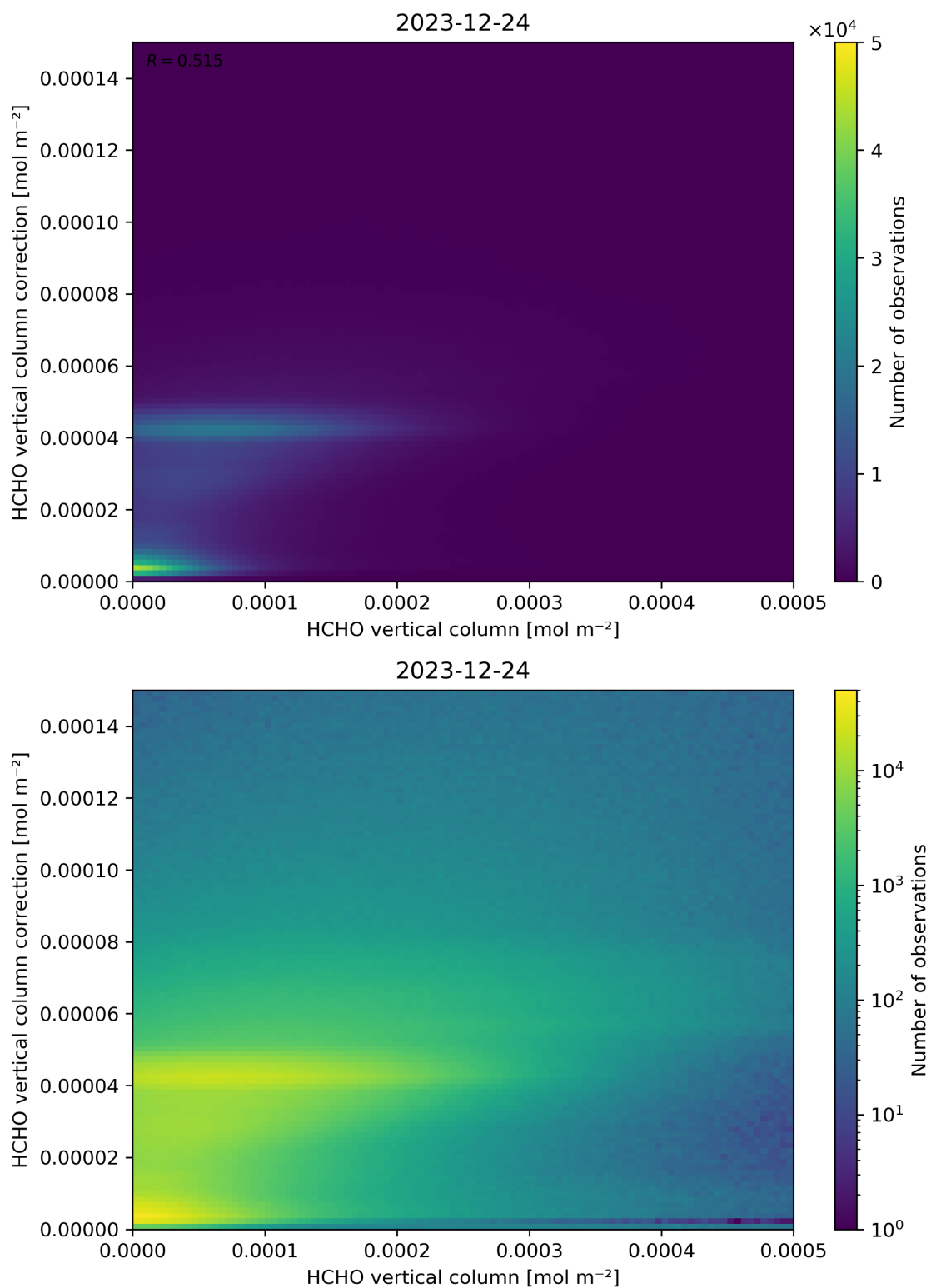
Figure 133: Scatter density plot of “HCHO vertical column” against “HCHO vertical column correction” for 2023-12-23 to 2023-12-25.
