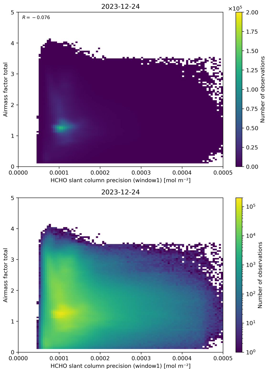
Figure 94: Scatter density plot of “HCHO slant column precision (window1)” against “Airmass factor total” for 2023-12-23 to 2023-12-25.
