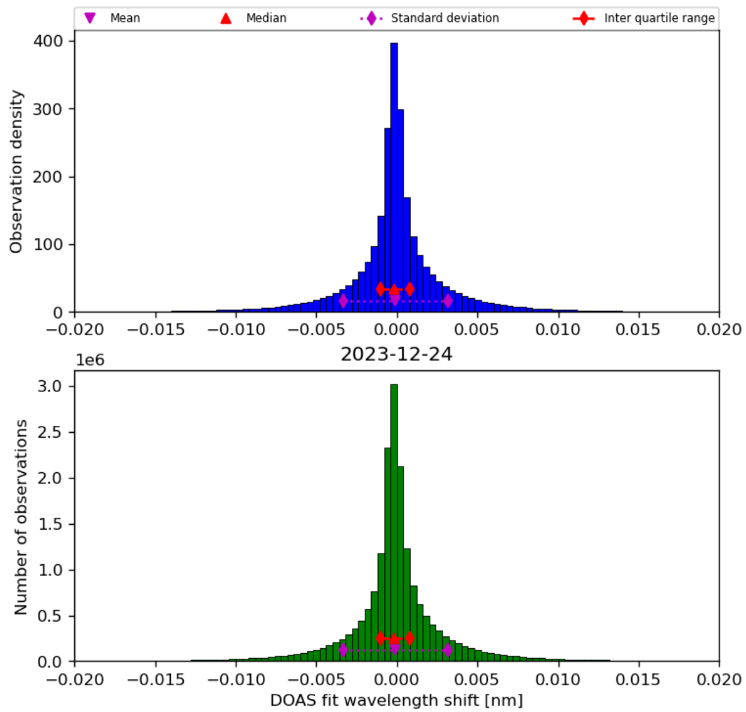
Figure 44: Histogram of “DOAS fit wavelength shift” for 2023-12-23 to 2023-12-25
