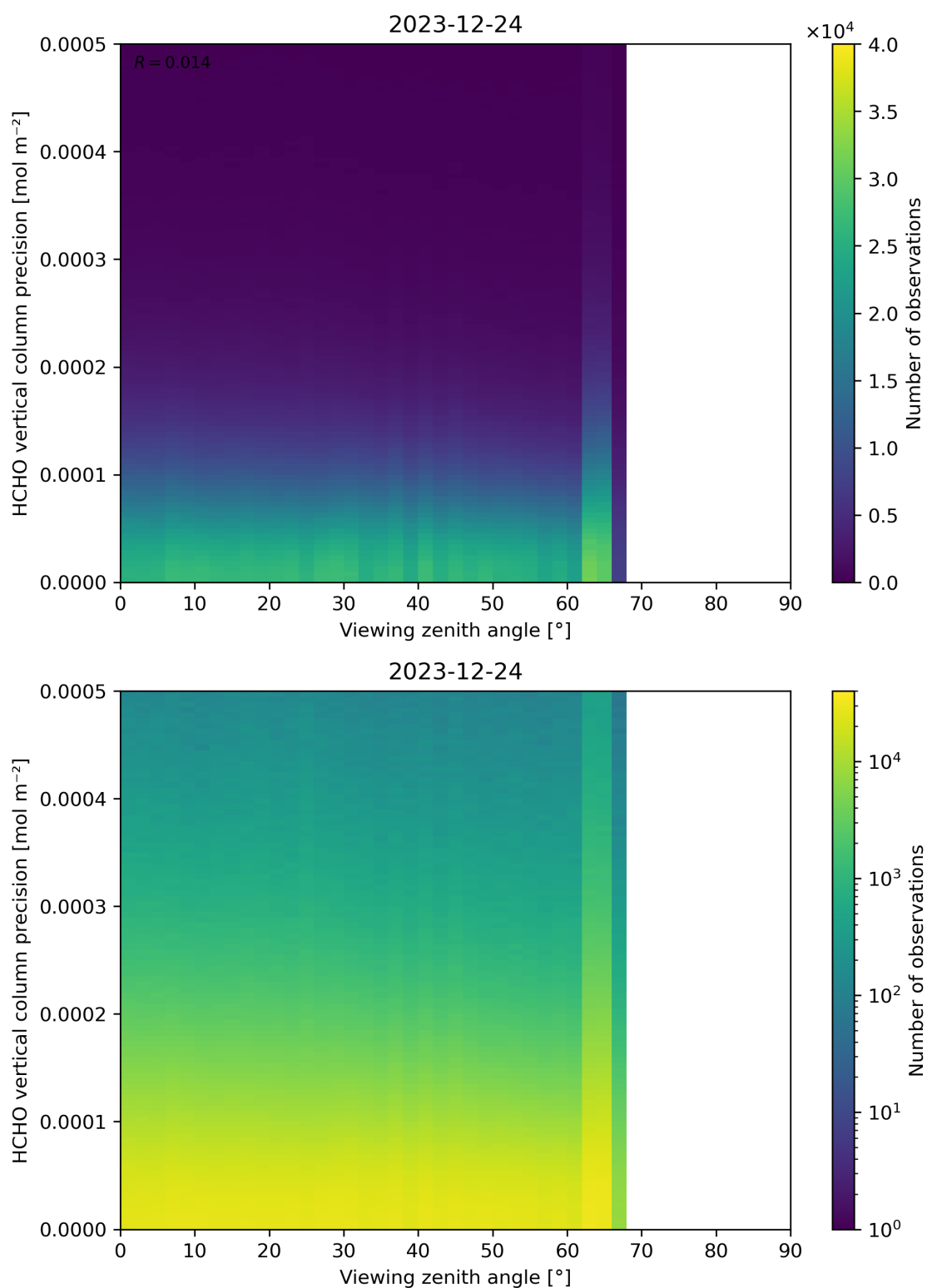
Figure 194: Scatter density plot of “Viewing zenith angle” against “HCHO vertical column precision” for 2023-12-23 to 2023-12-25.
