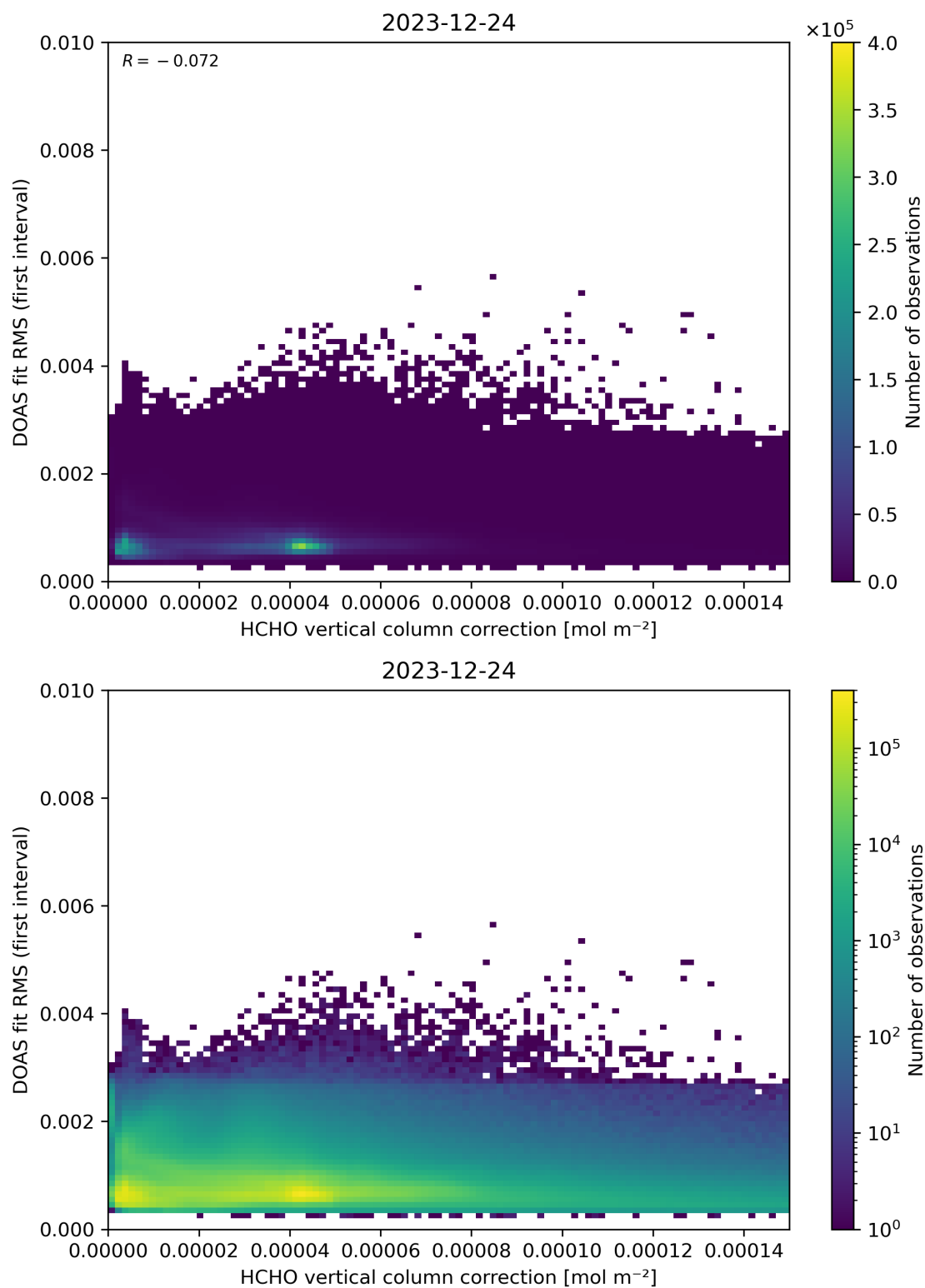
Figure 112: Scatter density plot of “HCHO vertical column correction” against “DOAS fit RMS (first interval)” for 2023-12-23 to 2023-12-25.
