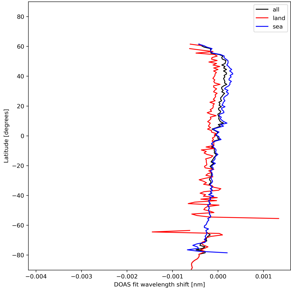
Figure 30: Zonal average of “DOAS fit wavelength shift” for 2023-12-23 to 2023-12-25.
