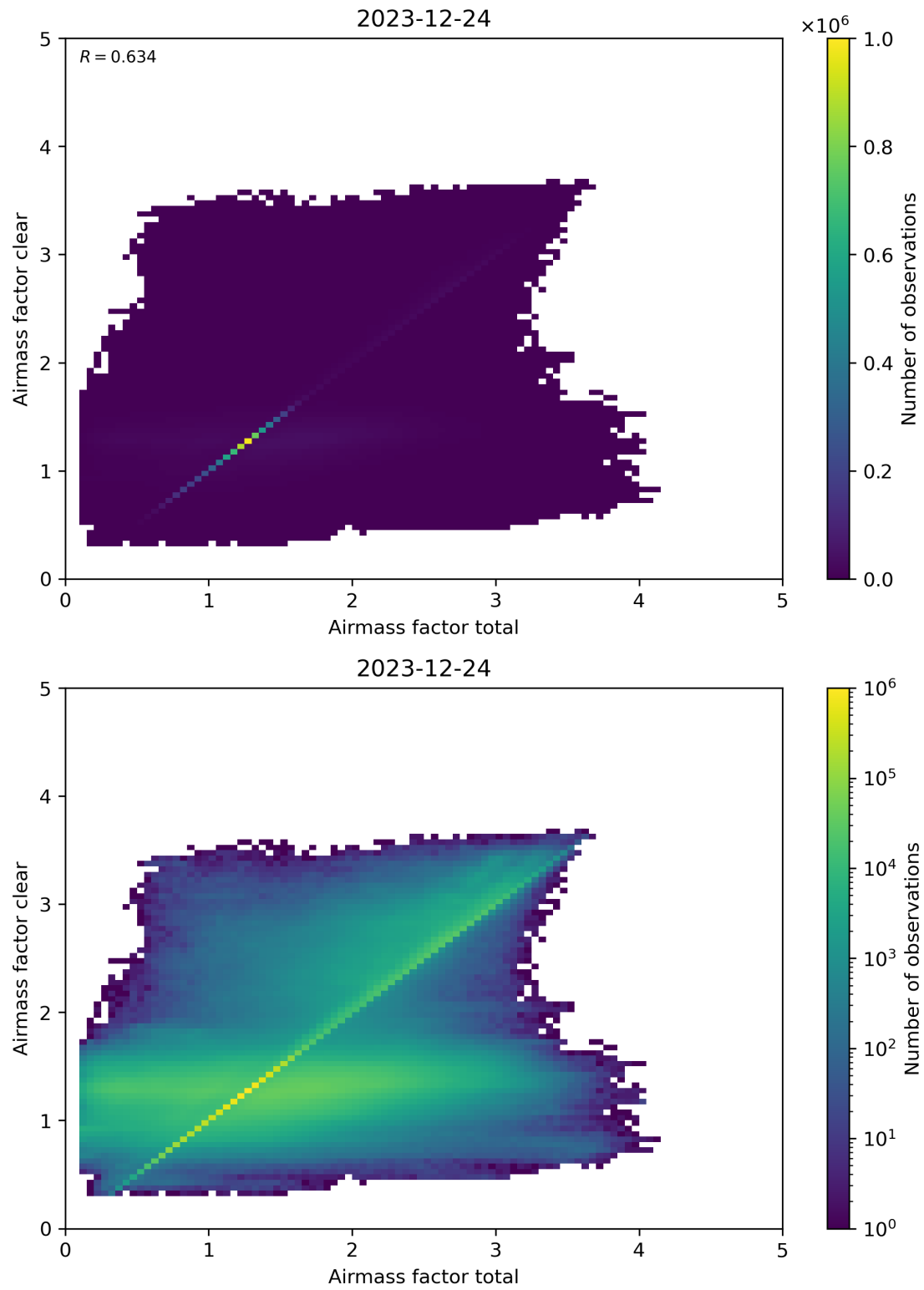
Figure 100: Scatter density plot of “Airmass factor total” against “Airmass factor clear” for 2023-12-23 to 2023-12-25.
