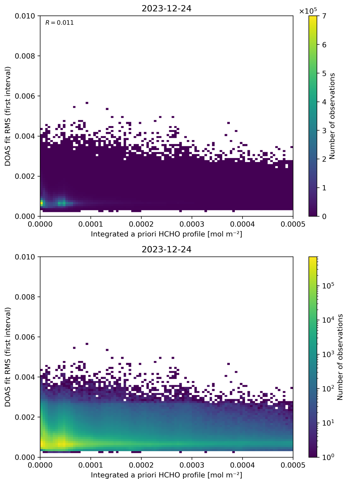
Figure 148: Scatter density plot of “Integrated a priori HCHO profile” against “DOAS fit RMS (first interval)” for 2023-12-23 to 2023-12-25.
