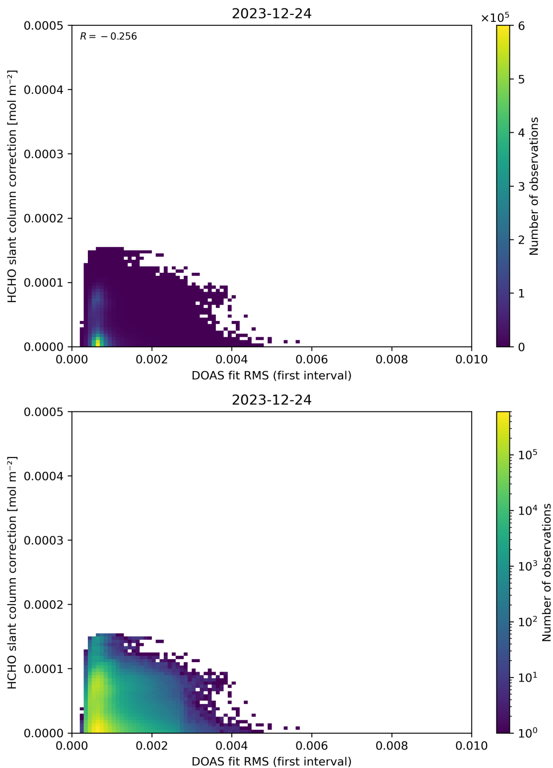
Figure 63: Scatter density plot of “DOAS fit RMS (first interval)” against “HCHO slant column correction” for 2023-12-23 to 2023-12-25.
