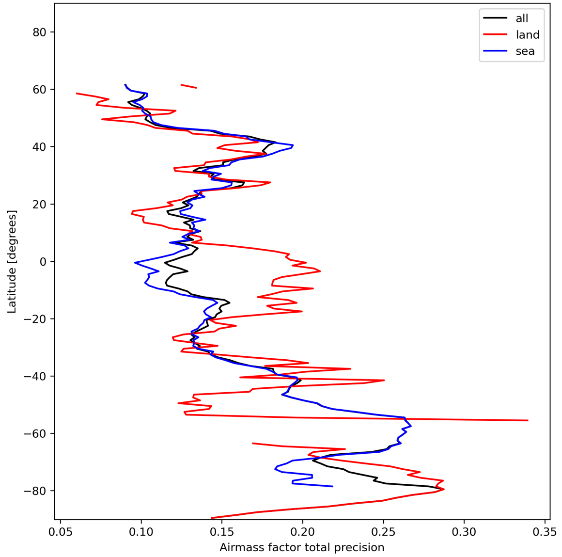
Figure 27: Zonal average of “Airmass factor total precision” for 2023-12-23 to 2023-12-25.
