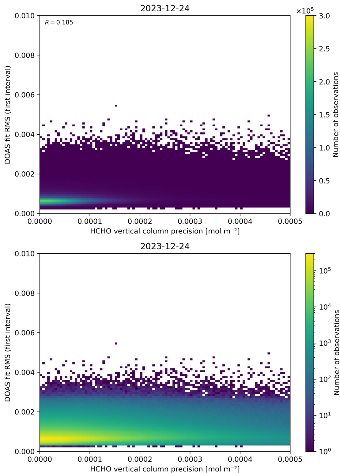
Figure 136: Scatter density plot of “HCHO vertical column precision” against “DOAS fit RMS (first interval)” for 2023-12-23 to 2023-12-25.
