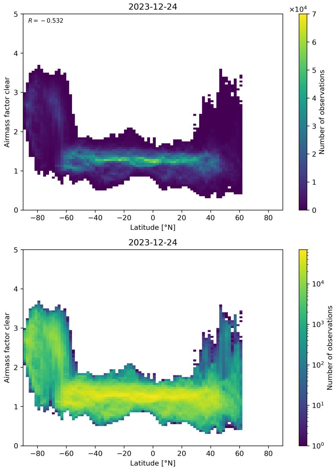
Figure 156: Scatter density plot of “Latitude” against “Airmass factor clear” for 2023-12-23 to 2023-12-25.
