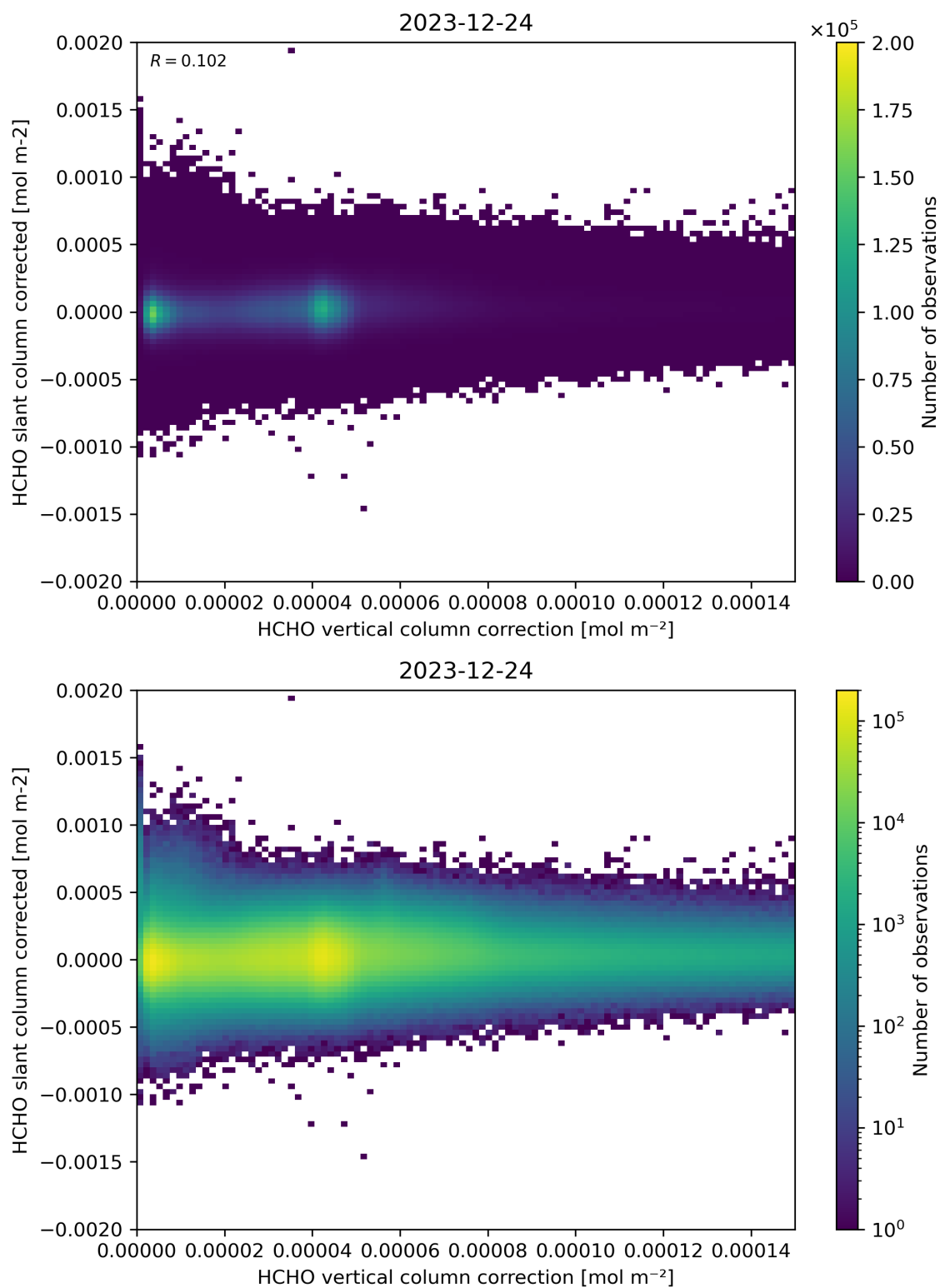
Figure 116: Scatter density plot of “HCHO vertical column correction” against “HCHO slant column corrected” for 2023-12-23 to 2023-12-25.
