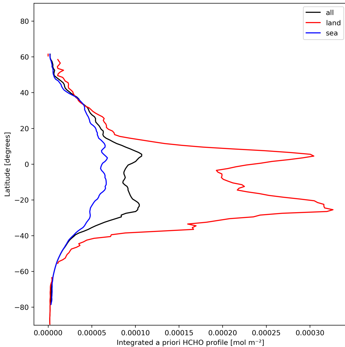
Figure 29: Zonal average of “Integrated a priori HCHO profile” for 2023-12-23 to 2023-12-25.
