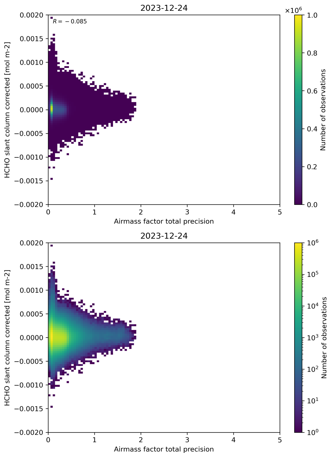
Figure 109: Scatter density plot of “Airmass factor total precision” against “HCHO slant column corrected” for 2023-12-23 to 2023-12-25.
