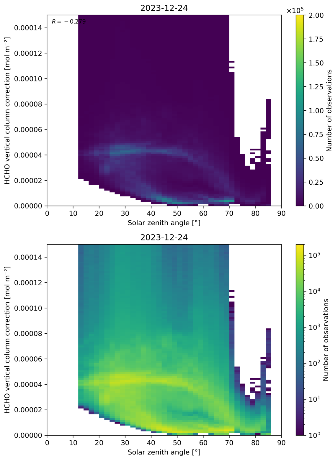
Figure 178: Scatter density plot of “Solar zenith angle” against “HCHO vertical column correction” for 2023-12-23 to 2023-12-25.
