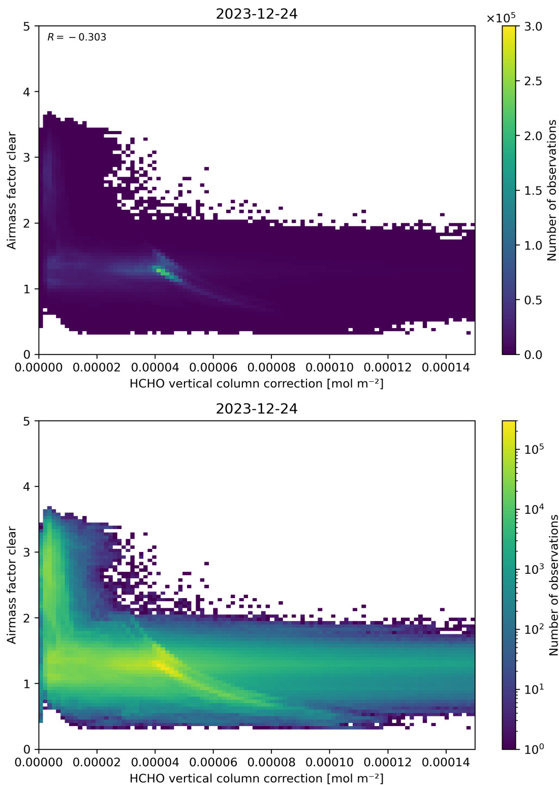
Figure 115: Scatter density plot of “HCHO vertical column correction” against “Airmass factor clear” for 2023-12-23 to 2023-12-25.
