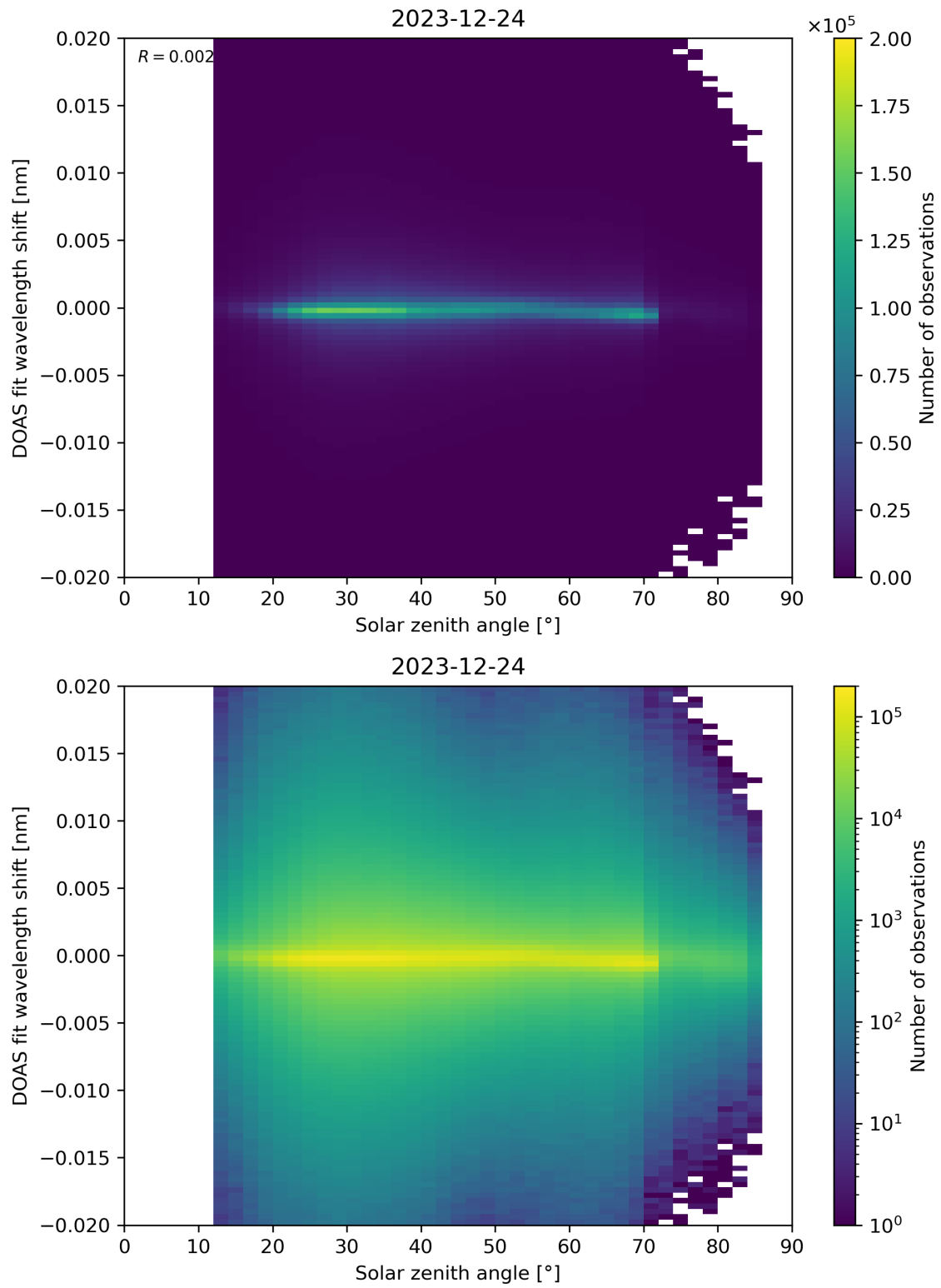
Figure 168: Scatter density plot of “Solar zenith angle” against “DOAS fit wavelength shift” for 2023-12-23 to 2023-12-25.
