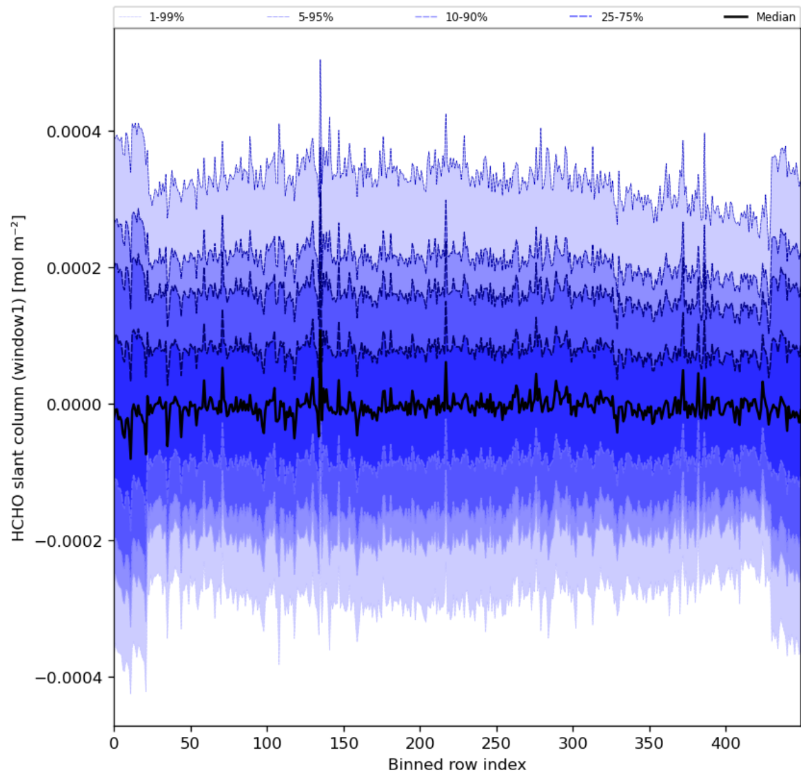
Figure 52: Along track statistics of “HCHO slant column (window1)” for 2023-12-23 to 2023-12-25
