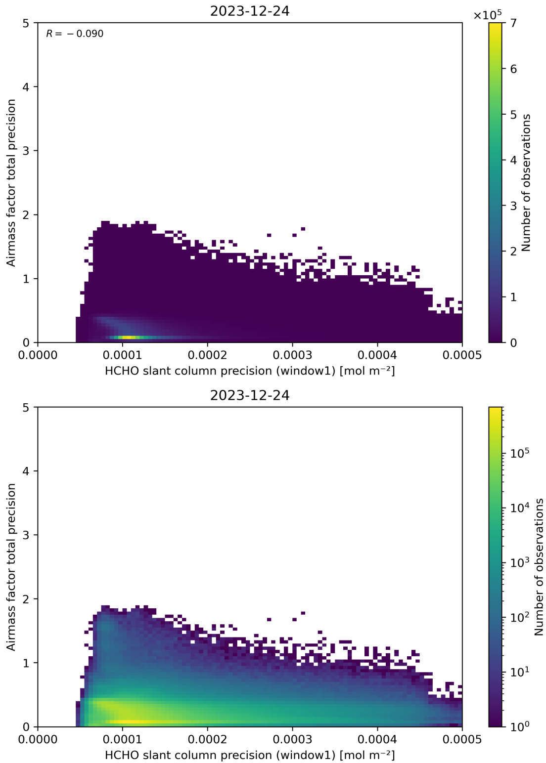
Figure 95: Scatter density plot of “HCHO slant column precision (window1)” against “Airmass factor total precision” for 2023-12-23 to 2023-12-25.
