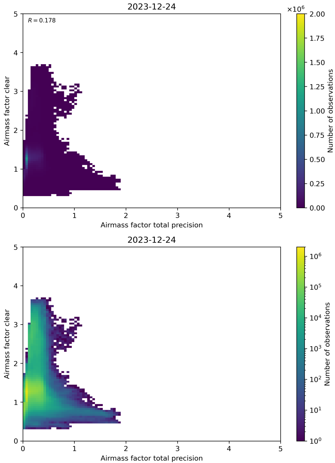
Figure 108: Scatter density plot of “Airmass factor total precision” against “Airmass factor clear” for 2023-12-23 to 2023-12-25.
