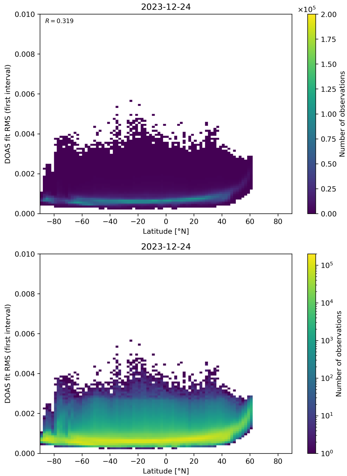
Figure 153: Scatter density plot of “Latitude” against “DOAS fit RMS (first interval)” for 2023-12-23 to 2023-12-25.
