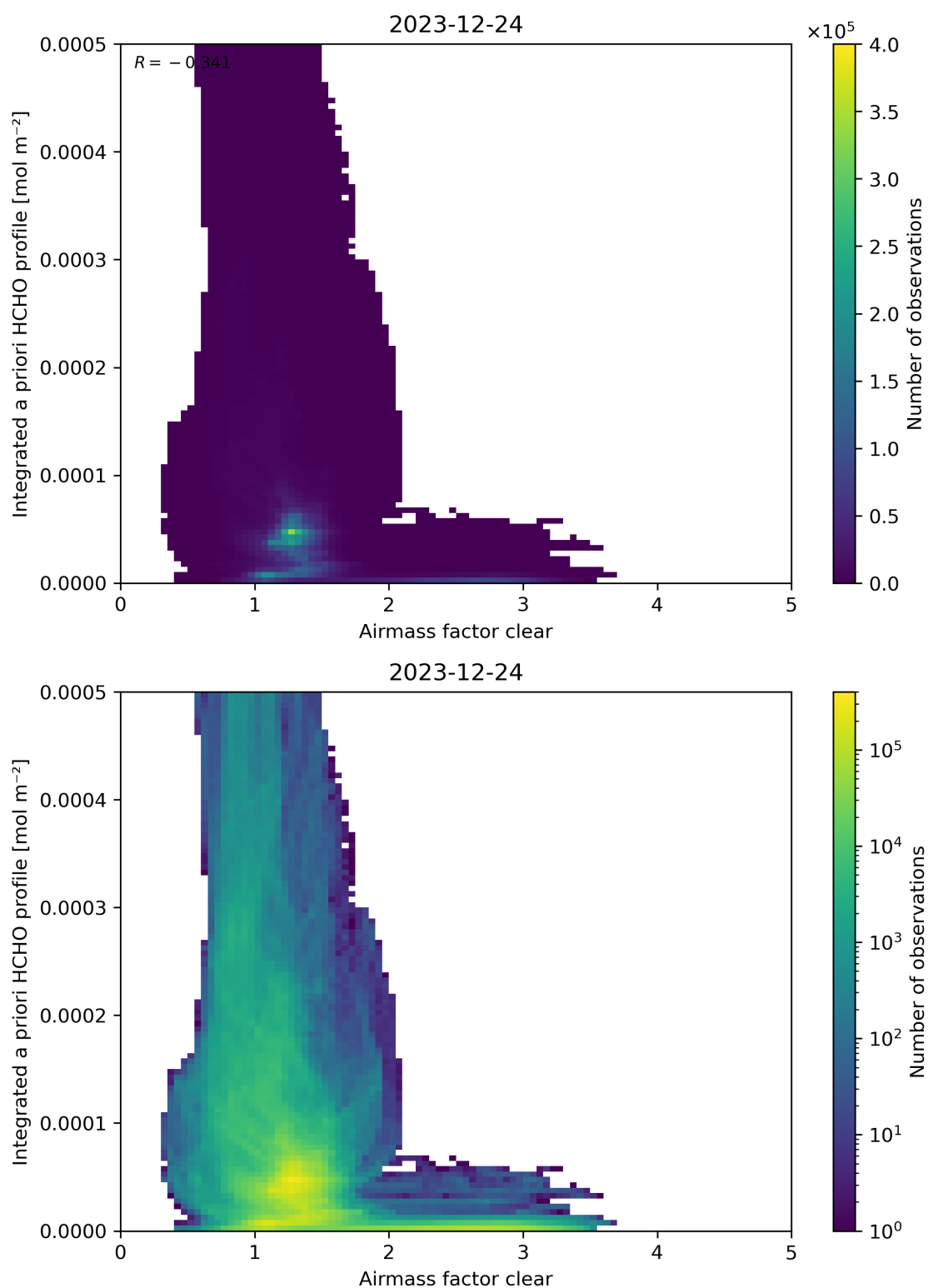
Figure 76: Scatter density plot of “Airmass factor clear” against “Integrated a priori HCHO profile” for 2023-12-23 to 2023-12-25.
