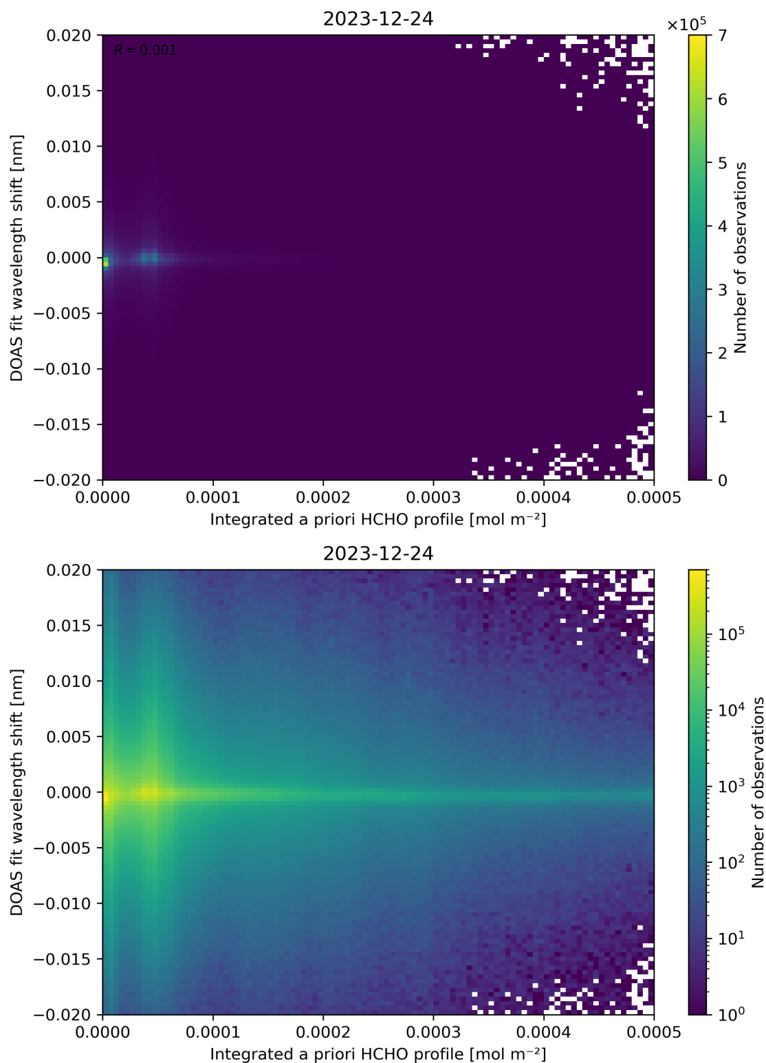
Figure 149: Scatter density plot of “Integrated a priori HCHO profile” against “DOAS fit wavelength shift” for 2023-12-23 to 2023-12-25.
