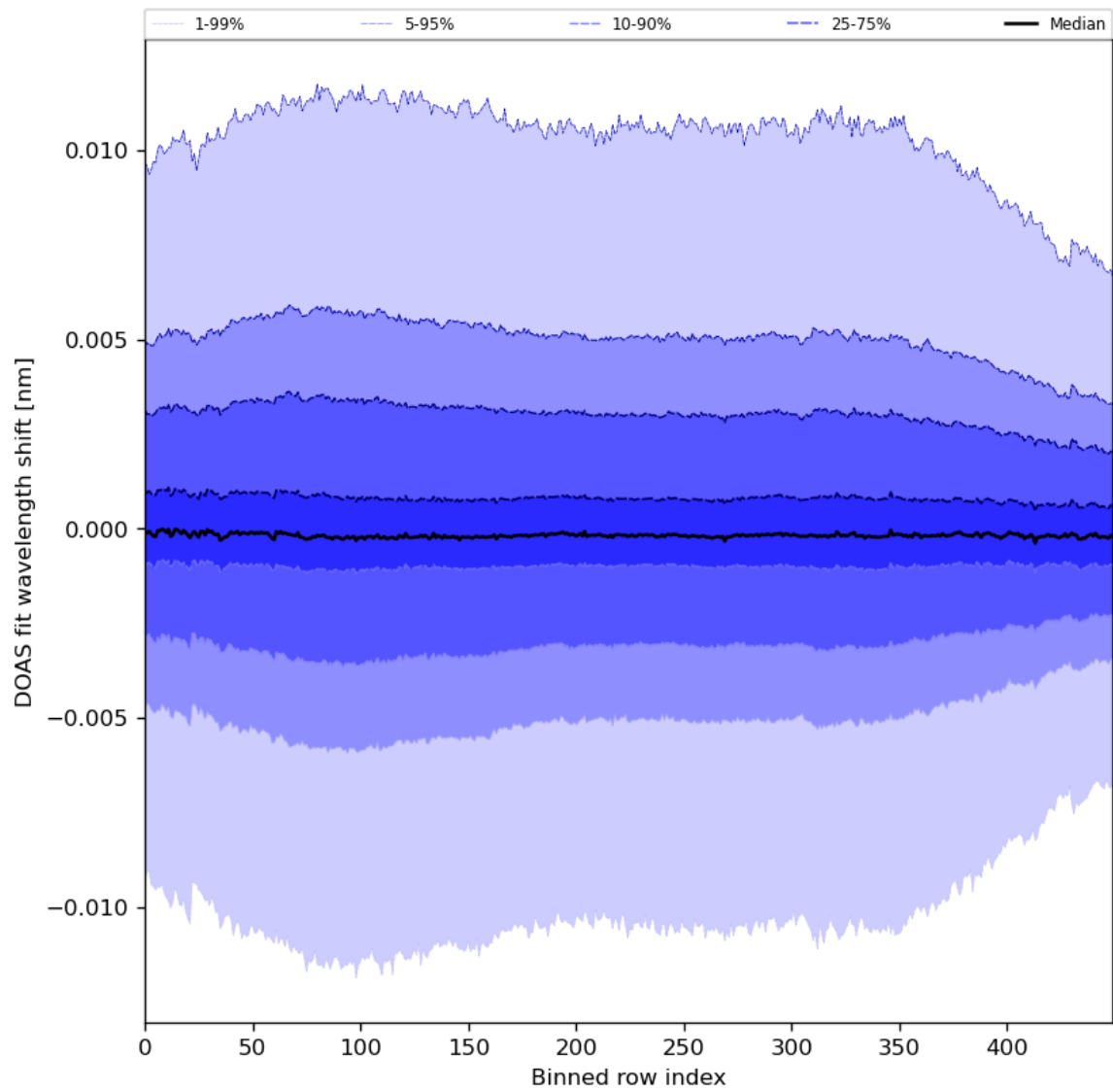
Figure 58: Along track statistics of “DOAS fit wavelength shift” for 2023-12-23 to 2023-12-25
