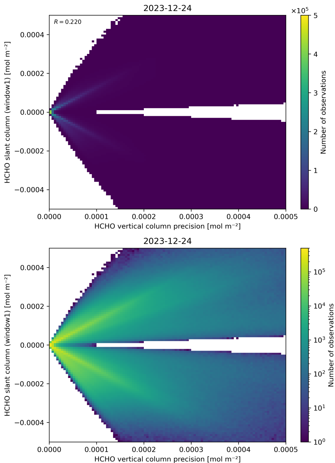
Figure 142: Scatter density plot of “HCHO vertical column precision” against “HCHO slant column (window1)” for 2023-12-23 to 2023-12-25.
