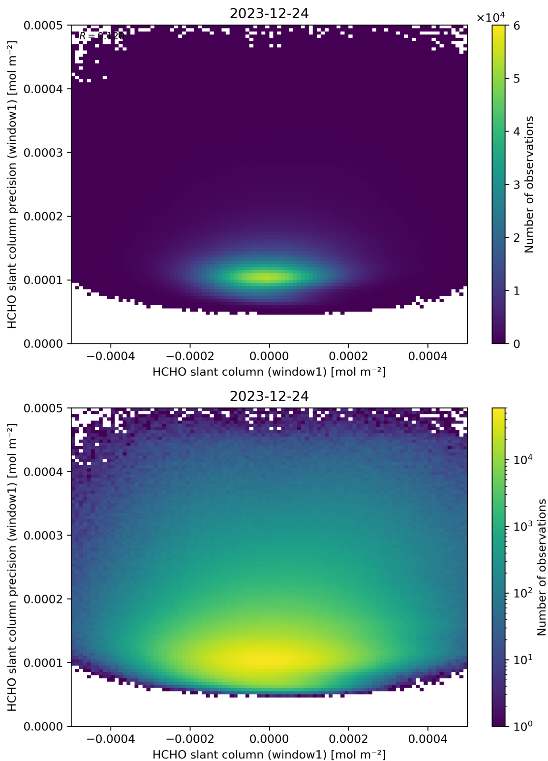
Figure 84: Scatter density plot of “HCHO slant column (window1)” against “HCHO slant column precision (window1)” for 2023-12-23 to 2023-12-25.
