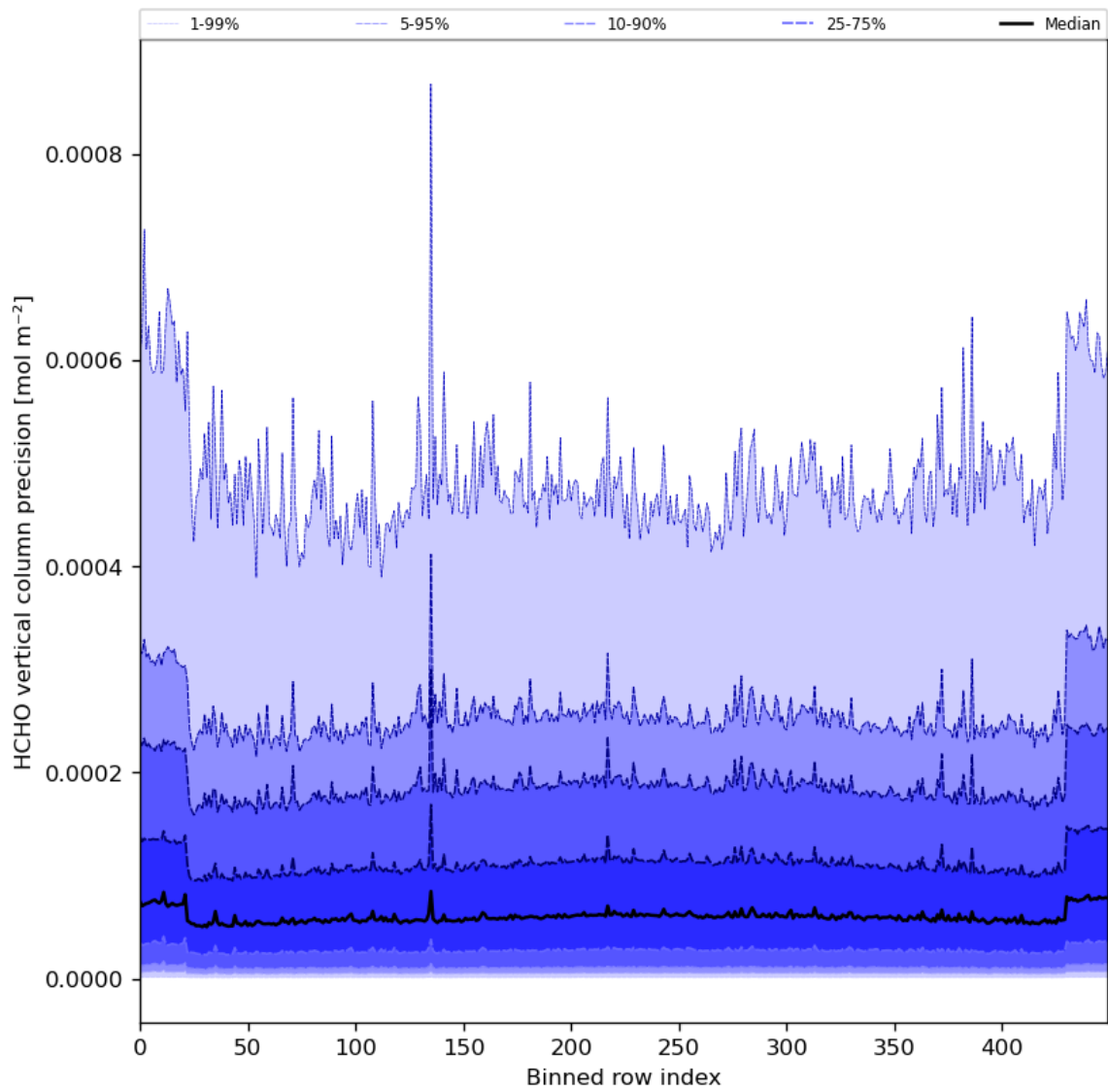
Figure 50: Along track statistics of “HCHO vertical column precision” for 2023-12-23 to 2023-12-25
