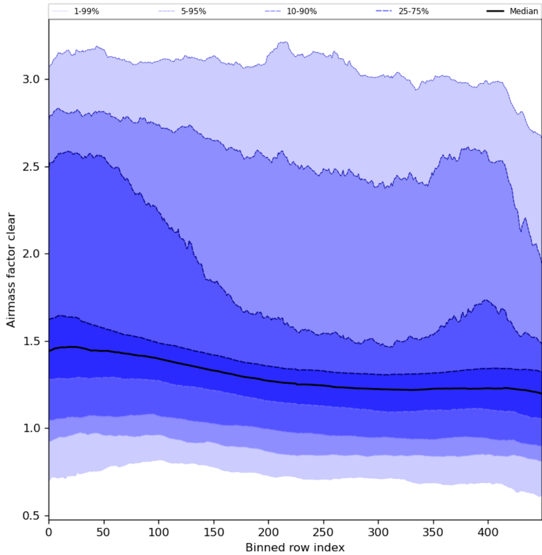
Figure 56: Along track statistics of “Airmass factor clear” for 2023-12-23 to 2023-12-25
