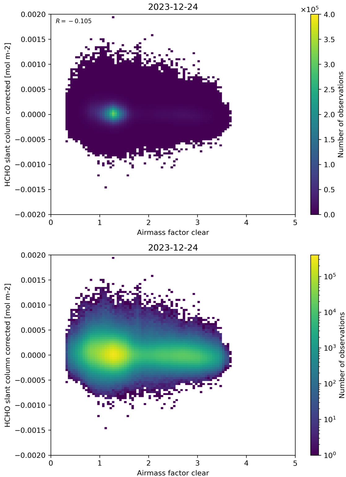
Figure 74: Scatter density plot of “Airmass factor clear” against “HCHO slant column corrected” for 2023-12-23 to 2023-12-25.
