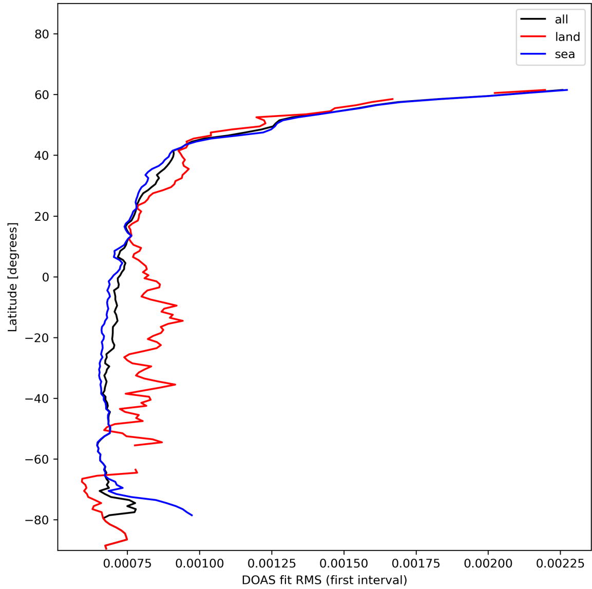
Figure 32: Zonal average of “DOAS fit RMS (first interval)” for 2023-12-23 to 2023-12-25.
