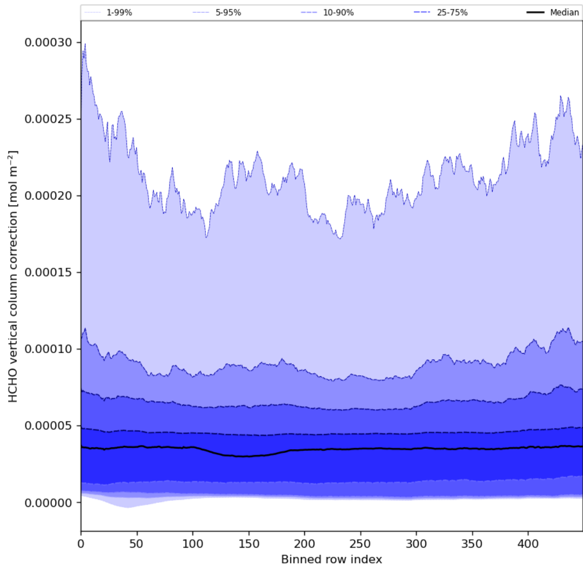
Figure 51: Along track statistics of “HCHO vertical column correction” for 2023-12-23 to 2023-12-25
