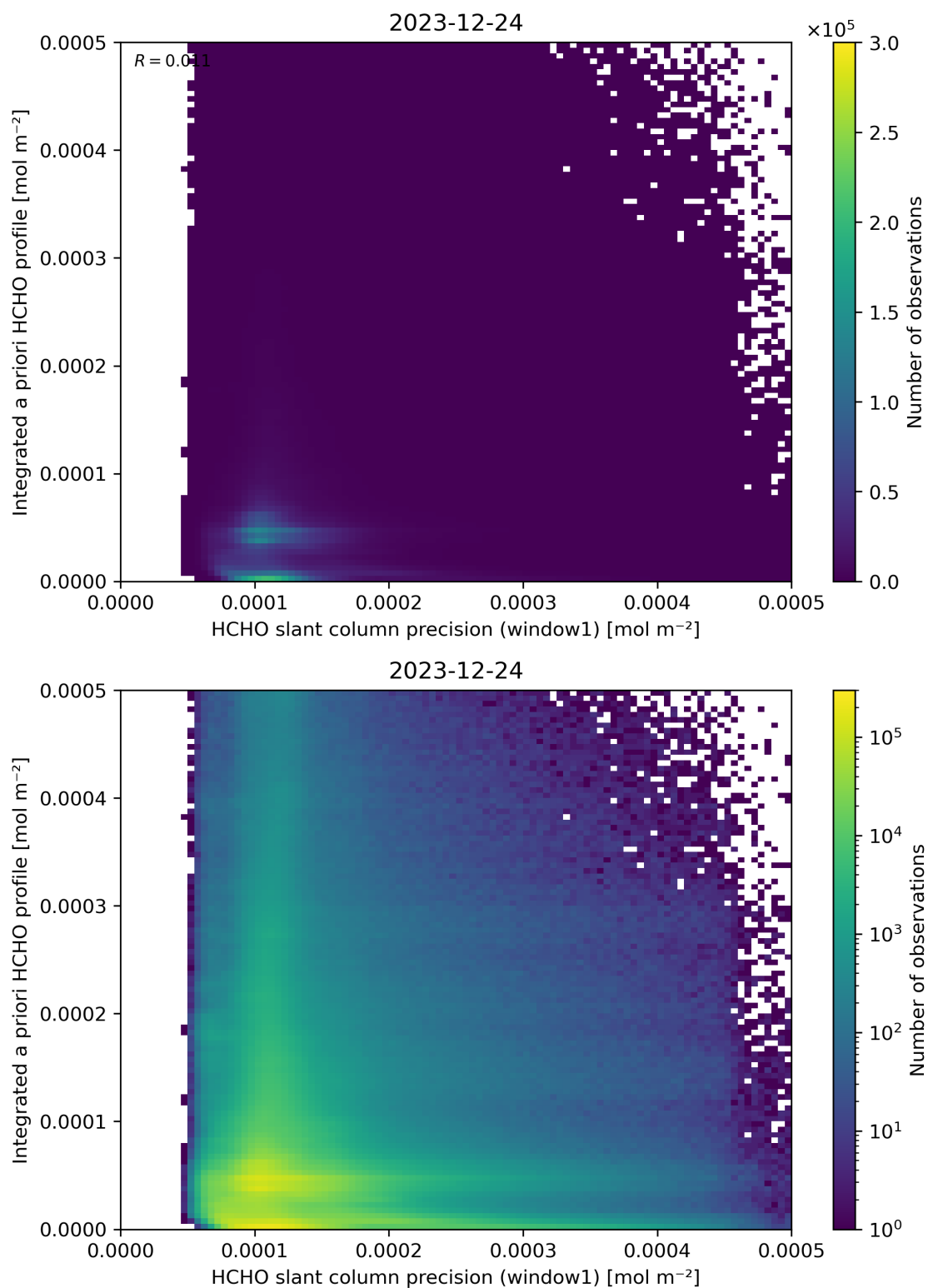
Figure 96: Scatter density plot of “HCHO slant column precision (window1)” against “Integrated a priori HCHO profile” for 2023-12-23 to 2023-12-25.
