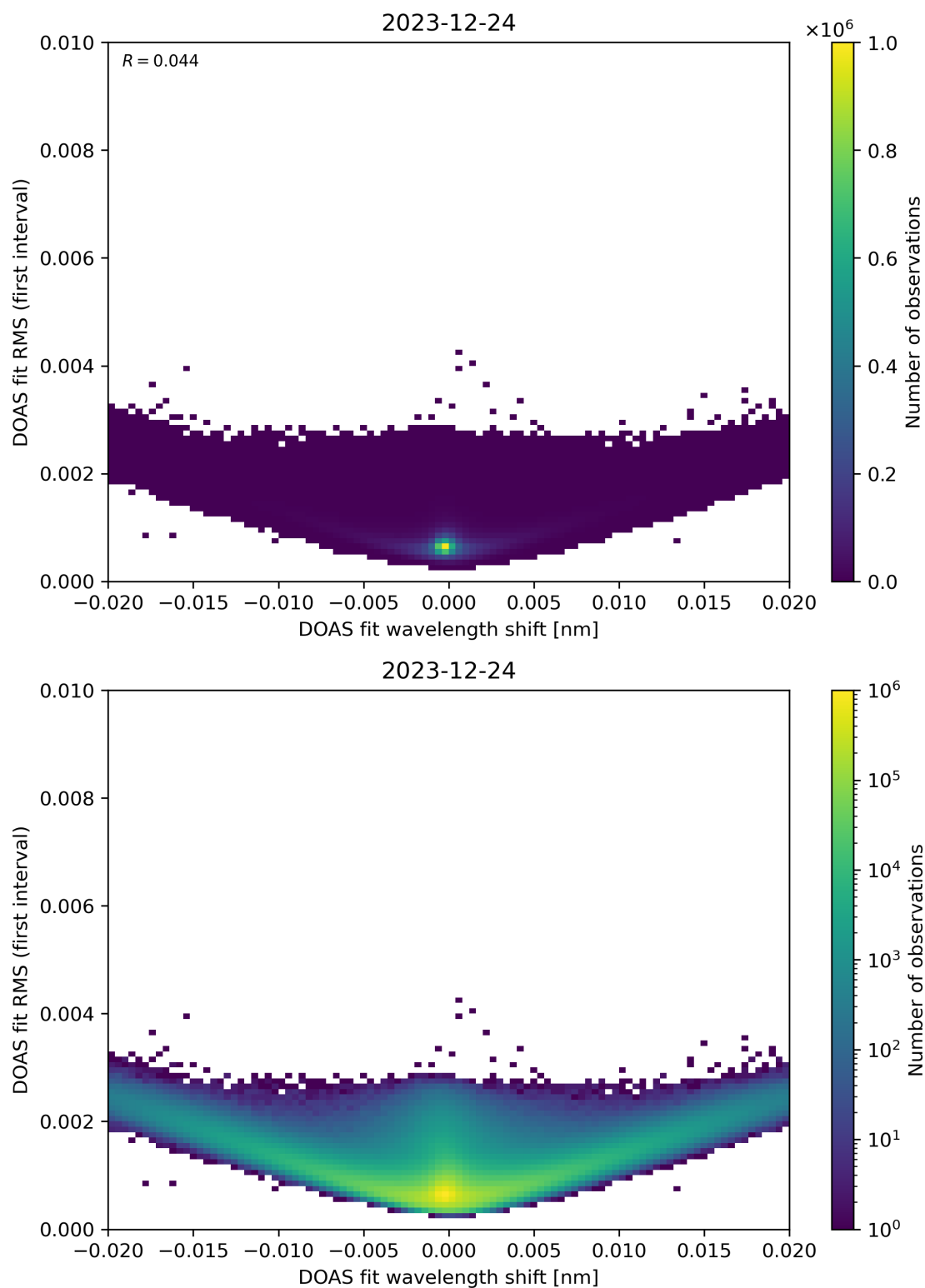
Figure 64: Scatter density plot of “DOAS fit wavelength shift” against “DOAS fit RMS (first interval)” for 2023-12-23 to 2023-12-25.
