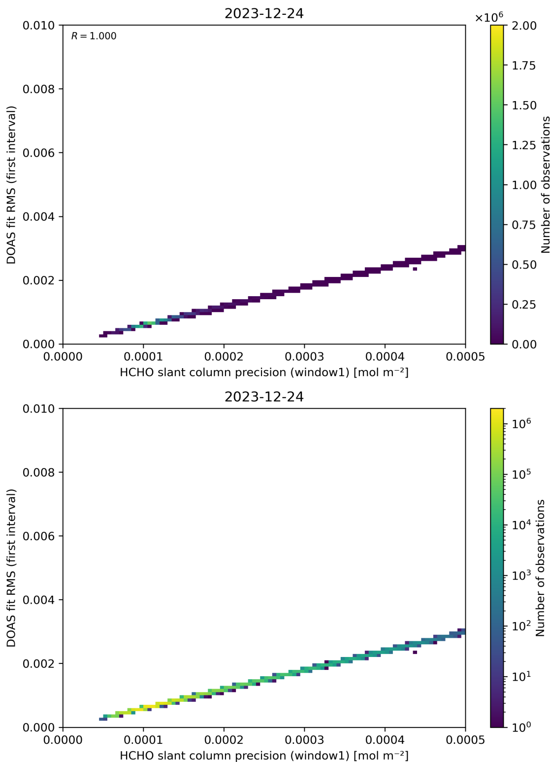
Figure 88: Scatter density plot of “HCHO slant column precision (window1)” against “DOAS fit RMS (first interval)” for 2023-12-23 to 2023-12-25.
