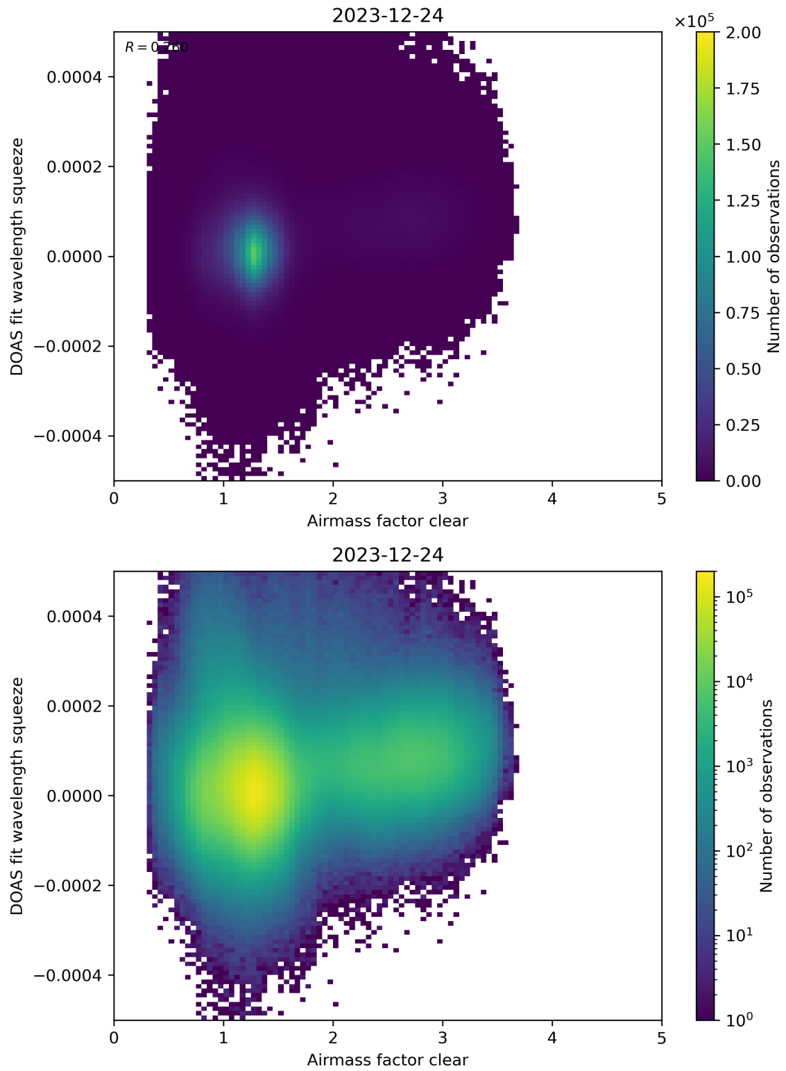
Figure 73: Scatter density plot of “Airmass factor clear” against “DOAS fit wavelength squeeze” for 2023-12-23 to 2023-12-25.
