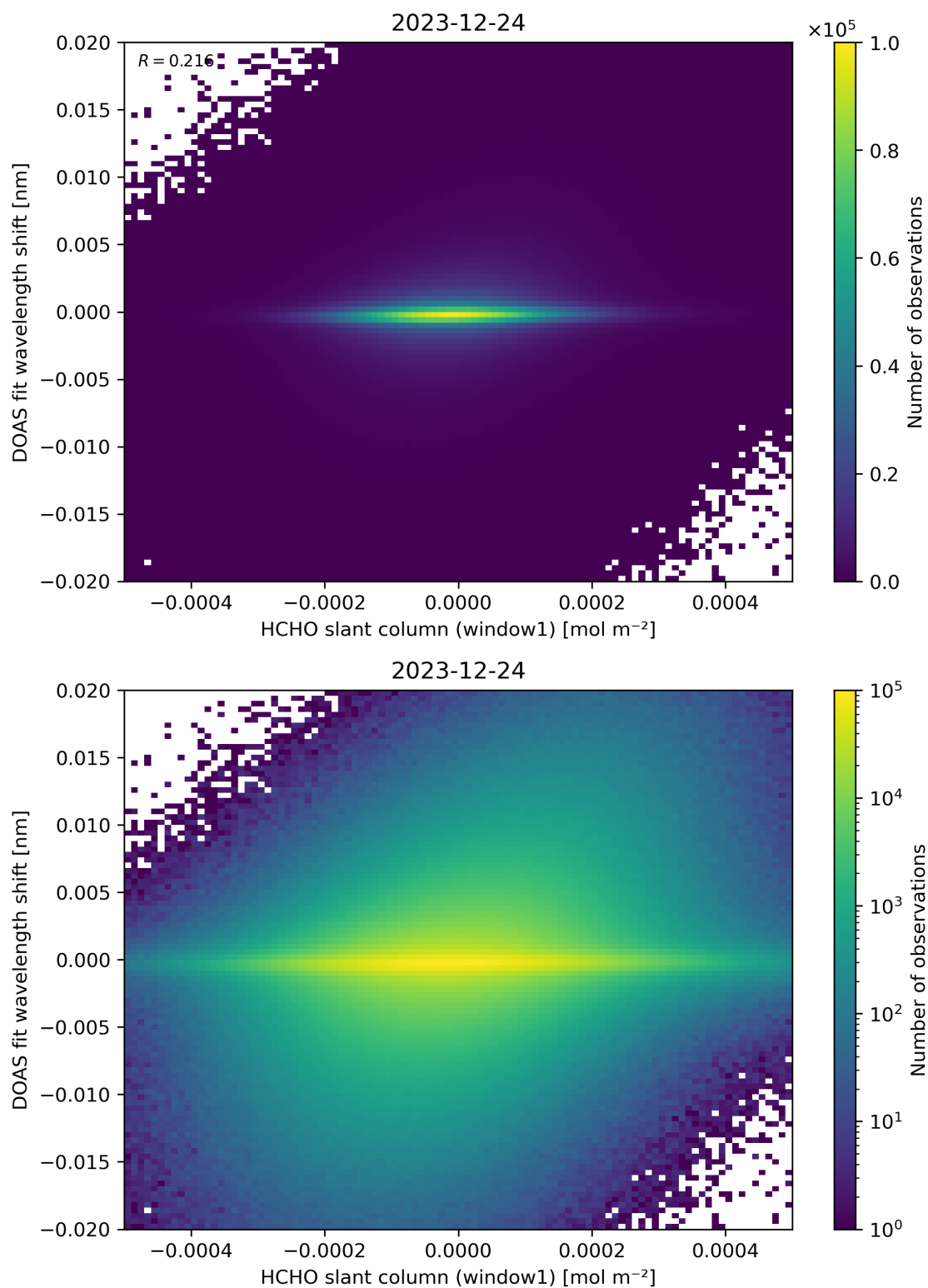
Figure 79: Scatter density plot of “HCHO slant column (window1)” against “DOAS fit wavelength shift” for 2023-12-23 to 2023-12-25.
