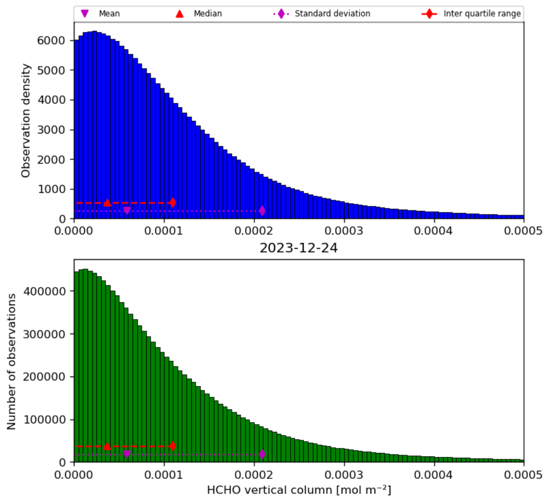
Figure 35: Histogram of “HCHO vertical column” for 2023-12-23 to 2023-12-25
