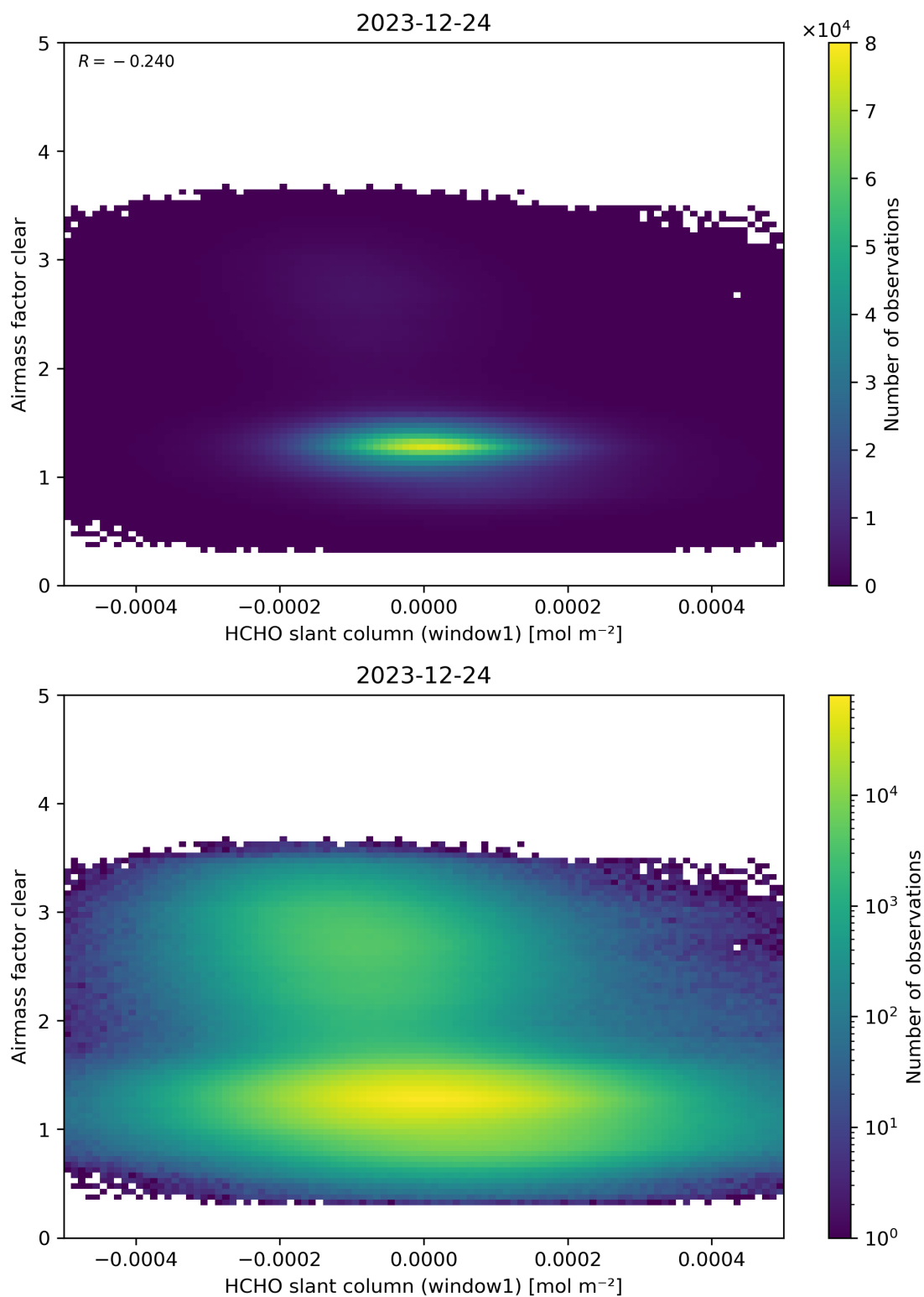
Figure 81: Scatter density plot of “HCHO slant column (window1)” against “Airmass factor clear” for 2023-12-23 to 2023-12-25.
