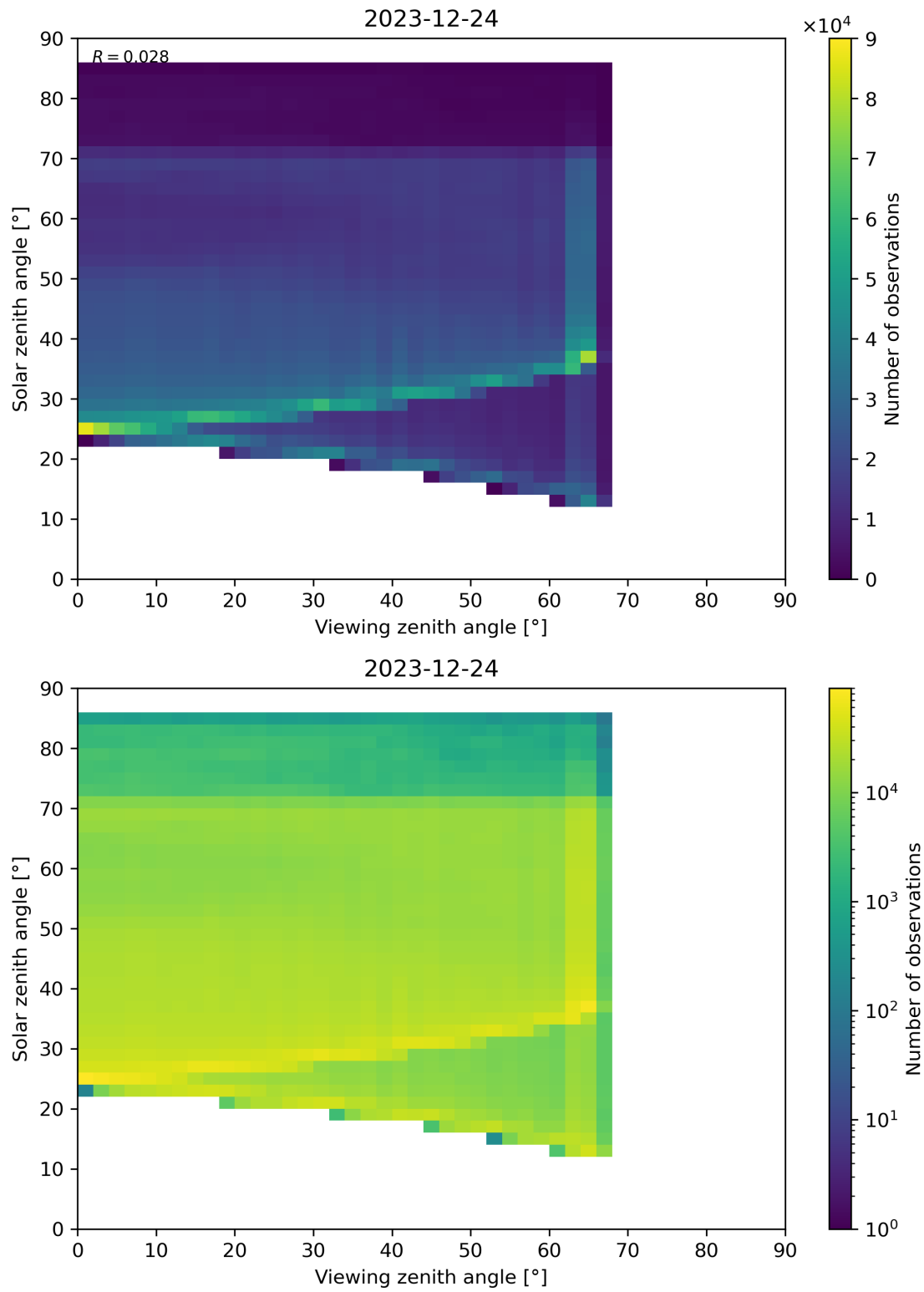
Figure 197: Scatter density plot of “Viewing zenith angle” against “Solar zenith angle” for 2023-12-23 to 2023-12-25.
