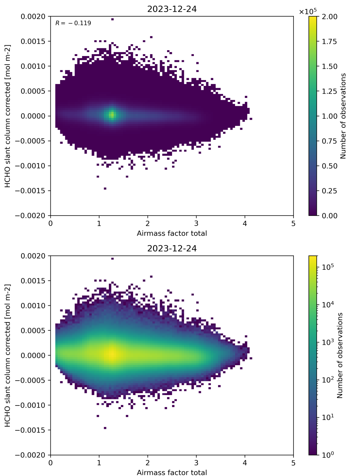
Figure 101: Scatter density plot of “Airmass factor total” against “HCHO slant column corrected” for 2023-12-23 to 2023-12-25.
