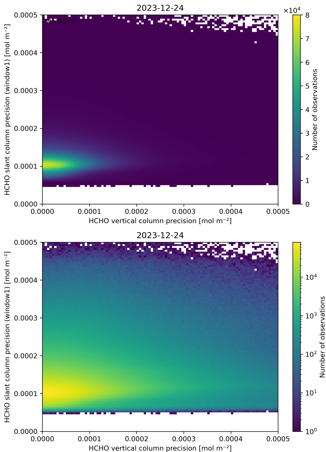
Figure 143: Scatter density plot of “HCHO vertical column precision” against “HCHO slant column precision (window1)” for 2023-12-23 to 2023-12-25.
