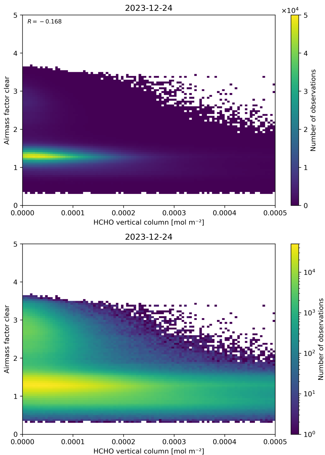
Figure 126: Scatter density plot of “HCHO vertical column” against “Airmass factor clear” for 2023-12-23 to 2023-12-25.
