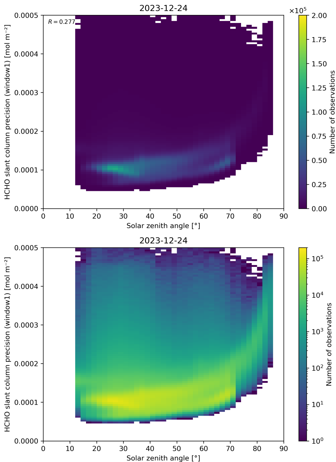
Figure 174: Scatter density plot of “Solar zenith angle” against “HCHO slant column precision (window1)” for 2023-12-23 to 2023-12-25.
