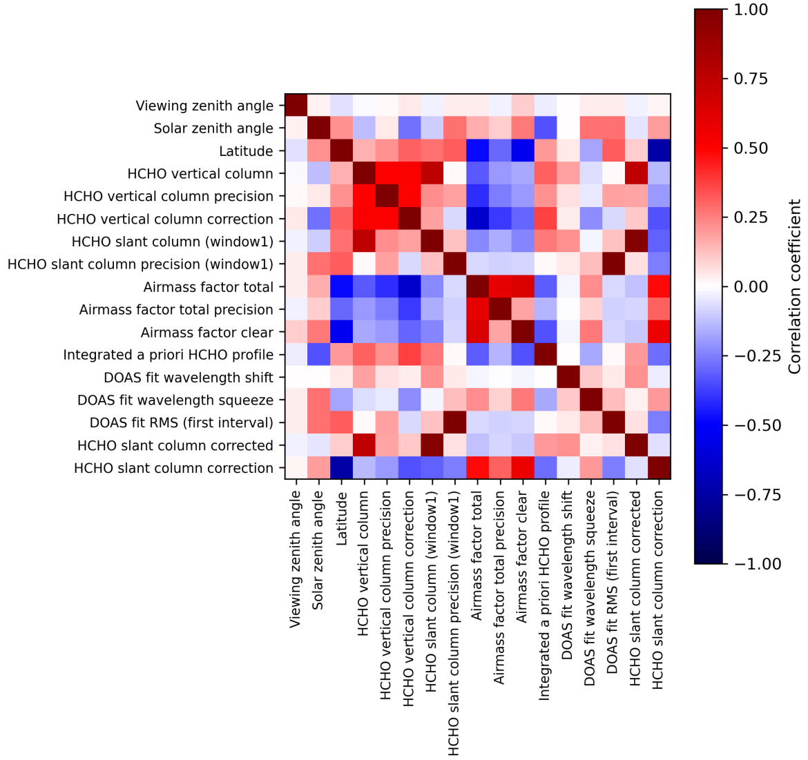
Figure 2: Map of correlation matrix for 2023-12-23 to 2023-12-25.
