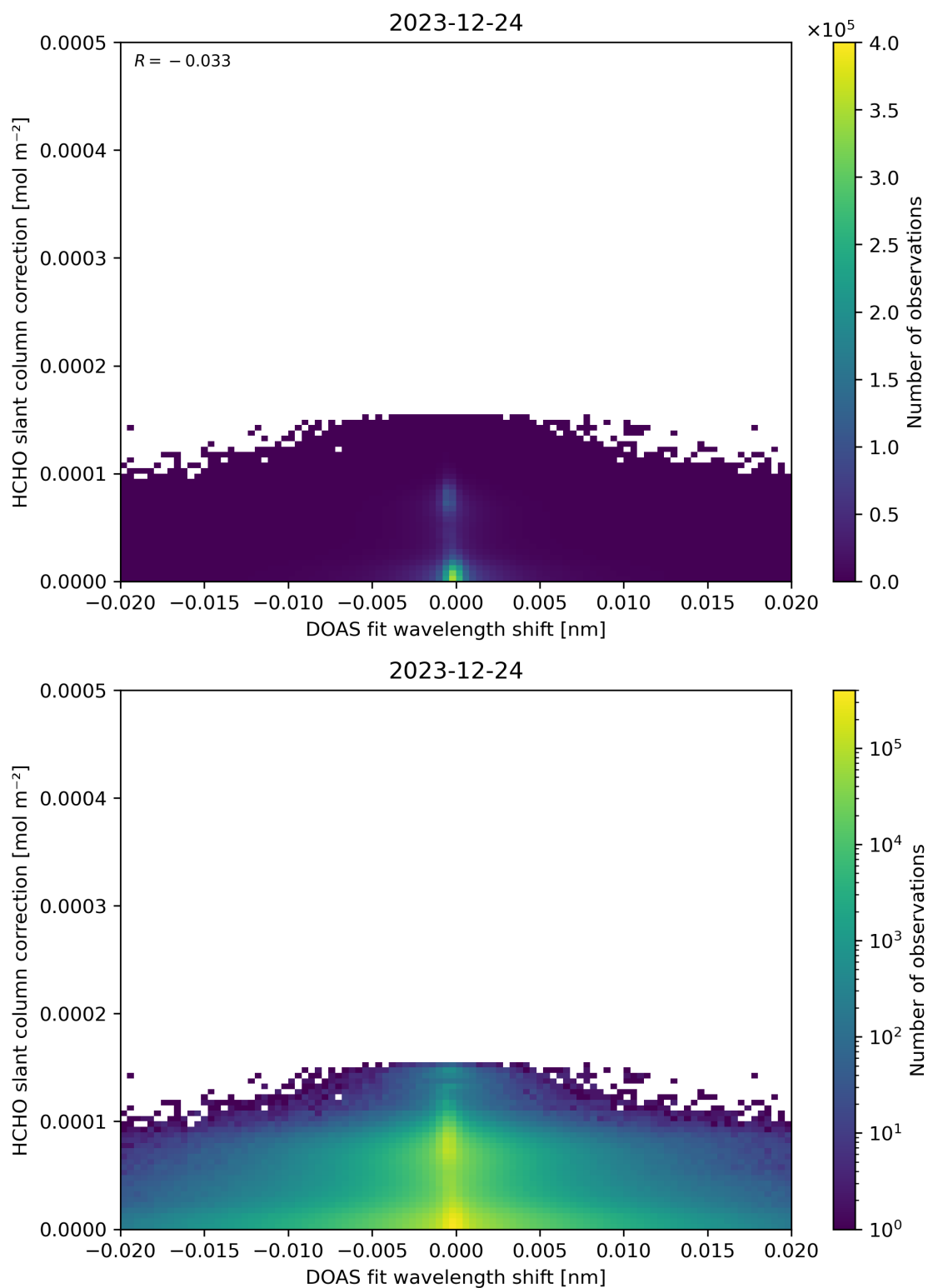
Figure 67: Scatter density plot of “DOAS fit wavelength shift” against “HCHO slant column correction” for 2023-12-23 to 2023-12-25.
