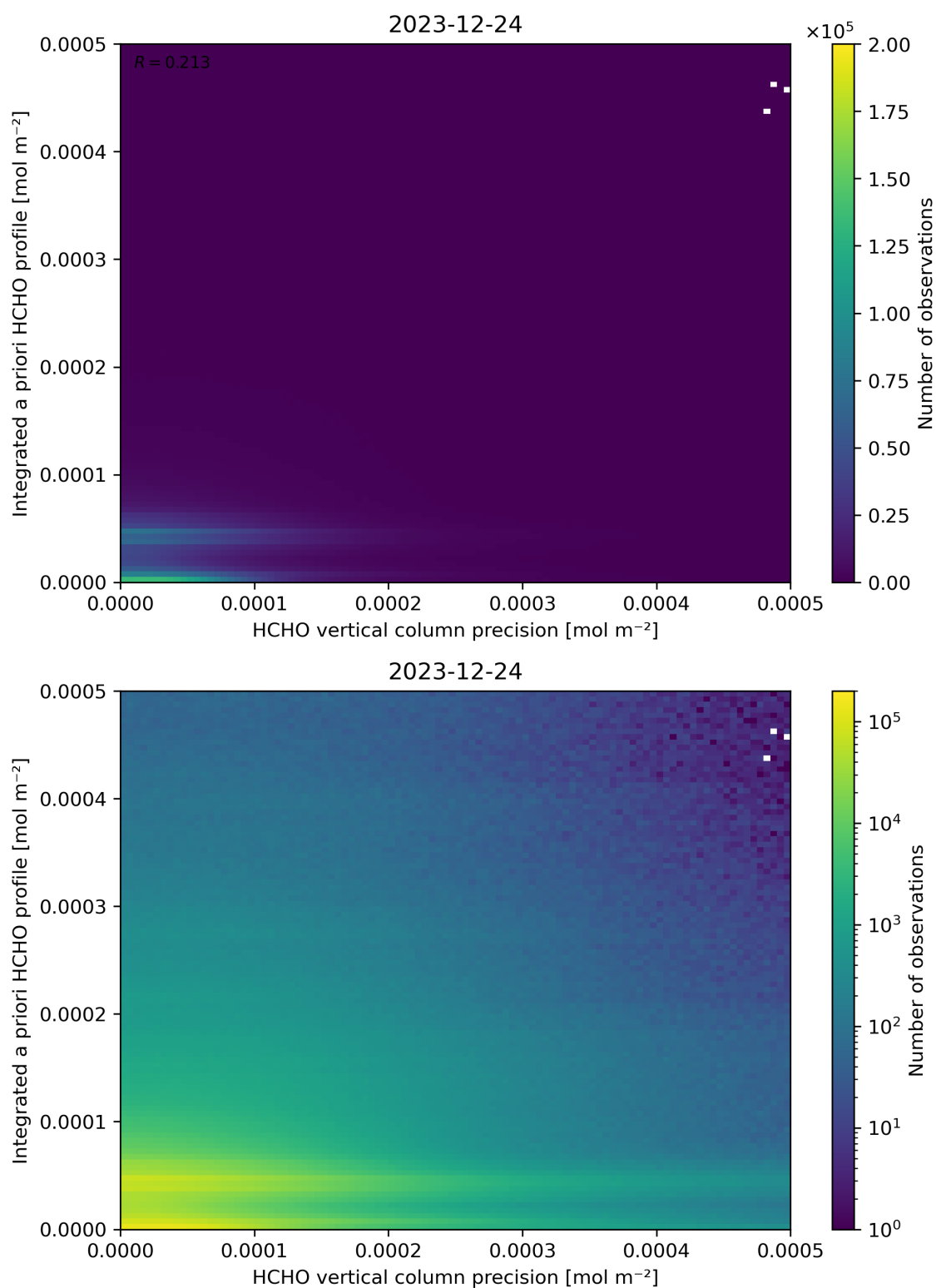
Figure 147: Scatter density plot of “HCHO vertical column precision” against “Integrated a priori HCHO profile” for 2023-12-23 to 2023-12-25.
