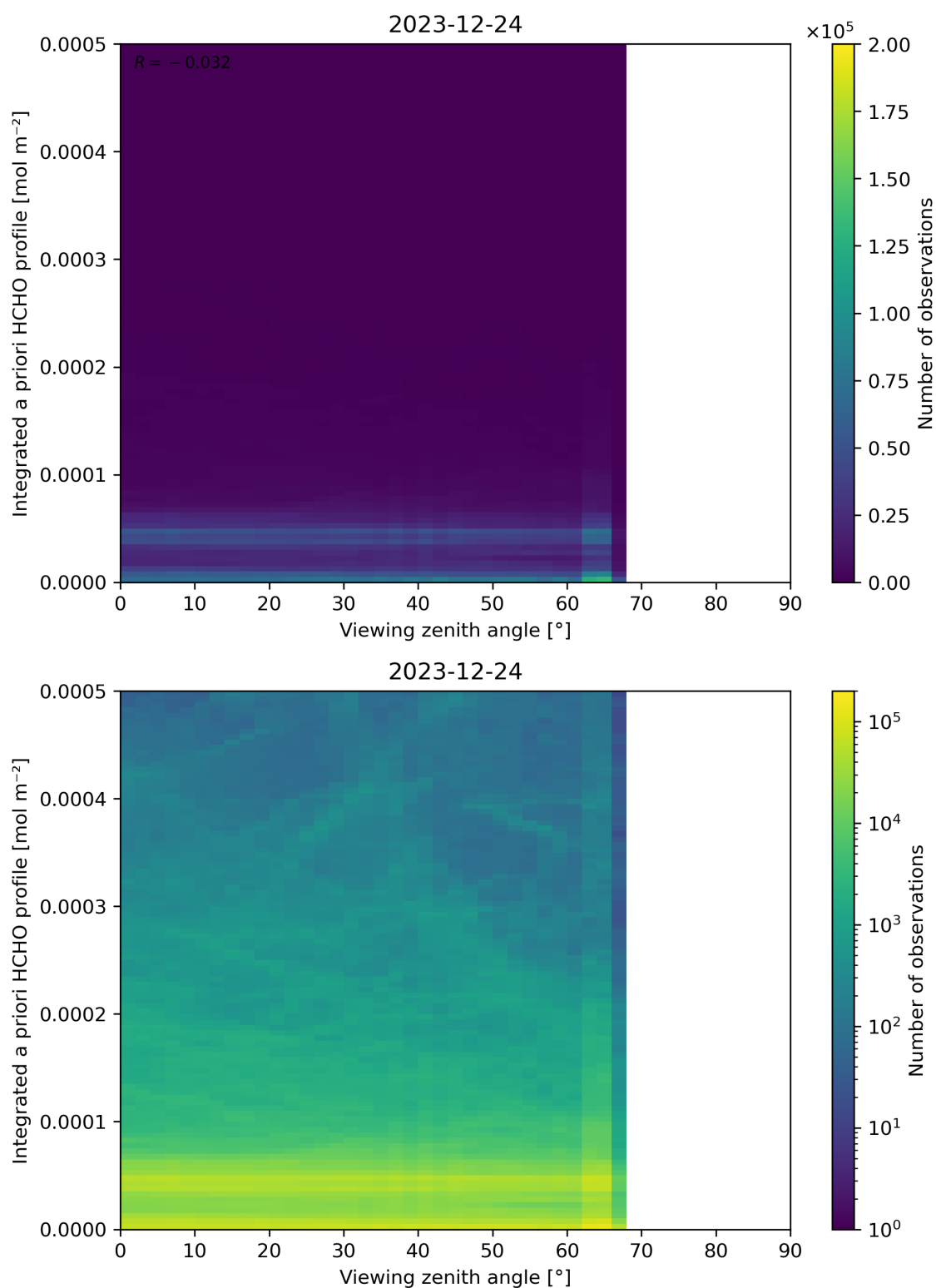
Figure 195: Scatter density plot of “Viewing zenith angle” against “Integrated a priori HCHO profile” for 2023-12-23 to 2023-12-25.
