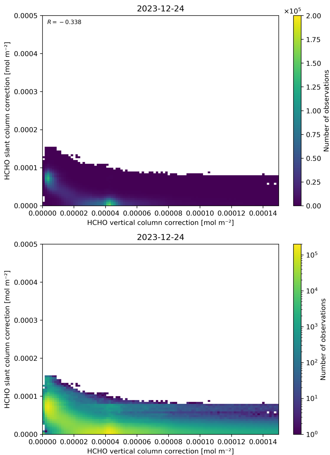
Figure 117: Scatter density plot of “HCHO vertical column correction” against “HCHO slant column correction” for 2023-12-23 to 2023-12-25.
