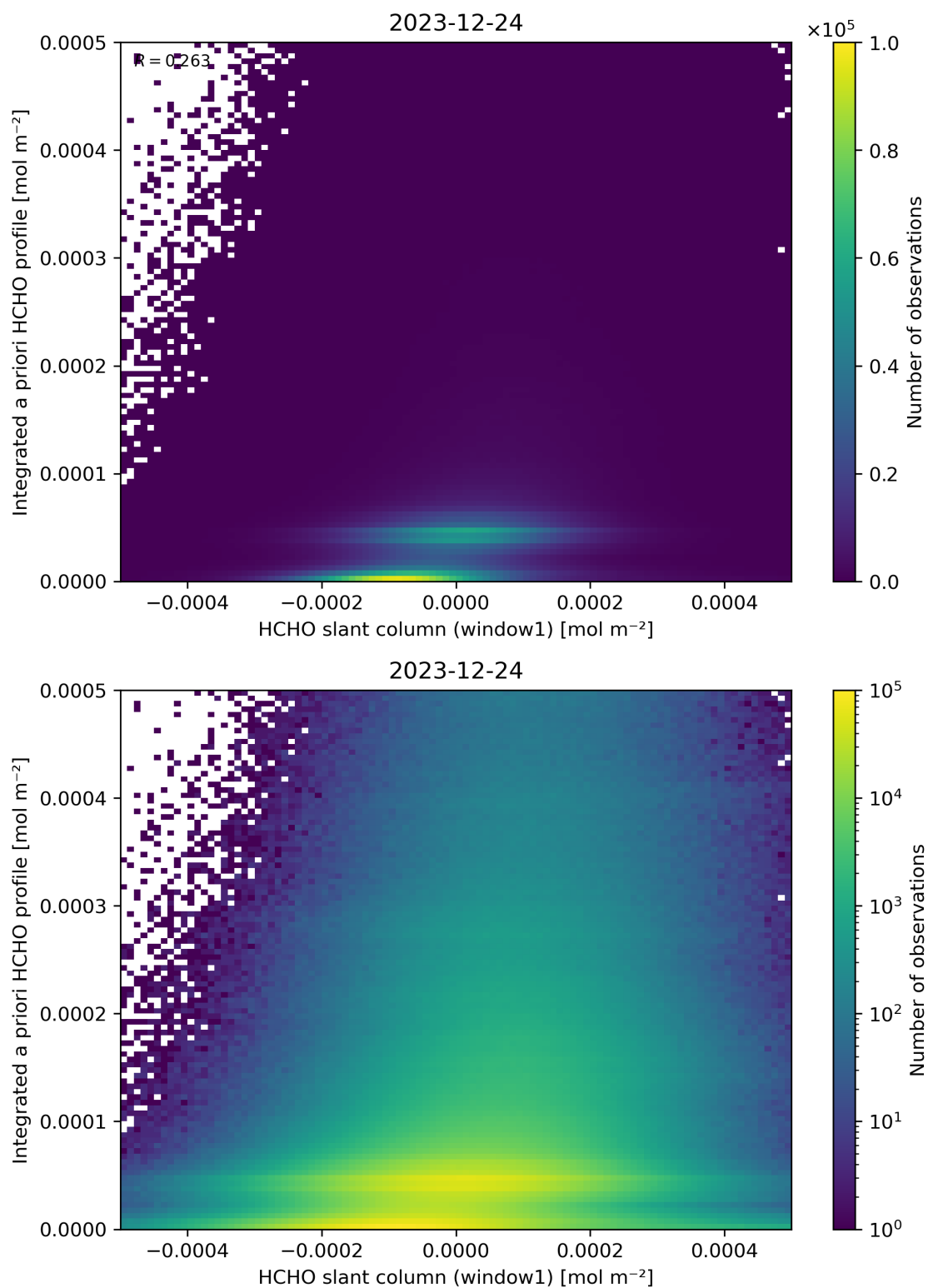
Figure 87: Scatter density plot of “HCHO slant column (window1)” against “Integrated a priori HCHO profile” for 2023-12-23 to 2023-12-25.
