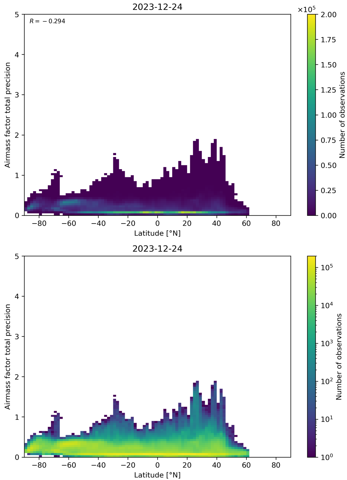
Figure 162: Scatter density plot of “Latitude” against “Airmass factor total precision” for 2023-12-23 to 2023-12-25.
