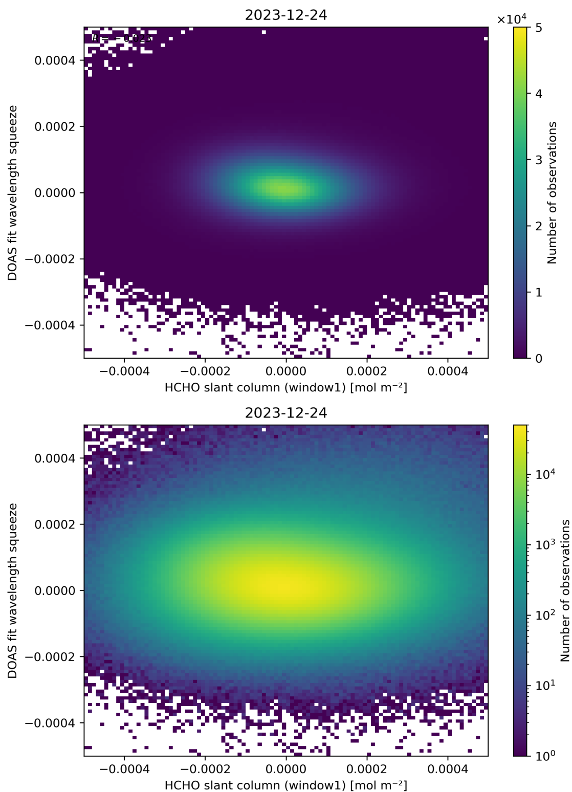
Figure 80: Scatter density plot of “HCHO slant column (window1)” against “DOAS fit wavelength squeeze” for 2023-12-23 to 2023-12-25.
