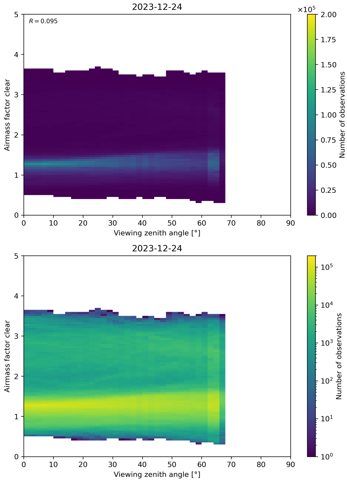
Figure 185: Scatter density plot of “Viewing zenith angle” against “Airmass factor clear” for 2023-12-23 to 2023-12-25.
