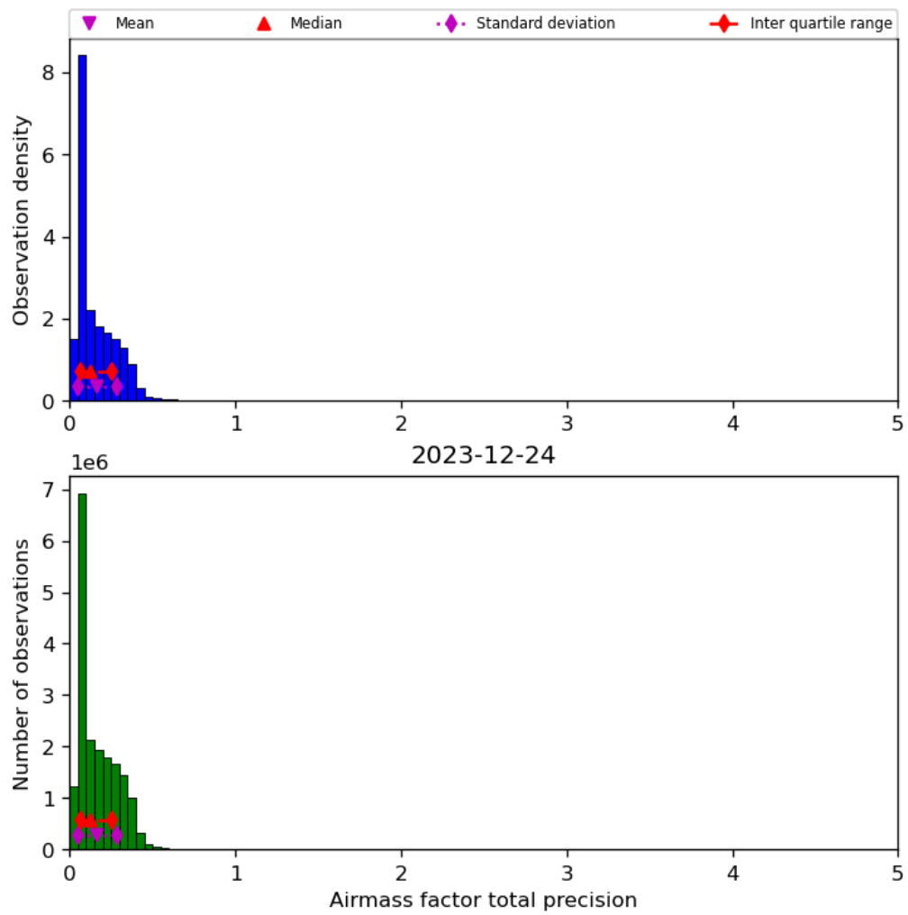
Figure 41: Histogram of “Airmass factor total precision” for 2023-12-23 to 2023-12-25
