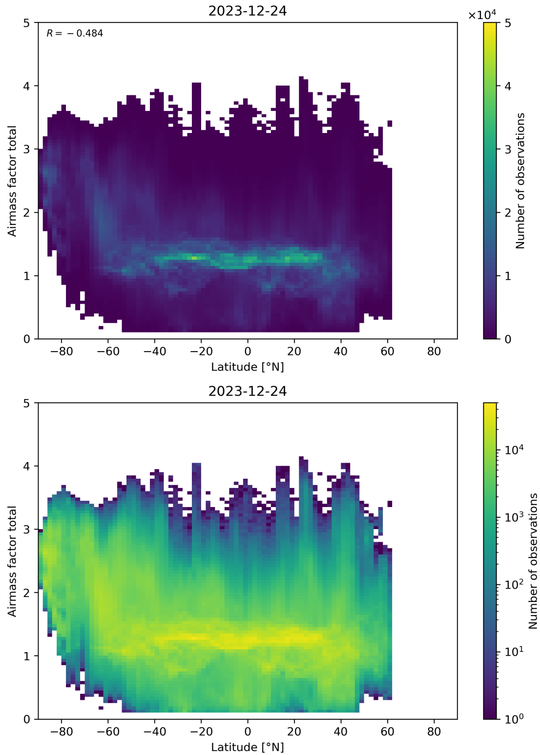
Figure 161: Scatter density plot of “Latitude” against “Airmass factor total” for 2023-12-23 to 2023-12-25.
