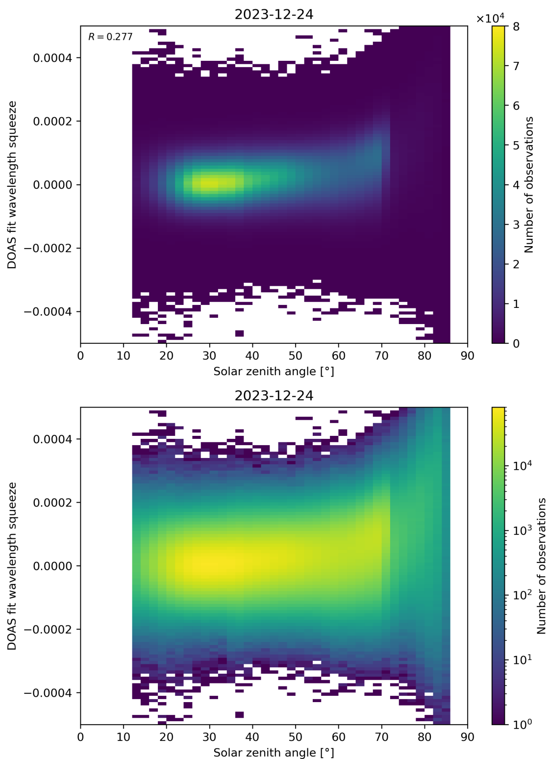
Figure 169: Scatter density plot of “Solar zenith angle” against “DOAS fit wavelength squeeze” for 2023-12-23 to 2023-12-25.
