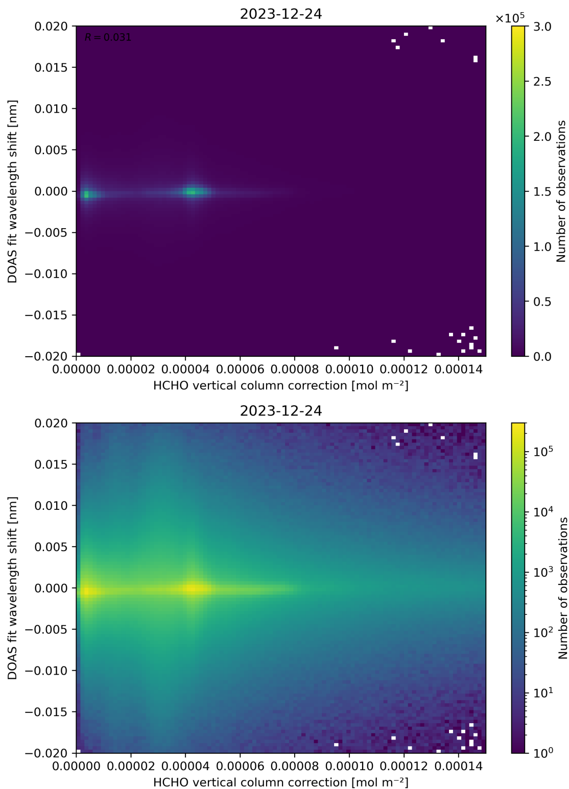
Figure 113: Scatter density plot of “HCHO vertical column correction” against “DOAS fit wavelength shift” for 2023-12-23 to 2023-12-25.
