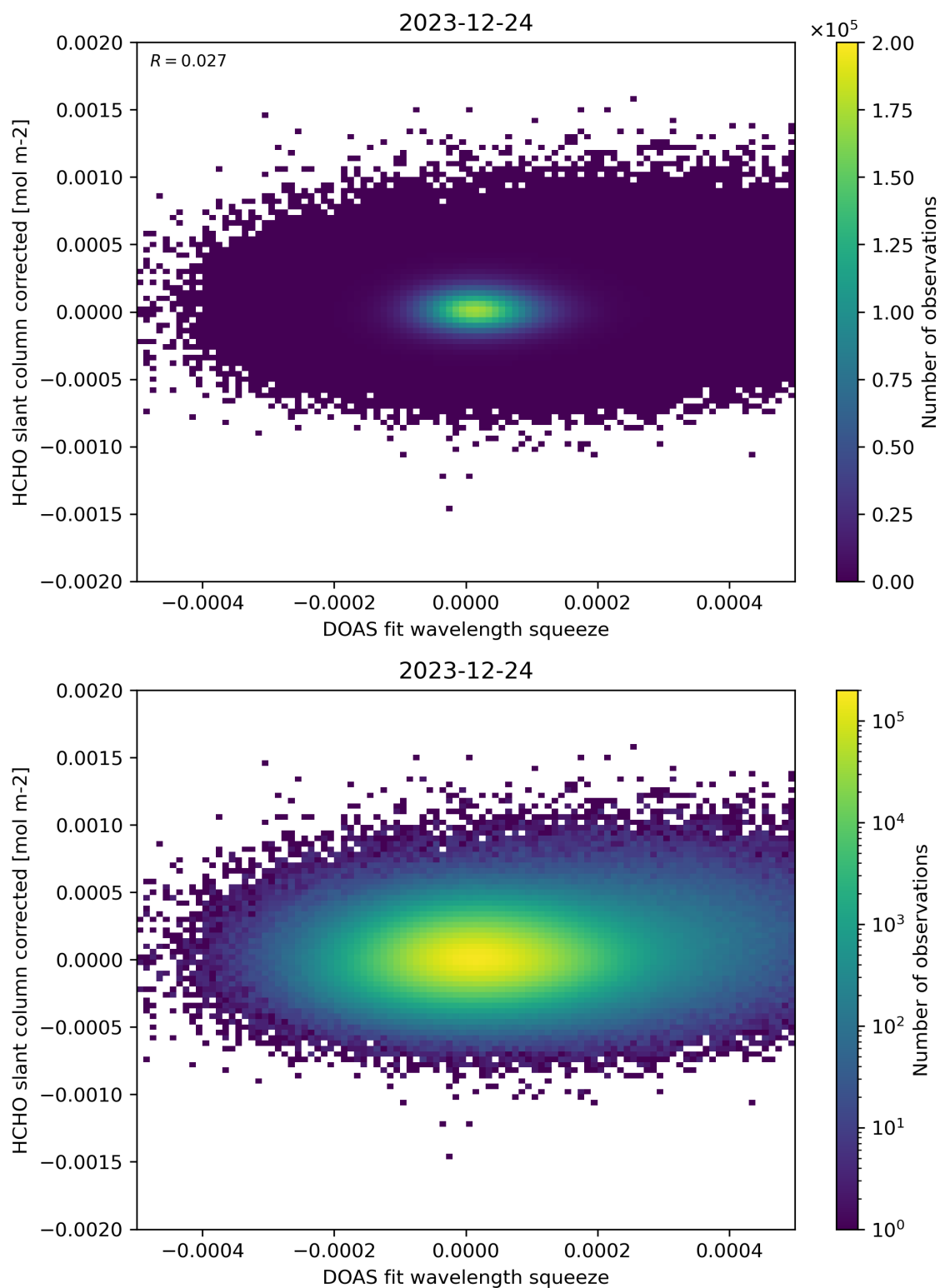
Figure 69: Scatter density plot of “DOAS fit wavelength squeeze” against “HCHO slant column corrected” for 2023-12-23 to 2023-12-25.
