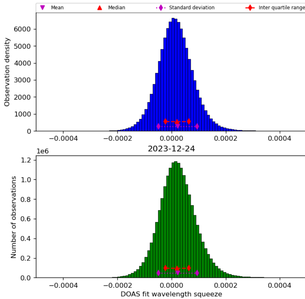
Figure 45: Histogram of “DOAS fit wavelength squeeze” for 2023-12-23 to 2023-12-25
