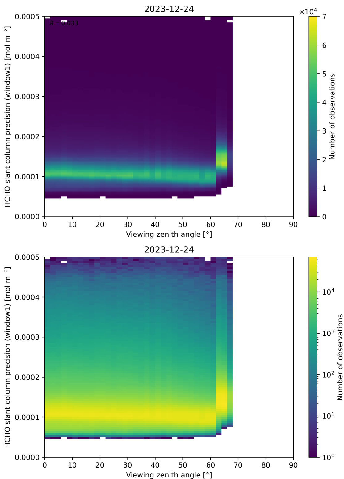
Figure 189: Scatter density plot of “Viewing zenith angle” against “HCHO slant column precision (window1)” for 2023-12-23 to 2023-12-25.
