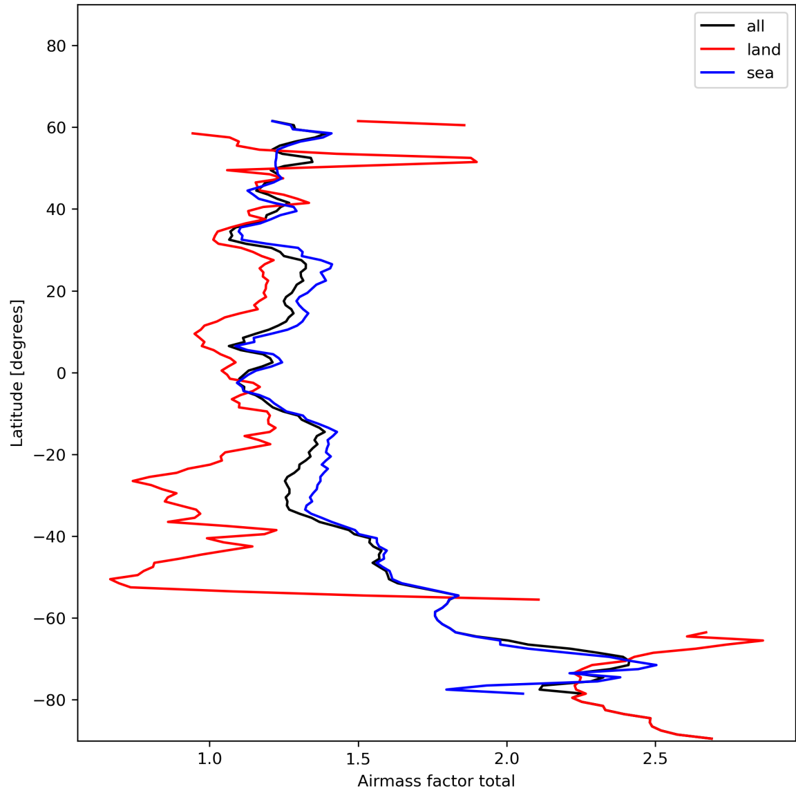
Figure 26: Zonal average of “Airmass factor total” for 2023-12-23 to 2023-12-25.
