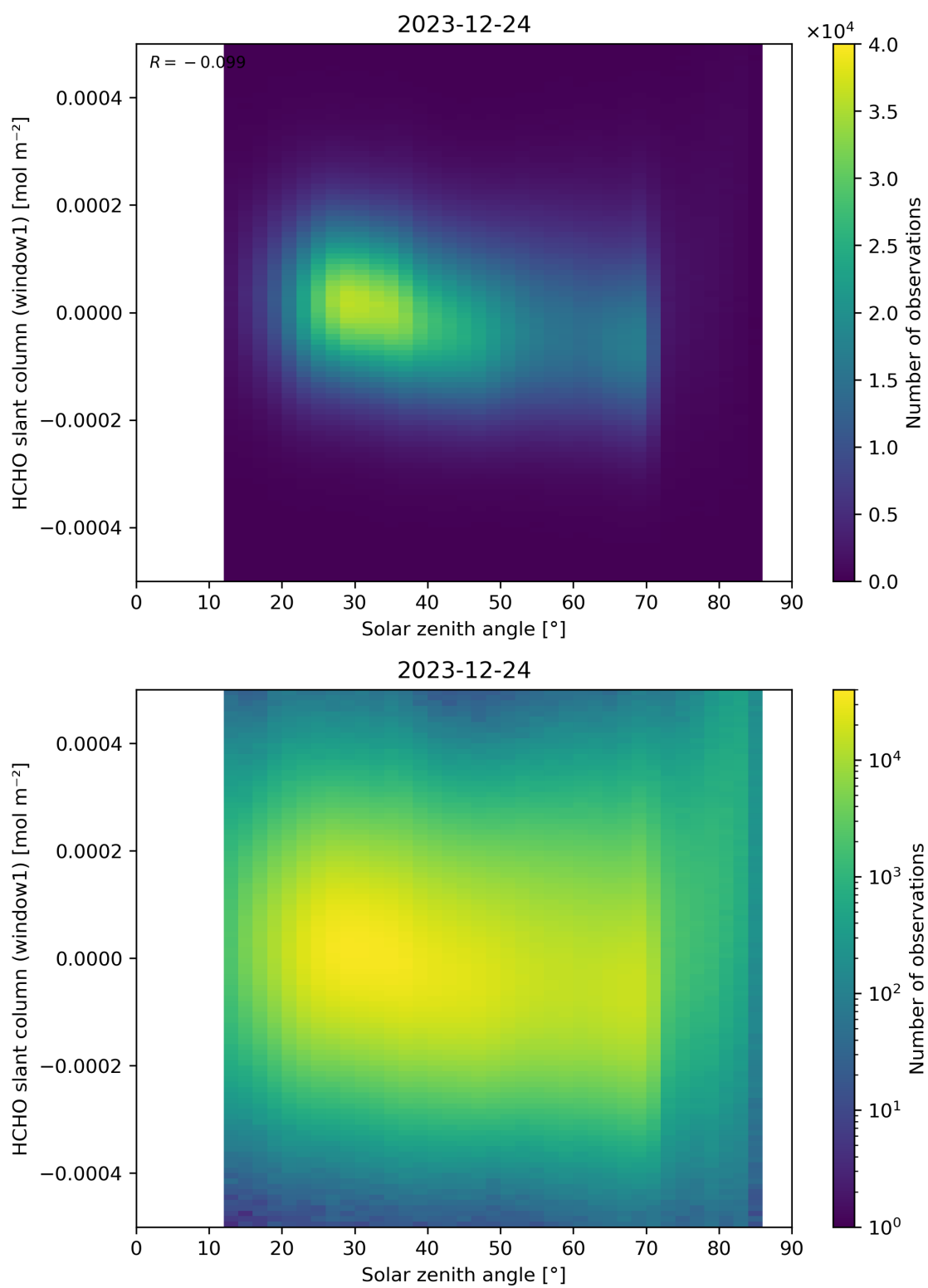
Figure 173: Scatter density plot of “Solar zenith angle” against “HCHO slant column (window1)” for 2023-12-23 to 2023-12-25.
