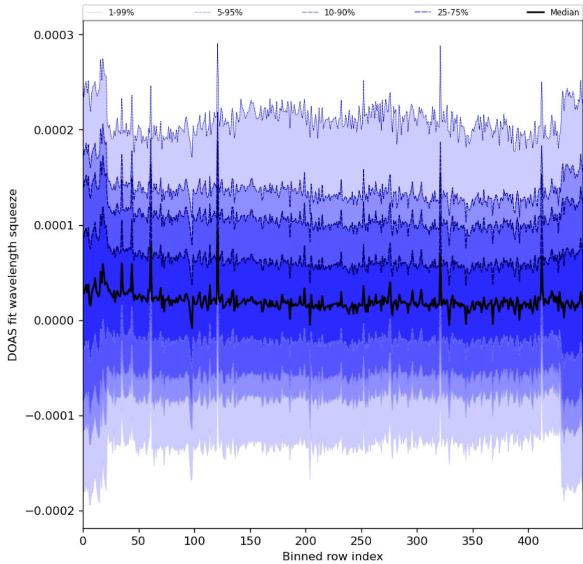
Figure 59: Along track statistics of “DOAS fit wavelength squeeze” for 2023-12-23 to 2023-12-25
