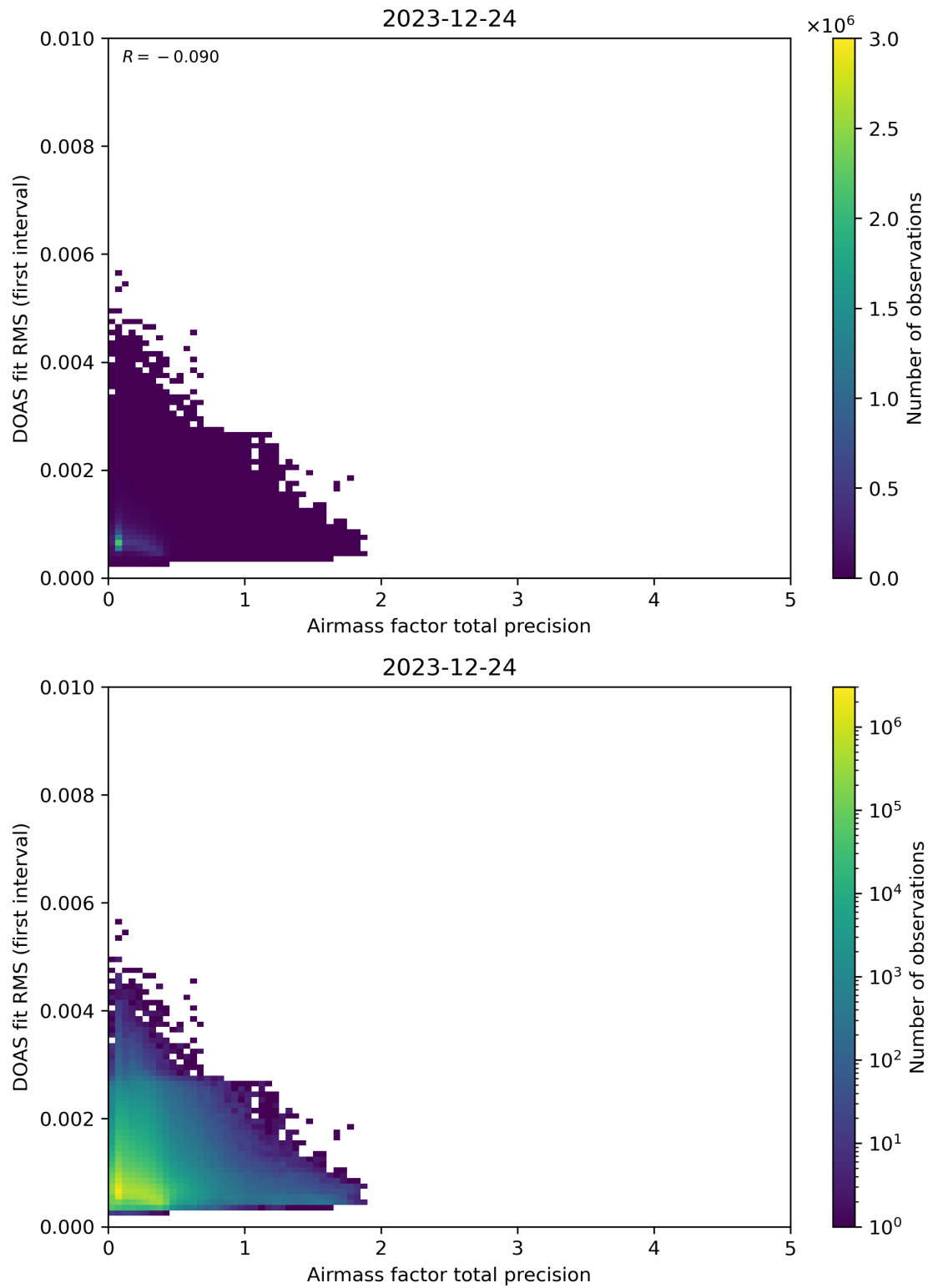
Figure 105: Scatter density plot of “Airmass factor total precision” against “DOAS fit RMS (first interval)” for 2023-12-23 to 2023-12-25.
