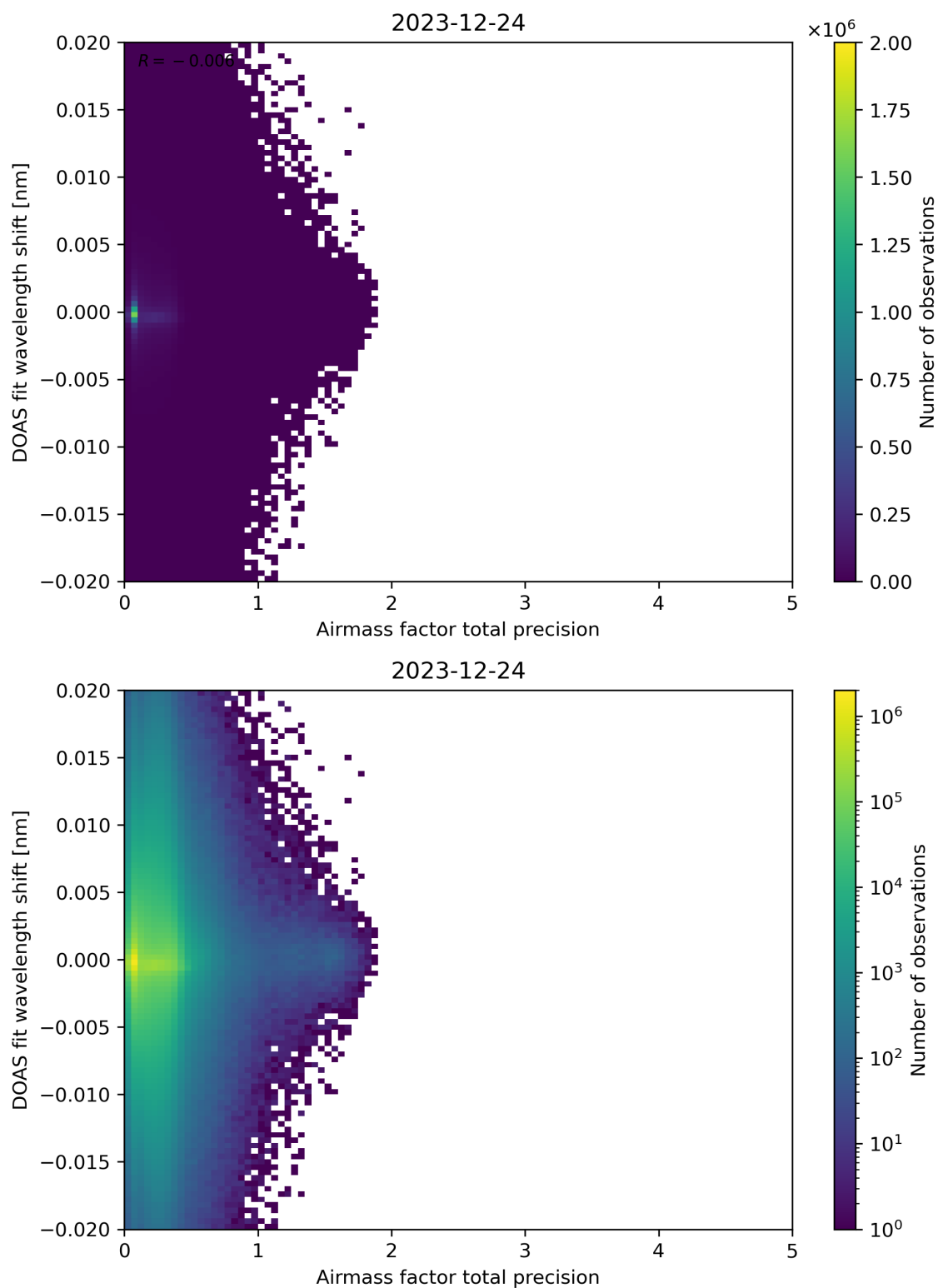
Figure 106: Scatter density plot of “Airmass factor total precision” against “DOAS fit wavelength shift” for 2023-12-23 to 2023-12-25.
