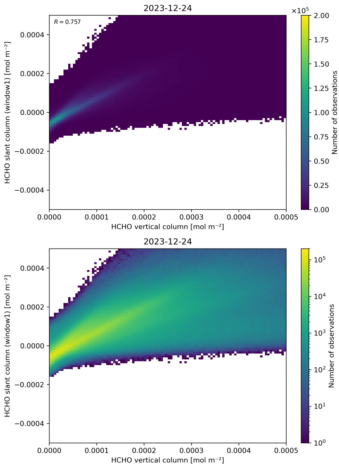
Figure 129: Scatter density plot of “HCHO vertical column” against “HCHO slant column (window1)” for 2023-12-23 to 2023-12-25.
