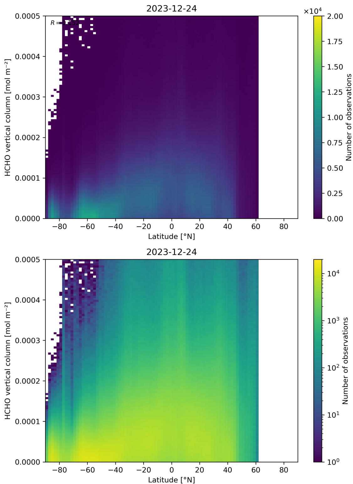
Figure 163: Scatter density plot of “Latitude” against “HCHO vertical column” for 2023-12-23 to 2023-12-25.
