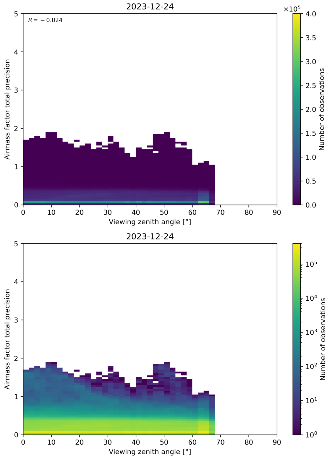
Figure 191: Scatter density plot of “Viewing zenith angle” against “Airmass factor total precision” for 2023-12-23 to 2023-12-25.
