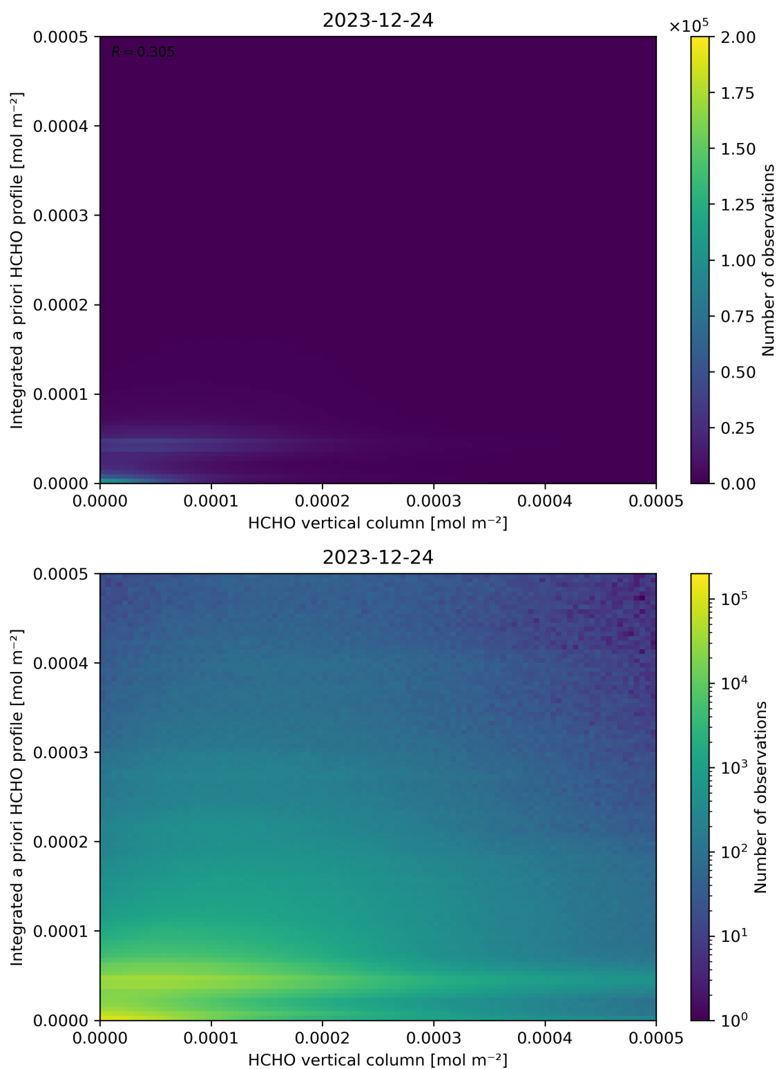
Figure 135: Scatter density plot of “HCHO vertical column” against “Integrated a priori HCHO profile” for 2023-12-23 to 2023-12-25.
