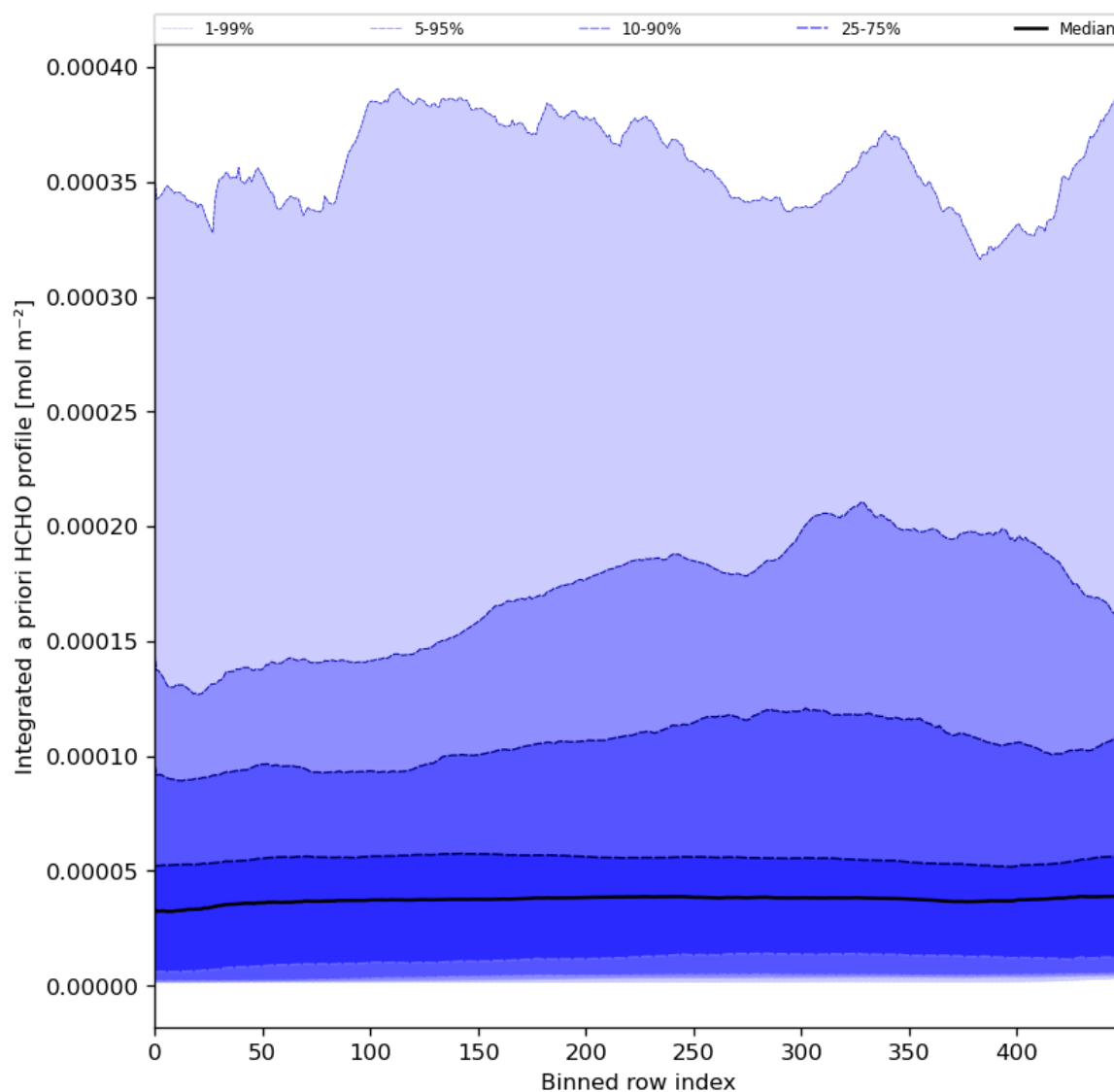
Figure 57: Along track statistics of “Integrated a priori HCHO profile” for 2023-12-23 to 2023-12-25
