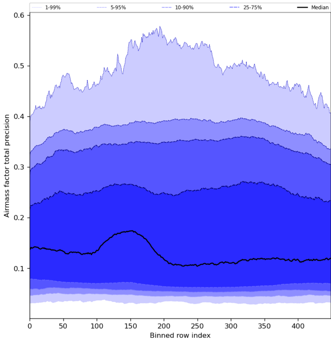
Figure 55: Along track statistics of “Airmass factor total precision” for 2023-12-23 to 2023-12-25
