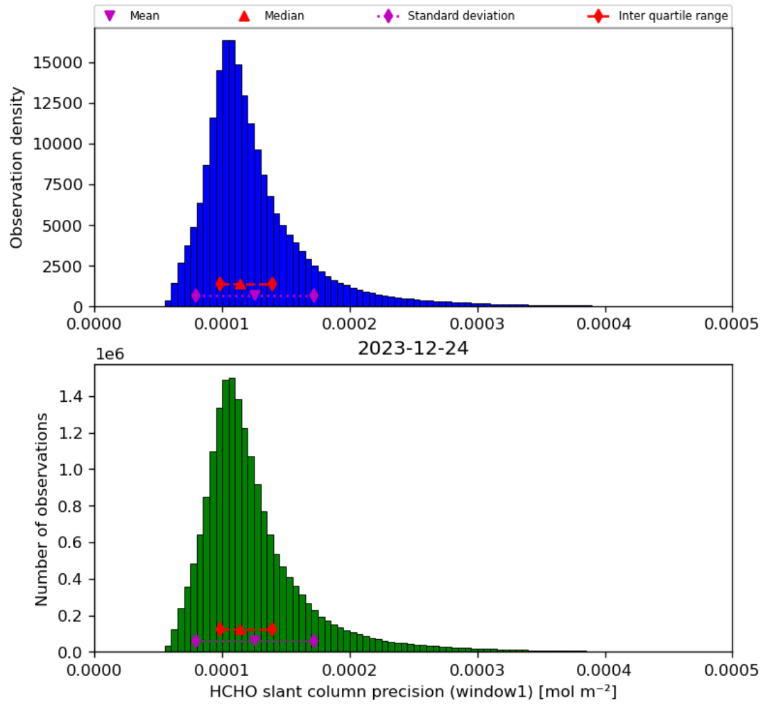
Figure 39: Histogram of “HCHO slant column precision (window1)” for 2023-12-23 to 2023-12-25
