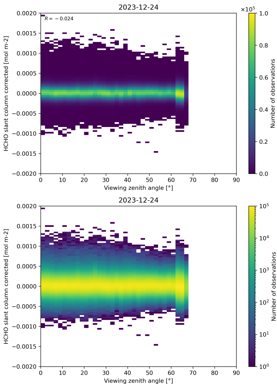
Figure 186: Scatter density plot of “Viewing zenith angle” against “HCHO slant column corrected” for 2023-12-23 to 2023-12-25.
