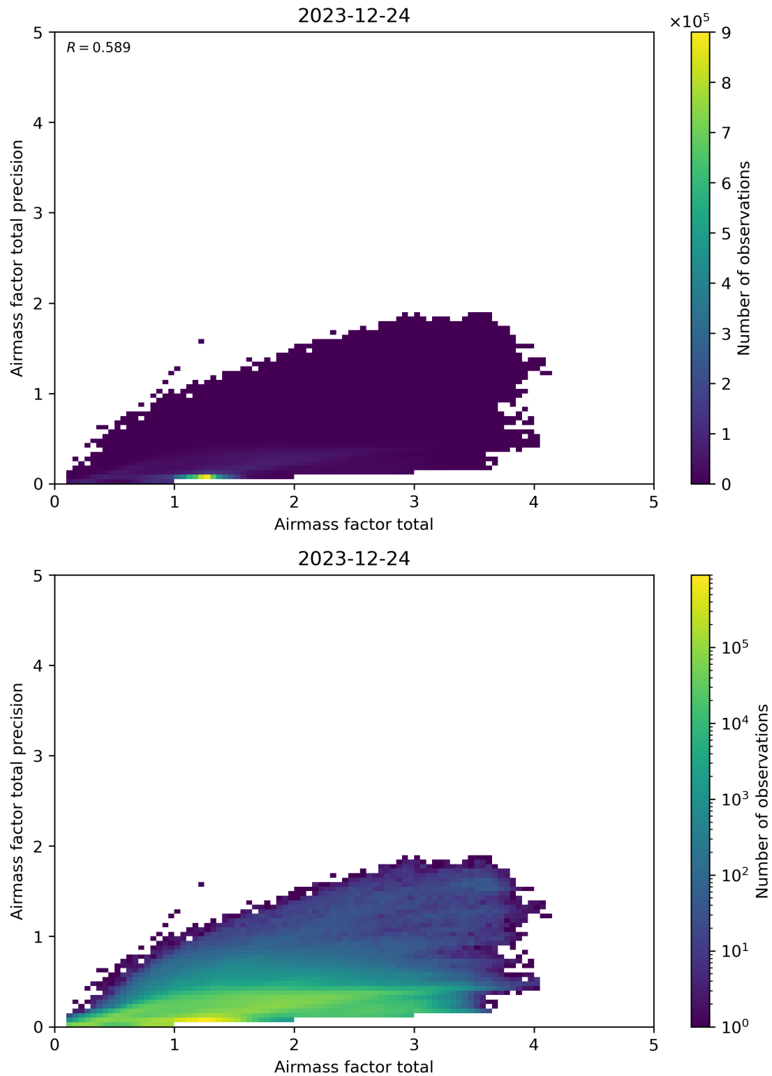
Figure 103: Scatter density plot of “Airmass factor total” against “Airmass factor total precision” for 2023-12-23 to 2023-12-25.
