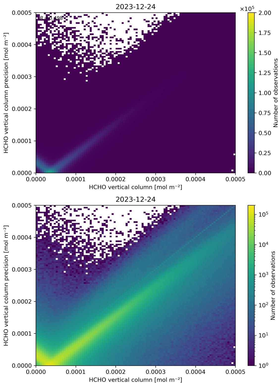
Figure 134: Scatter density plot of “HCHO vertical column” against “HCHO vertical column precision” for 2023-12-23 to 2023-12-25.
