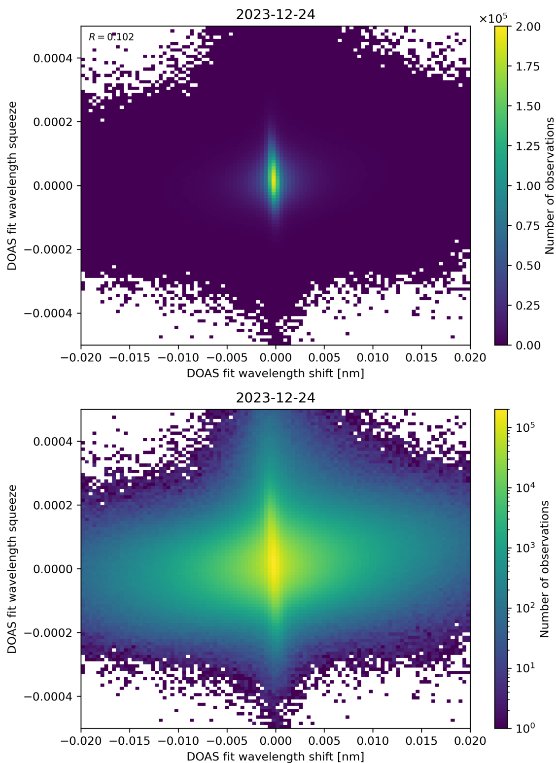
Figure 65: Scatter density plot of “DOAS fit wavelength shift” against “DOAS fit wavelength squeeze” for 2023-12-23 to 2023-12-25.
