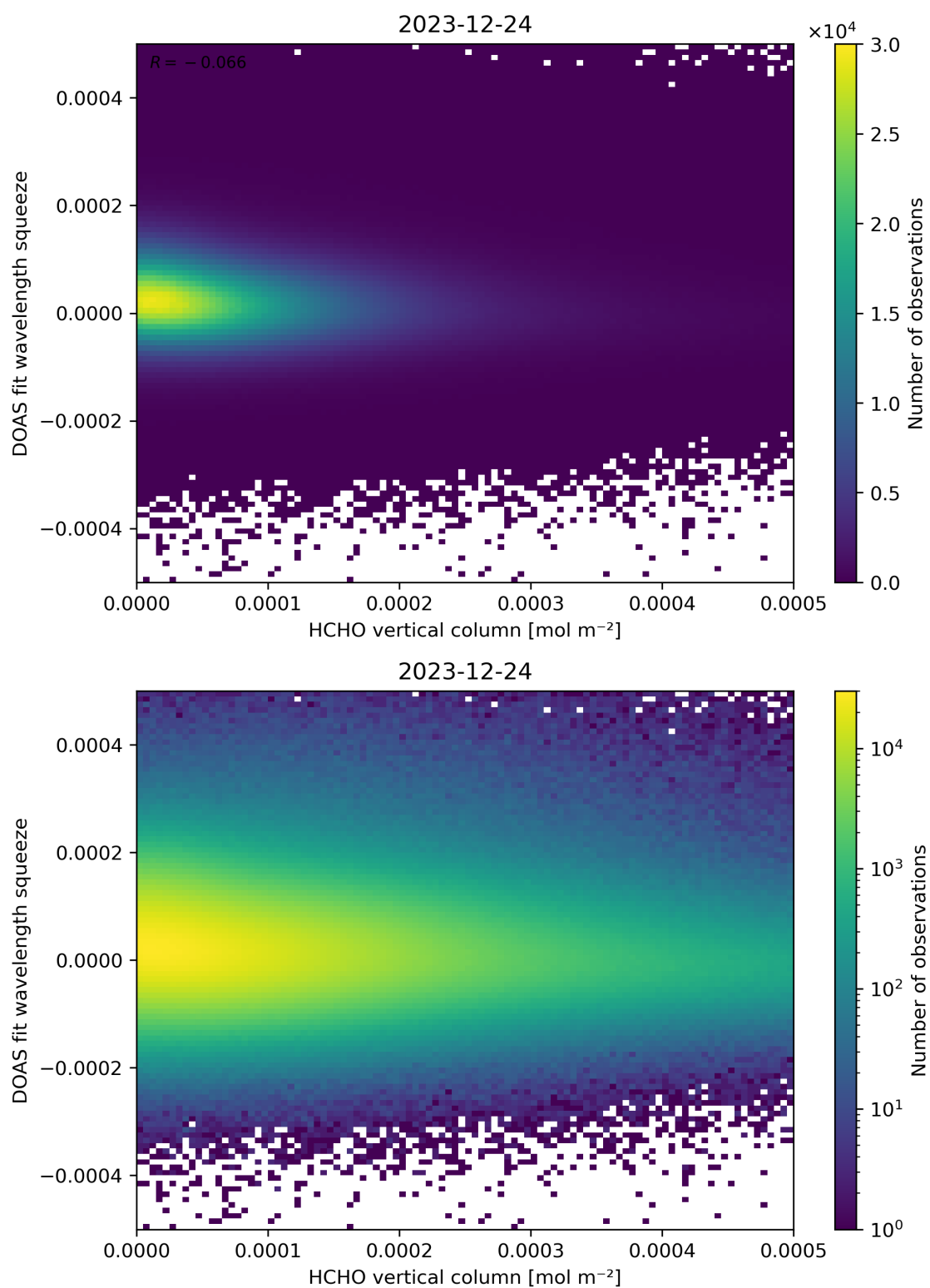
Figure 125: Scatter density plot of “HCHO vertical column” against “DOAS fit wavelength squeeze” for 2023-12-23 to 2023-12-25.
