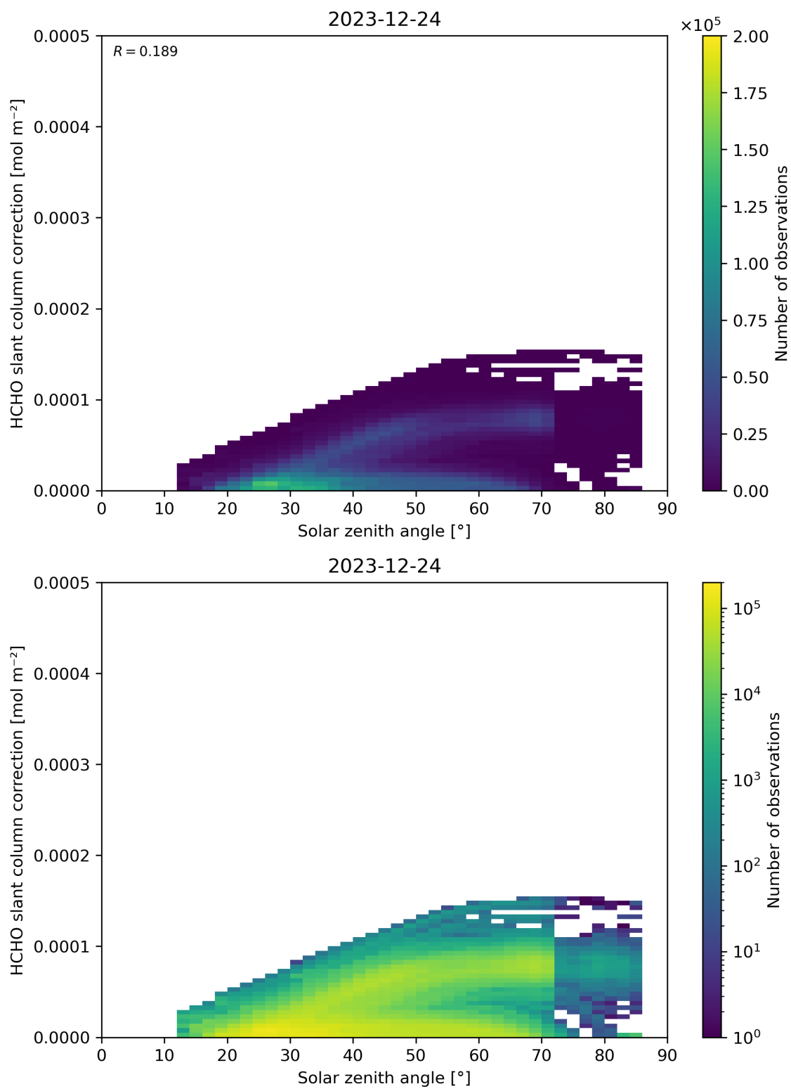
Figure 172: Scatter density plot of “Solar zenith angle” against “HCHO slant column correction” for 2023-12-23 to 2023-12-25.
