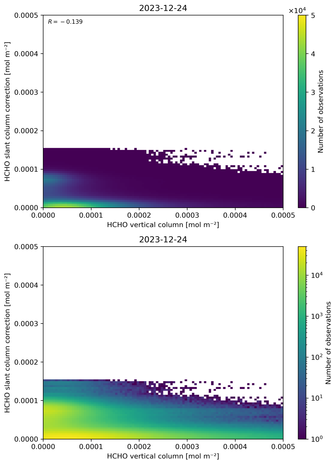
Figure 128: Scatter density plot of “HCHO vertical column” against “HCHO slant column correction” for 2023-12-23 to 2023-12-25.
