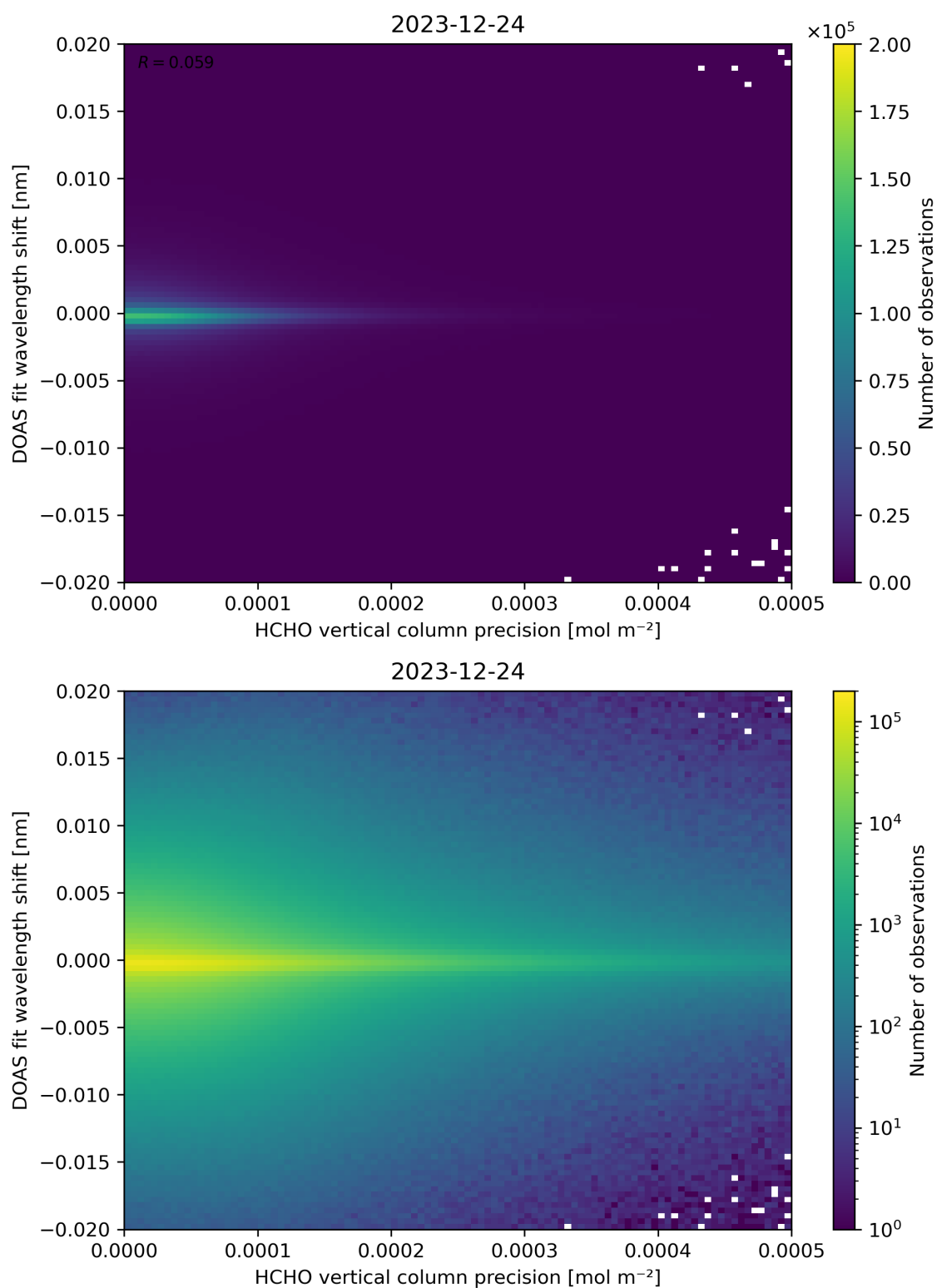
Figure 137: Scatter density plot of “HCHO vertical column precision” against “DOAS fit wavelength shift” for 2023-12-23 to 2023-12-25.
