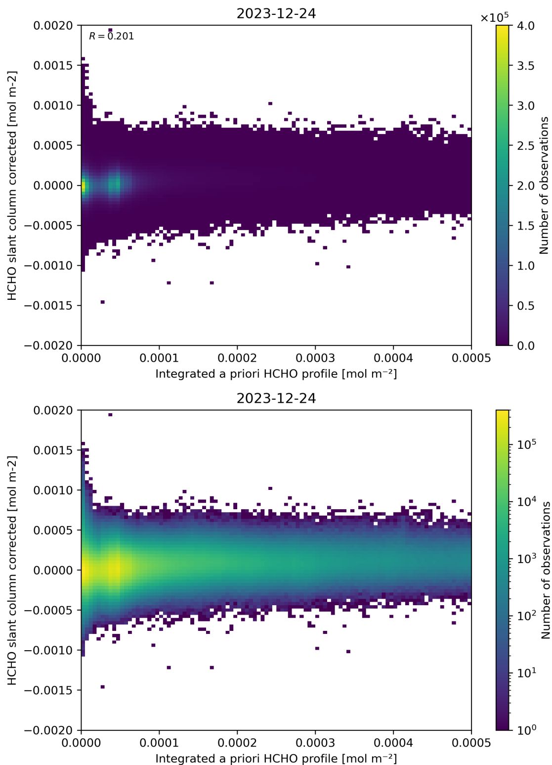
Figure 151: Scatter density plot of “Integrated a priori HCHO profile” against “HCHO slant column corrected” for 2023-12-23 to 2023-12-25.
