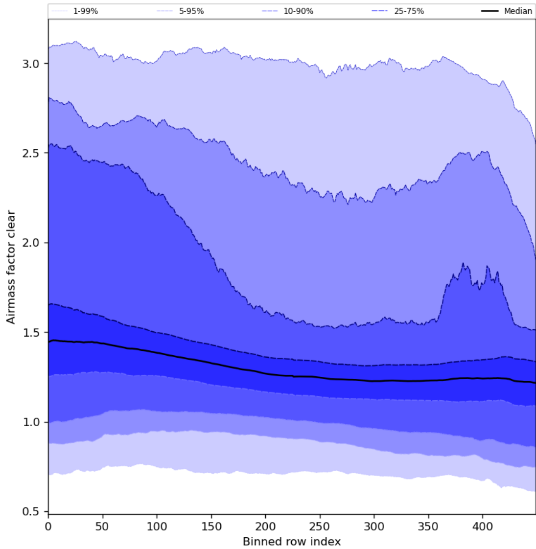
Figure 56: Along track statistics of “Airmass factor clear” for 2023-12-26 to 2023-12-28
