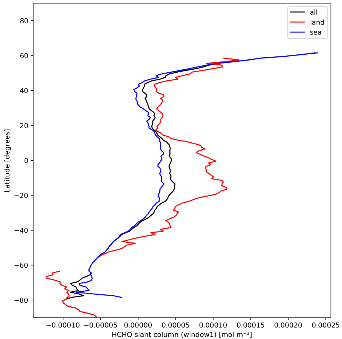
Figure 24: Zonal average of “HCHO slant column (window1)” for 2023-12-26 to 2023-12-28.
