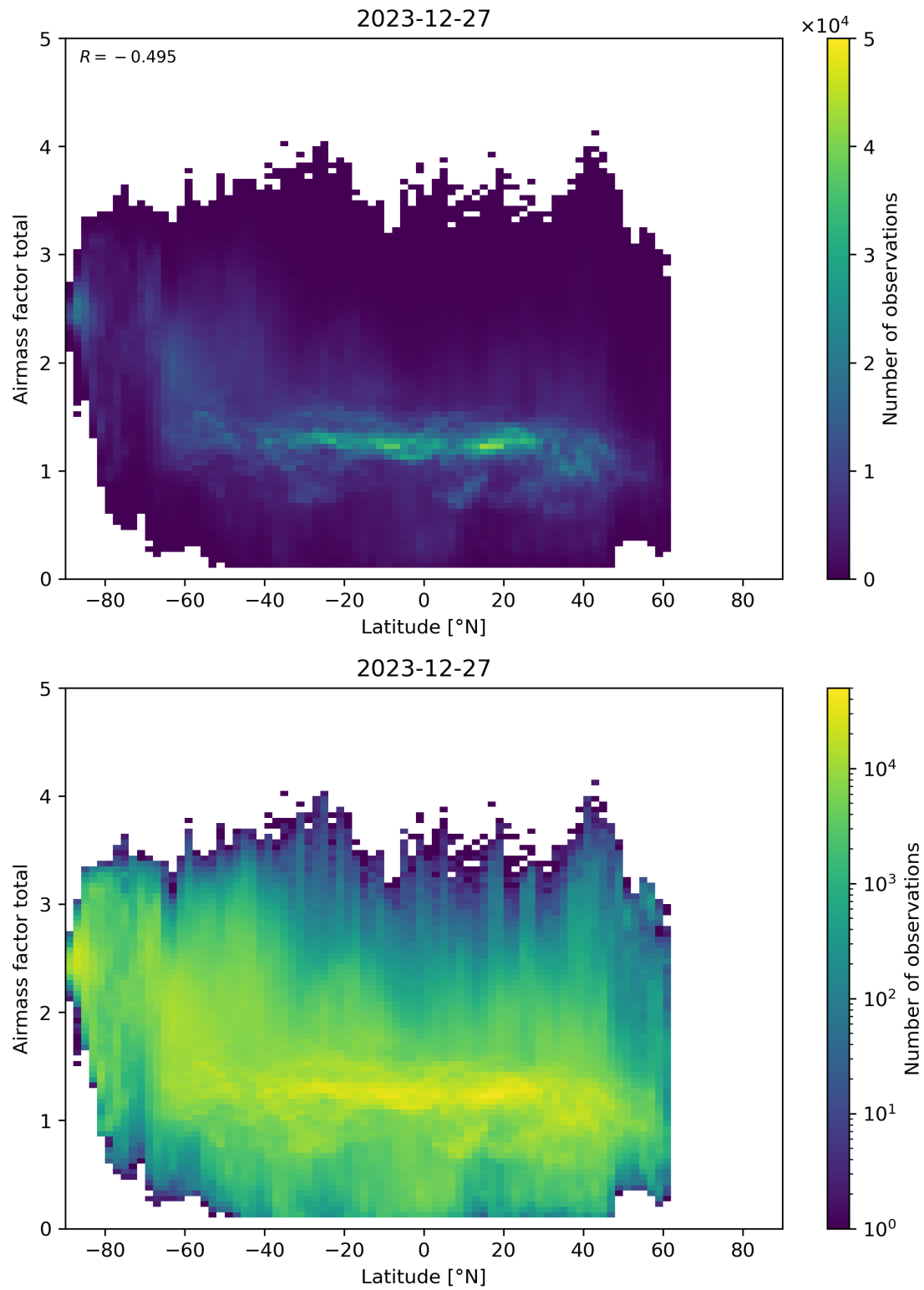
Figure 161: Scatter density plot of “Latitude” against “Airmass factor total” for 2023-12-26 to 2023-12-28.
