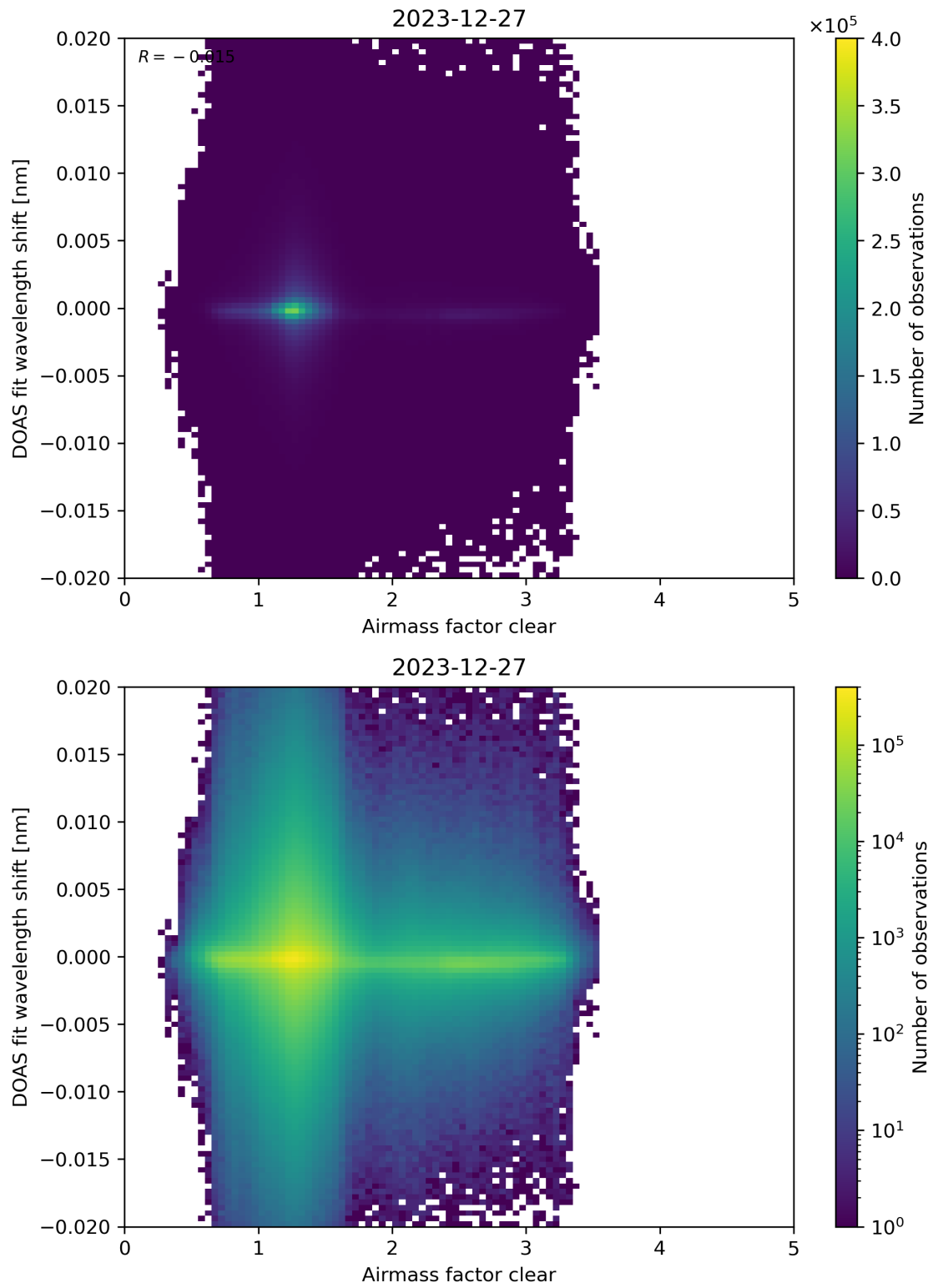
Figure 72: Scatter density plot of “Airmass factor clear” against “DOAS fit wavelength shift” for 2023-12-26 to 2023-12-28.
