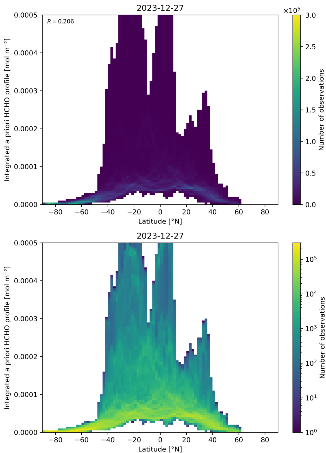
Figure 166: Scatter density plot of “Latitude” against “Integrated a priori HCHO profile” for 2023-12-26 to 2023-12-28.
