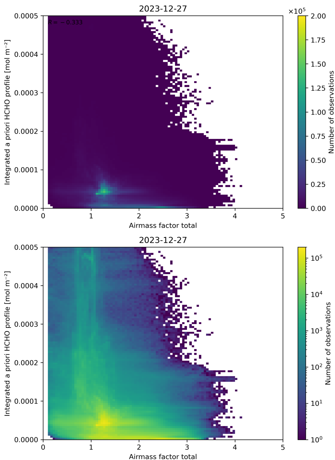
Figure 104: Scatter density plot of “Airmass factor total” against “Integrated a priori HCHO profile” for 2023-12-26 to 2023-12-28.
