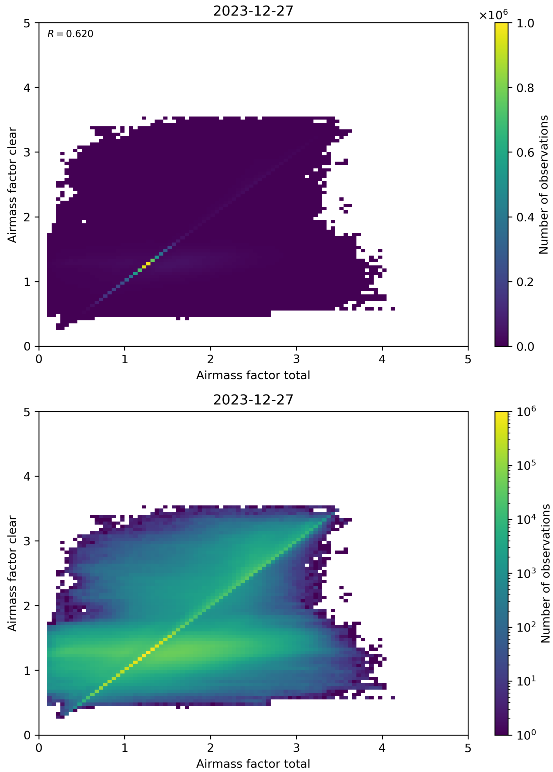
Figure 100: Scatter density plot of “Airmass factor total” against “Airmass factor clear” for 2023-12-26 to 2023-12-28.
