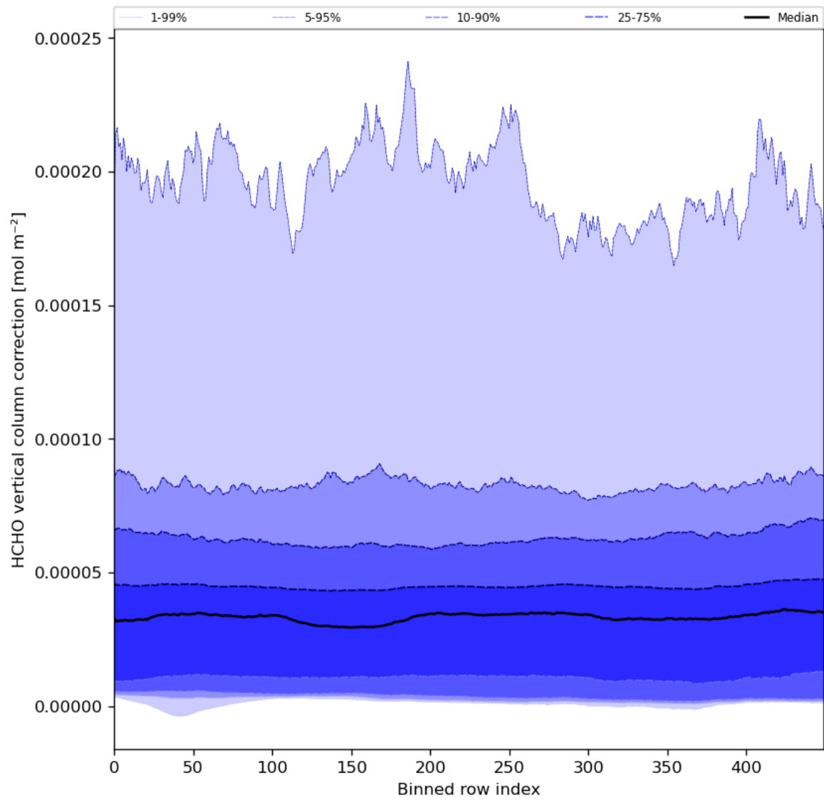
Figure 51: Along track statistics of “HCHO vertical column correction” for 2023-12-26 to 2023-12-28
