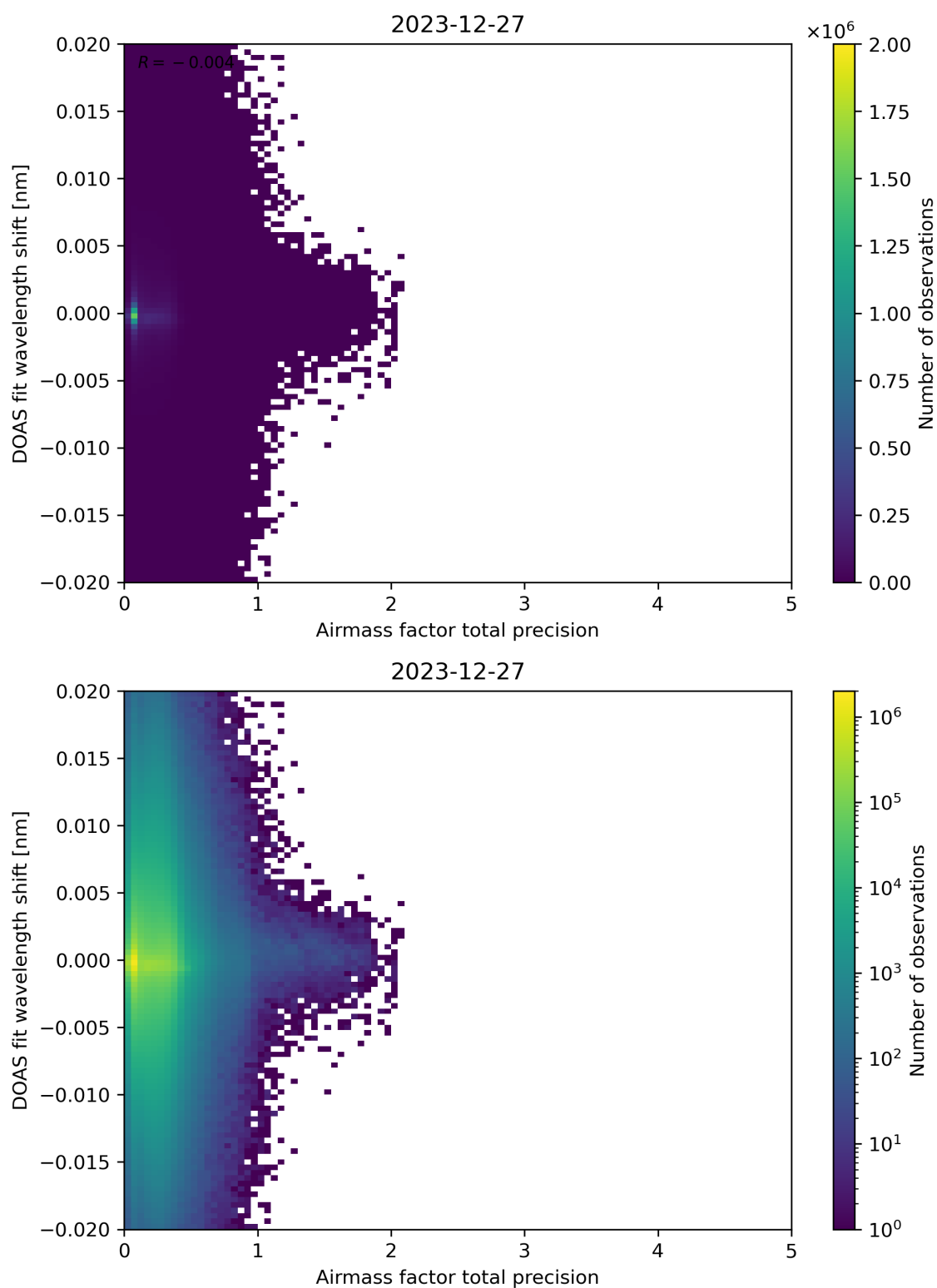
Figure 106: Scatter density plot of “Airmass factor total precision” against “DOAS fit wavelength shift” for 2023-12-26 to 2023-12-28.
