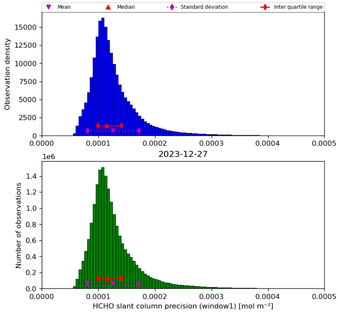
Figure 39: Histogram of “HCHO slant column precision (window1)” for 2023-12-26 to 2023-12-28
