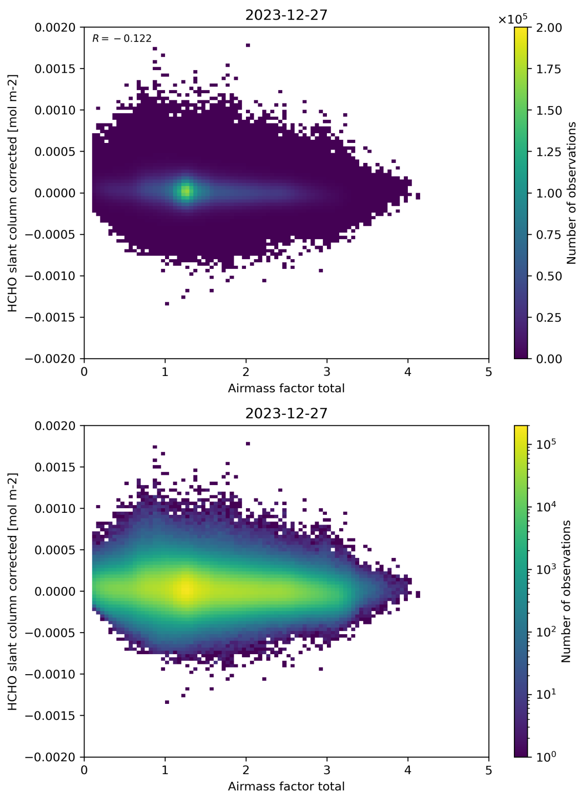
Figure 101: Scatter density plot of “Airmass factor total” against “HCHO slant column corrected” for 2023-12-26 to 2023-12-28.
