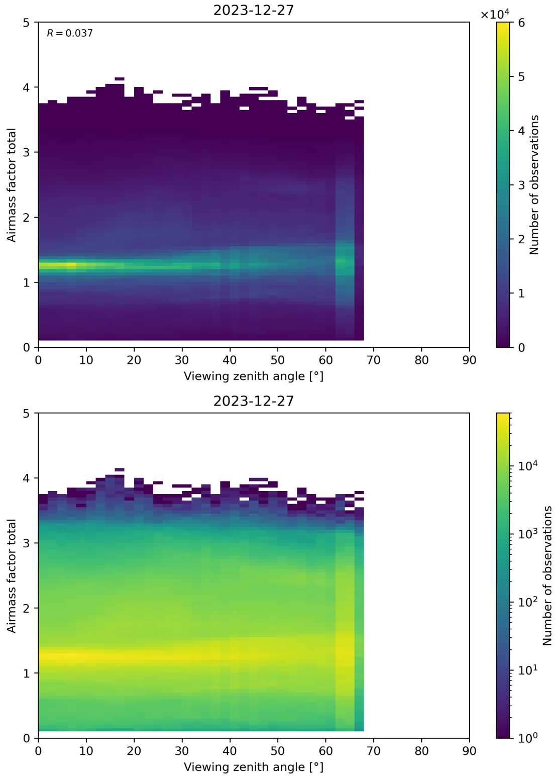
Figure 190: Scatter density plot of “Viewing zenith angle” against “Airmass factor total” for 2023-12-26 to 2023-12-28.
