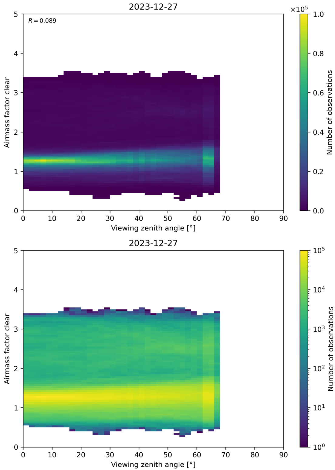
Figure 185: Scatter density plot of “Viewing zenith angle” against “Airmass factor clear” for 2023-12-26 to 2023-12-28.
