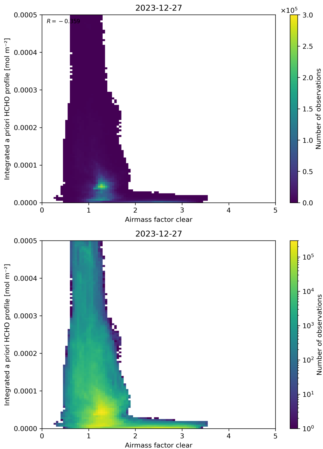
Figure 76: Scatter density plot of “Airmass factor clear” against “Integrated a priori HCHO profile” for 2023-12-26 to 2023-12-28.
