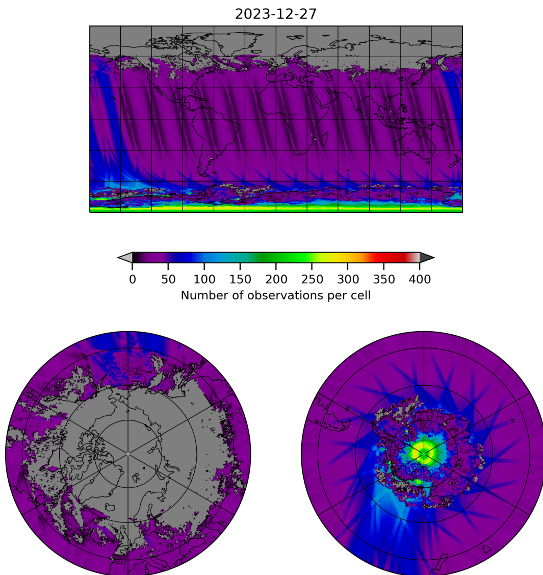
Figure 19: Map of the number of observations for 2023-12-26 to 2023-12-28
