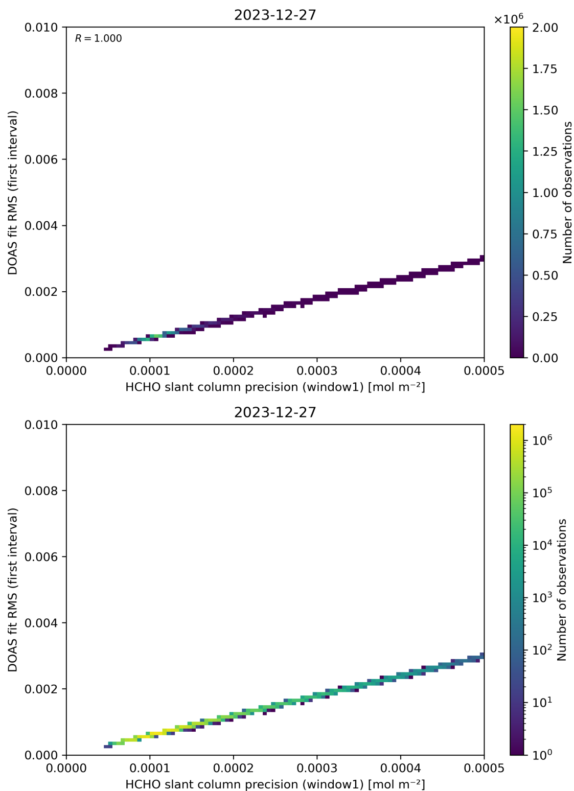
Figure 88: Scatter density plot of “HCHO slant column precision (window1)” against “DOAS fit RMS (first interval)” for 2023-12-26 to 2023-12-28.
