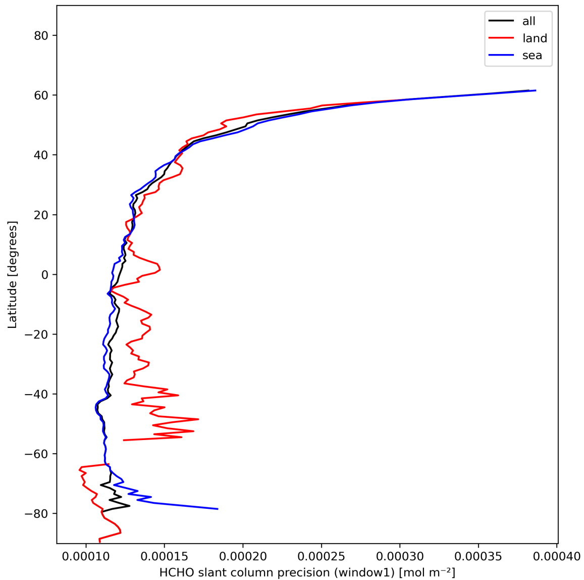
Figure 25: Zonal average of “HCHO slant column precision (window1)” for 2023-12-26 to 2023-12-28.
