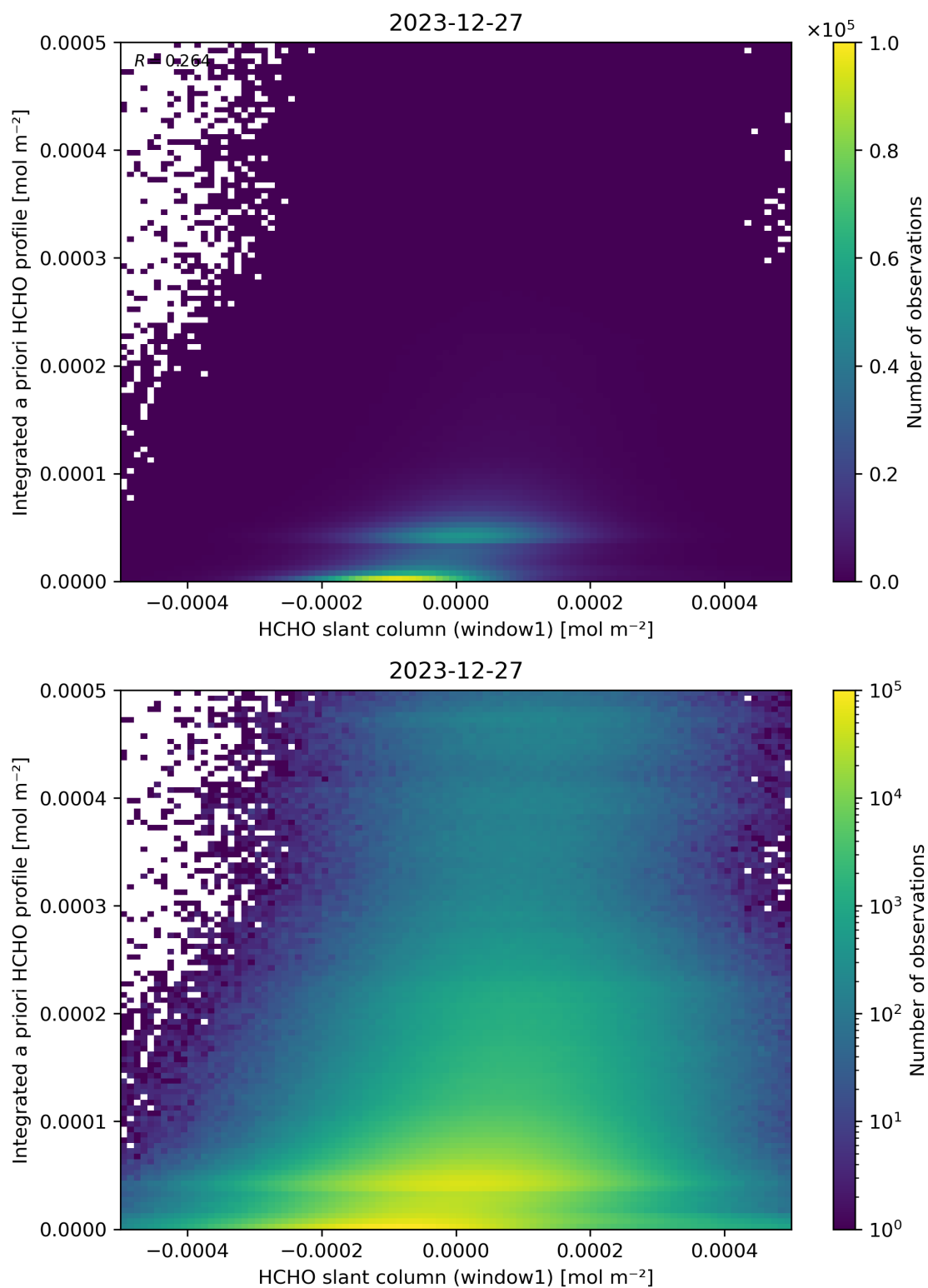
Figure 87: Scatter density plot of “HCHO slant column (window1)” against “Integrated a priori HCHO profile” for 2023-12-26 to 2023-12-28.
