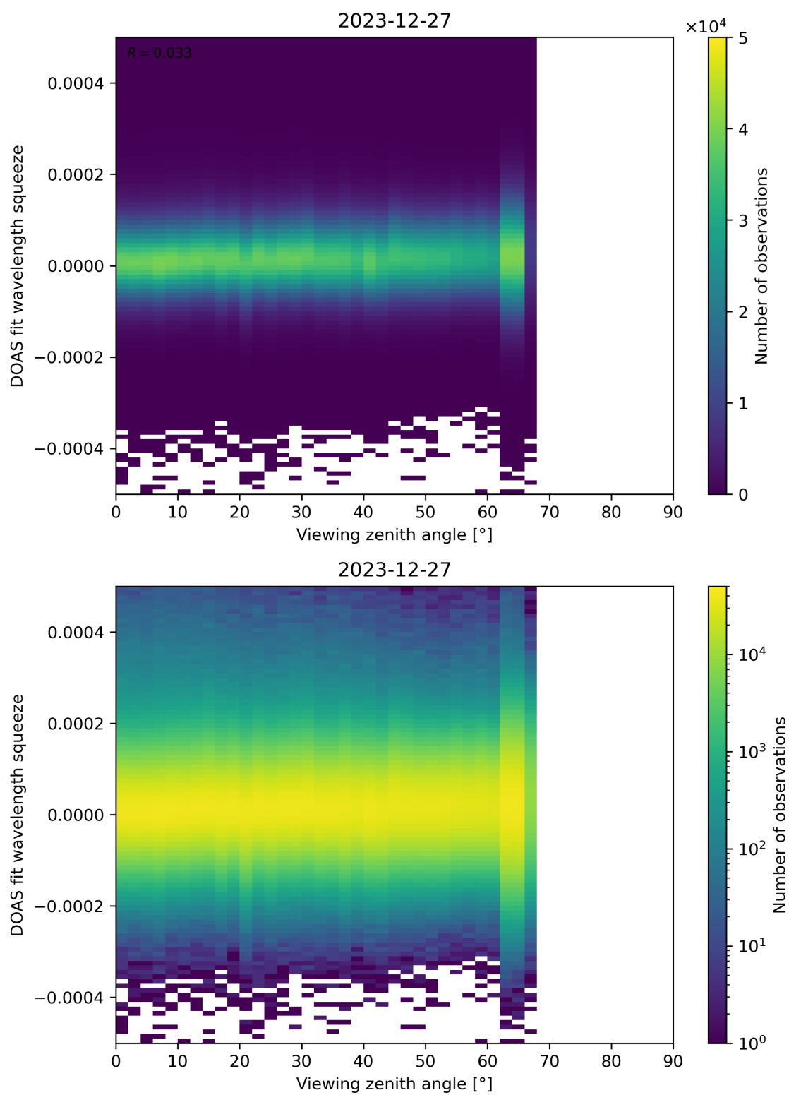
Figure 184: Scatter density plot of “Viewing zenith angle” against “DOAS fit wavelength squeeze” for 2023-12-26 to 2023-12-28.
