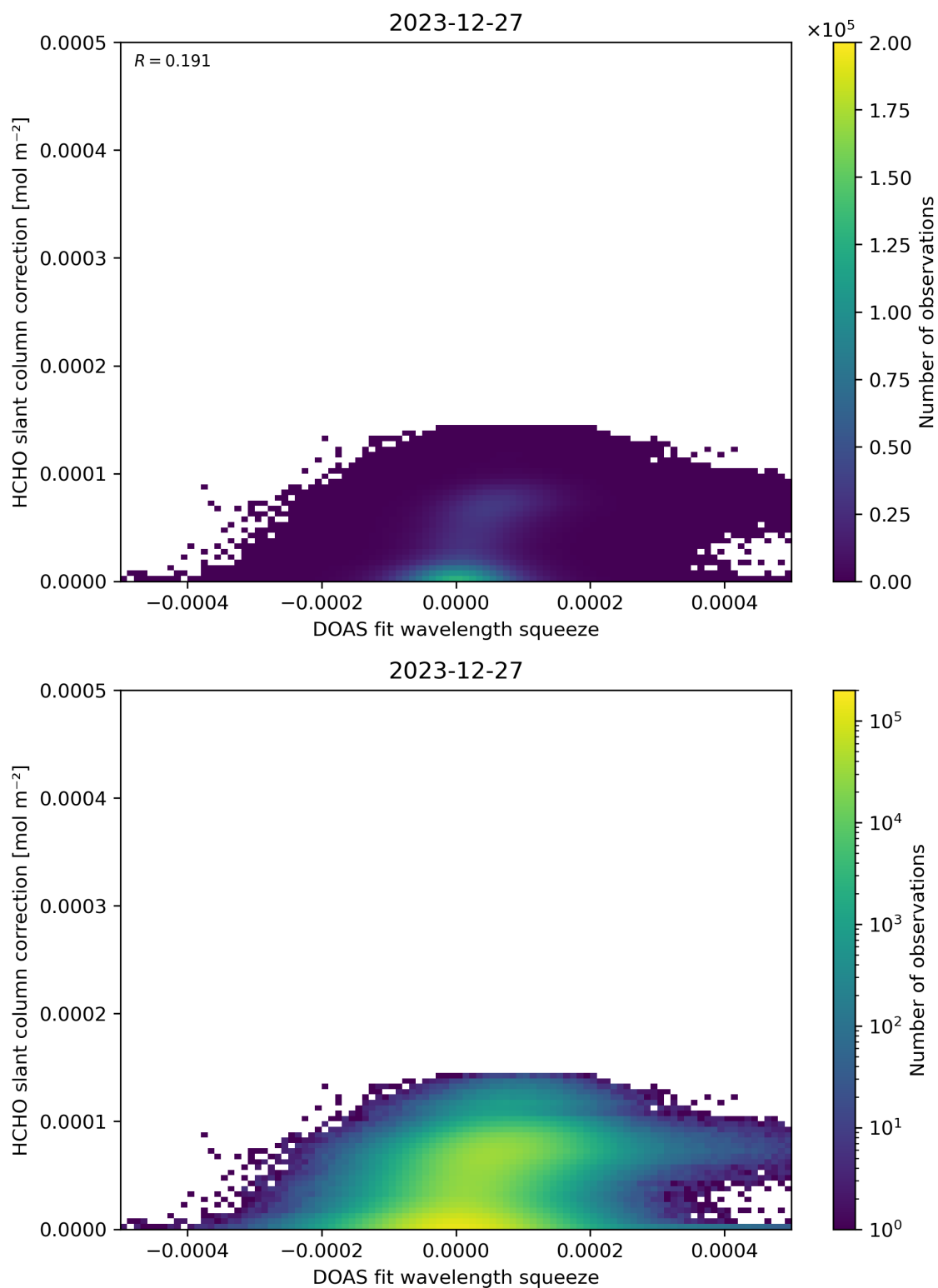
Figure 70: Scatter density plot of “DOAS fit wavelength squeeze” against “HCHO slant column correction” for 2023-12-26 to 2023-12-28.
