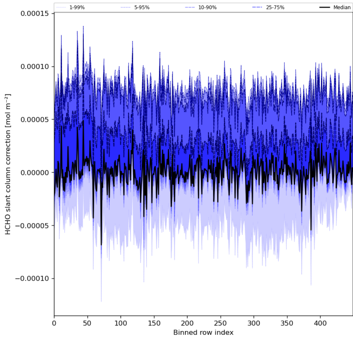
Figure 61: Along track statistics of “HCHO slant column correction” for 2023-12-26 to 2023-12-28
