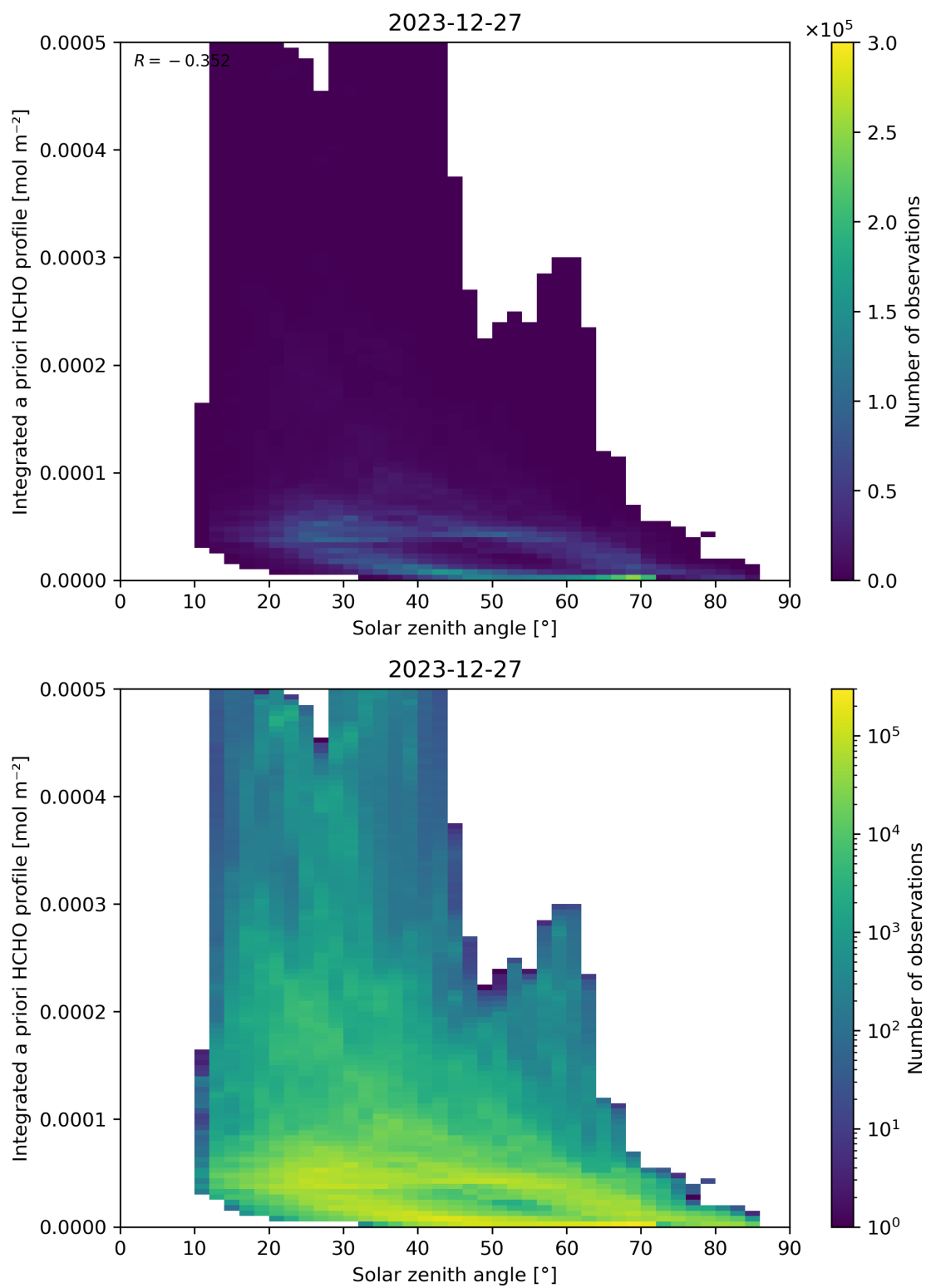
Figure 180: Scatter density plot of “Solar zenith angle” against “Integrated a priori HCHO profile” for 2023-12-26 to 2023-12-28.
