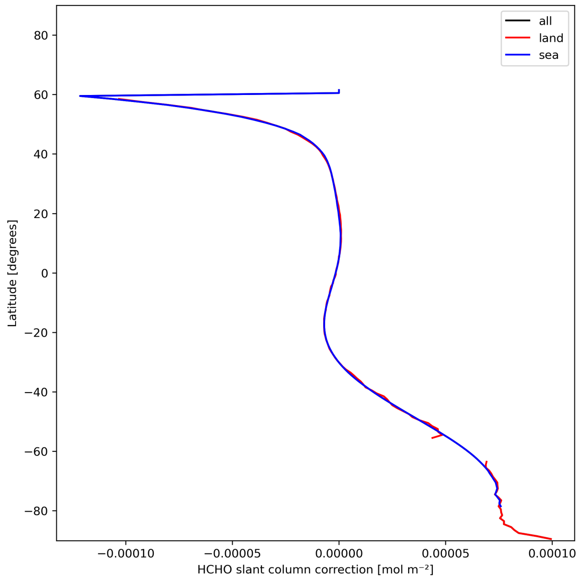
Figure 33: Zonal average of “HCHO slant column correction” for 2023-12-26 to 2023-12-28.
