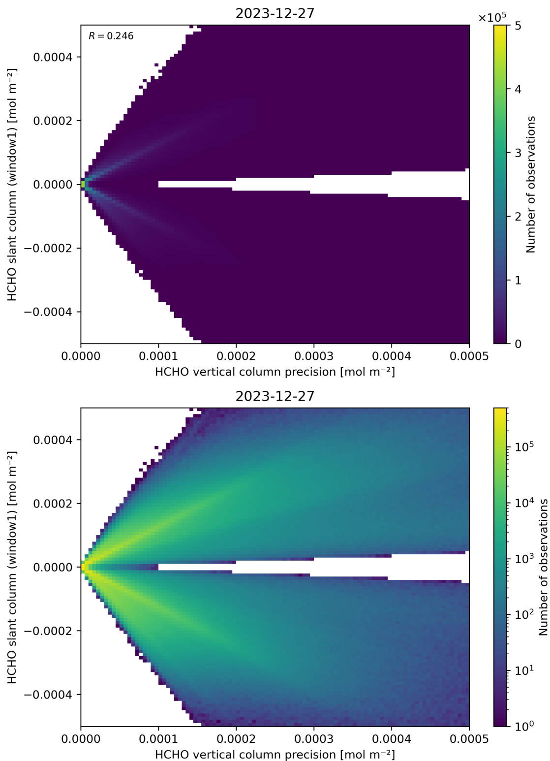
Figure 142: Scatter density plot of “HCHO vertical column precision” against “HCHO slant column (window1)” for 2023-12-26 to 2023-12-28.
