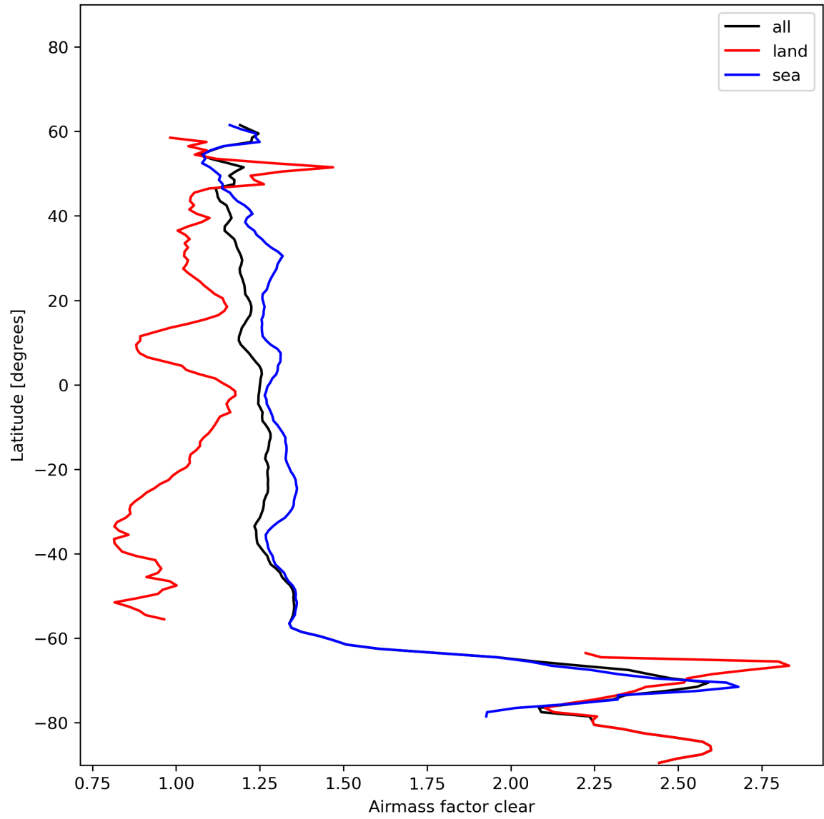
Figure 28: Zonal average of “Airmass factor clear” for 2023-12-26 to 2023-12-28.
