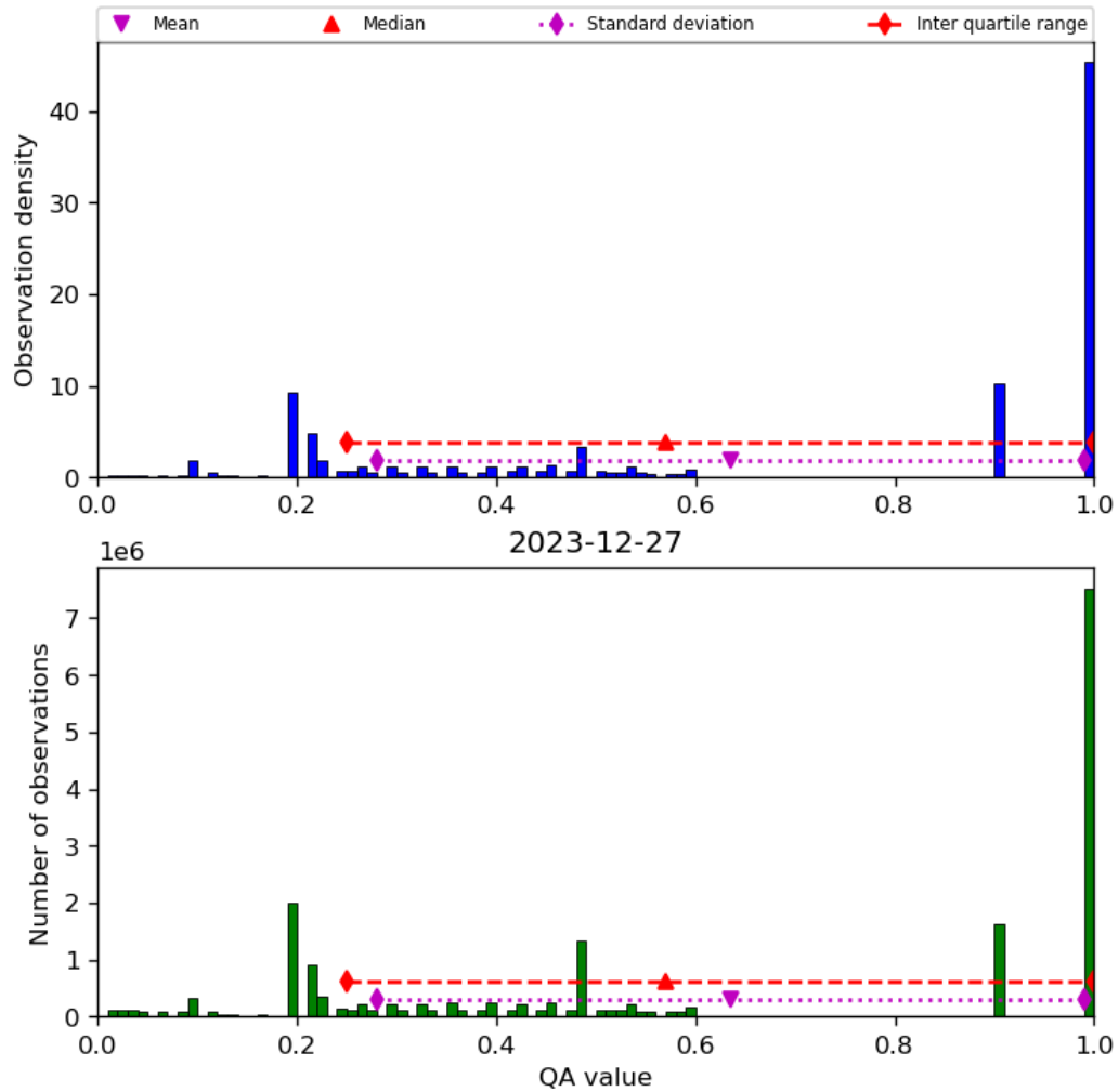
Figure 34: Histogram of “QA value” for 2023-12-26 to 2023-12-28
