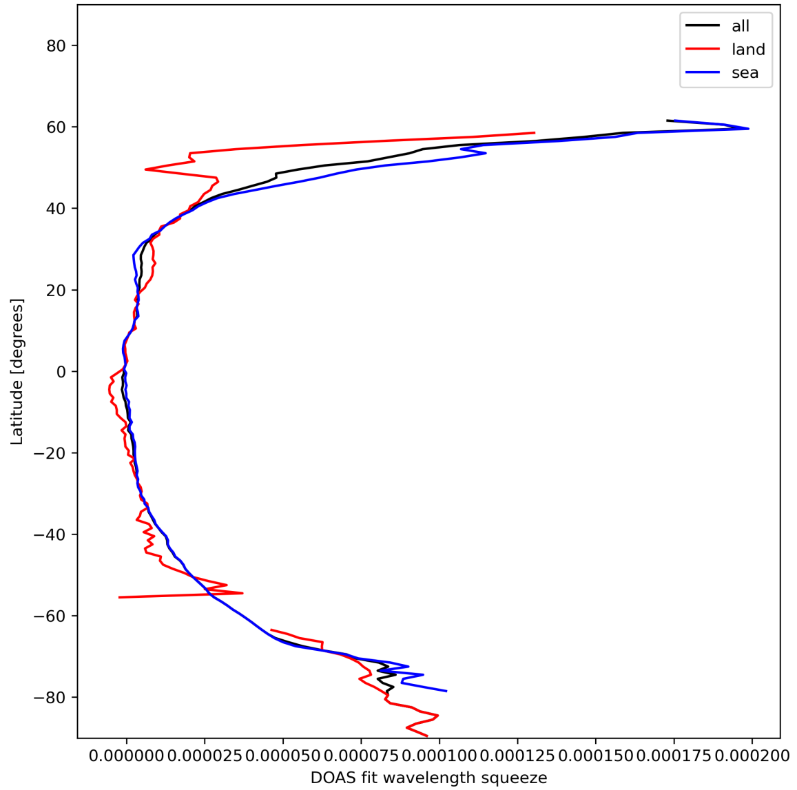
Figure 31: Zonal average of “DOAS fit wavelength squeeze” for 2023-12-26 to 2023-12-28.
