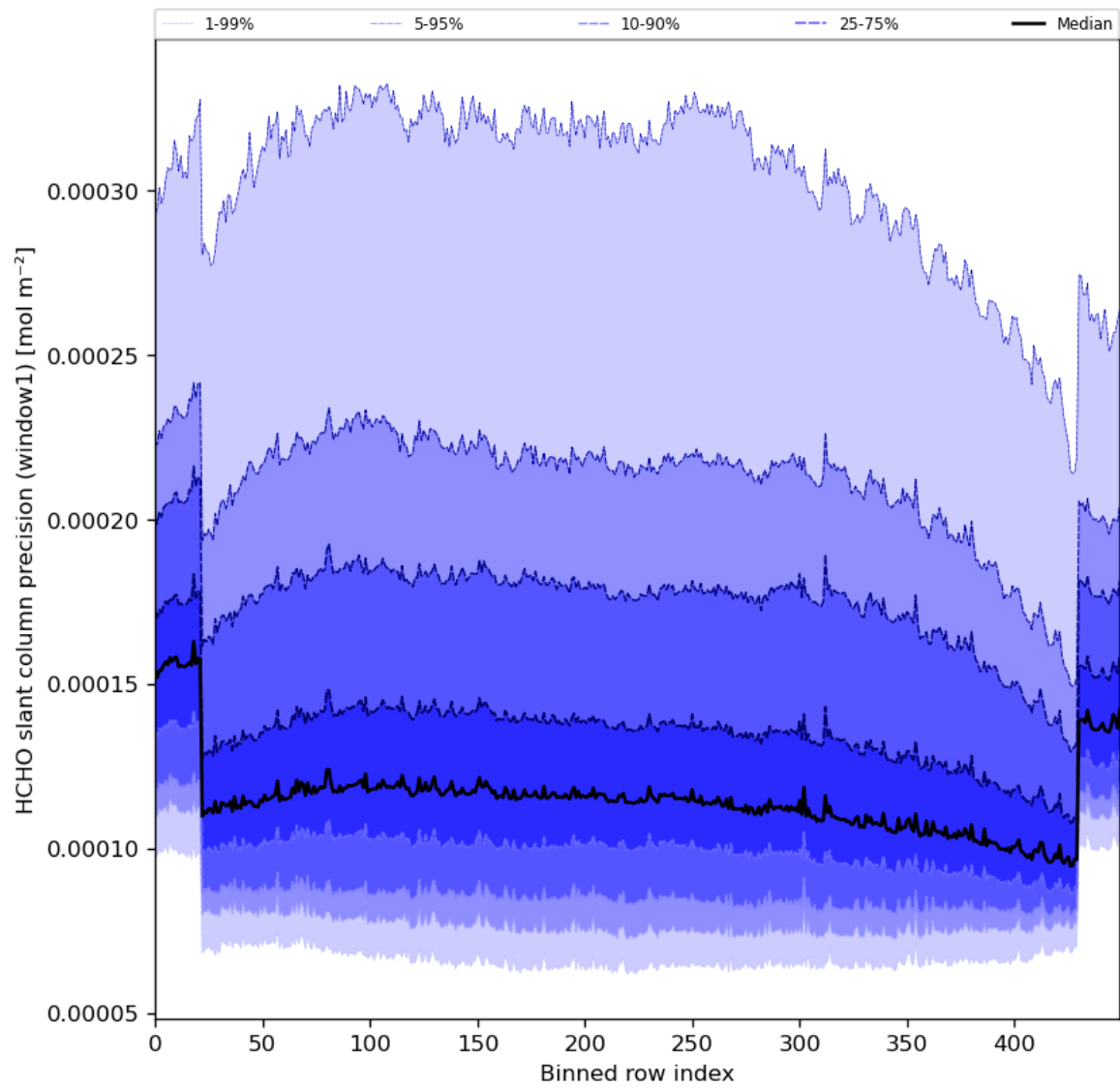
Figure 53: Along track statistics of “HCHO slant column precision (window1)” for 2023-12-26 to 2023-12-28
