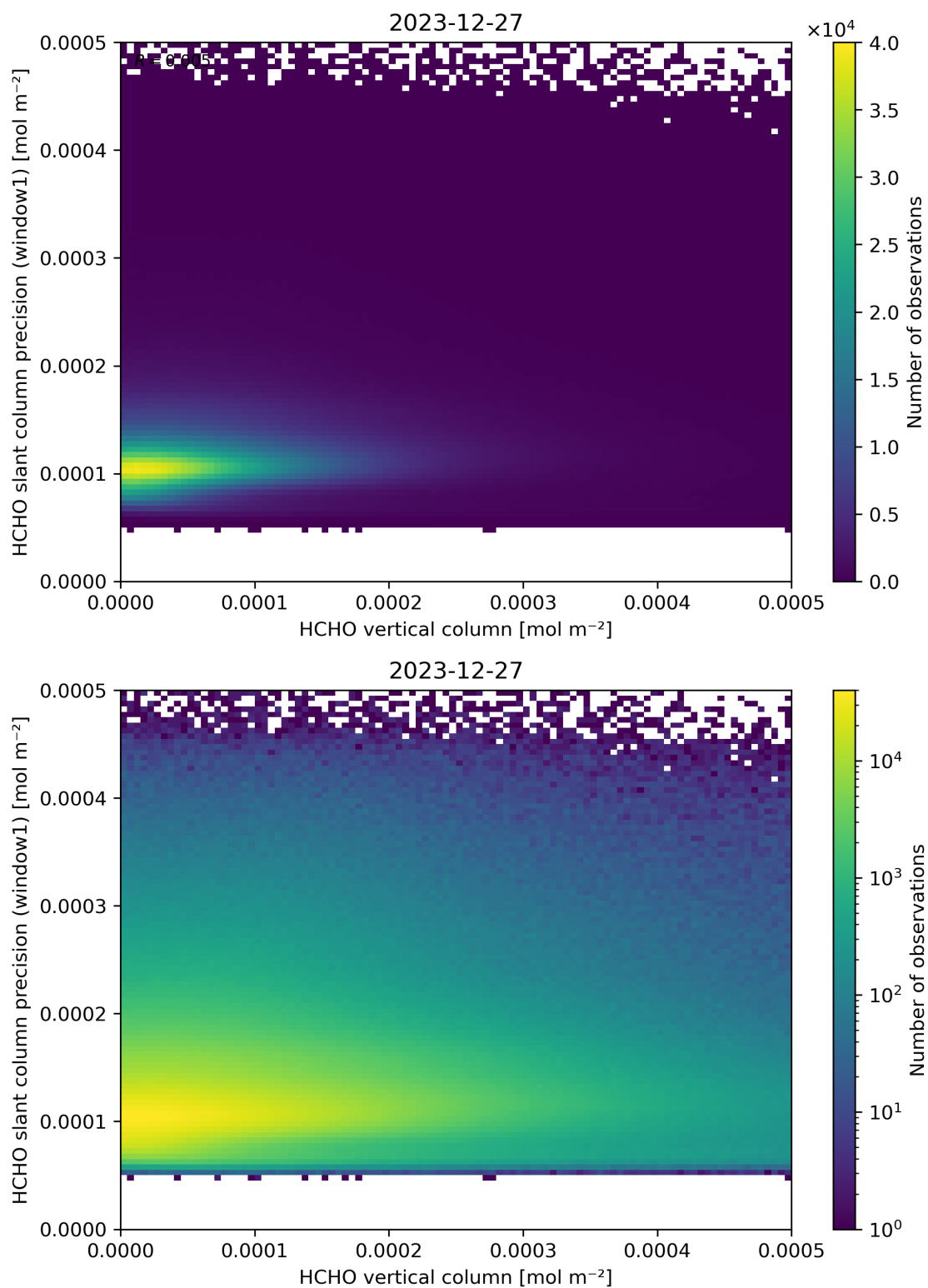
Figure 130: Scatter density plot of “HCHO vertical column” against “HCHO slant column precision (window1)” for 2023-12-26 to 2023-12-28.
