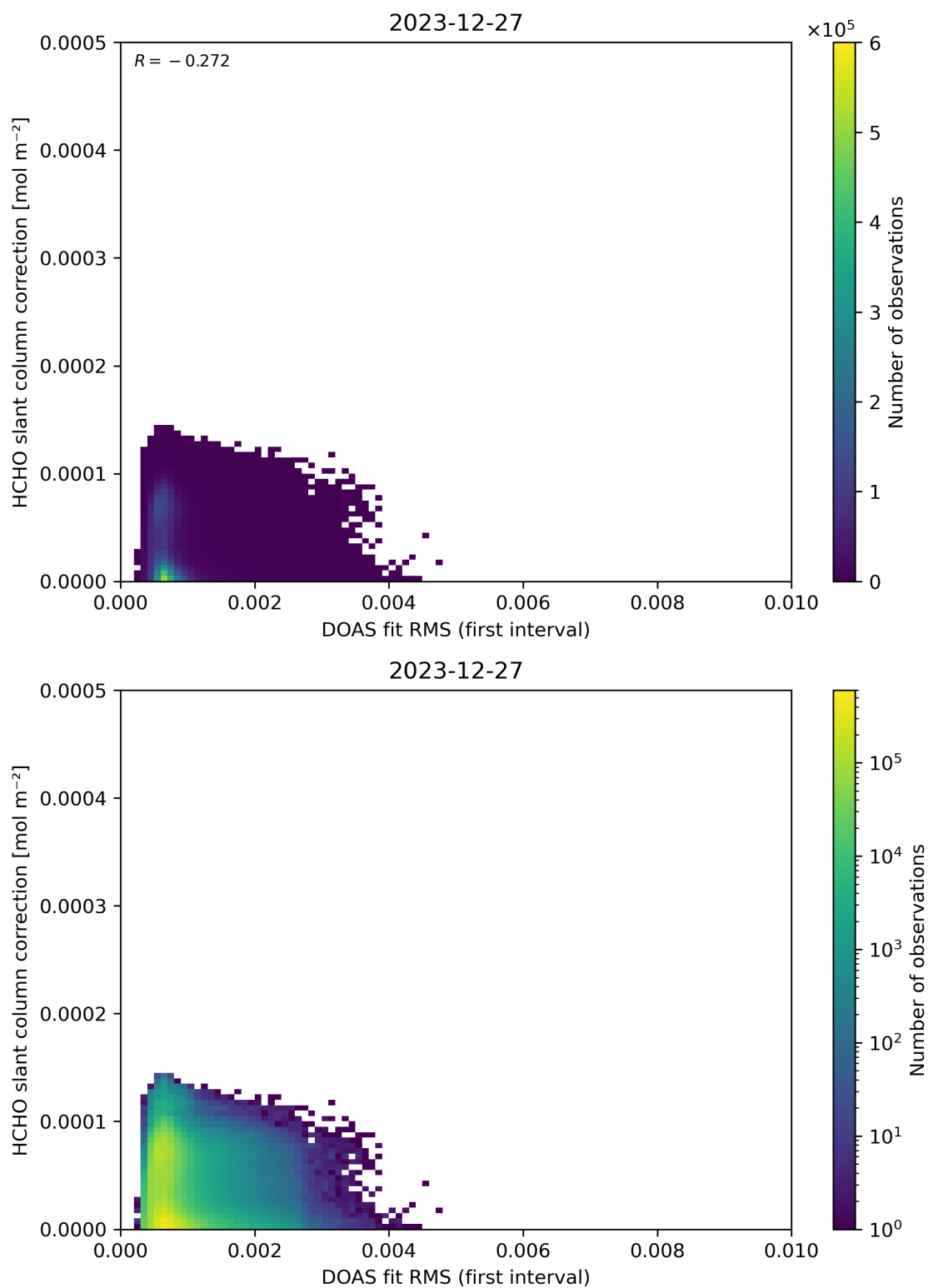
Figure 63: Scatter density plot of “DOAS fit RMS (first interval)” against “HCHO slant column correction” for 2023-12-26 to 2023-12-28.
