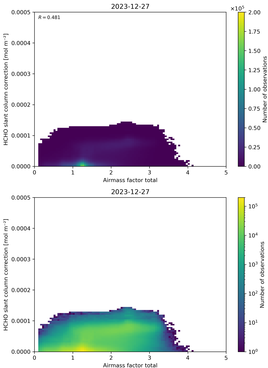
Figure 102: Scatter density plot of “Airmass factor total” against “HCHO slant column correction” for 2023-12-26 to 2023-12-28.
