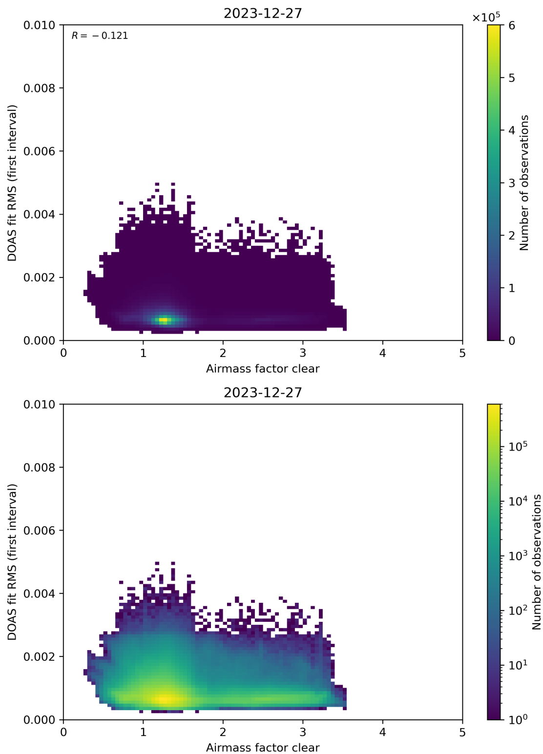
Figure 71: Scatter density plot of “Airmass factor clear” against “DOAS fit RMS (first interval)” for 2023-12-26 to 2023-12-28.
