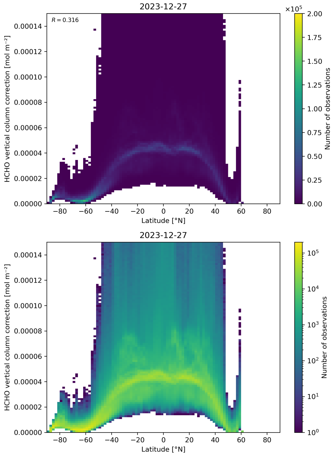
Figure 164: Scatter density plot of “Latitude” against “HCHO vertical column correction” for 2023-12-26 to 2023-12-28.
