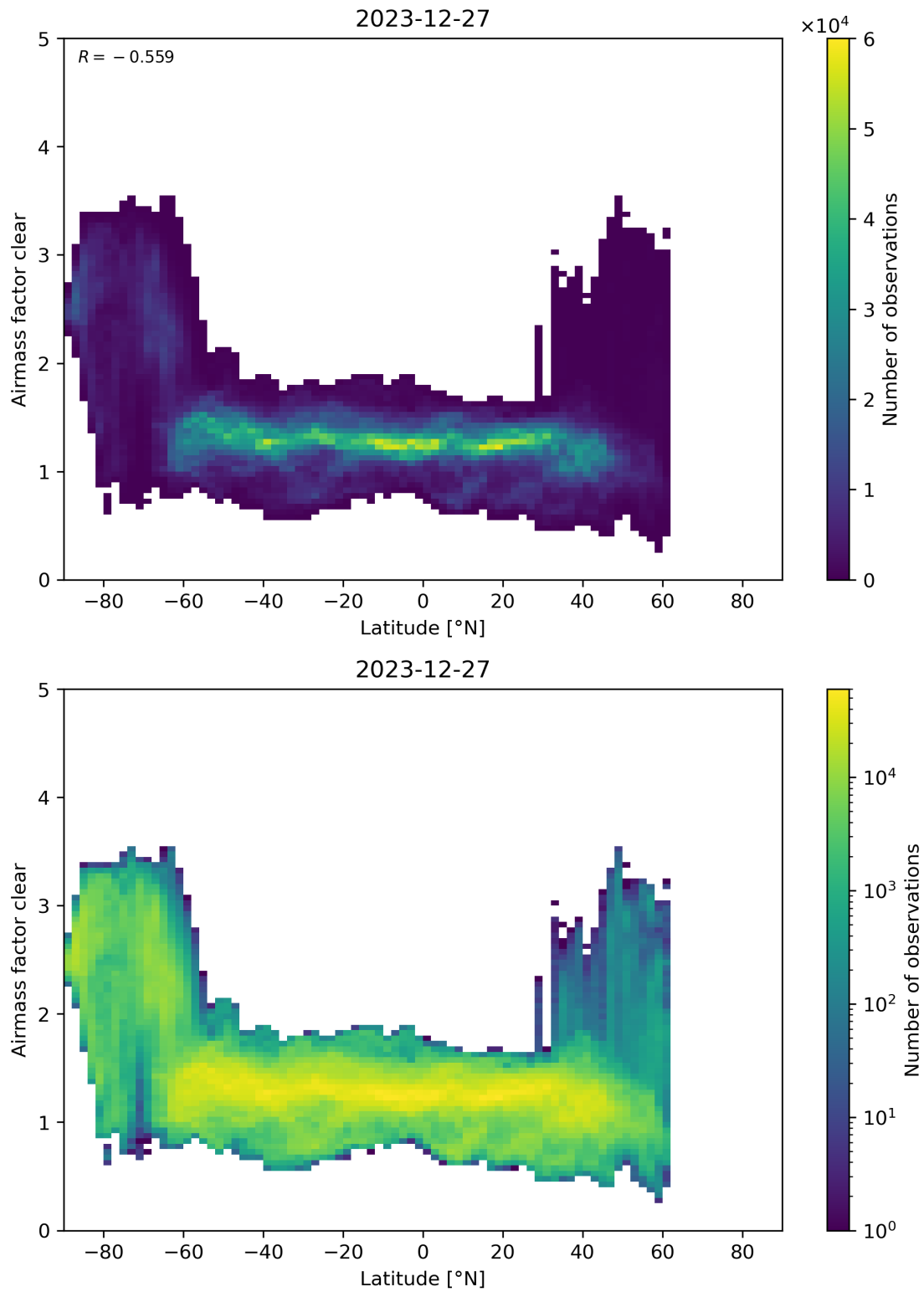
Figure 156: Scatter density plot of “Latitude” against “Airmass factor clear” for 2023-12-26 to 2023-12-28.
