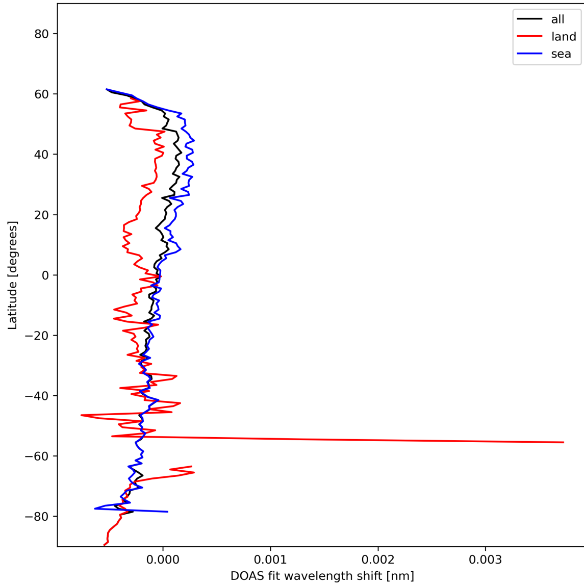
Figure 30: Zonal average of "DOAS fit wavelength shift" for 2023-12-26 to 2023-12-28.
