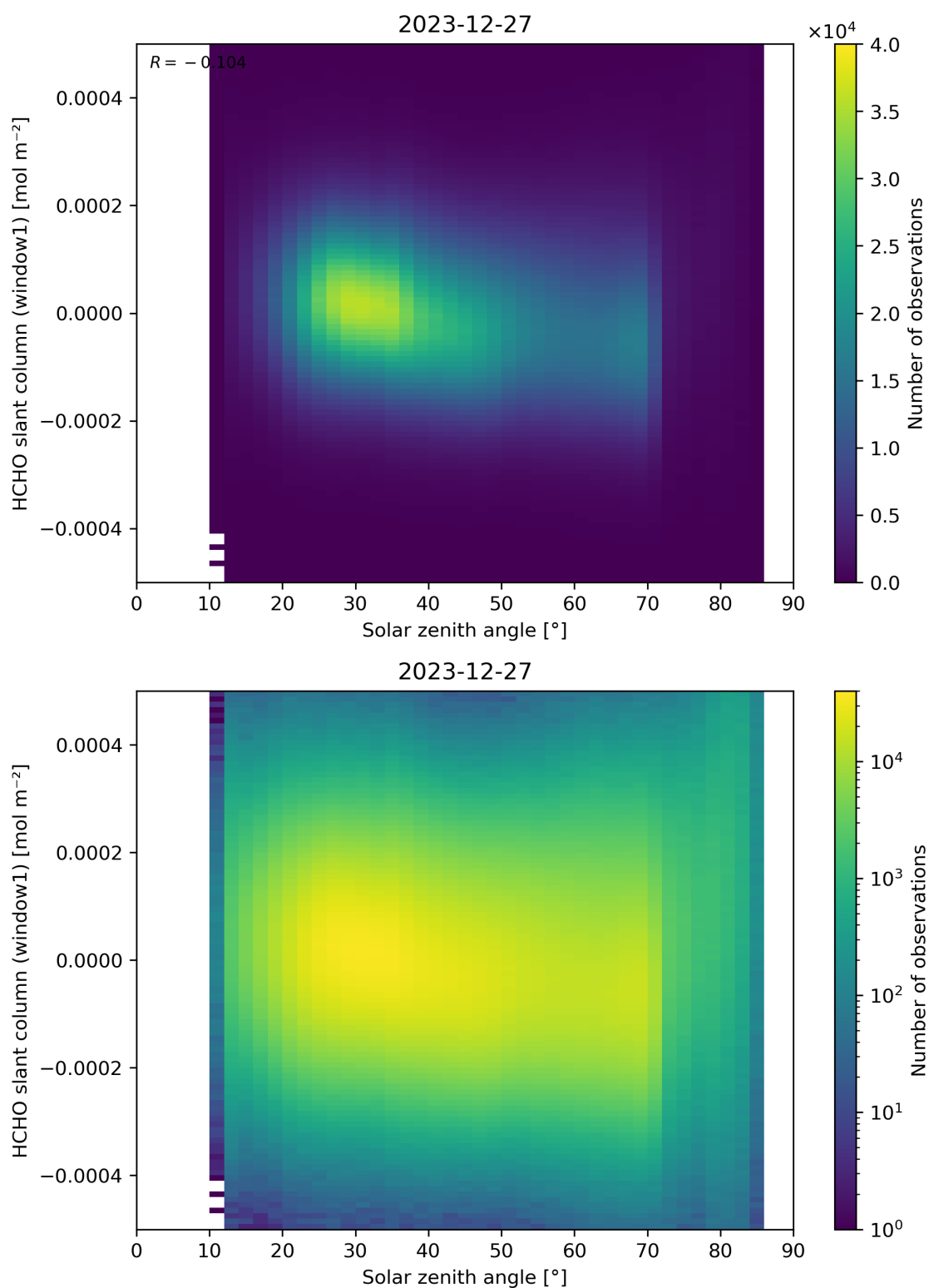
Figure 173: Scatter density plot of “Solar zenith angle” against “HCHO slant column (window1)” for 2023-12-26 to 2023-12-28.
