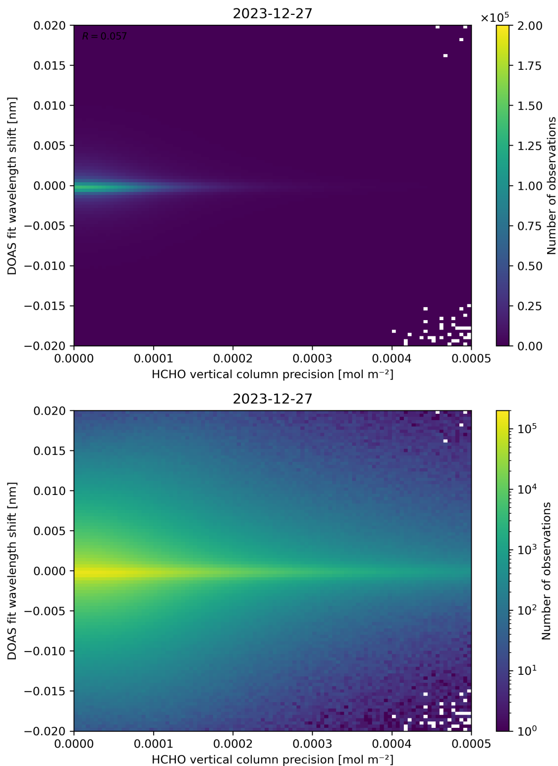
Figure 137: Scatter density plot of “HCHO vertical column precision” against “DOAS fit wavelength shift” for 2023-12-26 to 2023-12-28.
