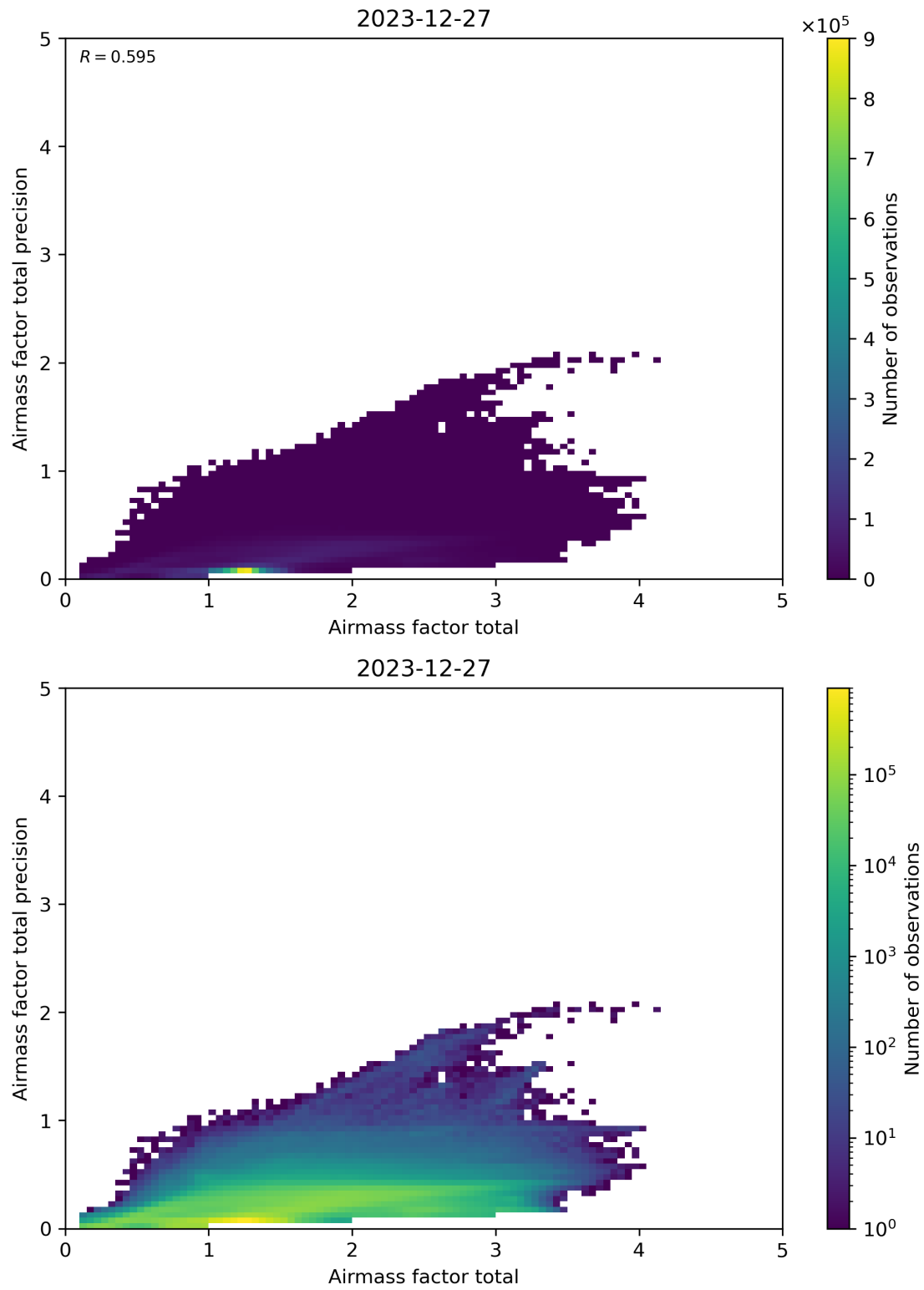
Figure 103: Scatter density plot of “Airmass factor total” against “Airmass factor total precision” for 2023-12-26 to 2023-12-28.
