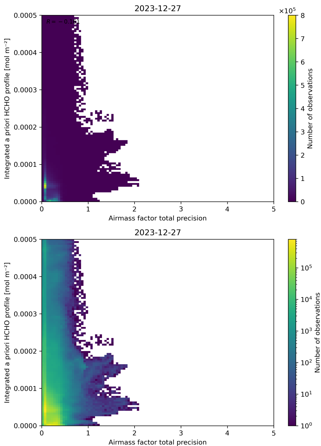
Figure 111: Scatter density plot of “Airmass factor total precision” against “Integrated a priori HCHO profile” for 2023-12-26 to 2023-12-28.
