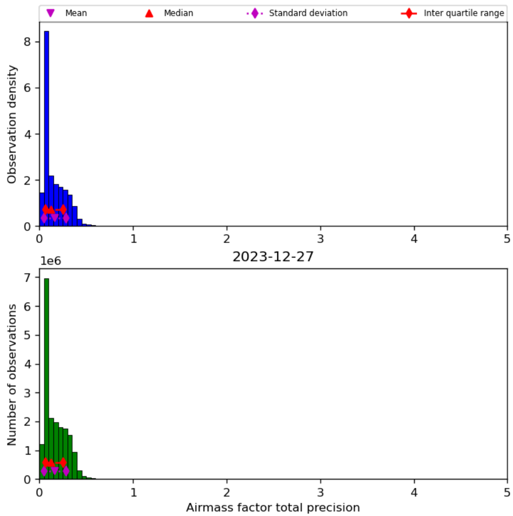
Figure 41: Histogram of “Airmass factor total precision” for 2023-12-26 to 2023-12-28
