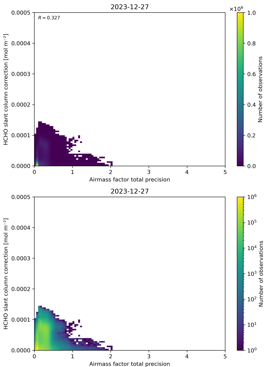
Figure 110: Scatter density plot of “Airmass factor total precision” against “HCHO slant column correction” for 2023-12-26 to 2023-12-28.
