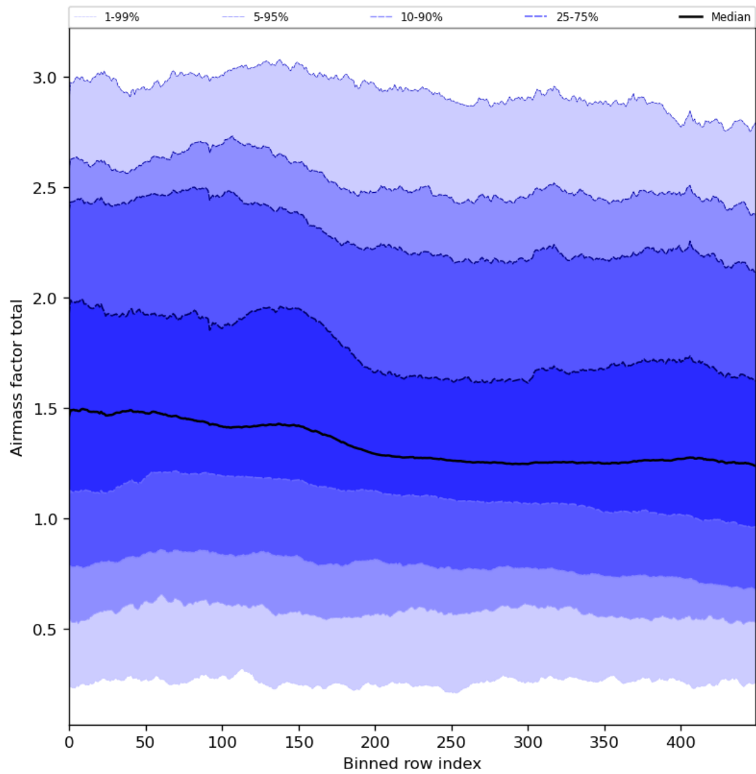
Figure 54: Along track statistics of “Airmass factor total” for 2023-12-26 to 2023-12-28
