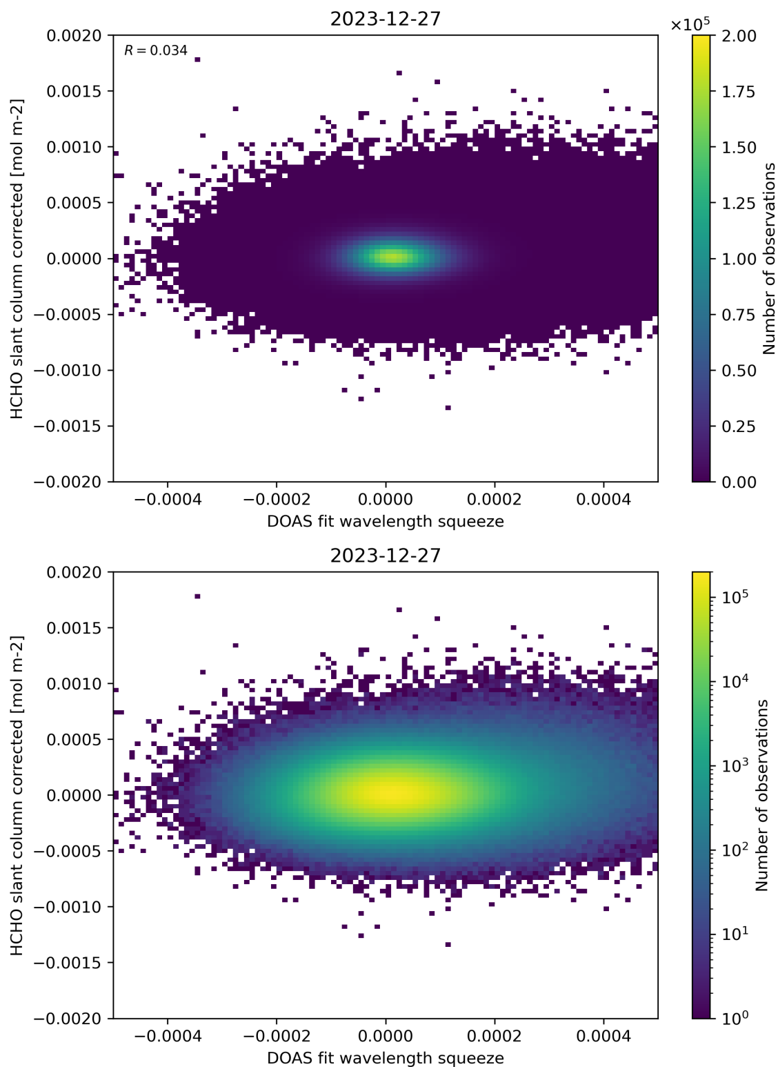
Figure 69: Scatter density plot of “DOAS fit wavelength squeeze” against “HCHO slant column corrected” for 2023-12-26 to 2023-12-28.
