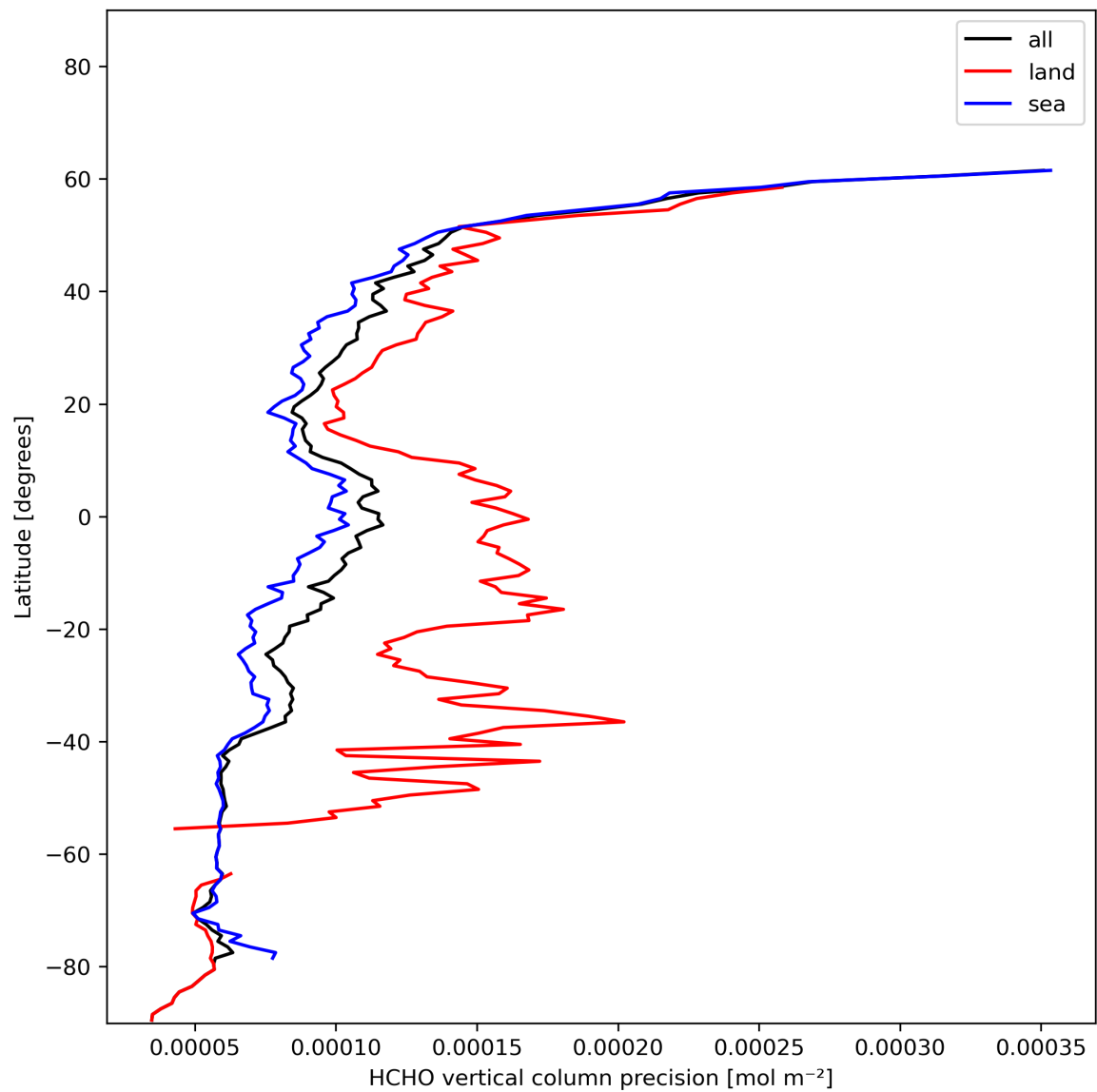
Figure 22: Zonal average of “HCHO vertical column precision” for 2023-12-26 to 2023-12-28.
