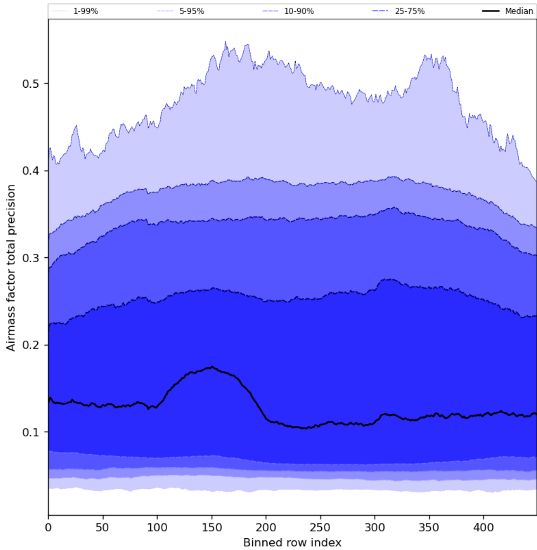
Figure 55: Along track statistics of “Airmass factor total precision” for 2023-12-26 to 2023-12-28
