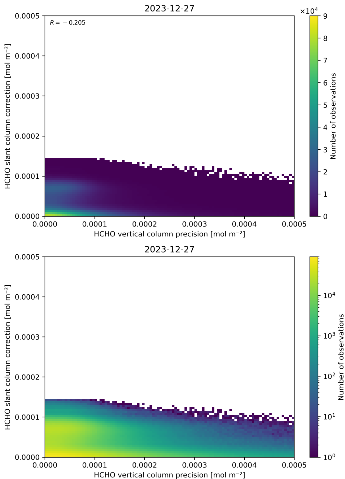
Figure 141: Scatter density plot of “HCHO vertical column precision” against “HCHO slant column correction” for 2023-12-26 to 2023-12-28.
