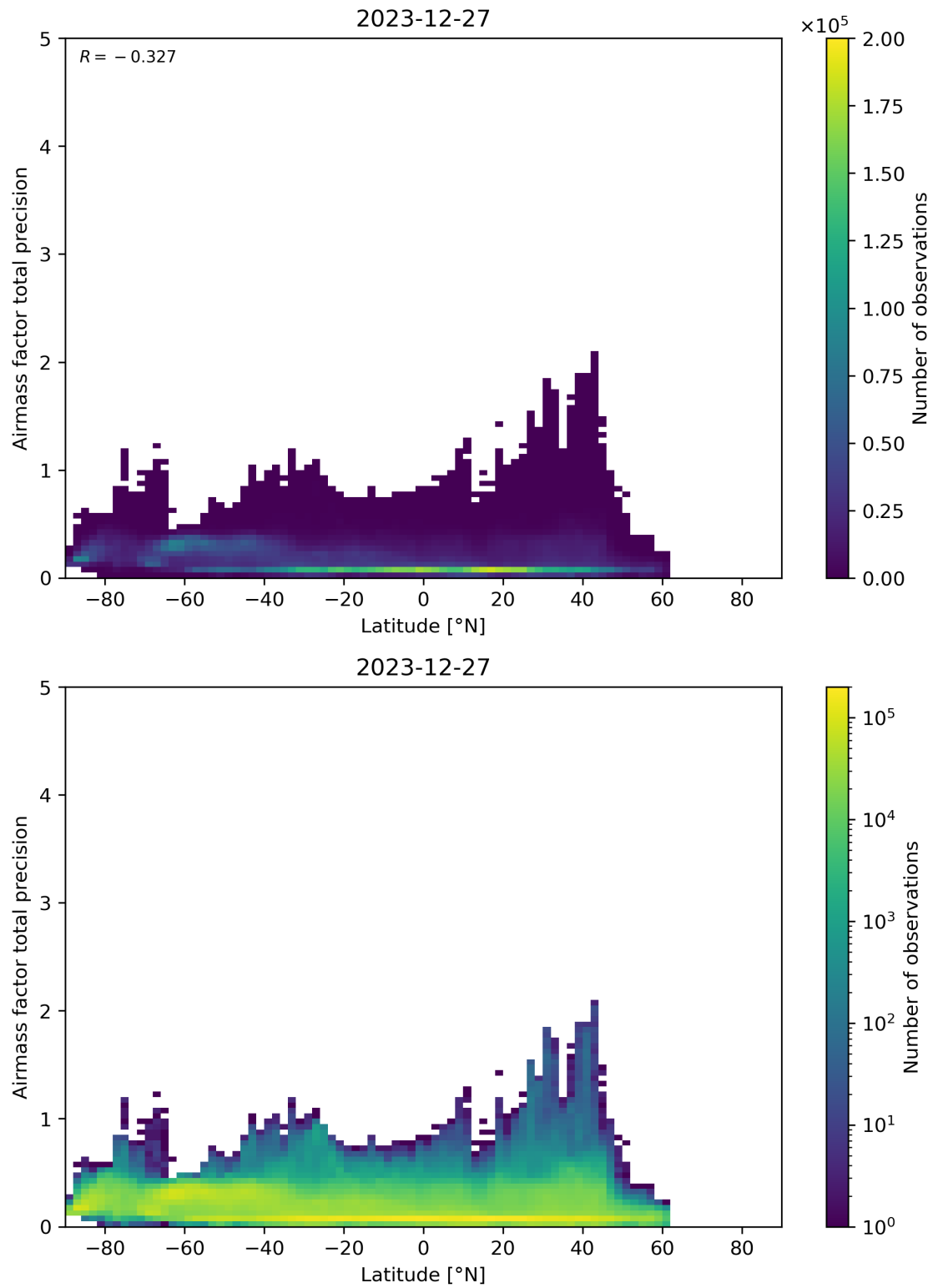
Figure 162: Scatter density plot of “Latitude” against “Airmass factor total precision” for 2023-12-26 to 2023-12-28.
