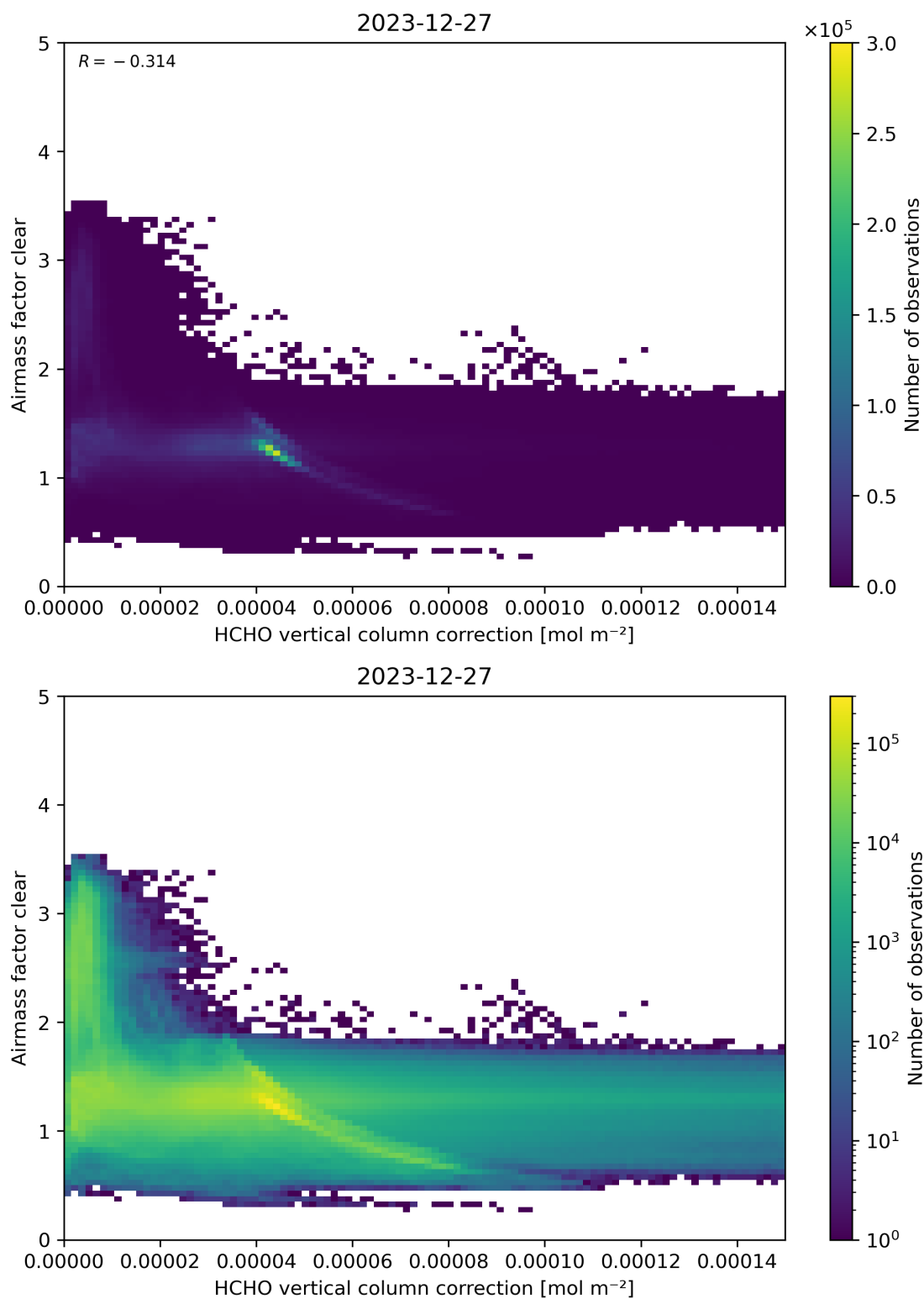
Figure 115: Scatter density plot of “HCHO vertical column correction” against “Airmass factor clear” for 2023-12-26 to 2023-12-28.
