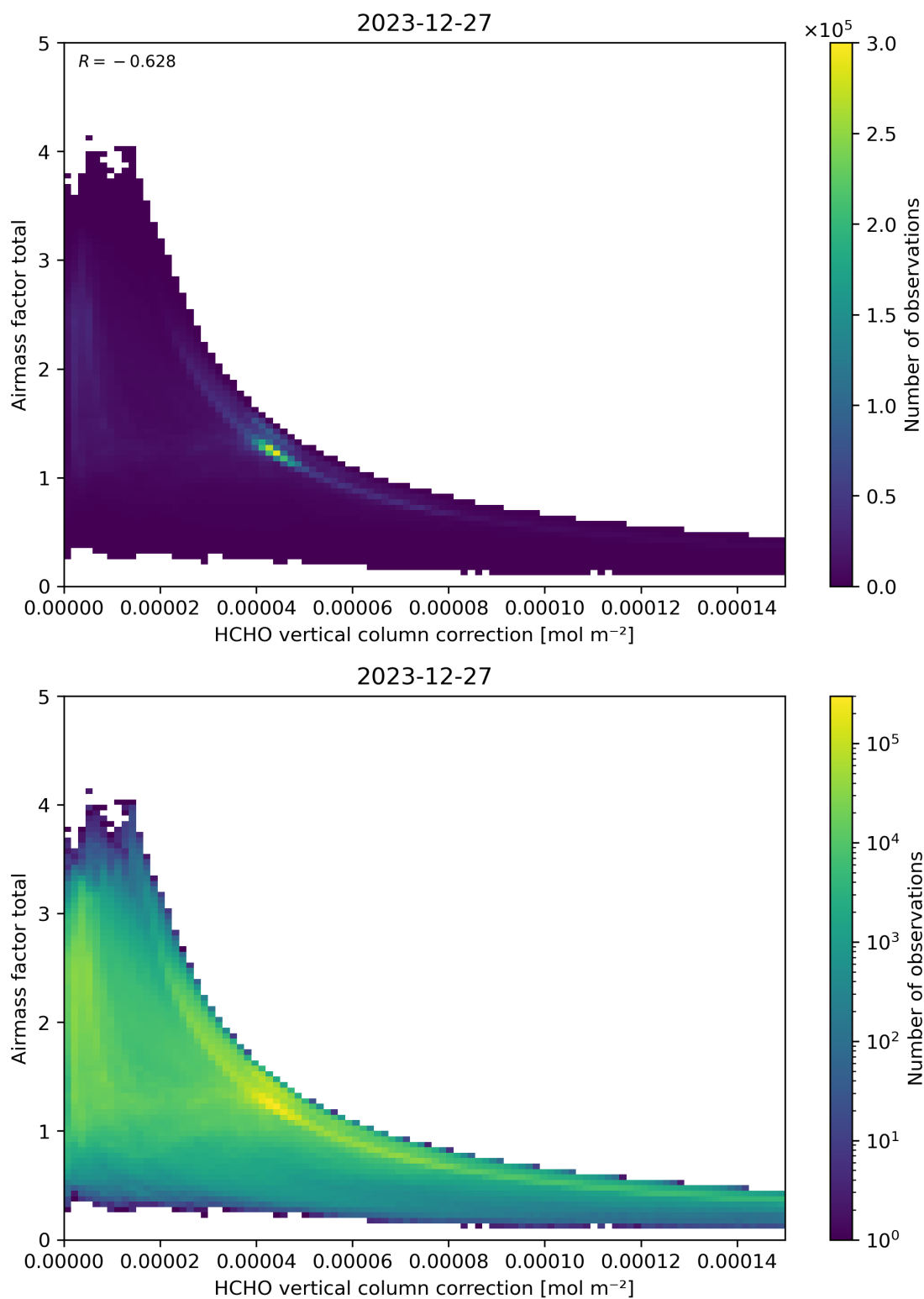
Figure 120: Scatter density plot of “HCHO vertical column correction” against “Airmass factor total” for 2023-12-26 to 2023-12-28.
