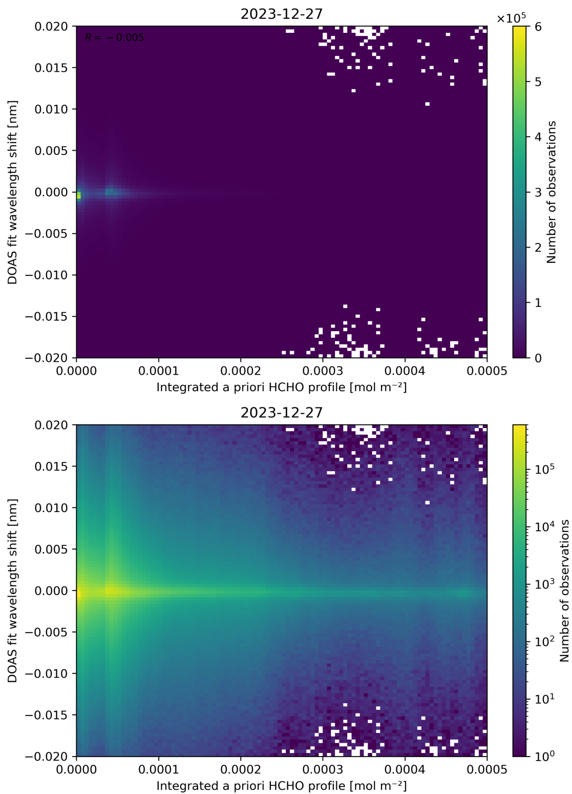
Figure 149: Scatter density plot of “Integrated a priori HCHO profile” against “DOAS fit wavelength shift” for 2023-12-26 to 2023-12-28.
