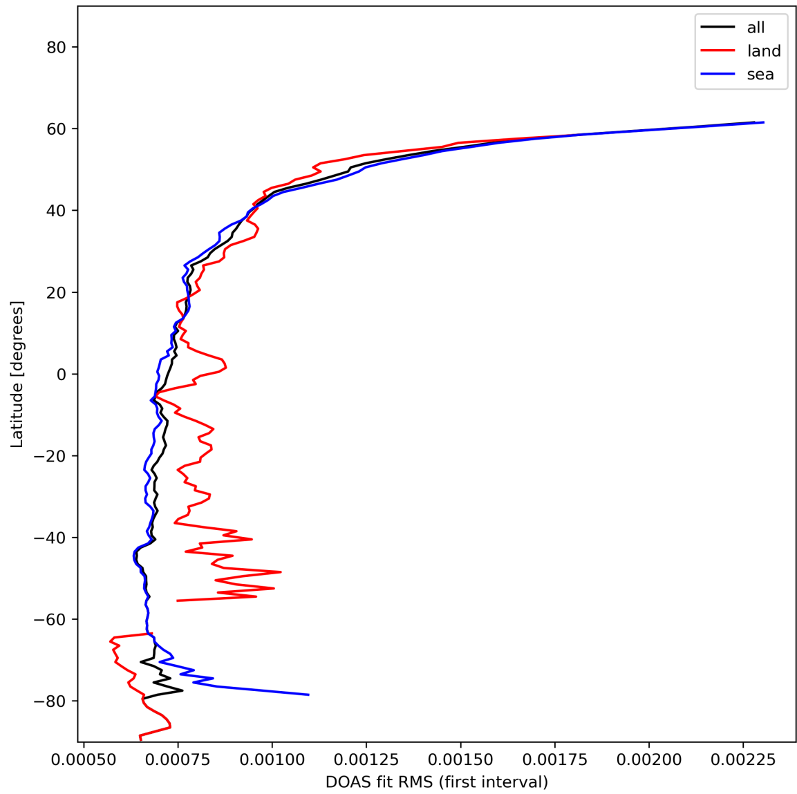
Figure 32: Zonal average of “DOAS fit RMS (first interval)” for 2023-12-26 to 2023-12-28.
