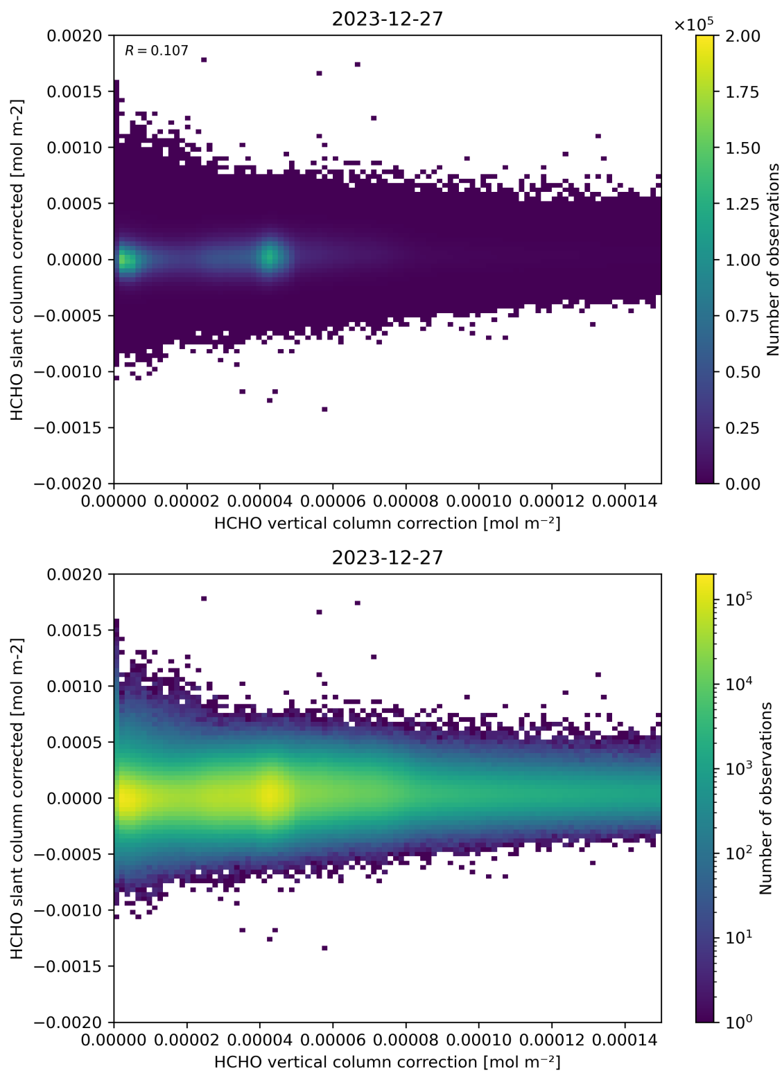
Figure 116: Scatter density plot of “HCHO vertical column correction” against “HCHO slant column corrected” for 2023-12-26 to 2023-12-28.
