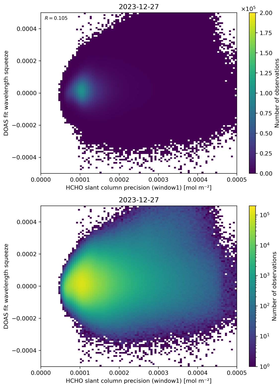
Figure 90: Scatter density plot of “HCHO slant column precision (window1)” against “DOAS fit wavelength squeeze” for 2023-12-26 to 2023-12-28.
