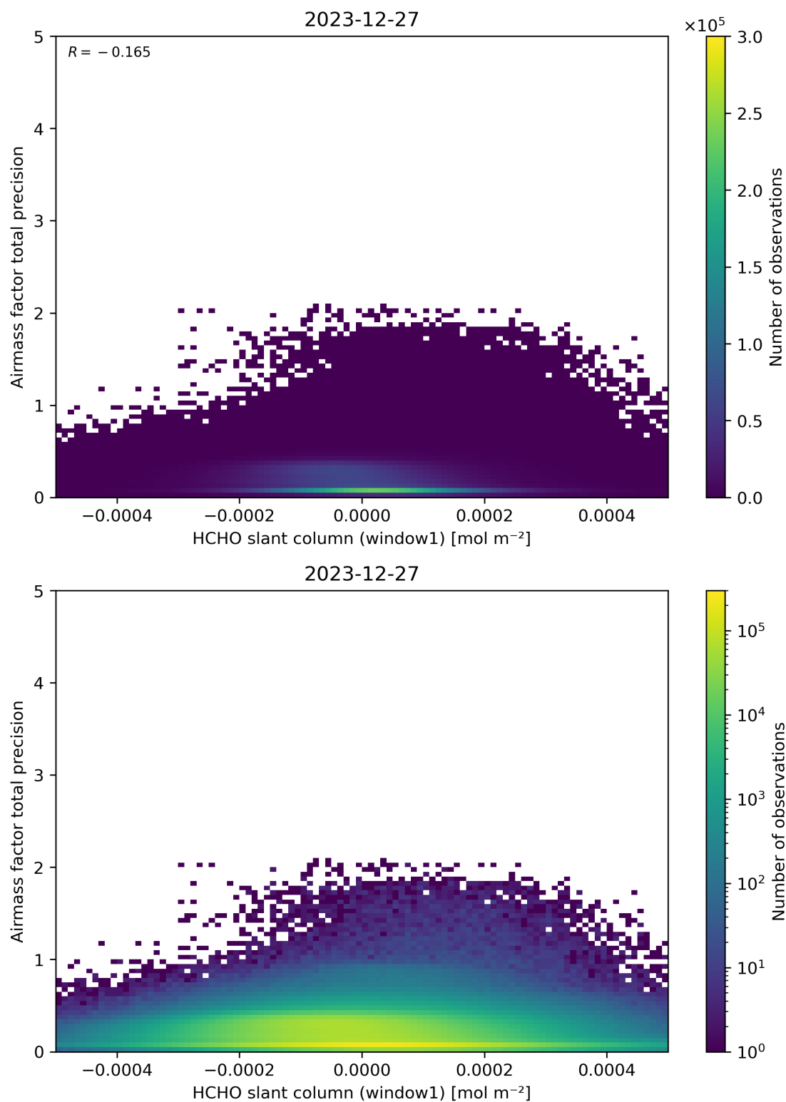
Figure 86: Scatter density plot of “HCHO slant column (window1)” against “Airmass factor total precision” for 2023-12-26 to 2023-12-28.
