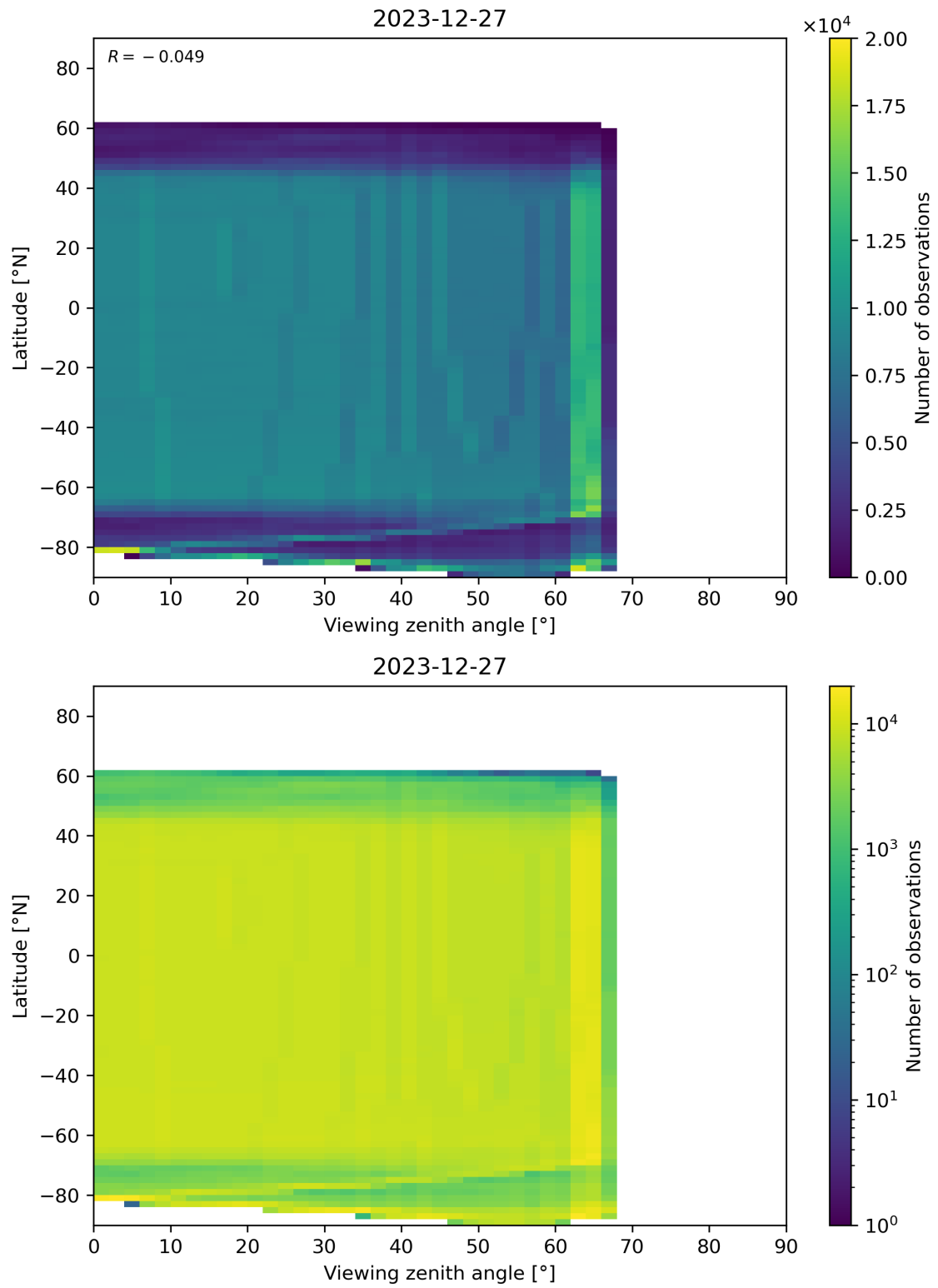
Figure 196: Scatter density plot of “Viewing zenith angle” against “Latitude” for 2023-12-26 to 2023-12-28.
