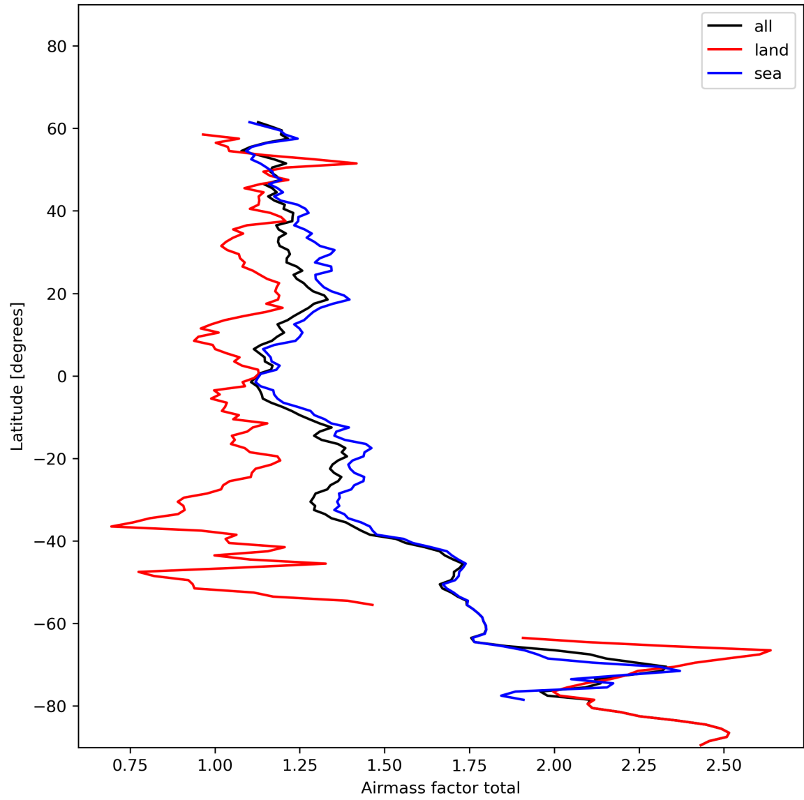
Figure 26: Zonal average of “Airmass factor total” for 2023-12-26 to 2023-12-28.
