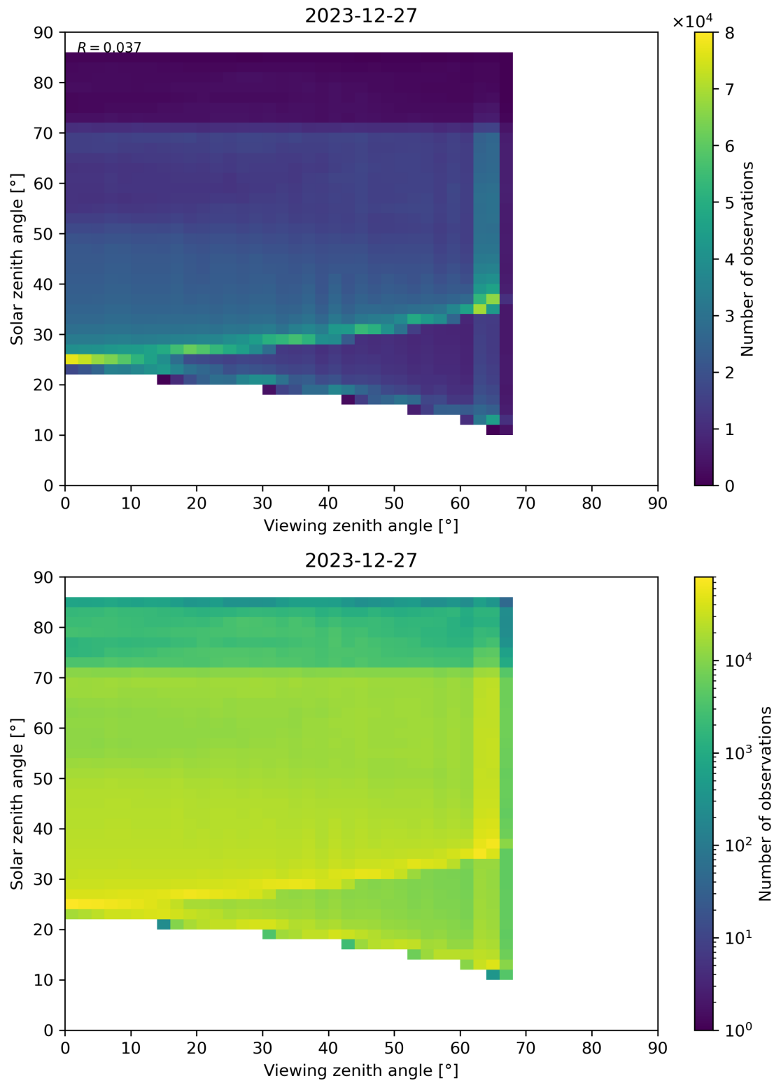
Figure 197: Scatter density plot of “Viewing zenith angle” against “Solar zenith angle” for 2023-12-26 to 2023-12-28.
