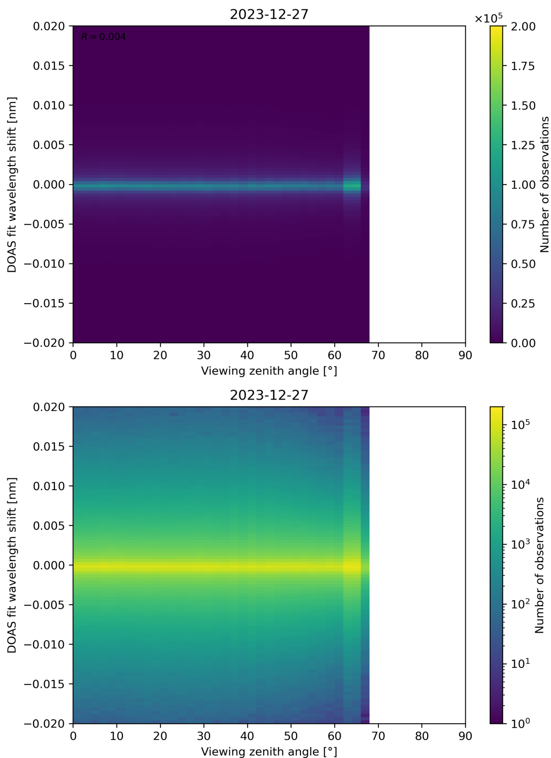
Figure 183: Scatter density plot of “Viewing zenith angle” against “DOAS fit wavelength shift” for 2023-12-26 to 2023-12-28.
