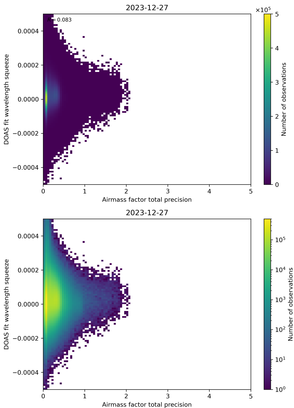
Figure 107: Scatter density plot of “Airmass factor total precision” against “DOAS fit wavelength squeeze” for 2023-12-26 to 2023-12-28.
