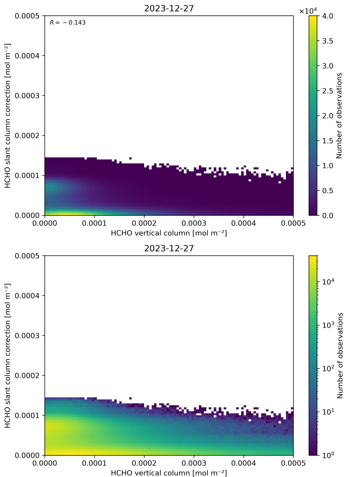
Figure 128: Scatter density plot of “HCHO vertical column” against “HCHO slant column correction” for 2023-12-26 to 2023-12-28.
