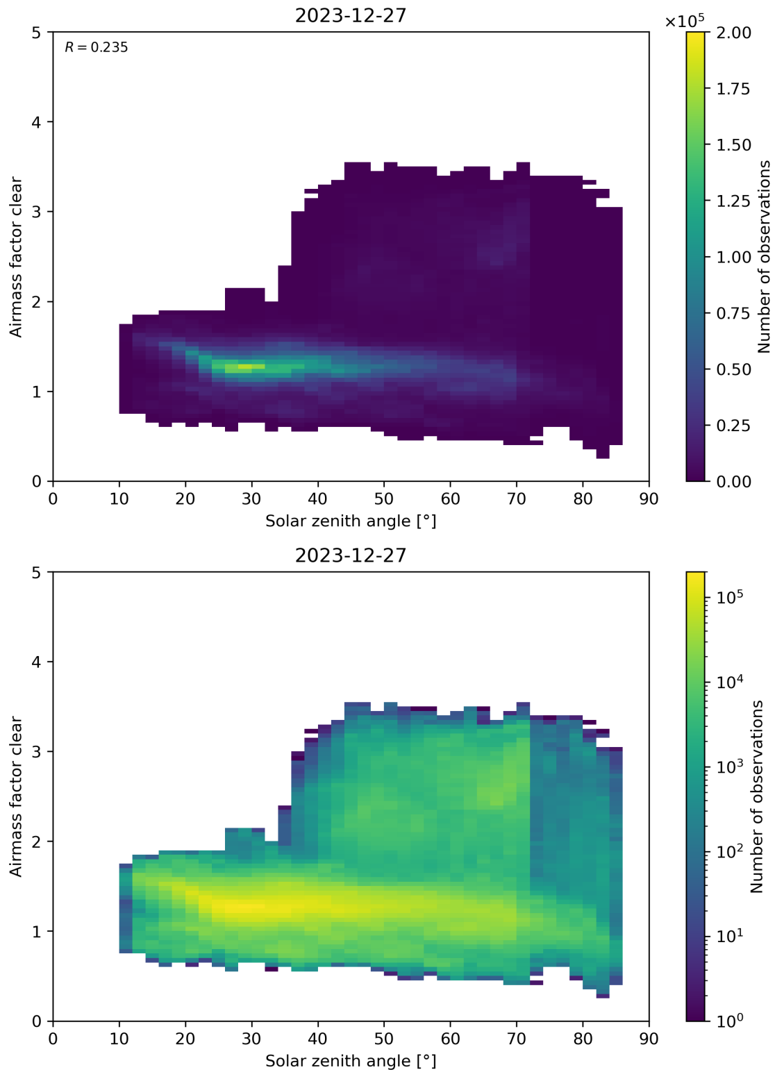
Figure 170: Scatter density plot of “Solar zenith angle” against “Airmass factor clear” for 2023-12-26 to 2023-12-28.
