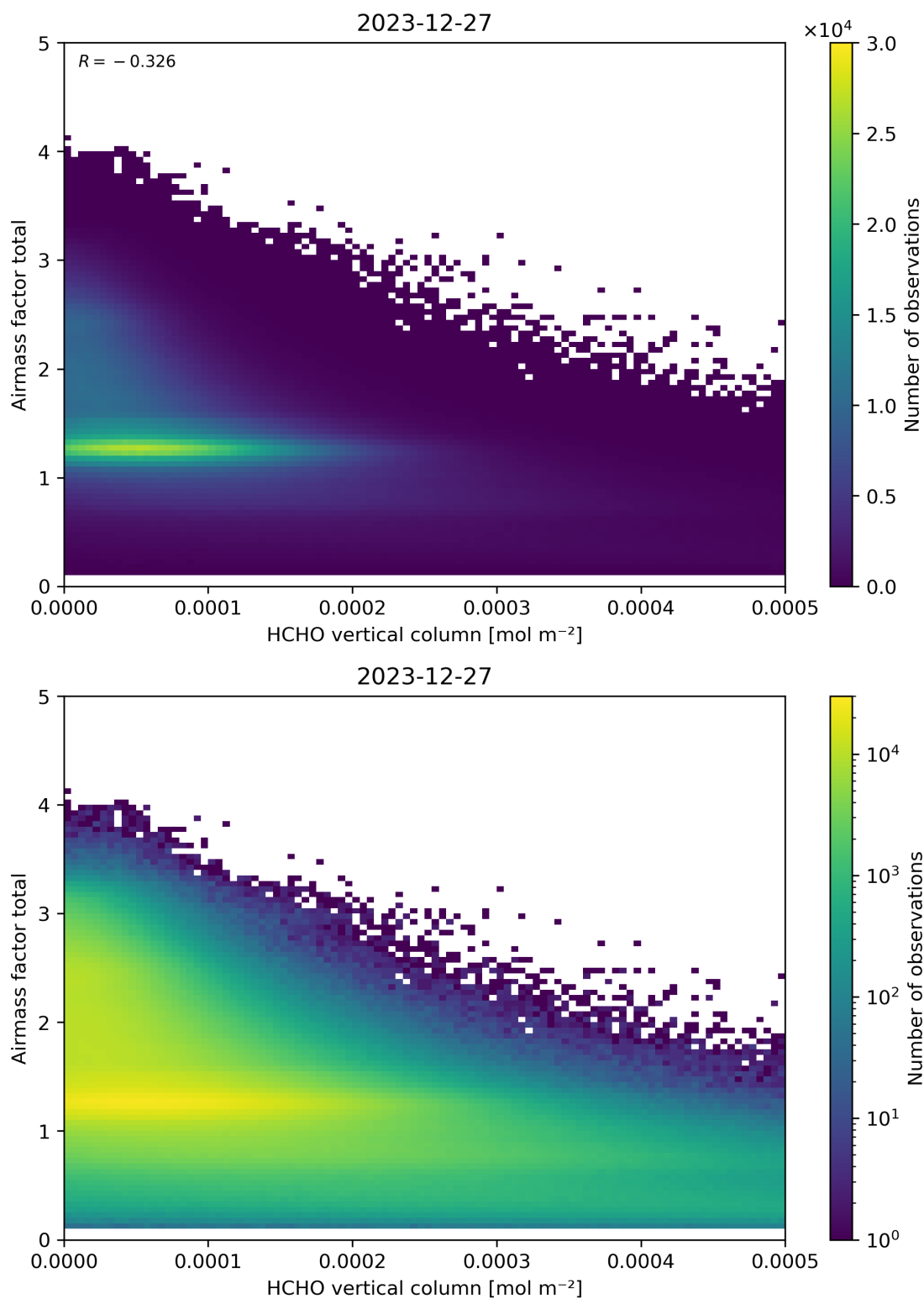
Figure 131: Scatter density plot of “HCHO vertical column” against “Airmass factor total” for 2023-12-26 to 2023-12-28.
