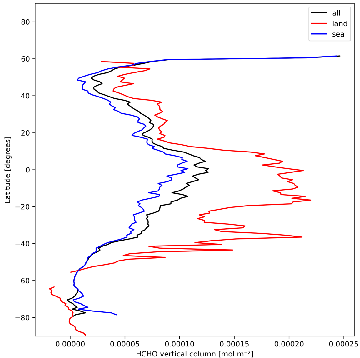
Figure 21: Zonal average of “HCHO vertical column” for 2023-12-26 to 2023-12-28.
