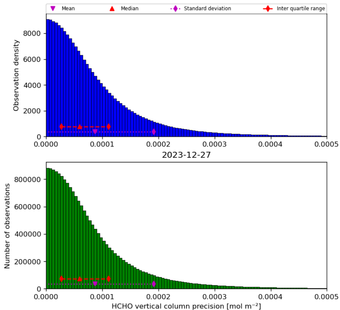
Figure 36: Histogram of “HCHO vertical column precision” for 2023-12-26 to 2023-12-28
