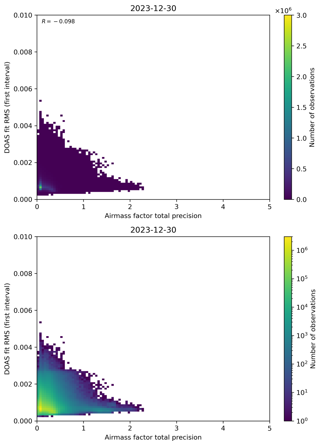
Figure 105: Scatter density plot of “Airmass factor total precision” against “DOAS fit RMS (first interval)” for 2023-12-30 to 2023-12-31.
