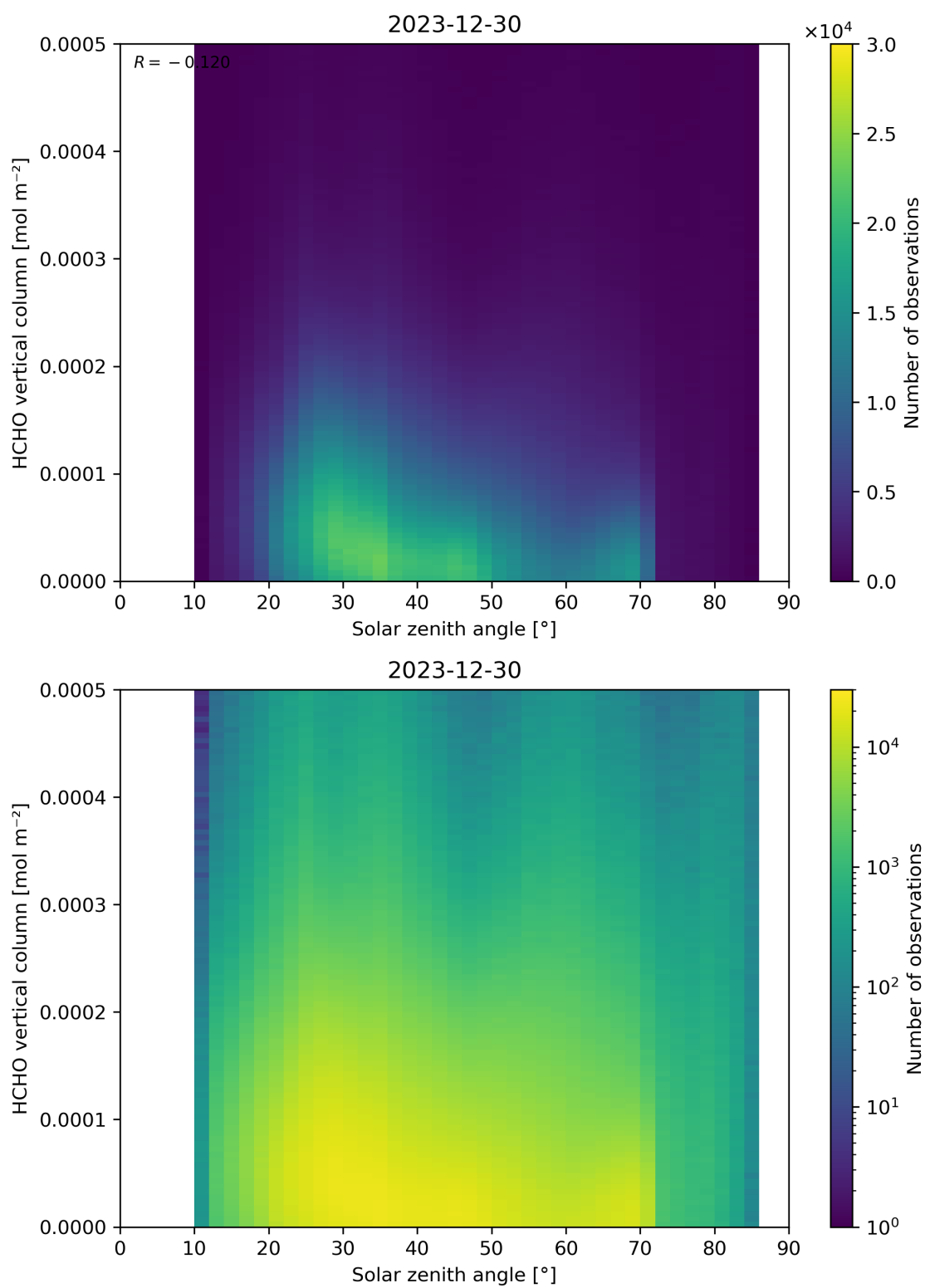
Figure 177: Scatter density plot of “Solar zenith angle” against “HCHO vertical column” for 2023-12-30 to 2023-12-31.
