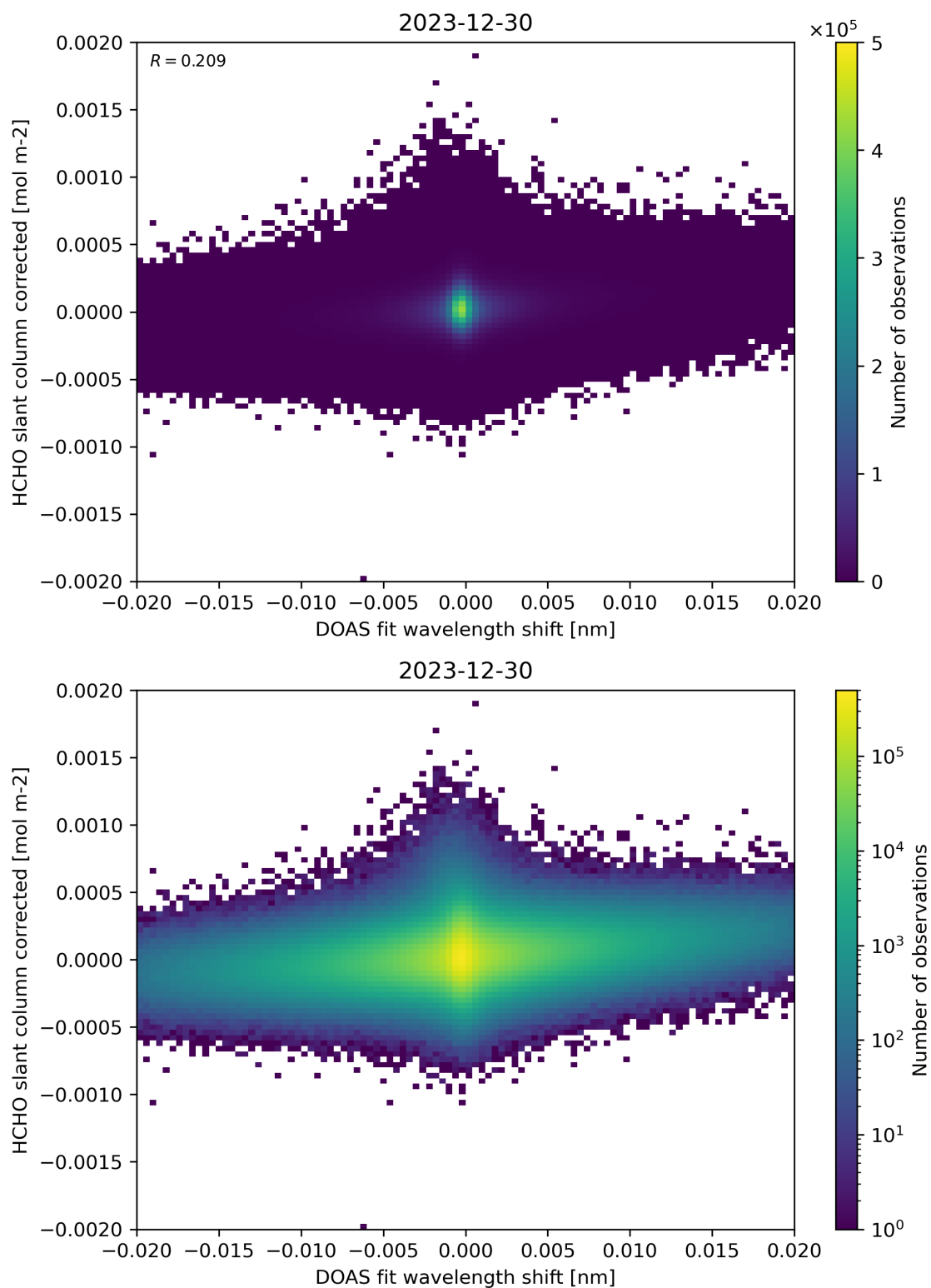
Figure 66: Scatter density plot of “DOAS fit wavelength shift” against “HCHO slant column corrected” for 2023-12-30 to 2023-12-31.
