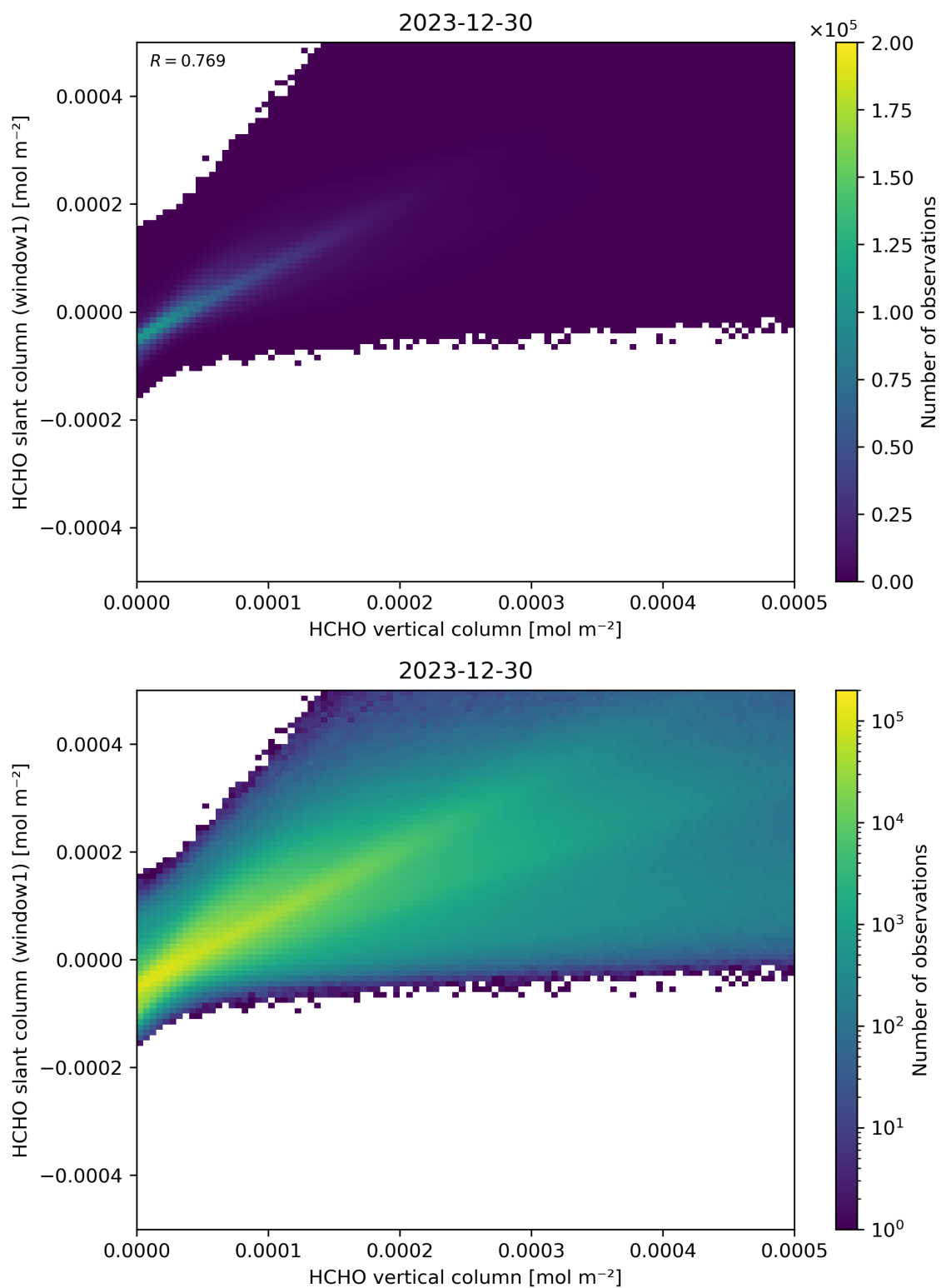
Figure 129: Scatter density plot of “HCHO vertical column” against “HCHO slant column (window1)” for 2023-12-30 to 2023-12-31.
