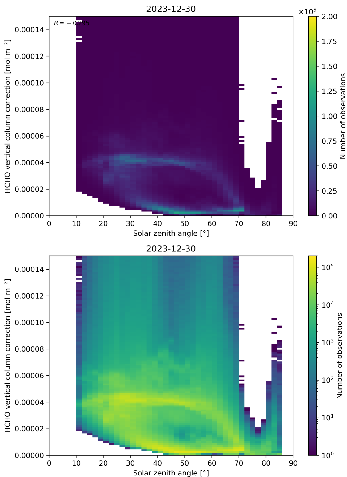
Figure 178: Scatter density plot of “Solar zenith angle” against “HCHO vertical column correction” for 2023-12-30 to 2023-12-31.
