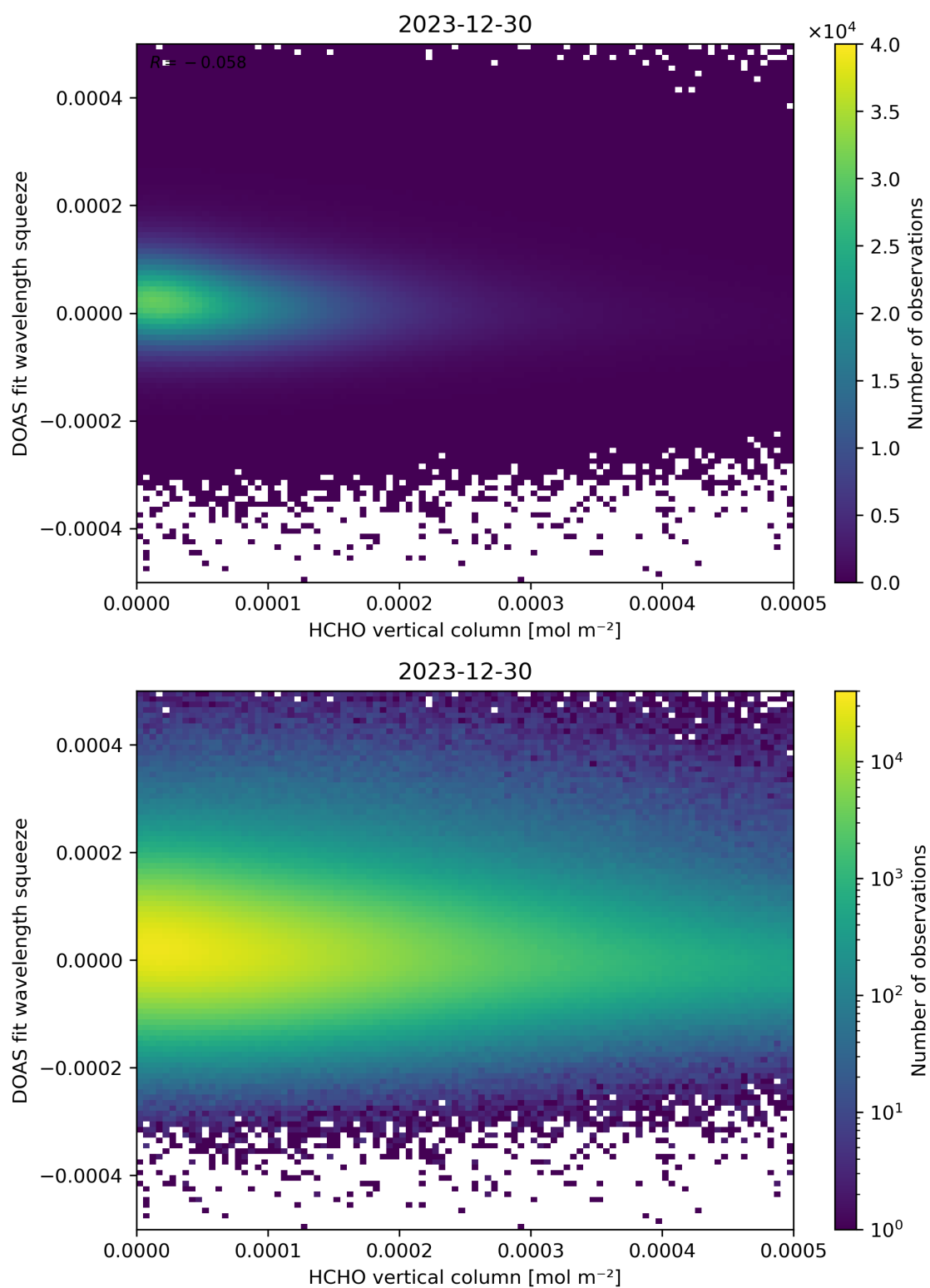
Figure 125: Scatter density plot of “HCHO vertical column” against “DOAS fit wavelength squeeze” for 2023-12-30 to 2023-12-31.
