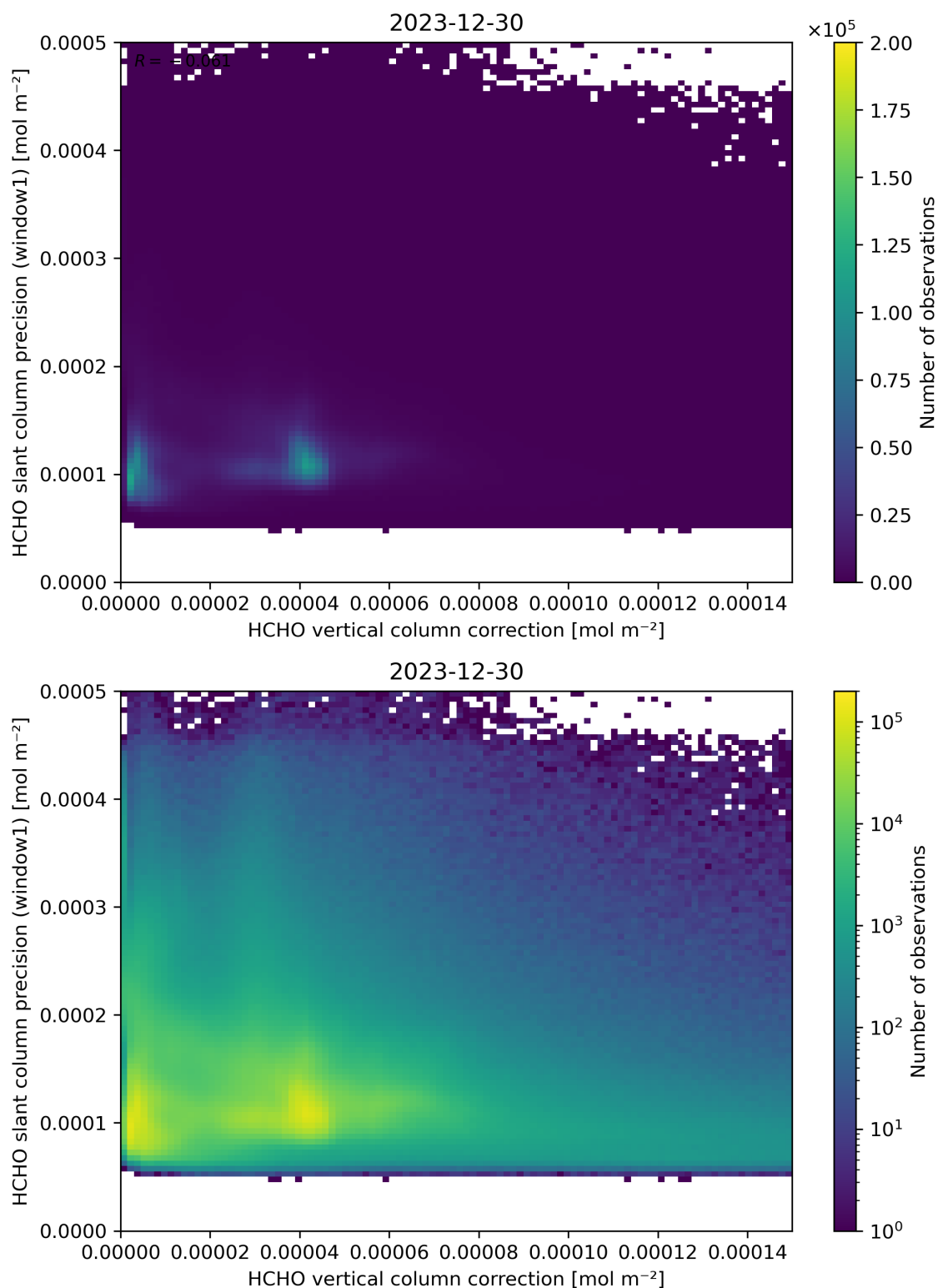
Figure 119: Scatter density plot of “HCHO vertical column correction” against “HCHO slant column precision (window1)” for 2023-12-30 to 2023-12-31.
