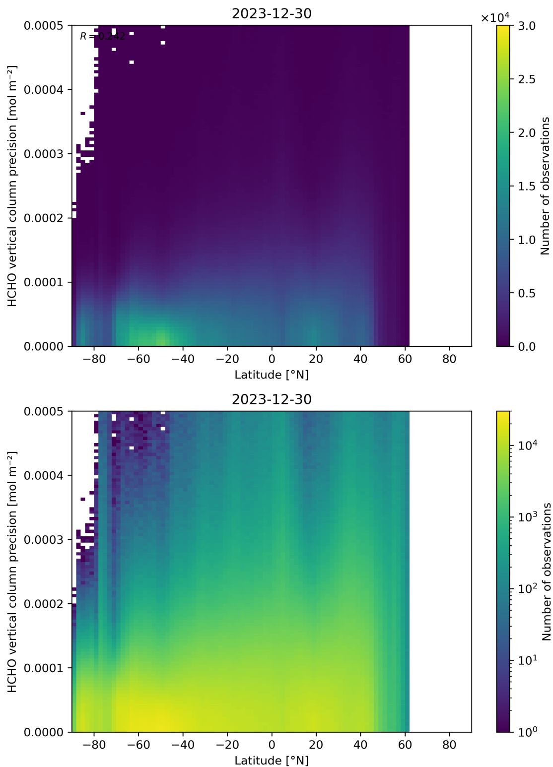
Figure 165: Scatter density plot of “Latitude” against “HCHO vertical column precision” for 2023-12-30 to 2023-12-31.
