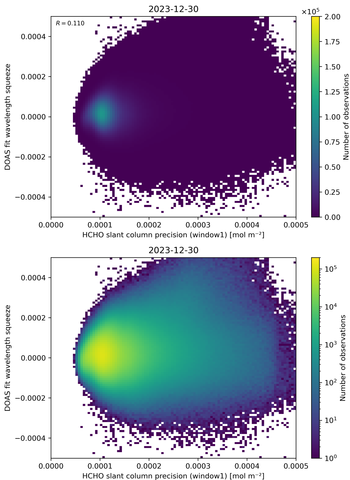
Figure 90: Scatter density plot of “HCHO slant column precision (window1)” against “DOAS fit wavelength squeeze” for 2023-12-30 to 2023-12-31.
