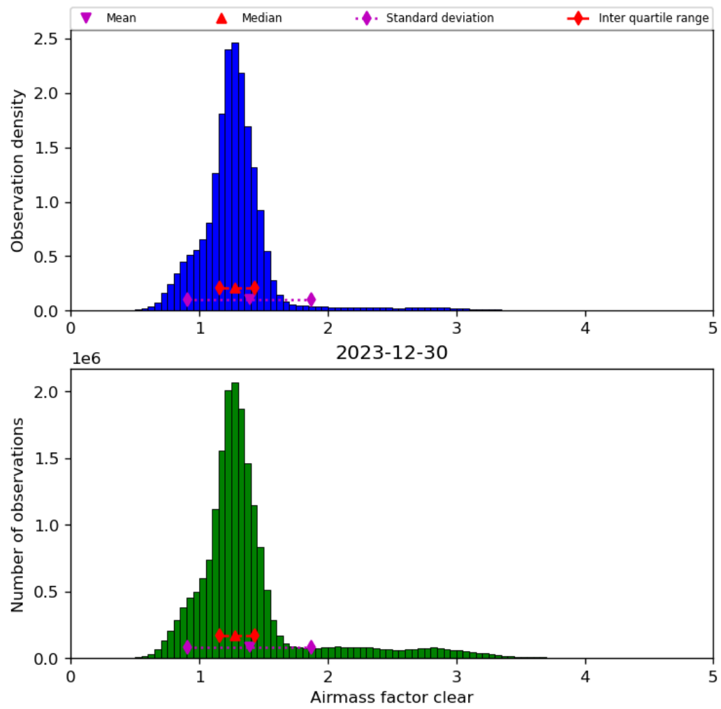
Figure 42: Histogram of “Airmass factor clear” for 2023-12-30 to 2023-12-31
