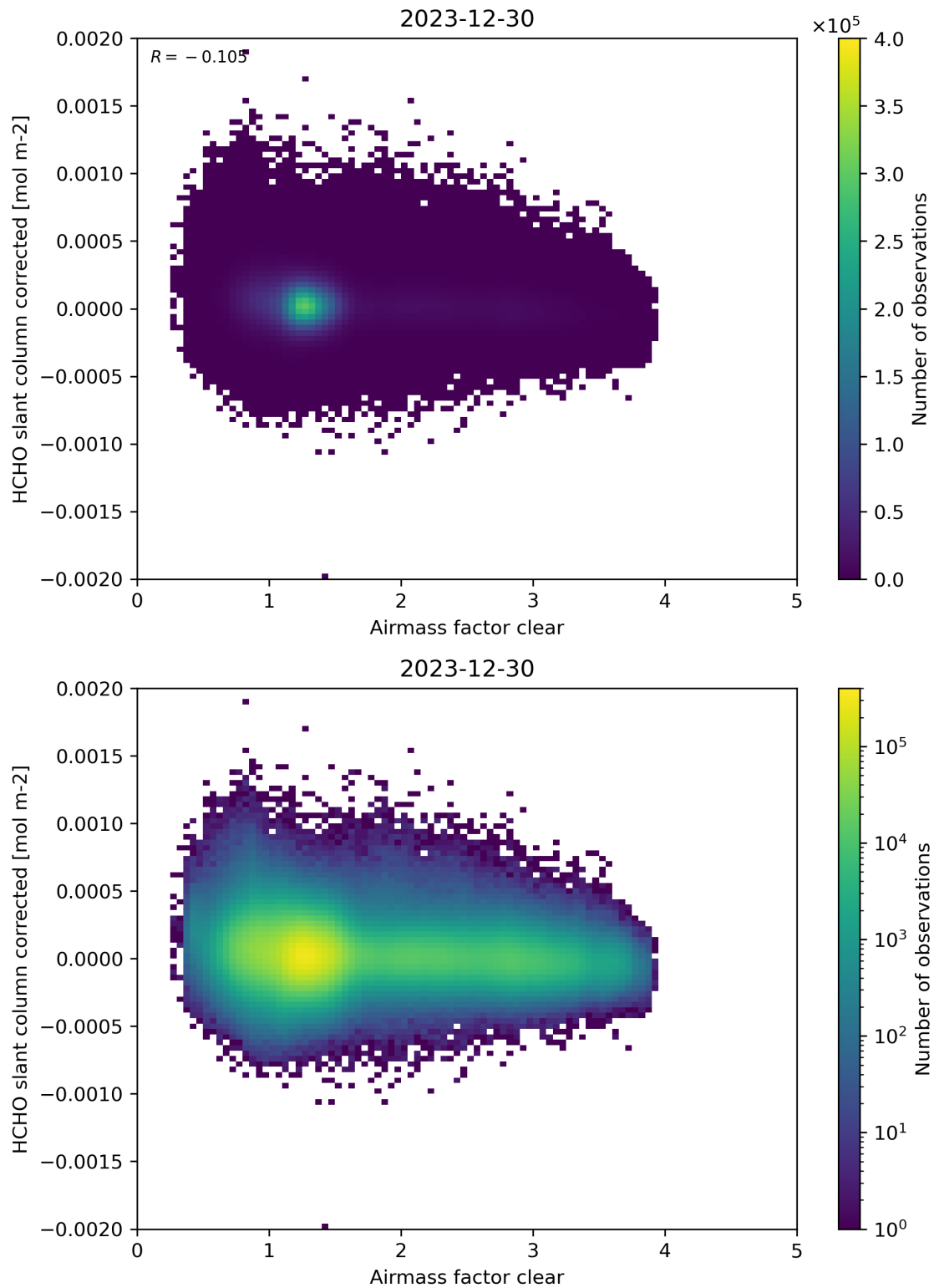
Figure 74: Scatter density plot of “Airmass factor clear” against “HCHO slant column corrected” for 2023-12-30 to 2023-12-31.
