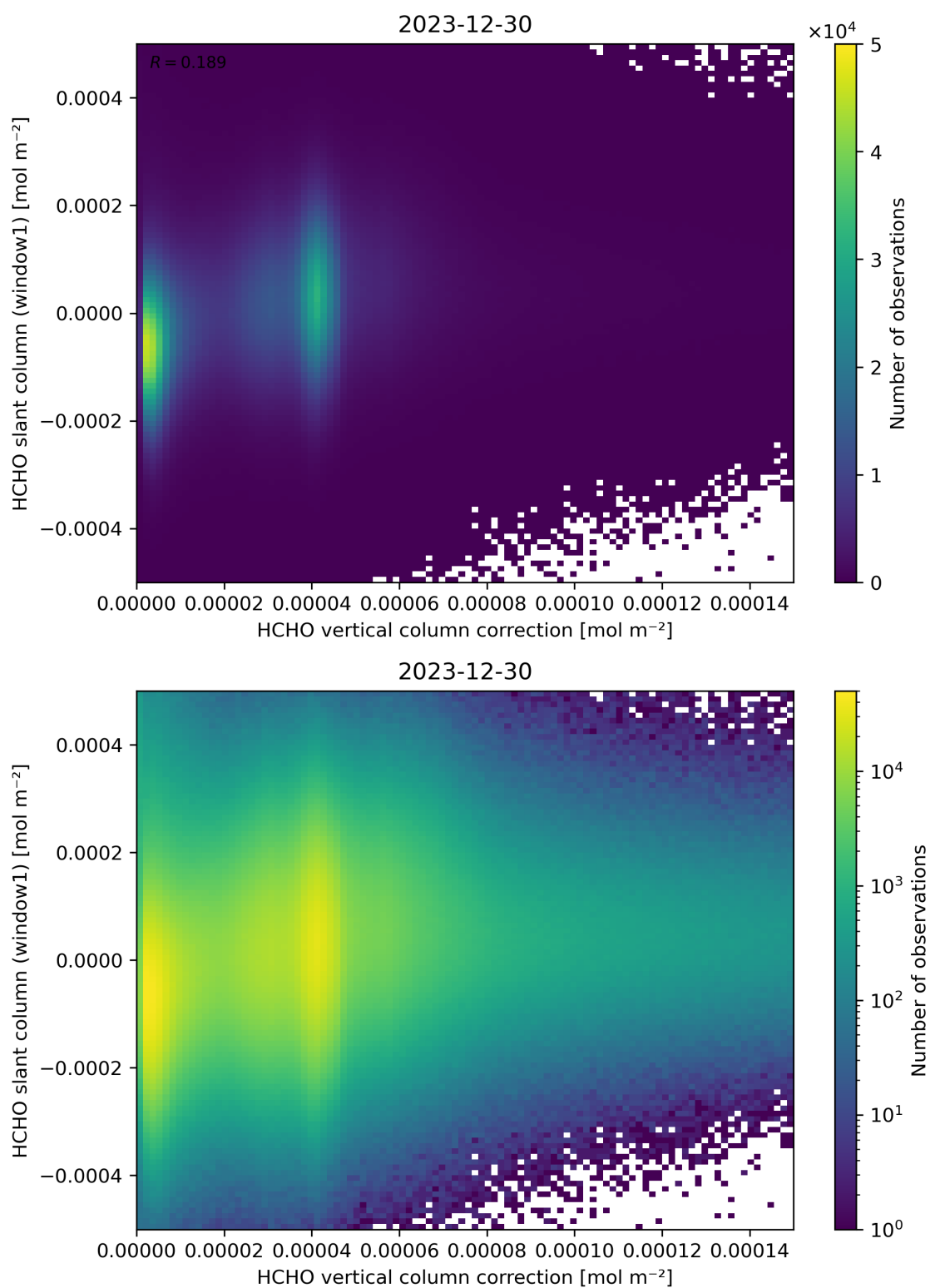
Figure 118: Scatter density plot of “HCHO vertical column correction” against “HCHO slant column (window1)” for 2023-12-30 to 2023-12-31.
