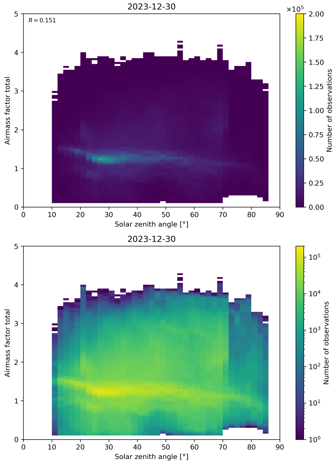
Figure 175: Scatter density plot of “Solar zenith angle” against “Airmass factor total” for 2023-12-30 to 2023-12-31.
