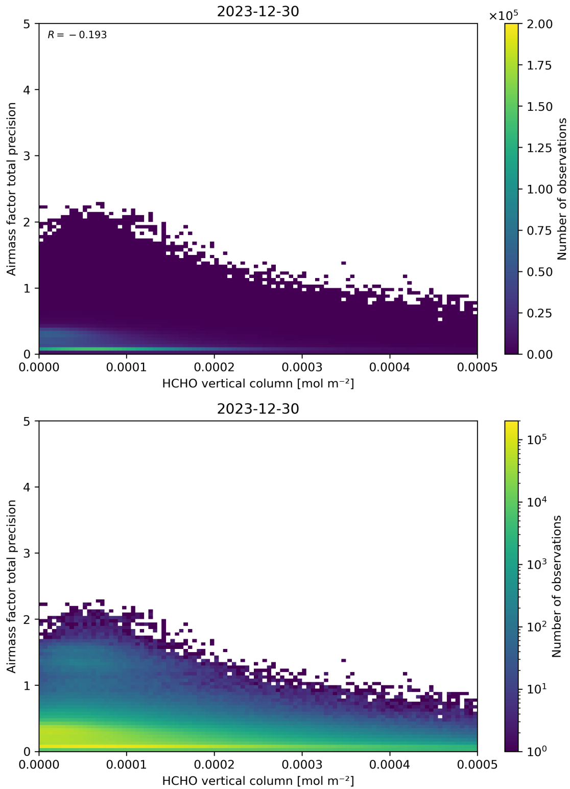
Figure 132: Scatter density plot of “HCHO vertical column” against “Airmass factor total precision” for 2023-12-30 to 2023-12-31.
