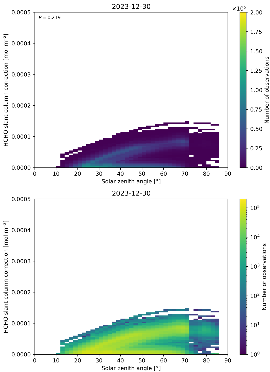
Figure 172: Scatter density plot of “Solar zenith angle” against “HCHO slant column correction” for 2023-12-30 to 2023-12-31.
