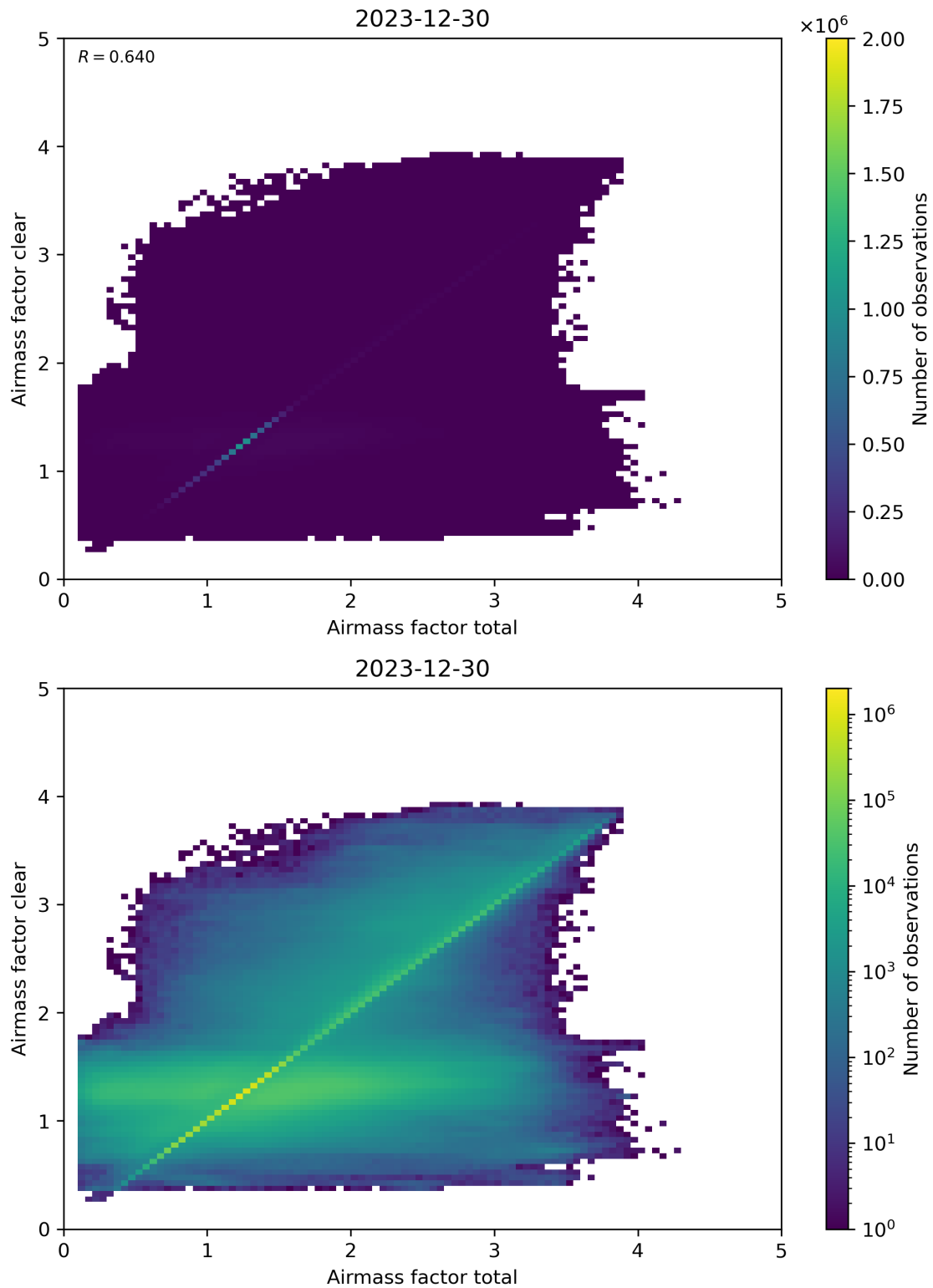
Figure 100: Scatter density plot of “Airmass factor total” against “Airmass factor clear” for 2023-12-30 to 2023-12-31.
