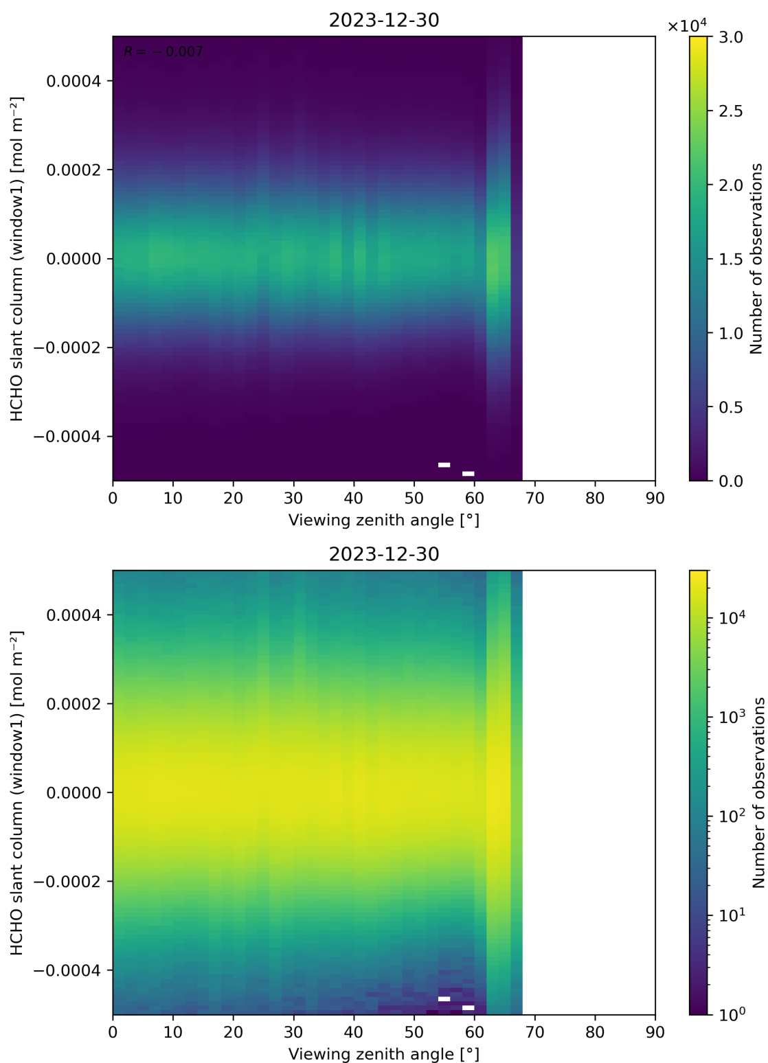
Figure 188: Scatter density plot of “Viewing zenith angle” against “HCHO slant column (window1)” for 2023-12-30 to 2023-12-31.
