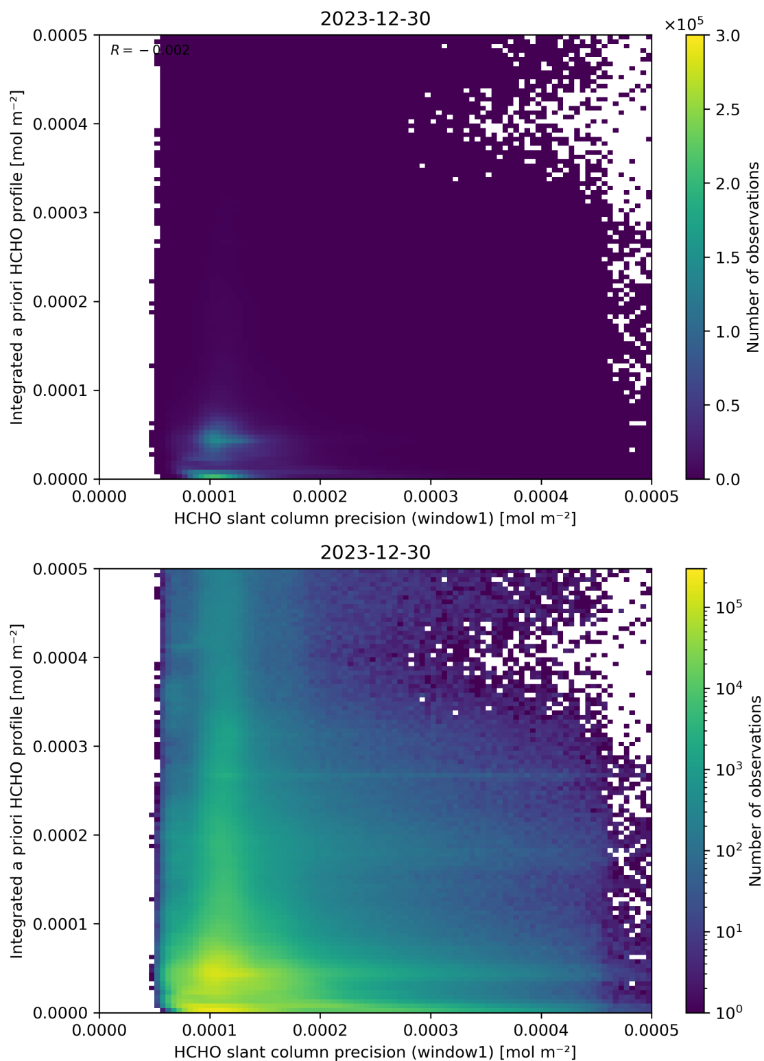
Figure 96: Scatter density plot of “HCHO slant column precision (window1)” against “Integrated a priori HCHO profile” for 2023-12-30 to 2023-12-31.
