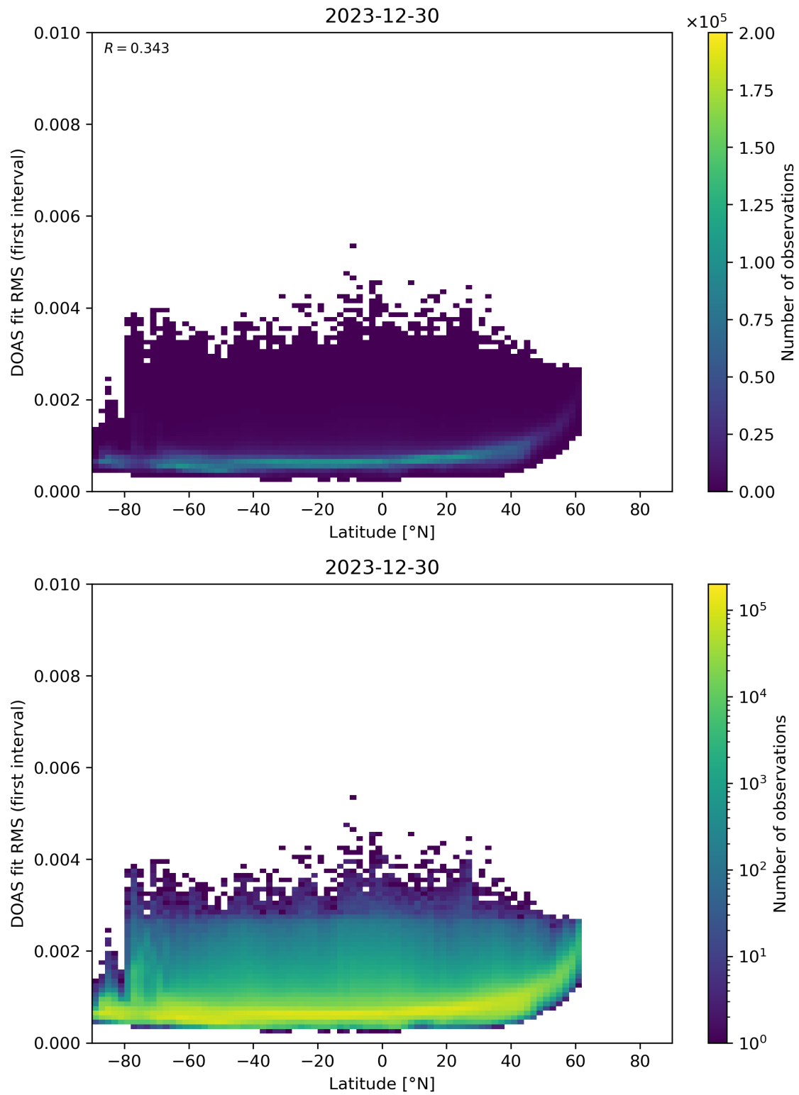
Figure 153: Scatter density plot of “Latitude” against “DOAS fit RMS (first interval)” for 2023-12-30 to 2023-12-31.
