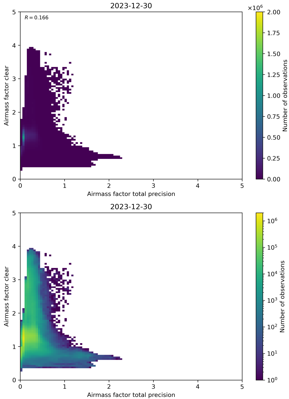
Figure 108: Scatter density plot of “Airmass factor total precision” against “Airmass factor clear” for 2023-12-30 to 2023-12-31.
