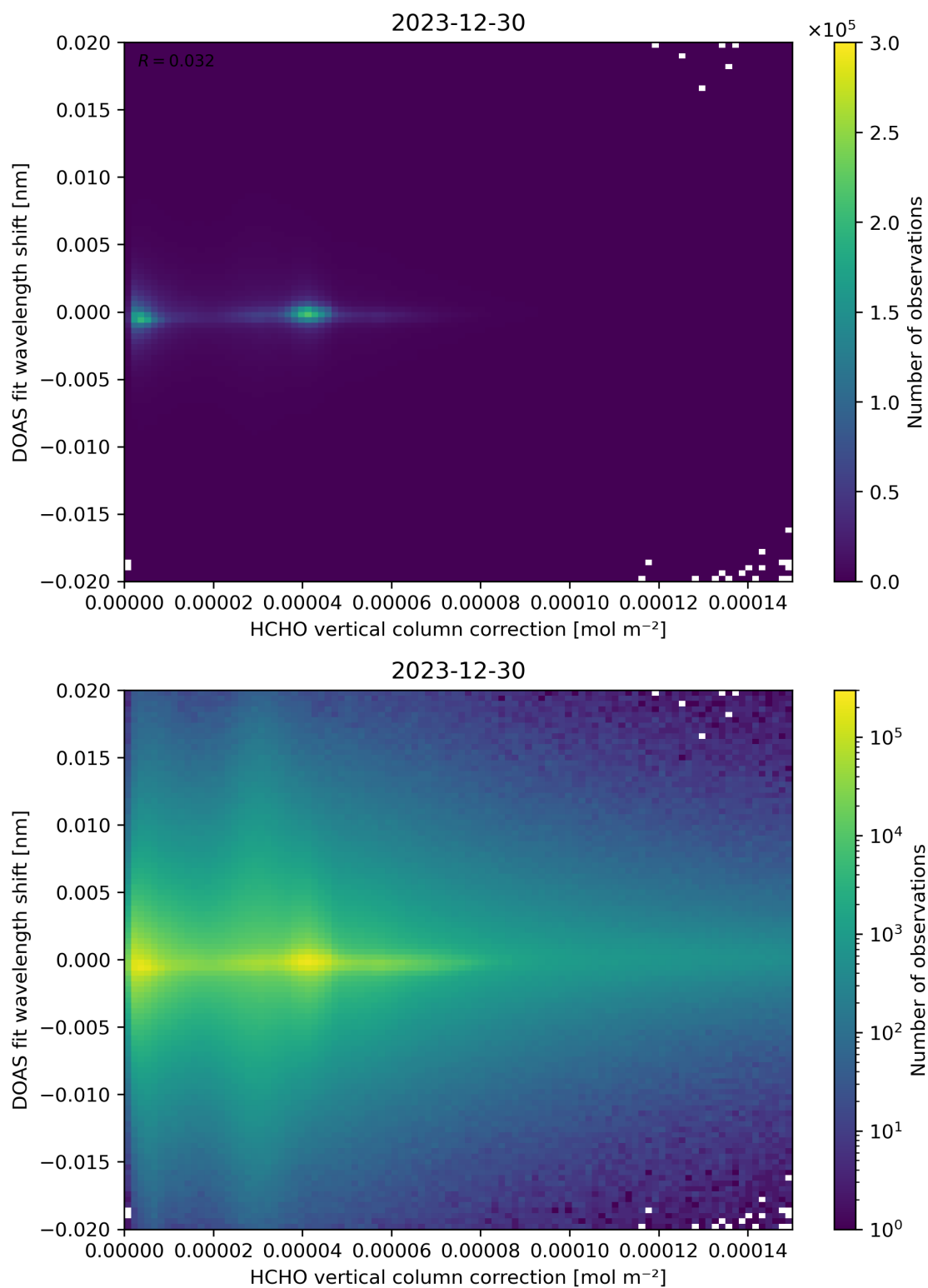
Figure 113: Scatter density plot of “HCHO vertical column correction” against “DOAS fit wavelength shift” for 2023-12-30 to 2023-12-31.
