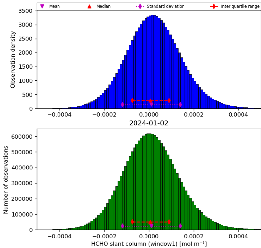
Figure 38: Histogram of “HCHO slant column (window1)” for 2024-01-01 to 2024-01-03
