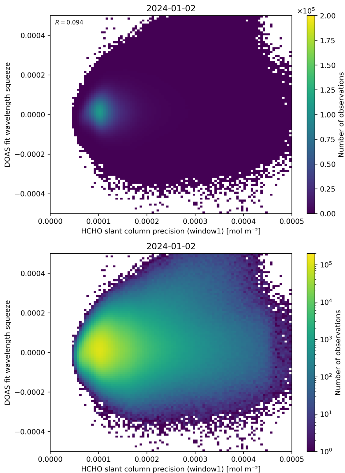
Figure 90: Scatter density plot of “HCHO slant column precision (window1)” against “DOAS fit wavelength squeeze” for 2024-01-01 to 2024-01-03.
