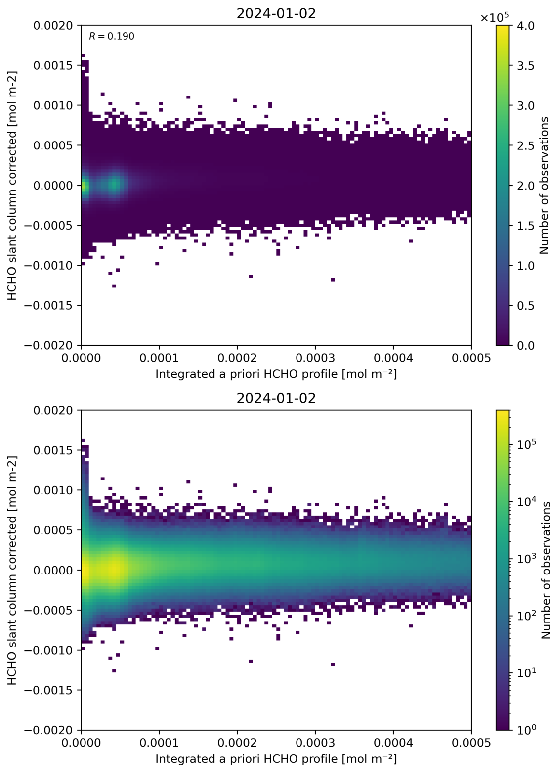
Figure 151: Scatter density plot of “Integrated a priori HCHO profile” against “HCHO slant column corrected” for 2024-01-01 to 2024-01-03.
