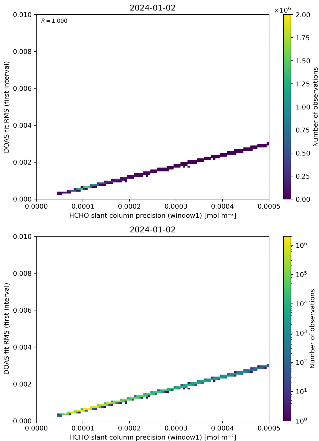
Figure 88: Scatter density plot of “HCHO slant column precision (window1)” against “DOAS fit RMS (first interval)” for 2024-01-01 to 2024-01-03.
