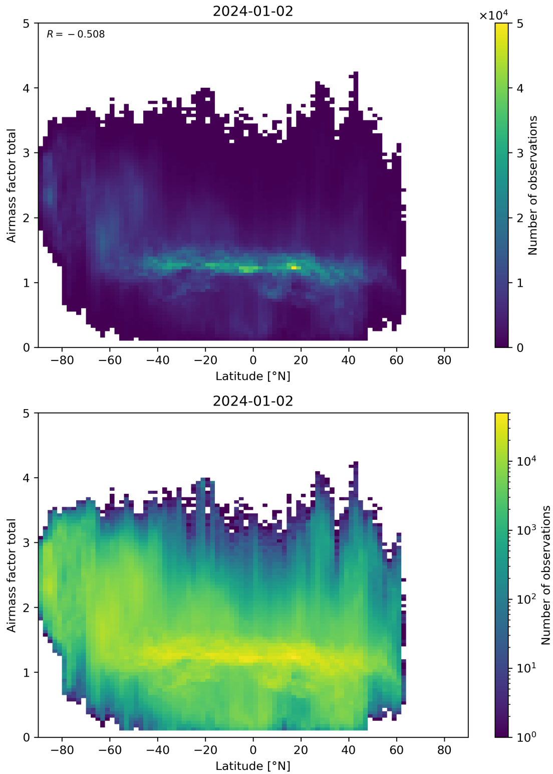
Figure 161: Scatter density plot of “Latitude” against “Airmass factor total” for 2024-01-01 to 2024-01-03.
