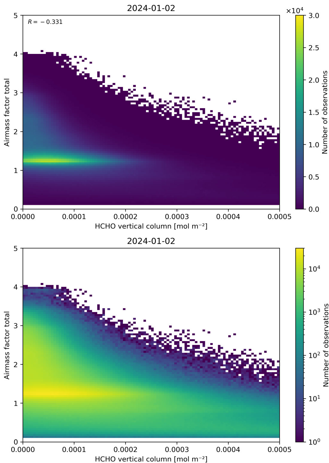
Figure 131: Scatter density plot of “HCHO vertical column” against “Airmass factor total” for 2024-01-01 to 2024-01-03.
