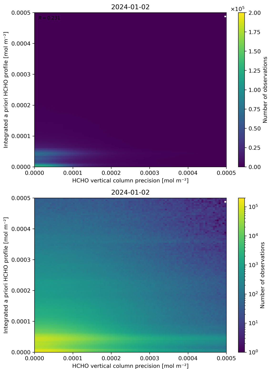
Figure 147: Scatter density plot of “HCHO vertical column precision” against “Integrated a priori HCHO profile” for 2024-01-01 to 2024-01-03.
