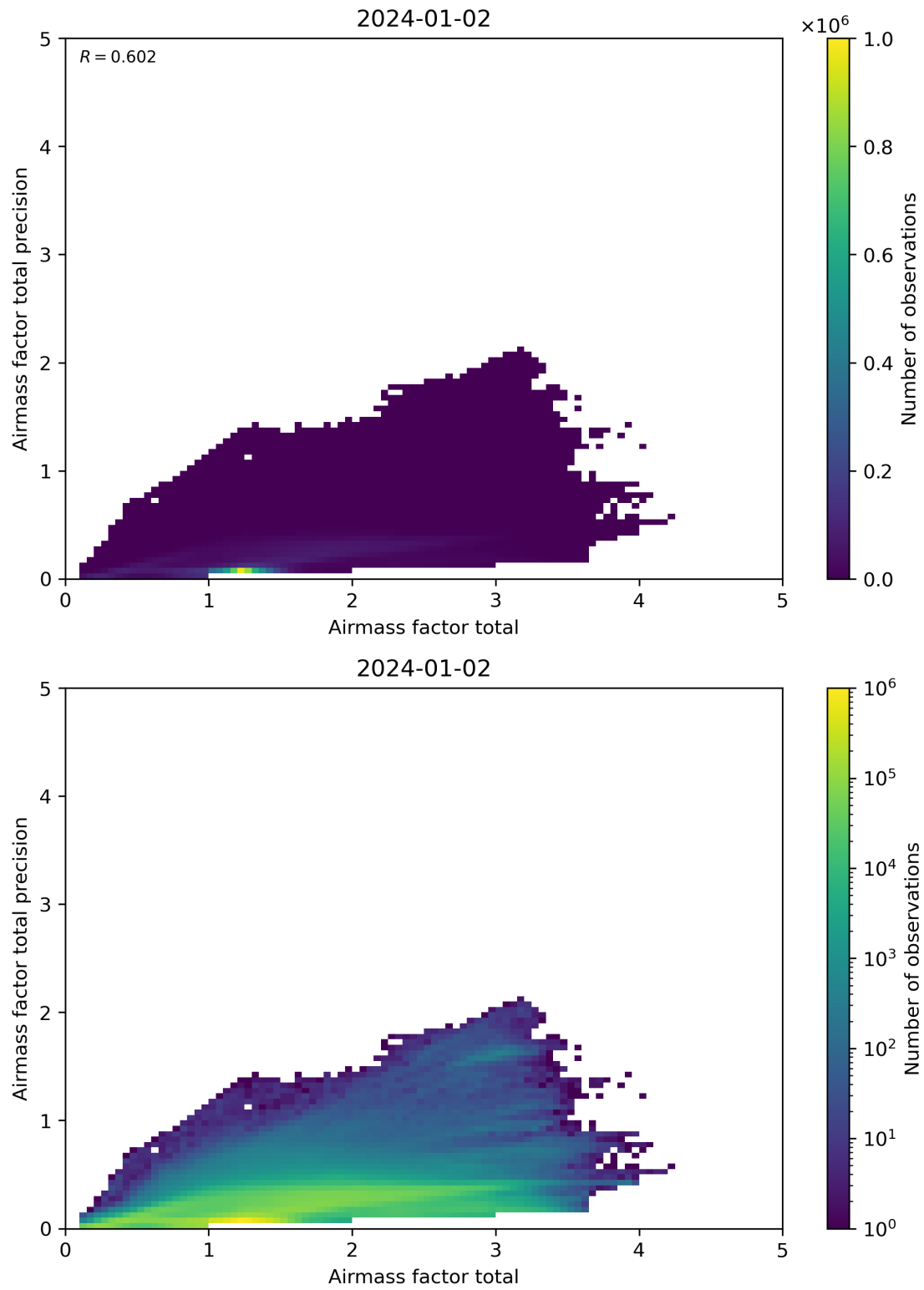
Figure 103: Scatter density plot of “Airmass factor total” against “Airmass factor total precision” for 2024-01-01 to 2024-01-03.
