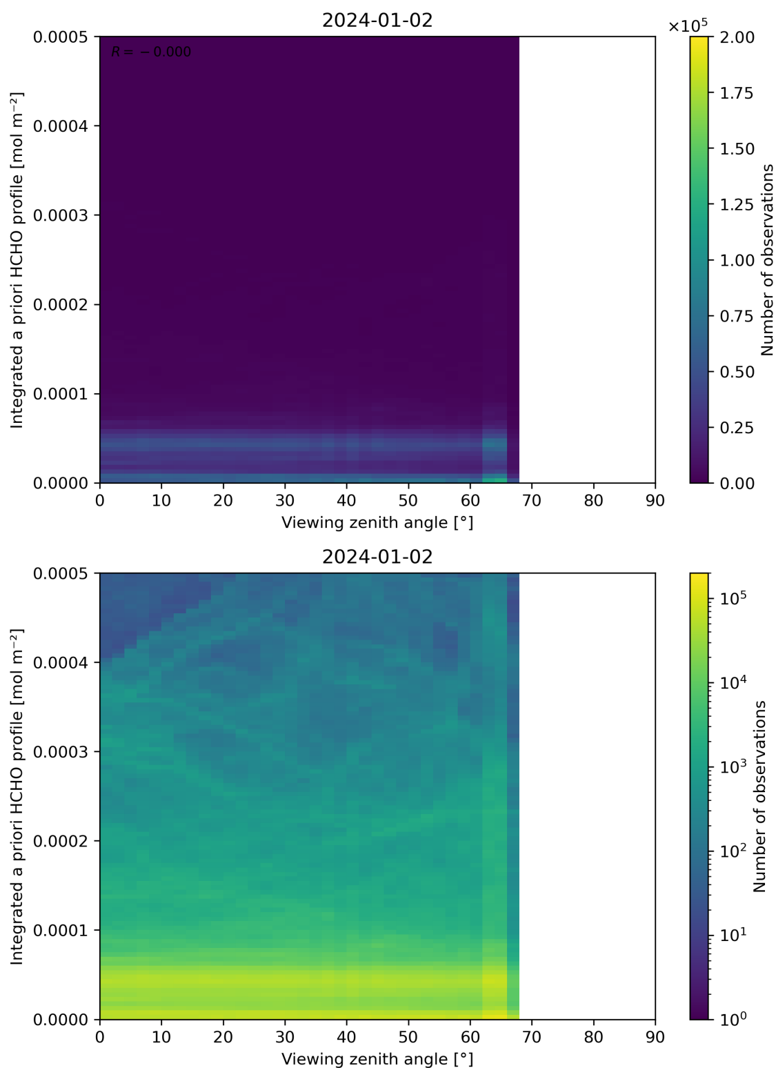
Figure 195: Scatter density plot of “Viewing zenith angle” against “Integrated a priori HCHO profile” for 2024-01-01 to 2024-01-03.
