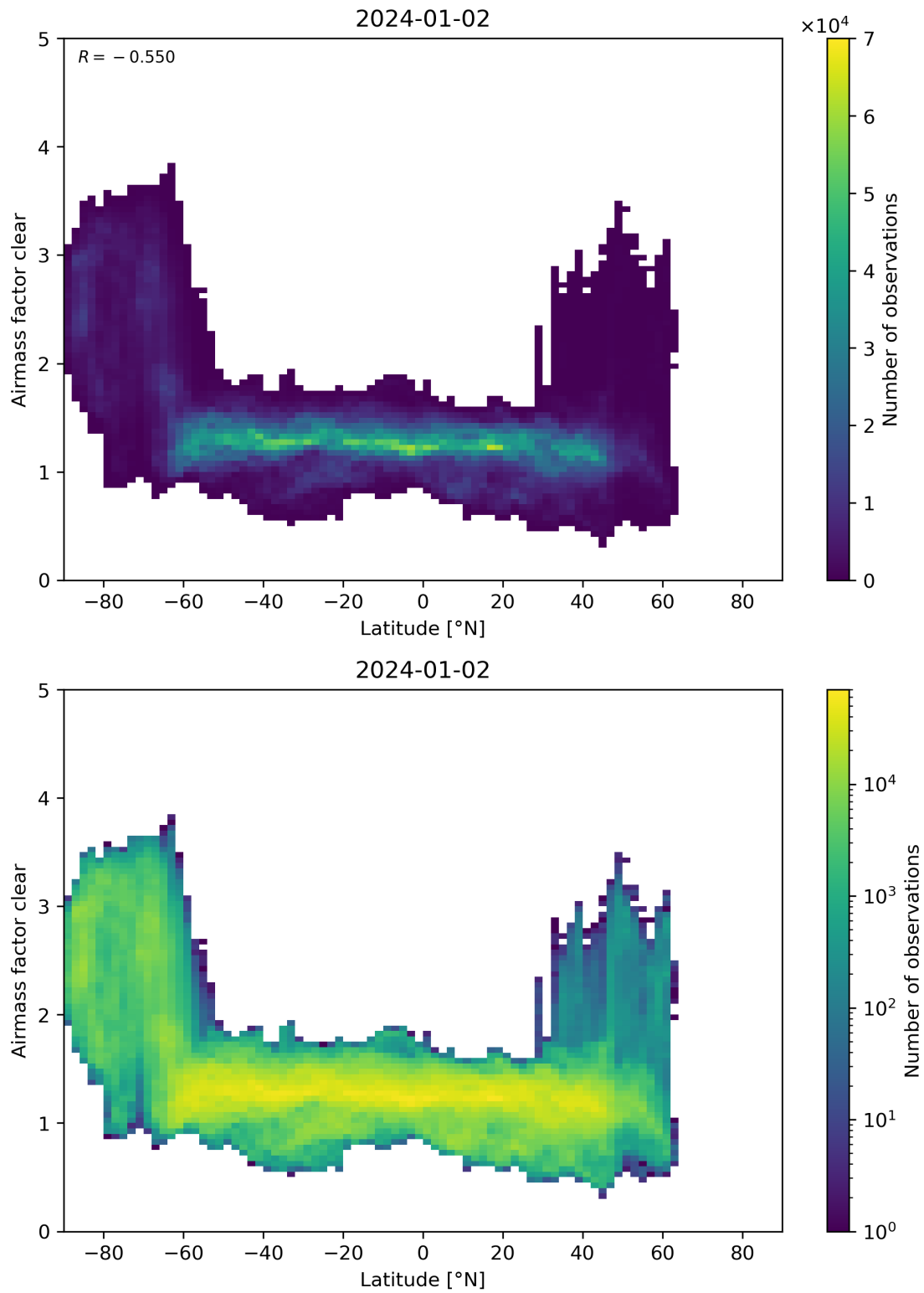
Figure 156: Scatter density plot of “Latitude” against “Airmass factor clear” for 2024-01-01 to 2024-01-03.
