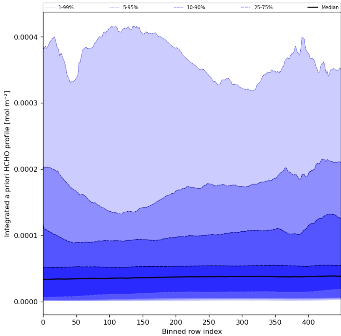
Figure 57: Along track statistics of “Integrated a priori HCHO profile” for 2024-01-01 to 2024-01-03
