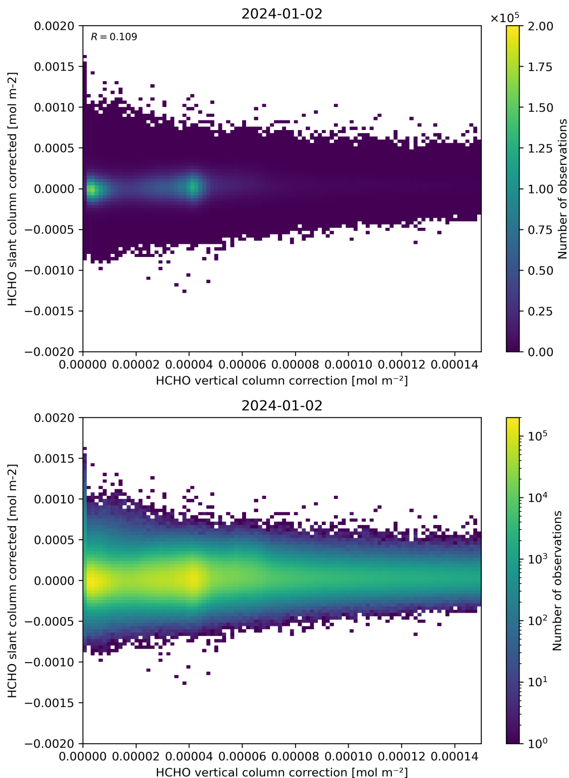
Figure 116: Scatter density plot of “HCHO vertical column correction” against “HCHO slant column corrected” for 2024-01-01 to 2024-01-03.
