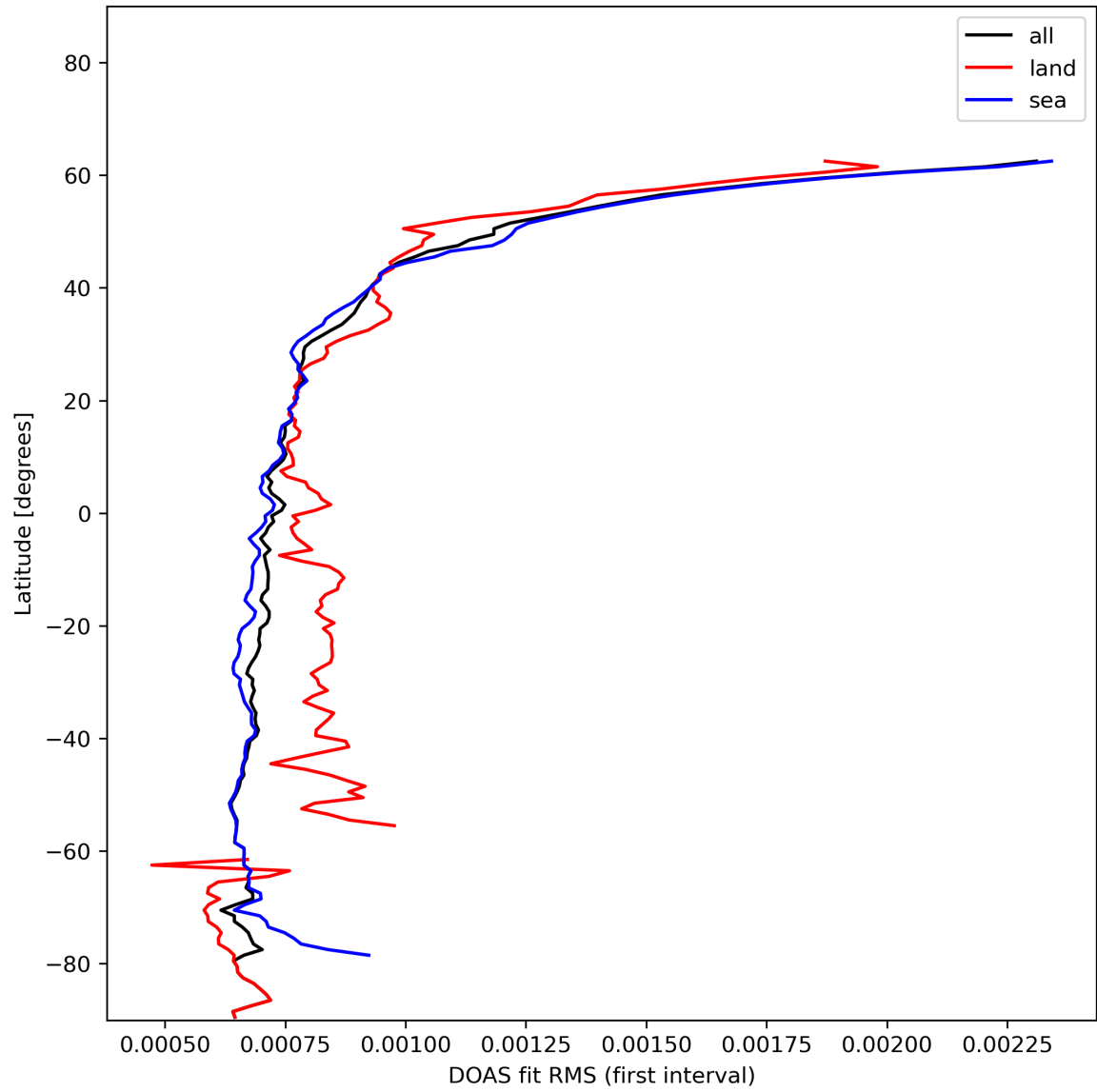
Figure 32: Zonal average of “DOAS fit RMS (first interval)” for 2024-01-01 to 2024-01-03.
