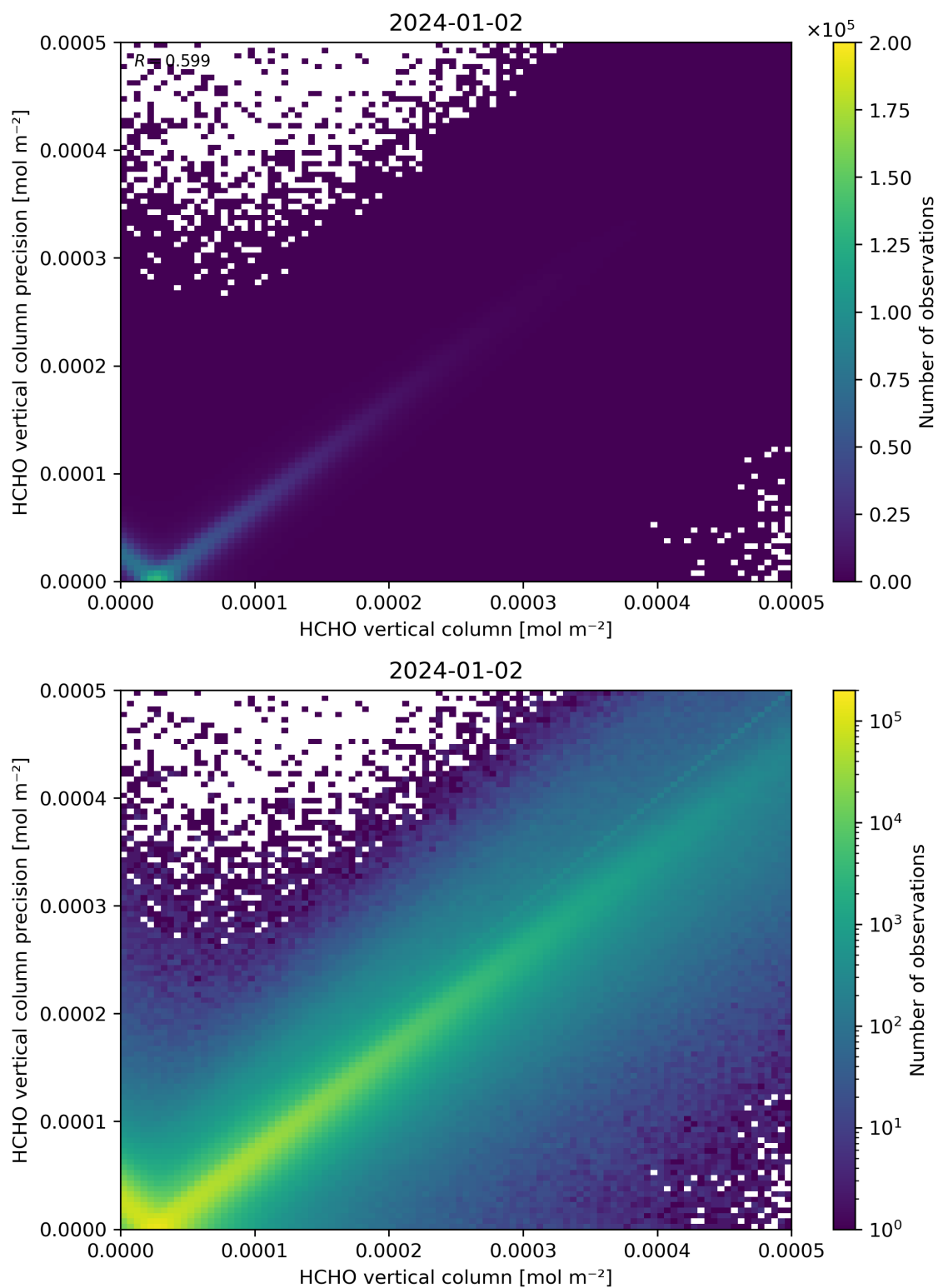
Figure 134: Scatter density plot of “HCHO vertical column” against “HCHO vertical column precision” for 2024-01-01 to 2024-01-03.
