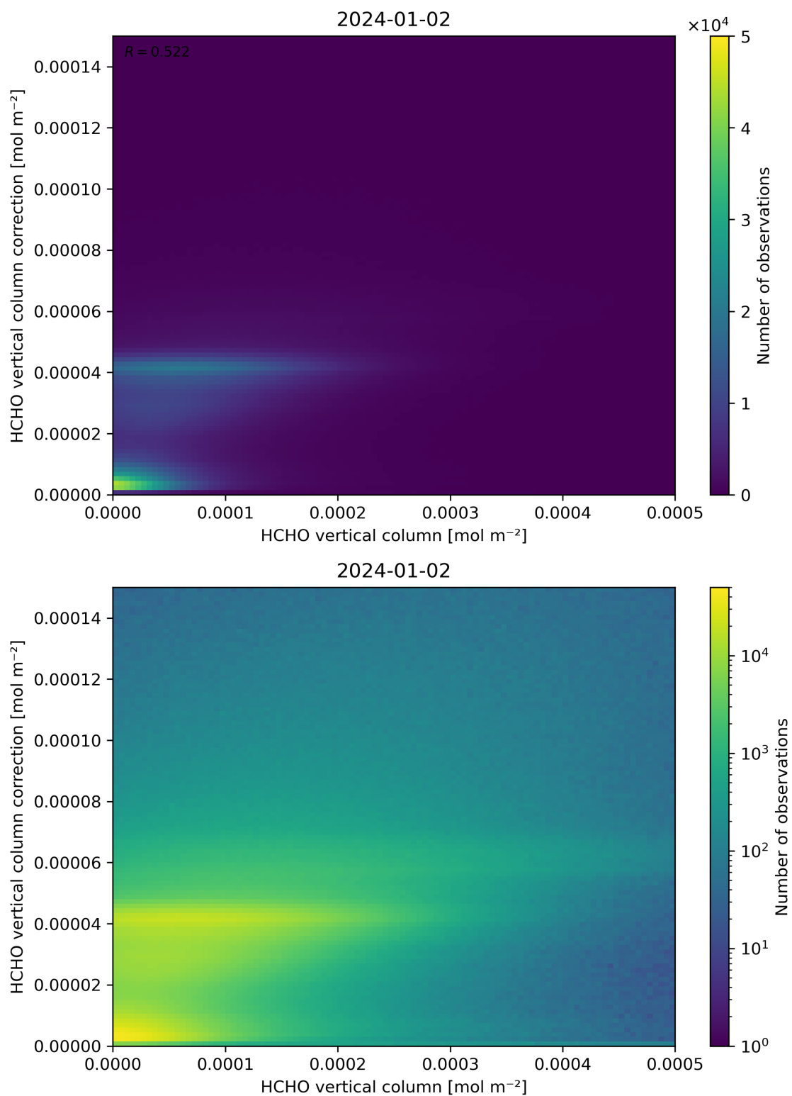
Figure 133: Scatter density plot of “HCHO vertical column” against “HCHO vertical column correction” for 2024-01-01 to 2024-01-03.
