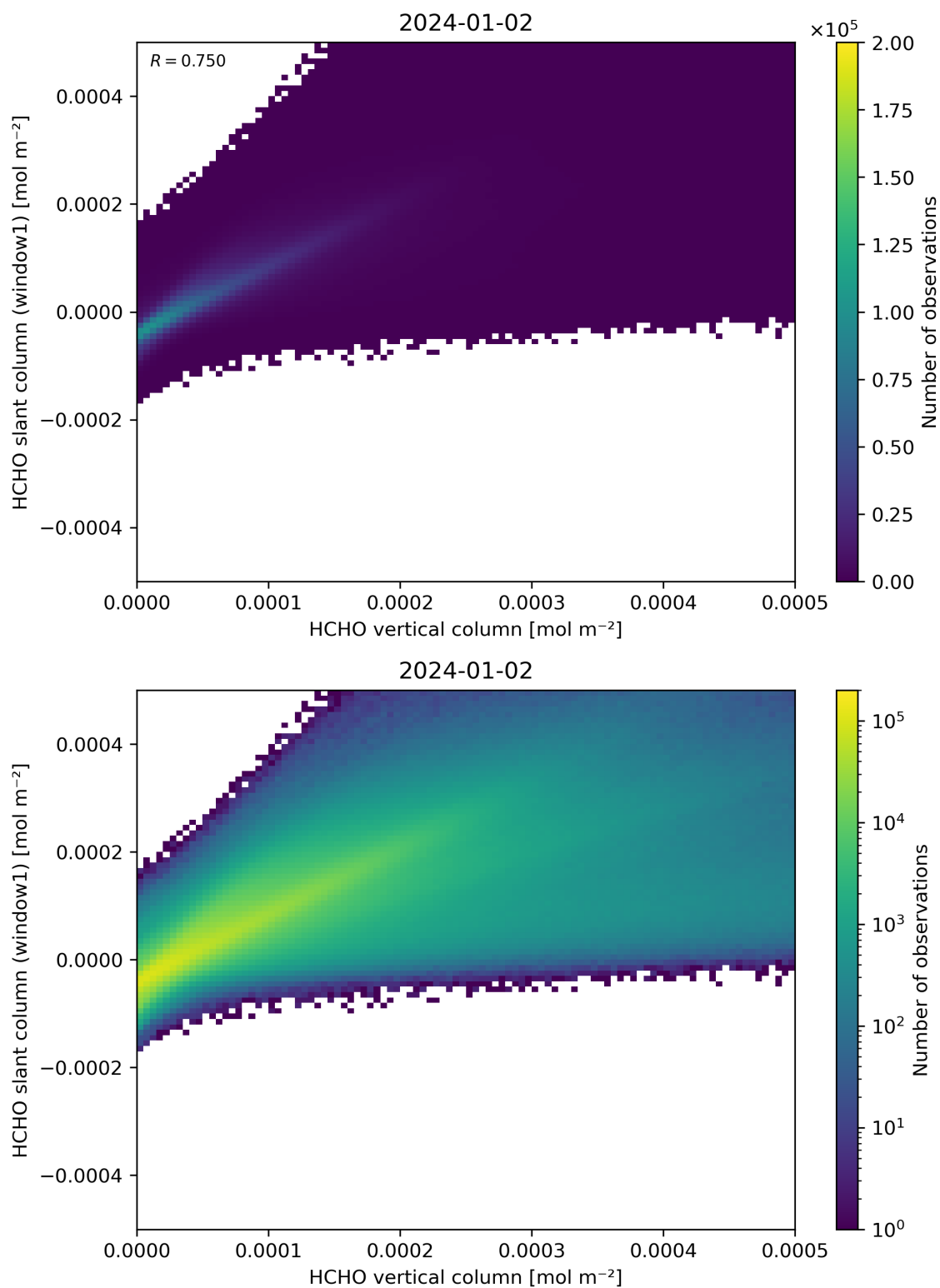
Figure 129: Scatter density plot of “HCHO vertical column” against “HCHO slant column (window1)” for 2024-01-01 to 2024-01-03.
