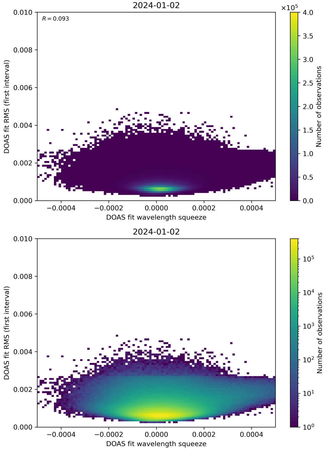
Figure 68: Scatter density plot of “DOAS fit wavelength squeeze” against “DOAS fit RMS (first interval)” for 2024-01-01 to 2024-01-03.
