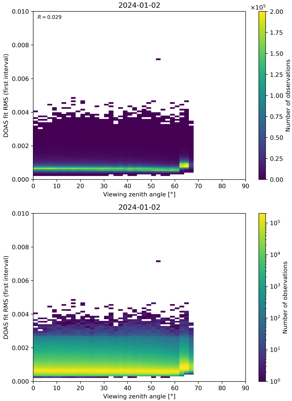
Figure 182: Scatter density plot of “Viewing zenith angle” against “DOAS fit RMS (first interval)” for 2024-01-01 to 2024-01-03.
