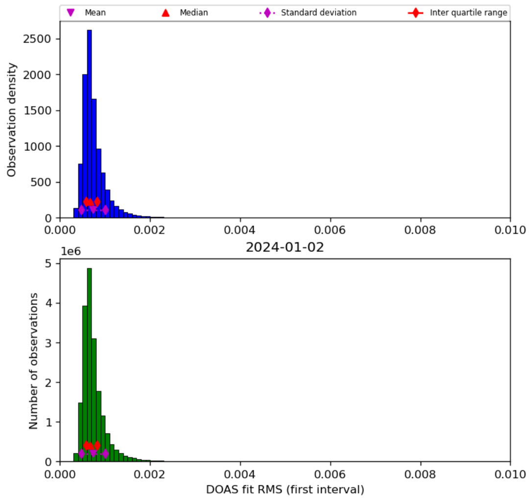
Figure 46: Histogram of “DOAS fit RMS (first interval)” for 2024-01-01 to 2024-01-03
