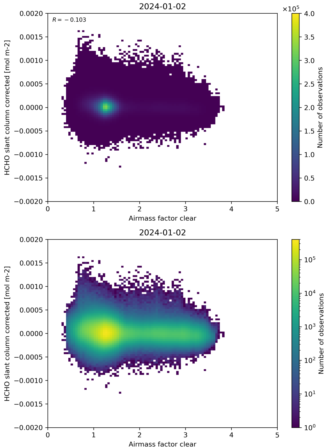
Figure 74: Scatter density plot of “Airmass factor clear” against “HCHO slant column corrected” for 2024-01-01 to 2024-01-03.
