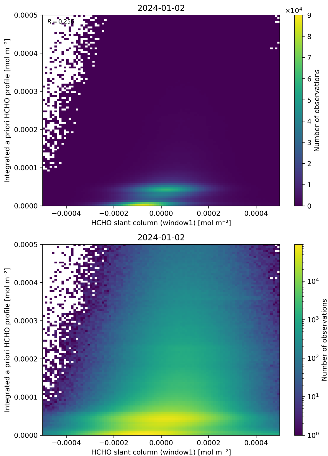
Figure 87: Scatter density plot of “HCHO slant column (window1)” against “Integrated a priori HCHO profile” for 2024-01-01 to 2024-01-03.
