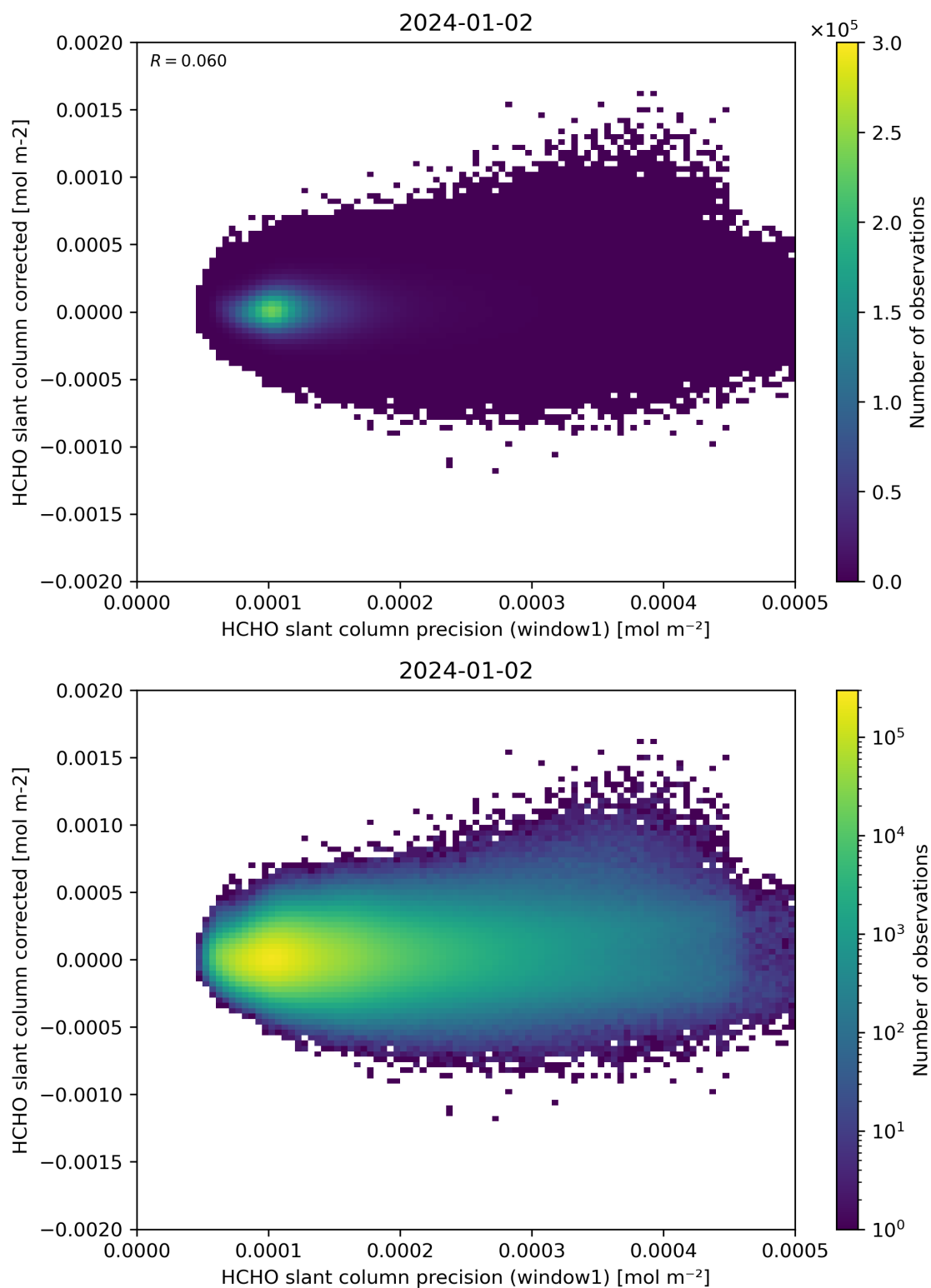
Figure 92: Scatter density plot of “HCHO slant column precision (window1)” against “HCHO slant column corrected” for 2024-01-01 to 2024-01-03.
