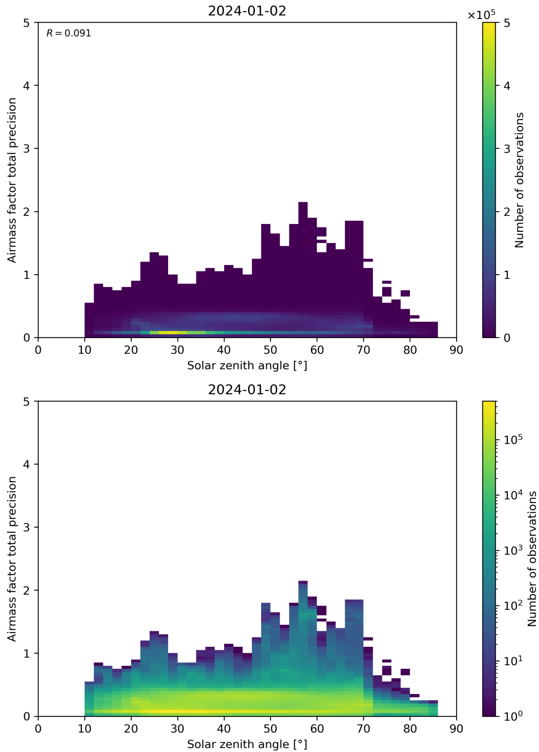
Figure 176: Scatter density plot of “Solar zenith angle” against “Airmass factor total precision” for 2024-01-01 to 2024-01-03.
