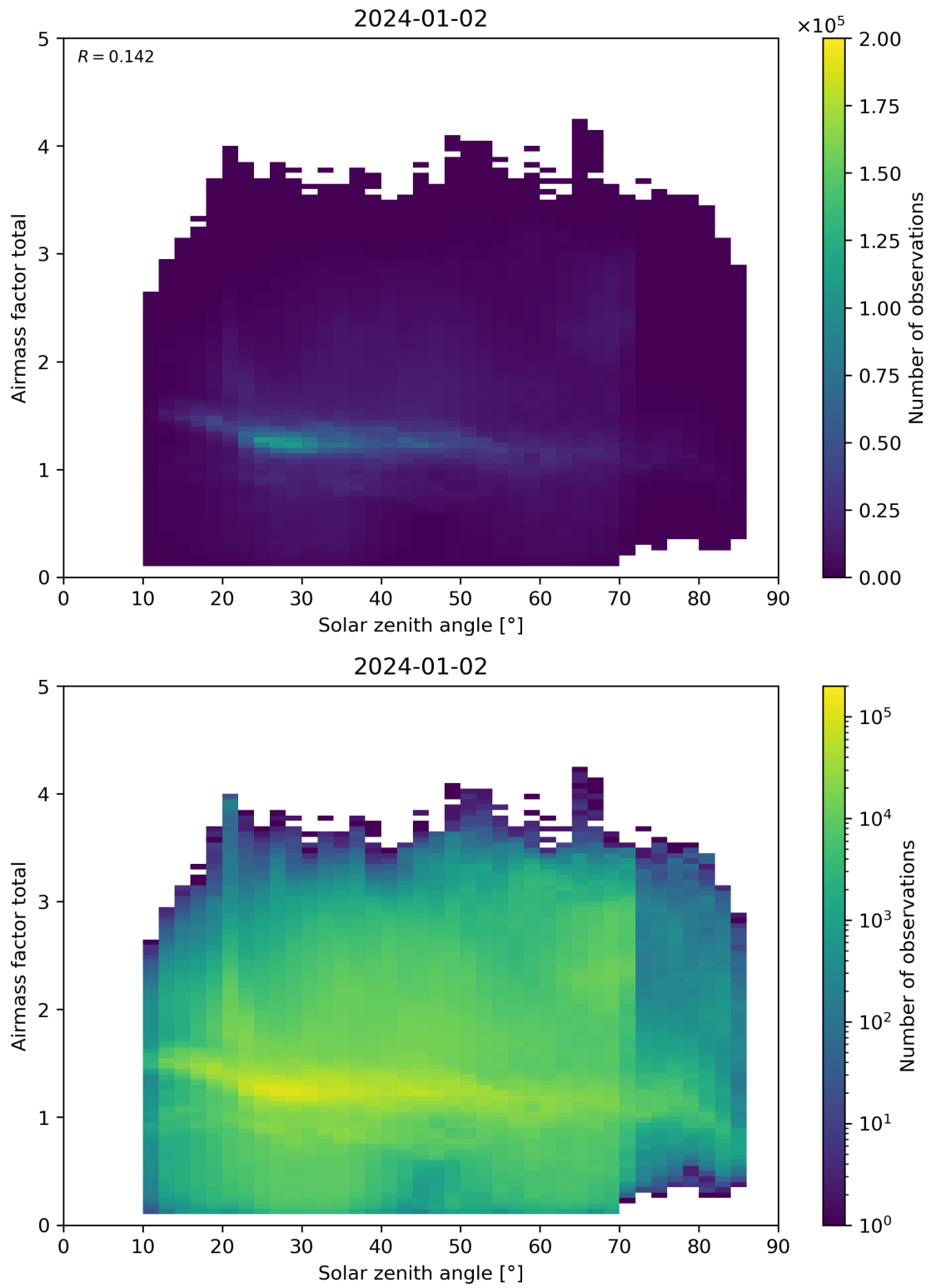
Figure 175: Scatter density plot of “Solar zenith angle” against “Airmass factor total” for 2024-01-01 to 2024-01-03.
