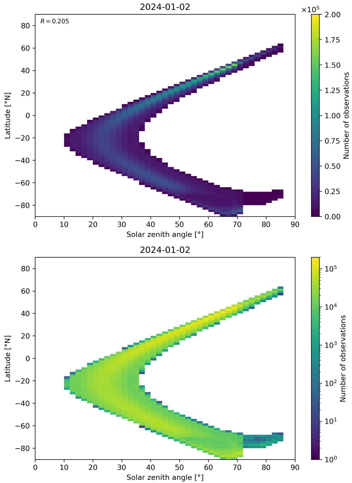
Figure 181: Scatter density plot of “Solar zenith angle” against “Latitude” for 2024-01-01 to 2024-01-03.
