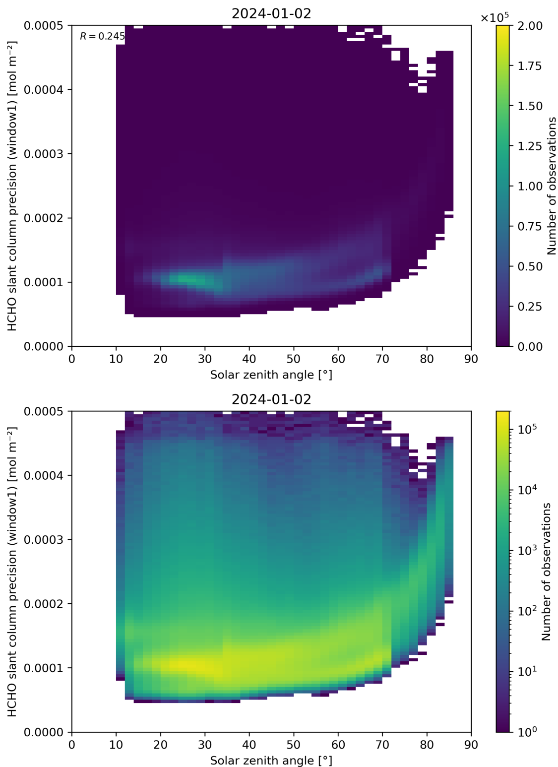
Figure 174: Scatter density plot of “Solar zenith angle” against “HCHO slant column precision (window1)” for 2024-01-01 to 2024-01-03.
