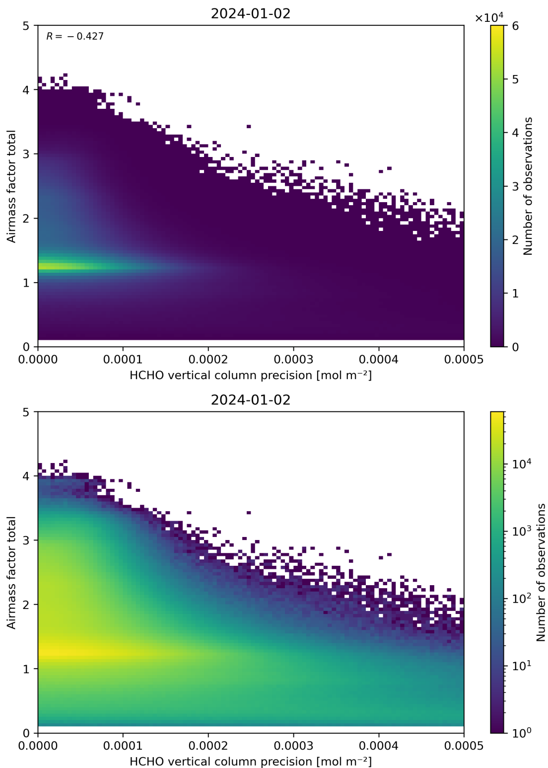
Figure 144: Scatter density plot of “HCHO vertical column precision” against “Airmass factor total” for 2024-01-01 to 2024-01-03.
