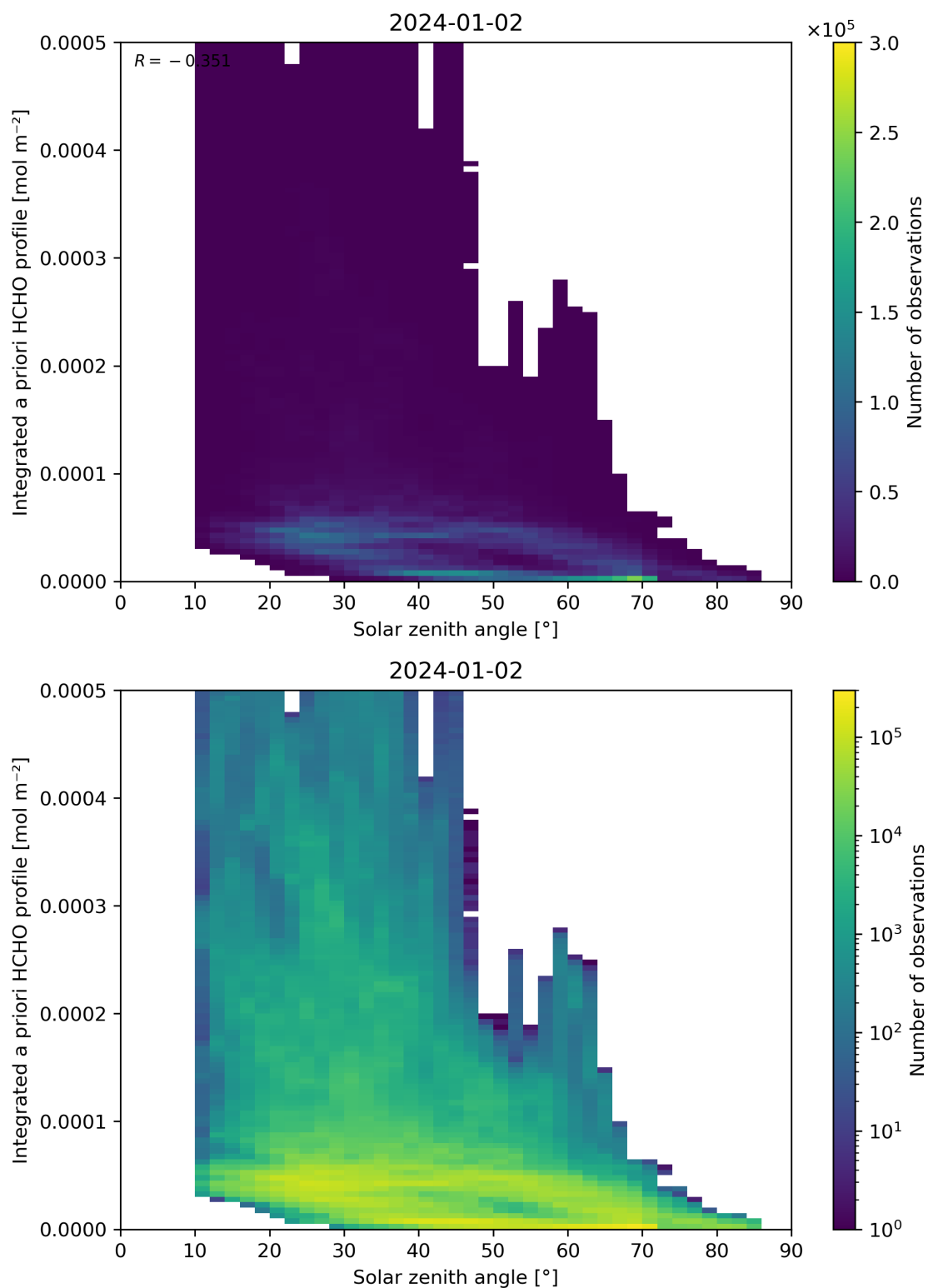
Figure 180: Scatter density plot of “Solar zenith angle” against “Integrated a priori HCHO profile” for 2024-01-01 to 2024-01-03.
