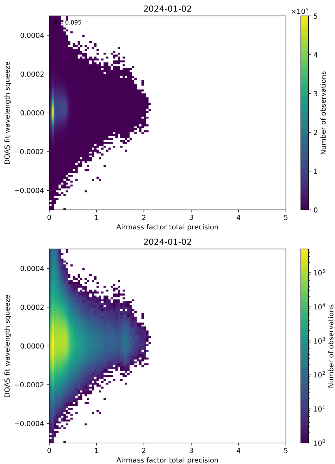
Figure 107: Scatter density plot of “Airmass factor total precision” against “DOAS fit wavelength squeeze” for 2024-01-01 to 2024-01-03.
