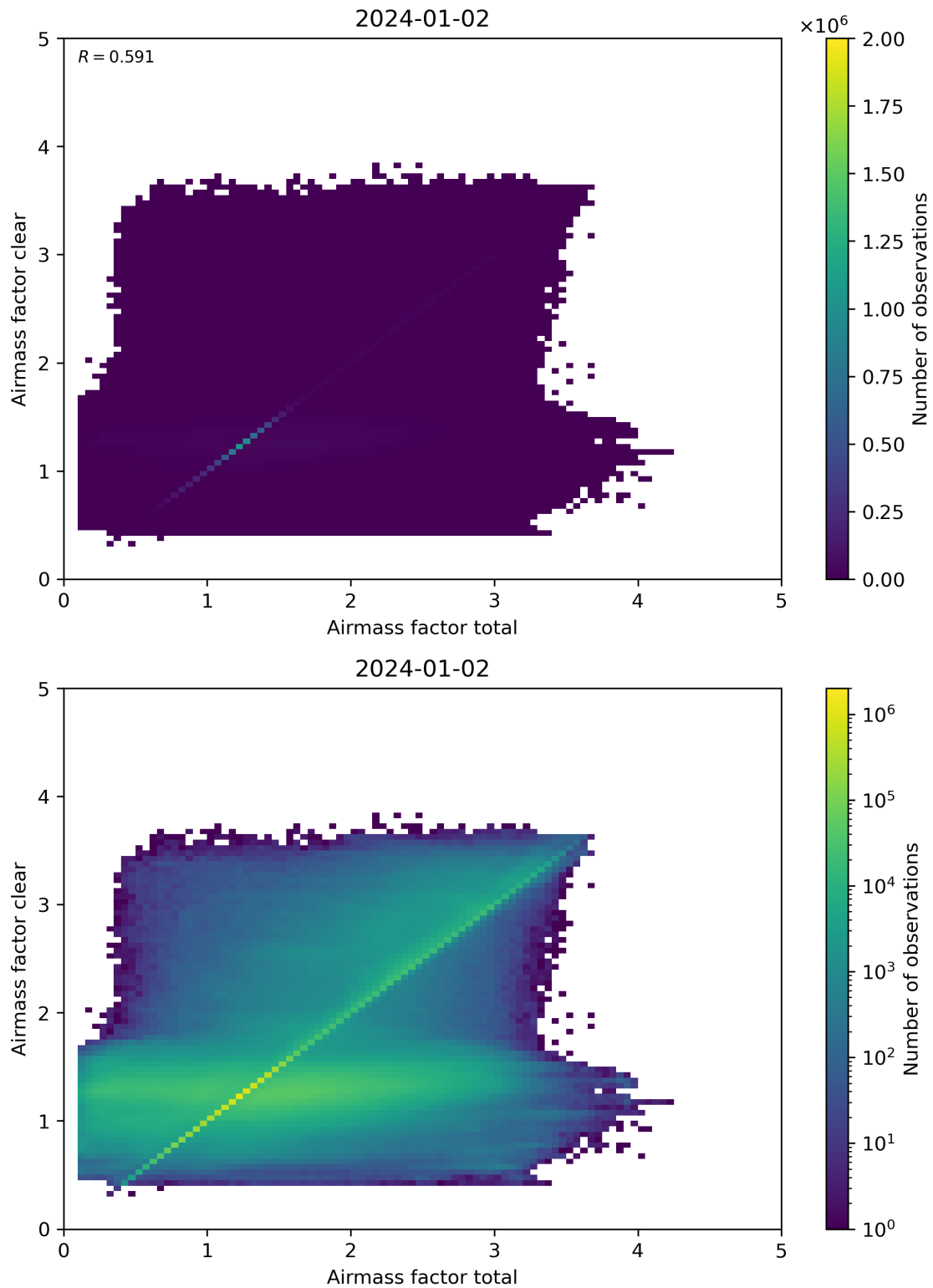
Figure 100: Scatter density plot of “Airmass factor total” against “Airmass factor clear” for 2024-01-01 to 2024-01-03.
