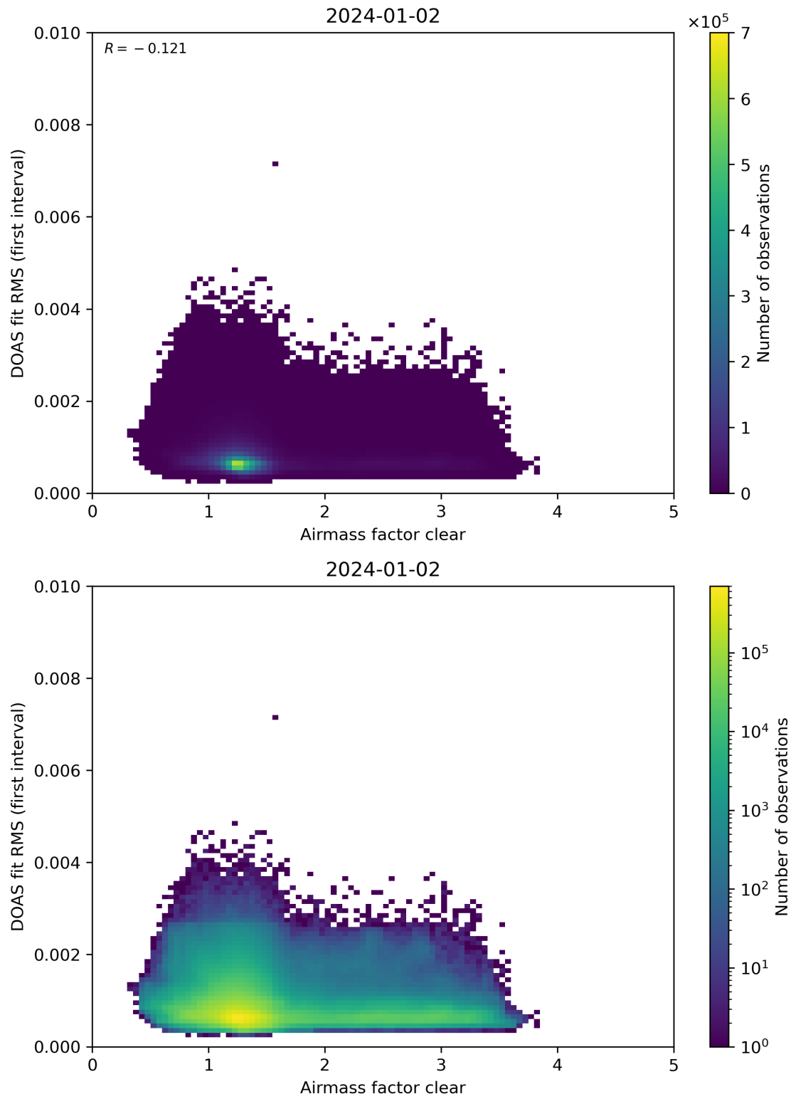
Figure 71: Scatter density plot of “Airmass factor clear” against “DOAS fit RMS (first interval)” for 2024-01-01 to 2024-01-03.
