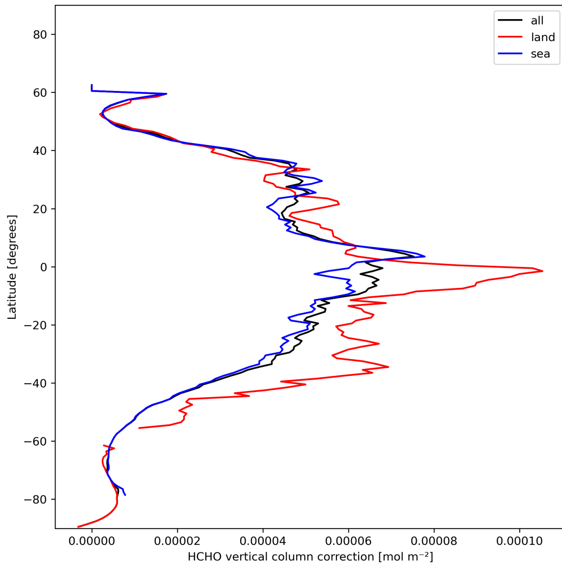
Figure 23: Zonal average of “HCHO vertical column correction” for 2024-01-01 to 2024-01-03.
