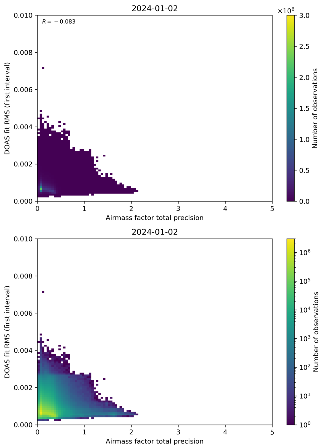
Figure 105: Scatter density plot of “Airmass factor total precision” against “DOAS fit RMS (first interval)” for 2024-01-01 to 2024-01-03.
