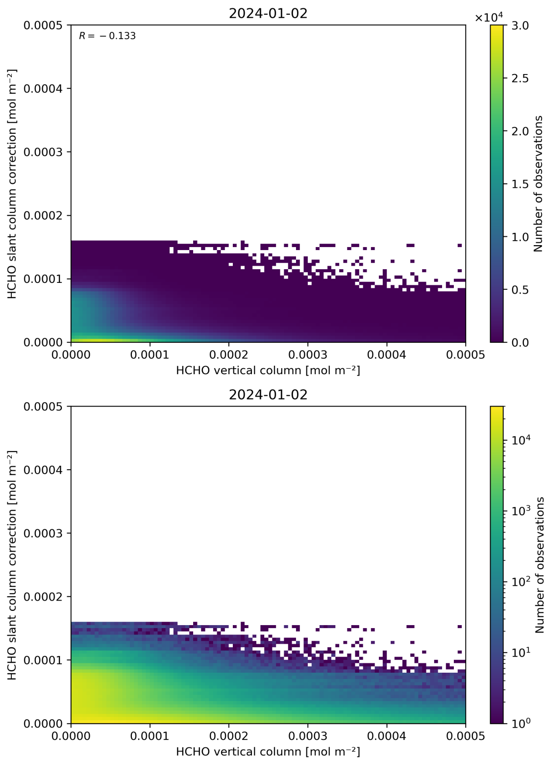
Figure 128: Scatter density plot of “HCHO vertical column” against “HCHO slant column correction” for 2024-01-01 to 2024-01-03.
