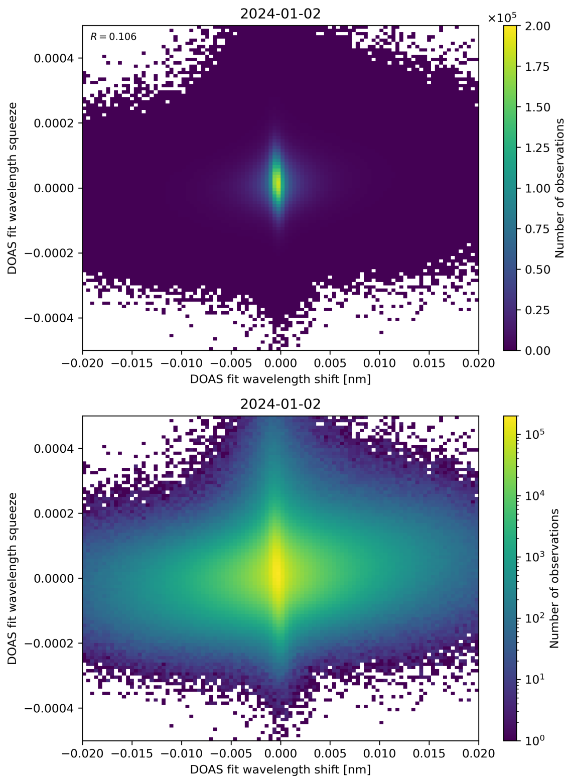
Figure 65: Scatter density plot of “DOAS fit wavelength shift” against “DOAS fit wavelength squeeze” for 2024-01-01 to 2024-01-03.
