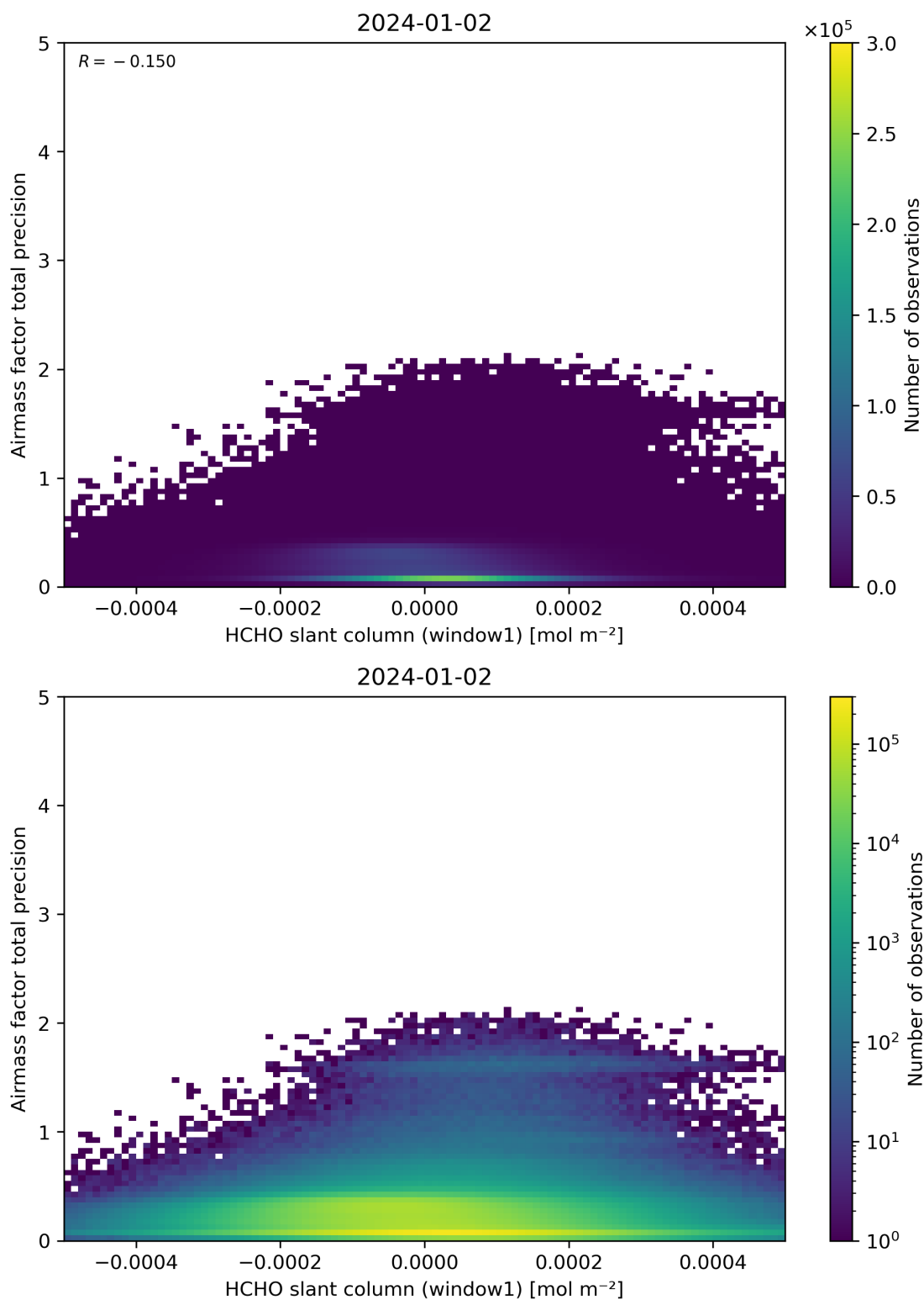
Figure 86: Scatter density plot of “HCHO slant column (window1)” against “Airmass factor total precision” for 2024-01-01 to 2024-01-03.
