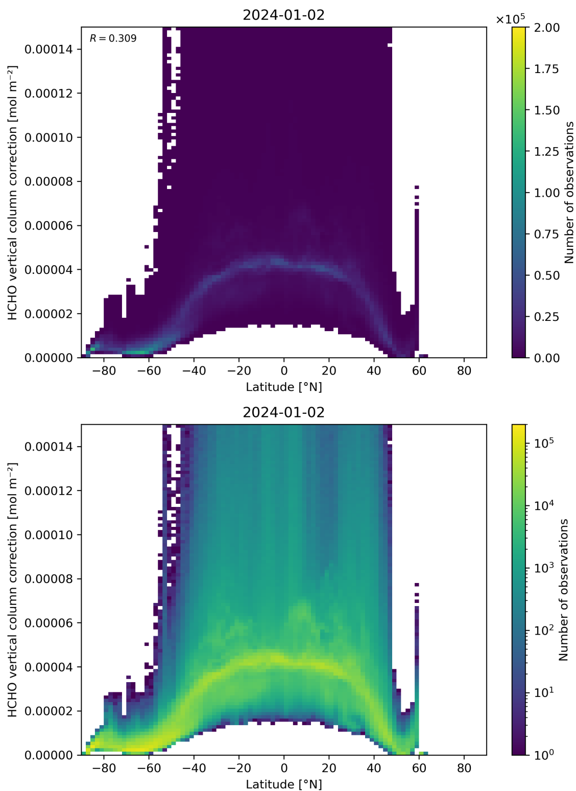
Figure 164: Scatter density plot of “Latitude” against “HCHO vertical column correction” for 2024-01-01 to 2024-01-03.
