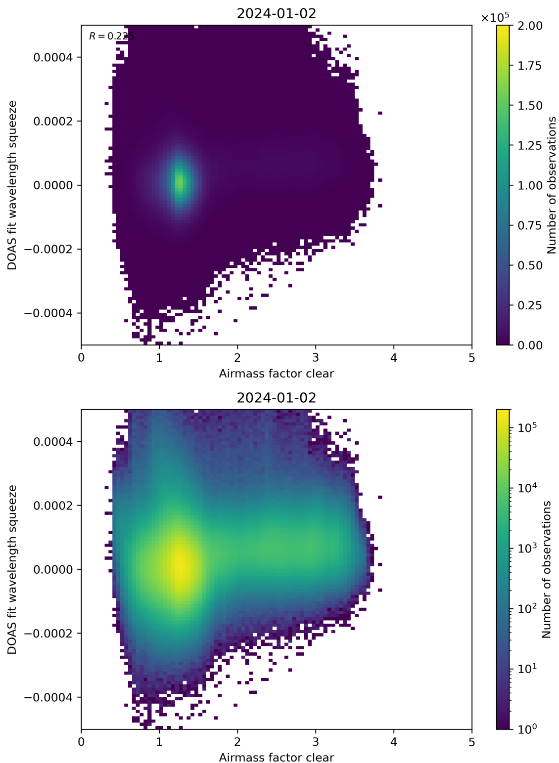
Figure 73: Scatter density plot of “Airmass factor clear” against “DOAS fit wavelength squeeze” for 2024-01-01 to 2024-01-03.
