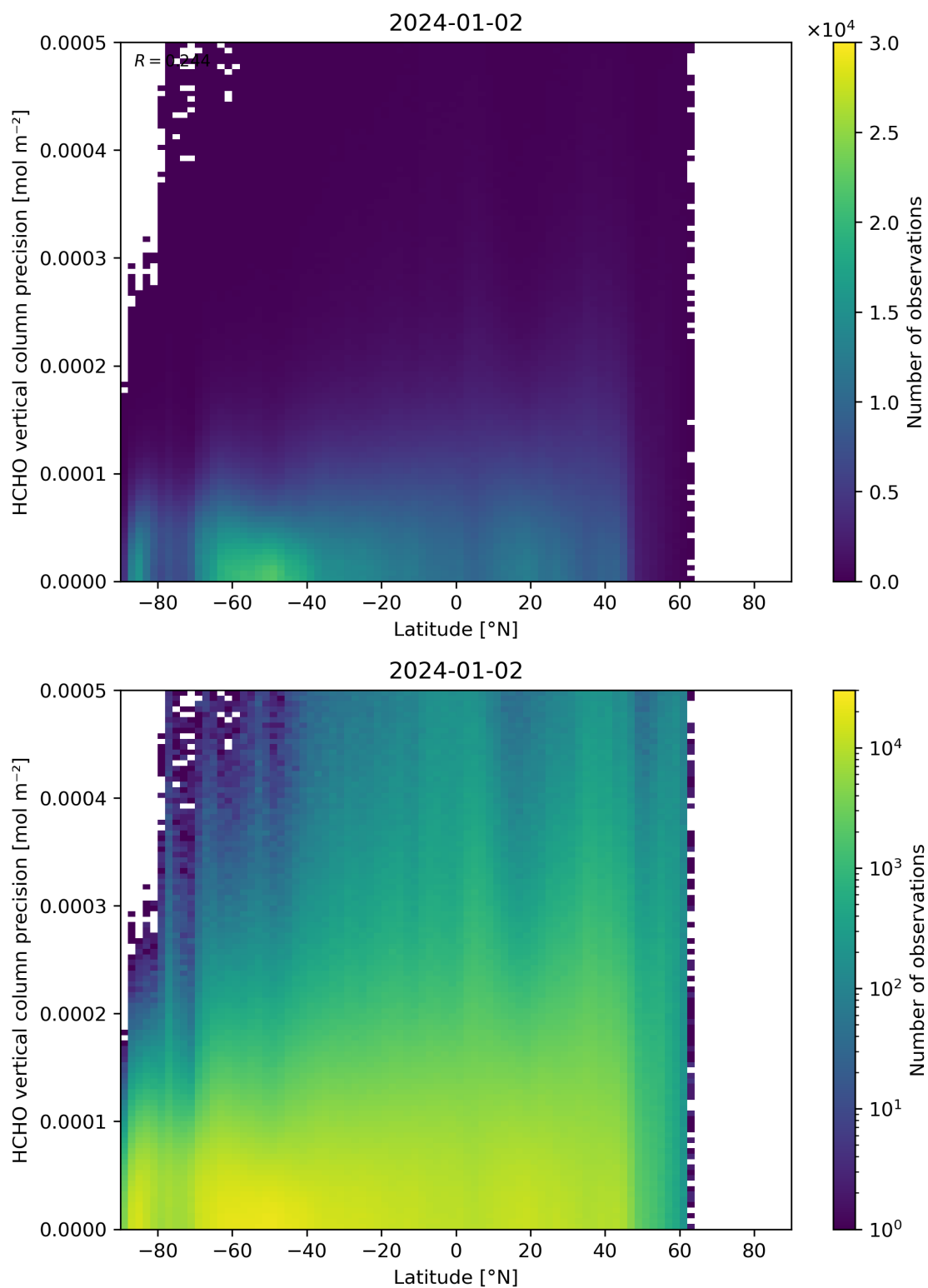
Figure 165: Scatter density plot of “Latitude” against “HCHO vertical column precision” for 2024-01-01 to 2024-01-03.
