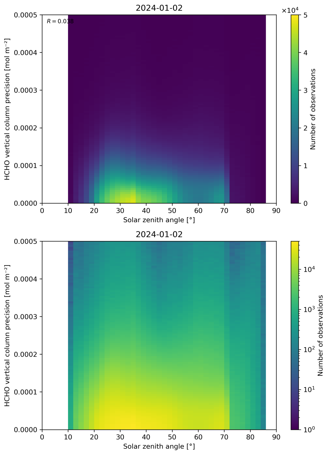
Figure 179: Scatter density plot of “Solar zenith angle” against “HCHO vertical column precision” for 2024-01-01 to 2024-01-03.
