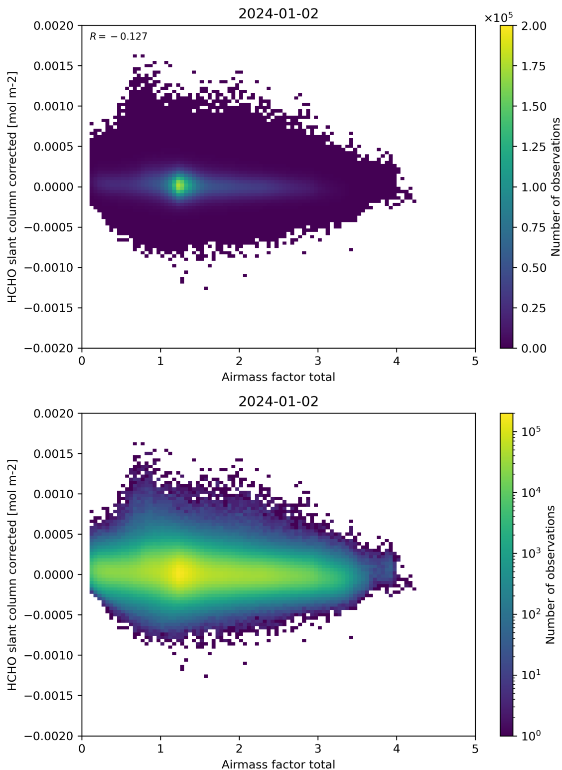
Figure 101: Scatter density plot of “Airmass factor total” against “HCHO slant column corrected” for 2024-01-01 to 2024-01-03.
