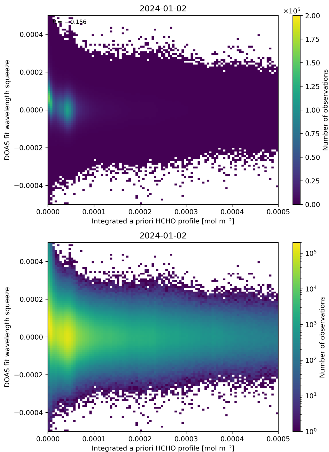
Figure 150: Scatter density plot of “Integrated a priori HCHO profile” against “DOAS fit wavelength squeeze” for 2024-01-01 to 2024-01-03.
