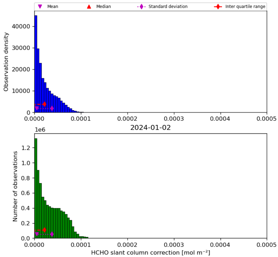
Figure 47: Histogram of “HCHO slant column correction” for 2024-01-01 to 2024-01-03
