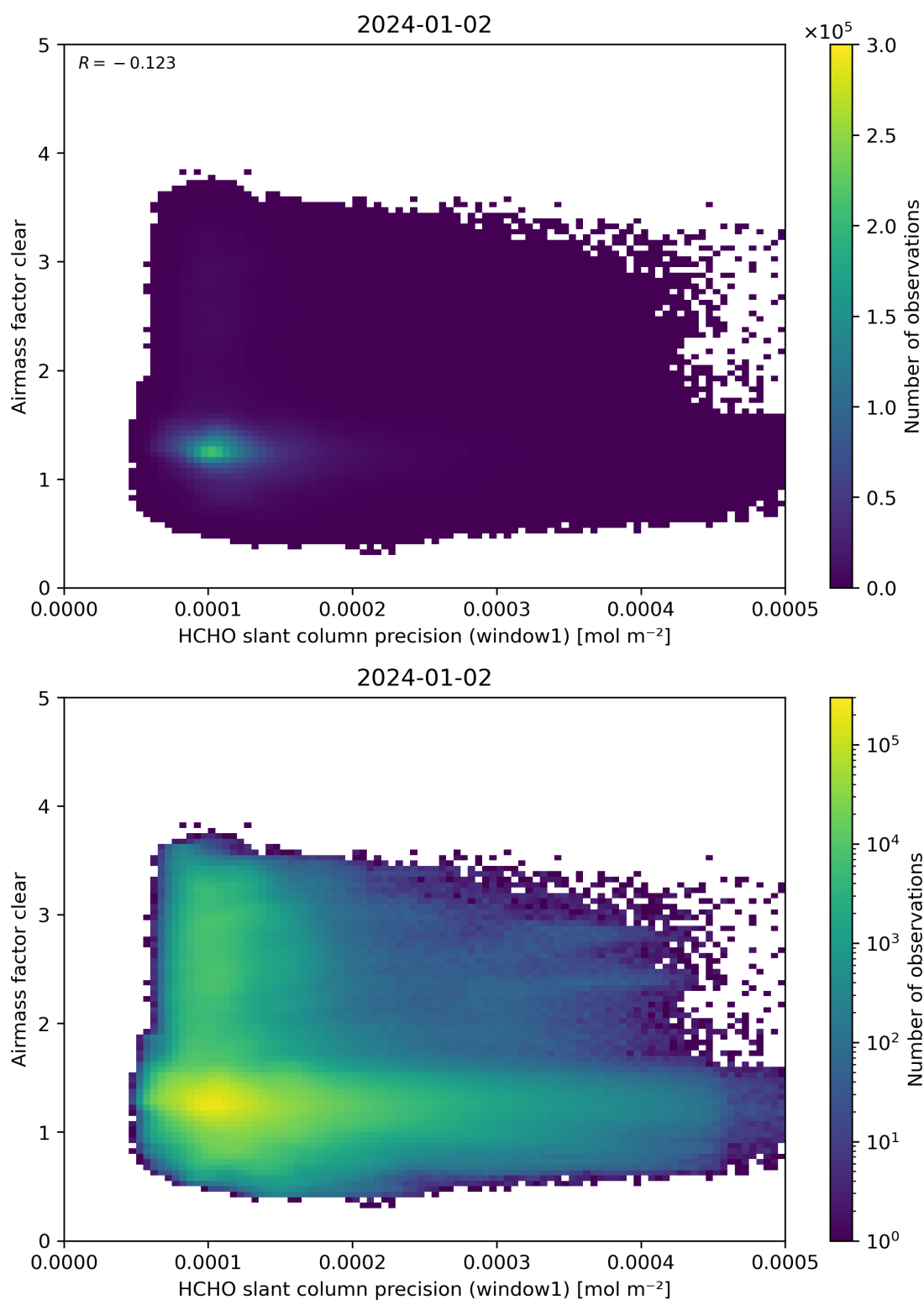
Figure 91: Scatter density plot of “HCHO slant column precision (window1)” against “Airmass factor clear” for 2024-01-01 to 2024-01-03.
