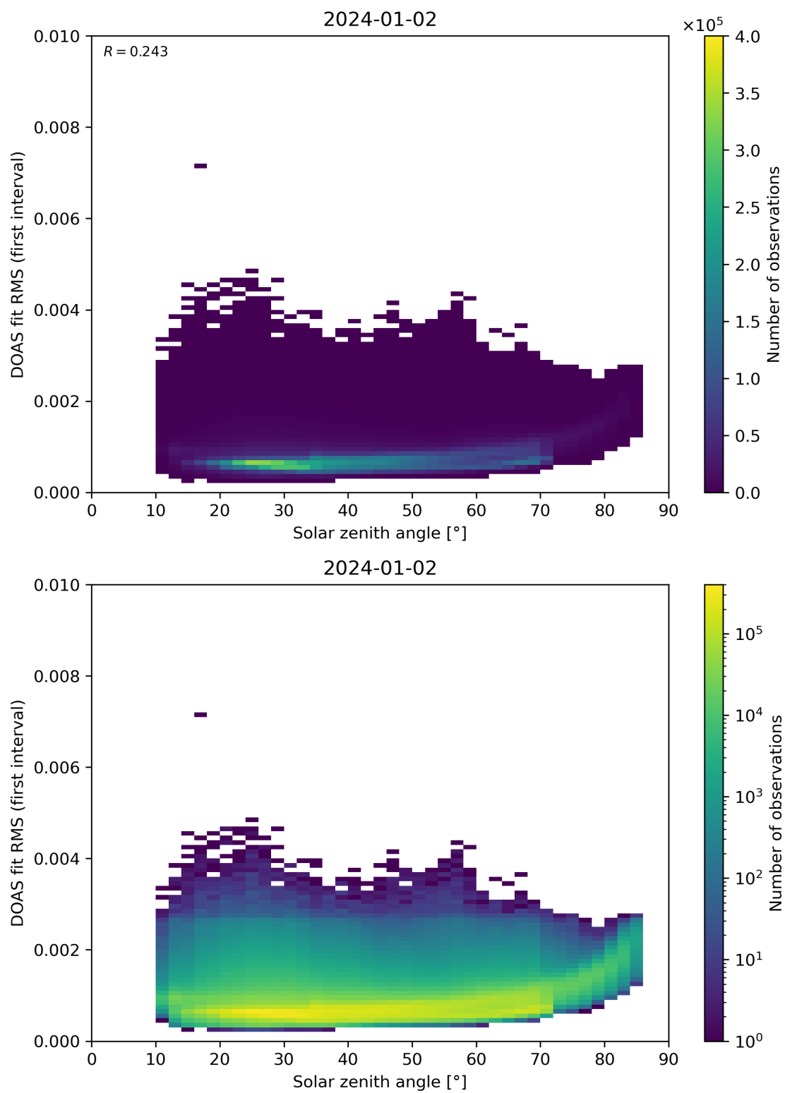
Figure 167: Scatter density plot of “Solar zenith angle” against “DOAS fit RMS (first interval)” for 2024-01-01 to 2024-01-03.
