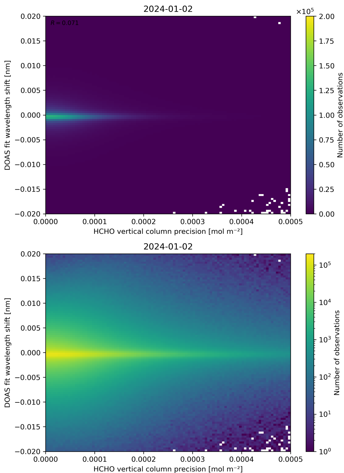
Figure 137: Scatter density plot of “HCHO vertical column precision” against “DOAS fit wavelength shift” for 2024-01-01 to 2024-01-03.
