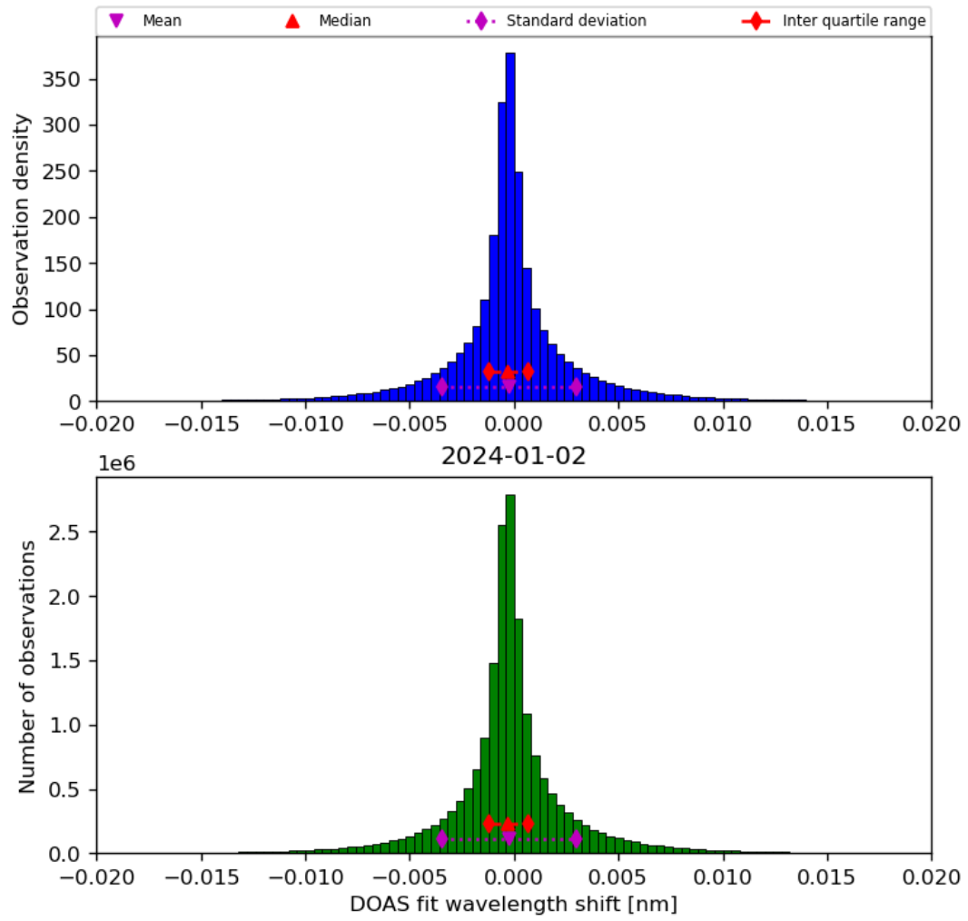
Figure 44: Histogram of “DOAS fit wavelength shift” for 2024-01-01 to 2024-01-03
