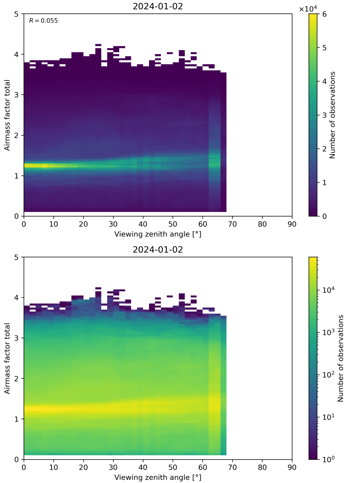
Figure 190: Scatter density plot of “Viewing zenith angle” against “Airmass factor total” for 2024-01-01 to 2024-01-03.
