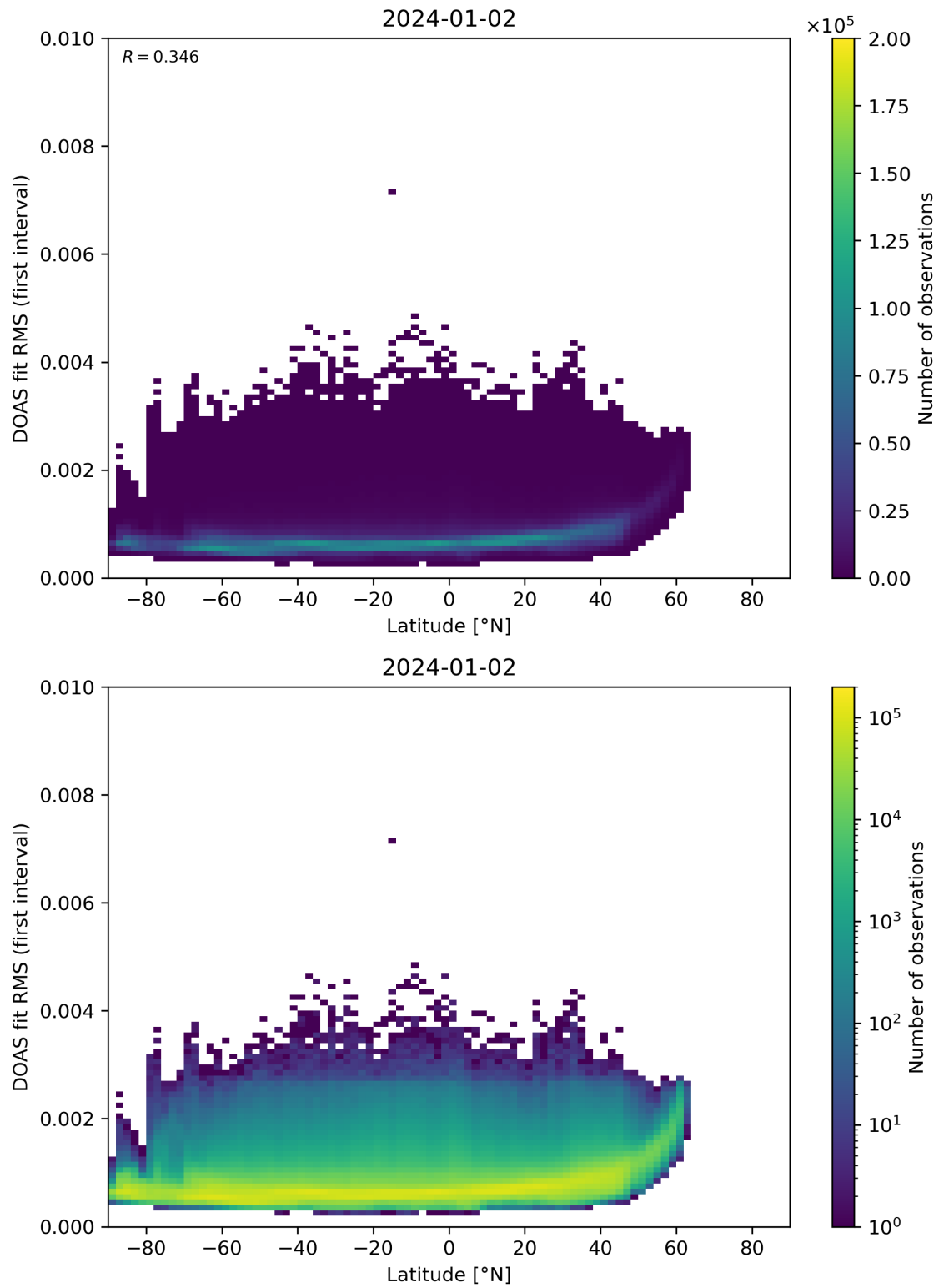
Figure 153: Scatter density plot of “Latitude” against “DOAS fit RMS (first interval)” for 2024-01-01 to 2024-01-03.
