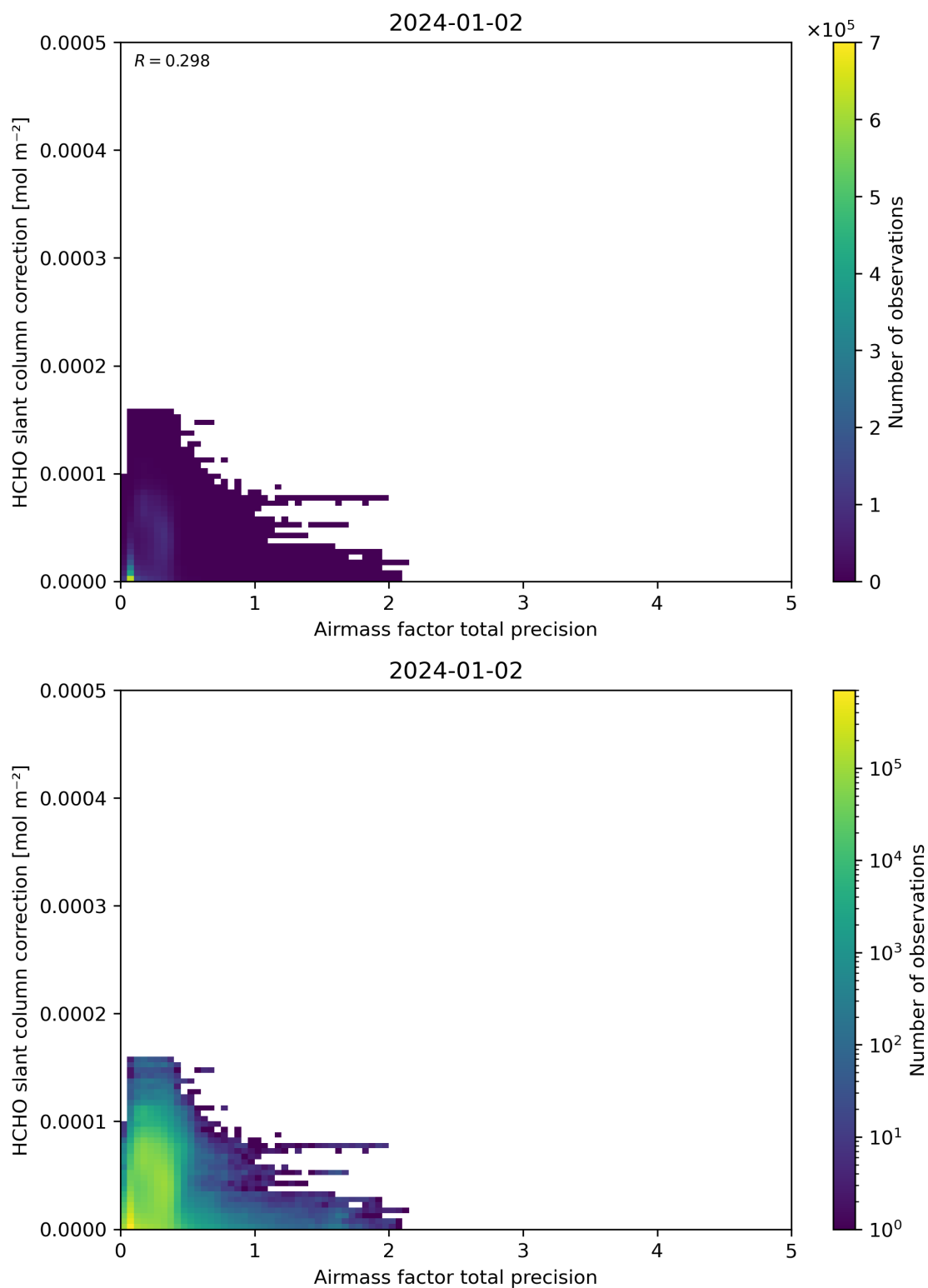
Figure 110: Scatter density plot of “Airmass factor total precision” against “HCHO slant column correction” for 2024-01-01 to 2024-01-03.
