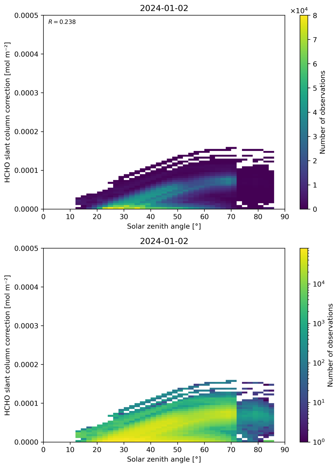
Figure 172: Scatter density plot of “Solar zenith angle” against “HCHO slant column correction” for 2024-01-01 to 2024-01-03.
