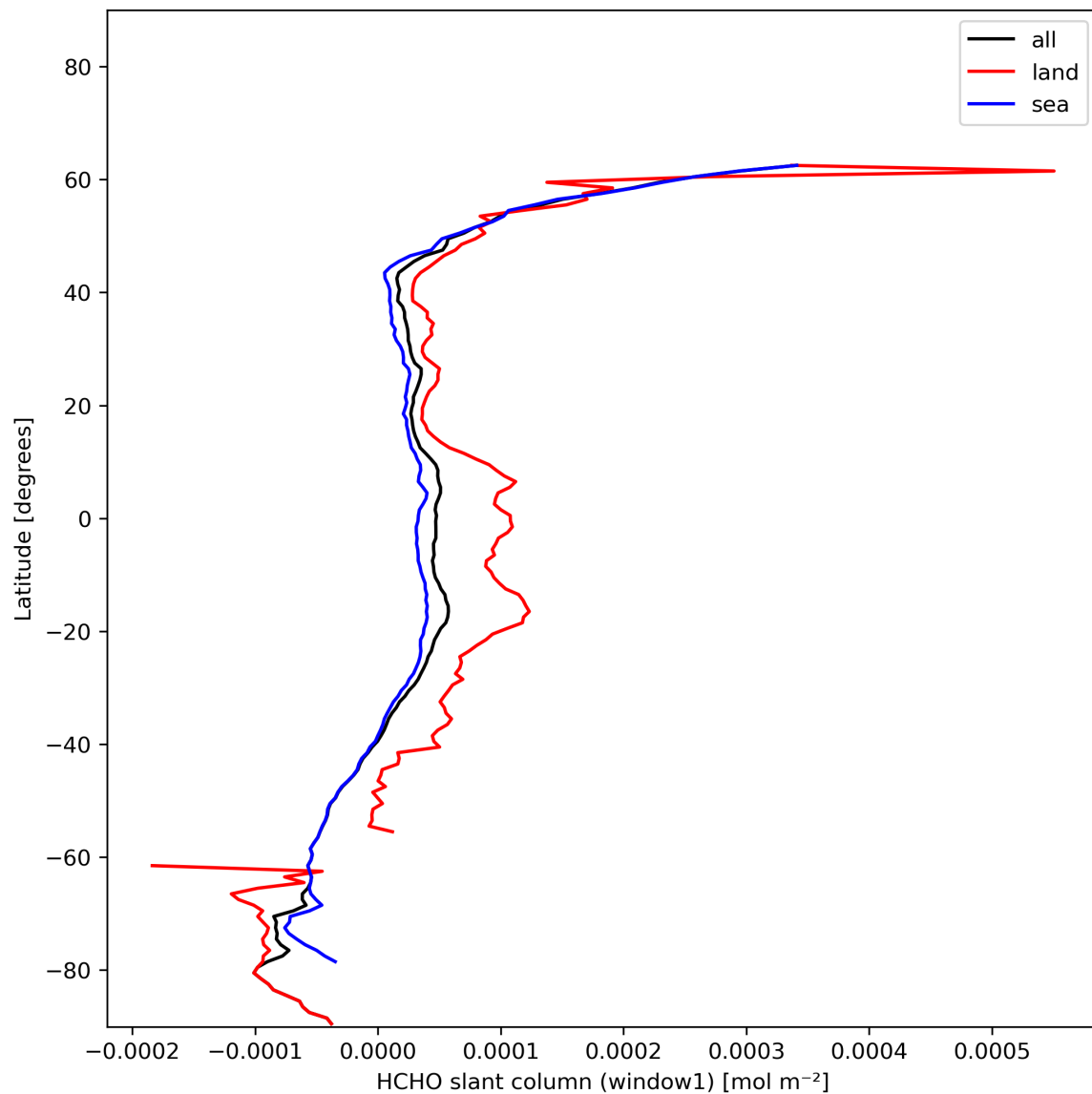
Figure 24: Zonal average of “HCHO slant column (window1)” for 2024-01-01 to 2024-01-03.
