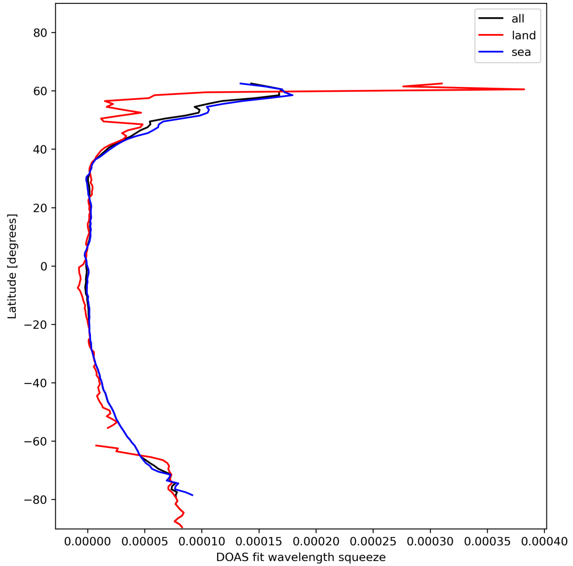
Figure 31: Zonal average of “DOAS fit wavelength squeeze” for 2024-01-01 to 2024-01-03.
