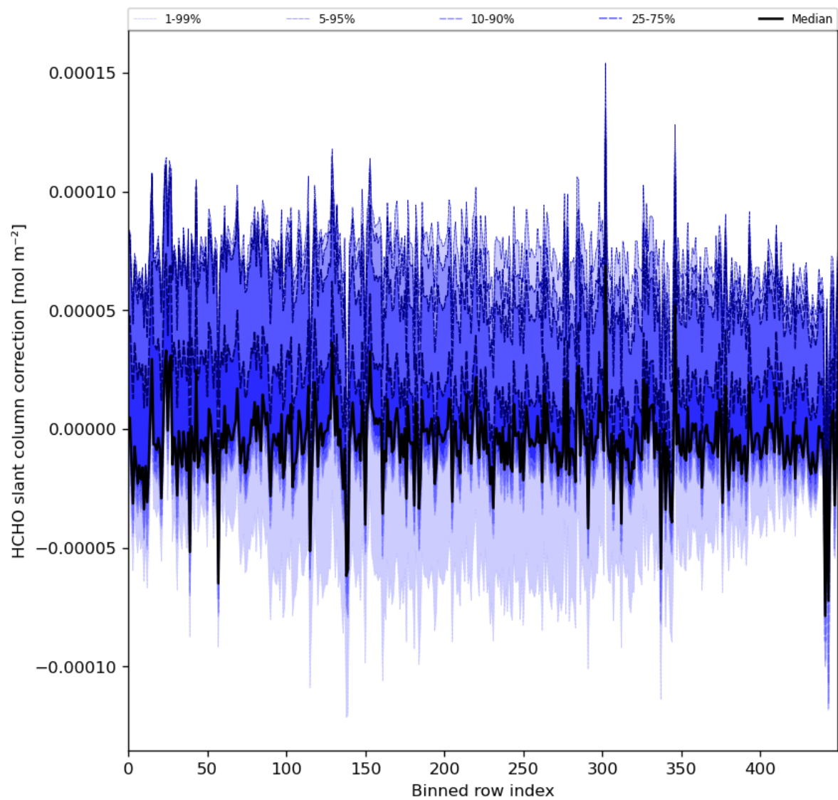
Figure 61: Along track statistics of “HCHO slant column correction” for 2024-01-01 to 2024-01-03
