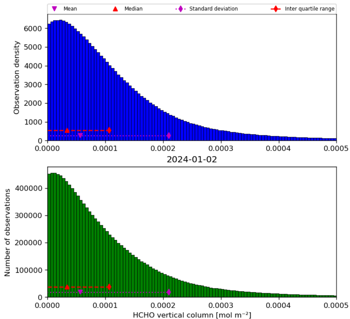
Figure 35: Histogram of “HCHO vertical column” for 2024-01-01 to 2024-01-03
