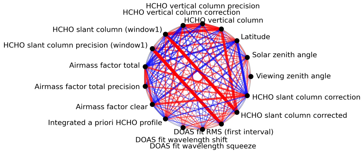
Figure 1: Map of correlation graph for 2024-01-01 to 2024-01-03.
