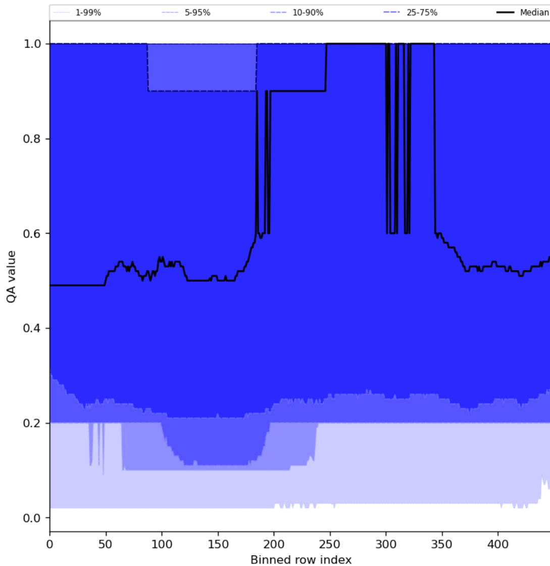
Figure 48: Along track statistics of “QA value” for 2024-01-01 to 2024-01-03
