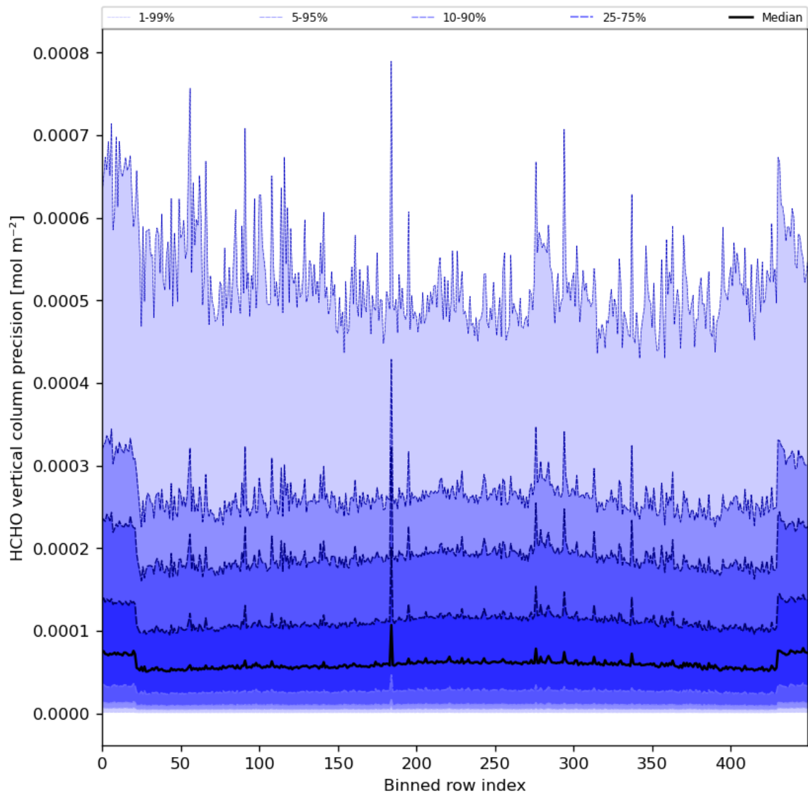
Figure 50: Along track statistics of "HCHO vertical column precision" for 2024-01-01 to 2024-01-03
