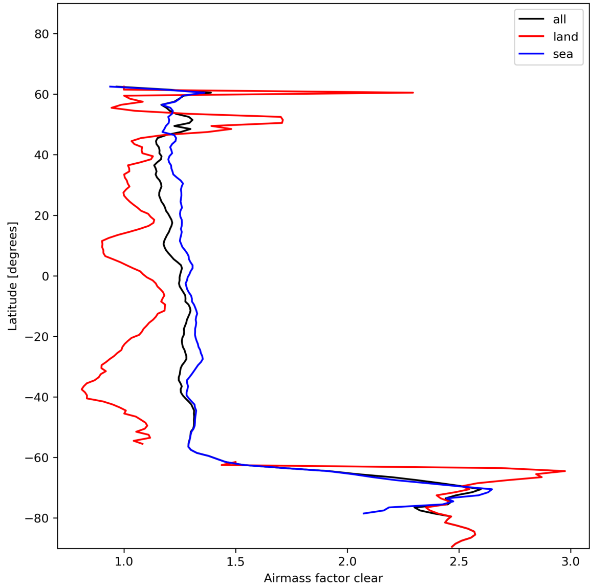
Figure 28: Zonal average of “Airmass factor clear” for 2024-01-01 to 2024-01-03.
