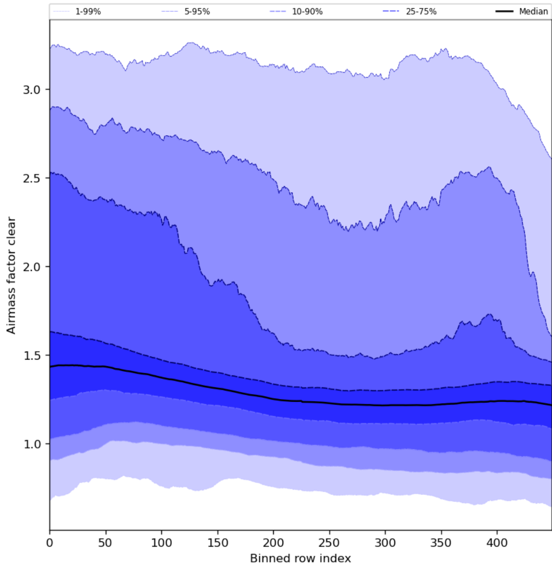
Figure 56: Along track statistics of “Airmass factor clear” for 2024-01-01 to 2024-01-03
