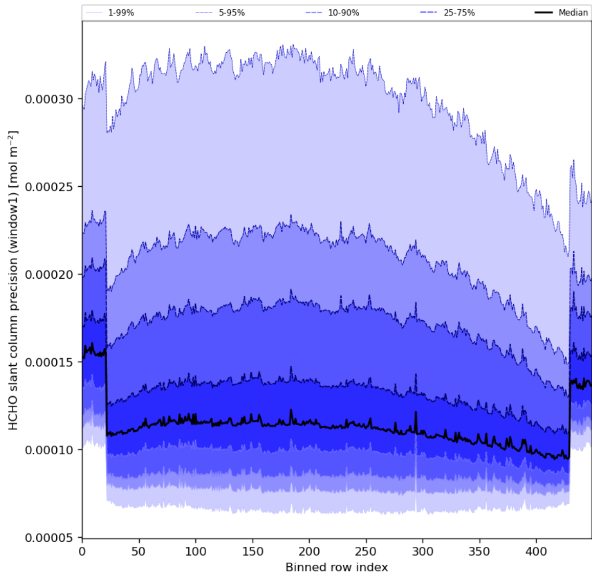
Figure 53: Along track statistics of “HCHO slant column precision (window1)” for 2024-01-01 to 2024-01-03
