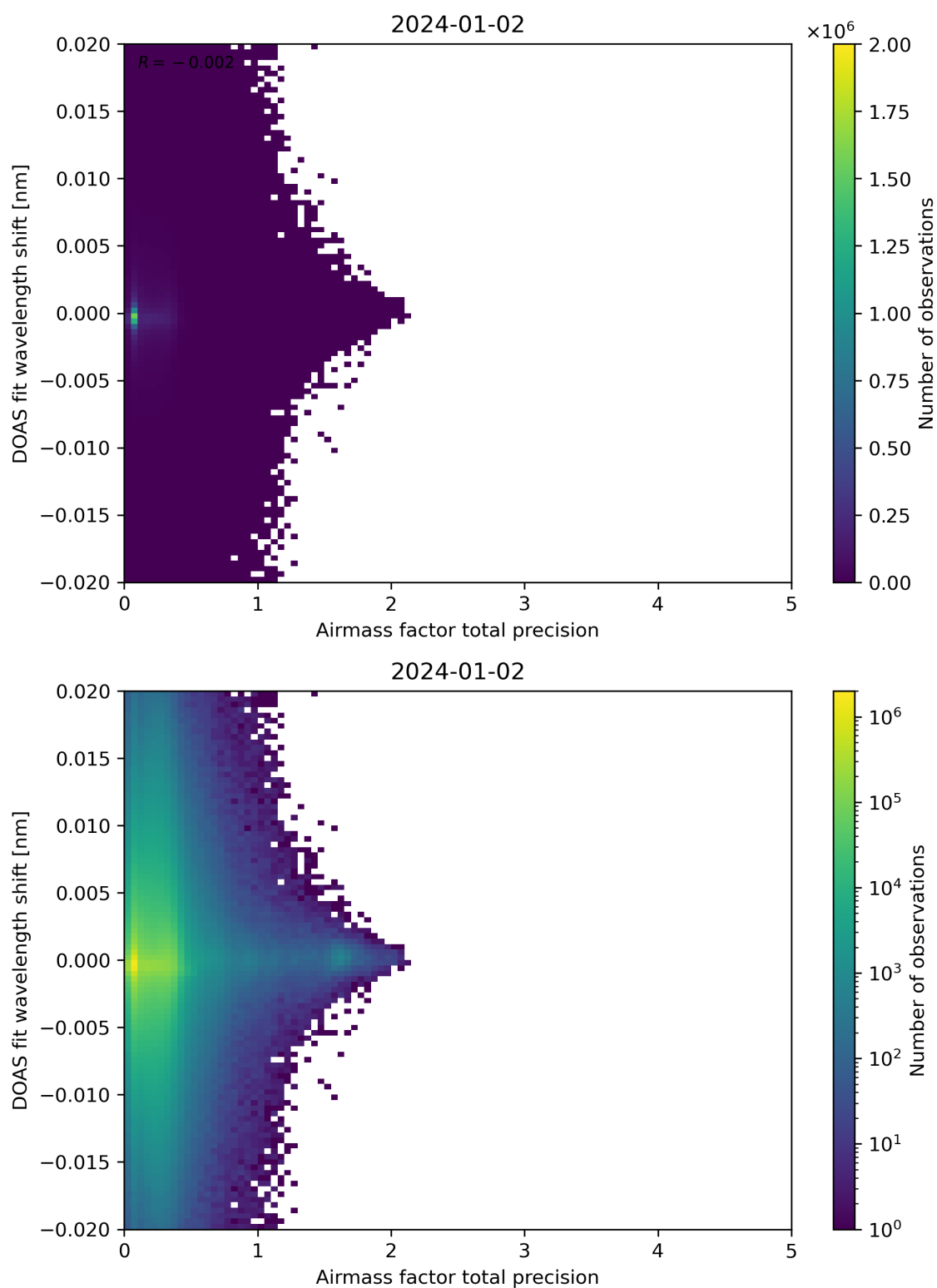
Figure 106: Scatter density plot of “Airmass factor total precision” against “DOAS fit wavelength shift” for 2024-01-01 to 2024-01-03.
