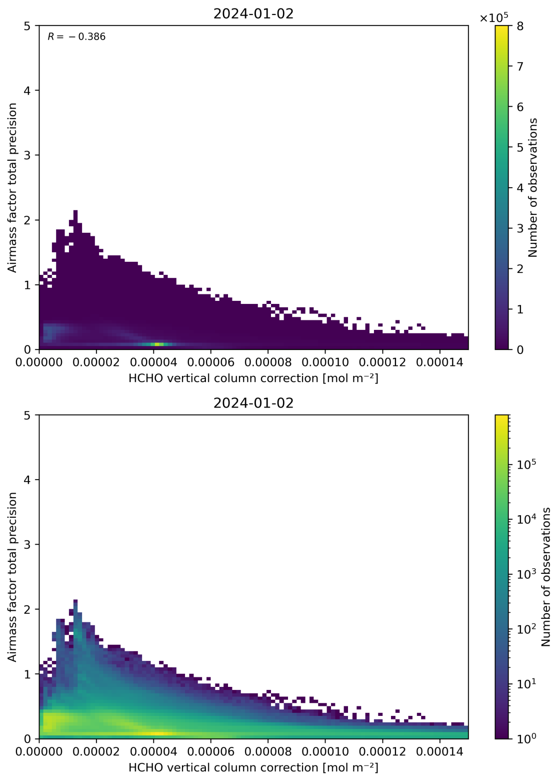
Figure 121: Scatter density plot of “HCHO vertical column correction” against “Airmass factor total precision” for 2024-01-01 to 2024-01-03.
