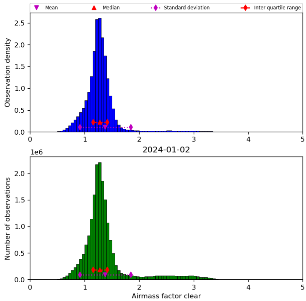
Figure 42: Histogram of “Airmass factor clear” for 2024-01-01 to 2024-01-03
