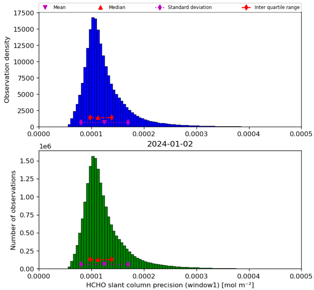
Figure 39: Histogram of “HCHO slant column precision (window1)” for 2024-01-01 to 2024-01-03
