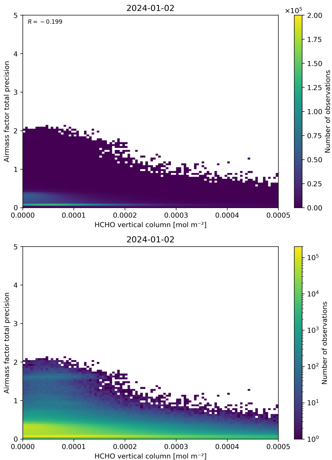
Figure 132: Scatter density plot of “HCHO vertical column” against “Airmass factor total precision” for 2024-01-01 to 2024-01-03.
