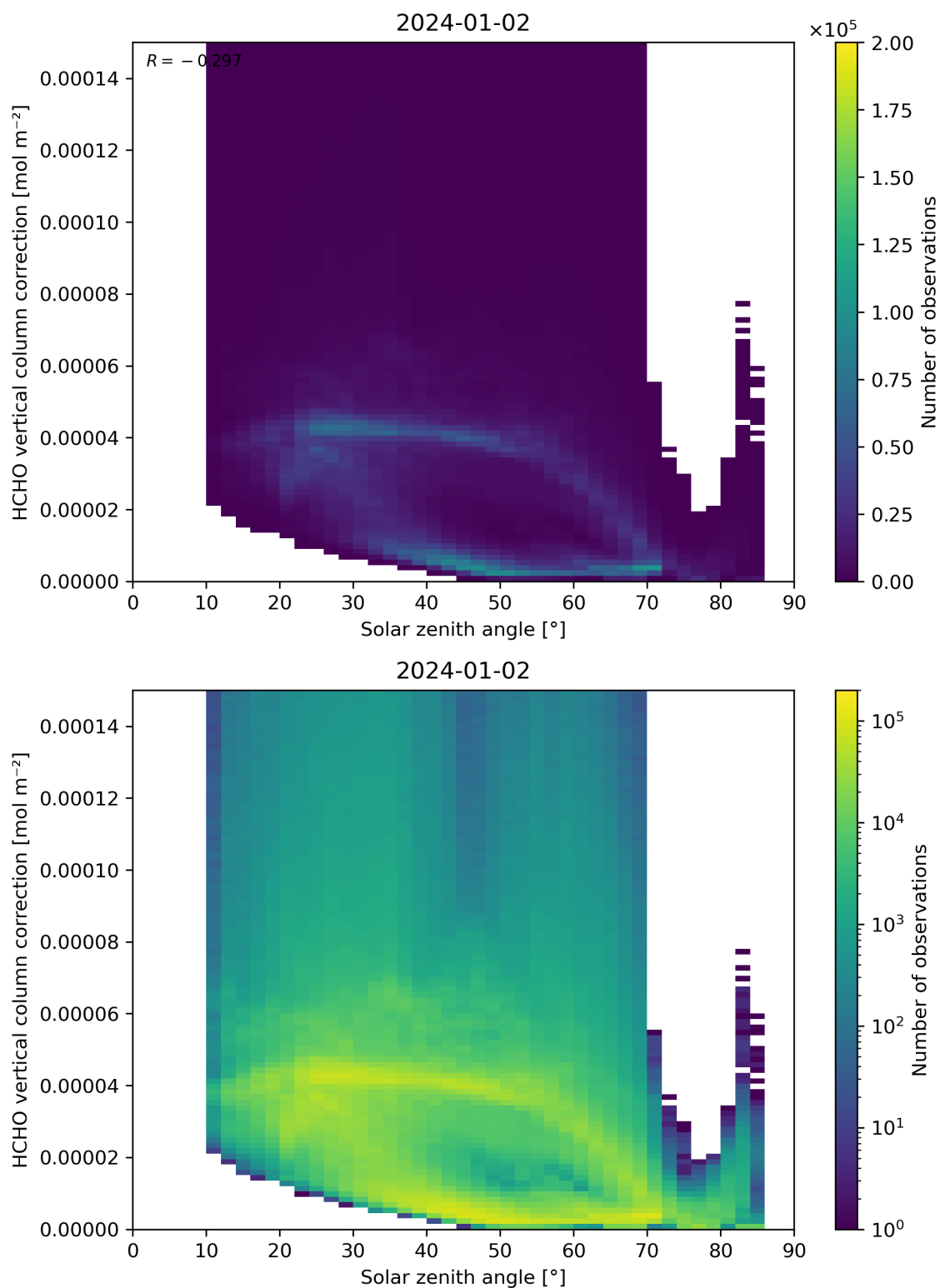
Figure 178: Scatter density plot of “Solar zenith angle” against “HCHO vertical column correction” for 2024-01-01 to 2024-01-03.
