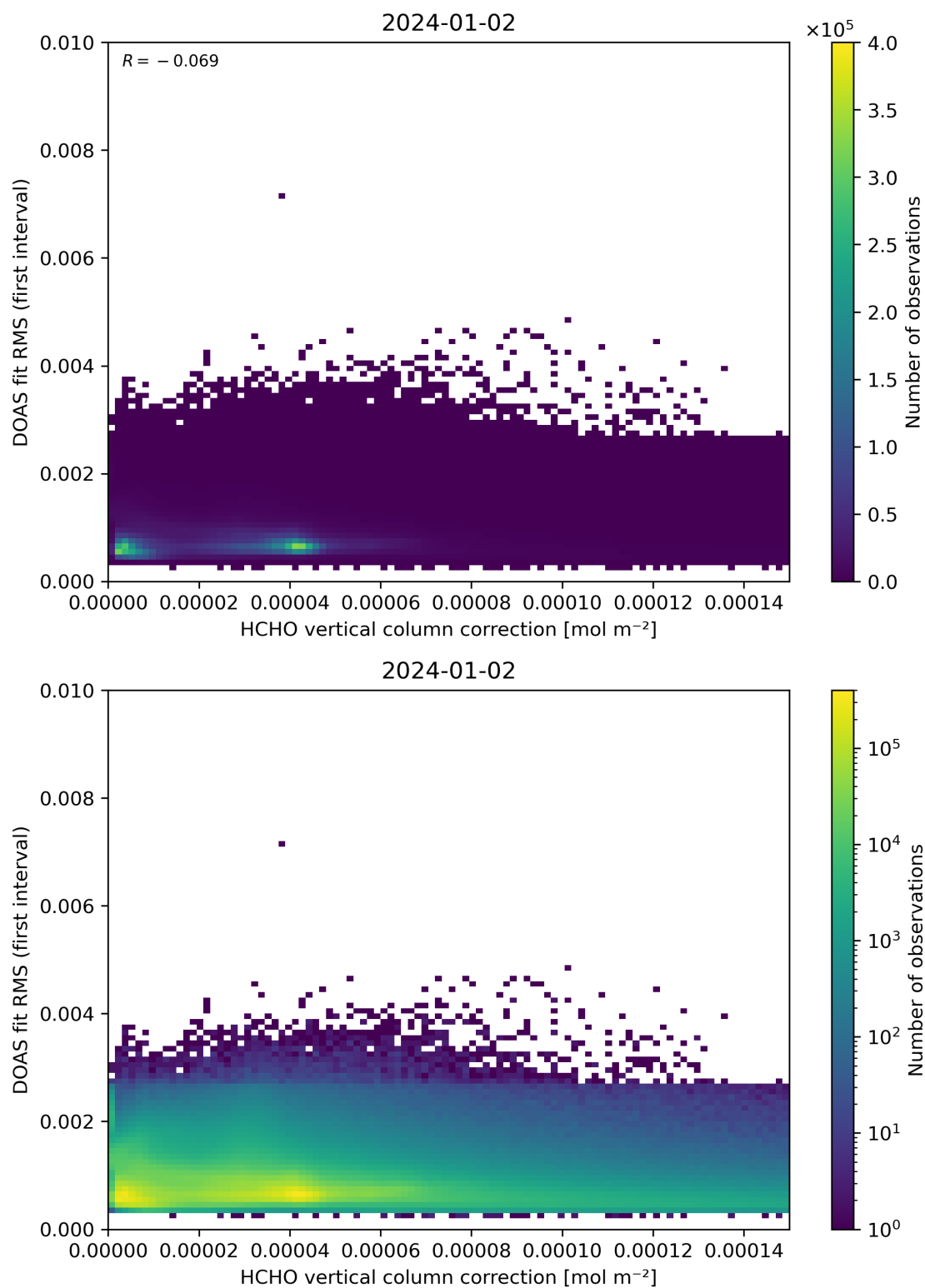
Figure 112: Scatter density plot of “HCHO vertical column correction” against “DOAS fit RMS (first interval)” for 2024-01-01 to 2024-01-03.
