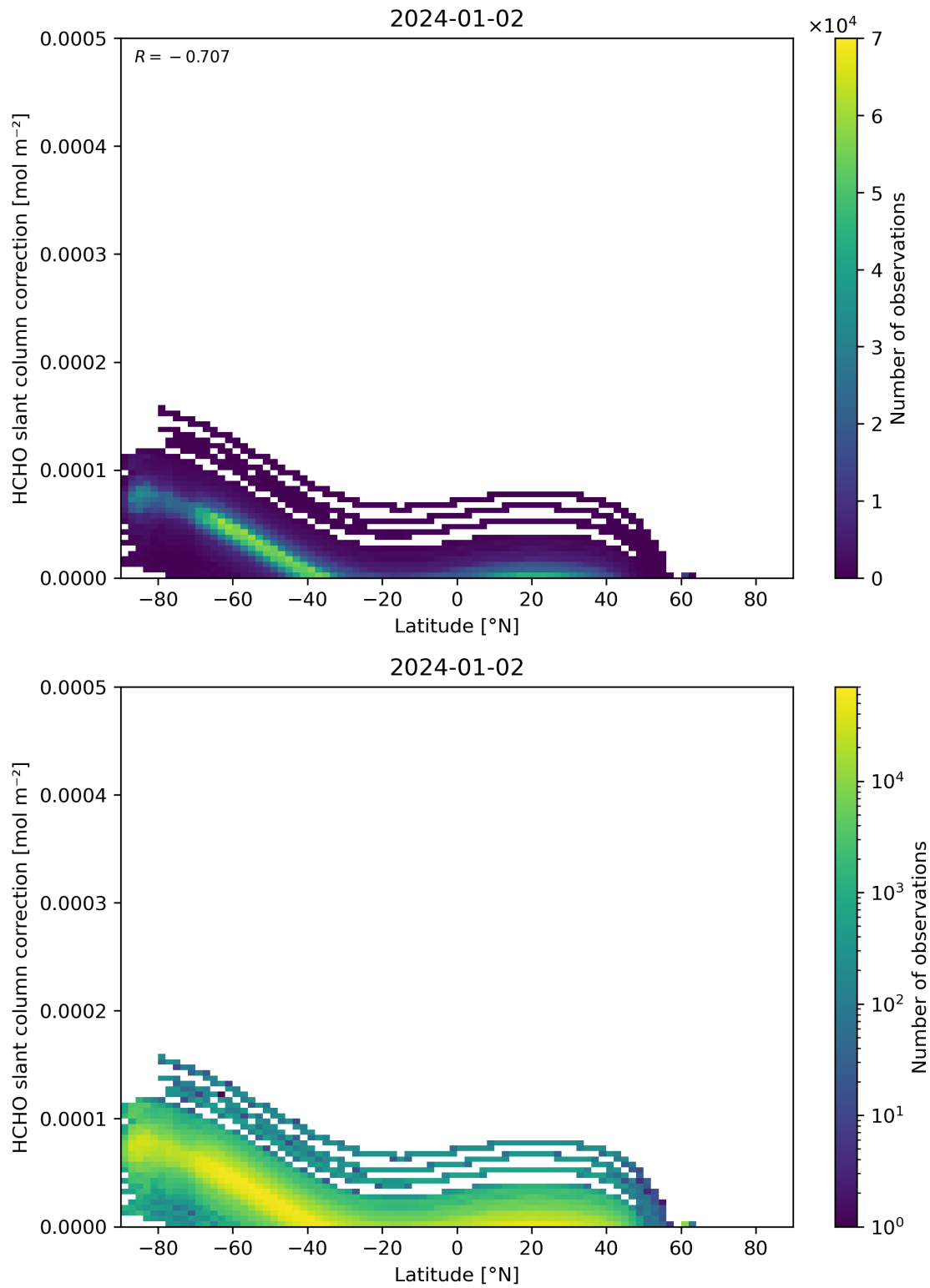
Figure 158: Scatter density plot of “Latitude” against “HCHO slant column correction” for 2024-01-01 to 2024-01-03.
