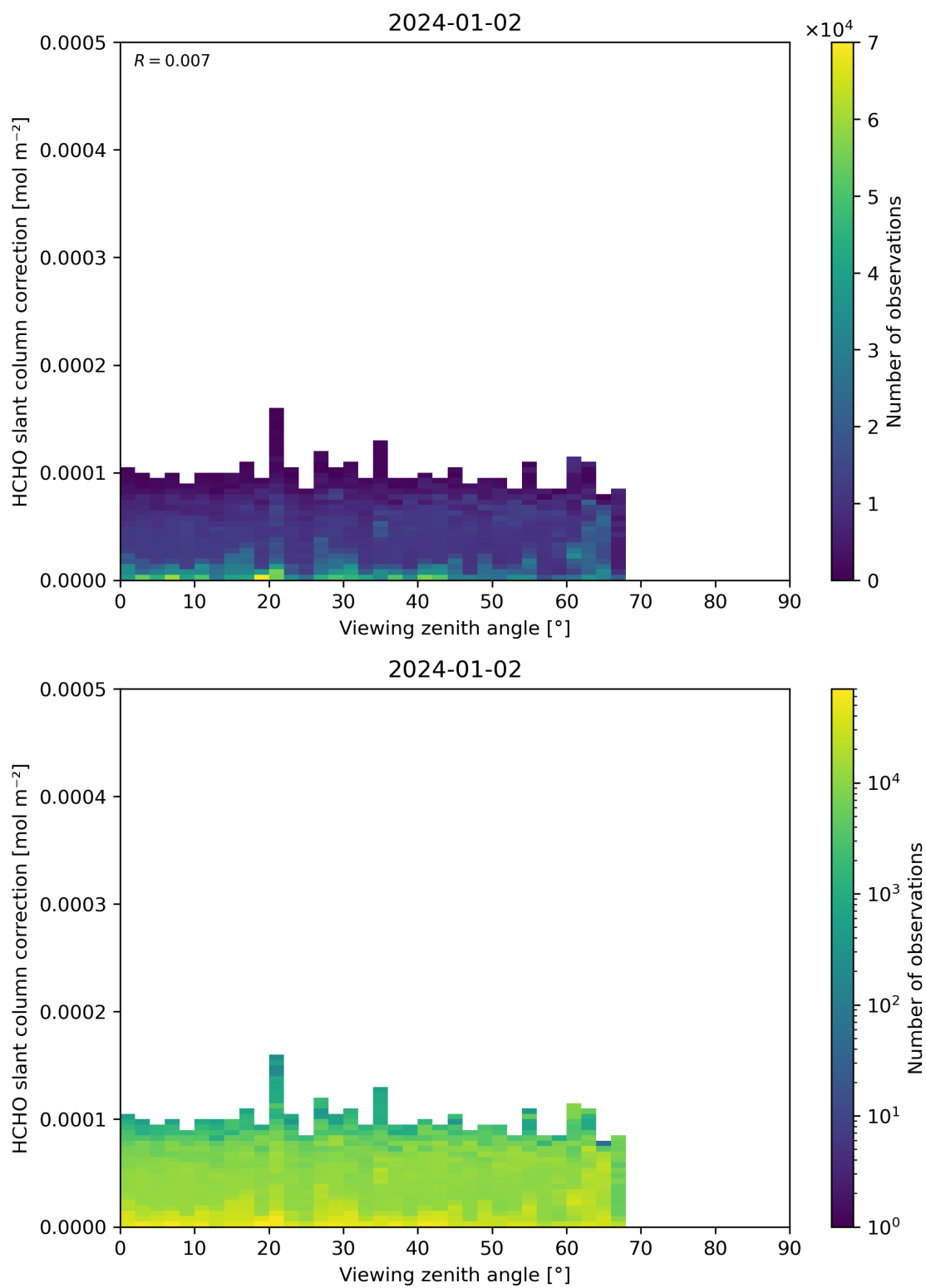
Figure 187: Scatter density plot of “Viewing zenith angle” against “HCHO slant column correction” for 2024-01-01 to 2024-01-03.
