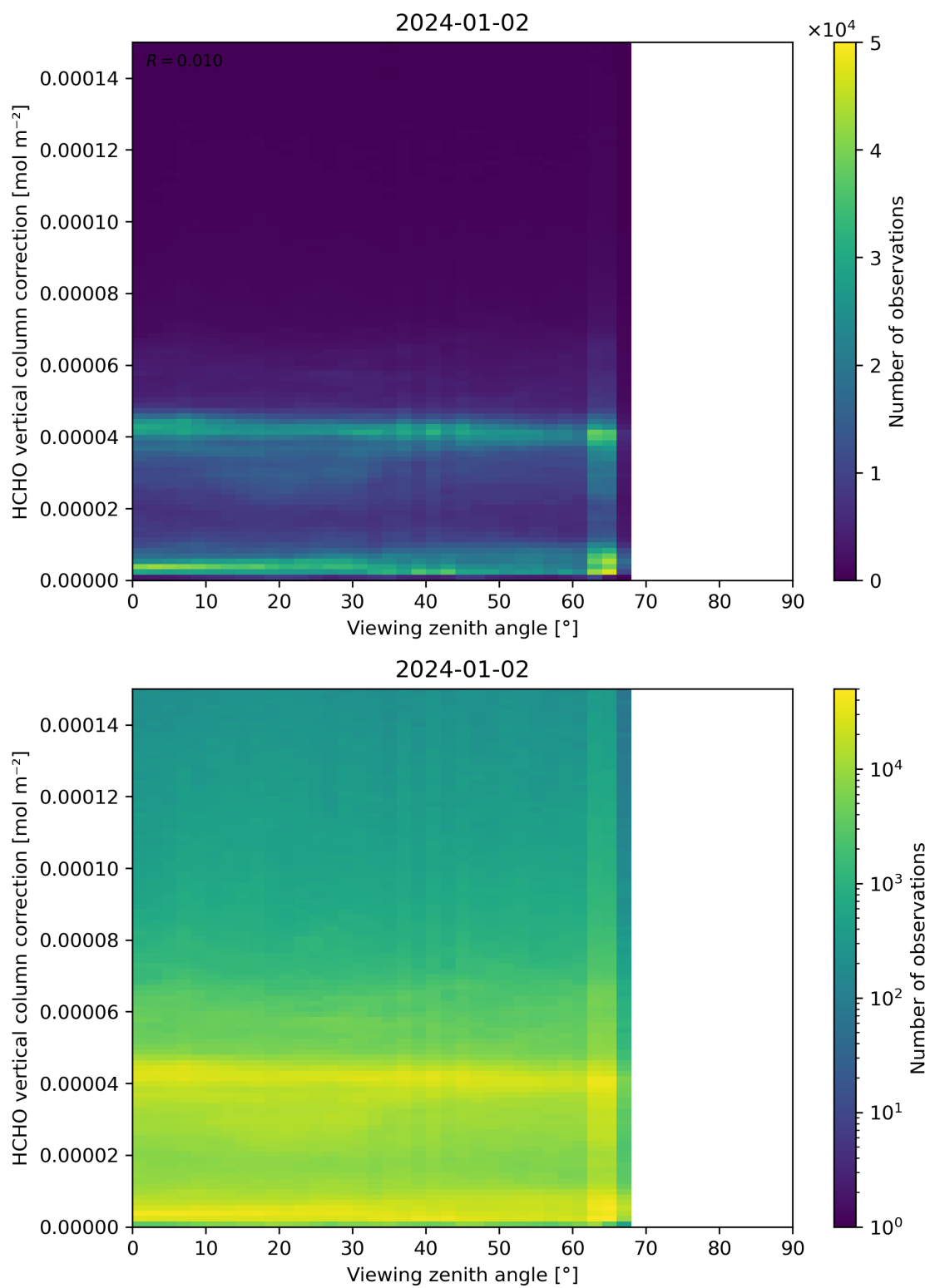
Figure 193: Scatter density plot of “Viewing zenith angle” against “HCHO vertical column correction” for 2024-01-01 to 2024-01-03.
