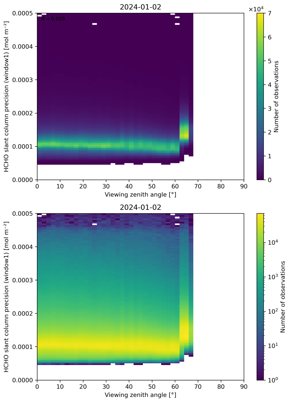
Figure 189: Scatter density plot of “Viewing zenith angle” against “HCHO slant column precision (window1)” for 2024-01-01 to 2024-01-03.
