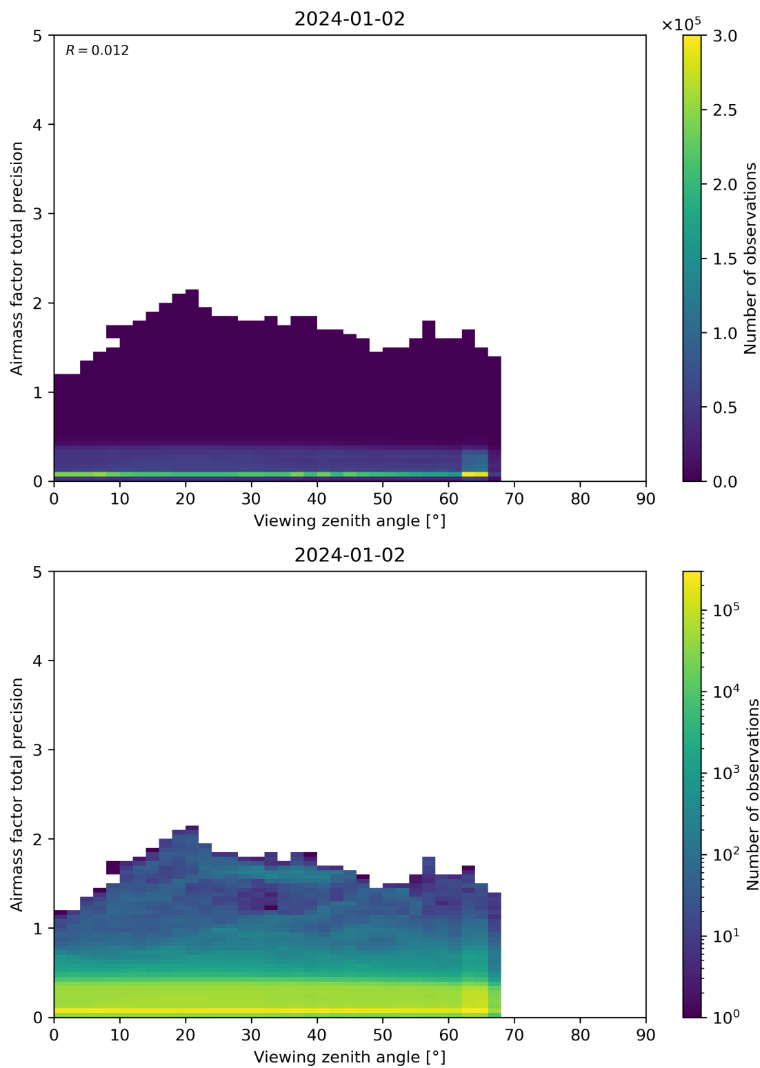
Figure 191: Scatter density plot of “Viewing zenith angle” against “Airmass factor total precision” for 2024-01-01 to 2024-01-03.
