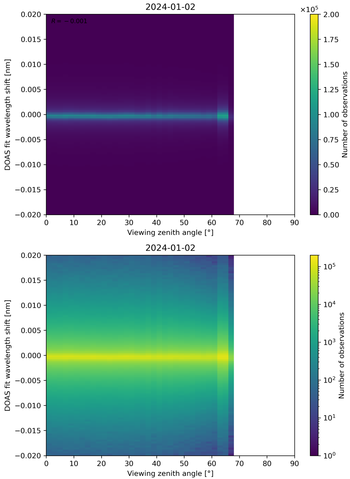
Figure 183: Scatter density plot of “Viewing zenith angle” against “DOAS fit wavelength shift” for 2024-01-01 to 2024-01-03.
