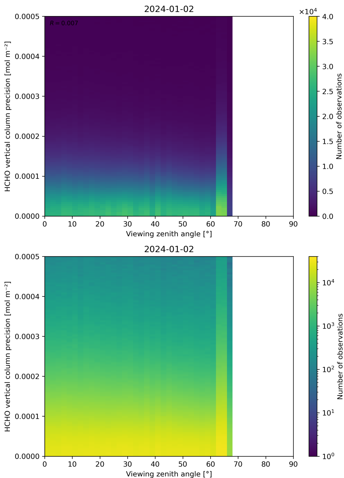
Figure 194: Scatter density plot of “Viewing zenith angle” against “HCHO vertical column precision” for 2024-01-01 to 2024-01-03.
