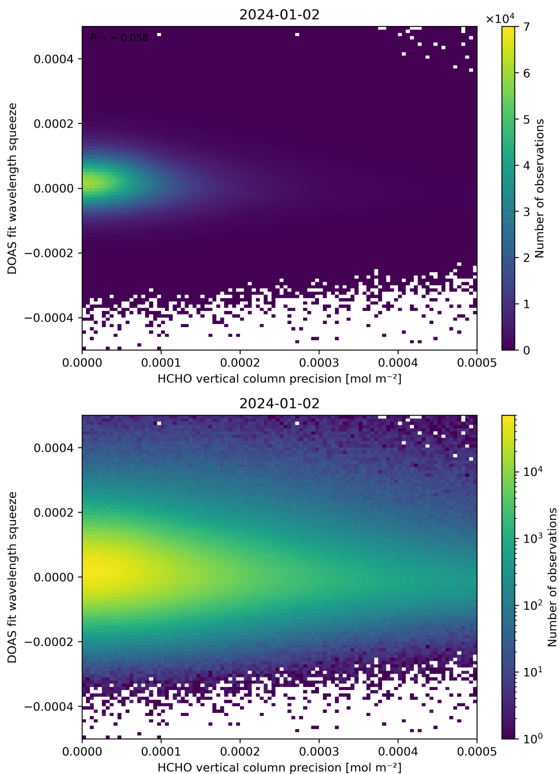
Figure 138: Scatter density plot of “HCHO vertical column precision” against “DOAS fit wavelength squeeze” for 2024-01-01 to 2024-01-03.
