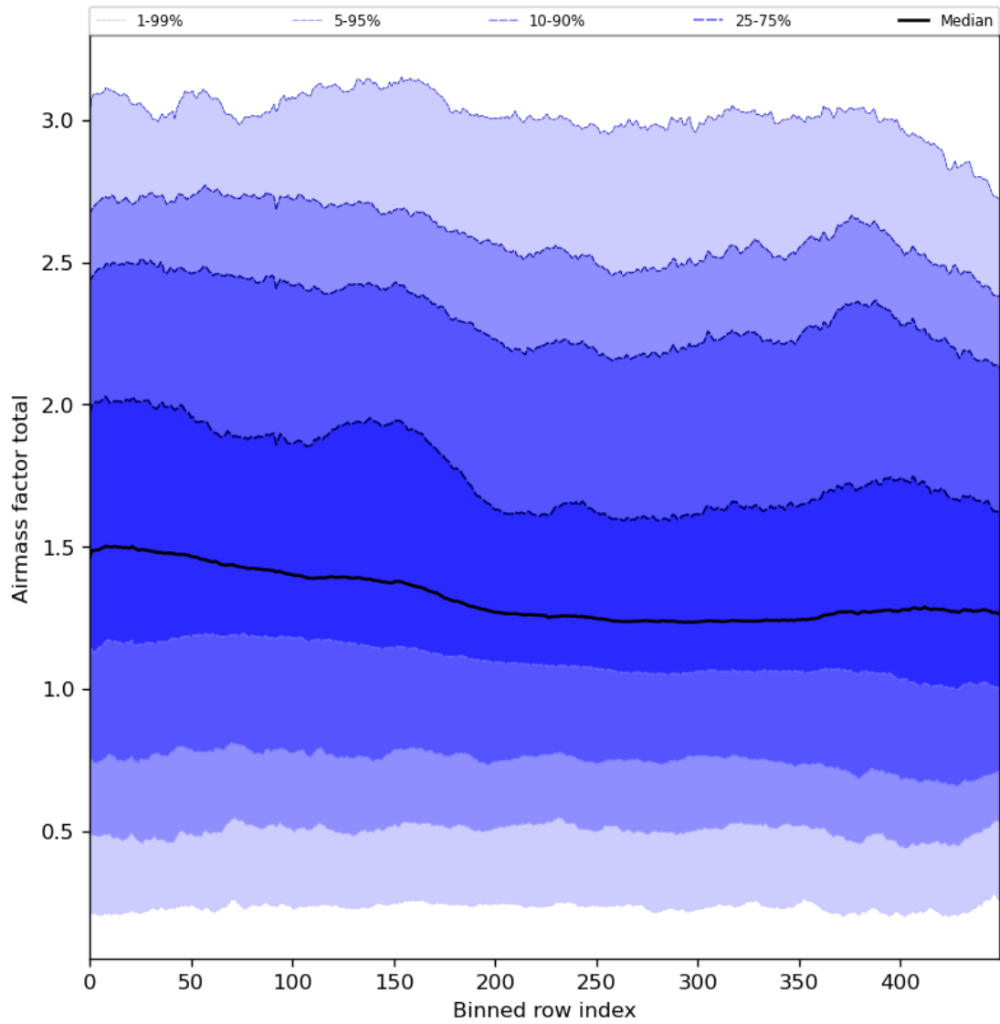
Figure 54: Along track statistics of “Airmass factor total” for 2024-01-01 to 2024-01-03
