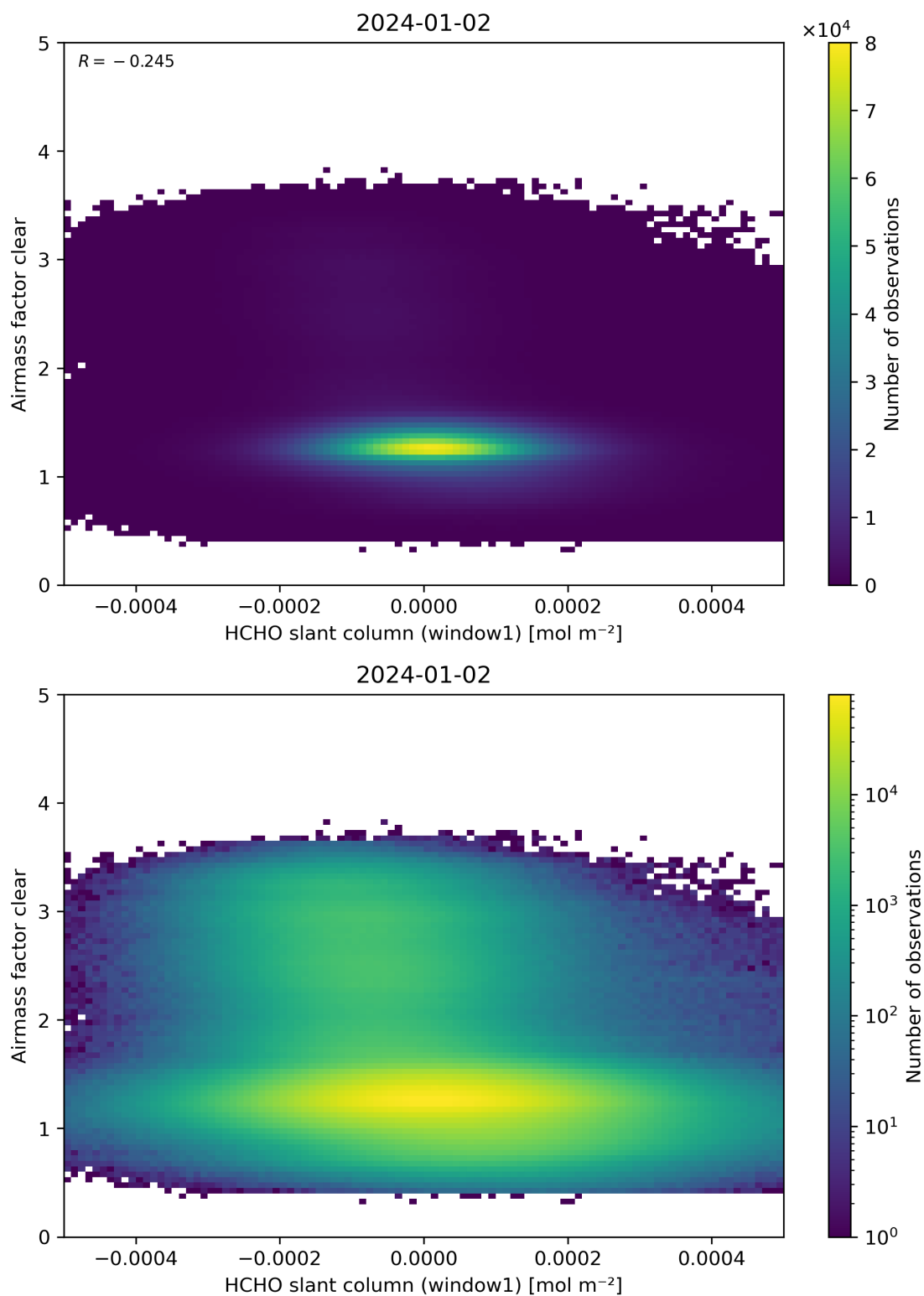
Figure 81: Scatter density plot of “HCHO slant column (window1)” against “Airmass factor clear” for 2024-01-01 to 2024-01-03.
