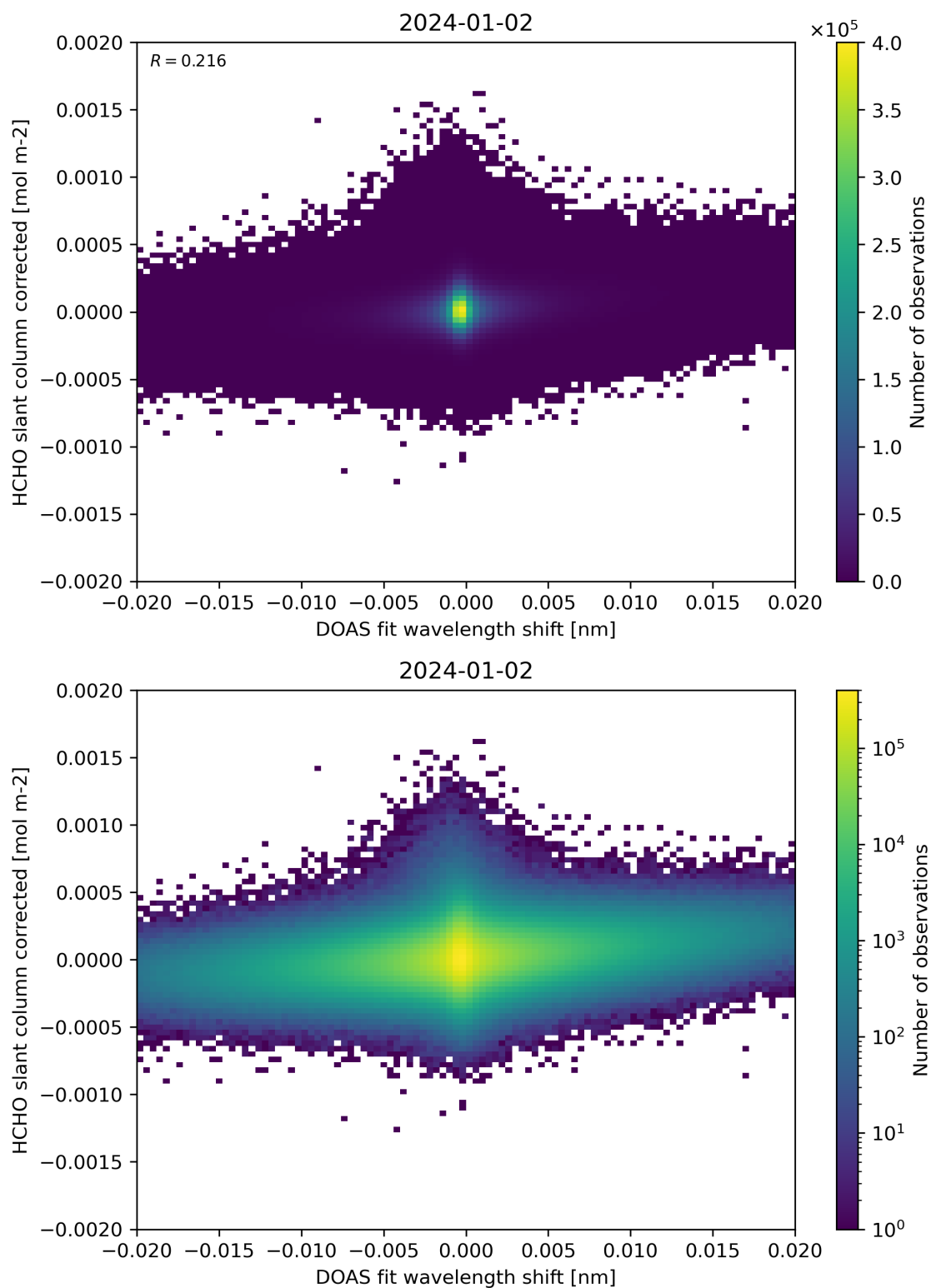
Figure 66: Scatter density plot of “DOAS fit wavelength shift” against “HCHO slant column corrected” for 2024-01-01 to 2024-01-03.
