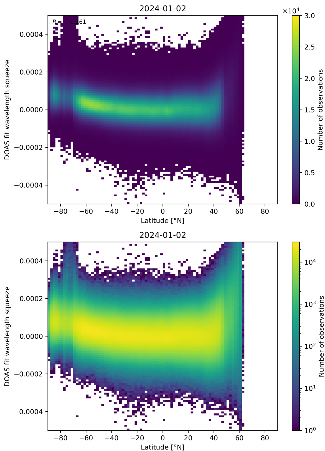
Figure 155: Scatter density plot of “Latitude” against “DOAS fit wavelength squeeze” for 2024-01-01 to 2024-01-03.
