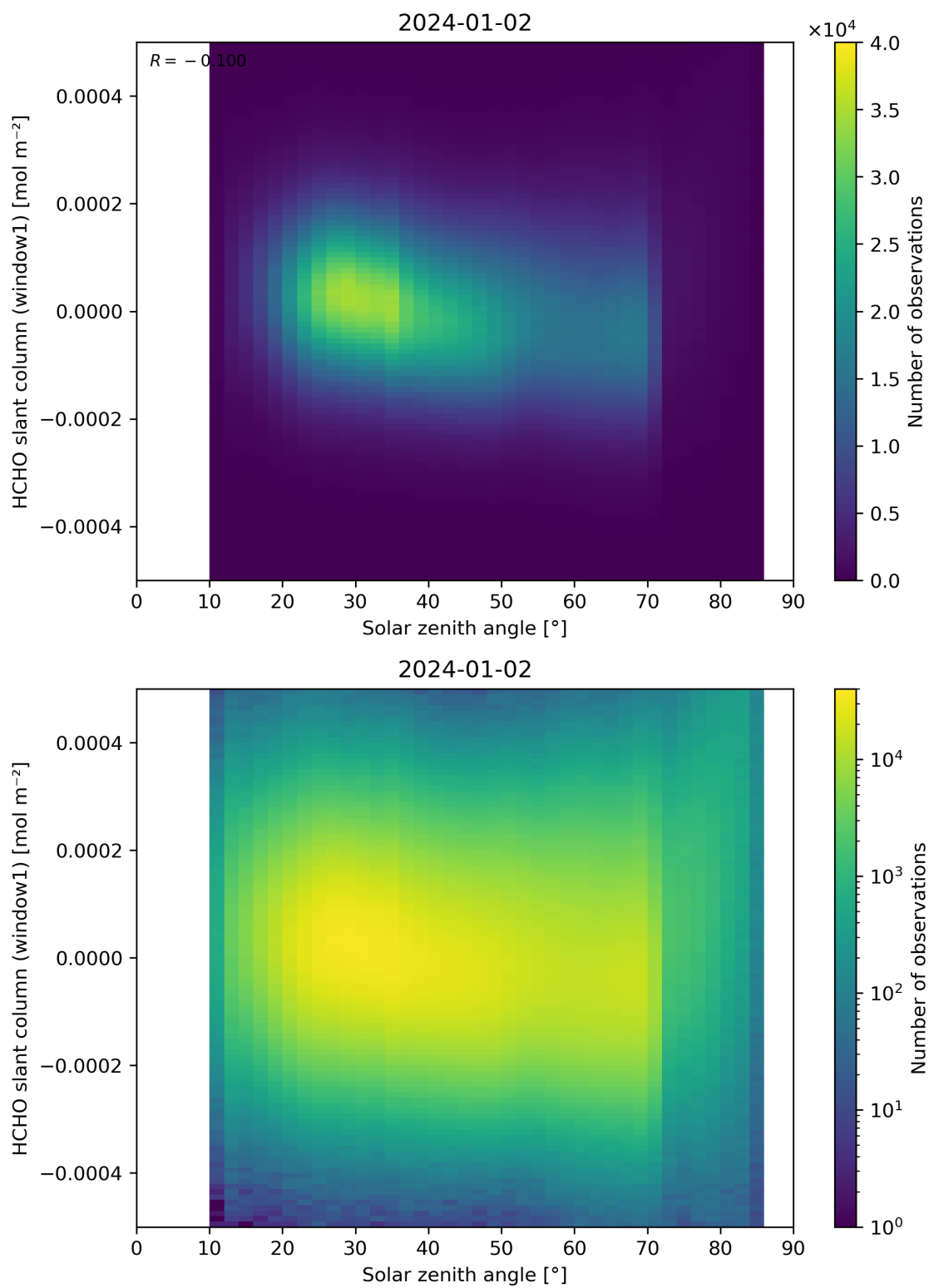
Figure 173: Scatter density plot of “Solar zenith angle” against “HCHO slant column (window1)” for 2024-01-01 to 2024-01-03.
