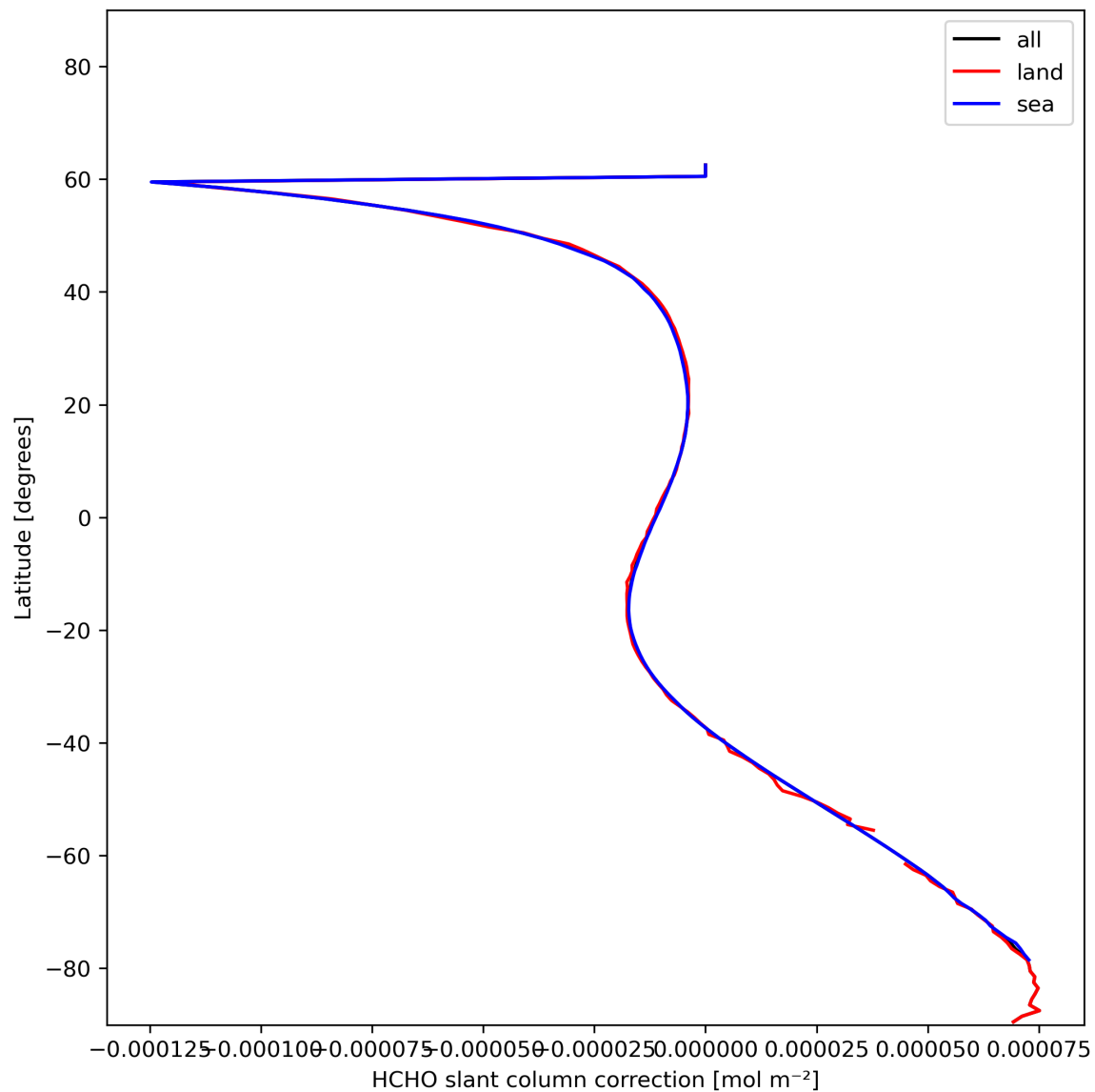
Figure 33: Zonal average of “HCHO slant column correction” for 2024-01-01 to 2024-01-03.
