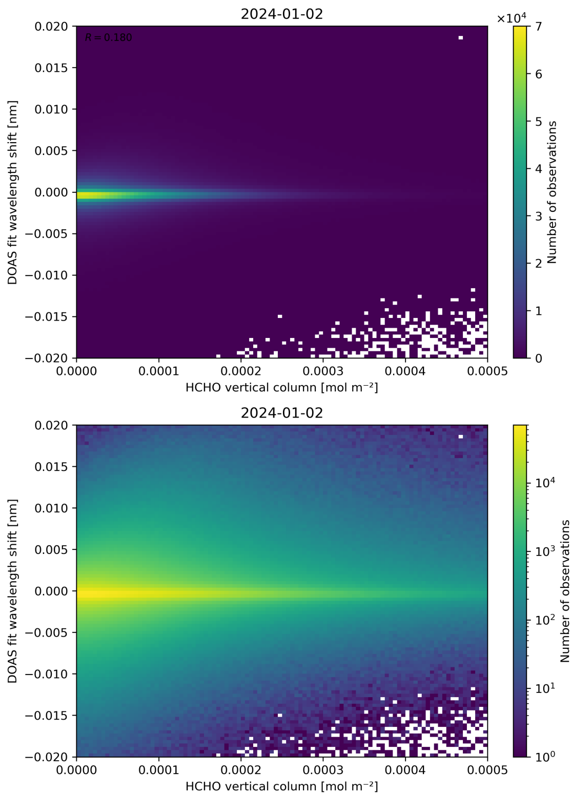
Figure 124: Scatter density plot of “HCHO vertical column” against “DOAS fit wavelength shift” for 2024-01-01 to 2024-01-03.
