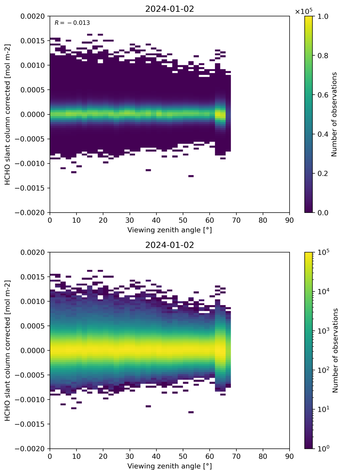
Figure 186: Scatter density plot of “Viewing zenith angle” against “HCHO slant column corrected” for 2024-01-01 to 2024-01-03.
