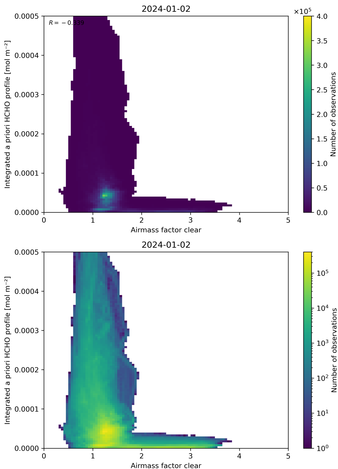
Figure 76: Scatter density plot of “Airmass factor clear” against “Integrated a priori HCHO profile” for 2024-01-01 to 2024-01-03.
