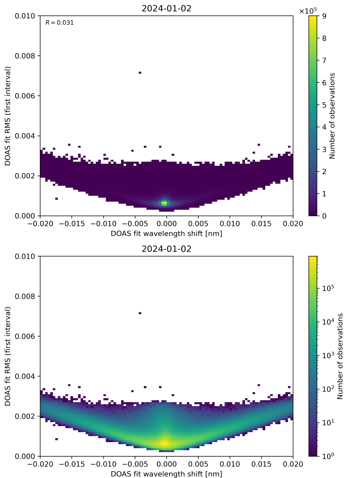
Figure 64: Scatter density plot of “DOAS fit wavelength shift” against “DOAS fit RMS (first interval)” for 2024-01-01 to 2024-01-03.
