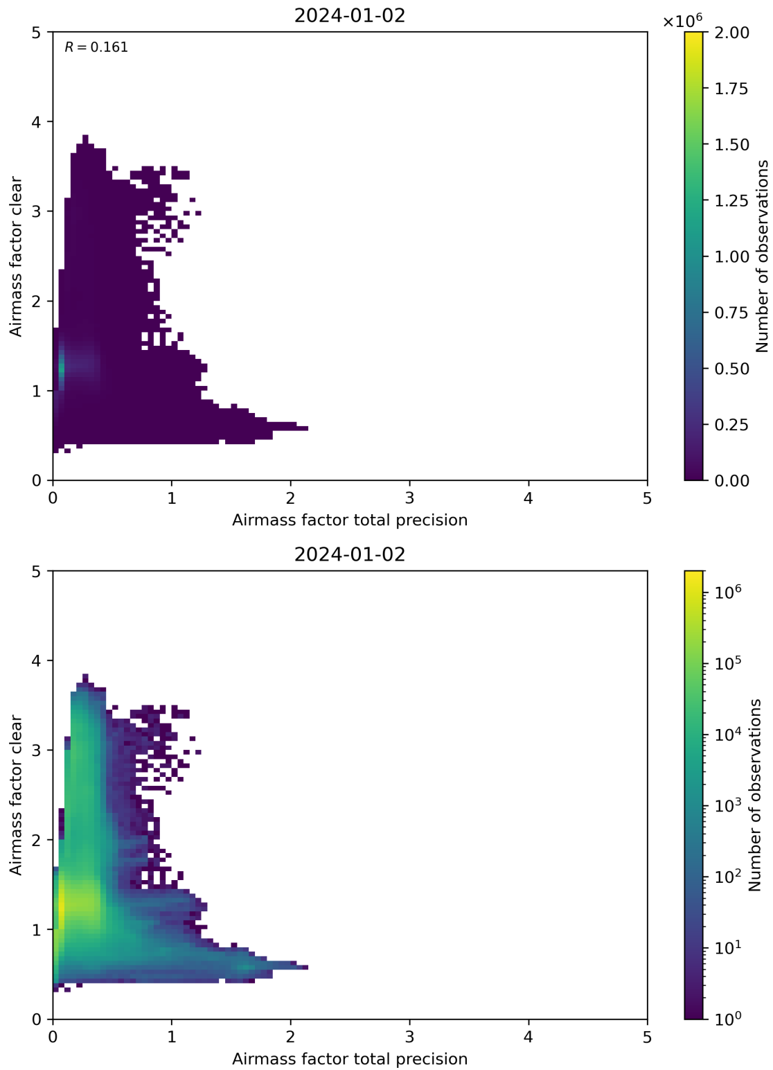
Figure 108: Scatter density plot of “Airmass factor total precision” against “Airmass factor clear” for 2024-01-01 to 2024-01-03.
