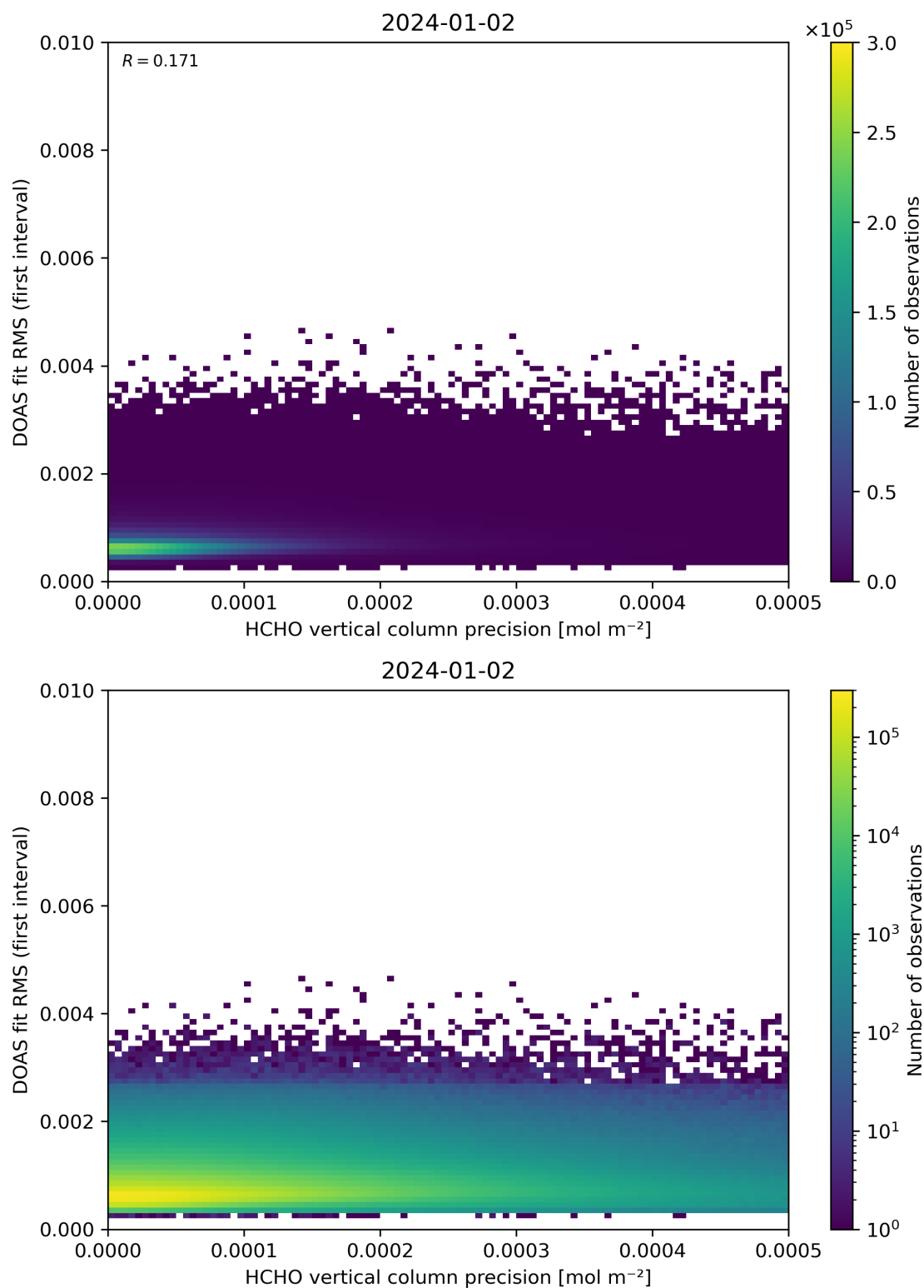
Figure 136: Scatter density plot of “HCHO vertical column precision” against “DOAS fit RMS (first interval)” for 2024-01-01 to 2024-01-03.
