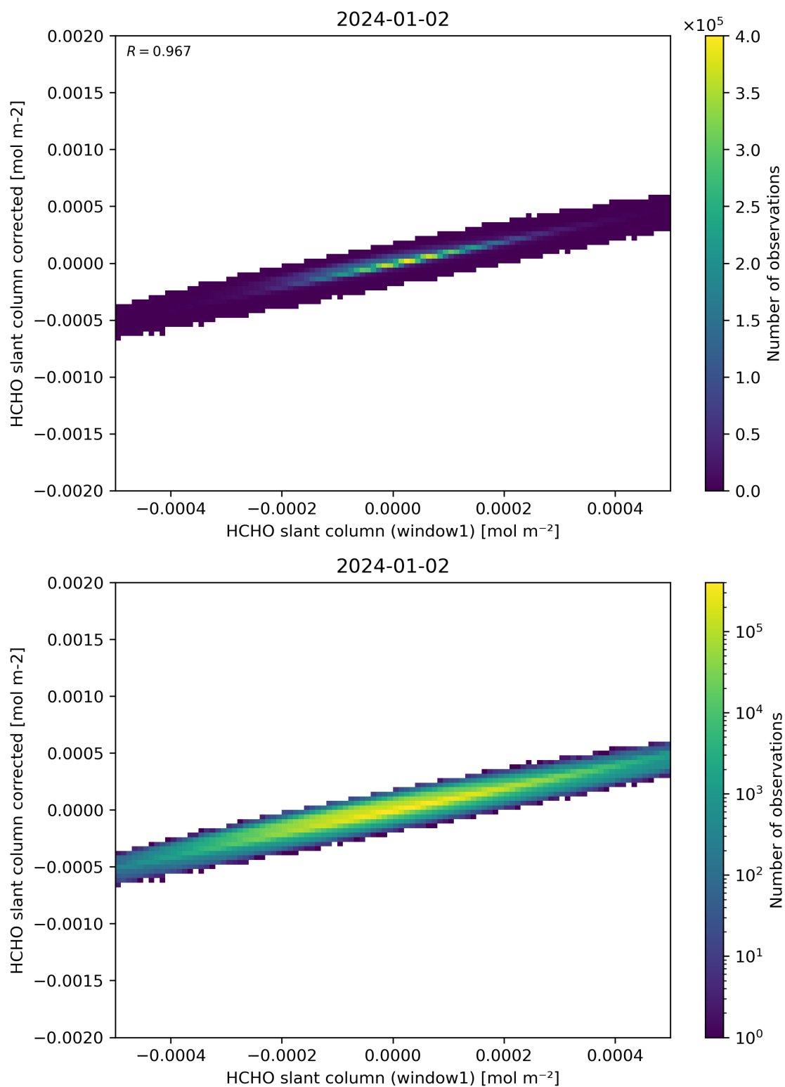
Figure 82: Scatter density plot of “HCHO slant column (window1)” against “HCHO slant column corrected” for 2024-01-01 to 2024-01-03.
