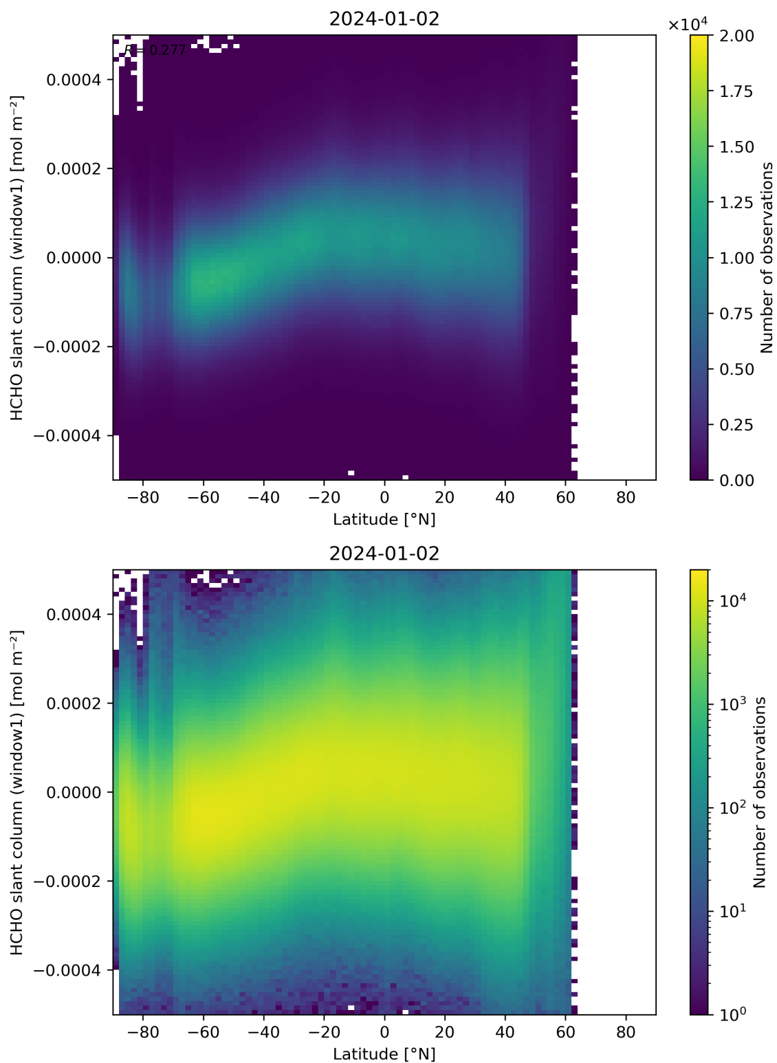
Figure 159: Scatter density plot of “Latitude” against “HCHO slant column (window1)” for 2024-01-01 to 2024-01-03.
