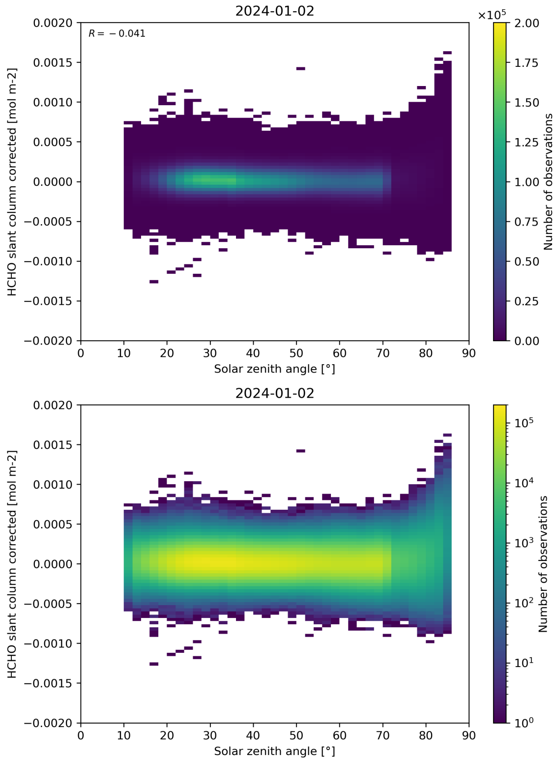
Figure 171: Scatter density plot of “Solar zenith angle” against “HCHO slant column corrected” for 2024-01-01 to 2024-01-03.
