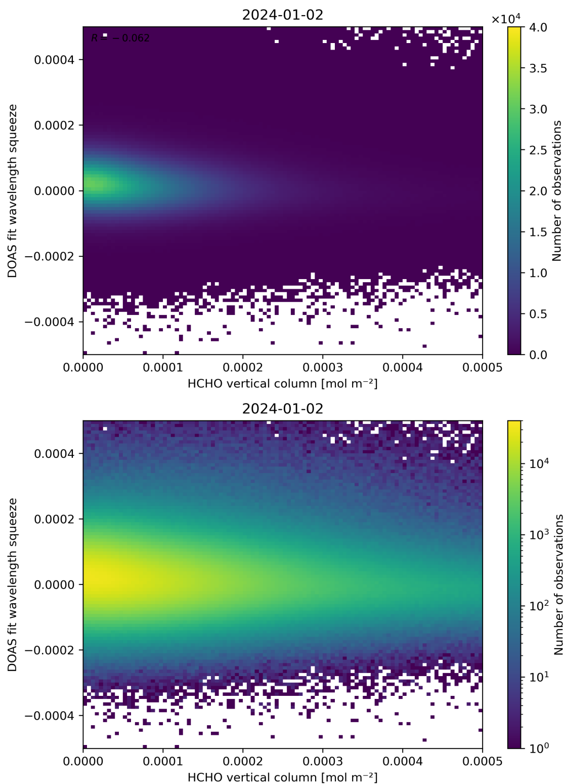
Figure 125: Scatter density plot of “HCHO vertical column” against “DOAS fit wavelength squeeze” for 2024-01-01 to 2024-01-03.
