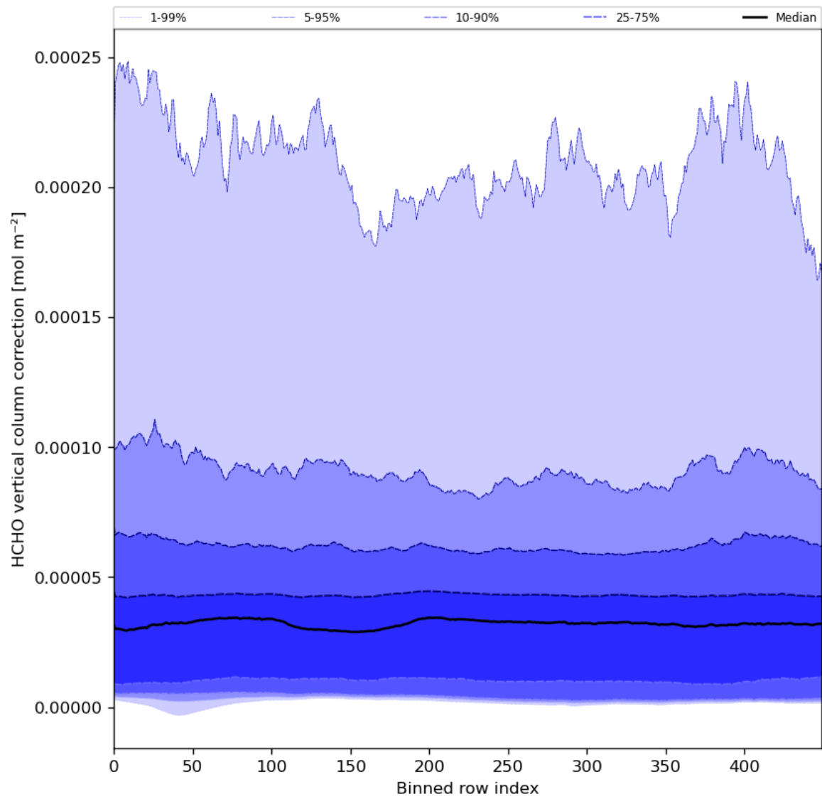
Figure 51: Along track statistics of “HCHO vertical column correction” for 2024-01-01 to 2024-01-03
