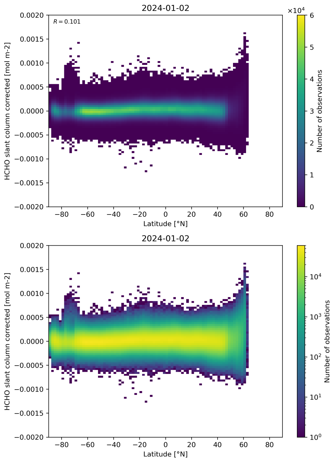
Figure 157: Scatter density plot of “Latitude” against “HCHO slant column corrected” for 2024-01-01 to 2024-01-03.
