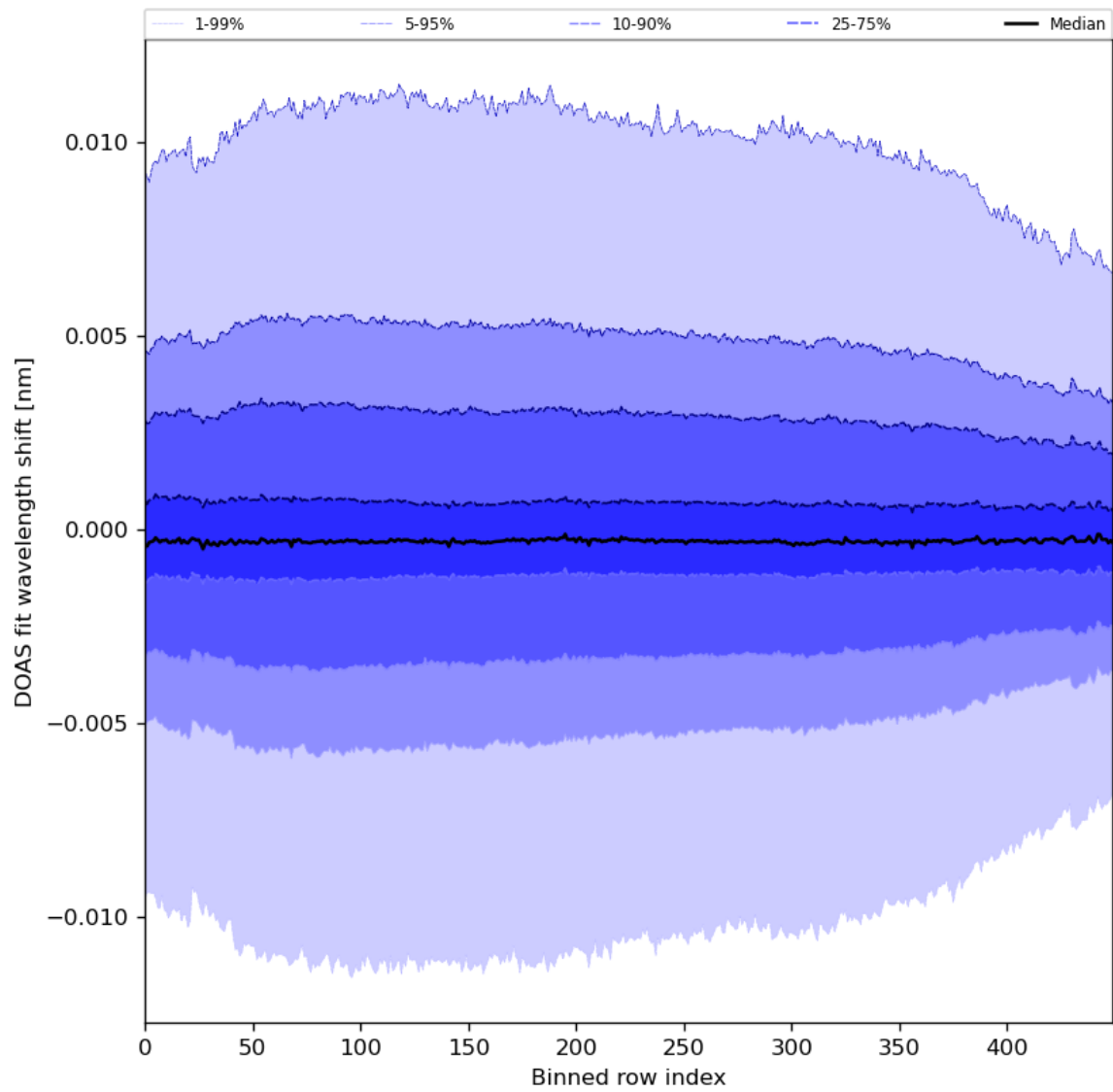
Figure 58: Along track statistics of “DOAS fit wavelength shift” for 2024-01-01 to 2024-01-03
