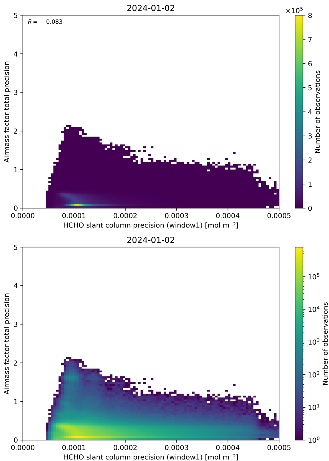
Figure 95: Scatter density plot of “HCHO slant column precision (window1)” against “Airmass factor total precision” for 2024-01-01 to 2024-01-03.
