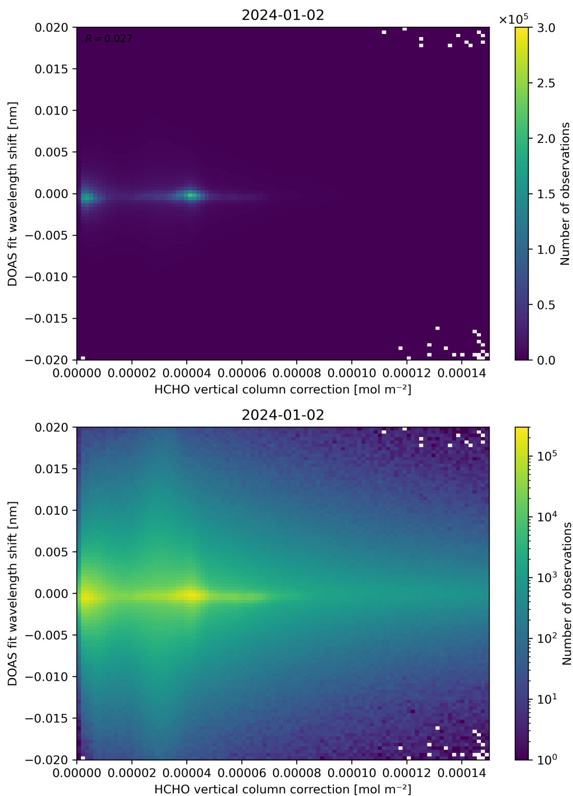
Figure 113: Scatter density plot of “HCHO vertical column correction” against “DOAS fit wavelength shift” for 2024-01-01 to 2024-01-03.
