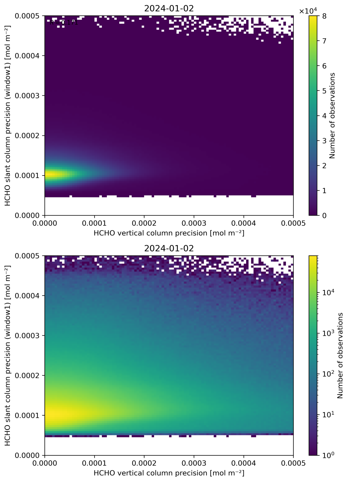
Figure 143: Scatter density plot of “HCHO vertical column precision” against “HCHO slant column precision (window1)” for 2024-01-01 to 2024-01-03.
