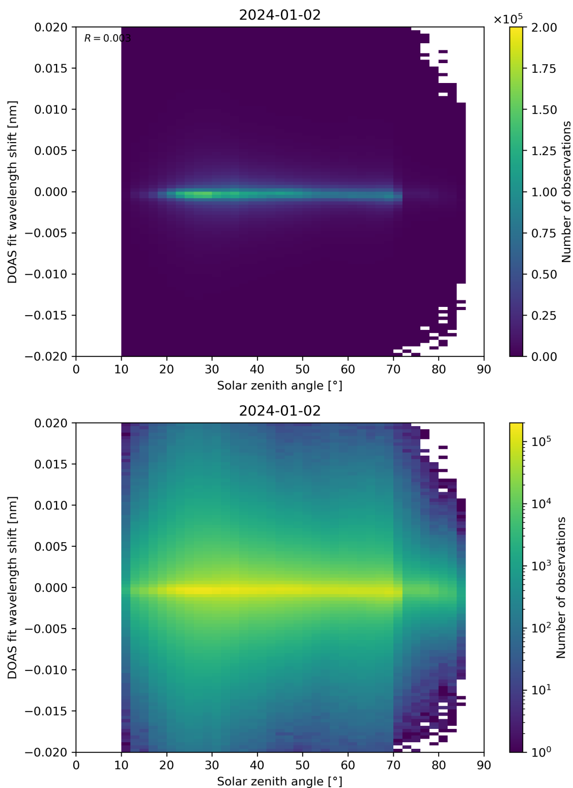
Figure 168: Scatter density plot of “Solar zenith angle” against “DOAS fit wavelength shift” for 2024-01-01 to 2024-01-03.
