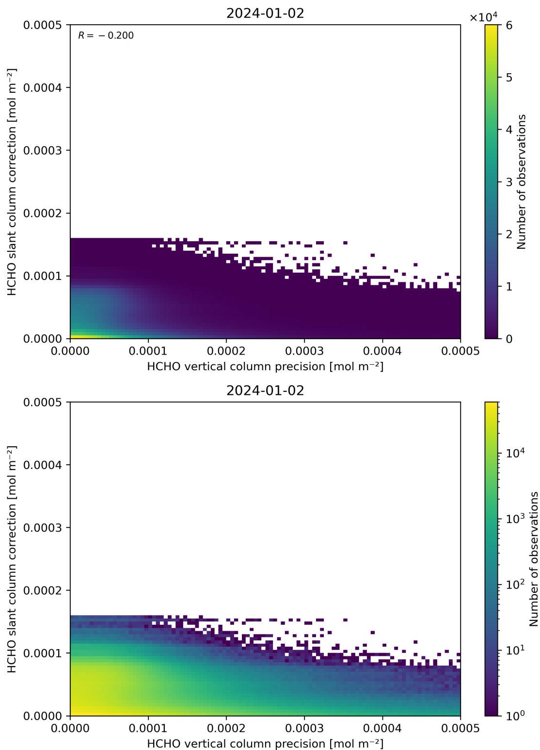
Figure 141: Scatter density plot of “HCHO vertical column precision” against “HCHO slant column correction” for 2024-01-01 to 2024-01-03.
