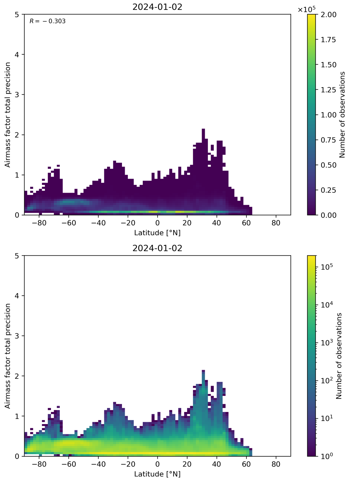
Figure 162: Scatter density plot of “Latitude” against “Airmass factor total precision” for 2024-01-01 to 2024-01-03.
