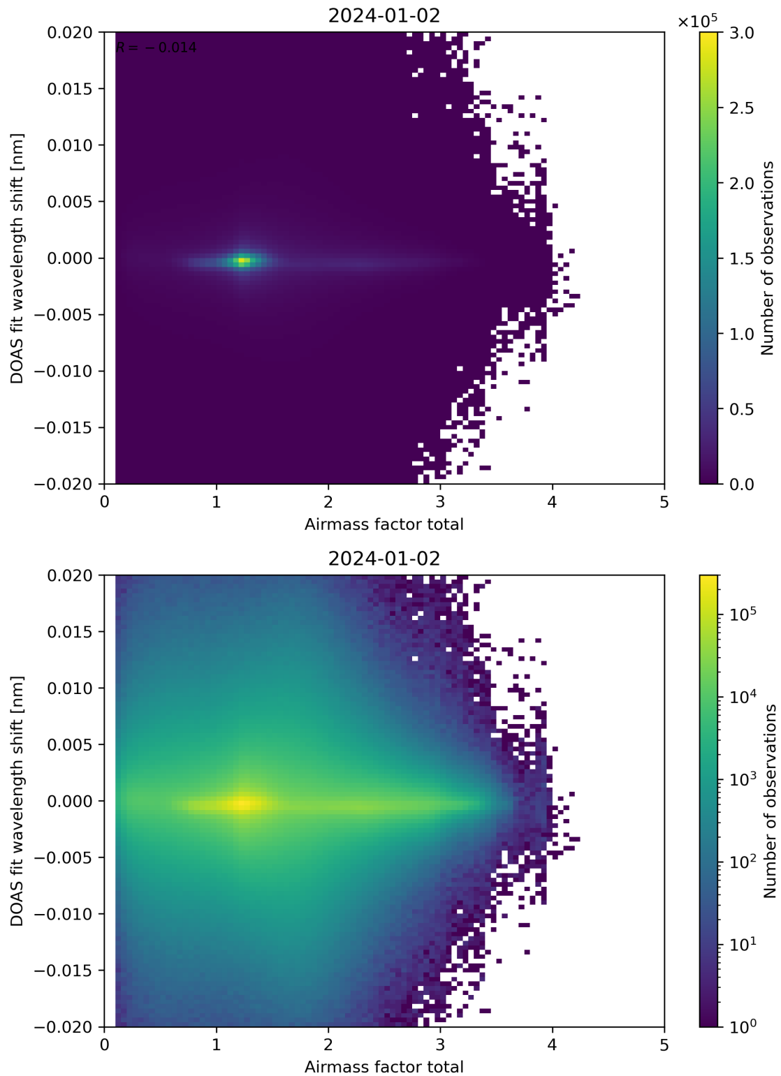
Figure 98: Scatter density plot of “Airmass factor total” against “DOAS fit wavelength shift” for 2024-01-01 to 2024-01-03.
