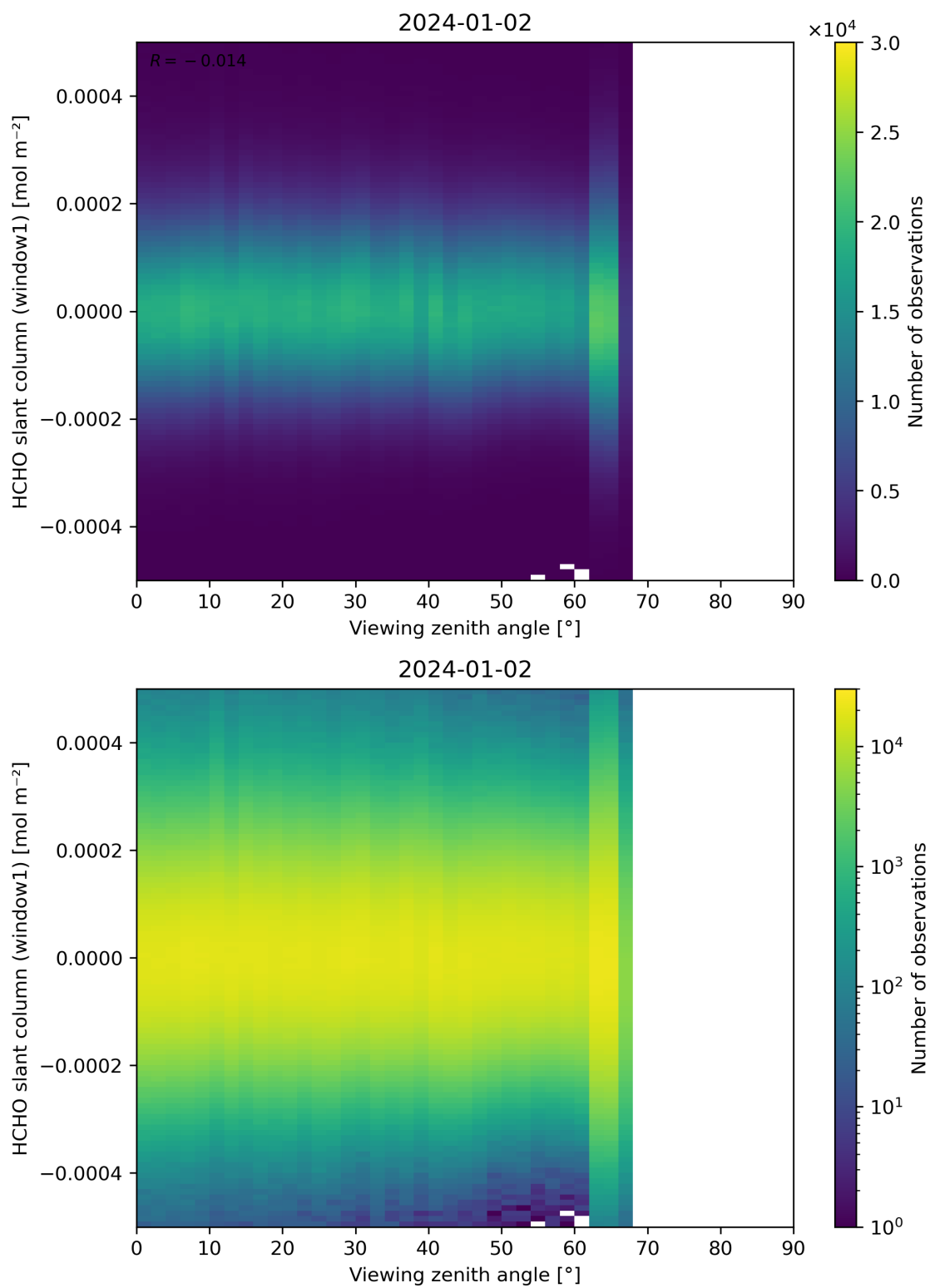
Figure 188: Scatter density plot of “Viewing zenith angle” against “HCHO slant column (window1)” for 2024-01-01 to 2024-01-03.
