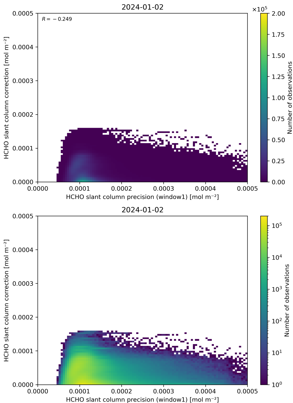
Figure 93: Scatter density plot of “HCHO slant column precision (window1)” against “HCHO slant column correction” for 2024-01-01 to 2024-01-03.
