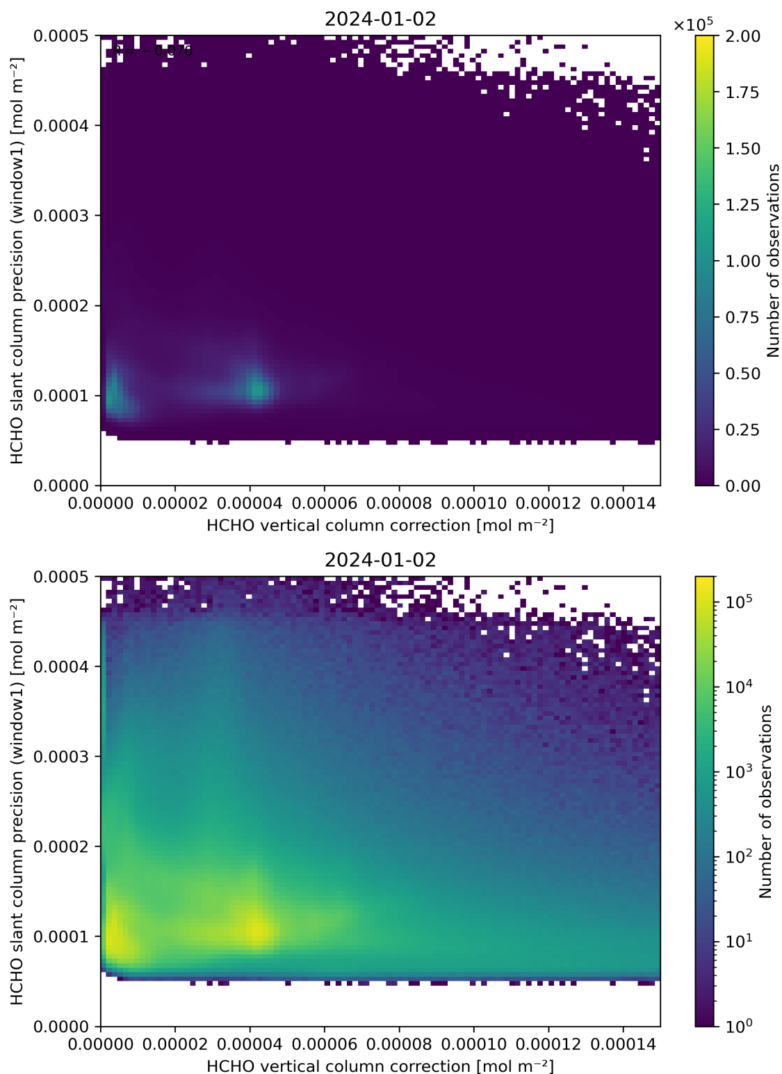
Figure 119: Scatter density plot of “HCHO vertical column correction” against “HCHO slant column precision (window1)” for 2024-01-01 to 2024-01-03.
