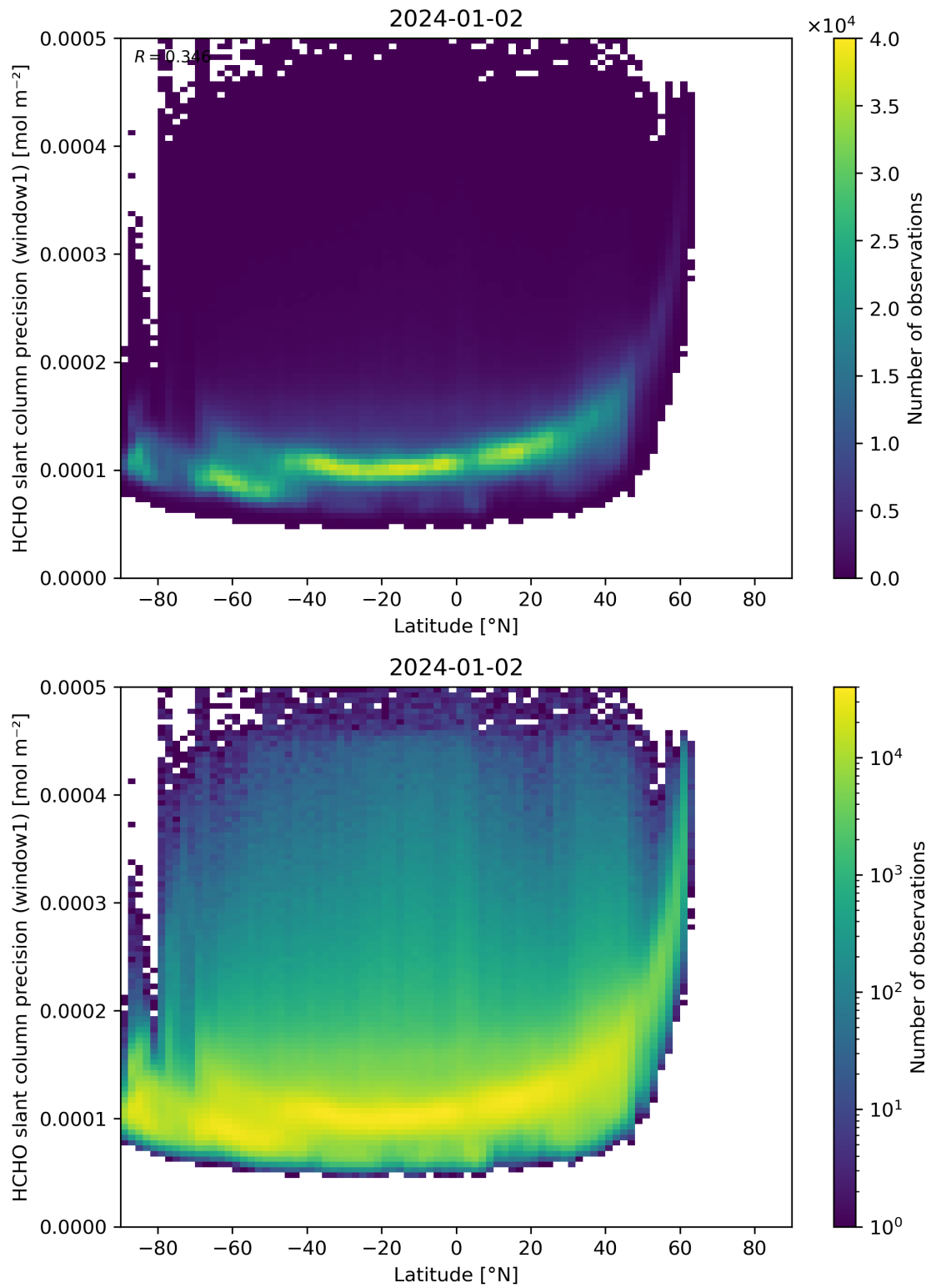
Figure 160: Scatter density plot of “Latitude” against “HCHO slant column precision (window1)” for 2024-01-01 to 2024-01-03.
