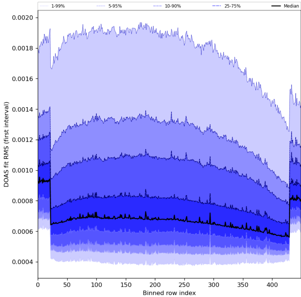
Figure 60: Along track statistics of “DOAS fit RMS (first interval)” for 2024-01-01 to 2024-01-03
