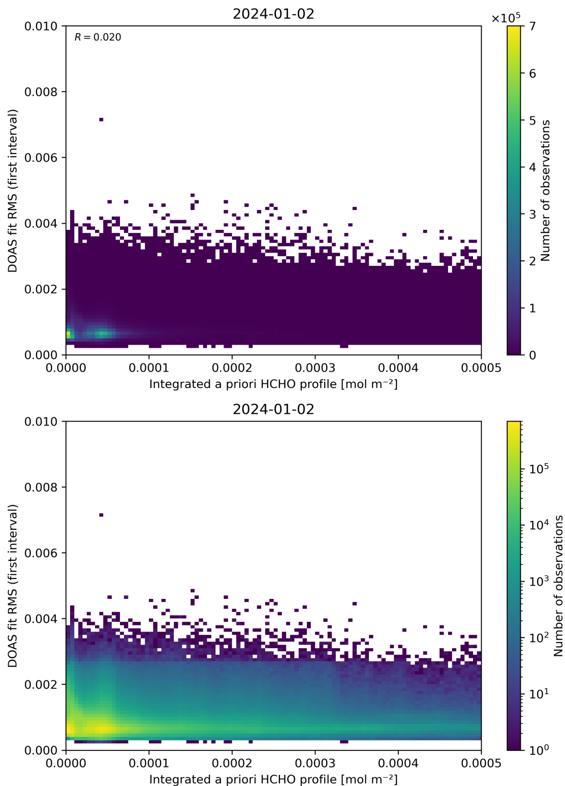
Figure 148: Scatter density plot of “Integrated a priori HCHO profile” against “DOAS fit RMS (first interval)” for 2024-01-01 to 2024-01-03.
