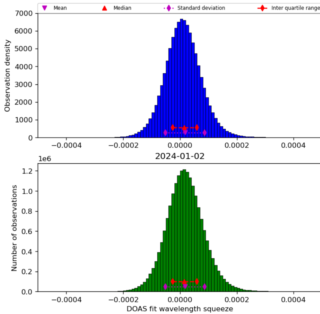
Figure 45: Histogram of “DOAS fit wavelength squeeze” for 2024-01-01 to 2024-01-03
