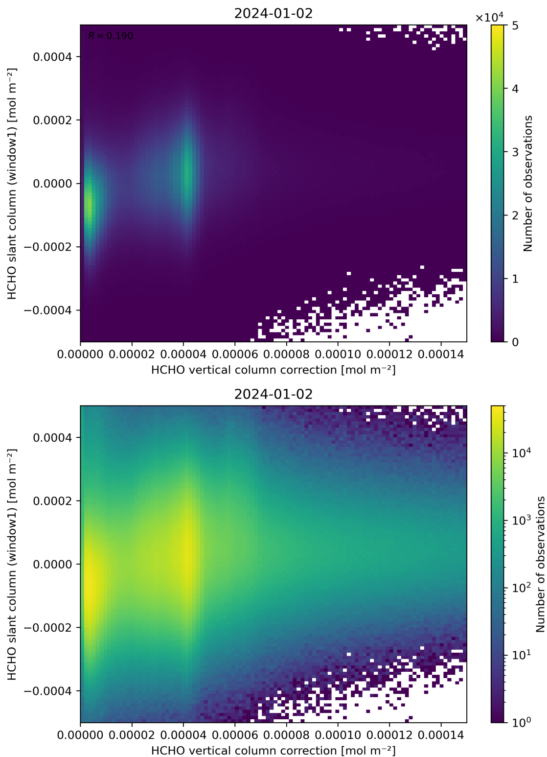
Figure 118: Scatter density plot of “HCHO vertical column correction” against “HCHO slant column (window1)” for 2024-01-01 to 2024-01-03.
