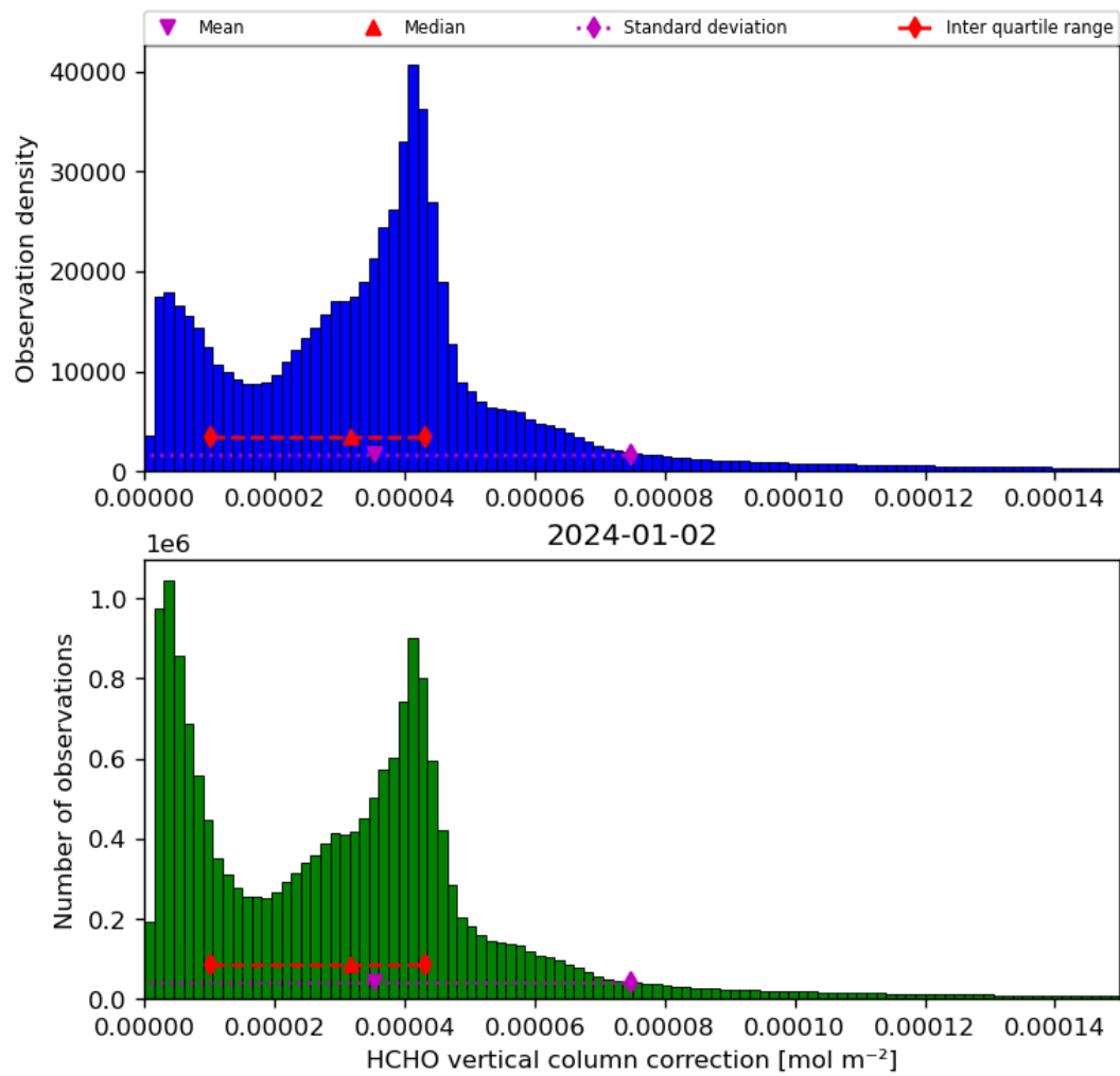
Figure 37: Histogram of “HCHO vertical column correction” for 2024-01-01 to 2024-01-03
