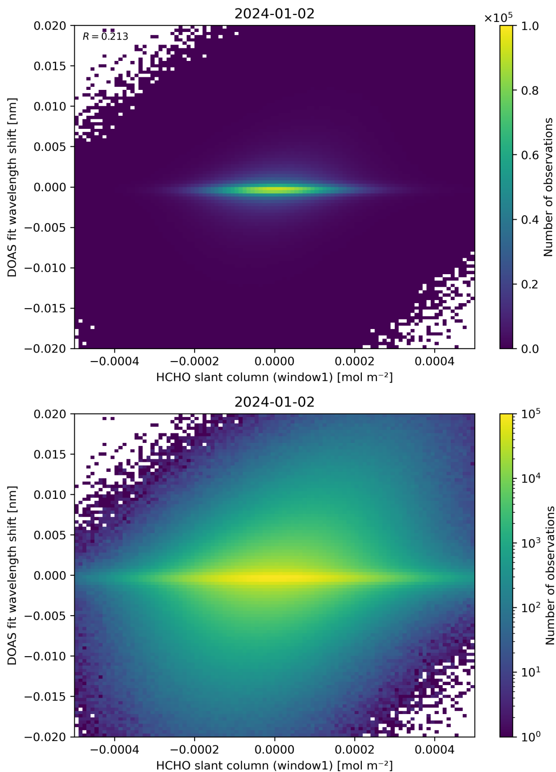
Figure 79: Scatter density plot of “HCHO slant column (window1)” against “DOAS fit wavelength shift” for 2024-01-01 to 2024-01-03.
