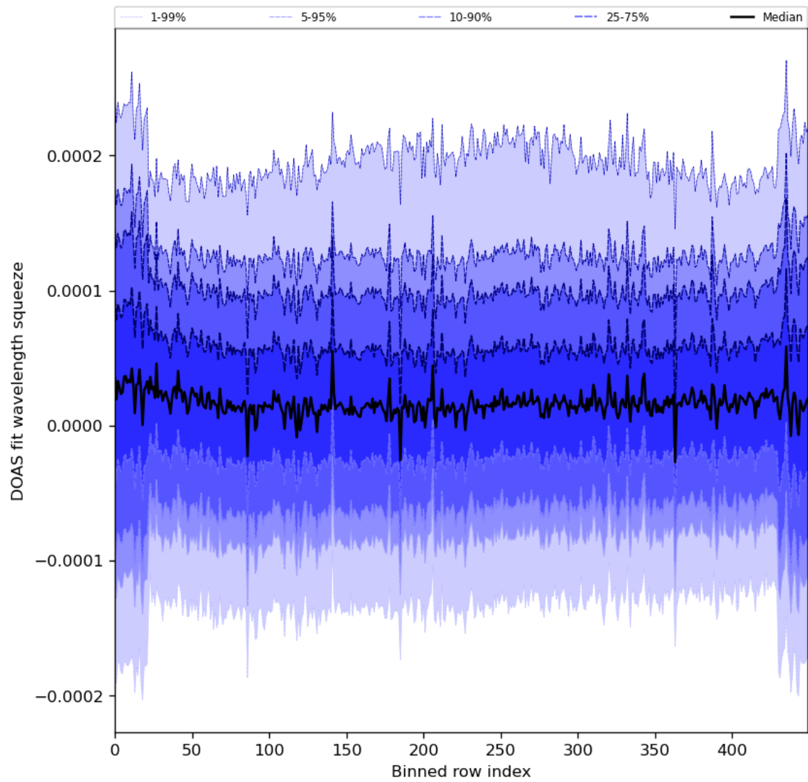
Figure 59: Along track statistics of “DOAS fit wavelength squeeze” for 2024-01-01 to 2024-01-03
