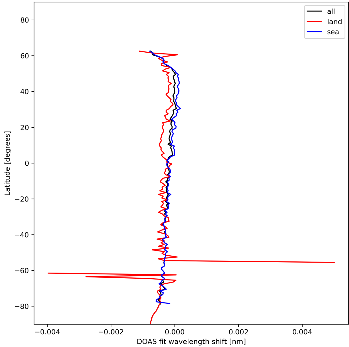
Figure 30: Zonal average of “DOAS fit wavelength shift” for 2024-01-01 to 2024-01-03.
