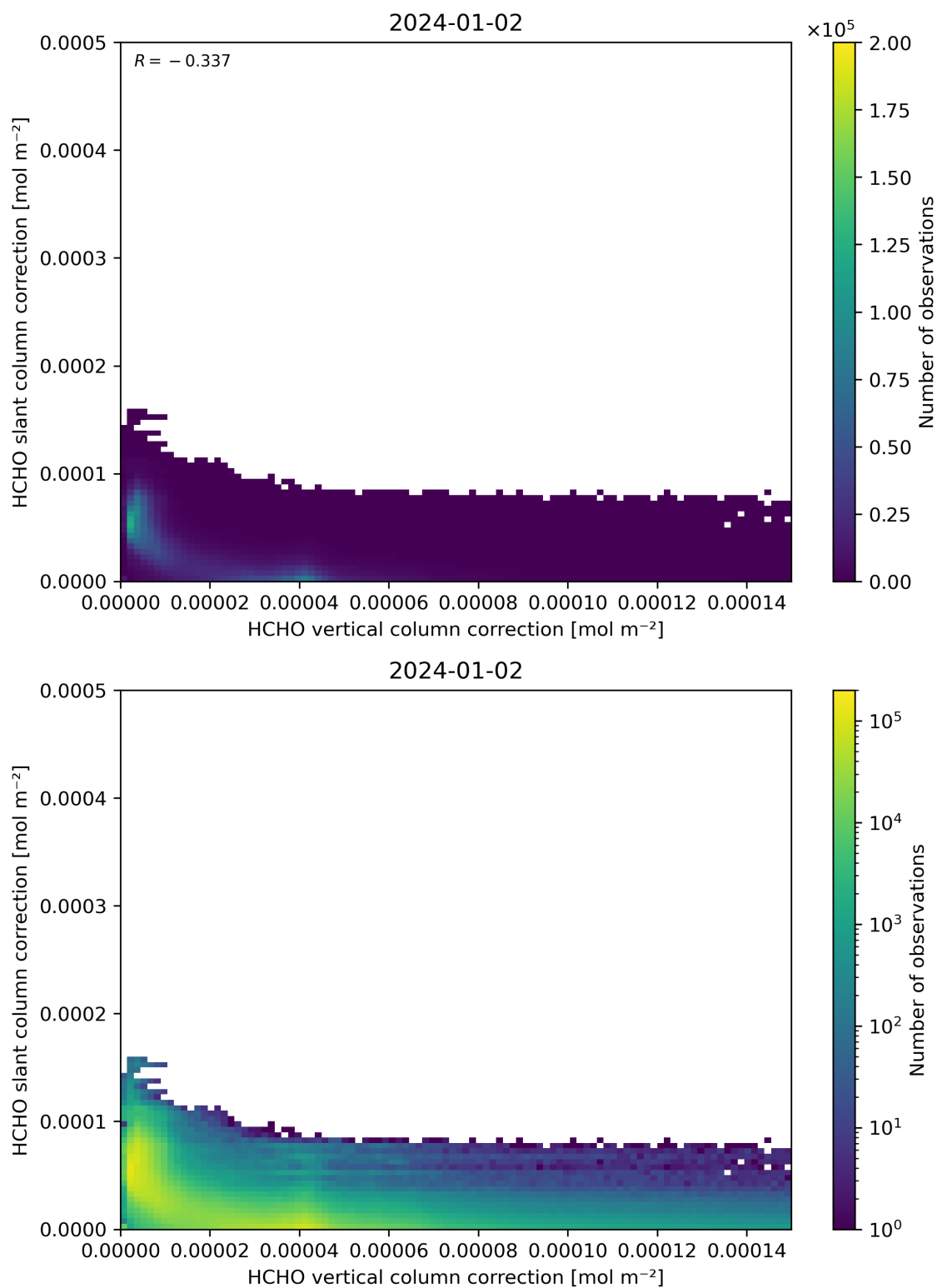
Figure 117: Scatter density plot of “HCHO vertical column correction” against “HCHO slant column correction” for 2024-01-01 to 2024-01-03.
