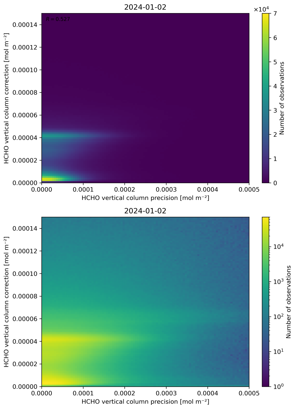
Figure 146: Scatter density plot of “HCHO vertical column precision” against “HCHO vertical column correction” for 2024-01-01 to 2024-01-03.
