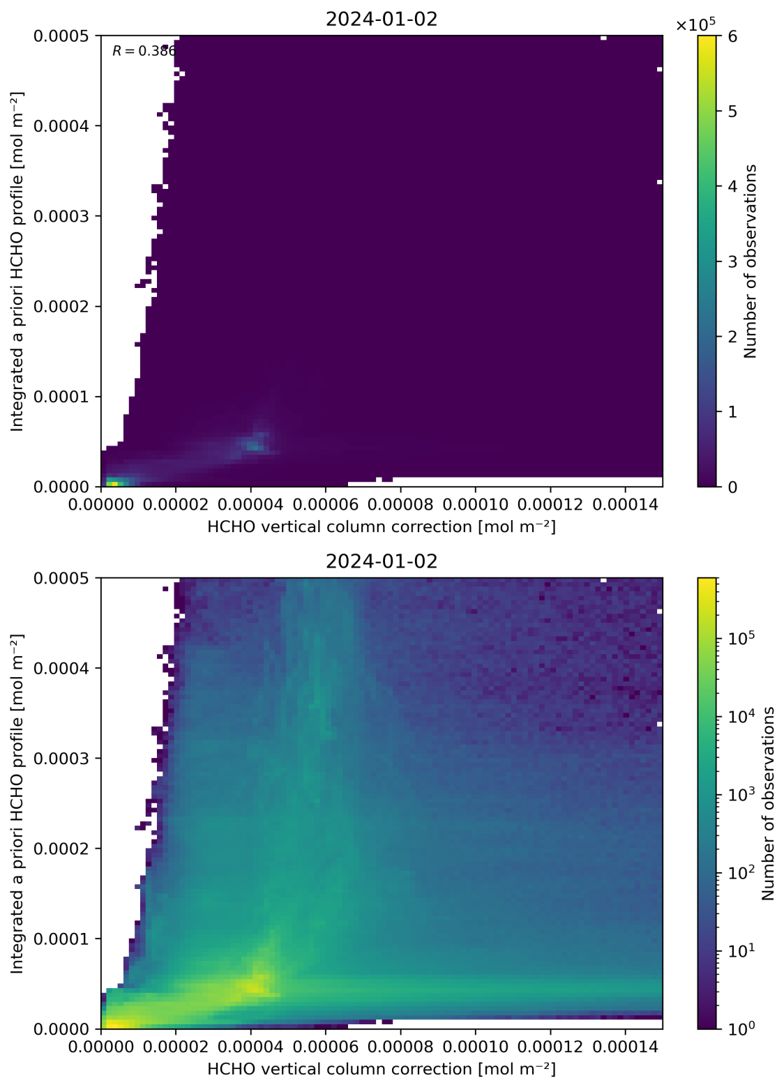
Figure 122: Scatter density plot of “HCHO vertical column correction” against “Integrated a priori HCHO profile” for 2024-01-01 to 2024-01-03.
