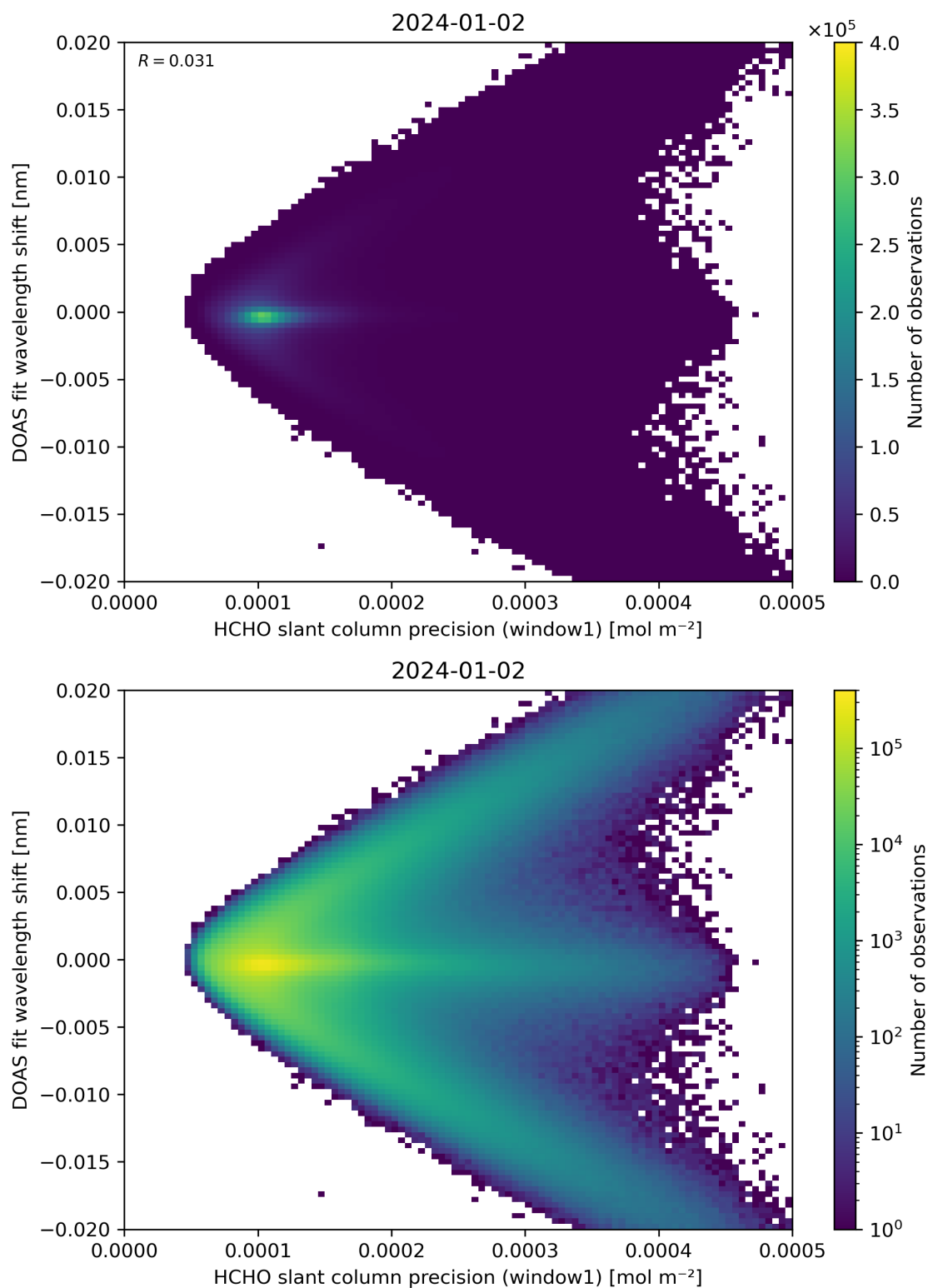
Figure 89: Scatter density plot of “HCHO slant column precision (window1)” against “DOAS fit wavelength shift” for 2024-01-01 to 2024-01-03.
