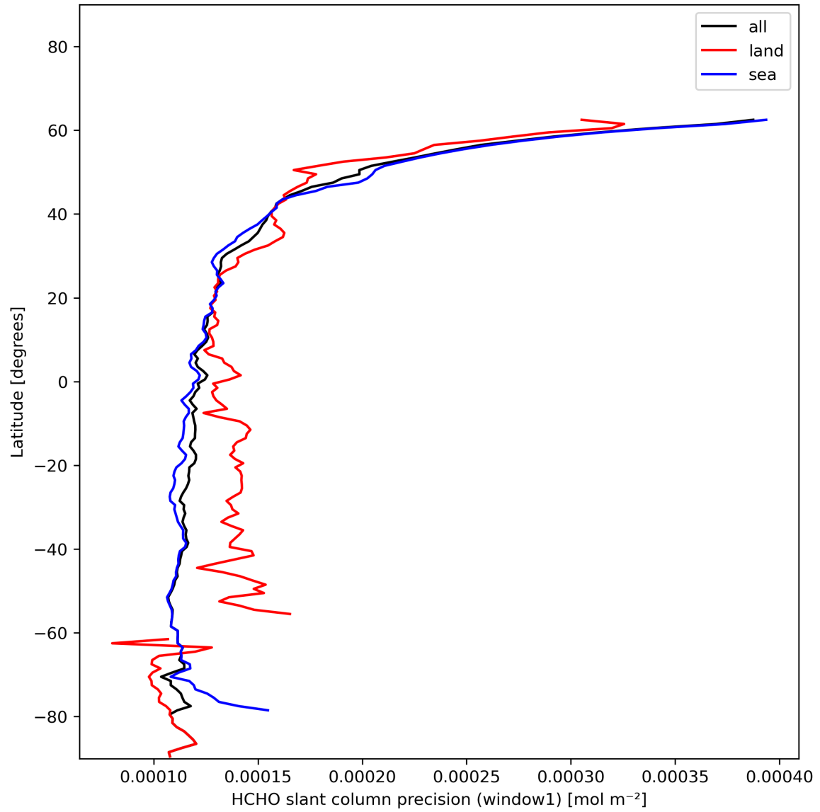
Figure 25: Zonal average of “HCHO slant column precision (window1)” for 2024-01-01 to 2024-01-03.
