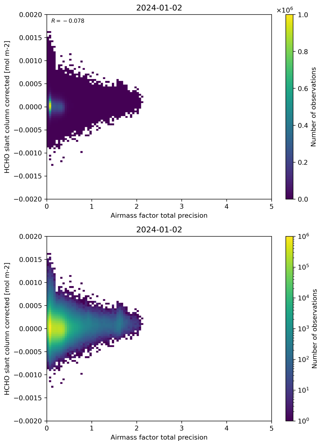
Figure 109: Scatter density plot of “Airmass factor total precision” against “HCHO slant column corrected” for 2024-01-01 to 2024-01-03.
