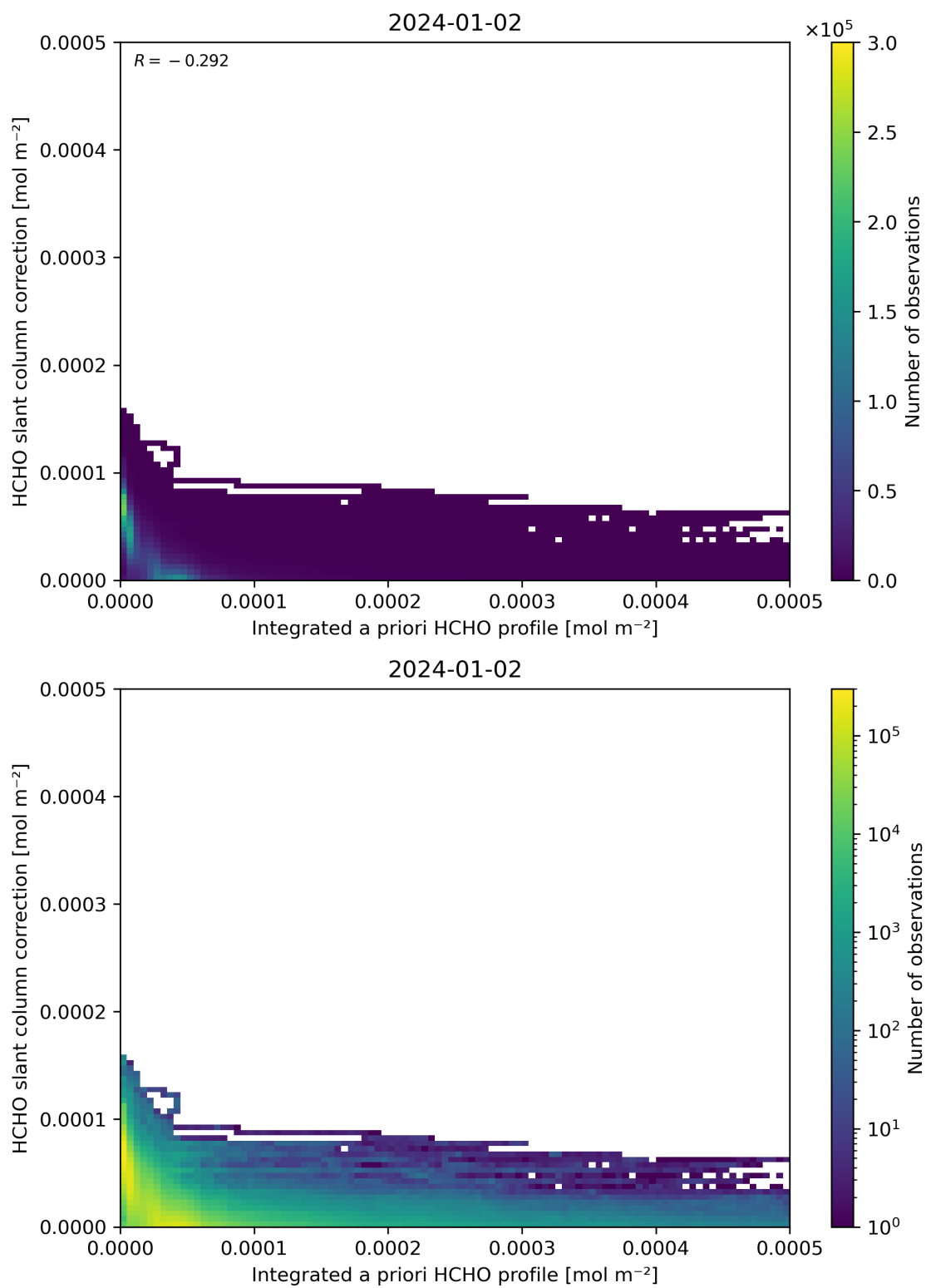
Figure 152: Scatter density plot of “Integrated a priori HCHO profile” against “HCHO slant column correction” for 2024-01-01 to 2024-01-03.
