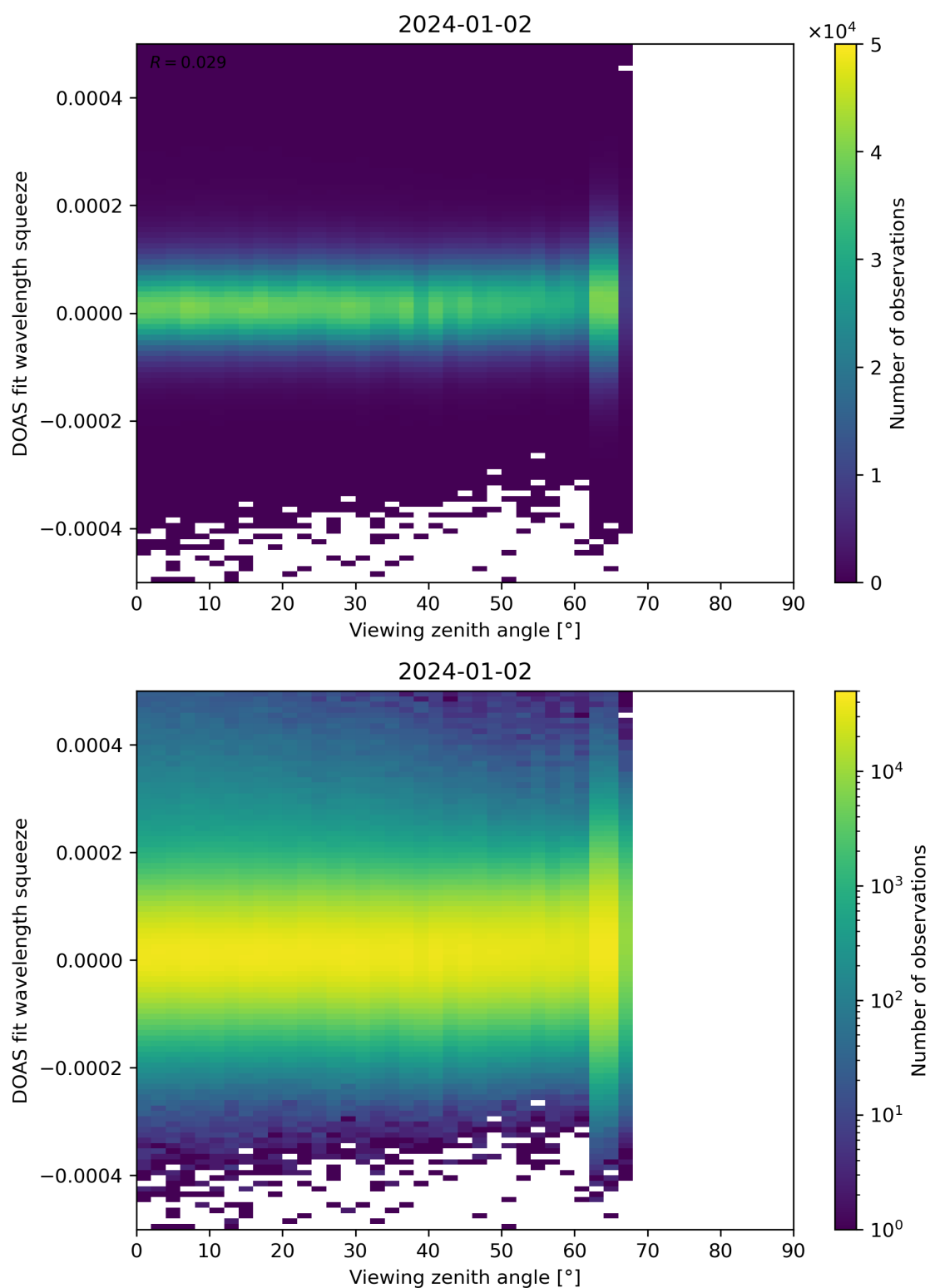
Figure 184: Scatter density plot of “Viewing zenith angle” against “DOAS fit wavelength squeeze” for 2024-01-01 to 2024-01-03.
