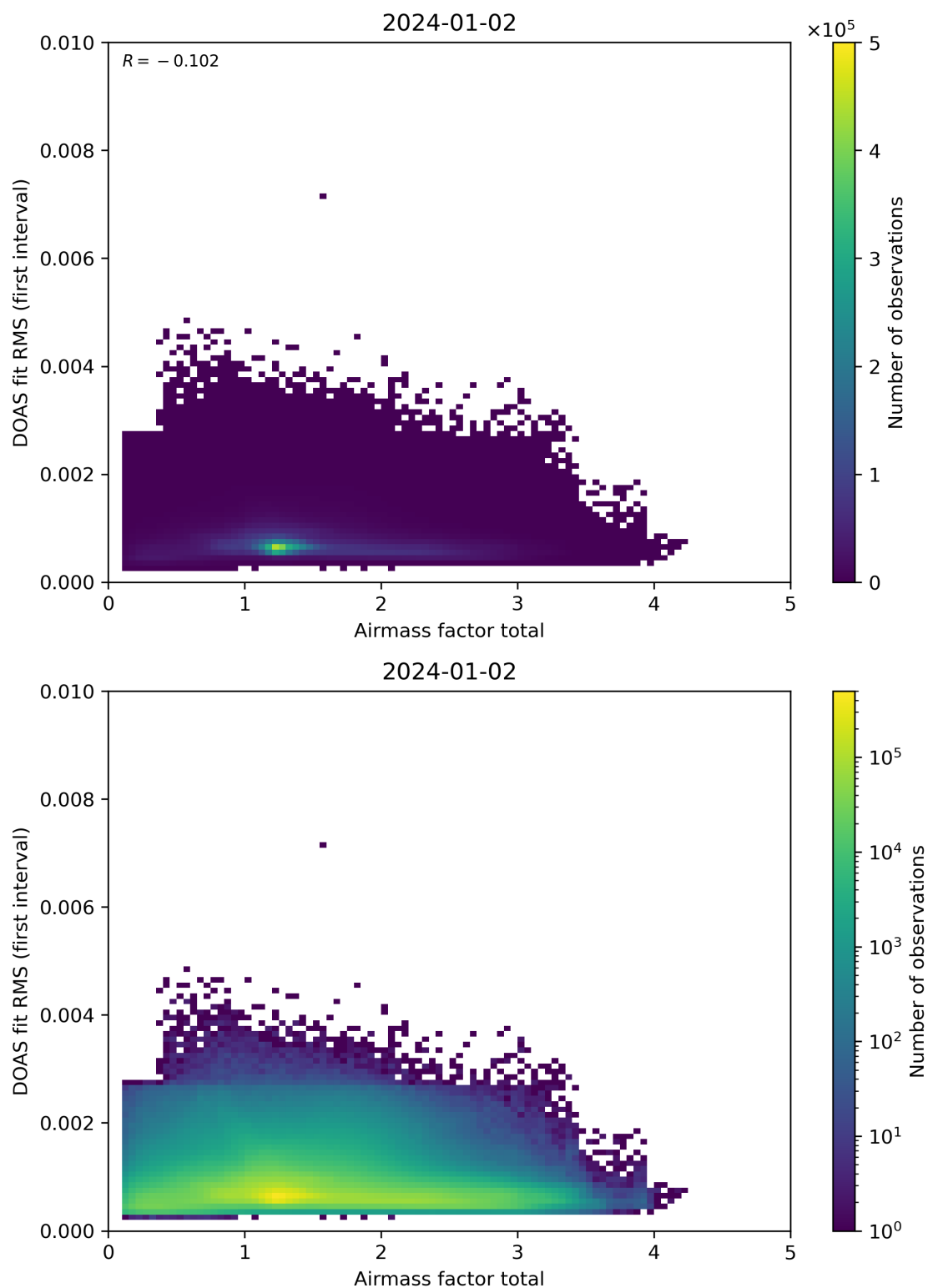
Figure 97: Scatter density plot of “Airmass factor total” against “DOAS fit RMS (first interval)” for 2024-01-01 to 2024-01-03.
