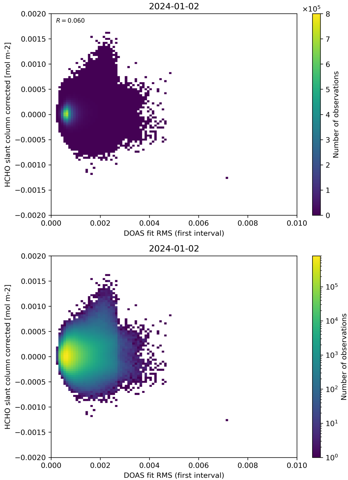
Figure 62: Scatter density plot of “DOAS fit RMS (first interval)” against “HCHO slant column corrected” for 2024-01-01 to 2024-01-03.
