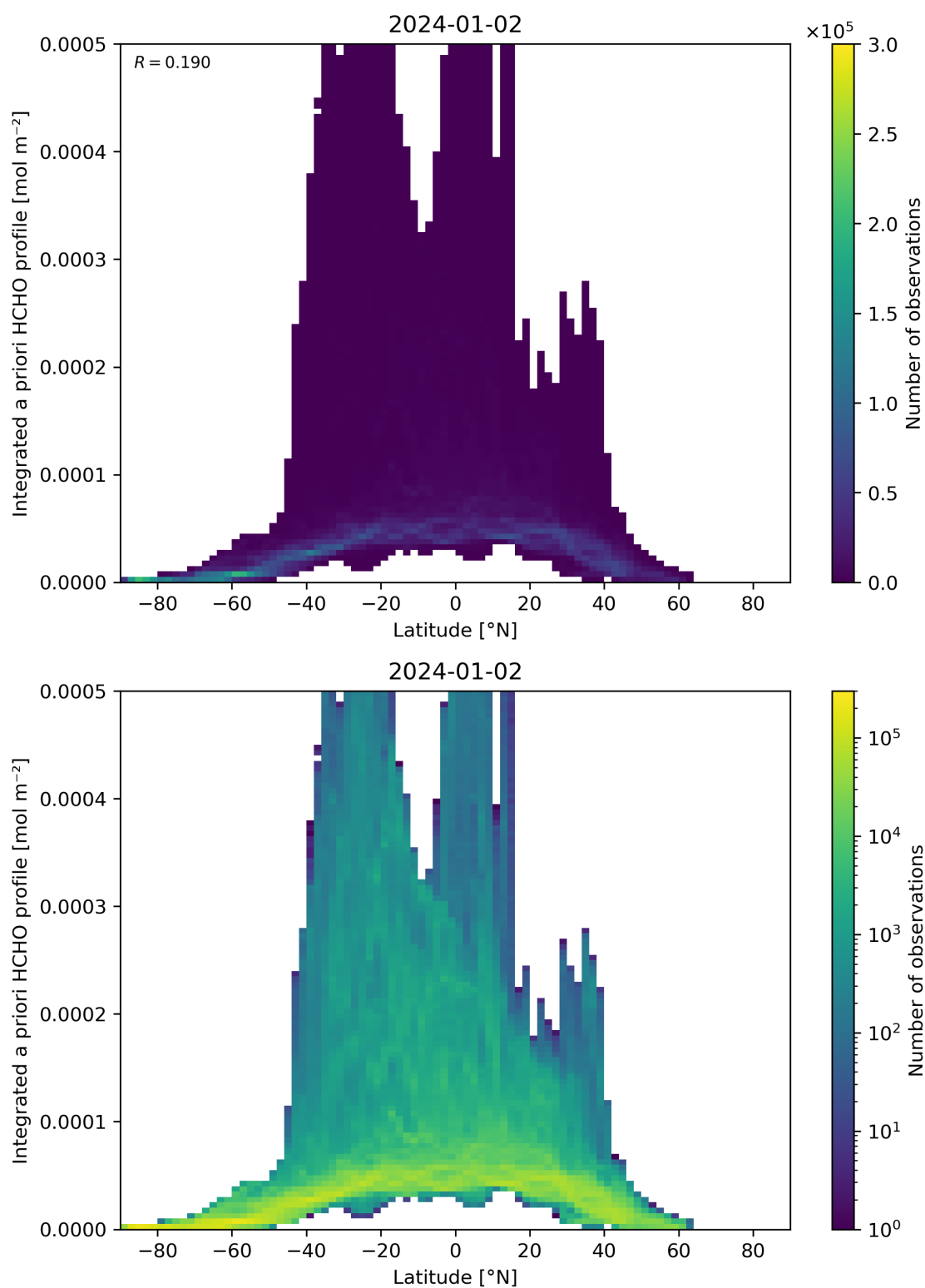
Figure 166: Scatter density plot of “Latitude” against “Integrated a priori HCHO profile” for 2024-01-01 to 2024-01-03.
