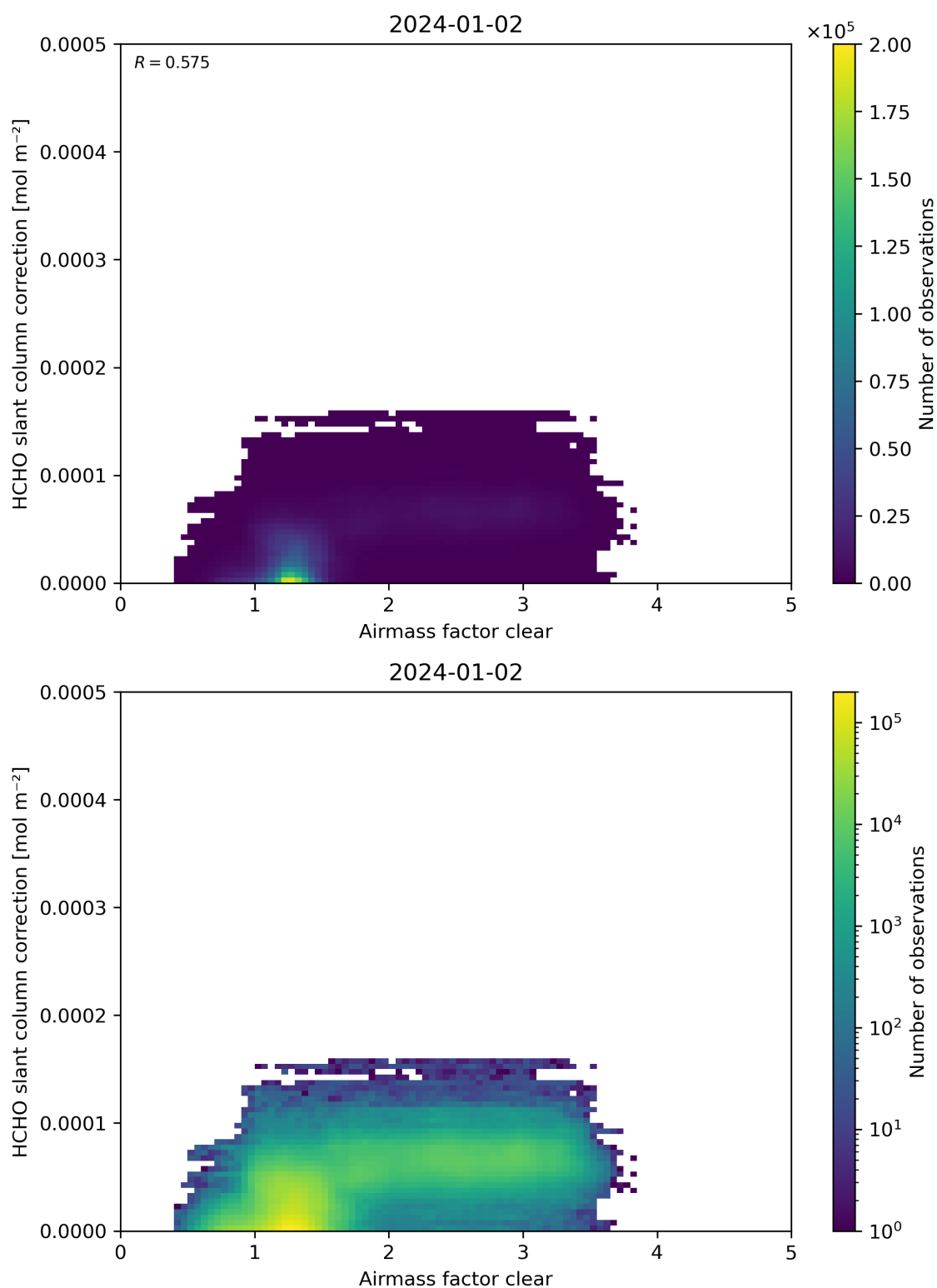
Figure 75: Scatter density plot of “Airmass factor clear” against “HCHO slant column correction” for 2024-01-01 to 2024-01-03.
