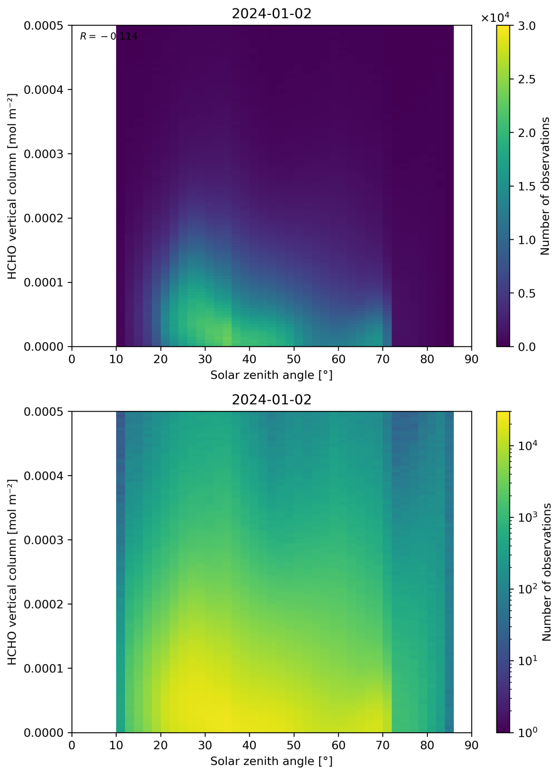
Figure 177: Scatter density plot of “Solar zenith angle” against “HCHO vertical column” for 2024-01-01 to 2024-01-03.
