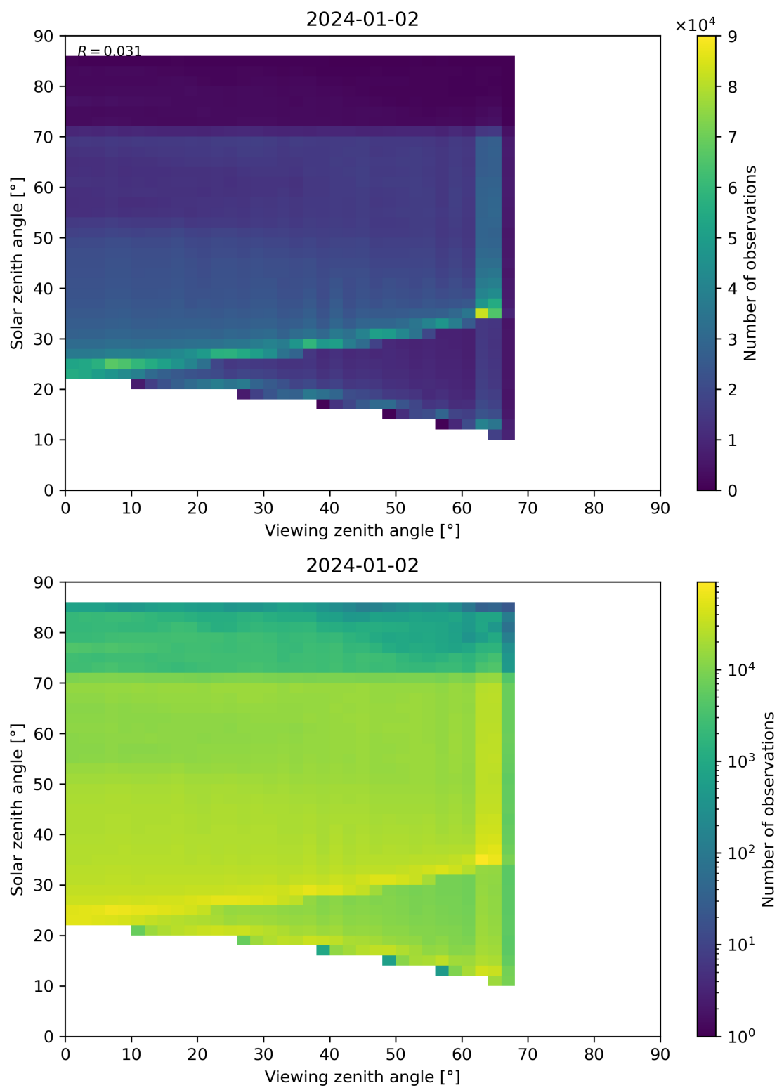
Figure 197: Scatter density plot of “Viewing zenith angle” against “Solar zenith angle” for 2024-01-01 to 2024-01-03.
