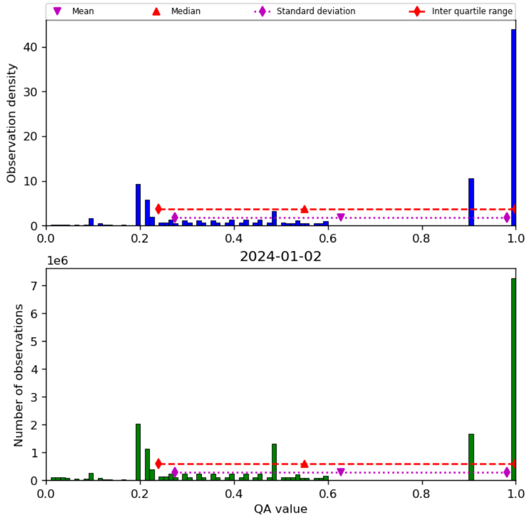
Figure 34: Histogram of “QA value” for 2024-01-01 to 2024-01-03
