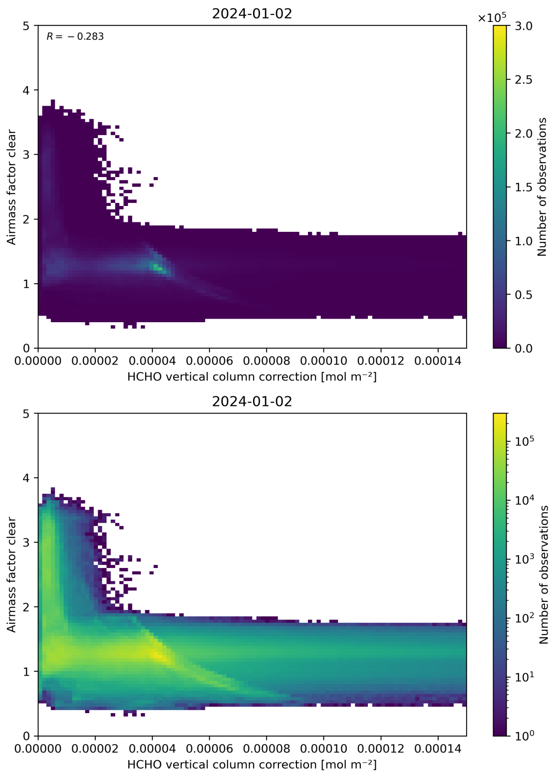
Figure 115: Scatter density plot of “HCHO vertical column correction” against “Airmass factor clear” for 2024-01-01 to 2024-01-03.
