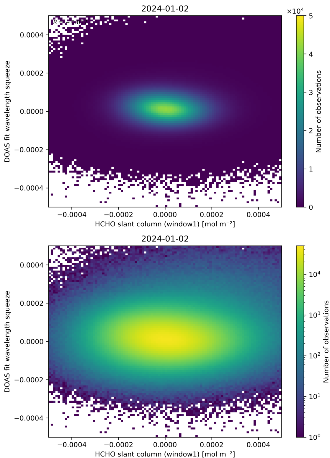
Figure 80: Scatter density plot of “HCHO slant column (window1)” against “DOAS fit wavelength squeeze” for 2024-01-01 to 2024-01-03.
