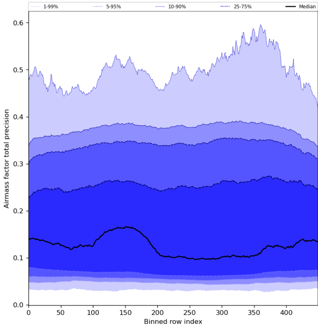
Figure 55: Along track statistics of “Airmass factor total precision” for 2024-01-01 to 2024-01-03
