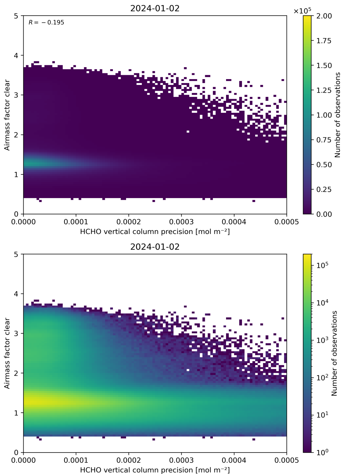
Figure 139: Scatter density plot of “HCHO vertical column precision” against “Airmass factor clear” for 2024-01-01 to 2024-01-03.
