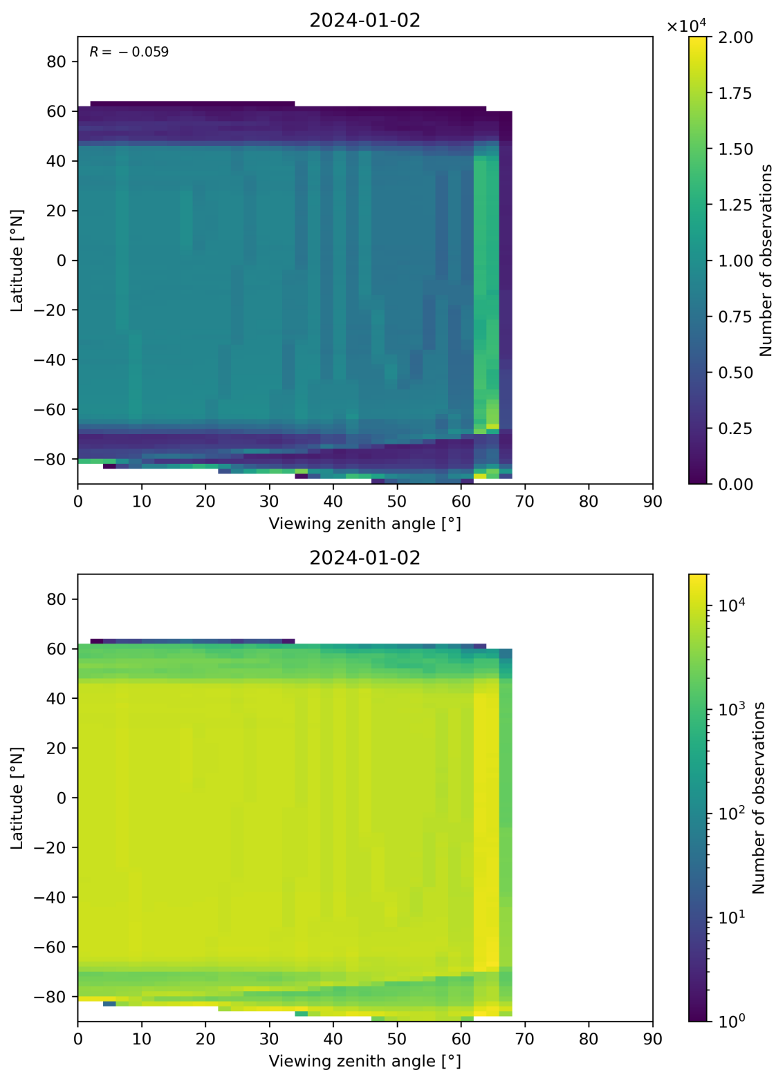
Figure 196: Scatter density plot of “Viewing zenith angle” against “Latitude” for 2024-01-01 to 2024-01-03.
