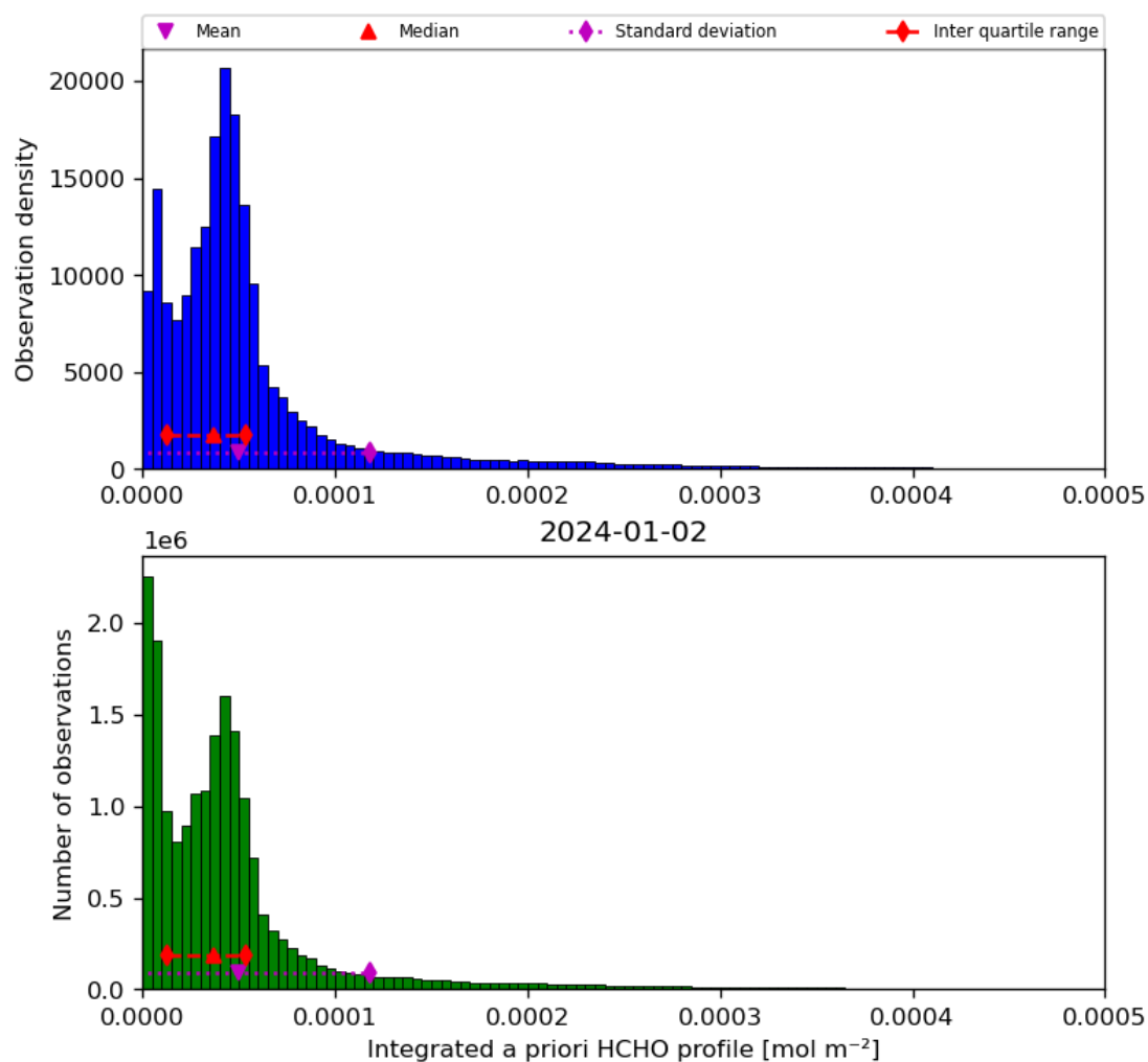
Figure 43: Histogram of “Integrated a priori HCHO profile” for 2024-01-01 to 2024-01-03
