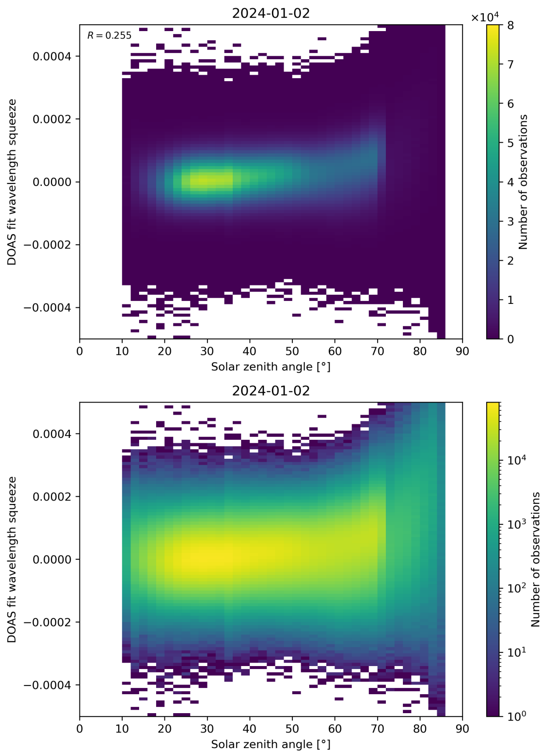
Figure 169: Scatter density plot of “Solar zenith angle” against “DOAS fit wavelength squeeze” for 2024-01-01 to 2024-01-03.
