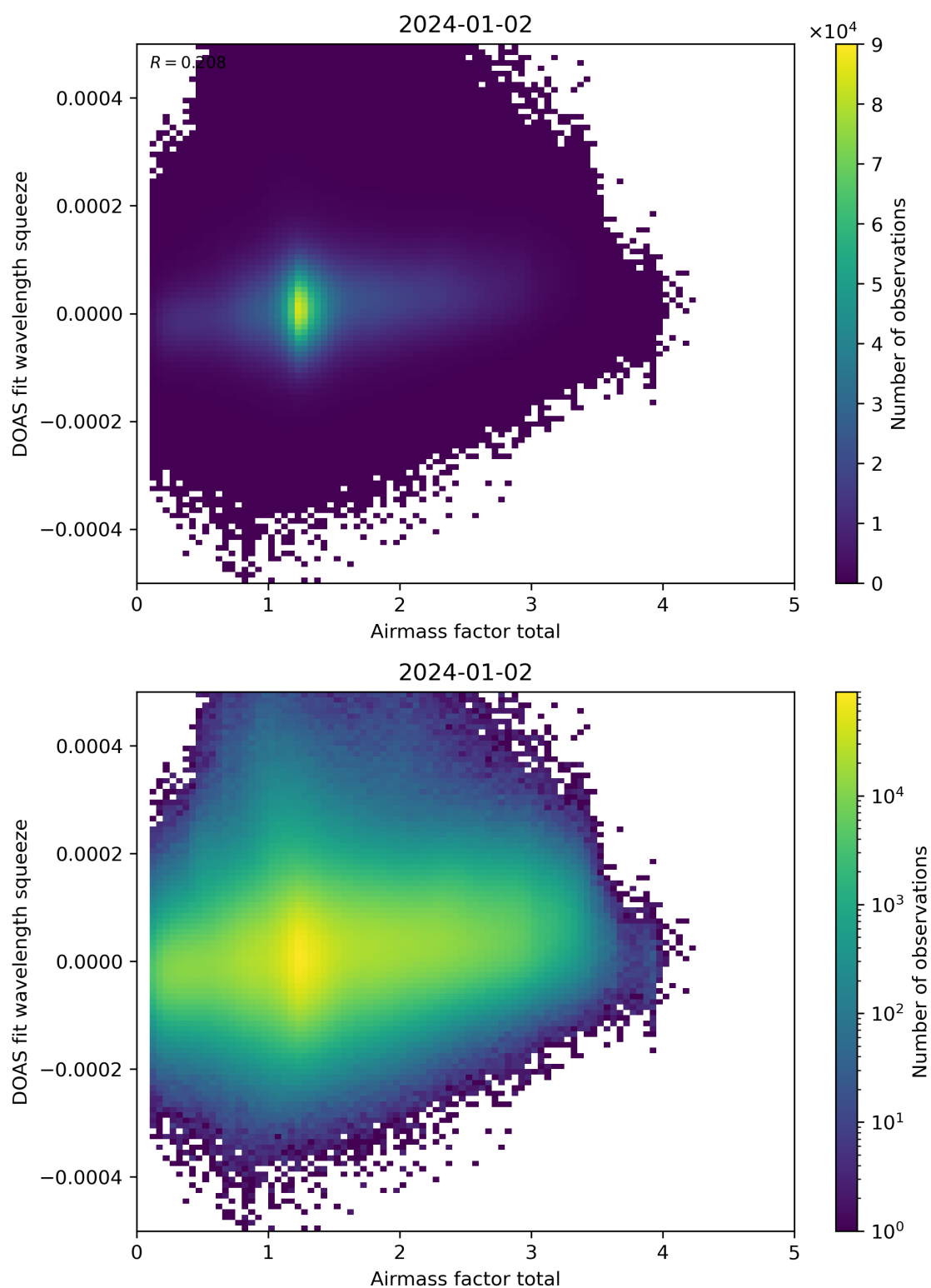
Figure 99: Scatter density plot of “Airmass factor total” against “DOAS fit wavelength squeeze” for 2024-01-01 to 2024-01-03.
