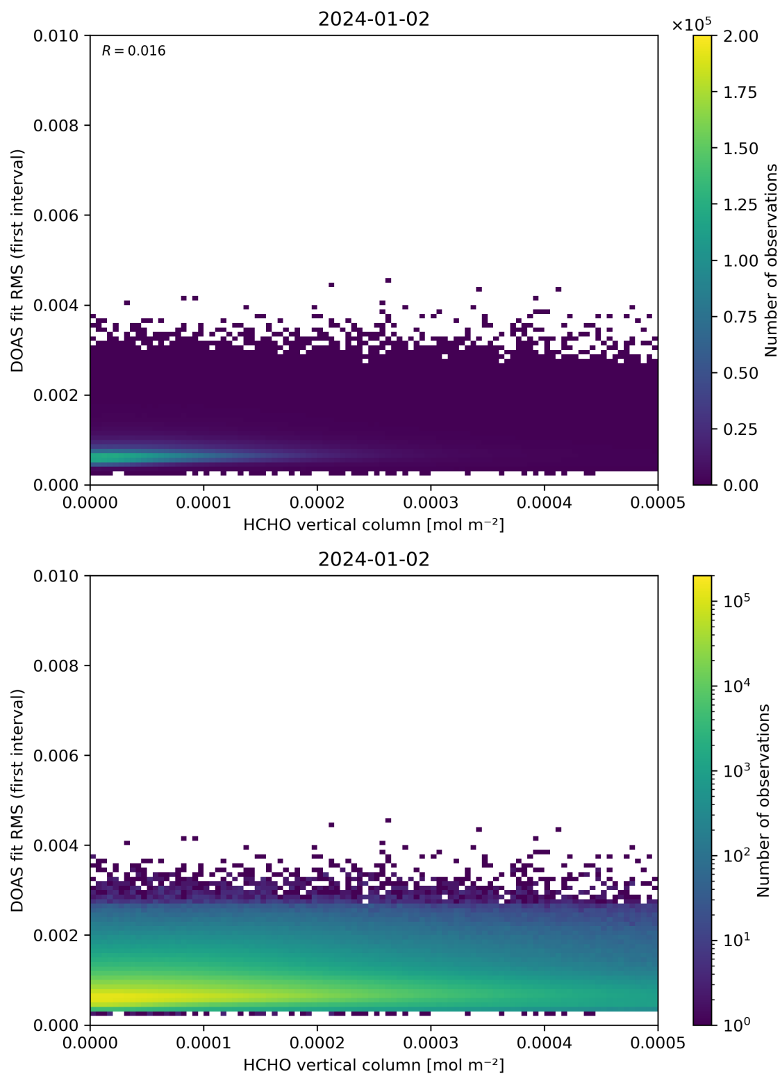
Figure 123: Scatter density plot of “HCHO vertical column” against “DOAS fit RMS (first interval)” for 2024-01-01 to 2024-01-03.
