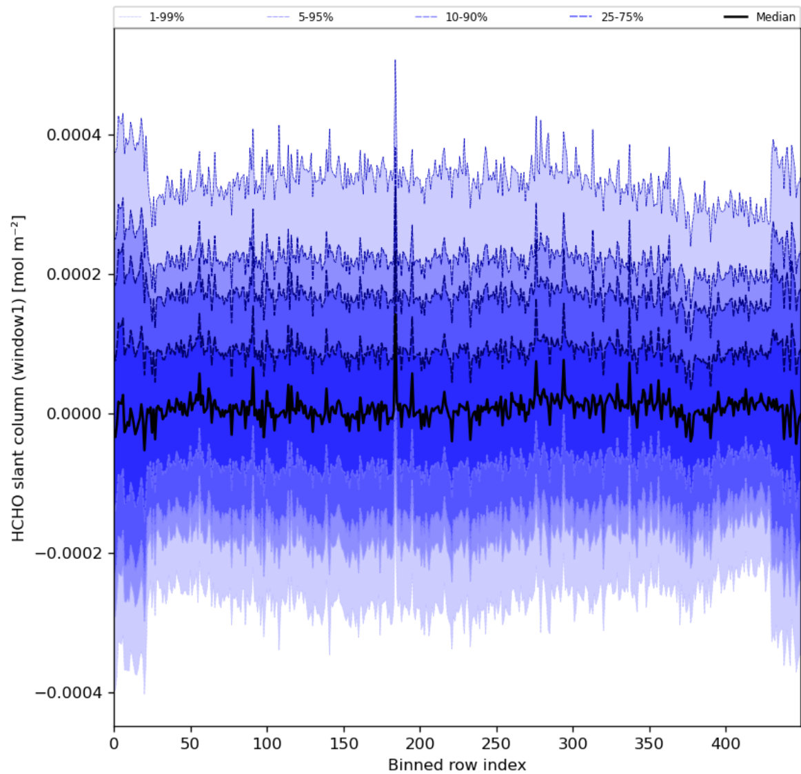
Figure 52: Along track statistics of “HCHO slant column (window1)” for 2024-01-01 to 2024-01-03
