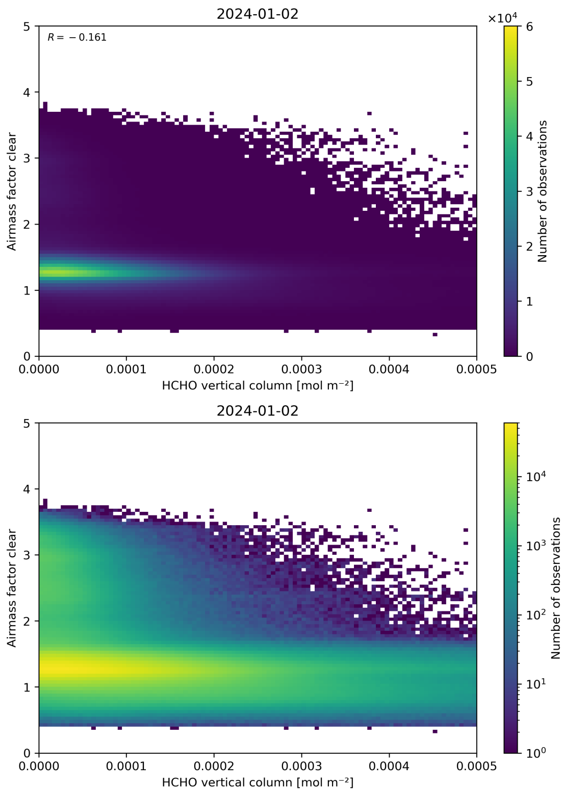
Figure 126: Scatter density plot of “HCHO vertical column” against “Airmass factor clear” for 2024-01-01 to 2024-01-03.
