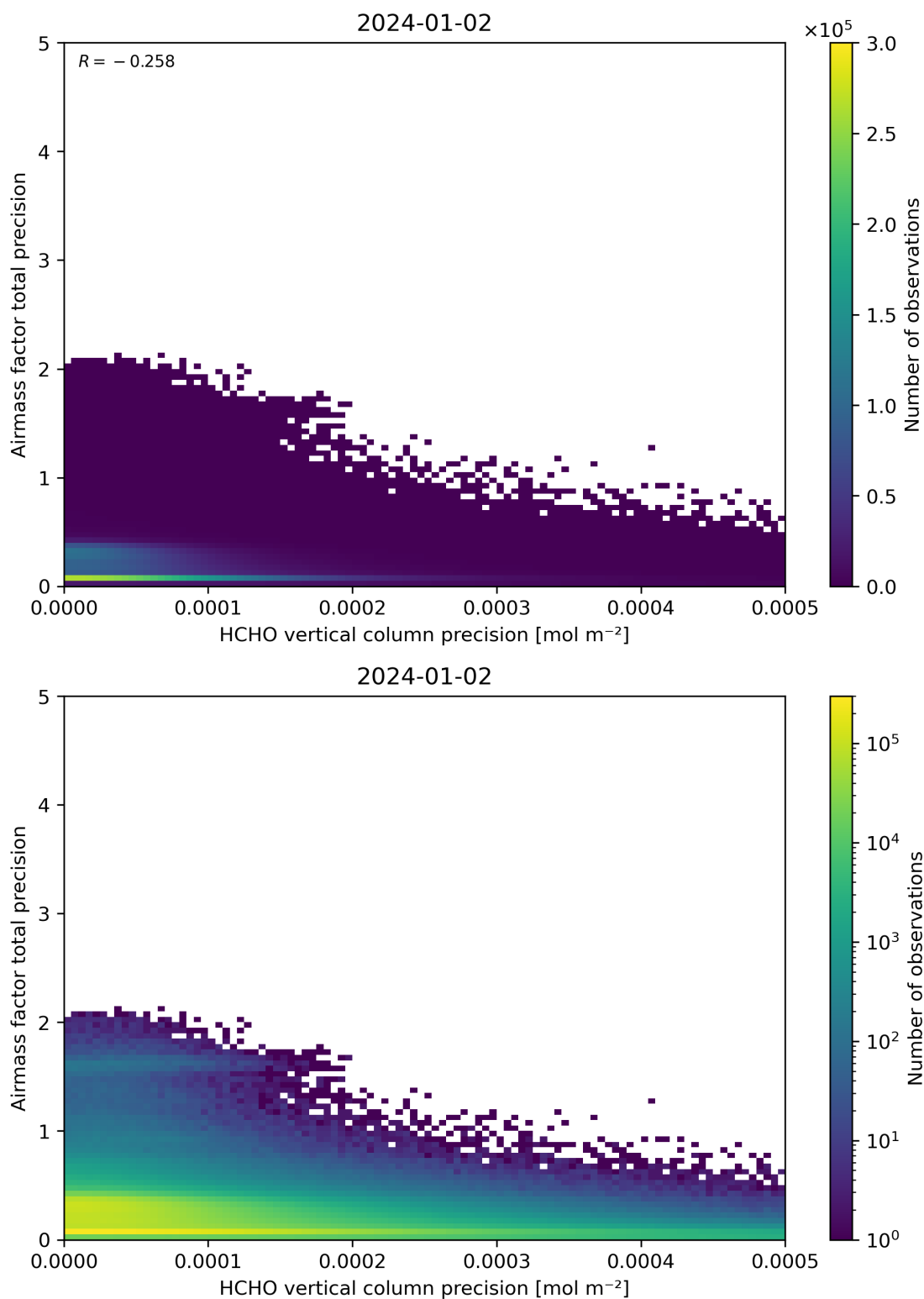
Figure 145: Scatter density plot of “HCHO vertical column precision” against “Airmass factor total precision” for 2024-01-01 to 2024-01-03.
