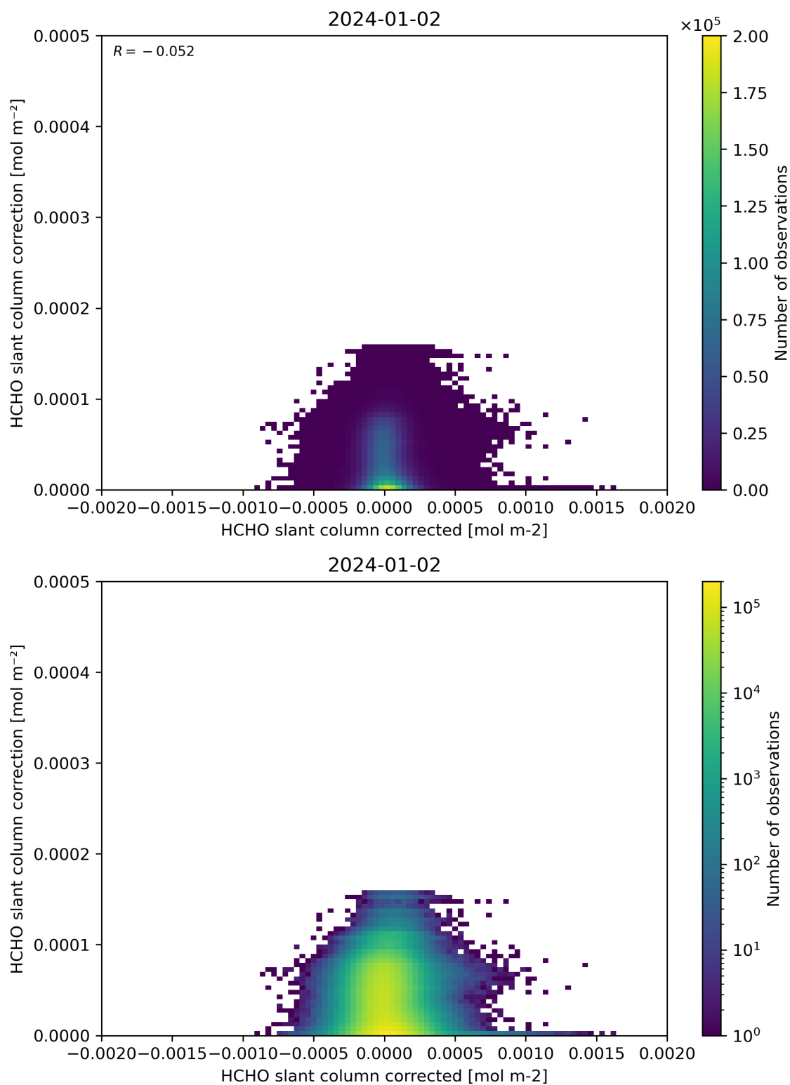
Figure 77: Scatter density plot of “HCHO slant column corrected” against “HCHO slant column correction” for 2024-01-01 to 2024-01-03.
