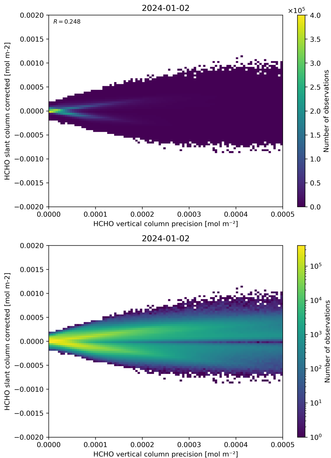
Figure 140: Scatter density plot of “HCHO vertical column precision” against “HCHO slant column corrected” for 2024-01-01 to 2024-01-03.
