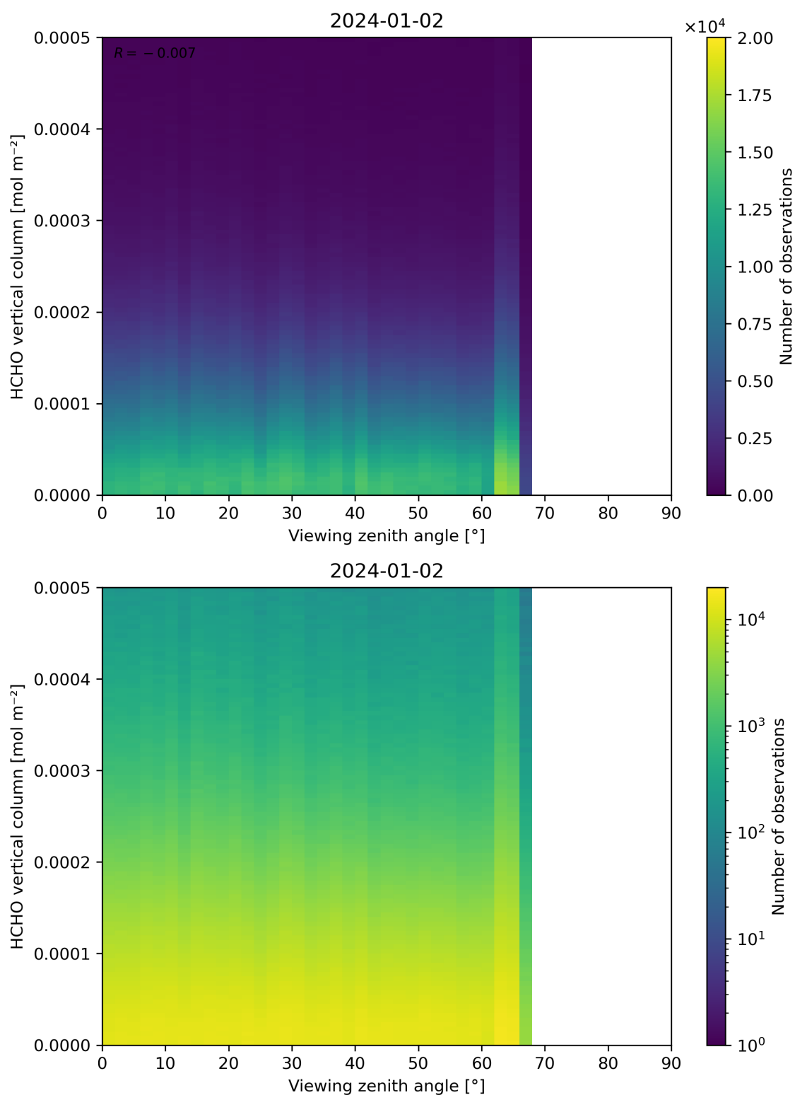
Figure 192: Scatter density plot of “Viewing zenith angle” against “HCHO vertical column” for 2024-01-01 to 2024-01-03.
