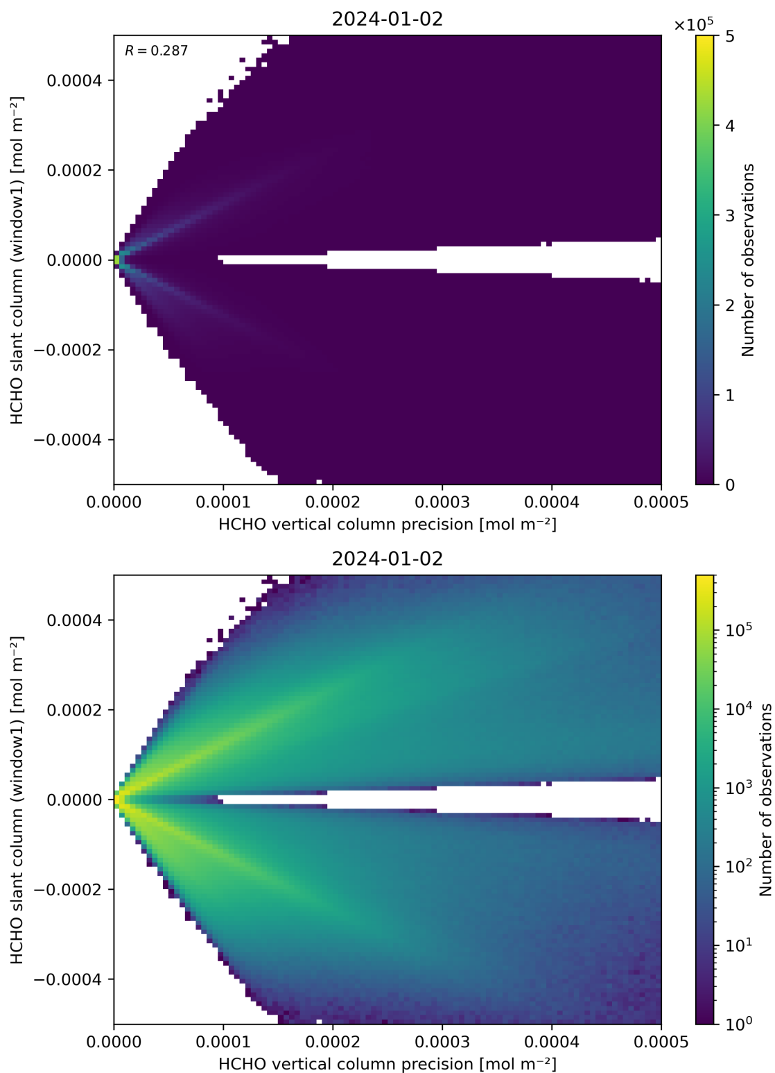
Figure 142: Scatter density plot of “HCHO vertical column precision” against “HCHO slant column (window1)” for 2024-01-01 to 2024-01-03.
