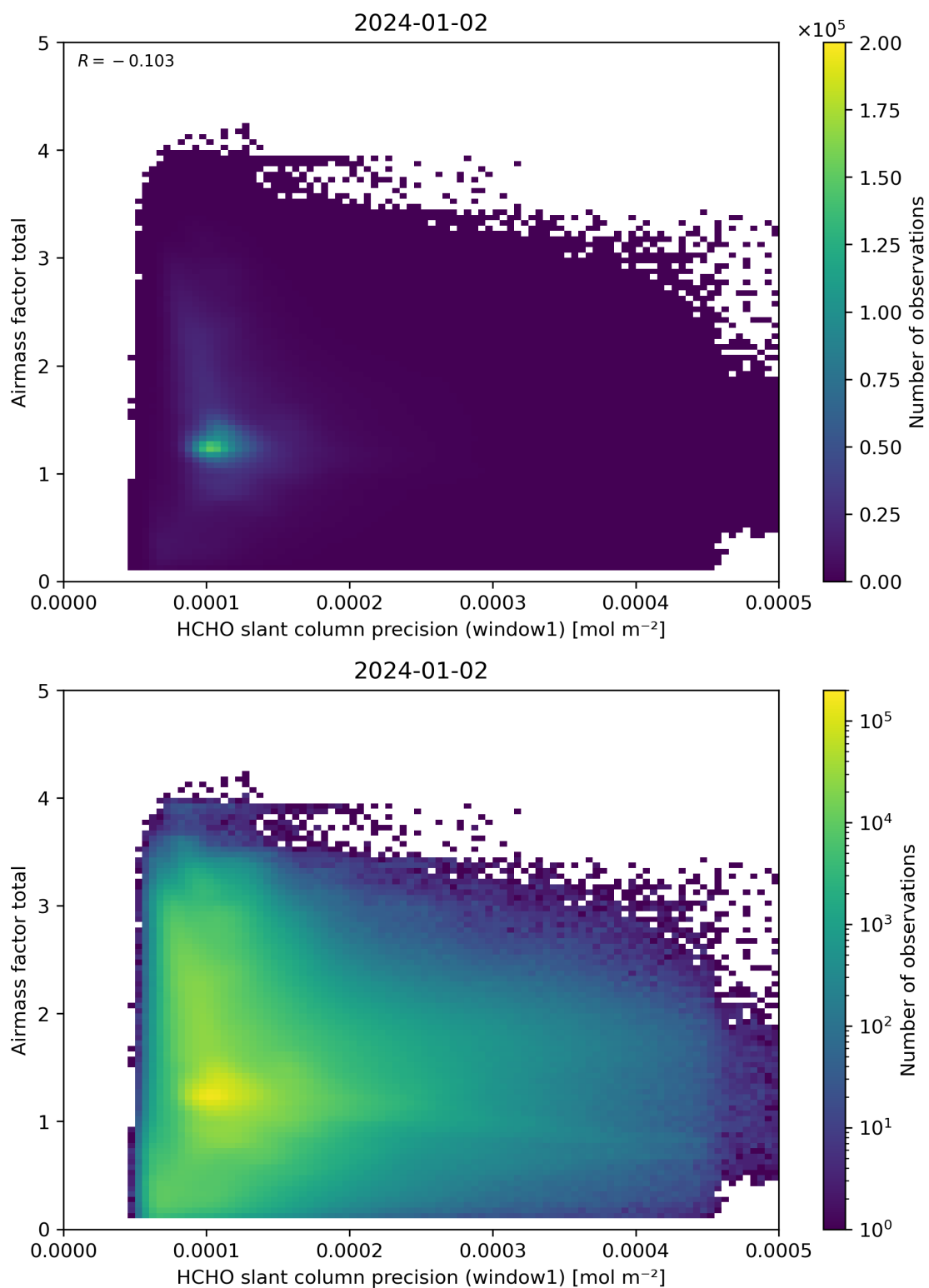
Figure 94: Scatter density plot of “HCHO slant column precision (window1)” against “Airmass factor total” for 2024-01-01 to 2024-01-03.
