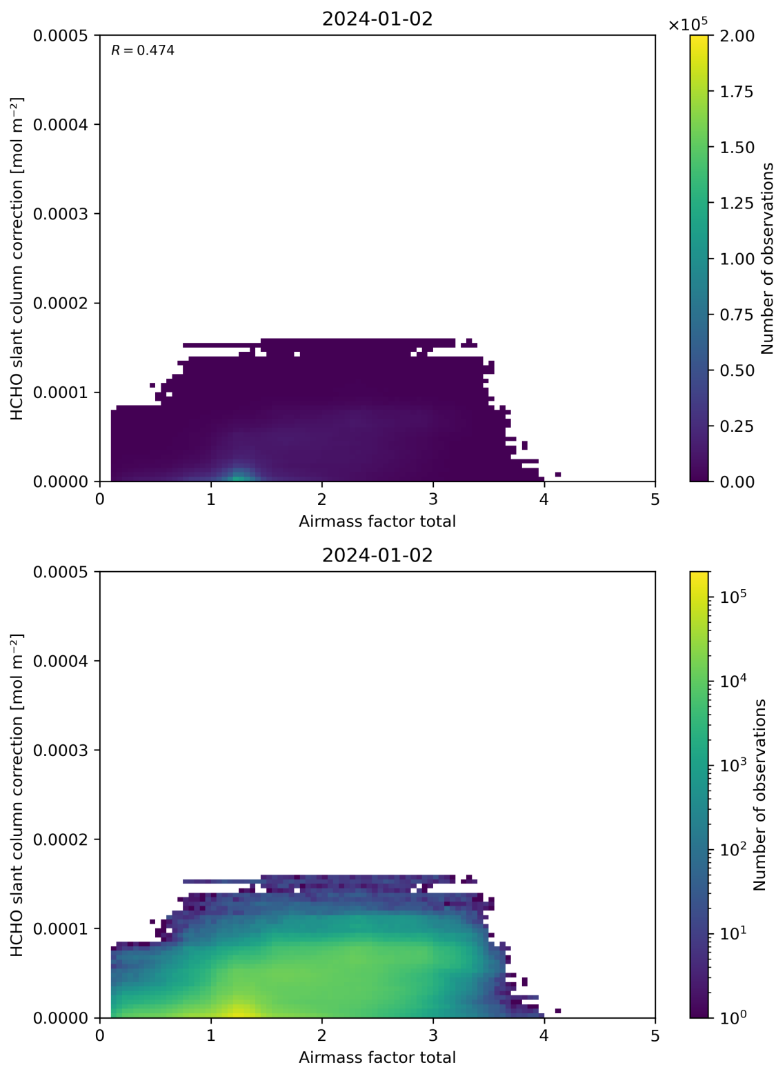
Figure 102: Scatter density plot of “Airmass factor total” against “HCHO slant column correction” for 2024-01-01 to 2024-01-03.
