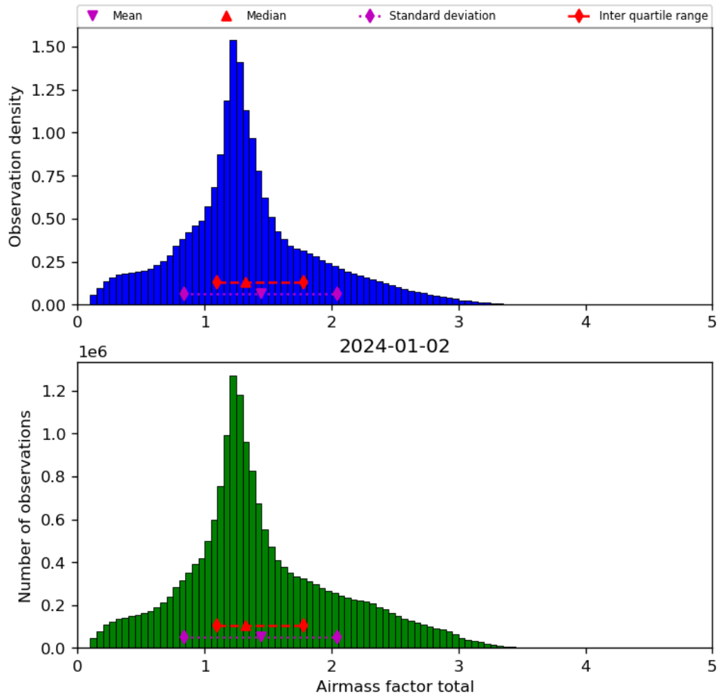
Figure 40: Histogram of “Airmass factor total” for 2024-01-01 to 2024-01-03
