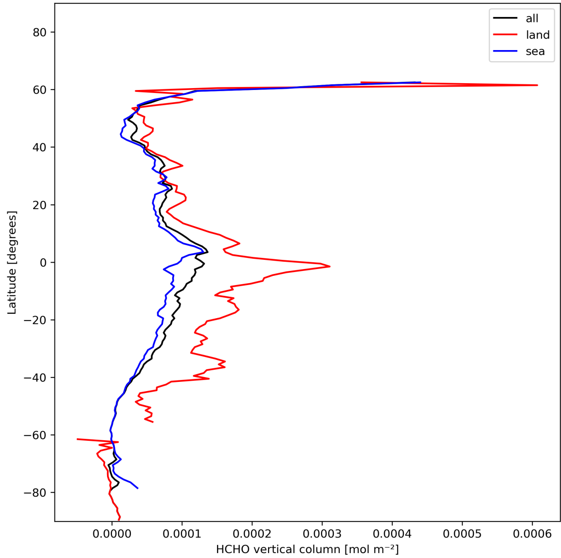
Figure 21: Zonal average of “HCHO vertical column” for 2024-01-01 to 2024-01-03.
