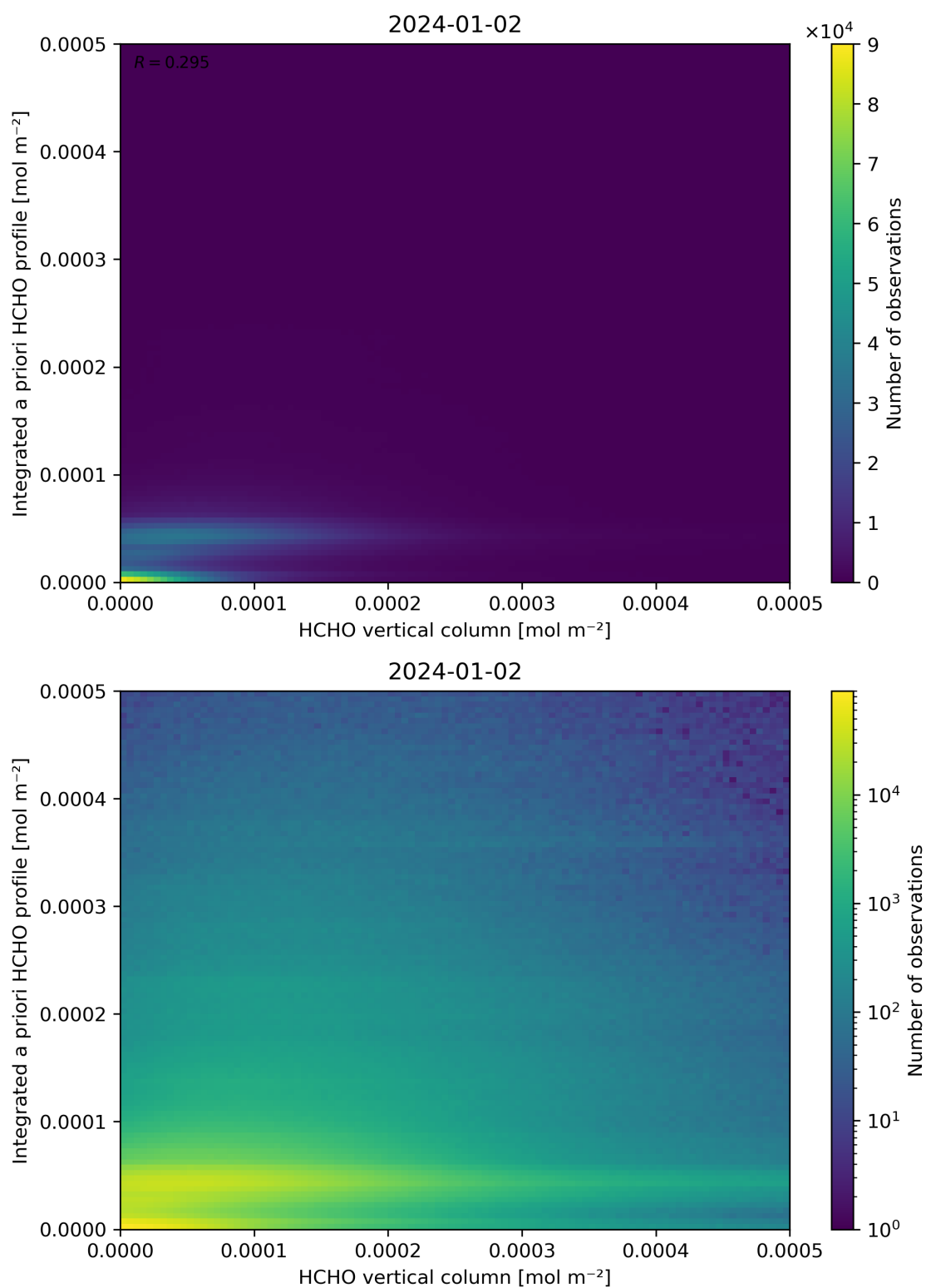
Figure 135: Scatter density plot of “HCHO vertical column” against “Integrated a priori HCHO profile” for 2024-01-01 to 2024-01-03.
