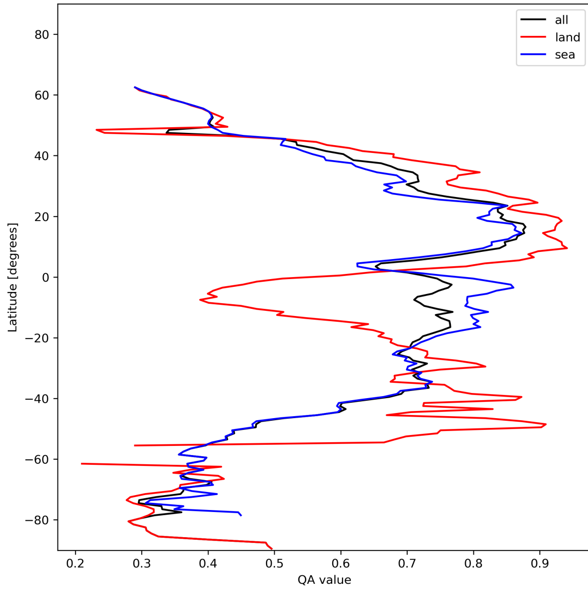
Figure 20: Zonal average of “QA value” for 2024-01-01 to 2024-01-03.
