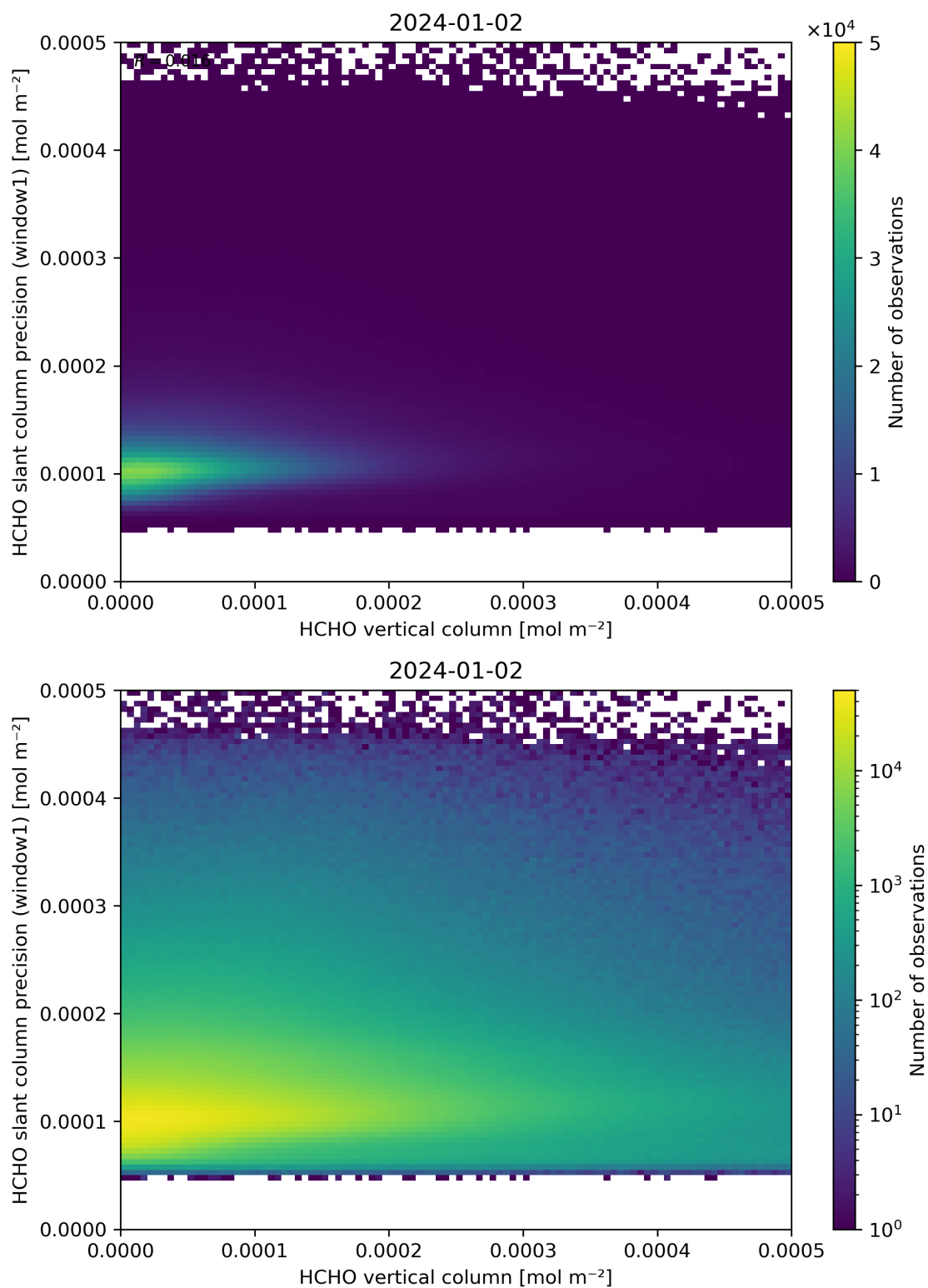
Figure 130: Scatter density plot of “HCHO vertical column” against “HCHO slant column precision (window1)” for 2024-01-01 to 2024-01-03.
