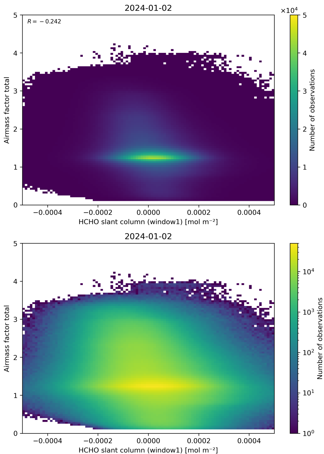
Figure 85: Scatter density plot of “HCHO slant column (window1)” against “Airmass factor total” for 2024-01-01 to 2024-01-03.
