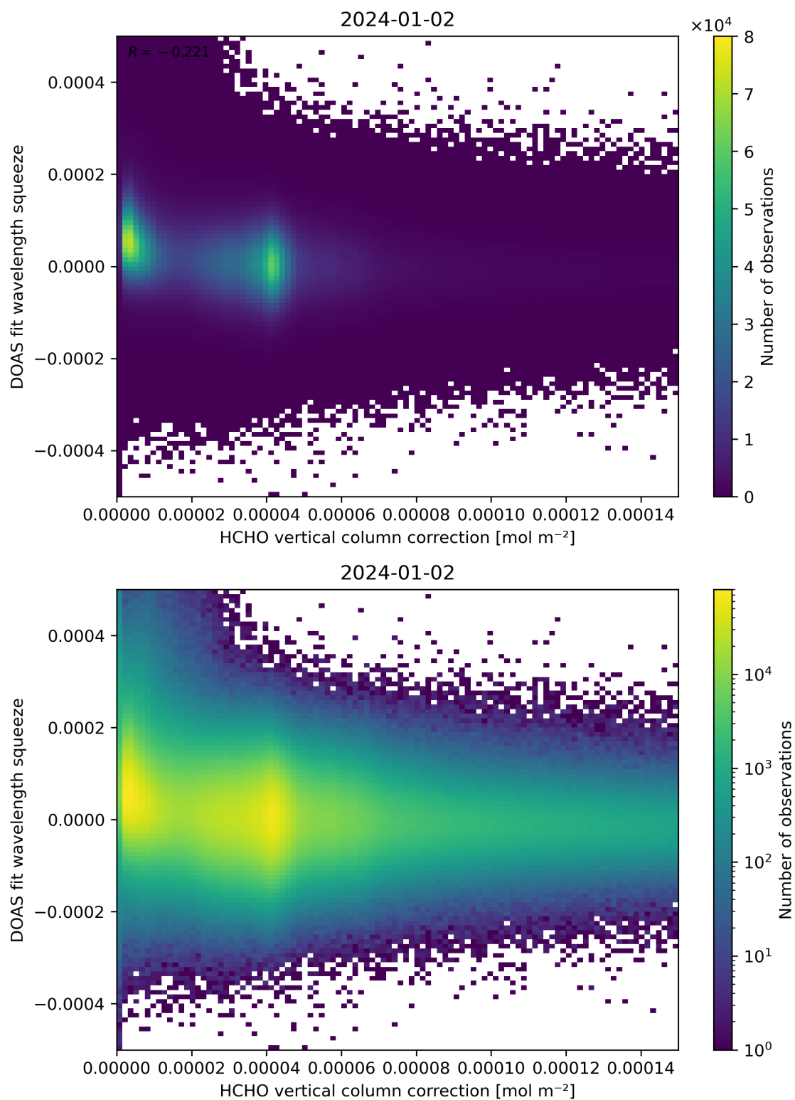
Figure 114: Scatter density plot of “HCHO vertical column correction” against “DOAS fit wavelength squeeze” for 2024-01-01 to 2024-01-03.
