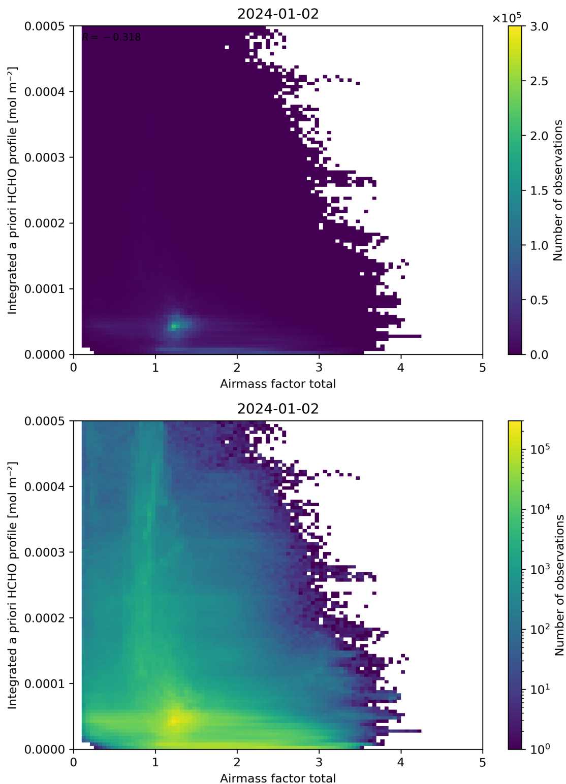
Figure 104: Scatter density plot of “Air mass factor total” against “Integrated a priori HCHO profile” for 2024-01-01 to 2024-01-03.
