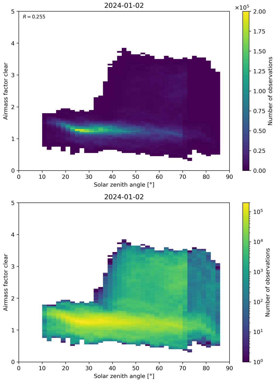
Figure 170: Scatter density plot of “Solar zenith angle” against “Airmass factor clear” for 2024-01-01 to 2024-01-03.
