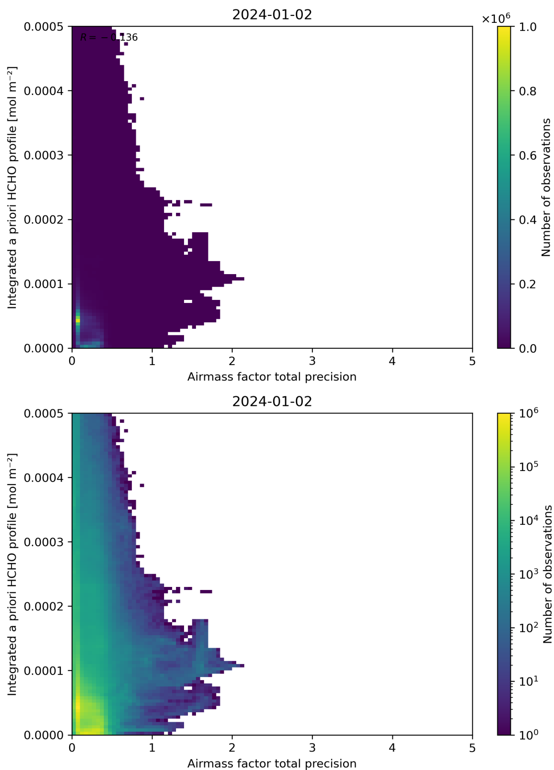
Figure 111: Scatter density plot of “Airmass factor total precision” against “Integrated a priori HCHO profile” for 2024-01-01 to 2024-01-03.
