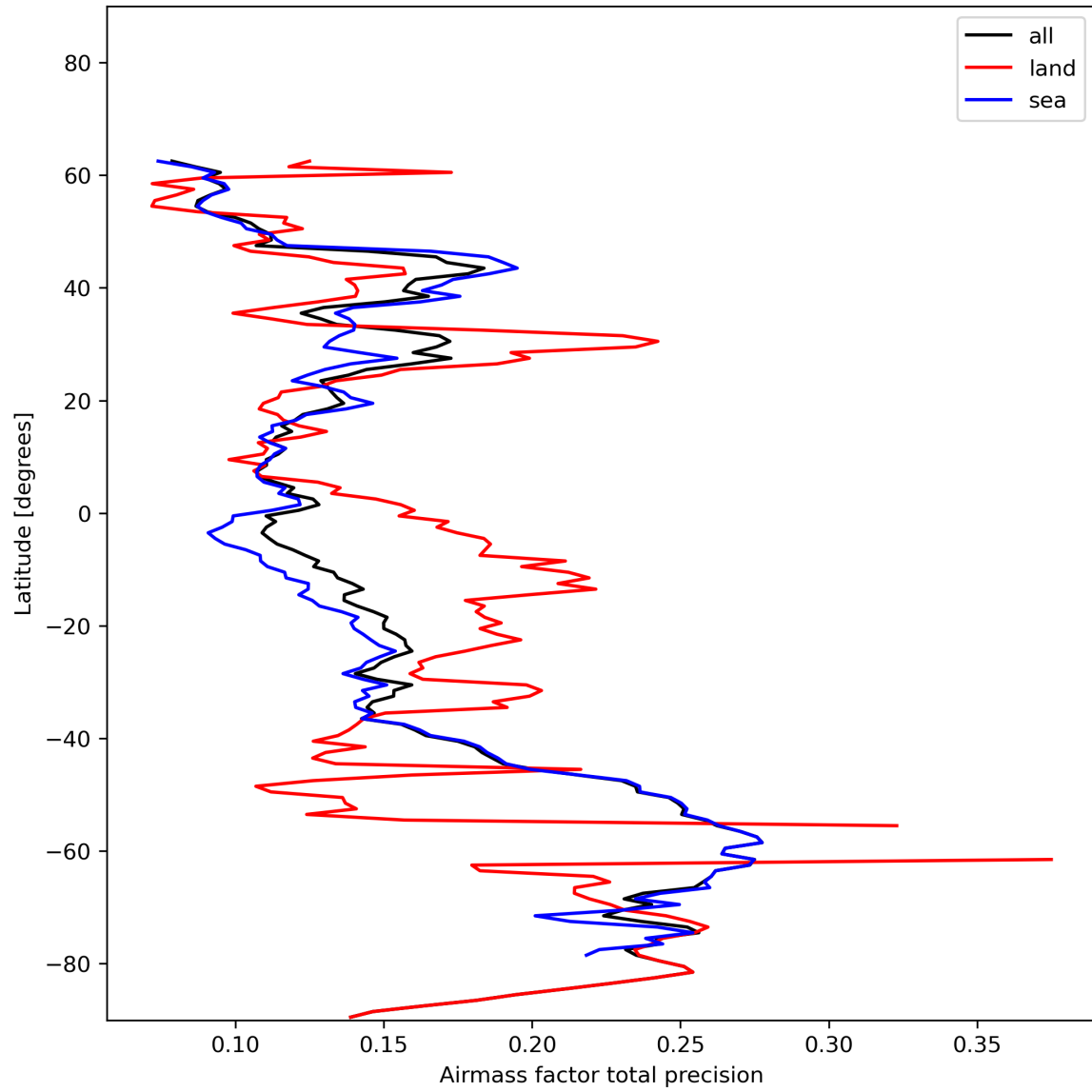
Figure 27: Zonal average of “Airmass factor total precision” for 2024-01-01 to 2024-01-03.
