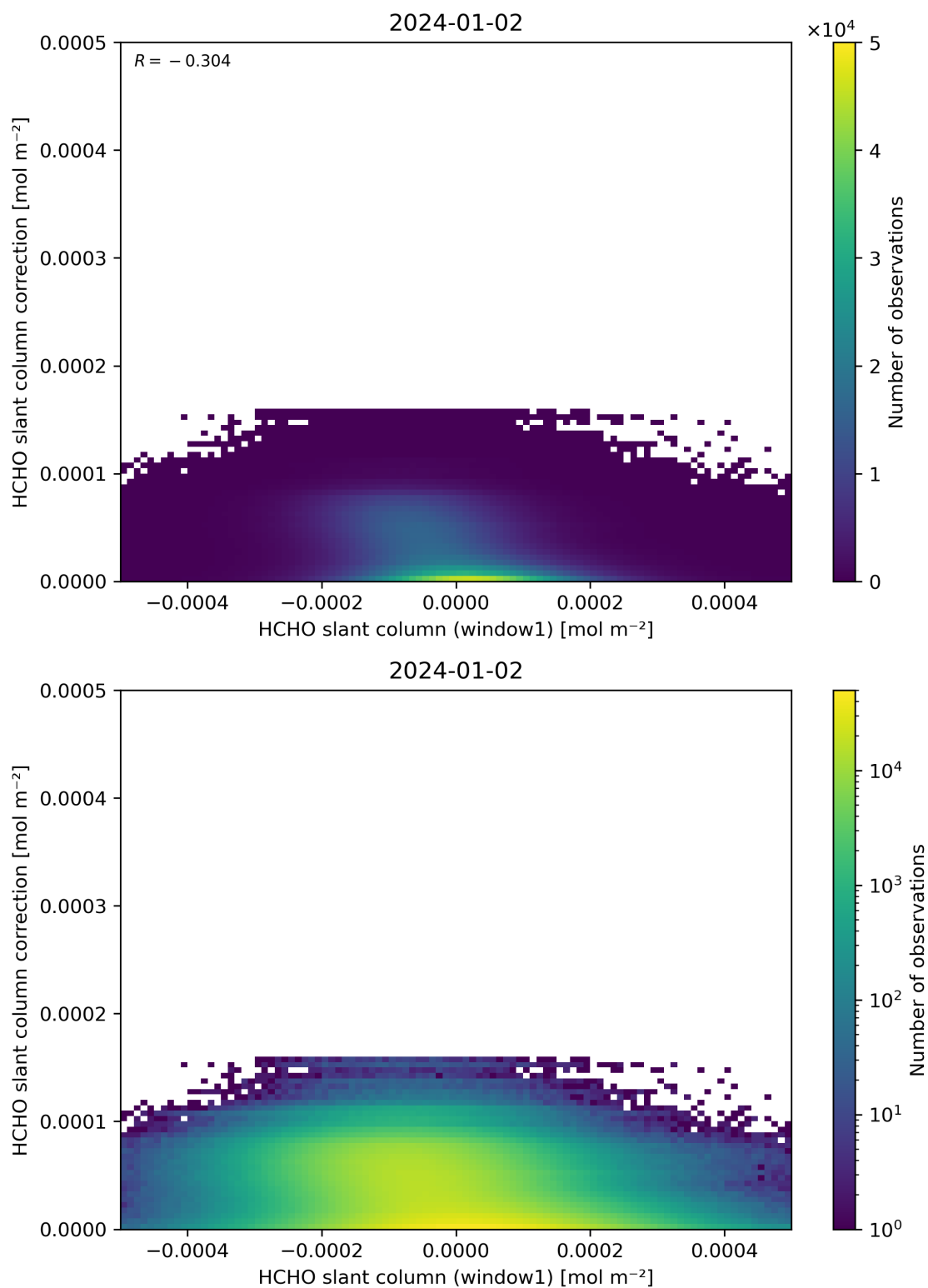
Figure 83: Scatter density plot of “HCHO slant column (window1)” against “HCHO slant column correction” for 2024-01-01 to 2024-01-03.
