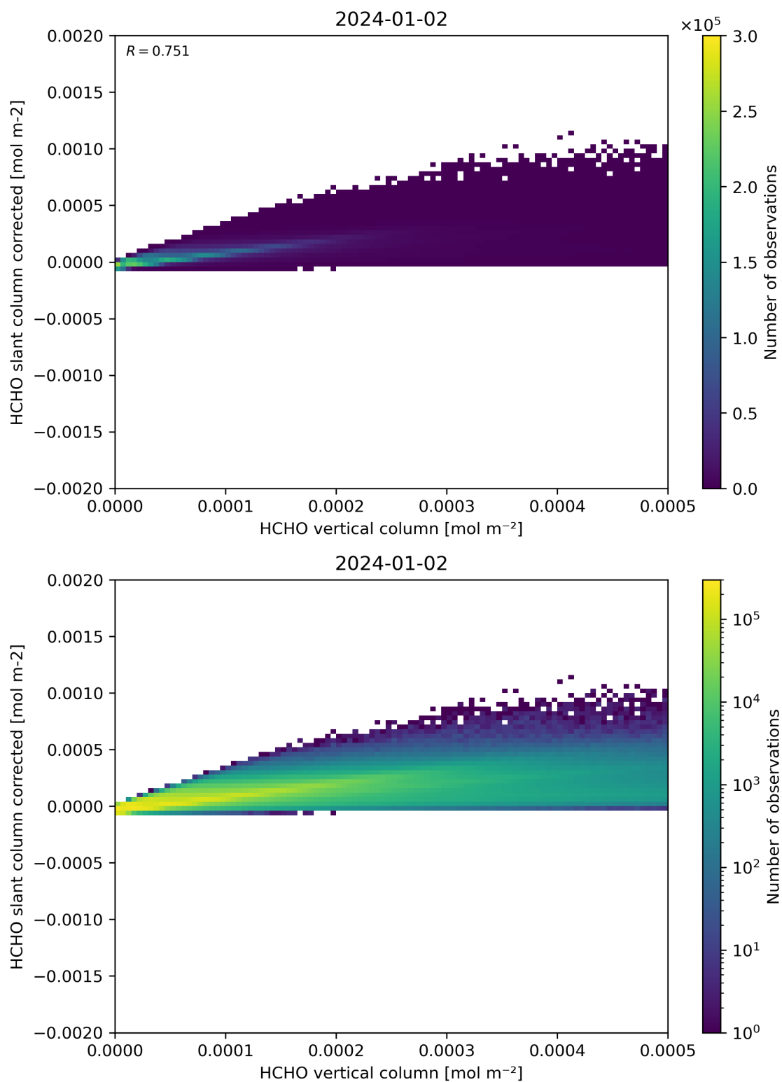
Figure 127: Scatter density plot of “HCHO vertical column” against “HCHO slant column corrected” for 2024-01-01 to 2024-01-03.
