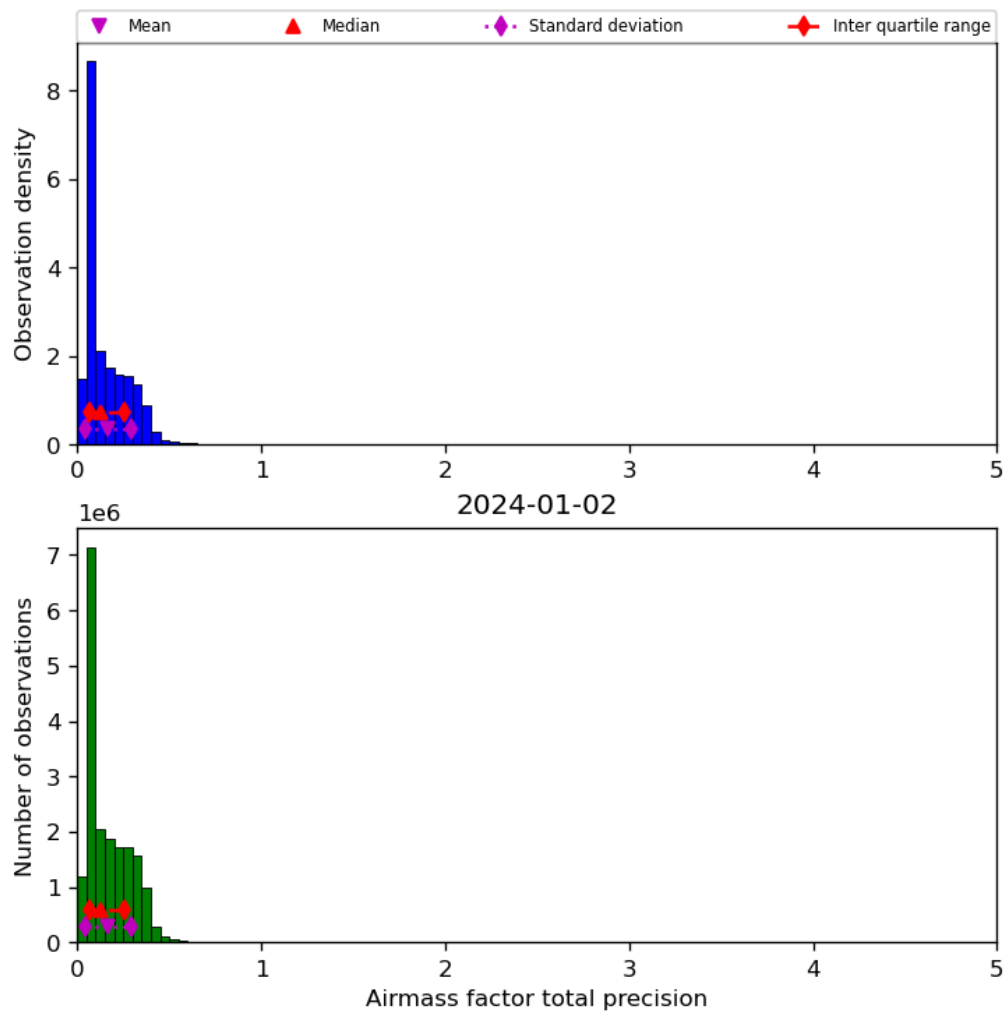
Figure 41: Histogram of “Airmass factor total precision” for 2024-01-01 to 2024-01-03
