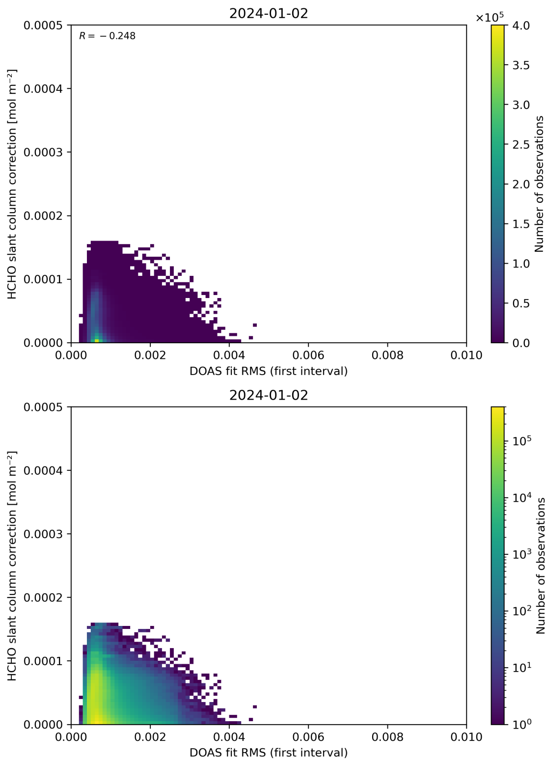
Figure 63: Scatter density plot of “DOAS fit RMS (first interval)” against “HCHO slant column correction” for 2024-01-01 to 2024-01-03.
