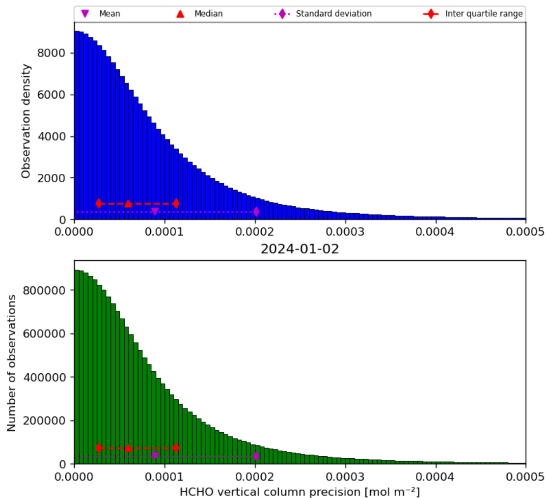
Figure 36: Histogram of “HCHO vertical column precision” for 2024-01-01 to 2024-01-03
