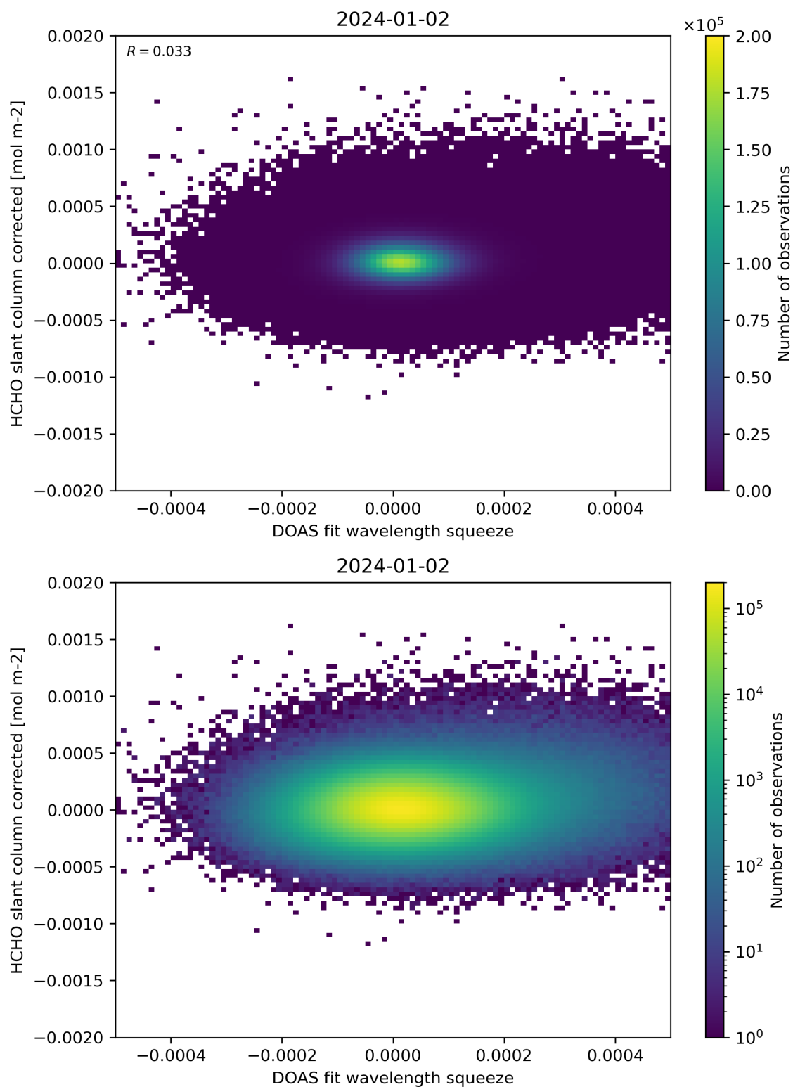
Figure 69: Scatter density plot of “DOAS fit wavelength squeeze” against “HCHO slant column corrected” for 2024-01-01 to 2024-01-03.
