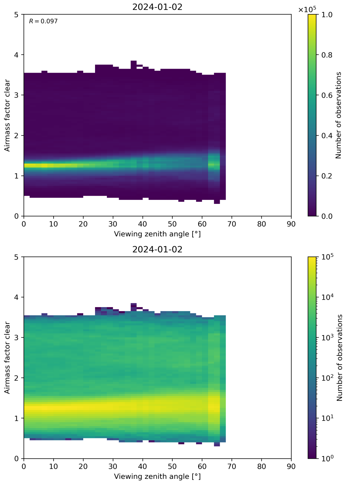
Figure 185: Scatter density plot of “Viewing zenith angle” against “Airmass factor clear” for 2024-01-01 to 2024-01-03.
