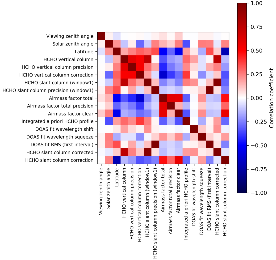
Figure 2: Map of correlation matrix for 2024-01-01 to 2024-01-03.
