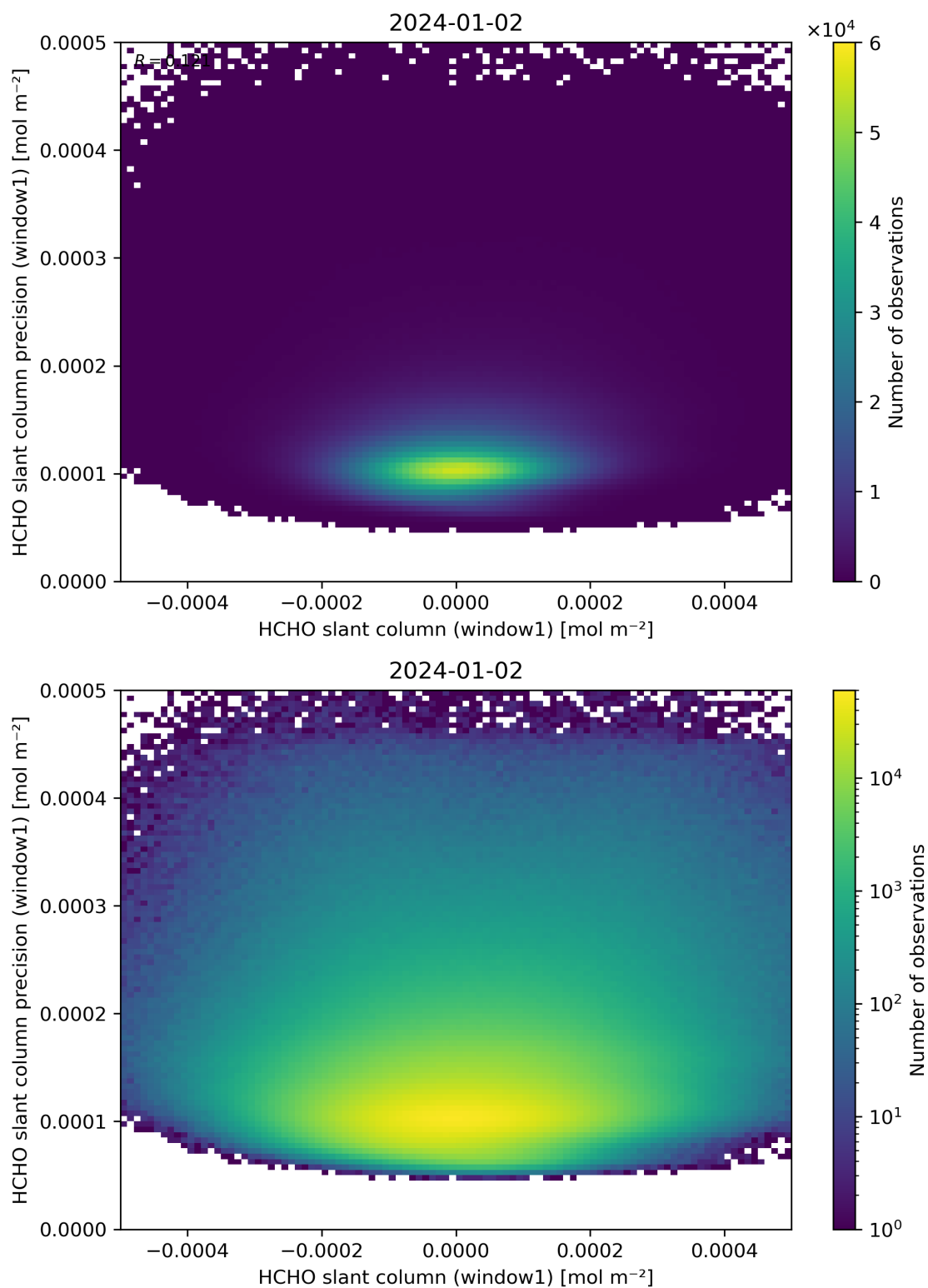
Figure 84: Scatter density plot of “HCHO slant column (window1)” against “HCHO slant column precision (window1)” for 2024-01-01 to 2024-01-03.
