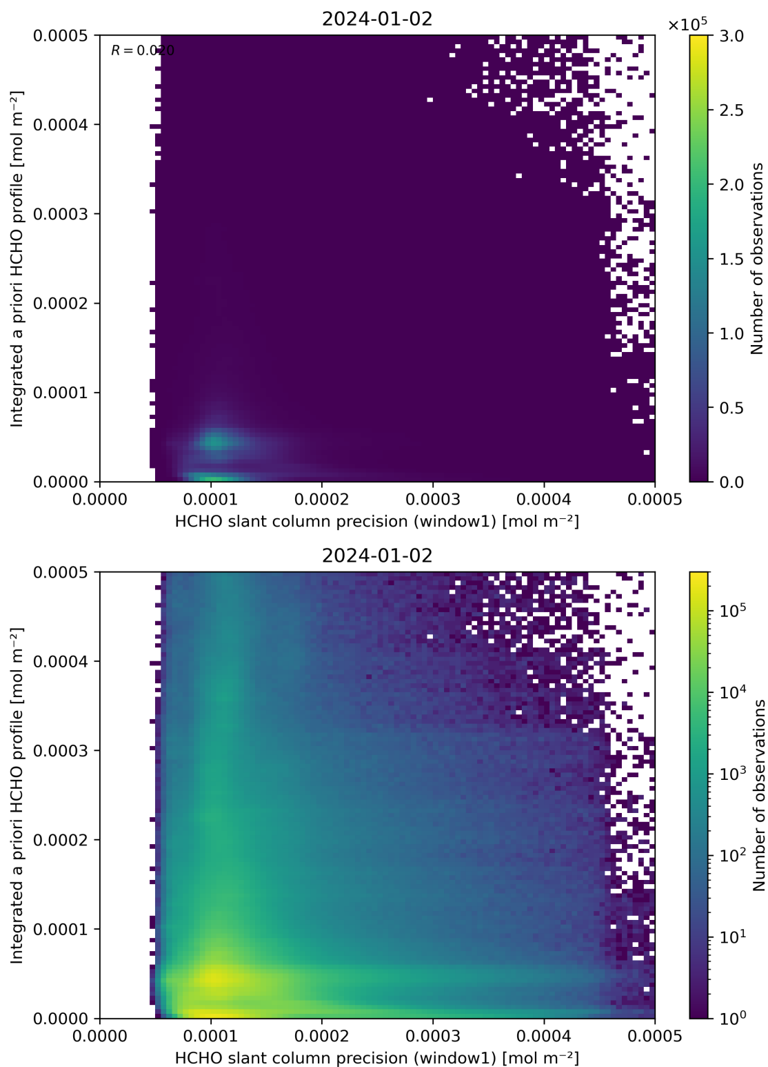
Figure 96: Scatter density plot of “HCHO slant column precision (window1)” against “Integrated a priori HCHO profile” for 2024-01-01 to 2024-01-03.
