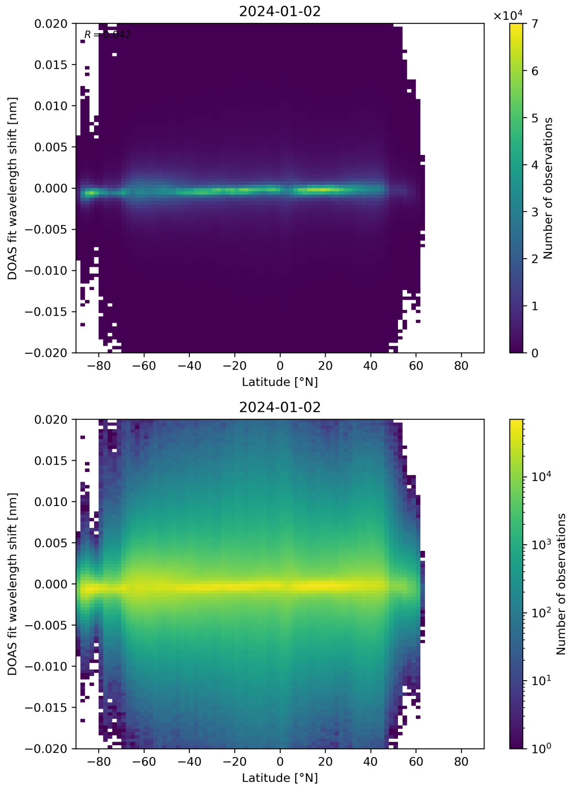
Figure 154: Scatter density plot of “Latitude” against “DOAS fit wavelength shift” for 2024-01-01 to 2024-01-03.
