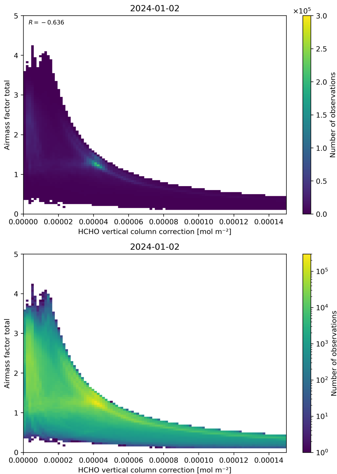
Figure 120: Scatter density plot of “HCHO vertical column correction” against “Airmass factor total” for 2024-01-01 to 2024-01-03.
