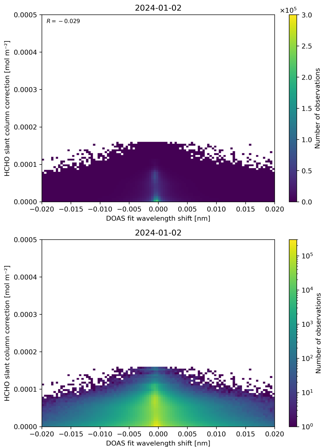
Figure 67: Scatter density plot of “DOAS fit wavelength shift” against “HCHO slant column correction” for 2024-01-01 to 2024-01-03.
