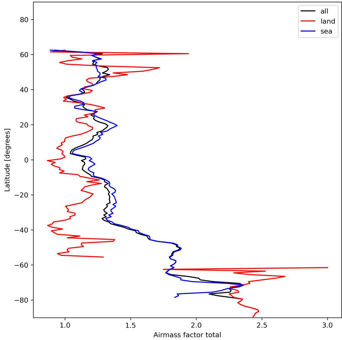
Figure 26: Zonal average of “Airmass factor total” for 2024-01-01 to 2024-01-03.
