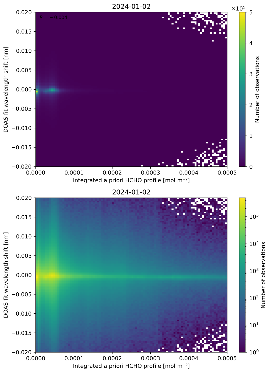
Figure 149: Scatter density plot of “Integrated a priori HCHO profile” against “DOAS fit wavelength shift” for 2024-01-01 to 2024-01-03.
