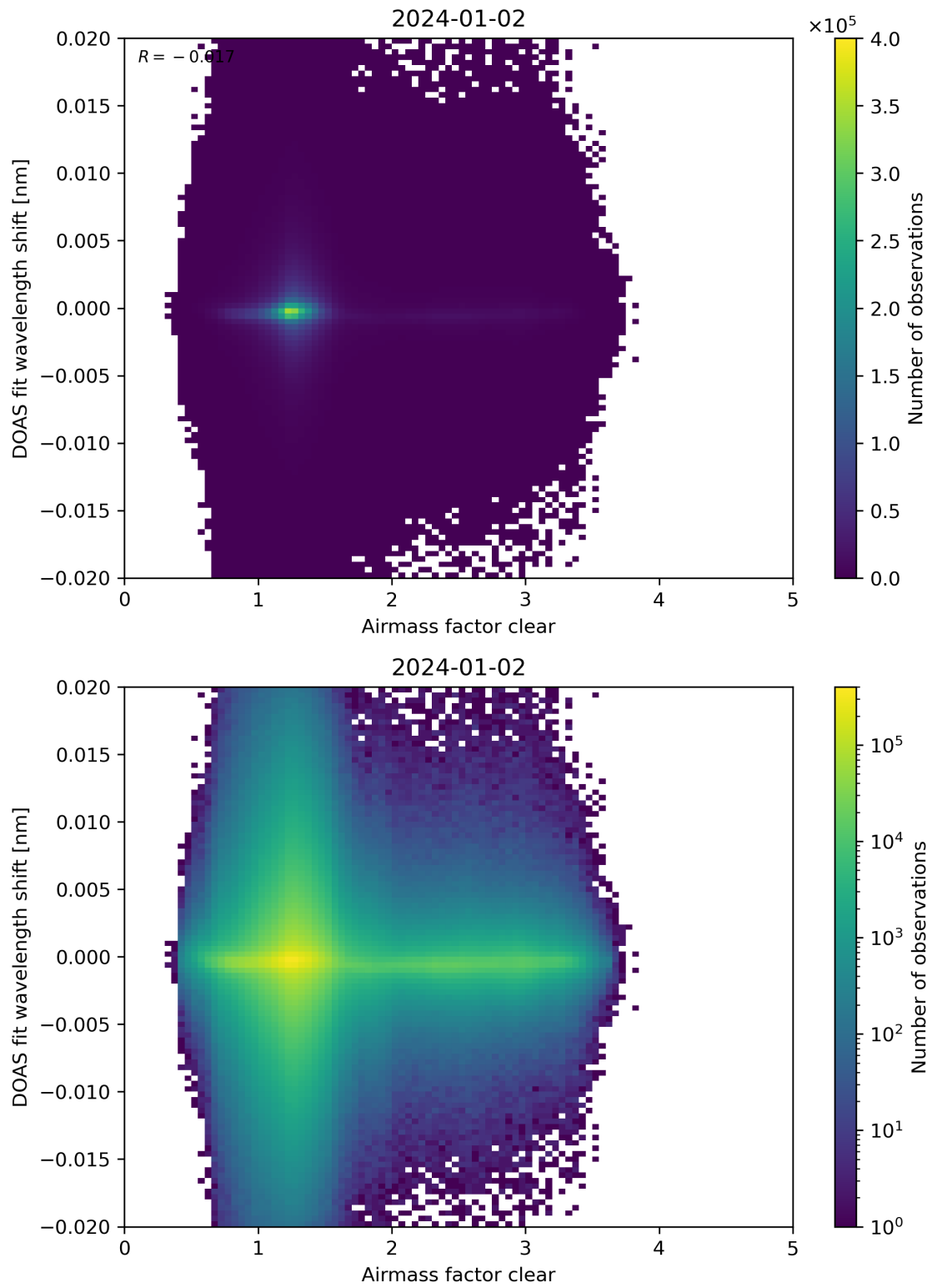
Figure 72: Scatter density plot of “Airmass factor clear” against “DOAS fit wavelength shift” for 2024-01-01 to 2024-01-03.
