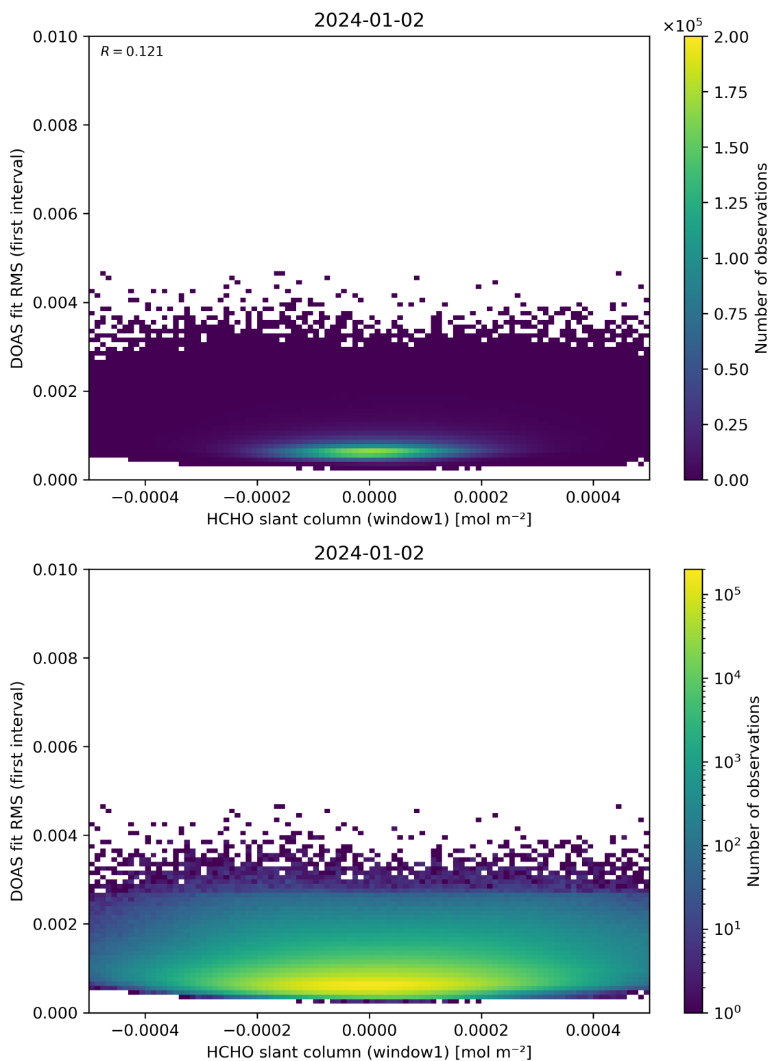
Figure 78: Scatter density plot of “HCHO slant column (window1)” against “DOAS fit RMS (first interval)” for 2024-01-01 to 2024-01-03.
