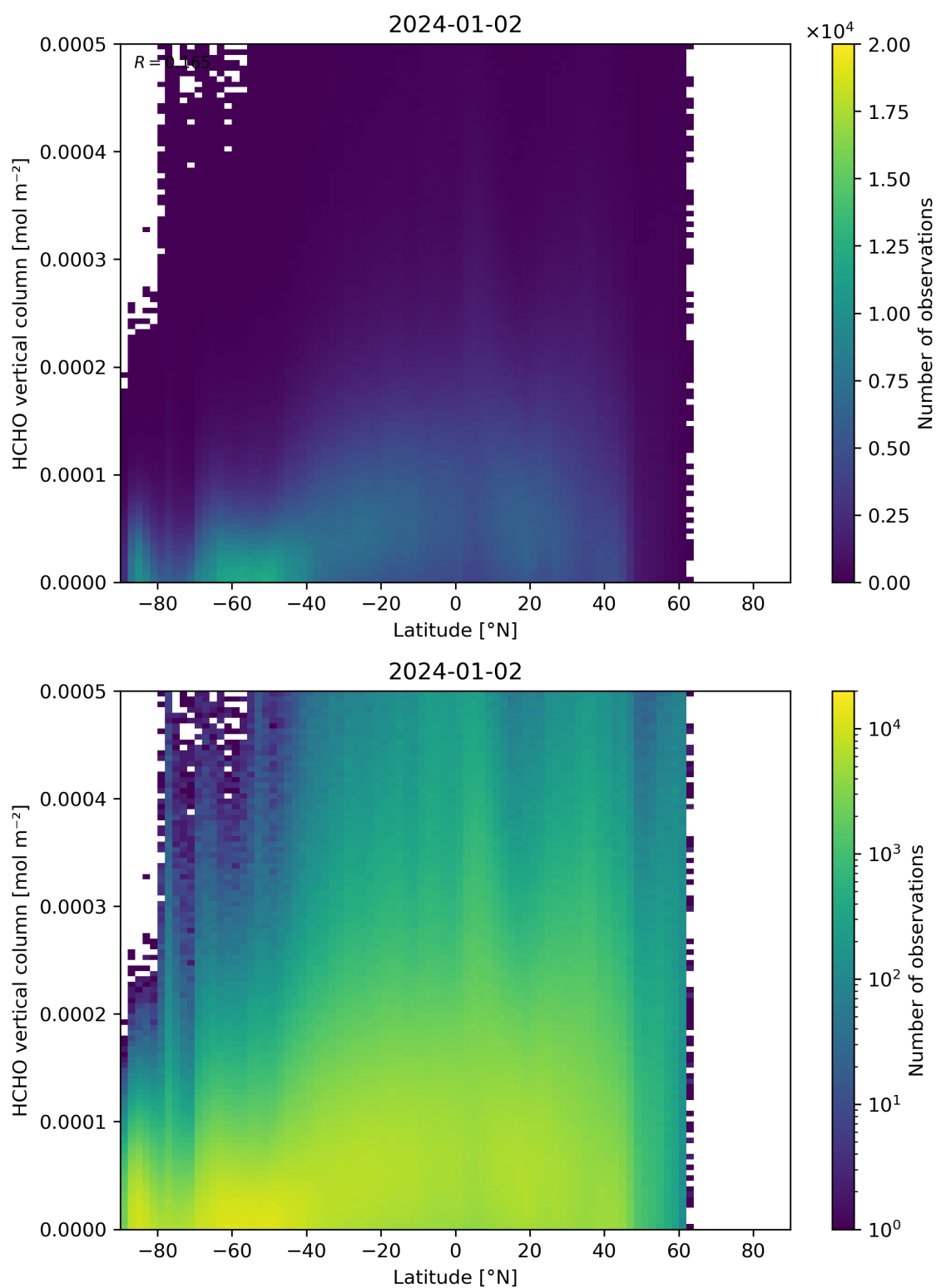
Figure 163: Scatter density plot of “Latitude” against “HCHO vertical column” for 2024-01-01 to 2024-01-03.
