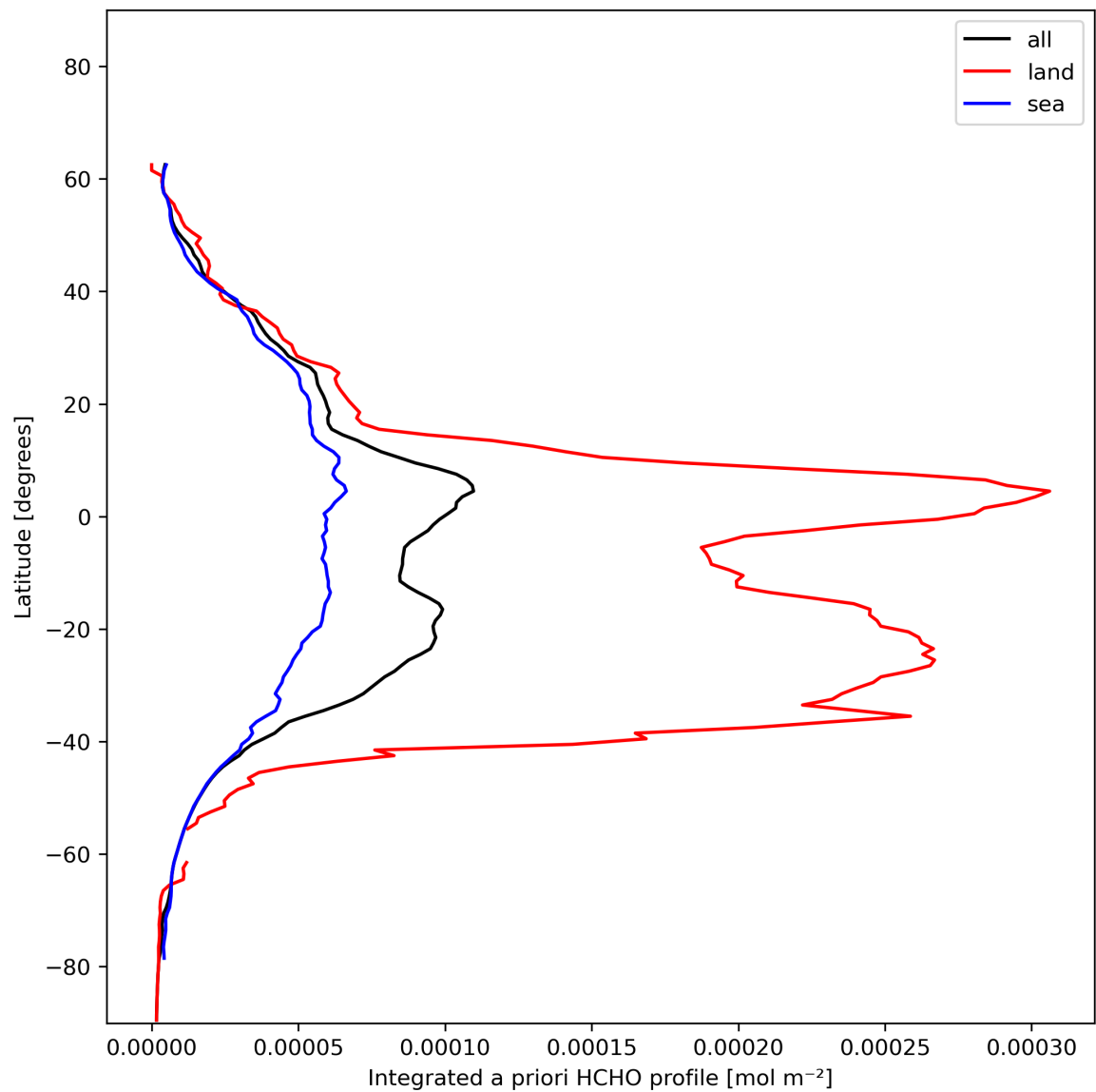
Figure 29: Zonal average of “Integrated a priori HCHO profile” for 2024-01-01 to 2024-01-03.
