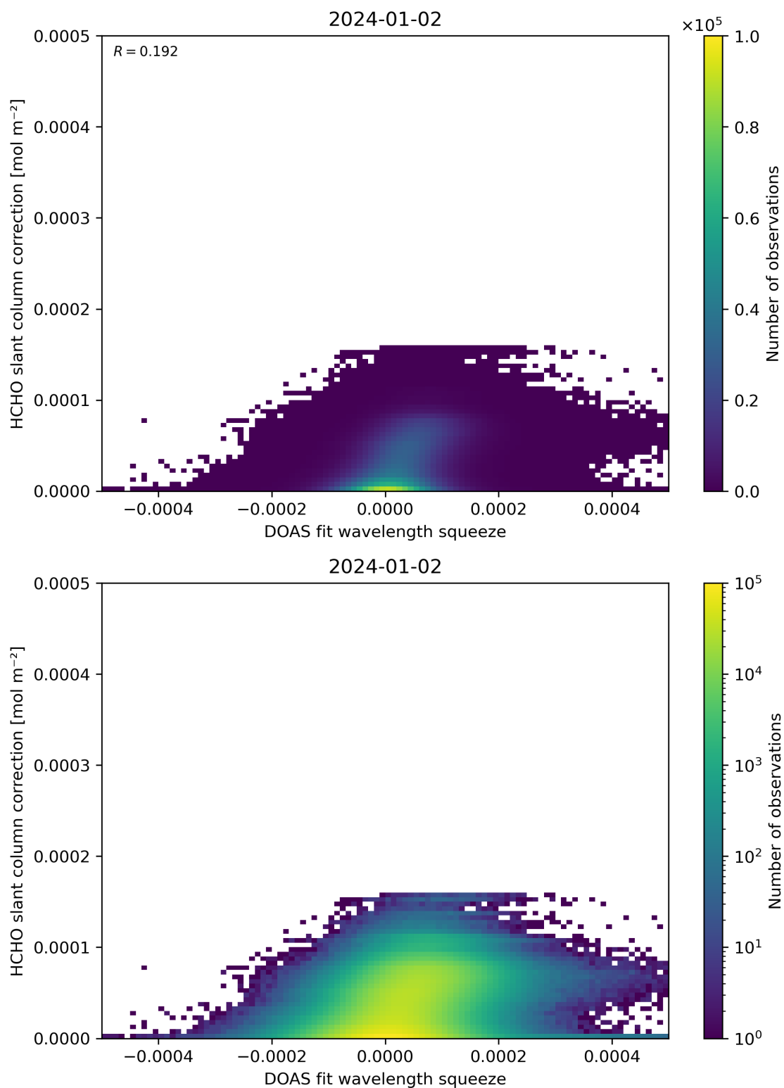
Figure 70: Scatter density plot of “DOAS fit wavelength squeeze” against “HCHO slant column correction” for 2024-01-01 to 2024-01-03.
