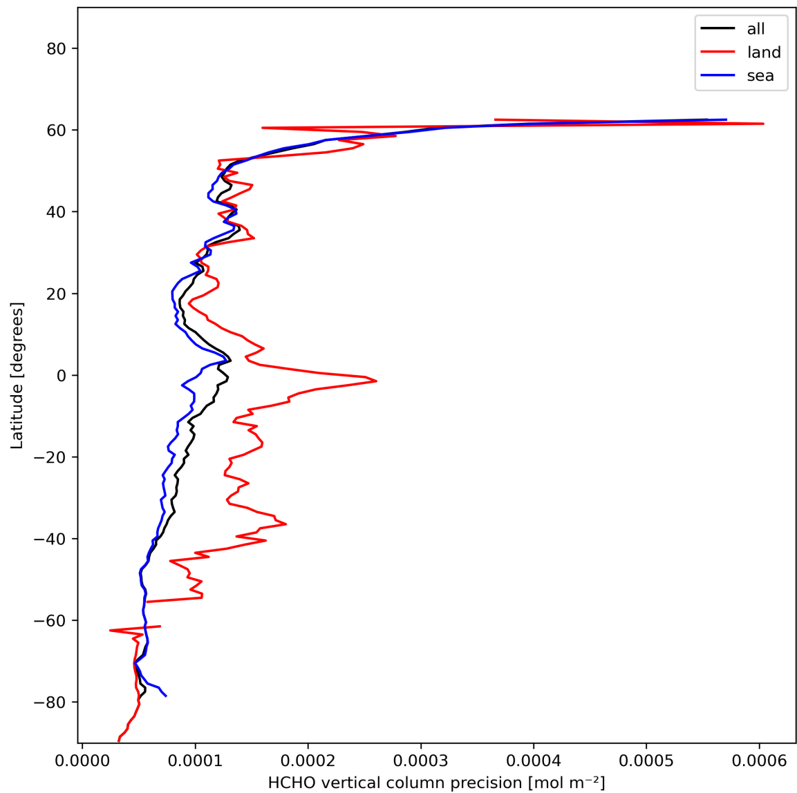
Figure 22: Zonal average of “HCHO vertical column precision” for 2024-01-01 to 2024-01-03.
