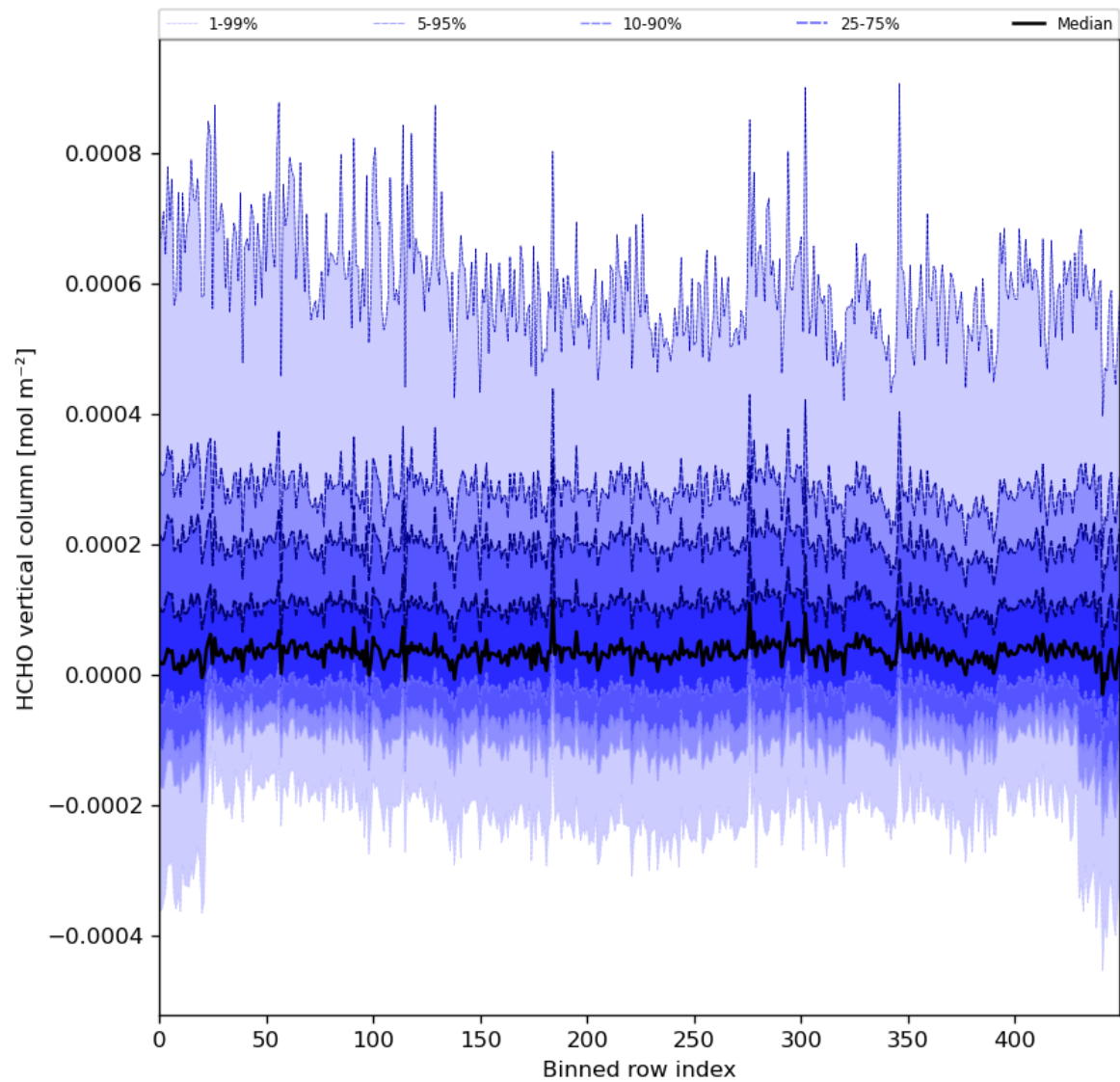
Figure 49: Along track statistics of “HCHO vertical column” for 2024-01-01 to 2024-01-03
