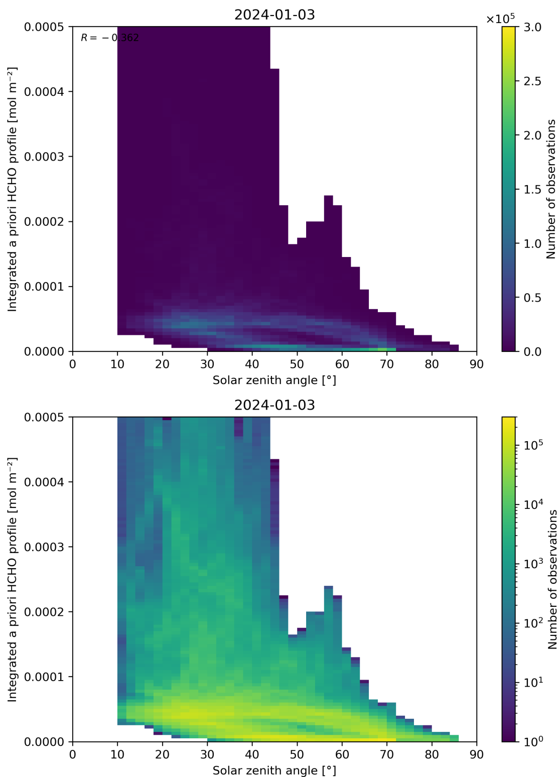
Figure 180: Scatter density plot of “Solar zenith angle” against “Integrated a priori HCHO profile” for 2024-01-02 to 2024-01-04.
