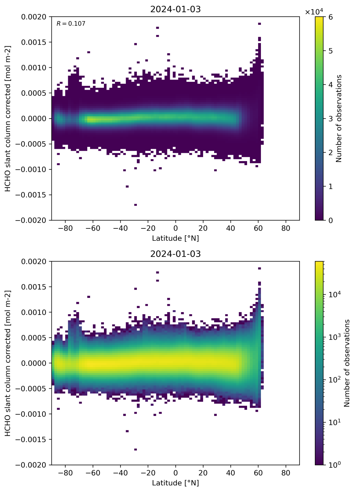
Figure 157: Scatter density plot of “Latitude” against “HCHO slant column corrected” for 2024-01-02 to 2024-01-04.
