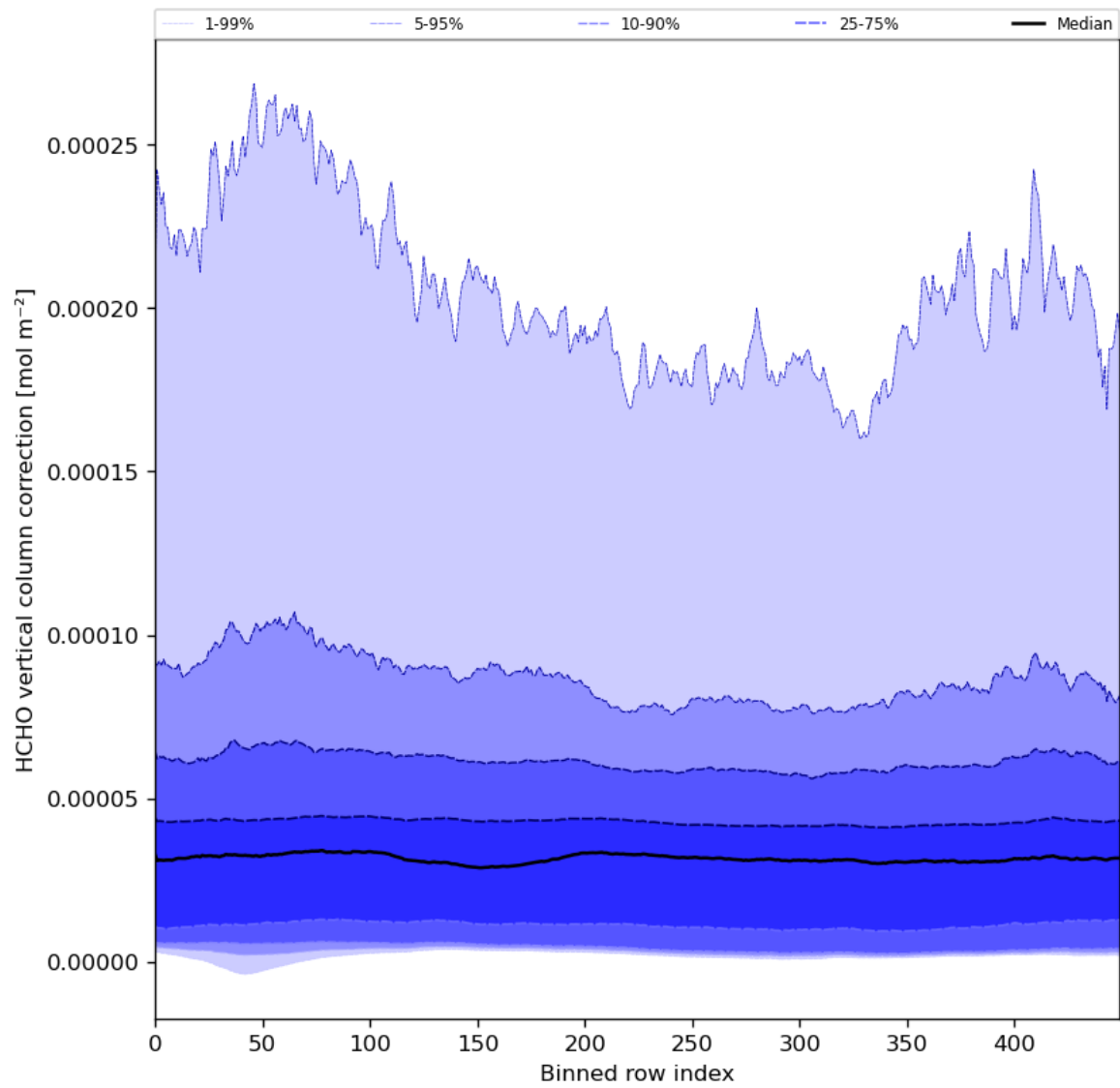
Figure 51: Along track statistics of “HCHO vertical column correction” for 2024-01-02 to 2024-01-04
