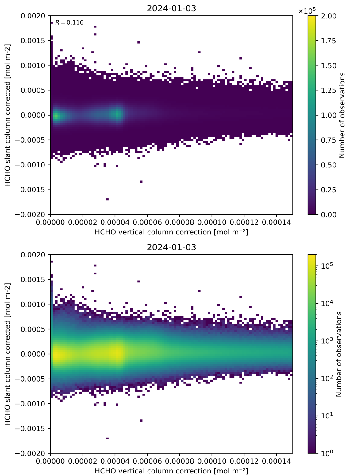
Figure 116: Scatter density plot of “HCHO vertical column correction” against “HCHO slant column corrected” for 2024-01-02 to 2024-01-04.
