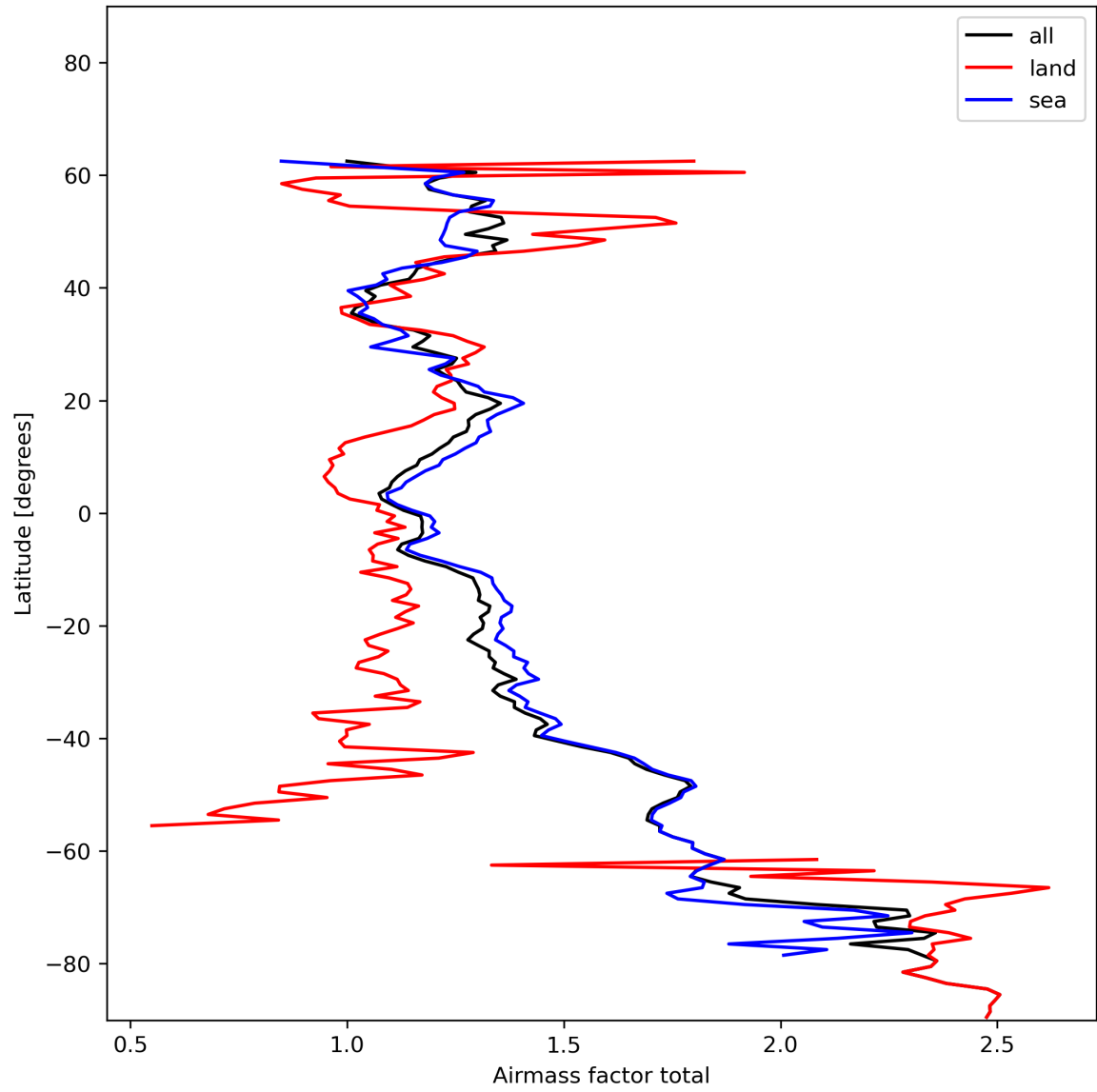
Figure 26: Zonal average of “Airmass factor total” for 2024-01-02 to 2024-01-04.
