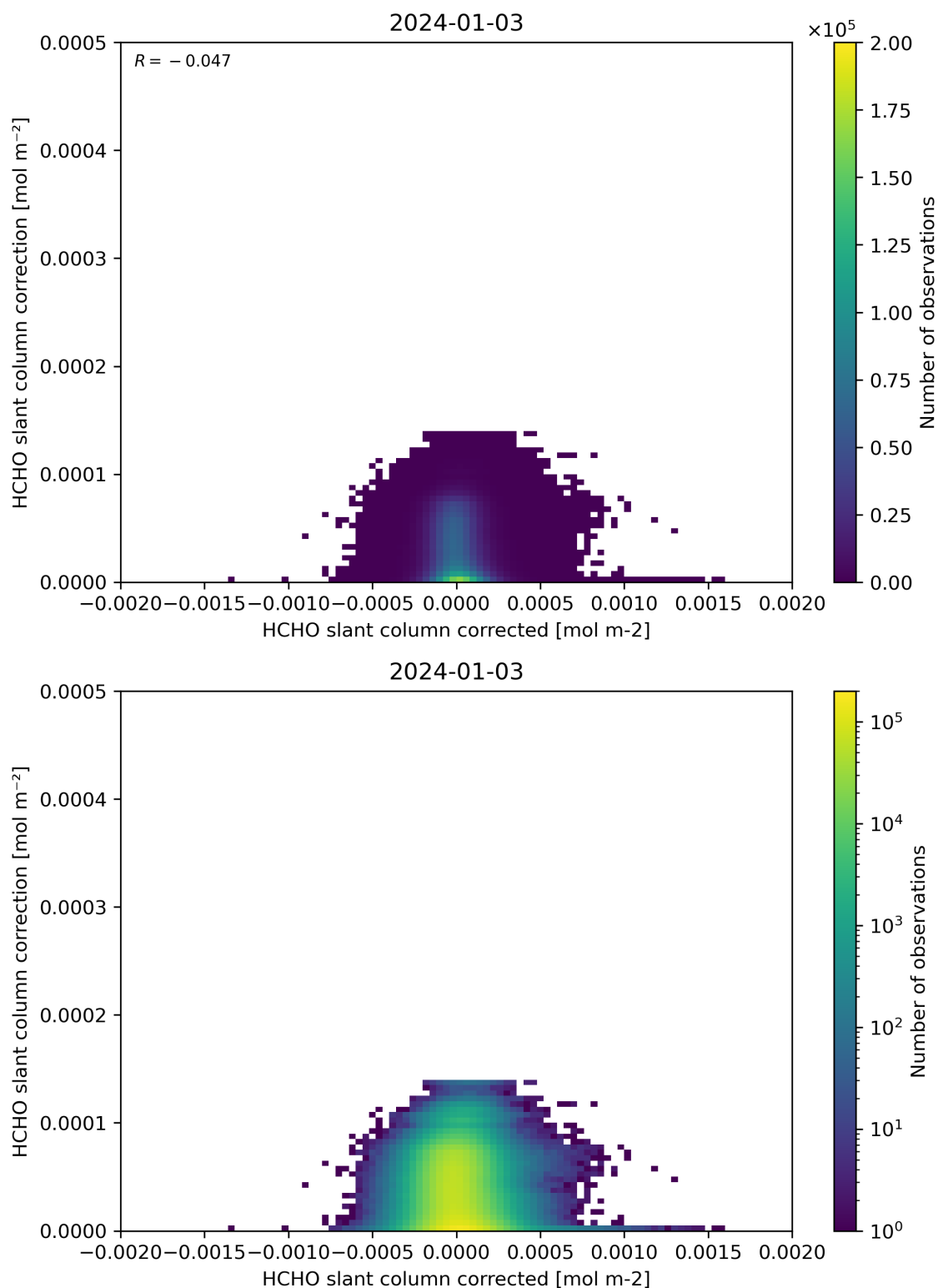
Figure 77: Scatter density plot of “HCHO slant column corrected” against “HCHO slant column correction” for 2024-01-02 to 2024-01-04.
