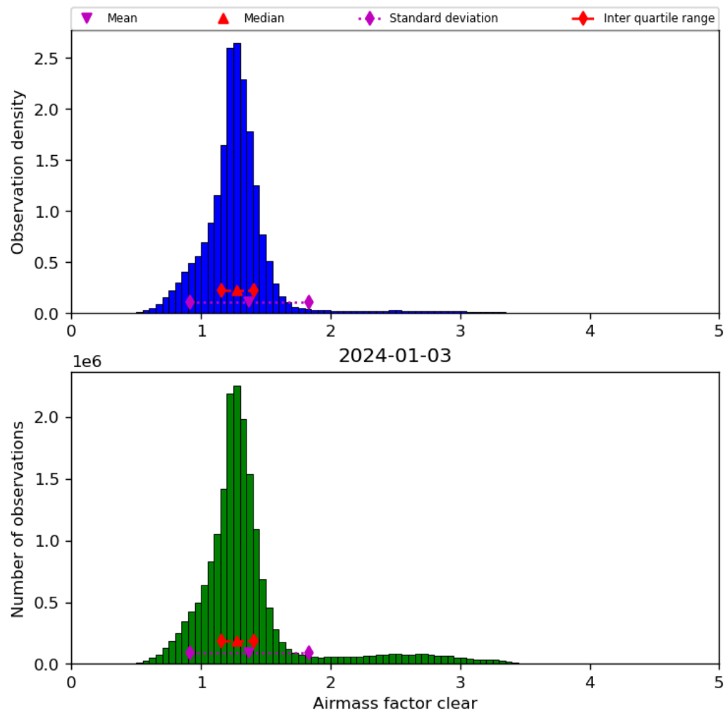
Figure 42: Histogram of "Airmass factor clear" for 2024-01-02 to 2024-01-04
