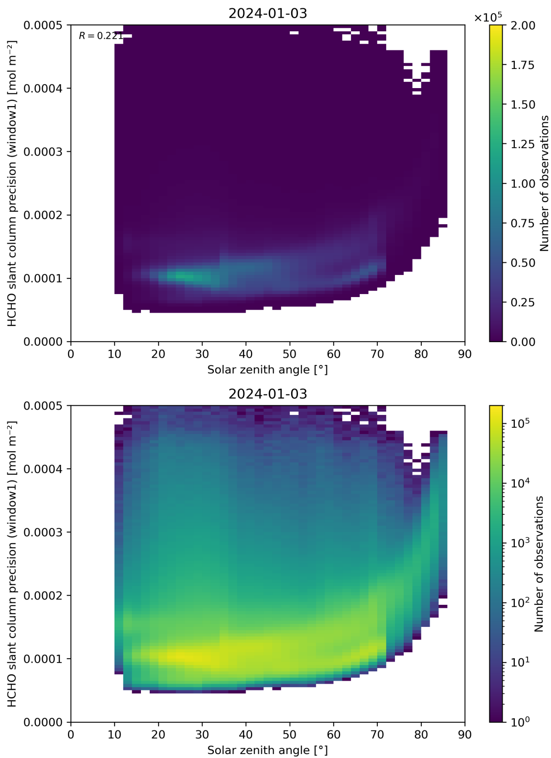
Figure 174: Scatter density plot of “Solar zenith angle” against “HCHO slant column precision (window1)” for 2024-01-02 to 2024-01-04.
