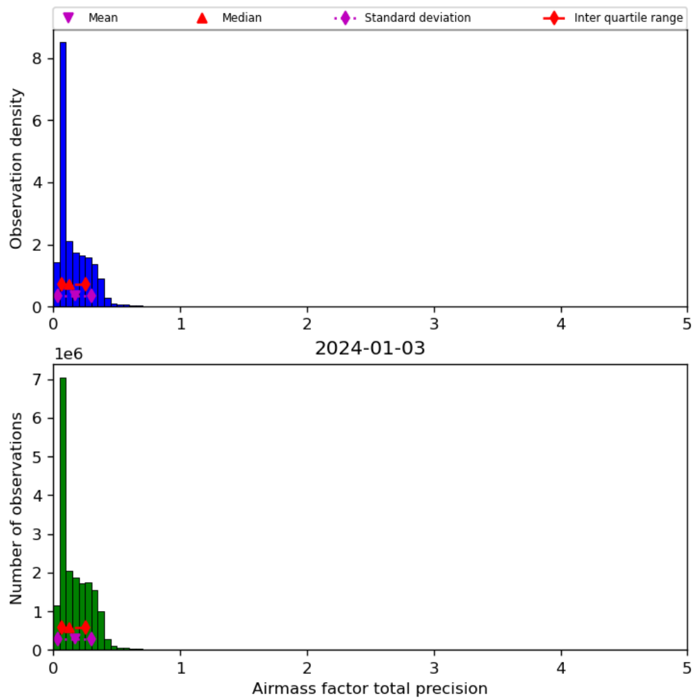
Figure 41: Histogram of “Airmass factor total precision” for 2024-01-02 to 2024-01-04
