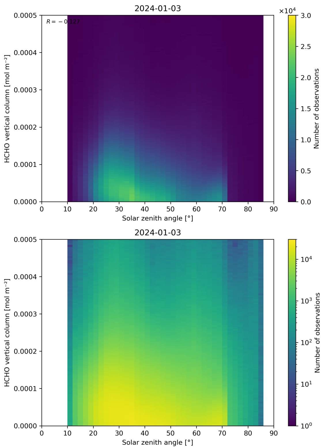
Figure 177: Scatter density plot of “Solar zenith angle” against “HCHO vertical column” for 2024-01-02 to 2024-01-04.
