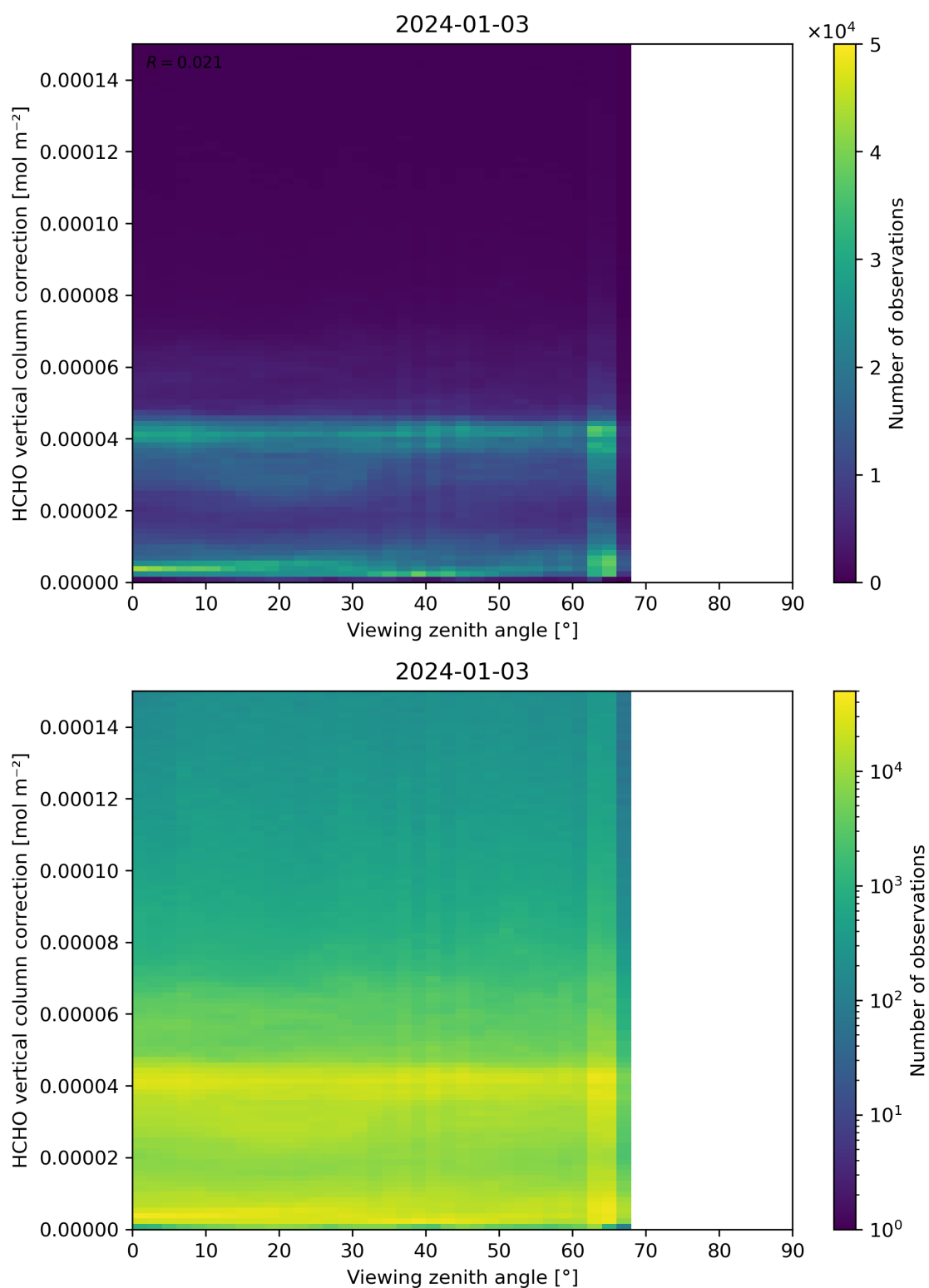
Figure 193: Scatter density plot of “Viewing zenith angle” against “HCHO vertical column correction” for 2024-01-02 to 2024-01-04.
