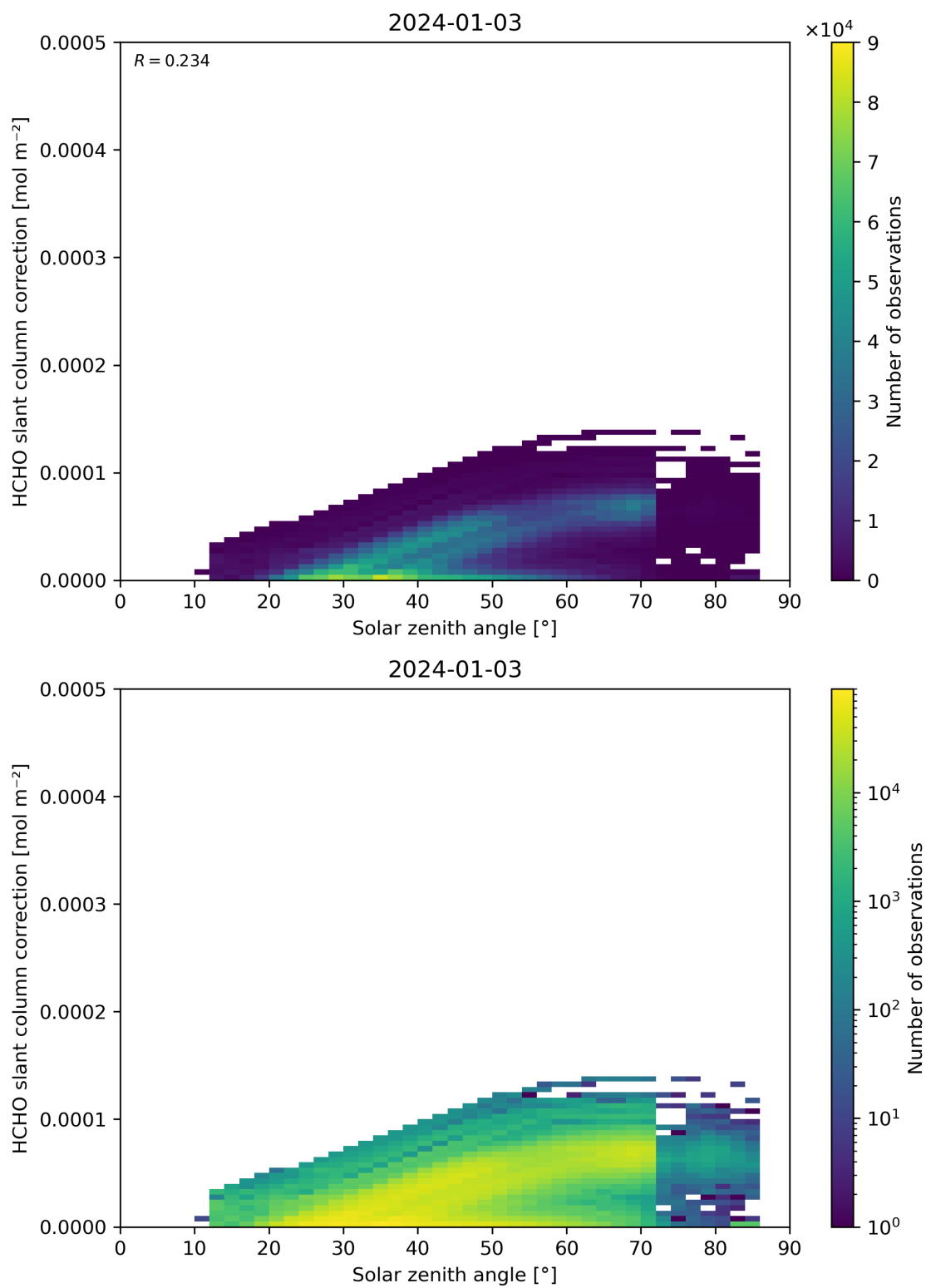
Figure 172: Scatter density plot of “Solar zenith angle” against “HCHO slant column correction” for 2024-01-02 to 2024-01-04.
