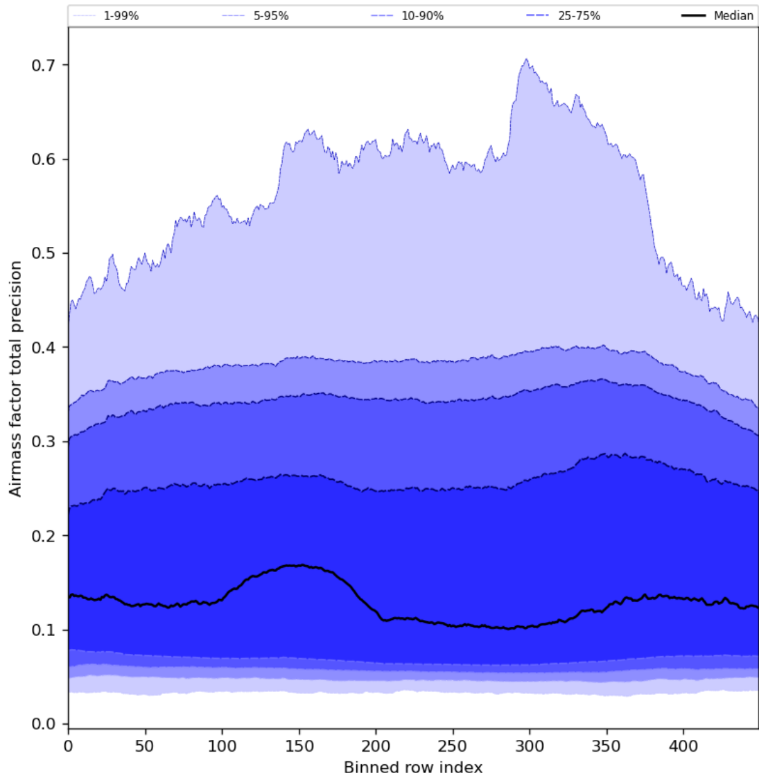
Figure 55: Along track statistics of “Airmass factor total precision” for 2024-01-02 to 2024-01-04
