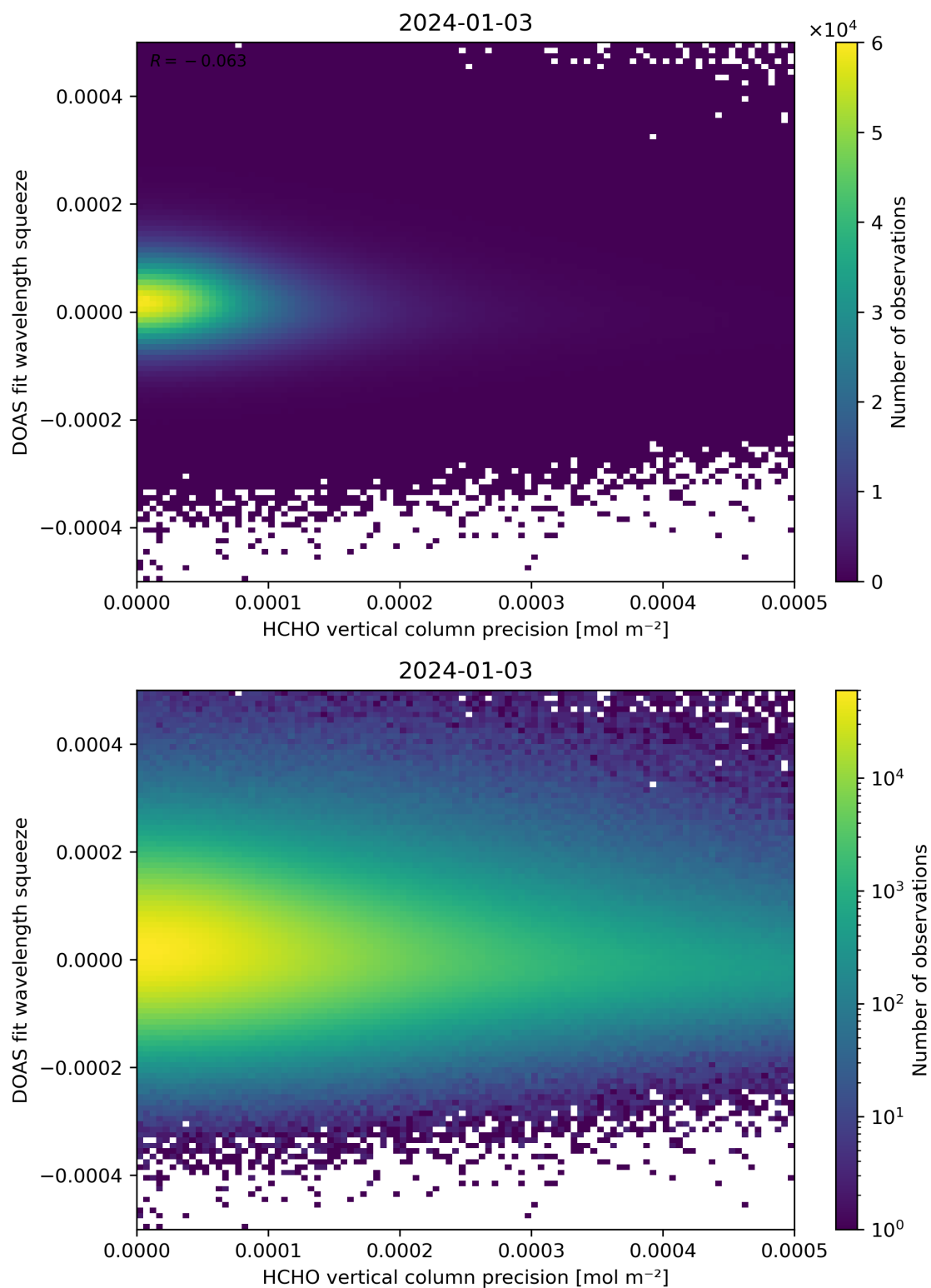
Figure 138: Scatter density plot of “HCHO vertical column precision” against “DOAS fit wavelength squeeze” for 2024-01-02 to 2024-01-04.
