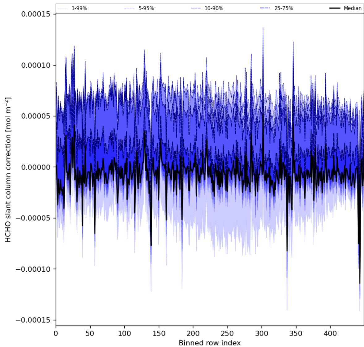
Figure 61: Along track statistics of “HCHO slant column correction” for 2024-01-02 to 2024-01-04
