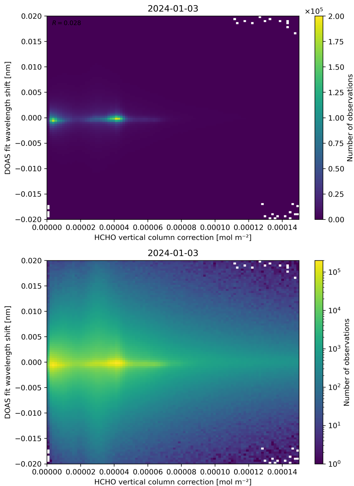
Figure 113: Scatter density plot of “HCHO vertical column correction” against “DOAS fit wavelength shift” for 2024-01-02 to 2024-01-04.
