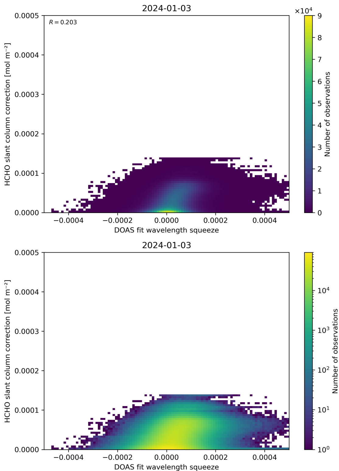
Figure 70: Scatter density plot of “DOAS fit wavelength squeeze” against “HCHO slant column correction” for 2024-01-02 to 2024-01-04.
