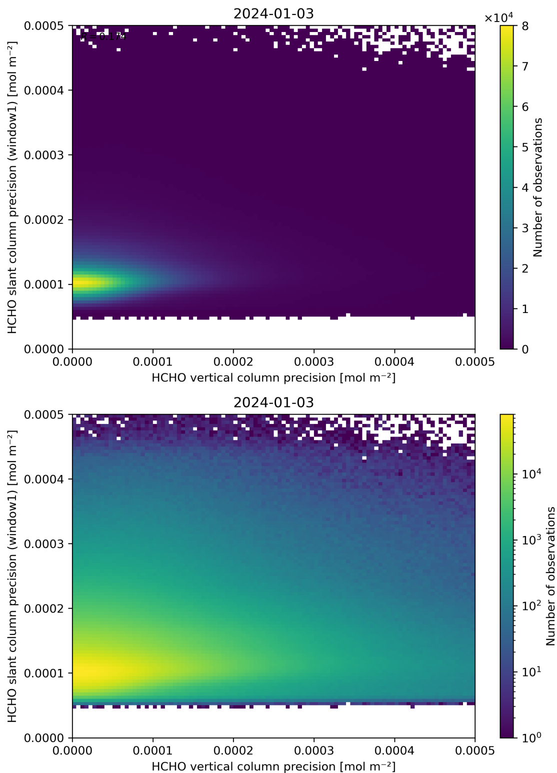
Figure 143: Scatter density plot of “HCHO vertical column precision” against “HCHO slant column precision (window1)” for 2024-01-02 to 2024-01-04.
