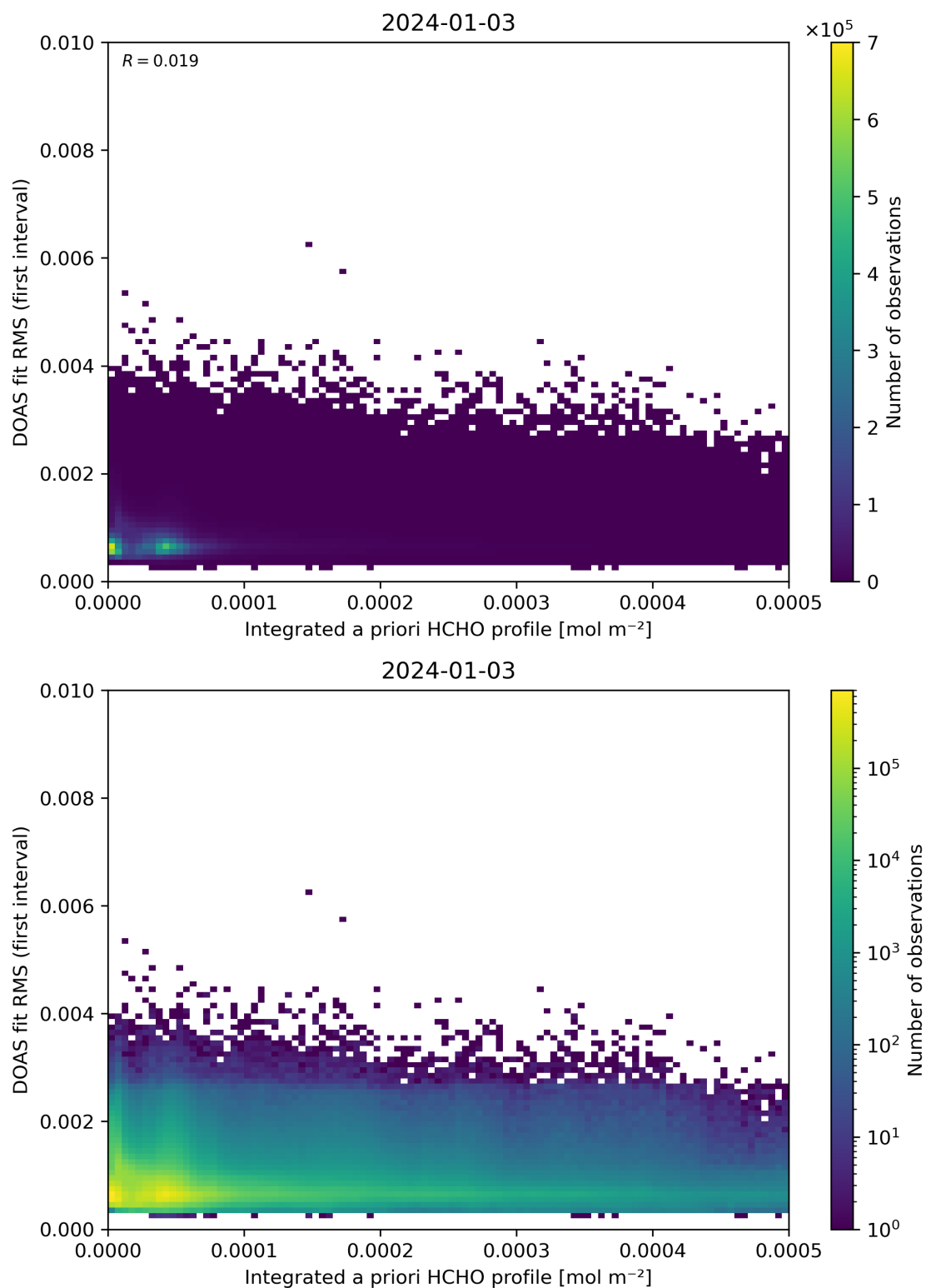
Figure 148: Scatter density plot of “Integrated a priori HCHO profile” against “DOAS fit RMS (first interval)” for 2024-01-02 to 2024-01-04.
