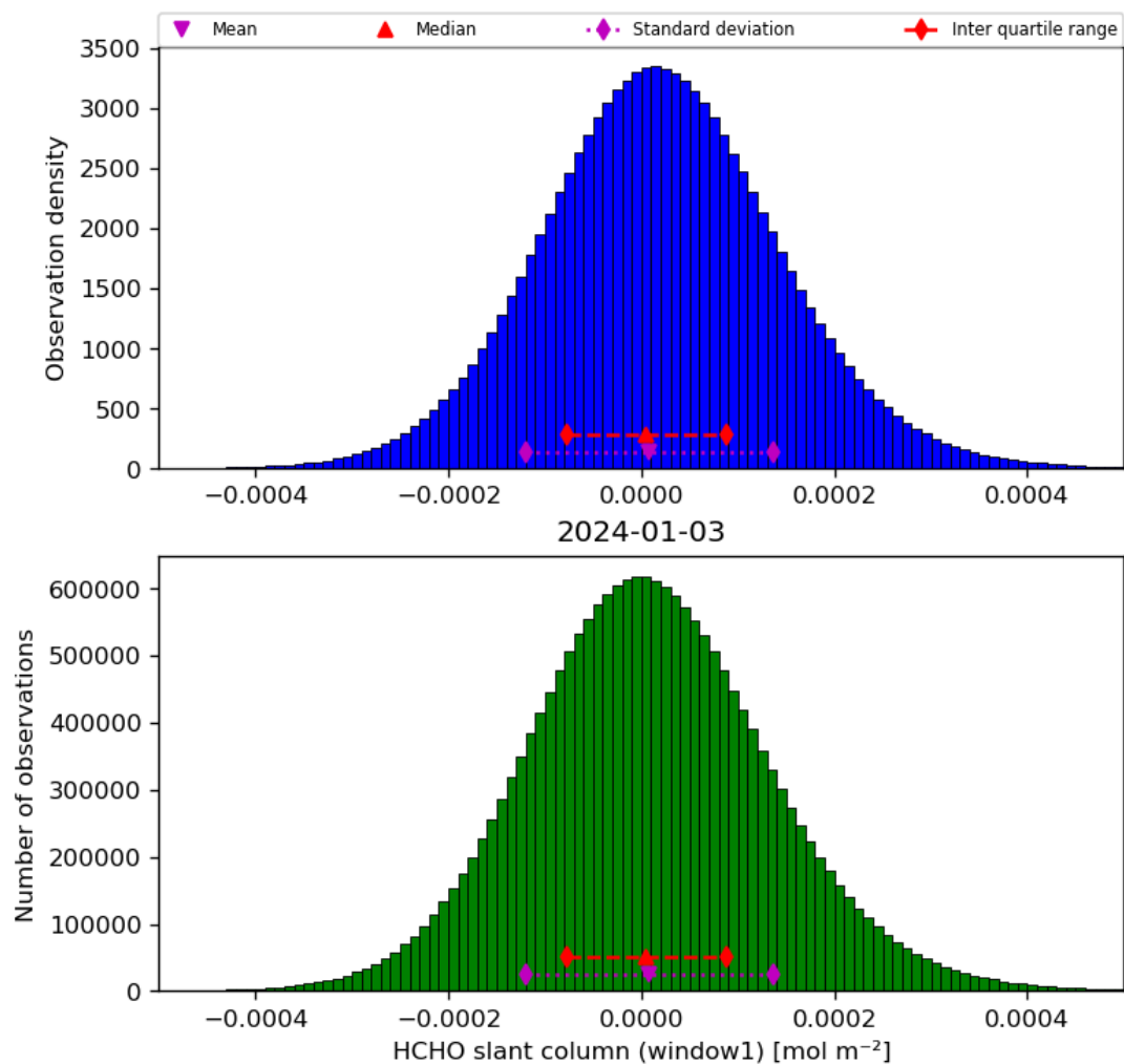
Figure 38: Histogram of “HCHO slant column (window1)” for 2024-01-02 to 2024-01-04
