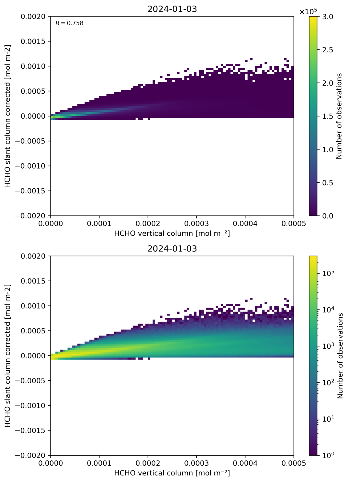
Figure 127: Scatter density plot of “HCHO vertical column” against “HCHO slant column corrected” for 2024-01-02 to 2024-01-04.
