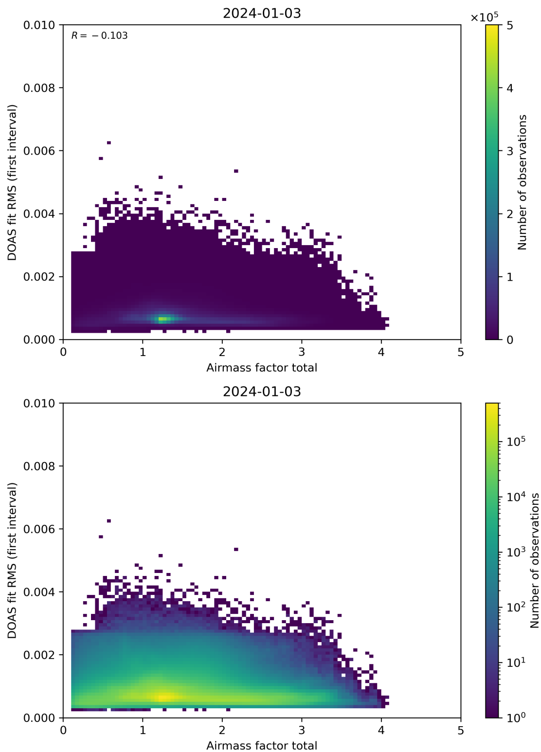
Figure 97: Scatter density plot of “Airmass factor total” against “DOAS fit RMS (first interval)” for 2024-01-02 to 2024-01-04.
