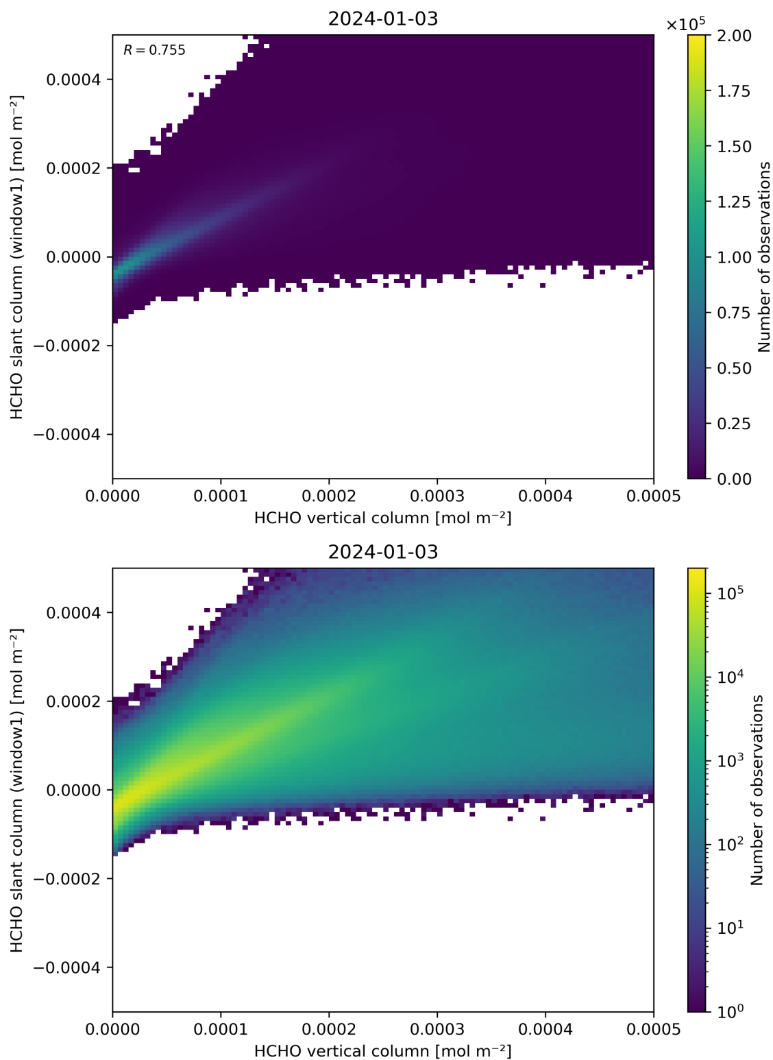
Figure 129: Scatter density plot of “HCHO vertical column” against “HCHO slant column (window1)” for 2024-01-02 to 2024-01-04.
