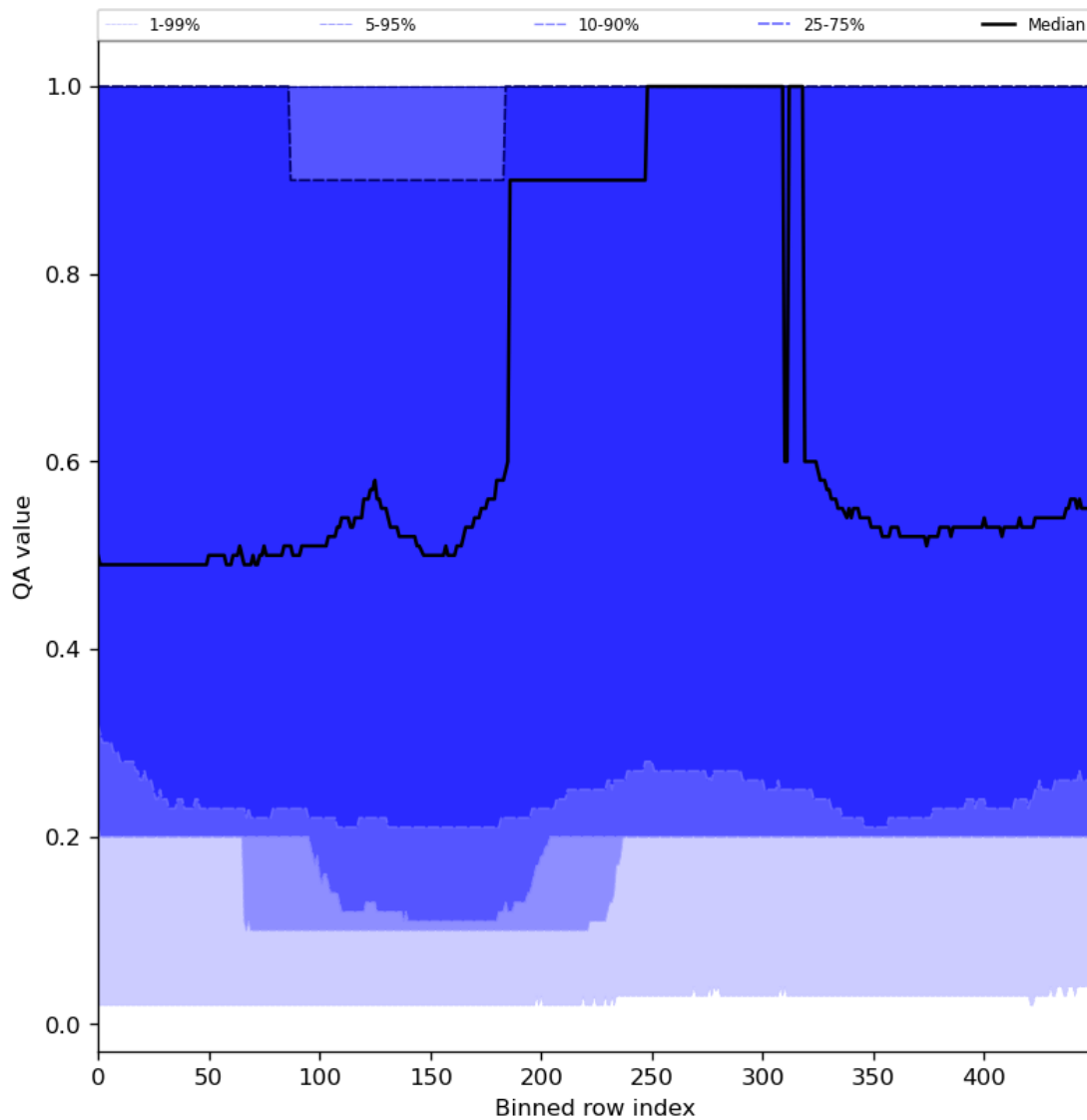
Figure 48: Along track statistics of “QA value” for 2024-01-02 to 2024-01-04
