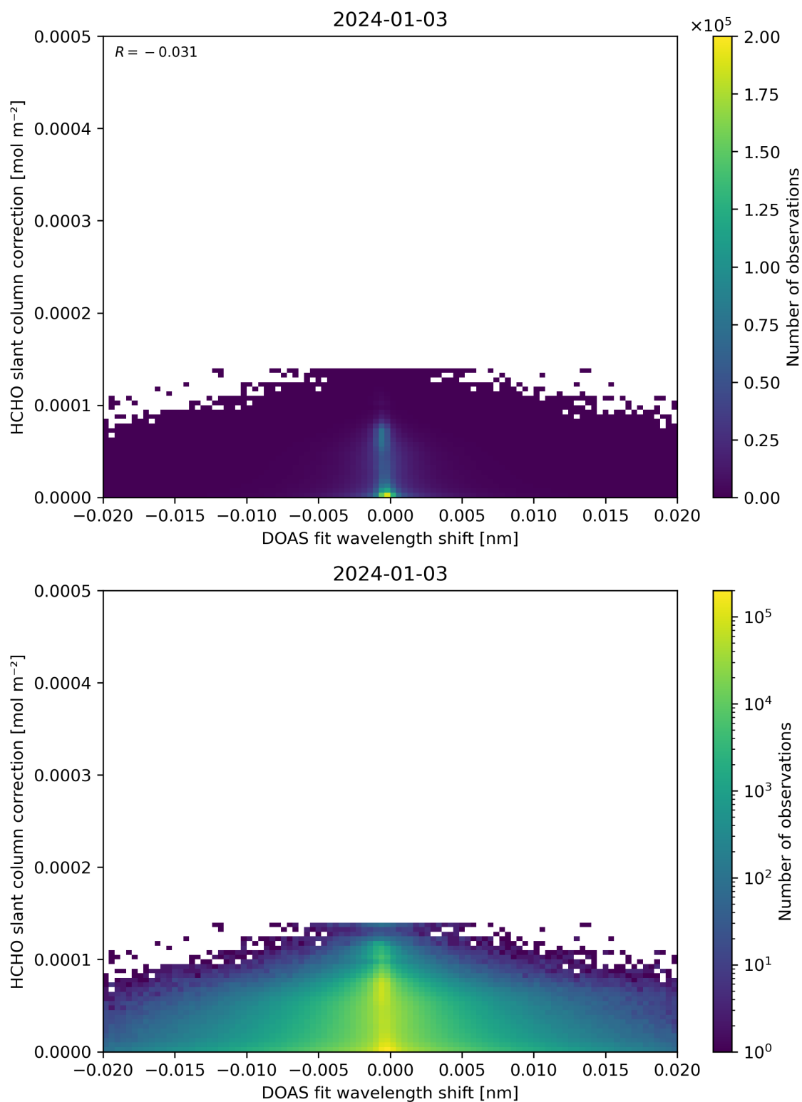
Figure 67: Scatter density plot of “DOAS fit wavelength shift” against “HCHO slant column correction” for 2024-01-02 to 2024-01-04.
