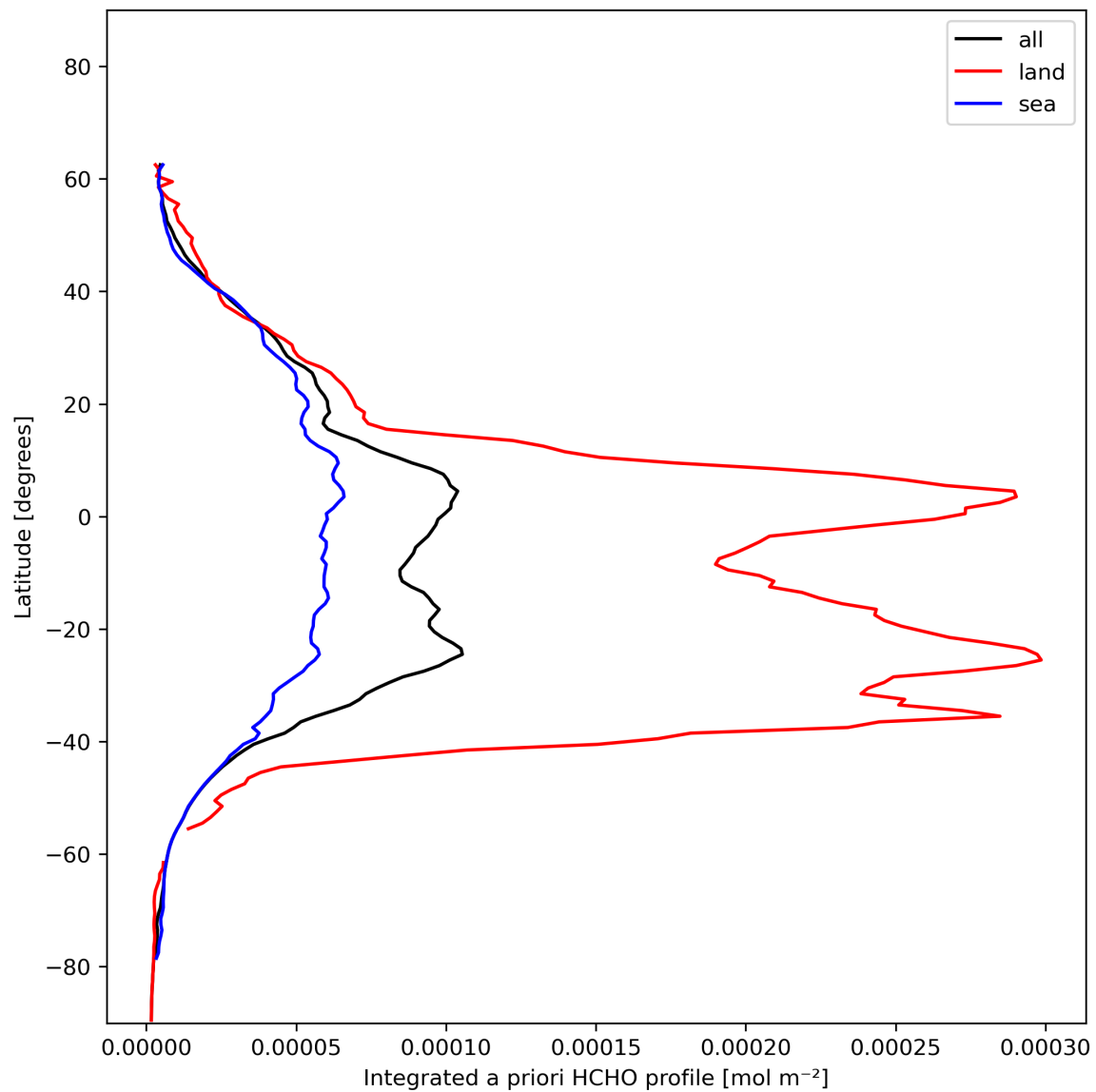
Figure 29: Zonal average of “Integrated a priori HCHO profile” for 2024-01-02 to 2024-01-04.
