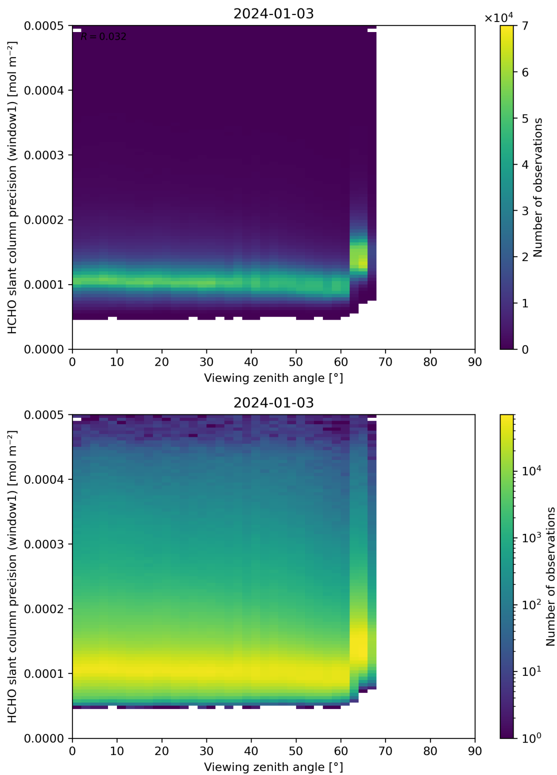
Figure 189: Scatter density plot of “Viewing zenith angle” against “HCHO slant column precision (window1)” for 2024-01-02 to 2024-01-04.
