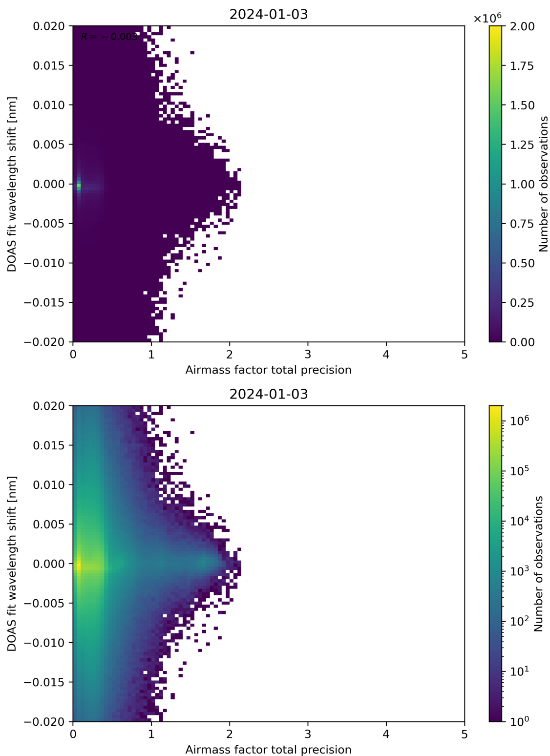
Figure 106: Scatter density plot of “Airmass factor total precision” against “DOAS fit wavelength shift” for 2024-01-02 to 2024-01-04.
