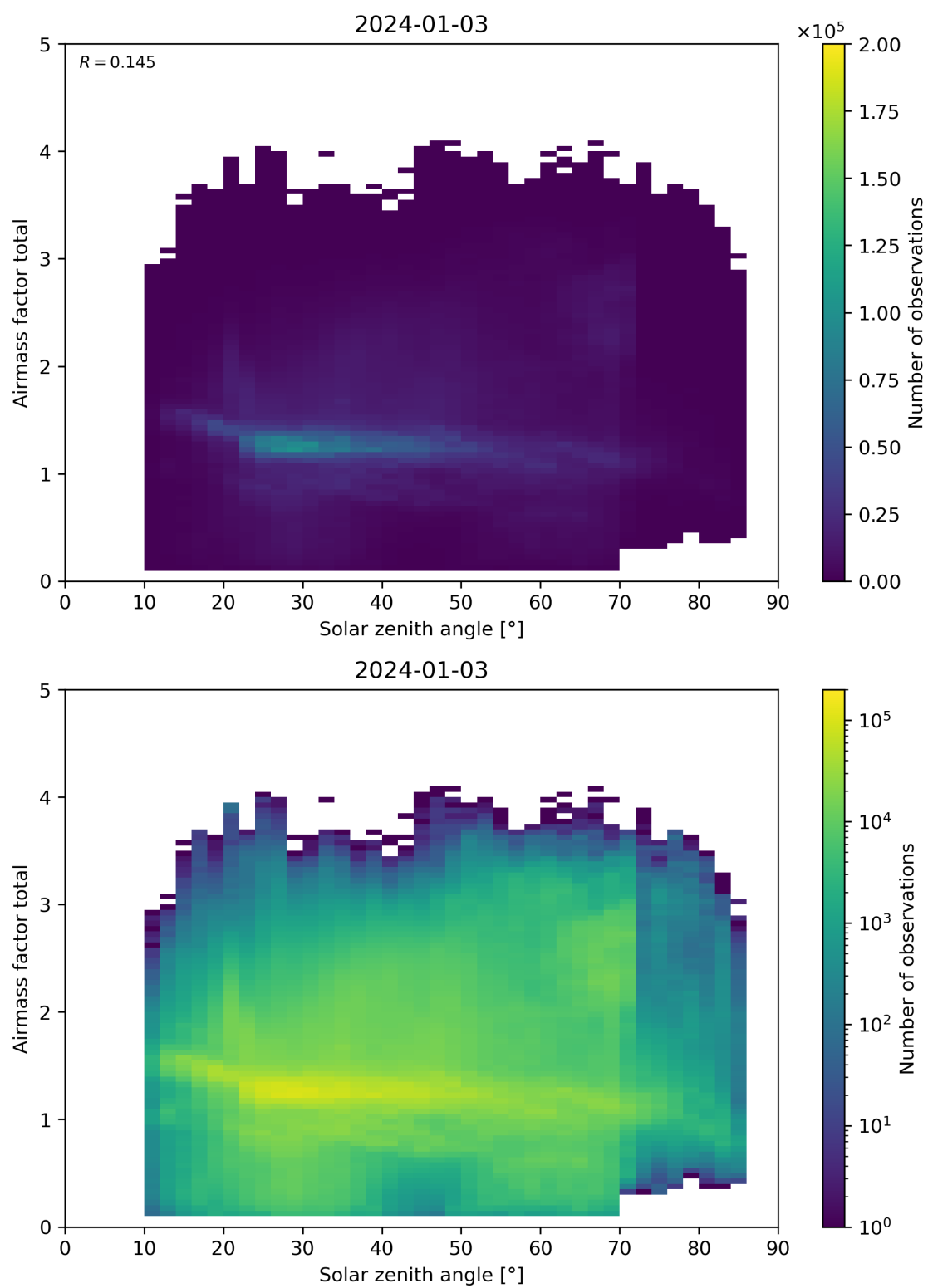
Figure 175: Scatter density plot of “Solar zenith angle” against “Airmass factor total” for 2024-01-02 to 2024-01-04.
