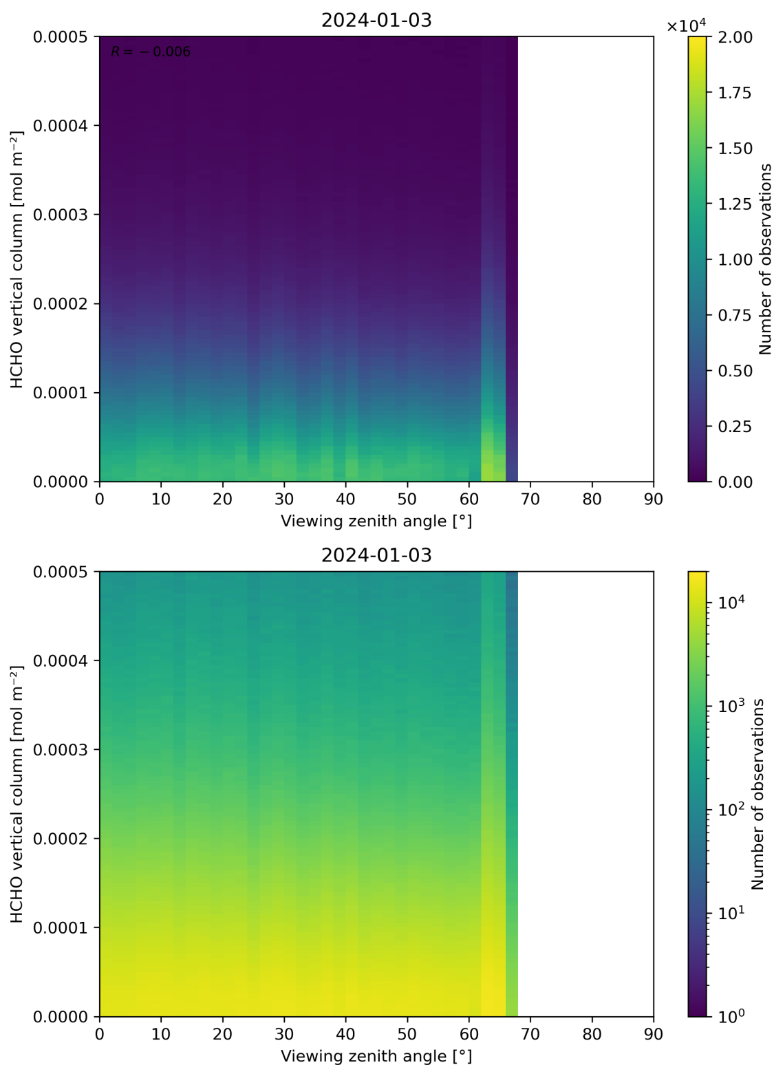
Figure 192: Scatter density plot of “Viewing zenith angle” against “HCHO vertical column” for 2024-01-02 to 2024-01-04.
