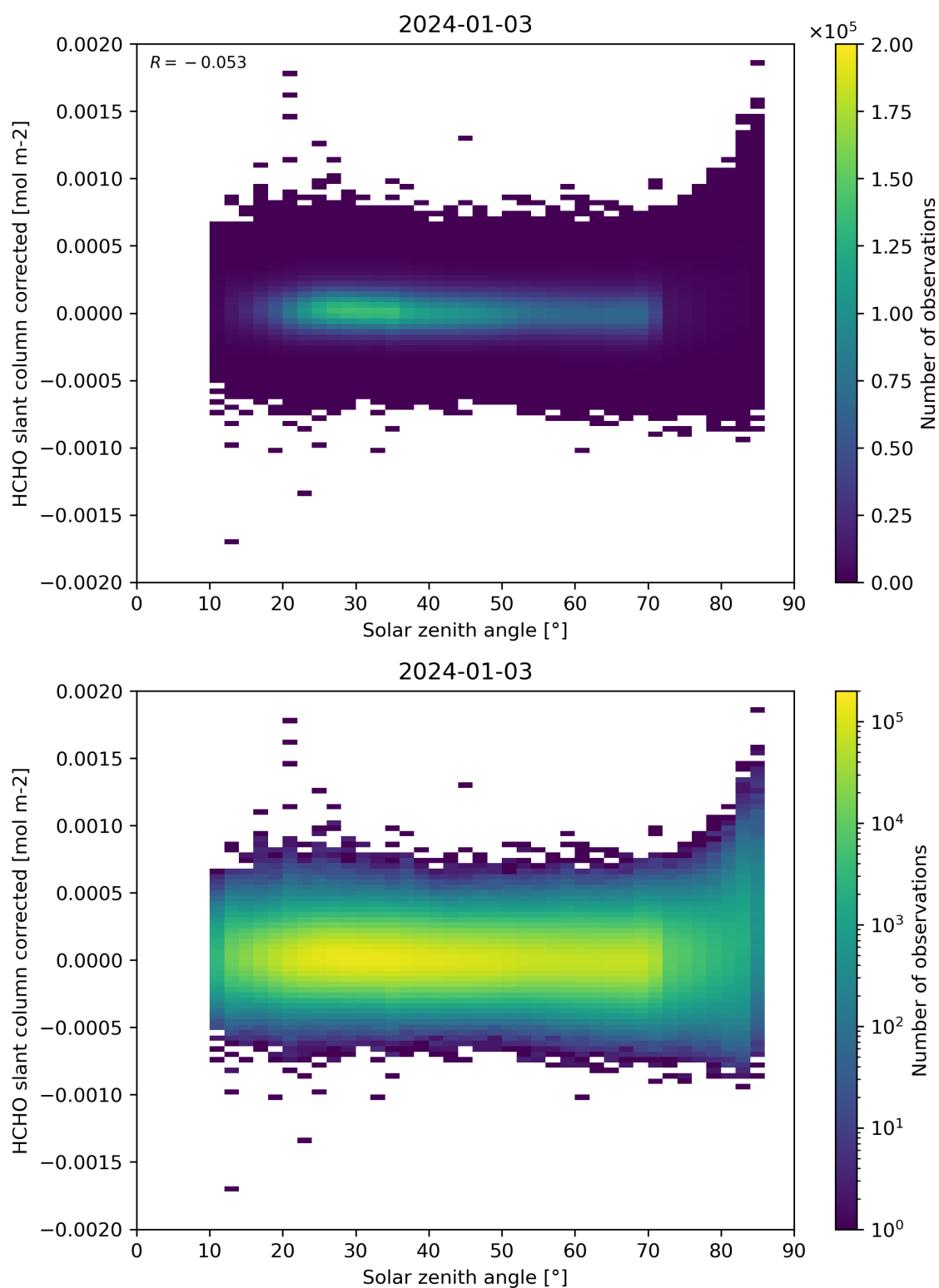
Figure 171: Scatter density plot of “Solar zenith angle” against “HCHO slant column corrected” for 2024-01-02 to 2024-01-04.
