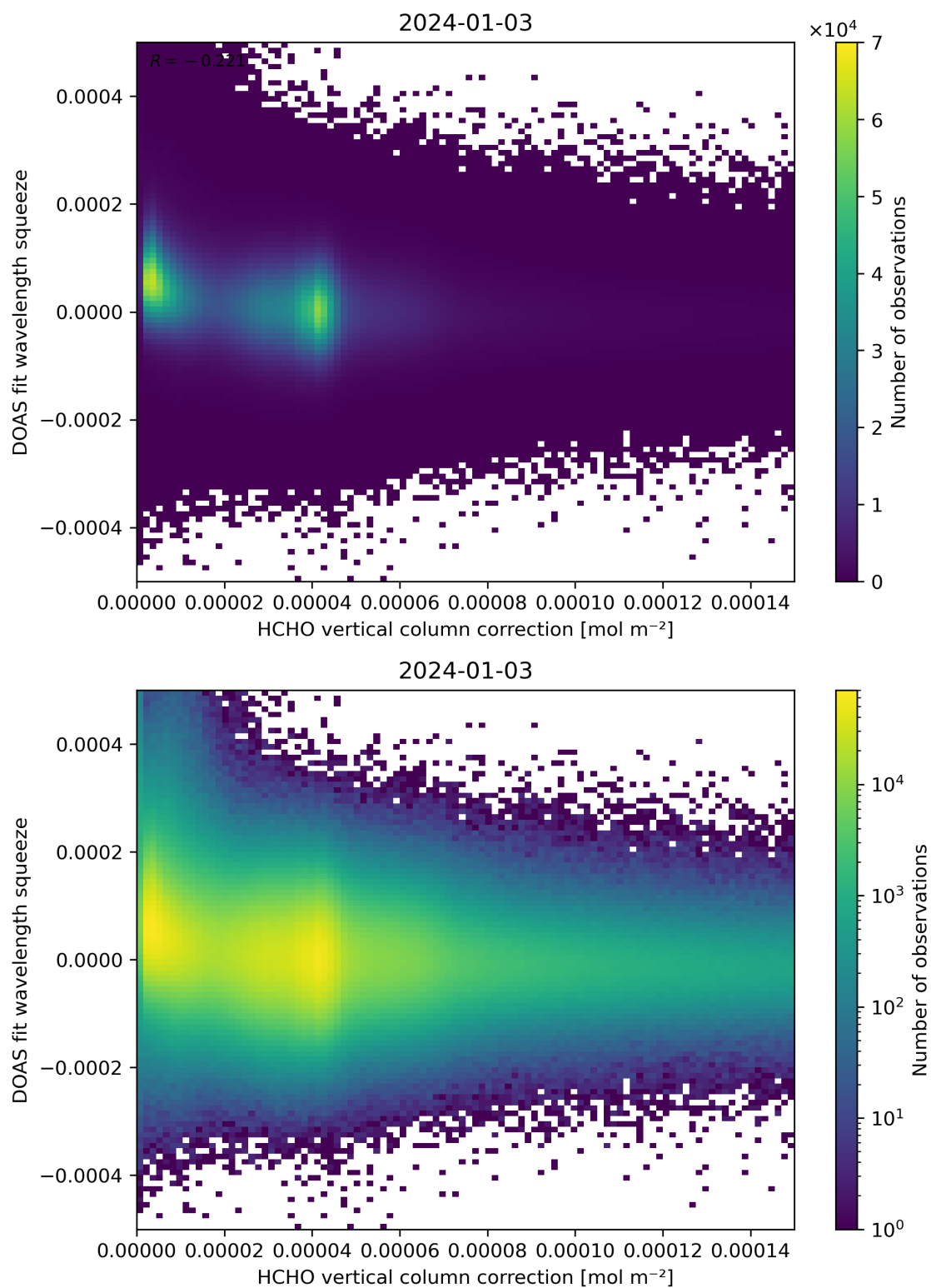
Figure 114: Scatter density plot of “HCHO vertical column correction” against “DOAS fit wavelength squeeze” for 2024-01-02 to 2024-01-04.
