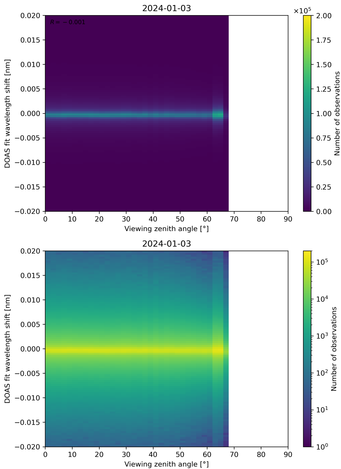
Figure 183: Scatter density plot of “Viewing zenith angle” against “DOAS fit wavelength shift” for 2024-01-02 to 2024-01-04.
