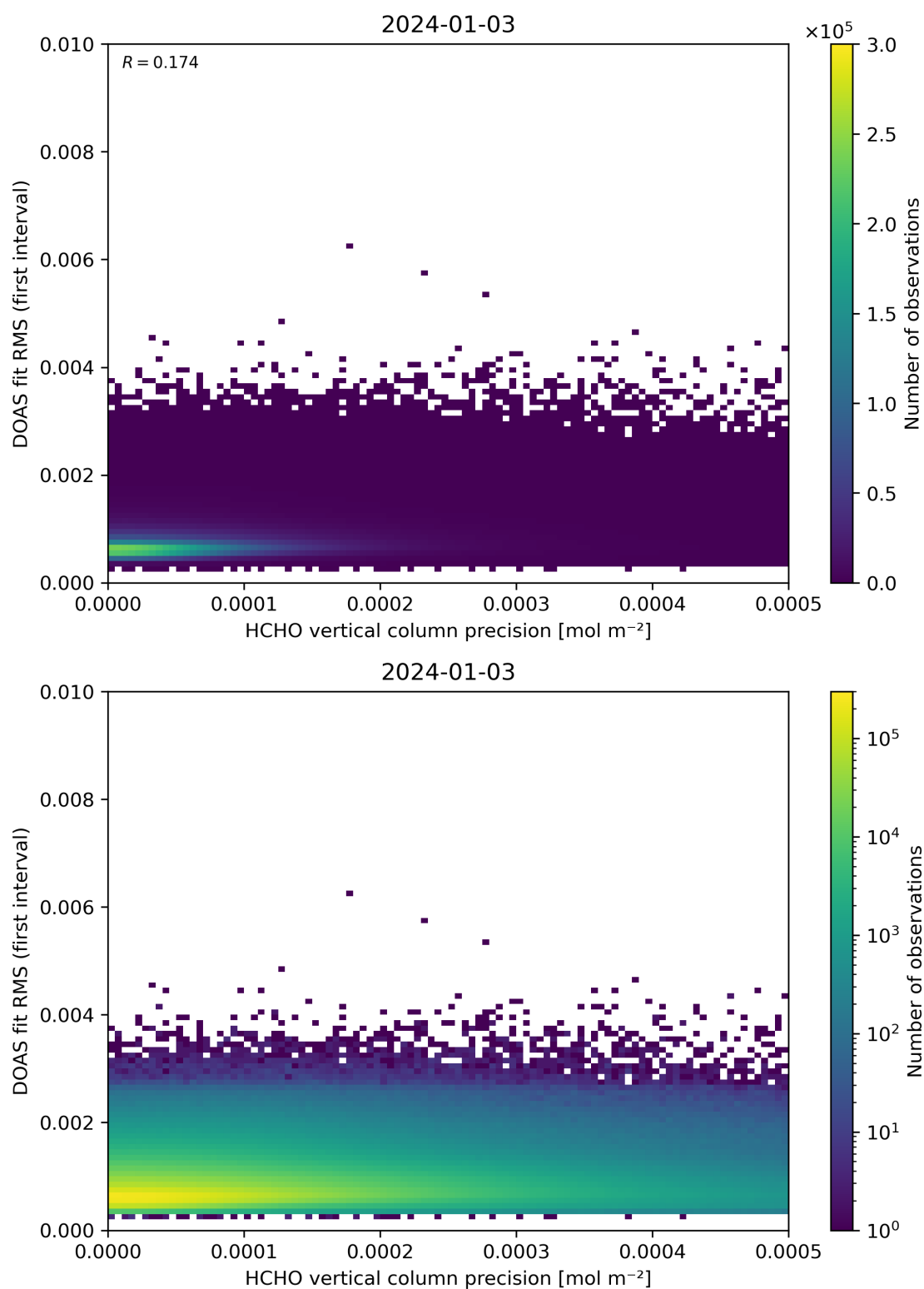
Figure 136: Scatter density plot of “HCHO vertical column precision” against “DOAS fit RMS (first interval)” for 2024-01-02 to 2024-01-04.
