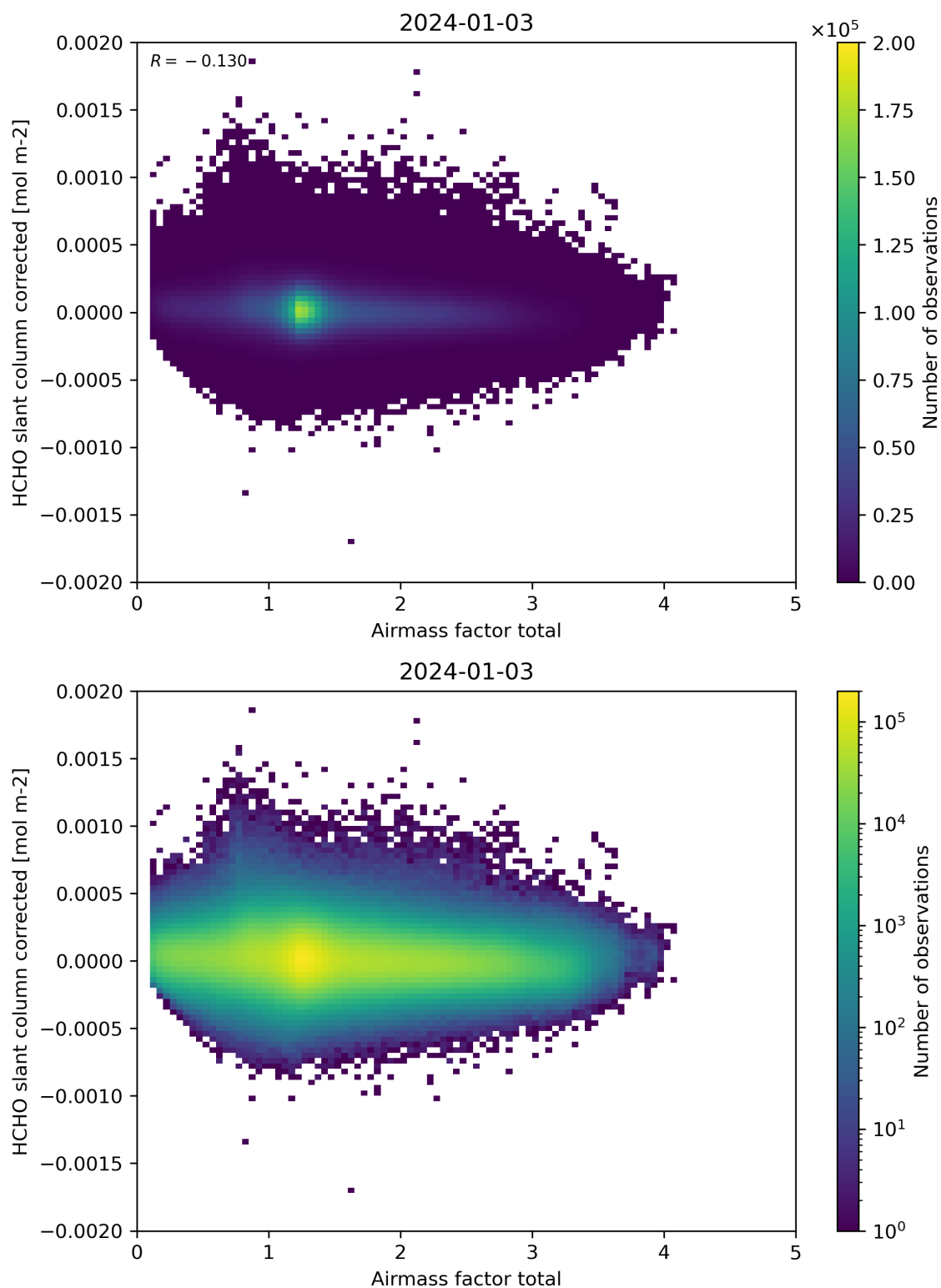
Figure 101: Scatter density plot of “Airmass factor total” against “HCHO slant column corrected” for 2024-01-02 to 2024-01-04.
