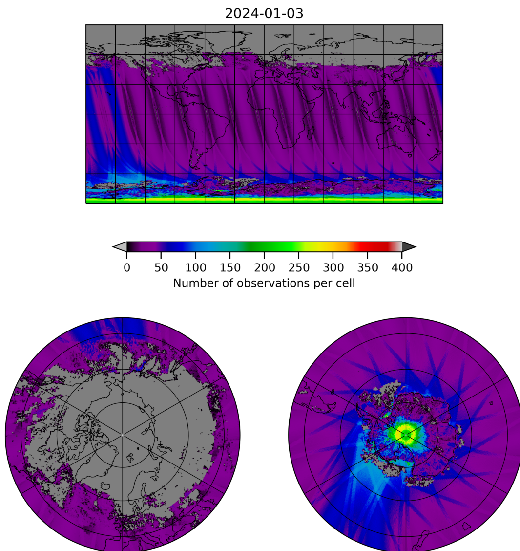
Figure 19: Map of the number of observations for 2024-01-02 to 2024-01-04
