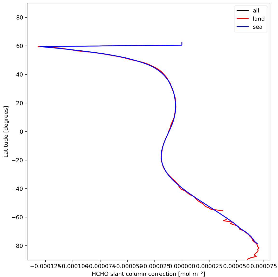
Figure 33: Zonal average of “HCHO slant column correction” for 2024-01-02 to 2024-01-04.
