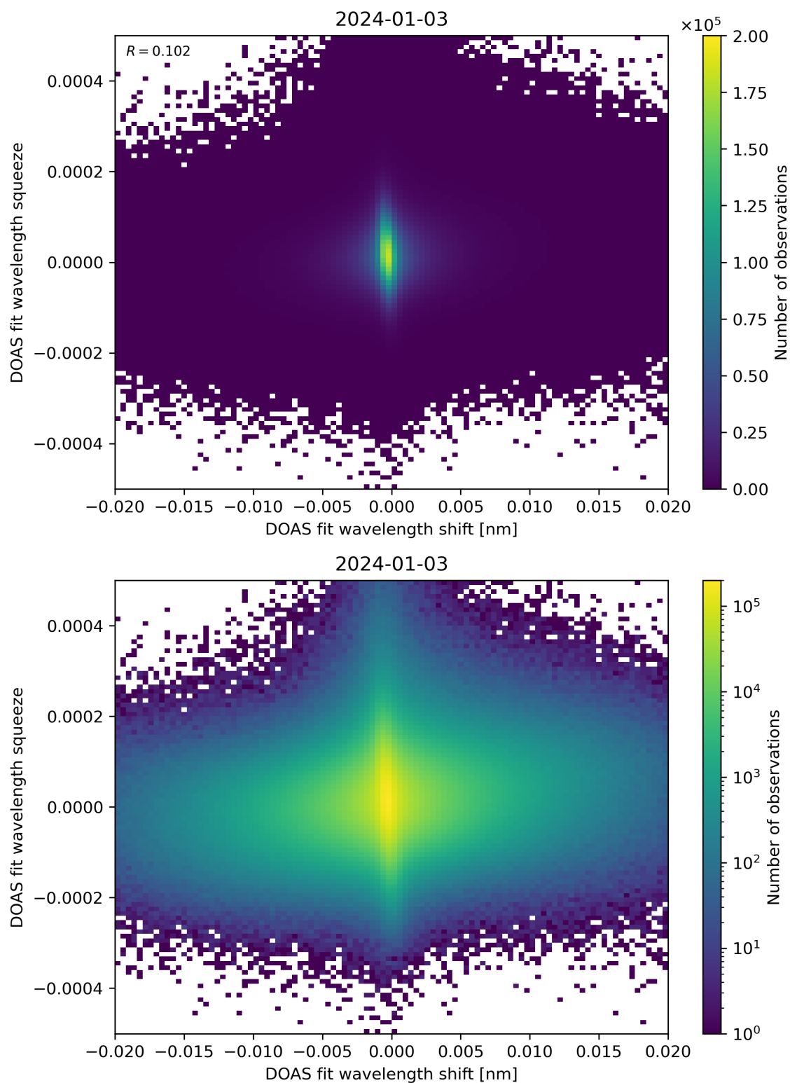
Figure 65: Scatter density plot of “DOAS fit wavelength shift” against “DOAS fit wavelength squeeze” for 2024-01-02 to 2024-01-04.
