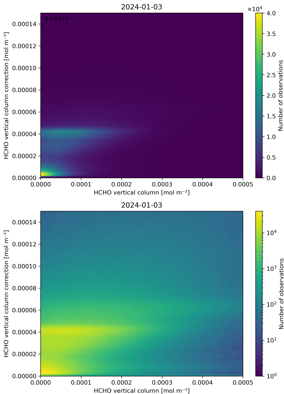
Figure 133: Scatter density plot of “HCHO vertical column” against “HCHO vertical column correction” for 2024-01-02 to 2024-01-04.
