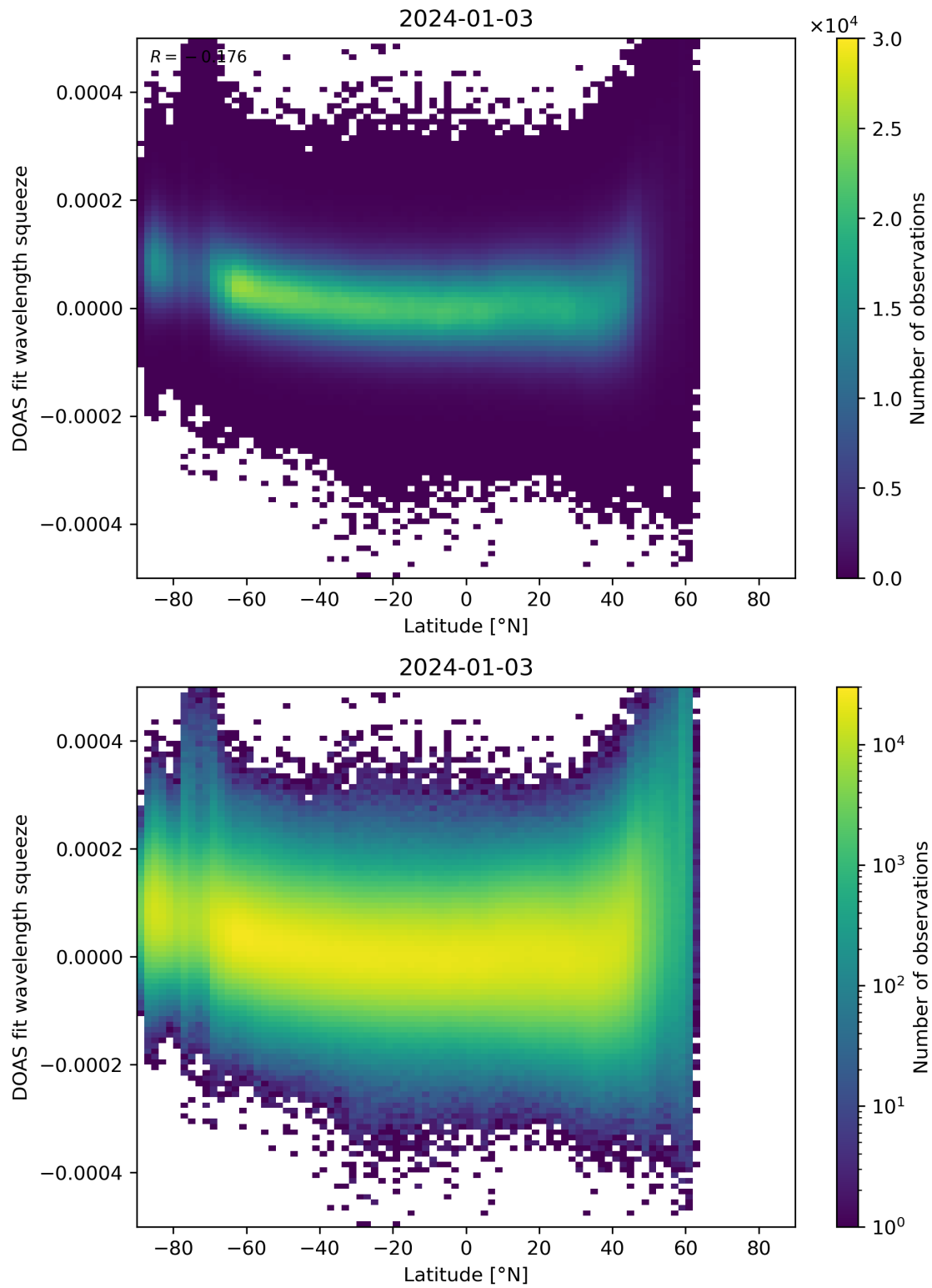
Figure 155: Scatter density plot of “Latitude” against “DOAS fit wavelength squeeze” for 2024-01-02 to 2024-01-04.
