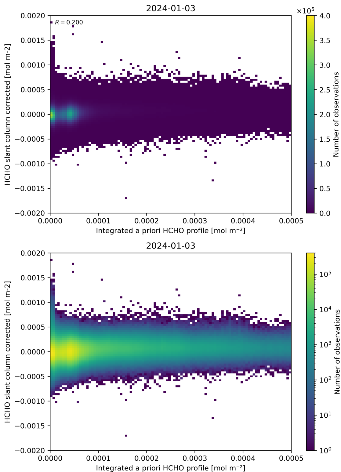
Figure 151: Scatter density plot of “Integrated a priori HCHO profile” against “HCHO slant column corrected” for 2024-01-02 to 2024-01-04.
