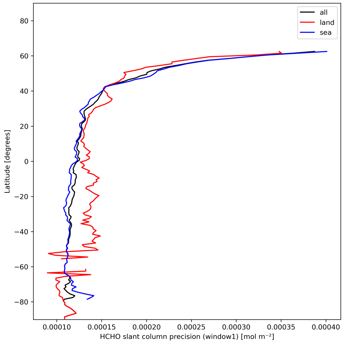
Figure 25: Zonal average of “HCHO slant column precision (window1)” for 2024-01-02 to 2024-01-04.
