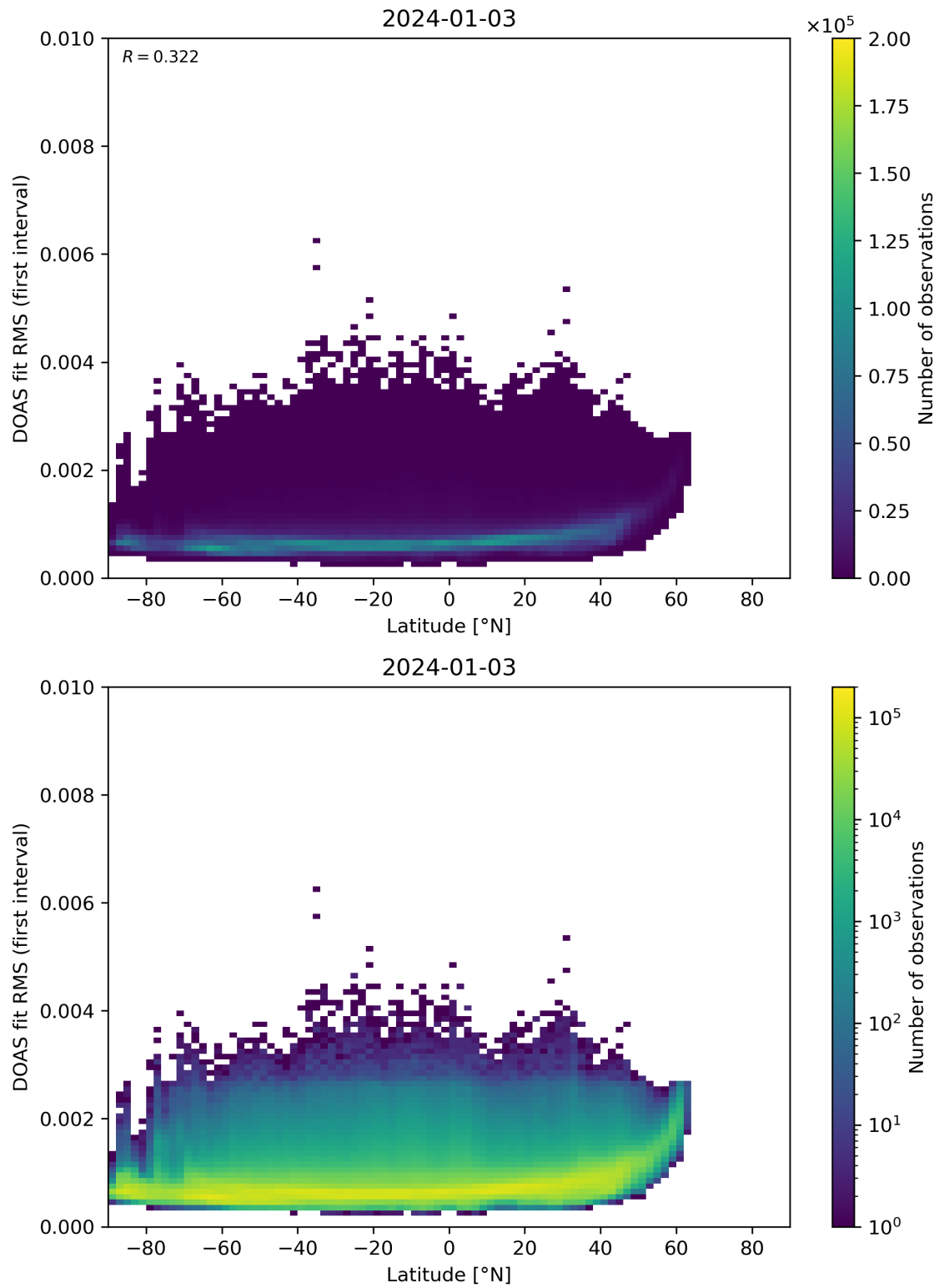
Figure 153: Scatter density plot of “Latitude” against “DOAS fit RMS (first interval)” for 2024-01-02 to 2024-01-04.
