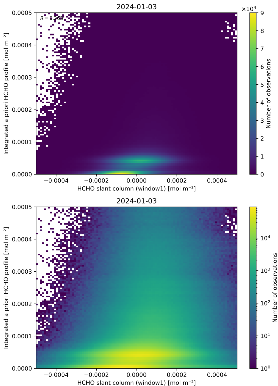
Figure 87: Scatter density plot of “HCHO slant column (window1)” against “Integrated a priori HCHO profile” for 2024-01-02 to 2024-01-04.
