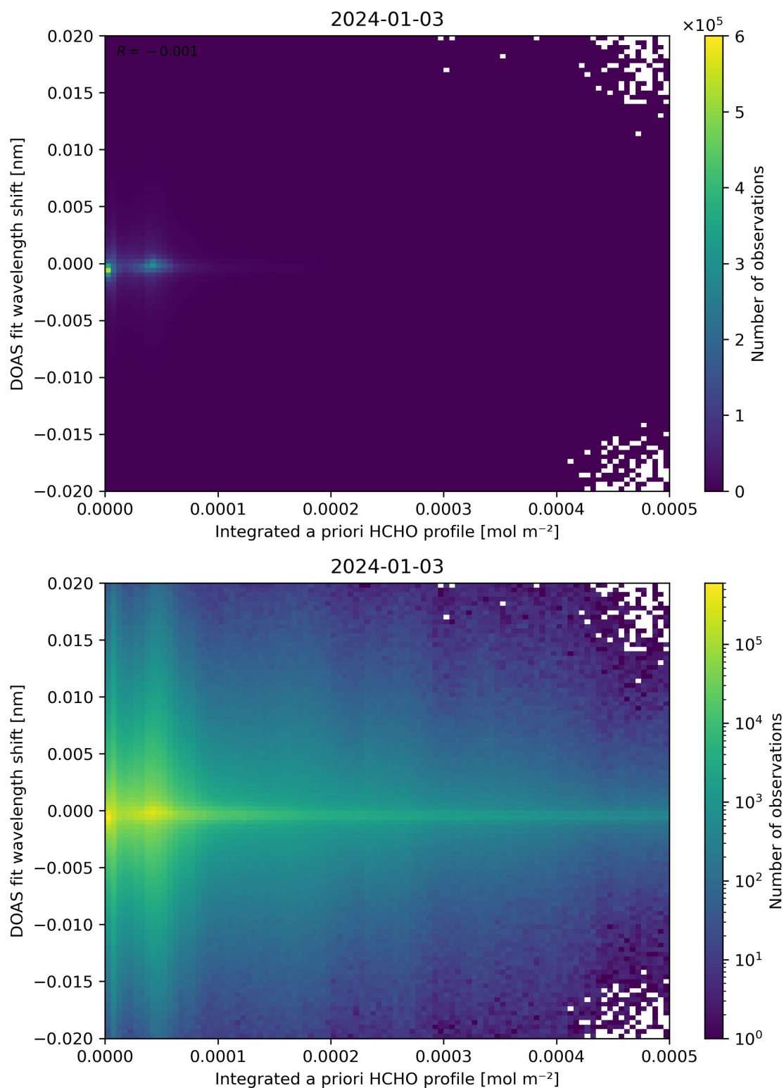
Figure 149: Scatter density plot of “Integrated a priori HCHO profile” against “DOAS fit wavelength shift” for 2024-01-02 to 2024-01-04.
