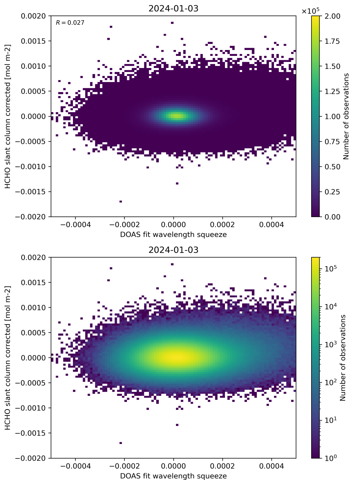
Figure 69: Scatter density plot of “DOAS fit wavelength squeeze” against “HCHO slant column corrected” for 2024-01-02 to 2024-01-04.
