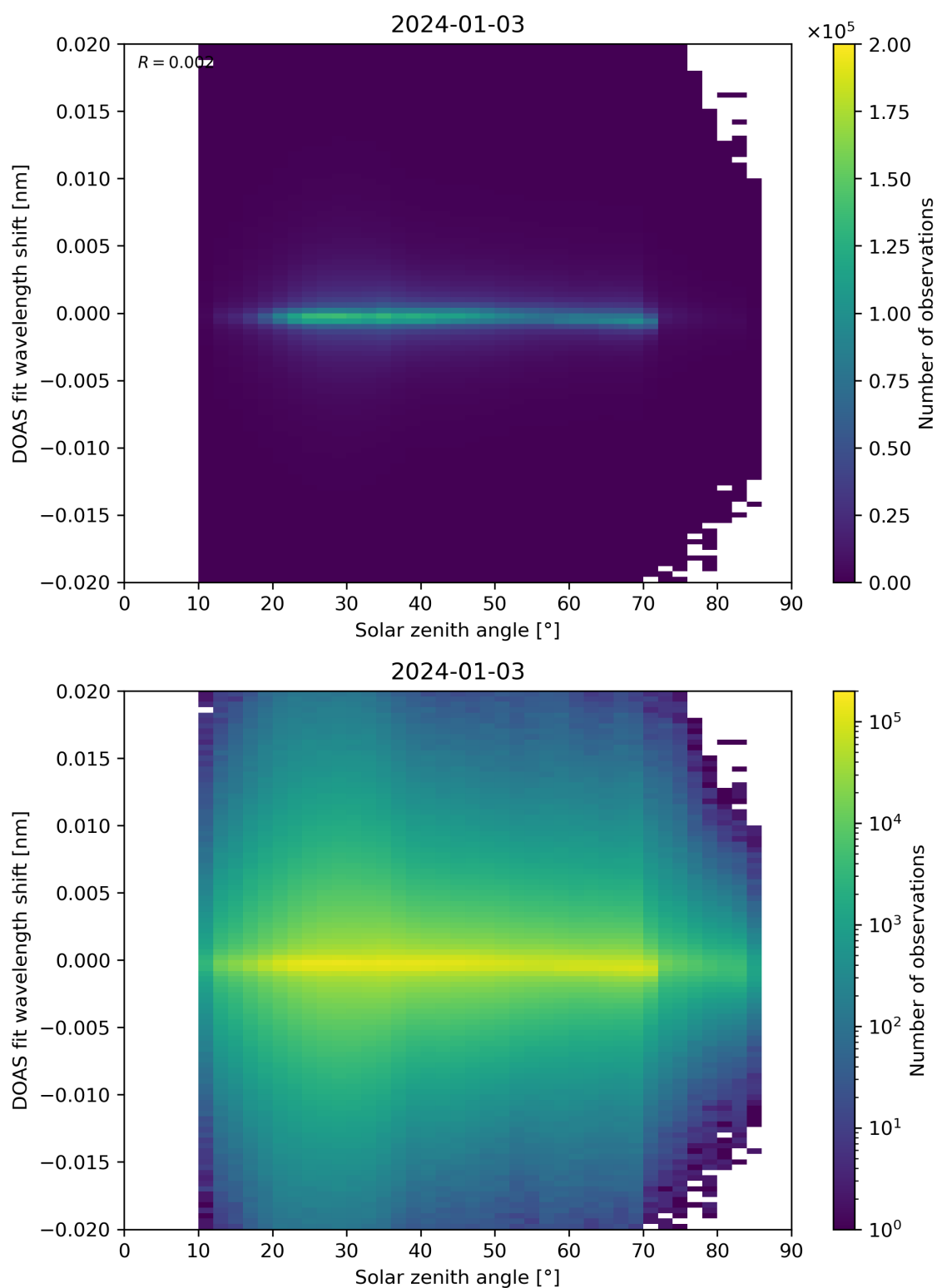
Figure 168: Scatter density plot of “Solar zenith angle” against “DOAS fit wavelength shift” for 2024-01-02 to 2024-01-04.
