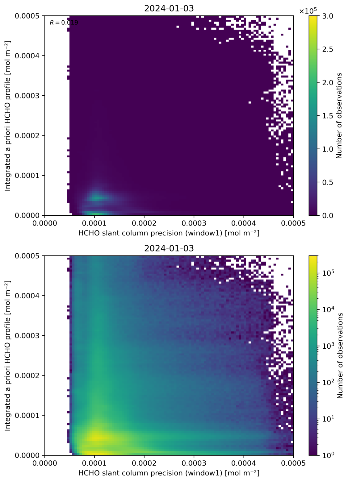
Figure 96: Scatter density plot of “HCHO slant column precision (window1)” against “Integrated a priori HCHO profile” for 2024-01-02 to 2024-01-04.
