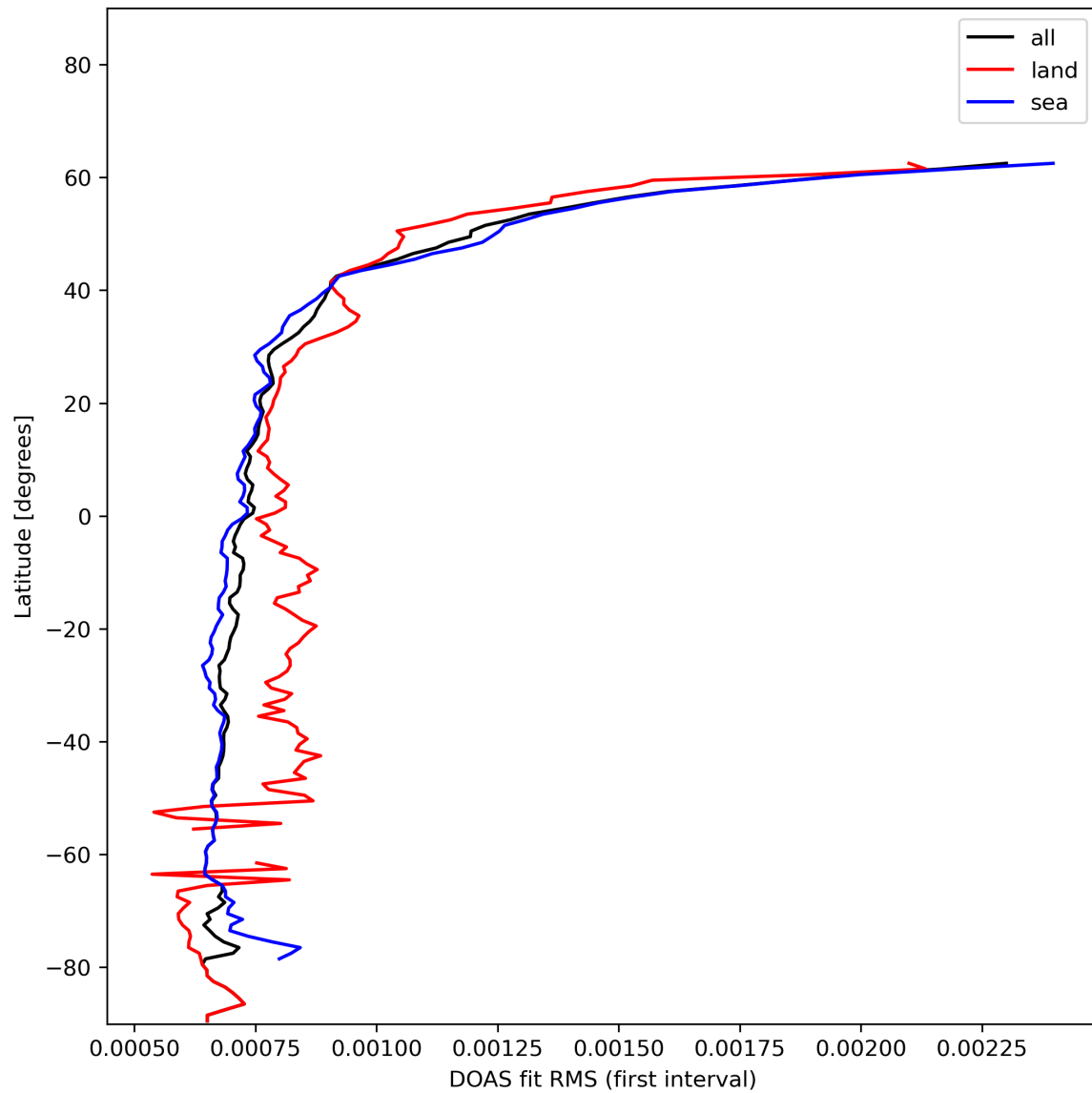
Figure 32: Zonal average of “DOAS fit RMS (first interval)” for 2024-01-02 to 2024-01-04.
