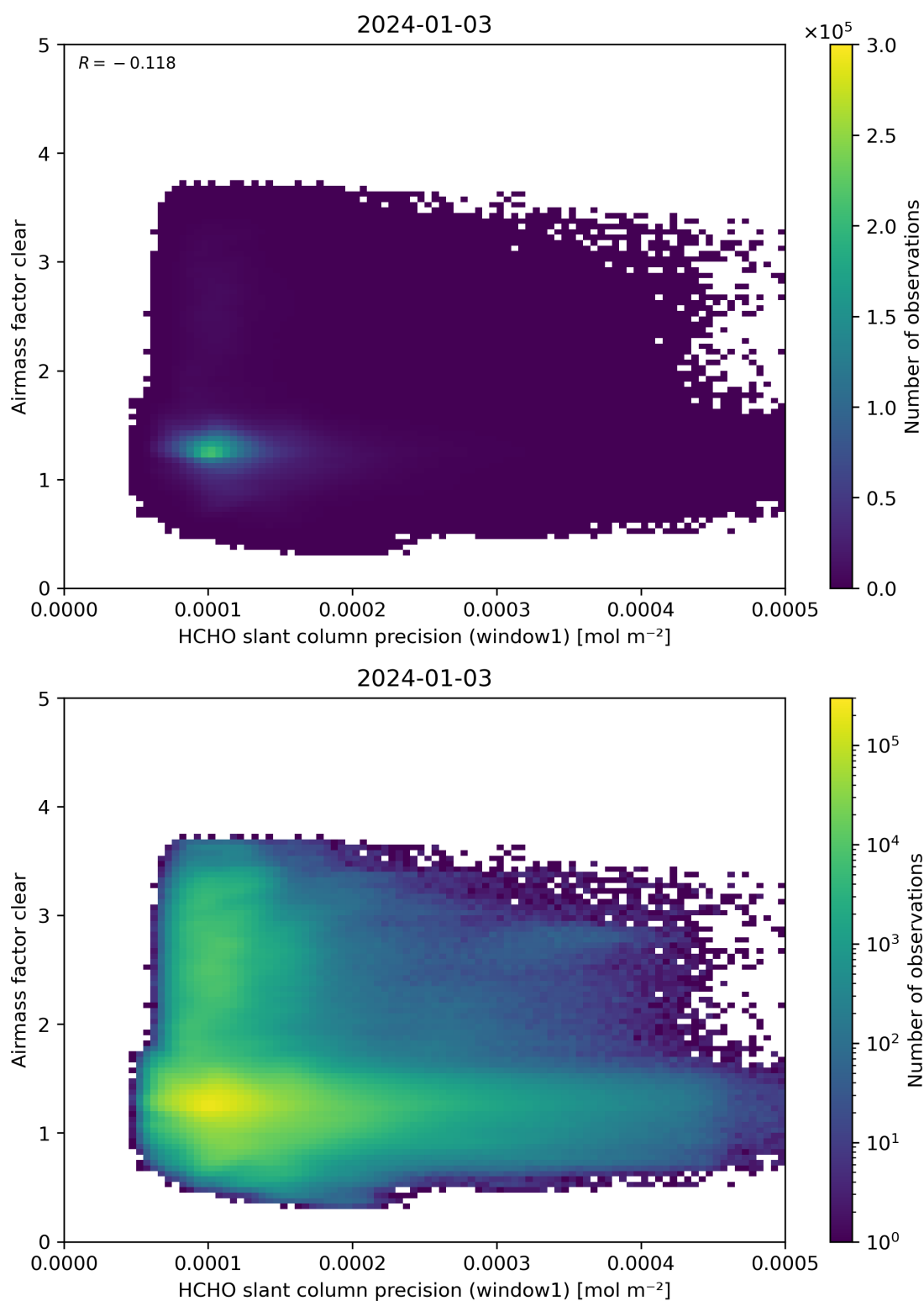
Figure 91: Scatter density plot of “HCHO slant column precision (window1)” against “Airmass factor clear” for 2024-01-02 to 2024-01-04.
