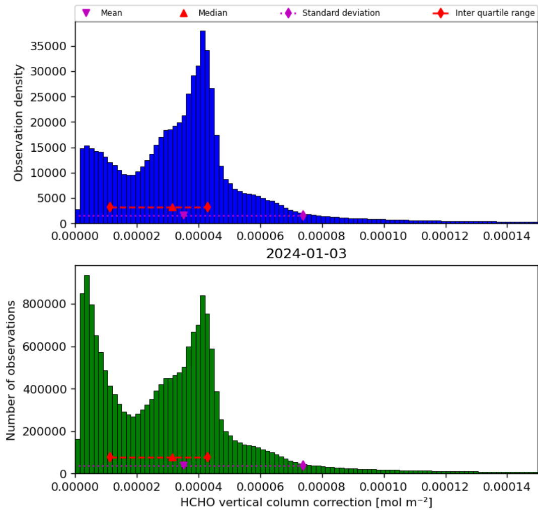
Figure 37: Histogram of “HCHO vertical column correction” for 2024-01-02 to 2024-01-04
