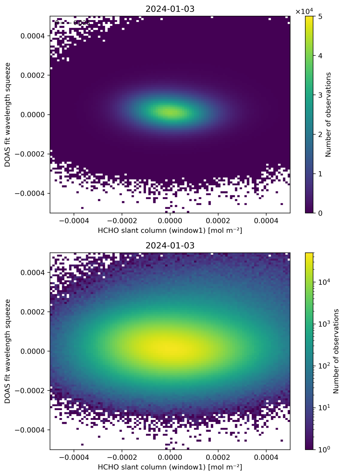
Figure 80: Scatter density plot of “HCHO slant column (window1)” against “DOAS fit wavelength squeeze” for 2024-01-02 to 2024-01-04.
