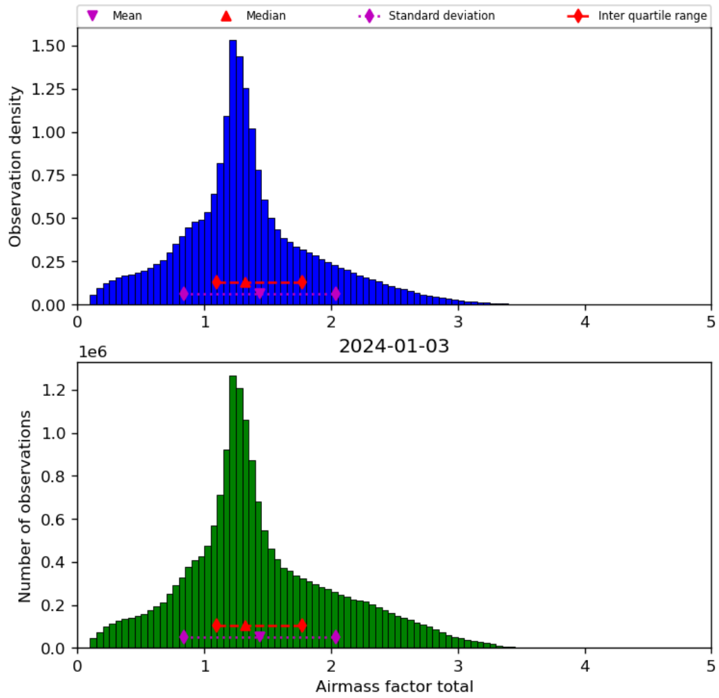
Figure 40: Histogram of “Airmass factor total” for 2024-01-02 to 2024-01-04
