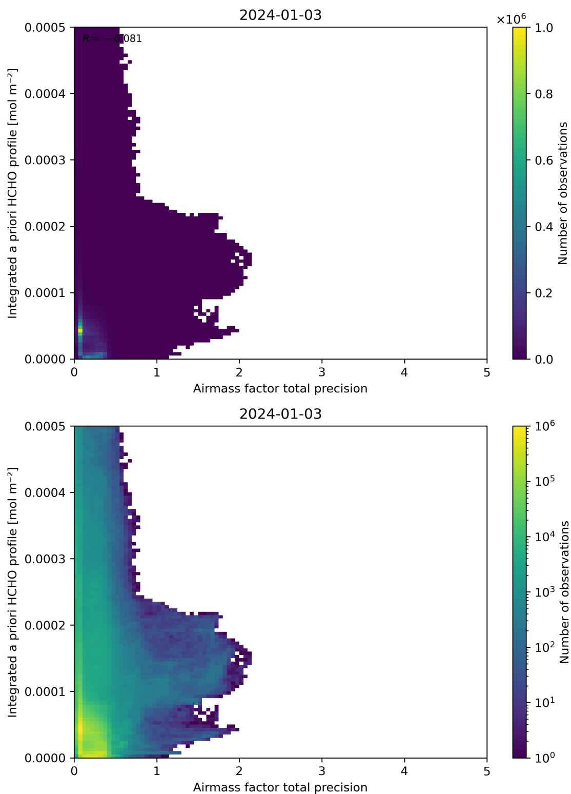
Figure 111: Scatter density plot of “Airmass factor total precision” against “Integrated a priori HCHO profile” for 2024-01-02 to 2024-01-04.
