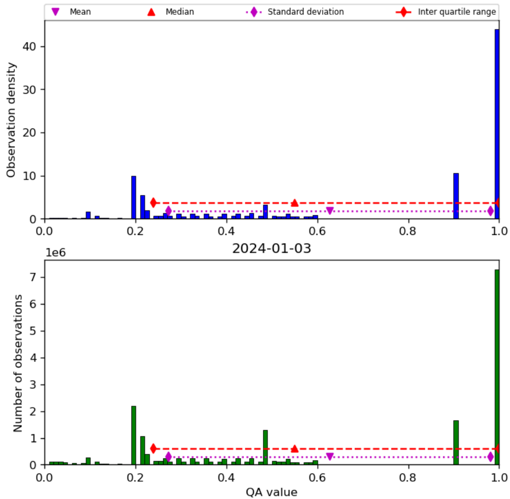
Figure 34: Histogram of “QA value” for 2024-01-02 to 2024-01-04
