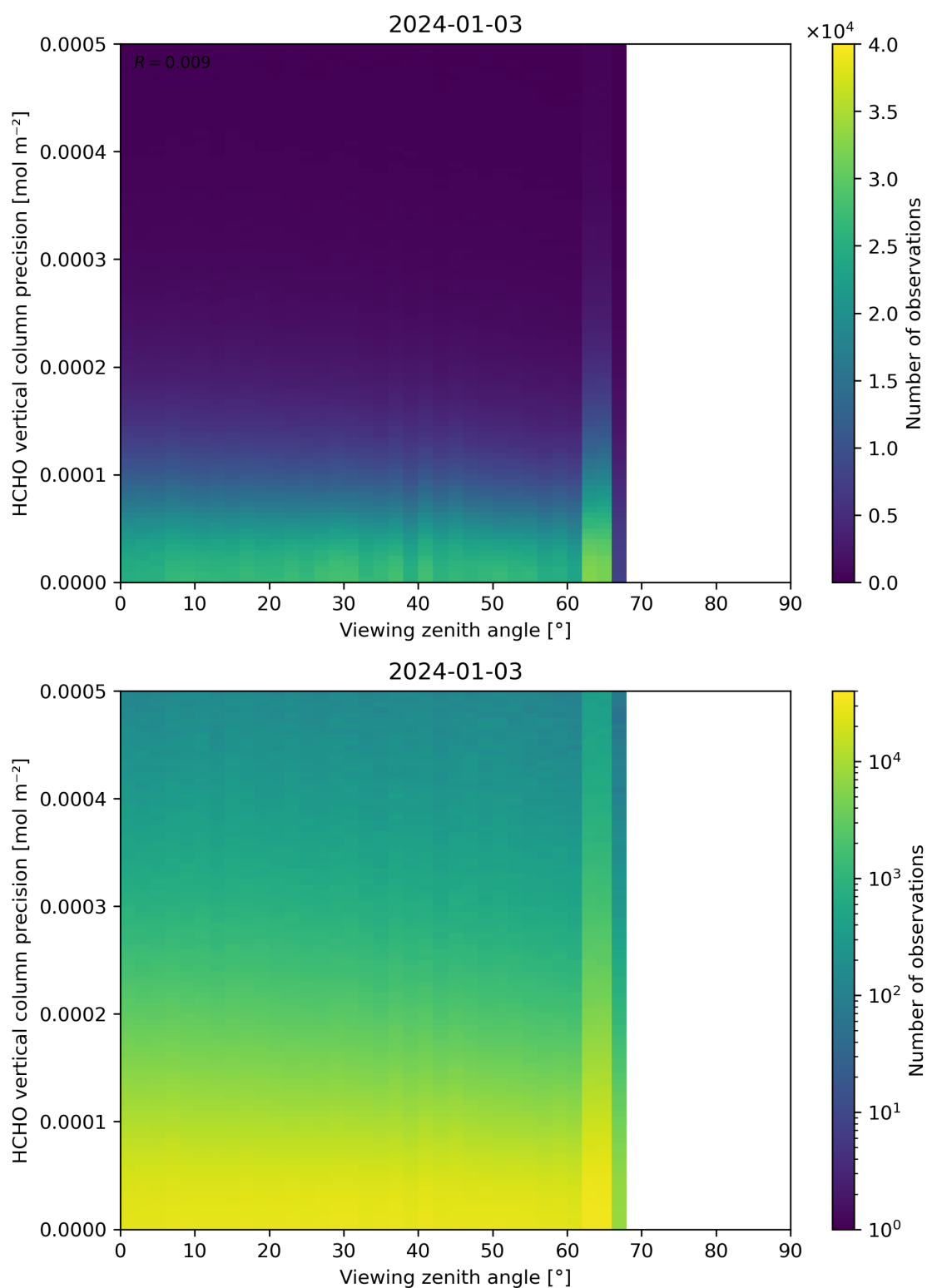
Figure 194: Scatter density plot of “Viewing zenith angle” against “HCHO vertical column precision” for 2024-01-02 to 2024-01-04.
