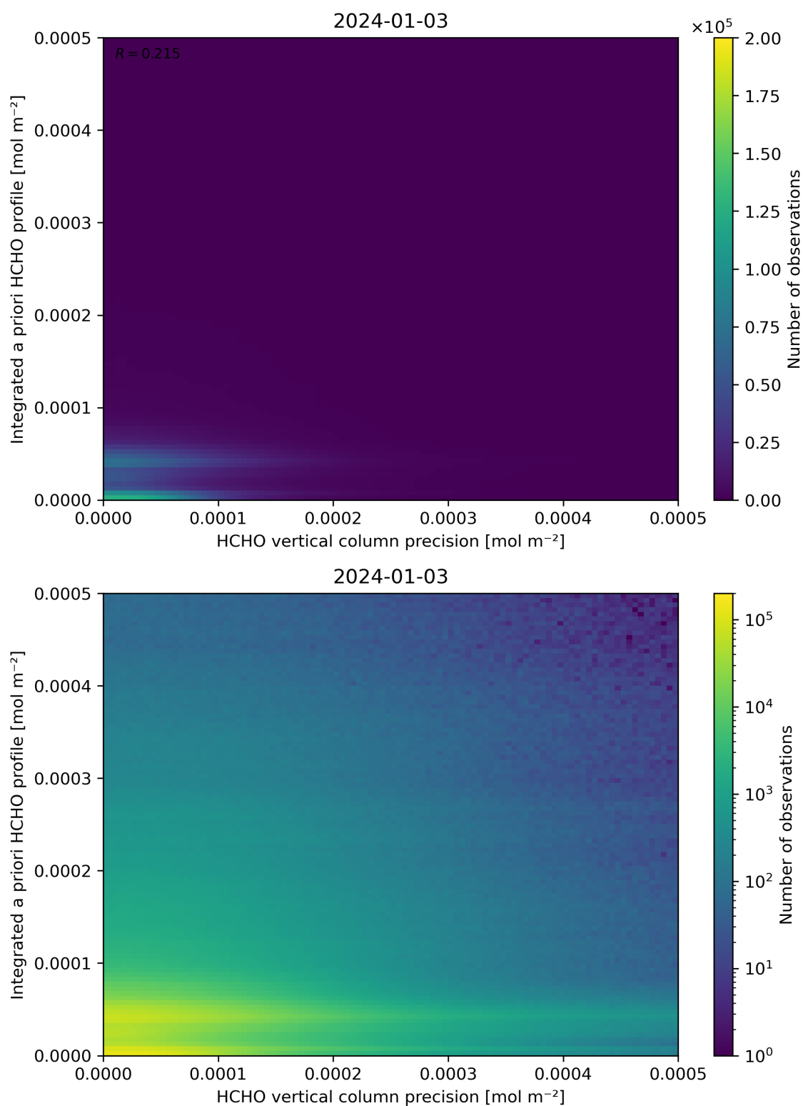
Figure 147: Scatter density plot of “HCHO vertical column precision” against “Integrated a priori HCHO profile” for 2024-01-02 to 2024-01-04.
