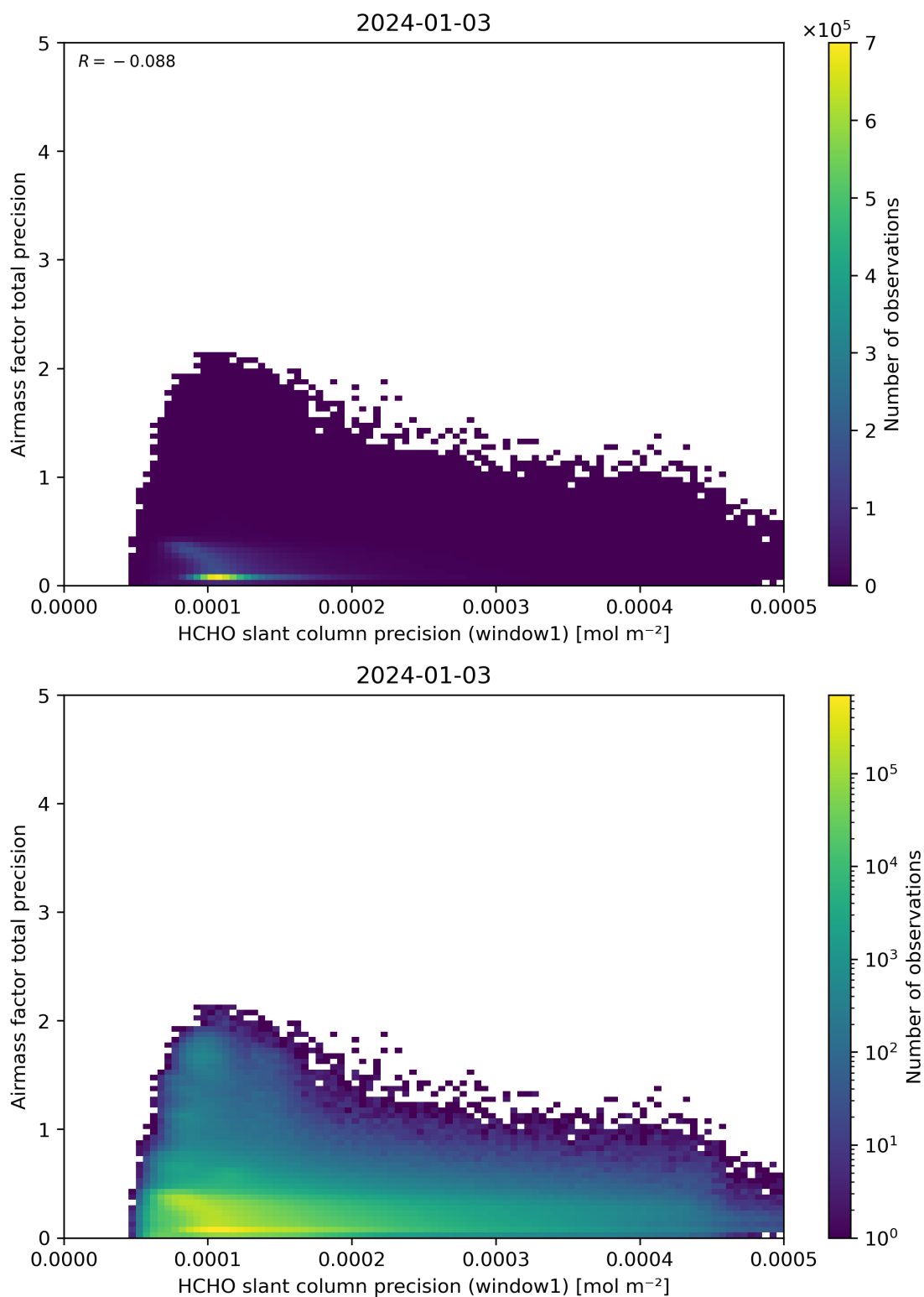
Figure 95: Scatter density plot of “HCHO slant column precision (window1)” against “Airmass factor total precision” for 2024-01-02 to 2024-01-04.
