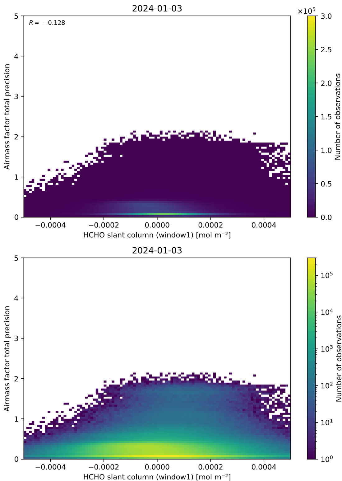
Figure 86: Scatter density plot of “HCHO slant column (window1)” against “Airmass factor total precision” for 2024-01-02 to 2024-01-04.
