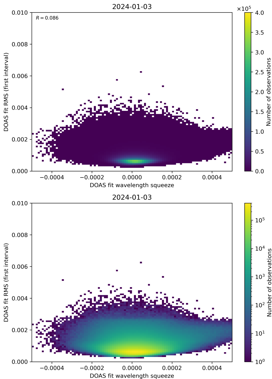
Figure 68: Scatter density plot of “DOAS fit wavelength squeeze” against “DOAS fit RMS (first interval)” for 2024-01-02 to 2024-01-04.
