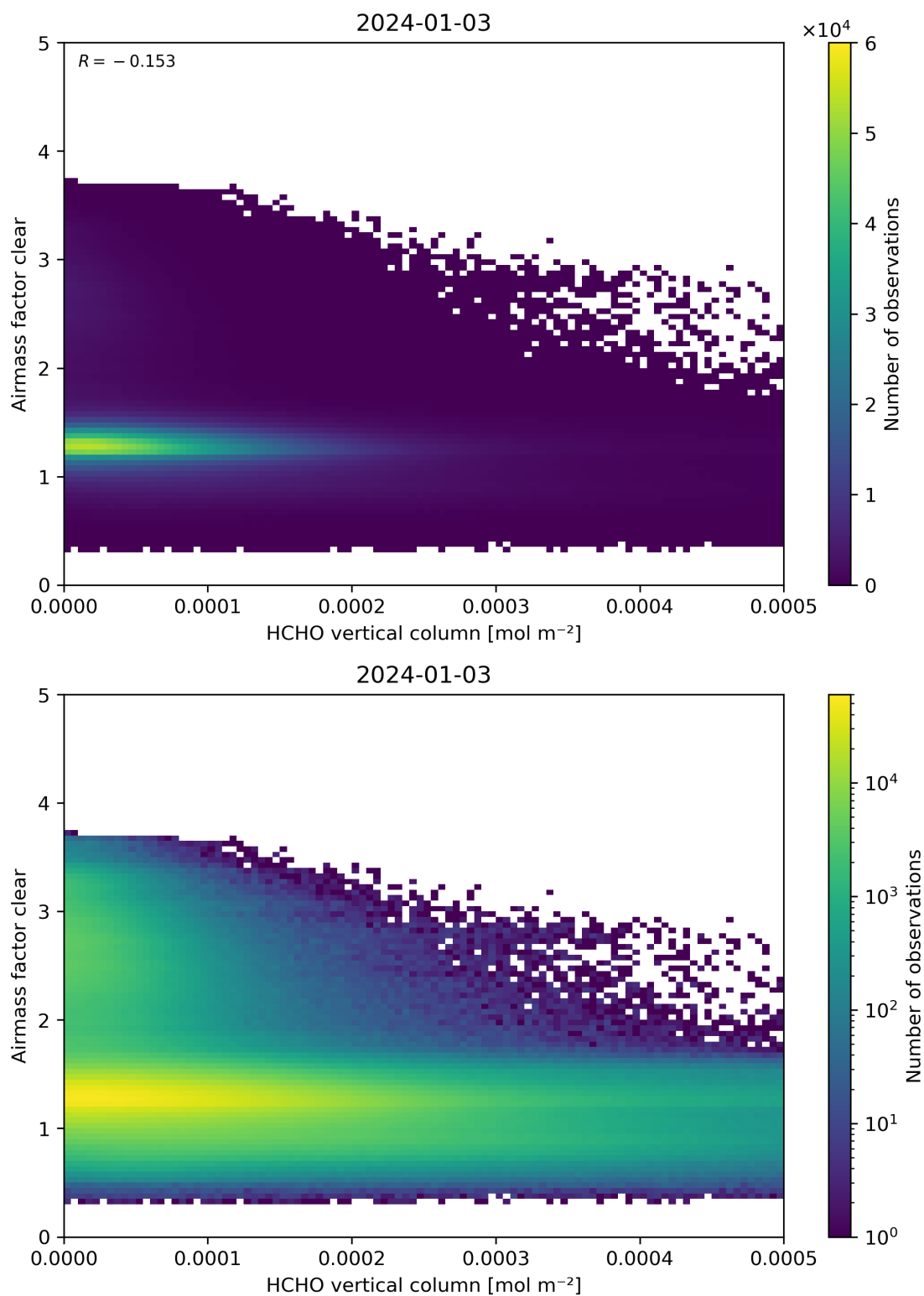
Figure 126: Scatter density plot of “HCHO vertical column” against “Airmass factor clear” for 2024-01-02 to 2024-01-04.
