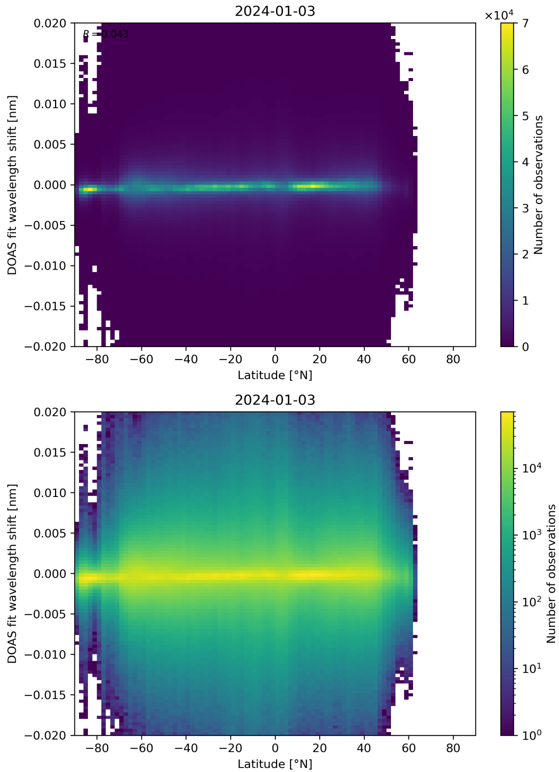
Figure 154: Scatter density plot of “Latitude” against “DOAS fit wavelength shift” for 2024-01-02 to 2024-01-04.
