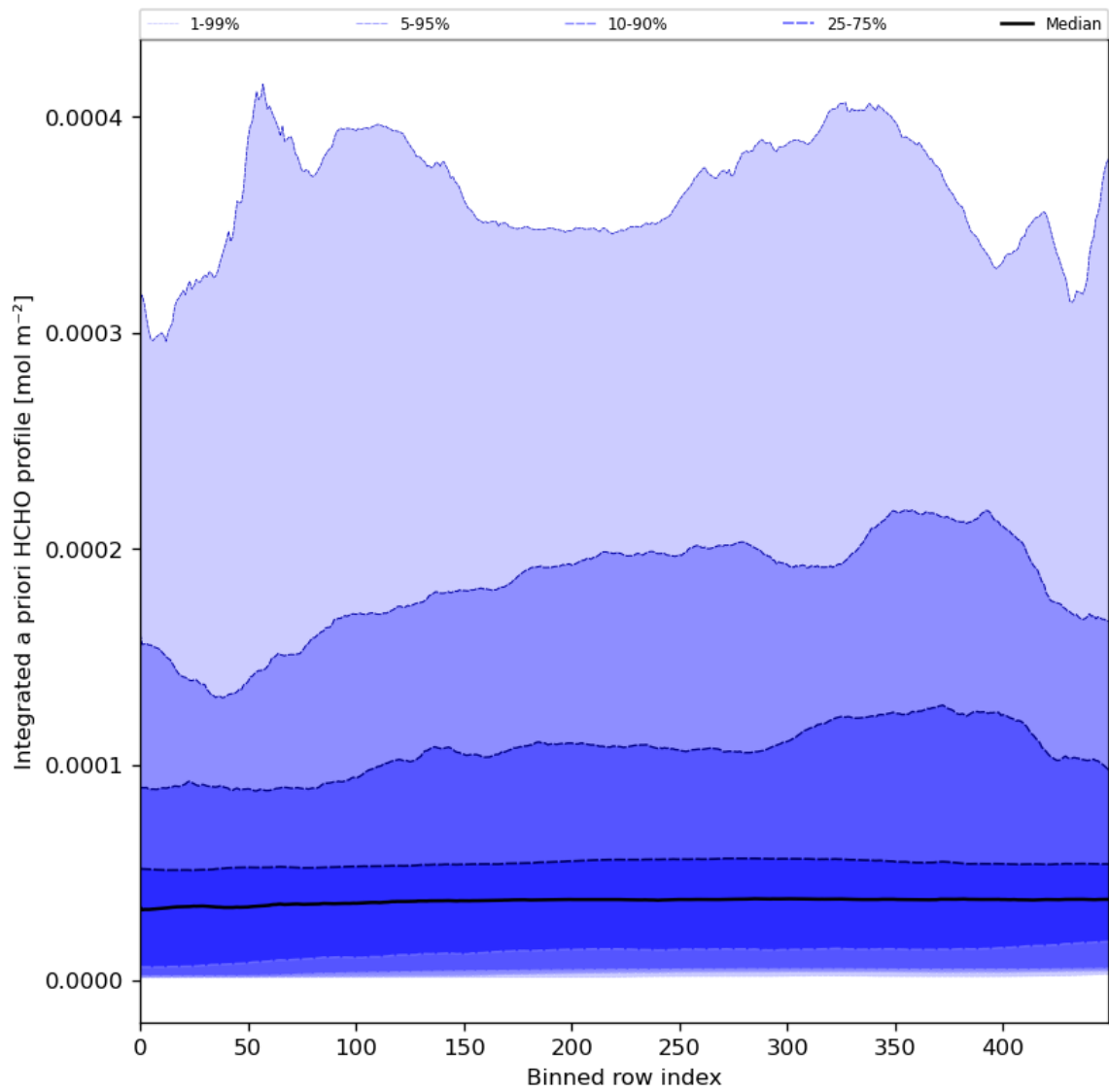
Figure 57: Along track statistics of "Integrated a priori HCHO profile" for 2024-01-02 to 2024-01-04
