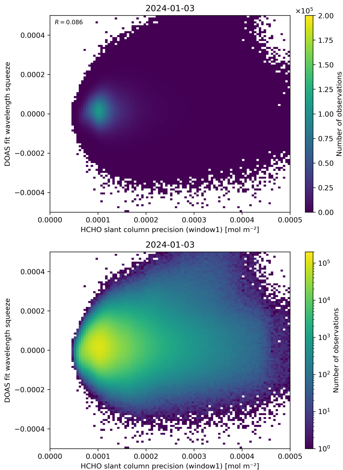
Figure 90: Scatter density plot of “HCHO slant column precision (window1)” against “DOAS fit wavelength squeeze” for 2024-01-02 to 2024-01-04.
