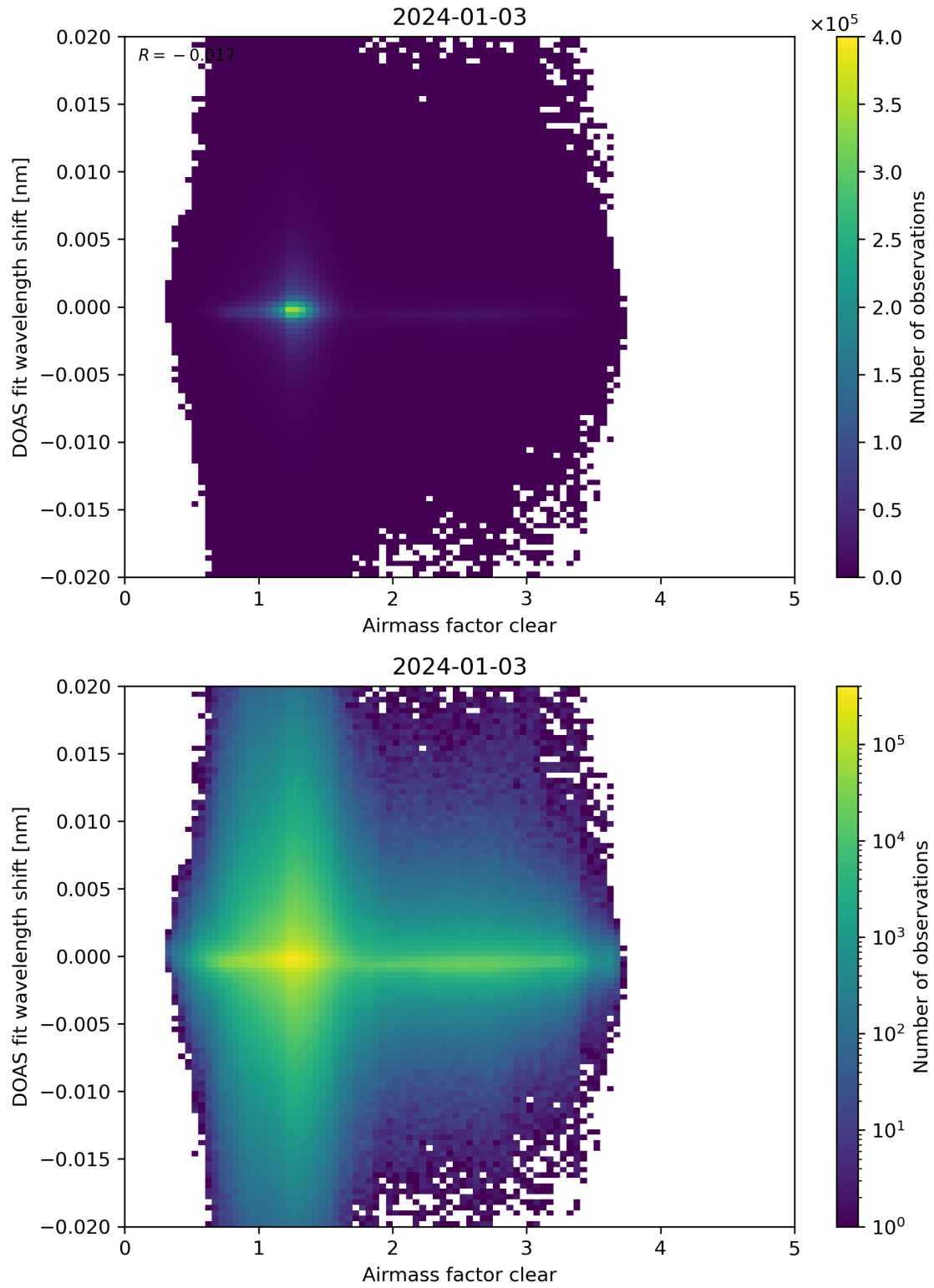
Figure 72: Scatter density plot of “Airmass factor clear” against “DOAS fit wavelength shift” for 2024-01-02 to 2024-01-04.
