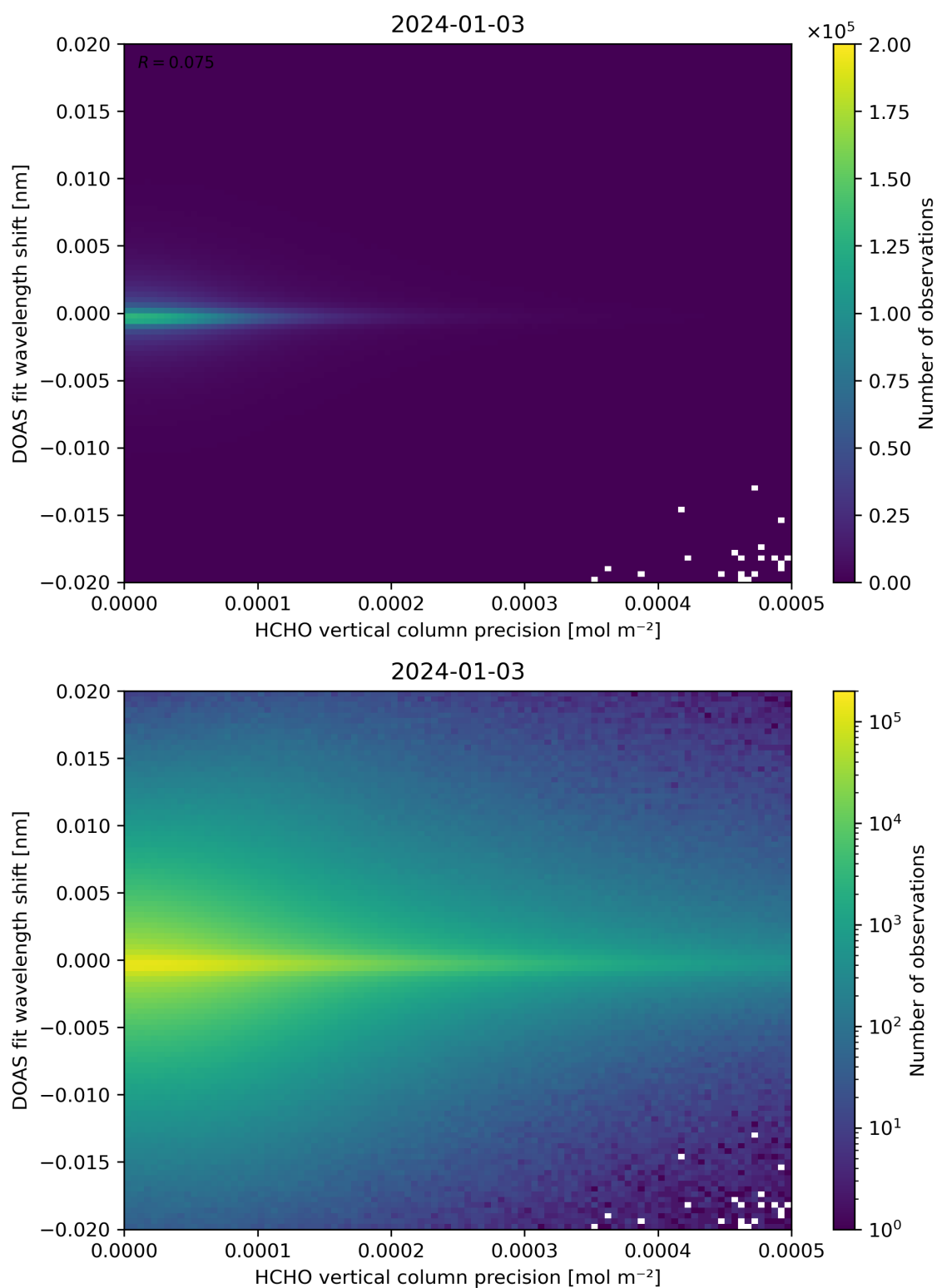
Figure 137: Scatter density plot of “HCHO vertical column precision” against “DOAS fit wavelength shift” for 2024-01-02 to 2024-01-04.
