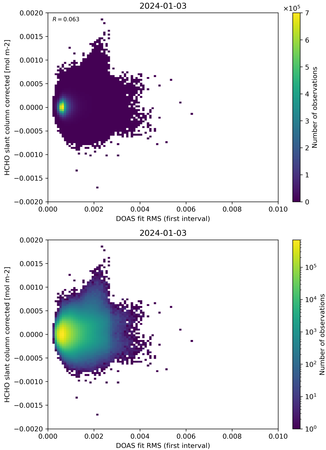
Figure 62: Scatter density plot of “DOAS fit RMS (first interval)” against “HCHO slant column corrected” for 2024-01-02 to 2024-01-04.
