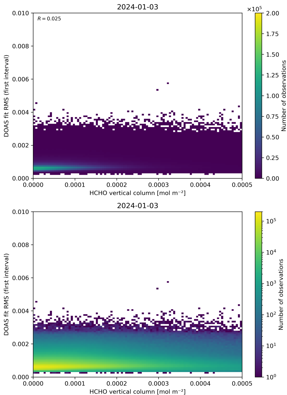
Figure 123: Scatter density plot of “HCHO vertical column” against “DOAS fit RMS (first interval)” for 2024-01-02 to 2024-01-04.
