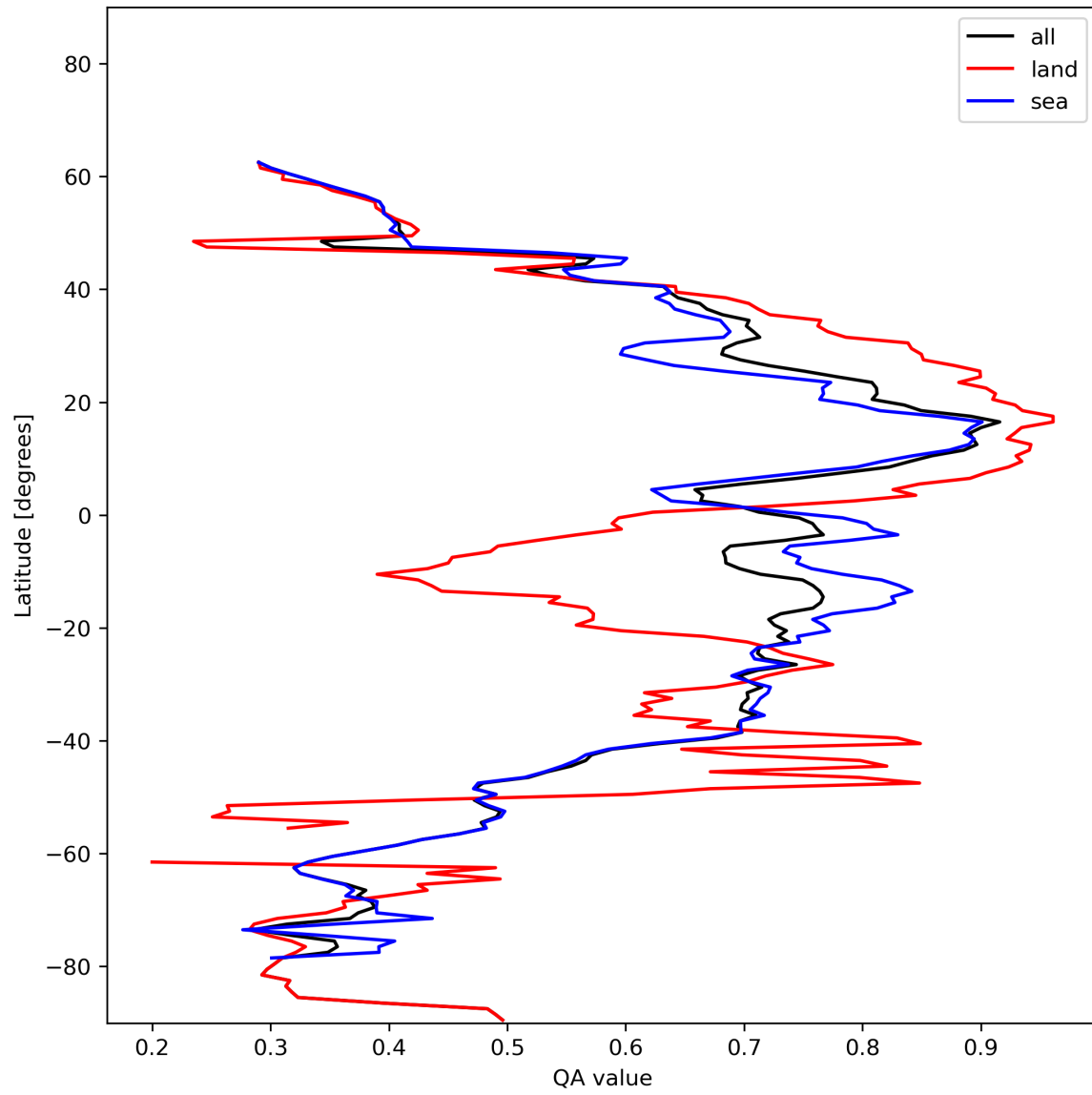
Figure 20: Zonal average of “QA value” for 2024-01-02 to 2024-01-04.
