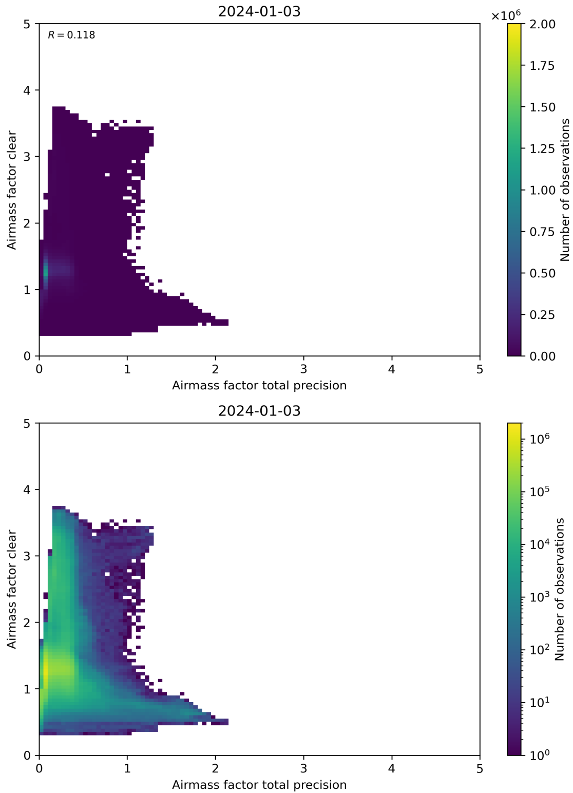
Figure 108: Scatter density plot of “Airmass factor total precision” against “Airmass factor clear” for 2024-01-02 to 2024-01-04.
