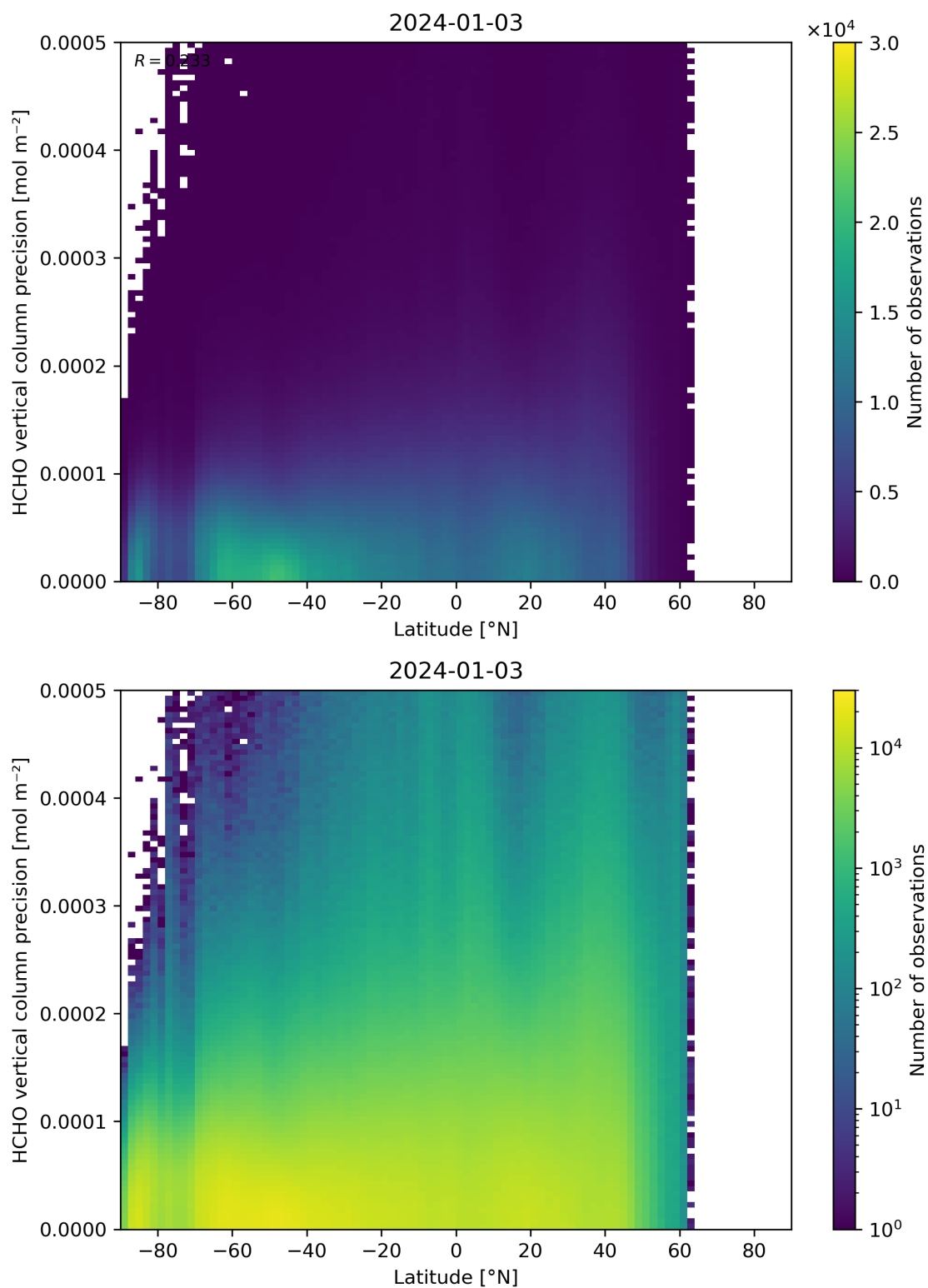
Figure 165: Scatter density plot of “Latitude” against “HCHO vertical column precision” for 2024-01-02 to 2024-01-04.
