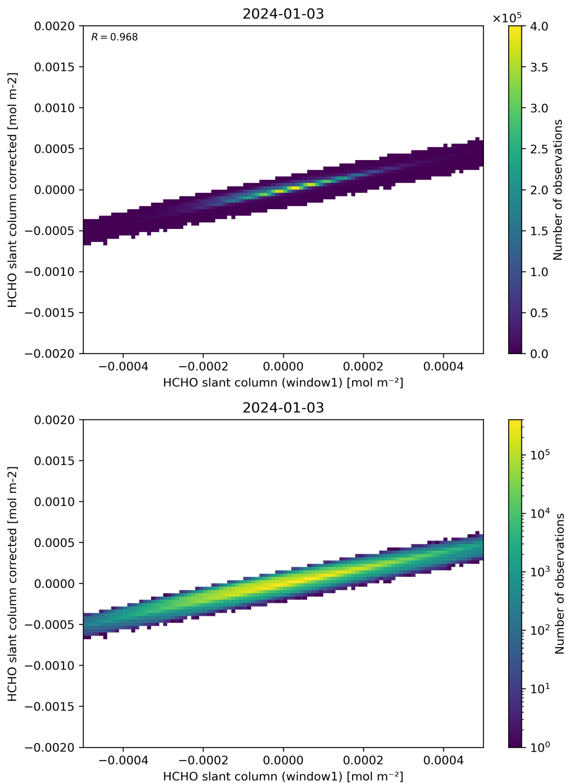
Figure 82: Scatter density plot of “HCHO slant column (window1)” against “HCHO slant column corrected” for 2024-01-02 to 2024-01-04.
