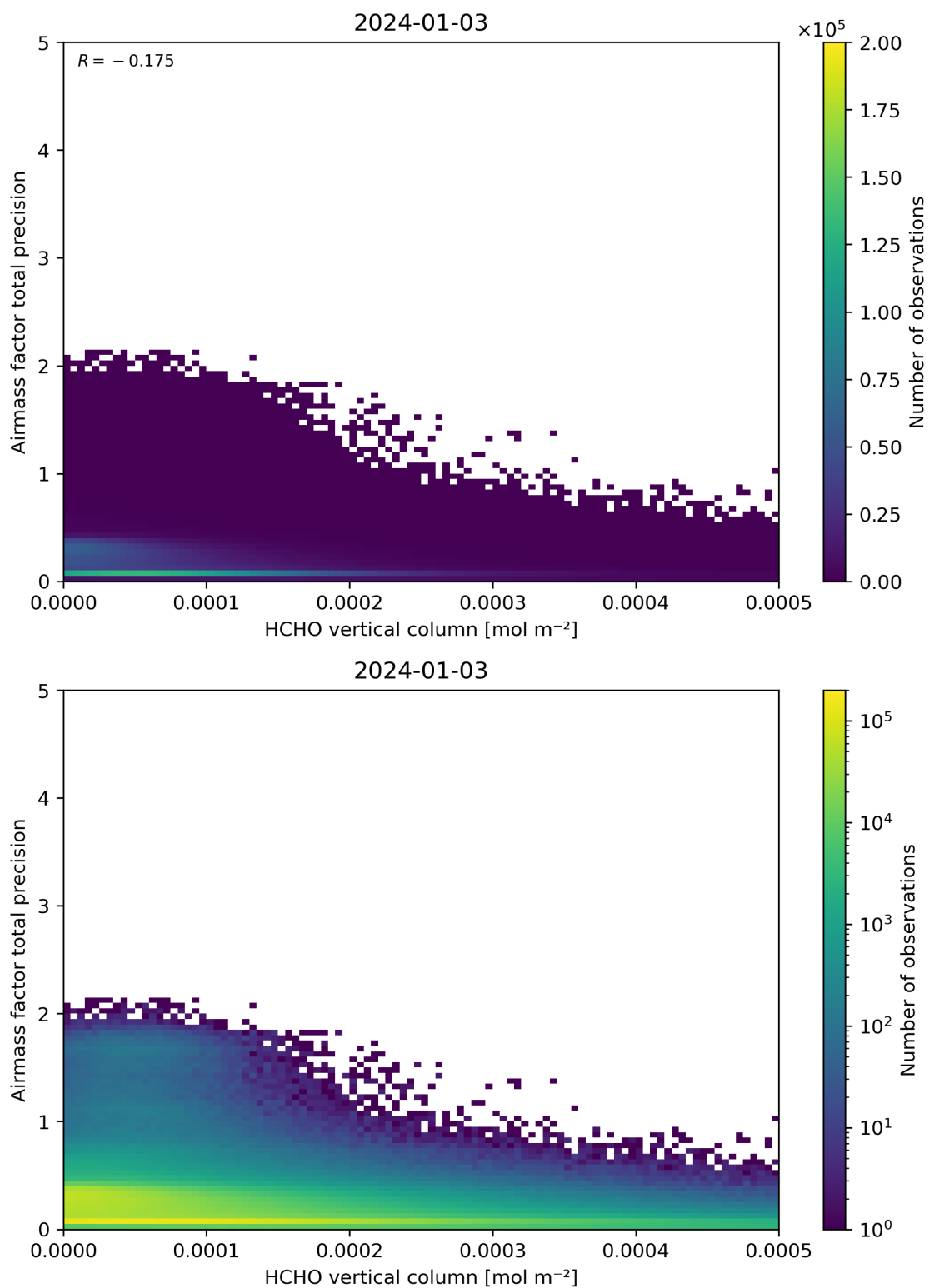
Figure 132: Scatter density plot of “HCHO vertical column” against “Airmass factor total precision” for 2024-01-02 to 2024-01-04.
