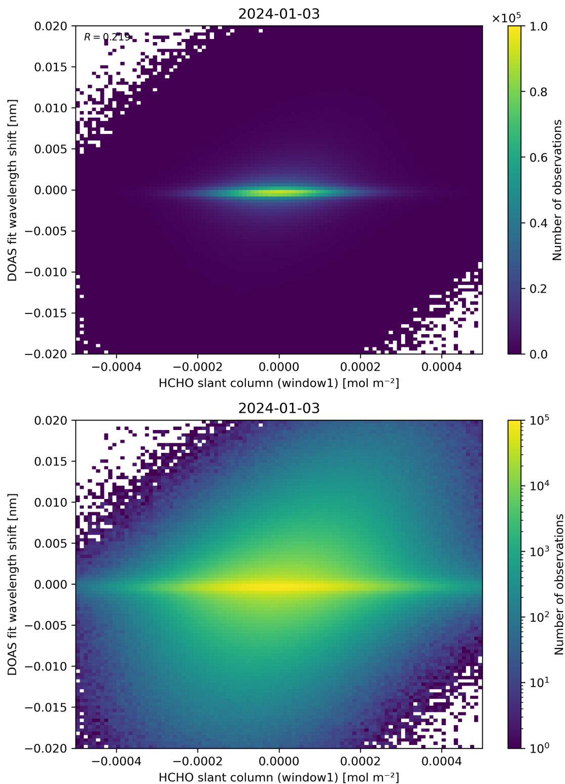
Figure 79: Scatter density plot of “HCHO slant column (window1)” against “DOAS fit wavelength shift” for 2024-01-02 to 2024-01-04.
