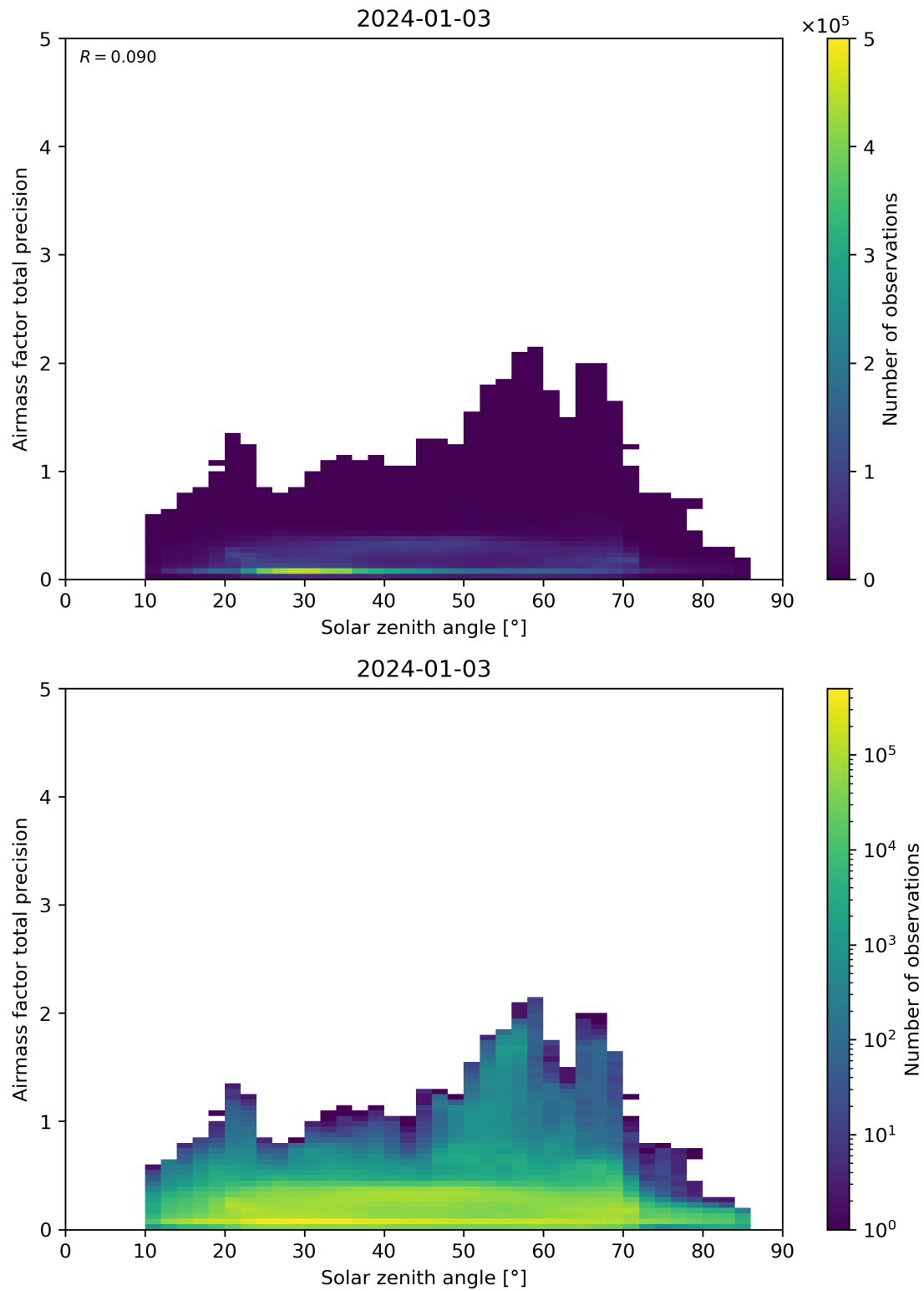
Figure 176: Scatter density plot of “Solar zenith angle” against “Airmass factor total precision” for 2024-01-02 to 2024-01-04.
