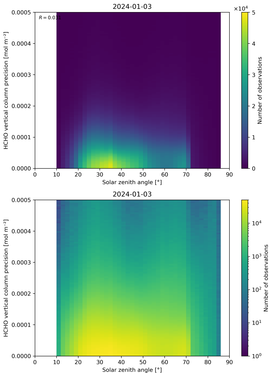
Figure 179: Scatter density plot of “Solar zenith angle” against “HCHO vertical column precision” for 2024-01-02 to 2024-01-04.
