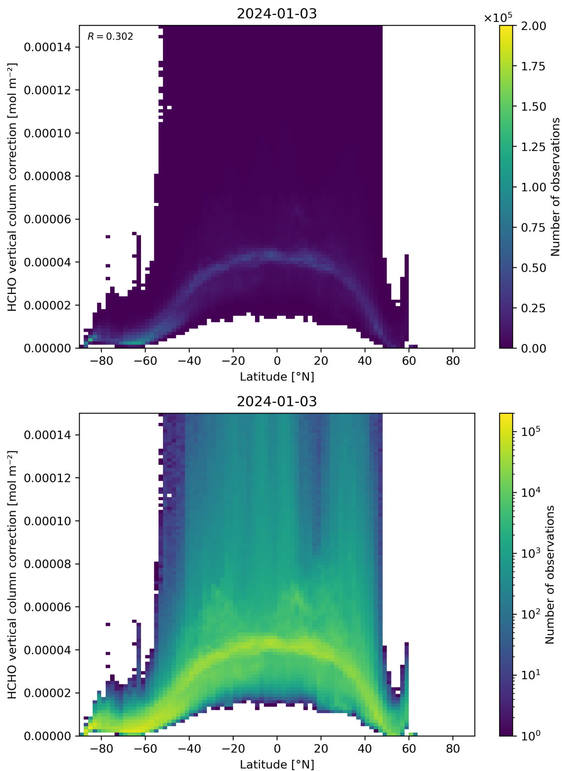
Figure 164: Scatter density plot of “Latitude” against “HCHO vertical column correction” for 2024-01-02 to 2024-01-04.
