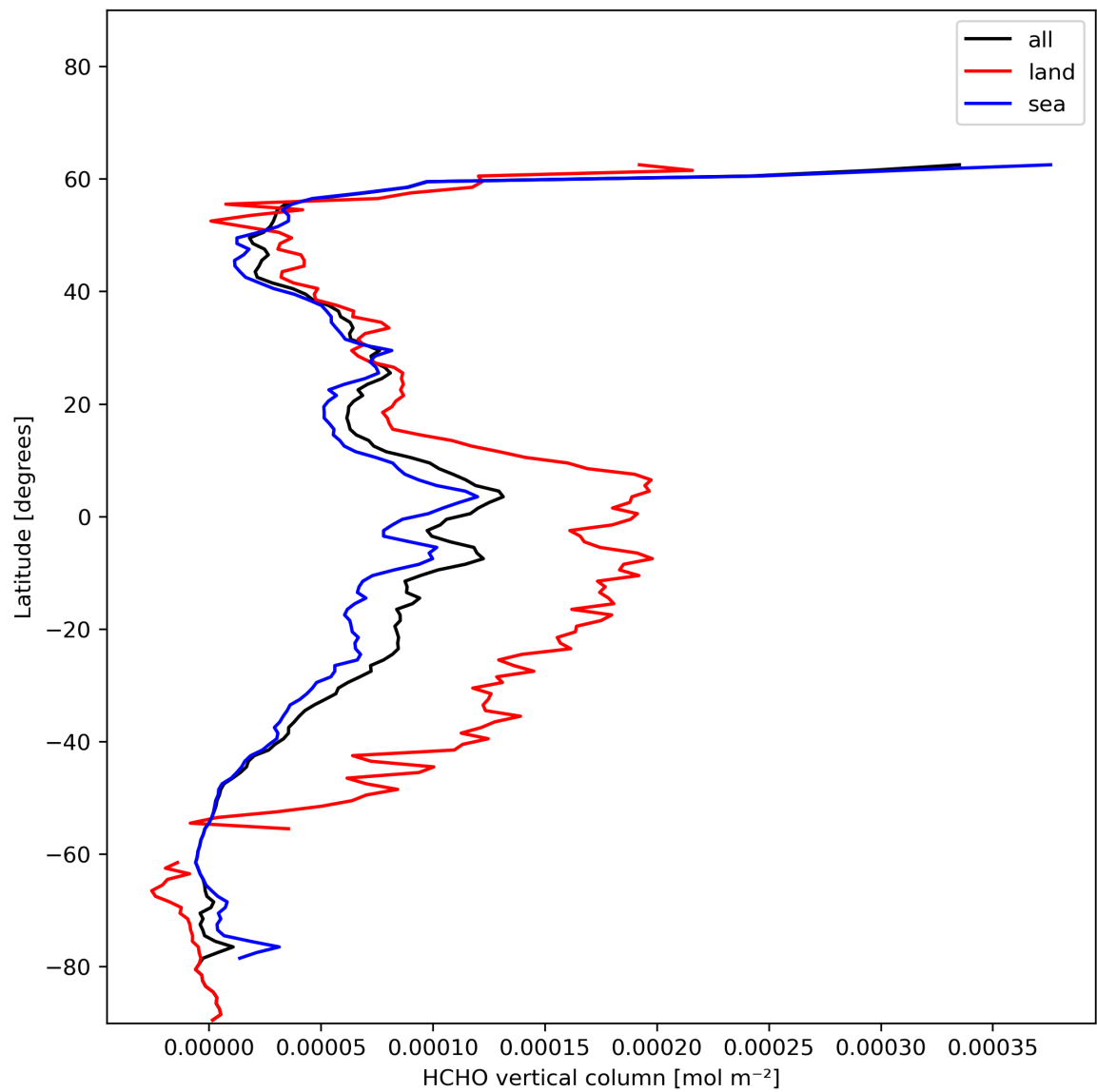
Figure 21: Zonal average of “HCHO vertical column” for 2024-01-02 to 2024-01-04.
