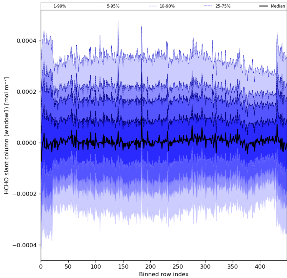
Figure 52: Along track statistics of “HCHO slant column (window1)” for 2024-01-02 to 2024-01-04
