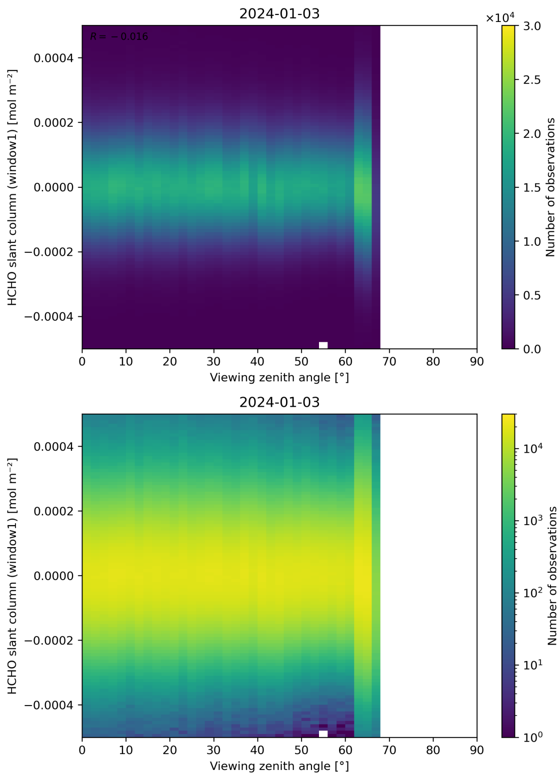
Figure 188: Scatter density plot of “Viewing zenith angle” against “HCHO slant column (window1)” for 2024-01-02 to 2024-01-04.
