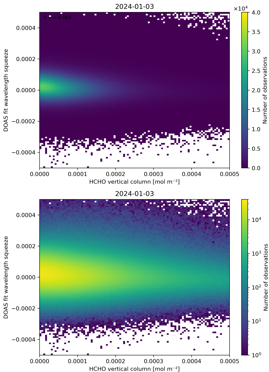
Figure 125: Scatter density plot of “HCHO vertical column” against “DOAS fit wavelength squeeze” for 2024-01-02 to 2024-01-04.
