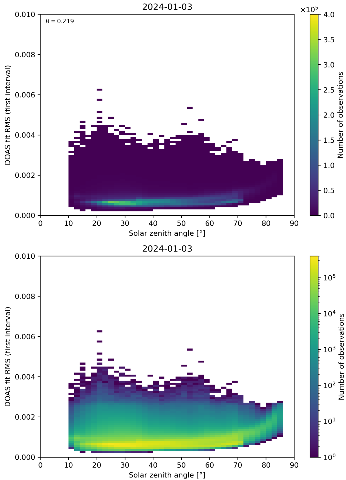
Figure 167: Scatter density plot of “Solar zenith angle” against “DOAS fit RMS (first interval)” for 2024-01-02 to 2024-01-04.
