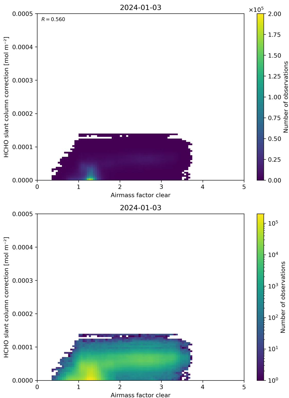
Figure 75: Scatter density plot of “Airmass factor clear” against “HCHO slant column correction” for 2024-01-02 to 2024-01-04.
