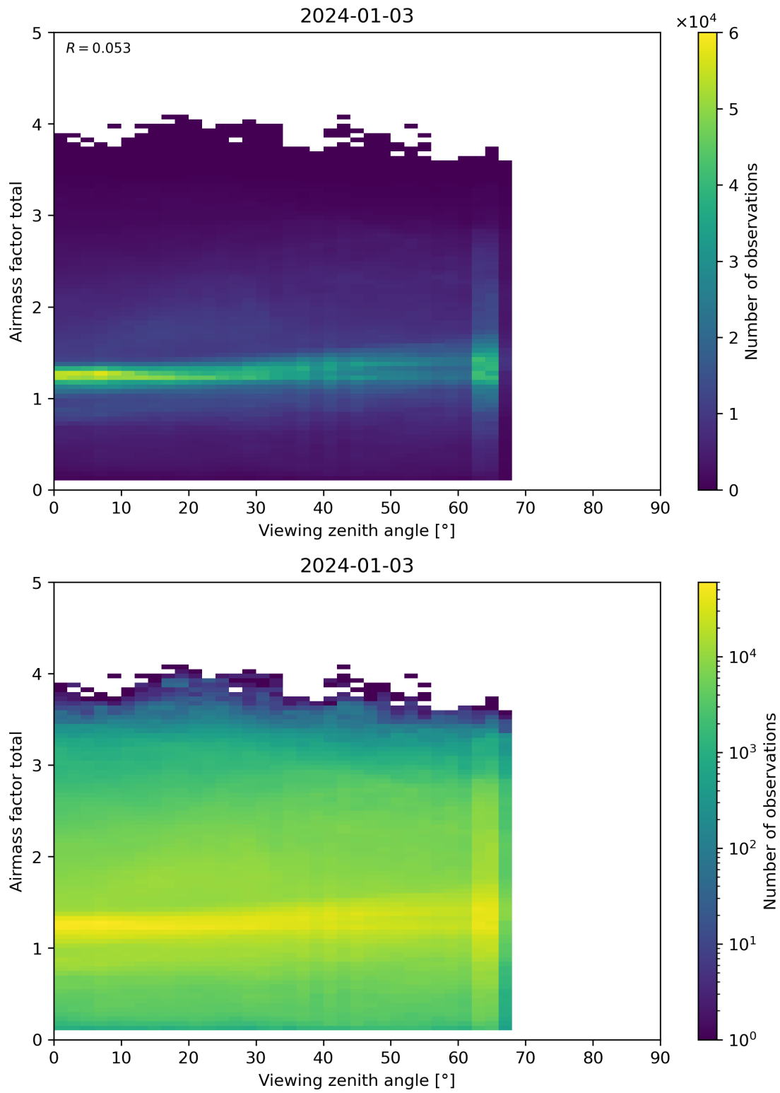
Figure 190: Scatter density plot of “Viewing zenith angle” against “Airmass factor total” for 2024-01-02 to 2024-01-04.
