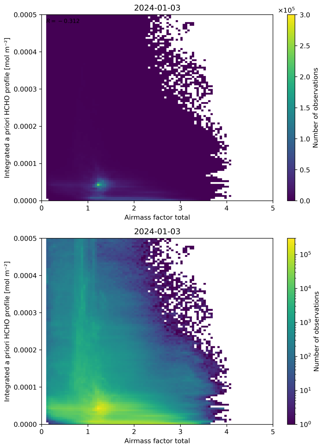
Figure 104: Scatter density plot of “Air mass factor total” against “Integrated a priori HCHO profile” for 2024-01-02 to 2024-01-04.
