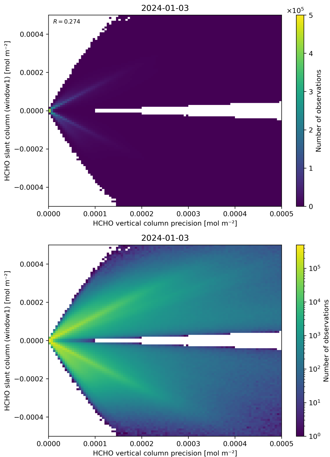
Figure 142: Scatter density plot of “HCHO vertical column precision” against “HCHO slant column (window1)” for 2024-01-02 to 2024-01-04.
