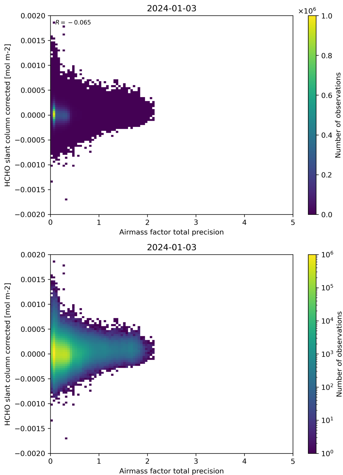
Figure 109: Scatter density plot of “Airmass factor total precision” against “HCHO slant column corrected” for 2024-01-02 to 2024-01-04.
