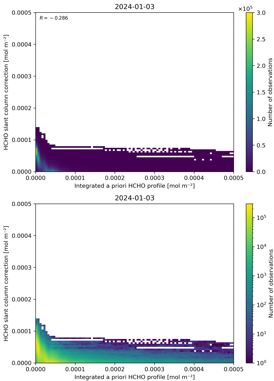
Figure 152: Scatter density plot of “Integrated a priori HCHO profile” against “HCHO slant column correction” for 2024-01-02 to 2024-01-04.
