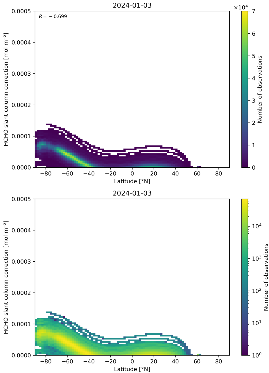
Figure 158: Scatter density plot of “Latitude” against “HCHO slant column correction” for 2024-01-02 to 2024-01-04.
