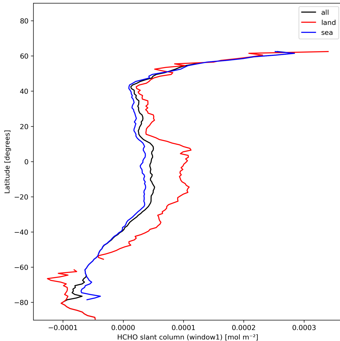
Figure 24: Zonal average of “HCHO slant column (window1)” for 2024-01-02 to 2024-01-04.
