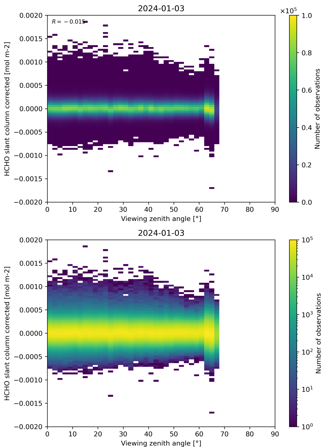
Figure 186: Scatter density plot of “Viewing zenith angle” against “HCHO slant column corrected” for 2024-01-02 to 2024-01-04.
