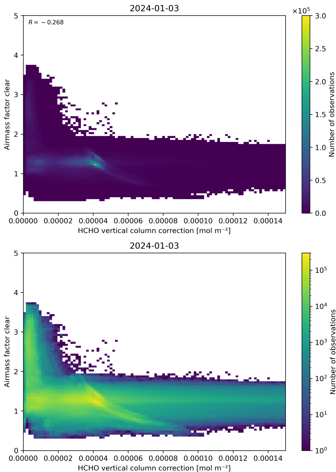
Figure 115: Scatter density plot of “HCHO vertical column correction” against “Airmass factor clear” for 2024-01-02 to 2024-01-04.
