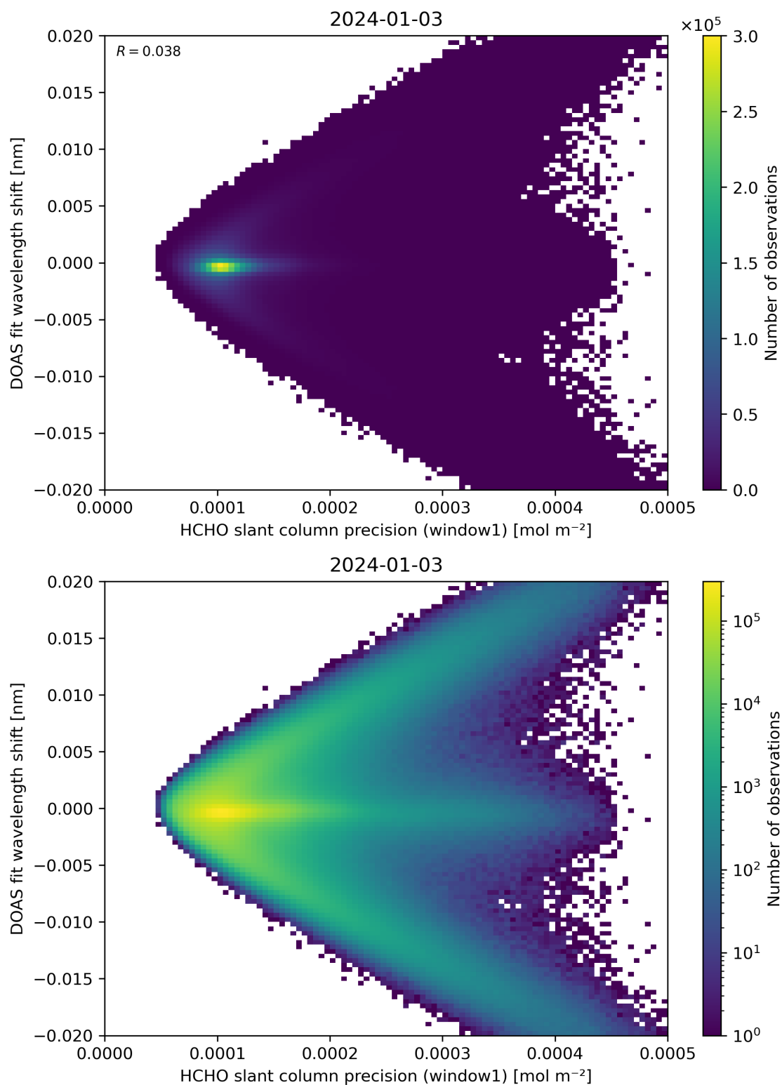
Figure 89: Scatter density plot of “HCHO slant column precision (window1)” against “DOAS fit wavelength shift” for 2024-01-02 to 2024-01-04.
