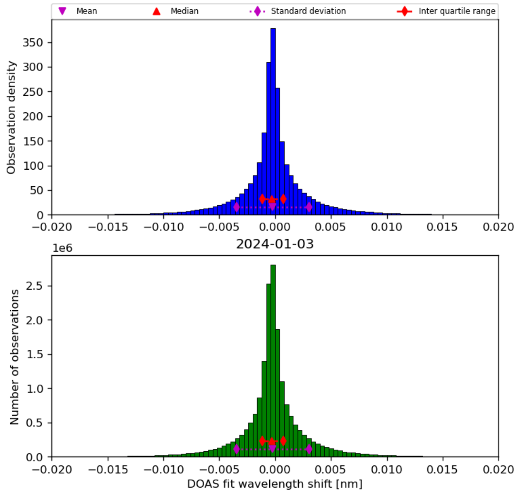
Figure 44: Histogram of “DOAS fit wavelength shift” for 2024-01-02 to 2024-01-04
