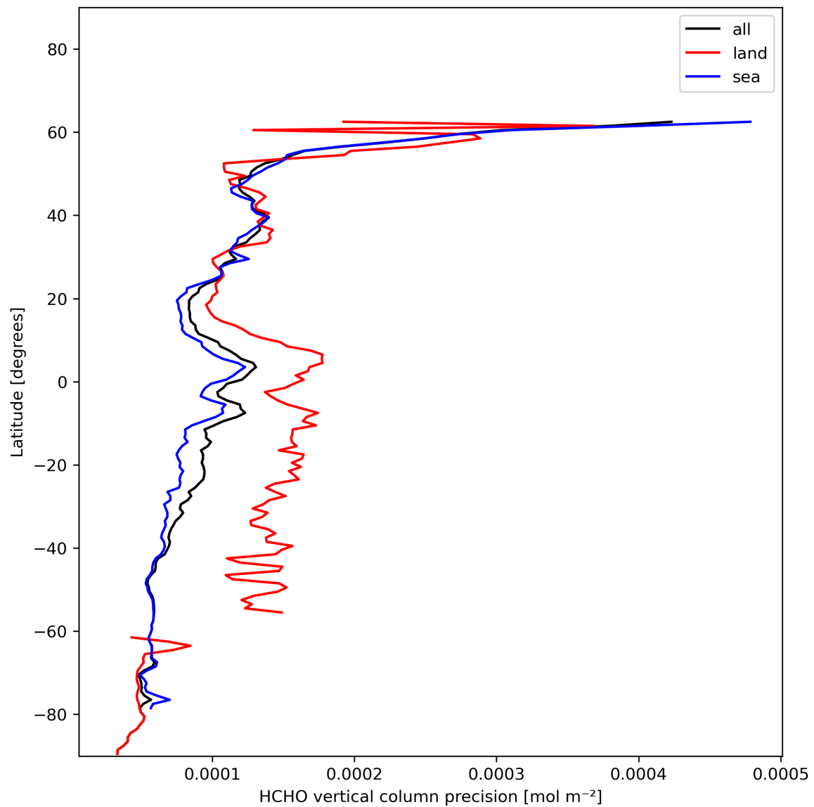
Figure 22: Zonal average of “HCHO vertical column precision” for 2024-01-02 to 2024-01-04.
