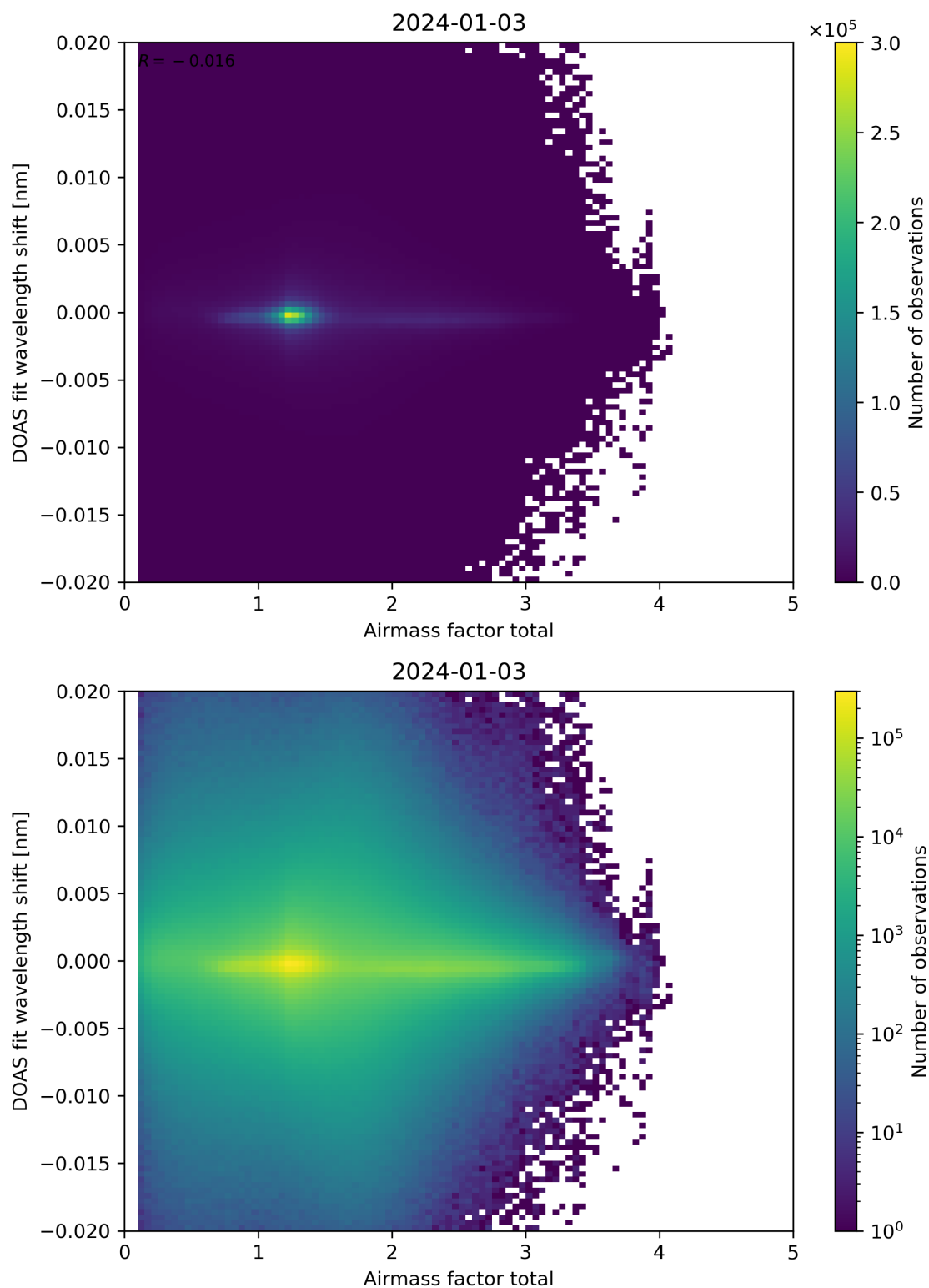
Figure 98: Scatter density plot of “Airmass factor total” against “DOAS fit wavelength shift” for 2024-01-02 to 2024-01-04.
