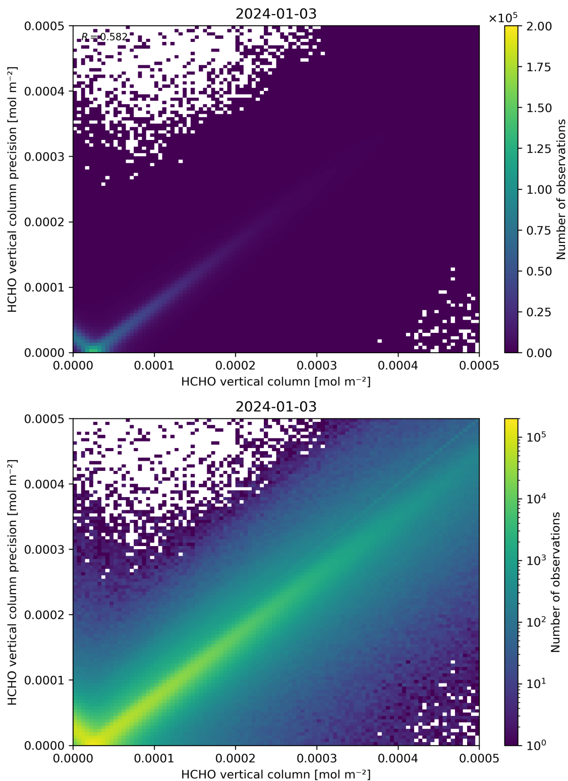
Figure 134: Scatter density plot of “HCHO vertical column” against “HCHO vertical column precision” for 2024-01-02 to 2024-01-04.
