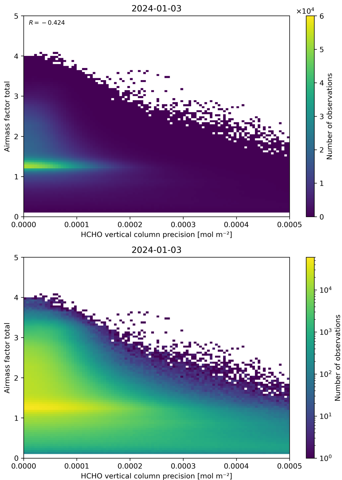
Figure 144: Scatter density plot of “HCHO vertical column precision” against “Airmass factor total” for 2024-01-02 to 2024-01-04.
