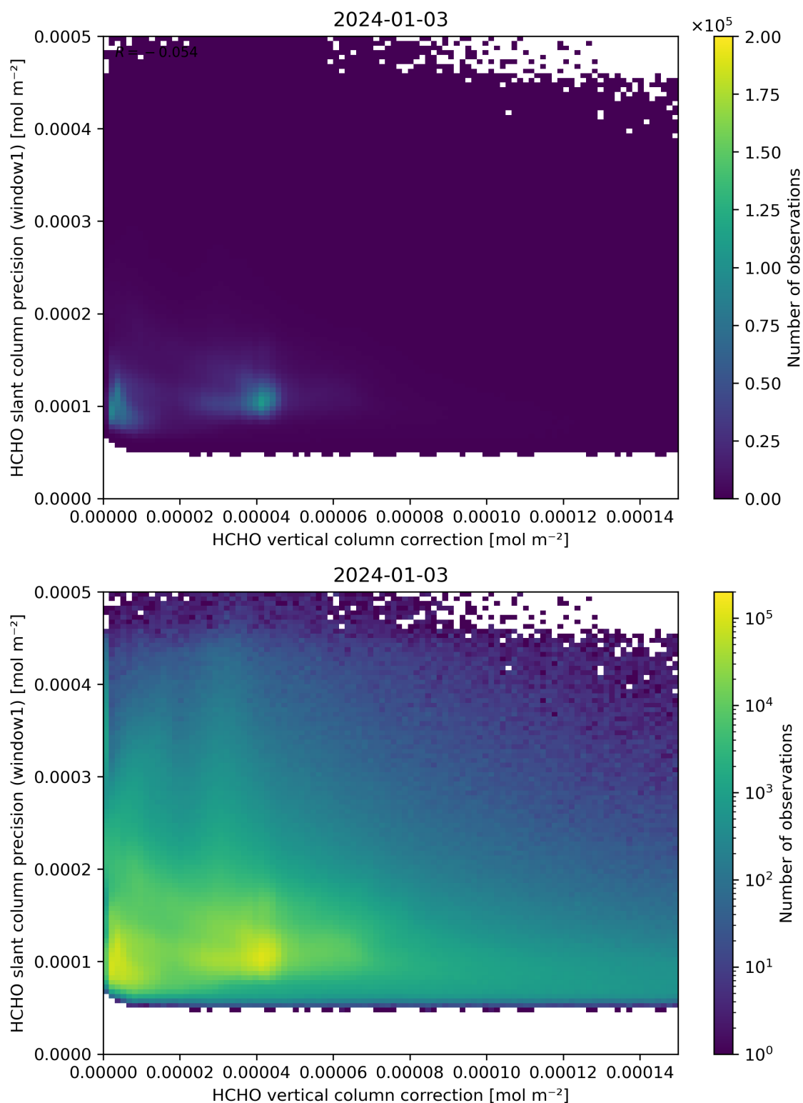
Figure 119: Scatter density plot of “HCHO vertical column correction” against “HCHO slant column precision (window1)” for 2024-01-02 to 2024-01-04.
