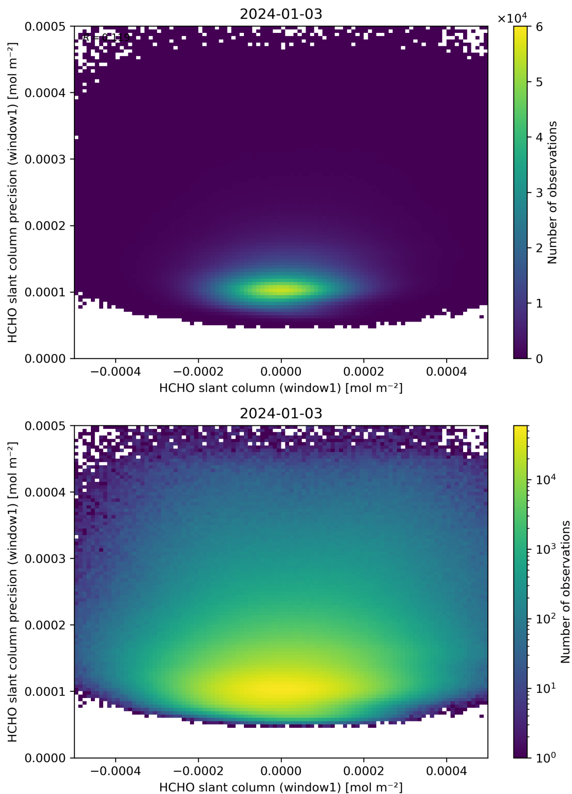
Figure 84: Scatter density plot of “HCHO slant column (window1)” against “HCHO slant column precision (window1)” for 2024-01-02 to 2024-01-04.
