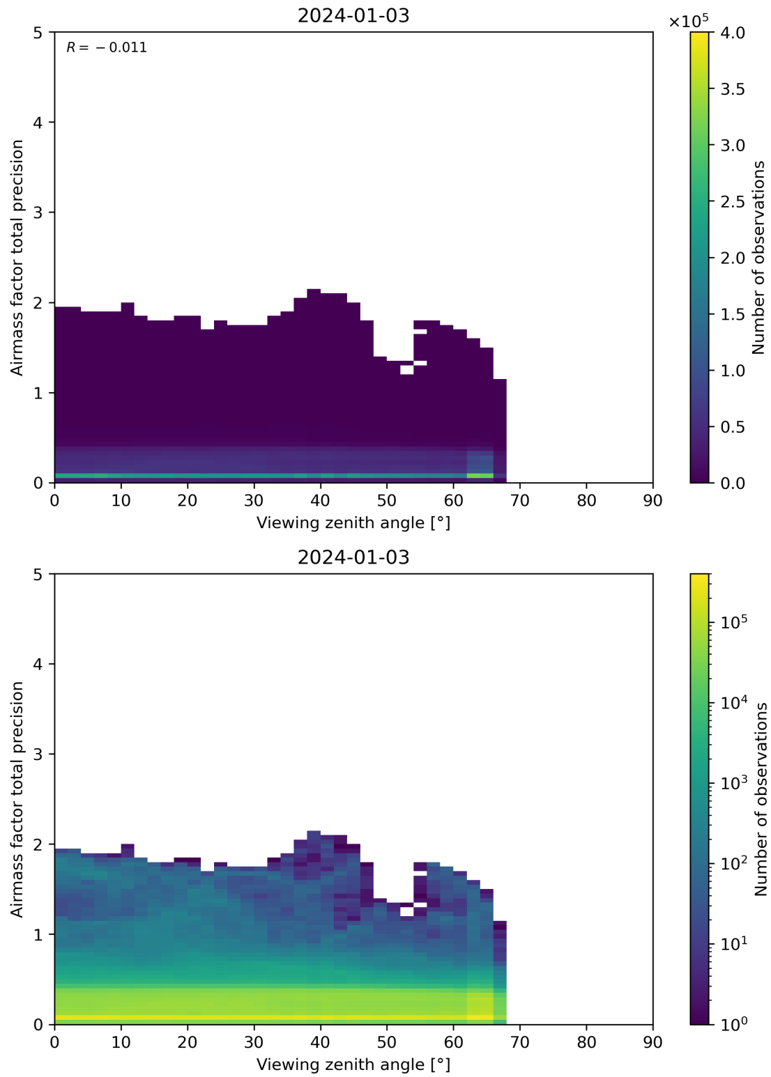
Figure 191: Scatter density plot of “Viewing zenith angle” against “Airmass factor total precision” for 2024-01-02 to 2024-01-04.
