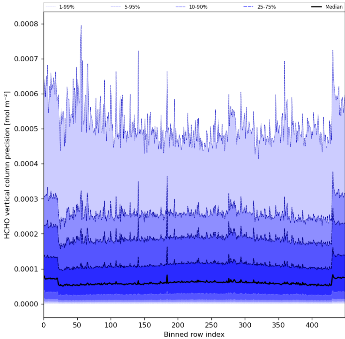
Figure 50: Along track statistics of “HCHO vertical column precision” for 2024-01-02 to 2024-01-04
