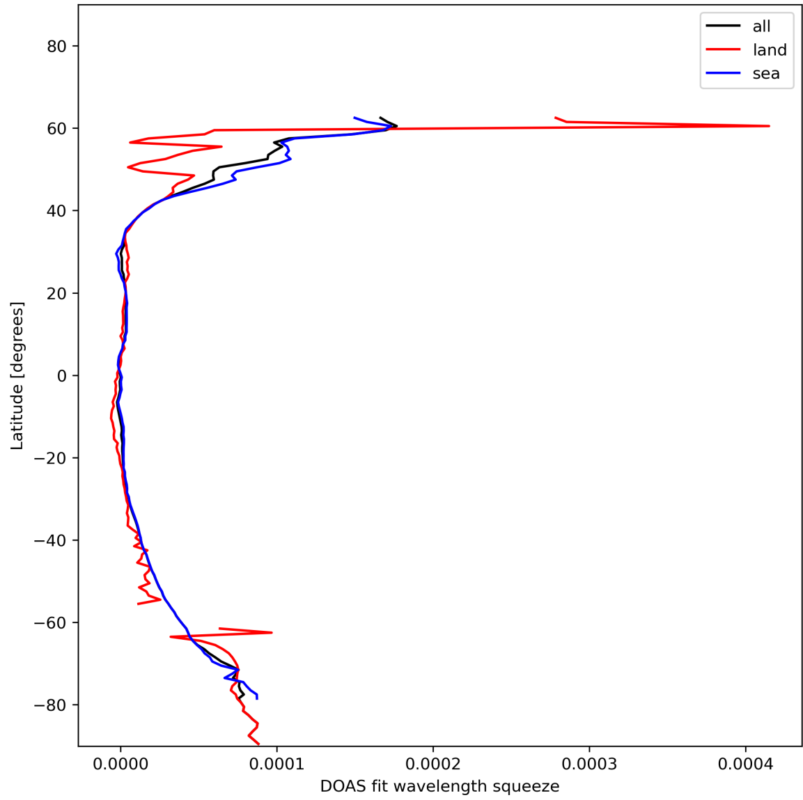
Figure 31: Zonal average of “DOAS fit wavelength squeeze” for 2024-01-02 to 2024-01-04.
