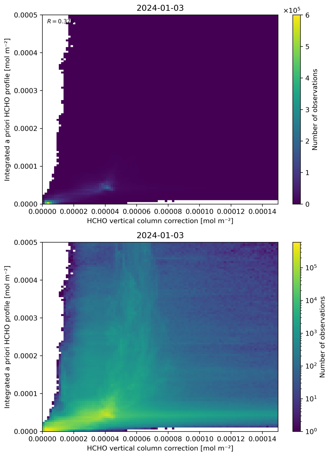
Figure 122: Scatter density plot of “HCHO vertical column correction” against “Integrated a priori HCHO profile” for 2024-01-02 to 2024-01-04.
