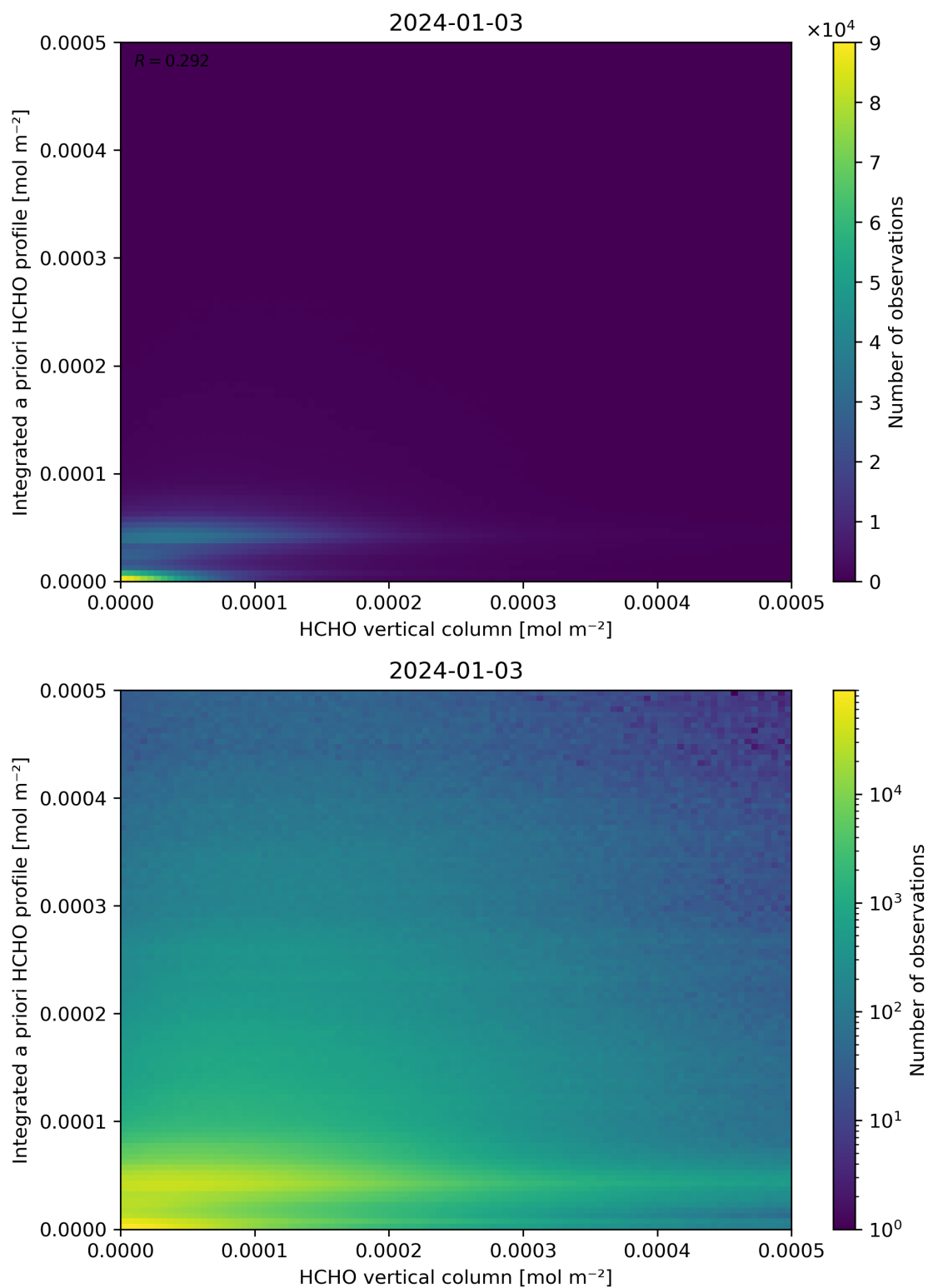
Figure 135: Scatter density plot of “HCHO vertical column” against “Integrated a priori HCHO profile” for 2024-01-02 to 2024-01-04.
