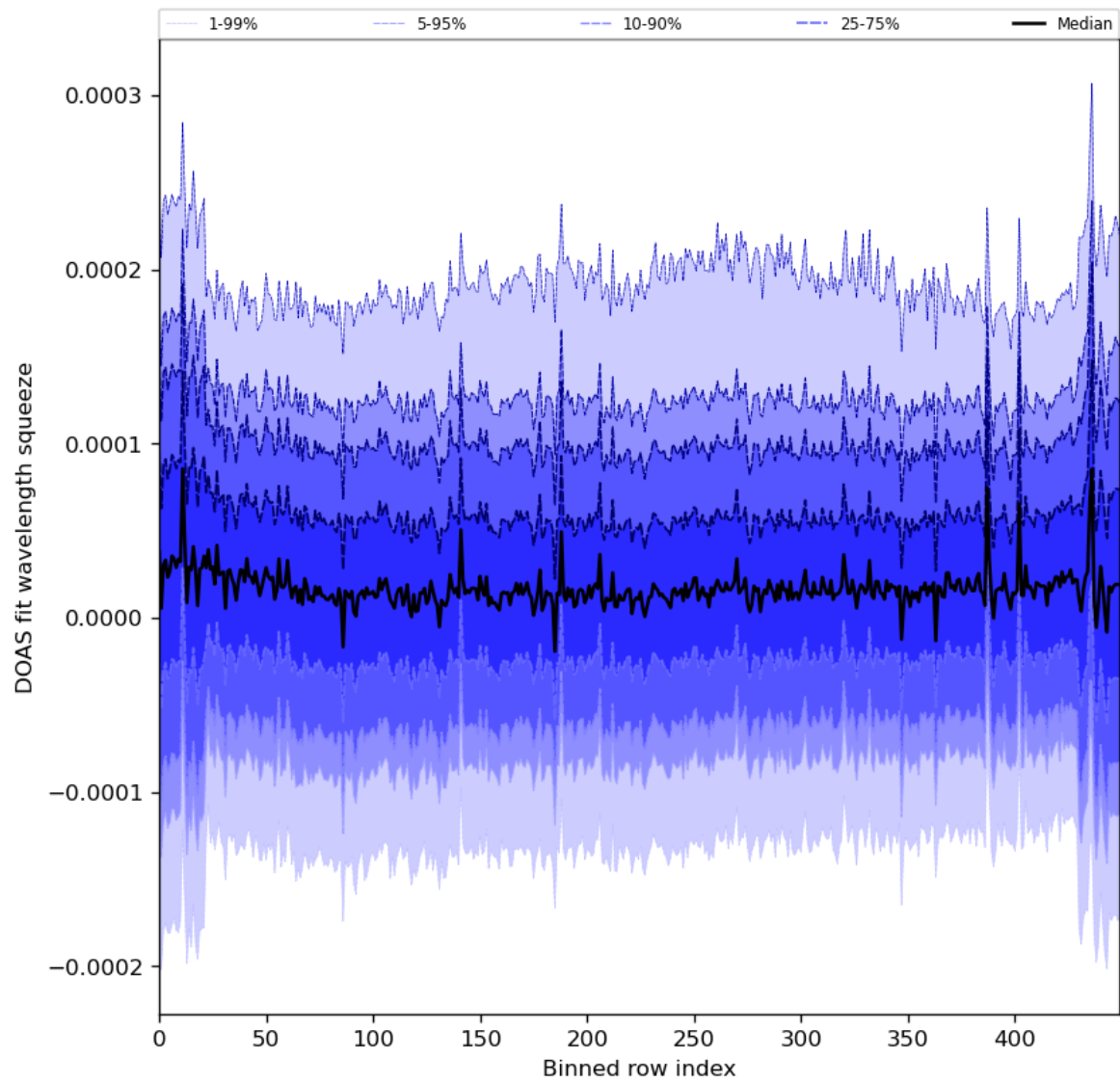
Figure 59: Along track statistics of “DOAS fit wavelength squeeze” for 2024-01-02 to 2024-01-04
