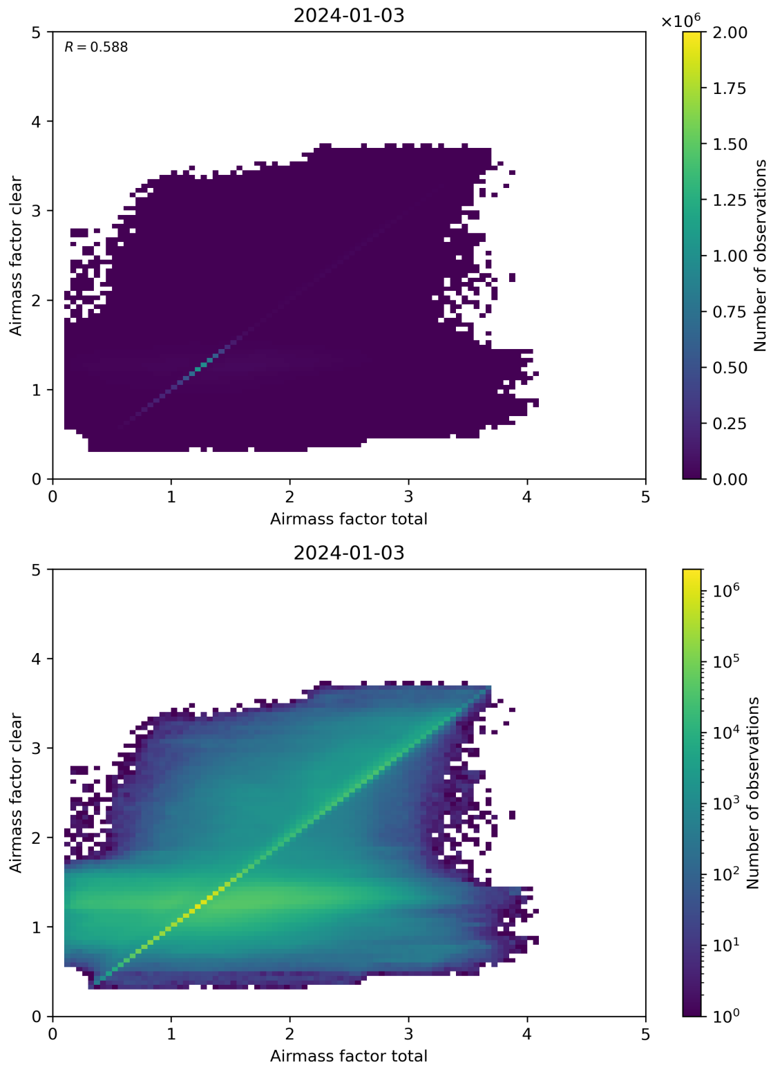
Figure 100: Scatter density plot of “Airmass factor total” against “Airmass factor clear” for 2024-01-02 to 2024-01-04.
