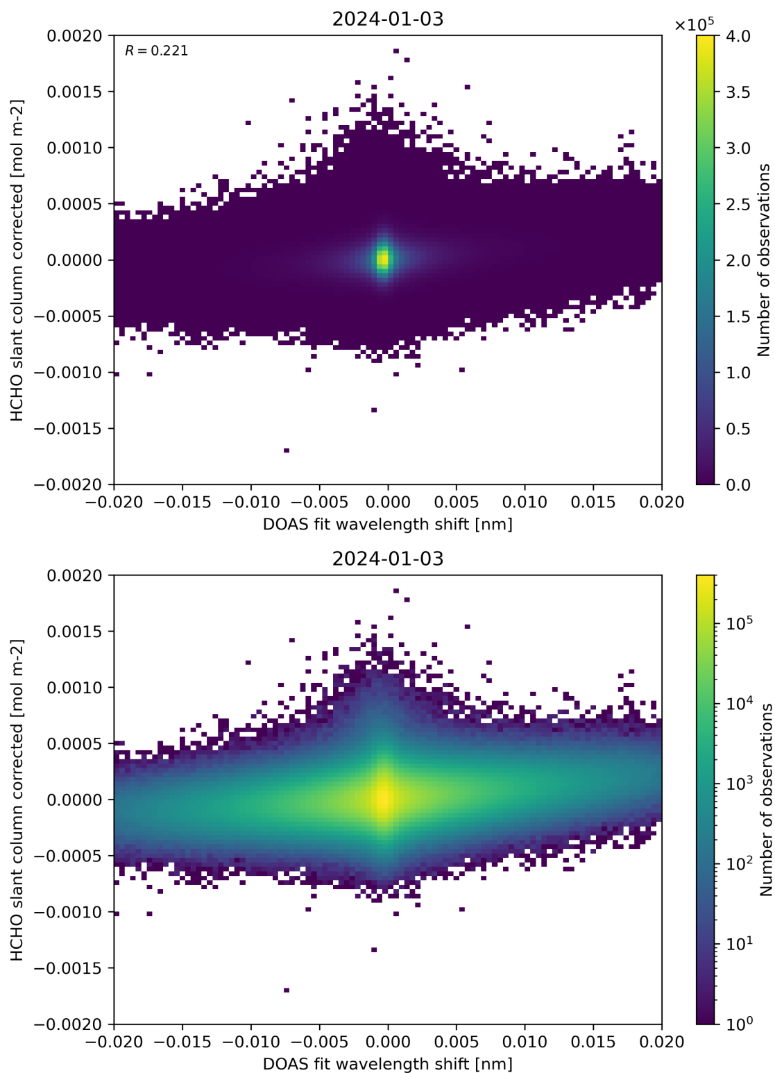
Figure 66: Scatter density plot of “DOAS fit wavelength shift” against “HCHO slant column corrected” for 2024-01-02 to 2024-01-04.
