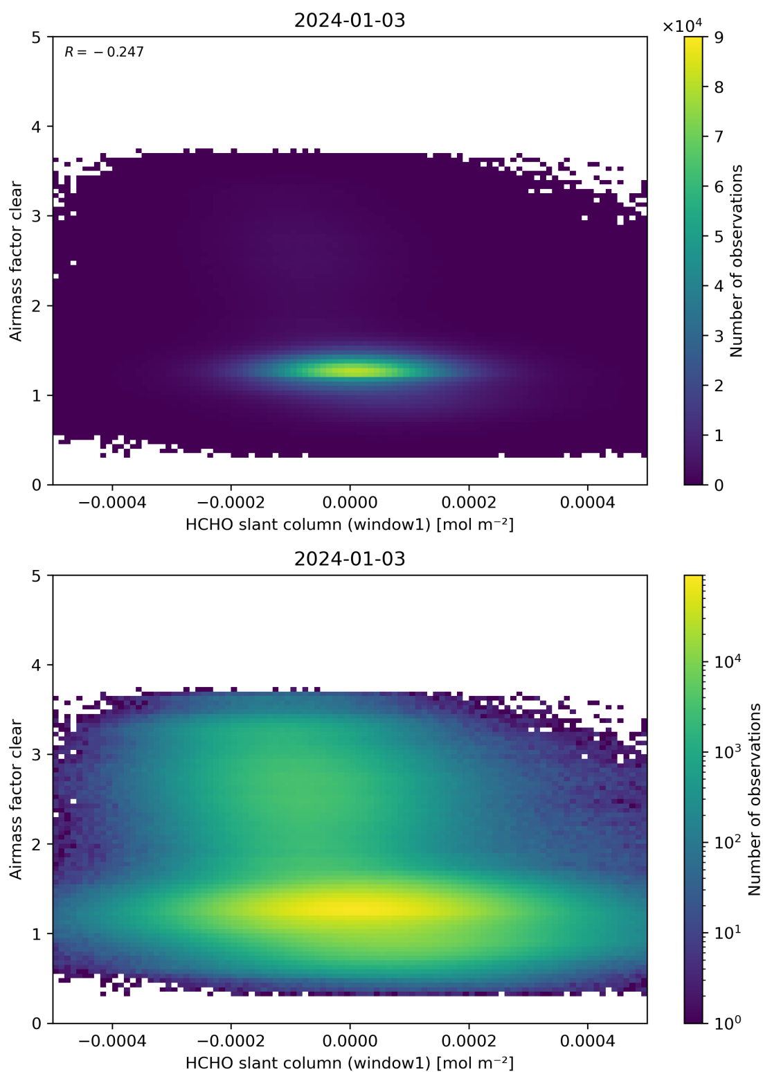
Figure 81: Scatter density plot of “HCHO slant column (window1)” against “Airmass factor clear” for 2024-01-02 to 2024-01-04.
