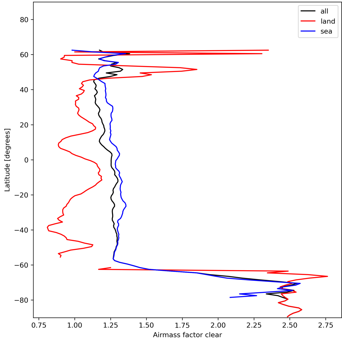
Figure 28: Zonal average of “Airmass factor clear” for 2024-01-02 to 2024-01-04.
