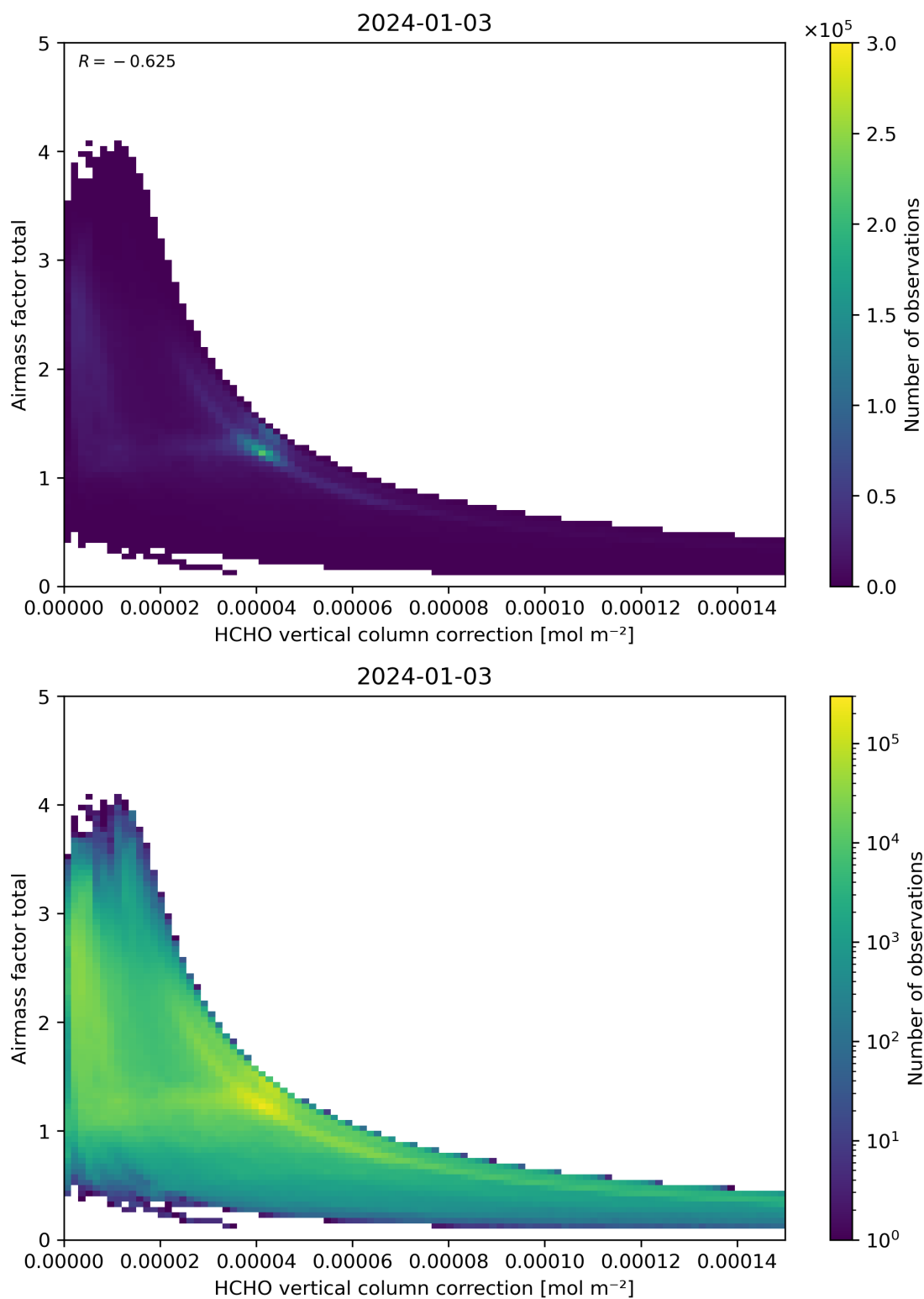
Figure 120: Scatter density plot of “HCHO vertical column correction” against “Airmass factor total” for 2024-01-02 to 2024-01-04.
