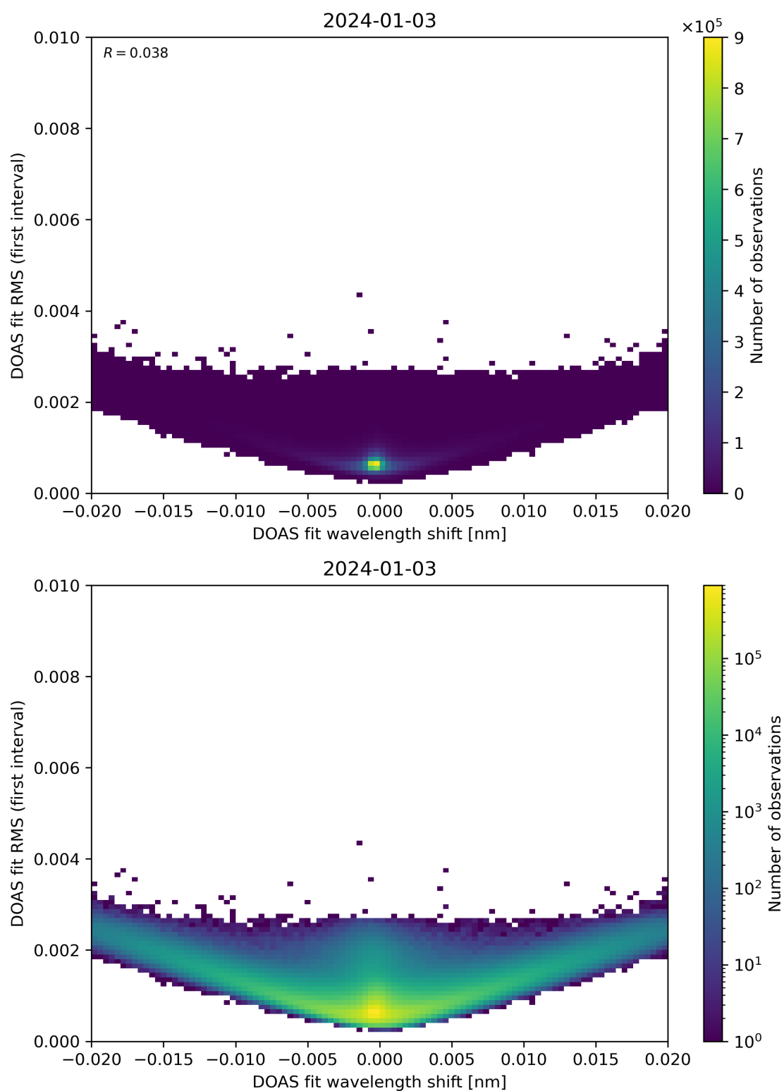
Figure 64: Scatter density plot of “DOAS fit wavelength shift” against “DOAS fit RMS (first interval)” for 2024-01-02 to 2024-01-04.
