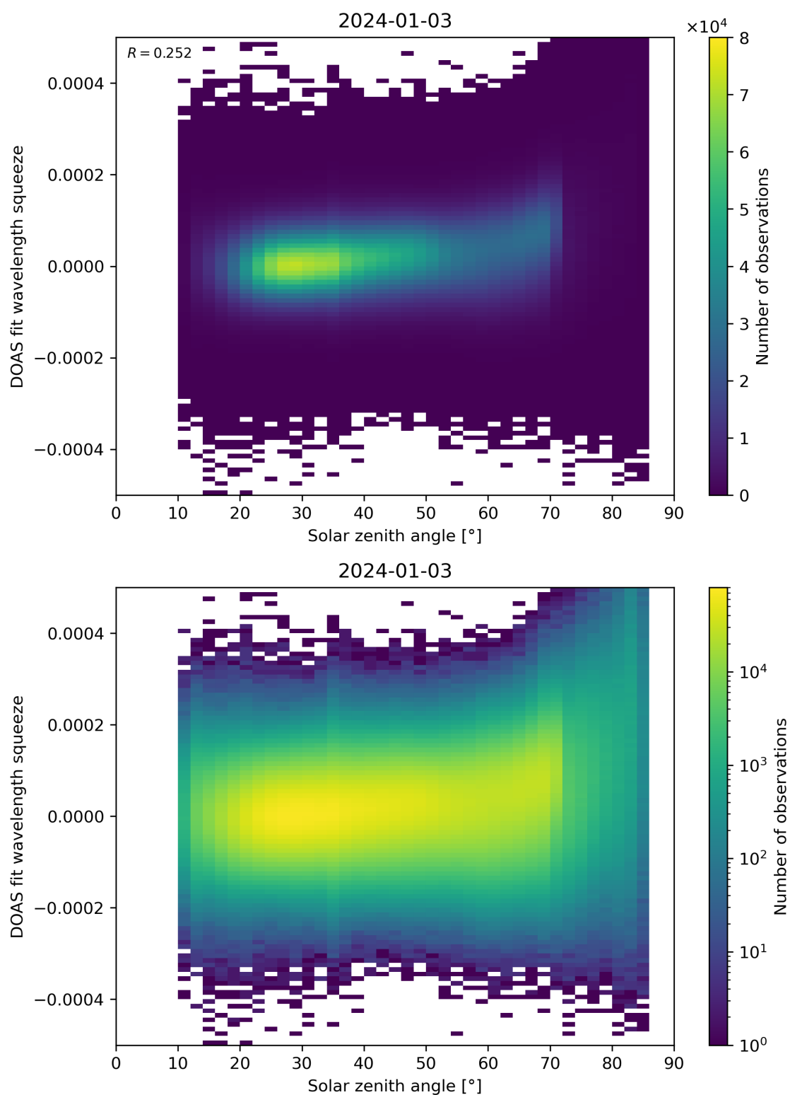
Figure 169: Scatter density plot of “Solar zenith angle” against “DOAS fit wavelength squeeze” for 2024-01-02 to 2024-01-04.
