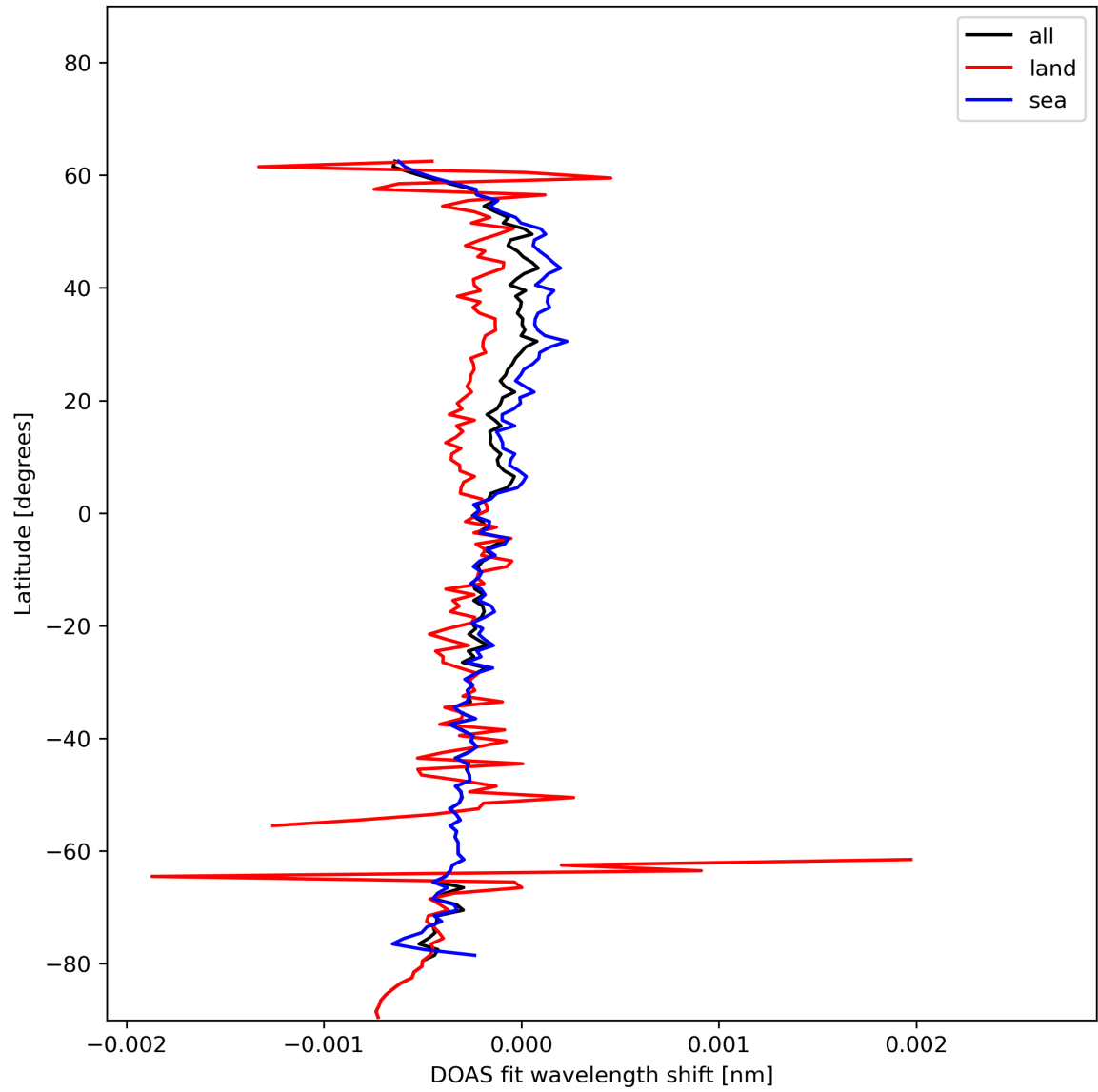
Figure 30: Zonal average of "DOAS fit wavelength shift" for 2024-01-02 to 2024-01-04.
