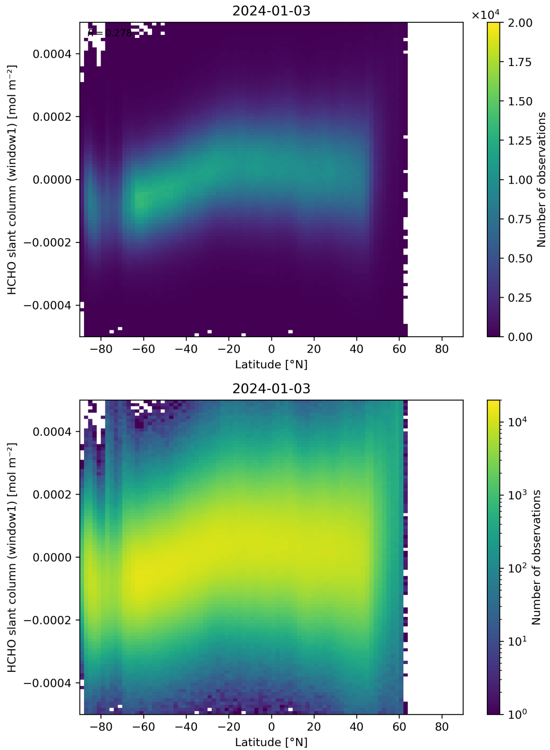
Figure 159: Scatter density plot of “Latitude” against “HCHO slant column (window1)” for 2024-01-02 to 2024-01-04.
