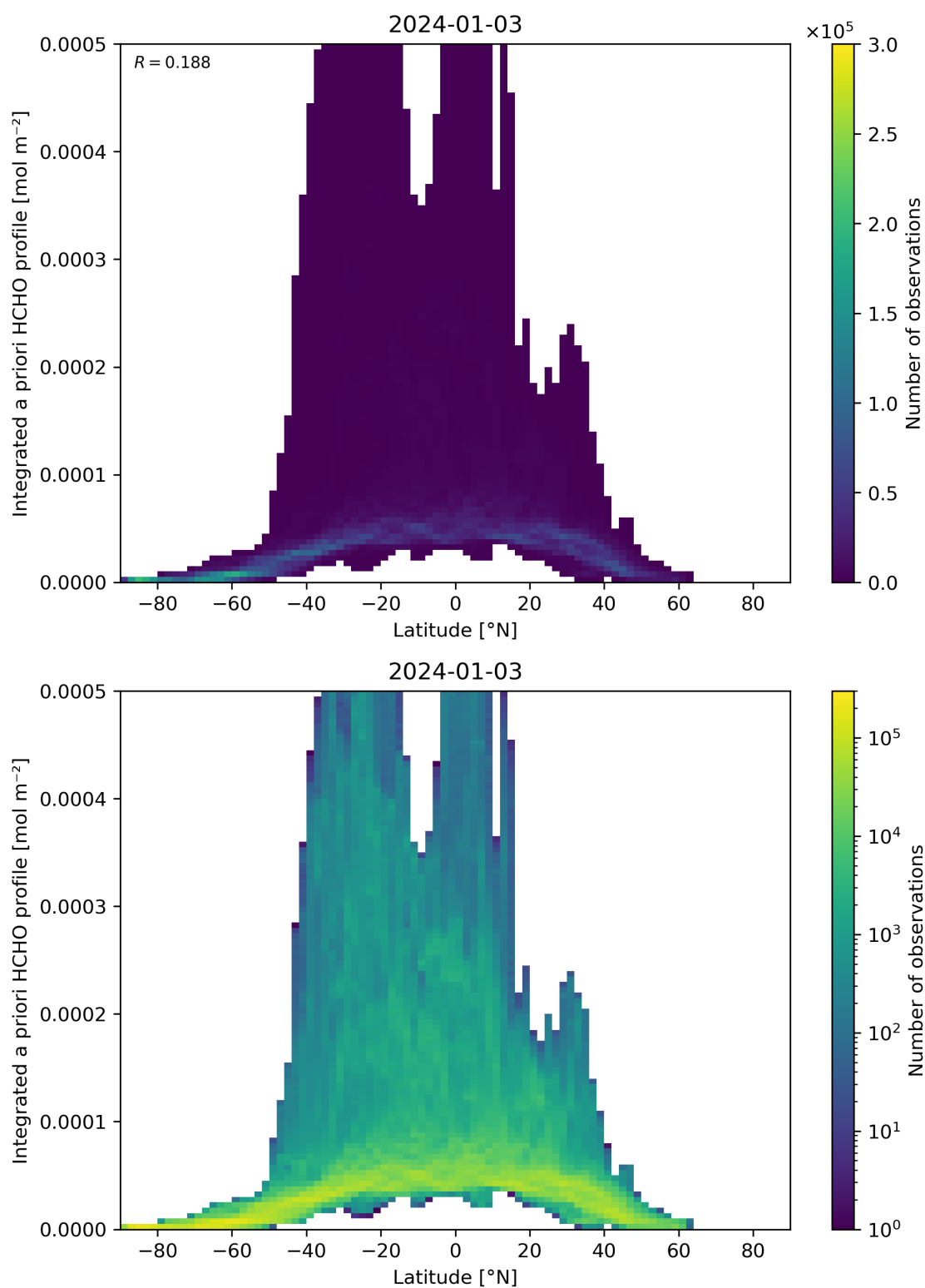
Figure 166: Scatter density plot of “Latitude” against “Integrated a priori HCHO profile” for 2024-01-02 to 2024-01-04.
