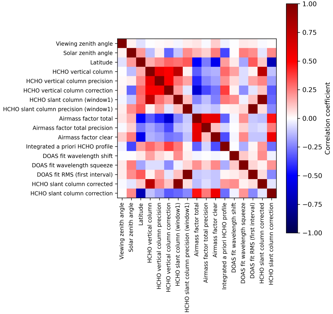
Figure 2: Map of correlation matrix for 2024-01-02 to 2024-01-04.
