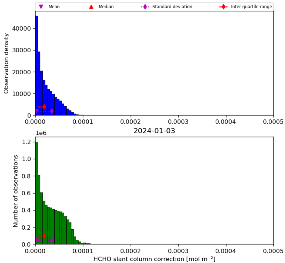
Figure 47: Histogram of “HCHO slant column correction” for 2024-01-02 to 2024-01-04
