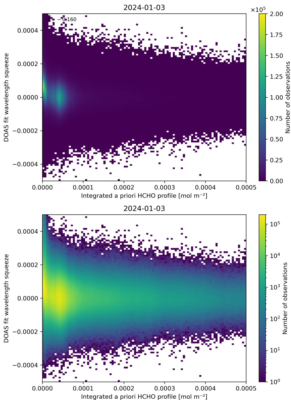
Figure 150: Scatter density plot of “Integrated a priori HCHO profile” against “DOAS fit wavelength squeeze” for 2024-01-02 to 2024-01-04.
