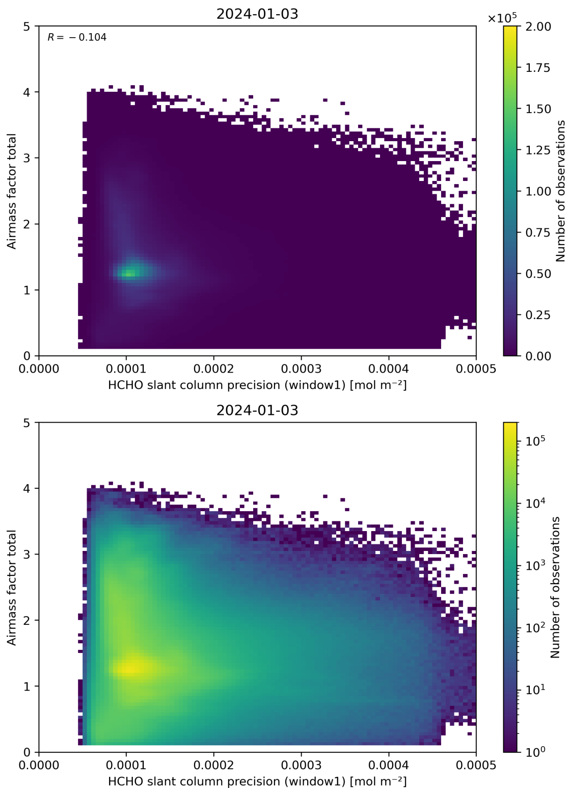
Figure 94: Scatter density plot of “HCHO slant column precision (window1)” against “Airmass factor total” for 2024-01-02 to 2024-01-04.
