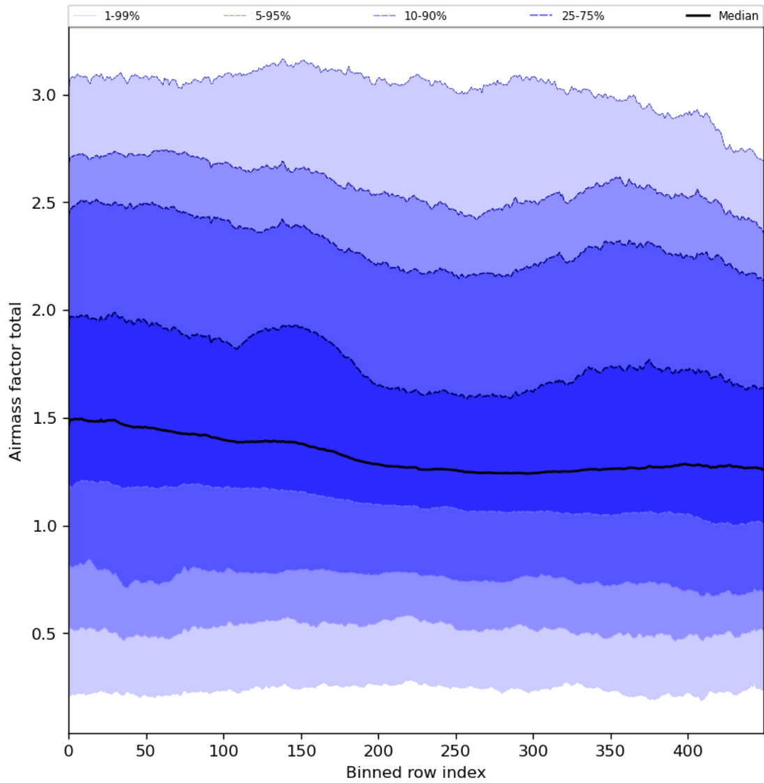
Figure 54: Along track statistics of “Airmass factor total” for 2024-01-02 to 2024-01-04
