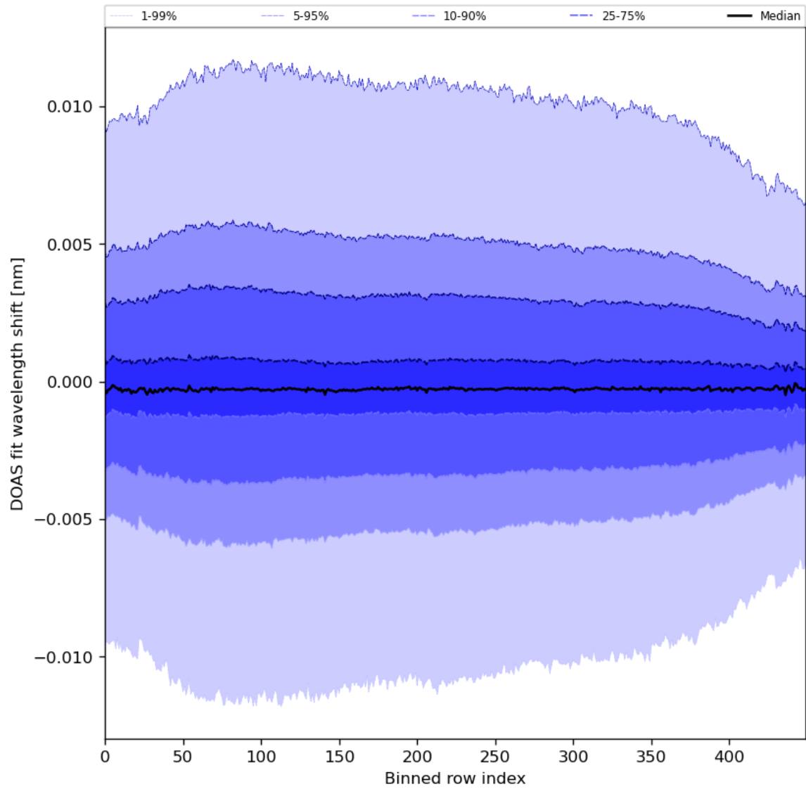
Figure 58: Along track statistics of “DOAS fit wavelength shift” for 2024-01-02 to 2024-01-04
