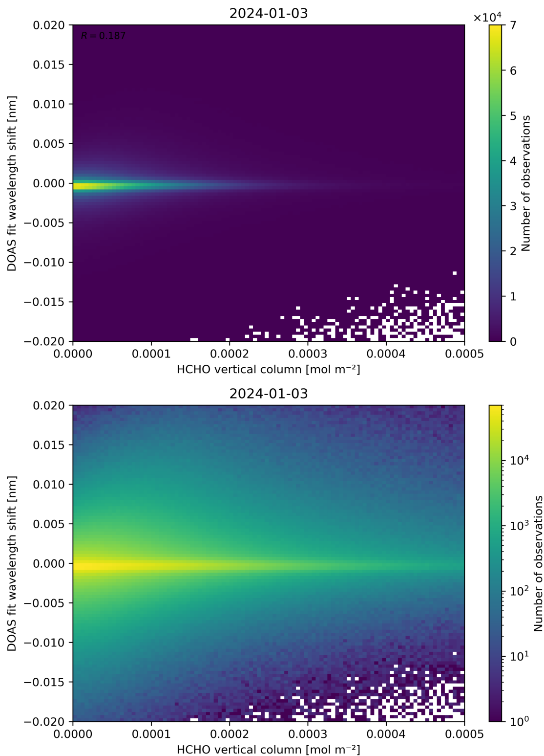
Figure 124: Scatter density plot of “HCHO vertical column” against “DOAS fit wavelength shift” for 2024-01-02 to 2024-01-04.
