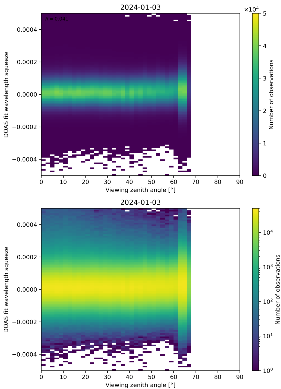
Figure 184: Scatter density plot of “Viewing zenith angle” against “DOAS fit wavelength squeeze” for 2024-01-02 to 2024-01-04.
