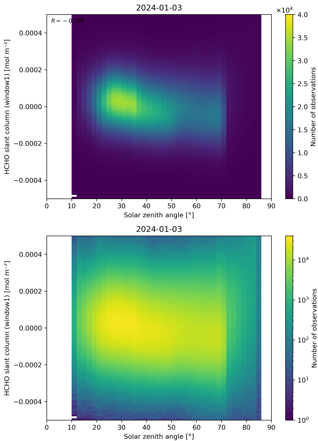
Figure 173: Scatter density plot of “Solar zenith angle” against “HCHO slant column (window1)” for 2024-01-02 to 2024-01-04.
