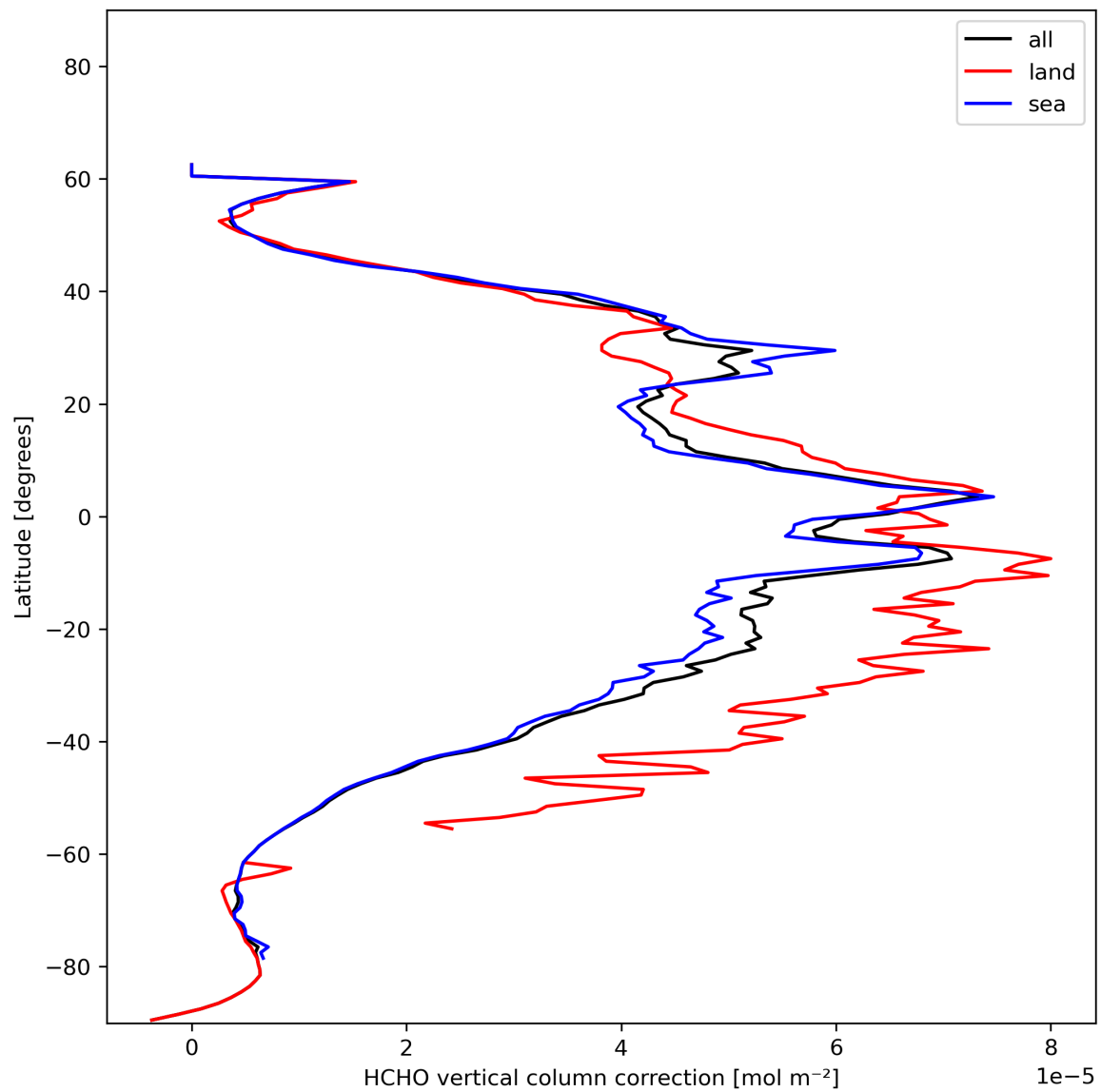
Figure 23: Zonal average of “HCHO vertical column correction” for 2024-01-02 to 2024-01-04.
