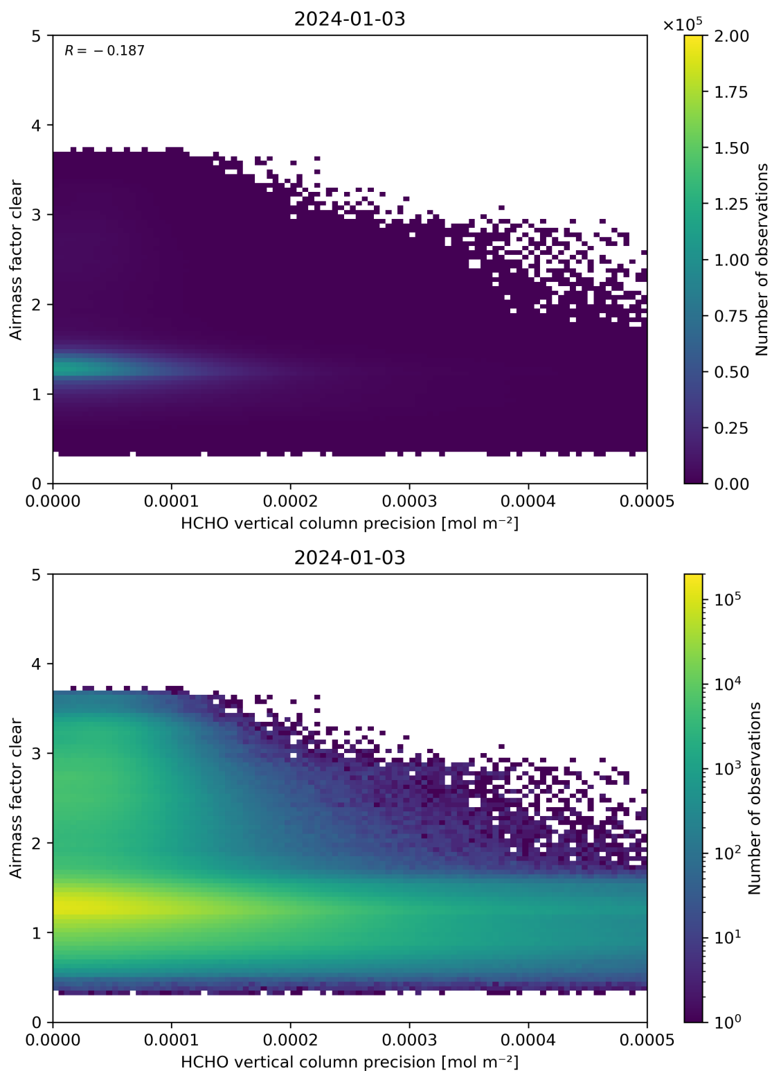
Figure 139: Scatter density plot of “HCHO vertical column precision” against “Airmass factor clear” for 2024-01-02 to 2024-01-04.
