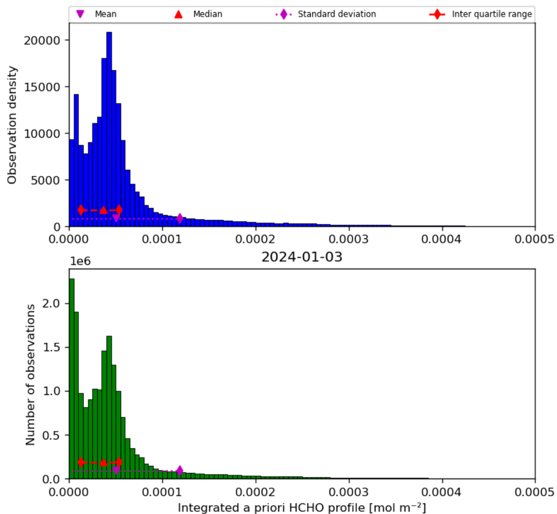
Figure 43: Histogram of “Integrated a priori HCHO profile” for 2024-01-02 to 2024-01-04
