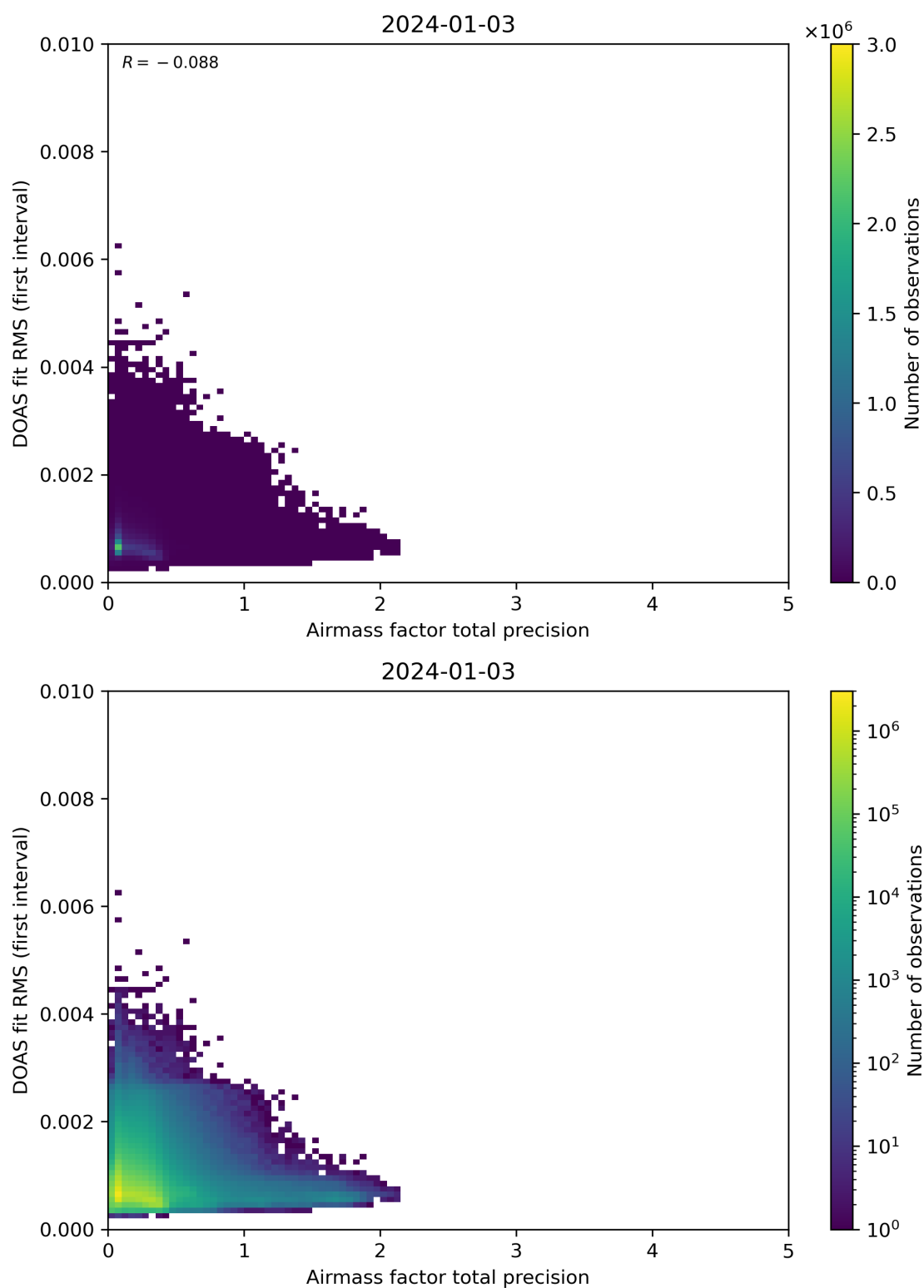
Figure 105: Scatter density plot of “Airmass factor total precision” against “DOAS fit RMS (first interval)” for 2024-01-02 to 2024-01-04.
