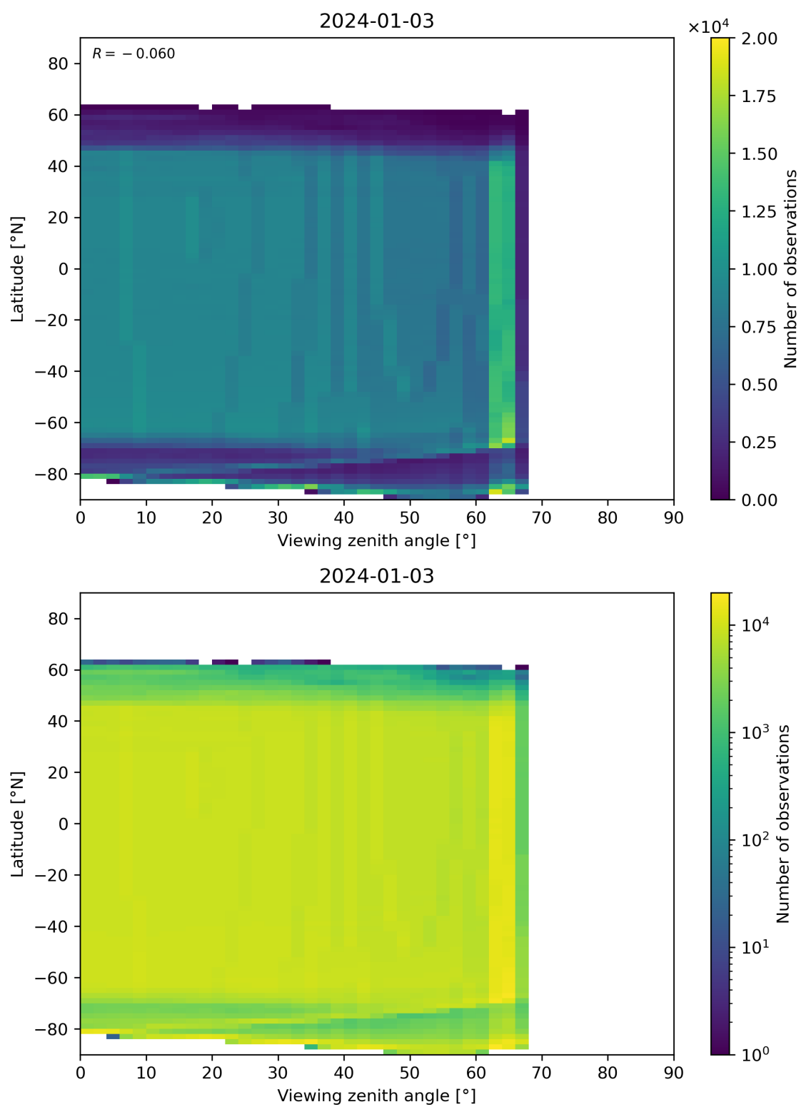
Figure 196: Scatter density plot of “Viewing zenith angle” against “Latitude” for 2024-01-02 to 2024-01-04.
