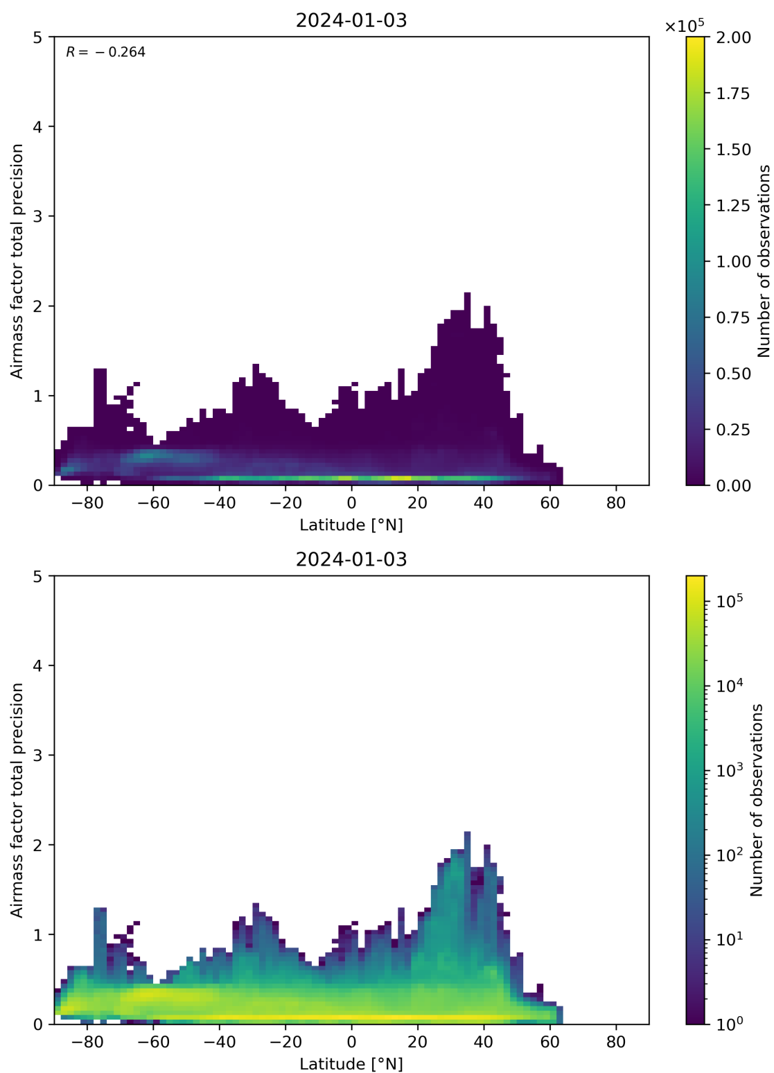
Figure 162: Scatter density plot of “Latitude” against “Airmass factor total precision” for 2024-01-02 to 2024-01-04.
