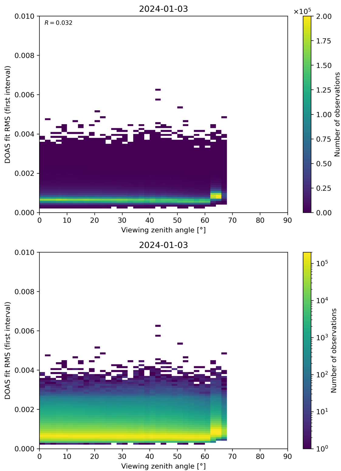
Figure 182: Scatter density plot of “Viewing zenith angle” against “DOAS fit RMS (first interval)” for 2024-01-02 to 2024-01-04.
