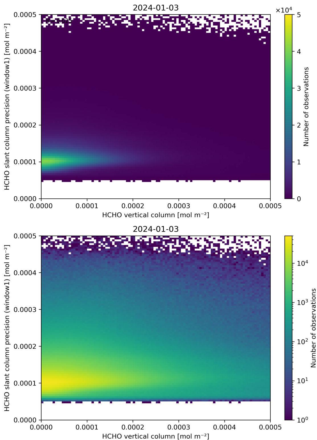
Figure 130: Scatter density plot of “HCHO vertical column” against “HCHO slant column precision (window1)” for 2024-01-02 to 2024-01-04.
