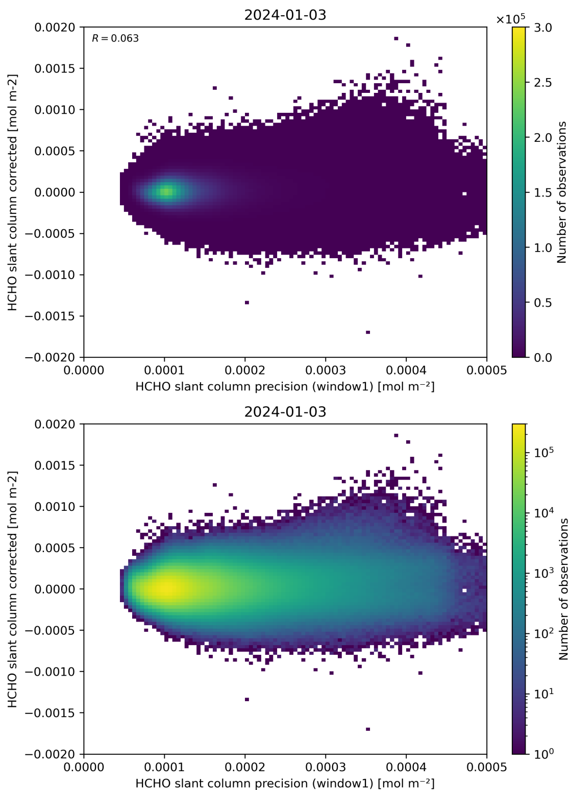
Figure 92: Scatter density plot of “HCHO slant column precision (window1)” against “HCHO slant column corrected” for 2024-01-02 to 2024-01-04.
