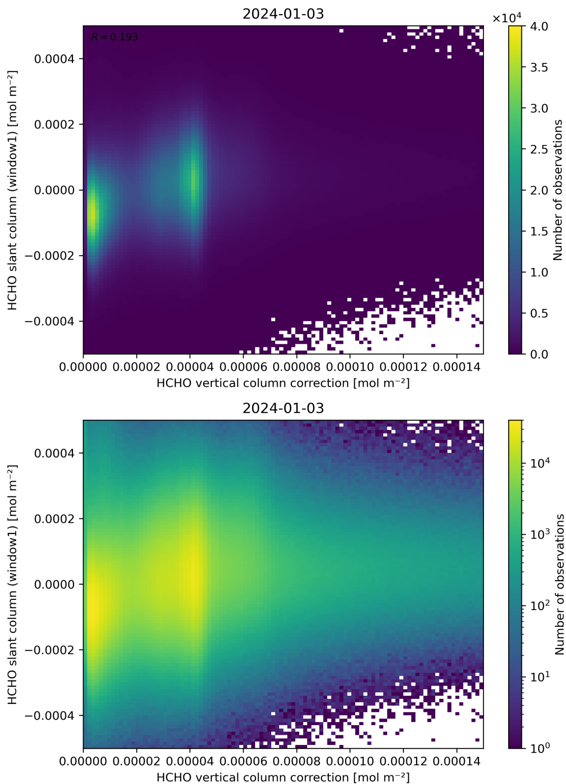
Figure 118: Scatter density plot of “HCHO vertical column correction” against “HCHO slant column (window1)” for 2024-01-02 to 2024-01-04.
