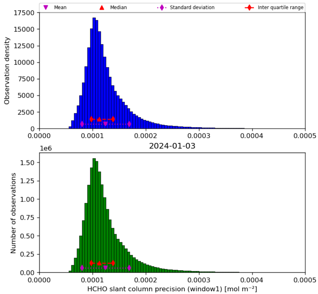
Figure 39: Histogram of “HCHO slant column precision (window1)” for 2024-01-02 to 2024-01-04
