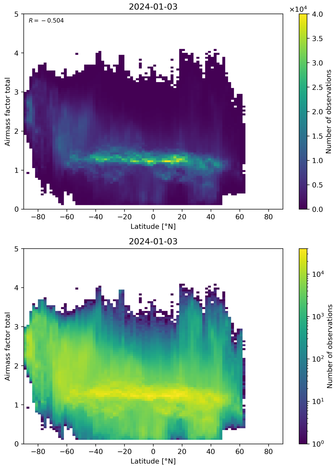
Figure 161: Scatter density plot of “Latitude” against “Airmass factor total” for 2024-01-02 to 2024-01-04.
