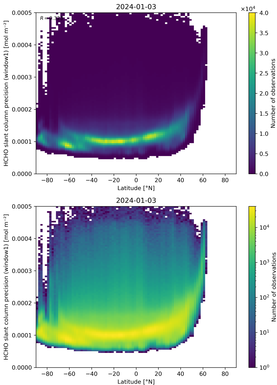
Figure 160: Scatter density plot of “Latitude” against “HCHO slant column precision (window1)” for 2024-01-02 to 2024-01-04.
