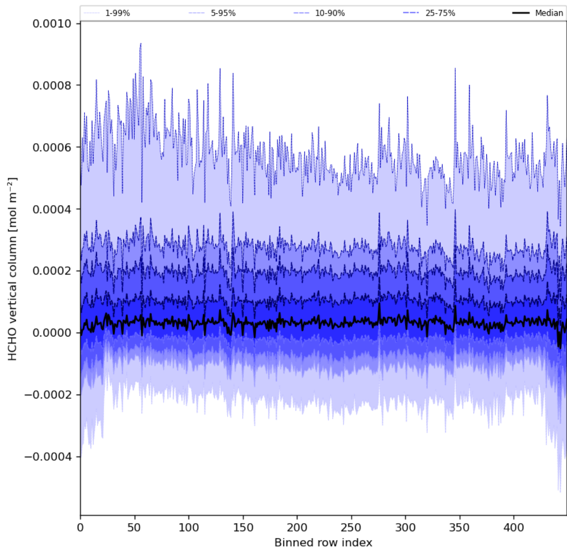
Figure 49: Along track statistics of “HCHO vertical column” for 2024-01-02 to 2024-01-04
