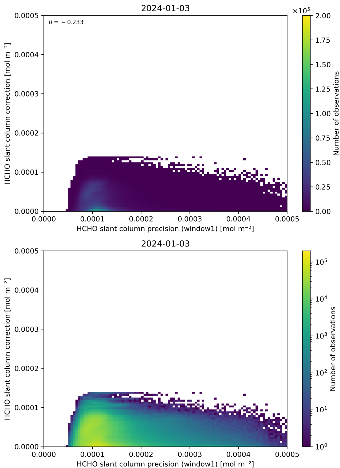
Figure 93: Scatter density plot of “HCHO slant column precision (window1)” against “HCHO slant column correction” for 2024-01-02 to 2024-01-04.
