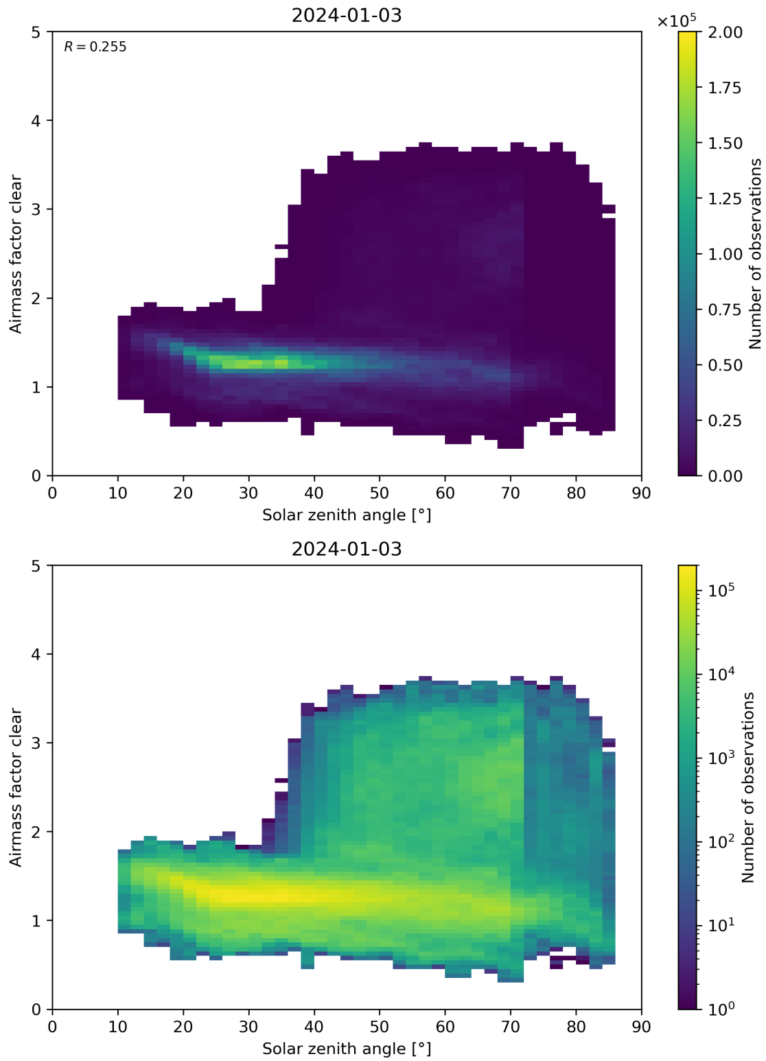
Figure 170: Scatter density plot of “Solar zenith angle” against “Airmass factor clear” for 2024-01-02 to 2024-01-04.
