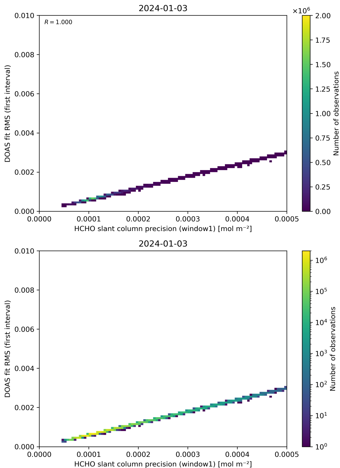
Figure 88: Scatter density plot of “HCHO slant column precision (window1)” against “DOAS fit RMS (first interval)” for 2024-01-02 to 2024-01-04.
