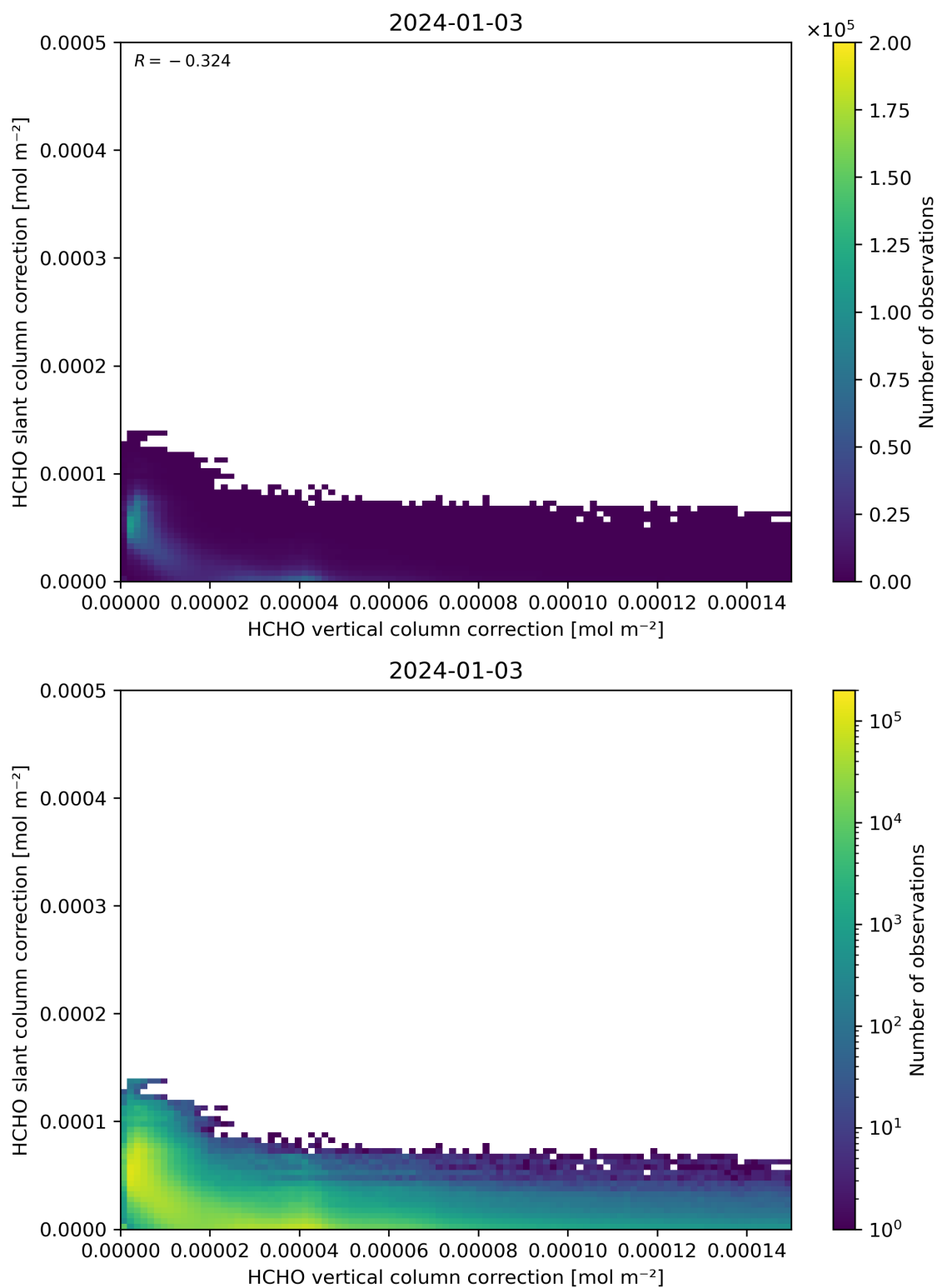
Figure 117: Scatter density plot of “HCHO vertical column correction” against “HCHO slant column correction” for 2024-01-02 to 2024-01-04.
