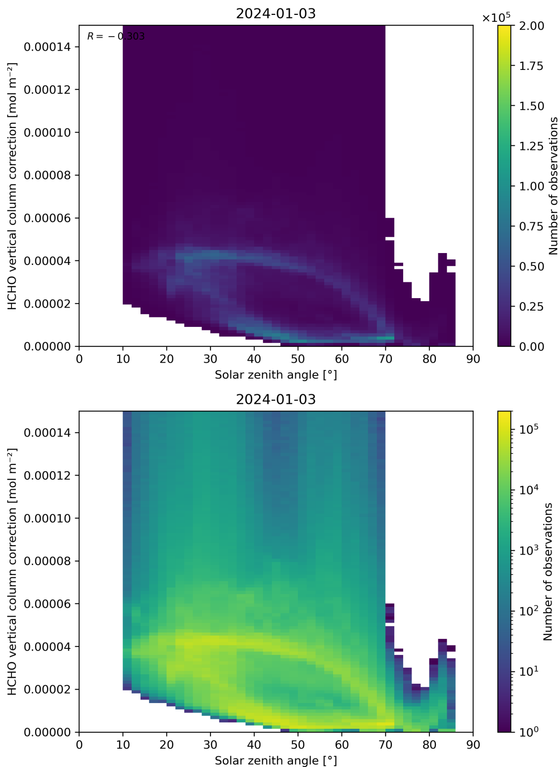
Figure 178: Scatter density plot of “Solar zenith angle” against “HCHO vertical column correction” for 2024-01-02 to 2024-01-04.
