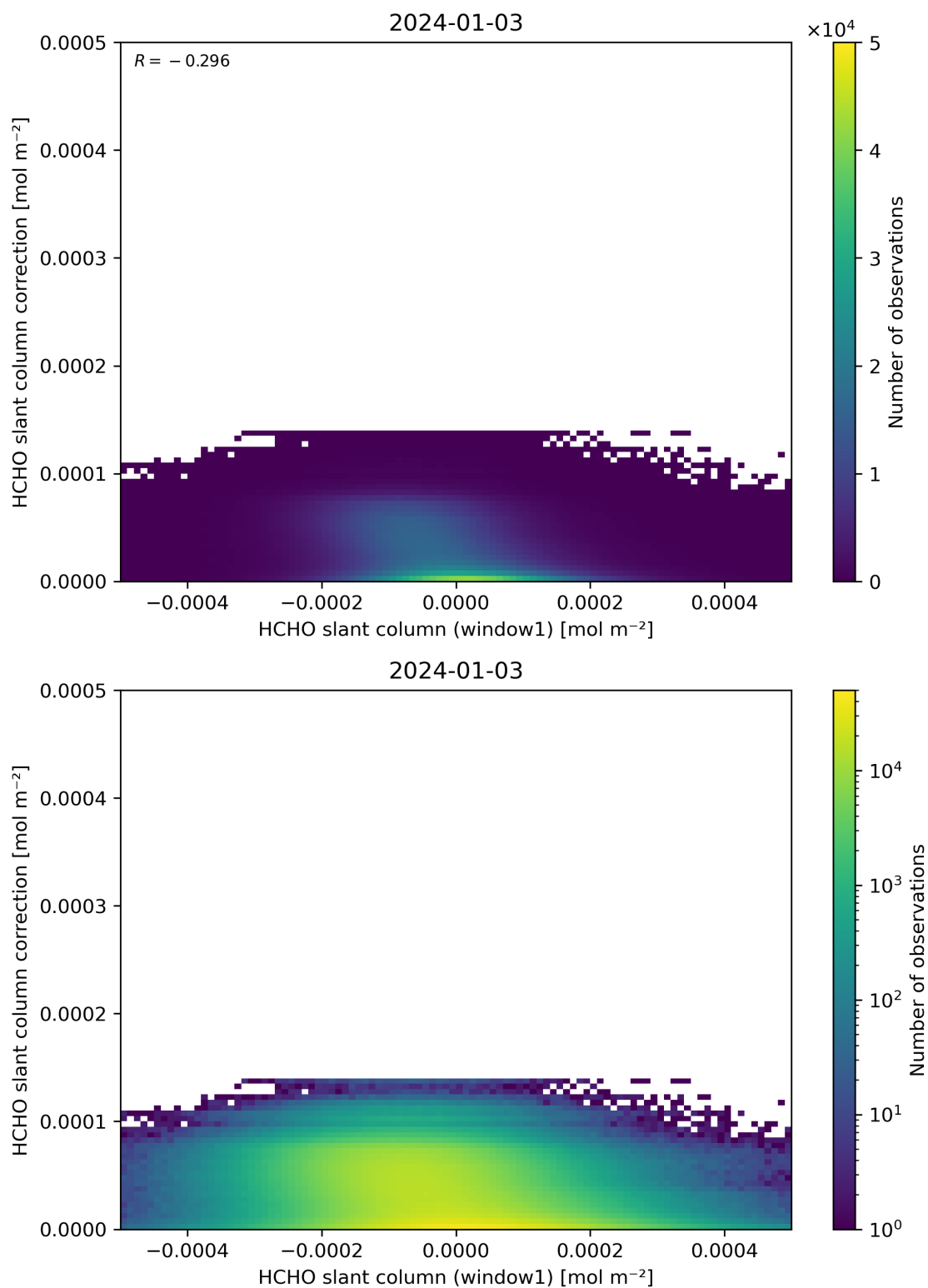
Figure 83: Scatter density plot of “HCHO slant column (window1)” against “HCHO slant column correction” for 2024-01-02 to 2024-01-04.
