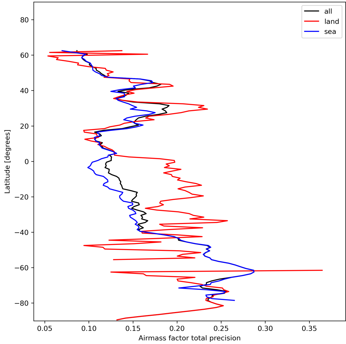
Figure 27: Zonal average of “Airmass factor total precision” for 2024-01-02 to 2024-01-04.
