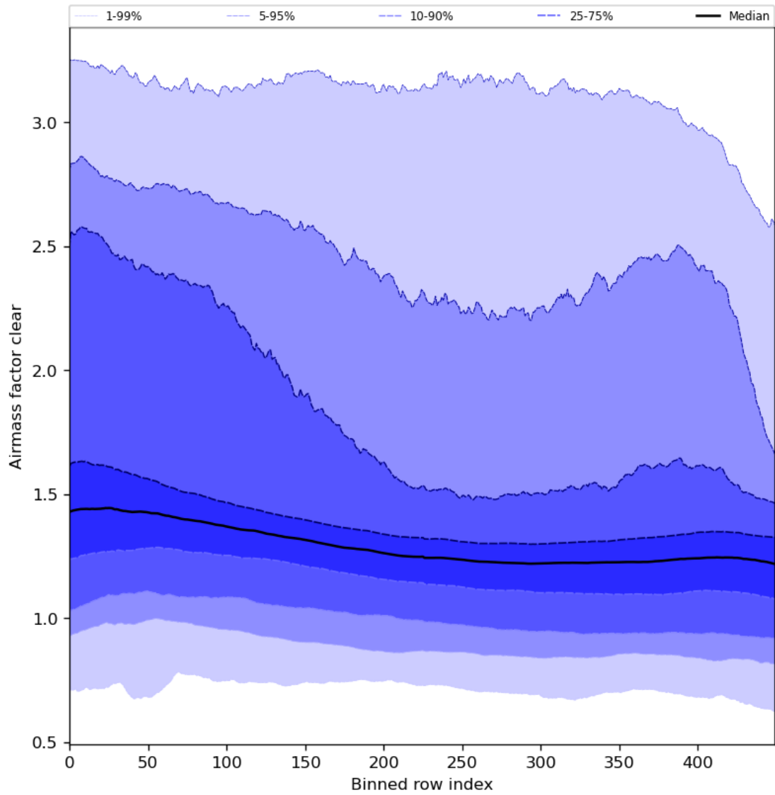
Figure 56: Along track statistics of “Airmass factor clear” for 2024-01-02 to 2024-01-04
