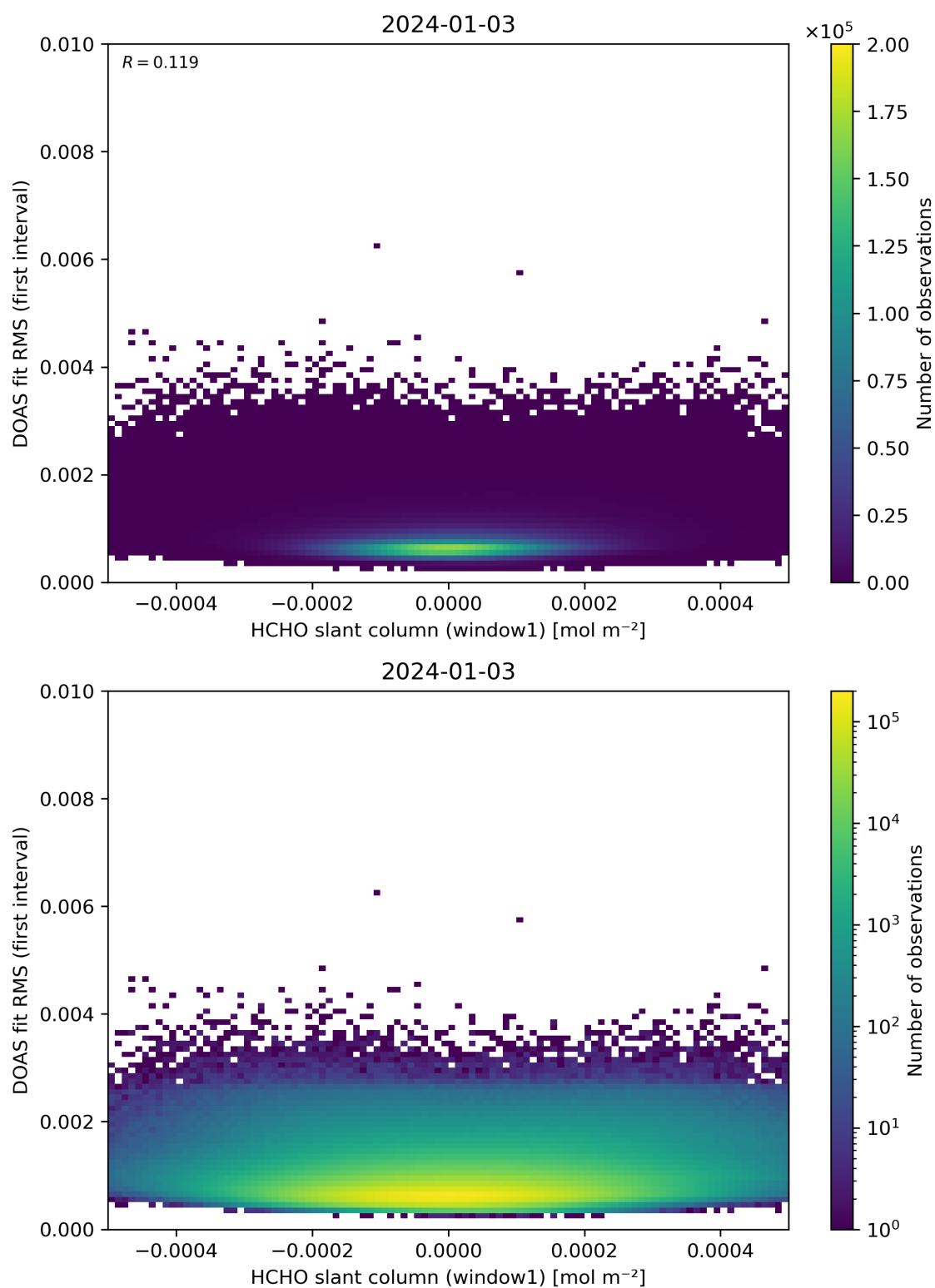
Figure 78: Scatter density plot of “HCHO slant column (window1)” against “DOAS fit RMS (first interval)” for 2024-01-02 to 2024-01-04.
