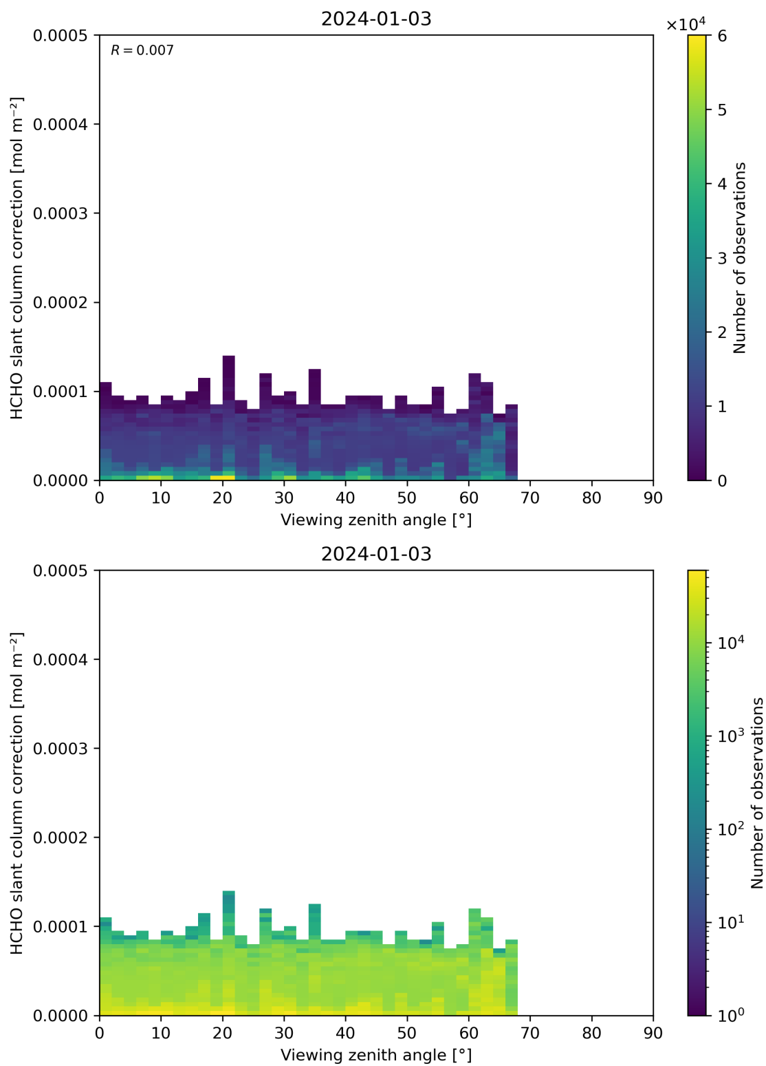
Figure 187: Scatter density plot of “Viewing zenith angle” against “HCHO slant column correction” for 2024-01-02 to 2024-01-04.
