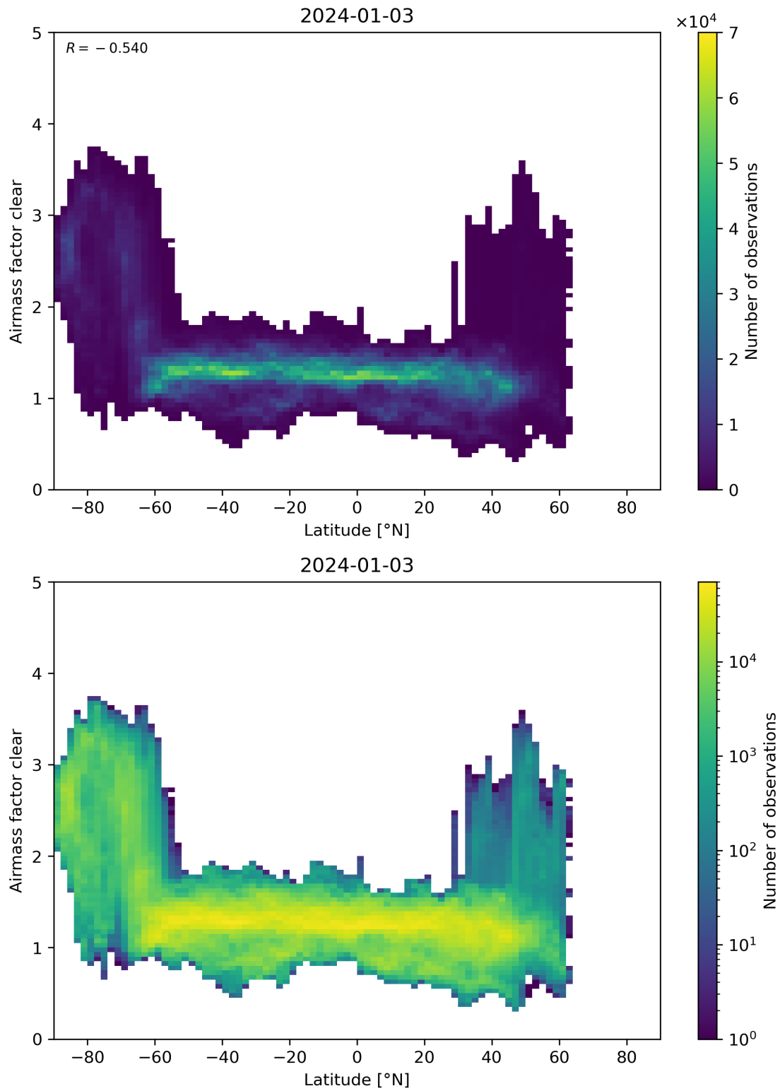
Figure 156: Scatter density plot of “Latitude” against “Airmass factor clear” for 2024-01-02 to 2024-01-04.
