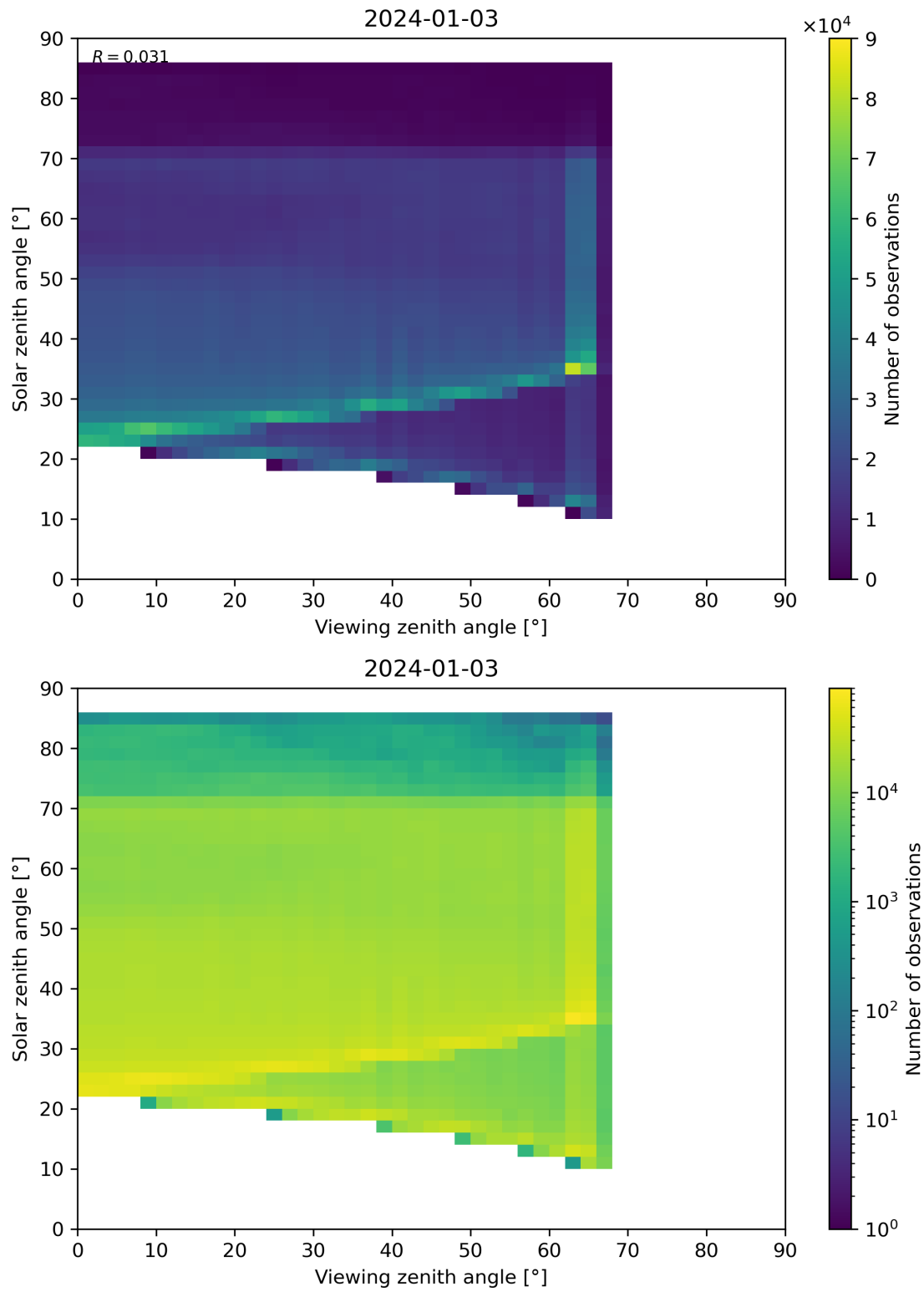
Figure 197: Scatter density plot of “Viewing zenith angle” against “Solar zenith angle” for 2024-01-02 to 2024-01-04.
