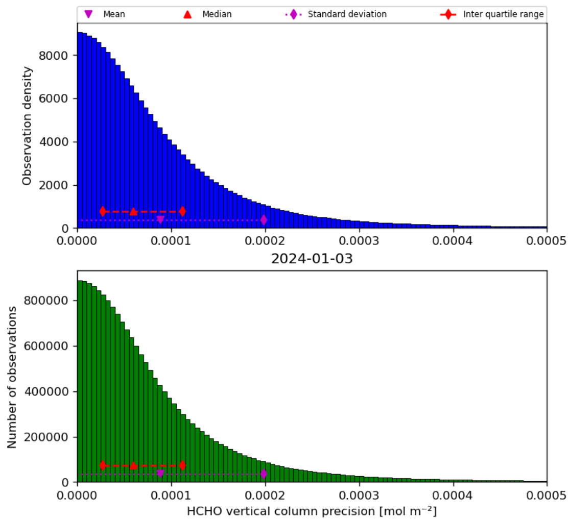
Figure 36: Histogram of “HCHO vertical column precision” for 2024-01-02 to 2024-01-04
