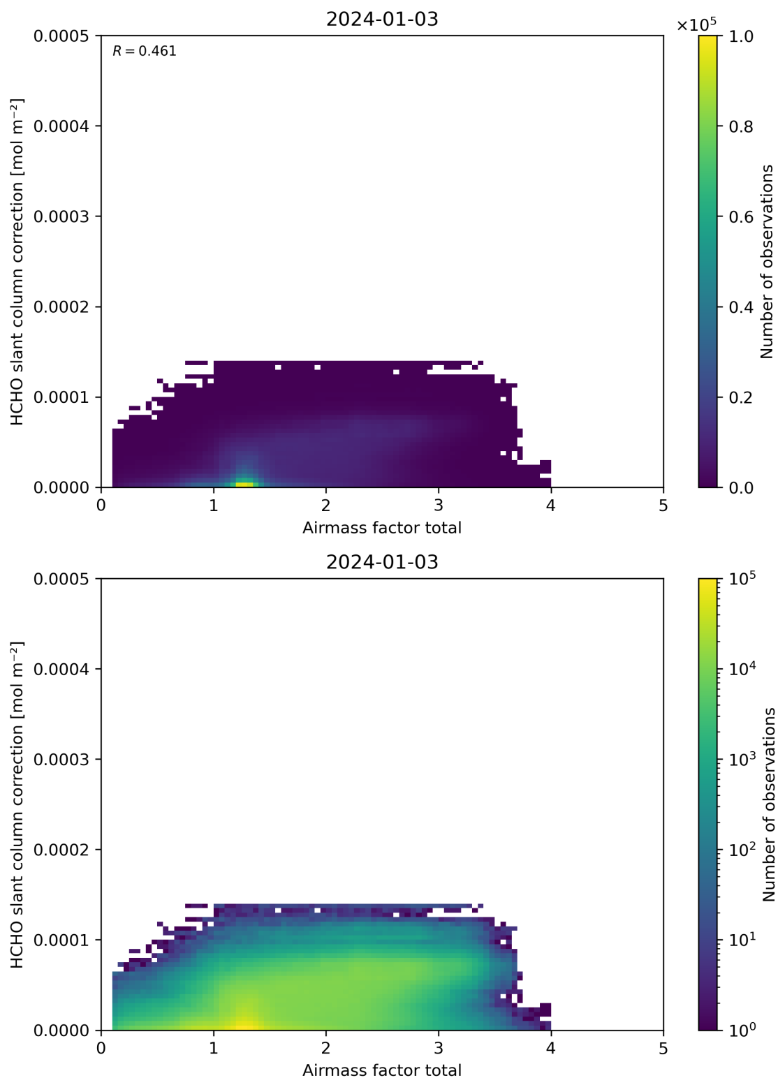
Figure 102: Scatter density plot of “Airmass factor total” against “HCHO slant column correction” for 2024-01-02 to 2024-01-04.
