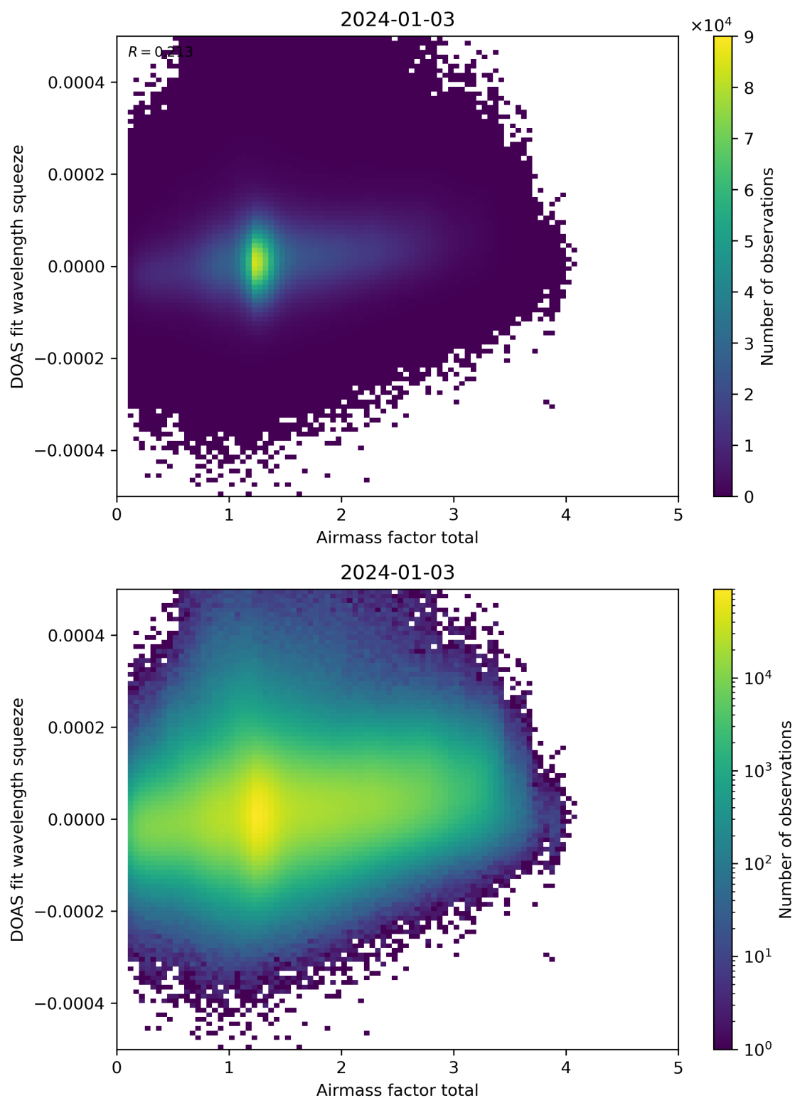
Figure 99: Scatter density plot of “Airmass factor total” against “DOAS fit wavelength squeeze” for 2024-01-02 to 2024-01-04.
