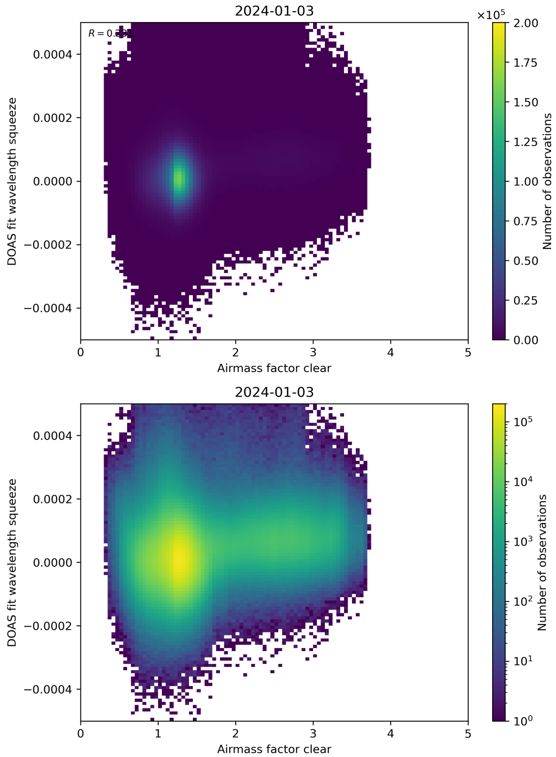
Figure 73: Scatter density plot of “Airmass factor clear” against “DOAS fit wavelength squeeze” for 2024-01-02 to 2024-01-04.
