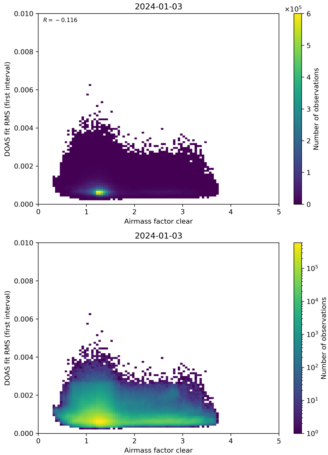
Figure 71: Scatter density plot of “Airmass factor clear” against “DOAS fit RMS (first interval)” for 2024-01-02 to 2024-01-04.
