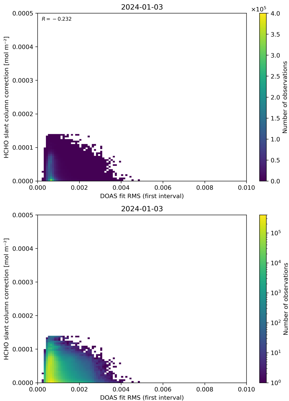
Figure 63: Scatter density plot of “DOAS fit RMS (first interval)” against “HCHO slant column correction” for 2024-01-02 to 2024-01-04.
