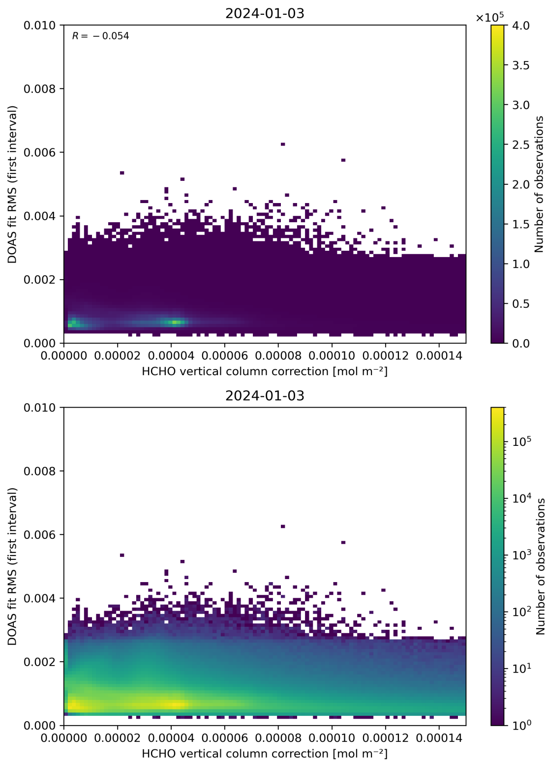
Figure 112: Scatter density plot of “HCHO vertical column correction” against “DOAS fit RMS (first interval)” for 2024-01-02 to 2024-01-04.
