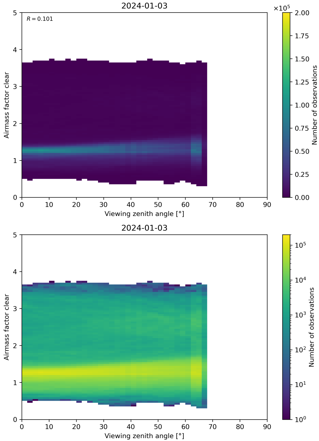
Figure 185: Scatter density plot of “Viewing zenith angle” against “Airmass factor clear” for 2024-01-02 to 2024-01-04.
