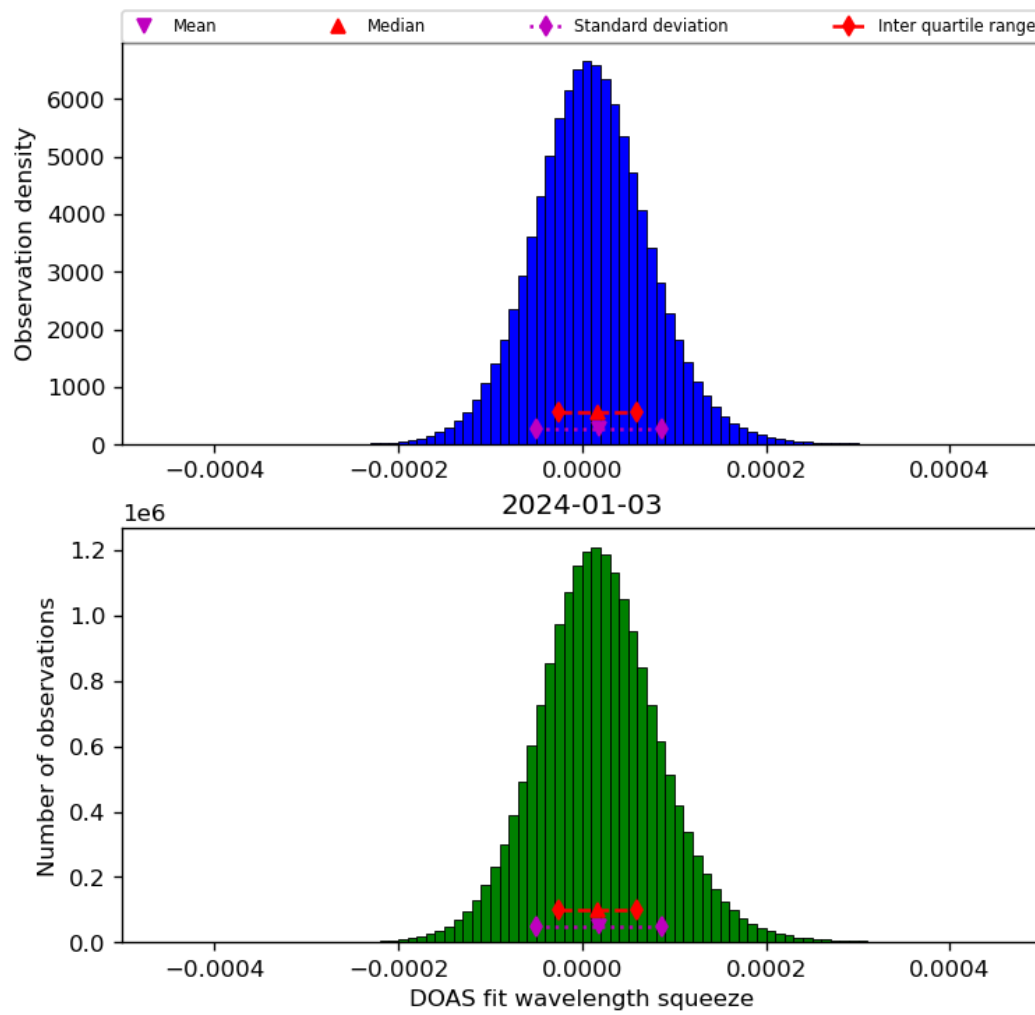
Figure 45: Histogram of “DOAS fit wavelength squeeze” for 2024-01-02 to 2024-01-04
