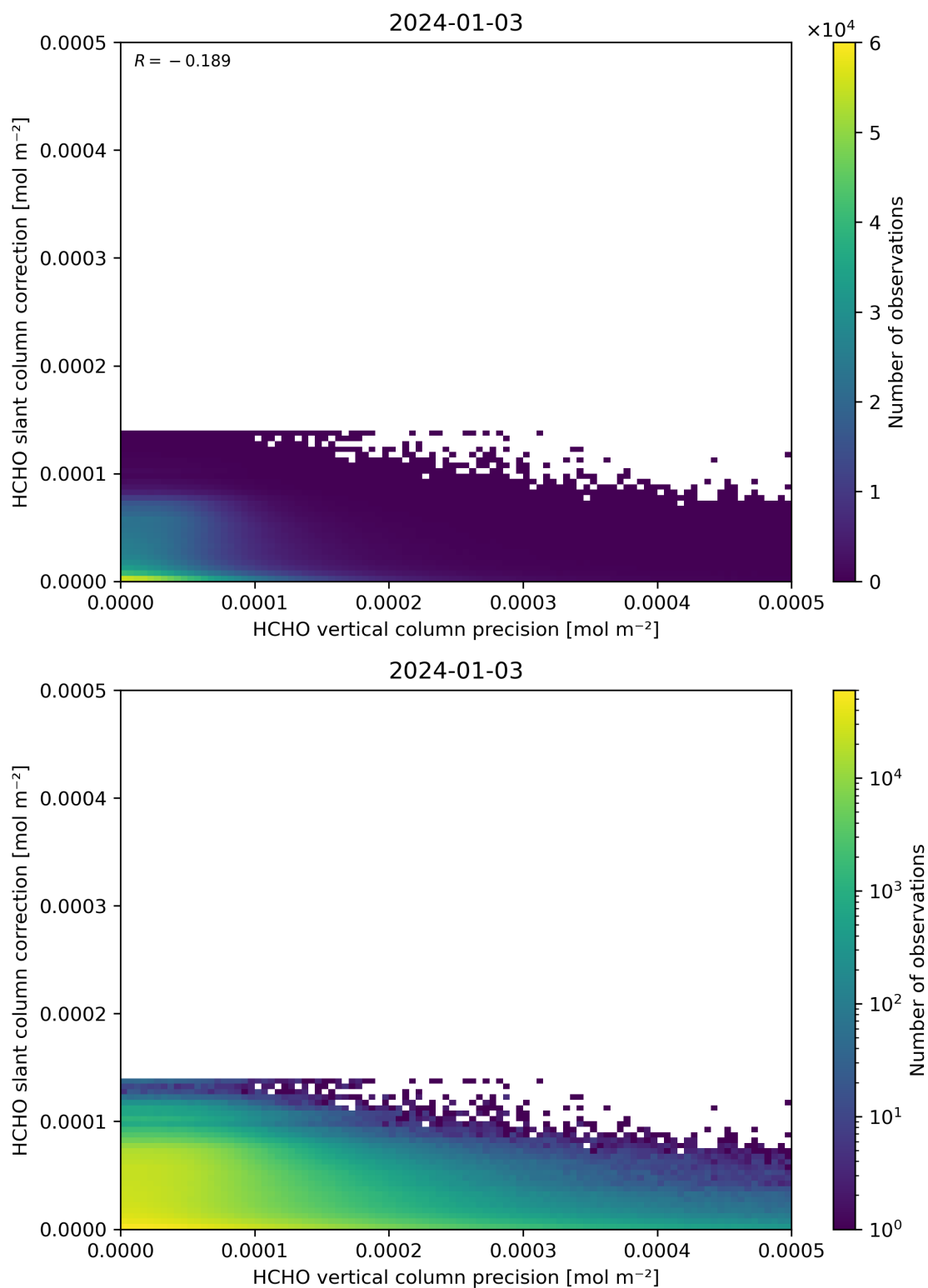
Figure 141: Scatter density plot of “HCHO vertical column precision” against “HCHO slant column correction” for 2024-01-02 to 2024-01-04.
