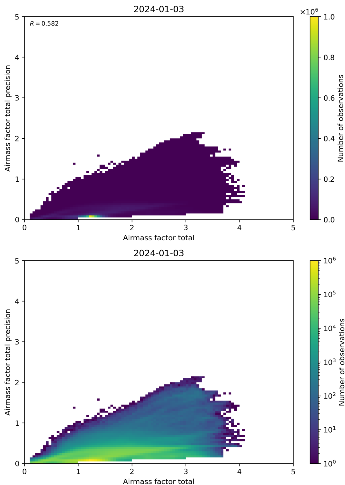
Figure 103: Scatter density plot of “Airmass factor total” against “Airmass factor total precision” for 2024-01-02 to 2024-01-04.
