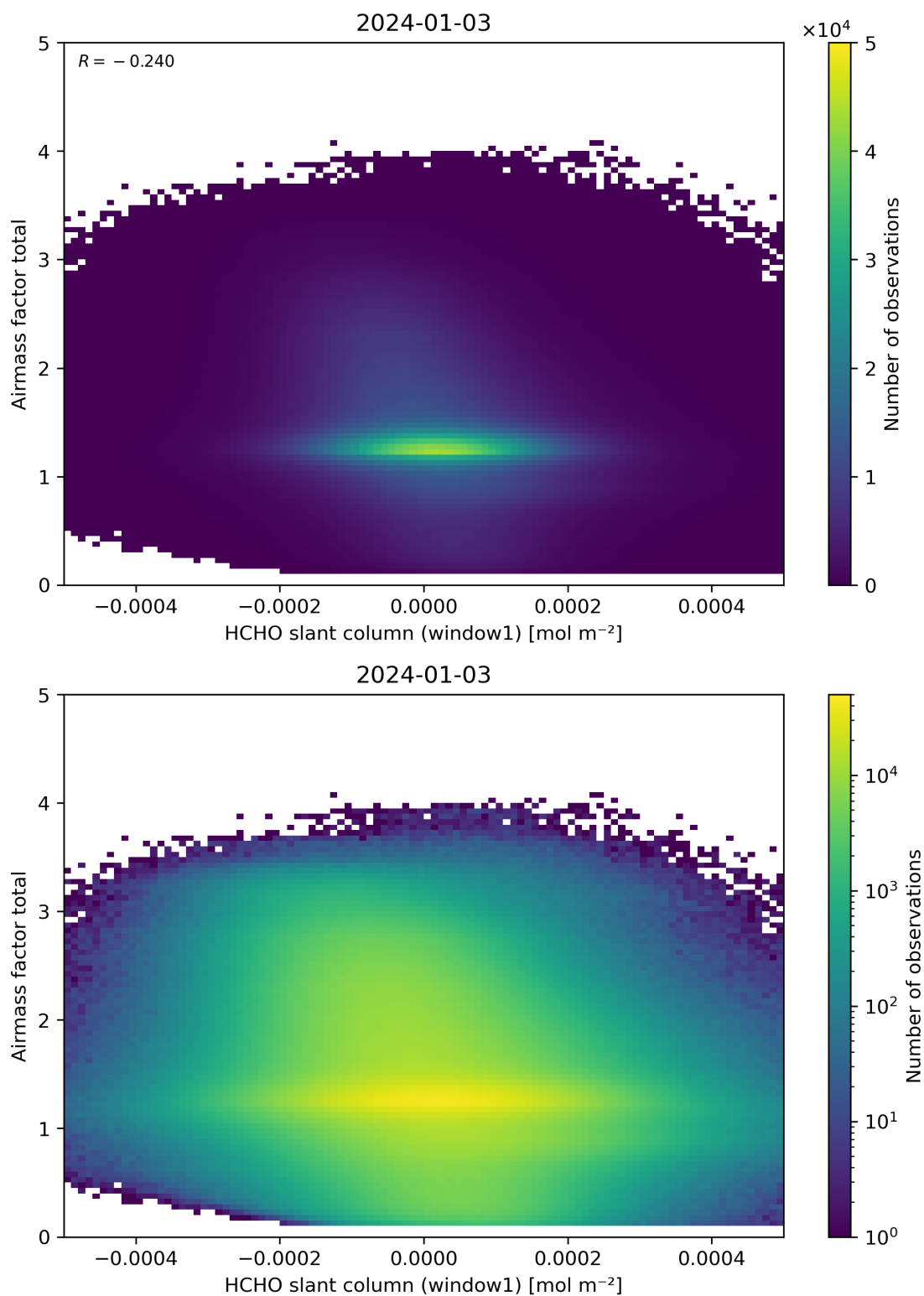
Figure 85: Scatter density plot of “HCHO slant column (window1)” against “Airmass factor total” for 2024-01-02 to 2024-01-04.
