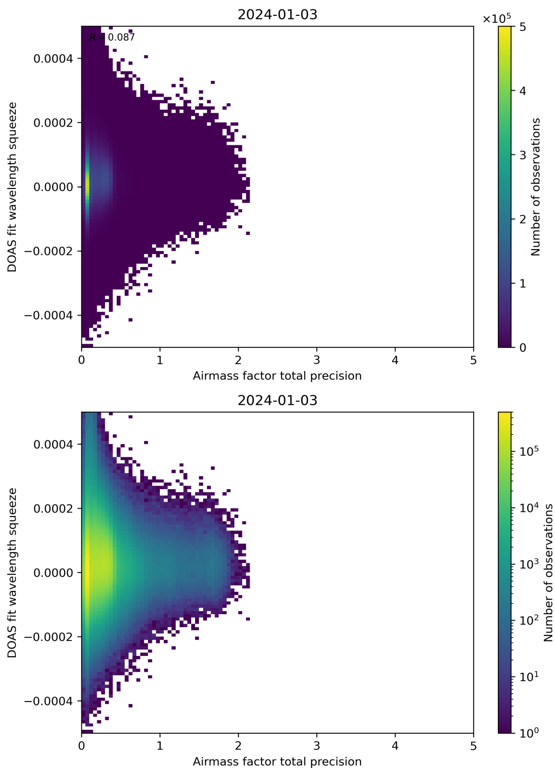
Figure 107: Scatter density plot of “Airmass factor total precision” against “DOAS fit wavelength squeeze” for 2024-01-02 to 2024-01-04.
