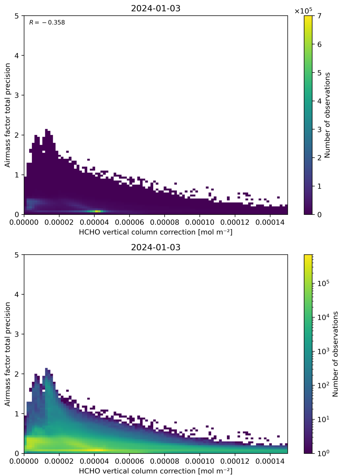
Figure 121: Scatter density plot of “HCHO vertical column correction” against “Airmass factor total precision” for 2024-01-02 to 2024-01-04.
