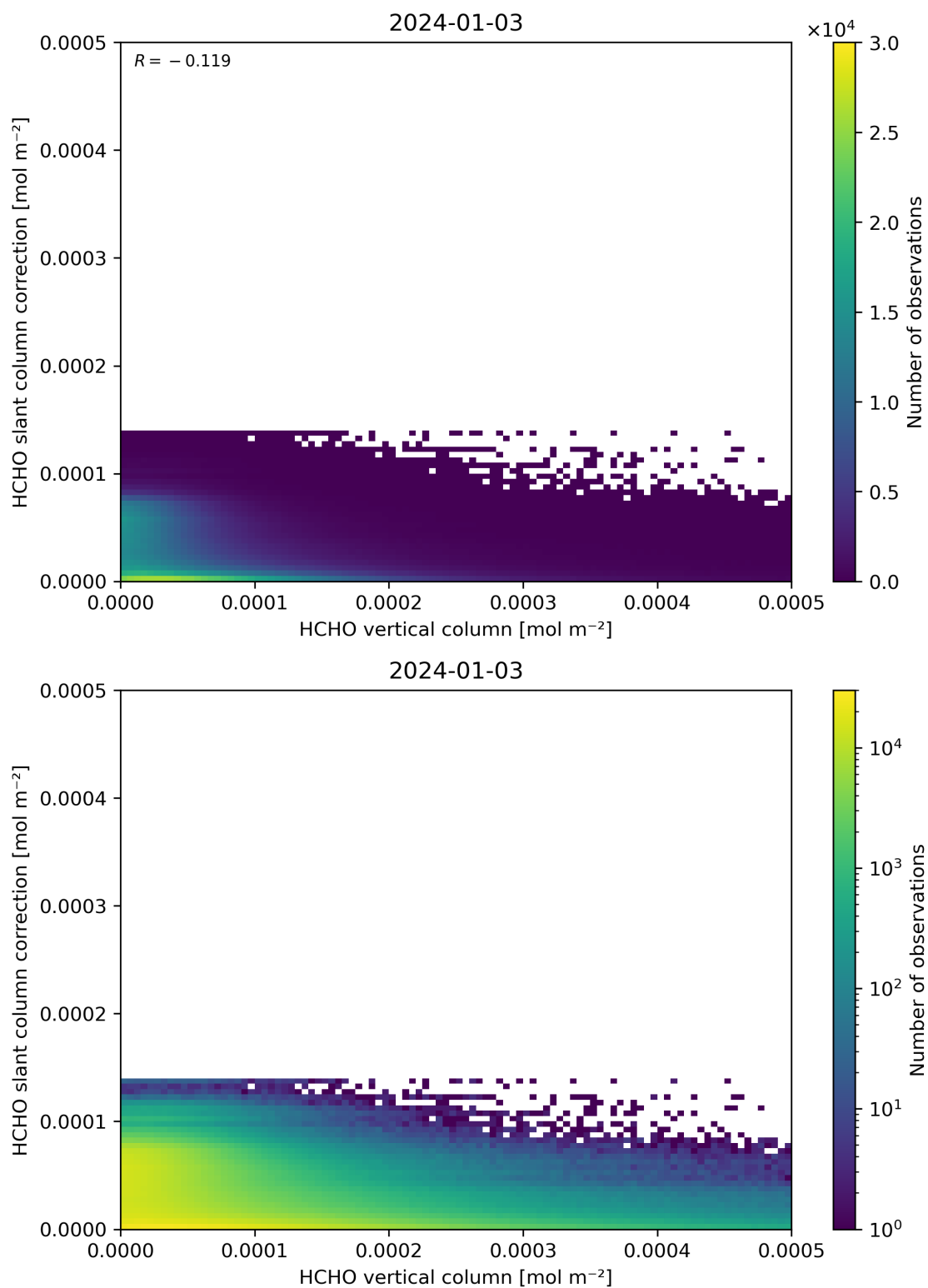
Figure 128: Scatter density plot of “HCHO vertical column” against “HCHO slant column correction” for 2024-01-02 to 2024-01-04.
