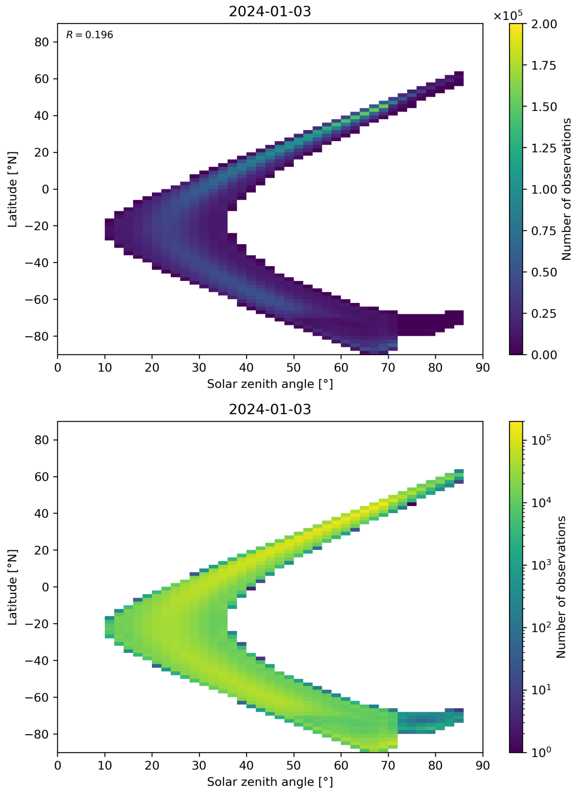
Figure 181: Scatter density plot of “Solar zenith angle” against “Latitude” for 2024-01-02 to 2024-01-04.
