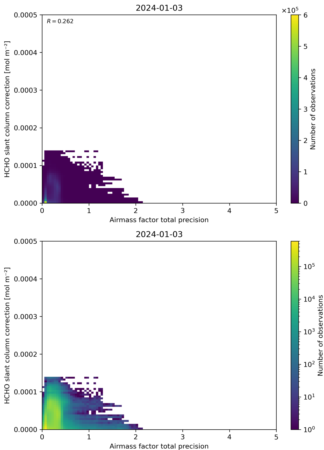
Figure 110: Scatter density plot of “Airmass factor total precision” against “HCHO slant column correction” for 2024-01-02 to 2024-01-04.
