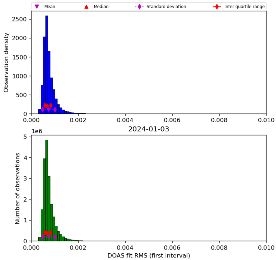
Figure 46: Histogram of “DOAS fit RMS (first interval)” for 2024-01-02 to 2024-01-04
