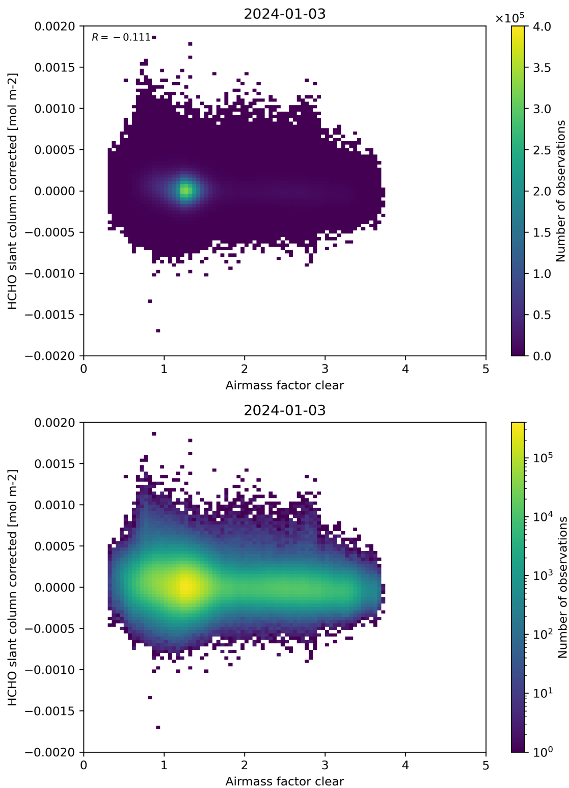
Figure 74: Scatter density plot of “Airmass factor clear” against “HCHO slant column corrected” for 2024-01-02 to 2024-01-04.
