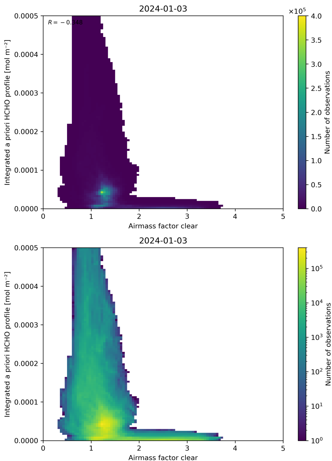
Figure 76: Scatter density plot of “Airmass factor clear” against “Integrated a priori HCHO profile” for 2024-01-02 to 2024-01-04.
