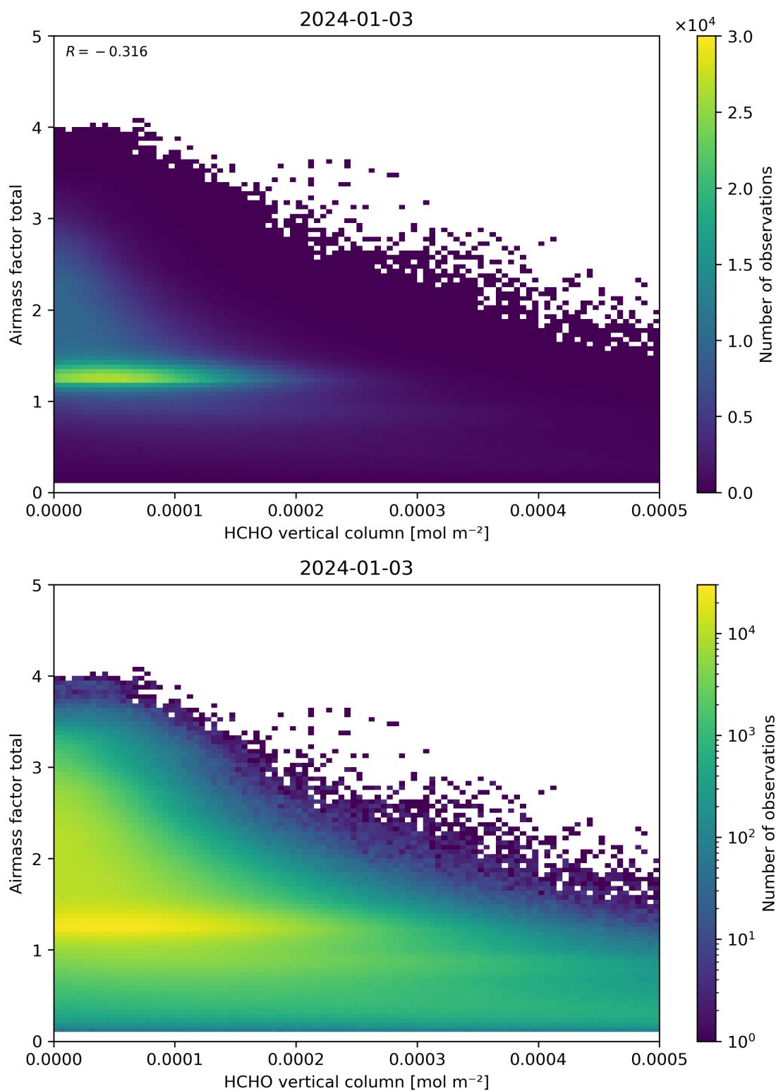
Figure 131: Scatter density plot of “HCHO vertical column” against “Airmass factor total” for 2024-01-02 to 2024-01-04.
