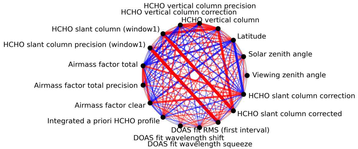
Figure 1: Map of correlation graph for 2024-01-02 to 2024-01-04.
