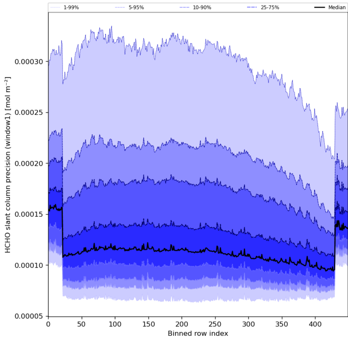
Figure 53: Along track statistics of “HCHO slant column precision (window1)” for 2024-01-02 to 2024-01-04
