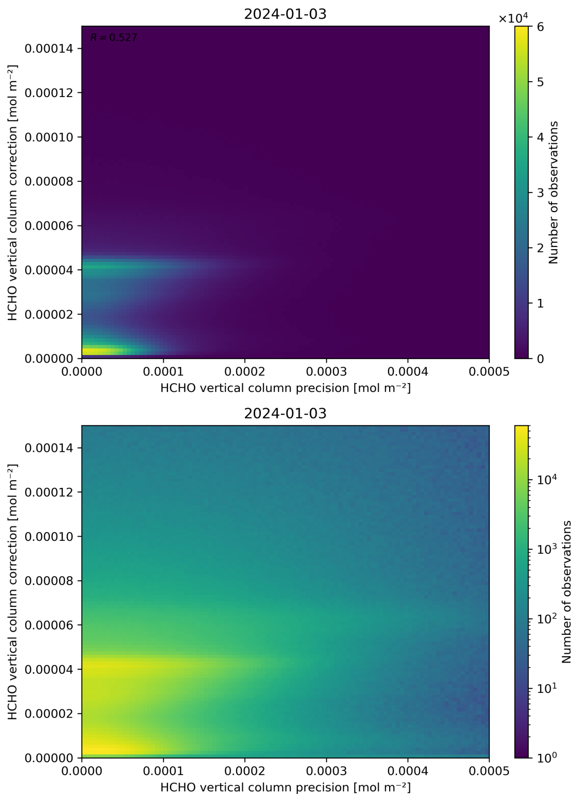
Figure 146: Scatter density plot of “HCHO vertical column precision” against “HCHO vertical column correction” for 2024-01-02 to 2024-01-04.
