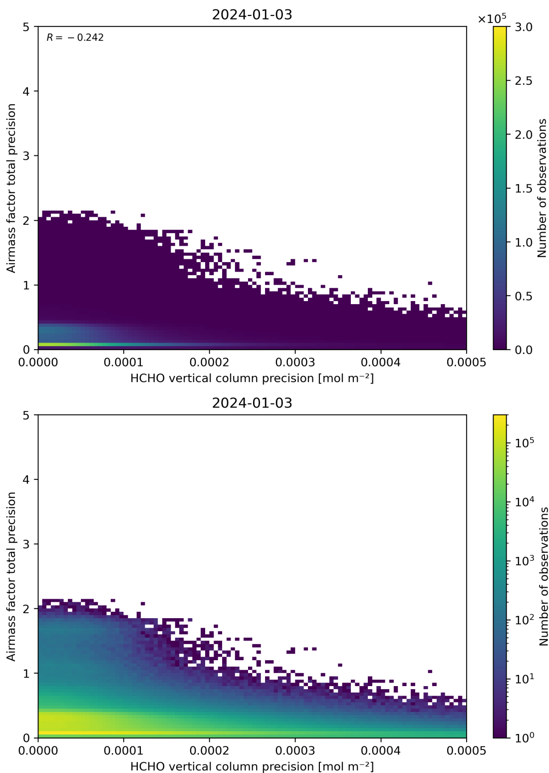
Figure 145: Scatter density plot of “HCHO vertical column precision” against “Airmass factor total precision” for 2024-01-02 to 2024-01-04.
