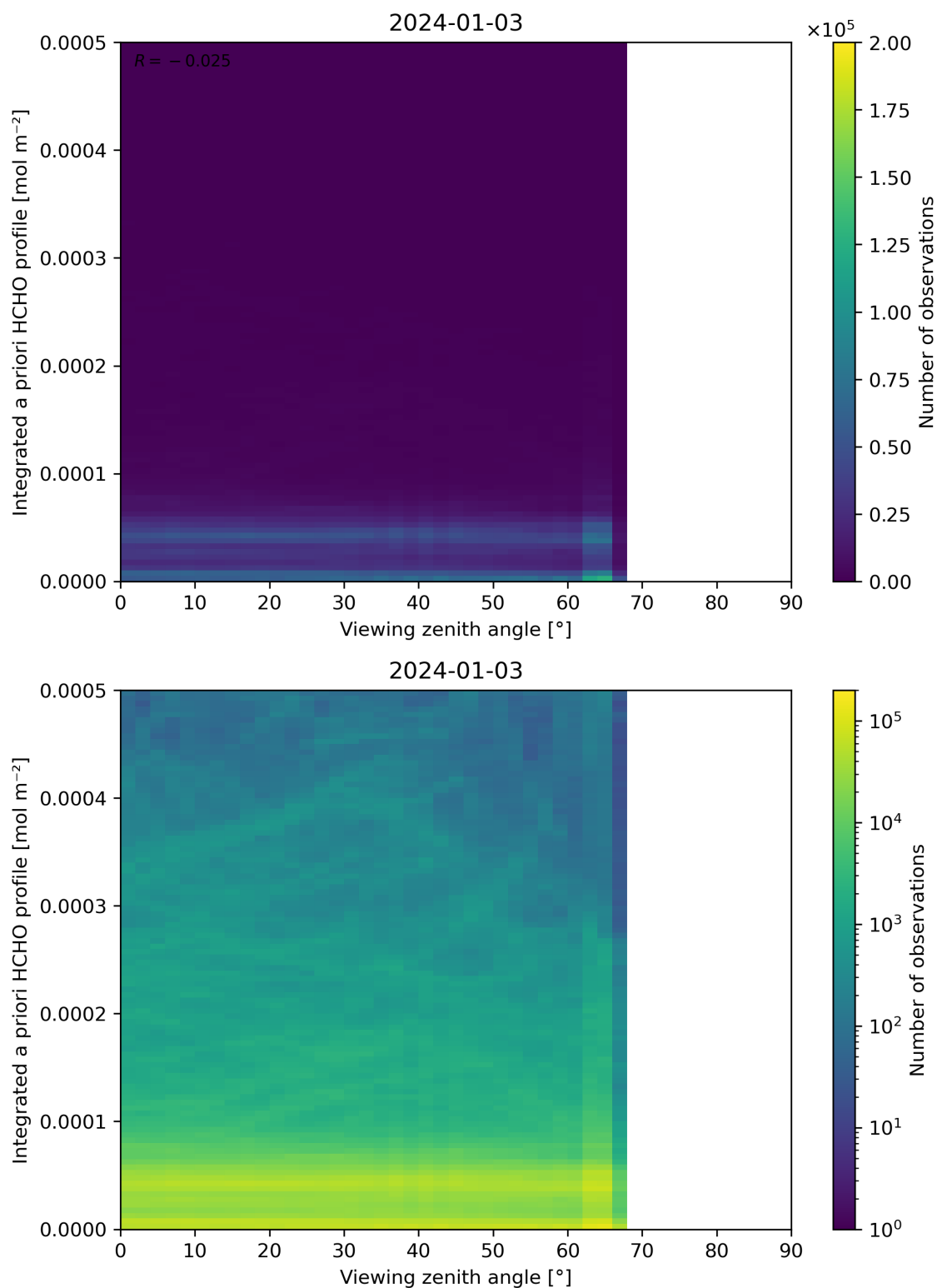
Figure 195: Scatter density plot of “Viewing zenith angle” against “Integrated a priori HCHO profile” for 2024-01-02 to 2024-01-04.
