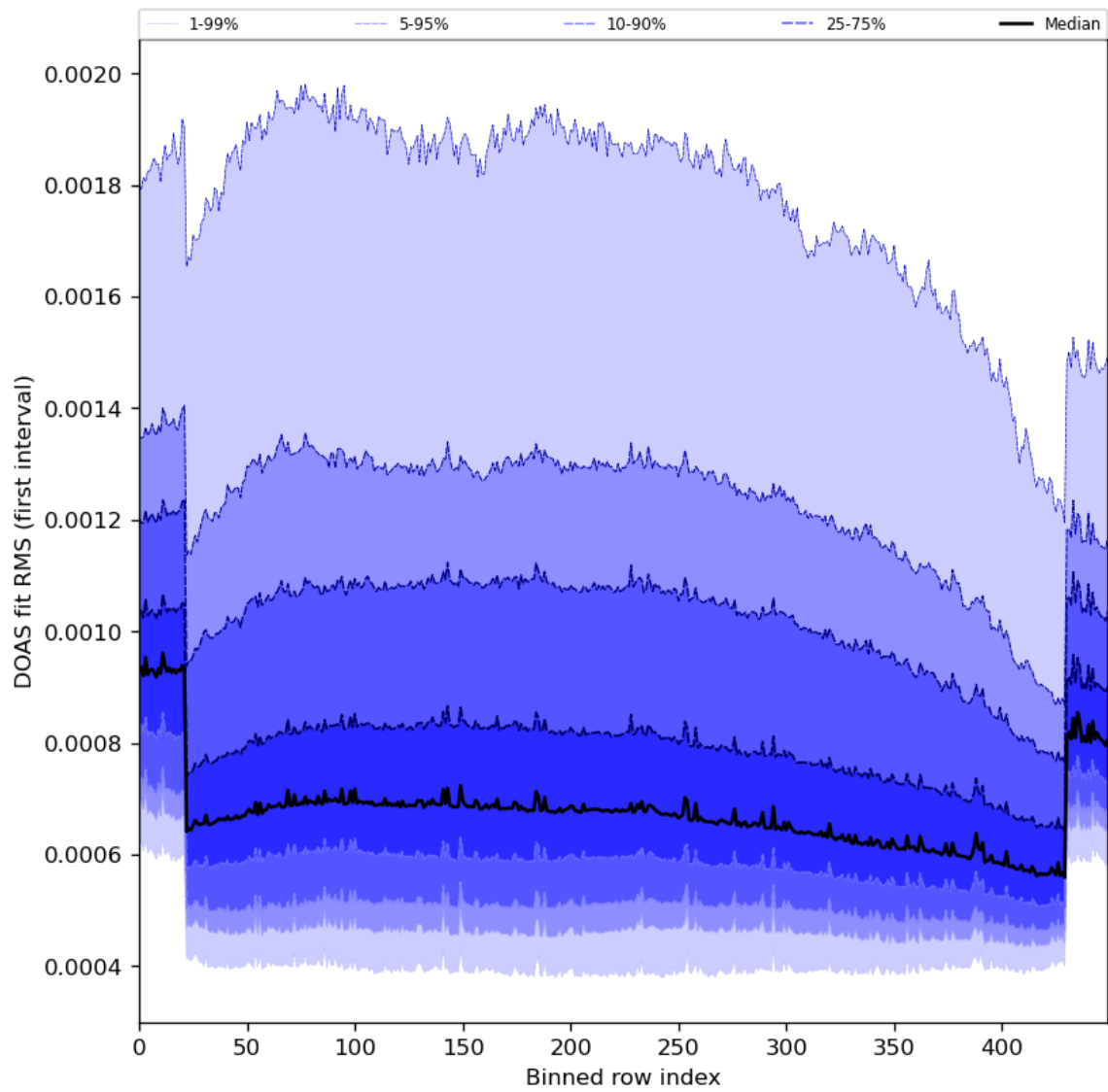
Figure 60: Along track statistics of “DOAS fit RMS (first interval)” for 2024-01-02 to 2024-01-04
