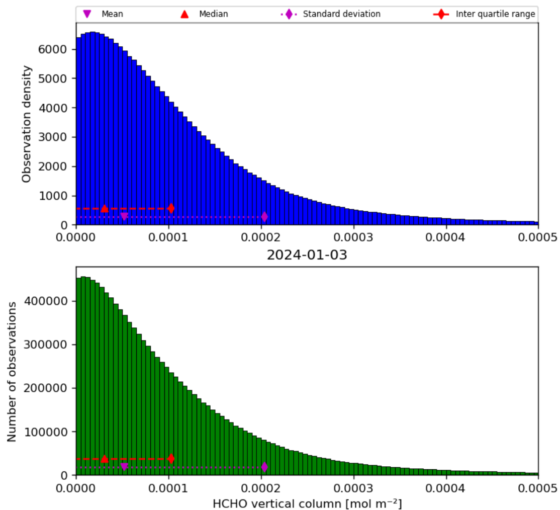
Figure 35: Histogram of “HCHO vertical column” for 2024-01-02 to 2024-01-04
