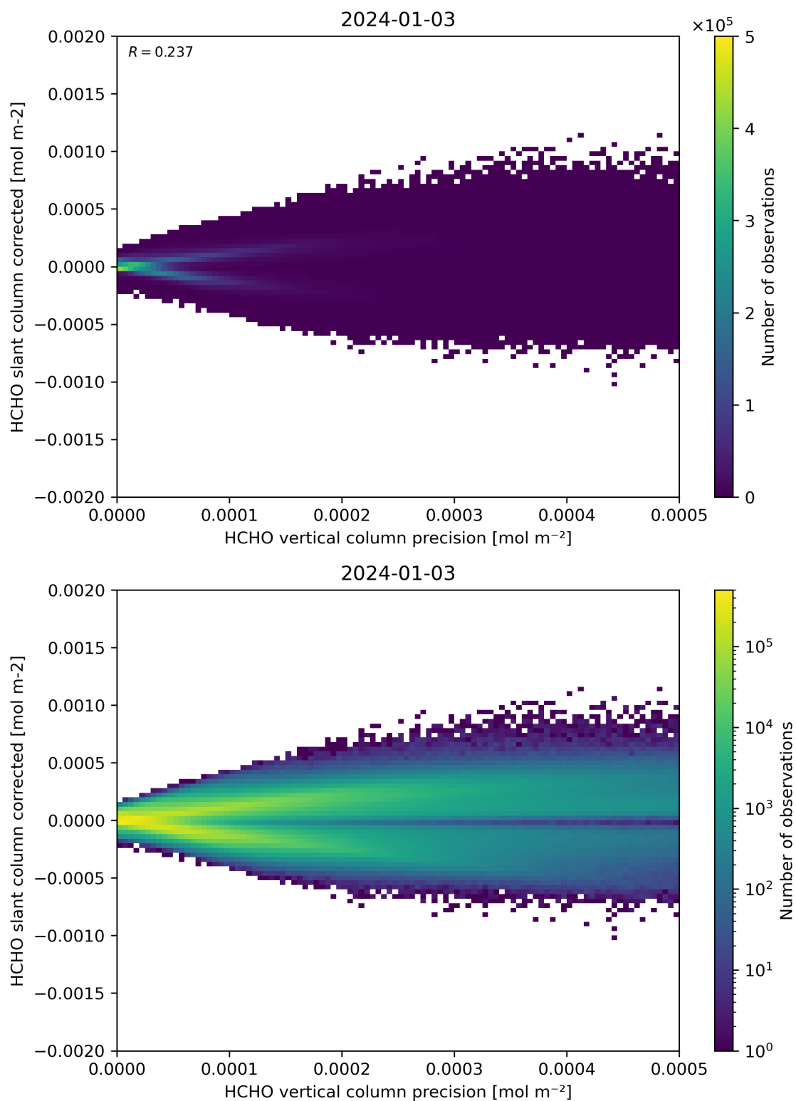
Figure 140: Scatter density plot of “HCHO vertical column precision” against “HCHO slant column corrected” for 2024-01-02 to 2024-01-04.
