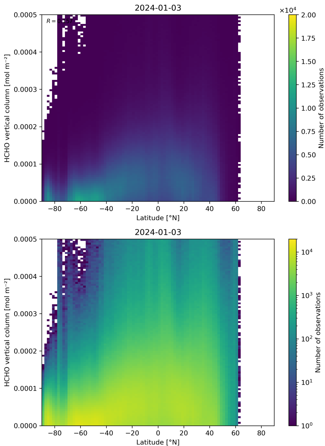
Figure 163: Scatter density plot of “Latitude” against “HCHO vertical column” for 2024-01-02 to 2024-01-04.
