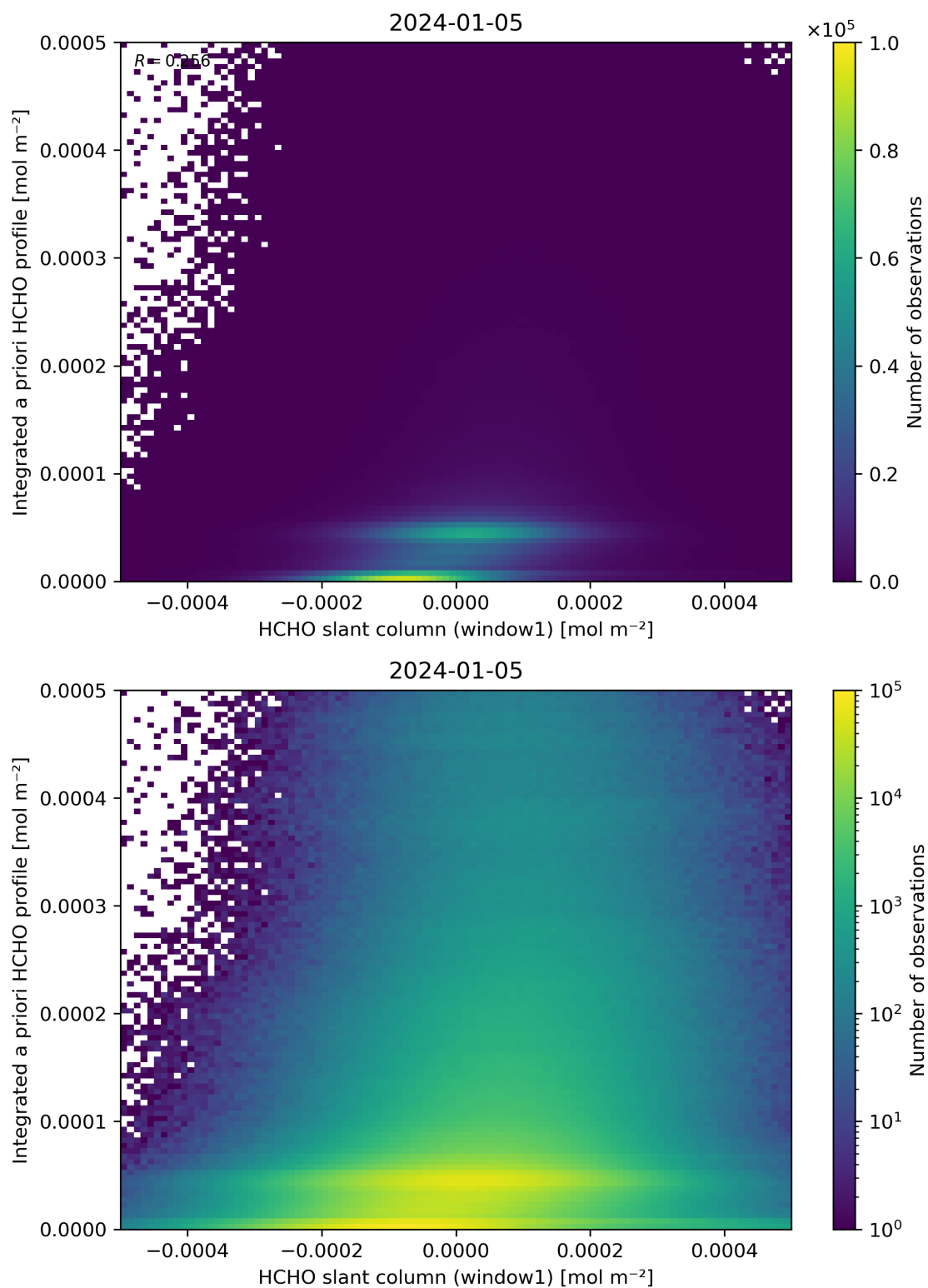
Figure 87: Scatter density plot of “HCHO slant column (window1)” against “Integrated a priori HCHO profile” for 2024-01-05 to 2024-01-06.
