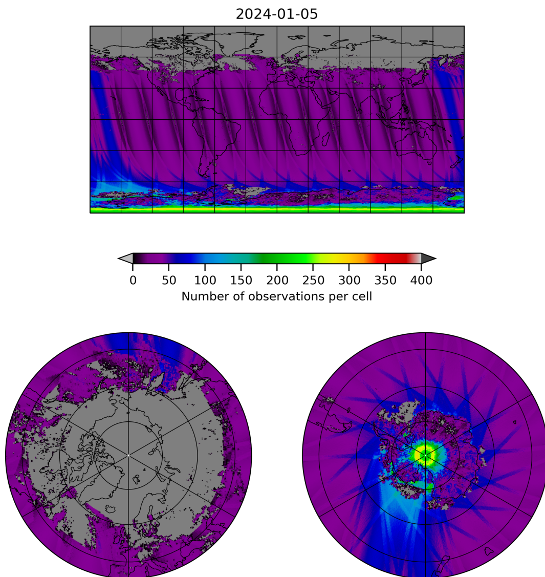
Figure 19: Map of the number of observations for 2024-01-05 to 2024-01-06
