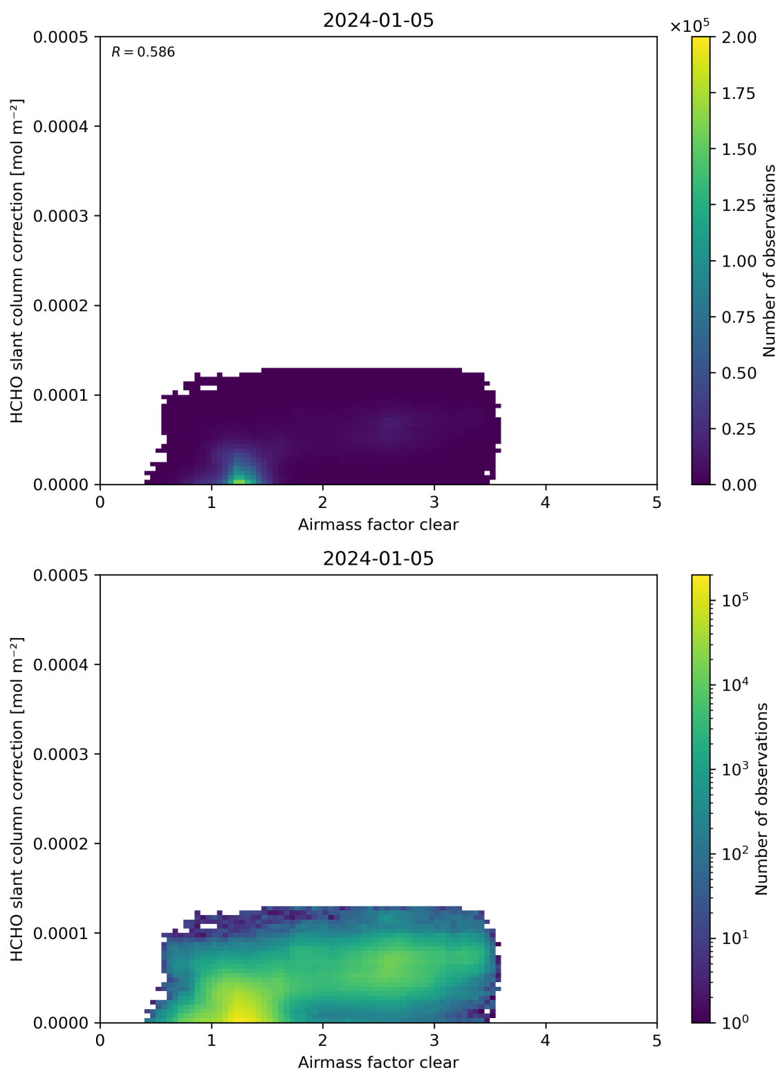
Figure 75: Scatter density plot of “Airmass factor clear” against “HCHO slant column correction” for 2024-01-05 to 2024-01-06.
