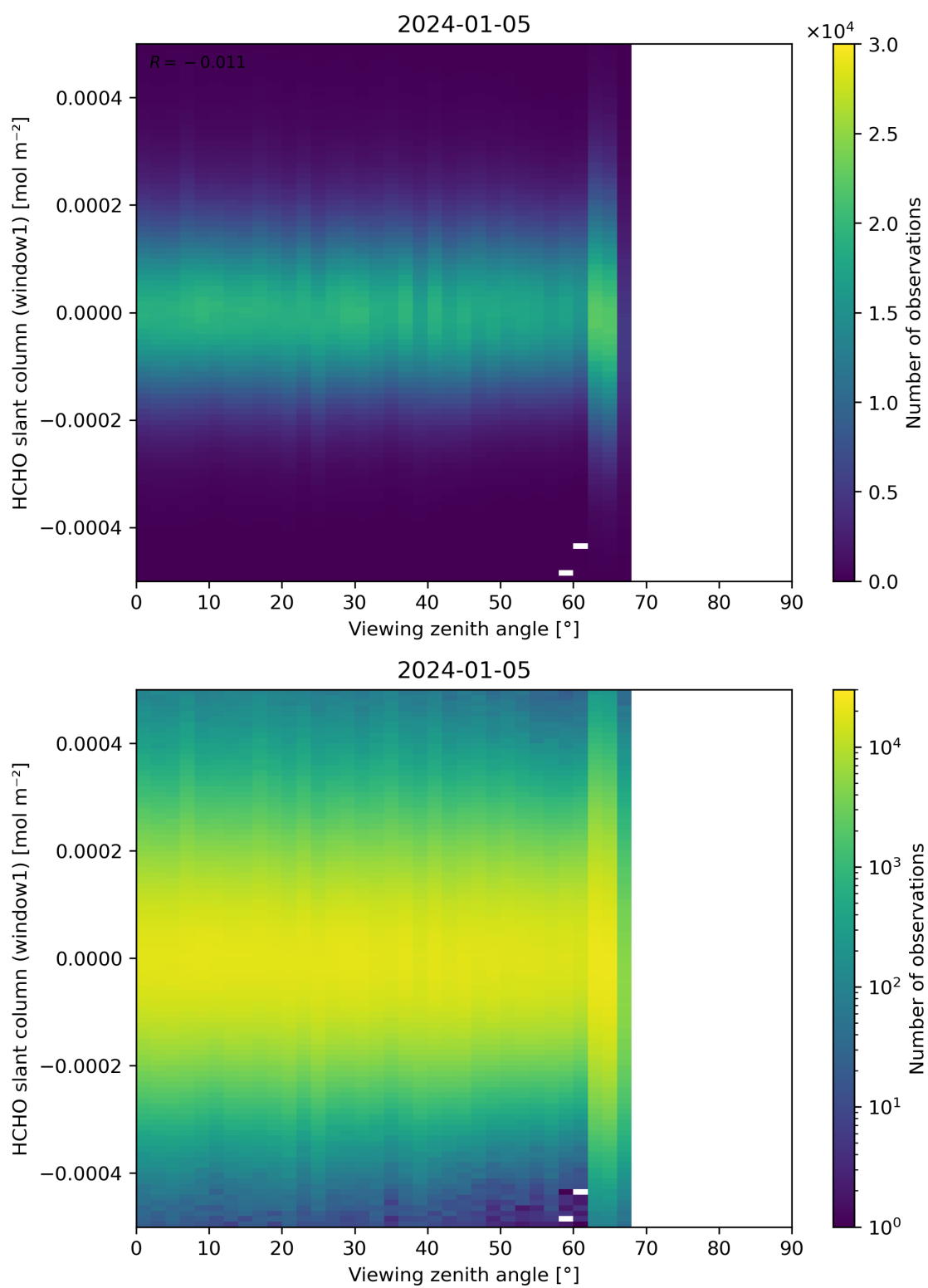
Figure 188: Scatter density plot of “Viewing zenith angle” against “HCHO slant column (window1)” for 2024-01-05 to 2024-01-06.
