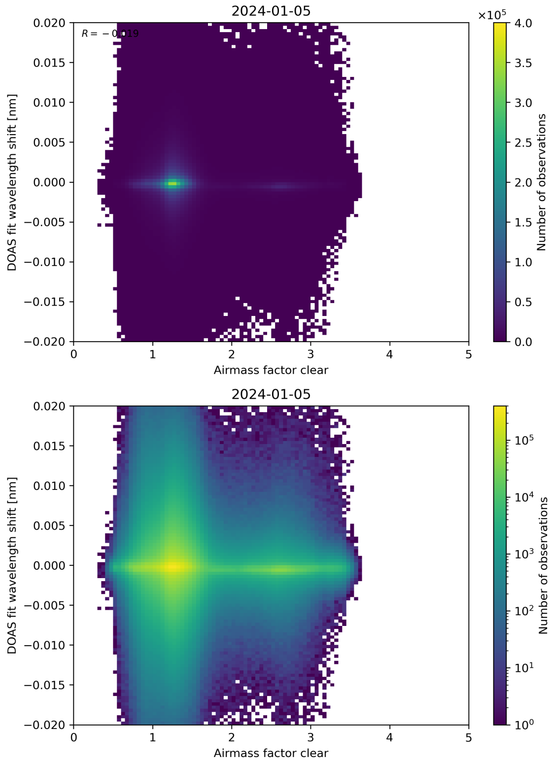
Figure 72: Scatter density plot of “Airmass factor clear” against “DOAS fit wavelength shift” for 2024-01-05 to 2024-01-06.
