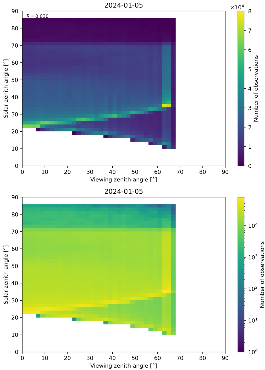
Figure 197: Scatter density plot of “Viewing zenith angle” against “Solar zenith angle” for 2024-01-05 to 2024-01-06.
