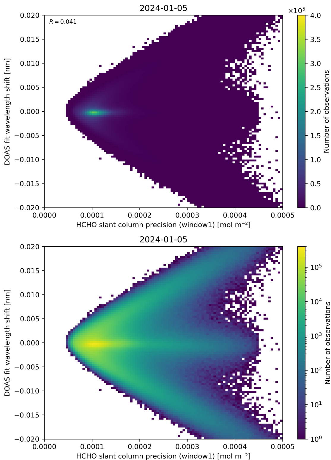
Figure 89: Scatter density plot of “HCHO slant column precision (window1)” against “DOAS fit wavelength shift” for 2024-01-05 to 2024-01-06.
