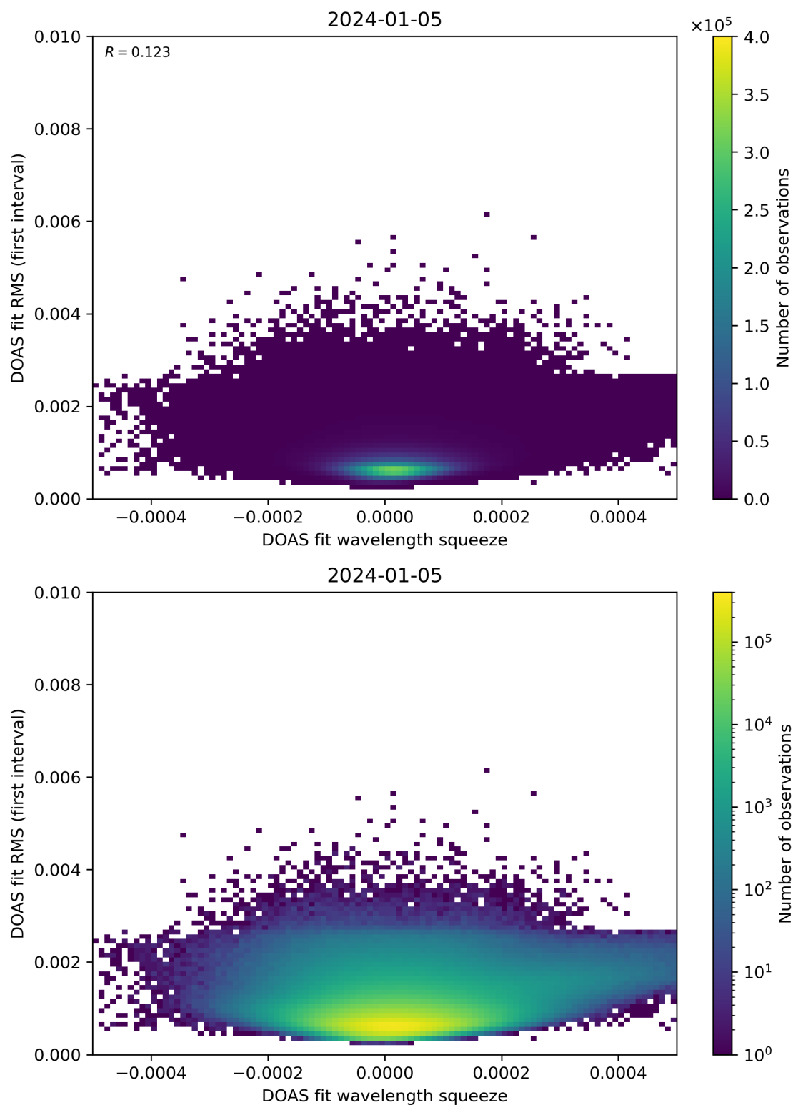
Figure 68: Scatter density plot of “DOAS fit wavelength squeeze” against “DOAS fit RMS (first interval)” for 2024-01-05 to 2024-01-06.
