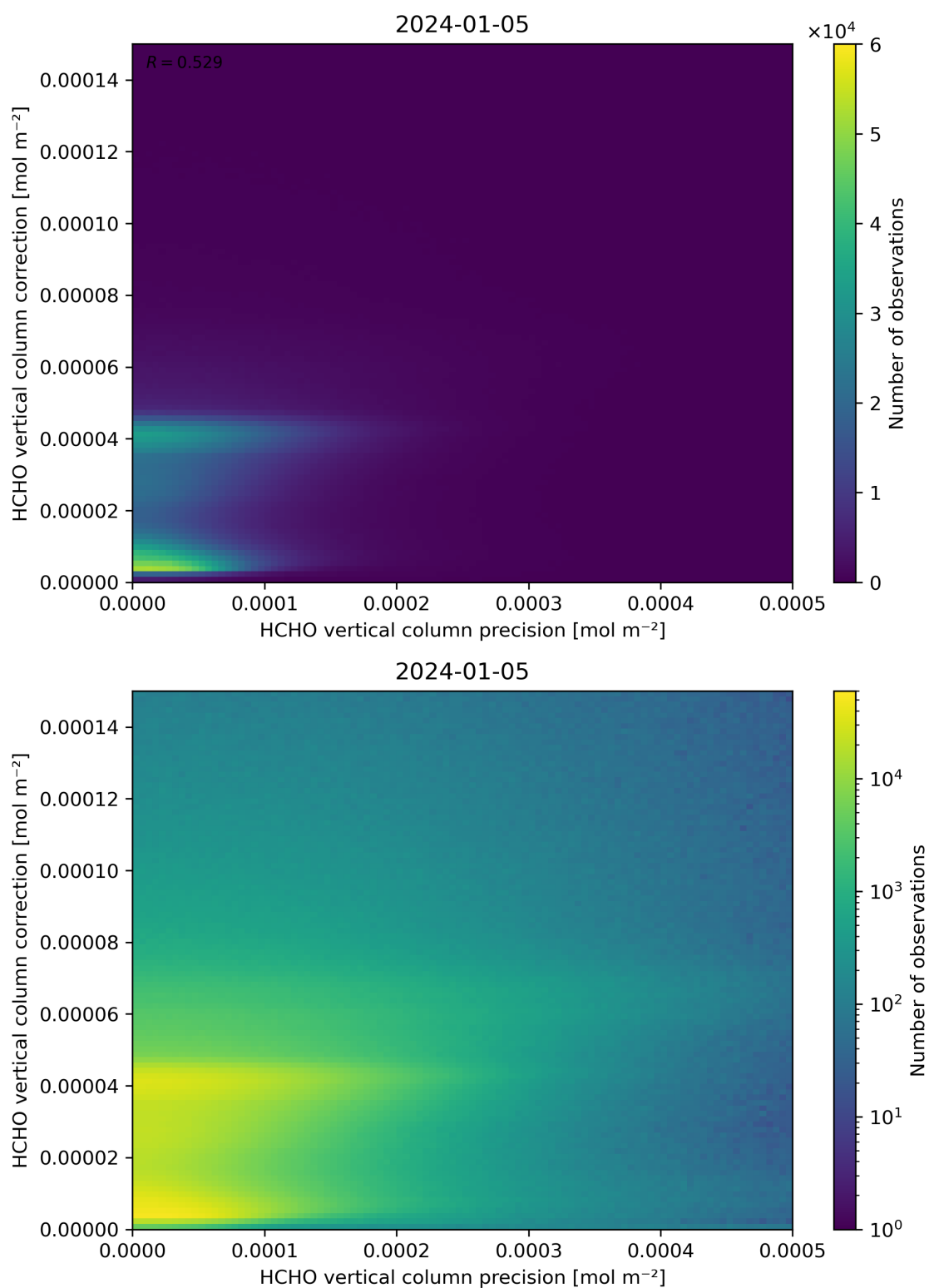
Figure 146: Scatter density plot of “HCHO vertical column precision” against “HCHO vertical column correction” for 2024-01-05 to 2024-01-06.
