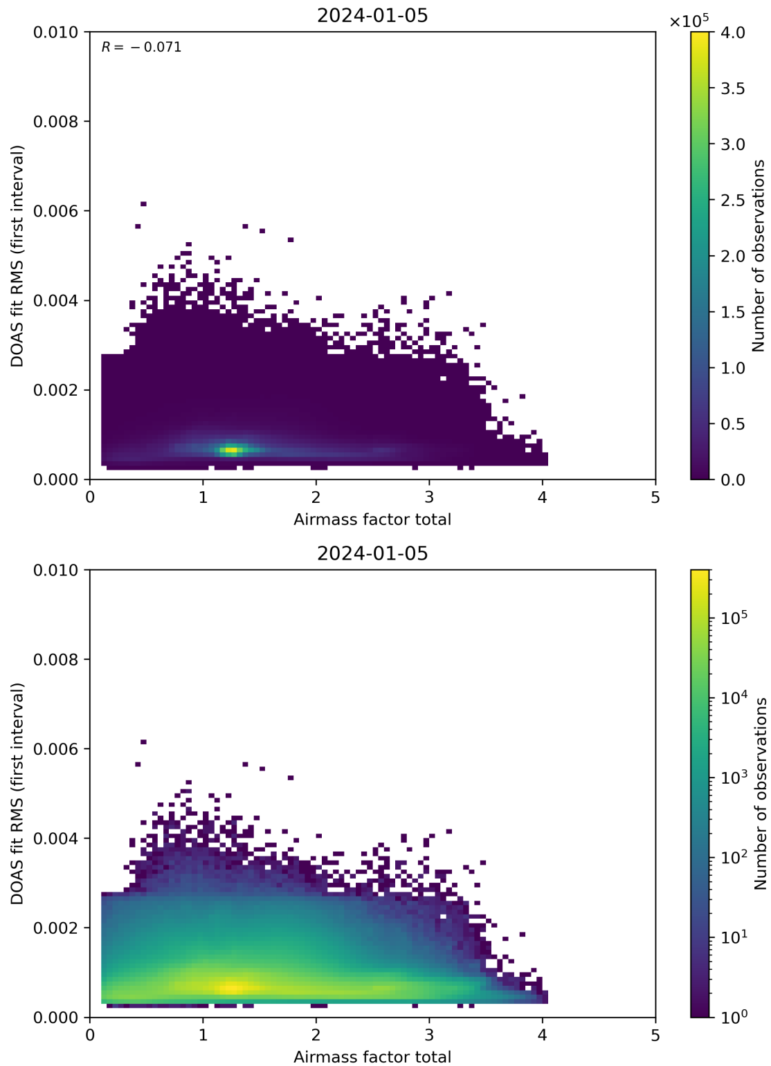
Figure 97: Scatter density plot of “Airmass factor total” against “DOAS fit RMS (first interval)” for 2024-01-05 to 2024-01-06.
