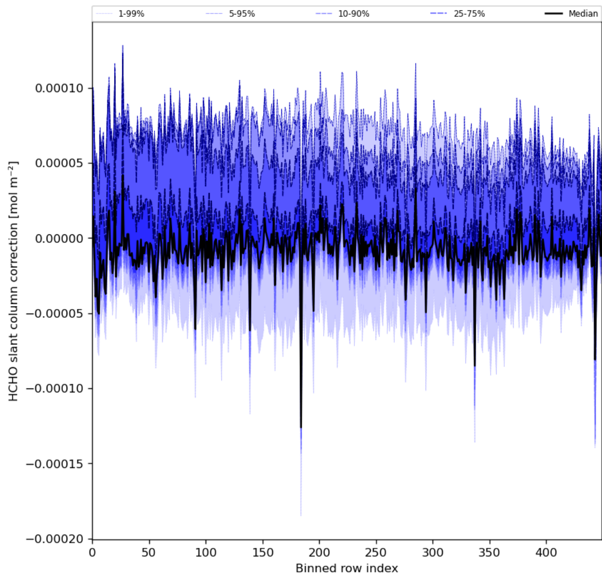
Figure 61: Along track statistics of “HCHO slant column correction” for 2024-01-05 to 2024-01-06
