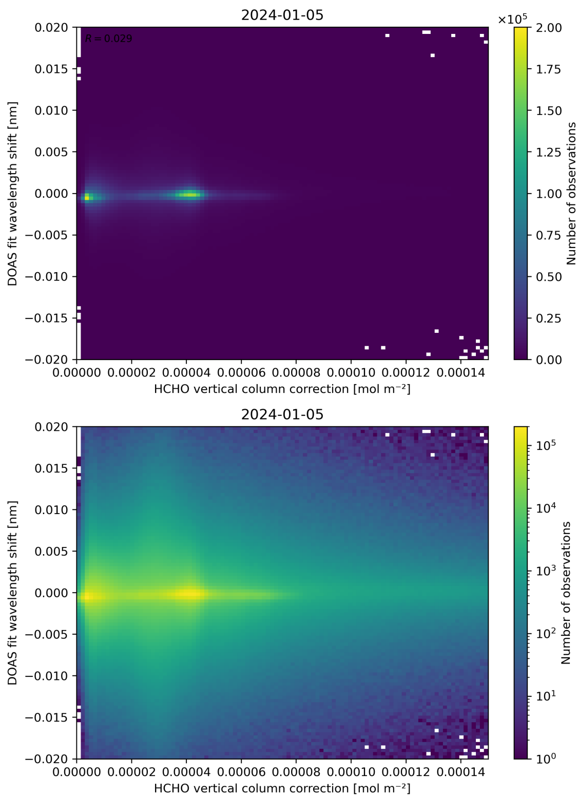
Figure 113: Scatter density plot of “HCHO vertical column correction” against “DOAS fit wavelength shift” for 2024-01-05 to 2024-01-06.
