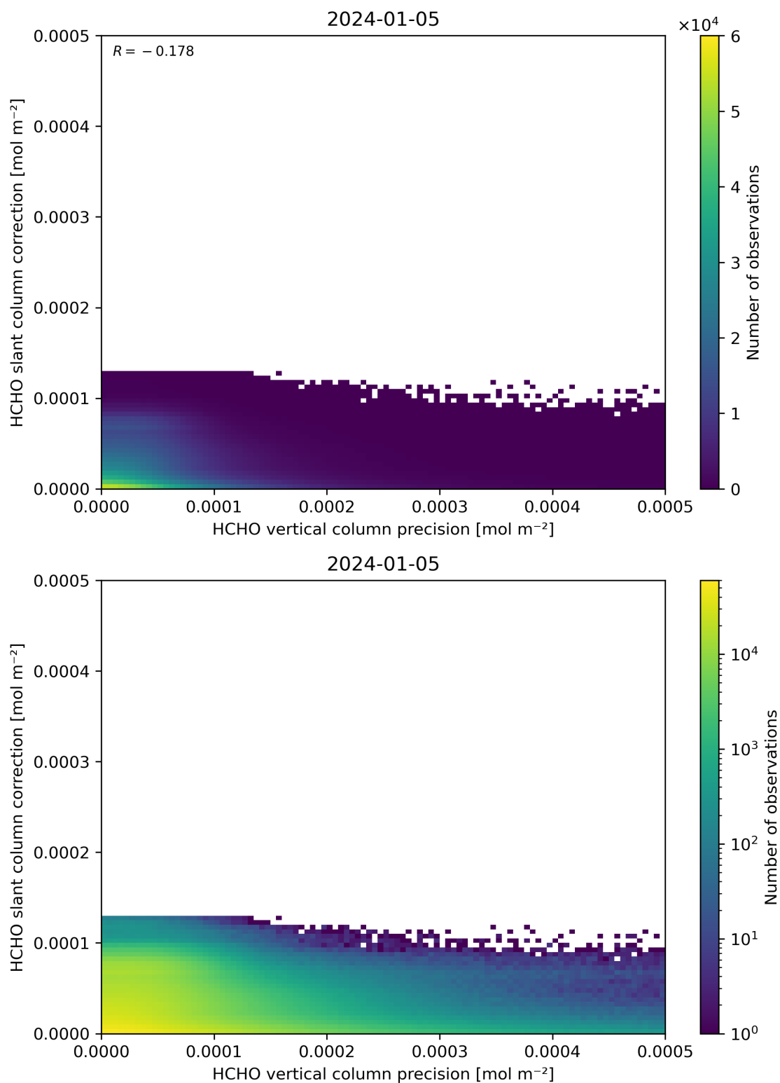
Figure 141: Scatter density plot of “HCHO vertical column precision” against “HCHO slant column correction” for 2024-01-05 to 2024-01-06.
