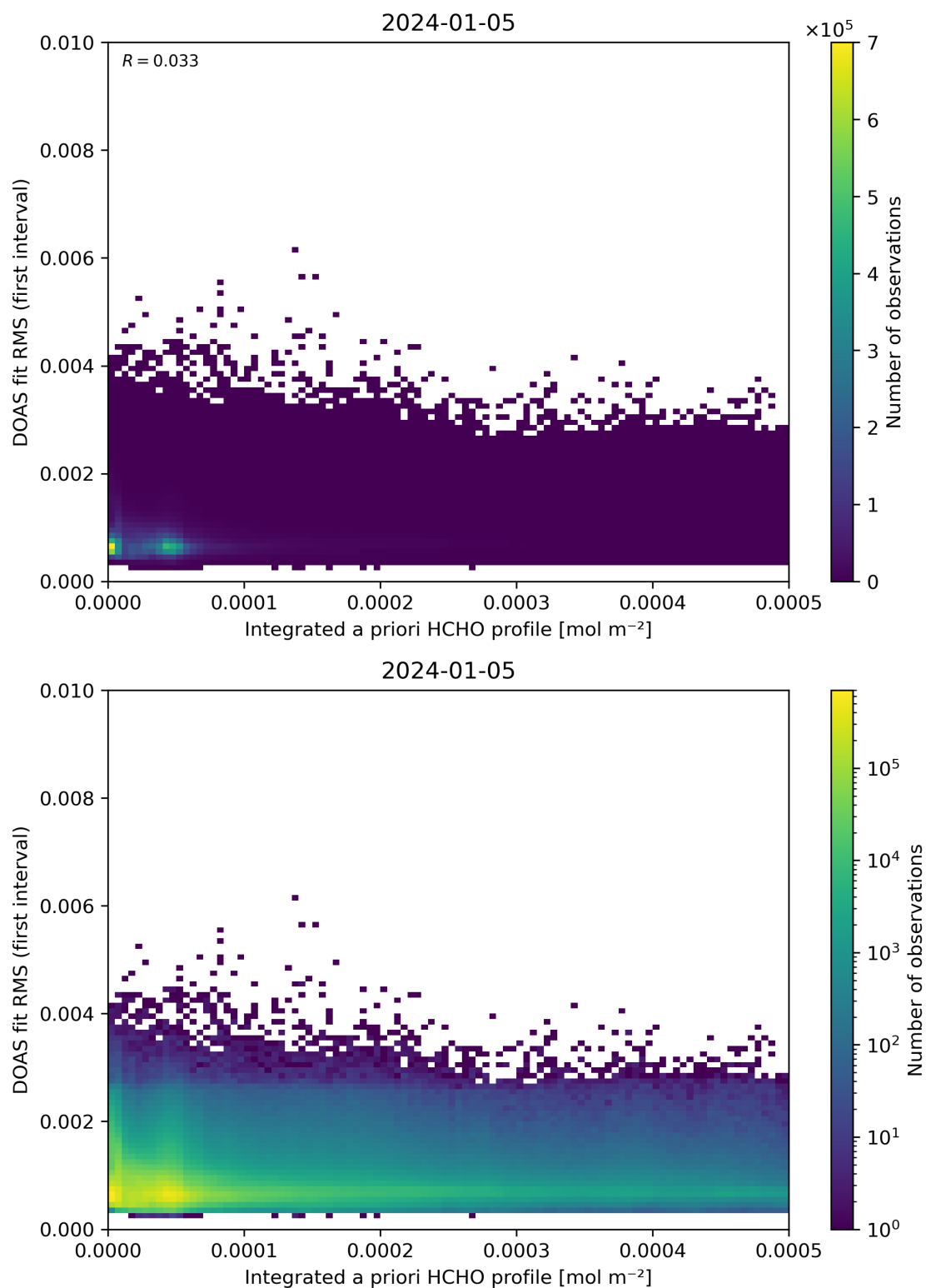
Figure 148: Scatter density plot of “Integrated a priori HCHO profile” against “DOAS fit RMS (first interval)” for 2024-01-05 to 2024-01-06.
