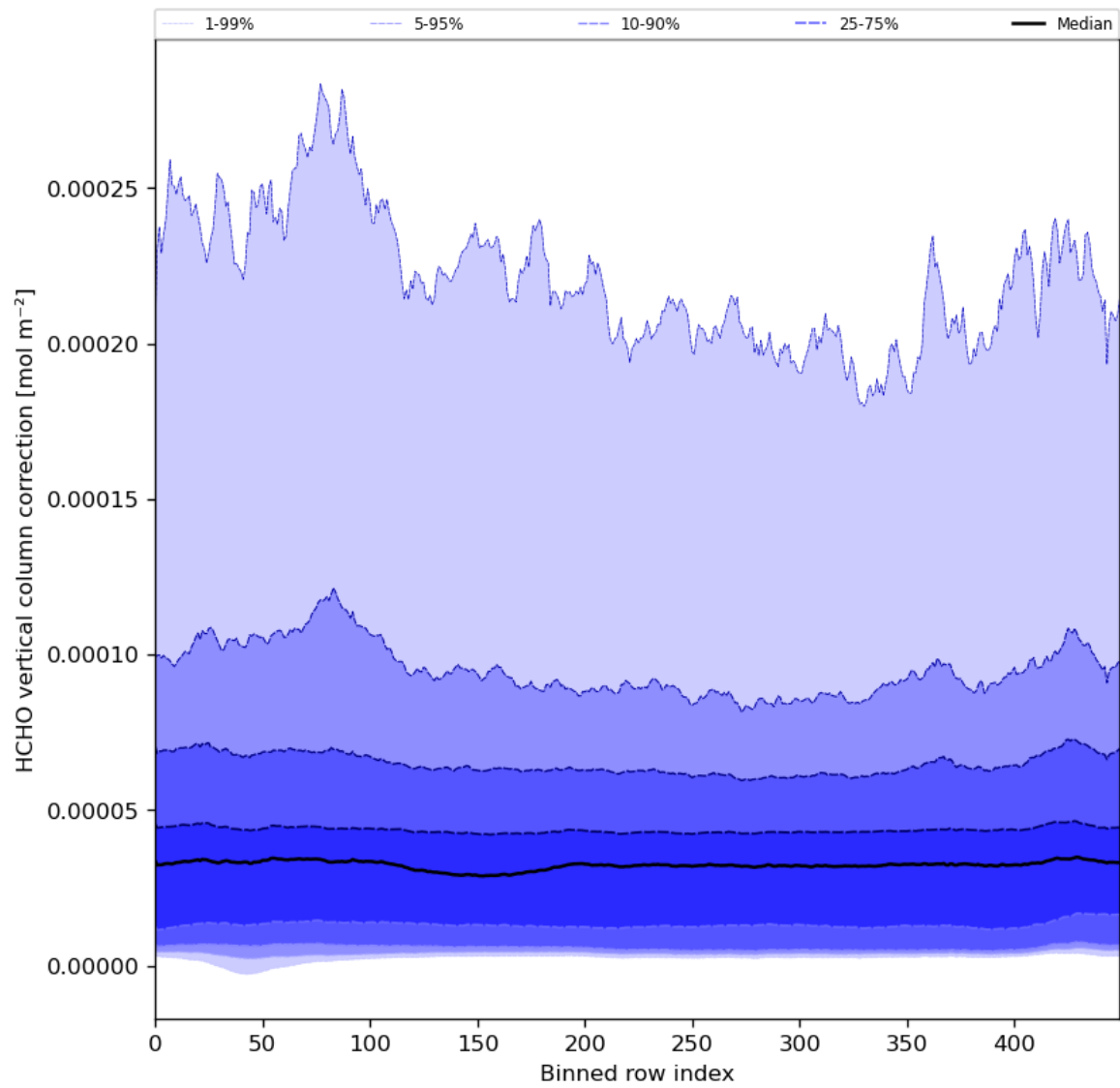
Figure 51: Along track statistics of "HCHO vertical column correction" for 2024-01-05 to 2024-01-06
