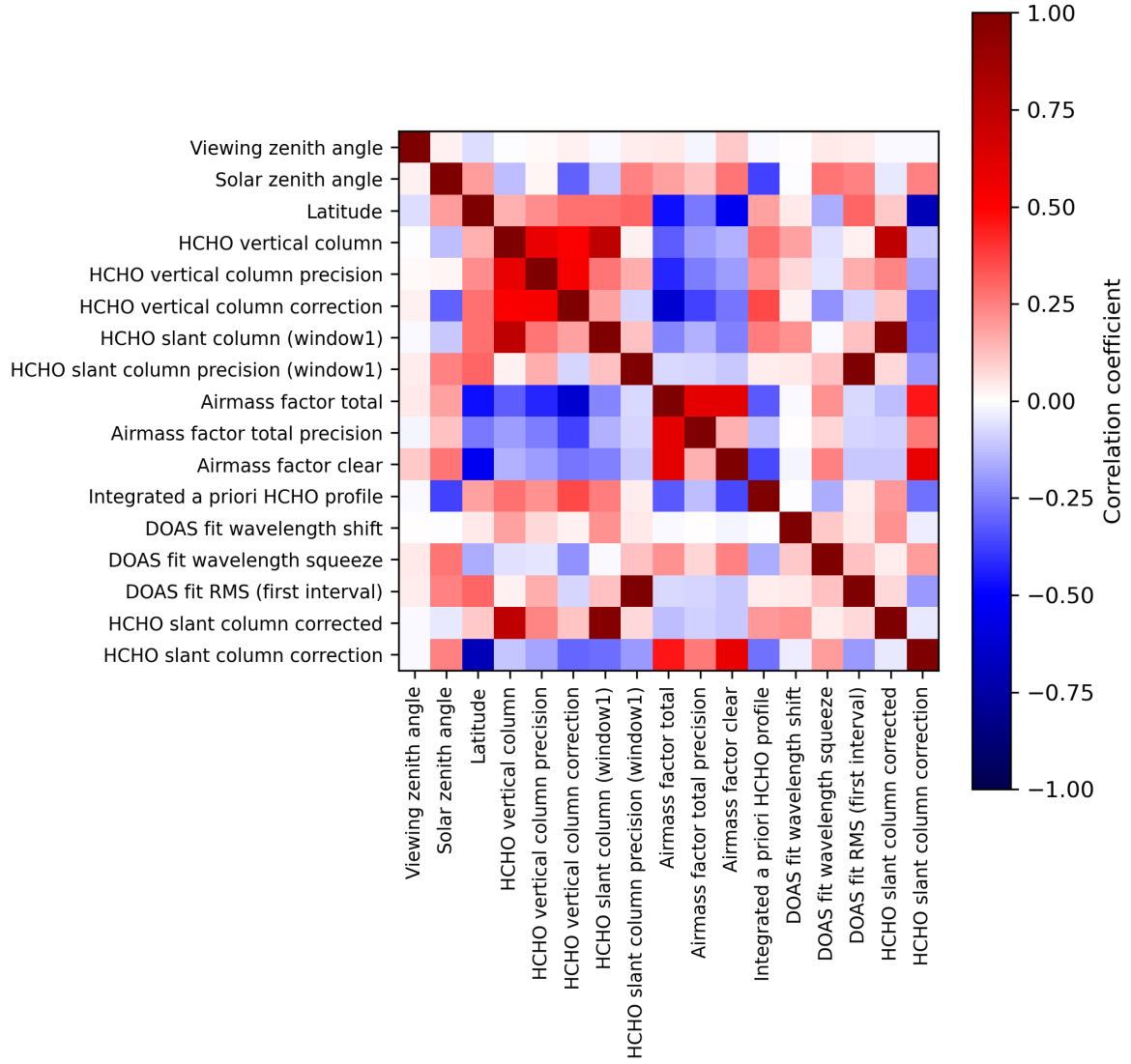
Figure 2: Map of correlation matrix for 2024-01-05 to 2024-01-06.
