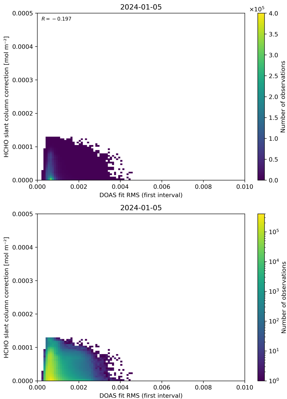
Figure 63: Scatter density plot of “DOAS fit RMS (first interval)” against “HCHO slant column correction” for 2024-01-05 to 2024-01-06.
