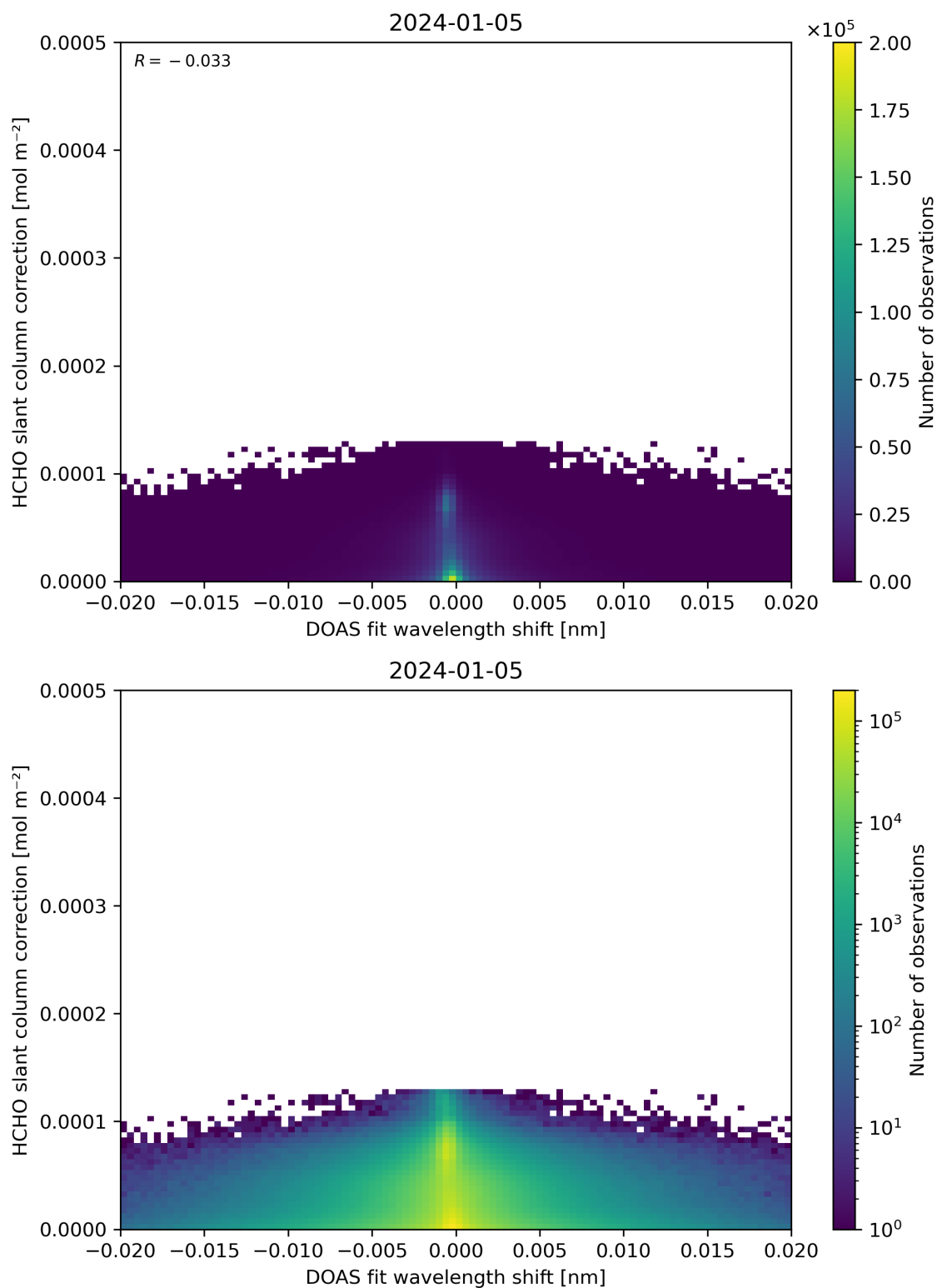
Figure 67: Scatter density plot of “DOAS fit wavelength shift” against “HCHO slant column correction” for 2024-01-05 to 2024-01-06.
