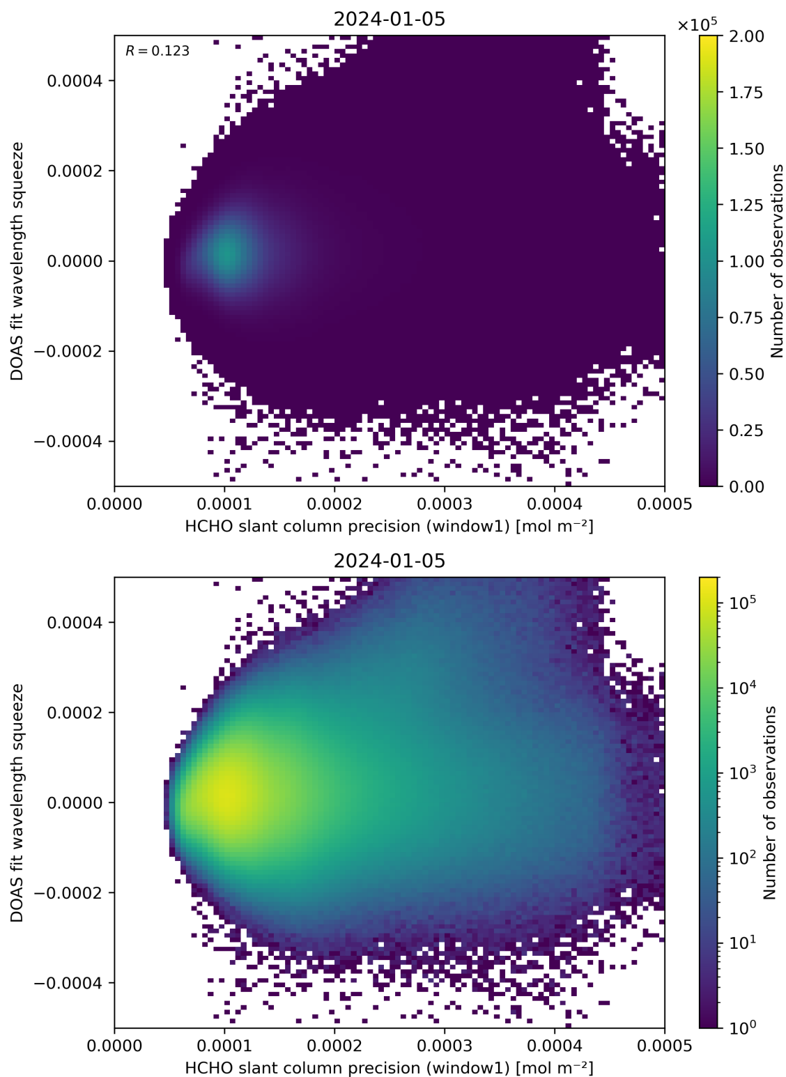
Figure 90: Scatter density plot of “HCHO slant column precision (window1)” against “DOAS fit wavelength squeeze” for 2024-01-05 to 2024-01-06.
