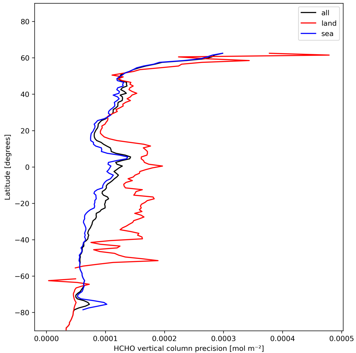
Figure 22: Zonal average of “HCHO vertical column precision” for 2024-01-05 to 2024-01-06.
