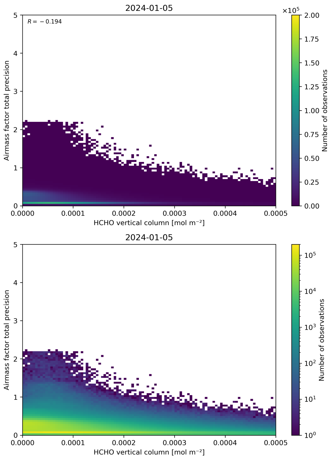
Figure 132: Scatter density plot of “HCHO vertical column” against “Airmass factor total precision” for 2024-01-05 to 2024-01-06.
