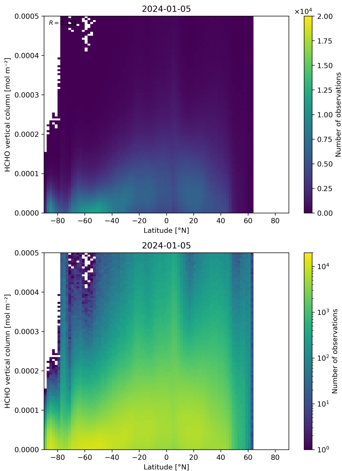
Figure 163: Scatter density plot of “Latitude” against “HCHO vertical column” for 2024-01-05 to 2024-01-06.
