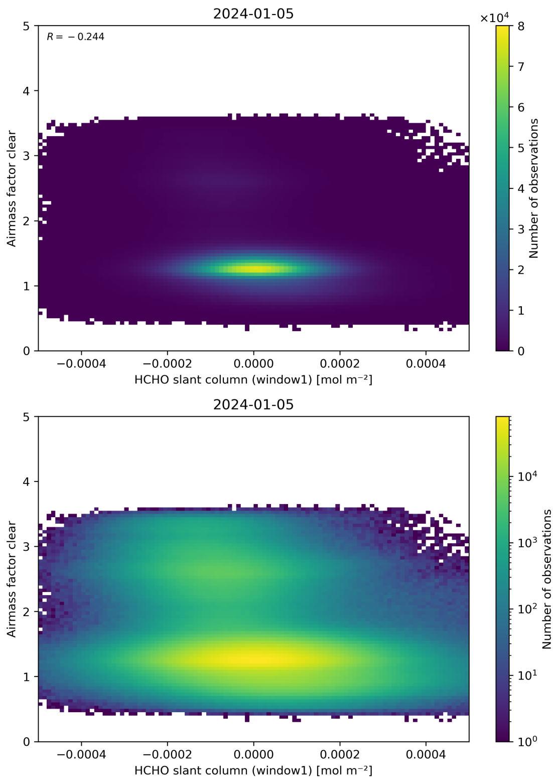
Figure 81: Scatter density plot of “HCHO slant column (window1)” against “Airmass factor clear” for 2024-01-05 to 2024-01-06.
