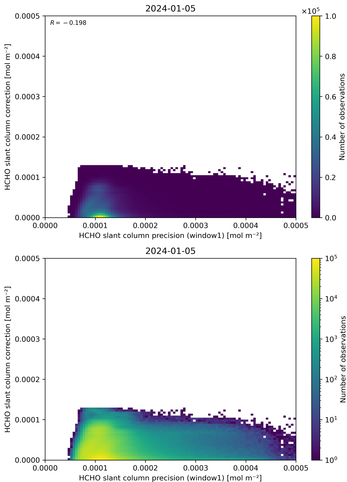
Figure 93: Scatter density plot of “HCHO slant column precision (window1)” against “HCHO slant column correction” for 2024-01-05 to 2024-01-06.
