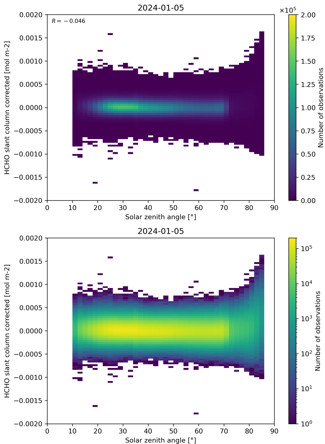
Figure 171: Scatter density plot of “Solar zenith angle” against “HCHO slant column corrected” for 2024-01-05 to 2024-01-06.
