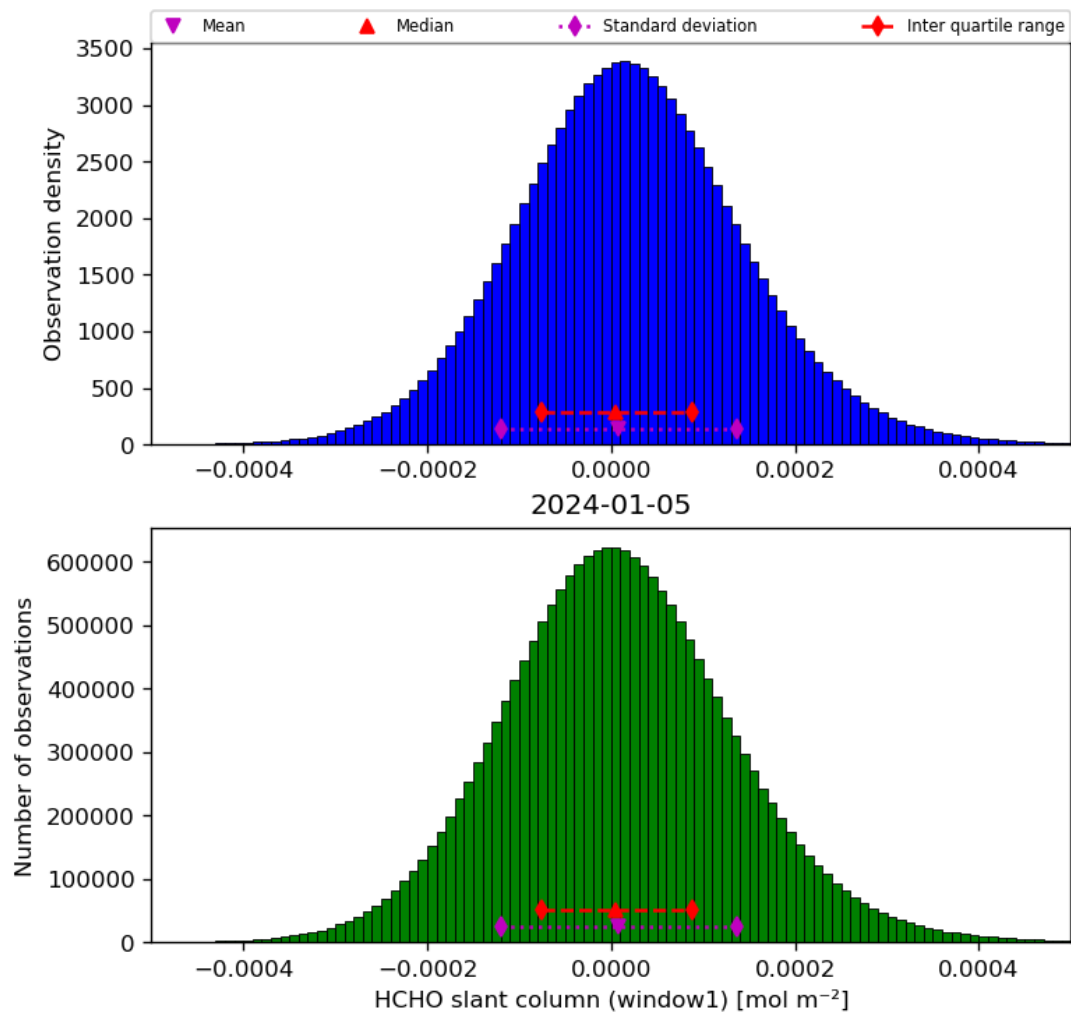
Figure 38: Histogram of “HCHO slant column (window1)” for 2024-01-05 to 2024-01-06
