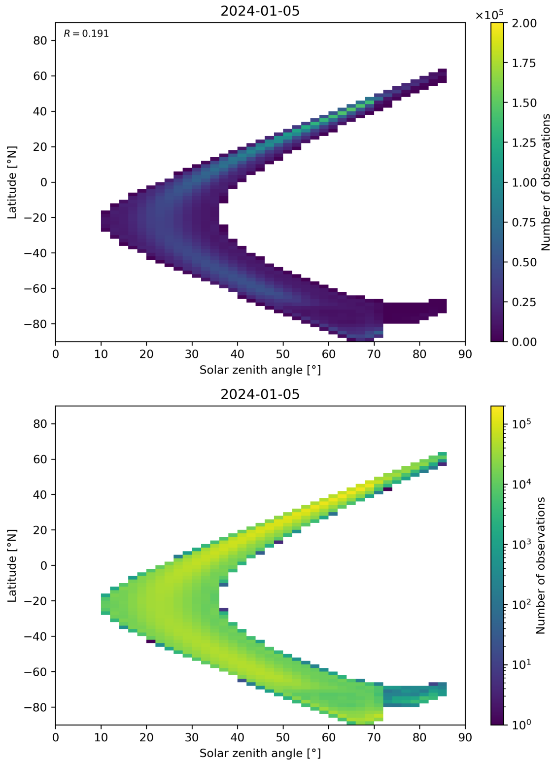
Figure 181: Scatter density plot of “Solar zenith angle” against “Latitude” for 2024-01-05 to 2024-01-06.
