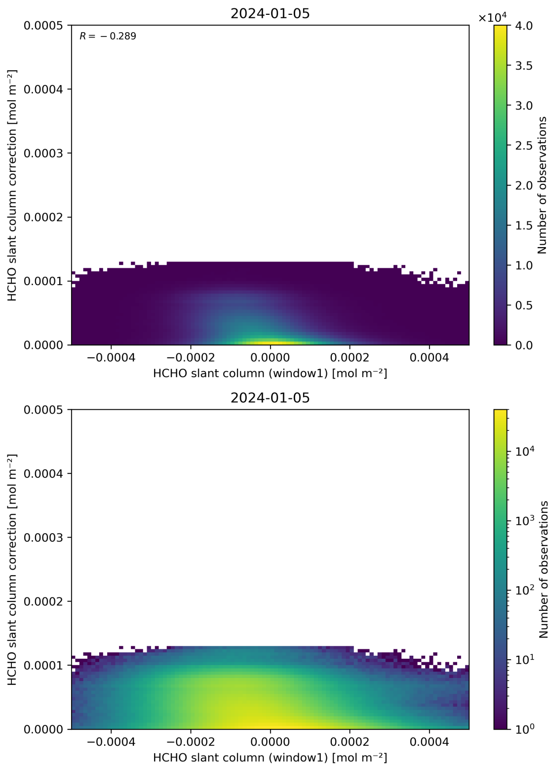
Figure 83: Scatter density plot of “HCHO slant column (window1)” against “HCHO slant column correction” for 2024-01-05 to 2024-01-06.
