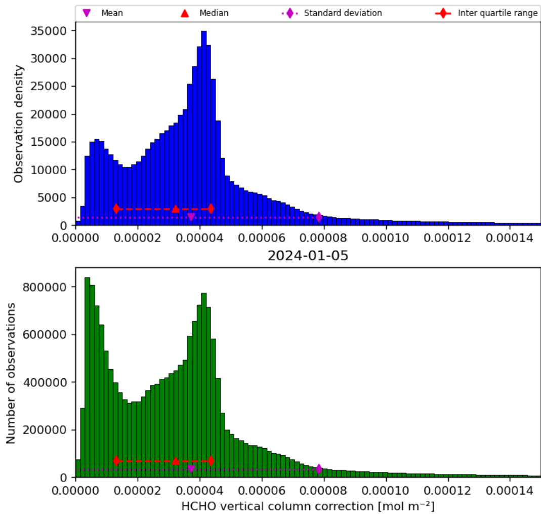
Figure 37: Histogram of “HCHO vertical column correction” for 2024-01-05 to 2024-01-06
