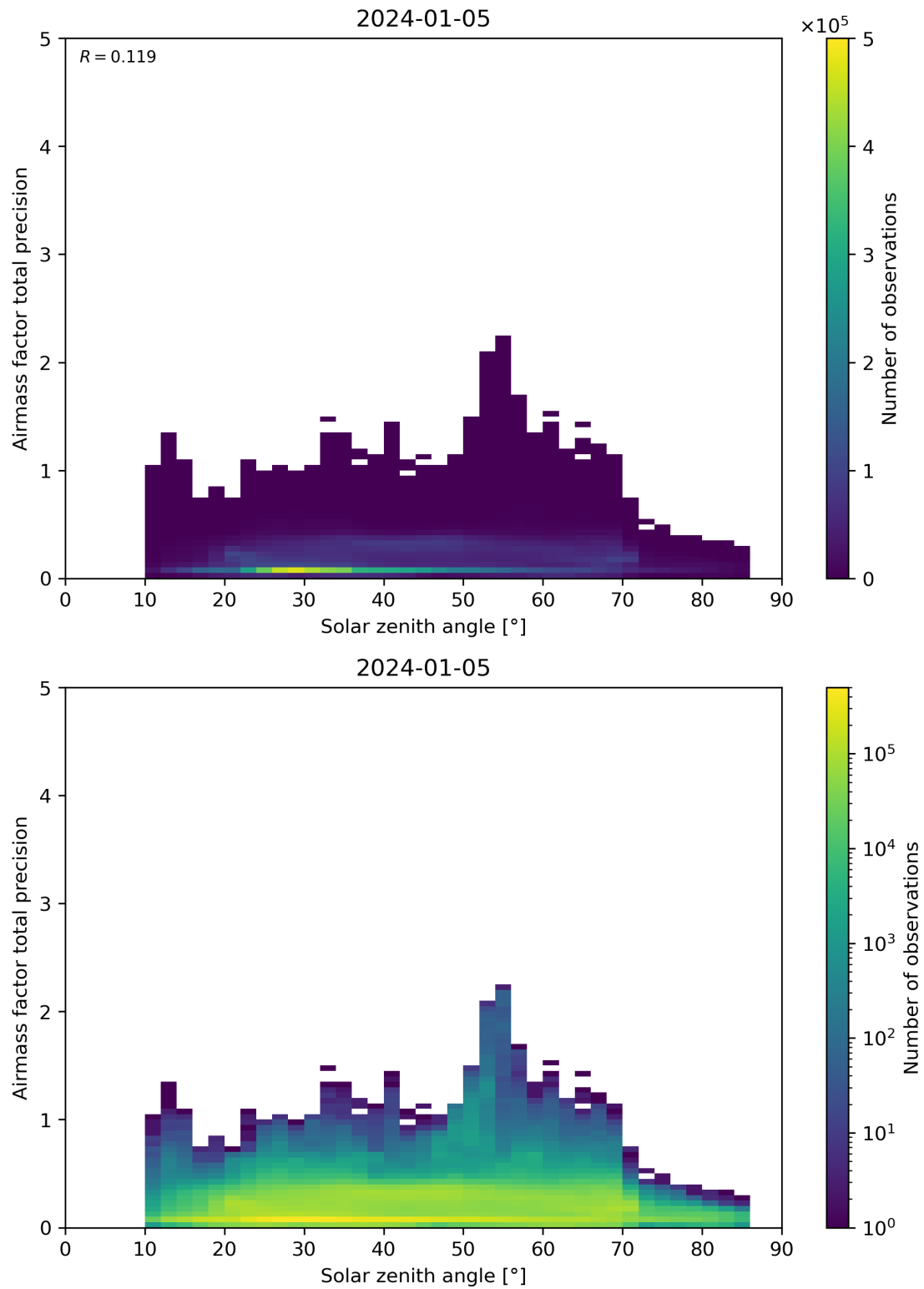
Figure 176: Scatter density plot of “Solar zenith angle” against “Airmass factor total precision” for 2024-01-05 to 2024-01-06.
