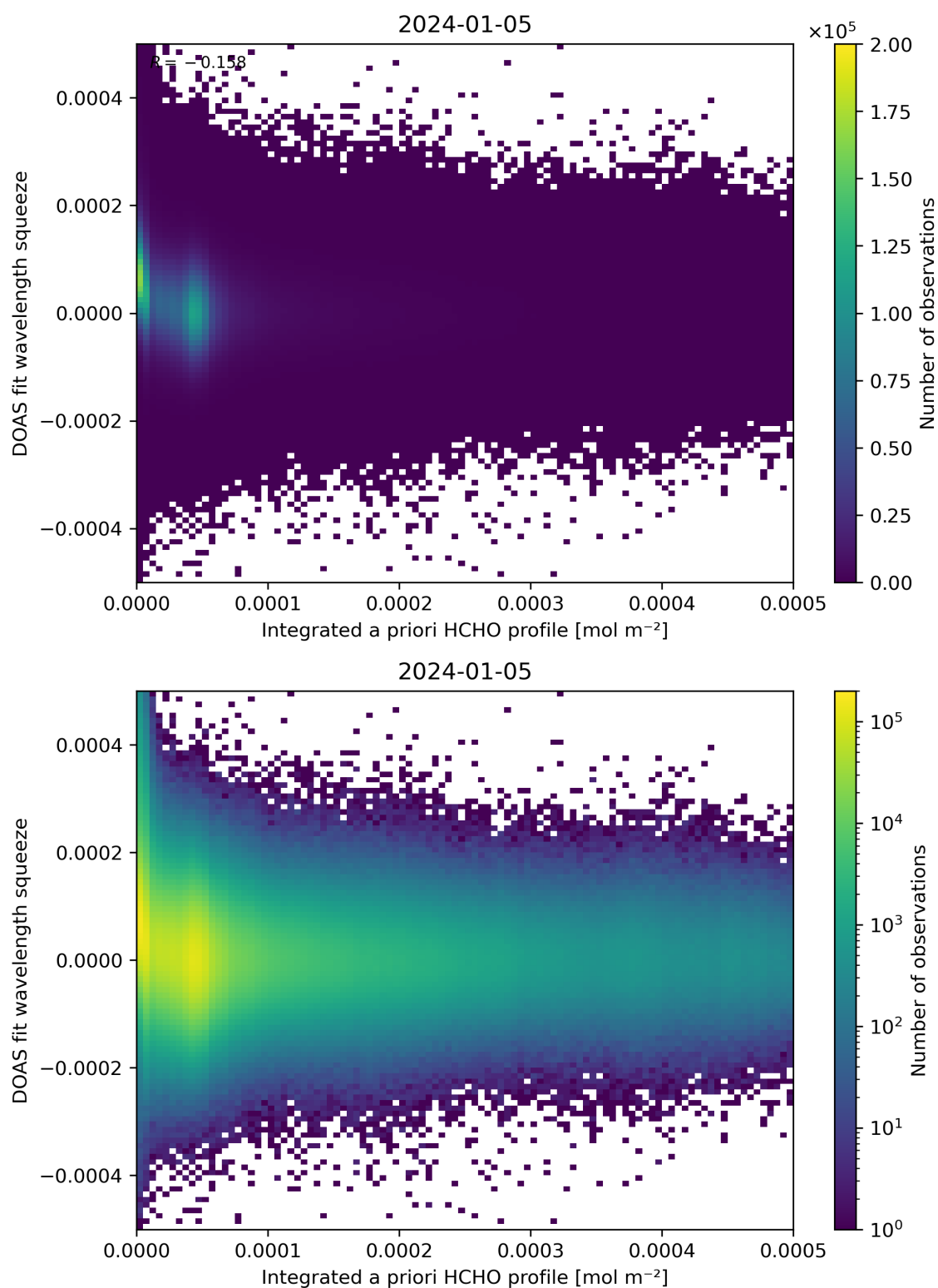
Figure 150: Scatter density plot of “Integrated a priori HCHO profile” against “DOAS fit wavelength squeeze” for 2024-01-05 to 2024-01-06.
