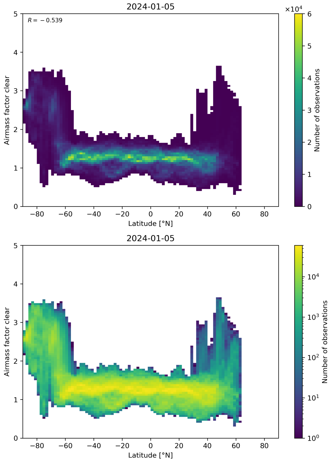
Figure 156: Scatter density plot of “Latitude” against “Airmass factor clear” for 2024-01-05 to 2024-01-06.
