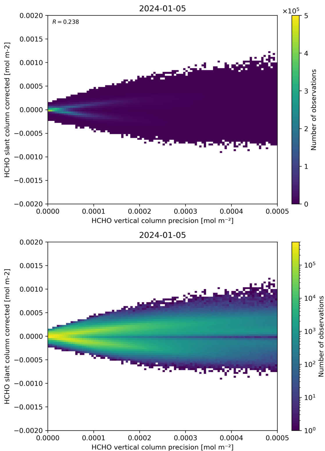
Figure 140: Scatter density plot of “HCHO vertical column precision” against “HCHO slant column corrected” for 2024-01-05 to 2024-01-06.
