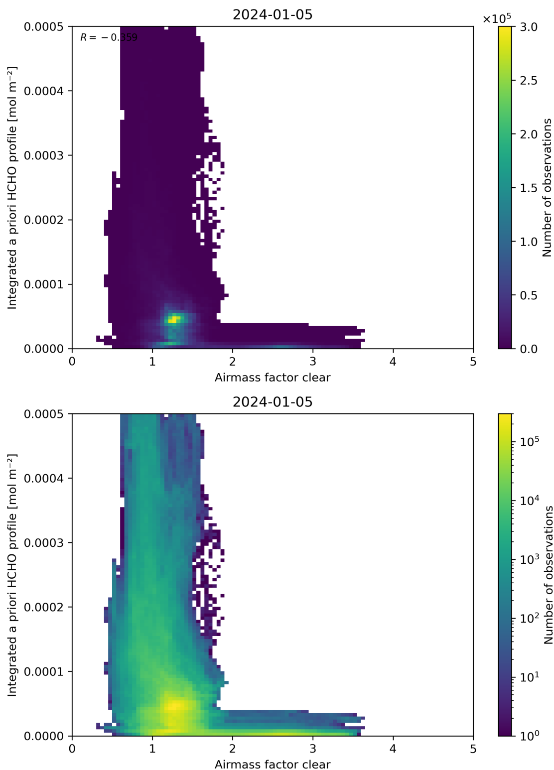
Figure 76: Scatter density plot of “Airmass factor clear” against “Integrated a priori HCHO profile” for 2024-01-05 to 2024-01-06.
