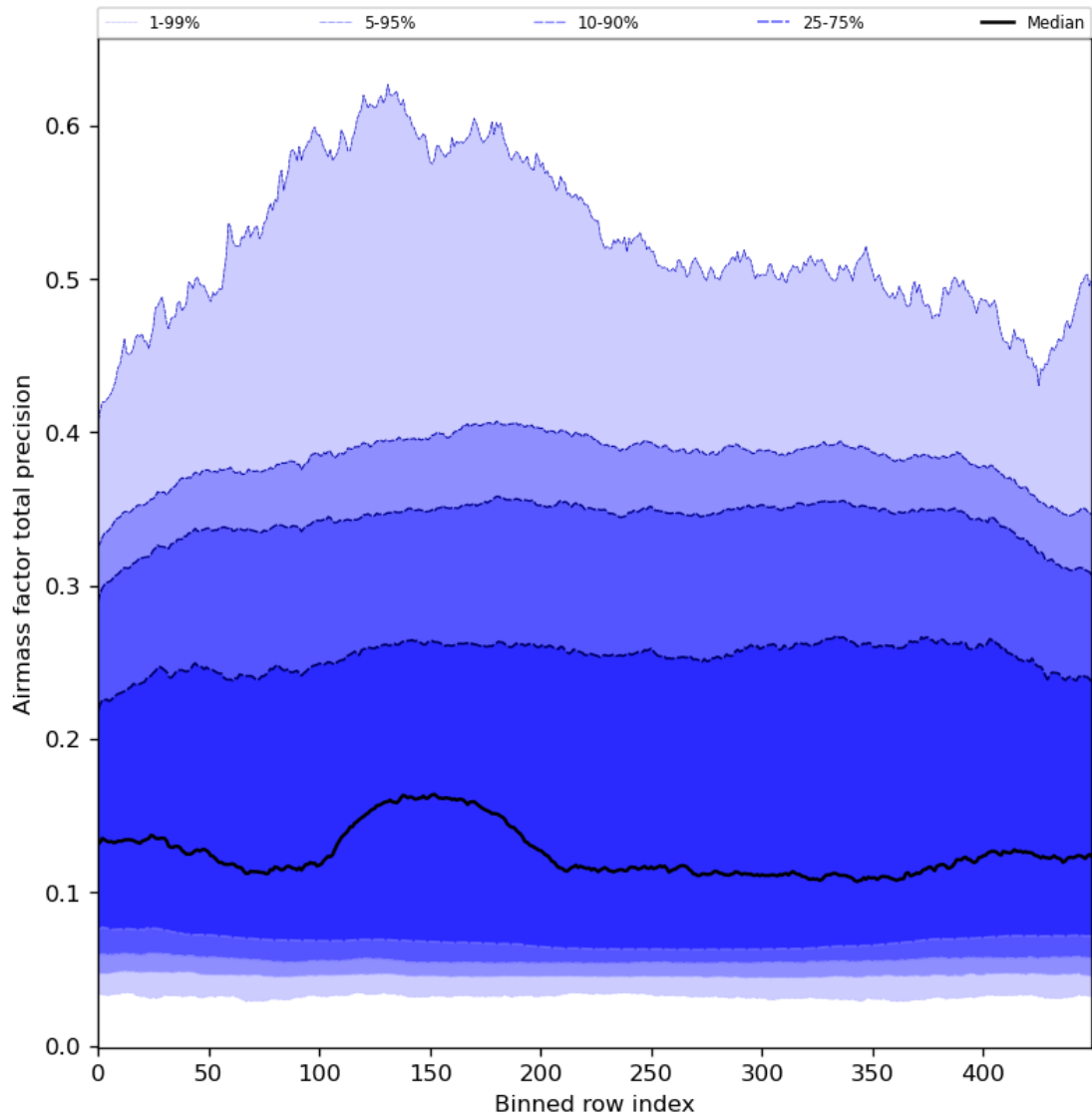
Figure 55: Along track statistics of “Airmass factor total precision” for 2024-01-05 to 2024-01-06
