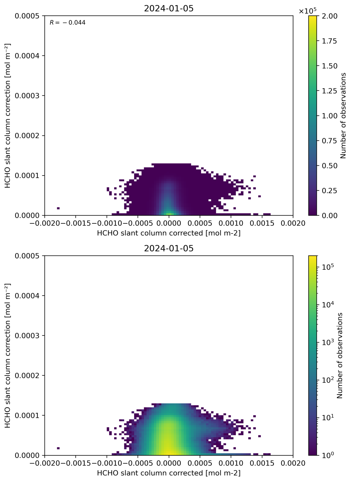
Figure 77: Scatter density plot of “HCHO slant column corrected” against “HCHO slant column correction” for 2024-01-05 to 2024-01-06.
