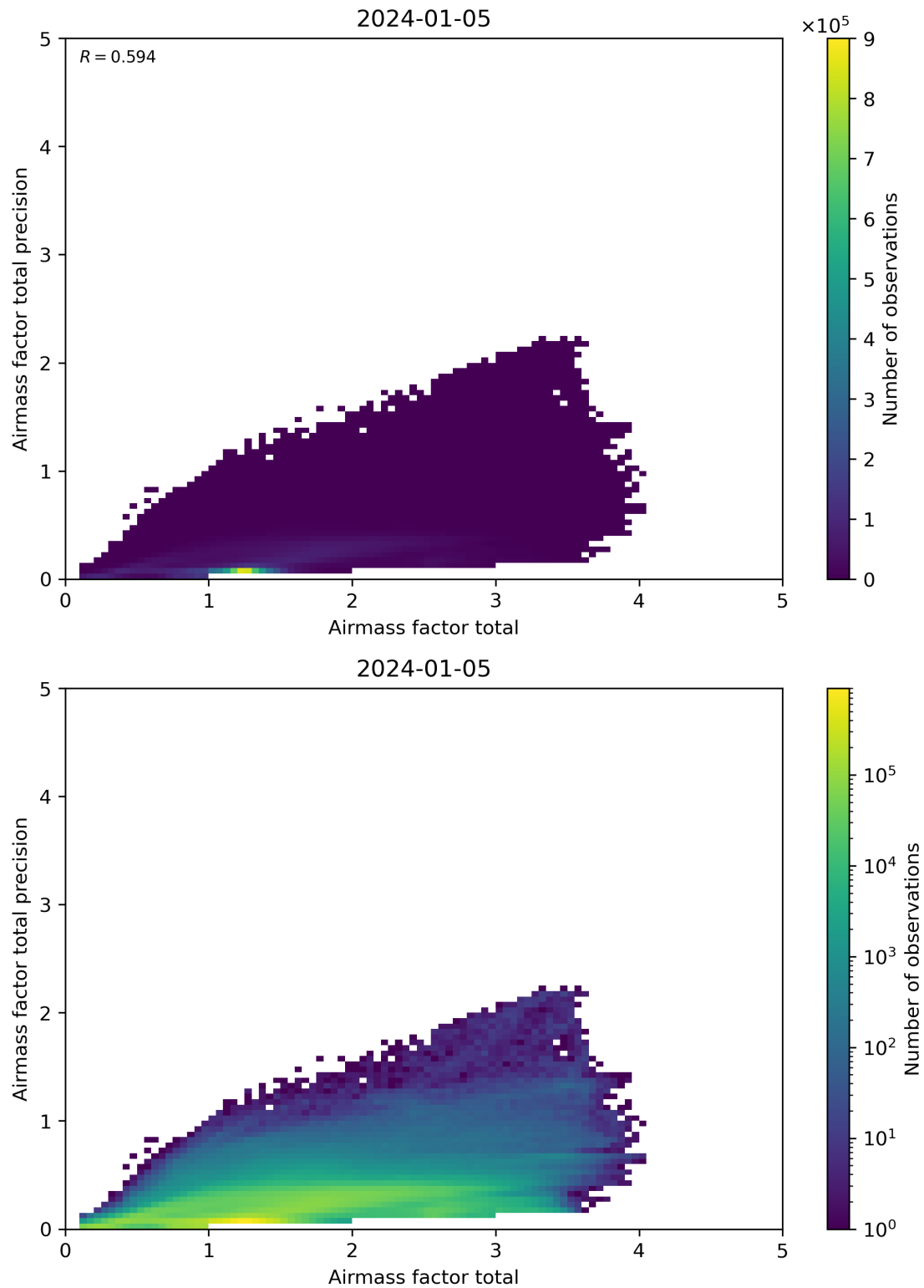
Figure 103: Scatter density plot of “Airmass factor total” against “Airmass factor total precision” for 2024-01-05 to 2024-01-06.
