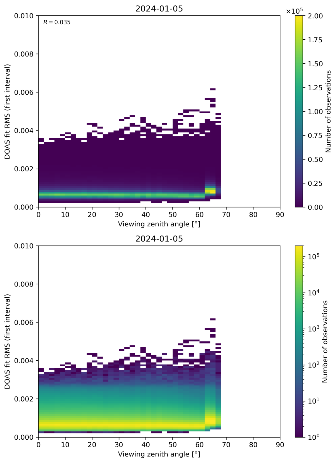
Figure 182: Scatter density plot of “Viewing zenith angle” against “DOAS fit RMS (first interval)” for 2024-01-05 to 2024-01-06.
