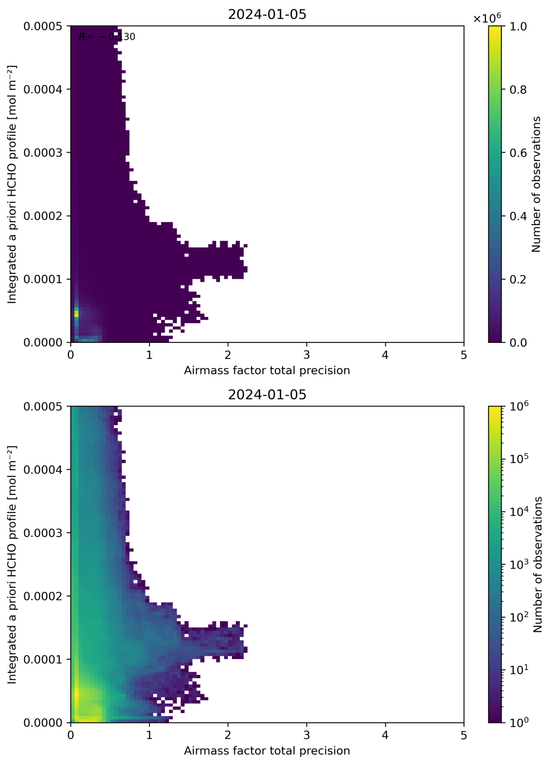
Figure 111: Scatter density plot of “Airmass factor total precision” against “Integrated a priori HCHO profile” for 2024-01-05 to 2024-01-06.
