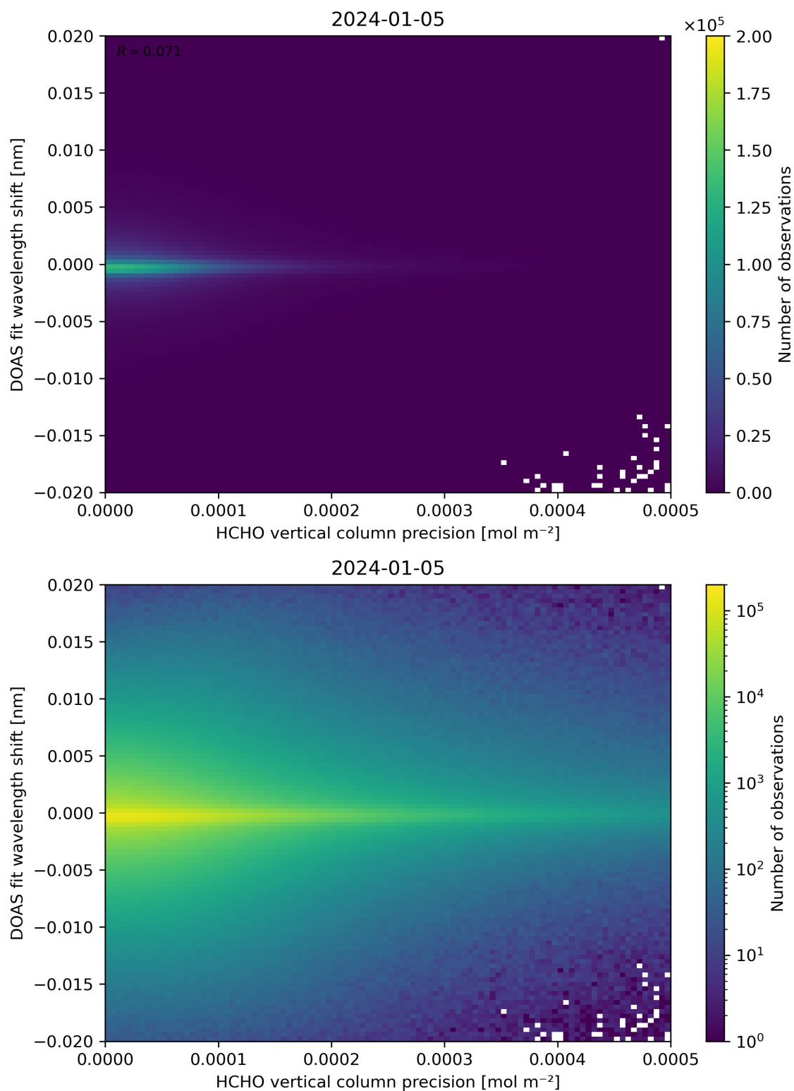
Figure 137: Scatter density plot of “HCHO vertical column precision” against “DOAS fit wavelength shift” for 2024-01-05 to 2024-01-06.
