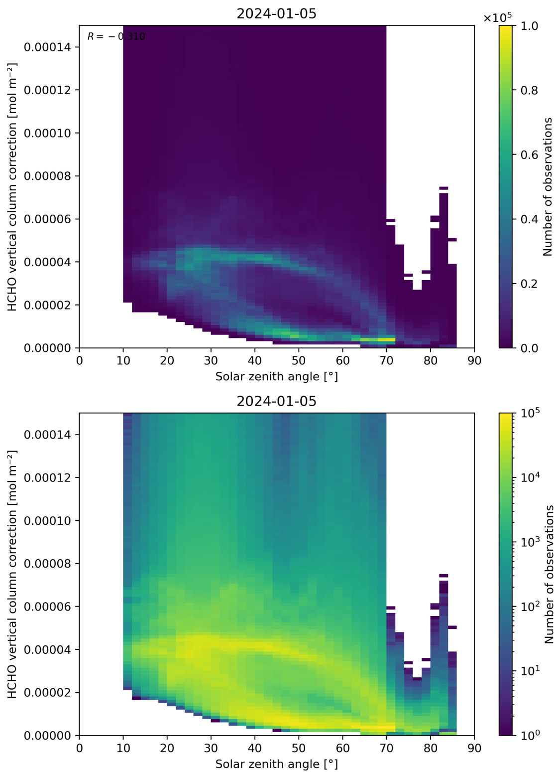
Figure 178: Scatter density plot of “Solar zenith angle” against “HCHO vertical column correction” for 2024-01-05 to 2024-01-06.
