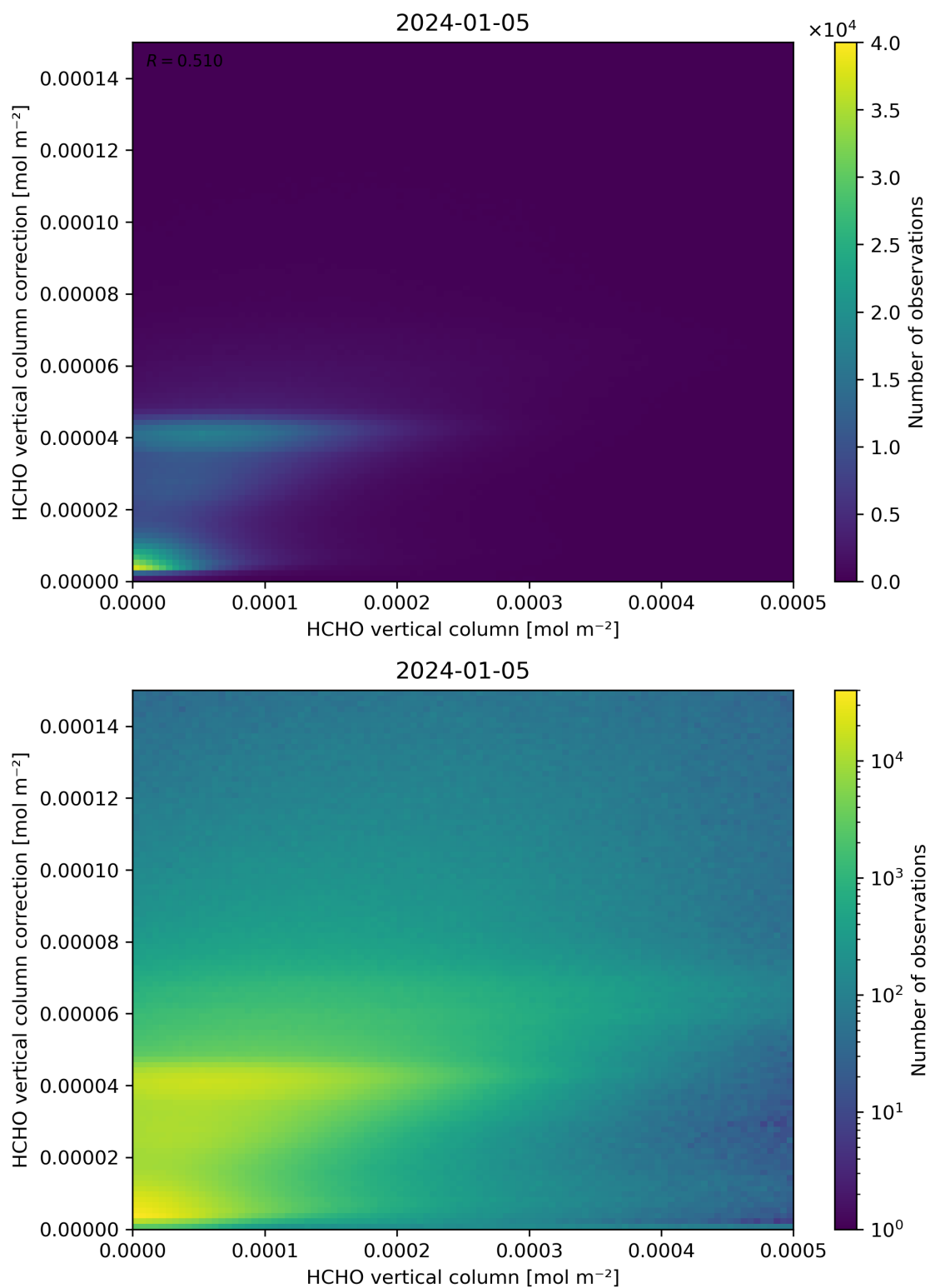
Figure 133: Scatter density plot of “HCHO vertical column” against “HCHO vertical column correction” for 2024-01-05 to 2024-01-06.
