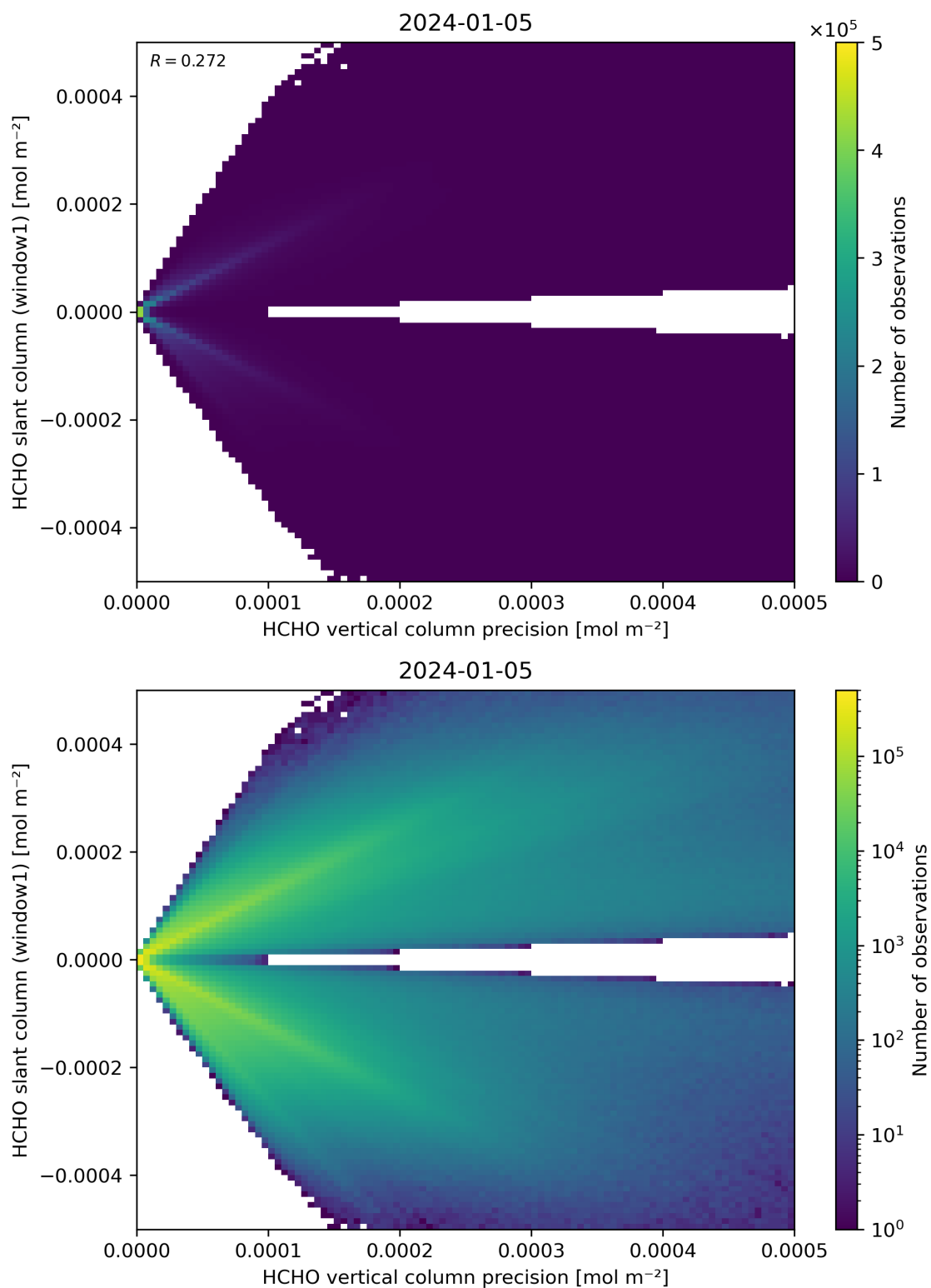
Figure 142: Scatter density plot of “HCHO vertical column precision” against “HCHO slant column (window1)” for 2024-01-05 to 2024-01-06.
