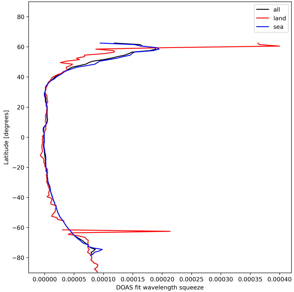
Figure 31: Zonal average of “DOAS fit wavelength squeeze” for 2024-01-05 to 2024-01-06.
