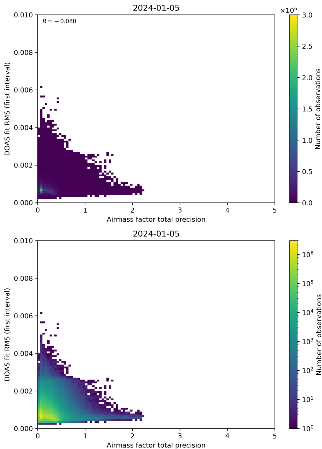
Figure 105: Scatter density plot of “Airmass factor total precision” against “DOAS fit RMS (first interval)” for 2024-01-05 to 2024-01-06.
