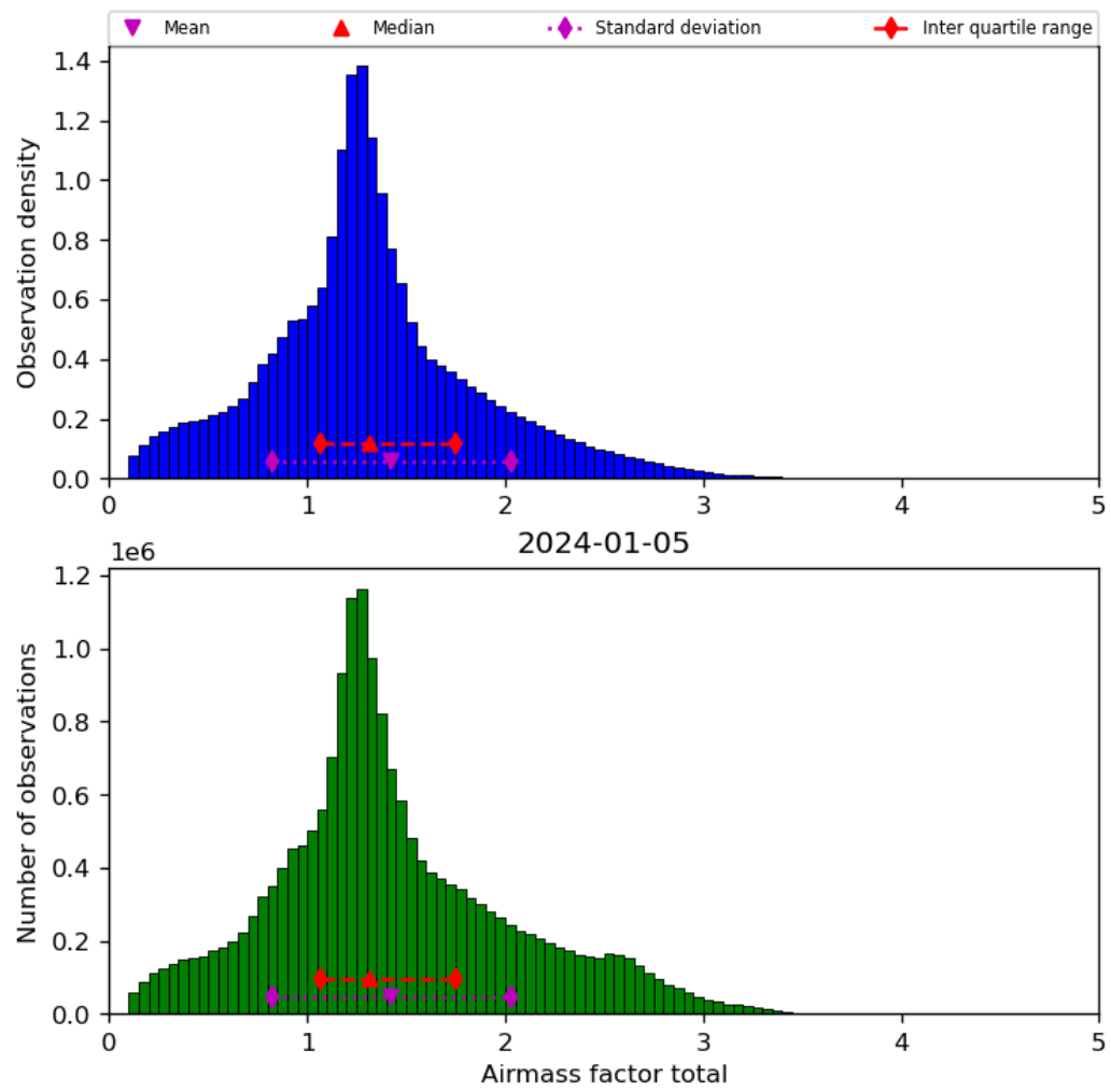
Figure 40: Histogram of “Airmass factor total” for 2024-01-05 to 2024-01-06
