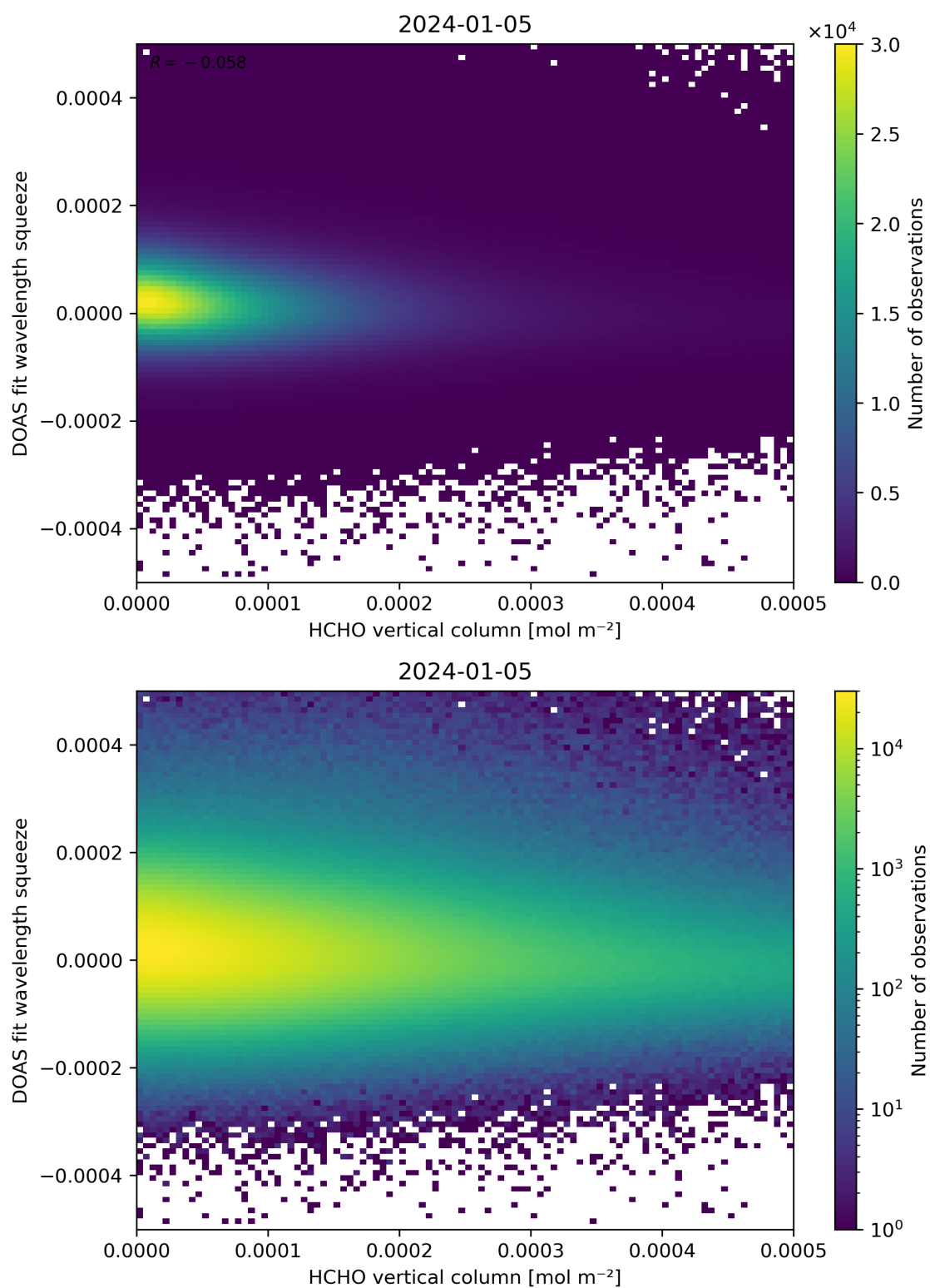
Figure 125: Scatter density plot of “HCHO vertical column” against “DOAS fit wavelength squeeze” for 2024-01-05 to 2024-01-06.
