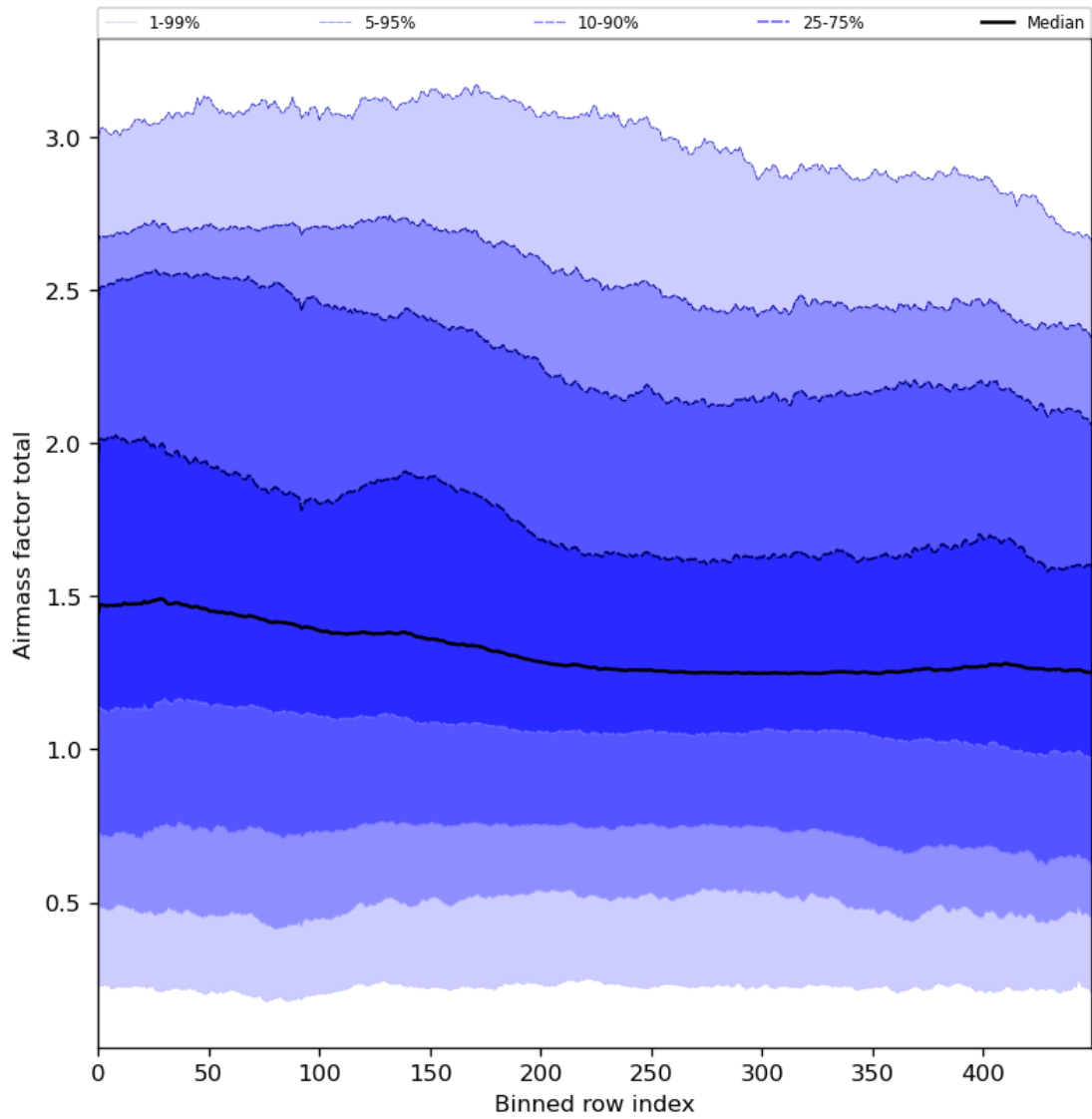
Figure 54: Along track statistics of “Airmass factor total” for 2024-01-05 to 2024-01-06
