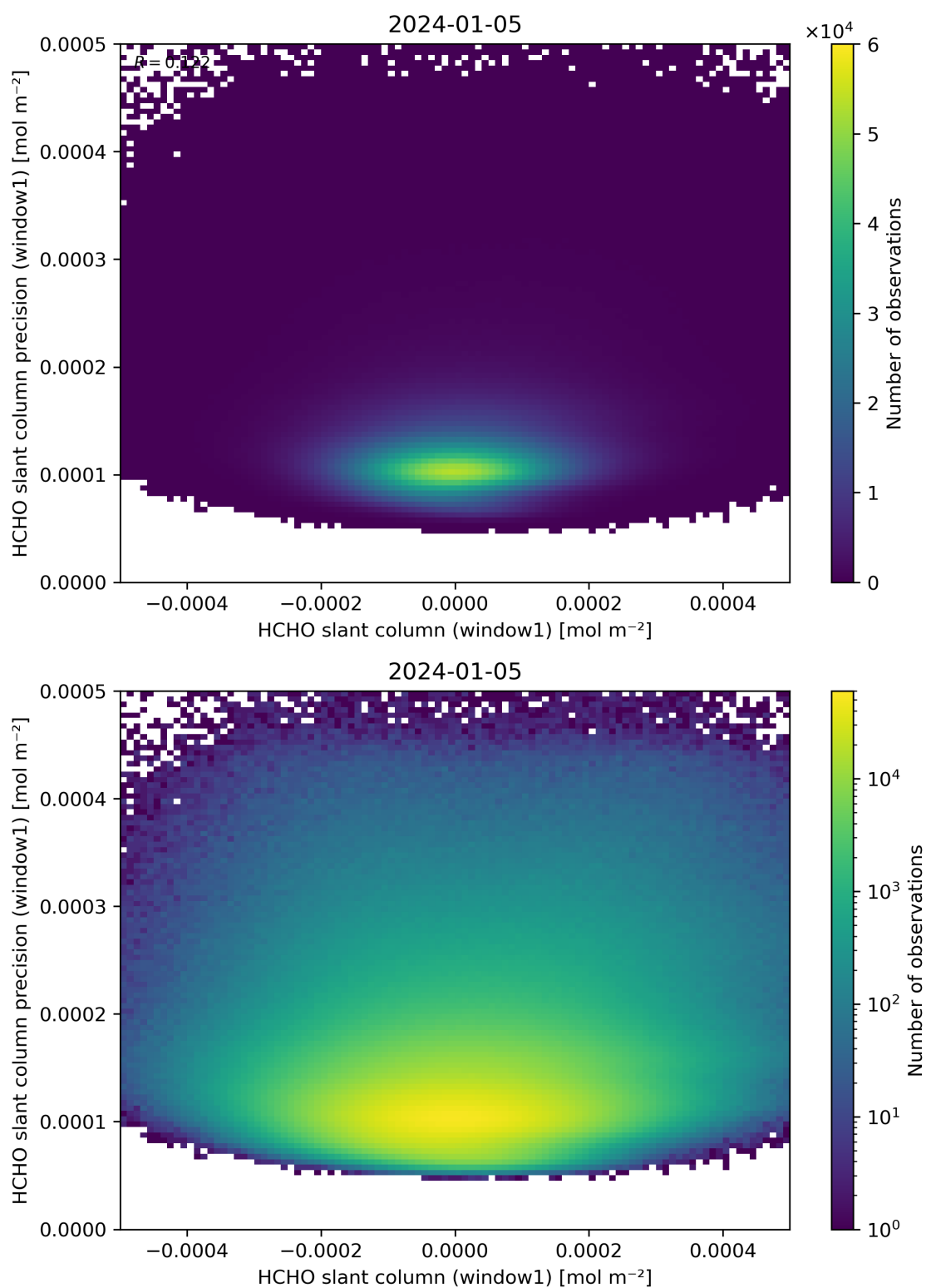
Figure 84: Scatter density plot of “HCHO slant column (window1)” against “HCHO slant column precision (window1)” for 2024-01-05 to 2024-01-06.
