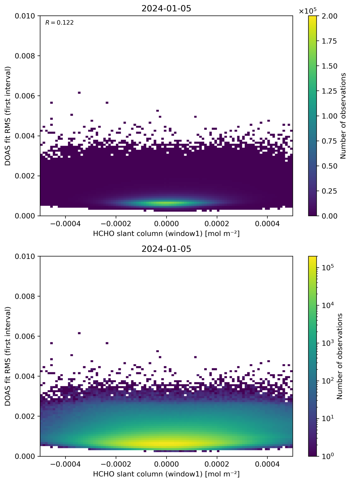
Figure 78: Scatter density plot of “HCHO slant column (window1)” against “DOAS fit RMS (first interval)” for 2024-01-05 to 2024-01-06.
