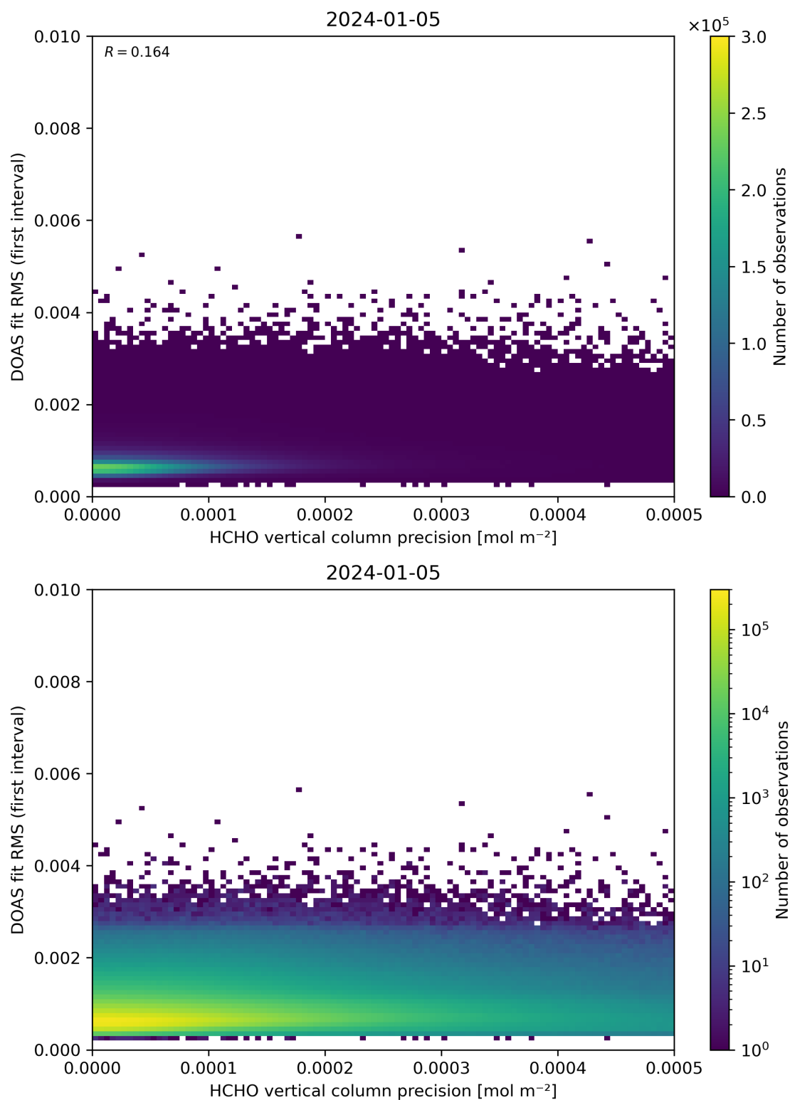
Figure 136: Scatter density plot of “HCHO vertical column precision” against “DOAS fit RMS (first interval)” for 2024-01-05 to 2024-01-06.
