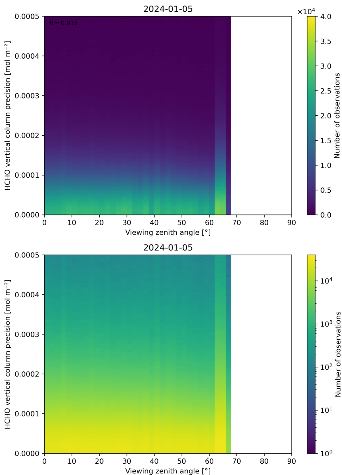
Figure 194: Scatter density plot of “Viewing zenith angle” against “HCHO vertical column precision” for 2024-01-05 to 2024-01-06.
