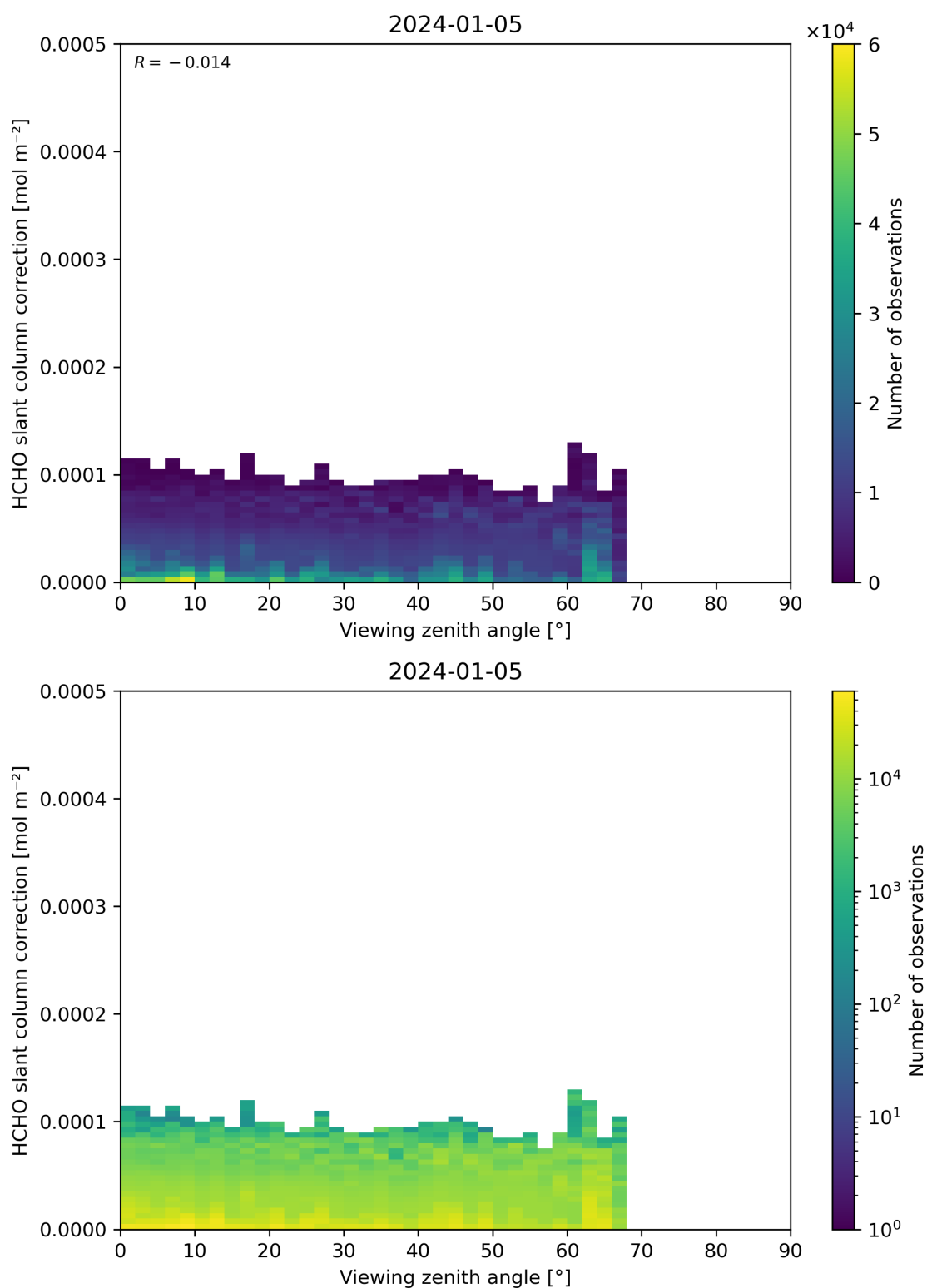
Figure 187: Scatter density plot of “Viewing zenith angle” against “HCHO slant column correction” for 2024-01-05 to 2024-01-06.
