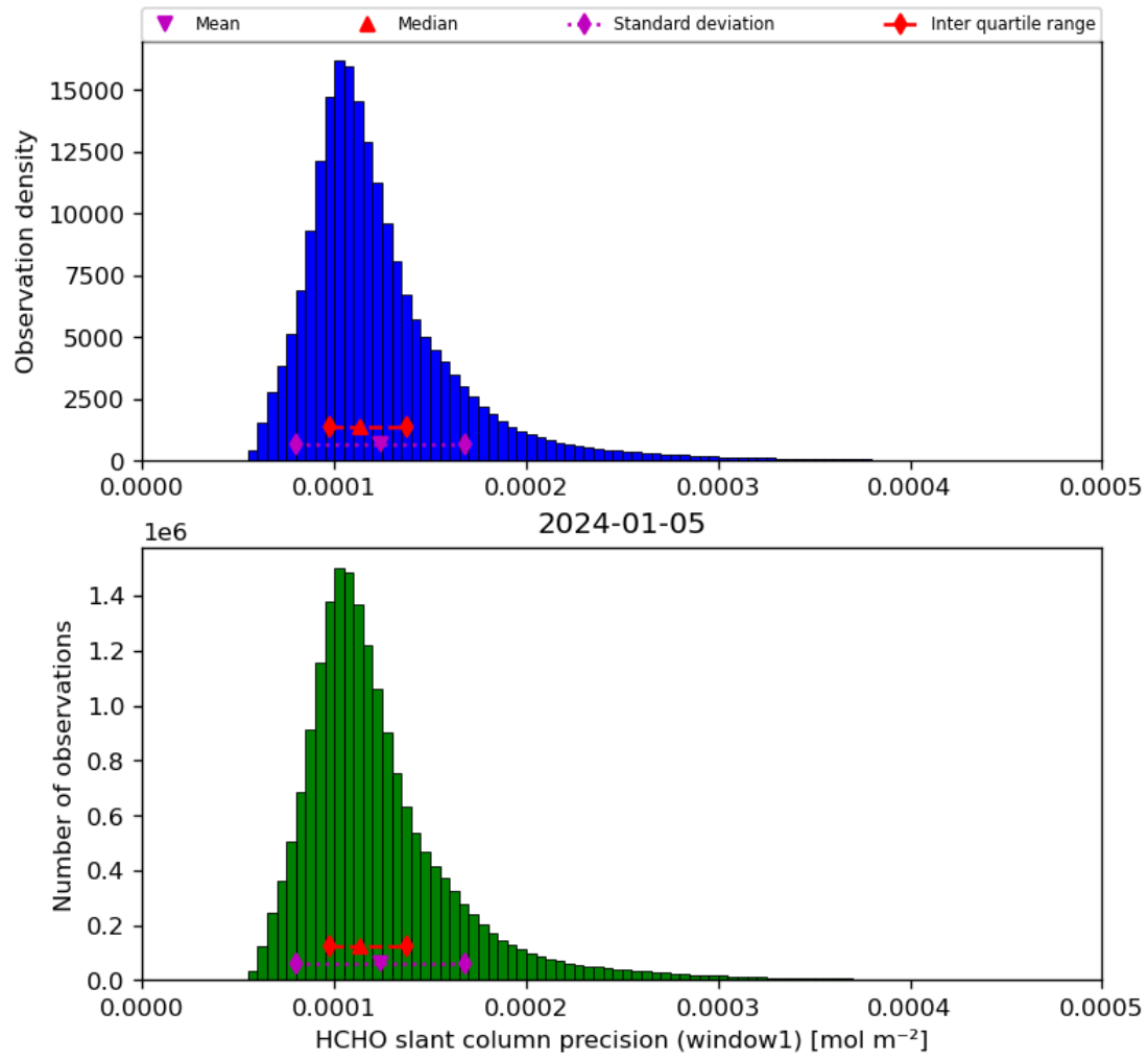
Figure 39: Histogram of “HCHO slant column precision (window1)” for 2024-01-05 to 2024-01-06
