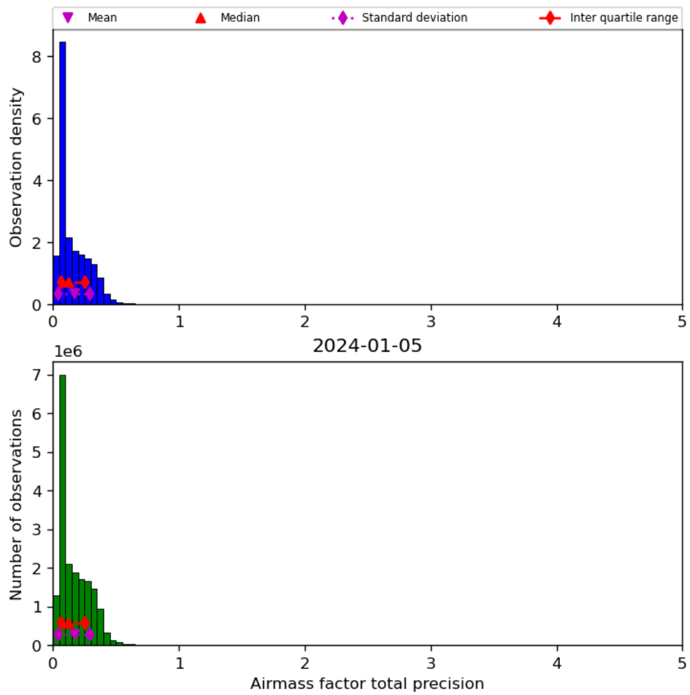
Figure 41: Histogram of “Airmass factor total precision” for 2024-01-05 to 2024-01-06
