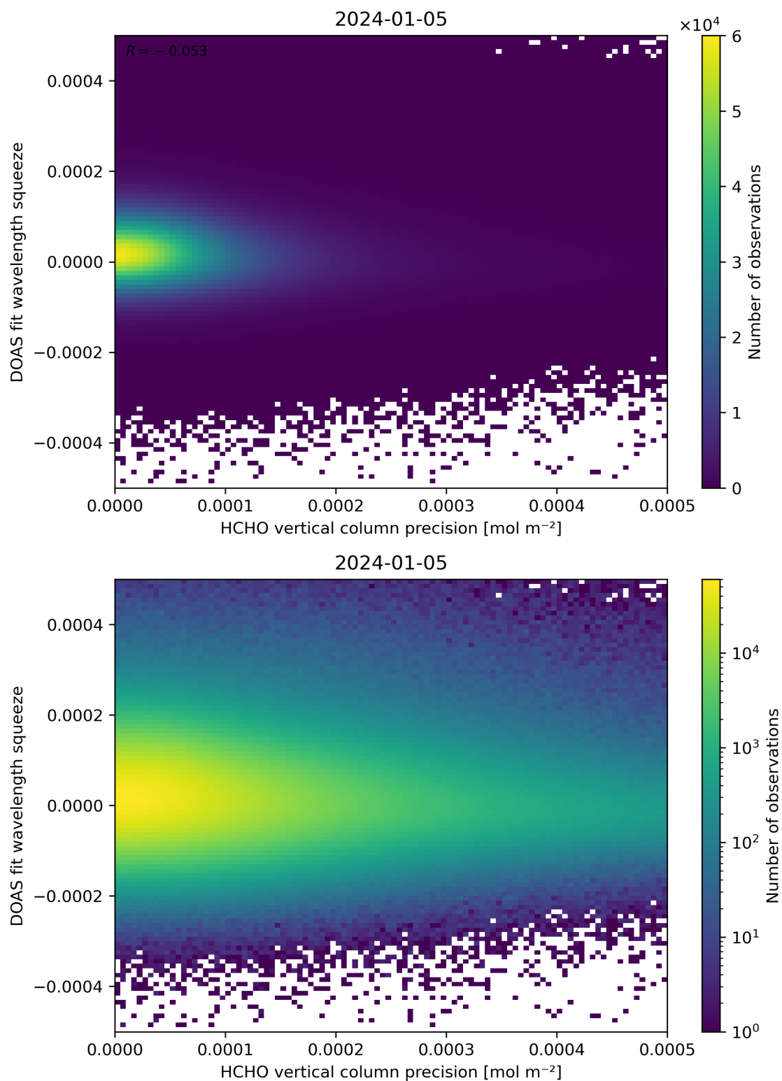
Figure 138: Scatter density plot of “HCHO vertical column precision” against “DOAS fit wavelength squeeze” for 2024-01-05 to 2024-01-06.
