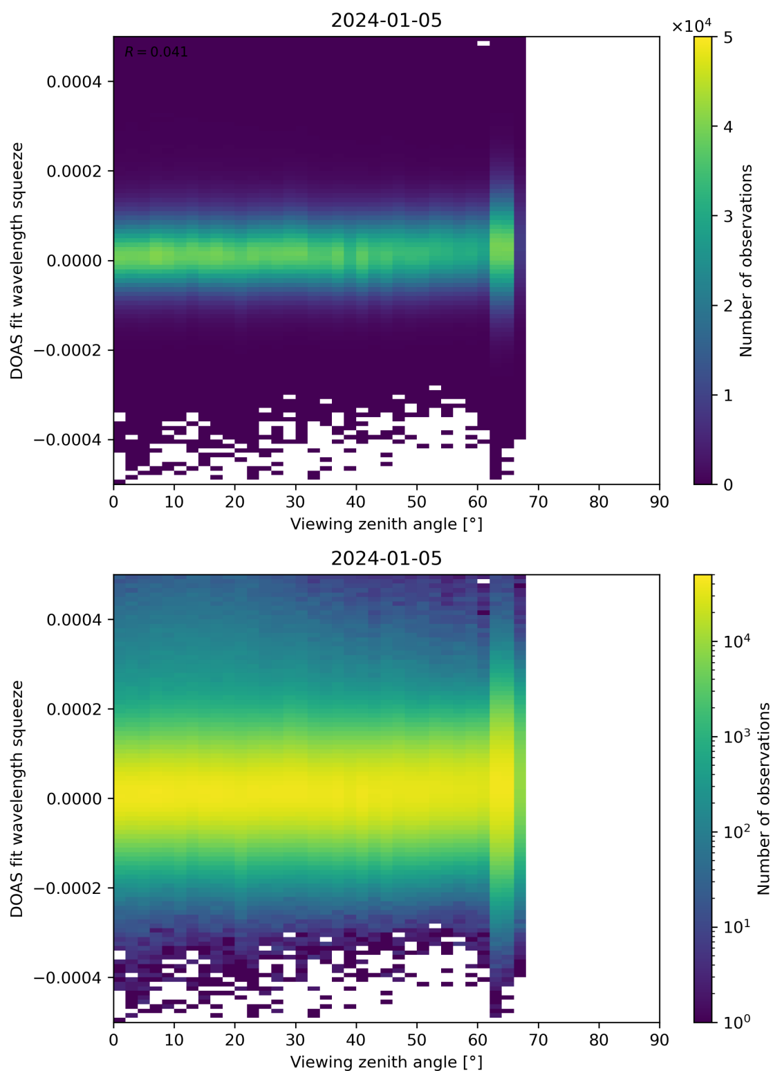
Figure 184: Scatter density plot of “Viewing zenith angle” against “DOAS fit wavelength squeeze” for 2024-01-05 to 2024-01-06.
