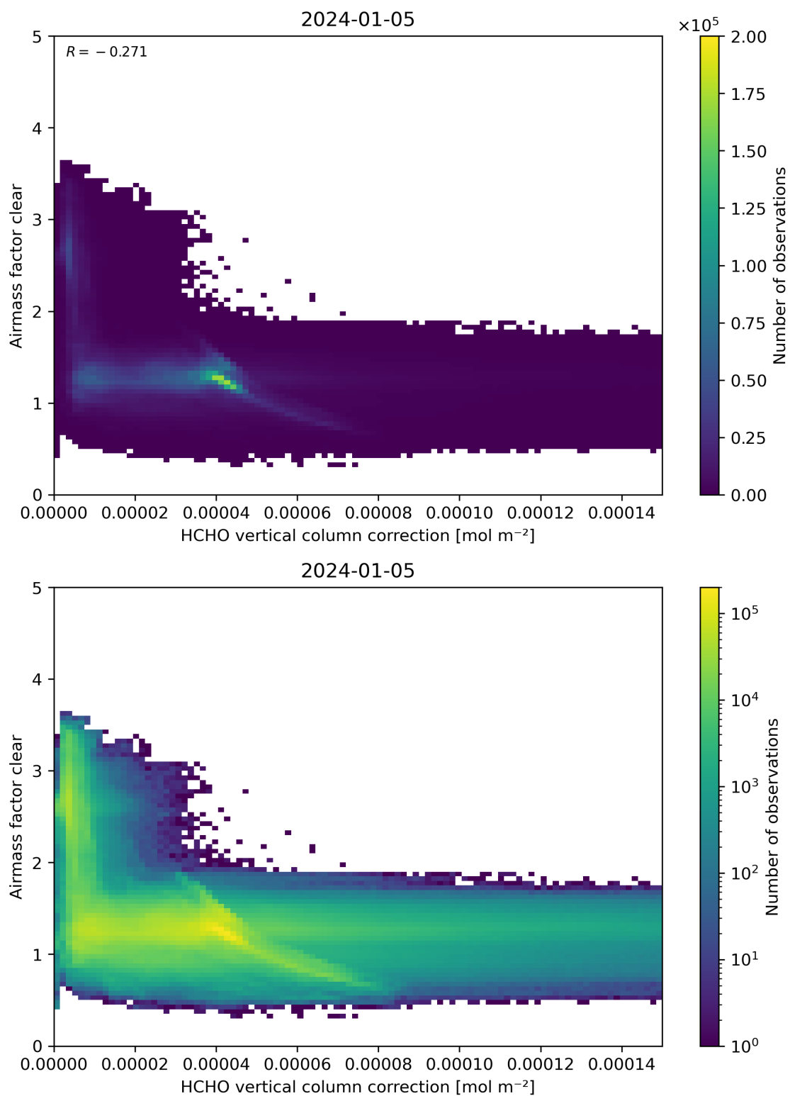
Figure 115: Scatter density plot of “HCHO vertical column correction” against “Airmass factor clear” for 2024-01-05 to 2024-01-06.
