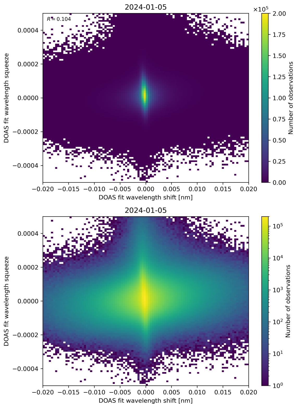
Figure 65: Scatter density plot of “DOAS fit wavelength shift” against “DOAS fit wavelength squeeze” for 2024-01-05 to 2024-01-06.
