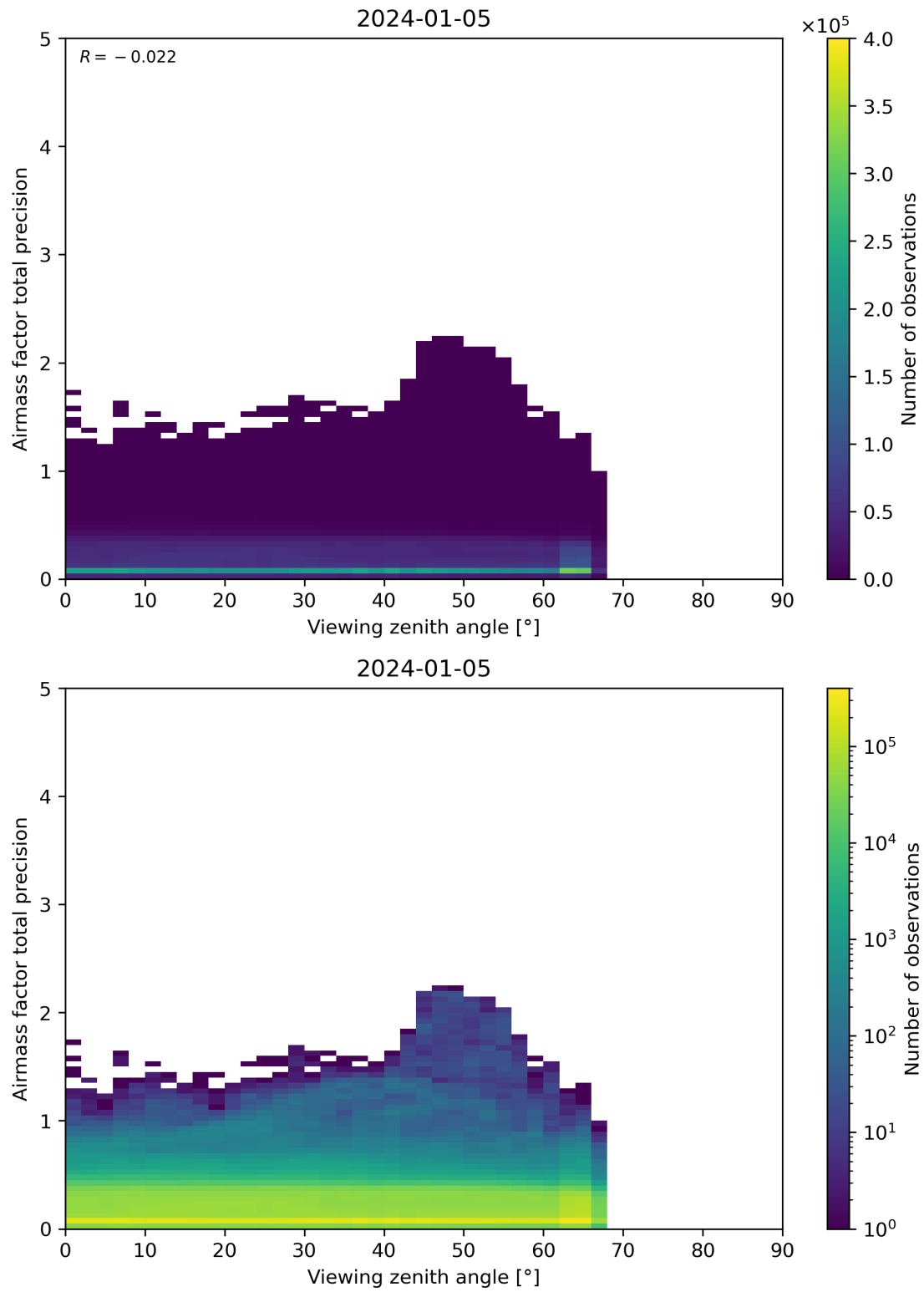
Figure 191: Scatter density plot of “Viewing zenith angle” against “Airmass factor total precision” for 2024-01-05 to 2024-01-06.
