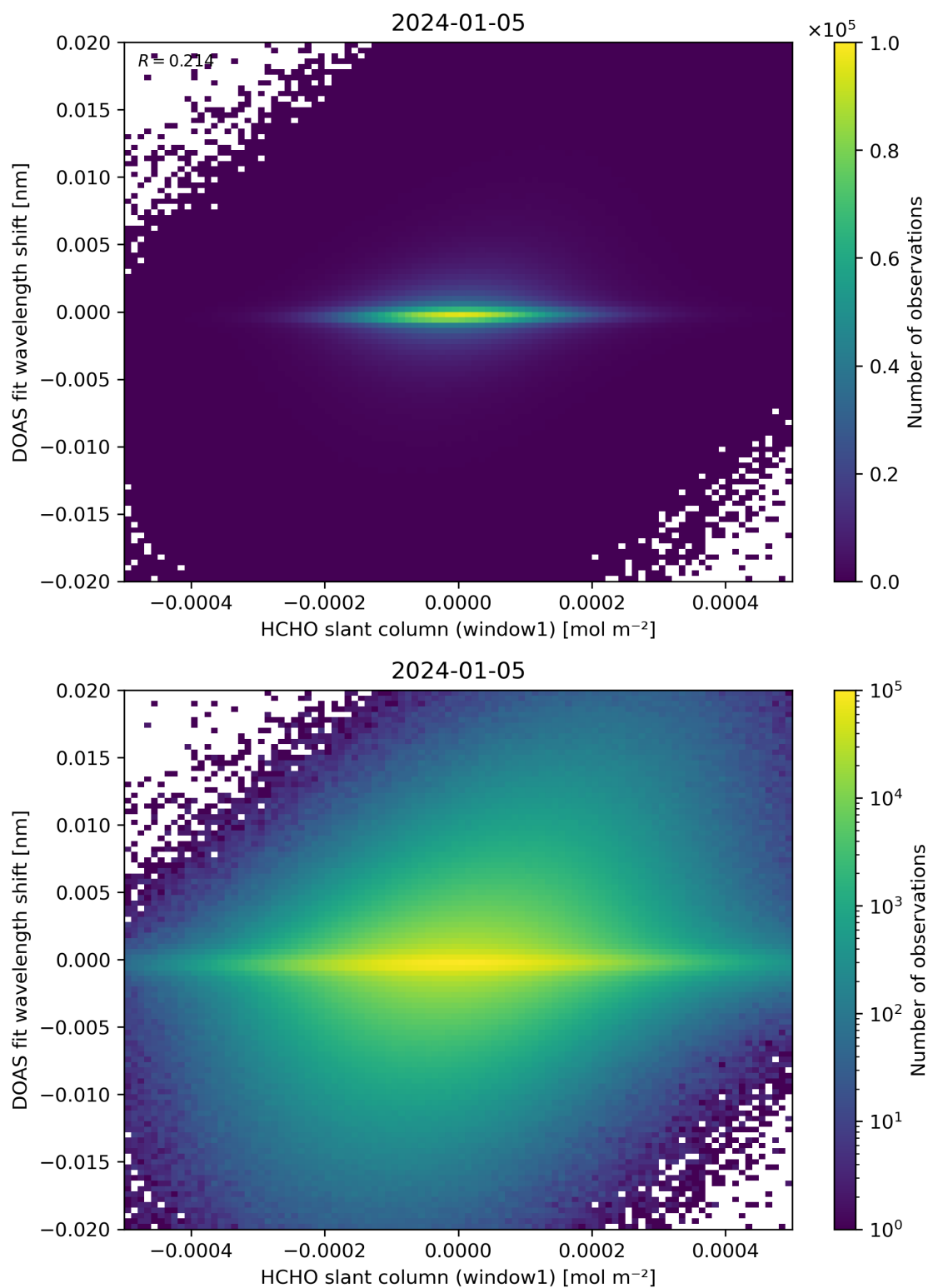
Figure 79: Scatter density plot of “HCHO slant column (window1)” against “DOAS fit wavelength shift” for 2024-01-05 to 2024-01-06.
