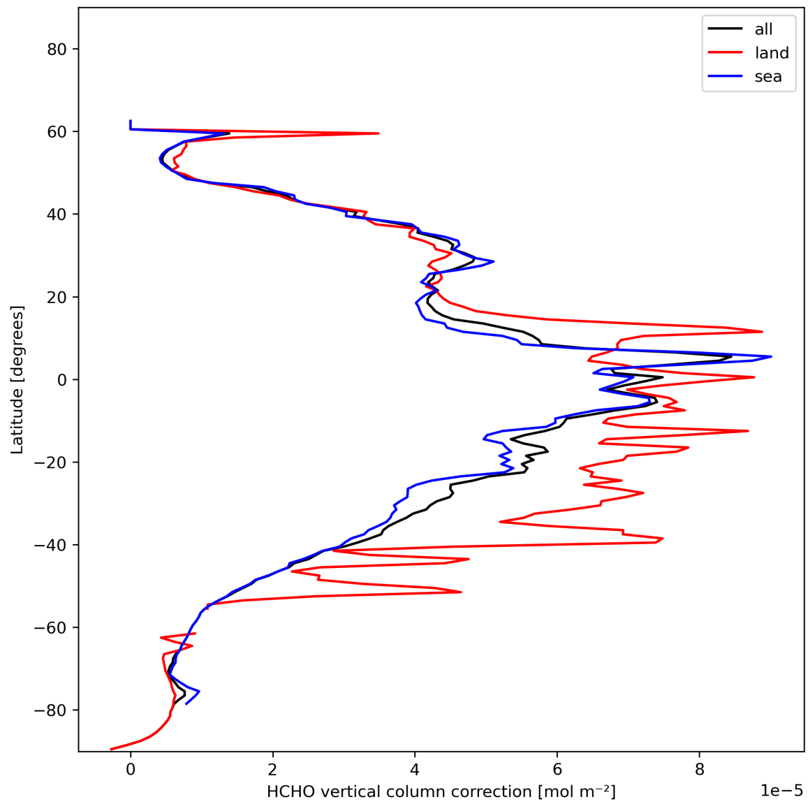
Figure 23: Zonal average of “HCHO vertical column correction” for 2024-01-05 to 2024-01-06.
