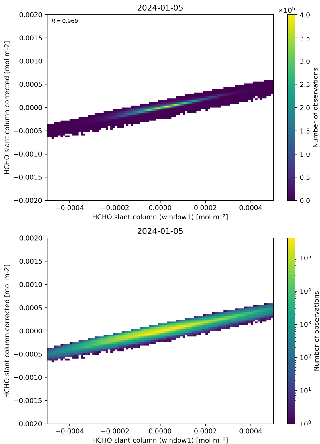
Figure 82: Scatter density plot of “HCHO slant column (window1)” against “HCHO slant column corrected” for 2024-01-05 to 2024-01-06.
