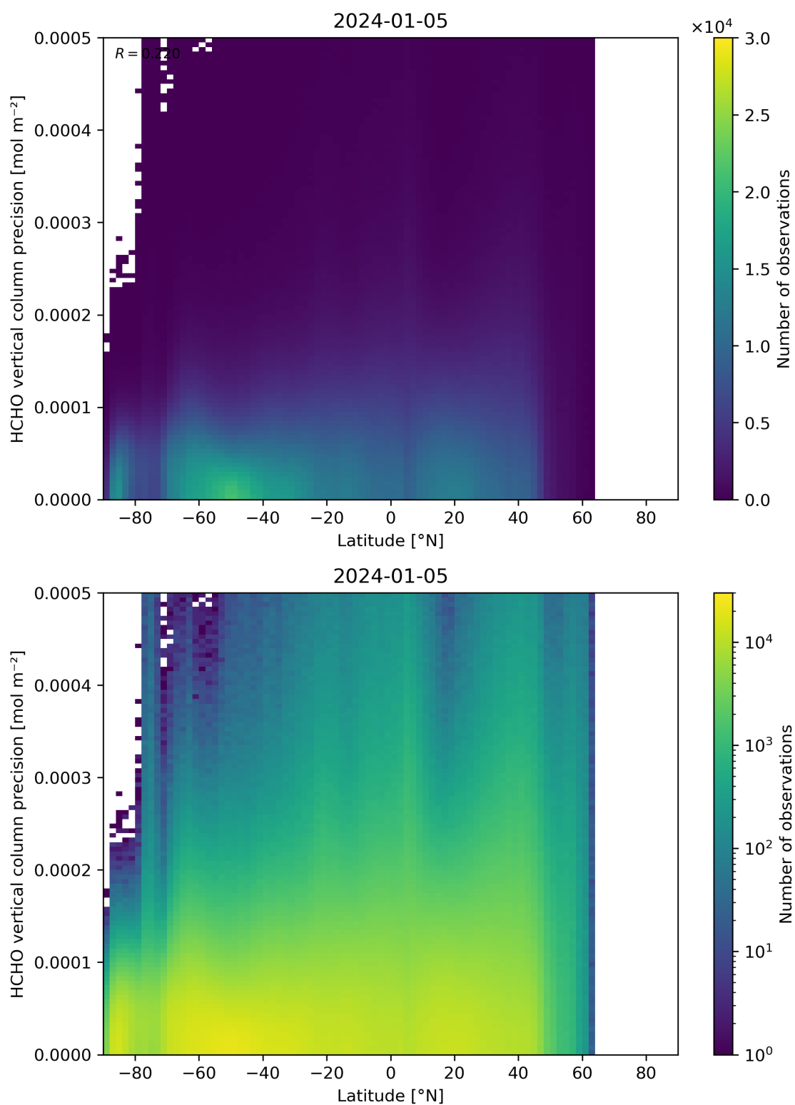
Figure 165: Scatter density plot of “Latitude” against “HCHO vertical column precision” for 2024-01-05 to 2024-01-06.
