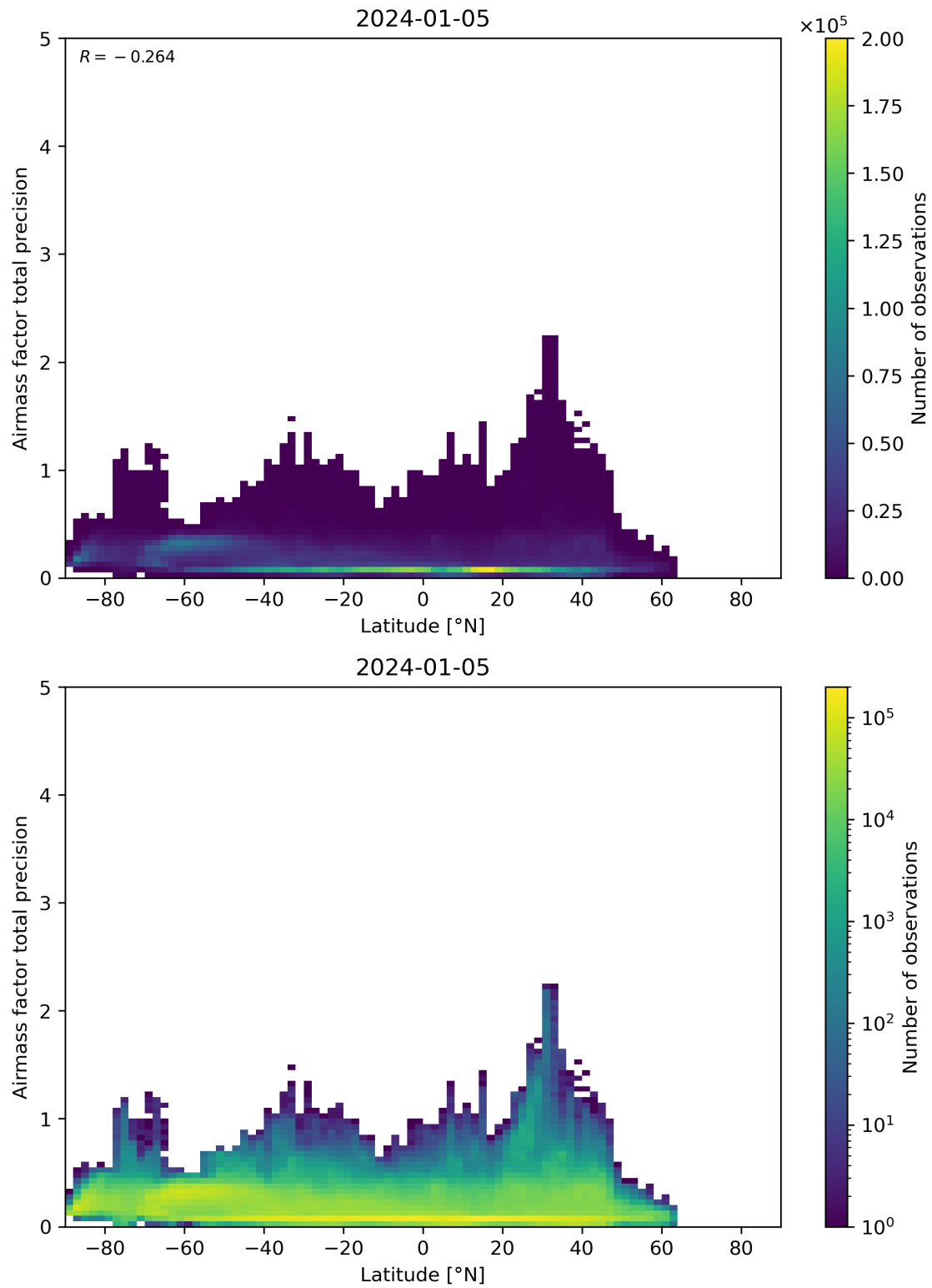
Figure 162: Scatter density plot of “Latitude” against “Airmass factor total precision” for 2024-01-05 to 2024-01-06.
