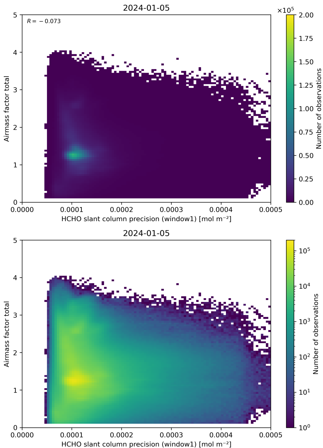
Figure 94: Scatter density plot of “HCHO slant column precision (window1)” against “Airmass factor total” for 2024-01-05 to 2024-01-06.
