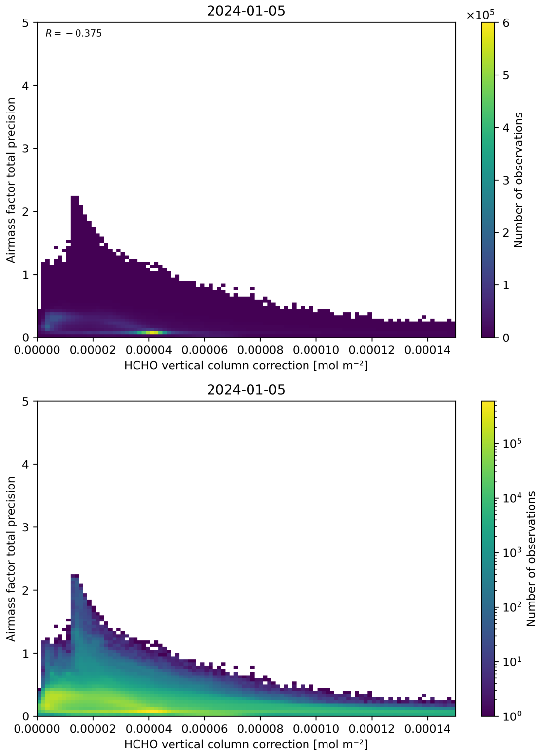
Figure 121: Scatter density plot of “HCHO vertical column correction” against “Airmass factor total precision” for 2024-01-05 to 2024-01-06.
