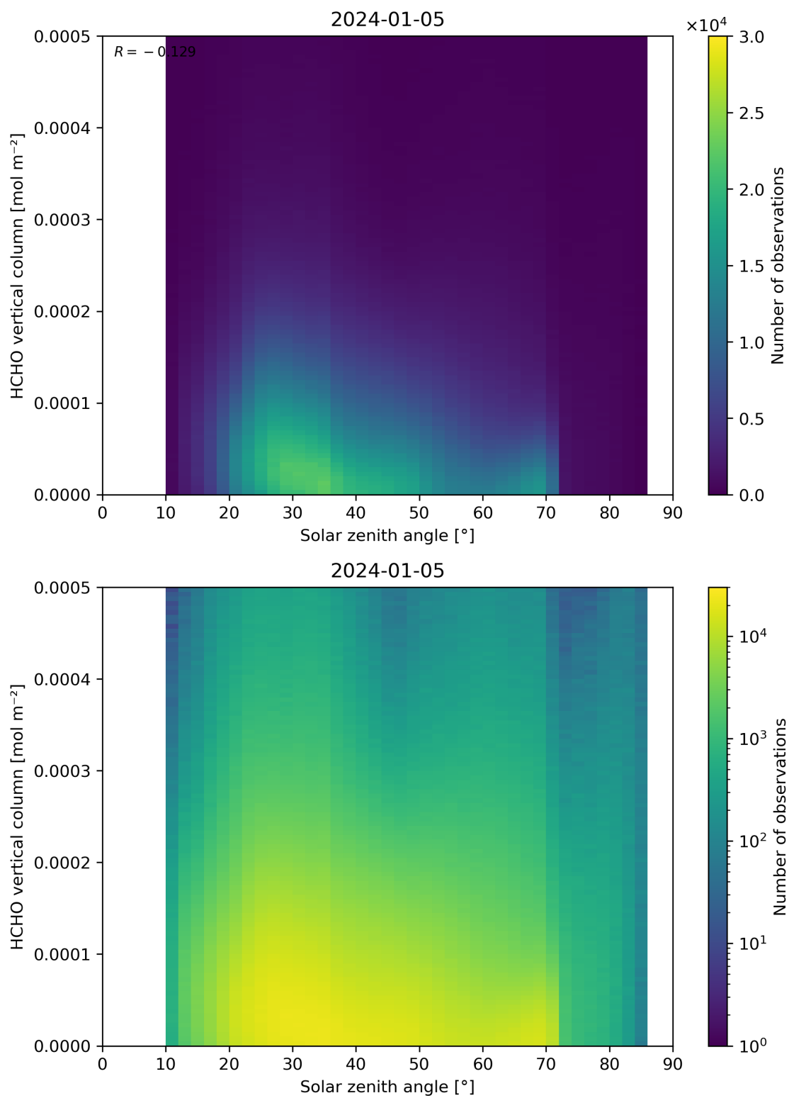
Figure 177: Scatter density plot of “Solar zenith angle” against “HCHO vertical column” for 2024-01-05 to 2024-01-06.
