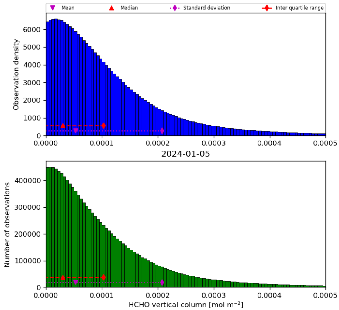
Figure 35: Histogram of “HCHO vertical column” for 2024-01-05 to 2024-01-06
