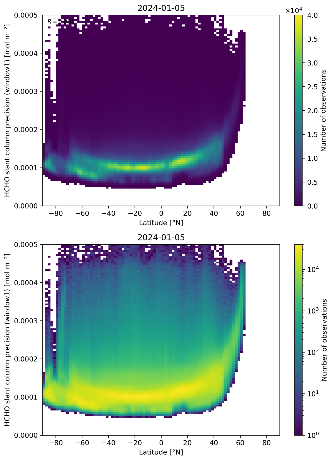
Figure 160: Scatter density plot of “Latitude” against “HCHO slant column precision (window1)” for 2024-01-05 to 2024-01-06.
