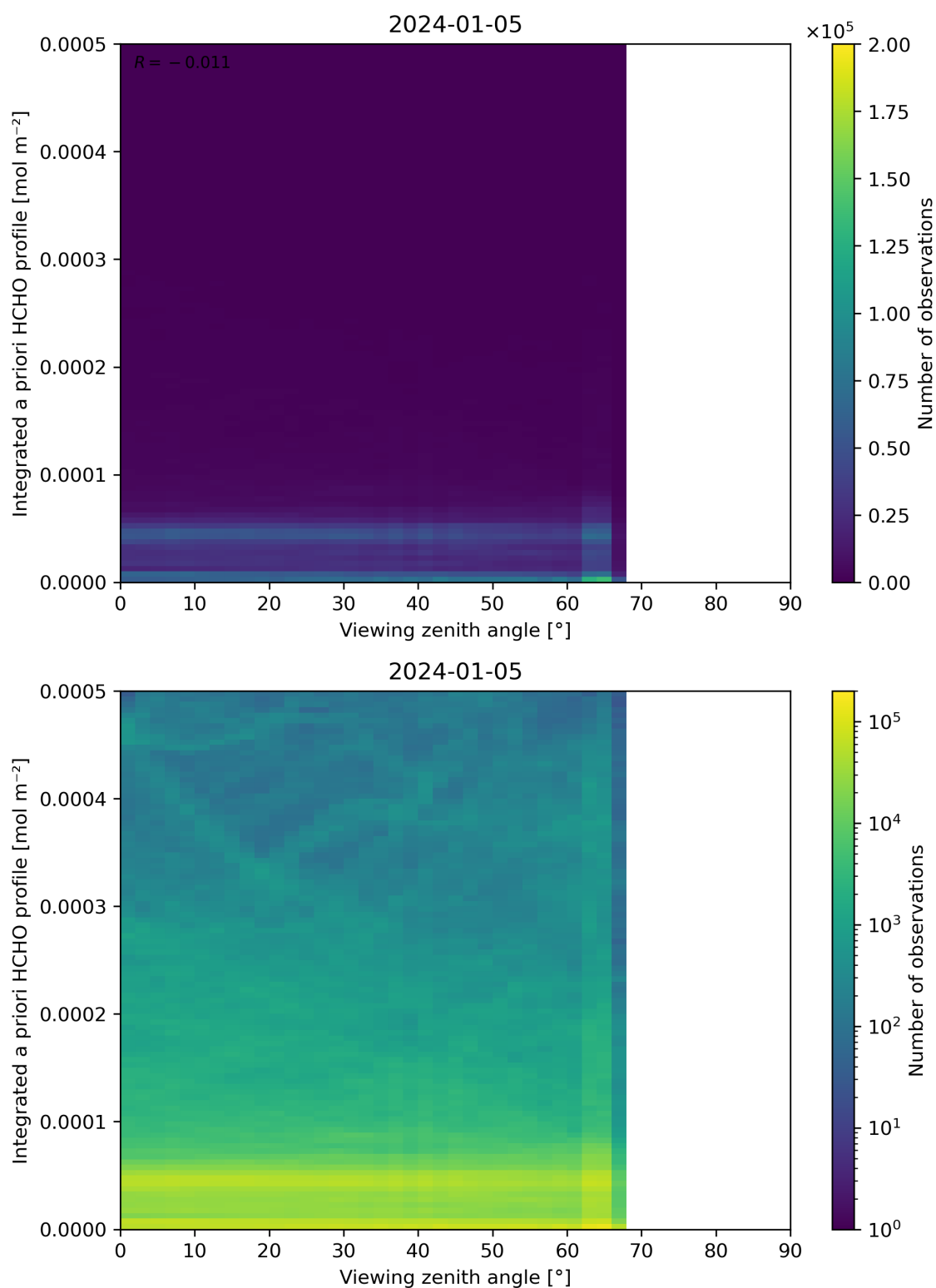
Figure 195: Scatter density plot of “Viewing zenith angle” against “Integrated a priori HCHO profile” for 2024-01-05 to 2024-01-06.
