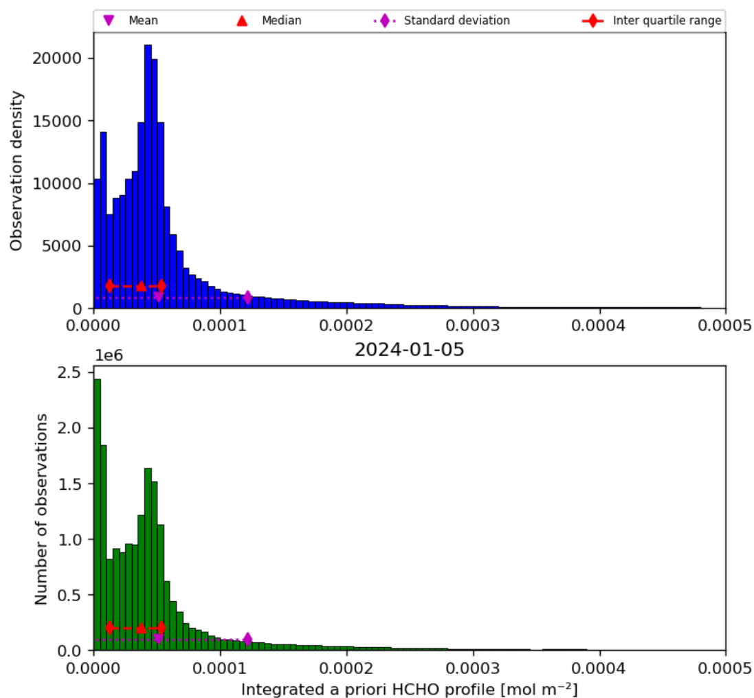
Figure 43: Histogram of “Integrated a priori HCHO profile” for 2024-01-05 to 2024-01-06
