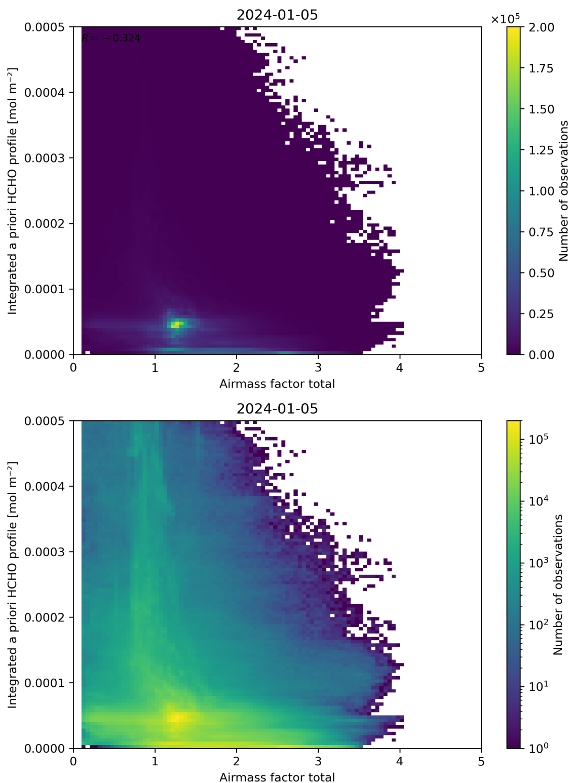
Figure 104: Scatter density plot of “Air mass factor total” against “Integrated a priori HCHO profile” for 2024-01-05 to 2024-01-06.
