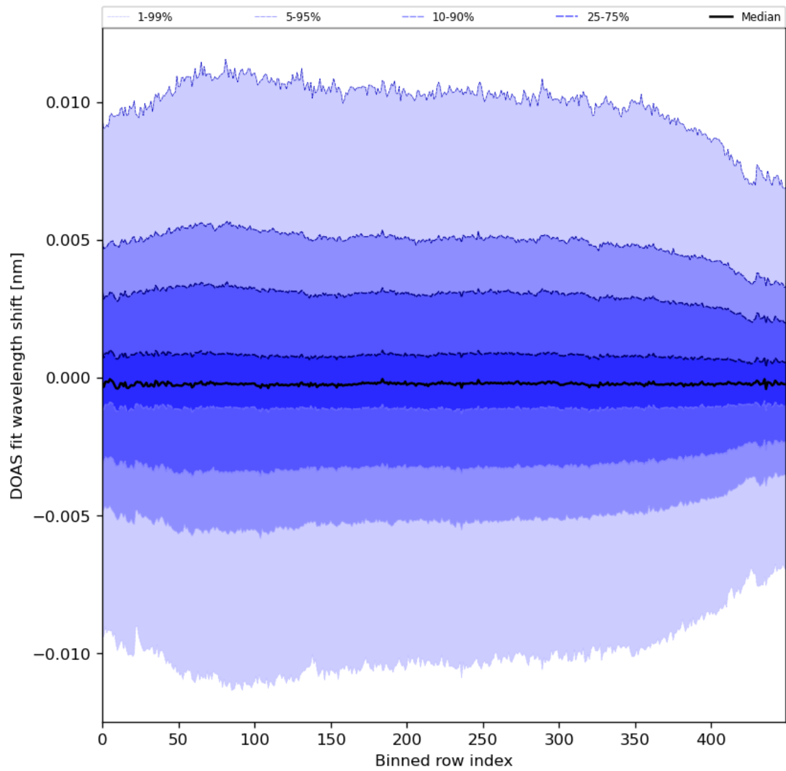
Figure 58: Along track statistics of “DOAS fit wavelength shift” for 2024-01-05 to 2024-01-06
