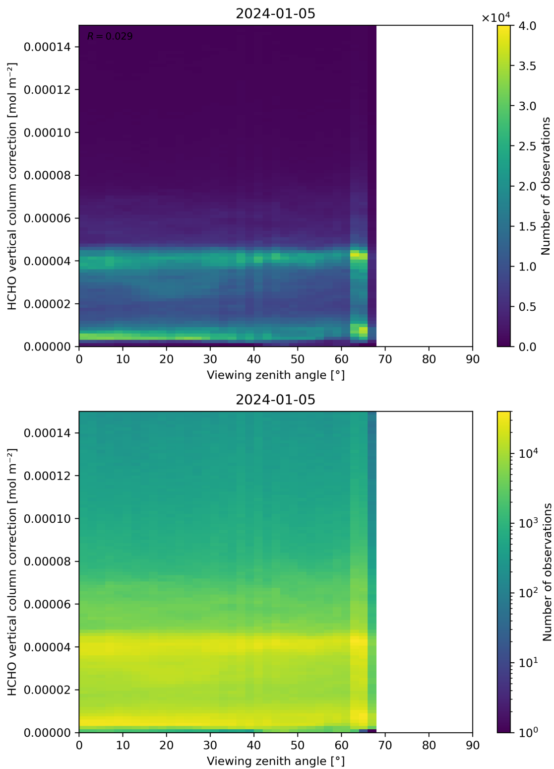
Figure 193: Scatter density plot of “Viewing zenith angle” against “HCHO vertical column correction” for 2024-01-05 to 2024-01-06.
