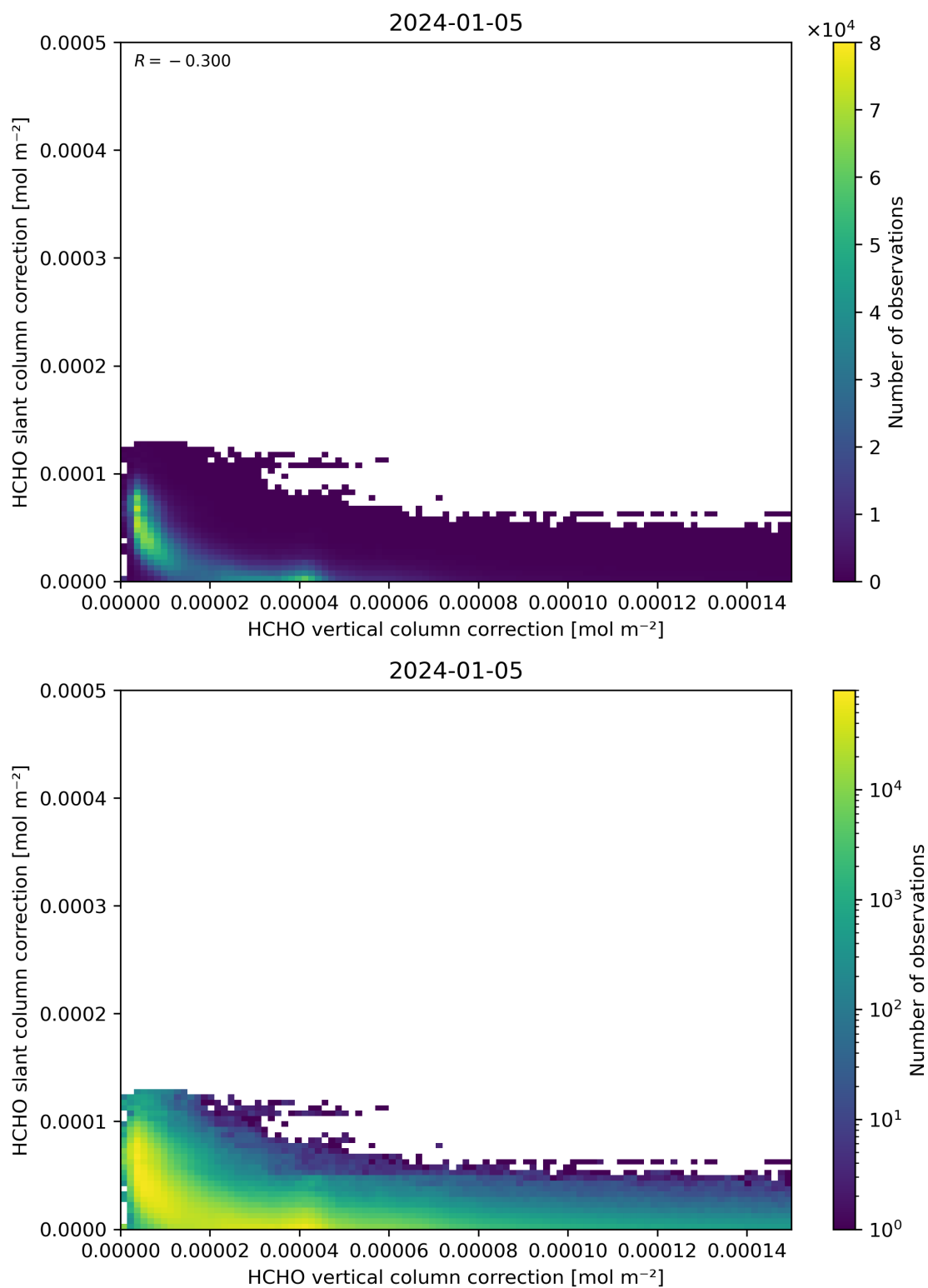
Figure 117: Scatter density plot of “HCHO vertical column correction” against “HCHO slant column correction” for 2024-01-05 to 2024-01-06.
