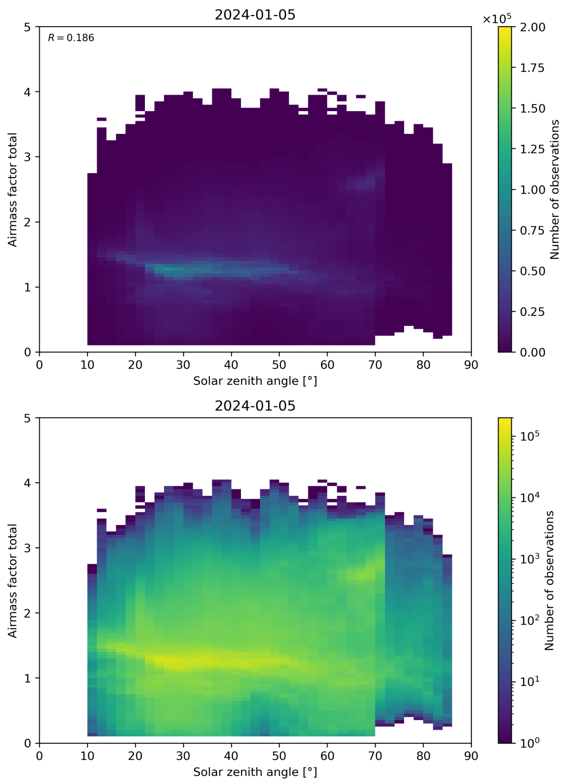
Figure 175: Scatter density plot of “Solar zenith angle” against “Airmass factor total” for 2024-01-05 to 2024-01-06.
