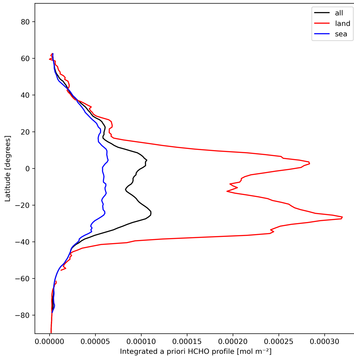
Figure 29: Zonal average of “Integrated a priori HCHO profile” for 2024-01-05 to 2024-01-06.
