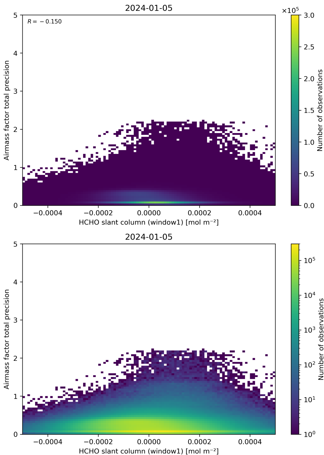
Figure 86: Scatter density plot of “HCHO slant column (window1)” against “Airmass factor total precision” for 2024-01-05 to 2024-01-06.
