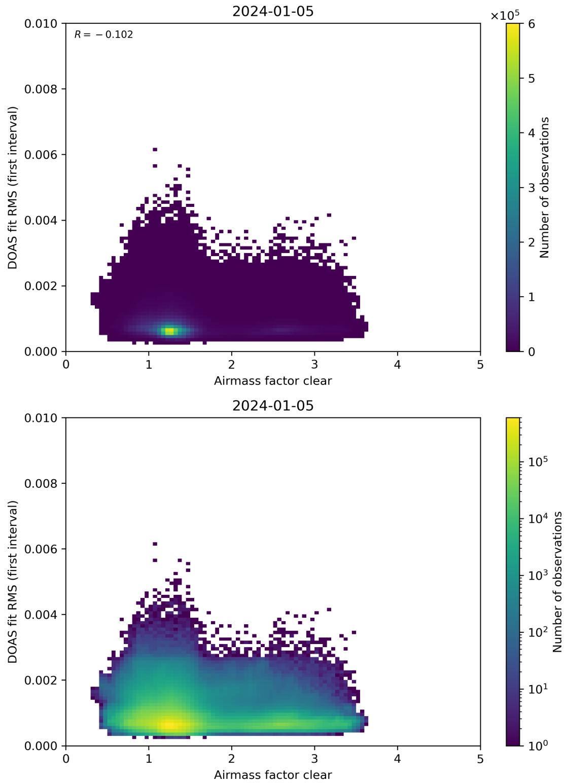
Figure 71: Scatter density plot of “Airmass factor clear” against “DOAS fit RMS (first interval)” for 2024-01-05 to 2024-01-06.
