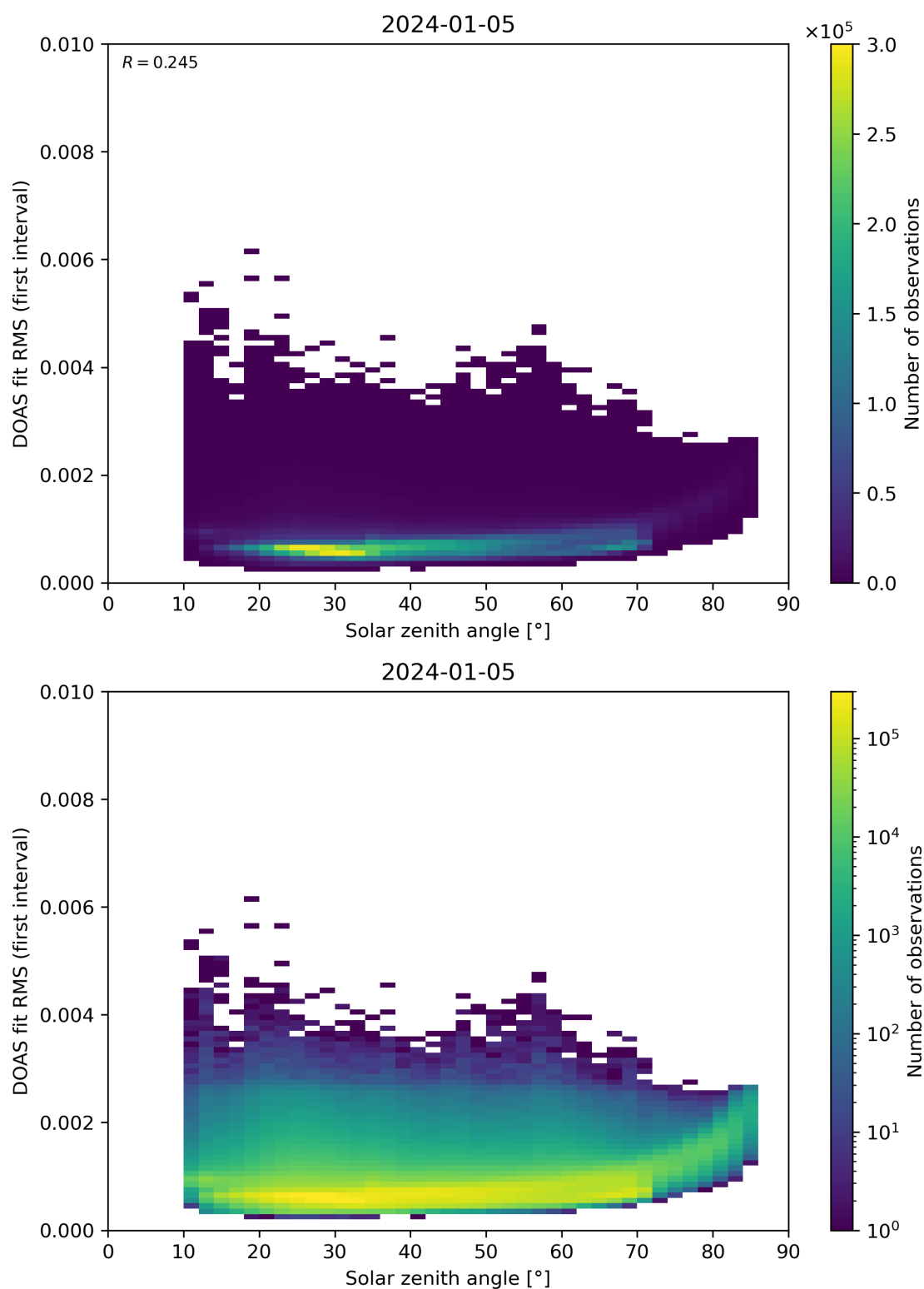
Figure 167: Scatter density plot of “Solar zenith angle” against “DOAS fit RMS (first interval)” for 2024-01-05 to 2024-01-06.
