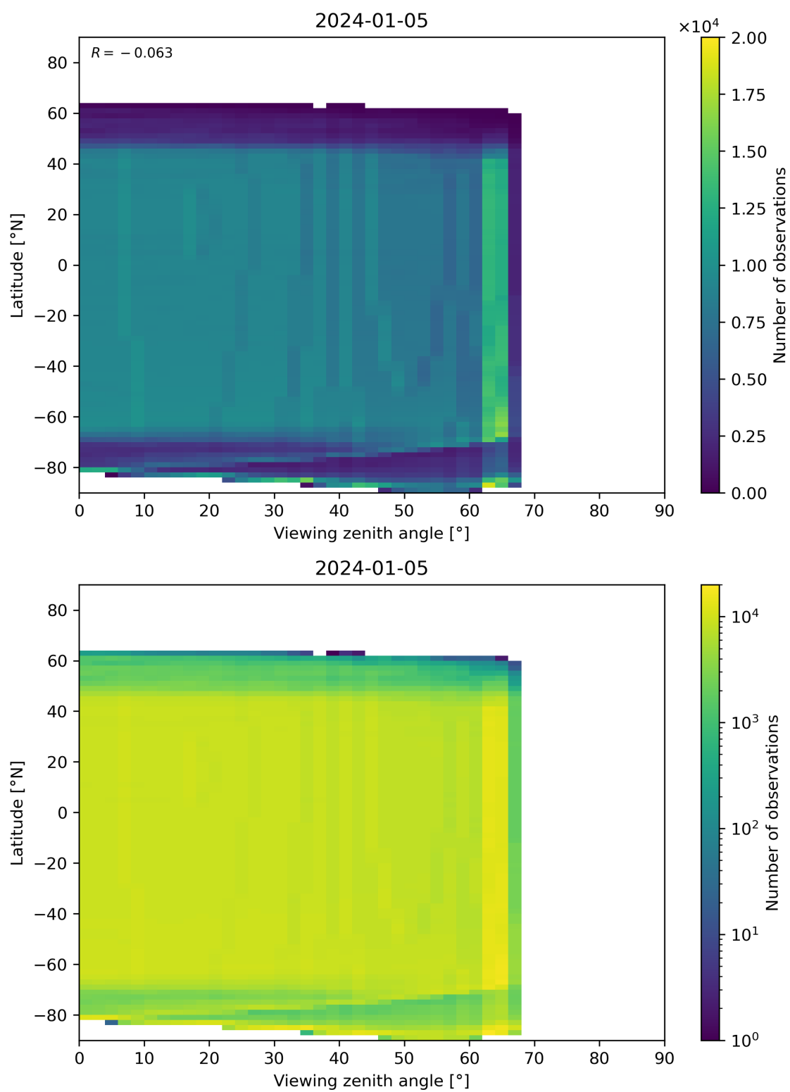
Figure 196: Scatter density plot of “Viewing zenith angle” against “Latitude” for 2024-01-05 to 2024-01-06.
