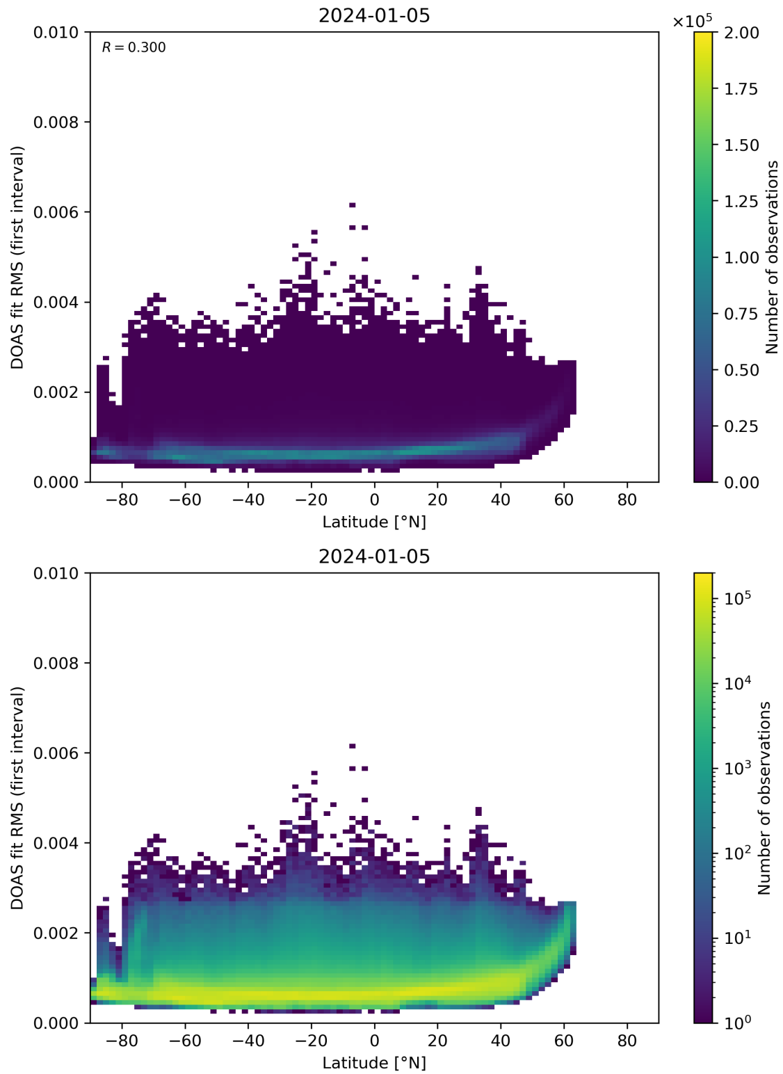
Figure 153: Scatter density plot of “Latitude” against “DOAS fit RMS (first interval)” for 2024-01-05 to 2024-01-06.
