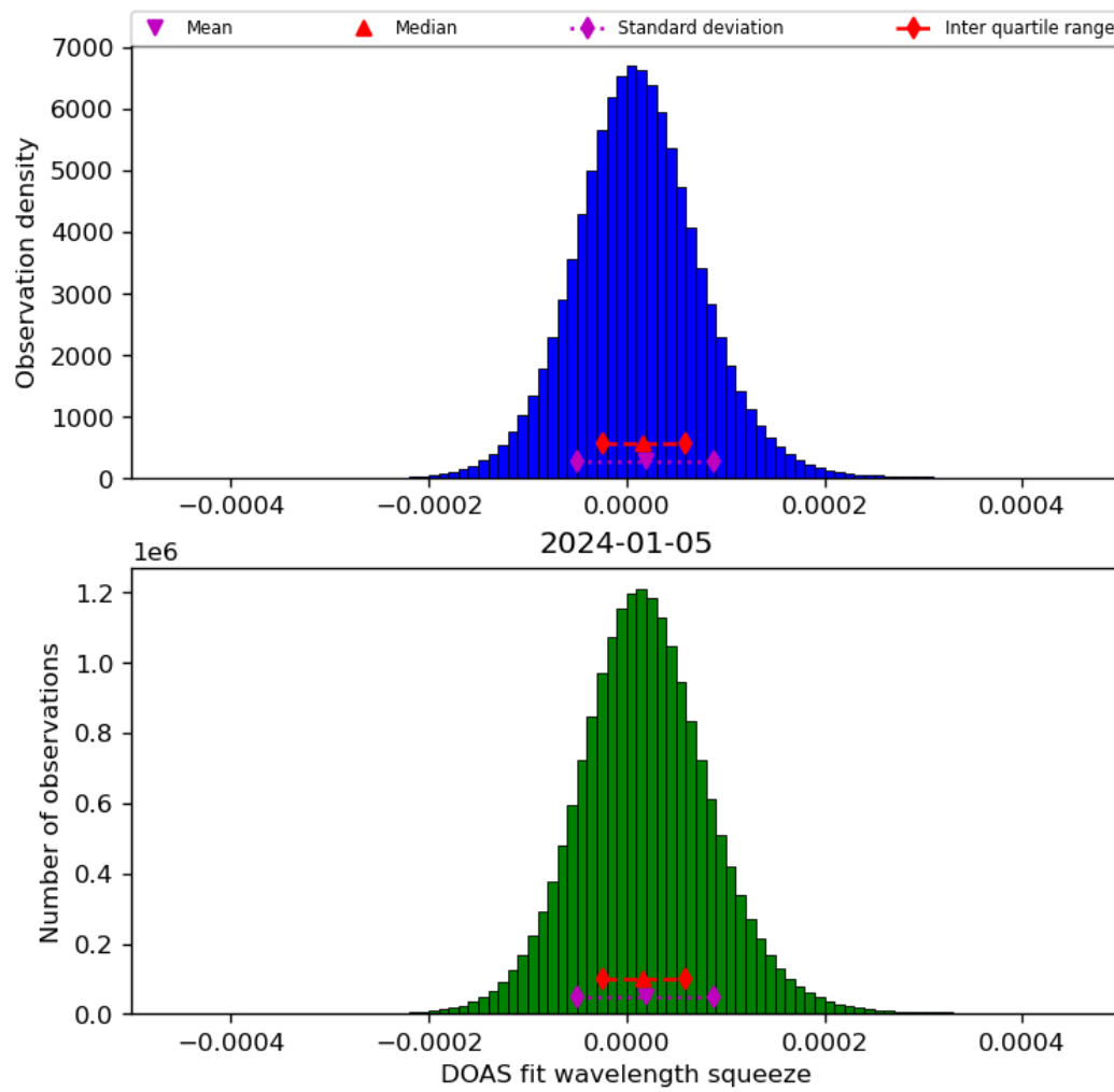
Figure 45: Histogram of “DOAS fit wavelength squeeze” for 2024-01-05 to 2024-01-06
