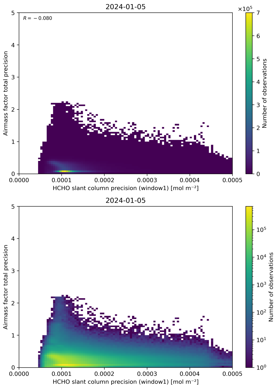
Figure 95: Scatter density plot of “HCHO slant column precision (window1)” against “Airmass factor total precision” for 2024-01-05 to 2024-01-06.
