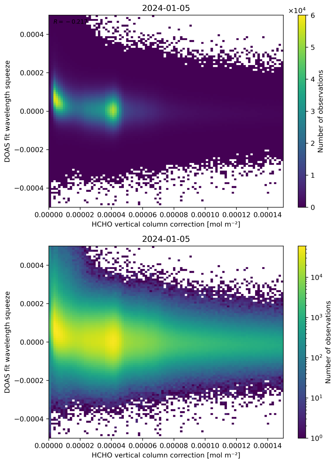
Figure 114: Scatter density plot of “HCHO vertical column correction” against “DOAS fit wavelength squeeze” for 2024-01-05 to 2024-01-06.
