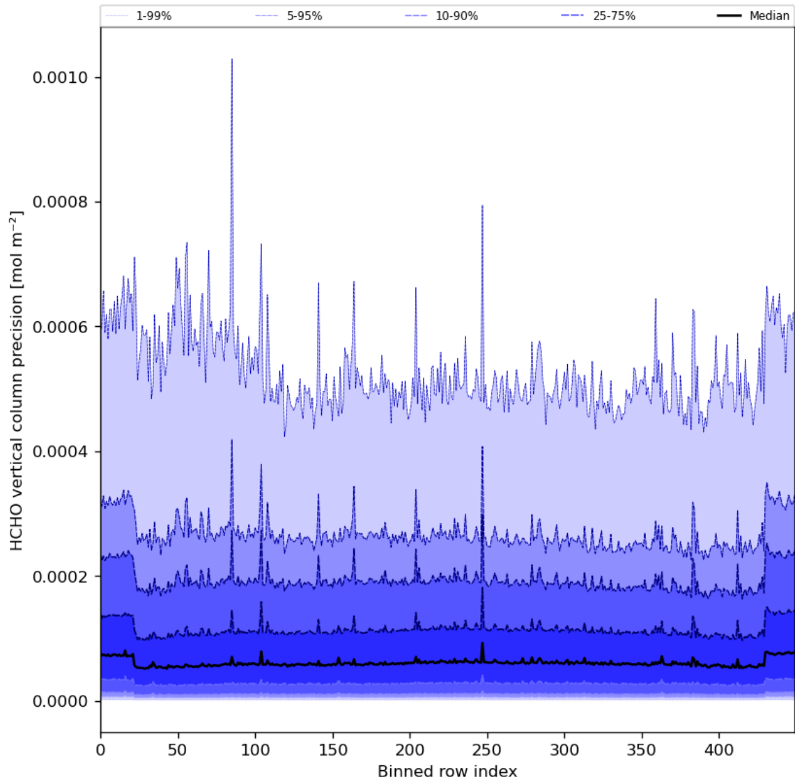
Figure 50: Along track statistics of "HCHO vertical column precision" for 2024-01-05 to 2024-01-06
