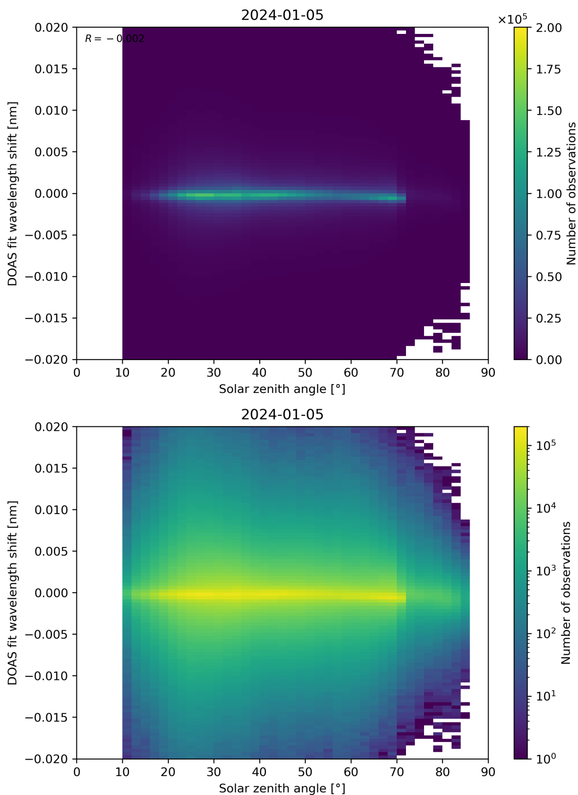
Figure 168: Scatter density plot of “Solar zenith angle” against “DOAS fit wavelength shift” for 2024-01-05 to 2024-01-06.
