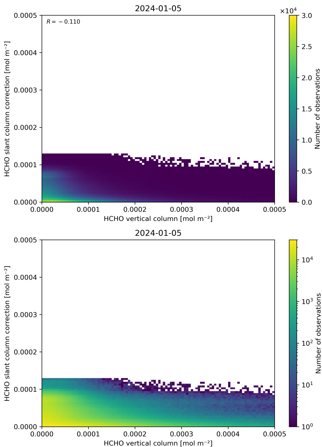
Figure 128: Scatter density plot of “HCHO vertical column” against “HCHO slant column correction” for 2024-01-05 to 2024-01-06.
