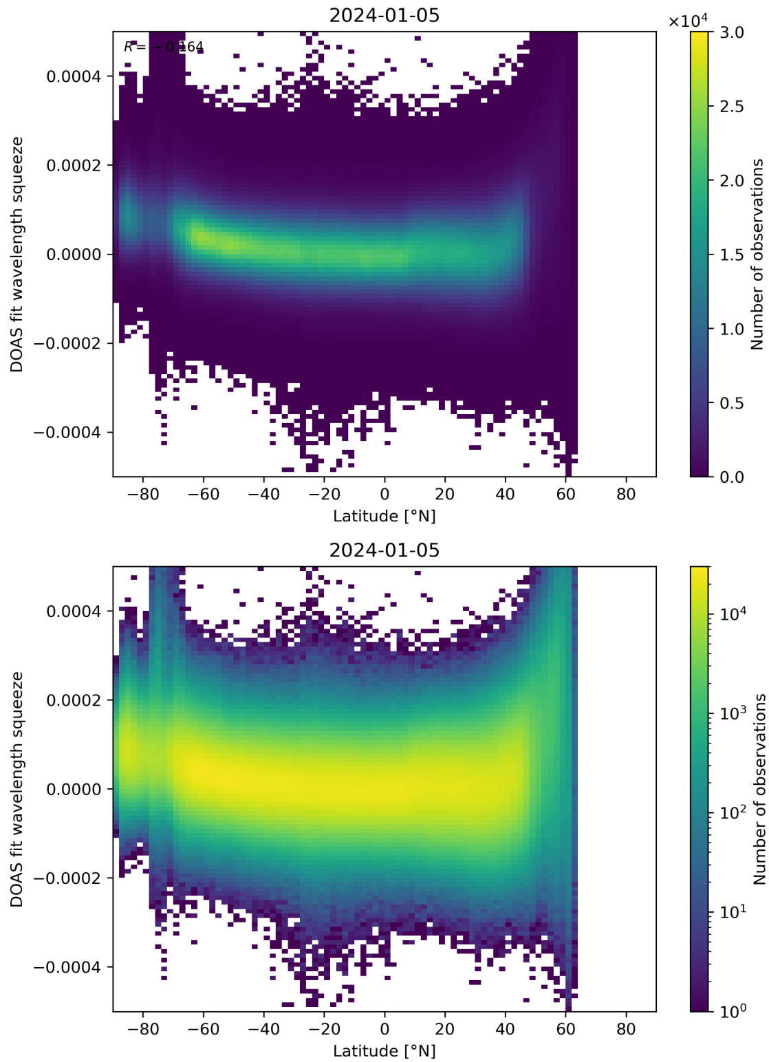
Figure 155: Scatter density plot of “Latitude” against “DOAS fit wavelength squeeze” for 2024-01-05 to 2024-01-06.
