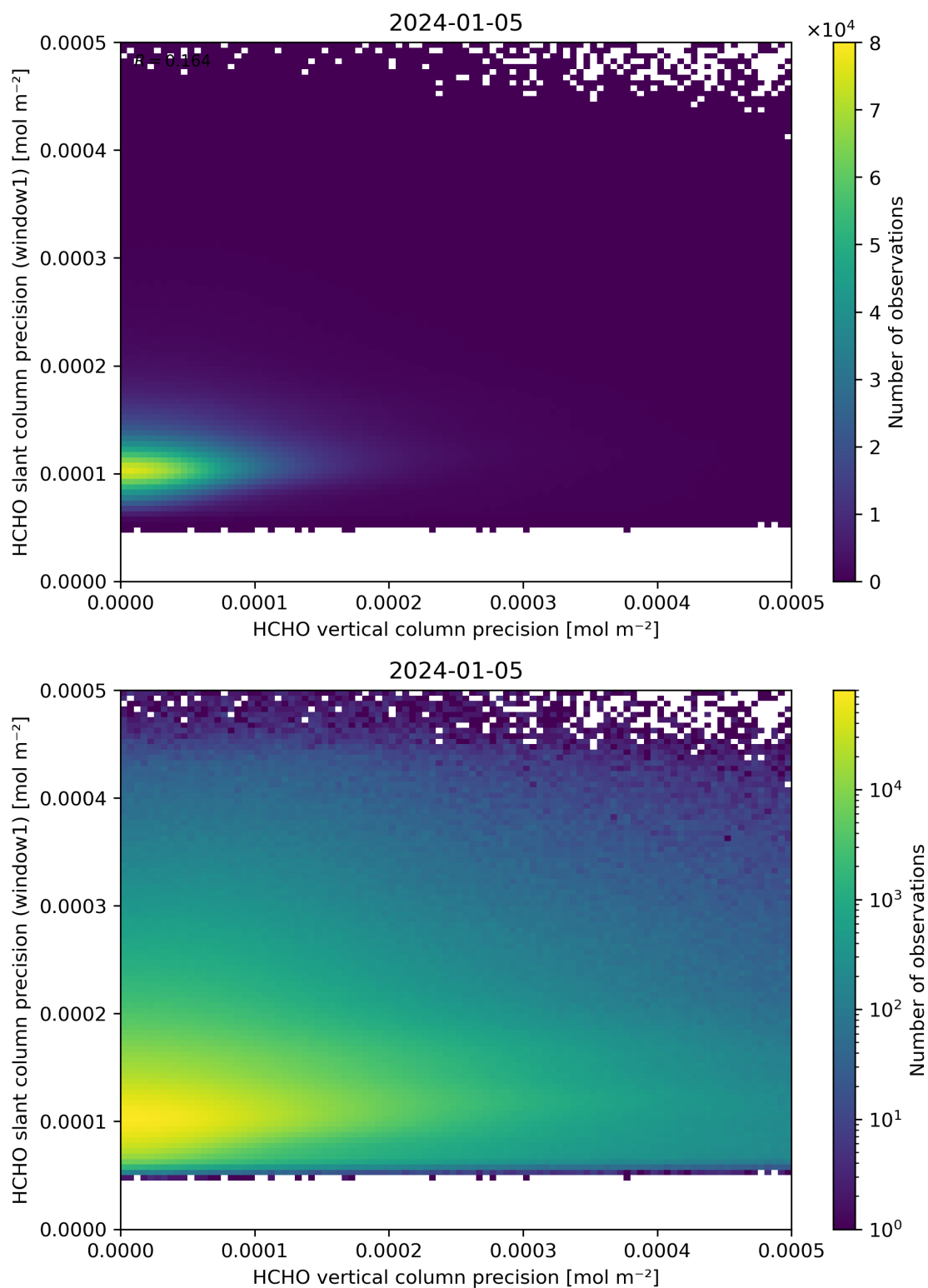
Figure 143: Scatter density plot of “HCHO vertical column precision” against “HCHO slant column precision (window1)” for 2024-01-05 to 2024-01-06.
