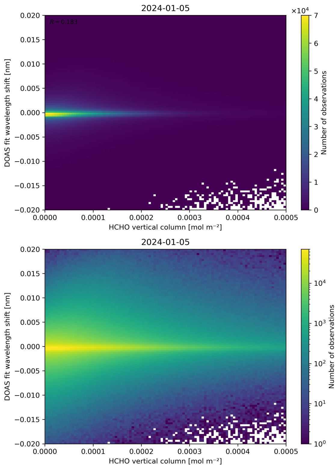
Figure 124: Scatter density plot of “HCHO vertical column” against “DOAS fit wavelength shift” for 2024-01-05 to 2024-01-06.
