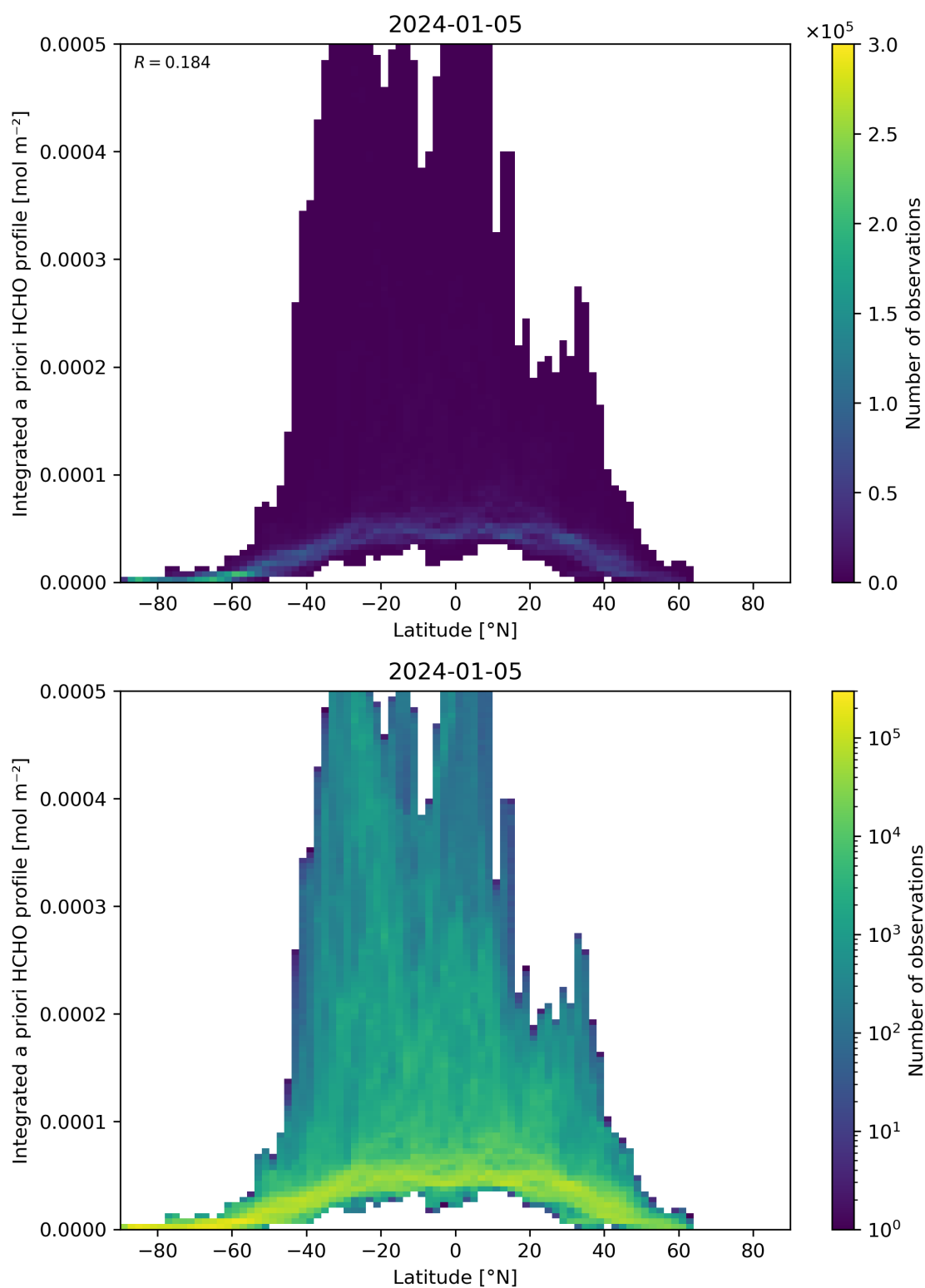
Figure 166: Scatter density plot of “Latitude” against “Integrated a priori HCHO profile” for 2024-01-05 to 2024-01-06.
