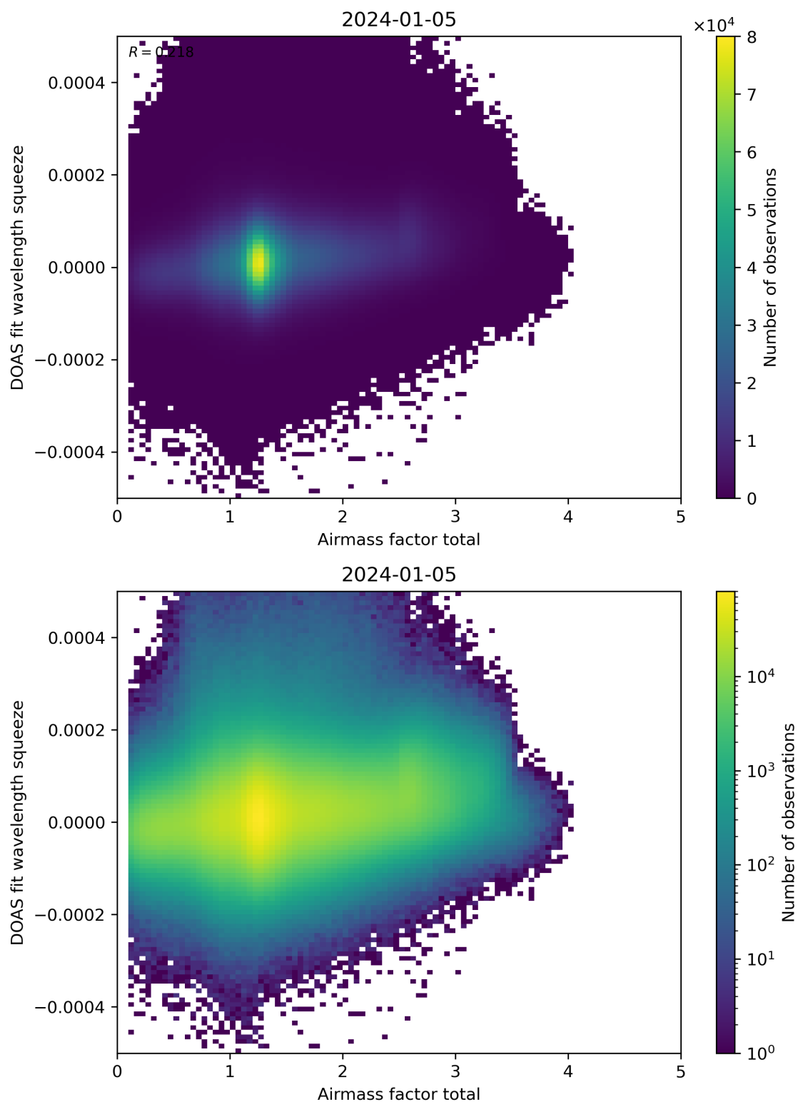
Figure 99: Scatter density plot of “Airmass factor total” against “DOAS fit wavelength squeeze” for 2024-01-05 to 2024-01-06.
