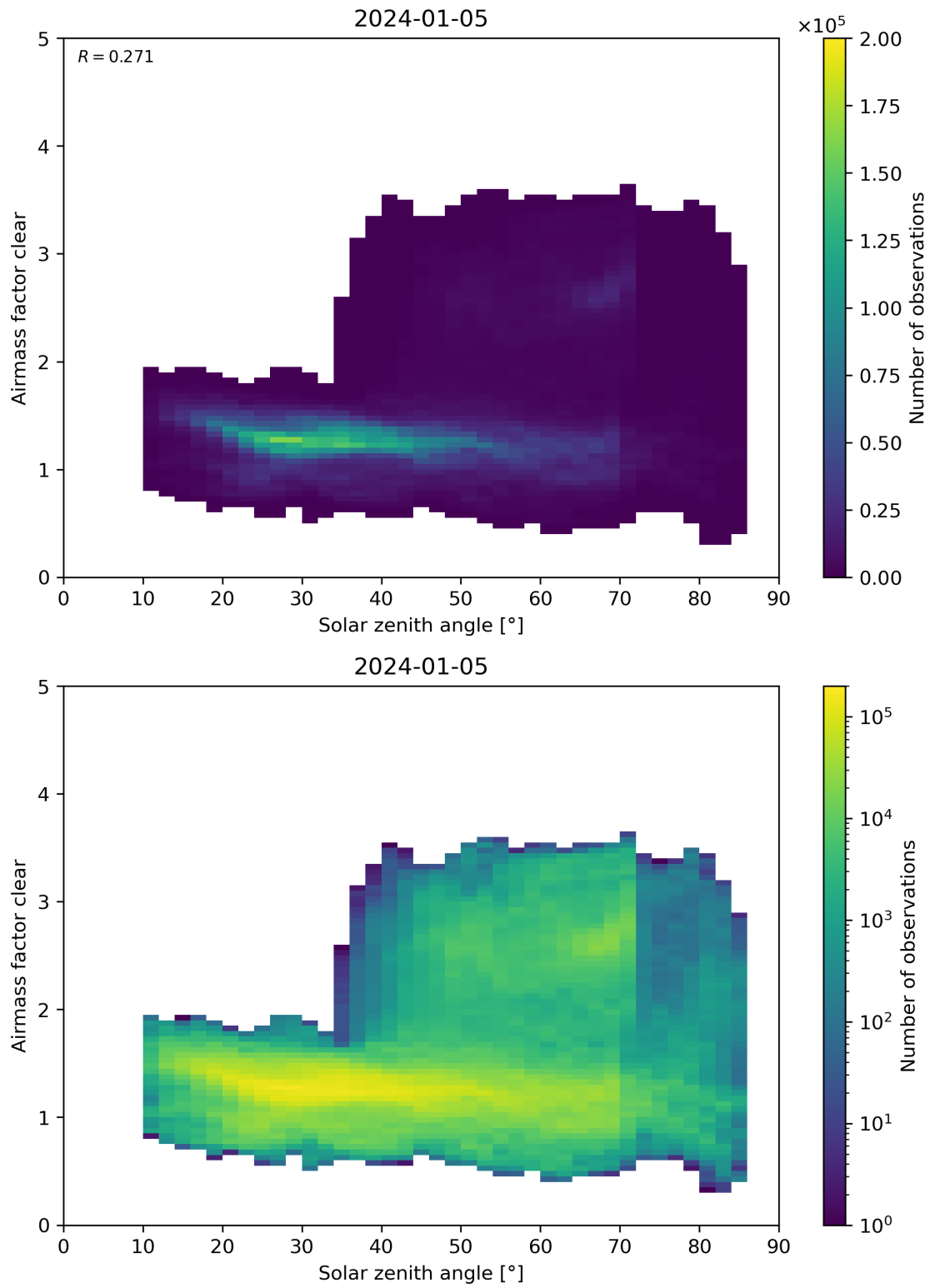
Figure 170: Scatter density plot of “Solar zenith angle” against “Airmass factor clear” for 2024-01-05 to 2024-01-06.
