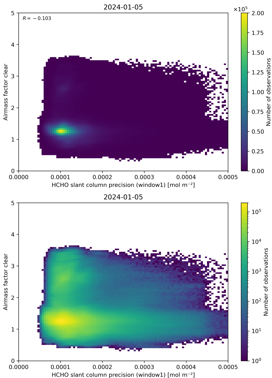
Figure 91: Scatter density plot of “HCHO slant column precision (window1)” against “Airmass factor clear” for 2024-01-05 to 2024-01-06.
