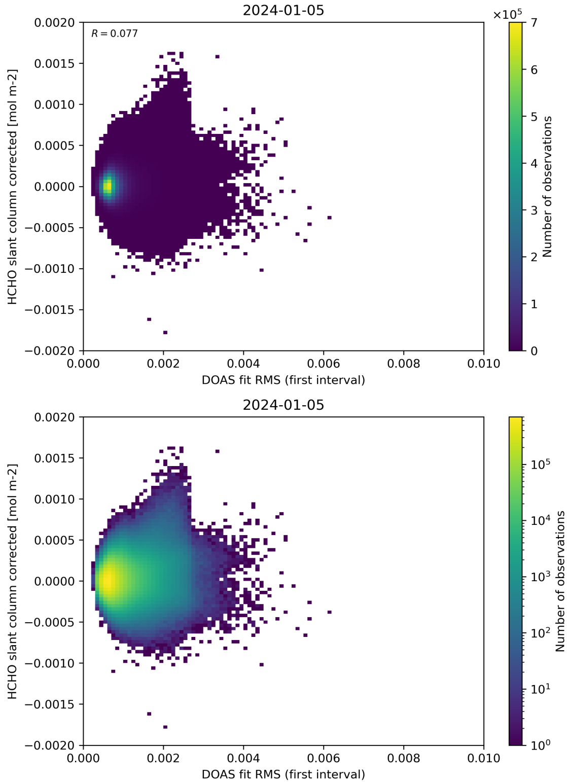
Figure 62: Scatter density plot of “DOAS fit RMS (first interval)” against “HCHO slant column corrected” for 2024-01-05 to 2024-01-06.
