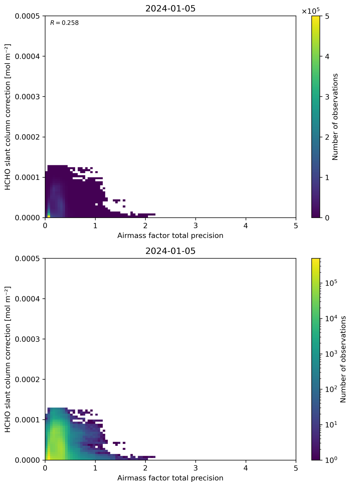
Figure 110: Scatter density plot of “Airmass factor total precision” against “HCHO slant column correction” for 2024-01-05 to 2024-01-06.
