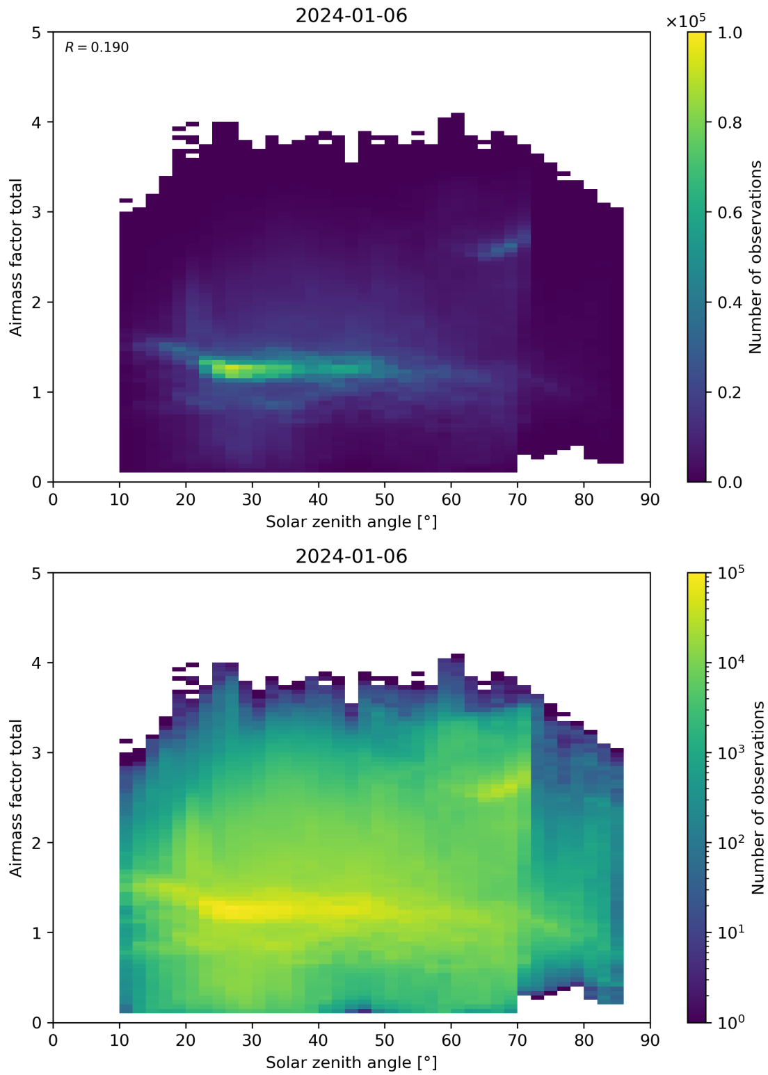
Figure 175: Scatter density plot of “Solar zenith angle” against “Airmass factor total” for 2024-01-05 to 2024-01-07.
