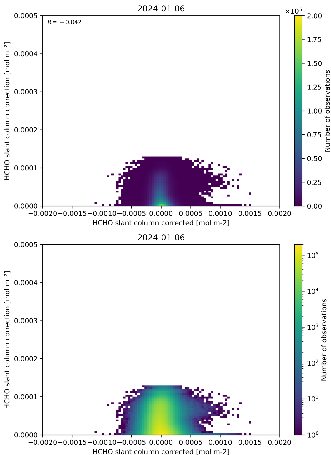
Figure 77: Scatter density plot of “HCHO slant column corrected” against “HCHO slant column correction” for 2024-01-05 to 2024-01-07.
