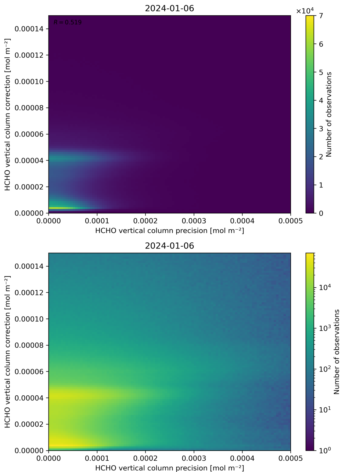
Figure 146: Scatter density plot of “HCHO vertical column precision” against “HCHO vertical column correction” for 2024-01-05 to 2024-01-07.
