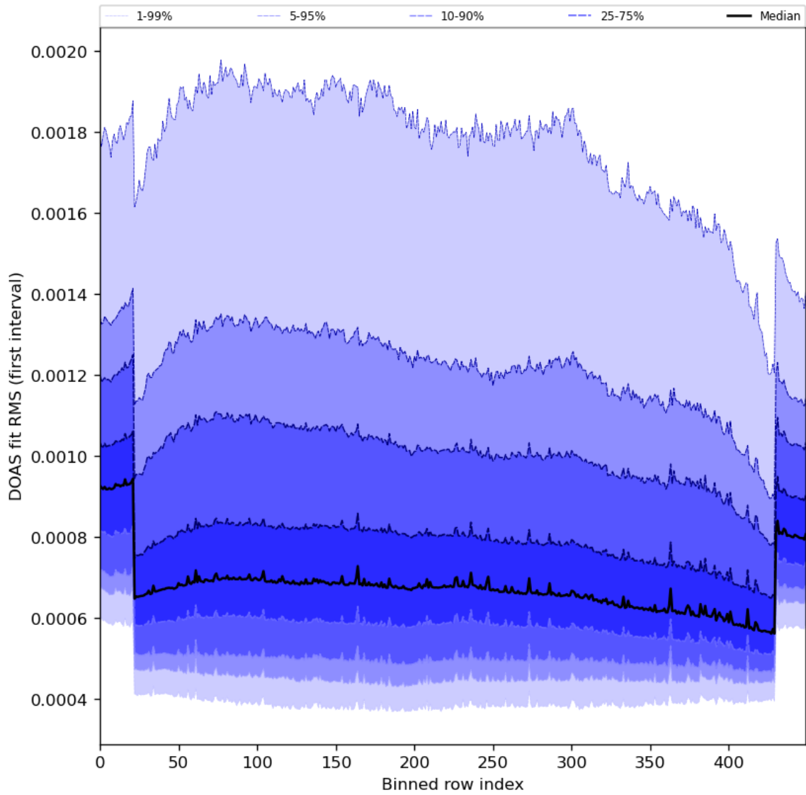
Figure 60: Along track statistics of “DOAS fit RMS (first interval)” for 2024-01-05 to 2024-01-07
