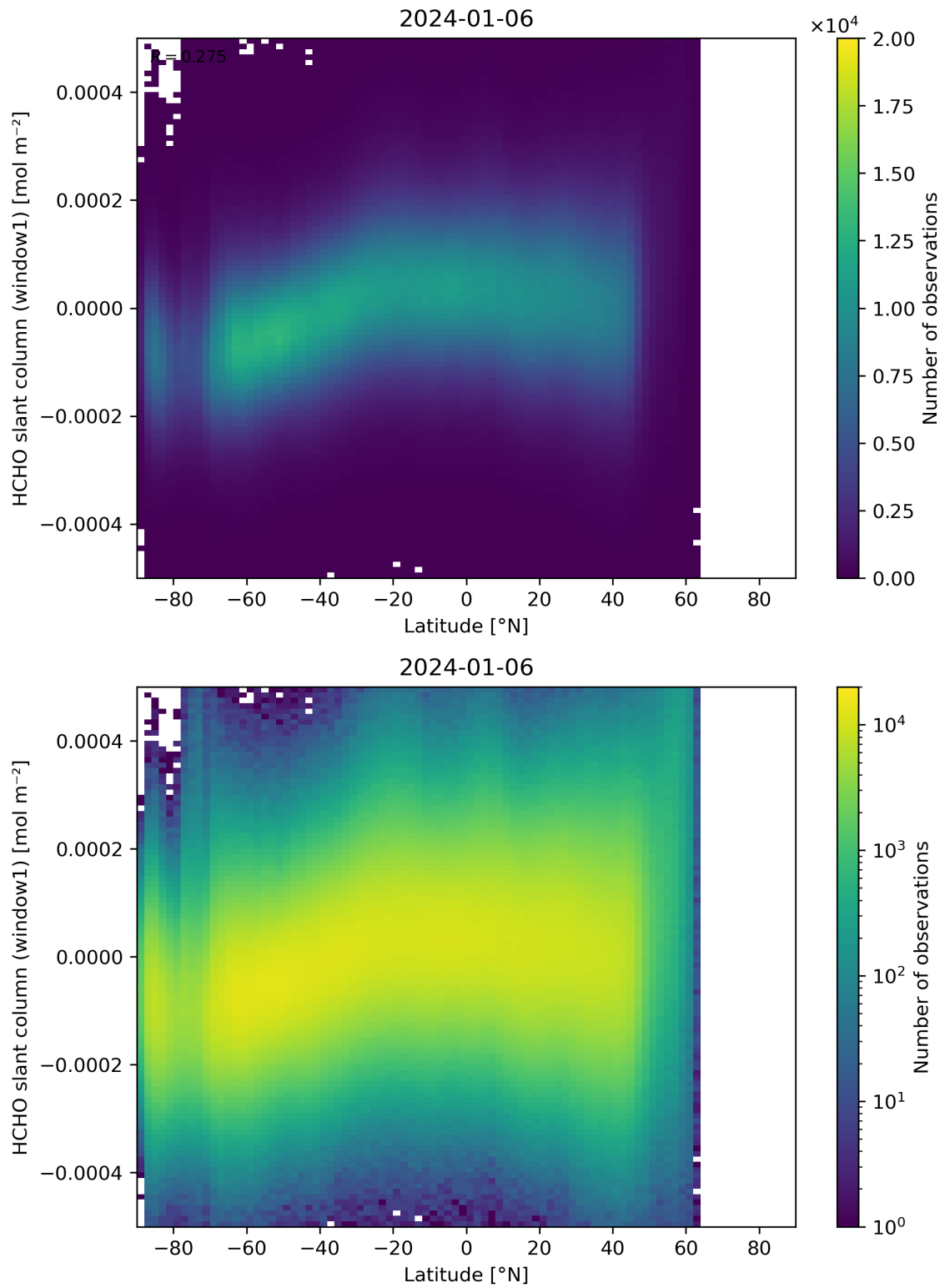
Figure 159: Scatter density plot of “Latitude” against “HCHO slant column (window1)” for 2024-01-05 to 2024-01-07.
