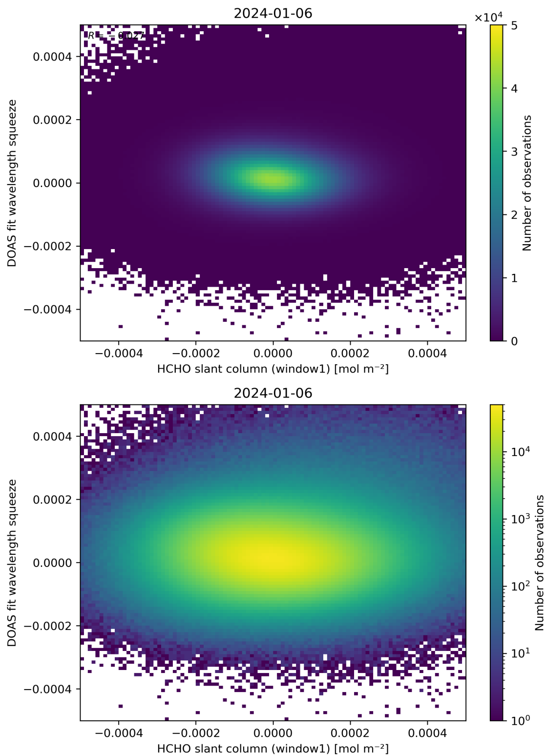
Figure 80: Scatter density plot of “HCHO slant column (window1)” against “DOAS fit wavelength squeeze” for 2024-01-05 to 2024-01-07.
