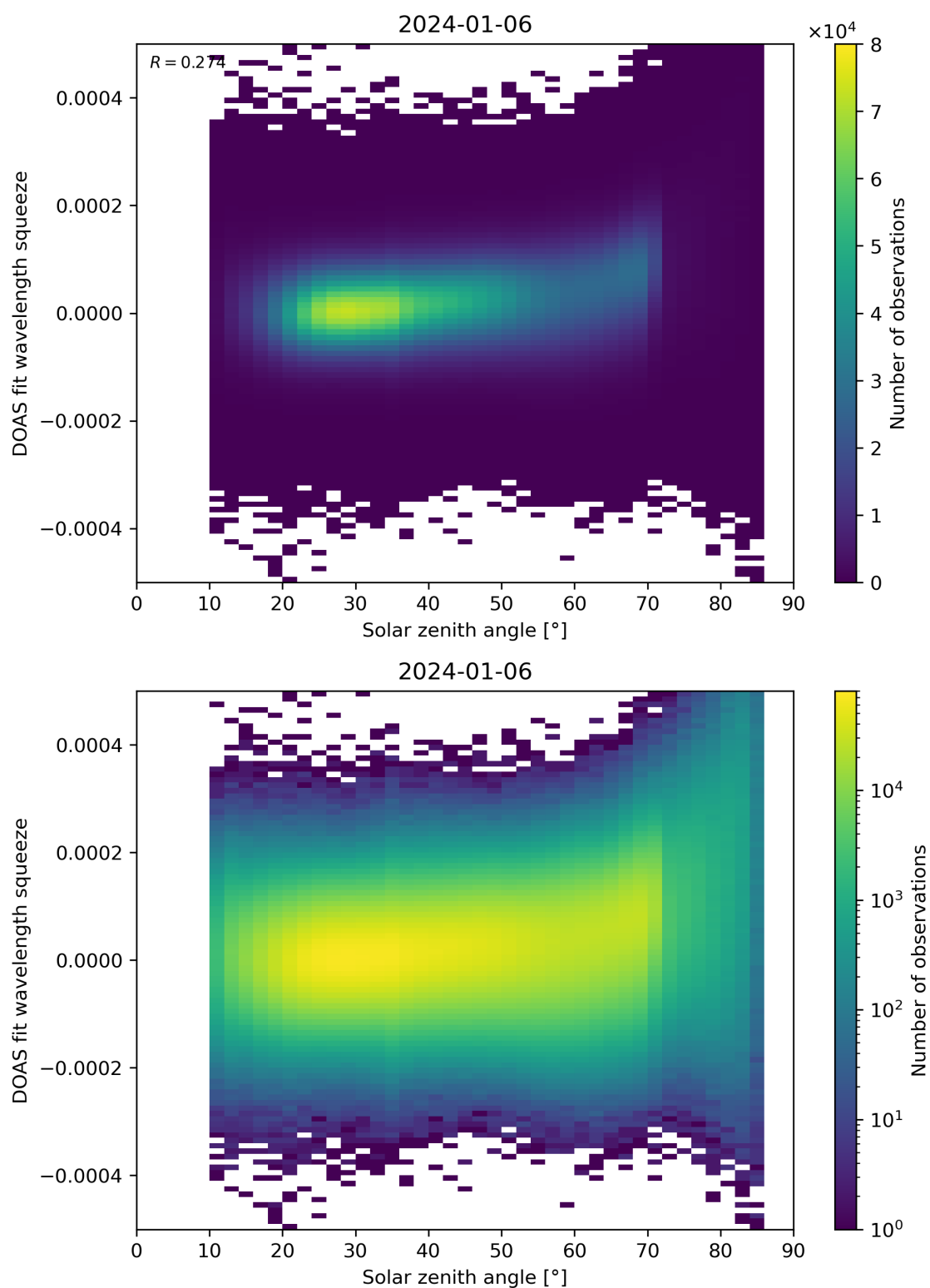
Figure 169: Scatter density plot of “Solar zenith angle” against “DOAS fit wavelength squeeze” for 2024-01-05 to 2024-01-07.
