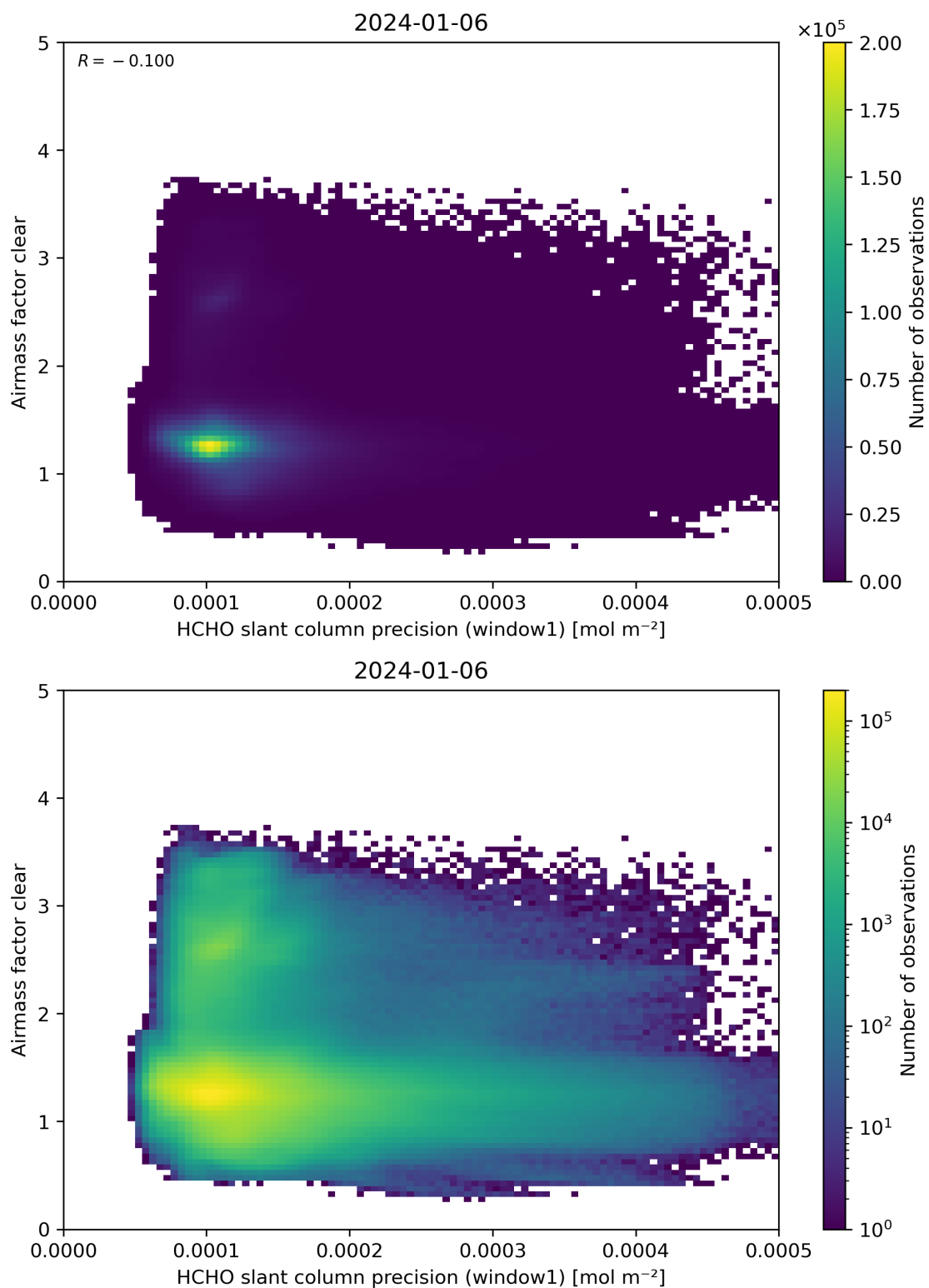
Figure 91: Scatter density plot of “HCHO slant column precision (window1)” against “Airmass factor clear” for 2024-01-05 to 2024-01-07.
