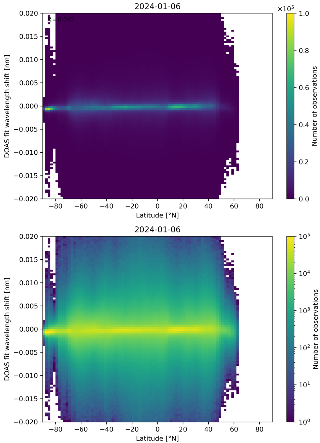
Figure 154: Scatter density plot of “Latitude” against “DOAS fit wavelength shift” for 2024-01-05 to 2024-01-07.
