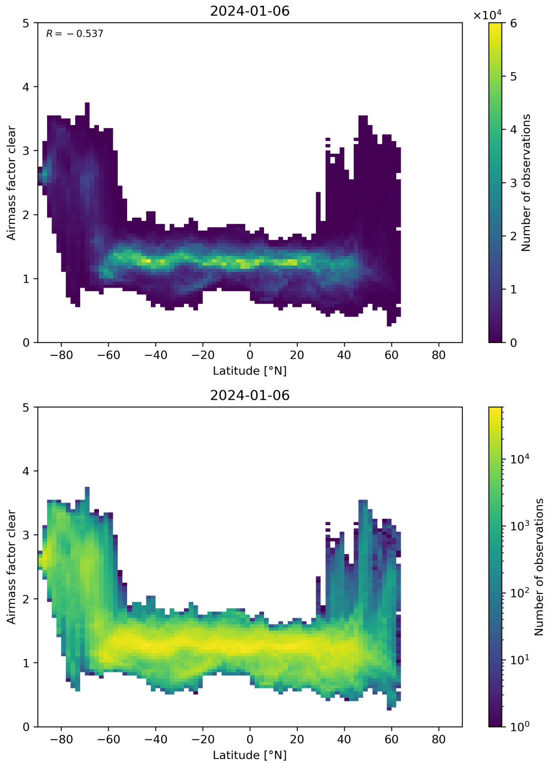
Figure 156: Scatter density plot of “Latitude” against “Airmass factor clear” for 2024-01-05 to 2024-01-07.
