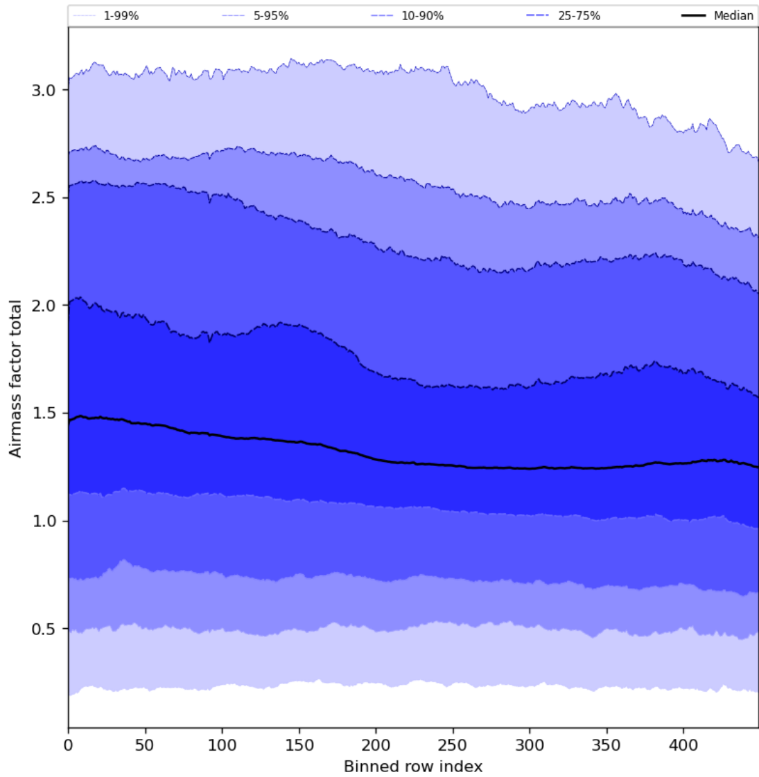
Figure 54: Along track statistics of “Airmass factor total” for 2024-01-05 to 2024-01-07
