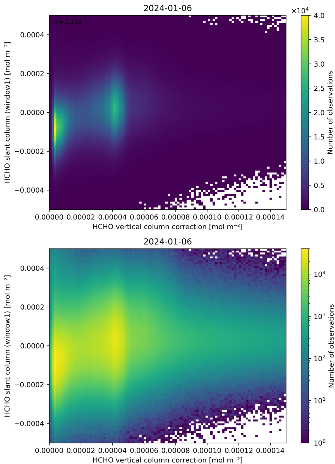
Figure 118: Scatter density plot of “HCHO vertical column correction” against “HCHO slant column (window1)” for 2024-01-05 to 2024-01-07.
