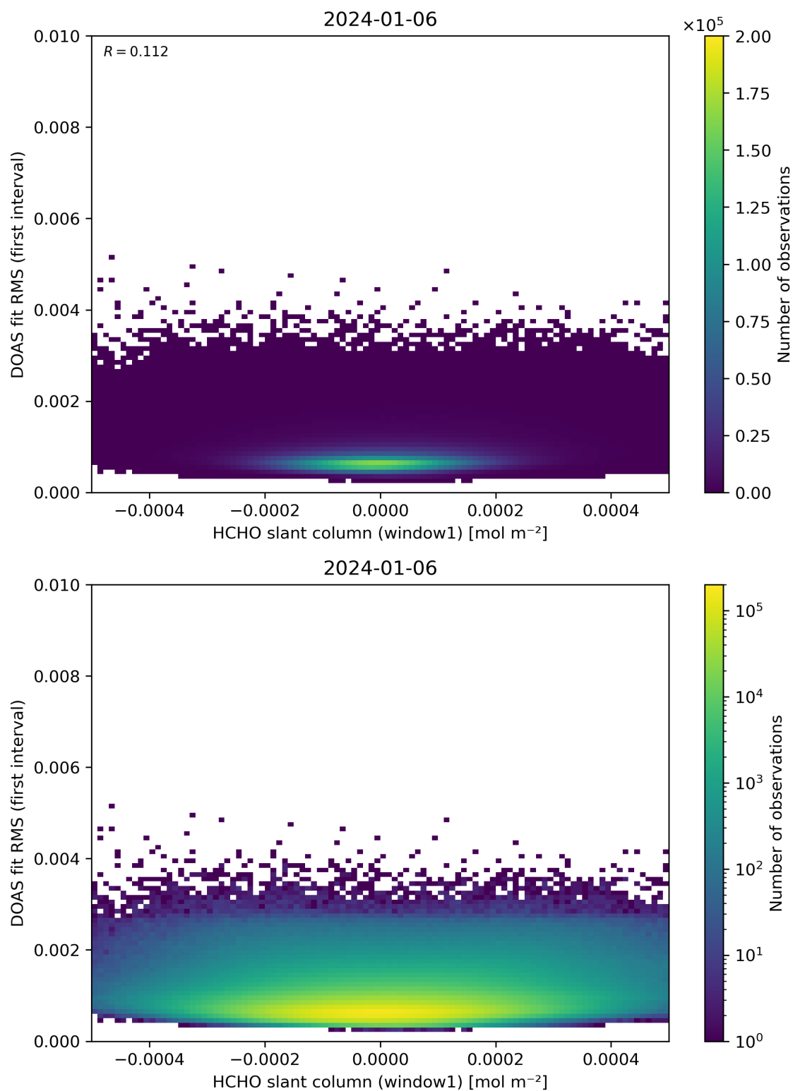
Figure 78: Scatter density plot of “HCHO slant column (window1)” against “DOAS fit RMS (first interval)” for 2024-01-05 to 2024-01-07.
