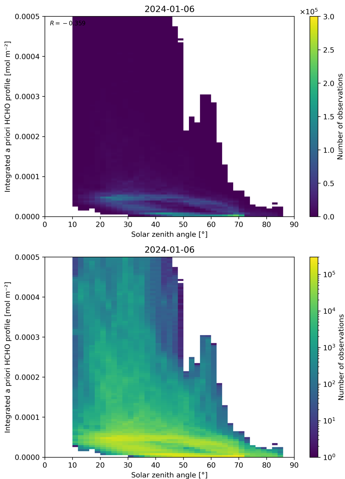
Figure 180: Scatter density plot of “Solar zenith angle” against “Integrated a priori HCHO profile” for 2024-01-05 to 2024-01-07.
