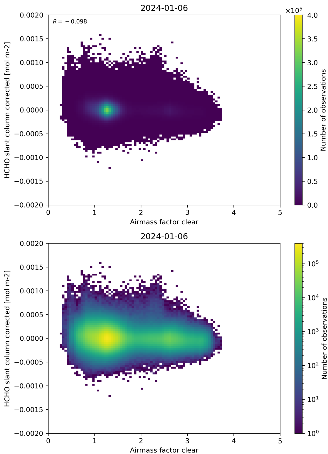
Figure 74: Scatter density plot of “Airmass factor clear” against “HCHO slant column corrected” for 2024-01-05 to 2024-01-07.
