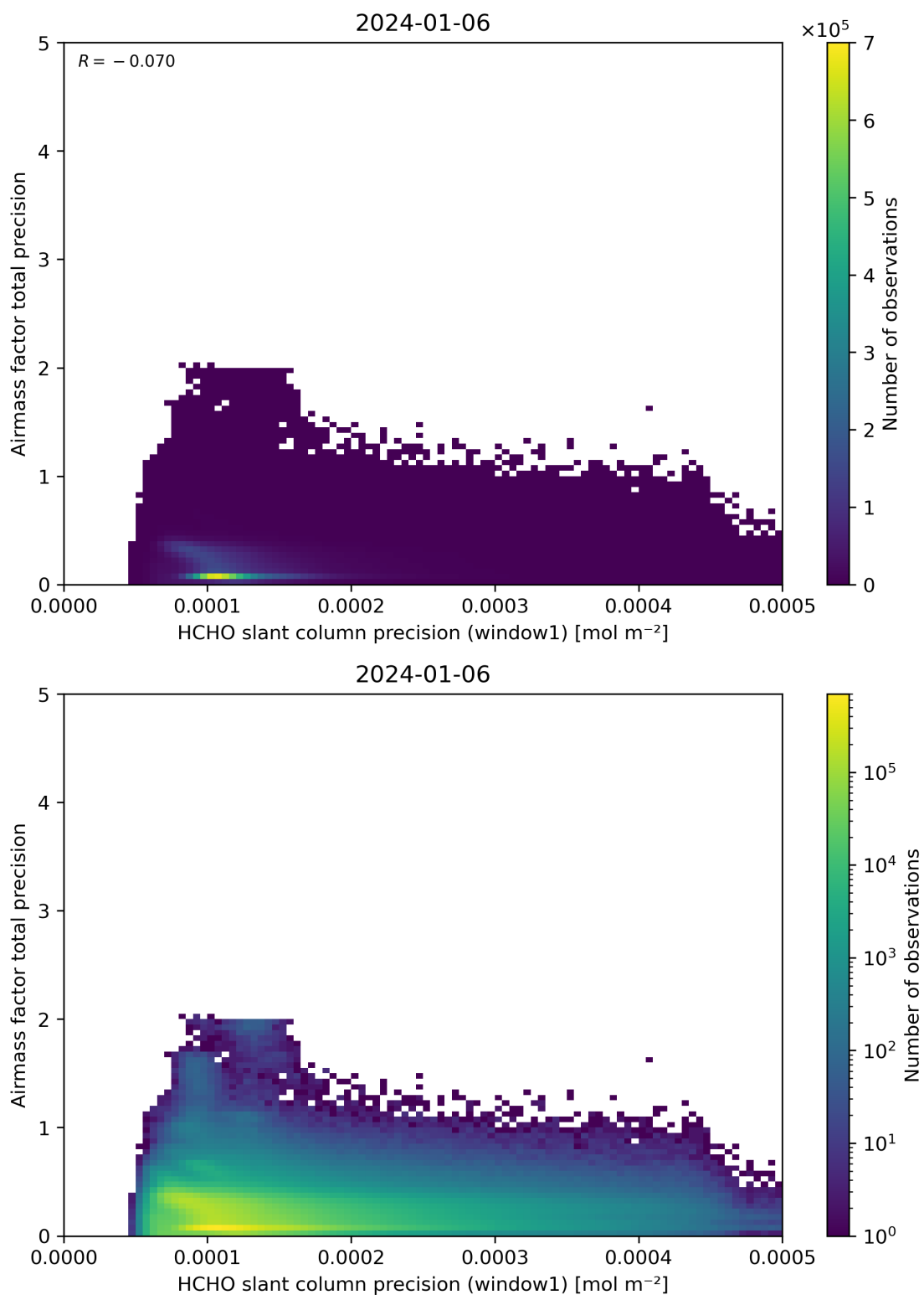
Figure 95: Scatter density plot of “HCHO slant column precision (window1)” against “Airmass factor total precision” for 2024-01-05 to 2024-01-07.
