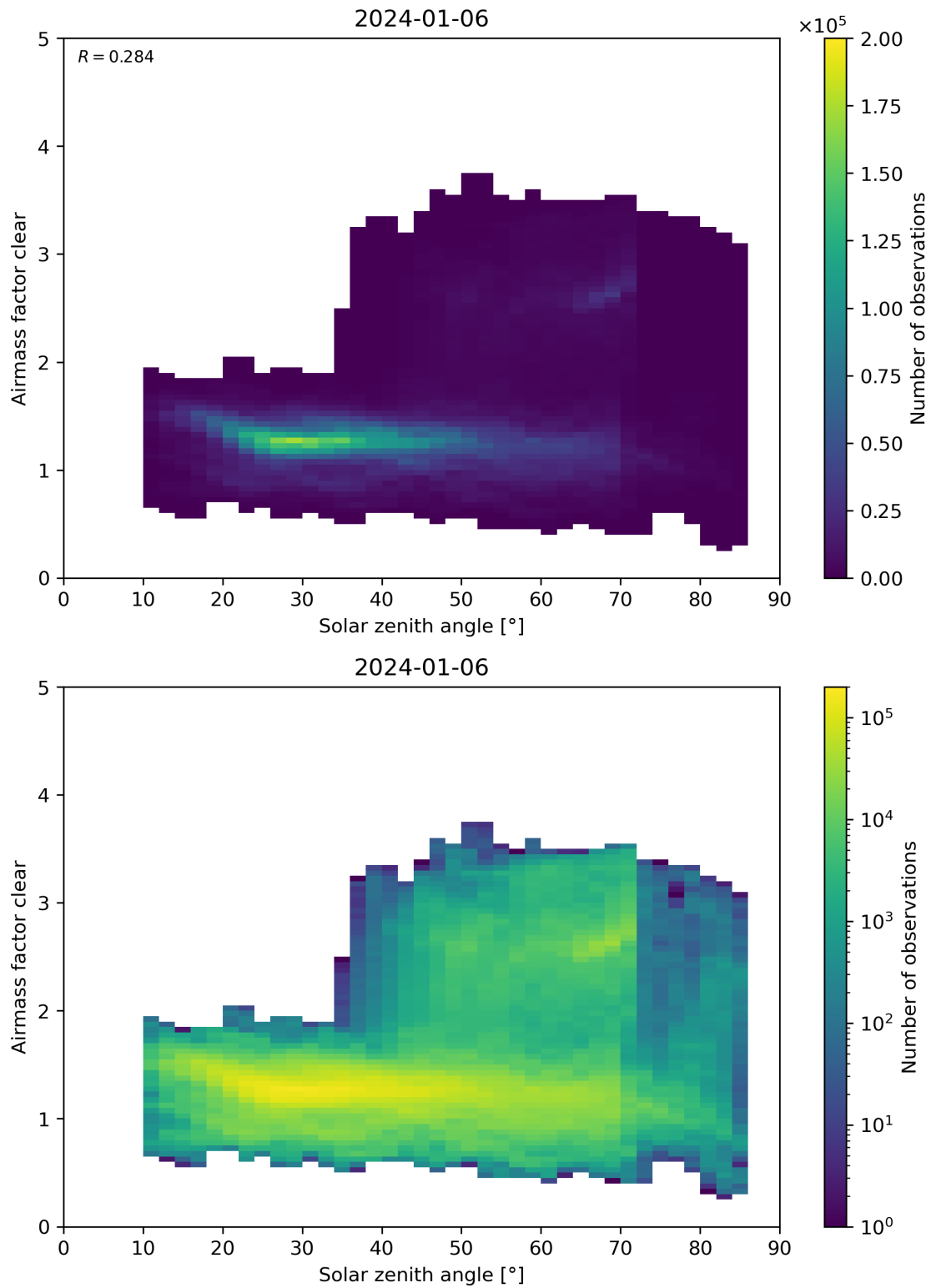
Figure 170: Scatter density plot of “Solar zenith angle” against “Airmass factor clear” for 2024-01-05 to 2024-01-07.
