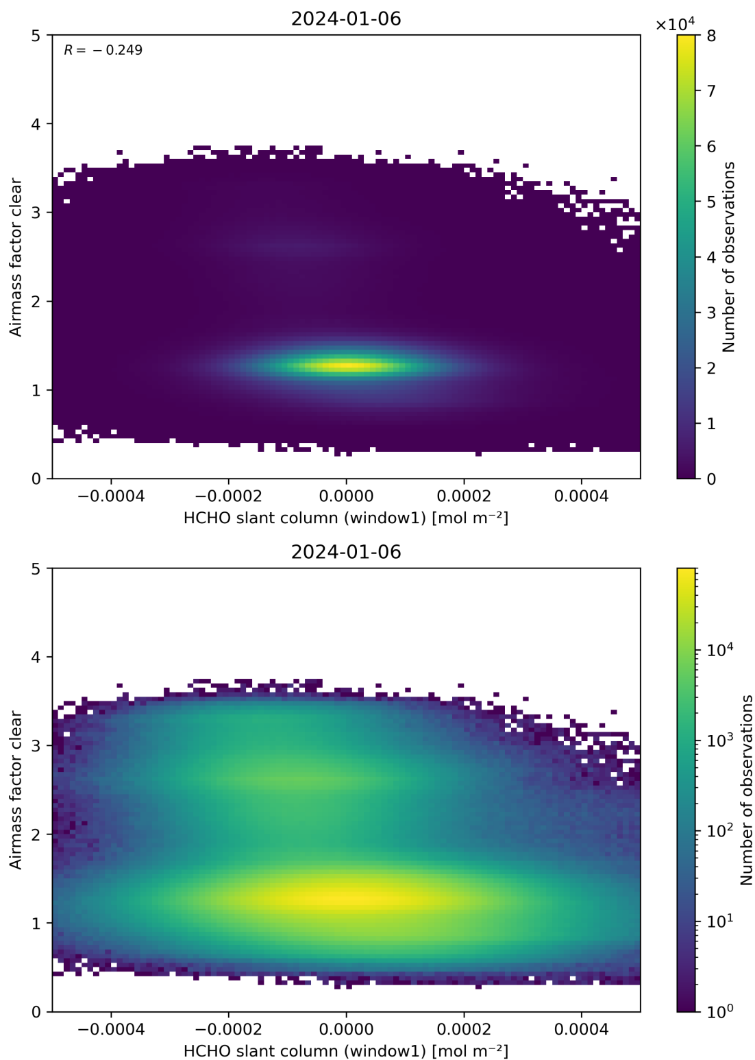
Figure 81: Scatter density plot of “HCHO slant column (window1)” against “Airmass factor clear” for 2024-01-05 to 2024-01-07.
