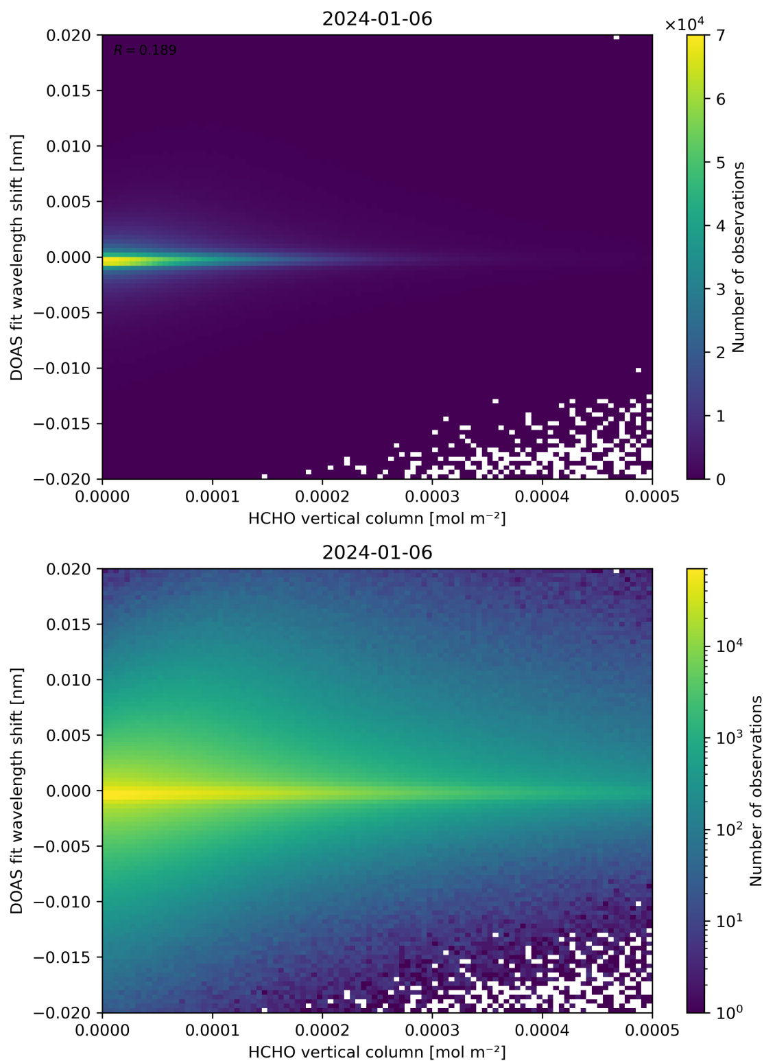
Figure 124: Scatter density plot of “HCHO vertical column” against “DOAS fit wavelength shift” for 2024-01-05 to 2024-01-07.
