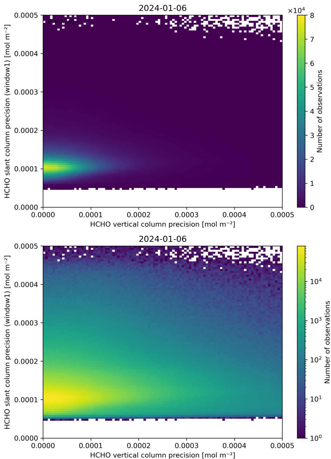
Figure 143: Scatter density plot of “HCHO vertical column precision” against “HCHO slant column precision (window1)” for 2024-01-05 to 2024-01-07.
