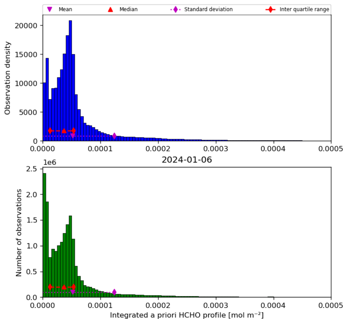
Figure 43: Histogram of “Integrated a priori HCHO profile” for 2024-01-05 to 2024-01-07
