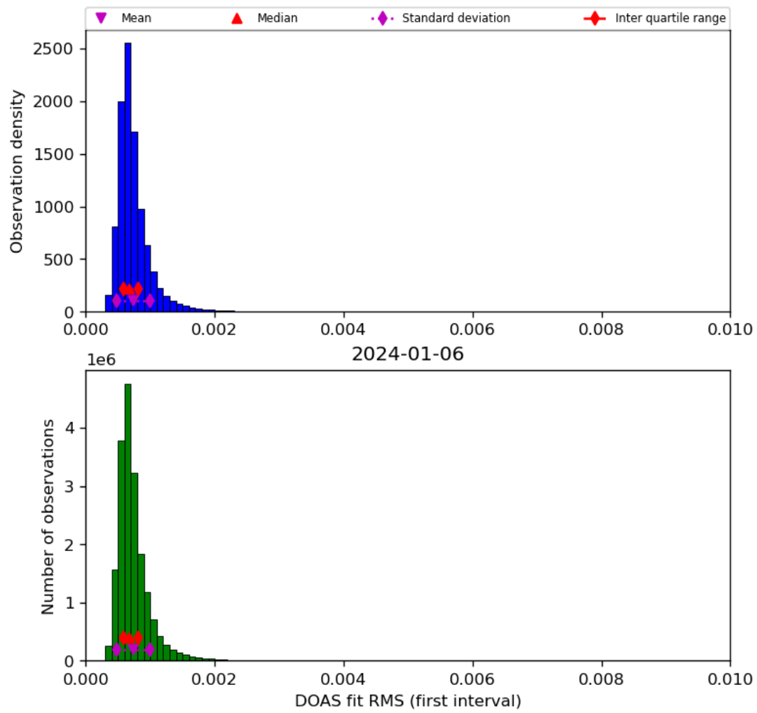
Figure 46: Histogram of “DOAS fit RMS (first interval)” for 2024-01-05 to 2024-01-07
