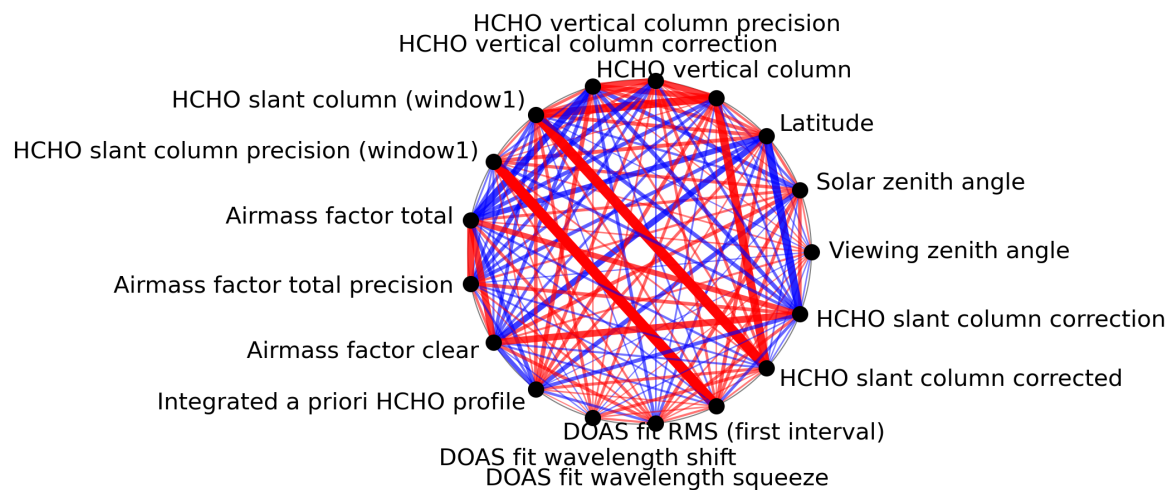
Figure 1: Map of correlation graph for 2024-01-05 to 2024-01-07.
