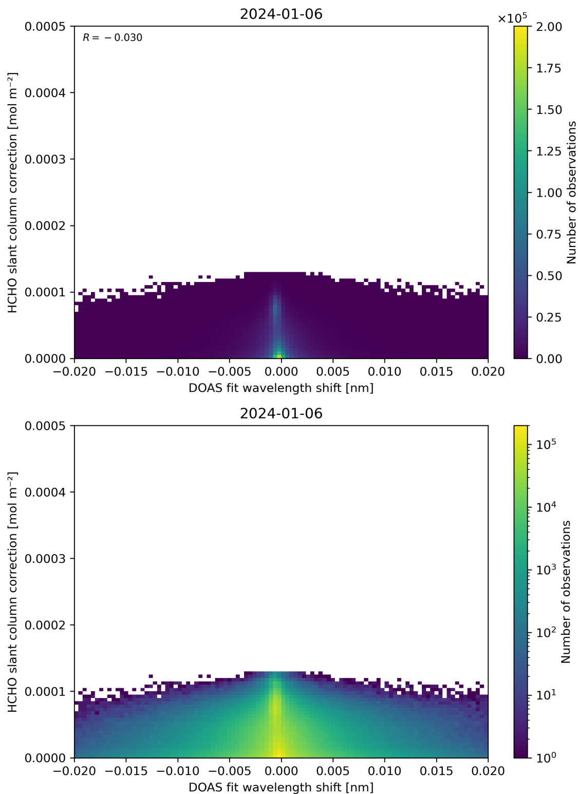
Figure 67: Scatter density plot of “DOAS fit wavelength shift” against “HCHO slant column correction” for 2024-01-05 to 2024-01-07.
