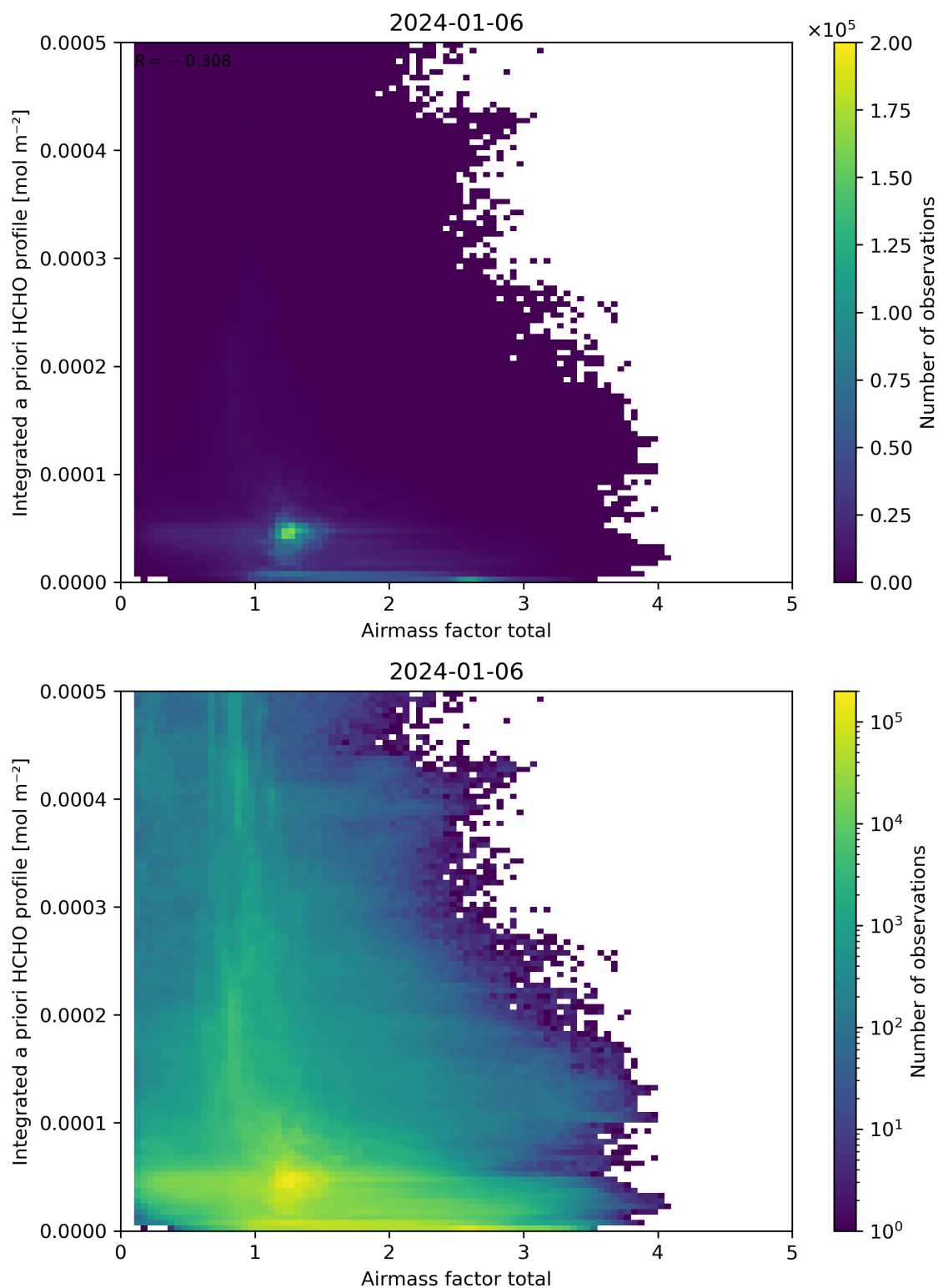
Figure 104: Scatter density plot of “Airmass factor total” against “Integrated a priori HCHO profile” for 2024-01-05 to 2024-01-07.
