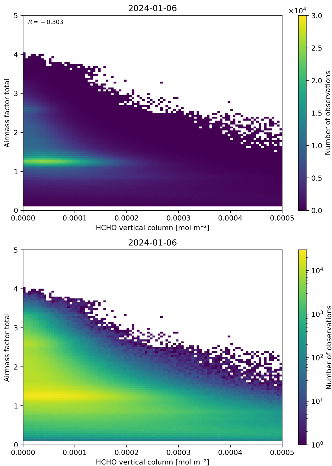
Figure 131: Scatter density plot of “HCHO vertical column” against “Airmass factor total” for 2024-01-05 to 2024-01-07.
