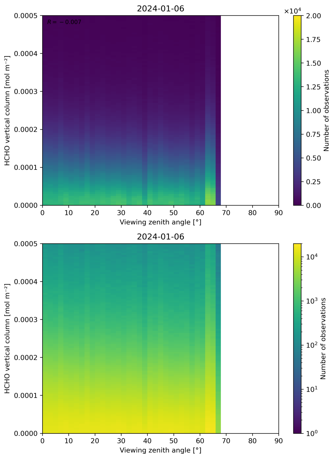
Figure 192: Scatter density plot of “Viewing zenith angle” against “HCHO vertical column” for 2024-01-05 to 2024-01-07.
