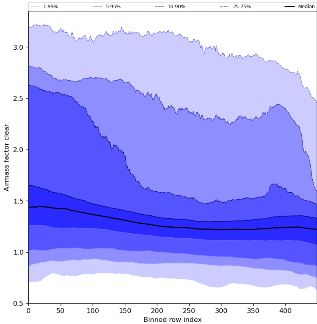
Figure 56: Along track statistics of “Airmass factor clear” for 2024-01-05 to 2024-01-07
