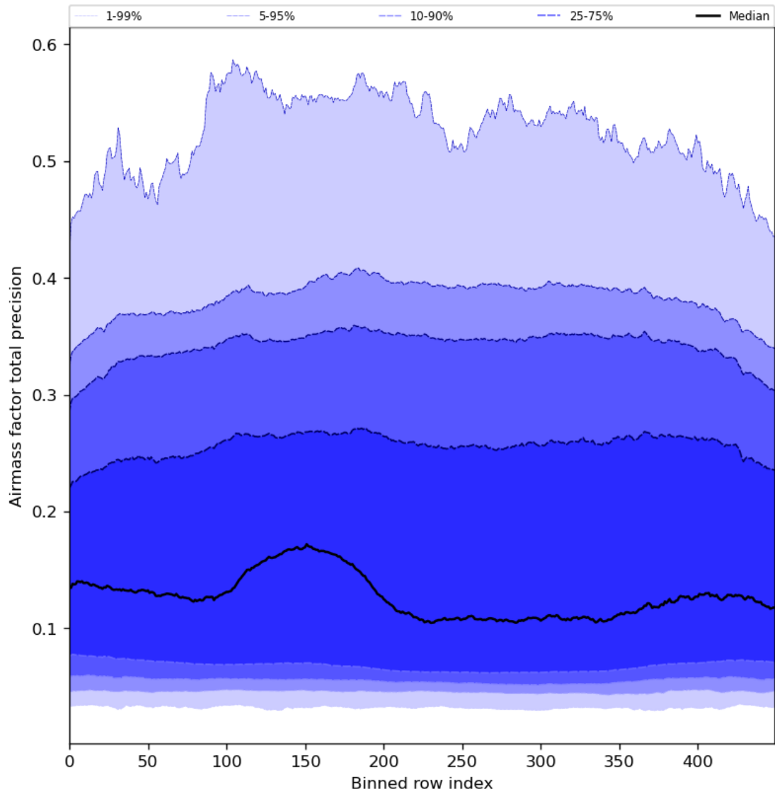
Figure 55: Along track statistics of “Airmass factor total precision” for 2024-01-05 to 2024-01-07
