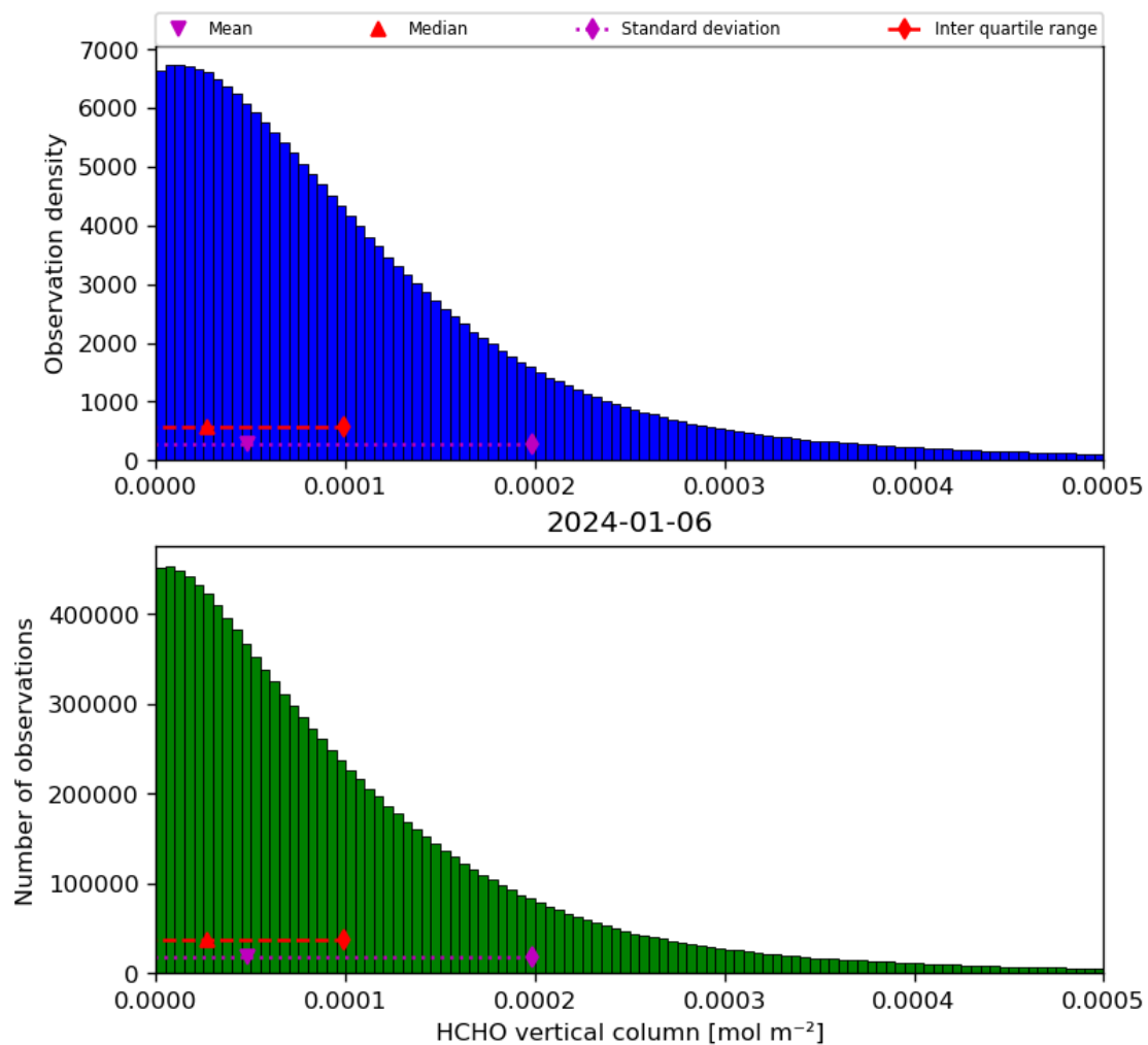
Figure 35: Histogram of “HCHO vertical column” for 2024-01-05 to 2024-01-07
