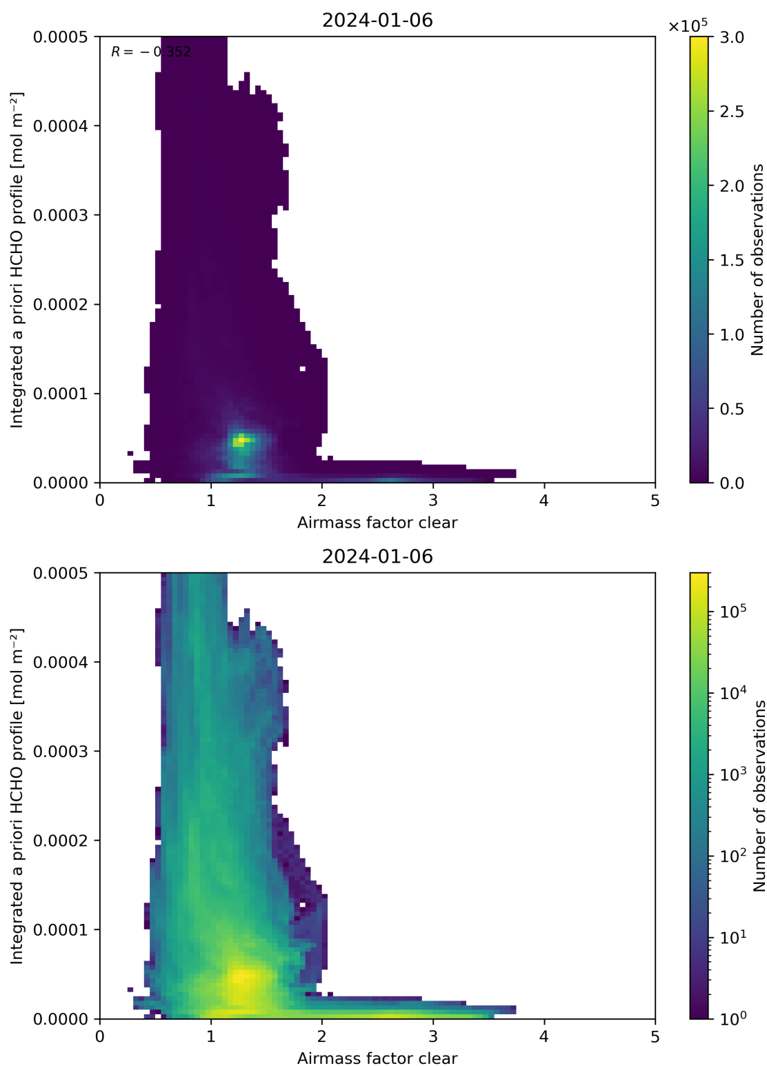
Figure 76: Scatter density plot of “Airmass factor clear” against “Integrated a priori HCHO profile” for 2024-01-05 to 2024-01-07.
