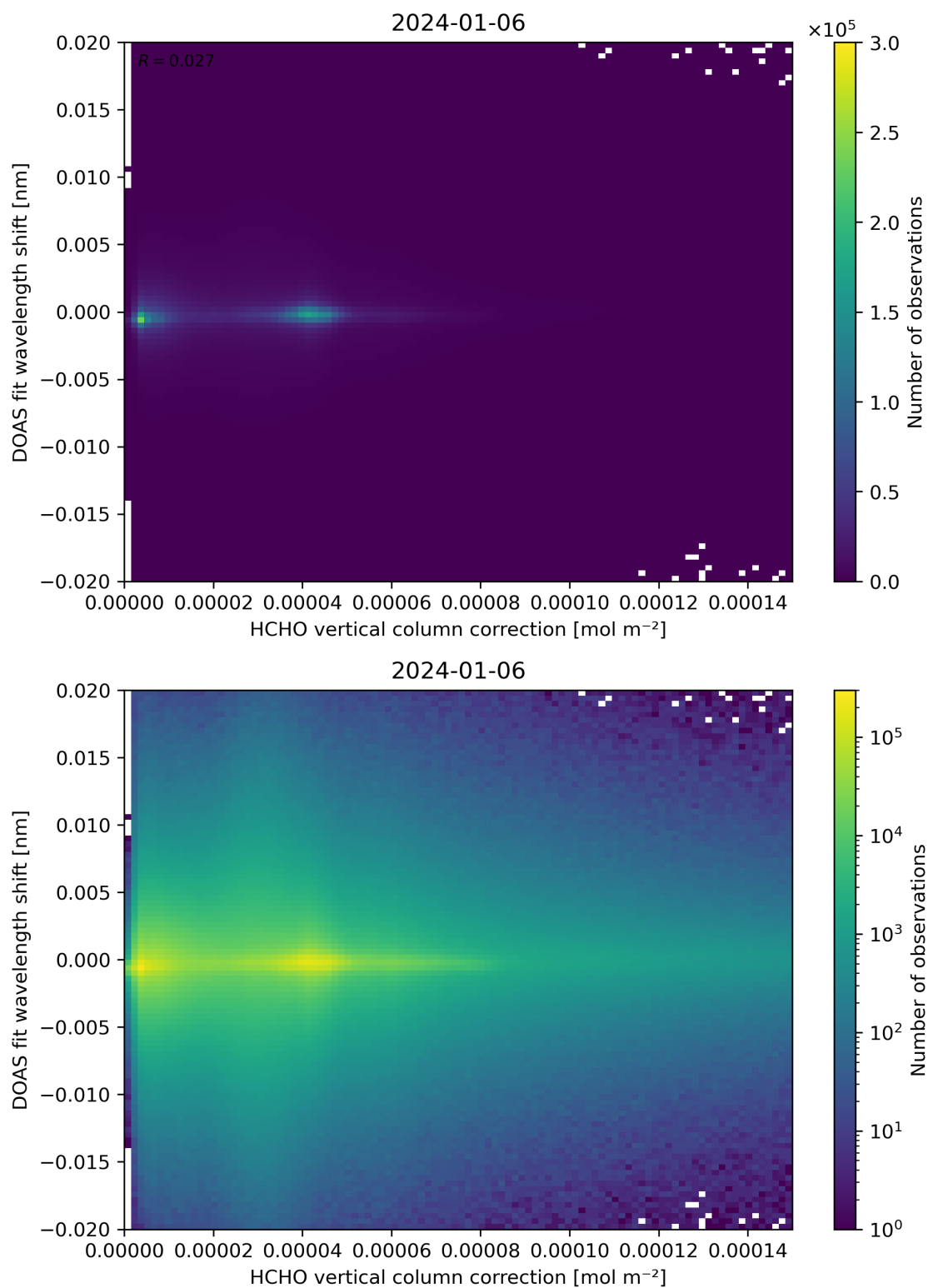
Figure 113: Scatter density plot of “HCHO vertical column correction” against “DOAS fit wavelength shift” for 2024-01-05 to 2024-01-07.
