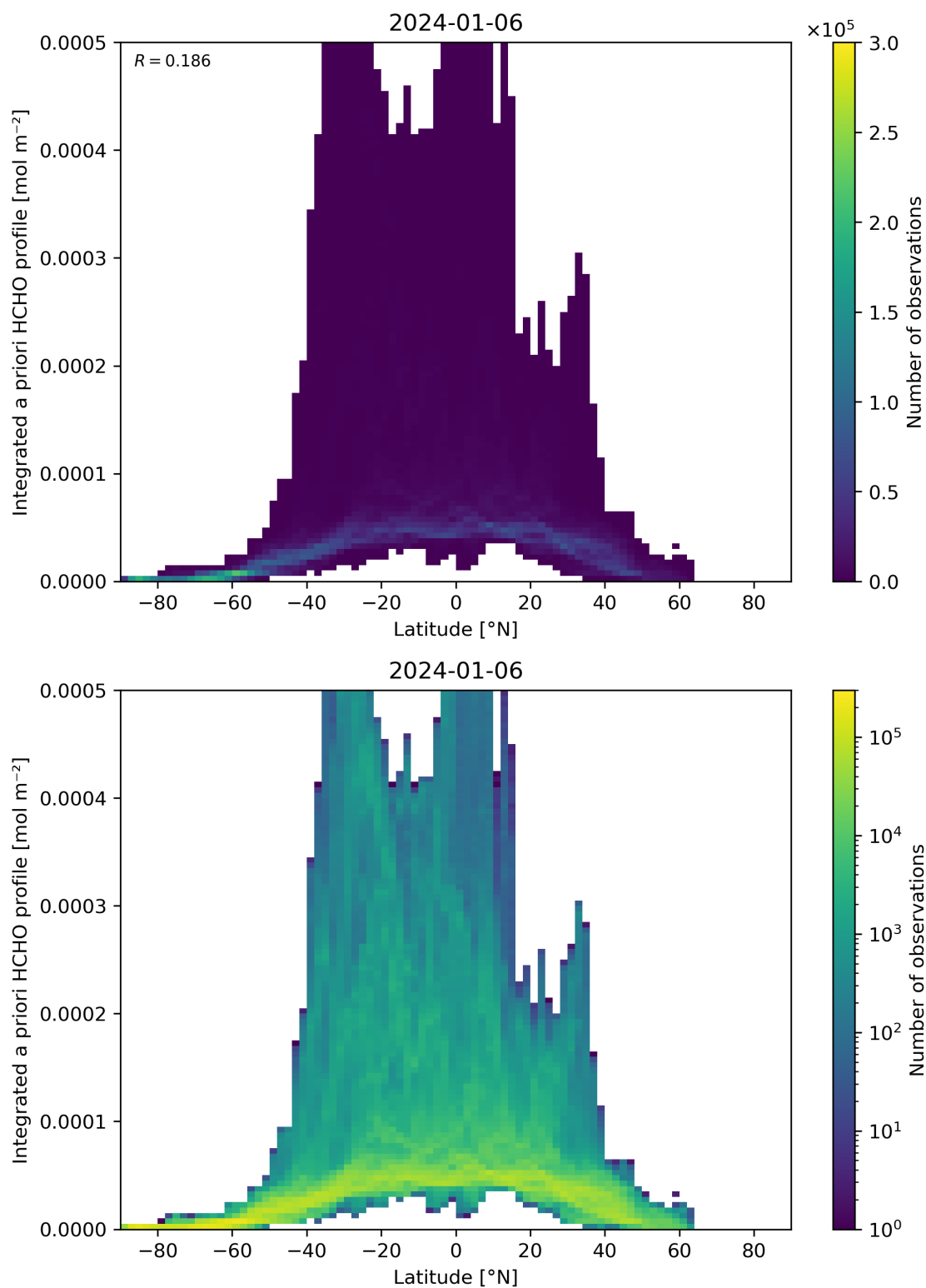
Figure 166: Scatter density plot of “Latitude” against “Integrated a priori HCHO profile” for 2024-01-05 to 2024-01-07.
