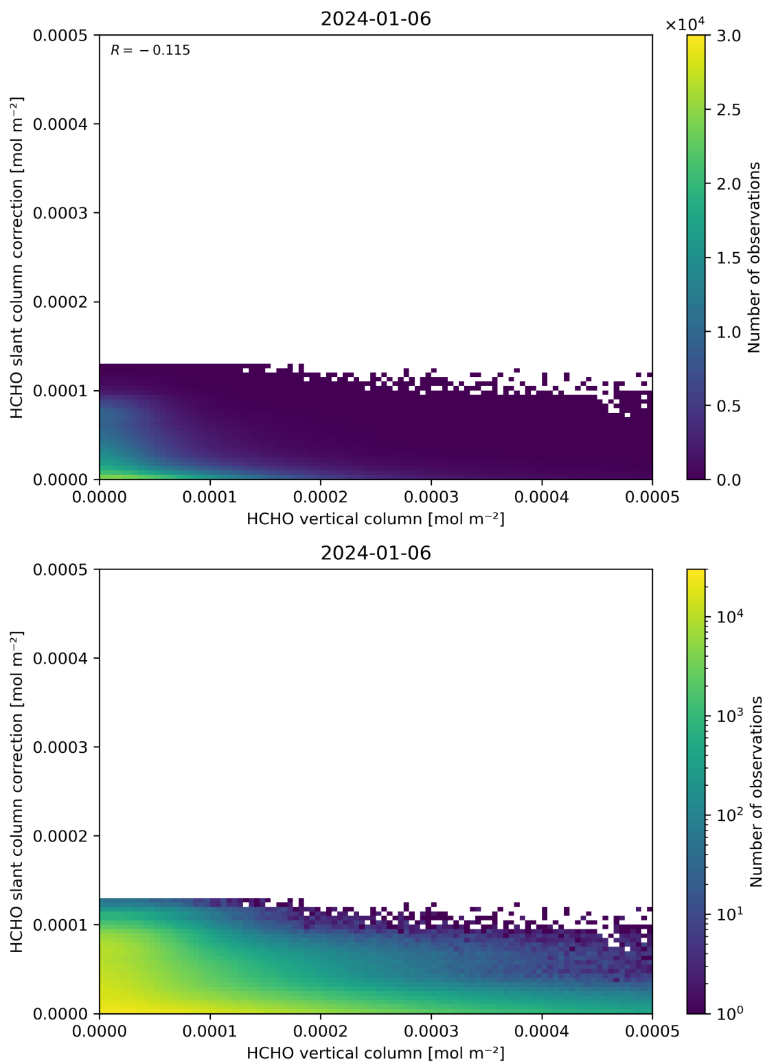
Figure 128: Scatter density plot of “HCHO vertical column” against “HCHO slant column correction” for 2024-01-05 to 2024-01-07.
