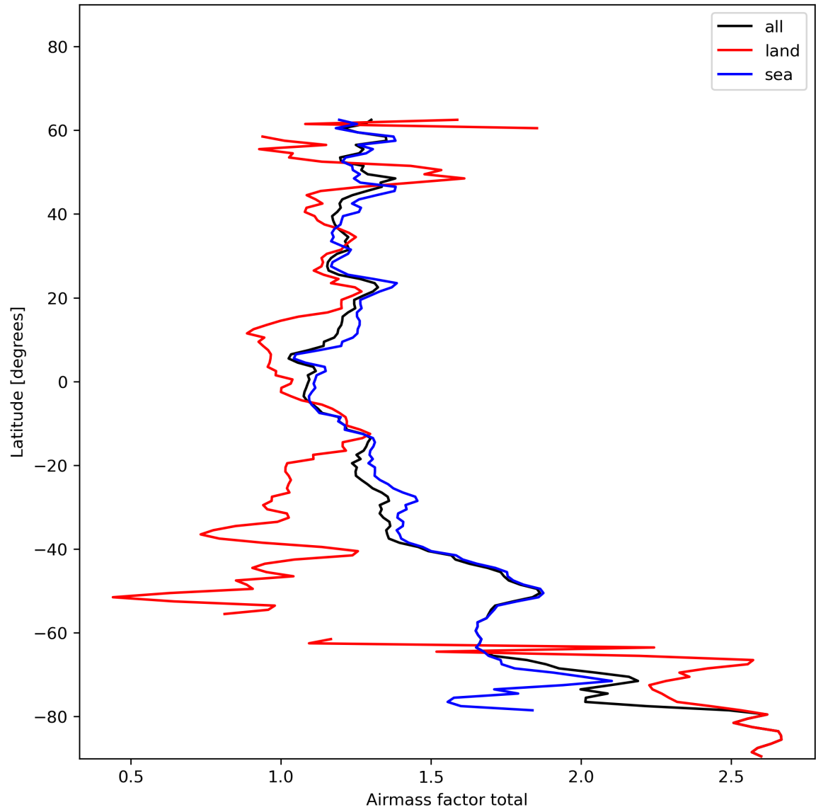
Figure 26: Zonal average of “Airmass factor total” for 2024-01-05 to 2024-01-07.
