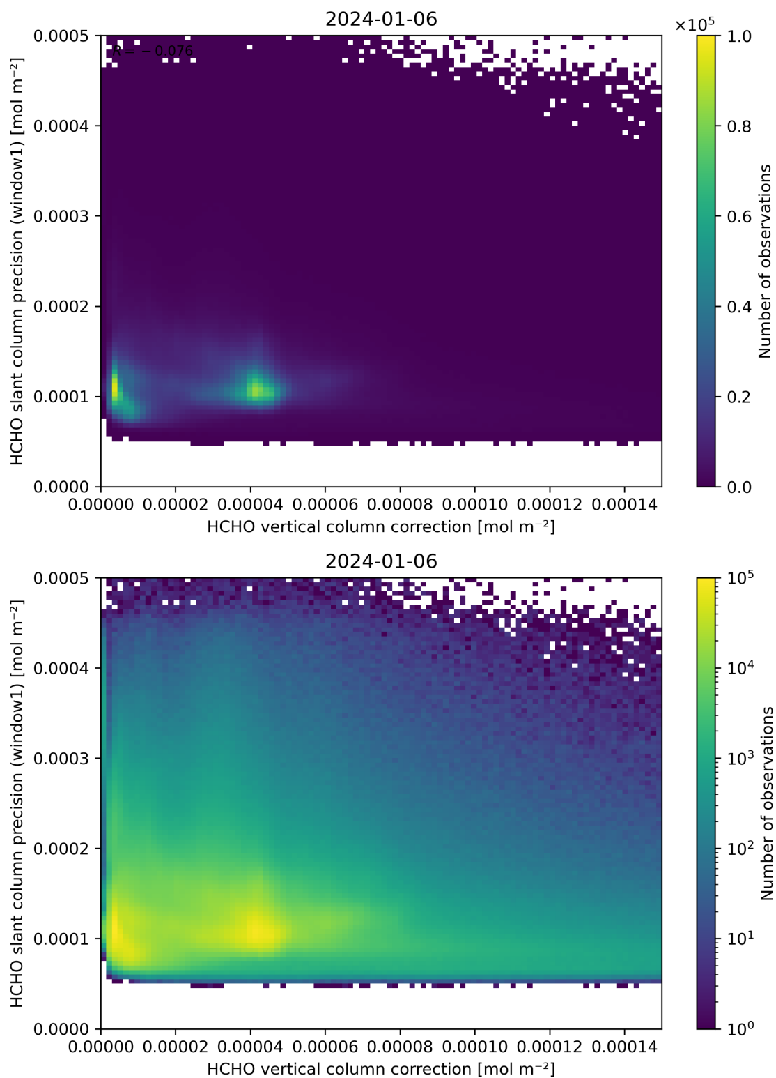
Figure 119: Scatter density plot of “HCHO vertical column correction” against “HCHO slant column precision (window1)” for 2024-01-05 to 2024-01-07.
