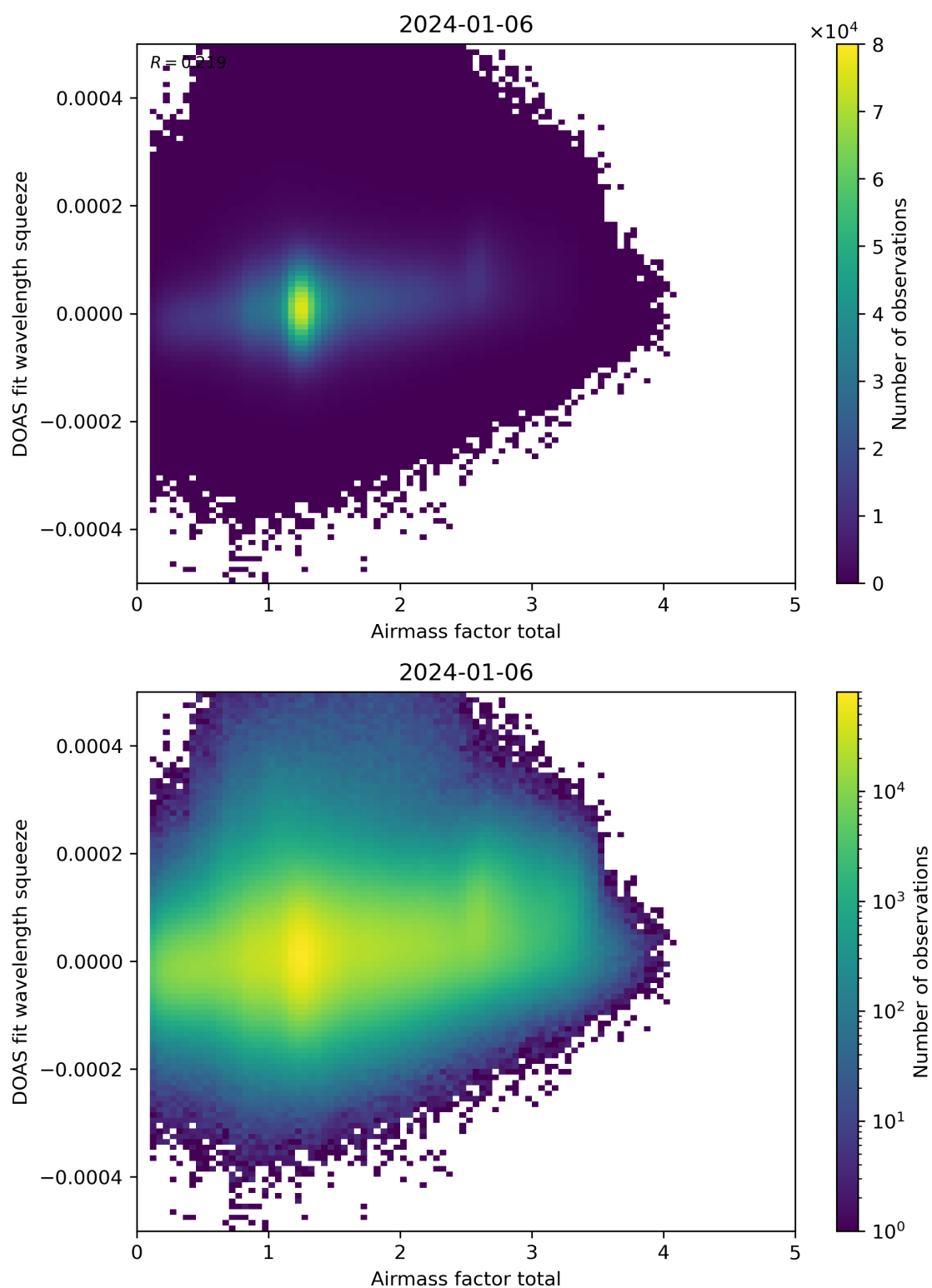
Figure 99: Scatter density plot of “Airmass factor total” against “DOAS fit wavelength squeeze” for 2024-01-05 to 2024-01-07.
