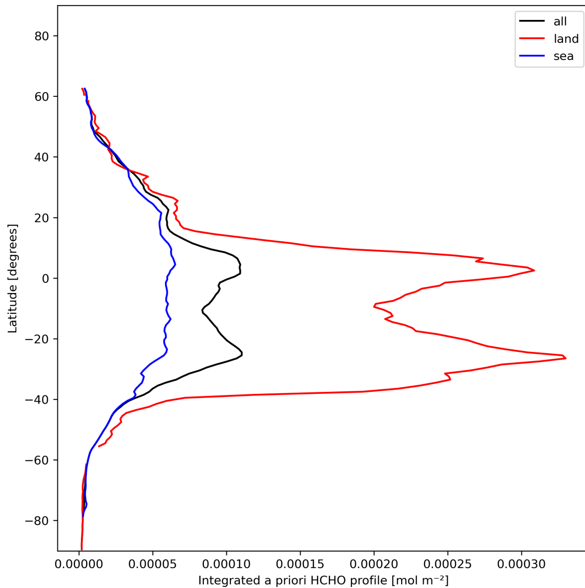
Figure 29: Zonal average of “Integrated a priori HCHO profile” for 2024-01-05 to 2024-01-07.
