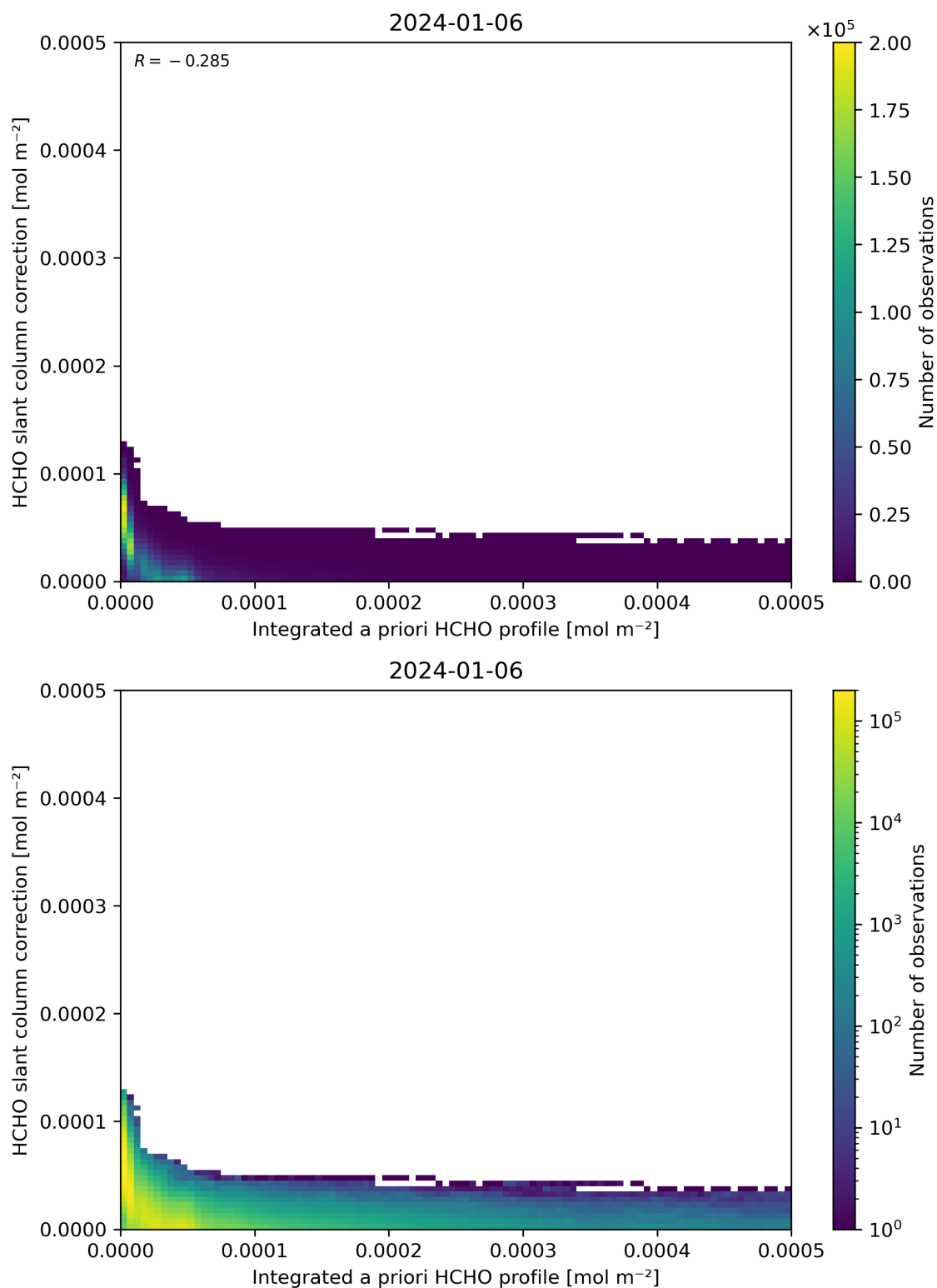
Figure 152: Scatter density plot of “Integrated a priori HCHO profile” against “HCHO slant column correction” for 2024-01-05 to 2024-01-07.
