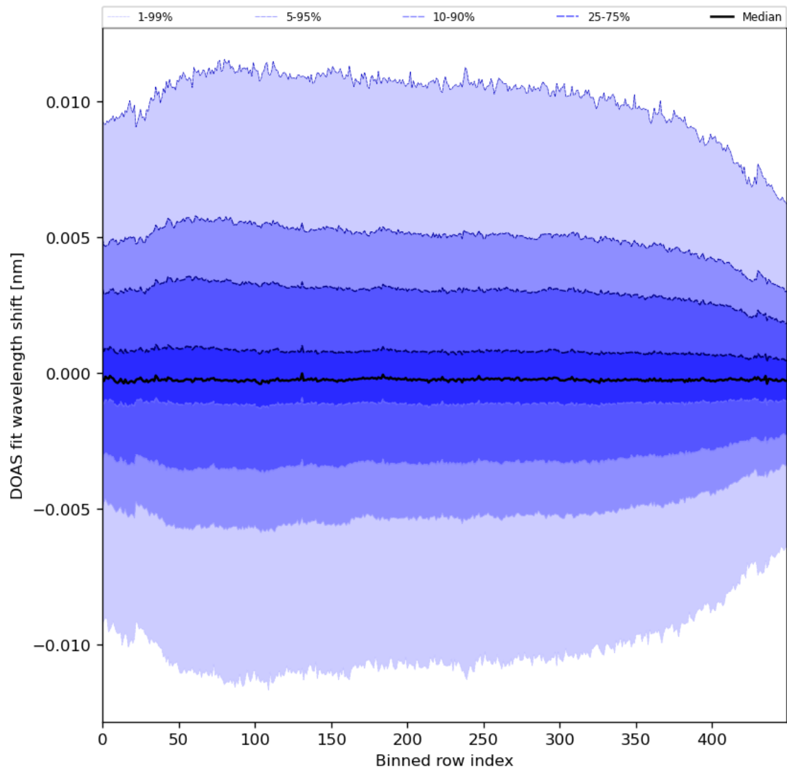
Figure 58: Along track statistics of “DOAS fit wavelength shift” for 2024-01-05 to 2024-01-07
