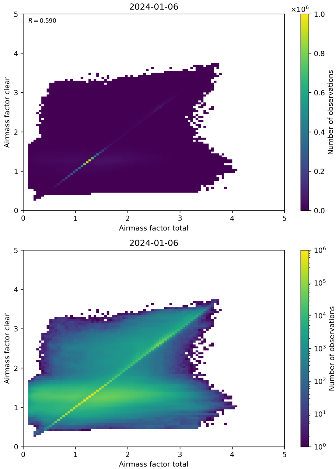
Figure 100: Scatter density plot of “Airmass factor total” against “Airmass factor clear” for 2024-01-05 to 2024-01-07.
