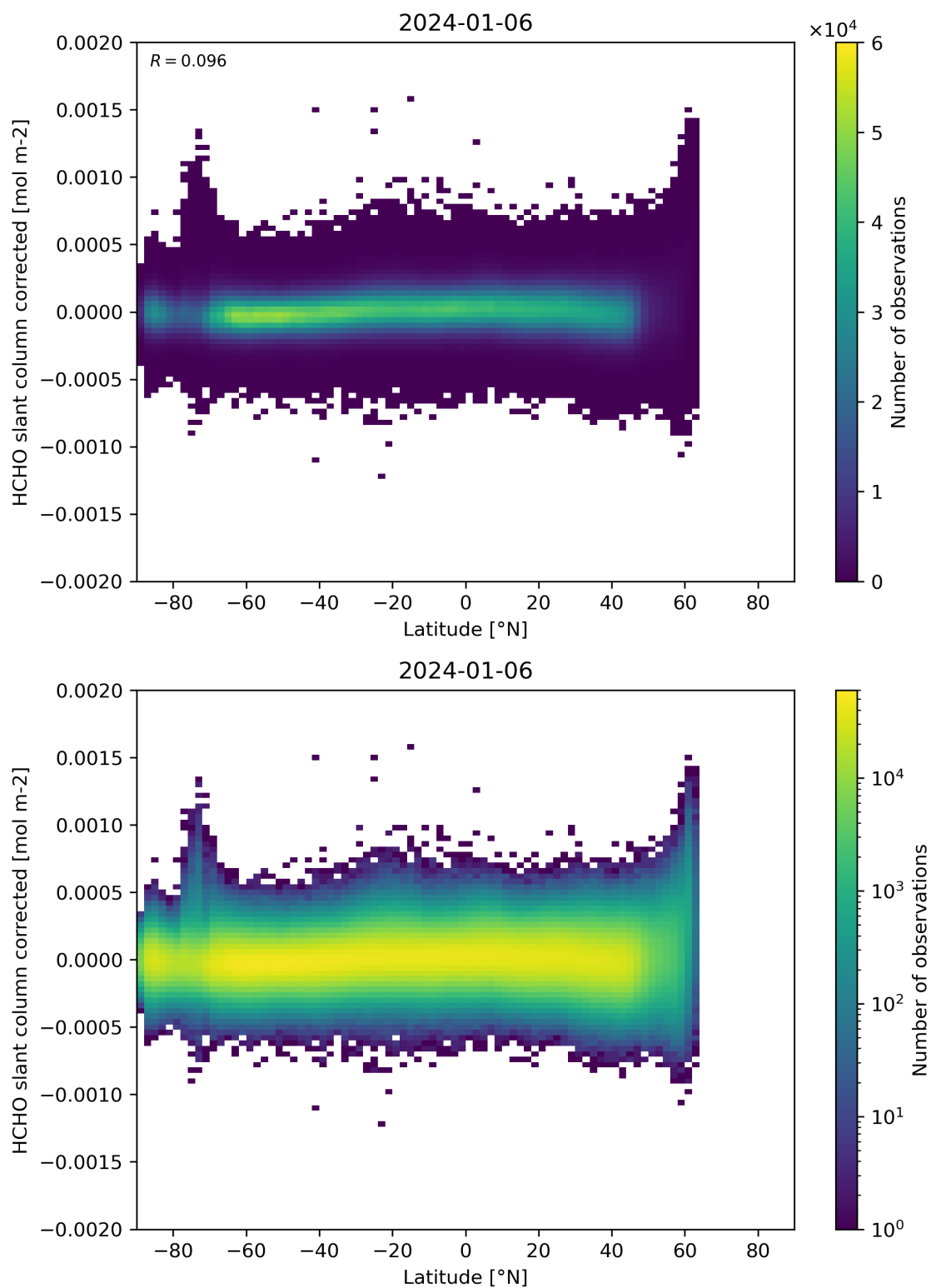
Figure 157: Scatter density plot of “Latitude” against “HCHO slant column corrected” for 2024-01-05 to 2024-01-07.
