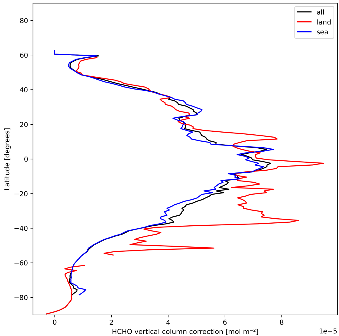
Figure 23: Zonal average of “HCHO vertical column correction” for 2024-01-05 to 2024-01-07.
