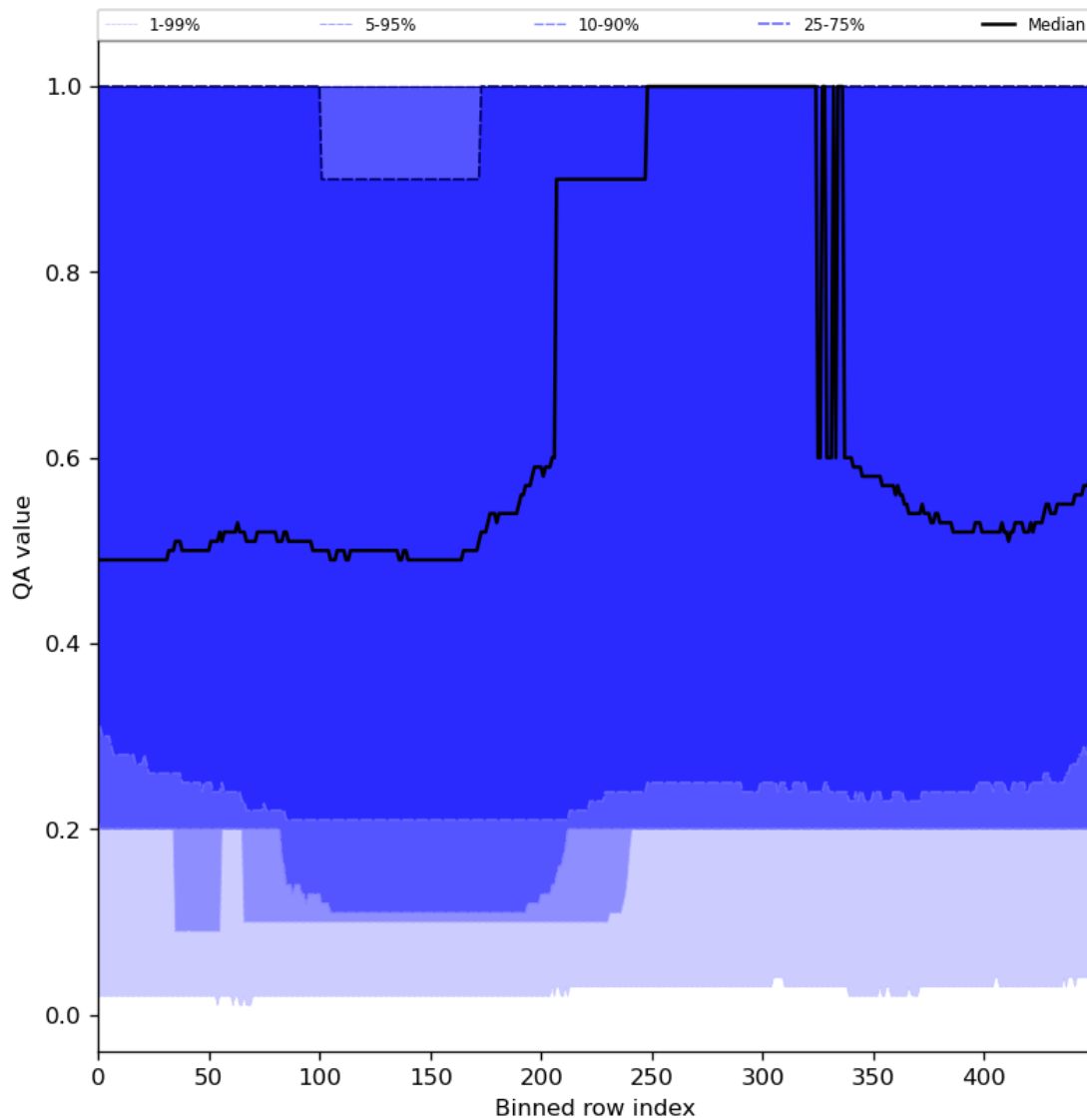
Figure 48: Along track statistics of “QA value” for 2024-01-05 to 2024-01-07
