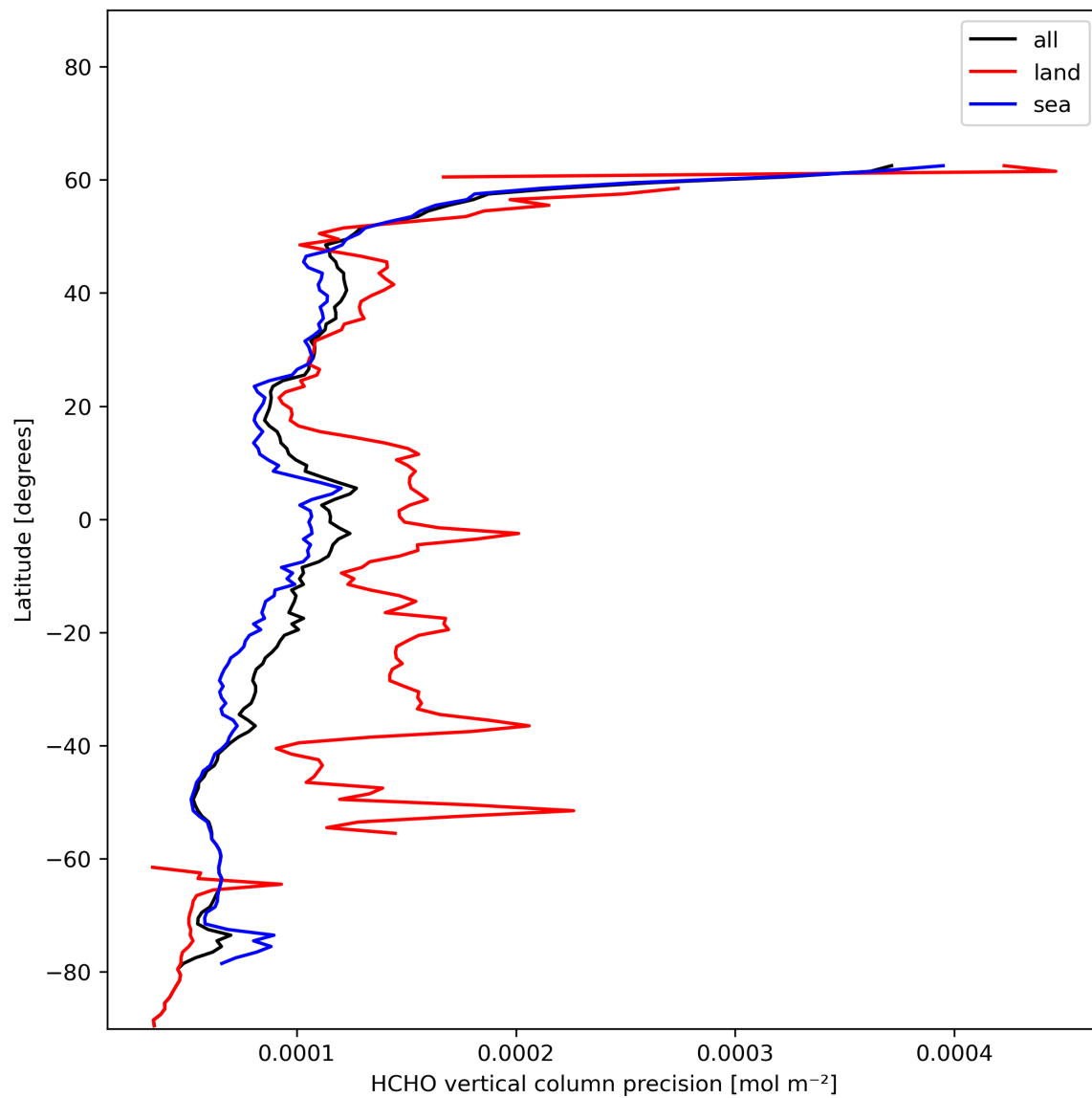
Figure 22: Zonal average of “HCHO vertical column precision” for 2024-01-05 to 2024-01-07.
