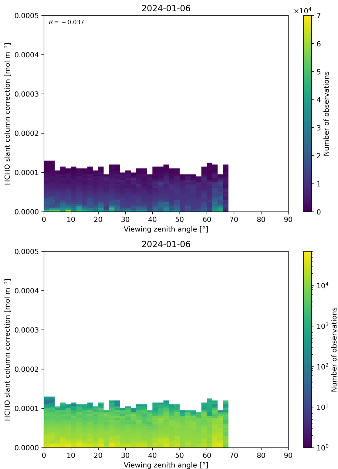
Figure 187: Scatter density plot of “Viewing zenith angle” against “HCHO slant column correction” for 2024-01-05 to 2024-01-07.
