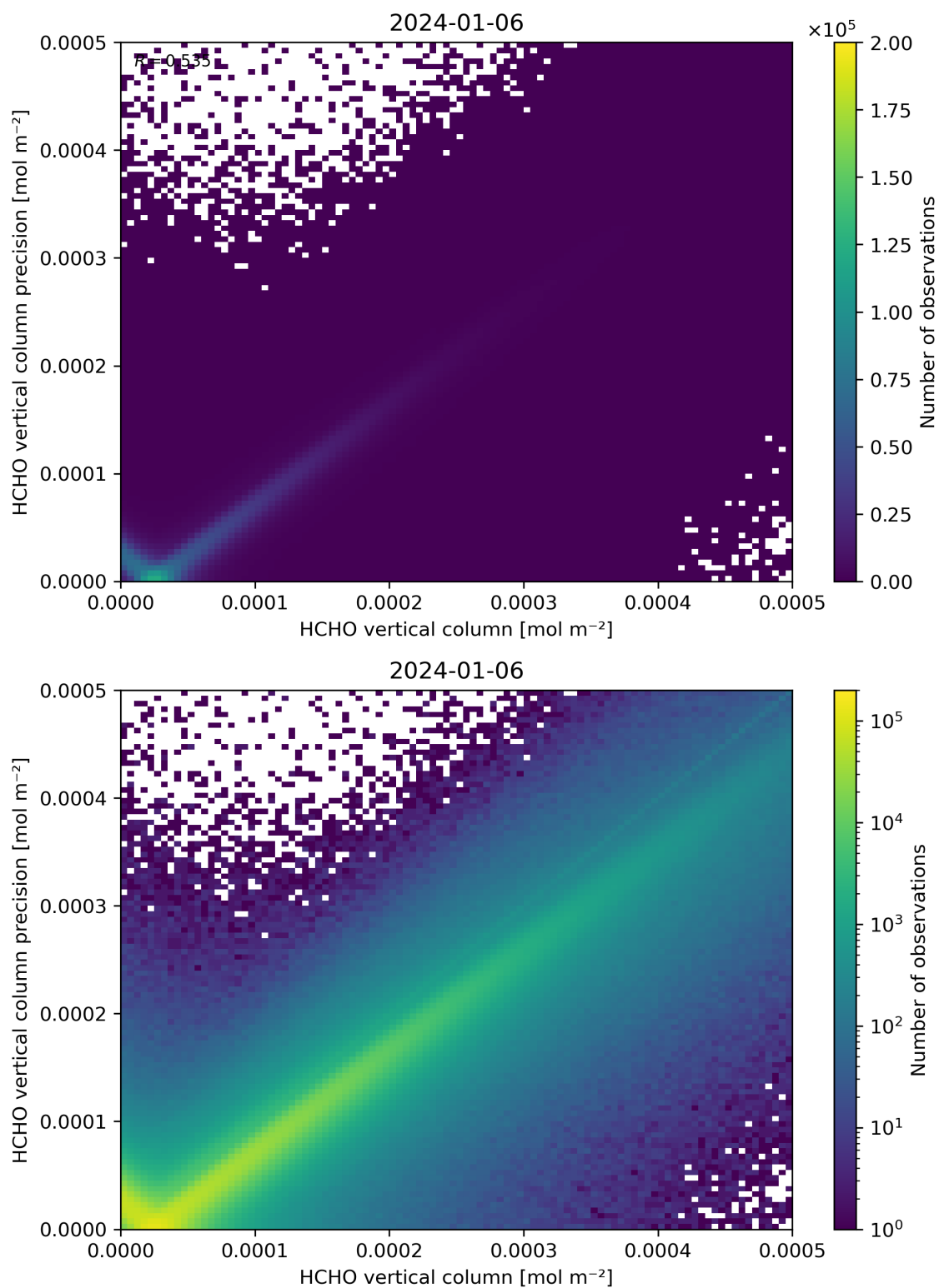
Figure 134: Scatter density plot of “HCHO vertical column” against “HCHO vertical column precision” for 2024-01-05 to 2024-01-07.
