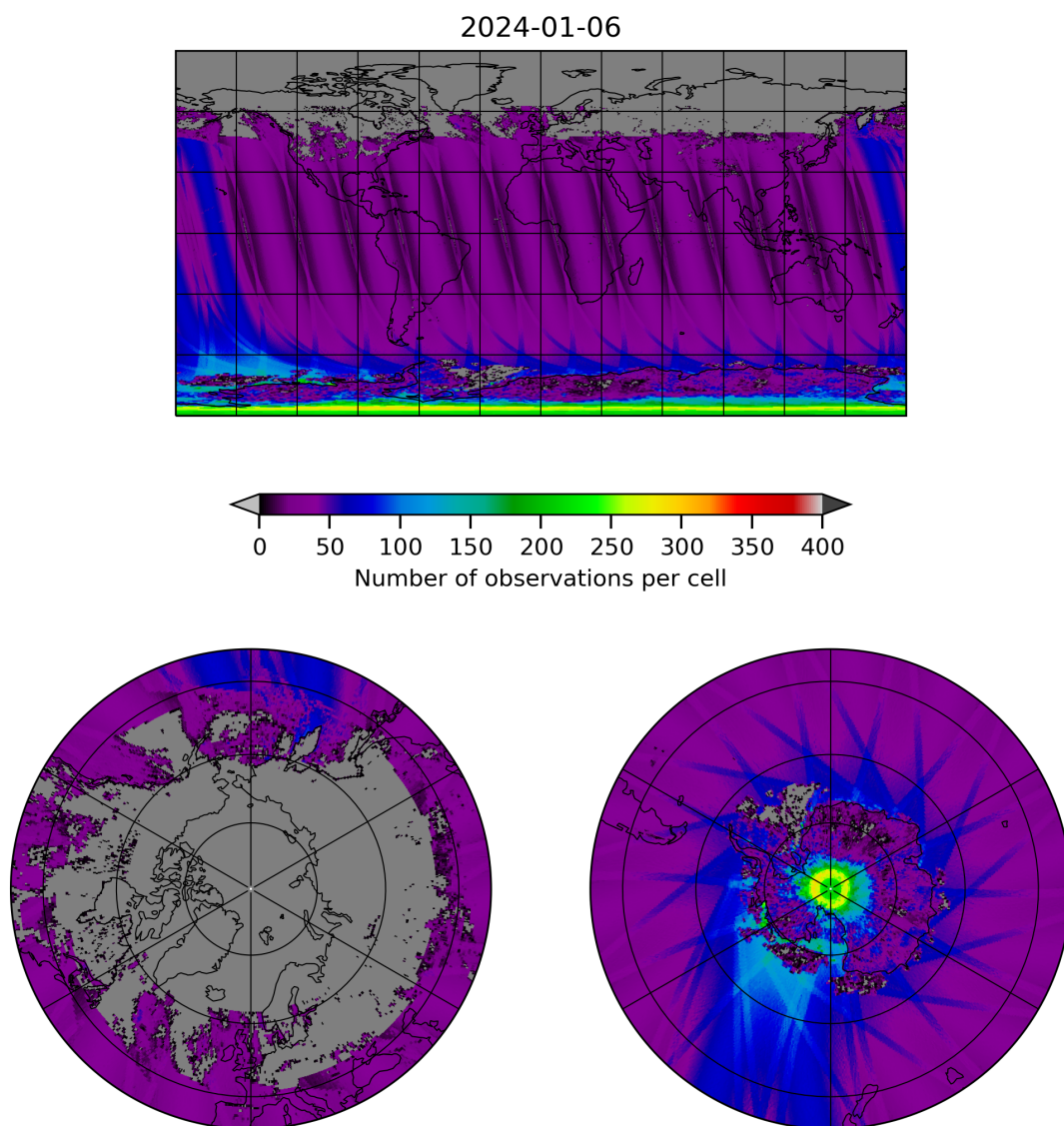
Figure 19: Map of the number of observations for 2024-01-05 to 2024-01-07
