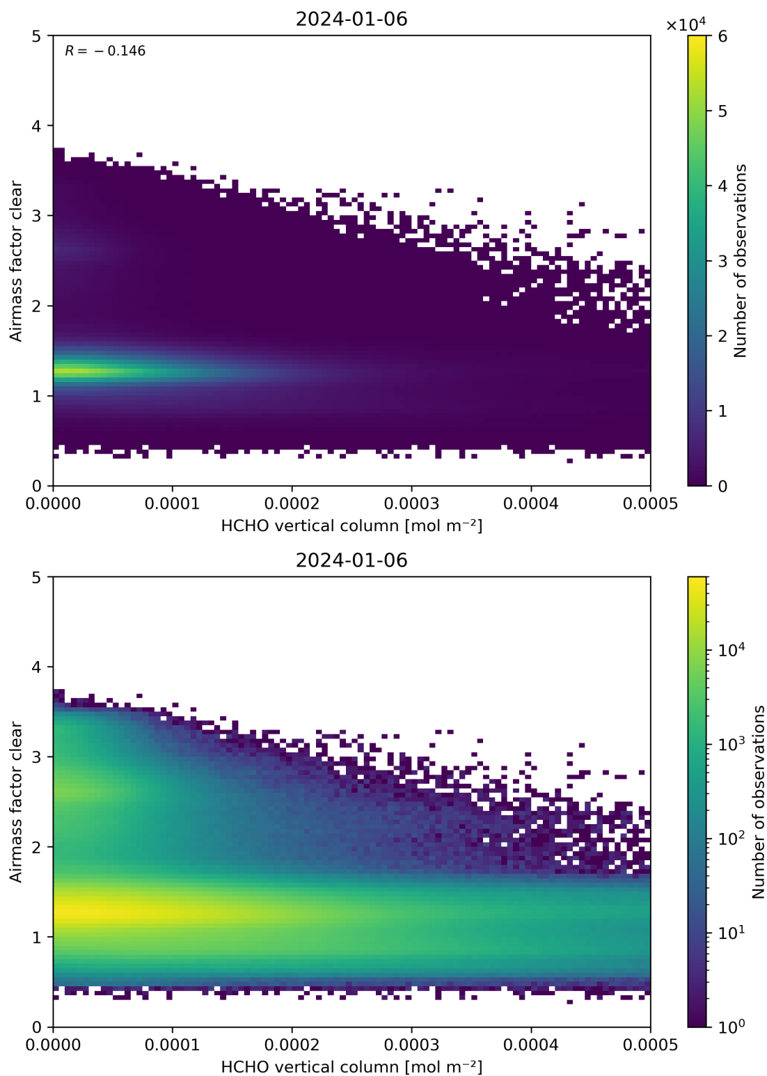
Figure 126: Scatter density plot of “HCHO vertical column” against “Airmass factor clear” for 2024-01-05 to 2024-01-07.
