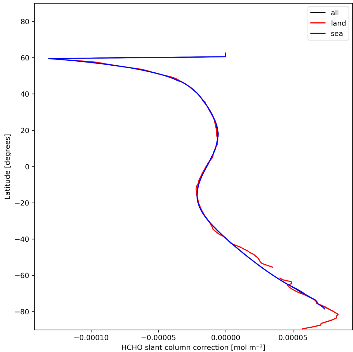
Figure 33: Zonal average of “HCHO slant column correction” for 2024-01-05 to 2024-01-07.
