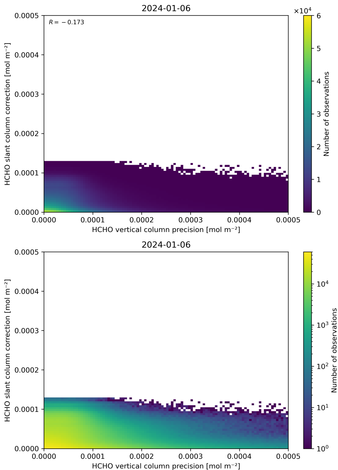
Figure 141: Scatter density plot of “HCHO vertical column precision” against “HCHO slant column correction” for 2024-01-05 to 2024-01-07.
