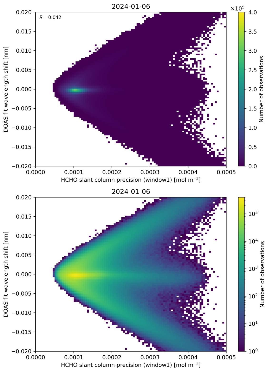
Figure 89: Scatter density plot of “HCHO slant column precision (window1)” against “DOAS fit wavelength shift” for 2024-01-05 to 2024-01-07.
