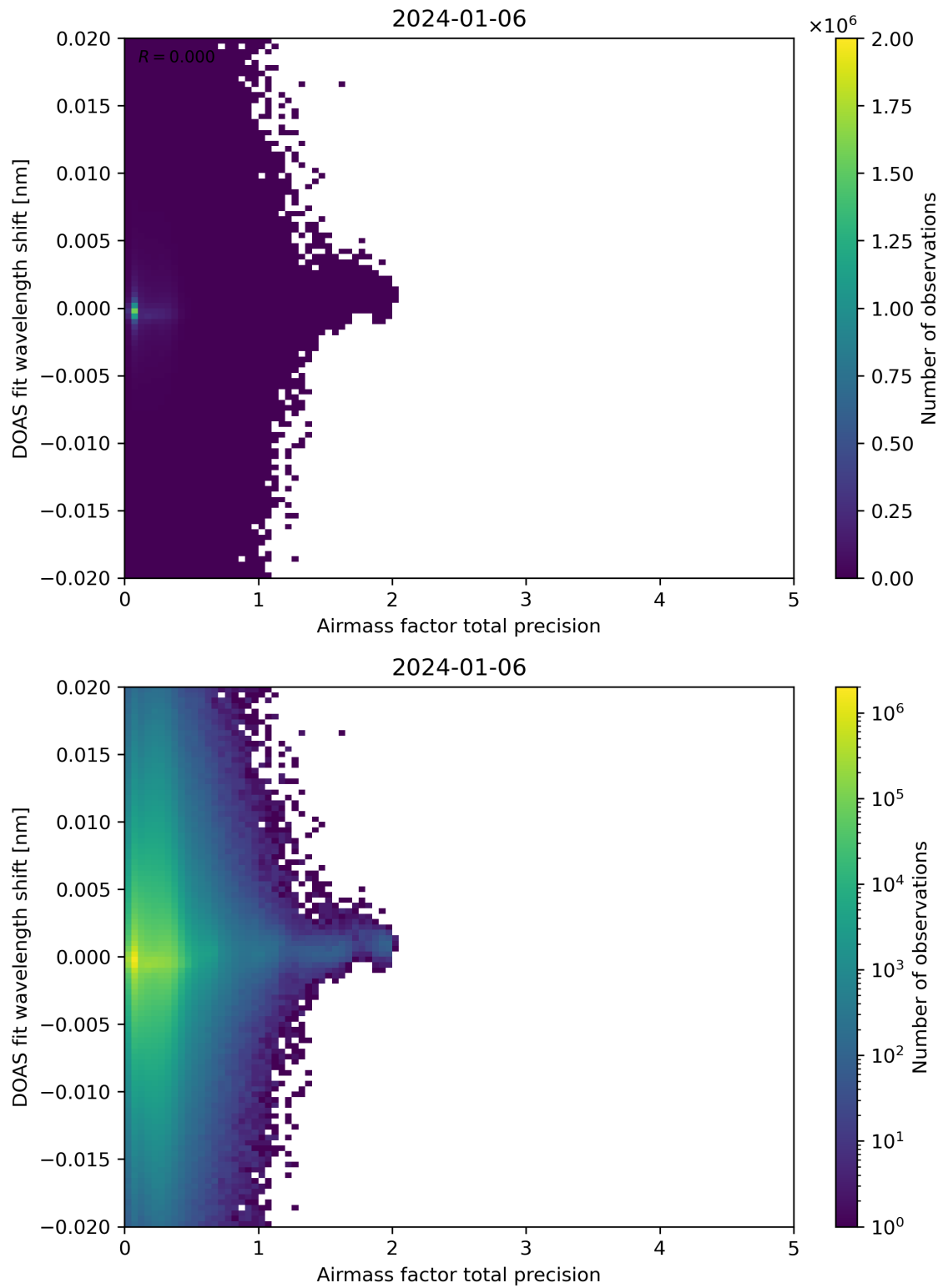
Figure 106: Scatter density plot of “Airmass factor total precision” against “DOAS fit wavelength shift” for 2024-01-05 to 2024-01-07.
