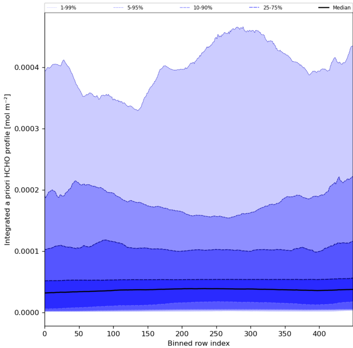
Figure 57: Along track statistics of “Integrated a priori HCHO profile” for 2024-01-05 to 2024-01-07
