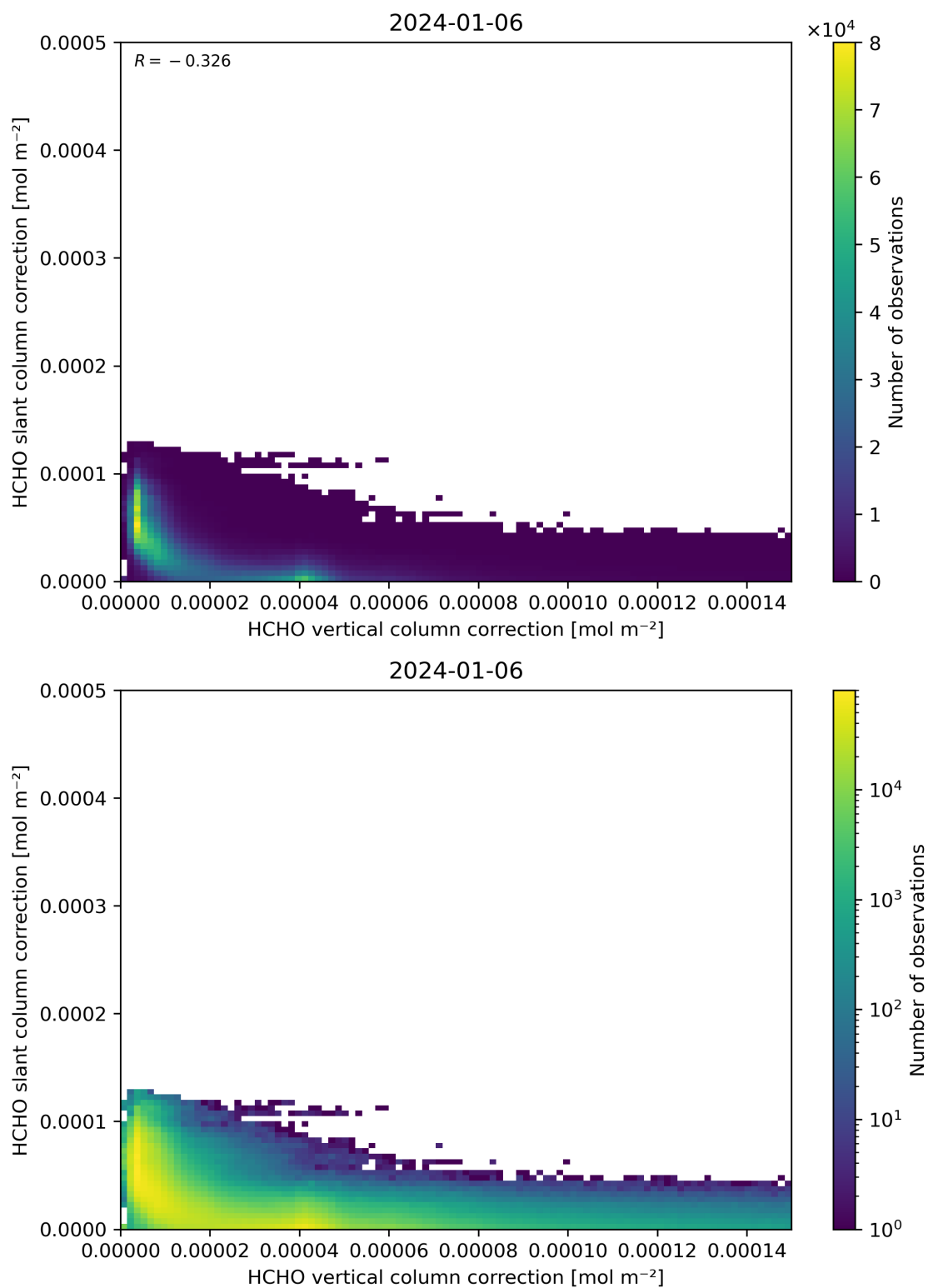
Figure 117: Scatter density plot of “HCHO vertical column correction” against “HCHO slant column correction” for 2024-01-05 to 2024-01-07.
