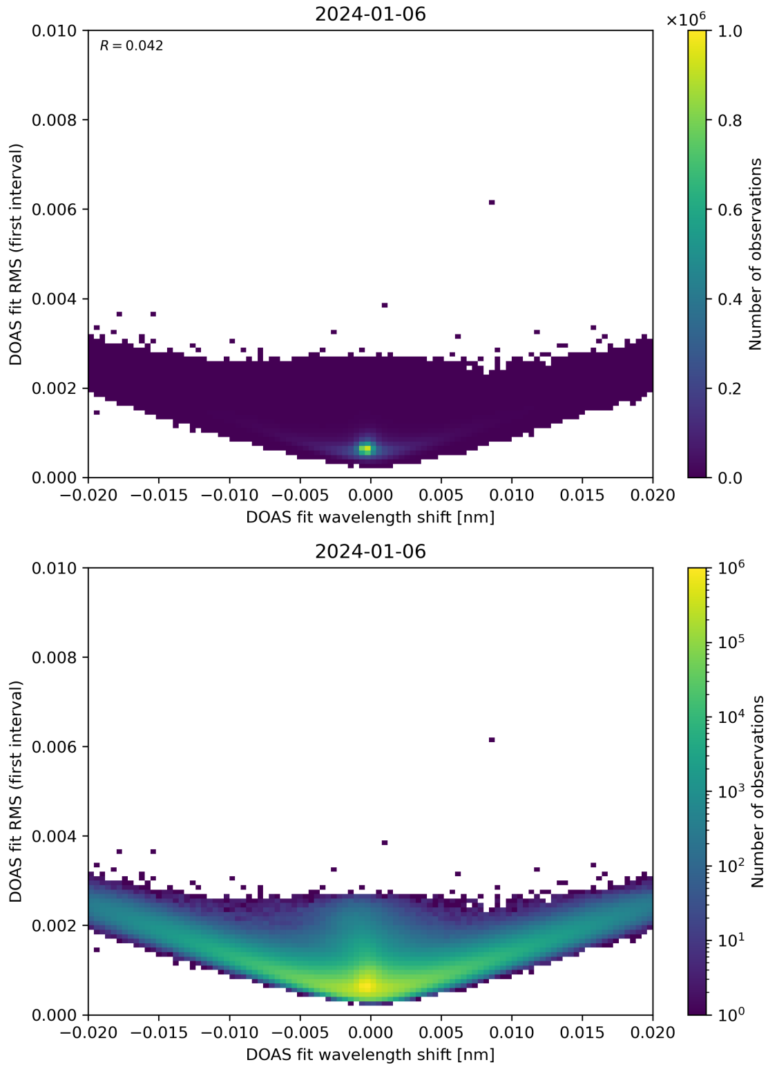
Figure 64: Scatter density plot of “DOAS fit wavelength shift” against “DOAS fit RMS (first interval)” for 2024-01-05 to 2024-01-07.
