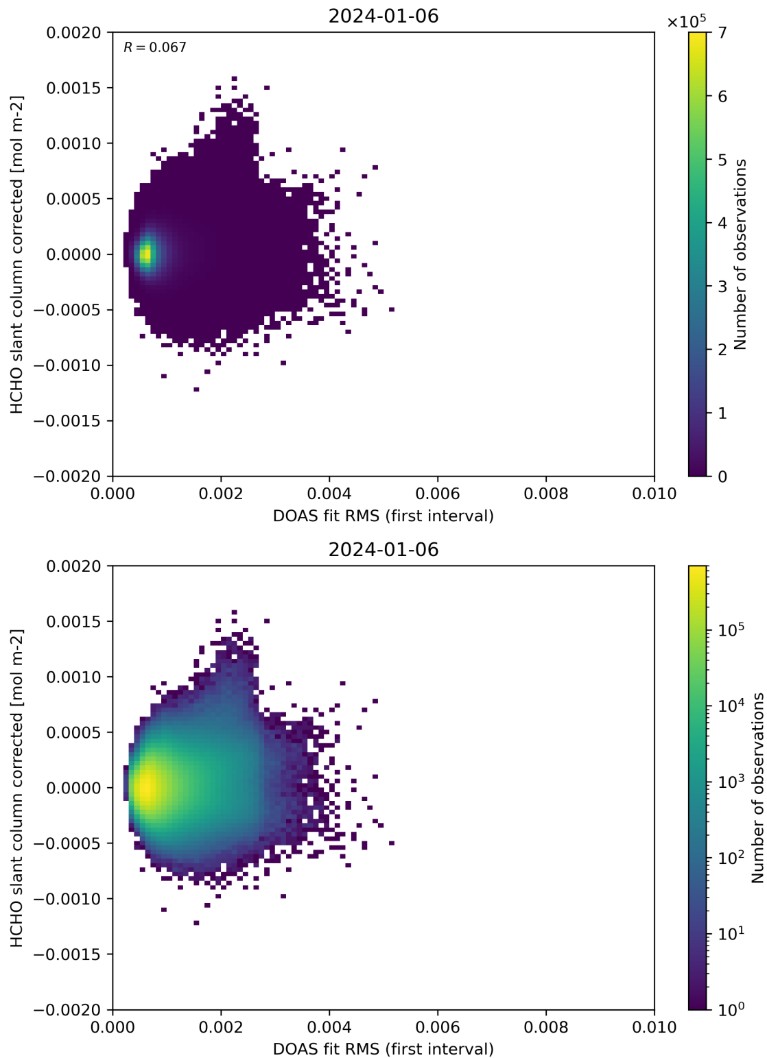
Figure 62: Scatter density plot of “DOAS fit RMS (first interval)” against “HCHO slant column corrected” for 2024-01-05 to 2024-01-07.
