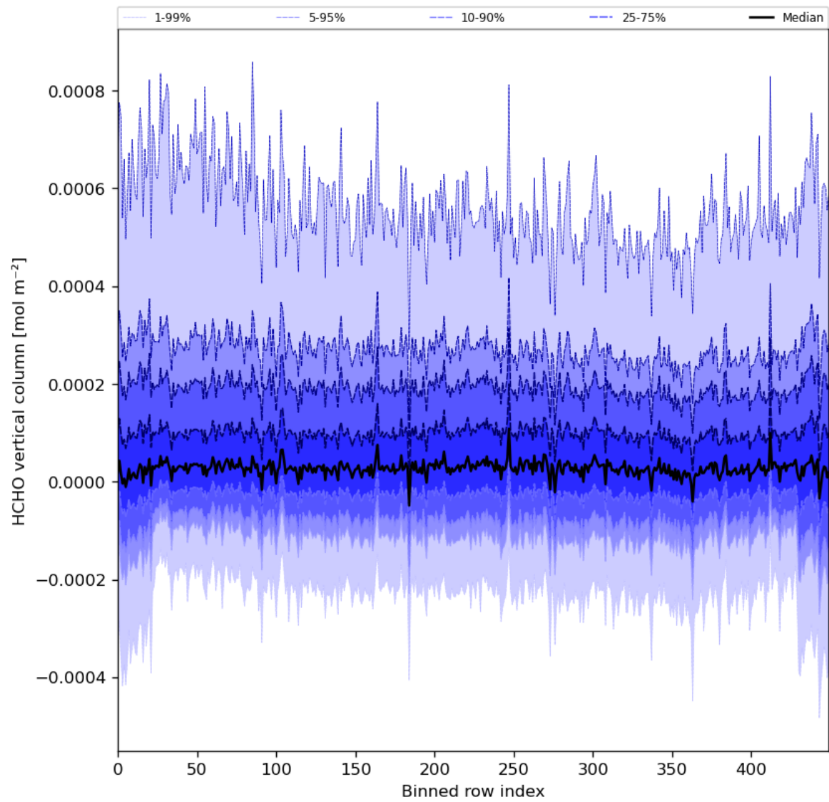
Figure 49: Along track statistics of “HCHO vertical column” for 2024-01-05 to 2024-01-07
