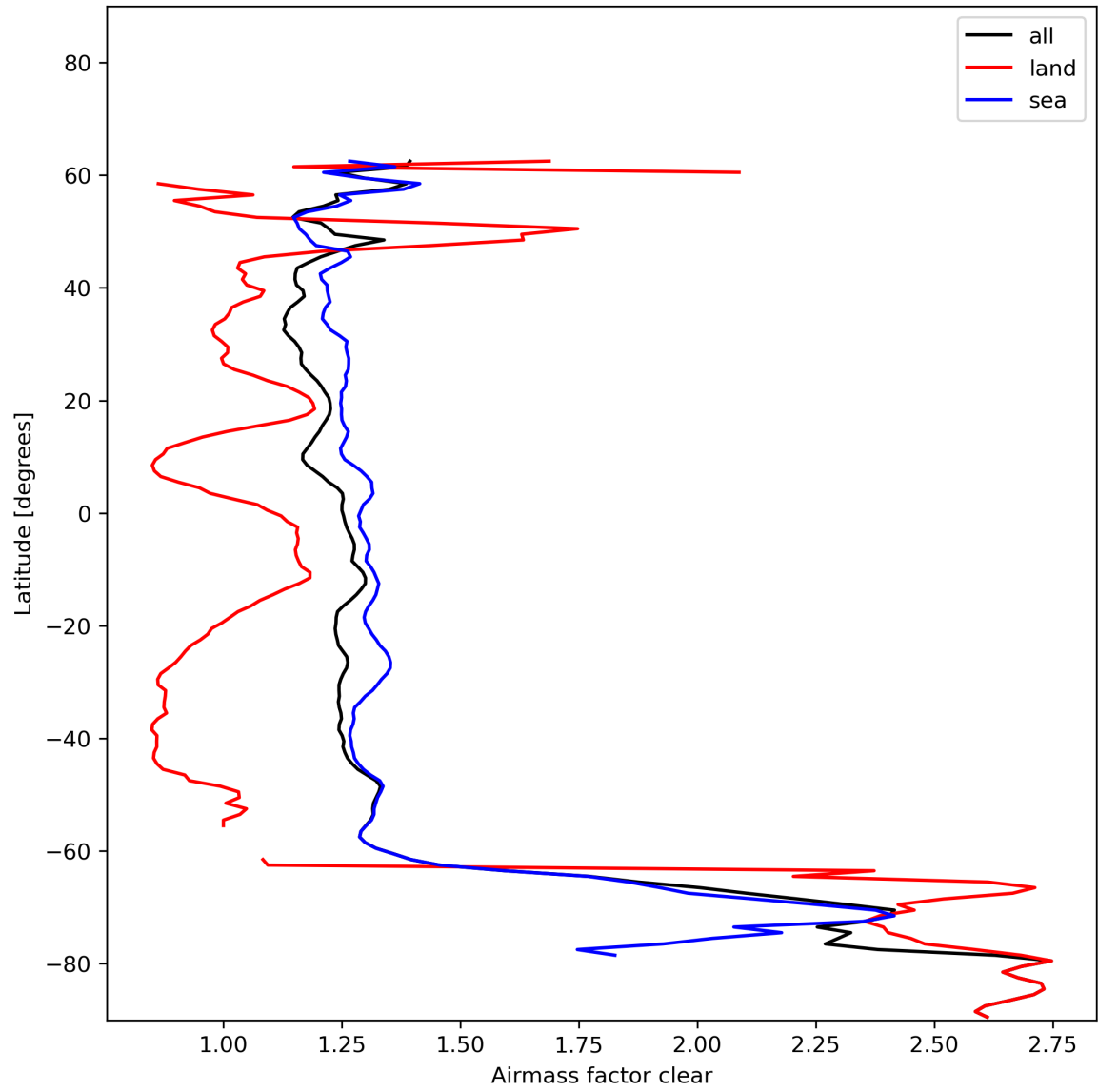
Figure 28: Zonal average of “Airmass factor clear” for 2024-01-05 to 2024-01-07.
