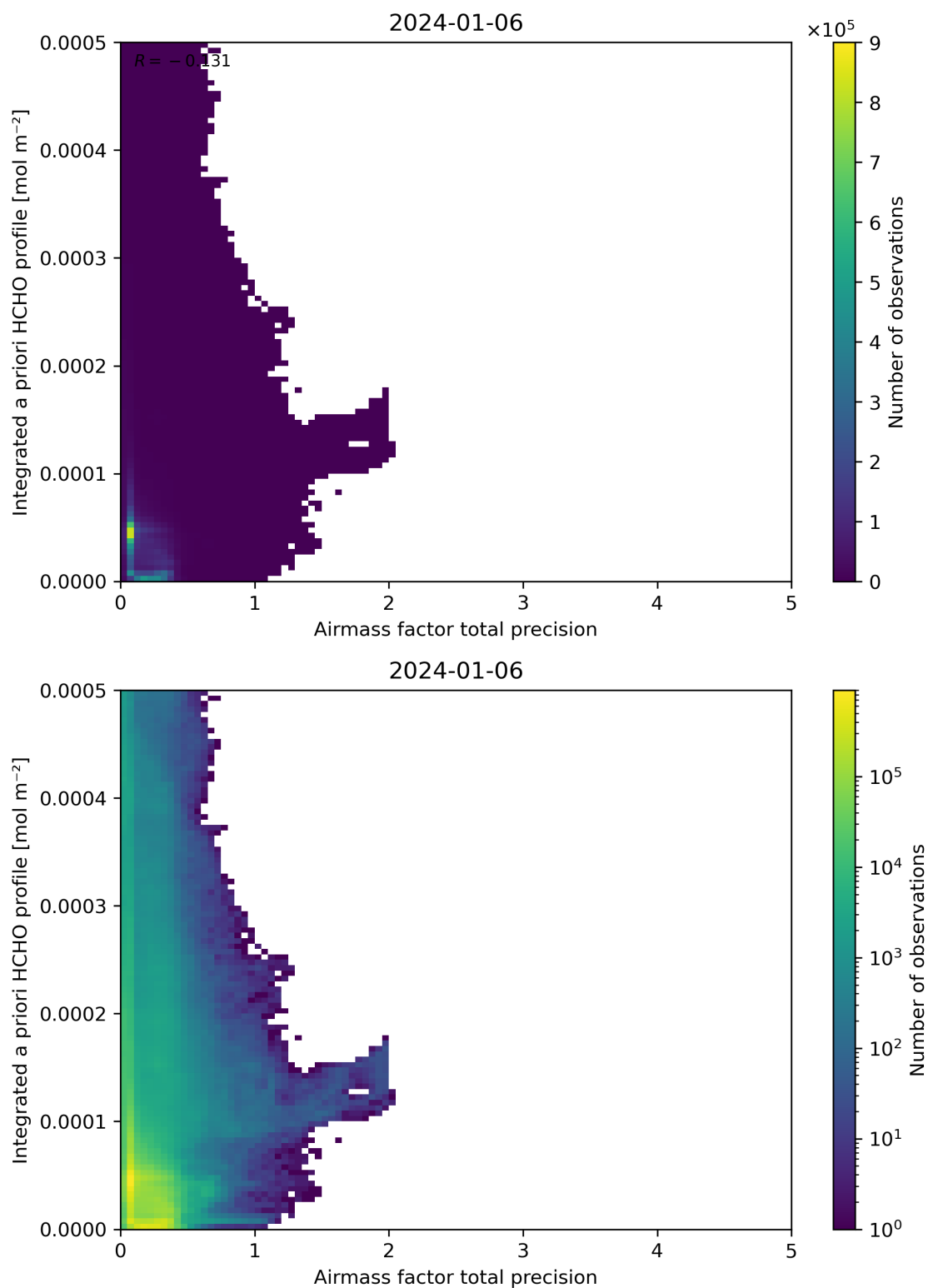
Figure 111: Scatter density plot of “Airmass factor total precision” against “Integrated a priori HCHO profile” for 2024-01-05 to 2024-01-07.
