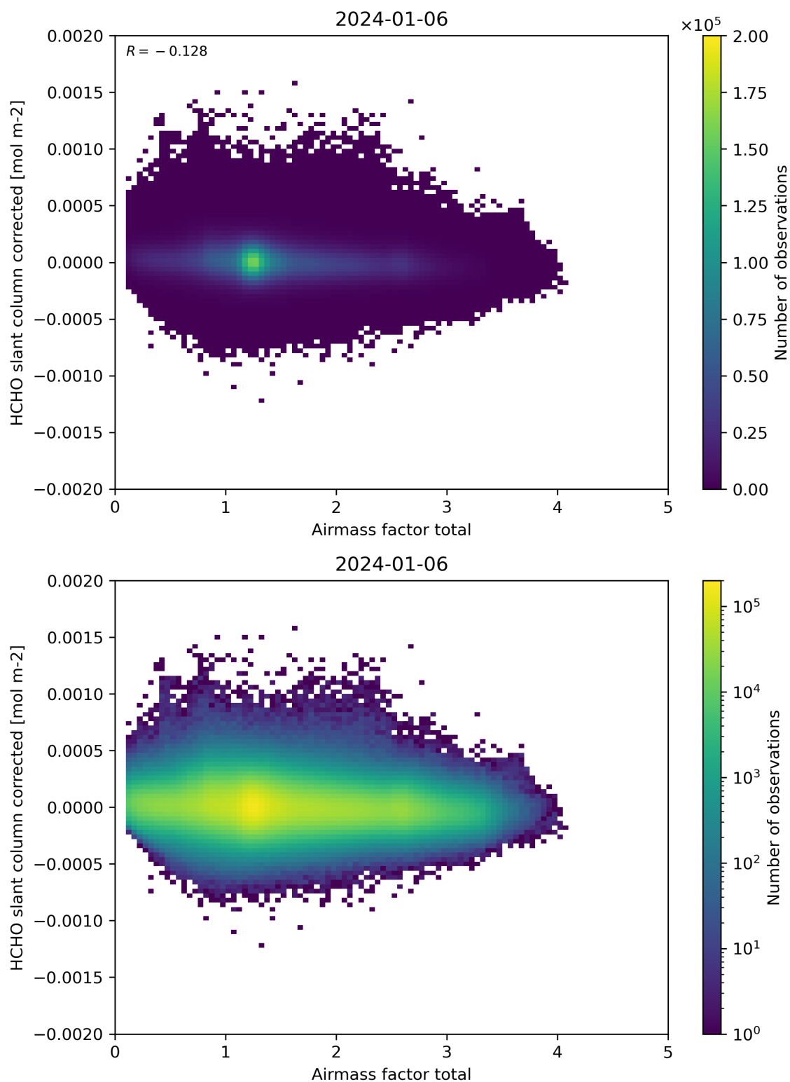
Figure 101: Scatter density plot of “Airmass factor total” against “HCHO slant column corrected” for 2024-01-05 to 2024-01-07.
