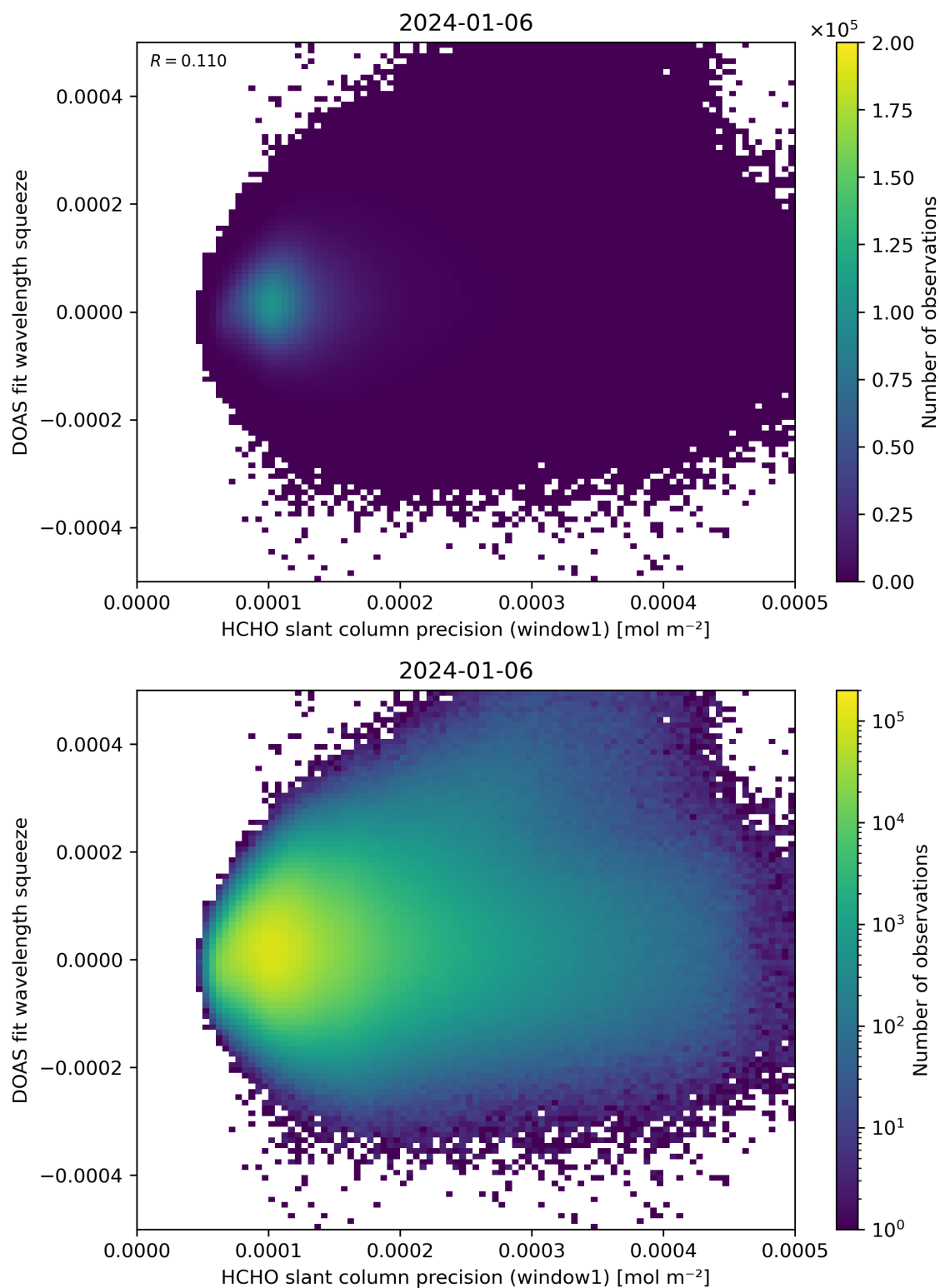
Figure 90: Scatter density plot of “HCHO slant column precision (window1)” against “DOAS fit wavelength squeeze” for 2024-01-05 to 2024-01-07.
