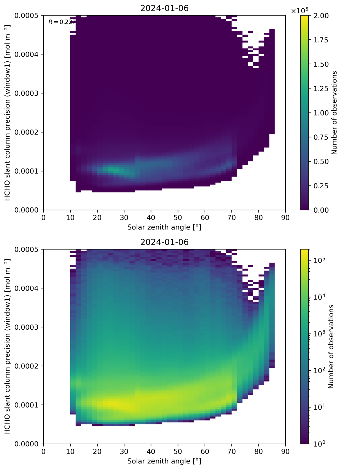
Figure 174: Scatter density plot of “Solar zenith angle” against “HCHO slant column precision (window1)” for 2024-01-05 to 2024-01-07.
