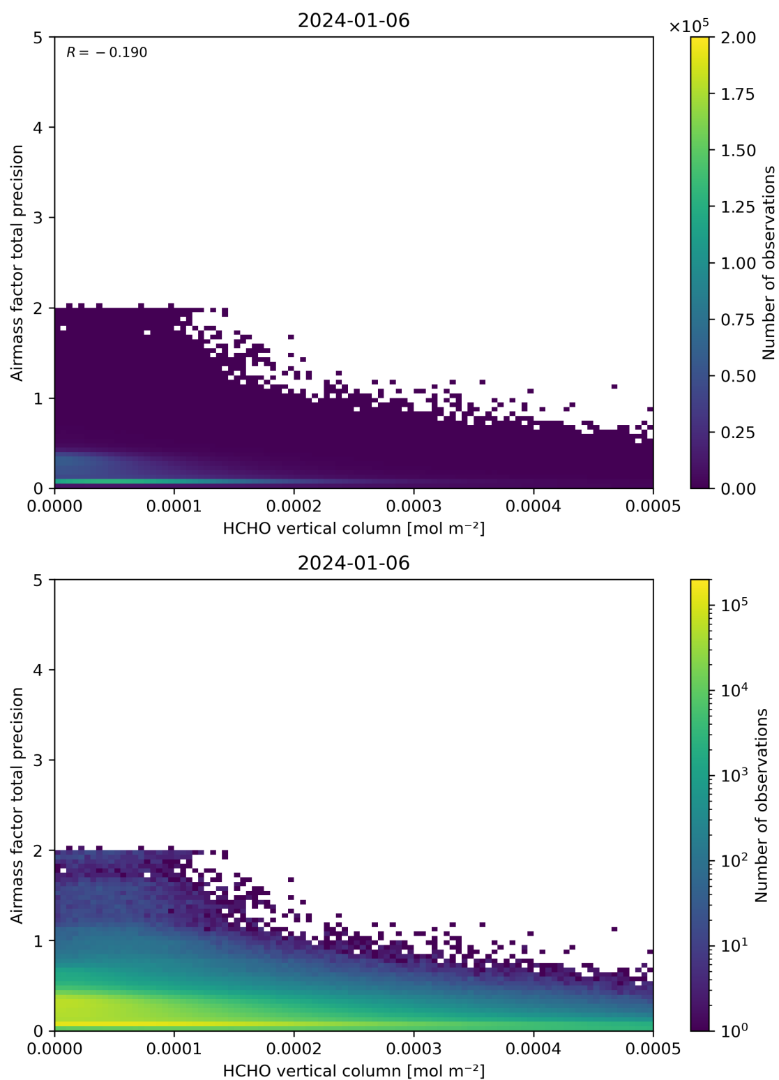
Figure 132: Scatter density plot of “HCHO vertical column” against “Airmass factor total precision” for 2024-01-05 to 2024-01-07.
