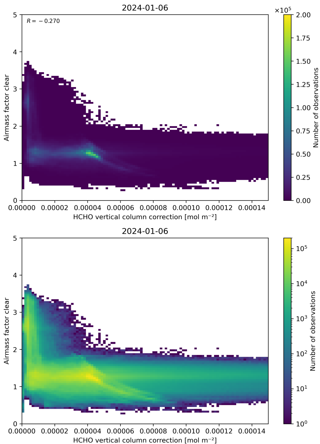
Figure 115: Scatter density plot of “HCHO vertical column correction” against “Airmass factor clear” for 2024-01-05 to 2024-01-07.
