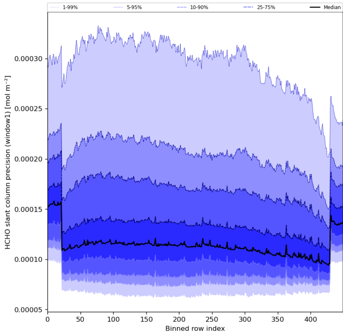
Figure 53: Along track statistics of “HCHO slant column precision (window1)” for 2024-01-05 to 2024-01-07
