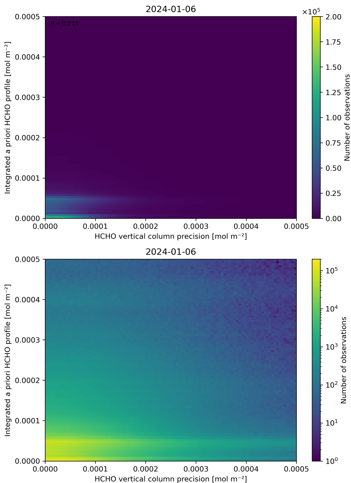
Figure 147: Scatter density plot of “HCHO vertical column precision” against “Integrated a priori HCHO profile” for 2024-01-05 to 2024-01-07.
