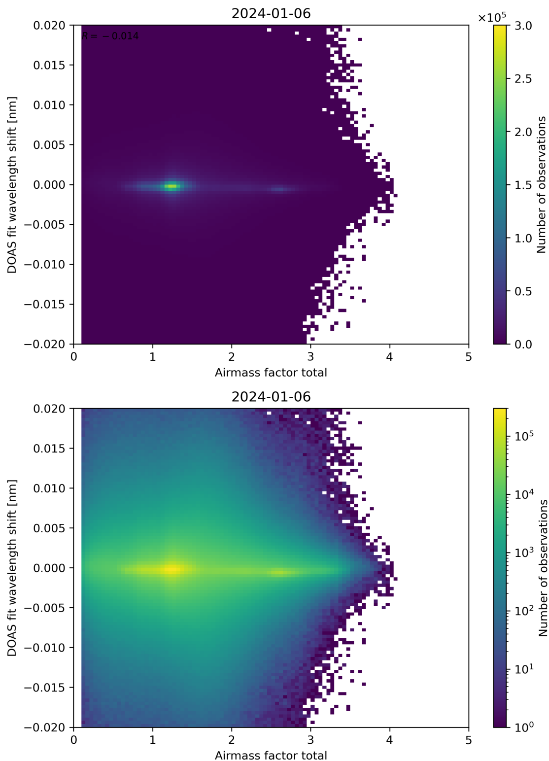
Figure 98: Scatter density plot of “Airmass factor total” against “DOAS fit wavelength shift” for 2024-01-05 to 2024-01-07.
