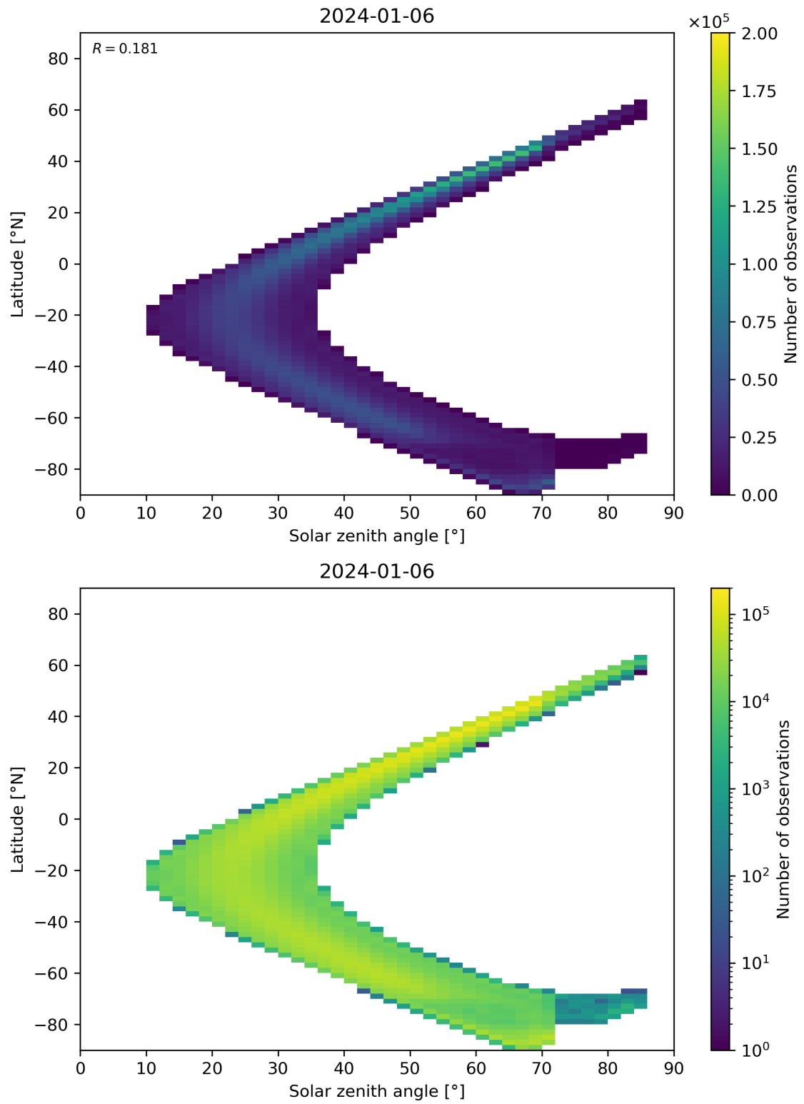
Figure 181: Scatter density plot of “Solar zenith angle” against “Latitude” for 2024-01-05 to 2024-01-07.
