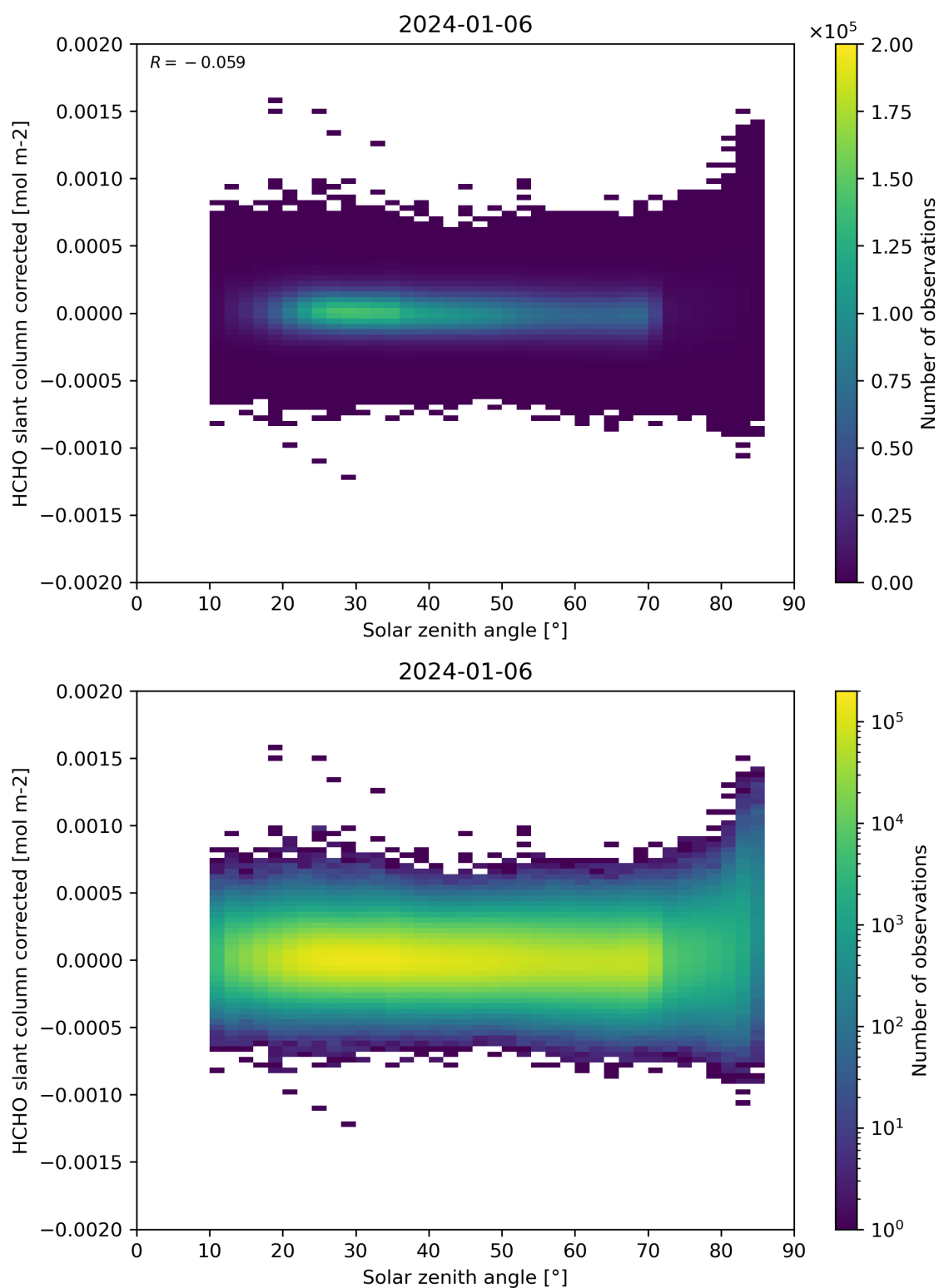
Figure 171: Scatter density plot of “Solar zenith angle” against “HCHO slant column corrected” for 2024-01-05 to 2024-01-07.
