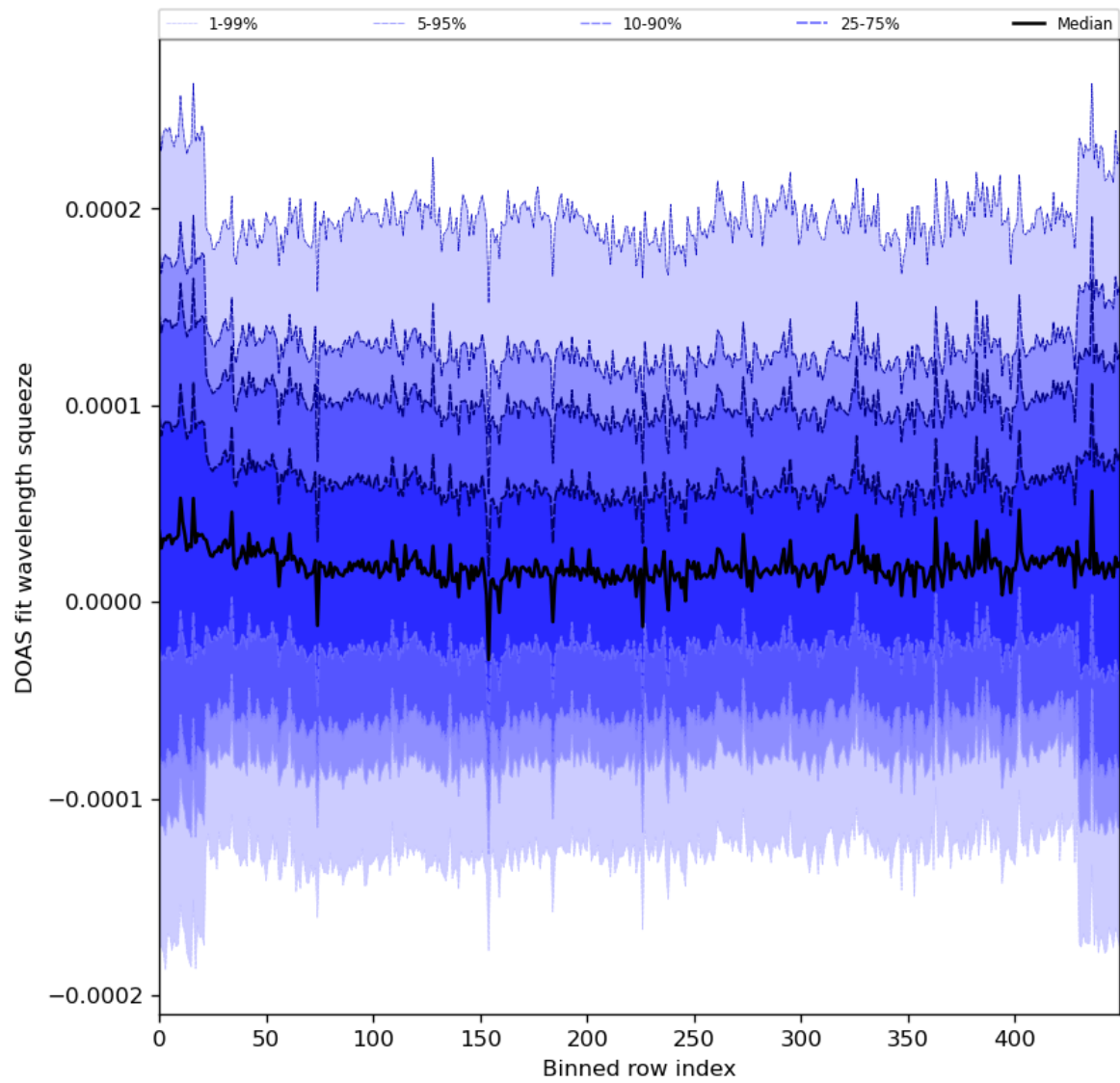
Figure 59: Along track statistics of “DOAS fit wavelength squeeze” for 2024-01-05 to 2024-01-07
