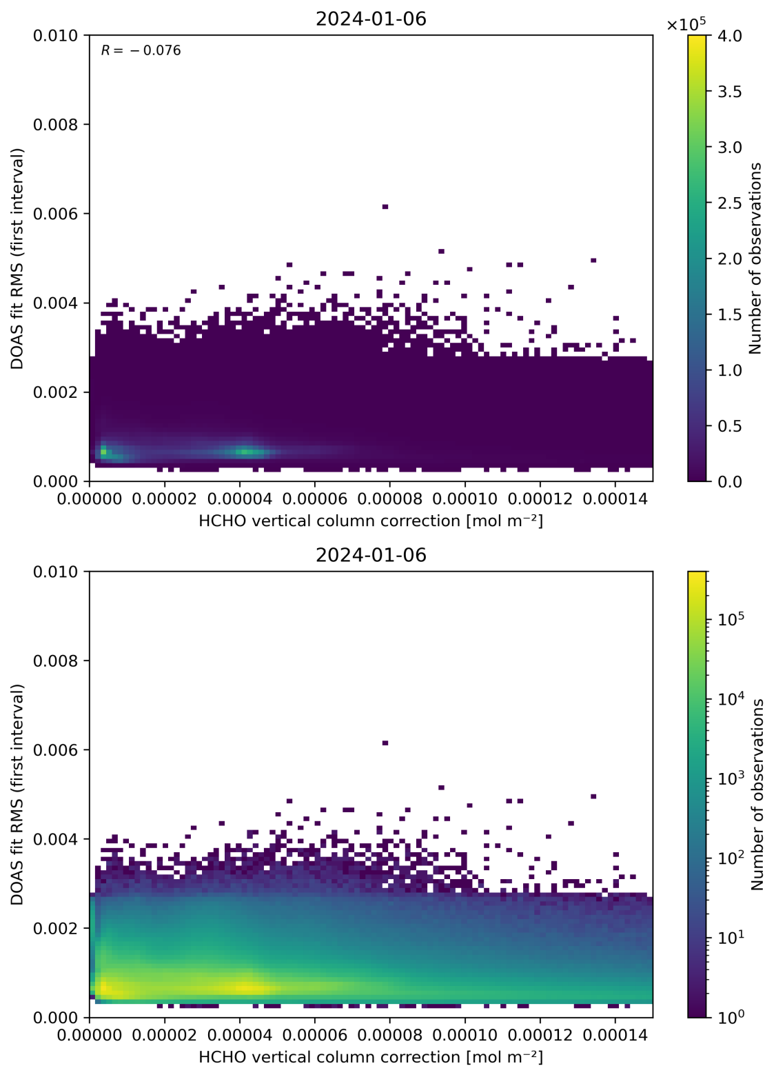
Figure 112: Scatter density plot of “HCHO vertical column correction” against “DOAS fit RMS (first interval)” for 2024-01-05 to 2024-01-07.
