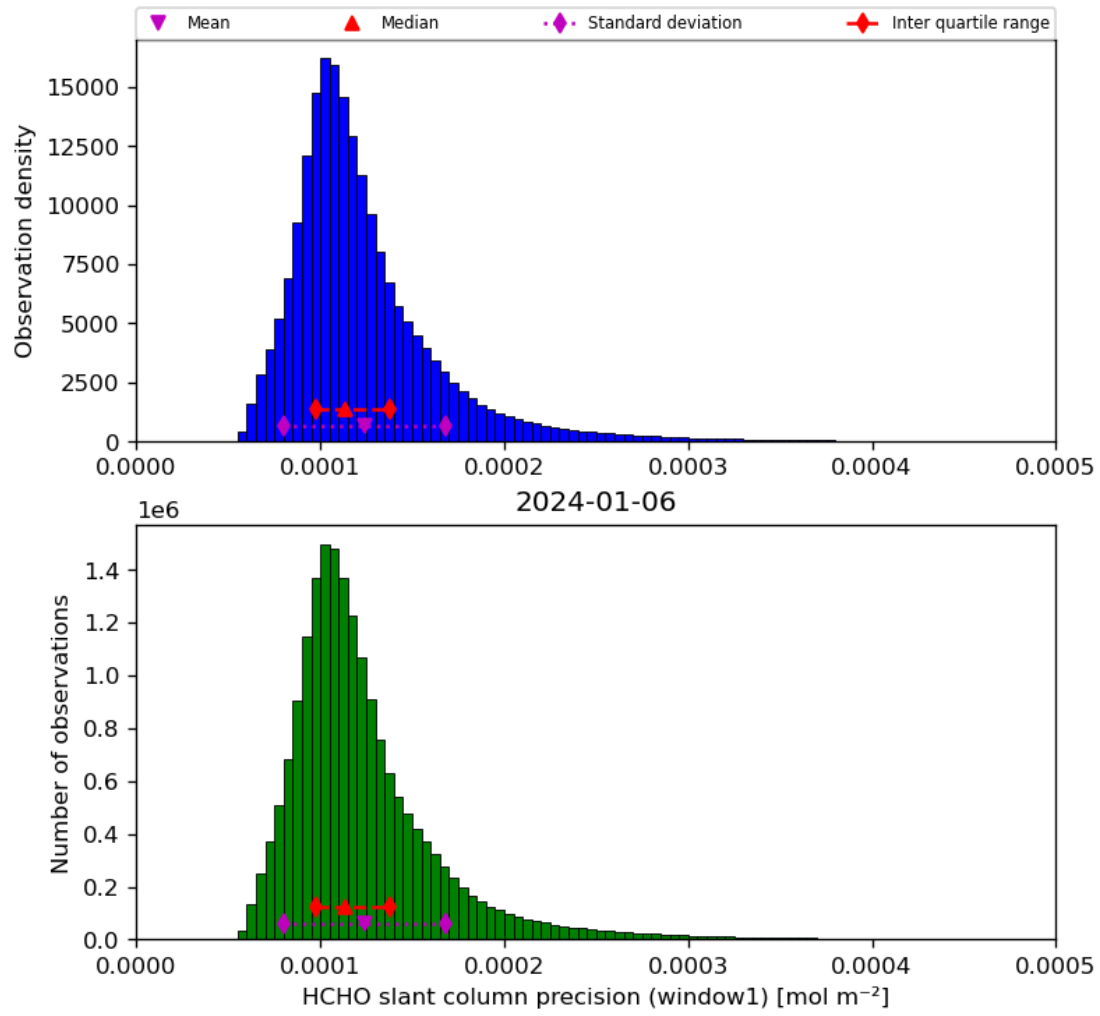
Figure 39: Histogram of “HCHO slant column precision (window1)” for 2024-01-05 to 2024-01-07
