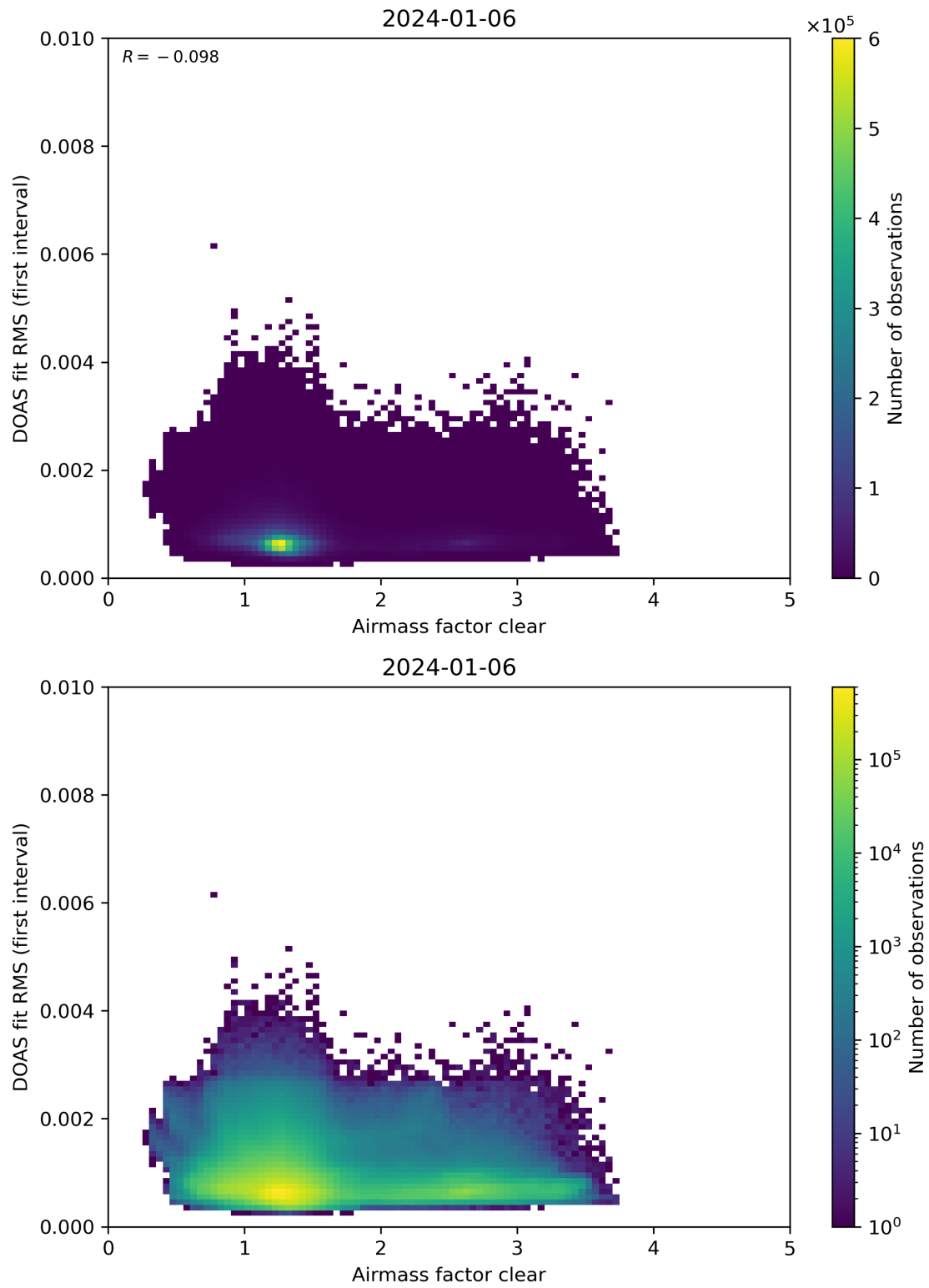
Figure 71: Scatter density plot of “Airmass factor clear” against “DOAS fit RMS (first interval)” for 2024-01-05 to 2024-01-07.
