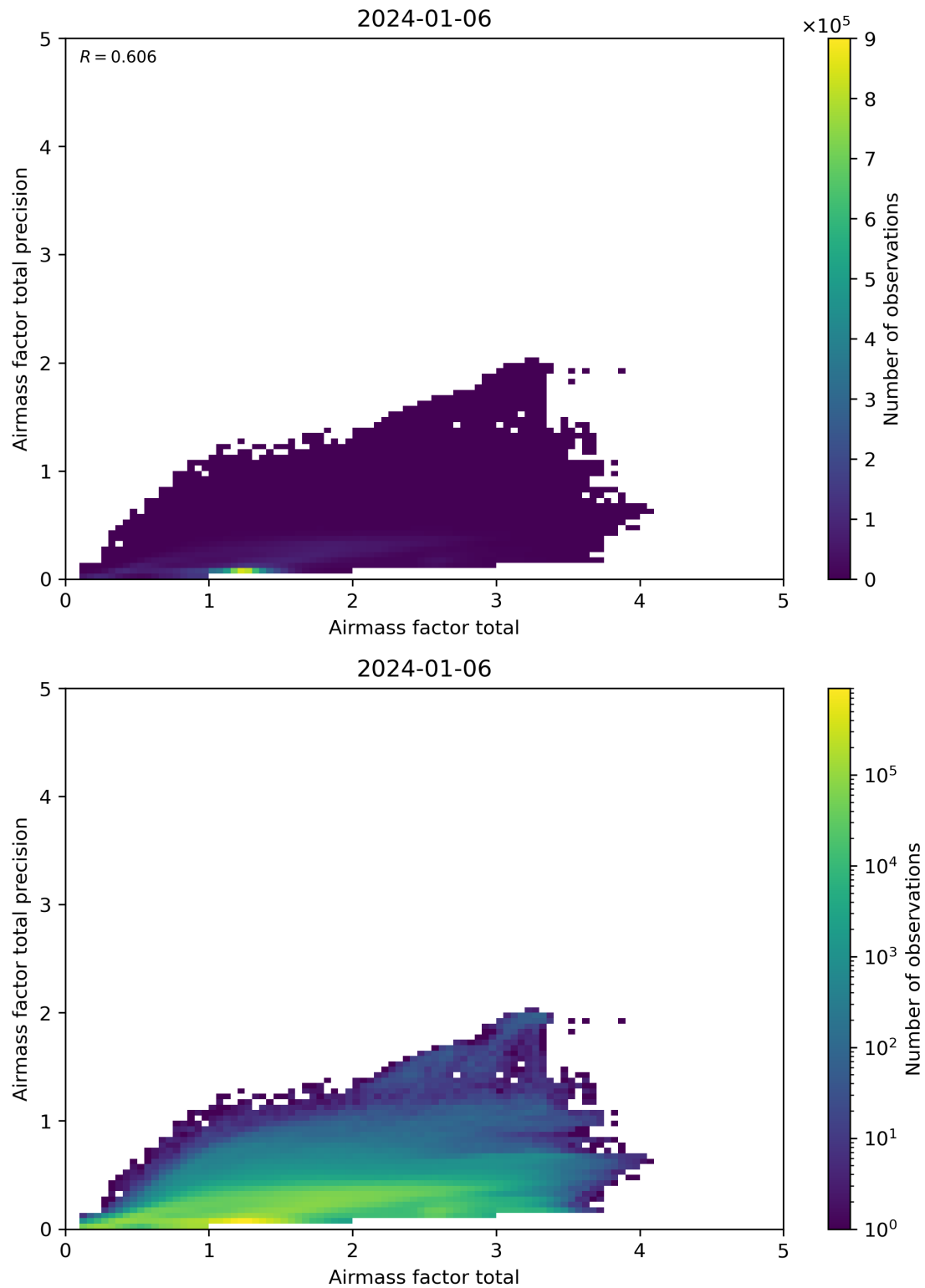
Figure 103: Scatter density plot of “Airmass factor total” against “Airmass factor total precision” for 2024-01-05 to 2024-01-07.
