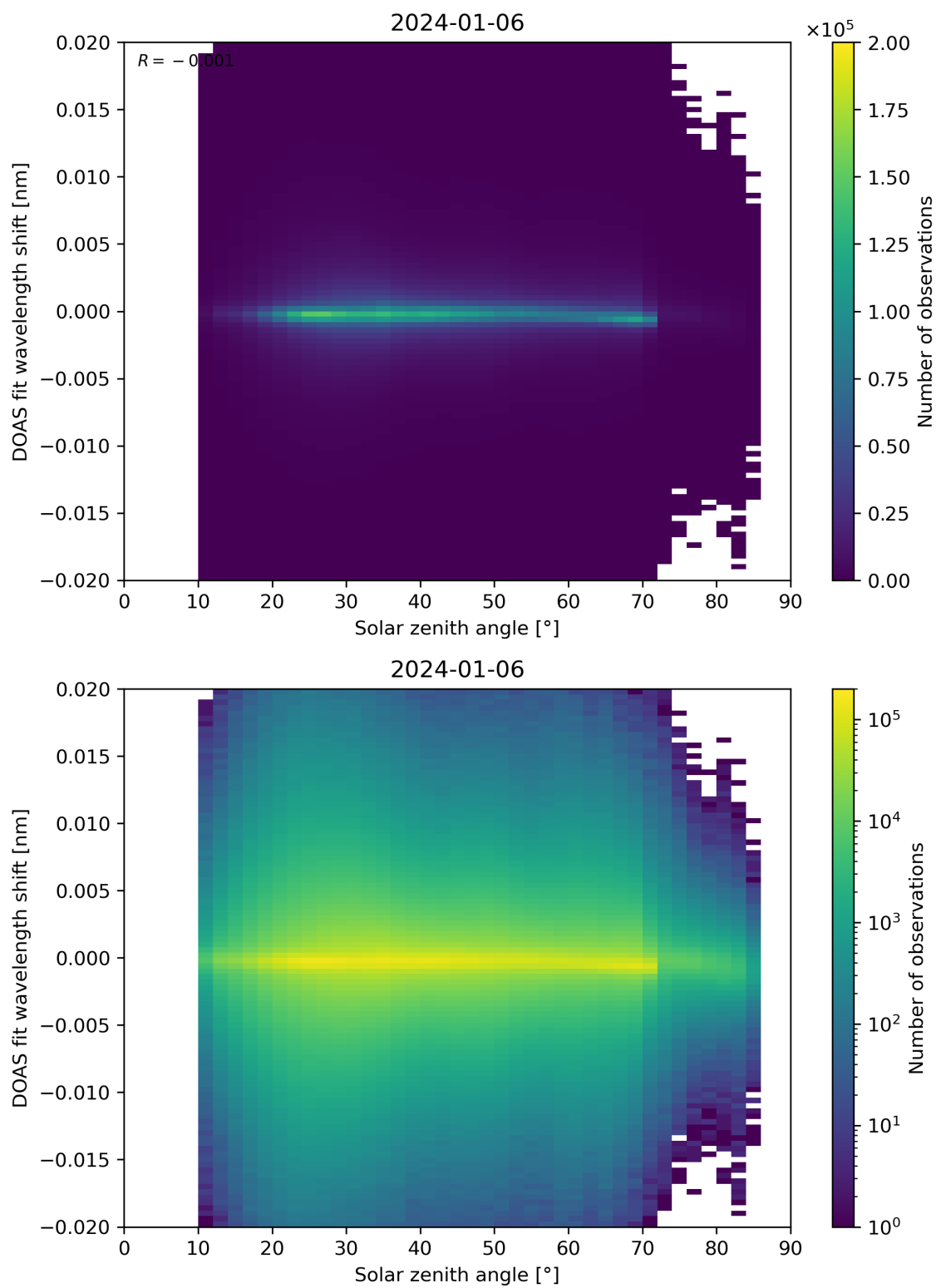
Figure 168: Scatter density plot of “Solar zenith angle” against “DOAS fit wavelength shift” for 2024-01-05 to 2024-01-07.
