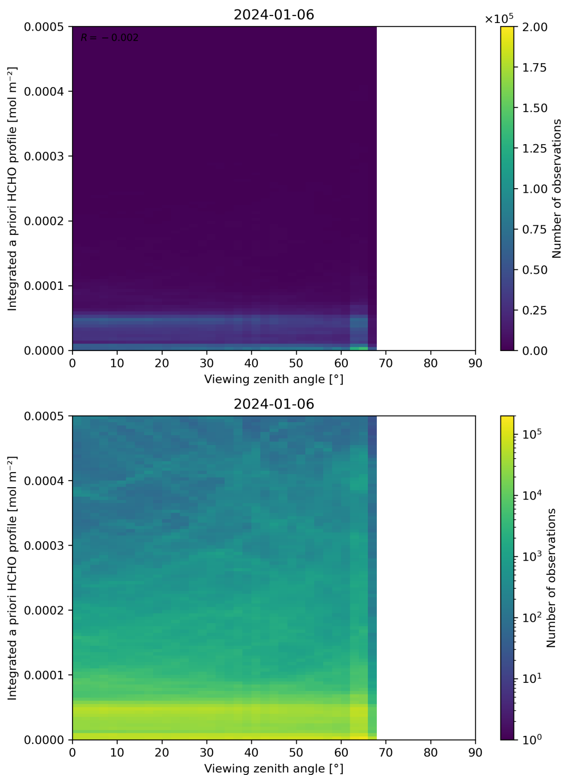
Figure 195: Scatter density plot of “Viewing zenith angle” against “Integrated a priori HCHO profile” for 2024-01-05 to 2024-01-07.
