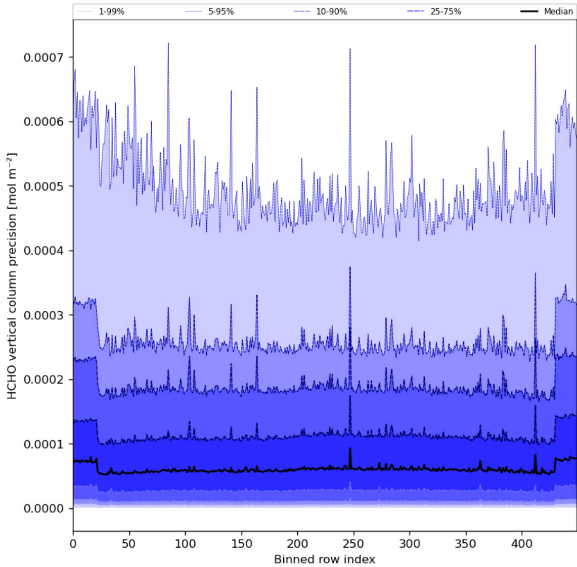
Figure 50: Along track statistics of “HCHO vertical column precision” for 2024-01-05 to 2024-01-07
