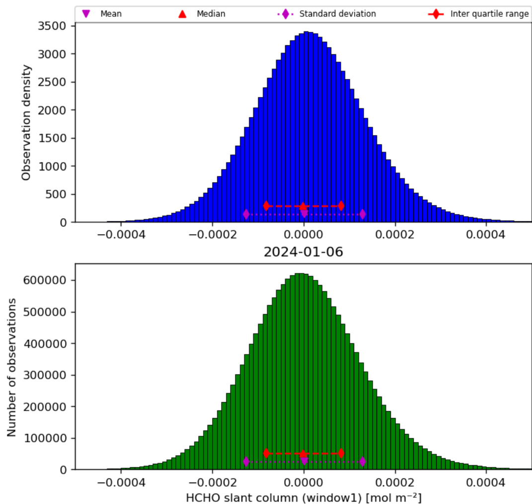
Figure 38: Histogram of “HCHO slant column (window1)” for 2024-01-05 to 2024-01-07
