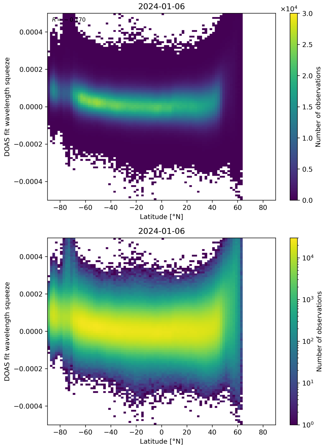
Figure 155: Scatter density plot of “Latitude” against “DOAS fit wavelength squeeze” for 2024-01-05 to 2024-01-07.
