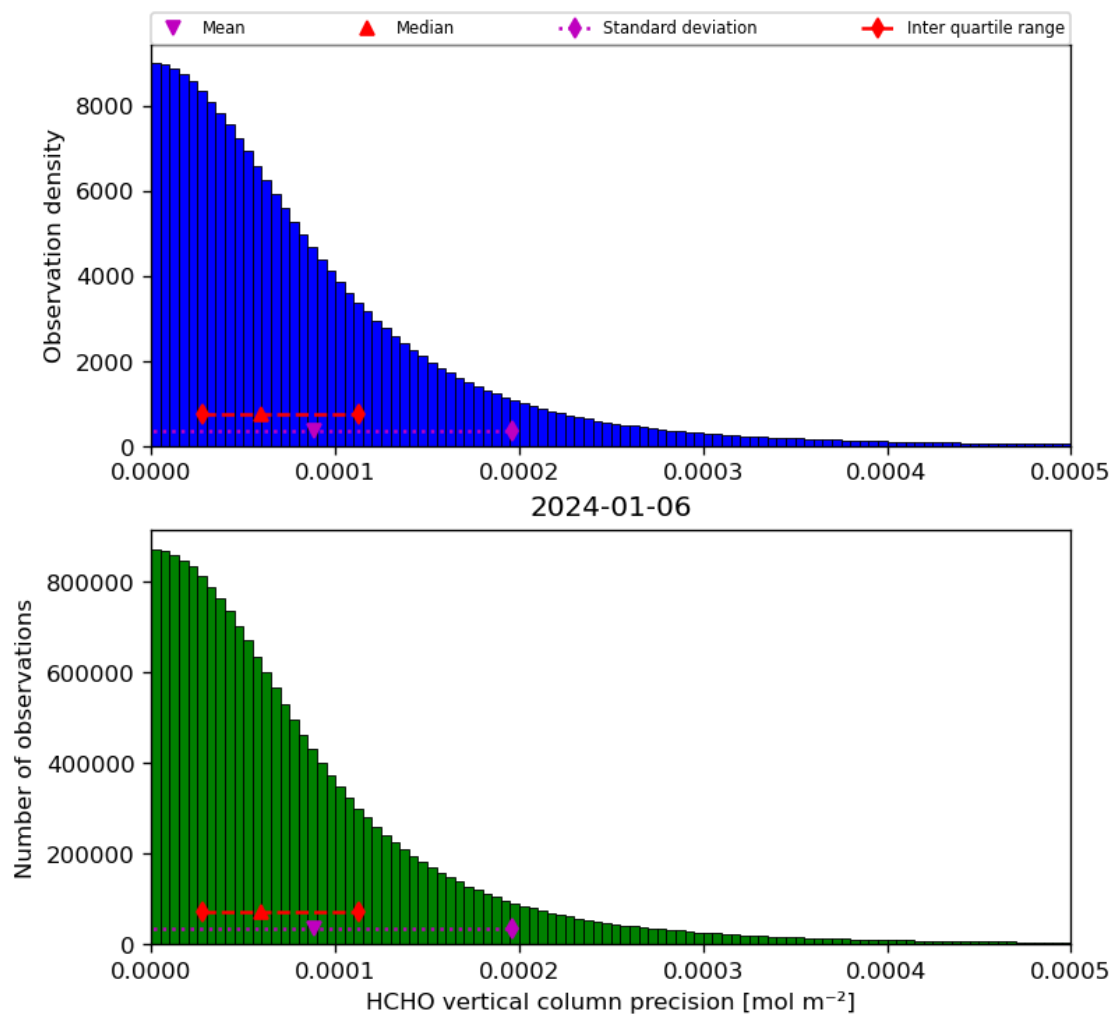
Figure 36: Histogram of “HCHO vertical column precision” for 2024-01-05 to 2024-01-07
