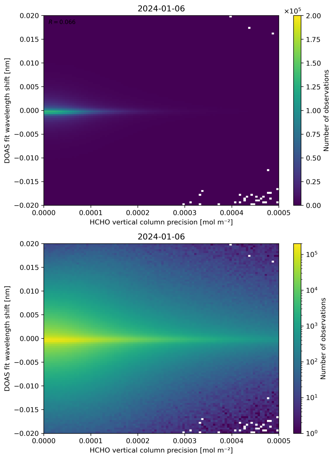
Figure 137: Scatter density plot of “HCHO vertical column precision” against “DOAS fit wavelength shift” for 2024-01-05 to 2024-01-07.
