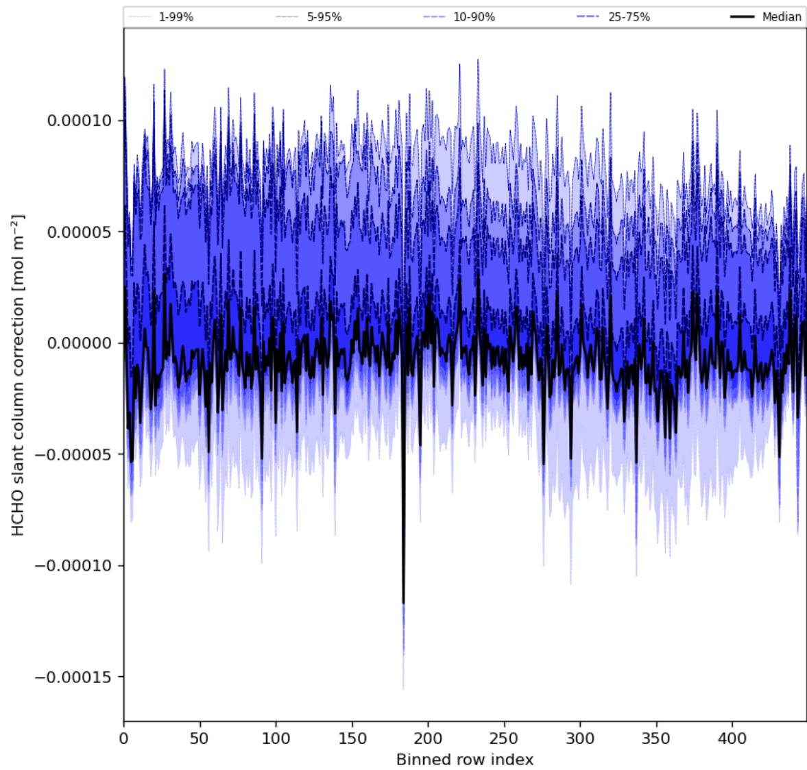
Figure 61: Along track statistics of “HCHO slant column correction” for 2024-01-05 to 2024-01-07
