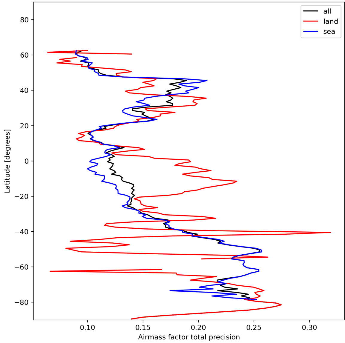
Figure 27: Zonal average of “Airmass factor total precision” for 2024-01-05 to 2024-01-07.
