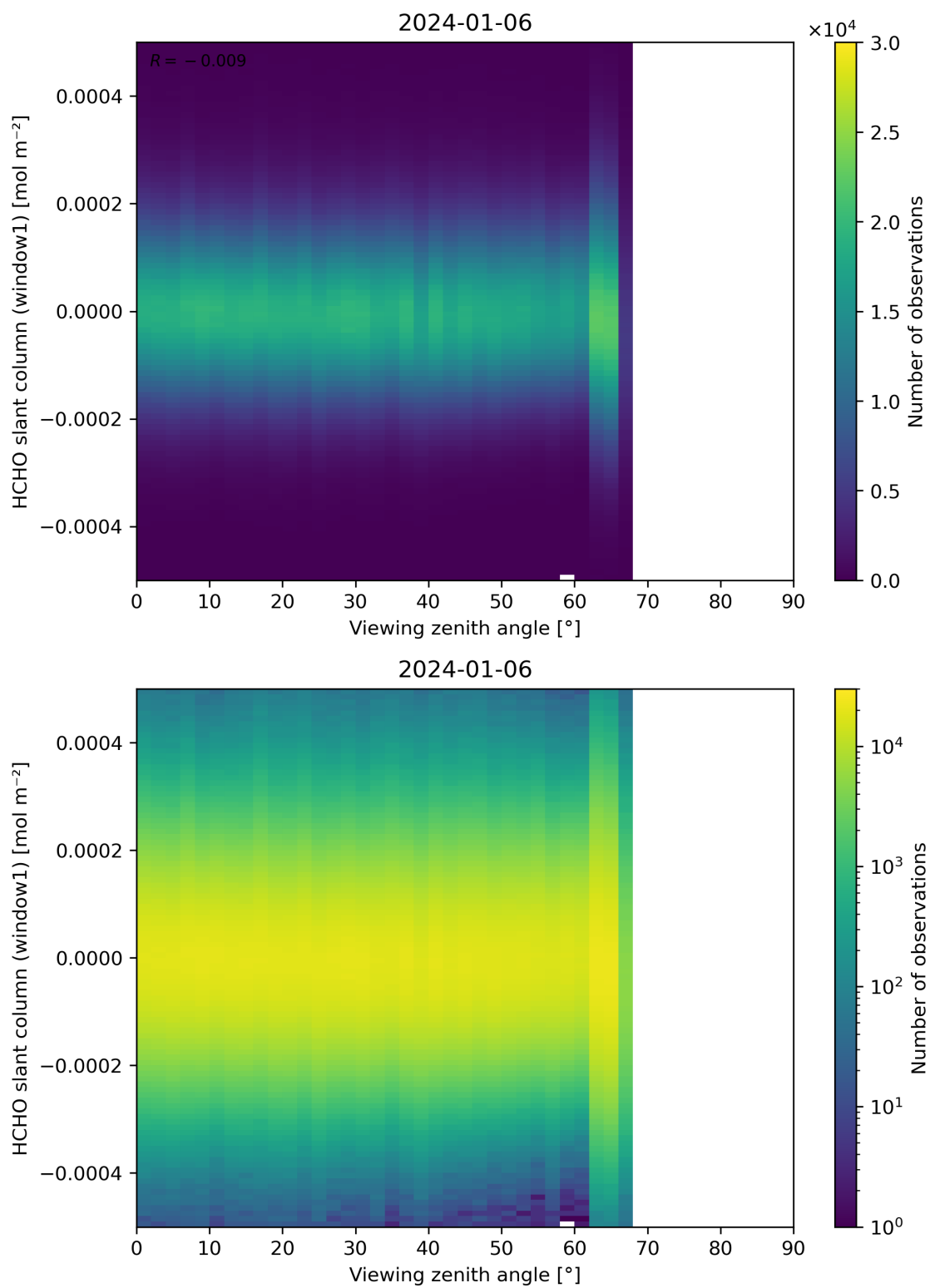
Figure 188: Scatter density plot of “Viewing zenith angle” against “HCHO slant column (window1)” for 2024-01-05 to 2024-01-07.
