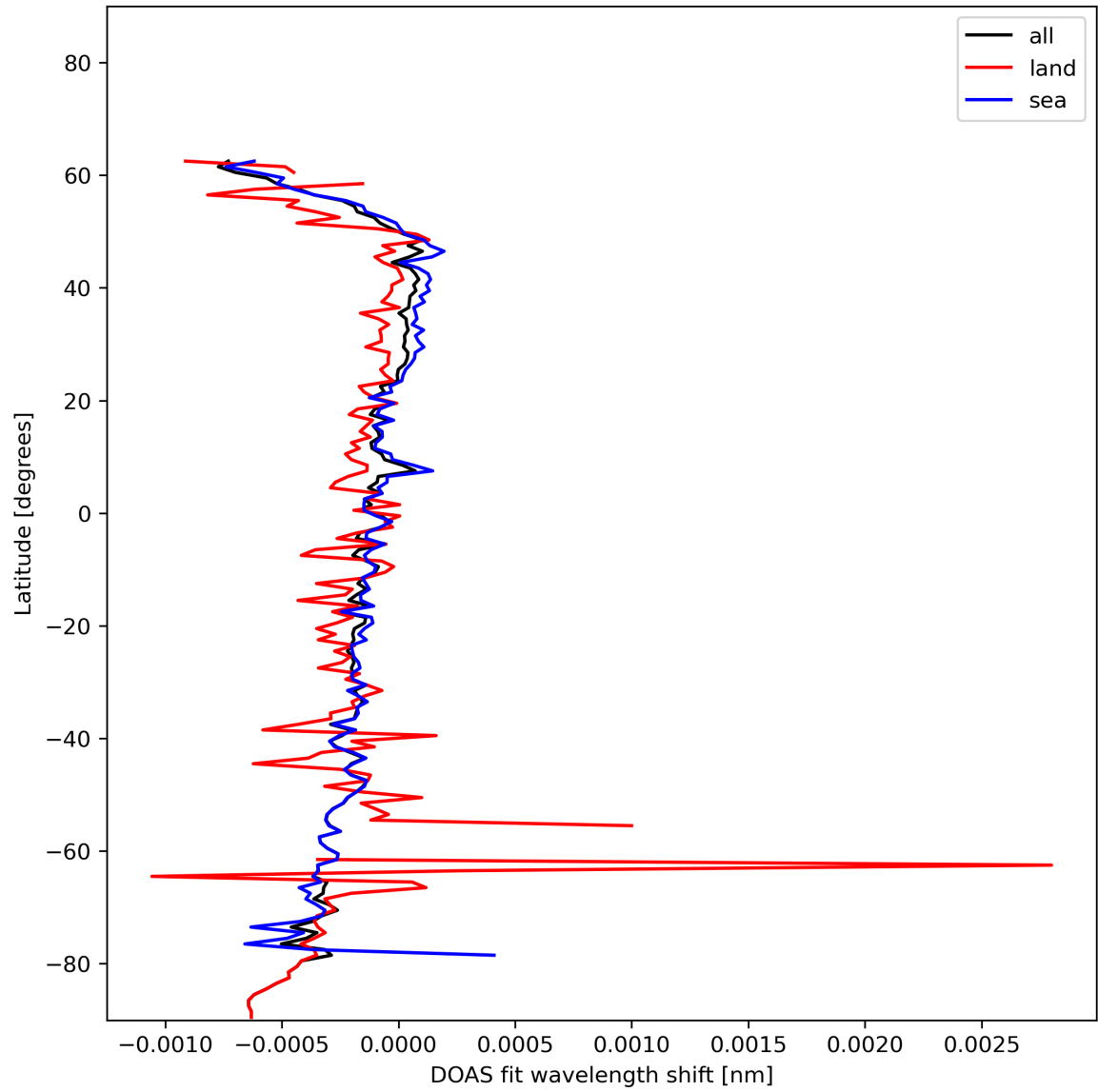
Figure 30: Zonal average of “DOAS fit wavelength shift” for 2024-01-05 to 2024-01-07.
