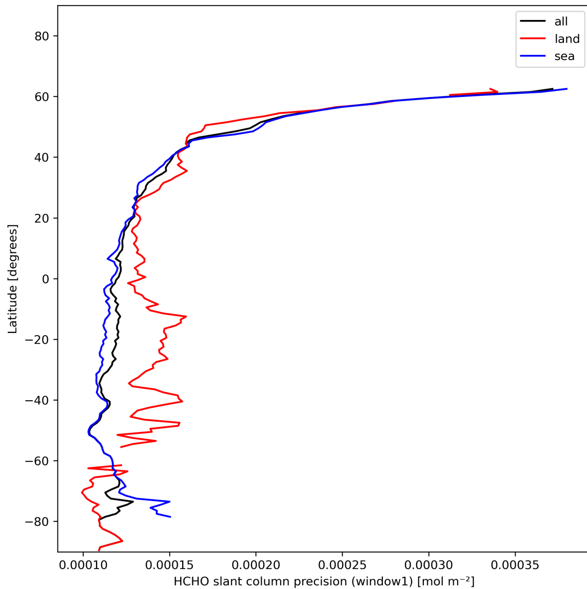
Figure 25: Zonal average of “HCHO slant column precision (window1)” for 2024-01-05 to 2024-01-07.
