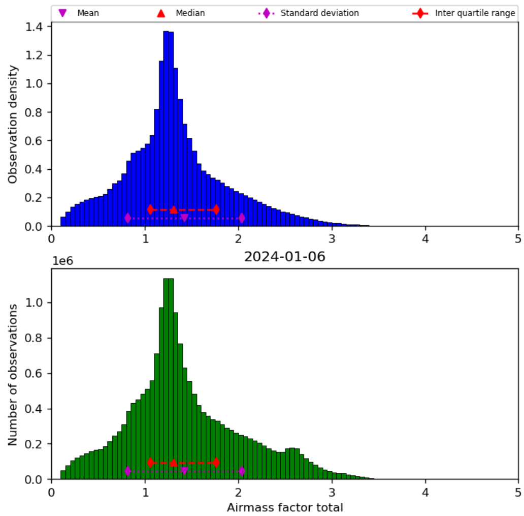
Figure 40: Histogram of “Airmass factor total” for 2024-01-05 to 2024-01-07
