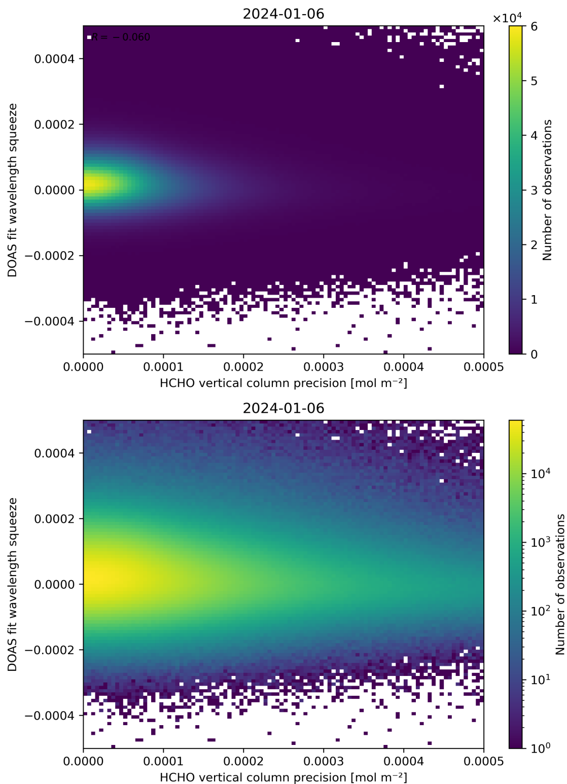
Figure 138: Scatter density plot of “HCHO vertical column precision” against “DOAS fit wavelength squeeze” for 2024-01-05 to 2024-01-07.
