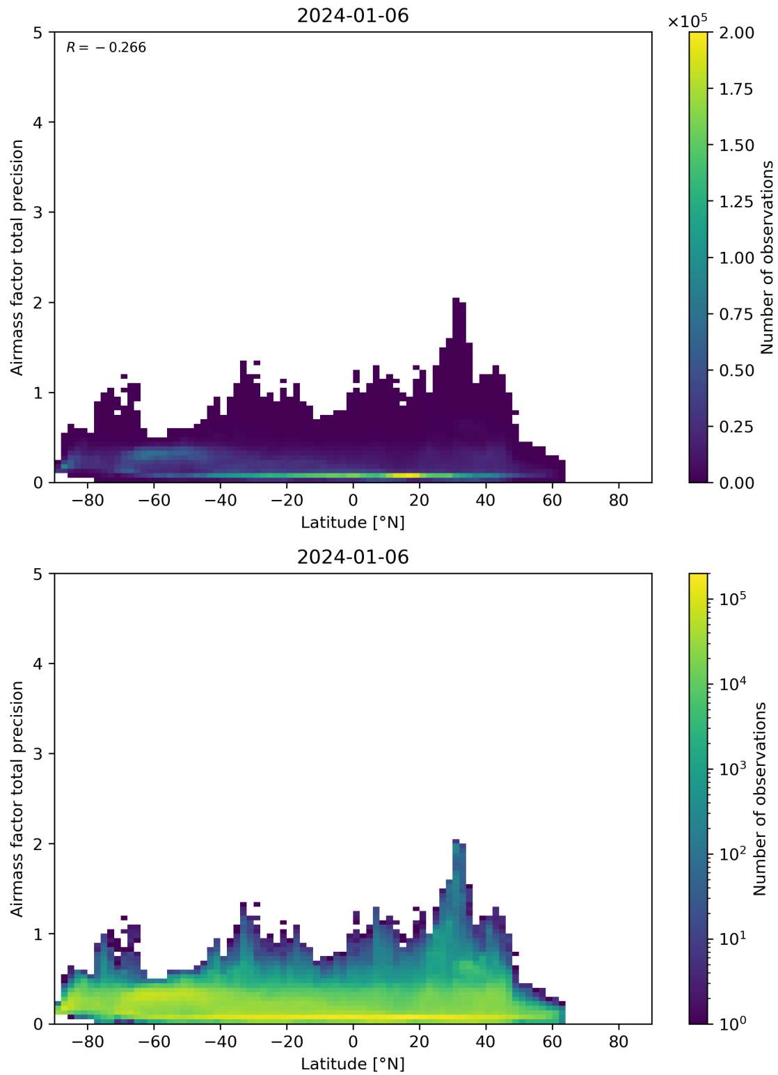
Figure 162: Scatter density plot of “Latitude” against “Airmass factor total precision” for 2024-01-05 to 2024-01-07.
