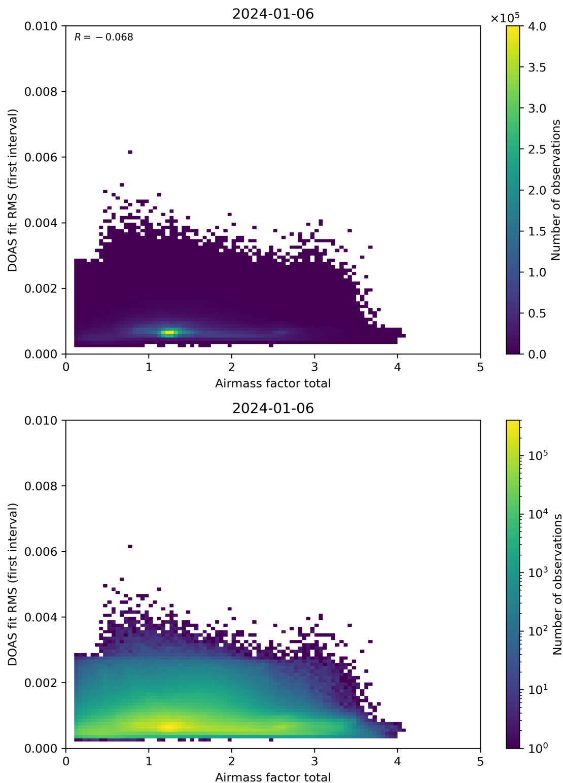
Figure 97: Scatter density plot of “Airmass factor total” against “DOAS fit RMS (first interval)” for 2024-01-05 to 2024-01-07.
