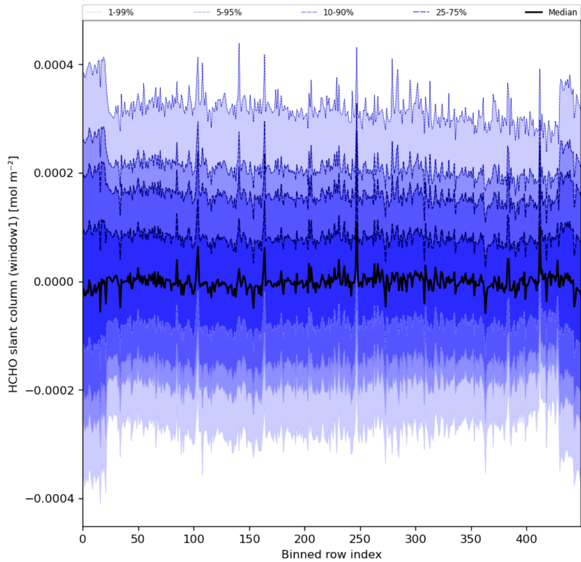
Figure 52: Along track statistics of “HCHO slant column (window1)” for 2024-01-05 to 2024-01-07
