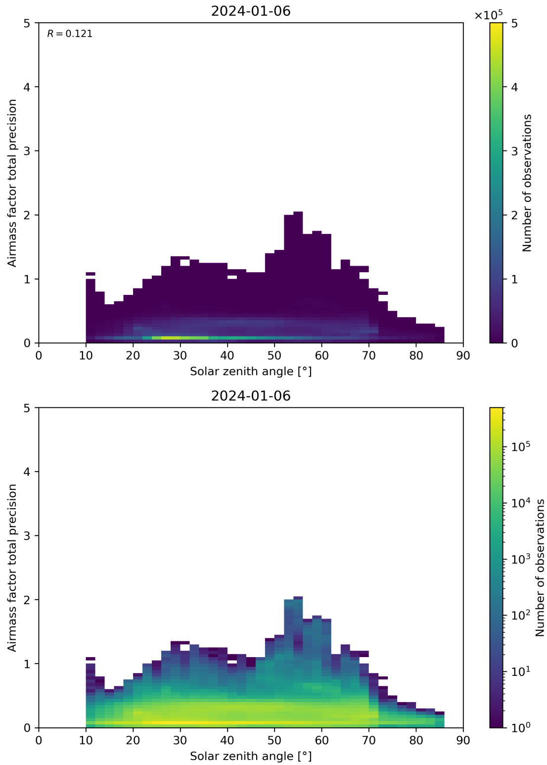
Figure 176: Scatter density plot of “Solar zenith angle” against “Airmass factor total precision” for 2024-01-05 to 2024-01-07.
