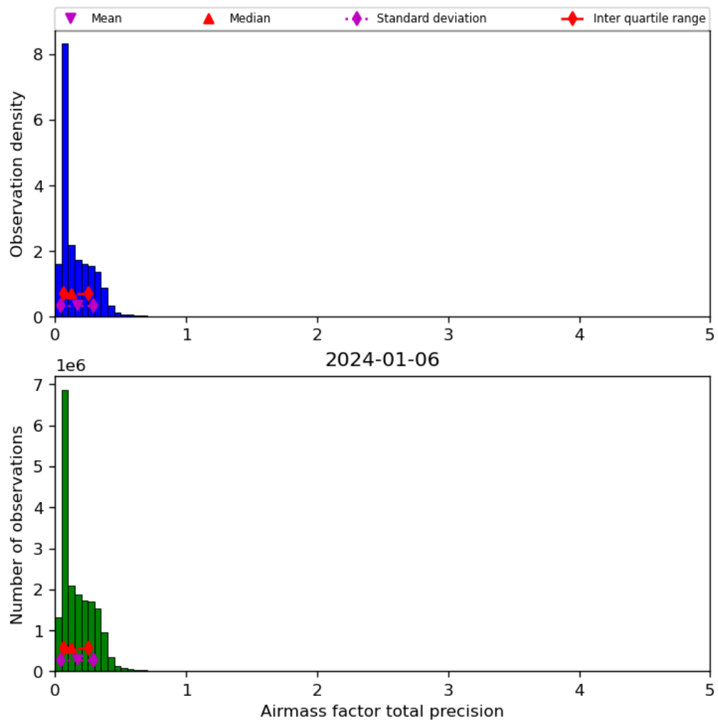
Figure 41: Histogram of “Airmass factor total precision” for 2024-01-05 to 2024-01-07
