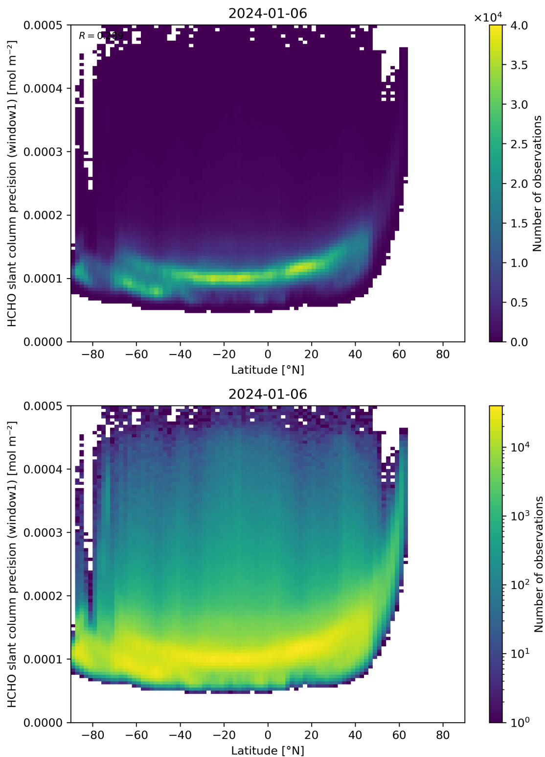
Figure 160: Scatter density plot of “Latitude” against “HCHO slant column precision (window1)” for 2024-01-05 to 2024-01-07.
