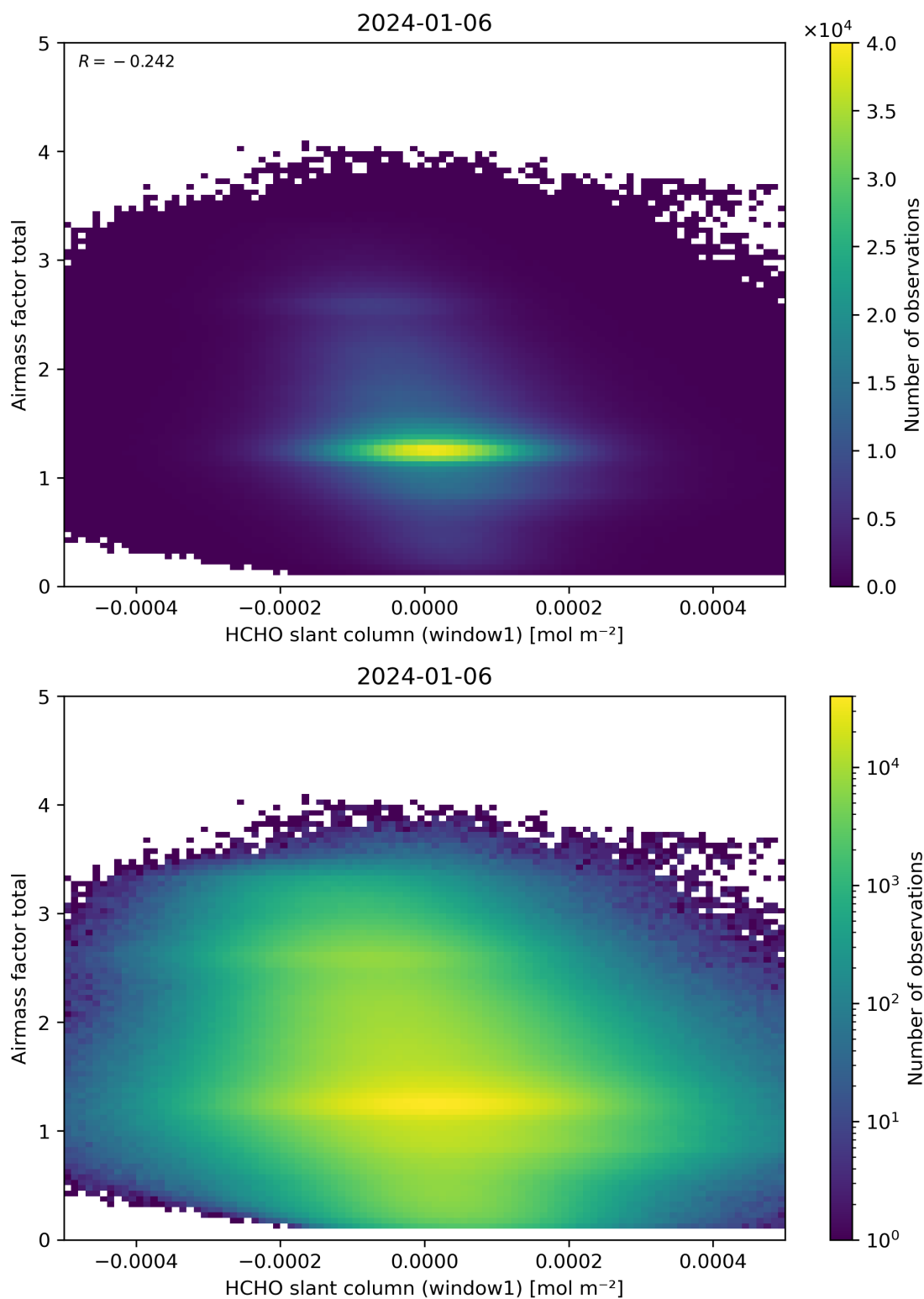
Figure 85: Scatter density plot of “HCHO slant column (window1)” against “Airmass factor total” for 2024-01-05 to 2024-01-07.
