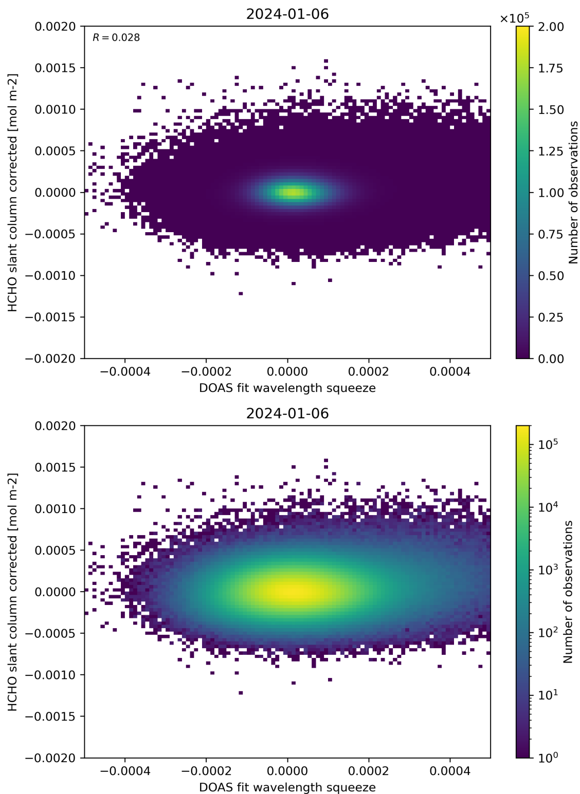
Figure 69: Scatter density plot of “DOAS fit wavelength squeeze” against “HCHO slant column corrected” for 2024-01-05 to 2024-01-07.
