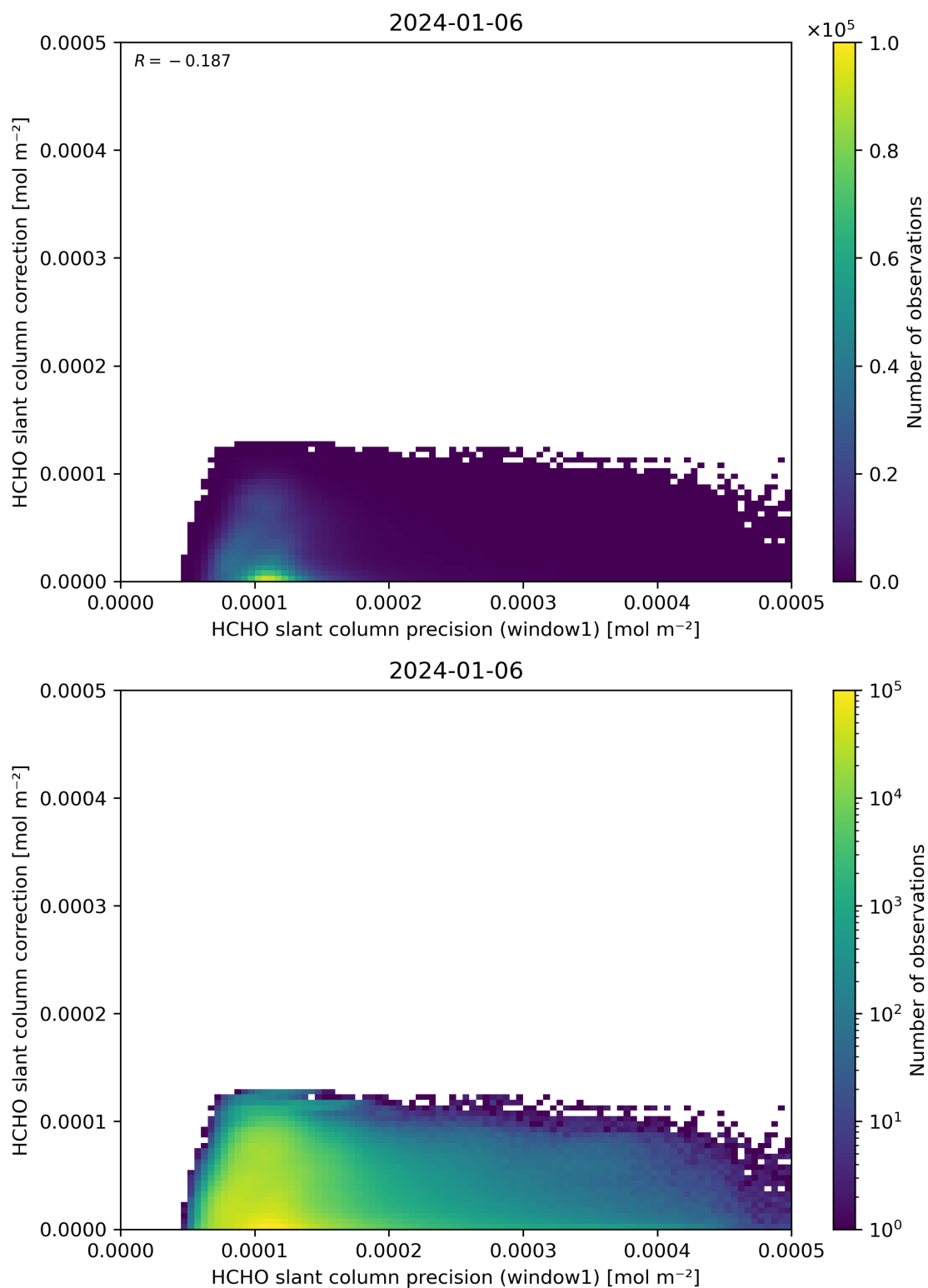
Figure 93: Scatter density plot of “HCHO slant column precision (window1)” against “HCHO slant column correction” for 2024-01-05 to 2024-01-07.
