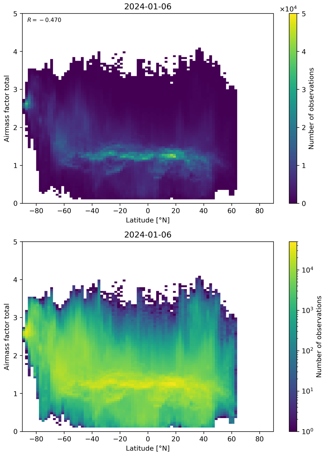
Figure 161: Scatter density plot of “Latitude” against “Airmass factor total” for 2024-01-05 to 2024-01-07.
