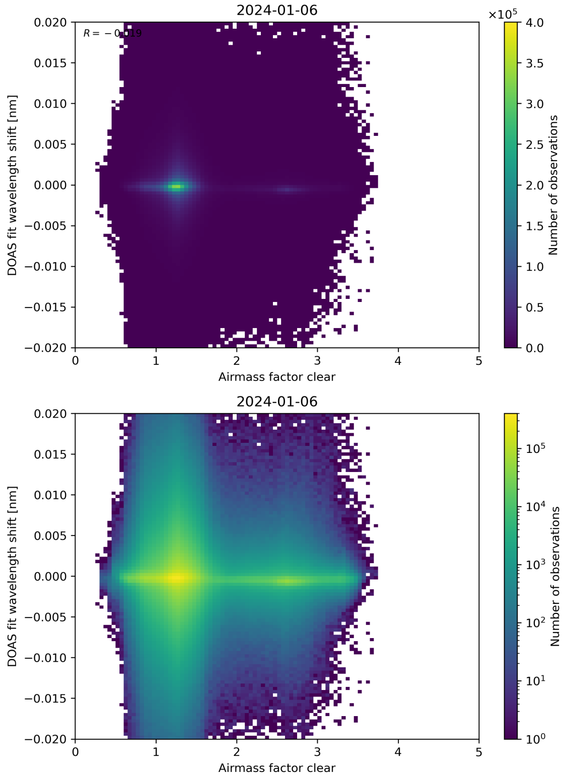
Figure 72: Scatter density plot of “Airmass factor clear” against “DOAS fit wavelength shift” for 2024-01-05 to 2024-01-07.
