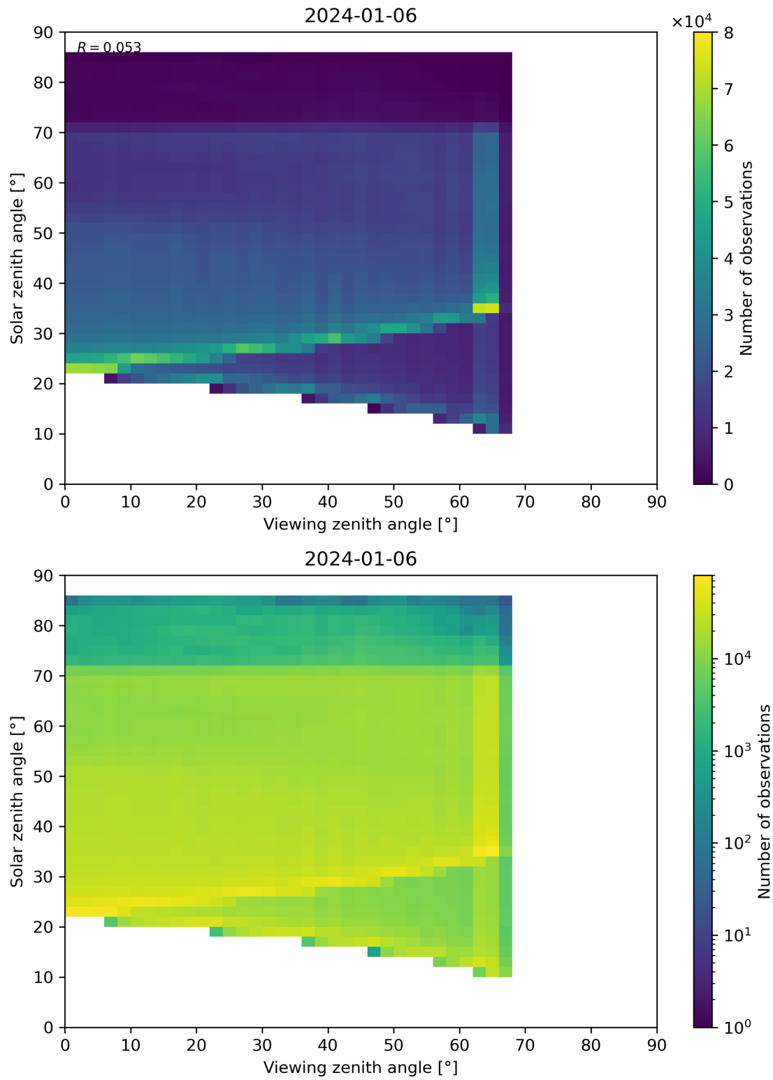
Figure 197: Scatter density plot of “Viewing zenith angle” against “Solar zenith angle” for 2024-01-05 to 2024-01-07.
