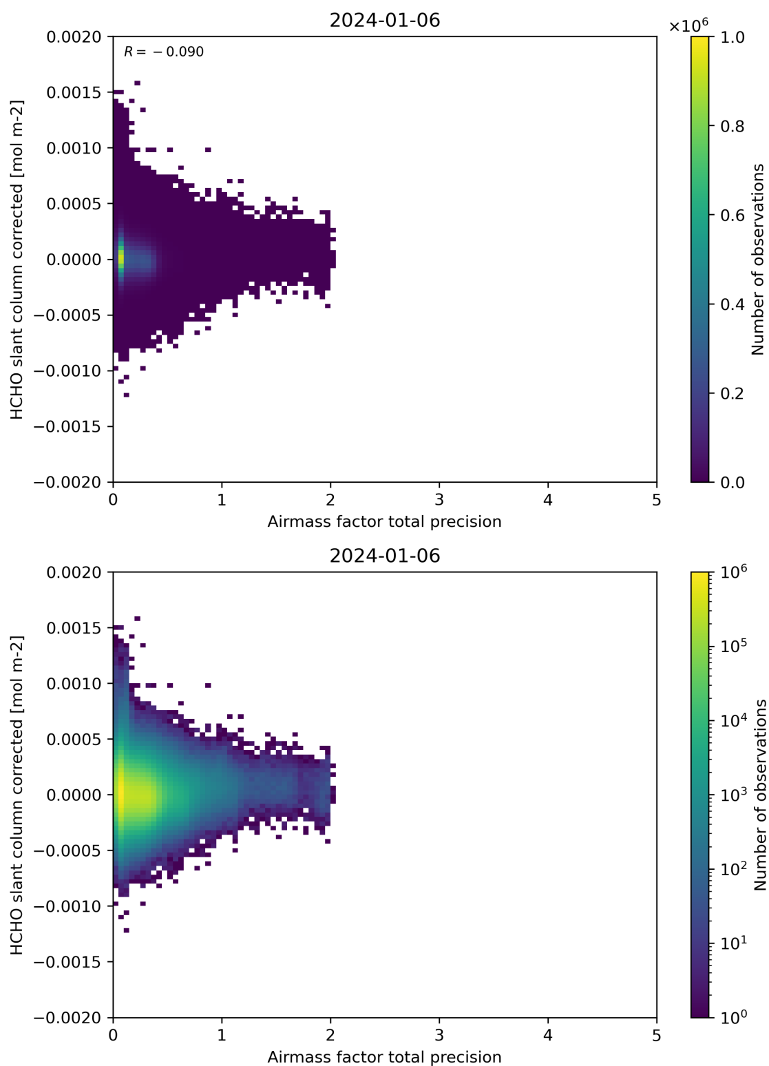
Figure 109: Scatter density plot of “Airmass factor total precision” against “HCHO slant column corrected” for 2024-01-05 to 2024-01-07.
