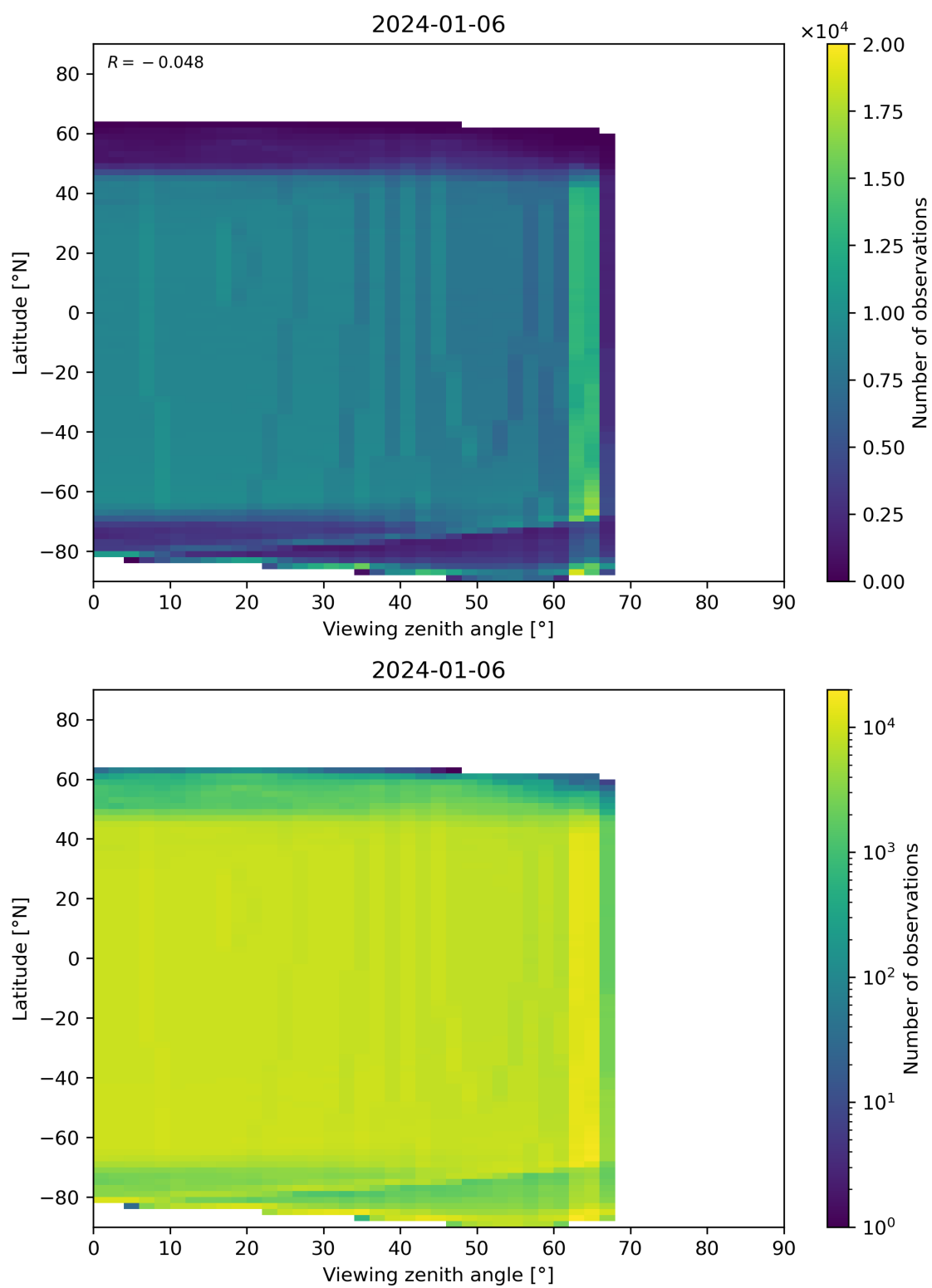
Figure 196: Scatter density plot of “Viewing zenith angle” against “Latitude” for 2024-01-05 to 2024-01-07.
