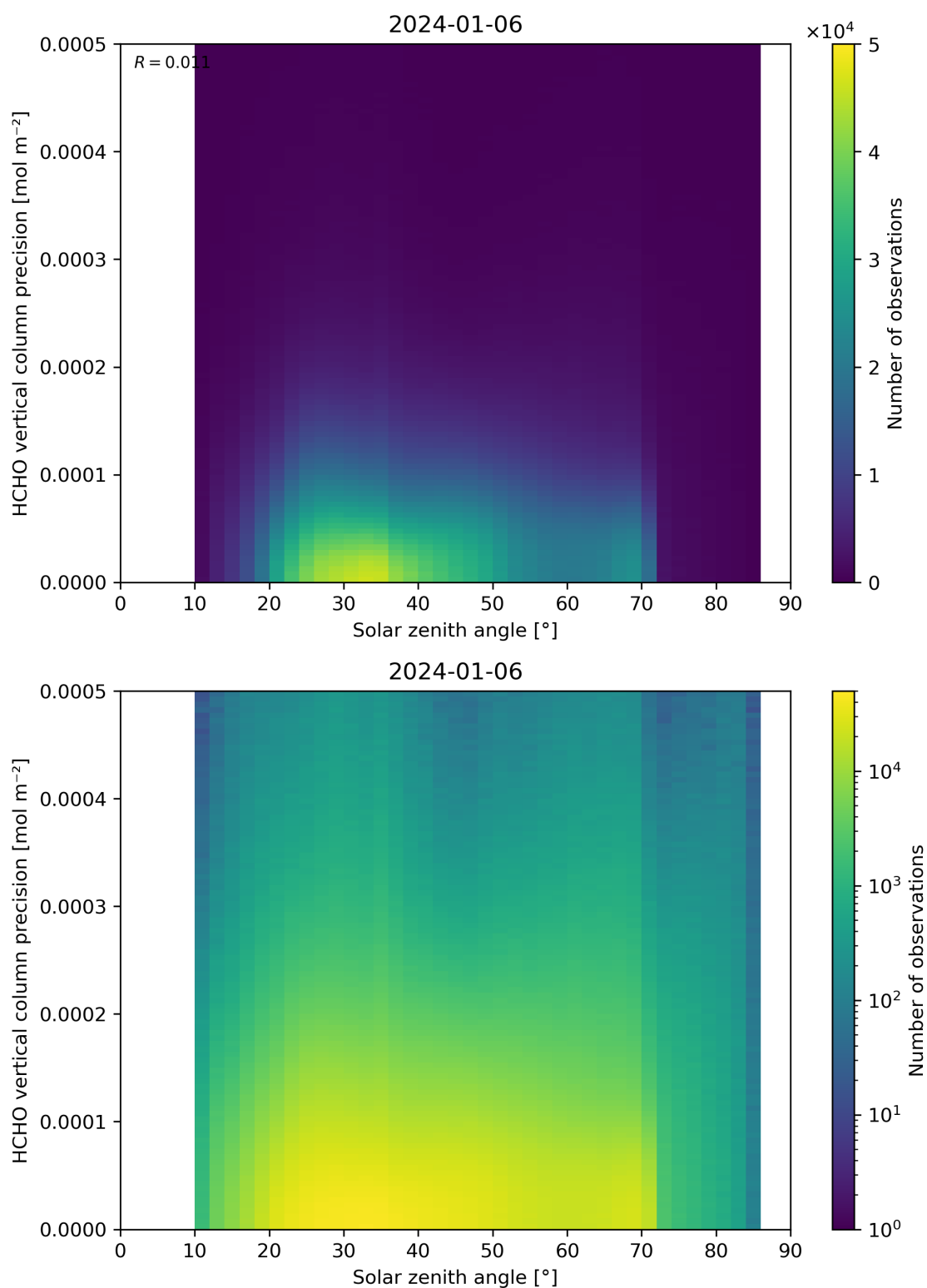
Figure 179: Scatter density plot of “Solar zenith angle” against “HCHO vertical column precision” for 2024-01-05 to 2024-01-07.
