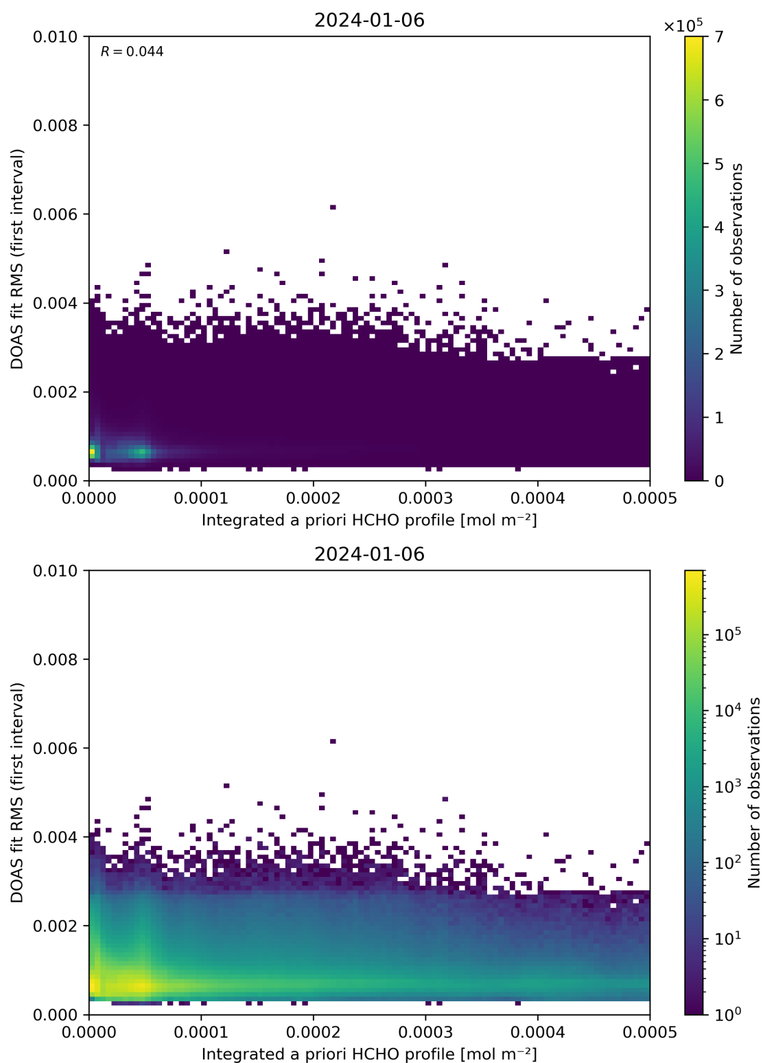
Figure 148: Scatter density plot of “Integrated a priori HCHO profile” against “DOAS fit RMS (first interval)” for 2024-01-05 to 2024-01-07.
