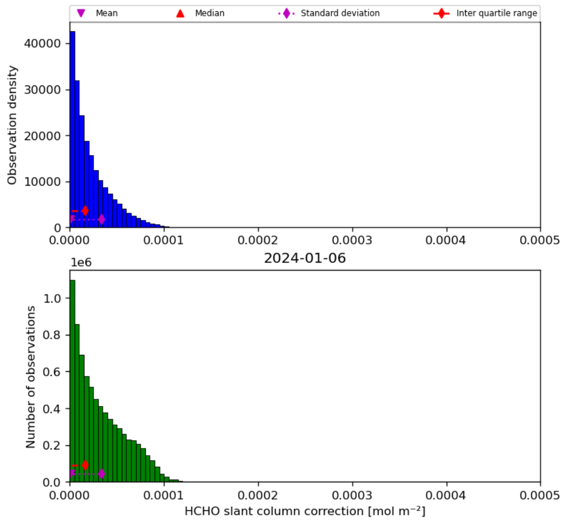
Figure 47: Histogram of “HCHO slant column correction” for 2024-01-05 to 2024-01-07
