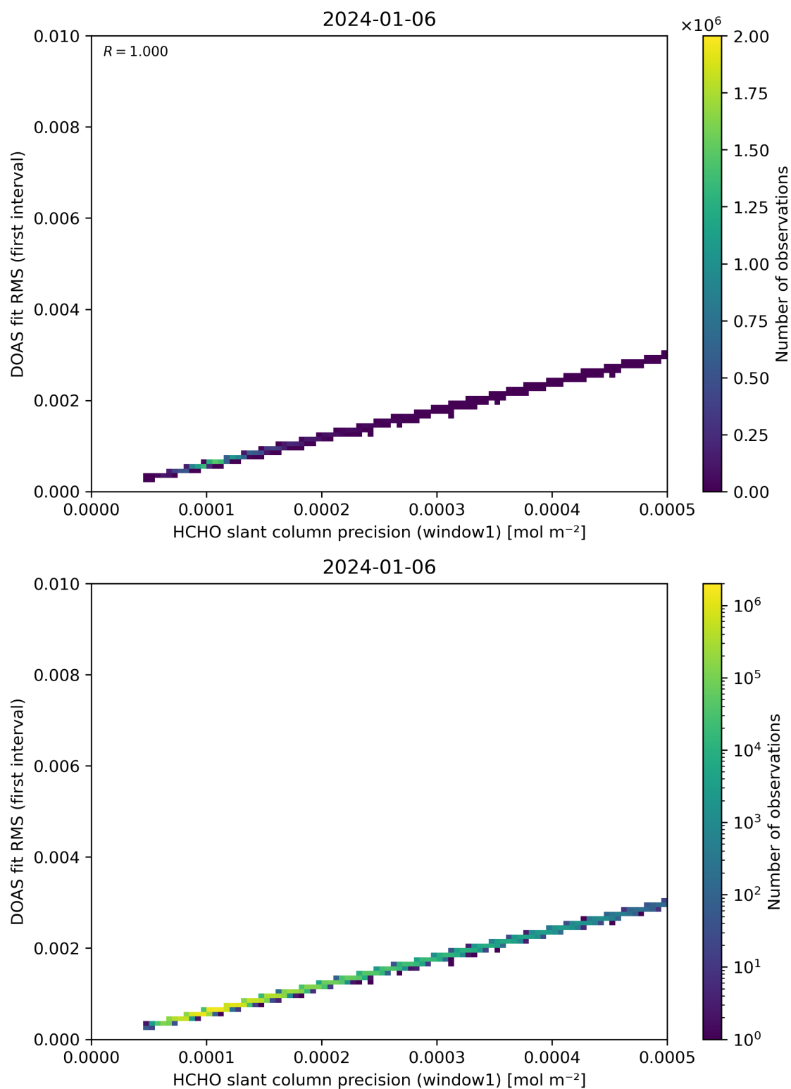
Figure 88: Scatter density plot of “HCHO slant column precision (window1)” against “DOAS fit RMS (first interval)” for 2024-01-05 to 2024-01-07.
