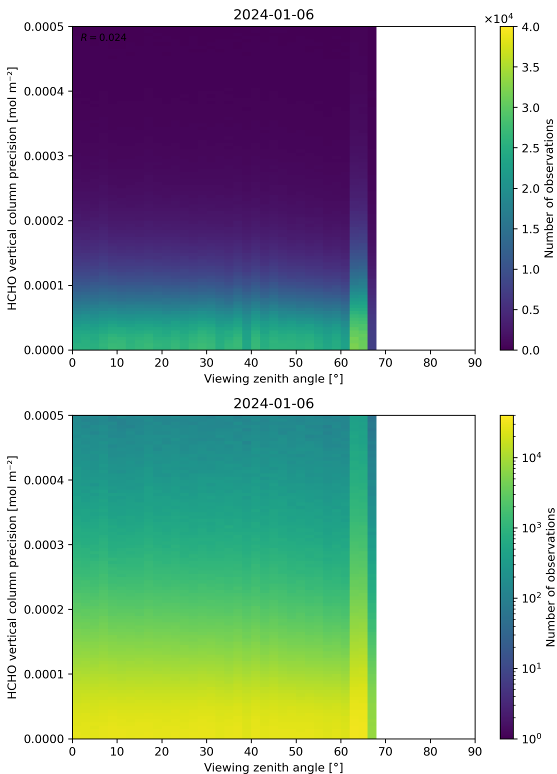
Figure 194: Scatter density plot of “Viewing zenith angle” against “HCHO vertical column precision” for 2024-01-05 to 2024-01-07.
