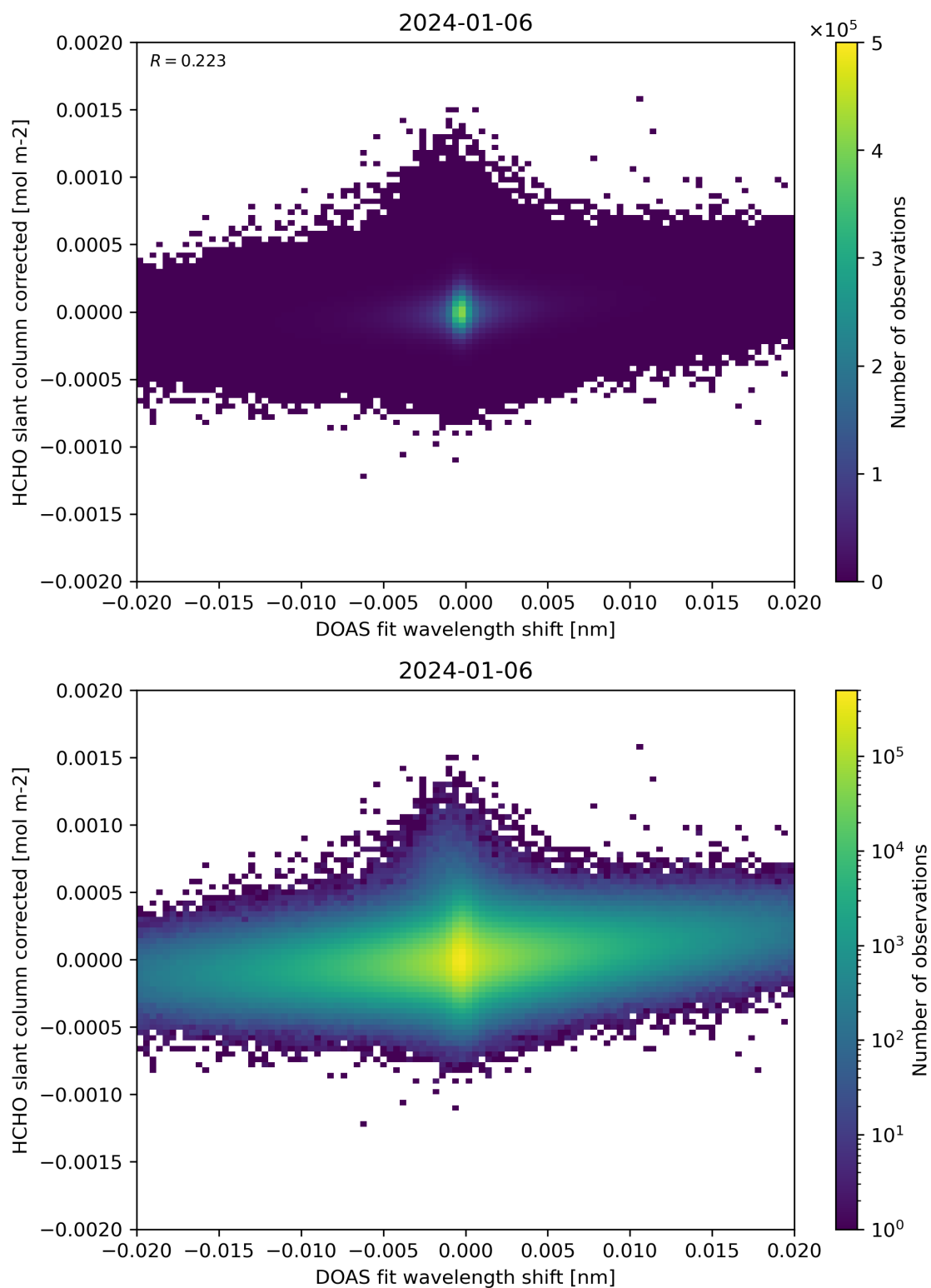
Figure 66: Scatter density plot of “DOAS fit wavelength shift” against “HCHO slant column corrected” for 2024-01-05 to 2024-01-07.
