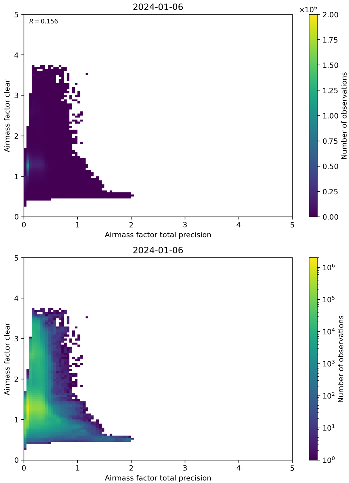
Figure 108: Scatter density plot of “Airmass factor total precision” against “Airmass factor clear” for 2024-01-05 to 2024-01-07.
