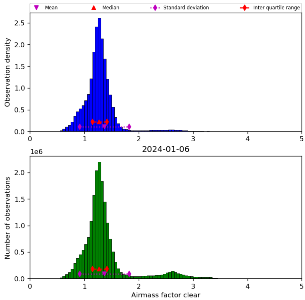
Figure 42: Histogram of “Airmass factor clear” for 2024-01-05 to 2024-01-07
