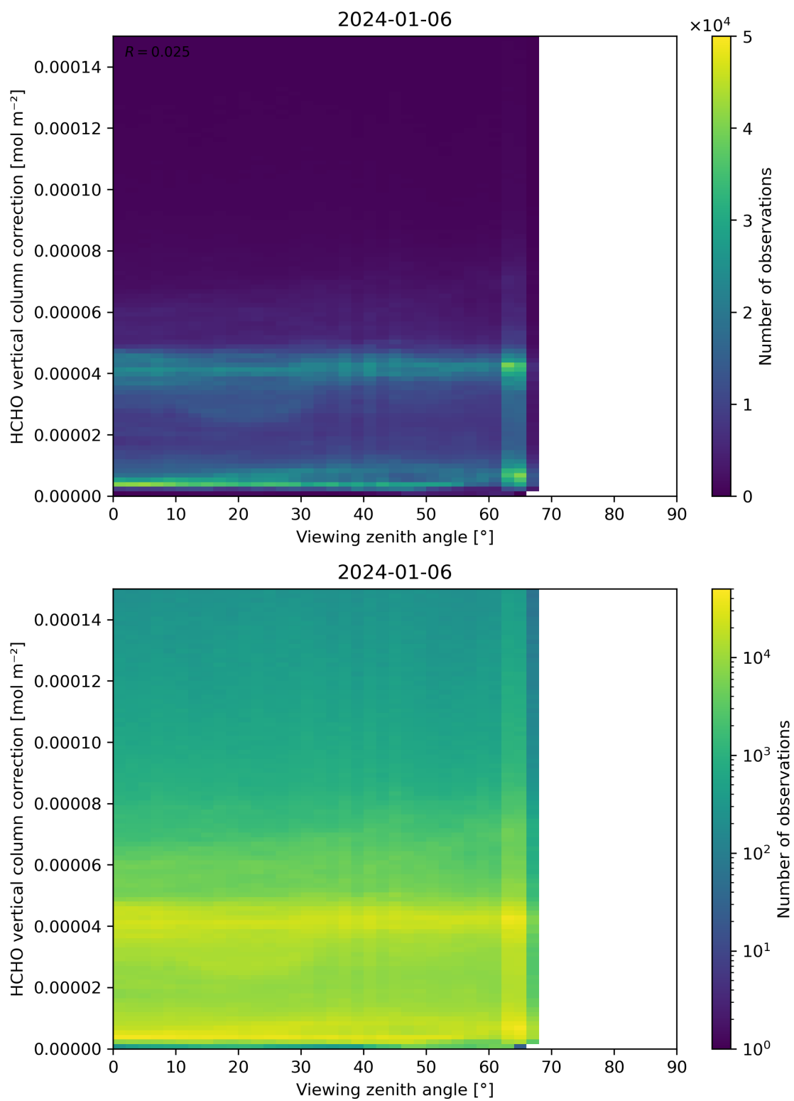
Figure 193: Scatter density plot of “Viewing zenith angle” against “HCHO vertical column correction” for 2024-01-05 to 2024-01-07.
