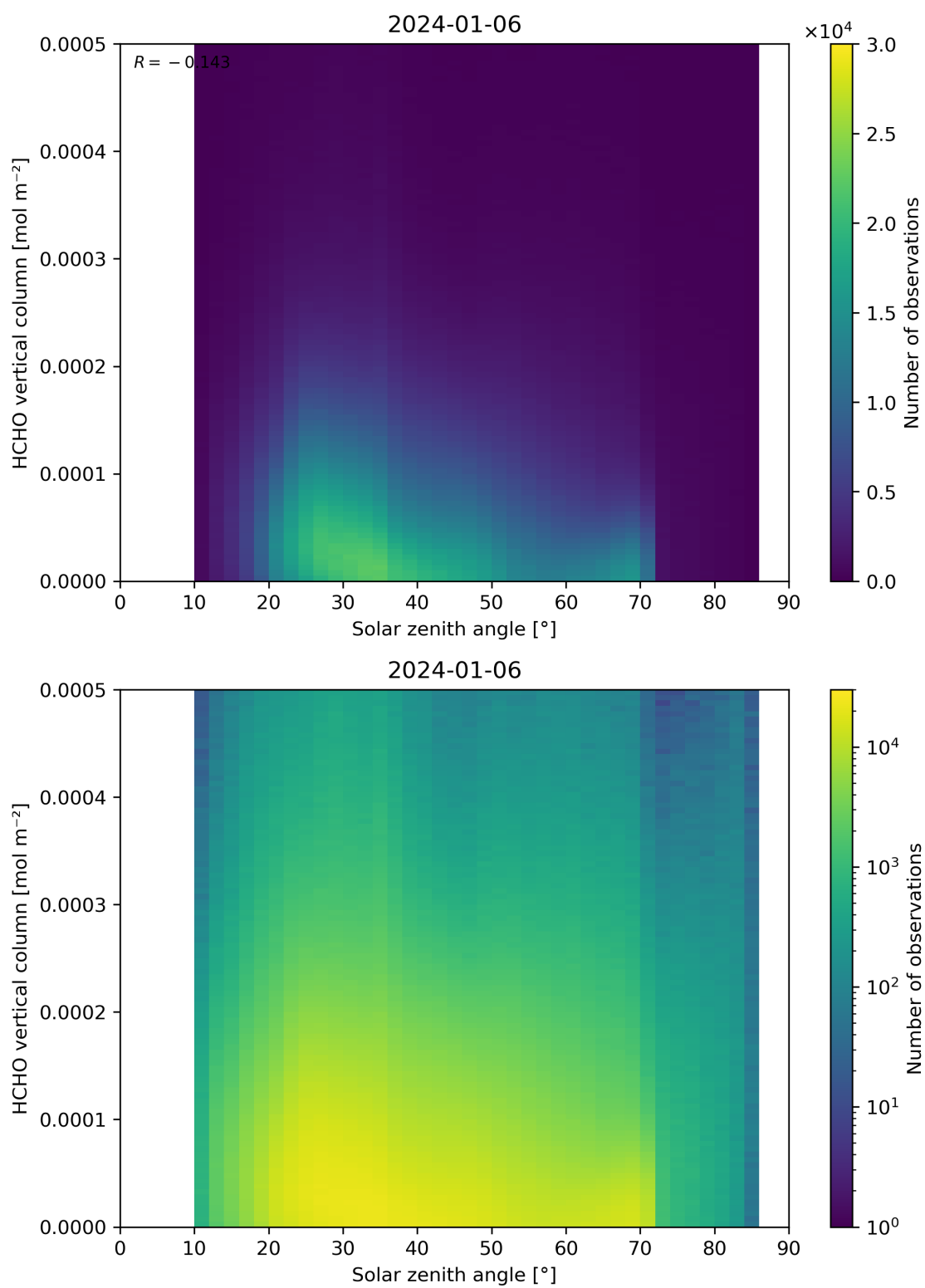
Figure 177: Scatter density plot of “Solar zenith angle” against “HCHO vertical column” for 2024-01-05 to 2024-01-07.
