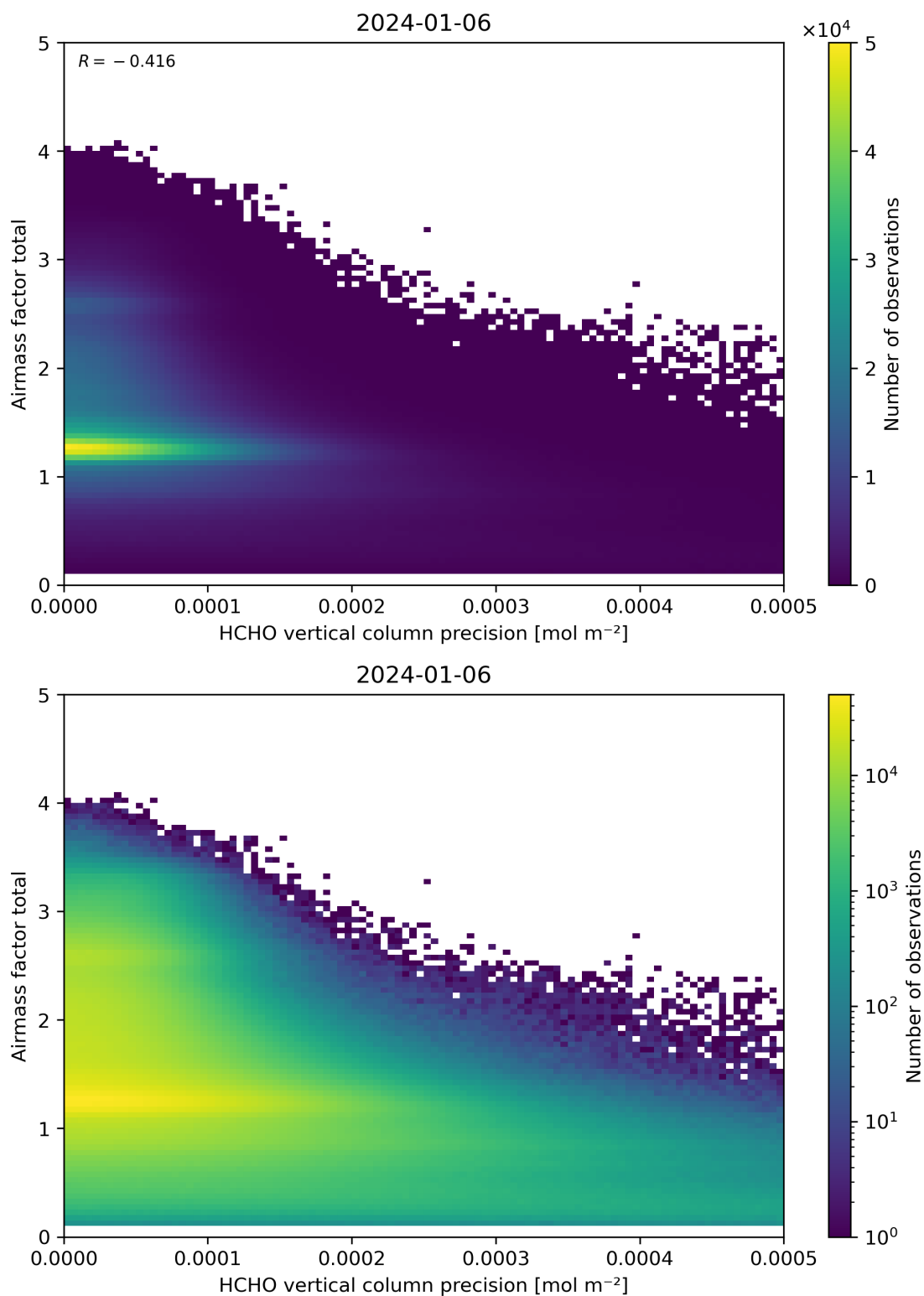
Figure 144: Scatter density plot of “HCHO vertical column precision” against “Airmass factor total” for 2024-01-05 to 2024-01-07.
