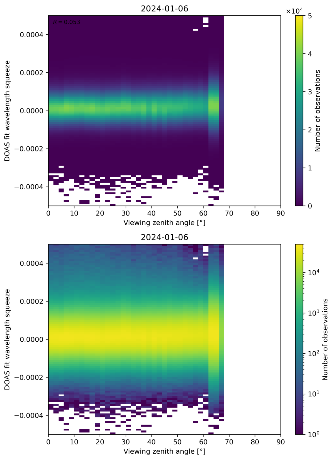
Figure 184: Scatter density plot of “Viewing zenith angle” against “DOAS fit wavelength squeeze” for 2024-01-05 to 2024-01-07.
