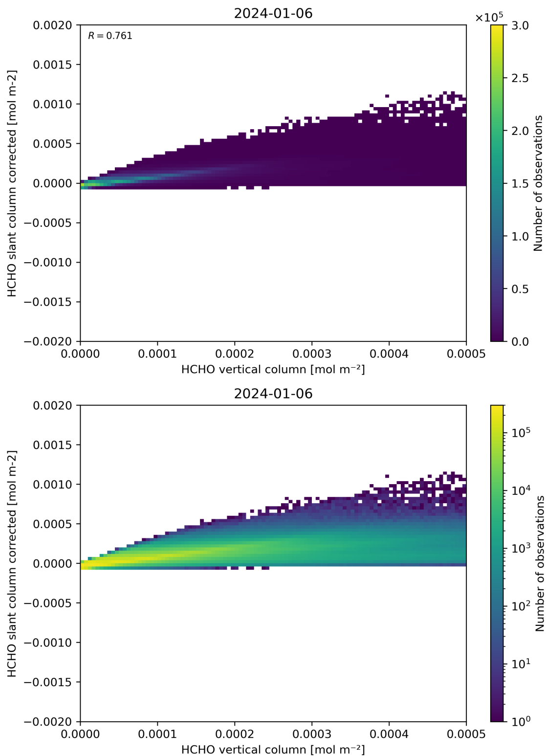
Figure 127: Scatter density plot of “HCHO vertical column” against “HCHO slant column corrected” for 2024-01-05 to 2024-01-07.
