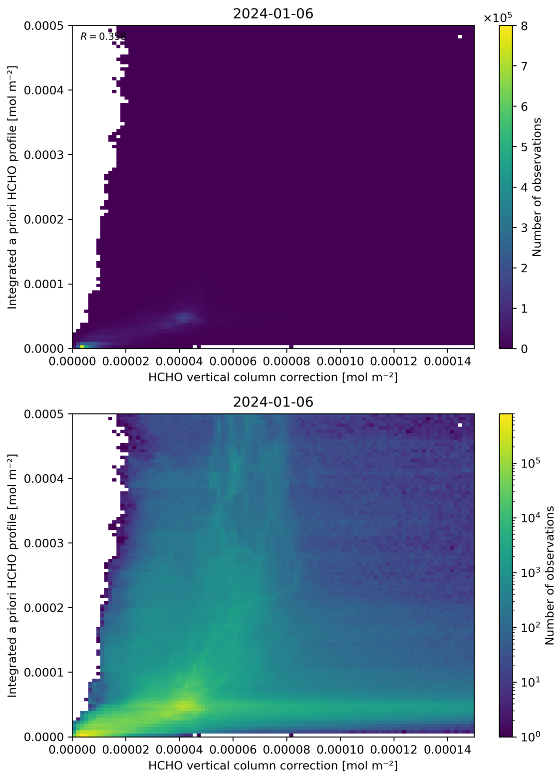
Figure 122: Scatter density plot of “HCHO vertical column correction” against “Integrated a priori HCHO profile” for 2024-01-05 to 2024-01-07.
