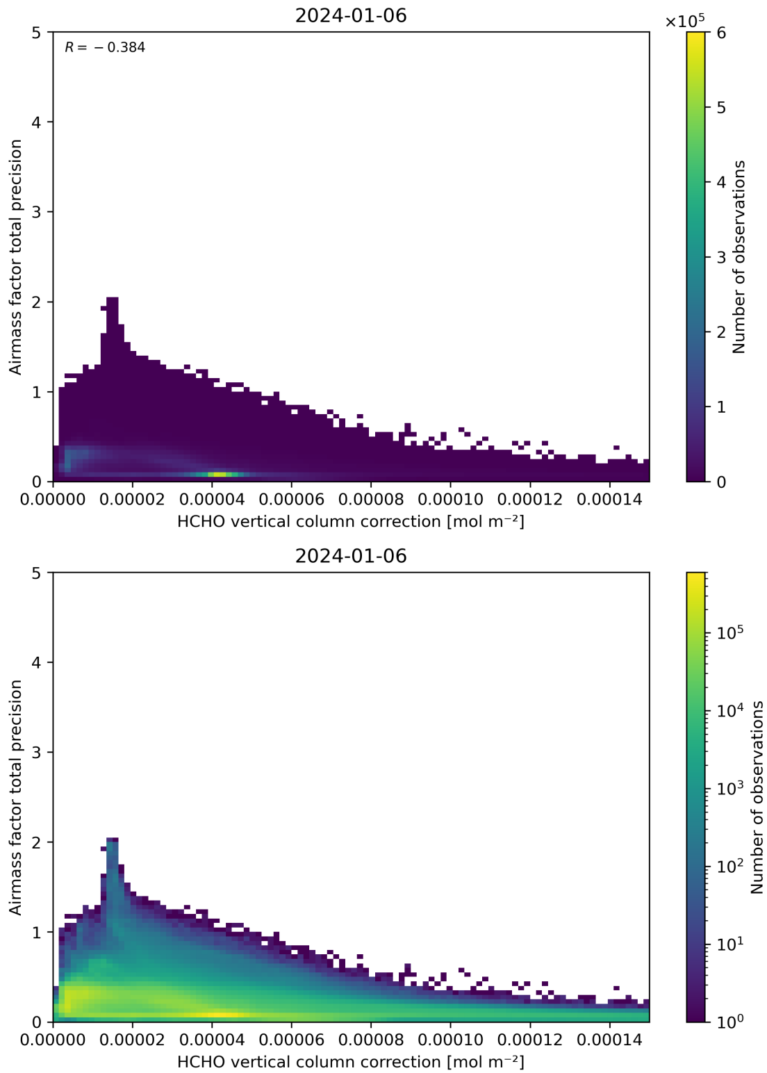
Figure 121: Scatter density plot of “HCHO vertical column correction” against “Airmass factor total precision” for 2024-01-05 to 2024-01-07.
