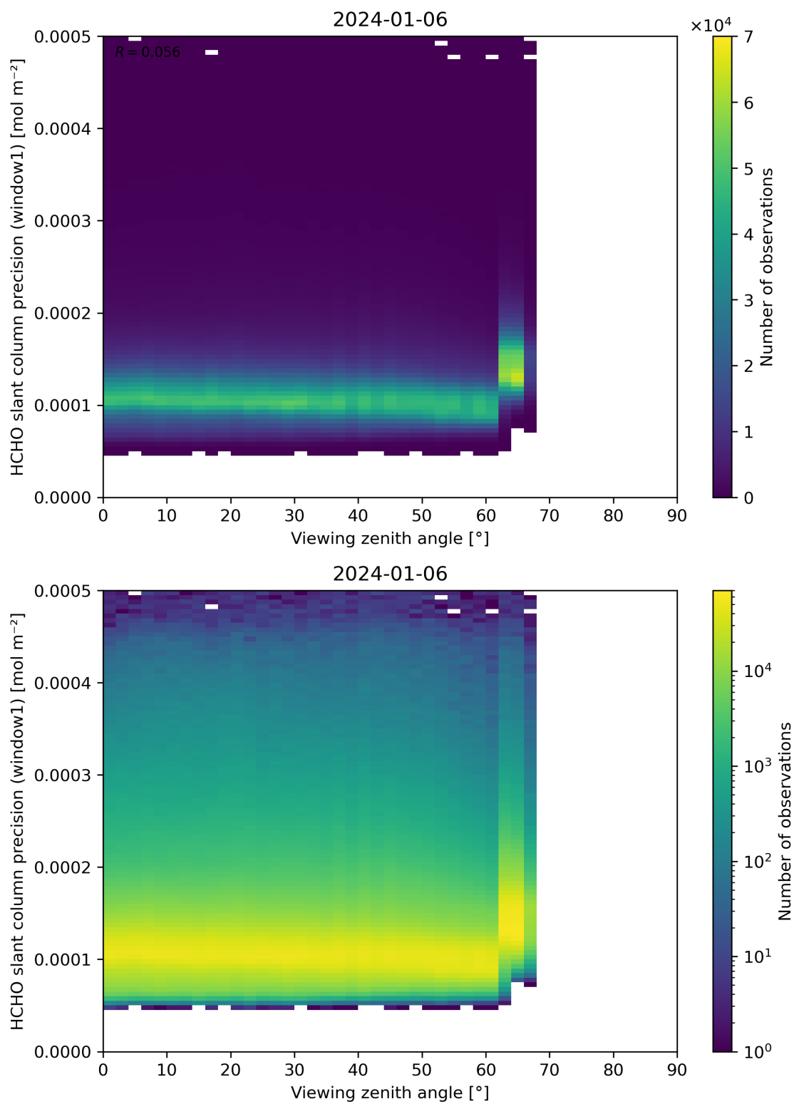
Figure 189: Scatter density plot of “Viewing zenith angle” against “HCHO slant column precision (window1)” for 2024-01-05 to 2024-01-07.
