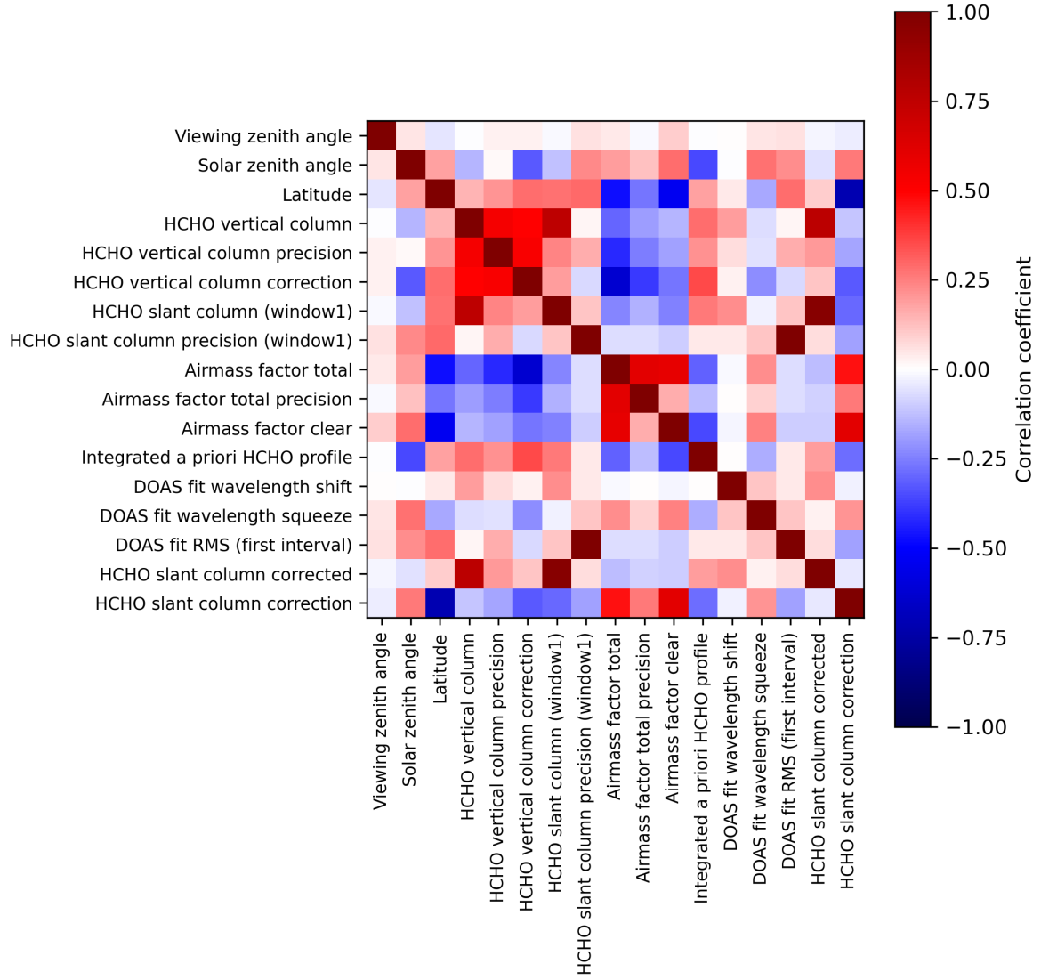
Figure 2: Map of correlation matrix for 2024-01-05 to 2024-01-07.
