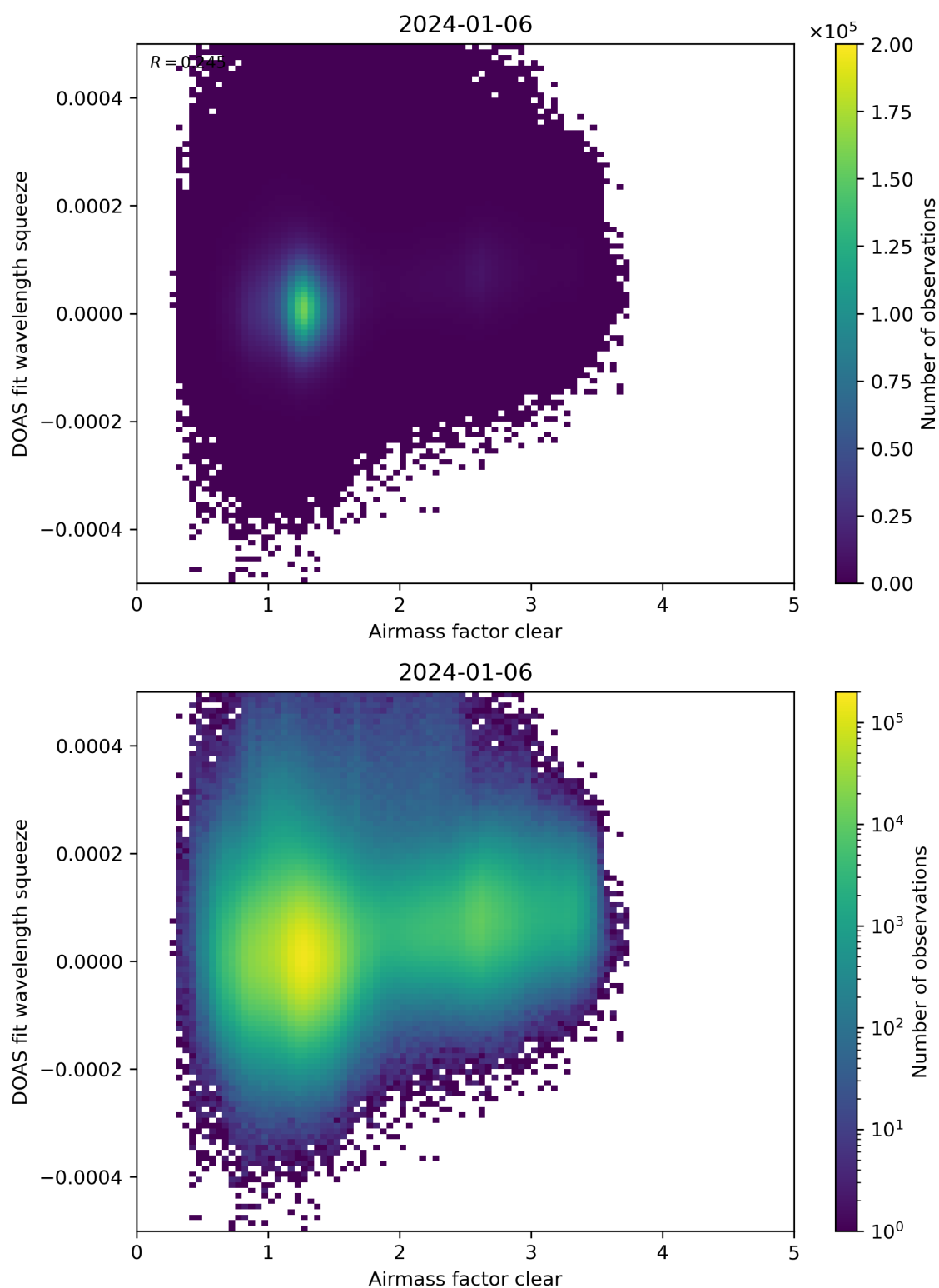
Figure 73: Scatter density plot of “Airmass factor clear” against “DOAS fit wavelength squeeze” for 2024-01-05 to 2024-01-07.
