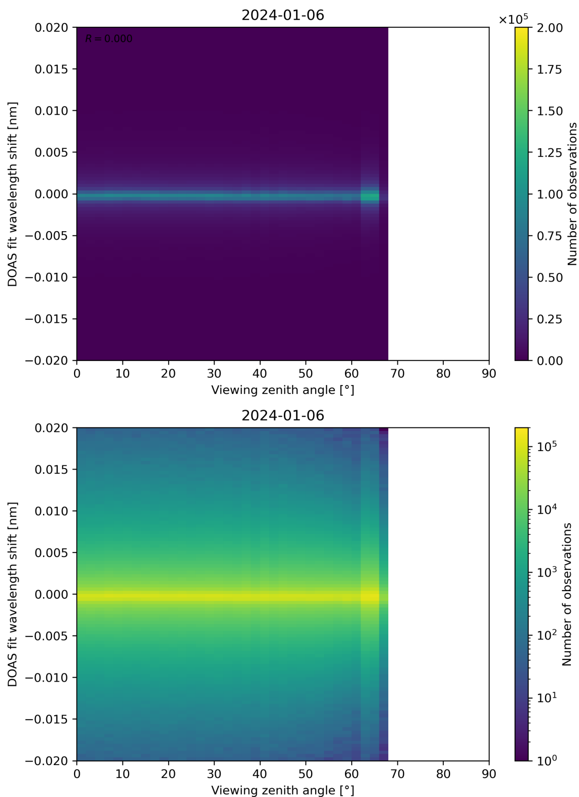
Figure 183: Scatter density plot of “Viewing zenith angle” against “DOAS fit wavelength shift” for 2024-01-05 to 2024-01-07.
