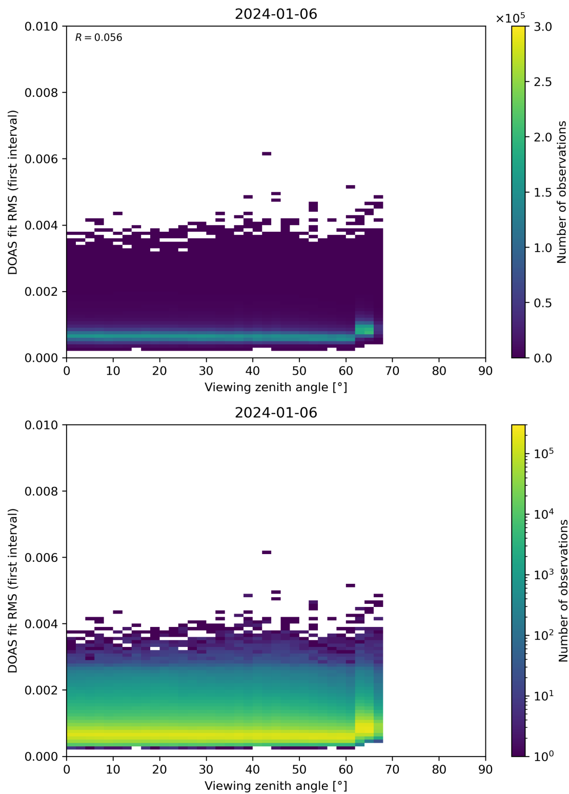
Figure 182: Scatter density plot of “Viewing zenith angle” against “DOAS fit RMS (first interval)” for 2024-01-05 to 2024-01-07.
