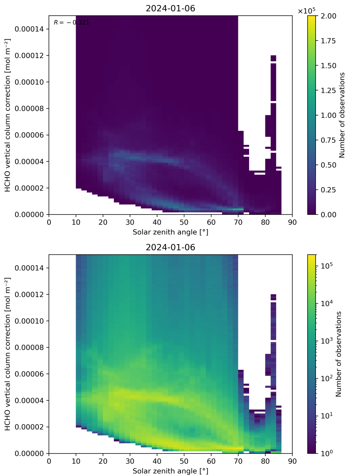
Figure 178: Scatter density plot of “Solar zenith angle” against “HCHO vertical column correction” for 2024-01-05 to 2024-01-07.
