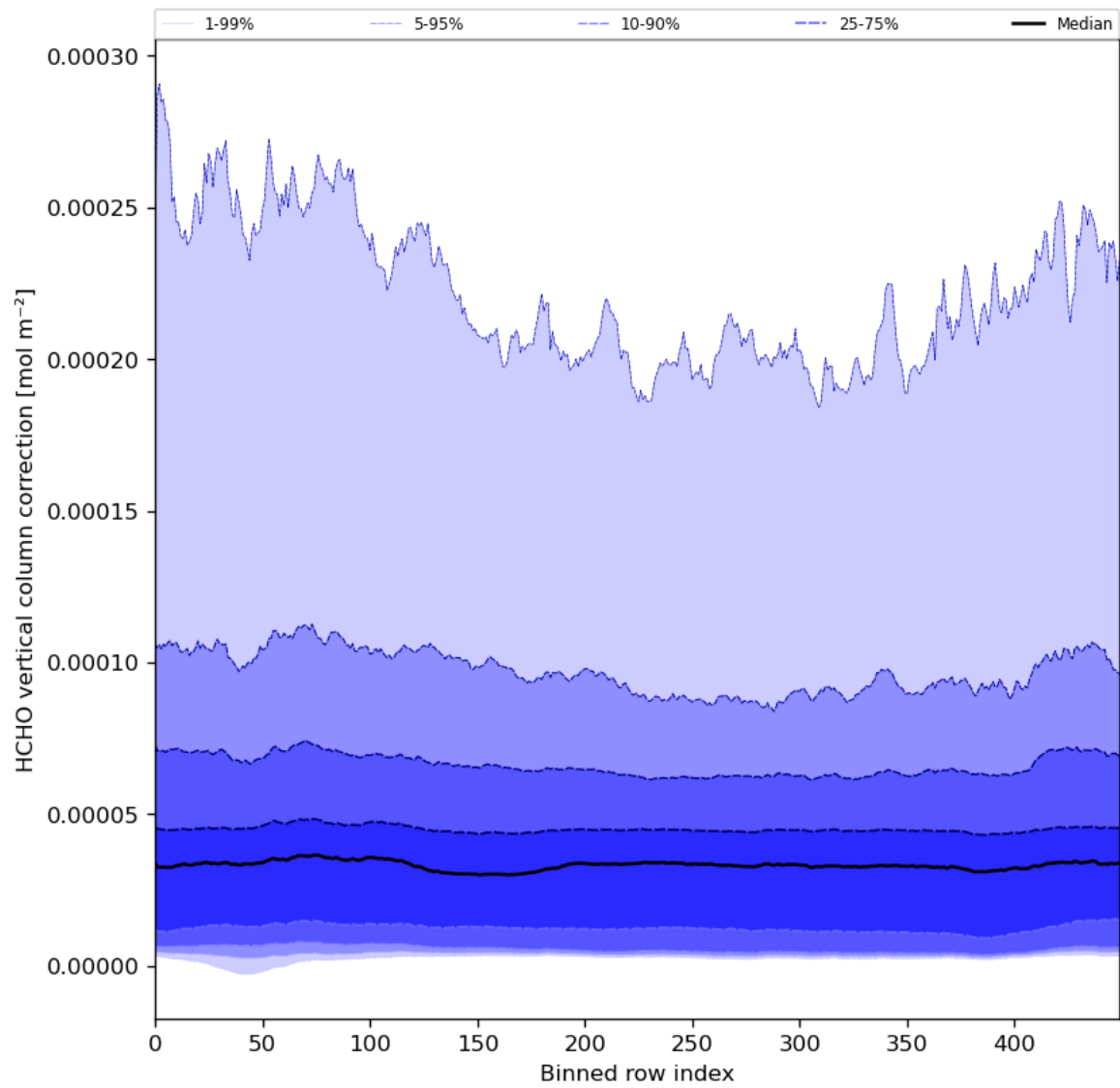
Figure 51: Along track statistics of “HCHO vertical column correction” for 2024-01-05 to 2024-01-07
