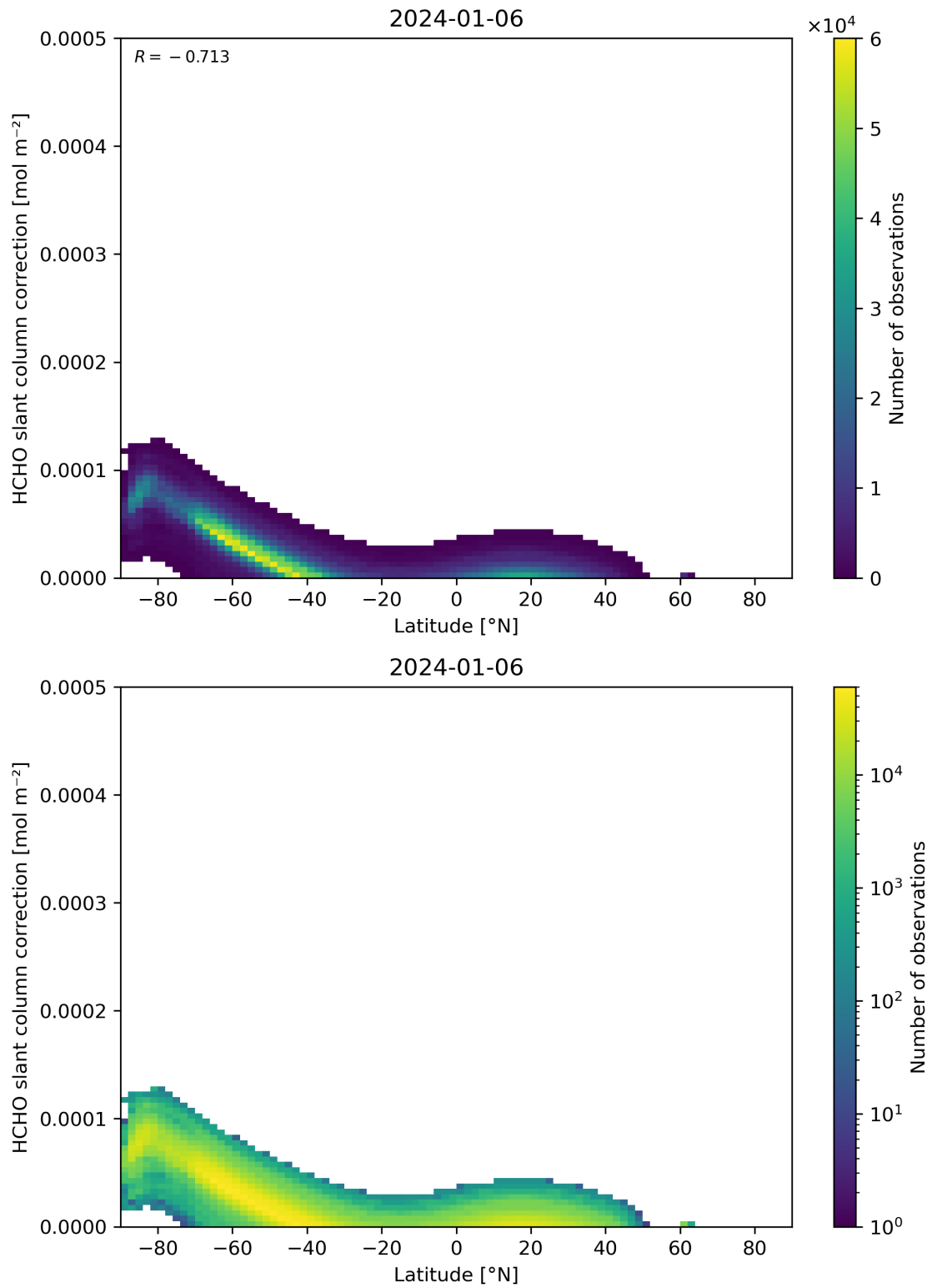
Figure 158: Scatter density plot of “Latitude” against “HCHO slant column correction” for 2024-01-05 to 2024-01-07.
