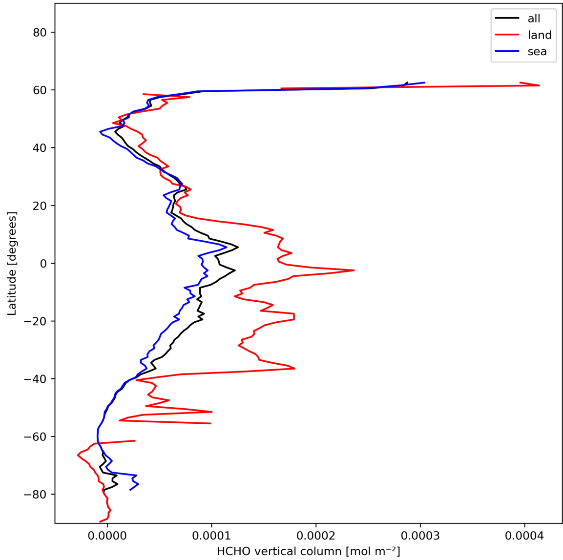
Figure 21: Zonal average of “HCHO vertical column” for 2024-01-05 to 2024-01-07.
