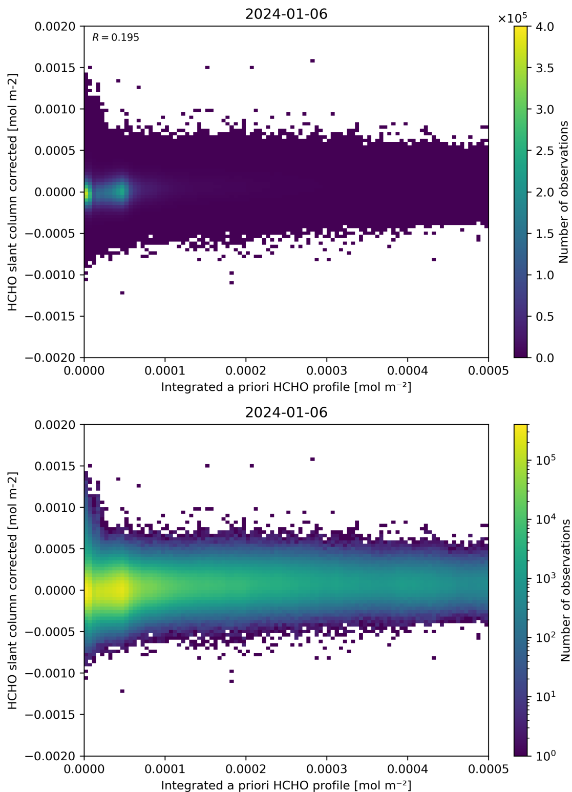
Figure 151: Scatter density plot of “Integrated a priori HCHO profile” against “HCHO slant column corrected” for 2024-01-05 to 2024-01-07.
