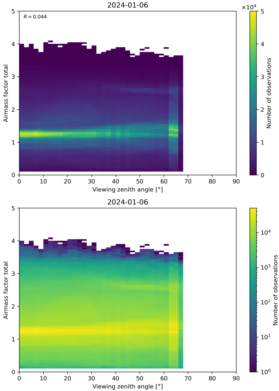
Figure 190: Scatter density plot of “Viewing zenith angle” against “Airmass factor total” for 2024-01-05 to 2024-01-07.
