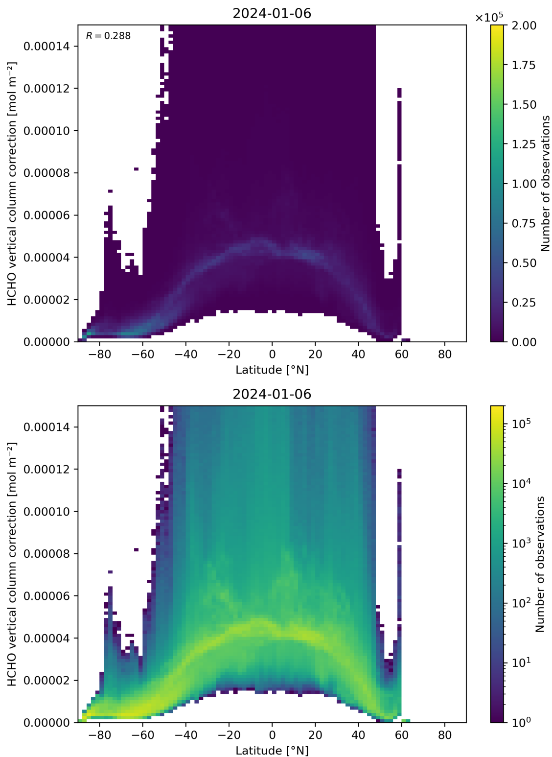
Figure 164: Scatter density plot of “Latitude” against “HCHO vertical column correction” for 2024-01-05 to 2024-01-07.
