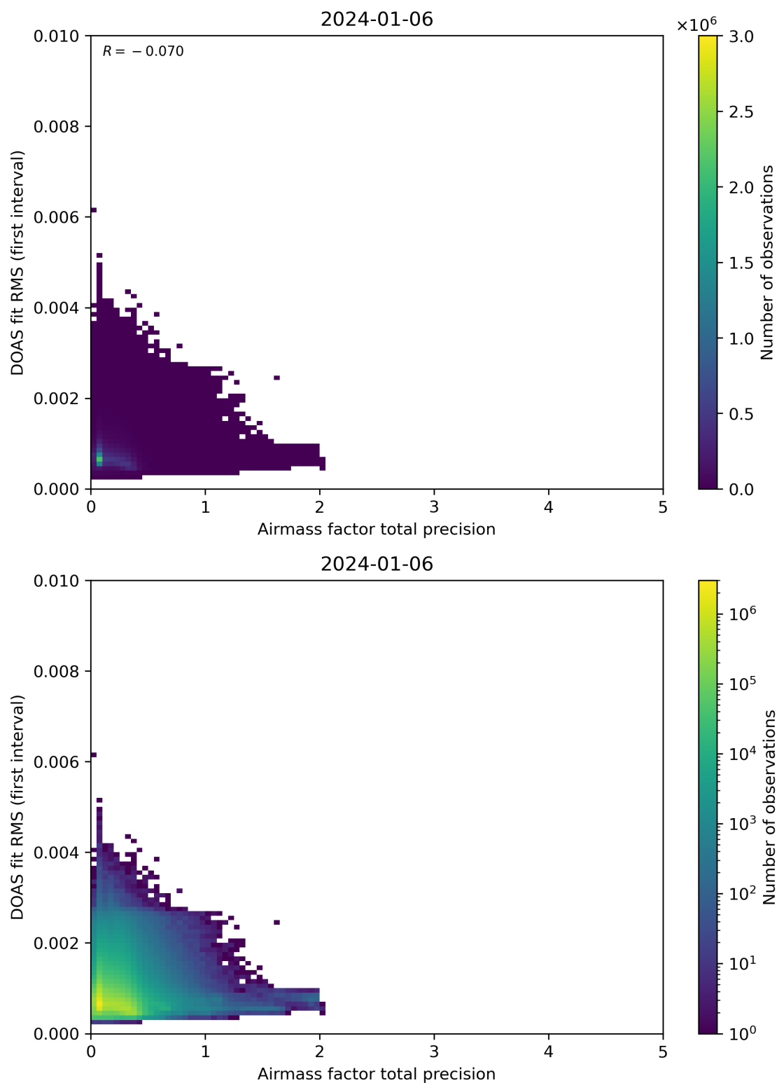
Figure 105: Scatter density plot of “Airmass factor total precision” against “DOAS fit RMS (first interval)” for 2024-01-05 to 2024-01-07.
