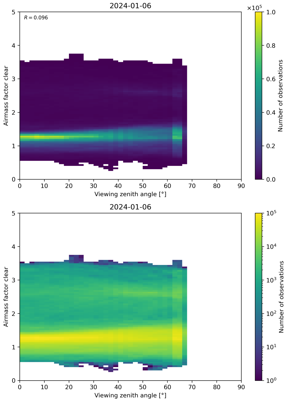
Figure 185: Scatter density plot of “Viewing zenith angle” against “Airmass factor clear” for 2024-01-05 to 2024-01-07.
