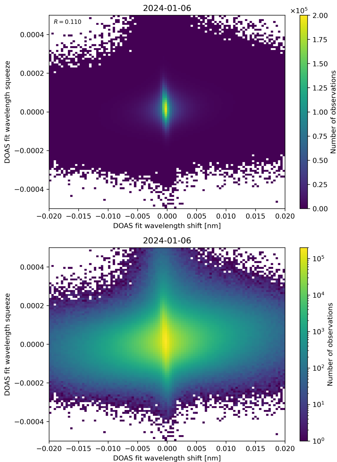
Figure 65: Scatter density plot of “DOAS fit wavelength shift” against “DOAS fit wavelength squeeze” for 2024-01-05 to 2024-01-07.
