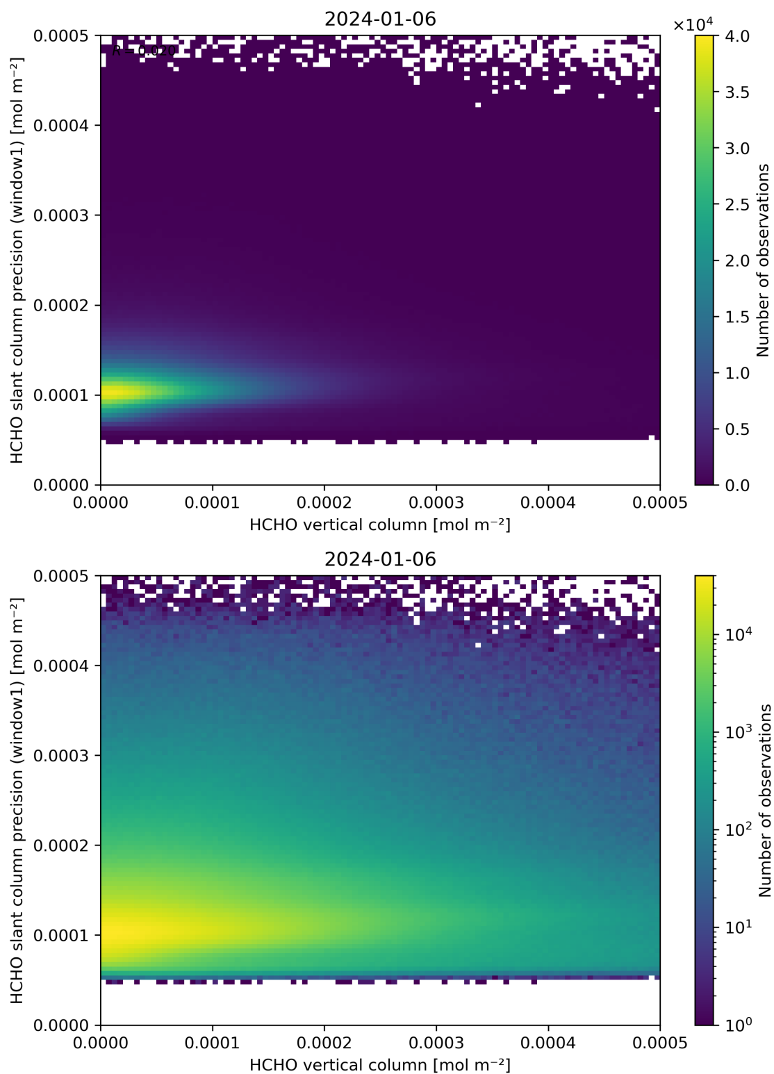
Figure 130: Scatter density plot of “HCHO vertical column” against “HCHO slant column precision (window1)” for 2024-01-05 to 2024-01-07.
