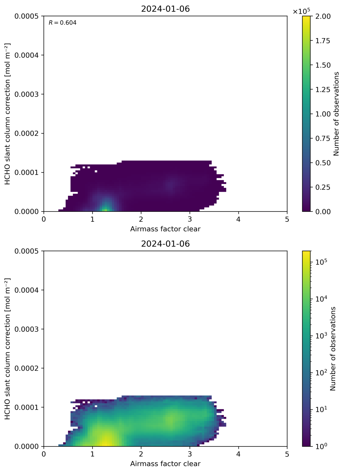
Figure 75: Scatter density plot of “Airmass factor clear” against “HCHO slant column correction” for 2024-01-05 to 2024-01-07.
