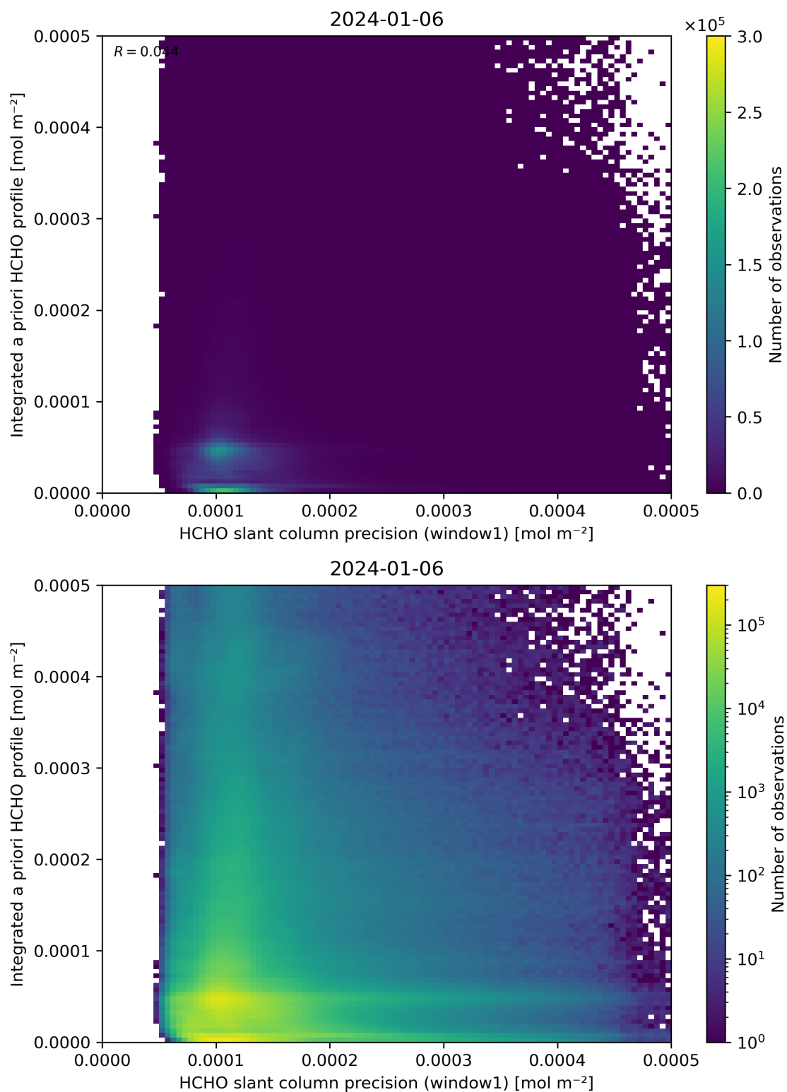
Figure 96: Scatter density plot of “HCHO slant column precision (window1)” against “Integrated a priori HCHO profile” for 2024-01-05 to 2024-01-07.
