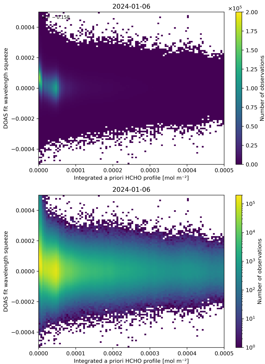
Figure 150: Scatter density plot of “Integrated a priori HCHO profile” against “DOAS fit wavelength squeeze” for 2024-01-05 to 2024-01-07.
