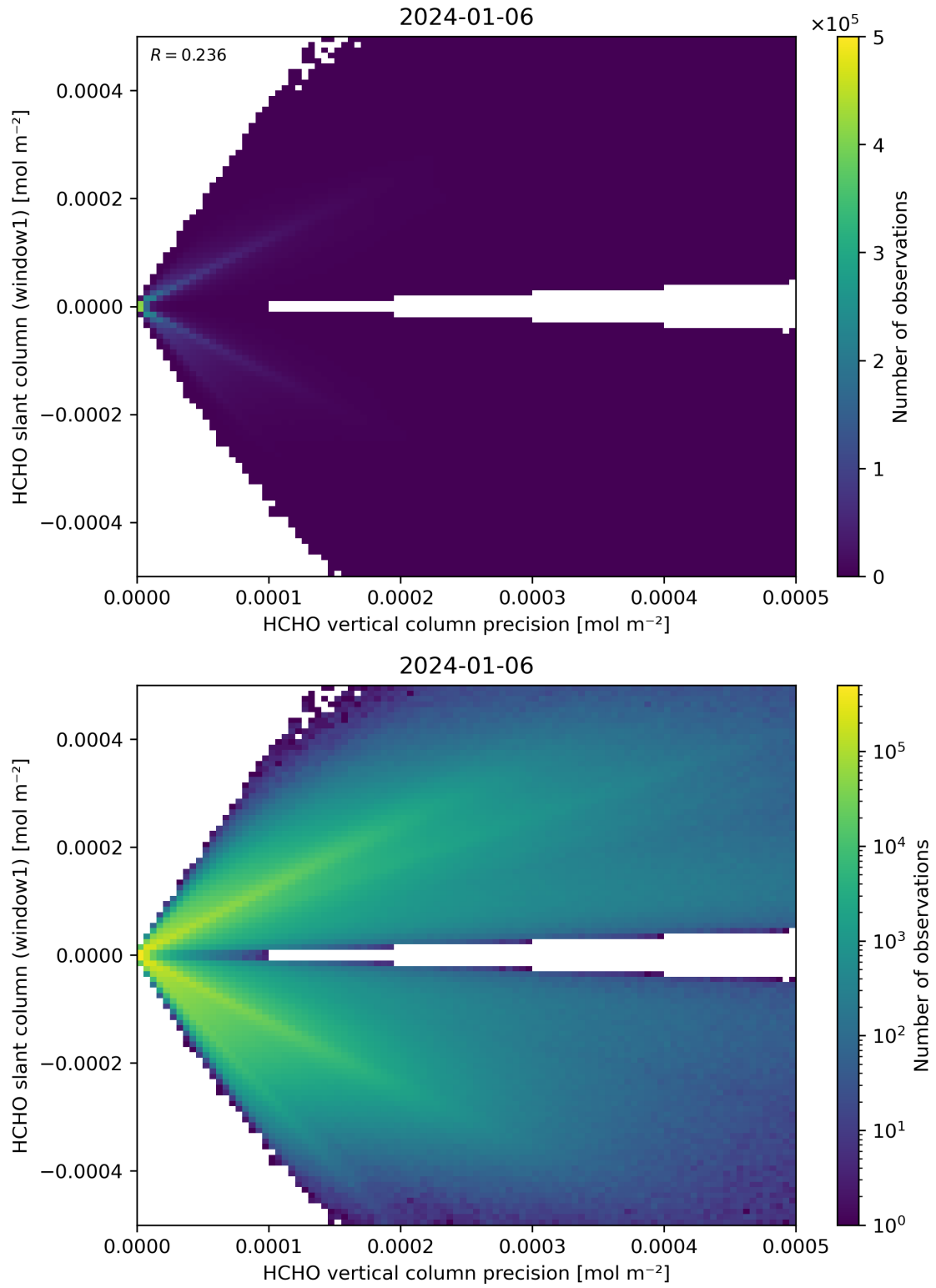
Figure 142: Scatter density plot of “HCHO vertical column precision” against “HCHO slant column (window1)” for 2024-01-05 to 2024-01-07.
