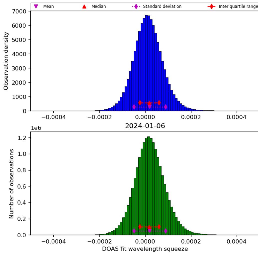
Figure 45: Histogram of “DOAS fit wavelength squeeze” for 2024-01-05 to 2024-01-07
