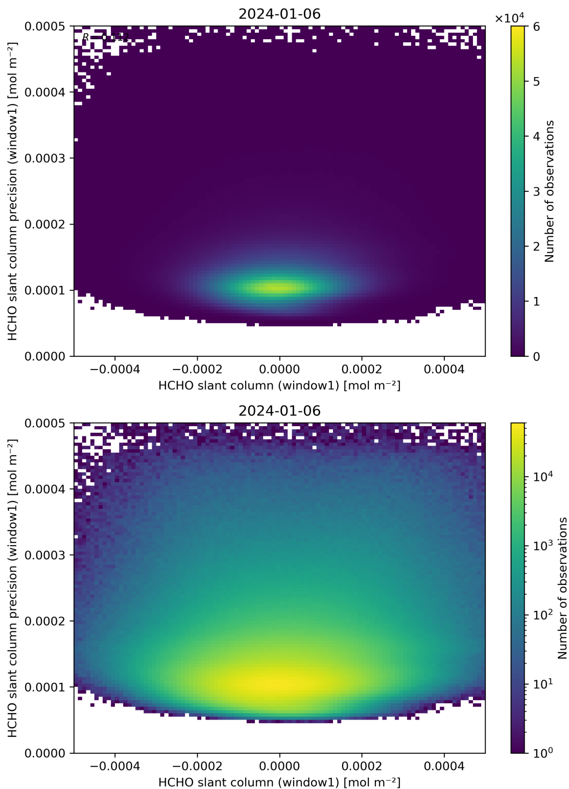
Figure 84: Scatter density plot of “HCHO slant column (window1)” against “HCHO slant column precision (window1)” for 2024-01-05 to 2024-01-07.
