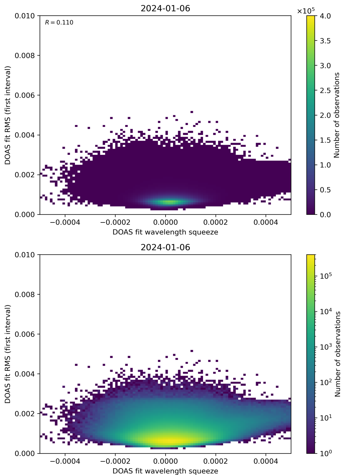
Figure 68: Scatter density plot of “DOAS fit wavelength squeeze” against “DOAS fit RMS (first interval)” for 2024-01-05 to 2024-01-07.
