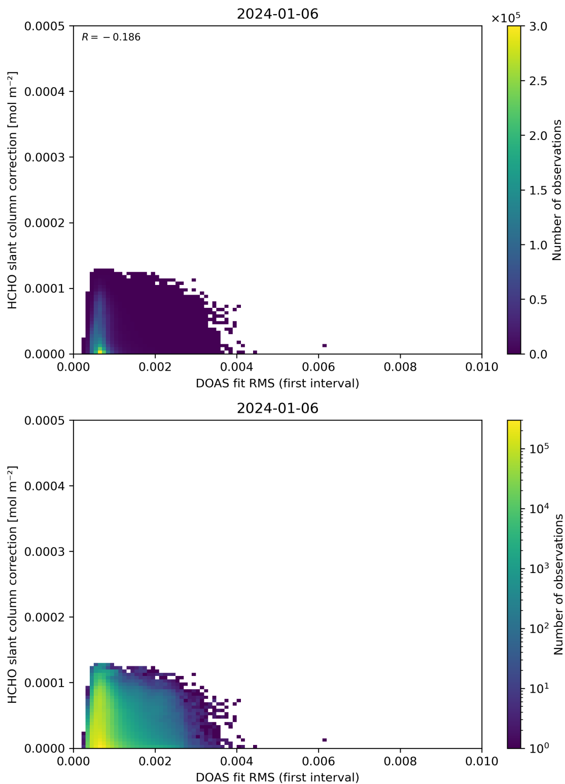
Figure 63: Scatter density plot of “DOAS fit RMS (first interval)” against “HCHO slant column correction” for 2024-01-05 to 2024-01-07.
