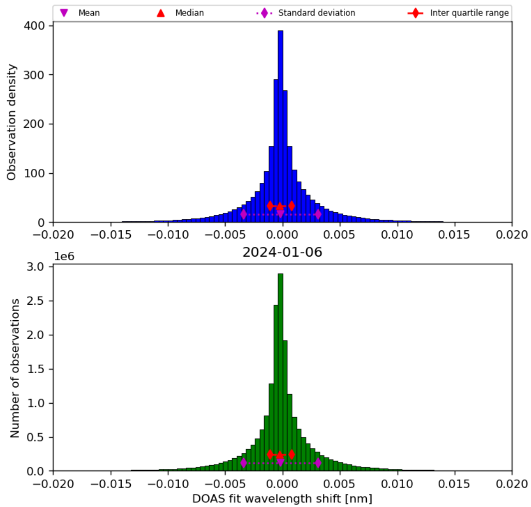
Figure 44: Histogram of “DOAS fit wavelength shift” for 2024-01-05 to 2024-01-07
