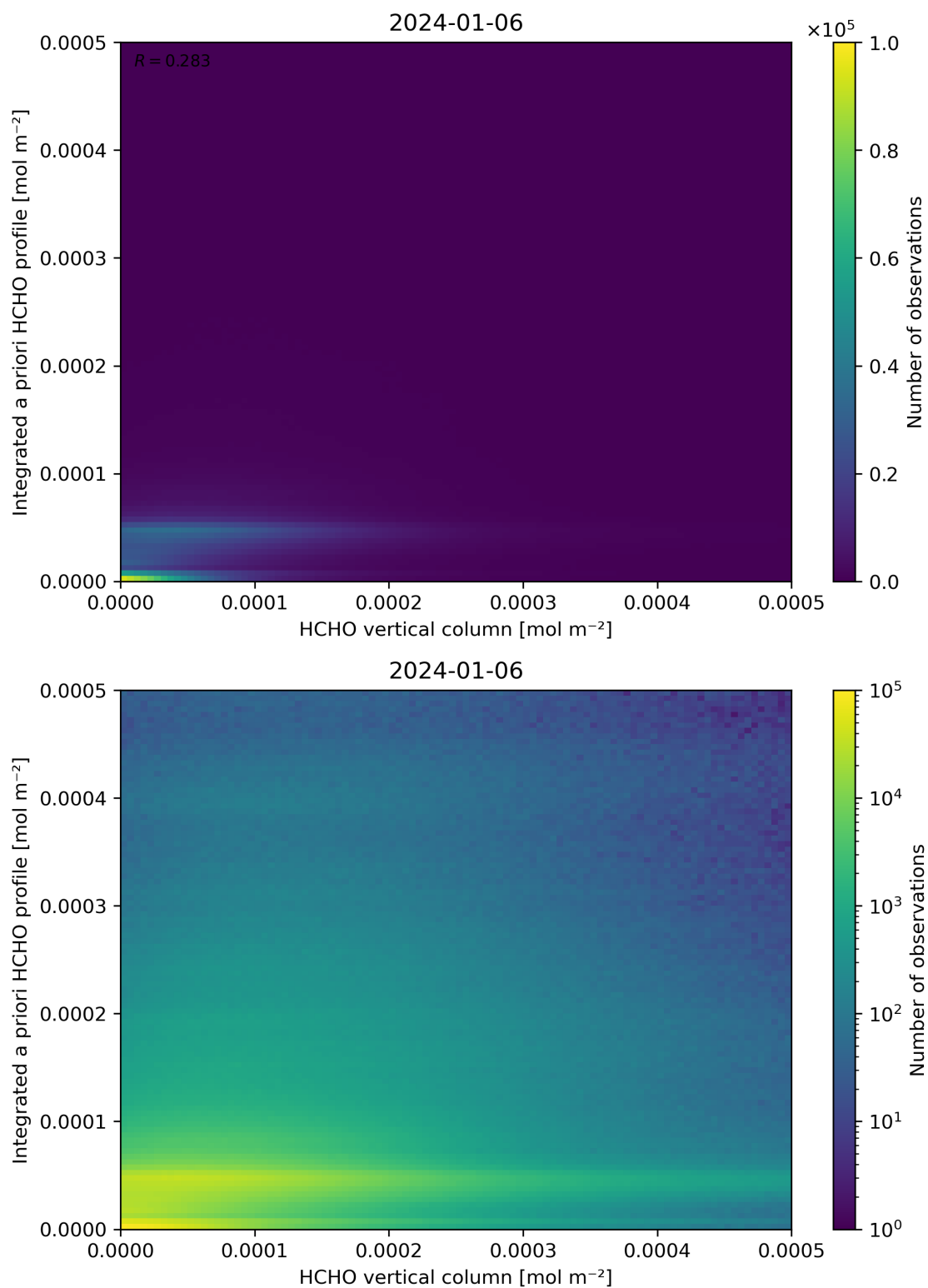
Figure 135: Scatter density plot of “HCHO vertical column” against “Integrated a priori HCHO profile” for 2024-01-05 to 2024-01-07.
