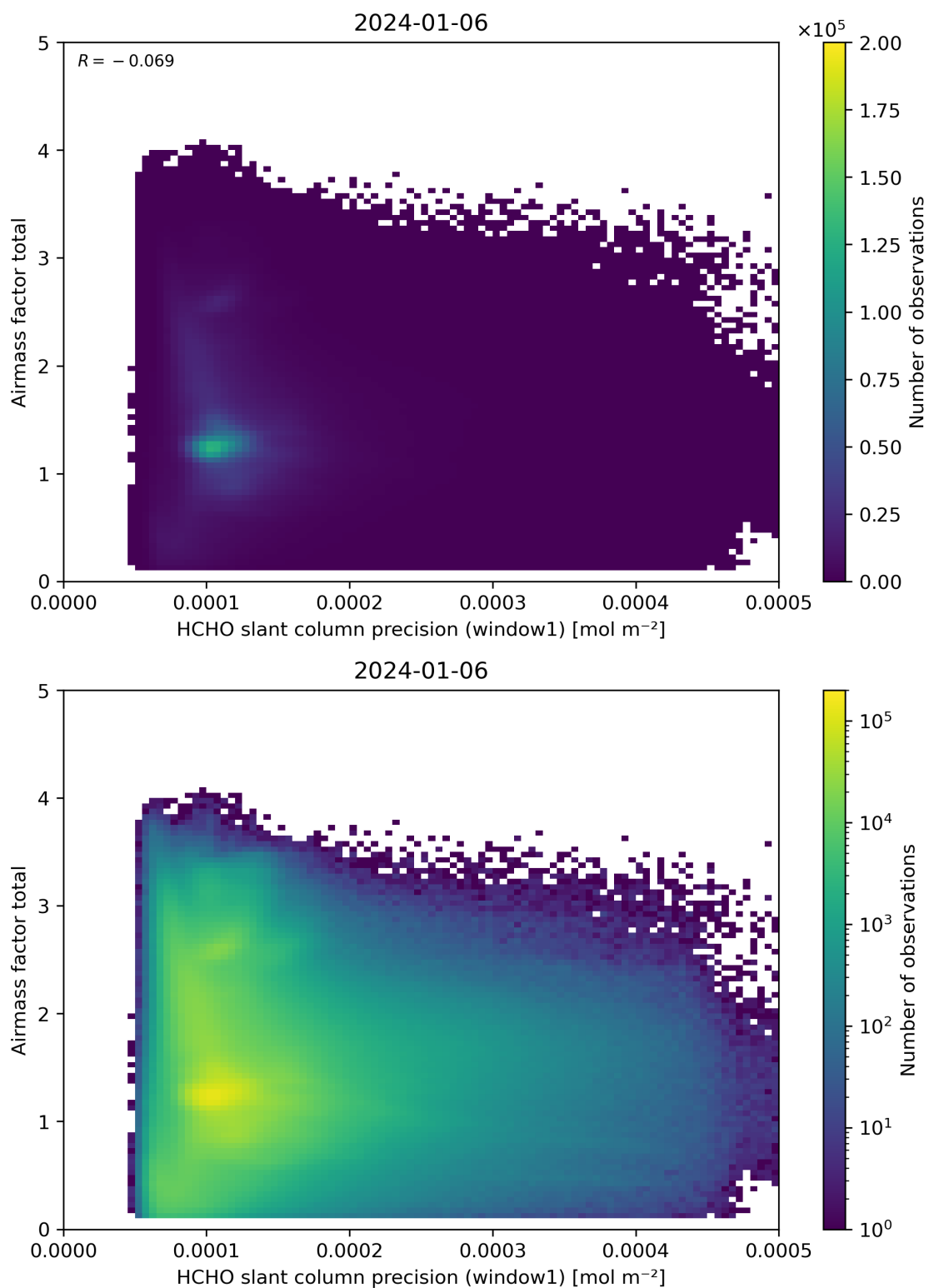
Figure 94: Scatter density plot of “HCHO slant column precision (window1)” against “Airmass factor total” for 2024-01-05 to 2024-01-07.
