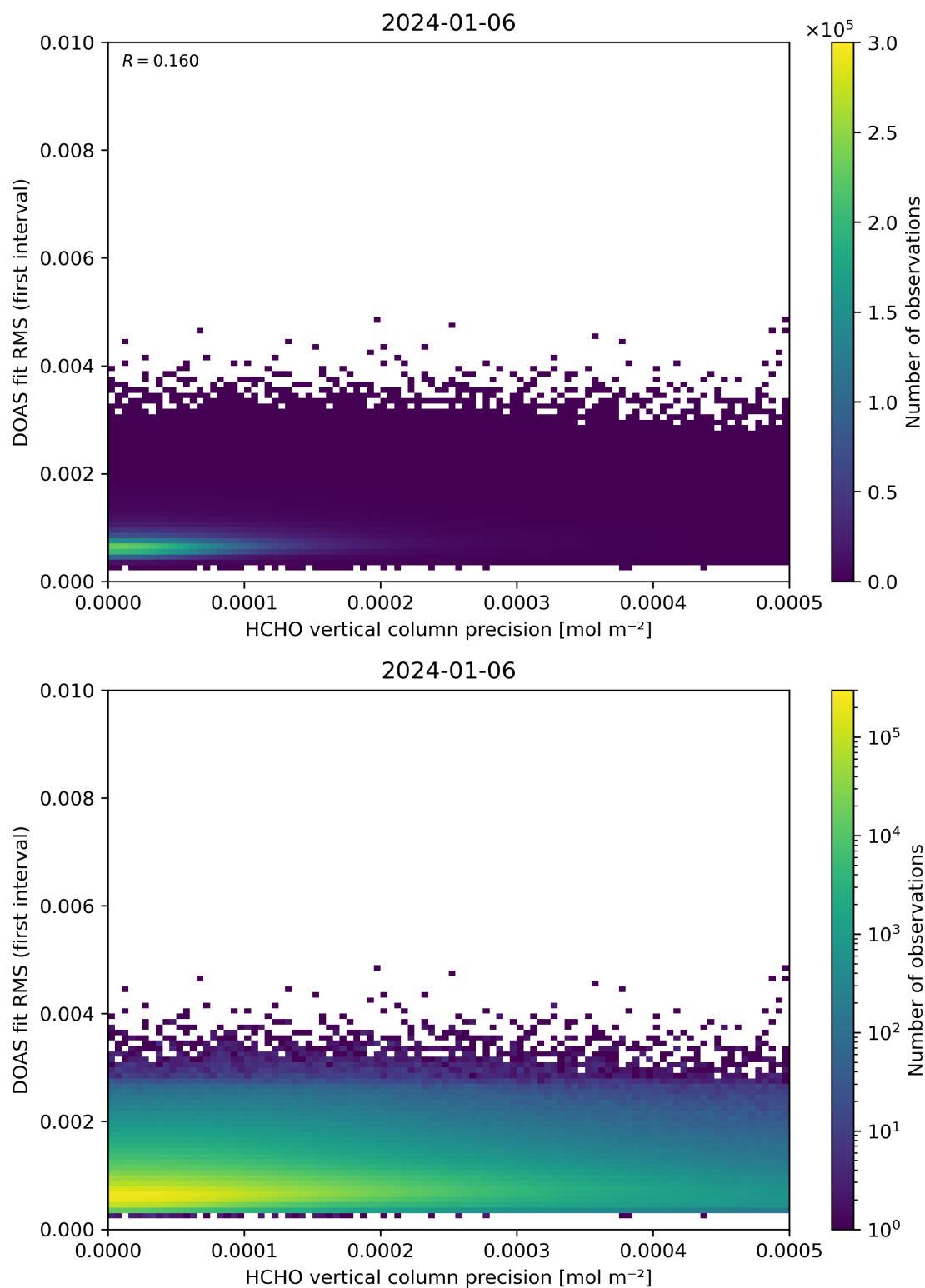
Figure 136: Scatter density plot of “HCHO vertical column precision” against “DOAS fit RMS (first interval)” for 2024-01-05 to 2024-01-07.
