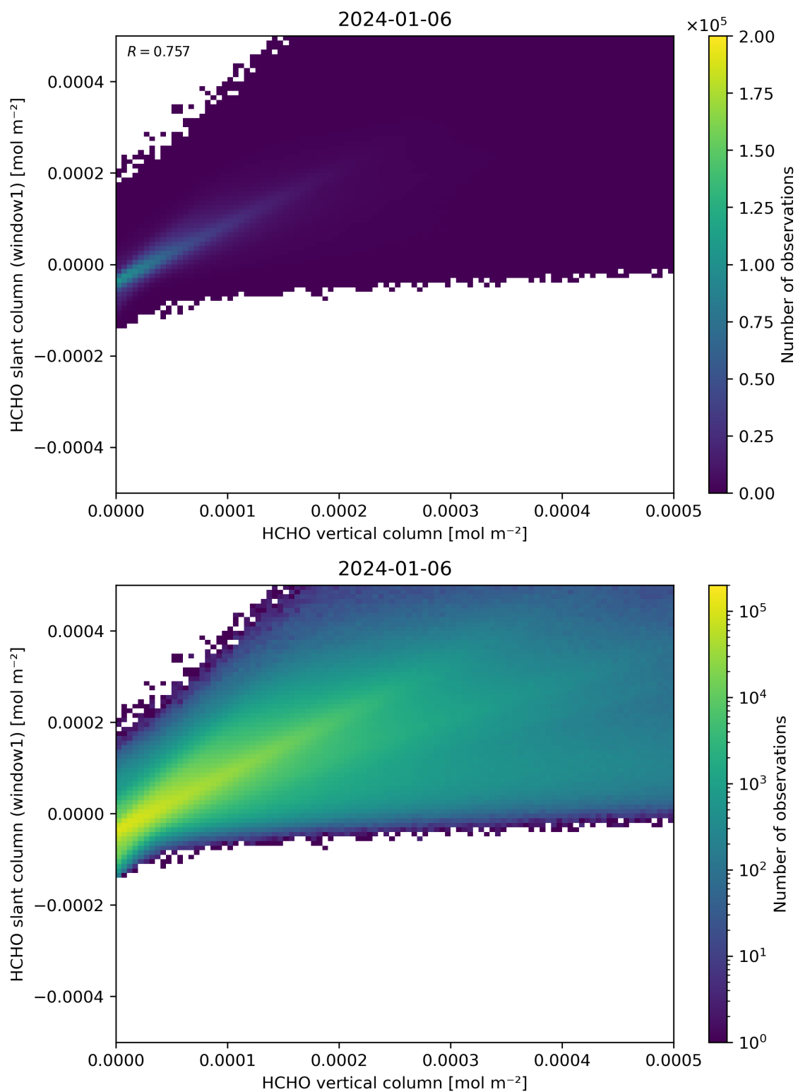
Figure 129: Scatter density plot of “HCHO vertical column” against “HCHO slant column (window1)” for 2024-01-05 to 2024-01-07.
