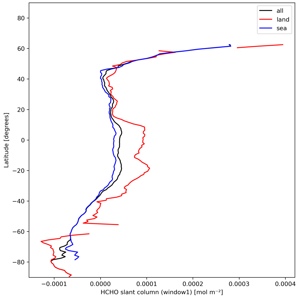
Figure 24: Zonal average of “HCHO slant column (window1)” for 2024-01-05 to 2024-01-07.
