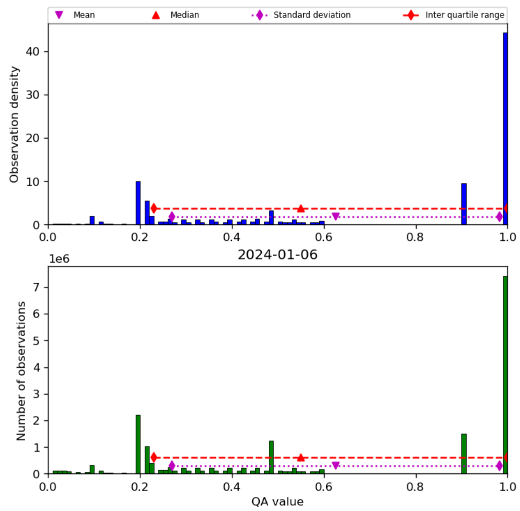
Figure 34: Histogram of “QA value” for 2024-01-05 to 2024-01-07
