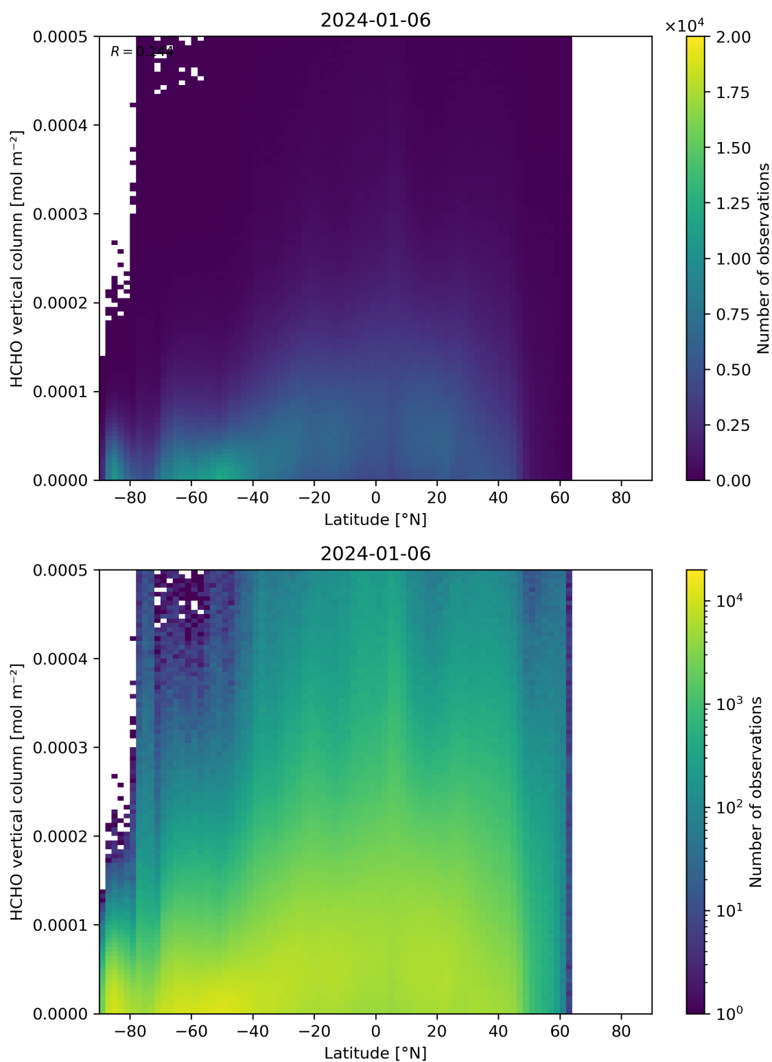
Figure 163: Scatter density plot of “Latitude” against “HCHO vertical column” for 2024-01-05 to 2024-01-07.
