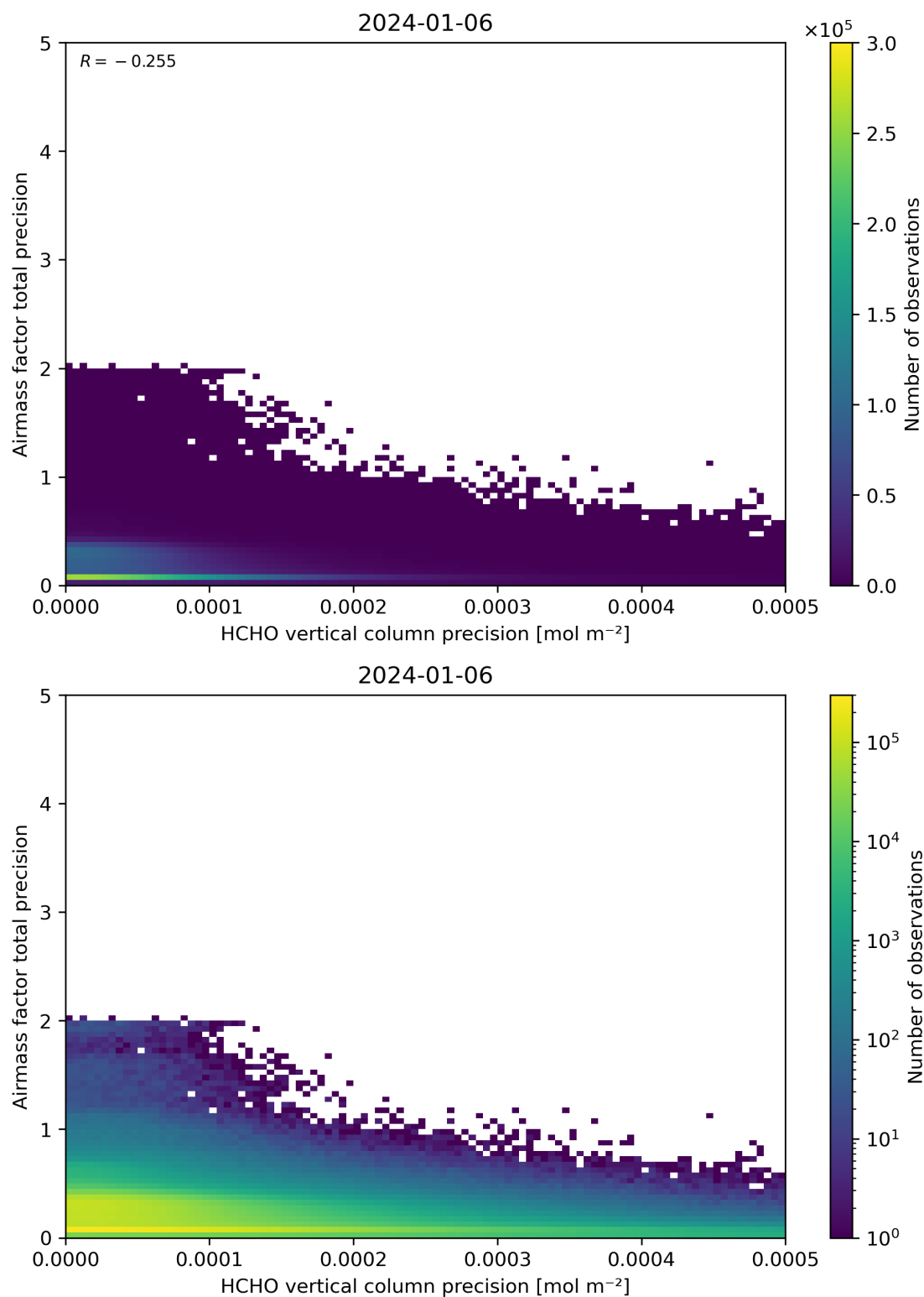
Figure 145: Scatter density plot of “HCHO vertical column precision” against “Airmass factor total precision” for 2024-01-05 to 2024-01-07.
