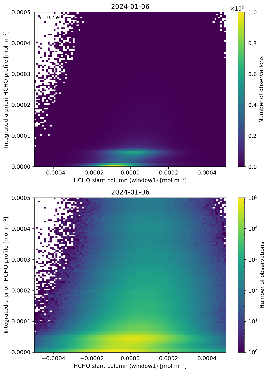
Figure 87: Scatter density plot of “HCHO slant column (window1)” against “Integrated a priori HCHO profile” for 2024-01-05 to 2024-01-07.
