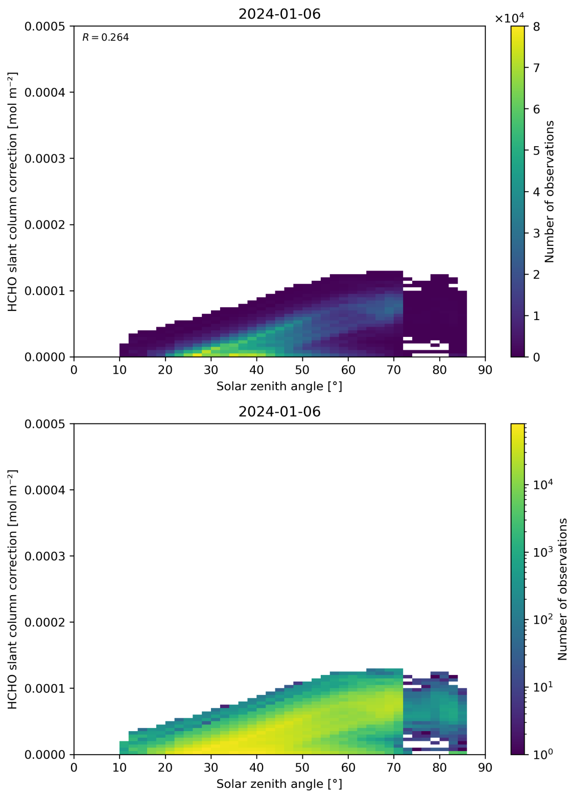
Figure 172: Scatter density plot of “Solar zenith angle” against “HCHO slant column correction” for 2024-01-05 to 2024-01-07.
