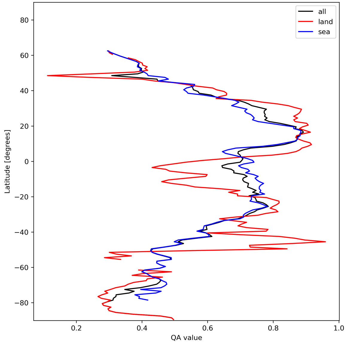
Figure 20: Zonal average of “QA value” for 2024-01-05 to 2024-01-07.
