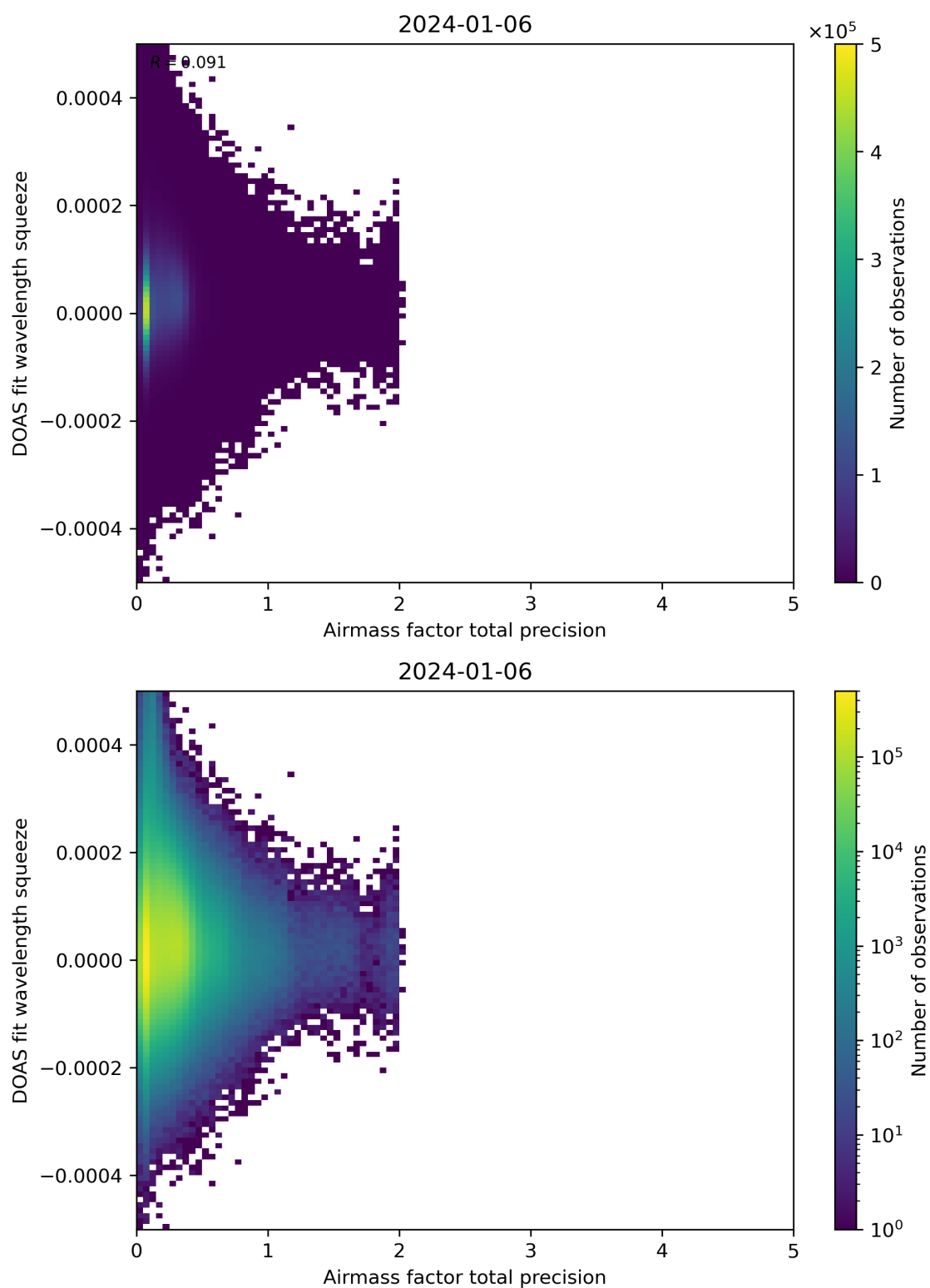
Figure 107: Scatter density plot of “Airmass factor total precision” against “DOAS fit wavelength squeeze” for 2024-01-05 to 2024-01-07.
