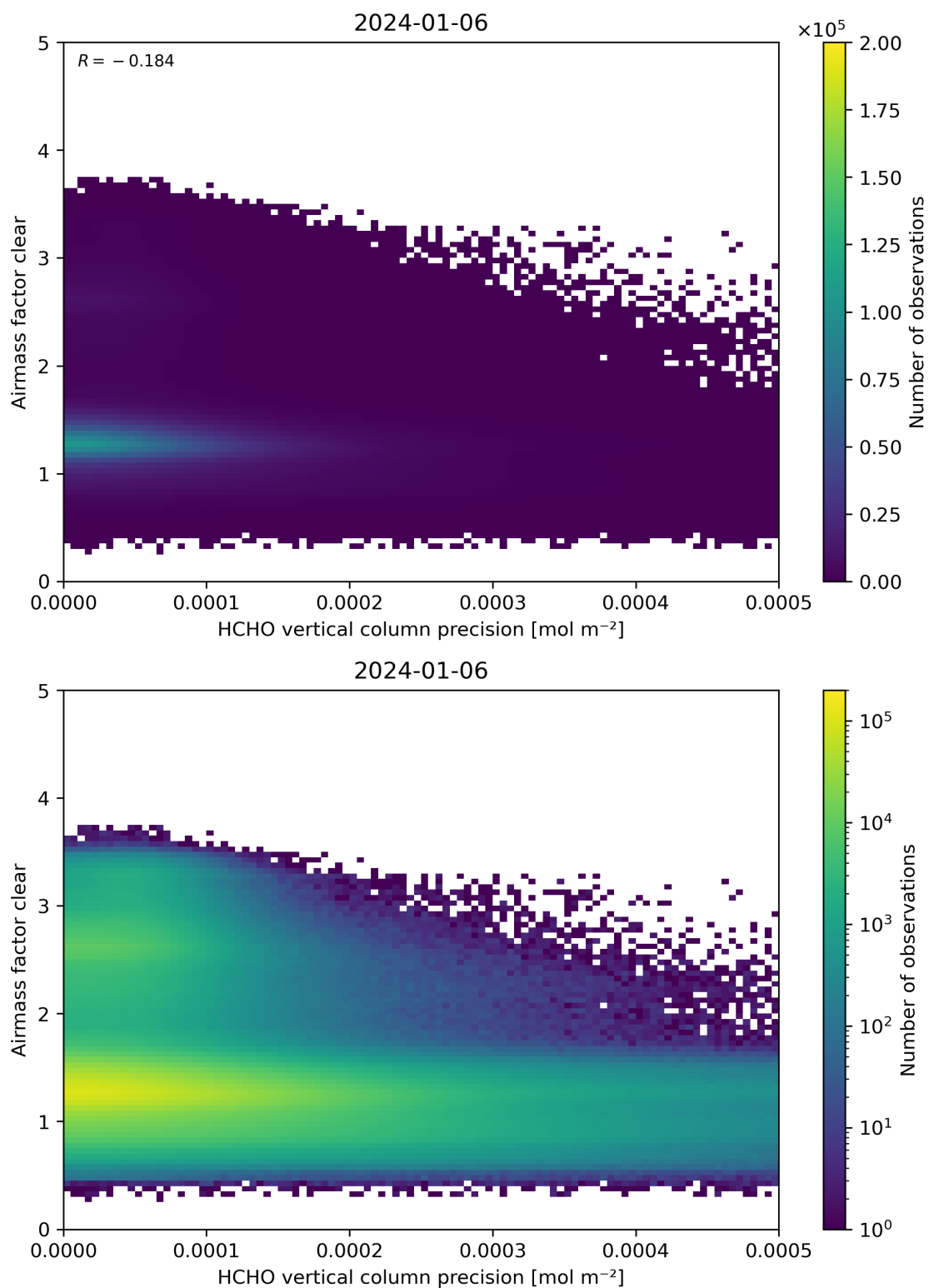
Figure 139: Scatter density plot of “HCHO vertical column precision” against “Airmass factor clear” for 2024-01-05 to 2024-01-07.
