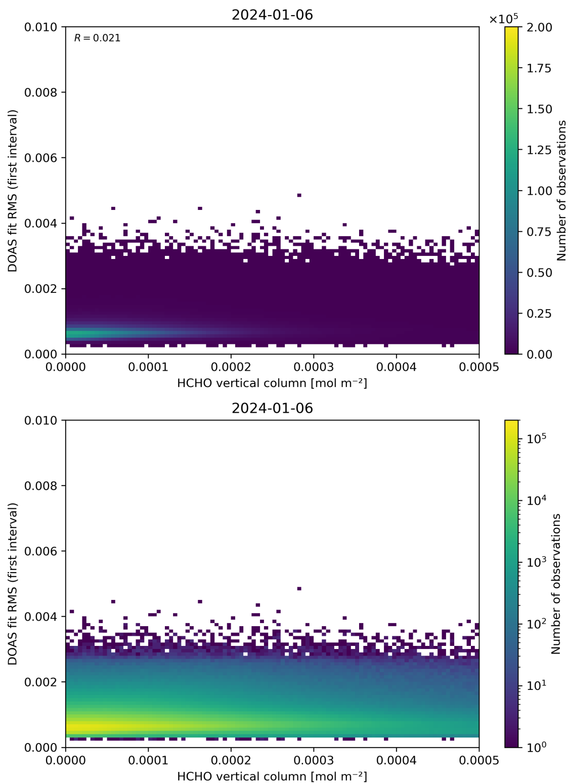
Figure 123: Scatter density plot of “HCHO vertical column” against “DOAS fit RMS (first interval)” for 2024-01-05 to 2024-01-07.
