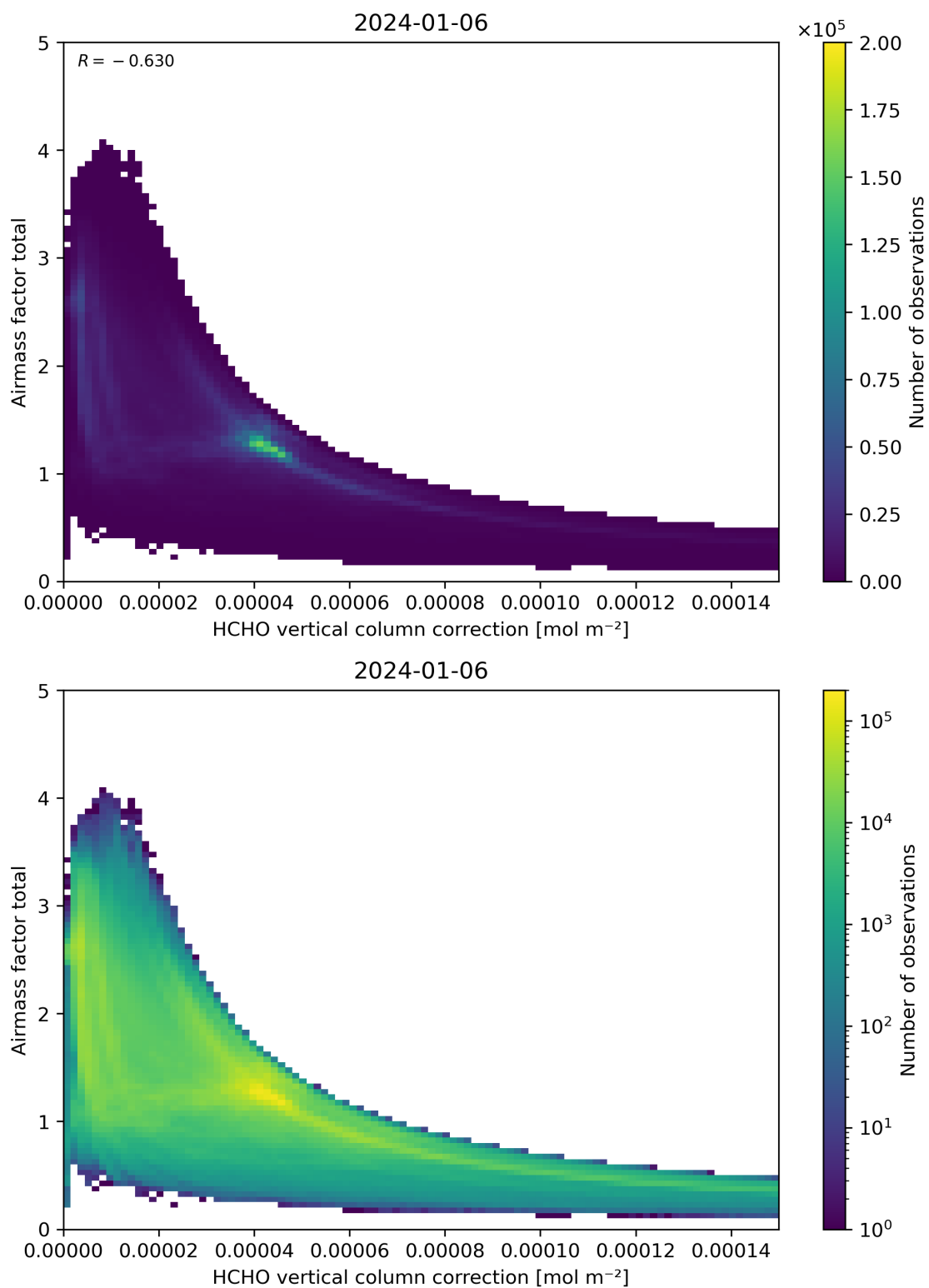
Figure 120: Scatter density plot of “HCHO vertical column correction” against “Airmass factor total” for 2024-01-05 to 2024-01-07.
