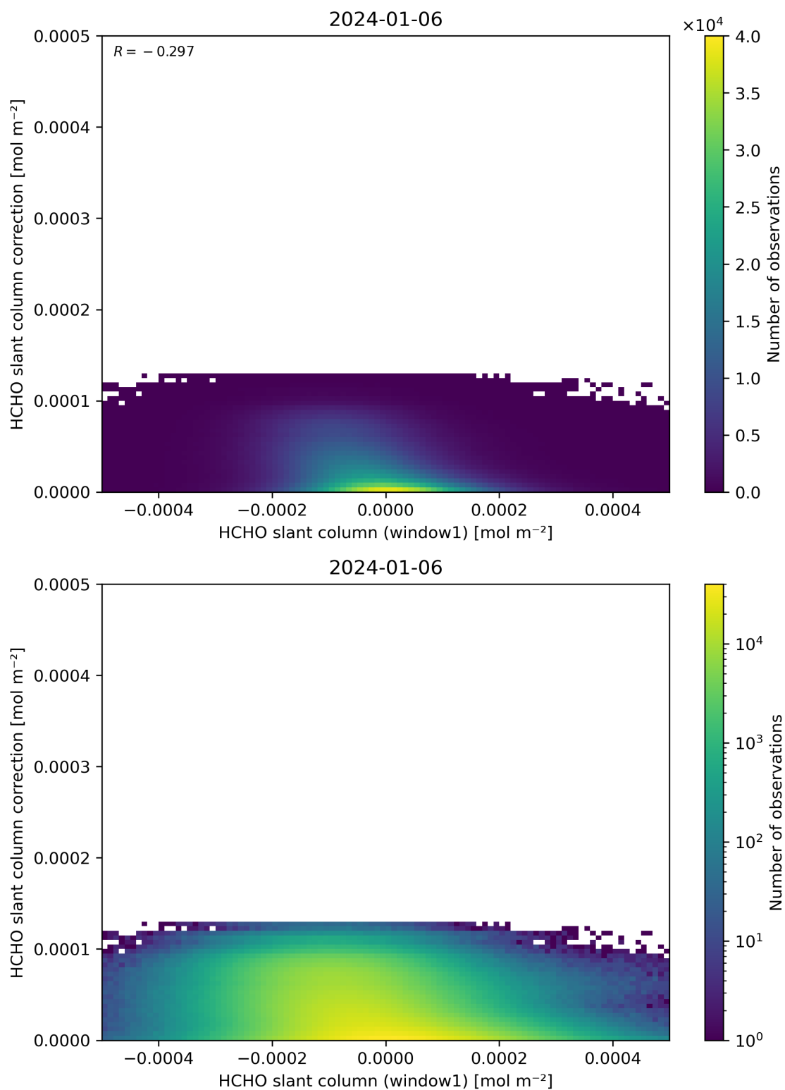
Figure 83: Scatter density plot of “HCHO slant column (window1)” against “HCHO slant column correction” for 2024-01-05 to 2024-01-07.
