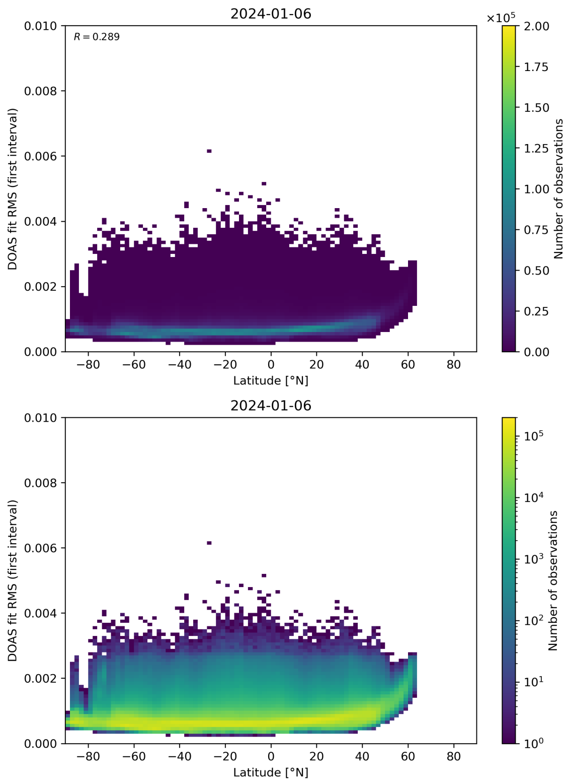
Figure 153: Scatter density plot of “Latitude” against “DOAS fit RMS (first interval)” for 2024-01-05 to 2024-01-07.
