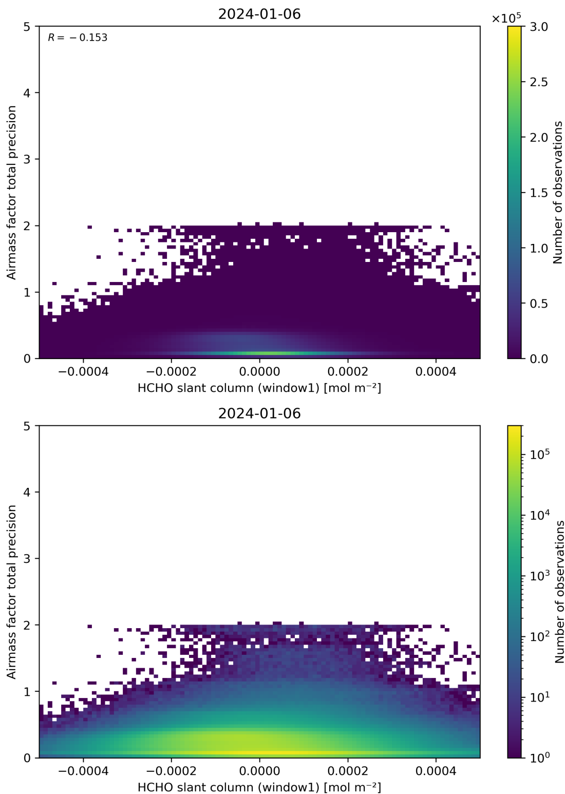
Figure 86: Scatter density plot of “HCHO slant column (window1)” against “Airmass factor total precision” for 2024-01-05 to 2024-01-07.
