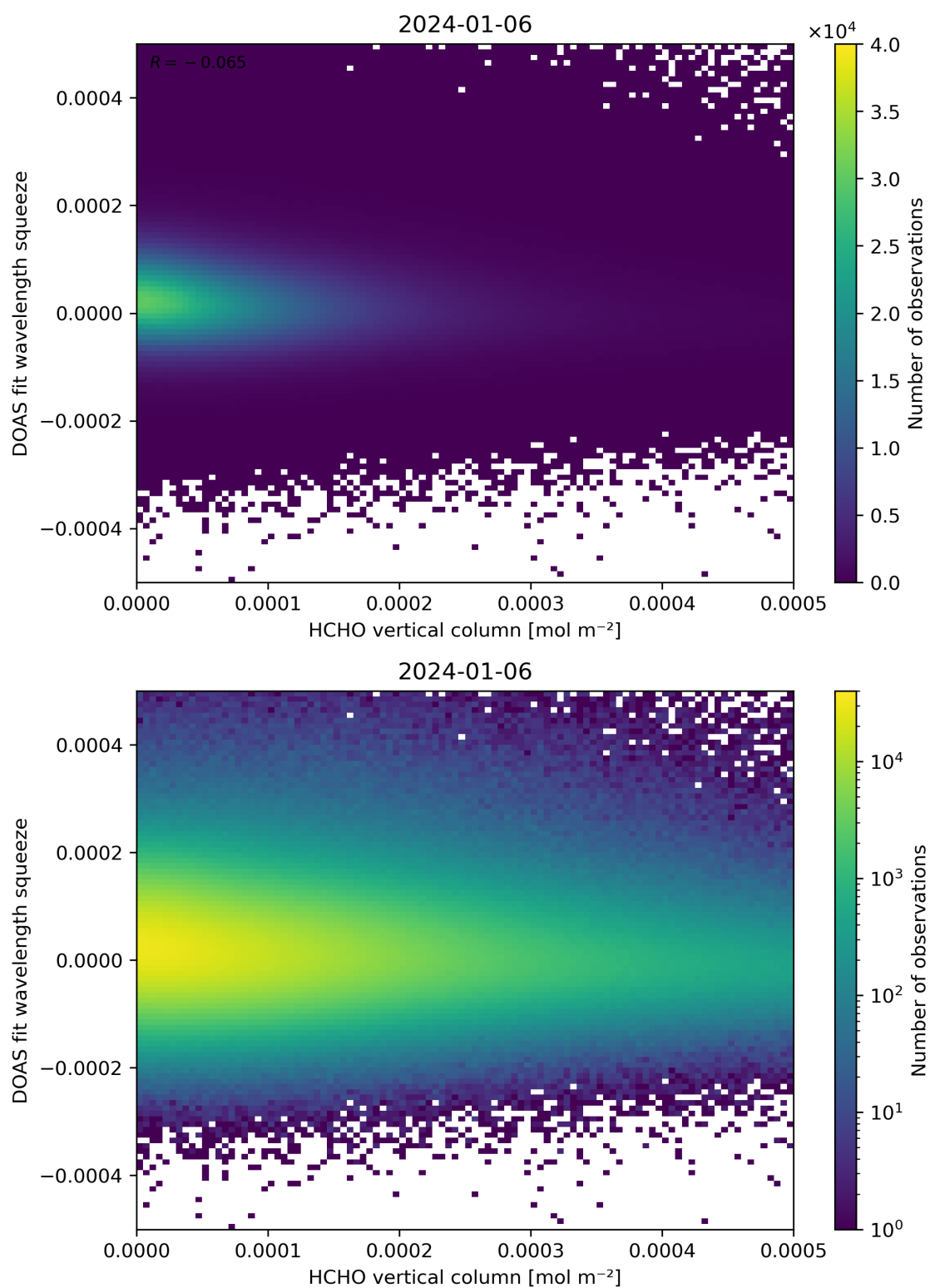
Figure 125: Scatter density plot of “HCHO vertical column” against “DOAS fit wavelength squeeze” for 2024-01-05 to 2024-01-07.
