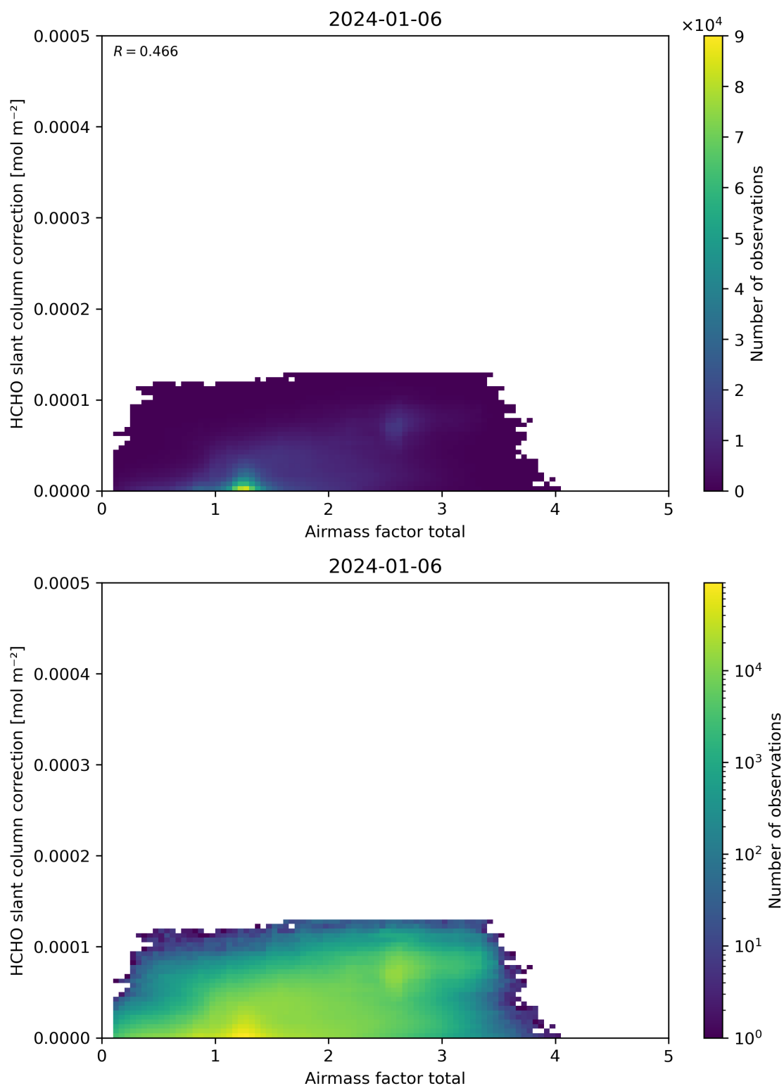
Figure 102: Scatter density plot of “Airmass factor total” against “HCHO slant column correction” for 2024-01-05 to 2024-01-07.
