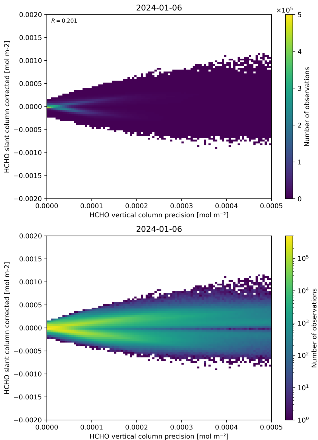
Figure 140: Scatter density plot of “HCHO vertical column precision” against “HCHO slant column corrected” for 2024-01-05 to 2024-01-07.
