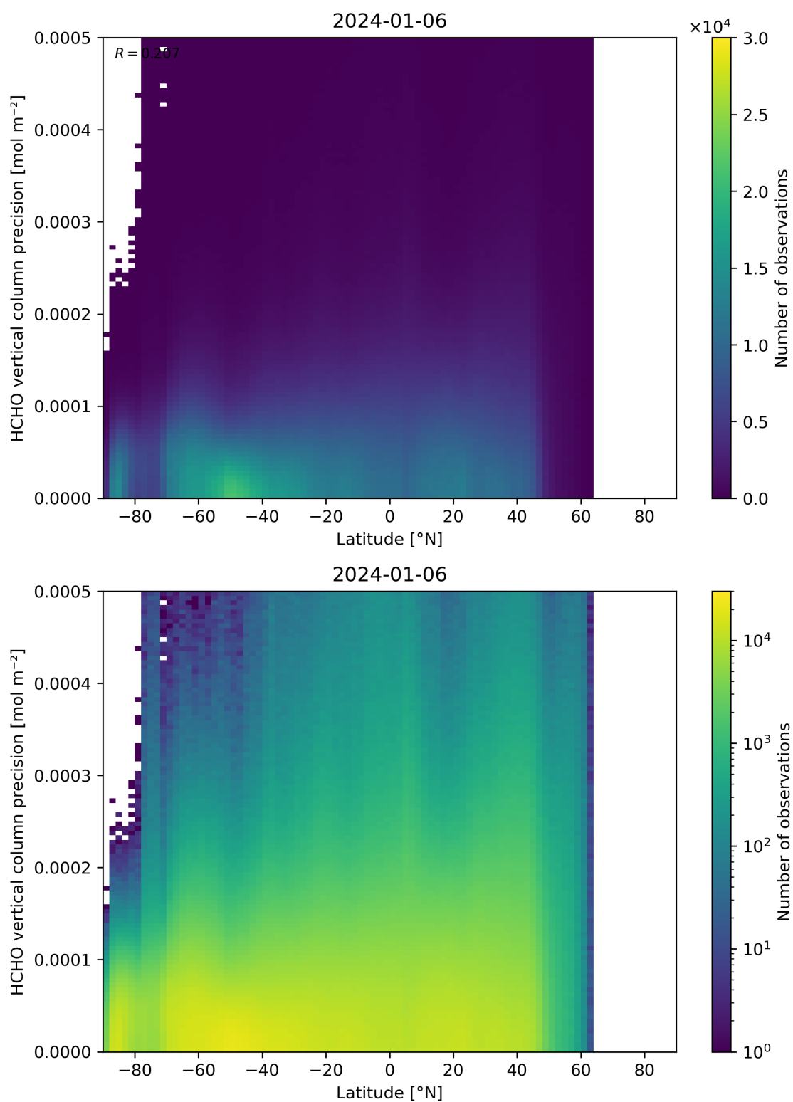
Figure 165: Scatter density plot of “Latitude” against “HCHO vertical column precision” for 2024-01-05 to 2024-01-07.
