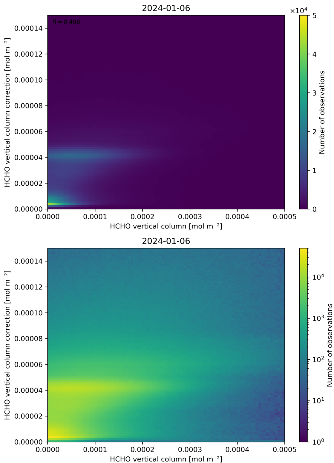
Figure 133: Scatter density plot of “HCHO vertical column” against “HCHO vertical column correction” for 2024-01-05 to 2024-01-07.
