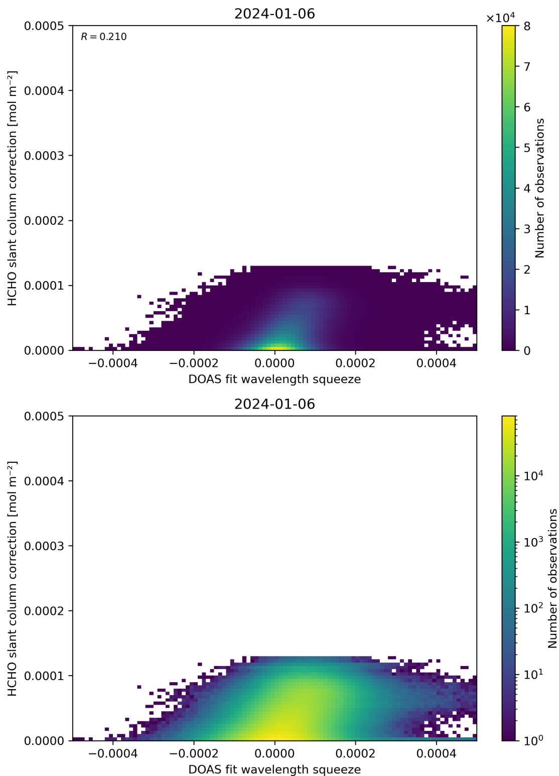
Figure 70: Scatter density plot of “DOAS fit wavelength squeeze” against “HCHO slant column correction” for 2024-01-05 to 2024-01-07.
