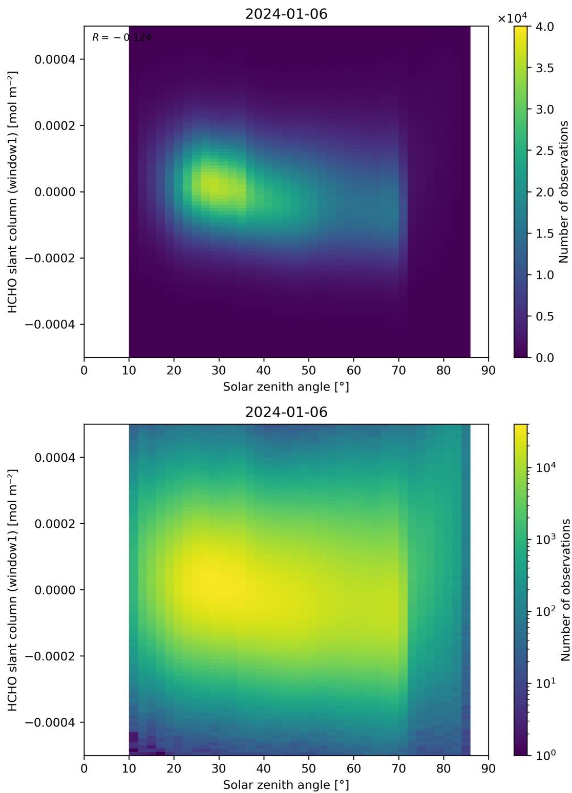
Figure 173: Scatter density plot of “Solar zenith angle” against “HCHO slant column (window1)” for 2024-01-05 to 2024-01-07.
