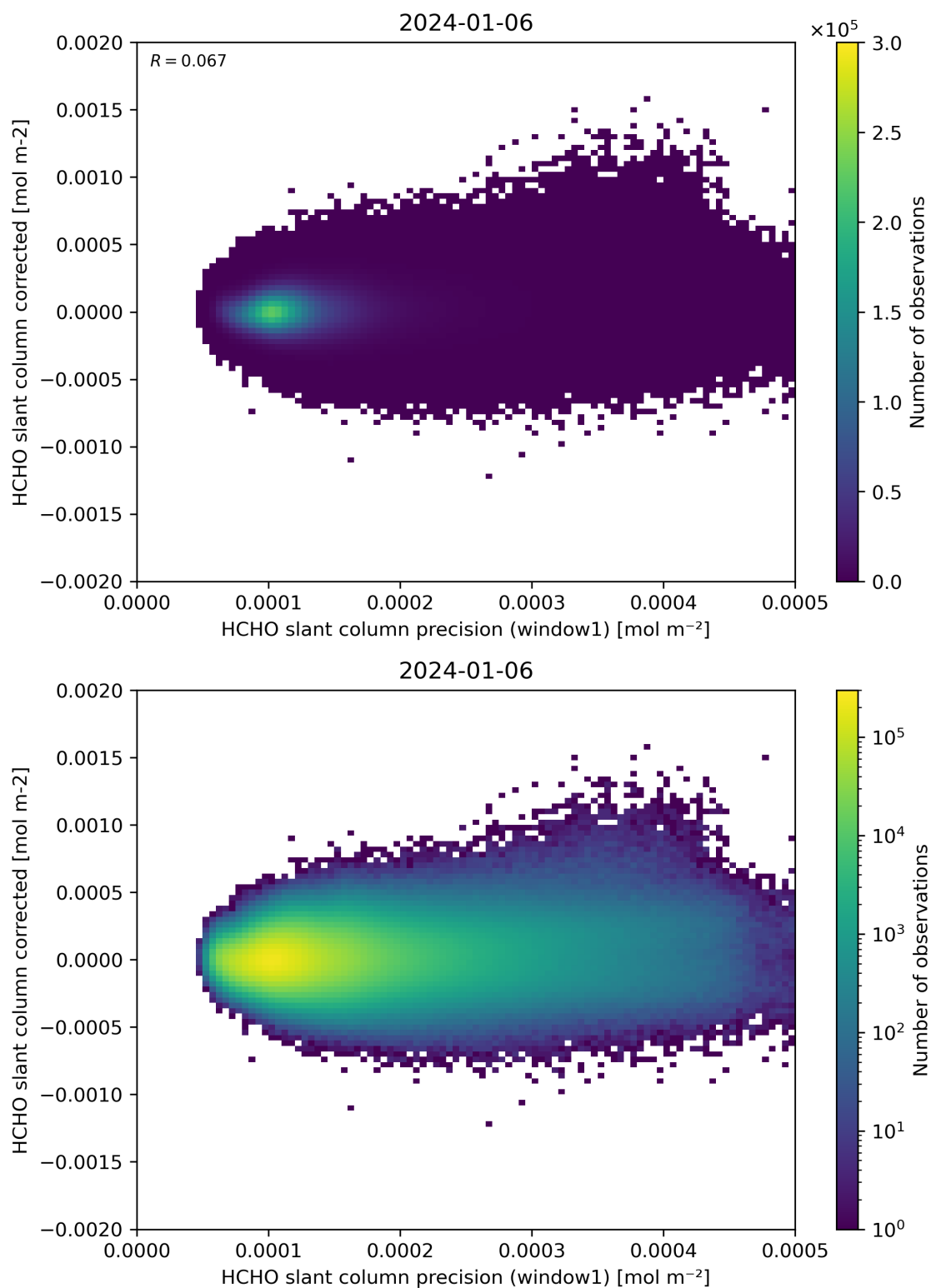
Figure 92: Scatter density plot of “HCHO slant column precision (window1)” against “HCHO slant column corrected” for 2024-01-05 to 2024-01-07.
