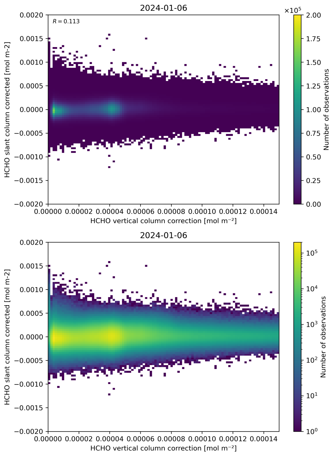
Figure 116: Scatter density plot of “HCHO vertical column correction” against “HCHO slant column corrected” for 2024-01-05 to 2024-01-07.
