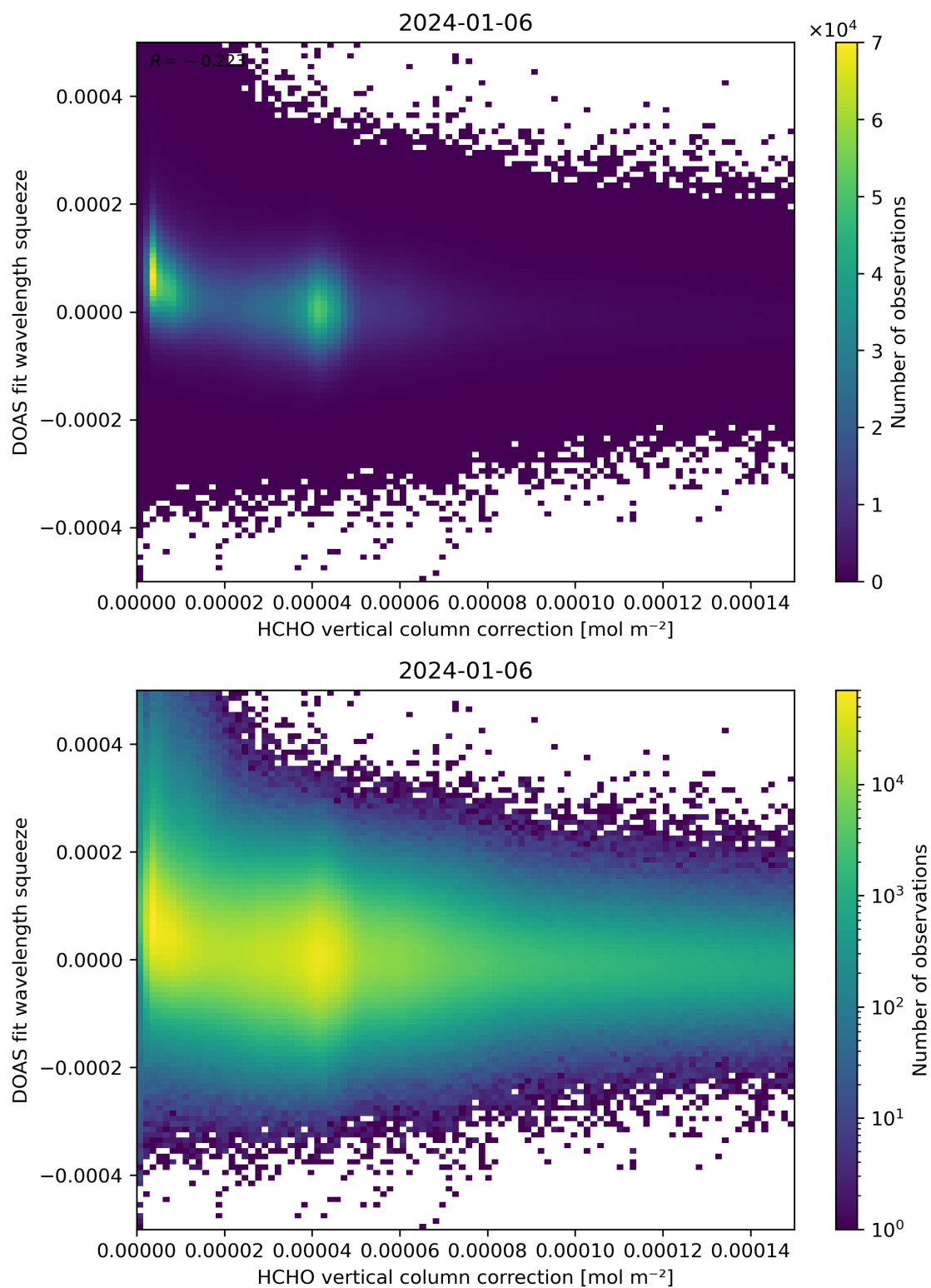
Figure 114: Scatter density plot of “HCHO vertical column correction” against “DOAS fit wavelength squeeze” for 2024-01-05 to 2024-01-07.
