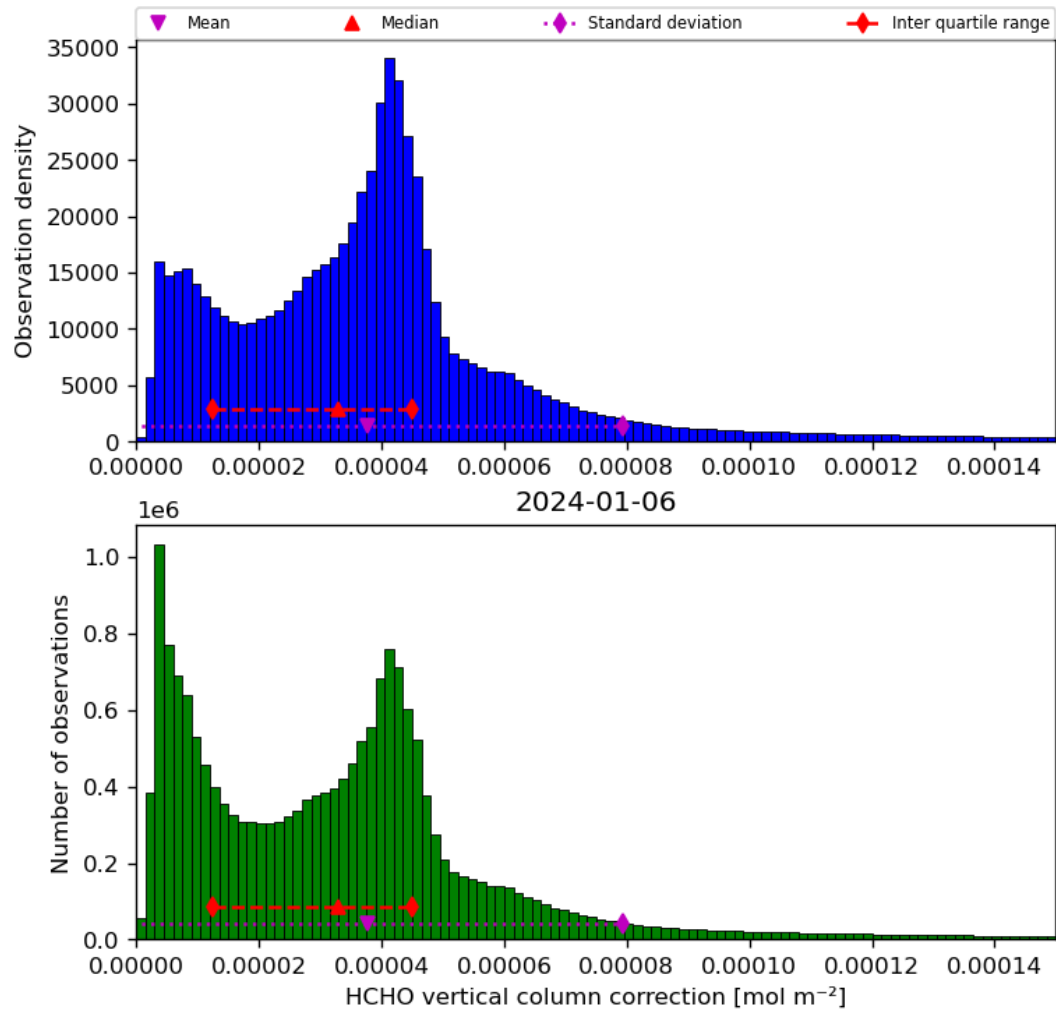
Figure 37: Histogram of “HCHO vertical column correction” for 2024-01-05 to 2024-01-07
