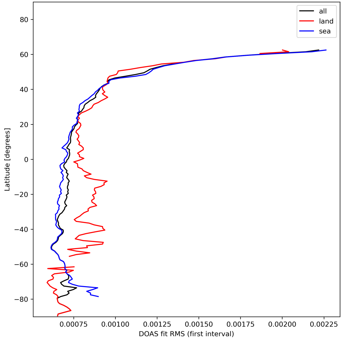
Figure 32: Zonal average of “DOAS fit RMS (first interval)” for 2024-01-05 to 2024-01-07.
