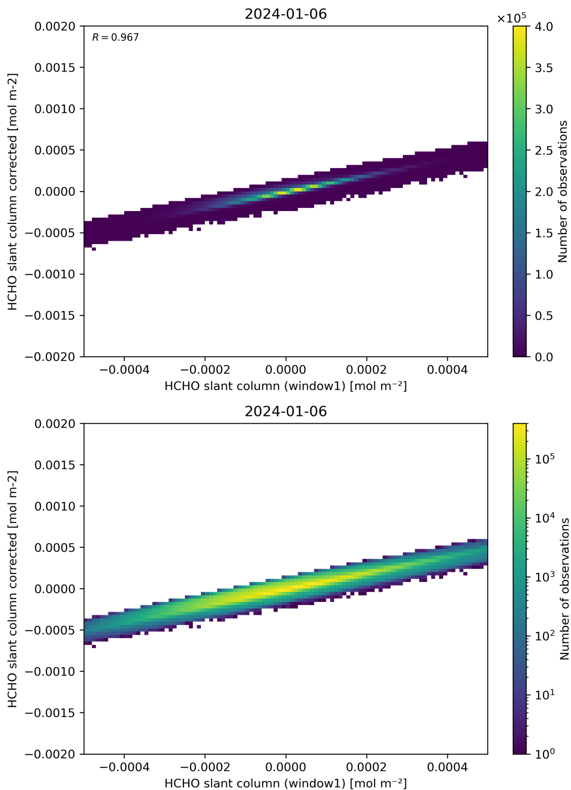
Figure 82: Scatter density plot of “HCHO slant column (window1)” against “HCHO slant column corrected” for 2024-01-05 to 2024-01-07.
