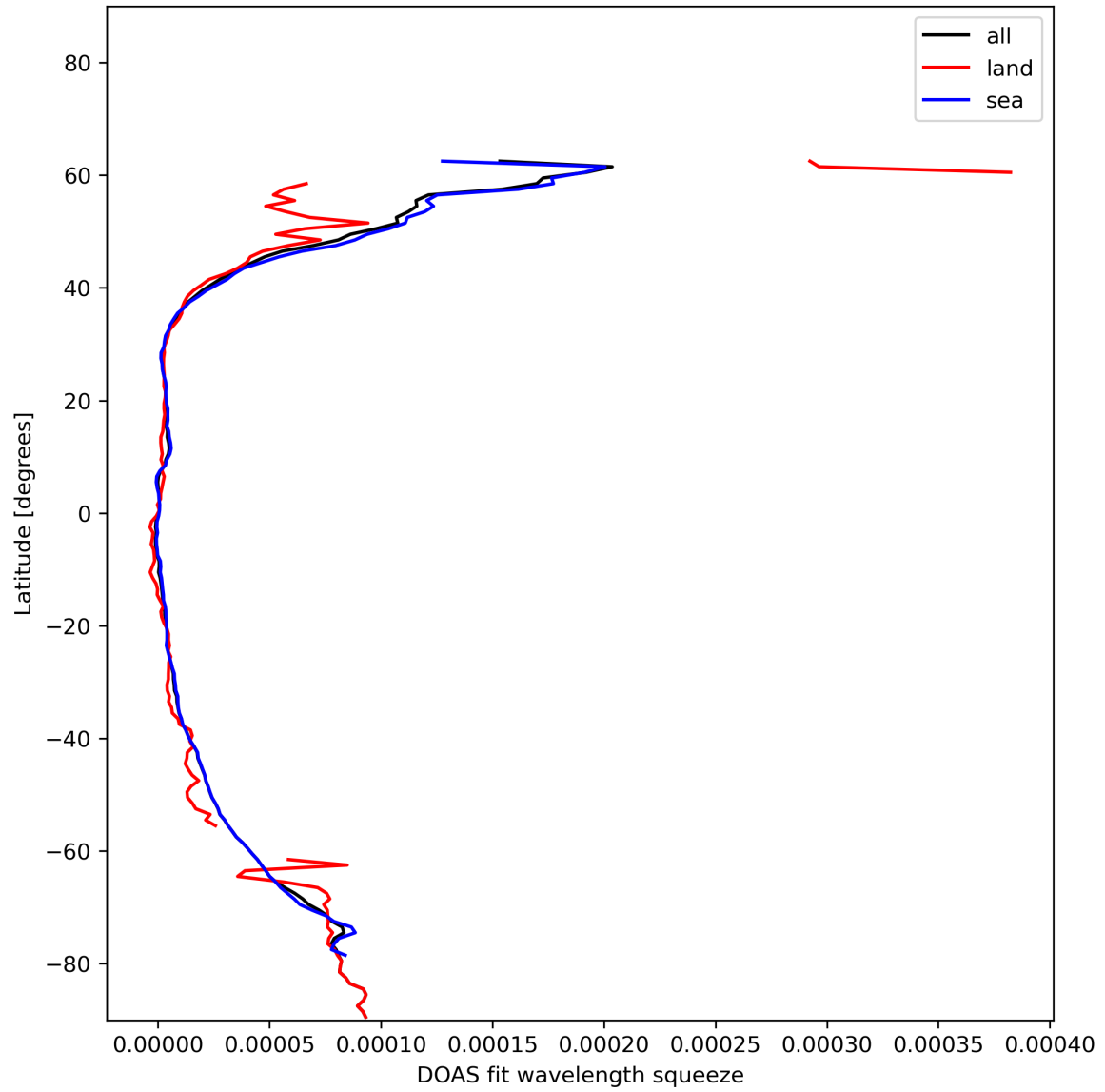
Figure 31: Zonal average of “DOAS fit wavelength squeeze” for 2024-01-05 to 2024-01-07.
