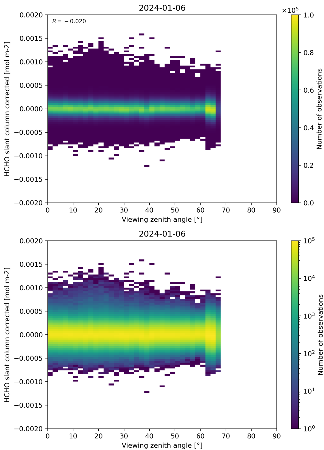
Figure 186: Scatter density plot of “Viewing zenith angle” against “HCHO slant column corrected” for 2024-01-05 to 2024-01-07.
