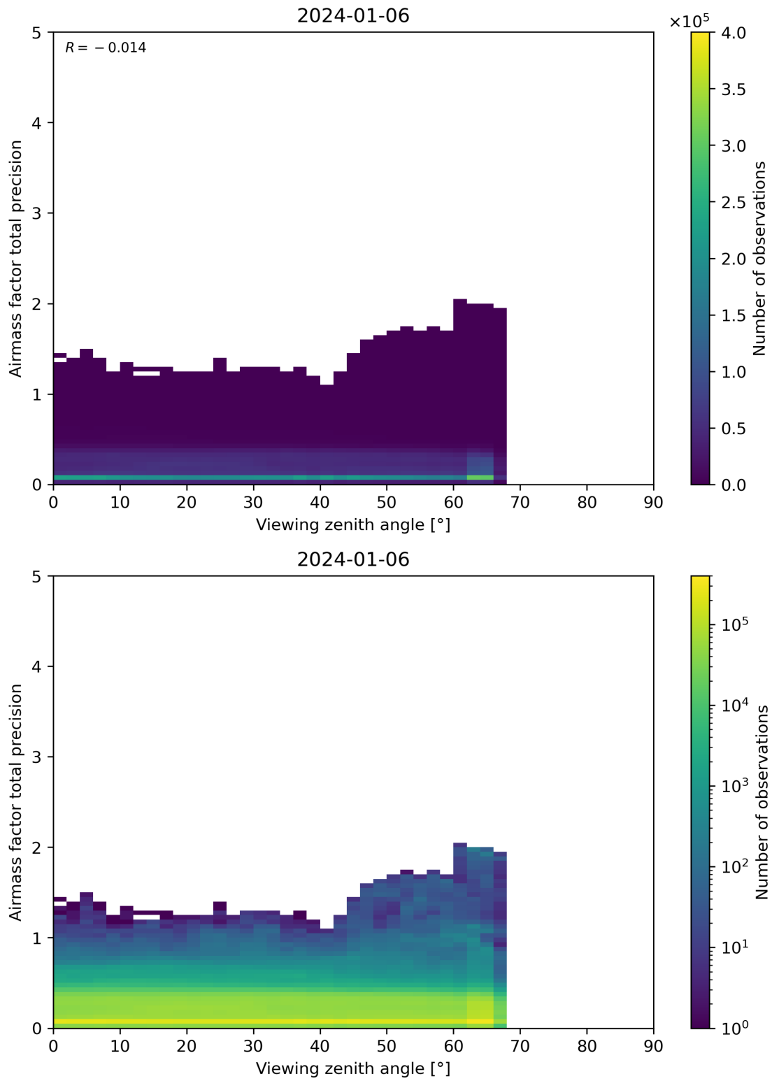
Figure 191: Scatter density plot of “Viewing zenith angle” against “Airmass factor total precision” for 2024-01-05 to 2024-01-07.
