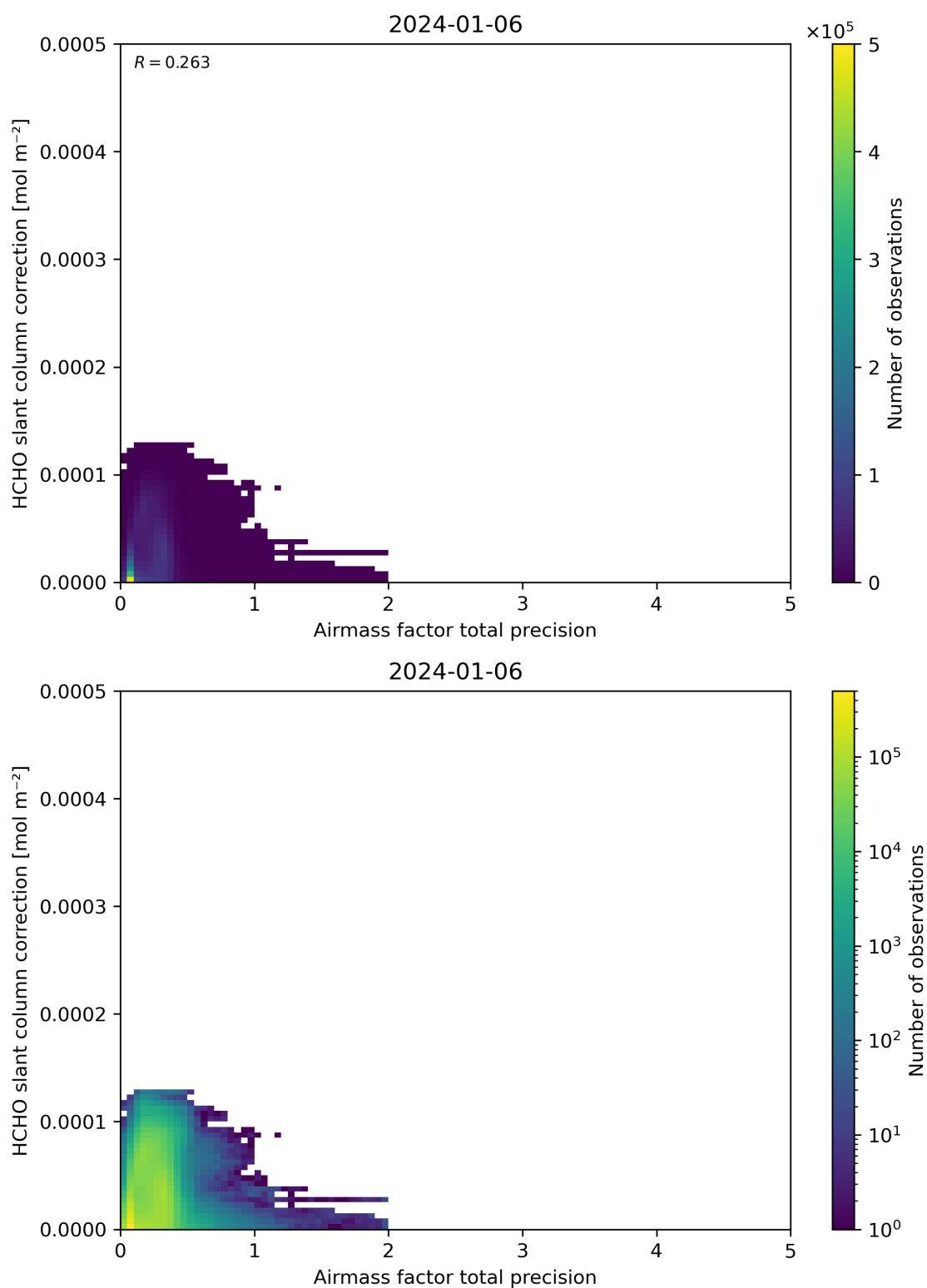
Figure 110: Scatter density plot of “Airmass factor total precision” against “HCHO slant column correction” for 2024-01-05 to 2024-01-07.
