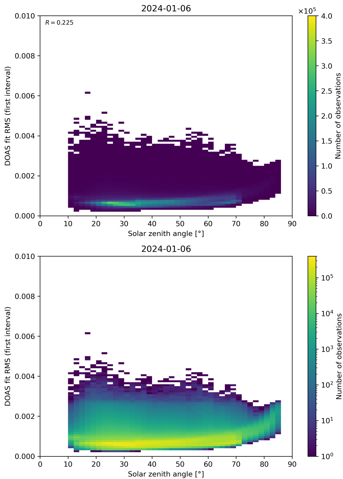
Figure 167: Scatter density plot of “Solar zenith angle” against “DOAS fit RMS (first interval)” for 2024-01-05 to 2024-01-07.
