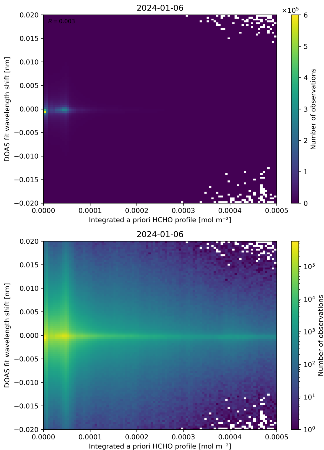
Figure 149: Scatter density plot of “Integrated a priori HCHO profile” against “DOAS fit wavelength shift” for 2024-01-05 to 2024-01-07.
