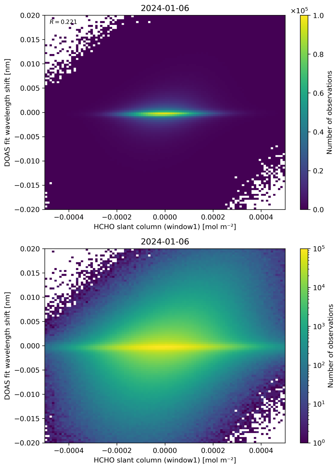
Figure 79: Scatter density plot of “HCHO slant column (window1)” against “DOAS fit wavelength shift” for 2024-01-05 to 2024-01-07.
