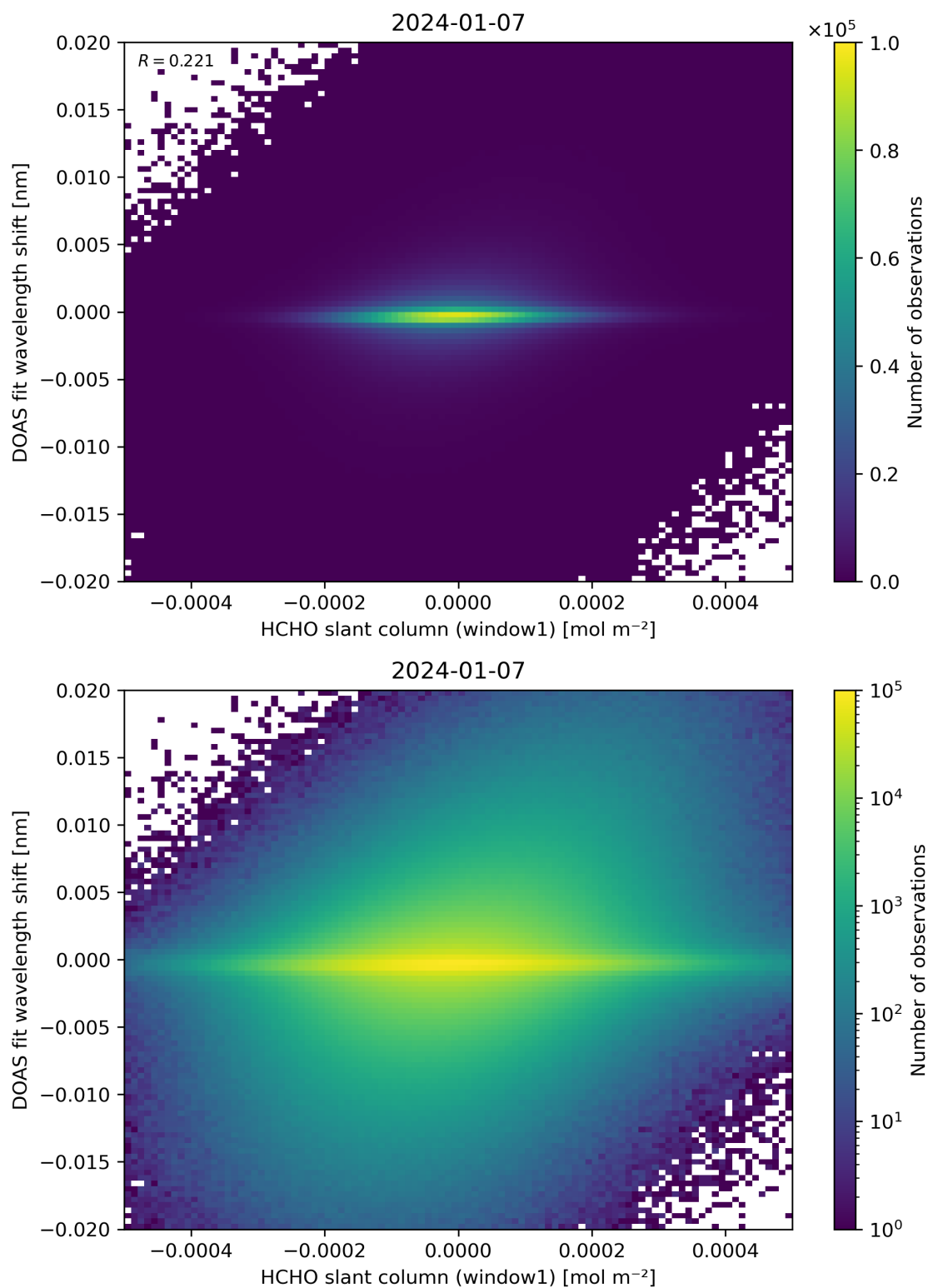
Figure 79: Scatter density plot of “HCHO slant column (window1)” against “DOAS fit wavelength shift” for 2024-01-06 to 2024-01-08.
