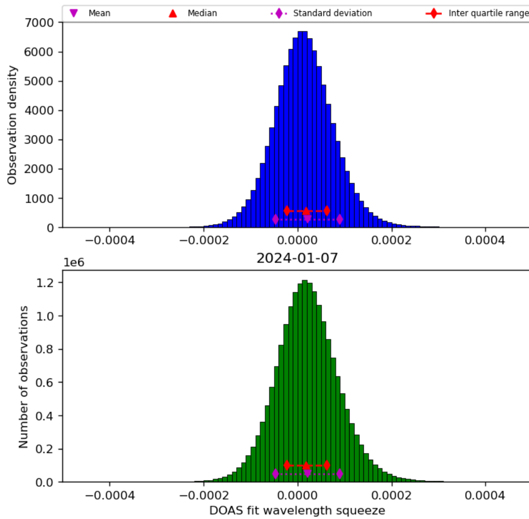
Figure 45: Histogram of “DOAS fit wavelength squeeze” for 2024-01-06 to 2024-01-08
