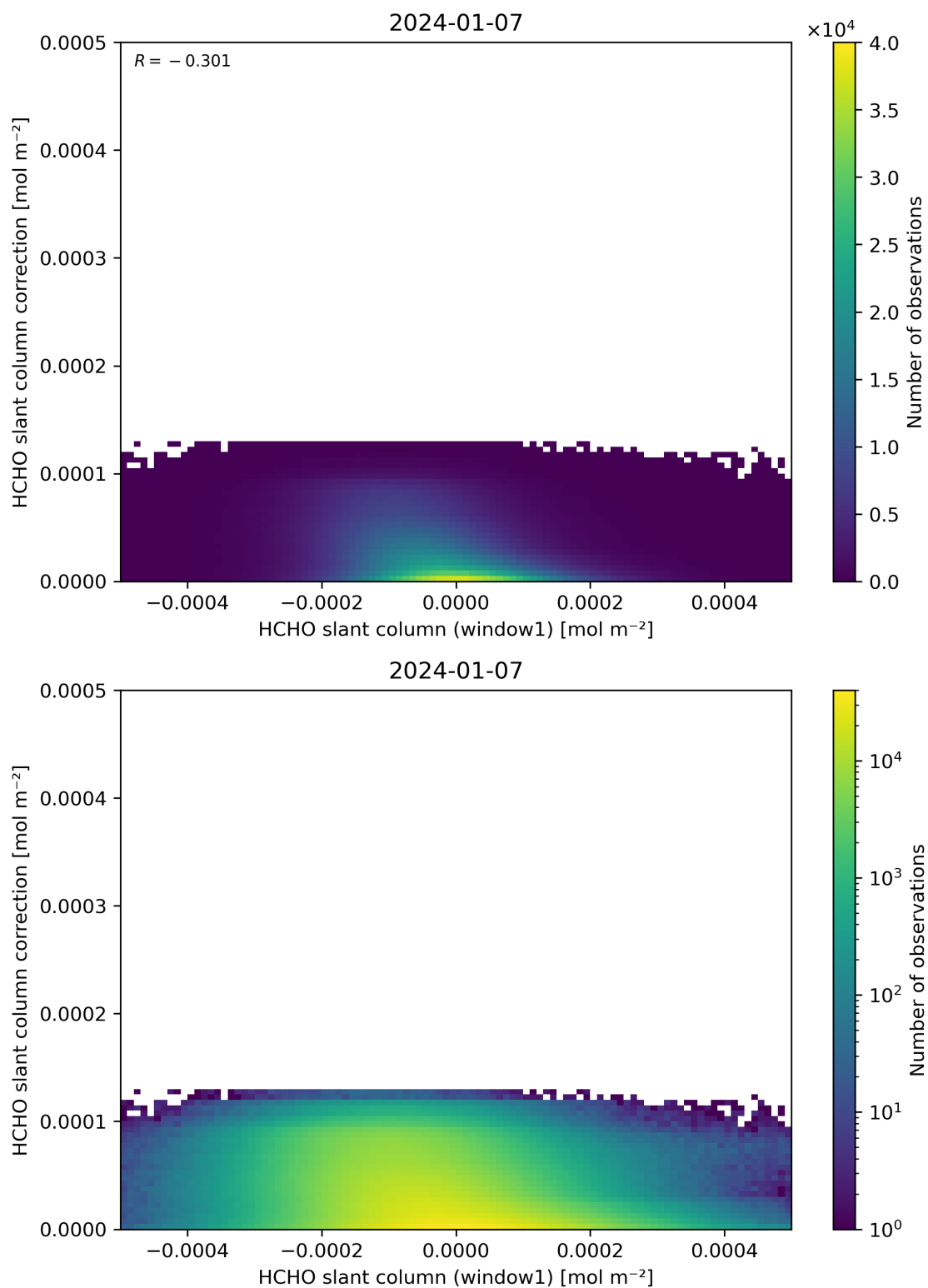
Figure 83: Scatter density plot of “HCHO slant column (window1)” against “HCHO slant column correction” for 2024-01-06 to 2024-01-08.
