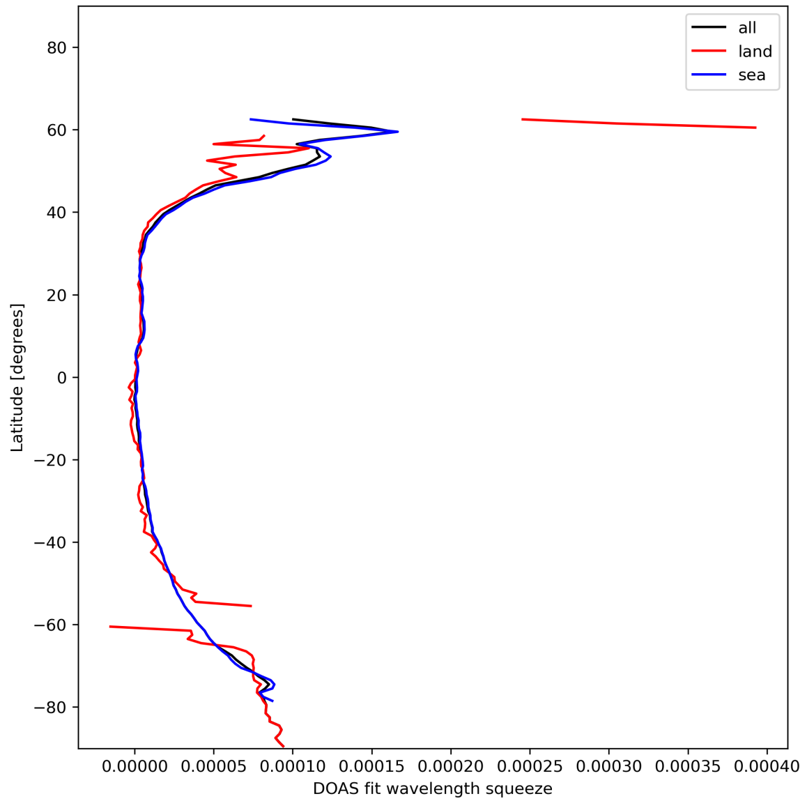
Figure 31: Zonal average of “DOAS fit wavelength squeeze” for 2024-01-06 to 2024-01-08.
