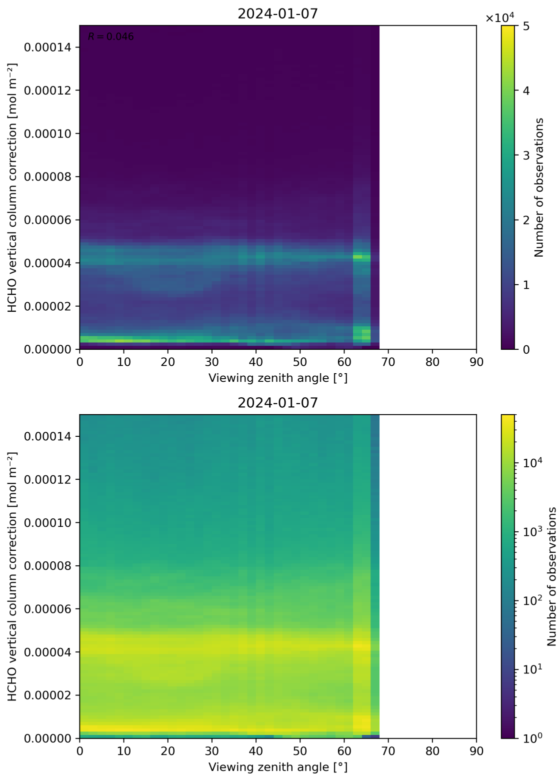
Figure 193: Scatter density plot of “Viewing zenith angle” against “HCHO vertical column correction” for 2024-01-06 to 2024-01-08.
