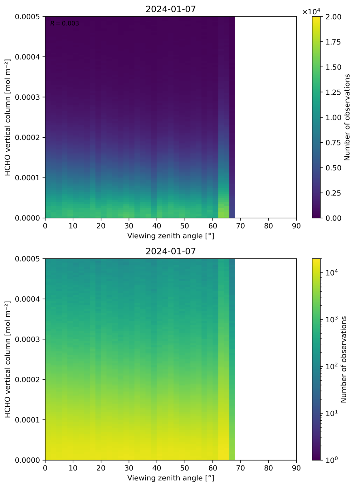
Figure 192: Scatter density plot of “Viewing zenith angle” against “HCHO vertical column” for 2024-01-06 to 2024-01-08.
