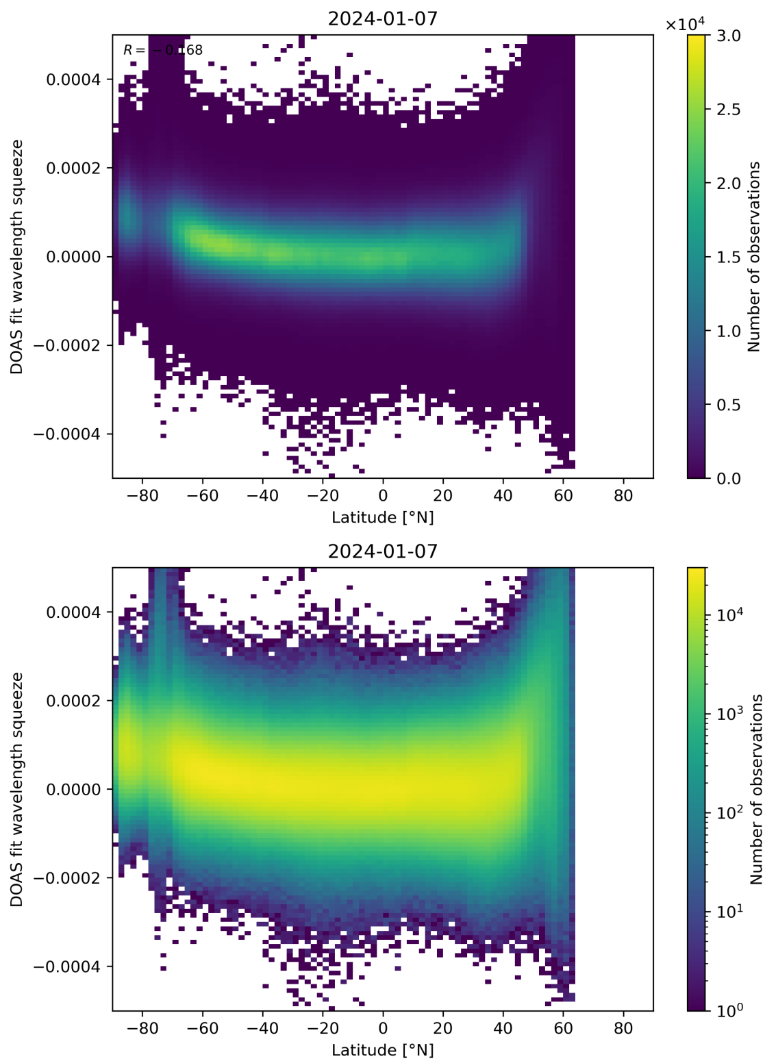
Figure 155: Scatter density plot of “Latitude” against “DOAS fit wavelength squeeze” for 2024-01-06 to 2024-01-08.
