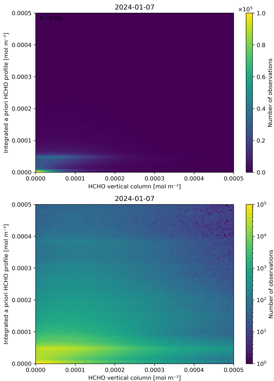
Figure 135: Scatter density plot of “HCHO vertical column” against “Integrated a priori HCHO profile” for 2024-01-06 to 2024-01-08.
