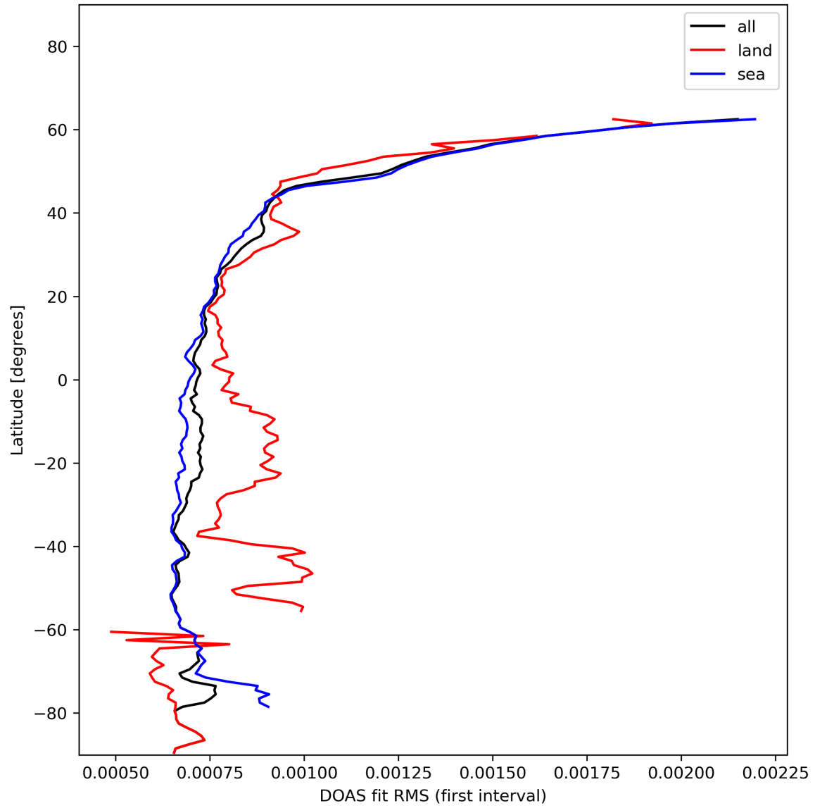
Figure 32: Zonal average of “DOAS fit RMS (first interval)” for 2024-01-06 to 2024-01-08.
