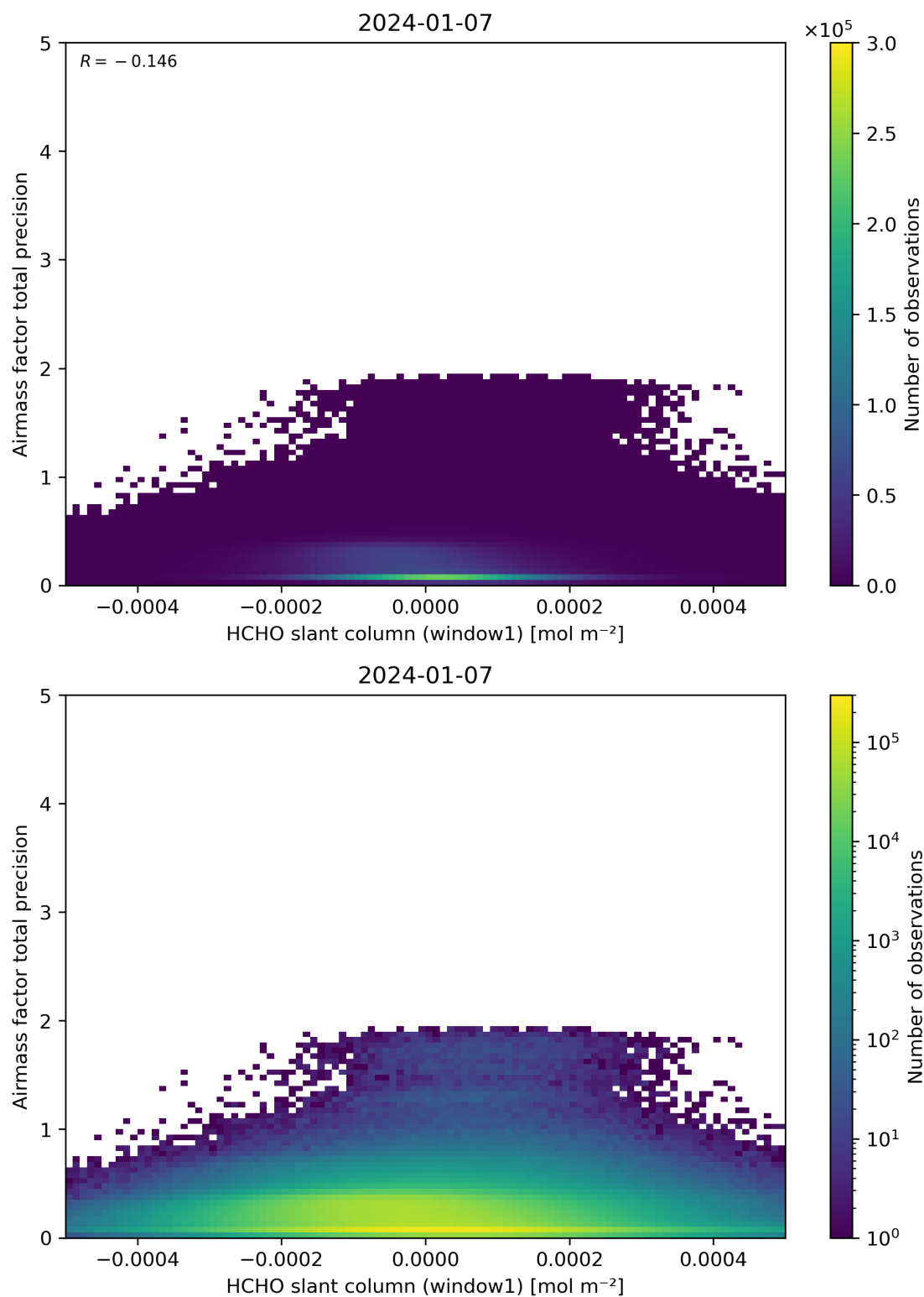
Figure 86: Scatter density plot of “HCHO slant column (window1)” against “Airmass factor total precision” for 2024-01-06 to 2024-01-08.
