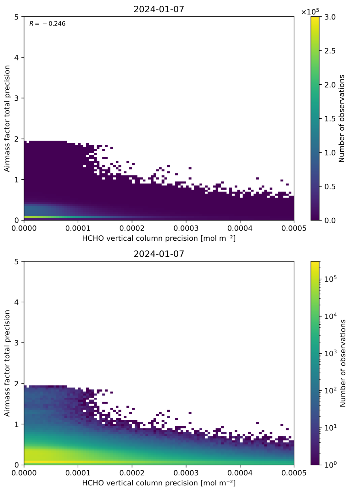
Figure 145: Scatter density plot of “HCHO vertical column precision” against “Airmass factor total precision” for 2024-01-06 to 2024-01-08.
