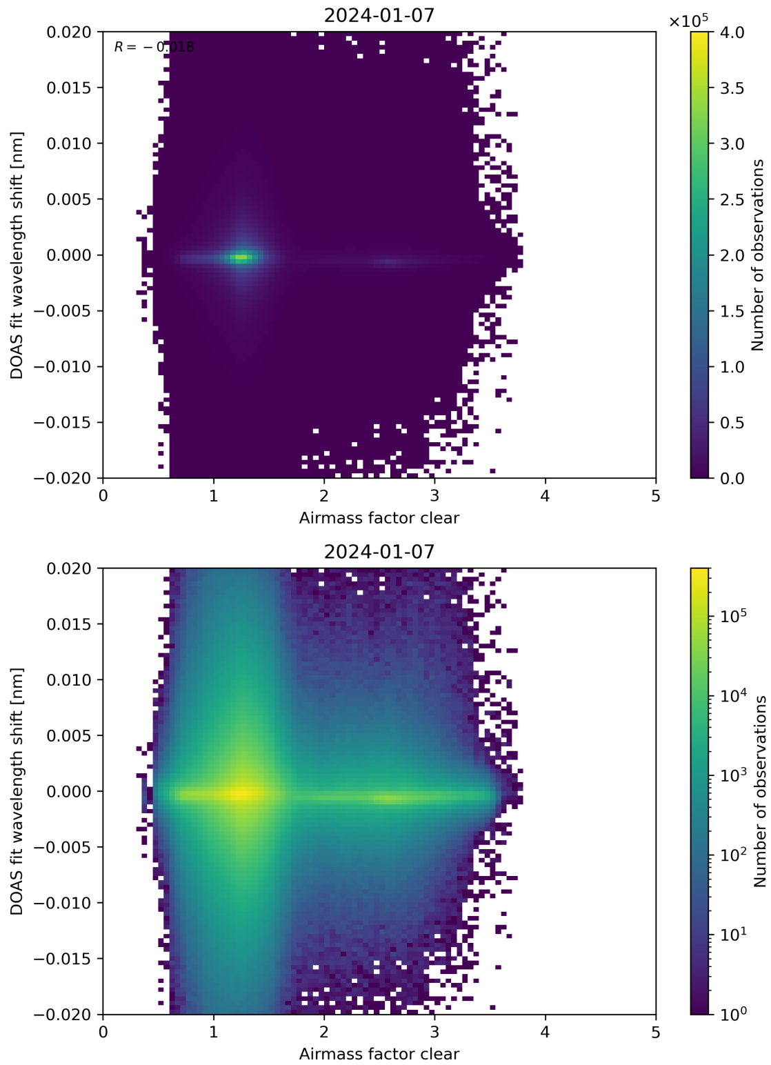
Figure 72: Scatter density plot of “Airmass factor clear” against “DOAS fit wavelength shift” for 2024-01-06 to 2024-01-08.
