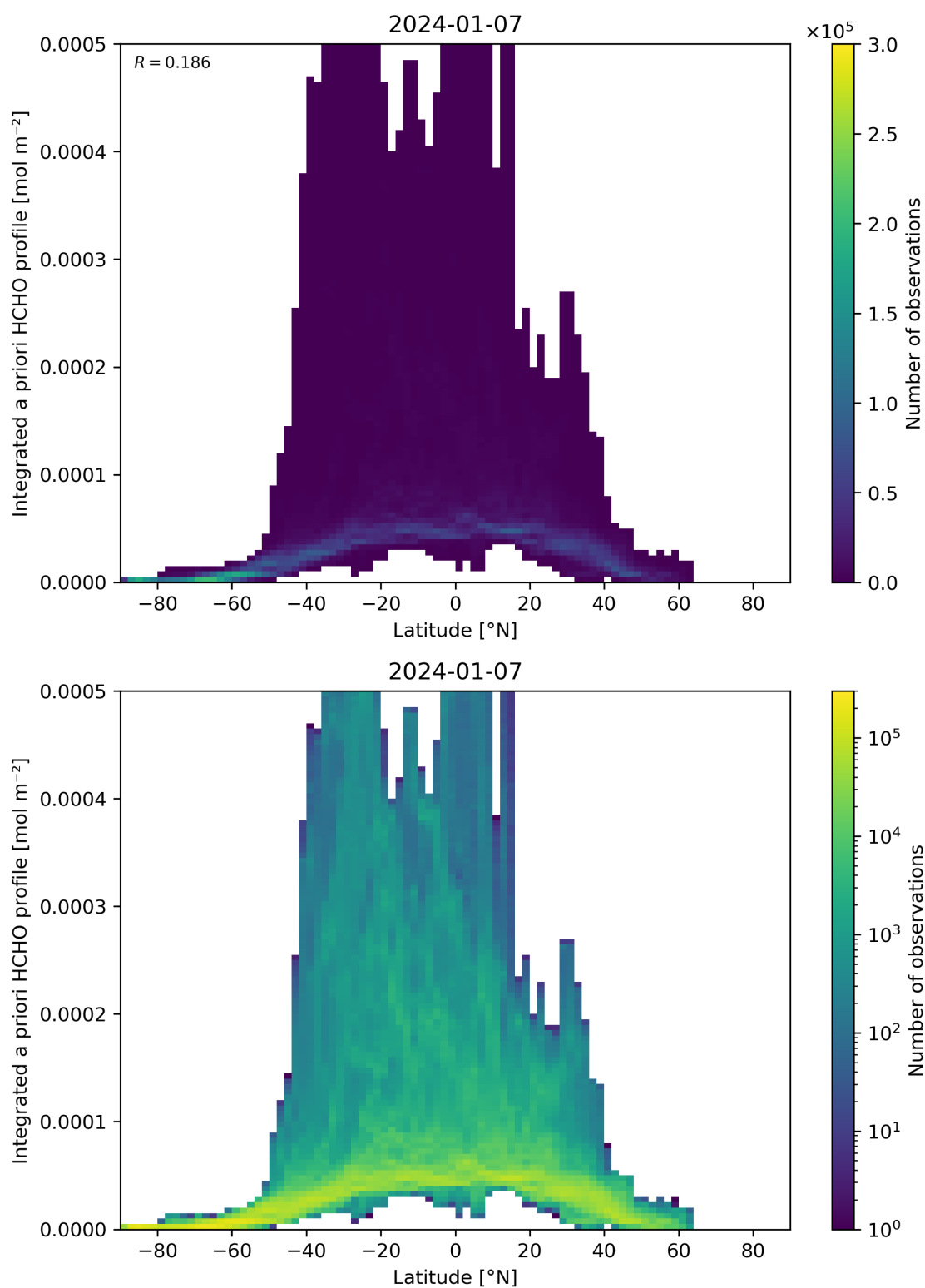
Figure 166: Scatter density plot of “Latitude” against “Integrated a priori HCHO profile” for 2024-01-06 to 2024-01-08.
