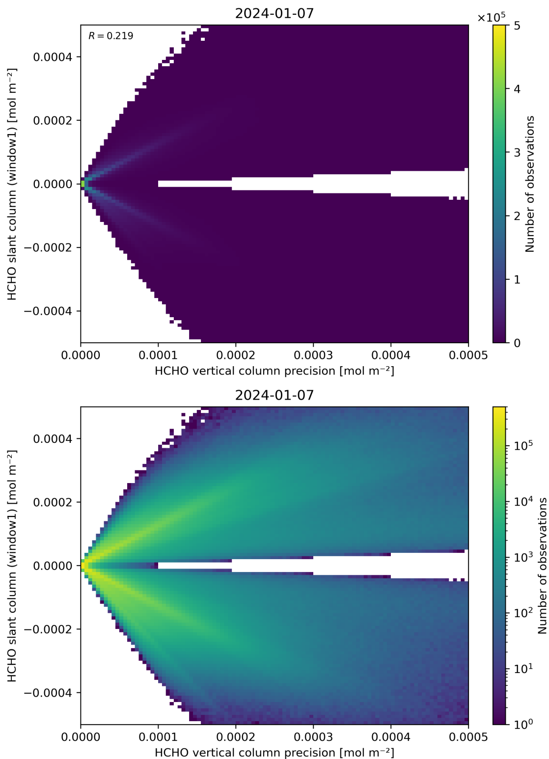
Figure 142: Scatter density plot of “HCHO vertical column precision” against “HCHO slant column (window1)” for 2024-01-06 to 2024-01-08.
