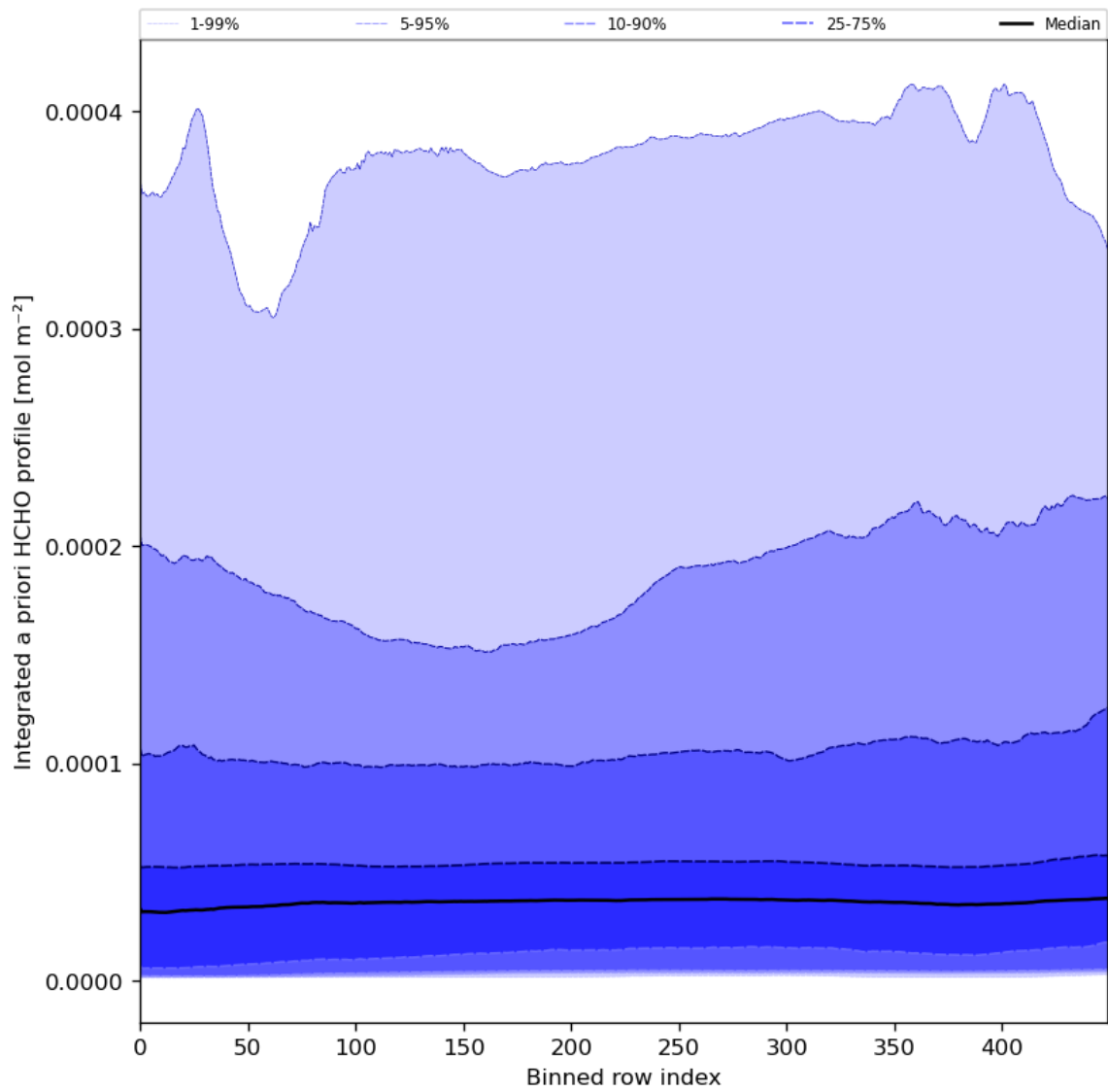
Figure 57: Along track statistics of “Integrated a priori HCHO profile” for 2024-01-06 to 2024-01-08
