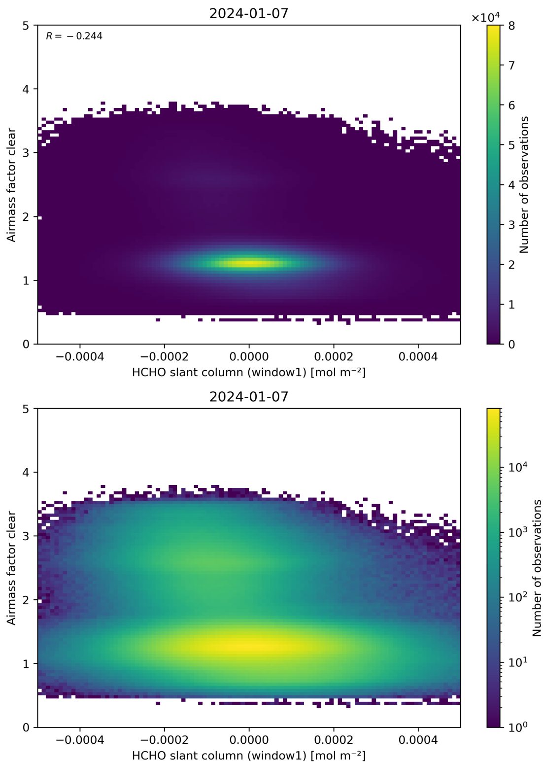
Figure 81: Scatter density plot of “HCHO slant column (window1)” against “Airmass factor clear” for 2024-01-06 to 2024-01-08.
