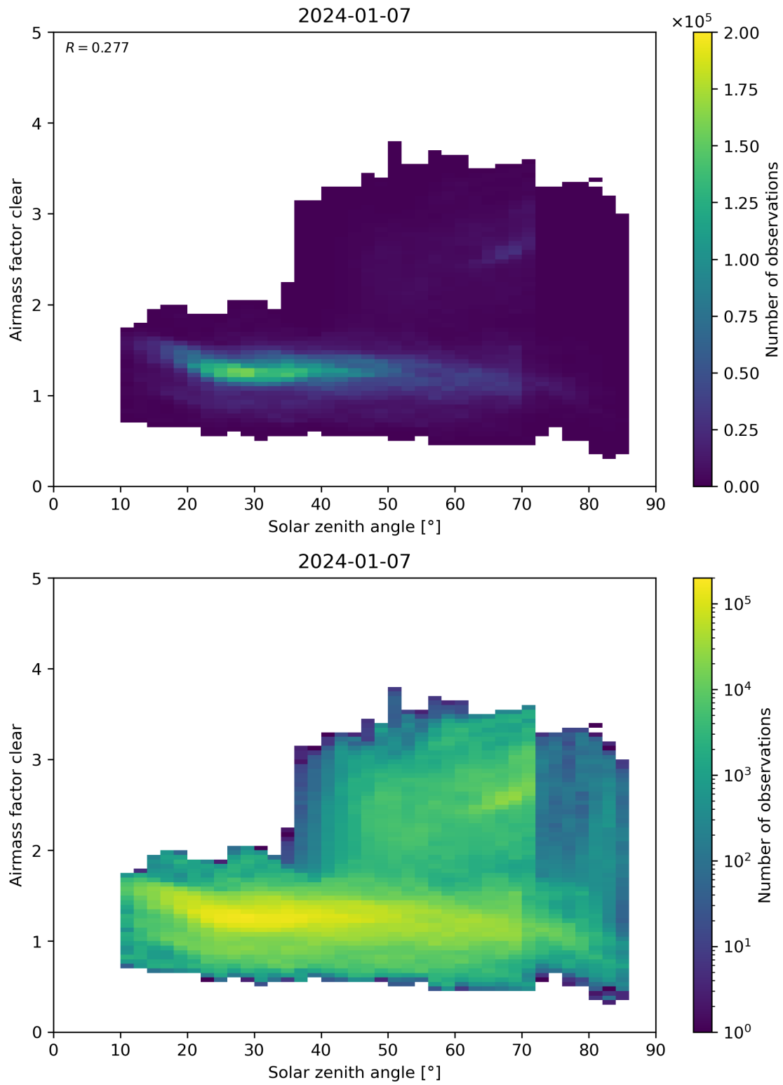
Figure 170: Scatter density plot of “Solar zenith angle” against “Airmass factor clear” for 2024-01-06 to 2024-01-08.
