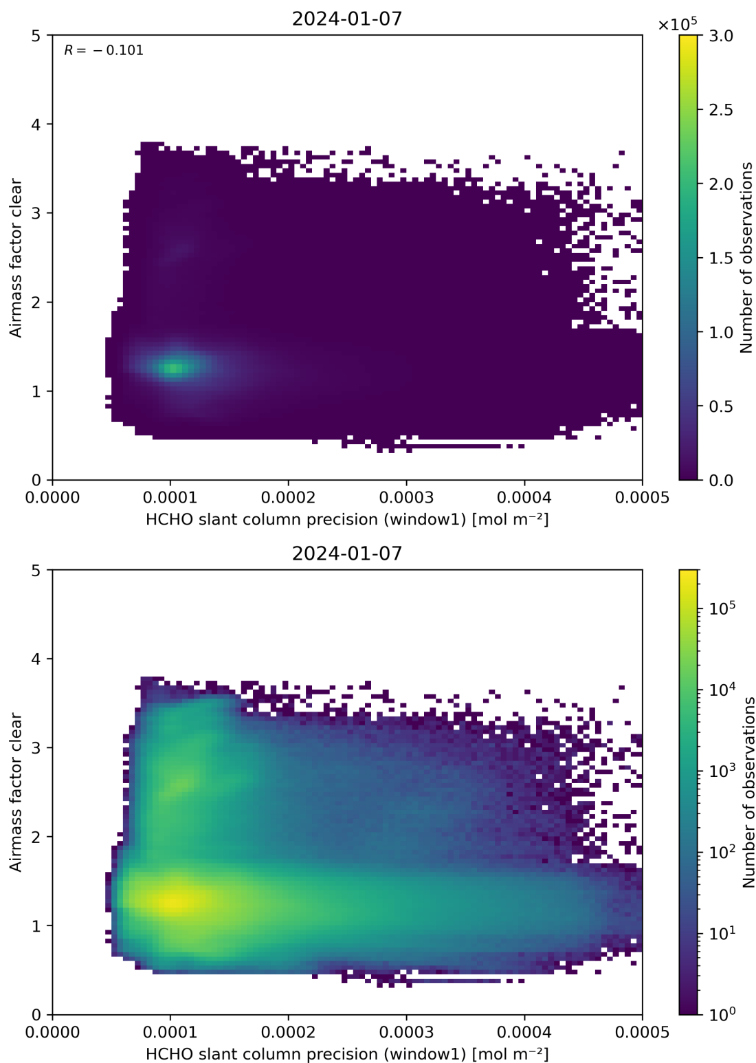
Figure 91: Scatter density plot of “HCHO slant column precision (window1)” against “Airmass factor clear” for 2024-01-06 to 2024-01-08.
