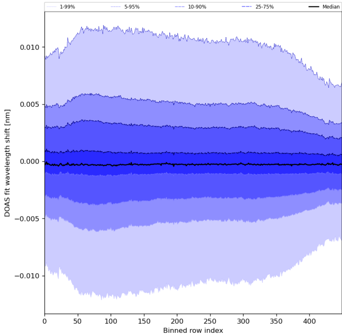
Figure 58: Along track statistics of “DOAS fit wavelength shift” for 2024-01-06 to 2024-01-08
