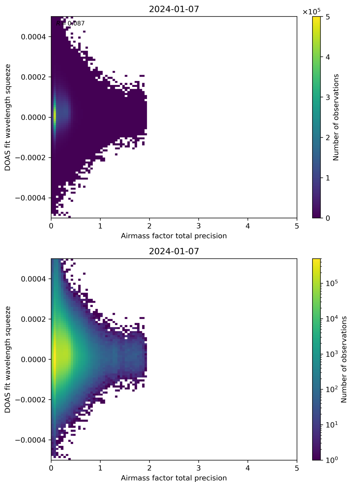
Figure 107: Scatter density plot of “Airmass factor total precision” against “DOAS fit wavelength squeeze” for 2024-01-06 to 2024-01-08.
