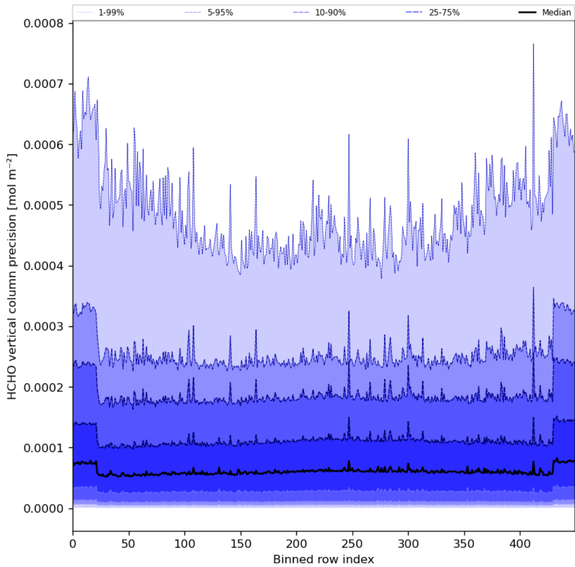
Figure 50: Along track statistics of “HCHO vertical column precision” for 2024-01-06 to 2024-01-08
