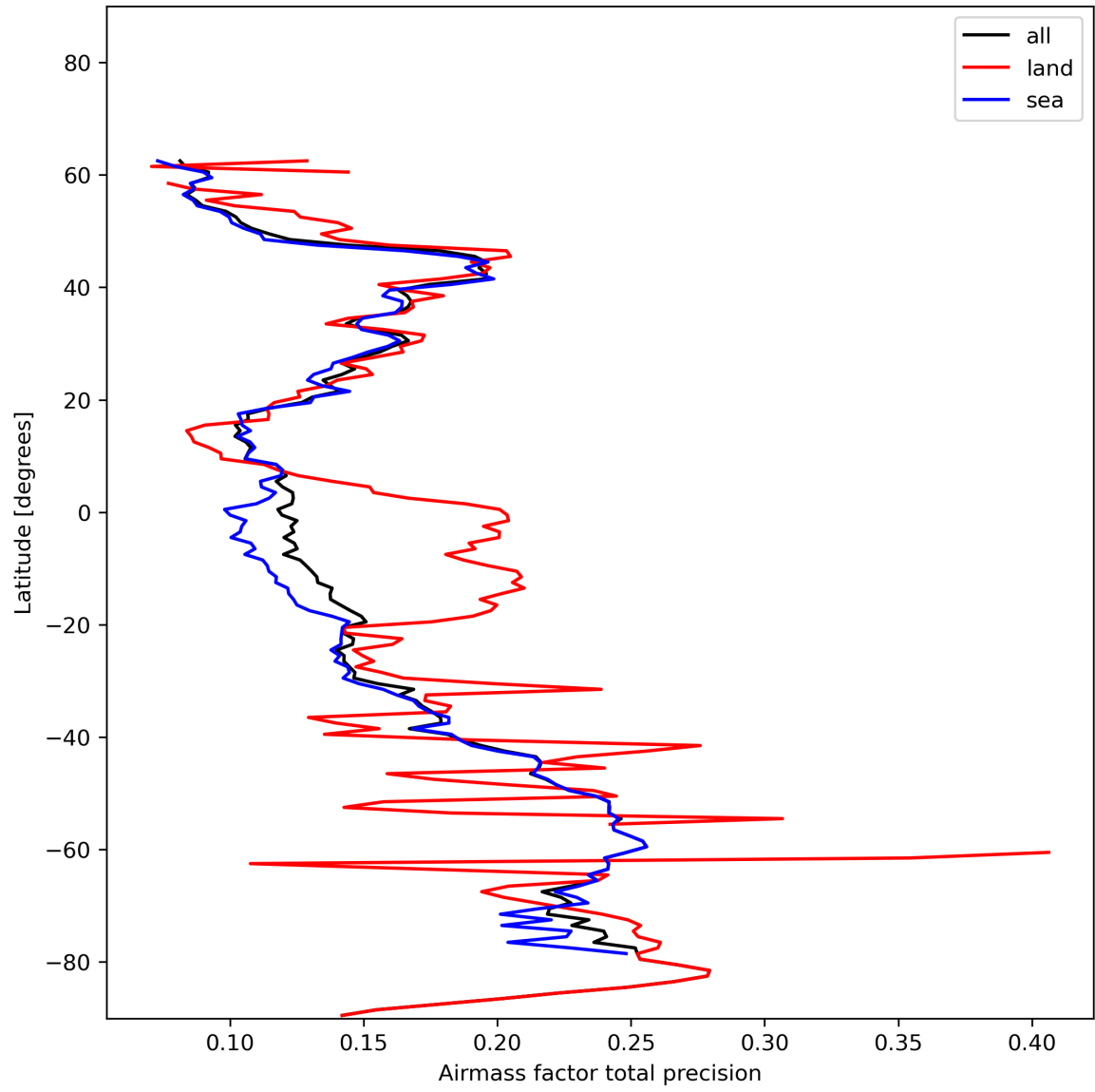
Figure 27: Zonal average of “Airmass factor total precision” for 2024-01-06 to 2024-01-08.
