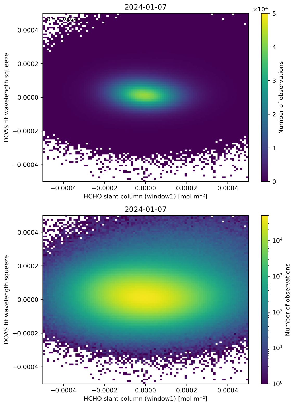
Figure 80: Scatter density plot of “HCHO slant column (window1)” against “DOAS fit wavelength squeeze” for 2024-01-06 to 2024-01-08.
