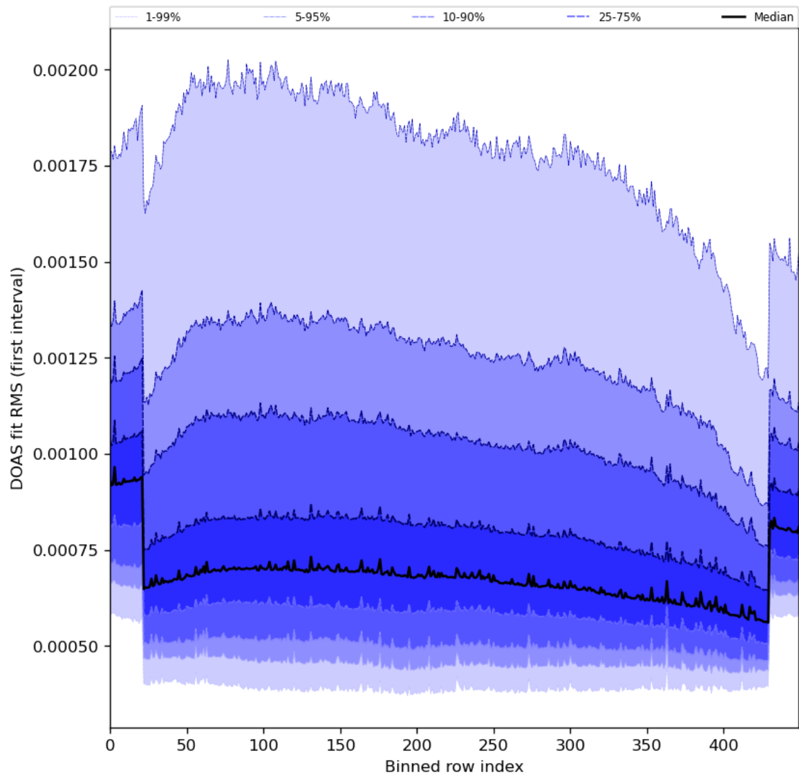
Figure 60: Along track statistics of “DOAS fit RMS (first interval)” for 2024-01-06 to 2024-01-08
