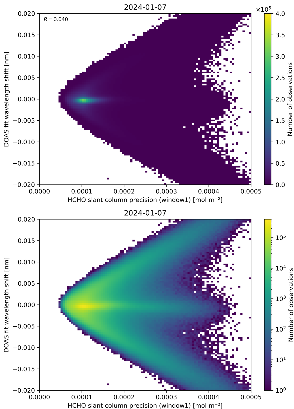
Figure 89: Scatter density plot of “HCHO slant column precision (window1)” against “DOAS fit wavelength shift” for 2024-01-06 to 2024-01-08.
