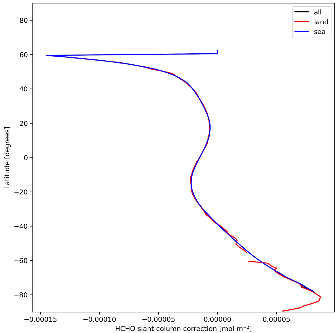
Figure 33: Zonal average of “HCHO slant column correction” for 2024-01-06 to 2024-01-08.
