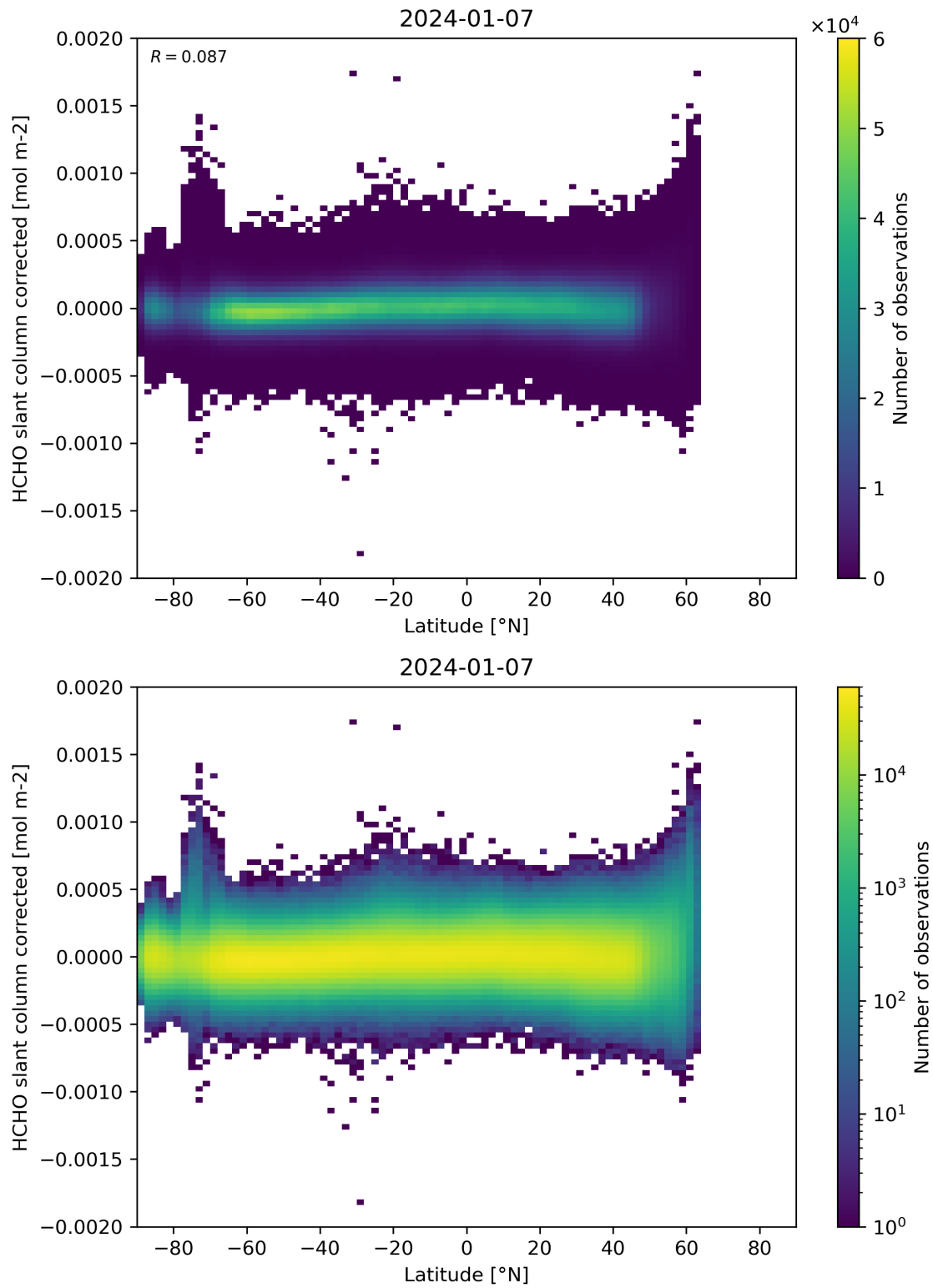
Figure 157: Scatter density plot of “Latitude” against “HCHO slant column corrected” for 2024-01-06 to 2024-01-08.
