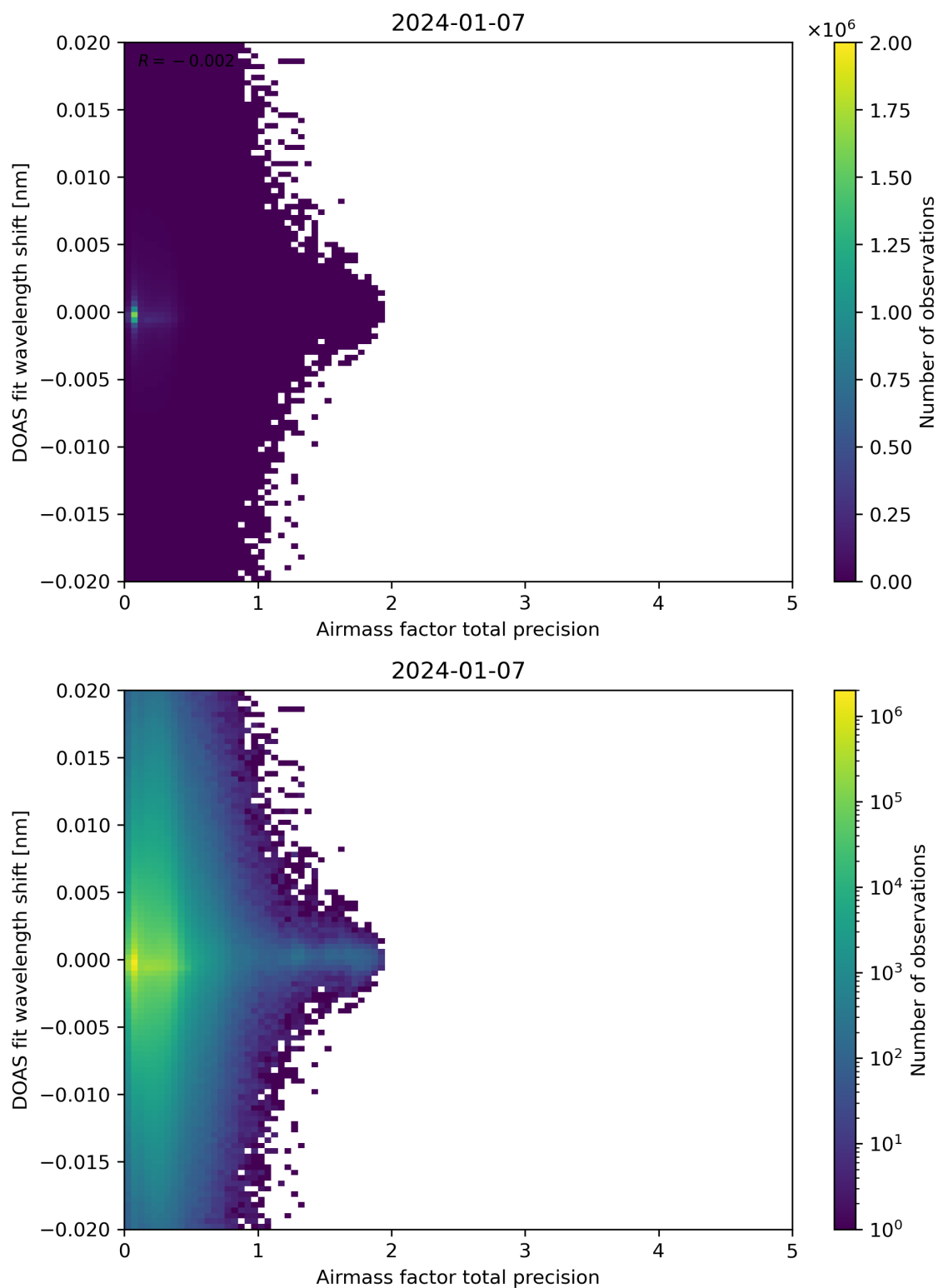
Figure 106: Scatter density plot of “Airmass factor total precision” against “DOAS fit wavelength shift” for 2024-01-06 to 2024-01-08.
