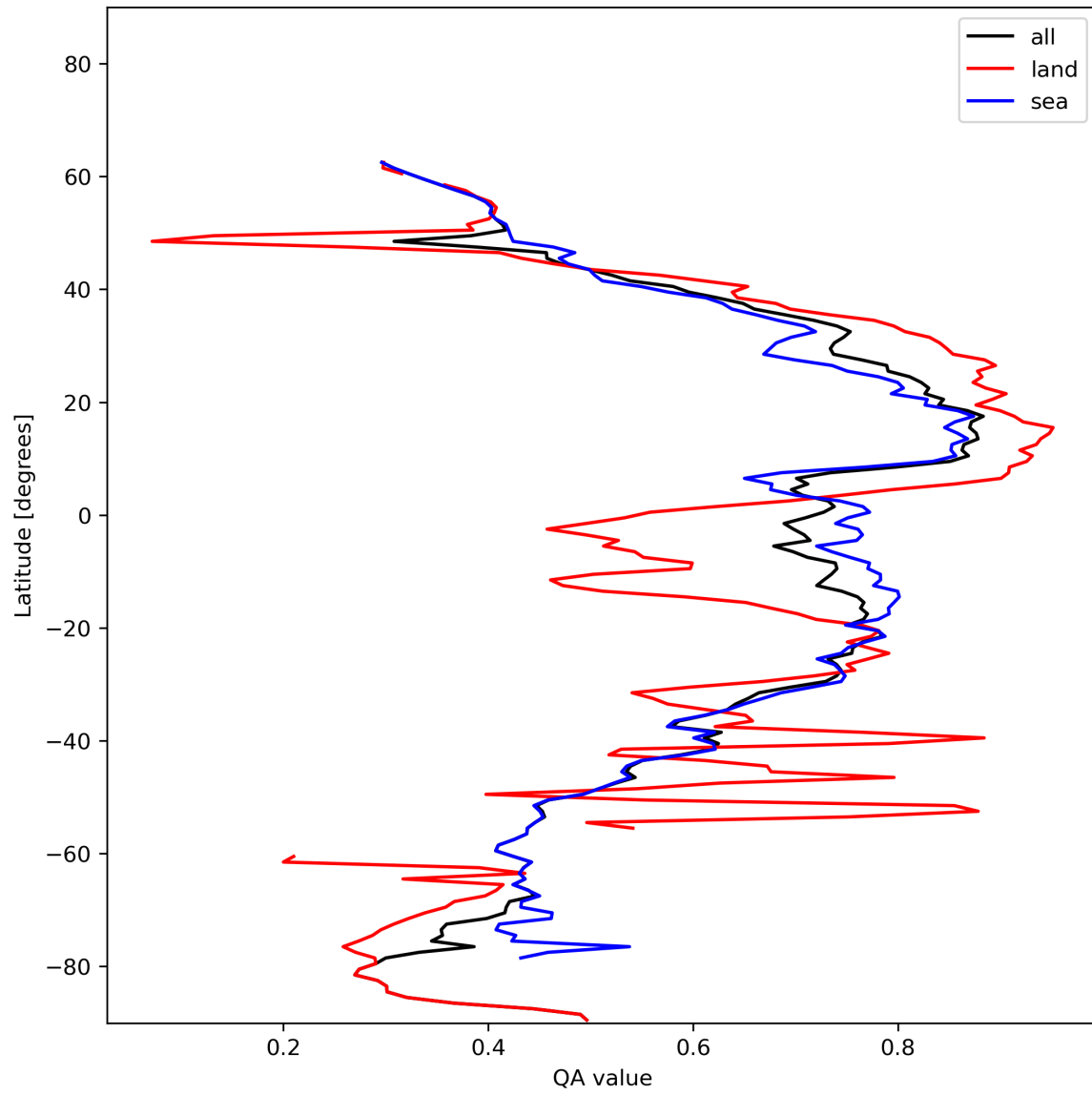
Figure 20: Zonal average of “QA value” for 2024-01-06 to 2024-01-08.
