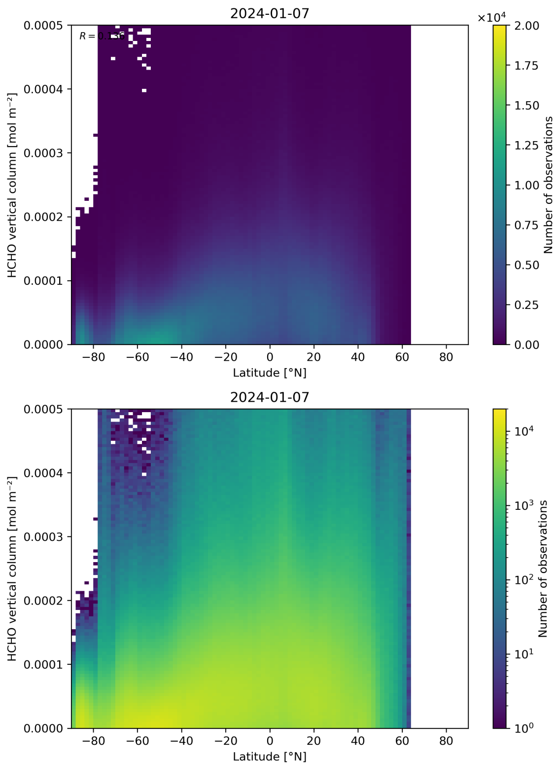
Figure 163: Scatter density plot of “Latitude” against “HCHO vertical column” for 2024-01-06 to 2024-01-08.
