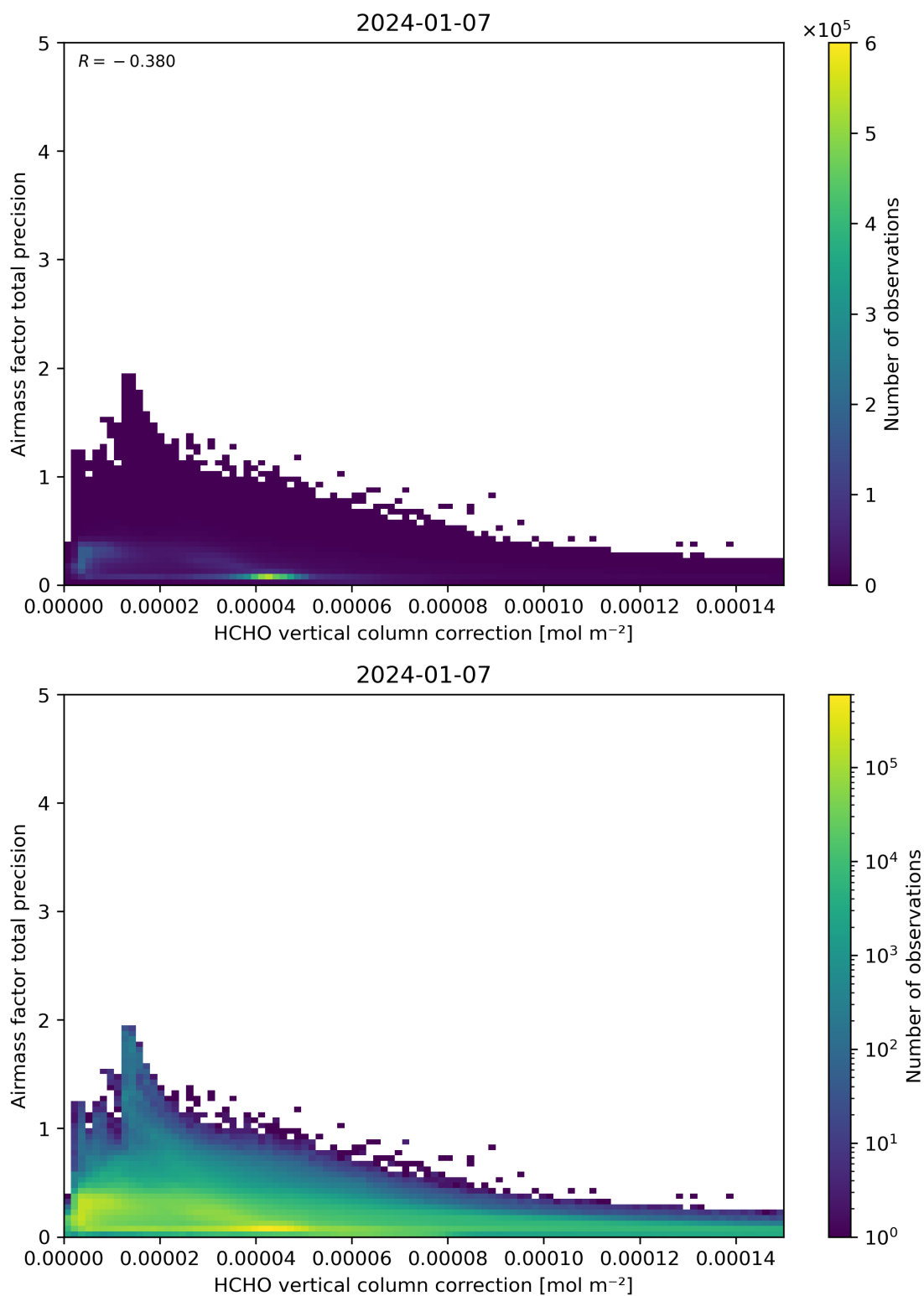
Figure 121: Scatter density plot of “HCHO vertical column correction” against “Airmass factor total precision” for 2024-01-06 to 2024-01-08.
