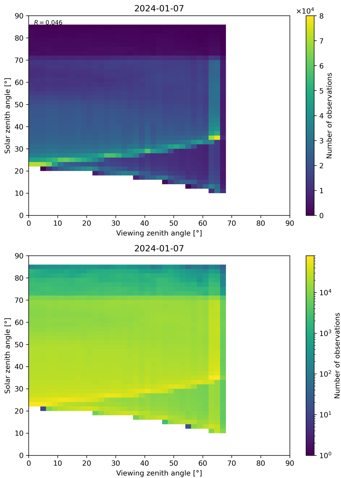
Figure 197: Scatter density plot of “Viewing zenith angle” against “Solar zenith angle” for 2024-01-06 to 2024-01-08.
