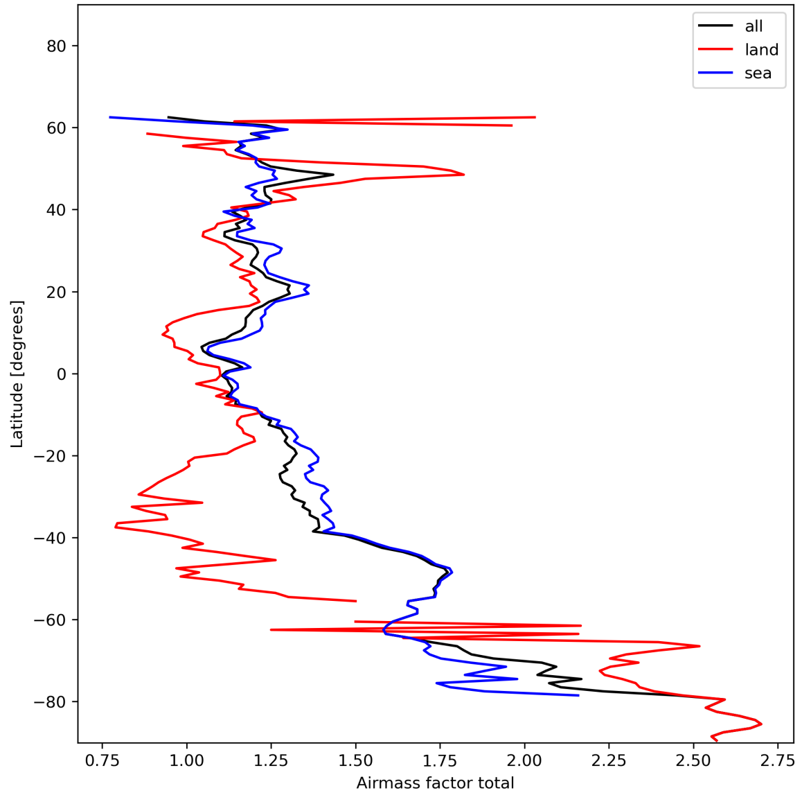
Figure 26: Zonal average of “Airmass factor total” for 2024-01-06 to 2024-01-08.
