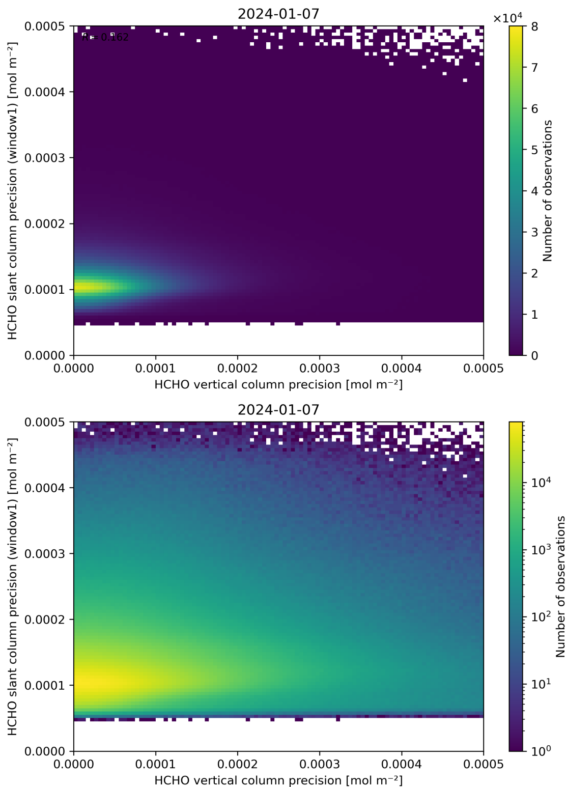
Figure 143: Scatter density plot of “HCHO vertical column precision” against “HCHO slant column precision (window1)” for 2024-01-06 to 2024-01-08.
