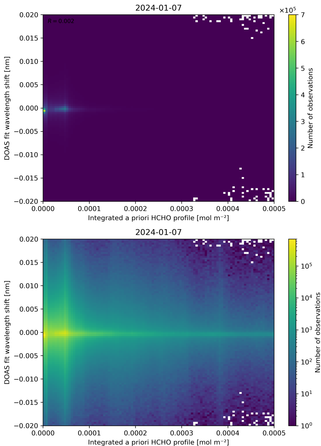
Figure 149: Scatter density plot of “Integrated a priori HCHO profile” against “DOAS fit wavelength shift” for 2024-01-06 to 2024-01-08.
