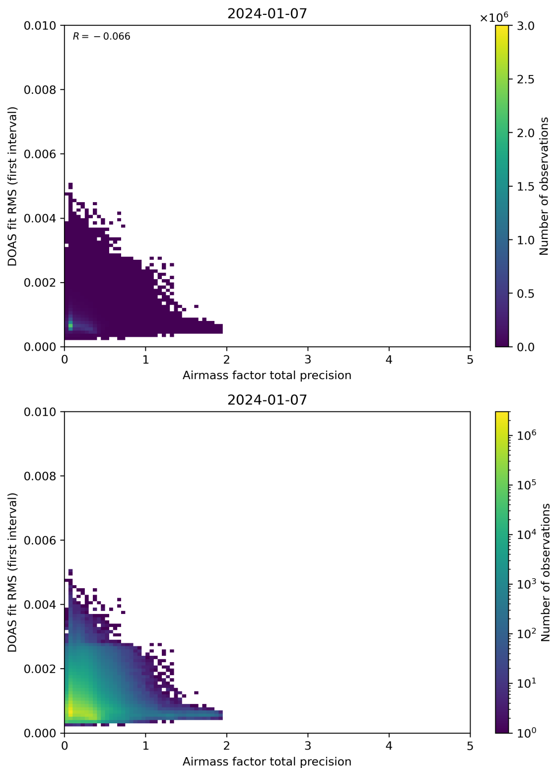
Figure 105: Scatter density plot of “Airmass factor total precision” against “DOAS fit RMS (first interval)” for 2024-01-06 to 2024-01-08.
