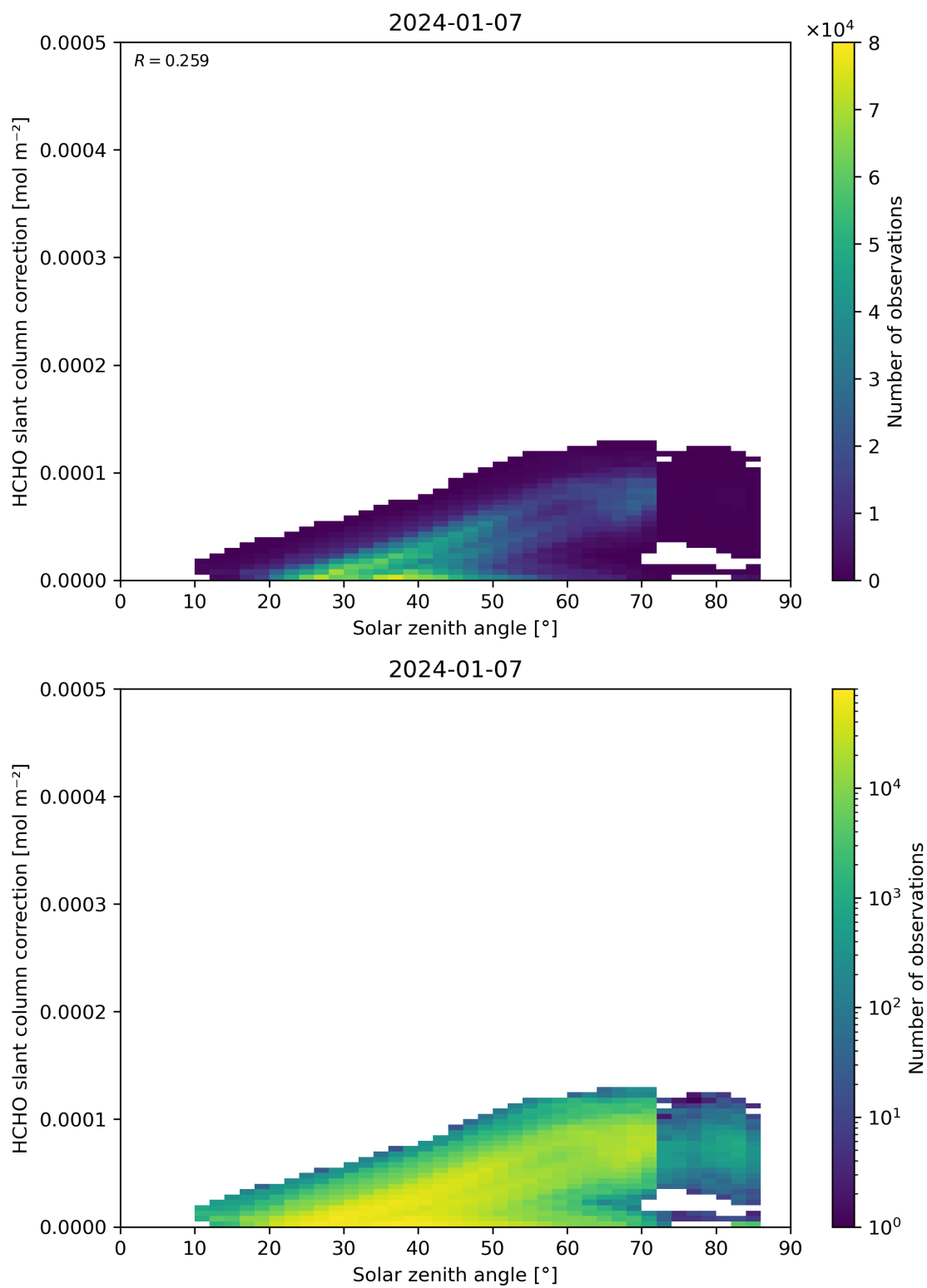
Figure 172: Scatter density plot of “Solar zenith angle” against “HCHO slant column correction” for 2024-01-06 to 2024-01-08.
