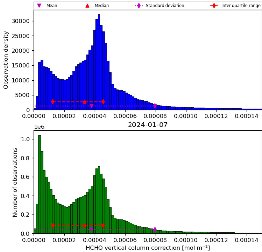
Figure 37: Histogram of “HCHO vertical column correction” for 2024-01-06 to 2024-01-08
