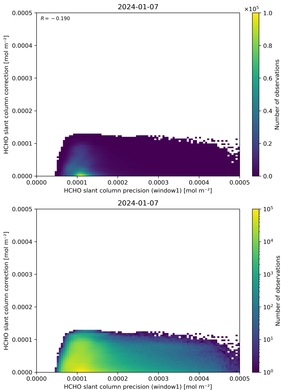
Figure 93: Scatter density plot of “HCHO slant column precision (window1)” against “HCHO slant column correction” for 2024-01-06 to 2024-01-08.
