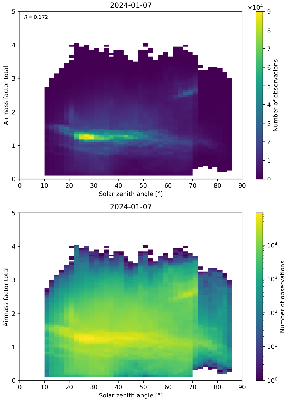
Figure 175: Scatter density plot of “Solar zenith angle” against “Airmass factor total” for 2024-01-06 to 2024-01-08.
