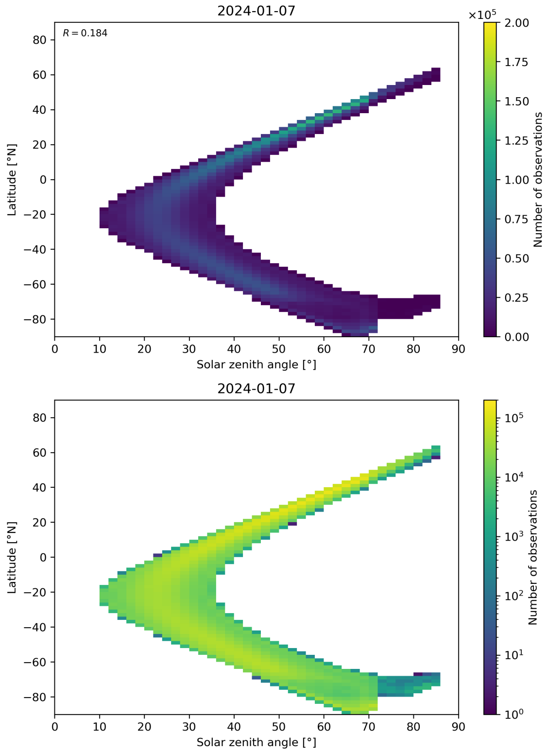
Figure 181: Scatter density plot of “Solar zenith angle” against “Latitude” for 2024-01-06 to 2024-01-08.
