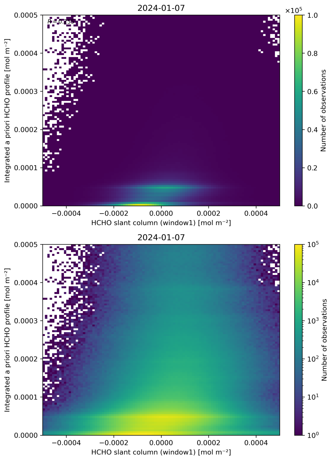
Figure 87: Scatter density plot of “HCHO slant column (window1)” against “Integrated a priori HCHO profile” for 2024-01-06 to 2024-01-08.
