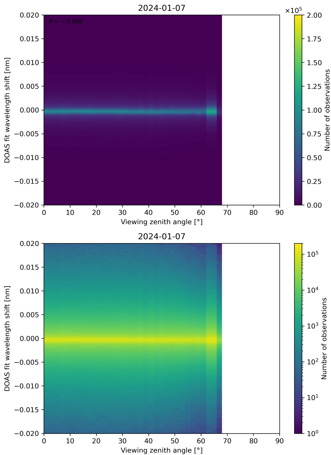
Figure 183: Scatter density plot of “Viewing zenith angle” against “DOAS fit wavelength shift” for 2024-01-06 to 2024-01-08.
