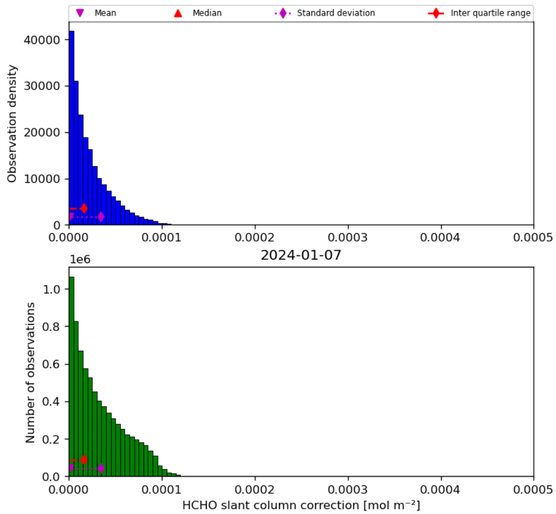
Figure 47: Histogram of “HCHO slant column correction” for 2024-01-06 to 2024-01-08
