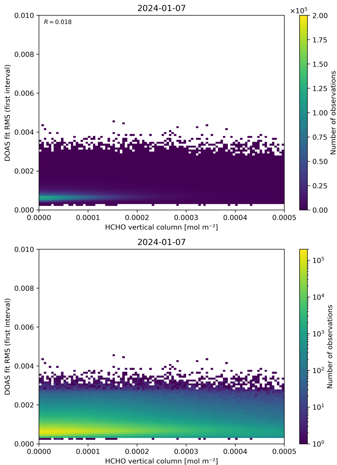
Figure 123: Scatter density plot of “HCHO vertical column” against “DOAS fit RMS (first interval)” for 2024-01-06 to 2024-01-08.
