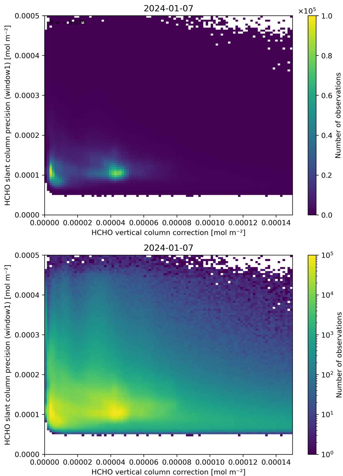
Figure 119: Scatter density plot of “HCHO vertical column correction” against “HCHO slant column precision (window1)” for 2024-01-06 to 2024-01-08.
