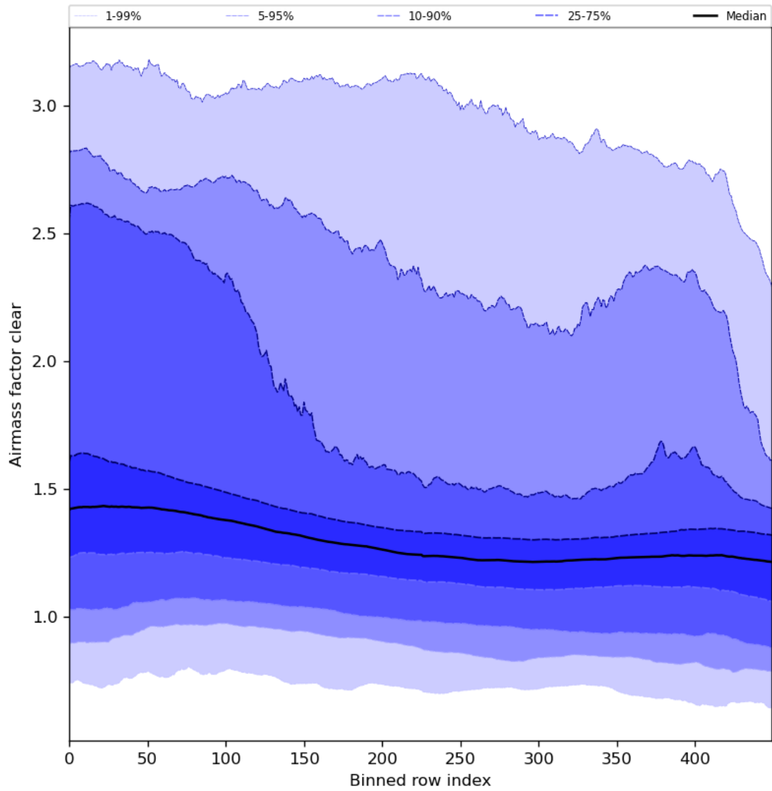
Figure 56: Along track statistics of “Airmass factor clear” for 2024-01-06 to 2024-01-08
