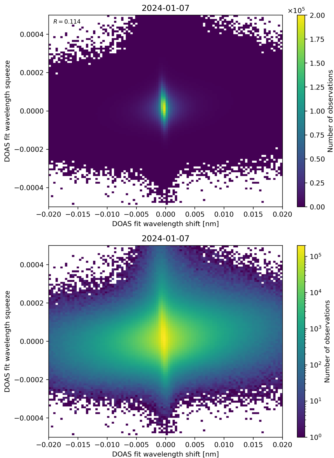
Figure 65: Scatter density plot of “DOAS fit wavelength shift” against “DOAS fit wavelength squeeze” for 2024-01-06 to 2024-01-08.
