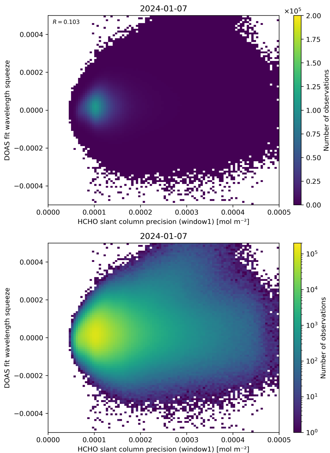
Figure 90: Scatter density plot of “HCHO slant column precision (window1)” against “DOAS fit wavelength squeeze” for 2024-01-06 to 2024-01-08.
