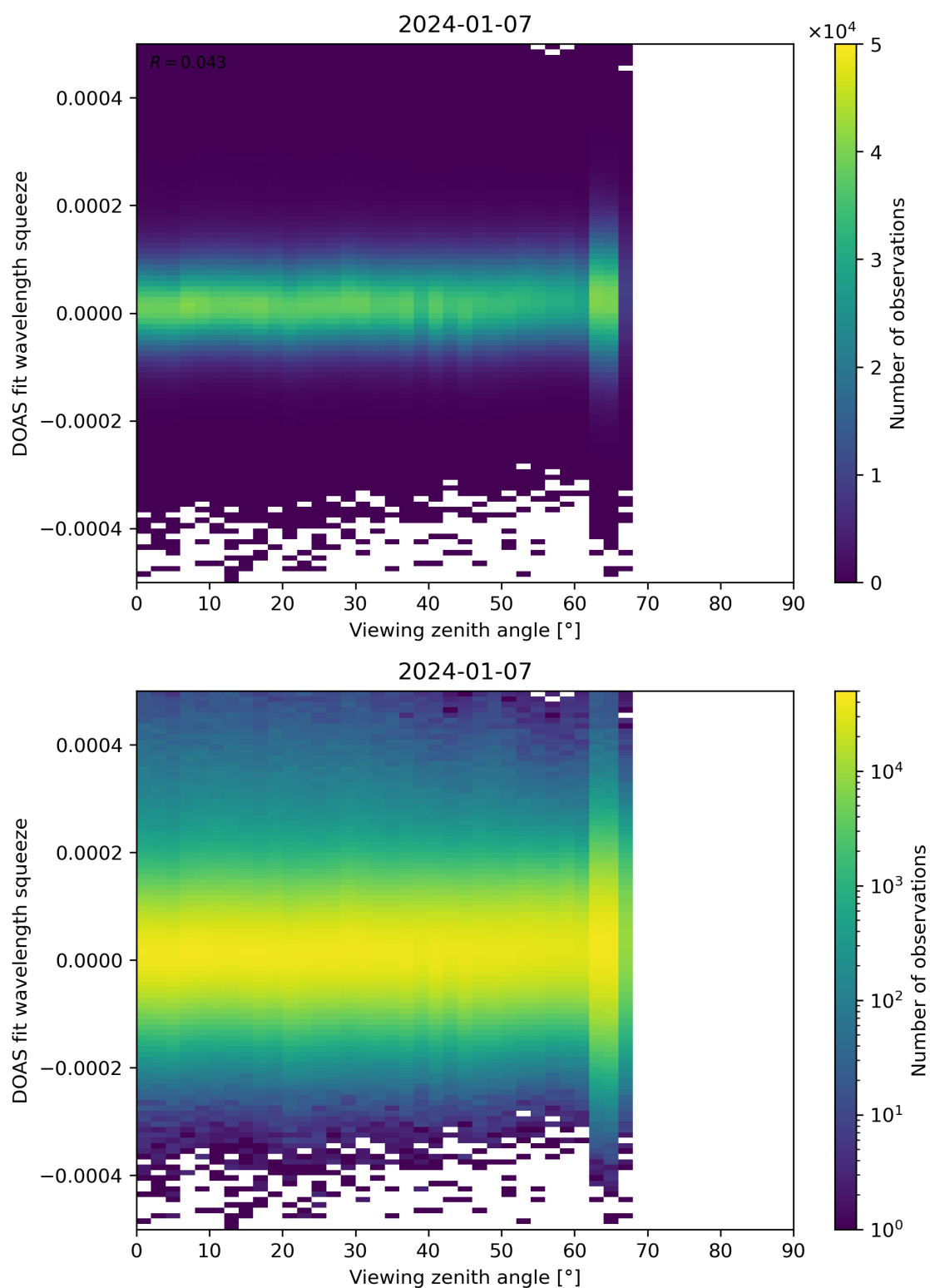
Figure 184: Scatter density plot of “Viewing zenith angle” against “DOAS fit wavelength squeeze” for 2024-01-06 to 2024-01-08.
