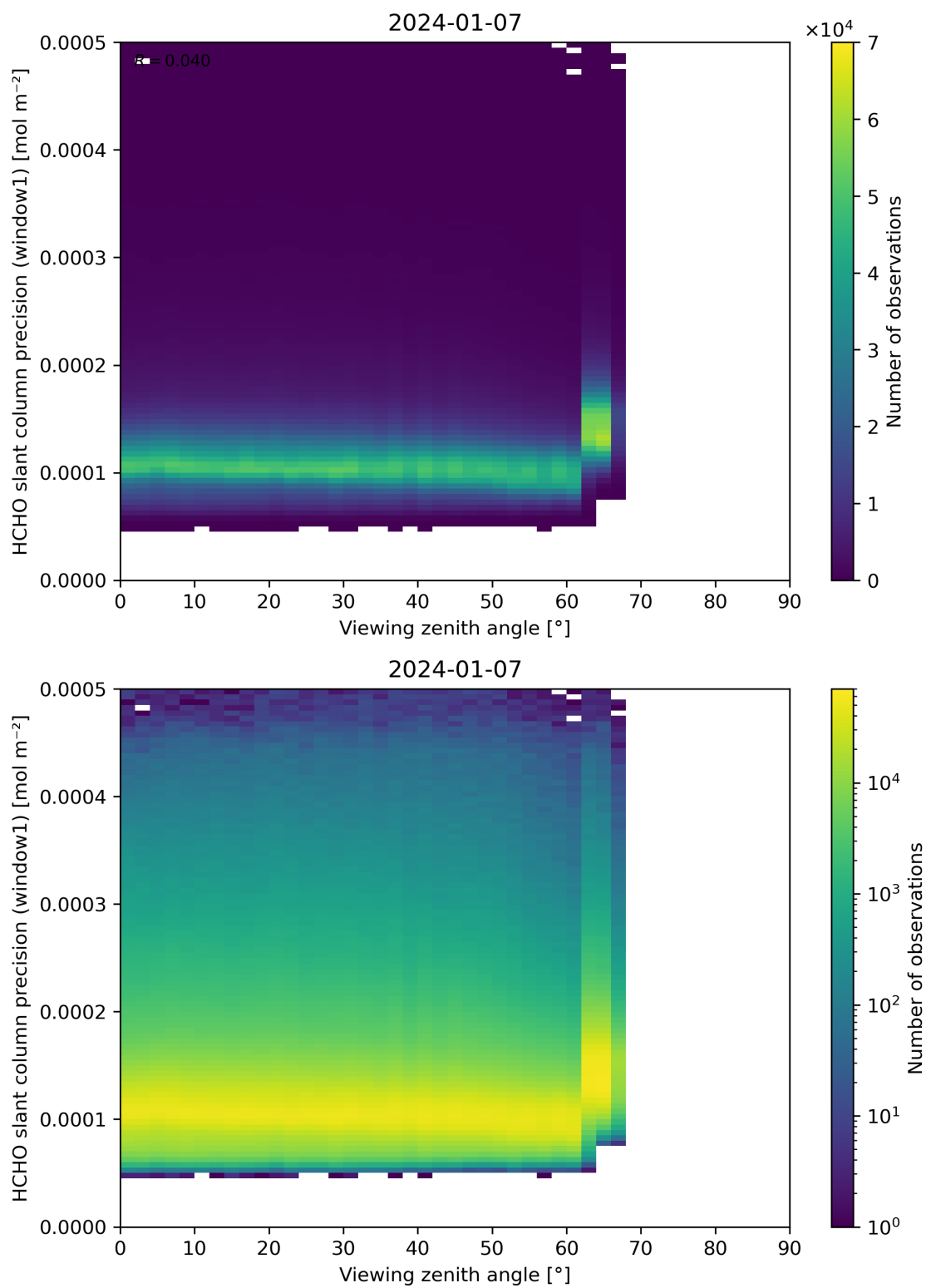
Figure 189: Scatter density plot of “Viewing zenith angle” against “HCHO slant column precision (window1)” for 2024-01-06 to 2024-01-08.
