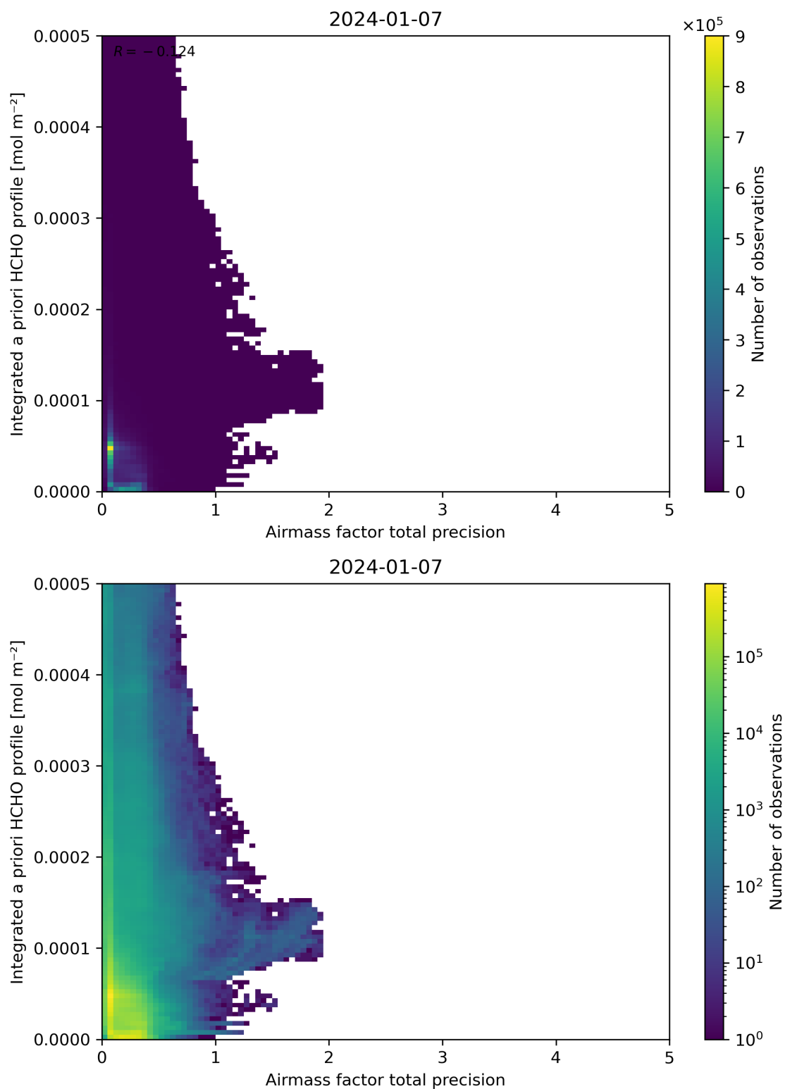
Figure 111: Scatter density plot of “Airmass factor total precision” against “Integrated a priori HCHO profile” for 2024-01-06 to 2024-01-08.
