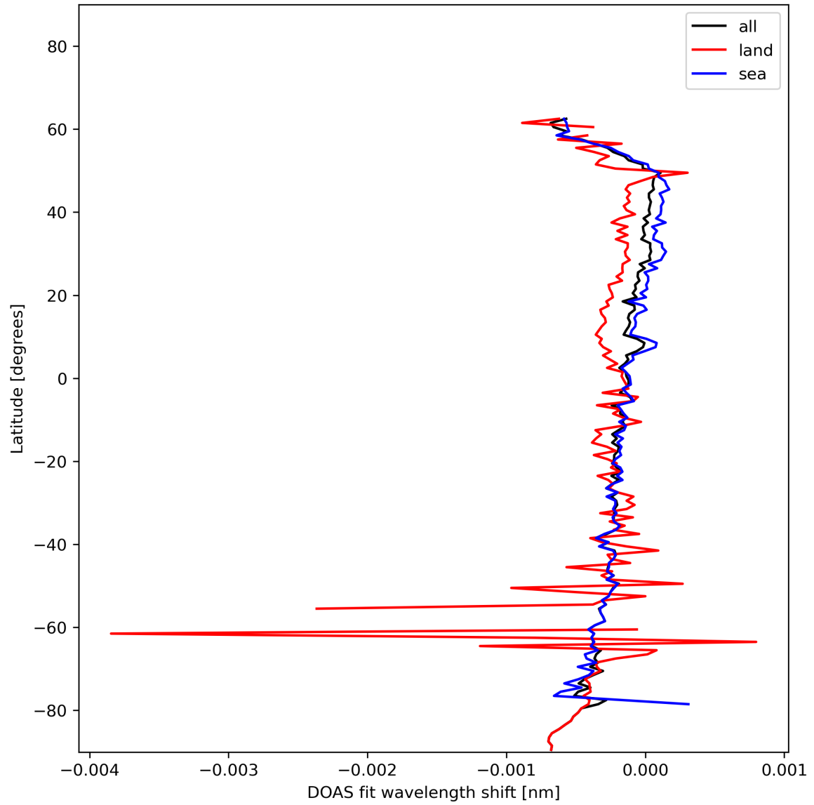
Figure 30: Zonal average of “DOAS fit wavelength shift” for 2024-01-06 to 2024-01-08.
