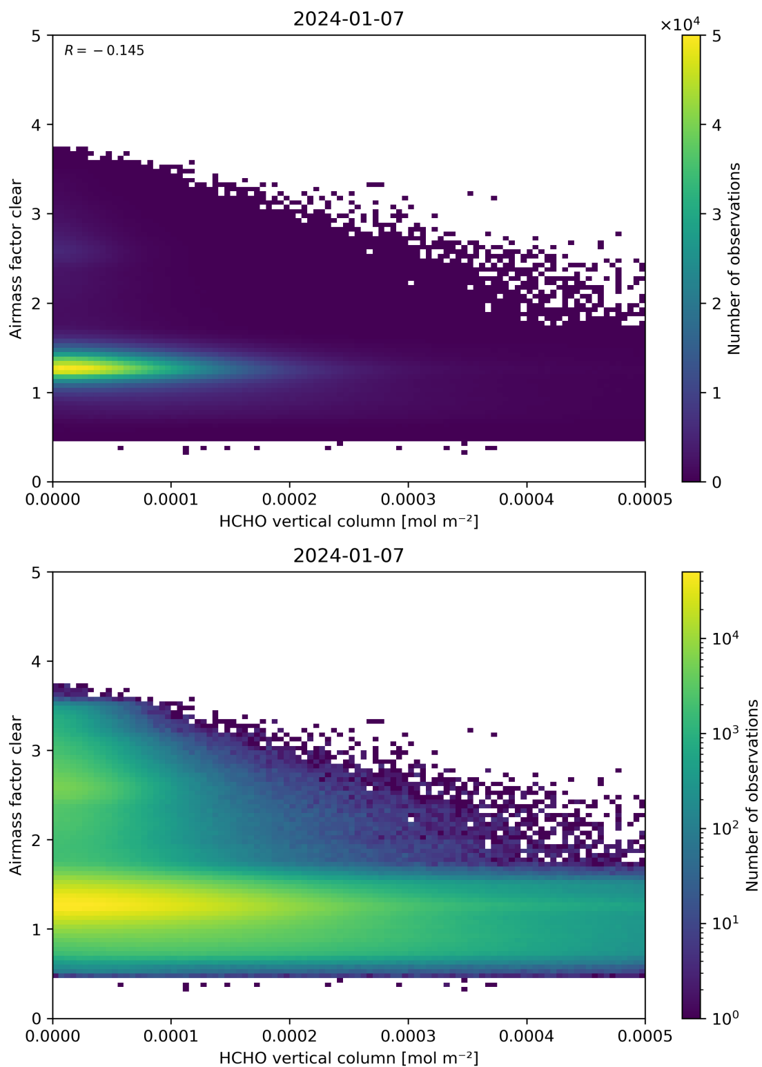
Figure 126: Scatter density plot of “HCHO vertical column” against “Airmass factor clear” for 2024-01-06 to 2024-01-08.
