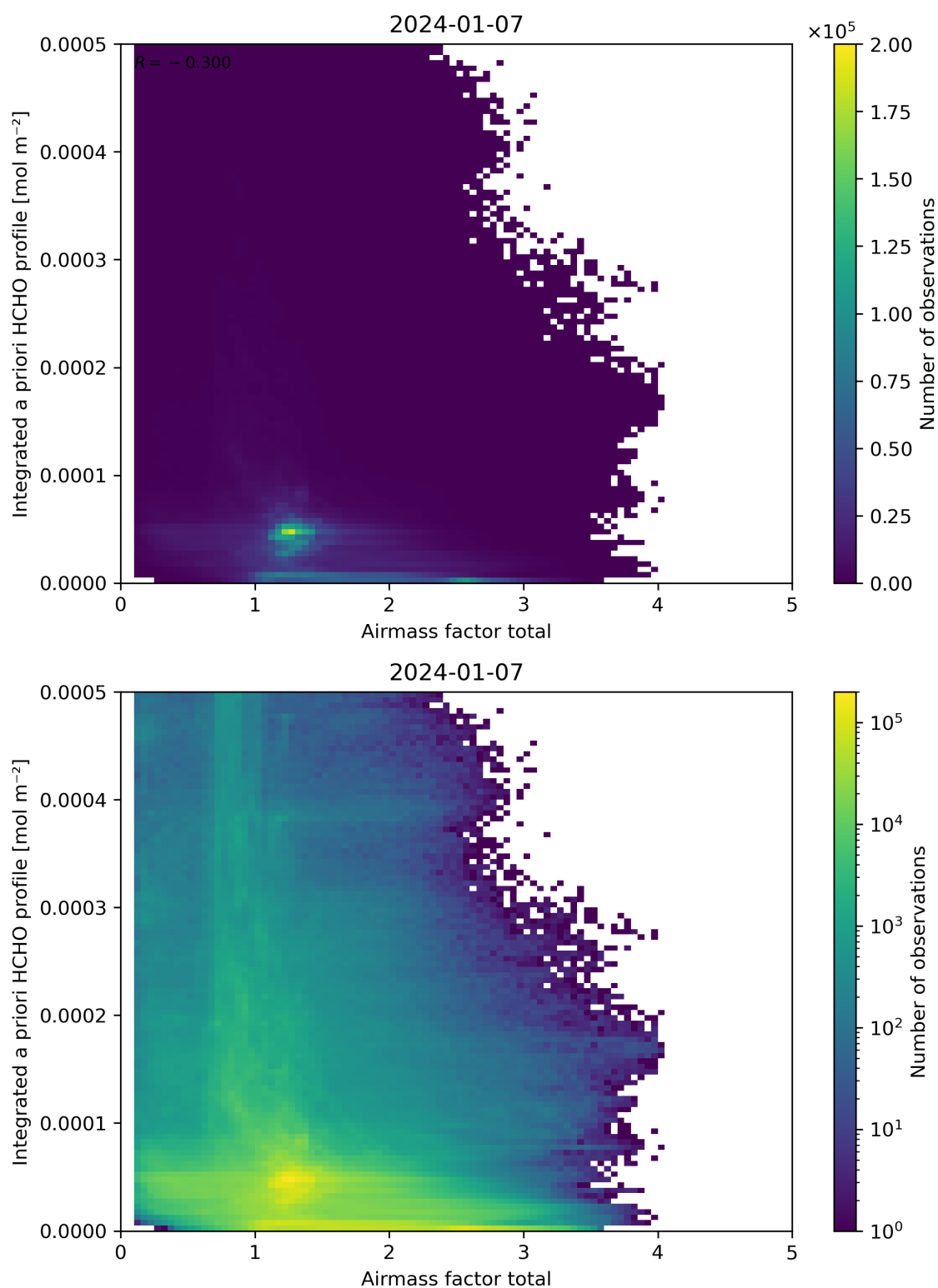
Figure 104: Scatter density plot of “Air mass factor total” against “Integrated a priori HCHO profile” for 2024-01-06 to 2024-01-08.
