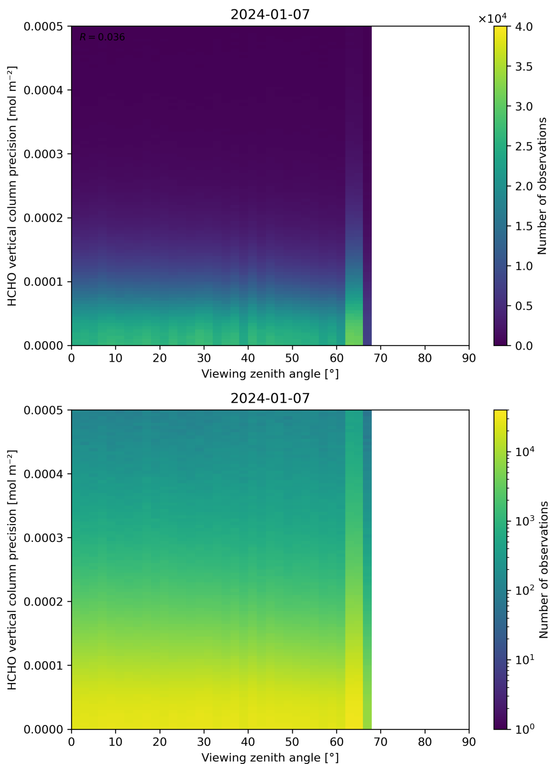
Figure 194: Scatter density plot of “Viewing zenith angle” against “HCHO vertical column precision” for 2024-01-06 to 2024-01-08.
