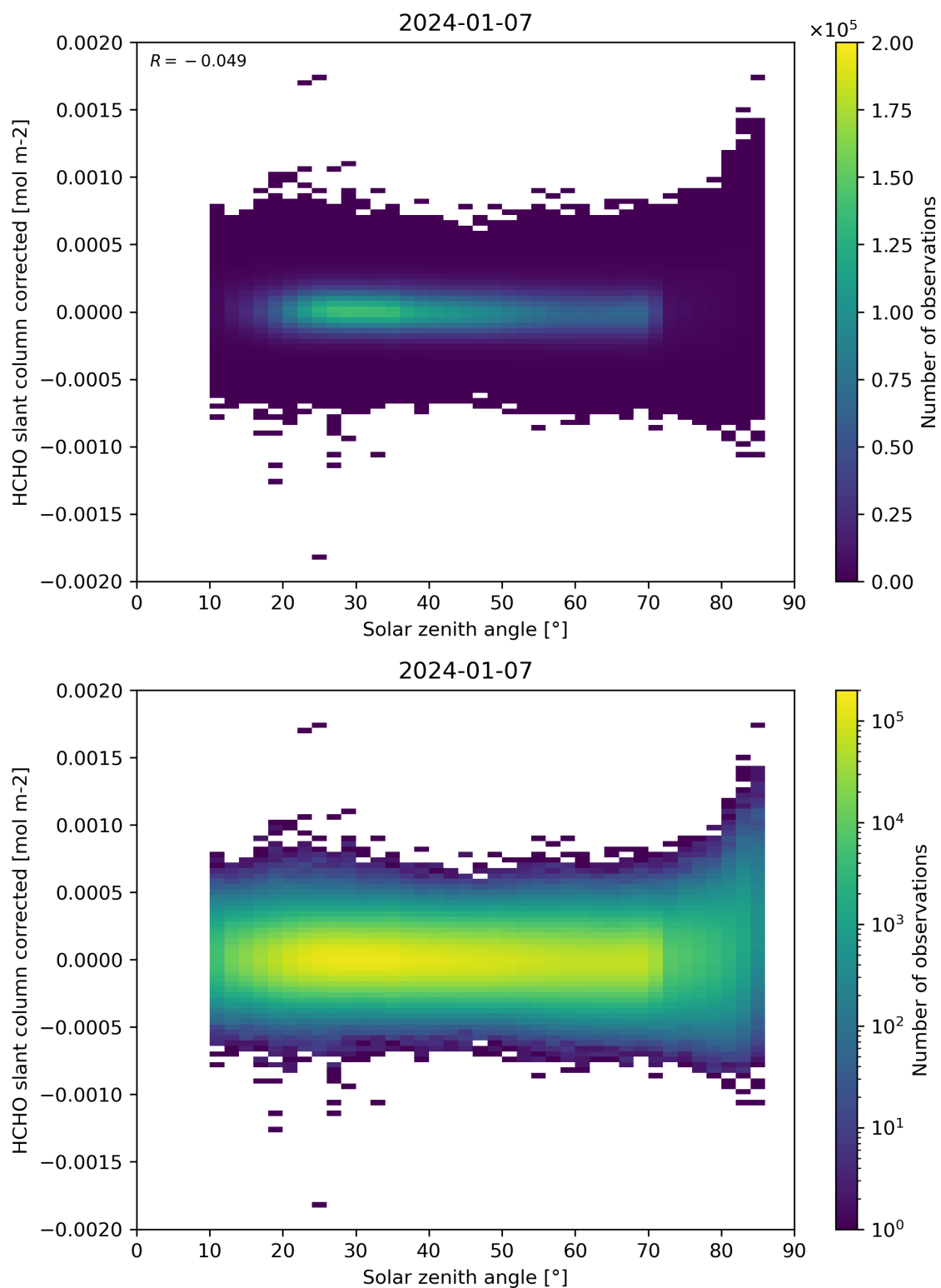
Figure 171: Scatter density plot of “Solar zenith angle” against “HCHO slant column corrected” for 2024-01-06 to 2024-01-08.
