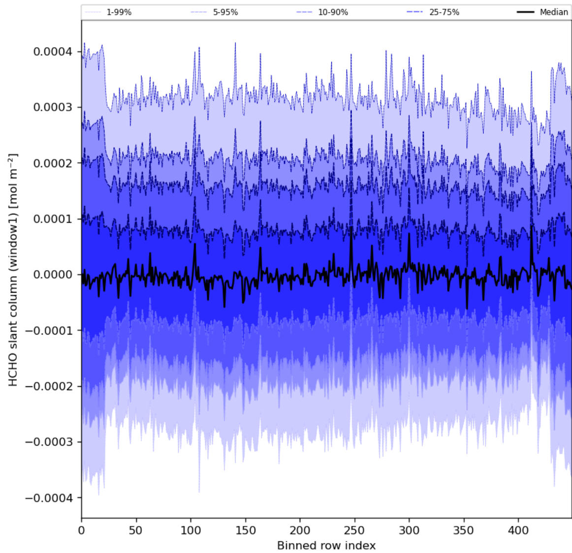
Figure 52: Along track statistics of “HCHO slant column (window1)” for 2024-01-06 to 2024-01-08
