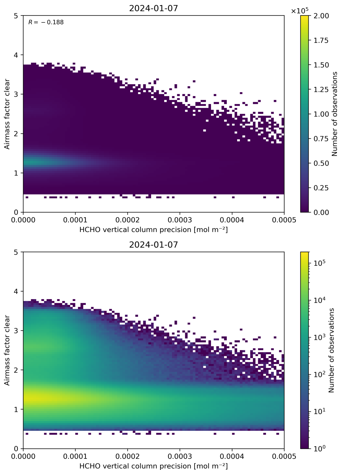
Figure 139: Scatter density plot of “HCHO vertical column precision” against “Airmass factor clear” for 2024-01-06 to 2024-01-08.
