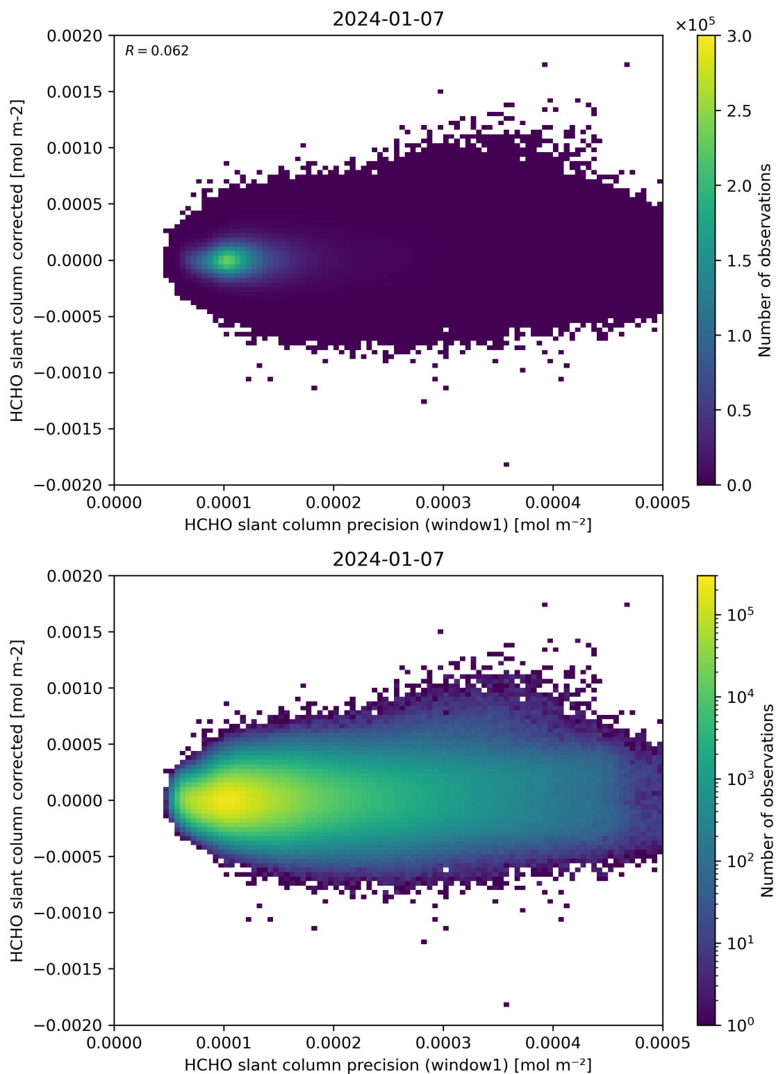
Figure 92: Scatter density plot of “HCHO slant column precision (window1)” against “HCHO slant column corrected” for 2024-01-06 to 2024-01-08.
