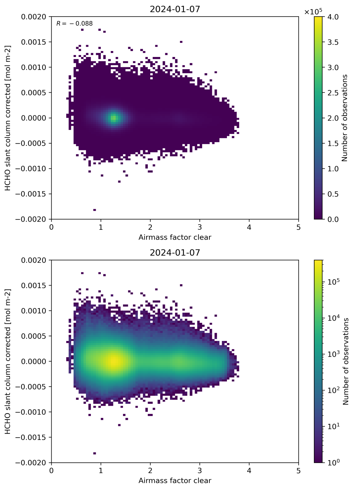
Figure 74: Scatter density plot of “Airmass factor clear” against “HCHO slant column corrected” for 2024-01-06 to 2024-01-08.
