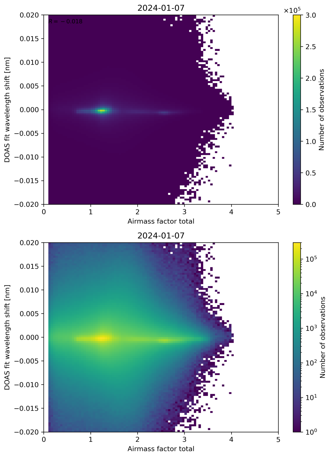
Figure 98: Scatter density plot of “Airmass factor total” against “DOAS fit wavelength shift” for 2024-01-06 to 2024-01-08.
