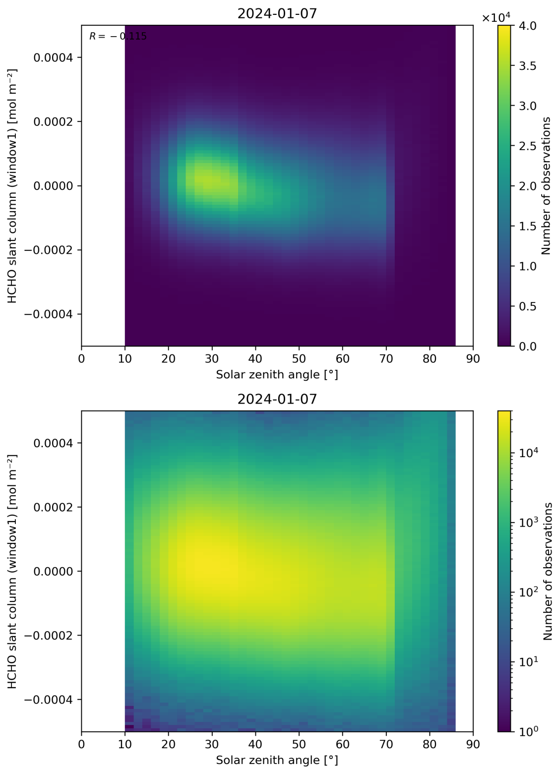
Figure 173: Scatter density plot of “Solar zenith angle” against “HCHO slant column (window1)” for 2024-01-06 to 2024-01-08.
