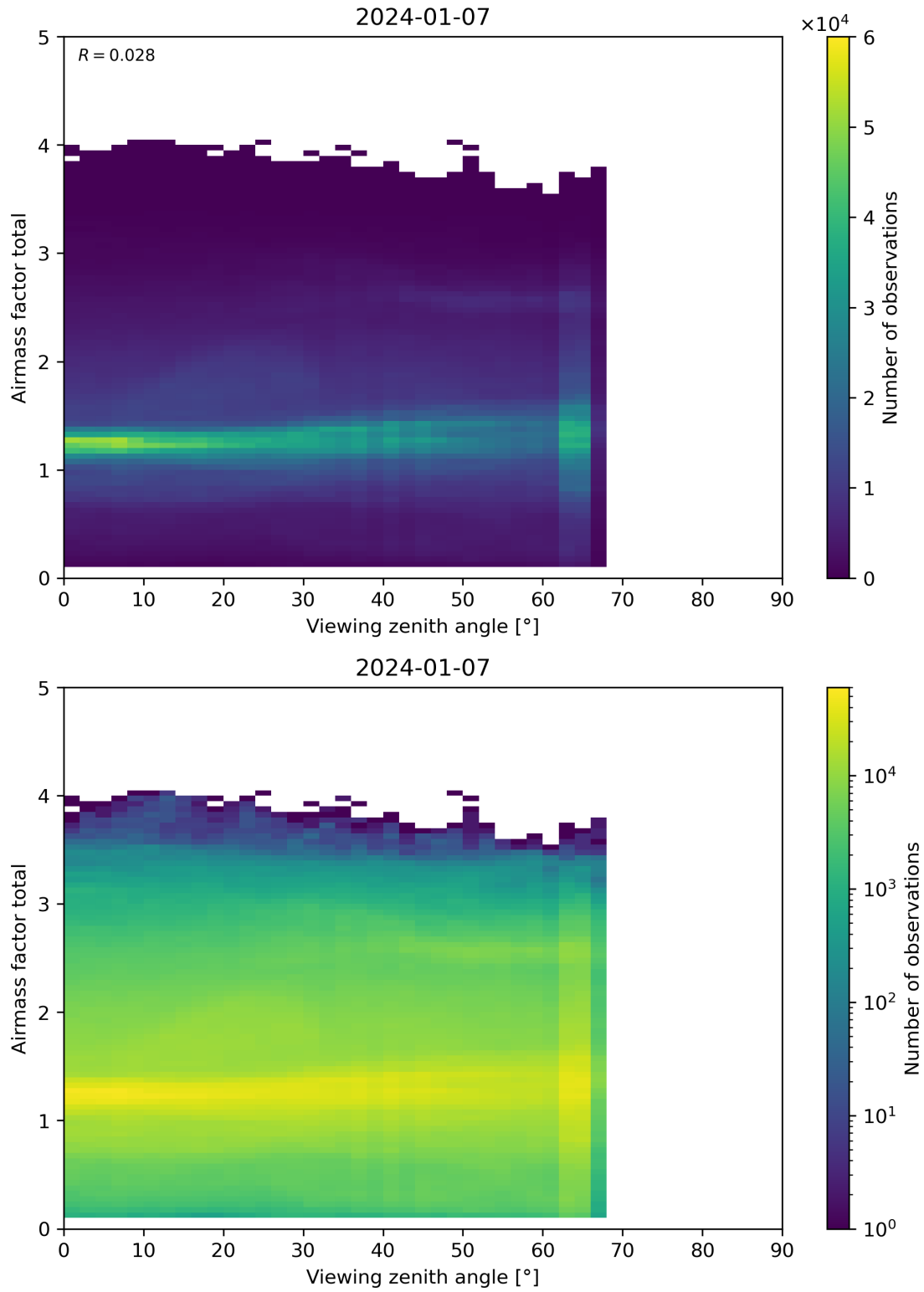
Figure 190: Scatter density plot of “Viewing zenith angle” against “Airmass factor total” for 2024-01-06 to 2024-01-08.
