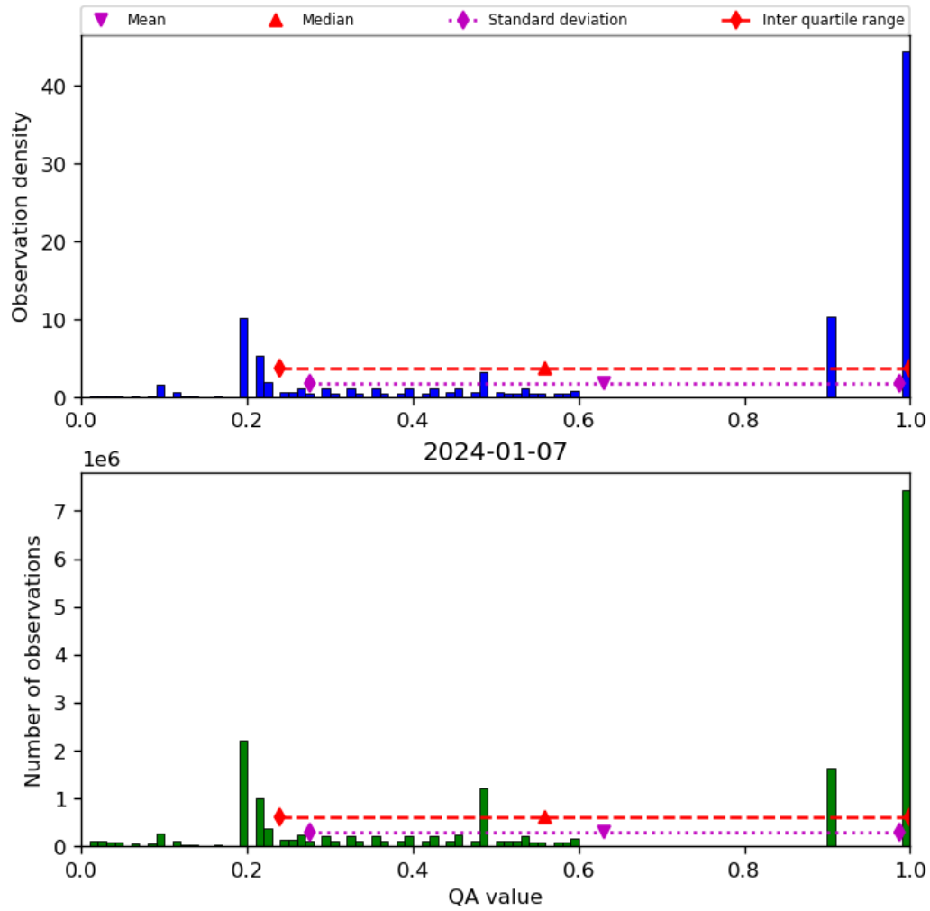
Figure 34: Histogram of “QA value” for 2024-01-06 to 2024-01-08
