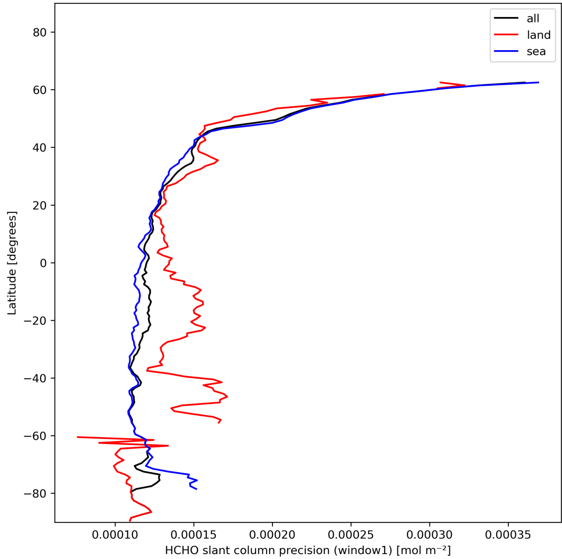
Figure 25: Zonal average of "HCHO slant column precision (window1)" for 2024-01-06 to 2024-01-08.
