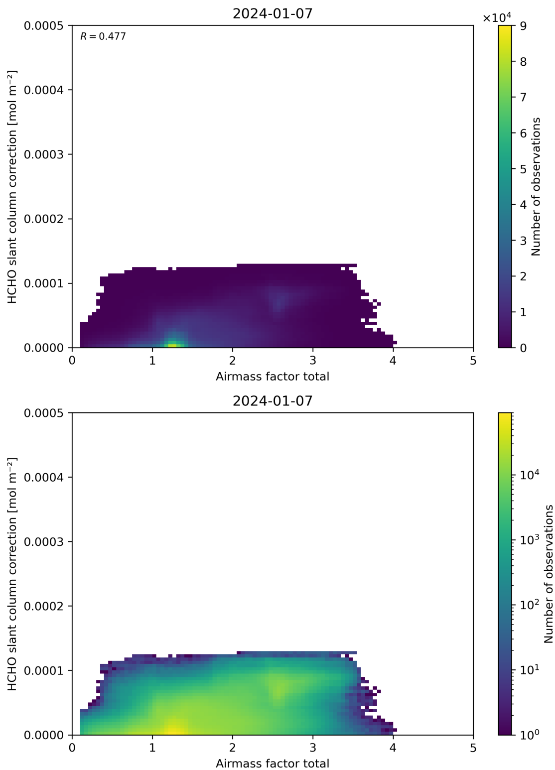
Figure 102: Scatter density plot of “Airmass factor total” against “HCHO slant column correction” for 2024-01-06 to 2024-01-08.
