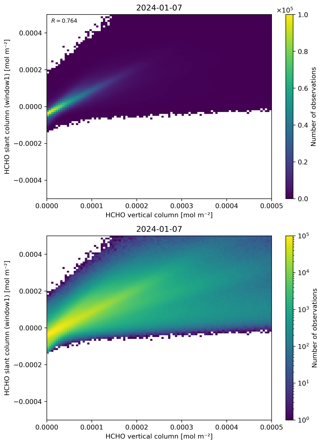
Figure 129: Scatter density plot of “HCHO vertical column” against “HCHO slant column (window1)” for 2024-01-06 to 2024-01-08.
