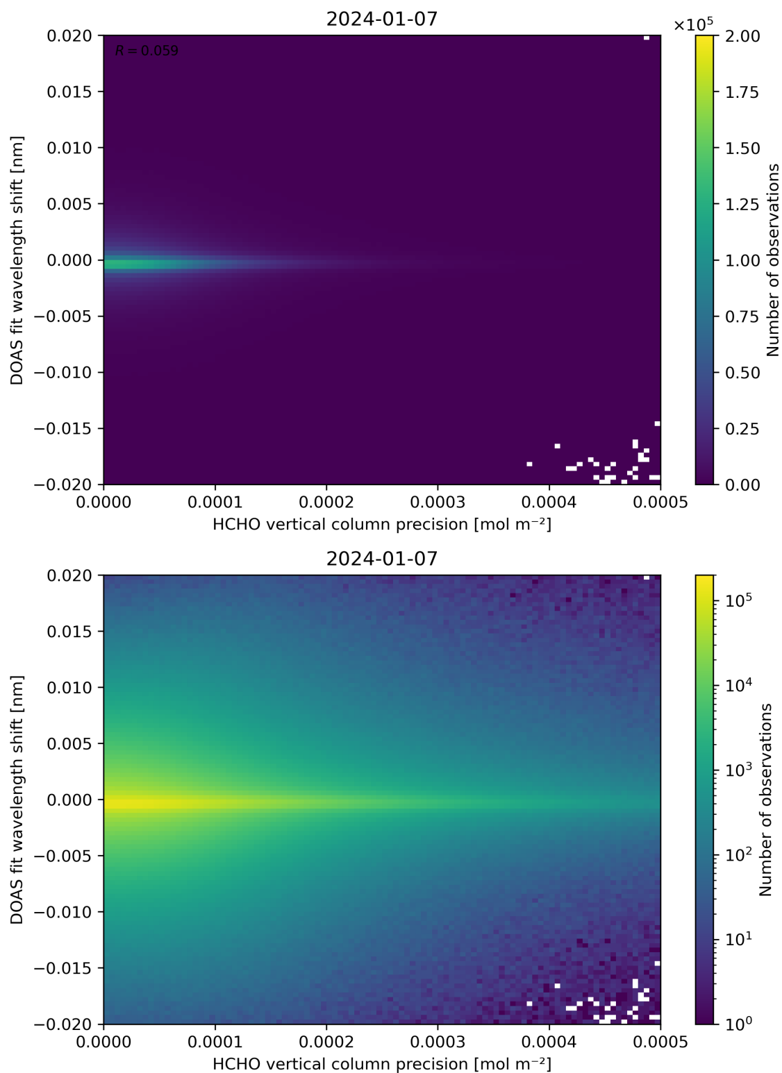
Figure 137: Scatter density plot of “HCHO vertical column precision” against “DOAS fit wavelength shift” for 2024-01-06 to 2024-01-08.
