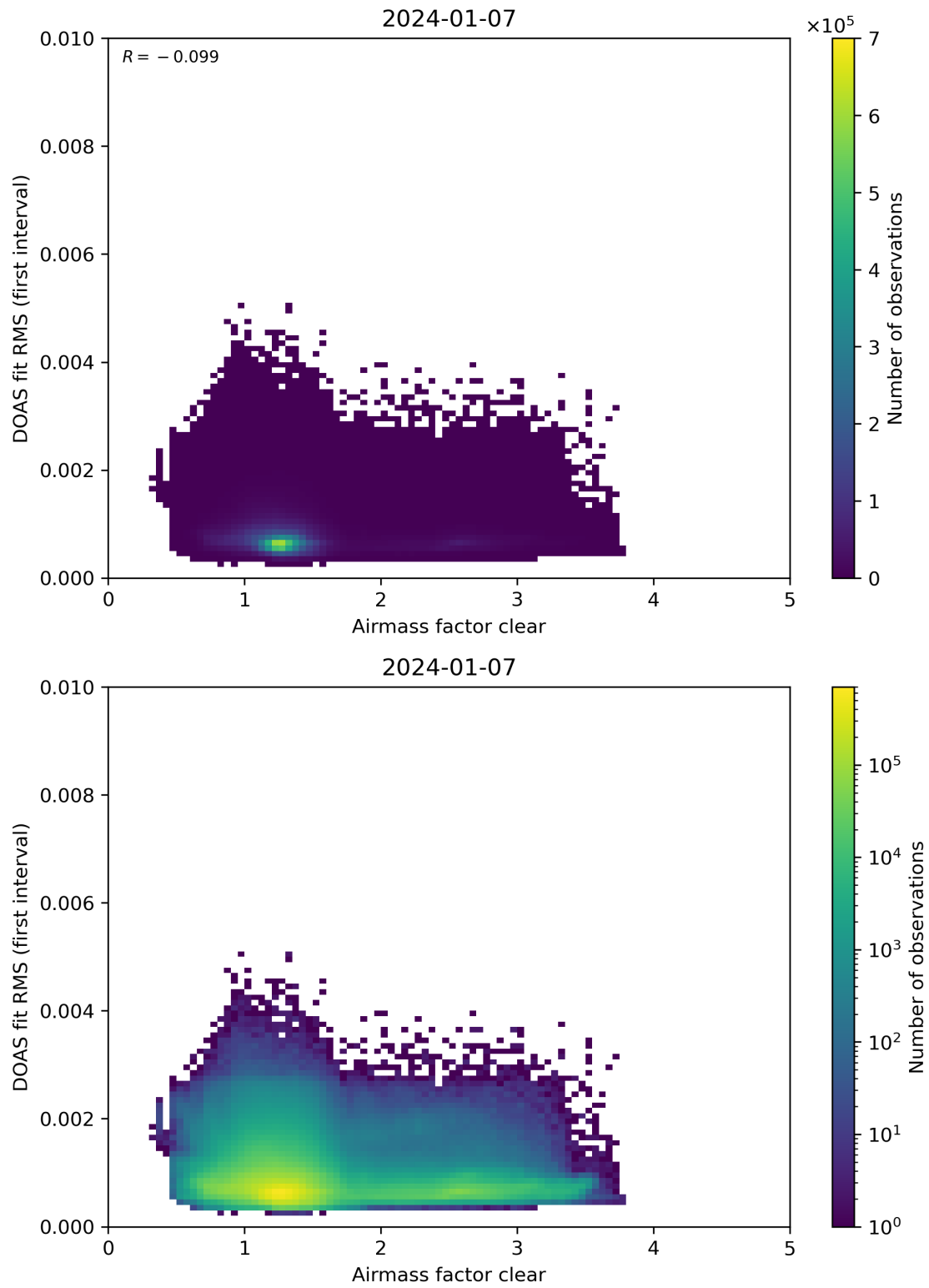
Figure 71: Scatter density plot of “Airmass factor clear” against “DOAS fit RMS (first interval)” for 2024-01-06 to 2024-01-08.
