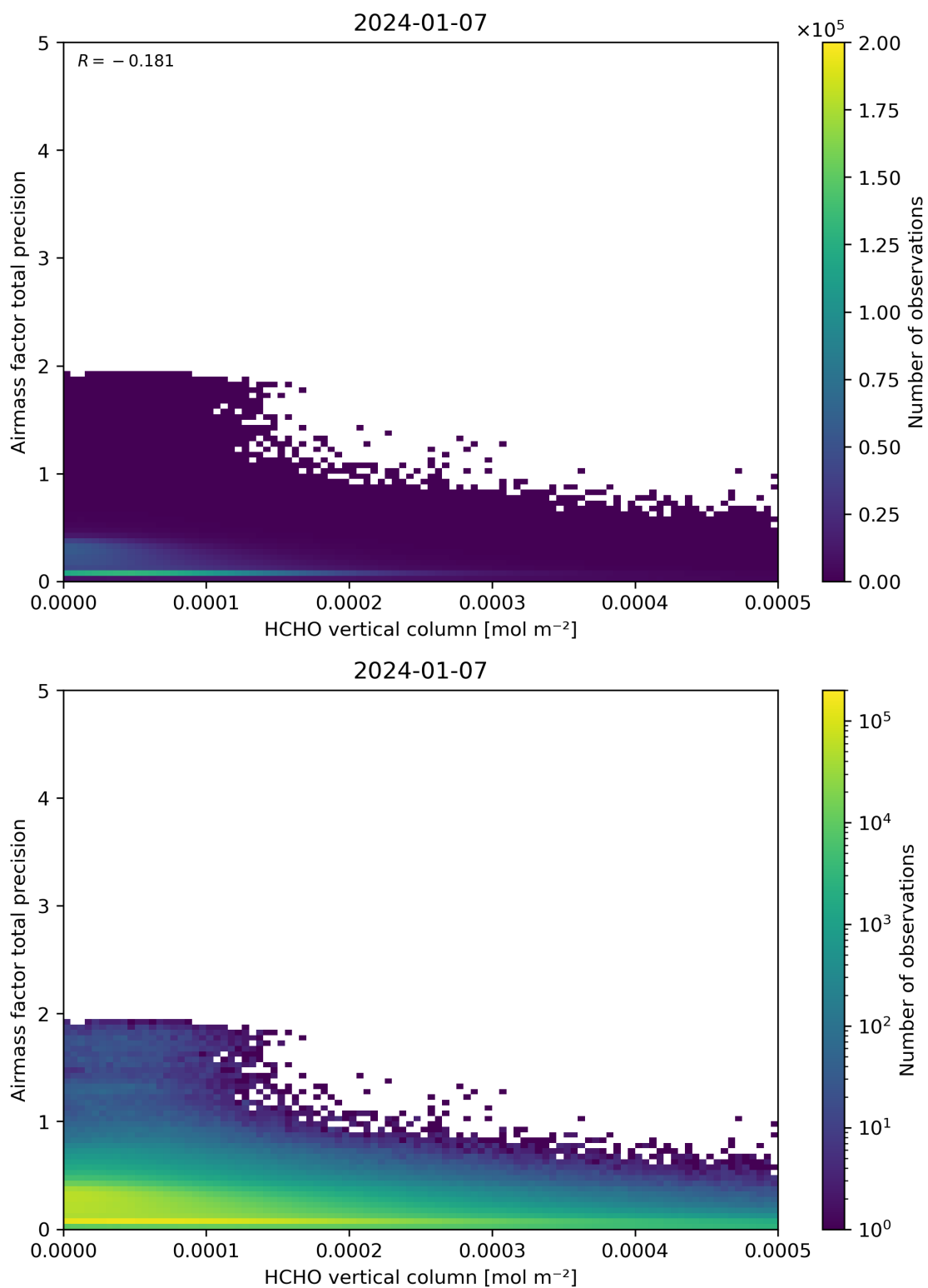
Figure 132: Scatter density plot of “HCHO vertical column” against “Airmass factor total precision” for 2024-01-06 to 2024-01-08.
