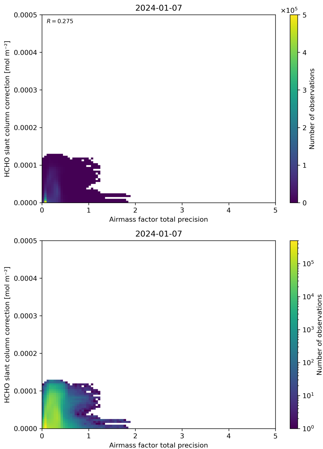
Figure 110: Scatter density plot of “Airmass factor total precision” against “HCHO slant column correction” for 2024-01-06 to 2024-01-08.
