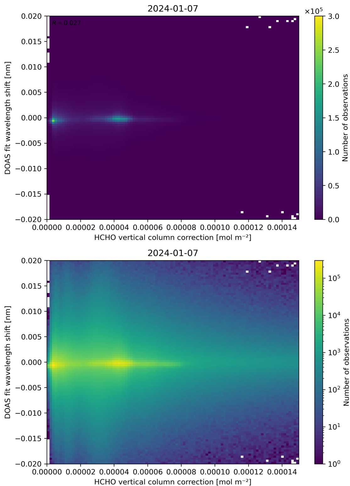
Figure 113: Scatter density plot of “HCHO vertical column correction” against “DOAS fit wavelength shift” for 2024-01-06 to 2024-01-08.
