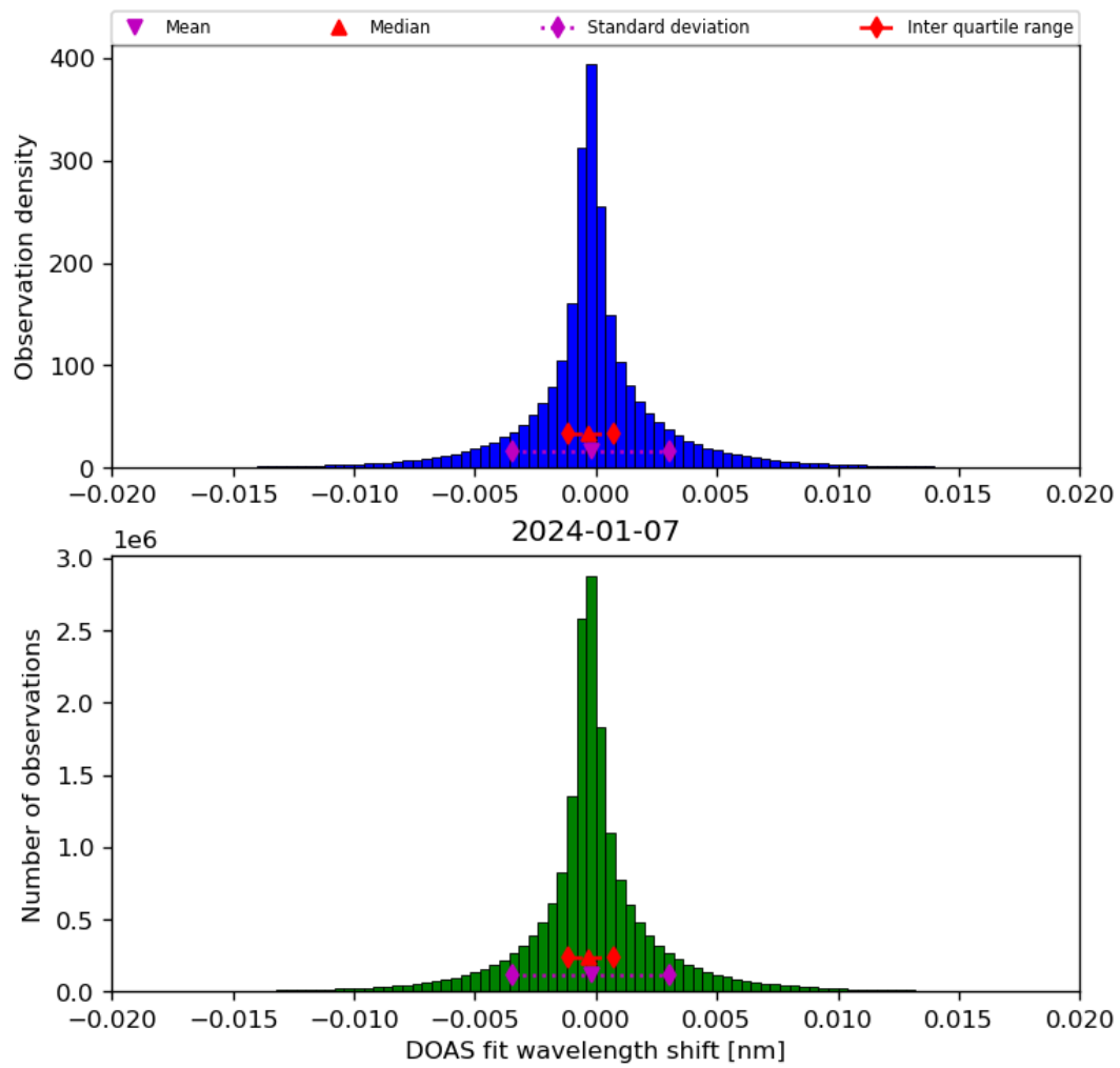
Figure 44: Histogram of “DOAS fit wavelength shift” for 2024-01-06 to 2024-01-08
