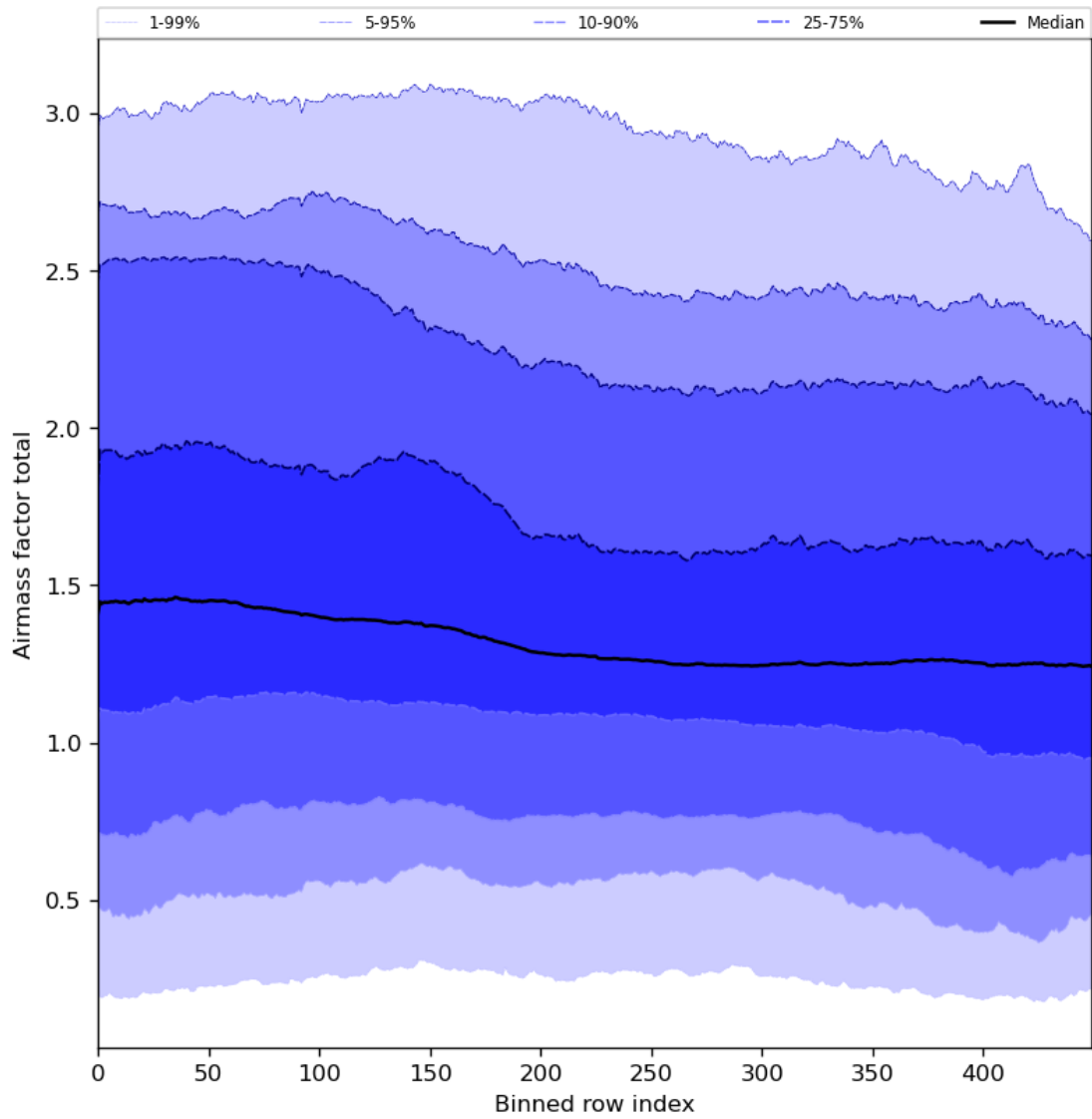
Figure 54: Along track statistics of “Airmass factor total” for 2024-01-06 to 2024-01-08
