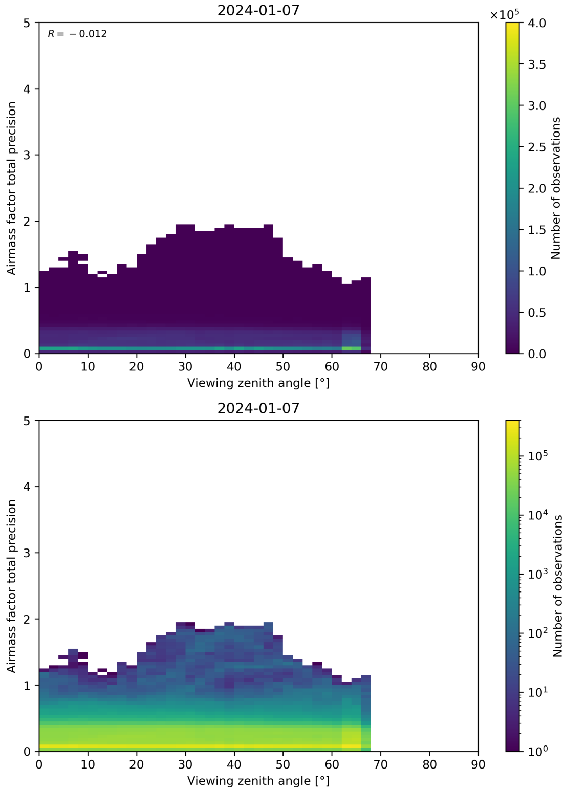
Figure 191: Scatter density plot of “Viewing zenith angle” against “Airmass factor total precision” for 2024-01-06 to 2024-01-08.
