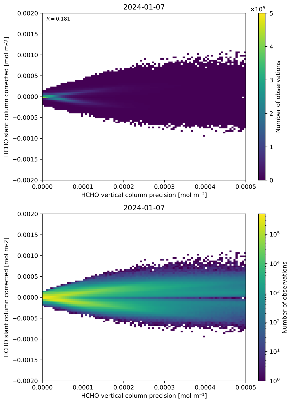
Figure 140: Scatter density plot of “HCHO vertical column precision” against “HCHO slant column corrected” for 2024-01-06 to 2024-01-08.
