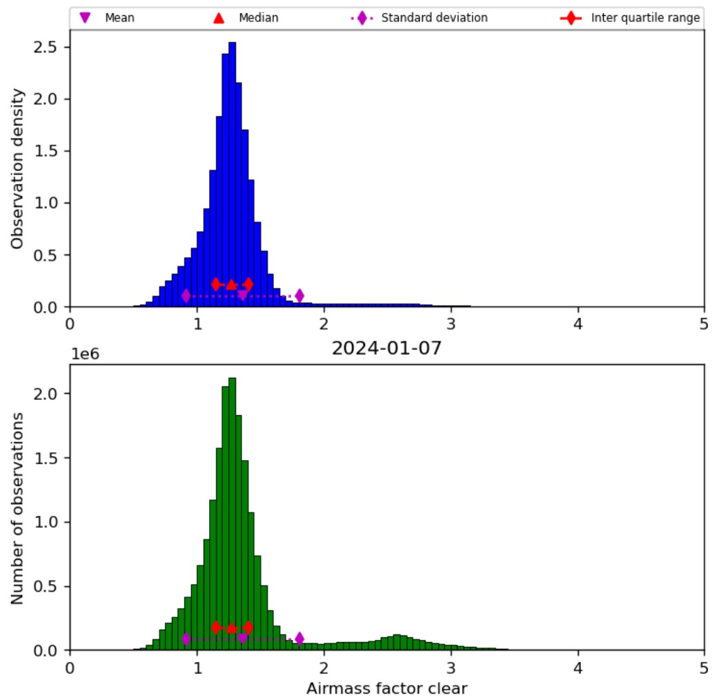
Figure 42: Histogram of “Airmass factor clear” for 2024-01-06 to 2024-01-08
