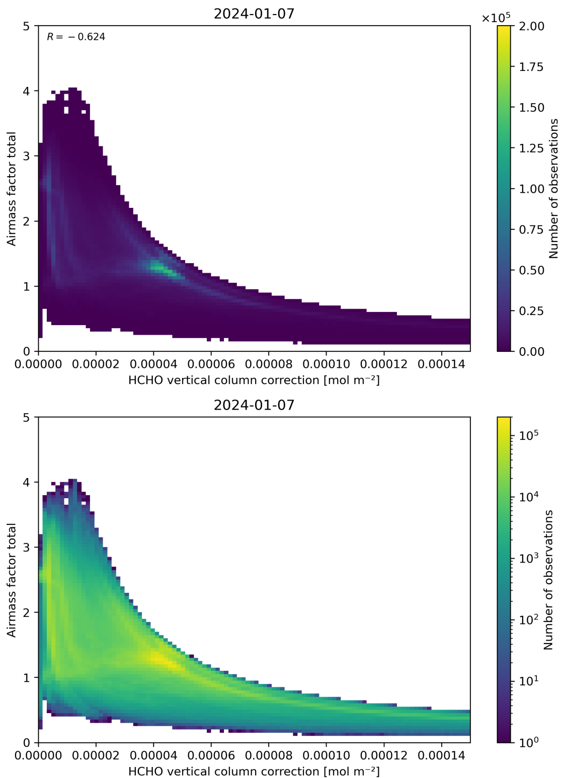
Figure 120: Scatter density plot of “HCHO vertical column correction” against “Airmass factor total” for 2024-01-06 to 2024-01-08.
