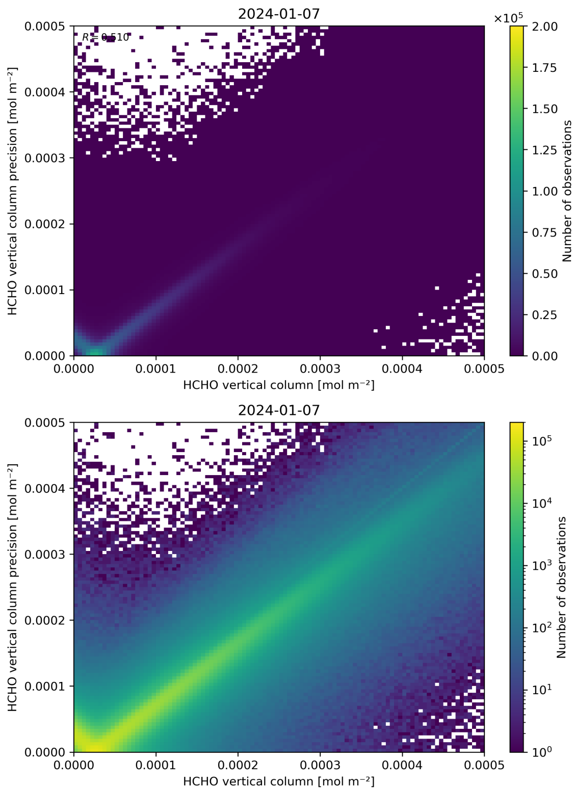
Figure 134: Scatter density plot of “HCHO vertical column” against “HCHO vertical column precision” for 2024-01-06 to 2024-01-08.
