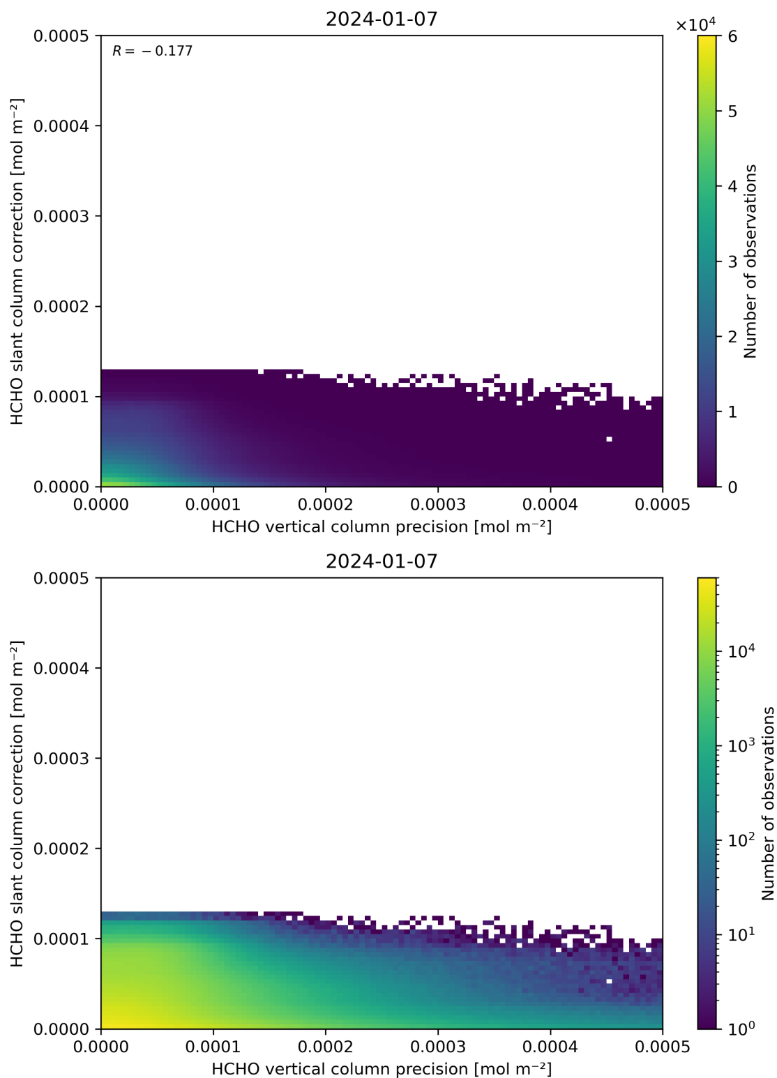
Figure 141: Scatter density plot of “HCHO vertical column precision” against “HCHO slant column correction” for 2024-01-06 to 2024-01-08.
