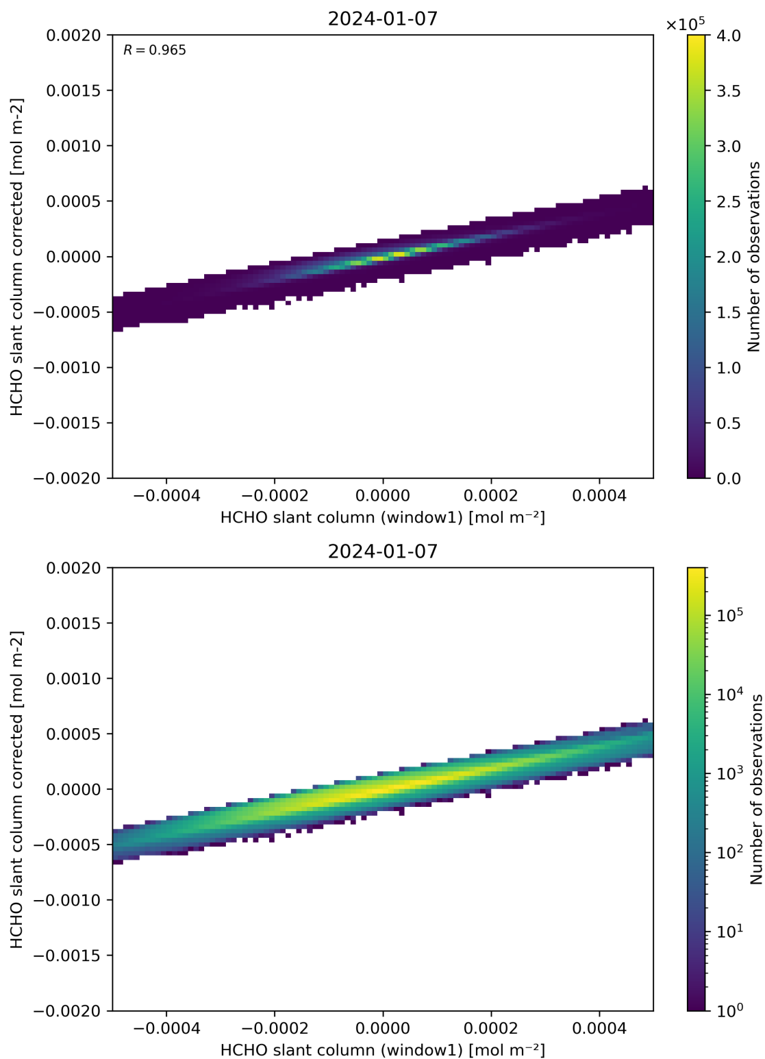
Figure 82: Scatter density plot of “HCHO slant column (window1)” against “HCHO slant column corrected” for 2024-01-06 to 2024-01-08.
