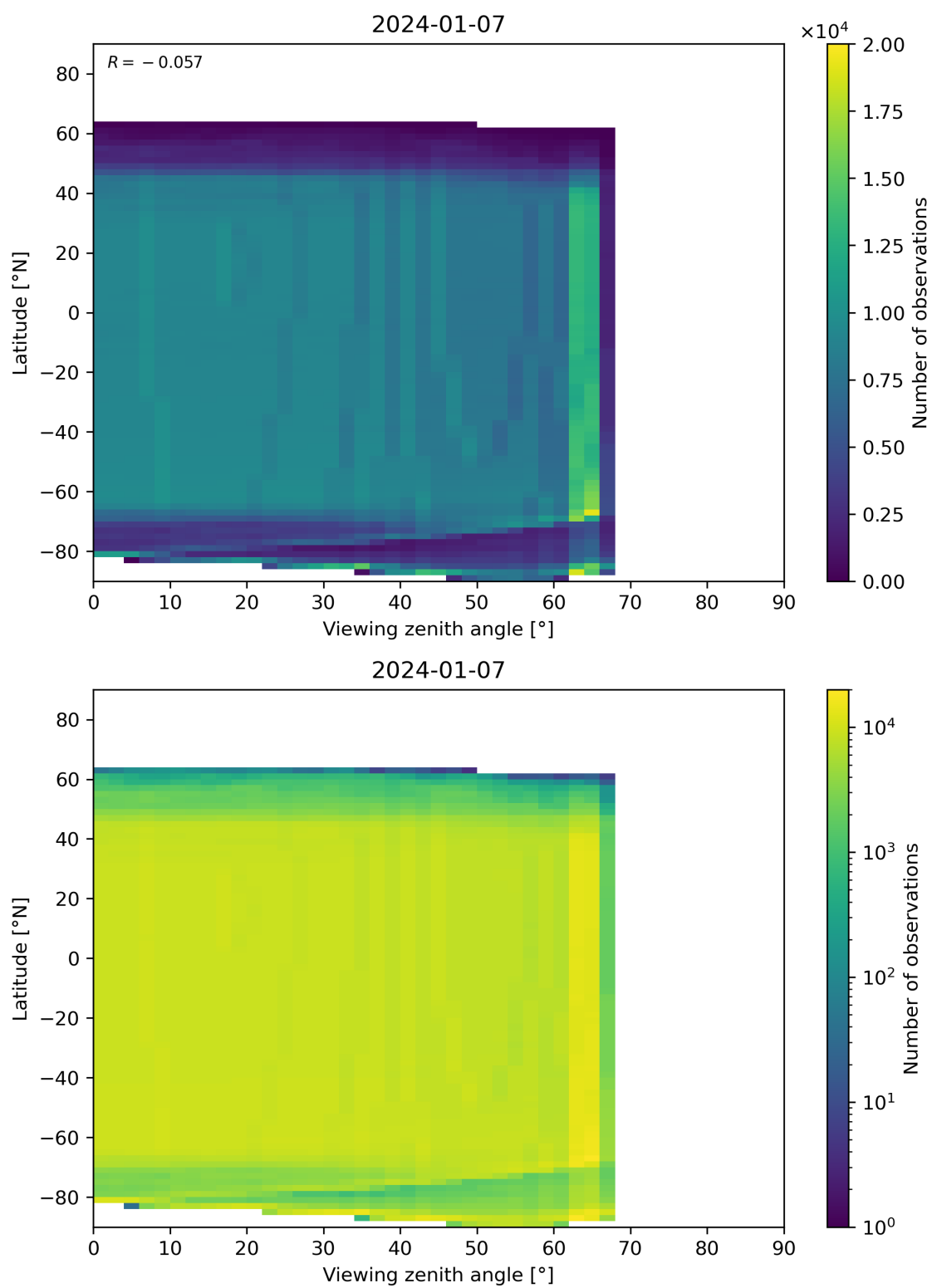
Figure 196: Scatter density plot of “Viewing zenith angle” against “Latitude” for 2024-01-06 to 2024-01-08.
