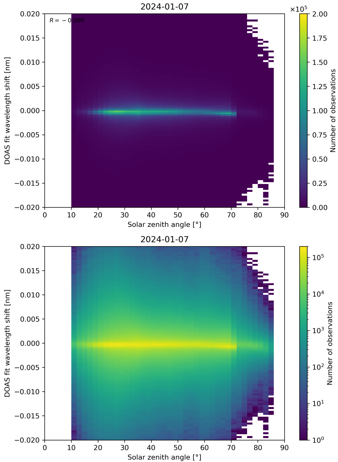
Figure 168: Scatter density plot of “Solar zenith angle” against “DOAS fit wavelength shift” for 2024-01-06 to 2024-01-08.
