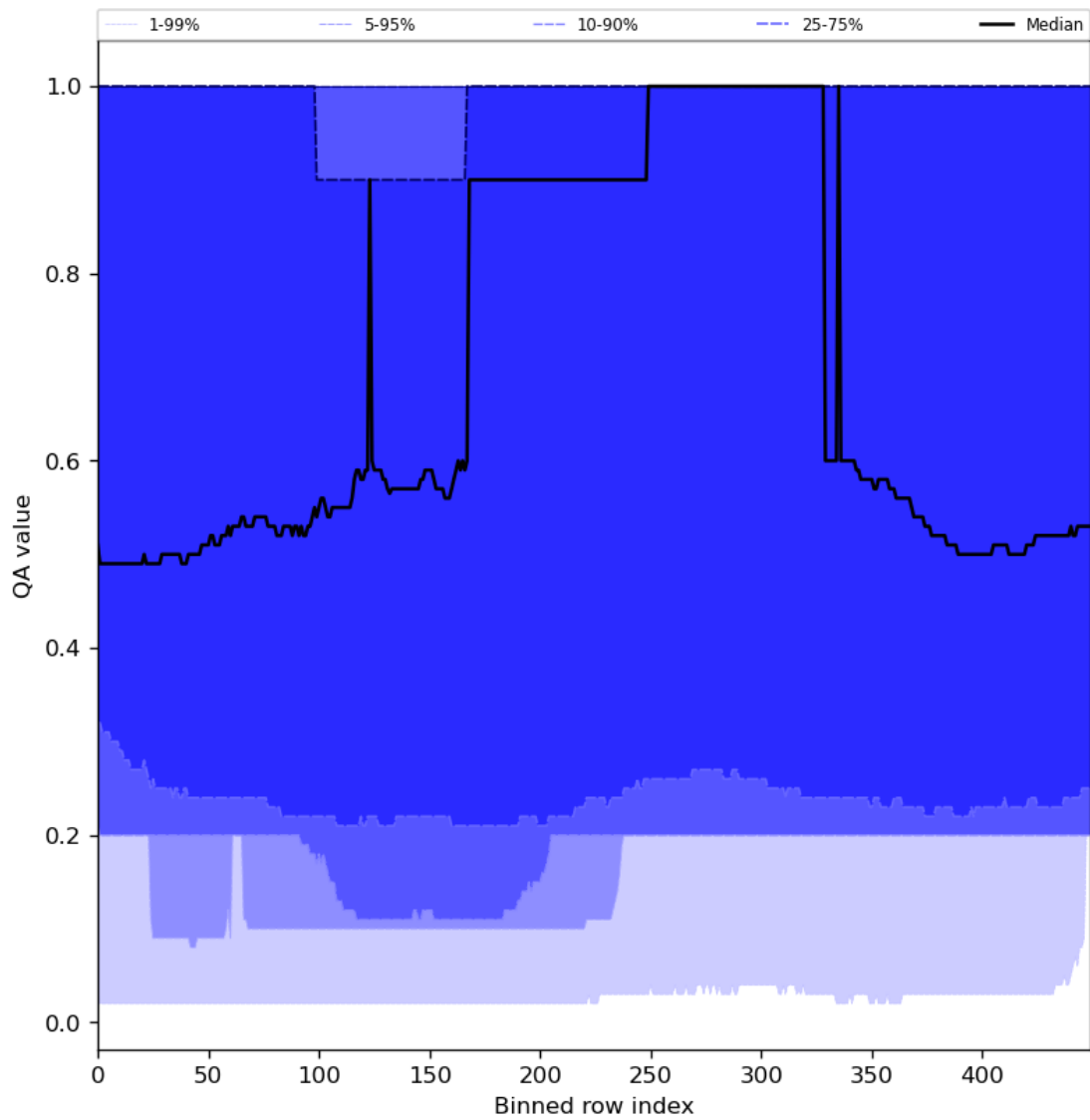
Figure 48: Along track statistics of “QA value” for 2024-01-06 to 2024-01-08
