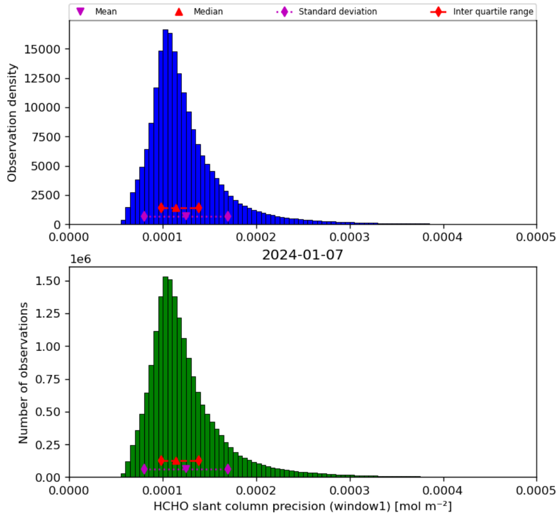
Figure 39: Histogram of “HCHO slant column precision (window1)” for 2024-01-06 to 2024-01-08
