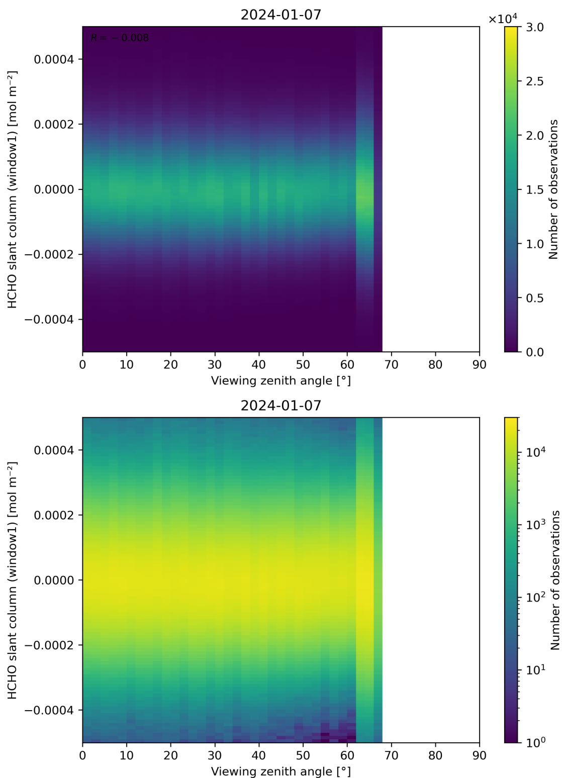
Figure 188: Scatter density plot of “Viewing zenith angle” against “HCHO slant column (window1)” for 2024-01-06 to 2024-01-08.
