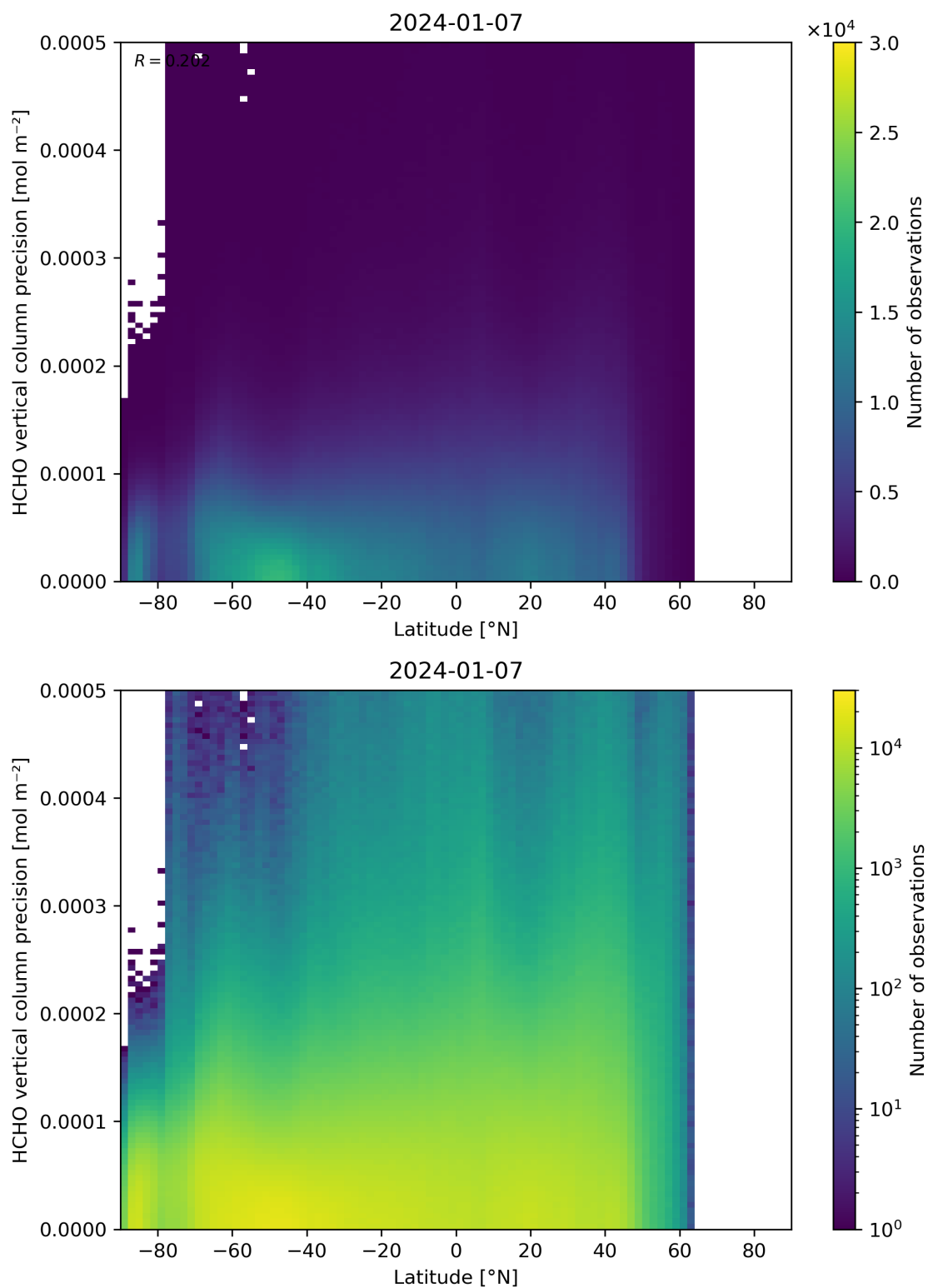
Figure 165: Scatter density plot of “Latitude” against “HCHO vertical column precision” for 2024-01-06 to 2024-01-08.
