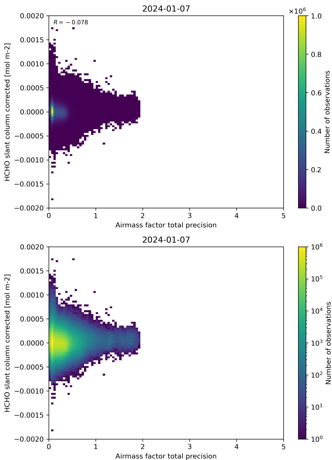
Figure 109: Scatter density plot of “Airmass factor total precision” against “HCHO slant column corrected” for 2024-01-06 to 2024-01-08.
