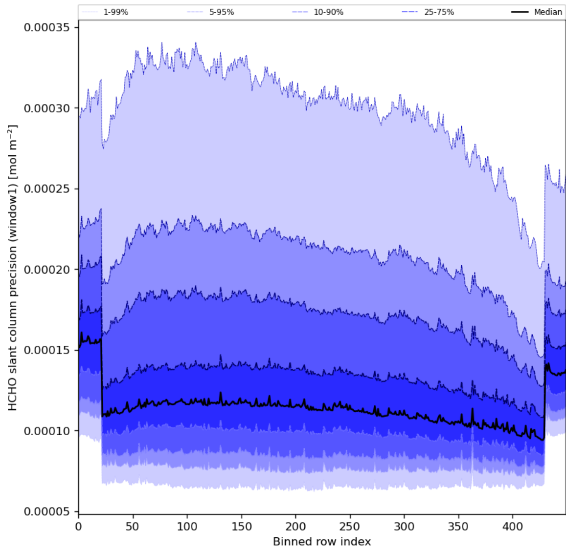
Figure 53: Along track statistics of “HCHO slant column precision (window1)” for 2024-01-06 to 2024-01-08
