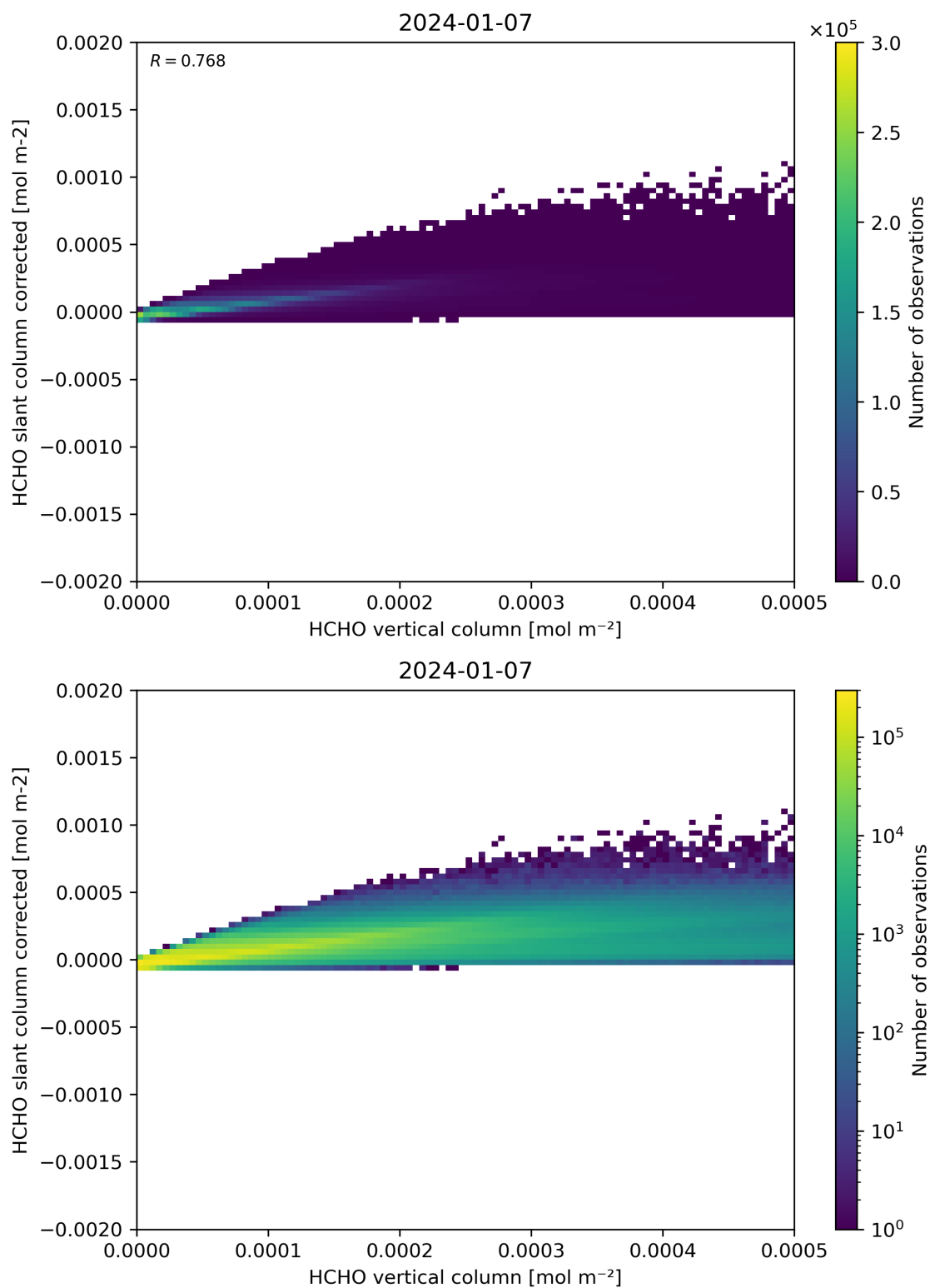
Figure 127: Scatter density plot of “HCHO vertical column” against “HCHO slant column corrected” for 2024-01-06 to 2024-01-08.
