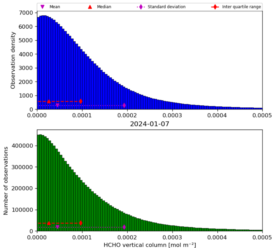
Figure 35: Histogram of “HCHO vertical column” for 2024-01-06 to 2024-01-08
