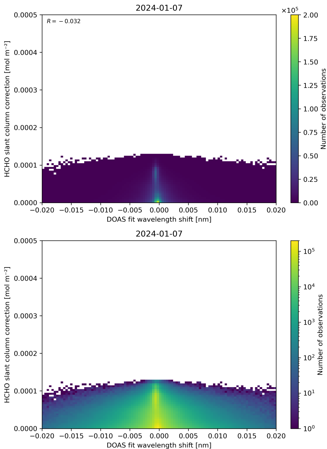
Figure 67: Scatter density plot of “DOAS fit wavelength shift” against “HCHO slant column correction” for 2024-01-06 to 2024-01-08.
