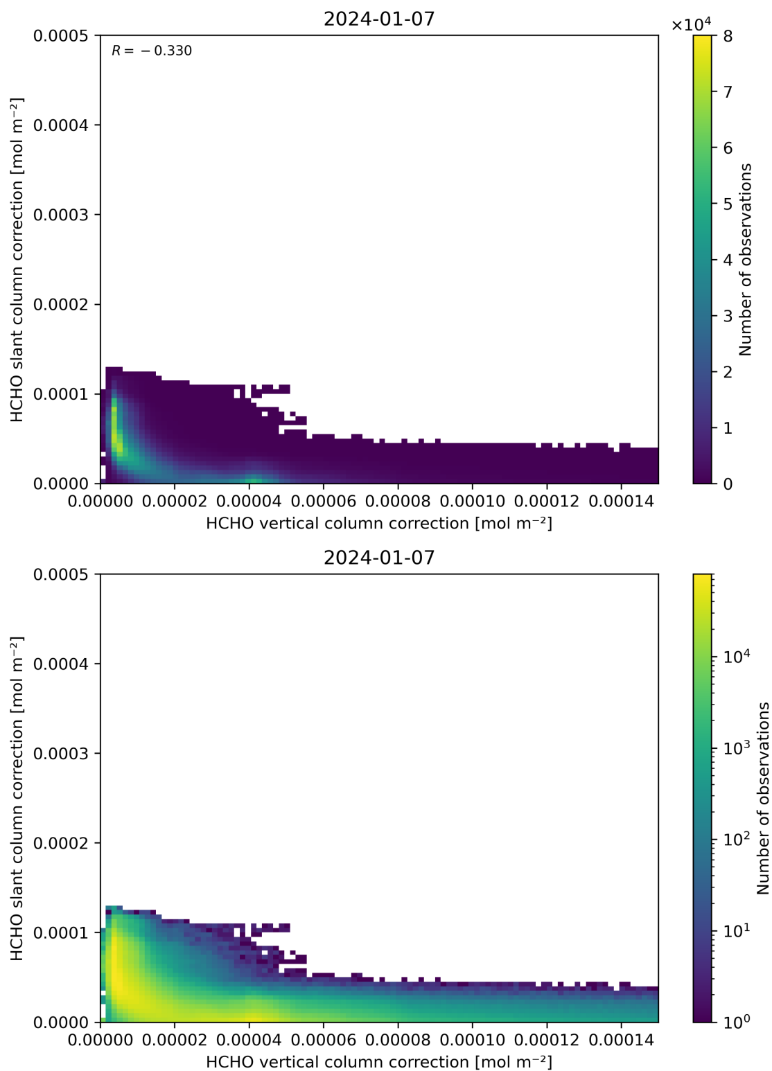
Figure 117: Scatter density plot of “HCHO vertical column correction” against “HCHO slant column correction” for 2024-01-06 to 2024-01-08.
