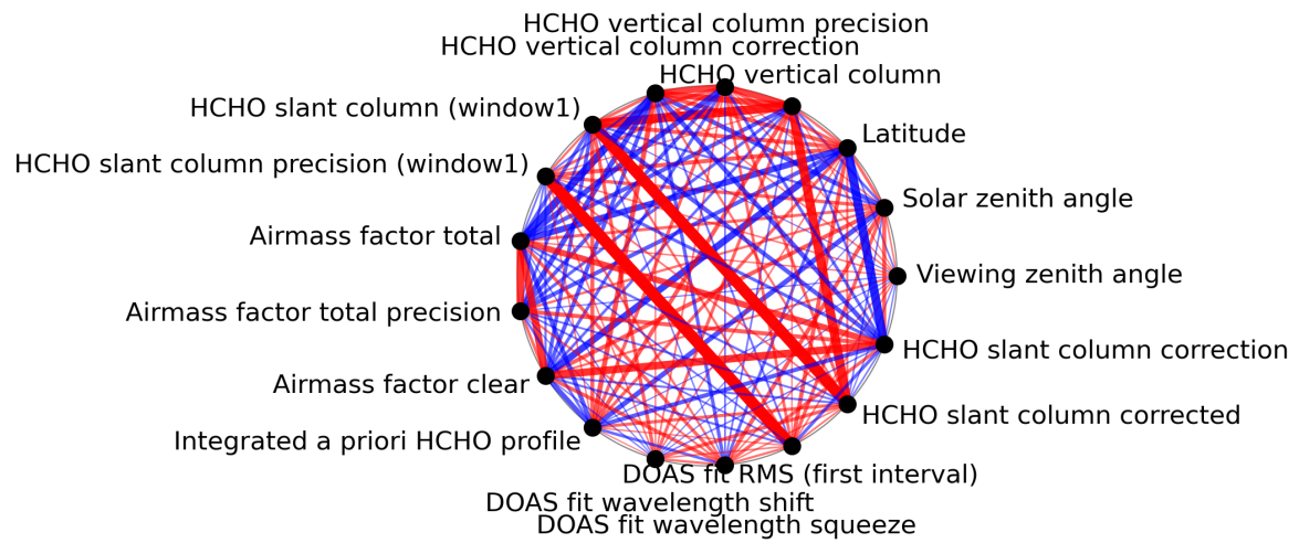
Figure 1: Map of correlation graph for 2024-01-06 to 2024-01-08.
