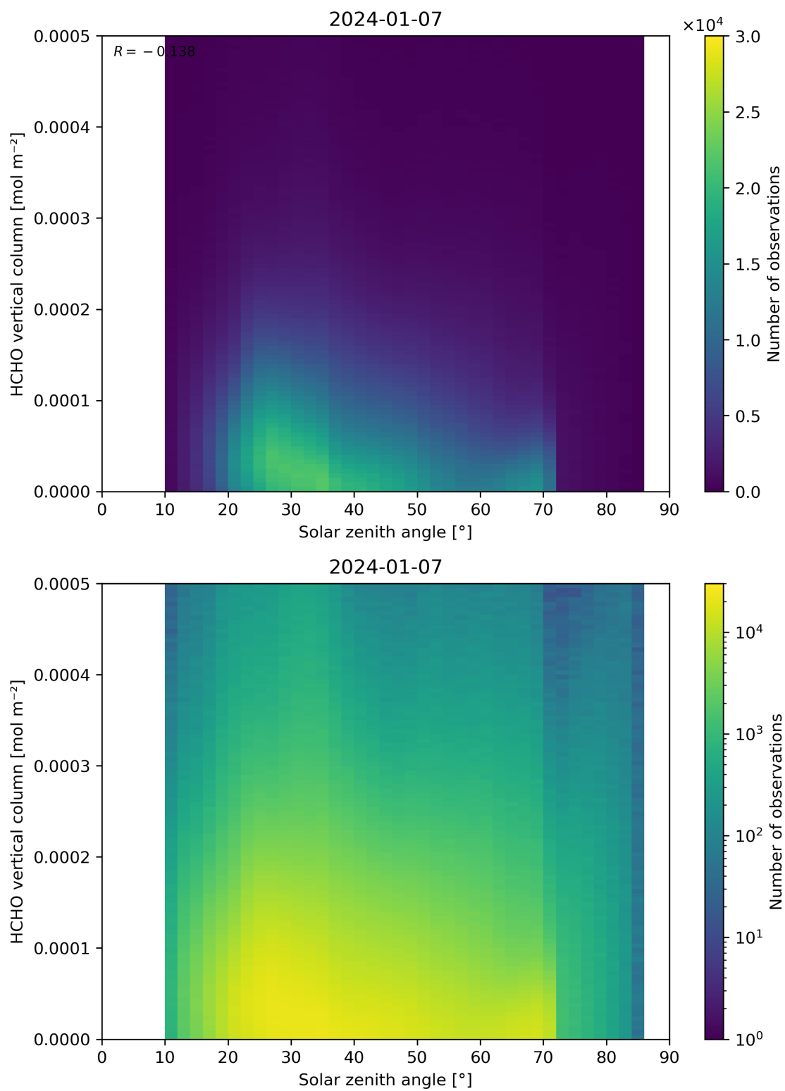
Figure 177: Scatter density plot of “Solar zenith angle” against “HCHO vertical column” for 2024-01-06 to 2024-01-08.
