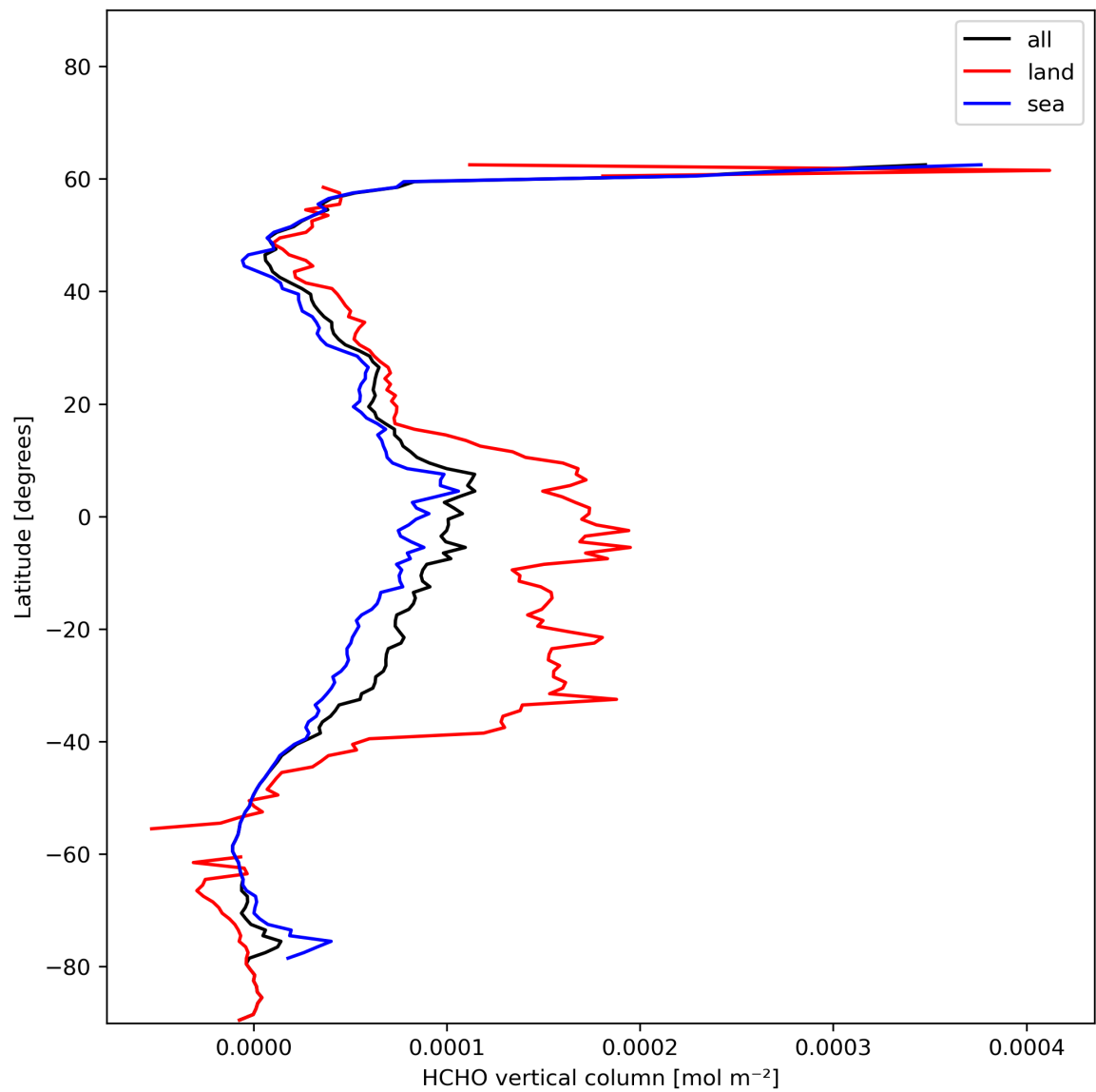
Figure 21: Zonal average of “HCHO vertical column” for 2024-01-06 to 2024-01-08.
