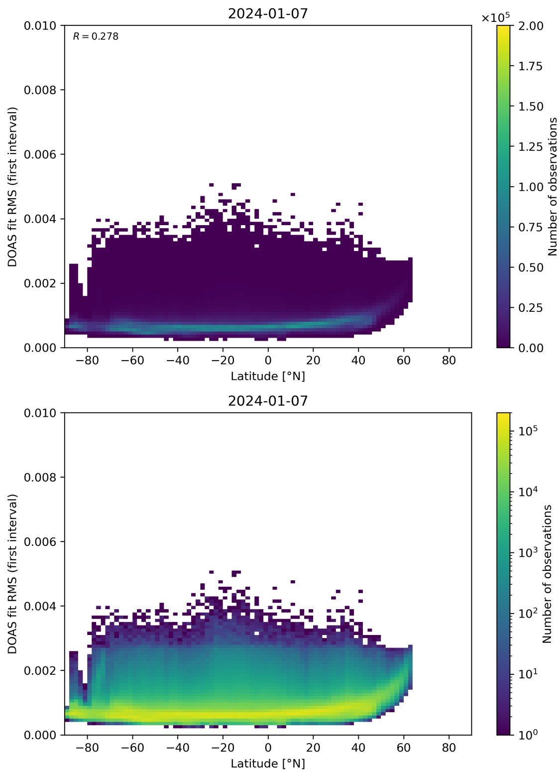
Figure 153: Scatter density plot of “Latitude” against “DOAS fit RMS (first interval)” for 2024-01-06 to 2024-01-08.
