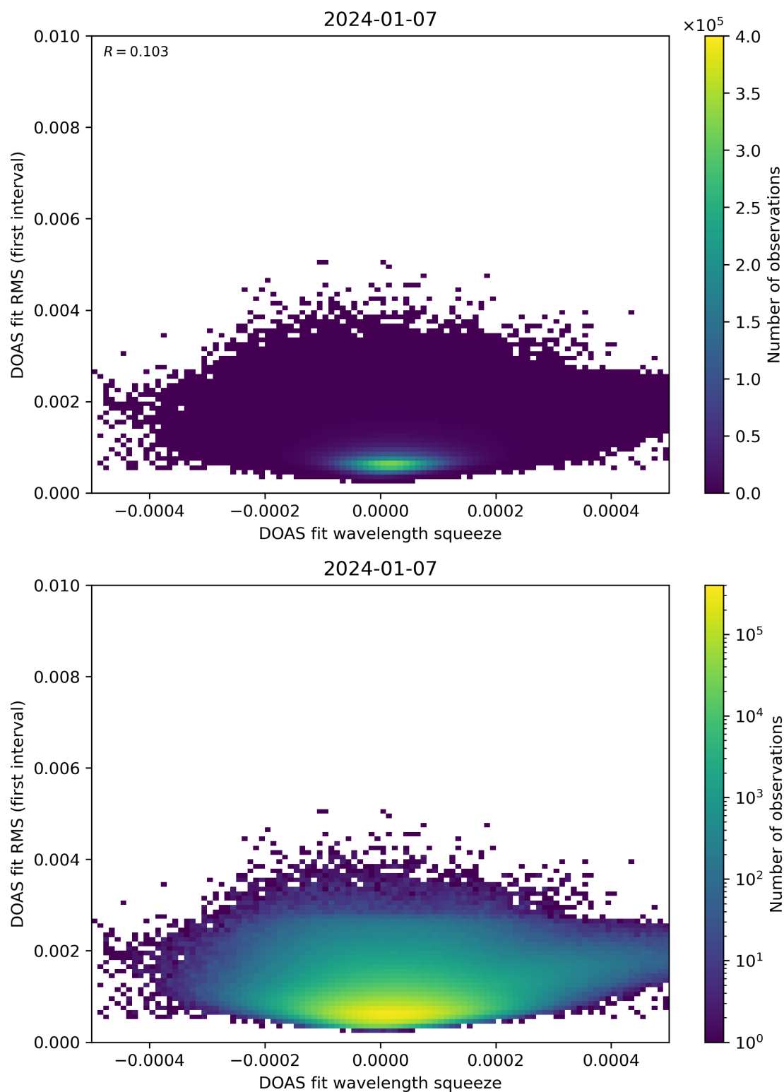
Figure 68: Scatter density plot of “DOAS fit wavelength squeeze” against “DOAS fit RMS (first interval)” for 2024-01-06 to 2024-01-08.
