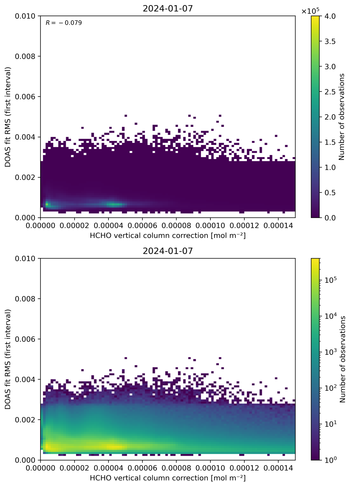
Figure 112: Scatter density plot of “HCHO vertical column correction” against “DOAS fit RMS (first interval)” for 2024-01-06 to 2024-01-08.
