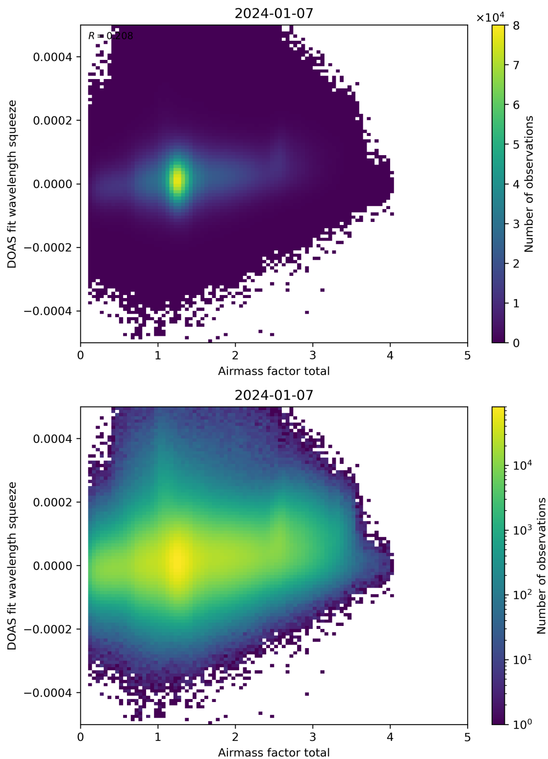
Figure 99: Scatter density plot of “Airmass factor total” against “DOAS fit wavelength squeeze” for 2024-01-06 to 2024-01-08.
