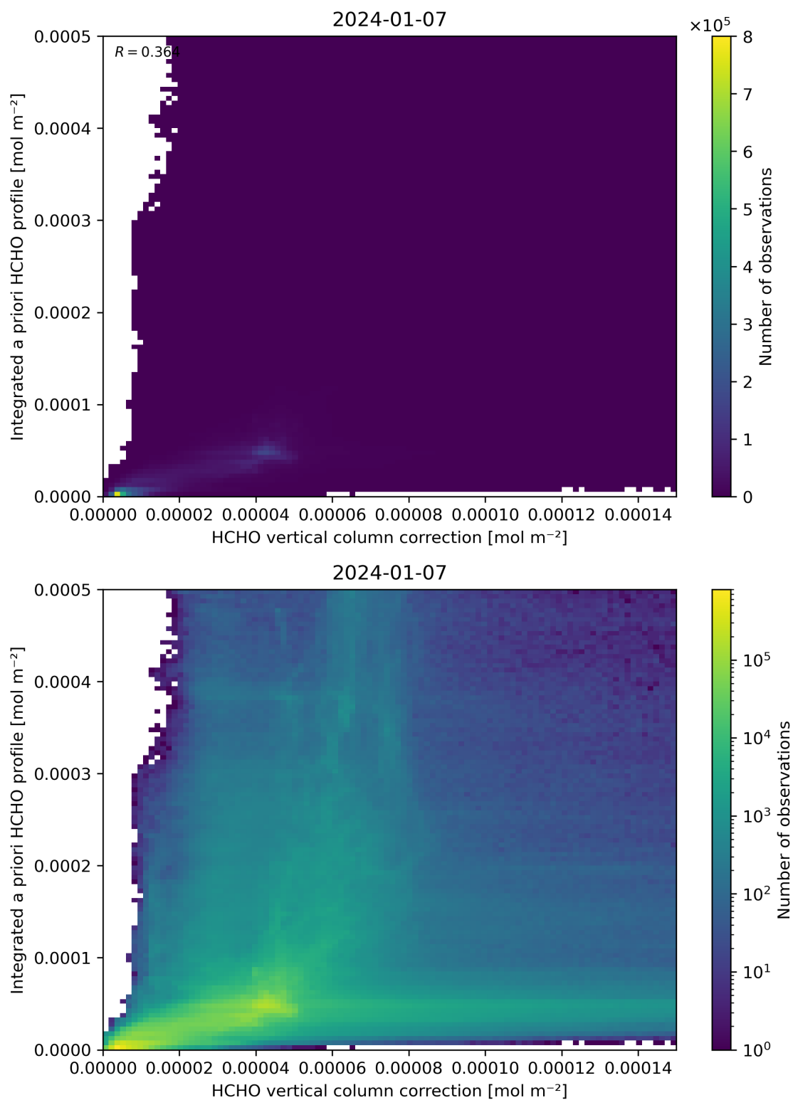
Figure 122: Scatter density plot of “HCHO vertical column correction” against “Integrated a priori HCHO profile” for 2024-01-06 to 2024-01-08.
