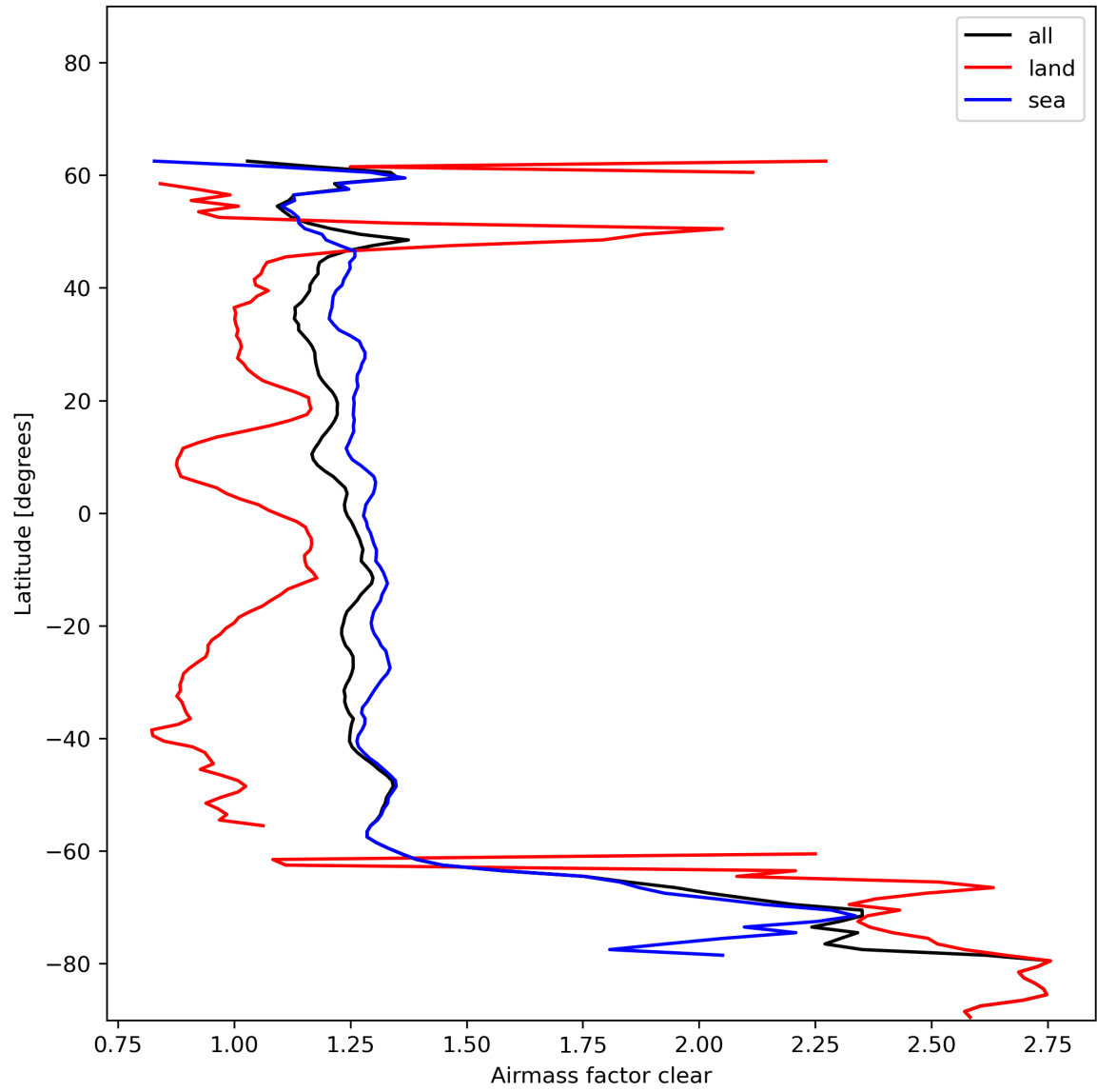
Figure 28: Zonal average of “Airmass factor clear” for 2024-01-06 to 2024-01-08.
