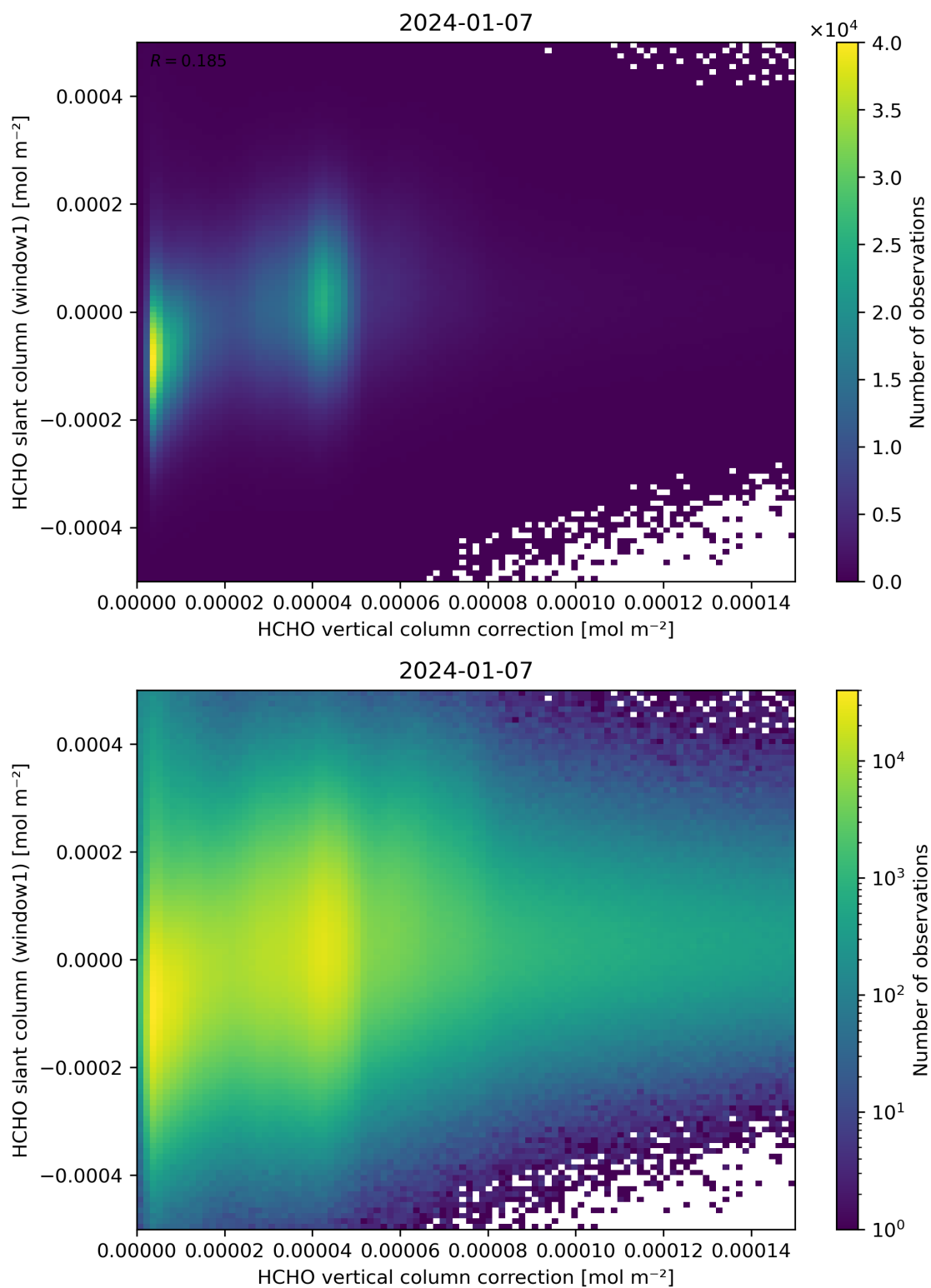
Figure 118: Scatter density plot of “HCHO vertical column correction” against “HCHO slant column (window1)” for 2024-01-06 to 2024-01-08.
