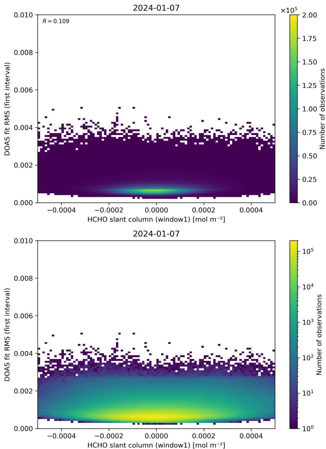
Figure 78: Scatter density plot of “HCHO slant column (window1)” against “DOAS fit RMS (first interval)” for 2024-01-06 to 2024-01-08.
