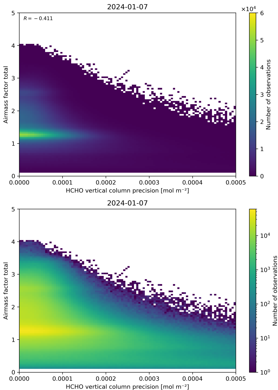
Figure 144: Scatter density plot of “HCHO vertical column precision” against “Airmass factor total” for 2024-01-06 to 2024-01-08.
