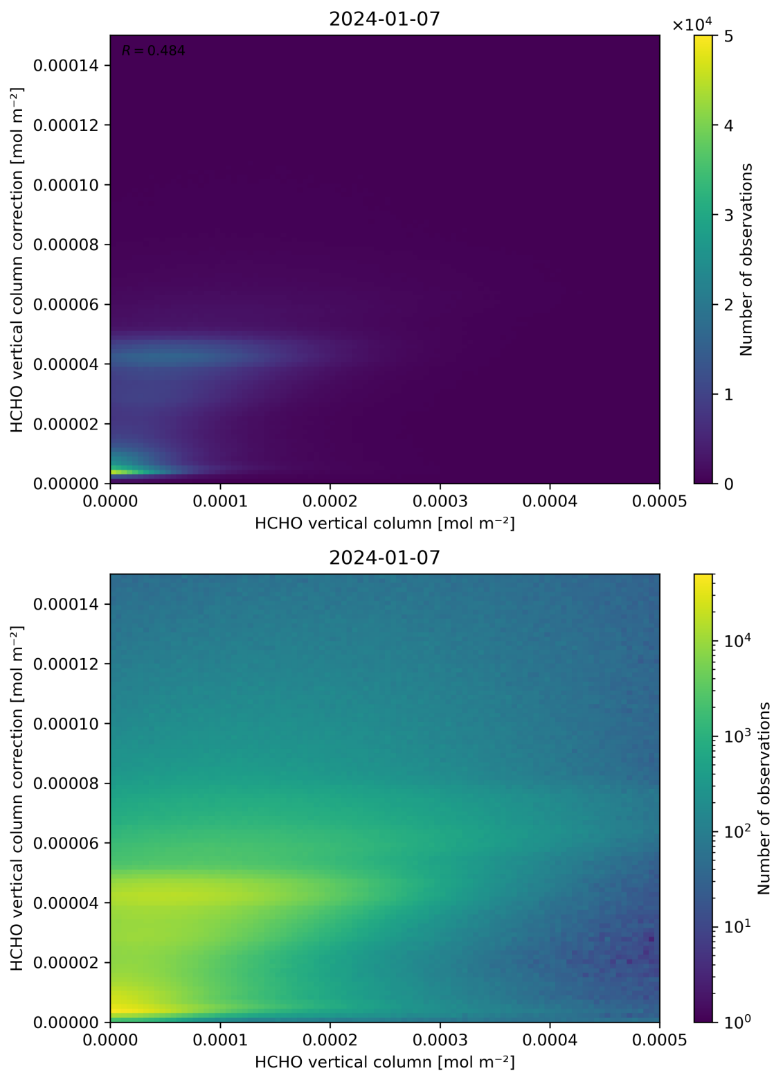
Figure 133: Scatter density plot of “HCHO vertical column” against “HCHO vertical column correction” for 2024-01-06 to 2024-01-08.
