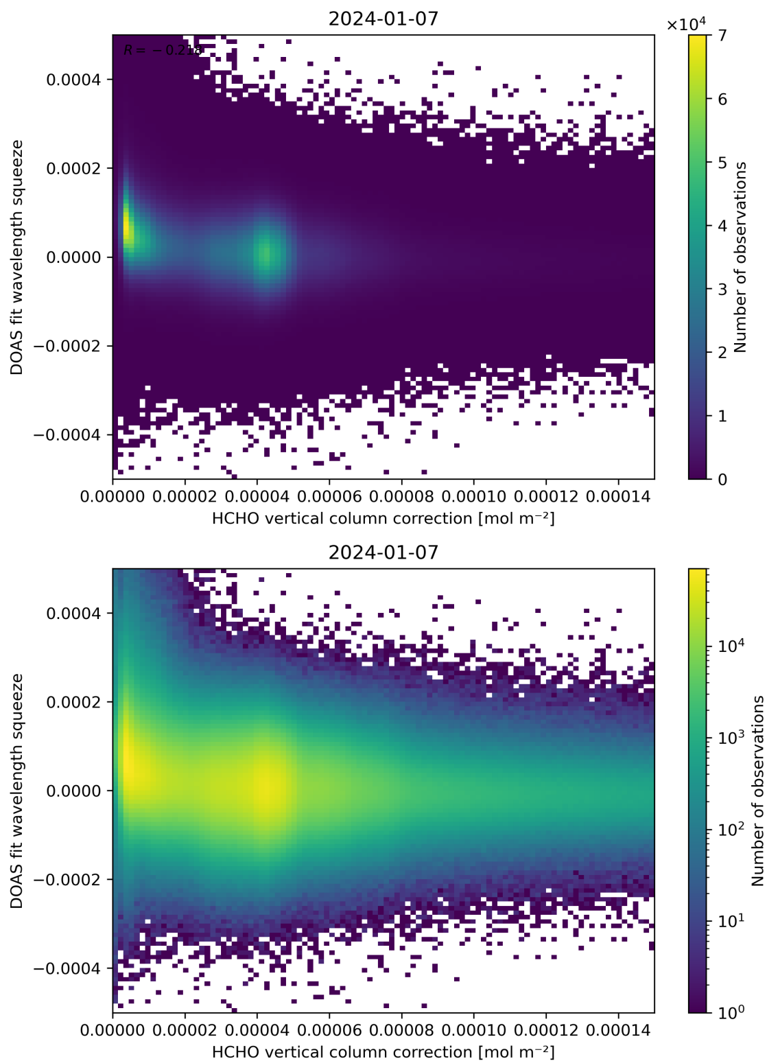
Figure 114: Scatter density plot of “HCHO vertical column correction” against “DOAS fit wavelength squeeze” for 2024-01-06 to 2024-01-08.
