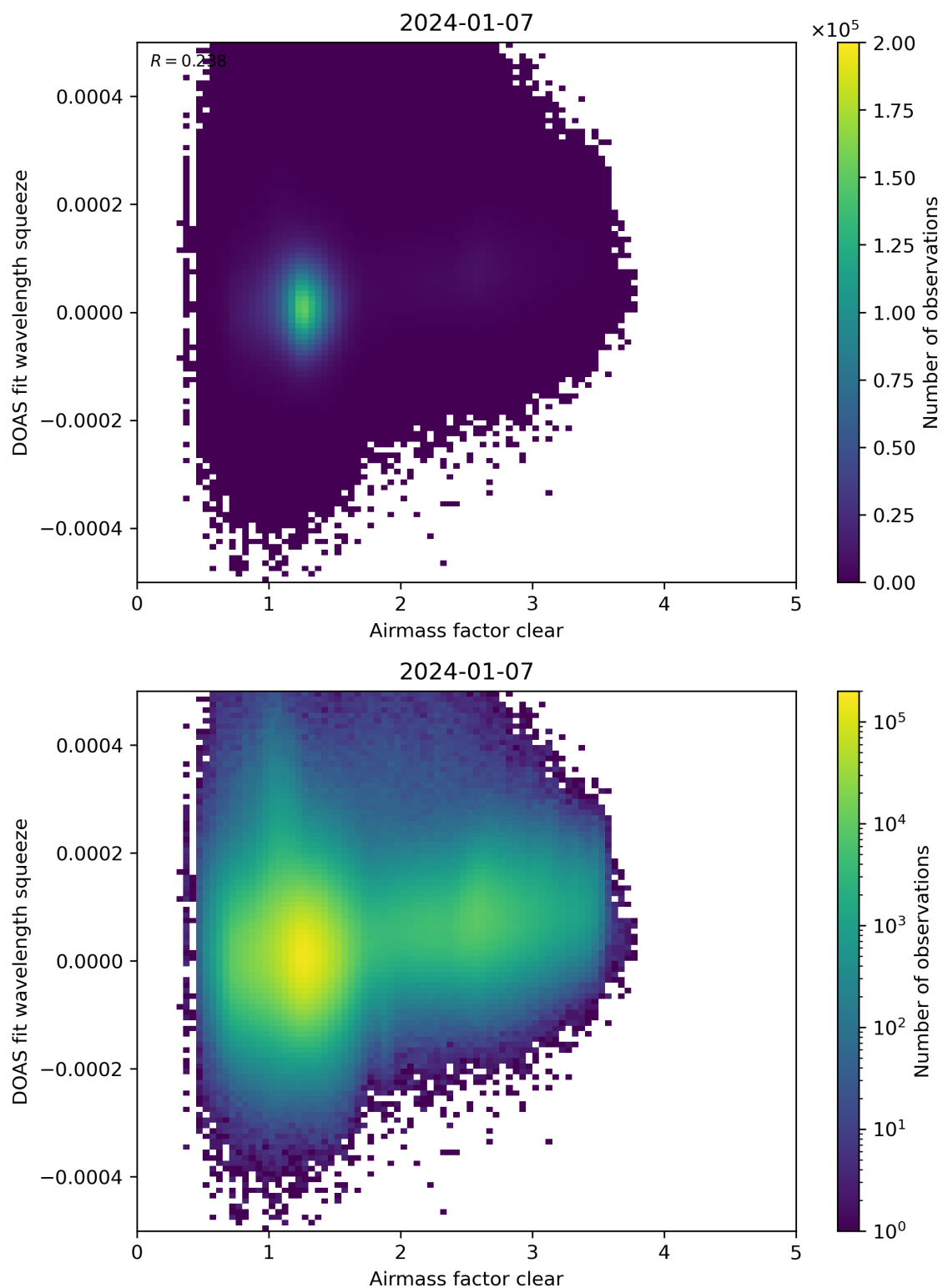
Figure 73: Scatter density plot of “Airmass factor clear” against “DOAS fit wavelength squeeze” for 2024-01-06 to 2024-01-08.
