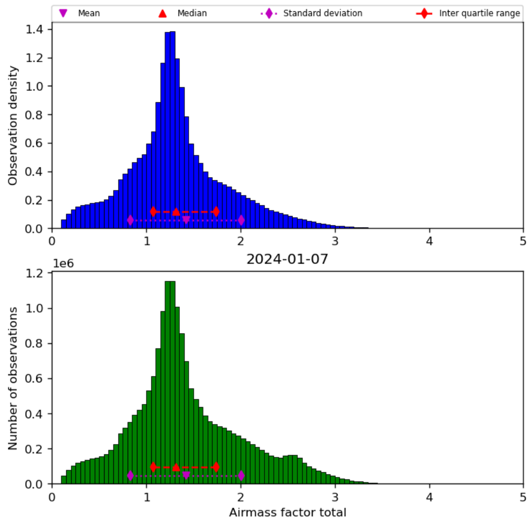
Figure 40: Histogram of “Airmass factor total” for 2024-01-06 to 2024-01-08
