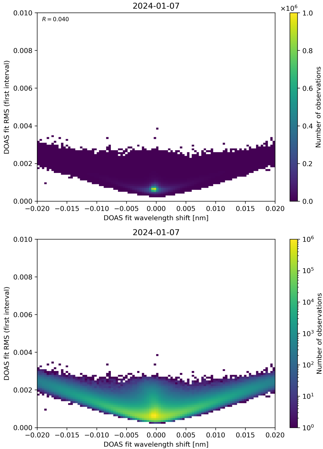
Figure 64: Scatter density plot of “DOAS fit wavelength shift” against “DOAS fit RMS (first interval)” for 2024-01-06 to 2024-01-08.
