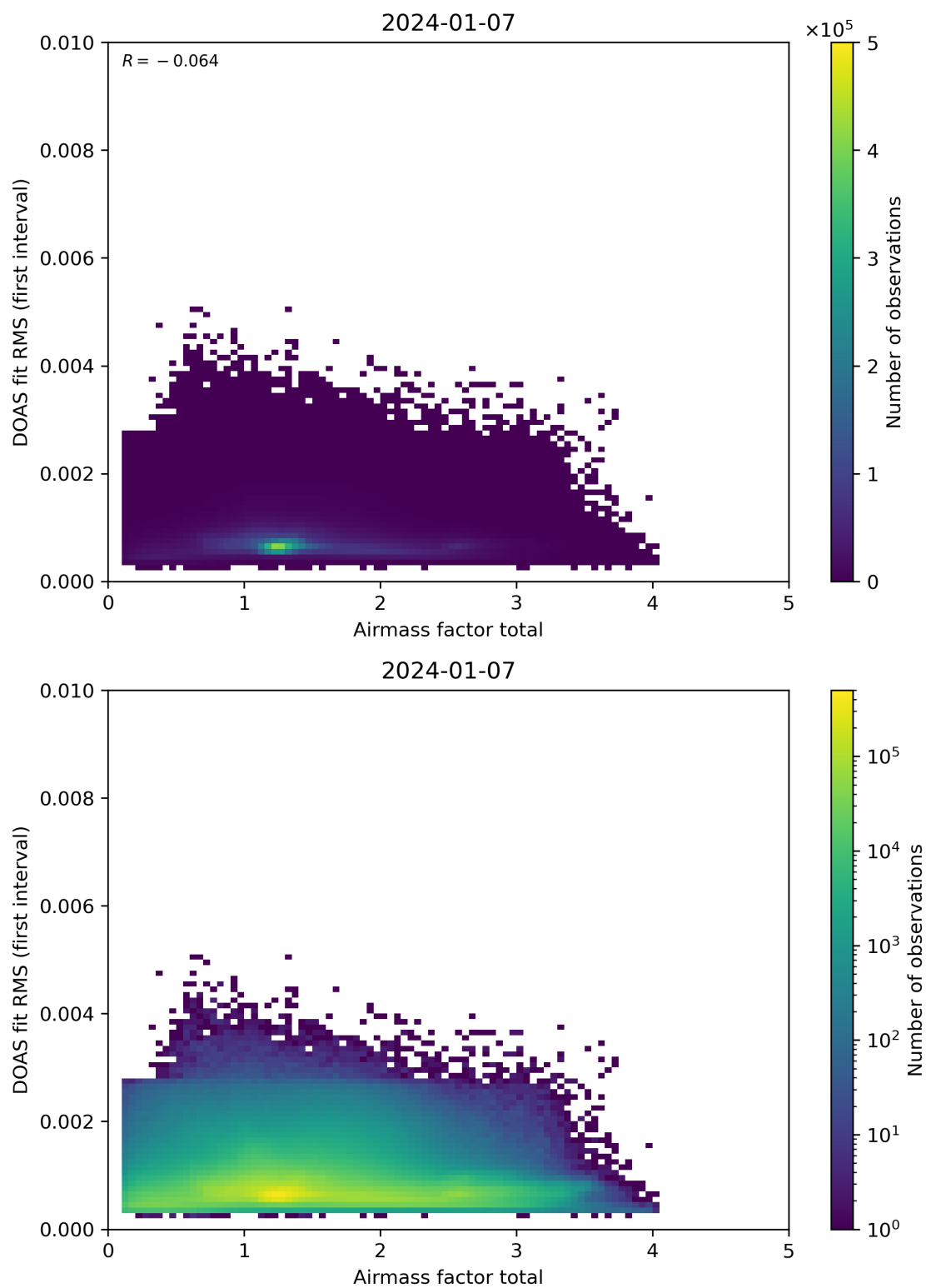
Figure 97: Scatter density plot of “Airmass factor total” against “DOAS fit RMS (first interval)” for 2024-01-06 to 2024-01-08.
