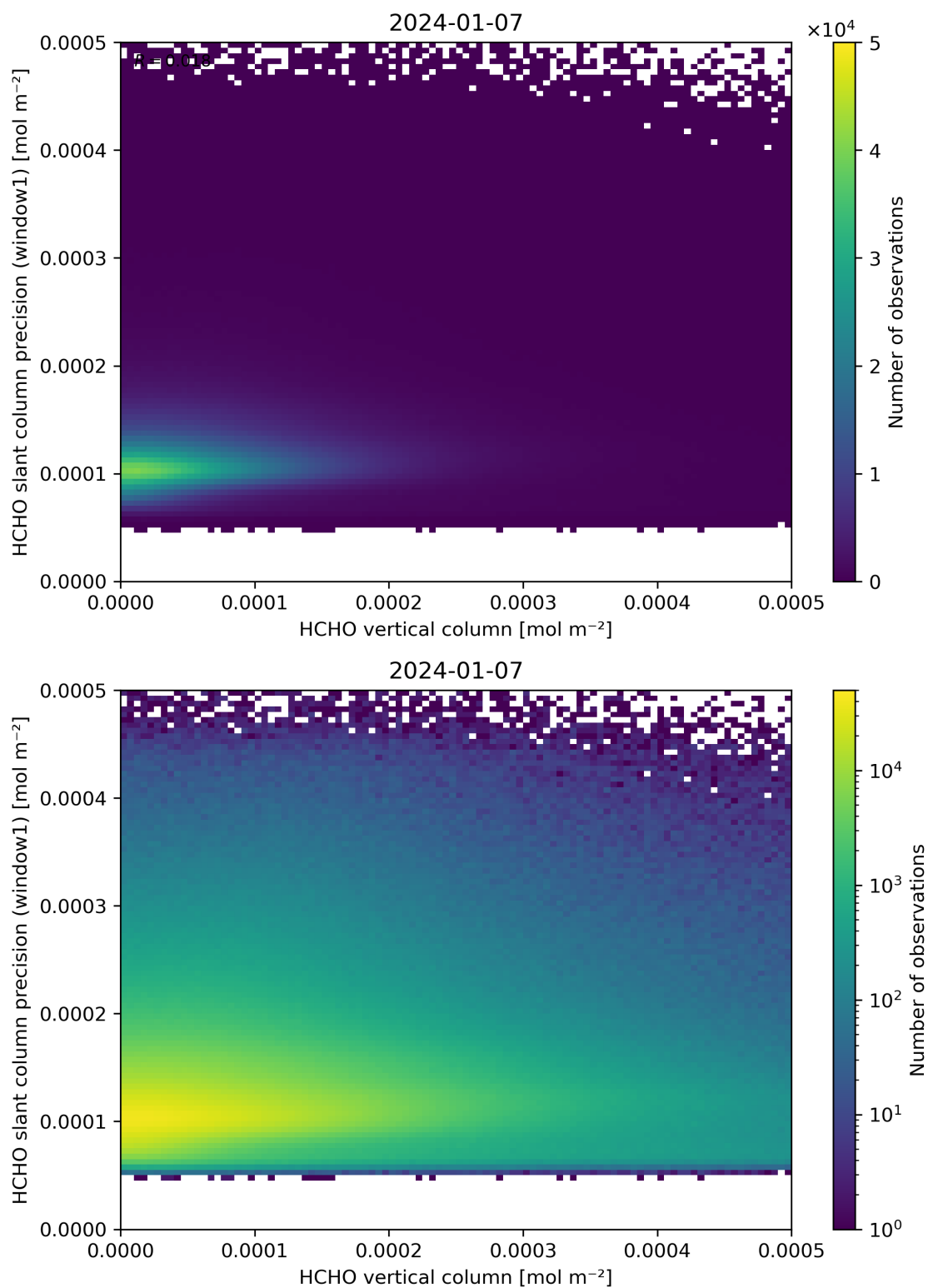
Figure 130: Scatter density plot of “HCHO vertical column” against “HCHO slant column precision (window1)” for 2024-01-06 to 2024-01-08.
