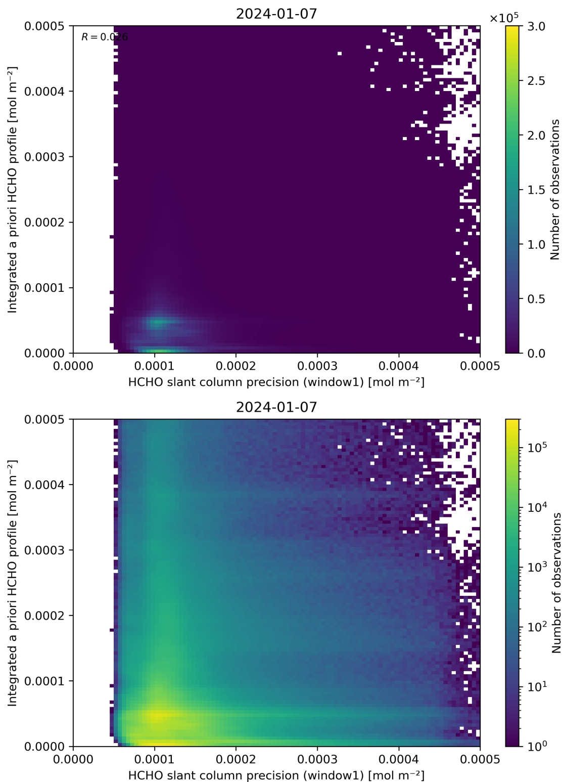
Figure 96: Scatter density plot of “HCHO slant column precision (window1)” against “Integrated a priori HCHO profile” for 2024-01-06 to 2024-01-08.
