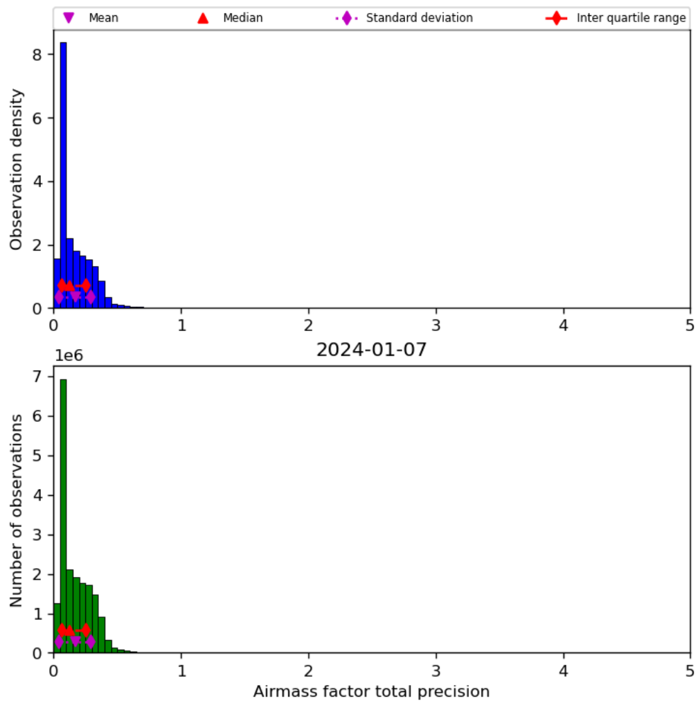
Figure 41: Histogram of “Airmass factor total precision” for 2024-01-06 to 2024-01-08
