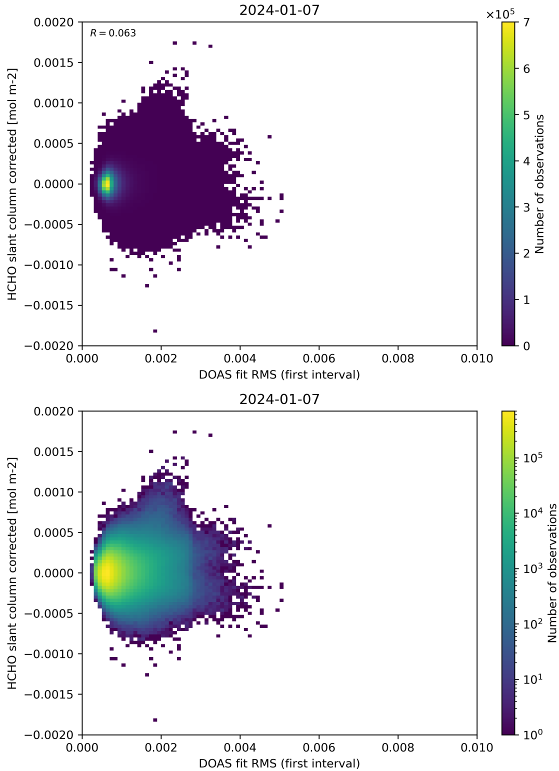
Figure 62: Scatter density plot of “DOAS fit RMS (first interval)” against “HCHO slant column corrected” for 2024-01-06 to 2024-01-08.
