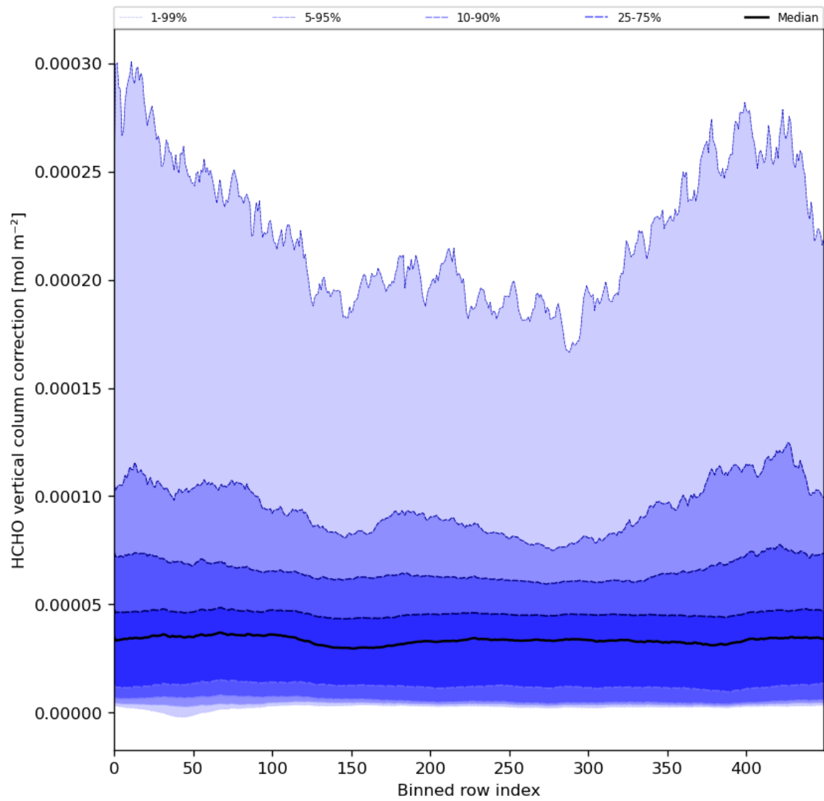
Figure 51: Along track statistics of “HCHO vertical column correction” for 2024-01-06 to 2024-01-08
