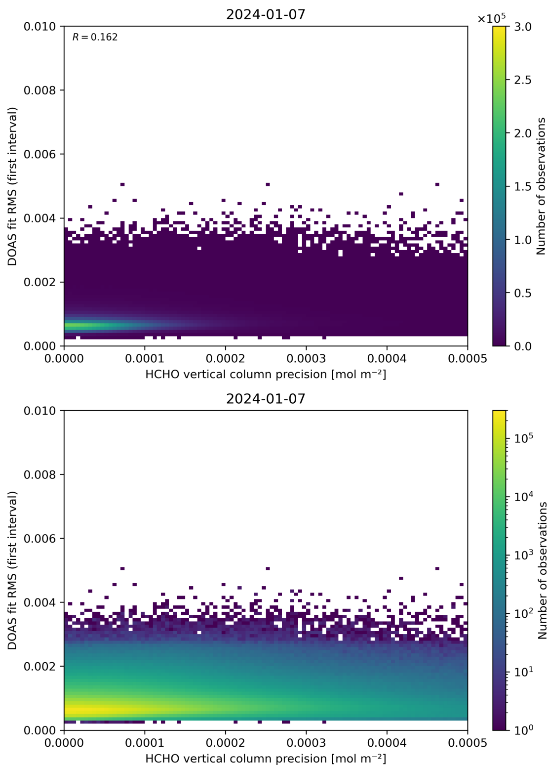
Figure 136: Scatter density plot of “HCHO vertical column precision” against “DOAS fit RMS (first interval)” for 2024-01-06 to 2024-01-08.
