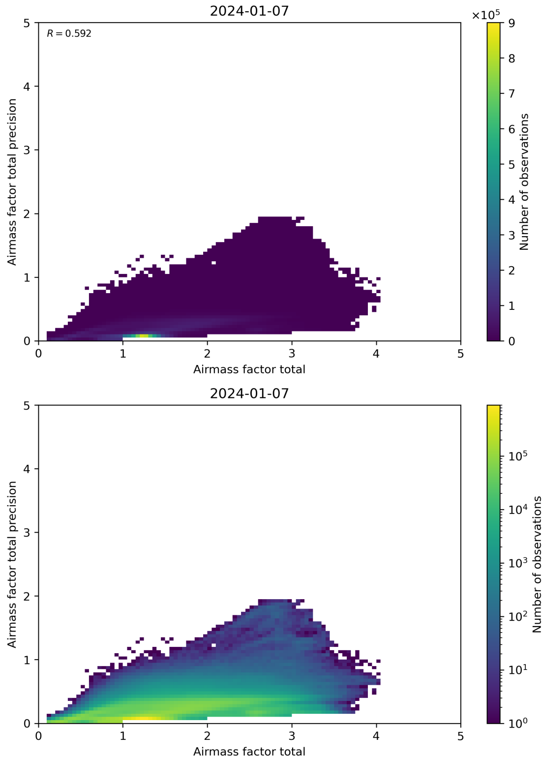
Figure 103: Scatter density plot of “Airmass factor total” against “Airmass factor total precision” for 2024-01-06 to 2024-01-08.
