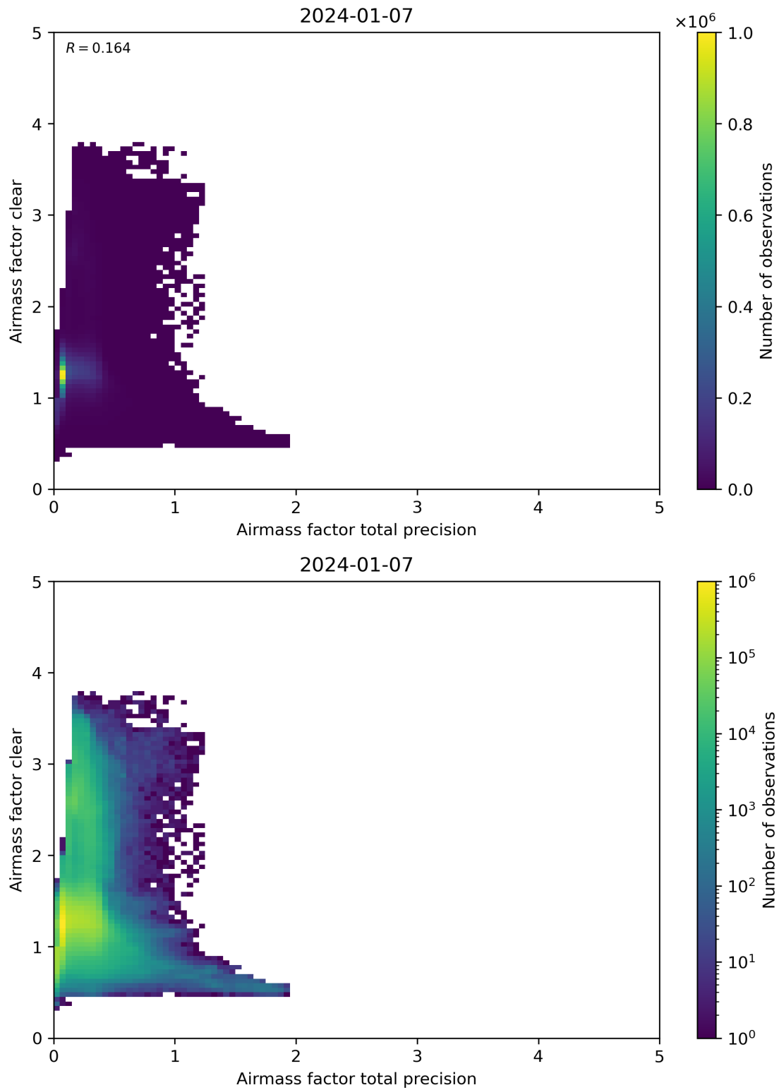
Figure 108: Scatter density plot of “Airmass factor total precision” against “Airmass factor clear” for 2024-01-06 to 2024-01-08.
