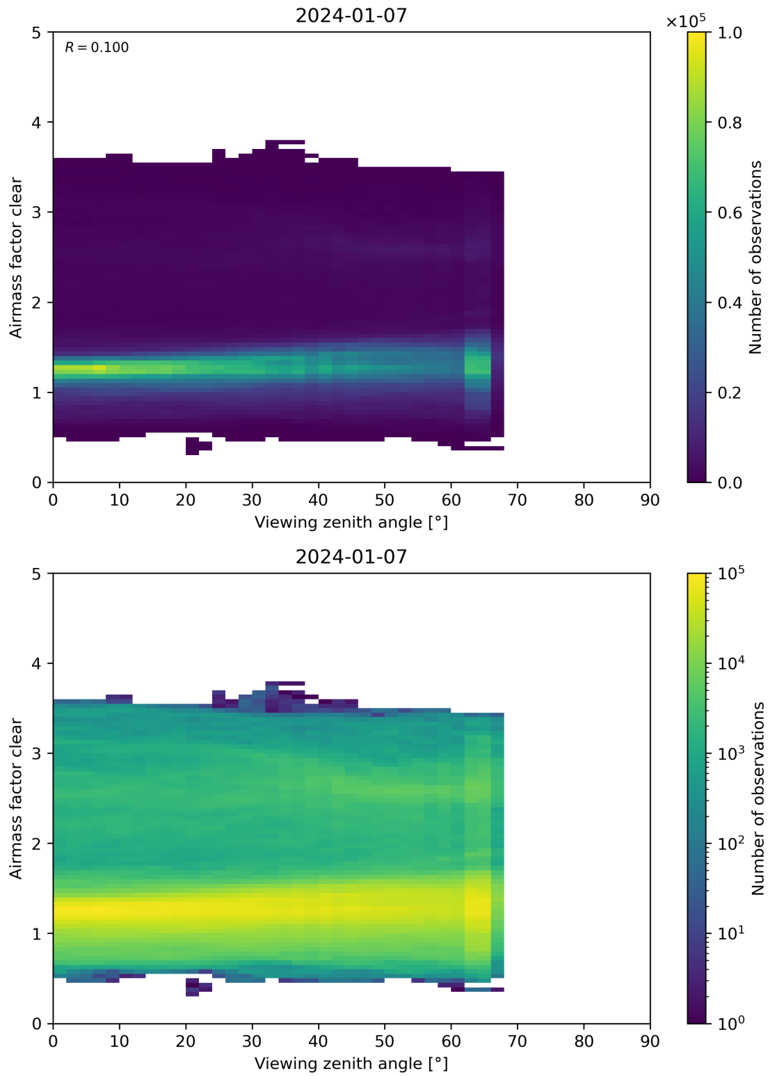
Figure 185: Scatter density plot of “Viewing zenith angle” against “Airmass factor clear” for 2024-01-06 to 2024-01-08.
