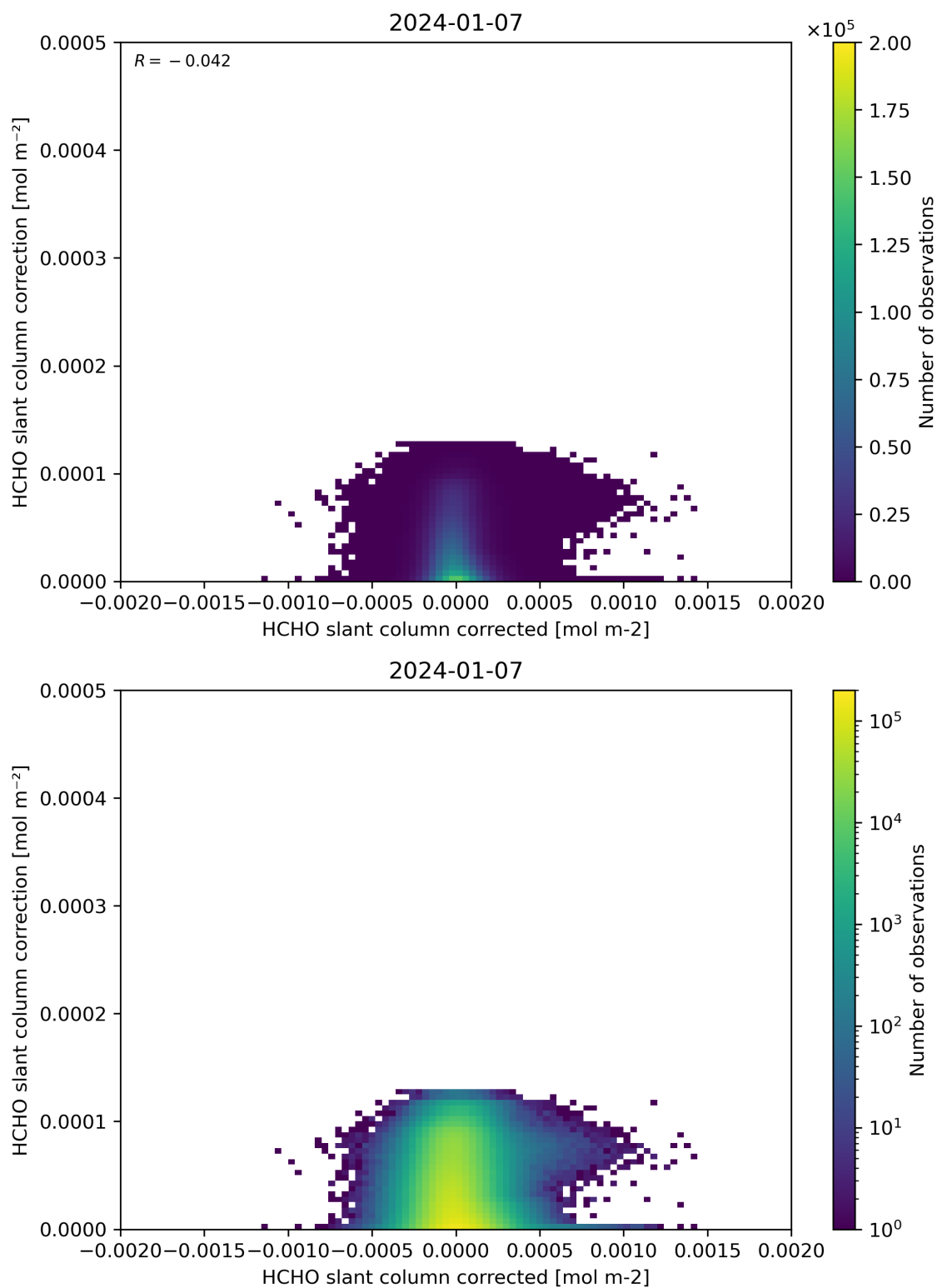
Figure 77: Scatter density plot of “HCHO slant column corrected” against “HCHO slant column correction” for 2024-01-06 to 2024-01-08.
