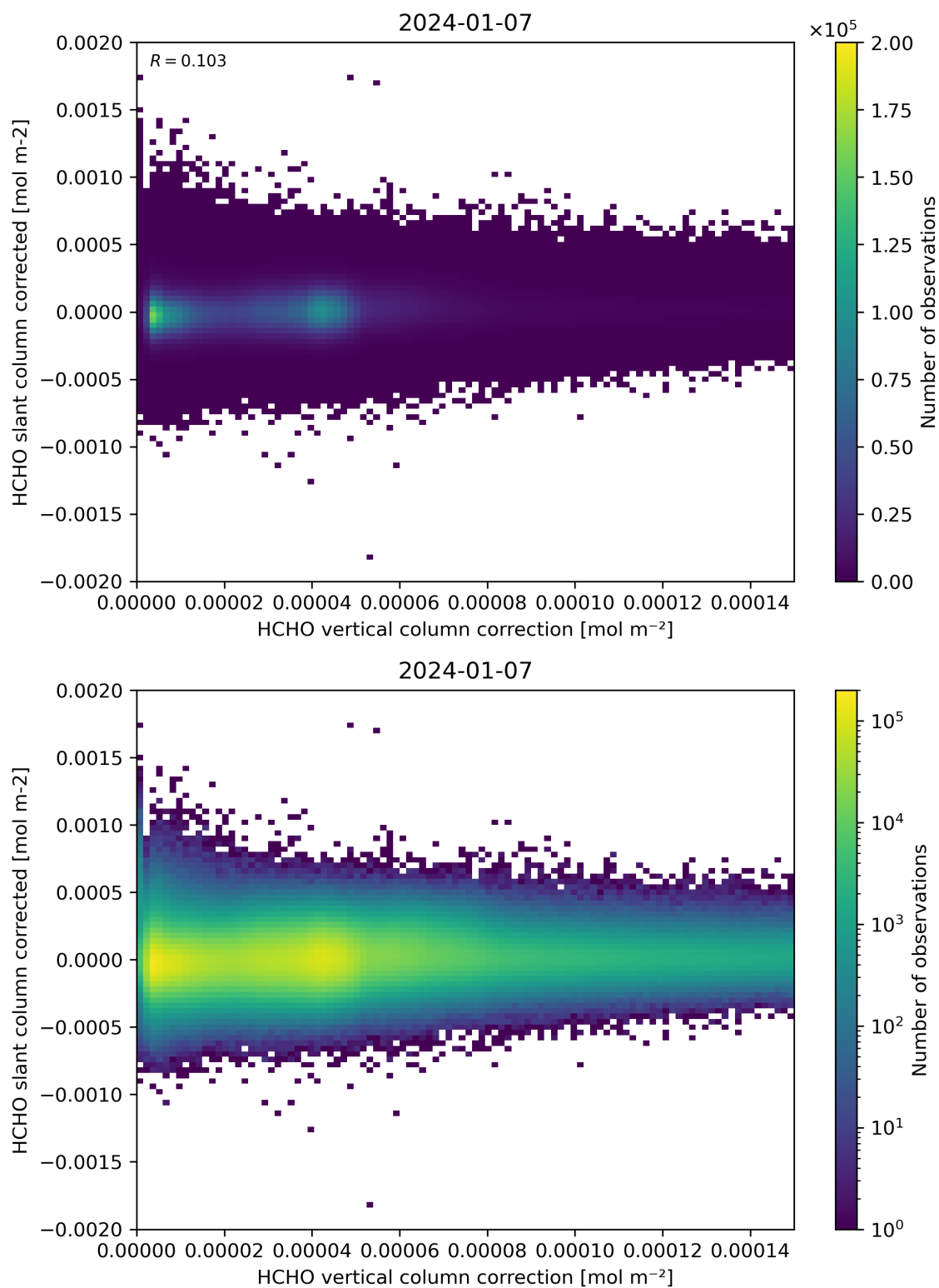
Figure 116: Scatter density plot of “HCHO vertical column correction” against “HCHO slant column corrected” for 2024-01-06 to 2024-01-08.
