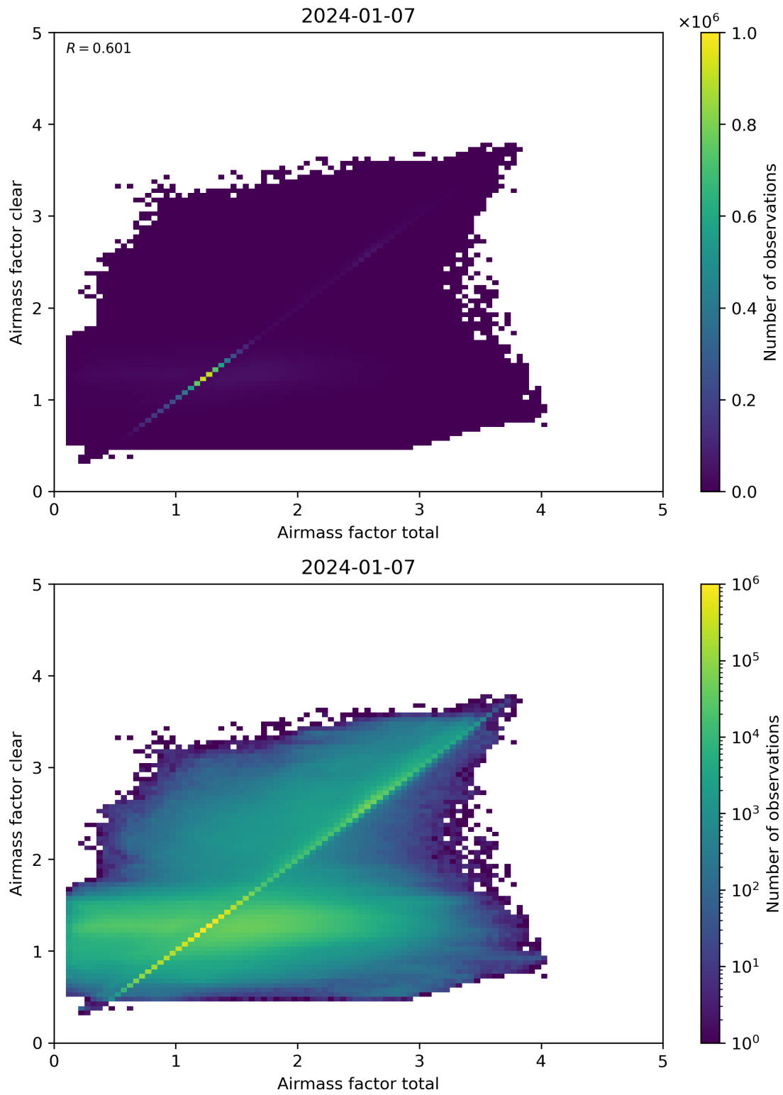
Figure 100: Scatter density plot of “Airmass factor total” against “Airmass factor clear” for 2024-01-06 to 2024-01-08.
