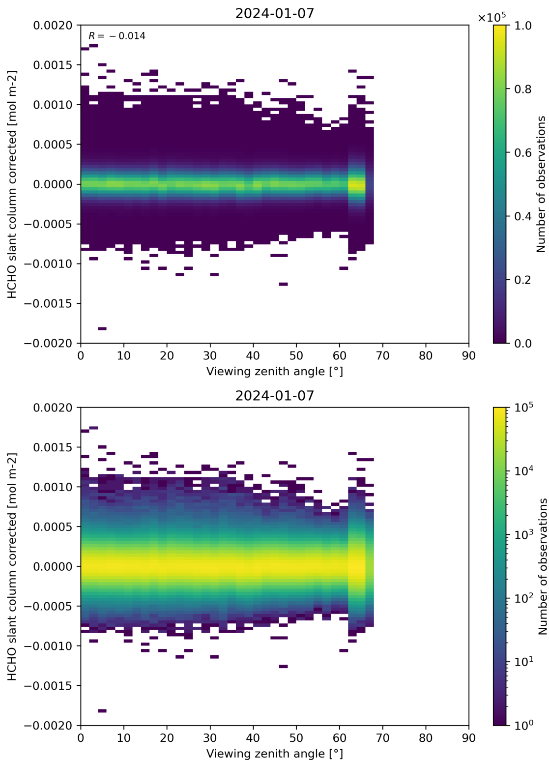
Figure 186: Scatter density plot of “Viewing zenith angle” against “HCHO slant column corrected” for 2024-01-06 to 2024-01-08.
