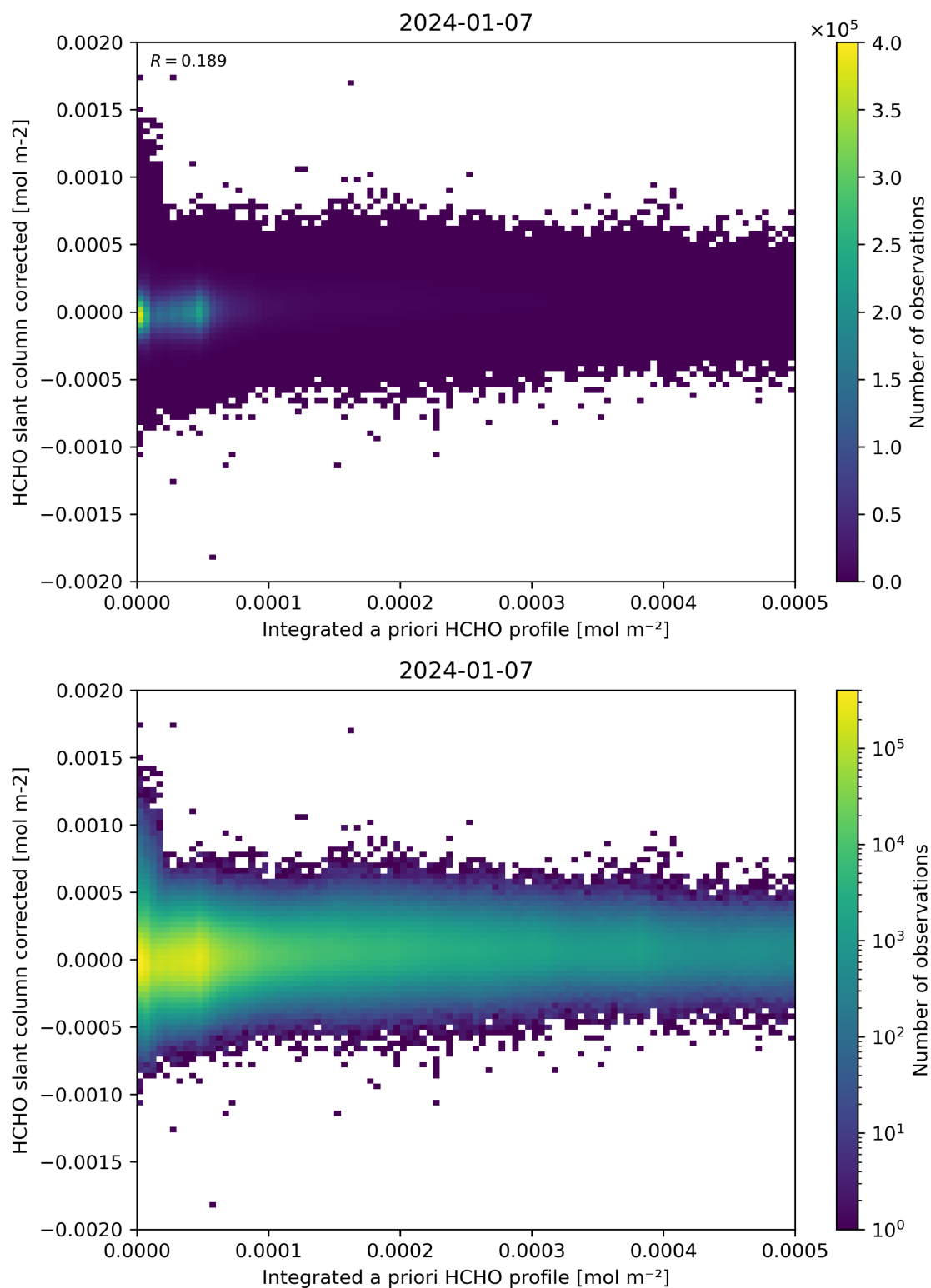
Figure 151: Scatter density plot of “Integrated a priori HCHO profile” against “HCHO slant column corrected” for 2024-01-06 to 2024-01-08.
