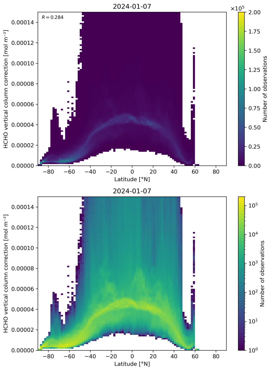
Figure 164: Scatter density plot of “Latitude” against “HCHO vertical column correction” for 2024-01-06 to 2024-01-08.
