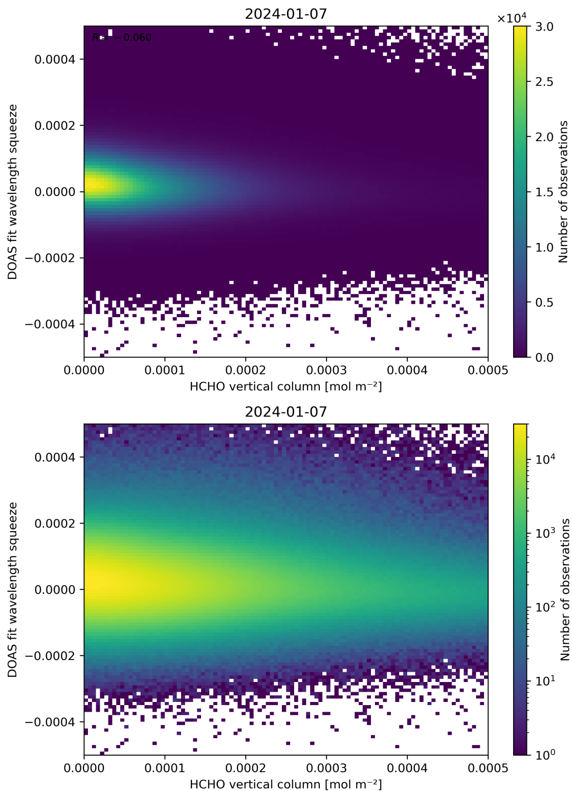
Figure 125: Scatter density plot of “HCHO vertical column” against “DOAS fit wavelength squeeze” for 2024-01-06 to 2024-01-08.
