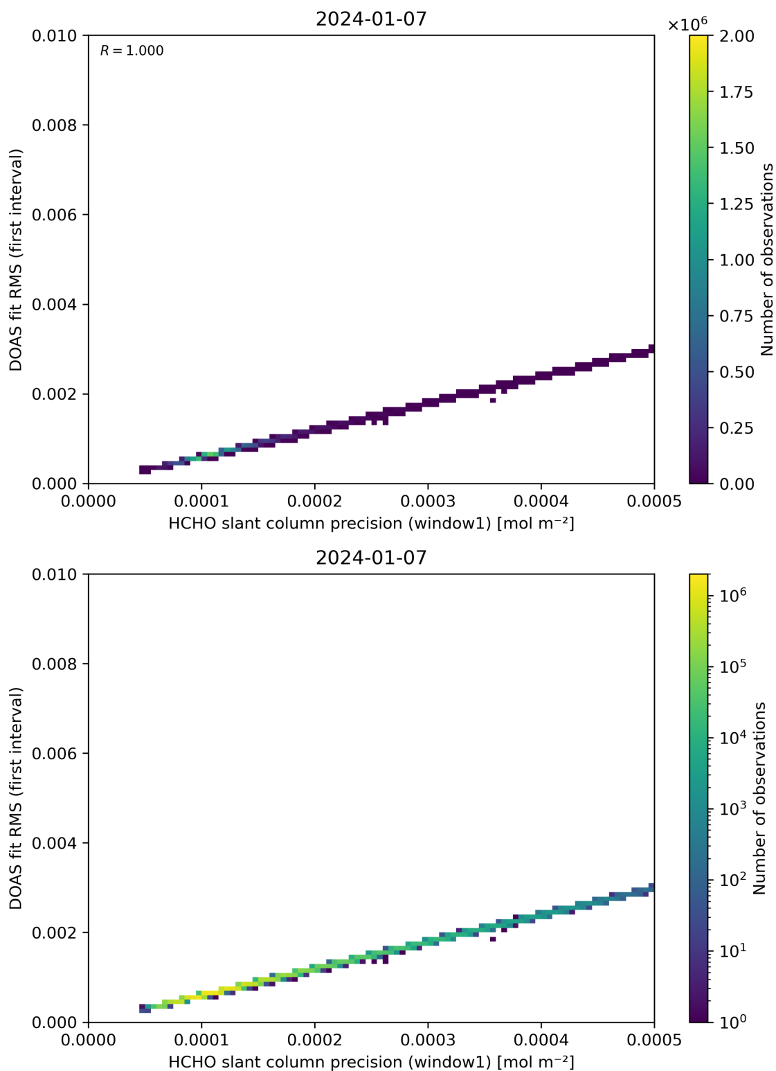
Figure 88: Scatter density plot of “HCHO slant column precision (window1)” against “DOAS fit RMS (first interval)” for 2024-01-06 to 2024-01-08.
