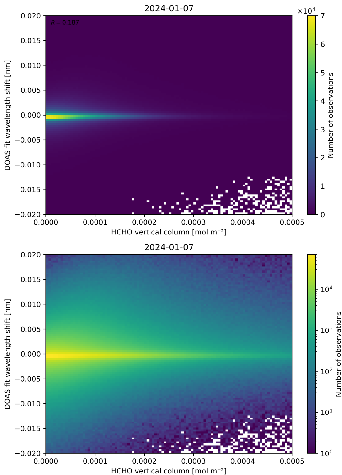
Figure 124: Scatter density plot of “HCHO vertical column” against “DOAS fit wavelength shift” for 2024-01-06 to 2024-01-08.
