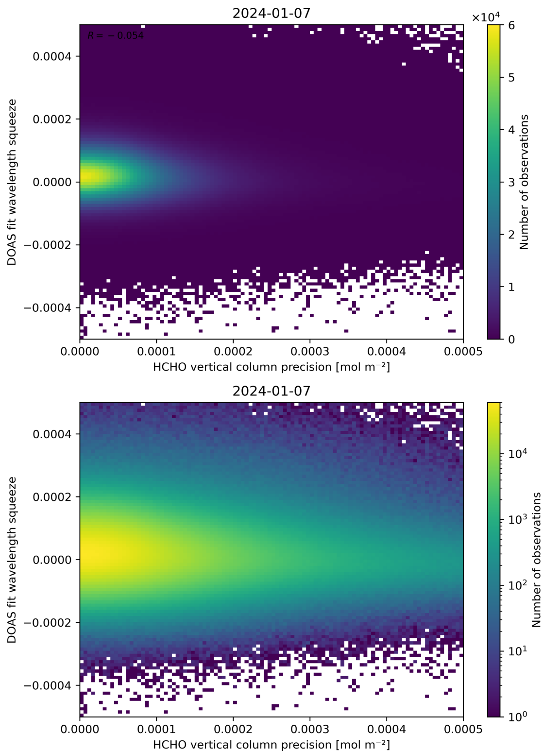
Figure 138: Scatter density plot of “HCHO vertical column precision” against “DOAS fit wavelength squeeze” for 2024-01-06 to 2024-01-08.
