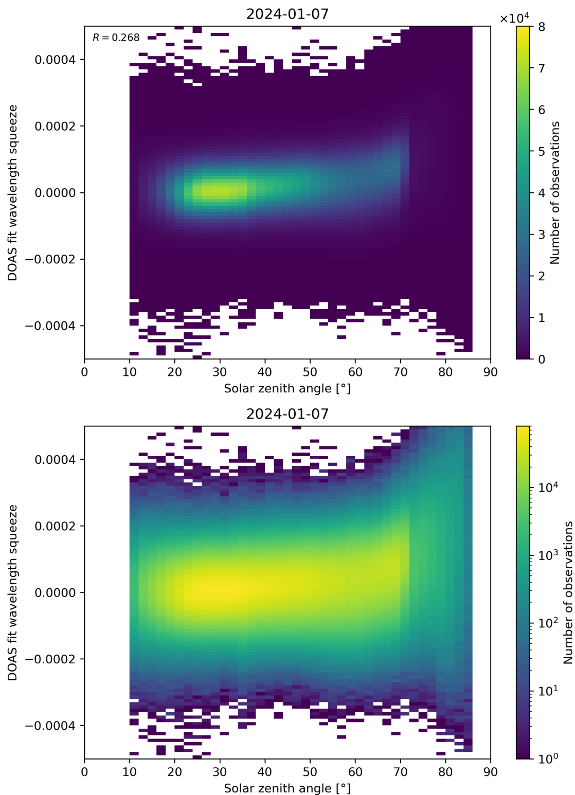
Figure 169: Scatter density plot of “Solar zenith angle” against “DOAS fit wavelength squeeze” for 2024-01-06 to 2024-01-08.
