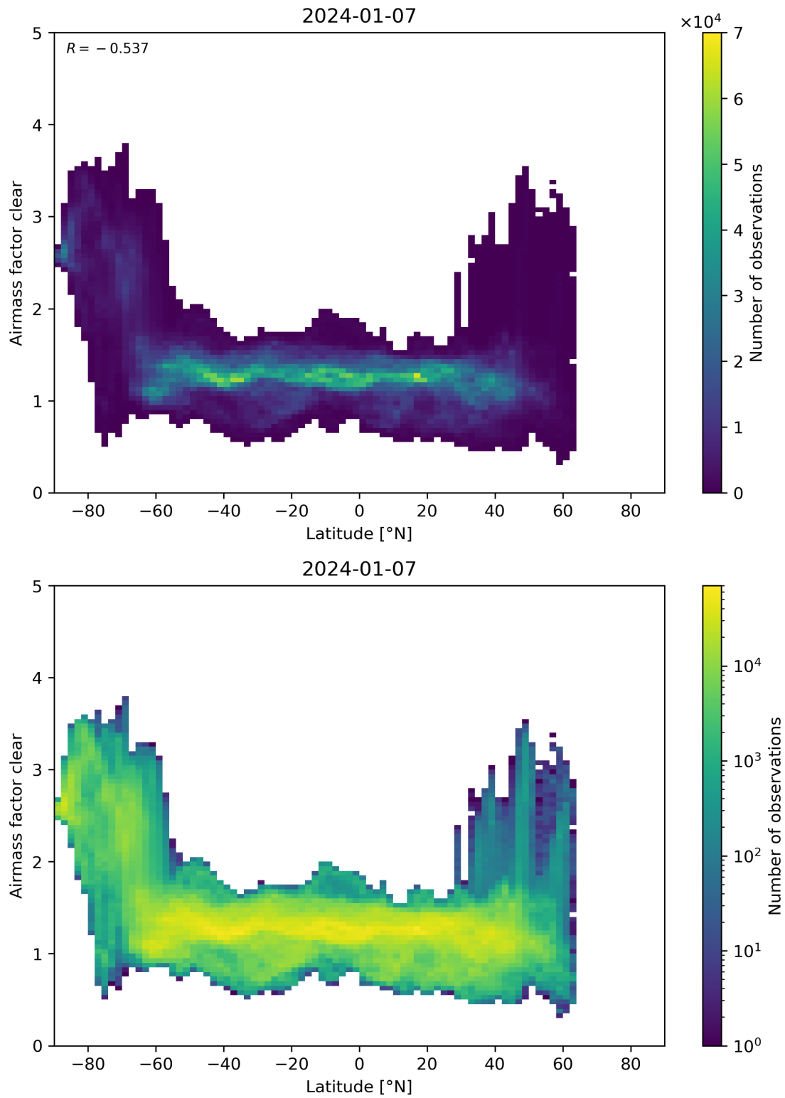
Figure 156: Scatter density plot of “Latitude” against “Airmass factor clear” for 2024-01-06 to 2024-01-08.
