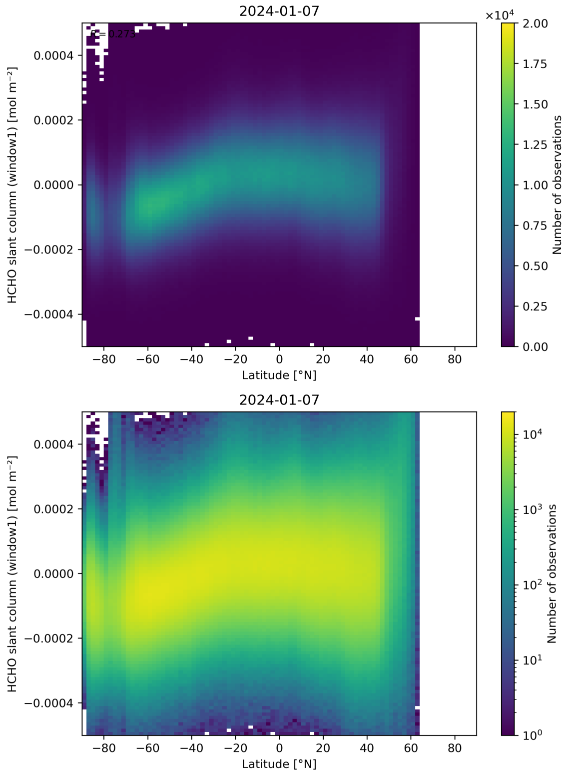
Figure 159: Scatter density plot of “Latitude” against “HCHO slant column (window1)” for 2024-01-06 to 2024-01-08.
