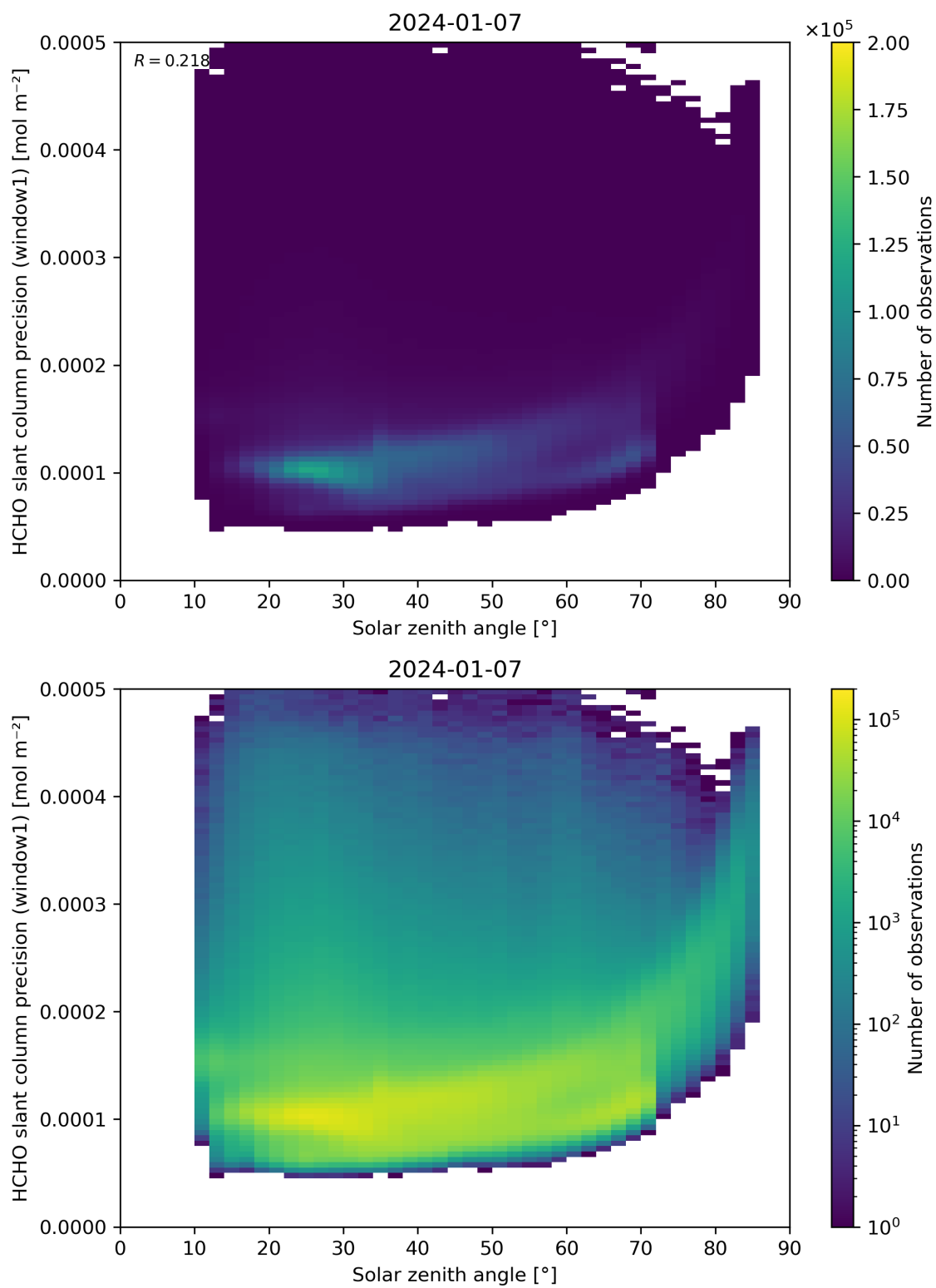
Figure 174: Scatter density plot of “Solar zenith angle” against “HCHO slant column precision (window1)” for 2024-01-06 to 2024-01-08.
