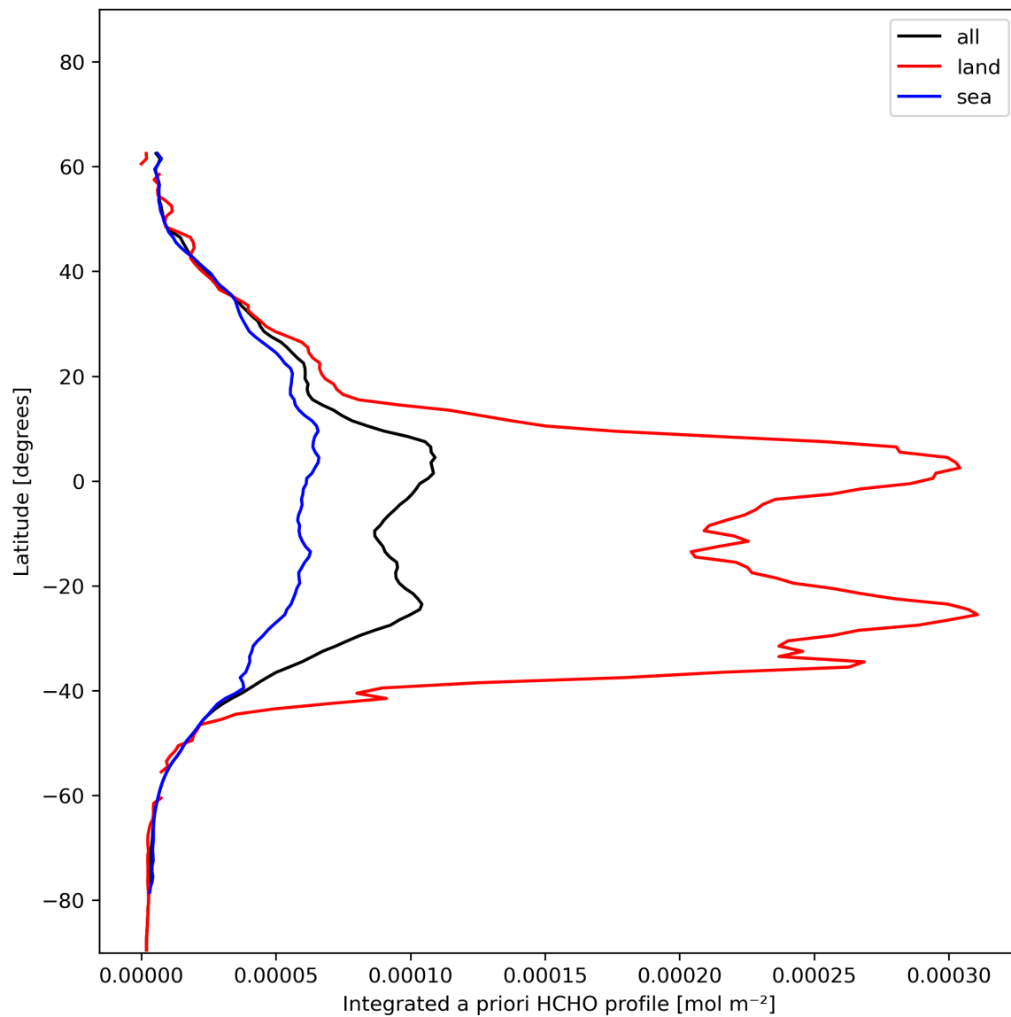
Figure 29: Zonal average of “Integrated a priori HCHO profile” for 2024-01-06 to 2024-01-08.
