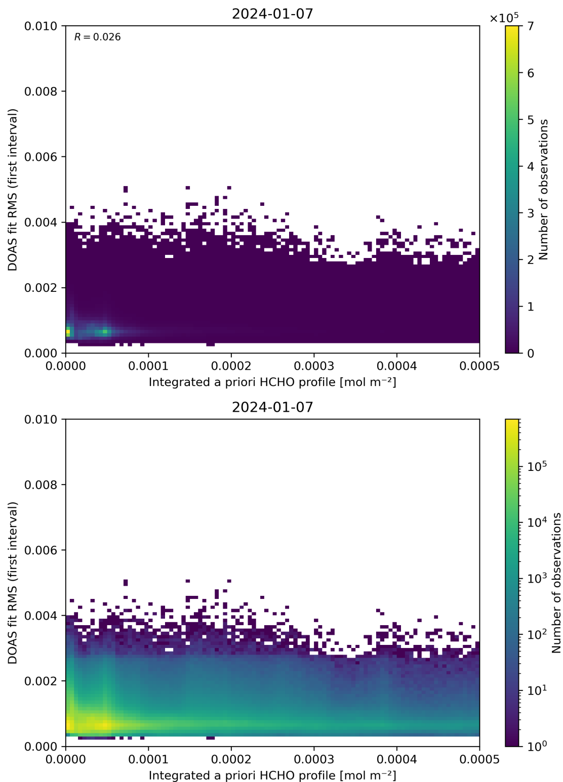
Figure 148: Scatter density plot of “Integrated a priori HCHO profile” against “DOAS fit RMS (first interval)” for 2024-01-06 to 2024-01-08.
