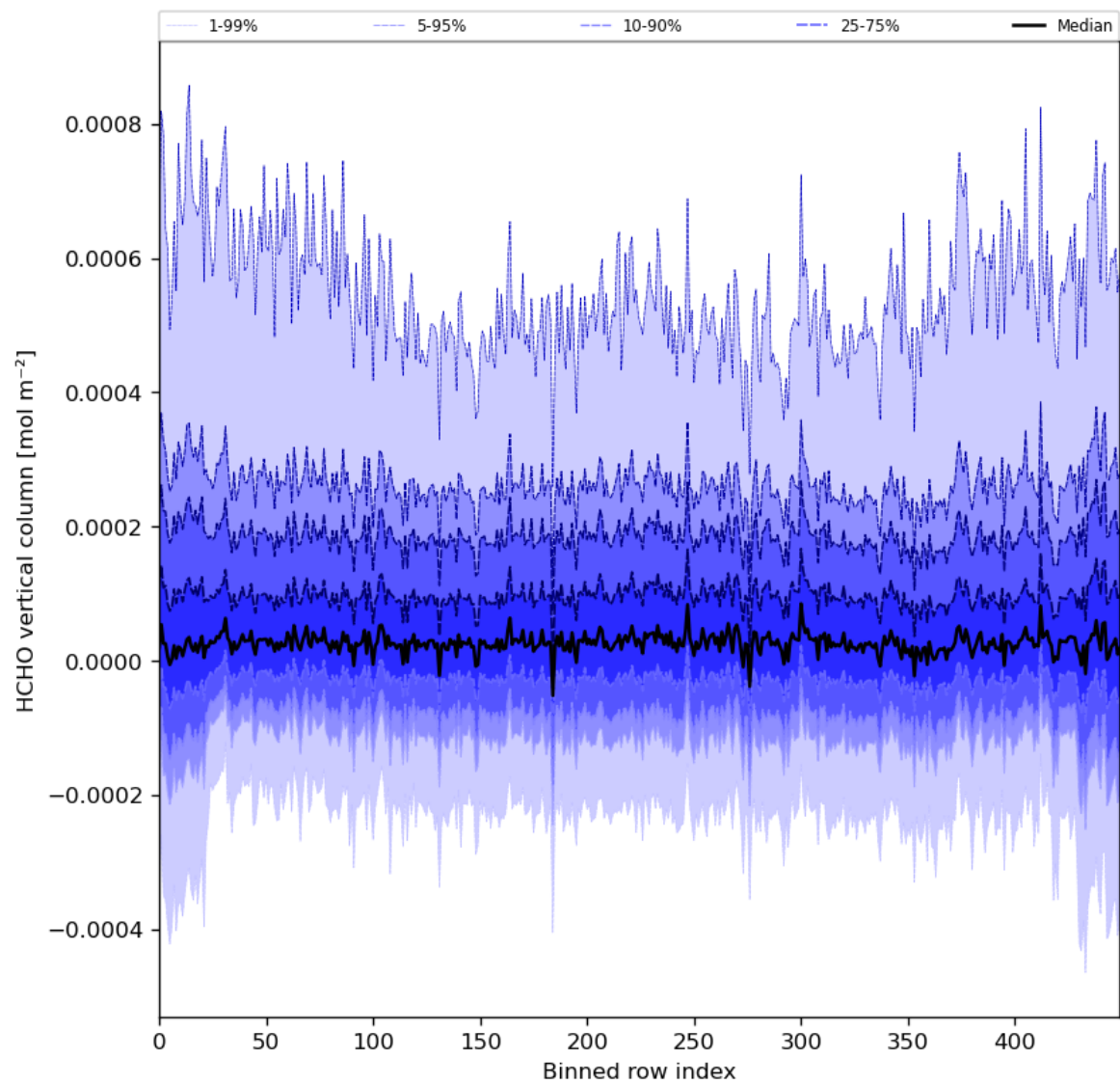
Figure 49: Along track statistics of “HCHO vertical column” for 2024-01-06 to 2024-01-08
