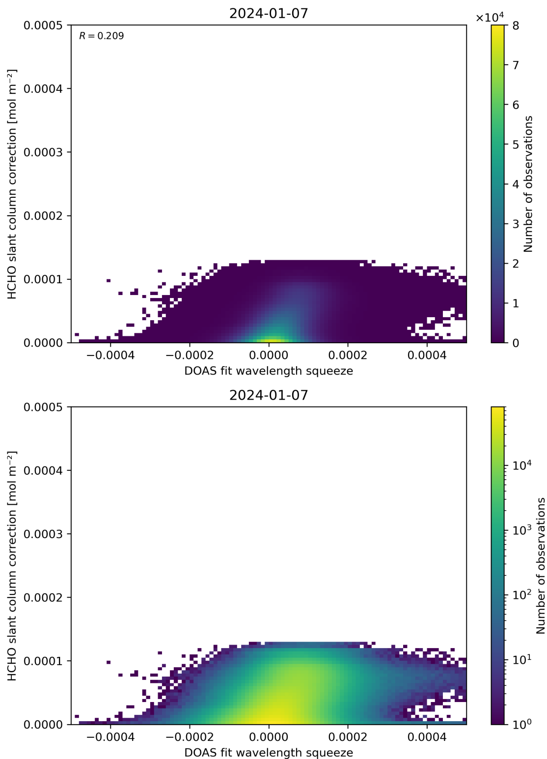
Figure 70: Scatter density plot of “DOAS fit wavelength squeeze” against “HCHO slant column correction” for 2024-01-06 to 2024-01-08.
