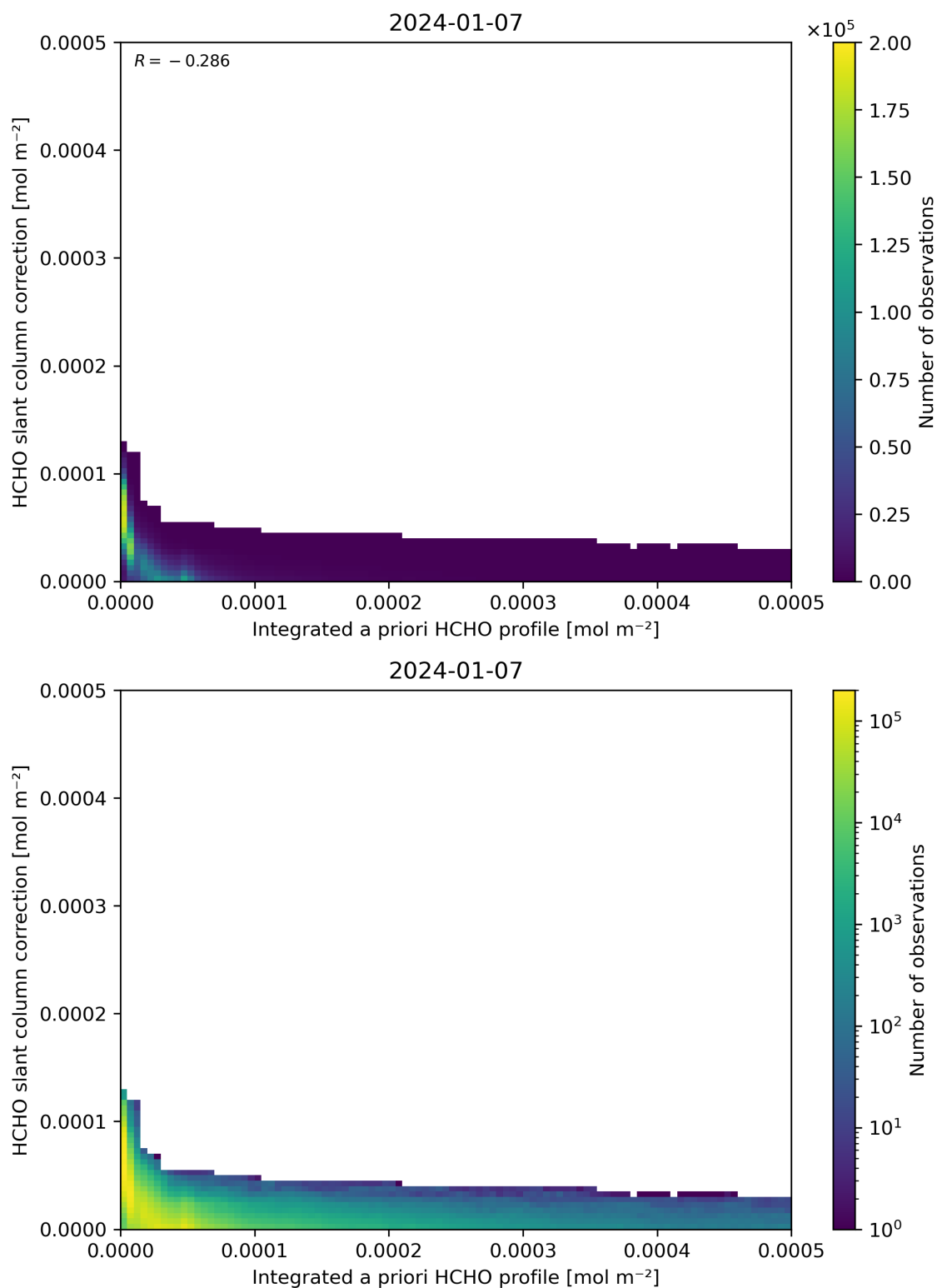
Figure 152: Scatter density plot of “Integrated a priori HCHO profile” against “HCHO slant column correction” for 2024-01-06 to 2024-01-08.
