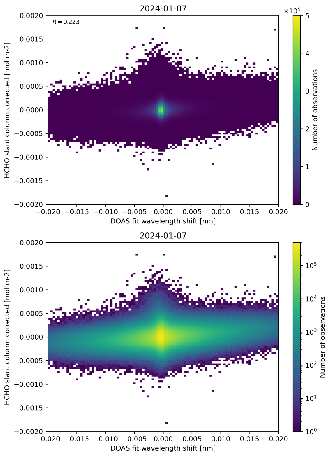
Figure 66: Scatter density plot of “DOAS fit wavelength shift” against “HCHO slant column corrected” for 2024-01-06 to 2024-01-08.
