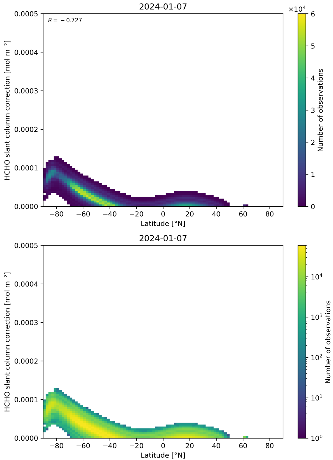
Figure 158: Scatter density plot of “Latitude” against “HCHO slant column correction” for 2024-01-06 to 2024-01-08.
