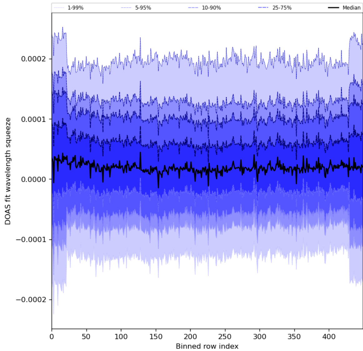
Figure 59: Along track statistics of “DOAS fit wavelength squeeze” for 2024-01-06 to 2024-01-08
