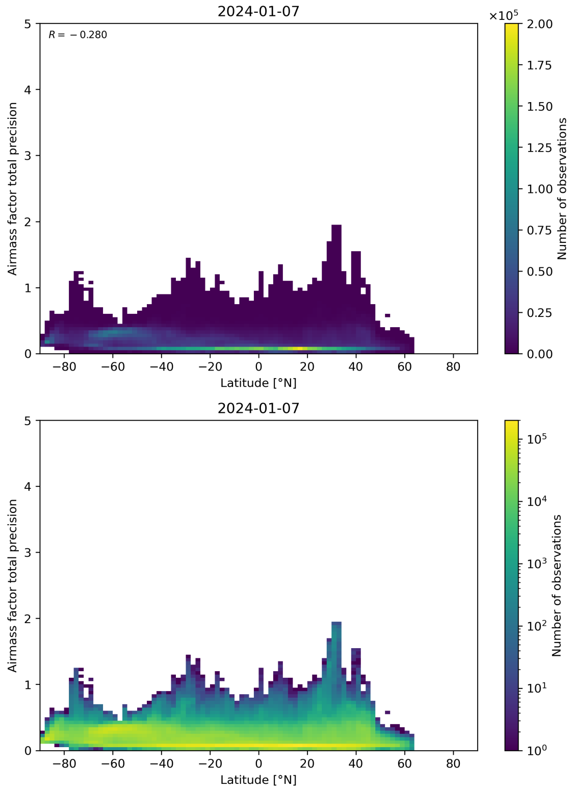
Figure 162: Scatter density plot of “Latitude” against “Airmass factor total precision” for 2024-01-06 to 2024-01-08.
