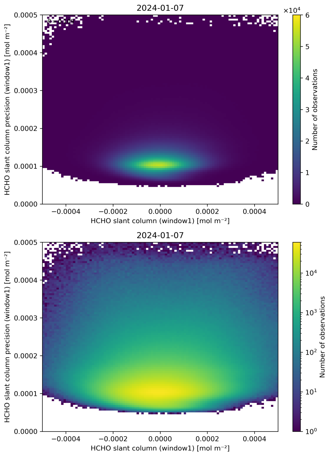
Figure 84: Scatter density plot of “HCHO slant column (window1)” against “HCHO slant column precision (window1)” for 2024-01-06 to 2024-01-08.
