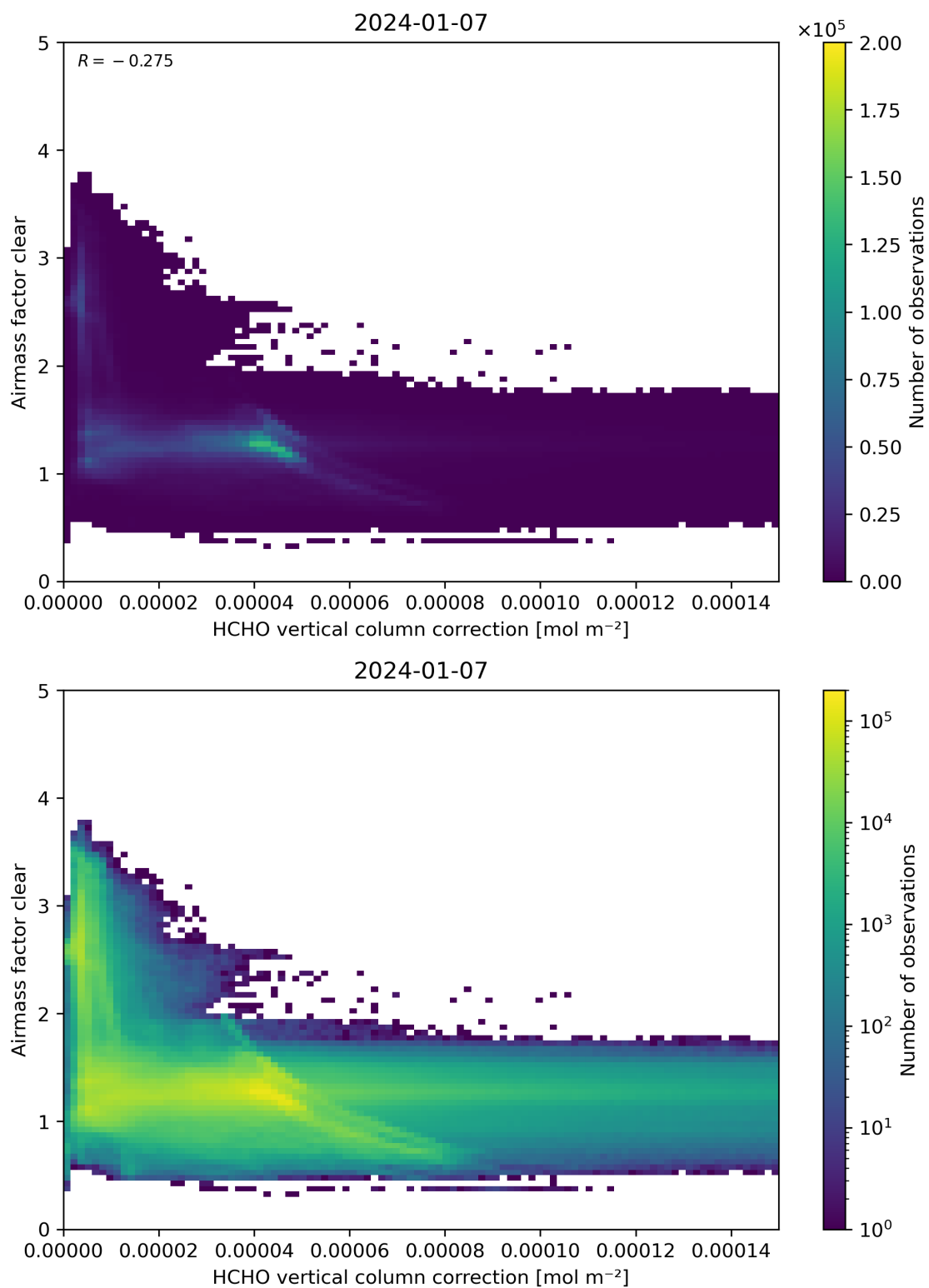
Figure 115: Scatter density plot of “HCHO vertical column correction” against “Airmass factor clear” for 2024-01-06 to 2024-01-08.
