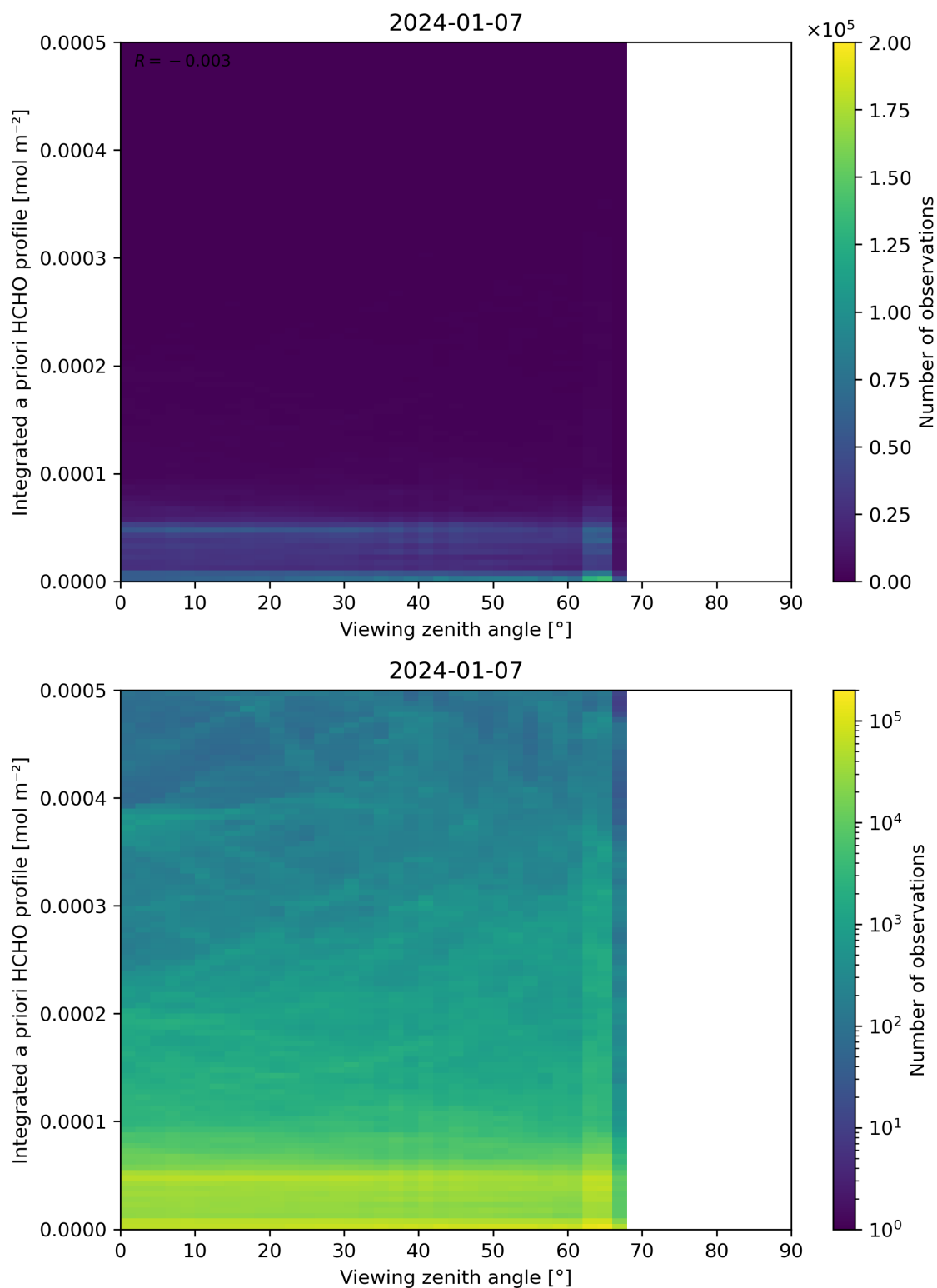
Figure 195: Scatter density plot of “Viewing zenith angle” against “Integrated a priori HCHO profile” for 2024-01-06 to 2024-01-08.
