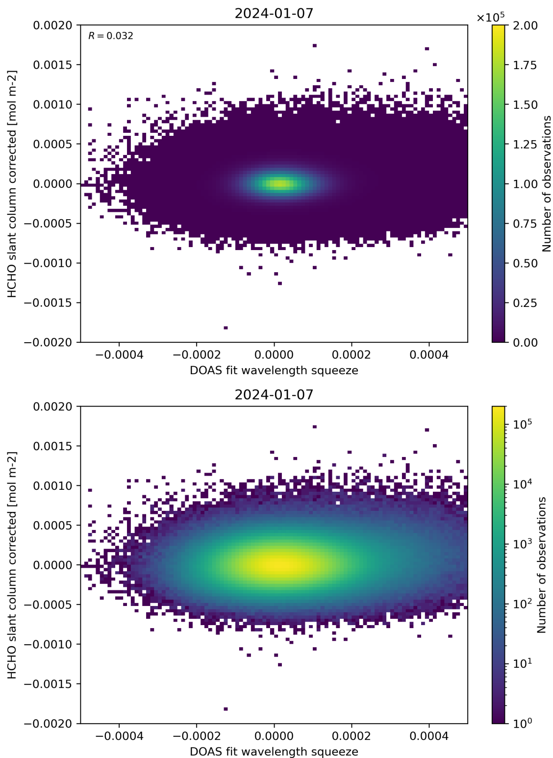
Figure 69: Scatter density plot of “DOAS fit wavelength squeeze” against “HCHO slant column corrected” for 2024-01-06 to 2024-01-08.
