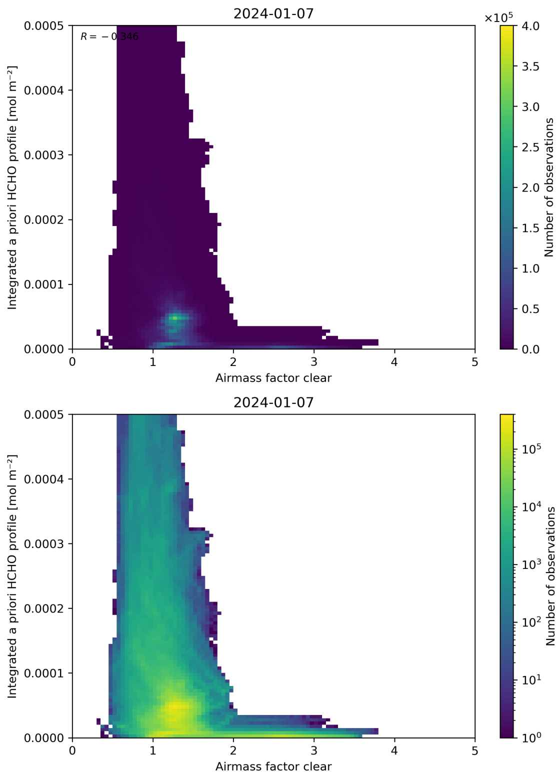
Figure 76: Scatter density plot of “Airmass factor clear” against “Integrated a priori HCHO profile” for 2024-01-06 to 2024-01-08.
