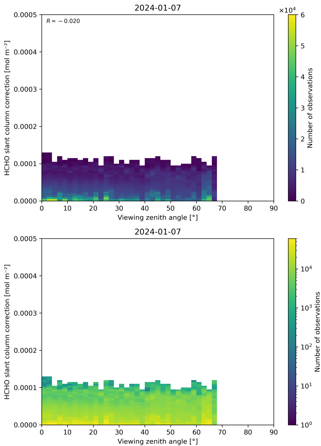
Figure 187: Scatter density plot of “Viewing zenith angle” against “HCHO slant column correction” for 2024-01-06 to 2024-01-08.
