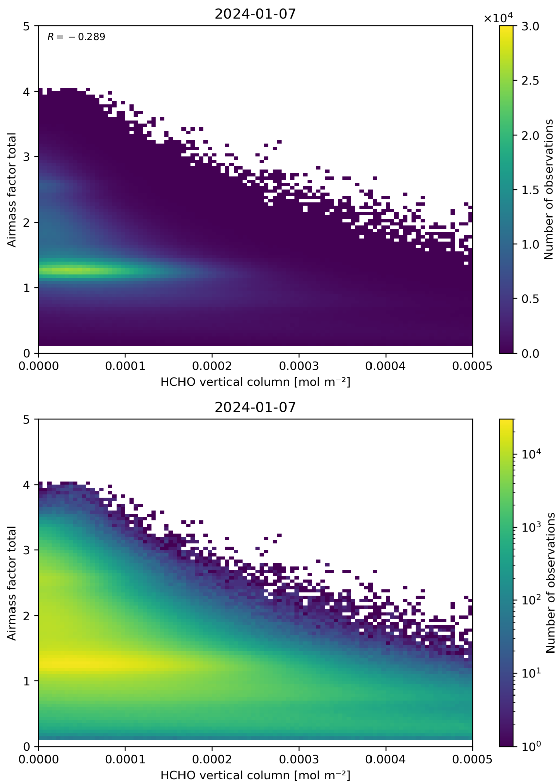
Figure 131: Scatter density plot of “HCHO vertical column” against “Airmass factor total” for 2024-01-06 to 2024-01-08.
