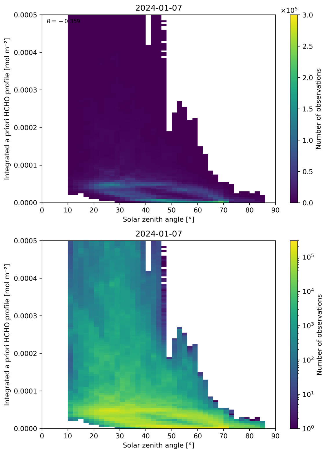
Figure 180: Scatter density plot of “Solar zenith angle” against “Integrated a priori HCHO profile” for 2024-01-06 to 2024-01-08.
