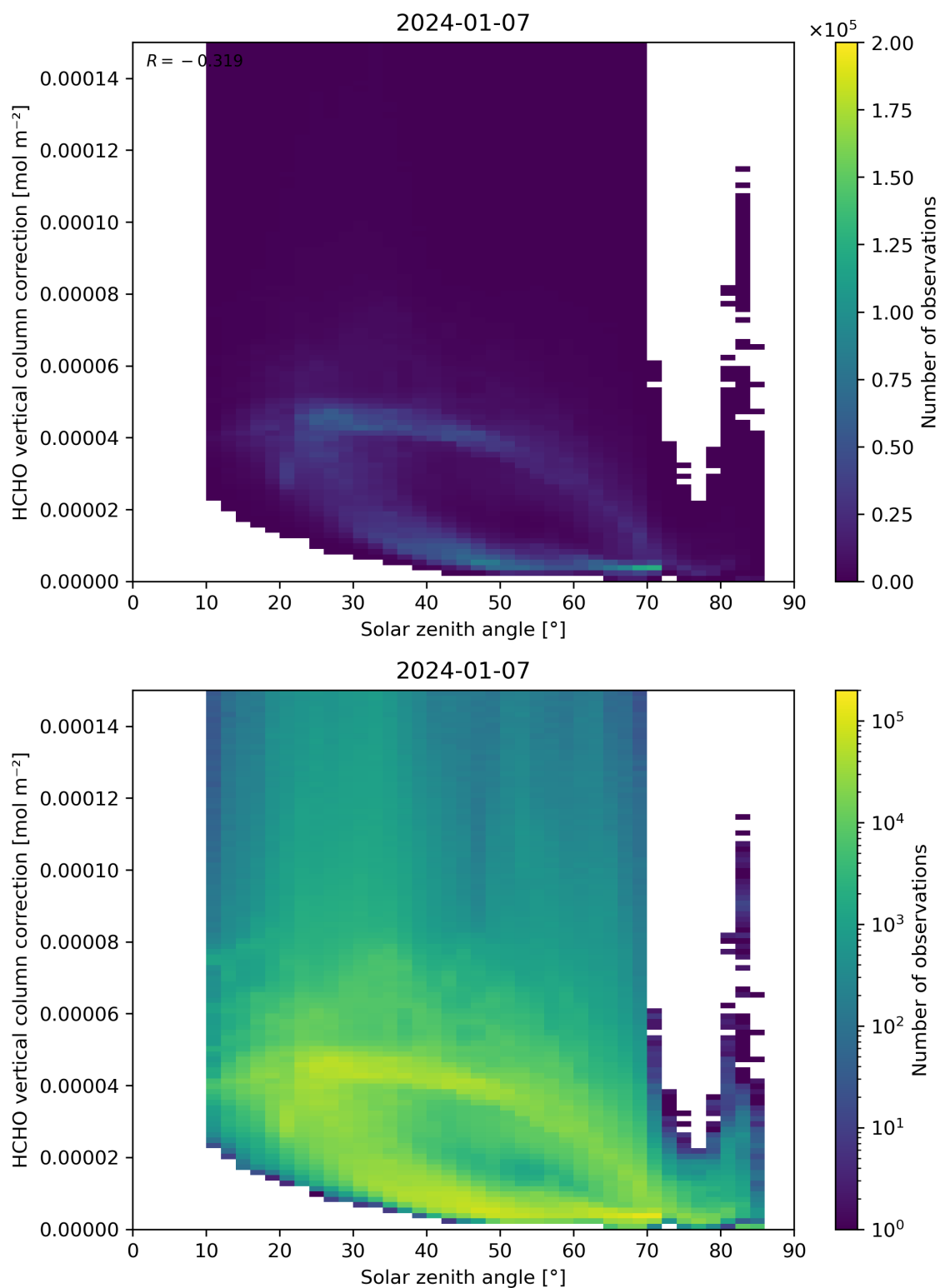
Figure 178: Scatter density plot of “Solar zenith angle” against “HCHO vertical column correction” for 2024-01-06 to 2024-01-08.
