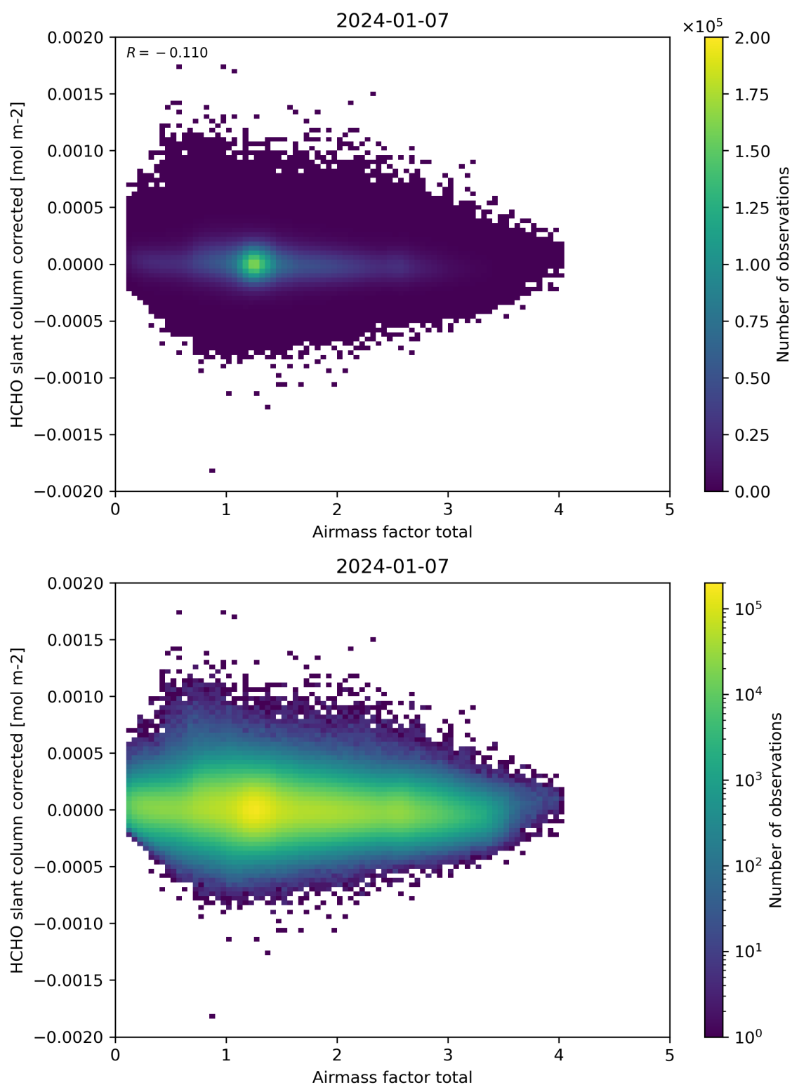
Figure 101: Scatter density plot of “Airmass factor total” against “HCHO slant column corrected” for 2024-01-06 to 2024-01-08.
