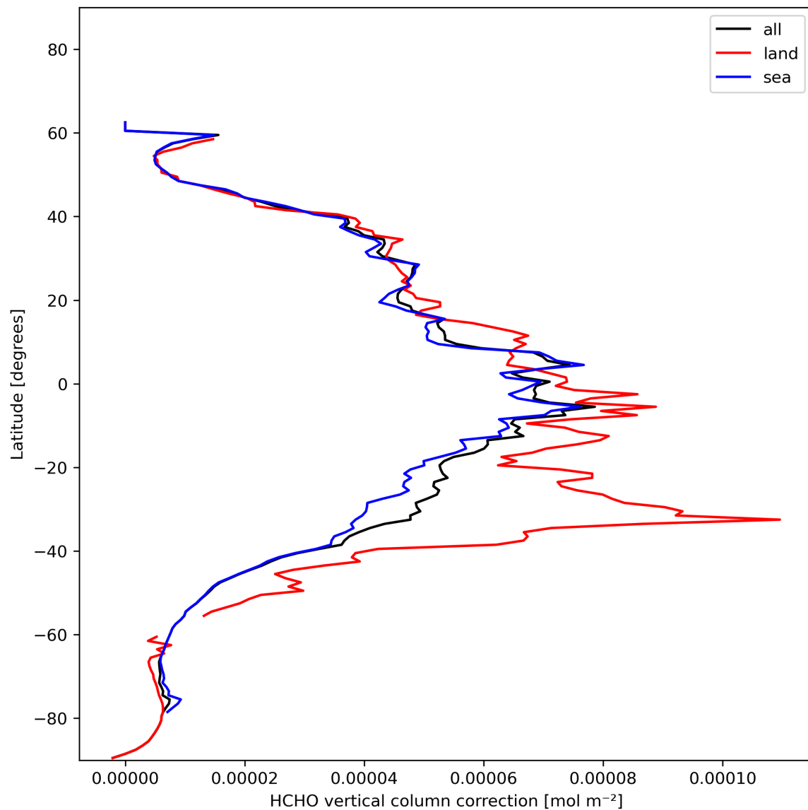
Figure 23: Zonal average of “HCHO vertical column correction” for 2024-01-06 to 2024-01-08.
