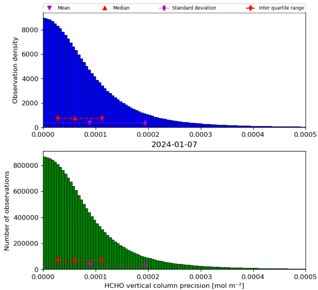
Figure 36: Histogram of “HCHO vertical column precision” for 2024-01-06 to 2024-01-08
