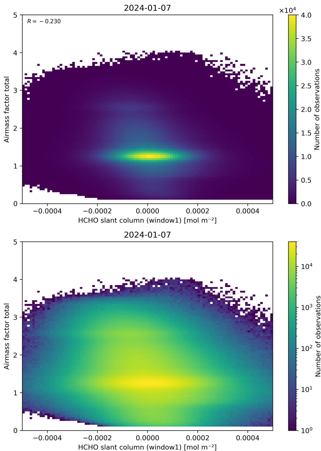
Figure 85: Scatter density plot of “HCHO slant column (window1)” against “Airmass factor total” for 2024-01-06 to 2024-01-08.
