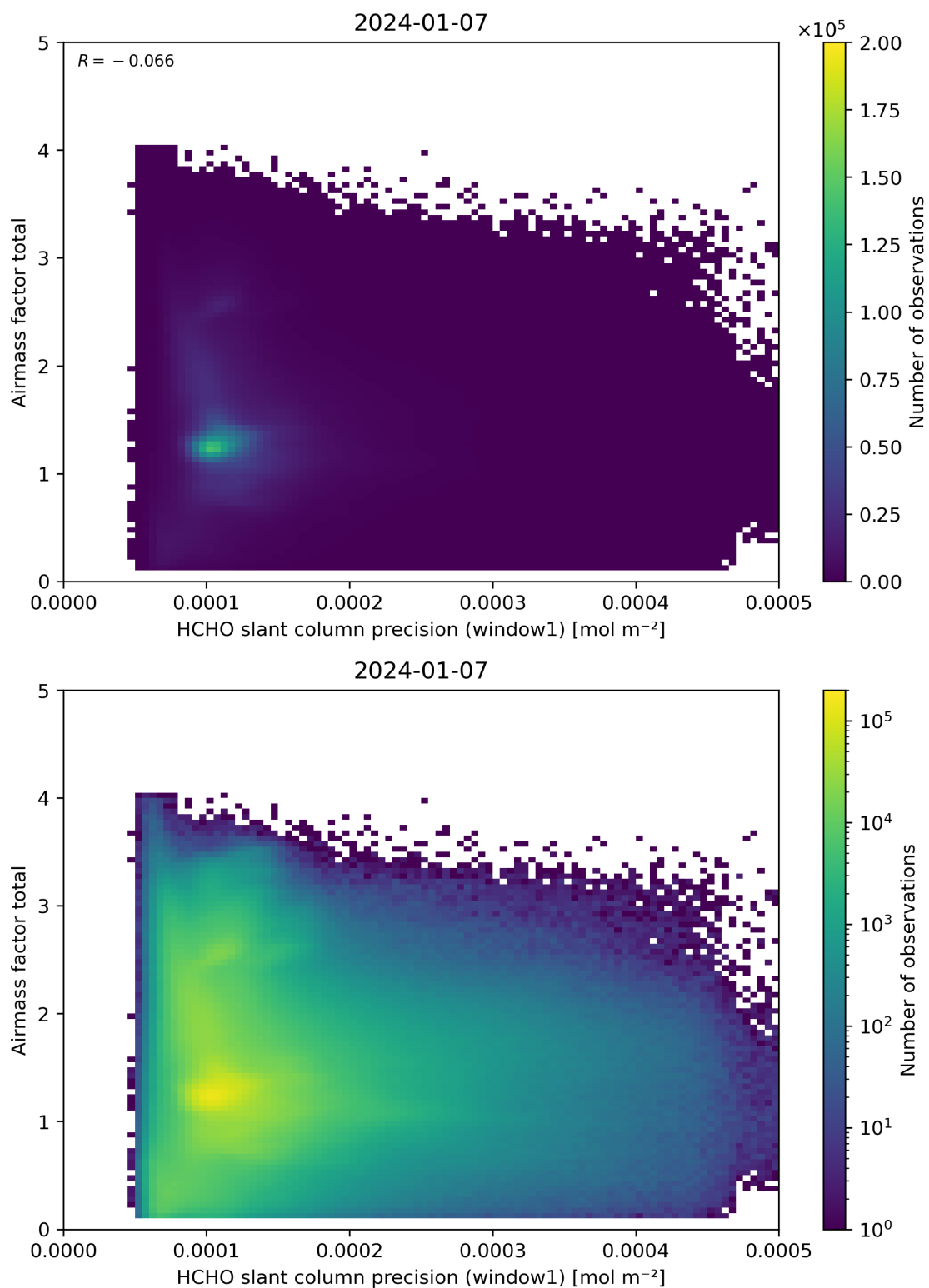
Figure 94: Scatter density plot of “HCHO slant column precision (window1)” against “Airmass factor total” for 2024-01-06 to 2024-01-08.
