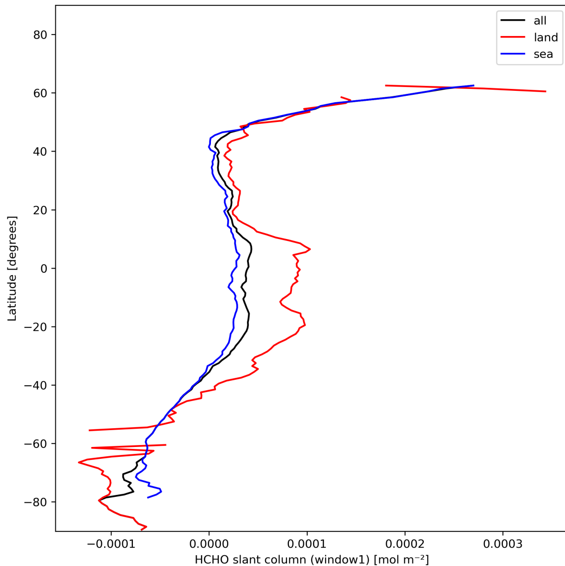
Figure 24: Zonal average of “HCHO slant column (window1)” for 2024-01-06 to 2024-01-08.
