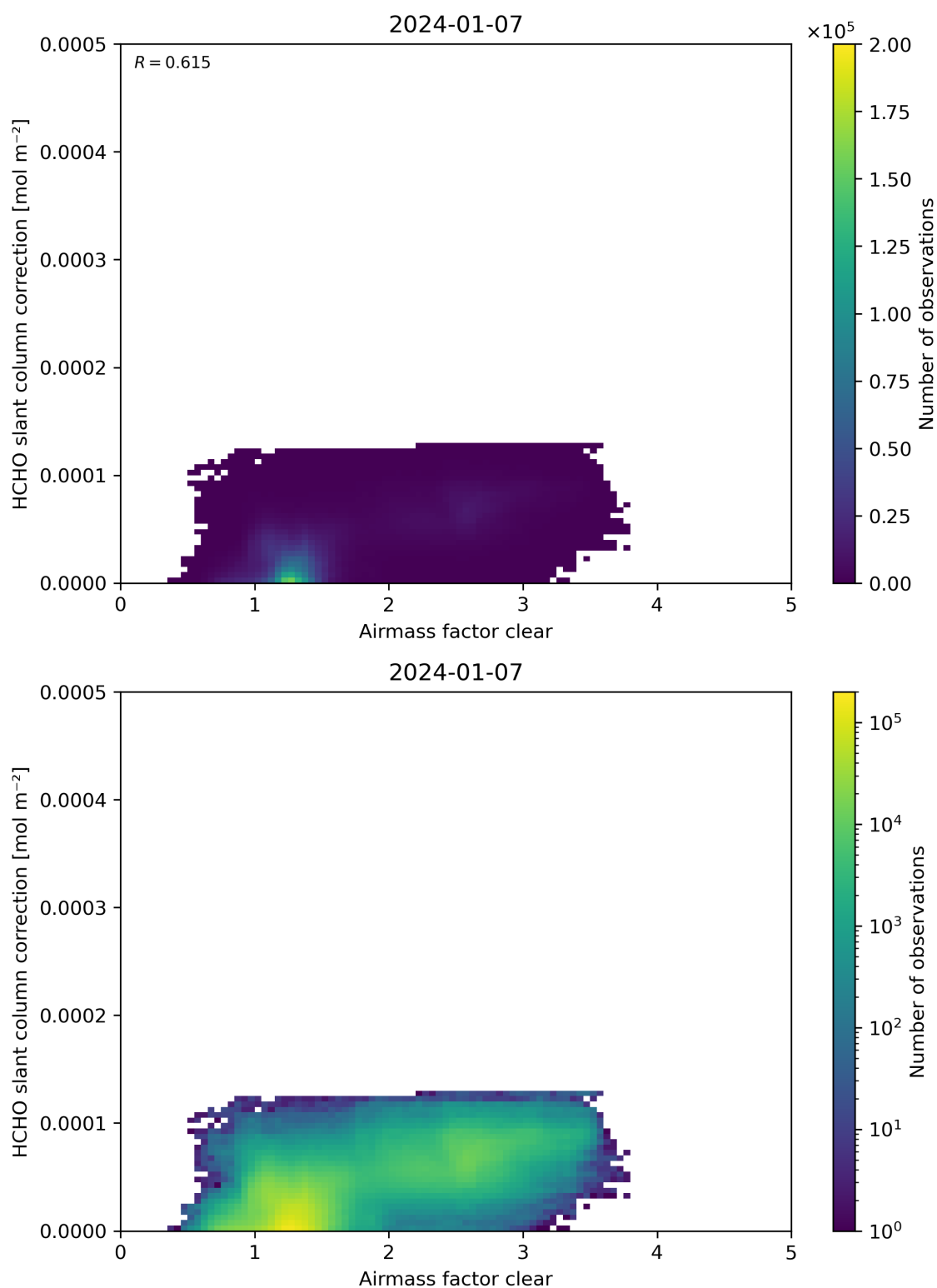
Figure 75: Scatter density plot of “Airmass factor clear” against “HCHO slant column correction” for 2024-01-06 to 2024-01-08.
