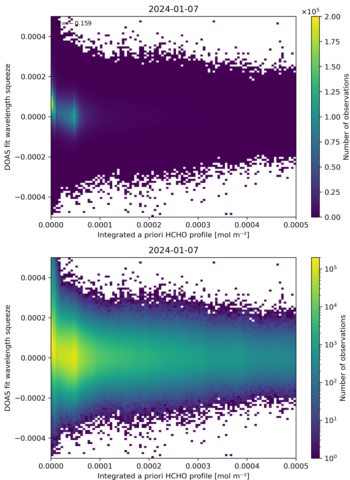
Figure 150: Scatter density plot of “Integrated a priori HCHO profile” against “DOAS fit wavelength squeeze” for 2024-01-06 to 2024-01-08.
