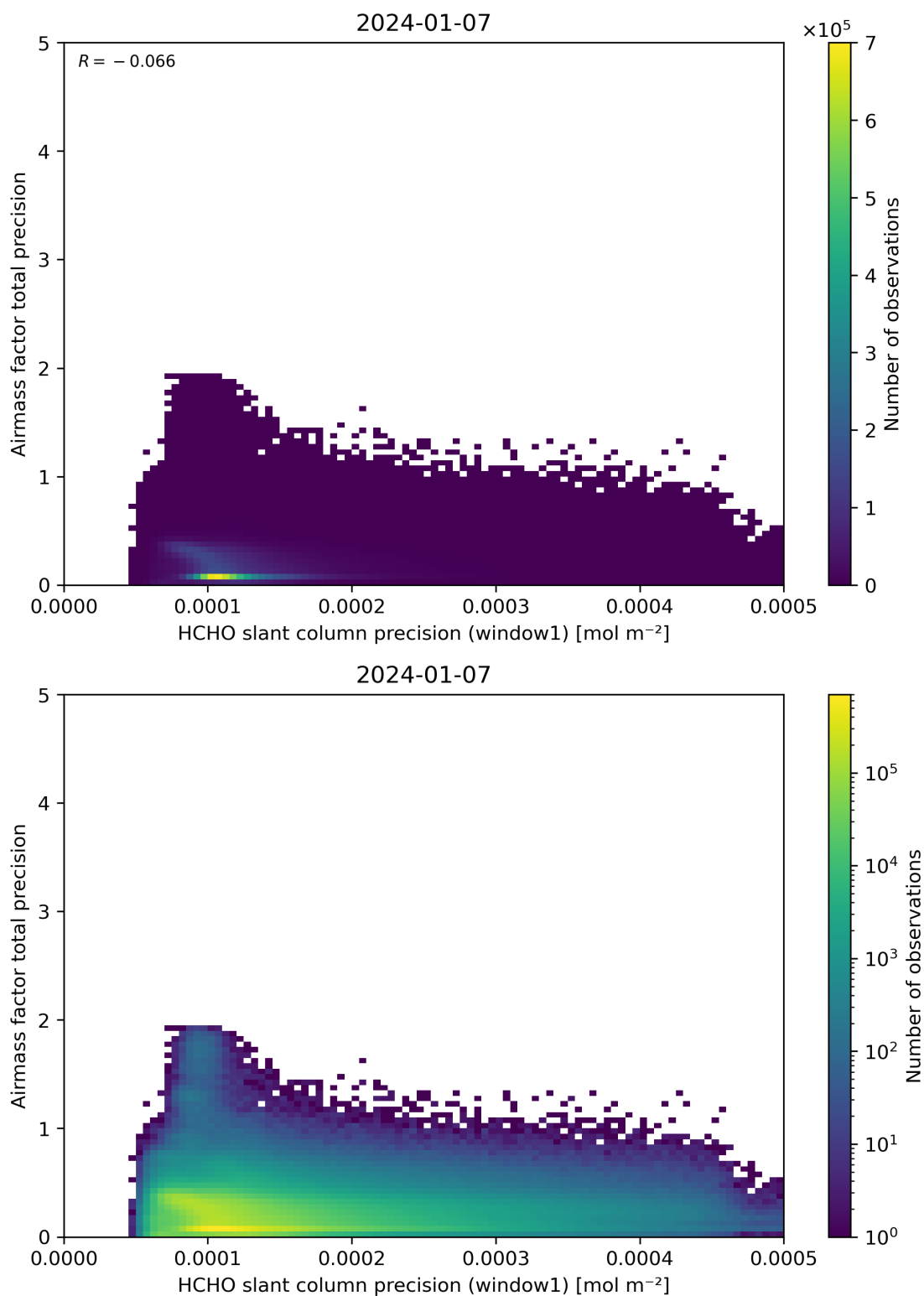
Figure 95: Scatter density plot of “HCHO slant column precision (window1)” against “Airmass factor total precision” for 2024-01-06 to 2024-01-08.
