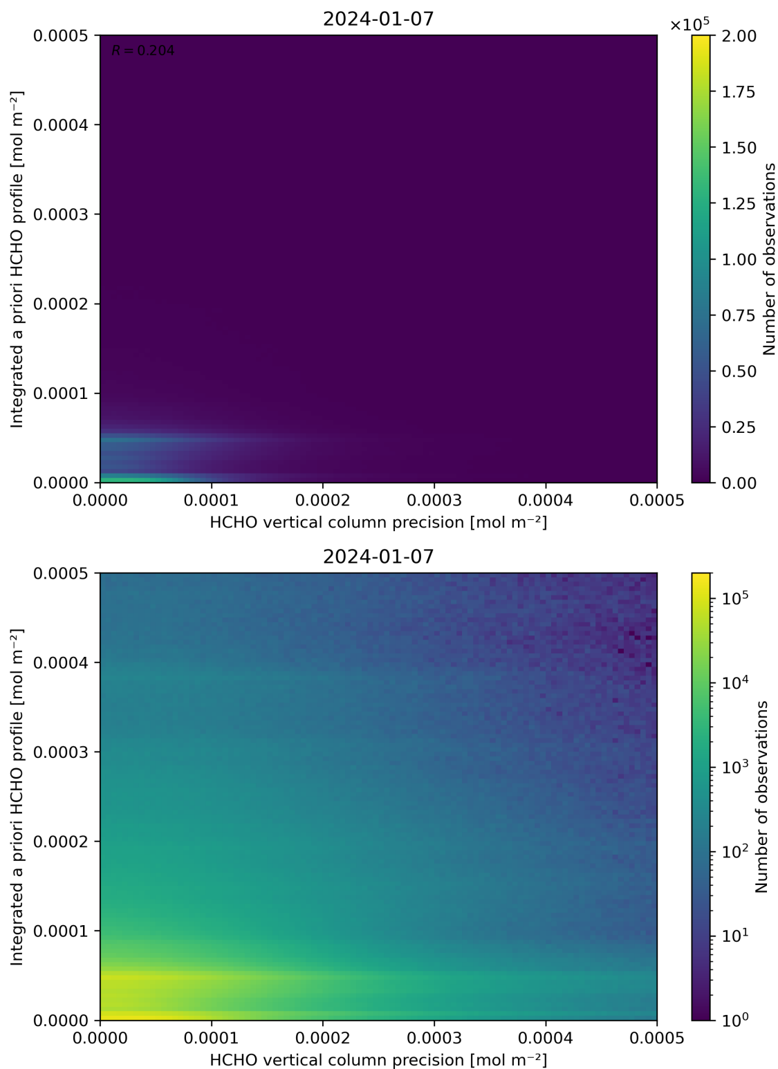
Figure 147: Scatter density plot of “HCHO vertical column precision” against “Integrated a priori HCHO profile” for 2024-01-06 to 2024-01-08.
