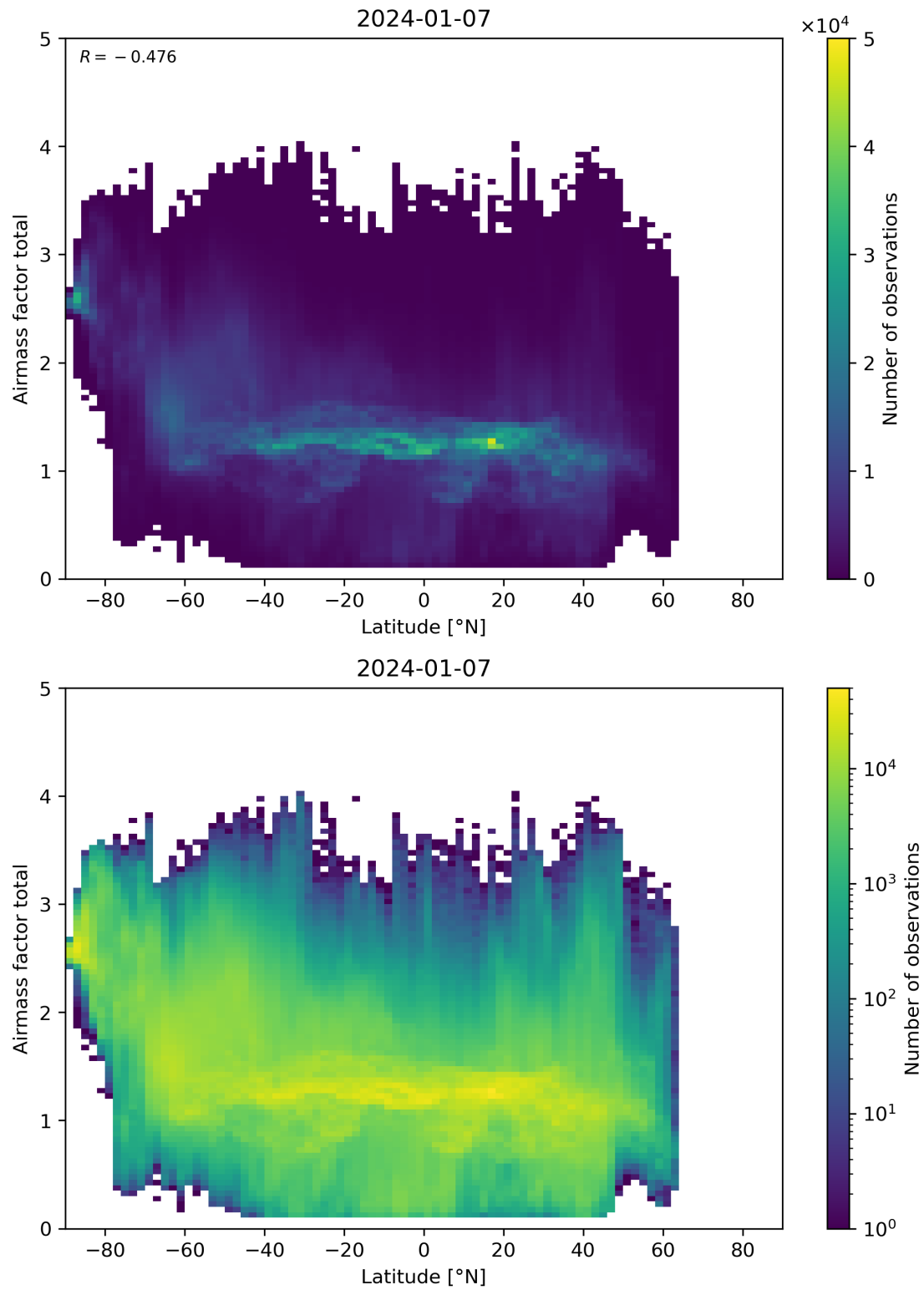
Figure 161: Scatter density plot of “Latitude” against “Airmass factor total” for 2024-01-06 to 2024-01-08.
