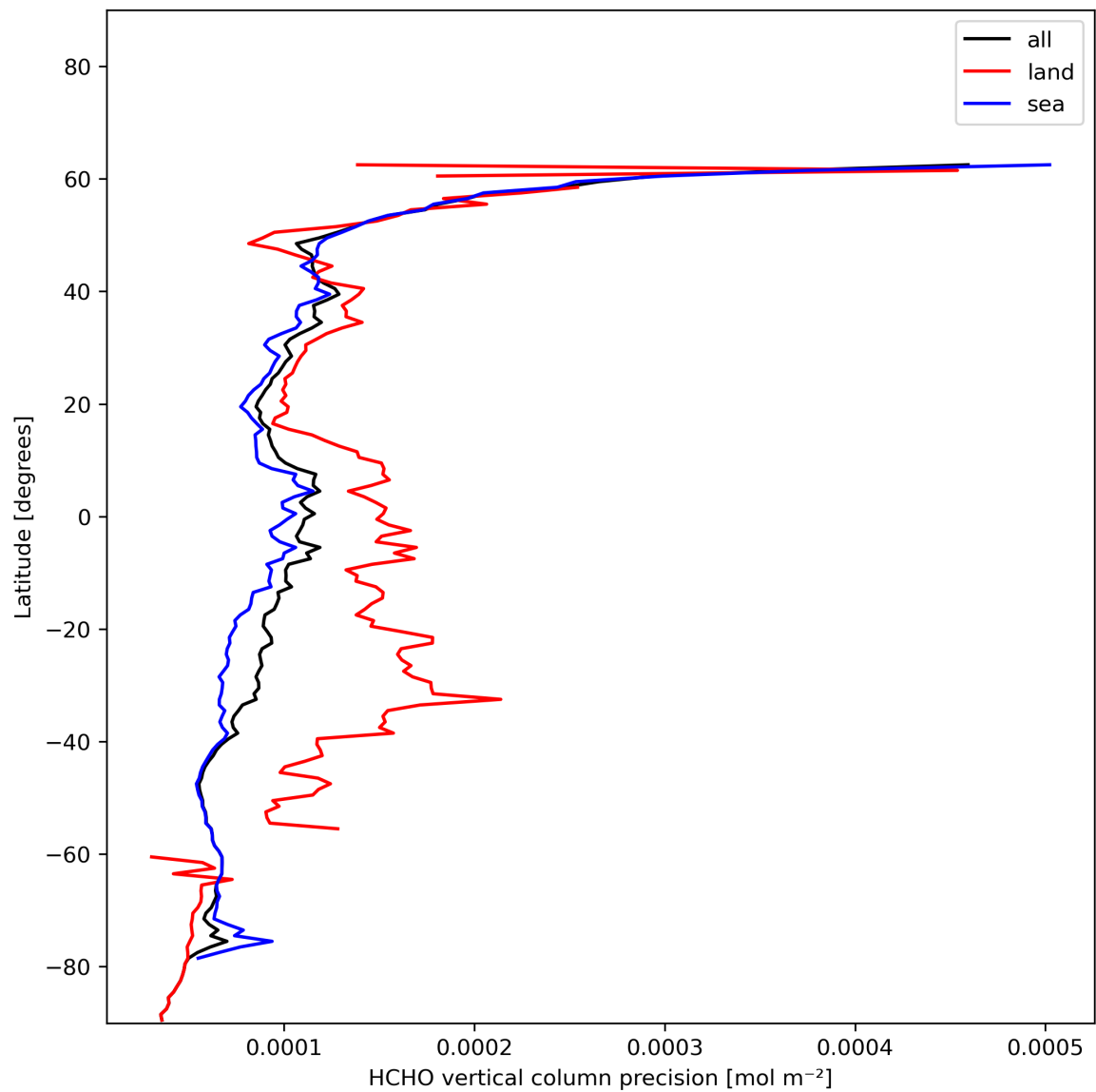
Figure 22: Zonal average of “HCHO vertical column precision” for 2024-01-06 to 2024-01-08.
