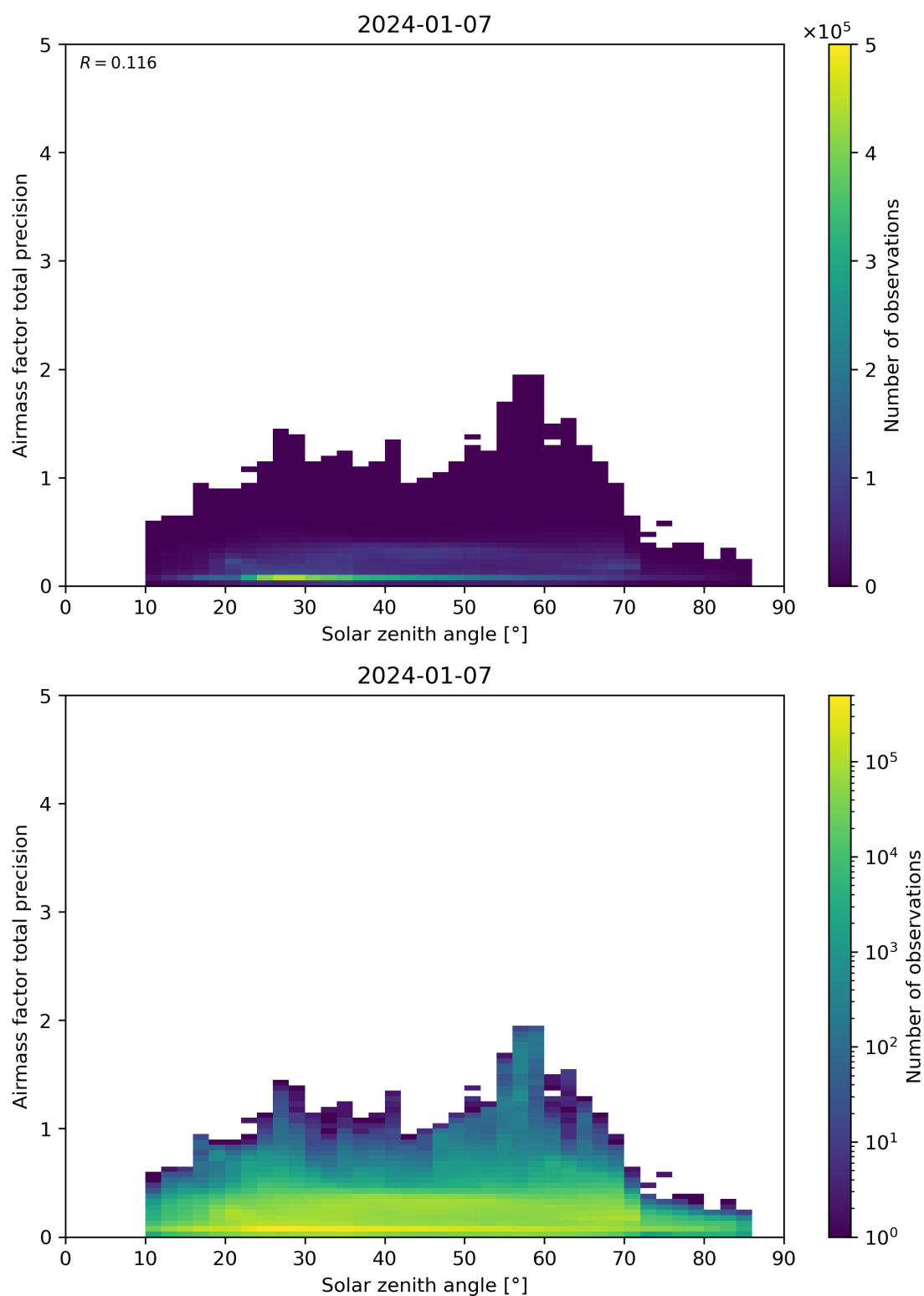
Figure 176: Scatter density plot of “Solar zenith angle” against “Airmass factor total precision” for 2024-01-06 to 2024-01-08.
