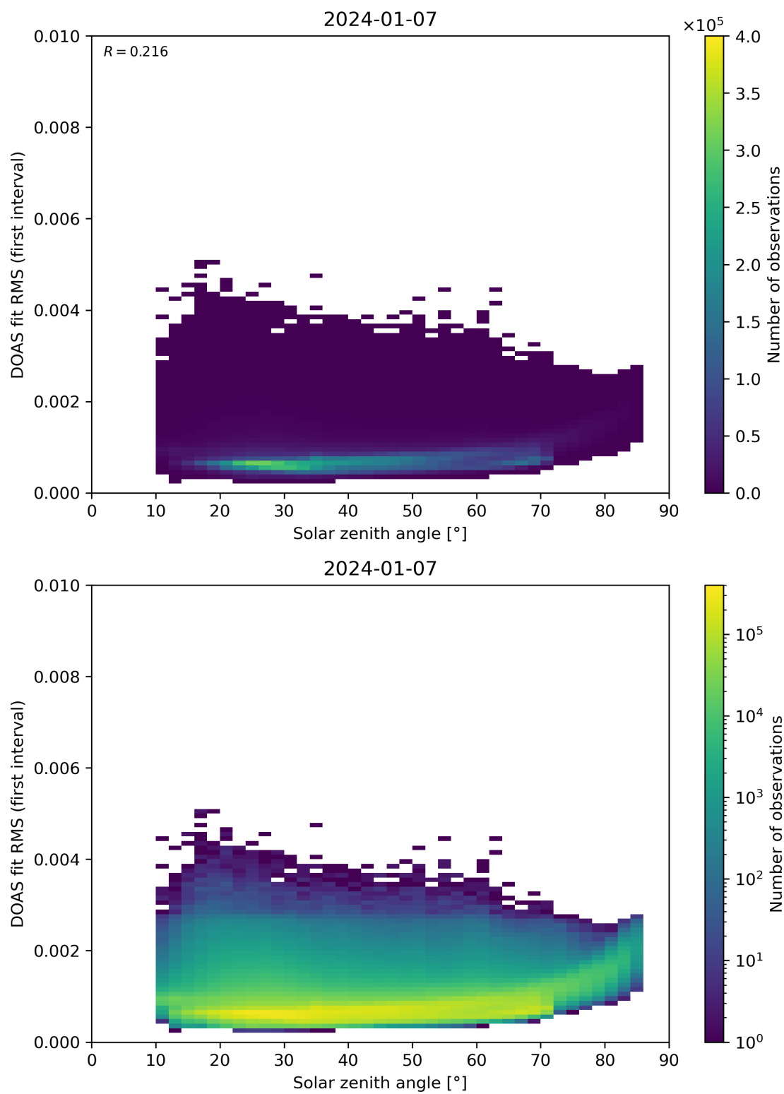
Figure 167: Scatter density plot of “Solar zenith angle” against “DOAS fit RMS (first interval)” for 2024-01-06 to 2024-01-08.
