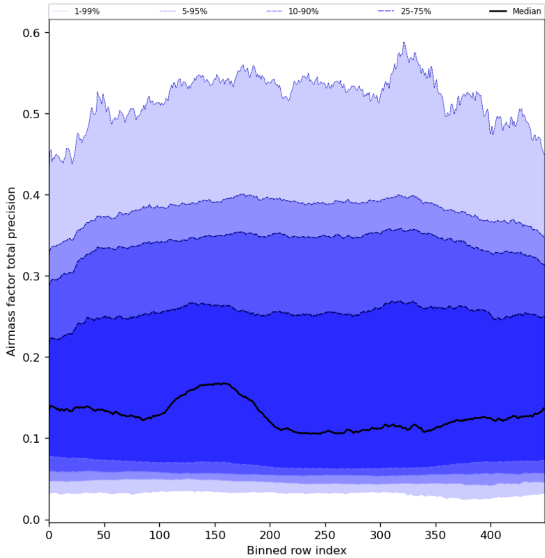
Figure 55: Along track statistics of “Airmass factor total precision” for 2024-01-06 to 2024-01-08
