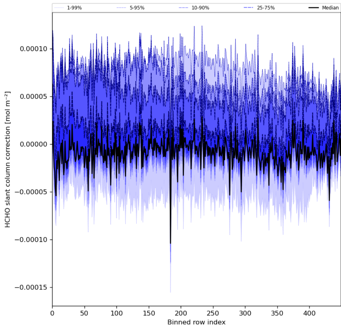
Figure 61: Along track statistics of “HCHO slant column correction” for 2024-01-06 to 2024-01-08
