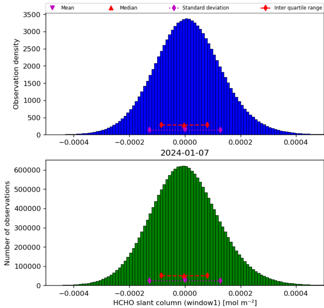
Figure 38: Histogram of “HCHO slant column (window1)” for 2024-01-06 to 2024-01-08
