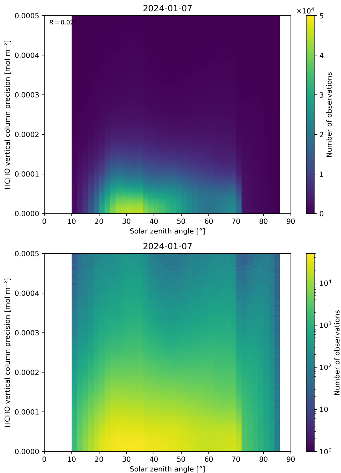
Figure 179: Scatter density plot of “Solar zenith angle” against “HCHO vertical column precision” for 2024-01-06 to 2024-01-08.
