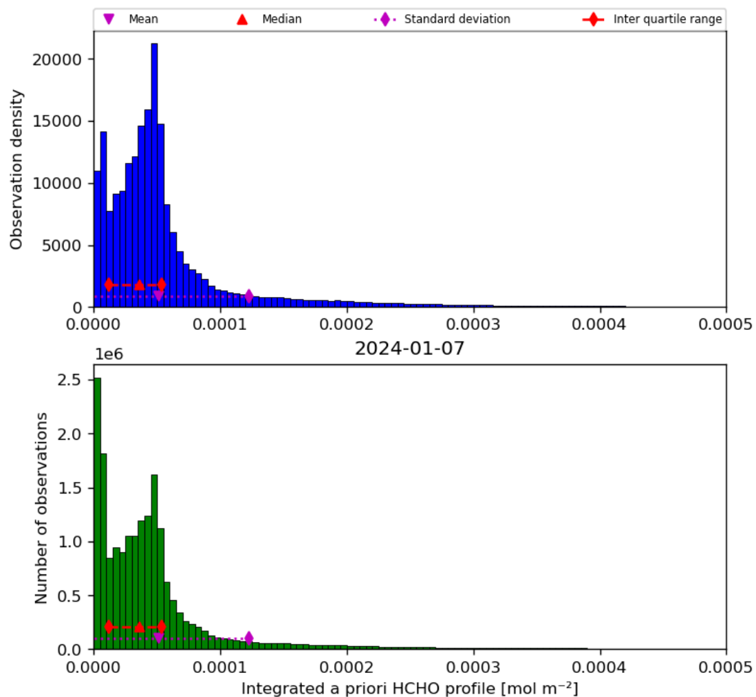
Figure 43: Histogram of “Integrated a priori HCHO profile” for 2024-01-06 to 2024-01-08
