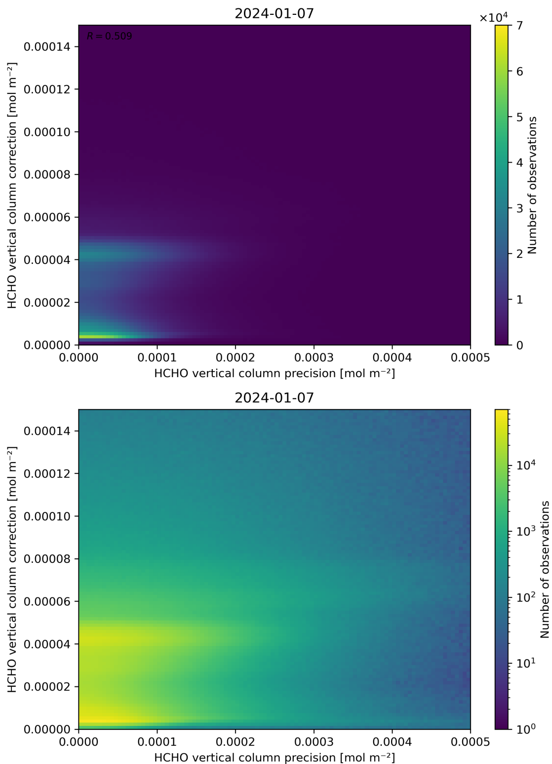
Figure 146: Scatter density plot of “HCHO vertical column precision” against “HCHO vertical column correction” for 2024-01-06 to 2024-01-08.
