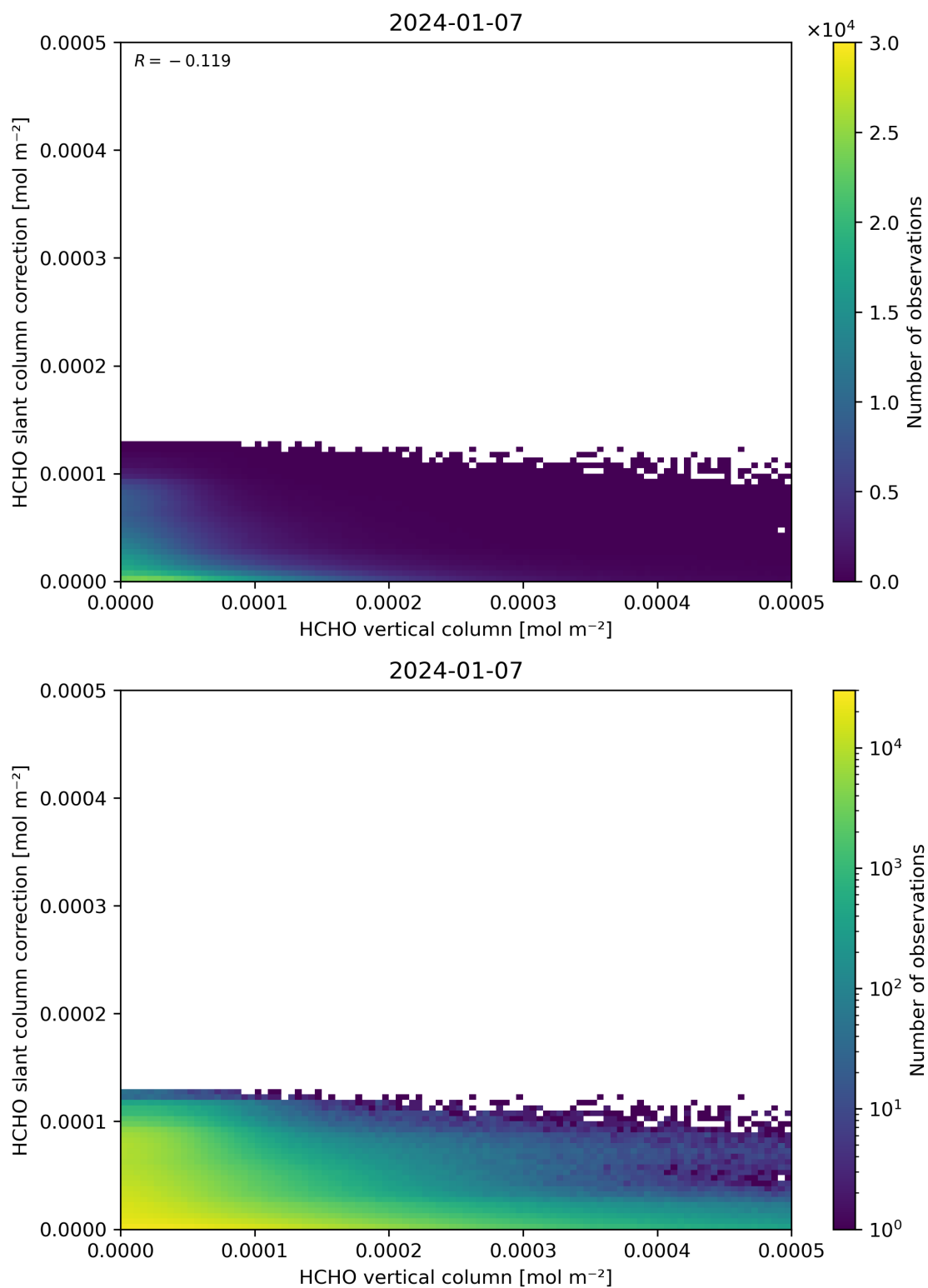
Figure 128: Scatter density plot of “HCHO vertical column” against “HCHO slant column correction” for 2024-01-06 to 2024-01-08.
