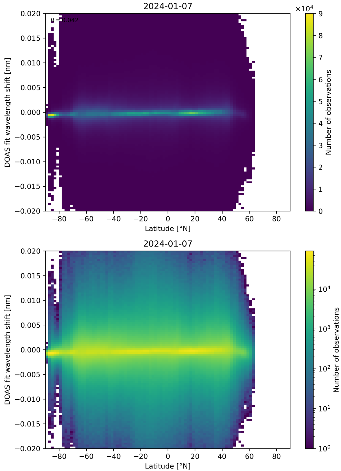
Figure 154: Scatter density plot of “Latitude” against “DOAS fit wavelength shift” for 2024-01-06 to 2024-01-08.
