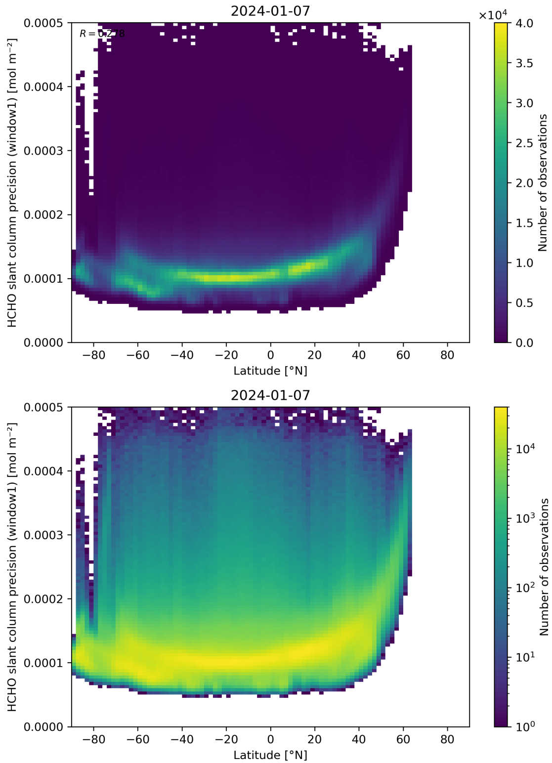
Figure 160: Scatter density plot of “Latitude” against “HCHO slant column precision (window1)” for 2024-01-06 to 2024-01-08.
