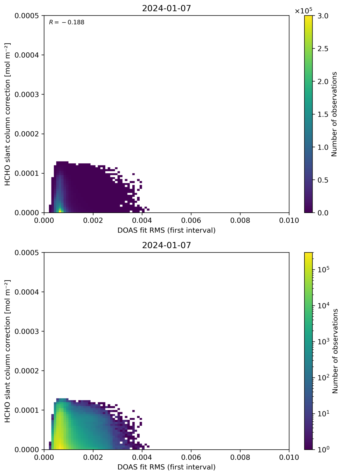
Figure 63: Scatter density plot of “DOAS fit RMS (first interval)” against “HCHO slant column correction” for 2024-01-06 to 2024-01-08.
