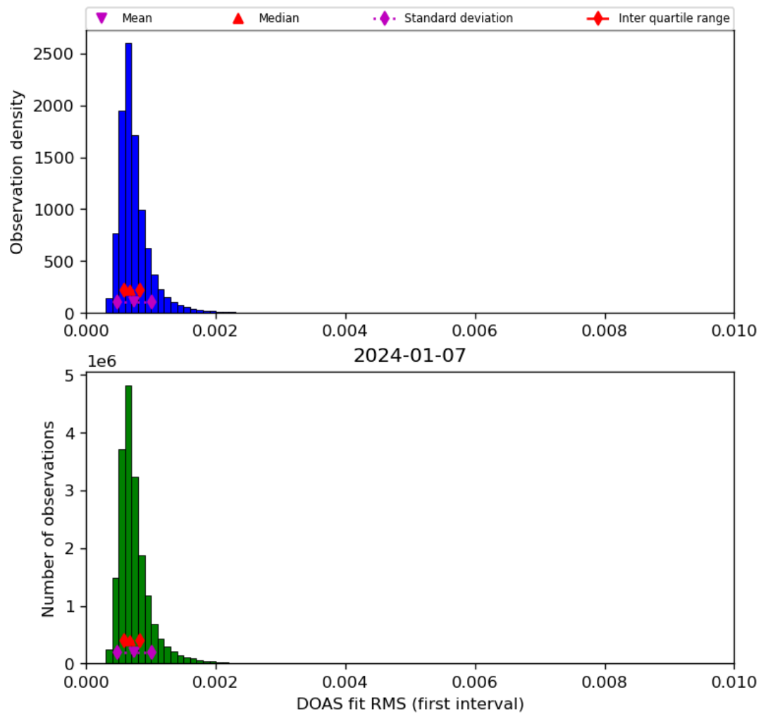
Figure 46: Histogram of “DOAS fit RMS (first interval)” for 2024-01-06 to 2024-01-08
