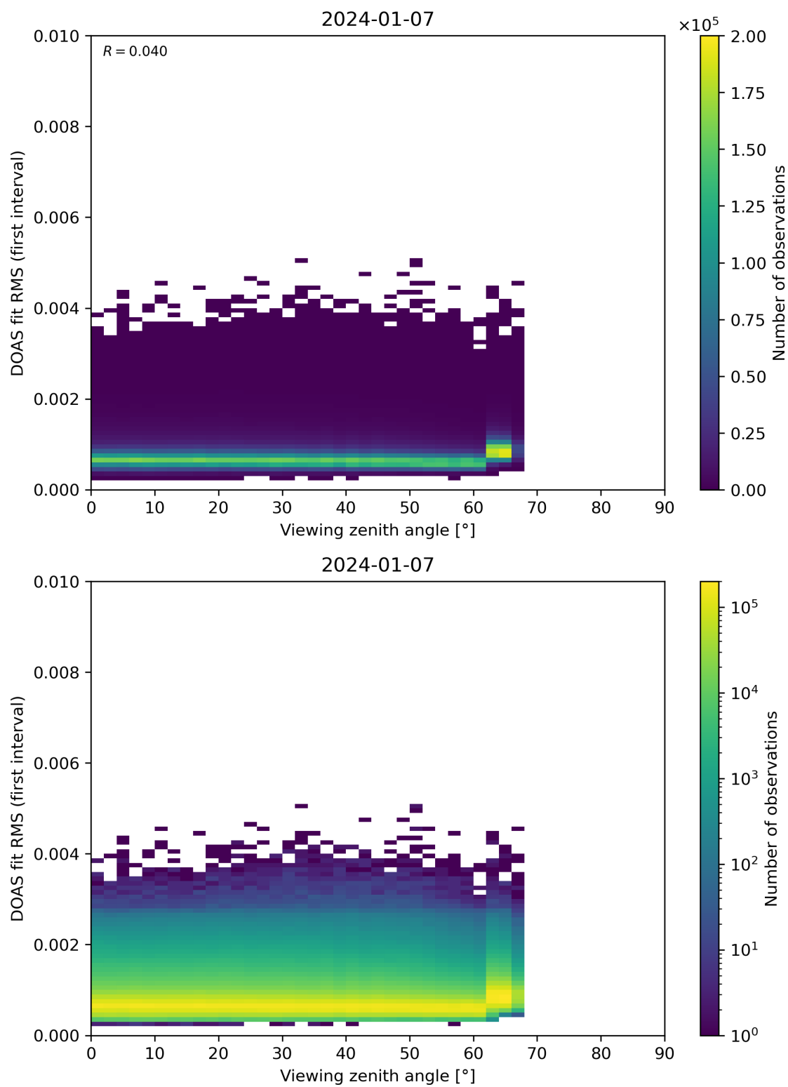
Figure 182: Scatter density plot of “Viewing zenith angle” against “DOAS fit RMS (first interval)” for 2024-01-06 to 2024-01-08.
