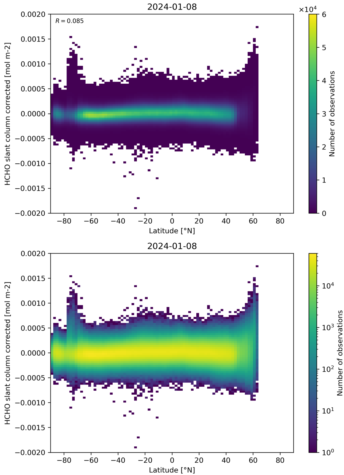
Figure 157: Scatter density plot of “Latitude” against “HCHO slant column corrected” for 2024-01-07 to 2024-01-09.
