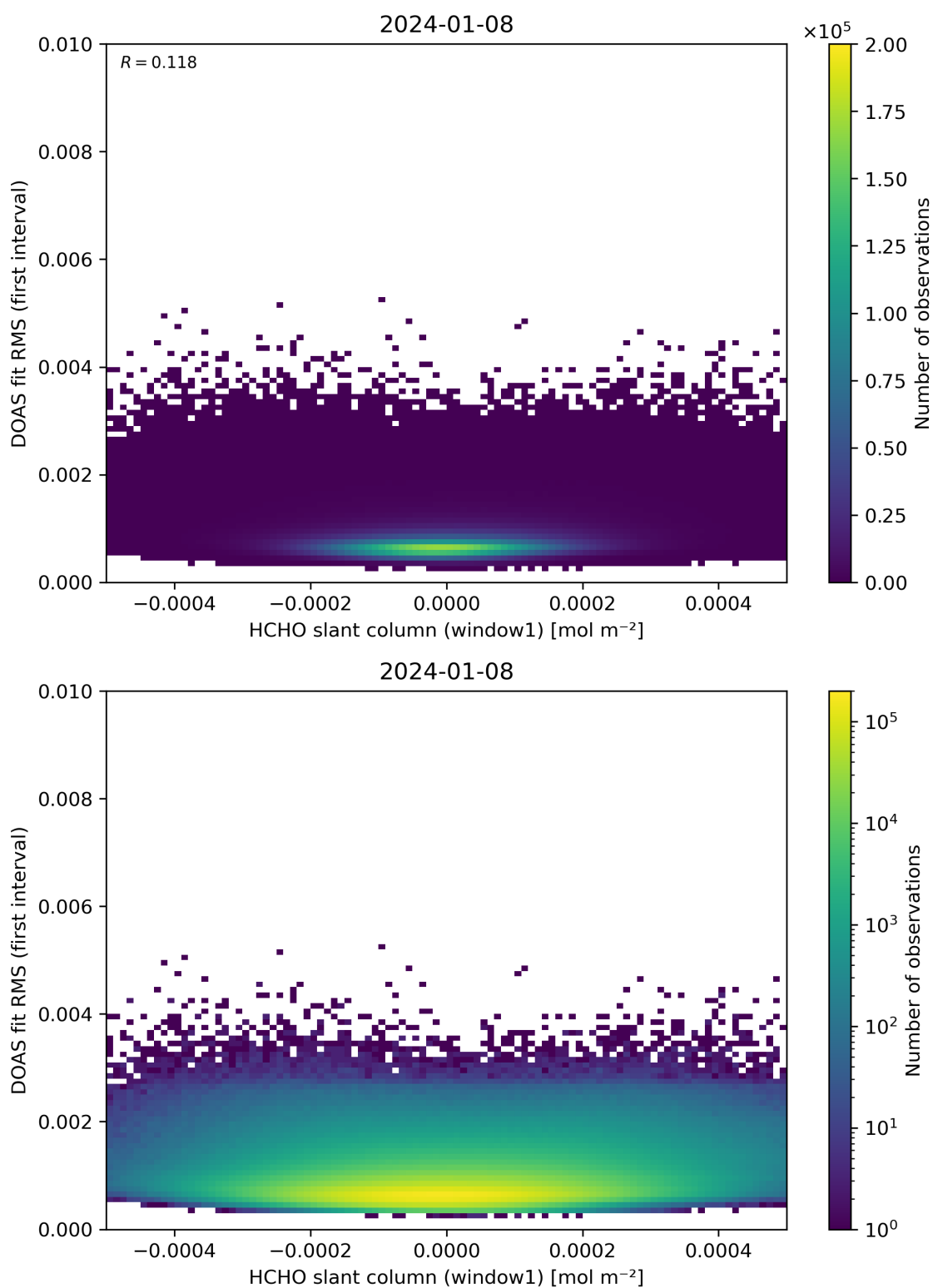
Figure 78: Scatter density plot of “HCHO slant column (window1)” against “DOAS fit RMS (first interval)” for 2024-01-07 to 2024-01-09.
