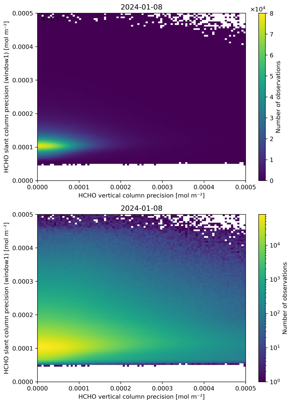
Figure 143: Scatter density plot of “HCHO vertical column precision” against “HCHO slant column precision (window1)” for 2024-01-07 to 2024-01-09.
