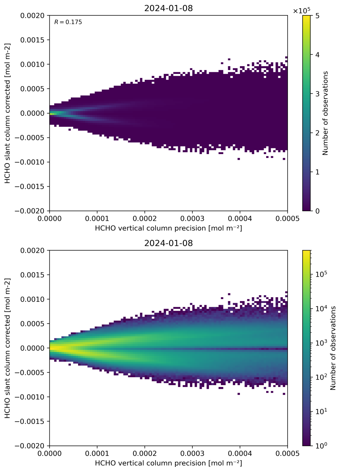
Figure 140: Scatter density plot of “HCHO vertical column precision” against “HCHO slant column corrected” for 2024-01-07 to 2024-01-09.
