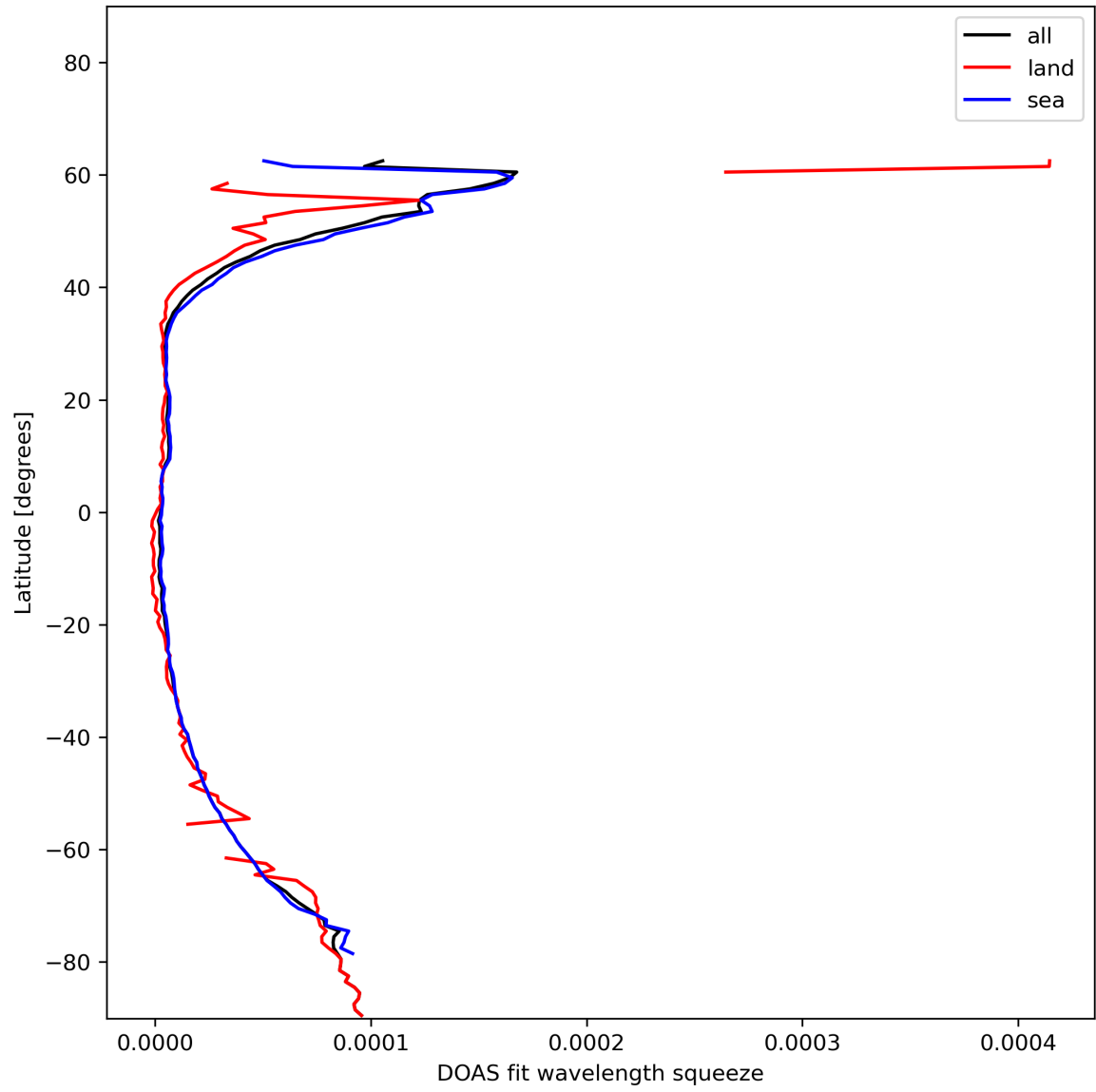
Figure 31: Zonal average of “DOAS fit wavelength squeeze” for 2024-01-07 to 2024-01-09.
