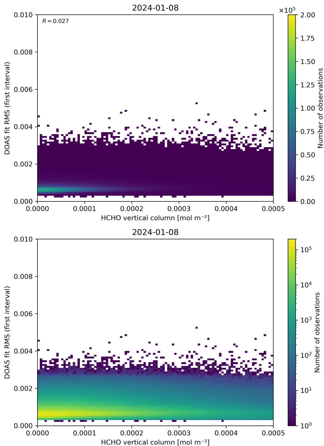
Figure 123: Scatter density plot of “HCHO vertical column” against “DOAS fit RMS (first interval)” for 2024-01-07 to 2024-01-09.
