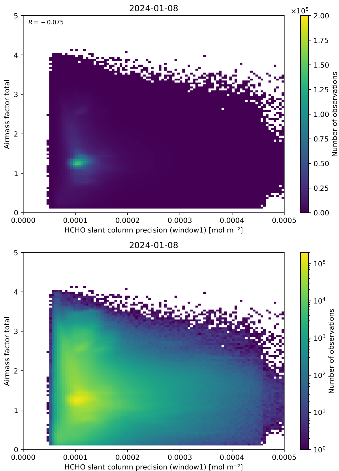
Figure 94: Scatter density plot of “HCHO slant column precision (window1)” against “Airmass factor total” for 2024-01-07 to 2024-01-09.
