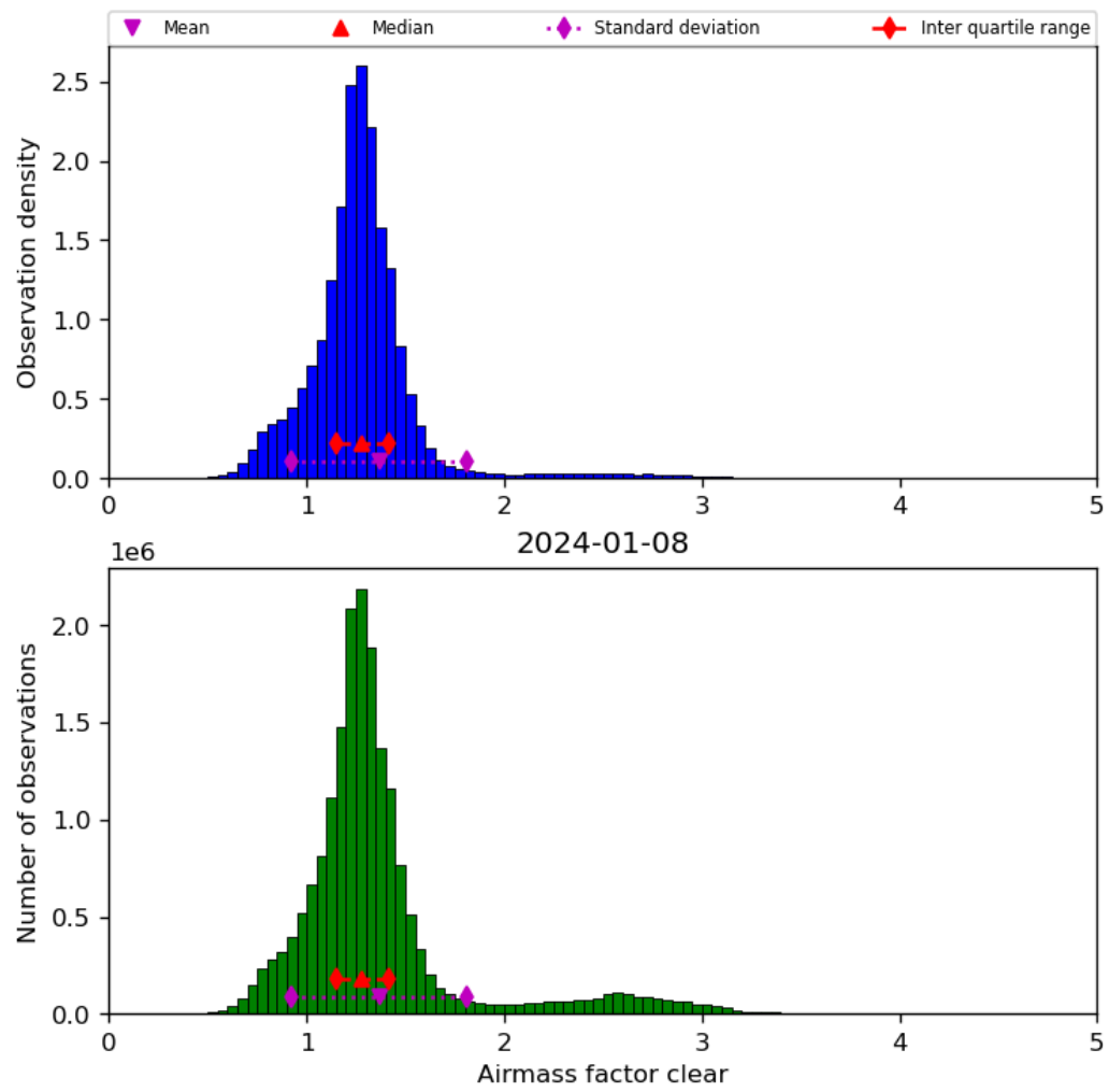
Figure 42: Histogram of “Airmass factor clear” for 2024-01-07 to 2024-01-09
