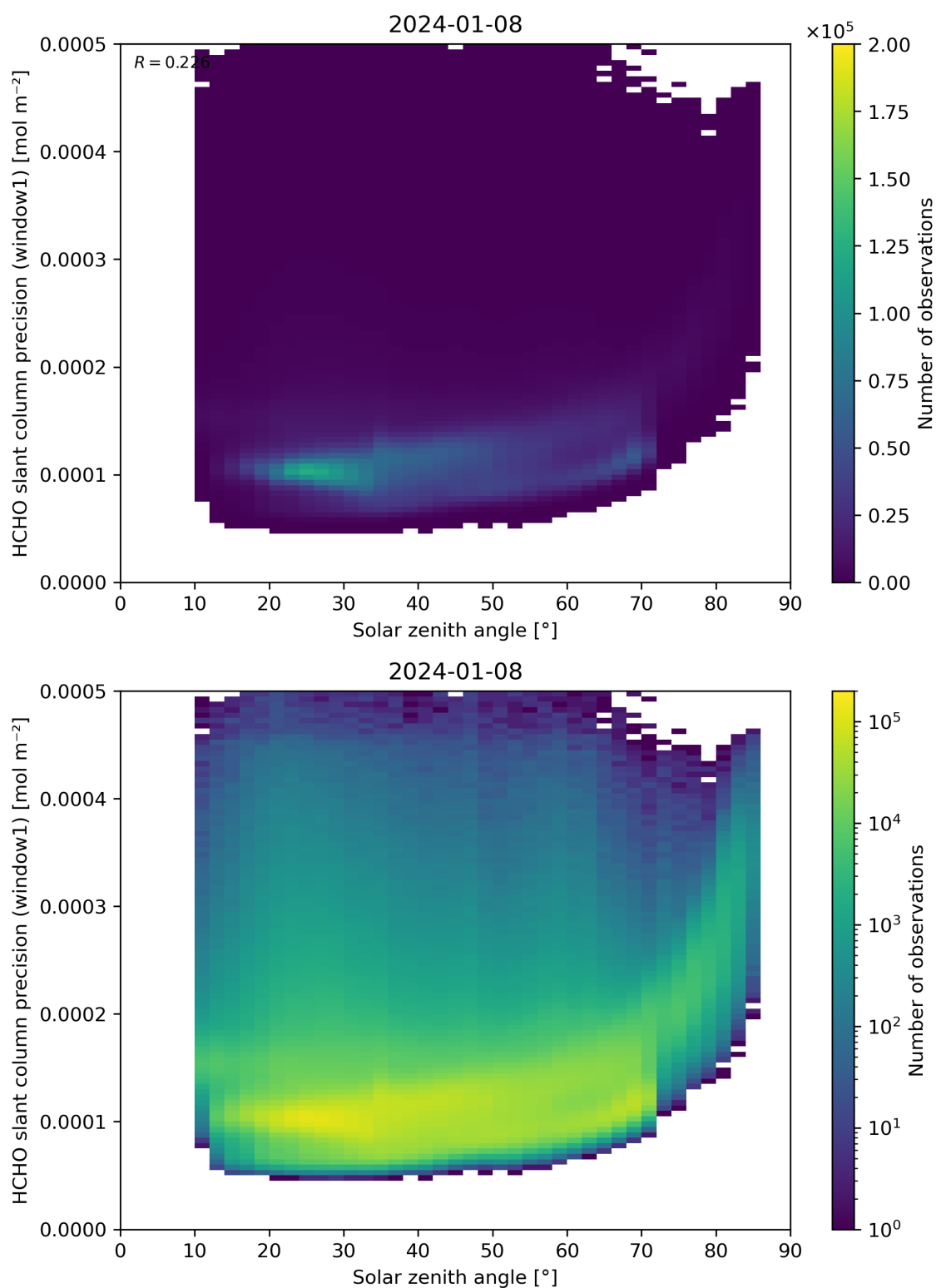
Figure 174: Scatter density plot of “Solar zenith angle” against “HCHO slant column precision (window1)” for 2024-01-07 to 2024-01-09.
