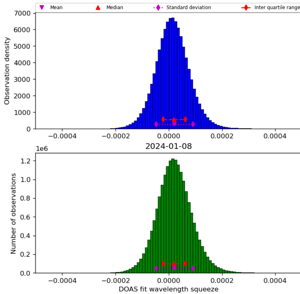
Figure 45: Histogram of “DOAS fit wavelength squeeze” for 2024-01-07 to 2024-01-09
