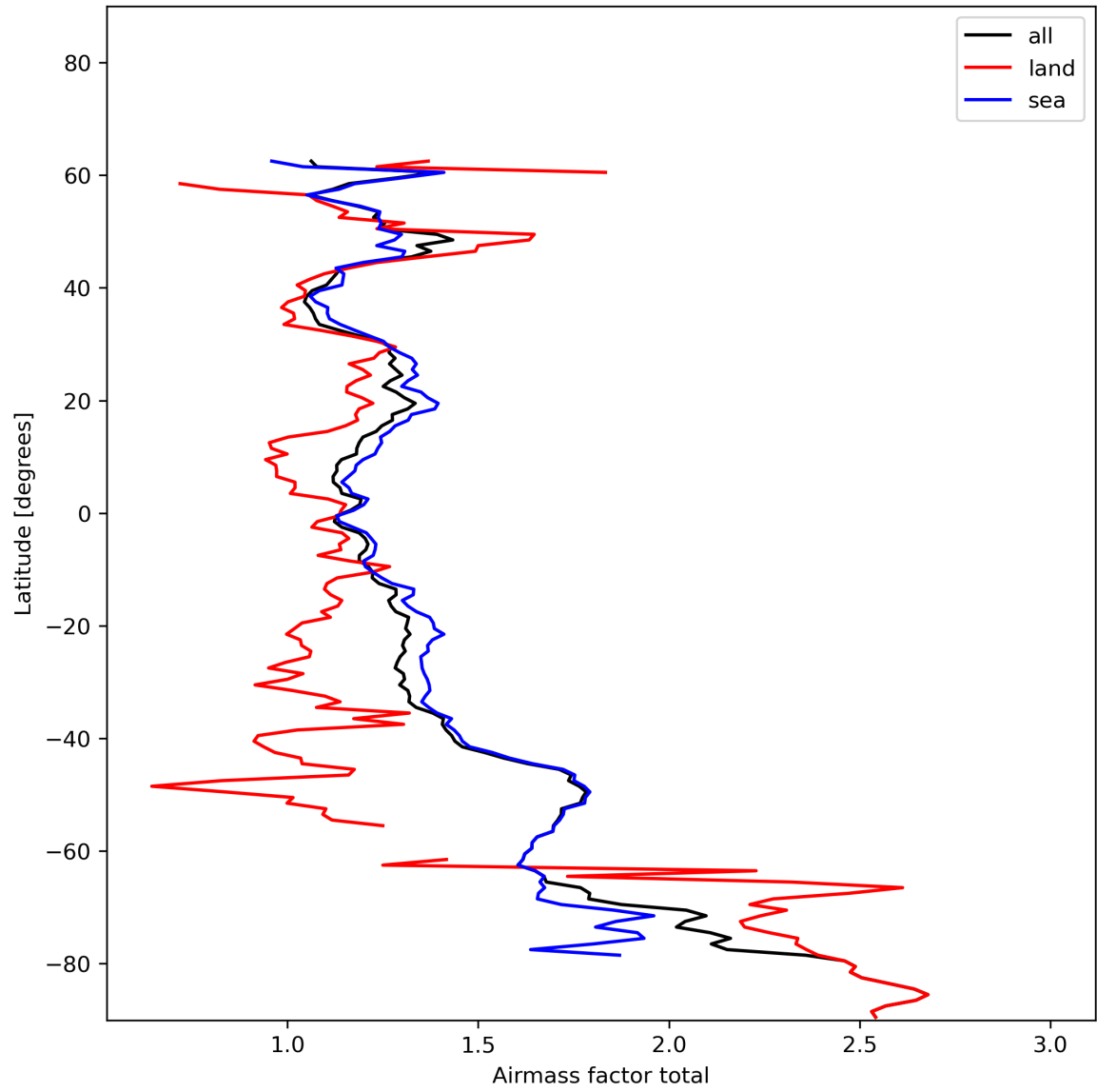
Figure 26: Zonal average of “Airmass factor total” for 2024-01-07 to 2024-01-09.
