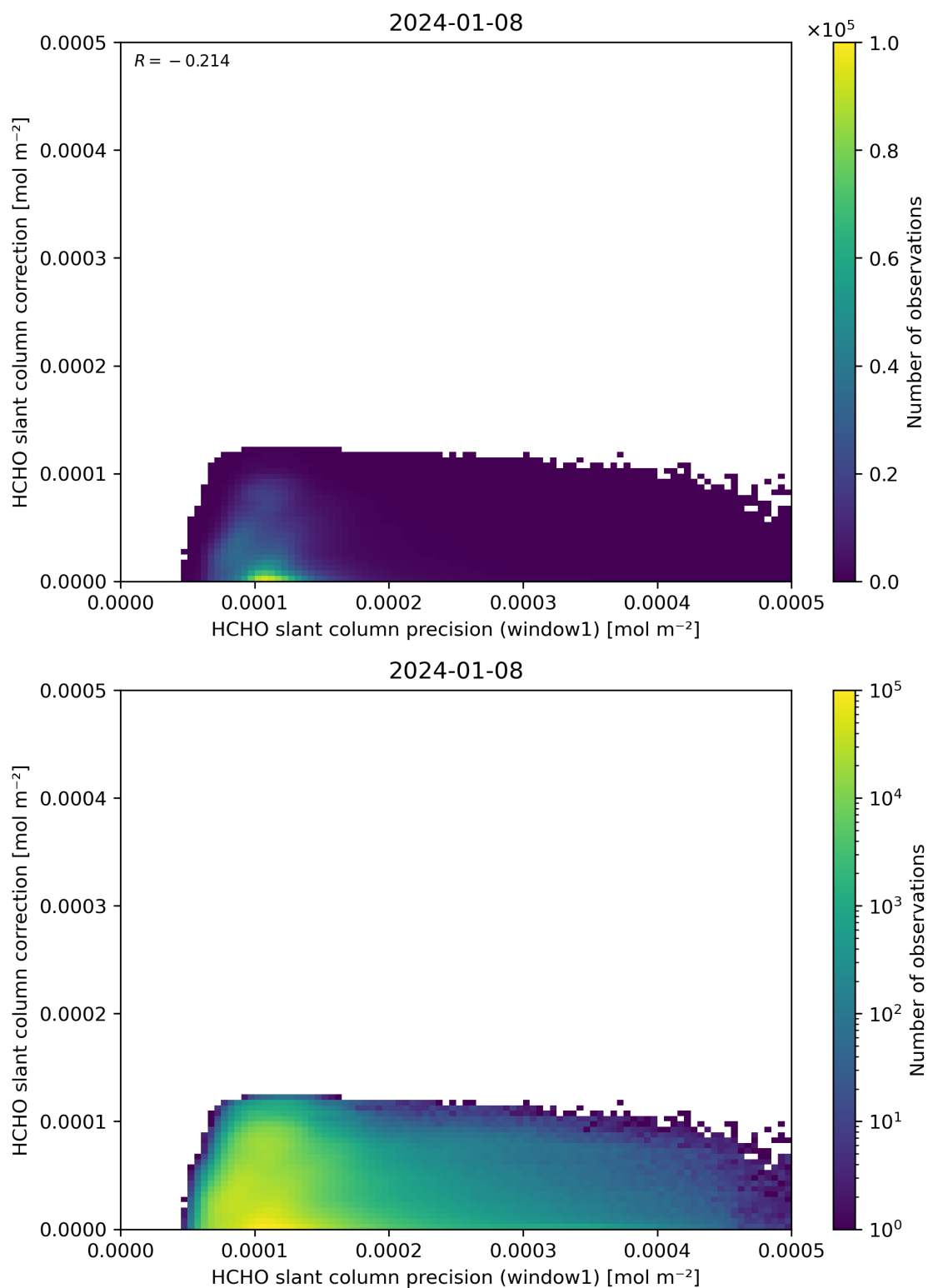
Figure 93: Scatter density plot of “HCHO slant column precision (window1)” against “HCHO slant column correction” for 2024-01-07 to 2024-01-09.
