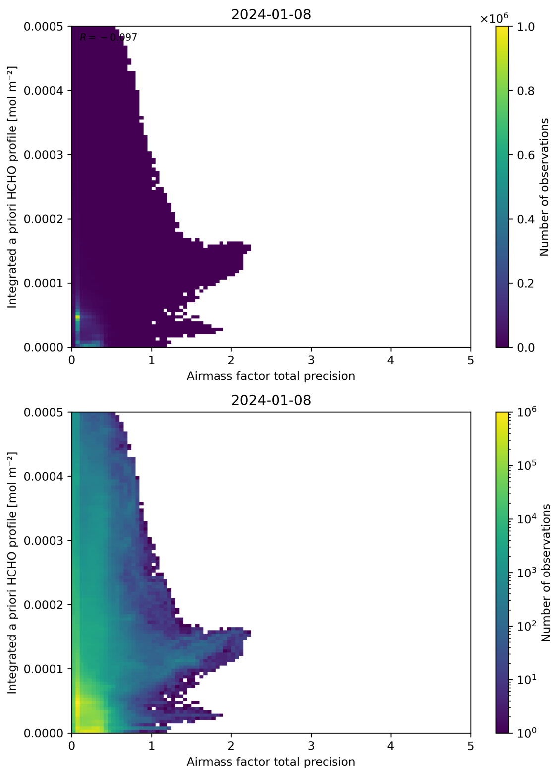
Figure 111: Scatter density plot of “Airmass factor total precision” against “Integrated a priori HCHO profile” for 2024-01-07 to 2024-01-09.
