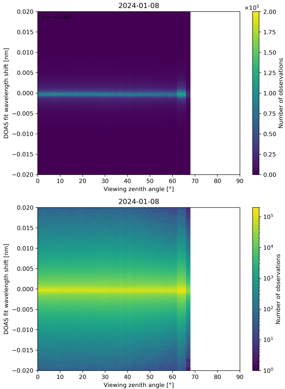
Figure 183: Scatter density plot of “Viewing zenith angle” against “DOAS fit wavelength shift” for 2024-01-07 to 2024-01-09.
