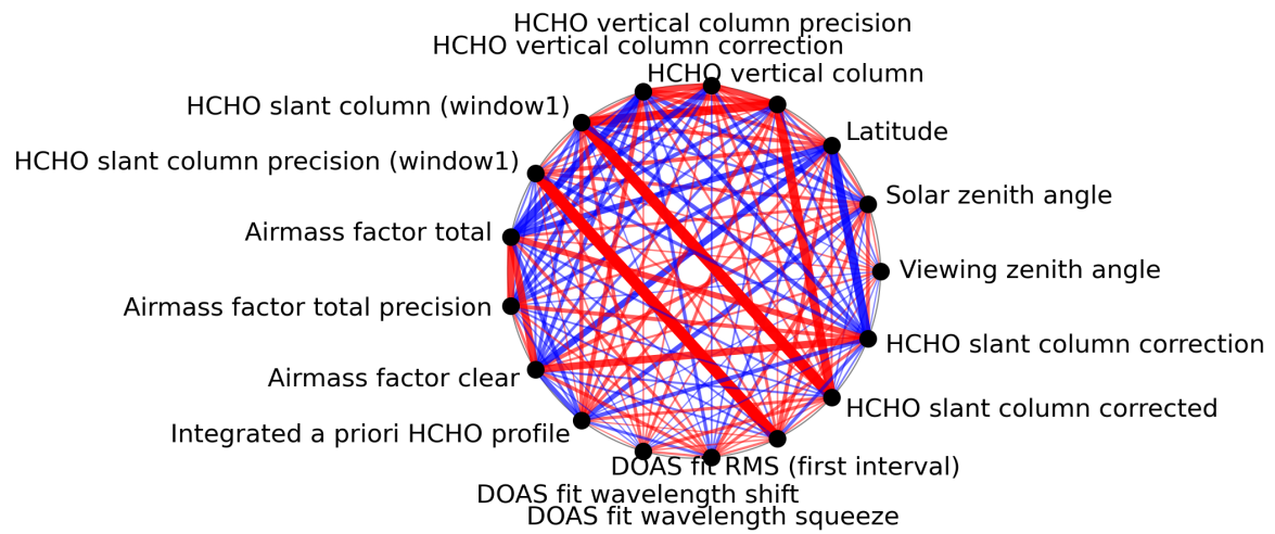
Figure 1: Map of correlation graph for 2024-01-07 to 2024-01-09.
