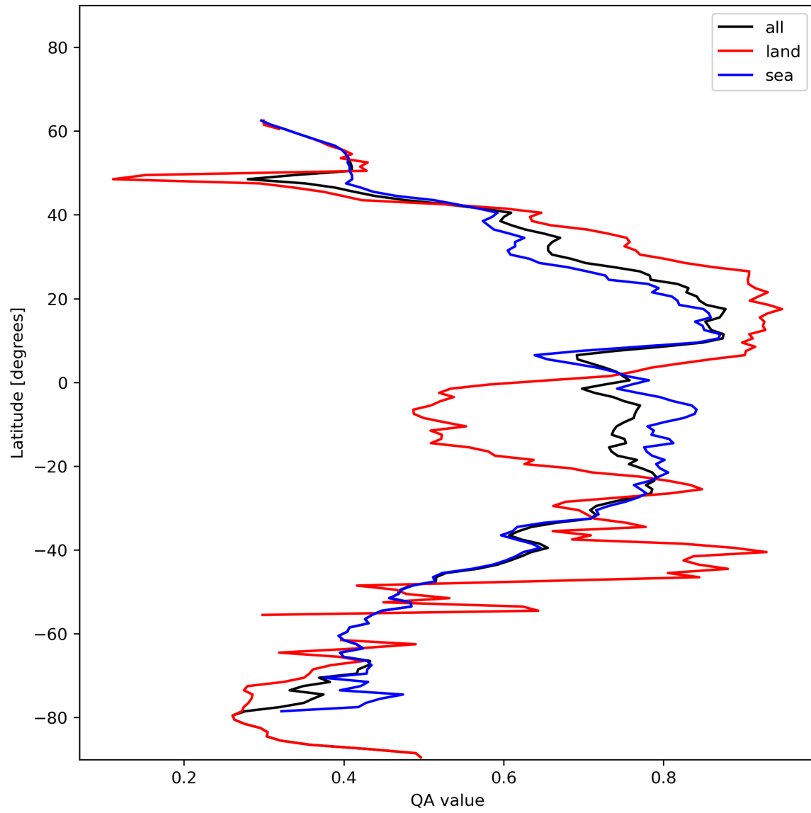
Figure 20: Zonal average of “QA value” for 2024-01-07 to 2024-01-09.
