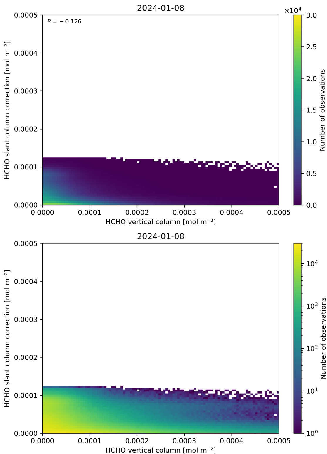
Figure 128: Scatter density plot of “HCHO vertical column” against “HCHO slant column correction” for 2024-01-07 to 2024-01-09.
