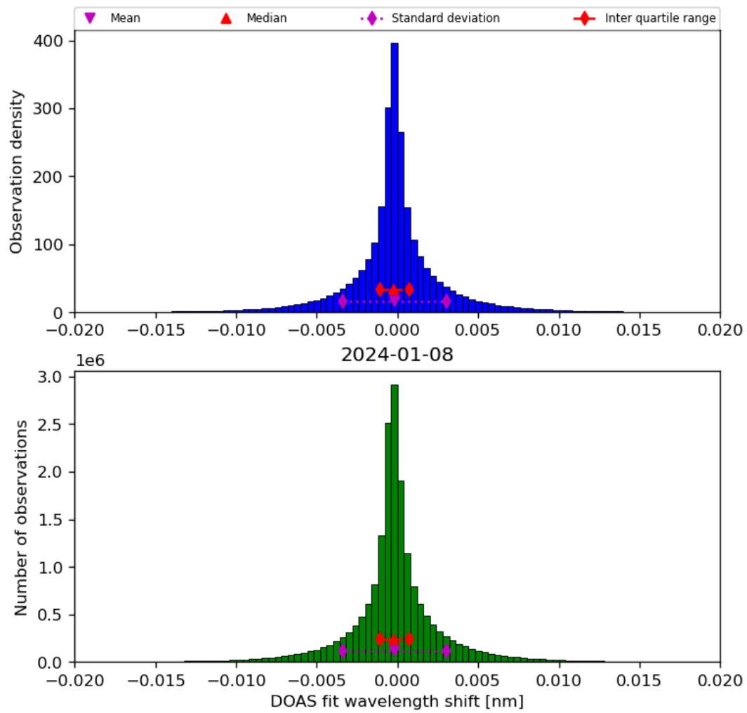
Figure 44: Histogram of “DOAS fit wavelength shift” for 2024-01-07 to 2024-01-09
