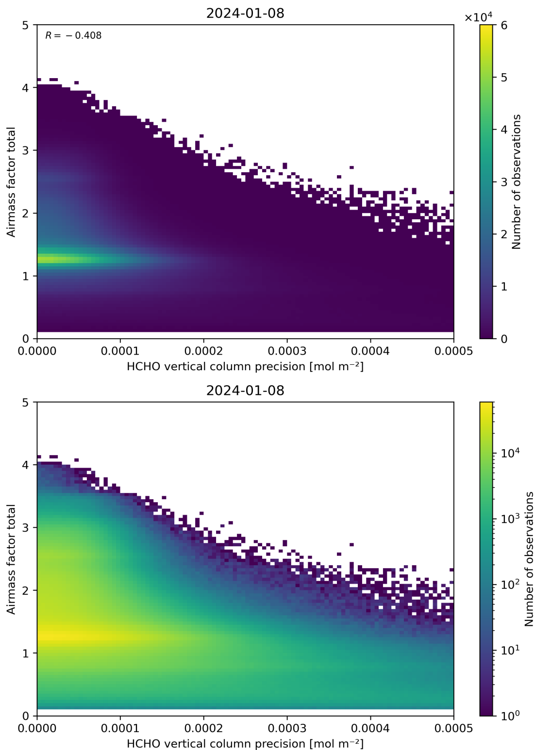
Figure 144: Scatter density plot of “HCHO vertical column precision” against “Airmass factor total” for 2024-01-07 to 2024-01-09.
