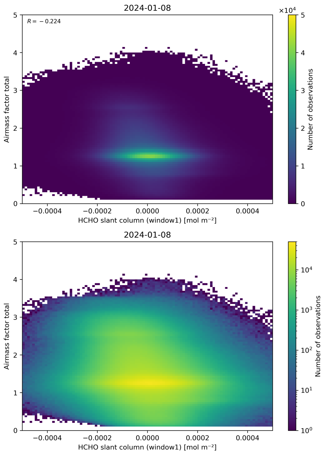
Figure 85: Scatter density plot of “HCHO slant column (window1)” against “Airmass factor total” for 2024-01-07 to 2024-01-09.
