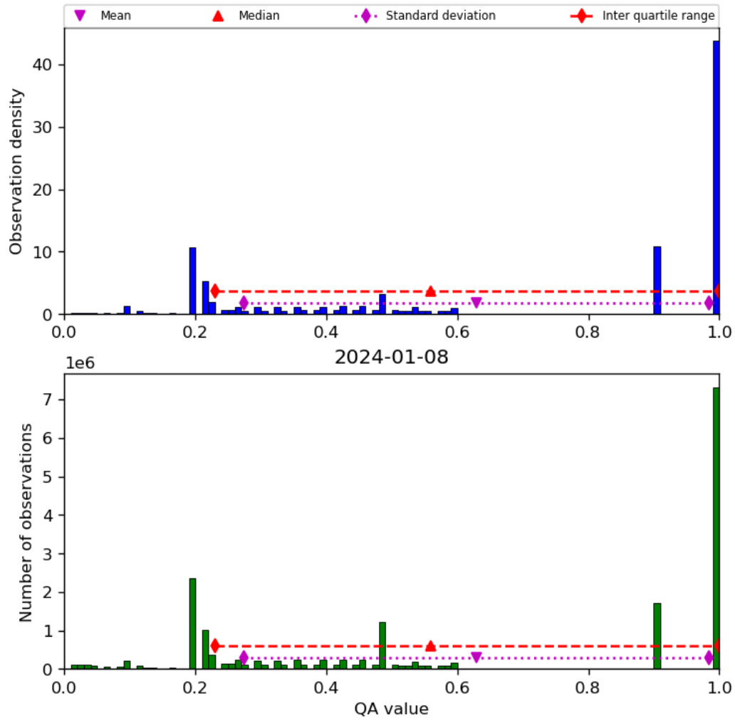
Figure 34: Histogram of “QA value” for 2024-01-07 to 2024-01-09
