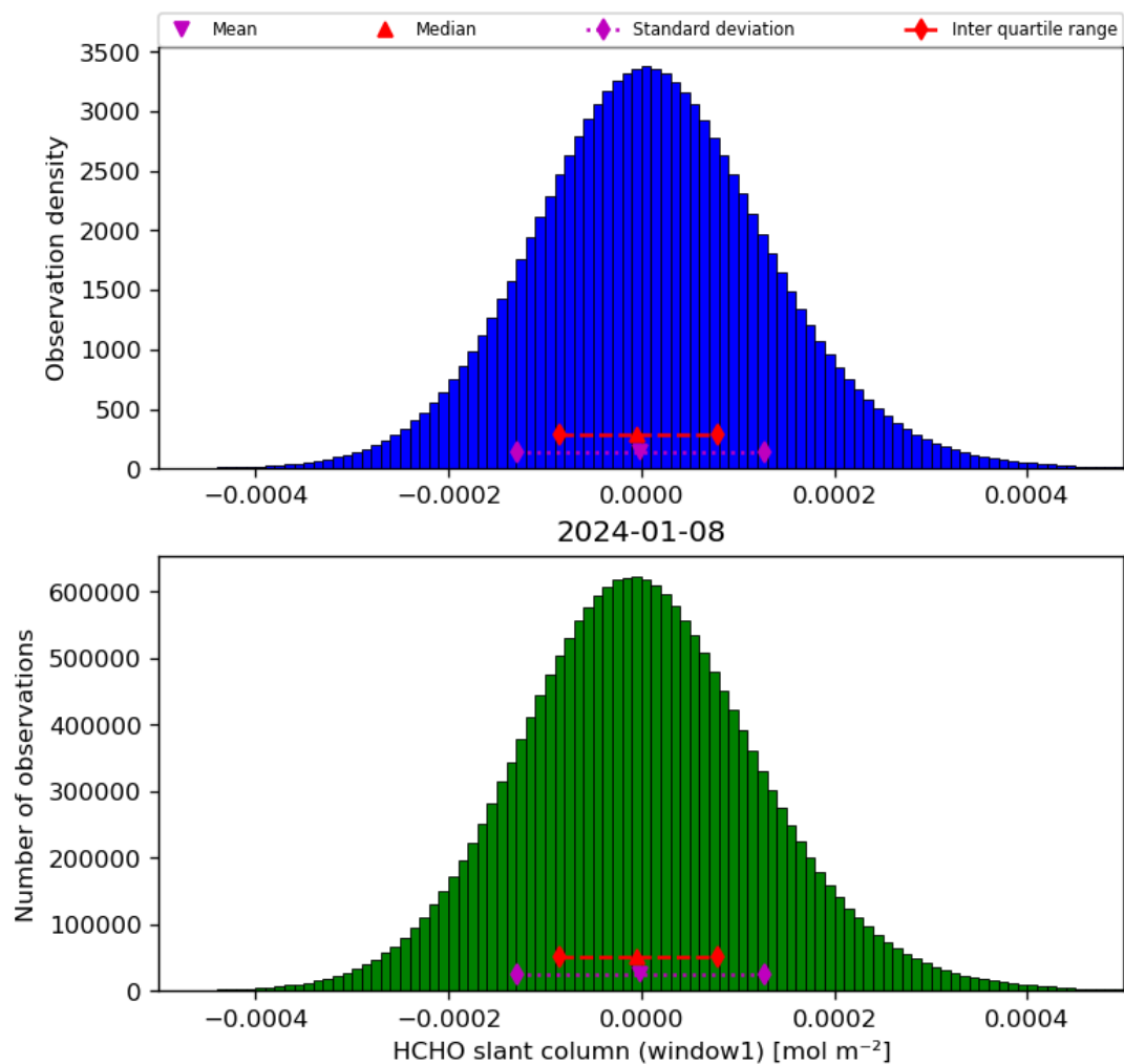
Figure 38: Histogram of “HCHO slant column (window1)” for 2024-01-07 to 2024-01-09
