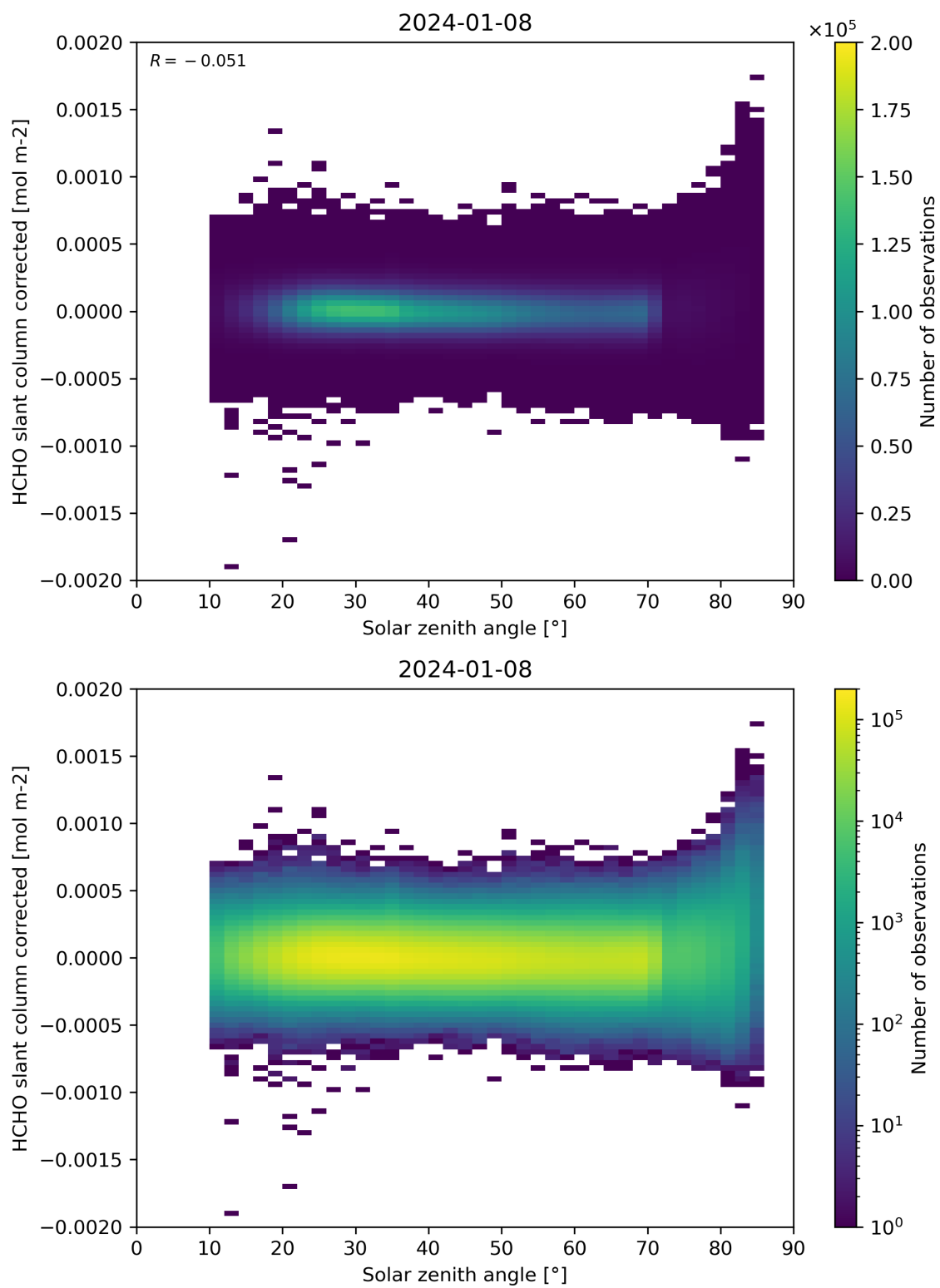
Figure 171: Scatter density plot of “Solar zenith angle” against “HCHO slant column corrected” for 2024-01-07 to 2024-01-09.
