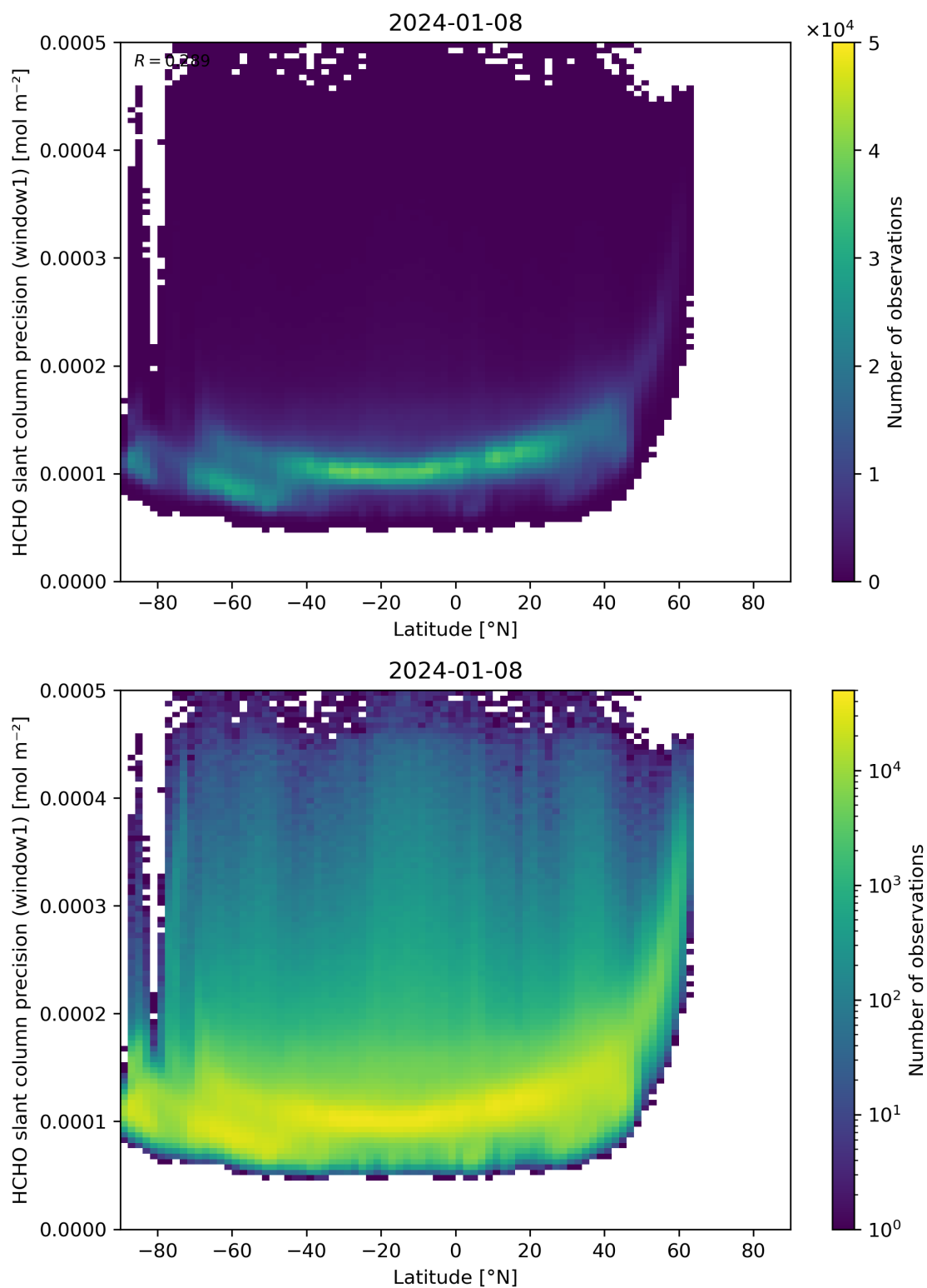
Figure 160: Scatter density plot of “Latitude” against “HCHO slant column precision (window1)” for 2024-01-07 to 2024-01-09.
