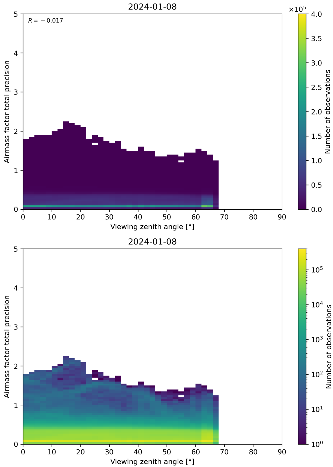
Figure 191: Scatter density plot of “Viewing zenith angle” against “Airmass factor total precision” for 2024-01-07 to 2024-01-09.
