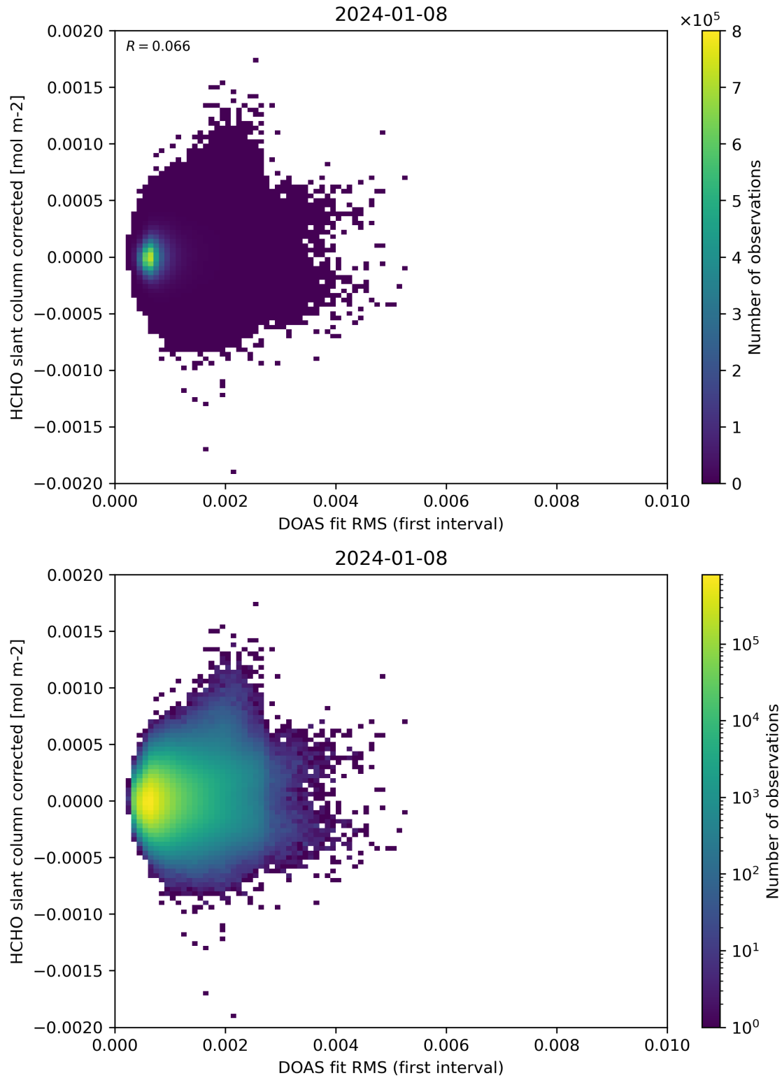
Figure 62: Scatter density plot of “DOAS fit RMS (first interval)” against “HCHO slant column corrected” for 2024-01-07 to 2024-01-09.
