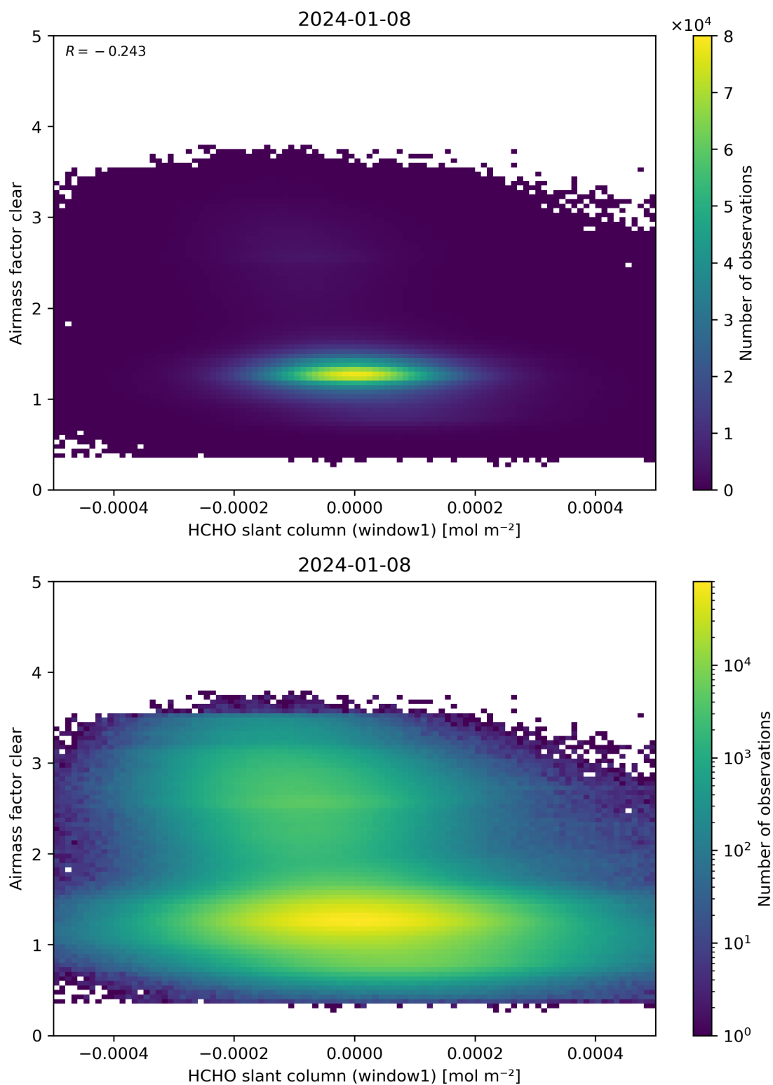
Figure 81: Scatter density plot of “HCHO slant column (window1)” against “Airmass factor clear” for 2024-01-07 to 2024-01-09.
