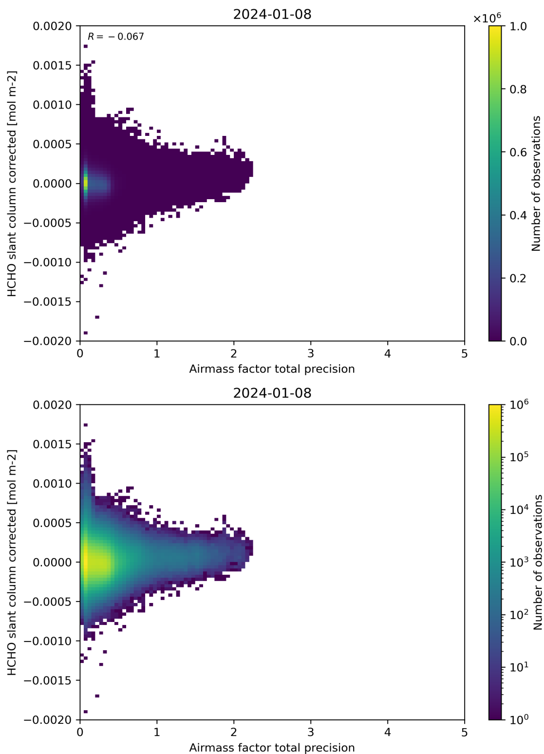
Figure 109: Scatter density plot of “Airmass factor total precision” against “HCHO slant column corrected” for 2024-01-07 to 2024-01-09.
