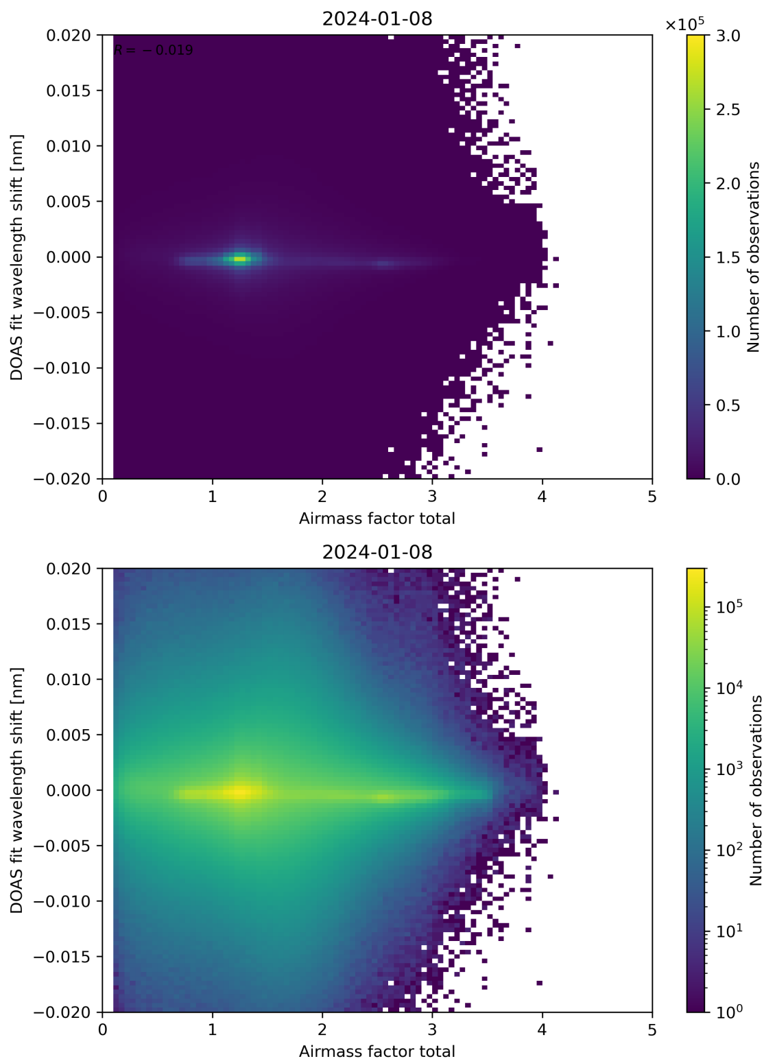
Figure 98: Scatter density plot of “Airmass factor total” against “DOAS fit wavelength shift” for 2024-01-07 to 2024-01-09.
