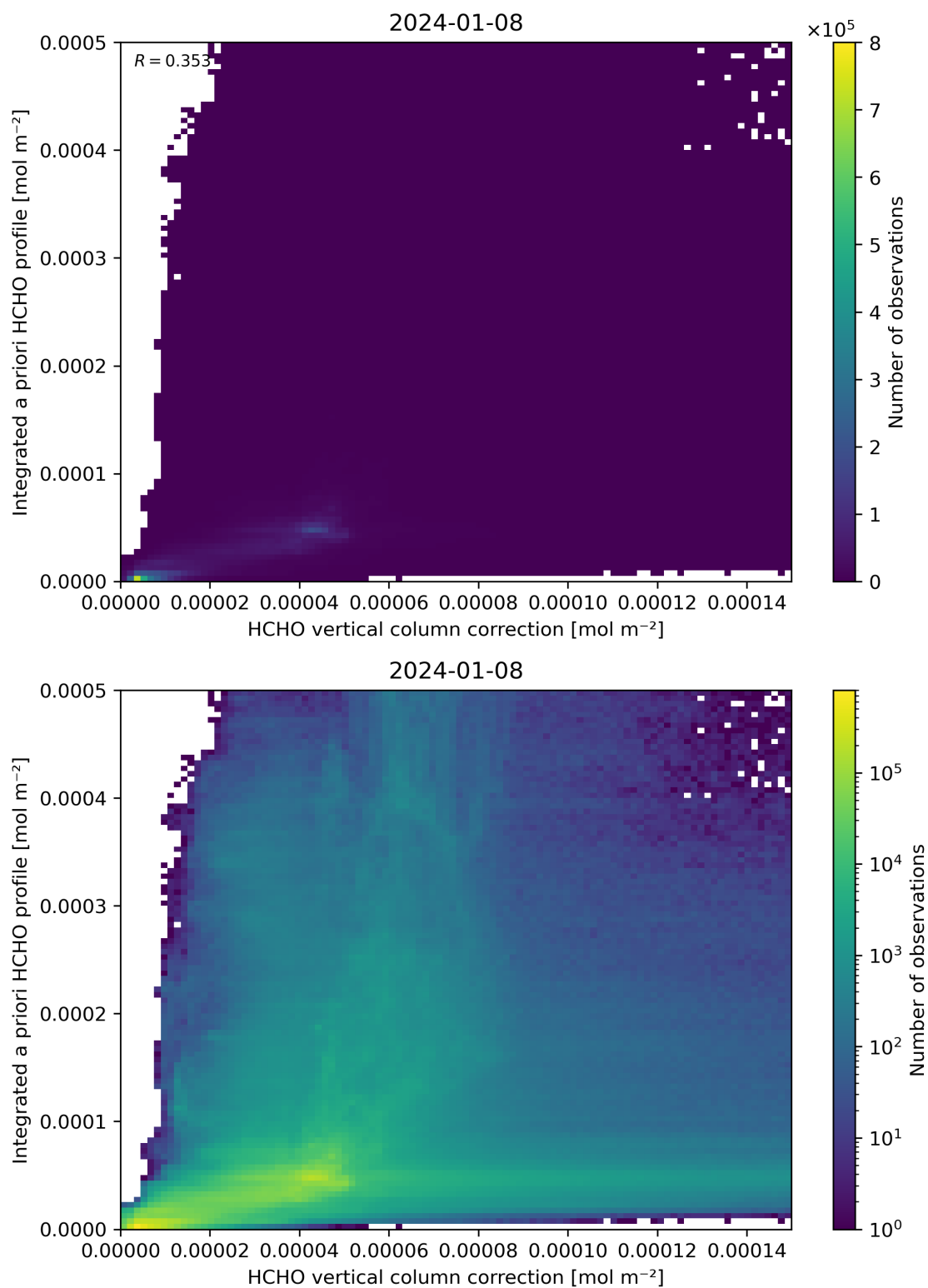
Figure 122: Scatter density plot of “HCHO vertical column correction” against “Integrated a priori HCHO profile” for 2024-01-07 to 2024-01-09.
