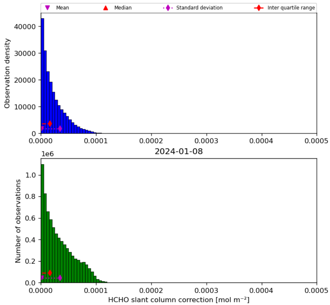
Figure 47: Histogram of “HCHO slant column correction” for 2024-01-07 to 2024-01-09
