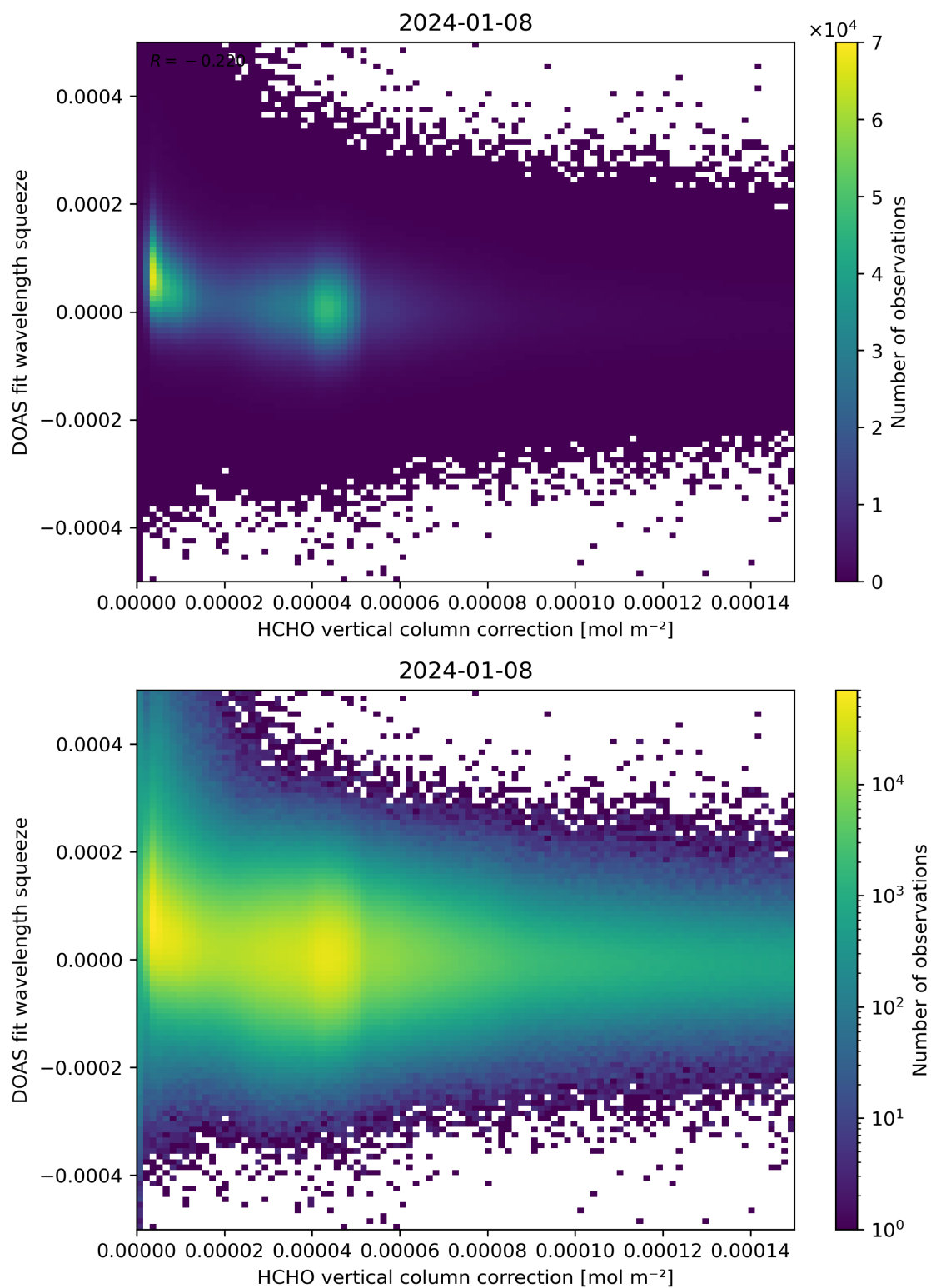
Figure 114: Scatter density plot of “HCHO vertical column correction” against “DOAS fit wavelength squeeze” for 2024-01-07 to 2024-01-09.
