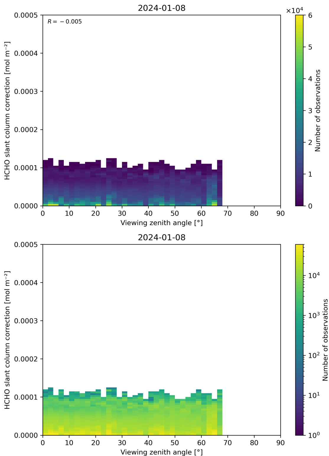
Figure 187: Scatter density plot of “Viewing zenith angle” against “HCHO slant column correction” for 2024-01-07 to 2024-01-09.
