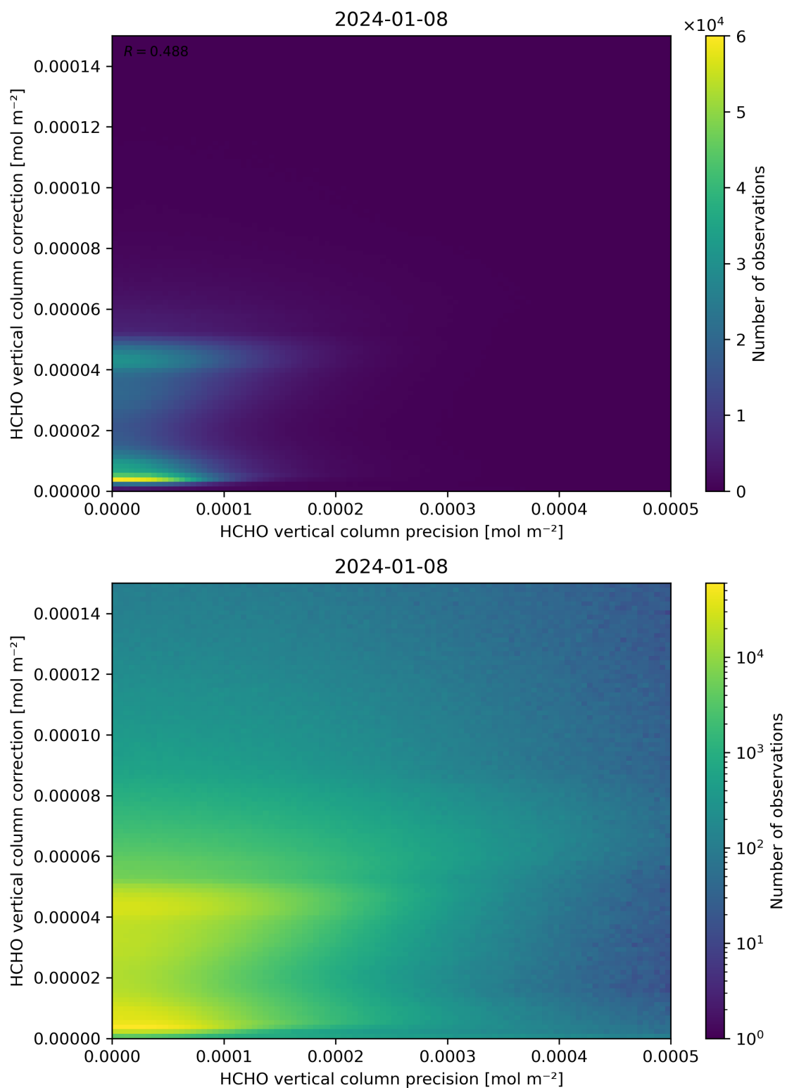
Figure 146: Scatter density plot of “HCHO vertical column precision” against “HCHO vertical column correction” for 2024-01-07 to 2024-01-09.
