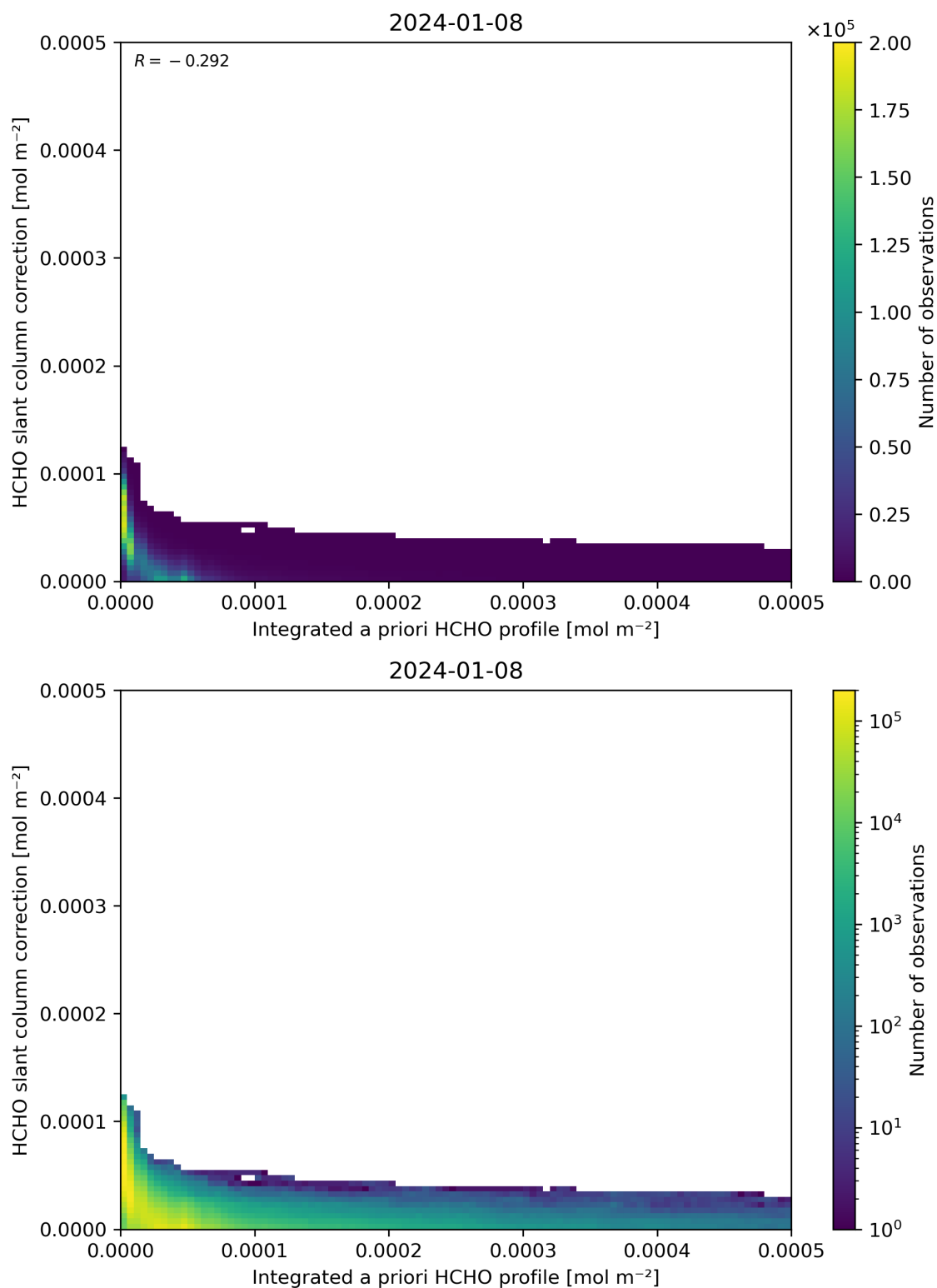
Figure 152: Scatter density plot of “Integrated a priori HCHO profile” against “HCHO slant column correction” for 2024-01-07 to 2024-01-09.
