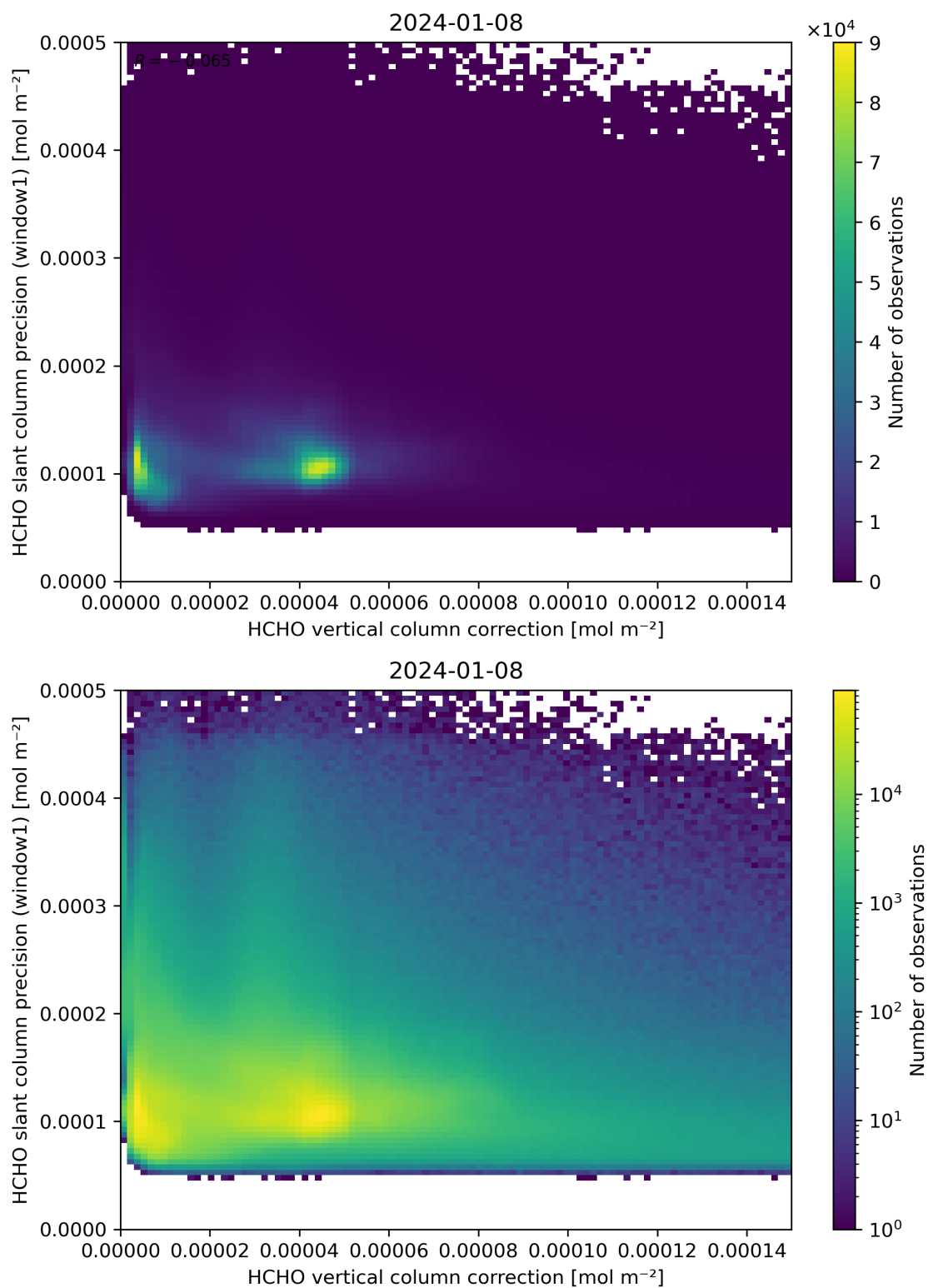
Figure 119: Scatter density plot of “HCHO vertical column correction” against “HCHO slant column precision (window1)” for 2024-01-07 to 2024-01-09.
