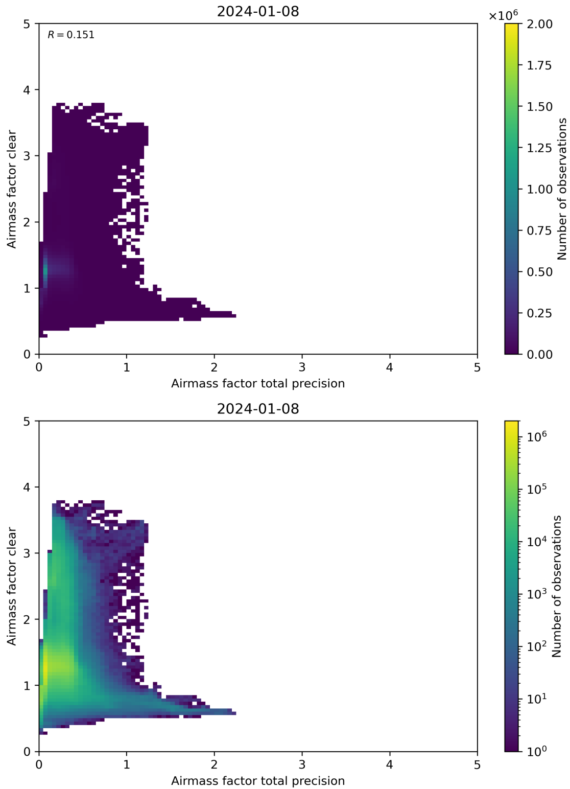
Figure 108: Scatter density plot of “Airmass factor total precision” against “Airmass factor clear” for 2024-01-07 to 2024-01-09.
