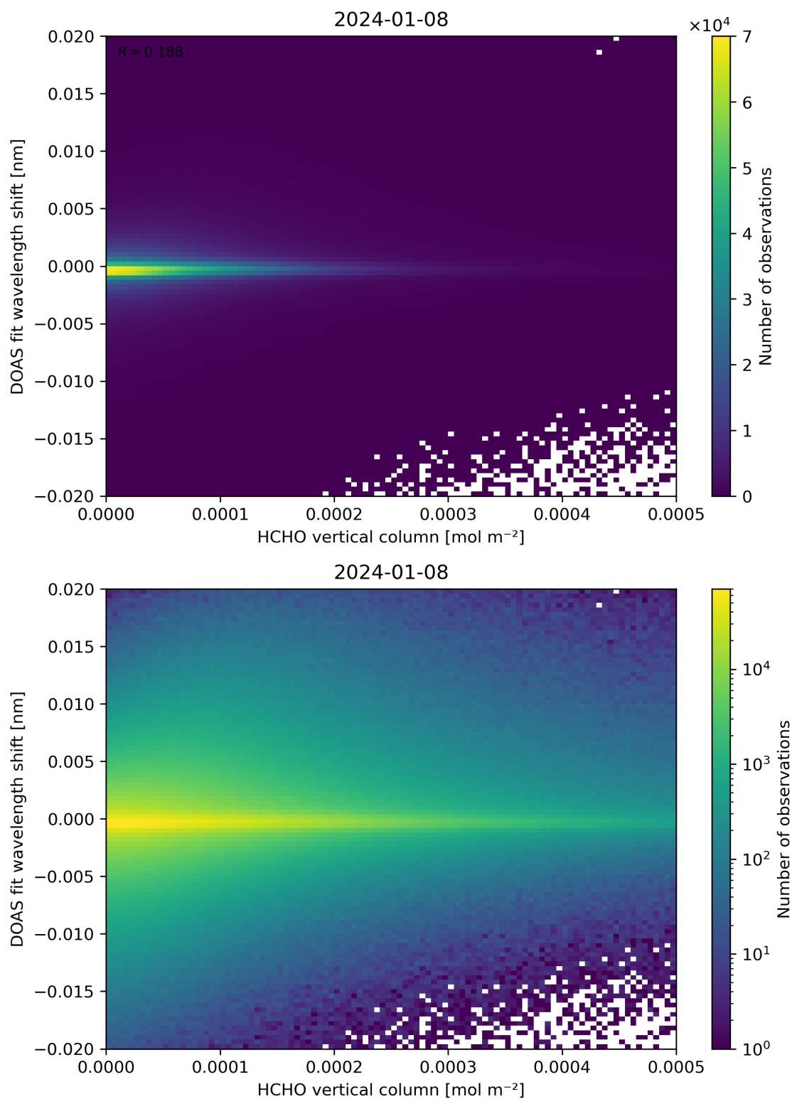
Figure 124: Scatter density plot of “HCHO vertical column” against “DOAS fit wavelength shift” for 2024-01-07 to 2024-01-09.
