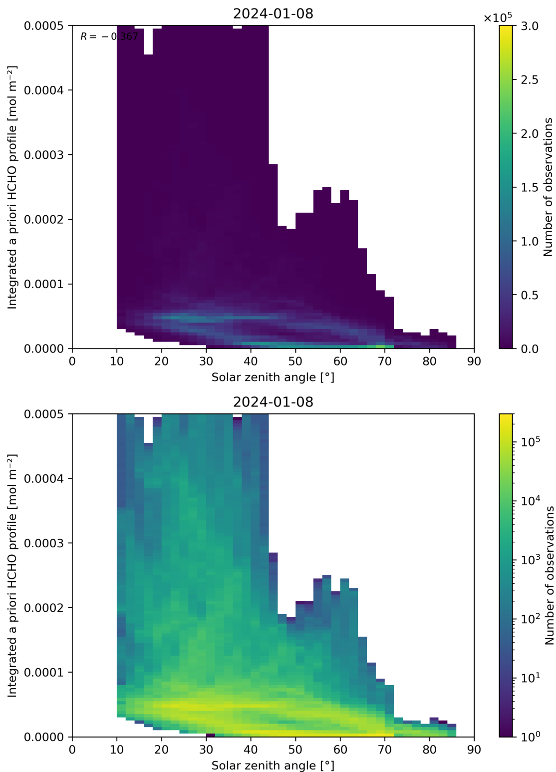
Figure 180: Scatter density plot of “Solar zenith angle” against “Integrated a priori HCHO profile” for 2024-01-07 to 2024-01-09.
