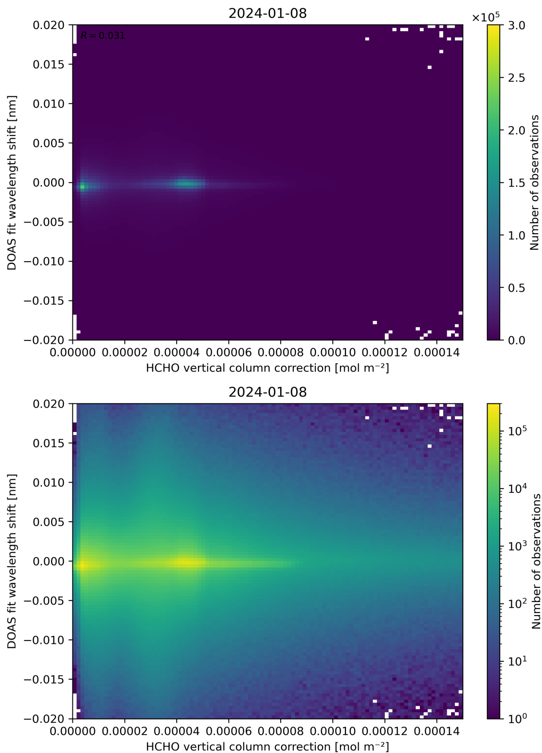
Figure 113: Scatter density plot of “HCHO vertical column correction” against “DOAS fit wavelength shift” for 2024-01-07 to 2024-01-09.
