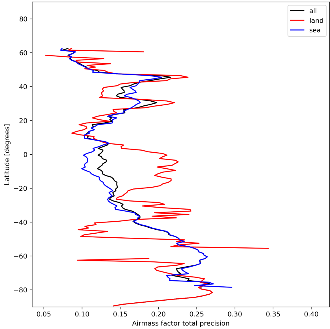
Figure 27: Zonal average of “Airmass factor total precision” for 2024-01-07 to 2024-01-09.
