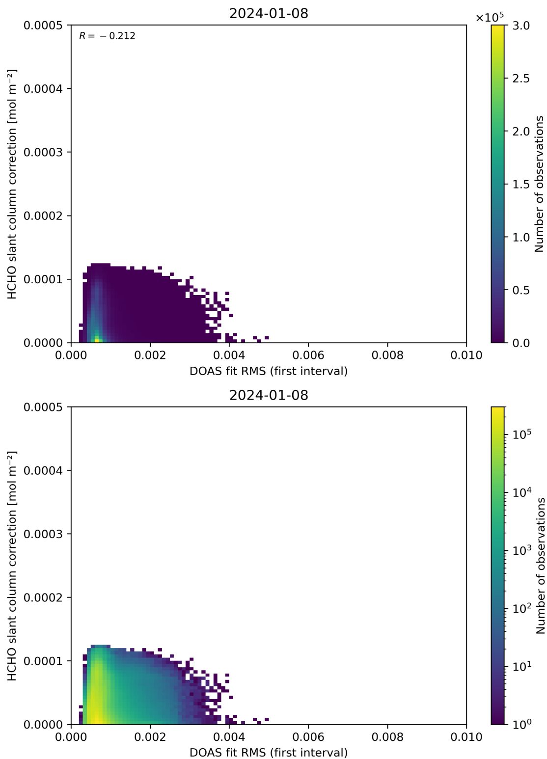
Figure 63: Scatter density plot of “DOAS fit RMS (first interval)” against “HCHO slant column correction” for 2024-01-07 to 2024-01-09.
