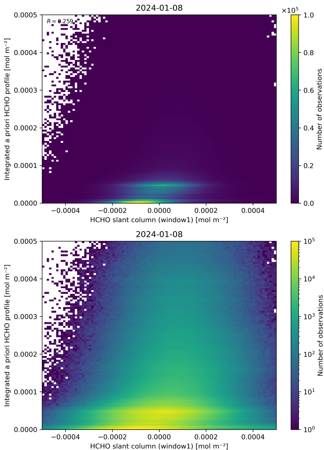
Figure 87: Scatter density plot of “HCHO slant column (window1)” against “Integrated a priori HCHO profile” for 2024-01-07 to 2024-01-09.
