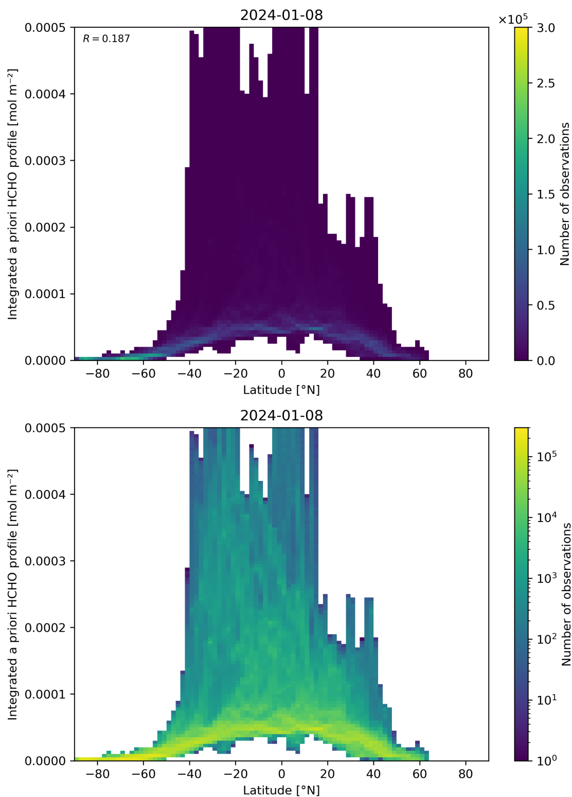
Figure 166: Scatter density plot of “Latitude” against “Integrated a priori HCHO profile” for 2024-01-07 to 2024-01-09.
