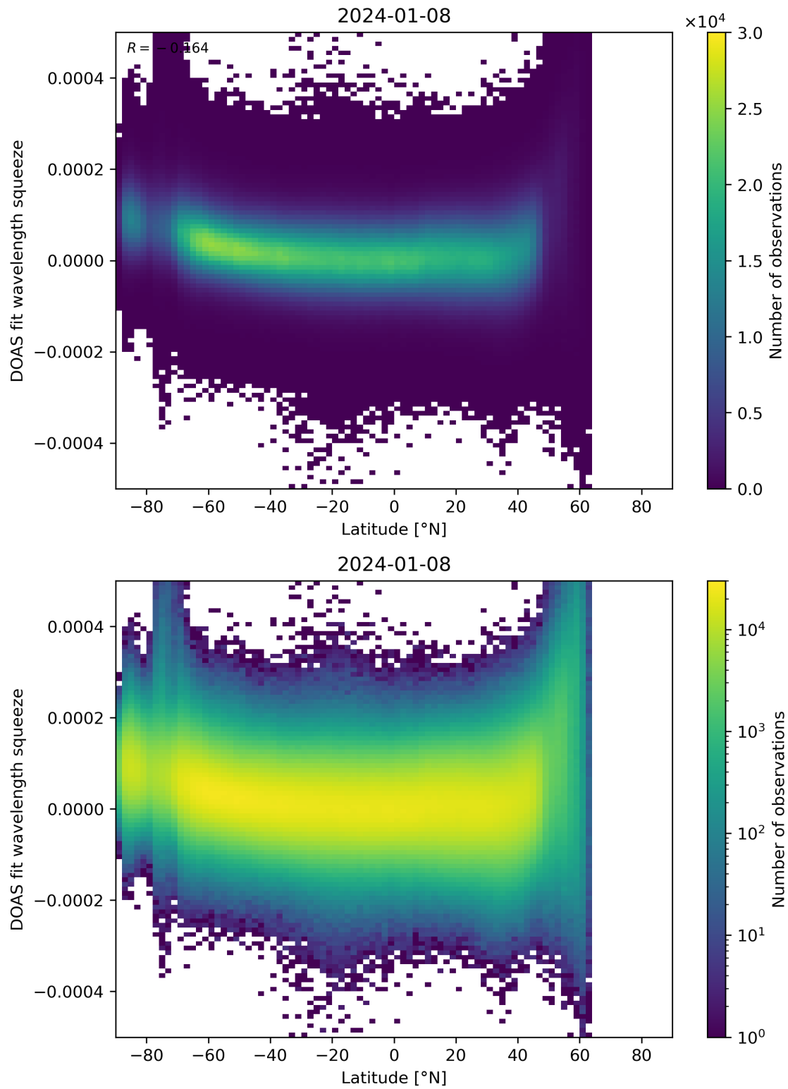
Figure 155: Scatter density plot of “Latitude” against “DOAS fit wavelength squeeze” for 2024-01-07 to 2024-01-09.
