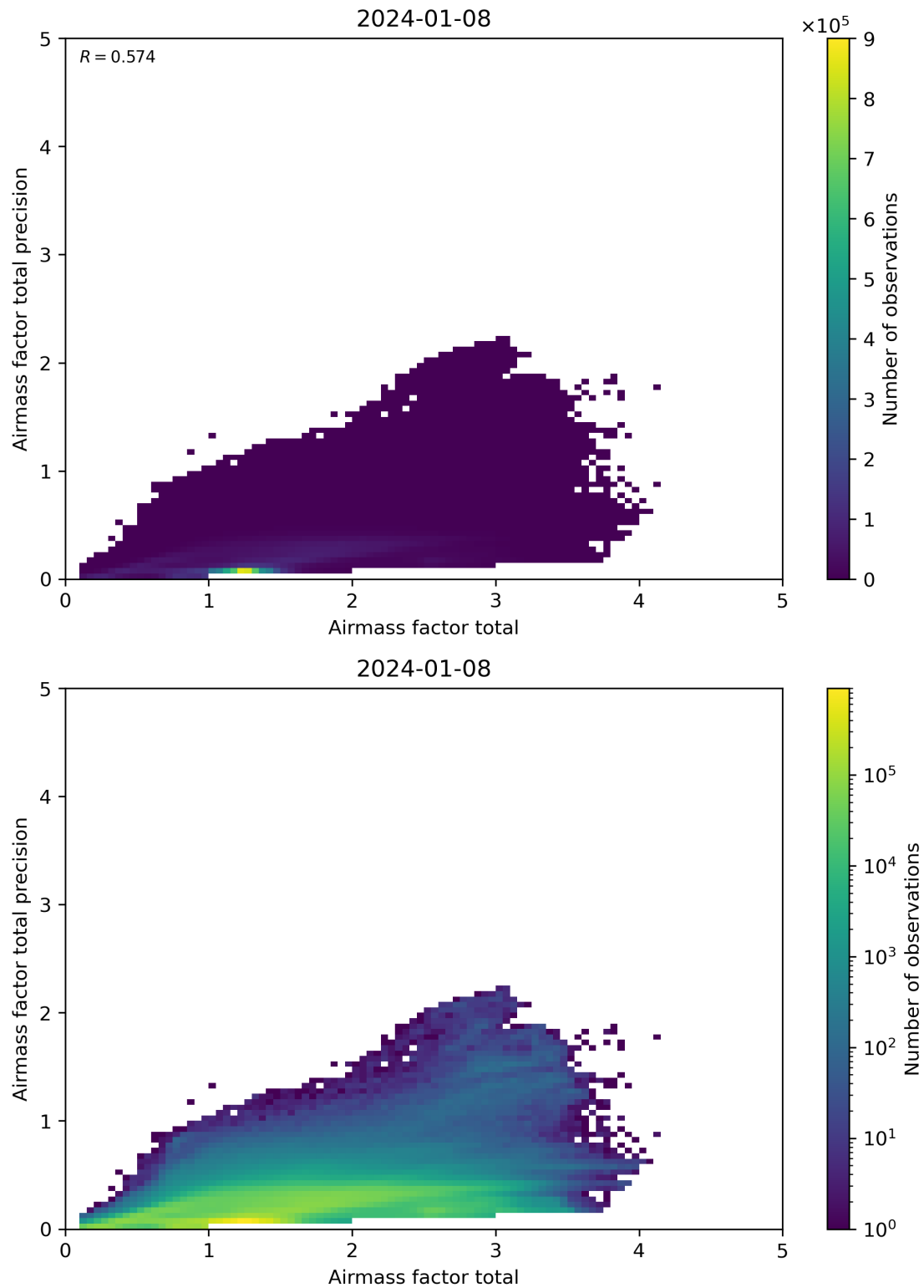
Figure 103: Scatter density plot of “Airmass factor total” against “Airmass factor total precision” for 2024-01-07 to 2024-01-09.
