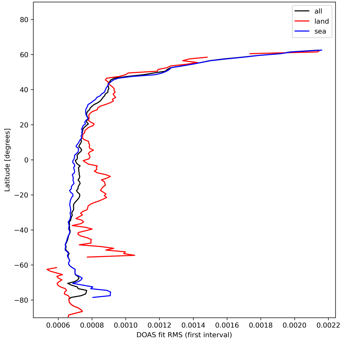
Figure 32: Zonal average of “DOAS fit RMS (first interval)” for 2024-01-07 to 2024-01-09.
