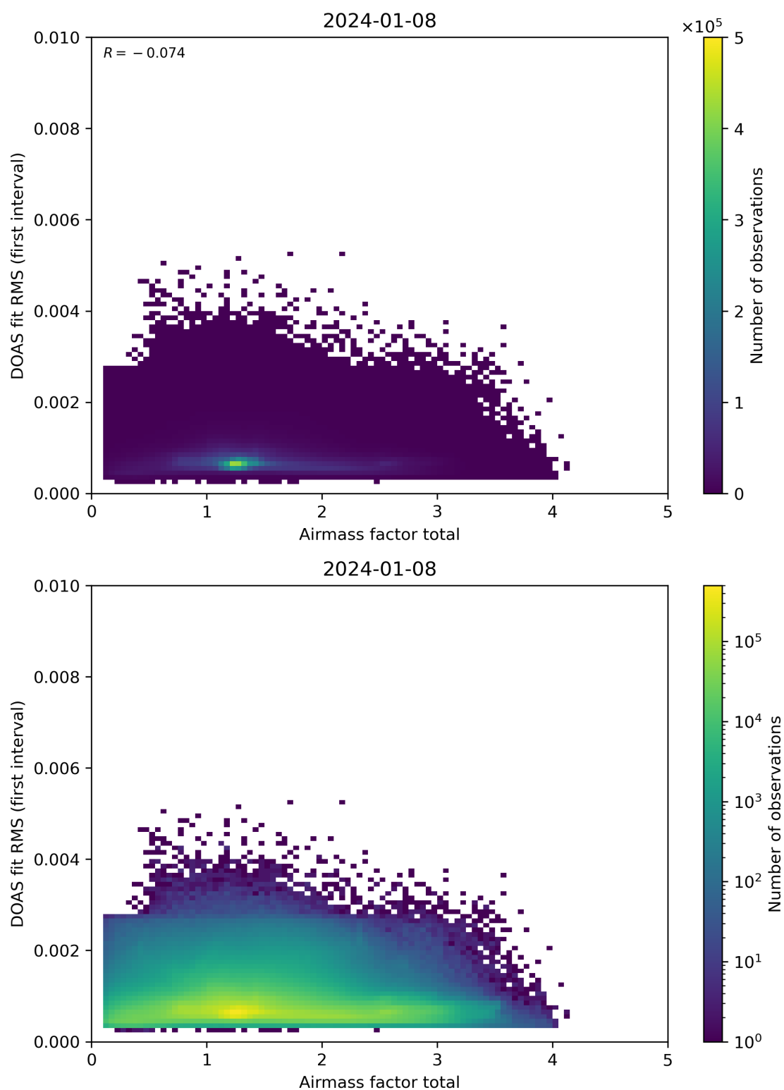
Figure 97: Scatter density plot of “Airmass factor total” against “DOAS fit RMS (first interval)” for 2024-01-07 to 2024-01-09.
