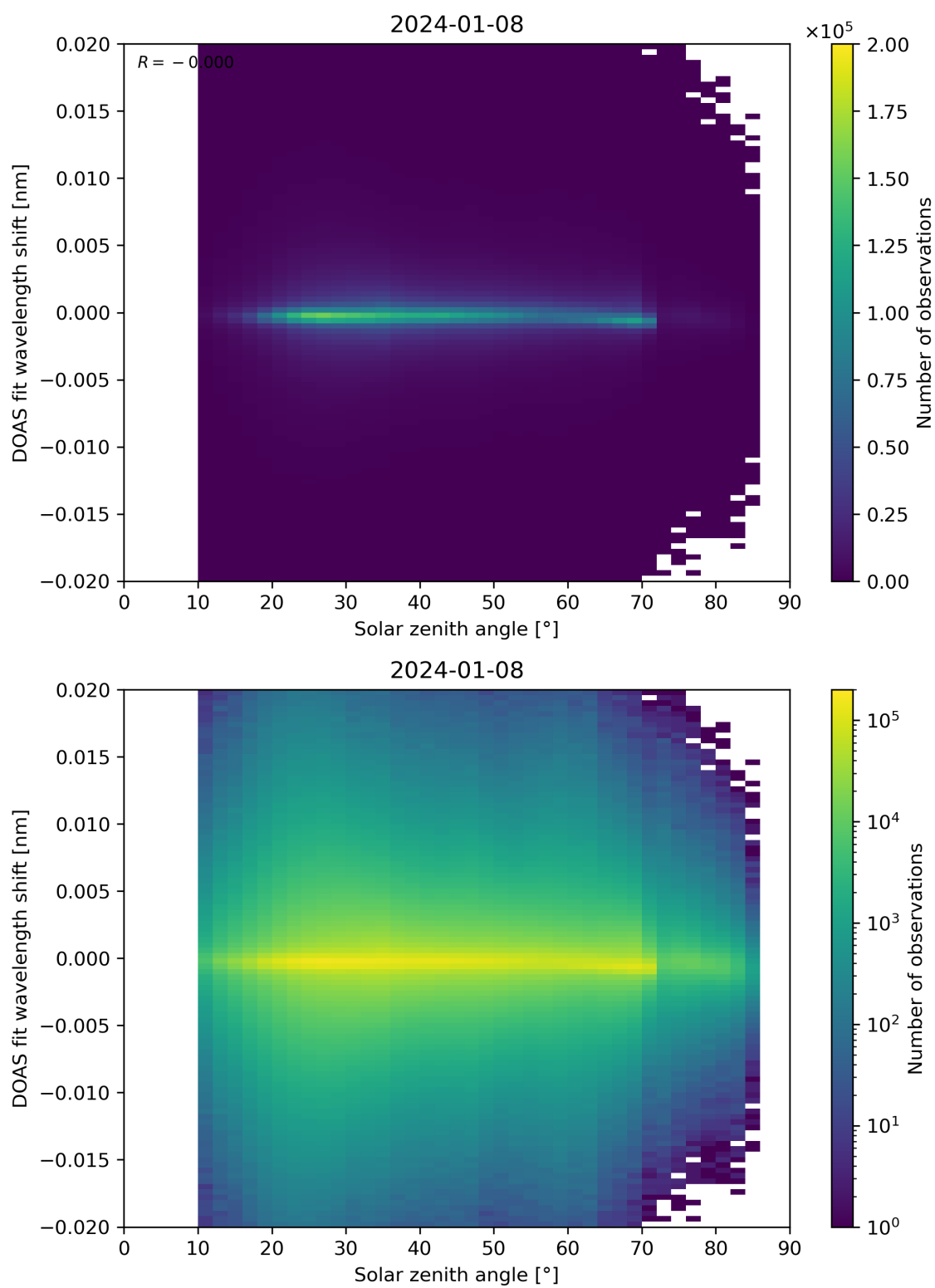
Figure 168: Scatter density plot of “Solar zenith angle” against “DOAS fit wavelength shift” for 2024-01-07 to 2024-01-09.
