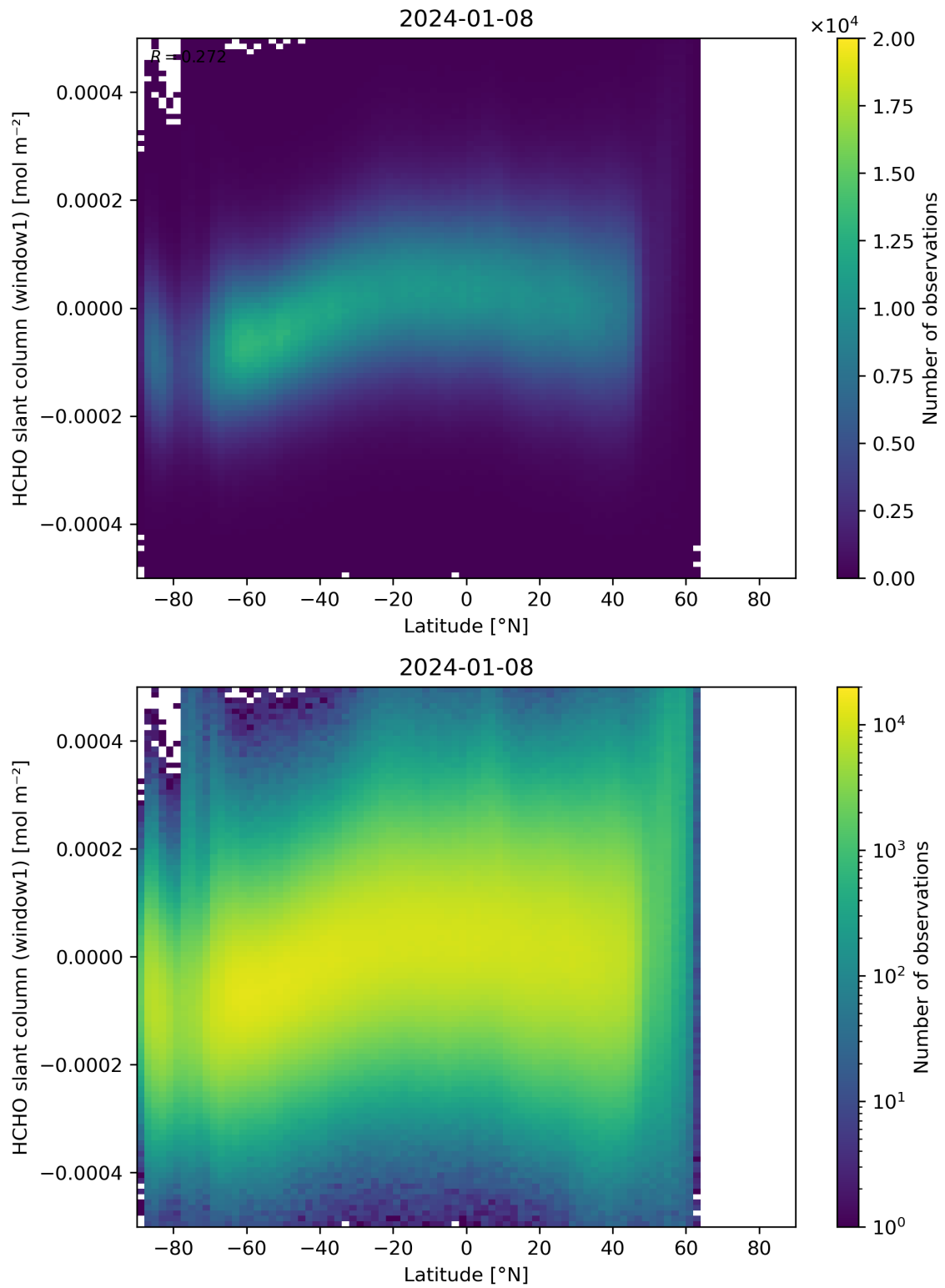
Figure 159: Scatter density plot of “Latitude” against “HCHO slant column (window1)” for 2024-01-07 to 2024-01-09.
