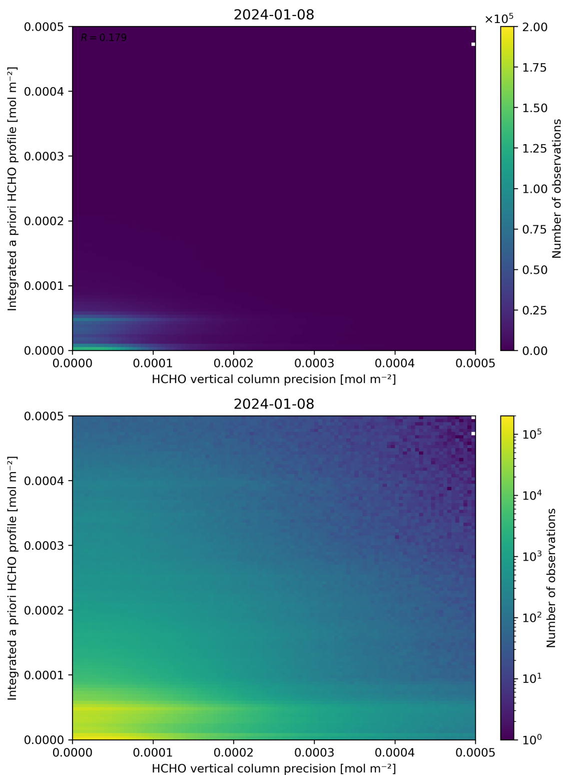
Figure 147: Scatter density plot of “HCHO vertical column precision” against “Integrated a priori HCHO profile” for 2024-01-07 to 2024-01-09.
