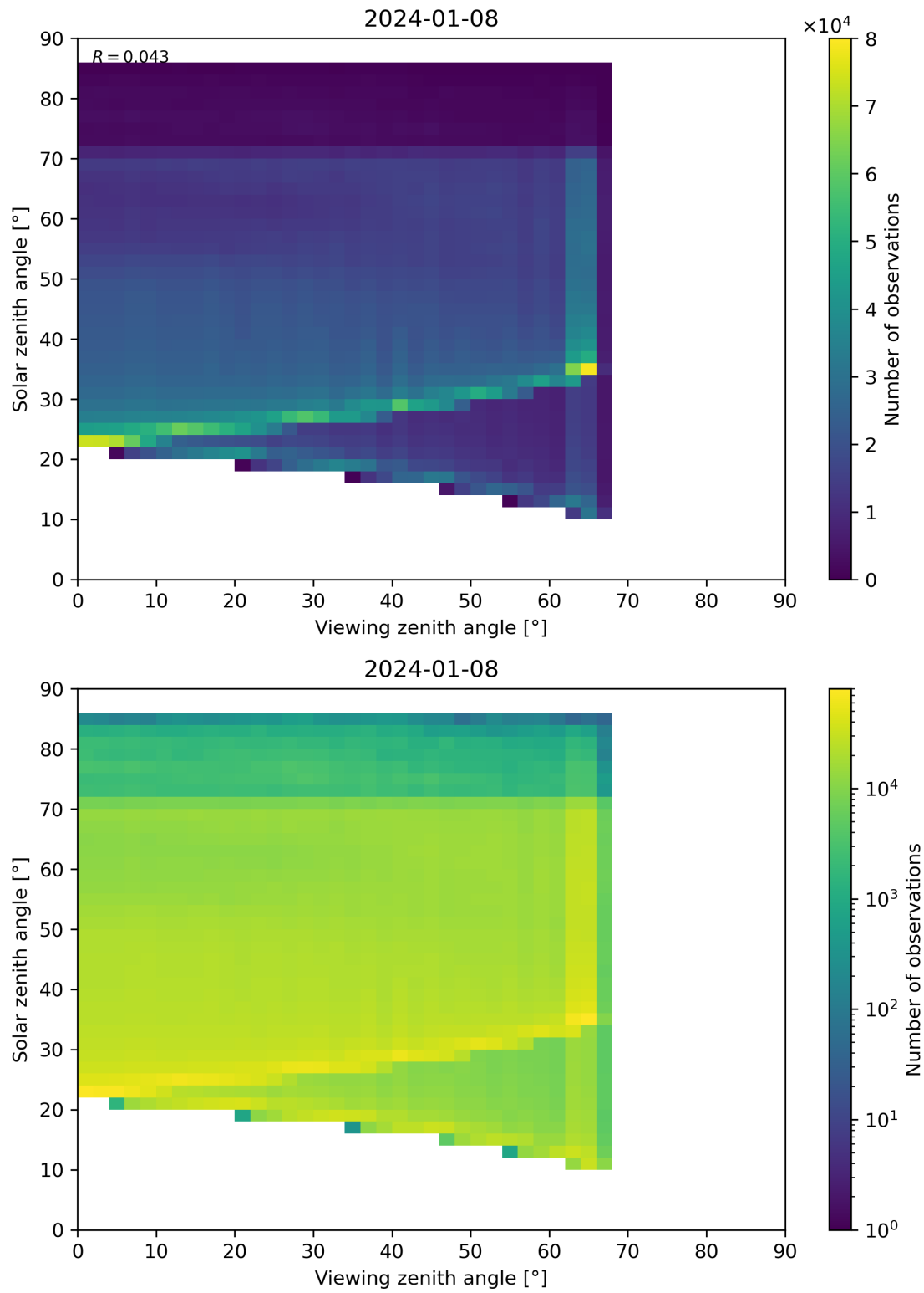
Figure 197: Scatter density plot of “Viewing zenith angle” against “Solar zenith angle” for 2024-01-07 to 2024-01-09.
