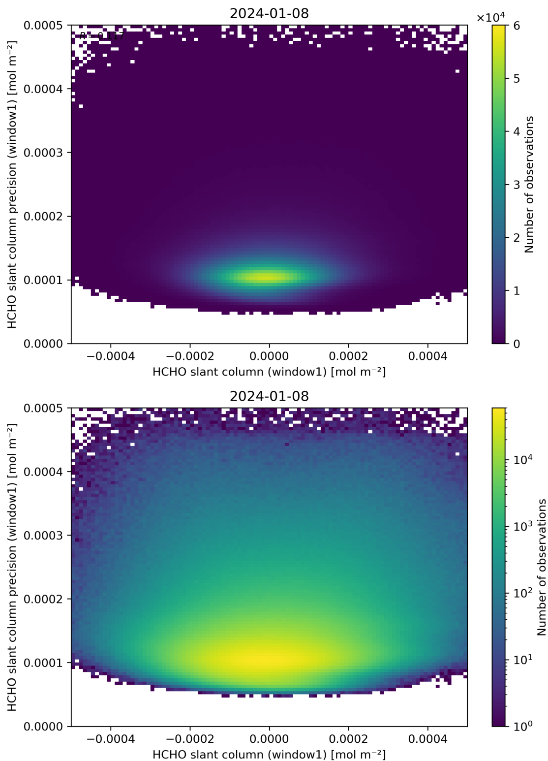
Figure 84: Scatter density plot of “HCHO slant column (window1)” against “HCHO slant column precision (window1)” for 2024-01-07 to 2024-01-09.
