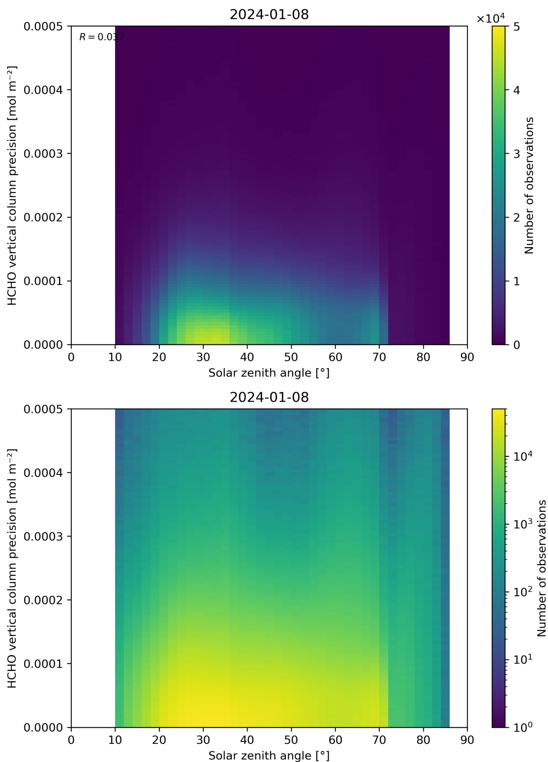
Figure 179: Scatter density plot of “Solar zenith angle” against “HCHO vertical column precision” for 2024-01-07 to 2024-01-09.
