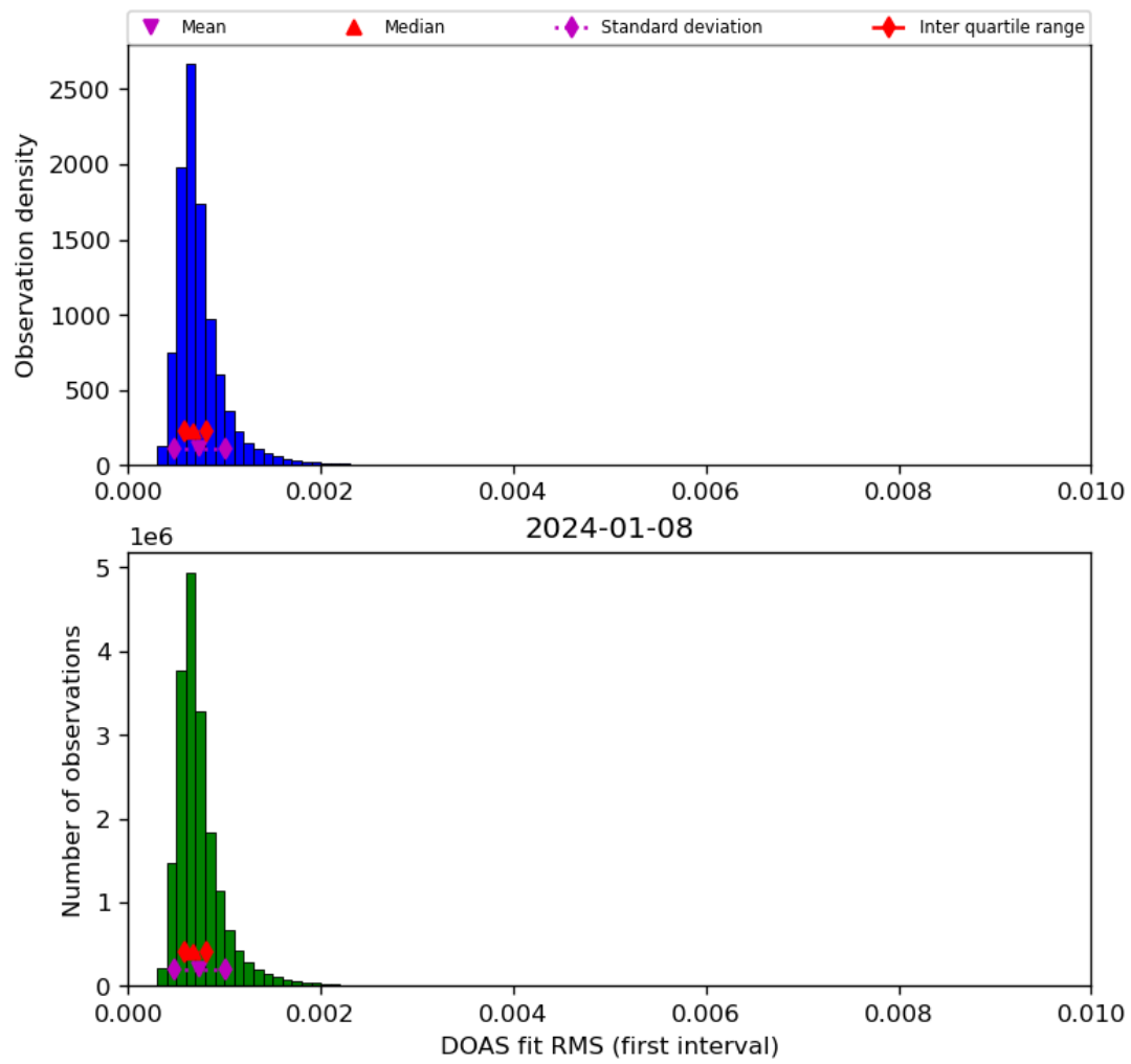
Figure 46: Histogram of “DOAS fit RMS (first interval)” for 2024-01-07 to 2024-01-09
