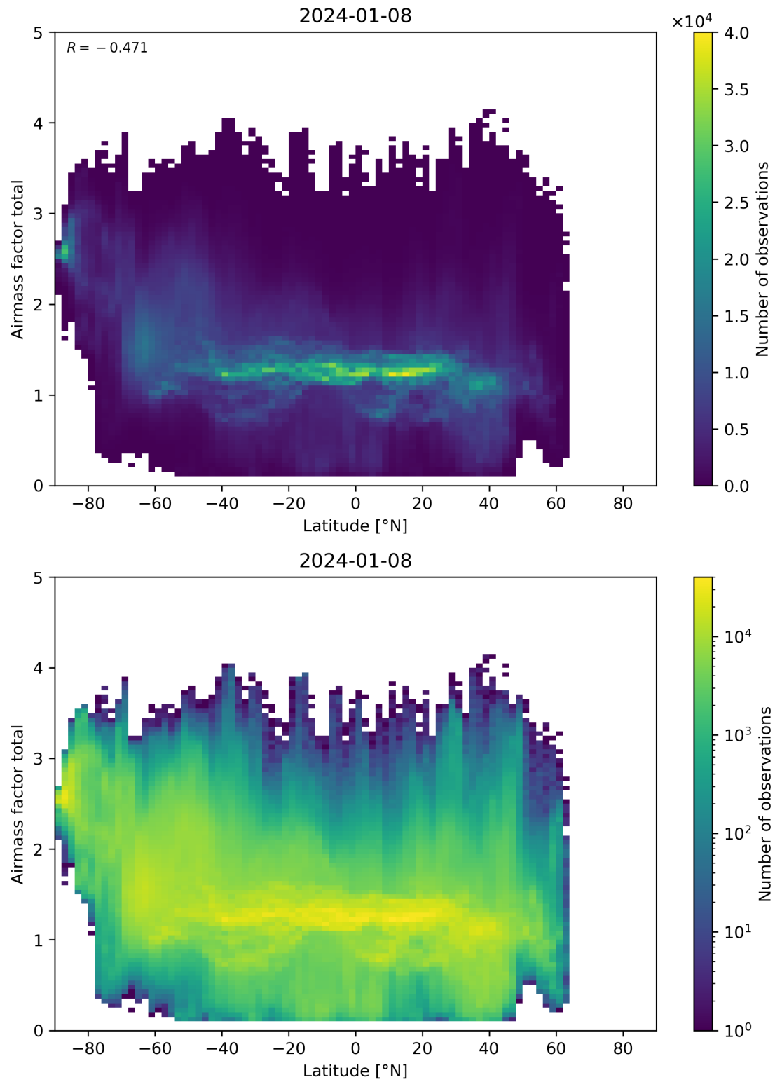
Figure 161: Scatter density plot of “Latitude” against “Airmass factor total” for 2024-01-07 to 2024-01-09.
