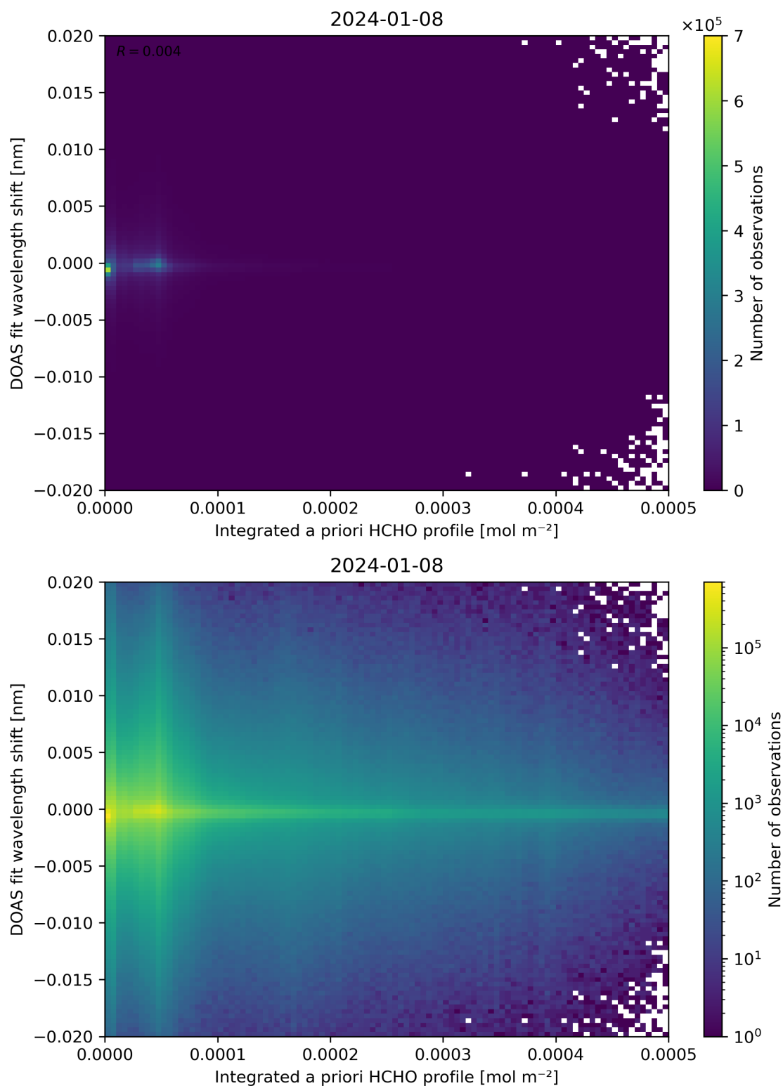
Figure 149: Scatter density plot of “Integrated a priori HCHO profile” against “DOAS fit wavelength shift” for 2024-01-07 to 2024-01-09.
