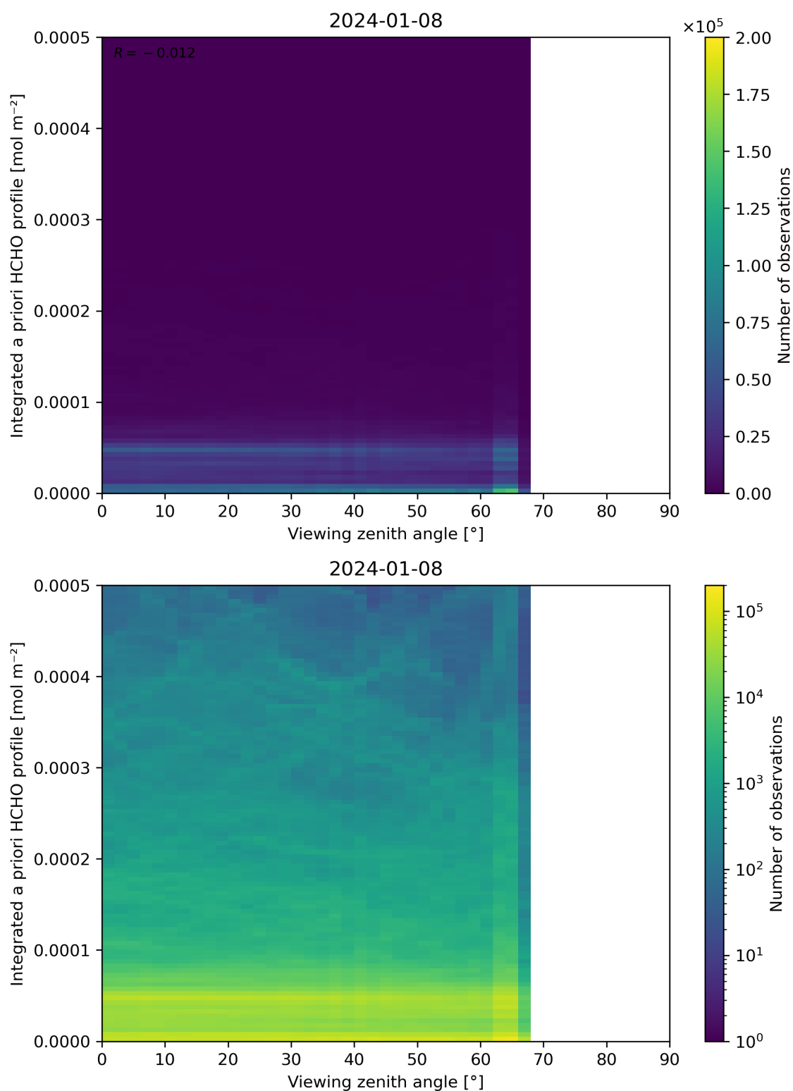
Figure 195: Scatter density plot of “Viewing zenith angle” against “Integrated a priori HCHO profile” for 2024-01-07 to 2024-01-09.
