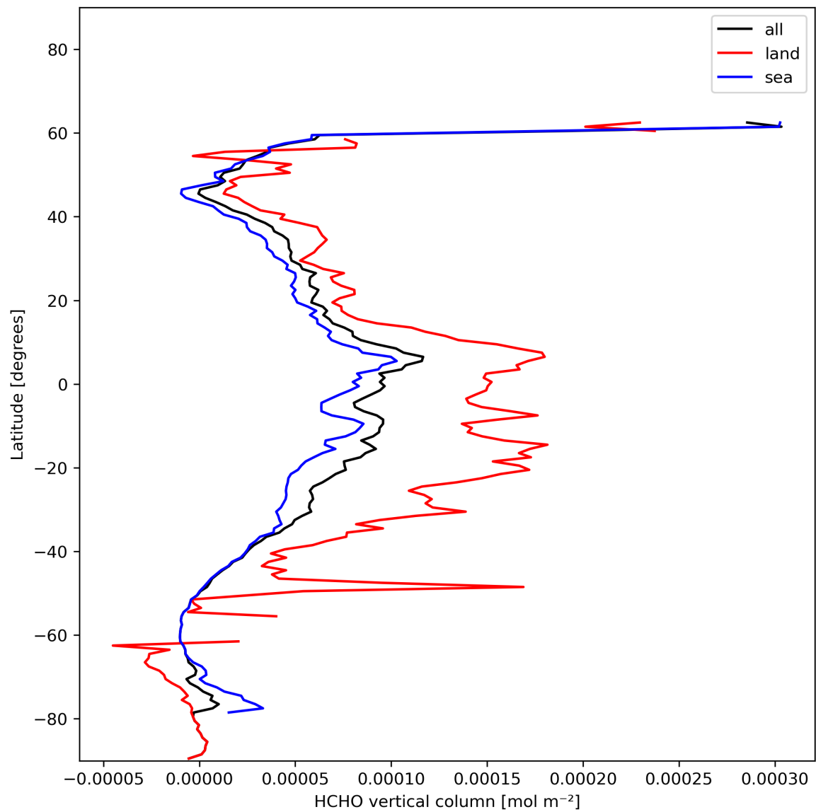
Figure 21: Zonal average of “HCHO vertical column” for 2024-01-07 to 2024-01-09.
