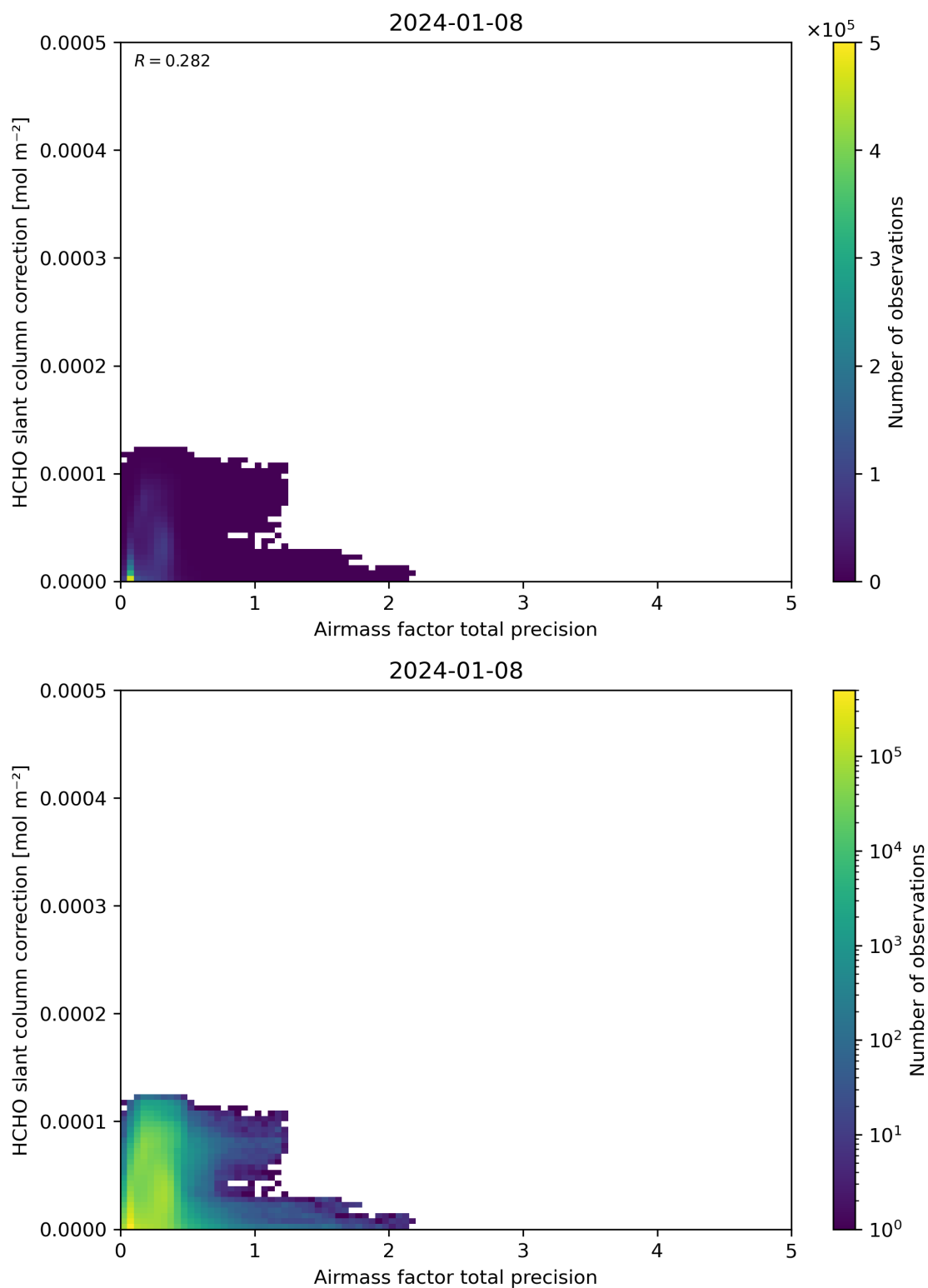
Figure 110: Scatter density plot of “Airmass factor total precision” against “HCHO slant column correction” for 2024-01-07 to 2024-01-09.
