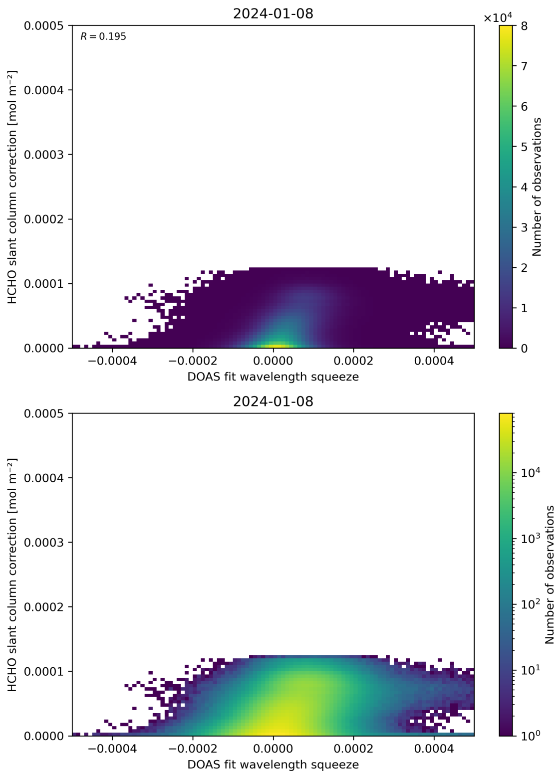
Figure 70: Scatter density plot of “DOAS fit wavelength squeeze” against “HCHO slant column correction” for 2024-01-07 to 2024-01-09.
