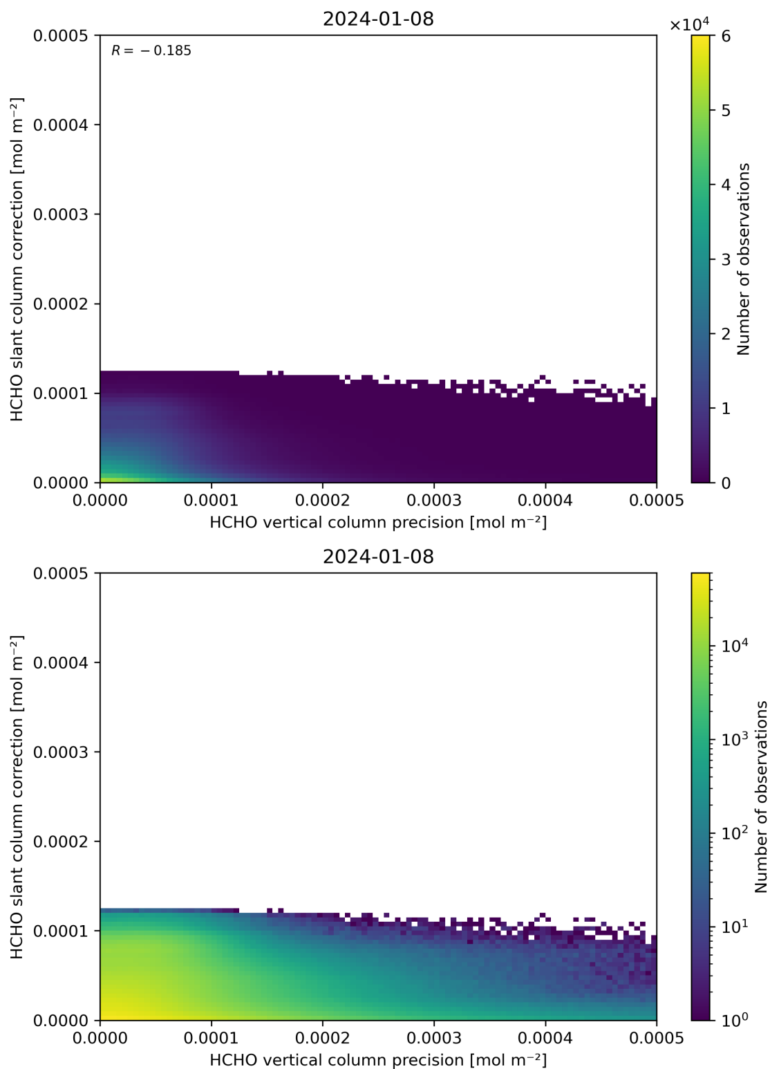
Figure 141: Scatter density plot of “HCHO vertical column precision” against “HCHO slant column correction” for 2024-01-07 to 2024-01-09.
