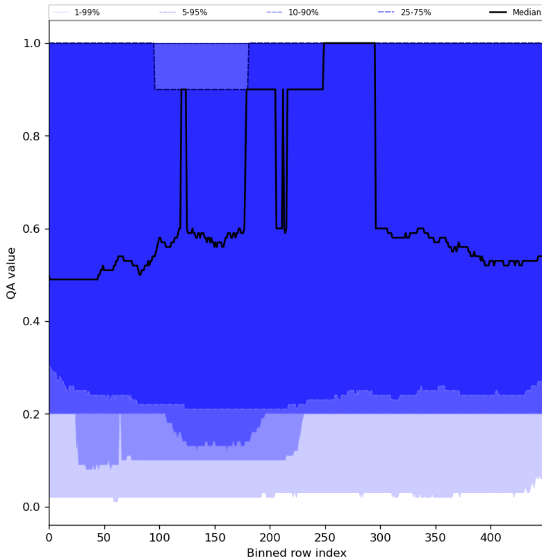
Figure 48: Along track statistics of “QA value” for 2024-01-07 to 2024-01-09
