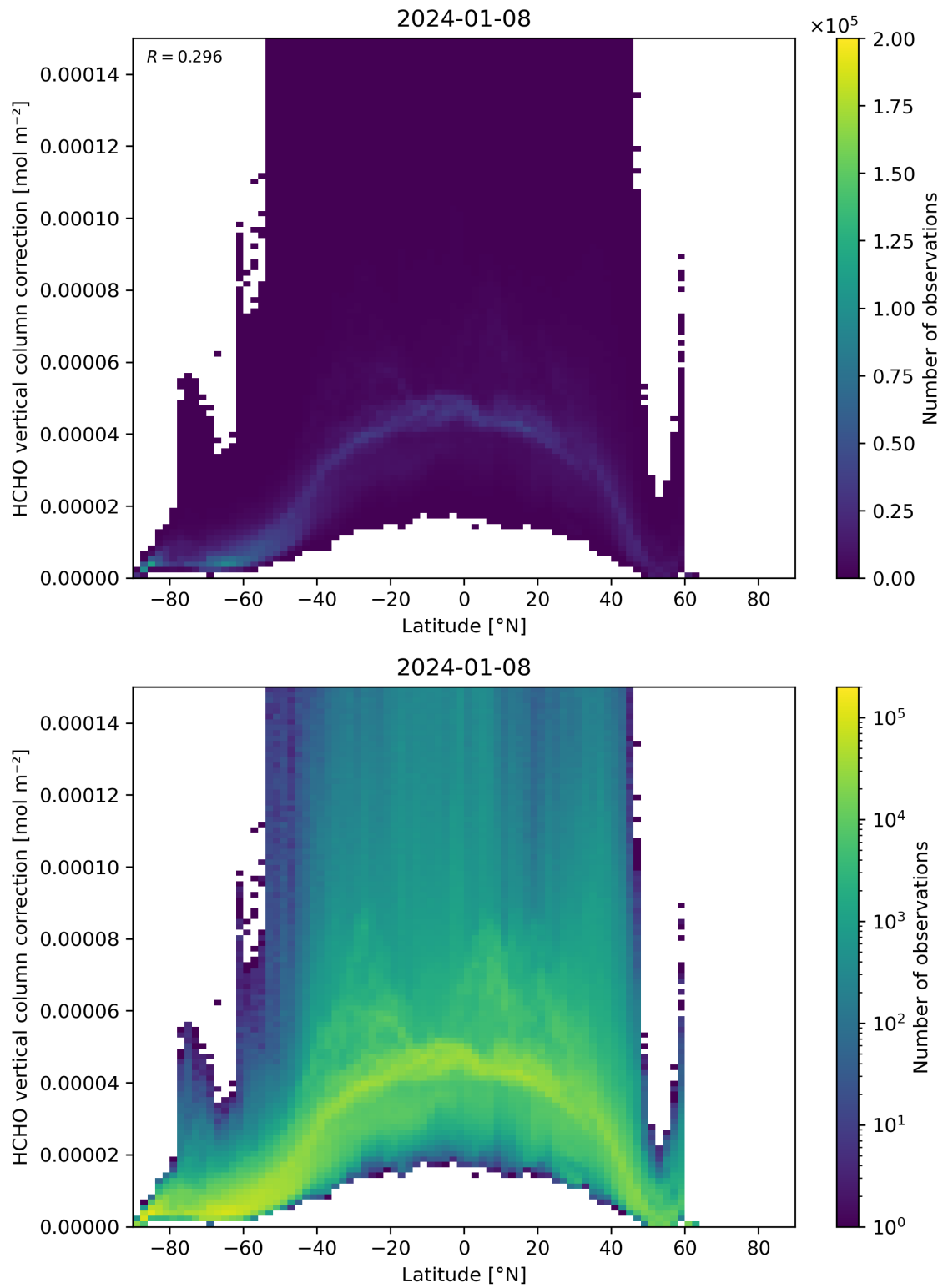
Figure 164: Scatter density plot of “Latitude” against “HCHO vertical column correction” for 2024-01-07 to 2024-01-09.
