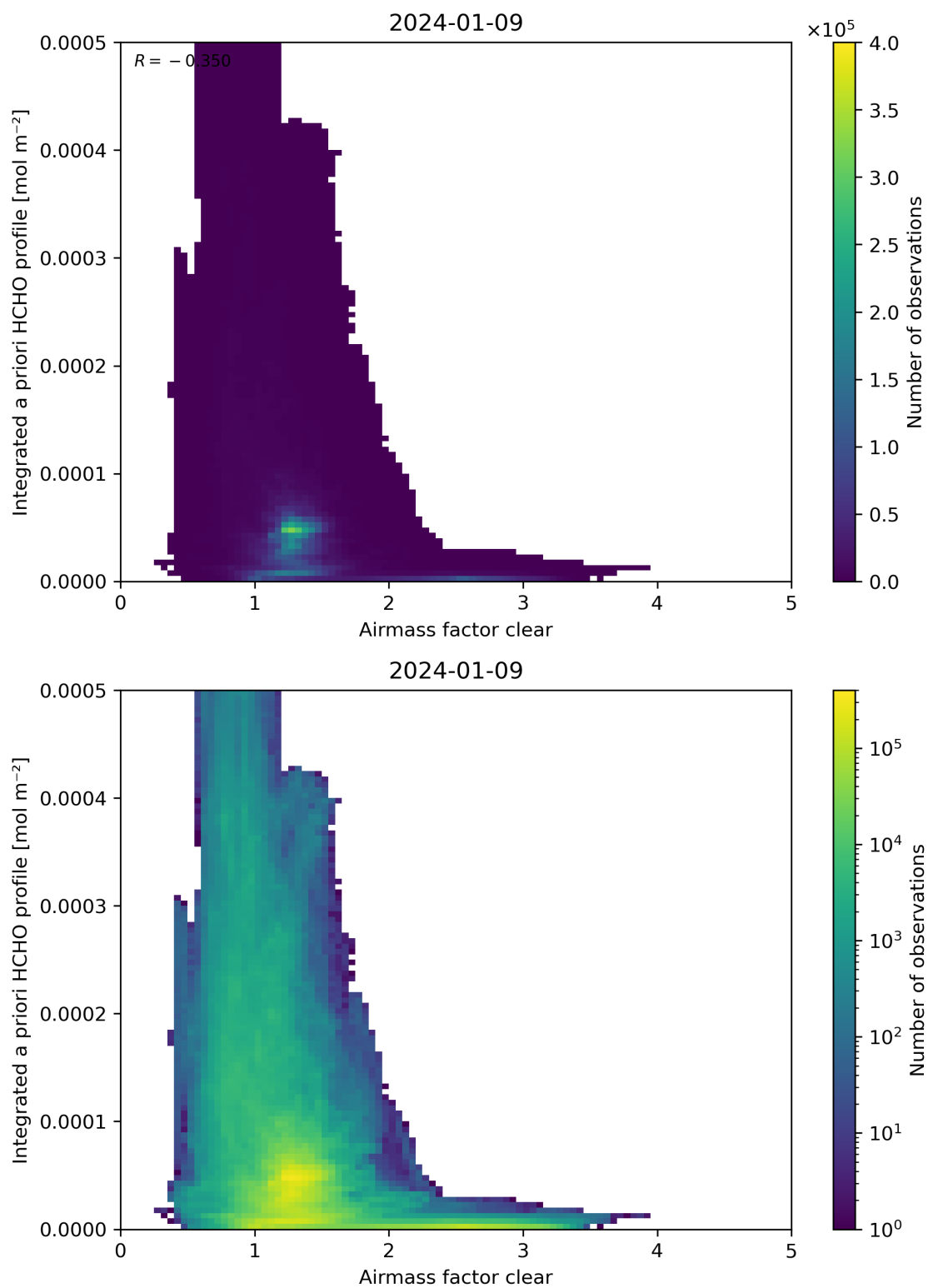
Figure 76: Scatter density plot of “Airmass factor clear” against “Integrated a priori HCHO profile” for 2024-01-08 to 2024-01-10.
