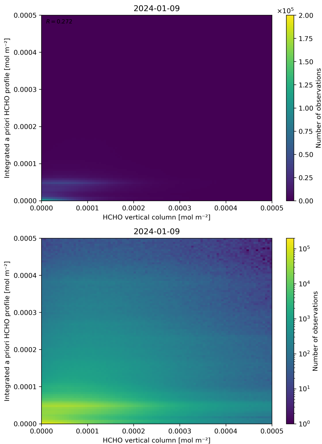
Figure 135: Scatter density plot of “HCHO vertical column” against “Integrated a priori HCHO profile” for 2024-01-08 to 2024-01-10.
