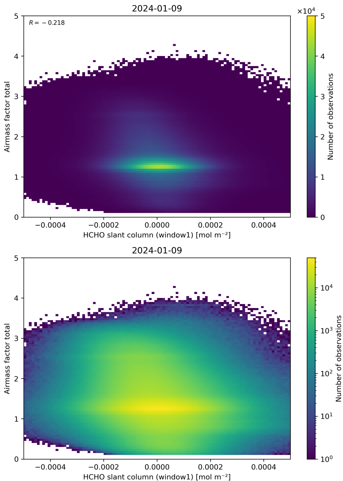
Figure 85: Scatter density plot of “HCHO slant column (window1)” against “Airmass factor total” for 2024-01-08 to 2024-01-10.
