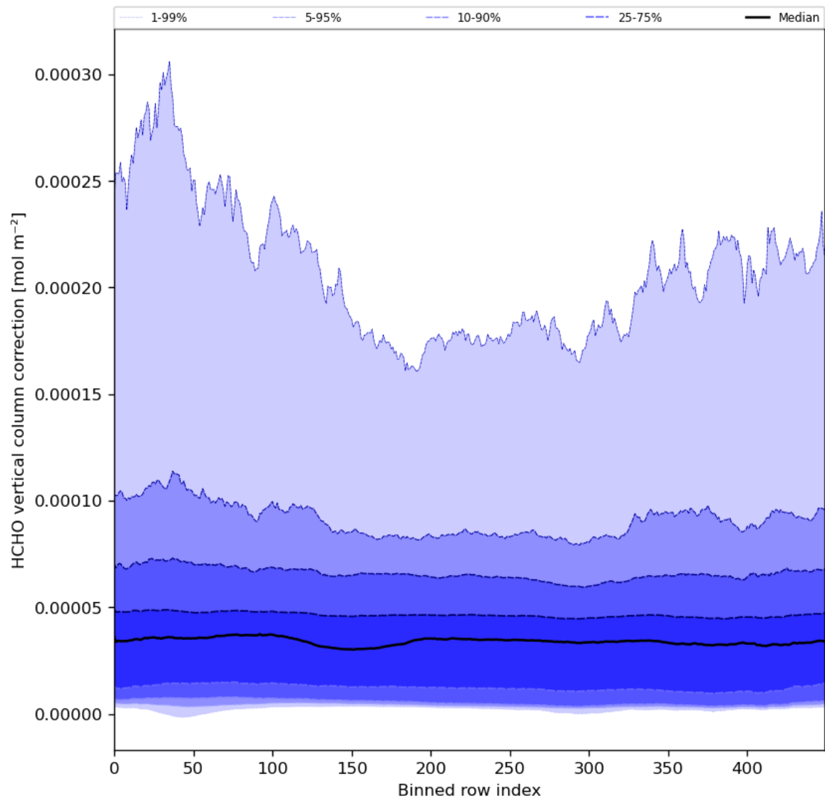
Figure 51: Along track statistics of “HCHO vertical column correction” for 2024-01-08 to 2024-01-10
