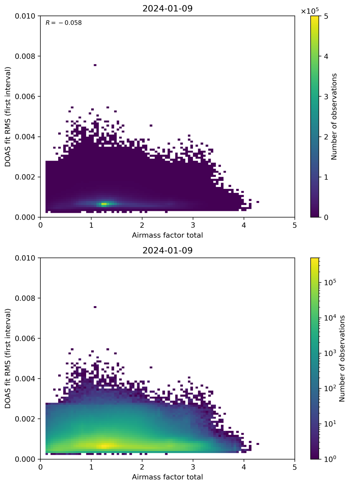
Figure 97: Scatter density plot of “Airmass factor total” against “DOAS fit RMS (first interval)” for 2024-01-08 to 2024-01-10.
