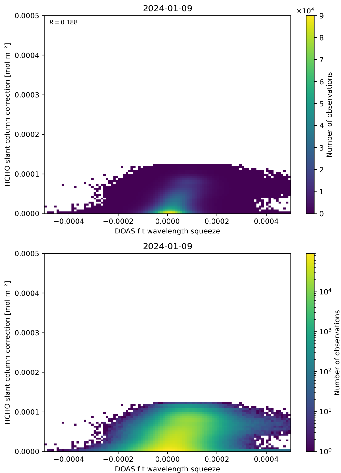
Figure 70: Scatter density plot of “DOAS fit wavelength squeeze” against “HCHO slant column correction” for 2024-01-08 to 2024-01-10.
