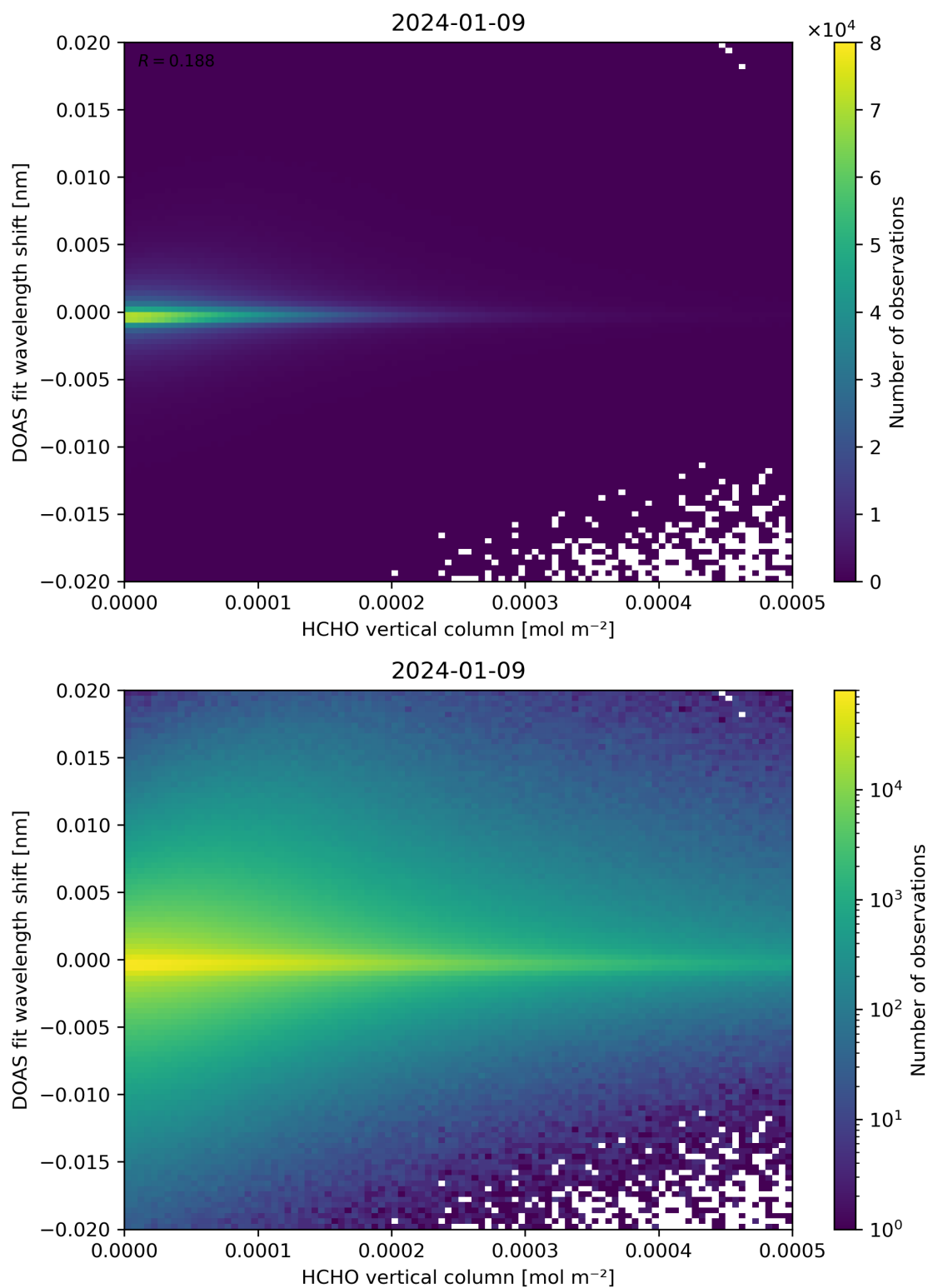
Figure 124: Scatter density plot of “HCHO vertical column” against “DOAS fit wavelength shift” for 2024-01-08 to 2024-01-10.
