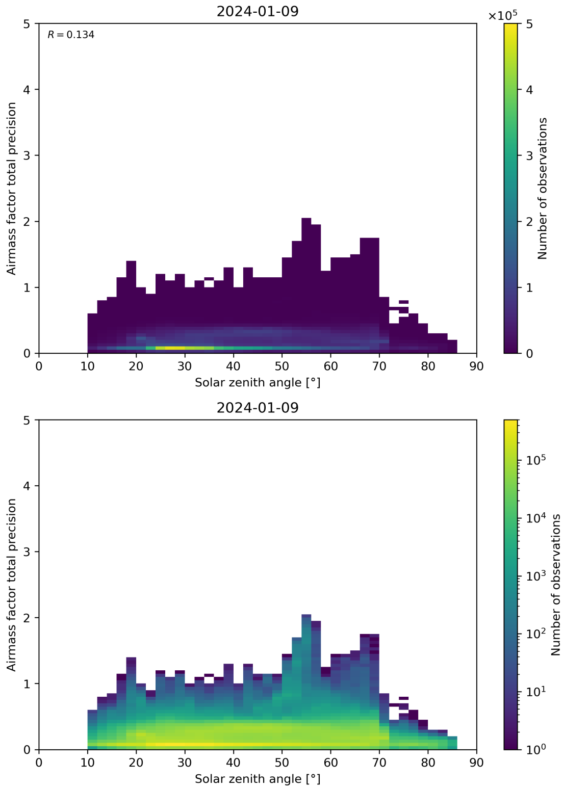
Figure 176: Scatter density plot of “Solar zenith angle” against “Airmass factor total precision” for 2024-01-08 to 2024-01-10.
