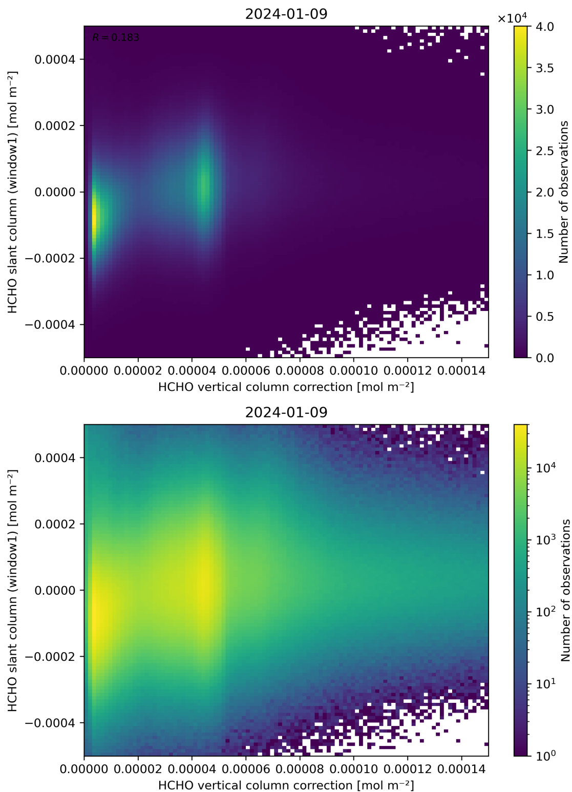
Figure 118: Scatter density plot of “HCHO vertical column correction” against “HCHO slant column (window1)” for 2024-01-08 to 2024-01-10.
