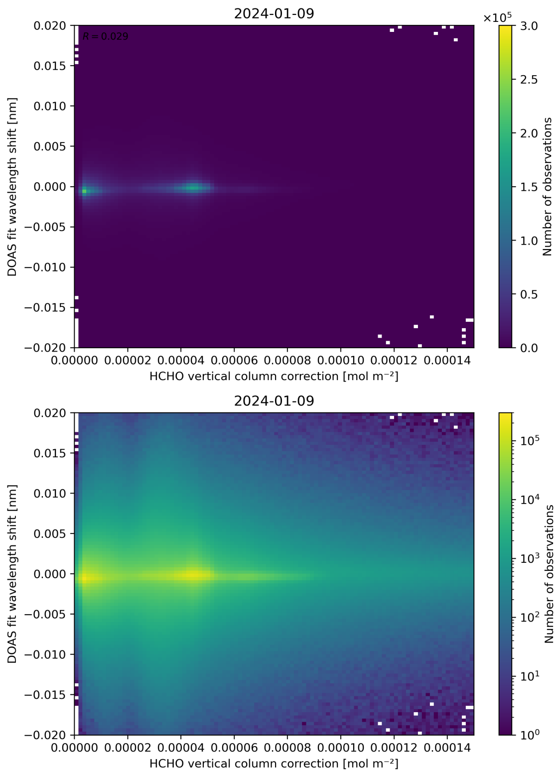
Figure 113: Scatter density plot of “HCHO vertical column correction” against “DOAS fit wavelength shift” for 2024-01-08 to 2024-01-10.
