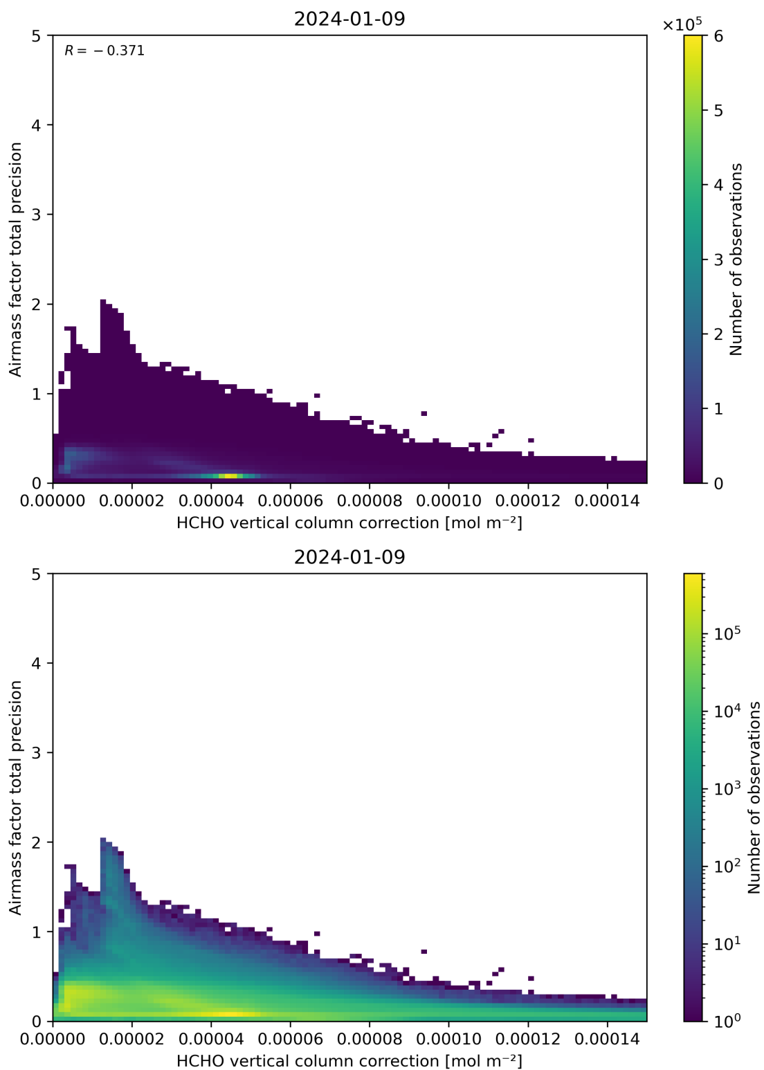
Figure 121: Scatter density plot of “HCHO vertical column correction” against “Airmass factor total precision” for 2024-01-08 to 2024-01-10.
