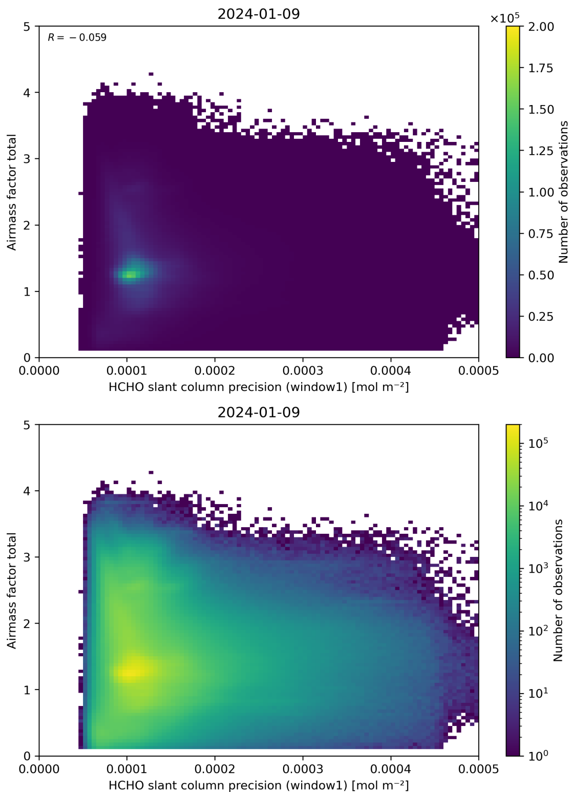
Figure 94: Scatter density plot of “HCHO slant column precision (window1)” against “Airmass factor total” for 2024-01-08 to 2024-01-10.
