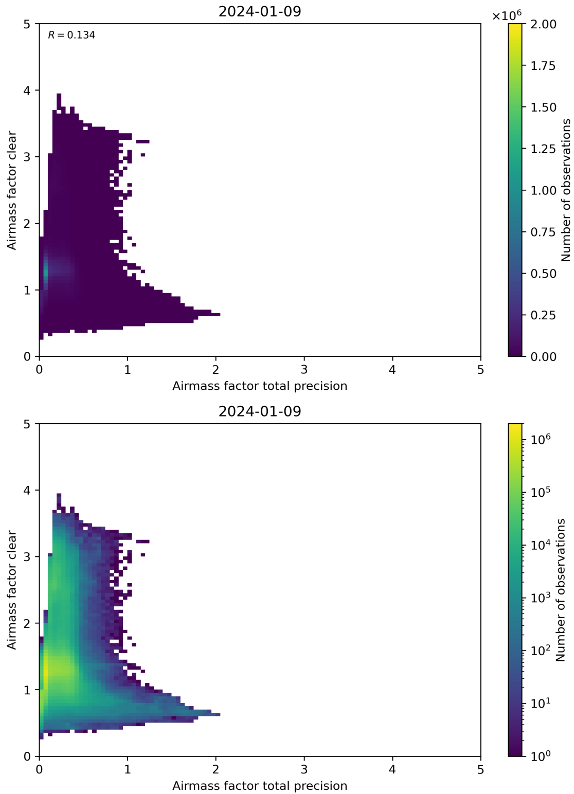
Figure 108: Scatter density plot of “Airmass factor total precision” against “Airmass factor clear” for 2024-01-08 to 2024-01-10.
