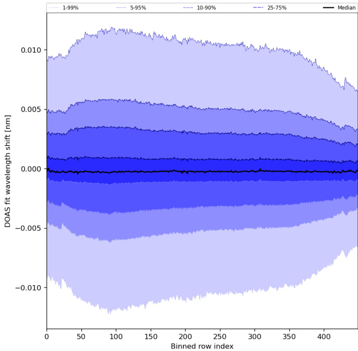
Figure 58: Along track statistics of “DOAS fit wavelength shift” for 2024-01-08 to 2024-01-10
