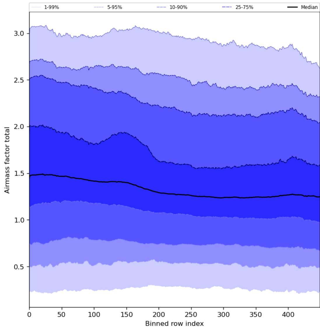
Figure 54: Along track statistics of “Airmass factor total” for 2024-01-08 to 2024-01-10
