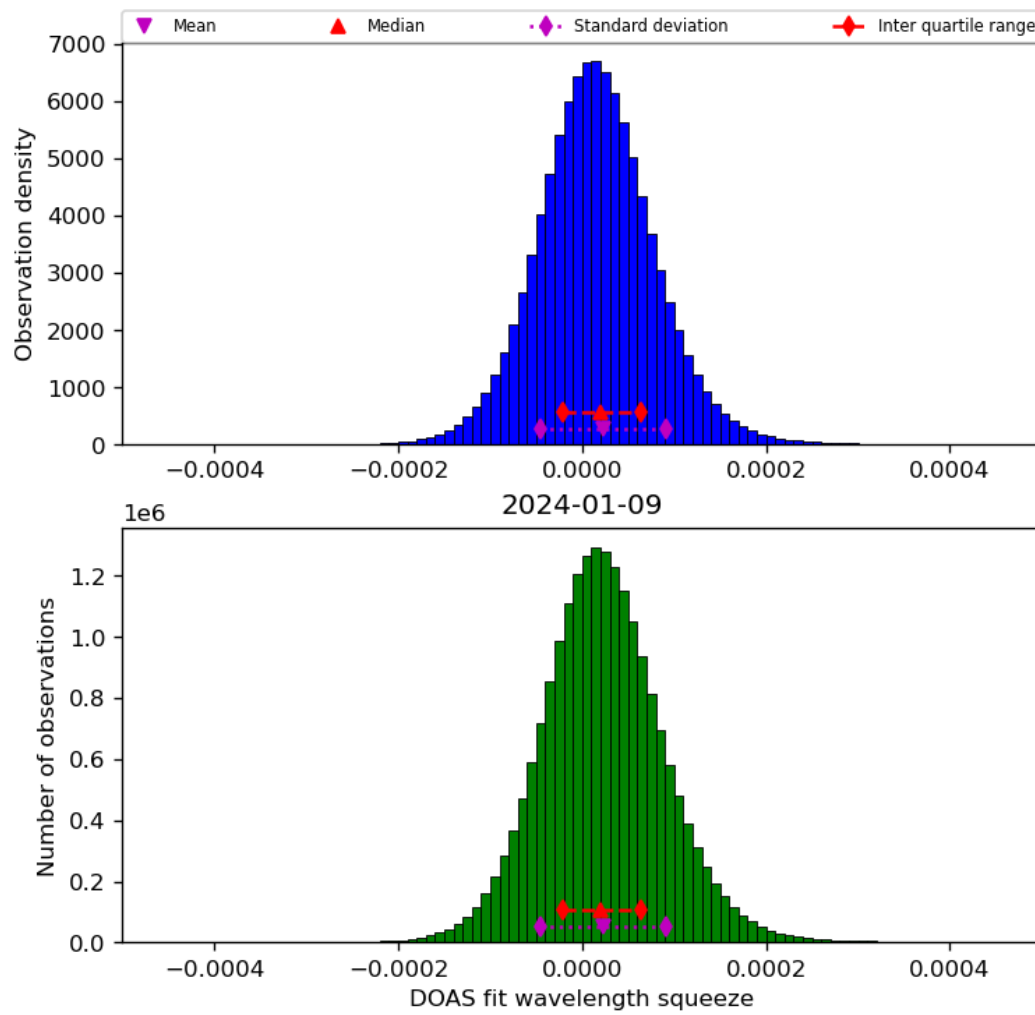
Figure 45: Histogram of “DOAS fit wavelength squeeze” for 2024-01-08 to 2024-01-10
