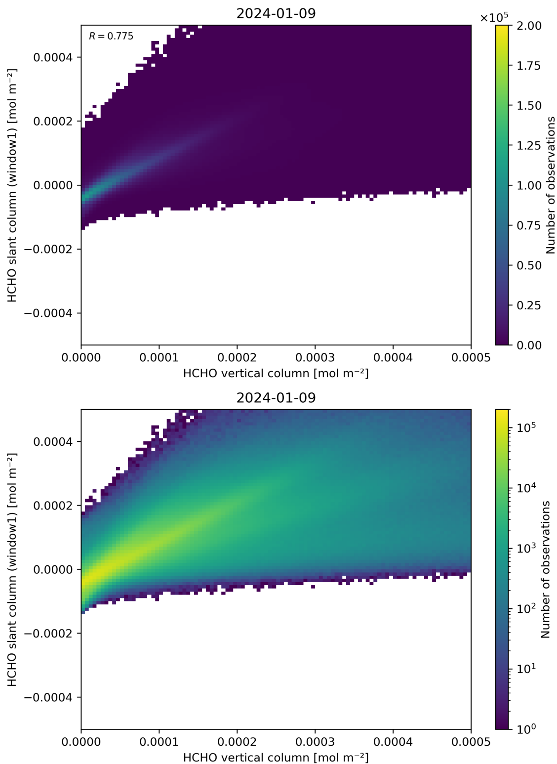
Figure 129: Scatter density plot of “HCHO vertical column” against “HCHO slant column (window1)” for 2024-01-08 to 2024-01-10.
