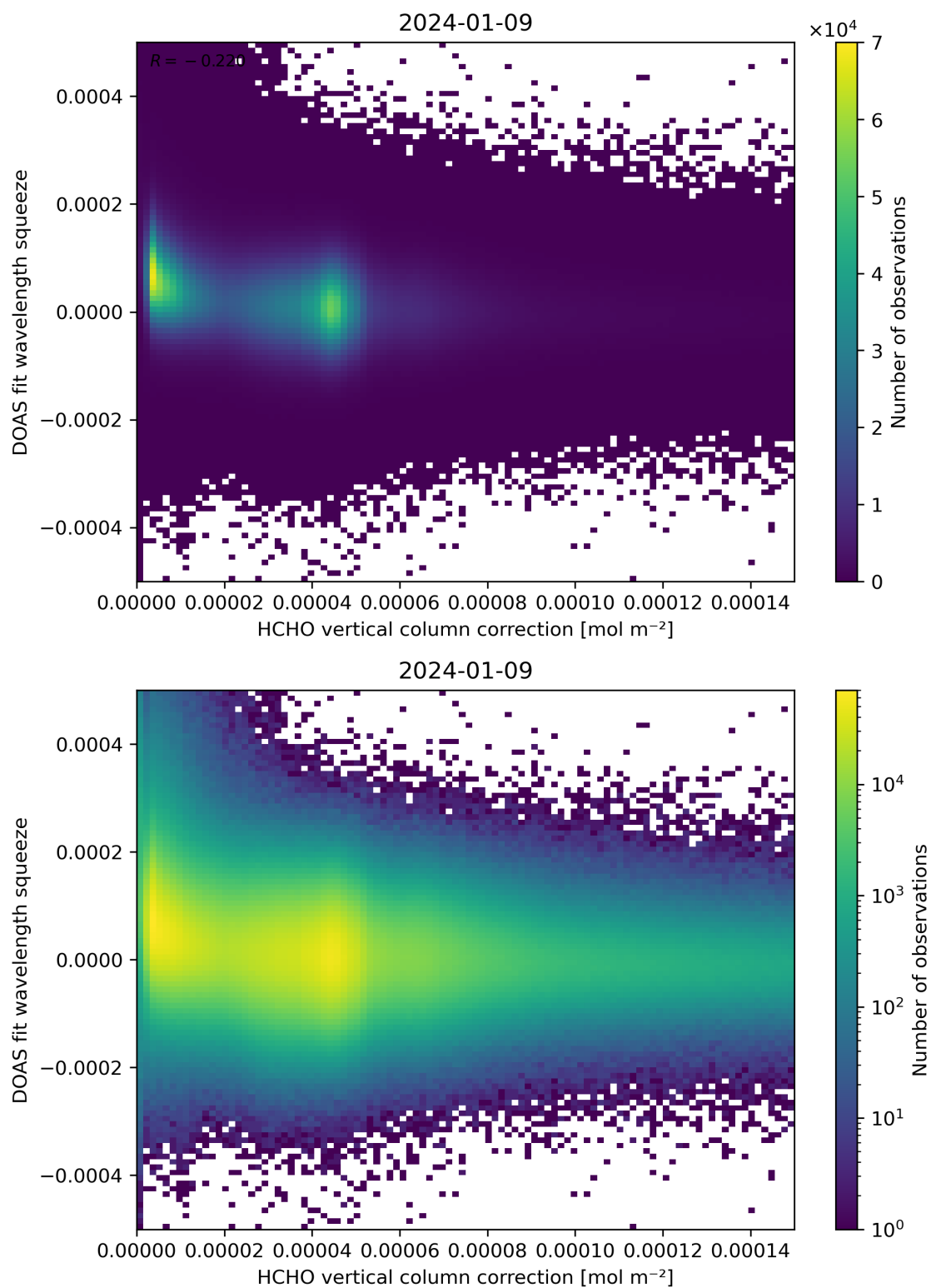
Figure 114: Scatter density plot of “HCHO vertical column correction” against “DOAS fit wavelength squeeze” for 2024-01-08 to 2024-01-10.
