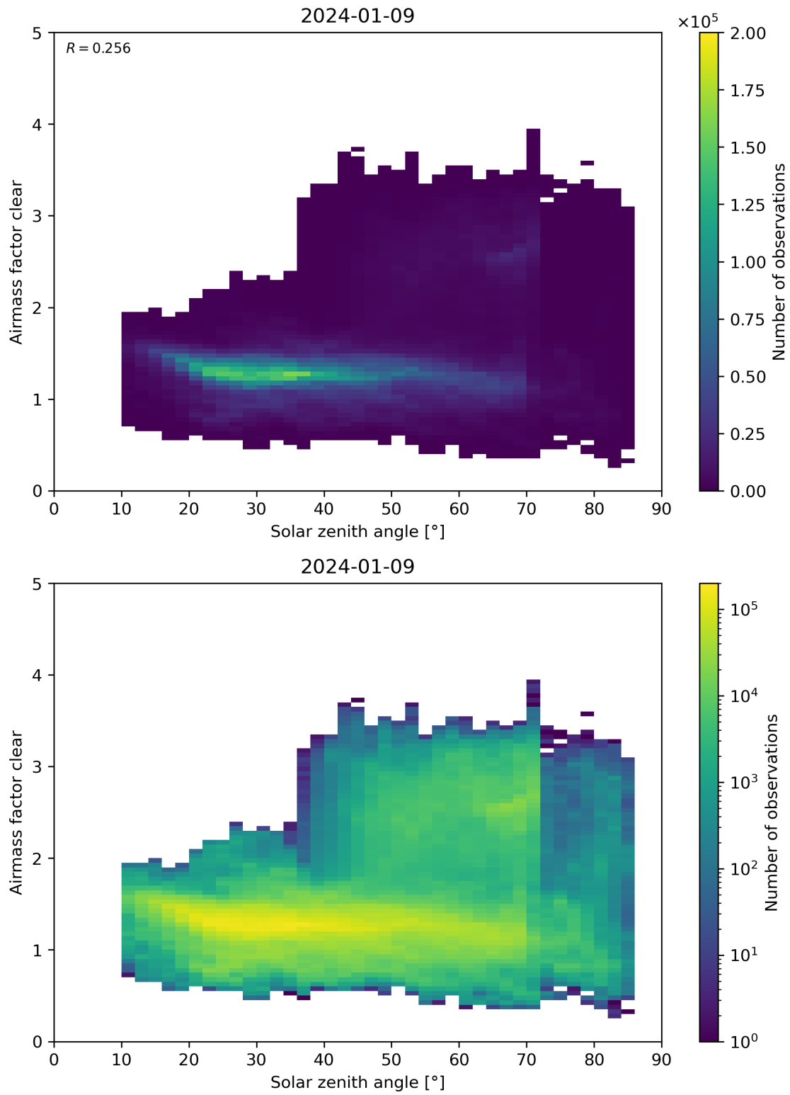
Figure 170: Scatter density plot of “Solar zenith angle” against “Airmass factor clear” for 2024-01-08 to 2024-01-10.
