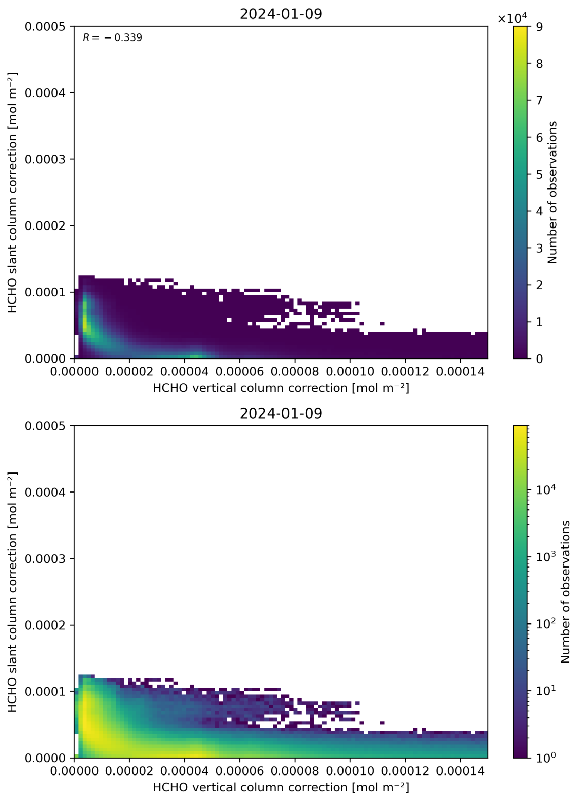
Figure 117: Scatter density plot of “HCHO vertical column correction” against “HCHO slant column correction” for 2024-01-08 to 2024-01-10.
