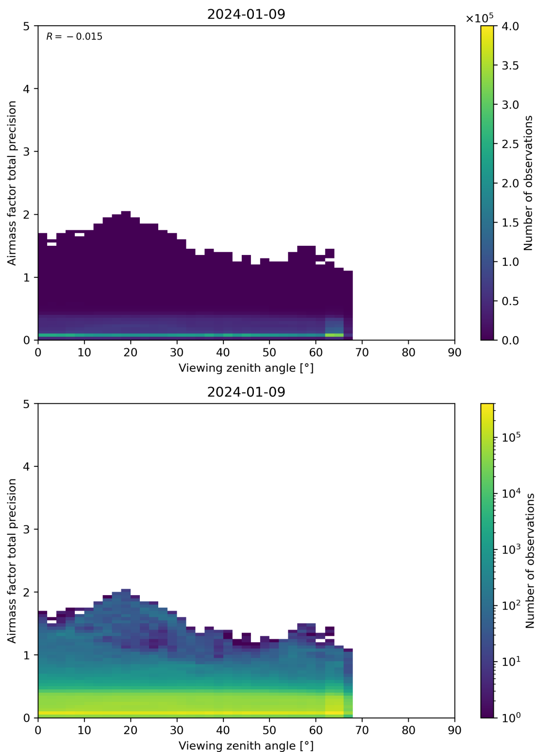
Figure 191: Scatter density plot of “Viewing zenith angle” against “Airmass factor total precision” for 2024-01-08 to 2024-01-10.
