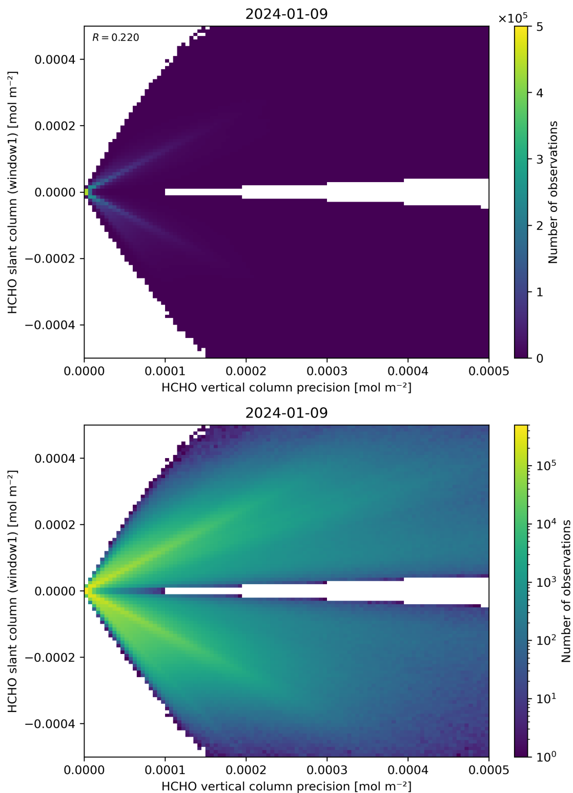
Figure 142: Scatter density plot of “HCHO vertical column precision” against “HCHO slant column (window1)” for 2024-01-08 to 2024-01-10.
