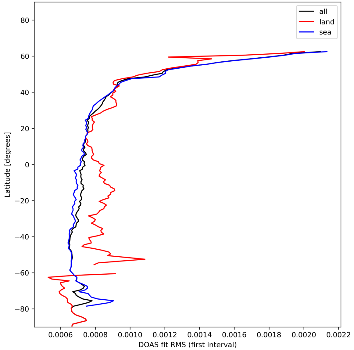
Figure 32: Zonal average of “DOAS fit RMS (first interval)” for 2024-01-08 to 2024-01-10.
