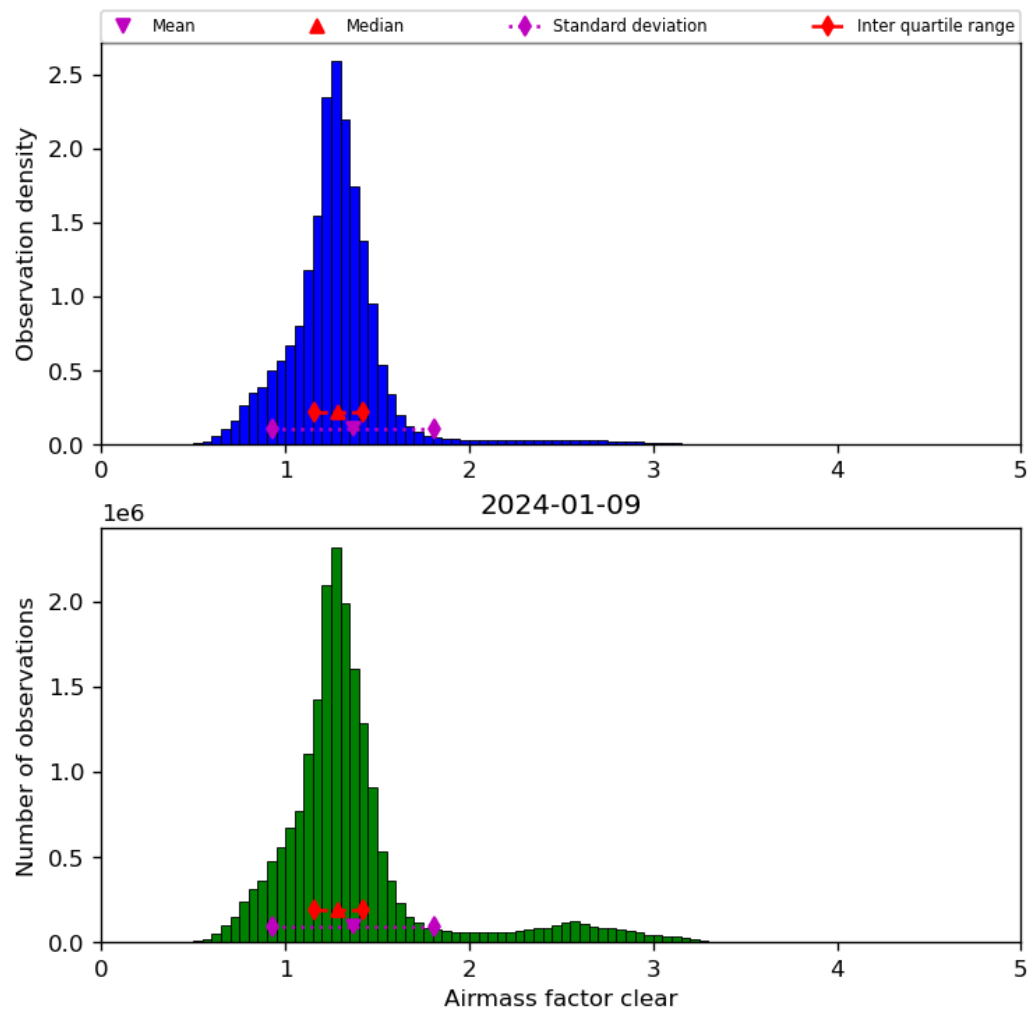
Figure 42: Histogram of “Airmass factor clear” for 2024-01-08 to 2024-01-10
