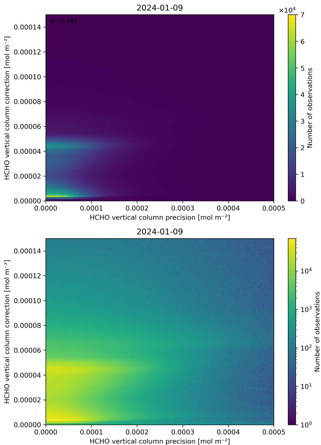
Figure 146: Scatter density plot of “HCHO vertical column precision” against “HCHO vertical column correction” for 2024-01-08 to 2024-01-10.
