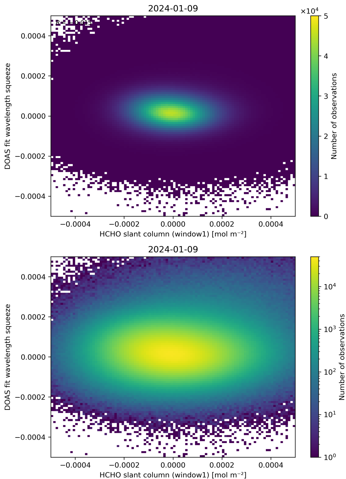
Figure 80: Scatter density plot of “HCHO slant column (window1)” against “DOAS fit wavelength squeeze” for 2024-01-08 to 2024-01-10.
