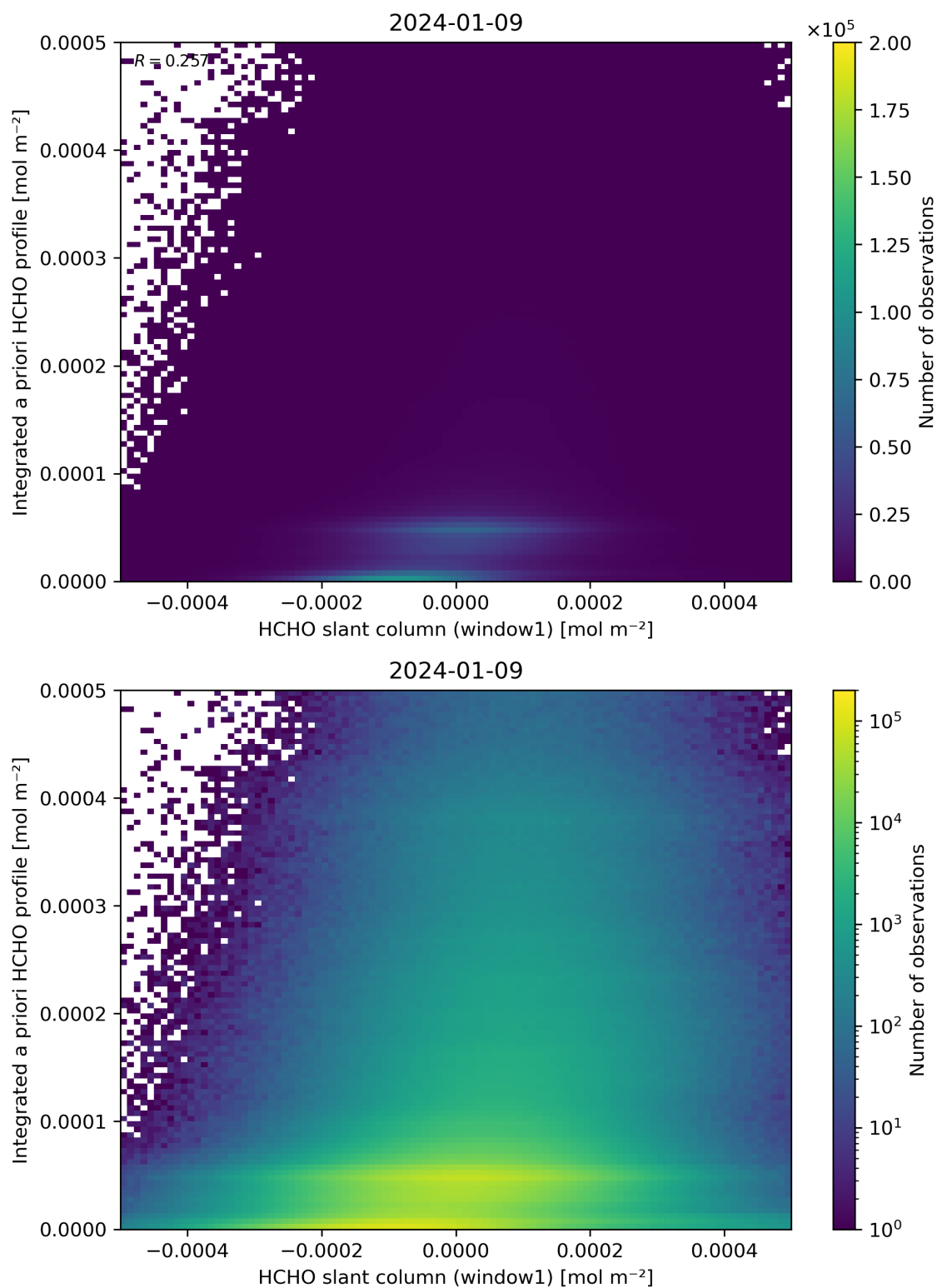
Figure 87: Scatter density plot of “HCHO slant column (window1)” against “Integrated a priori HCHO profile” for 2024-01-08 to 2024-01-10.
