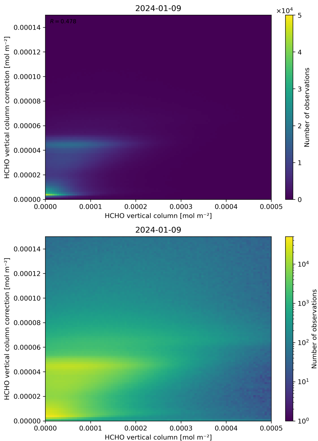
Figure 133: Scatter density plot of “HCHO vertical column” against “HCHO vertical column correction” for 2024-01-08 to 2024-01-10.
