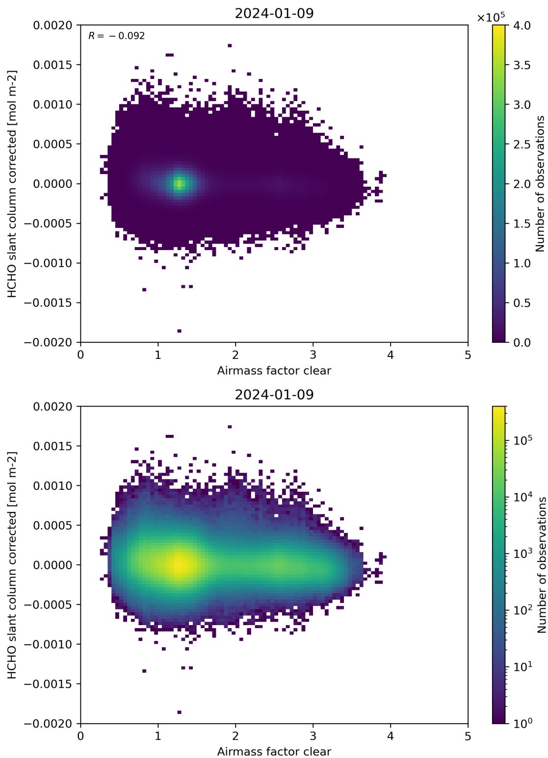
Figure 74: Scatter density plot of “Airmass factor clear” against “HCHO slant column corrected” for 2024-01-08 to 2024-01-10.
