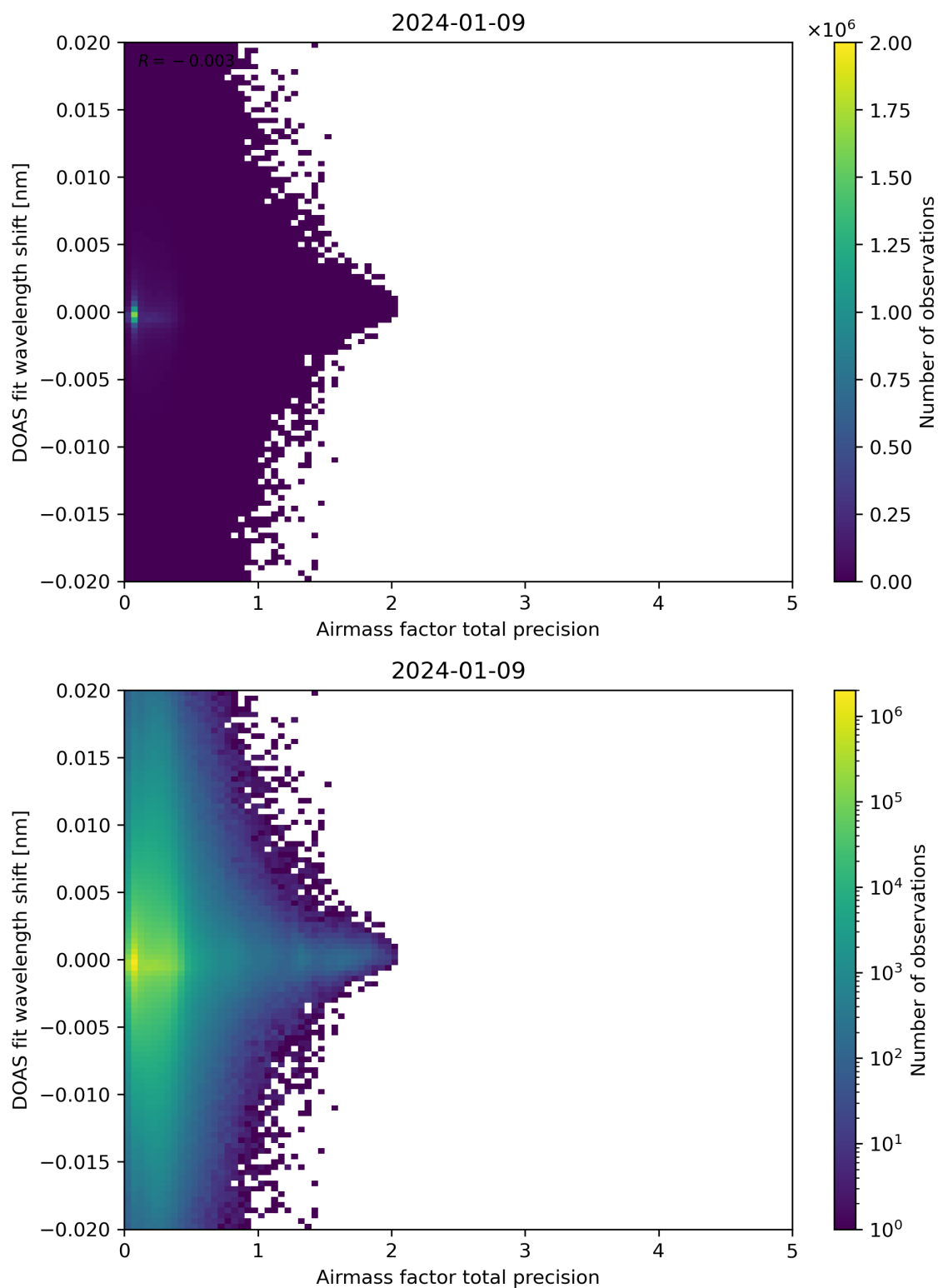
Figure 106: Scatter density plot of “Airmass factor total precision” against “DOAS fit wavelength shift” for 2024-01-08 to 2024-01-10.
