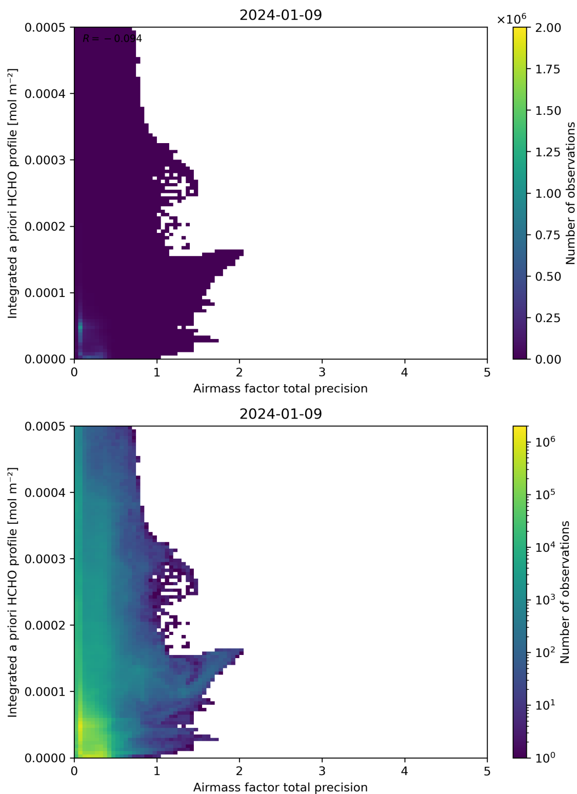
Figure 111: Scatter density plot of “Airmass factor total precision” against “Integrated a priori HCHO profile” for 2024-01-08 to 2024-01-10.
