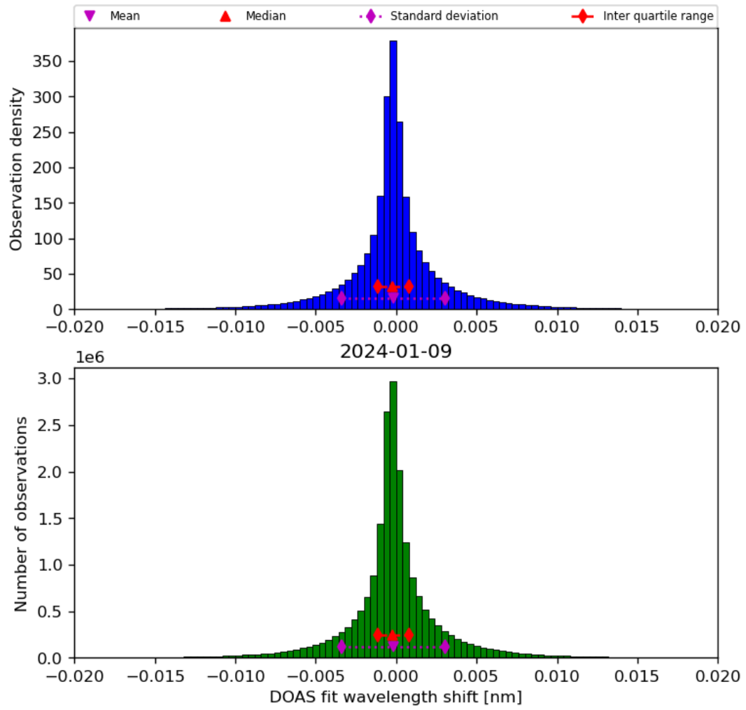
Figure 44: Histogram of “DOAS fit wavelength shift” for 2024-01-08 to 2024-01-10
