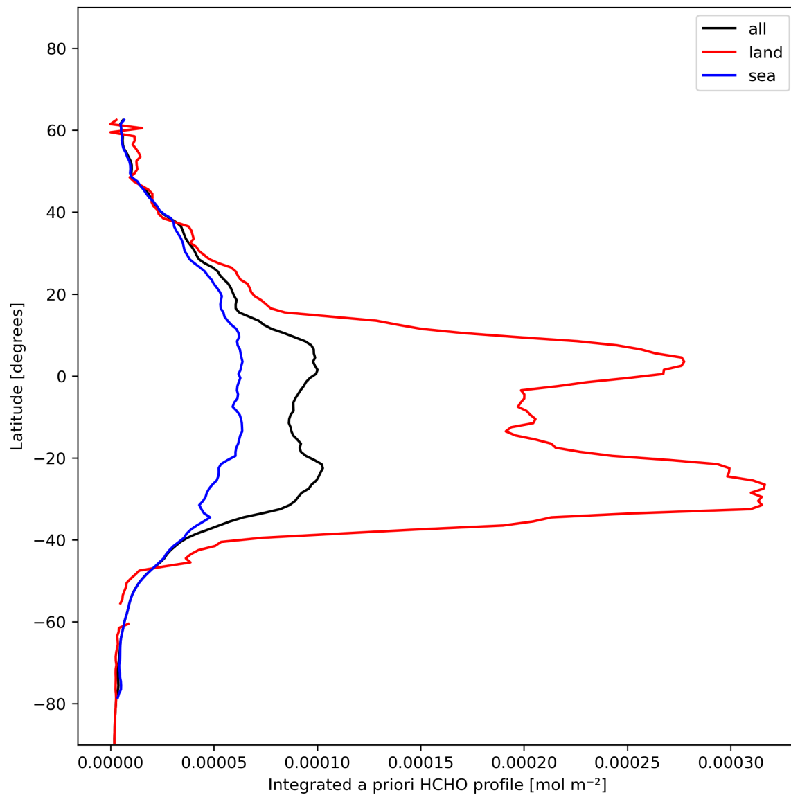
Figure 29: Zonal average of “Integrated a priori HCHO profile” for 2024-01-08 to 2024-01-10.
