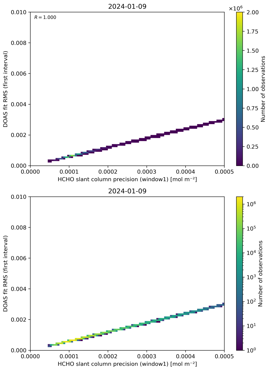
Figure 88: Scatter density plot of “HCHO slant column precision (window1)” against “DOAS fit RMS (first interval)” for 2024-01-08 to 2024-01-10.
