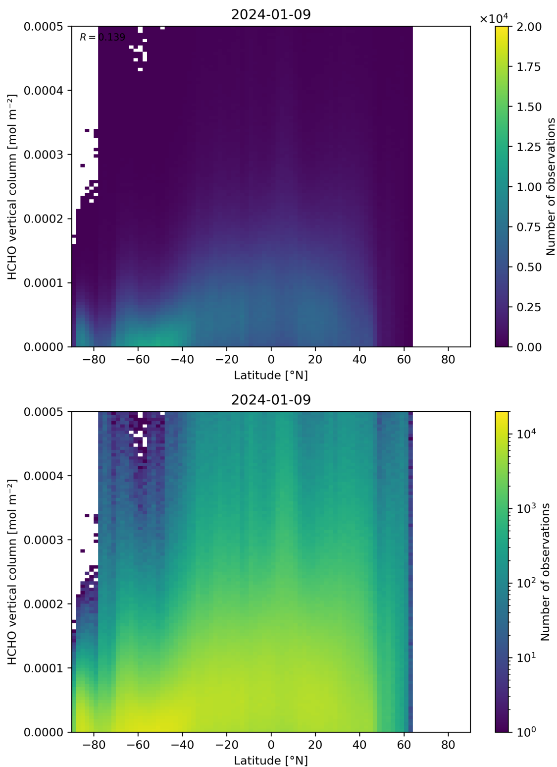
Figure 163: Scatter density plot of “Latitude” against “HCHO vertical column” for 2024-01-08 to 2024-01-10.
