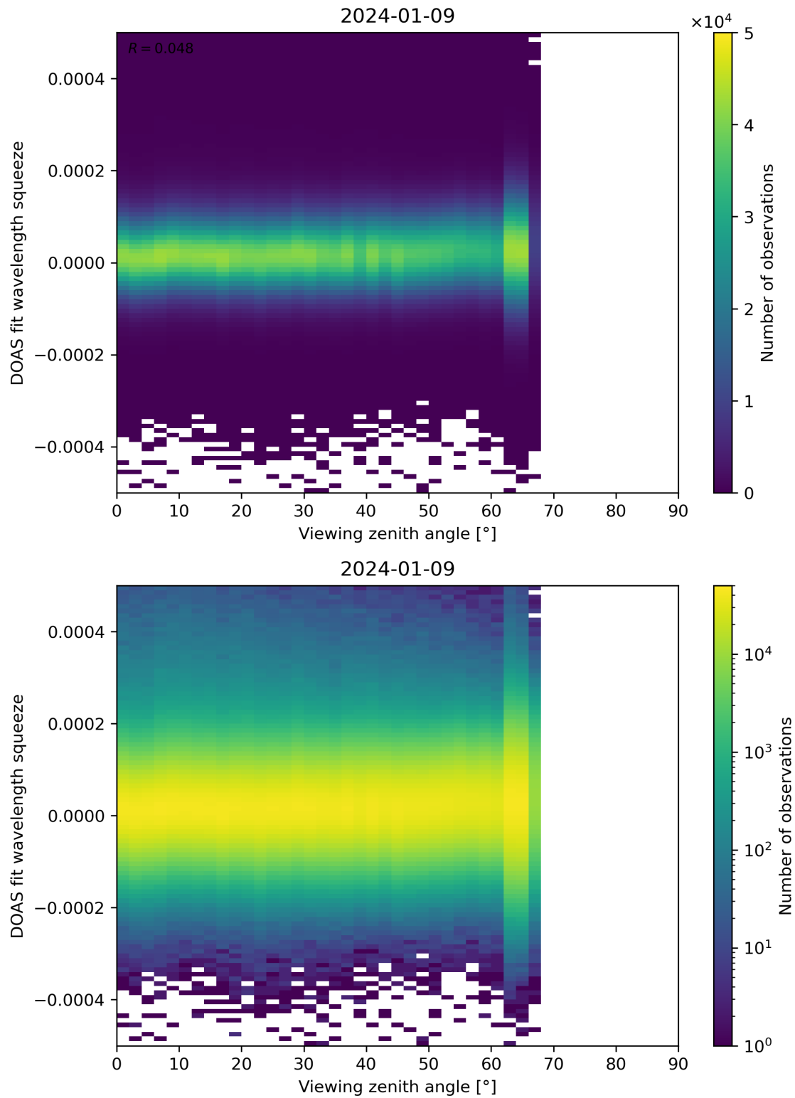
Figure 184: Scatter density plot of “Viewing zenith angle” against “DOAS fit wavelength squeeze” for 2024-01-08 to 2024-01-10.
