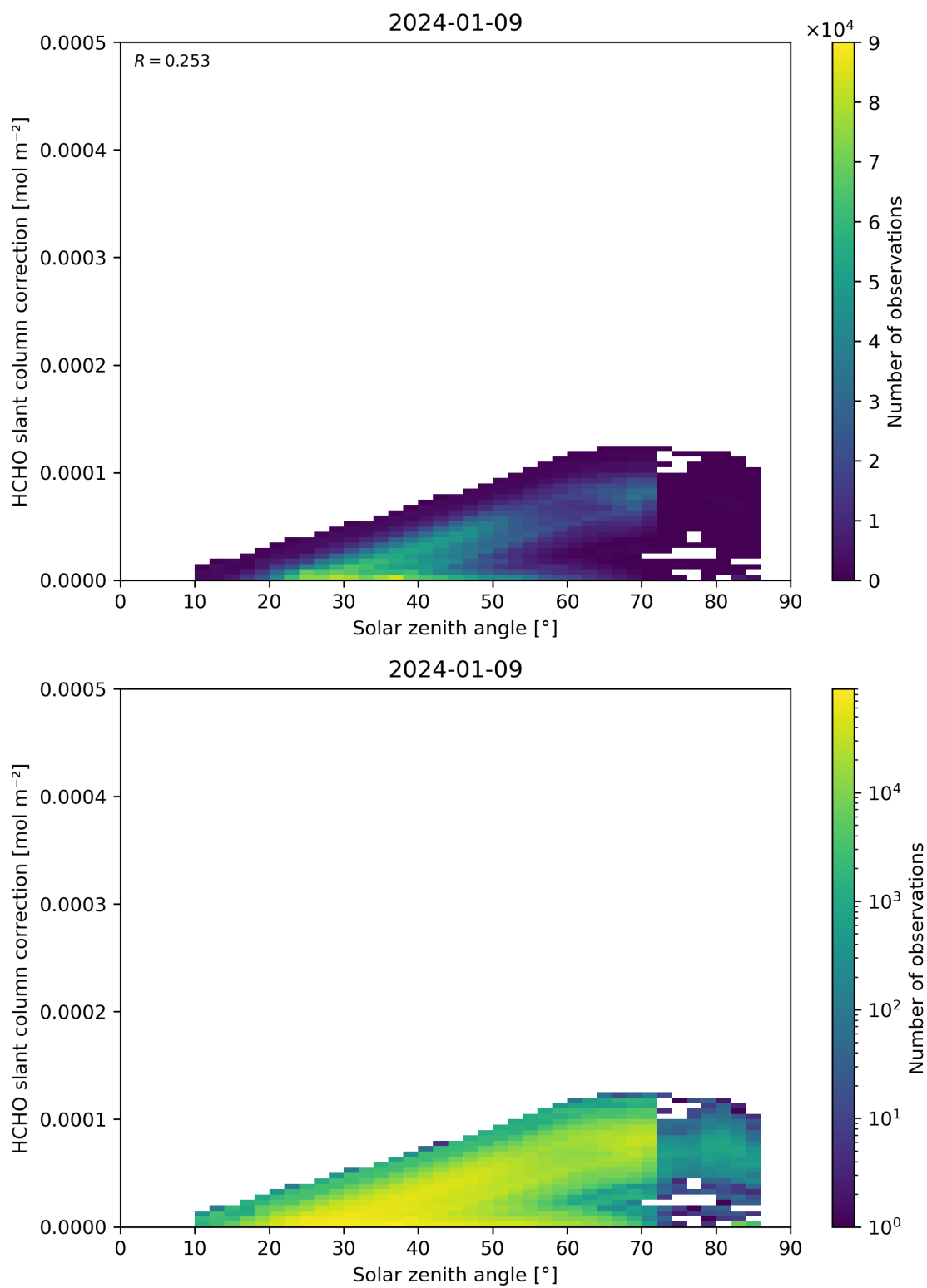
Figure 172: Scatter density plot of “Solar zenith angle” against “HCHO slant column correction” for 2024-01-08 to 2024-01-10.
