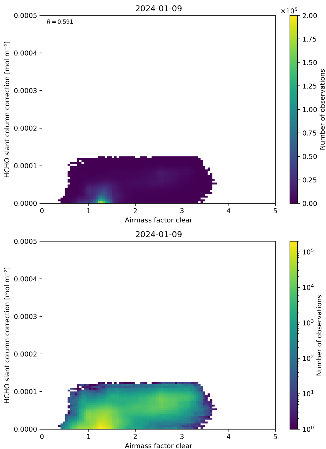
Figure 75: Scatter density plot of “Airmass factor clear” against “HCHO slant column correction” for 2024-01-08 to 2024-01-10.
