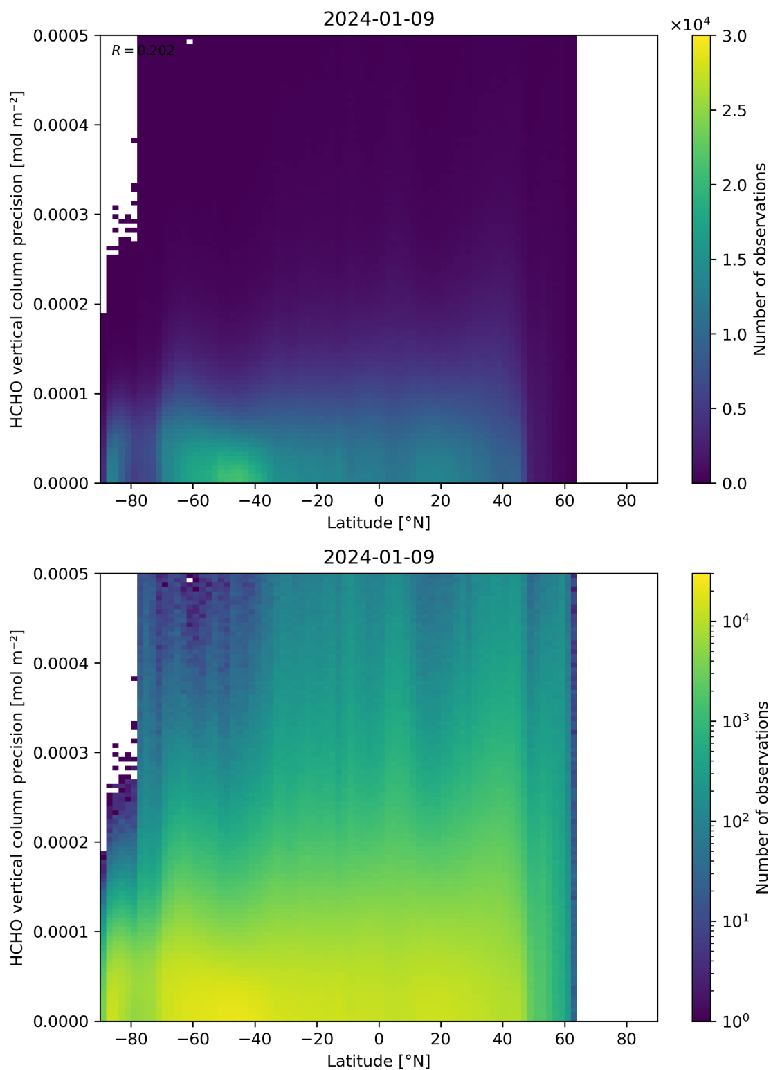
Figure 165: Scatter density plot of “Latitude” against “HCHO vertical column precision” for 2024-01-08 to 2024-01-10.
