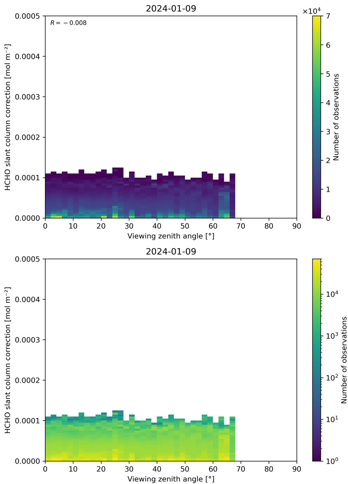
Figure 187: Scatter density plot of “Viewing zenith angle” against “HCHO slant column correction” for 2024-01-08 to 2024-01-10.
