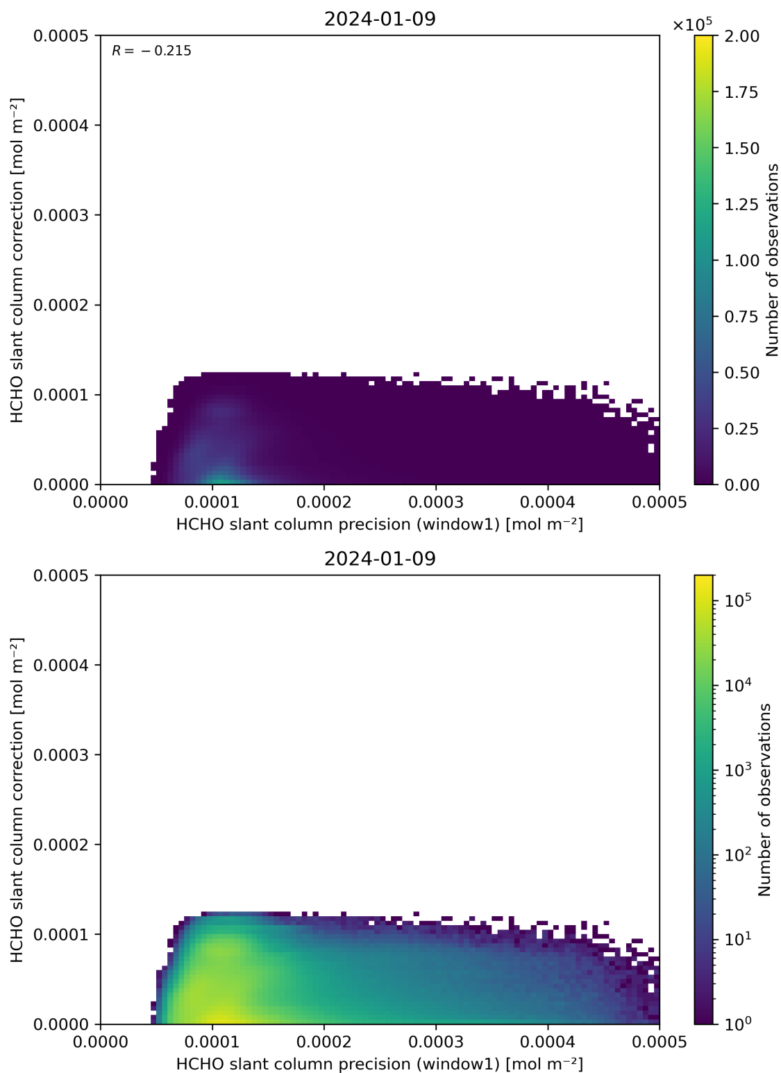
Figure 93: Scatter density plot of “HCHO slant column precision (window1)” against “HCHO slant column correction” for 2024-01-08 to 2024-01-10.
