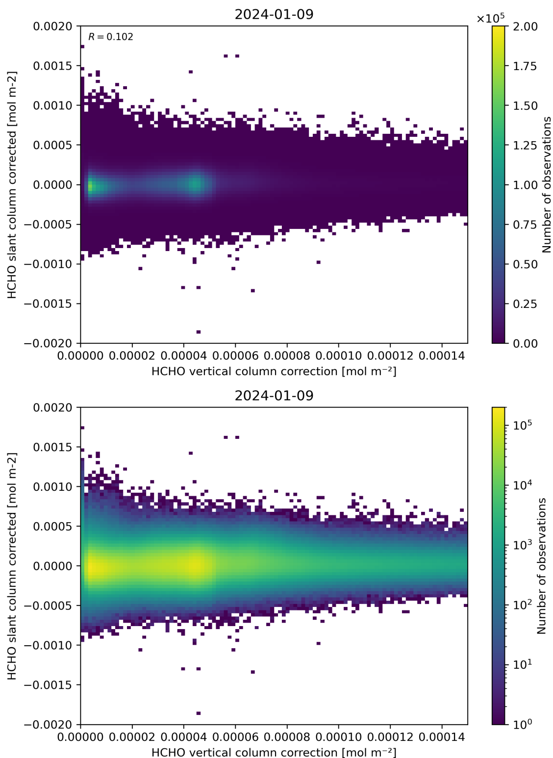
Figure 116: Scatter density plot of “HCHO vertical column correction” against “HCHO slant column corrected” for 2024-01-08 to 2024-01-10.
