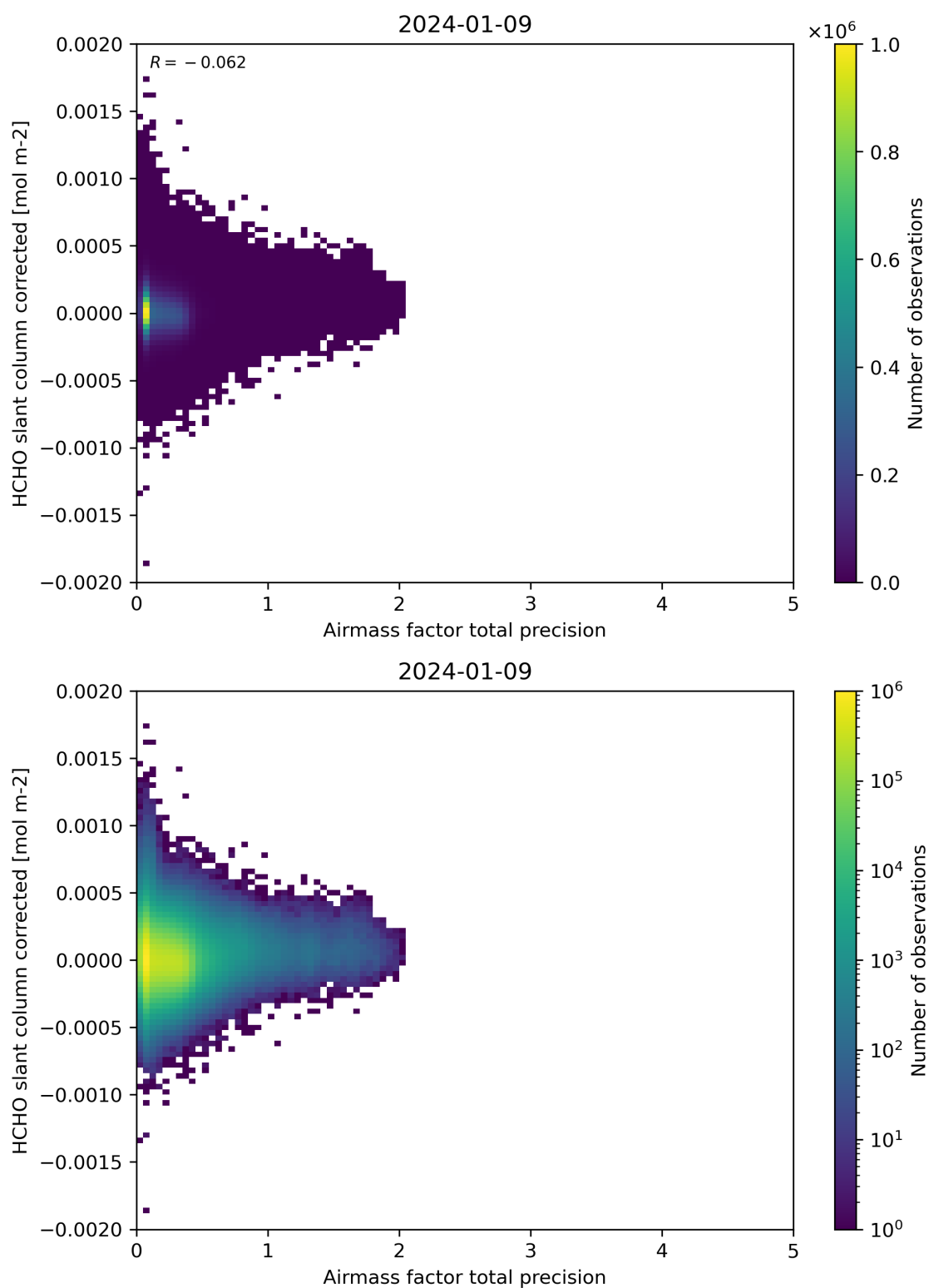
Figure 109: Scatter density plot of “Airmass factor total precision” against “HCHO slant column corrected” for 2024-01-08 to 2024-01-10.
