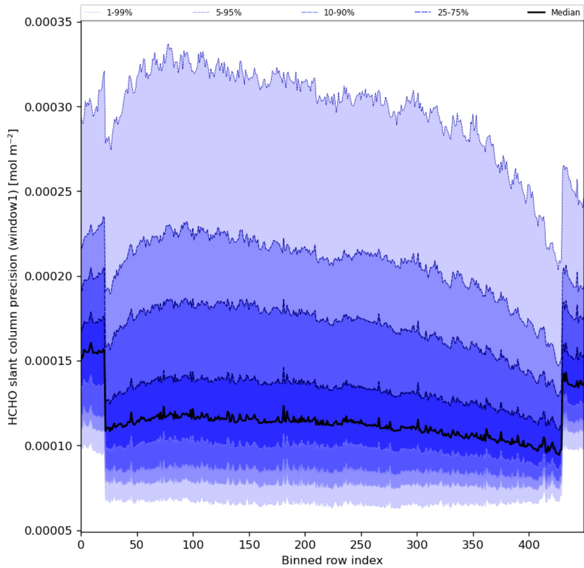
Figure 53: Along track statistics of “HCHO slant column precision (window1)” for 2024-01-08 to 2024-01-10
