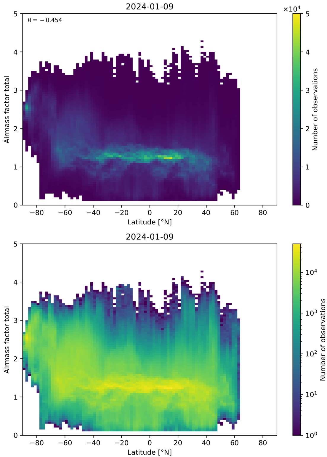
Figure 161: Scatter density plot of “Latitude” against “Airmass factor total” for 2024-01-08 to 2024-01-10.
