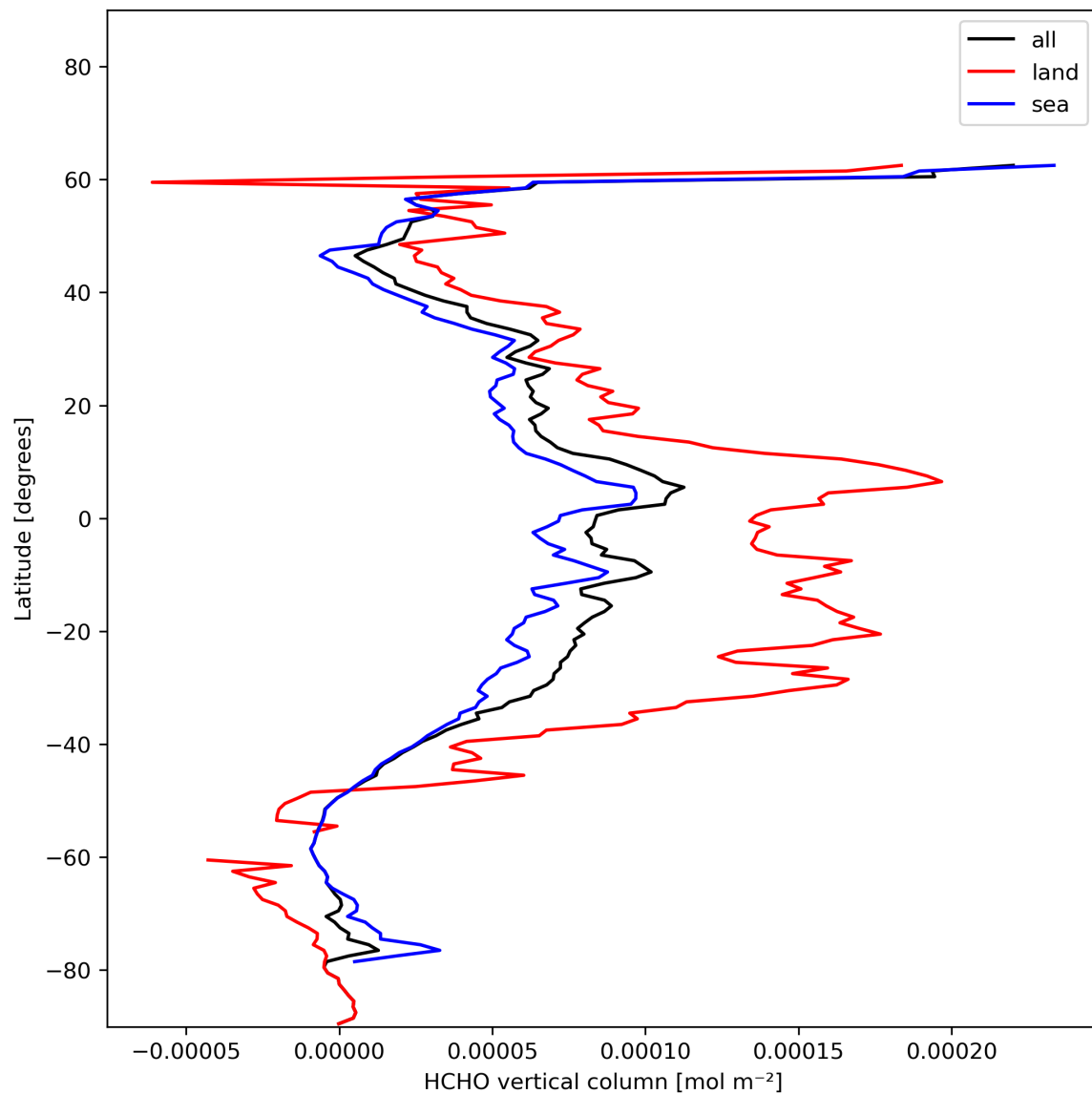
Figure 21: Zonal average of “HCHO vertical column” for 2024-01-08 to 2024-01-10.
