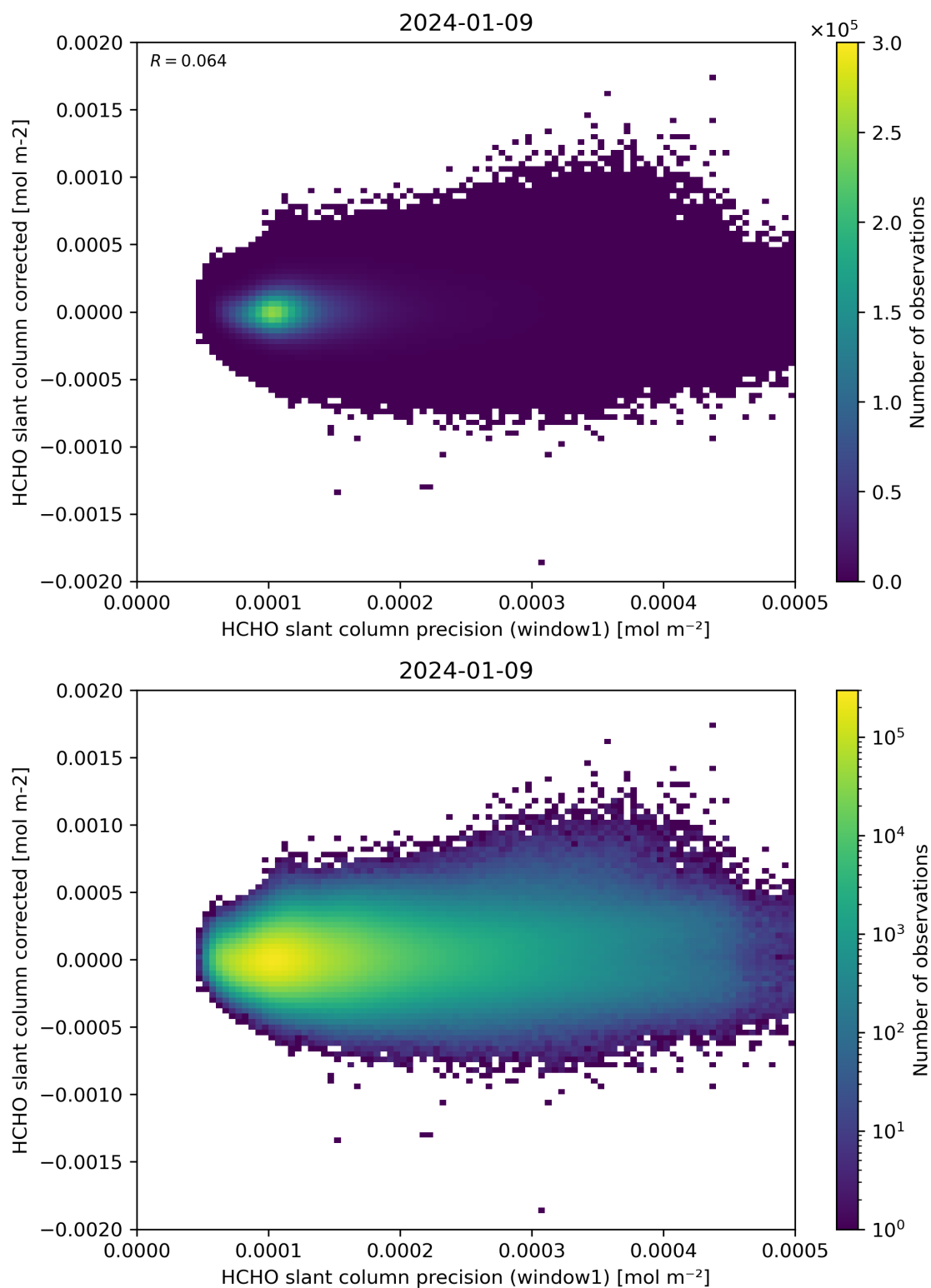
Figure 92: Scatter density plot of “HCHO slant column precision (window1)” against “HCHO slant column corrected” for 2024-01-08 to 2024-01-10.
