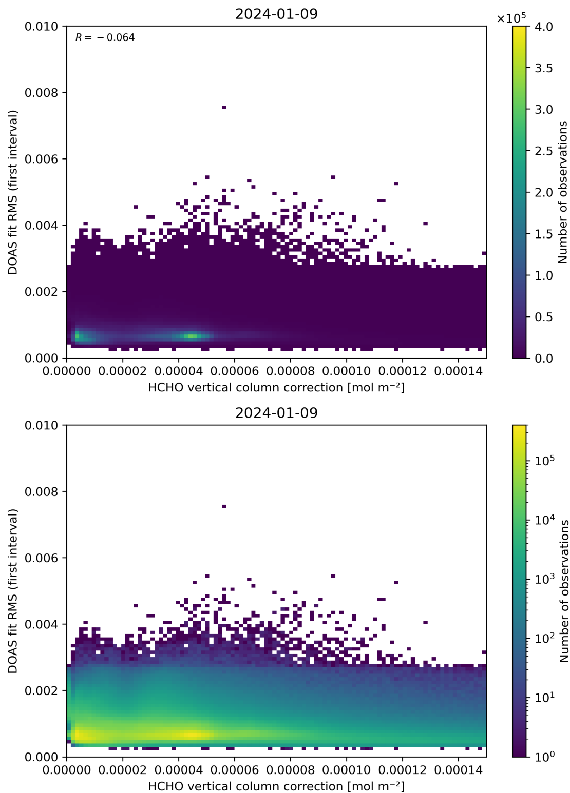
Figure 112: Scatter density plot of “HCHO vertical column correction” against “DOAS fit RMS (first interval)” for 2024-01-08 to 2024-01-10.
