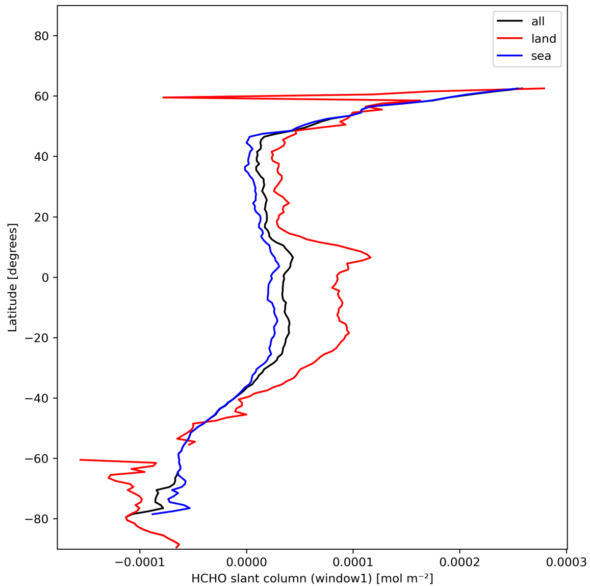
Figure 24: Zonal average of “HCHO slant column (window1)” for 2024-01-08 to 2024-01-10.
