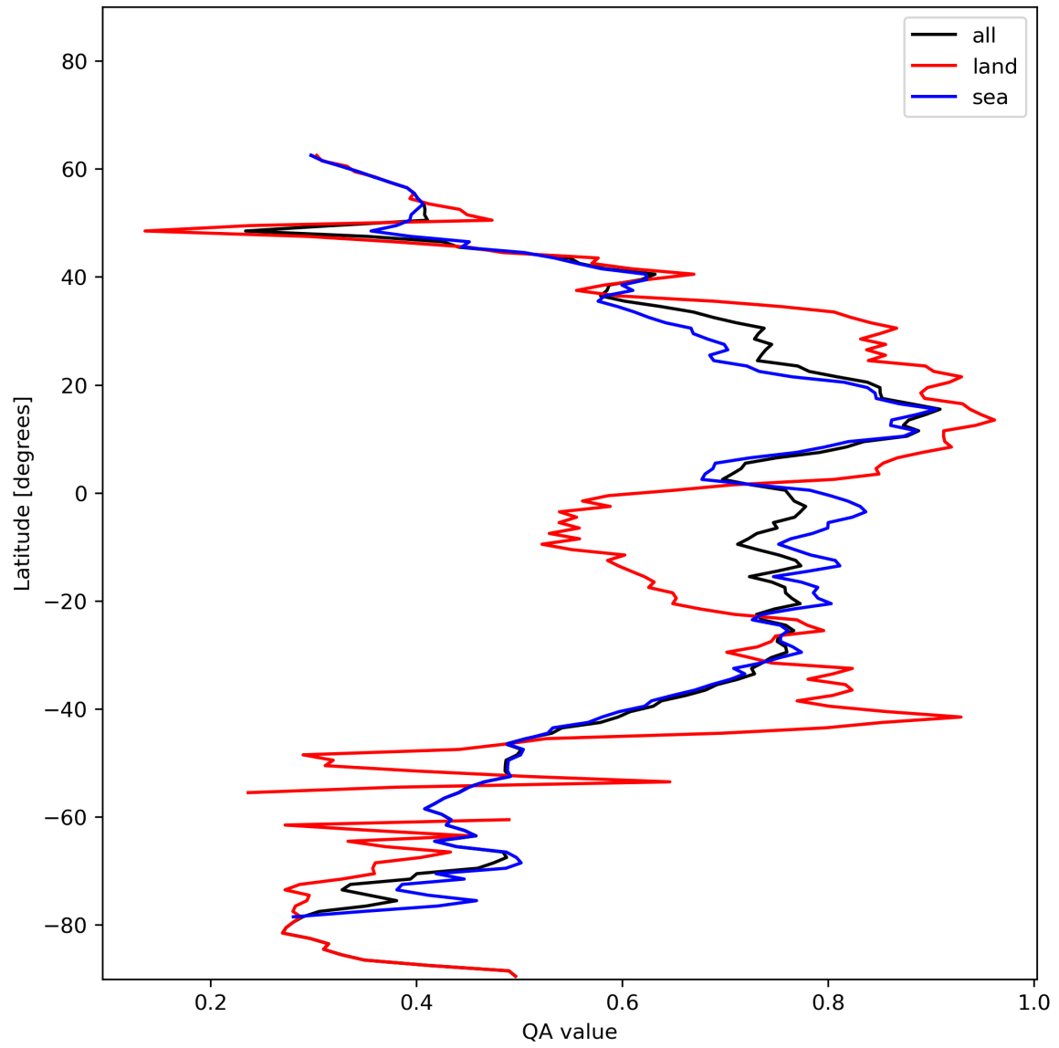
Figure 20: Zonal average of “QA value” for 2024-01-08 to 2024-01-10.
