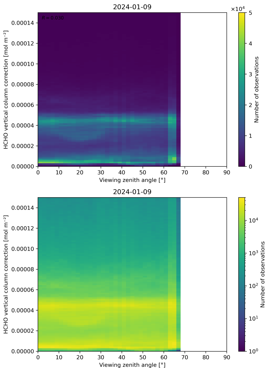
Figure 193: Scatter density plot of “Viewing zenith angle” against “HCHO vertical column correction” for 2024-01-08 to 2024-01-10.
