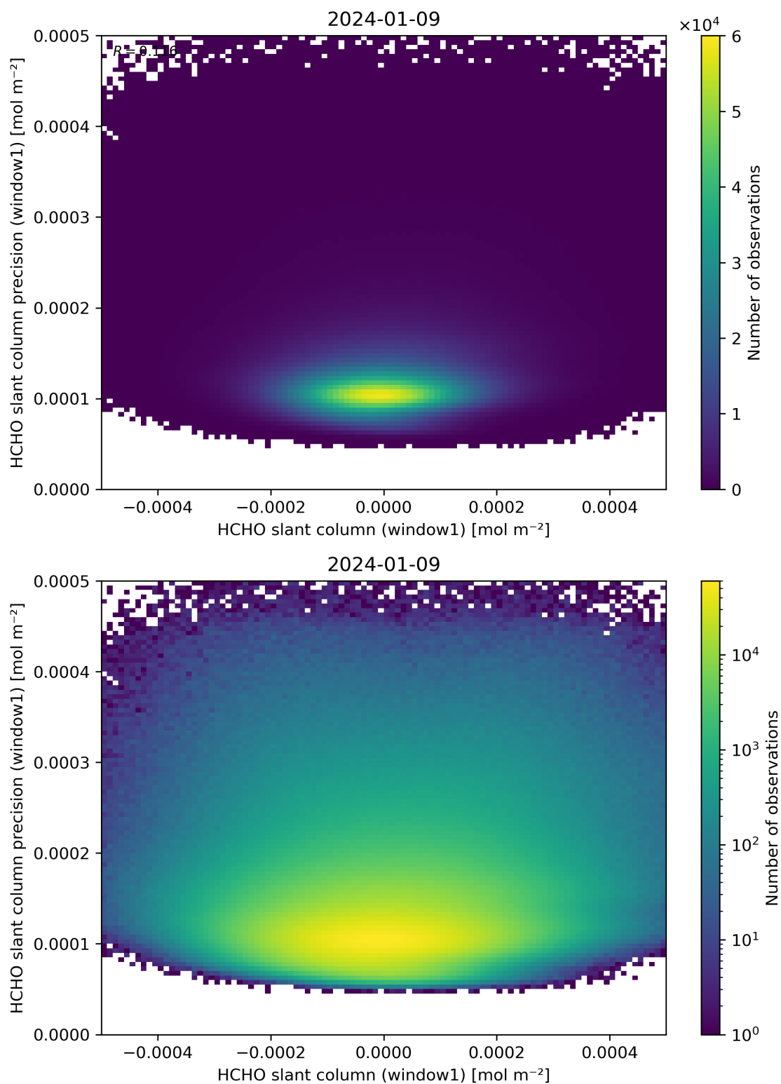
Figure 84: Scatter density plot of “HCHO slant column (window1)” against “HCHO slant column precision (window1)” for 2024-01-08 to 2024-01-10.
