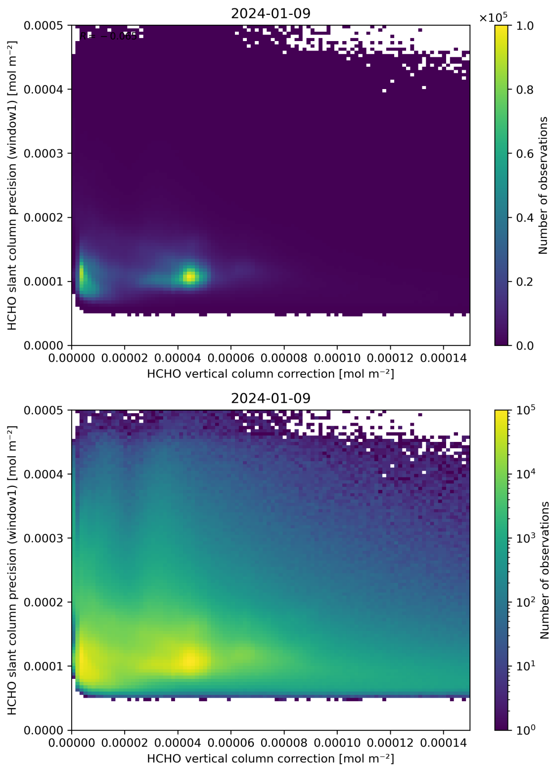
Figure 119: Scatter density plot of “HCHO vertical column correction” against “HCHO slant column precision (window1)” for 2024-01-08 to 2024-01-10.
