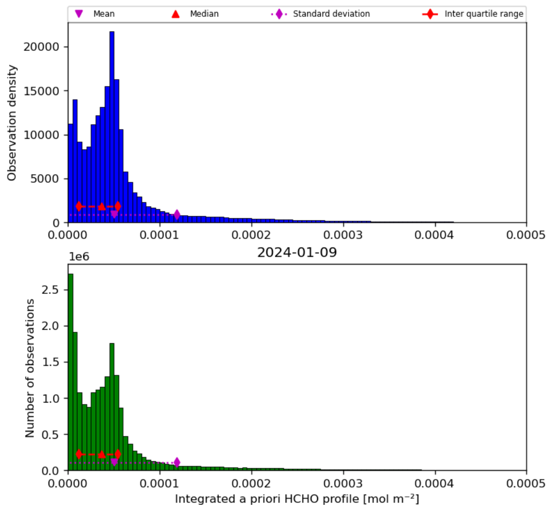
Figure 43: Histogram of “Integrated a priori HCHO profile” for 2024-01-08 to 2024-01-10
