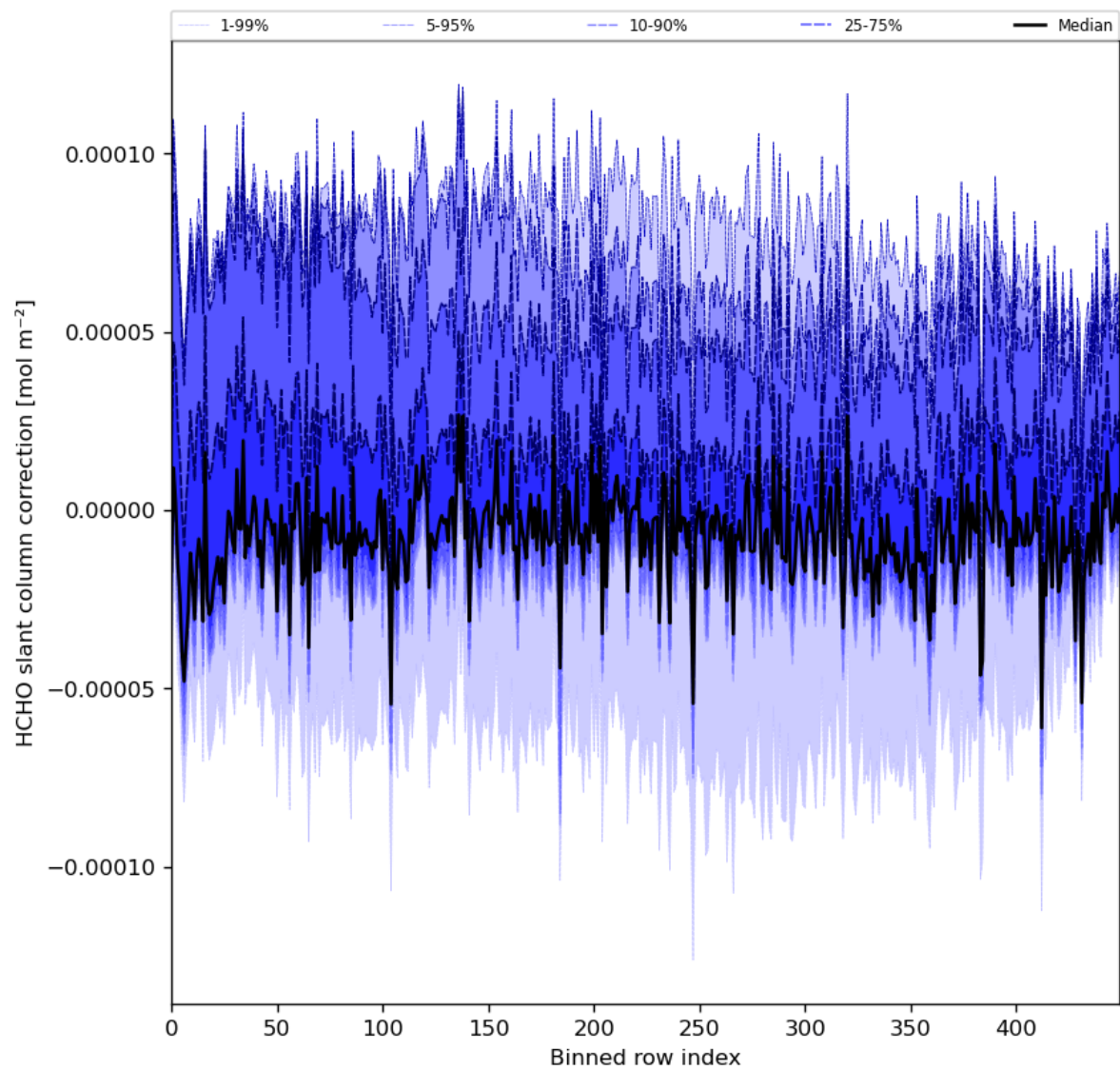
Figure 61: Along track statistics of “HCHO slant column correction” for 2024-01-08 to 2024-01-10
