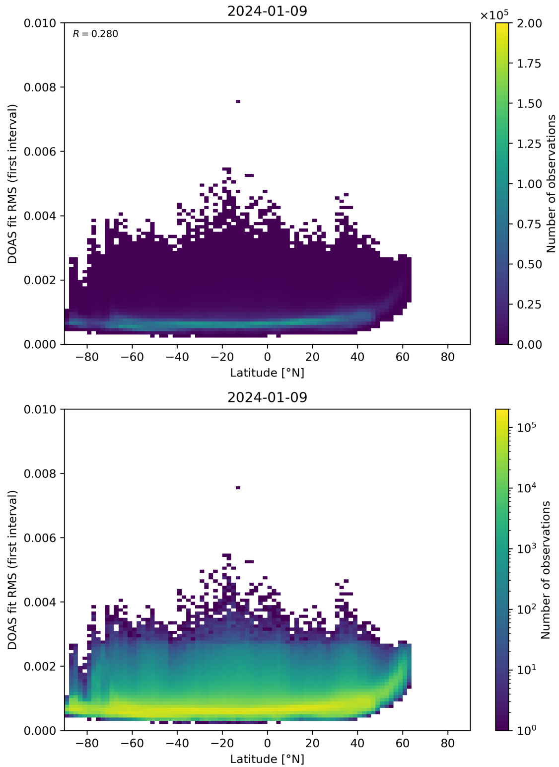
Figure 153: Scatter density plot of “Latitude” against “DOAS fit RMS (first interval)” for 2024-01-08 to 2024-01-10.
