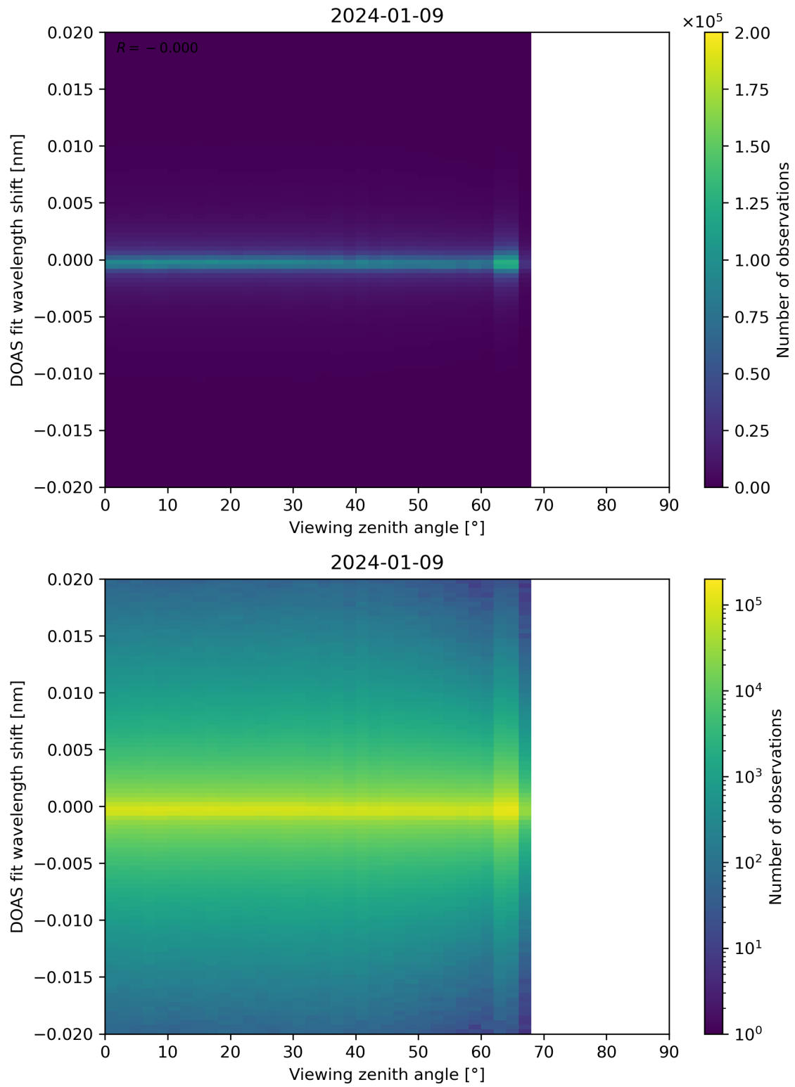
Figure 183: Scatter density plot of “Viewing zenith angle” against “DOAS fit wavelength shift” for 2024-01-08 to 2024-01-10.
