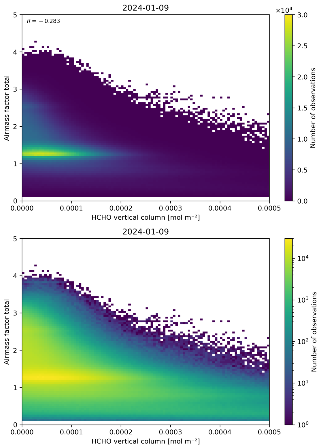
Figure 131: Scatter density plot of “HCHO vertical column” against “Airmass factor total” for 2024-01-08 to 2024-01-10.
