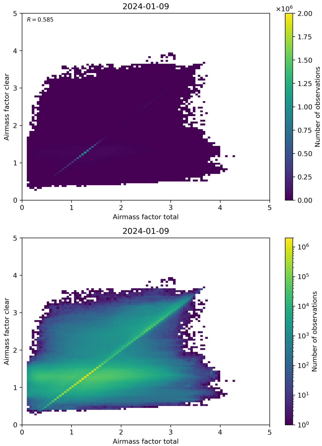
Figure 100: Scatter density plot of “Airmass factor total” against “Airmass factor clear” for 2024-01-08 to 2024-01-10.
