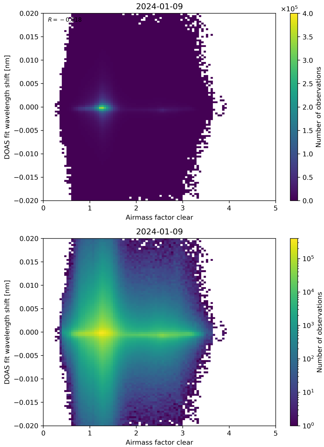
Figure 72: Scatter density plot of “Airmass factor clear” against “DOAS fit wavelength shift” for 2024-01-08 to 2024-01-10.
