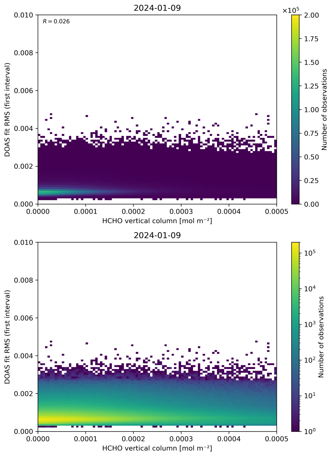
Figure 123: Scatter density plot of “HCHO vertical column” against “DOAS fit RMS (first interval)” for 2024-01-08 to 2024-01-10.
