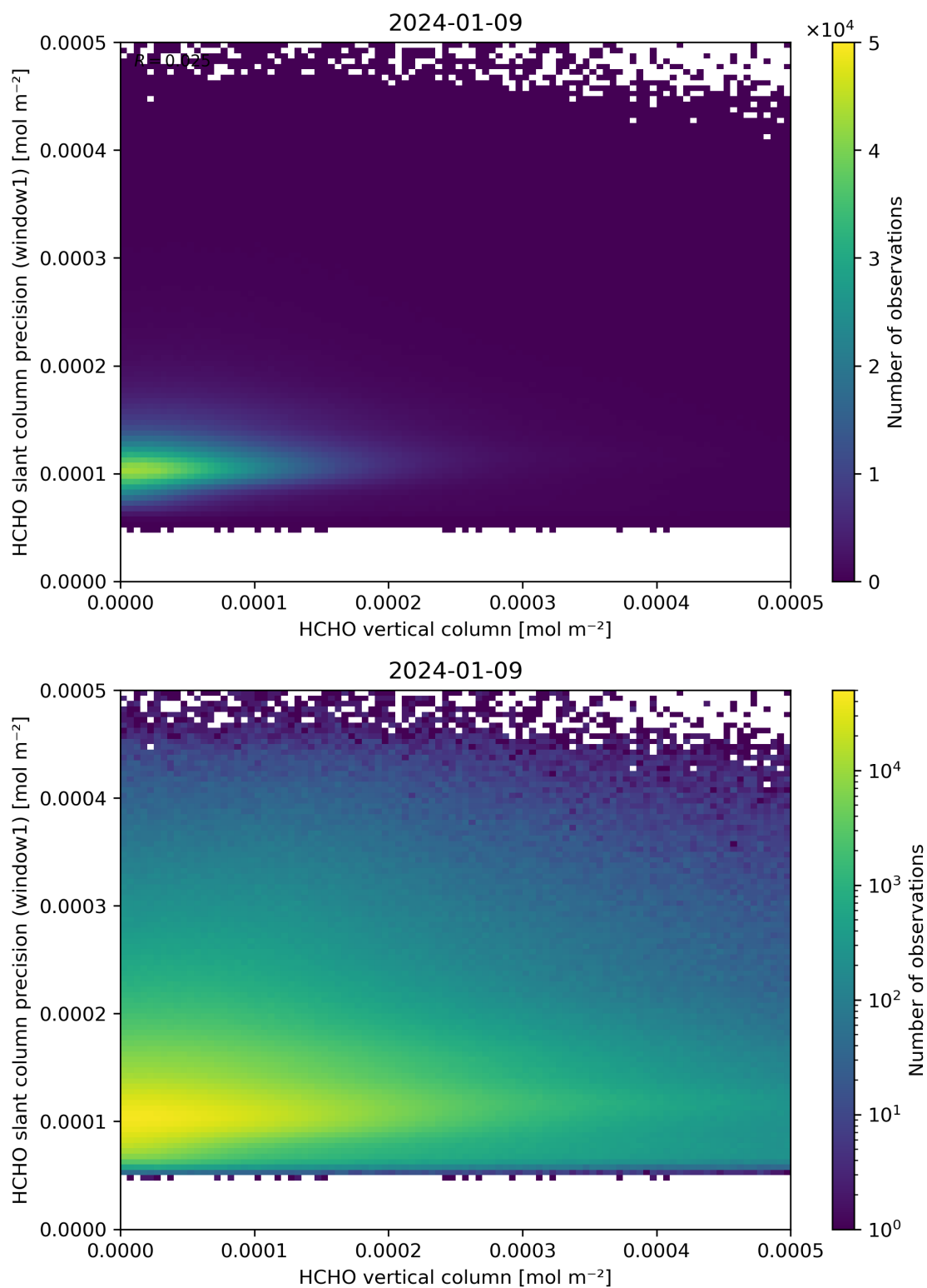
Figure 130: Scatter density plot of “HCHO vertical column” against “HCHO slant column precision (window1)” for 2024-01-08 to 2024-01-10.
