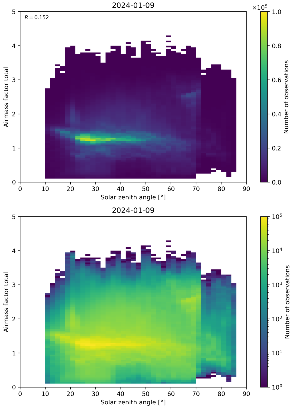
Figure 175: Scatter density plot of “Solar zenith angle” against “Airmass factor total” for 2024-01-08 to 2024-01-10.
