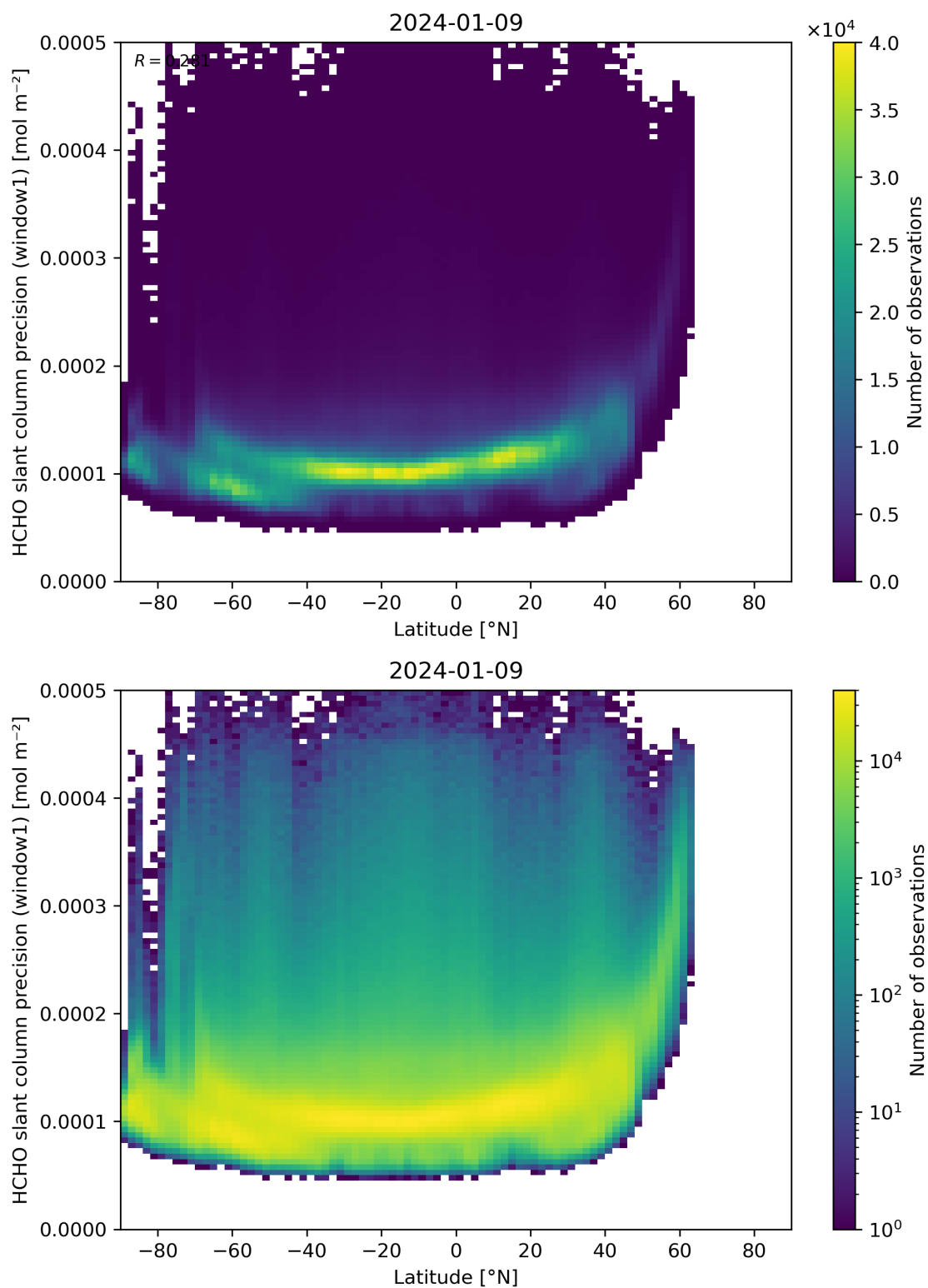
Figure 160: Scatter density plot of “Latitude” against “HCHO slant column precision (window1)” for 2024-01-08 to 2024-01-10.
