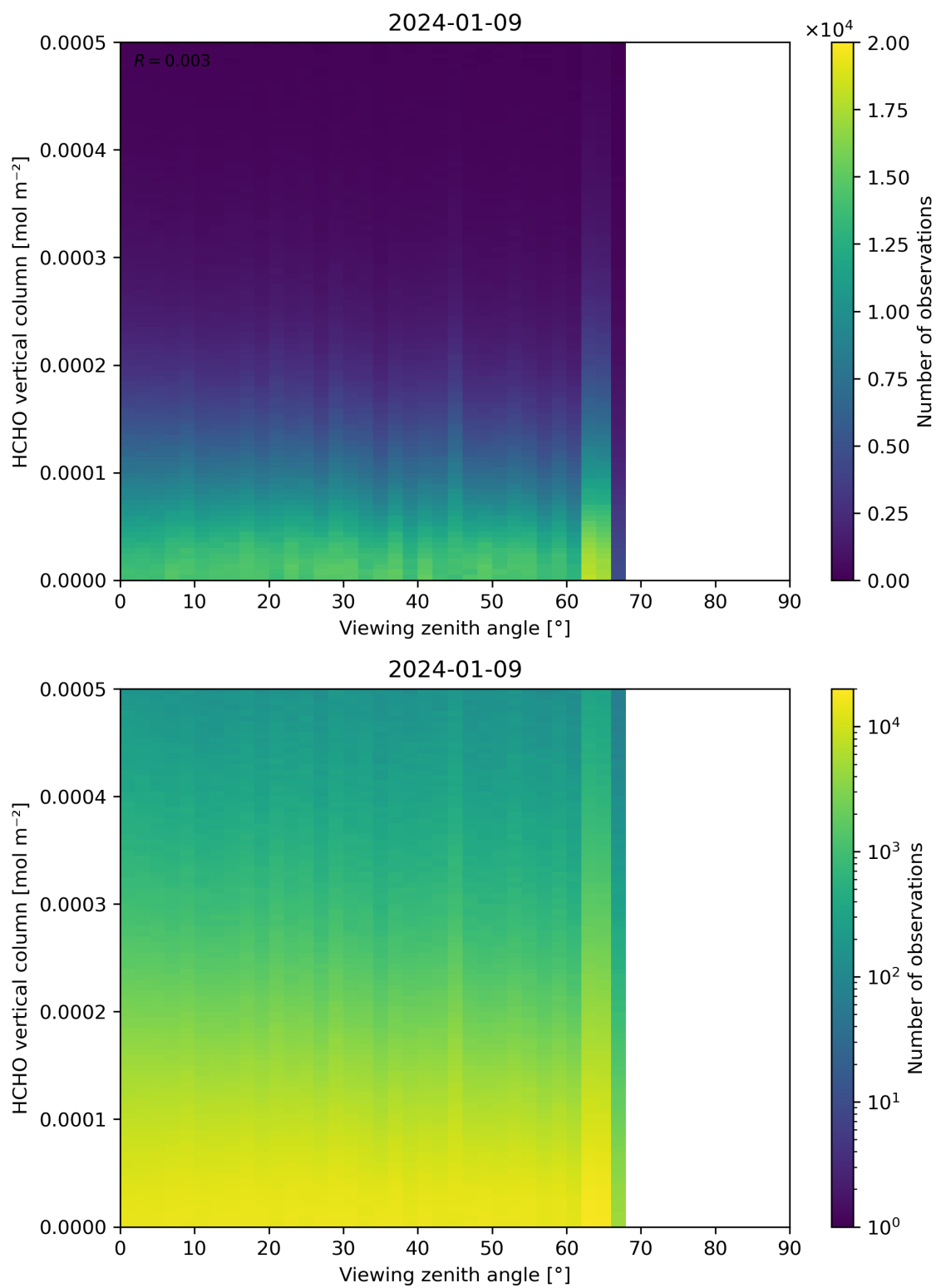
Figure 192: Scatter density plot of “Viewing zenith angle” against “HCHO vertical column” for 2024-01-08 to 2024-01-10.
