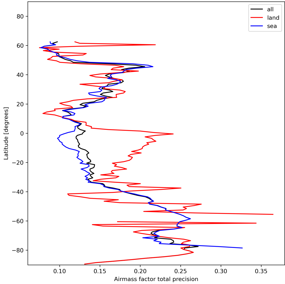
Figure 27: Zonal average of “Airmass factor total precision” for 2024-01-08 to 2024-01-10.
