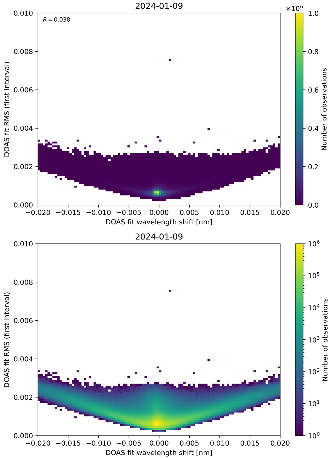
Figure 64: Scatter density plot of “DOAS fit wavelength shift” against “DOAS fit RMS (first interval)” for 2024-01-08 to 2024-01-10.
