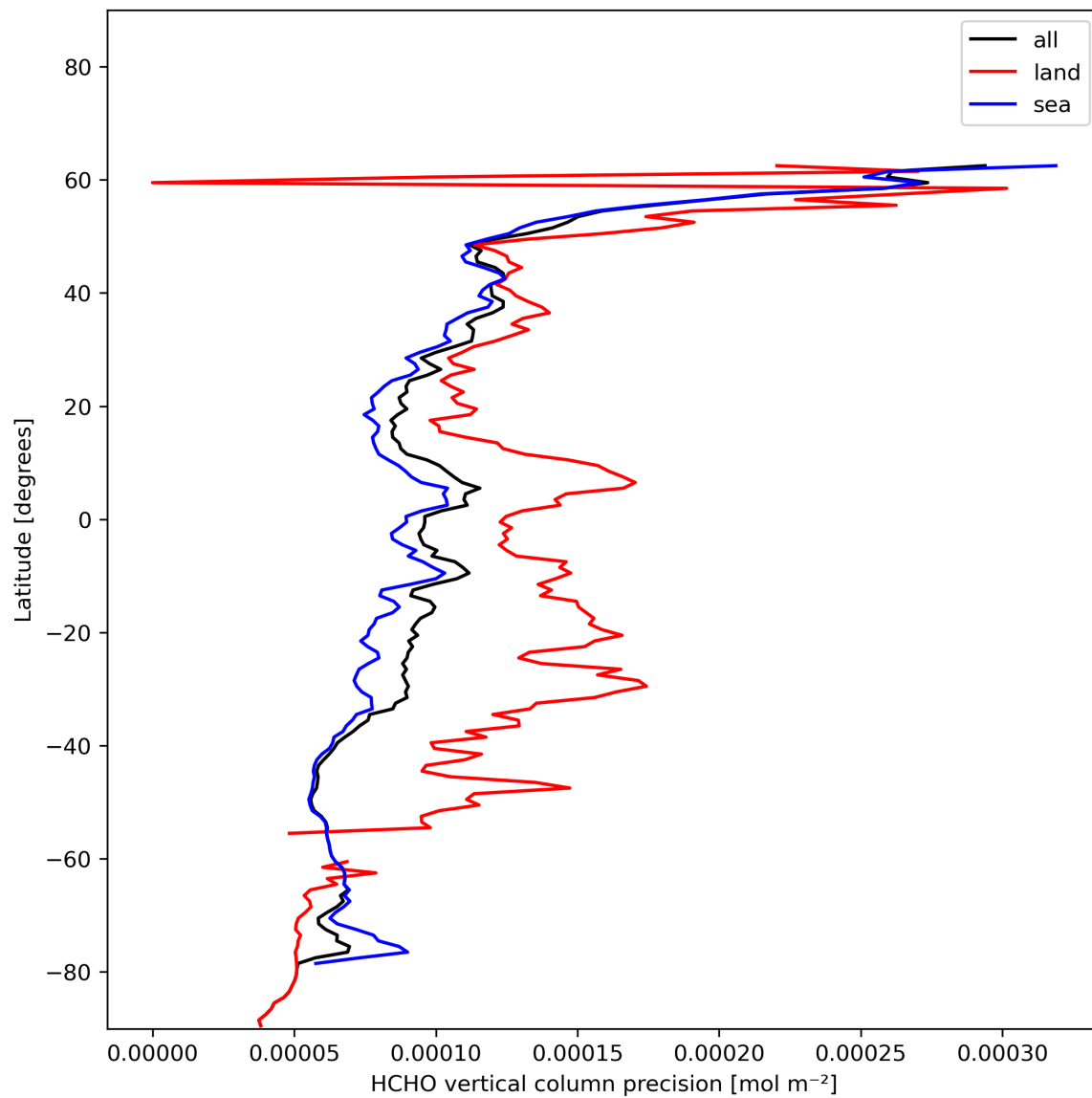
Figure 22: Zonal average of “HCHO vertical column precision” for 2024-01-08 to 2024-01-10.
