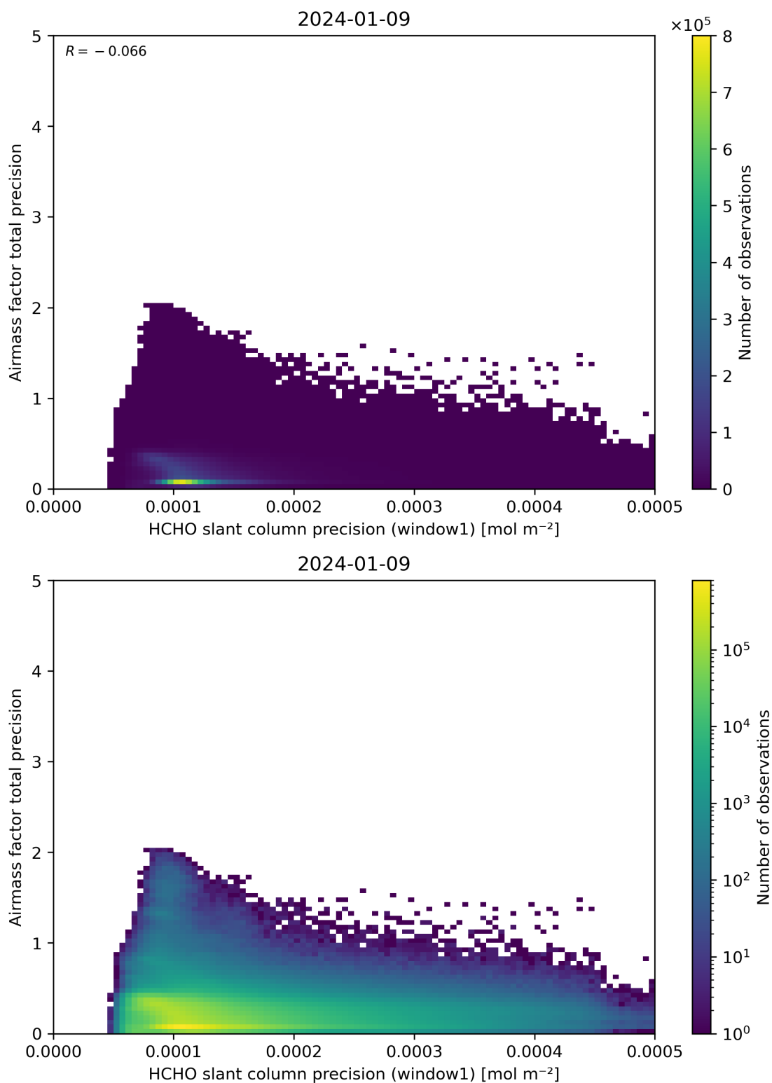
Figure 95: Scatter density plot of “HCHO slant column precision (window1)” against “Airmass factor total precision” for 2024-01-08 to 2024-01-10.
