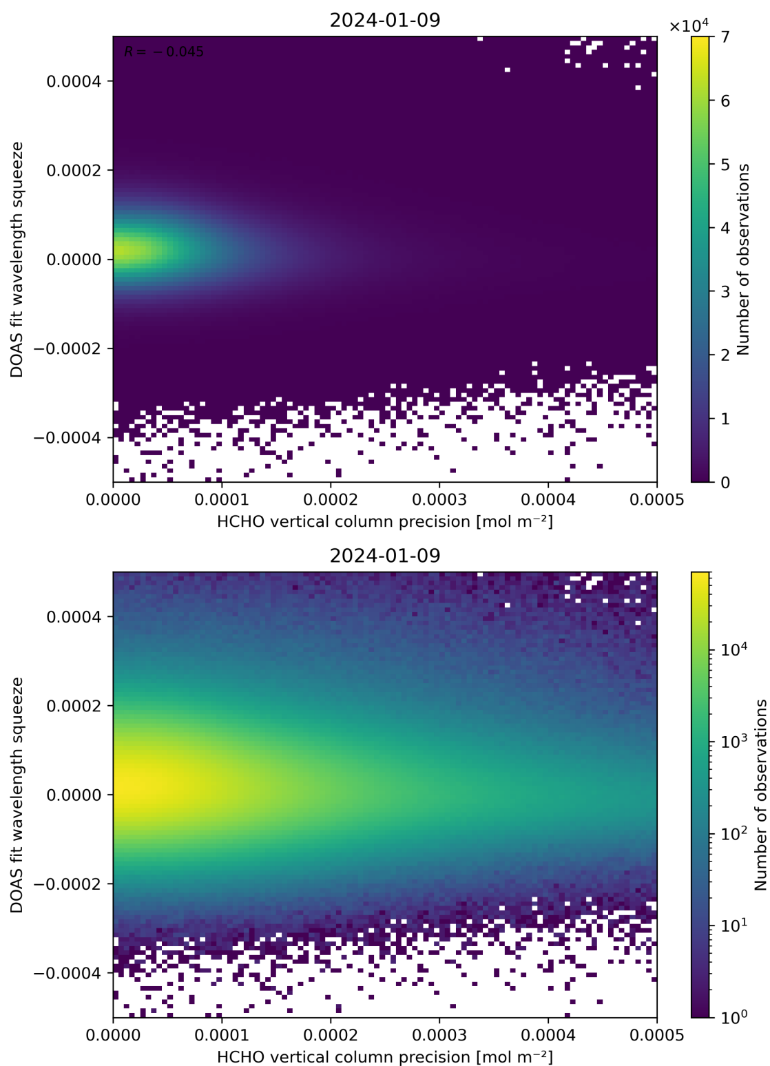
Figure 138: Scatter density plot of “HCHO vertical column precision” against “DOAS fit wavelength squeeze” for 2024-01-08 to 2024-01-10.
