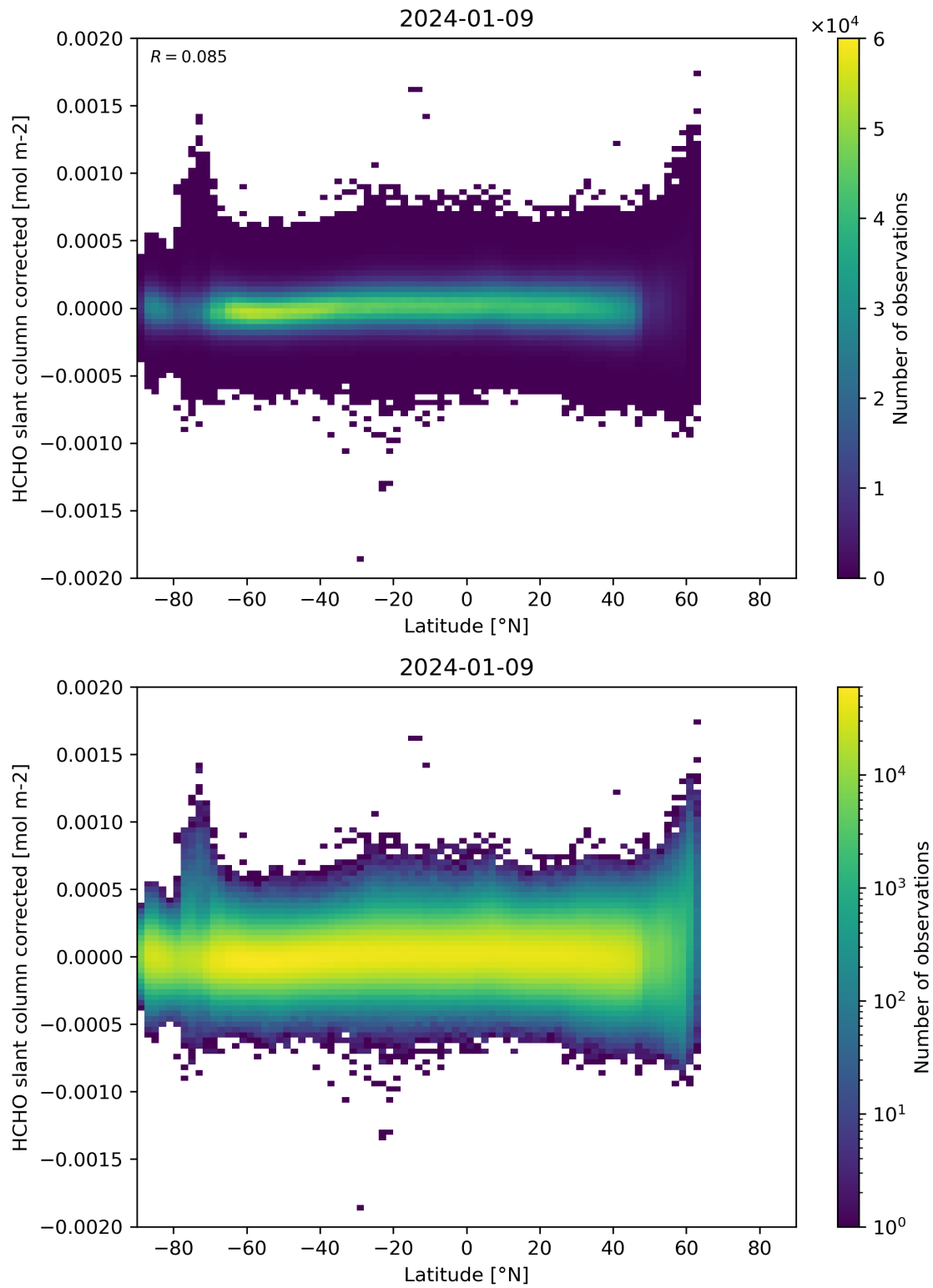
Figure 157: Scatter density plot of “Latitude” against “HCHO slant column corrected” for 2024-01-08 to 2024-01-10.
