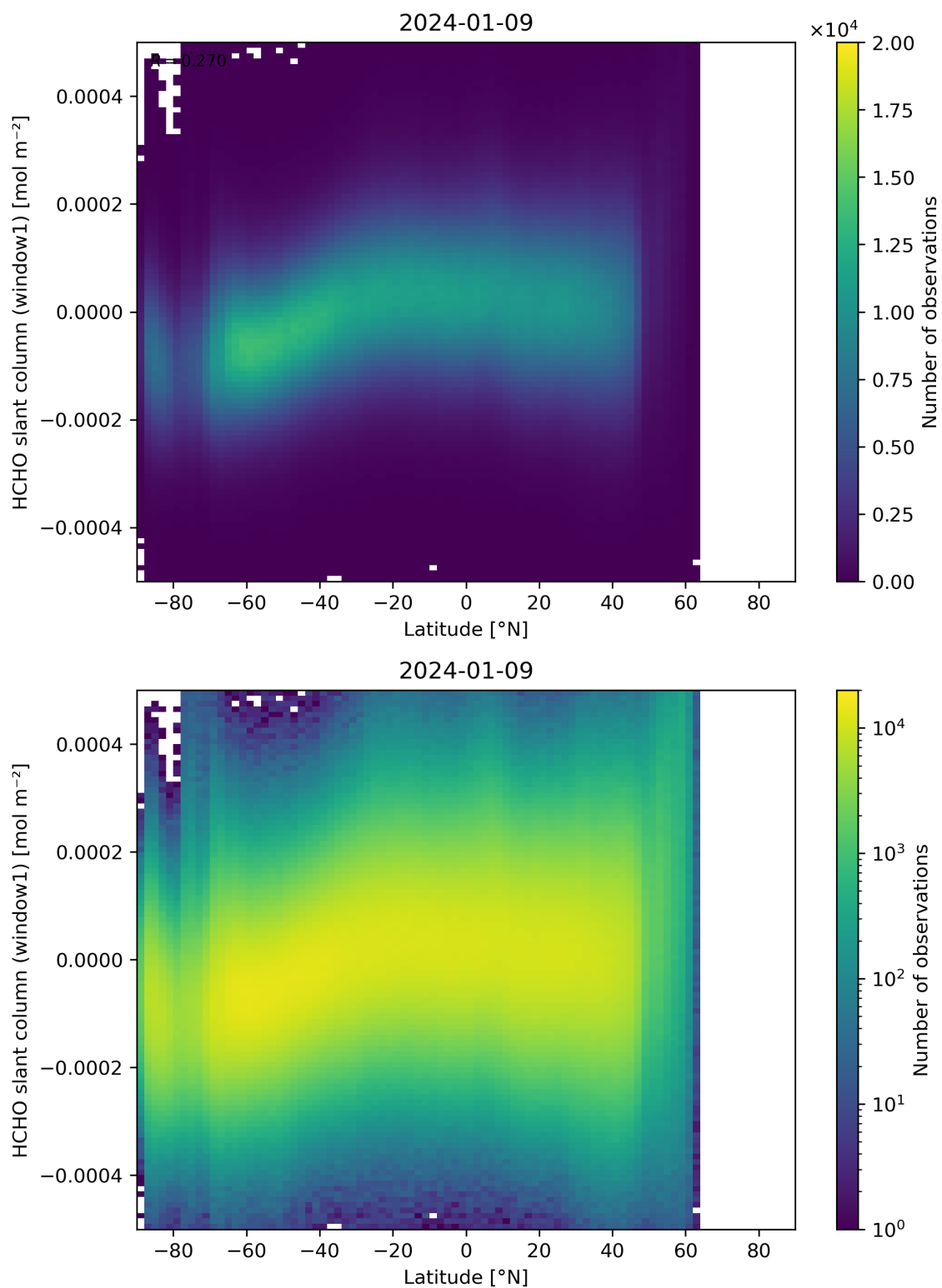
Figure 159: Scatter density plot of “Latitude” against “HCHO slant column (window1)” for 2024-01-08 to 2024-01-10.
