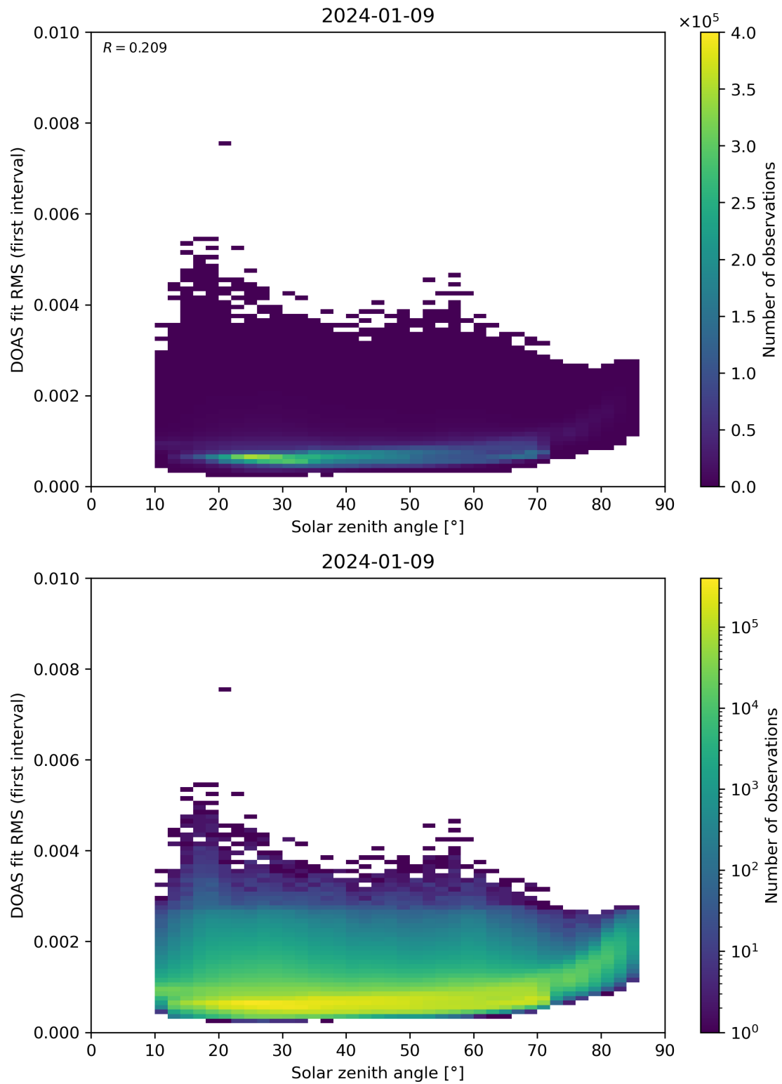
Figure 167: Scatter density plot of “Solar zenith angle” against “DOAS fit RMS (first interval)” for 2024-01-08 to 2024-01-10.
