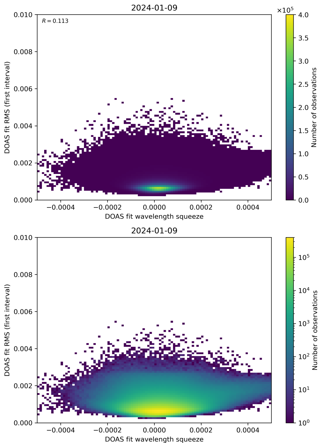
Figure 68: Scatter density plot of “DOAS fit wavelength squeeze” against “DOAS fit RMS (first interval)” for 2024-01-08 to 2024-01-10.
