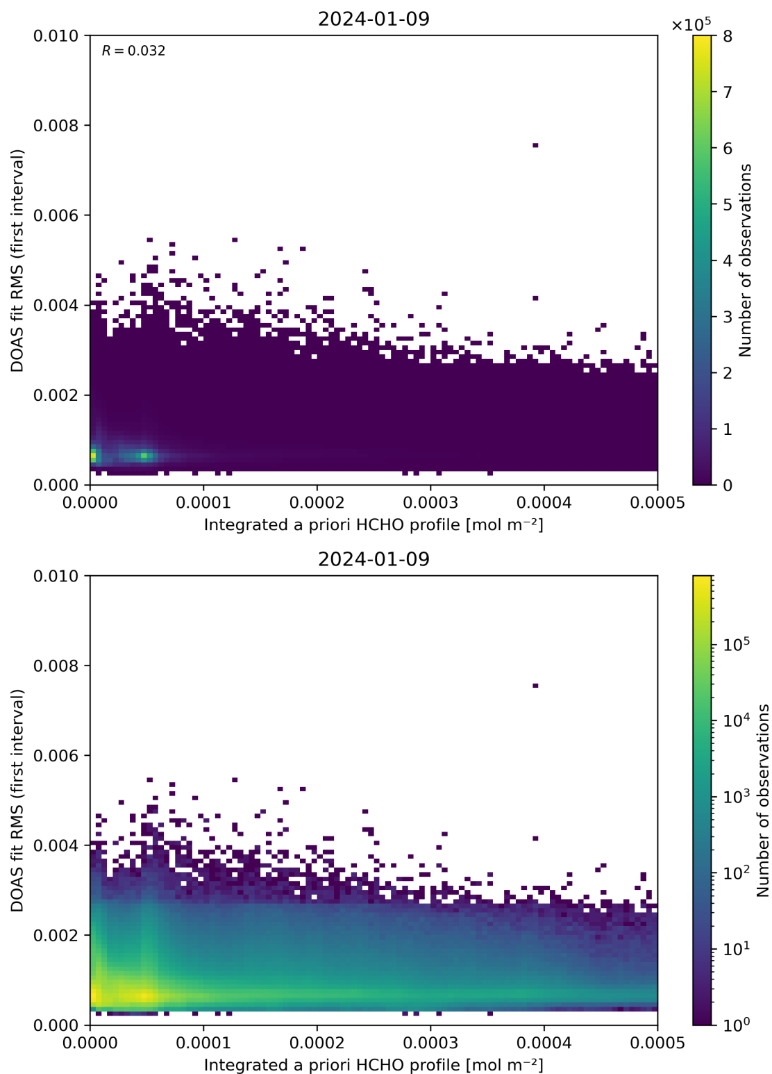
Figure 148: Scatter density plot of “Integrated a priori HCHO profile” against “DOAS fit RMS (first interval)” for 2024-01-08 to 2024-01-10.
