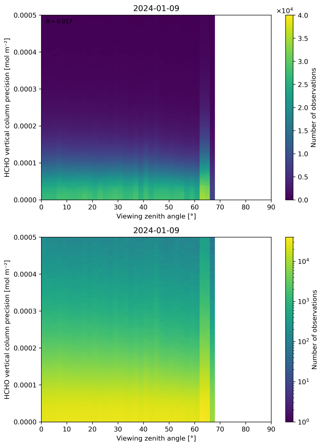
Figure 194: Scatter density plot of “Viewing zenith angle” against “HCHO vertical column precision” for 2024-01-08 to 2024-01-10.
