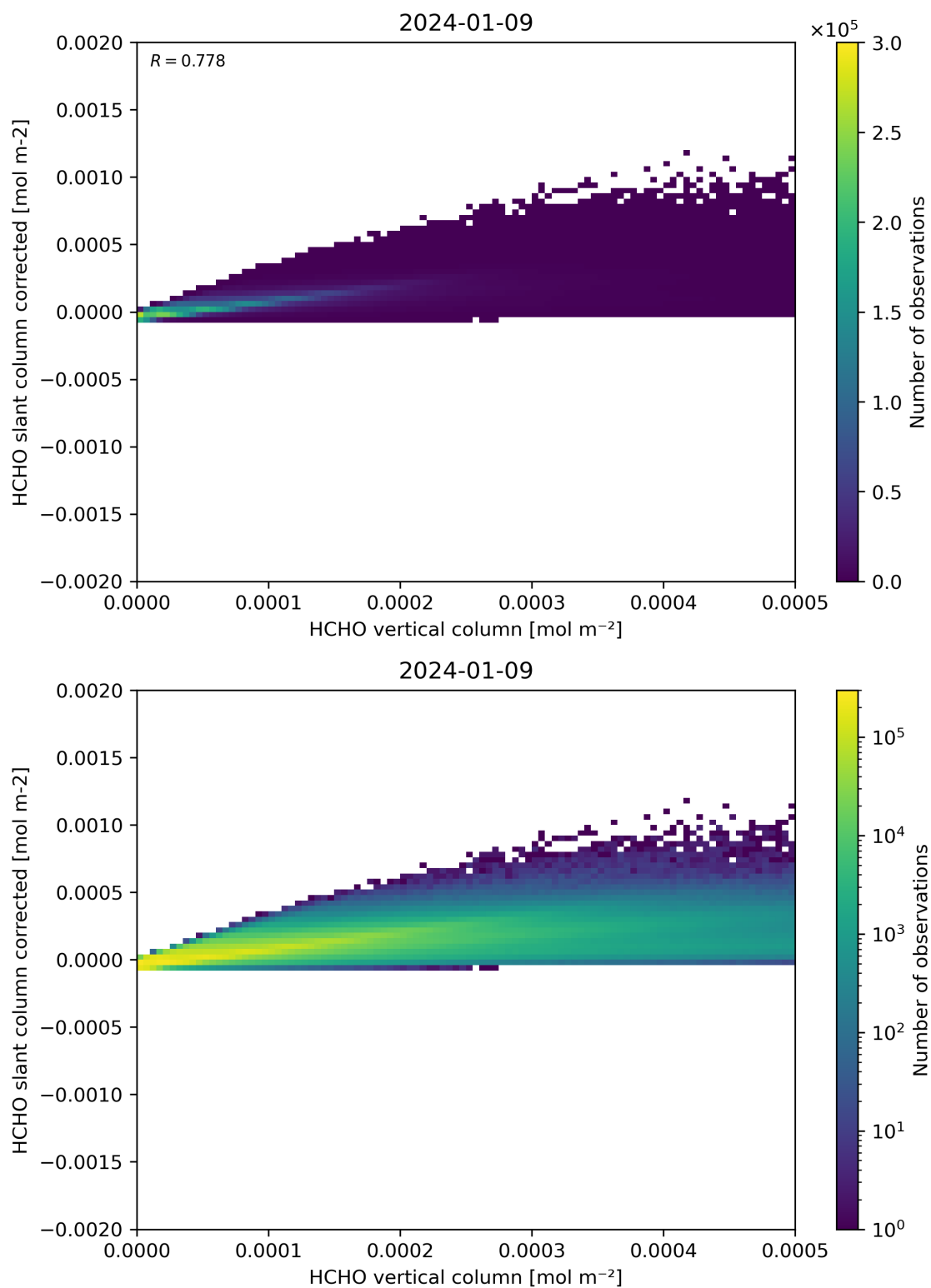
Figure 127: Scatter density plot of “HCHO vertical column” against “HCHO slant column corrected” for 2024-01-08 to 2024-01-10.
