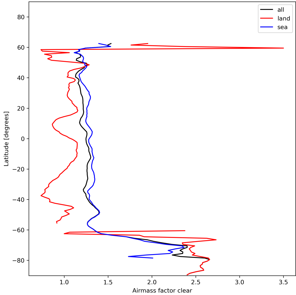
Figure 28: Zonal average of “Airmass factor clear” for 2024-01-08 to 2024-01-10.
