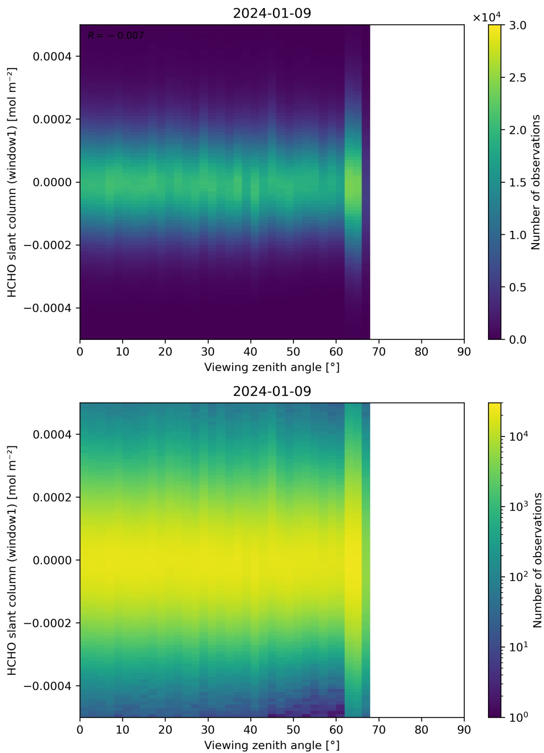
Figure 188: Scatter density plot of “Viewing zenith angle” against “HCHO slant column (window1)” for 2024-01-08 to 2024-01-10.
