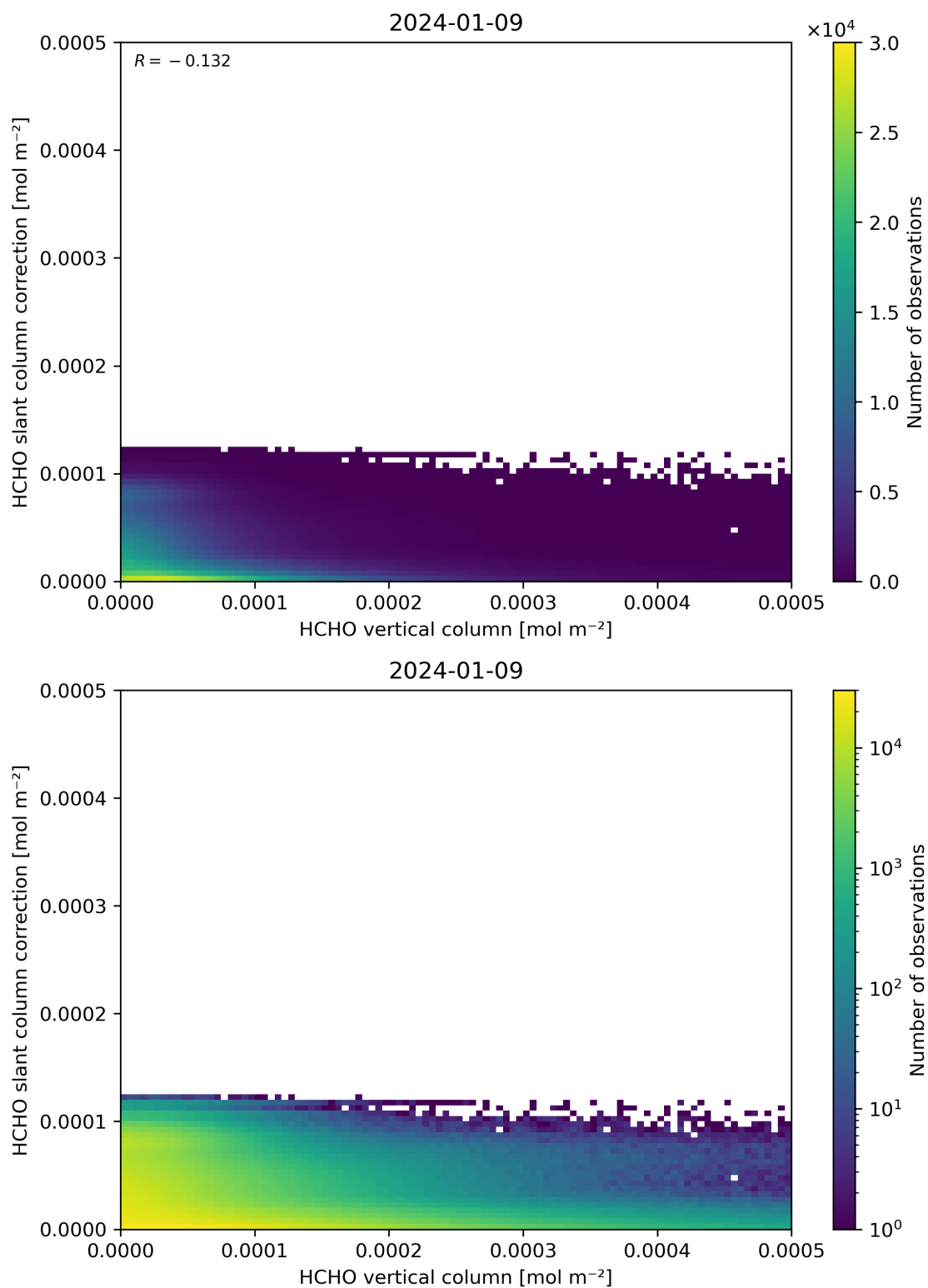
Figure 128: Scatter density plot of “HCHO vertical column” against “HCHO slant column correction” for 2024-01-08 to 2024-01-10.
