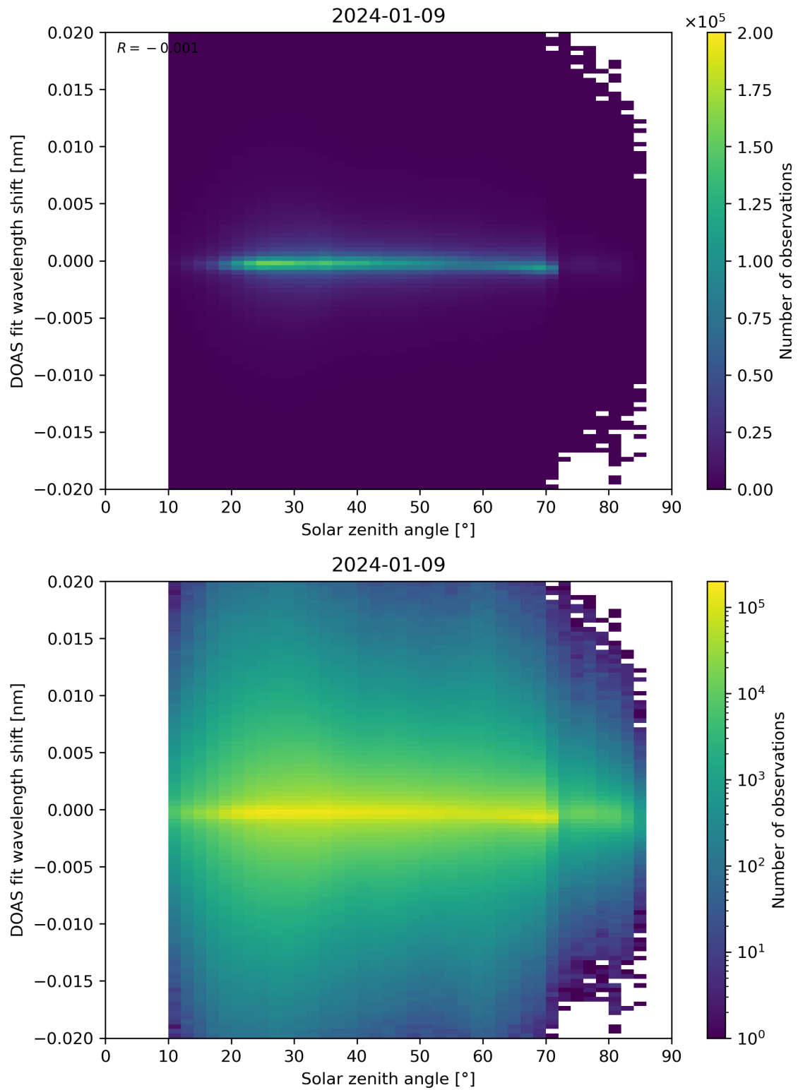
Figure 168: Scatter density plot of “Solar zenith angle” against “DOAS fit wavelength shift” for 2024-01-08 to 2024-01-10.
