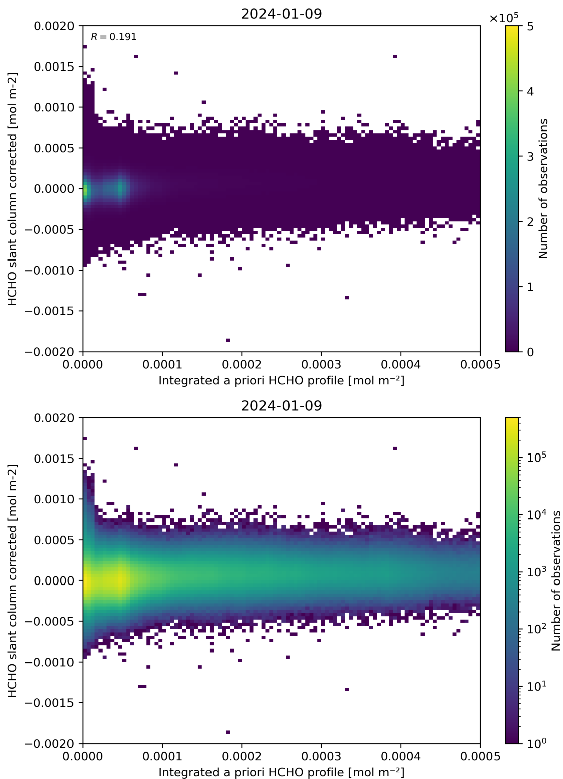
Figure 151: Scatter density plot of “Integrated a priori HCHO profile” against “HCHO slant column corrected” for 2024-01-08 to 2024-01-10.
