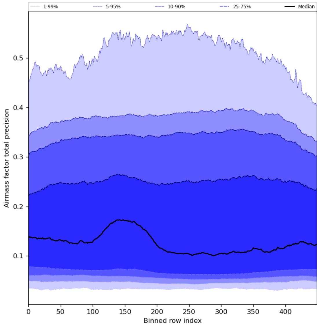
Figure 55: Along track statistics of “Airmass factor total precision” for 2024-01-08 to 2024-01-10
