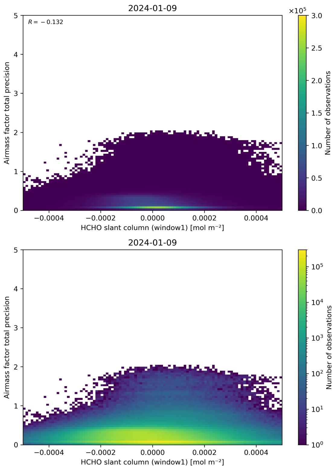
Figure 86: Scatter density plot of “HCHO slant column (window1)” against “Airmass factor total precision” for 2024-01-08 to 2024-01-10.
