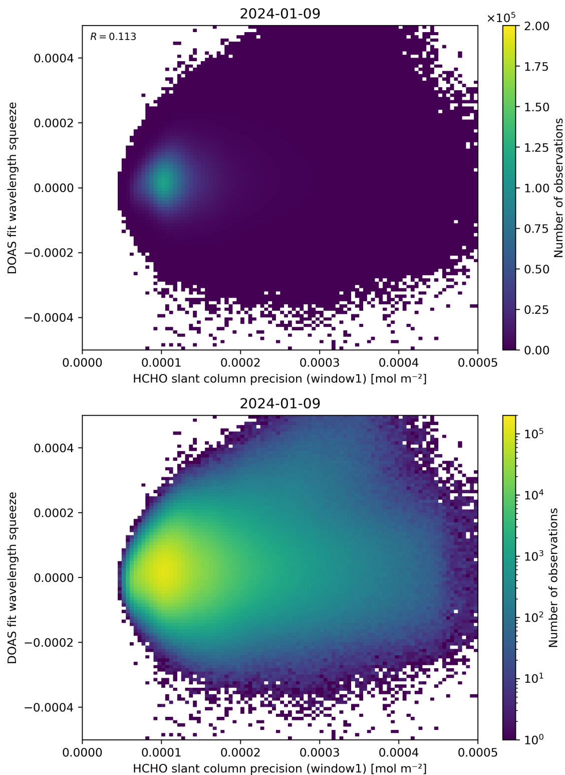
Figure 90: Scatter density plot of “HCHO slant column precision (window1)” against “DOAS fit wavelength squeeze” for 2024-01-08 to 2024-01-10.
