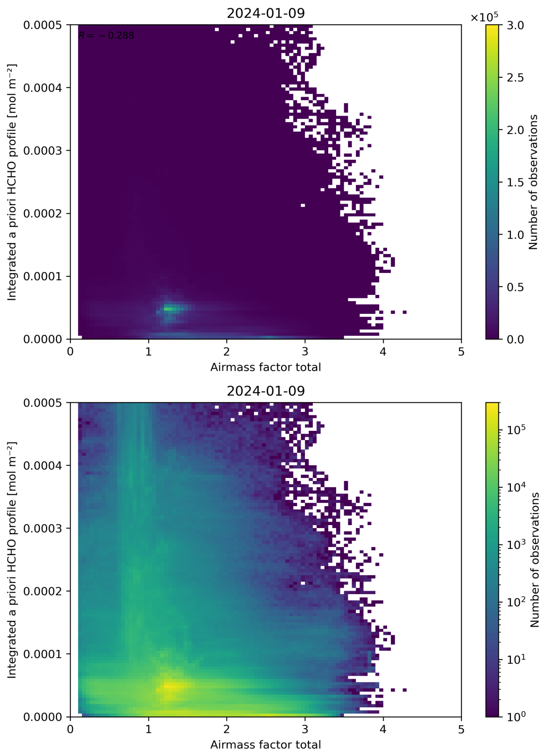
Figure 104: Scatter density plot of “Airmass factor total” against “Integrated a priori HCHO profile” for 2024-01-08 to 2024-01-10.
