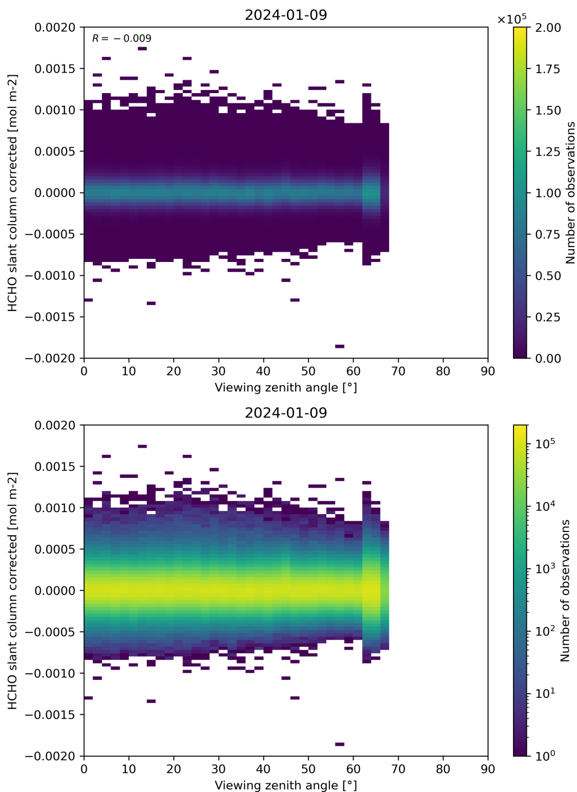
Figure 186: Scatter density plot of “Viewing zenith angle” against “HCHO slant column corrected” for 2024-01-08 to 2024-01-10.
