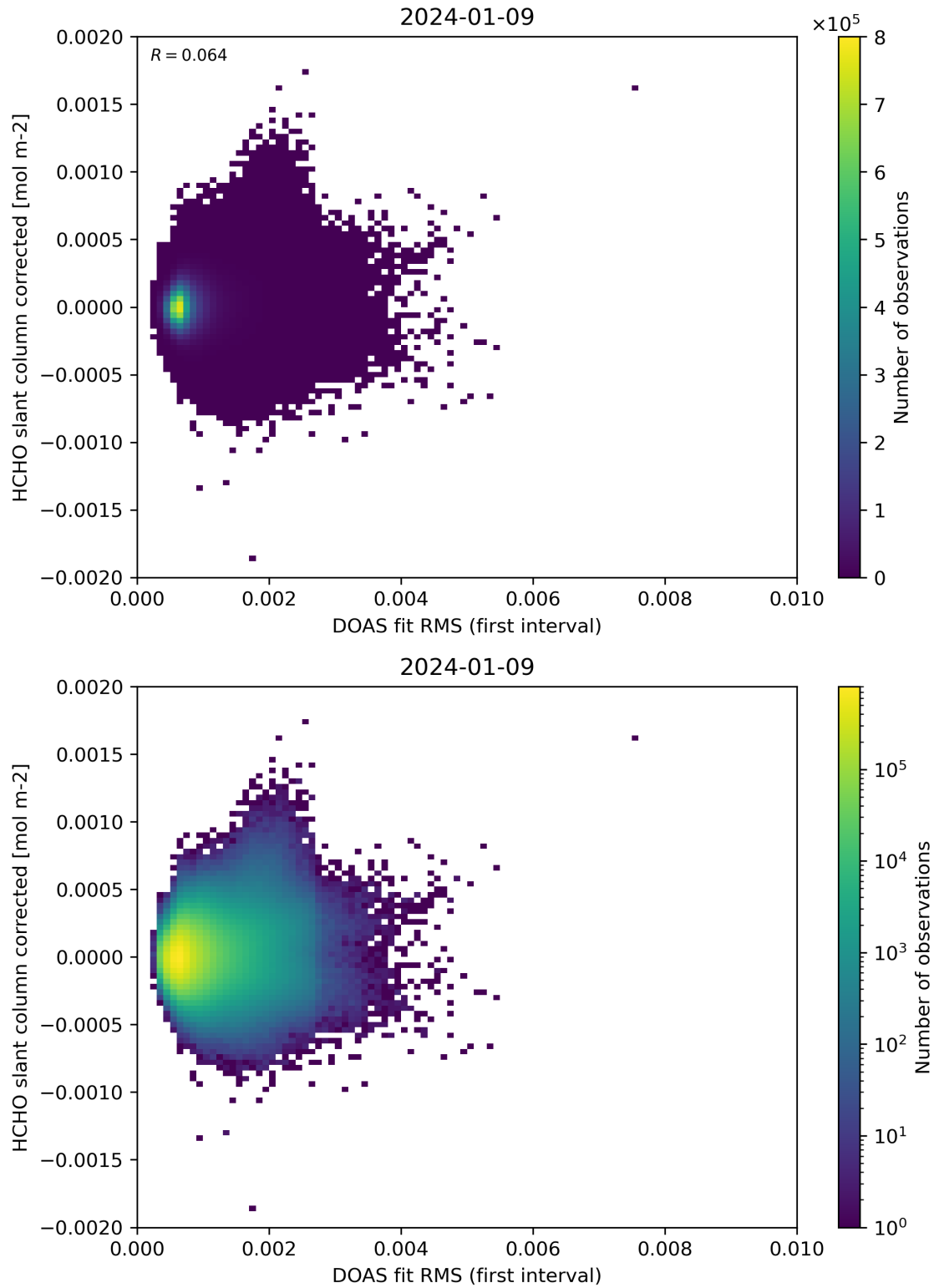
Figure 62: Scatter density plot of “DOAS fit RMS (first interval)” against “HCHO slant column corrected” for 2024-01-08 to 2024-01-10.
