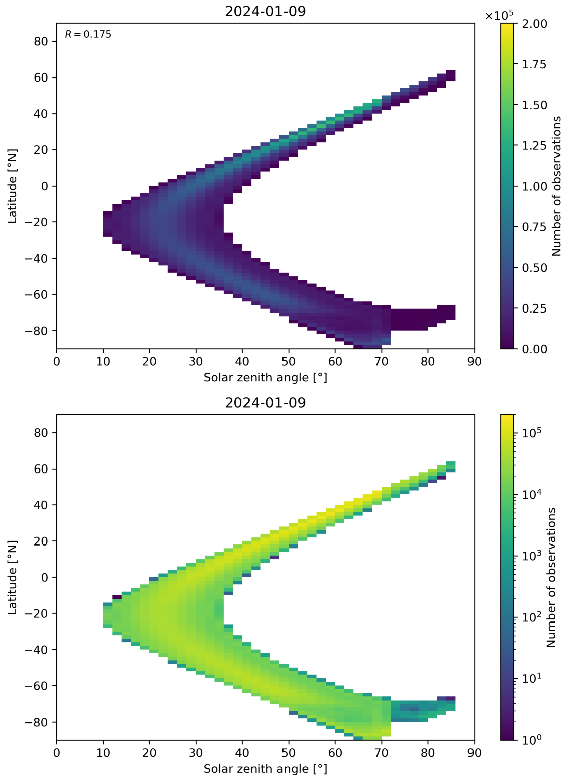
Figure 181: Scatter density plot of “Solar zenith angle” against “Latitude” for 2024-01-08 to 2024-01-10.
