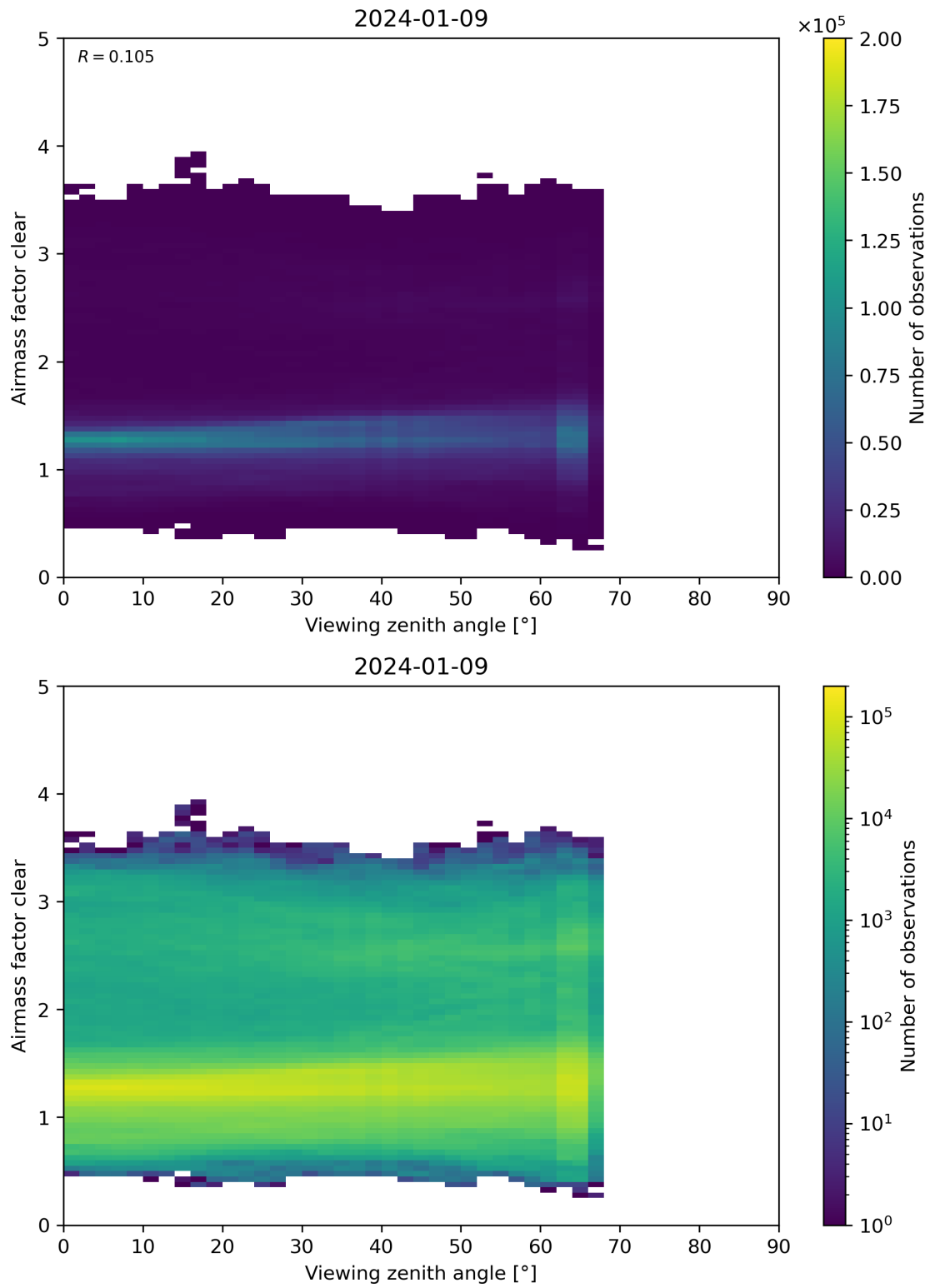
Figure 185: Scatter density plot of “Viewing zenith angle” against “Airmass factor clear” for 2024-01-08 to 2024-01-10.
