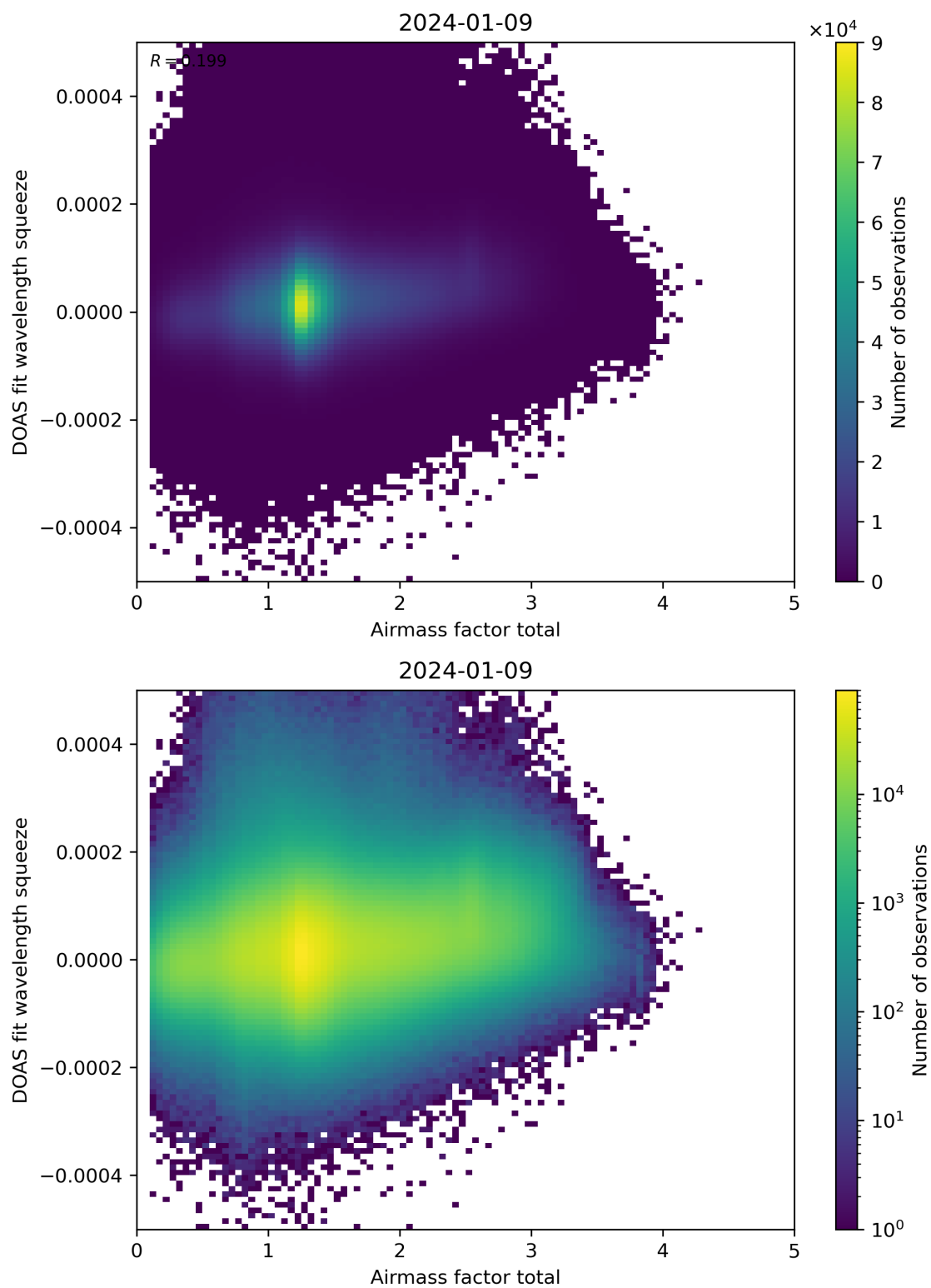
Figure 99: Scatter density plot of “Airmass factor total” against “DOAS fit wavelength squeeze” for 2024-01-08 to 2024-01-10.
