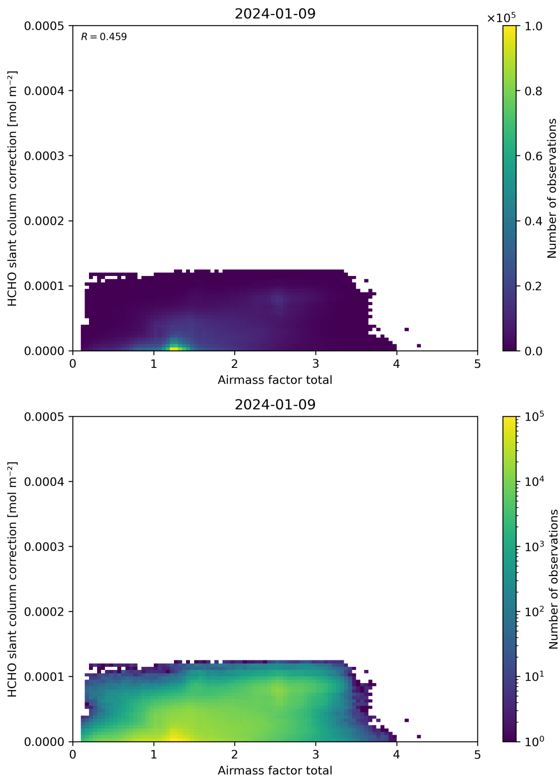
Figure 102: Scatter density plot of “Airmass factor total” against “HCHO slant column correction” for 2024-01-08 to 2024-01-10.
