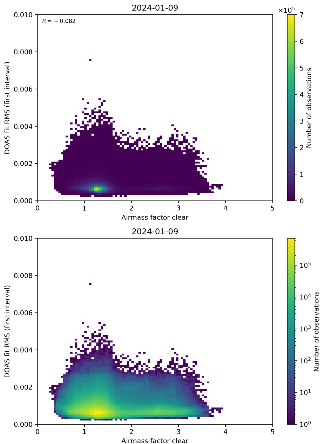
Figure 71: Scatter density plot of “Airmass factor clear” against “DOAS fit RMS (first interval)” for 2024-01-08 to 2024-01-10.
