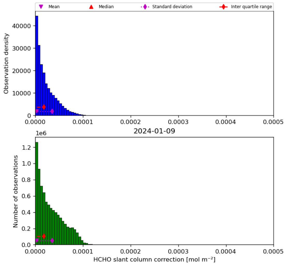
Figure 47: Histogram of “HCHO slant column correction” for 2024-01-08 to 2024-01-10
