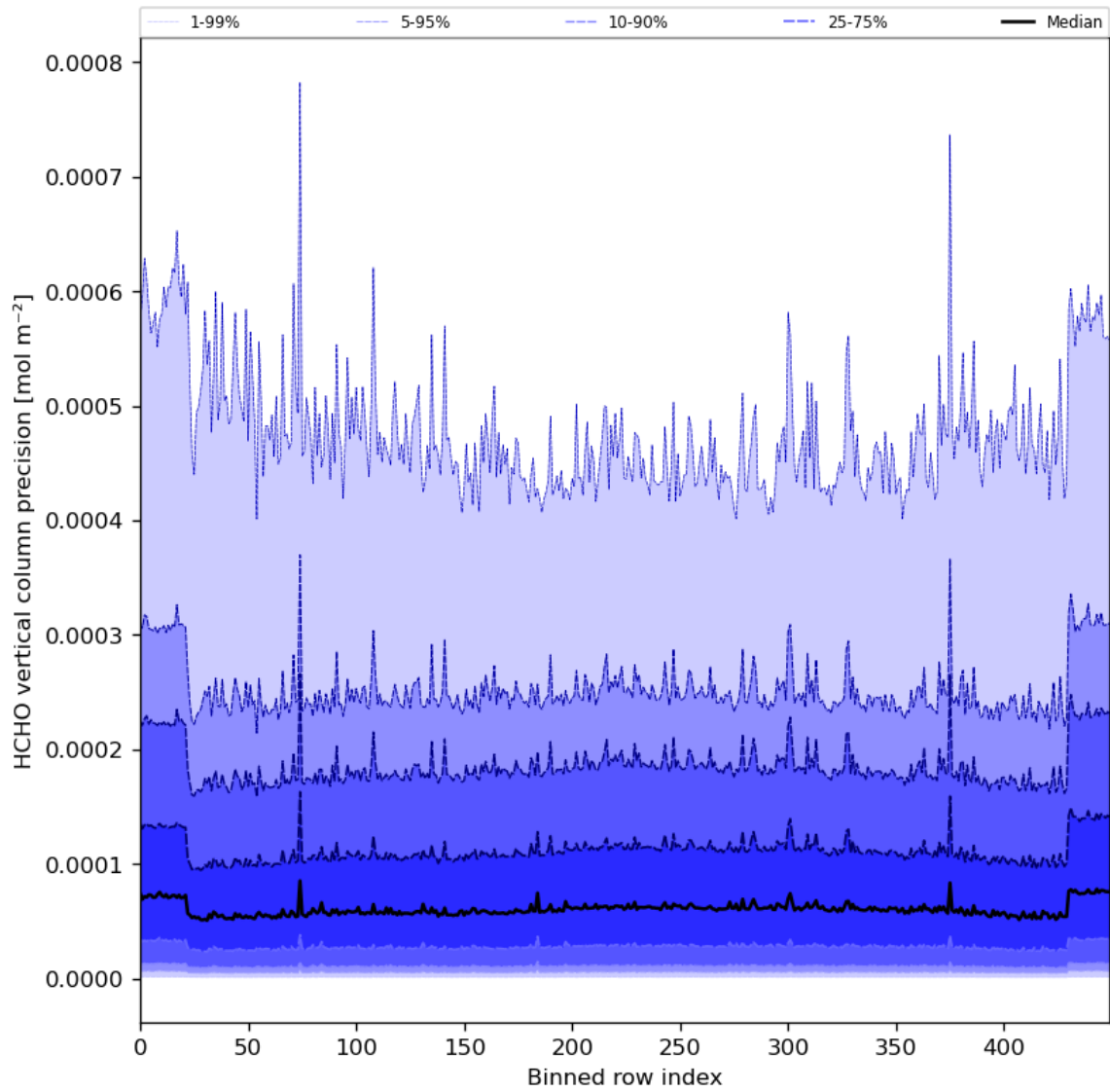
Figure 50: Along track statistics of "HCHO vertical column precision" for 2024-01-08 to 2024-01-10
