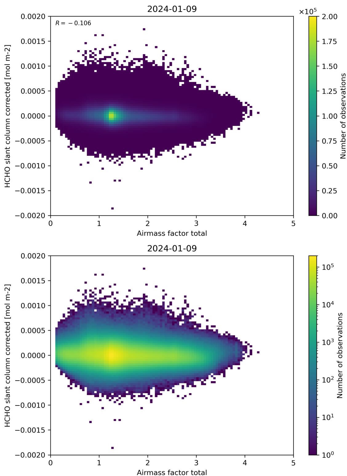
Figure 101: Scatter density plot of “Airmass factor total” against “HCHO slant column corrected” for 2024-01-08 to 2024-01-10.
