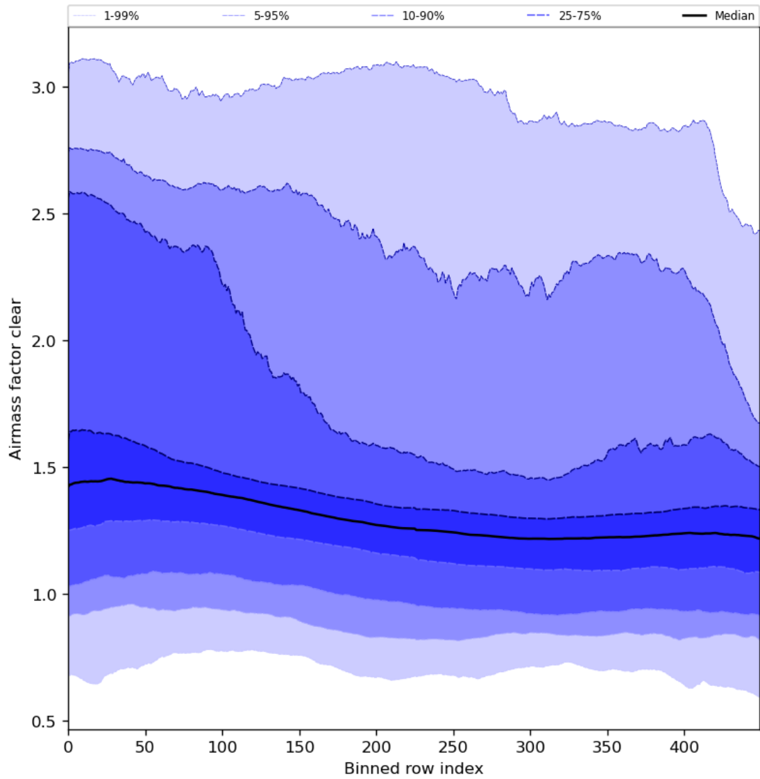
Figure 56: Along track statistics of “Airmass factor clear” for 2024-01-08 to 2024-01-10
