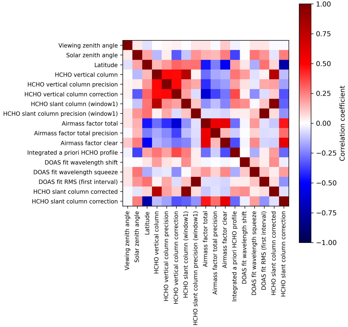
Figure 2: Map of correlation matrix for 2024-01-08 to 2024-01-10.
