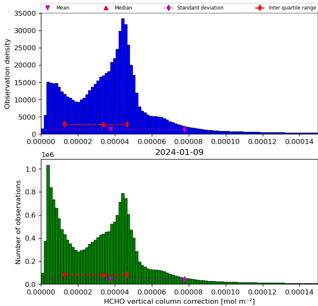
Figure 37: Histogram of “HCHO vertical column correction” for 2024-01-08 to 2024-01-10
