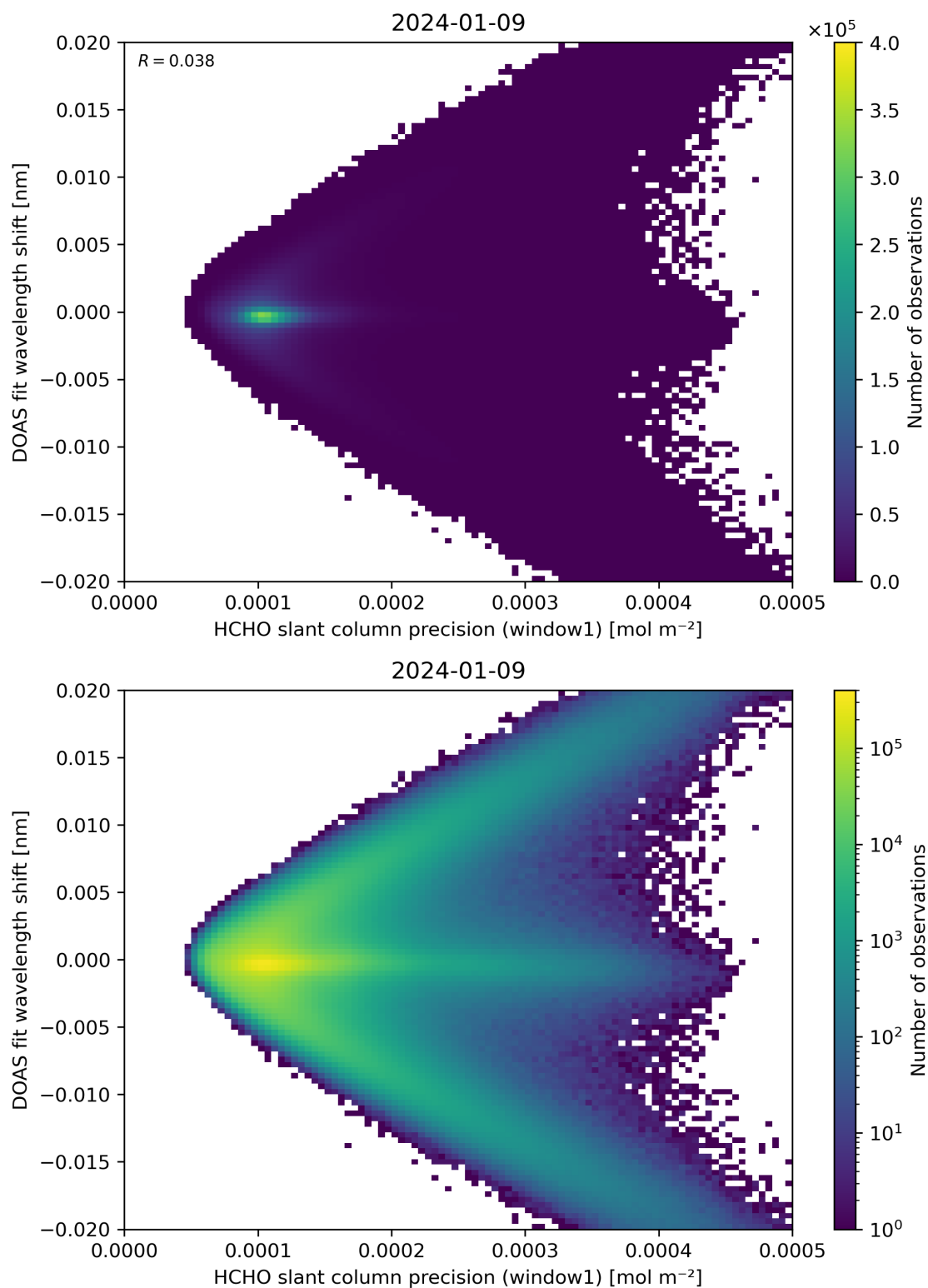
Figure 89: Scatter density plot of “HCHO slant column precision (window1)” against “DOAS fit wavelength shift” for 2024-01-08 to 2024-01-10.
