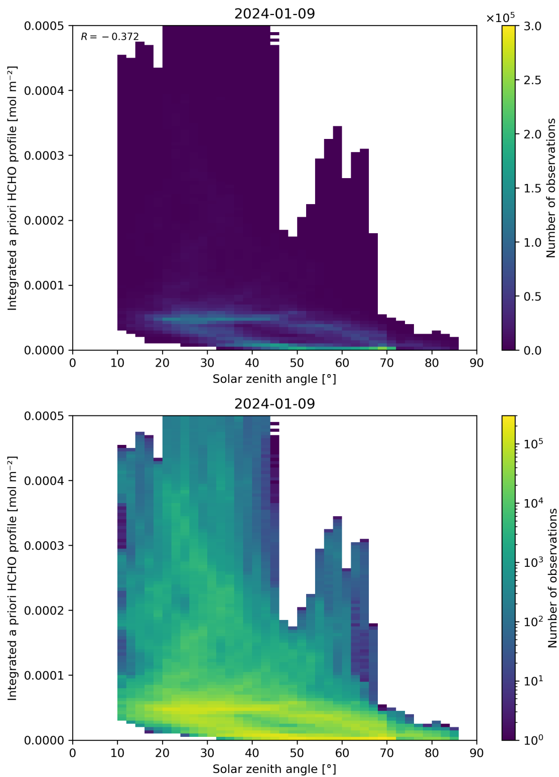
Figure 180: Scatter density plot of “Solar zenith angle” against “Integrated a priori HCHO profile” for 2024-01-08 to 2024-01-10.
