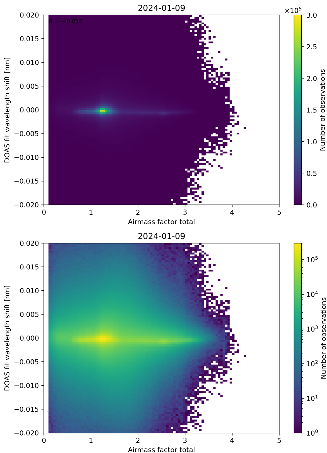
Figure 98: Scatter density plot of “Airmass factor total” against “DOAS fit wavelength shift” for 2024-01-08 to 2024-01-10.
