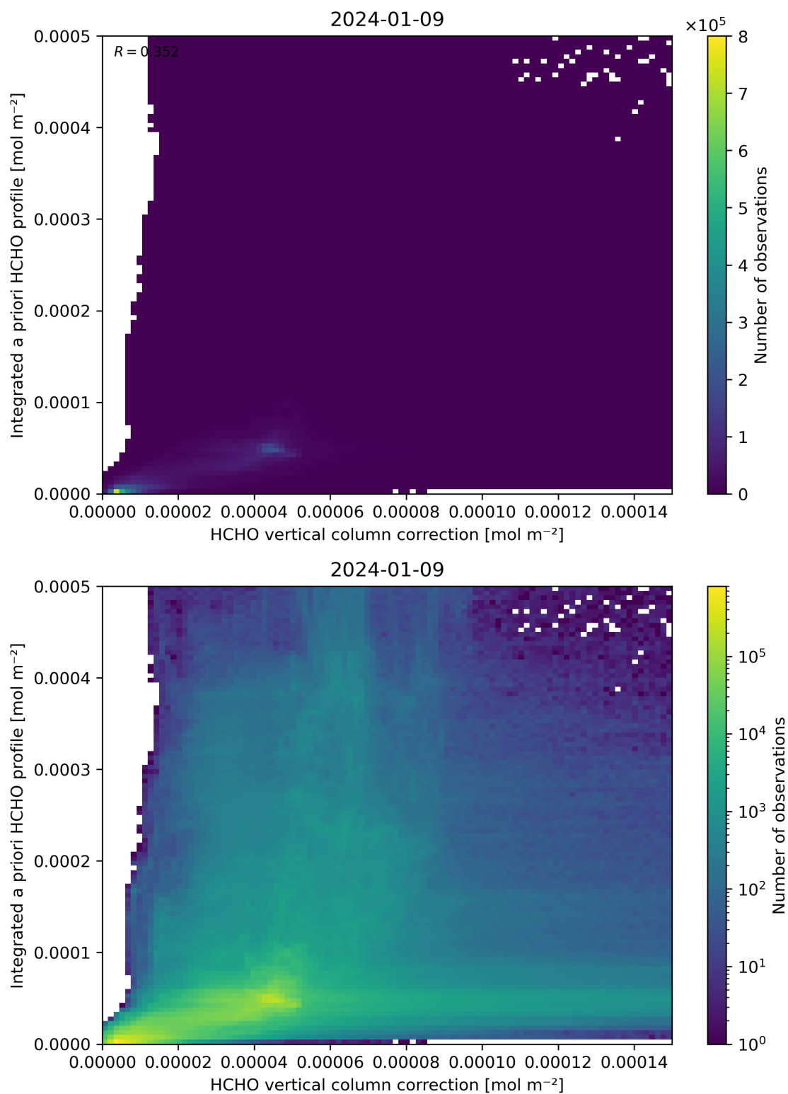
Figure 122: Scatter density plot of “HCHO vertical column correction” against “Integrated a priori HCHO profile” for 2024-01-08 to 2024-01-10.
