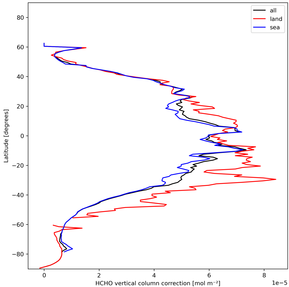
Figure 23: Zonal average of “HCHO vertical column correction” for 2024-01-08 to 2024-01-10.
