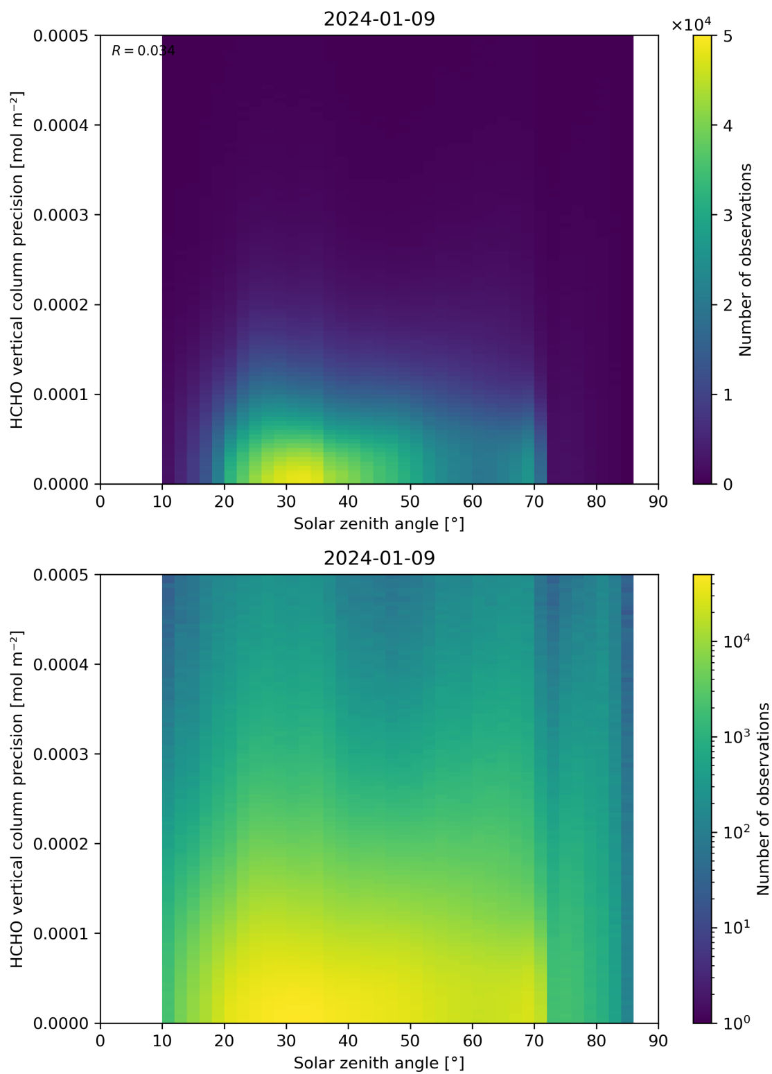
Figure 179: Scatter density plot of “Solar zenith angle” against “HCHO vertical column precision” for 2024-01-08 to 2024-01-10.
