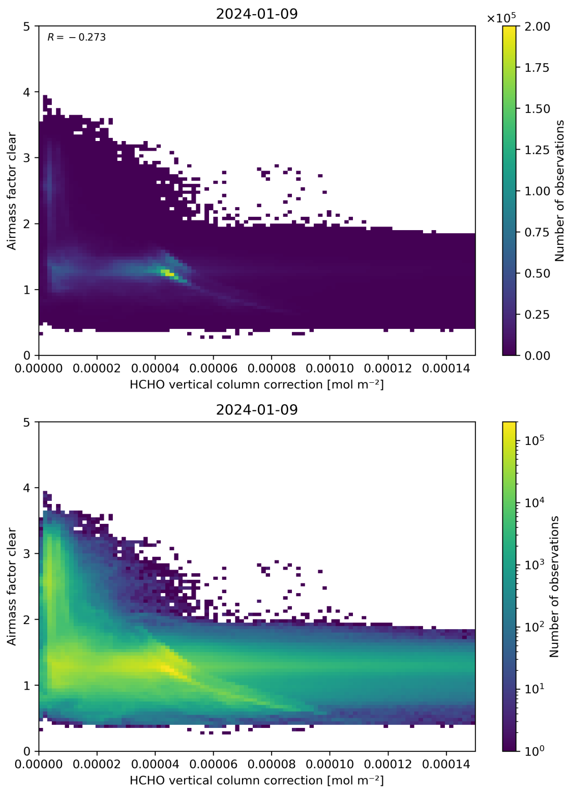
Figure 115: Scatter density plot of “HCHO vertical column correction” against “Airmass factor clear” for 2024-01-08 to 2024-01-10.
