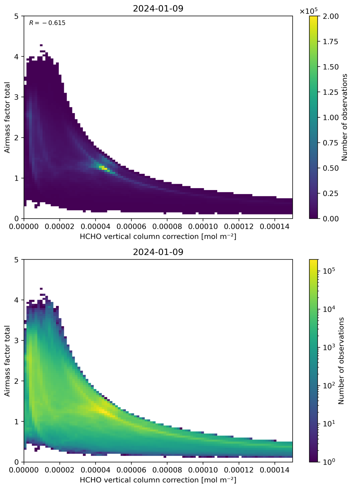
Figure 120: Scatter density plot of “HCHO vertical column correction” against “Airmass factor total” for 2024-01-08 to 2024-01-10.
