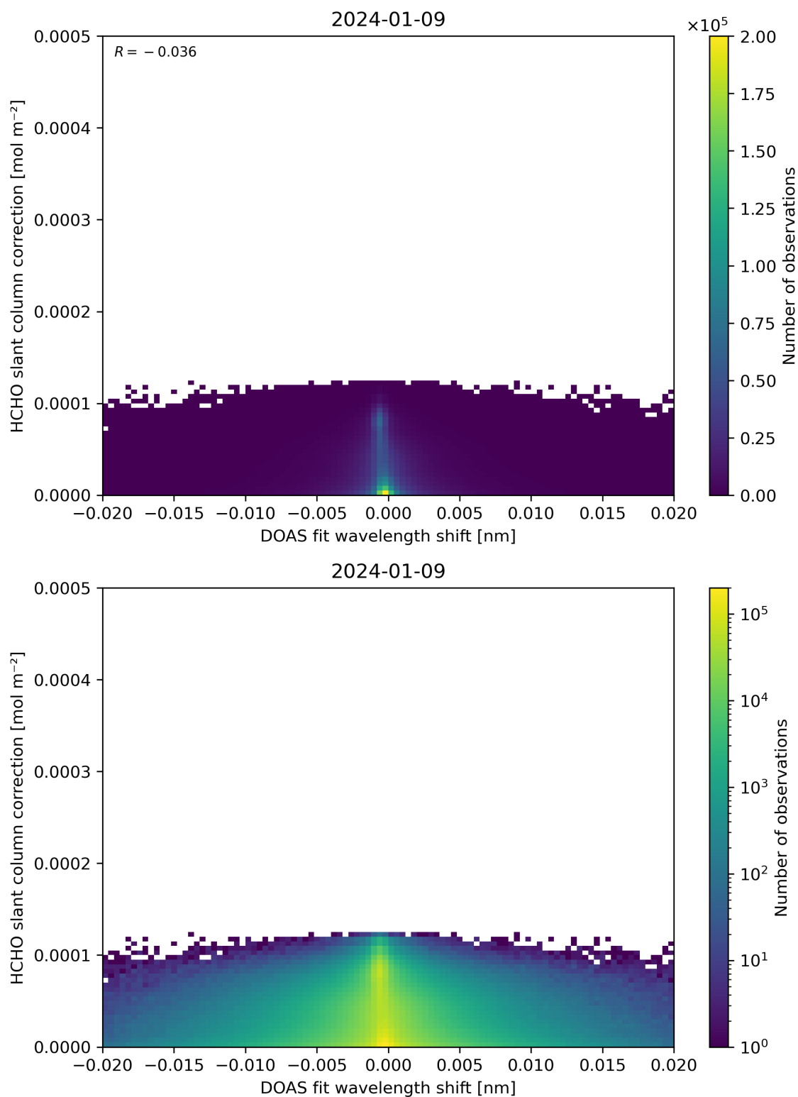
Figure 67: Scatter density plot of “DOAS fit wavelength shift” against “HCHO slant column correction” for 2024-01-08 to 2024-01-10.
