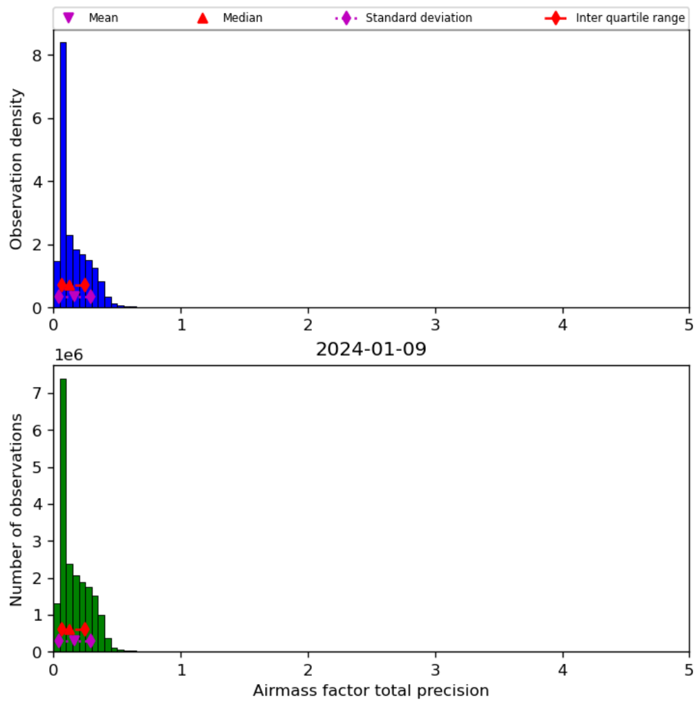
Figure 41: Histogram of “Airmass factor total precision” for 2024-01-08 to 2024-01-10
