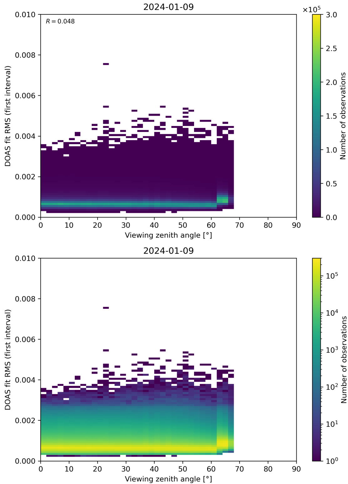
Figure 182: Scatter density plot of “Viewing zenith angle” against “DOAS fit RMS (first interval)” for 2024-01-08 to 2024-01-10.
