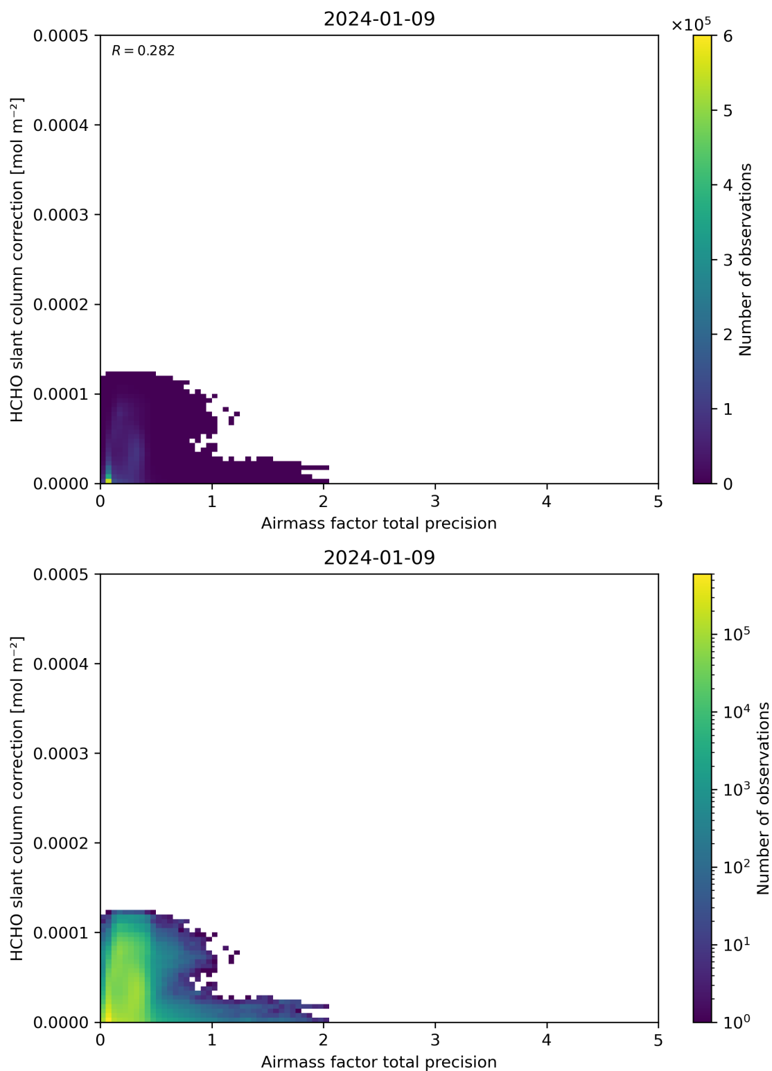
Figure 110: Scatter density plot of “Airmass factor total precision” against “HCHO slant column correction” for 2024-01-08 to 2024-01-10.
