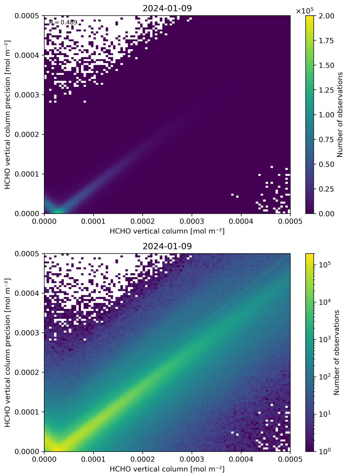
Figure 134: Scatter density plot of “HCHO vertical column” against “HCHO vertical column precision” for 2024-01-08 to 2024-01-10.
