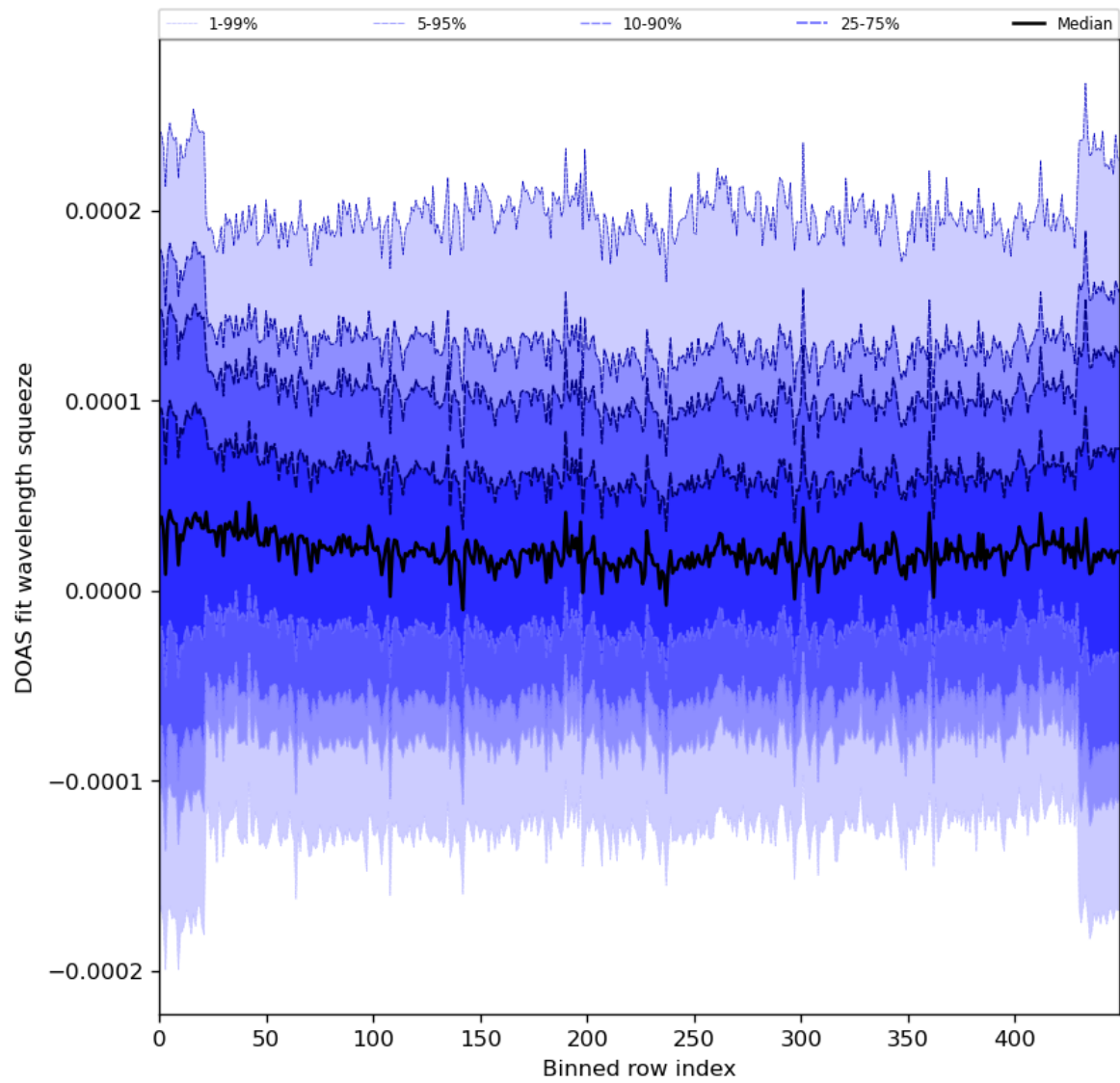
Figure 59: Along track statistics of “DOAS fit wavelength squeeze” for 2024-01-08 to 2024-01-10
