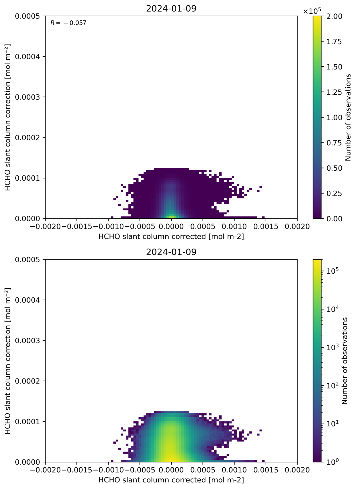
Figure 77: Scatter density plot of “HCHO slant column corrected” against “HCHO slant column correction” for 2024-01-08 to 2024-01-10.
