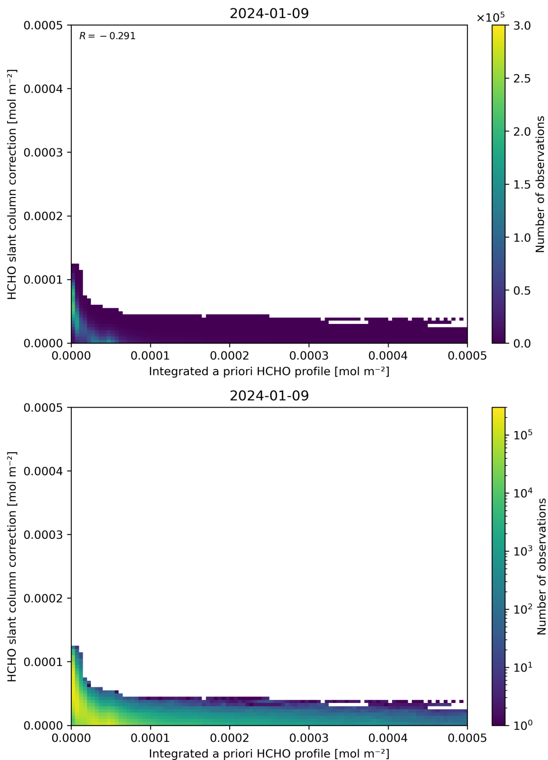
Figure 152: Scatter density plot of “Integrated a priori HCHO profile” against “HCHO slant column correction” for 2024-01-08 to 2024-01-10.
