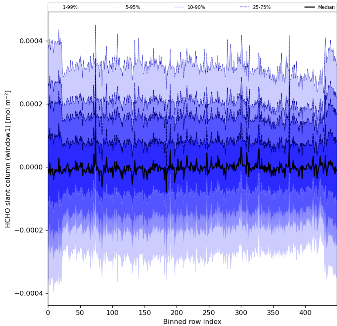
Figure 52: Along track statistics of “HCHO slant column (window1)” for 2024-01-08 to 2024-01-10
