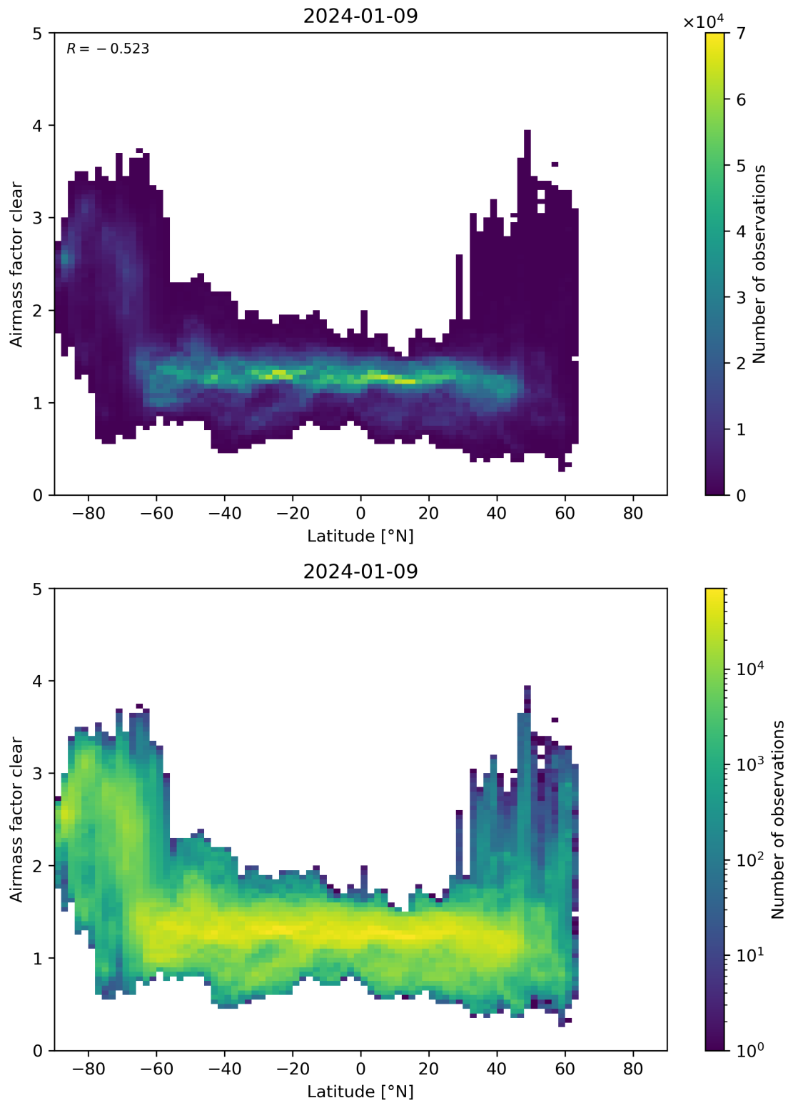
Figure 156: Scatter density plot of “Latitude” against “Airmass factor clear” for 2024-01-08 to 2024-01-10.
