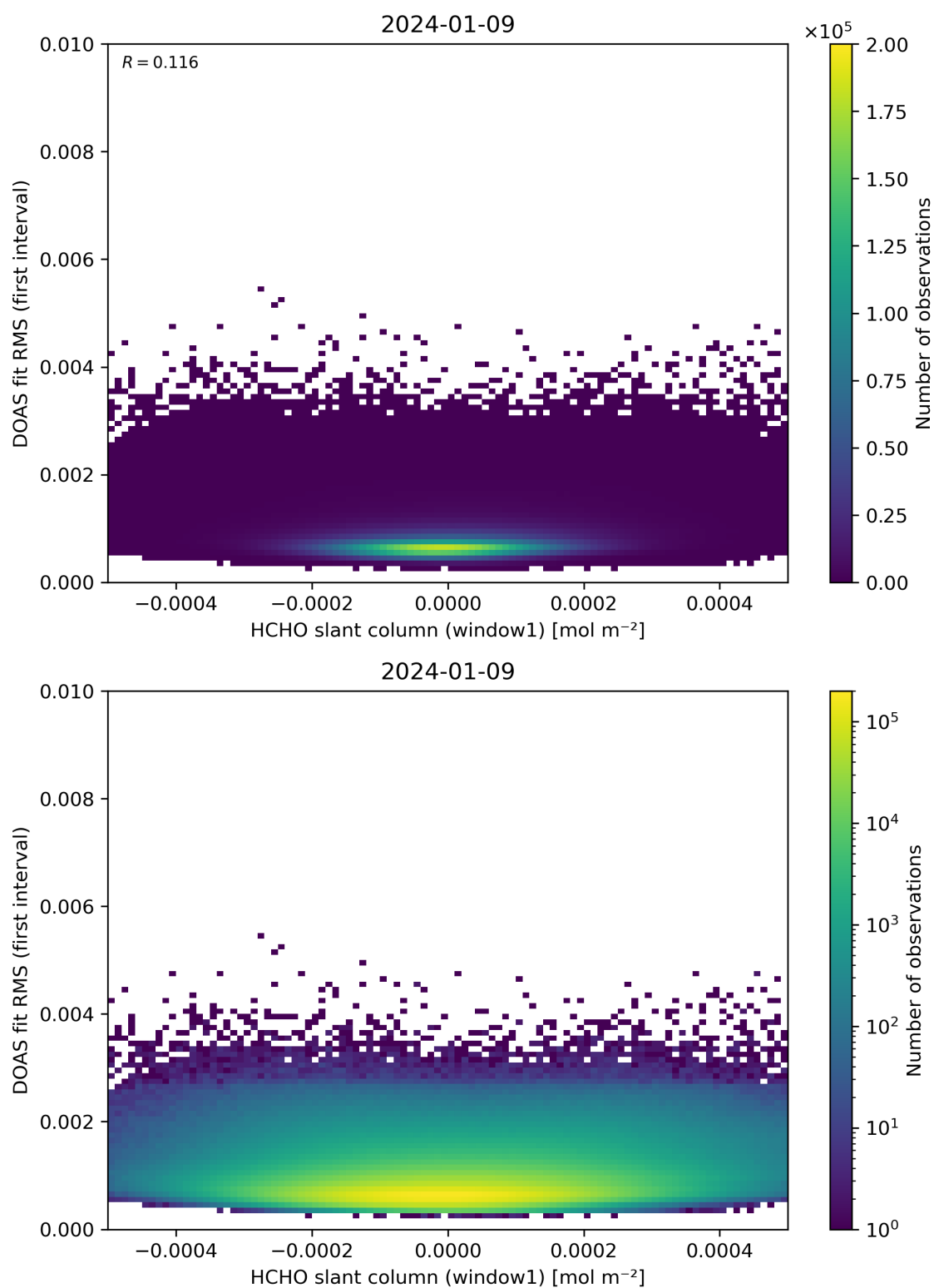
Figure 78: Scatter density plot of “HCHO slant column (window1)” against “DOAS fit RMS (first interval)” for 2024-01-08 to 2024-01-10.
