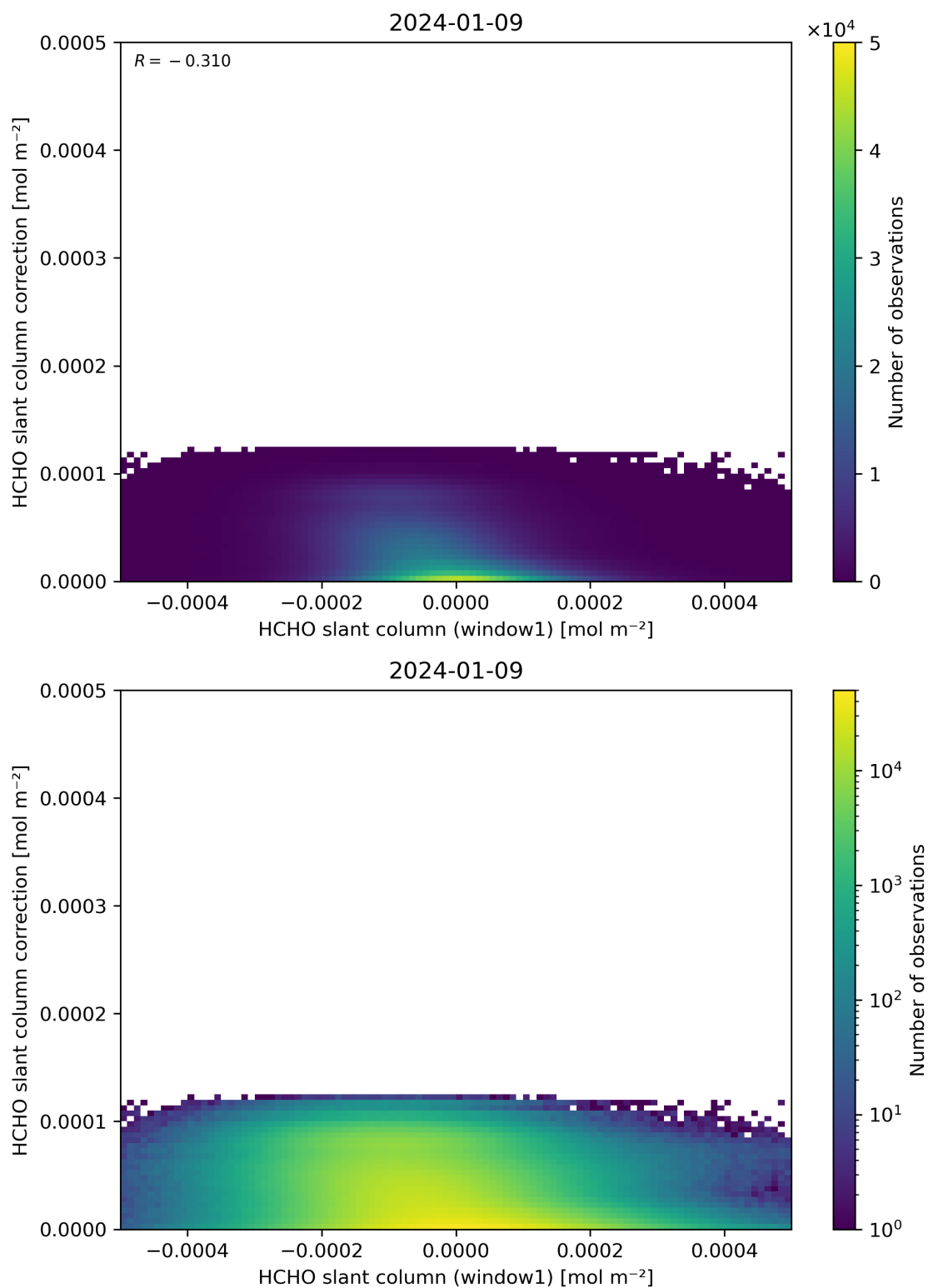
Figure 83: Scatter density plot of “HCHO slant column (window1)” against “HCHO slant column correction” for 2024-01-08 to 2024-01-10.
