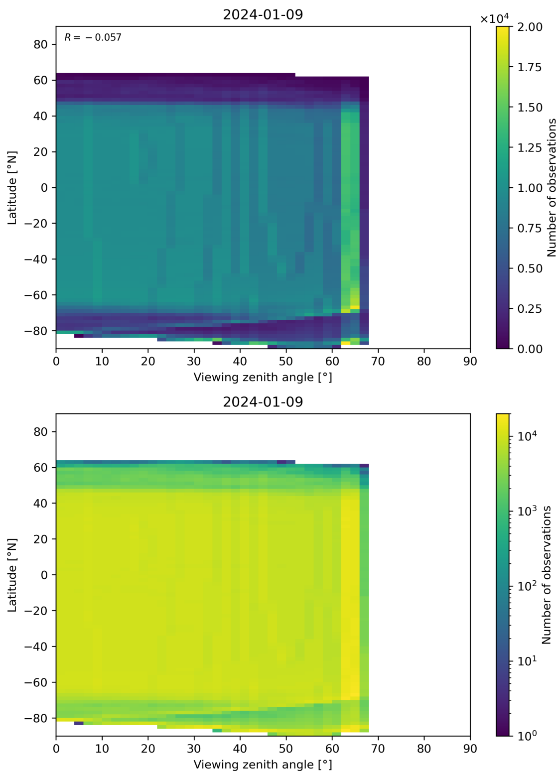
Figure 196: Scatter density plot of “Viewing zenith angle” against “Latitude” for 2024-01-08 to 2024-01-10.
