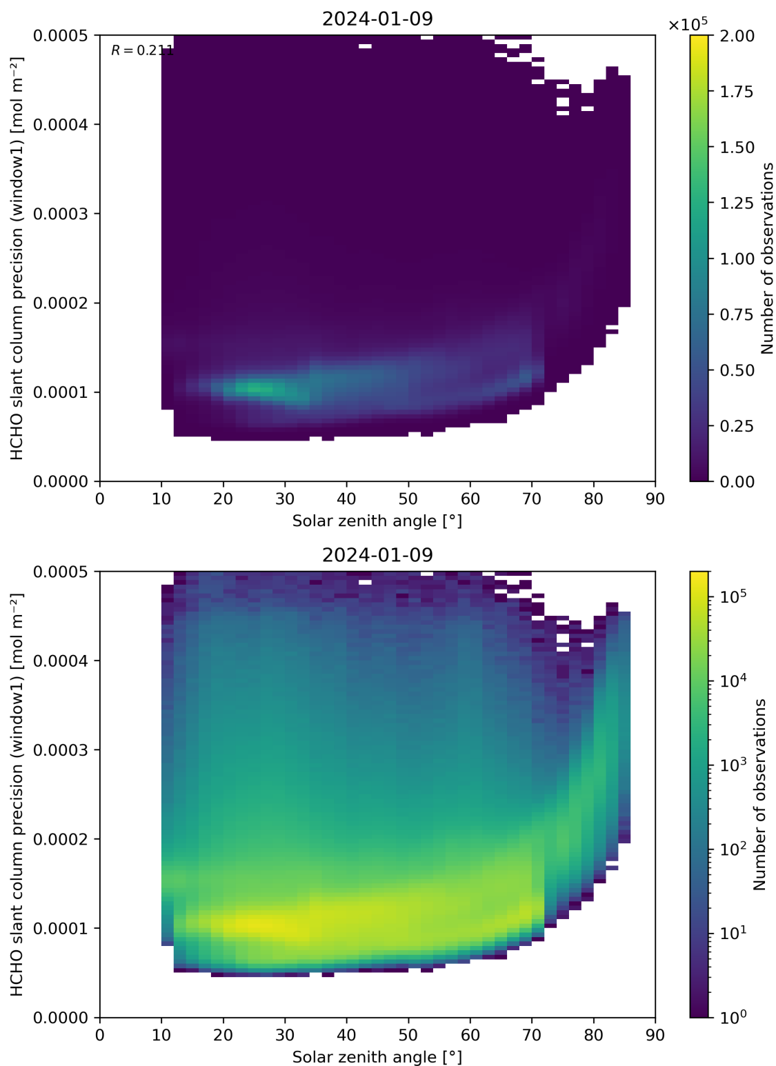
Figure 174: Scatter density plot of “Solar zenith angle” against “HCHO slant column precision (window1)” for 2024-01-08 to 2024-01-10.
