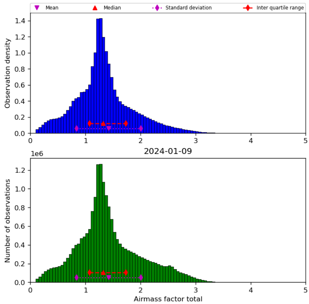
Figure 40: Histogram of “Airmass factor total” for 2024-01-08 to 2024-01-10
