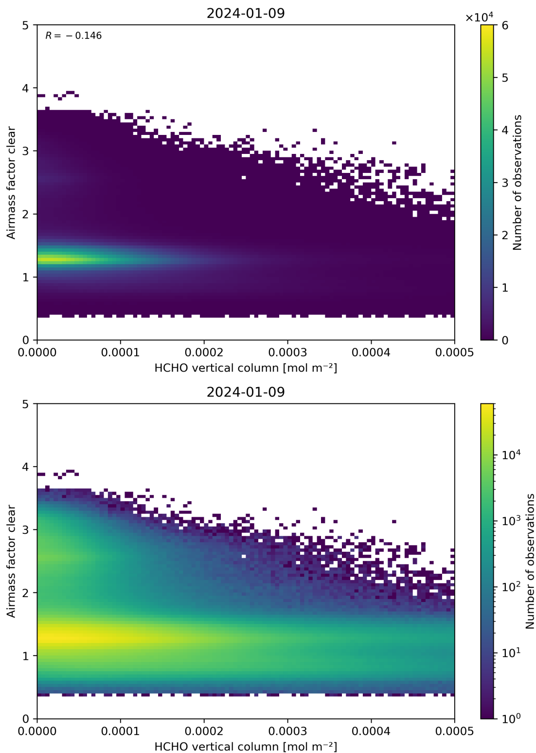
Figure 126: Scatter density plot of “HCHO vertical column” against “Airmass factor clear” for 2024-01-08 to 2024-01-10.
