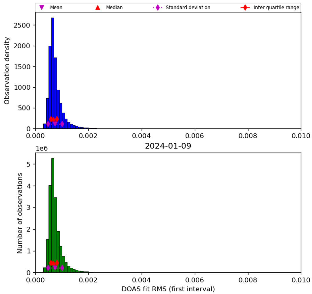
Figure 46: Histogram of “DOAS fit RMS (first interval)” for 2024-01-08 to 2024-01-10
