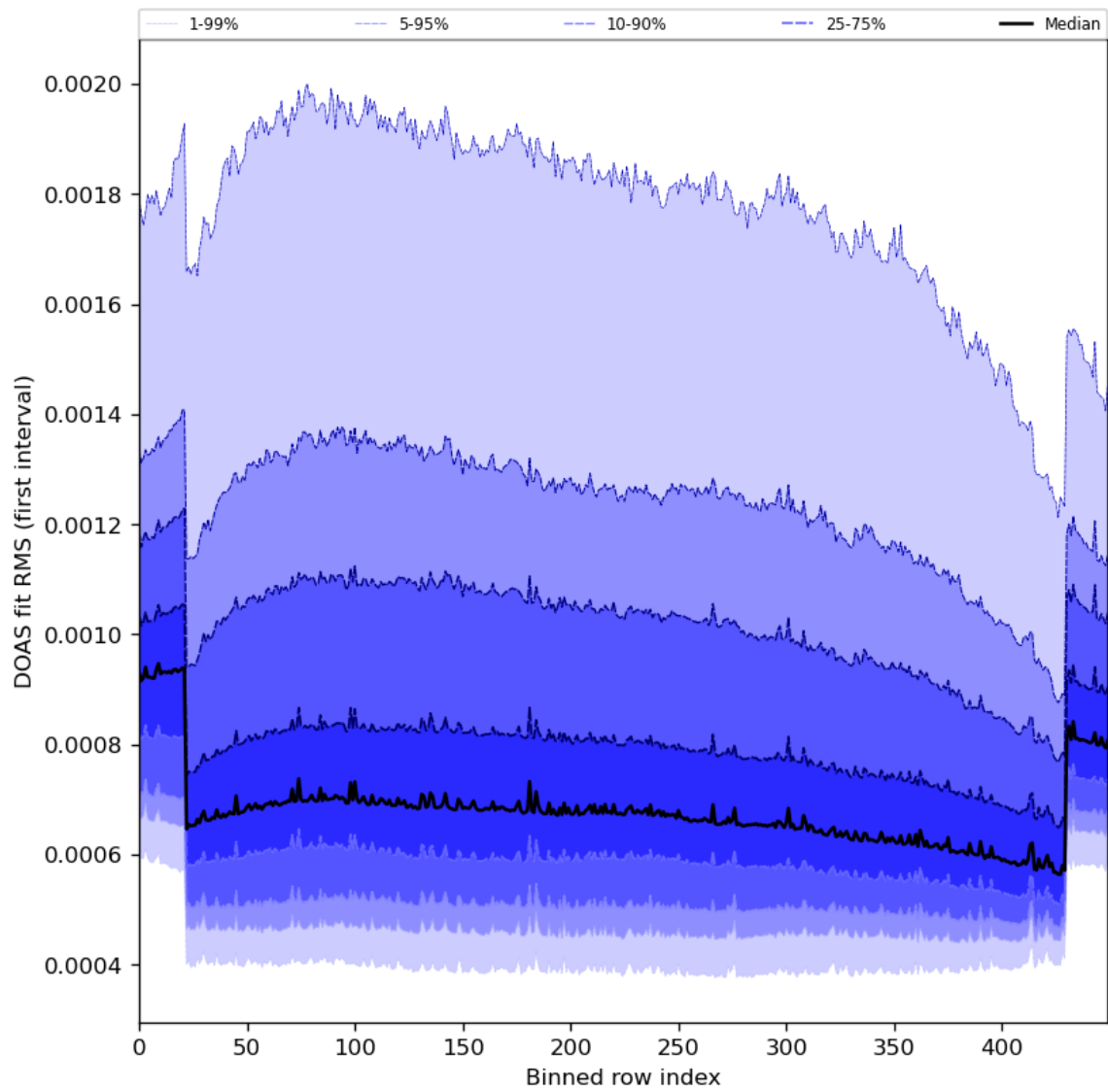
Figure 60: Along track statistics of “DOAS fit RMS (first interval)” for 2024-01-08 to 2024-01-10
