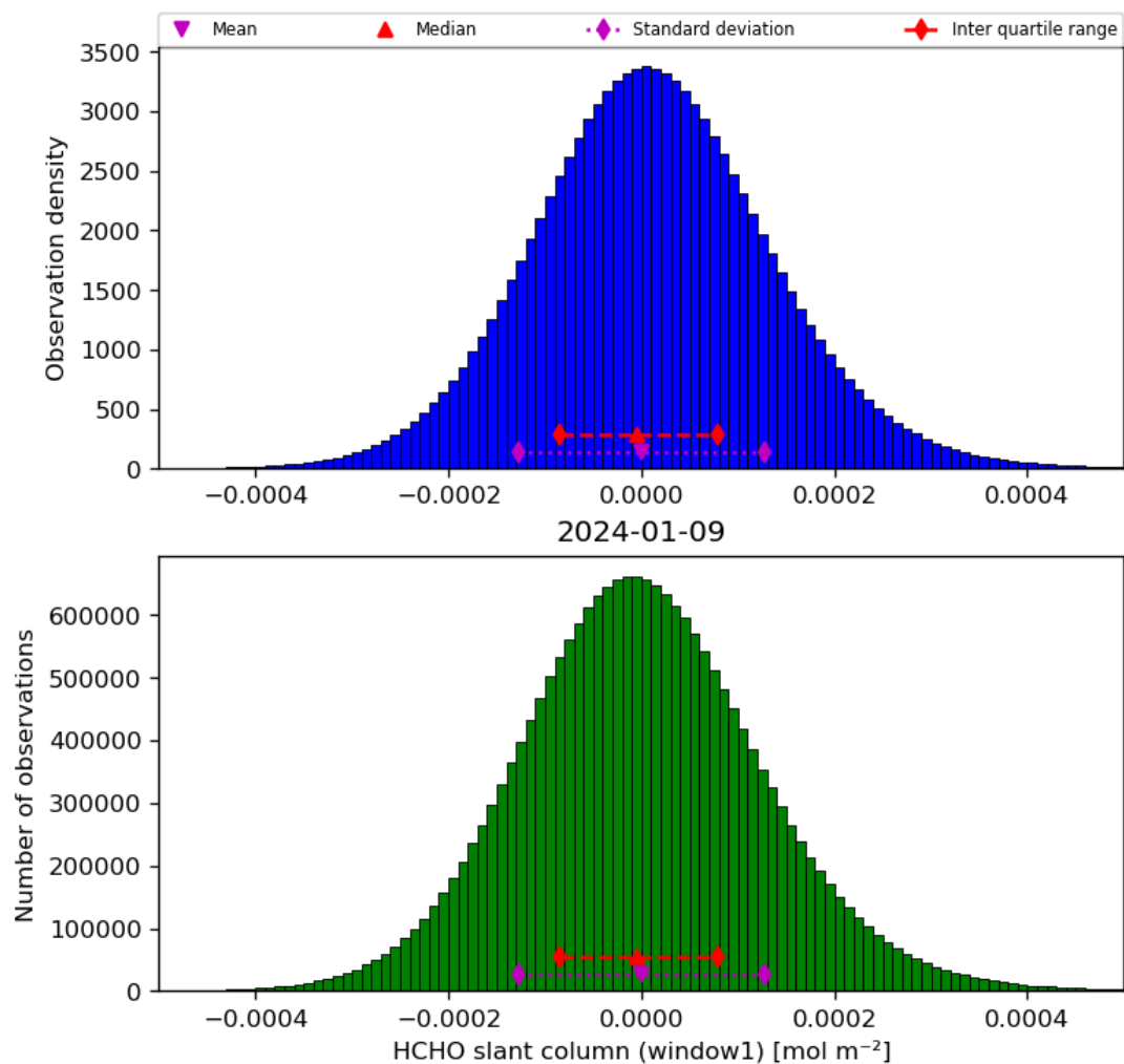
Figure 38: Histogram of “HCHO slant column (window1)” for 2024-01-08 to 2024-01-10
