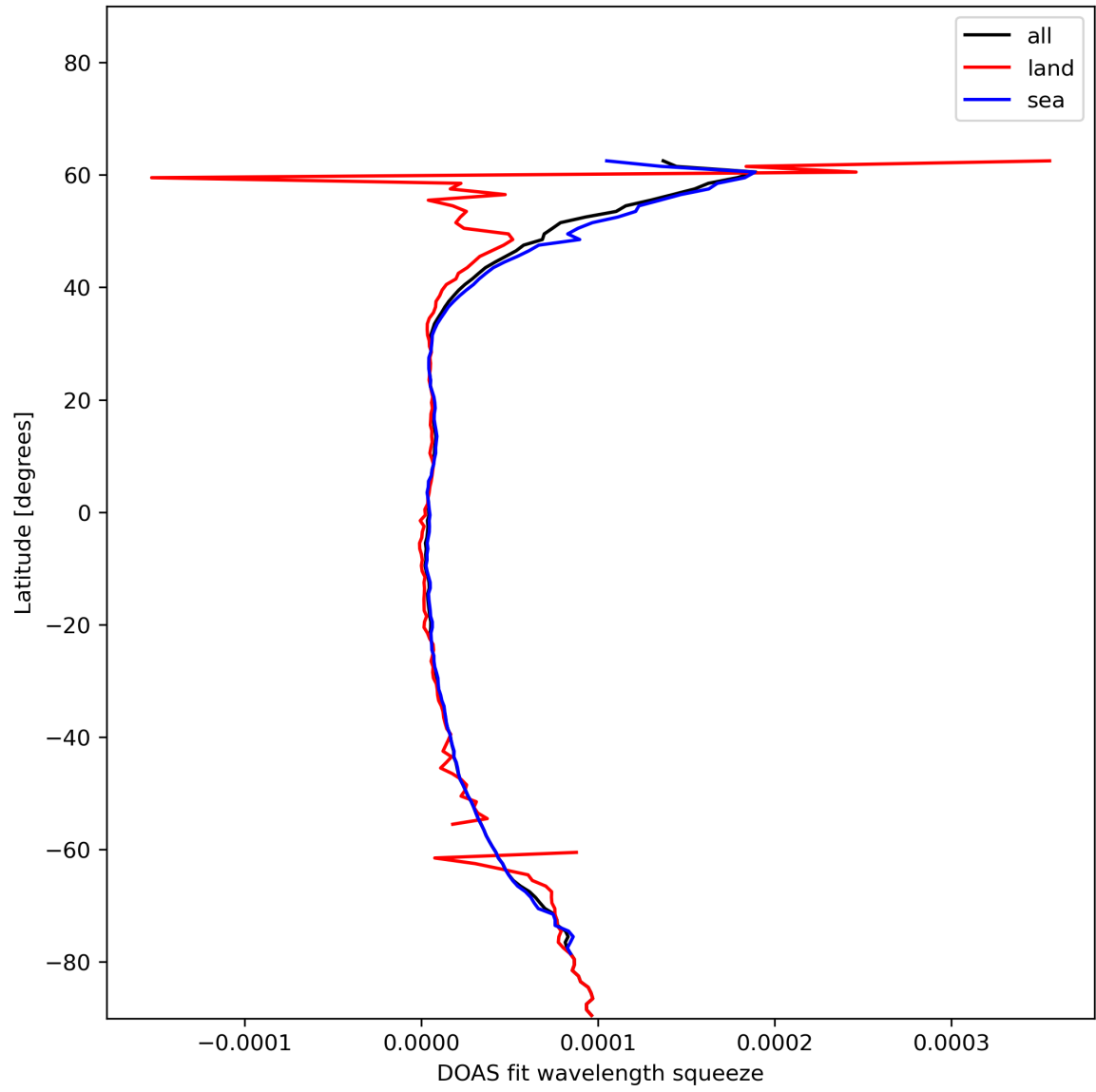
Figure 31: Zonal average of “DOAS fit wavelength squeeze” for 2024-01-08 to 2024-01-10.
