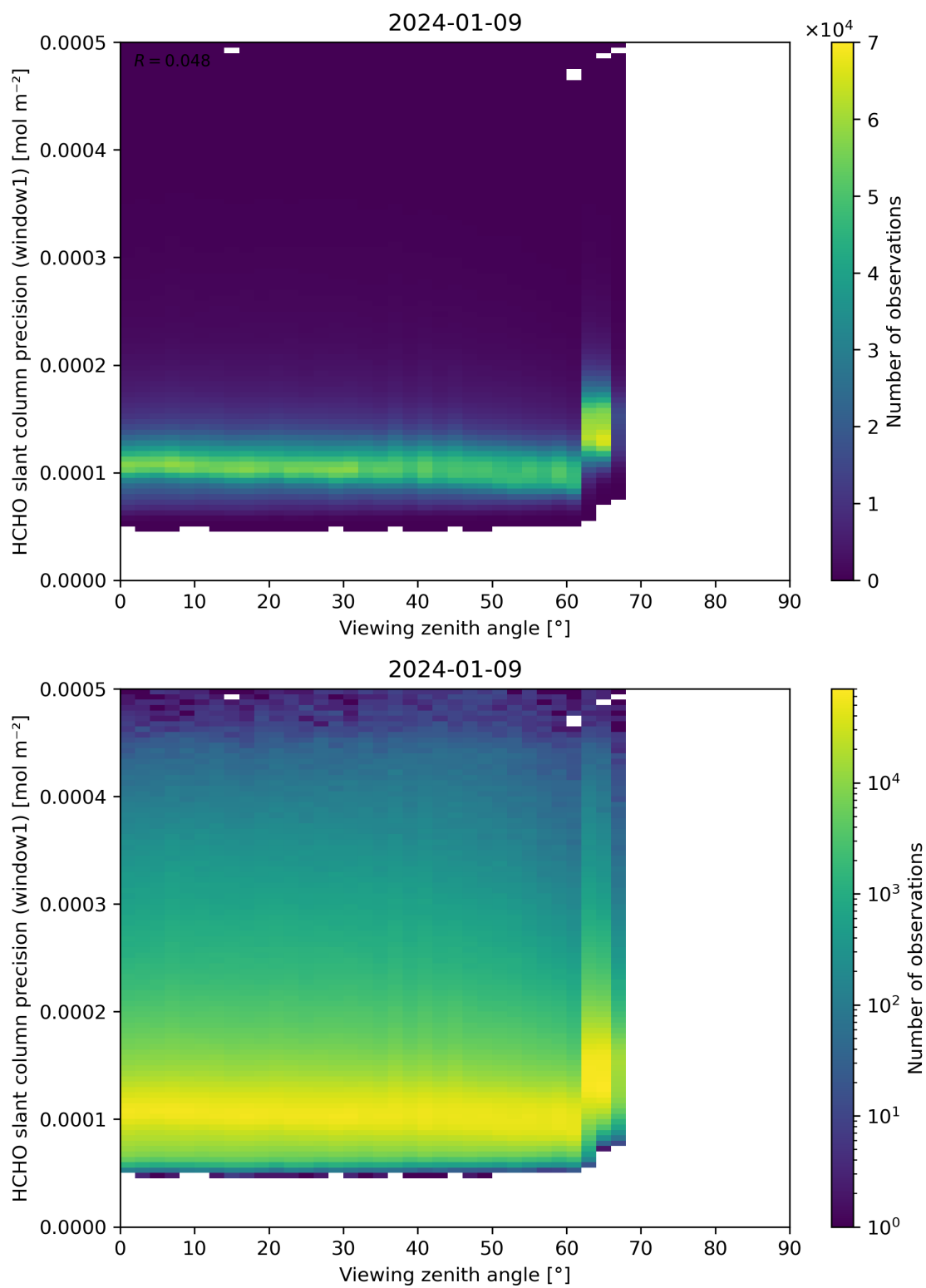
Figure 189: Scatter density plot of “Viewing zenith angle” against “HCHO slant column precision (window1)” for 2024-01-08 to 2024-01-10.
