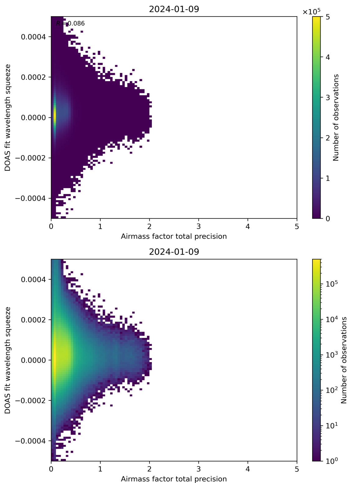
Figure 107: Scatter density plot of “Airmass factor total precision” against “DOAS fit wavelength squeeze” for 2024-01-08 to 2024-01-10.
