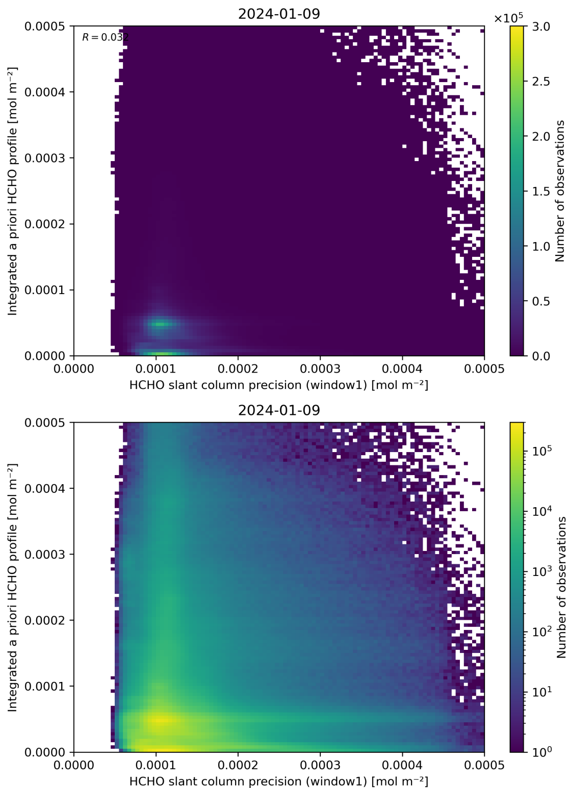
Figure 96: Scatter density plot of “HCHO slant column precision (window1)” against “Integrated a priori HCHO profile” for 2024-01-08 to 2024-01-10.
