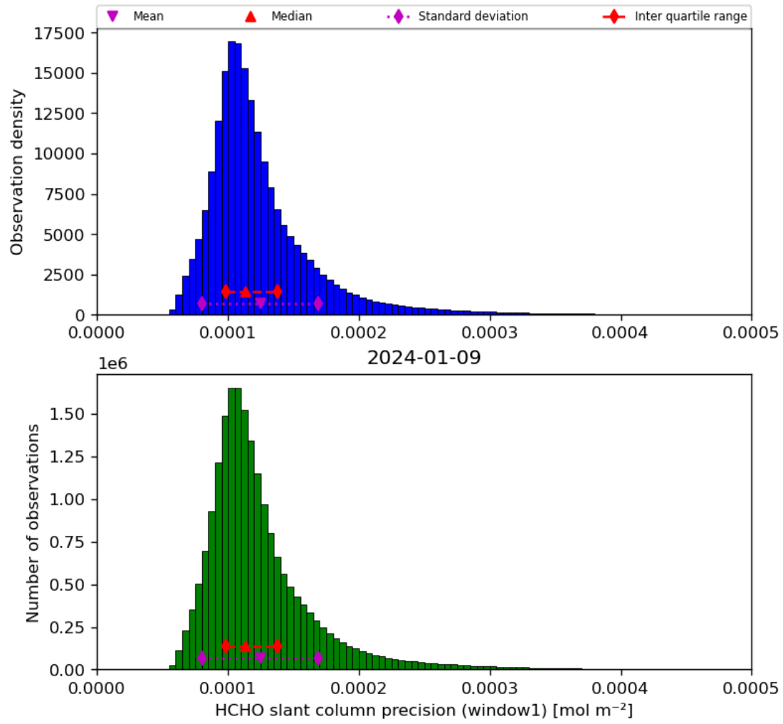
Figure 39: Histogram of “HCHO slant column precision (window1)” for 2024-01-08 to 2024-01-10
