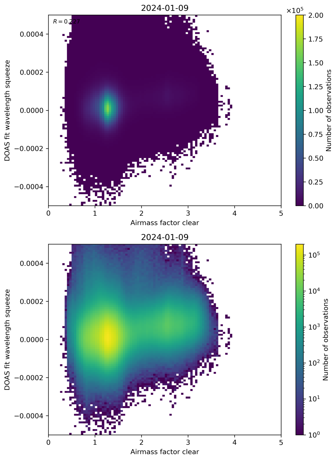
Figure 73: Scatter density plot of “Airmass factor clear” against “DOAS fit wavelength squeeze” for 2024-01-08 to 2024-01-10.
