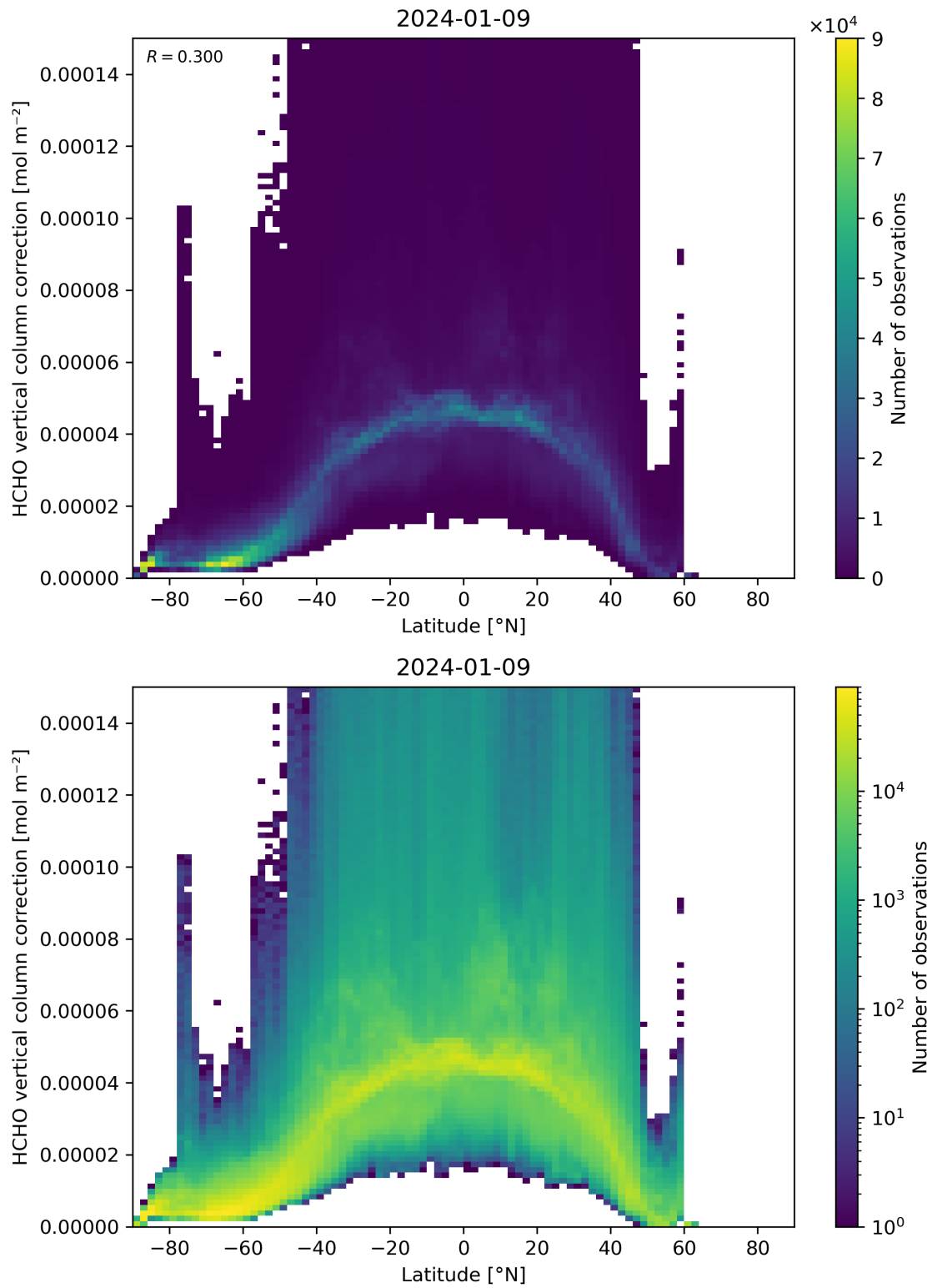
Figure 164: Scatter density plot of “Latitude” against “HCHO vertical column correction” for 2024-01-08 to 2024-01-10.
