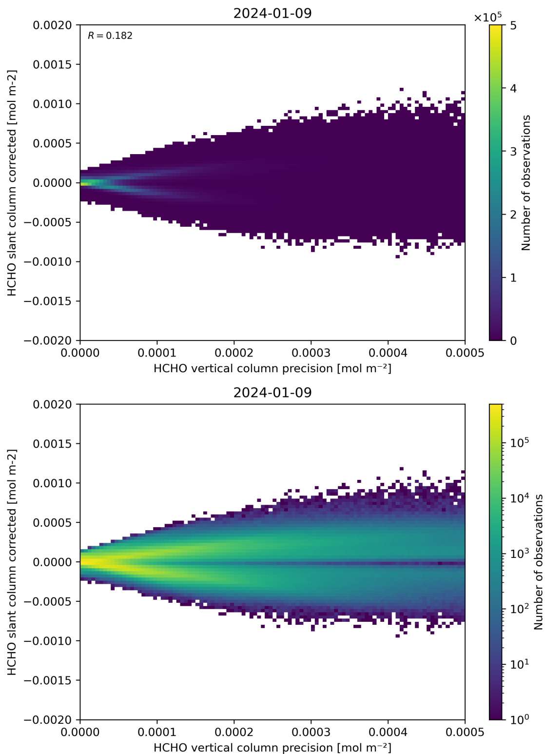
Figure 140: Scatter density plot of “HCHO vertical column precision” against “HCHO slant column corrected” for 2024-01-08 to 2024-01-10.
