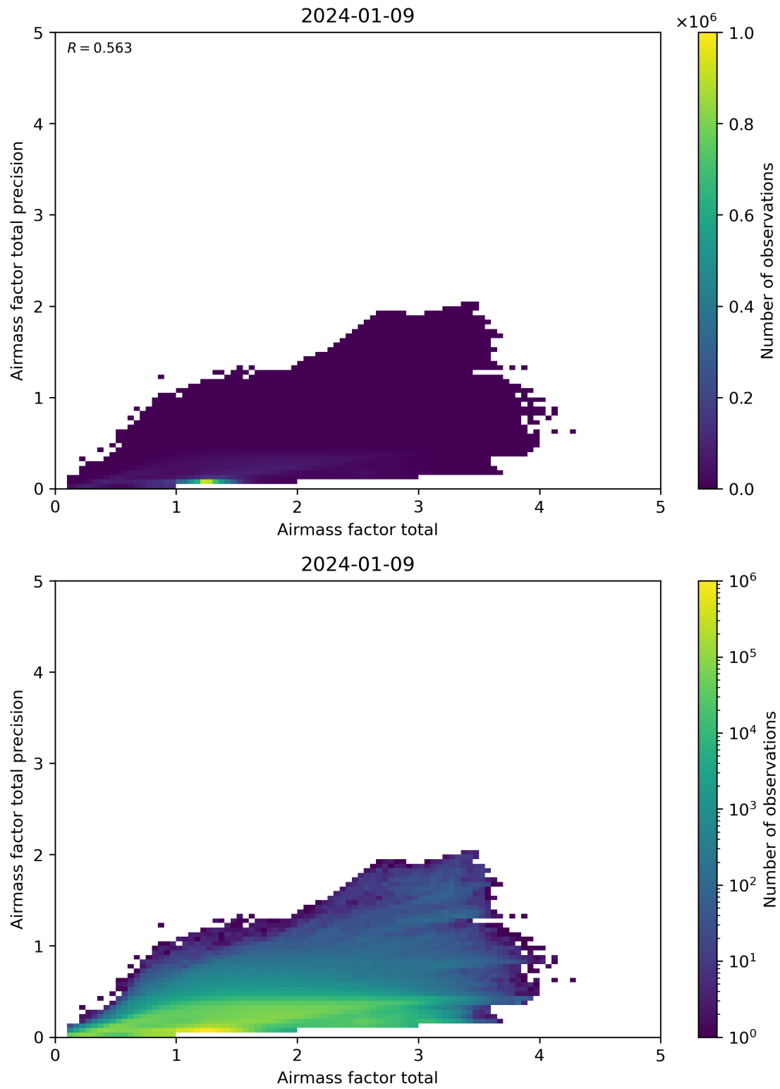
Figure 103: Scatter density plot of “Airmass factor total” against “Airmass factor total precision” for 2024-01-08 to 2024-01-10.
