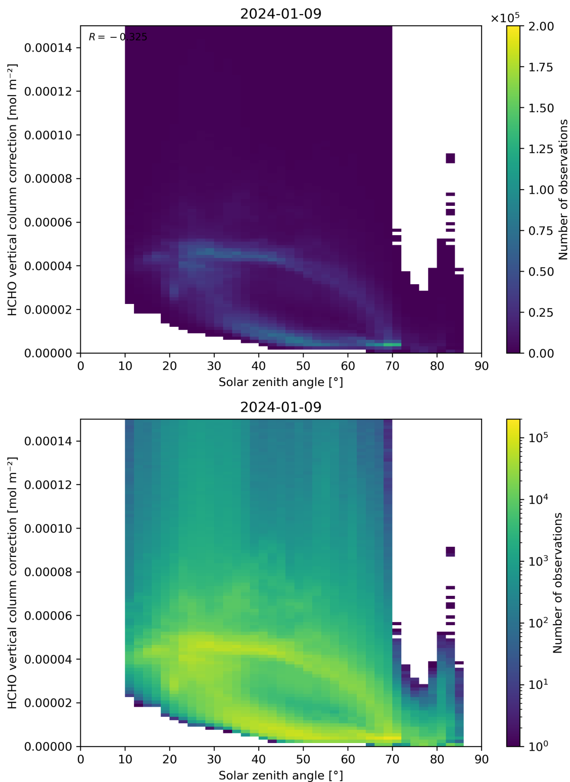
Figure 178: Scatter density plot of “Solar zenith angle” against “HCHO vertical column correction” for 2024-01-08 to 2024-01-10.
