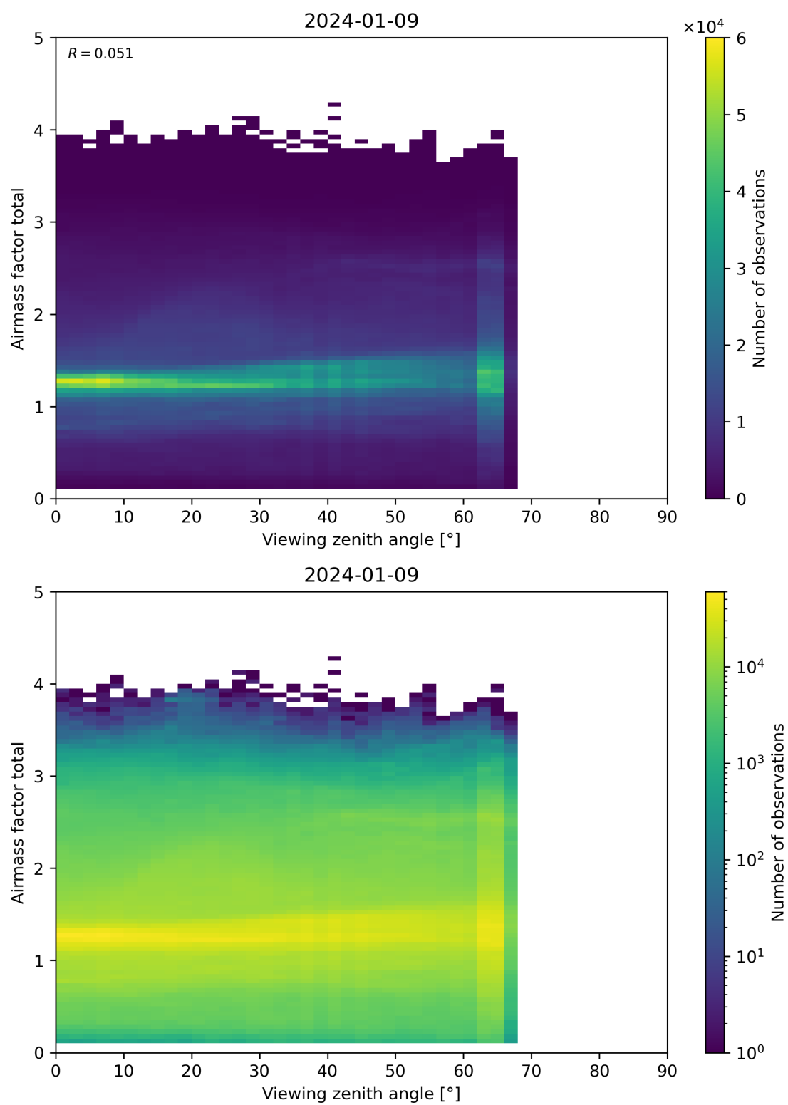
Figure 190: Scatter density plot of “Viewing zenith angle” against “Airmass factor total” for 2024-01-08 to 2024-01-10.
