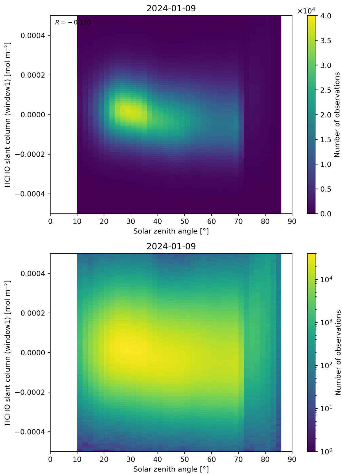
Figure 173: Scatter density plot of “Solar zenith angle” against “HCHO slant column (window1)” for 2024-01-08 to 2024-01-10.
