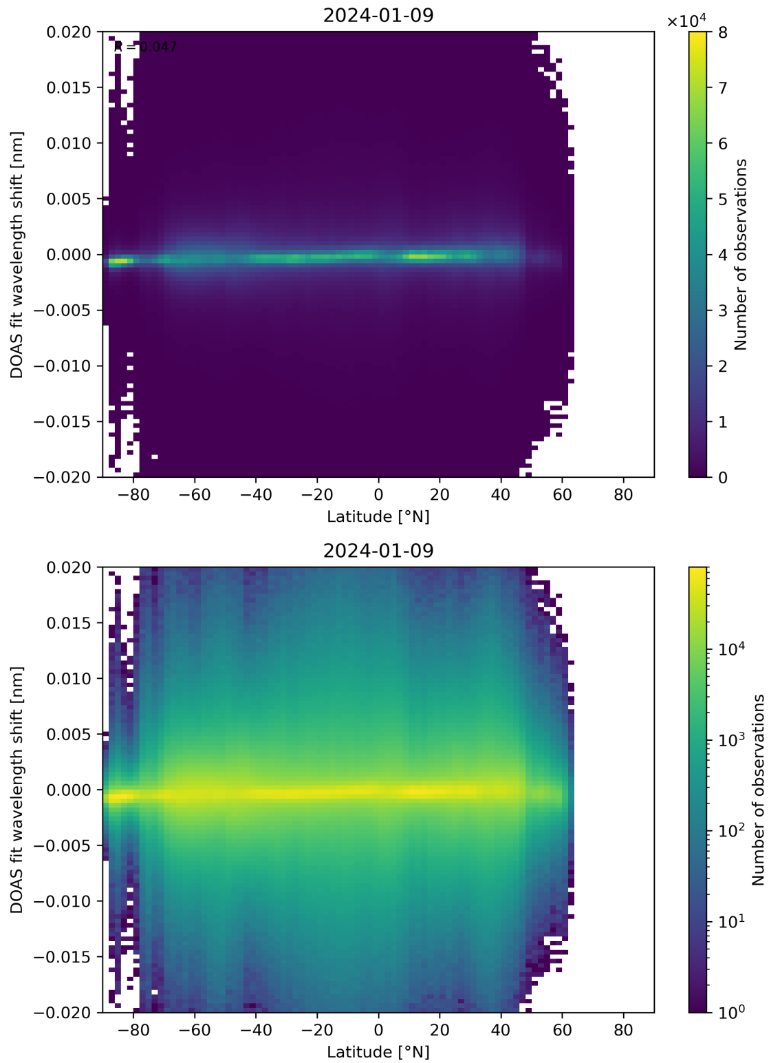
Figure 154: Scatter density plot of “Latitude” against “DOAS fit wavelength shift” for 2024-01-08 to 2024-01-10.
