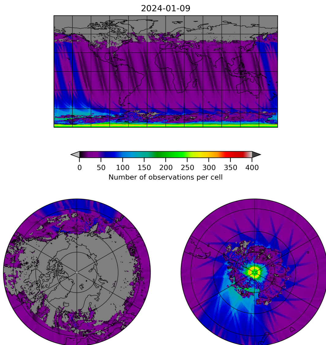
Figure 19: Map of the number of observations for 2024-01-08 to 2024-01-10
