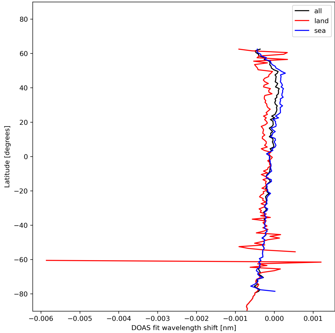
Figure 30: Zonal average of “DOAS fit wavelength shift” for 2024-01-08 to 2024-01-10.
