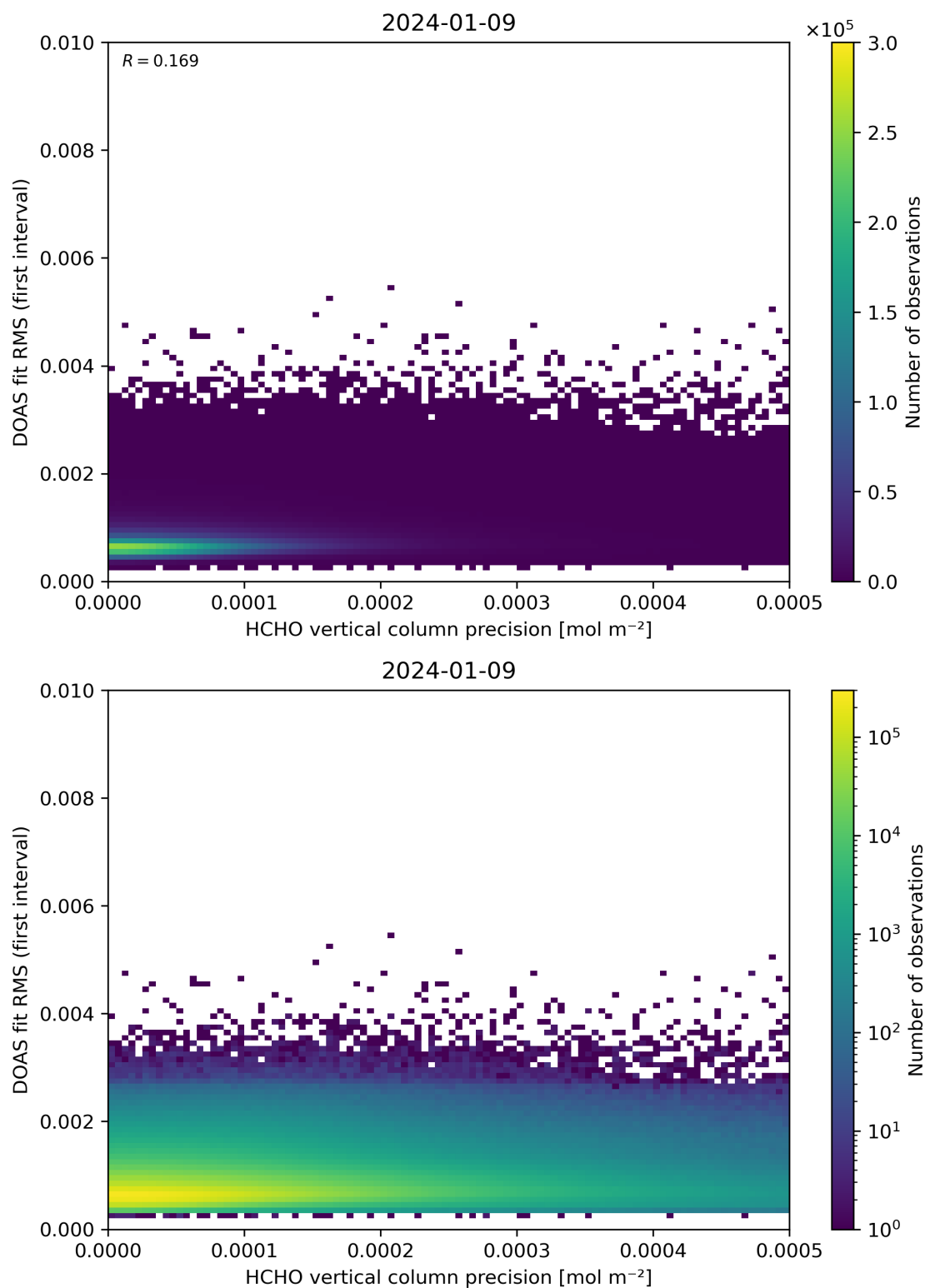
Figure 136: Scatter density plot of “HCHO vertical column precision” against “DOAS fit RMS (first interval)” for 2024-01-08 to 2024-01-10.
