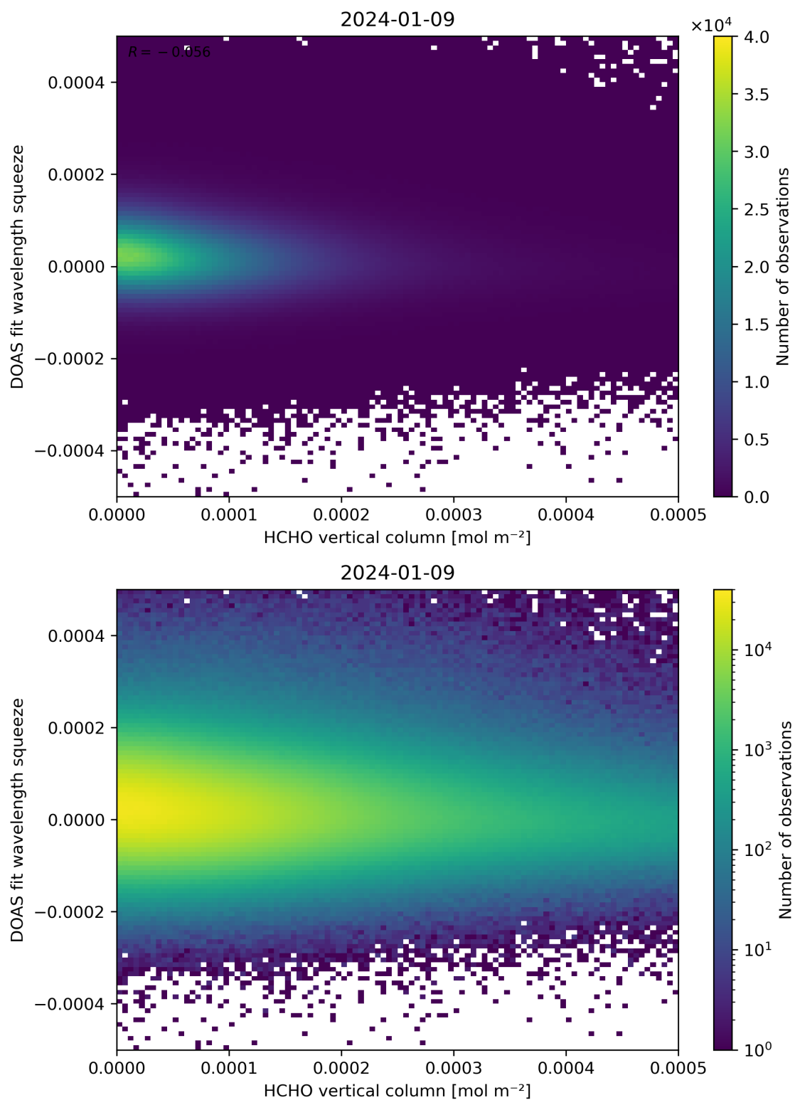
Figure 125: Scatter density plot of “HCHO vertical column” against “DOAS fit wavelength squeeze” for 2024-01-08 to 2024-01-10.
