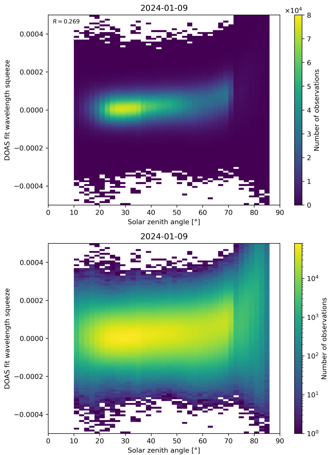
Figure 169: Scatter density plot of “Solar zenith angle” against “DOAS fit wavelength squeeze” for 2024-01-08 to 2024-01-10.
