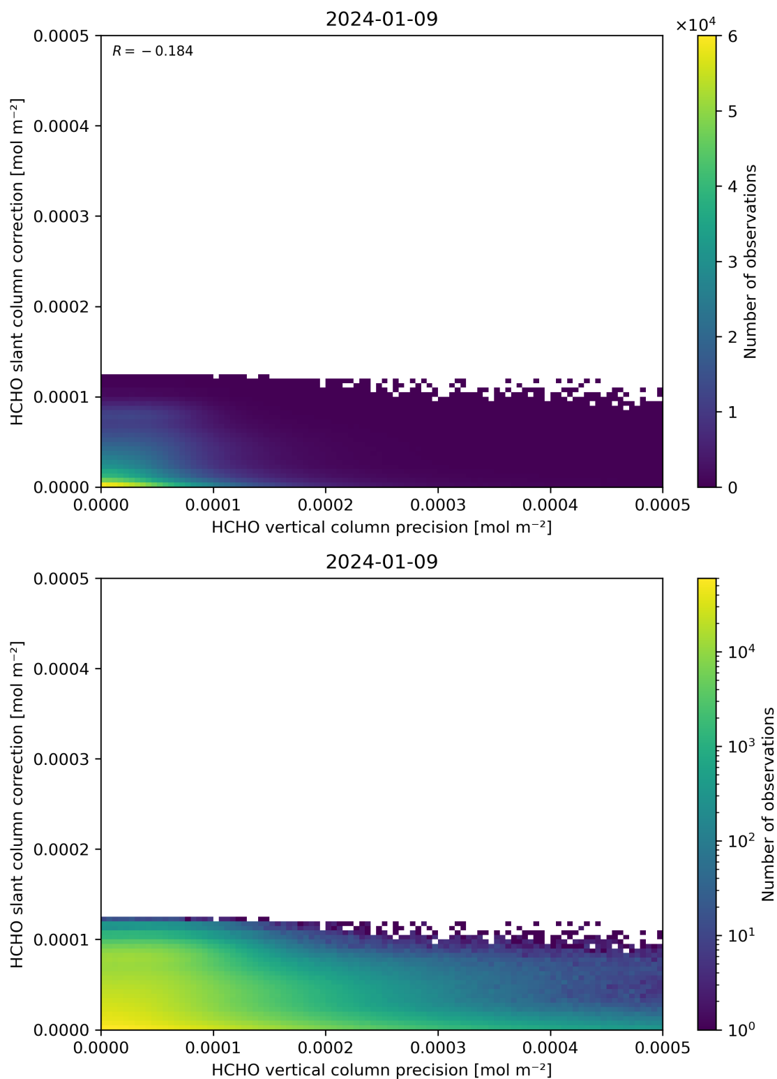
Figure 141: Scatter density plot of “HCHO vertical column precision” against “HCHO slant column correction” for 2024-01-08 to 2024-01-10.
