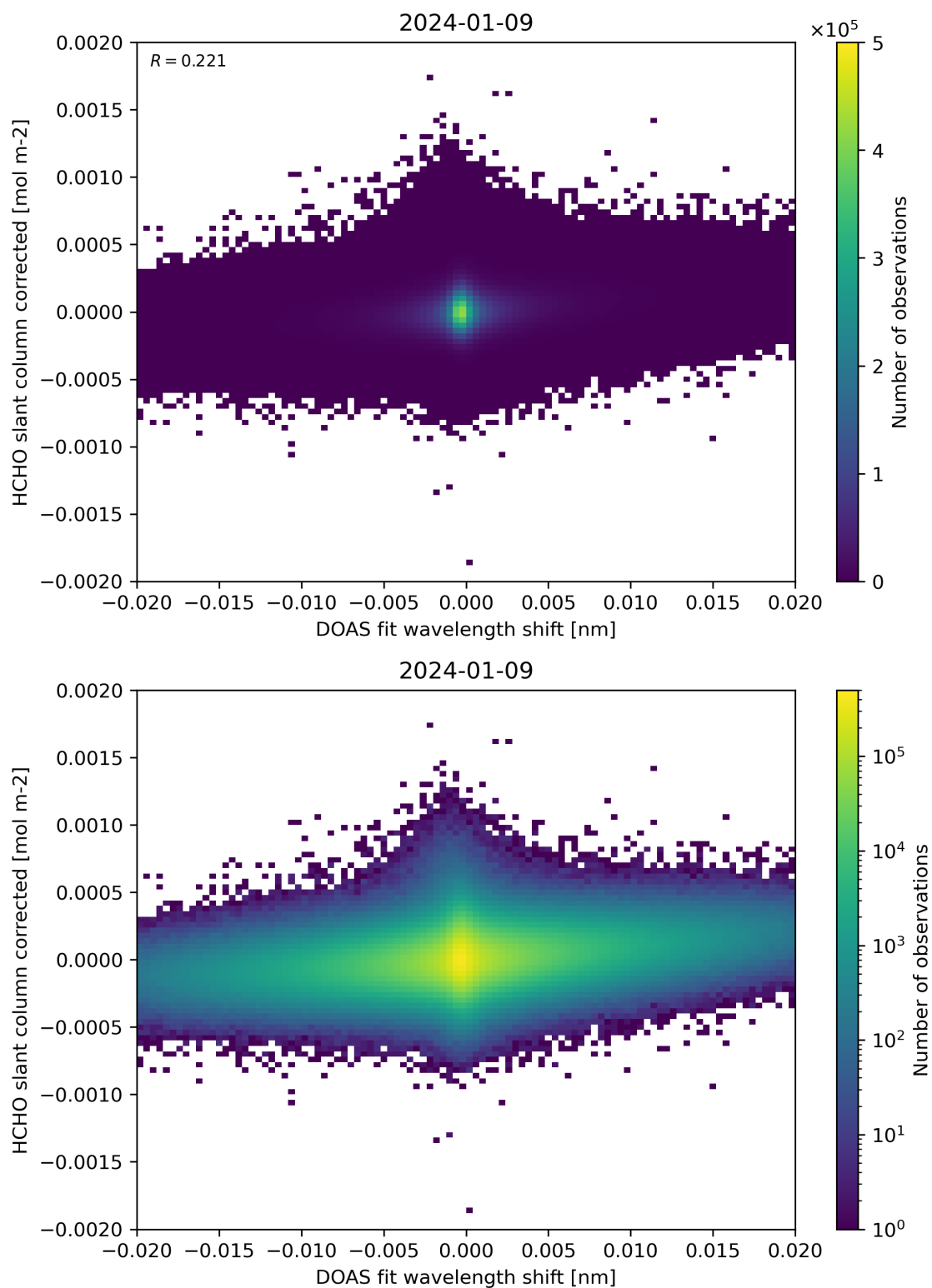
Figure 66: Scatter density plot of “DOAS fit wavelength shift” against “HCHO slant column corrected” for 2024-01-08 to 2024-01-10.
