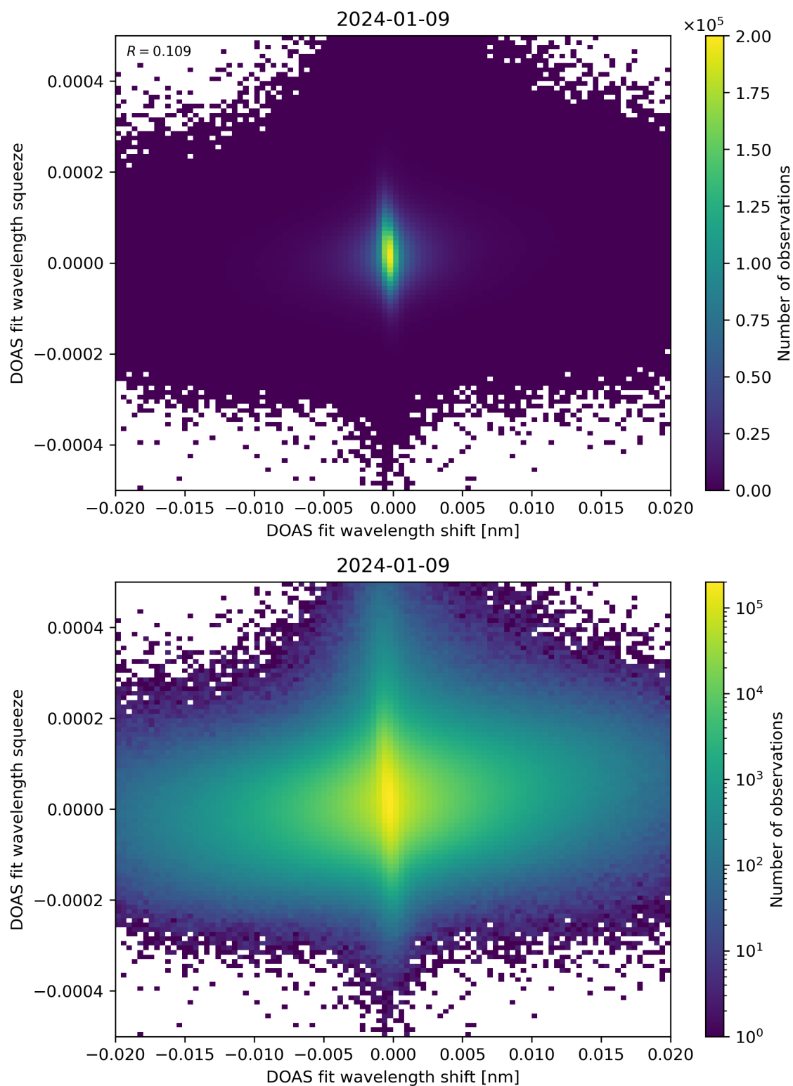
Figure 65: Scatter density plot of “DOAS fit wavelength shift” against “DOAS fit wavelength squeeze” for 2024-01-08 to 2024-01-10.
