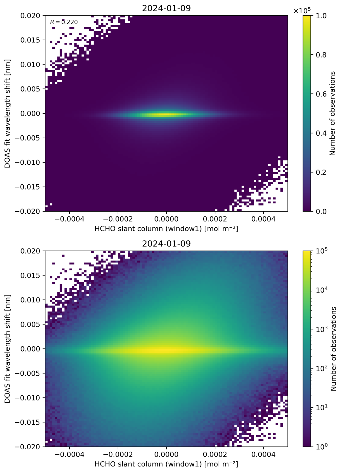
Figure 79: Scatter density plot of “HCHO slant column (window1)” against “DOAS fit wavelength shift” for 2024-01-08 to 2024-01-10.
