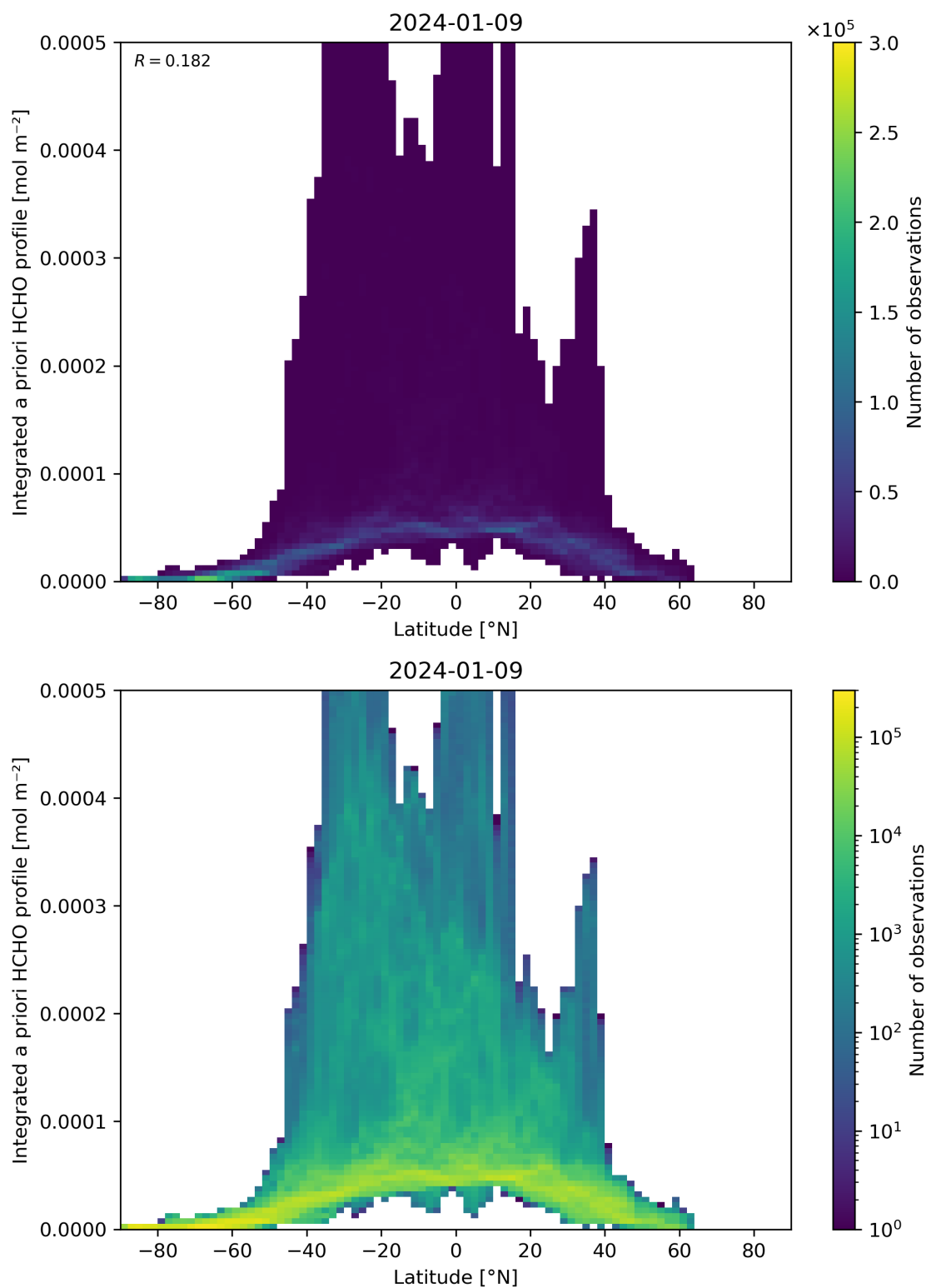
Figure 166: Scatter density plot of “Latitude” against “Integrated a priori HCHO profile” for 2024-01-08 to 2024-01-10.
