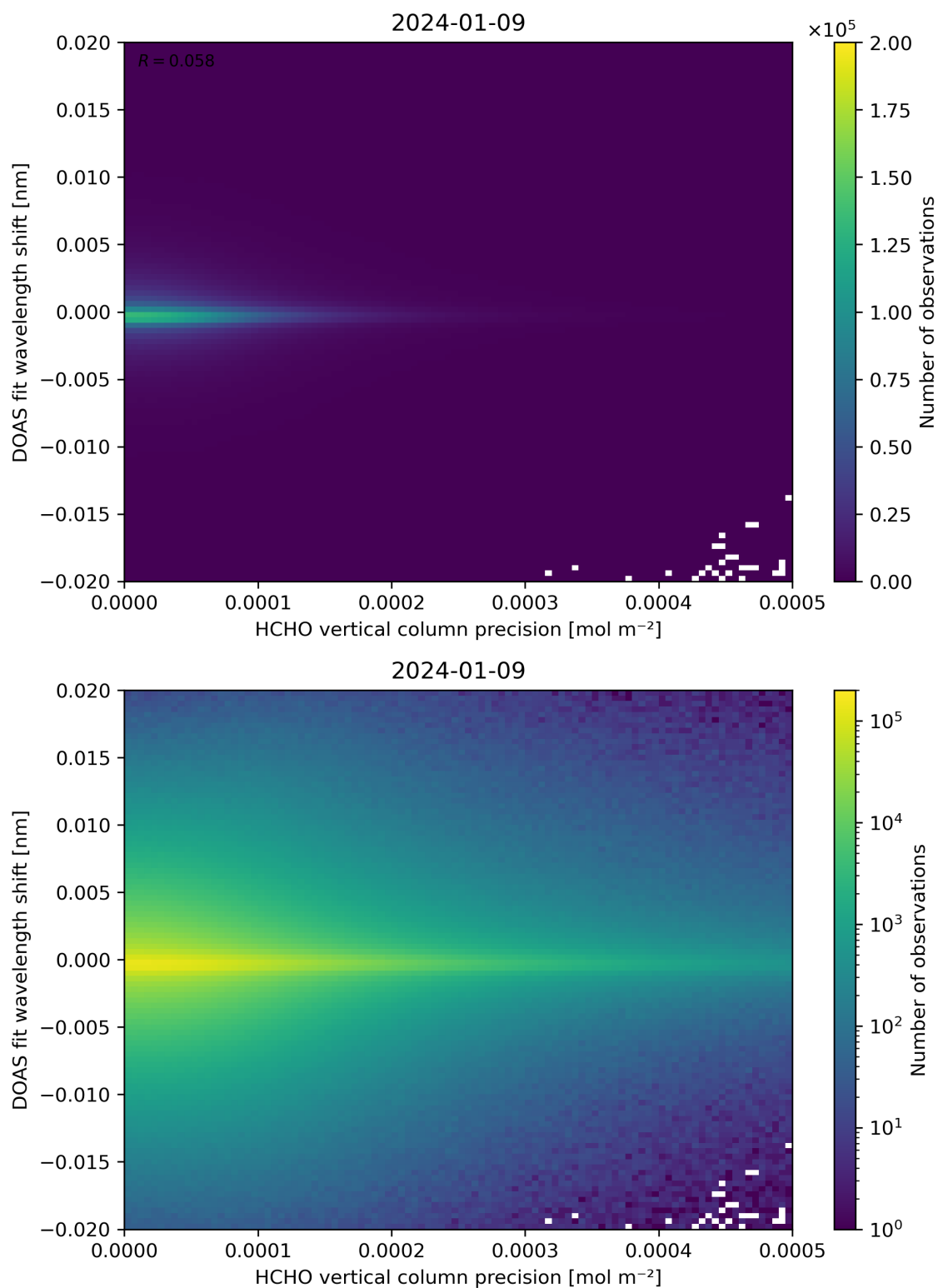
Figure 137: Scatter density plot of “HCHO vertical column precision” against “DOAS fit wavelength shift” for 2024-01-08 to 2024-01-10.
