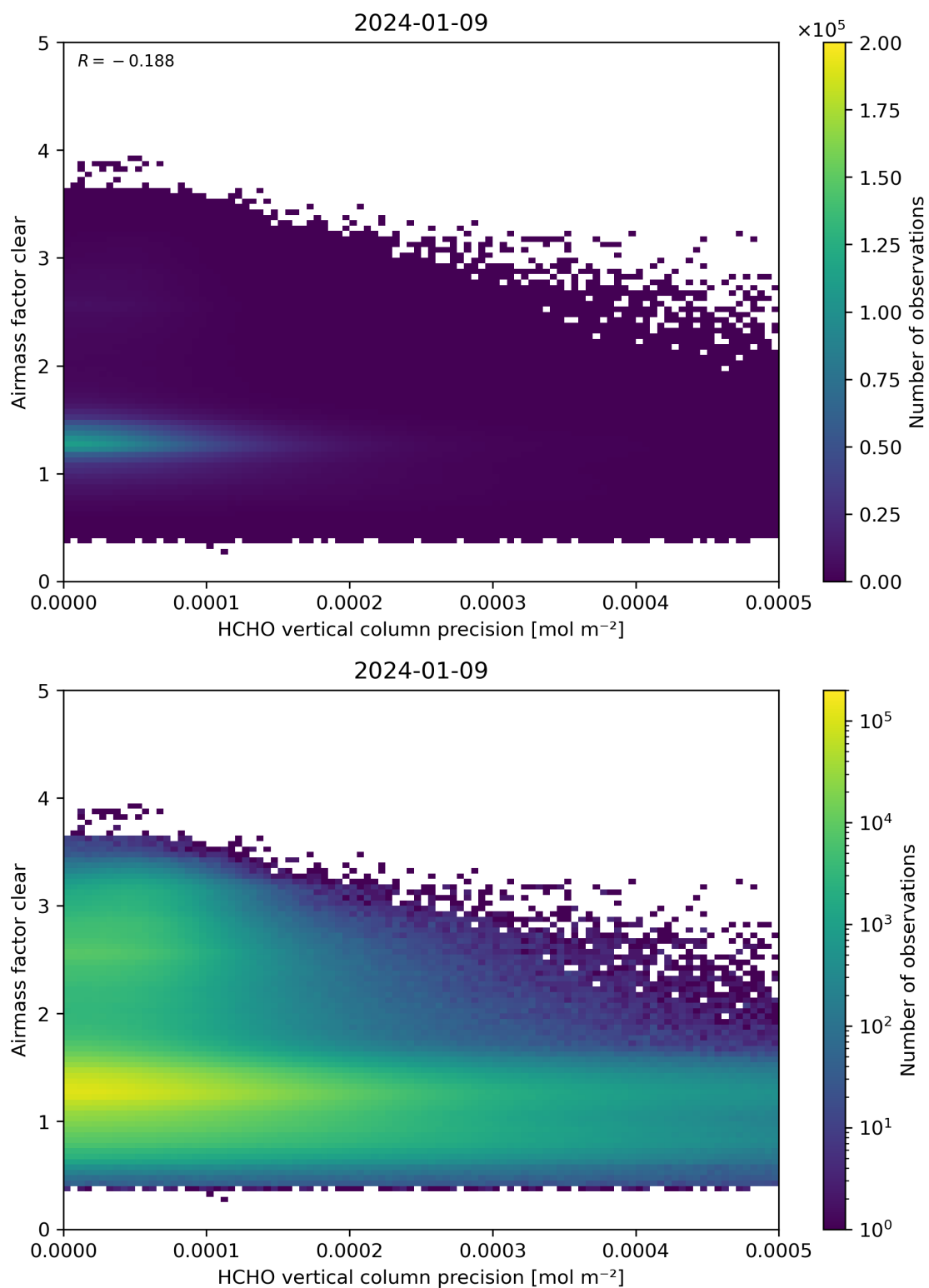
Figure 139: Scatter density plot of “HCHO vertical column precision” against “Airmass factor clear” for 2024-01-08 to 2024-01-10.
