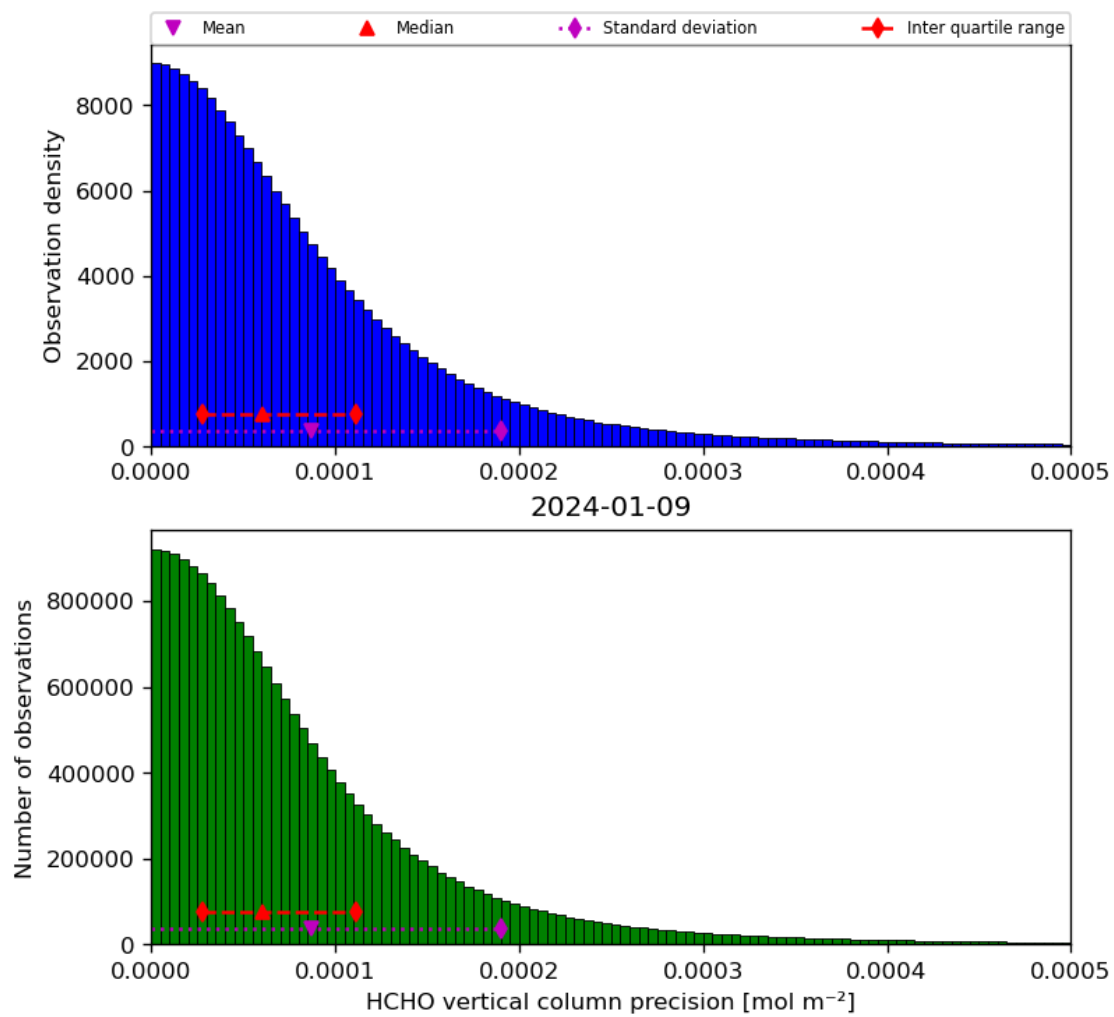
Figure 36: Histogram of “HCHO vertical column precision” for 2024-01-08 to 2024-01-10
