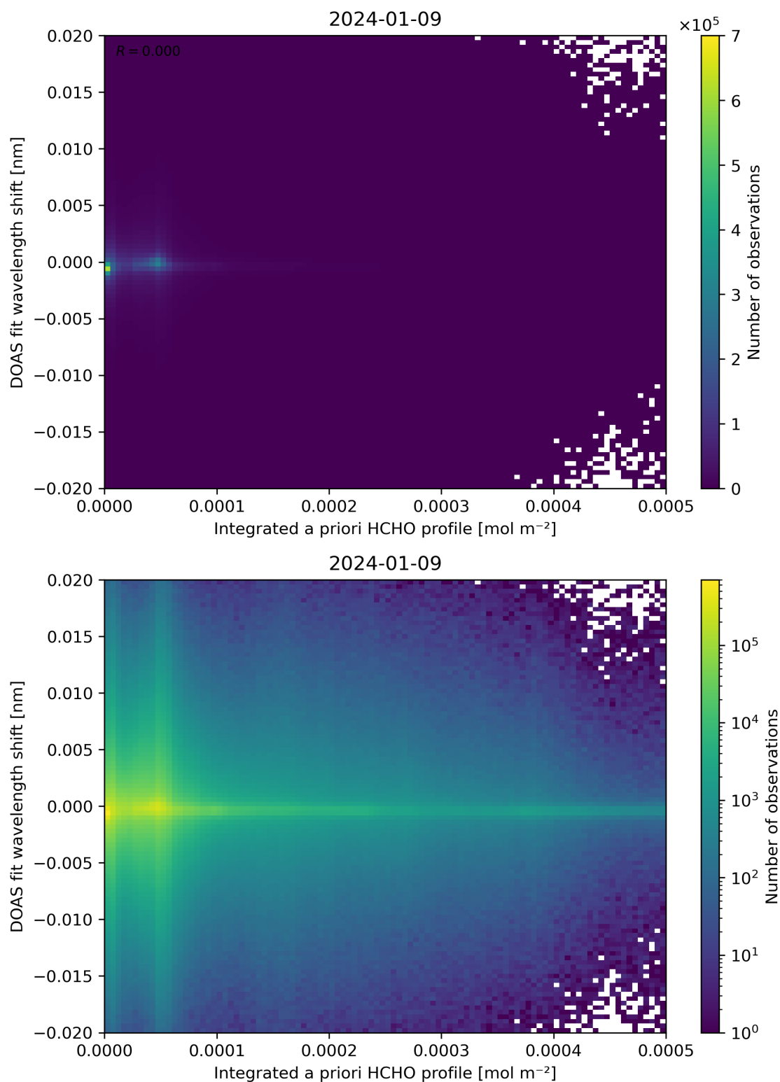
Figure 149: Scatter density plot of “Integrated a priori HCHO profile” against “DOAS fit wavelength shift” for 2024-01-08 to 2024-01-10.
