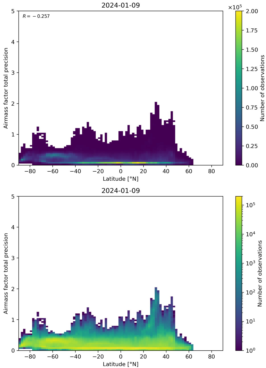
Figure 162: Scatter density plot of “Latitude” against “Airmass factor total precision” for 2024-01-08 to 2024-01-10.
