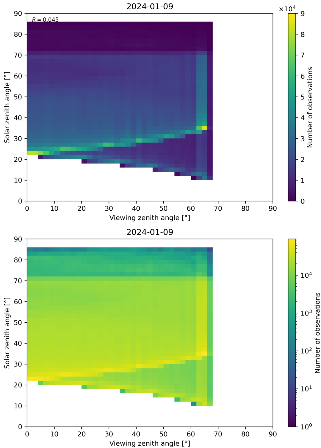
Figure 197: Scatter density plot of “Viewing zenith angle” against “Solar zenith angle” for 2024-01-08 to 2024-01-10.
