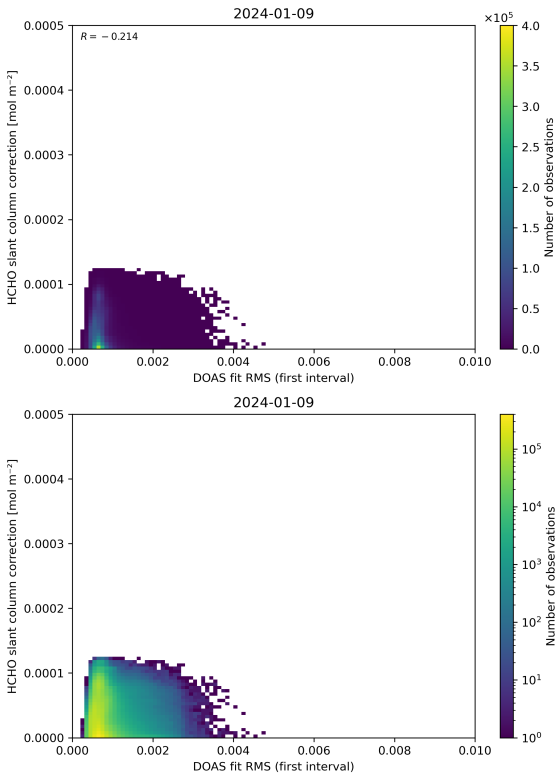
Figure 63: Scatter density plot of “DOAS fit RMS (first interval)” against “HCHO slant column correction” for 2024-01-08 to 2024-01-10.
