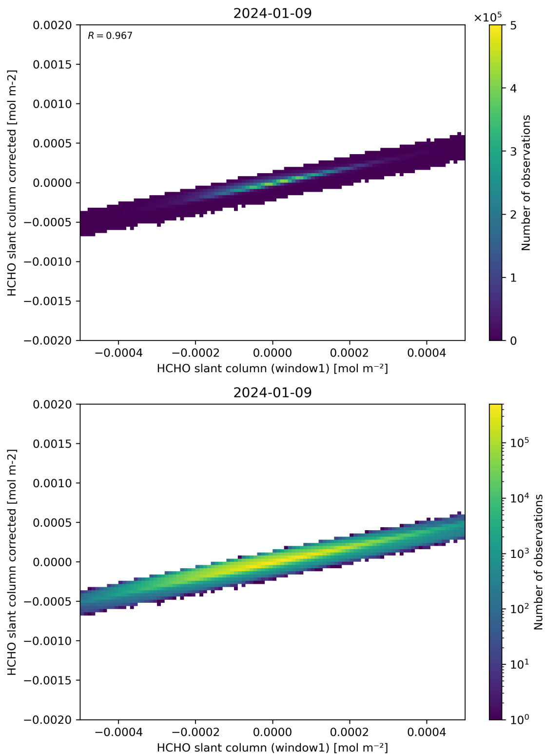
Figure 82: Scatter density plot of “HCHO slant column (window1)” against “HCHO slant column corrected” for 2024-01-08 to 2024-01-10.
