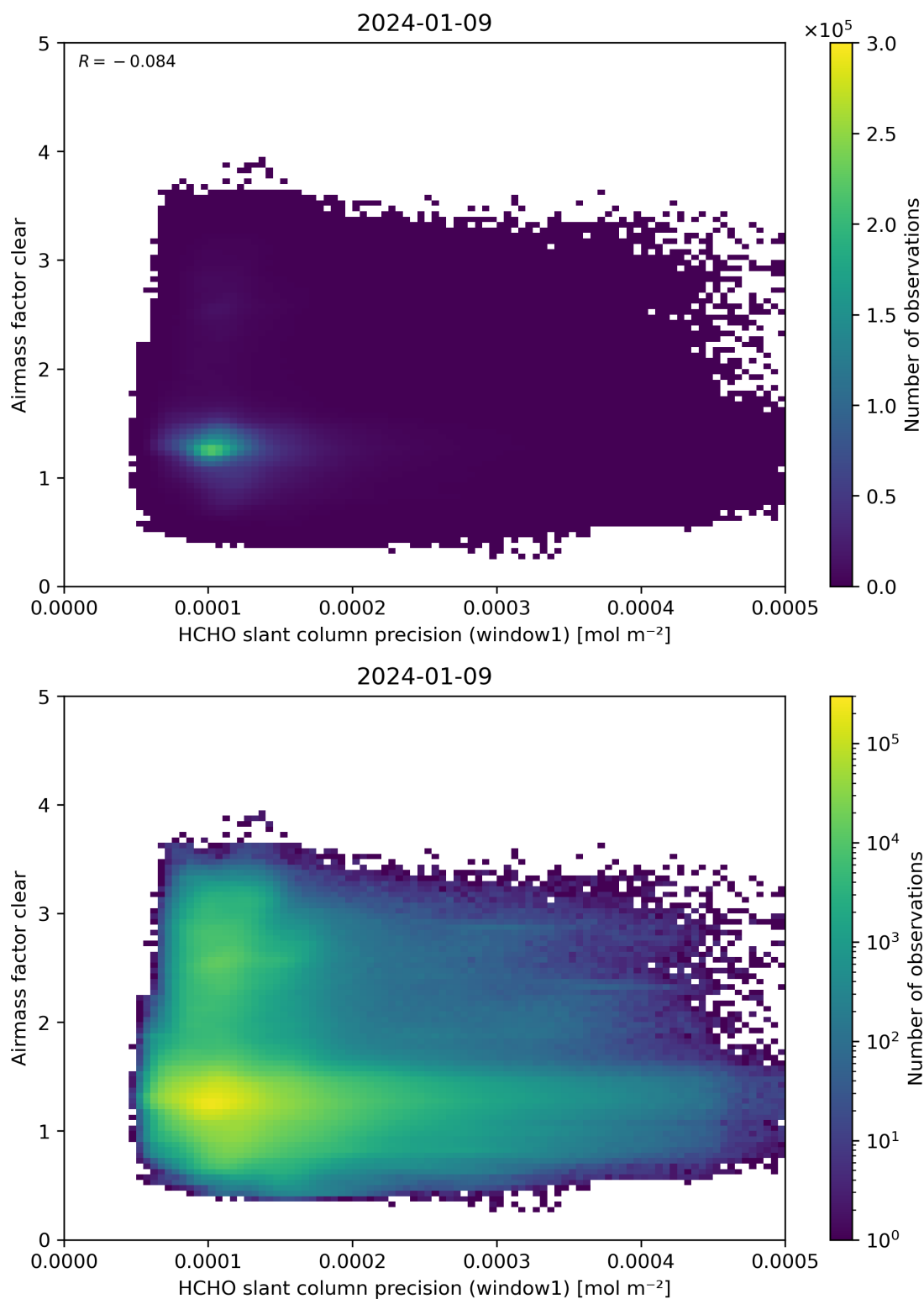
Figure 91: Scatter density plot of “HCHO slant column precision (window1)” against “Airmass factor clear” for 2024-01-08 to 2024-01-10.
