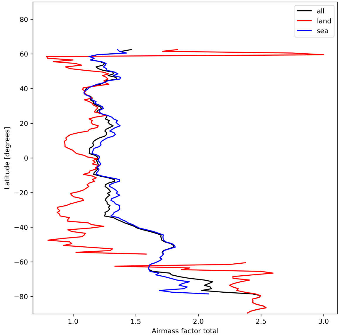
Figure 26: Zonal average of “Airmass factor total” for 2024-01-08 to 2024-01-10.
