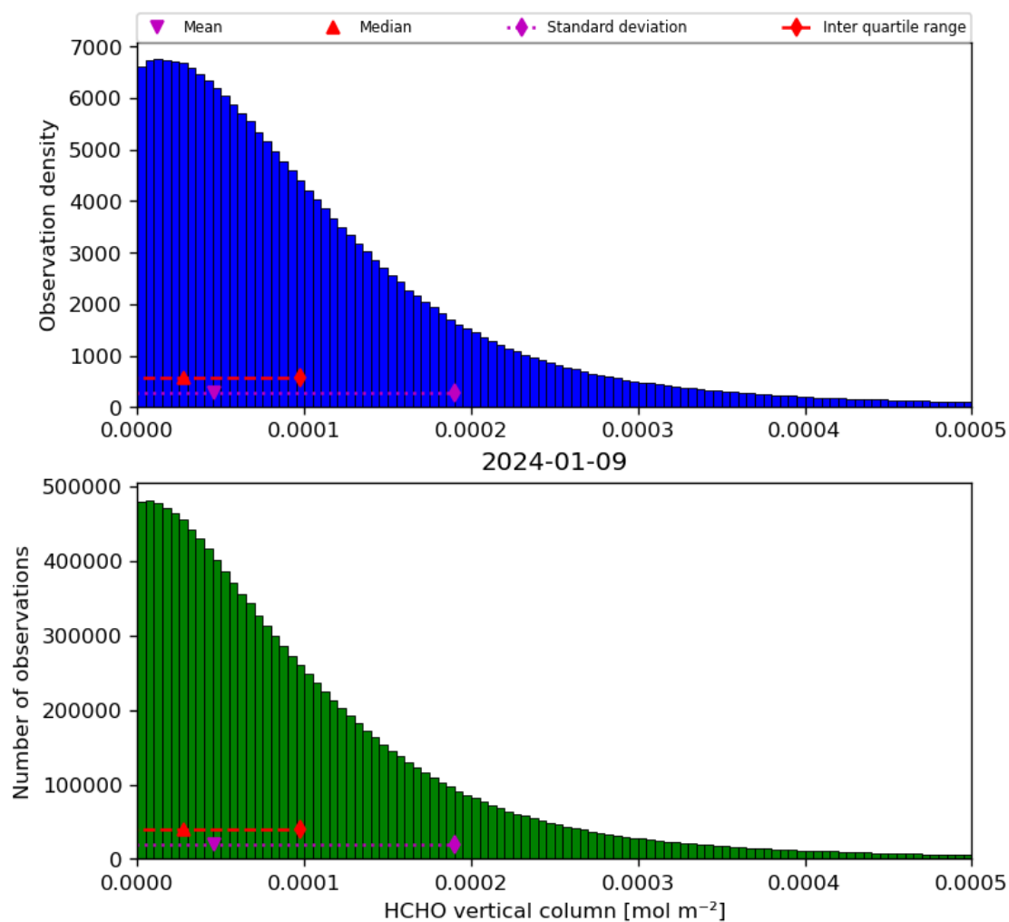
Figure 35: Histogram of “HCHO vertical column” for 2024-01-08 to 2024-01-10
