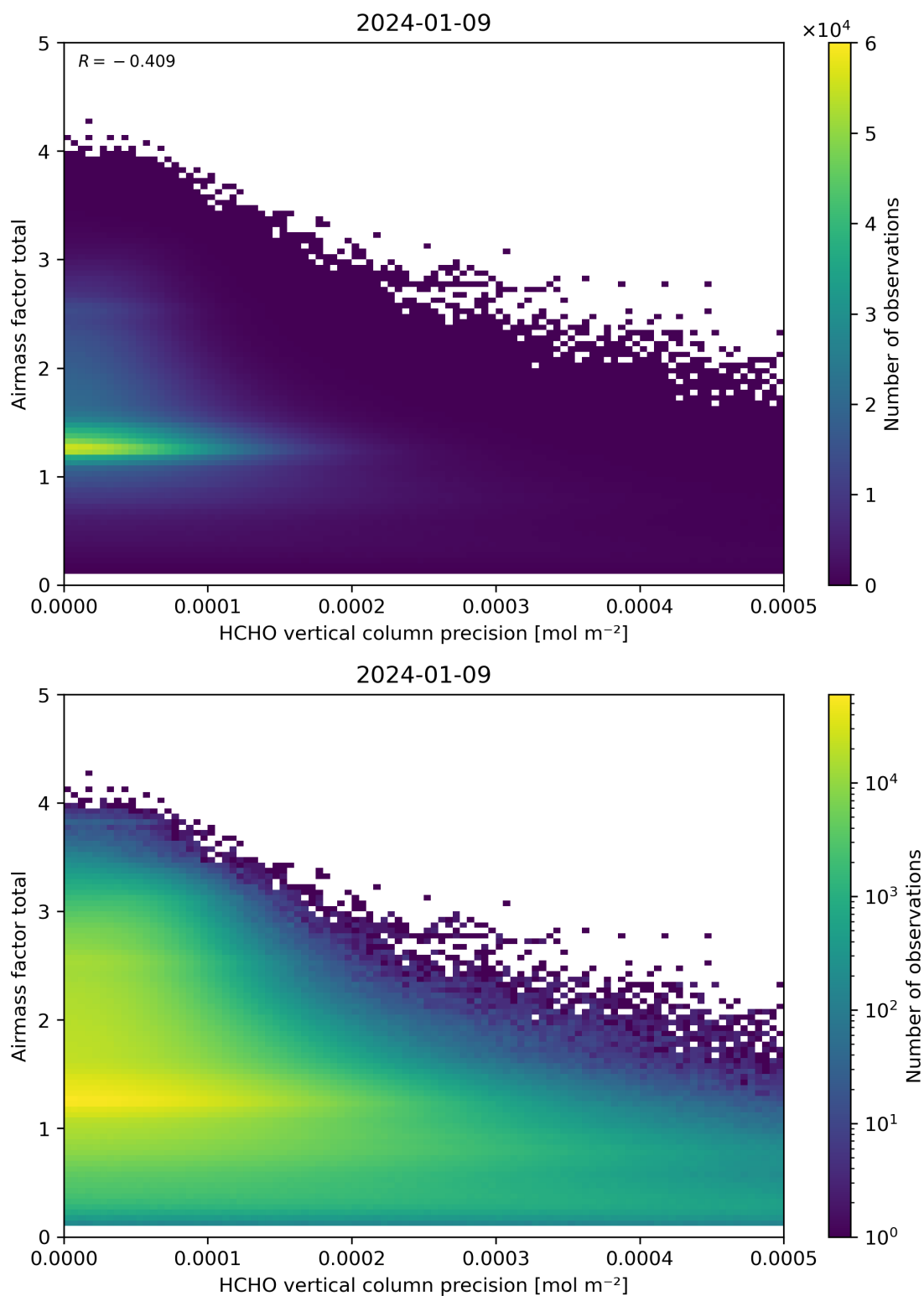
Figure 144: Scatter density plot of “HCHO vertical column precision” against “Airmass factor total” for 2024-01-08 to 2024-01-10.
