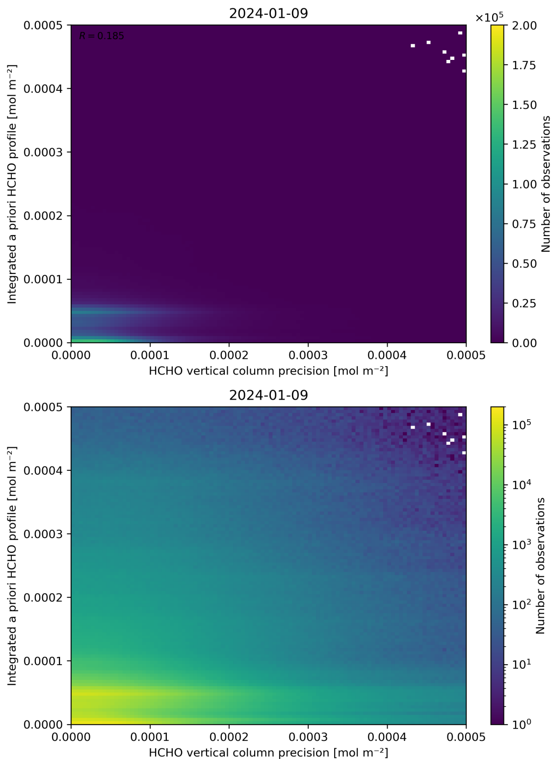
Figure 147: Scatter density plot of “HCHO vertical column precision” against “Integrated a priori HCHO profile” for 2024-01-08 to 2024-01-10.
