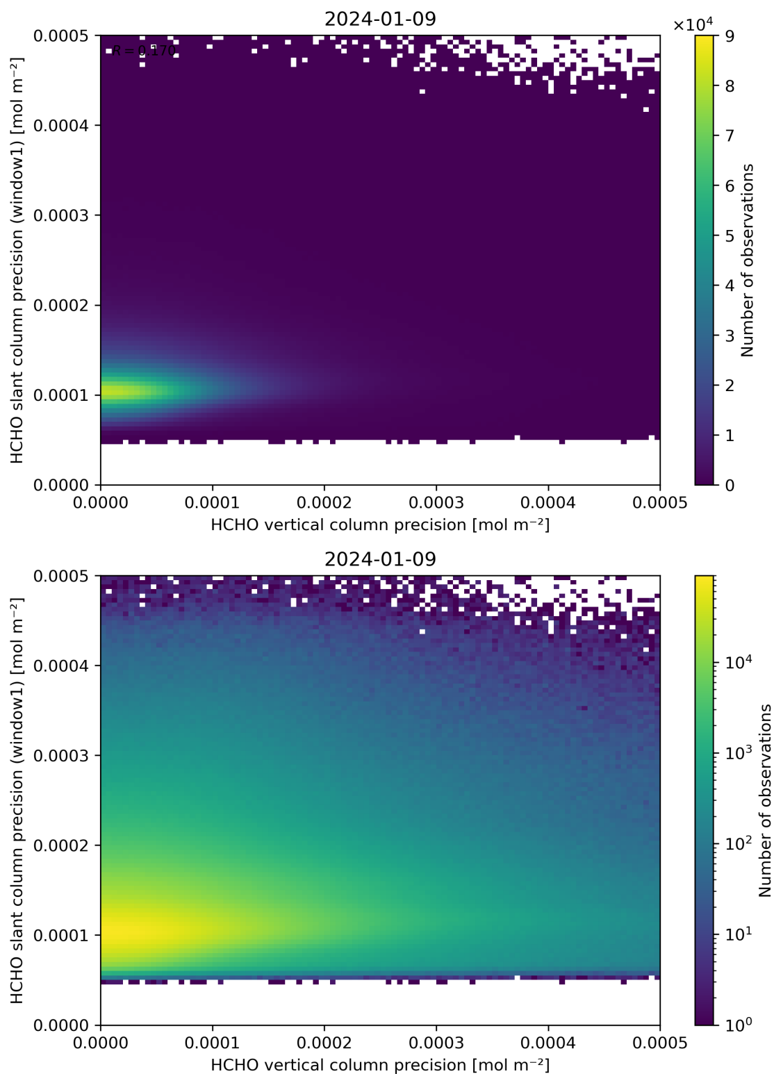
Figure 143: Scatter density plot of “HCHO vertical column precision” against “HCHO slant column precision (window1)” for 2024-01-08 to 2024-01-10.
