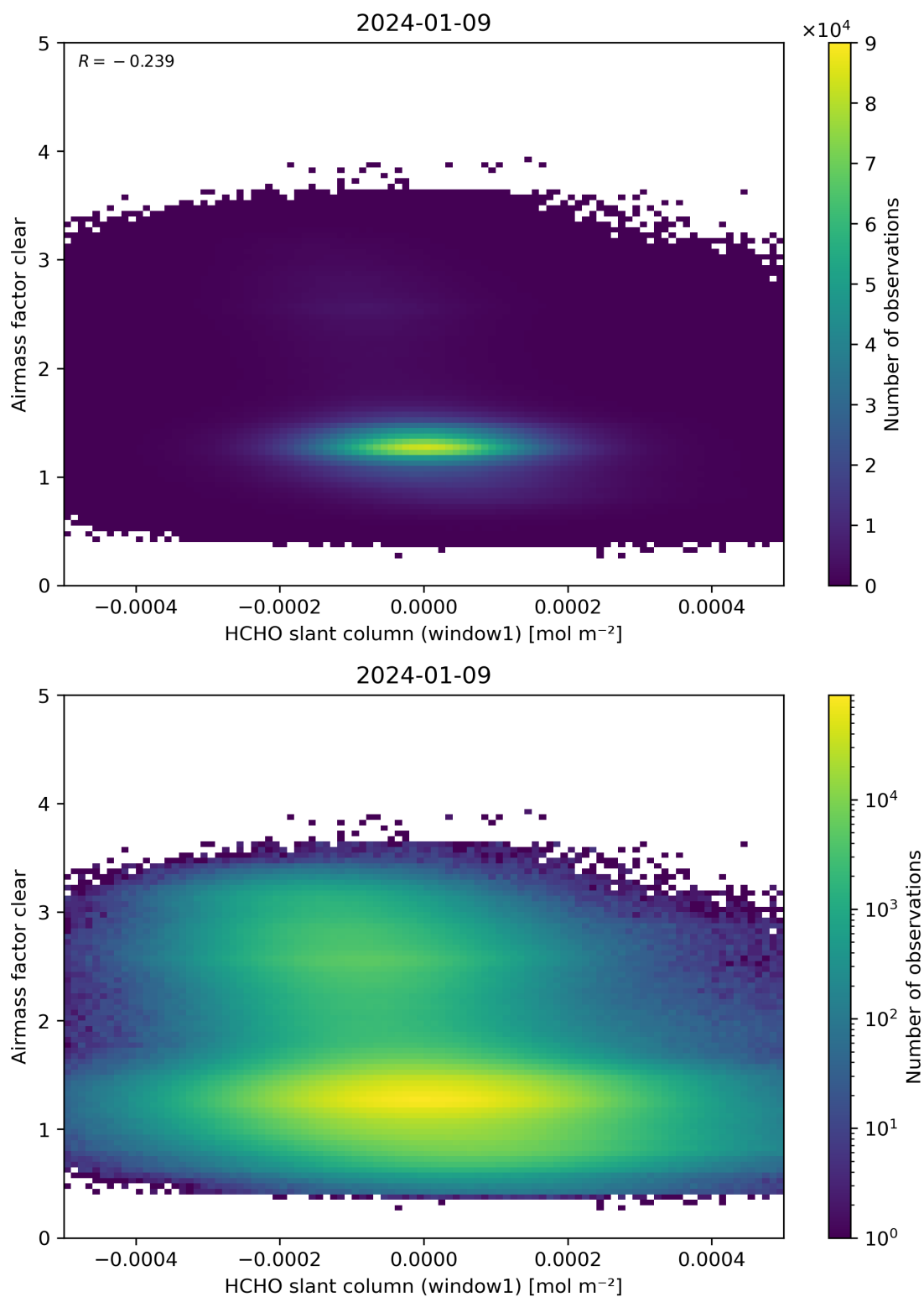
Figure 81: Scatter density plot of “HCHO slant column (window1)” against “Airmass factor clear” for 2024-01-08 to 2024-01-10.
