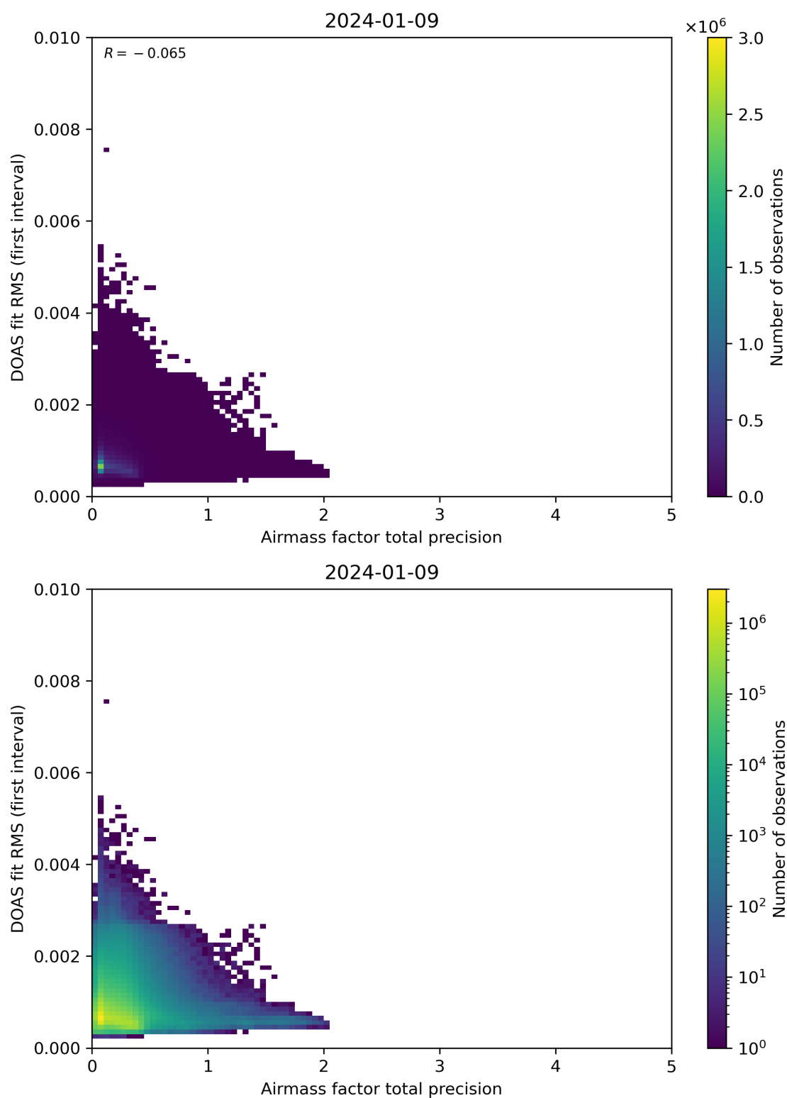
Figure 105: Scatter density plot of “Airmass factor total precision” against “DOAS fit RMS (first interval)” for 2024-01-08 to 2024-01-10.
