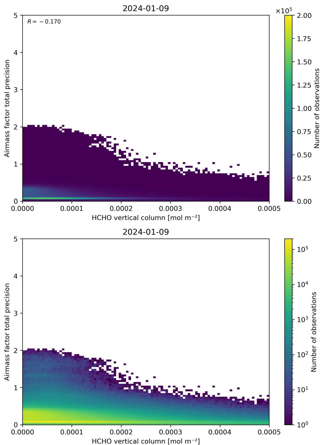
Figure 132: Scatter density plot of “HCHO vertical column” against “Airmass factor total precision” for 2024-01-08 to 2024-01-10.
