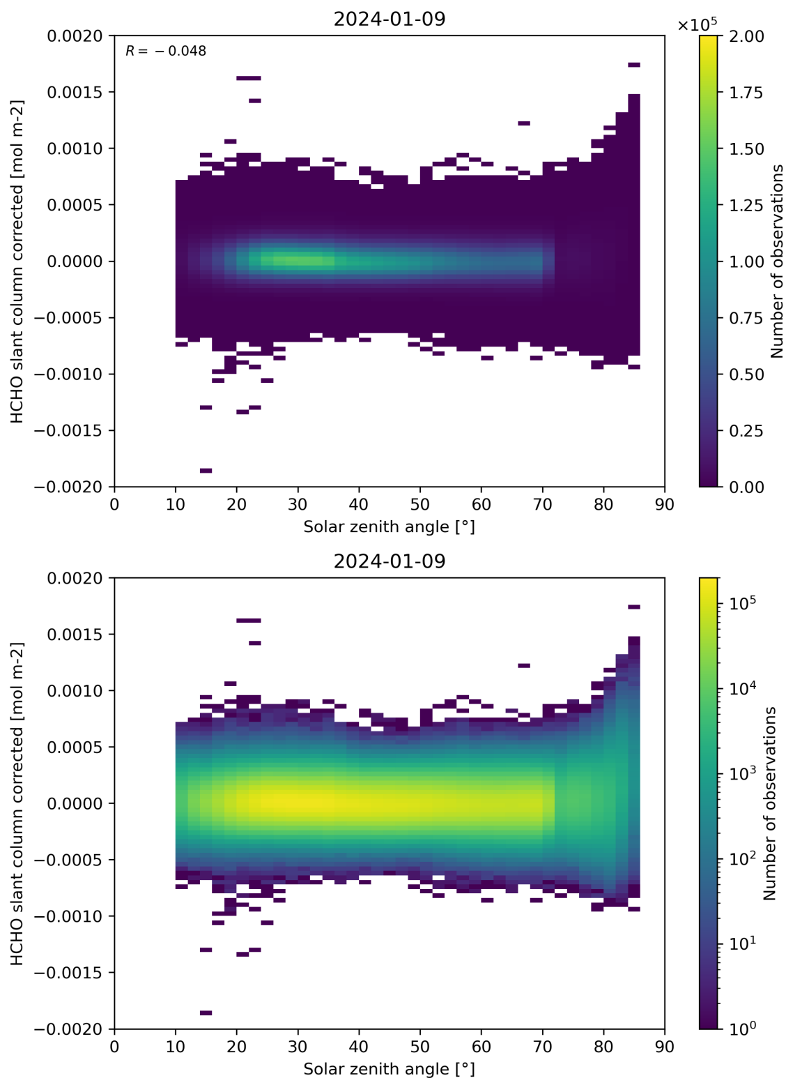
Figure 171: Scatter density plot of “Solar zenith angle” against “HCHO slant column corrected” for 2024-01-08 to 2024-01-10.
