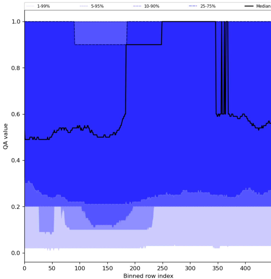
Figure 48: Along track statistics of “QA value” for 2024-01-08 to 2024-01-10
