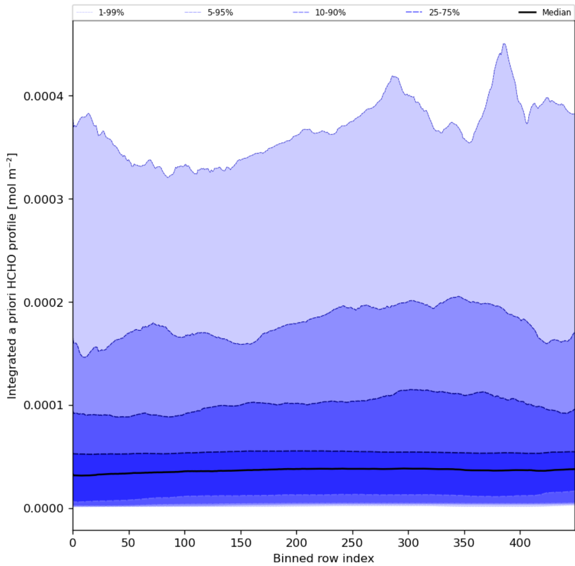
Figure 57: Along track statistics of “Integrated a priori HCHO profile” for 2024-01-08 to 2024-01-10
