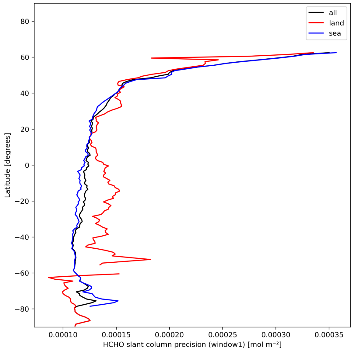
Figure 25: Zonal average of “HCHO slant column precision (window1)” for 2024-01-08 to 2024-01-10.
