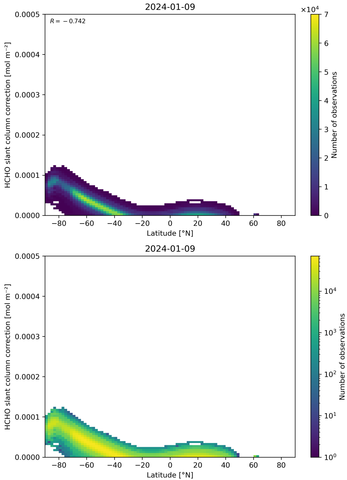
Figure 158: Scatter density plot of “Latitude” against “HCHO slant column correction” for 2024-01-08 to 2024-01-10.
