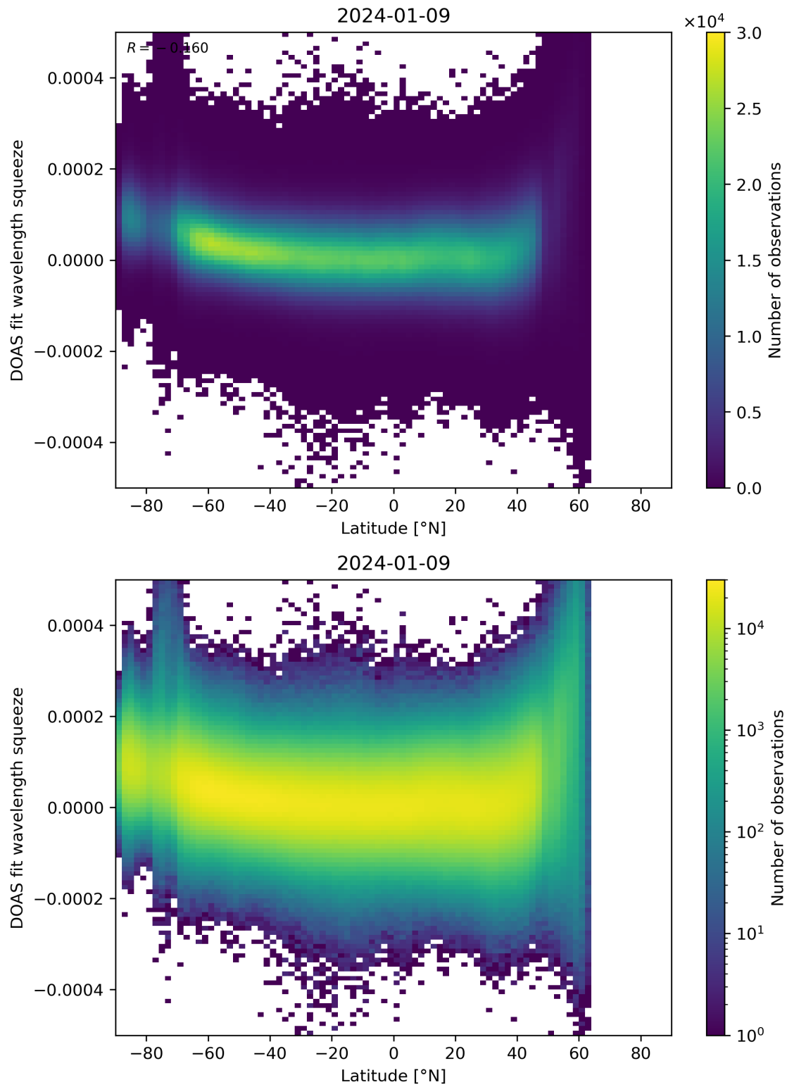
Figure 155: Scatter density plot of “Latitude” against “DOAS fit wavelength squeeze” for 2024-01-08 to 2024-01-10.
