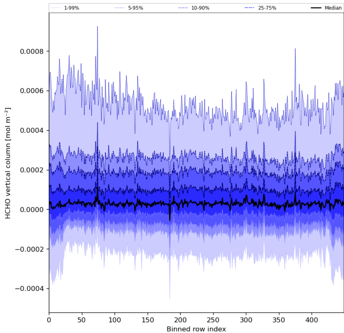
Figure 49: Along track statistics of “HCHO vertical column” for 2024-01-08 to 2024-01-10
