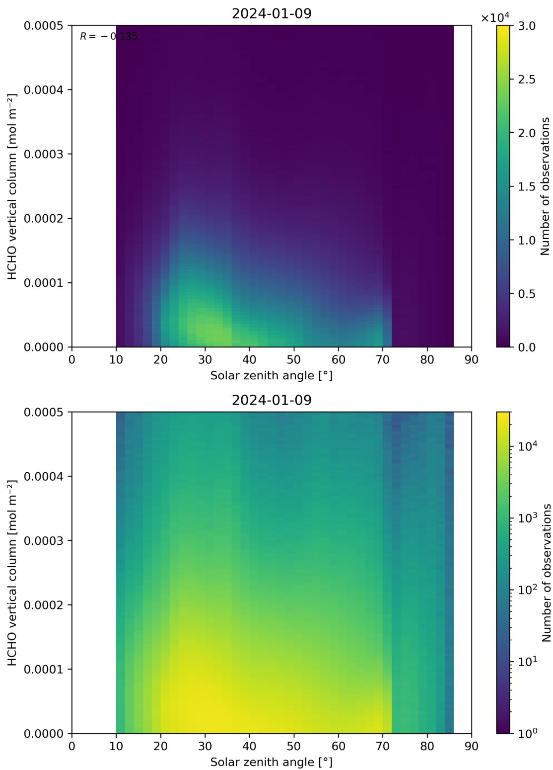
Figure 177: Scatter density plot of “Solar zenith angle” against “HCHO vertical column” for 2024-01-08 to 2024-01-10.
