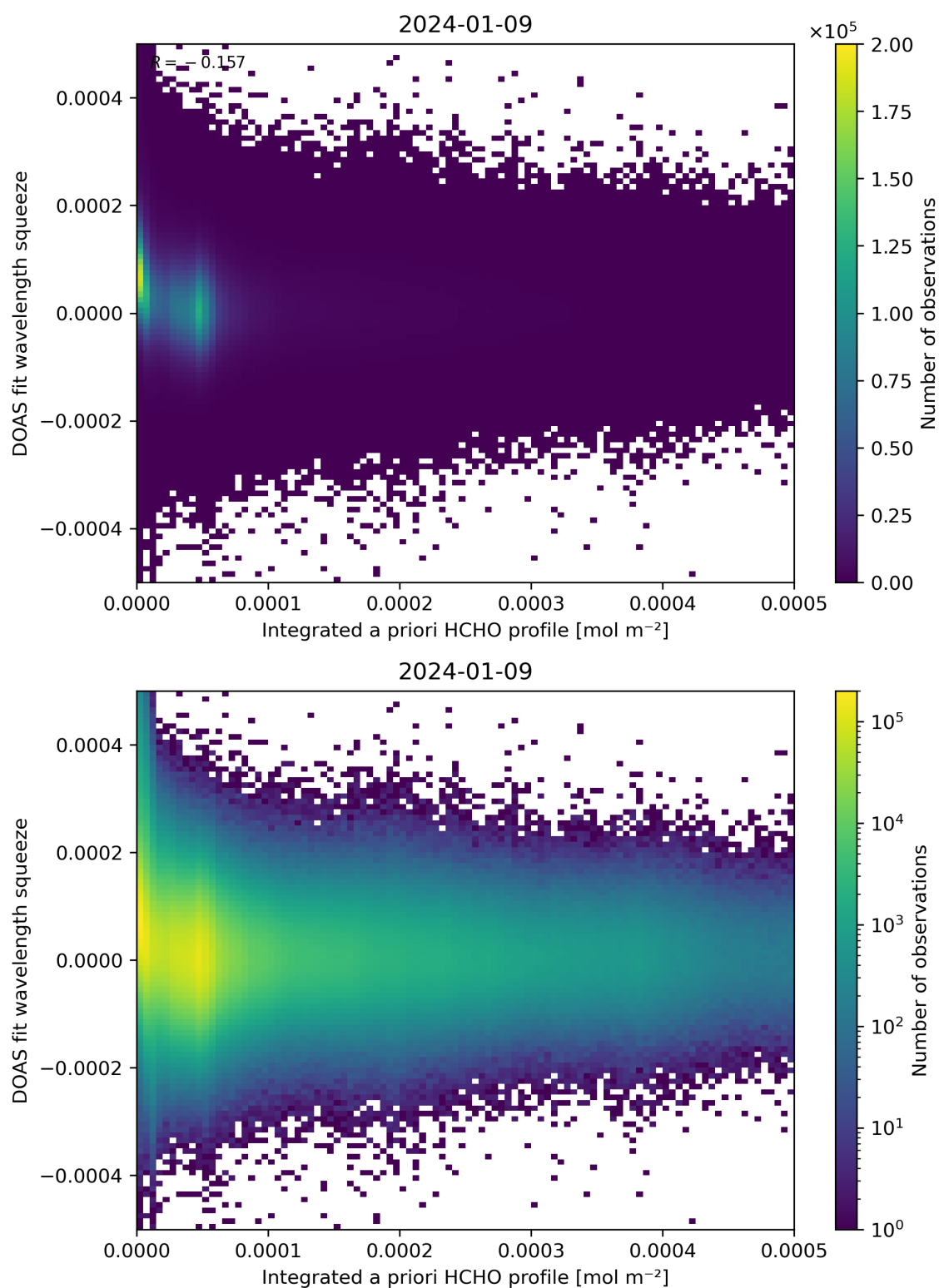
Figure 150: Scatter density plot of “Integrated a priori HCHO profile” against “DOAS fit wavelength squeeze” for 2024-01-08 to 2024-01-10.
