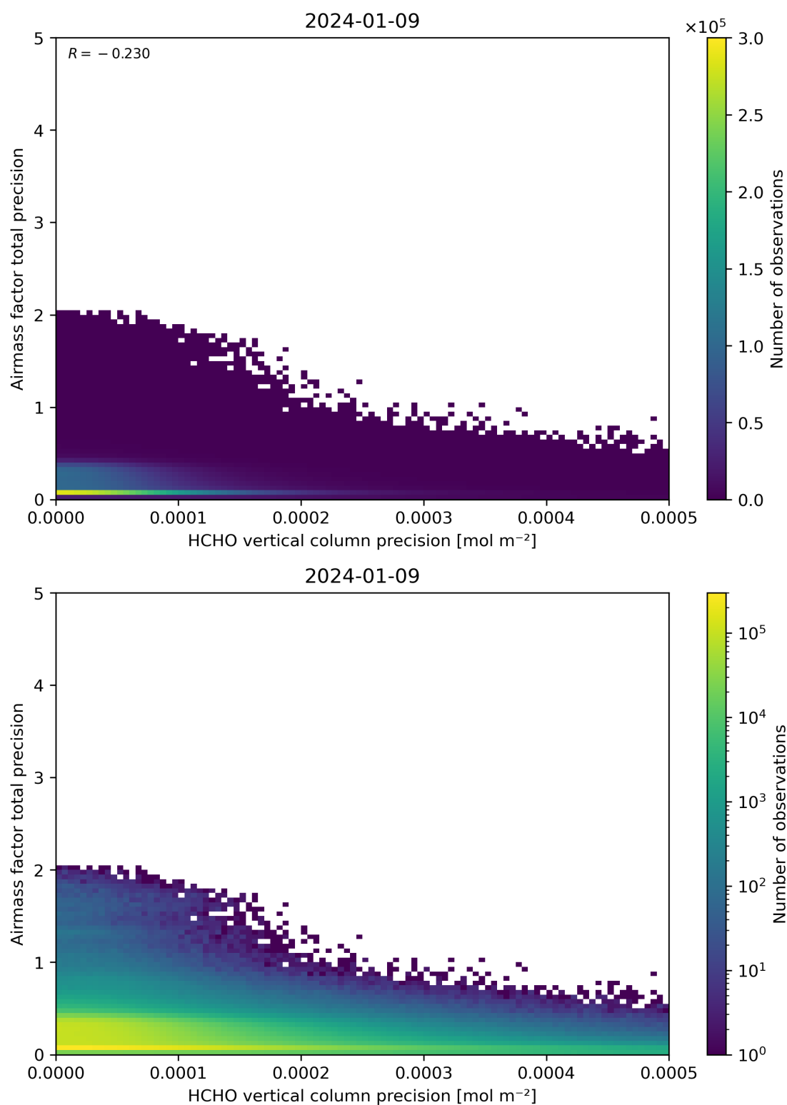
Figure 145: Scatter density plot of “HCHO vertical column precision” against “Airmass factor total precision” for 2024-01-08 to 2024-01-10.
