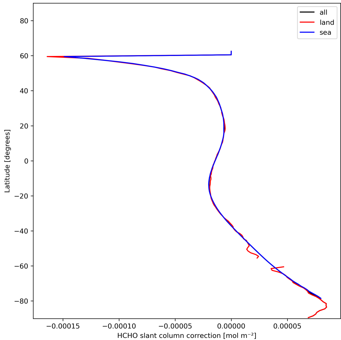
Figure 33: Zonal average of “HCHO slant column correction” for 2024-01-08 to 2024-01-10.
