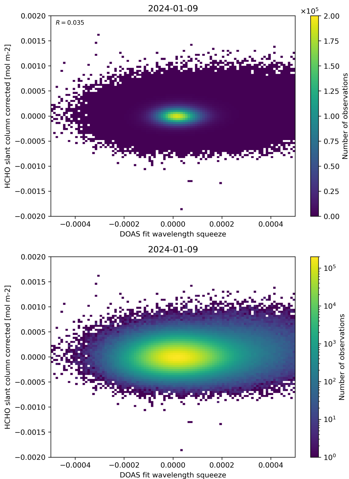
Figure 69: Scatter density plot of “DOAS fit wavelength squeeze” against “HCHO slant column corrected” for 2024-01-08 to 2024-01-10.
