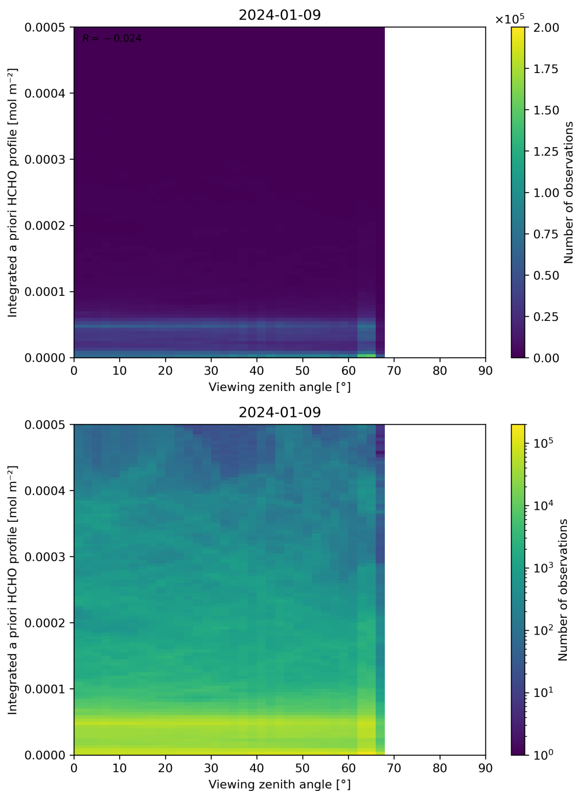
Figure 195: Scatter density plot of “Viewing zenith angle” against “Integrated a priori HCHO profile” for 2024-01-08 to 2024-01-10.
