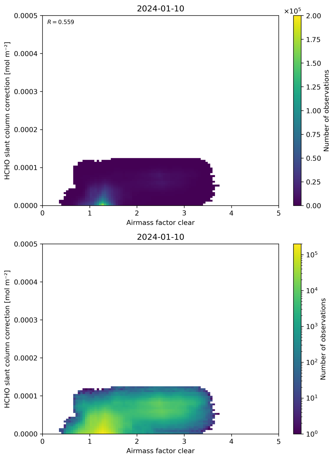
Figure 75: Scatter density plot of “Airmass factor clear” against “HCHO slant column correction” for 2024-01-10 to 2024-01-11.
