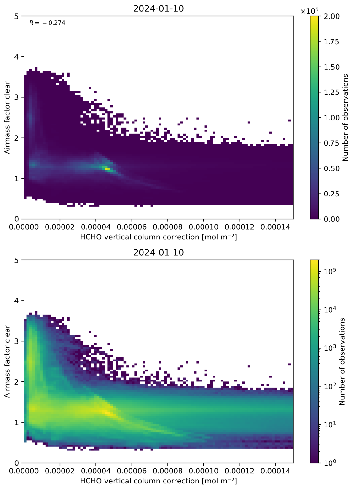
Figure 115: Scatter density plot of “HCHO vertical column correction” against “Airmass factor clear” for 2024-01-10 to 2024-01-11.
