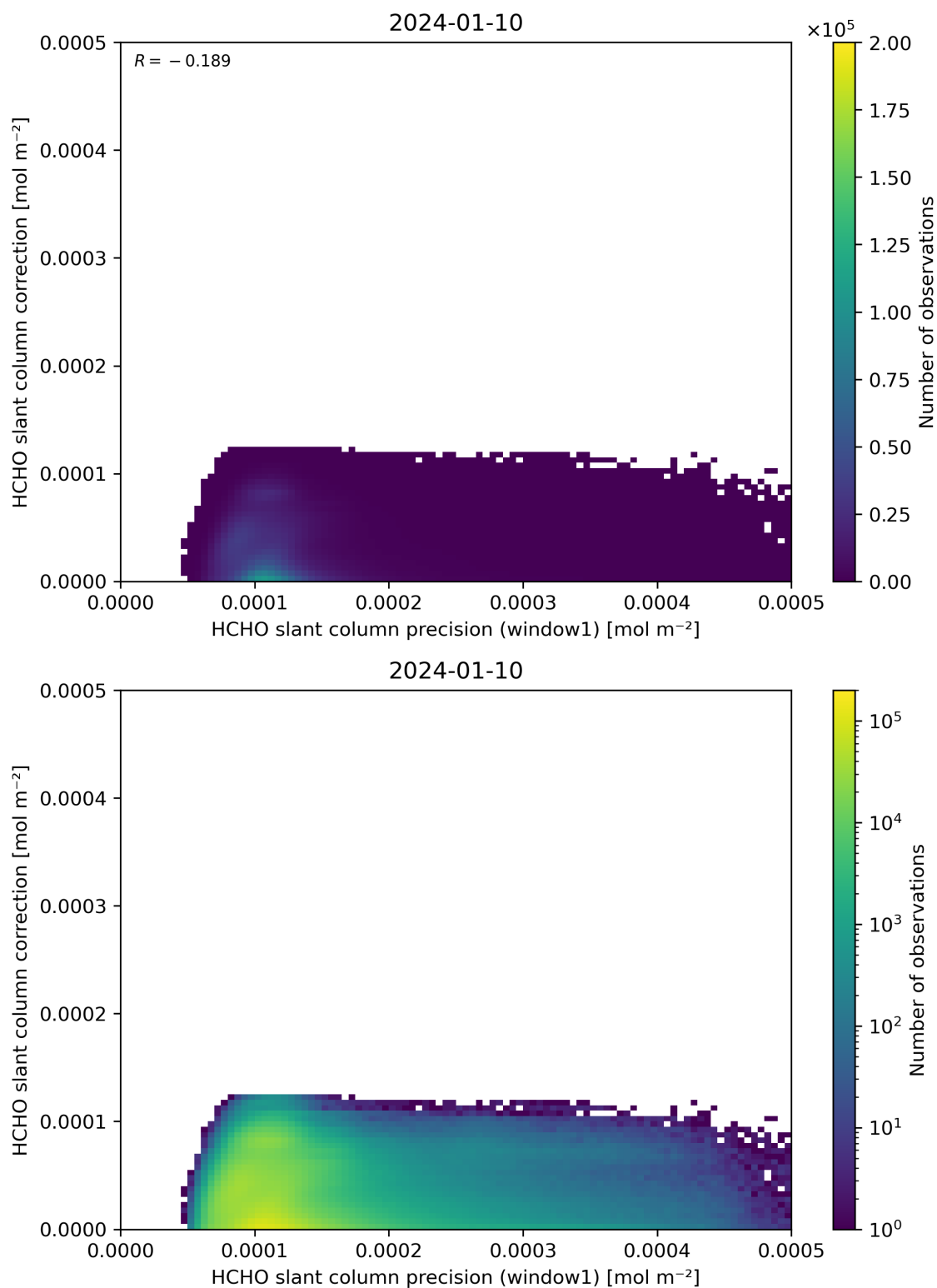
Figure 93: Scatter density plot of “HCHO slant column precision (window1)” against “HCHO slant column correction” for 2024-01-10 to 2024-01-11.
