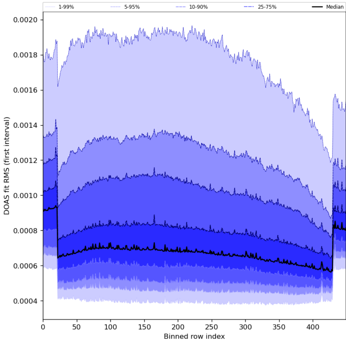
Figure 60: Along track statistics of “DOAS fit RMS (first interval)” for 2024-01-10 to 2024-01-11
