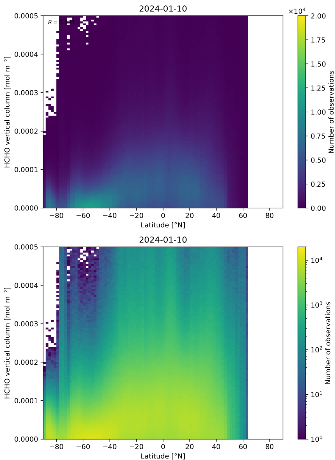
Figure 163: Scatter density plot of “Latitude” against “HCHO vertical column” for 2024-01-10 to 2024-01-11.
