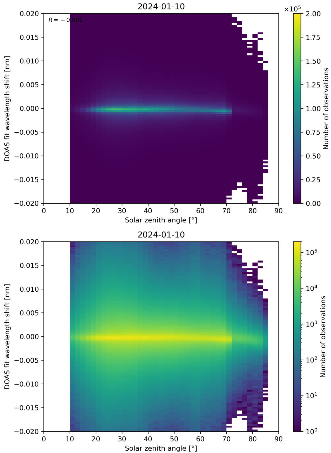
Figure 168: Scatter density plot of “Solar zenith angle” against “DOAS fit wavelength shift” for 2024-01-10 to 2024-01-11.
