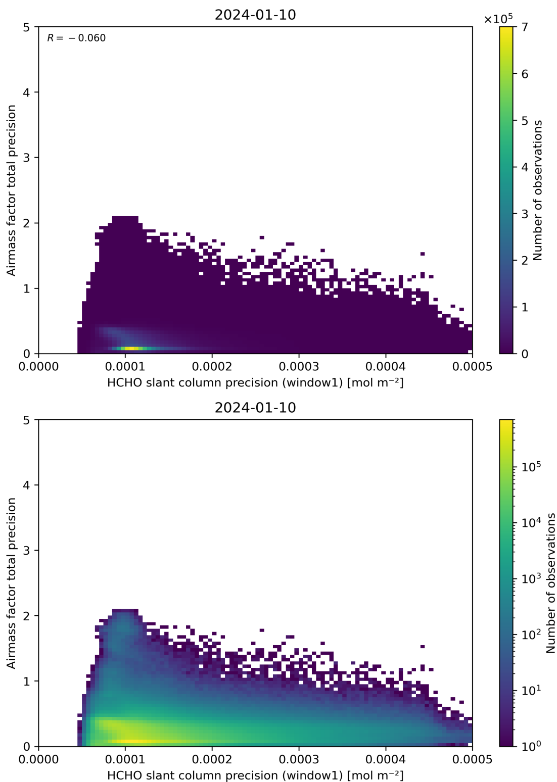
Figure 95: Scatter density plot of “HCHO slant column precision (window1)” against “Airmass factor total precision” for 2024-01-10 to 2024-01-11.
