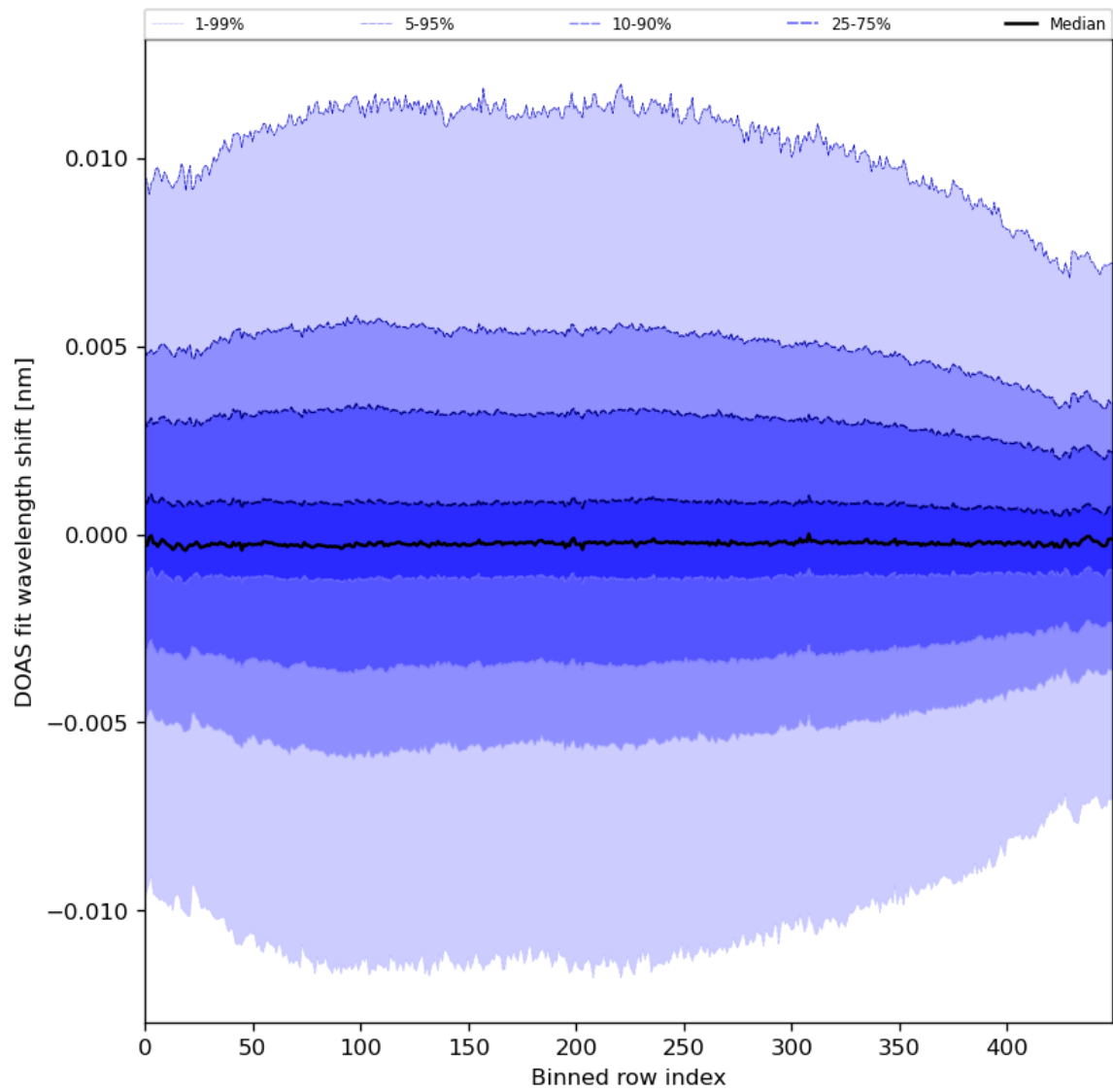
Figure 58: Along track statistics of “DOAS fit wavelength shift” for 2024-01-10 to 2024-01-11
