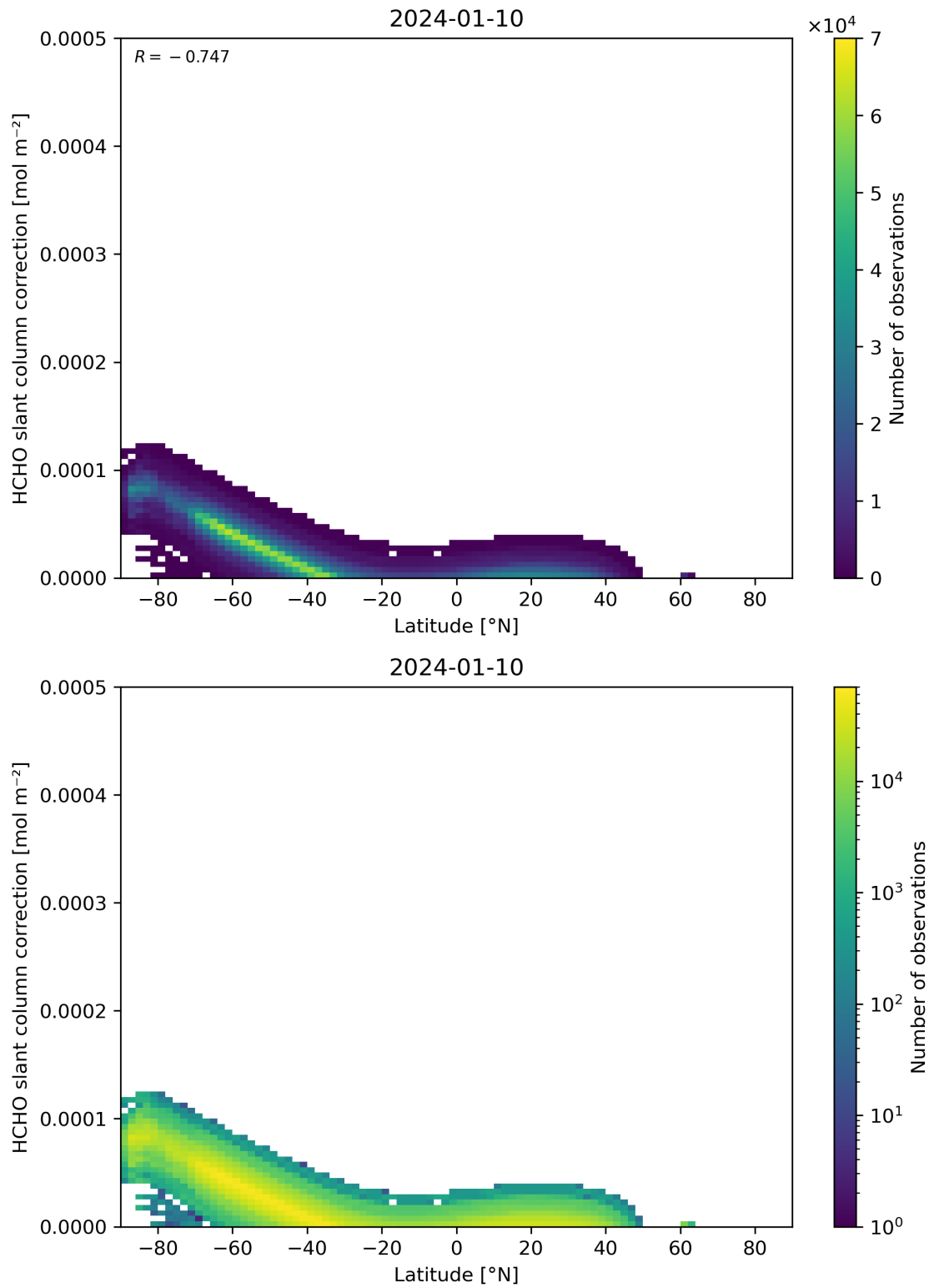
Figure 158: Scatter density plot of “Latitude” against “HCHO slant column correction” for 2024-01-10 to 2024-01-11.
