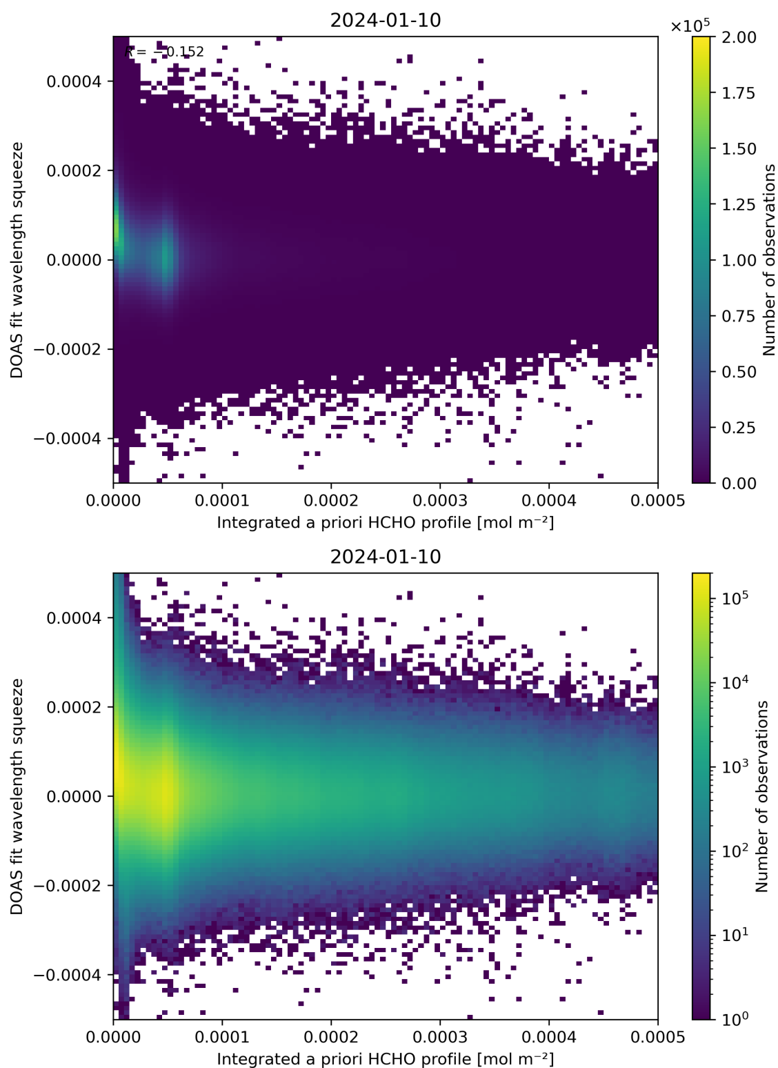
Figure 150: Scatter density plot of “Integrated a priori HCHO profile” against “DOAS fit wavelength squeeze” for 2024-01-10 to 2024-01-11.
