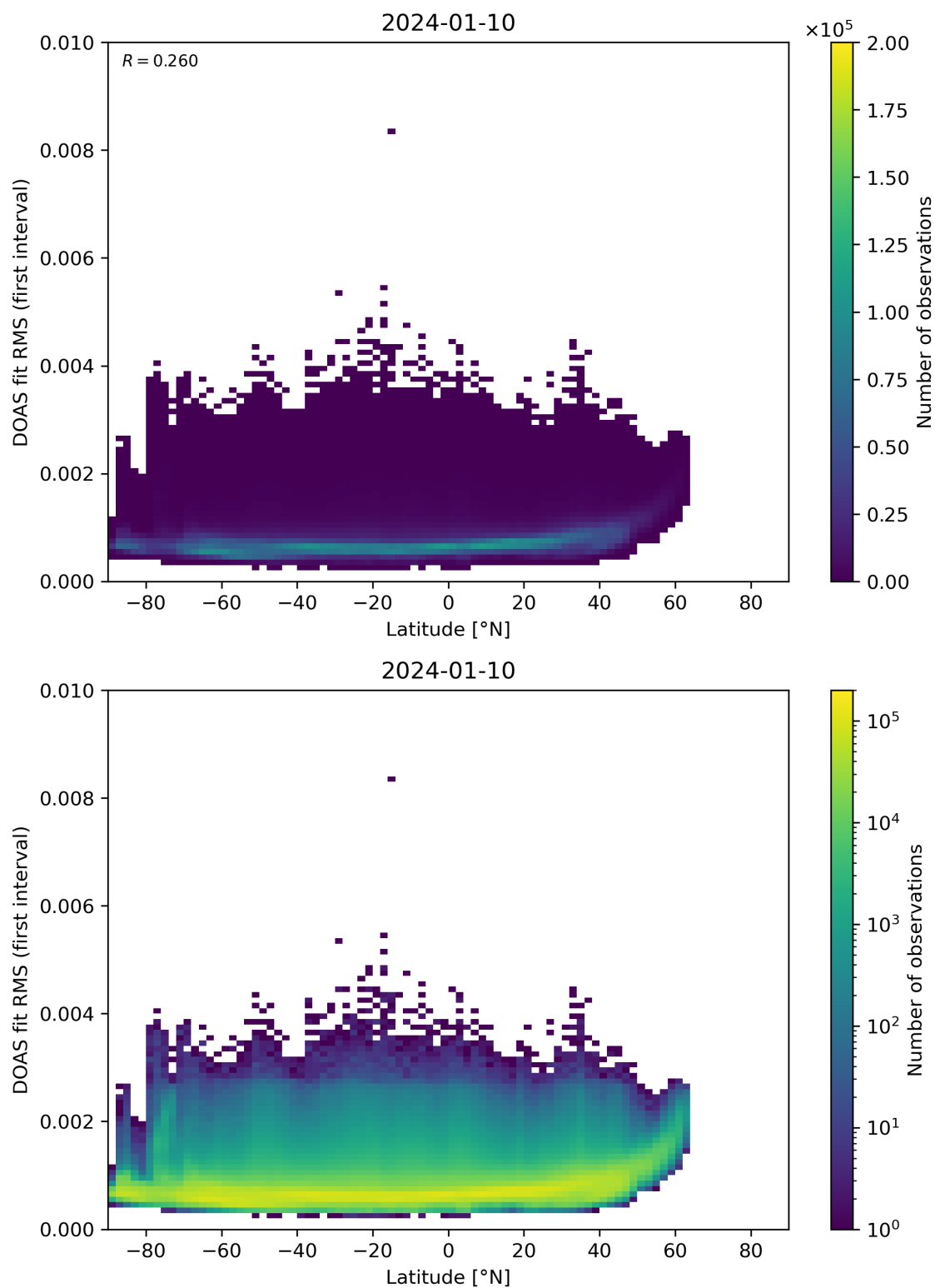
Figure 153: Scatter density plot of “Latitude” against “DOAS fit RMS (first interval)” for 2024-01-10 to 2024-01-11.
