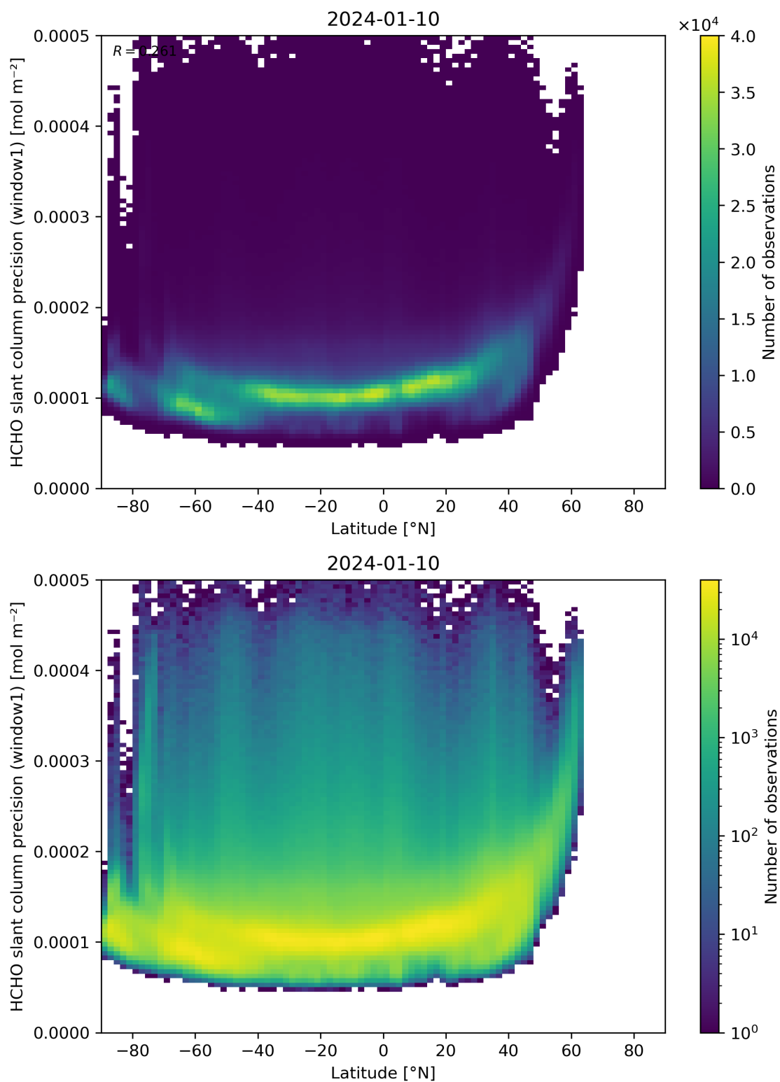
Figure 160: Scatter density plot of “Latitude” against “HCHO slant column precision (window1)” for 2024-01-10 to 2024-01-11.
