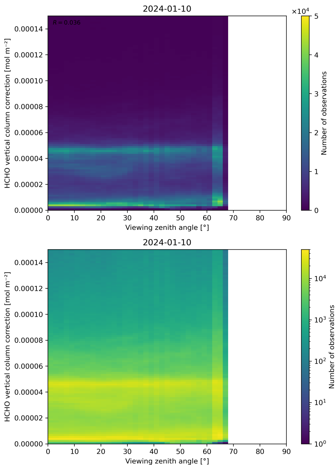
Figure 193: Scatter density plot of “Viewing zenith angle” against “HCHO vertical column correction” for 2024-01-10 to 2024-01-11.
