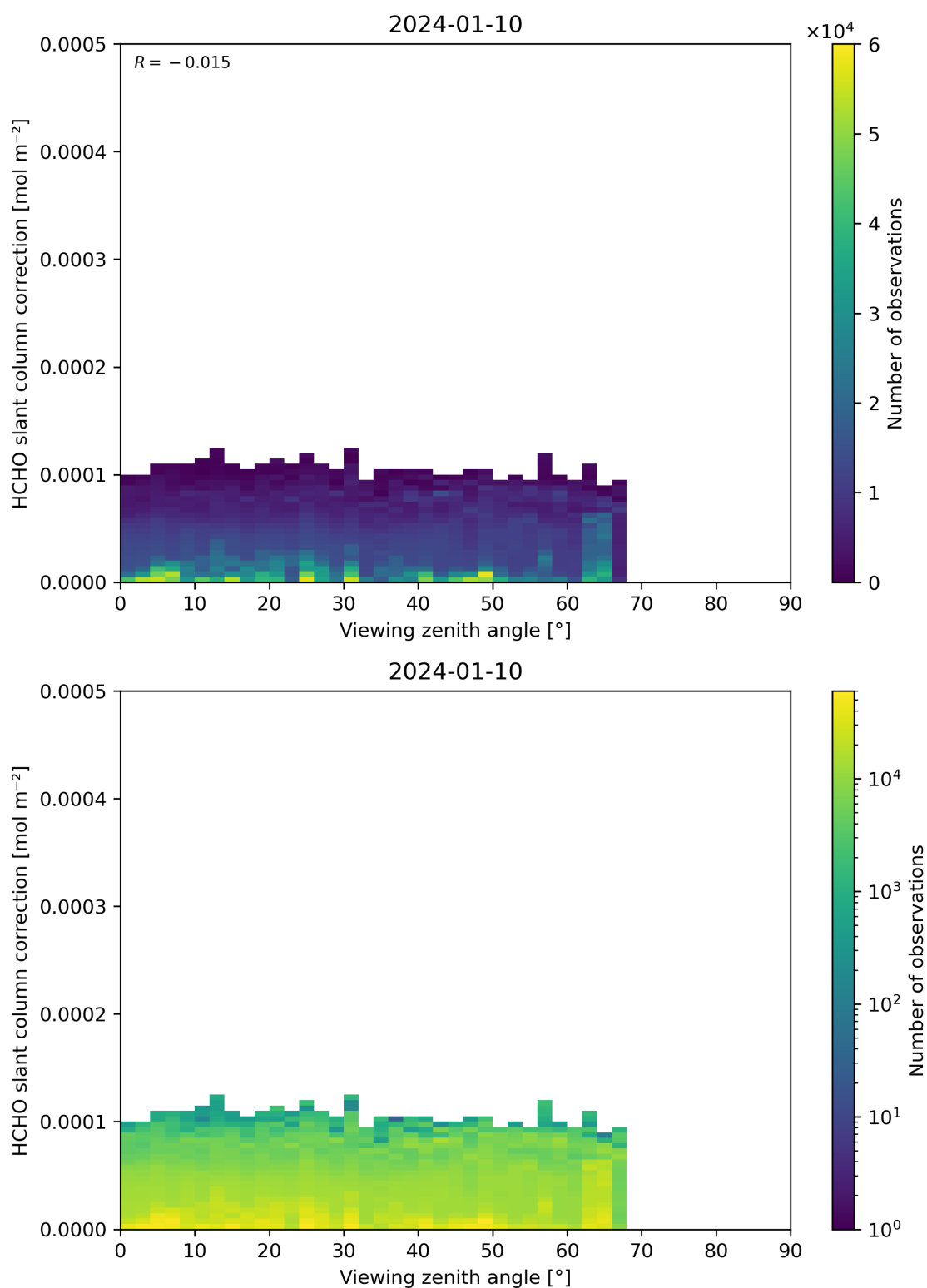
Figure 187: Scatter density plot of “Viewing zenith angle” against “HCHO slant column correction” for 2024-01-10 to 2024-01-11.
