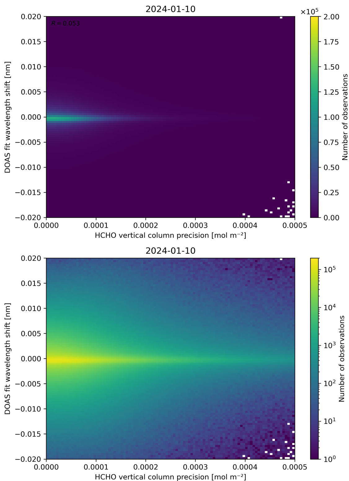
Figure 137: Scatter density plot of “HCHO vertical column precision” against “DOAS fit wavelength shift” for 2024-01-10 to 2024-01-11.
