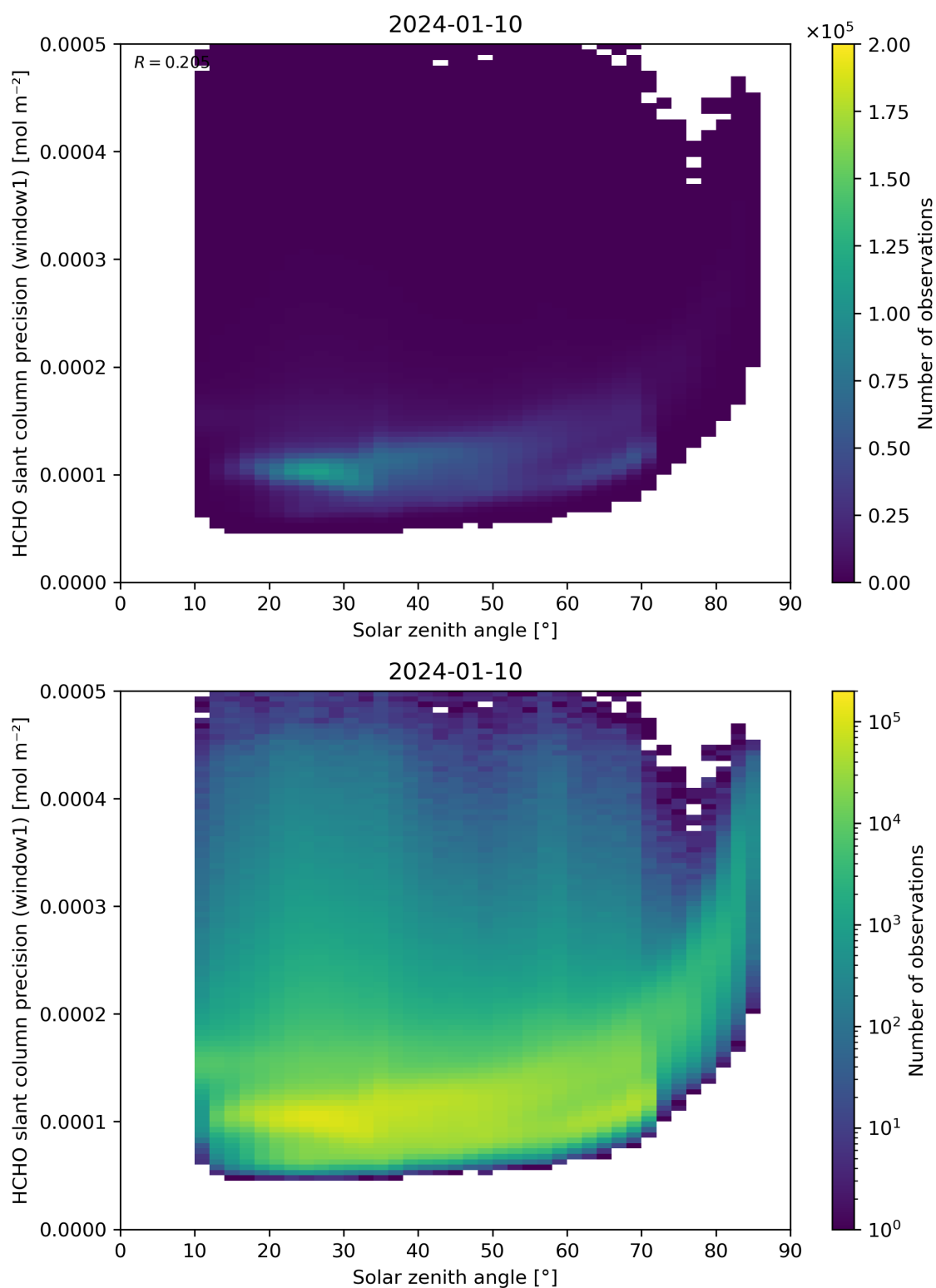
Figure 174: Scatter density plot of “Solar zenith angle” against “HCHO slant column precision (window1)” for 2024-01-10 to 2024-01-11.
