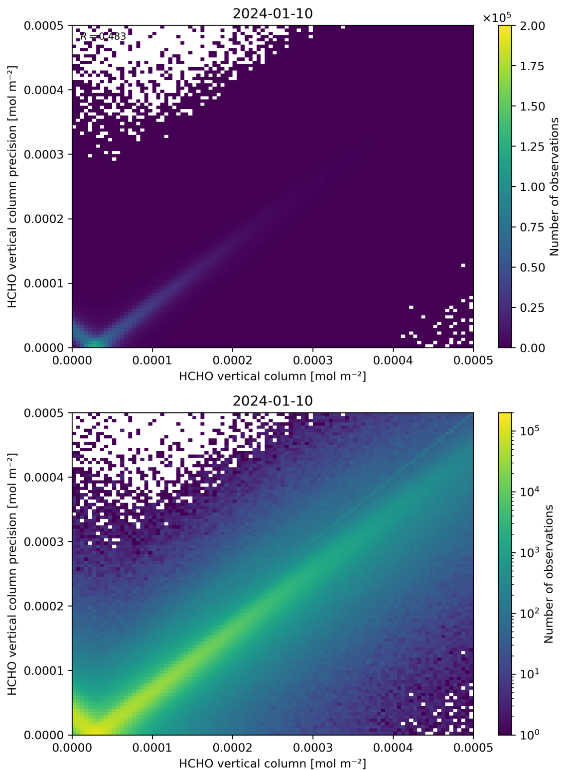
Figure 134: Scatter density plot of “HCHO vertical column” against “HCHO vertical column precision” for 2024-01-10 to 2024-01-11.
