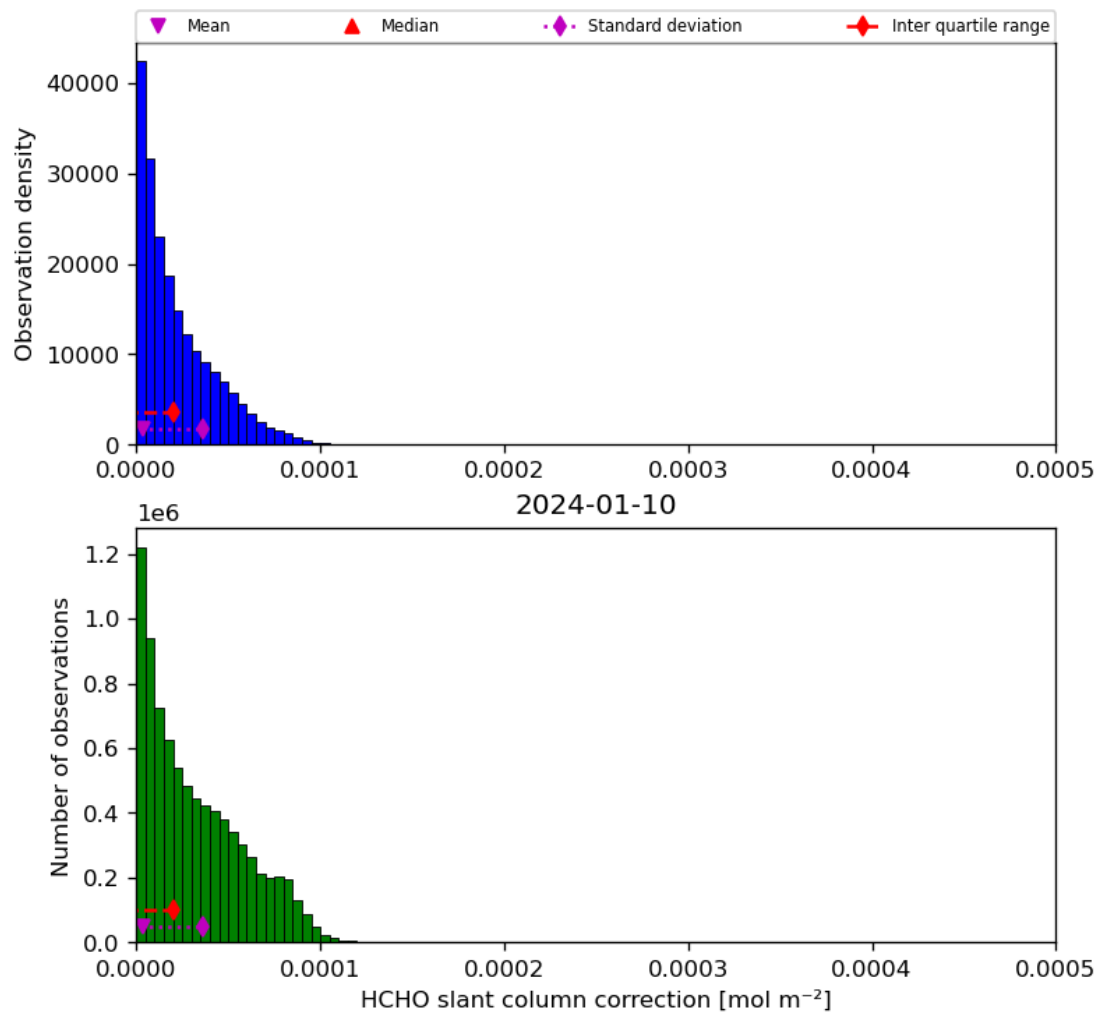
Figure 47: Histogram of “HCHO slant column correction” for 2024-01-10 to 2024-01-11
