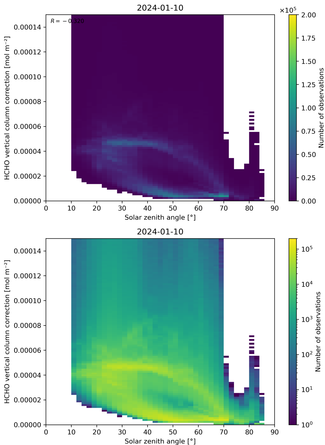
Figure 178: Scatter density plot of “Solar zenith angle” against “HCHO vertical column correction” for 2024-01-10 to 2024-01-11.
