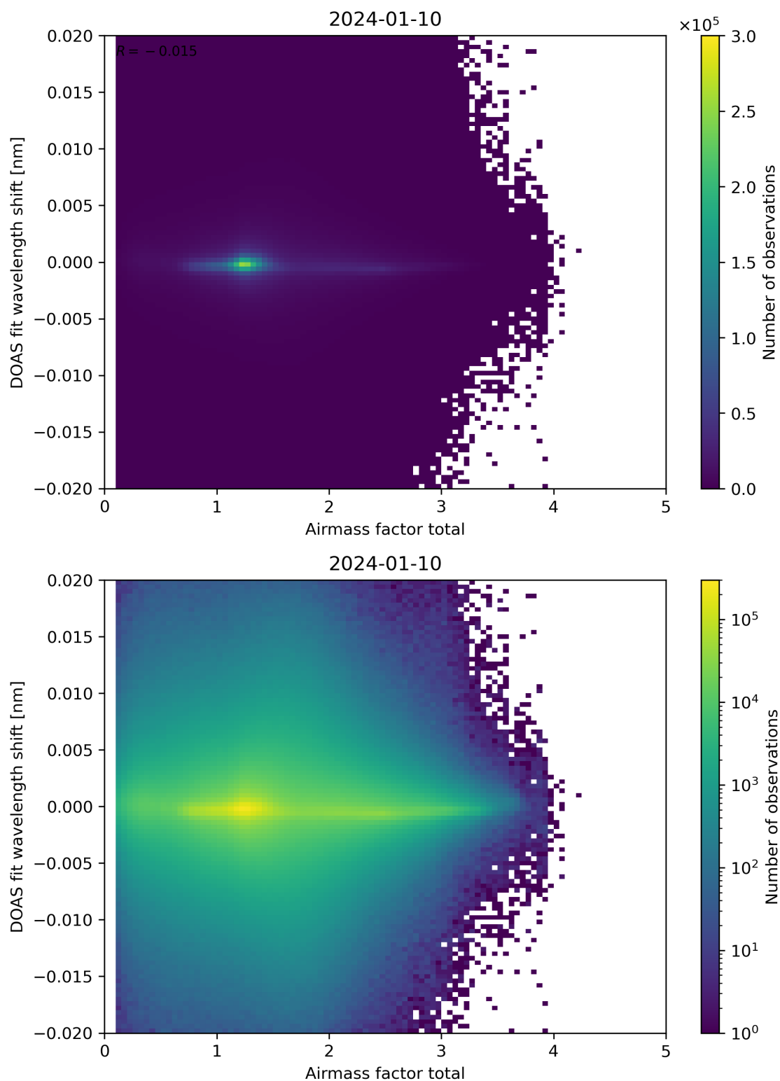
Figure 98: Scatter density plot of “Airmass factor total” against “DOAS fit wavelength shift” for 2024-01-10 to 2024-01-11.
