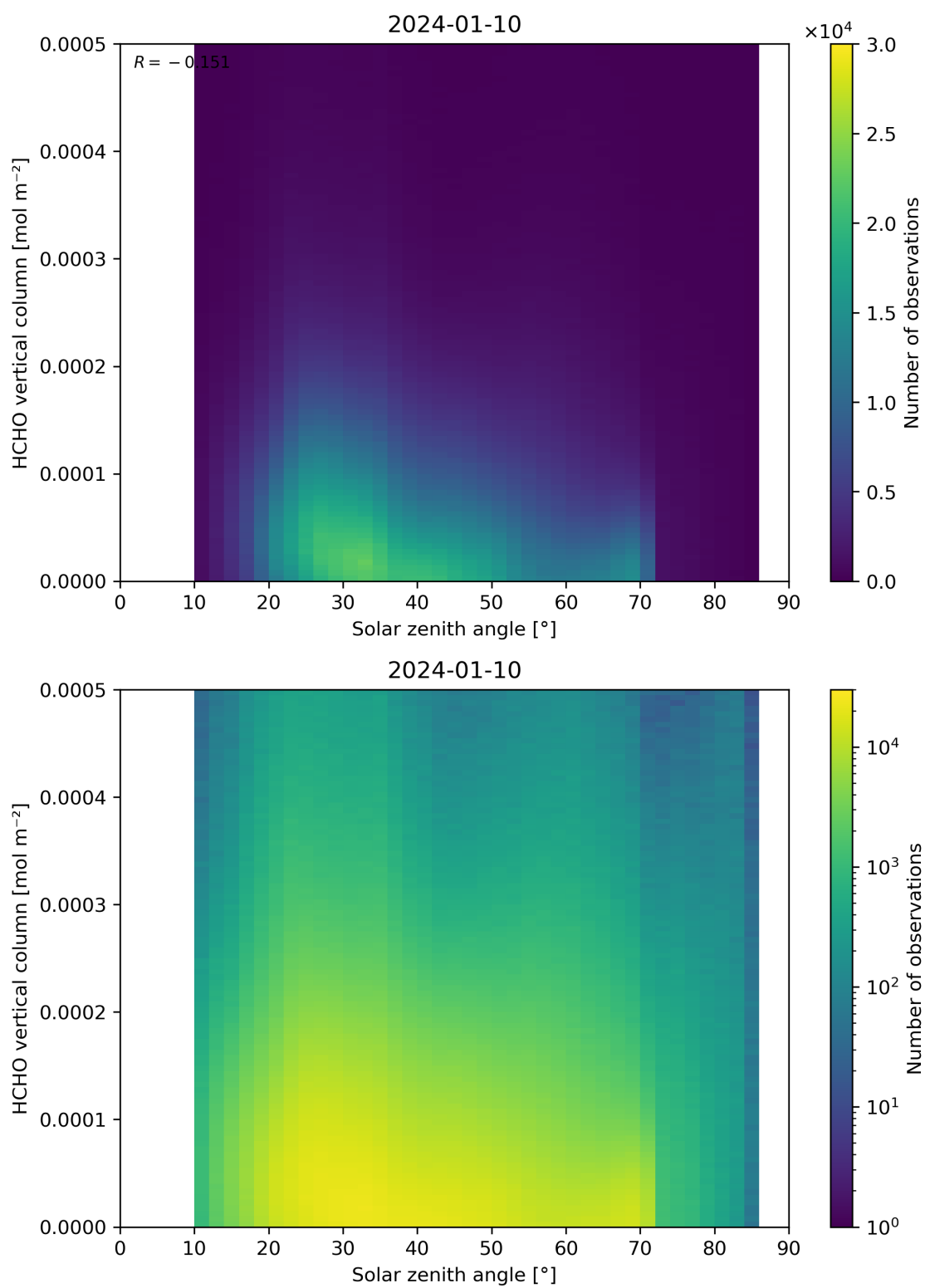
Figure 177: Scatter density plot of “Solar zenith angle” against “HCHO vertical column” for 2024-01-10 to 2024-01-11.
