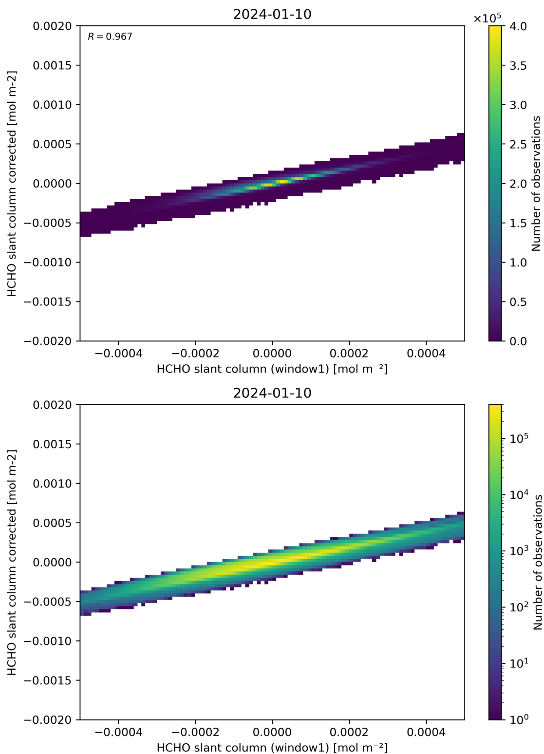
Figure 82: Scatter density plot of “HCHO slant column (window1)” against “HCHO slant column corrected” for 2024-01-10 to 2024-01-11.
