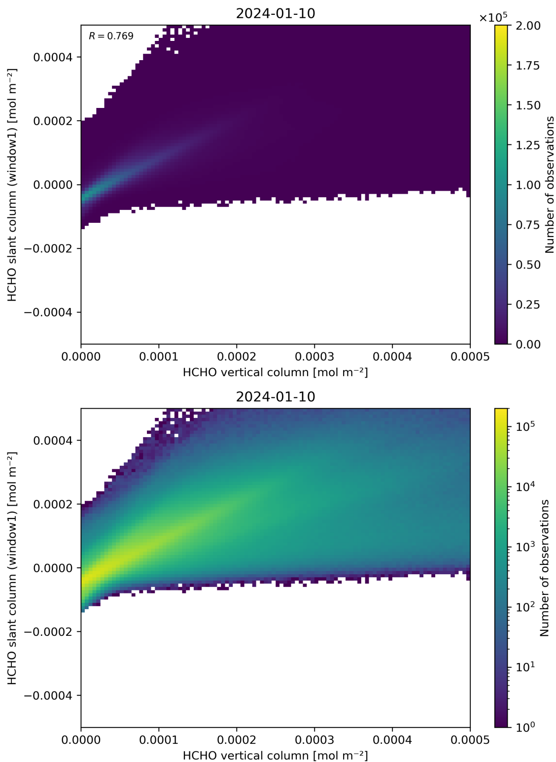
Figure 129: Scatter density plot of “HCHO vertical column” against “HCHO slant column (window1)” for 2024-01-10 to 2024-01-11.
