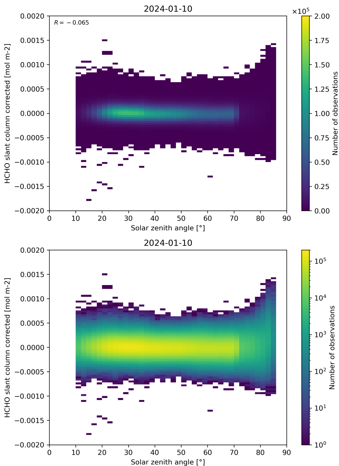
Figure 171: Scatter density plot of “Solar zenith angle” against “HCHO slant column corrected” for 2024-01-10 to 2024-01-11.
