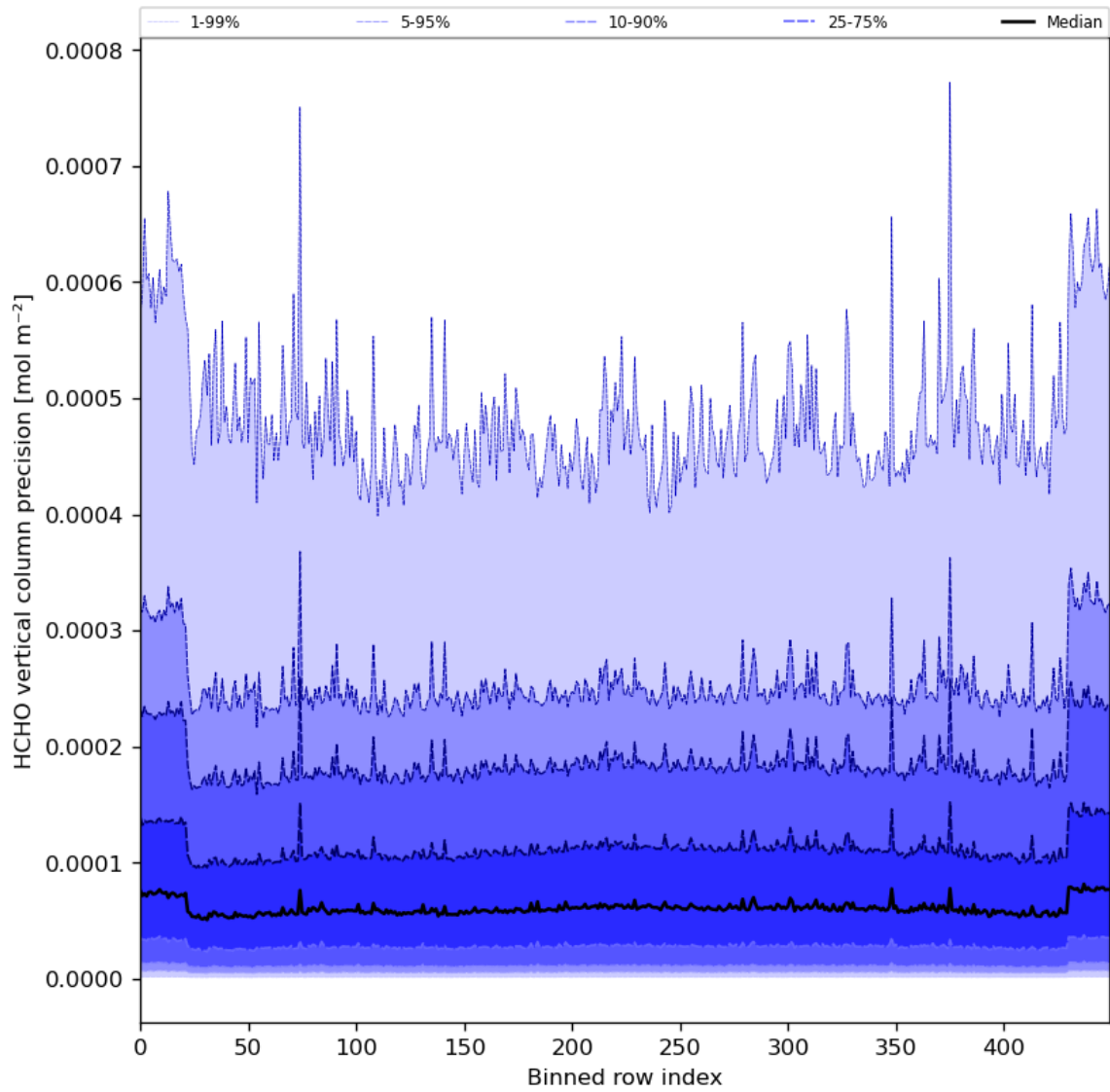
Figure 50: Along track statistics of "HCHO vertical column precision" for 2024-01-10 to 2024-01-11
