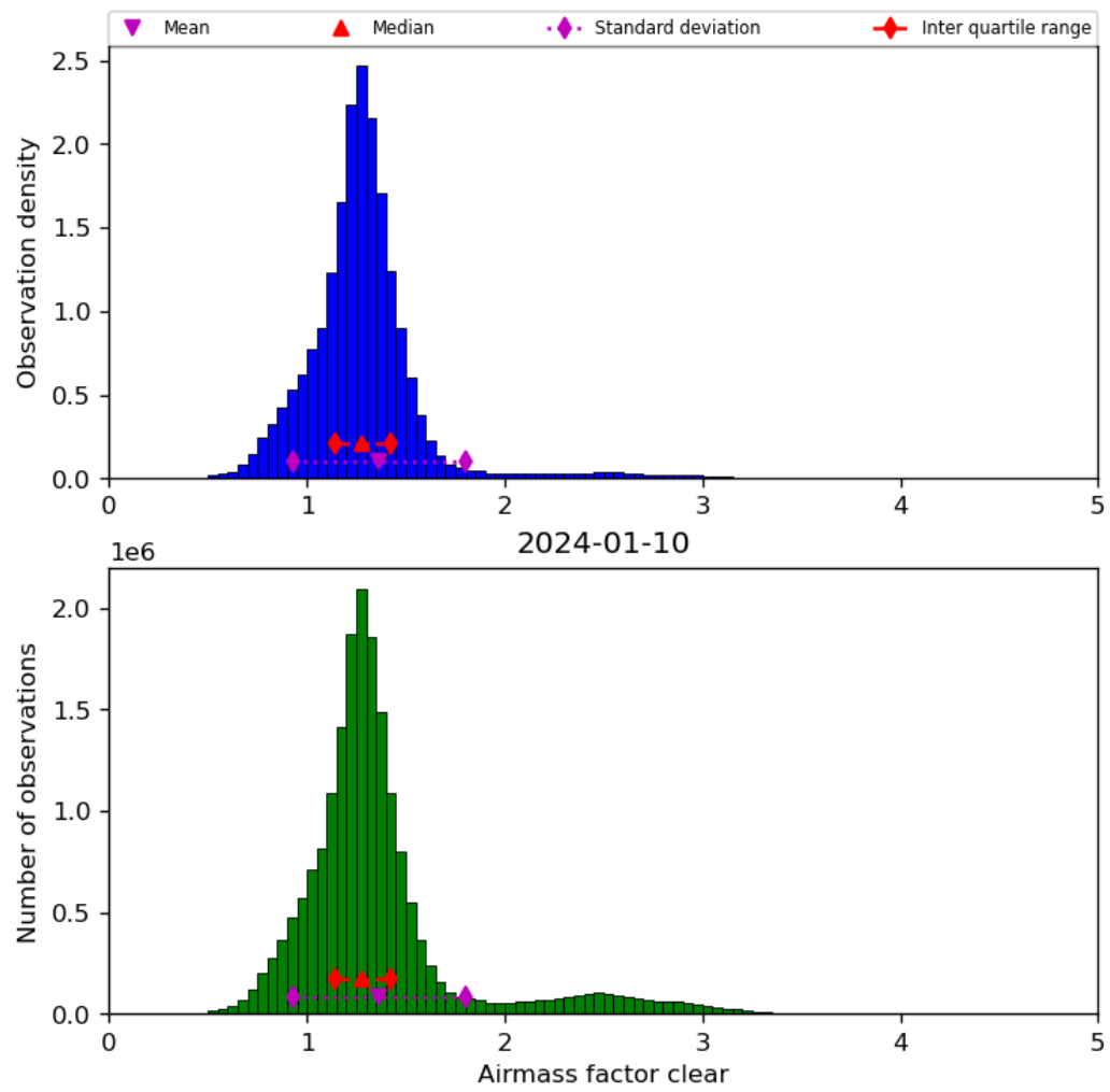
Figure 42: Histogram of “Airmass factor clear” for 2024-01-10 to 2024-01-11
