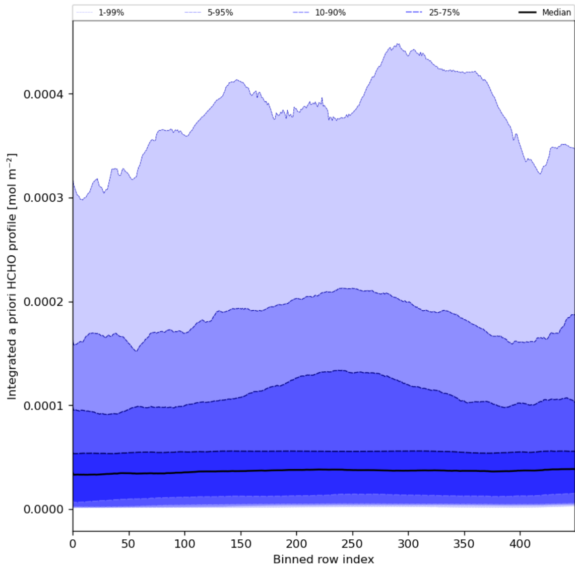
Figure 57: Along track statistics of “Integrated a priori HCHO profile” for 2024-01-10 to 2024-01-11
