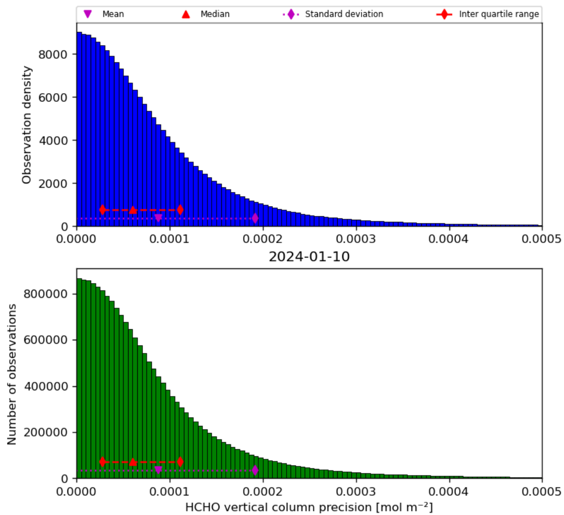
Figure 36: Histogram of “HCHO vertical column precision” for 2024-01-10 to 2024-01-11
