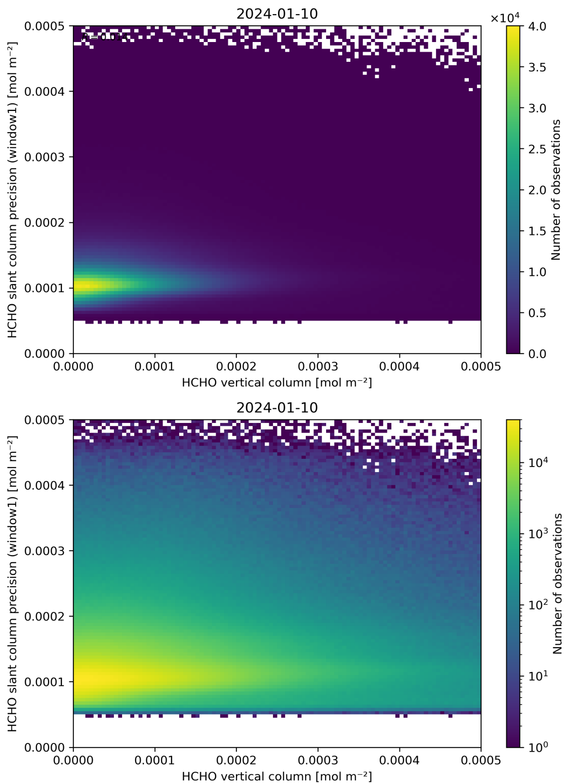
Figure 130: Scatter density plot of “HCHO vertical column” against “HCHO slant column precision (window1)” for 2024-01-10 to 2024-01-11.
