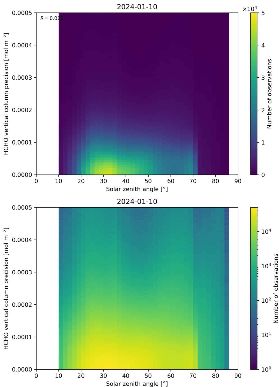
Figure 179: Scatter density plot of “Solar zenith angle” against “HCHO vertical column precision” for 2024-01-10 to 2024-01-11.
