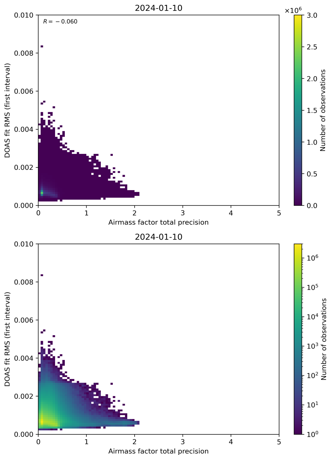
Figure 105: Scatter density plot of “Airmass factor total precision” against “DOAS fit RMS (first interval)” for 2024-01-10 to 2024-01-11.
