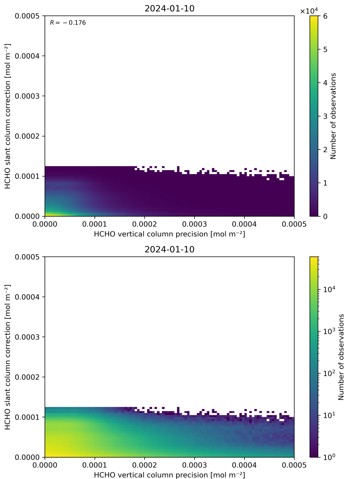
Figure 141: Scatter density plot of “HCHO vertical column precision” against “HCHO slant column correction” for 2024-01-10 to 2024-01-11.
