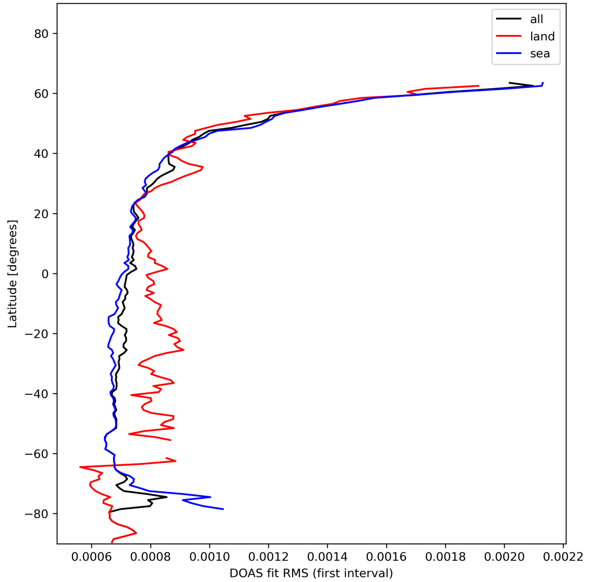
Figure 32: Zonal average of “DOAS fit RMS (first interval)” for 2024-01-10 to 2024-01-11.
