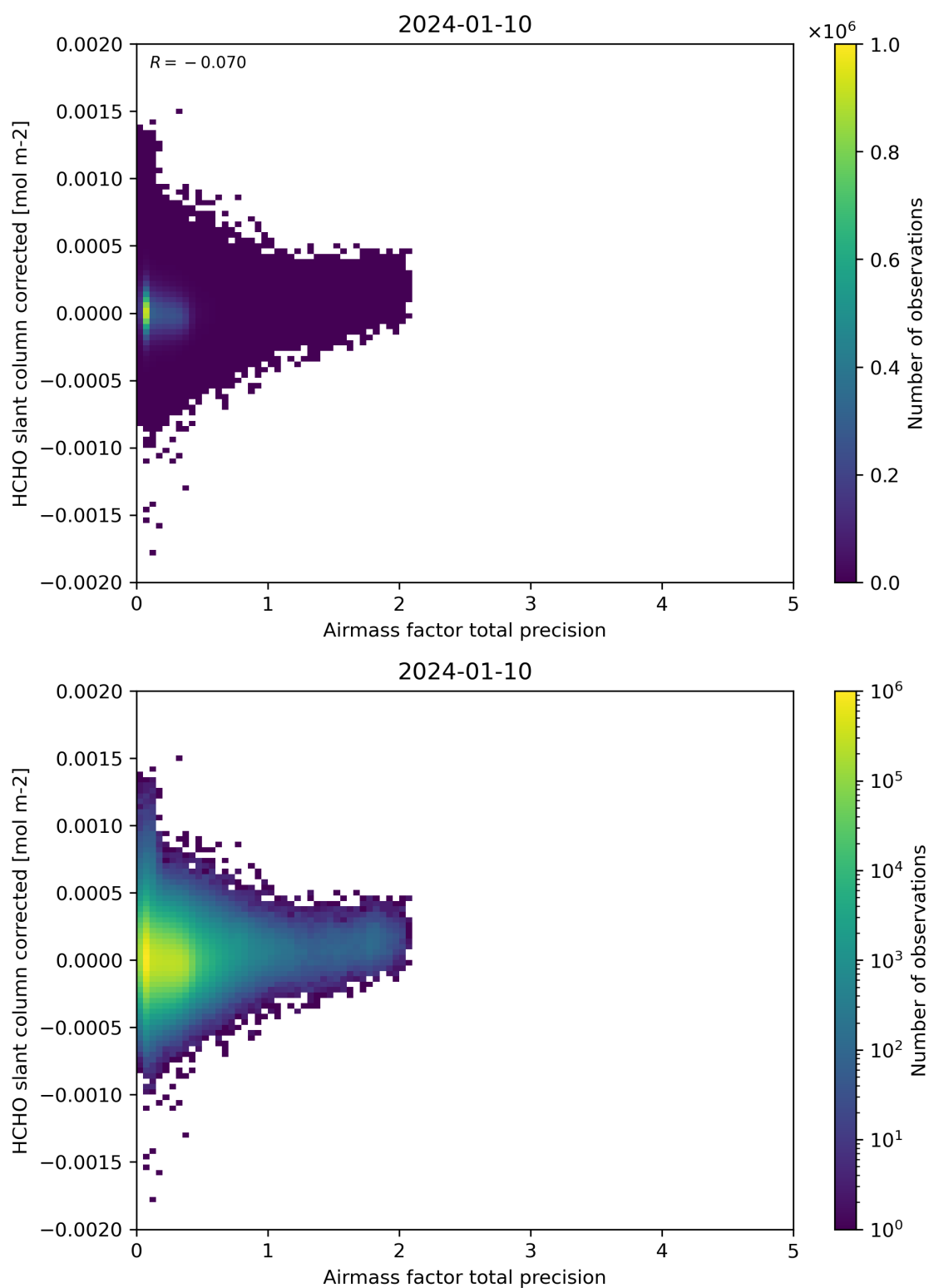
Figure 109: Scatter density plot of “Airmass factor total precision” against “HCHO slant column corrected” for 2024-01-10 to 2024-01-11.
