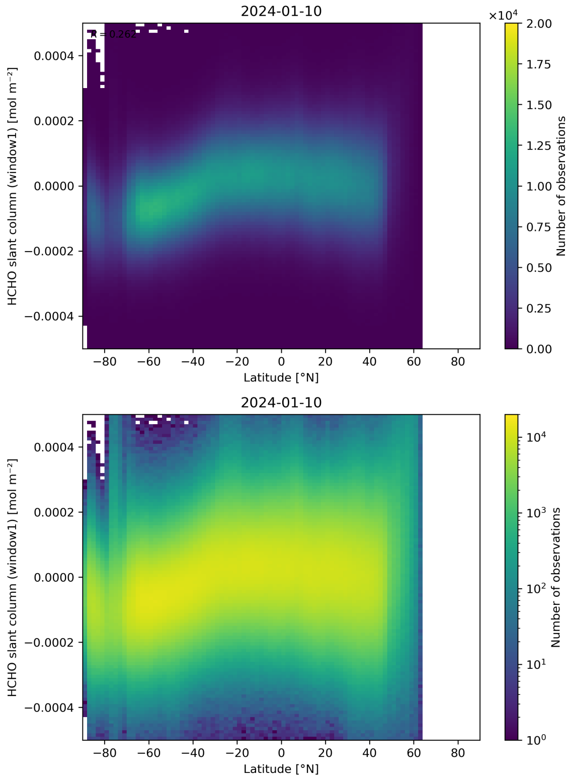
Figure 159: Scatter density plot of “Latitude” against “HCHO slant column (window1)” for 2024-01-10 to 2024-01-11.
