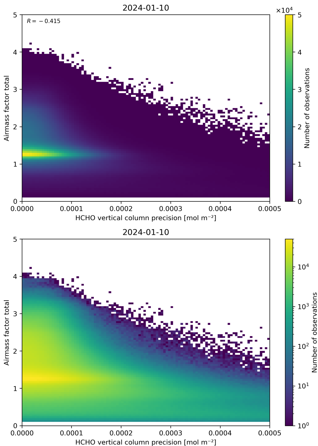
Figure 144: Scatter density plot of “HCHO vertical column precision” against “Airmass factor total” for 2024-01-10 to 2024-01-11.
