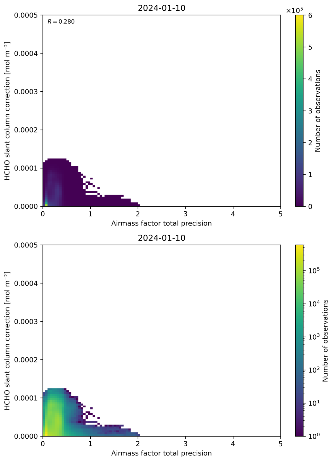
Figure 110: Scatter density plot of “Airmass factor total precision” against “HCHO slant column correction” for 2024-01-10 to 2024-01-11.
