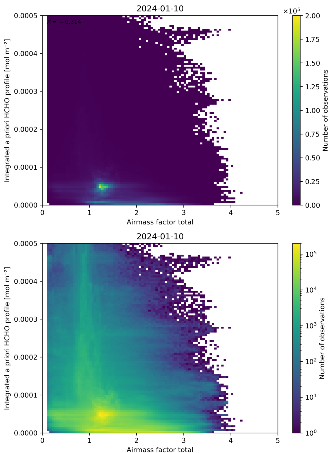
Figure 104: Scatter density plot of “Airmass factor total” against “Integrated a priori HCHO profile” for 2024-01-10 to 2024-01-11.
