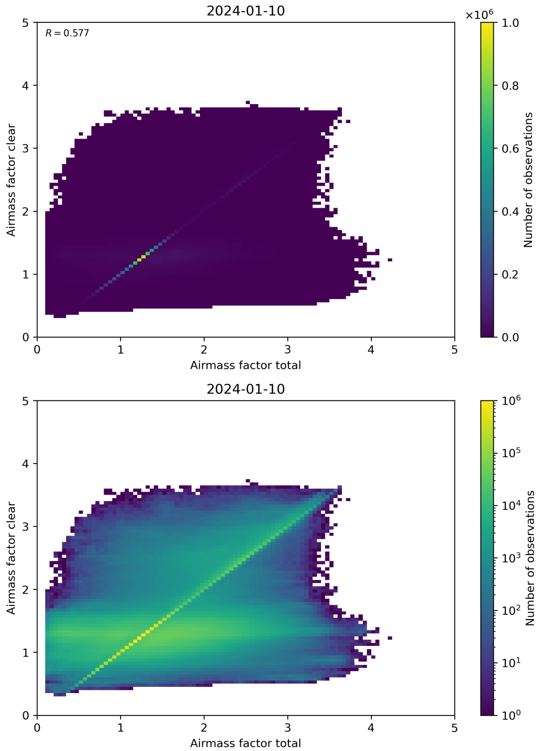
Figure 100: Scatter density plot of “Airmass factor total” against “Airmass factor clear” for 2024-01-10 to 2024-01-11.
