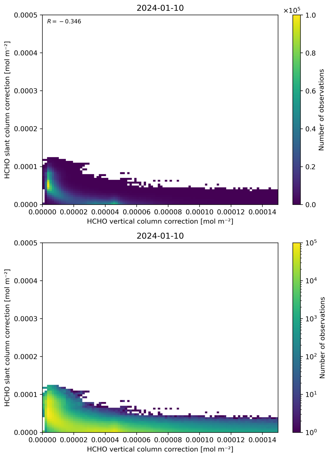
Figure 117: Scatter density plot of “HCHO vertical column correction” against “HCHO slant column correction” for 2024-01-10 to 2024-01-11.
