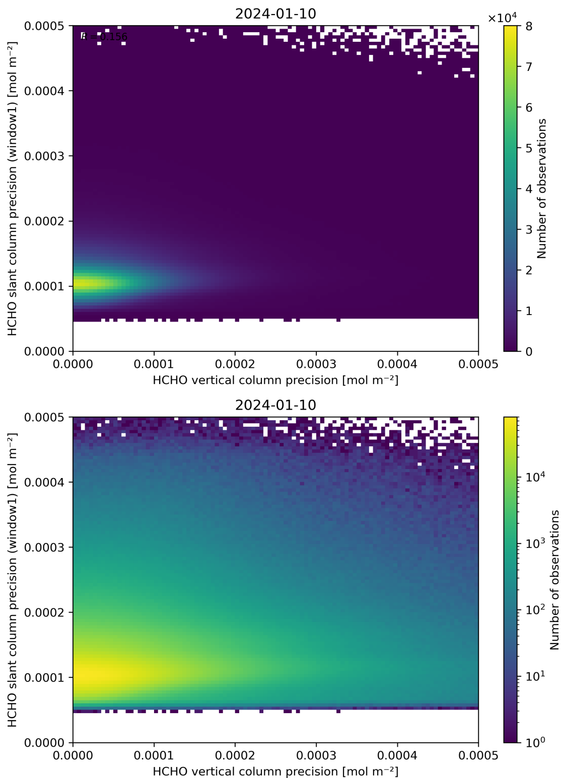
Figure 143: Scatter density plot of “HCHO vertical column precision” against “HCHO slant column precision (window1)” for 2024-01-10 to 2024-01-11.
