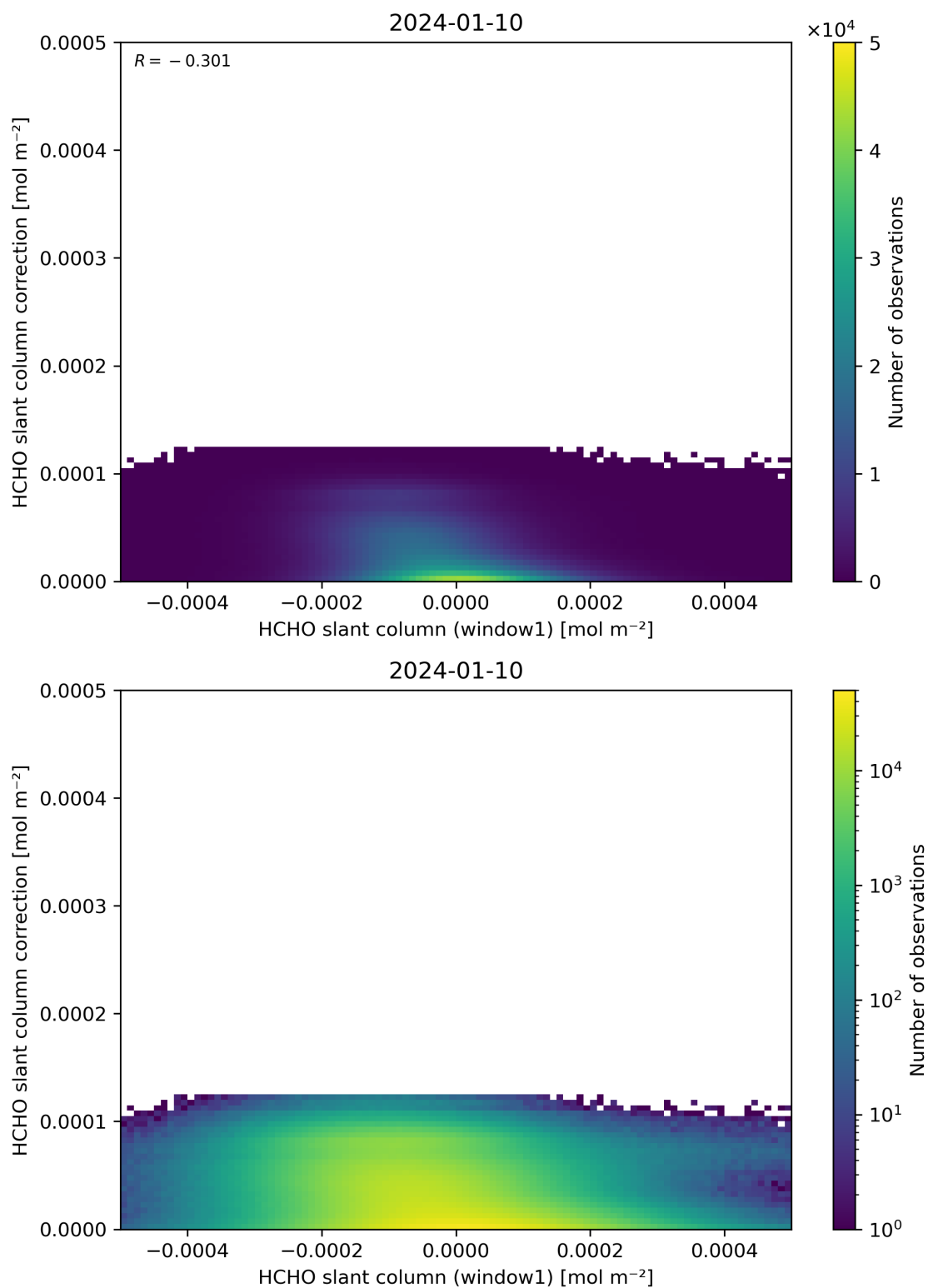
Figure 83: Scatter density plot of “HCHO slant column (window1)” against “HCHO slant column correction” for 2024-01-10 to 2024-01-11.
