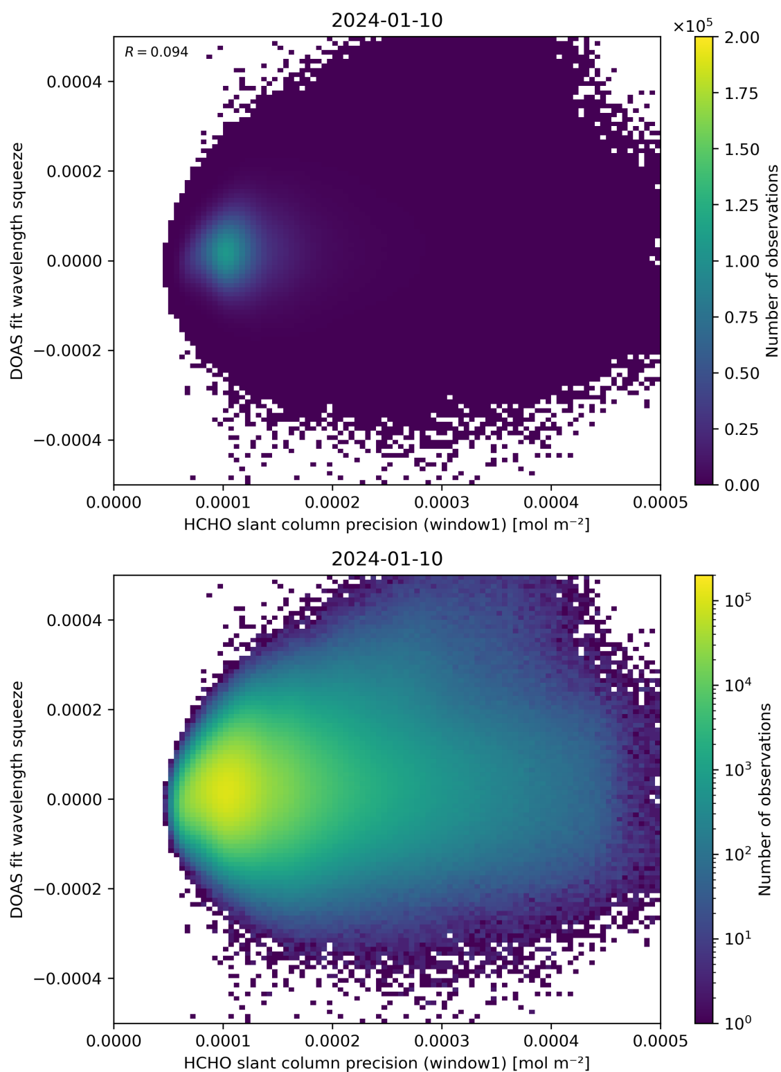
Figure 90: Scatter density plot of “HCHO slant column precision (window1)” against “DOAS fit wavelength squeeze” for 2024-01-10 to 2024-01-11.
