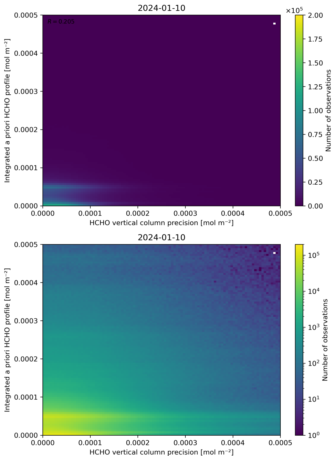
Figure 147: Scatter density plot of “HCHO vertical column precision” against “Integrated a priori HCHO profile” for 2024-01-10 to 2024-01-11.
