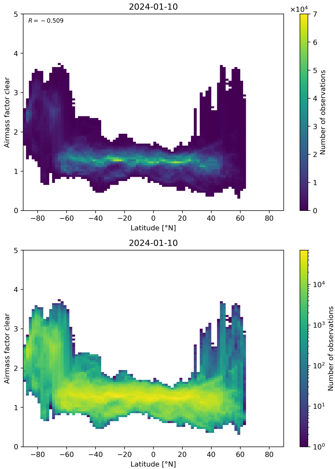
Figure 156: Scatter density plot of “Latitude” against “Airmass factor clear” for 2024-01-10 to 2024-01-11.
