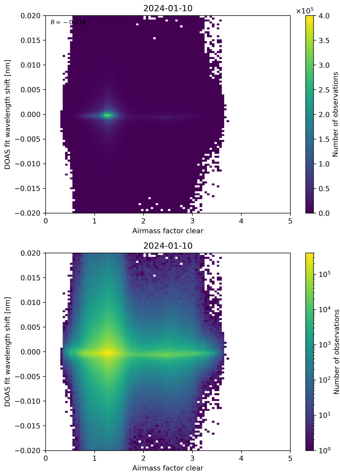
Figure 72: Scatter density plot of “Airmass factor clear” against “DOAS fit wavelength shift” for 2024-01-10 to 2024-01-11.
