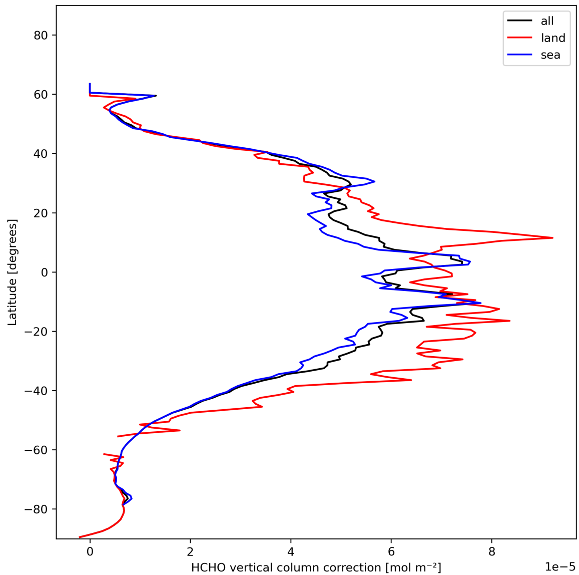
Figure 23: Zonal average of “HCHO vertical column correction” for 2024-01-10 to 2024-01-11.
