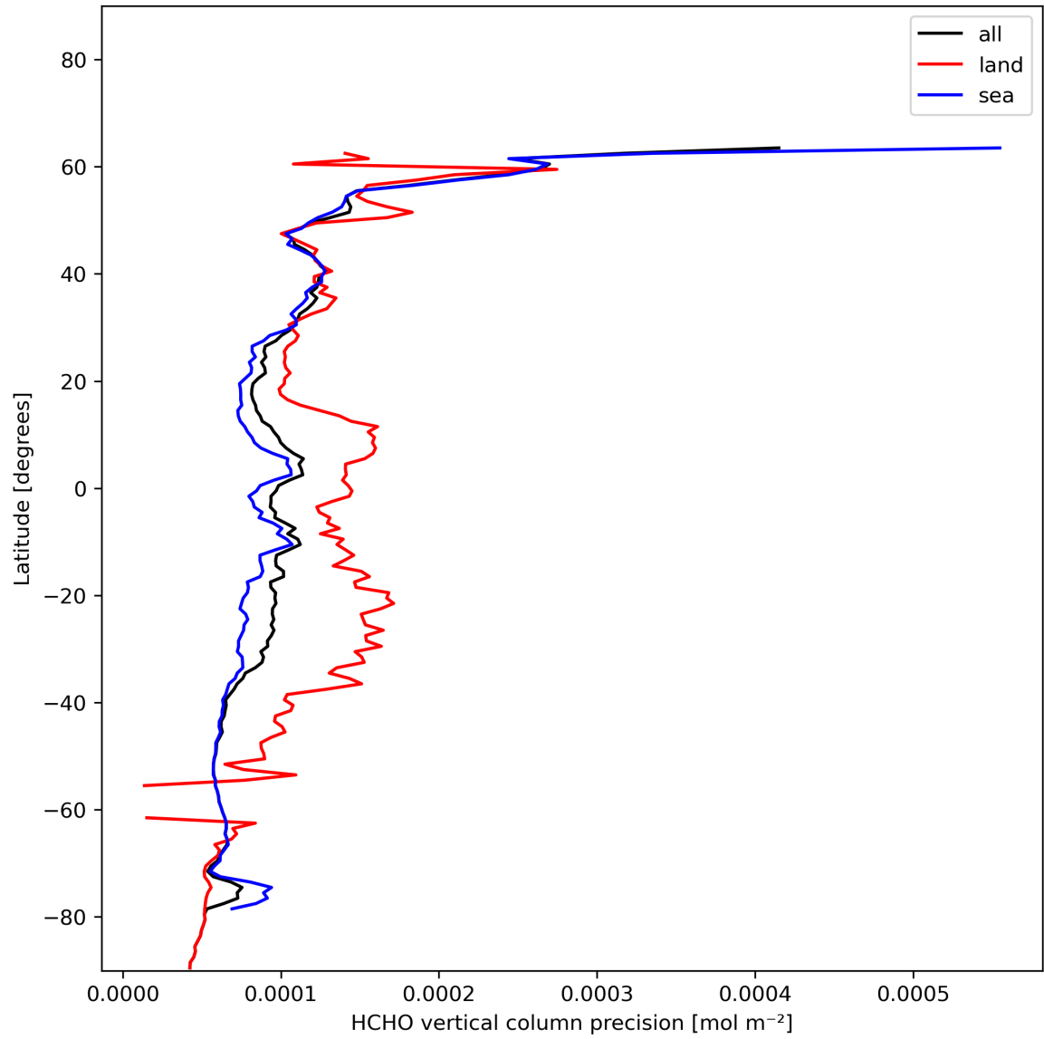
Figure 22: Zonal average of “HCHO vertical column precision” for 2024-01-10 to 2024-01-11.
