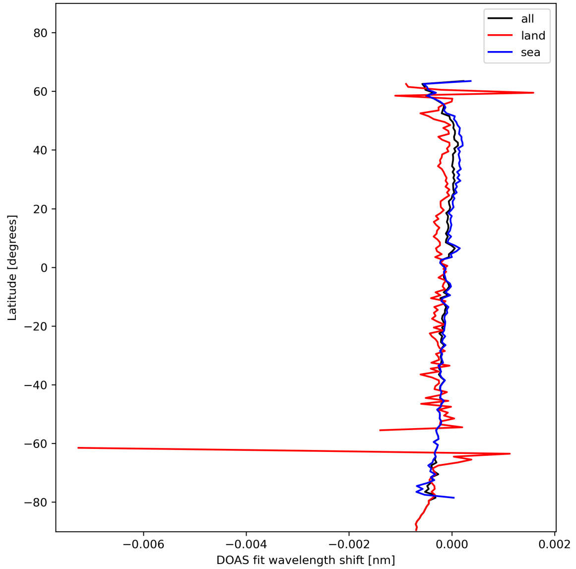
Figure 30: Zonal average of "DOAS fit wavelength shift" for 2024-01-10 to 2024-01-11.
