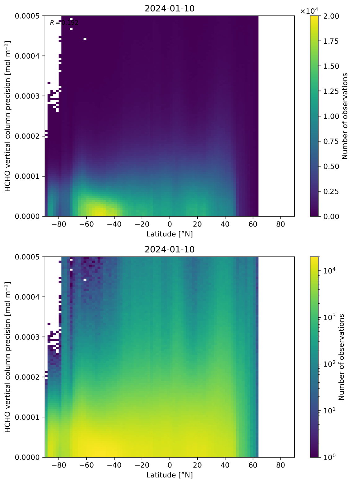
Figure 165: Scatter density plot of “Latitude” against “HCHO vertical column precision” for 2024-01-10 to 2024-01-11.
