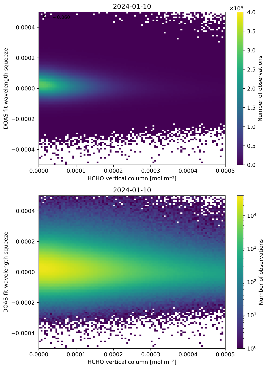
Figure 125: Scatter density plot of “HCHO vertical column” against “DOAS fit wavelength squeeze” for 2024-01-10 to 2024-01-11.
