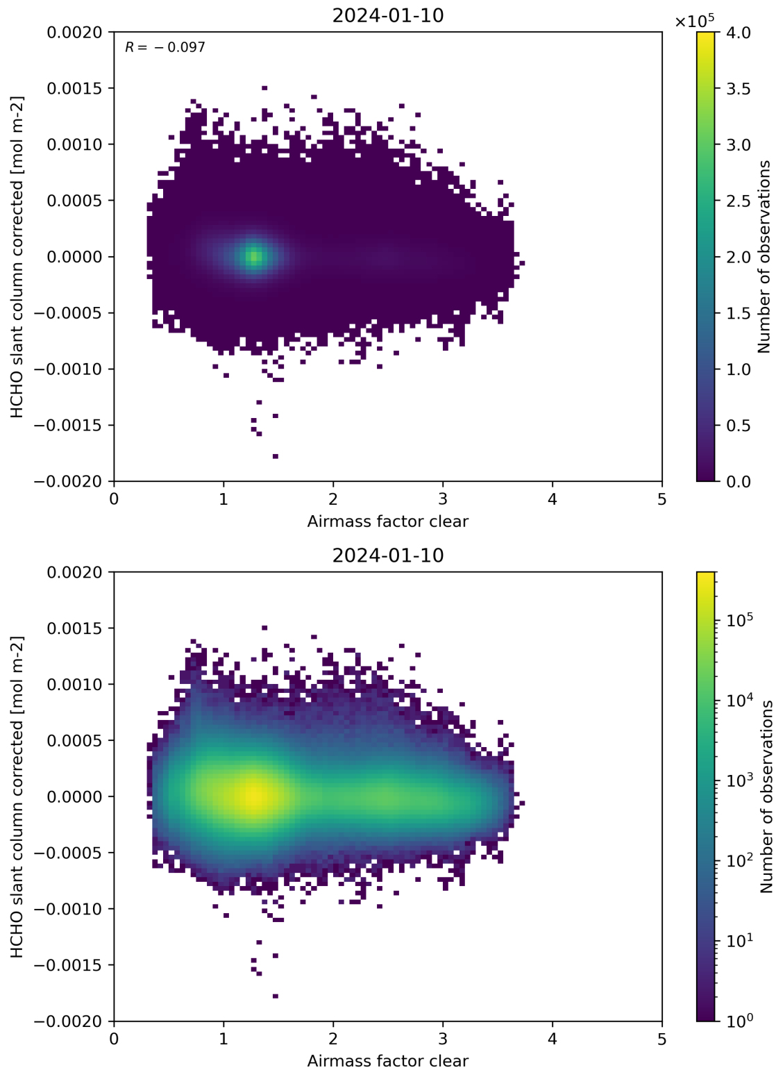
Figure 74: Scatter density plot of “Airmass factor clear” against “HCHO slant column corrected” for 2024-01-10 to 2024-01-11.
