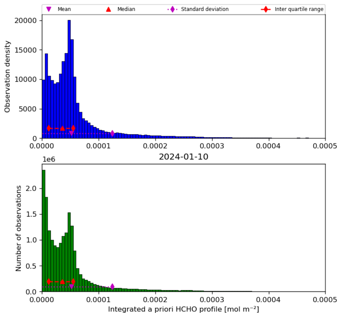
Figure 43: Histogram of “Integrated a priori HCHO profile” for 2024-01-10 to 2024-01-11
