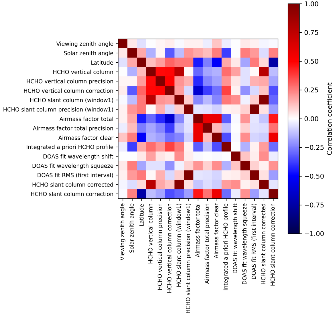
Figure 2: Map of correlation matrix for 2024-01-10 to 2024-01-11.
