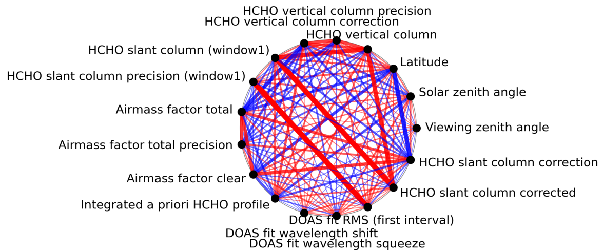
Figure 1: Map of correlation graph for 2024-01-10 to 2024-01-11.
