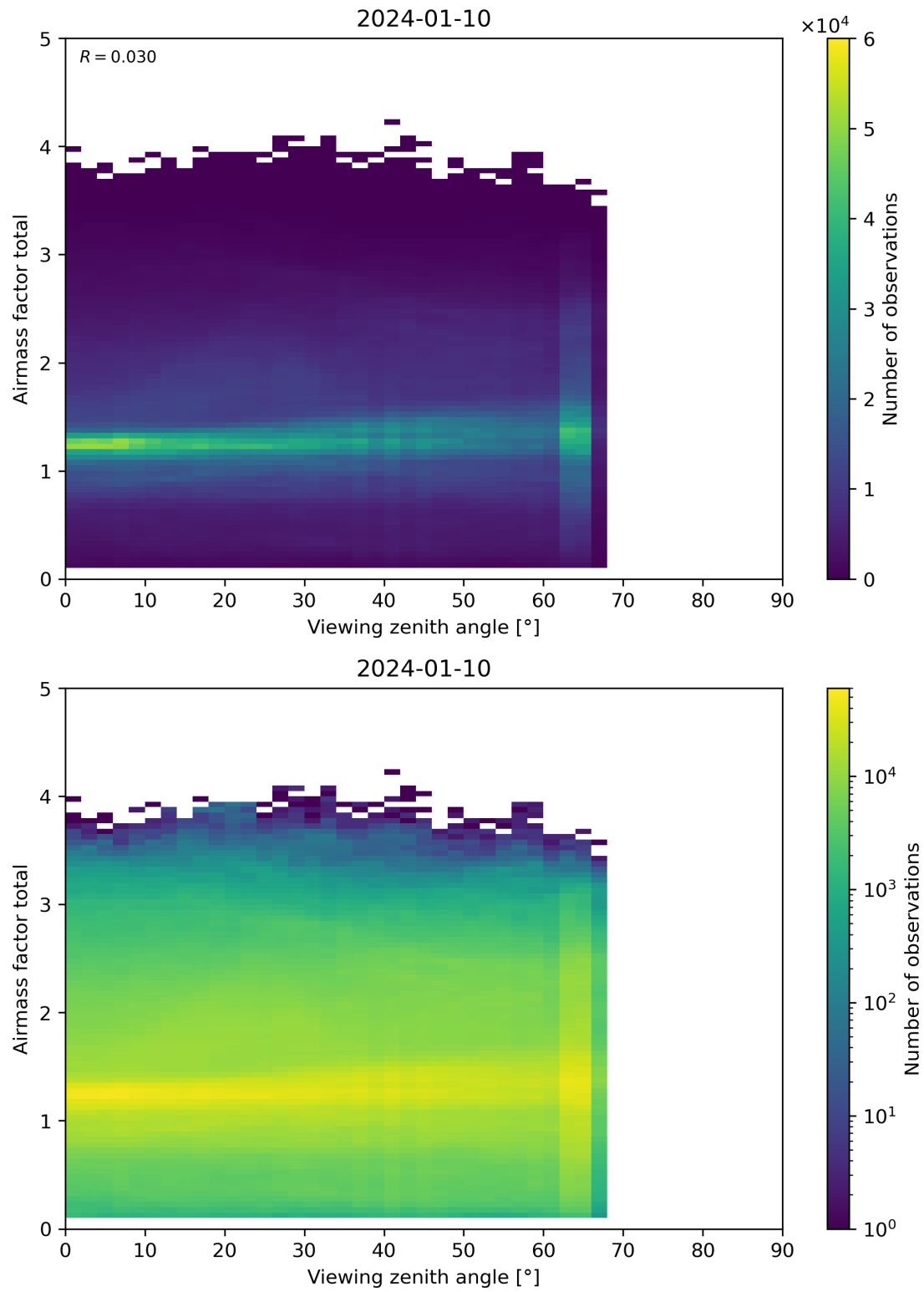
Figure 190: Scatter density plot of “Viewing zenith angle” against “Airmass factor total” for 2024-01-10 to 2024-01-11.
