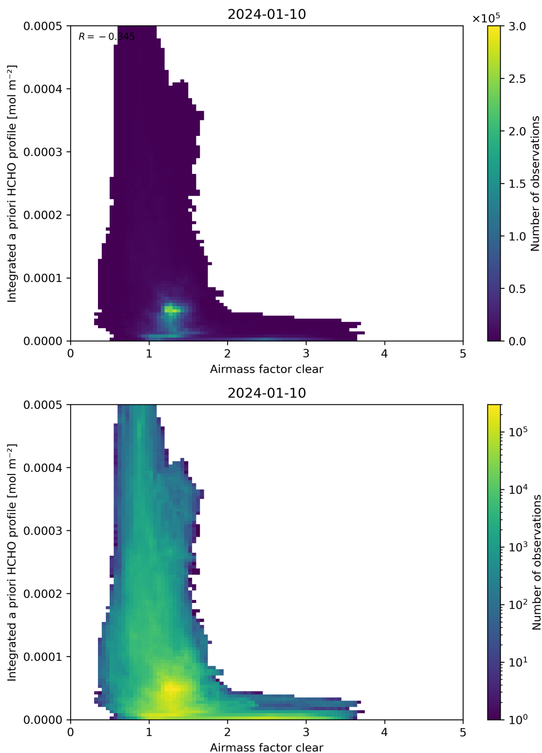
Figure 76: Scatter density plot of “Airmass factor clear” against “Integrated a priori HCHO profile” for 2024-01-10 to 2024-01-11.
