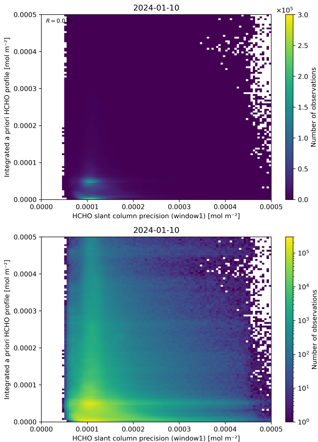
Figure 96: Scatter density plot of “HCHO slant column precision (window1)” against “Integrated a priori HCHO profile” for 2024-01-10 to 2024-01-11.
