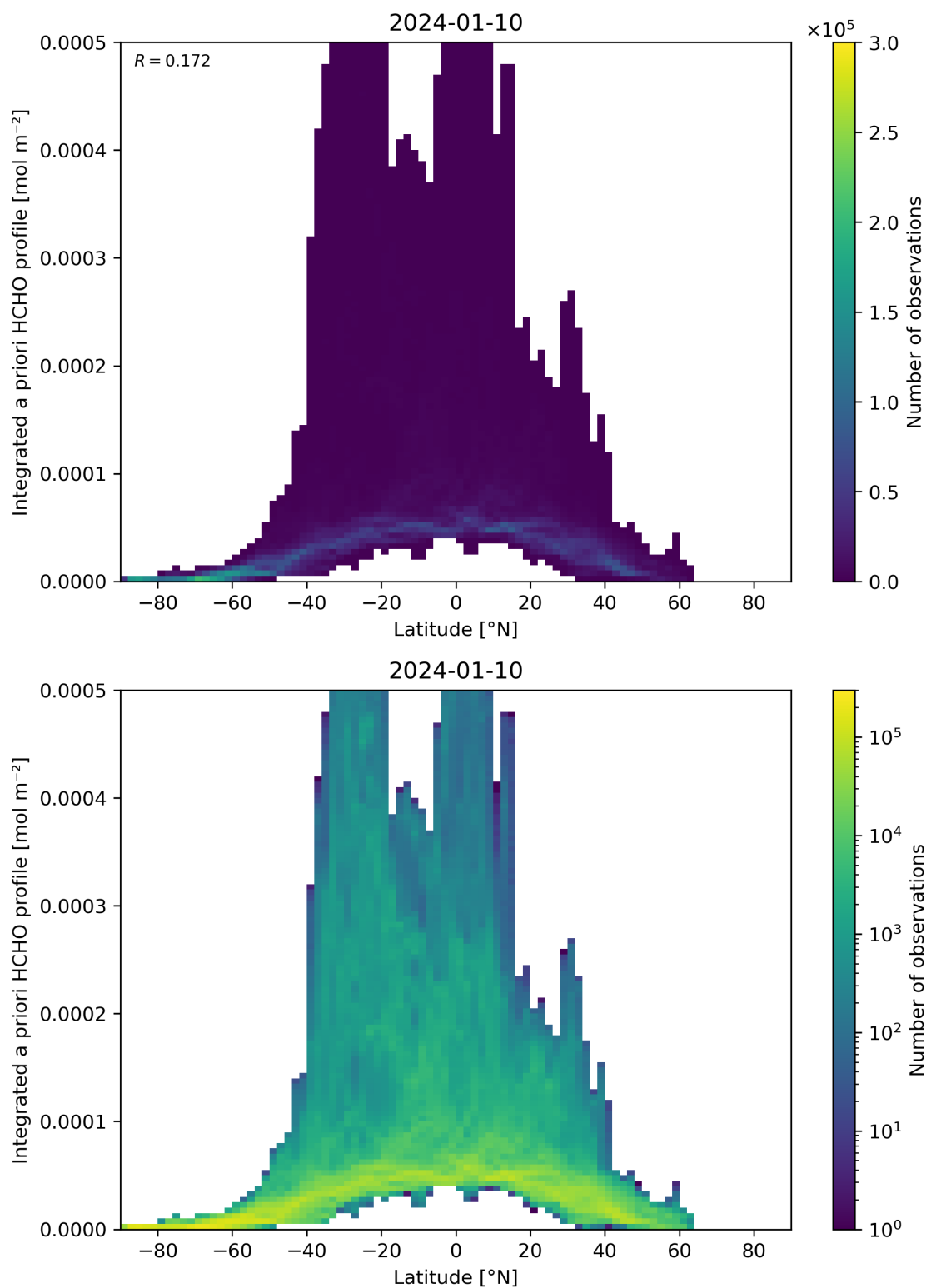
Figure 166: Scatter density plot of “Latitude” against “Integrated a priori HCHO profile” for 2024-01-10 to 2024-01-11.
