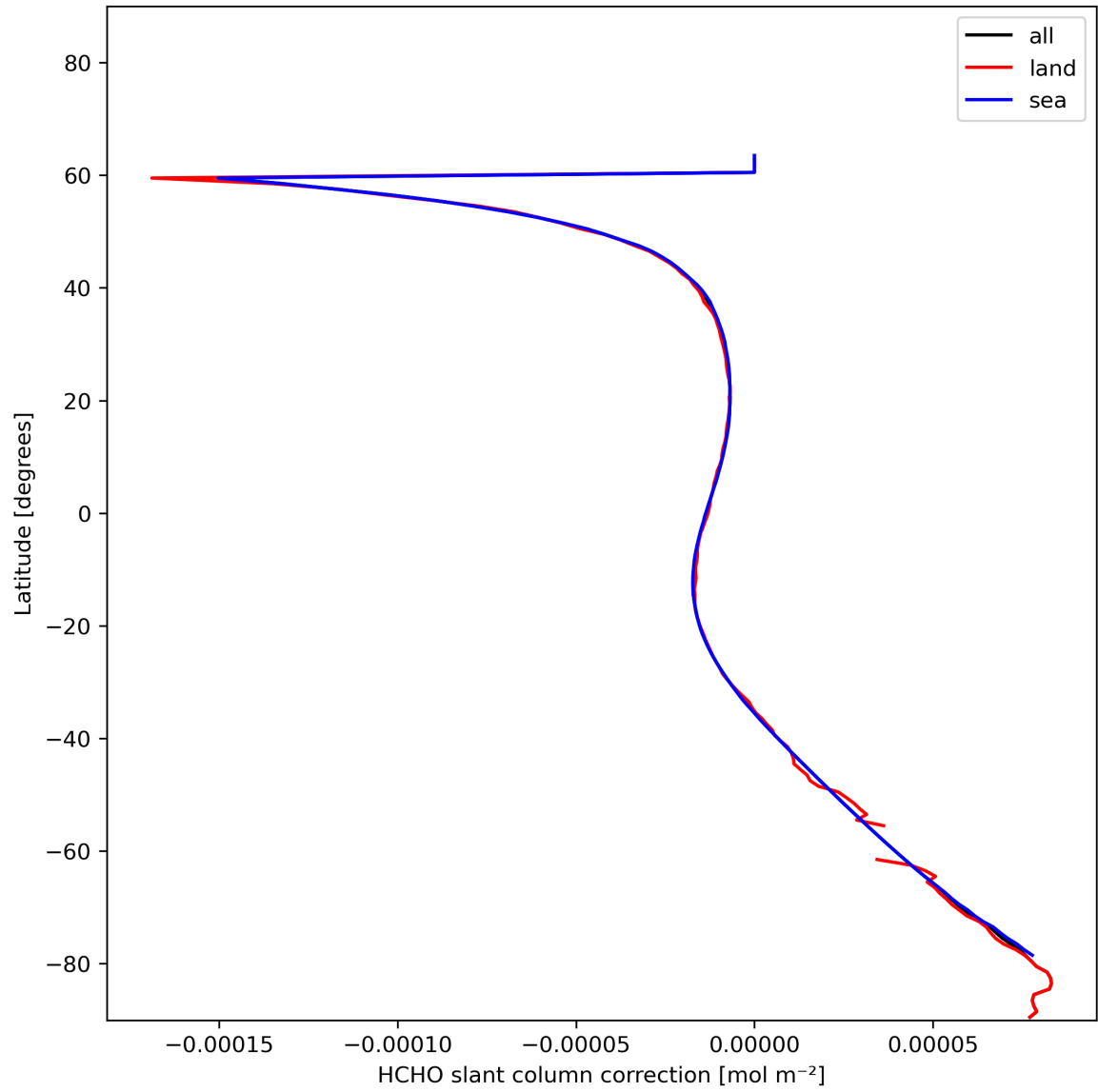
Figure 33: Zonal average of "HCHO slant column correction" for 2024-01-10 to 2024-01-11.
