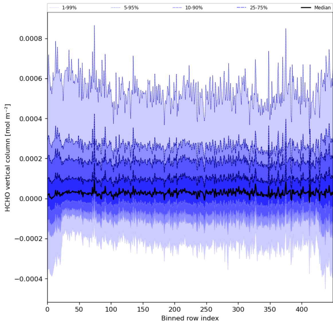
Figure 49: Along track statistics of “HCHO vertical column” for 2024-01-10 to 2024-01-11
