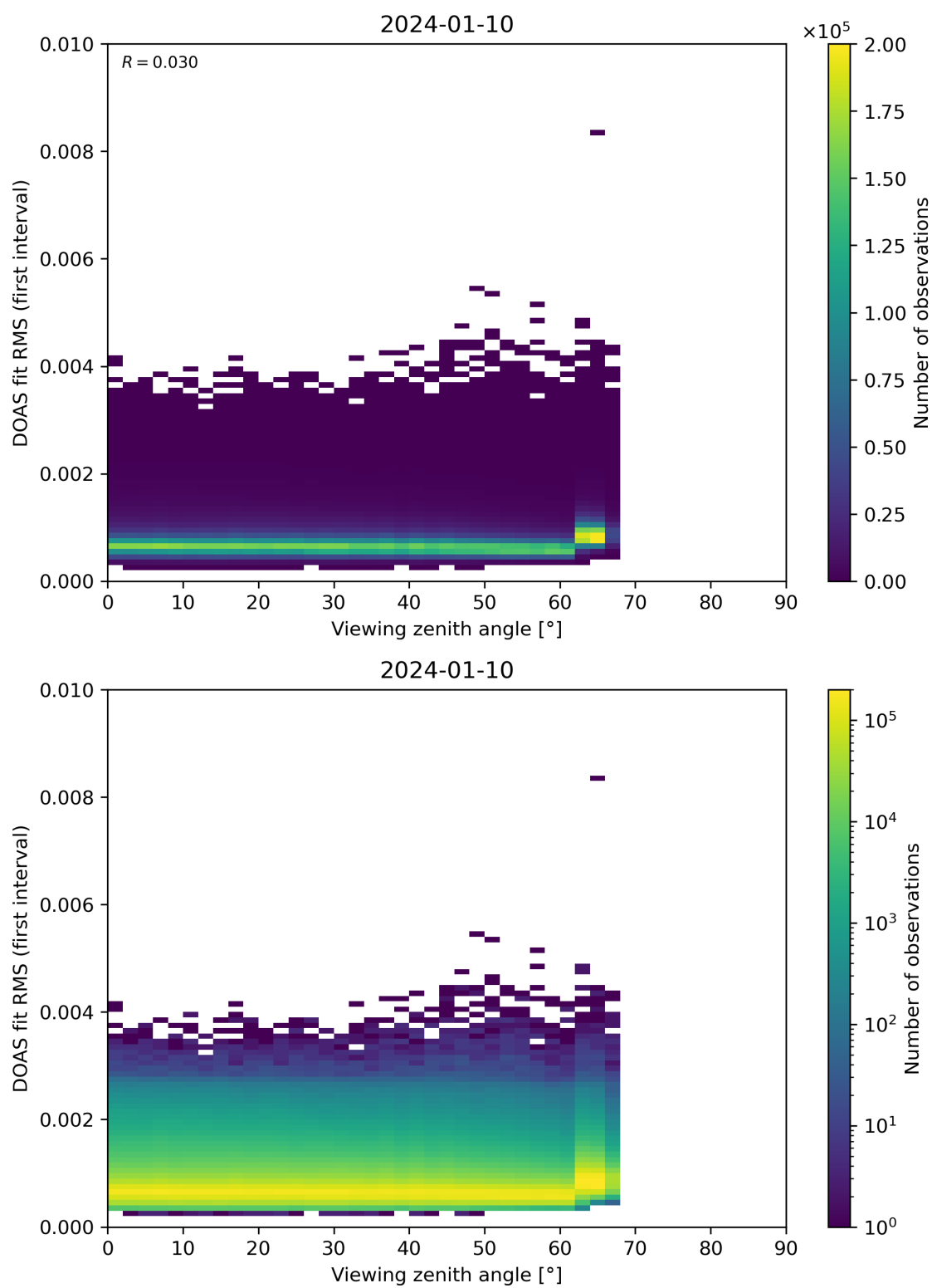
Figure 182: Scatter density plot of “Viewing zenith angle” against “DOAS fit RMS (first interval)” for 2024-01-10 to 2024-01-11.
