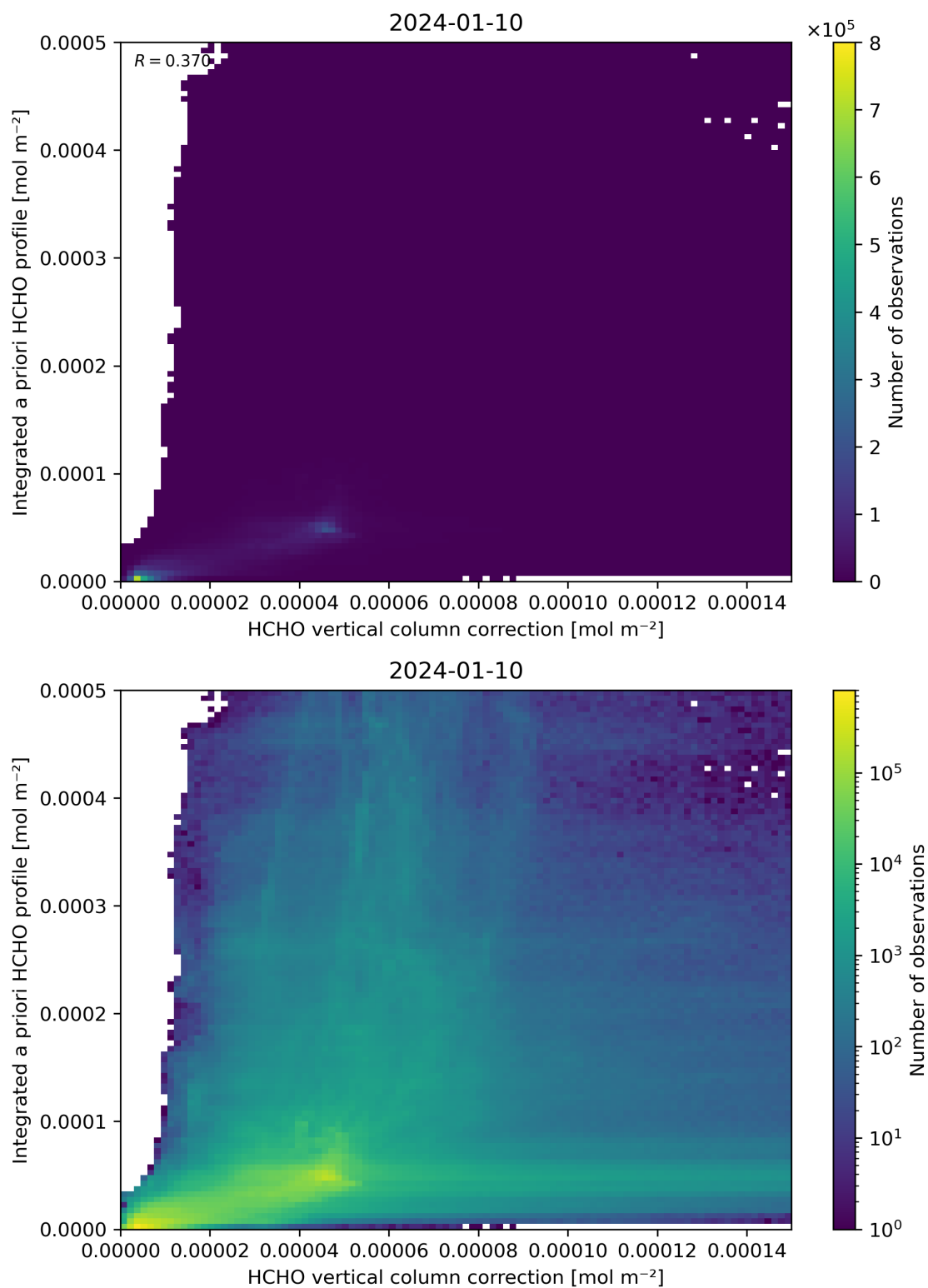
Figure 122: Scatter density plot of “HCHO vertical column correction” against “Integrated a priori HCHO profile” for 2024-01-10 to 2024-01-11.
