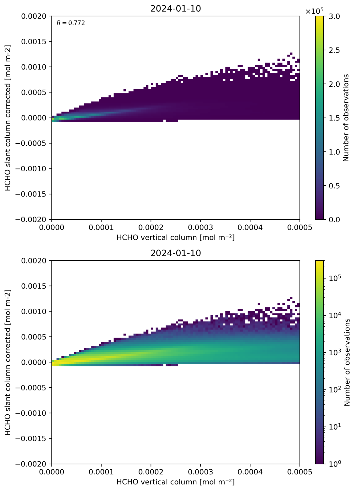
Figure 127: Scatter density plot of “HCHO vertical column” against “HCHO slant column corrected” for 2024-01-10 to 2024-01-11.
