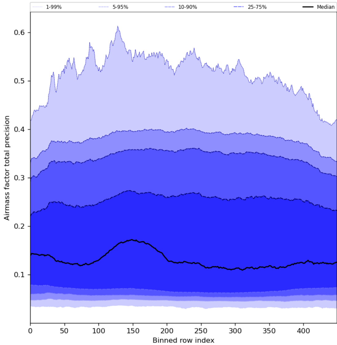
Figure 55: Along track statistics of “Airmass factor total precision” for 2024-01-10 to 2024-01-11
