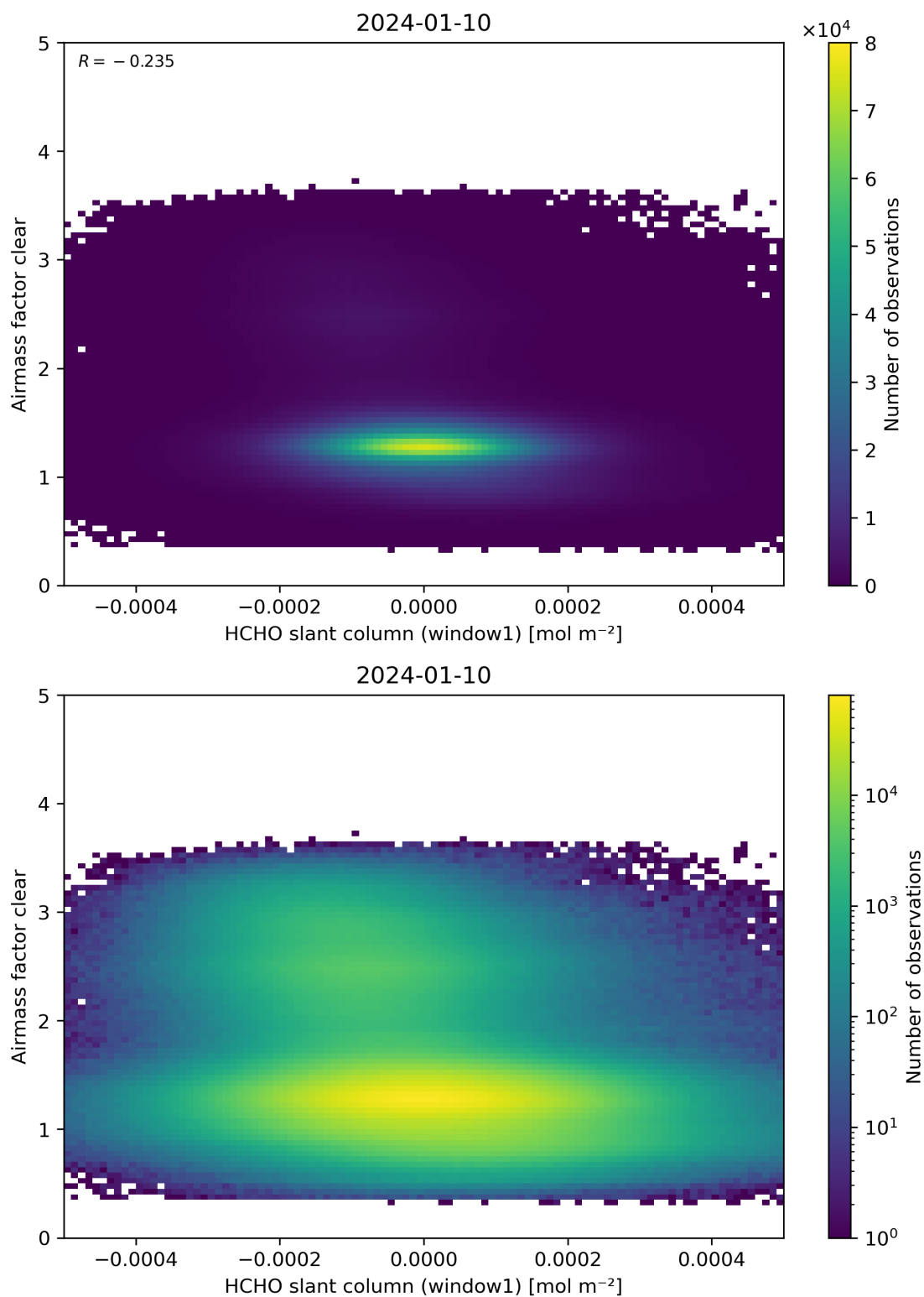
Figure 81: Scatter density plot of “HCHO slant column (window1)” against “Airmass factor clear” for 2024-01-10 to 2024-01-11.
