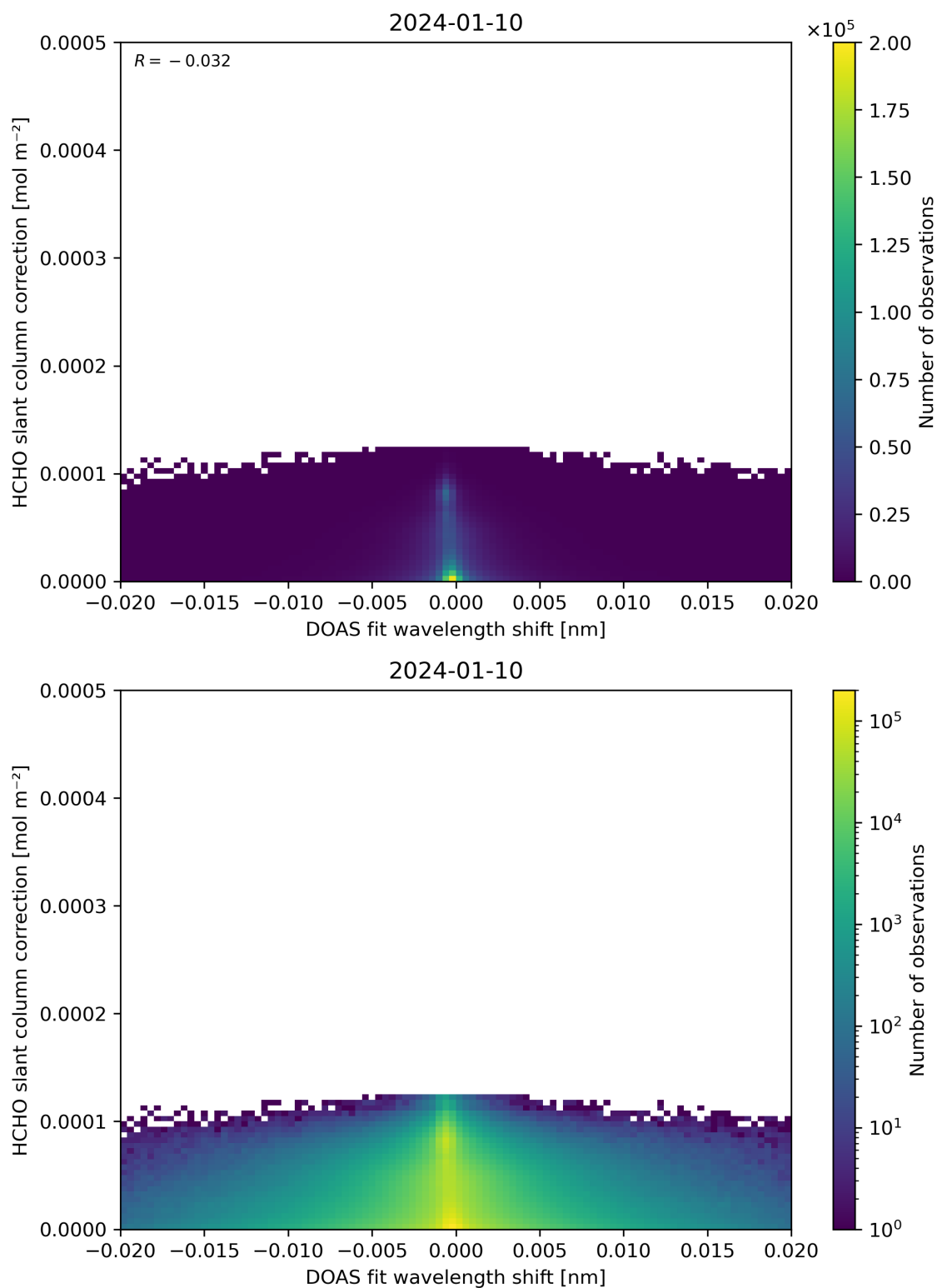
Figure 67: Scatter density plot of “DOAS fit wavelength shift” against “HCHO slant column correction” for 2024-01-10 to 2024-01-11.
