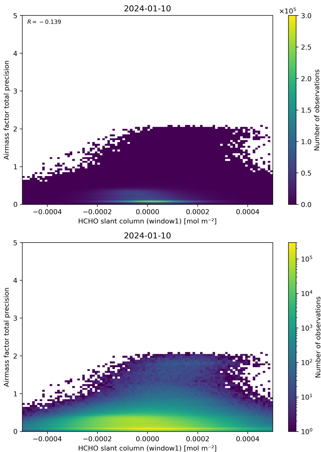
Figure 86: Scatter density plot of “HCHO slant column (window1)” against “Airmass factor total precision” for 2024-01-10 to 2024-01-11.
