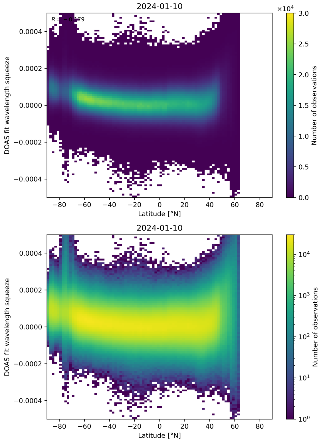
Figure 155: Scatter density plot of “Latitude” against “DOAS fit wavelength squeeze” for 2024-01-10 to 2024-01-11.
