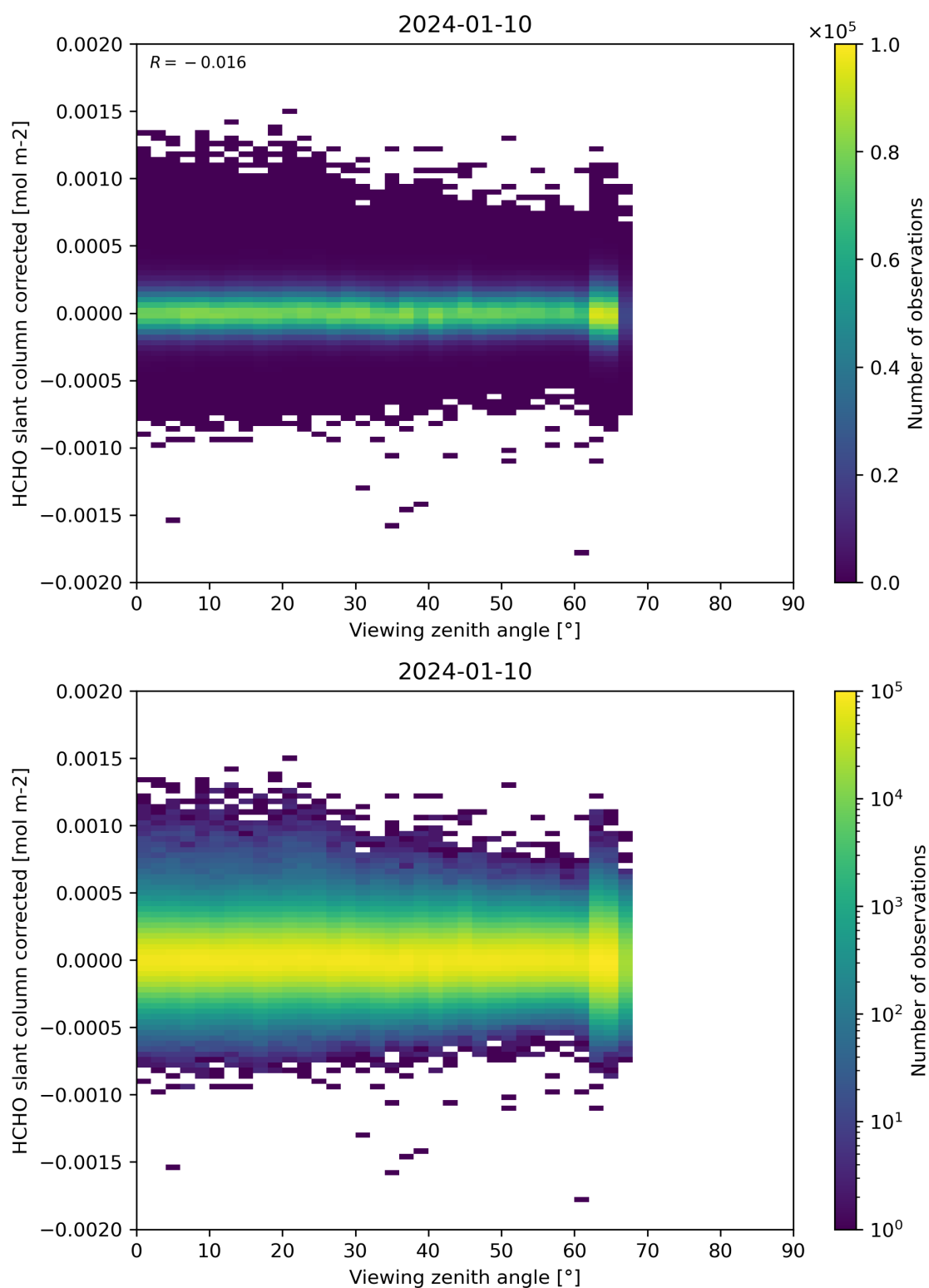
Figure 186: Scatter density plot of “Viewing zenith angle” against “HCHO slant column corrected” for 2024-01-10 to 2024-01-11.
