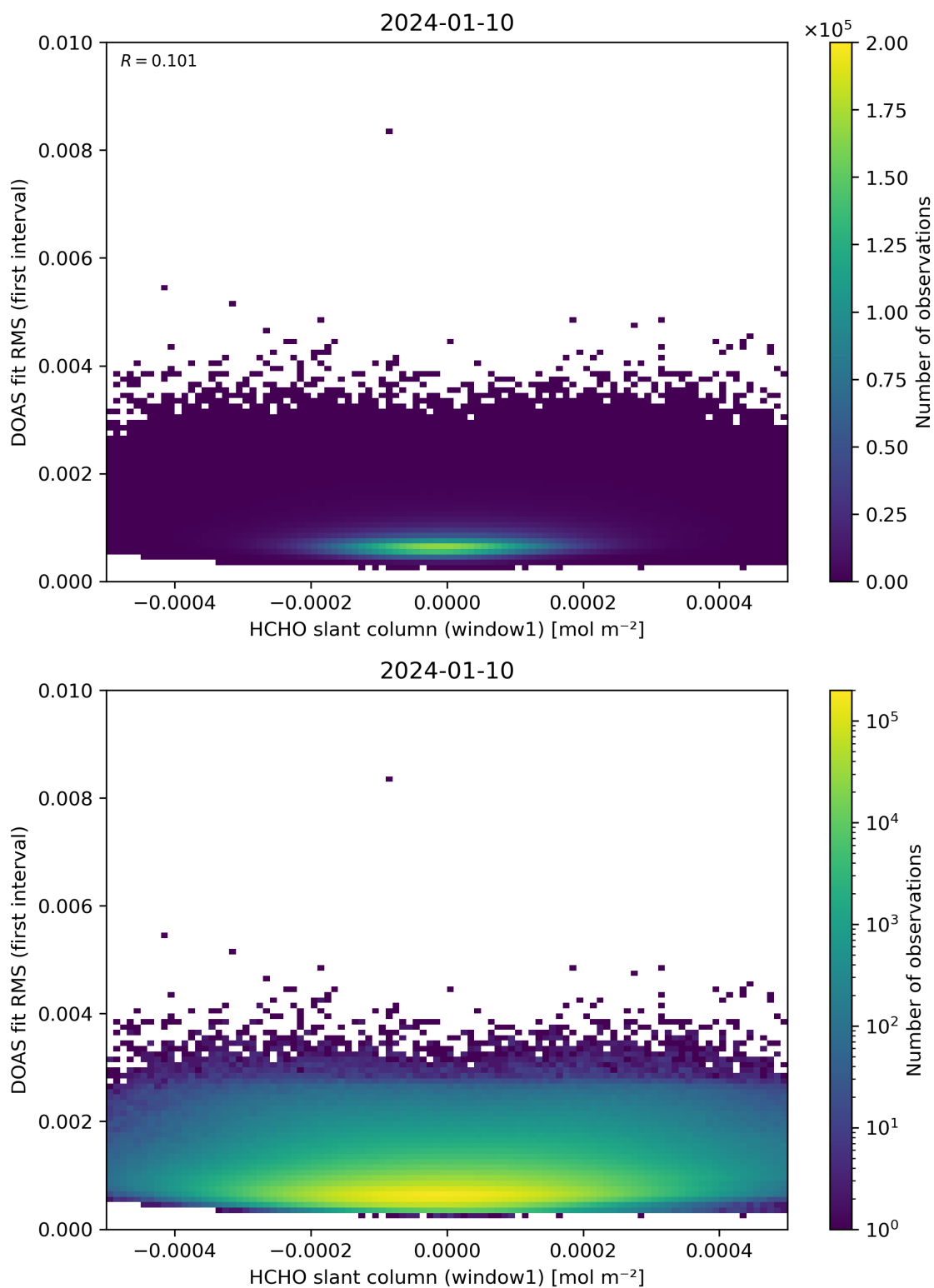
Figure 78: Scatter density plot of “HCHO slant column (window1)” against “DOAS fit RMS (first interval)” for 2024-01-10 to 2024-01-11.
