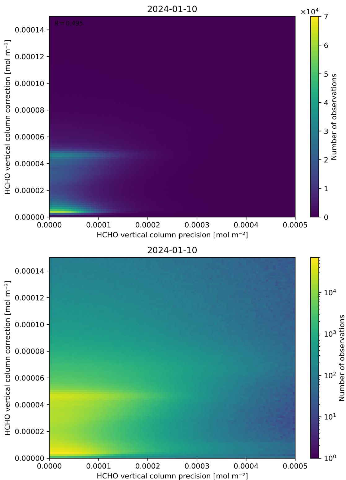
Figure 146: Scatter density plot of “HCHO vertical column precision” against “HCHO vertical column correction” for 2024-01-10 to 2024-01-11.
