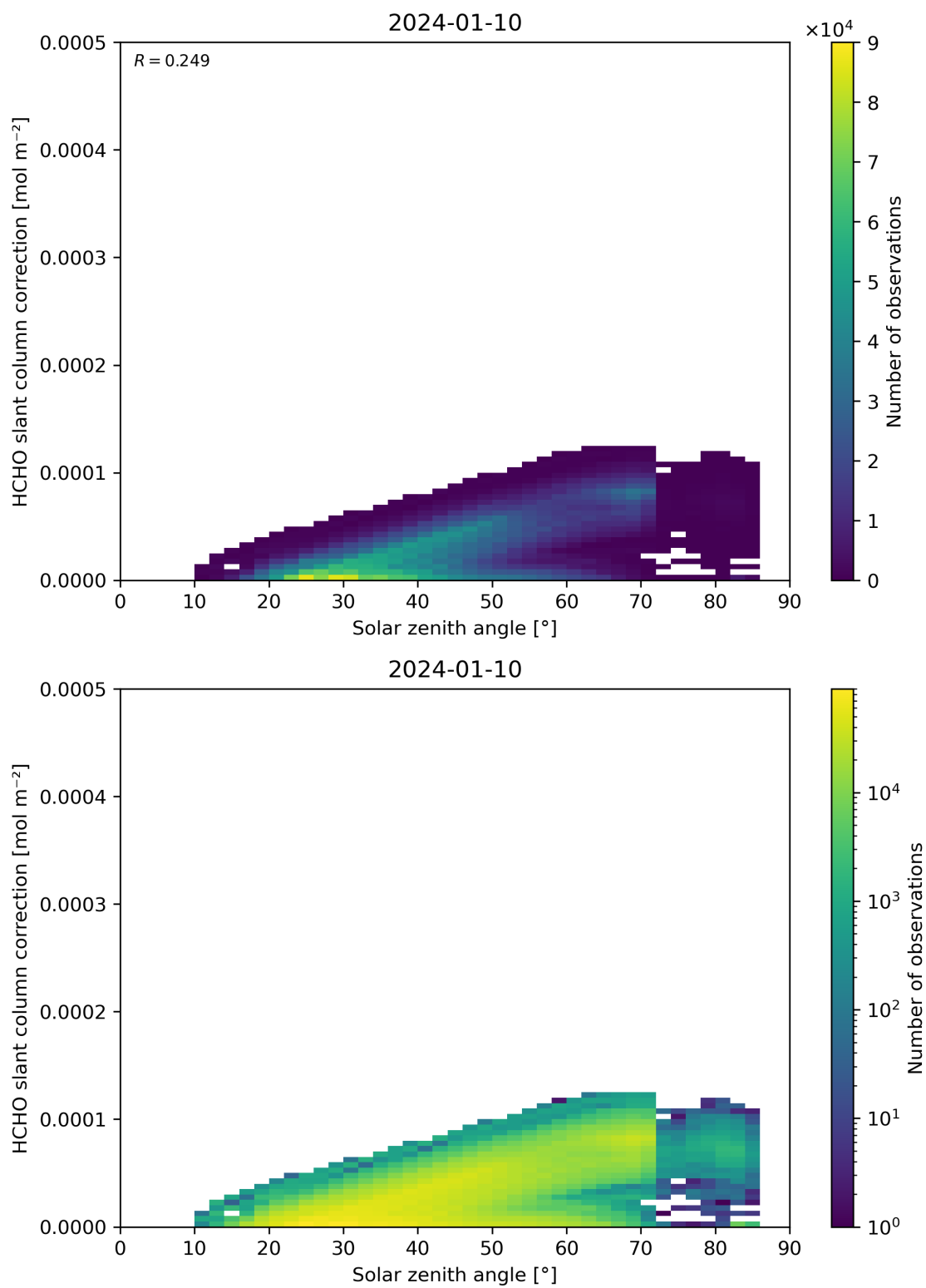
Figure 172: Scatter density plot of “Solar zenith angle” against “HCHO slant column correction” for 2024-01-10 to 2024-01-11.
