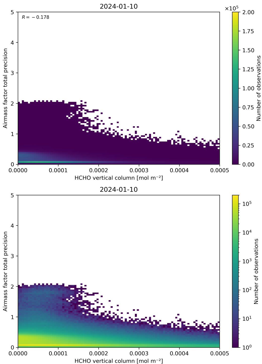
Figure 132: Scatter density plot of “HCHO vertical column” against “Airmass factor total precision” for 2024-01-10 to 2024-01-11.
