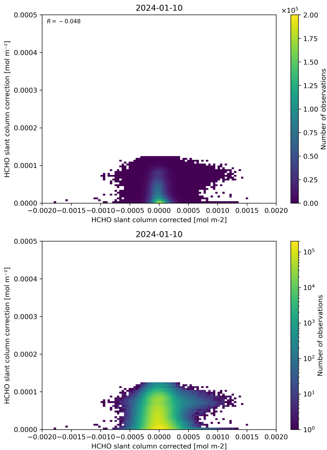
Figure 77: Scatter density plot of “HCHO slant column corrected” against “HCHO slant column correction” for 2024-01-10 to 2024-01-11.
