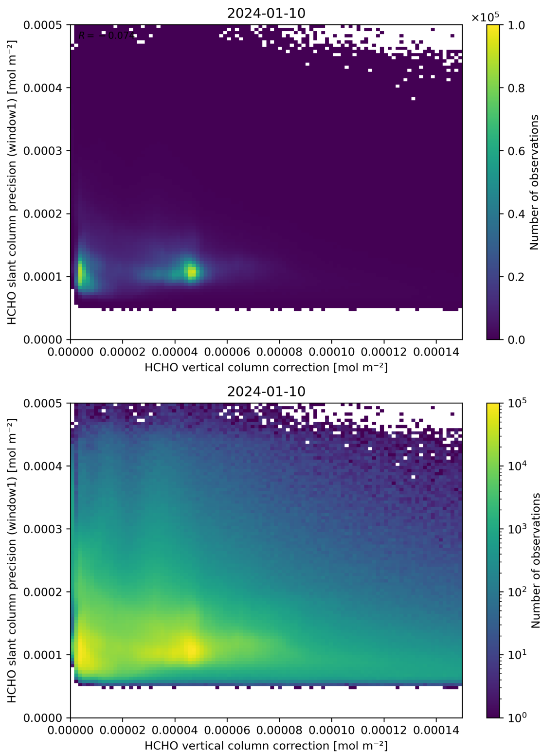
Figure 119: Scatter density plot of “HCHO vertical column correction” against “HCHO slant column precision (window1)” for 2024-01-10 to 2024-01-11.
