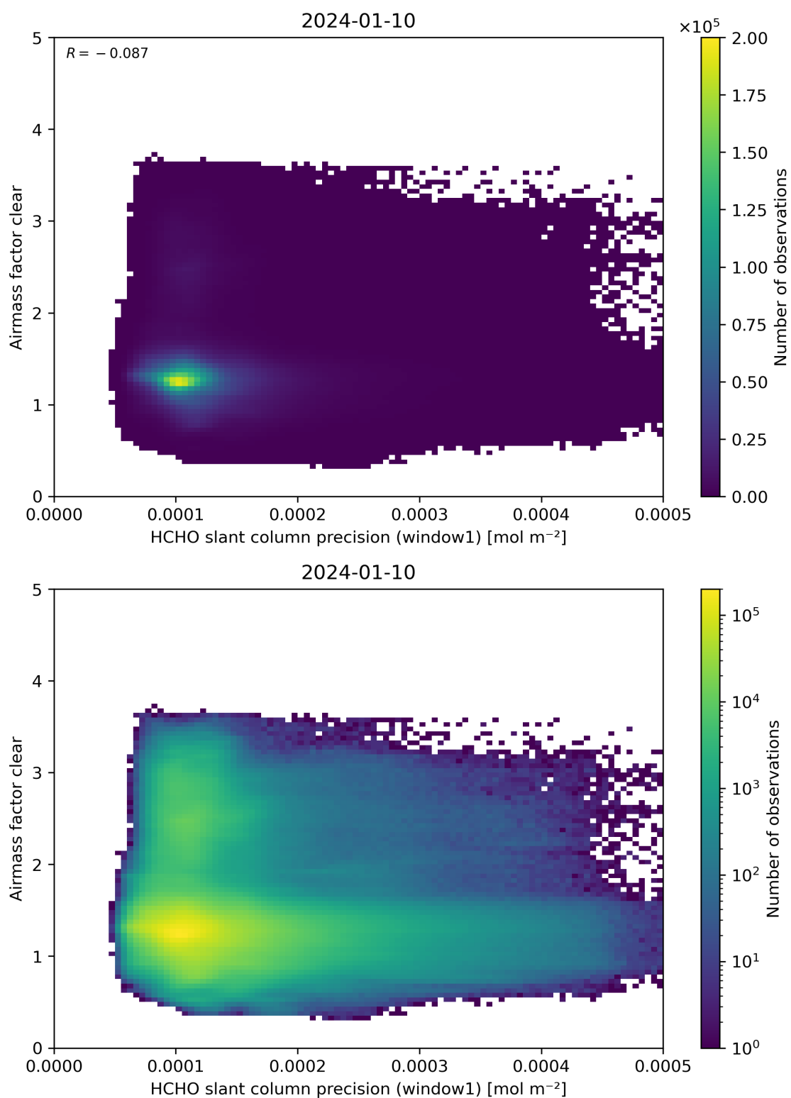
Figure 91: Scatter density plot of “HCHO slant column precision (window1)” against “Airmass factor clear” for 2024-01-10 to 2024-01-11.
