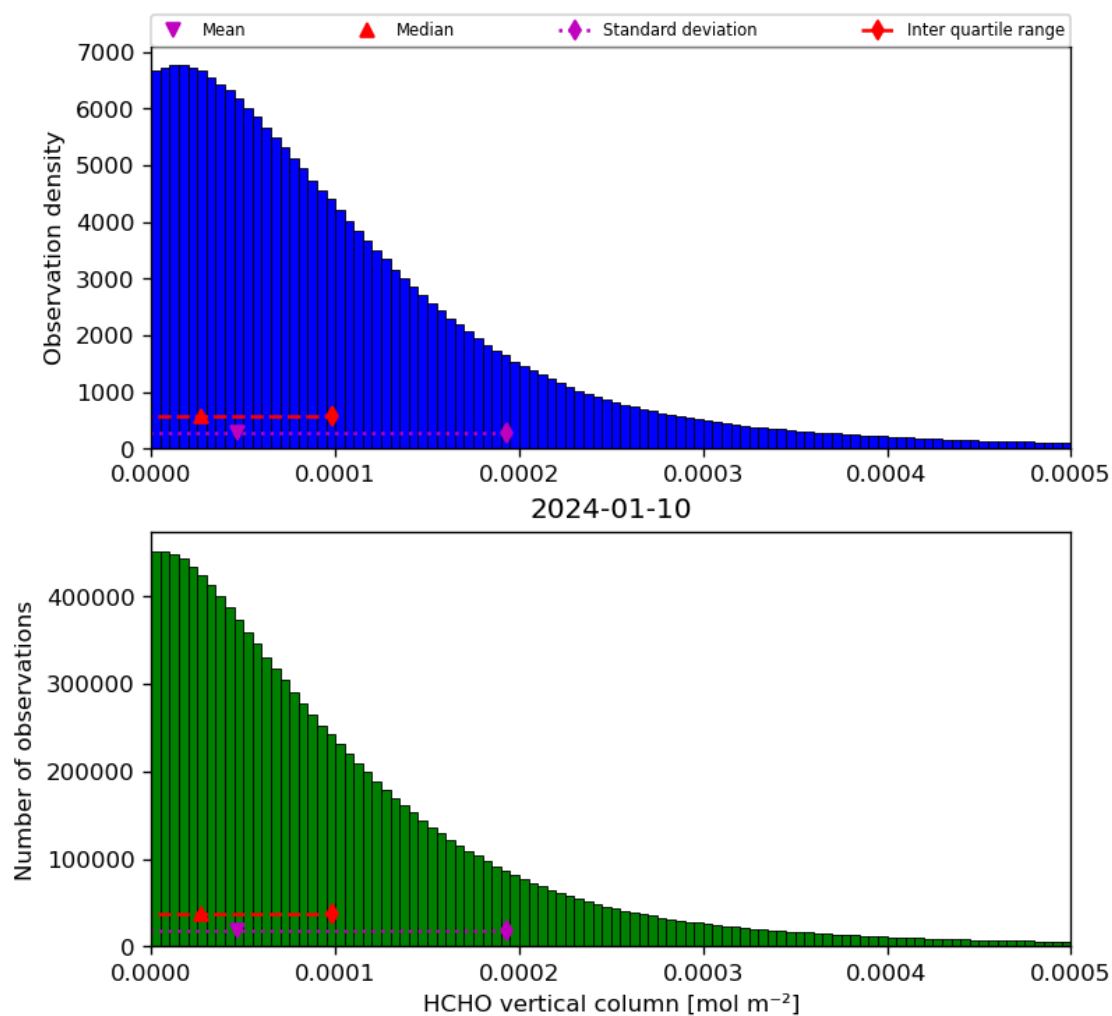
Figure 35: Histogram of “HCHO vertical column” for 2024-01-10 to 2024-01-11
