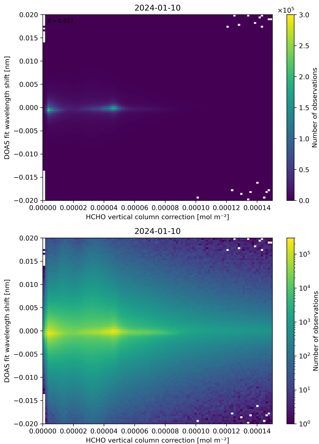
Figure 113: Scatter density plot of “HCHO vertical column correction” against “DOAS fit wavelength shift” for 2024-01-10 to 2024-01-11.
