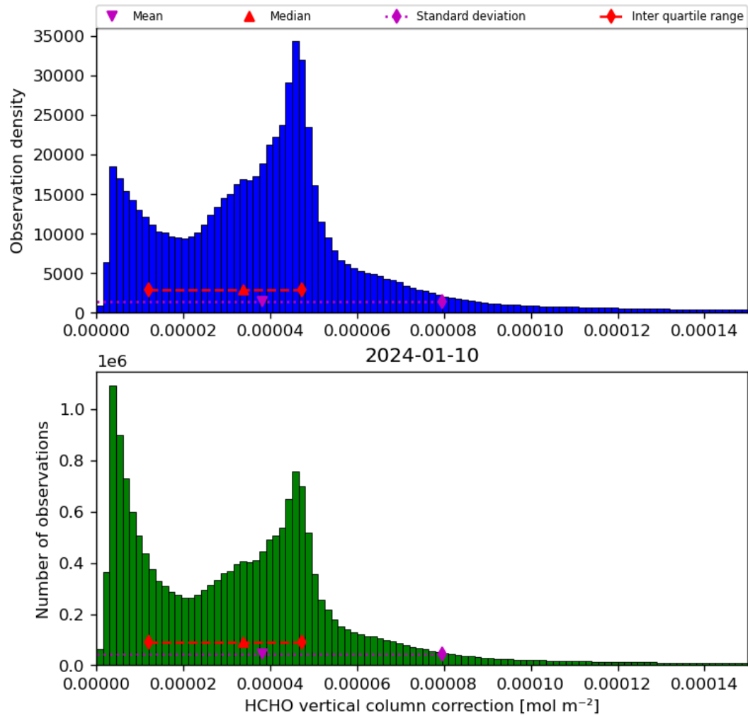
Figure 37: Histogram of “HCHO vertical column correction” for 2024-01-10 to 2024-01-11
