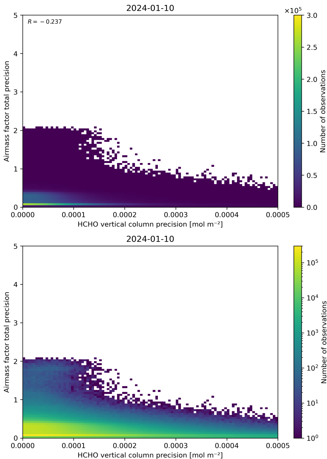
Figure 145: Scatter density plot of “HCHO vertical column precision” against “Airmass factor total precision” for 2024-01-10 to 2024-01-11.
