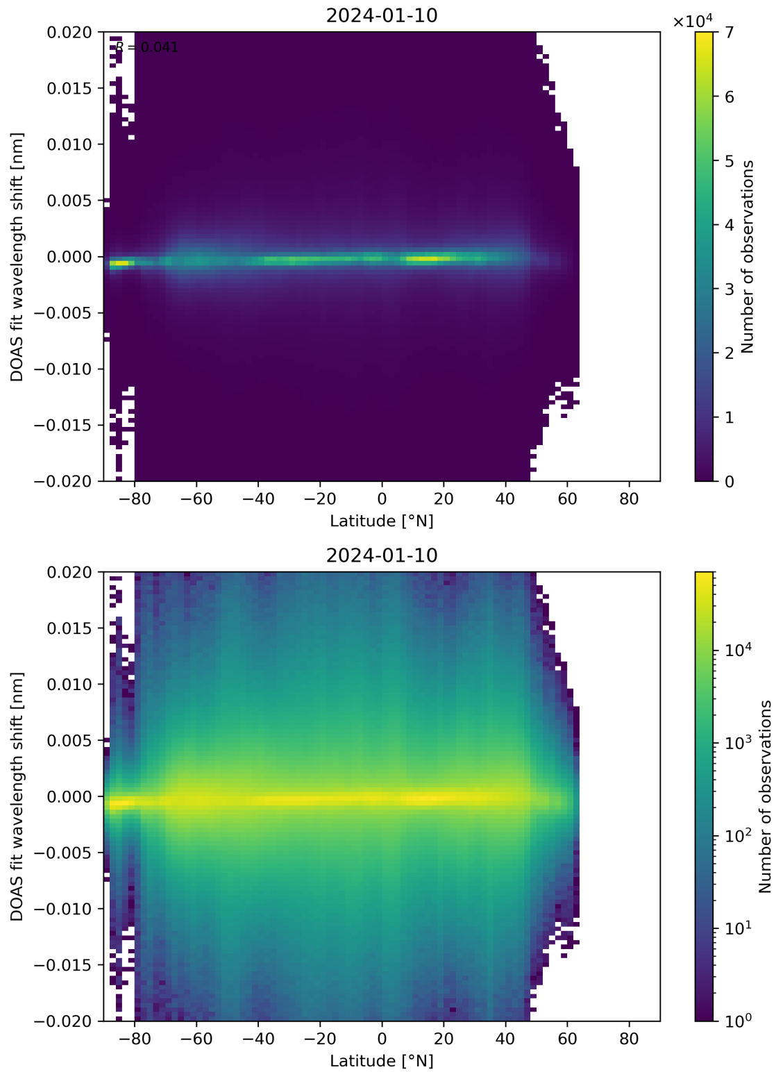
Figure 154: Scatter density plot of “Latitude” against “DOAS fit wavelength shift” for 2024-01-10 to 2024-01-11.
