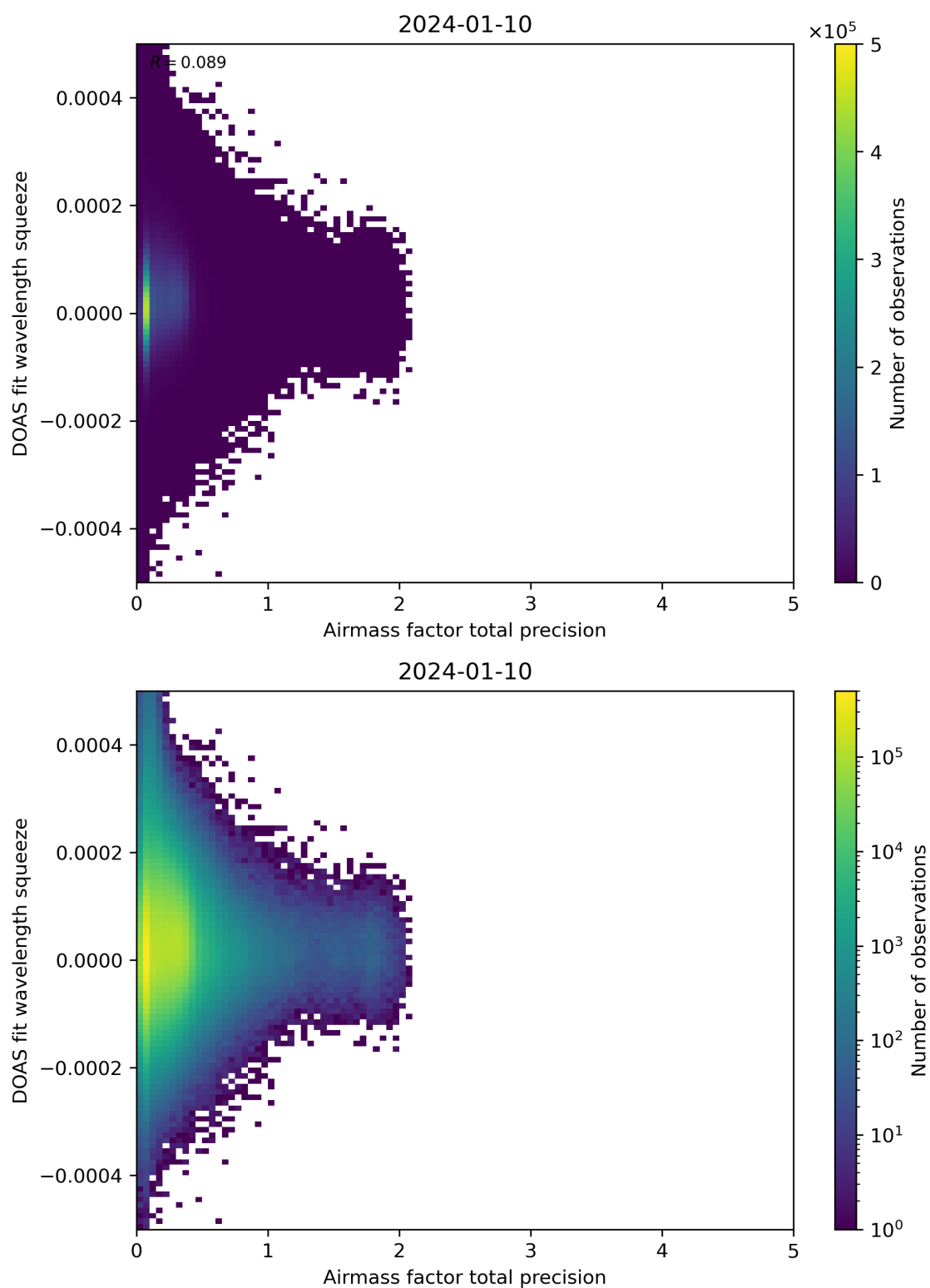
Figure 107: Scatter density plot of “Airmass factor total precision” against “DOAS fit wavelength squeeze” for 2024-01-10 to 2024-01-11.
