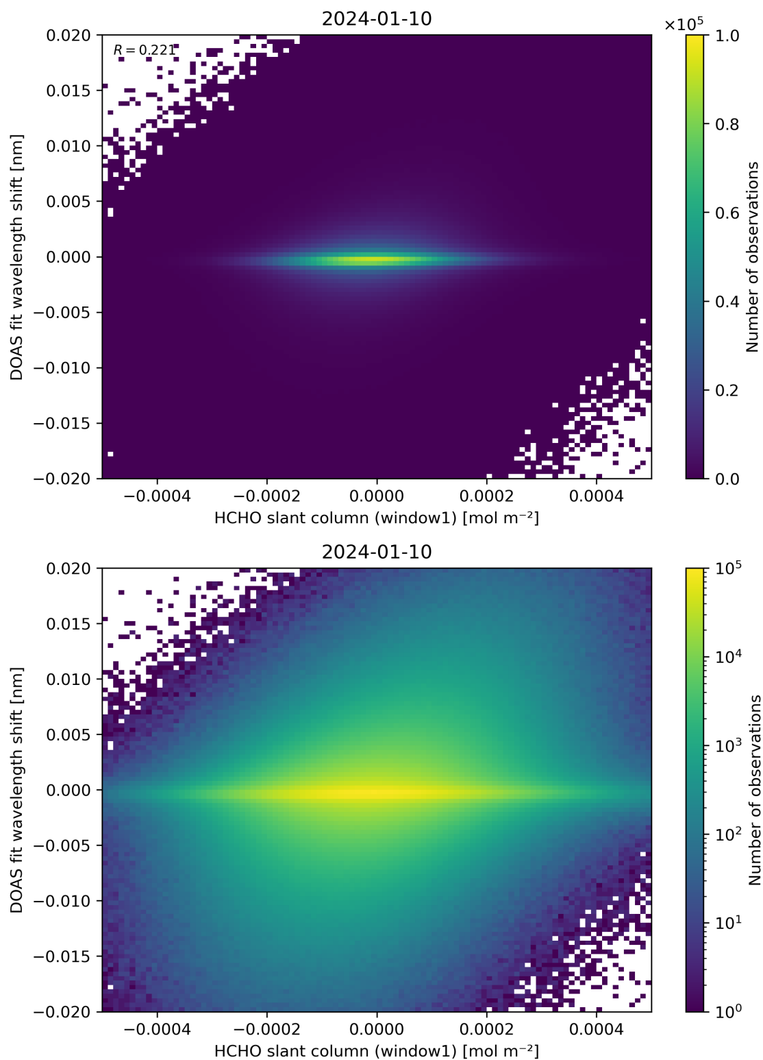
Figure 79: Scatter density plot of “HCHO slant column (window1)” against “DOAS fit wavelength shift” for 2024-01-10 to 2024-01-11.
