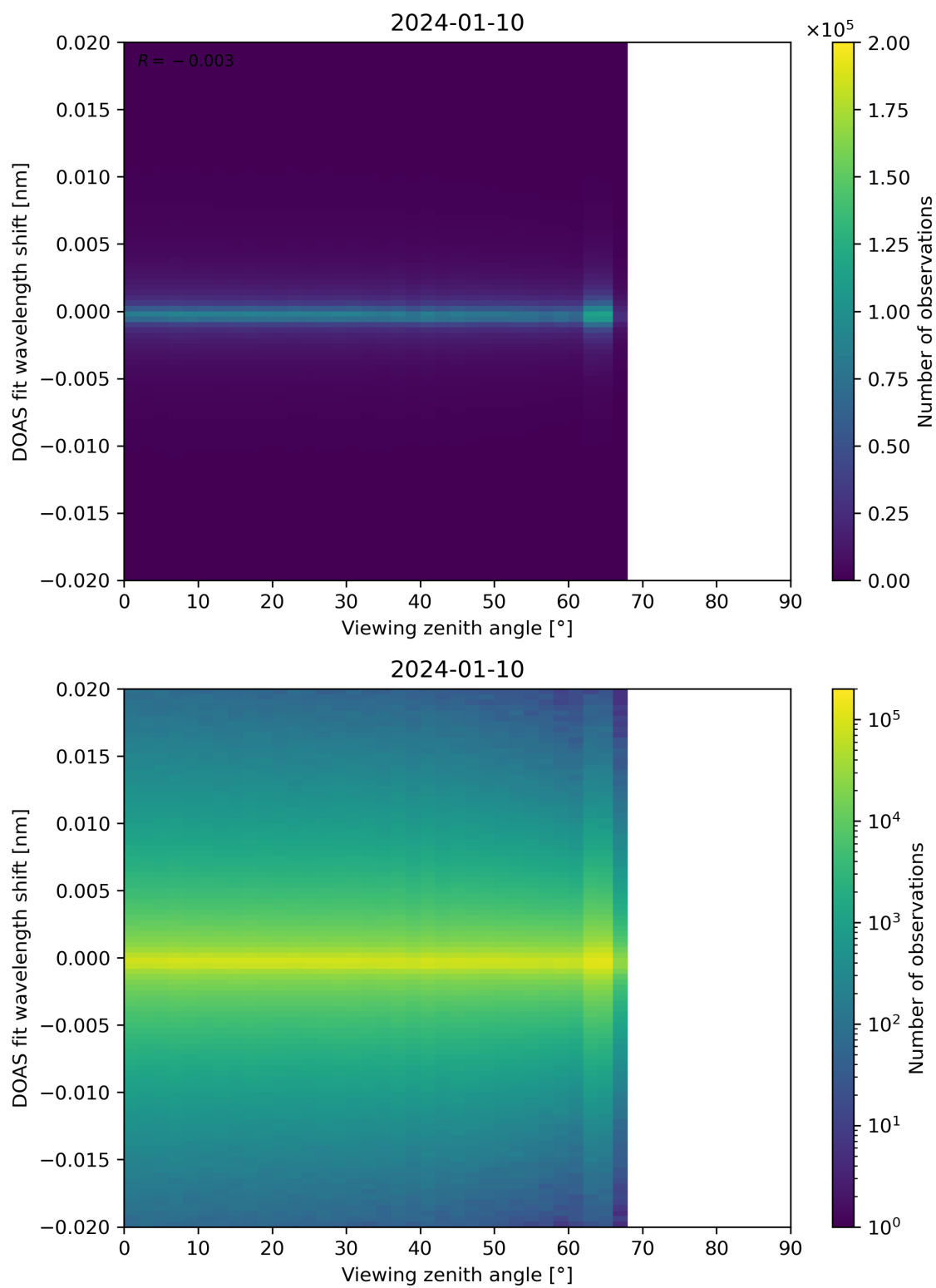
Figure 183: Scatter density plot of “Viewing zenith angle” against “DOAS fit wavelength shift” for 2024-01-10 to 2024-01-11.
