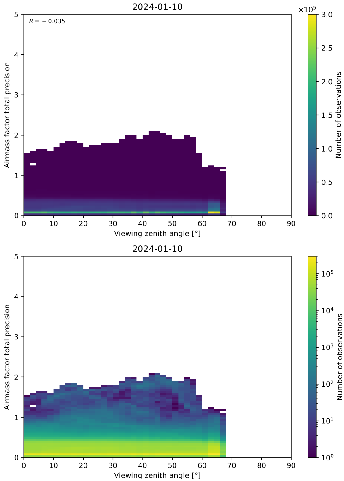
Figure 191: Scatter density plot of “Viewing zenith angle” against “Airmass factor total precision” for 2024-01-10 to 2024-01-11.
