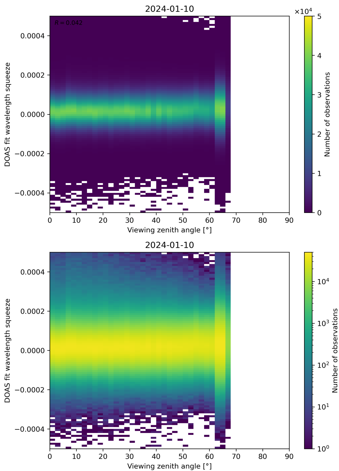
Figure 184: Scatter density plot of “Viewing zenith angle” against “DOAS fit wavelength squeeze” for 2024-01-10 to 2024-01-11.
