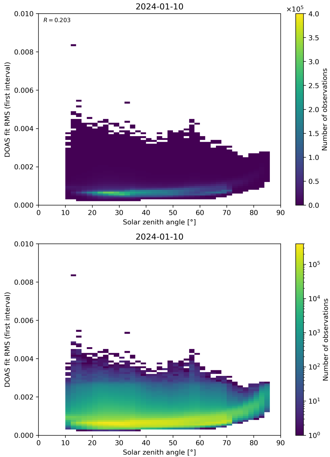
Figure 167: Scatter density plot of “Solar zenith angle” against “DOAS fit RMS (first interval)” for 2024-01-10 to 2024-01-11.
