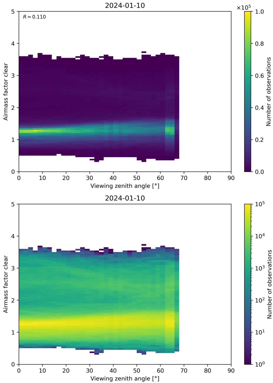
Figure 185: Scatter density plot of “Viewing zenith angle” against “Airmass factor clear” for 2024-01-10 to 2024-01-11.
