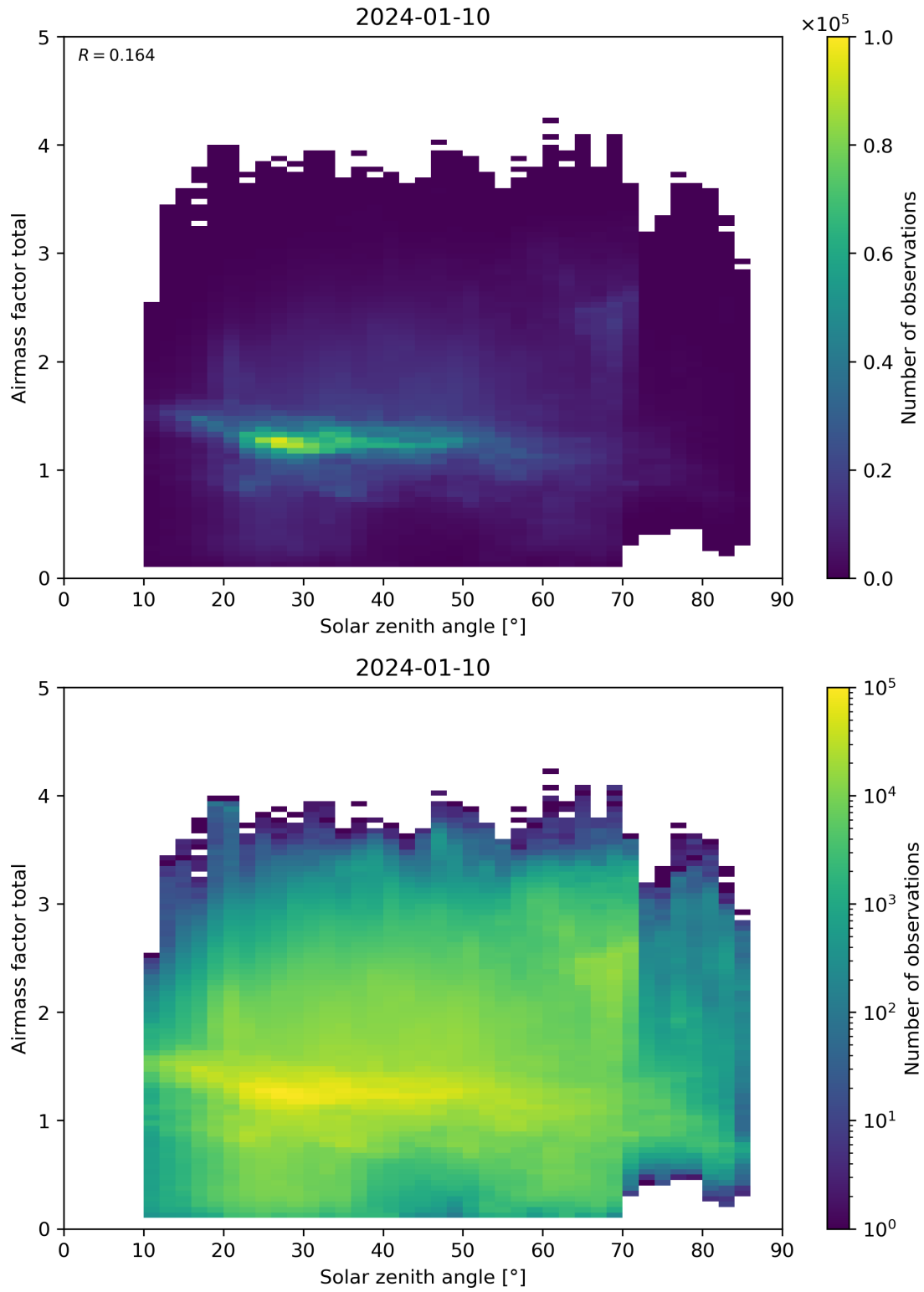
Figure 175: Scatter density plot of “Solar zenith angle” against “Airmass factor total” for 2024-01-10 to 2024-01-11.
