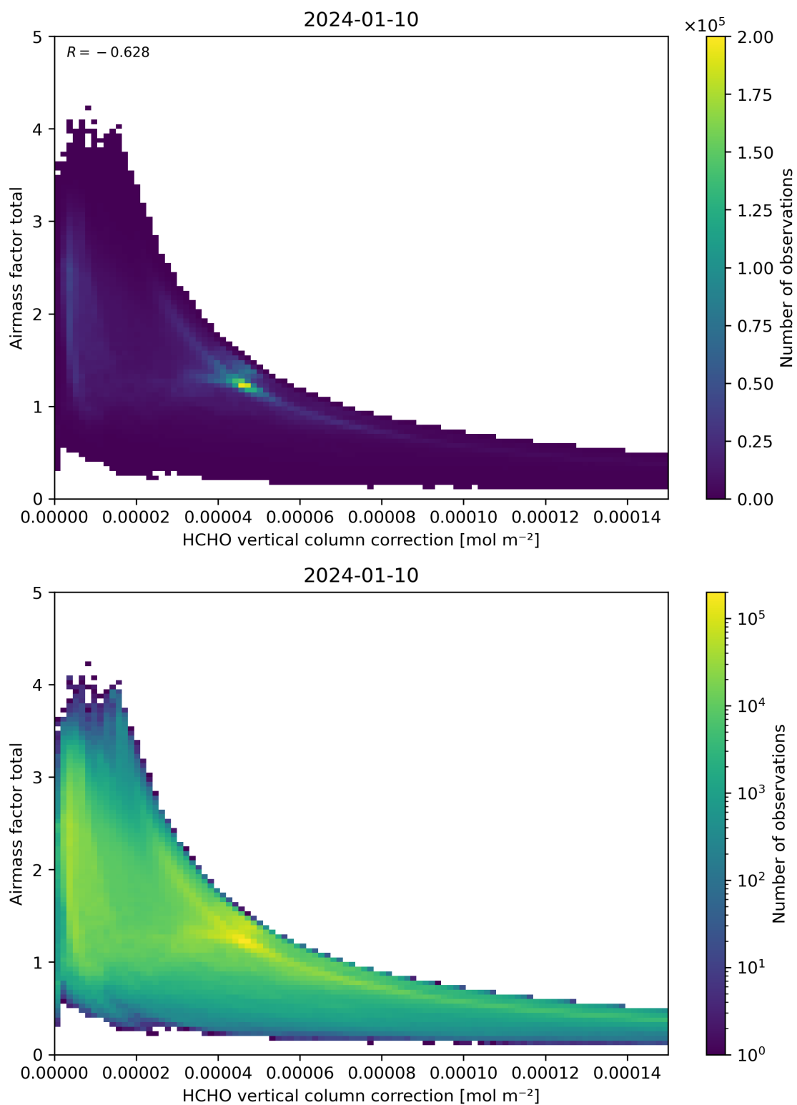
Figure 120: Scatter density plot of “HCHO vertical column correction” against “Airmass factor total” for 2024-01-10 to 2024-01-11.
