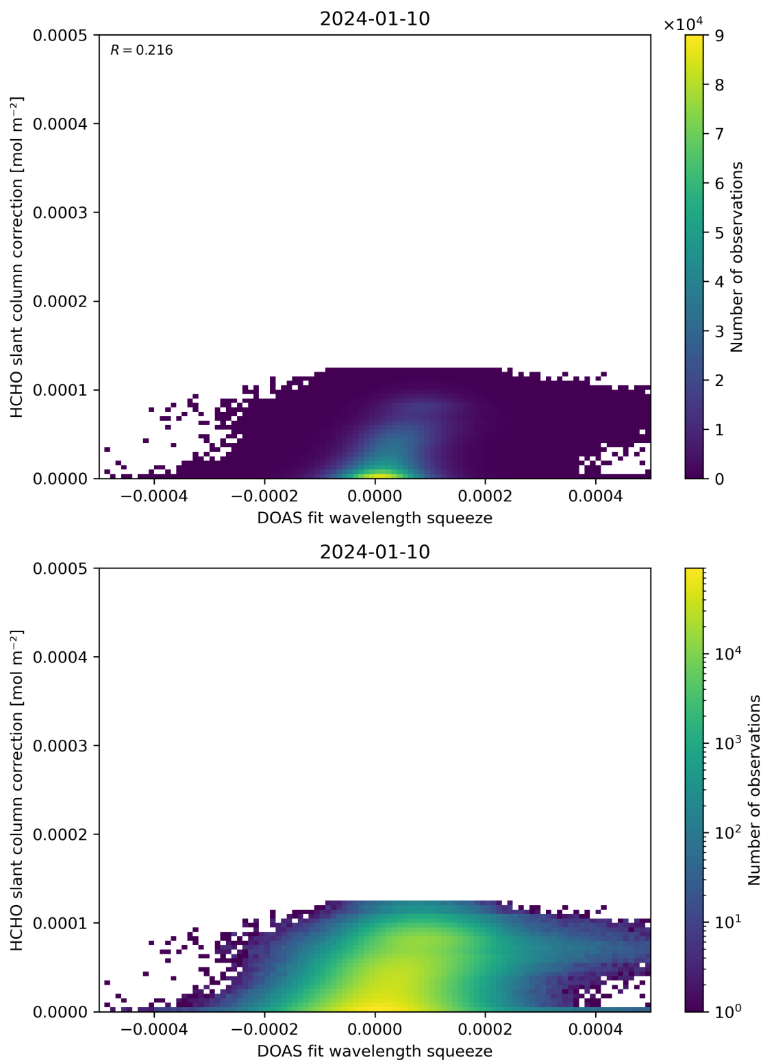
Figure 70: Scatter density plot of “DOAS fit wavelength squeeze” against “HCHO slant column correction” for 2024-01-10 to 2024-01-11.
