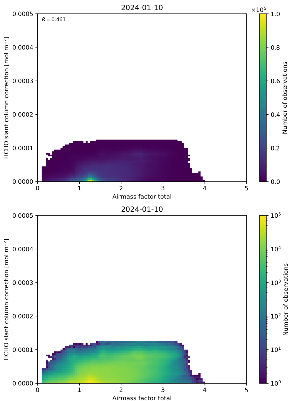
Figure 102: Scatter density plot of “Airmass factor total” against “HCHO slant column correction” for 2024-01-10 to 2024-01-11.
