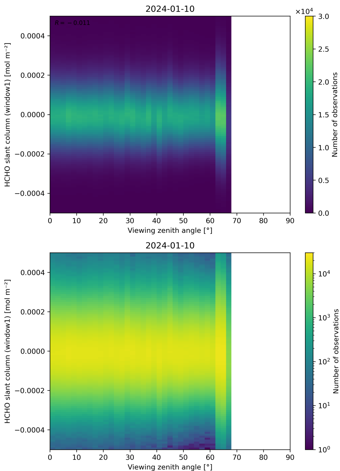
Figure 188: Scatter density plot of “Viewing zenith angle” against “HCHO slant column (window1)” for 2024-01-10 to 2024-01-11.
