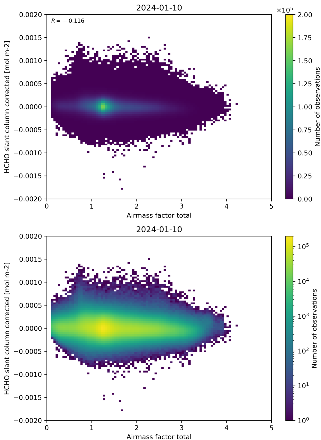
Figure 101: Scatter density plot of “Airmass factor total” against “HCHO slant column corrected” for 2024-01-10 to 2024-01-11.
