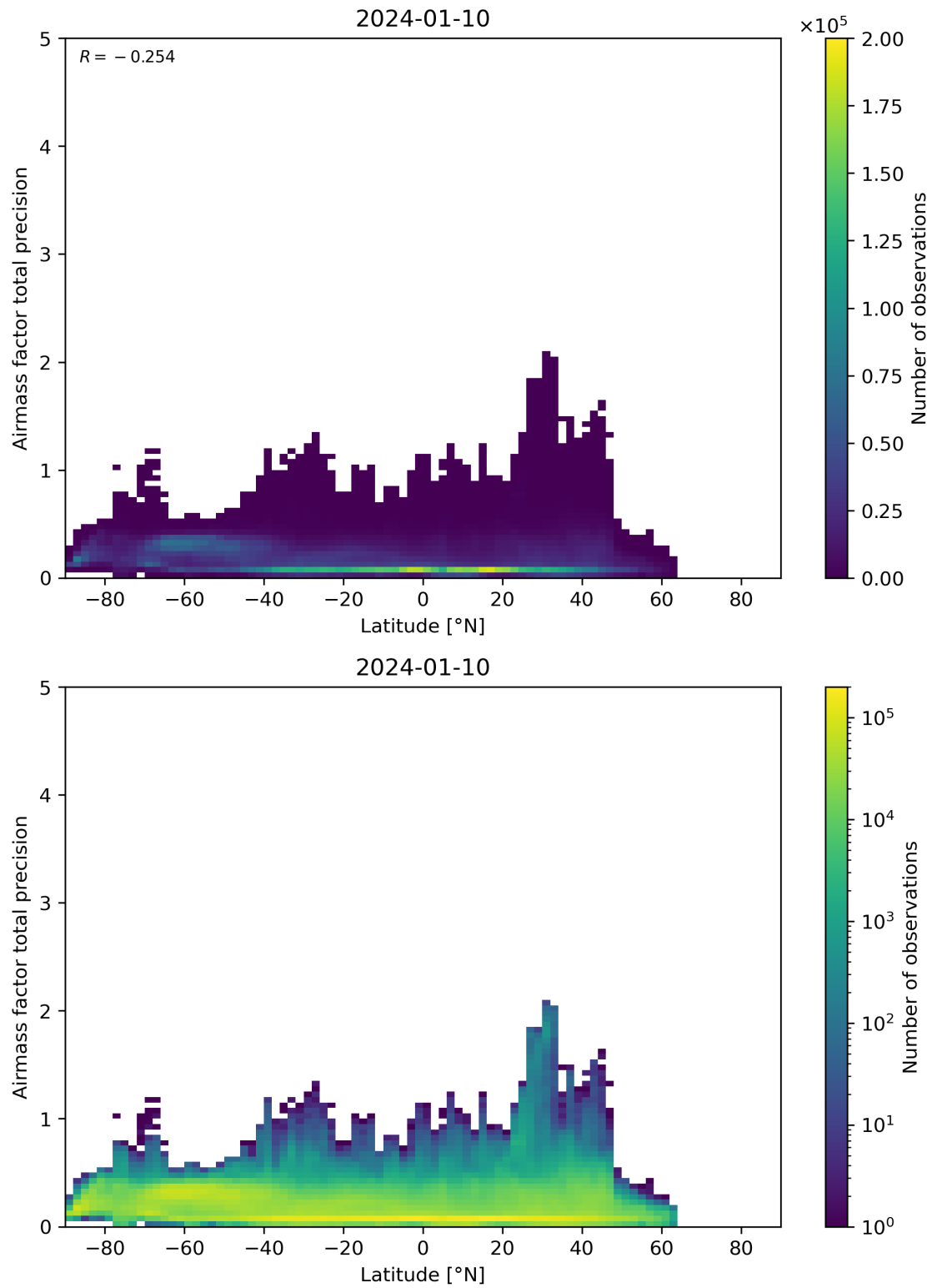
Figure 162: Scatter density plot of “Latitude” against “Airmass factor total precision” for 2024-01-10 to 2024-01-11.
