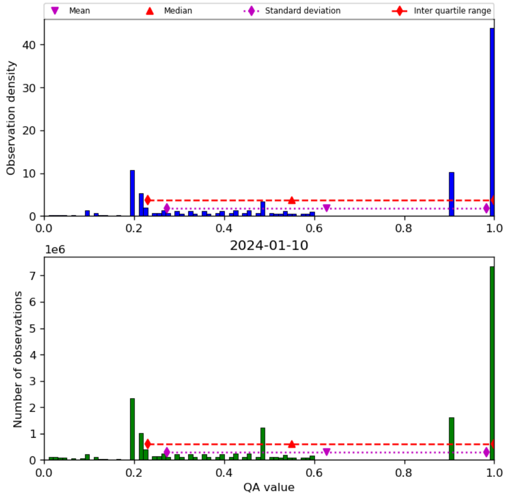
Figure 34: Histogram of “QA value” for 2024-01-10 to 2024-01-11
