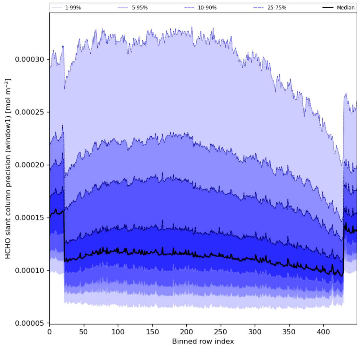
Figure 53: Along track statistics of “HCHO slant column precision (window1)” for 2024-01-10 to 2024-01-11
