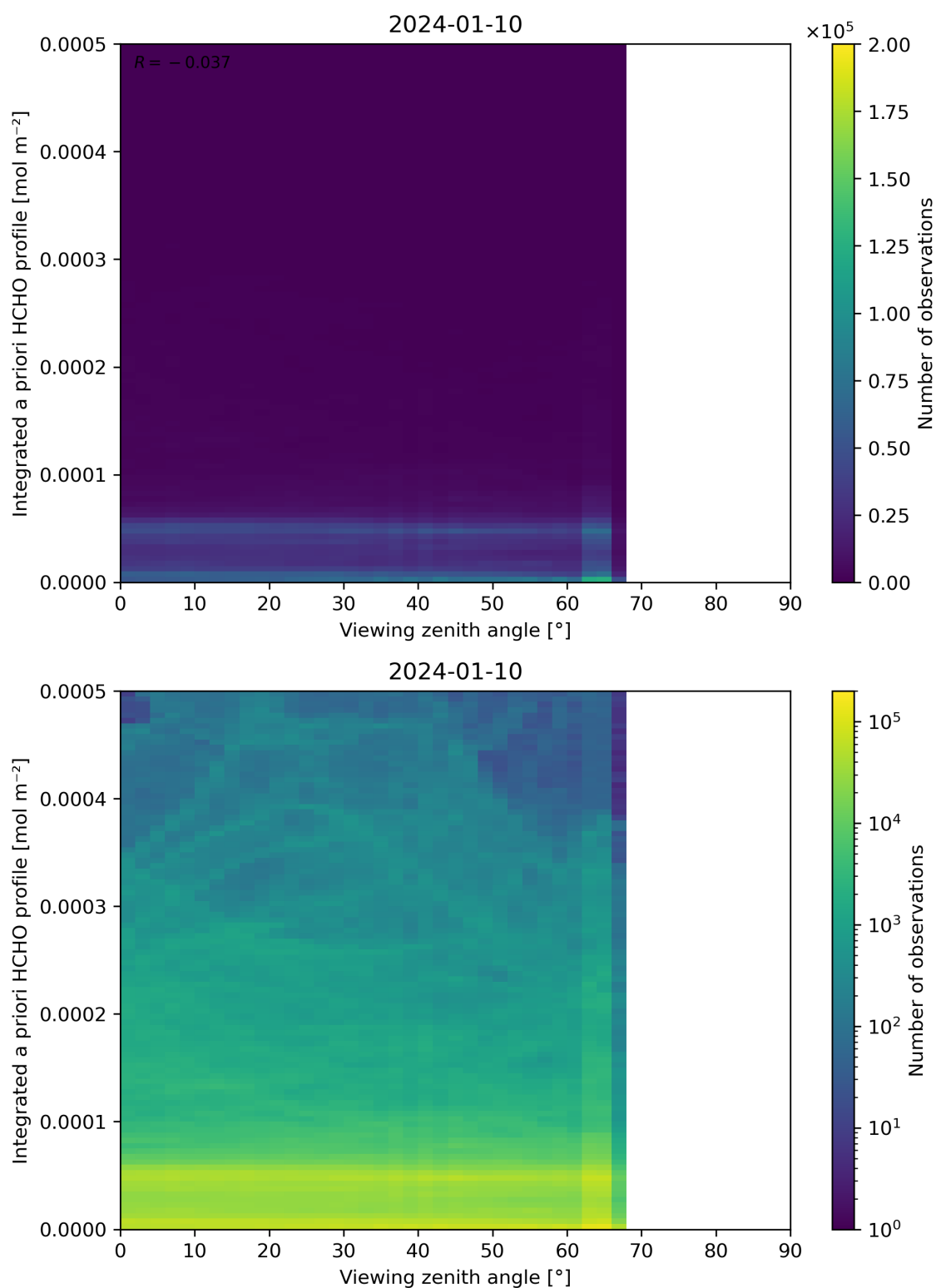
Figure 195: Scatter density plot of “Viewing zenith angle” against “Integrated a priori HCHO profile” for 2024-01-10 to 2024-01-11.
