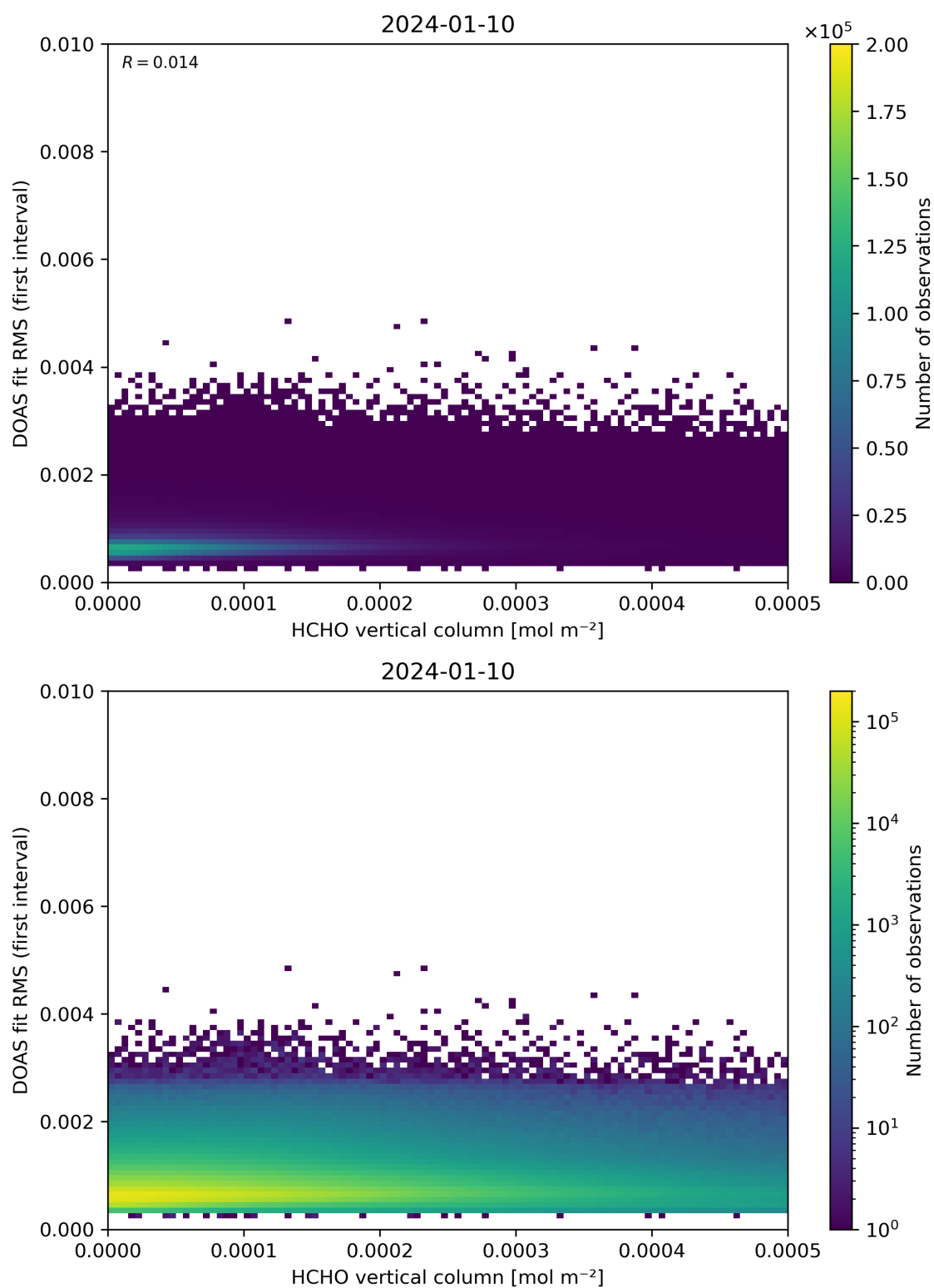
Figure 123: Scatter density plot of “HCHO vertical column” against “DOAS fit RMS (first interval)” for 2024-01-10 to 2024-01-11.
