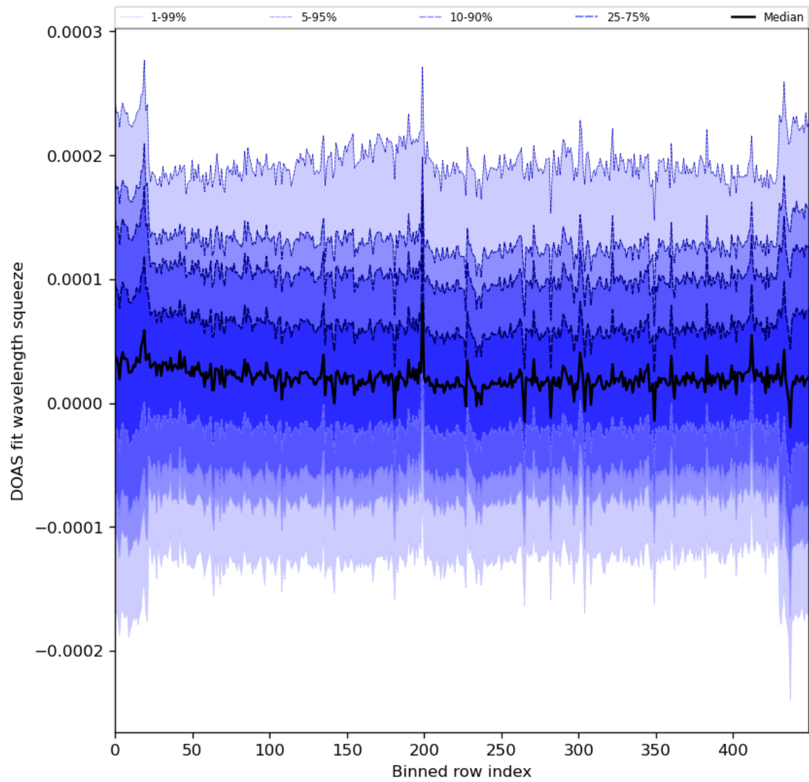
Figure 59: Along track statistics of “DOAS fit wavelength squeeze” for 2024-01-10 to 2024-01-11
