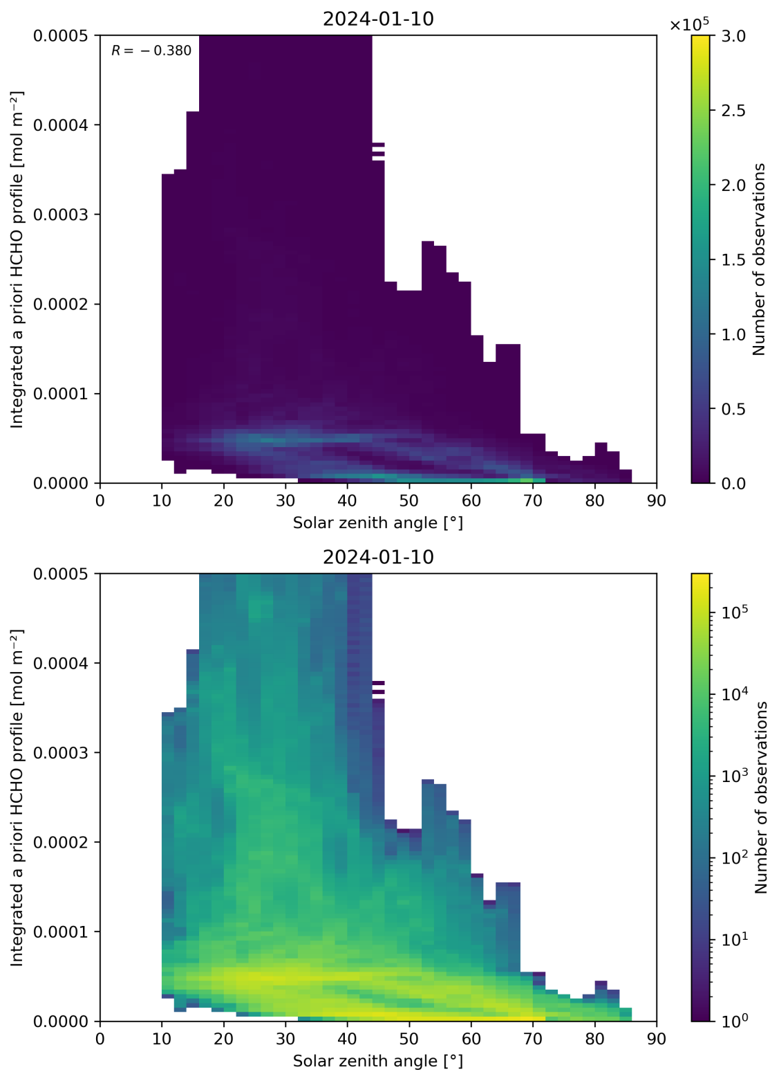
Figure 180: Scatter density plot of “Solar zenith angle” against “Integrated a priori HCHO profile” for 2024-01-10 to 2024-01-11.
