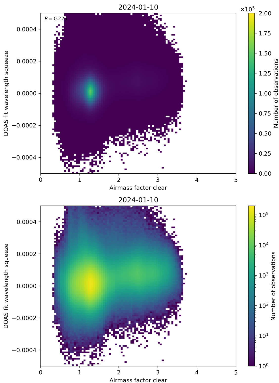
Figure 73: Scatter density plot of “Airmass factor clear” against “DOAS fit wavelength squeeze” for 2024-01-10 to 2024-01-11.
