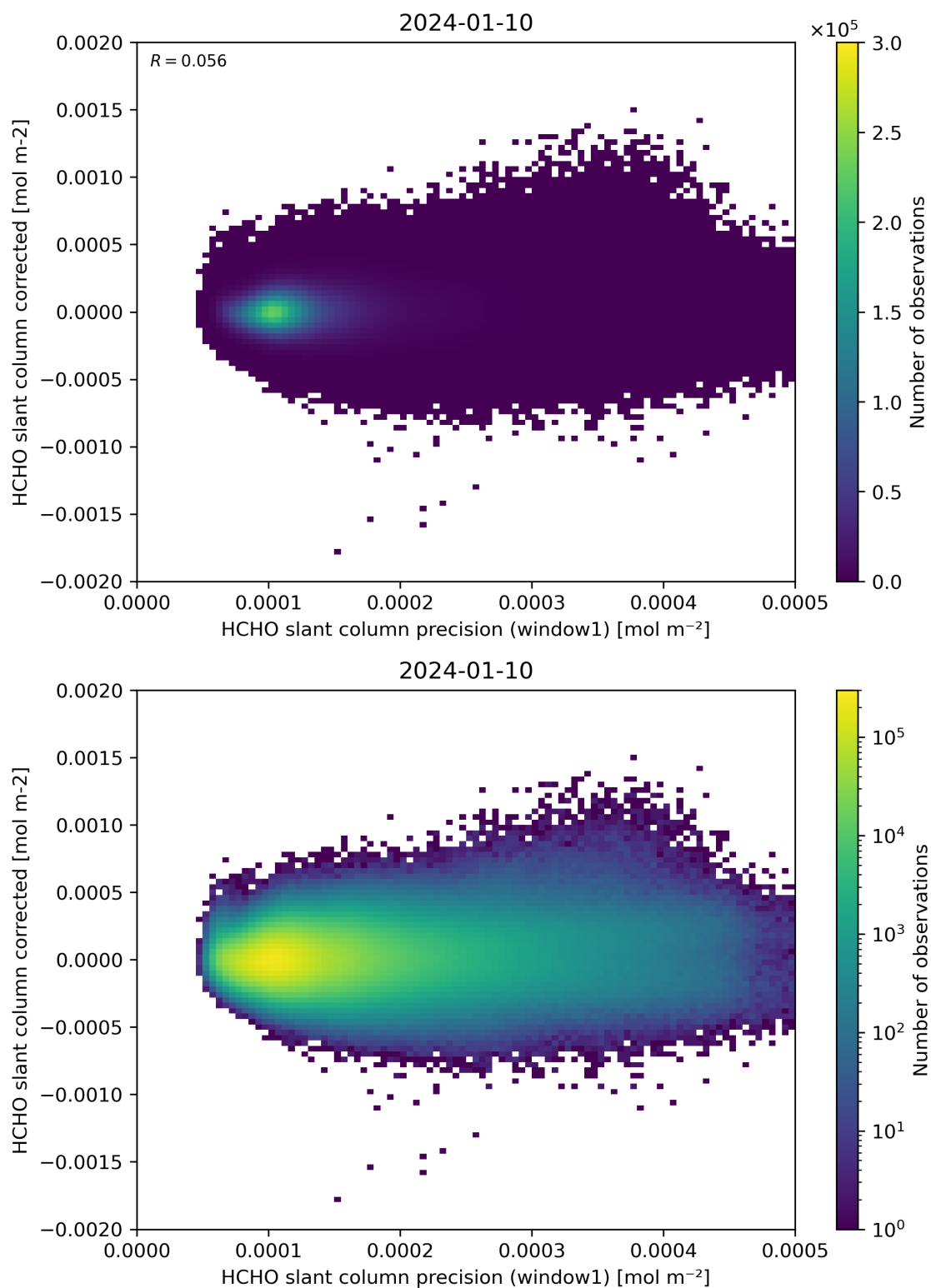
Figure 92: Scatter density plot of “HCHO slant column precision (window1)” against “HCHO slant column corrected” for 2024-01-10 to 2024-01-11.
