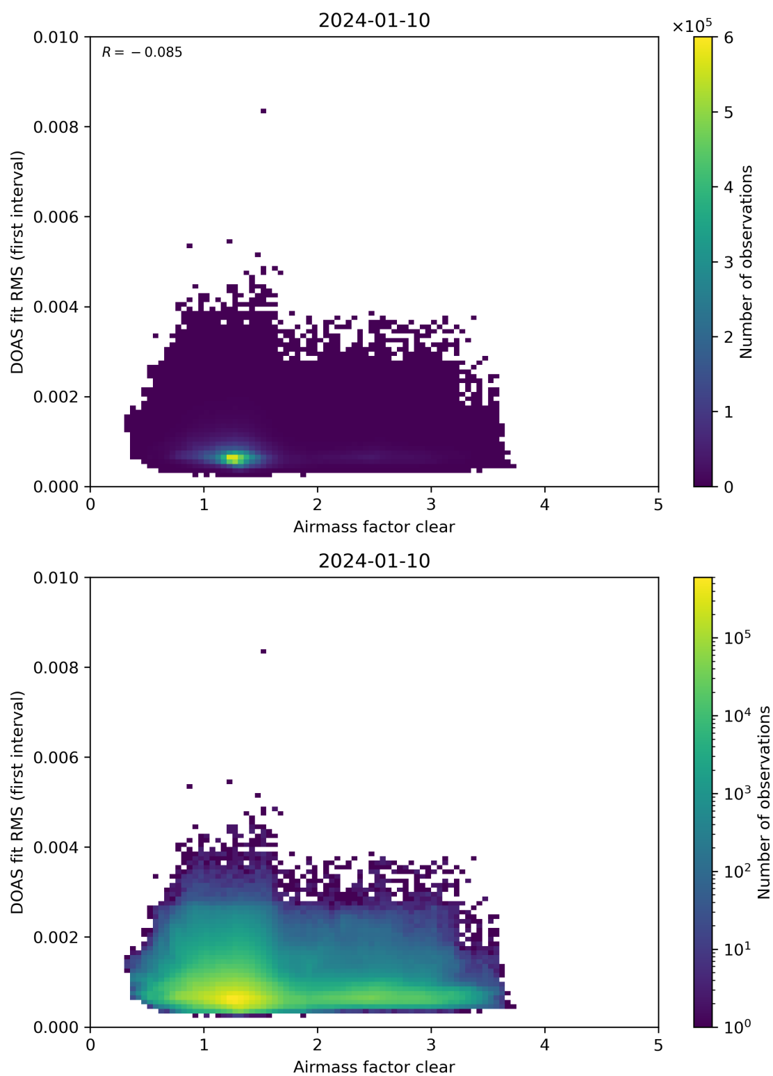
Figure 71: Scatter density plot of “Airmass factor clear” against “DOAS fit RMS (first interval)” for 2024-01-10 to 2024-01-11.
