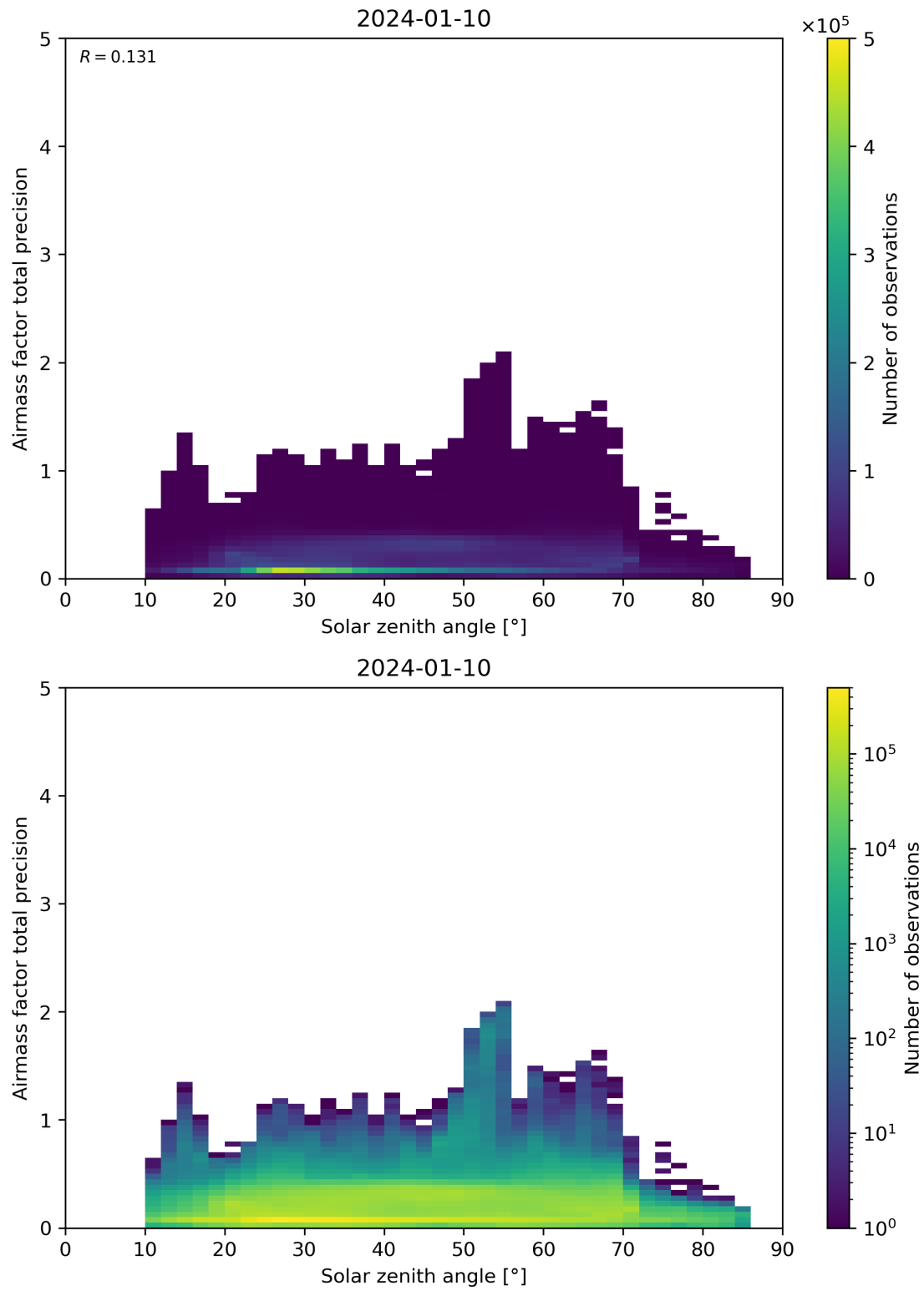
Figure 176: Scatter density plot of “Solar zenith angle” against “Airmass factor total precision” for 2024-01-10 to 2024-01-11.
