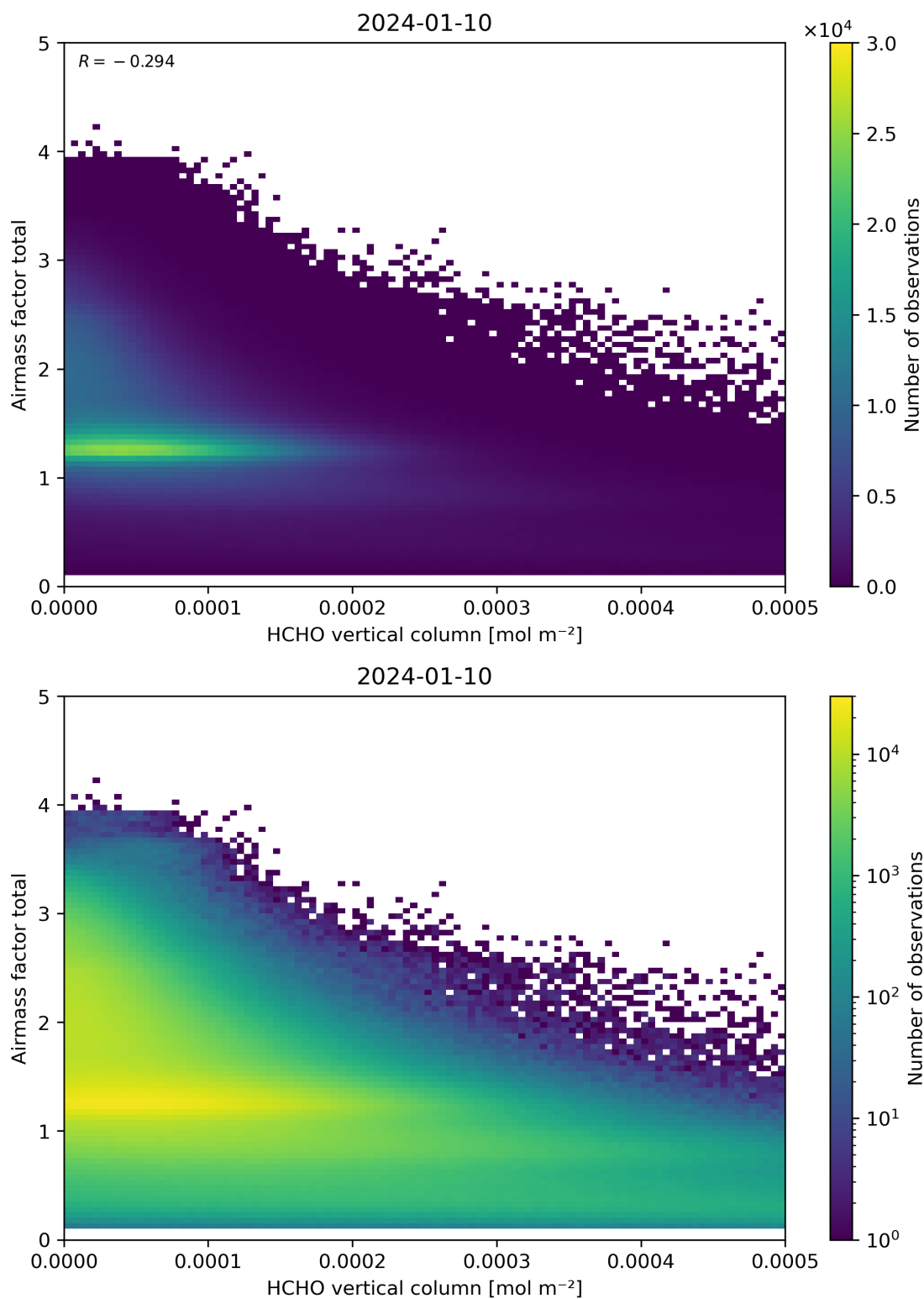
Figure 131: Scatter density plot of “HCHO vertical column” against “Airmass factor total” for 2024-01-10 to 2024-01-11.
