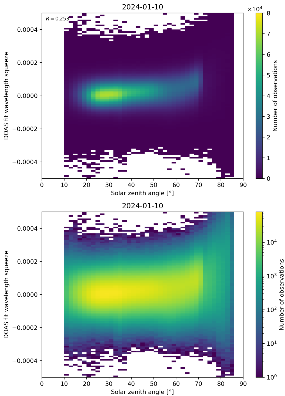
Figure 169: Scatter density plot of “Solar zenith angle” against “DOAS fit wavelength squeeze” for 2024-01-10 to 2024-01-11.
