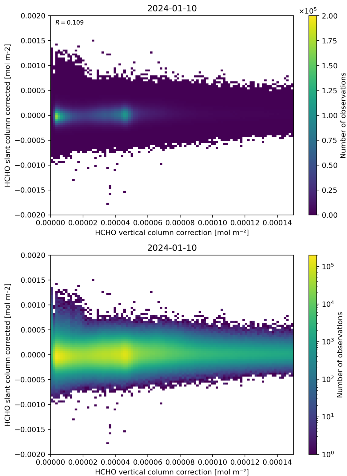
Figure 116: Scatter density plot of “HCHO vertical column correction” against “HCHO slant column corrected” for 2024-01-10 to 2024-01-11.
