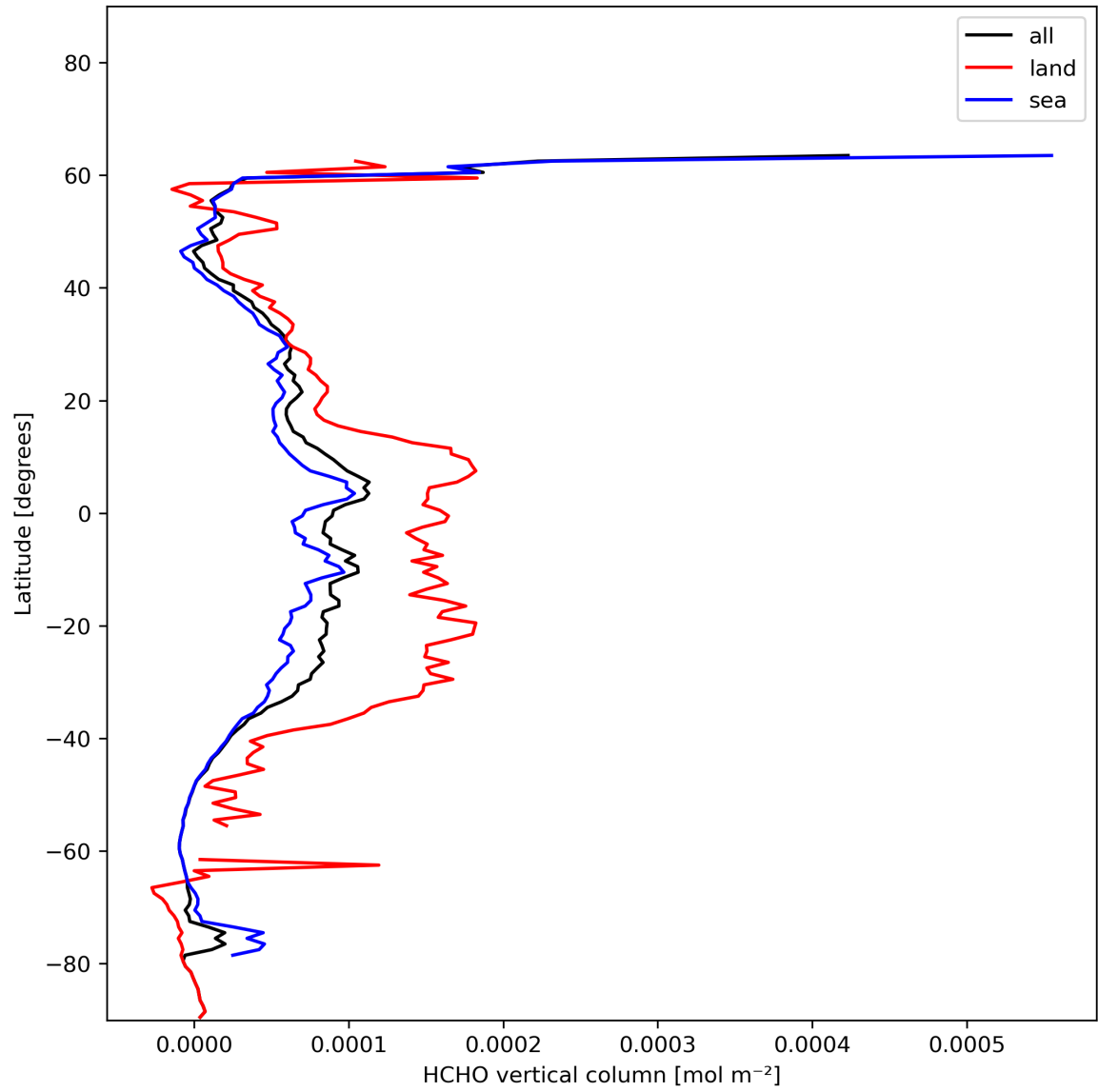
Figure 21: Zonal average of “HCHO vertical column” for 2024-01-10 to 2024-01-11.
