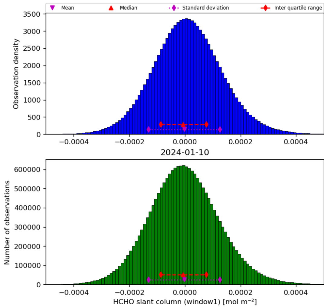
Figure 38: Histogram of “HCHO slant column (window1)” for 2024-01-10 to 2024-01-11
