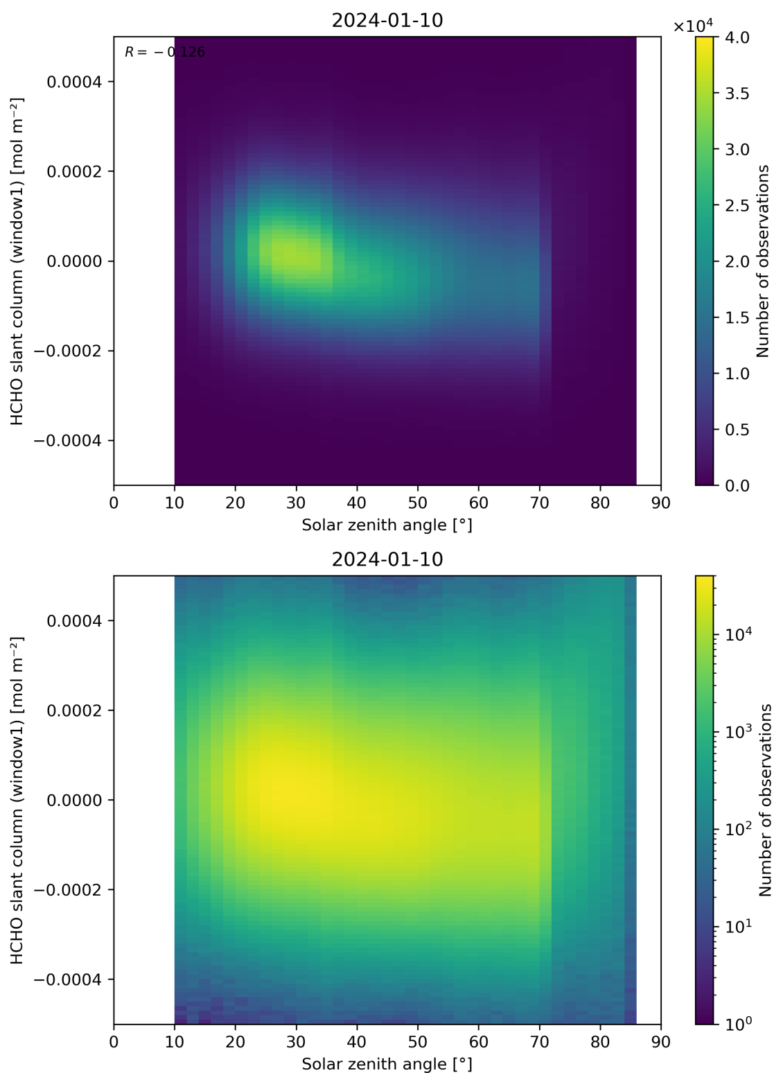
Figure 173: Scatter density plot of “Solar zenith angle” against “HCHO slant column (window1)” for 2024-01-10 to 2024-01-11.
