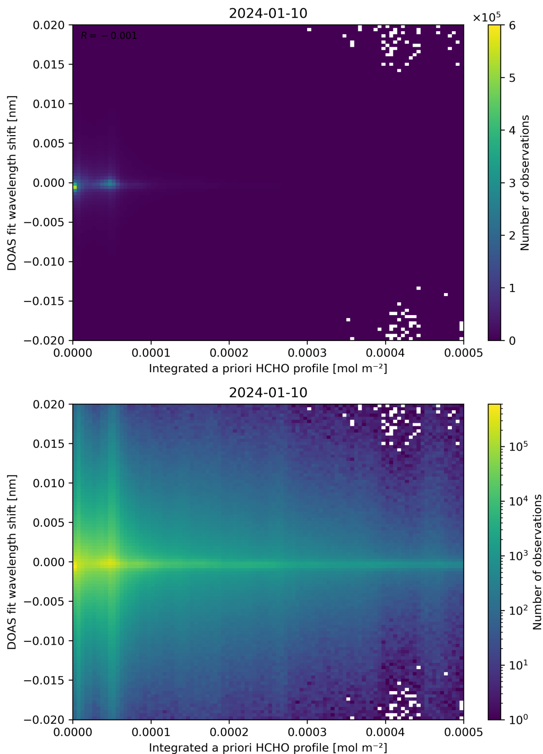
Figure 149: Scatter density plot of “Integrated a priori HCHO profile” against “DOAS fit wavelength shift” for 2024-01-10 to 2024-01-11.
