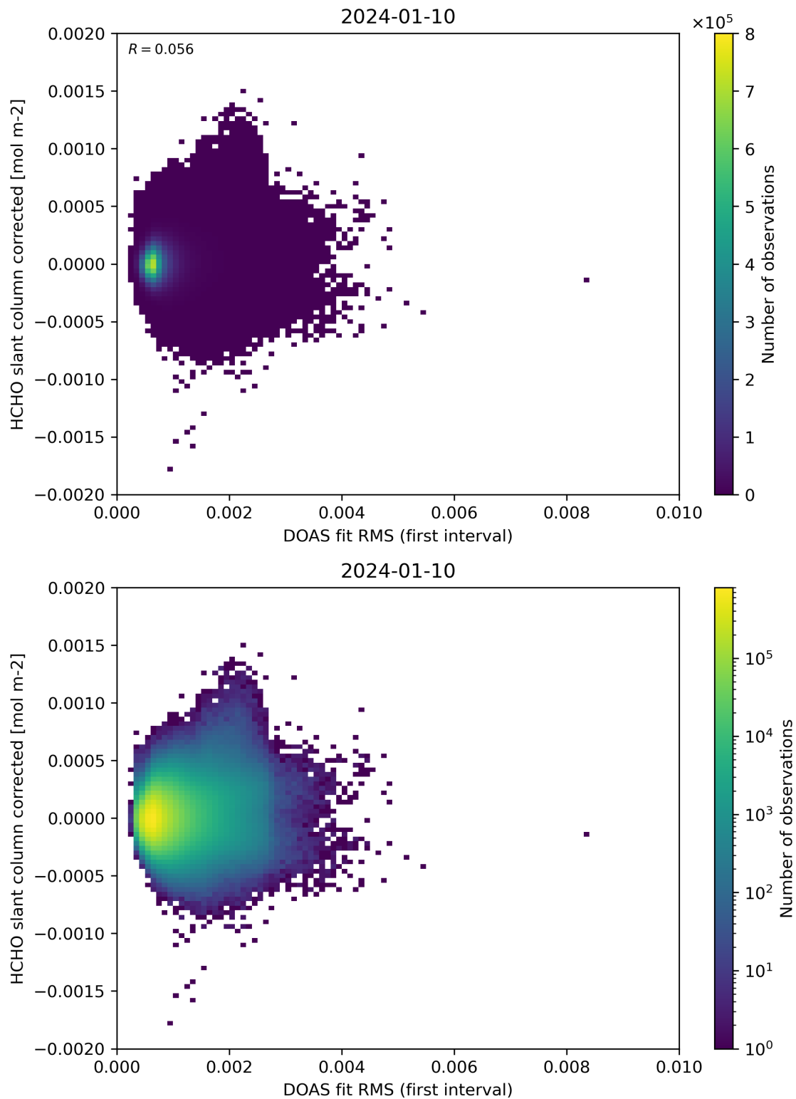
Figure 62: Scatter density plot of “DOAS fit RMS (first interval)” against “HCHO slant column corrected” for 2024-01-10 to 2024-01-11.
