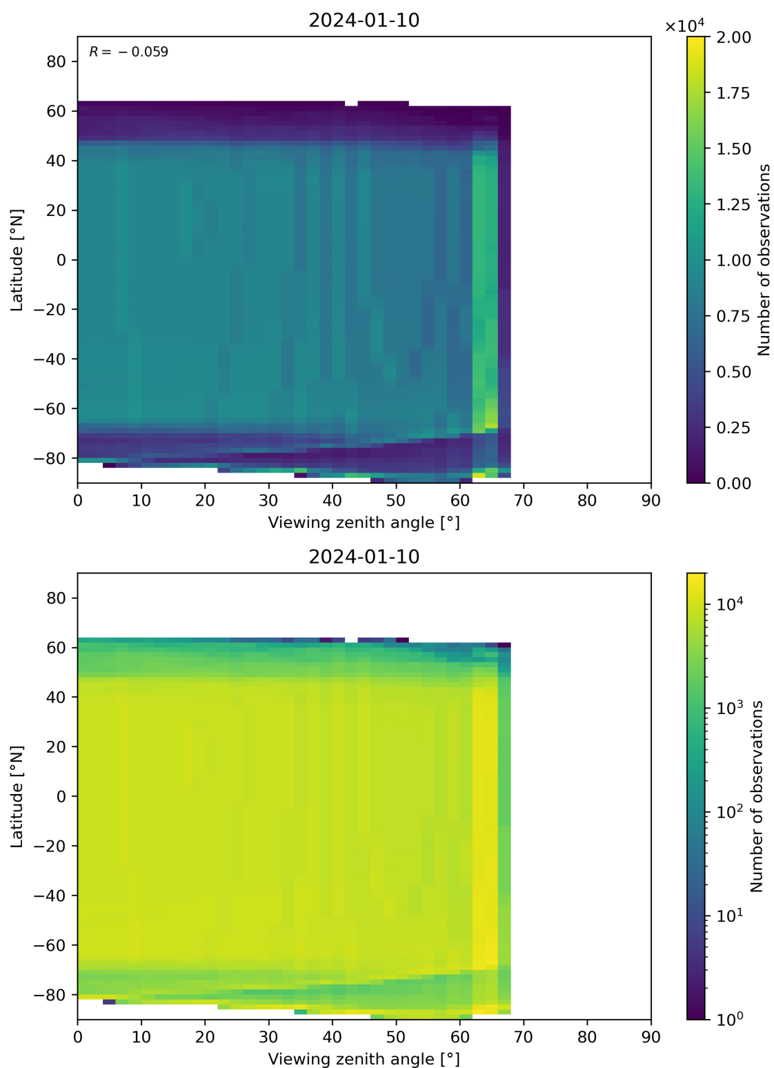
Figure 196: Scatter density plot of “Viewing zenith angle” against “Latitude” for 2024-01-10 to 2024-01-11.
