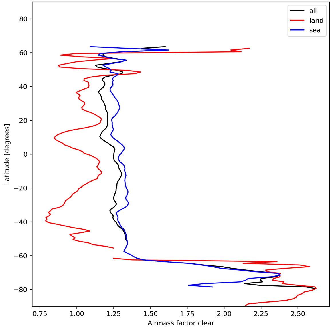
Figure 28: Zonal average of “Airmass factor clear” for 2024-01-10 to 2024-01-11.
