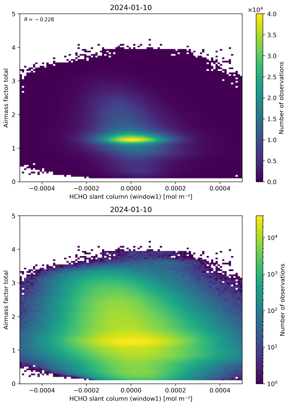
Figure 85: Scatter density plot of “HCHO slant column (window1)” against “Airmass factor total” for 2024-01-10 to 2024-01-11.
