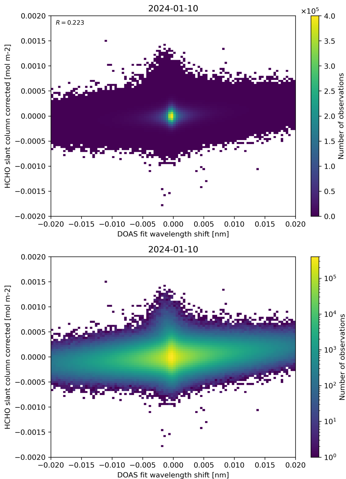
Figure 66: Scatter density plot of “DOAS fit wavelength shift” against “HCHO slant column corrected” for 2024-01-10 to 2024-01-11.
