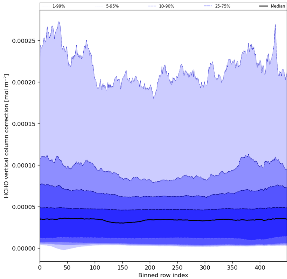
Figure 51: Along track statistics of “HCHO vertical column correction” for 2024-01-10 to 2024-01-11
