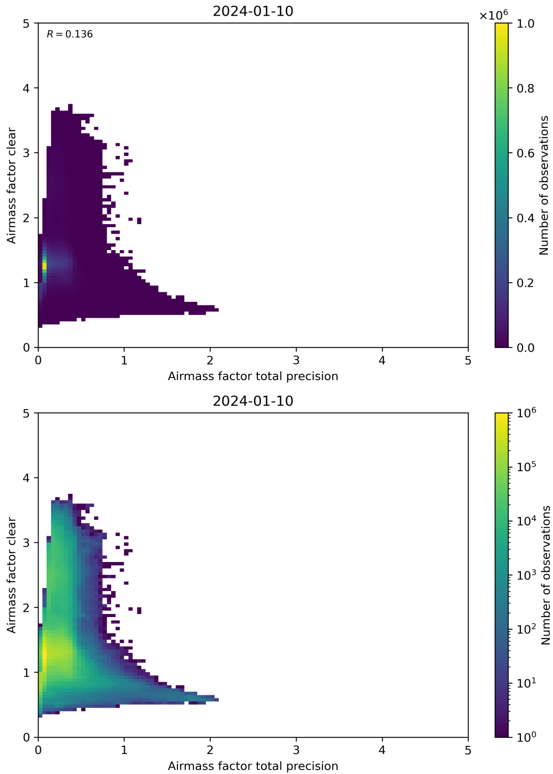
Figure 108: Scatter density plot of “Airmass factor total precision” against “Airmass factor clear” for 2024-01-10 to 2024-01-11.
