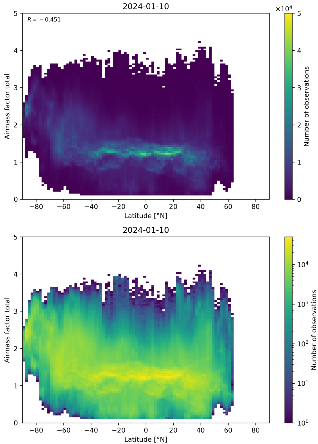
Figure 161: Scatter density plot of “Latitude” against “Airmass factor total” for 2024-01-10 to 2024-01-11.
