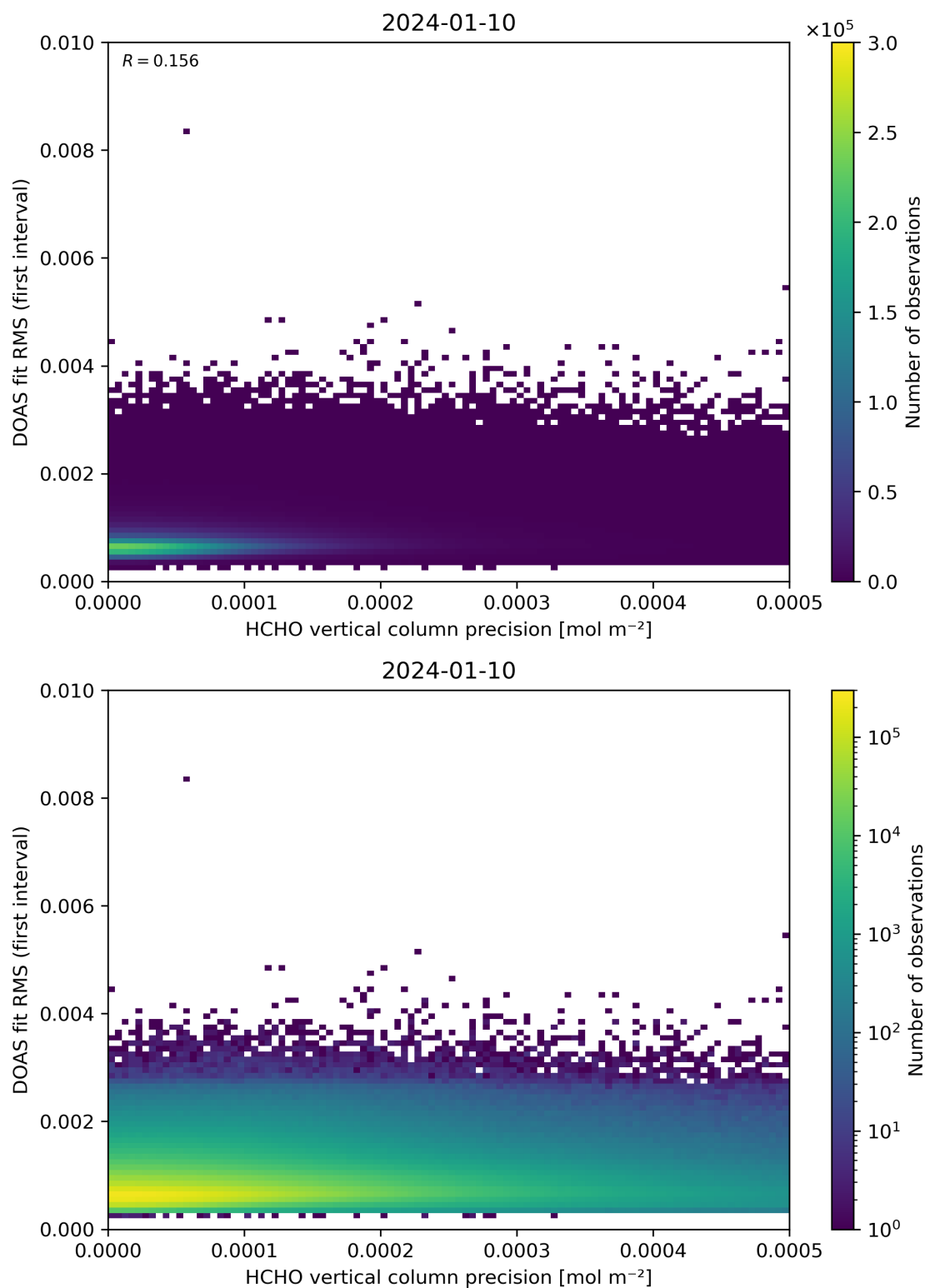
Figure 136: Scatter density plot of “HCHO vertical column precision” against “DOAS fit RMS (first interval)” for 2024-01-10 to 2024-01-11.
