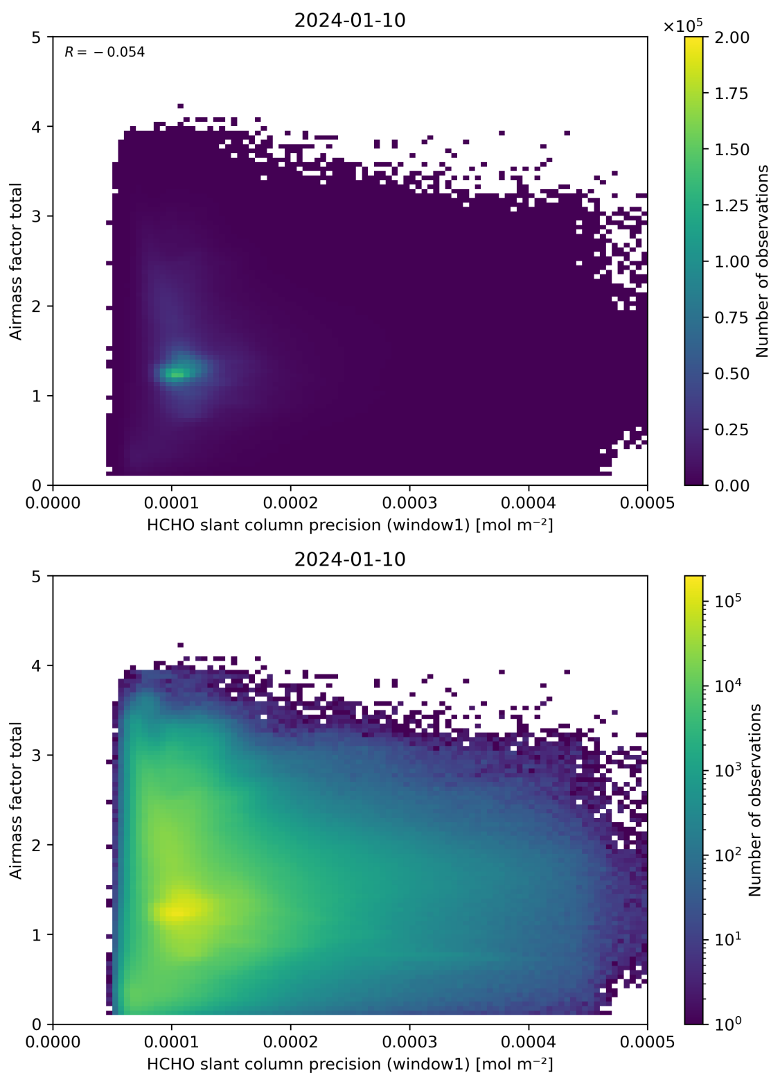
Figure 94: Scatter density plot of “HCHO slant column precision (window1)” against “Airmass factor total” for 2024-01-10 to 2024-01-11.
