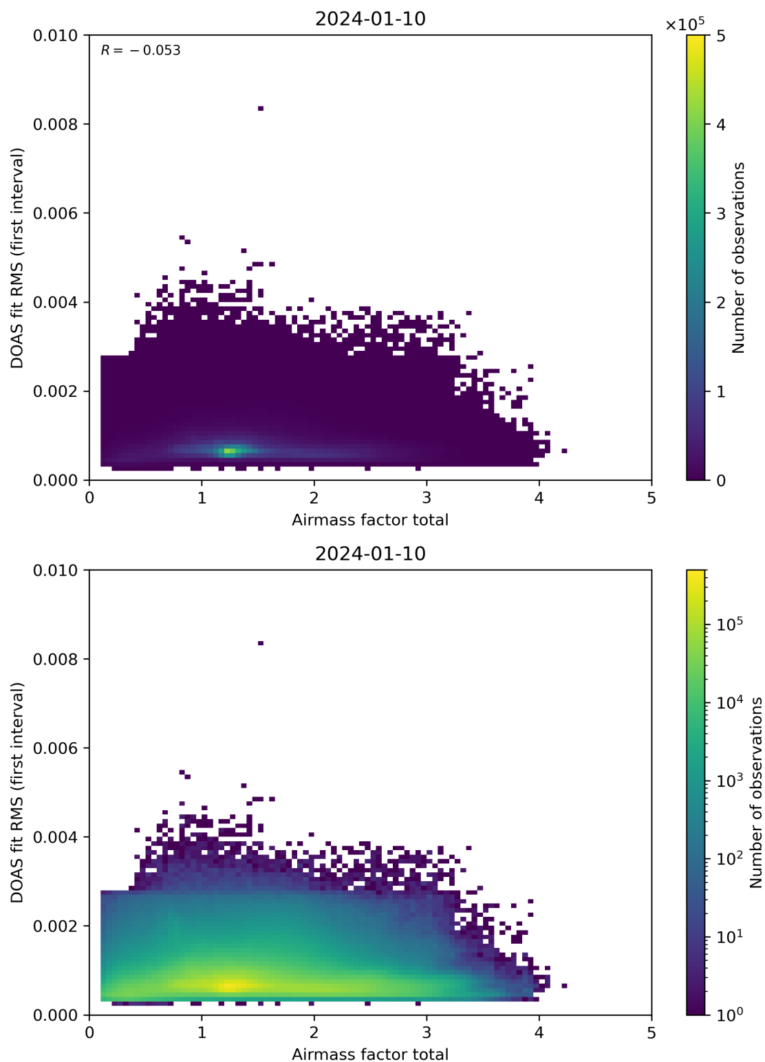
Figure 97: Scatter density plot of “Airmass factor total” against “DOAS fit RMS (first interval)” for 2024-01-10 to 2024-01-11.
