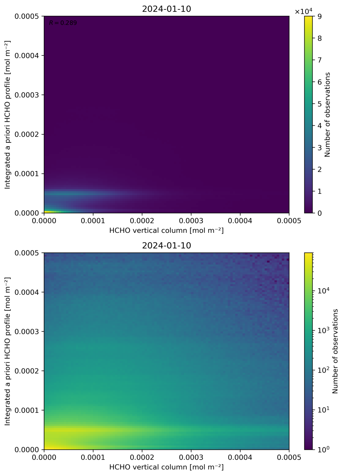
Figure 135: Scatter density plot of “HCHO vertical column” against “Integrated a priori HCHO profile” for 2024-01-10 to 2024-01-11.
