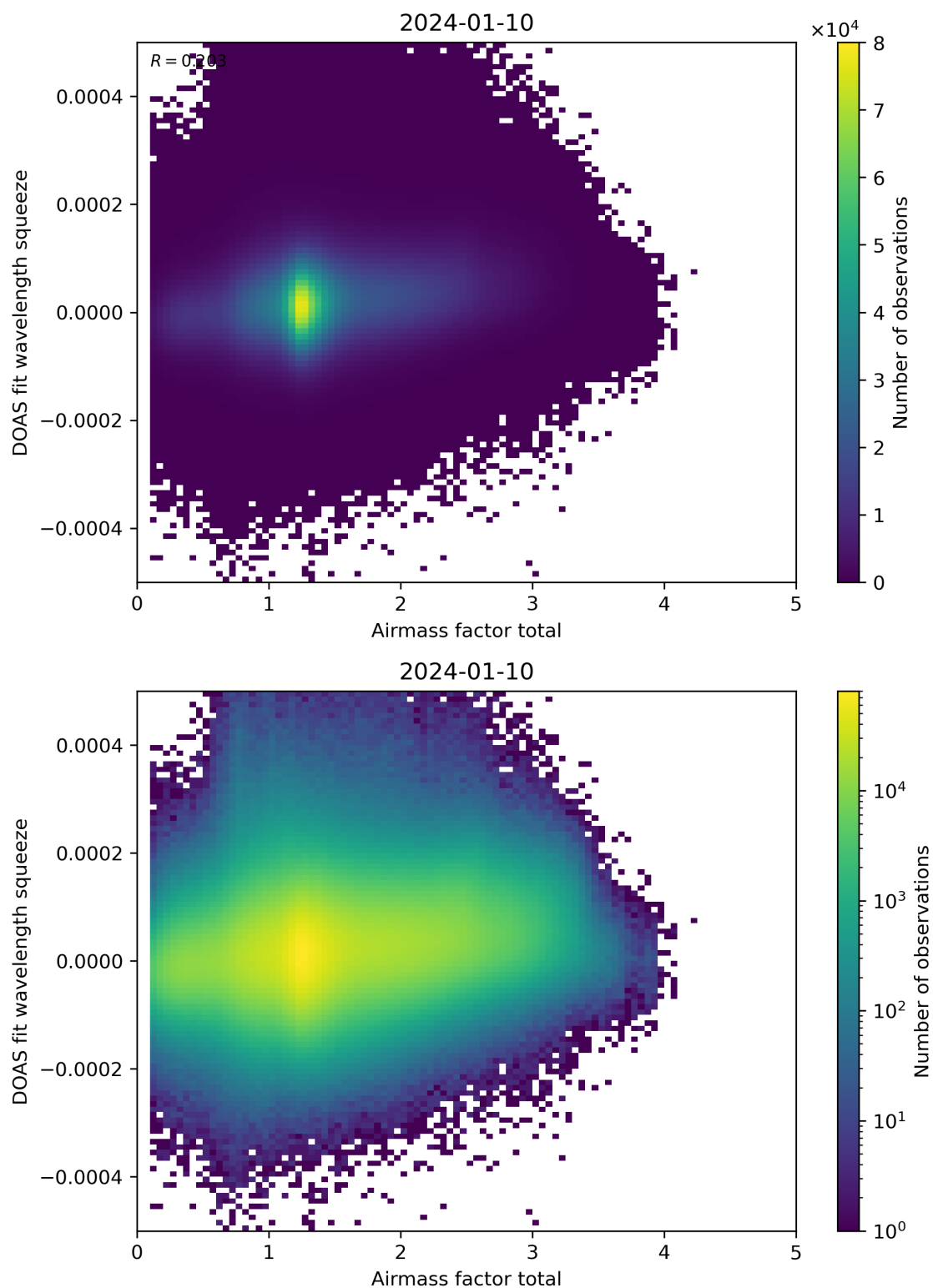
Figure 99: Scatter density plot of “Airmass factor total” against “DOAS fit wavelength squeeze” for 2024-01-10 to 2024-01-11.
