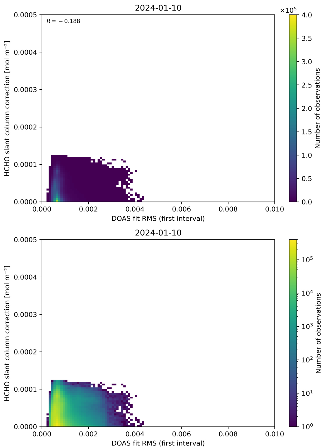
Figure 63: Scatter density plot of “DOAS fit RMS (first interval)” against “HCHO slant column correction” for 2024-01-10 to 2024-01-11.
