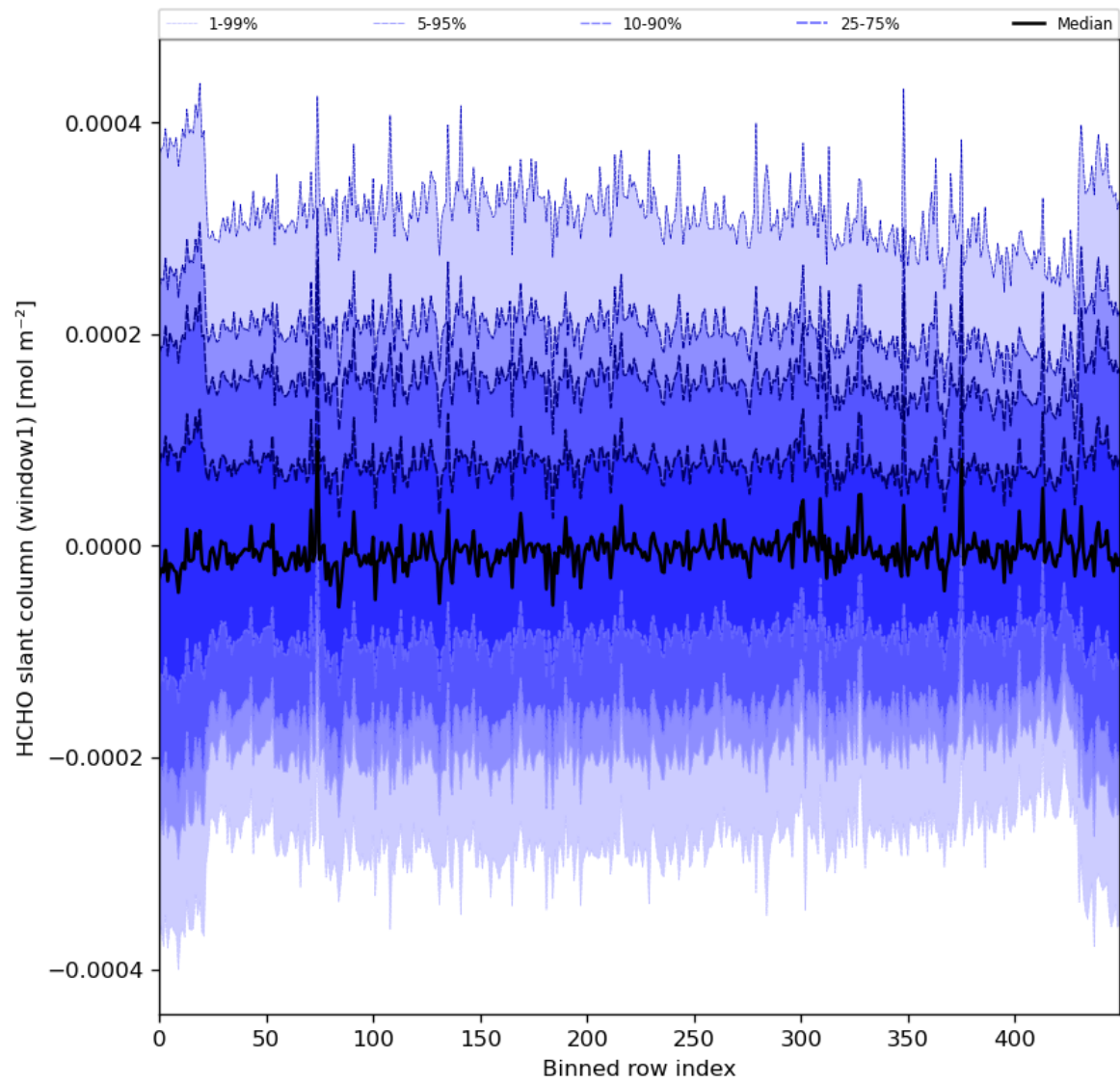
Figure 52: Along track statistics of “HCHO slant column (window1)” for 2024-01-10 to 2024-01-11
