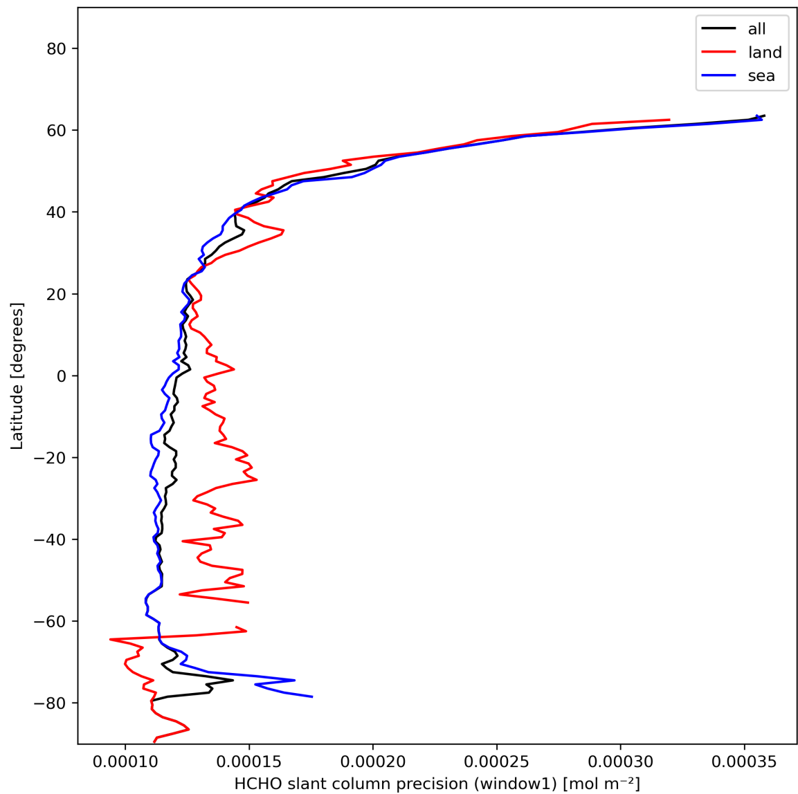
Figure 25: Zonal average of “HCHO slant column precision (window1)” for 2024-01-10 to 2024-01-11.
