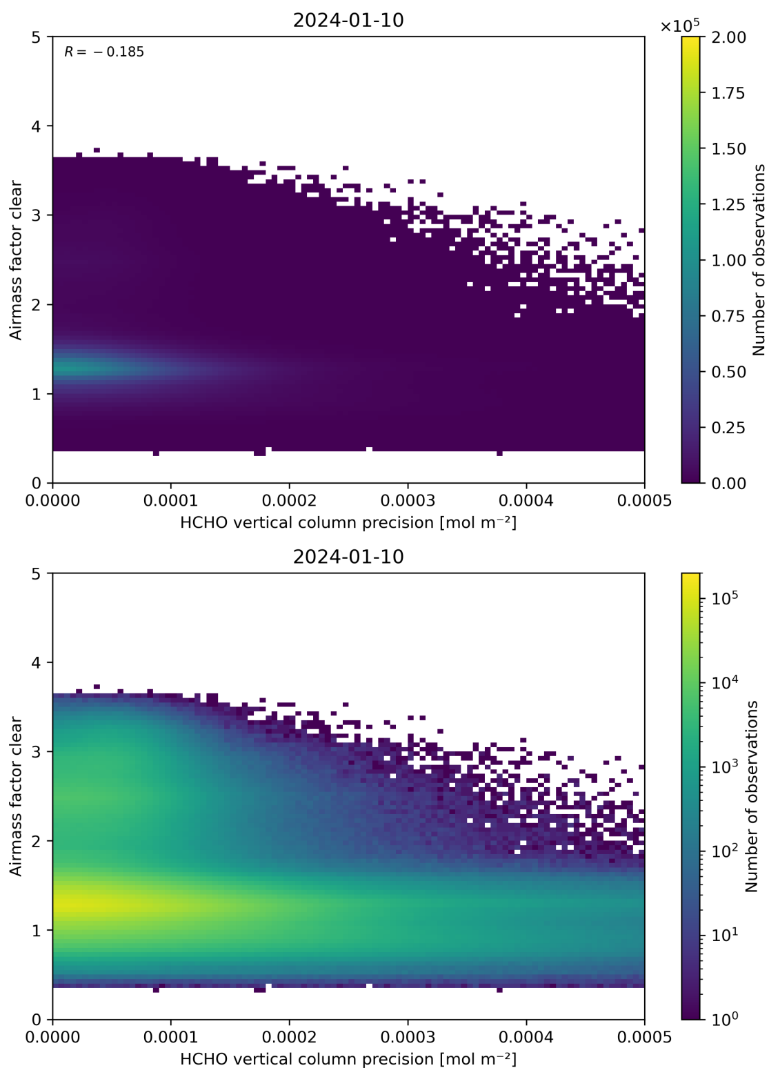
Figure 139: Scatter density plot of “HCHO vertical column precision” against “Airmass factor clear” for 2024-01-10 to 2024-01-11.
