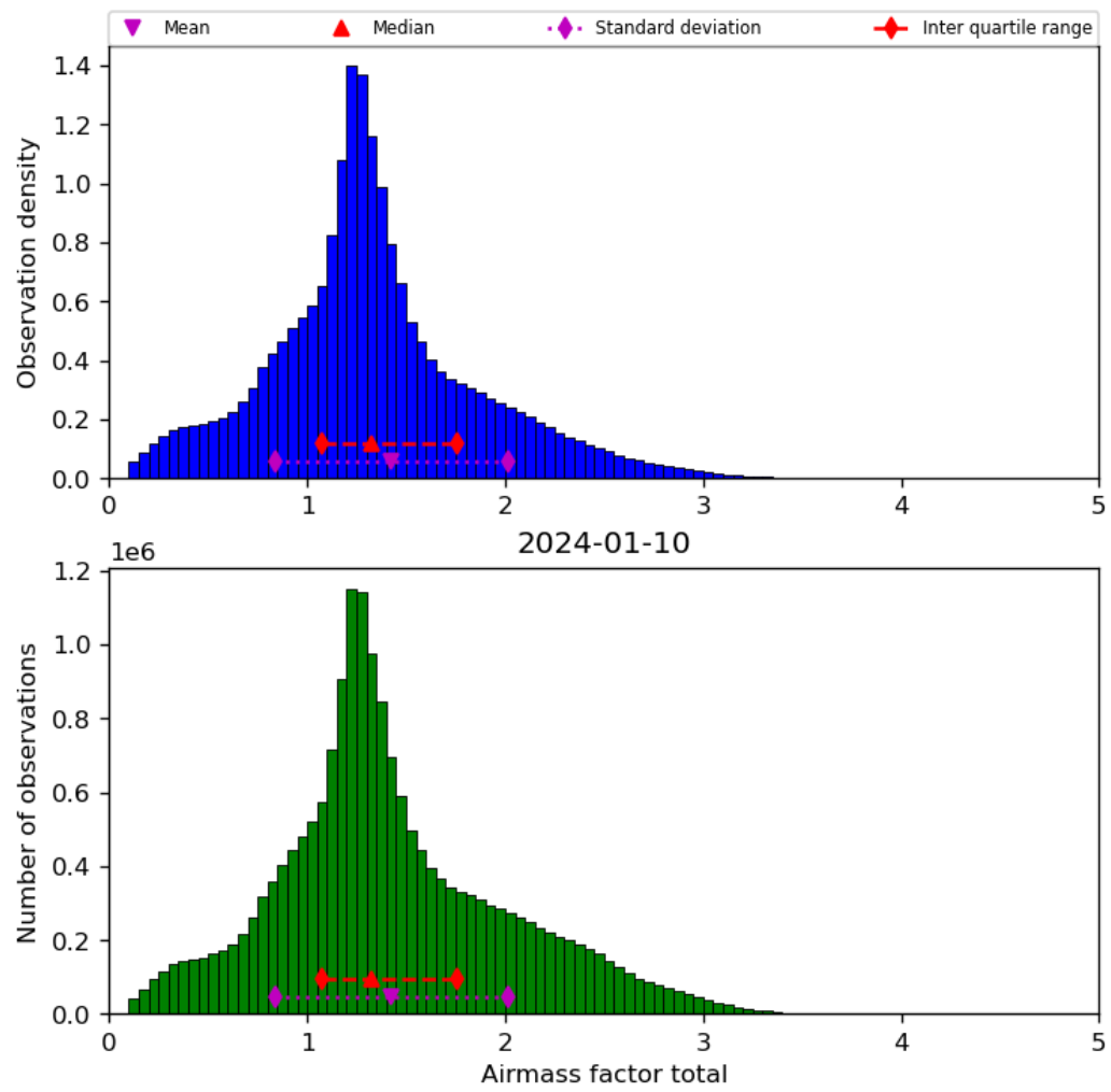
Figure 40: Histogram of “Airmass factor total” for 2024-01-10 to 2024-01-11
