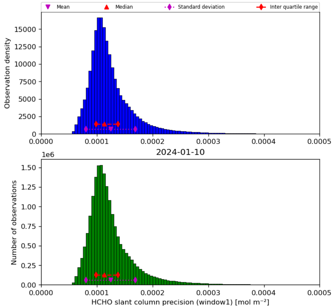
Figure 39: Histogram of “HCHO slant column precision (window1)” for 2024-01-10 to 2024-01-11
