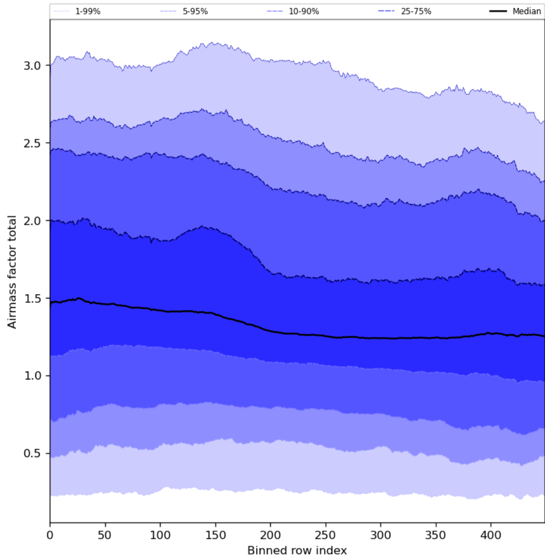
Figure 54: Along track statistics of “Airmass factor total” for 2024-01-10 to 2024-01-11
