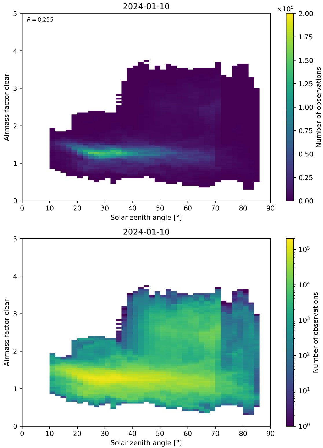
Figure 170: Scatter density plot of “Solar zenith angle” against “Airmass factor clear” for 2024-01-10 to 2024-01-11.
