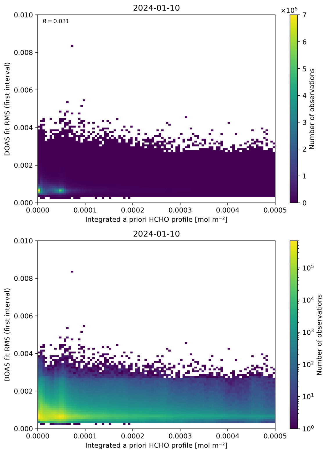
Figure 148: Scatter density plot of “Integrated a priori HCHO profile” against “DOAS fit RMS (first interval)” for 2024-01-10 to 2024-01-11.
