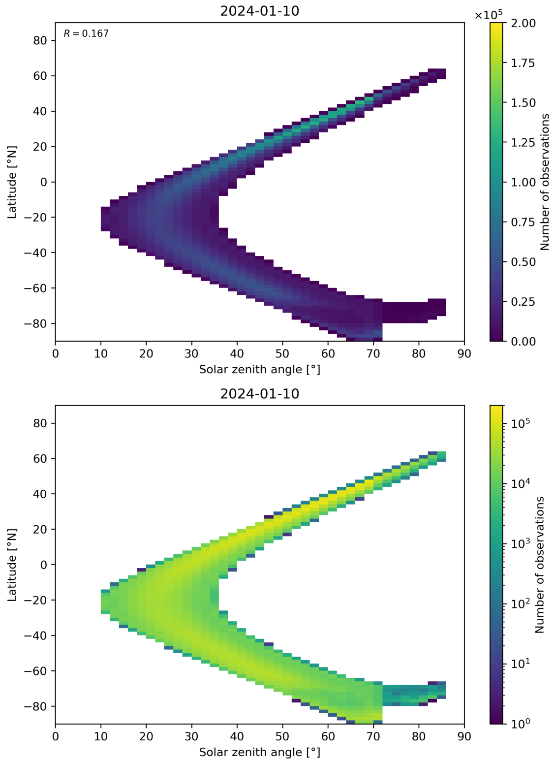
Figure 181: Scatter density plot of “Solar zenith angle” against “Latitude” for 2024-01-10 to 2024-01-11.
