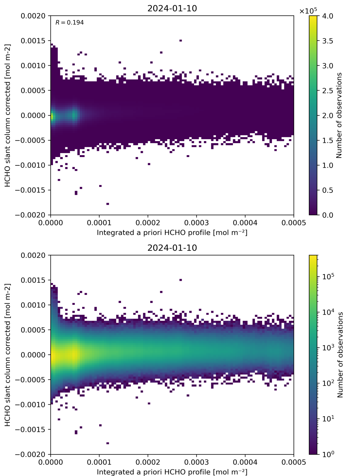
Figure 151: Scatter density plot of “Integrated a priori HCHO profile” against “HCHO slant column corrected” for 2024-01-10 to 2024-01-11.
