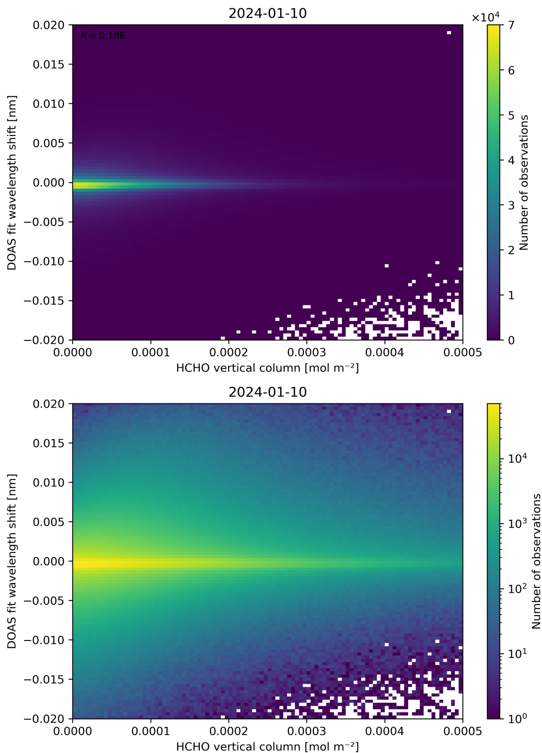
Figure 124: Scatter density plot of “HCHO vertical column” against “DOAS fit wavelength shift” for 2024-01-10 to 2024-01-11.
