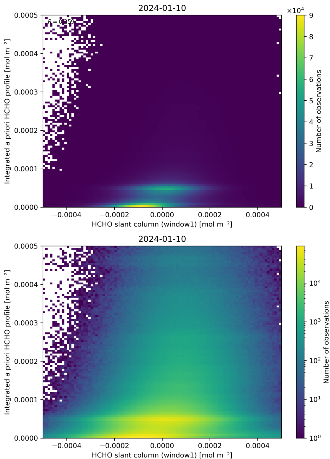
Figure 87: Scatter density plot of “HCHO slant column (window1)” against “Integrated a priori HCHO profile” for 2024-01-10 to 2024-01-11.
