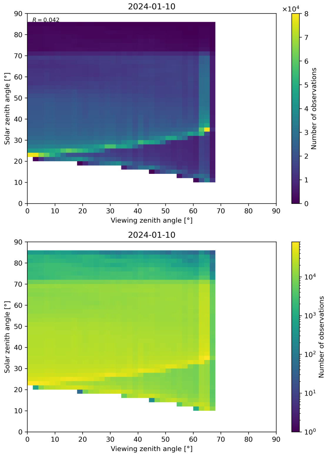
Figure 197: Scatter density plot of “Viewing zenith angle” against “Solar zenith angle” for 2024-01-10 to 2024-01-11.
