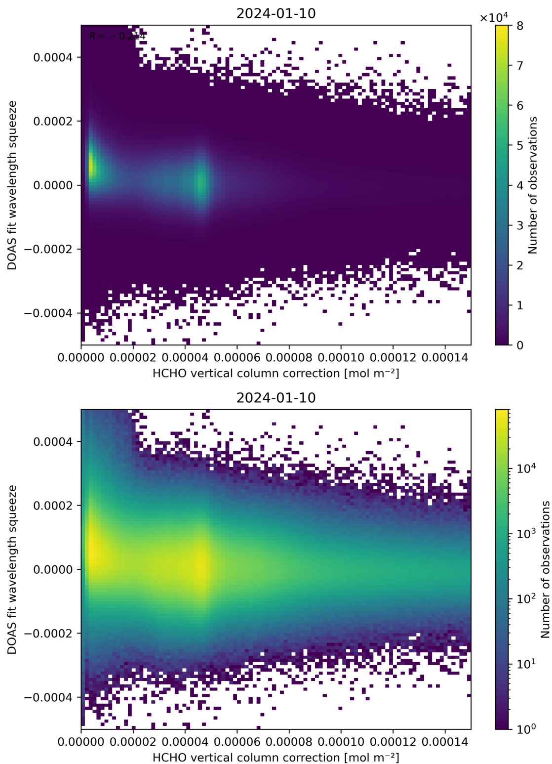
Figure 114: Scatter density plot of “HCHO vertical column correction” against “DOAS fit wavelength squeeze” for 2024-01-10 to 2024-01-11.
