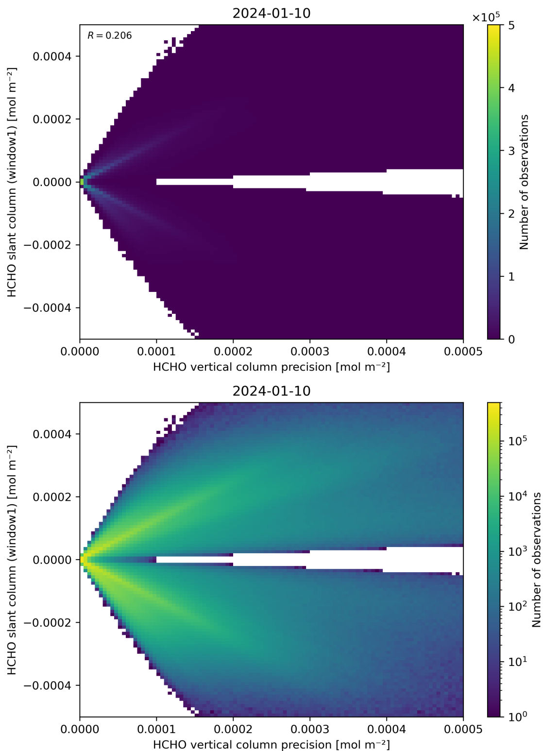
Figure 142: Scatter density plot of “HCHO vertical column precision” against “HCHO slant column (window1)” for 2024-01-10 to 2024-01-11.
