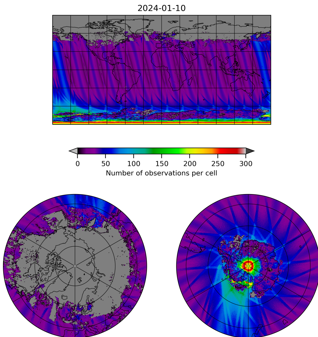
Figure 19: Map of the number of observations for 2024-01-10 to 2024-01-11
