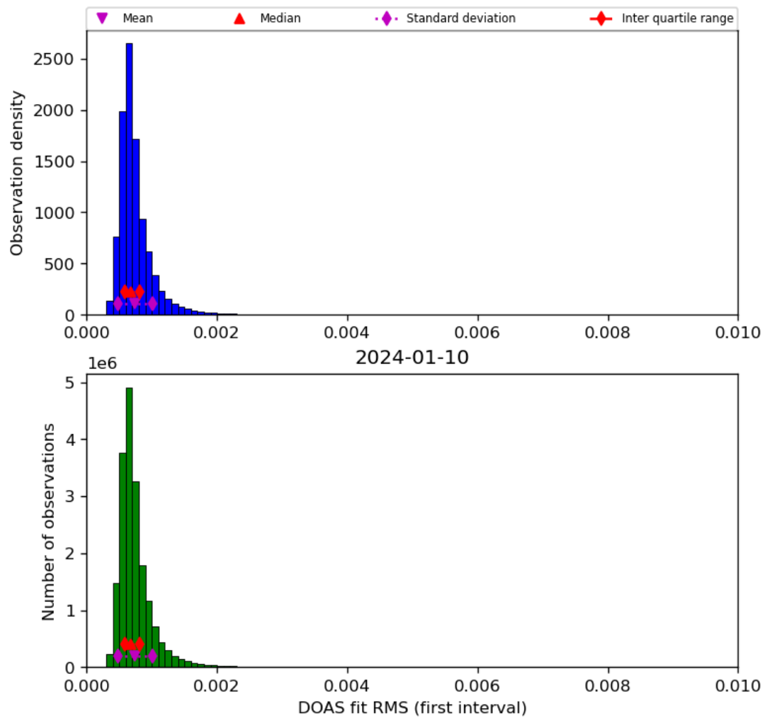
Figure 46: Histogram of “DOAS fit RMS (first interval)” for 2024-01-10 to 2024-01-11
