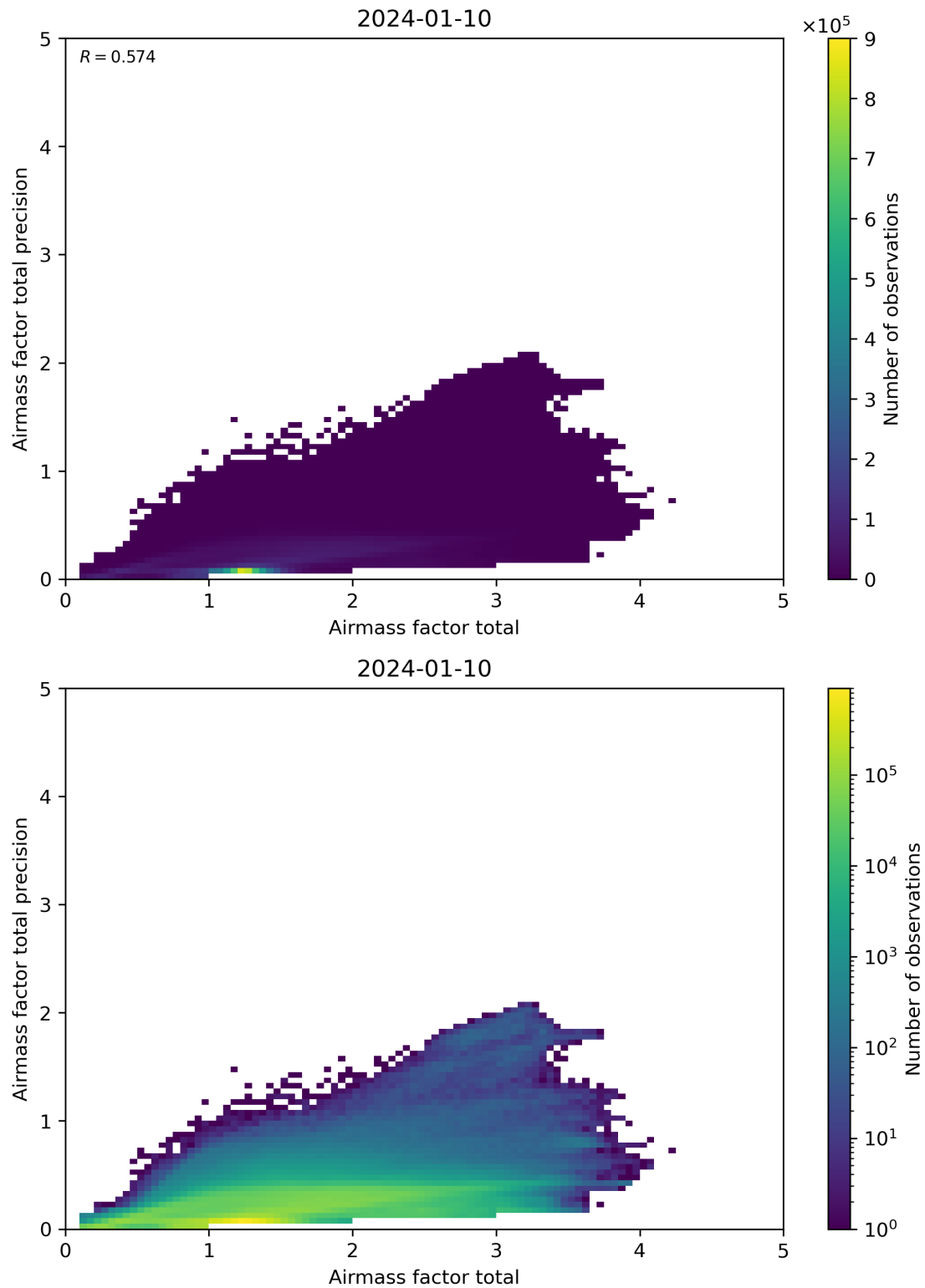
Figure 103: Scatter density plot of “Airmass factor total” against “Airmass factor total precision” for 2024-01-10 to 2024-01-11.
