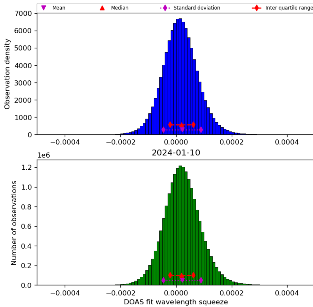
Figure 45: Histogram of “DOAS fit wavelength squeeze” for 2024-01-10 to 2024-01-11
