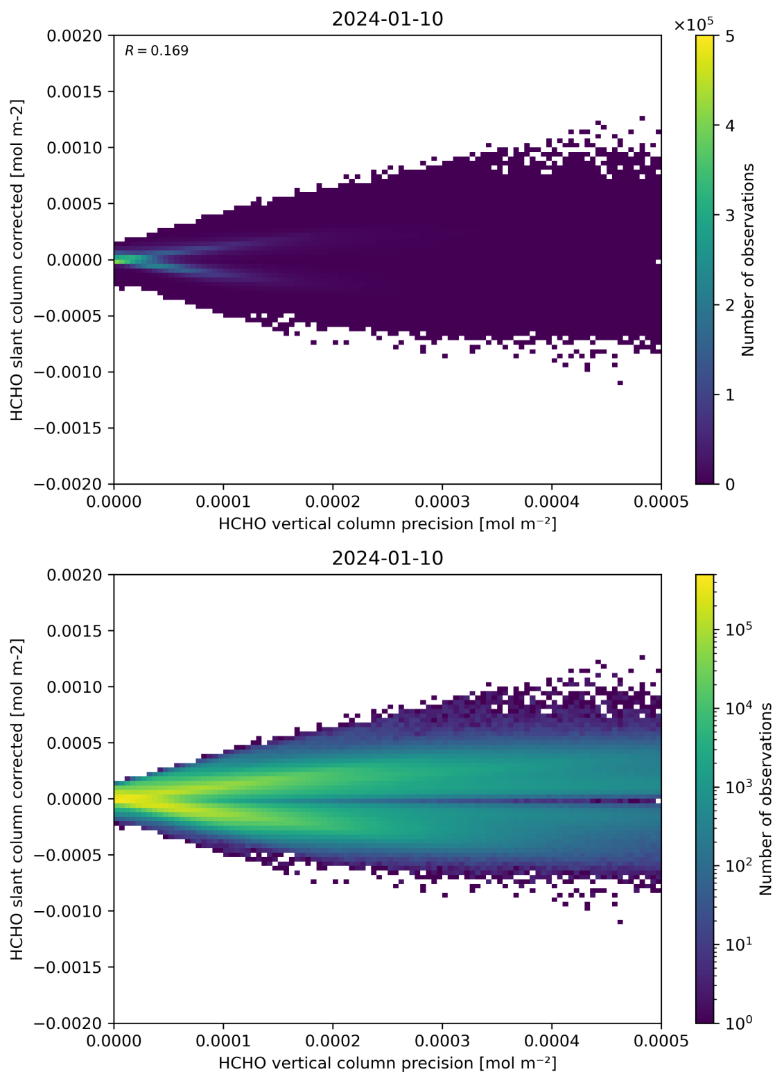
Figure 140: Scatter density plot of “HCHO vertical column precision” against “HCHO slant column corrected” for 2024-01-10 to 2024-01-11.
