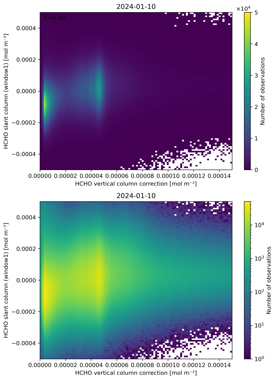
Figure 118: Scatter density plot of “HCHO vertical column correction” against “HCHO slant column (window1)” for 2024-01-10 to 2024-01-11.
