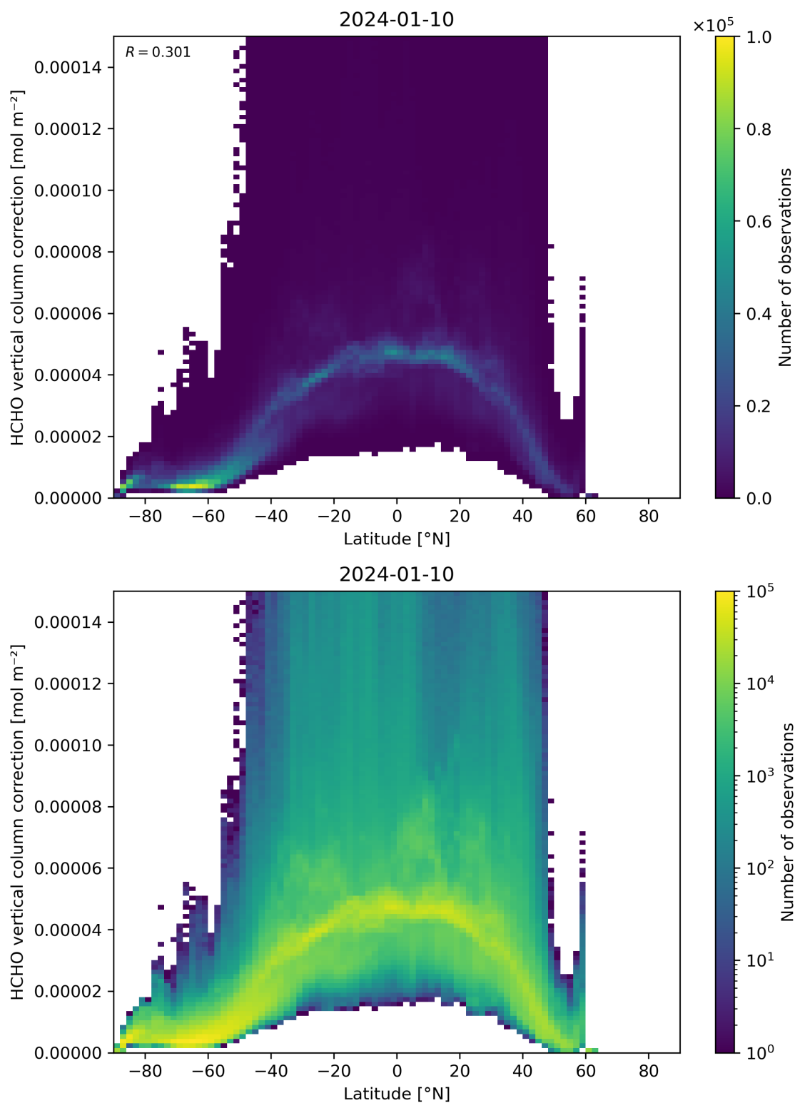
Figure 164: Scatter density plot of “Latitude” against “HCHO vertical column correction” for 2024-01-10 to 2024-01-11.
