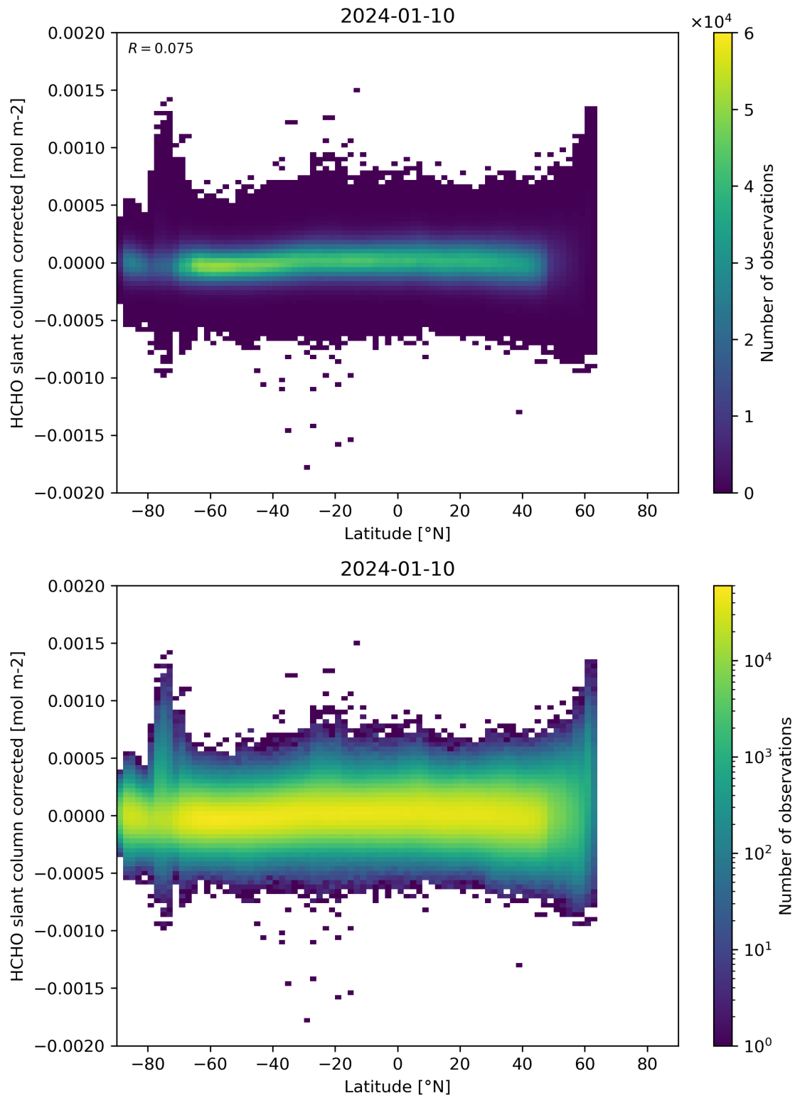
Figure 157: Scatter density plot of “Latitude” against “HCHO slant column corrected” for 2024-01-10 to 2024-01-11.
