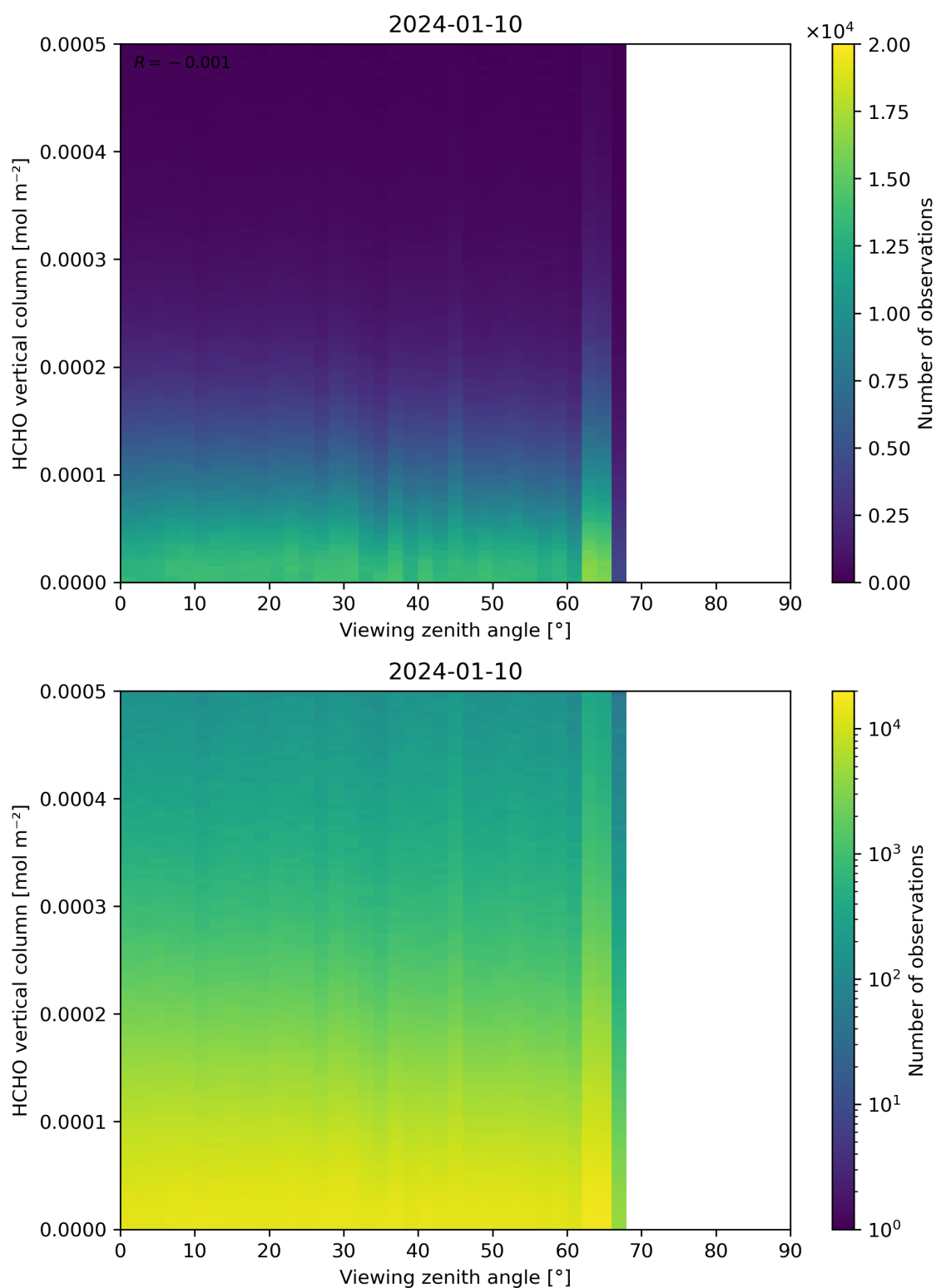
Figure 192: Scatter density plot of “Viewing zenith angle” against “HCHO vertical column” for 2024-01-10 to 2024-01-11.
