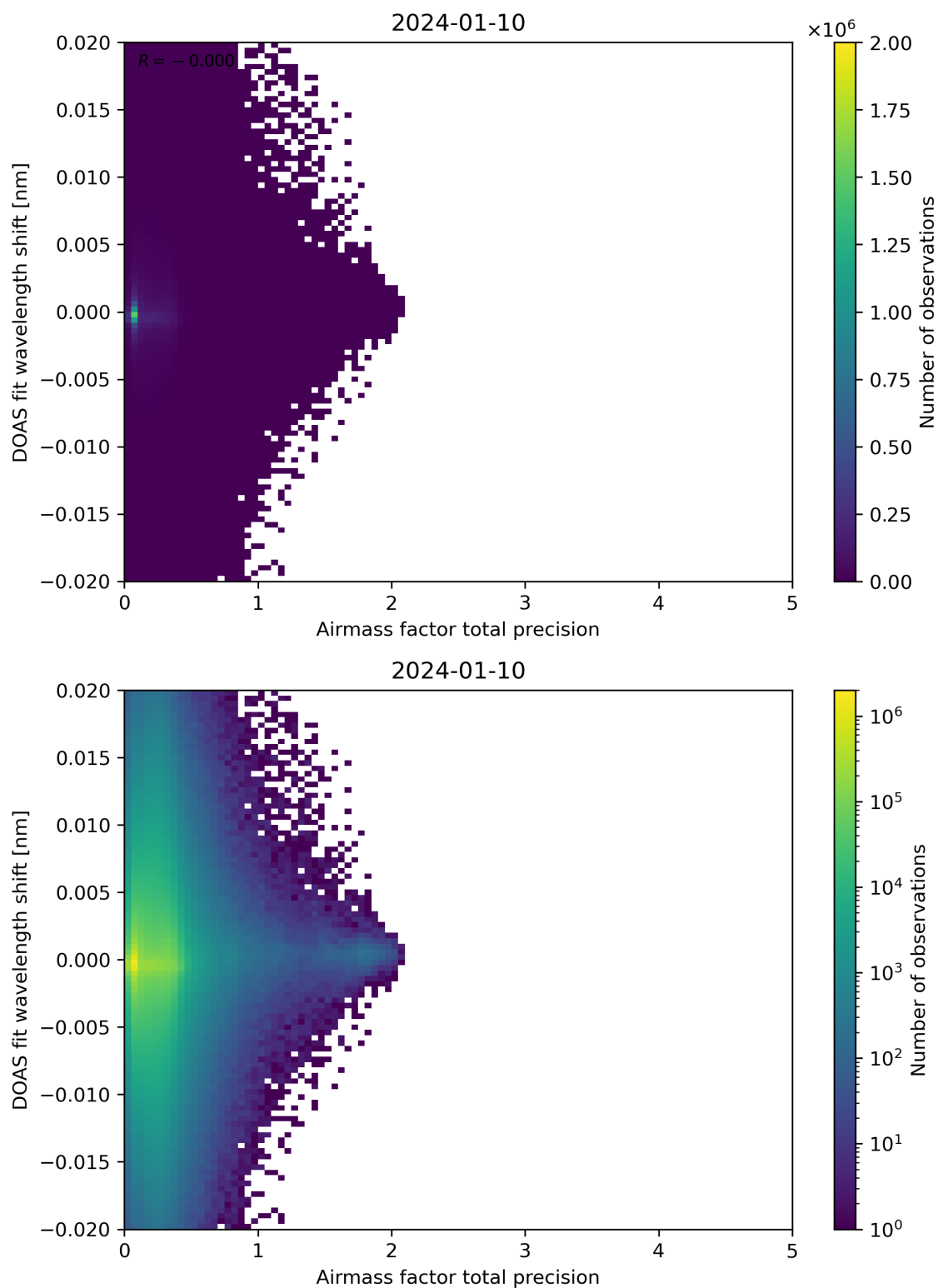
Figure 106: Scatter density plot of “Airmass factor total precision” against “DOAS fit wavelength shift” for 2024-01-10 to 2024-01-11.
