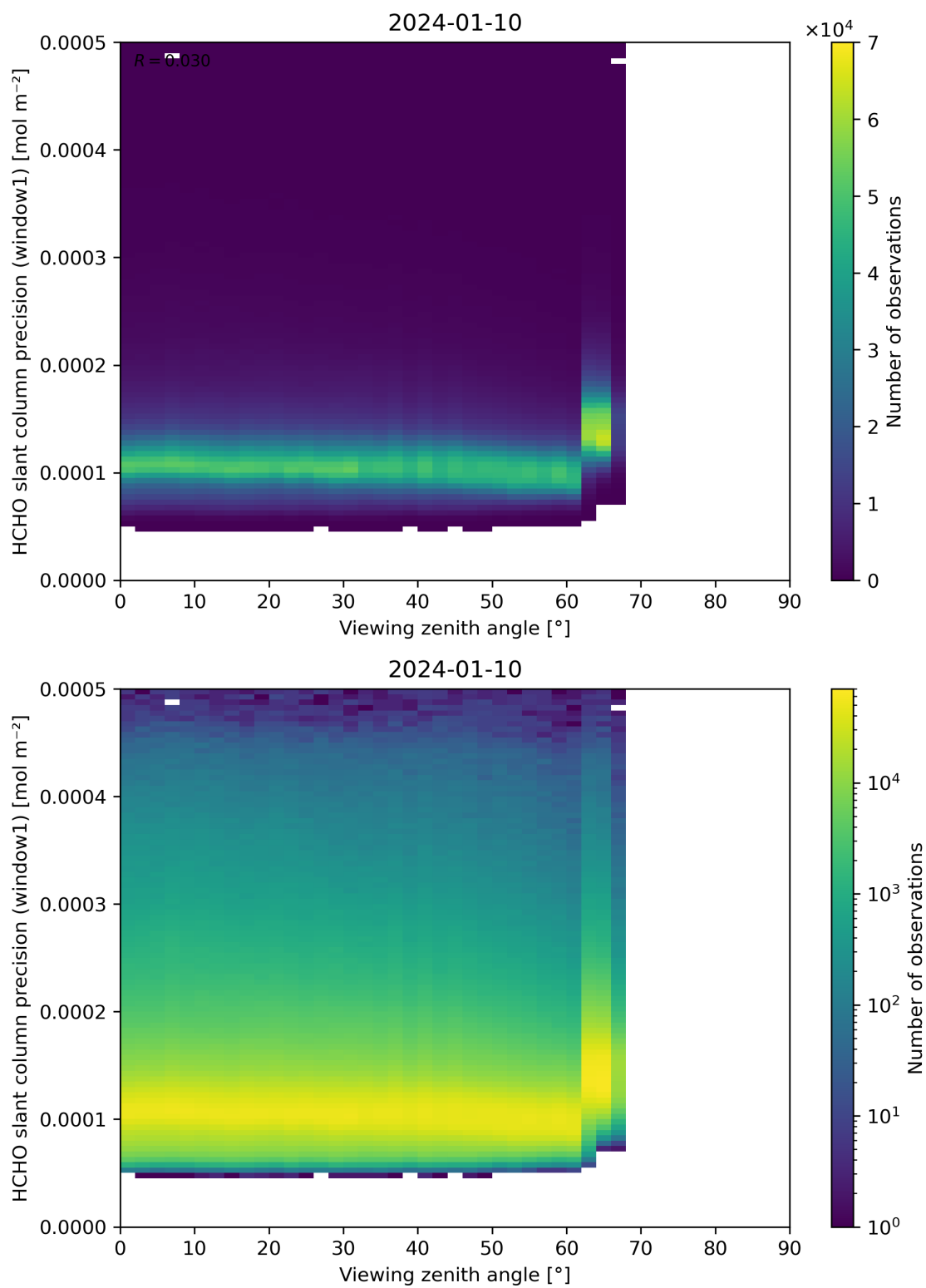
Figure 189: Scatter density plot of “Viewing zenith angle” against “HCHO slant column precision (window1)” for 2024-01-10 to 2024-01-11.
