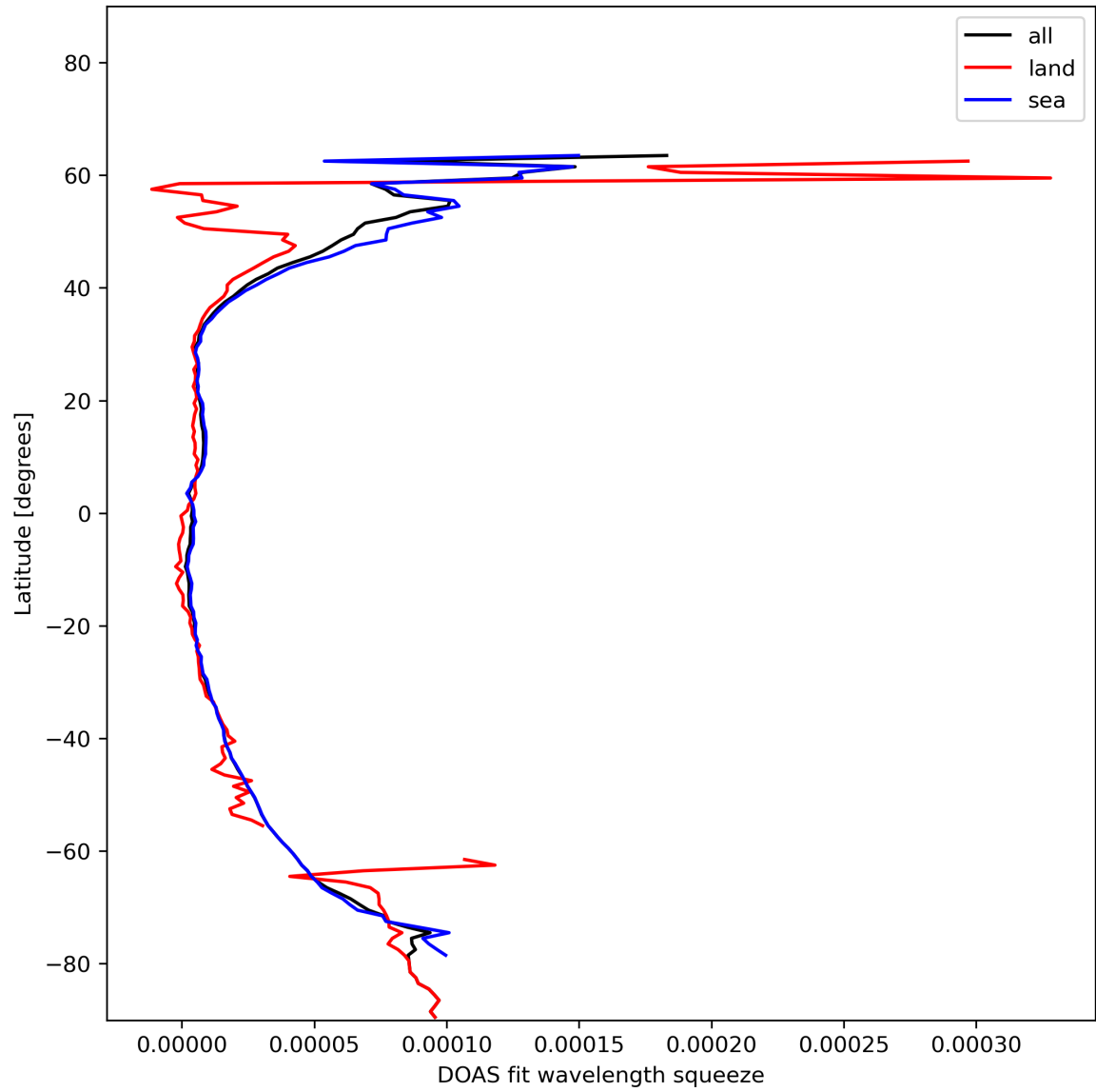
Figure 31: Zonal average of “DOAS fit wavelength squeeze” for 2024-01-10 to 2024-01-11.
