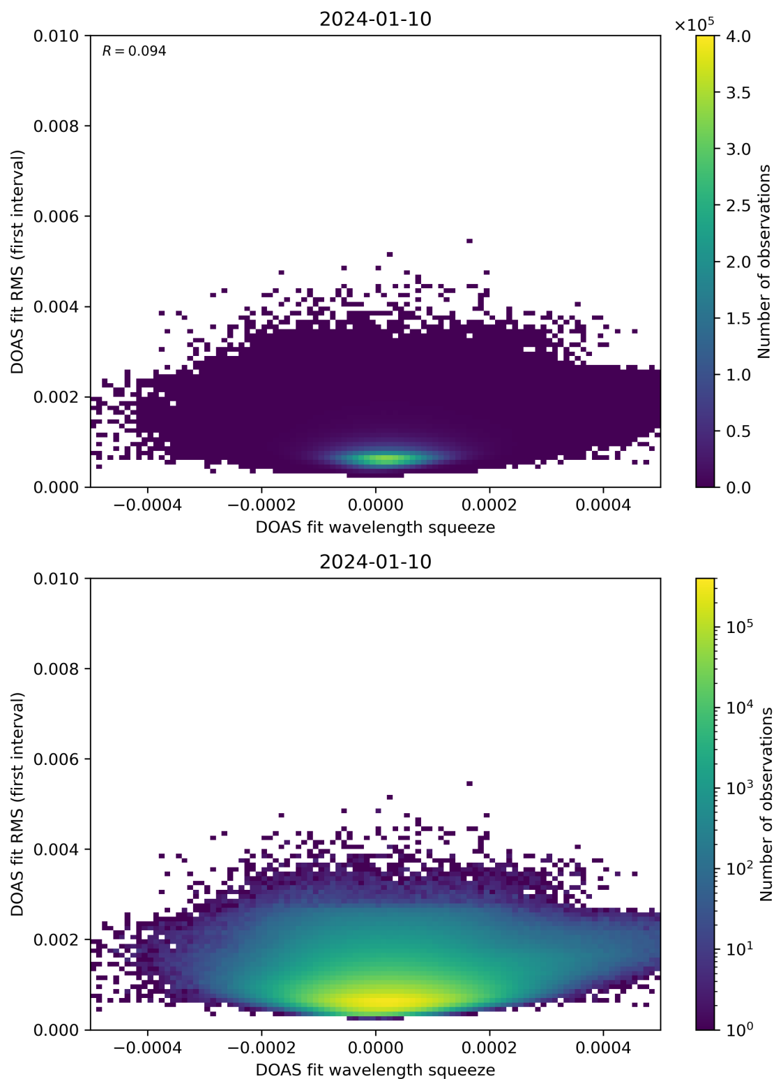
Figure 68: Scatter density plot of “DOAS fit wavelength squeeze” against “DOAS fit RMS (first interval)” for 2024-01-10 to 2024-01-11.
