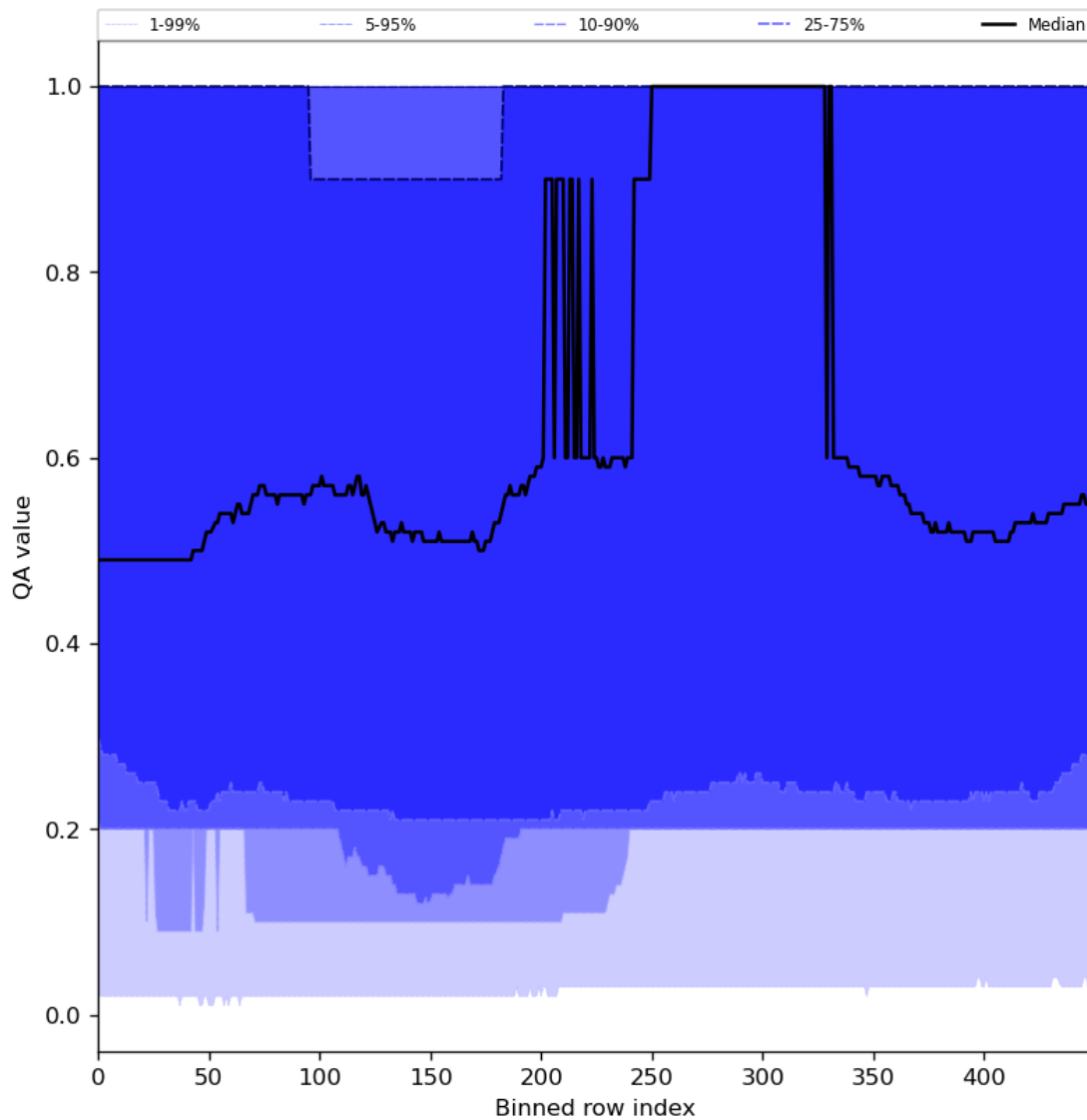
Figure 48: Along track statistics of “QA value” for 2024-01-10 to 2024-01-11
