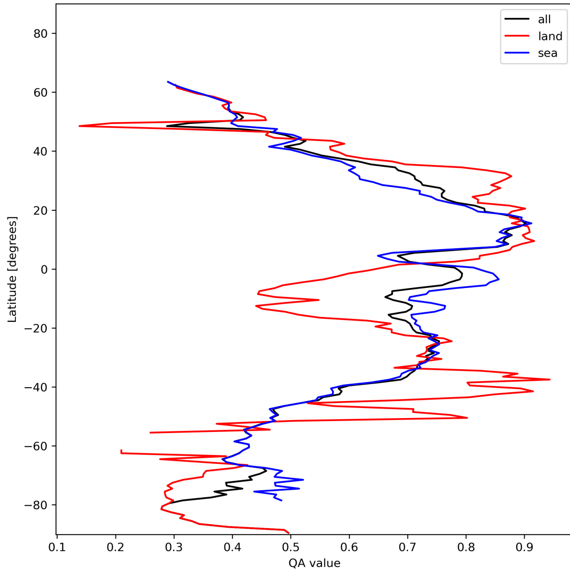
Figure 20: Zonal average of “QA value” for 2024-01-10 to 2024-01-11.
