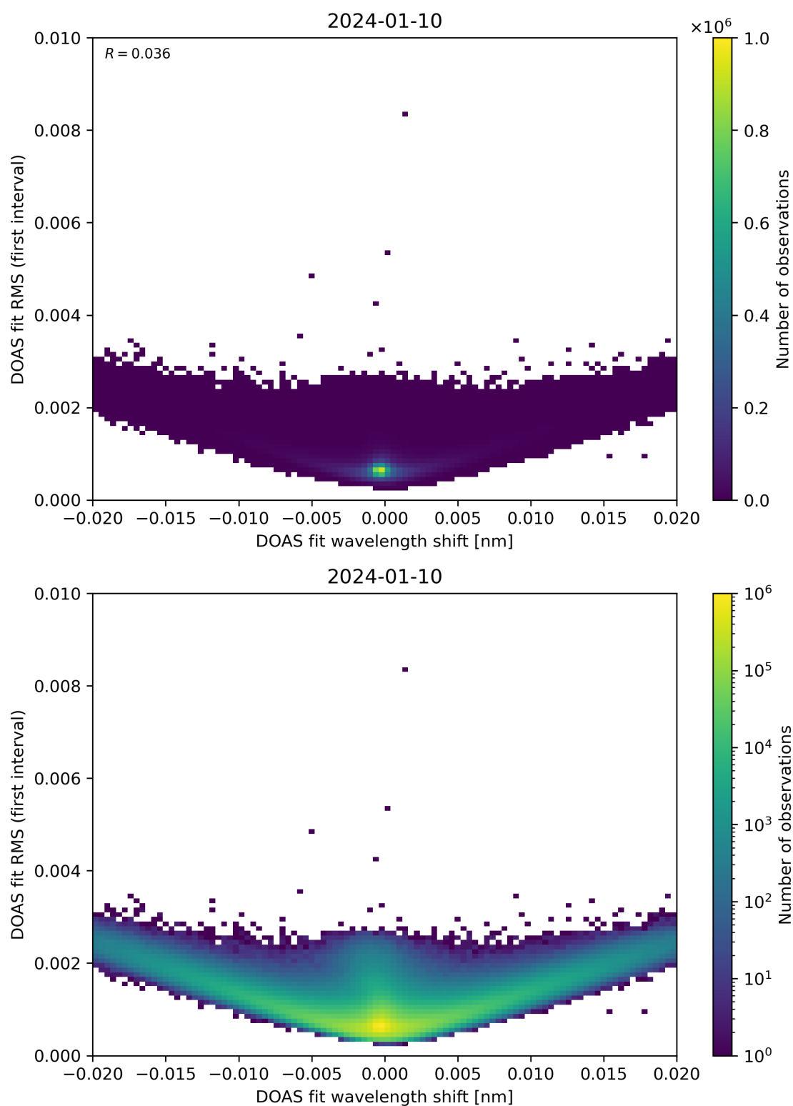
Figure 64: Scatter density plot of “DOAS fit wavelength shift” against “DOAS fit RMS (first interval)” for 2024-01-10 to 2024-01-11.
