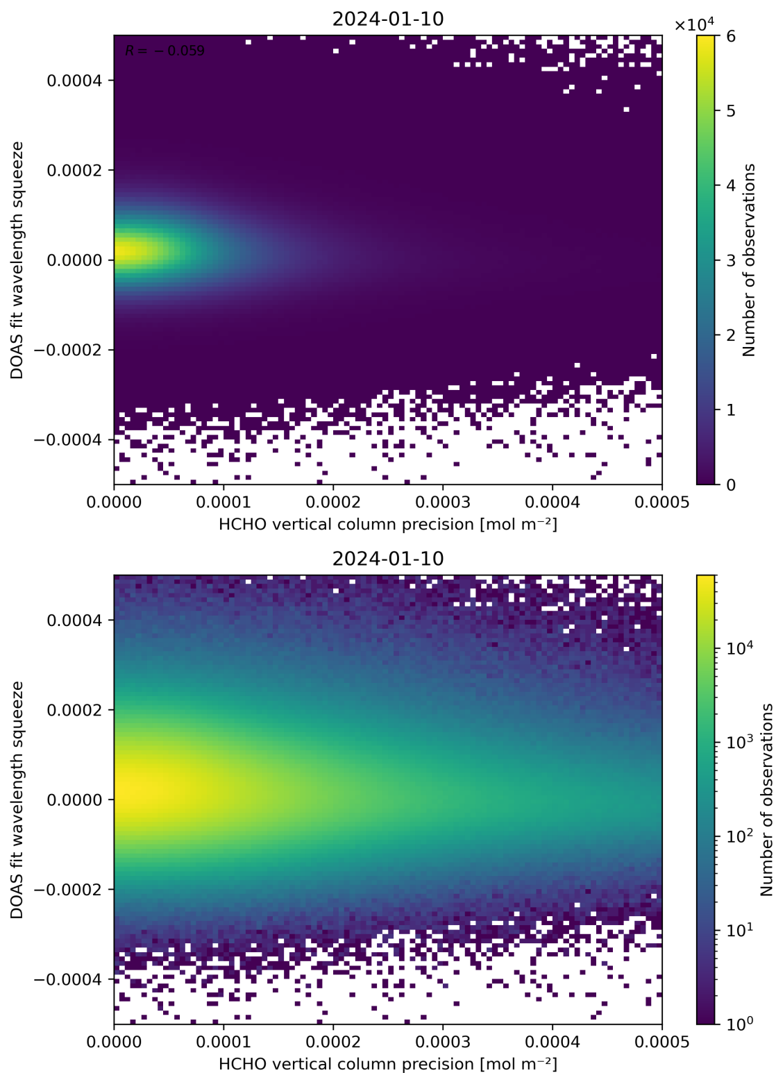
Figure 138: Scatter density plot of “HCHO vertical column precision” against “DOAS fit wavelength squeeze” for 2024-01-10 to 2024-01-11.
