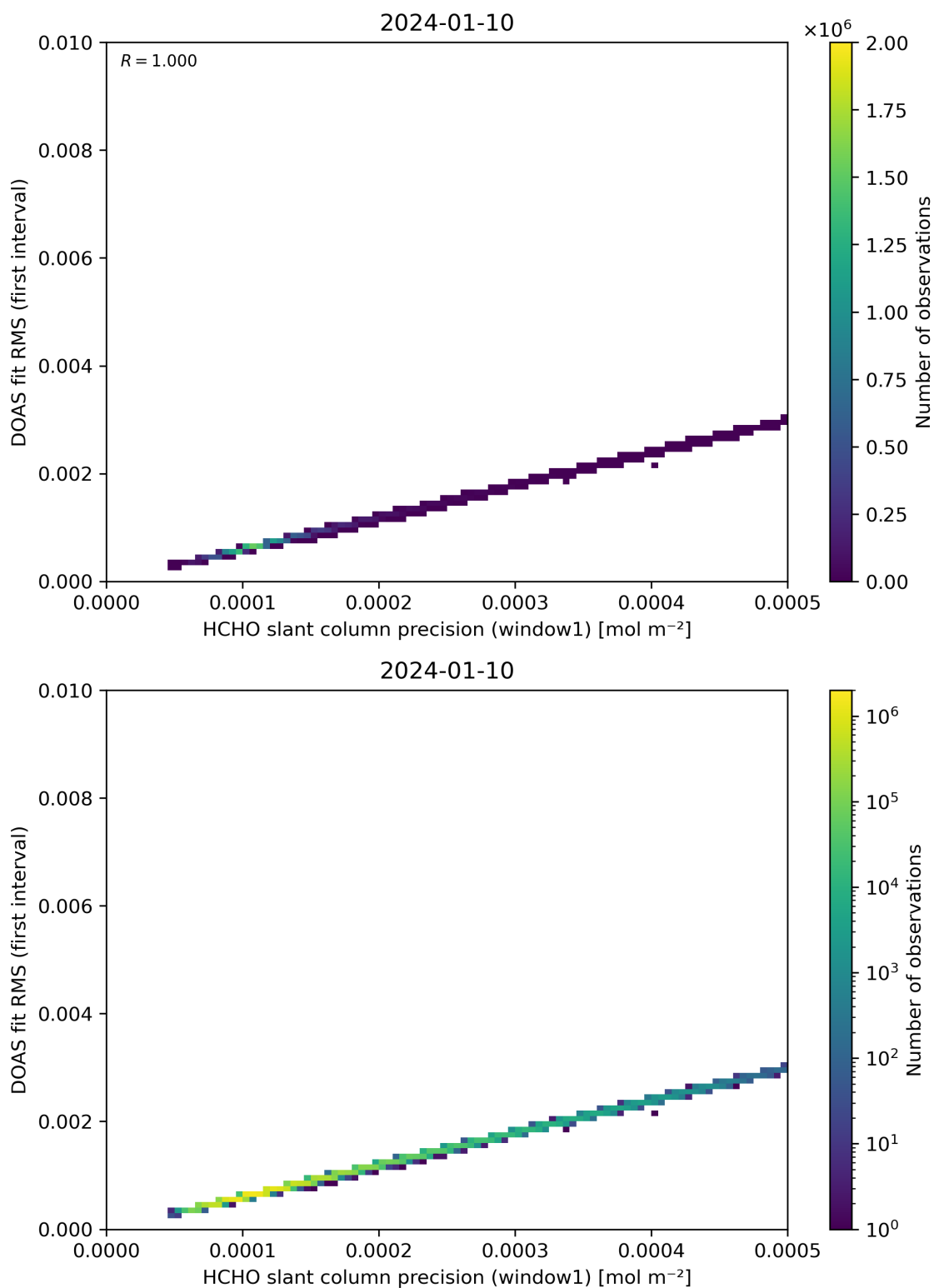
Figure 88: Scatter density plot of “HCHO slant column precision (window1)” against “DOAS fit RMS (first interval)” for 2024-01-10 to 2024-01-11.
