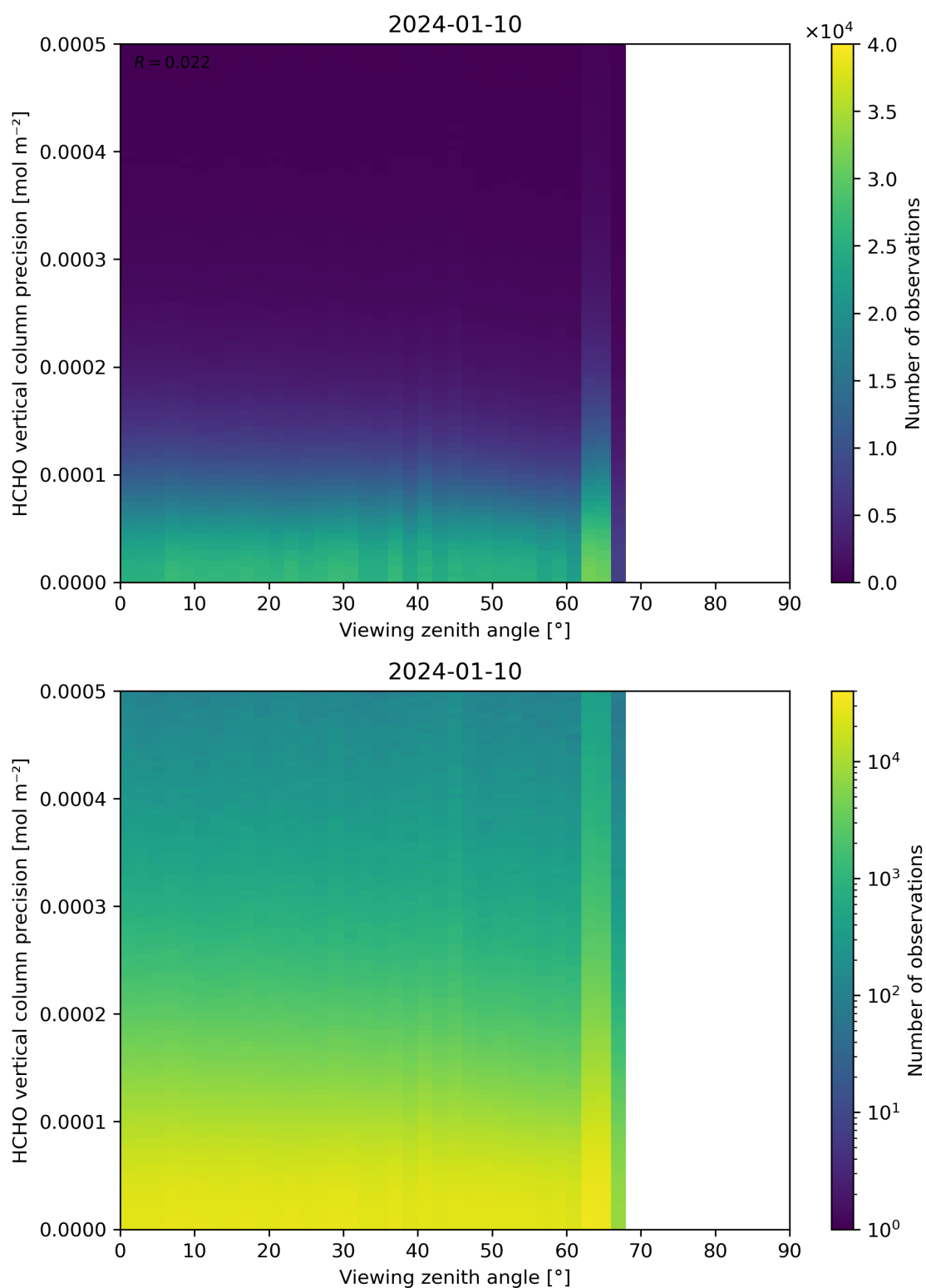
Figure 194: Scatter density plot of “Viewing zenith angle” against “HCHO vertical column precision” for 2024-01-10 to 2024-01-11.
