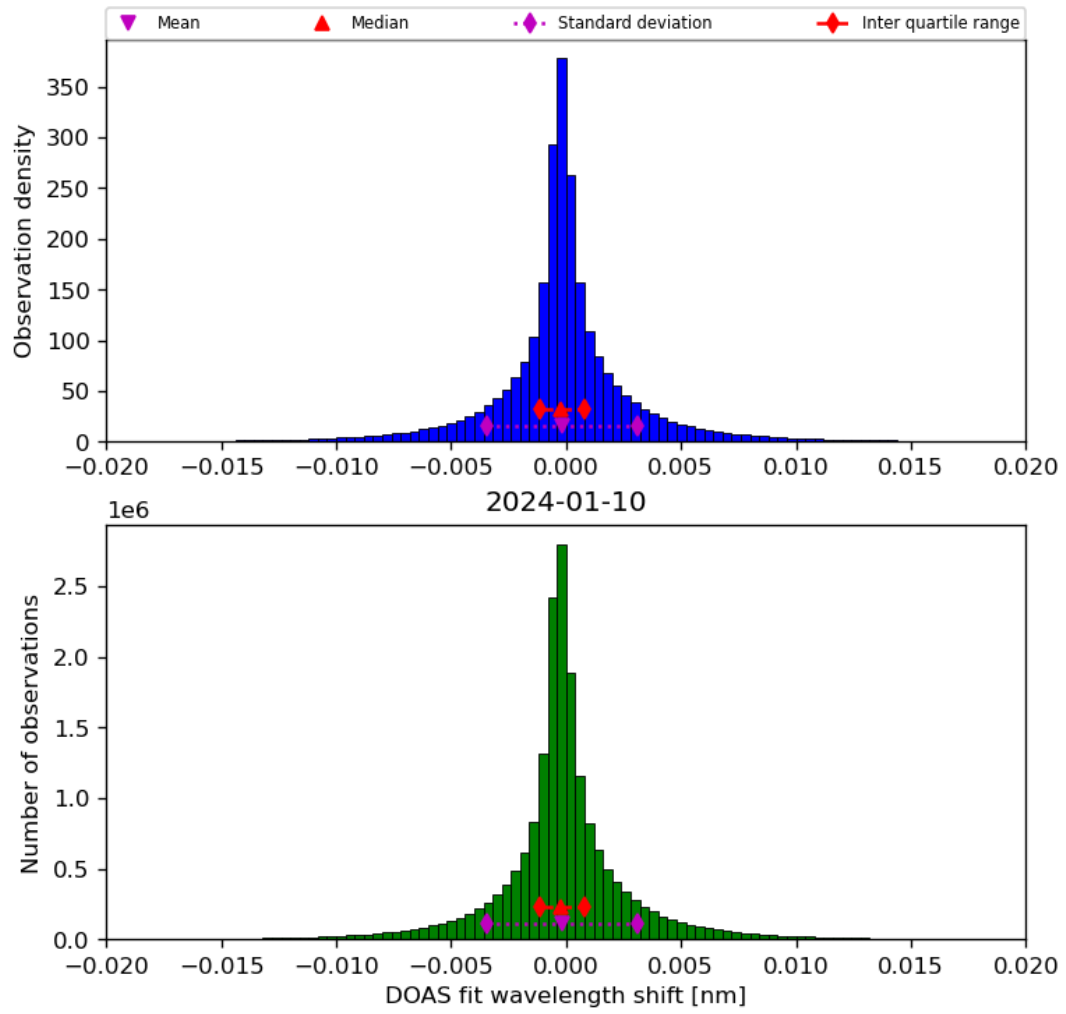
Figure 44: Histogram of “DOAS fit wavelength shift” for 2024-01-10 to 2024-01-11
