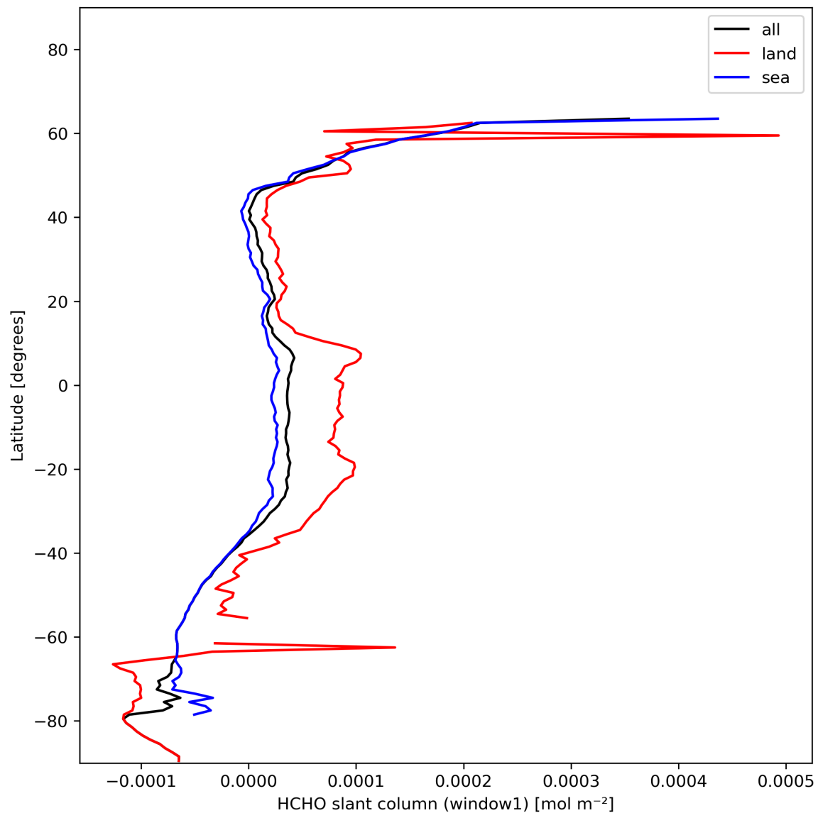
Figure 24: Zonal average of “HCHO slant column (window1)” for 2024-01-10 to 2024-01-11.
