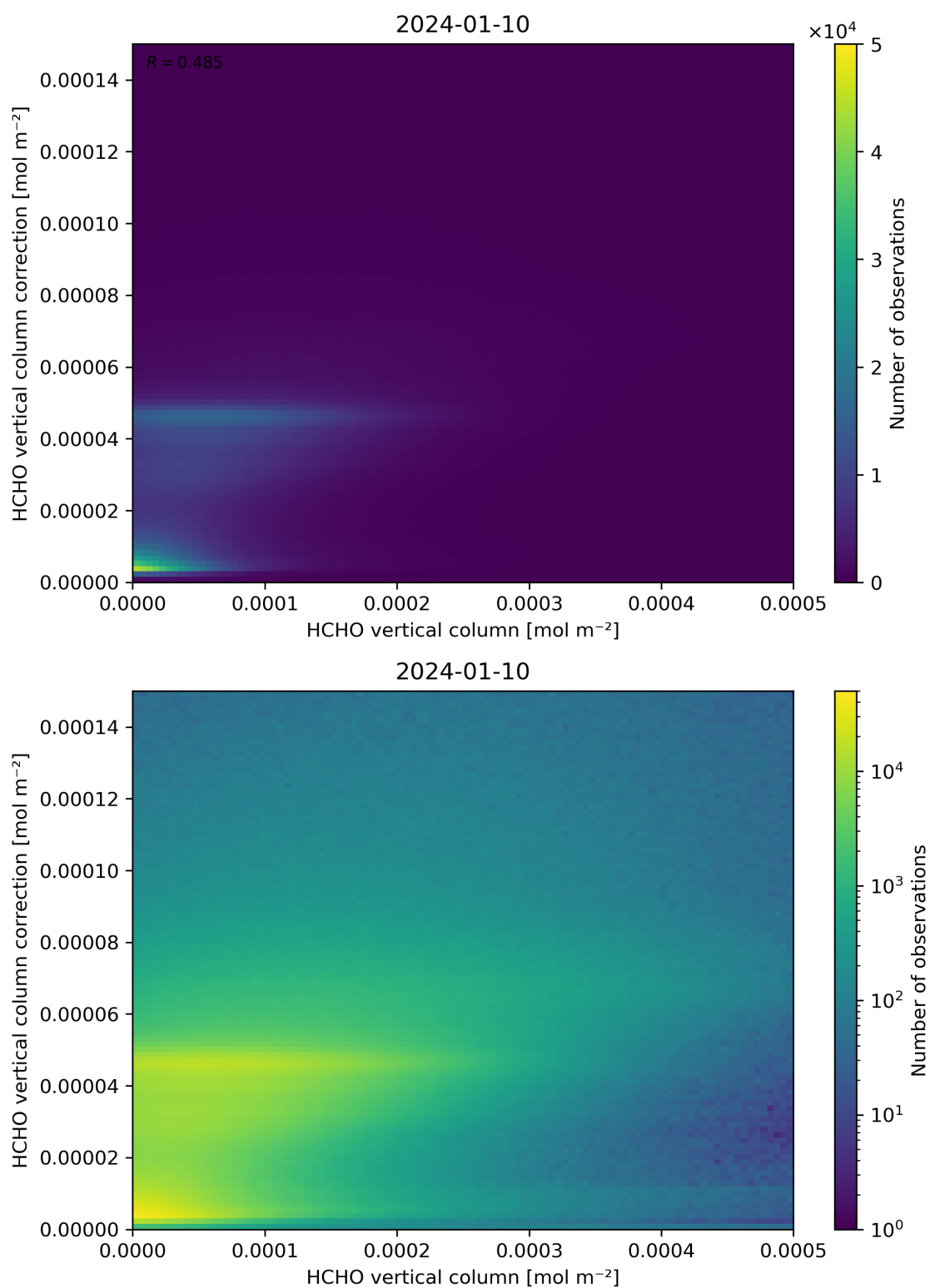
Figure 133: Scatter density plot of “HCHO vertical column” against “HCHO vertical column correction” for 2024-01-10 to 2024-01-11.
