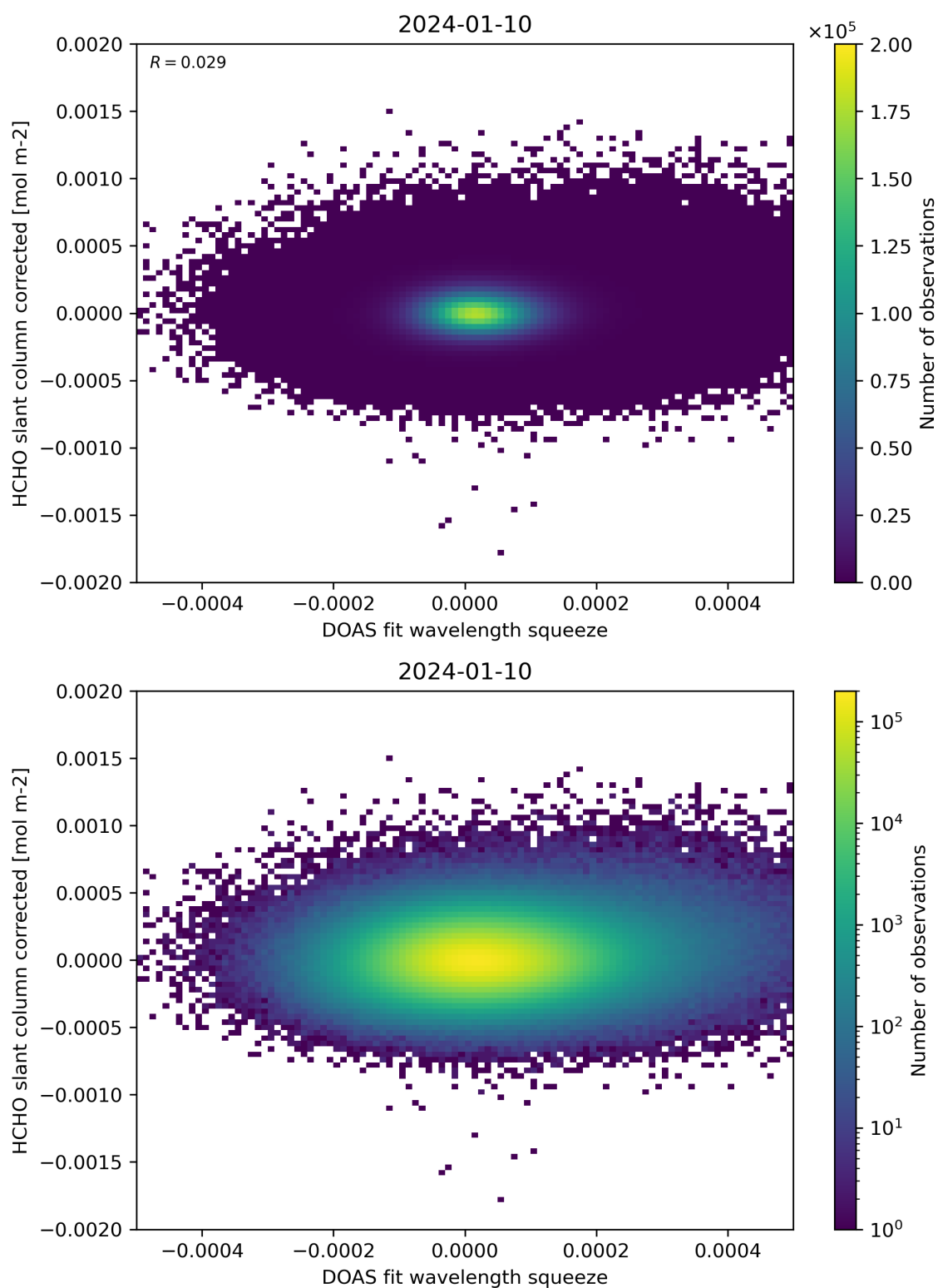
Figure 69: Scatter density plot of “DOAS fit wavelength squeeze” against “HCHO slant column corrected” for 2024-01-10 to 2024-01-11.
