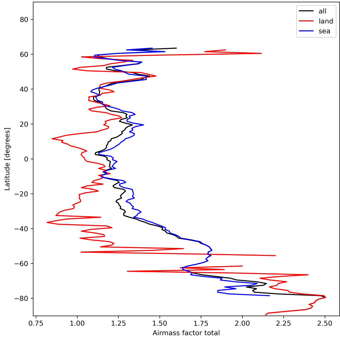
Figure 26: Zonal average of “Airmass factor total” for 2024-01-10 to 2024-01-11.
