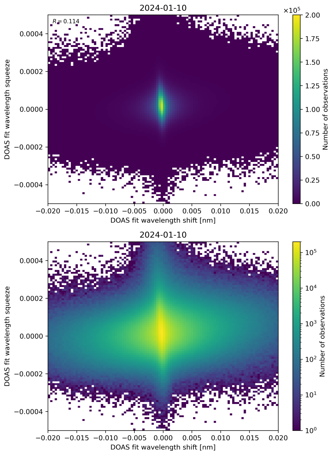
Figure 65: Scatter density plot of “DOAS fit wavelength shift” against “DOAS fit wavelength squeeze” for 2024-01-10 to 2024-01-11.
