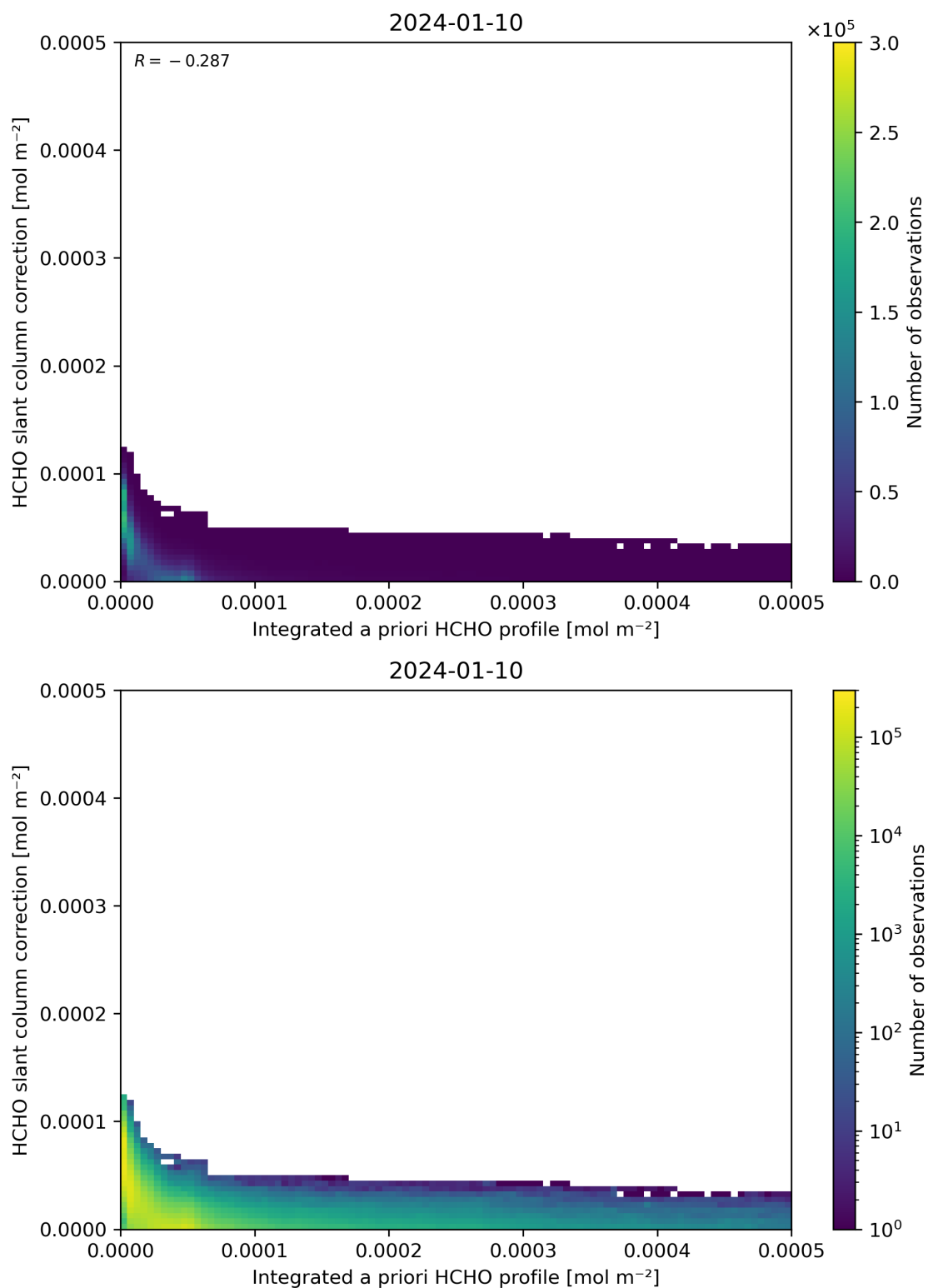
Figure 152: Scatter density plot of “Integrated a priori HCHO profile” against “HCHO slant column correction” for 2024-01-10 to 2024-01-11.
