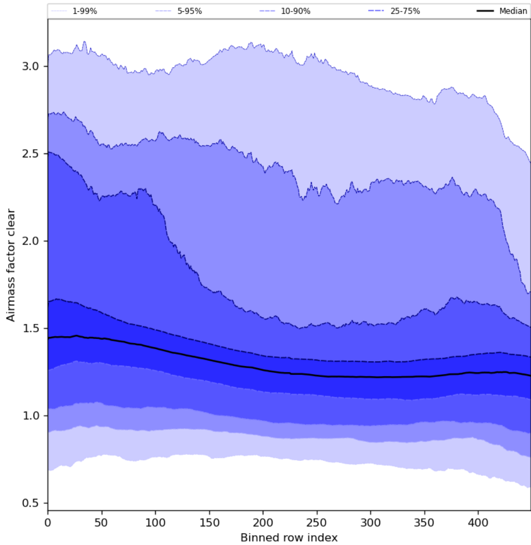
Figure 56: Along track statistics of “Airmass factor clear” for 2024-01-10 to 2024-01-11
