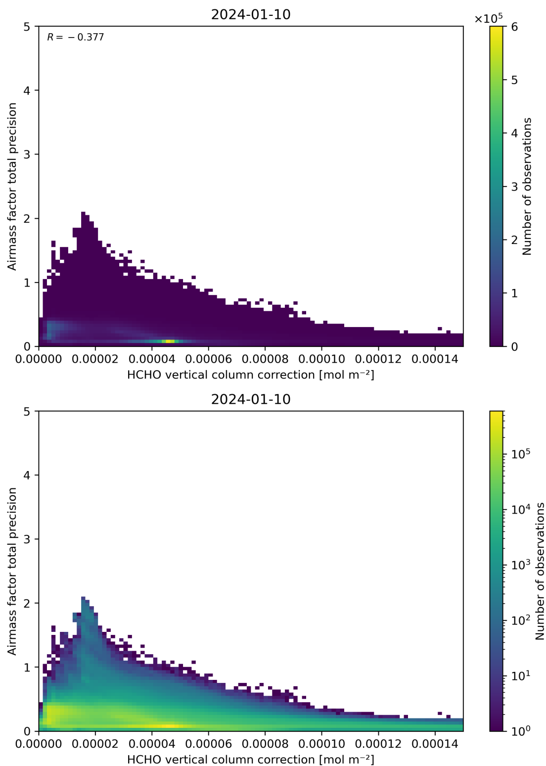
Figure 121: Scatter density plot of “HCHO vertical column correction” against “Airmass factor total precision” for 2024-01-10 to 2024-01-11.
