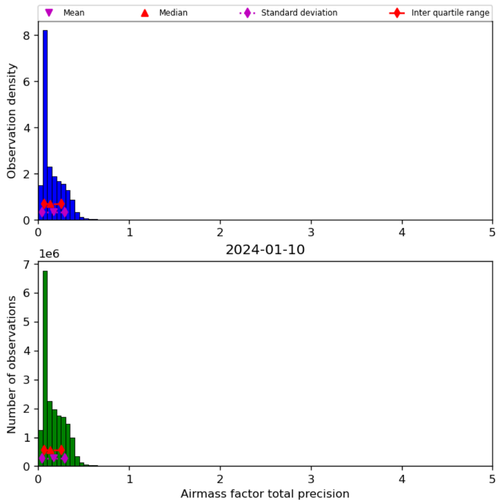
Figure 41: Histogram of “Airmass factor total precision” for 2024-01-10 to 2024-01-11
