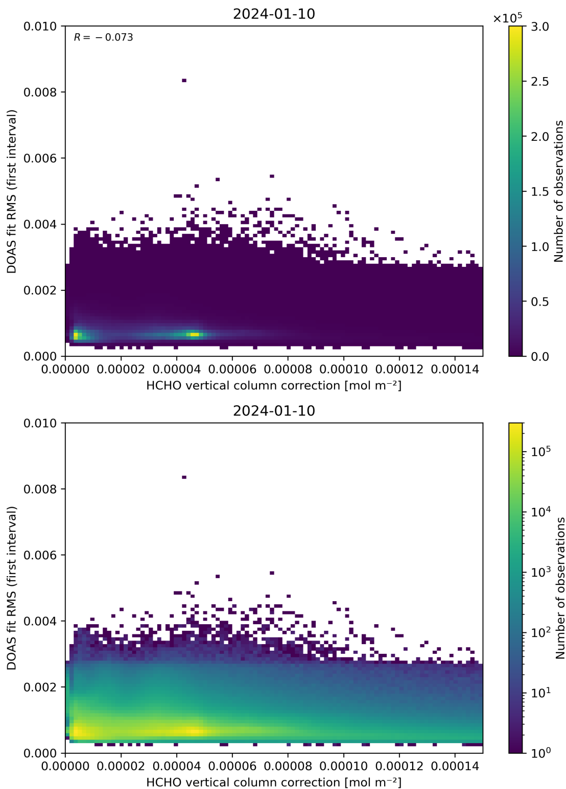
Figure 112: Scatter density plot of “HCHO vertical column correction” against “DOAS fit RMS (first interval)” for 2024-01-10 to 2024-01-11.
