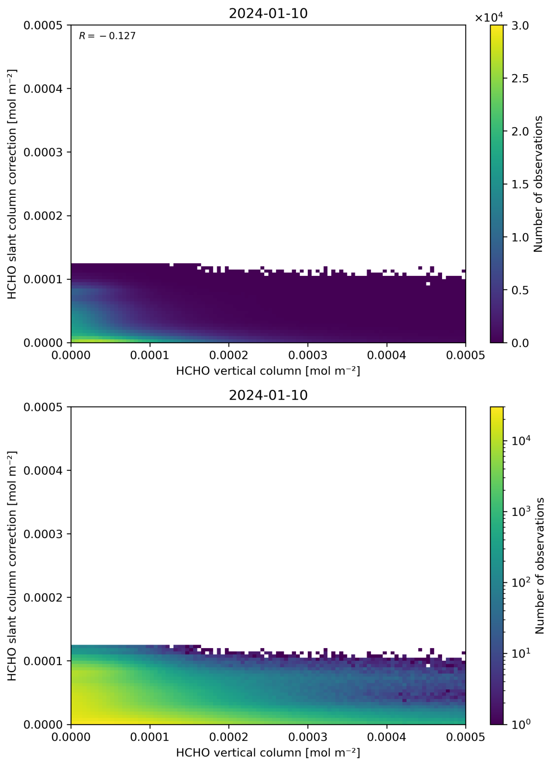
Figure 128: Scatter density plot of “HCHO vertical column” against “HCHO slant column correction” for 2024-01-10 to 2024-01-11.
