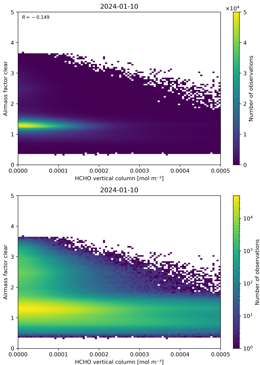
Figure 126: Scatter density plot of “HCHO vertical column” against “Airmass factor clear” for 2024-01-10 to 2024-01-11.
