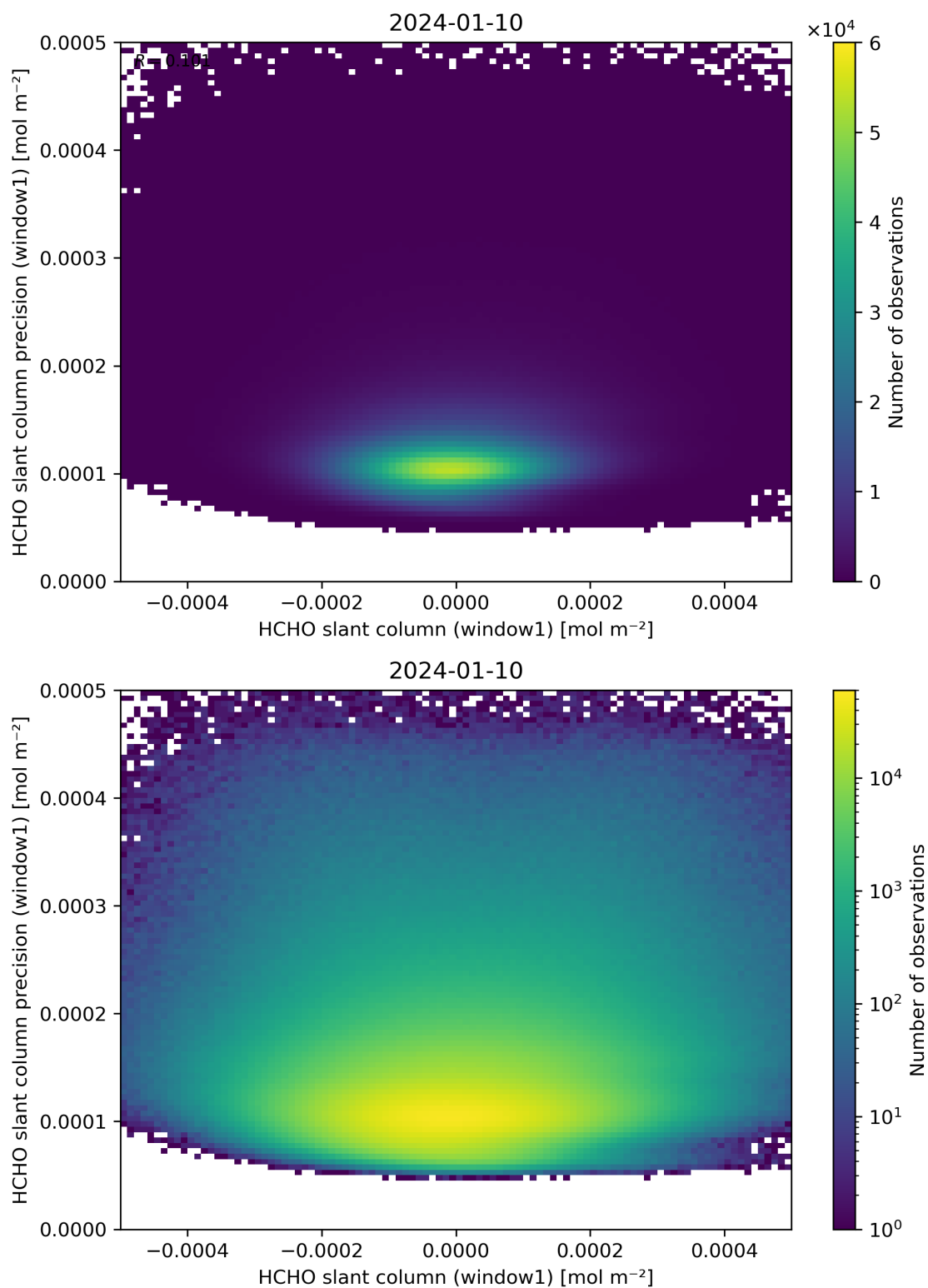
Figure 84: Scatter density plot of “HCHO slant column (window1)” against “HCHO slant column precision (window1)” for 2024-01-10 to 2024-01-11.
