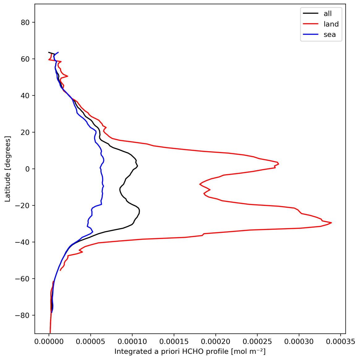
Figure 29: Zonal average of “Integrated a priori HCHO profile” for 2024-01-10 to 2024-01-11.
