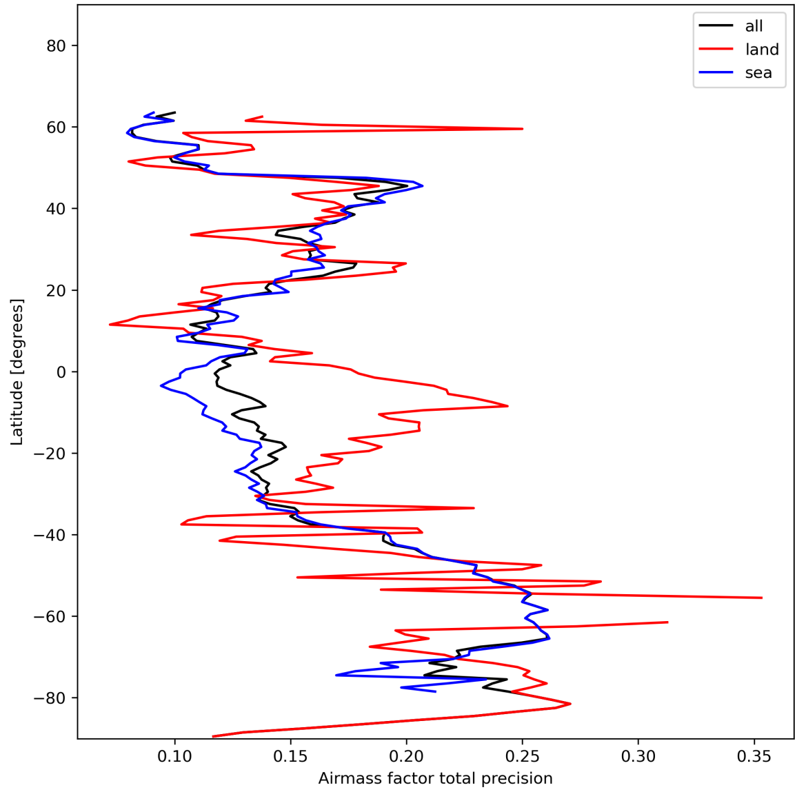
Figure 27: Zonal average of “Airmass factor total precision” for 2024-01-10 to 2024-01-11.
