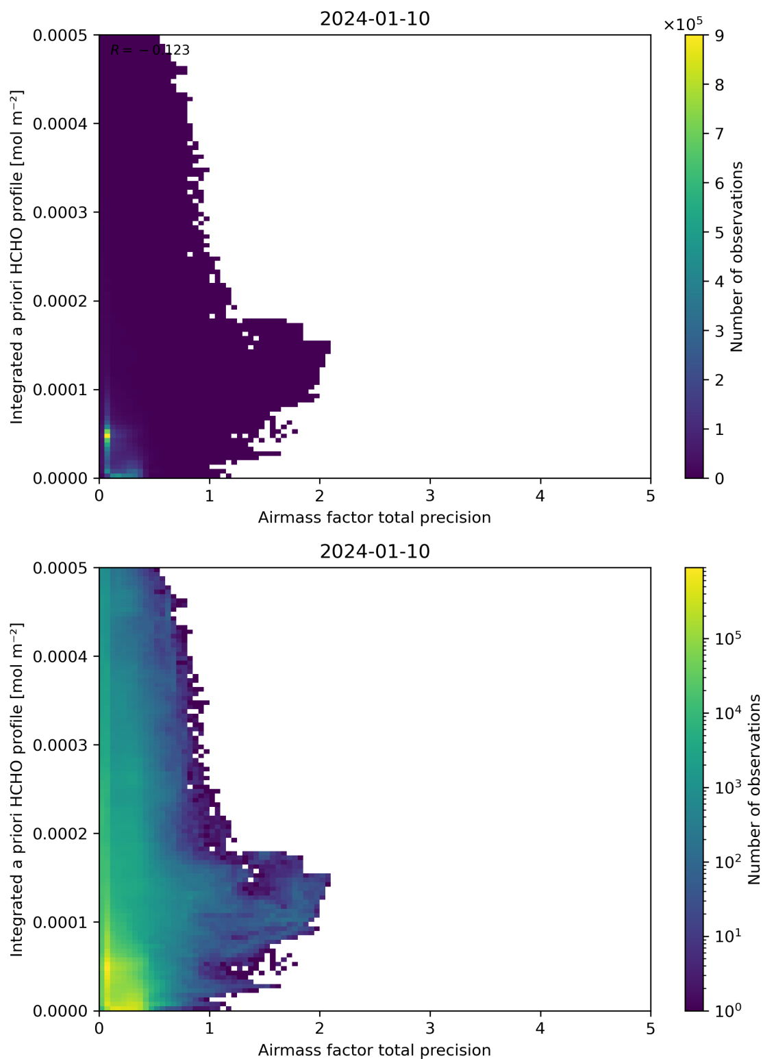
Figure 111: Scatter density plot of “Airmass factor total precision” against “Integrated a priori HCHO profile” for 2024-01-10 to 2024-01-11.
