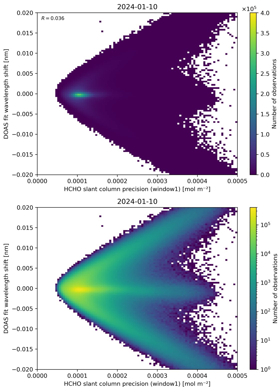
Figure 89: Scatter density plot of “HCHO slant column precision (window1)” against “DOAS fit wavelength shift” for 2024-01-10 to 2024-01-11.
