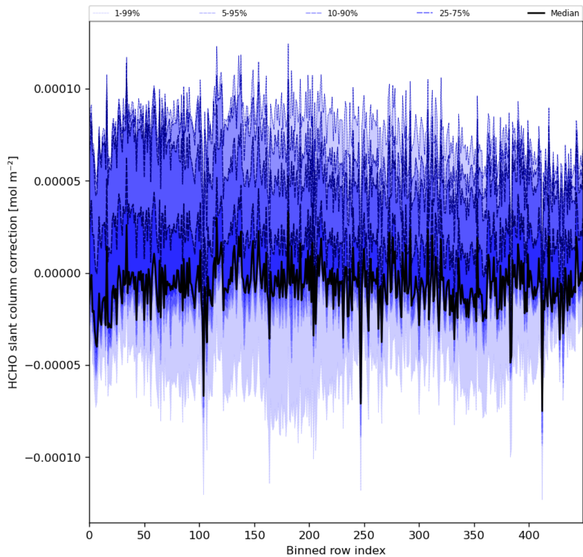
Figure 61: Along track statistics of “HCHO slant column correction” for 2024-01-10 to 2024-01-11
