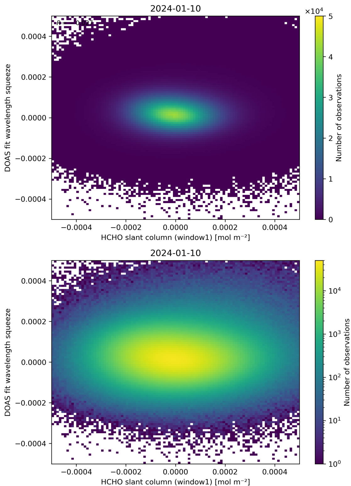
Figure 80: Scatter density plot of “HCHO slant column (window1)” against “DOAS fit wavelength squeeze” for 2024-01-10 to 2024-01-11.
