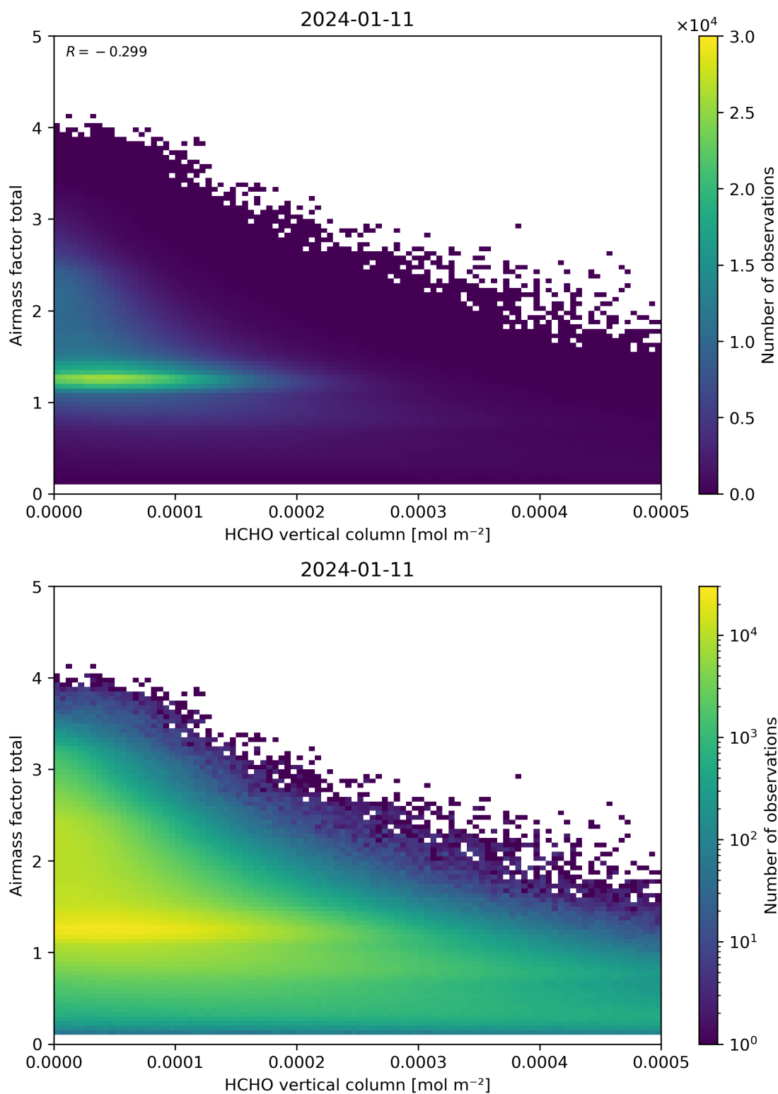
Figure 131: Scatter density plot of “HCHO vertical column” against “Airmass factor total” for 2024-01-10 to 2024-01-12.
