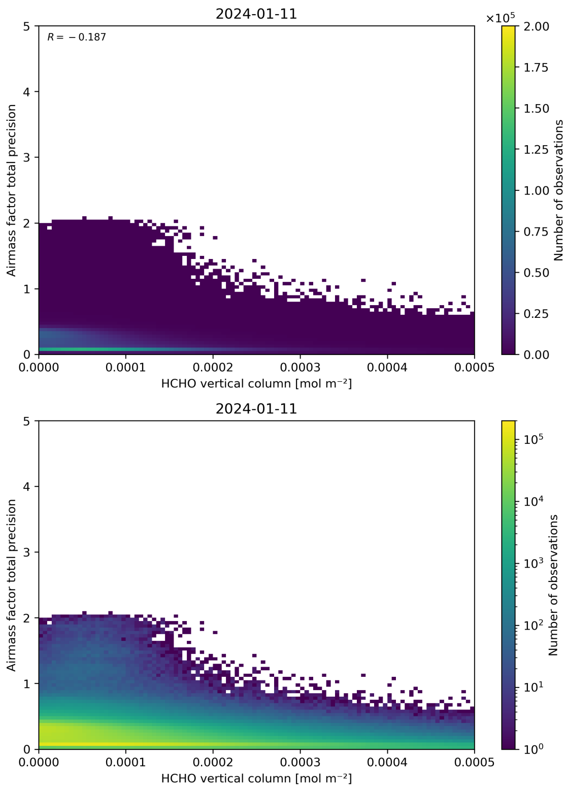
Figure 132: Scatter density plot of “HCHO vertical column” against “Airmass factor total precision” for 2024-01-10 to 2024-01-12.
