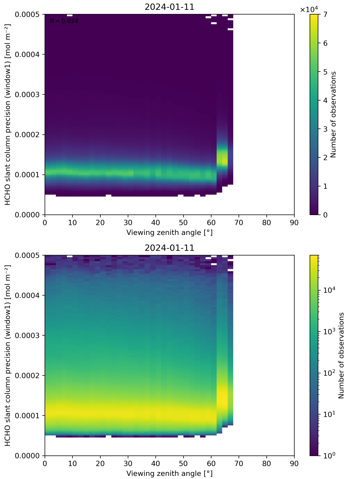
Figure 189: Scatter density plot of “Viewing zenith angle” against “HCHO slant column precision (window1)” for 2024-01-10 to 2024-01-12.
