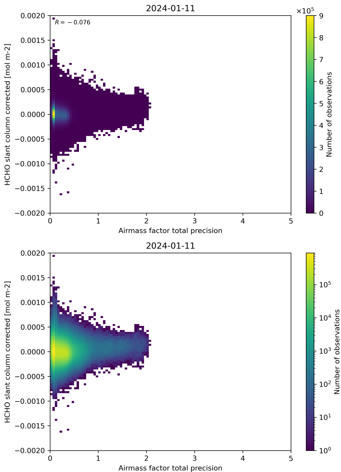
Figure 109: Scatter density plot of “Airmass factor total precision” against “HCHO slant column corrected” for 2024-01-10 to 2024-01-12.
