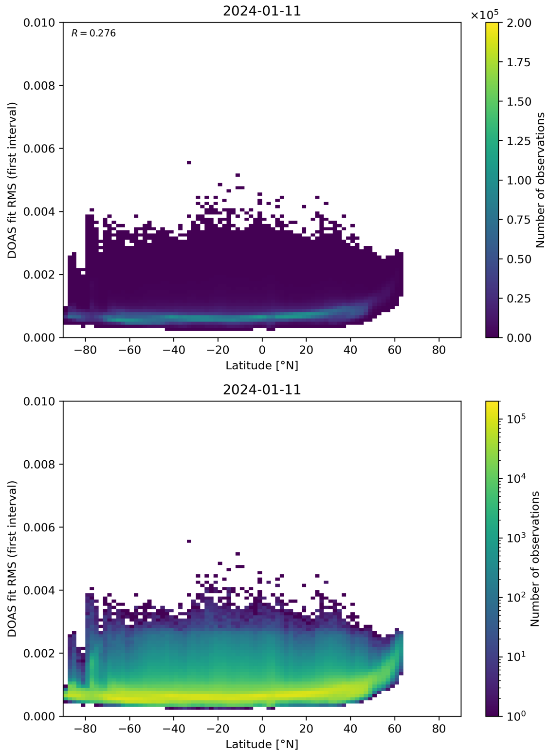
Figure 153: Scatter density plot of “Latitude” against “DOAS fit RMS (first interval)” for 2024-01-10 to 2024-01-12.
