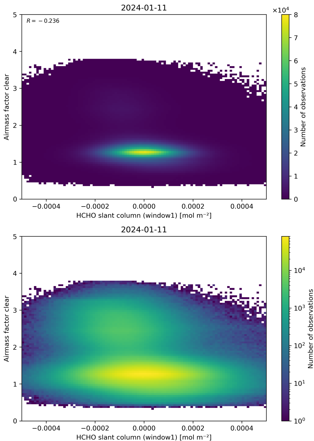
Figure 81: Scatter density plot of “HCHO slant column (window1)” against “Airmass factor clear” for 2024-01-10 to 2024-01-12.
