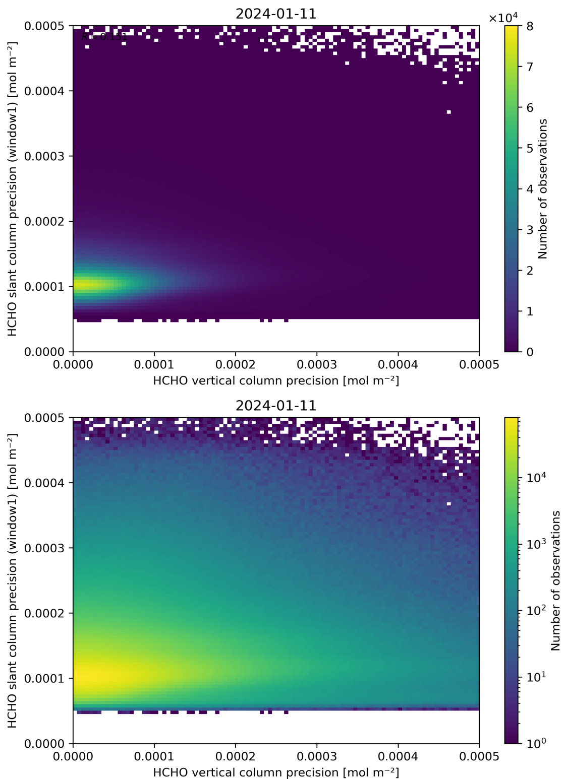
Figure 143: Scatter density plot of “HCHO vertical column precision” against “HCHO slant column precision (window1)” for 2024-01-10 to 2024-01-12.
