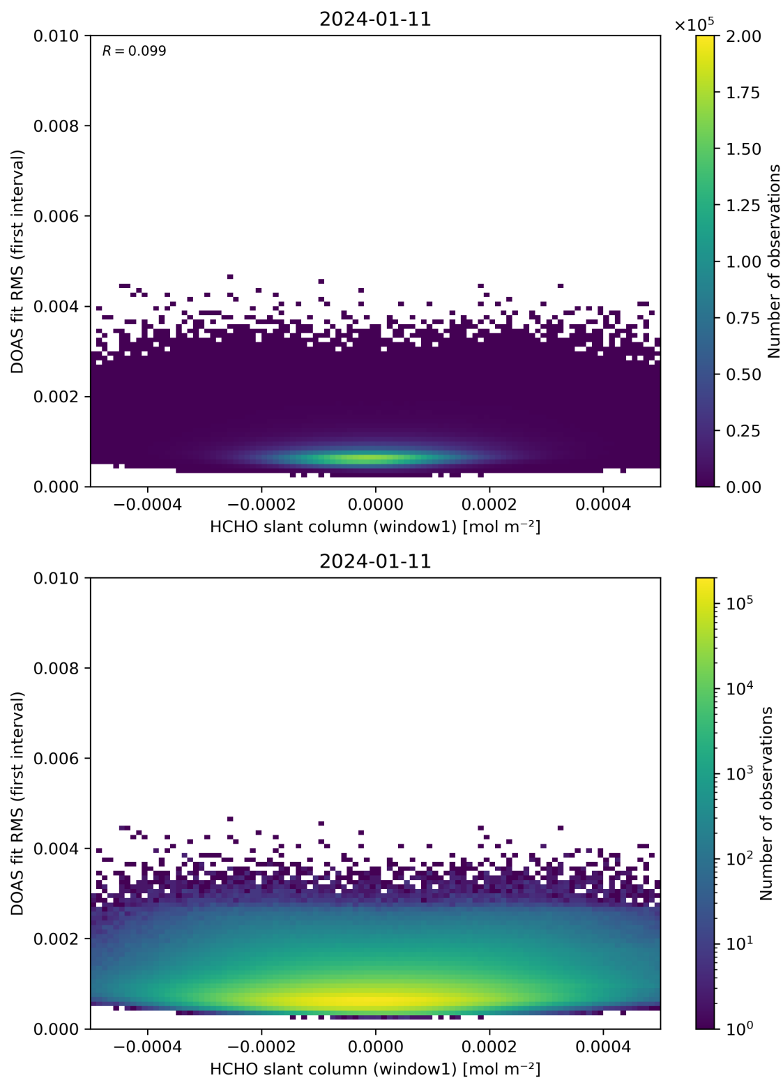
Figure 78: Scatter density plot of “HCHO slant column (window1)” against “DOAS fit RMS (first interval)” for 2024-01-10 to 2024-01-12.
