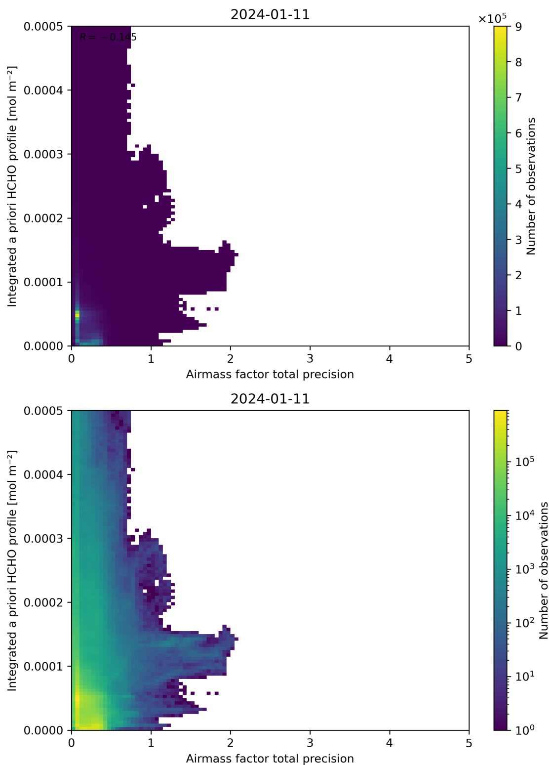
Figure 111: Scatter density plot of “Airmass factor total precision” against “Integrated a priori HCHO profile” for 2024-01-10 to 2024-01-12.
