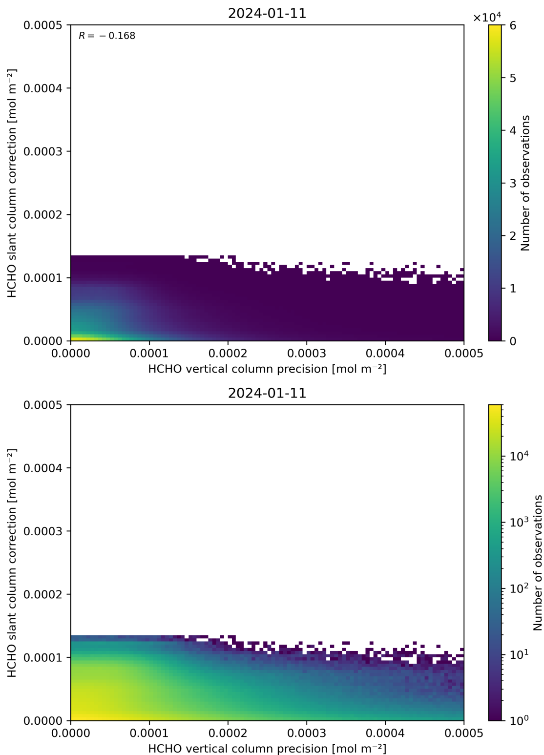
Figure 141: Scatter density plot of “HCHO vertical column precision” against “HCHO slant column correction” for 2024-01-10 to 2024-01-12.
