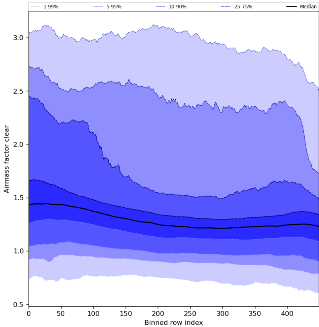
Figure 56: Along track statistics of “Airmass factor clear” for 2024-01-10 to 2024-01-12
