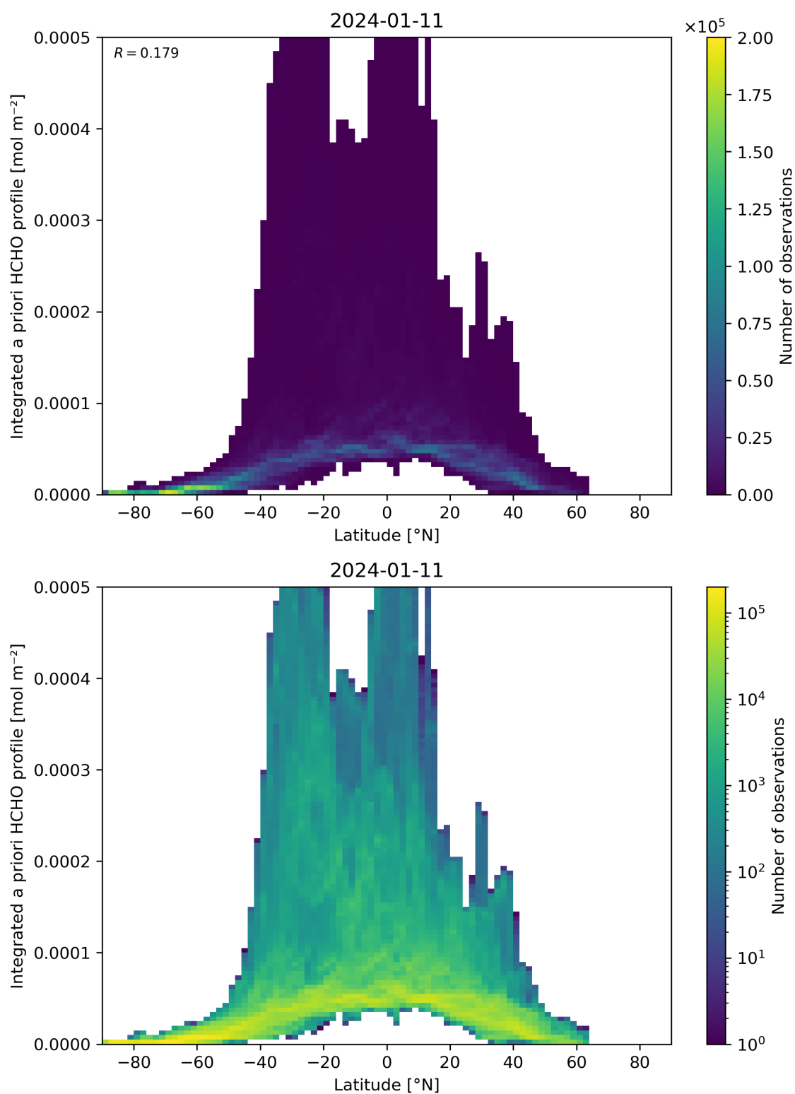
Figure 166: Scatter density plot of “Latitude” against “Integrated a priori HCHO profile” for 2024-01-10 to 2024-01-12.
