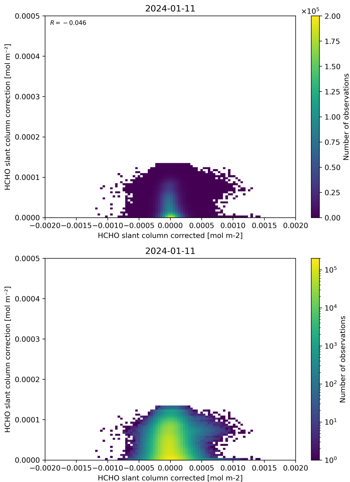
Figure 77: Scatter density plot of “HCHO slant column corrected” against “HCHO slant column correction” for 2024-01-10 to 2024-01-12.
