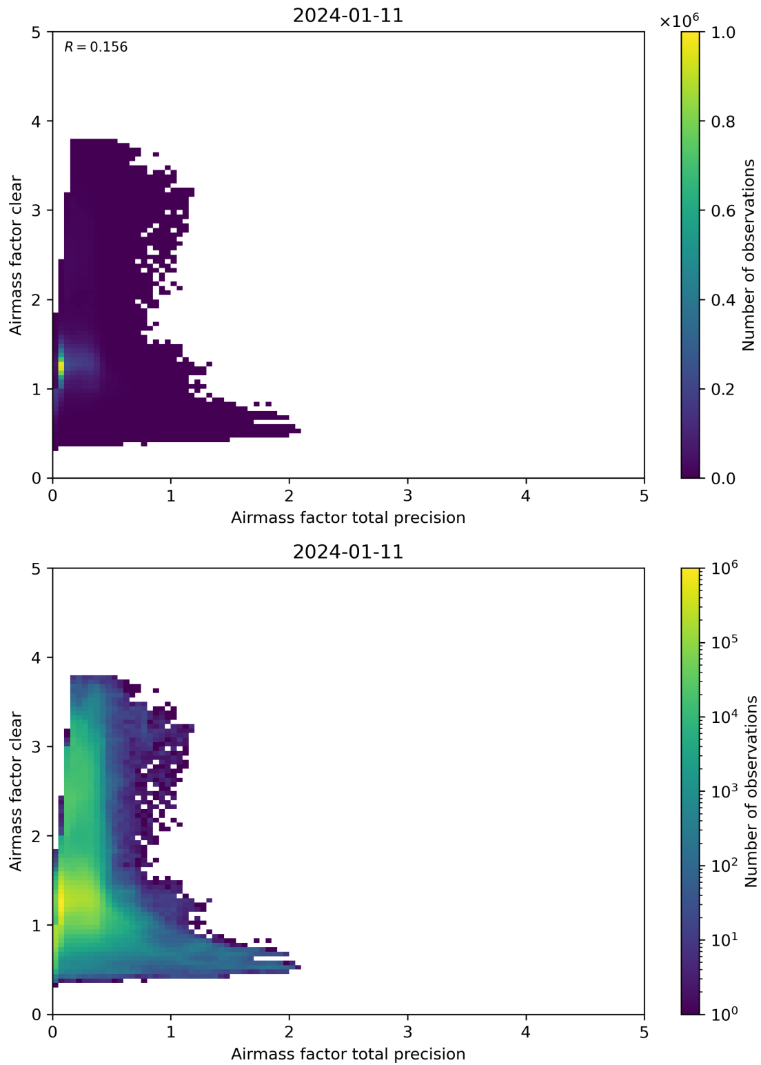
Figure 108: Scatter density plot of “Airmass factor total precision” against “Airmass factor clear” for 2024-01-10 to 2024-01-12.
