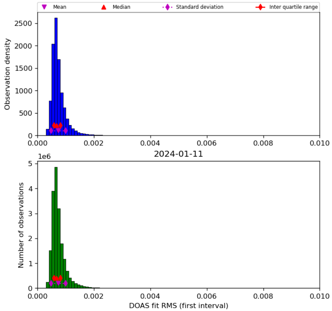
Figure 46: Histogram of “DOAS fit RMS (first interval)” for 2024-01-10 to 2024-01-12
