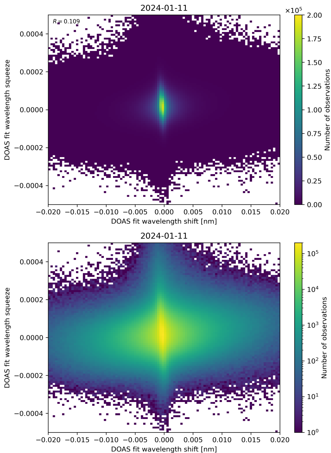
Figure 65: Scatter density plot of “DOAS fit wavelength shift” against “DOAS fit wavelength squeeze” for 2024-01-10 to 2024-01-12.
