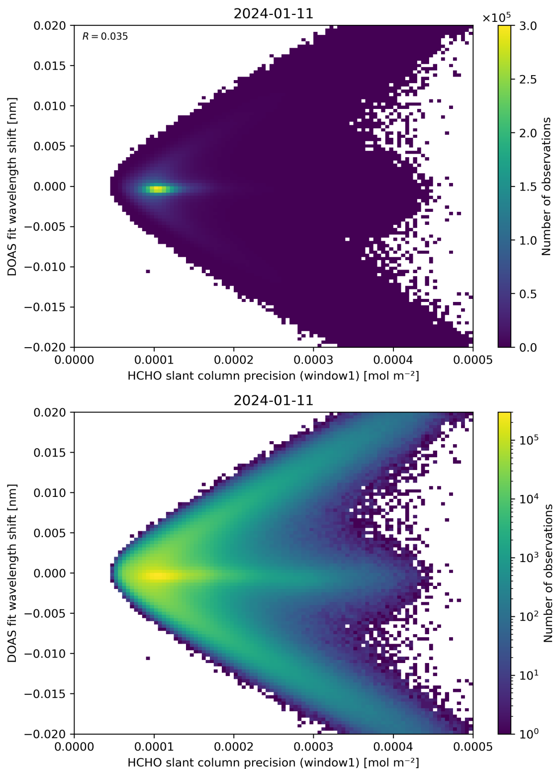
Figure 89: Scatter density plot of “HCHO slant column precision (window1)” against “DOAS fit wavelength shift” for 2024-01-10 to 2024-01-12.
