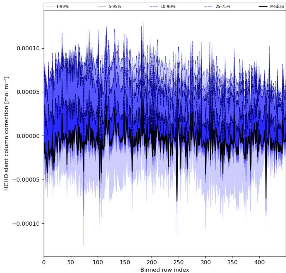
Figure 61: Along track statistics of “HCHO slant column correction” for 2024-01-10 to 2024-01-12
