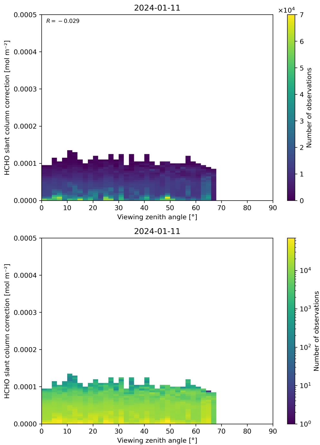
Figure 187: Scatter density plot of “Viewing zenith angle” against “HCHO slant column correction” for 2024-01-10 to 2024-01-12.
