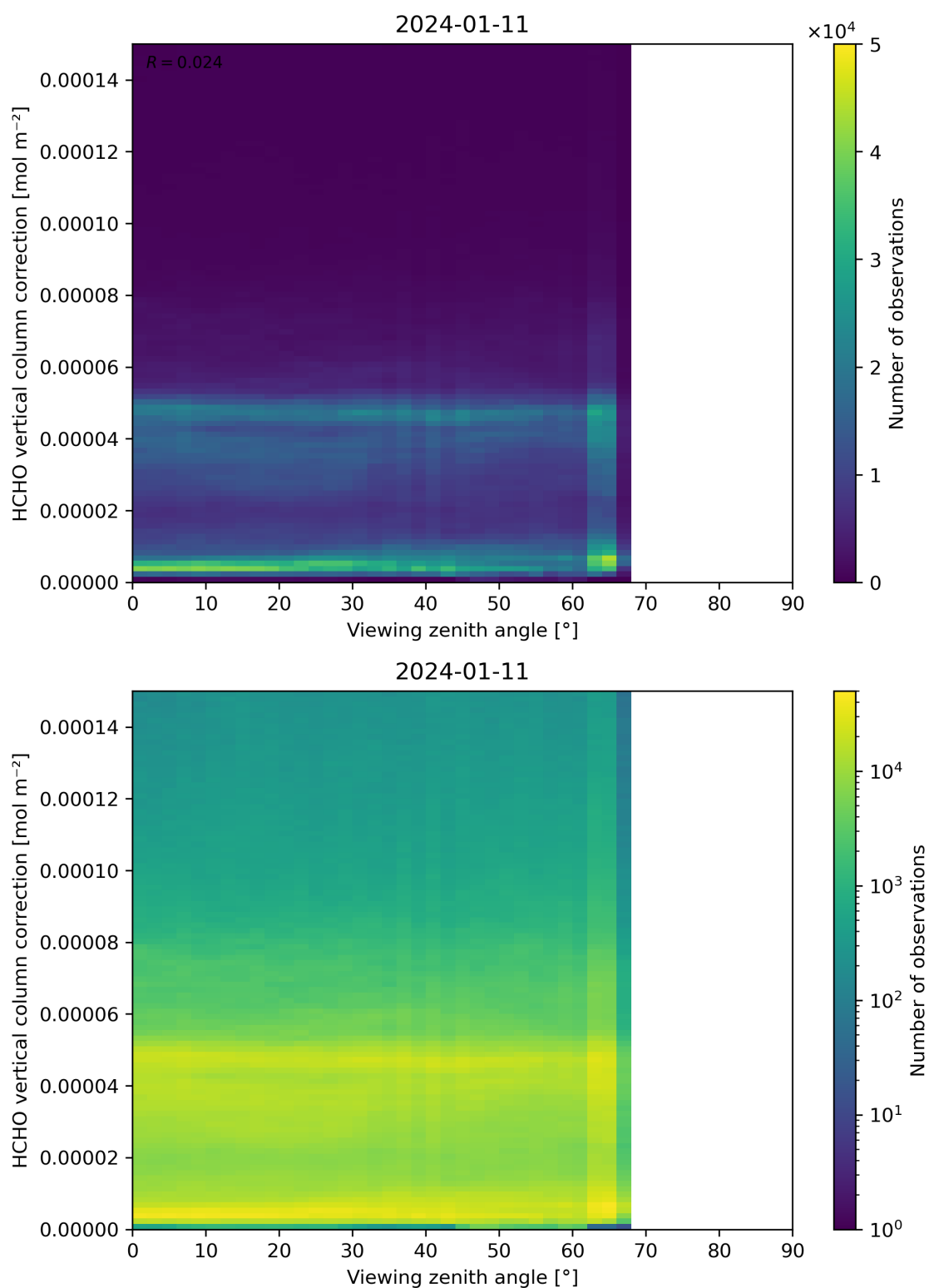
Figure 193: Scatter density plot of “Viewing zenith angle” against “HCHO vertical column correction” for 2024-01-10 to 2024-01-12.
