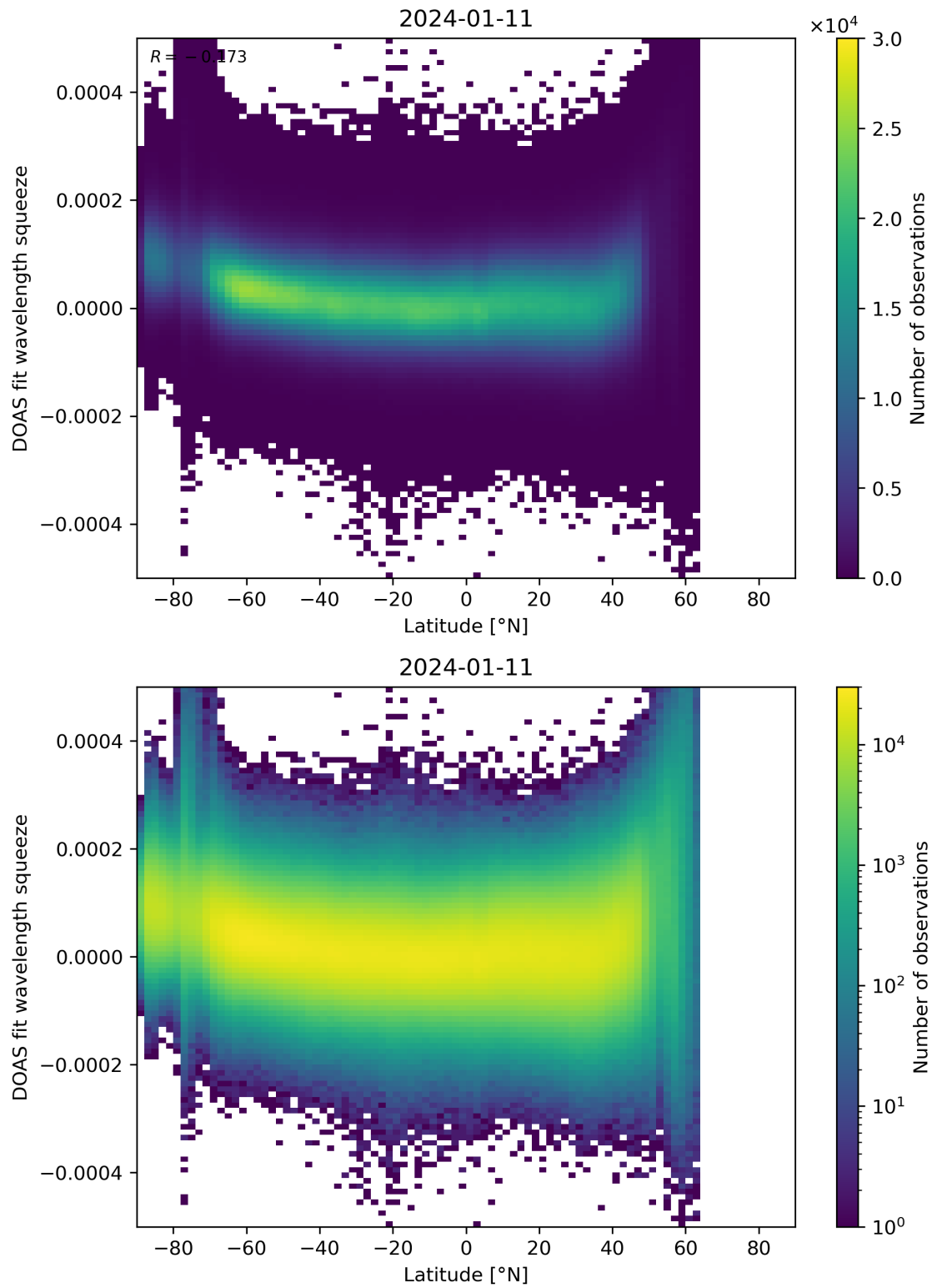
Figure 155: Scatter density plot of “Latitude” against “DOAS fit wavelength squeeze” for 2024-01-10 to 2024-01-12.
