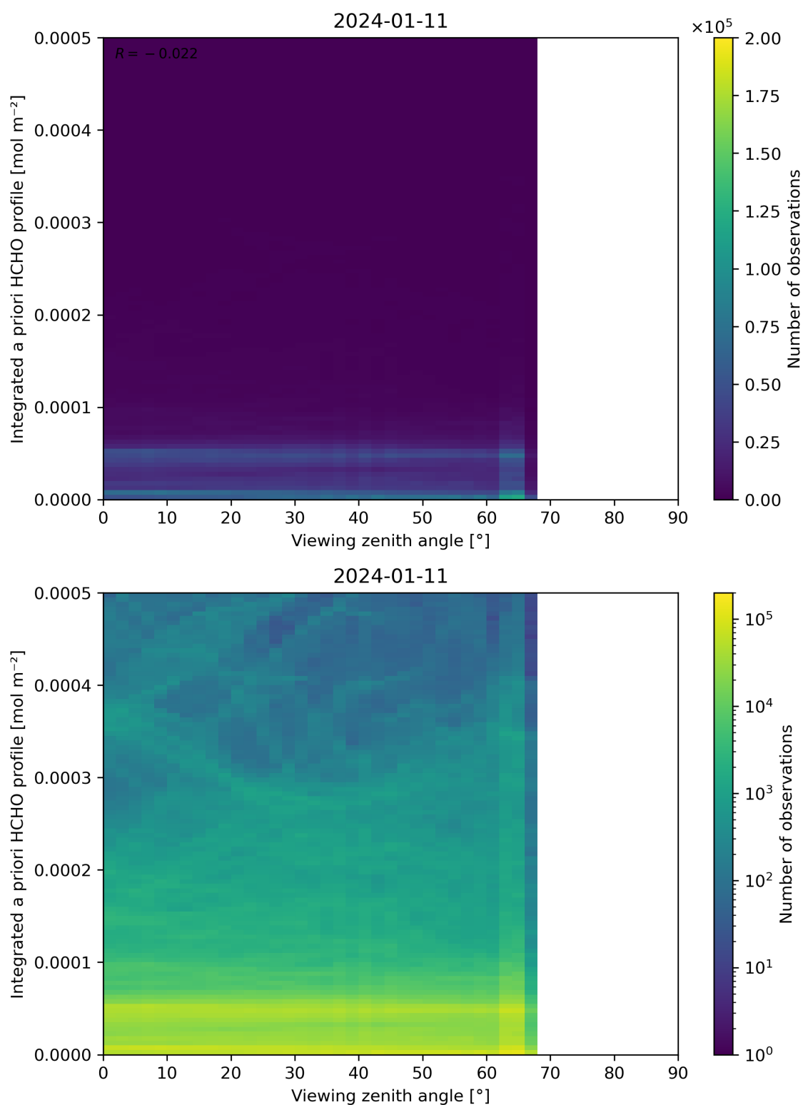
Figure 195: Scatter density plot of “Viewing zenith angle” against “Integrated a priori HCHO profile” for 2024-01-10 to 2024-01-12.
