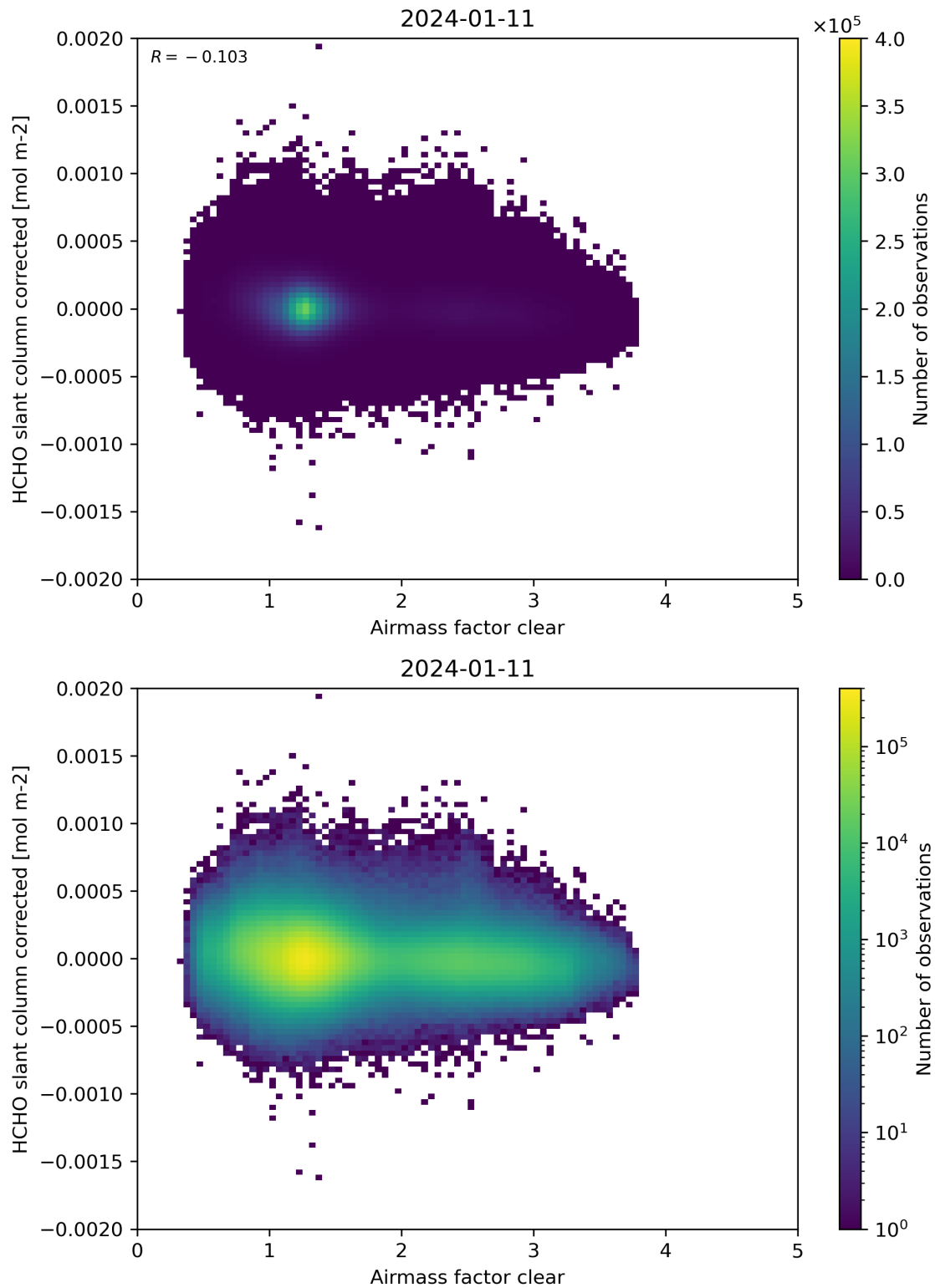
Figure 74: Scatter density plot of “Airmass factor clear” against “HCHO slant column corrected” for 2024-01-10 to 2024-01-12.
