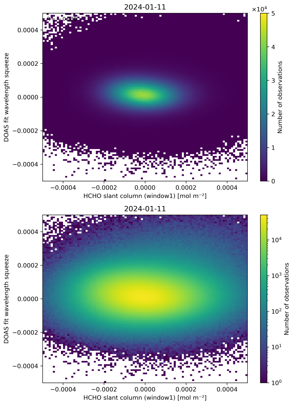
Figure 80: Scatter density plot of “HCHO slant column (window1)” against “DOAS fit wavelength squeeze” for 2024-01-10 to 2024-01-12.
