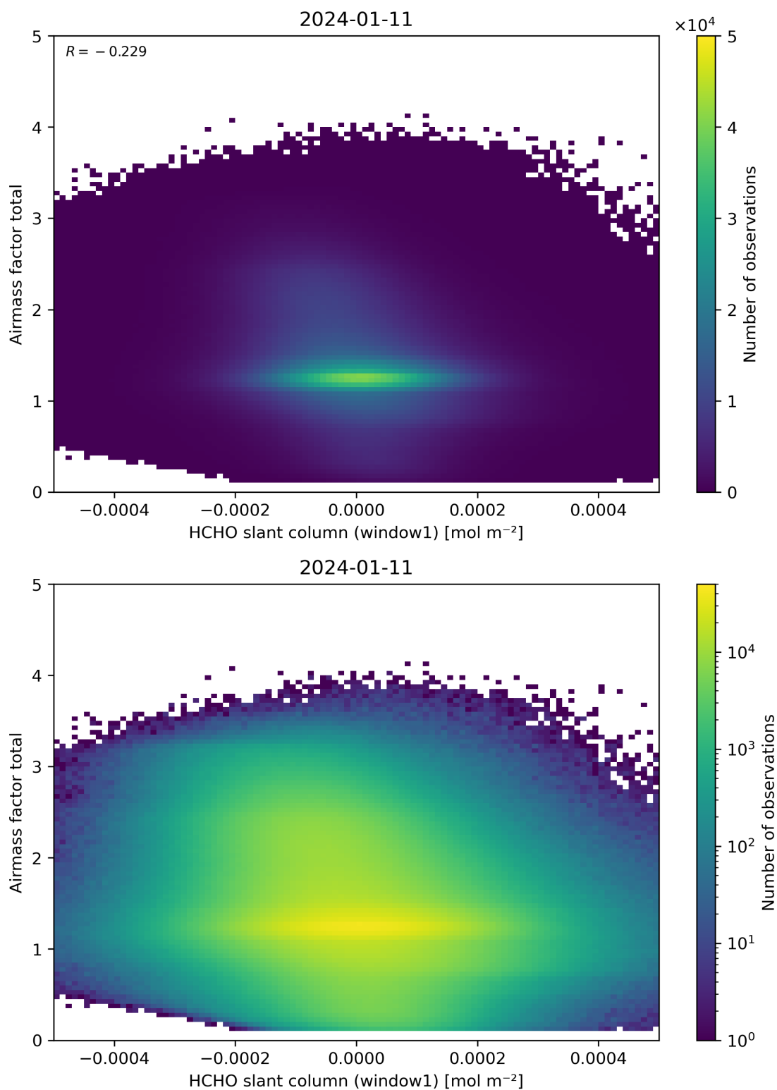
Figure 85: Scatter density plot of “HCHO slant column (window1)” against “Airmass factor total” for 2024-01-10 to 2024-01-12.
