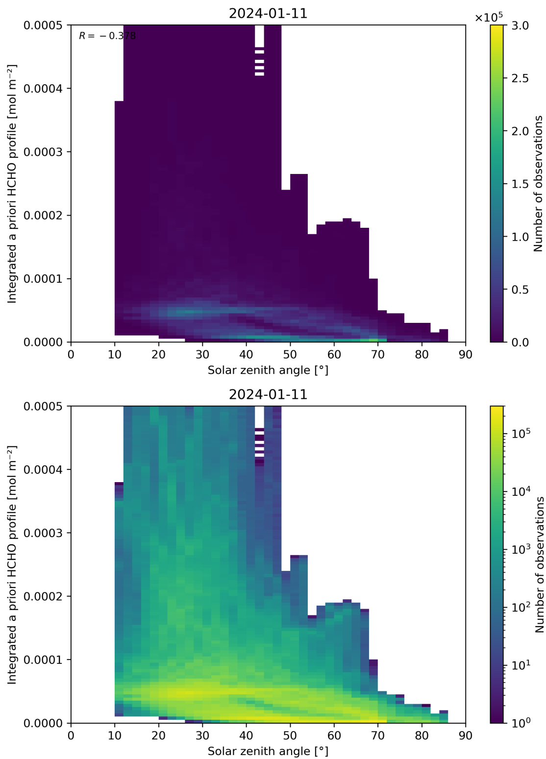
Figure 180: Scatter density plot of “Solar zenith angle” against “Integrated a priori HCHO profile” for 2024-01-10 to 2024-01-12.
