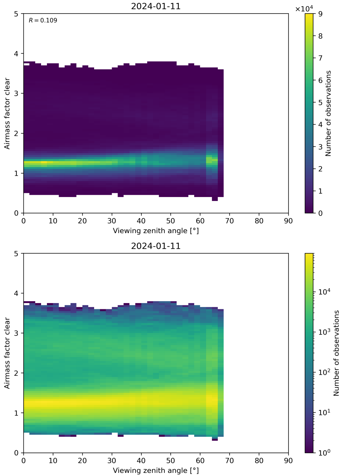
Figure 185: Scatter density plot of “Viewing zenith angle” against “Airmass factor clear” for 2024-01-10 to 2024-01-12.
