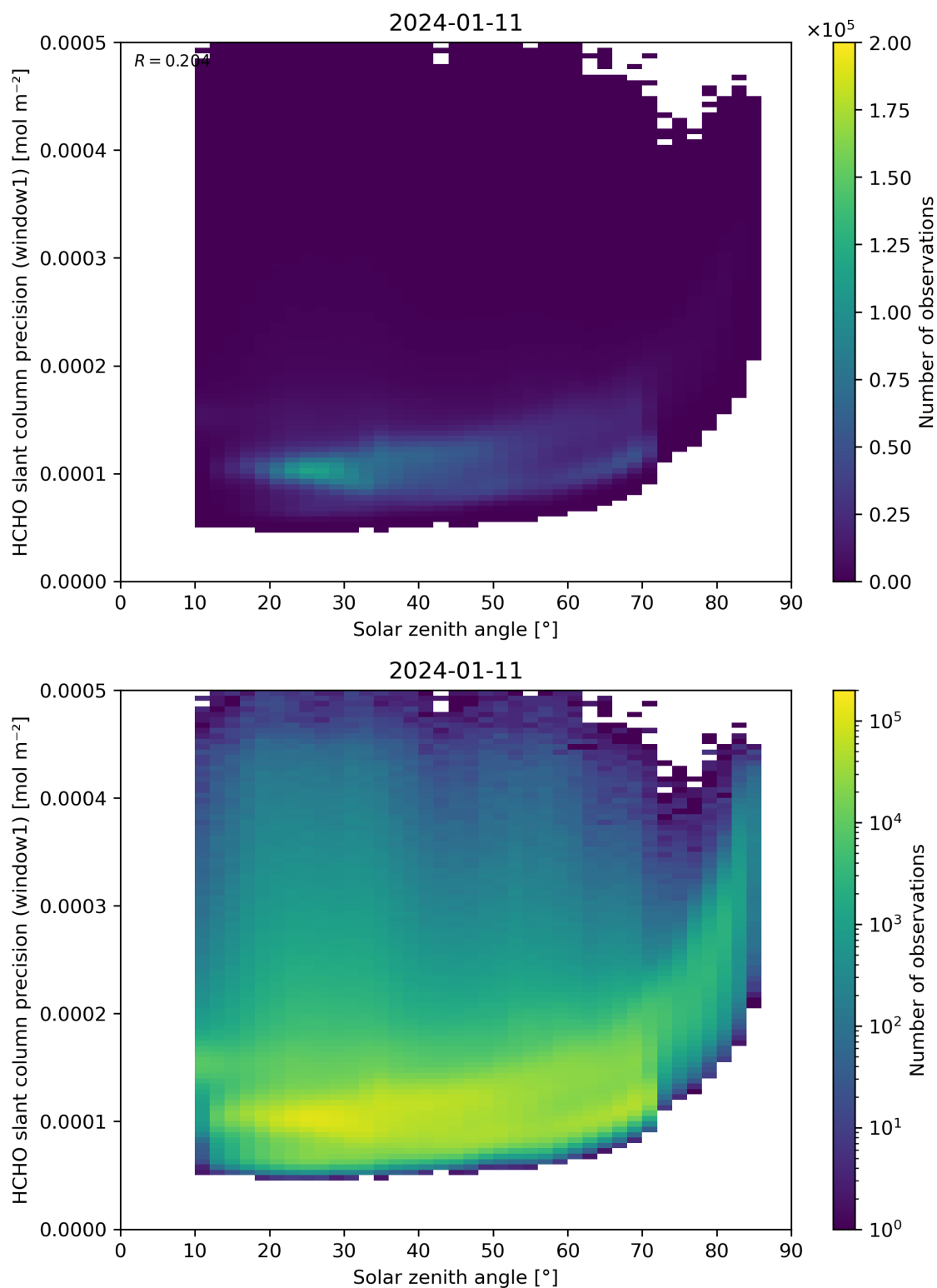
Figure 174: Scatter density plot of “Solar zenith angle” against “HCHO slant column precision (window1)” for 2024-01-10 to 2024-01-12.
