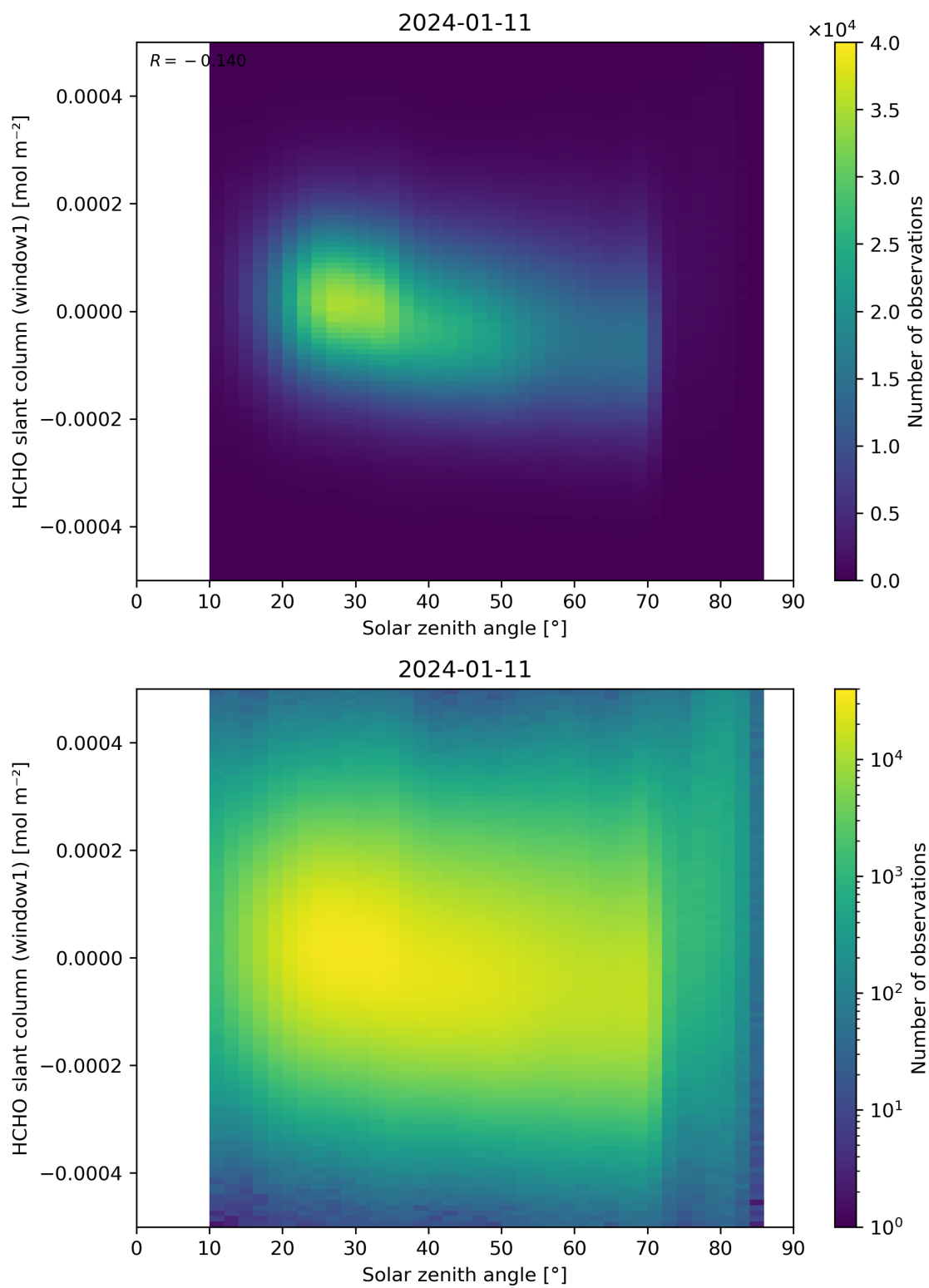
Figure 173: Scatter density plot of “Solar zenith angle” against “HCHO slant column (window1)” for 2024-01-10 to 2024-01-12.
