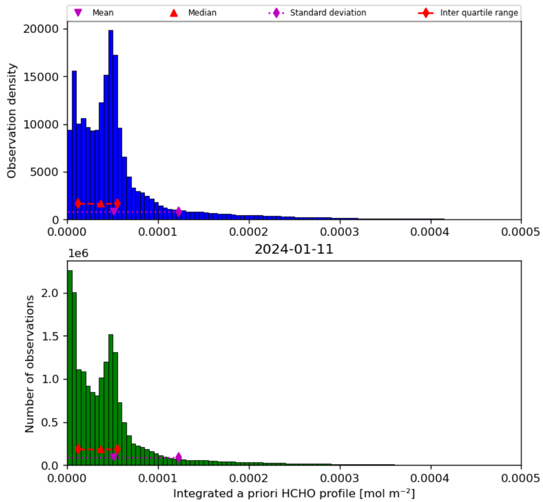
Figure 43: Histogram of “Integrated a priori HCHO profile” for 2024-01-10 to 2024-01-12
