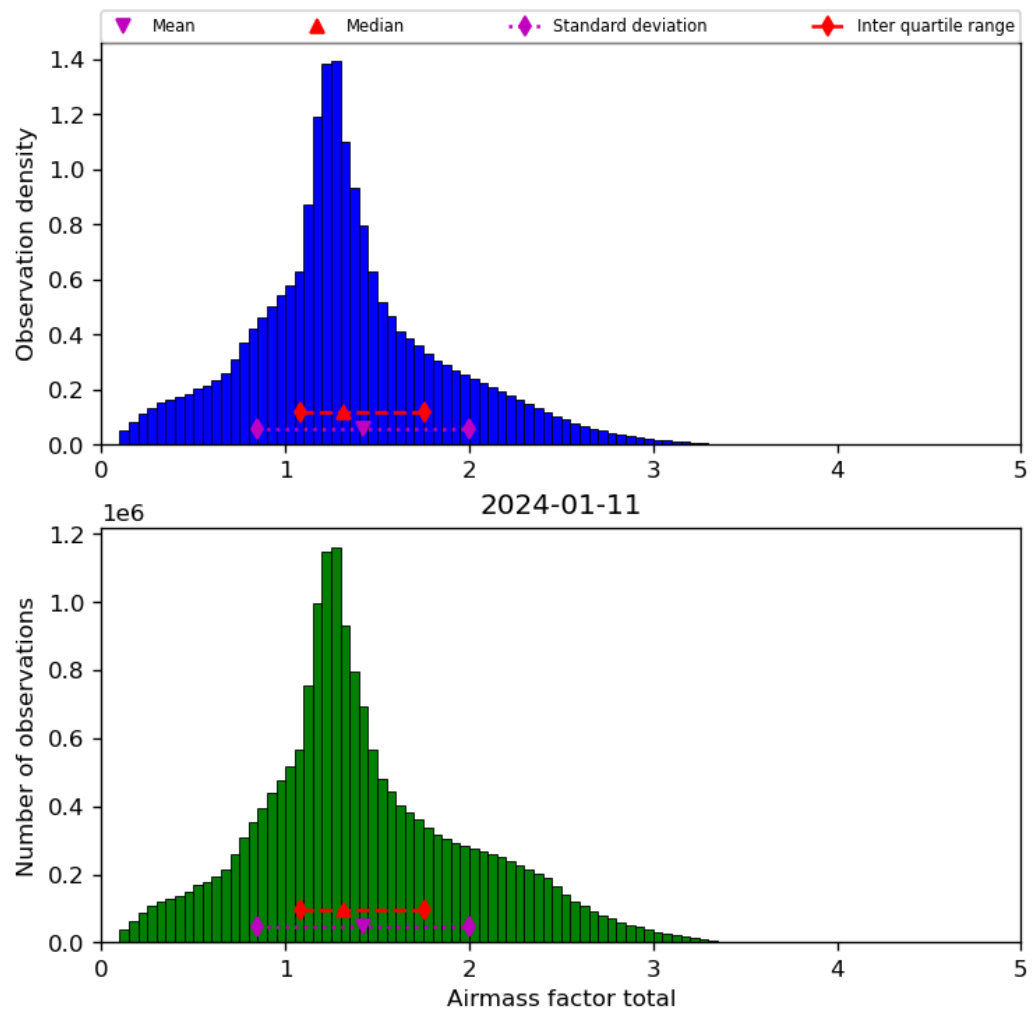
Figure 40: Histogram of “Airmass factor total” for 2024-01-10 to 2024-01-12
