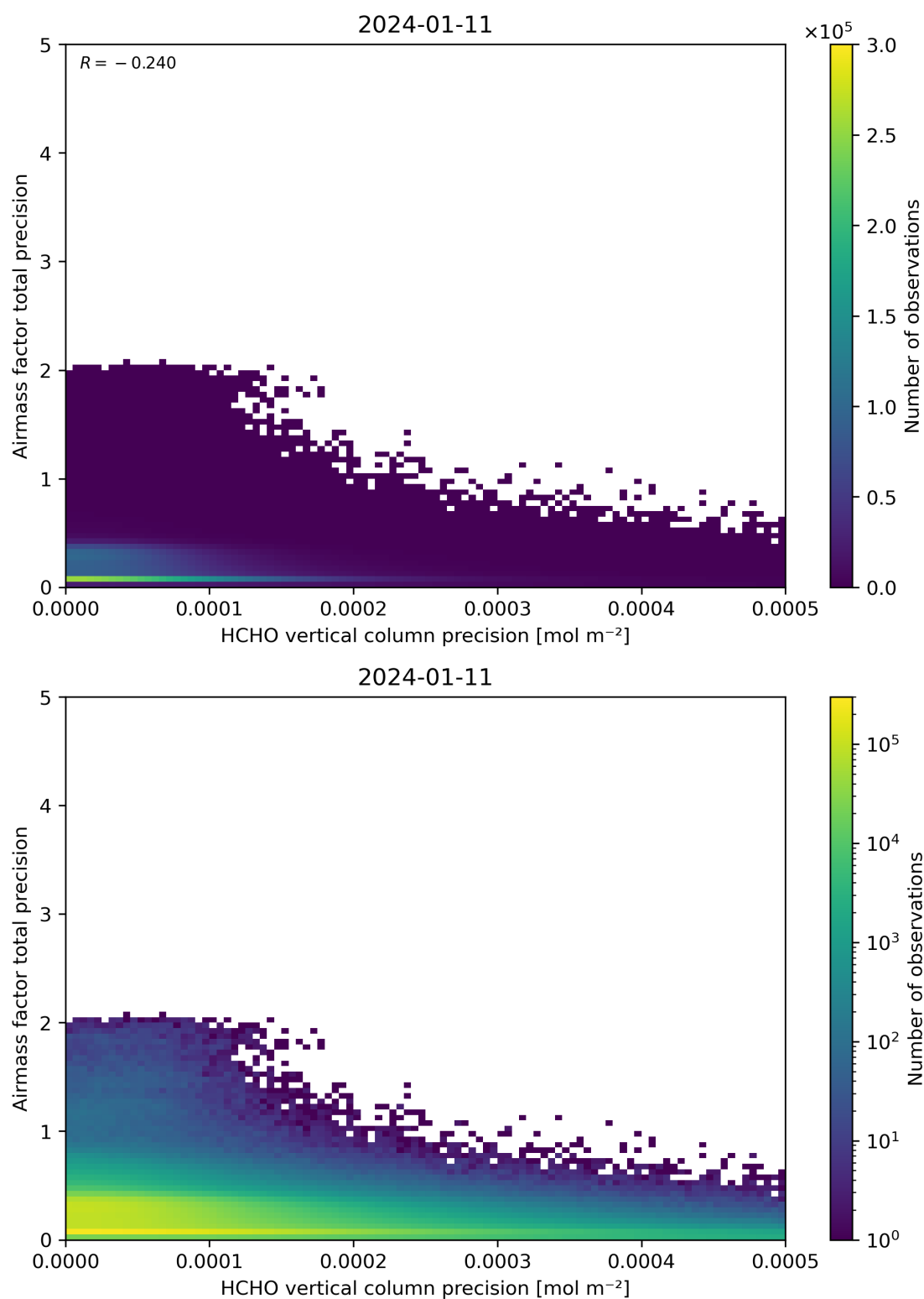
Figure 145: Scatter density plot of “HCHO vertical column precision” against “Airmass factor total precision” for 2024-01-10 to 2024-01-12.
