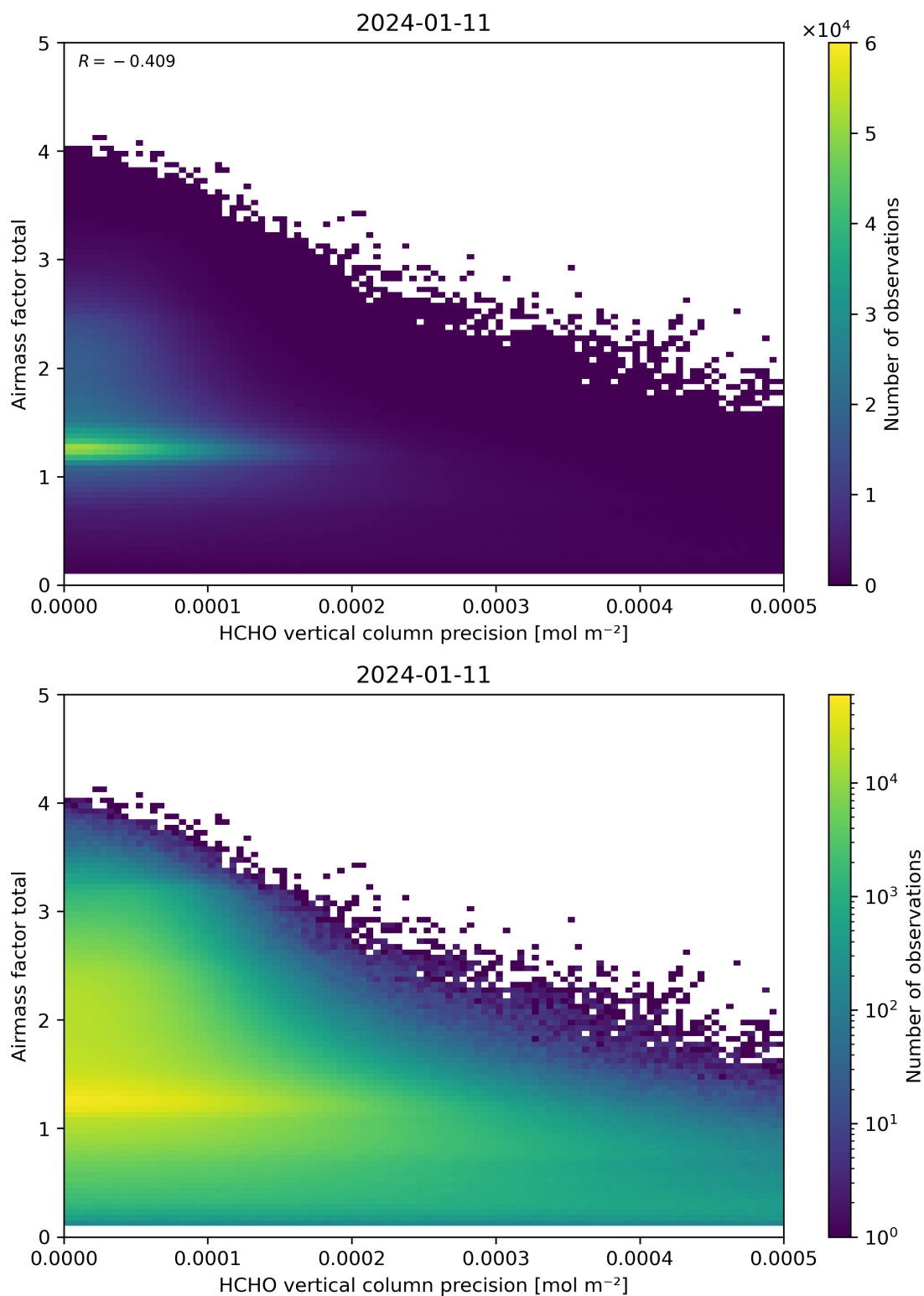
Figure 144: Scatter density plot of “HCHO vertical column precision” against “Airmass factor total” for 2024-01-10 to 2024-01-12.
