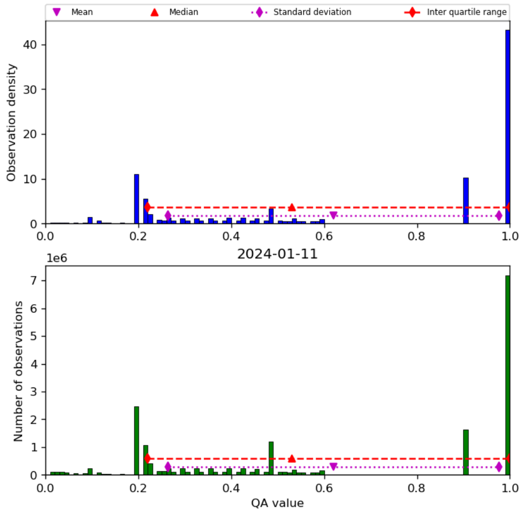
Figure 34: Histogram of “QA value” for 2024-01-10 to 2024-01-12
