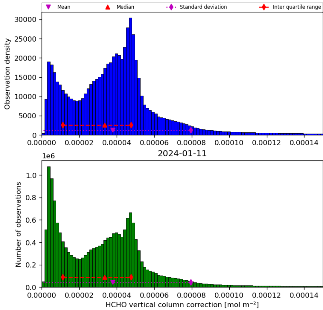
Figure 37: Histogram of “HCHO vertical column correction” for 2024-01-10 to 2024-01-12
