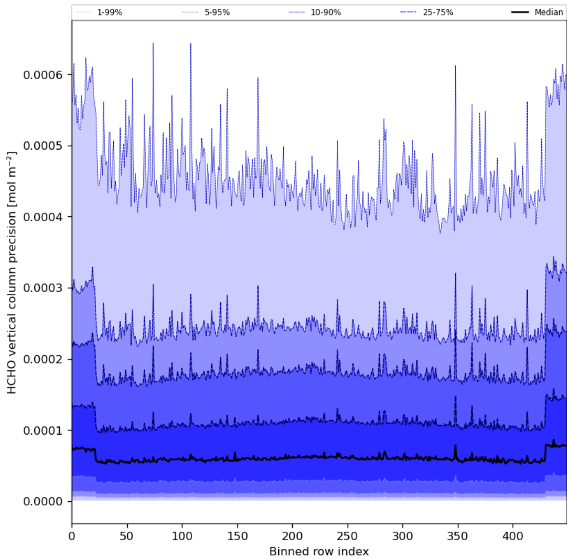
Figure 50: Along track statistics of “HCHO vertical column precision” for 2024-01-10 to 2024-01-12
