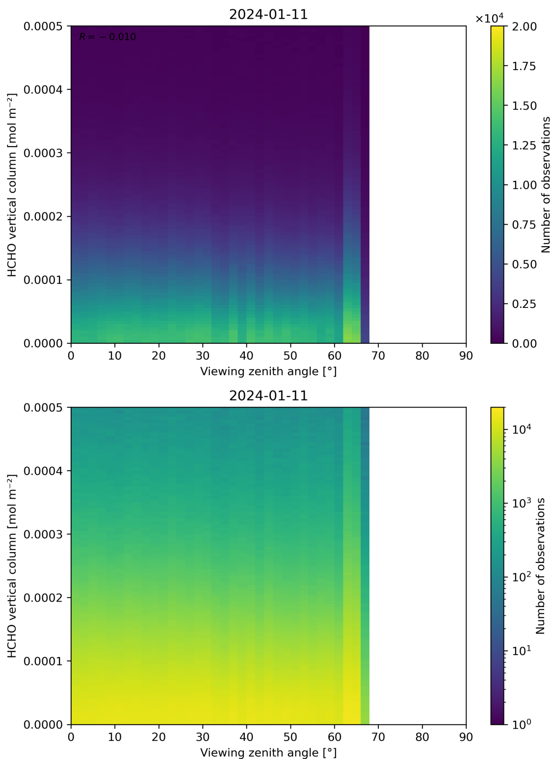
Figure 192: Scatter density plot of “Viewing zenith angle” against “HCHO vertical column” for 2024-01-10 to 2024-01-12.
