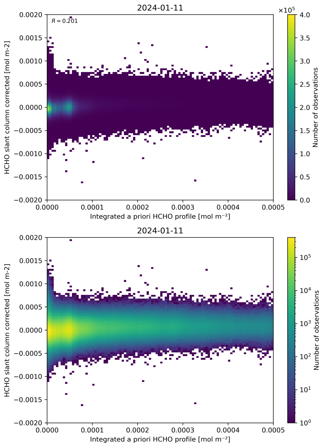
Figure 151: Scatter density plot of “Integrated a priori HCHO profile” against “HCHO slant column corrected” for 2024-01-10 to 2024-01-12.
