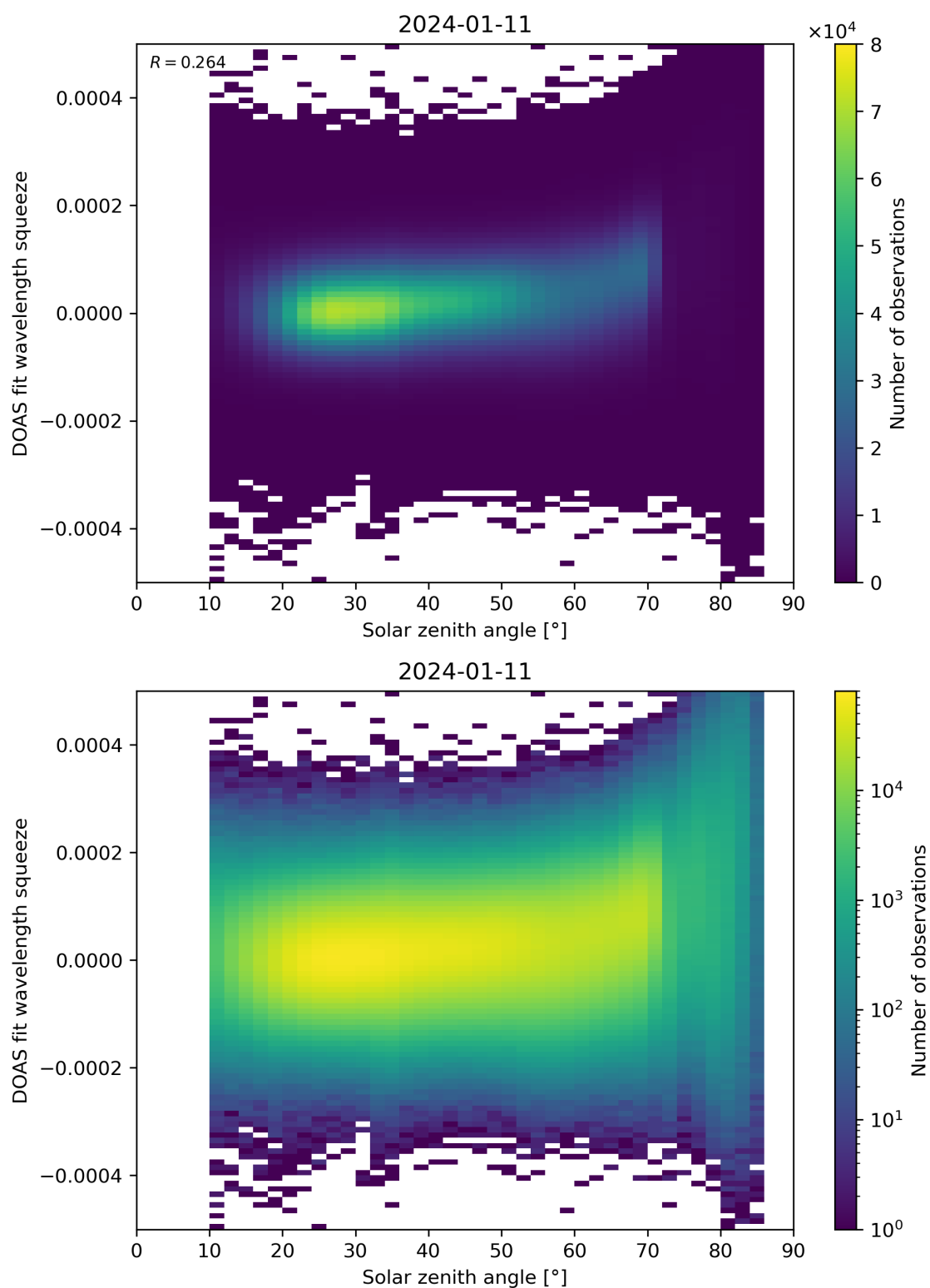
Figure 169: Scatter density plot of “Solar zenith angle” against “DOAS fit wavelength squeeze” for 2024-01-10 to 2024-01-12.
