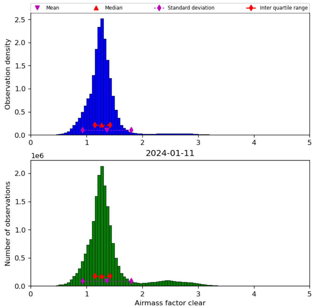
Figure 42: Histogram of “Airmass factor clear” for 2024-01-10 to 2024-01-12
