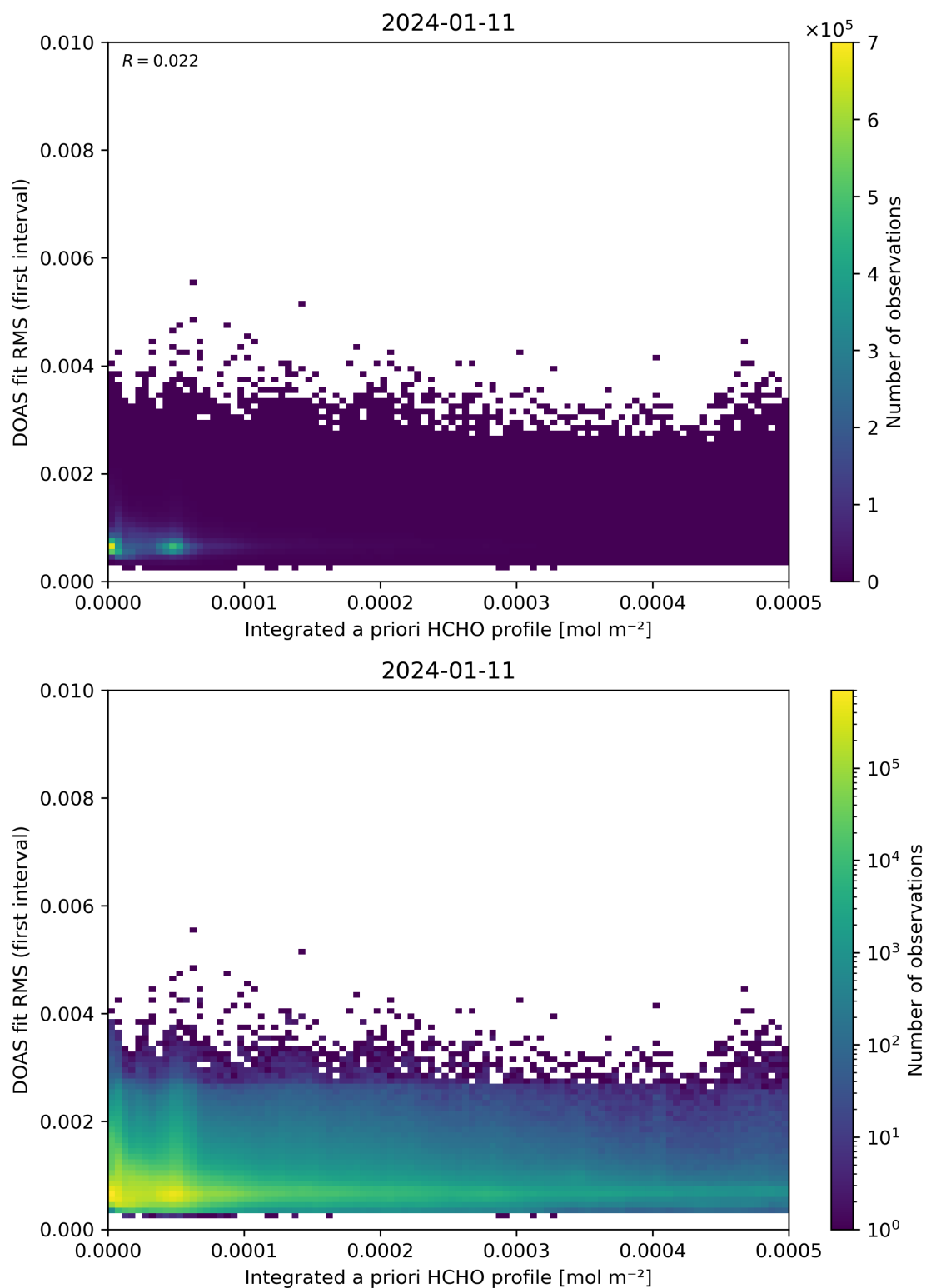
Figure 148: Scatter density plot of “Integrated a priori HCHO profile” against “DOAS fit RMS (first interval)” for 2024-01-10 to 2024-01-12.
