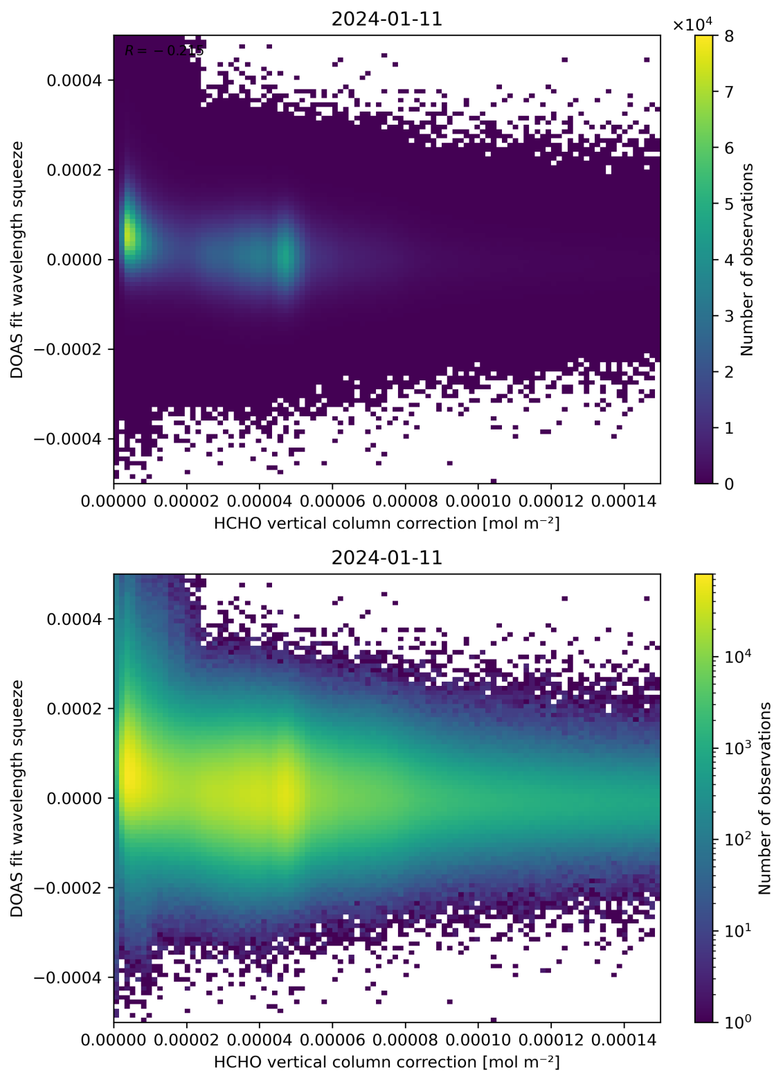
Figure 114: Scatter density plot of “HCHO vertical column correction” against “DOAS fit wavelength squeeze” for 2024-01-10 to 2024-01-12.
