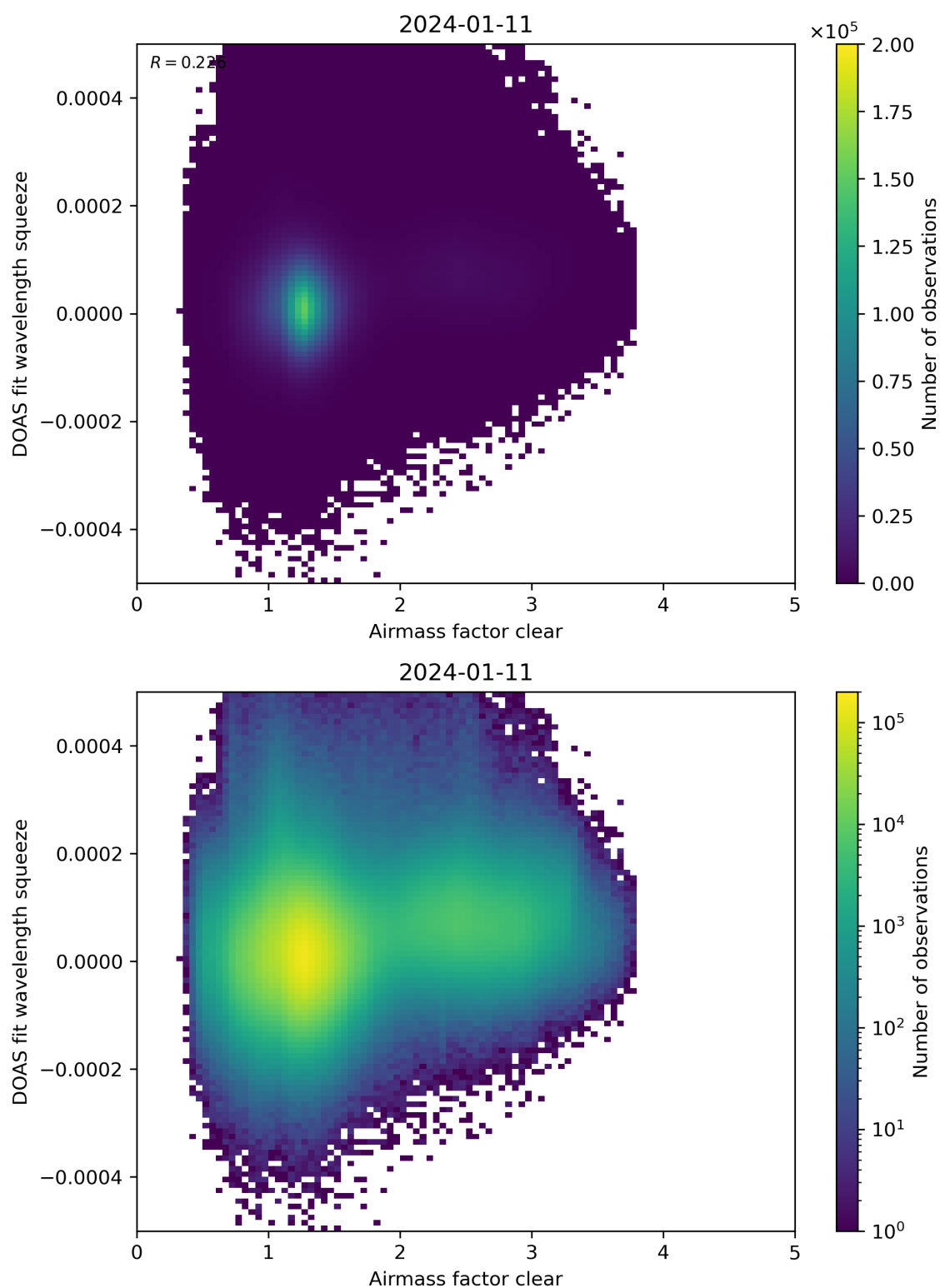
Figure 73: Scatter density plot of “Airmass factor clear” against “DOAS fit wavelength squeeze” for 2024-01-10 to 2024-01-12.
