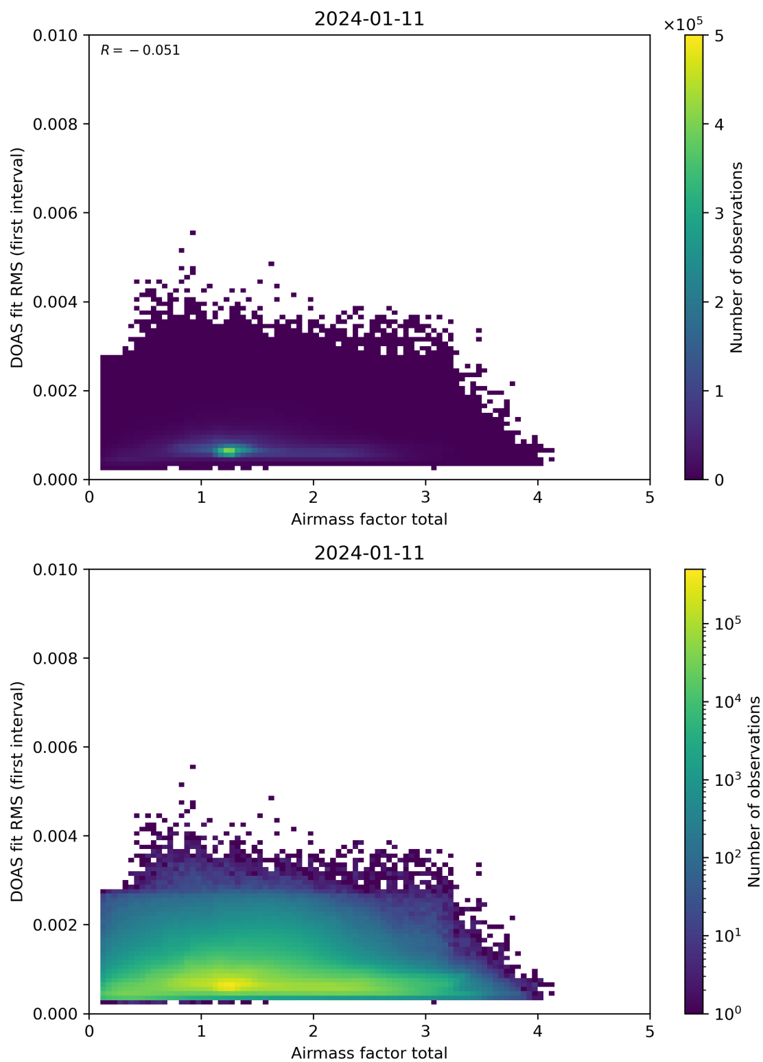
Figure 97: Scatter density plot of “Airmass factor total” against “DOAS fit RMS (first interval)” for 2024-01-10 to 2024-01-12.
