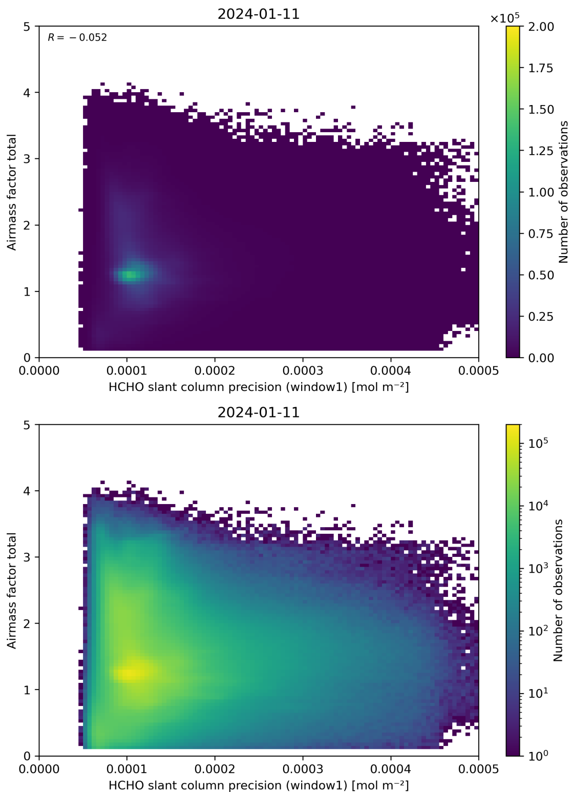
Figure 94: Scatter density plot of “HCHO slant column precision (window1)” against “Airmass factor total” for 2024-01-10 to 2024-01-12.
