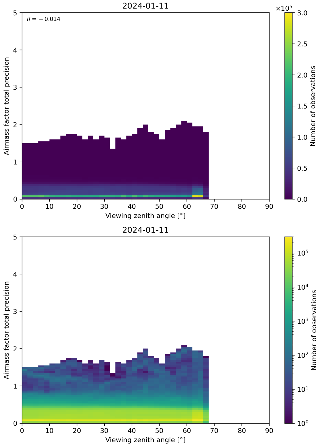
Figure 191: Scatter density plot of “Viewing zenith angle” against “Airmass factor total precision” for 2024-01-10 to 2024-01-12.
