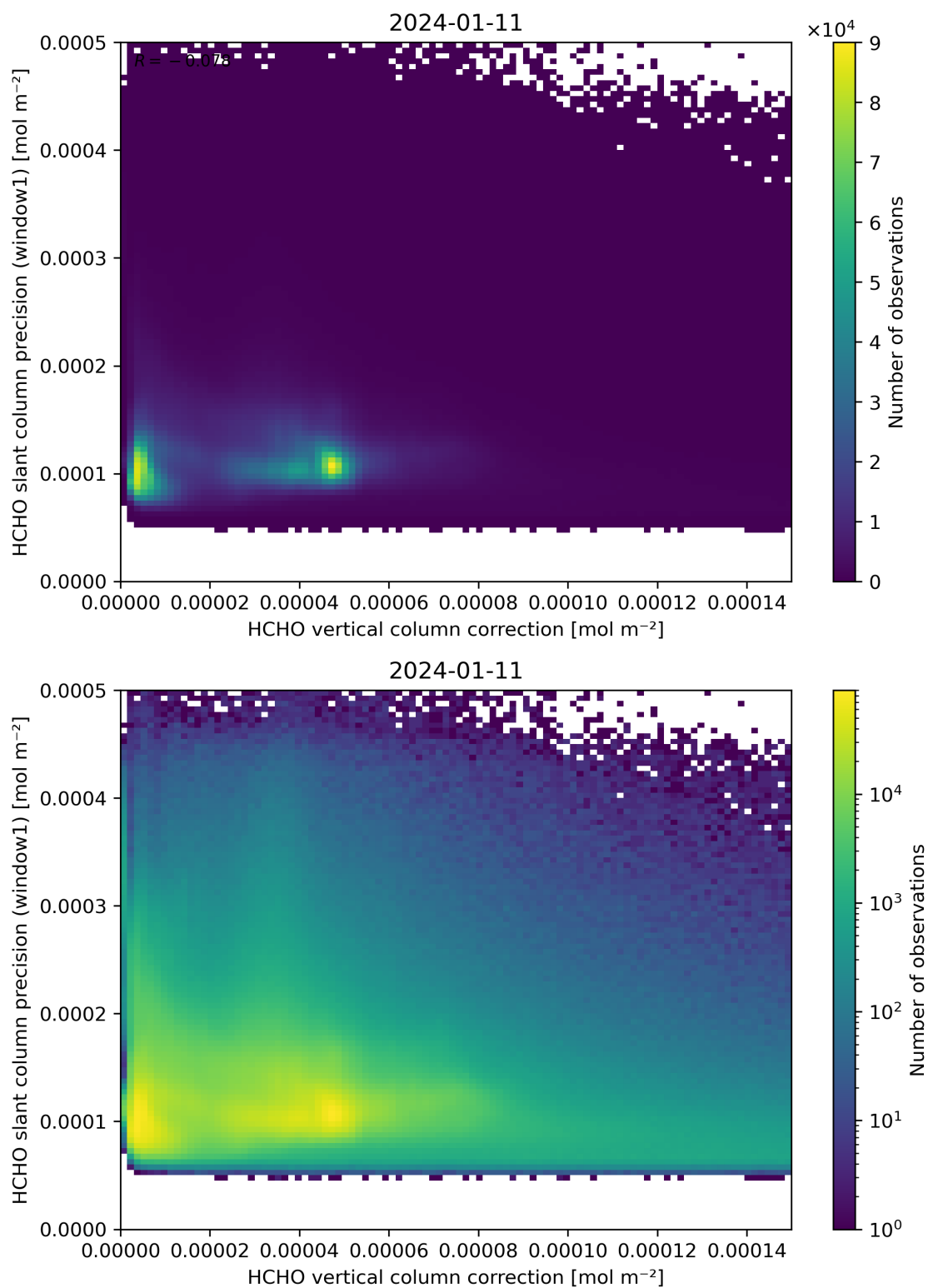
Figure 119: Scatter density plot of “HCHO vertical column correction” against “HCHO slant column precision (window1)” for 2024-01-10 to 2024-01-12.
