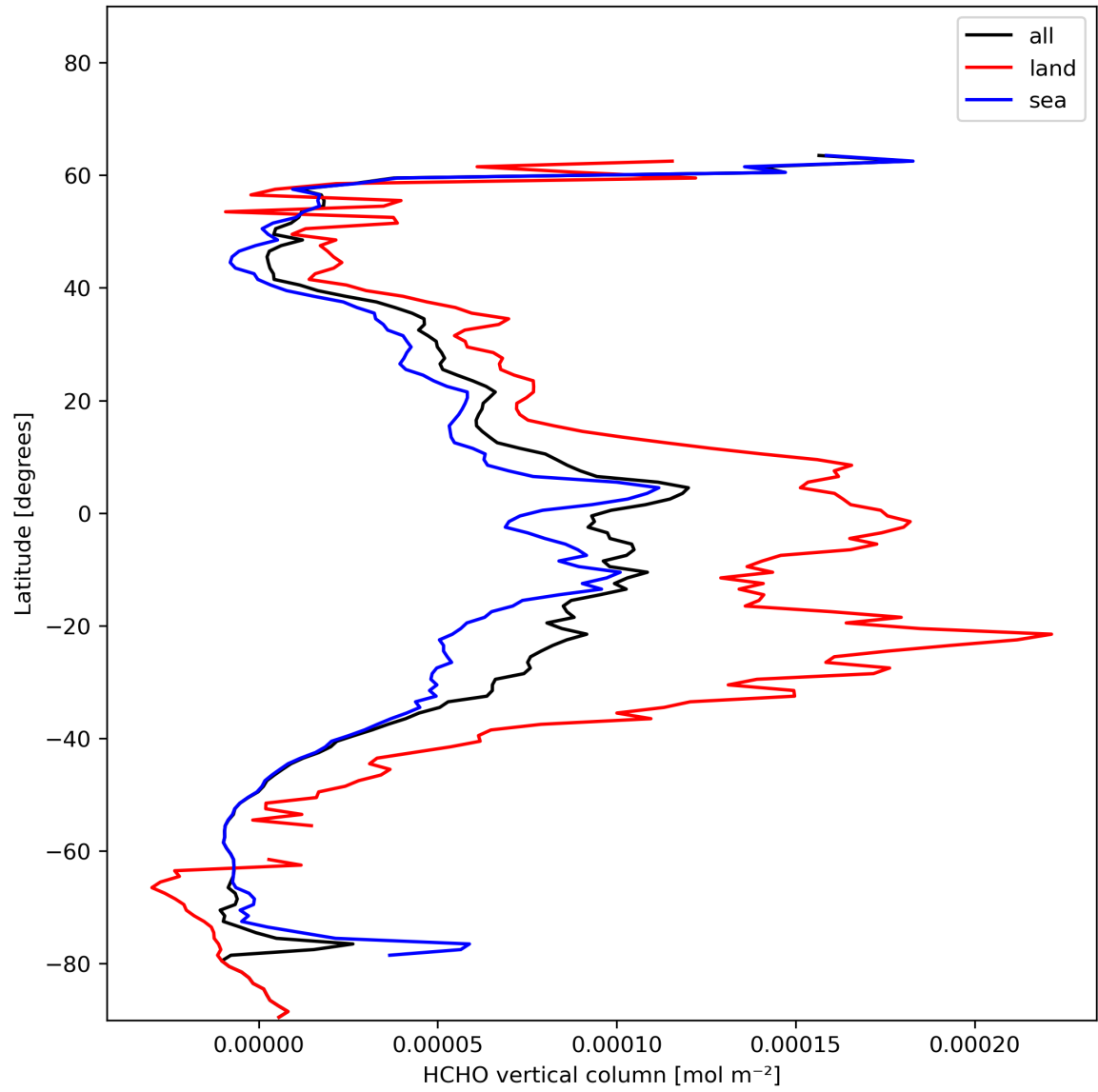
Figure 21: Zonal average of “HCHO vertical column” for 2024-01-10 to 2024-01-12.
