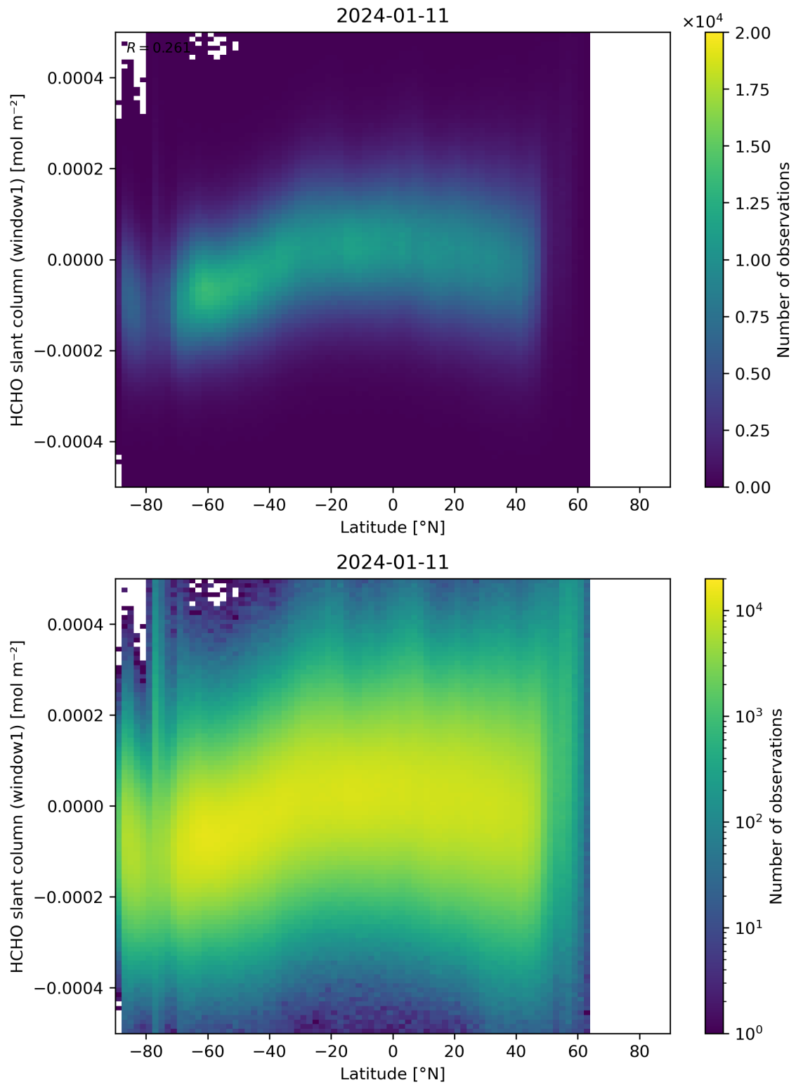
Figure 159: Scatter density plot of “Latitude” against “HCHO slant column (window1)” for 2024-01-10 to 2024-01-12.
