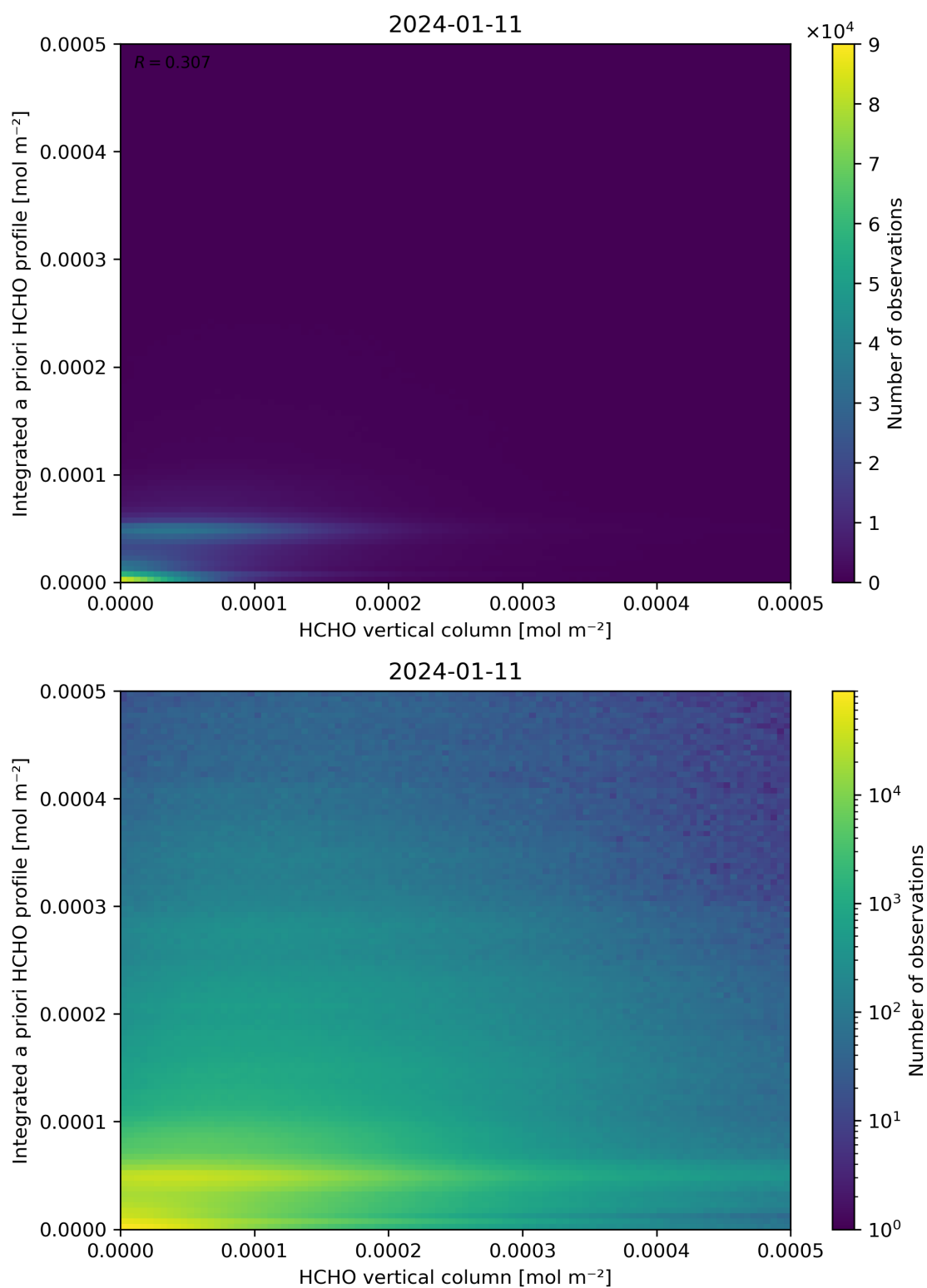
Figure 135: Scatter density plot of “HCHO vertical column” against “Integrated a priori HCHO profile” for 2024-01-10 to 2024-01-12.
