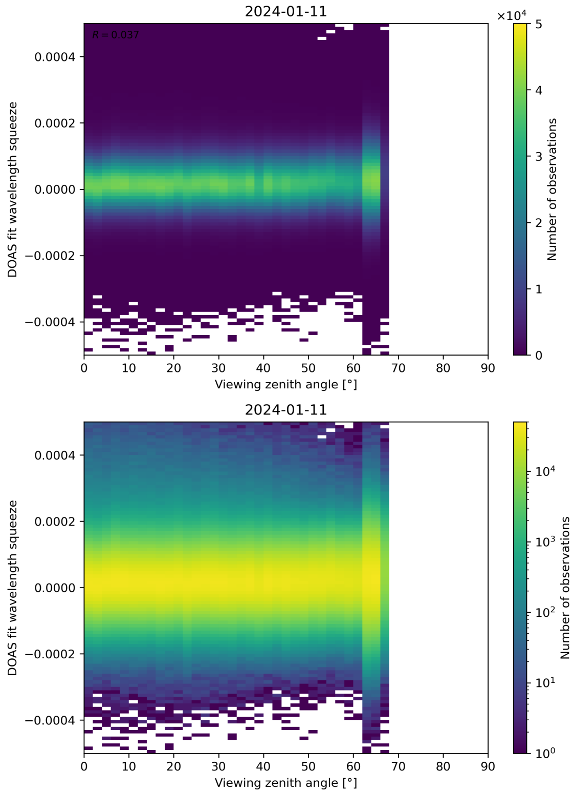
Figure 184: Scatter density plot of “Viewing zenith angle” against “DOAS fit wavelength squeeze” for 2024-01-10 to 2024-01-12.
