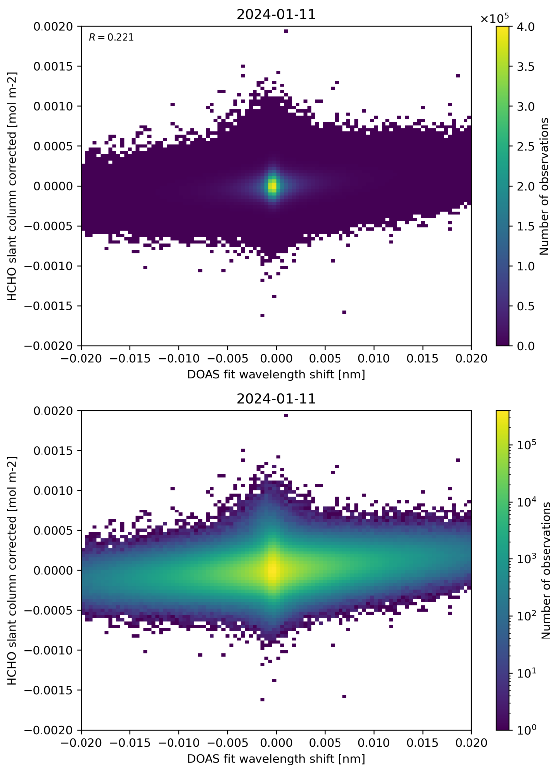
Figure 66: Scatter density plot of “DOAS fit wavelength shift” against “HCHO slant column corrected” for 2024-01-10 to 2024-01-12.
