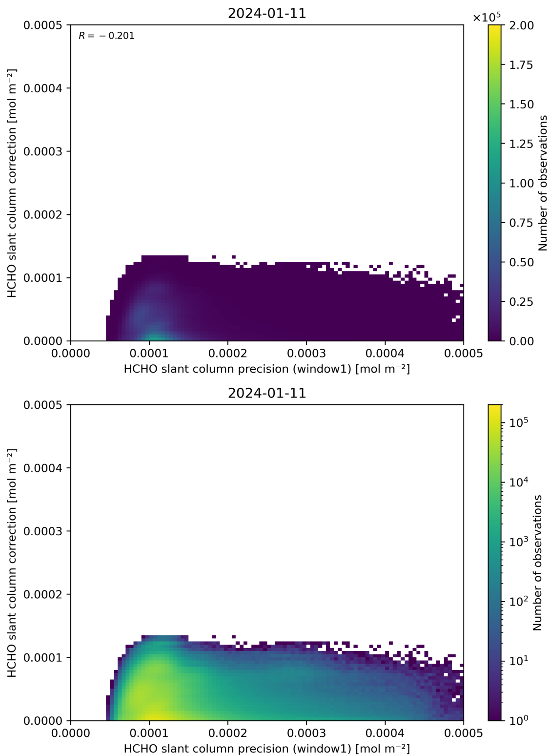
Figure 93: Scatter density plot of “HCHO slant column precision (window1)” against “HCHO slant column correction” for 2024-01-10 to 2024-01-12.
