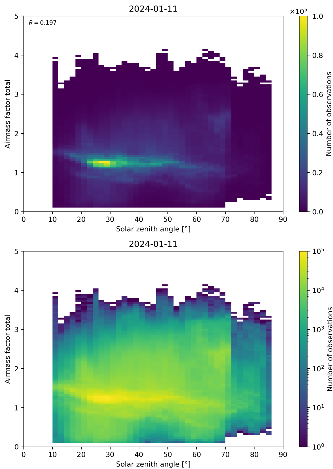
Figure 175: Scatter density plot of “Solar zenith angle” against “Airmass factor total” for 2024-01-10 to 2024-01-12.
