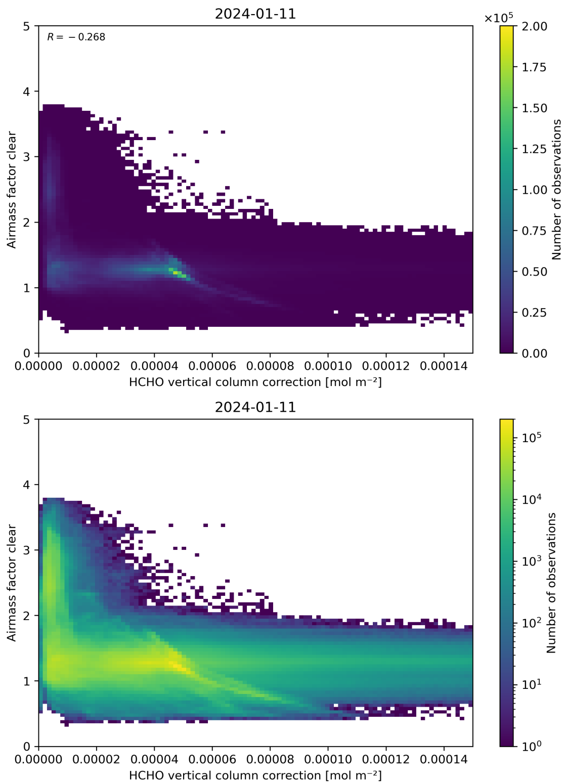
Figure 115: Scatter density plot of “HCHO vertical column correction” against “Airmass factor clear” for 2024-01-10 to 2024-01-12.
