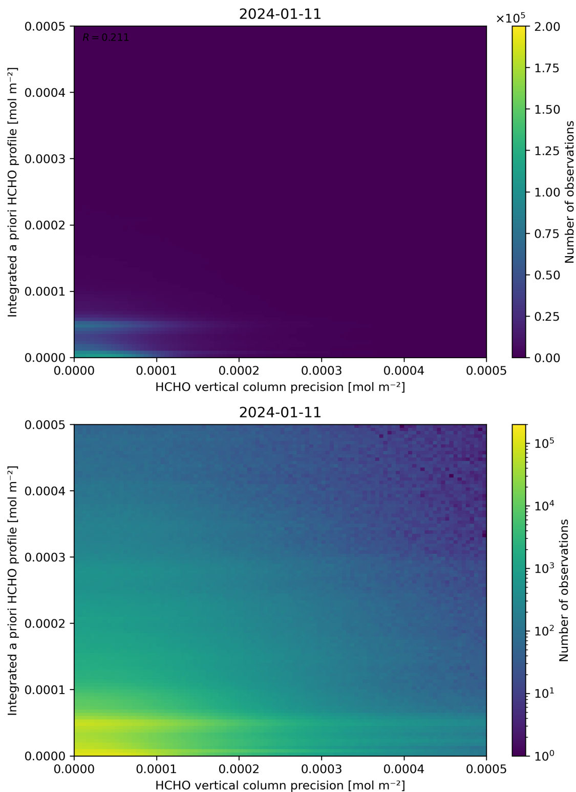
Figure 147: Scatter density plot of “HCHO vertical column precision” against “Integrated a priori HCHO profile” for 2024-01-10 to 2024-01-12.
