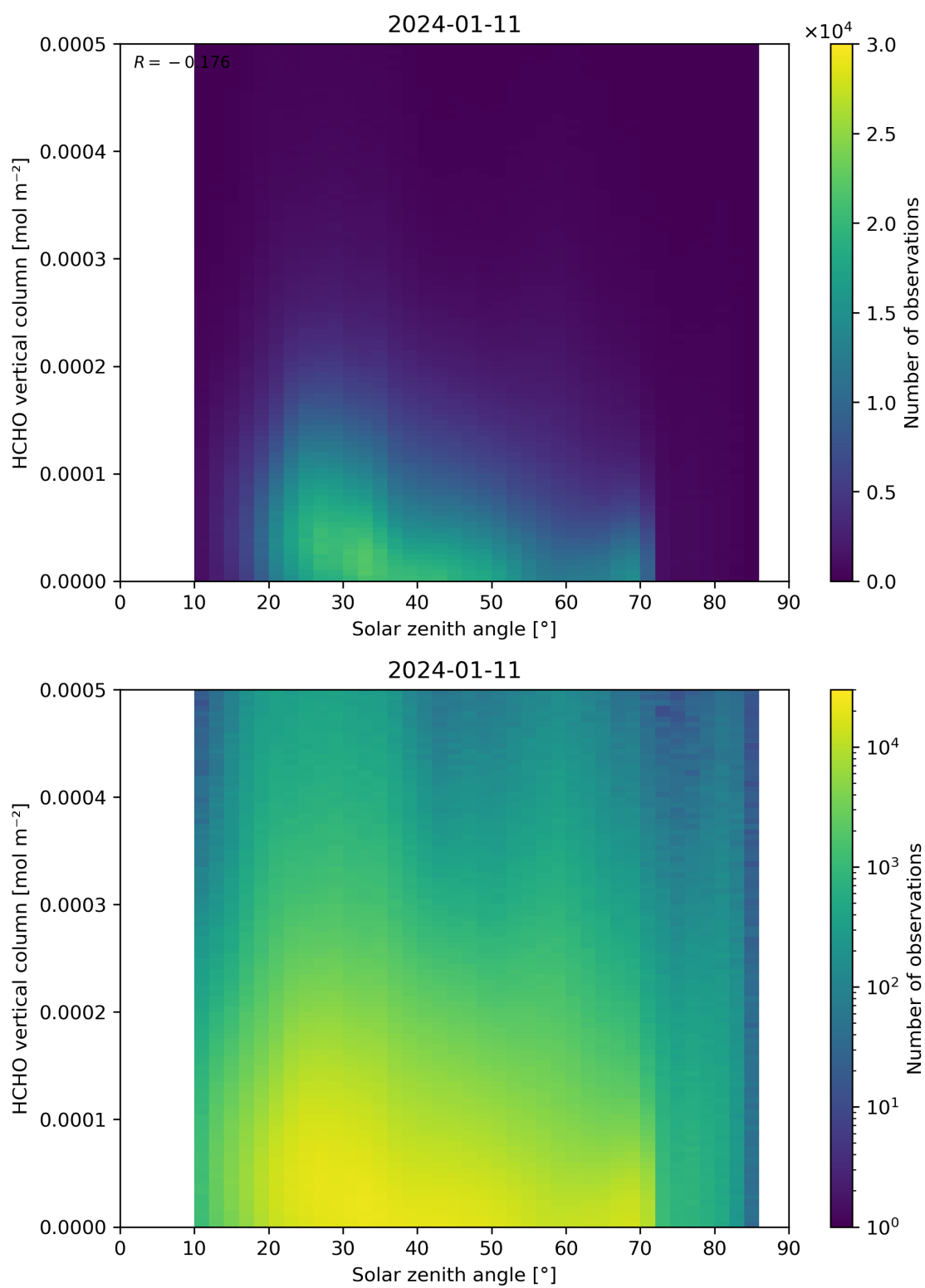
Figure 177: Scatter density plot of “Solar zenith angle” against “HCHO vertical column” for 2024-01-10 to 2024-01-12.
