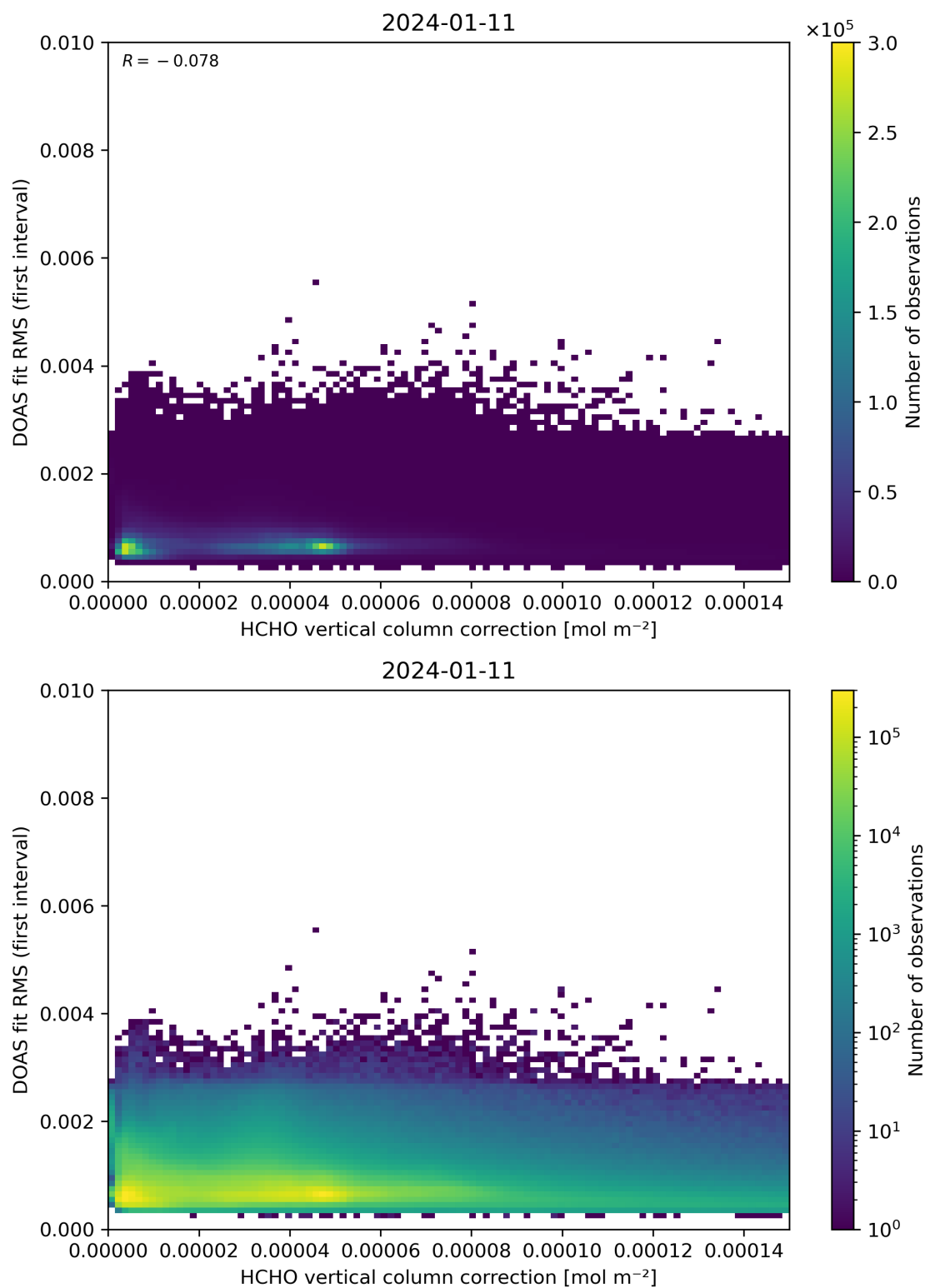
Figure 112: Scatter density plot of “HCHO vertical column correction” against “DOAS fit RMS (first interval)” for 2024-01-10 to 2024-01-12.
