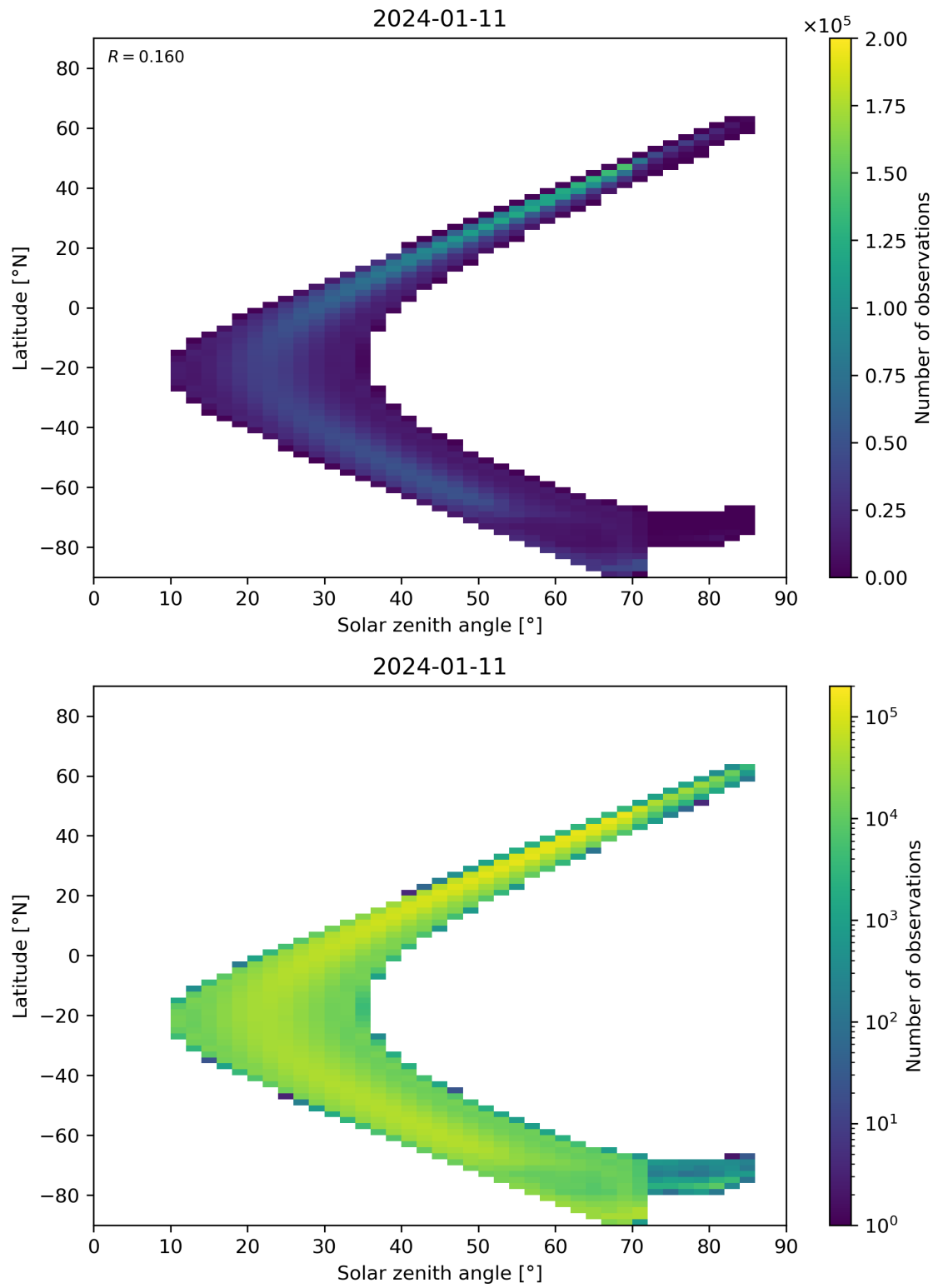
Figure 181: Scatter density plot of “Solar zenith angle” against “Latitude” for 2024-01-10 to 2024-01-12.
