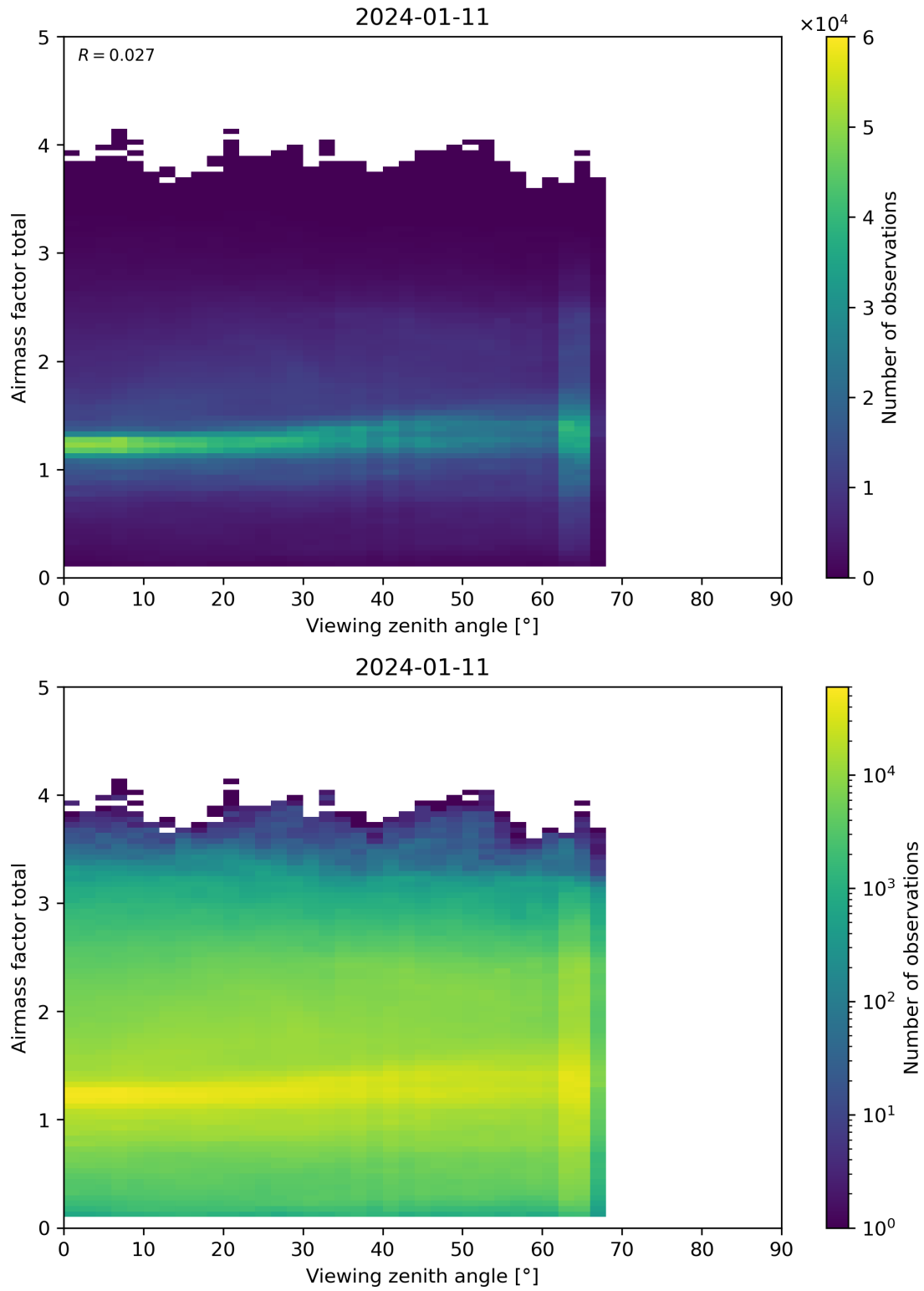
Figure 190: Scatter density plot of “Viewing zenith angle” against “Airmass factor total” for 2024-01-10 to 2024-01-12.
