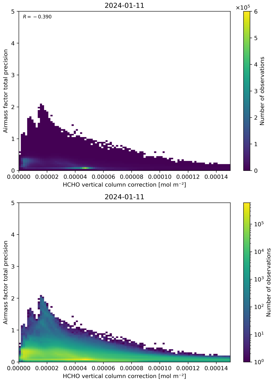
Figure 121: Scatter density plot of “HCHO vertical column correction” against “Airmass factor total precision” for 2024-01-10 to 2024-01-12.
