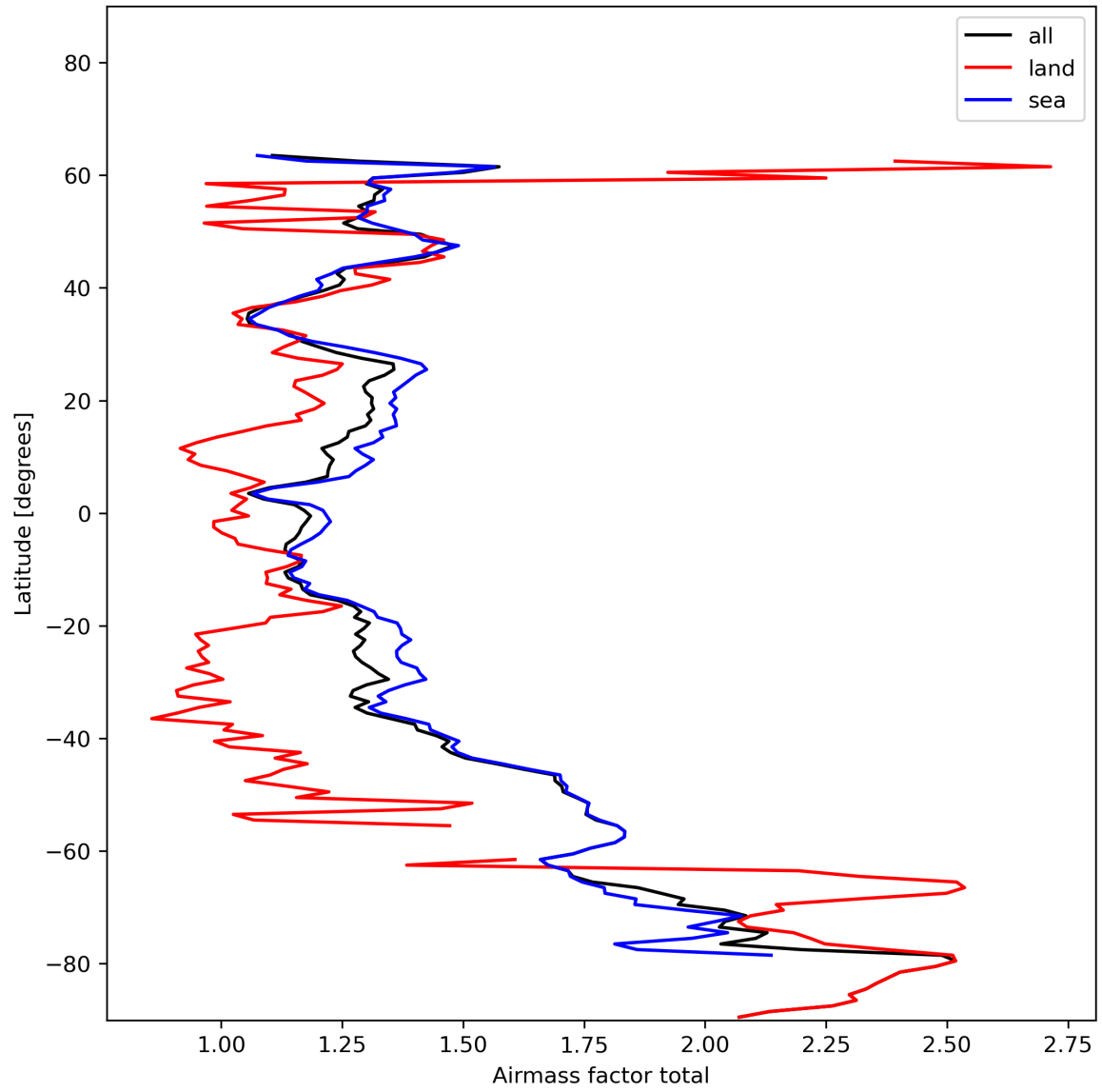
Figure 26: Zonal average of "Airmass factor total" for 2024-01-10 to 2024-01-12.
