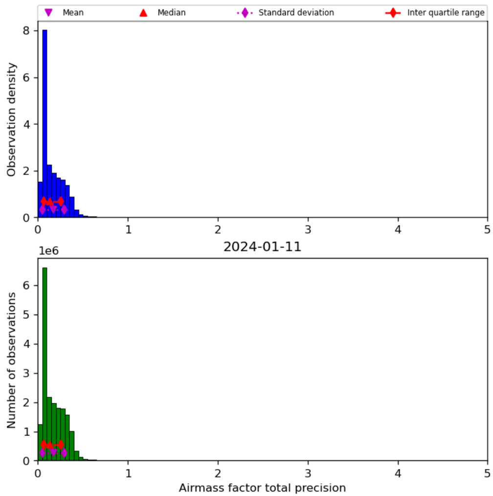
Figure 41: Histogram of “Airmass factor total precision” for 2024-01-10 to 2024-01-12
