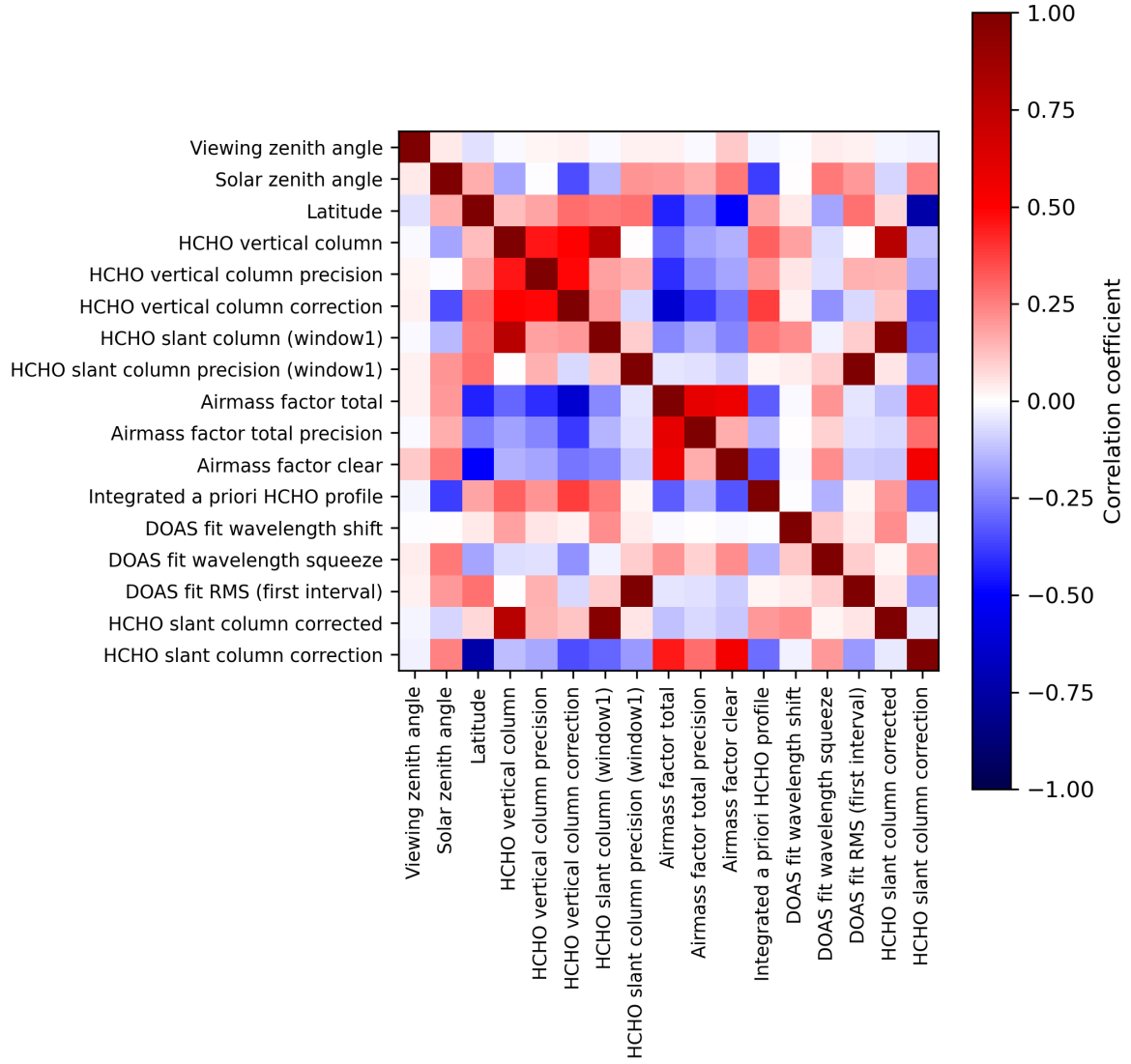
Figure 2: Map of correlation matrix for 2024-01-10 to 2024-01-12.
