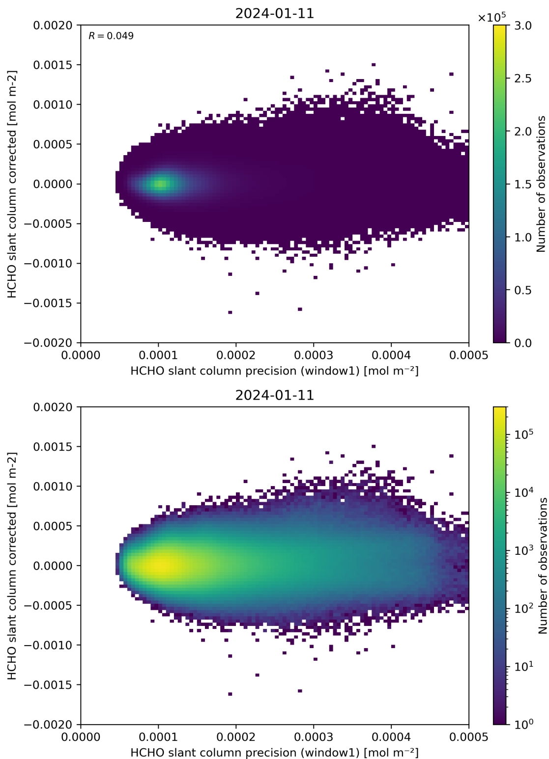
Figure 92: Scatter density plot of “HCHO slant column precision (window1)” against “HCHO slant column corrected” for 2024-01-10 to 2024-01-12.
