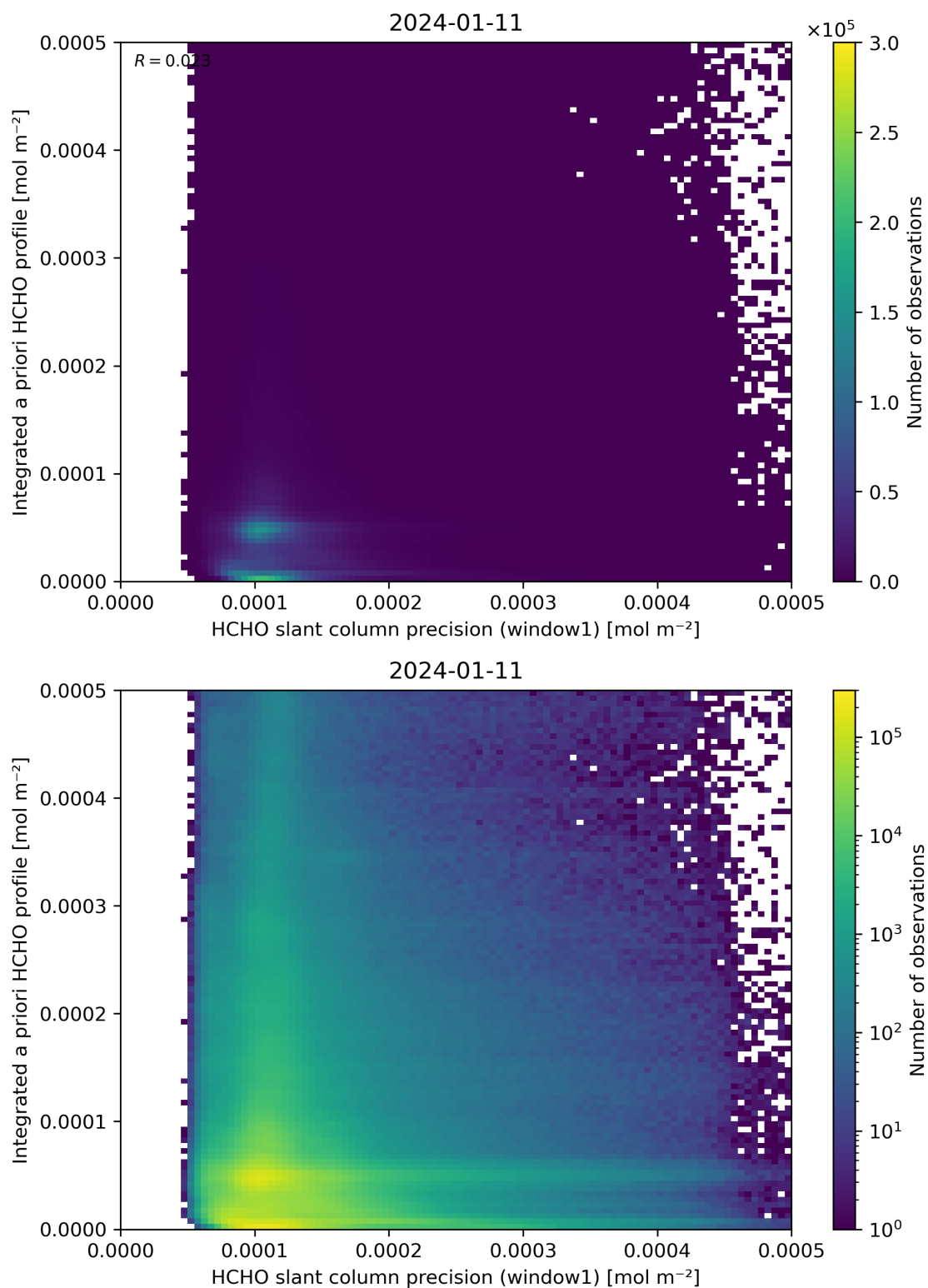
Figure 96: Scatter density plot of “HCHO slant column precision (window1)” against “Integrated a priori HCHO profile” for 2024-01-10 to 2024-01-12.
