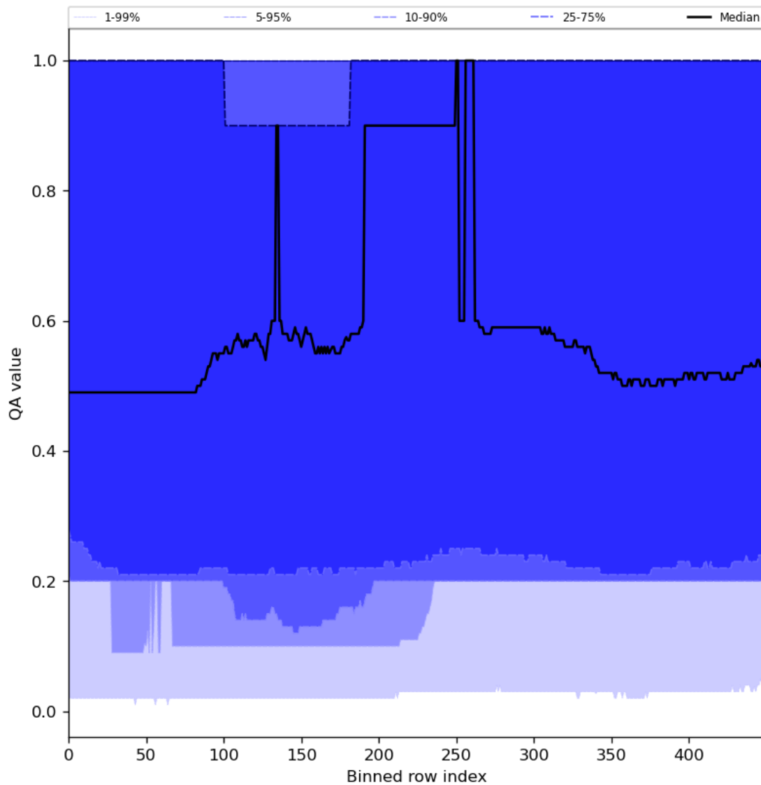
Figure 48: Along track statistics of “QA value” for 2024-01-10 to 2024-01-12
