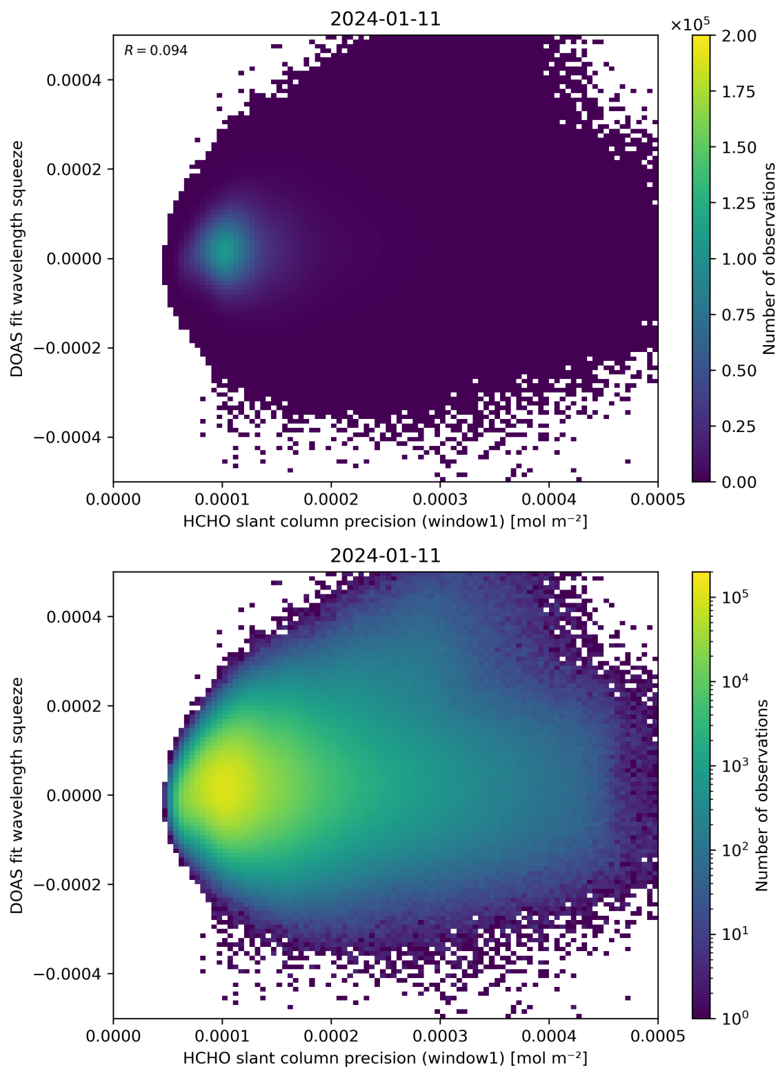
Figure 90: Scatter density plot of “HCHO slant column precision (window1)” against “DOAS fit wavelength squeeze” for 2024-01-10 to 2024-01-12.
