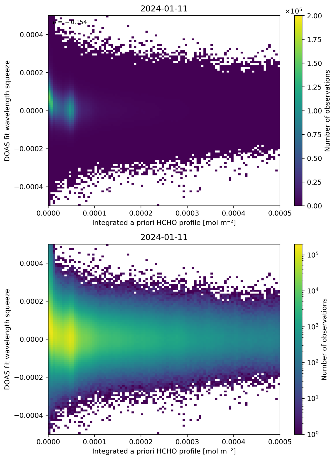
Figure 150: Scatter density plot of “Integrated a priori HCHO profile” against “DOAS fit wavelength squeeze” for 2024-01-10 to 2024-01-12.
