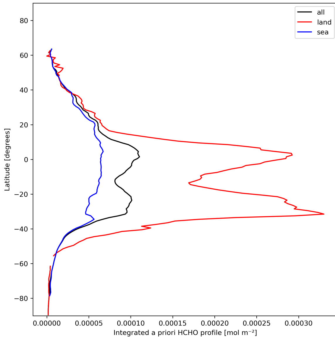
Figure 29: Zonal average of “Integrated a priori HCHO profile” for 2024-01-10 to 2024-01-12.
