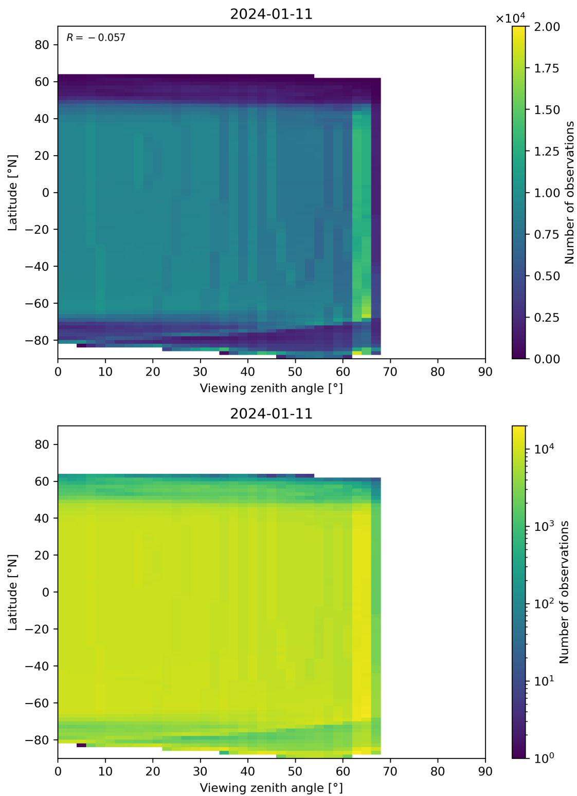
Figure 196: Scatter density plot of “Viewing zenith angle” against “Latitude” for 2024-01-10 to 2024-01-12.
