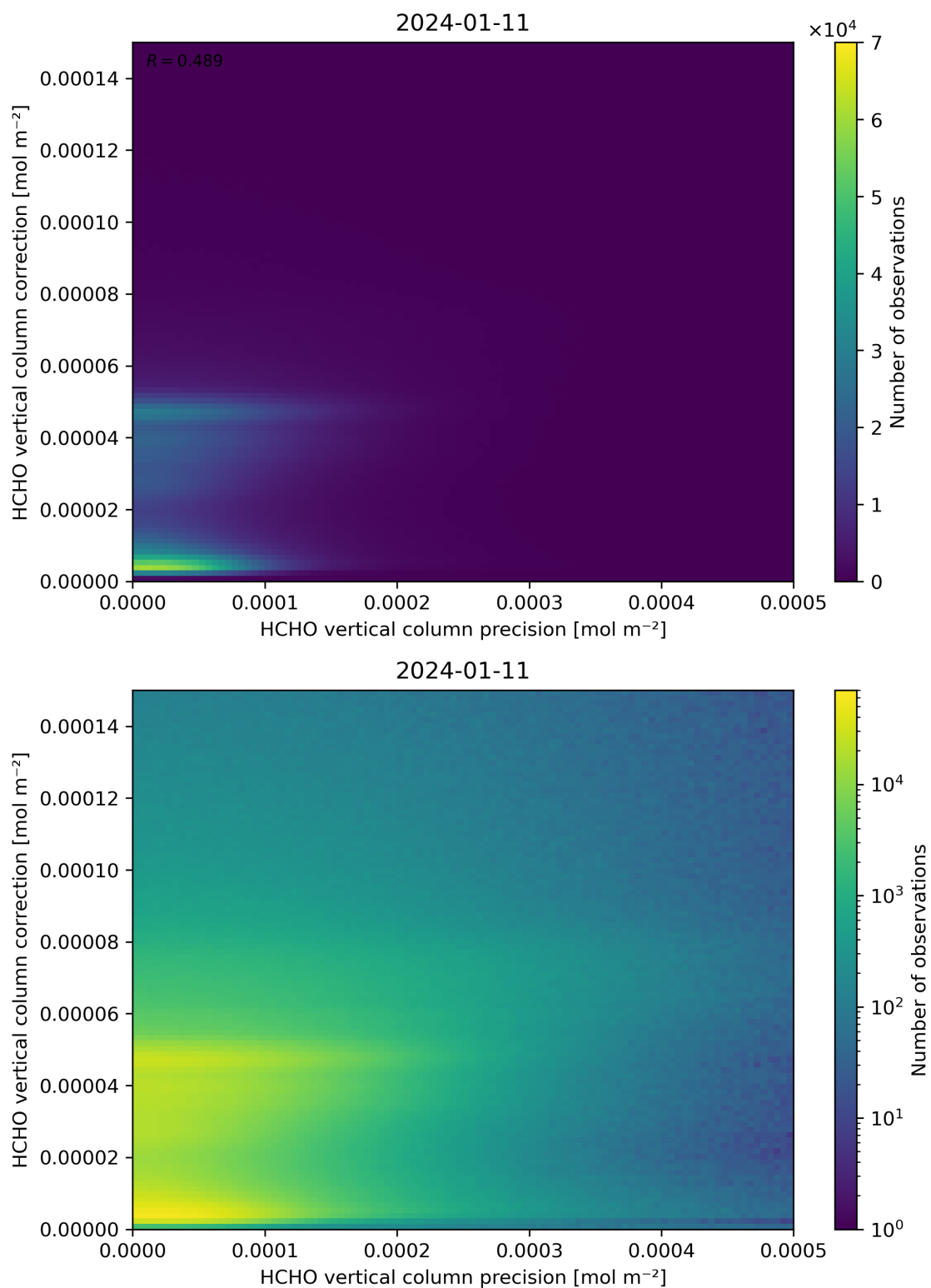
Figure 146: Scatter density plot of “HCHO vertical column precision” against “HCHO vertical column correction” for 2024-01-10 to 2024-01-12.
