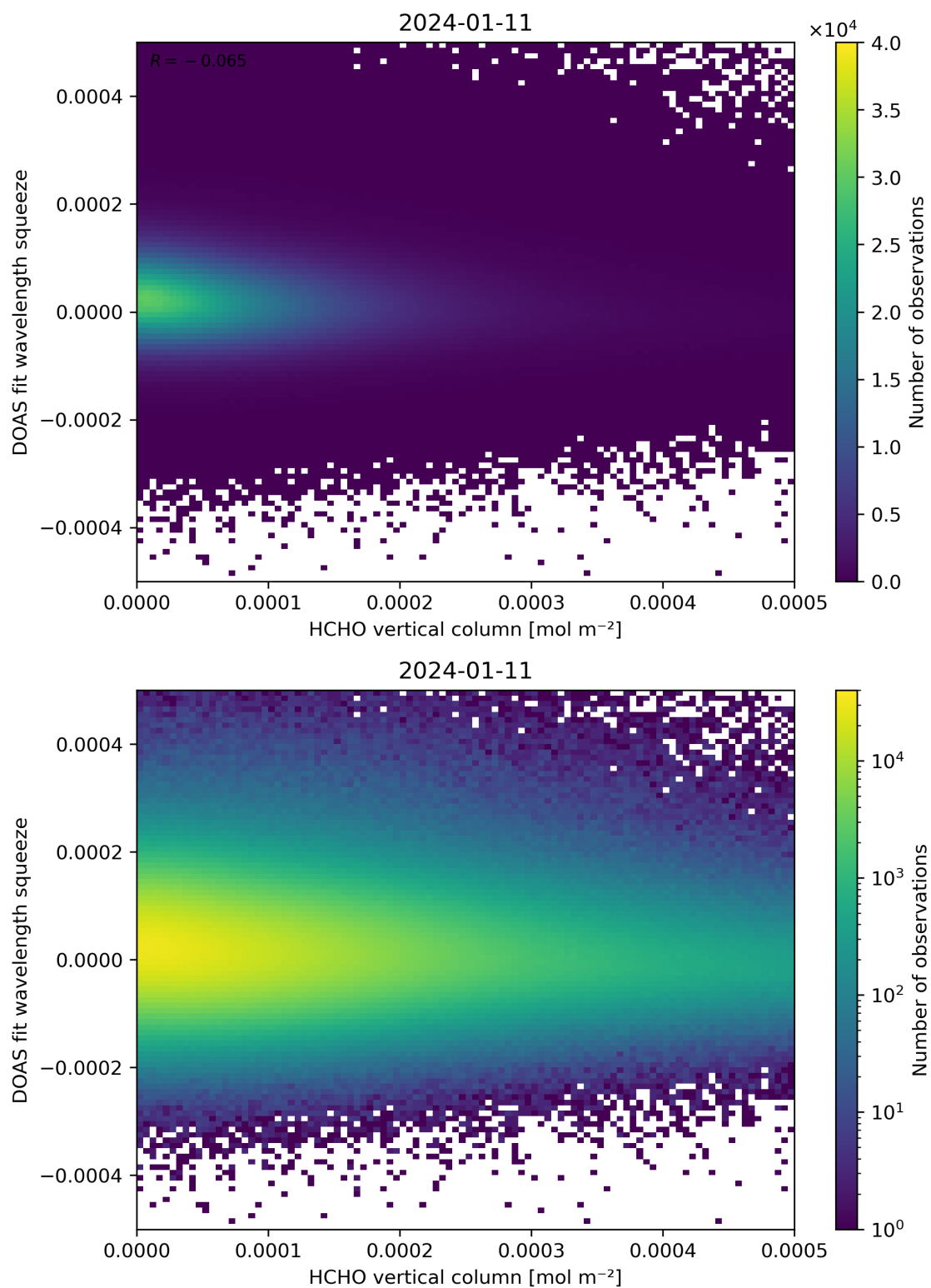
Figure 125: Scatter density plot of “HCHO vertical column” against “DOAS fit wavelength squeeze” for 2024-01-10 to 2024-01-12.
