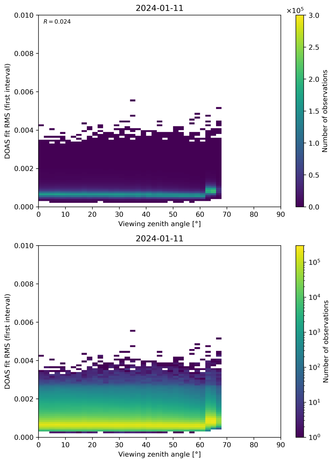
Figure 182: Scatter density plot of “Viewing zenith angle” against “DOAS fit RMS (first interval)” for 2024-01-10 to 2024-01-12.
