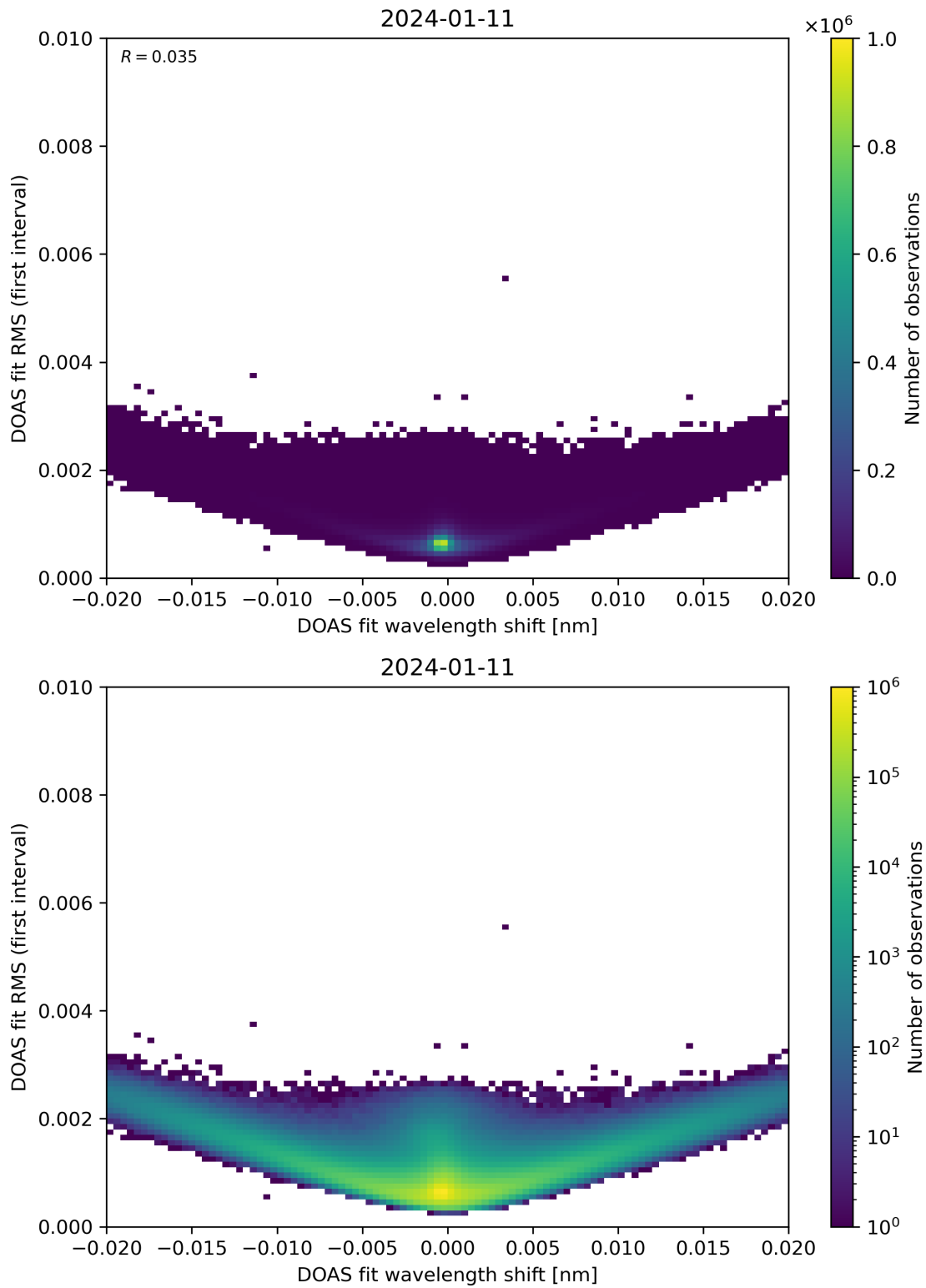
Figure 64: Scatter density plot of “DOAS fit wavelength shift” against “DOAS fit RMS (first interval)” for 2024-01-10 to 2024-01-12.
