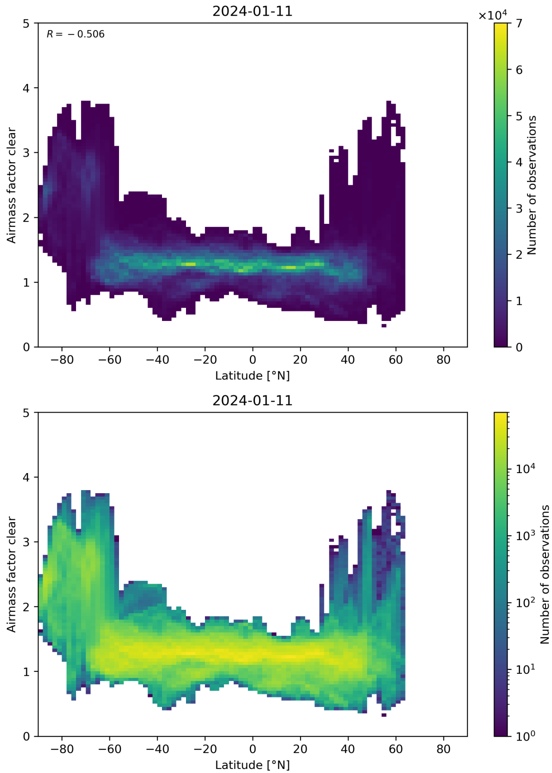
Figure 156: Scatter density plot of “Latitude” against “Airmass factor clear” for 2024-01-10 to 2024-01-12.
