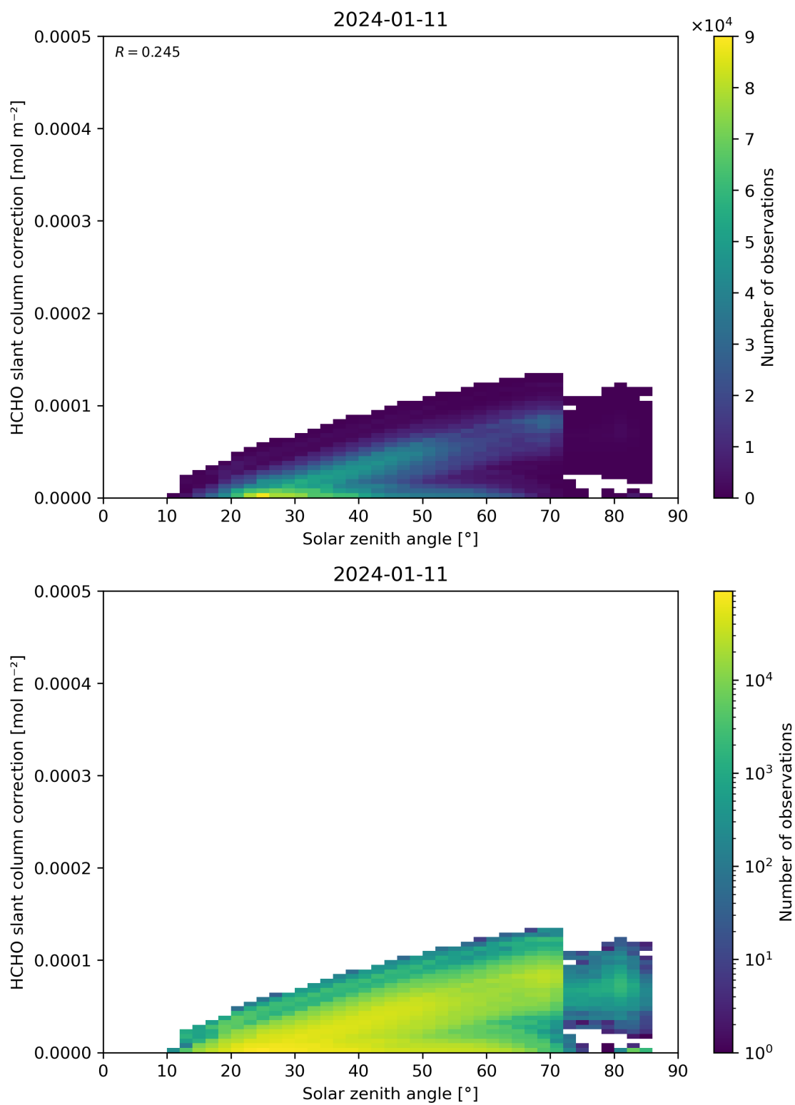
Figure 172: Scatter density plot of “Solar zenith angle” against “HCHO slant column correction” for 2024-01-10 to 2024-01-12.
