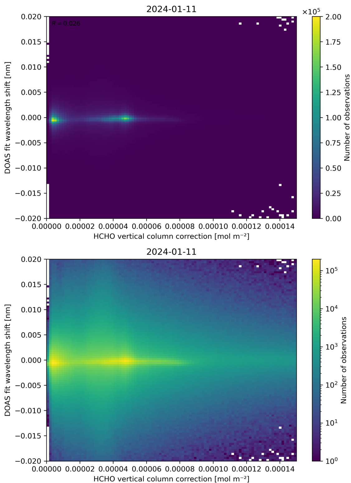
Figure 113: Scatter density plot of “HCHO vertical column correction” against “DOAS fit wavelength shift” for 2024-01-10 to 2024-01-12.
