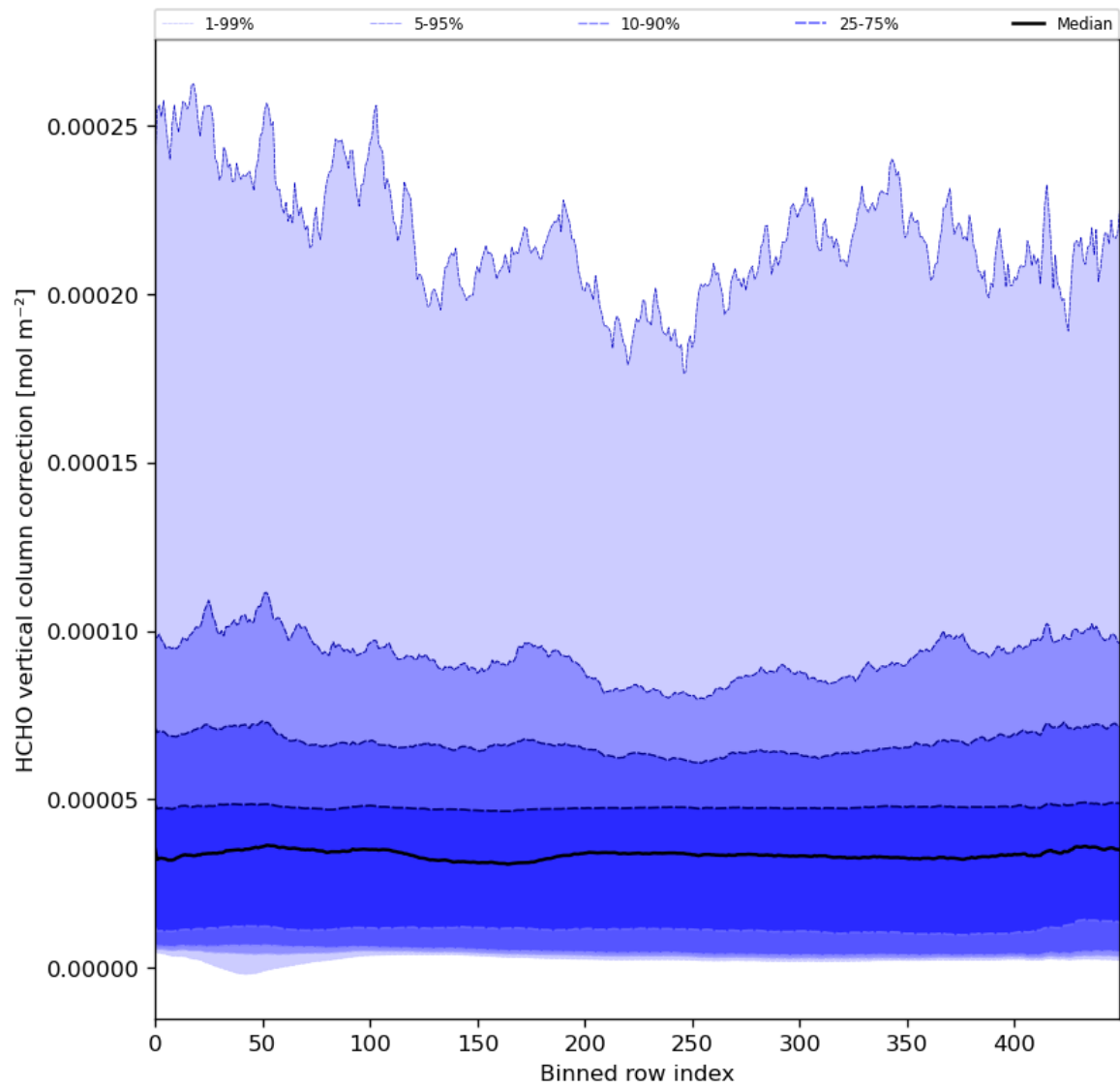
Figure 51: Along track statistics of “HCHO vertical column correction” for 2024-01-10 to 2024-01-12
