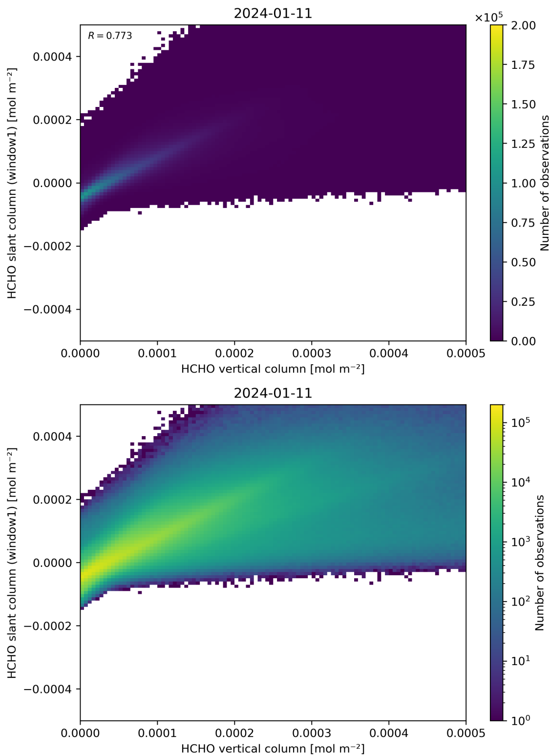
Figure 129: Scatter density plot of “HCHO vertical column” against “HCHO slant column (window1)” for 2024-01-10 to 2024-01-12.
