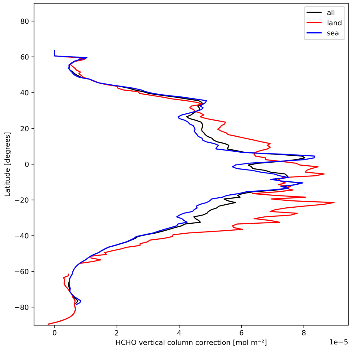
Figure 23: Zonal average of “HCHO vertical column correction” for 2024-01-10 to 2024-01-12.
