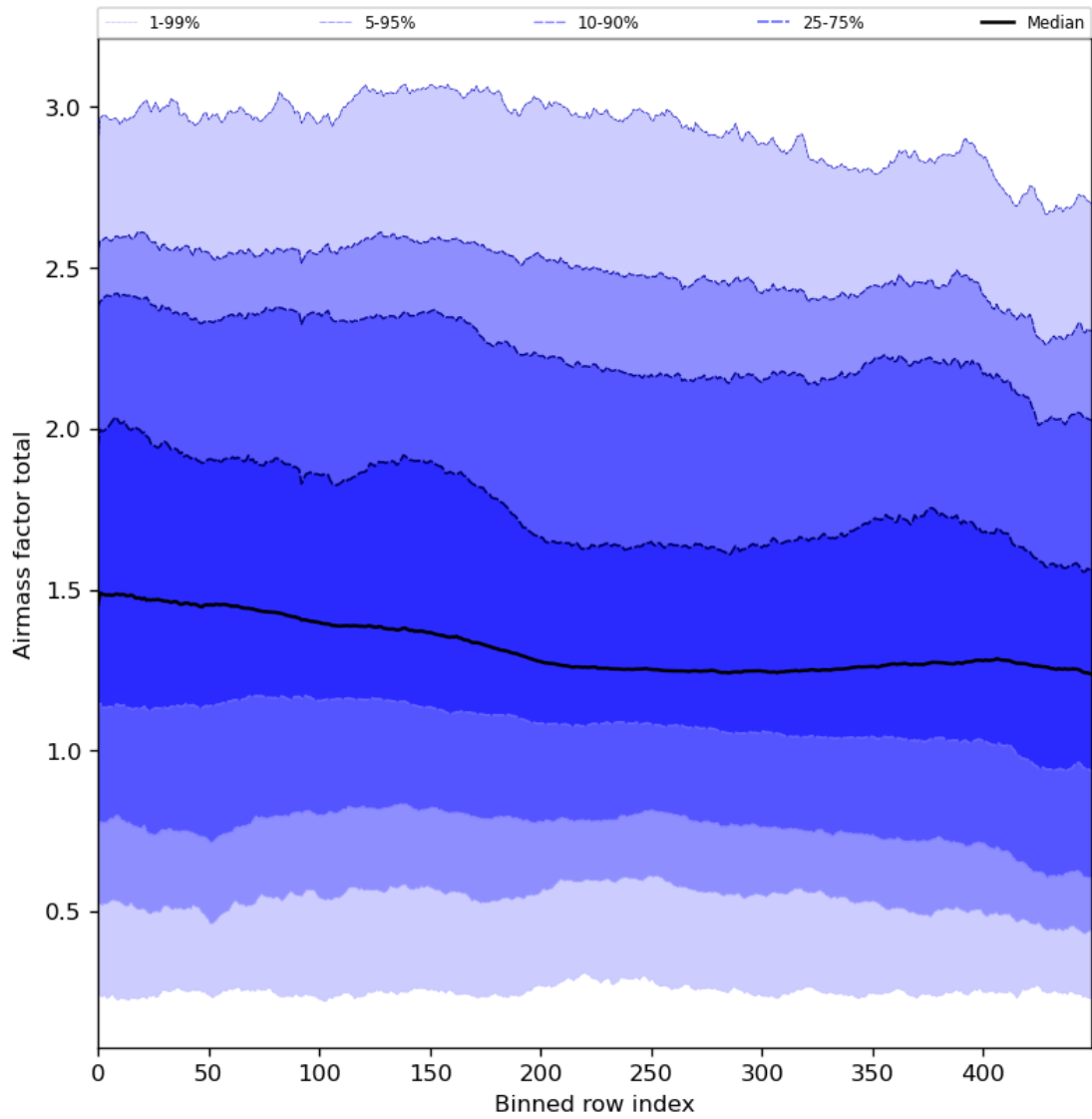
Figure 54: Along track statistics of “Airmass factor total” for 2024-01-10 to 2024-01-12
