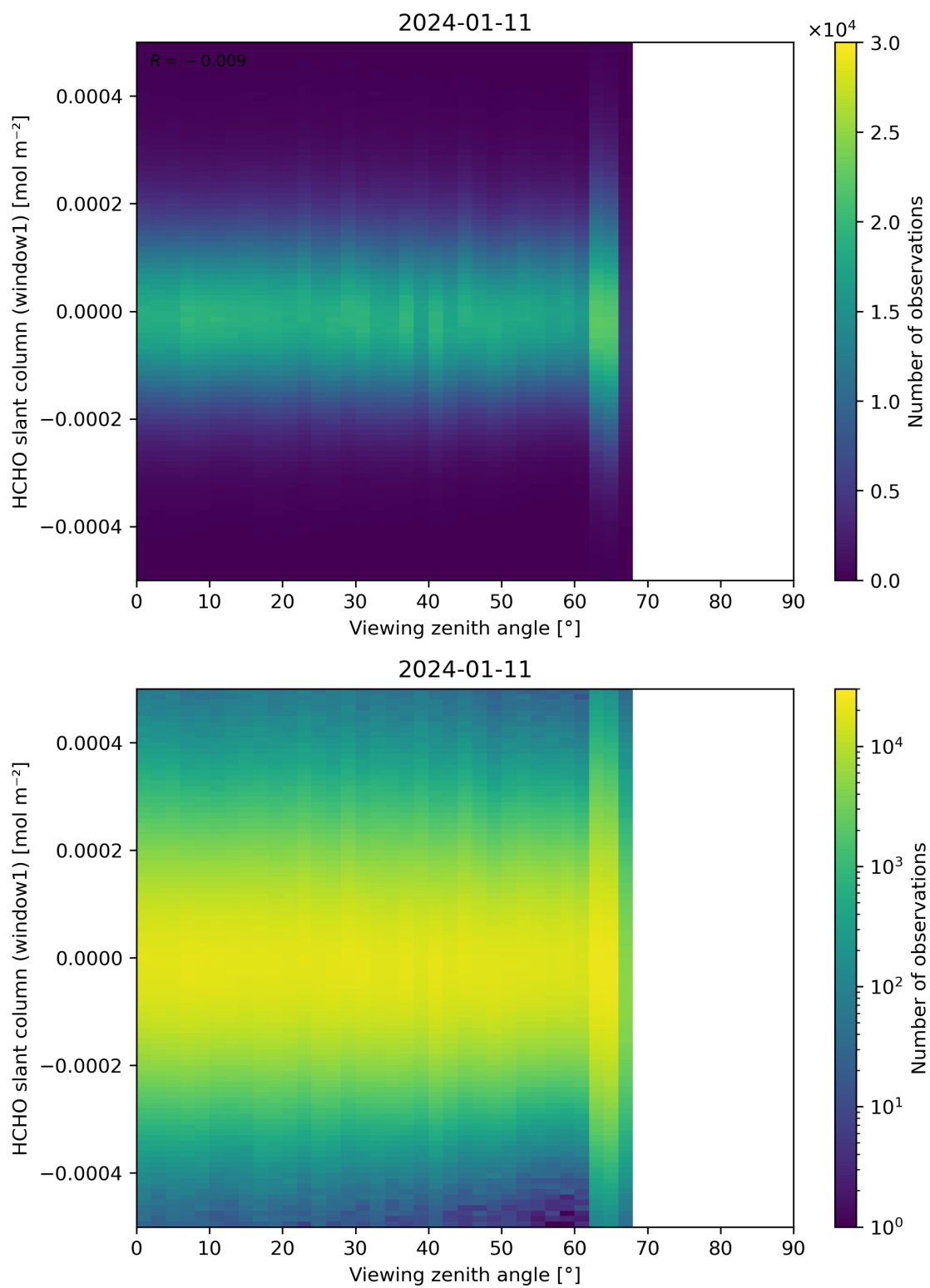
Figure 188: Scatter density plot of “Viewing zenith angle” against “HCHO slant column (window1)” for 2024-01-10 to 2024-01-12.
