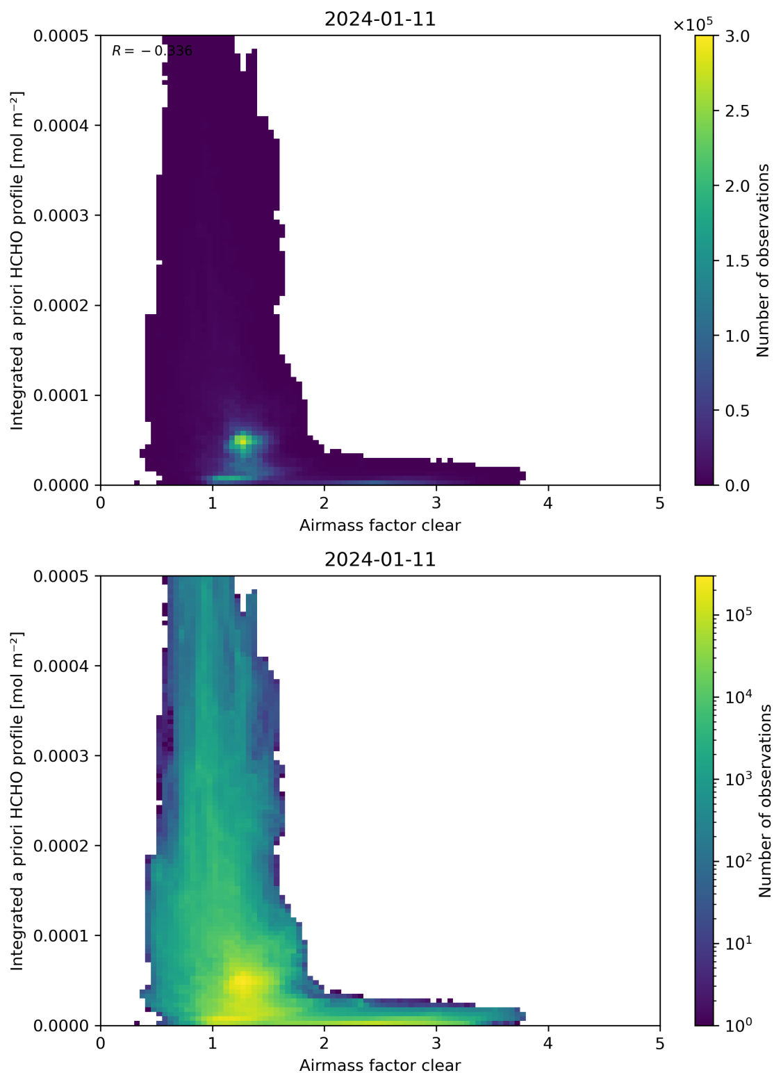
Figure 76: Scatter density plot of “Airmass factor clear” against “Integrated a priori HCHO profile” for 2024-01-10 to 2024-01-12.
