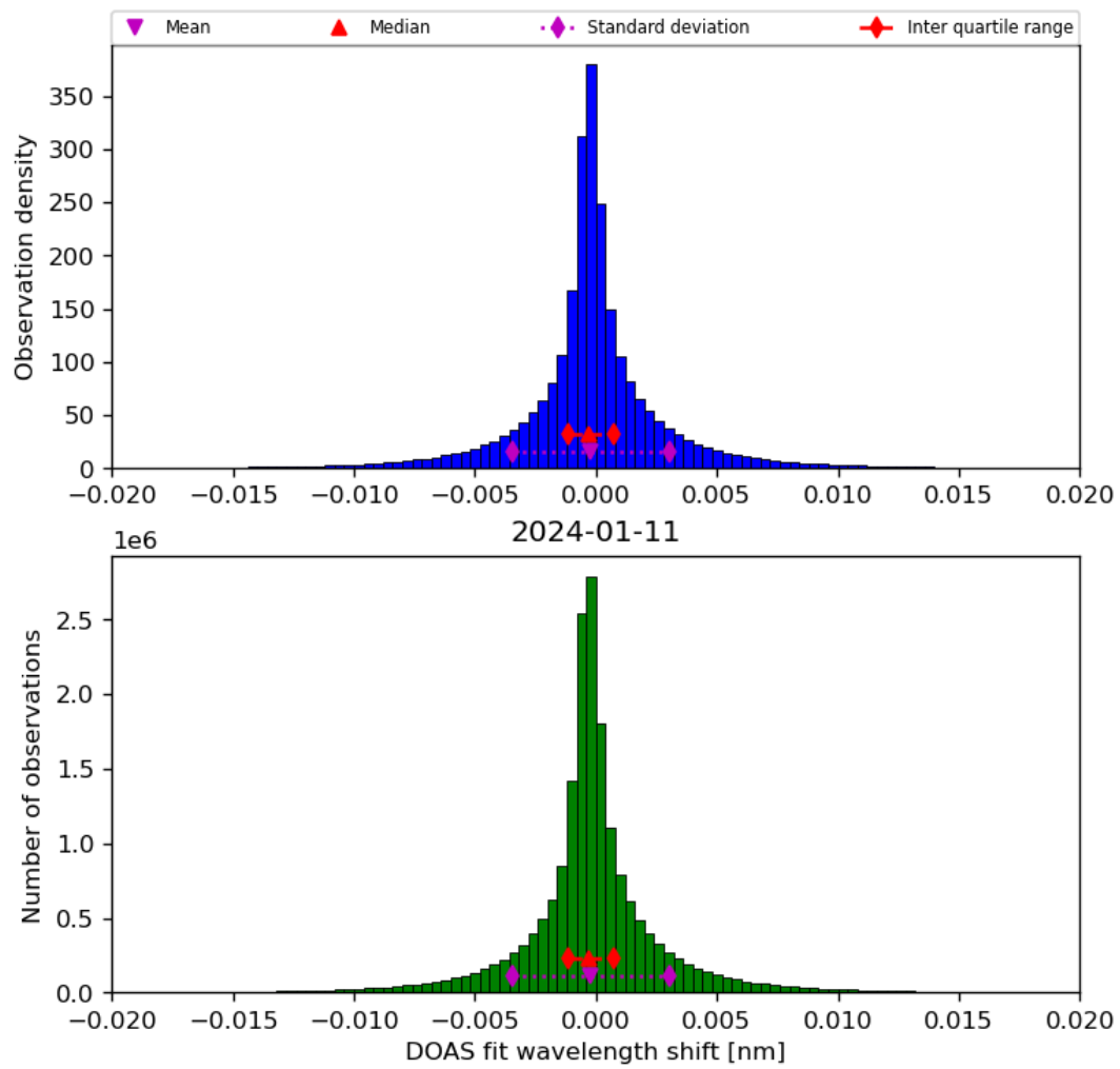
Figure 44: Histogram of “DOAS fit wavelength shift” for 2024-01-10 to 2024-01-12
