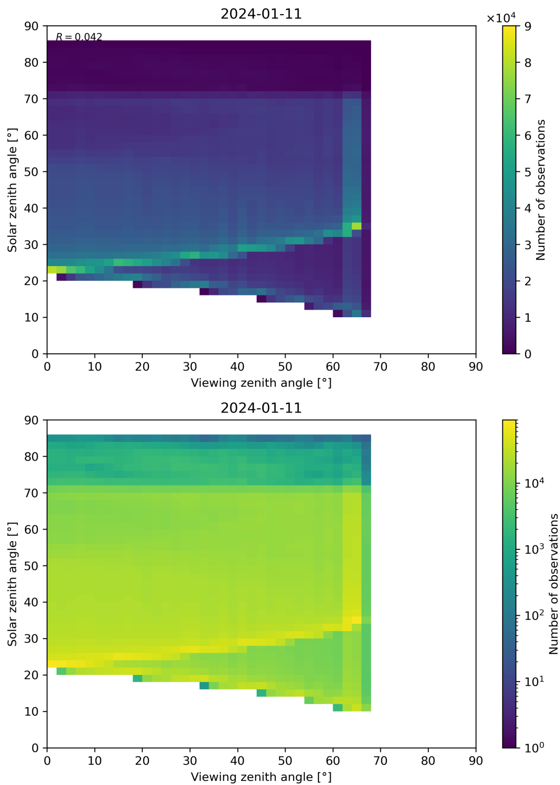
Figure 197: Scatter density plot of “Viewing zenith angle” against “Solar zenith angle” for 2024-01-10 to 2024-01-12.
