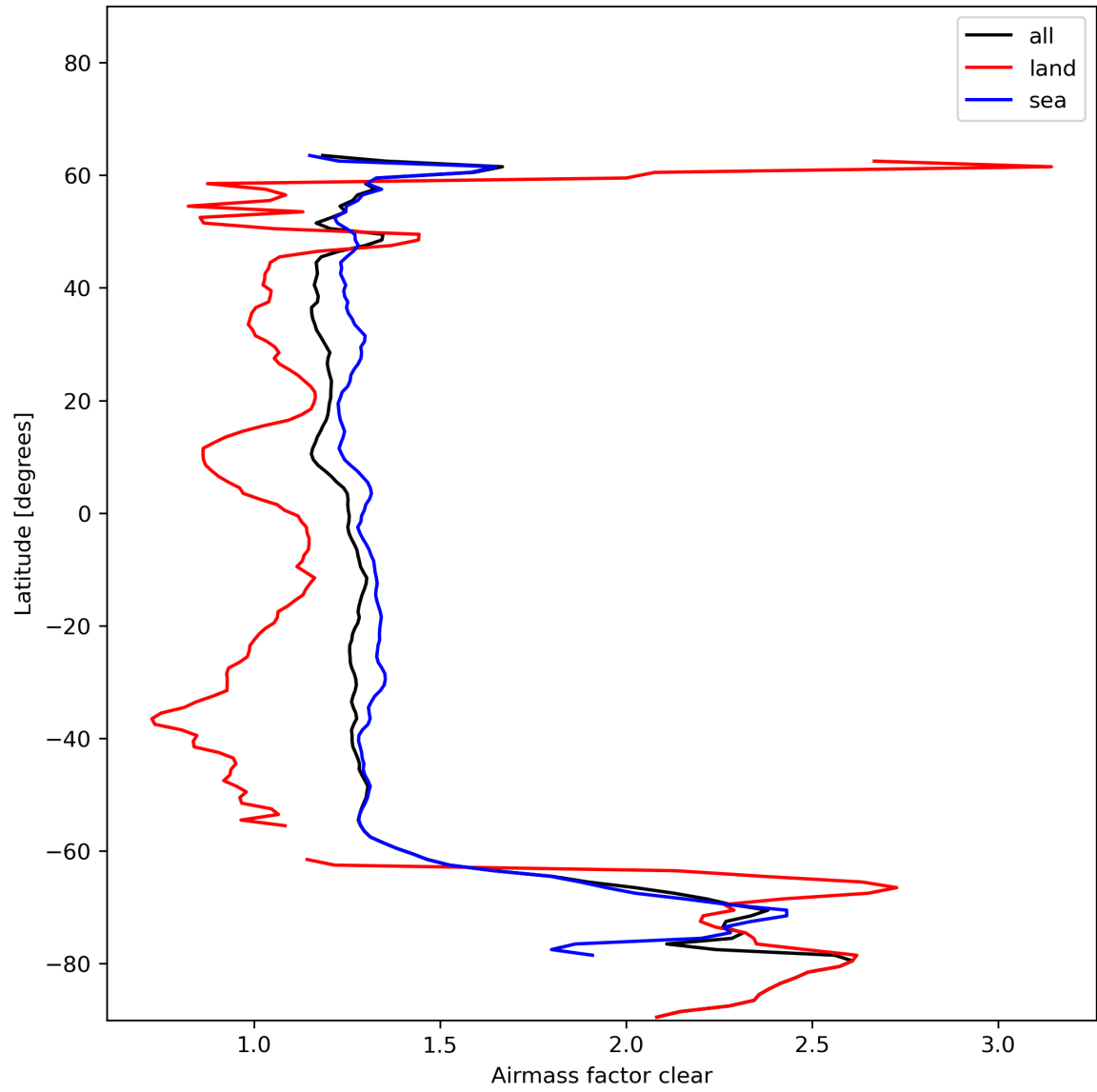
Figure 28: Zonal average of “Airmass factor clear” for 2024-01-10 to 2024-01-12.
