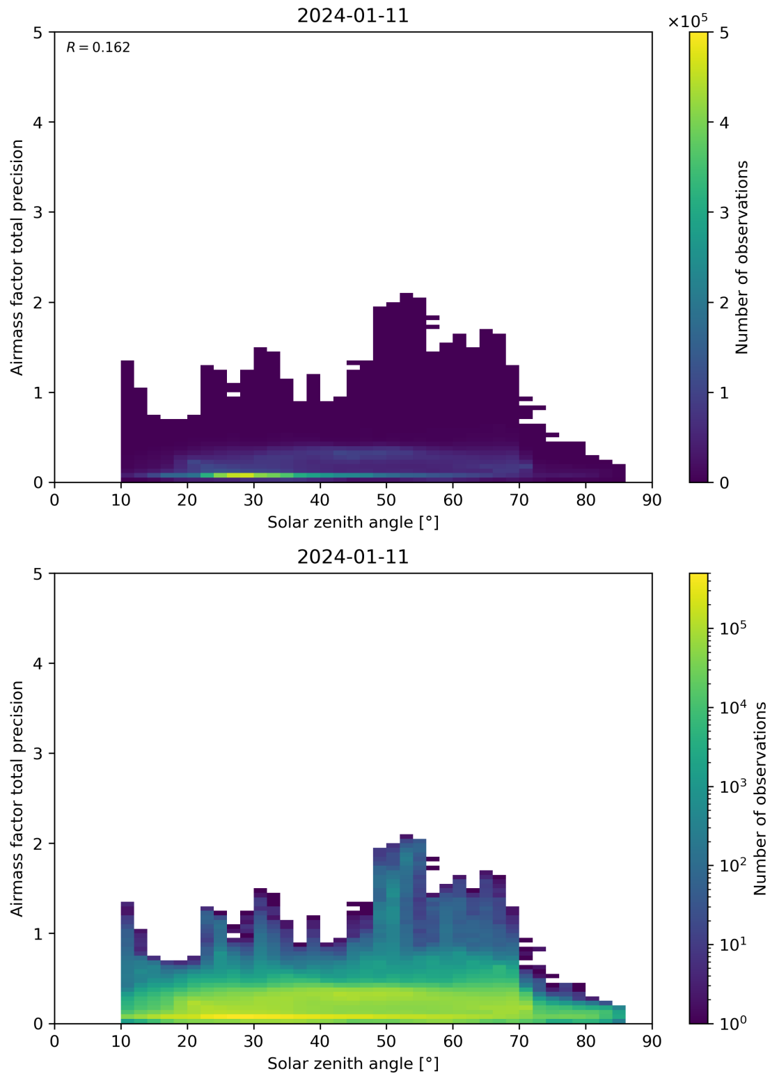
Figure 176: Scatter density plot of “Solar zenith angle” against “Airmass factor total precision” for 2024-01-10 to 2024-01-12.
