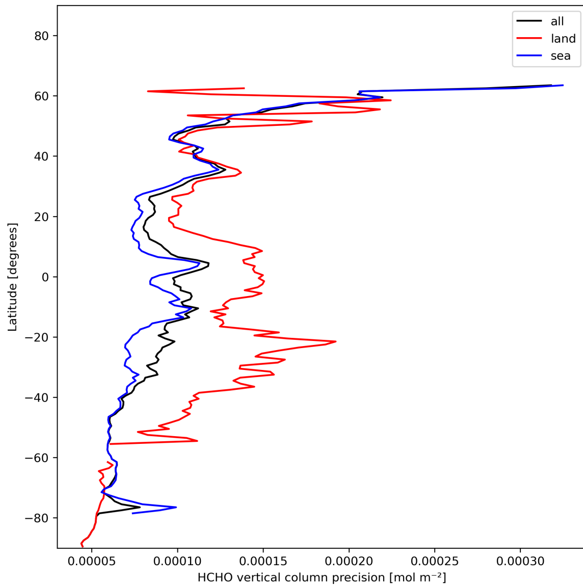
Figure 22: Zonal average of “HCHO vertical column precision” for 2024-01-10 to 2024-01-12.
