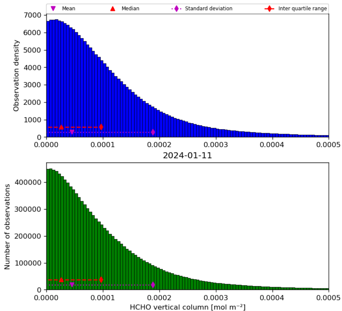
Figure 35: Histogram of “HCHO vertical column” for 2024-01-10 to 2024-01-12
