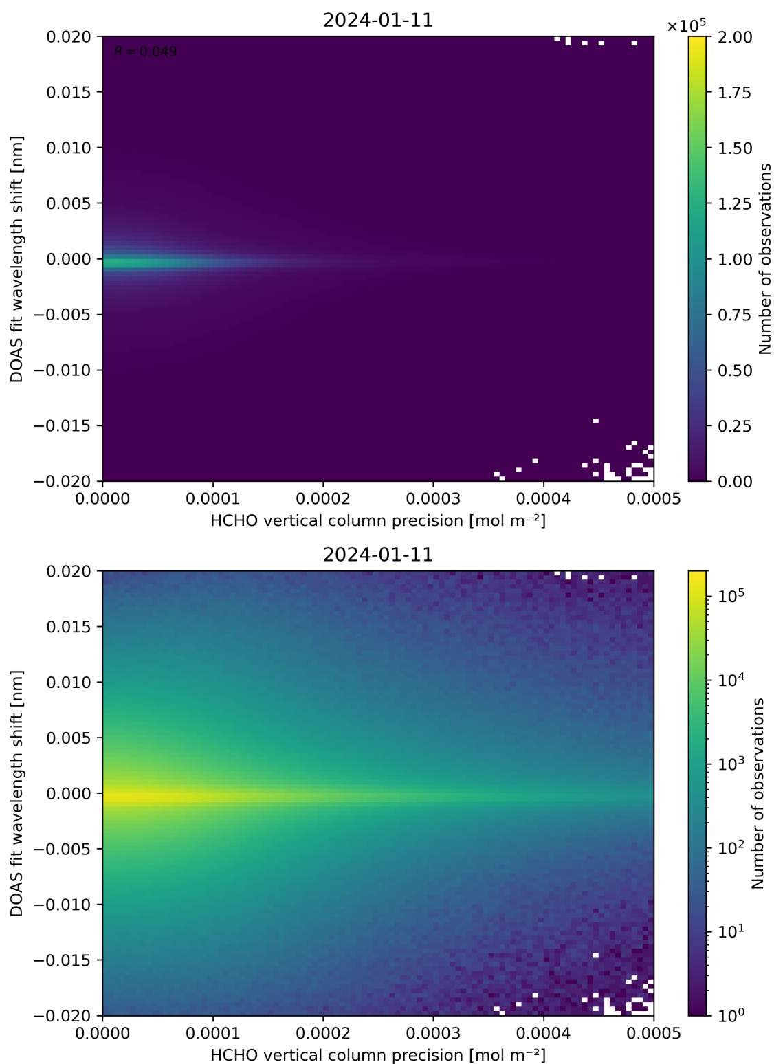
Figure 137: Scatter density plot of “HCHO vertical column precision” against “DOAS fit wavelength shift” for 2024-01-10 to 2024-01-12.
