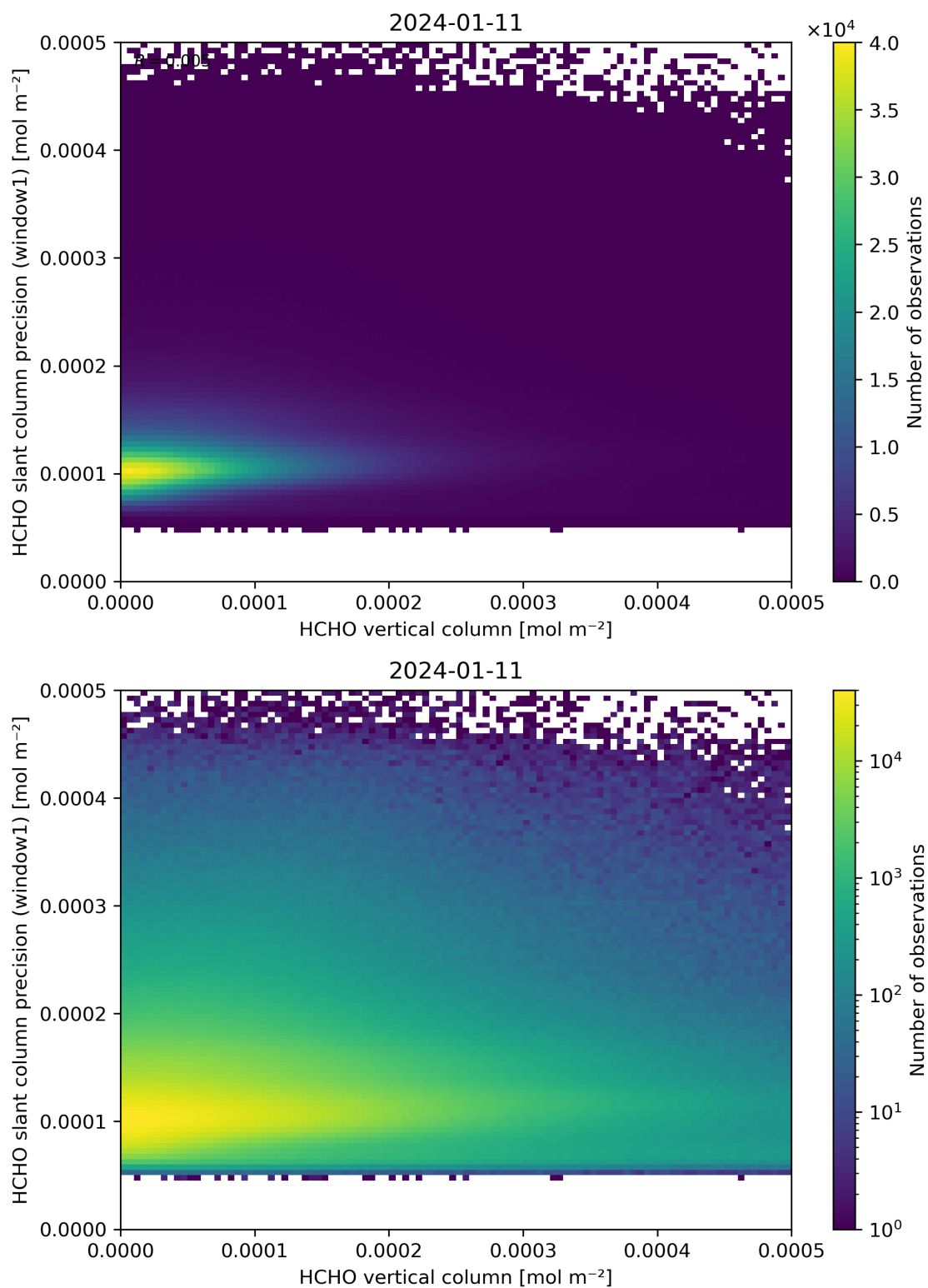
Figure 130: Scatter density plot of “HCHO vertical column” against “HCHO slant column precision (window1)” for 2024-01-10 to 2024-01-12.
