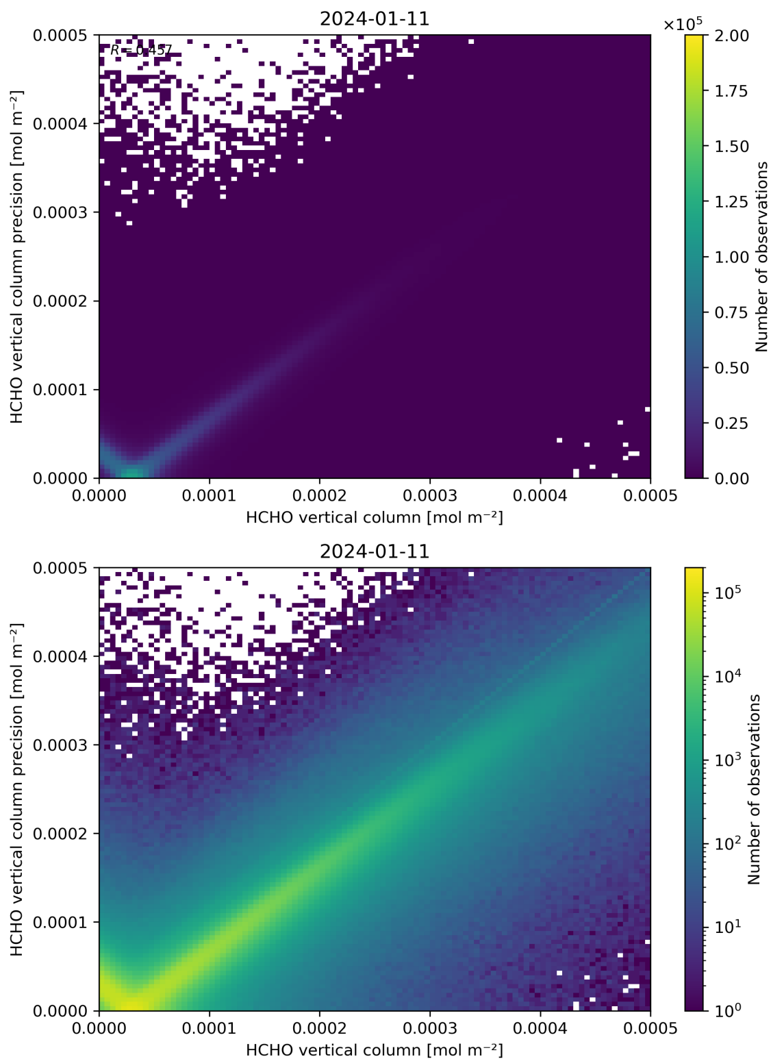
Figure 134: Scatter density plot of “HCHO vertical column” against “HCHO vertical column precision” for 2024-01-10 to 2024-01-12.
