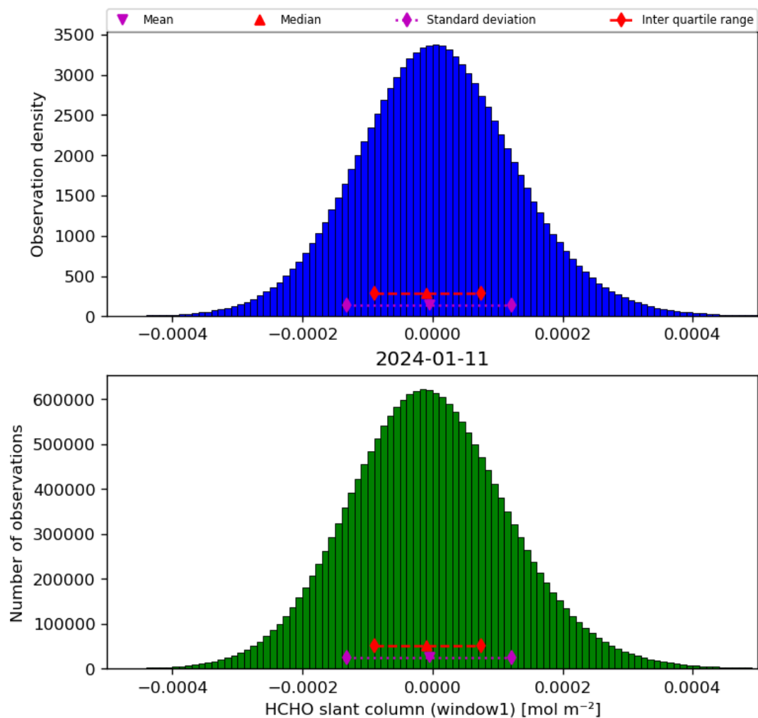
Figure 38: Histogram of “HCHO slant column (window1)” for 2024-01-10 to 2024-01-12
