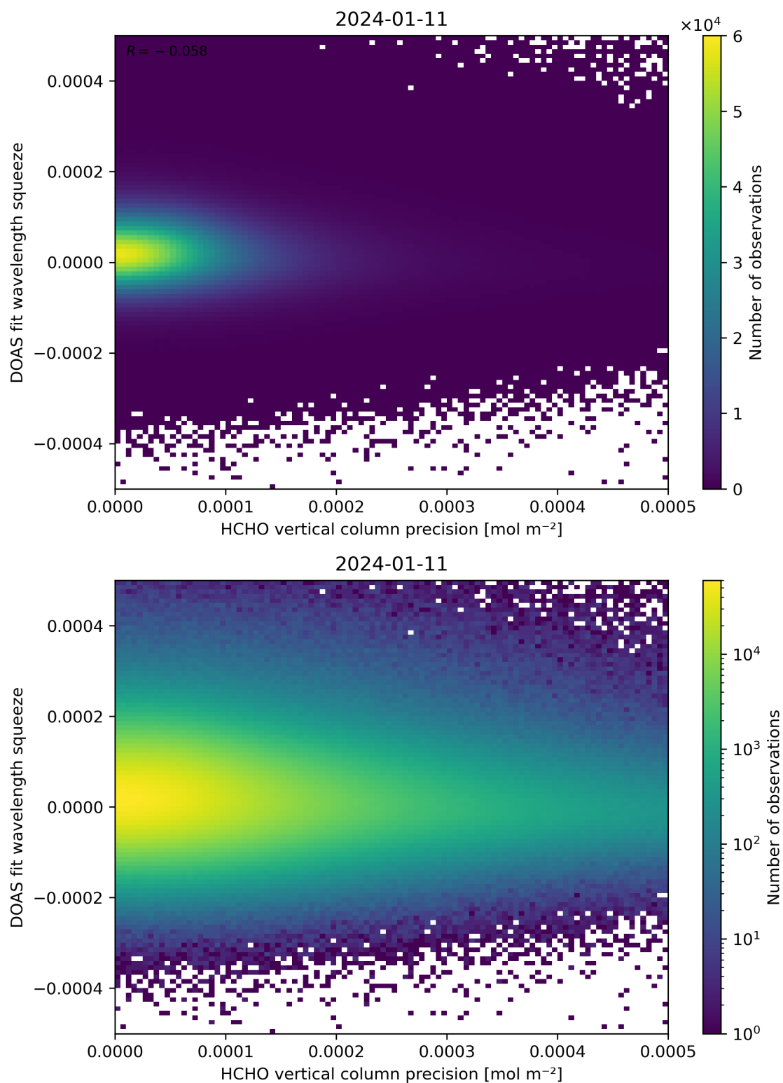
Figure 138: Scatter density plot of “HCHO vertical column precision” against “DOAS fit wavelength squeeze” for 2024-01-10 to 2024-01-12.
