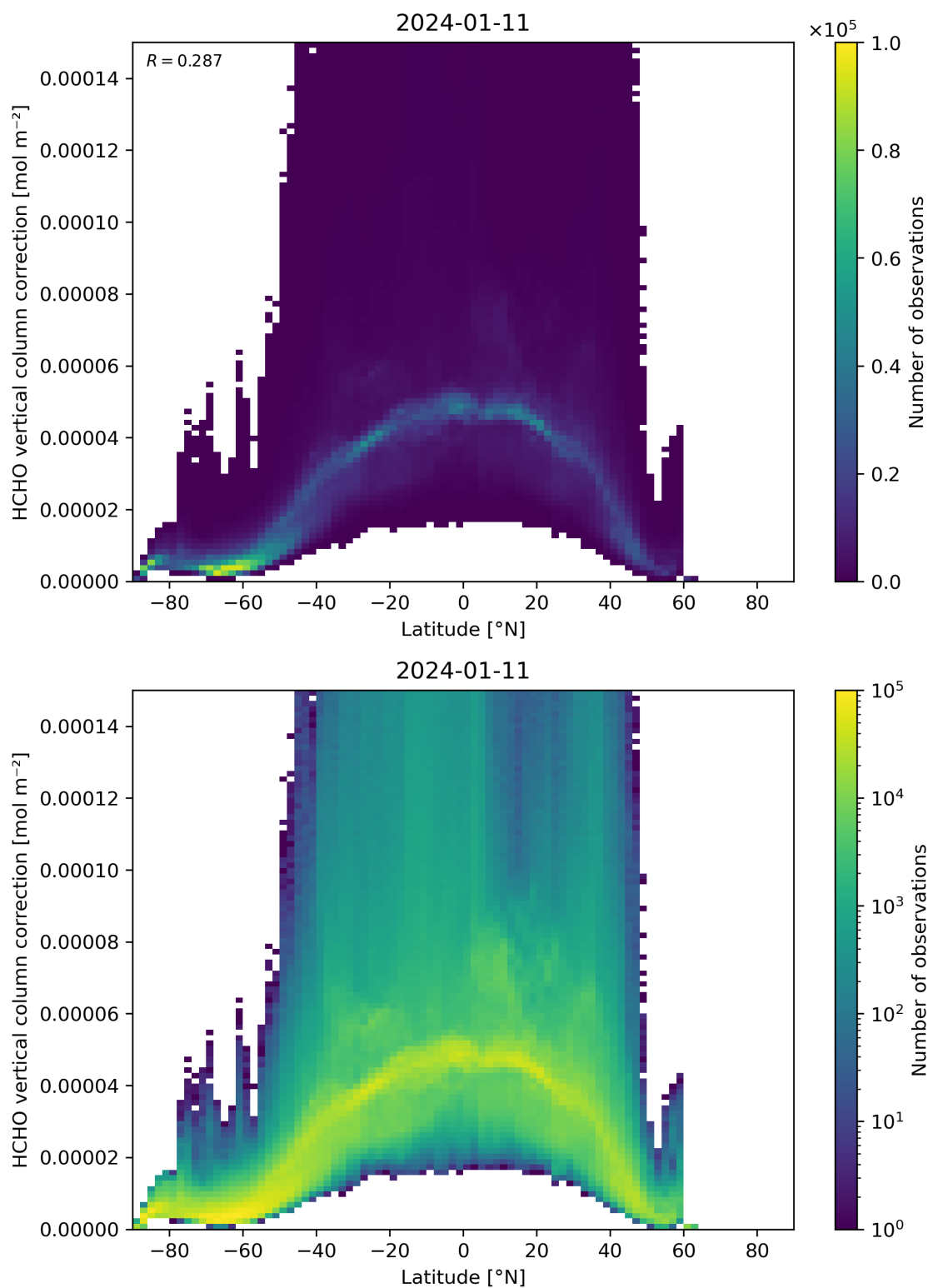
Figure 164: Scatter density plot of “Latitude” against “HCHO vertical column correction” for 2024-01-10 to 2024-01-12.
