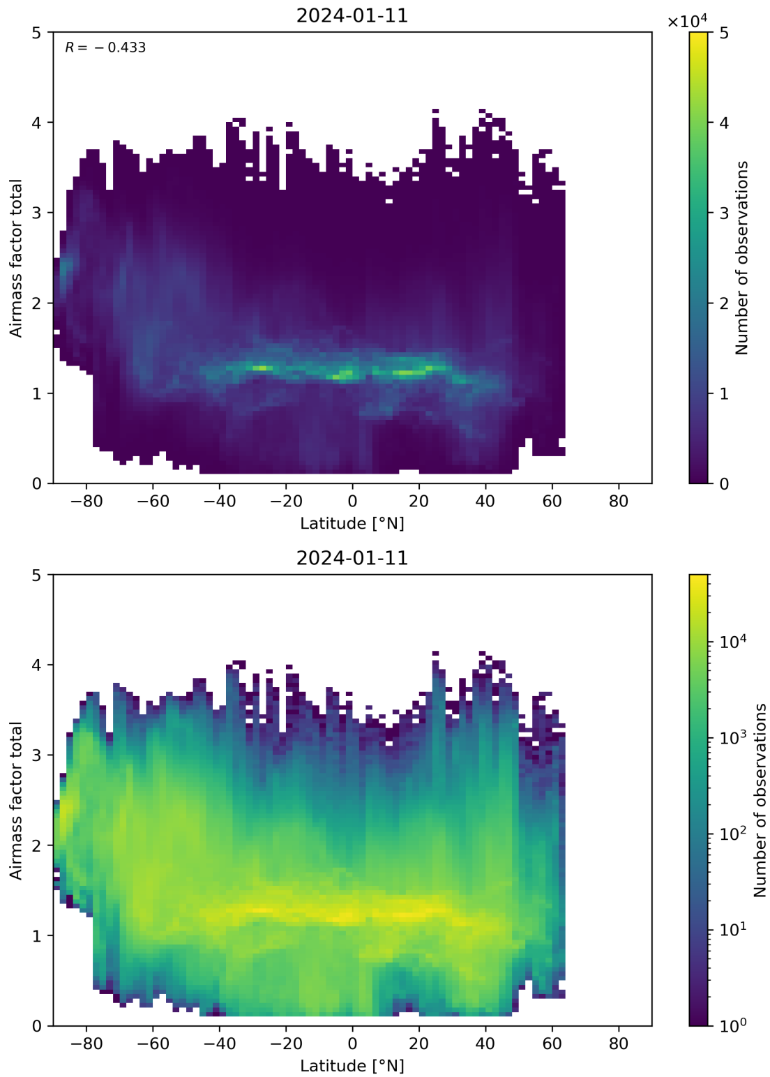
Figure 161: Scatter density plot of “Latitude” against “Airmass factor total” for 2024-01-10 to 2024-01-12.
