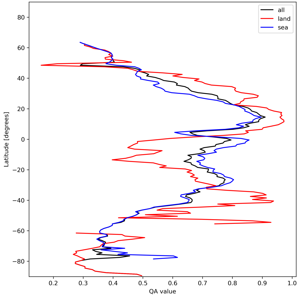
Figure 20: Zonal average of “QA value” for 2024-01-10 to 2024-01-12.
