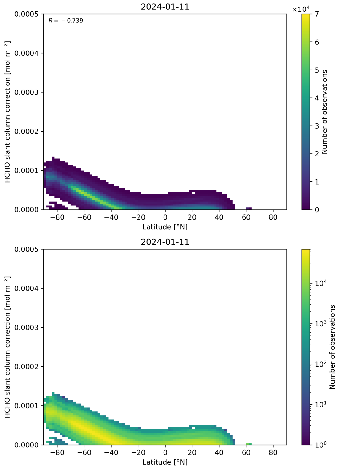
Figure 158: Scatter density plot of “Latitude” against “HCHO slant column correction” for 2024-01-10 to 2024-01-12.
