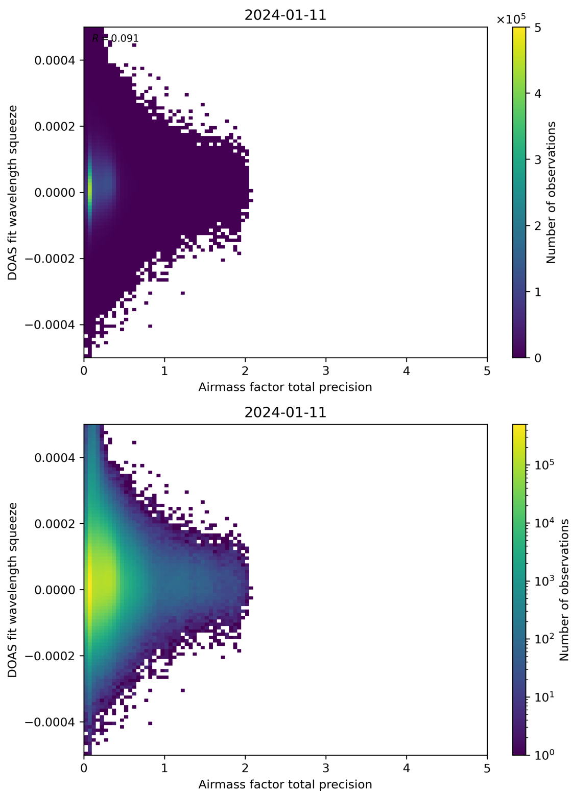
Figure 107: Scatter density plot of “Airmass factor total precision” against “DOAS fit wavelength squeeze” for 2024-01-10 to 2024-01-12.
