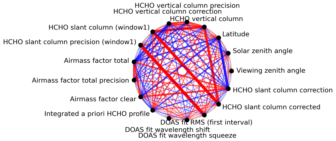
Figure 1: Map of correlation graph for 2024-01-10 to 2024-01-12.
