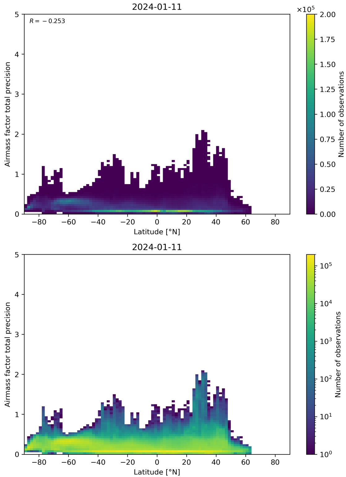
Figure 162: Scatter density plot of “Latitude” against “Airmass factor total precision” for 2024-01-10 to 2024-01-12.
