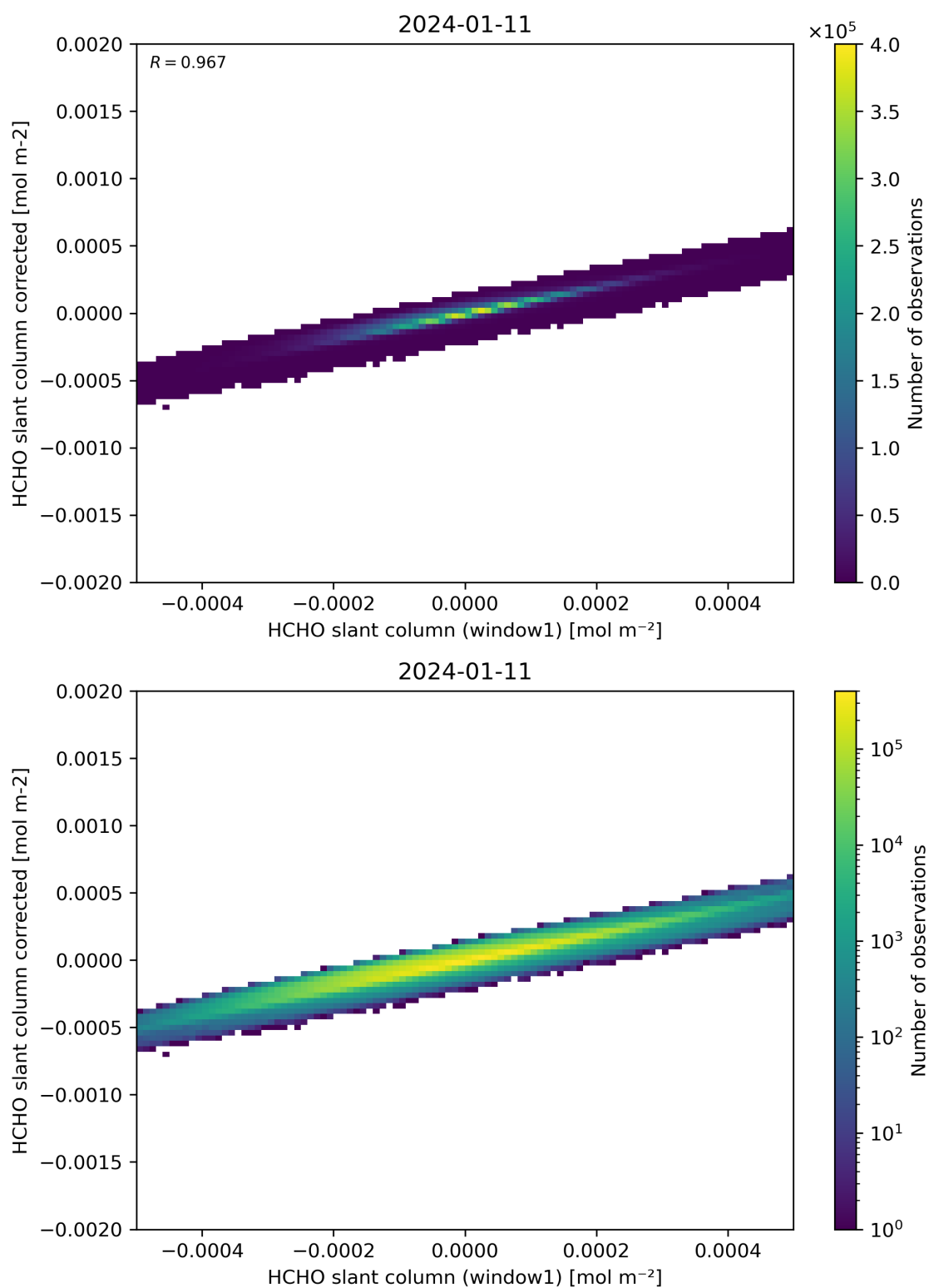
Figure 82: Scatter density plot of “HCHO slant column (window1)” against “HCHO slant column corrected” for 2024-01-10 to 2024-01-12.
