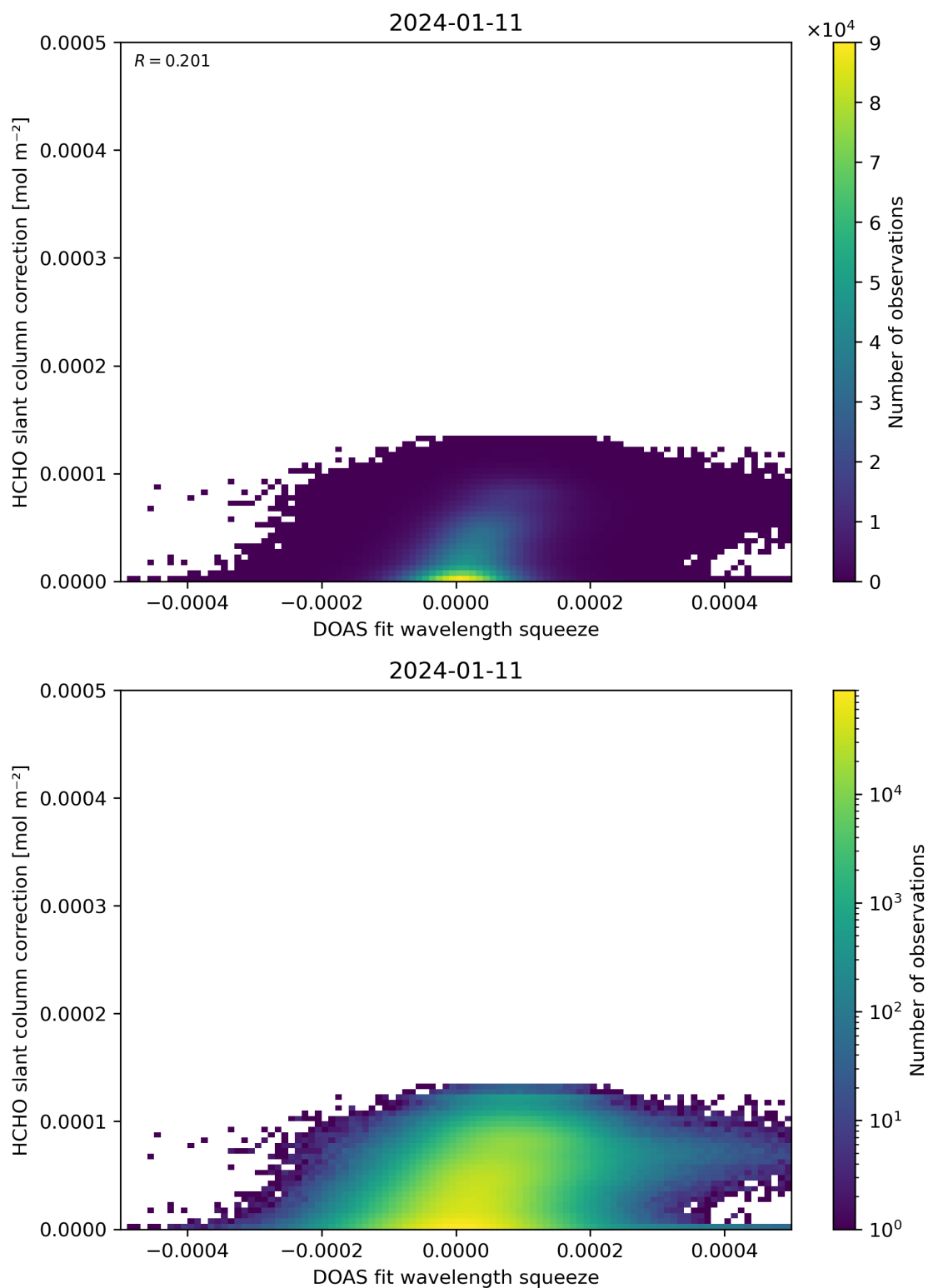
Figure 70: Scatter density plot of “DOAS fit wavelength squeeze” against “HCHO slant column correction” for 2024-01-10 to 2024-01-12.
