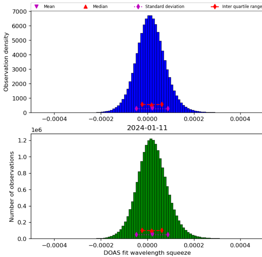
Figure 45: Histogram of “DOAS fit wavelength squeeze” for 2024-01-10 to 2024-01-12
