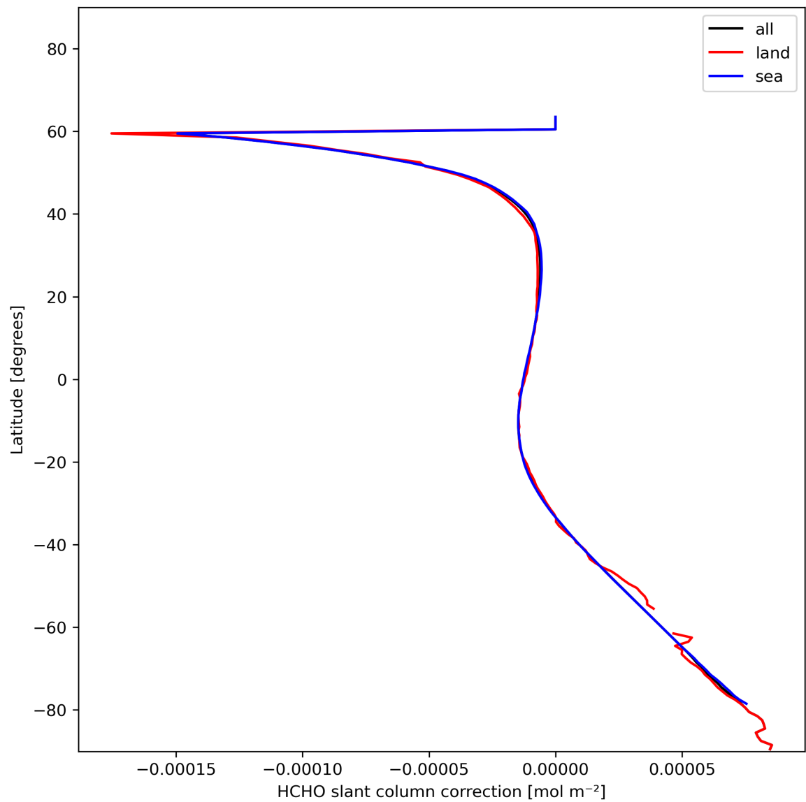
Figure 33: Zonal average of “HCHO slant column correction” for 2024-01-10 to 2024-01-12.
