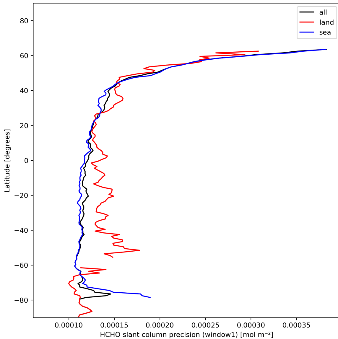
Figure 25: Zonal average of “HCHO slant column precision (window1)” for 2024-01-10 to 2024-01-12.
