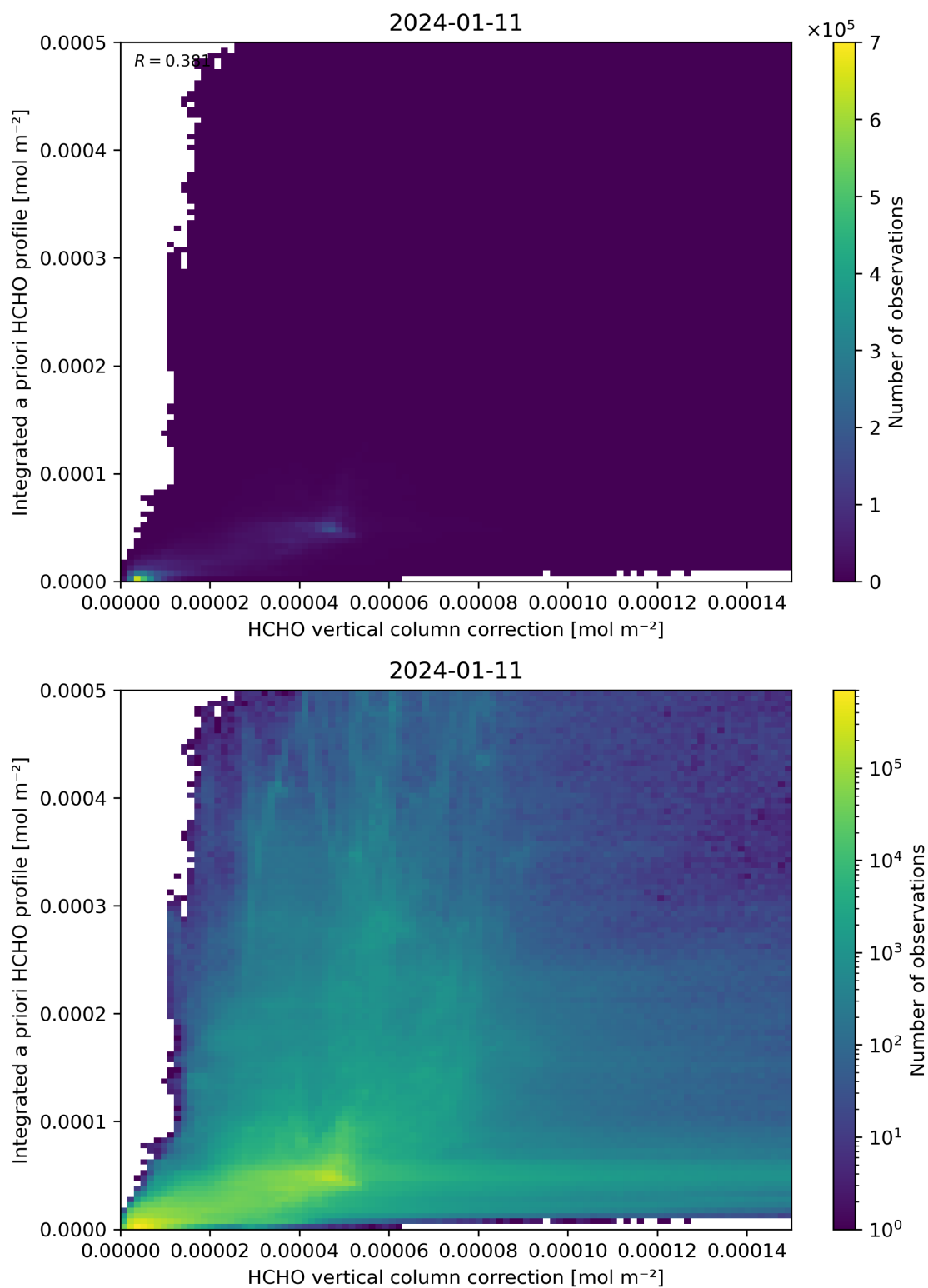
Figure 122: Scatter density plot of “HCHO vertical column correction” against “Integrated a priori HCHO profile” for 2024-01-10 to 2024-01-12.
