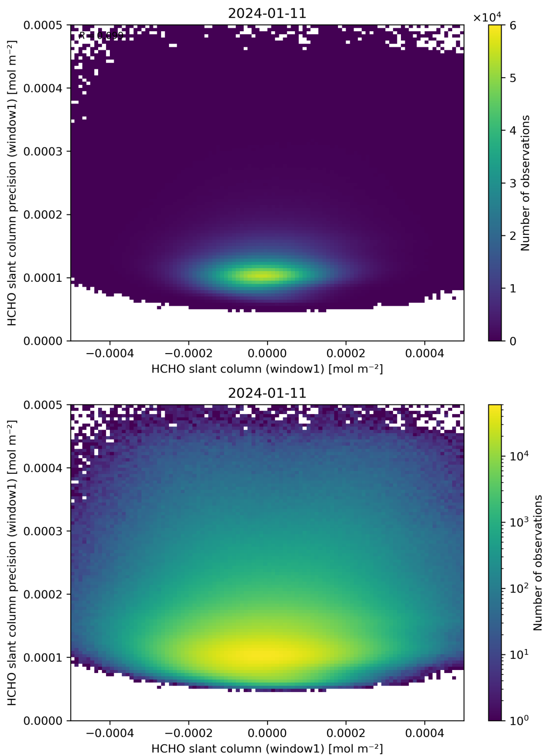
Figure 84: Scatter density plot of “HCHO slant column (window1)” against “HCHO slant column precision (window1)” for 2024-01-10 to 2024-01-12.
