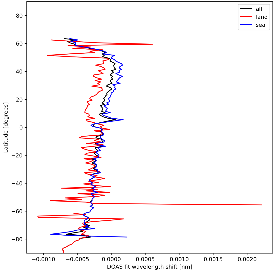
Figure 30: Zonal average of "DOAS fit wavelength shift" for 2024-01-10 to 2024-01-12.
