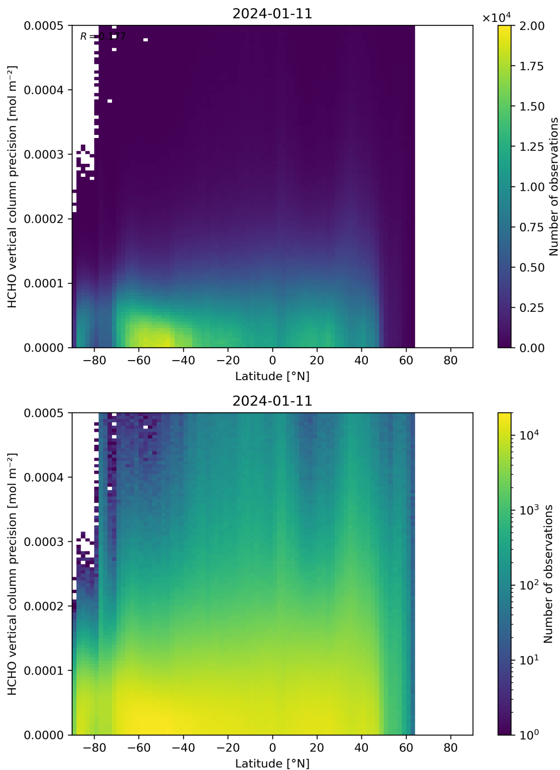
Figure 165: Scatter density plot of “Latitude” against “HCHO vertical column precision” for 2024-01-10 to 2024-01-12.
