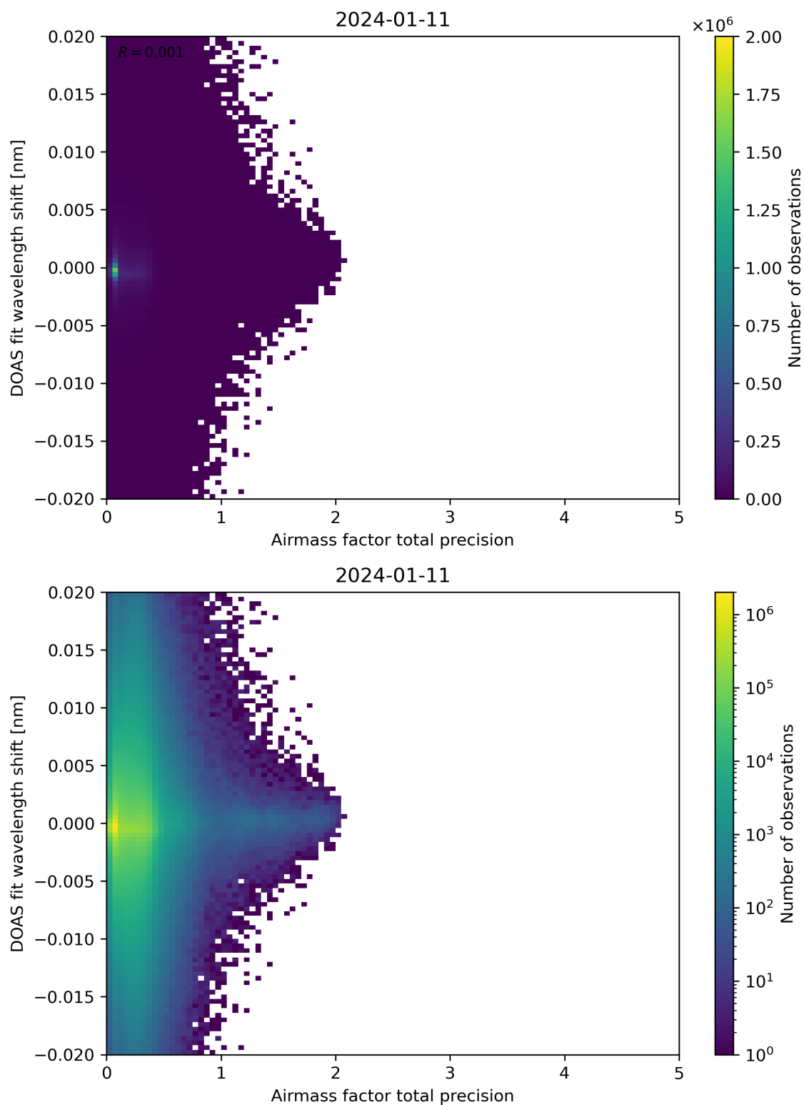
Figure 106: Scatter density plot of “Airmass factor total precision” against “DOAS fit wavelength shift” for 2024-01-10 to 2024-01-12.
