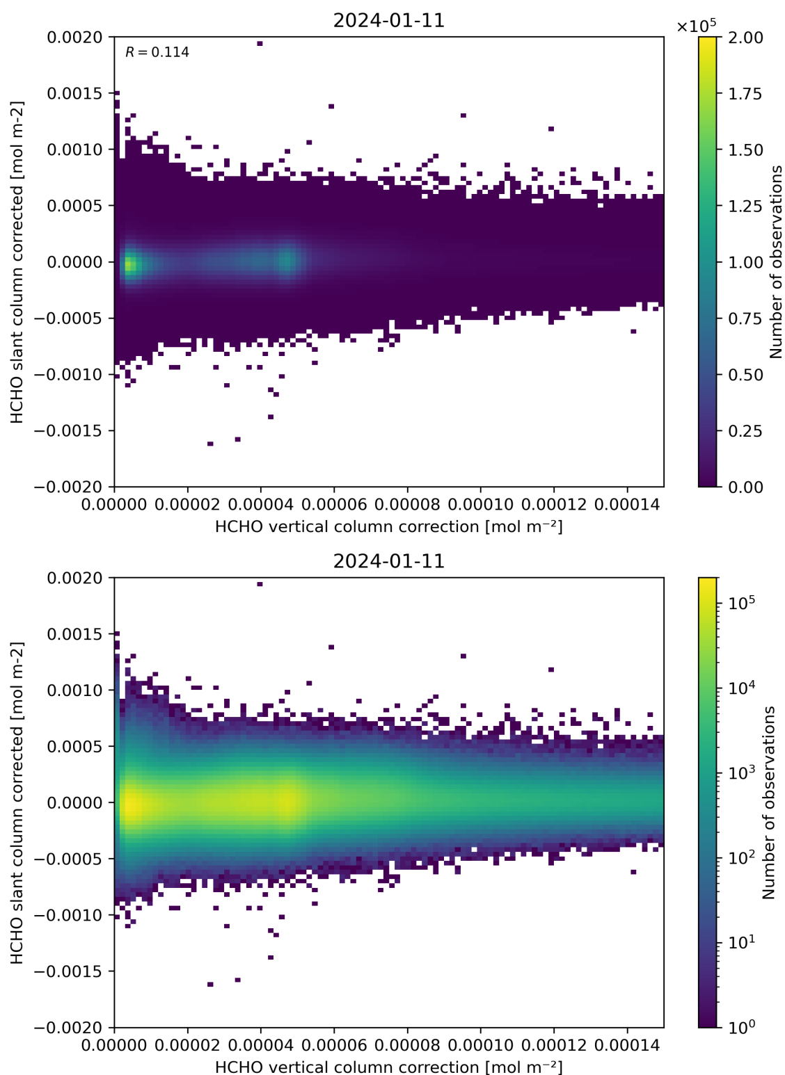
Figure 116: Scatter density plot of “HCHO vertical column correction” against “HCHO slant column corrected” for 2024-01-10 to 2024-01-12.
