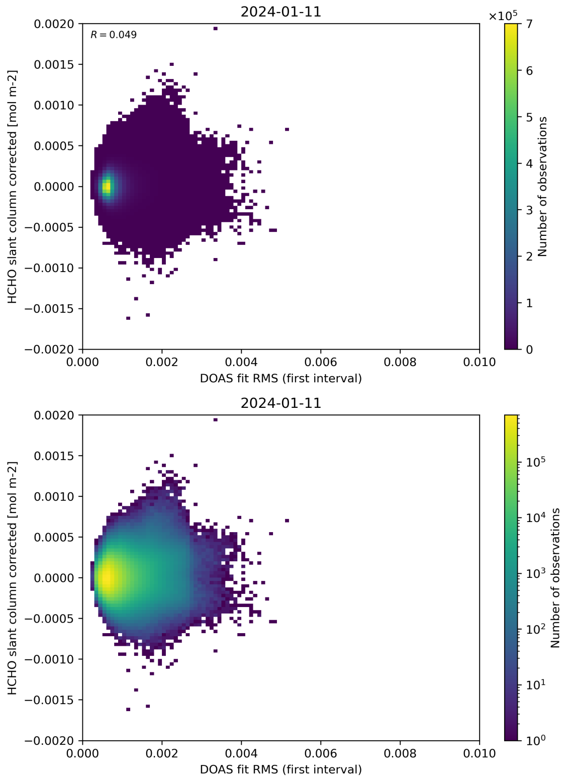
Figure 62: Scatter density plot of “DOAS fit RMS (first interval)” against “HCHO slant column corrected” for 2024-01-10 to 2024-01-12.
