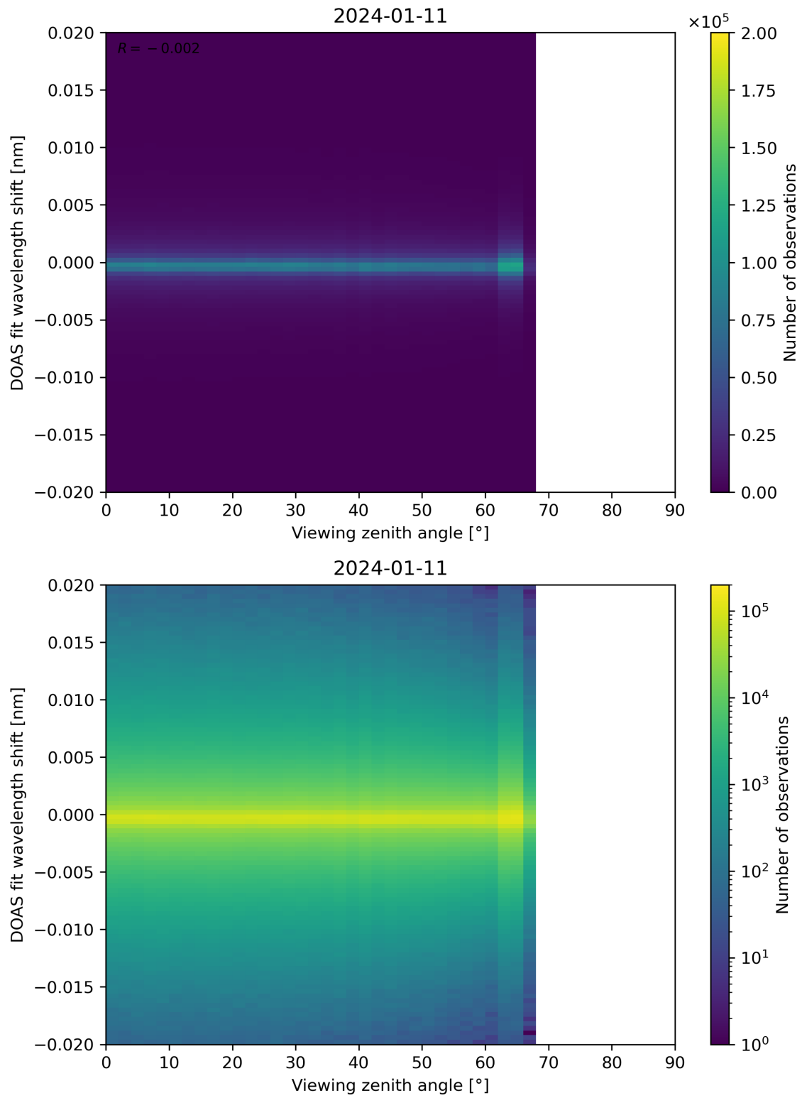
Figure 183: Scatter density plot of “Viewing zenith angle” against “DOAS fit wavelength shift” for 2024-01-10 to 2024-01-12.
