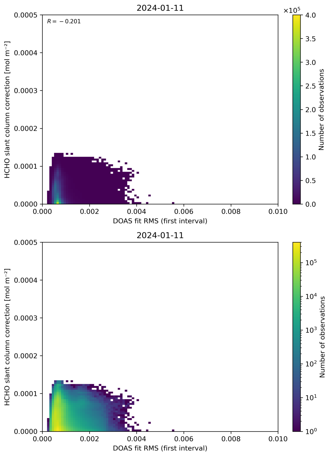
Figure 63: Scatter density plot of “DOAS fit RMS (first interval)” against “HCHO slant column correction” for 2024-01-10 to 2024-01-12.
