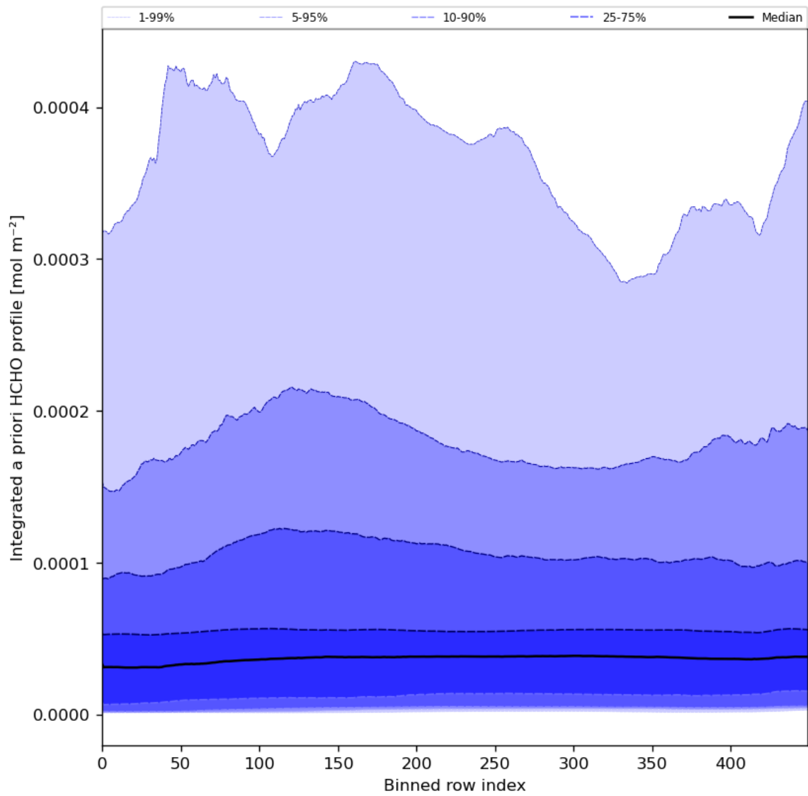
Figure 57: Along track statistics of “Integrated a priori HCHO profile” for 2024-01-10 to 2024-01-12
