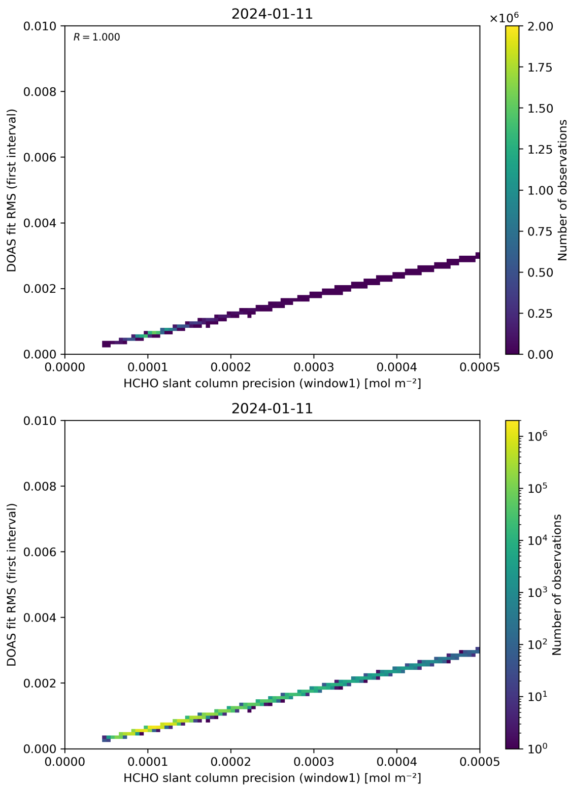
Figure 88: Scatter density plot of “HCHO slant column precision (window1)” against “DOAS fit RMS (first interval)” for 2024-01-10 to 2024-01-12.
