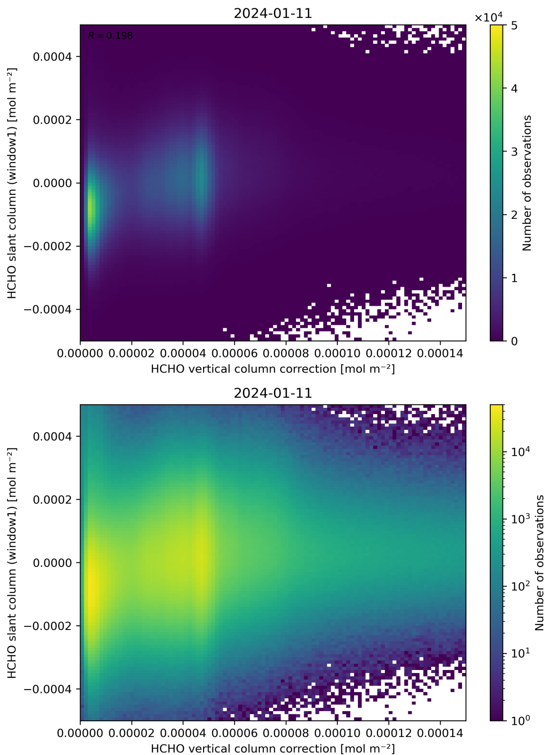
Figure 118: Scatter density plot of “HCHO vertical column correction” against “HCHO slant column (window1)” for 2024-01-10 to 2024-01-12.
