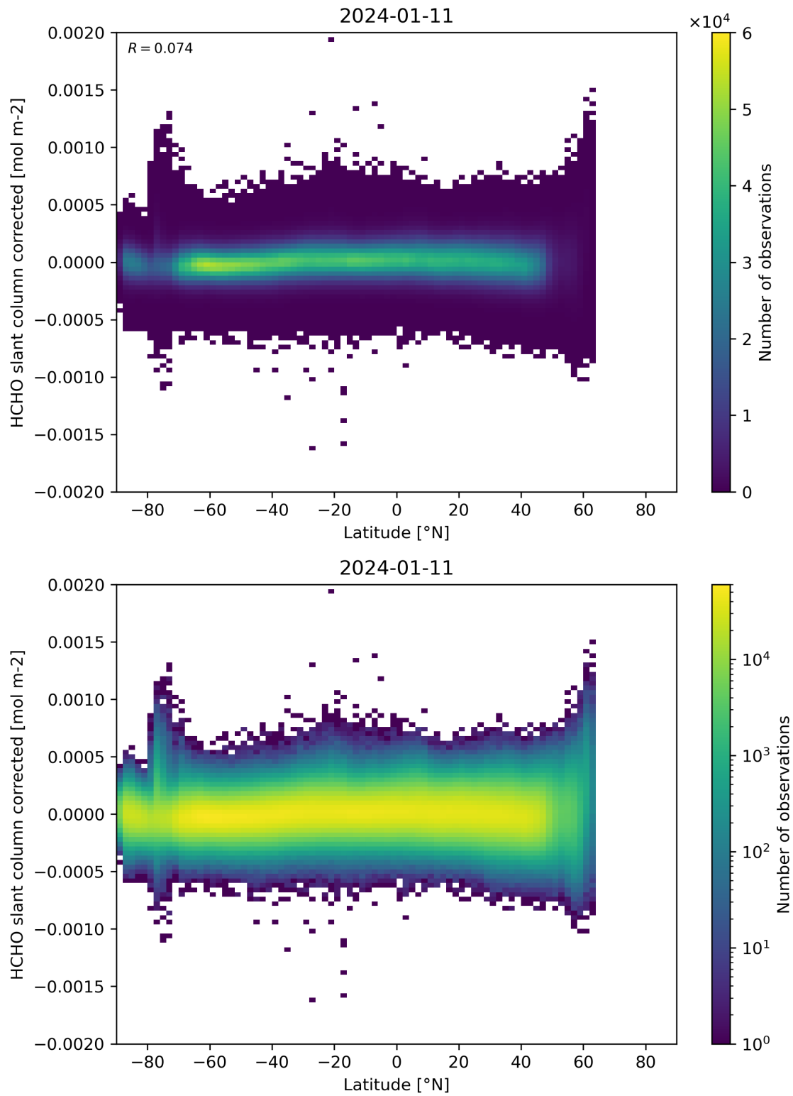
Figure 157: Scatter density plot of “Latitude” against “HCHO slant column corrected” for 2024-01-10 to 2024-01-12.
