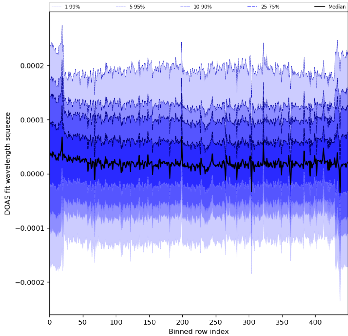
Figure 59: Along track statistics of “DOAS fit wavelength squeeze” for 2024-01-10 to 2024-01-12
