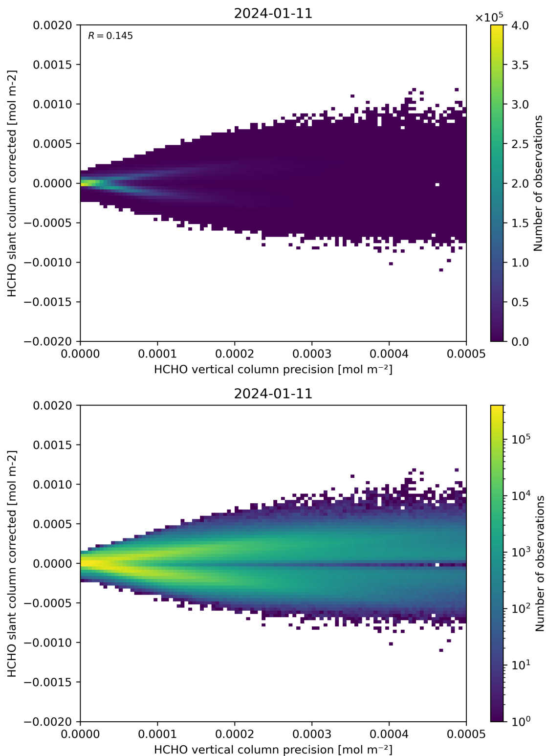
Figure 140: Scatter density plot of “HCHO vertical column precision” against “HCHO slant column corrected” for 2024-01-10 to 2024-01-12.
