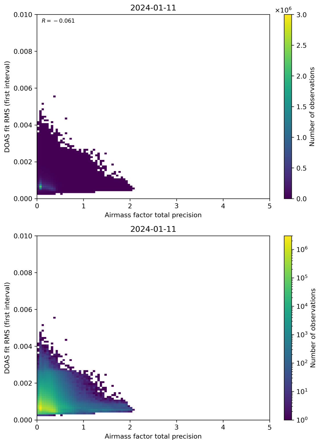
Figure 105: Scatter density plot of “Airmass factor total precision” against “DOAS fit RMS (first interval)” for 2024-01-10 to 2024-01-12.
