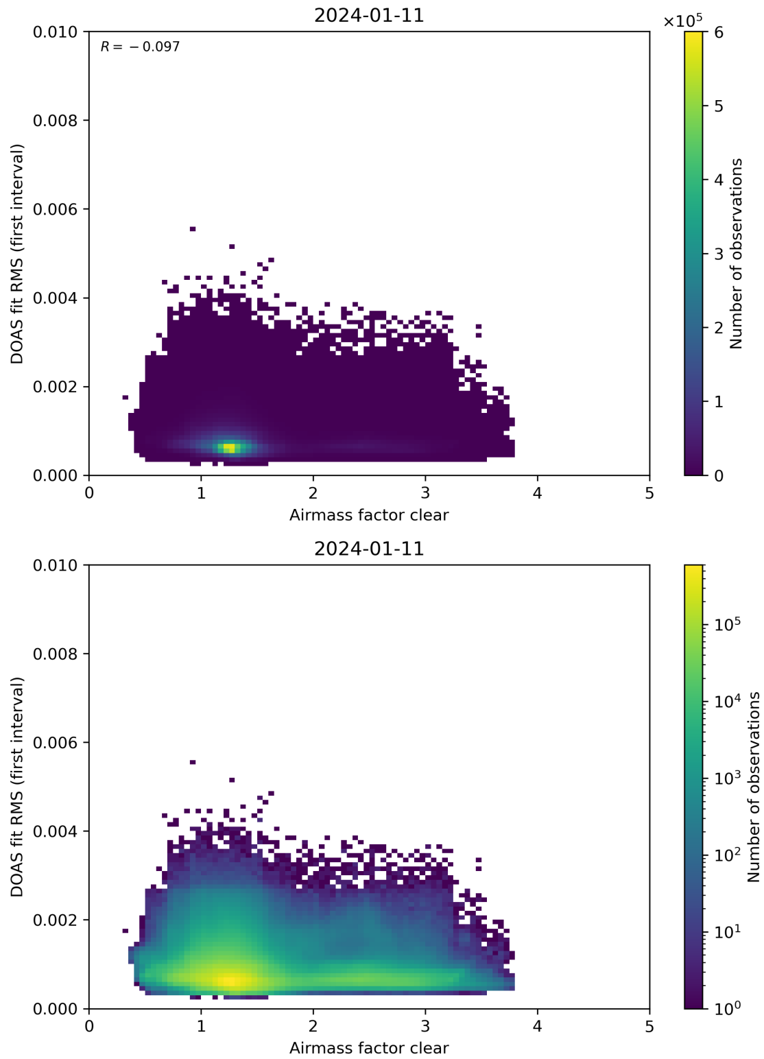
Figure 71: Scatter density plot of “Airmass factor clear” against “DOAS fit RMS (first interval)” for 2024-01-10 to 2024-01-12.
