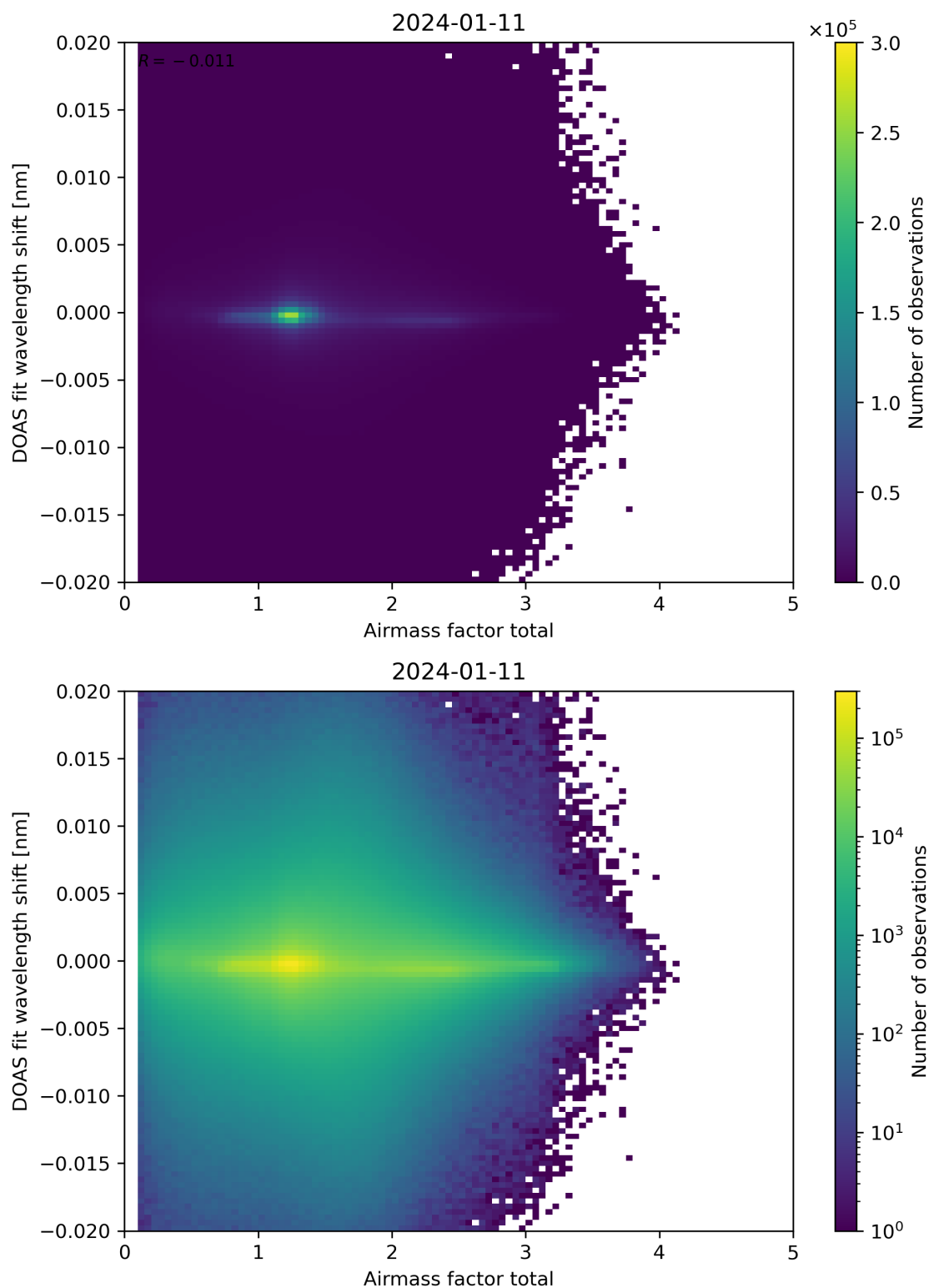
Figure 98: Scatter density plot of “Airmass factor total” against “DOAS fit wavelength shift” for 2024-01-10 to 2024-01-12.
