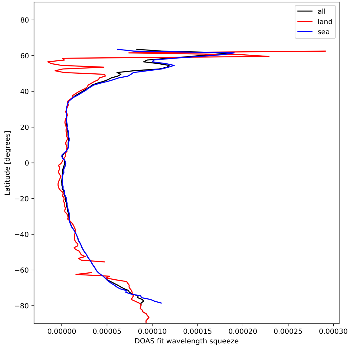
Figure 31: Zonal average of “DOAS fit wavelength squeeze” for 2024-01-10 to 2024-01-12.
