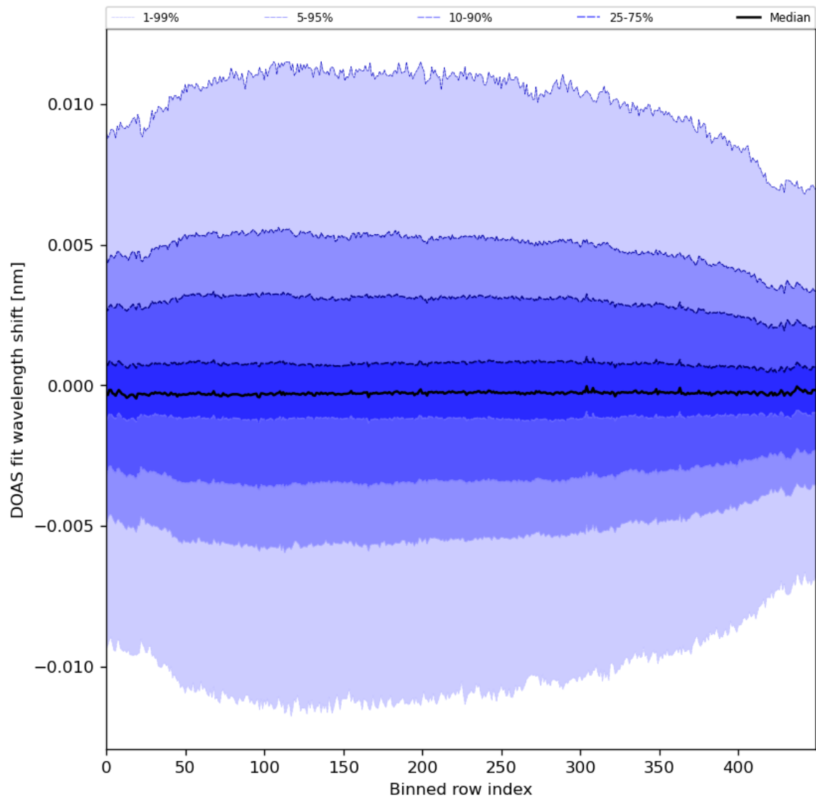
Figure 58: Along track statistics of “DOAS fit wavelength shift” for 2024-01-10 to 2024-01-12
