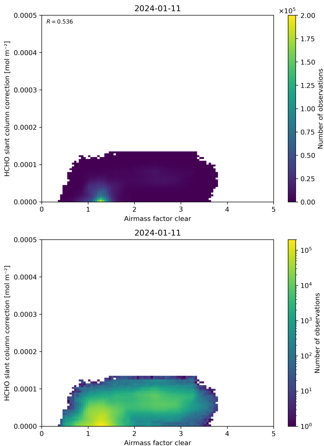
Figure 75: Scatter density plot of “Airmass factor clear” against “HCHO slant column correction” for 2024-01-10 to 2024-01-12.
