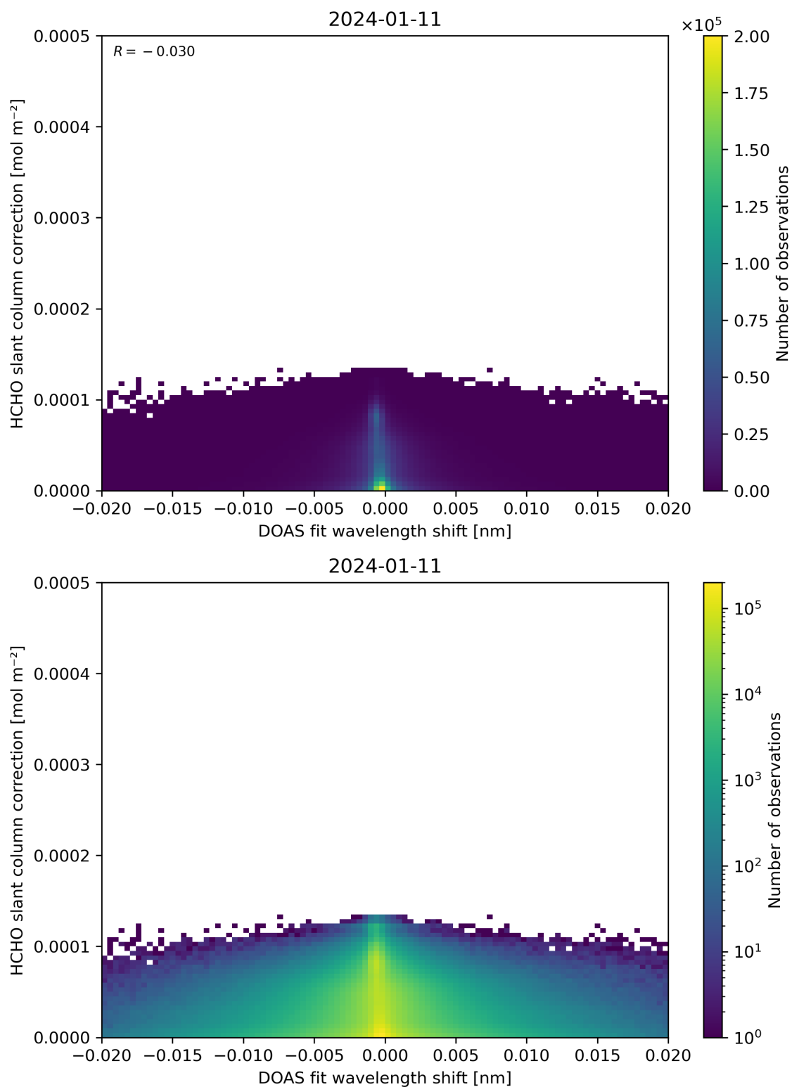
Figure 67: Scatter density plot of “DOAS fit wavelength shift” against “HCHO slant column correction” for 2024-01-10 to 2024-01-12.
