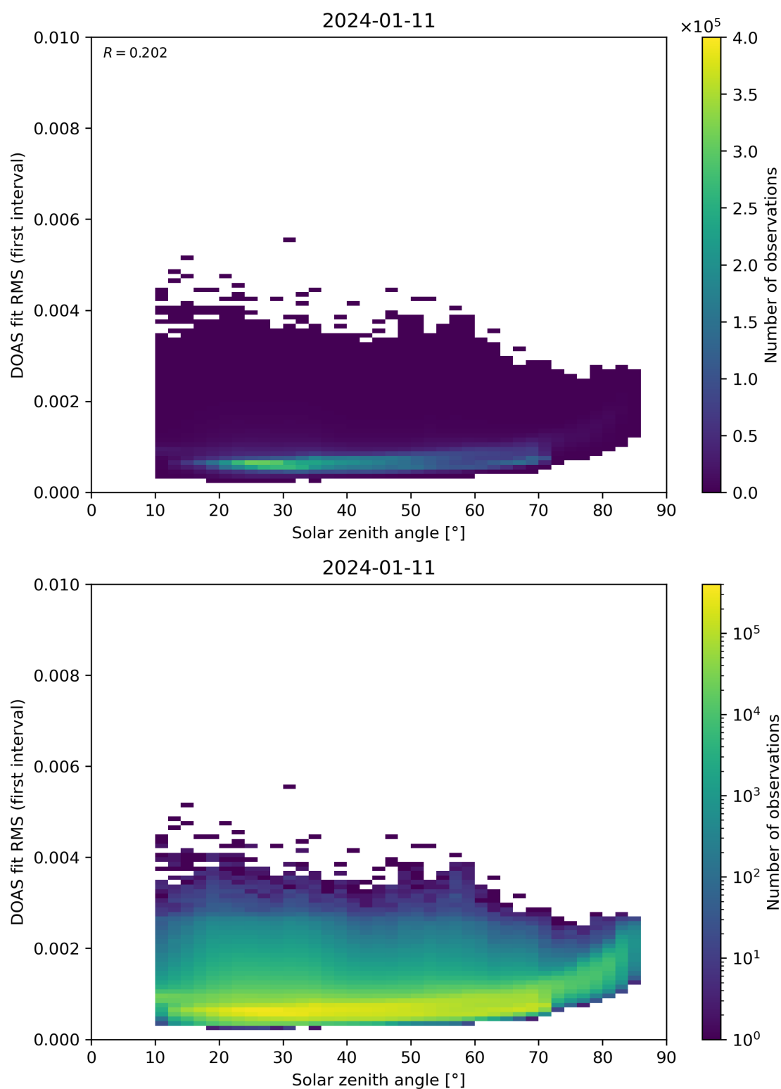
Figure 167: Scatter density plot of “Solar zenith angle” against “DOAS fit RMS (first interval)” for 2024-01-10 to 2024-01-12.
