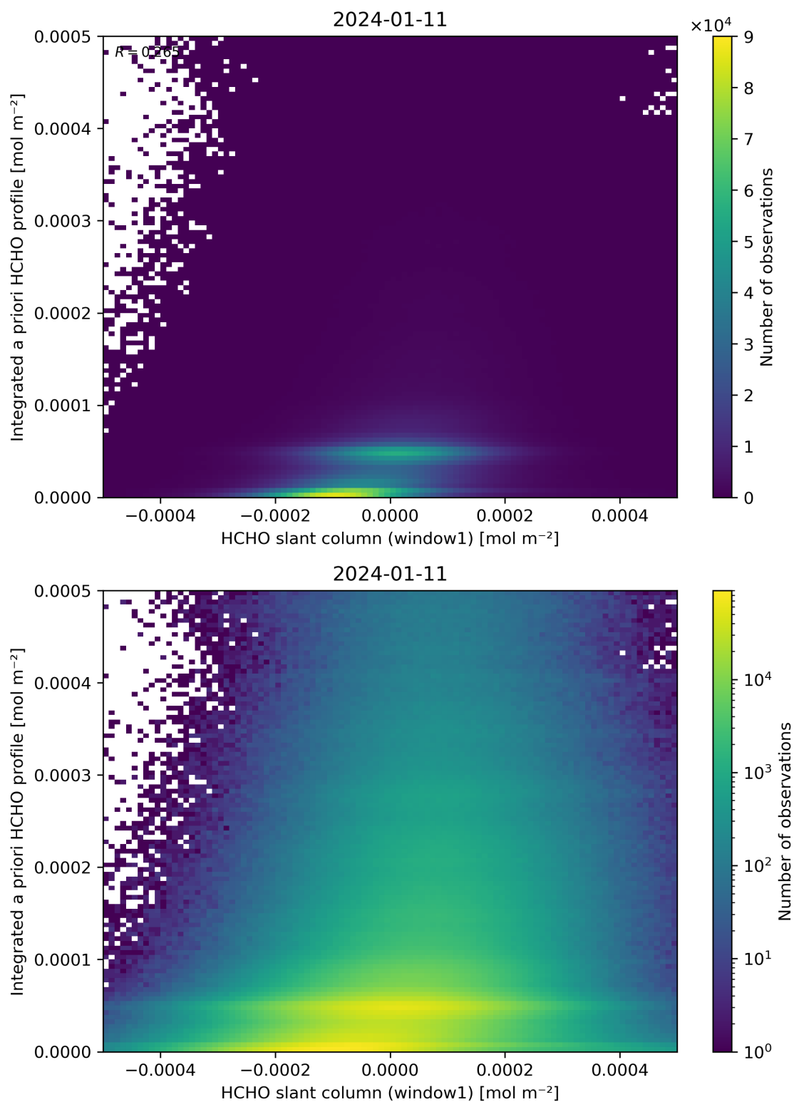
Figure 87: Scatter density plot of “HCHO slant column (window1)” against “Integrated a priori HCHO profile” for 2024-01-10 to 2024-01-12.
