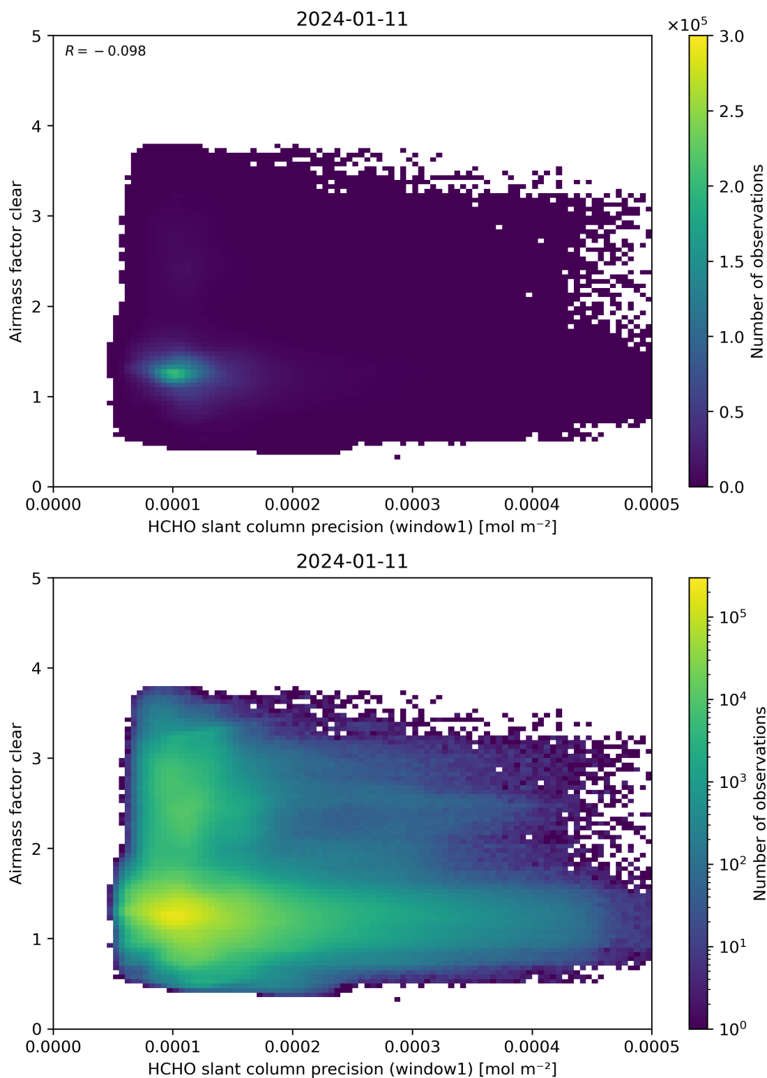
Figure 91: Scatter density plot of “HCHO slant column precision (window1)” against “Airmass factor clear” for 2024-01-10 to 2024-01-12.
