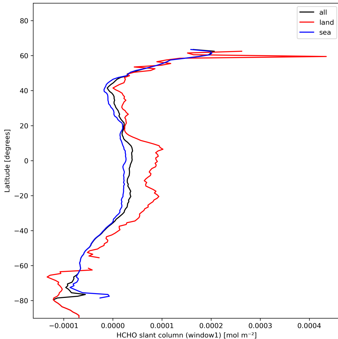
Figure 24: Zonal average of “HCHO slant column (window1)” for 2024-01-10 to 2024-01-12.
