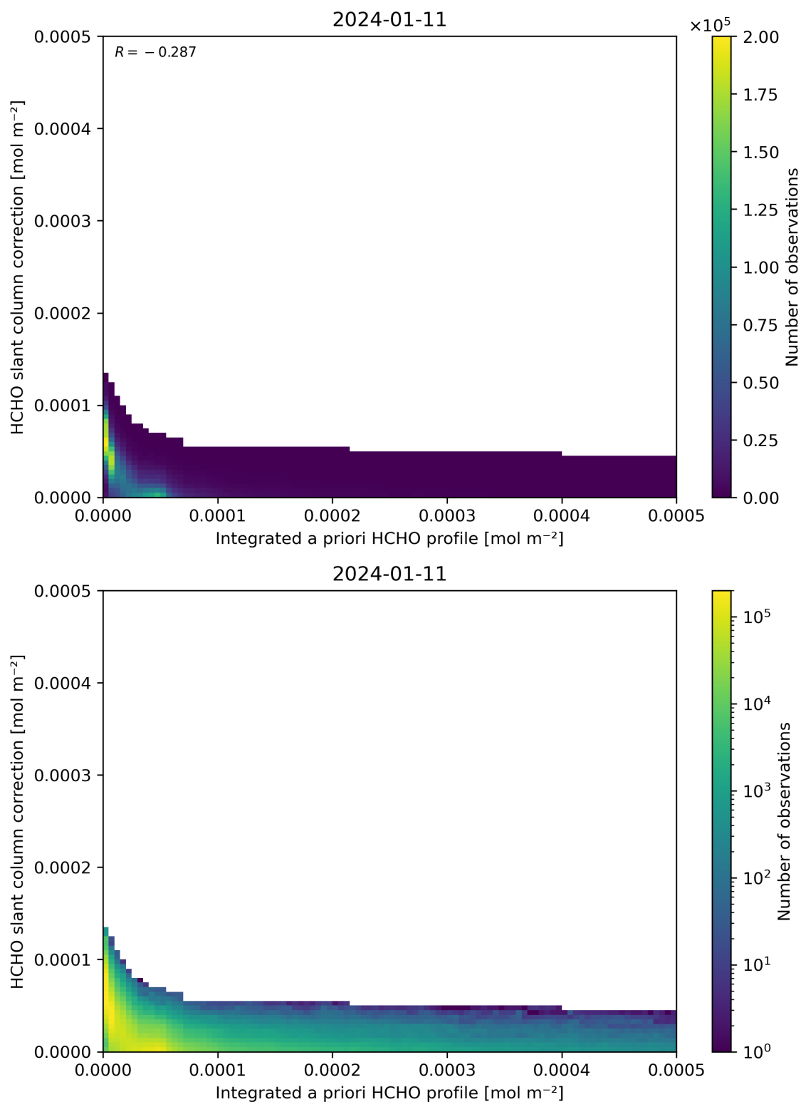
Figure 152: Scatter density plot of “Integrated a priori HCHO profile” against “HCHO slant column correction” for 2024-01-10 to 2024-01-12.
