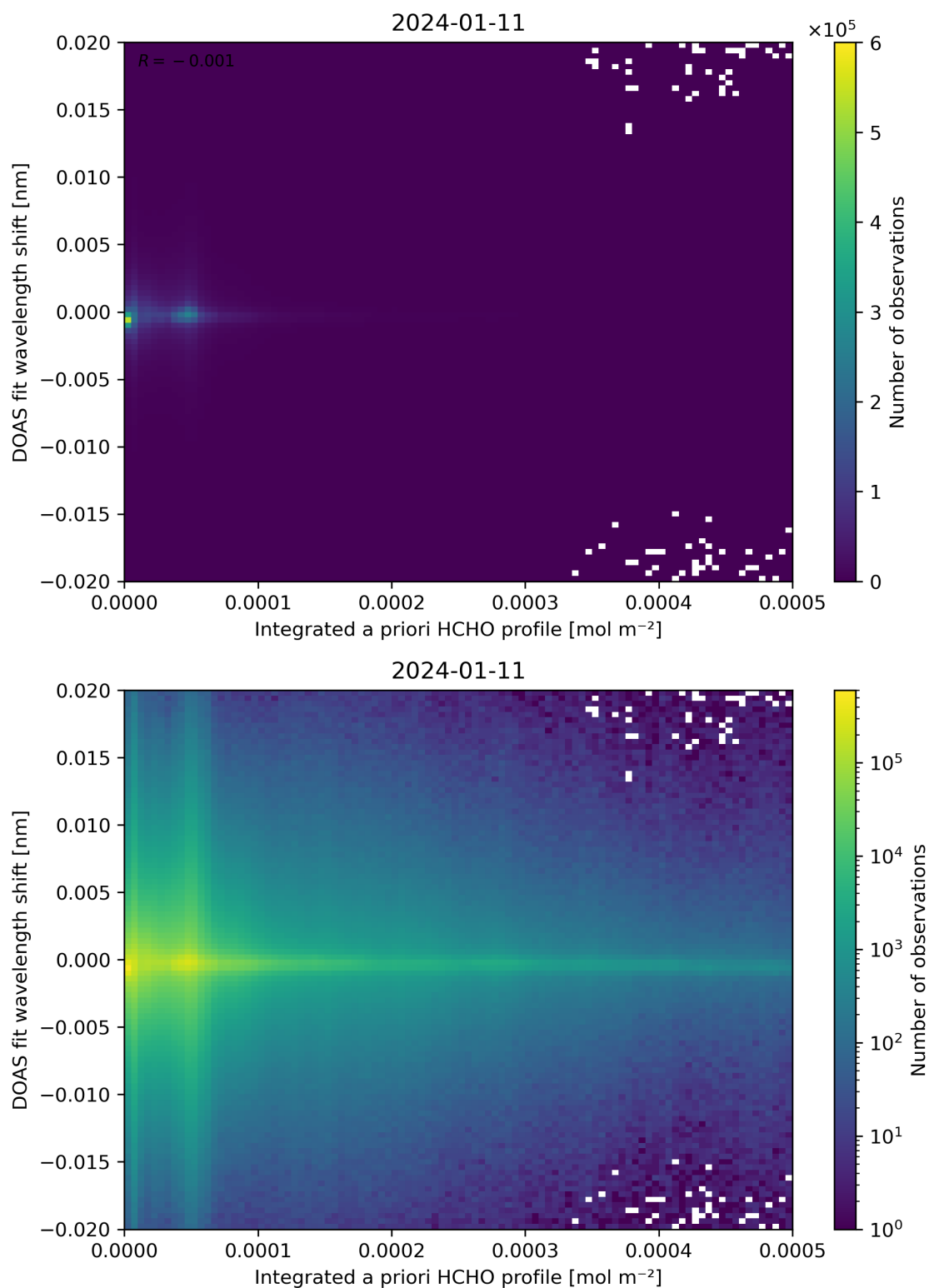
Figure 149: Scatter density plot of “Integrated a priori HCHO profile” against “DOAS fit wavelength shift” for 2024-01-10 to 2024-01-12.
