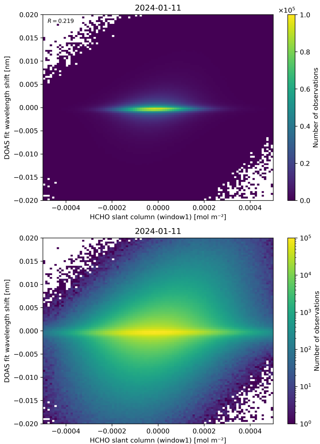
Figure 79: Scatter density plot of “HCHO slant column (window1)” against “DOAS fit wavelength shift” for 2024-01-10 to 2024-01-12.
