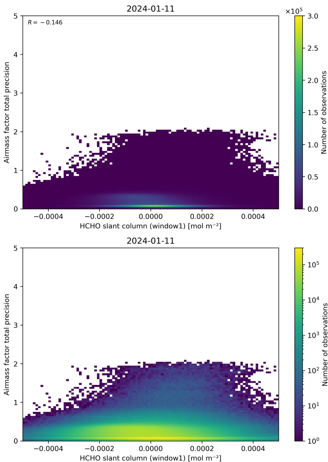
Figure 86: Scatter density plot of “HCHO slant column (window1)” against “Airmass factor total precision” for 2024-01-10 to 2024-01-12.
