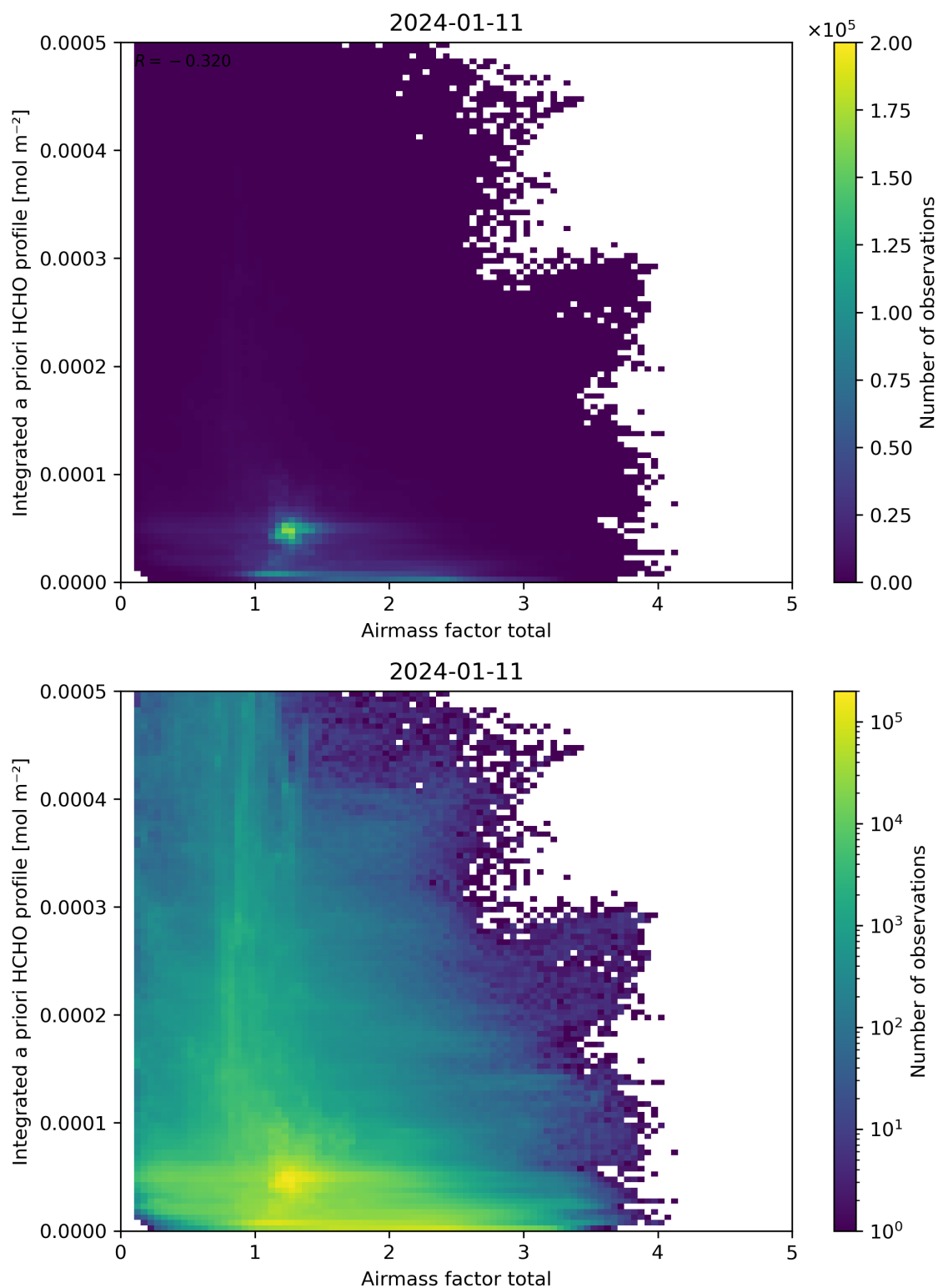
Figure 104: Scatter density plot of “Airmass factor total” against “Integrated a priori HCHO profile” for 2024-01-10 to 2024-01-12.
