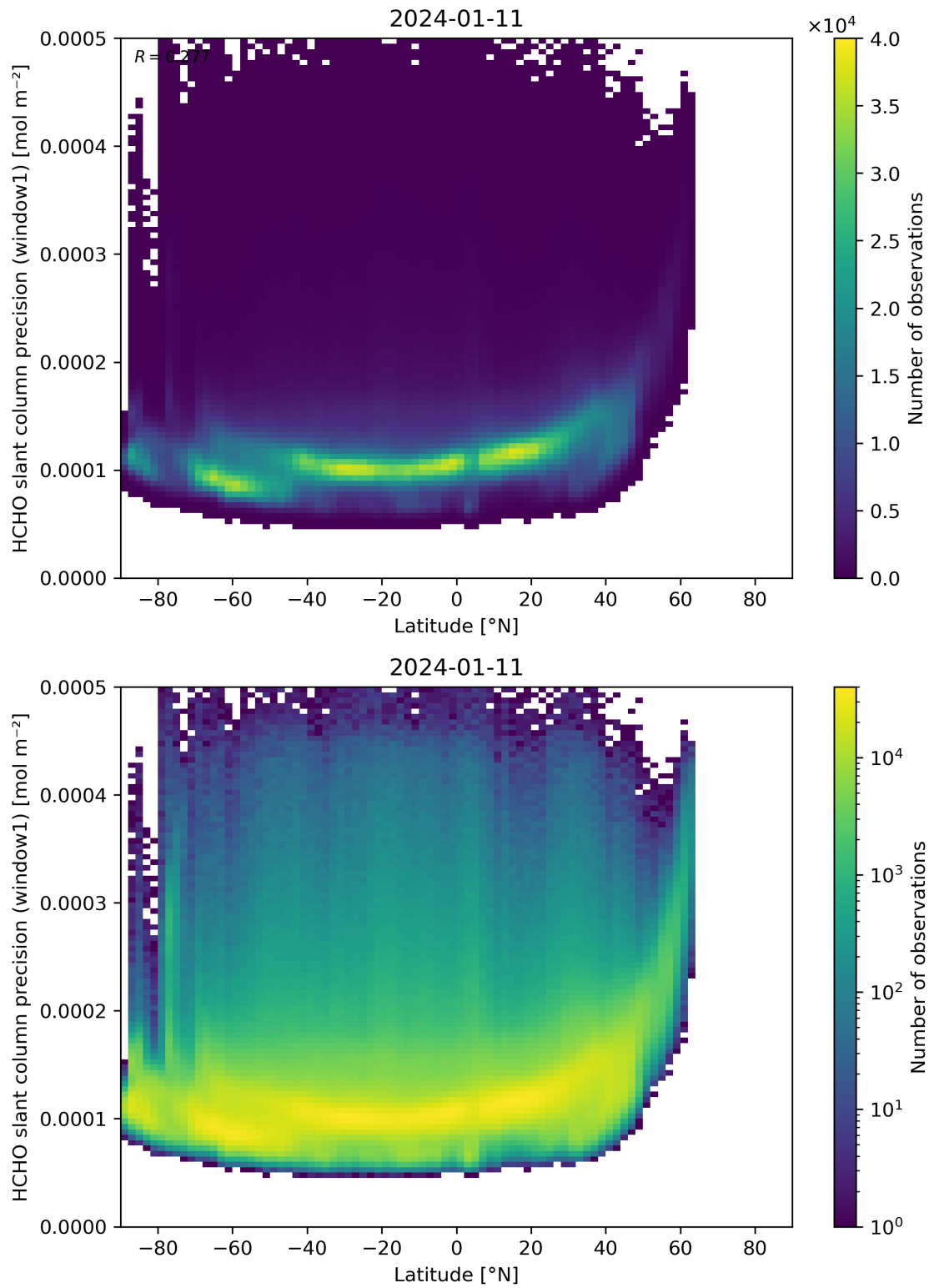
Figure 160: Scatter density plot of “Latitude” against “HCHO slant column precision (window1)” for 2024-01-10 to 2024-01-12.
