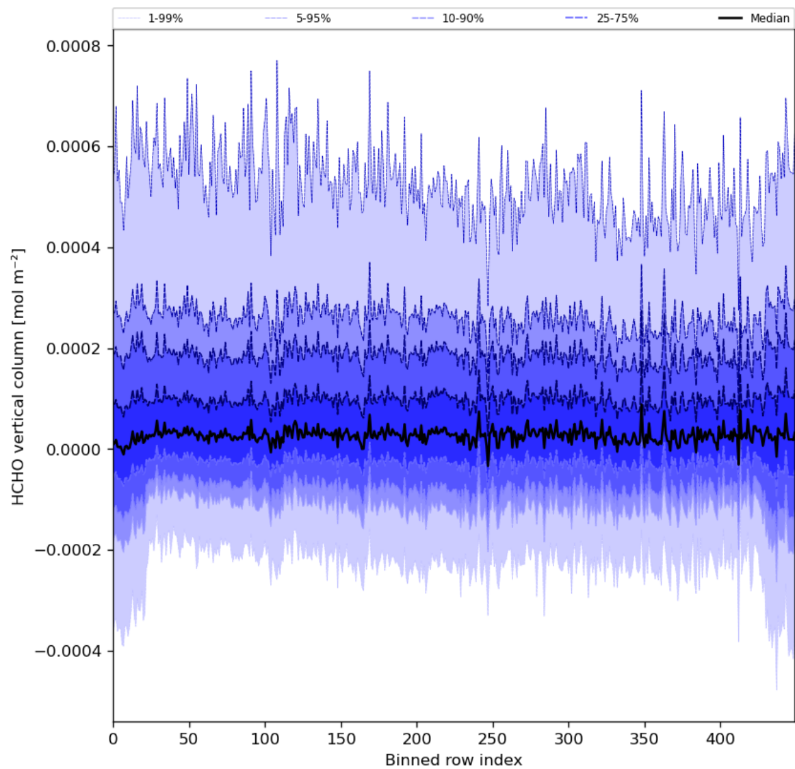
Figure 49: Along track statistics of “HCHO vertical column” for 2024-01-10 to 2024-01-12
