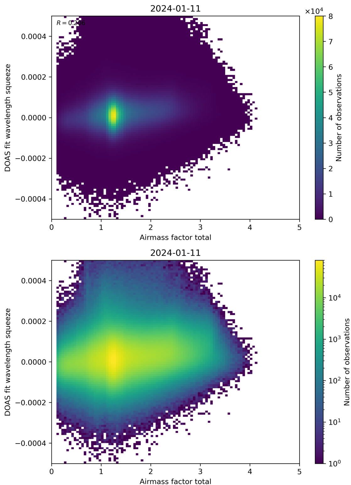
Figure 99: Scatter density plot of “Airmass factor total” against “DOAS fit wavelength squeeze” for 2024-01-10 to 2024-01-12.
