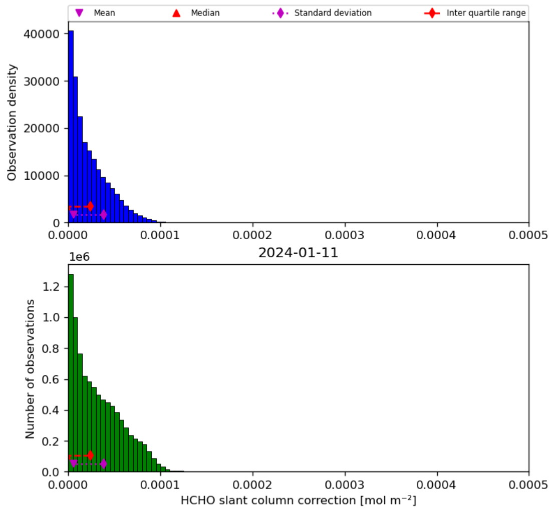
Figure 47: Histogram of “HCHO slant column correction” for 2024-01-10 to 2024-01-12
