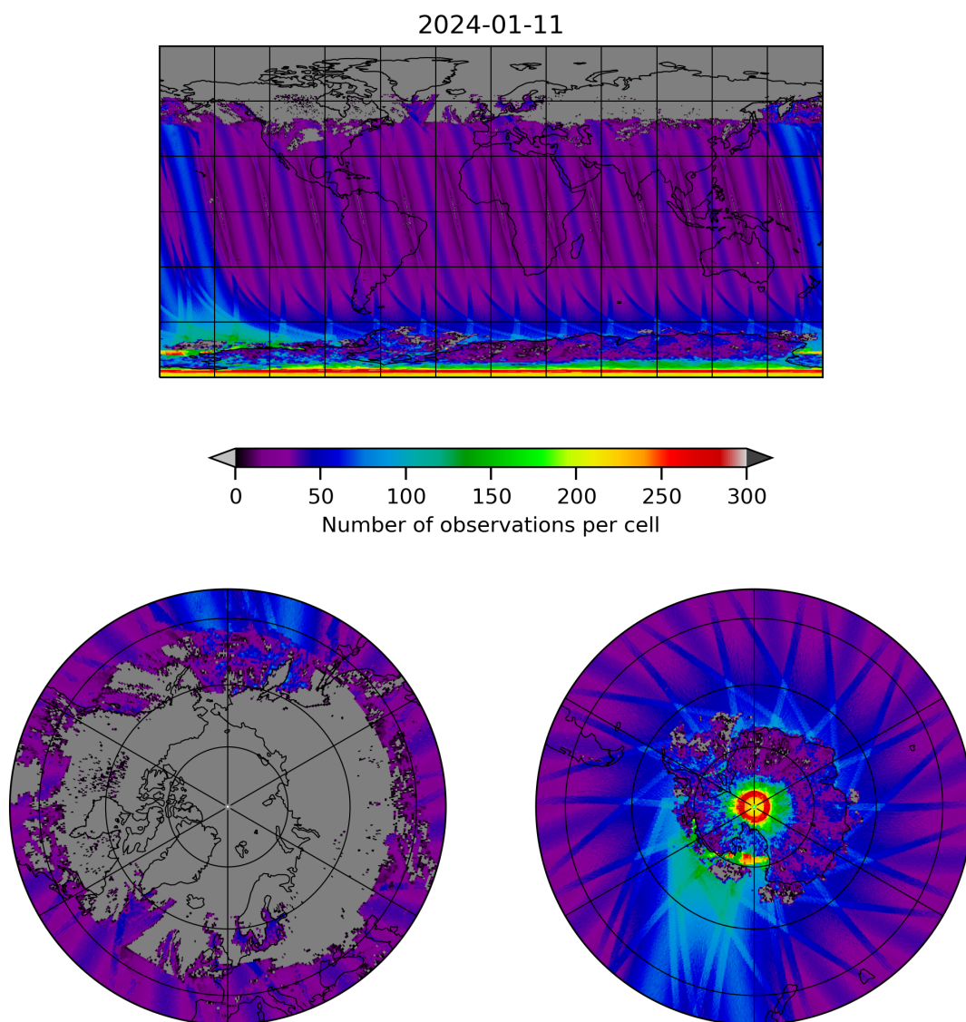
Figure 19: Map of the number of observations for 2024-01-10 to 2024-01-12
