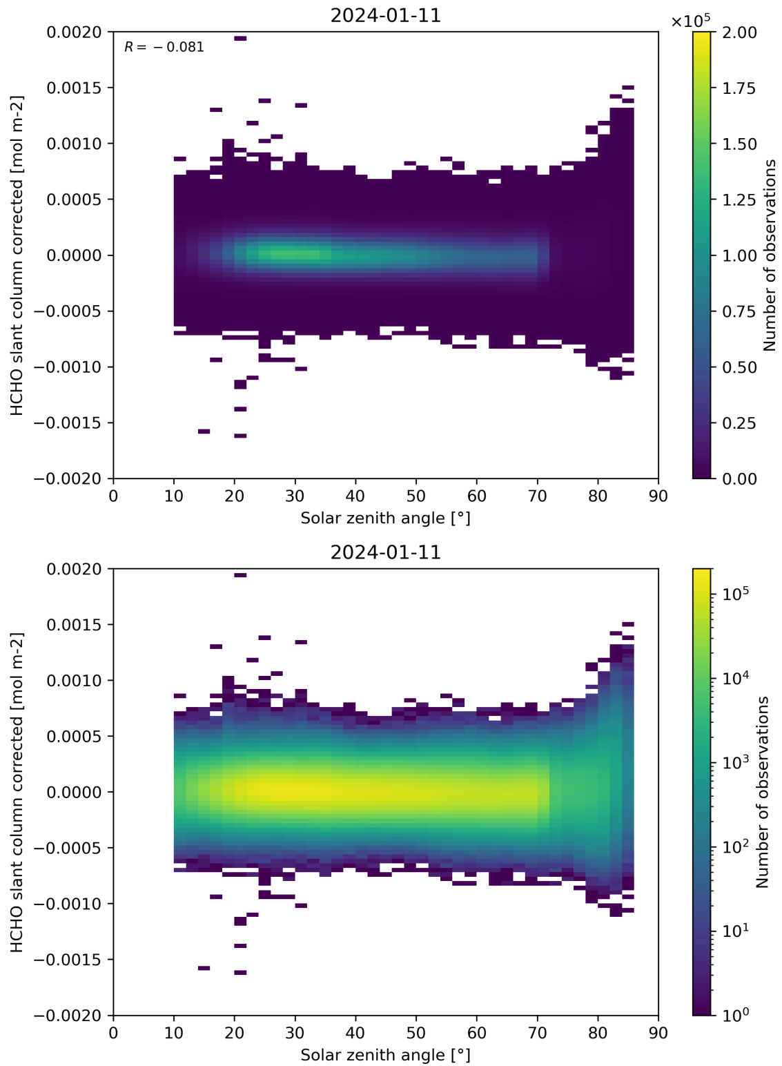
Figure 171: Scatter density plot of “Solar zenith angle” against “HCHO slant column corrected” for 2024-01-10 to 2024-01-12.
