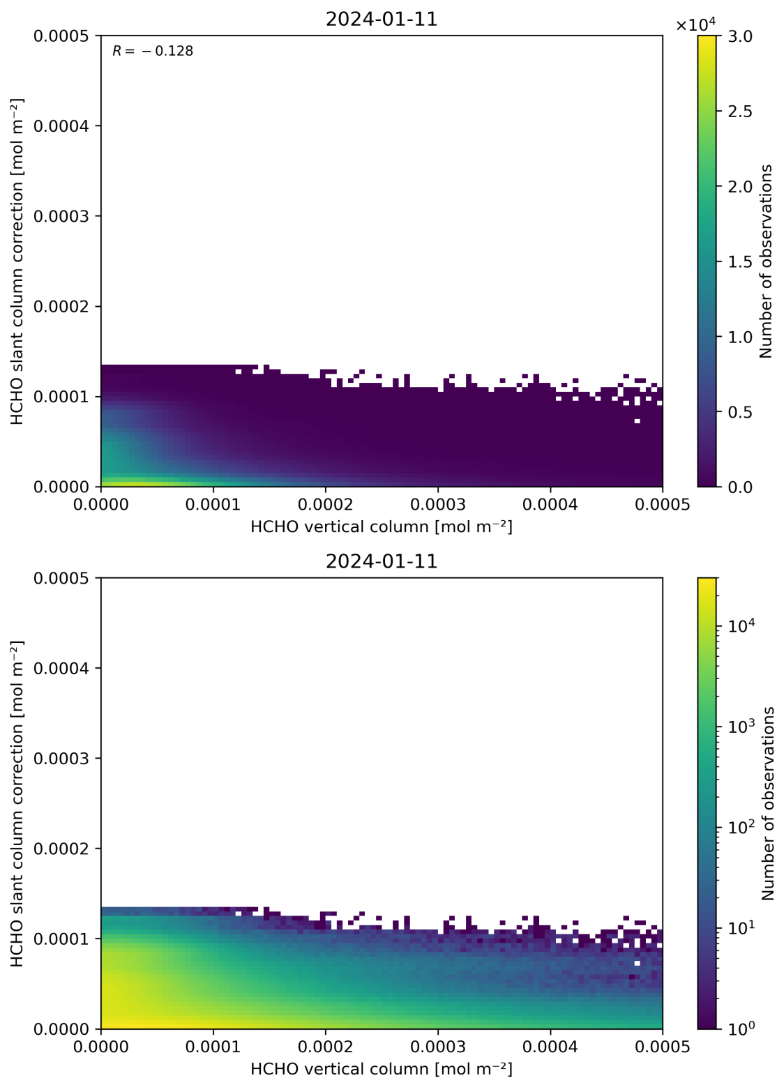
Figure 128: Scatter density plot of “HCHO vertical column” against “HCHO slant column correction” for 2024-01-10 to 2024-01-12.
