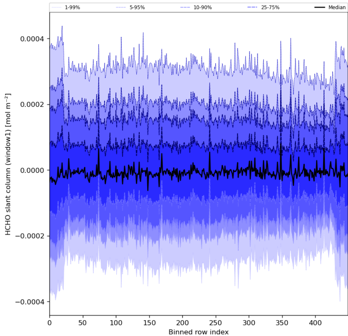
Figure 52: Along track statistics of “HCHO slant column (window1)” for 2024-01-10 to 2024-01-12
