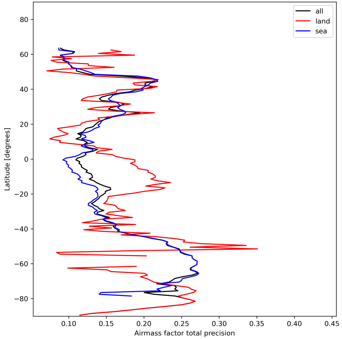
Figure 27: Zonal average of “Airmass factor total precision” for 2024-01-10 to 2024-01-12.
