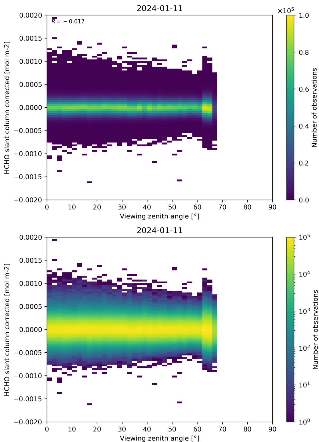
Figure 186: Scatter density plot of “Viewing zenith angle” against “HCHO slant column corrected” for 2024-01-10 to 2024-01-12.
