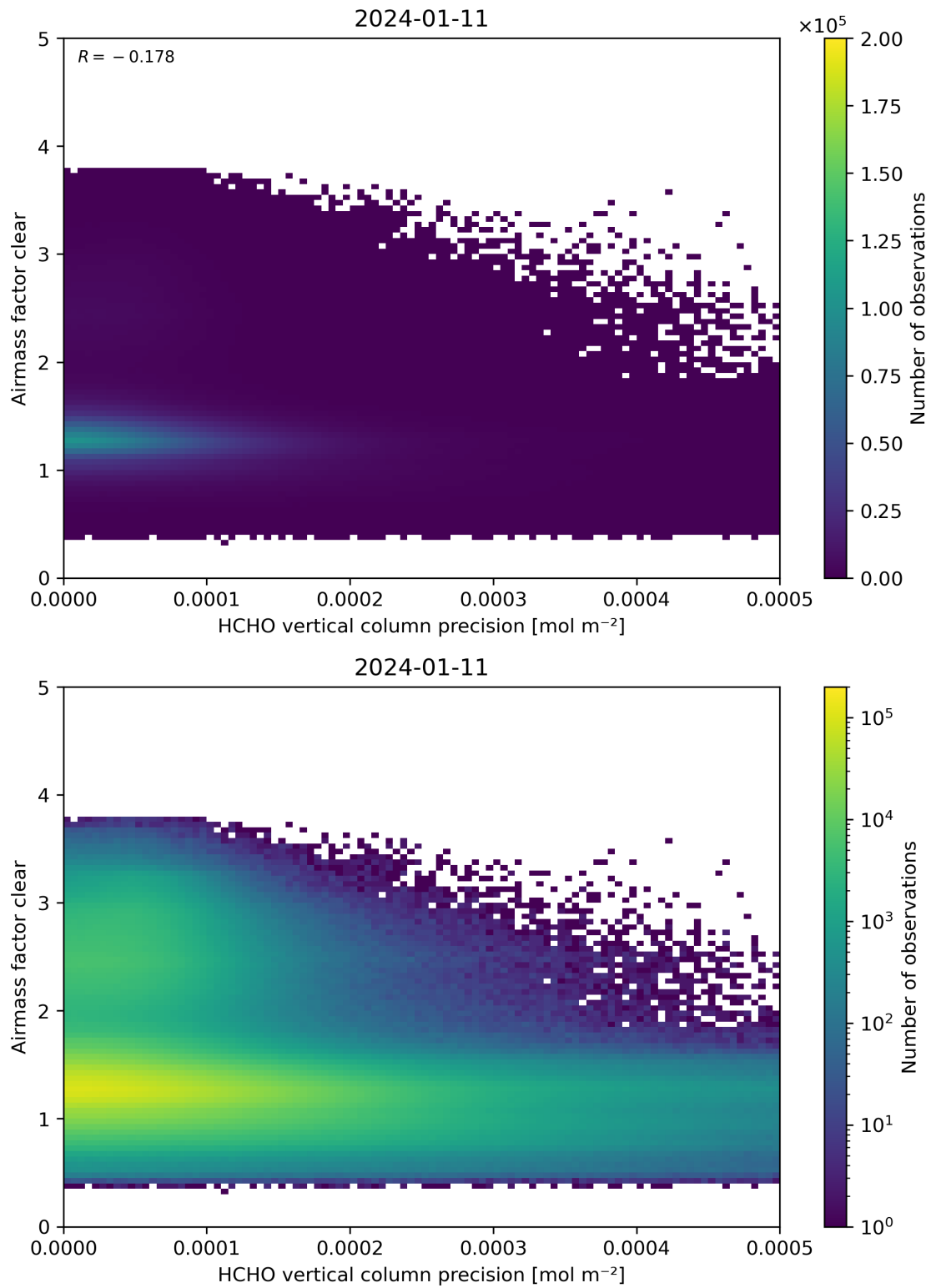
Figure 139: Scatter density plot of “HCHO vertical column precision” against “Airmass factor clear” for 2024-01-10 to 2024-01-12.
