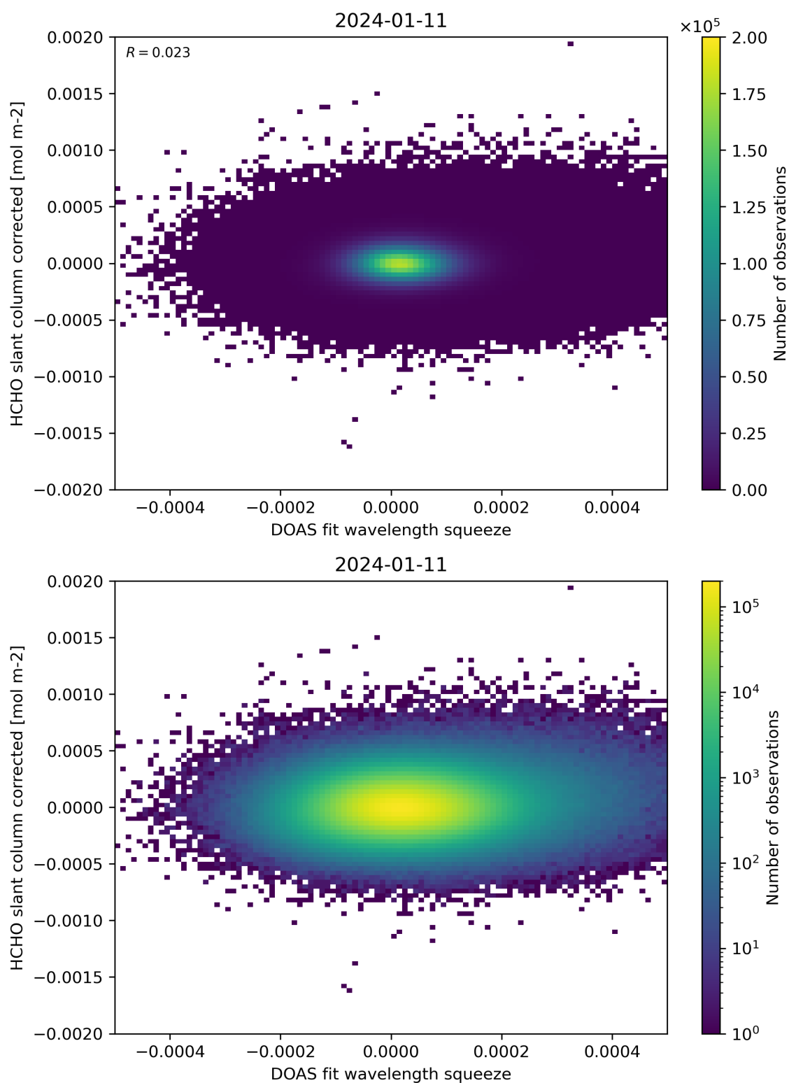
Figure 69: Scatter density plot of “DOAS fit wavelength squeeze” against “HCHO slant column corrected” for 2024-01-10 to 2024-01-12.
