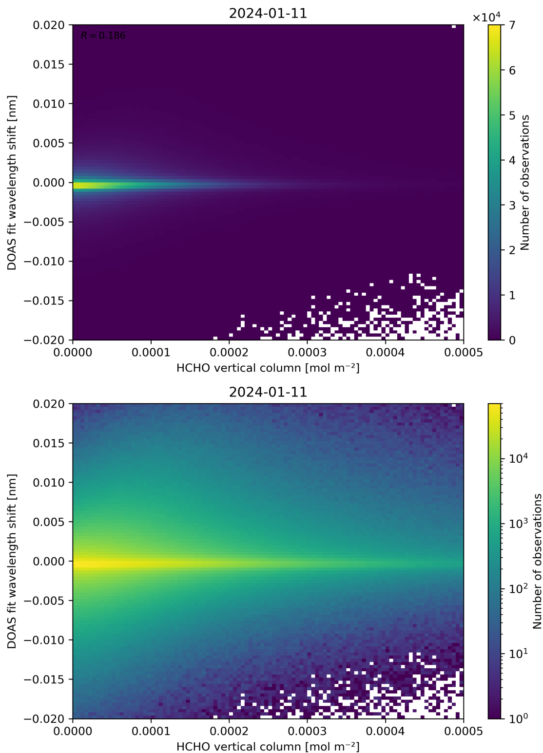
Figure 124: Scatter density plot of “HCHO vertical column” against “DOAS fit wavelength shift” for 2024-01-10 to 2024-01-12.
