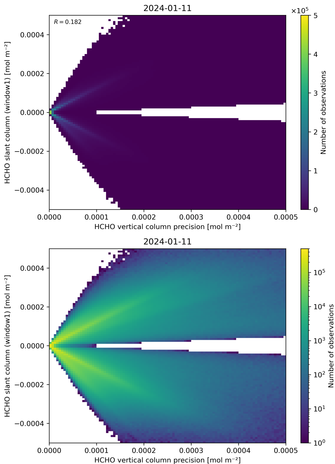
Figure 142: Scatter density plot of “HCHO vertical column precision” against “HCHO slant column (window1)” for 2024-01-10 to 2024-01-12.
