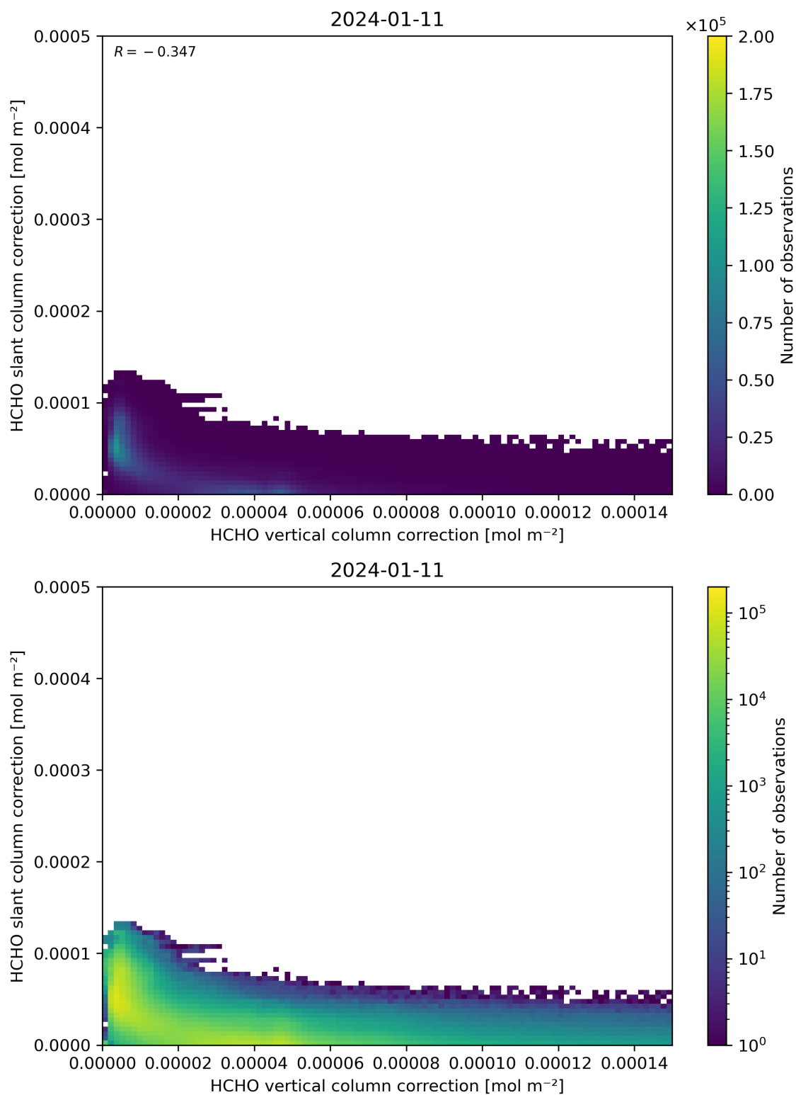
Figure 117: Scatter density plot of “HCHO vertical column correction” against “HCHO slant column correction” for 2024-01-10 to 2024-01-12.
