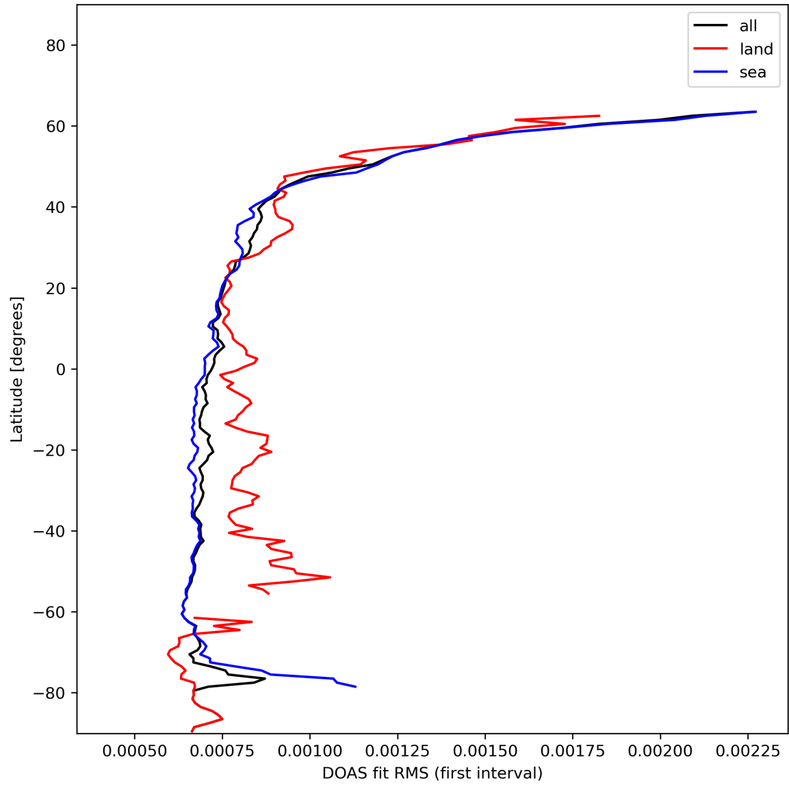
Figure 32: Zonal average of "DOAS fit RMS (first interval)" for 2024-01-10 to 2024-01-12.
