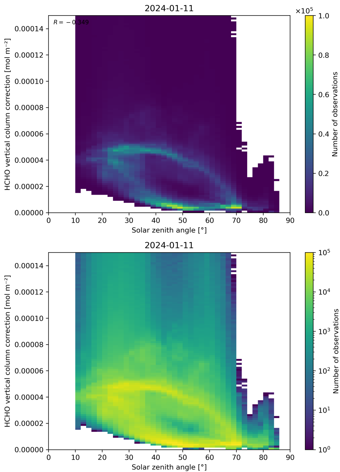
Figure 178: Scatter density plot of “Solar zenith angle” against “HCHO vertical column correction” for 2024-01-10 to 2024-01-12.
