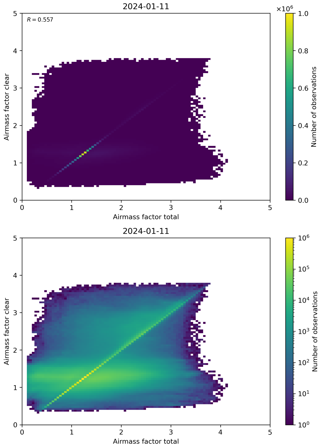
Figure 100: Scatter density plot of “Airmass factor total” against “Airmass factor clear” for 2024-01-10 to 2024-01-12.
