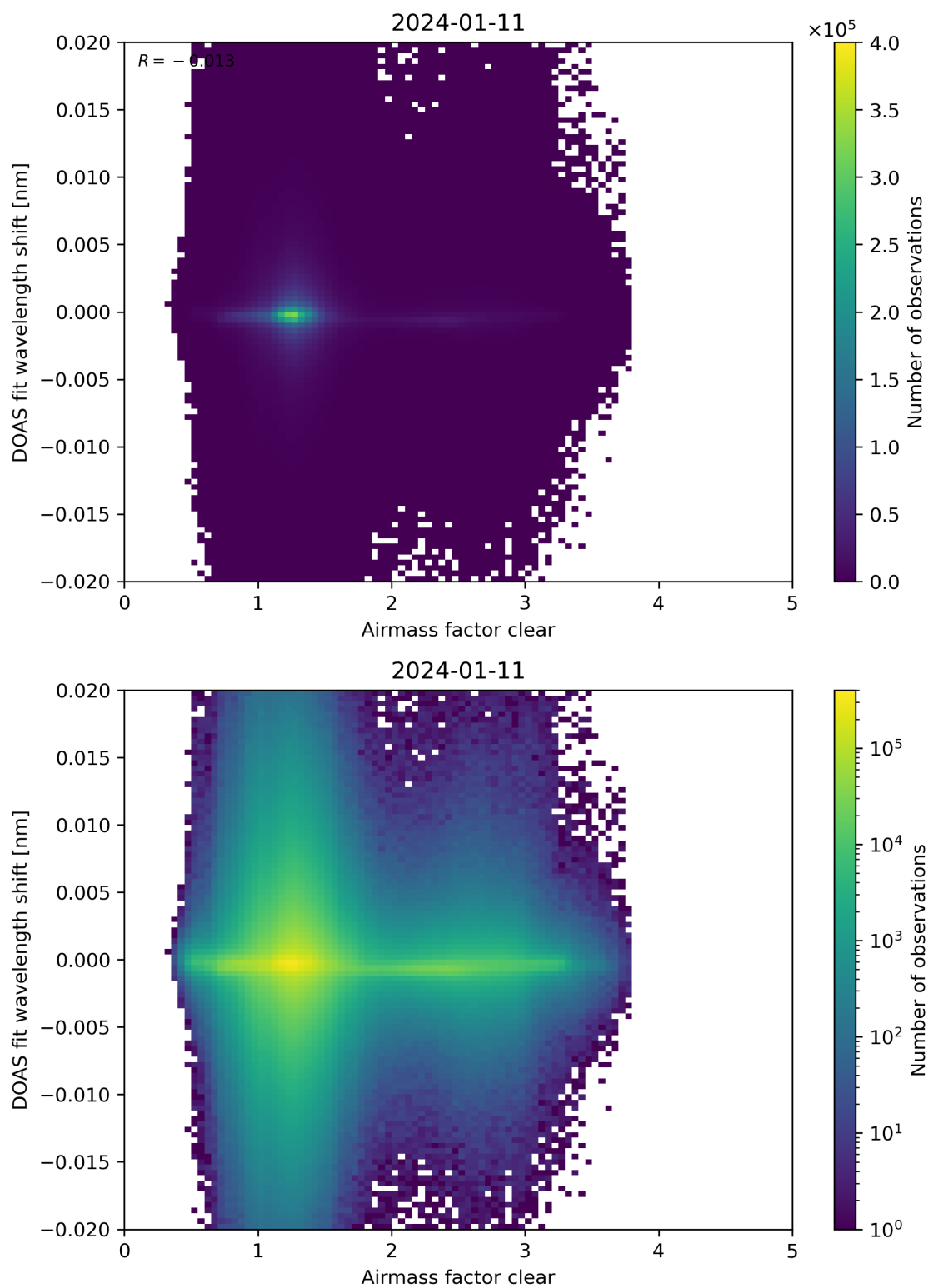
Figure 72: Scatter density plot of “Airmass factor clear” against “DOAS fit wavelength shift” for 2024-01-10 to 2024-01-12.
