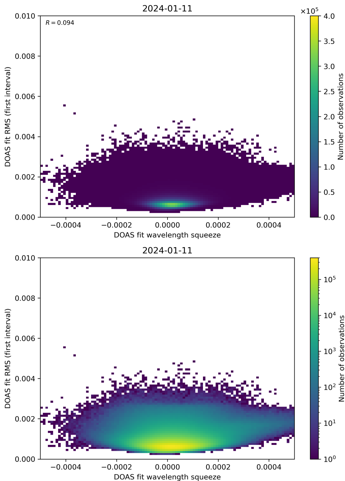
Figure 68: Scatter density plot of “DOAS fit wavelength squeeze” against “DOAS fit RMS (first interval)” for 2024-01-10 to 2024-01-12.
