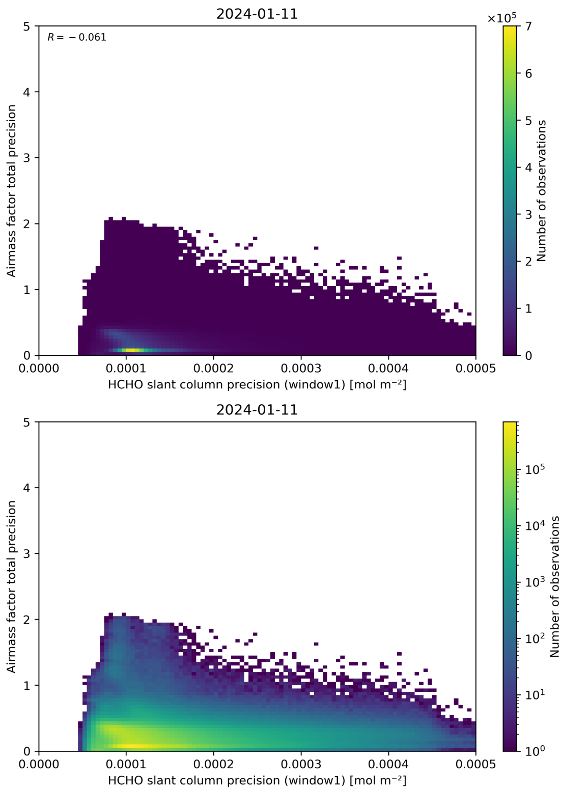
Figure 95: Scatter density plot of “HCHO slant column precision (window1)” against “Airmass factor total precision” for 2024-01-10 to 2024-01-12.
