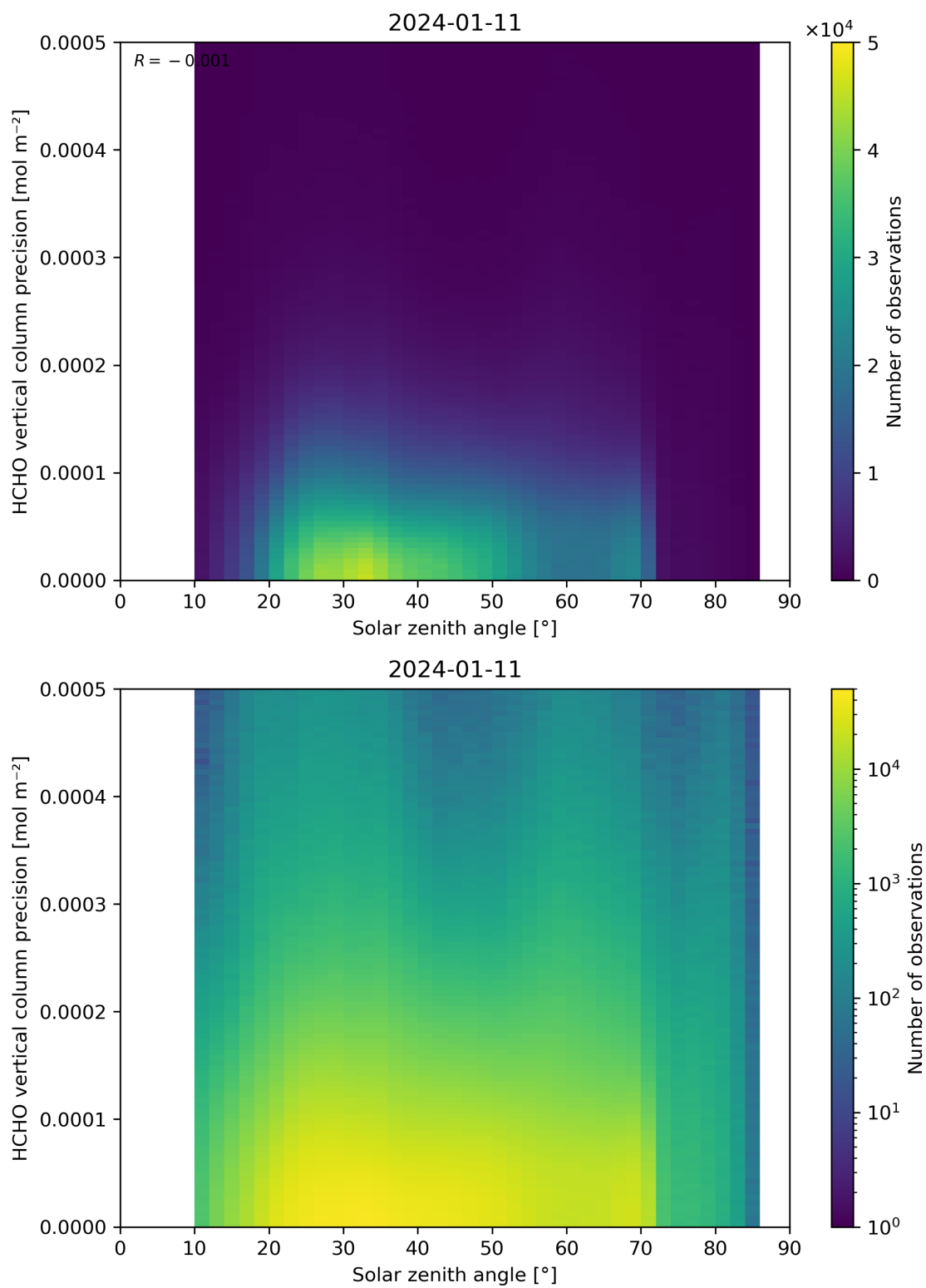
Figure 179: Scatter density plot of “Solar zenith angle” against “HCHO vertical column precision” for 2024-01-10 to 2024-01-12.
