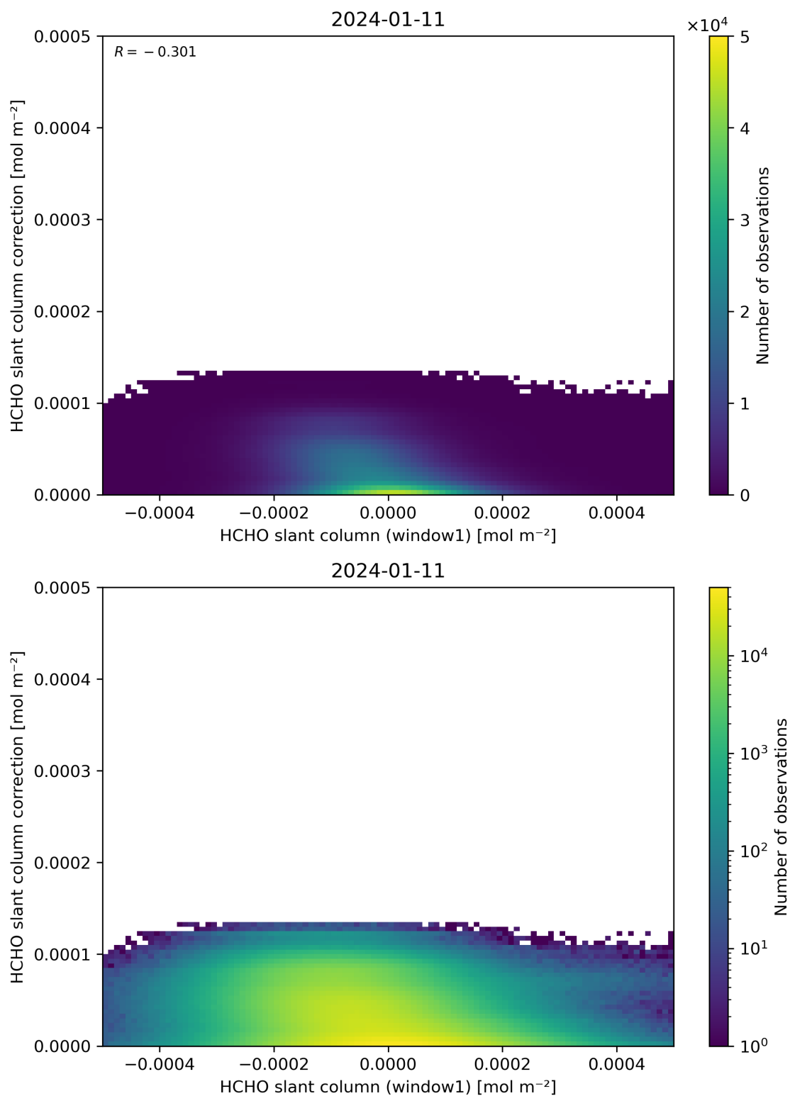
Figure 83: Scatter density plot of “HCHO slant column (window1)” against “HCHO slant column correction” for 2024-01-10 to 2024-01-12.
