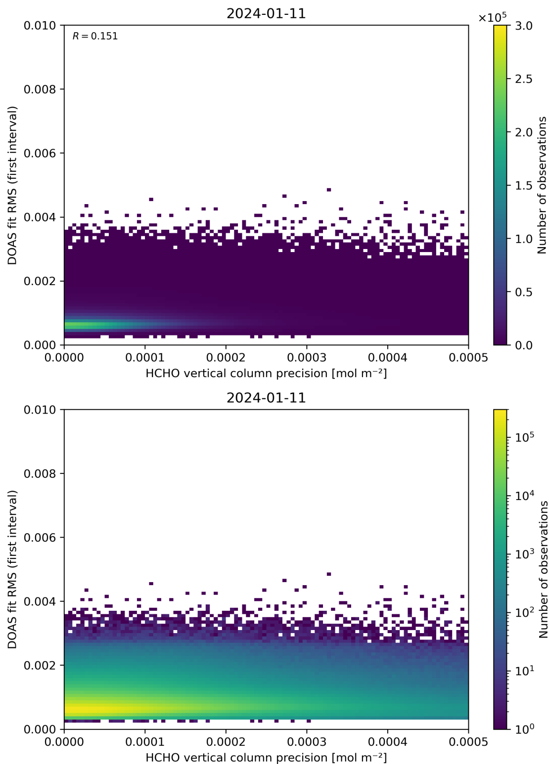
Figure 136: Scatter density plot of “HCHO vertical column precision” against “DOAS fit RMS (first interval)” for 2024-01-10 to 2024-01-12.
