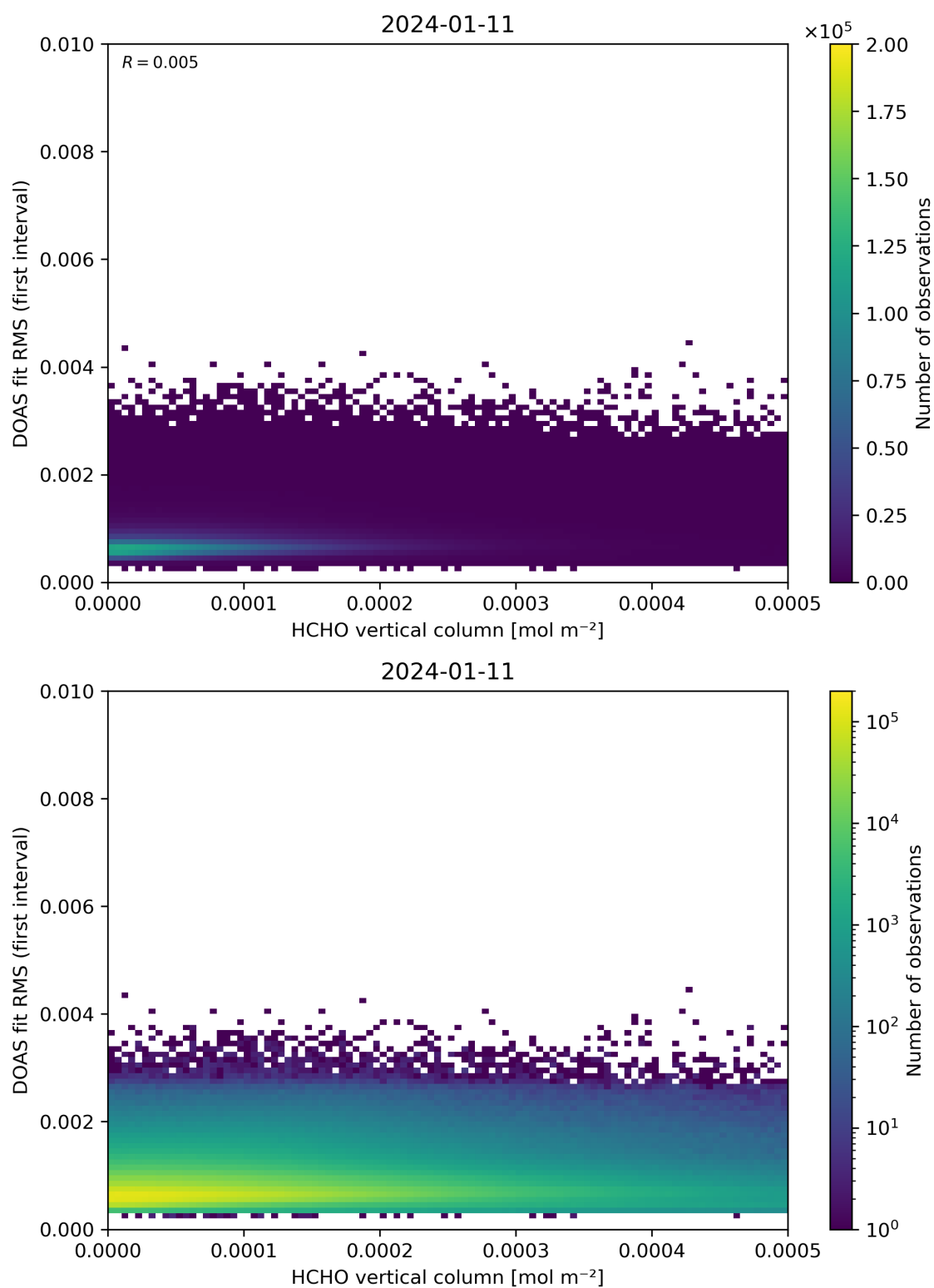
Figure 123: Scatter density plot of “HCHO vertical column” against “DOAS fit RMS (first interval)” for 2024-01-10 to 2024-01-12.
