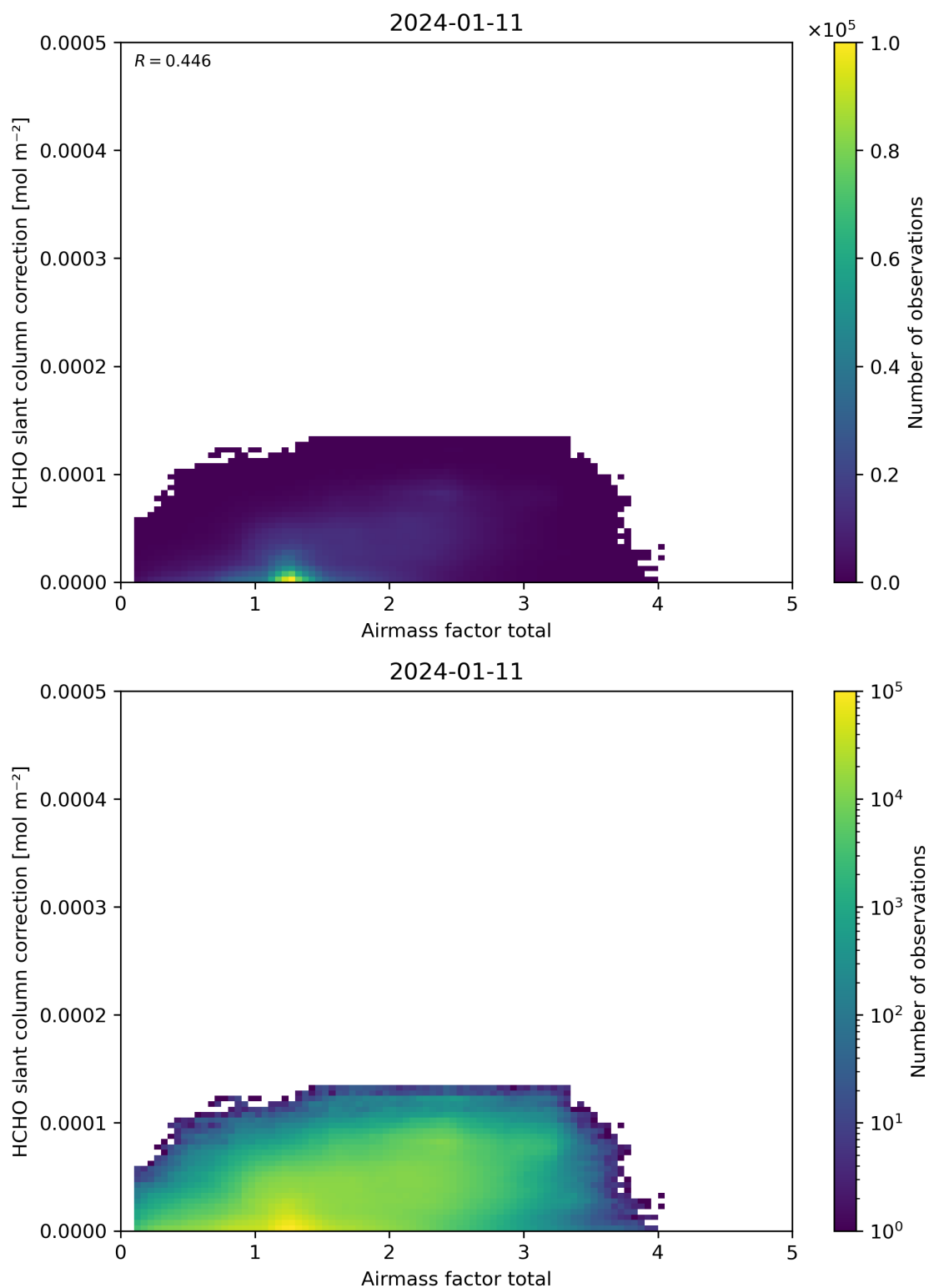
Figure 102: Scatter density plot of “Airmass factor total” against “HCHO slant column correction” for 2024-01-10 to 2024-01-12.
