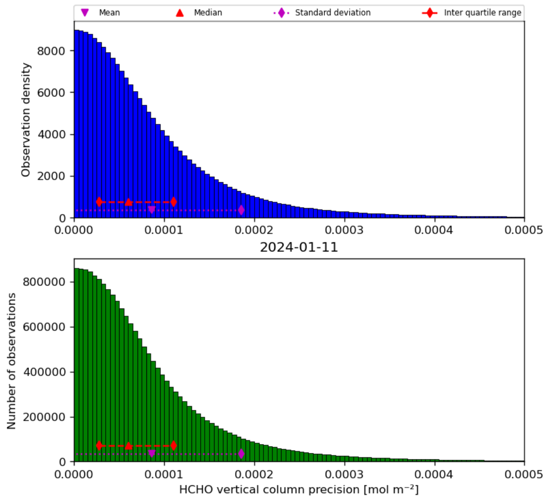
Figure 36: Histogram of “HCHO vertical column precision” for 2024-01-10 to 2024-01-12
