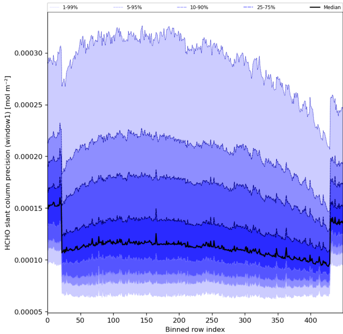
Figure 53: Along track statistics of “HCHO slant column precision (window1)” for 2024-01-10 to 2024-01-12
