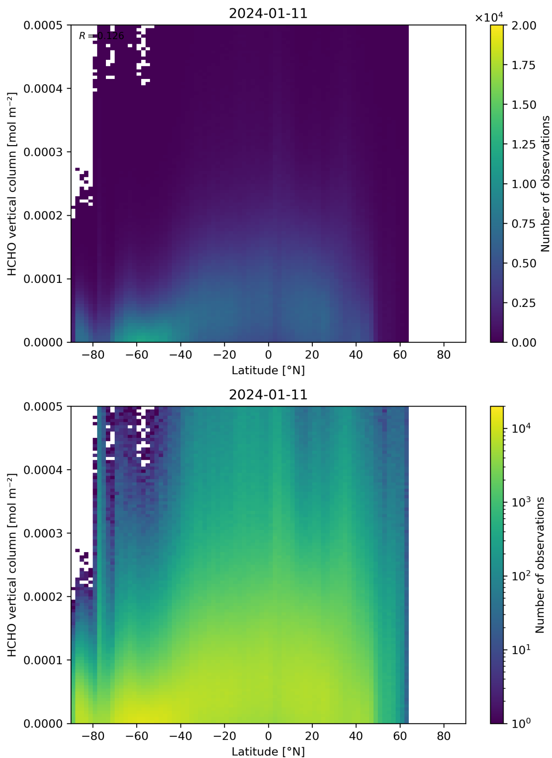
Figure 163: Scatter density plot of “Latitude” against “HCHO vertical column” for 2024-01-10 to 2024-01-12.
