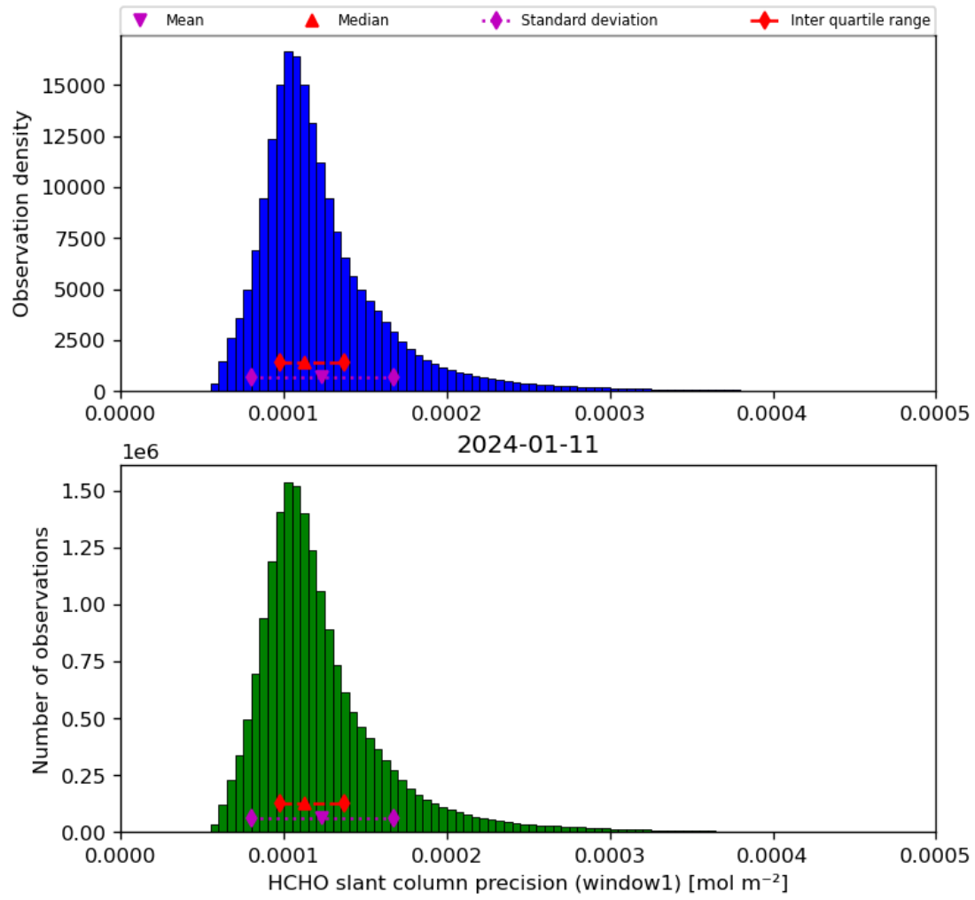
Figure 39: Histogram of “HCHO slant column precision (window1)” for 2024-01-10 to 2024-01-12
