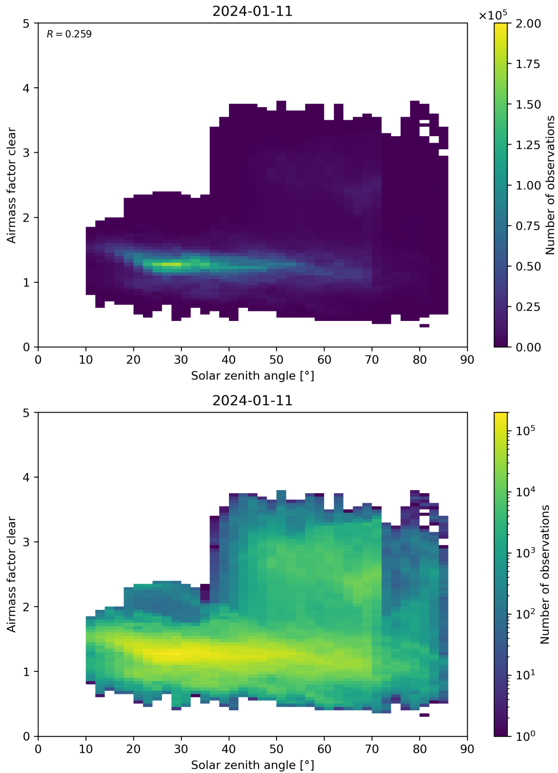
Figure 170: Scatter density plot of “Solar zenith angle” against “Airmass factor clear” for 2024-01-10 to 2024-01-12.
