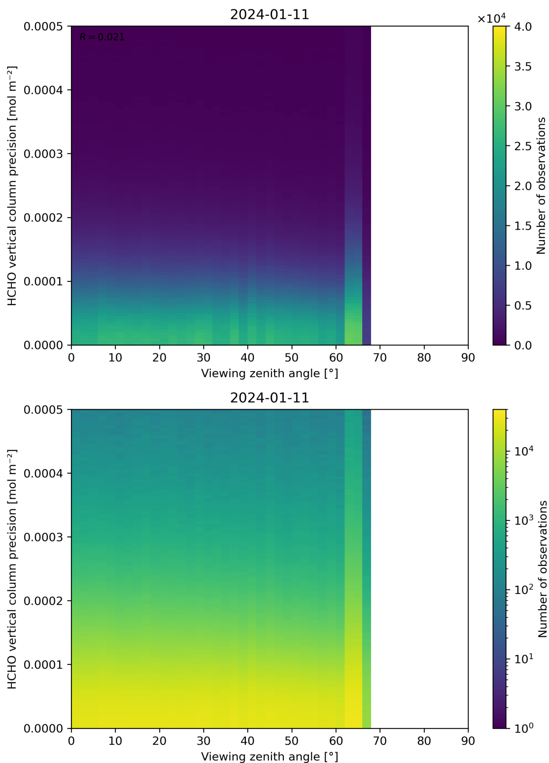
Figure 194: Scatter density plot of “Viewing zenith angle” against “HCHO vertical column precision” for 2024-01-10 to 2024-01-12.
