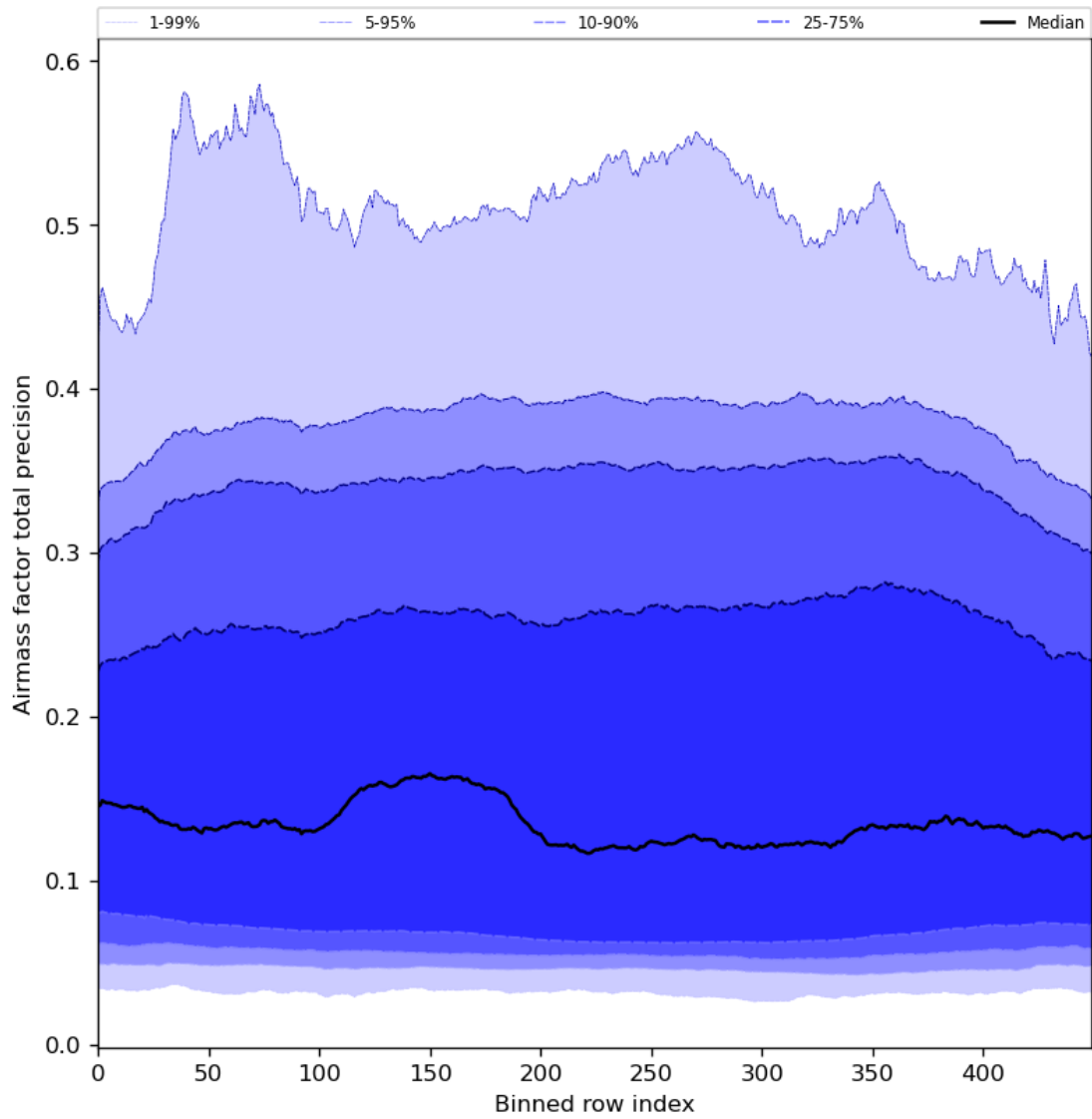
Figure 55: Along track statistics of “Airmass factor total precision” for 2024-01-10 to 2024-01-12
