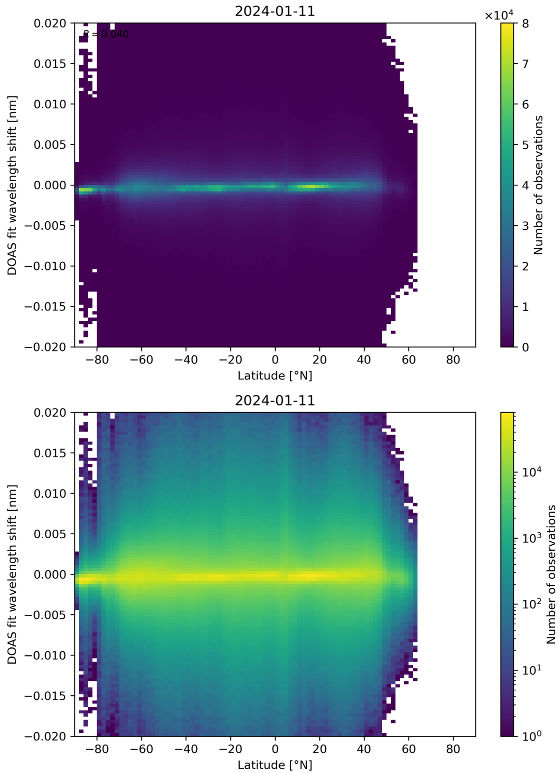
Figure 154: Scatter density plot of “Latitude” against “DOAS fit wavelength shift” for 2024-01-10 to 2024-01-12.
