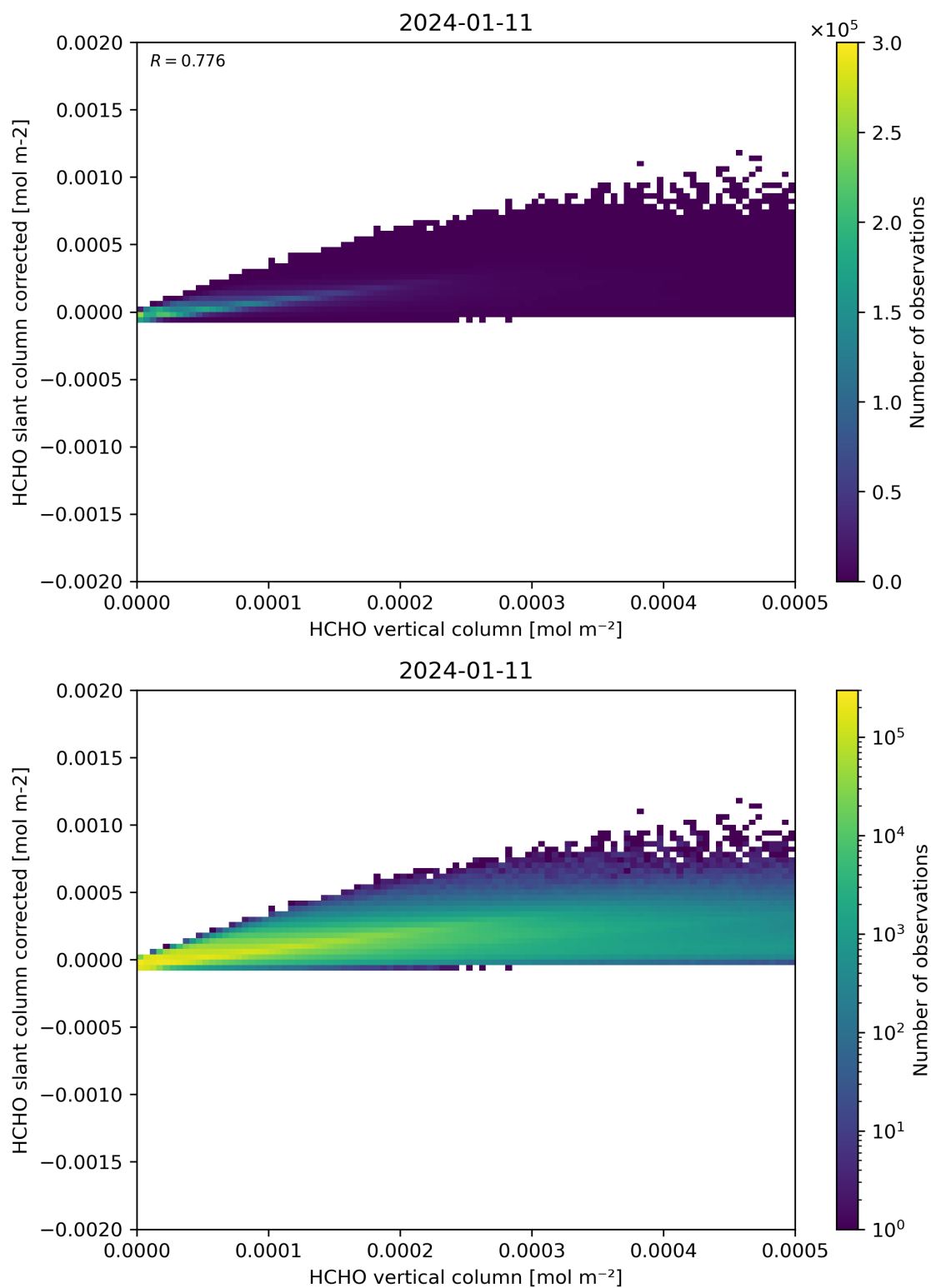
Figure 127: Scatter density plot of “HCHO vertical column” against “HCHO slant column corrected” for 2024-01-10 to 2024-01-12.
