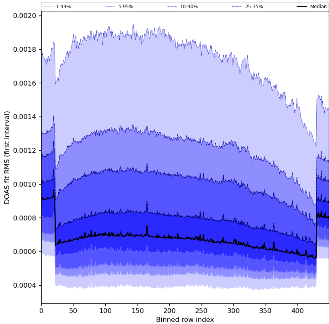
Figure 60: Along track statistics of “DOAS fit RMS (first interval)” for 2024-01-10 to 2024-01-12
