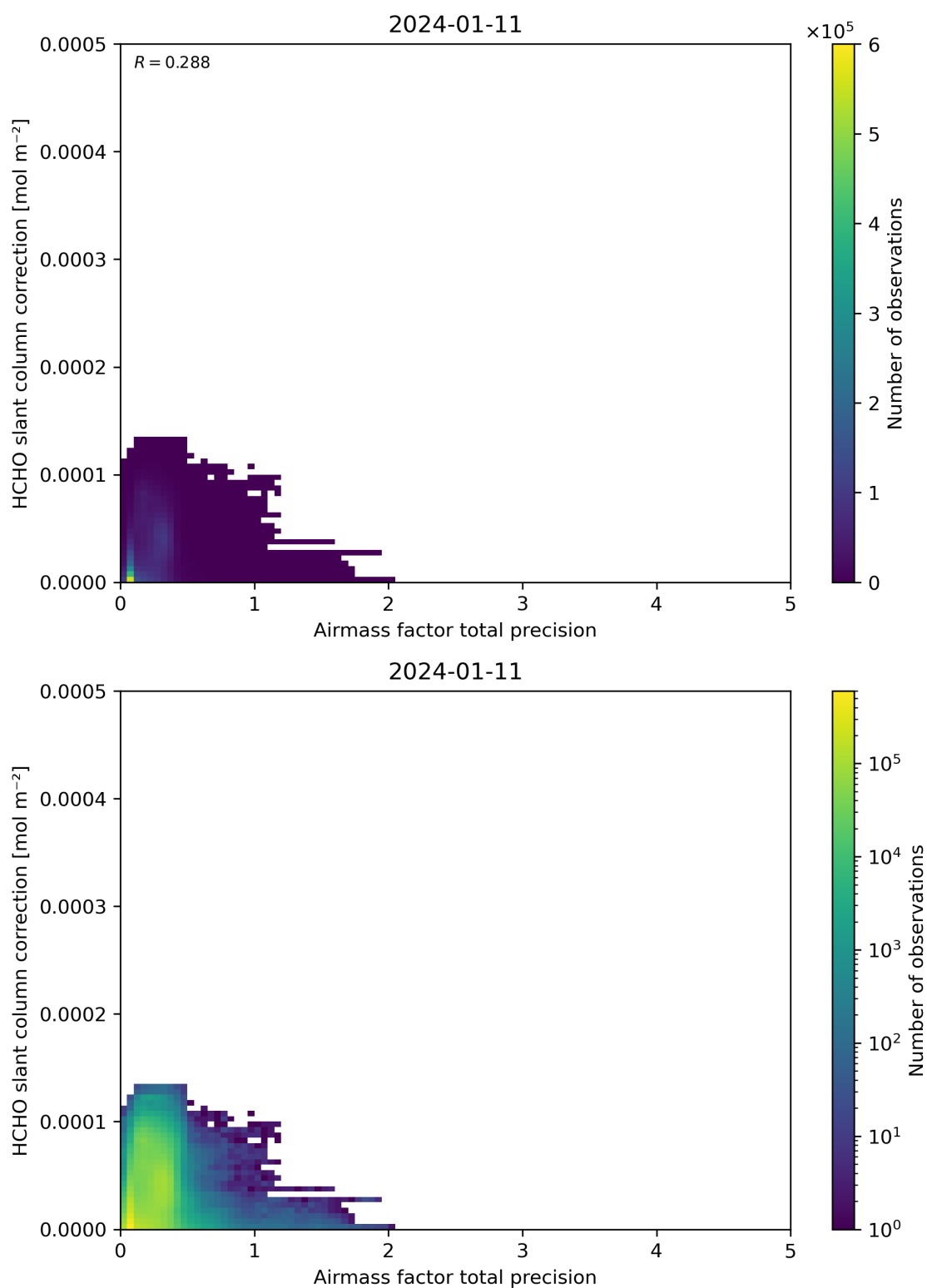
Figure 110: Scatter density plot of “Airmass factor total precision” against “HCHO slant column correction” for 2024-01-10 to 2024-01-12.
