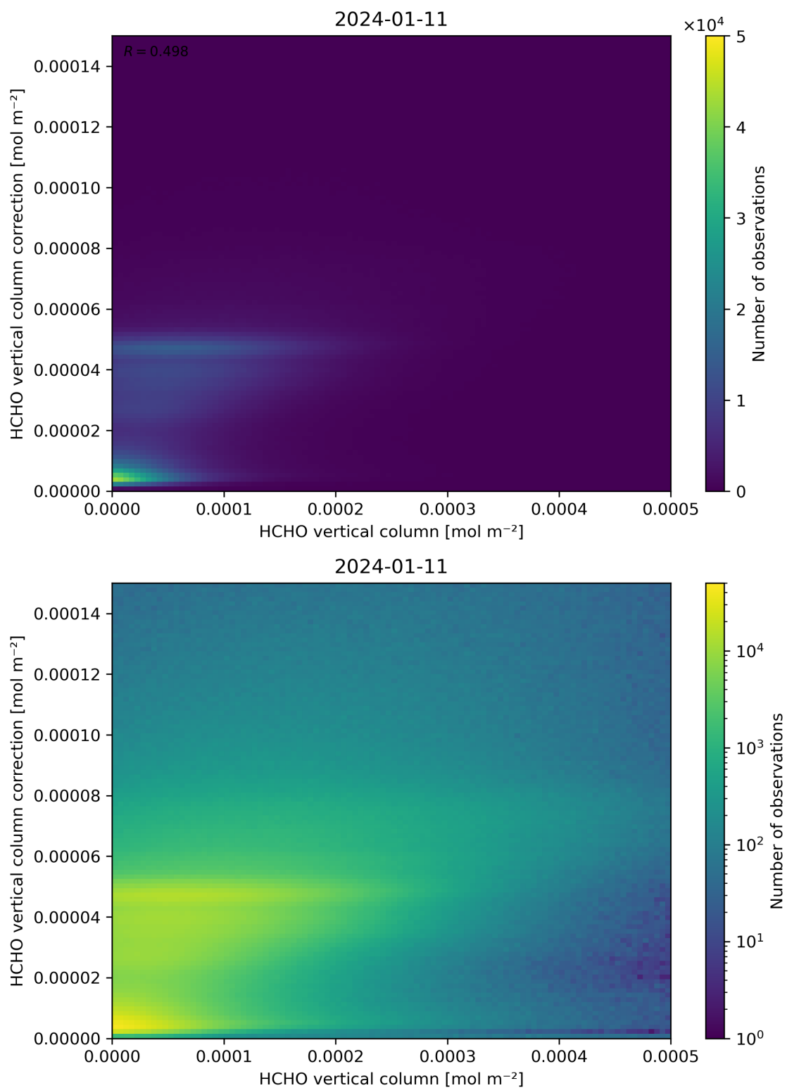
Figure 133: Scatter density plot of “HCHO vertical column” against “HCHO vertical column correction” for 2024-01-10 to 2024-01-12.
