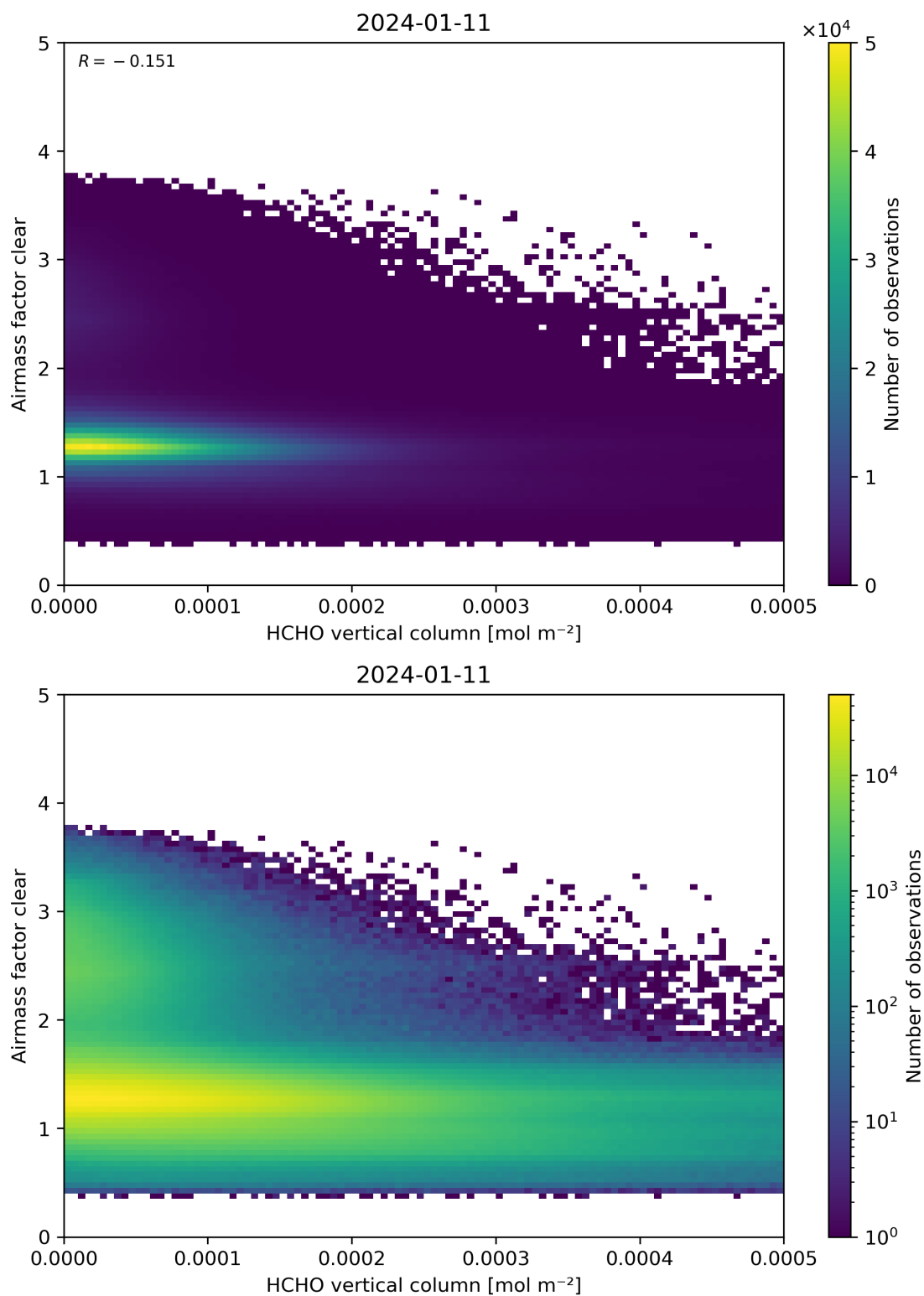
Figure 126: Scatter density plot of “HCHO vertical column” against “Airmass factor clear” for 2024-01-10 to 2024-01-12.
