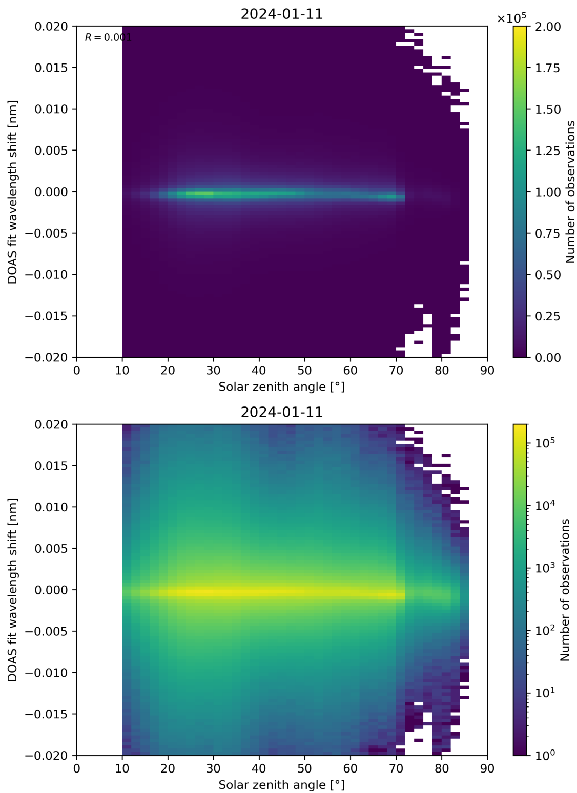
Figure 168: Scatter density plot of “Solar zenith angle” against “DOAS fit wavelength shift” for 2024-01-10 to 2024-01-12.
