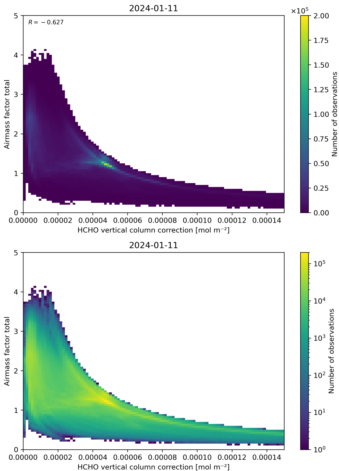
Figure 120: Scatter density plot of “HCHO vertical column correction” against “Airmass factor total” for 2024-01-10 to 2024-01-12.
