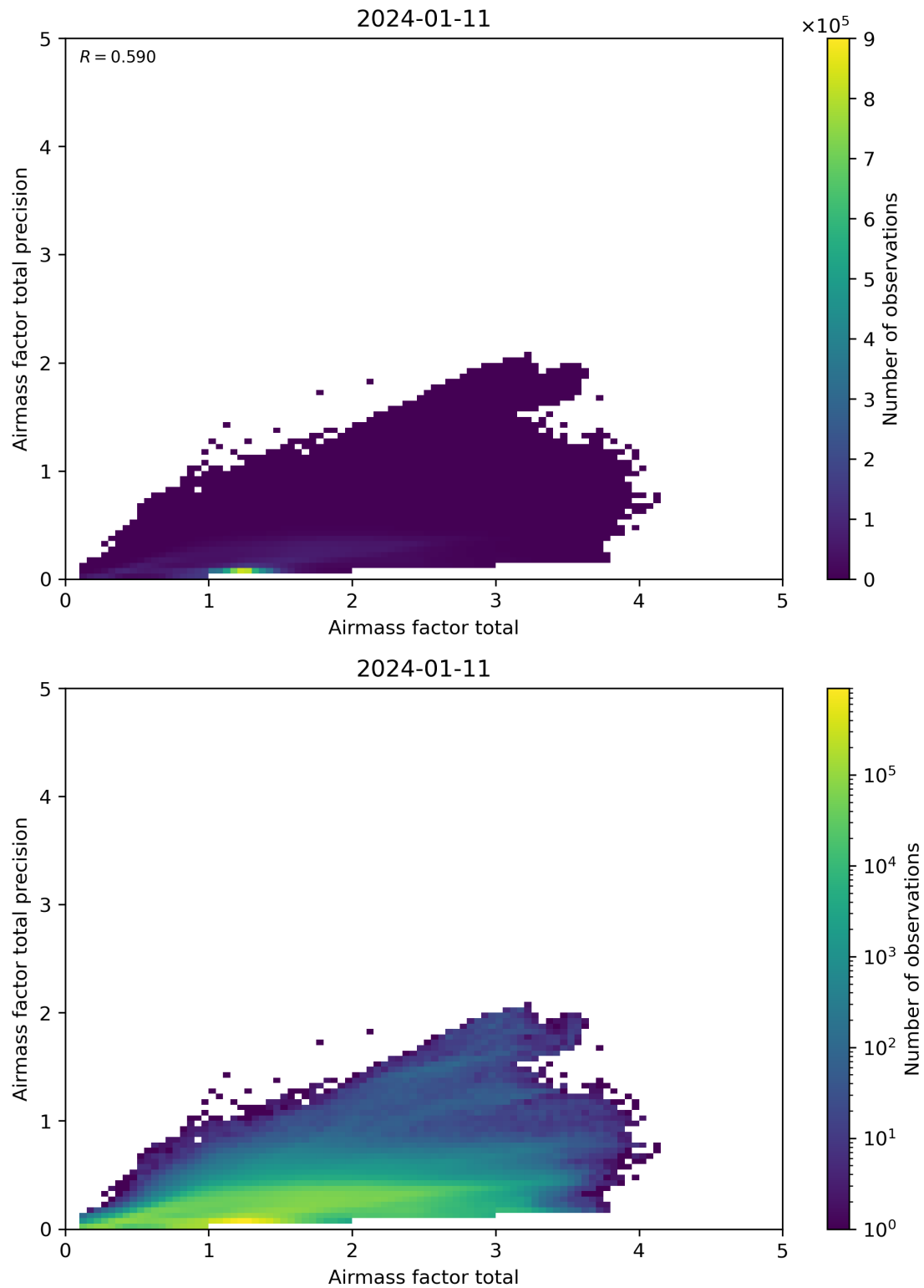
Figure 103: Scatter density plot of “Airmass factor total” against “Airmass factor total precision” for 2024-01-10 to 2024-01-12.
