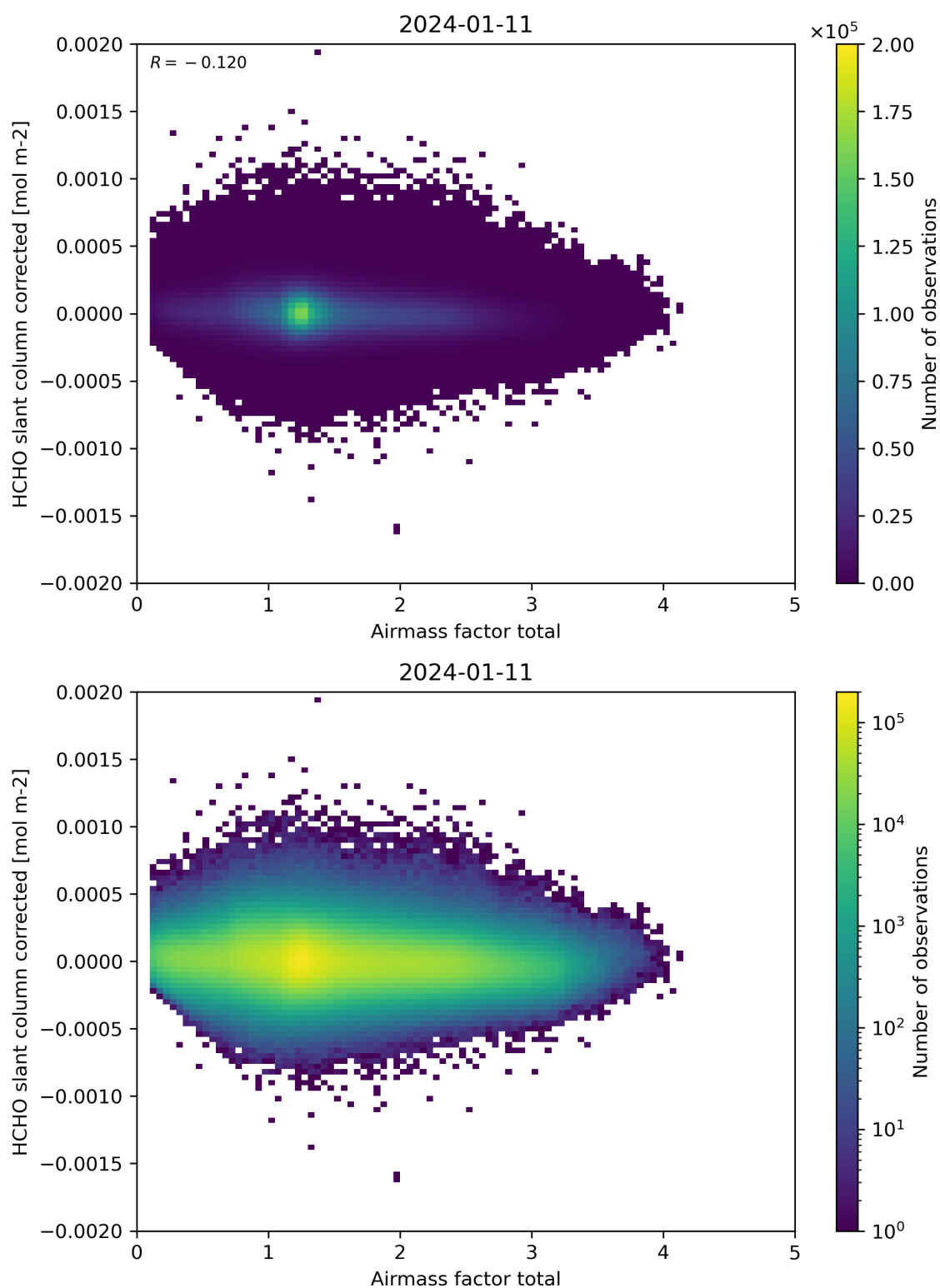
Figure 101: Scatter density plot of “Airmass factor total” against “HCHO slant column corrected” for 2024-01-10 to 2024-01-12.
