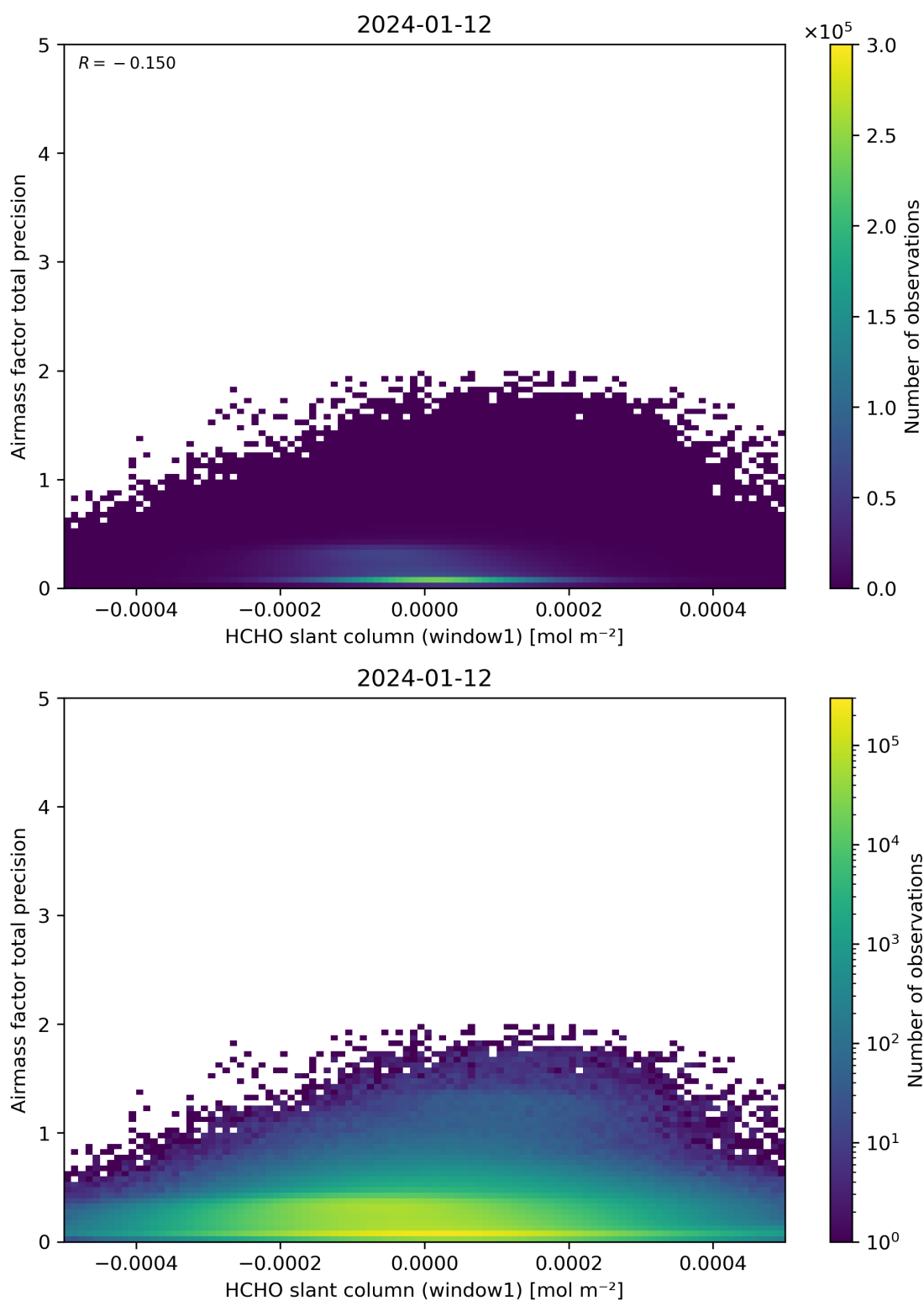
Figure 86: Scatter density plot of “HCHO slant column (window1)” against “Airmass factor total precision” for 2024-01-11 to 2024-01-13.
