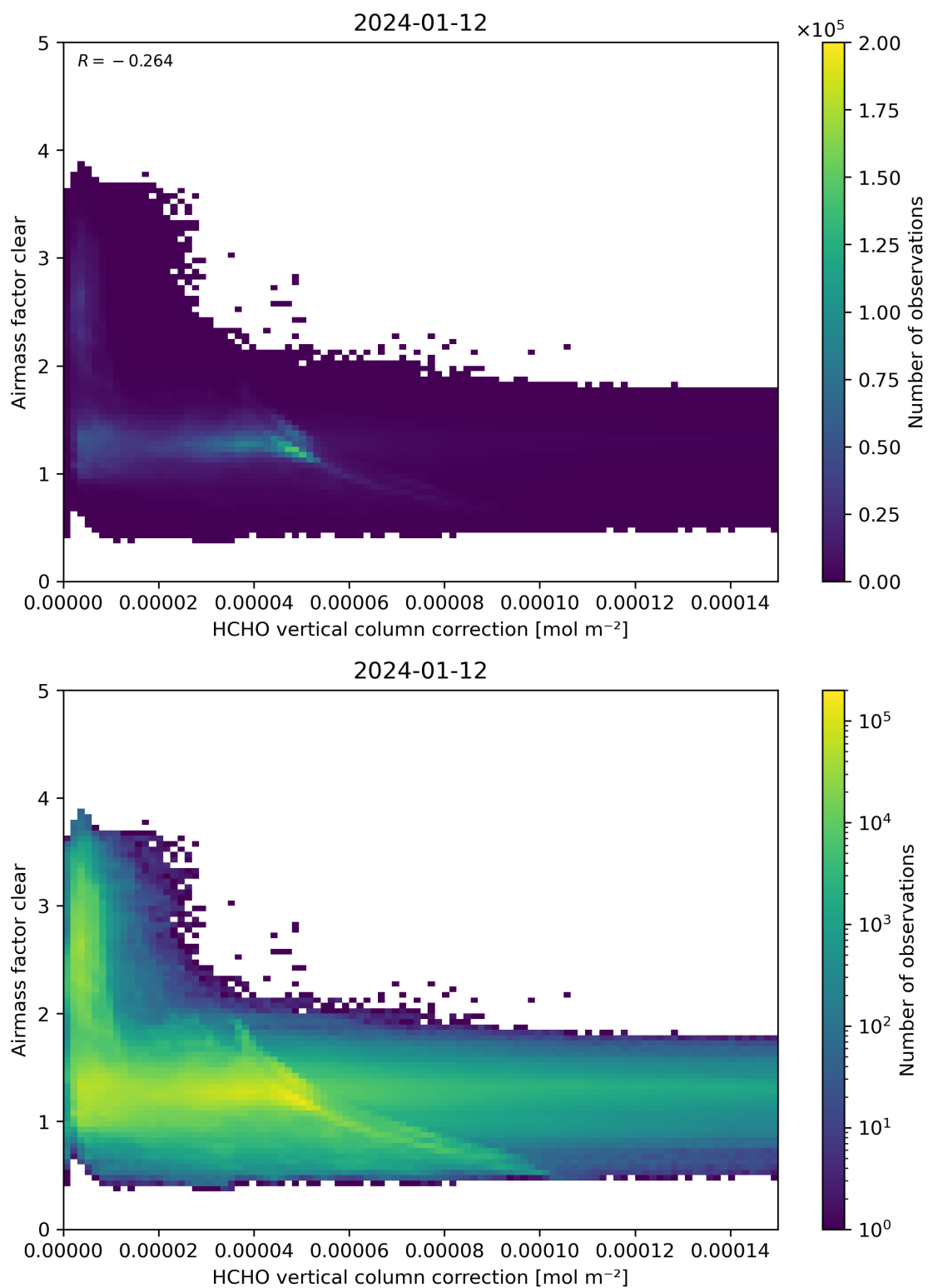
Figure 115: Scatter density plot of “HCHO vertical column correction” against “Airmass factor clear” for 2024-01-11 to 2024-01-13.
