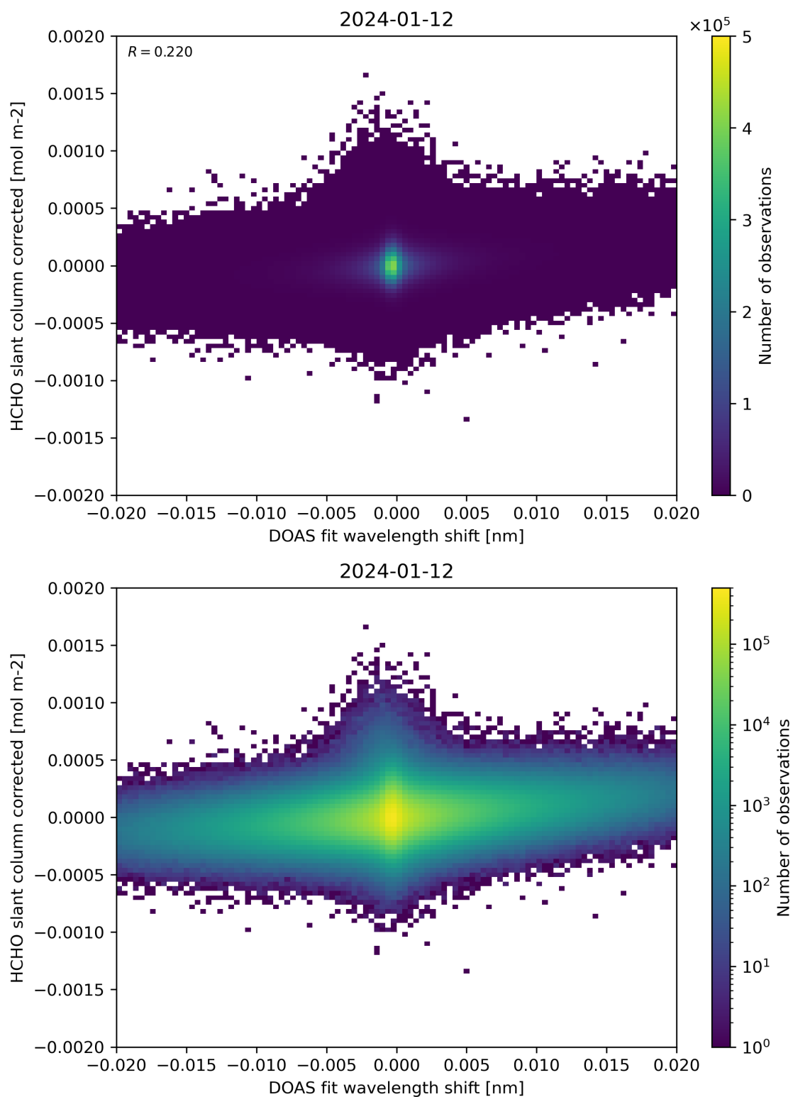
Figure 66: Scatter density plot of “DOAS fit wavelength shift” against “HCHO slant column corrected” for 2024-01-11 to 2024-01-13.
