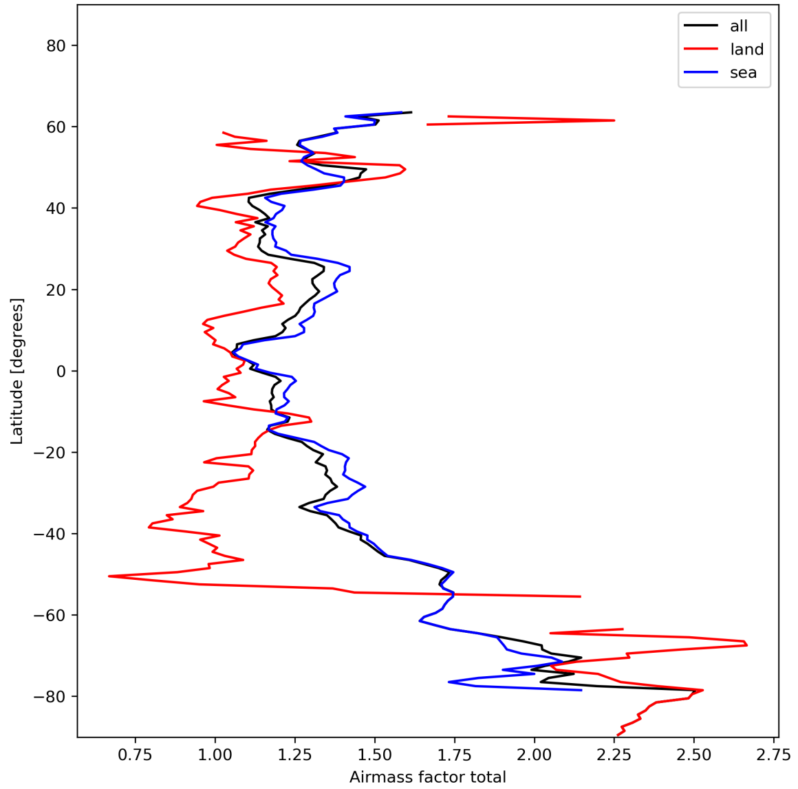
Figure 26: Zonal average of “Airmass factor total” for 2024-01-11 to 2024-01-13.
