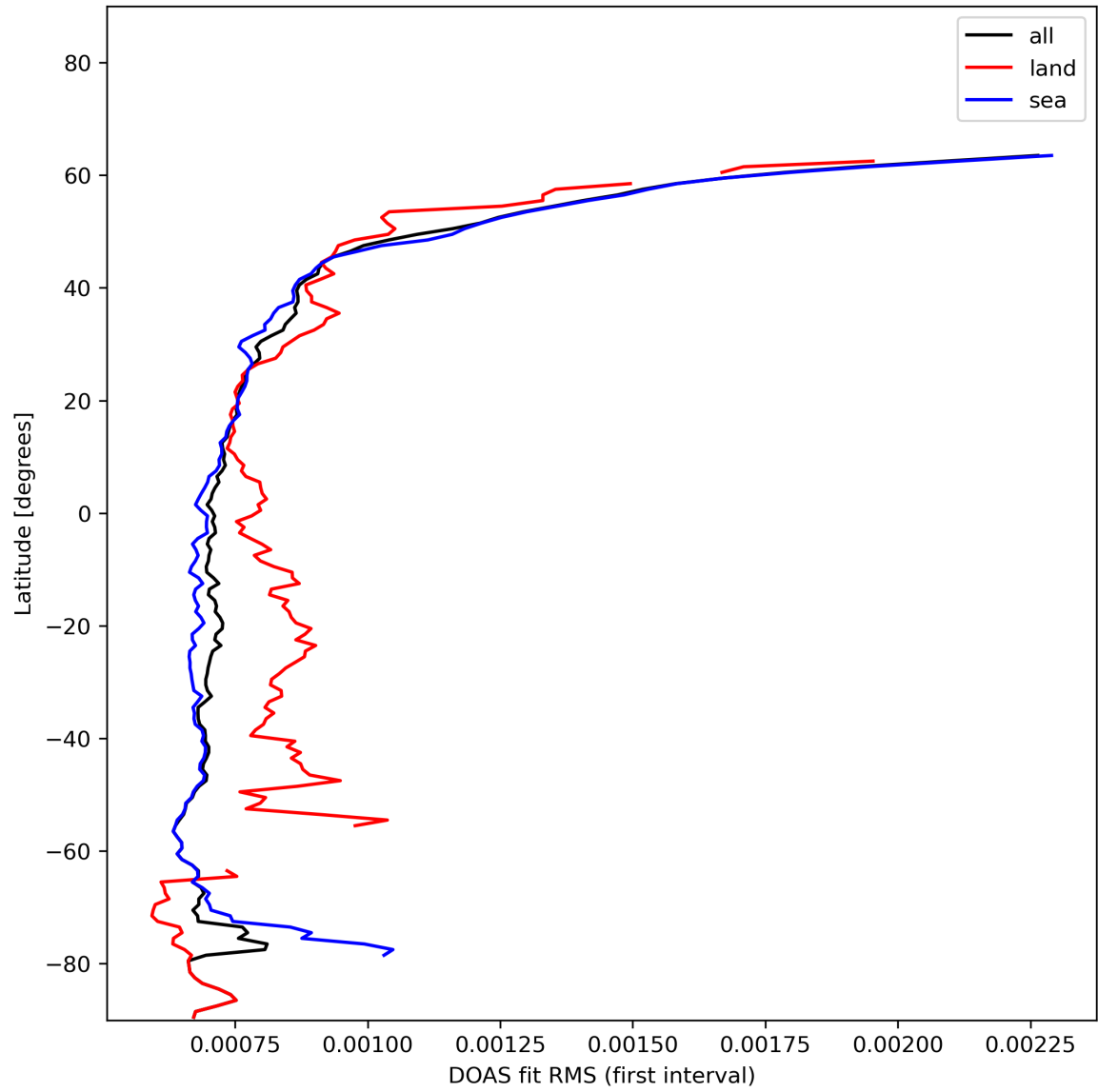
Figure 32: Zonal average of “DOAS fit RMS (first interval)” for 2024-01-11 to 2024-01-13.
