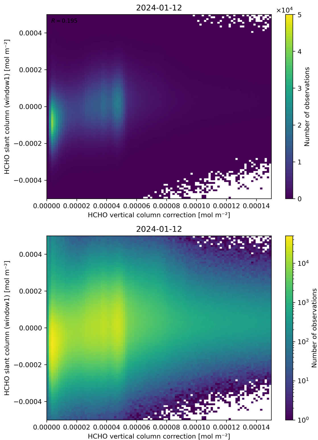
Figure 118: Scatter density plot of “HCHO vertical column correction” against “HCHO slant column (window1)” for 2024-01-11 to 2024-01-13.
