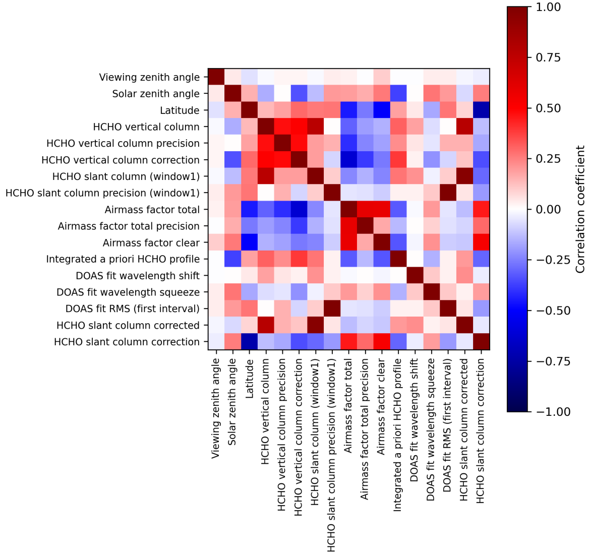
Figure 2: Map of correlation matrix for 2024-01-11 to 2024-01-13.
