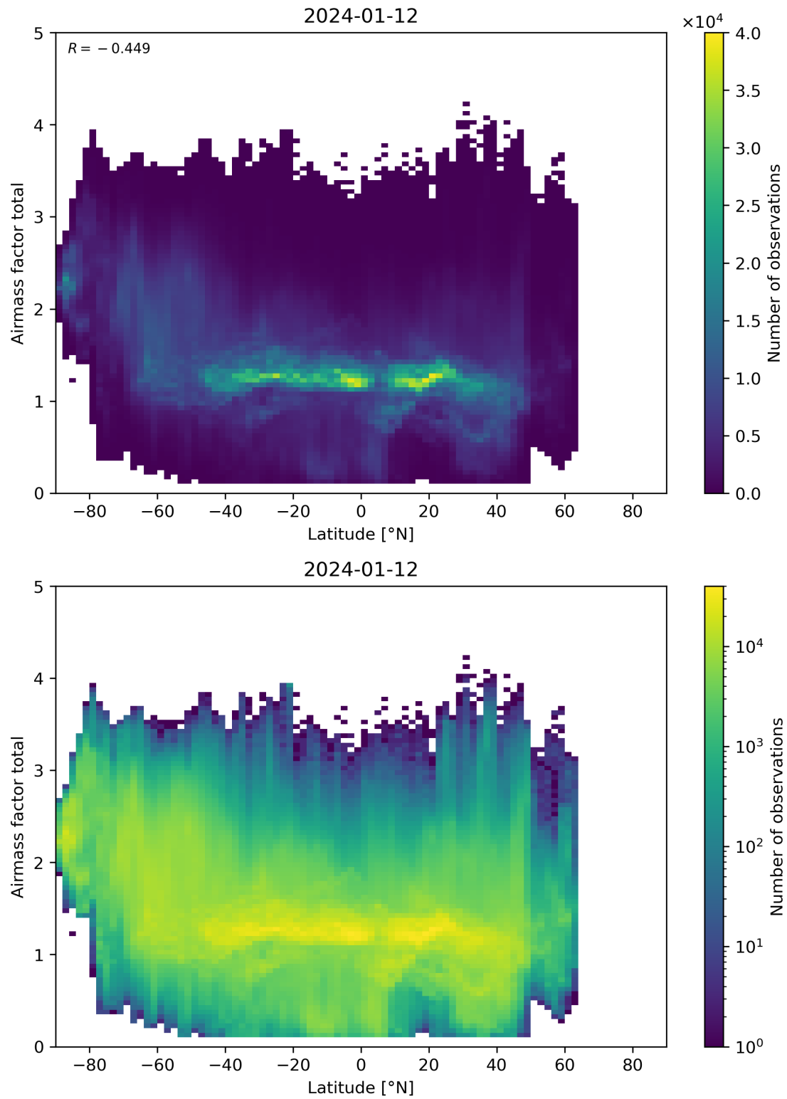
Figure 161: Scatter density plot of “Latitude” against “Airmass factor total” for 2024-01-11 to 2024-01-13.
