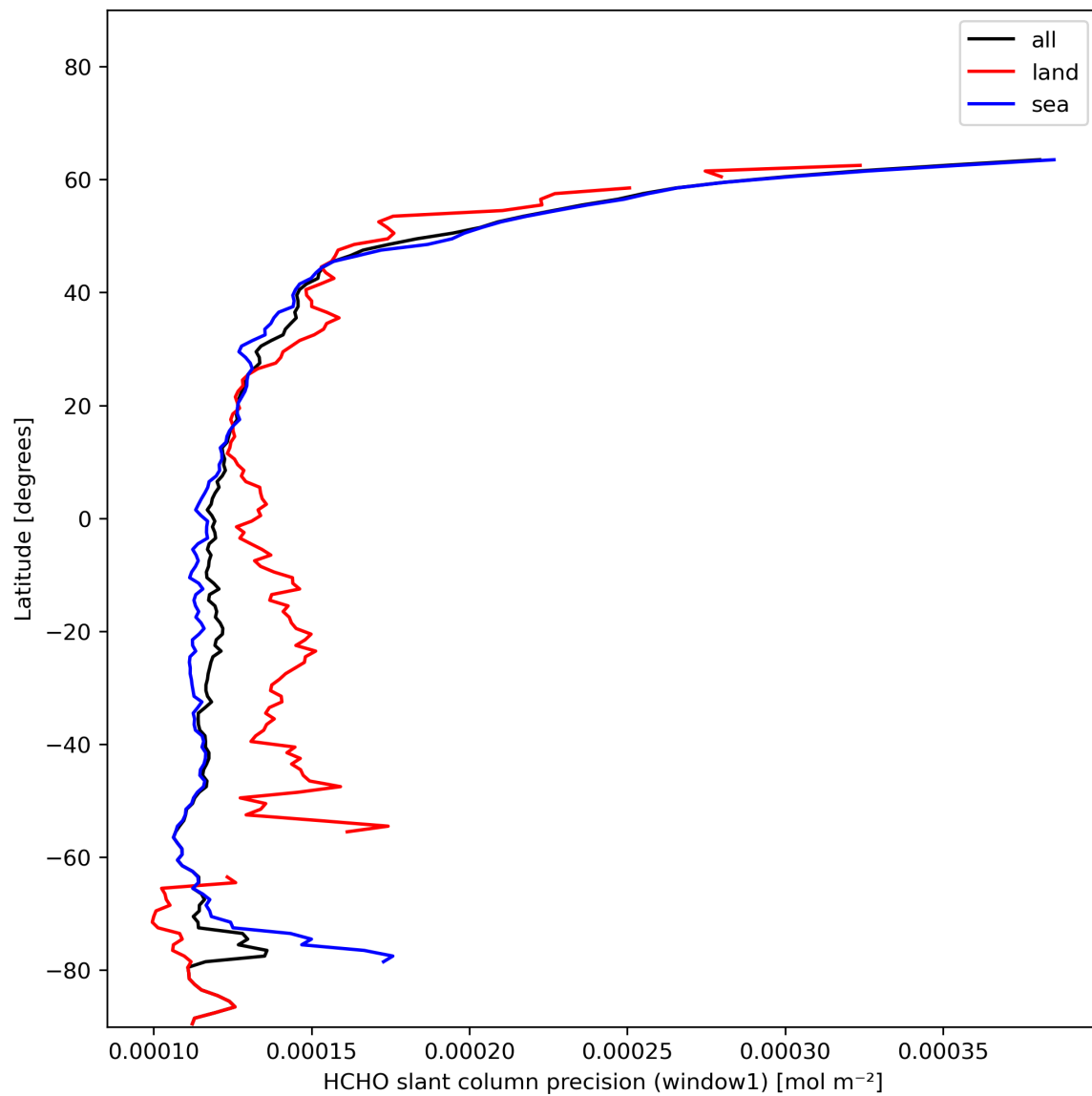
Figure 25: Zonal average of “HCHO slant column precision (window1)” for 2024-01-11 to 2024-01-13.
