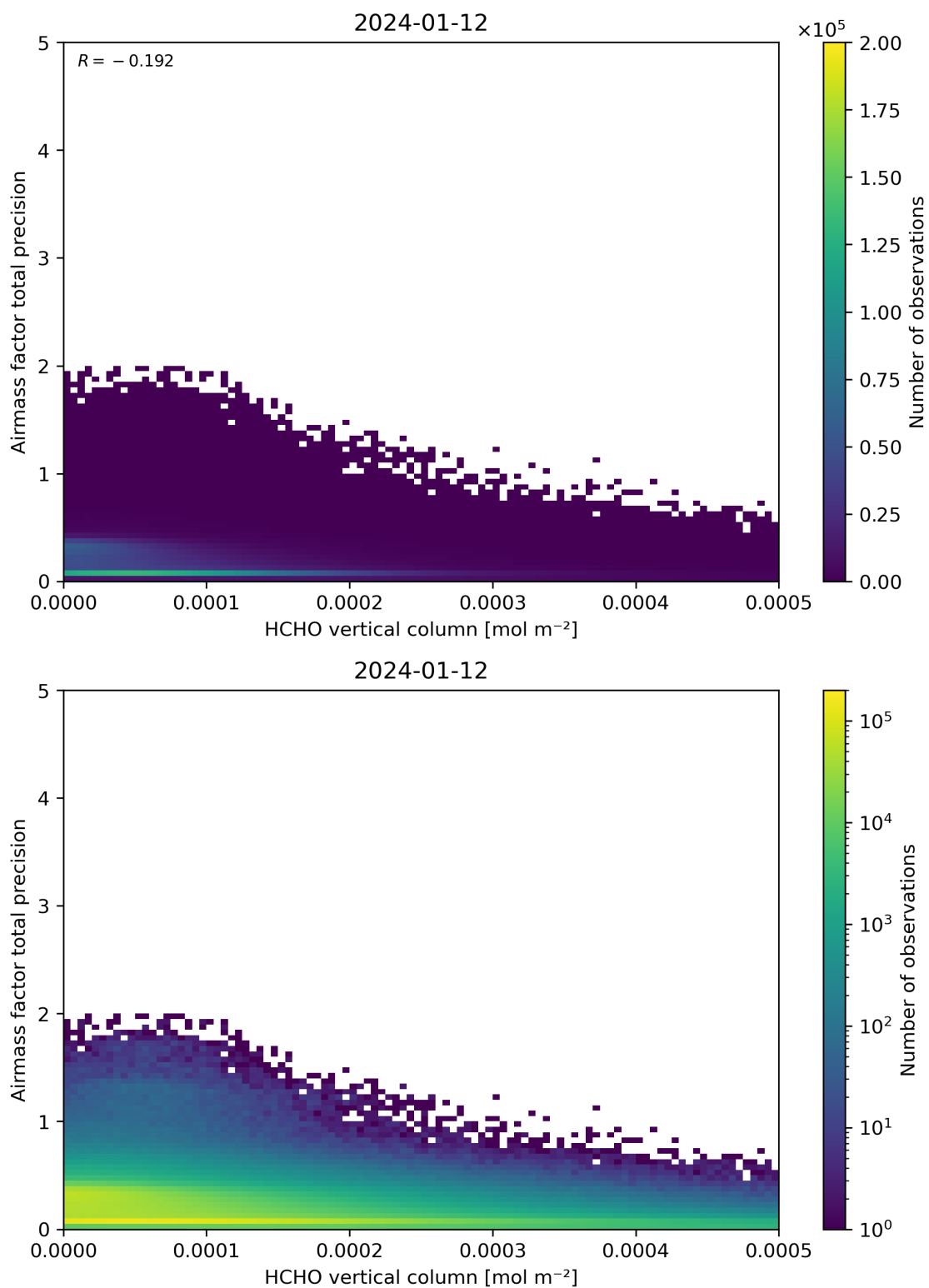
Figure 132: Scatter density plot of “HCHO vertical column” against “Airmass factor total precision” for 2024-01-11 to 2024-01-13.
