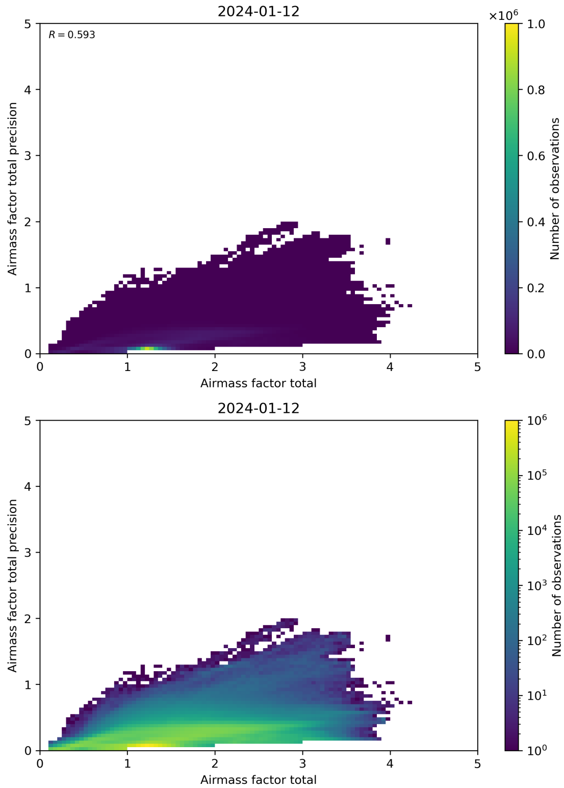
Figure 103: Scatter density plot of “Airmass factor total” against “Airmass factor total precision” for 2024-01-11 to 2024-01-13.
