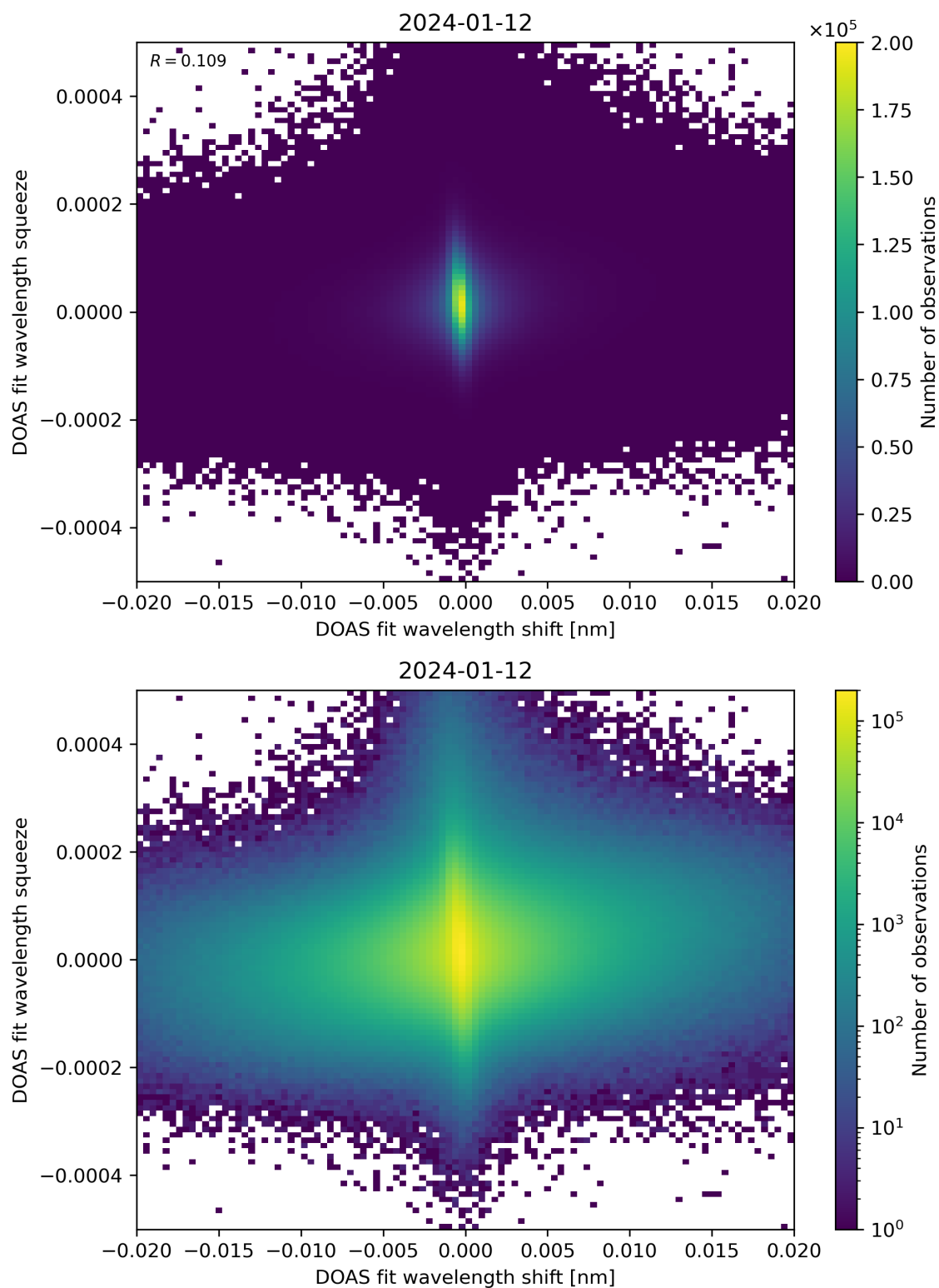
Figure 65: Scatter density plot of “DOAS fit wavelength shift” against “DOAS fit wavelength squeeze” for 2024-01-11 to 2024-01-13.
