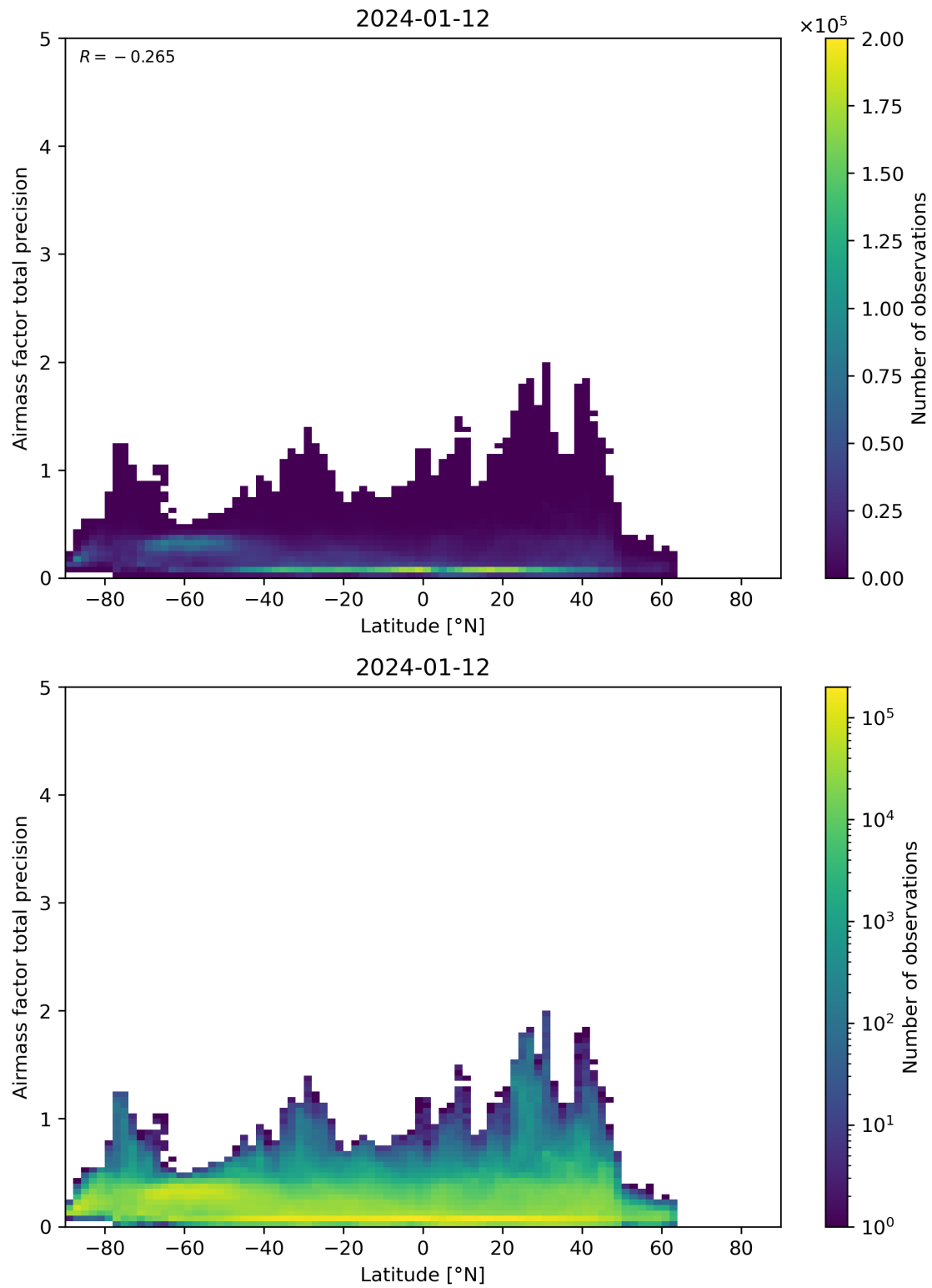
Figure 162: Scatter density plot of “Latitude” against “Airmass factor total precision” for 2024-01-11 to 2024-01-13.
