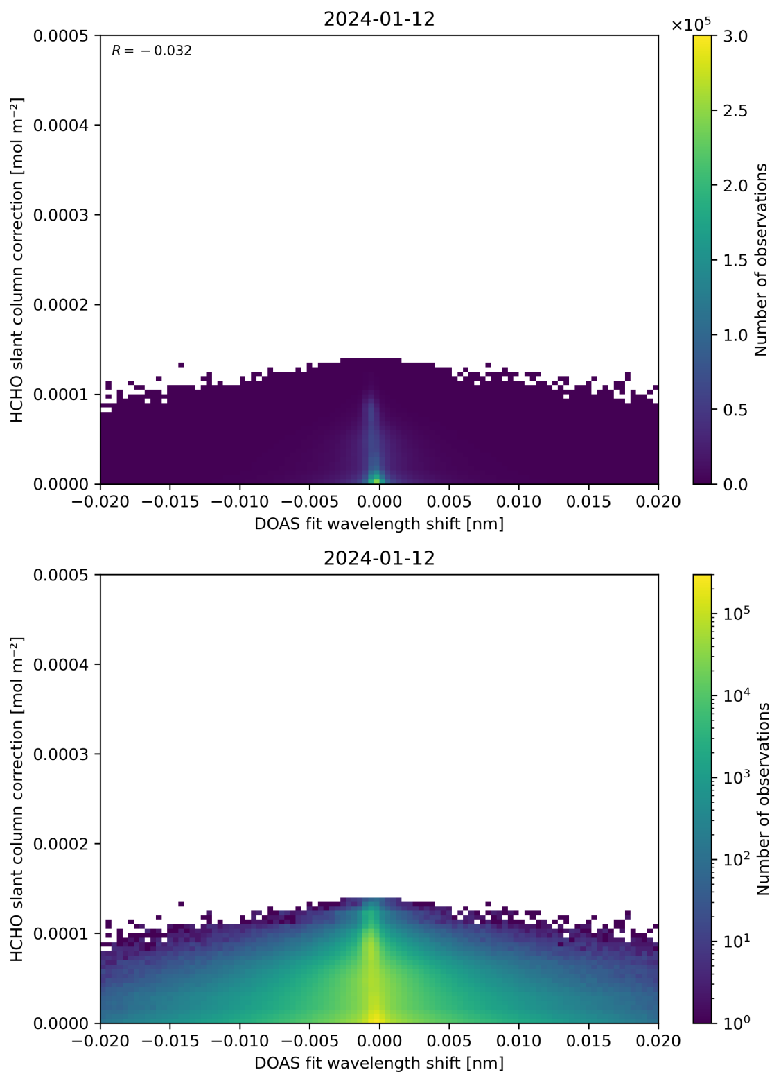
Figure 67: Scatter density plot of “DOAS fit wavelength shift” against “HCHO slant column correction” for 2024-01-11 to 2024-01-13.
