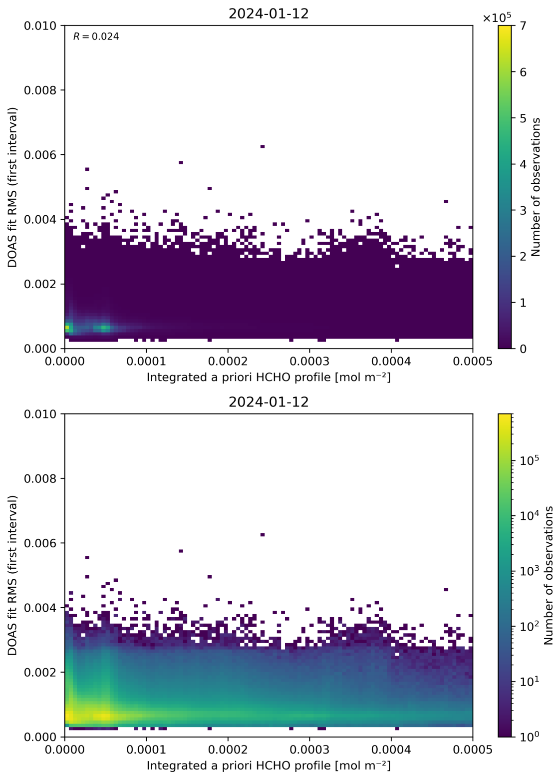
Figure 148: Scatter density plot of “Integrated a priori HCHO profile” against “DOAS fit RMS (first interval)” for 2024-01-11 to 2024-01-13.
