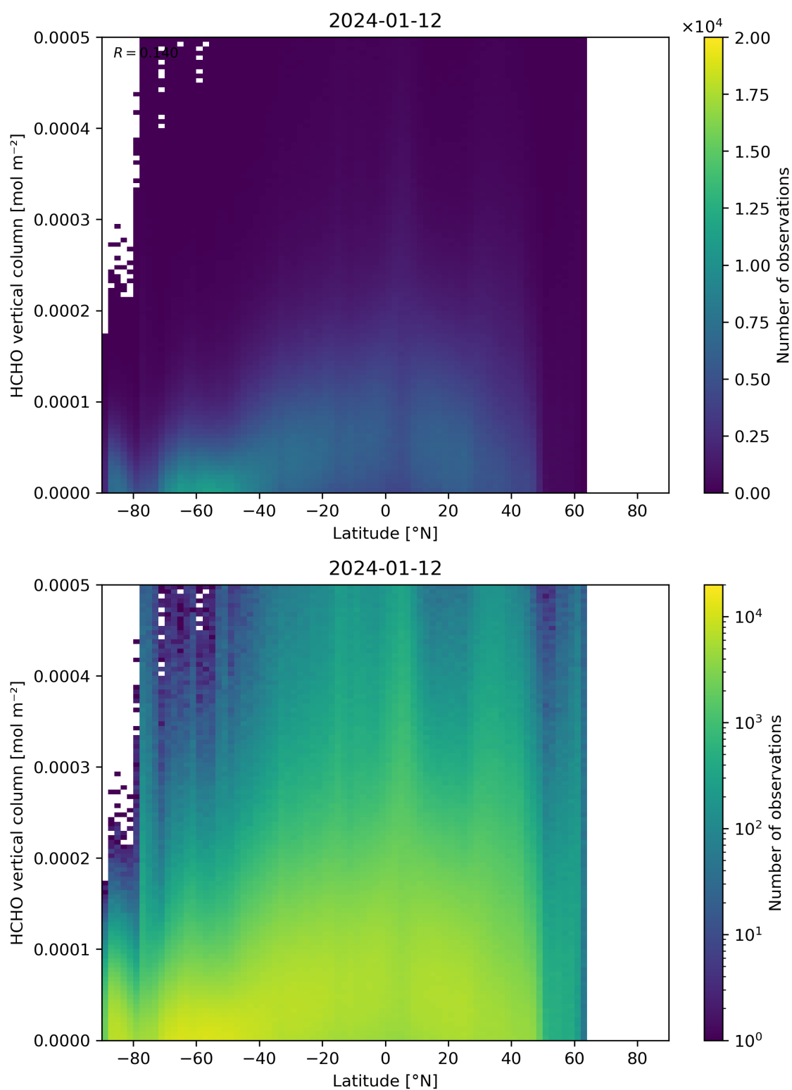
Figure 163: Scatter density plot of “Latitude” against “HCHO vertical column” for 2024-01-11 to 2024-01-13.
