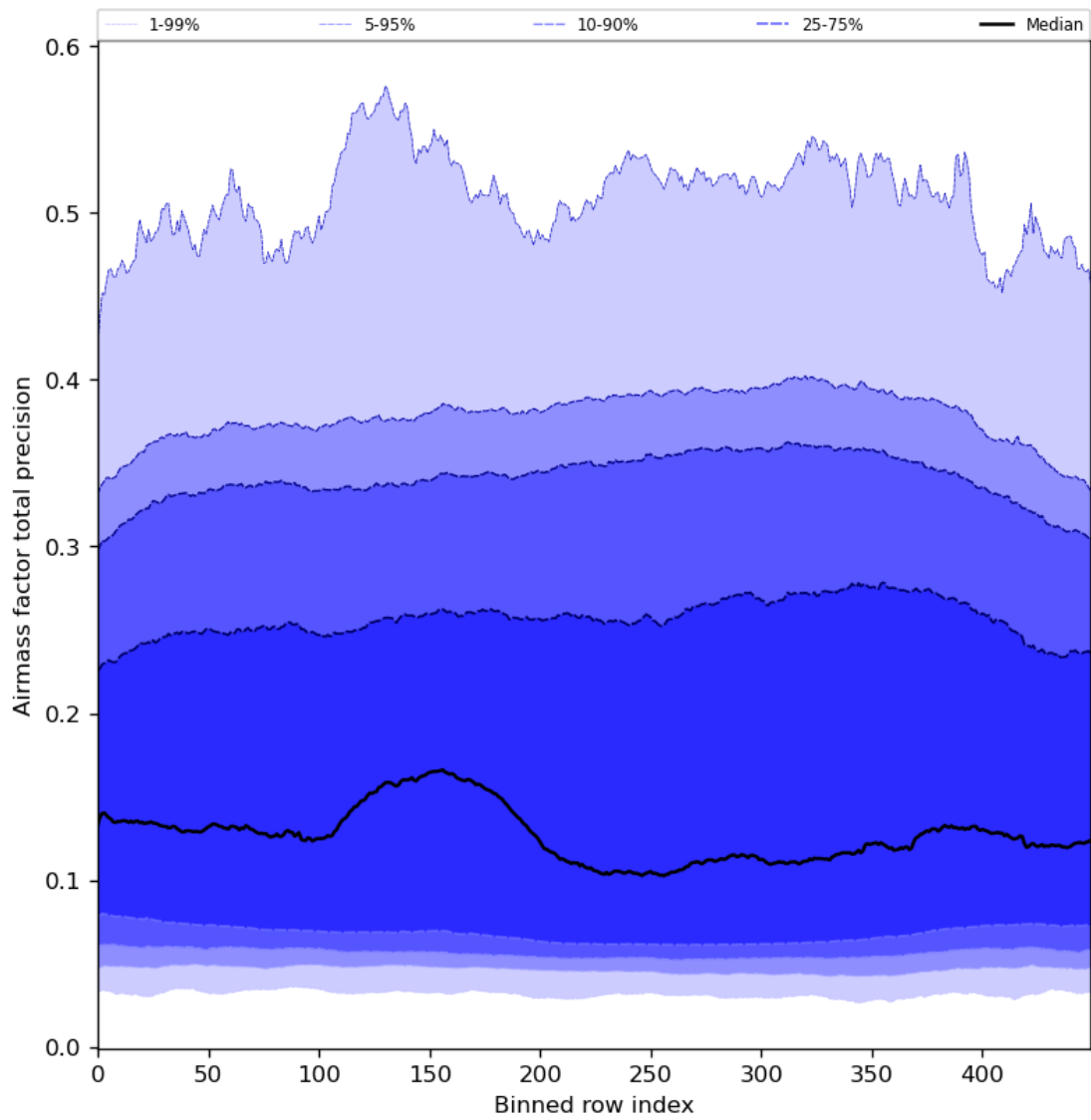
Figure 55: Along track statistics of “Airmass factor total precision” for 2024-01-11 to 2024-01-13
