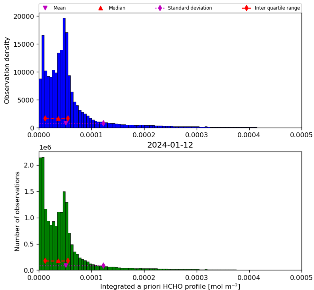
Figure 43: Histogram of “Integrated a priori HCHO profile” for 2024-01-11 to 2024-01-13
