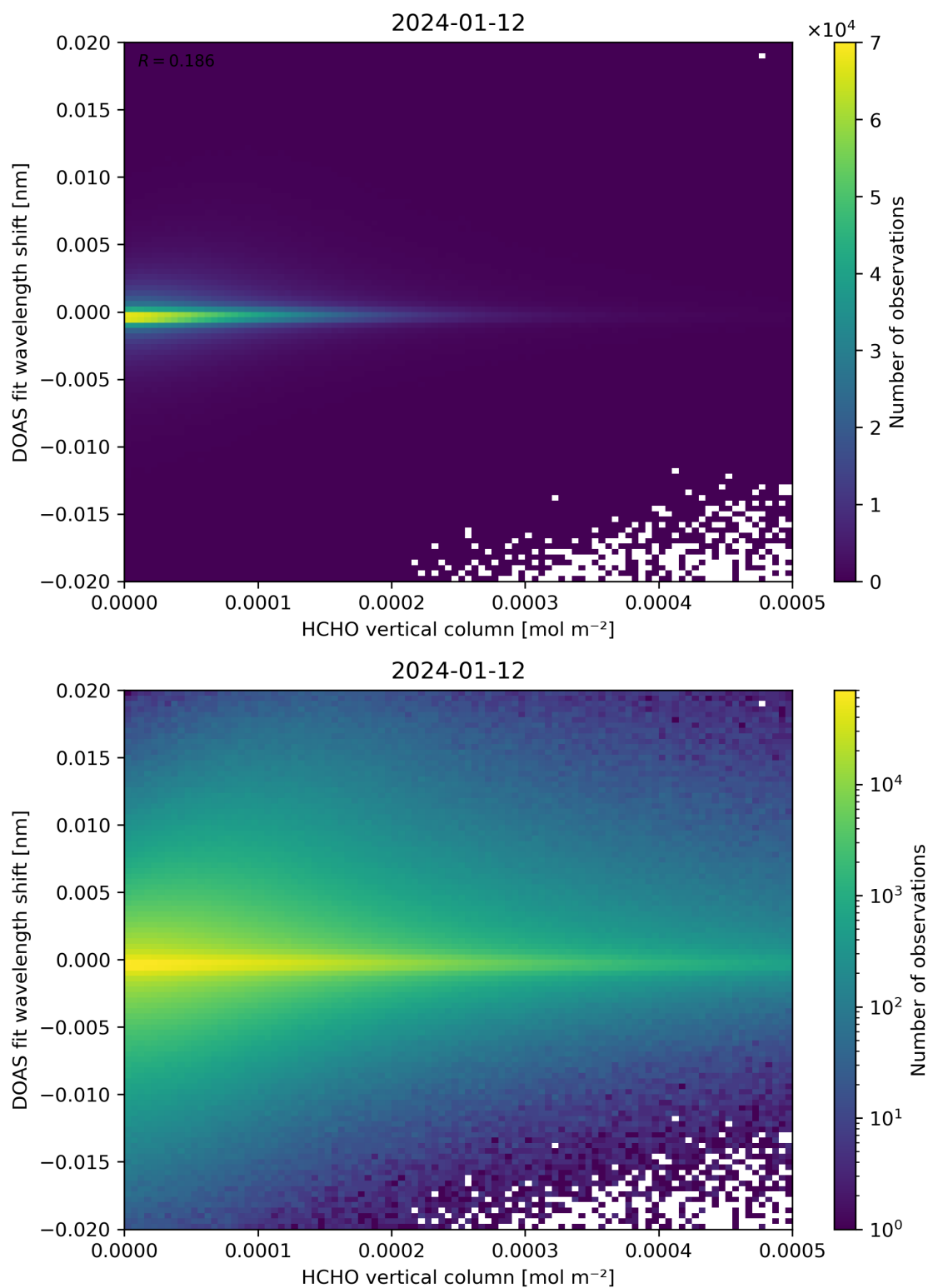
Figure 124: Scatter density plot of “HCHO vertical column” against “DOAS fit wavelength shift” for 2024-01-11 to 2024-01-13.
