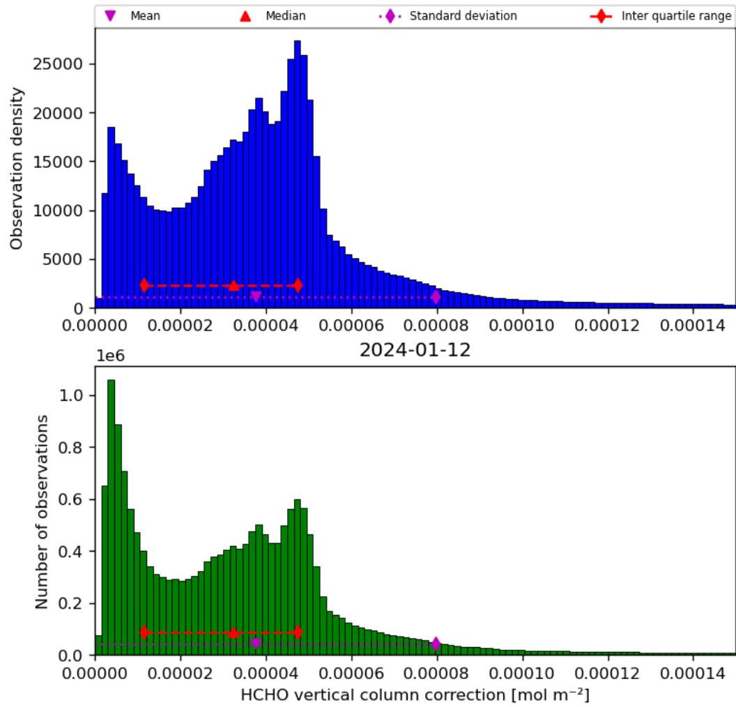
Figure 37: Histogram of “HCHO vertical column correction” for 2024-01-11 to 2024-01-13
