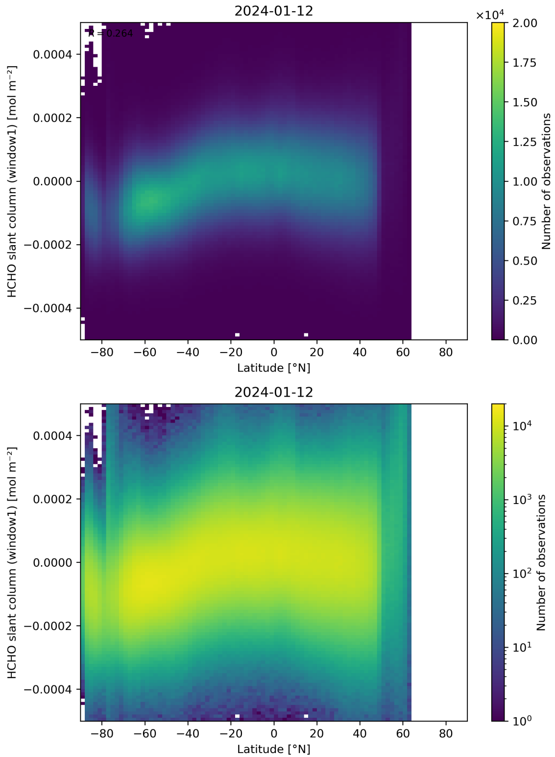
Figure 159: Scatter density plot of “Latitude” against “HCHO slant column (window1)” for 2024-01-11 to 2024-01-13.
