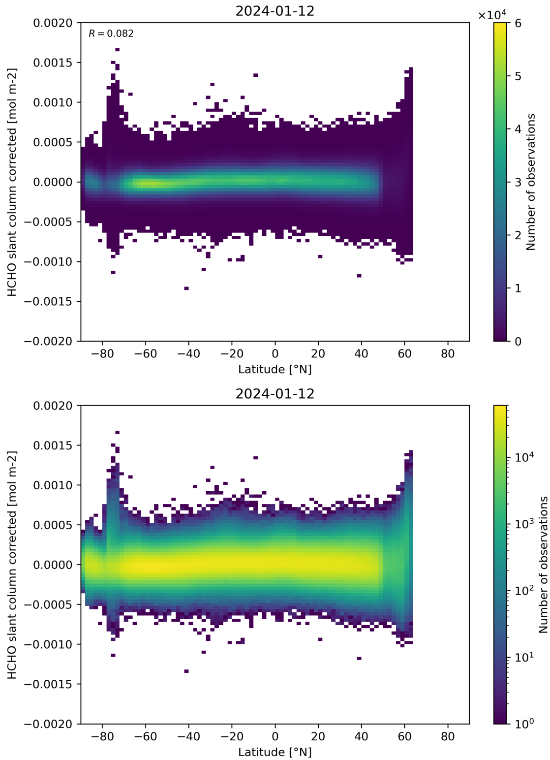
Figure 157: Scatter density plot of “Latitude” against “HCHO slant column corrected” for 2024-01-11 to 2024-01-13.
