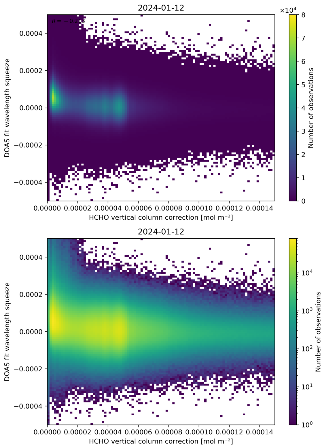
Figure 114: Scatter density plot of “HCHO vertical column correction” against “DOAS fit wavelength squeeze” for 2024-01-11 to 2024-01-13.
