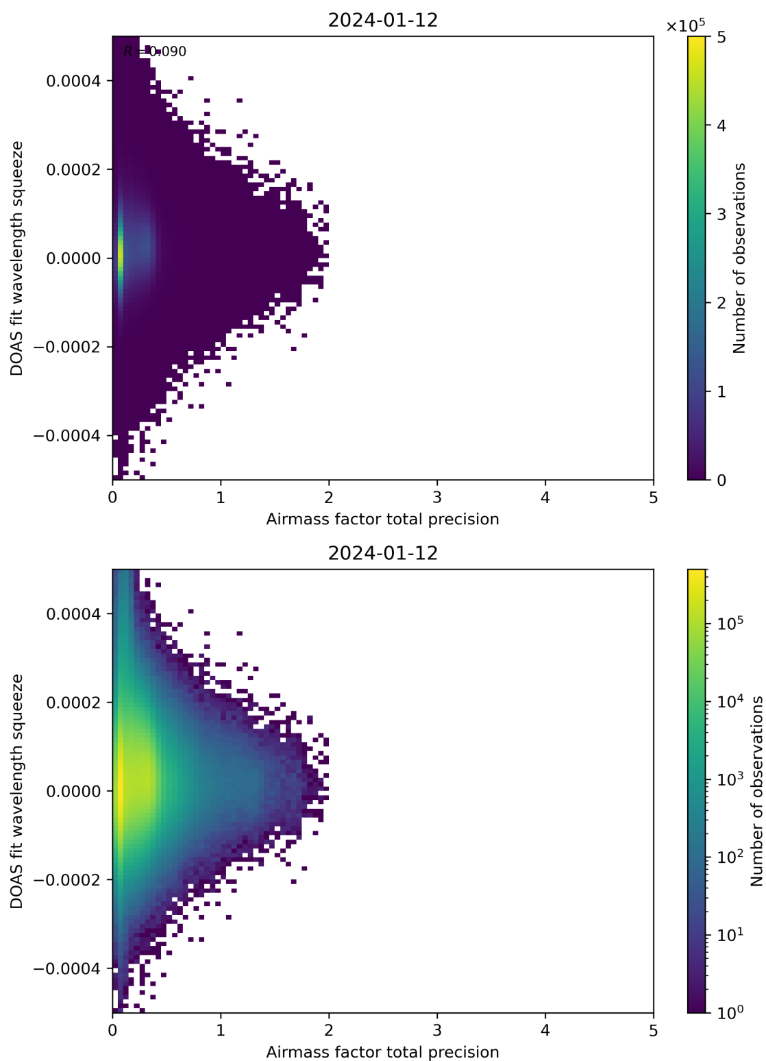
Figure 107: Scatter density plot of “Airmass factor total precision” against “DOAS fit wavelength squeeze” for 2024-01-11 to 2024-01-13.
