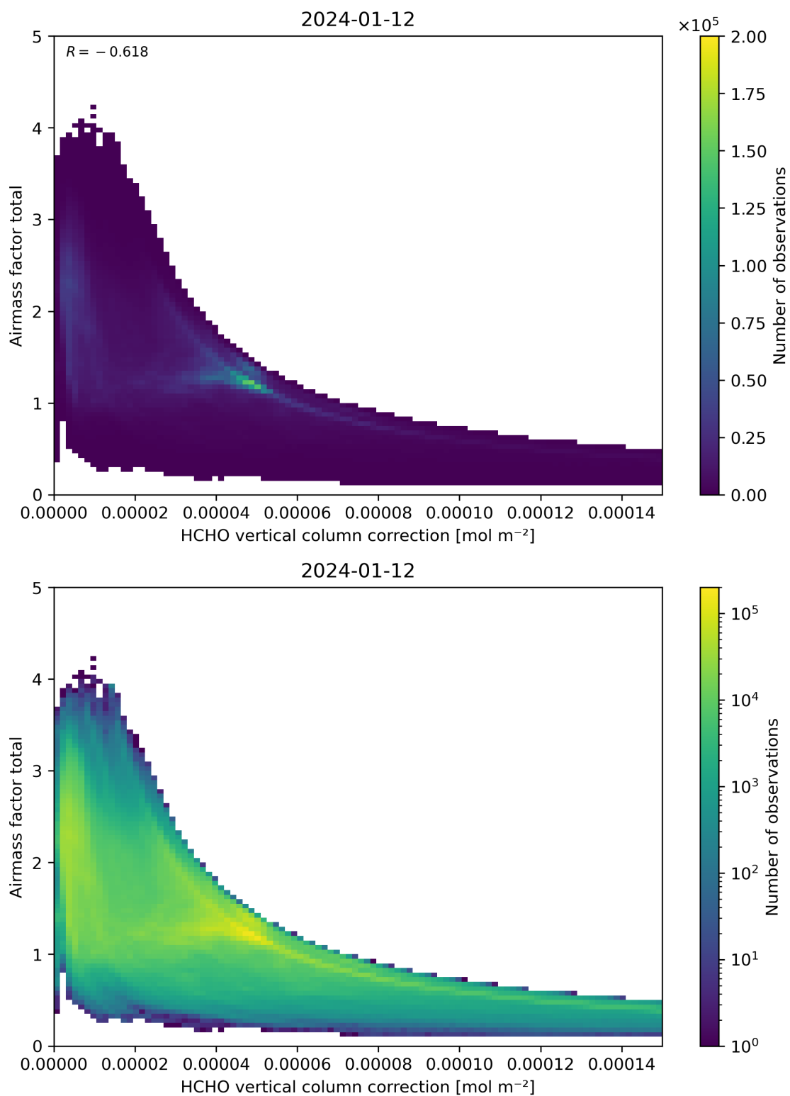
Figure 120: Scatter density plot of “HCHO vertical column correction” against “Airmass factor total” for 2024-01-11 to 2024-01-13.
