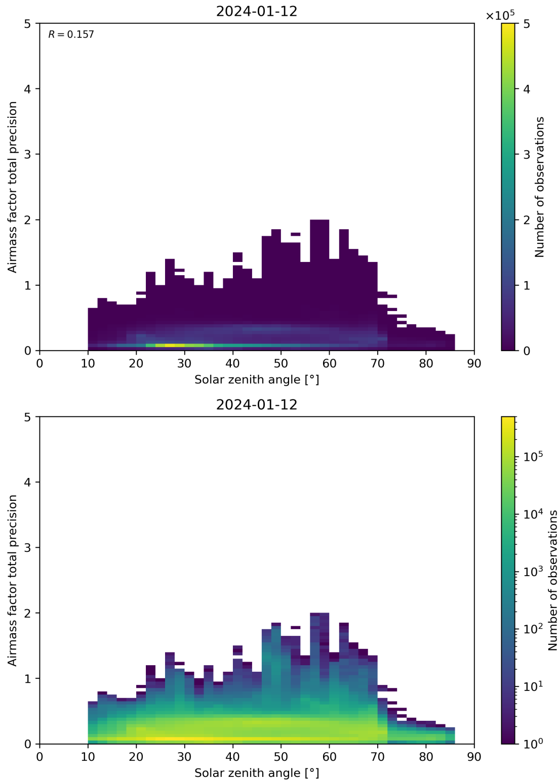
Figure 176: Scatter density plot of “Solar zenith angle” against “Airmass factor total precision” for 2024-01-11 to 2024-01-13.
