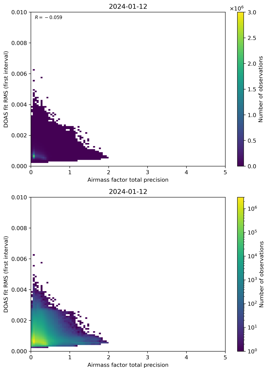
Figure 105: Scatter density plot of “Airmass factor total precision” against “DOAS fit RMS (first interval)” for 2024-01-11 to 2024-01-13.
