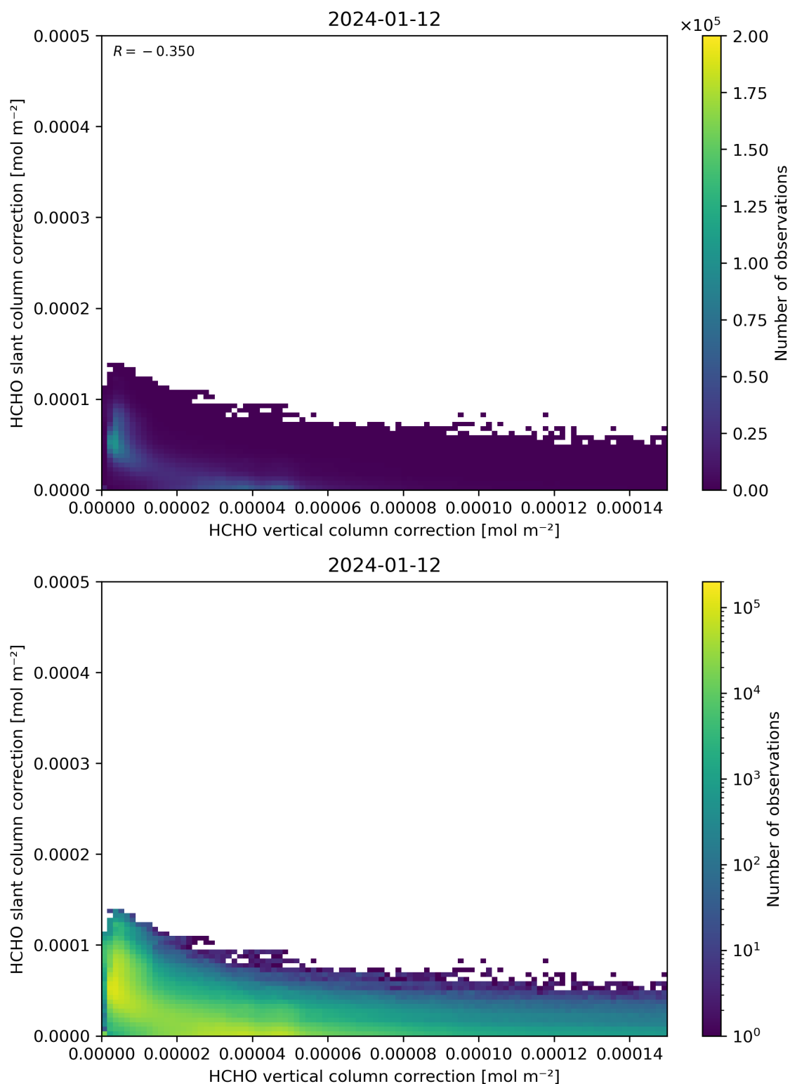
Figure 117: Scatter density plot of “HCHO vertical column correction” against “HCHO slant column correction” for 2024-01-11 to 2024-01-13.
