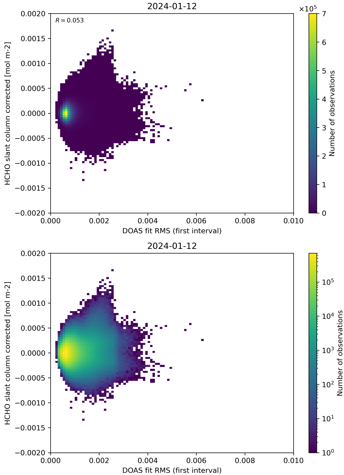
Figure 62: Scatter density plot of “DOAS fit RMS (first interval)” against “HCHO slant column corrected” for 2024-01-11 to 2024-01-13.
