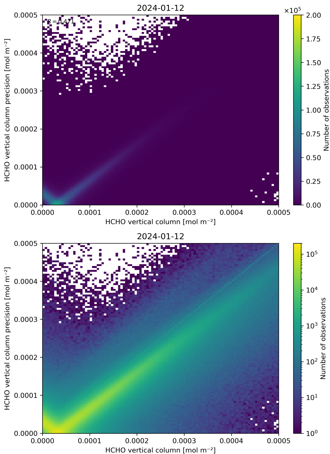
Figure 134: Scatter density plot of “HCHO vertical column” against “HCHO vertical column precision” for 2024-01-11 to 2024-01-13.
