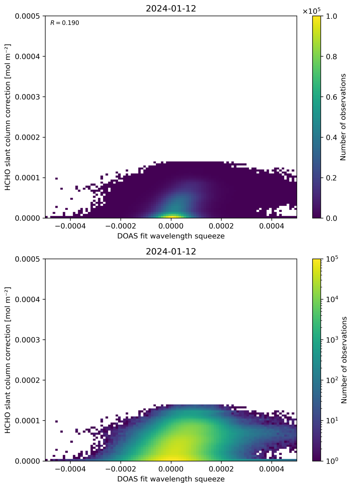
Figure 70: Scatter density plot of “DOAS fit wavelength squeeze” against “HCHO slant column correction” for 2024-01-11 to 2024-01-13.
