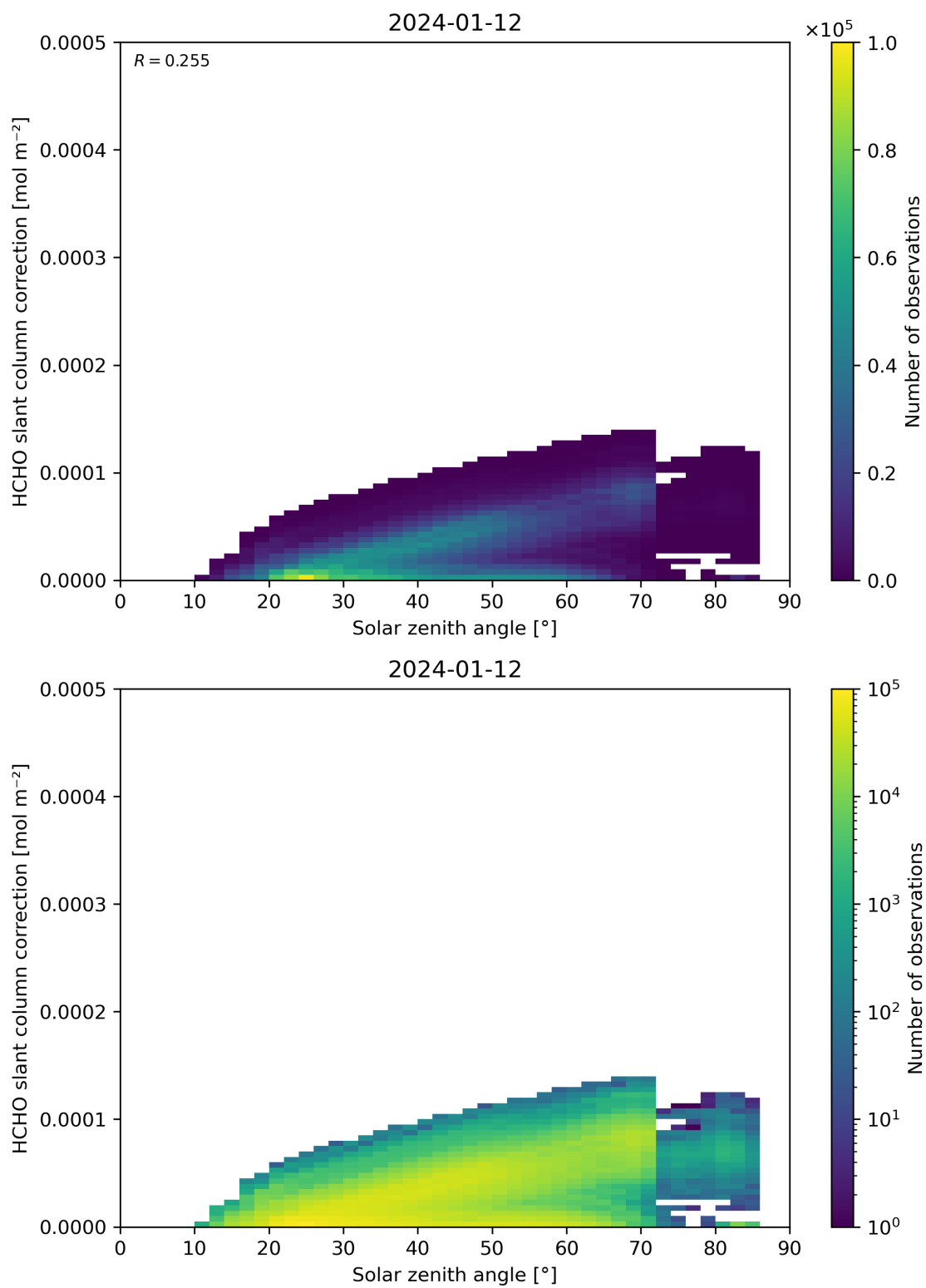
Figure 172: Scatter density plot of “Solar zenith angle” against “HCHO slant column correction” for 2024-01-11 to 2024-01-13.
