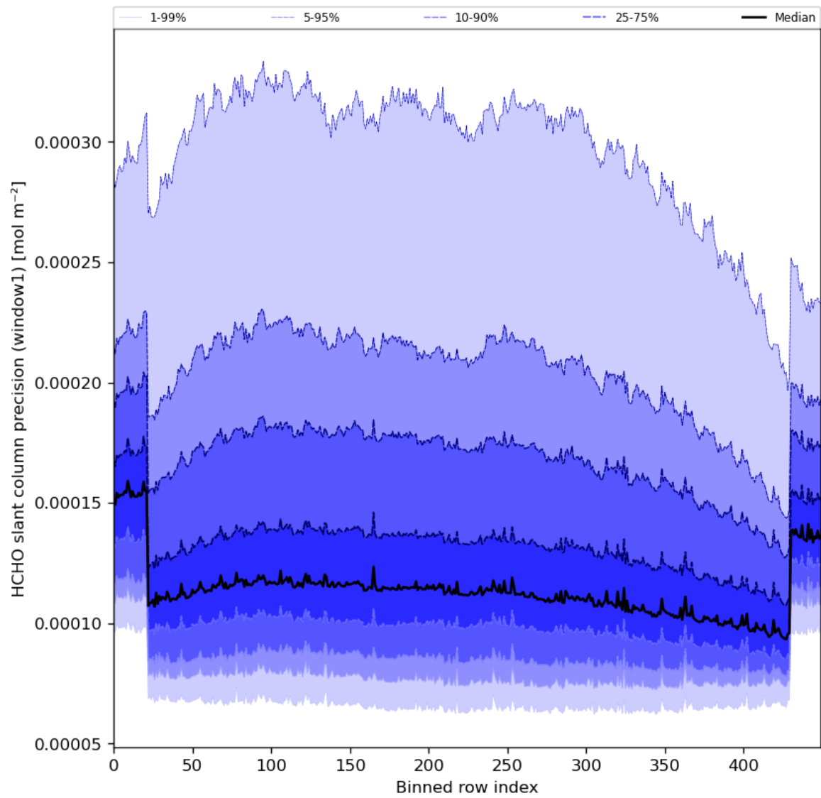
Figure 53: Along track statistics of “HCHO slant column precision (window1)” for 2024-01-11 to 2024-01-13
