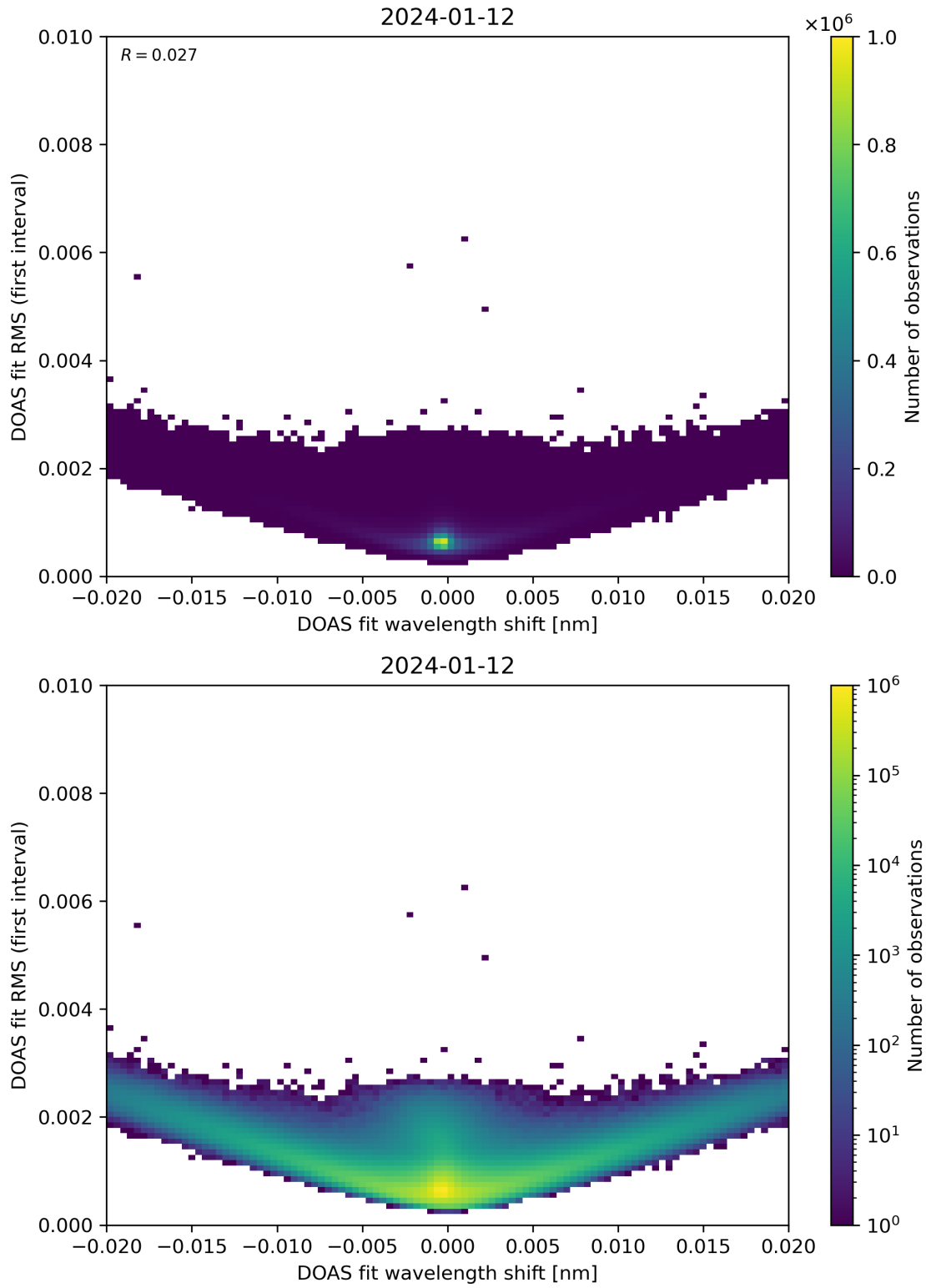
Figure 64: Scatter density plot of “DOAS fit wavelength shift” against “DOAS fit RMS (first interval)” for 2024-01-11 to 2024-01-13.
