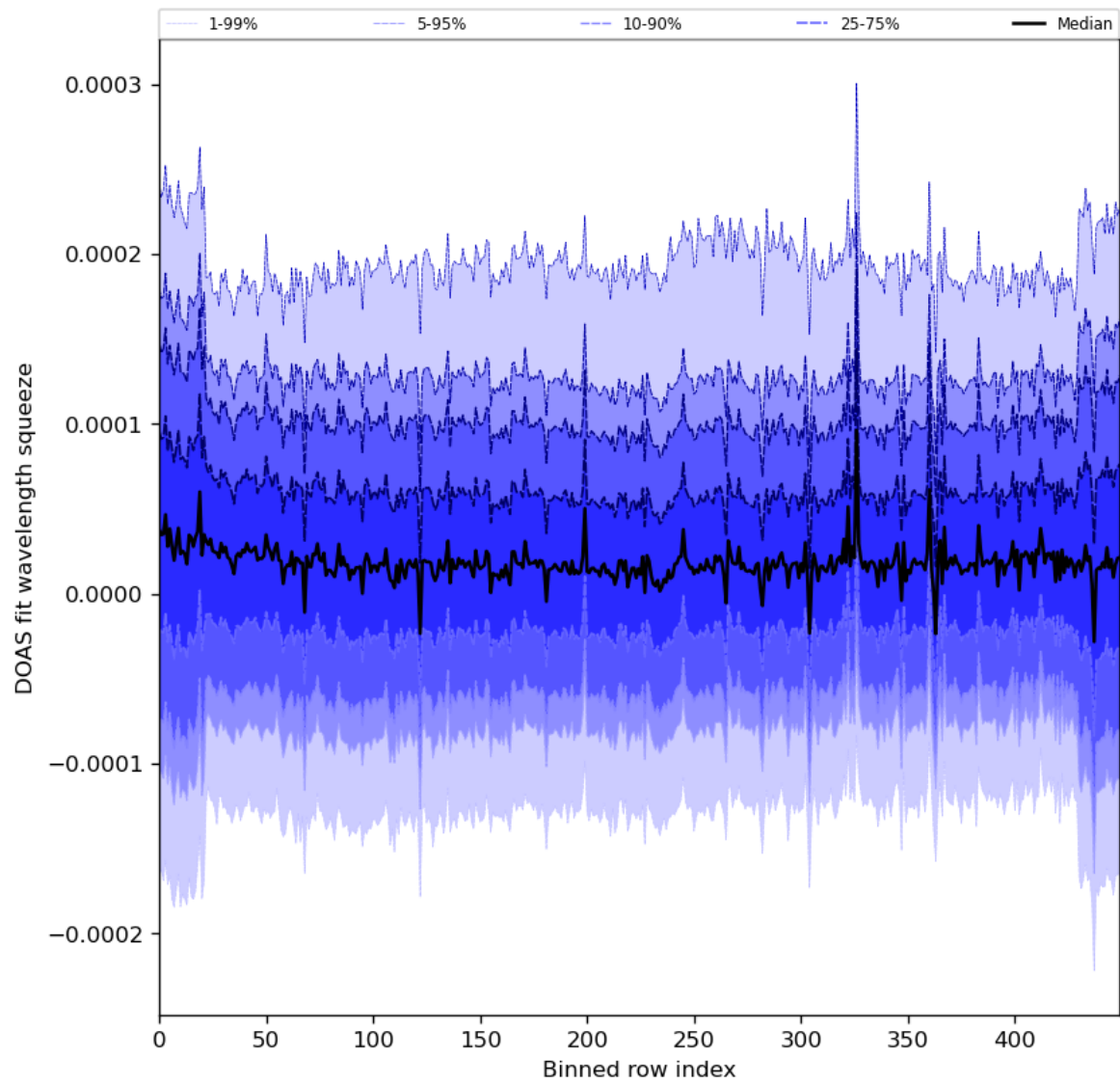
Figure 59: Along track statistics of “DOAS fit wavelength squeeze” for 2024-01-11 to 2024-01-13
