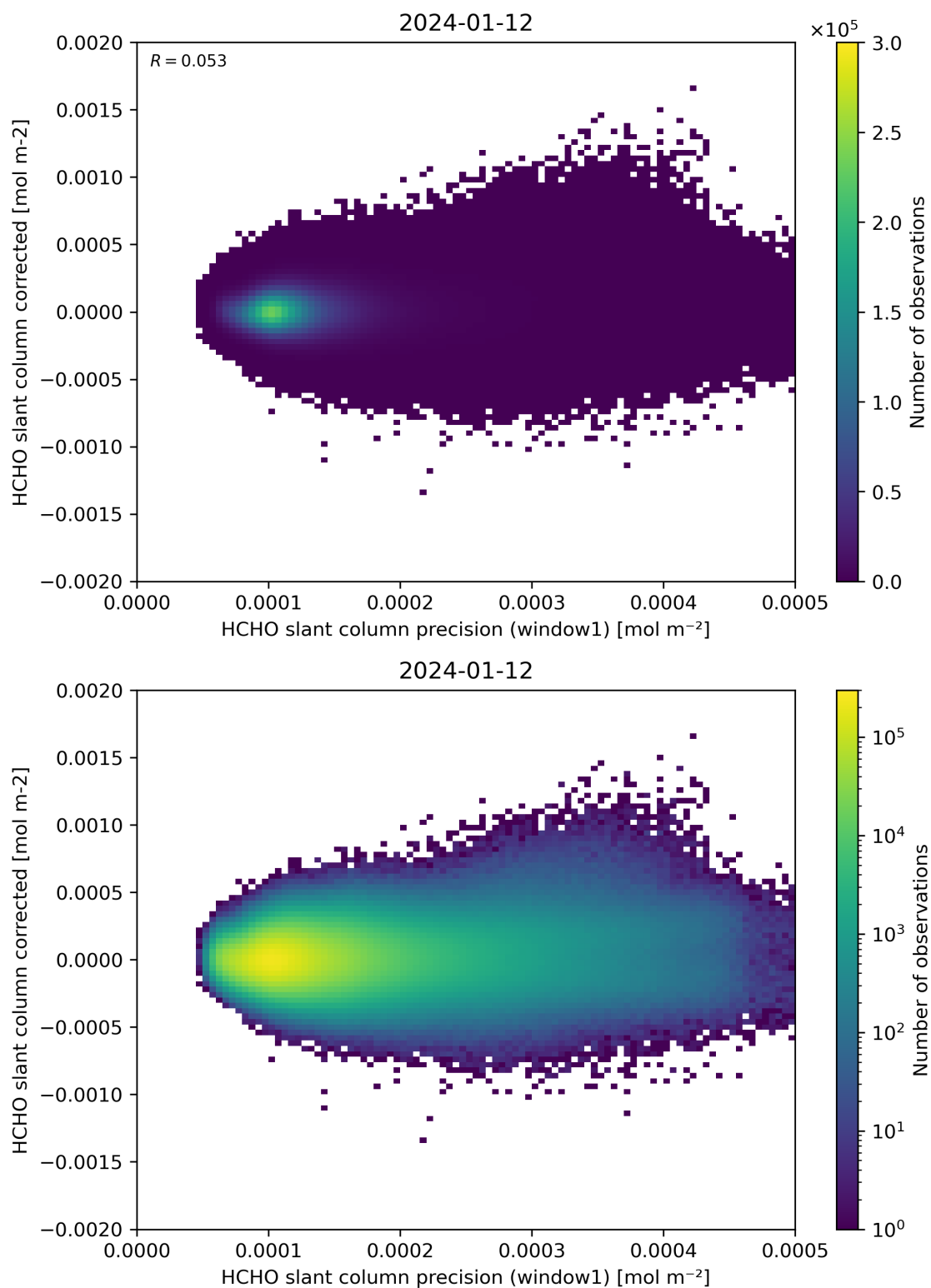
Figure 92: Scatter density plot of “HCHO slant column precision (window1)” against “HCHO slant column corrected” for 2024-01-11 to 2024-01-13.
