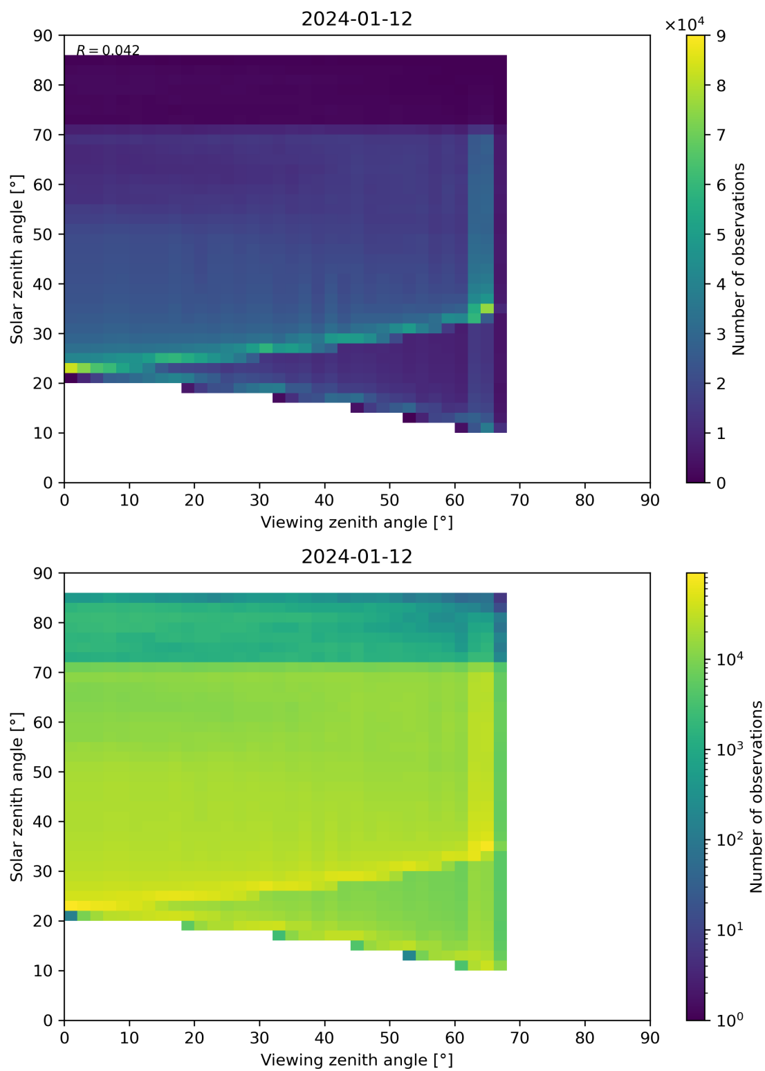
Figure 197: Scatter density plot of “Viewing zenith angle” against “Solar zenith angle” for 2024-01-11 to 2024-01-13.
