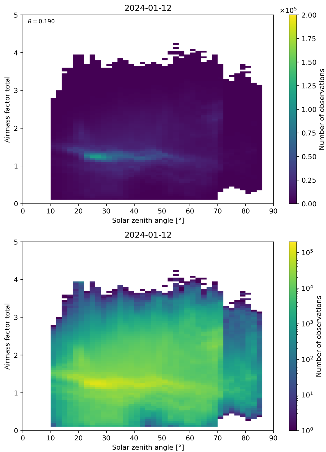
Figure 175: Scatter density plot of “Solar zenith angle” against “Airmass factor total” for 2024-01-11 to 2024-01-13.
