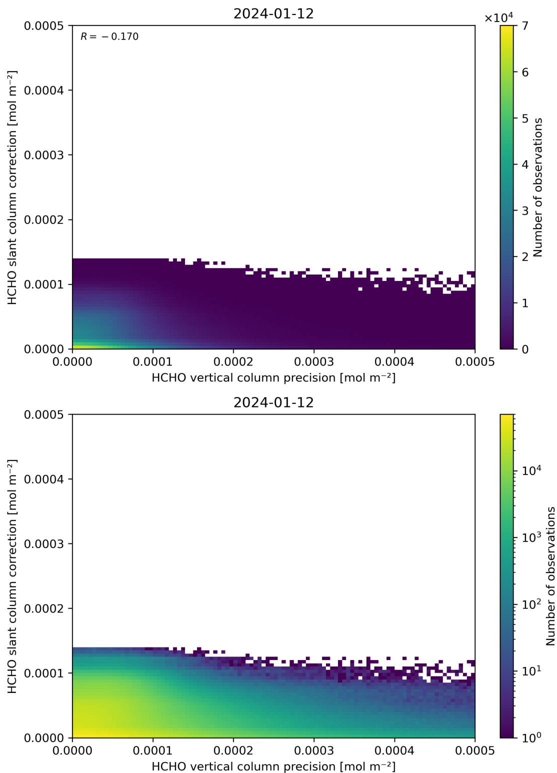
Figure 141: Scatter density plot of “HCHO vertical column precision” against “HCHO slant column correction” for 2024-01-11 to 2024-01-13.
