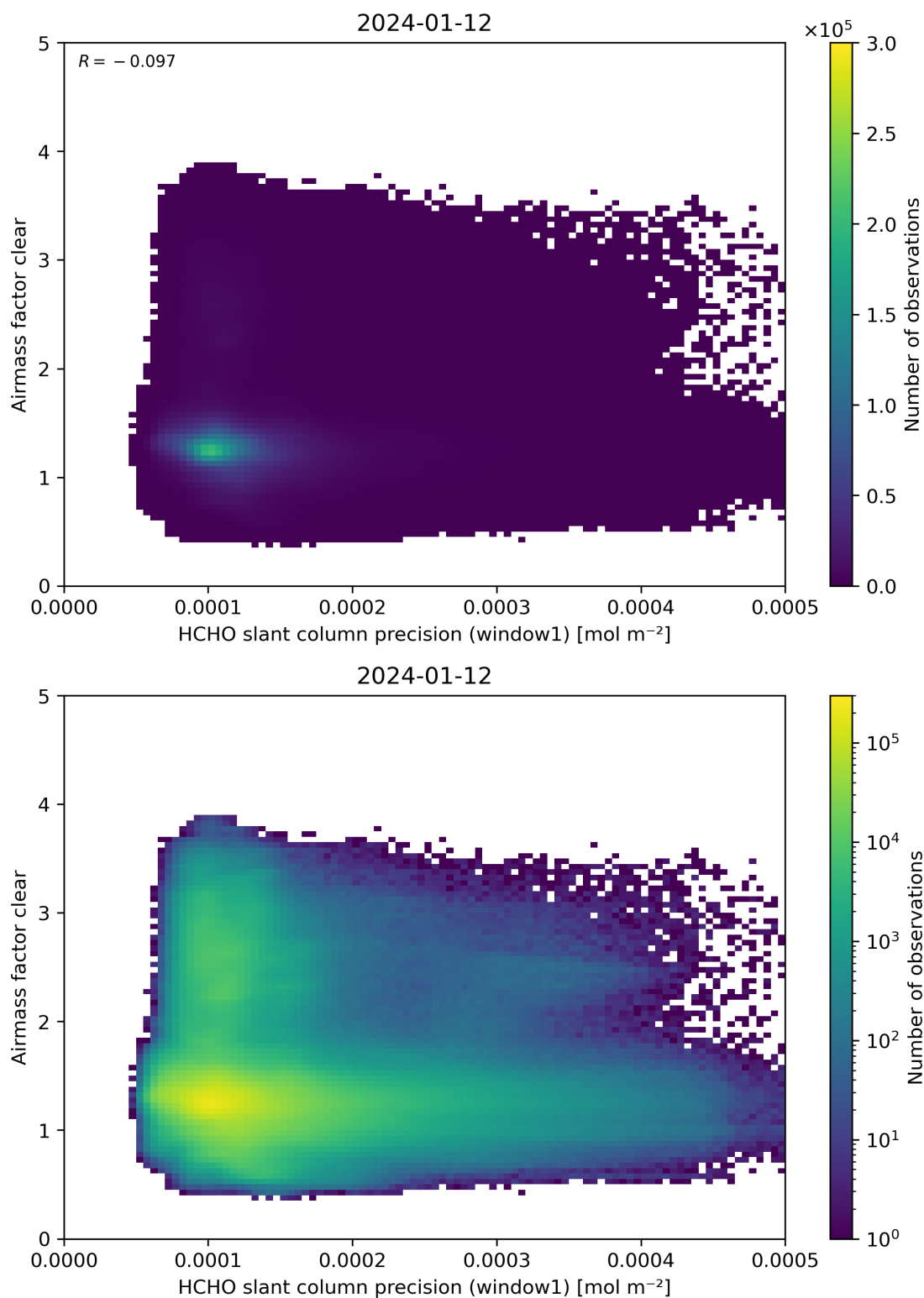
Figure 91: Scatter density plot of “HCHO slant column precision (window1)” against “Airmass factor clear” for 2024-01-11 to 2024-01-13.
