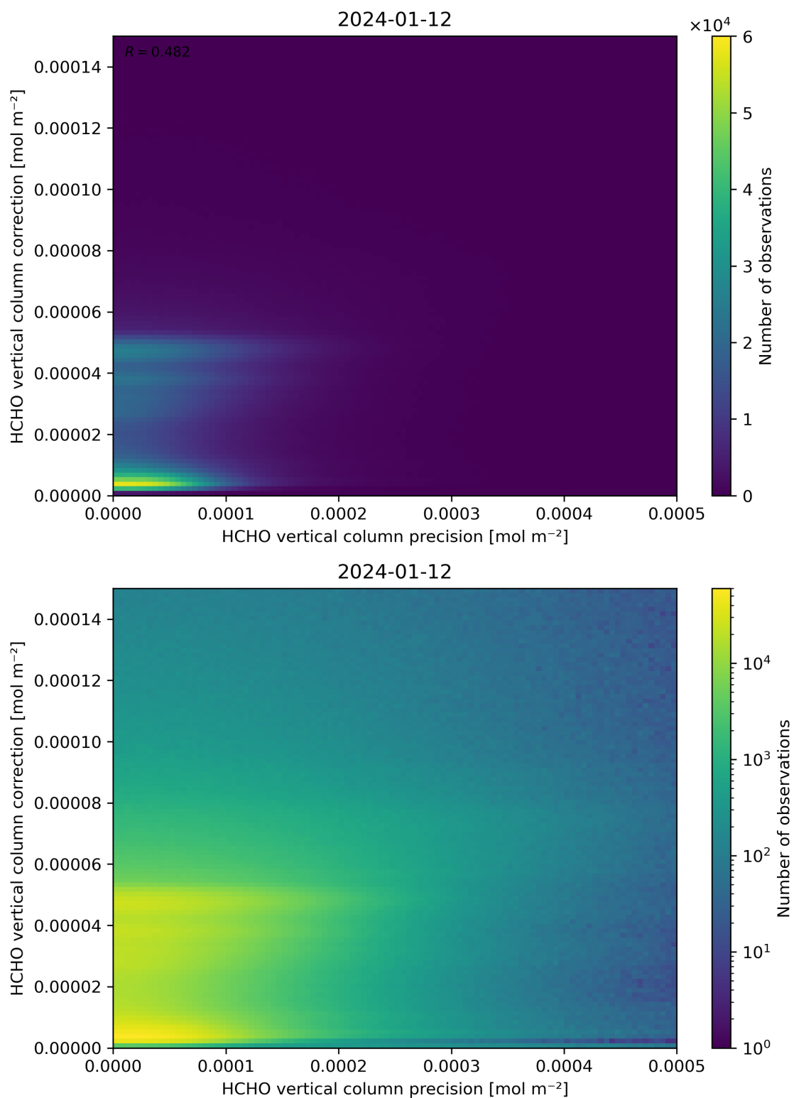
Figure 146: Scatter density plot of “HCHO vertical column precision” against “HCHO vertical column correction” for 2024-01-11 to 2024-01-13.
