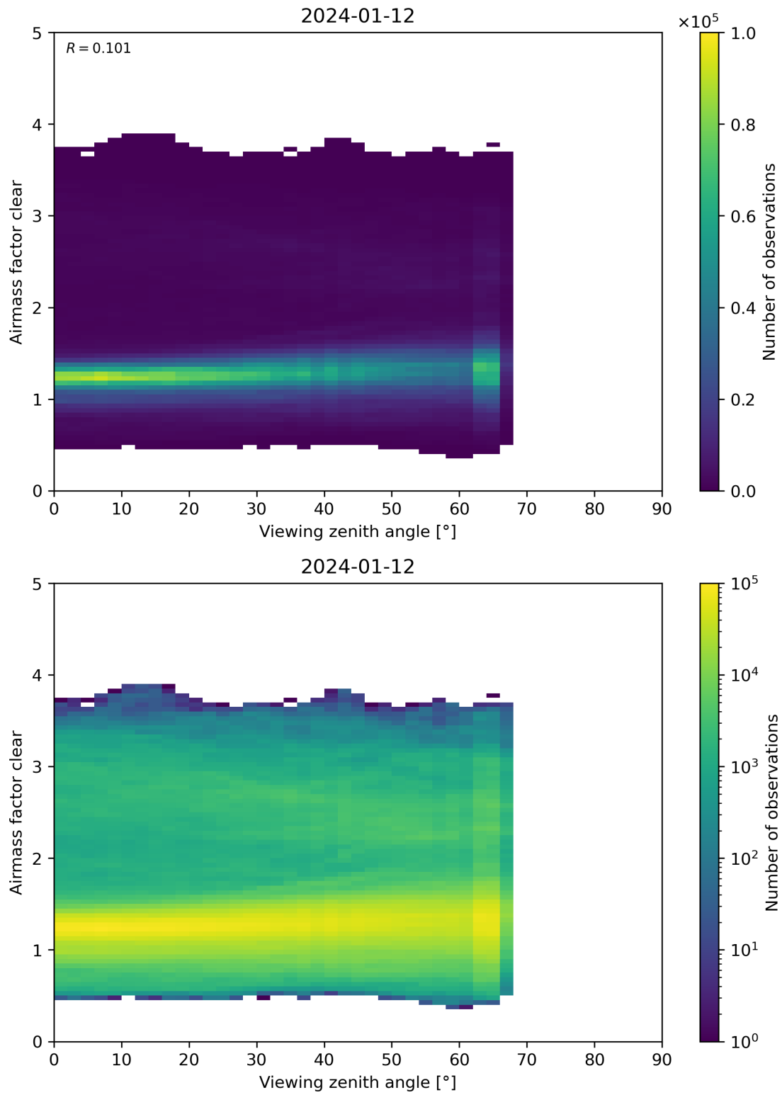
Figure 185: Scatter density plot of “Viewing zenith angle” against “Airmass factor clear” for 2024-01-11 to 2024-01-13.
