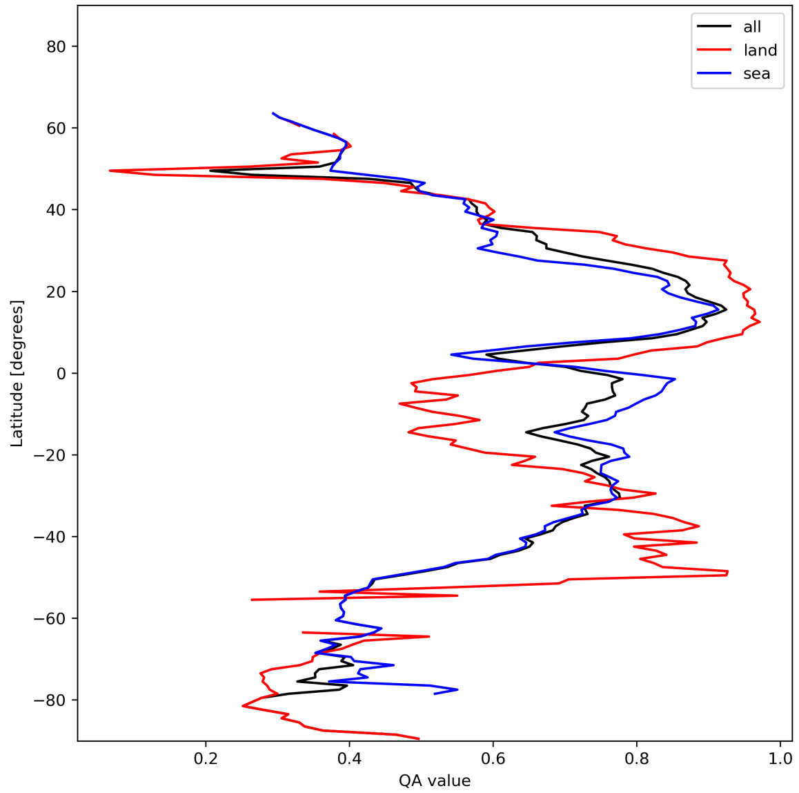
Figure 20: Zonal average of “QA value” for 2024-01-11 to 2024-01-13.
