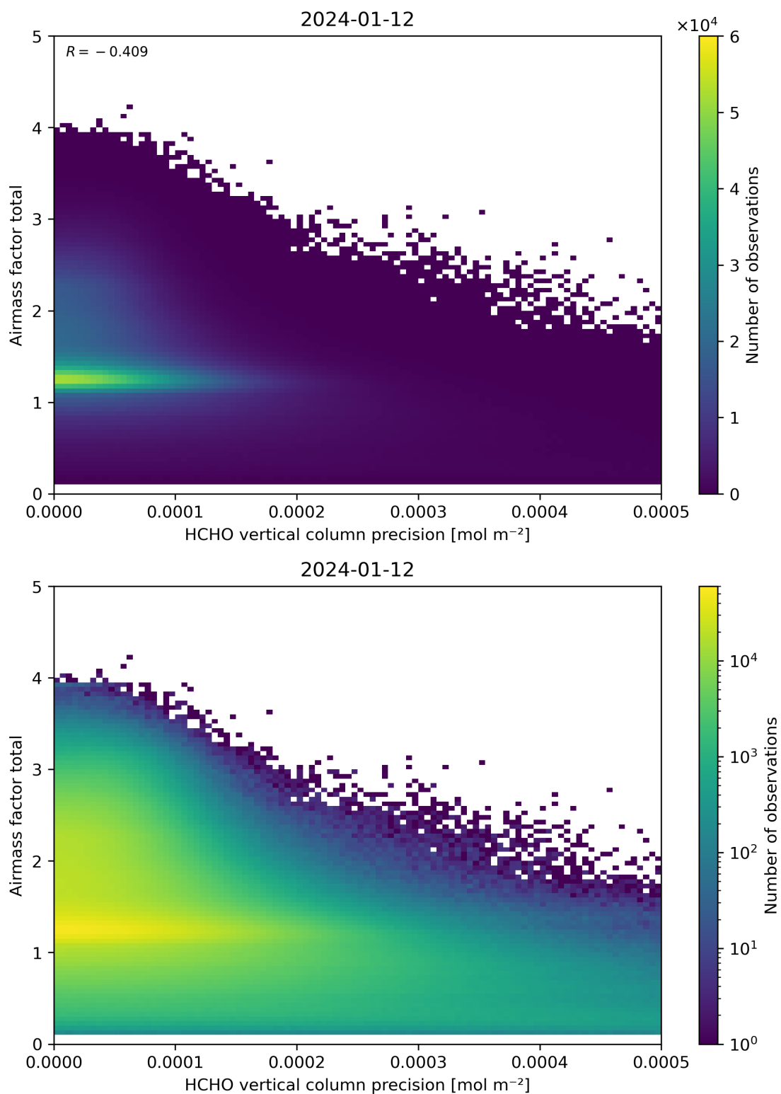
Figure 144: Scatter density plot of “HCHO vertical column precision” against “Airmass factor total” for 2024-01-11 to 2024-01-13.
