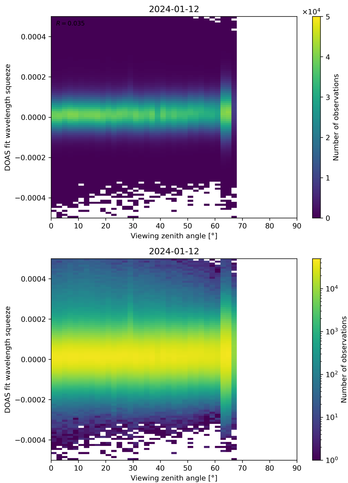
Figure 184: Scatter density plot of “Viewing zenith angle” against “DOAS fit wavelength squeeze” for 2024-01-11 to 2024-01-13.
