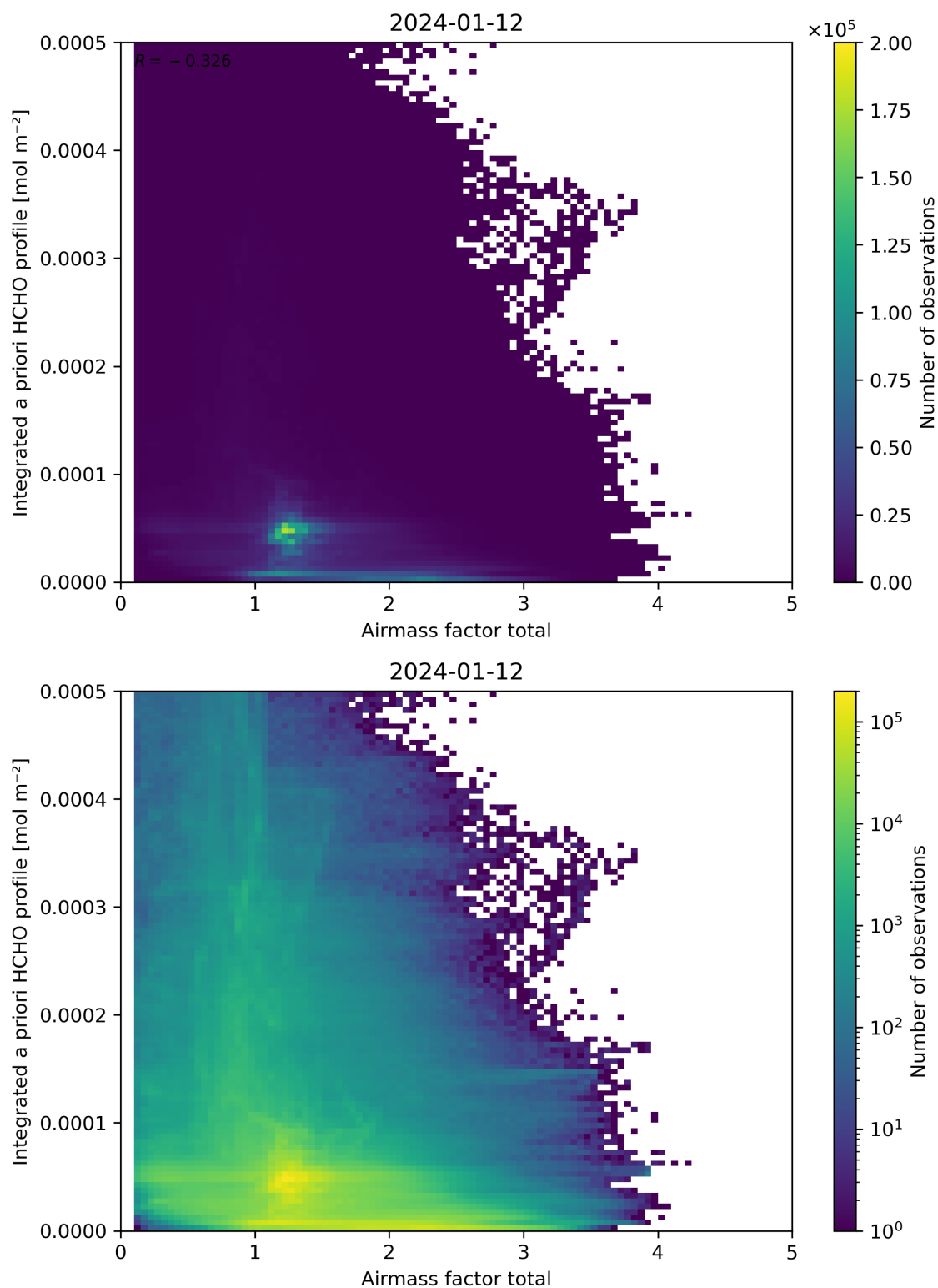
Figure 104: Scatter density plot of “Airmass factor total” against “Integrated a priori HCHO profile” for 2024-01-11 to 2024-01-13.
