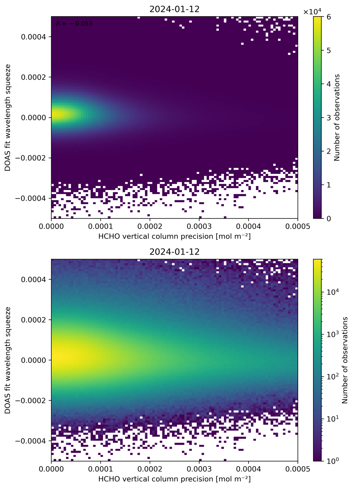
Figure 138: Scatter density plot of “HCHO vertical column precision” against “DOAS fit wavelength squeeze” for 2024-01-11 to 2024-01-13.
