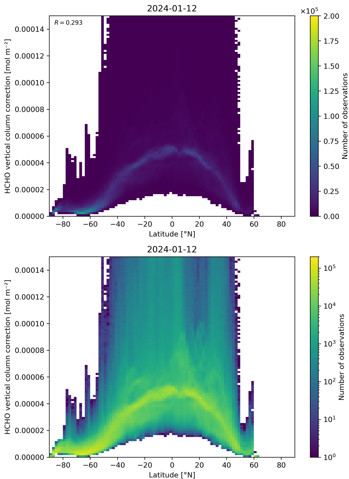
Figure 164: Scatter density plot of “Latitude” against “HCHO vertical column correction” for 2024-01-11 to 2024-01-13.
