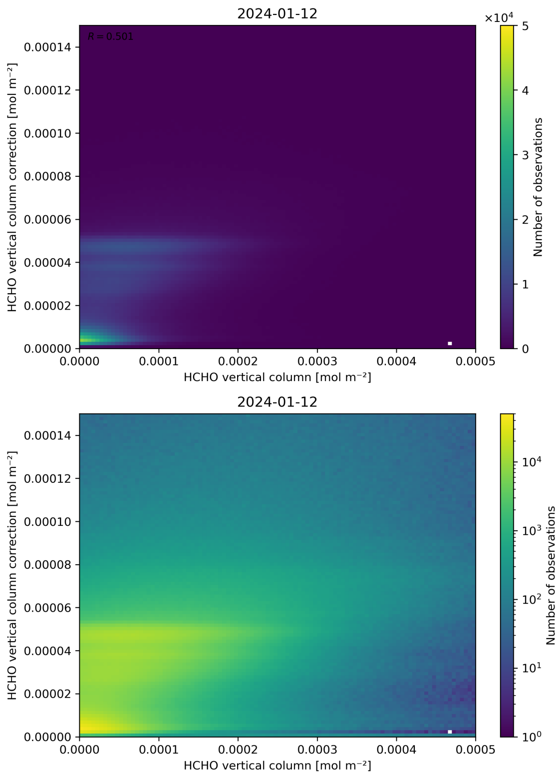
Figure 133: Scatter density plot of “HCHO vertical column” against “HCHO vertical column correction” for 2024-01-11 to 2024-01-13.
