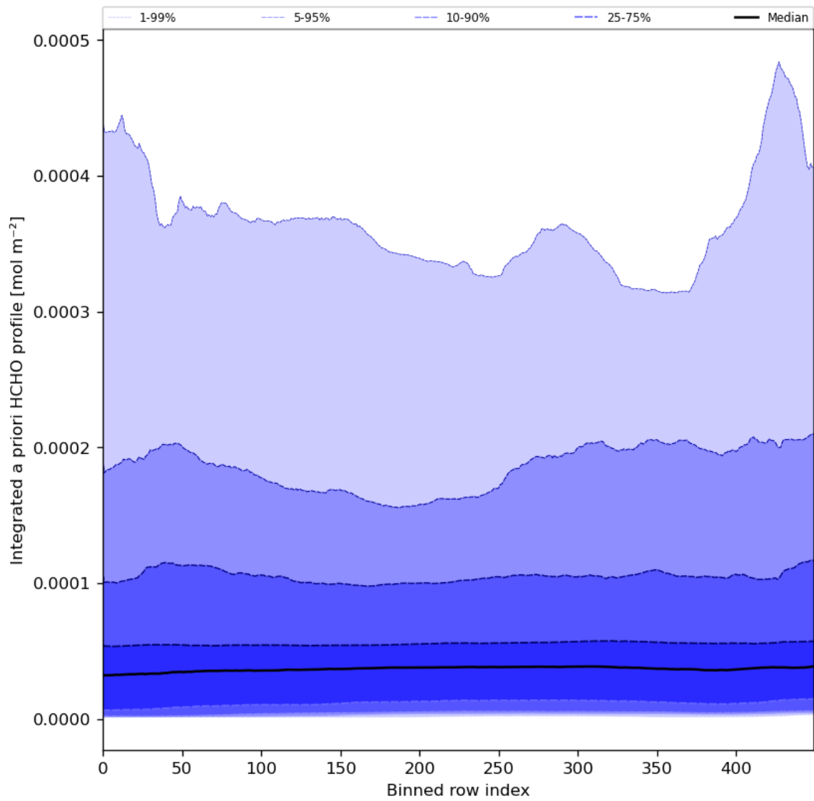
Figure 57: Along track statistics of “Integrated a priori HCHO profile” for 2024-01-11 to 2024-01-13
