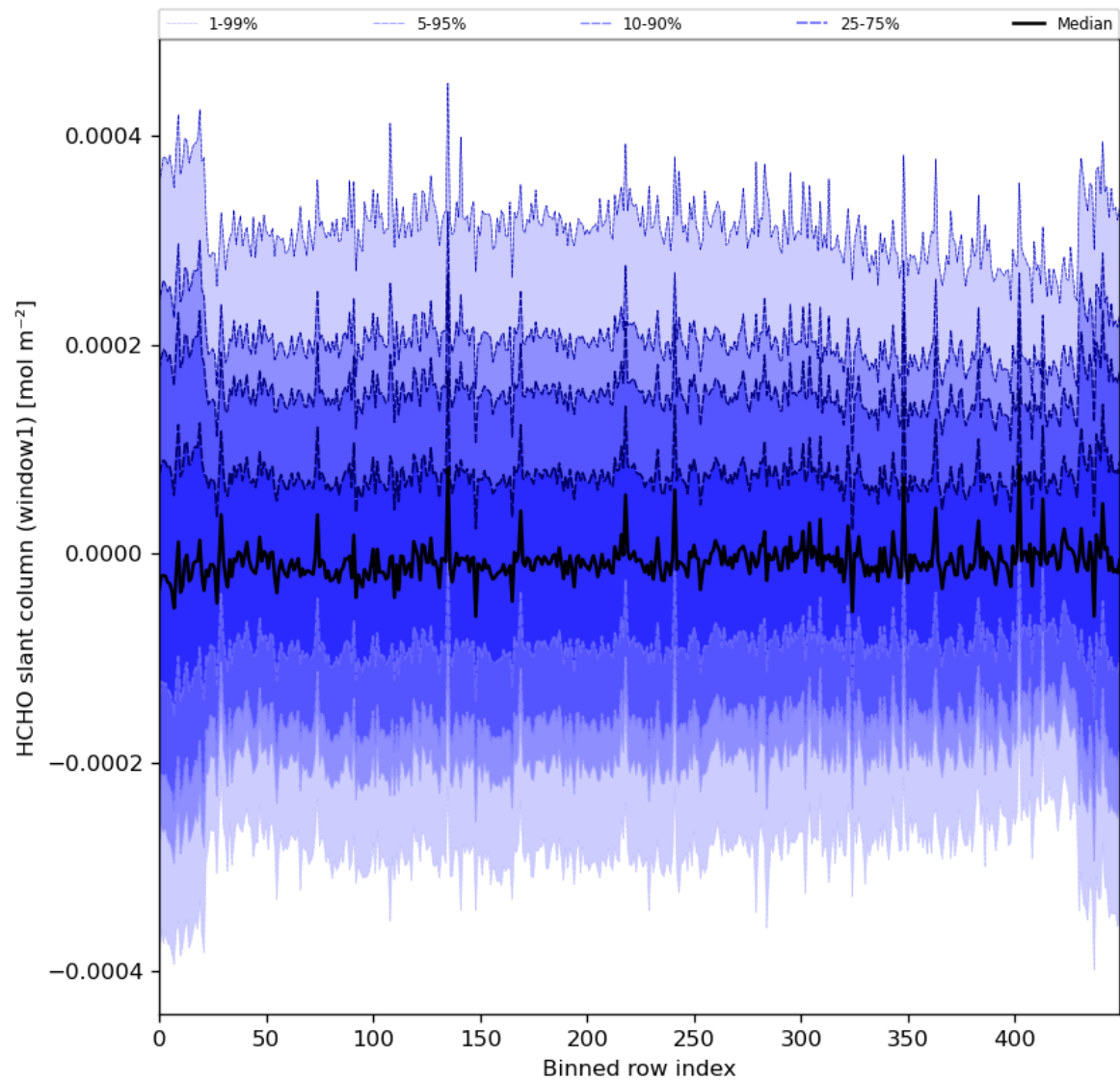
Figure 52: Along track statistics of “HCHO slant column (window1)” for 2024-01-11 to 2024-01-13
