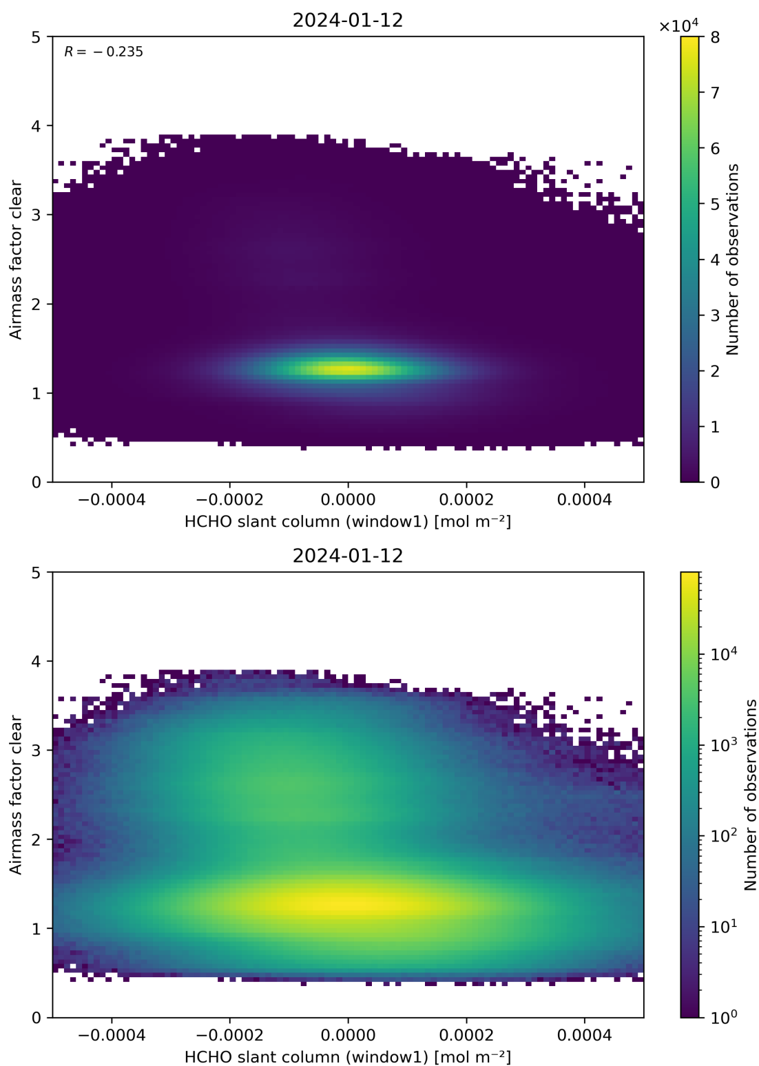
Figure 81: Scatter density plot of “HCHO slant column (window1)” against “Airmass factor clear” for 2024-01-11 to 2024-01-13.
