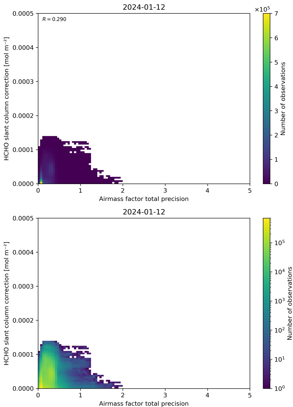
Figure 110: Scatter density plot of “Airmass factor total precision” against “HCHO slant column correction” for 2024-01-11 to 2024-01-13.
