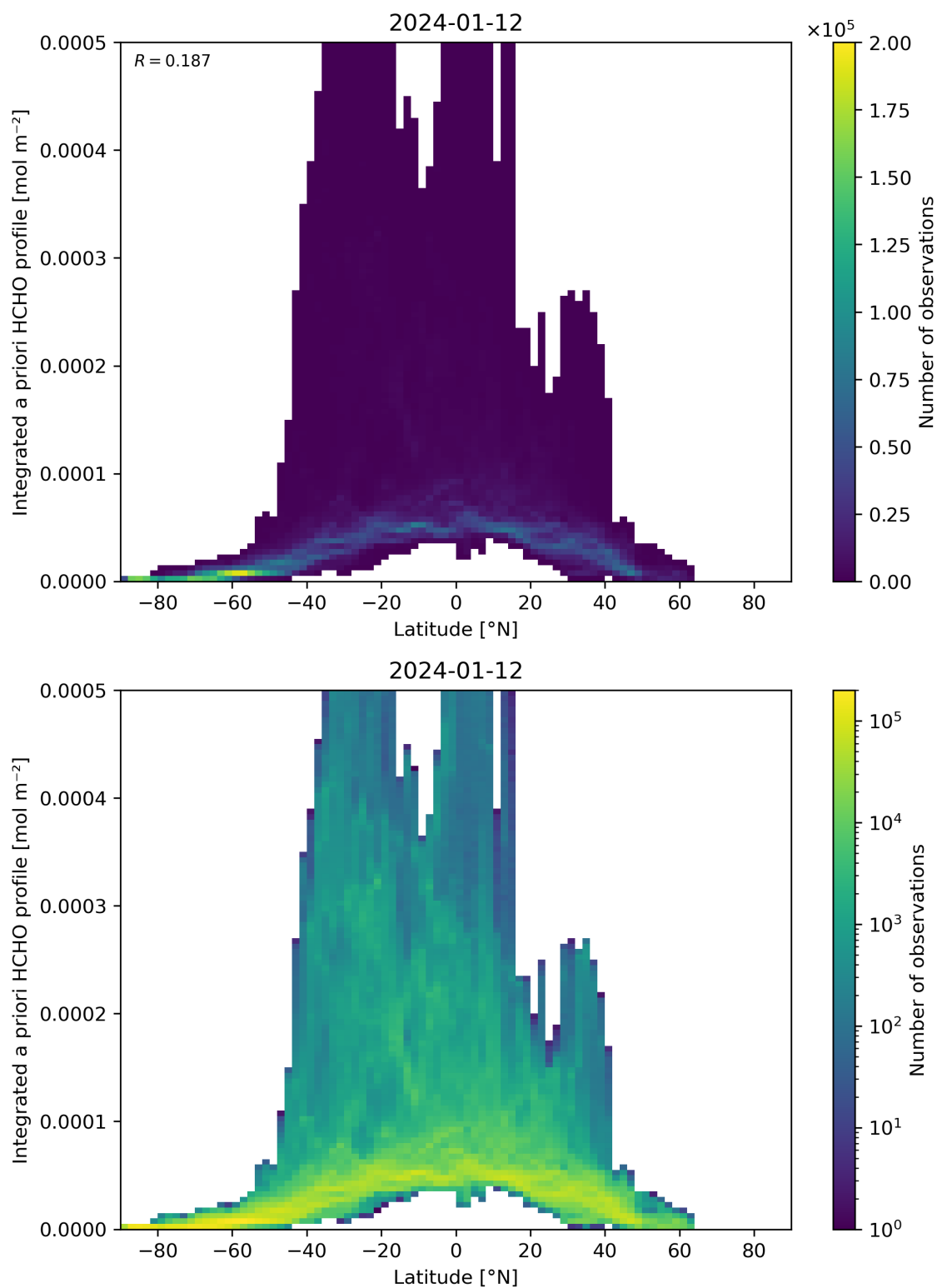
Figure 166: Scatter density plot of “Latitude” against “Integrated a priori HCHO profile” for 2024-01-11 to 2024-01-13.
