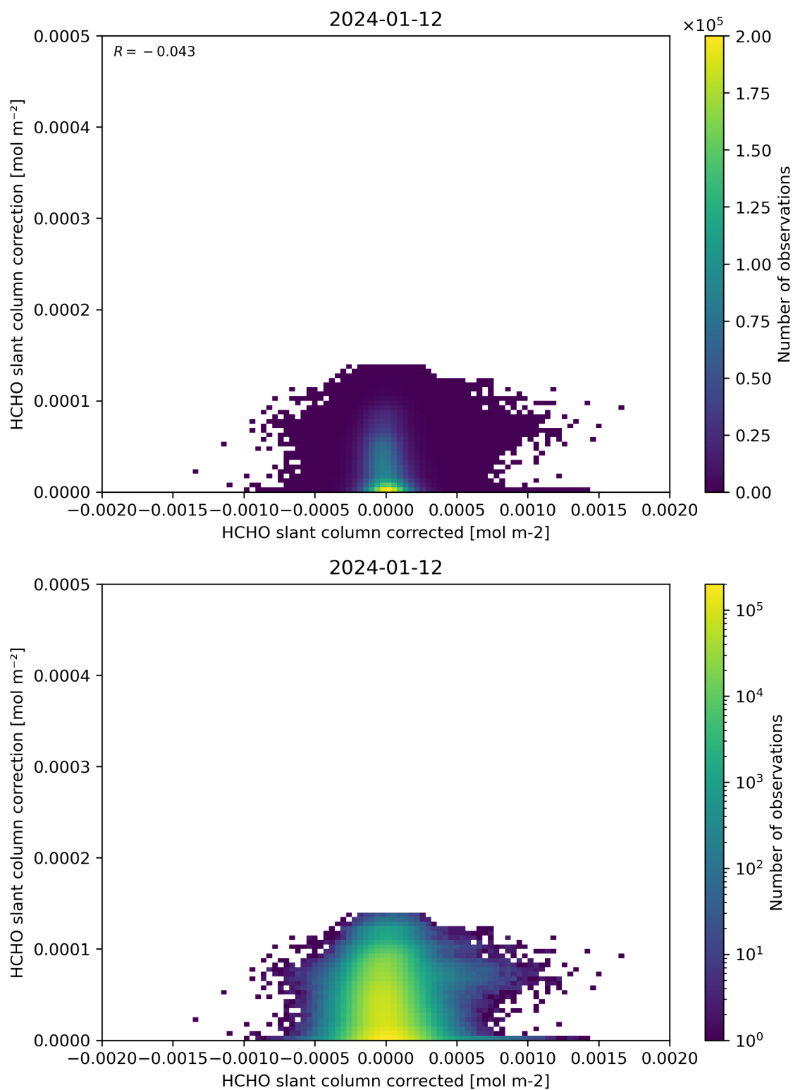
Figure 77: Scatter density plot of “HCHO slant column corrected” against “HCHO slant column correction” for 2024-01-11 to 2024-01-13.
