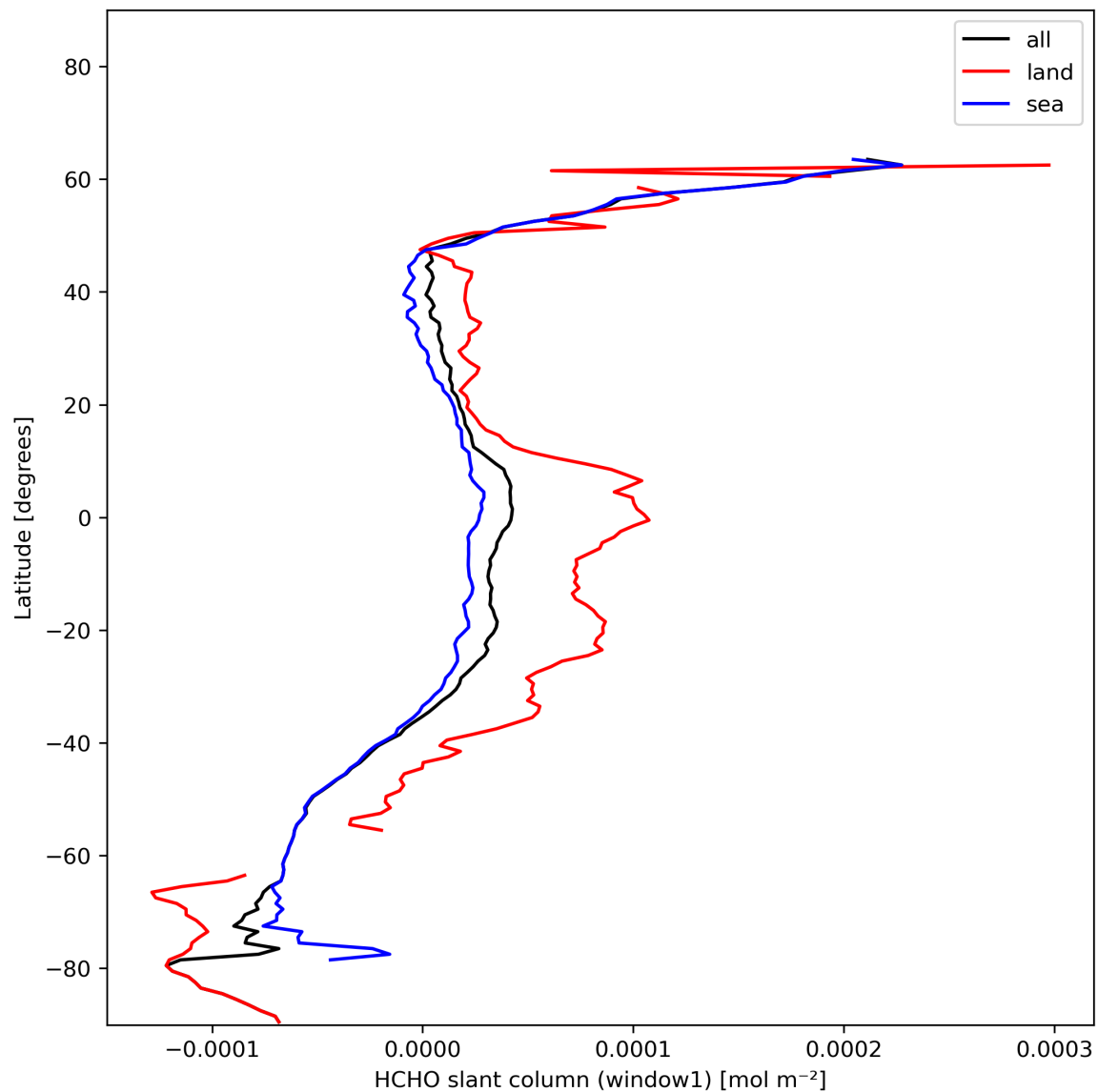
Figure 24: Zonal average of “HCHO slant column (window1)” for 2024-01-11 to 2024-01-13.
