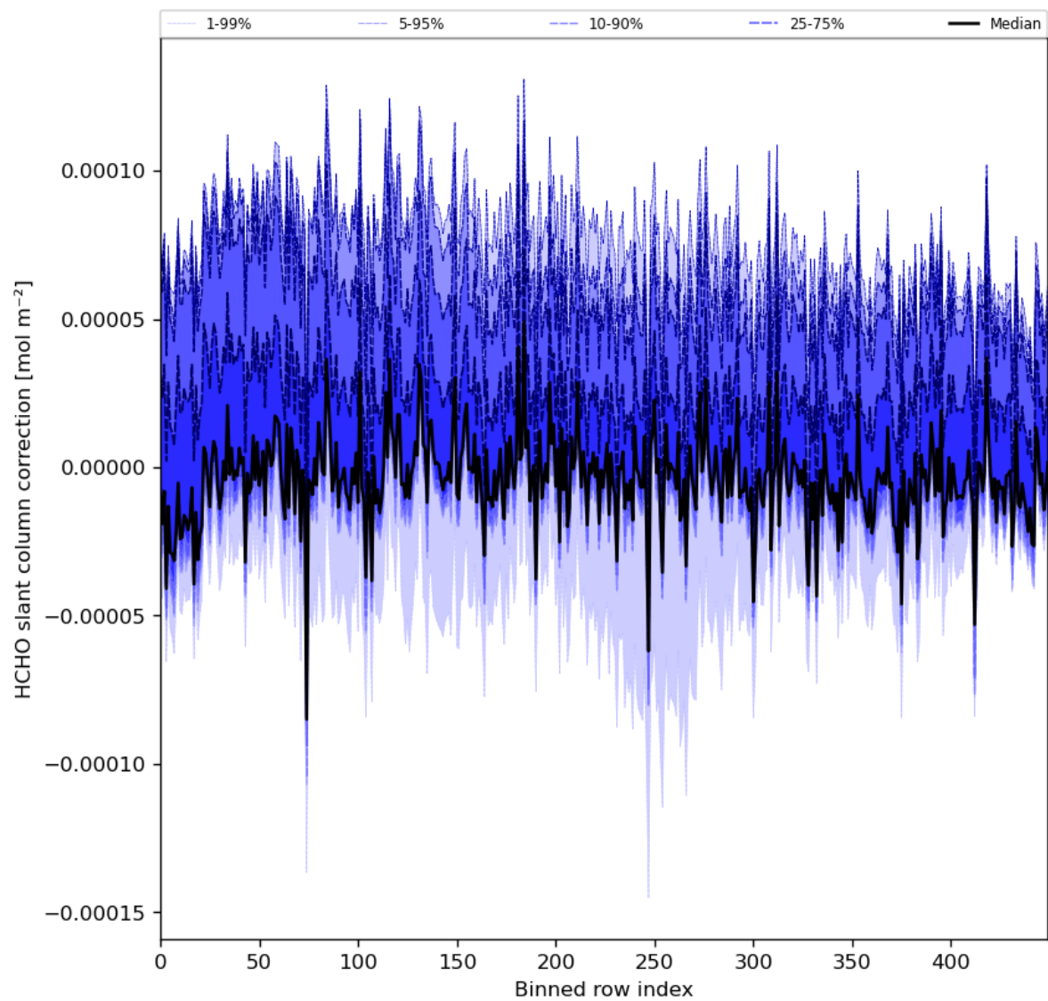
Figure 61: Along track statistics of “HCHO slant column correction” for 2024-01-11 to 2024-01-13
