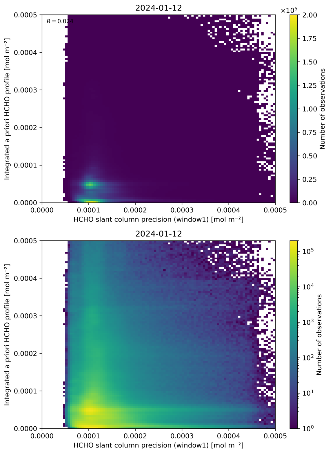
Figure 96: Scatter density plot of “HCHO slant column precision (window1)” against “Integrated a priori HCHO profile” for 2024-01-11 to 2024-01-13.
