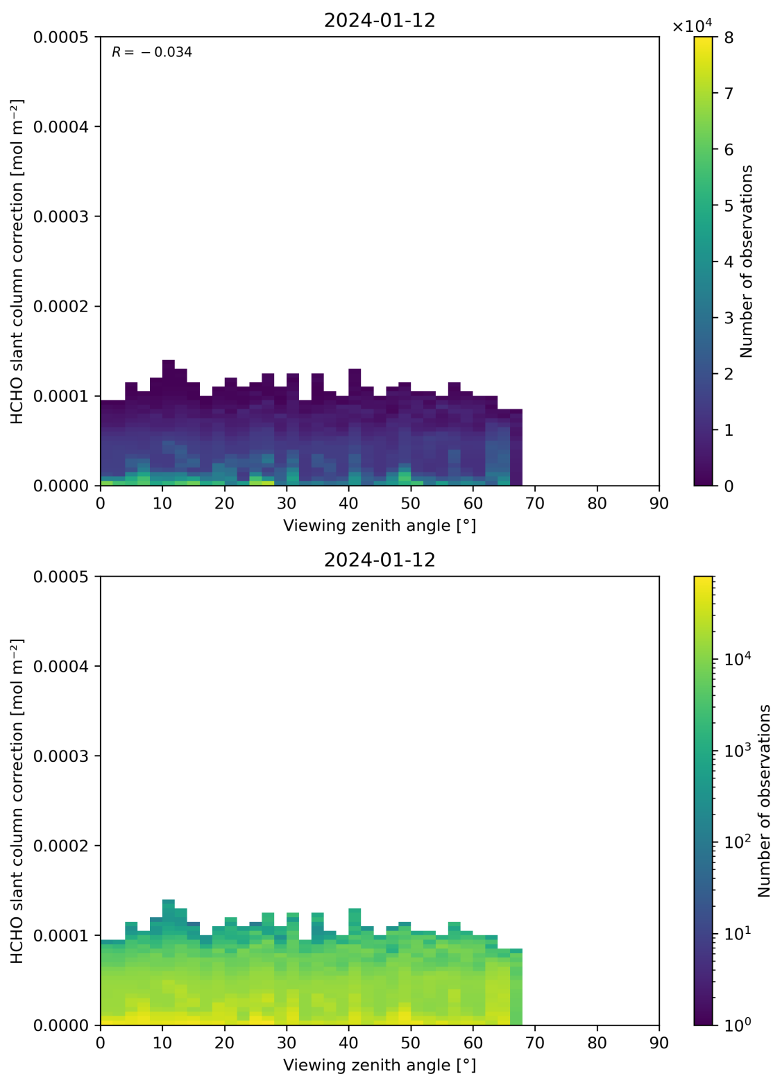
Figure 187: Scatter density plot of “Viewing zenith angle” against “HCHO slant column correction” for 2024-01-11 to 2024-01-13.
