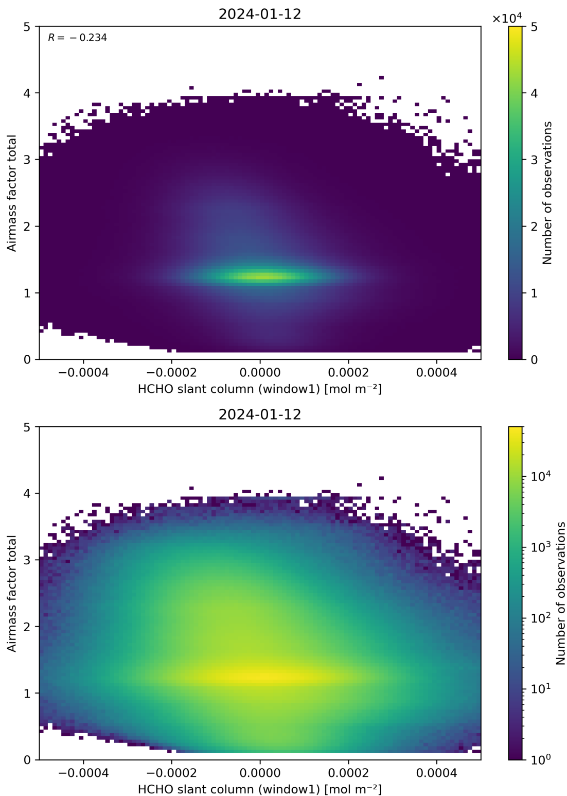
Figure 85: Scatter density plot of “HCHO slant column (window1)” against “Airmass factor total” for 2024-01-11 to 2024-01-13.
