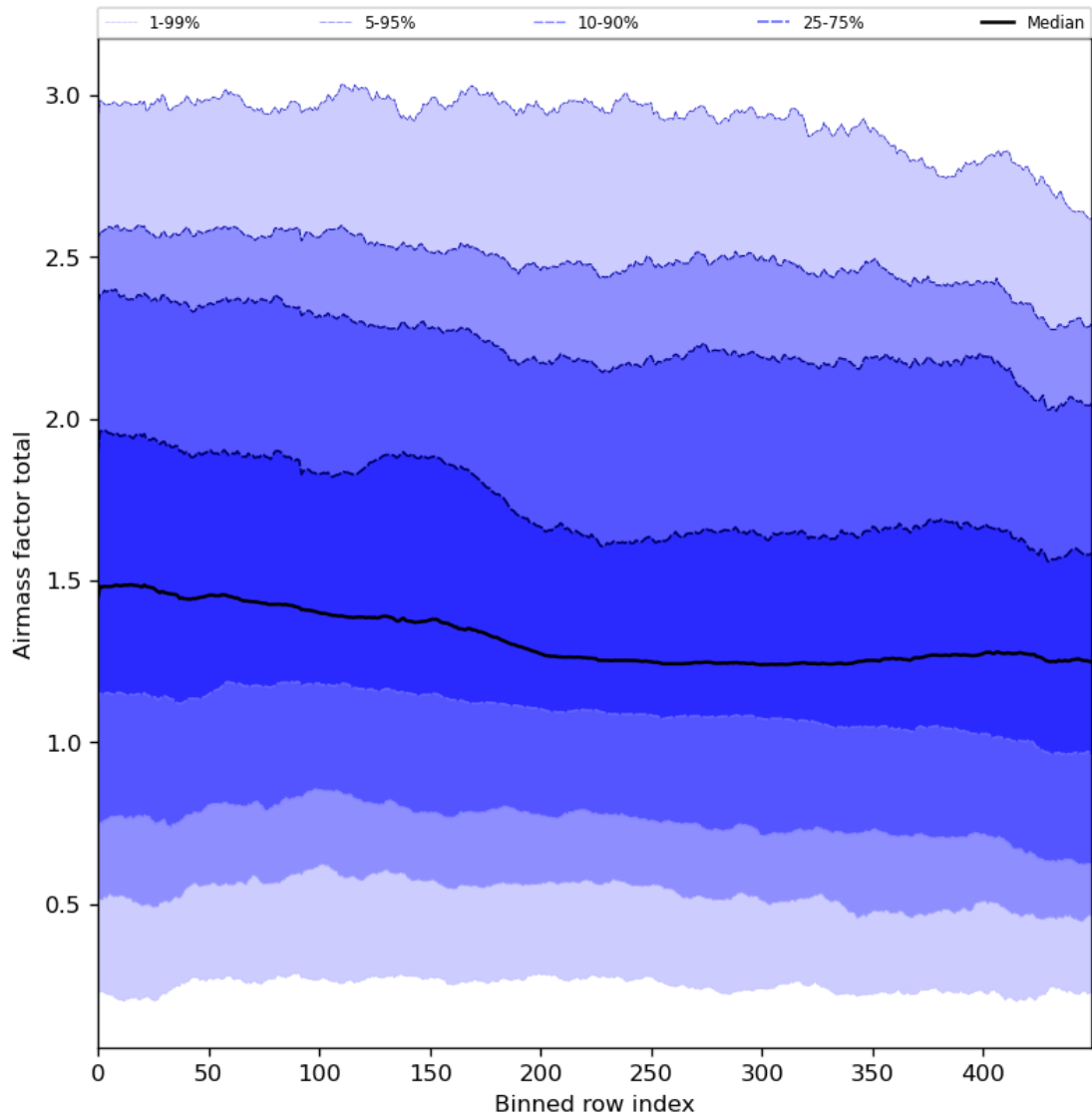
Figure 54: Along track statistics of “Airmass factor total” for 2024-01-11 to 2024-01-13
