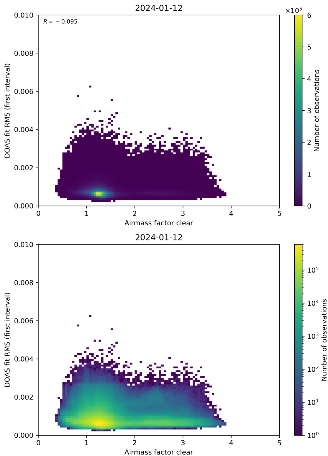
Figure 71: Scatter density plot of “Airmass factor clear” against “DOAS fit RMS (first interval)” for 2024-01-11 to 2024-01-13.
