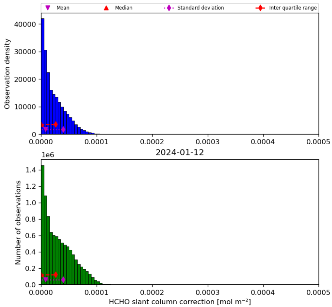
Figure 47: Histogram of “HCHO slant column correction” for 2024-01-11 to 2024-01-13
