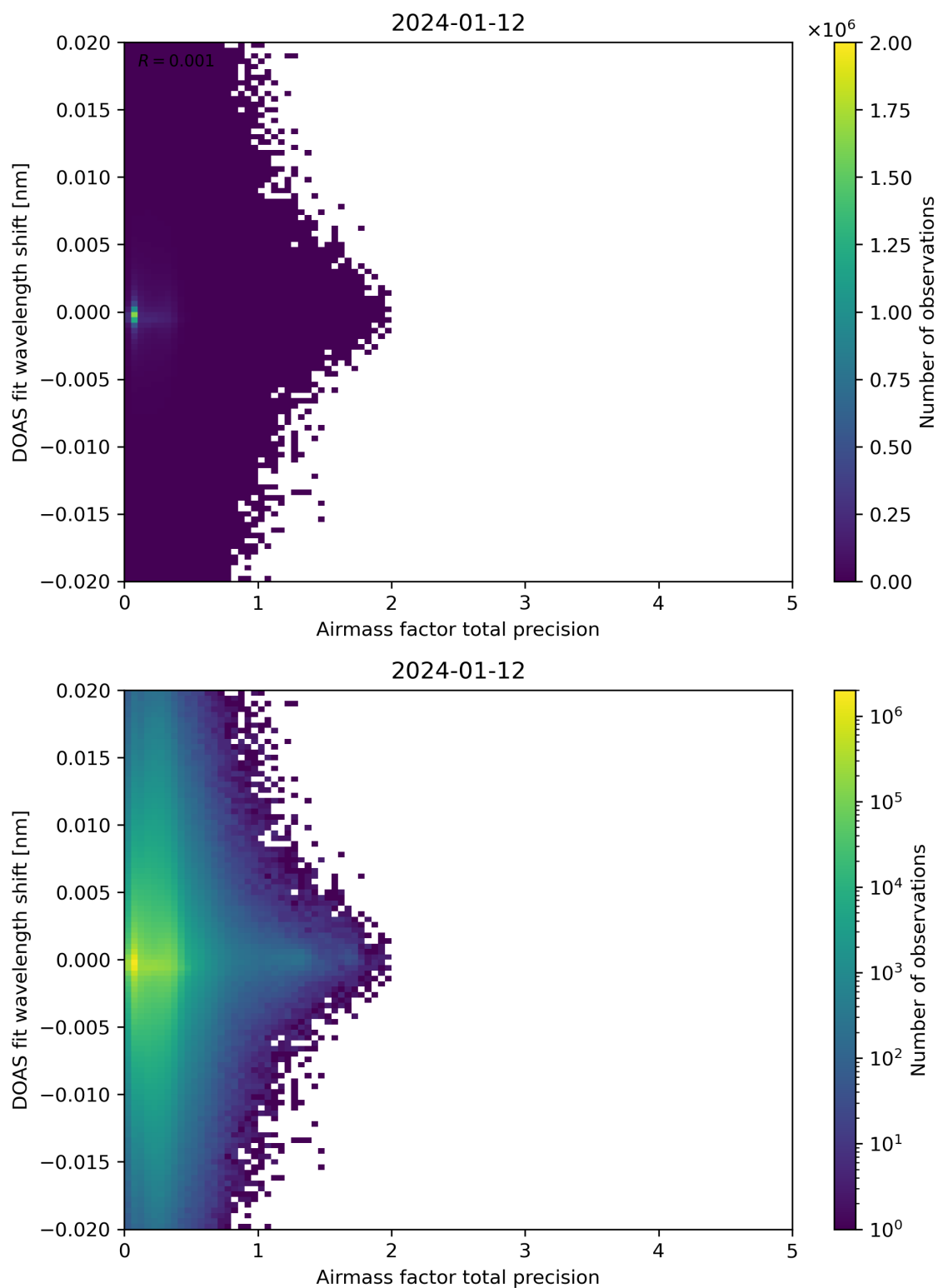
Figure 106: Scatter density plot of “Airmass factor total precision” against “DOAS fit wavelength shift” for 2024-01-11 to 2024-01-13.
