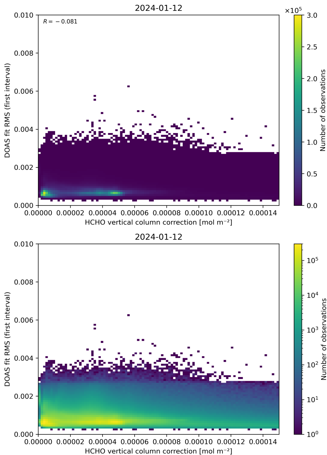
Figure 112: Scatter density plot of “HCHO vertical column correction” against “DOAS fit RMS (first interval)” for 2024-01-11 to 2024-01-13.
