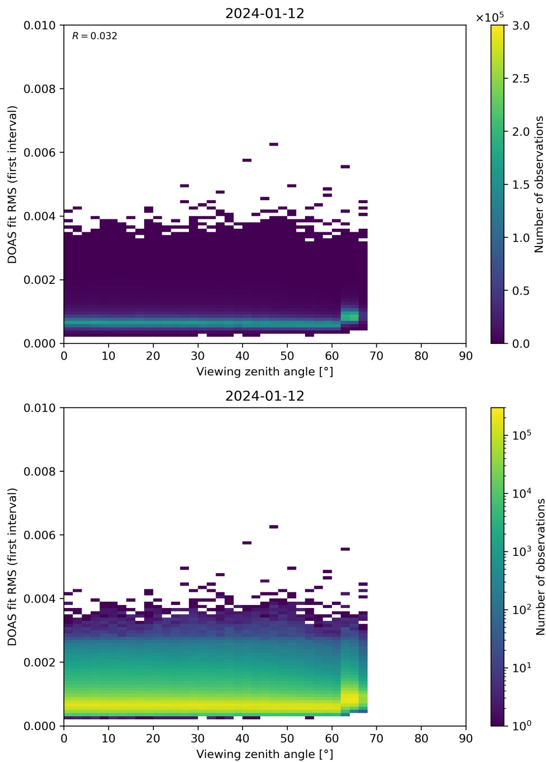
Figure 182: Scatter density plot of “Viewing zenith angle” against “DOAS fit RMS (first interval)” for 2024-01-11 to 2024-01-13.
