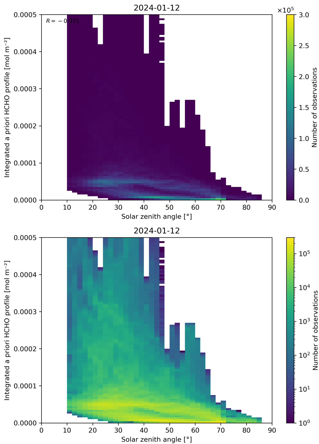
Figure 180: Scatter density plot of “Solar zenith angle” against “Integrated a priori HCHO profile” for 2024-01-11 to 2024-01-13.
