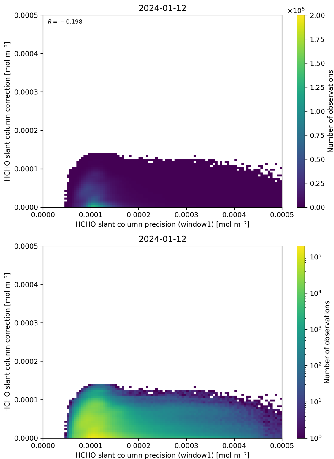
Figure 93: Scatter density plot of “HCHO slant column precision (window1)” against “HCHO slant column correction” for 2024-01-11 to 2024-01-13.
