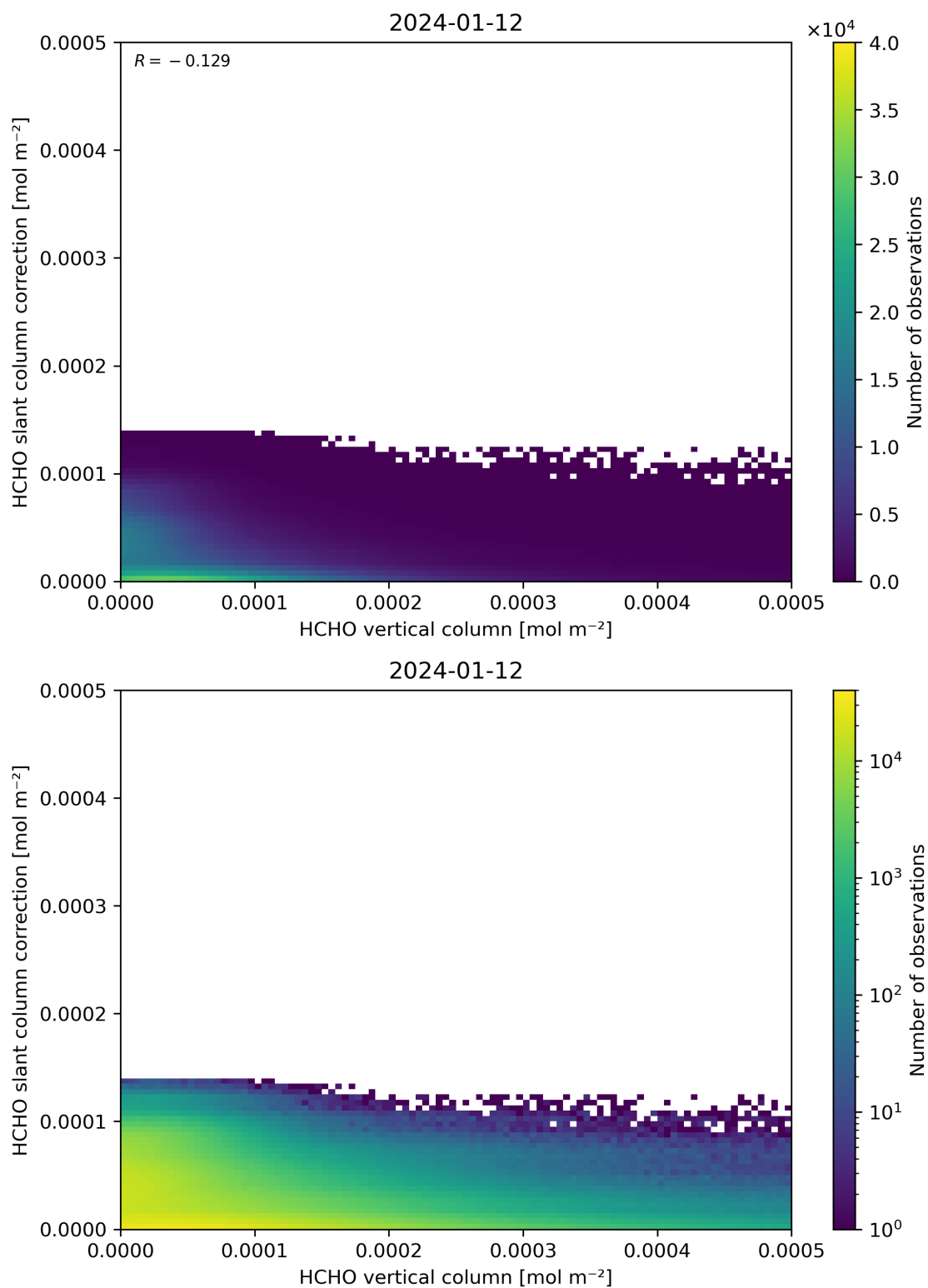
Figure 128: Scatter density plot of “HCHO vertical column” against “HCHO slant column correction” for 2024-01-11 to 2024-01-13.
