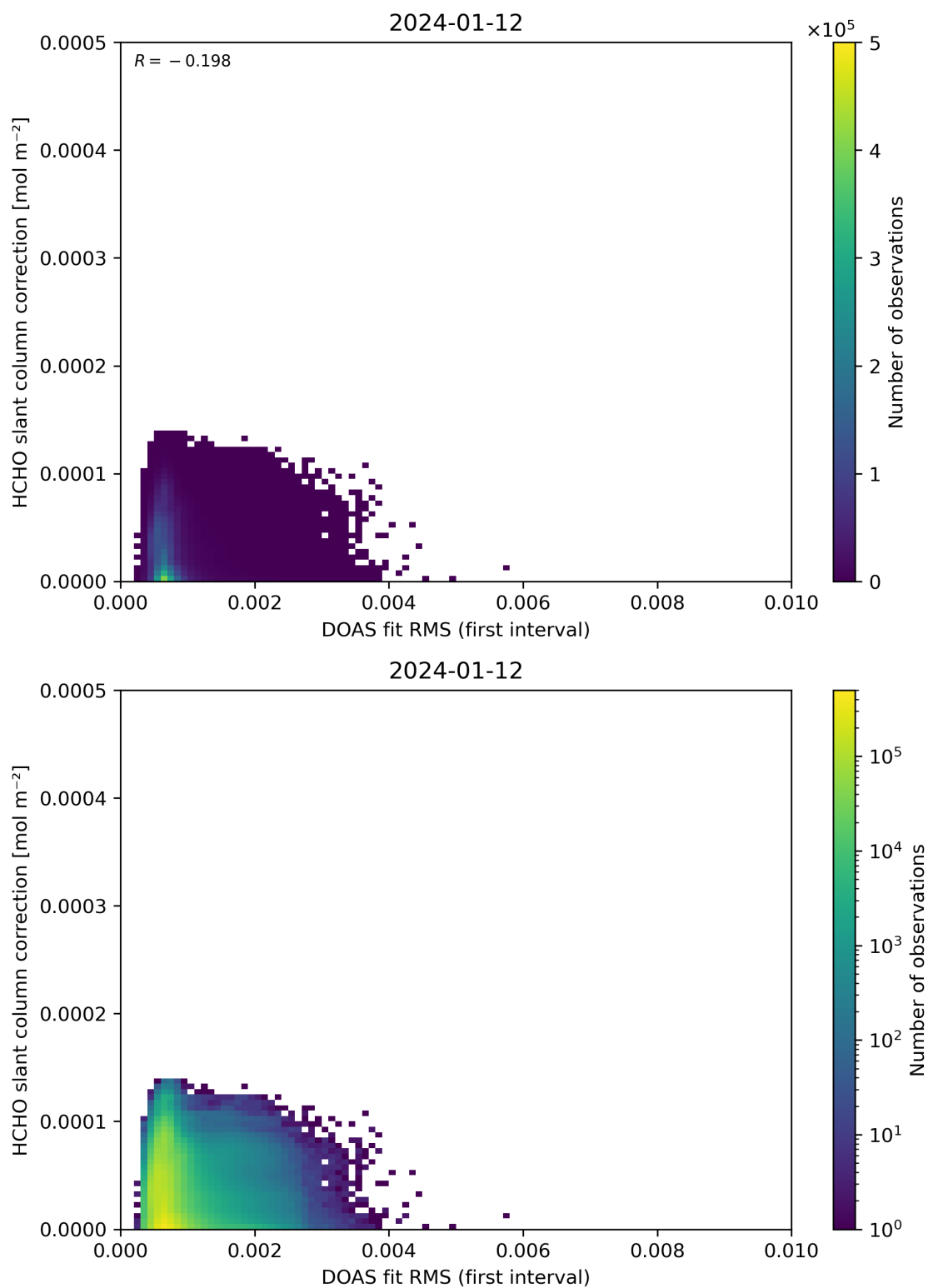
Figure 63: Scatter density plot of “DOAS fit RMS (first interval)” against “HCHO slant column correction” for 2024-01-11 to 2024-01-13.
