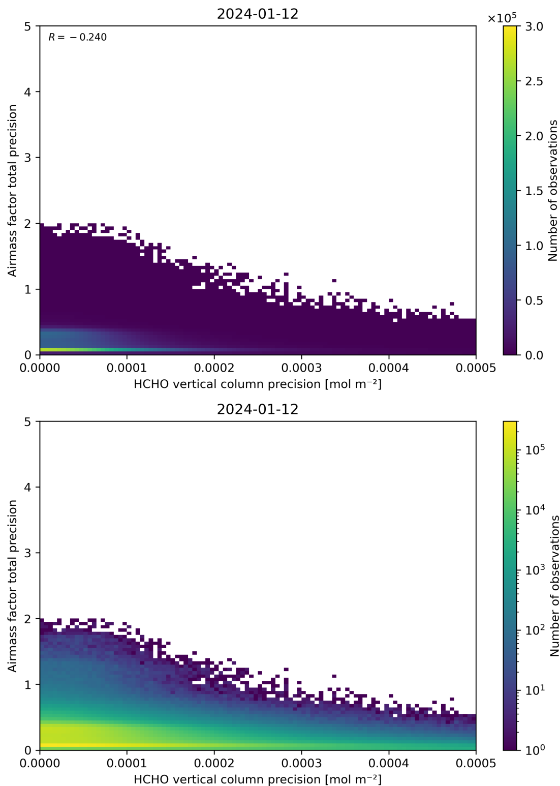
Figure 145: Scatter density plot of “HCHO vertical column precision” against “Airmass factor total precision” for 2024-01-11 to 2024-01-13.
