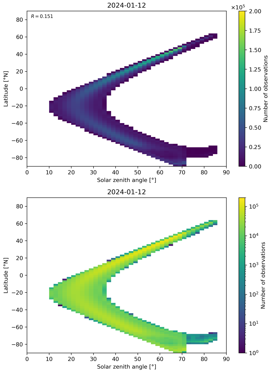
Figure 181: Scatter density plot of “Solar zenith angle” against “Latitude” for 2024-01-11 to 2024-01-13.
