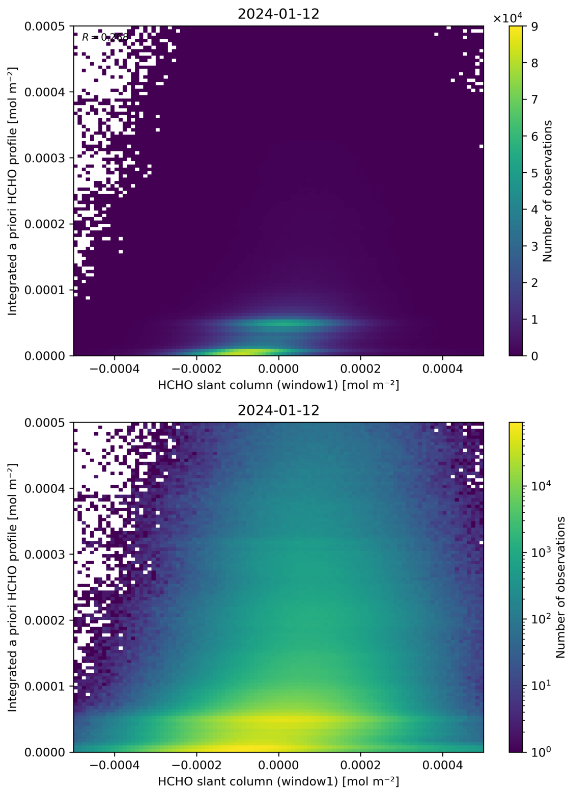
Figure 87: Scatter density plot of “HCHO slant column (window1)” against “Integrated a priori HCHO profile” for 2024-01-11 to 2024-01-13.
