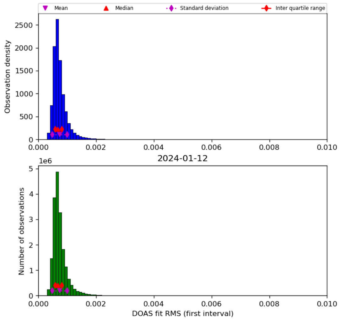
Figure 46: Histogram of “DOAS fit RMS (first interval)” for 2024-01-11 to 2024-01-13
