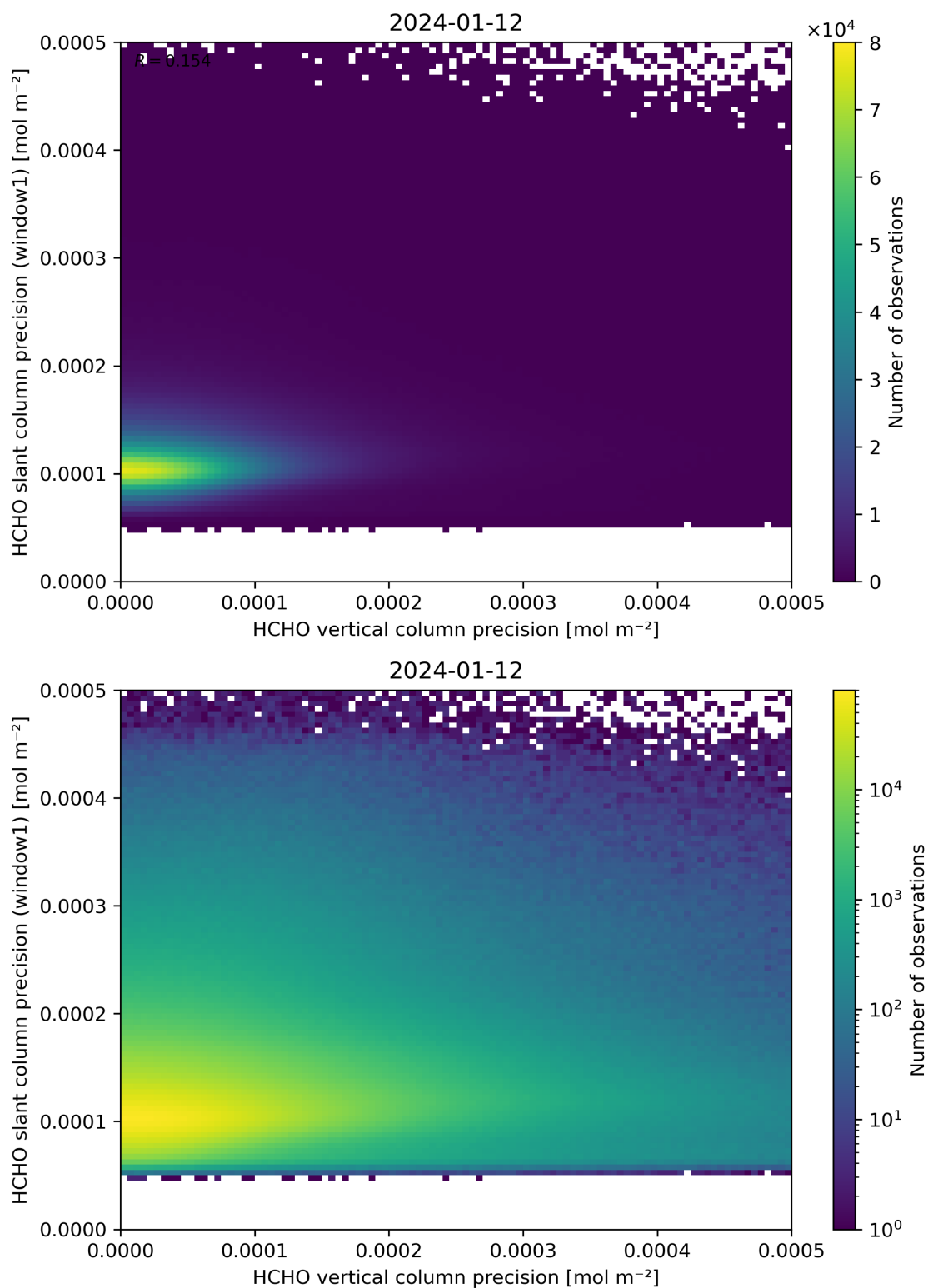
Figure 143: Scatter density plot of “HCHO vertical column precision” against “HCHO slant column precision (window1)” for 2024-01-11 to 2024-01-13.
