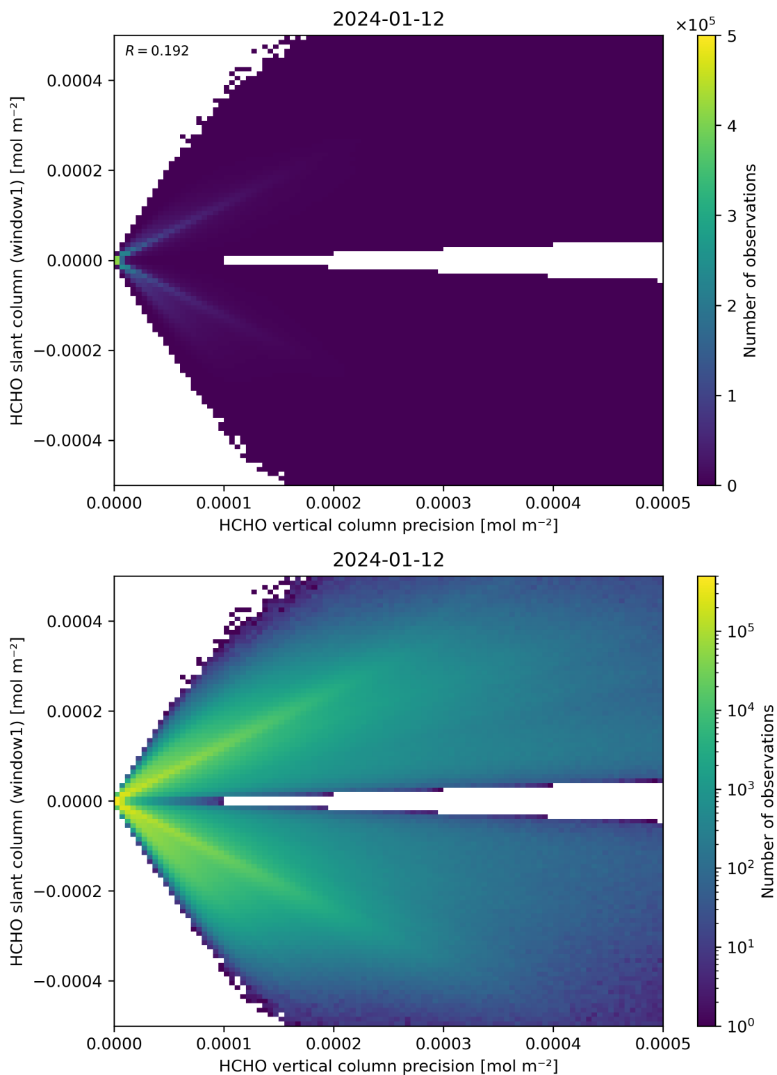
Figure 142: Scatter density plot of “HCHO vertical column precision” against “HCHO slant column (window1)” for 2024-01-11 to 2024-01-13.
