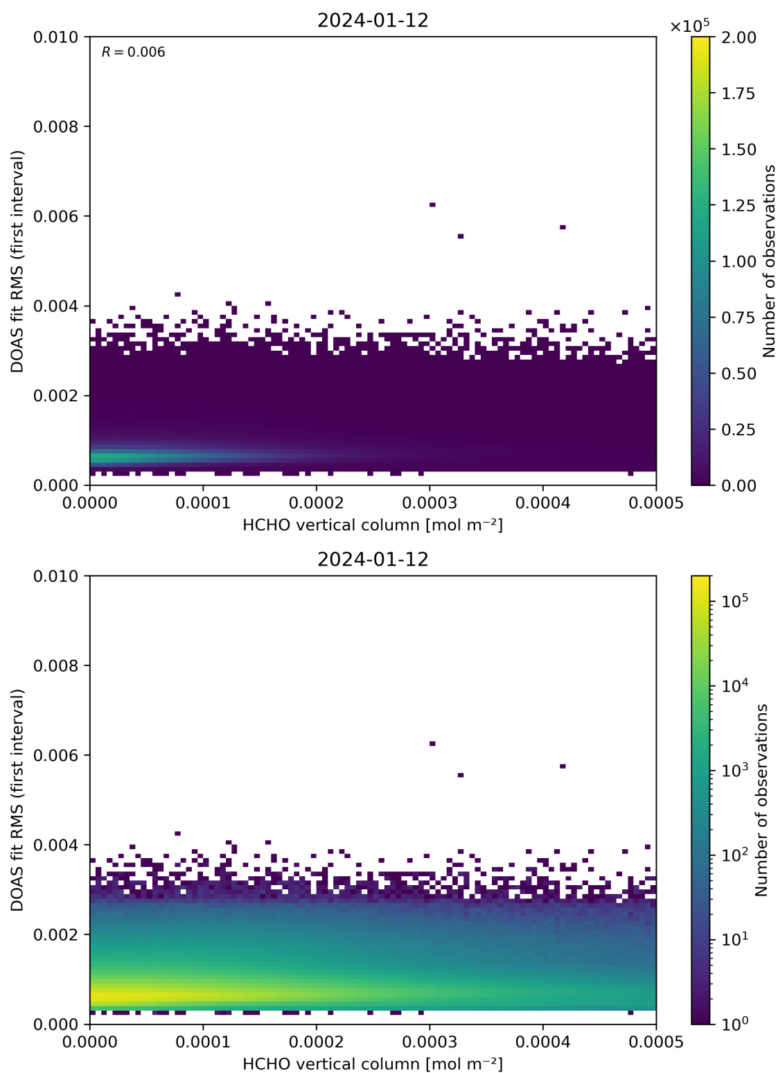
Figure 123: Scatter density plot of “HCHO vertical column” against “DOAS fit RMS (first interval)” for 2024-01-11 to 2024-01-13.
