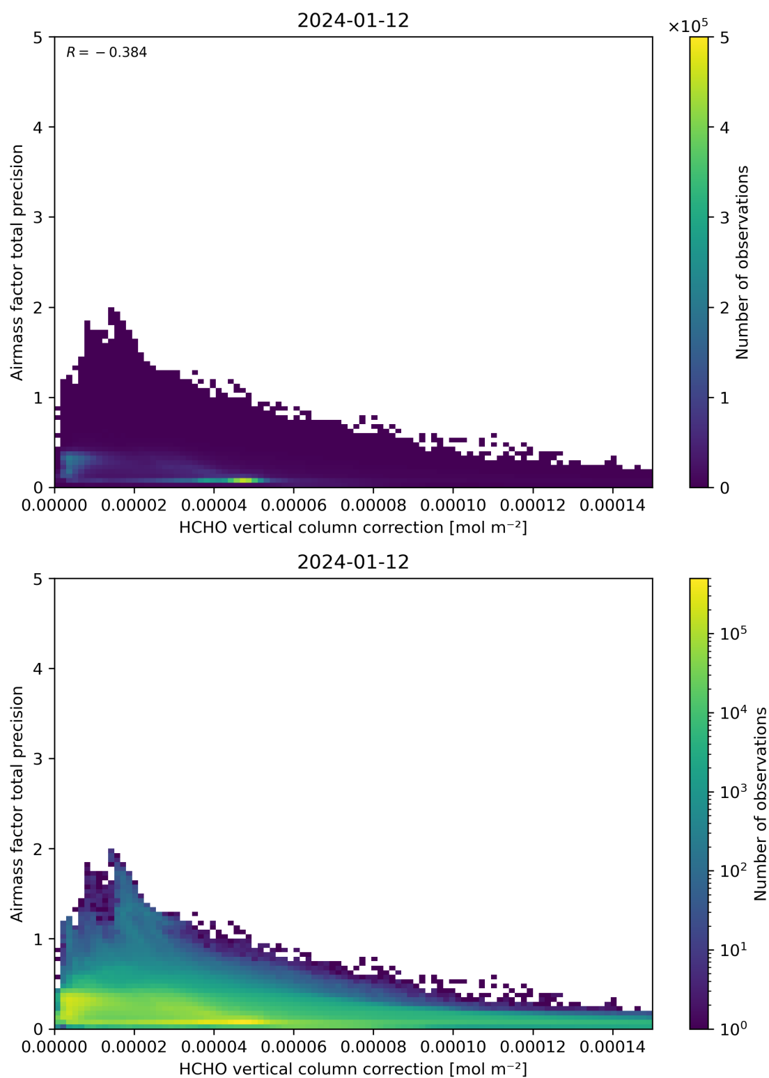
Figure 121: Scatter density plot of “HCHO vertical column correction” against “Airmass factor total precision” for 2024-01-11 to 2024-01-13.
