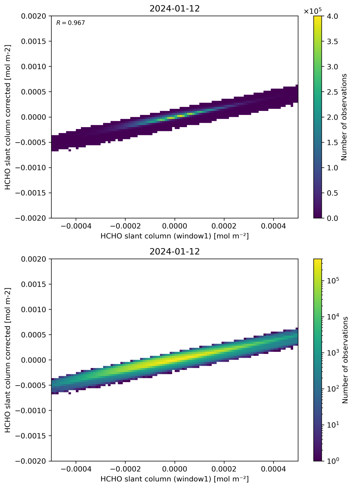
Figure 82: Scatter density plot of “HCHO slant column (window1)” against “HCHO slant column corrected” for 2024-01-11 to 2024-01-13.
