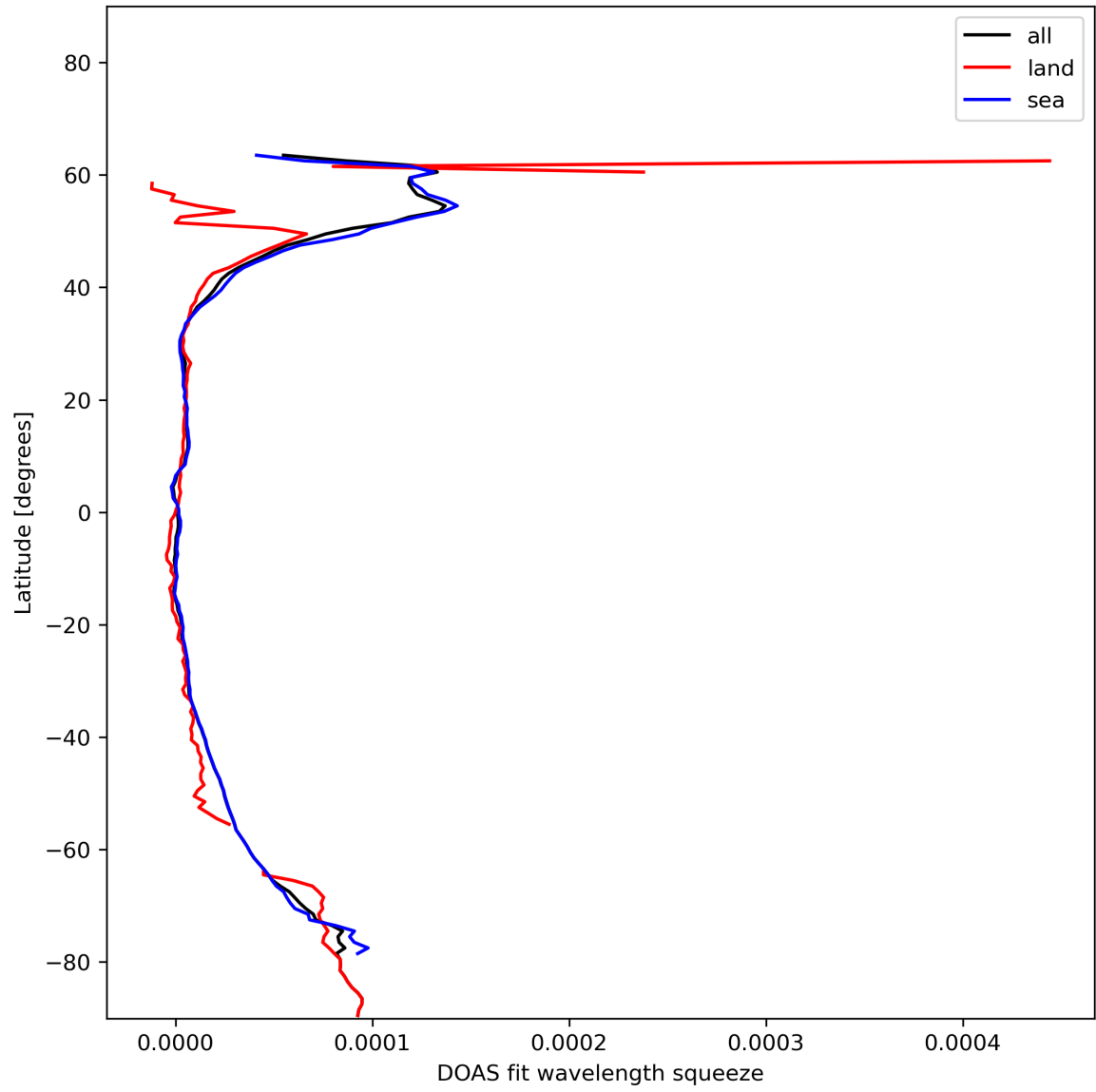
Figure 31: Zonal average of “DOAS fit wavelength squeeze” for 2024-01-11 to 2024-01-13.
