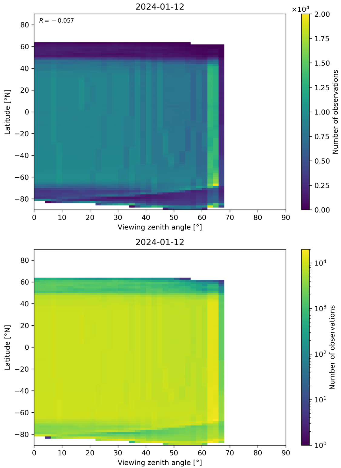
Figure 196: Scatter density plot of “Viewing zenith angle” against “Latitude” for 2024-01-11 to 2024-01-13.
