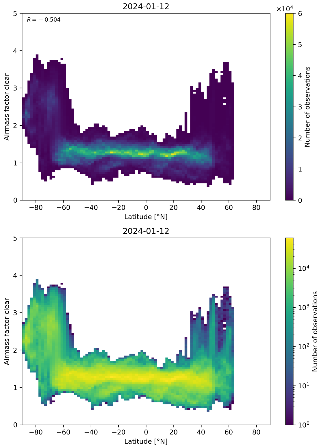
Figure 156: Scatter density plot of “Latitude” against “Airmass factor clear” for 2024-01-11 to 2024-01-13.
