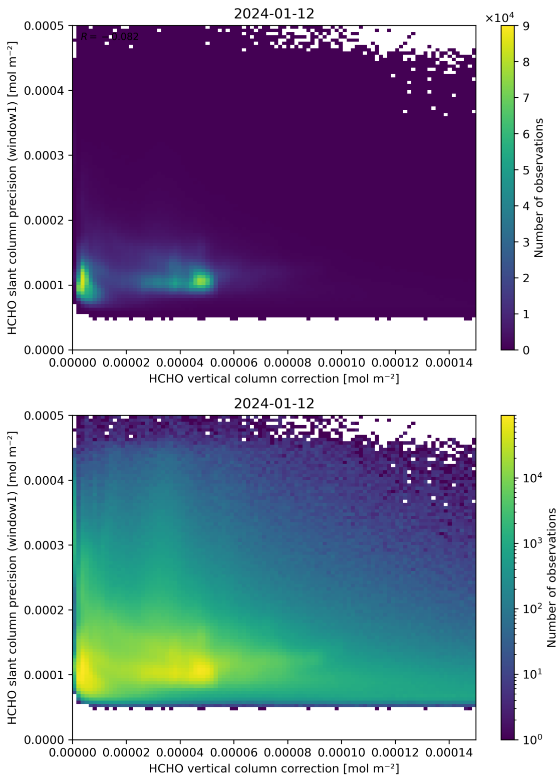
Figure 119: Scatter density plot of “HCHO vertical column correction” against “HCHO slant column precision (window1)” for 2024-01-11 to 2024-01-13.
