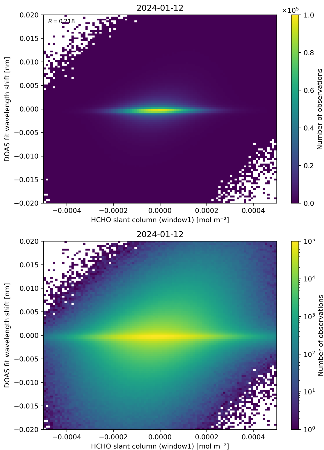
Figure 79: Scatter density plot of “HCHO slant column (window1)” against “DOAS fit wavelength shift” for 2024-01-11 to 2024-01-13.
