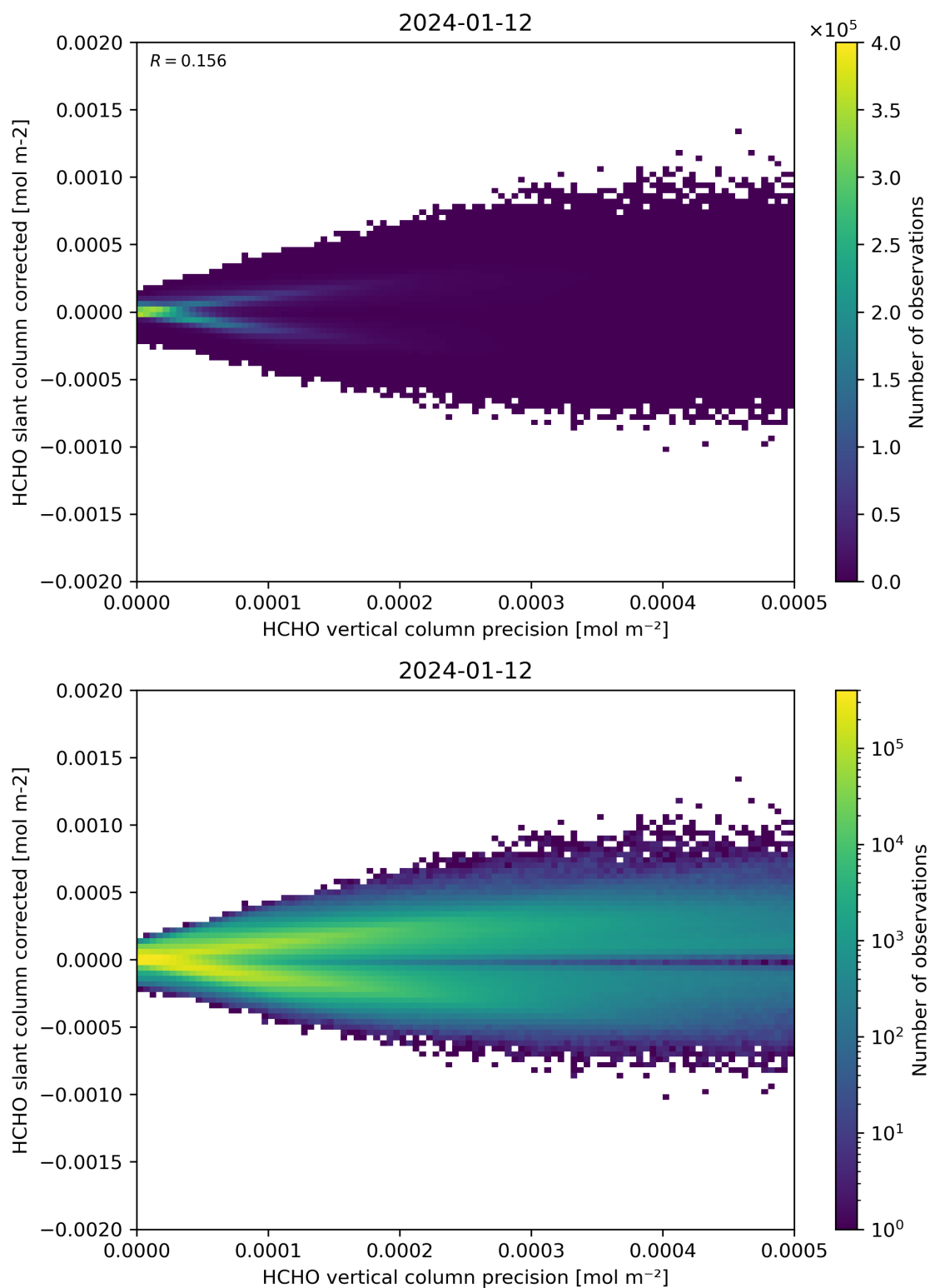
Figure 140: Scatter density plot of “HCHO vertical column precision” against “HCHO slant column corrected” for 2024-01-11 to 2024-01-13.
