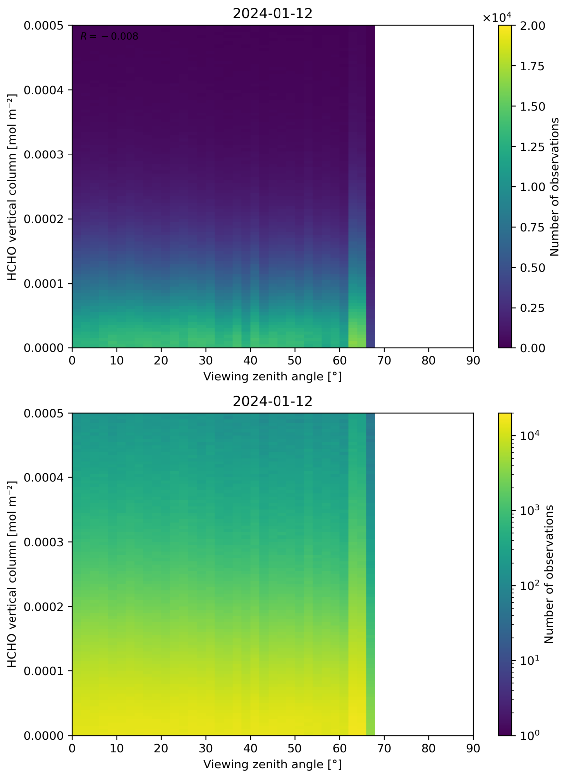
Figure 192: Scatter density plot of “Viewing zenith angle” against “HCHO vertical column” for 2024-01-11 to 2024-01-13.
