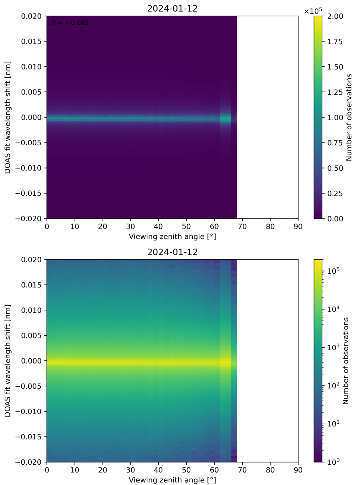
Figure 183: Scatter density plot of “Viewing zenith angle” against “DOAS fit wavelength shift” for 2024-01-11 to 2024-01-13.
