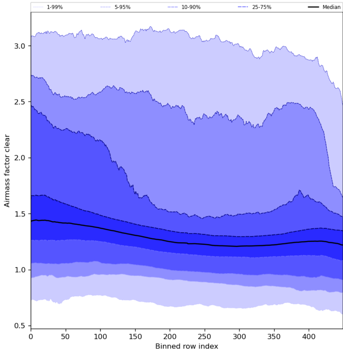
Figure 56: Along track statistics of “Airmass factor clear” for 2024-01-11 to 2024-01-13
