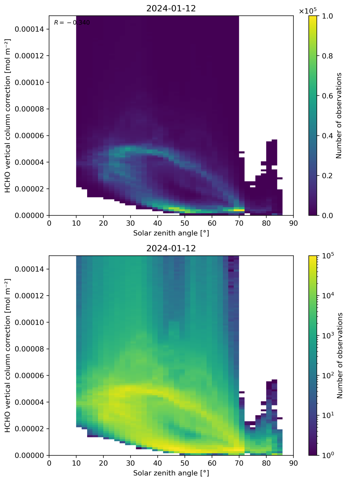
Figure 178: Scatter density plot of “Solar zenith angle” against “HCHO vertical column correction” for 2024-01-11 to 2024-01-13.
