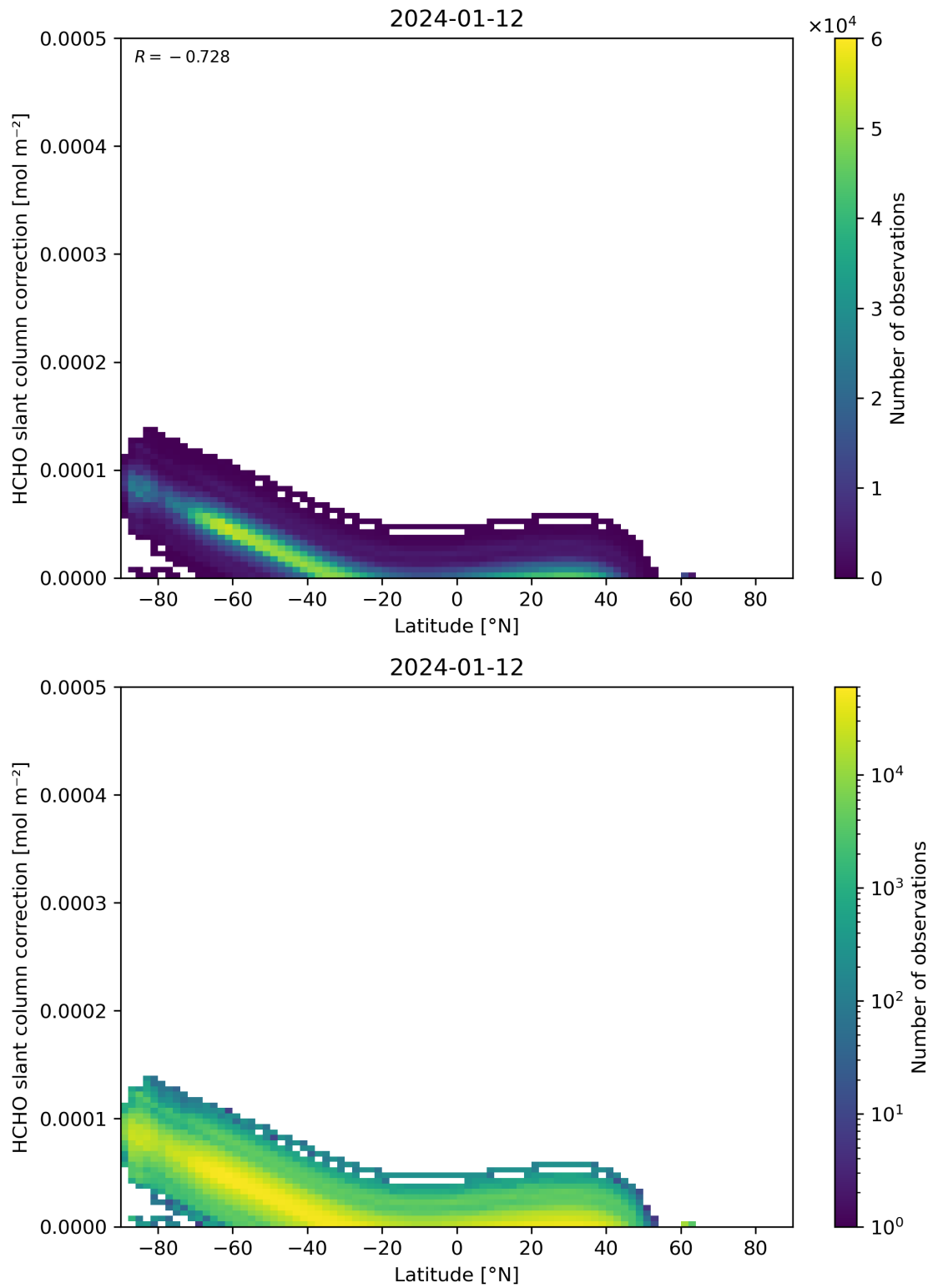
Figure 158: Scatter density plot of “Latitude” against “HCHO slant column correction” for 2024-01-11 to 2024-01-13.
