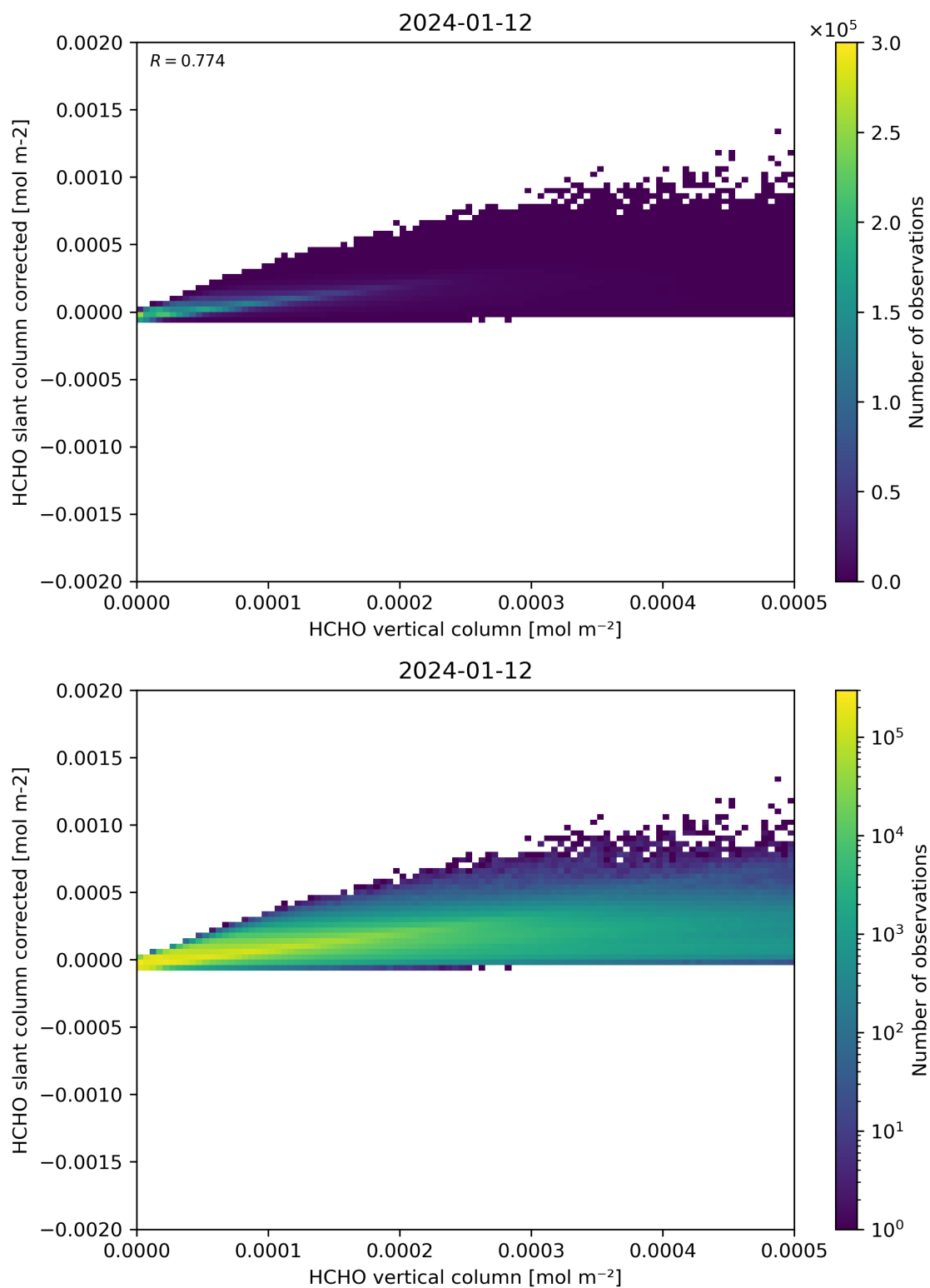
Figure 127: Scatter density plot of “HCHO vertical column” against “HCHO slant column corrected” for 2024-01-11 to 2024-01-13.
