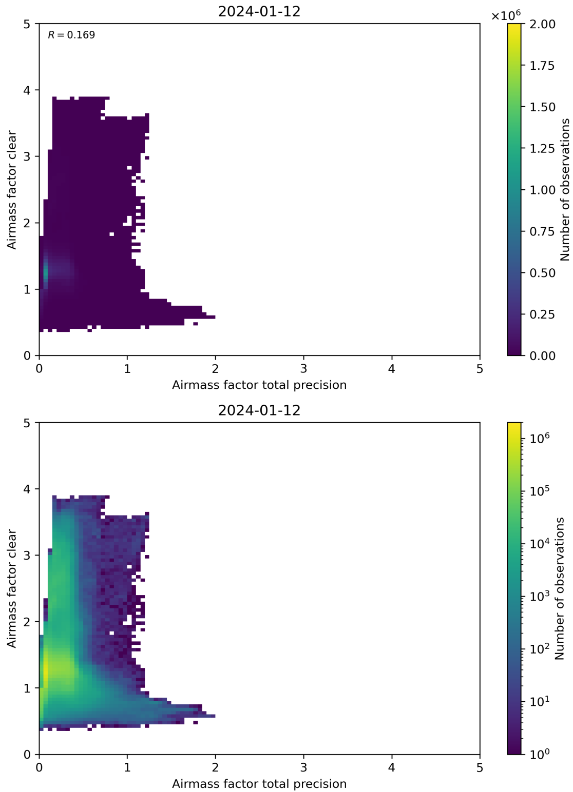
Figure 108: Scatter density plot of “Airmass factor total precision” against “Airmass factor clear” for 2024-01-11 to 2024-01-13.
