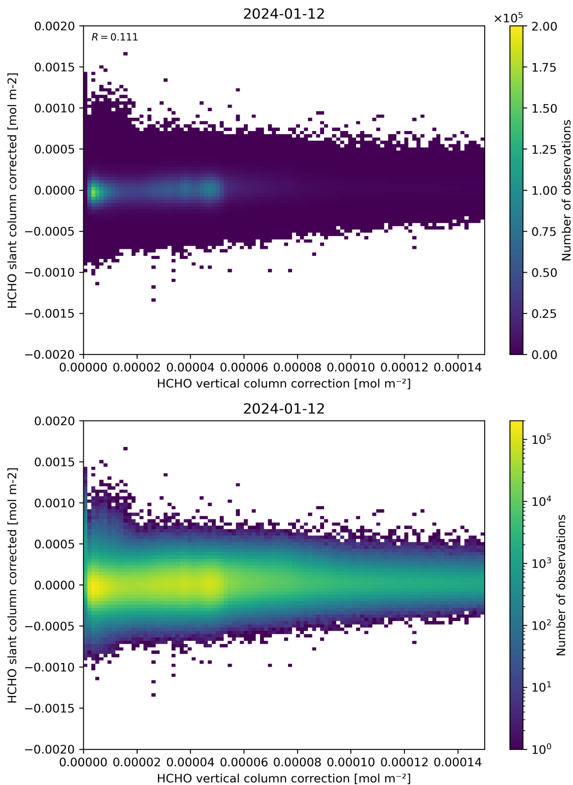
Figure 116: Scatter density plot of “HCHO vertical column correction” against “HCHO slant column corrected” for 2024-01-11 to 2024-01-13.
