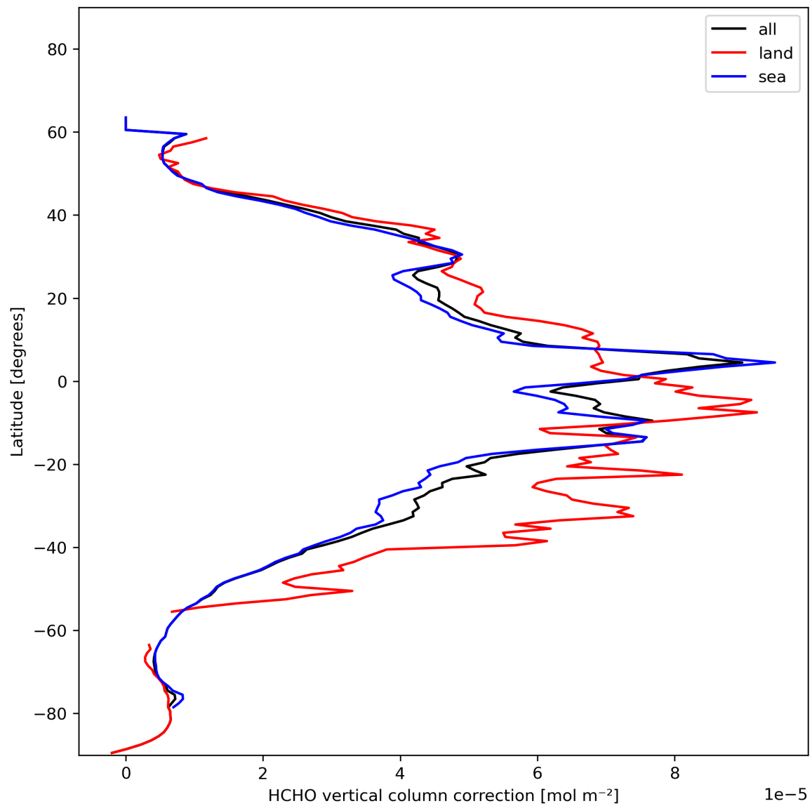
Figure 23: Zonal average of “HCHO vertical column correction” for 2024-01-11 to 2024-01-13.
