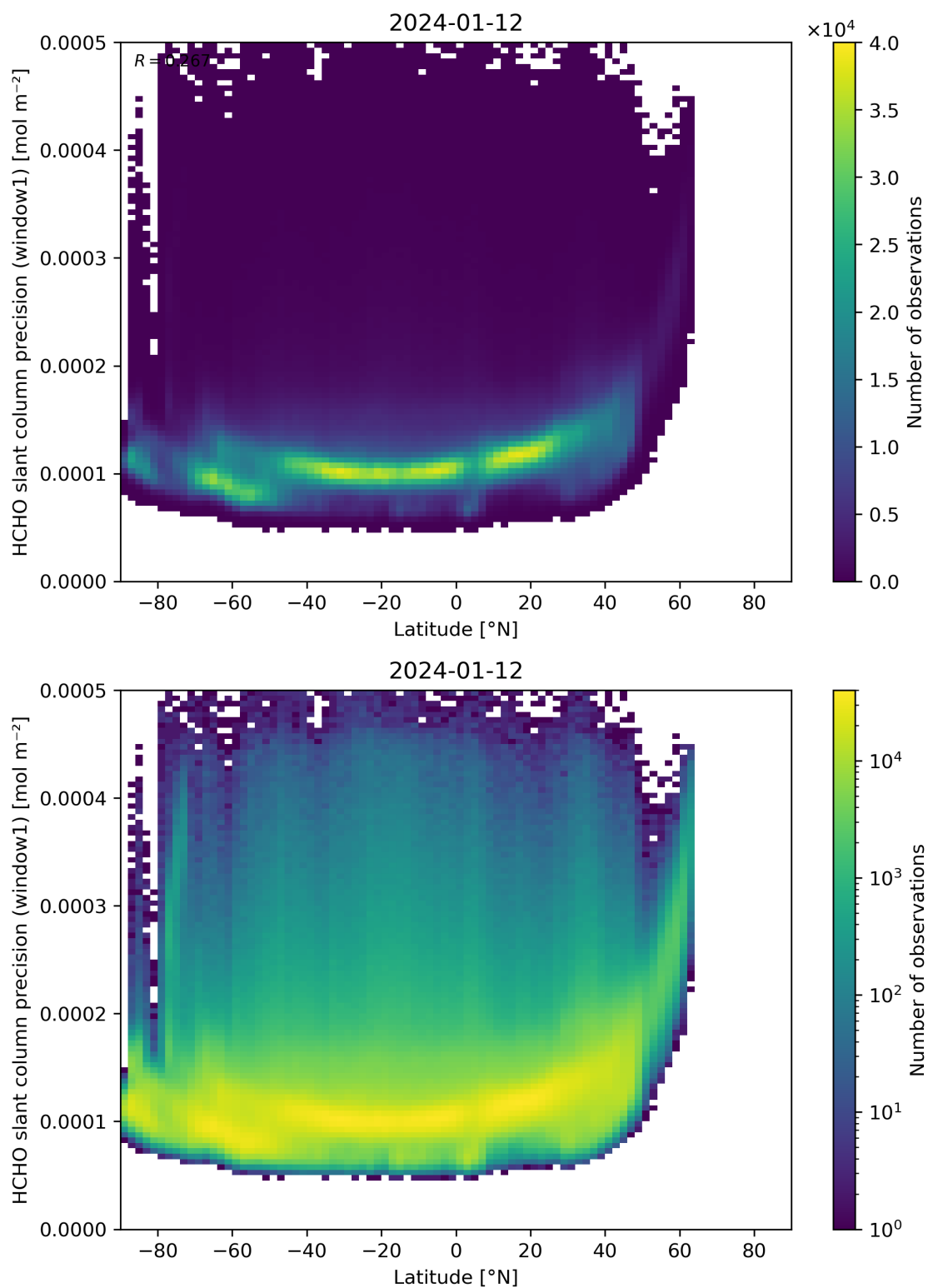
Figure 160: Scatter density plot of “Latitude” against “HCHO slant column precision (window1)” for 2024-01-11 to 2024-01-13.
