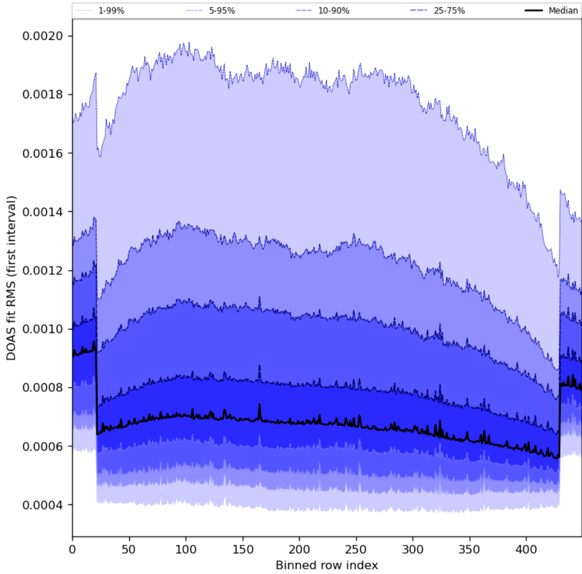
Figure 60: Along track statistics of “DOAS fit RMS (first interval)” for 2024-01-11 to 2024-01-13
