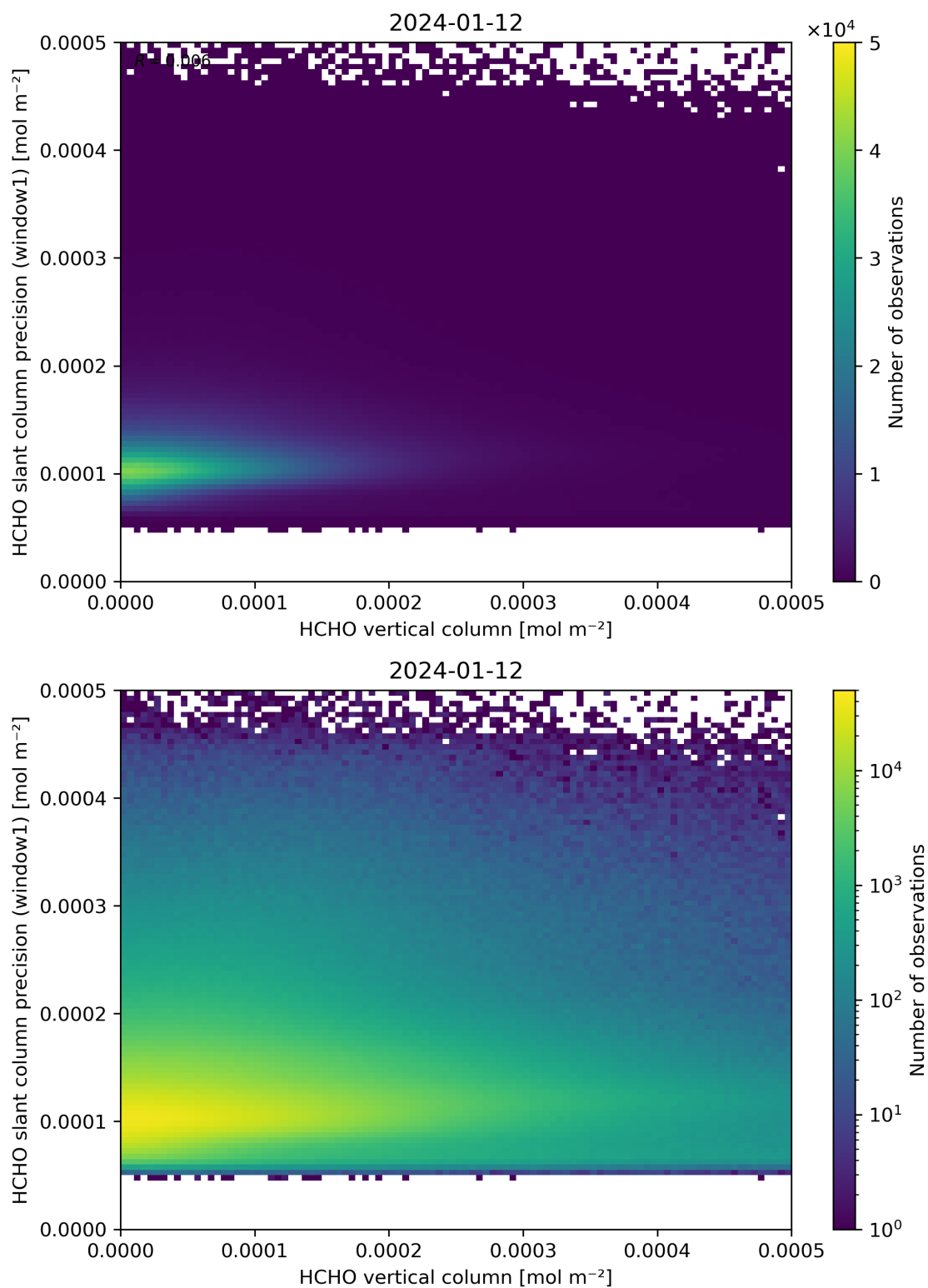
Figure 130: Scatter density plot of “HCHO vertical column” against “HCHO slant column precision (window1)” for 2024-01-11 to 2024-01-13.
