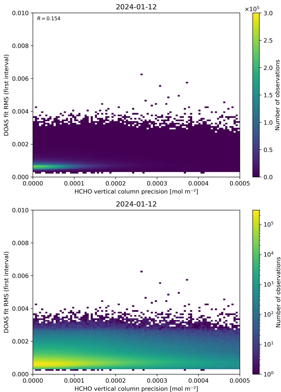
Figure 136: Scatter density plot of “HCHO vertical column precision” against “DOAS fit RMS (first interval)” for 2024-01-11 to 2024-01-13.
