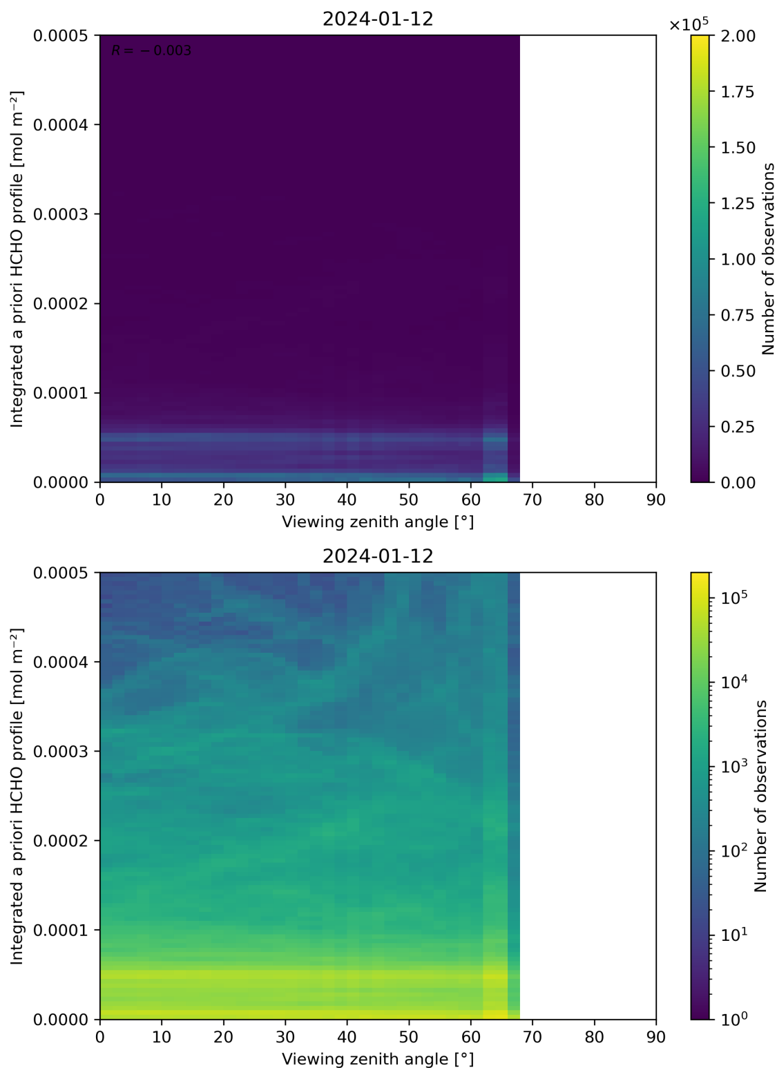
Figure 195: Scatter density plot of “Viewing zenith angle” against “Integrated a priori HCHO profile” for 2024-01-11 to 2024-01-13.
