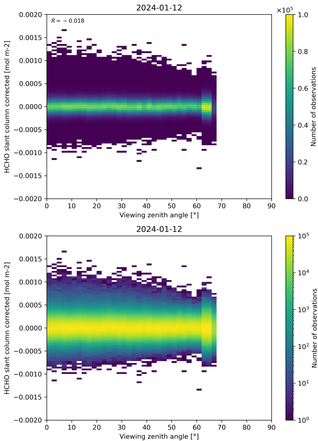
Figure 186: Scatter density plot of “Viewing zenith angle” against “HCHO slant column corrected” for 2024-01-11 to 2024-01-13.
