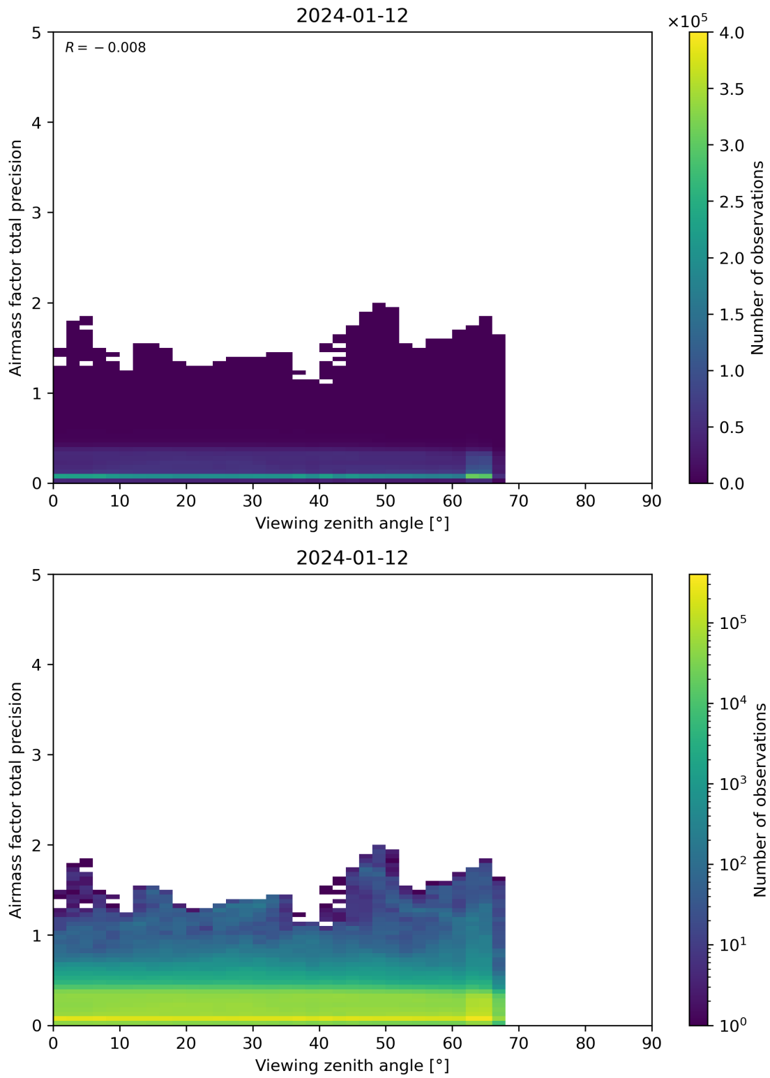
Figure 191: Scatter density plot of “Viewing zenith angle” against “Airmass factor total precision” for 2024-01-11 to 2024-01-13.
