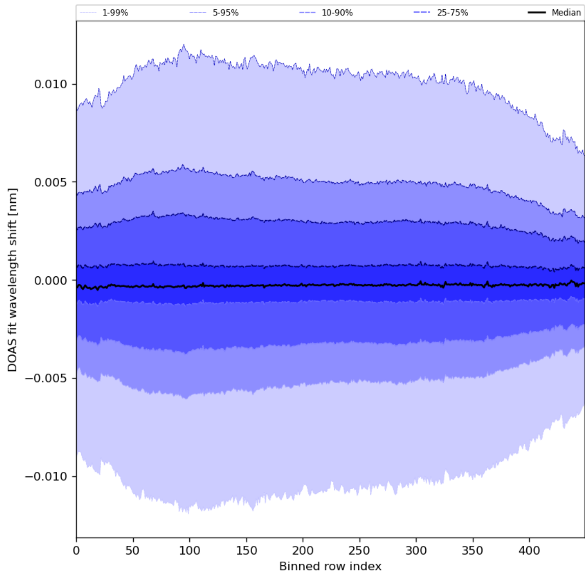
Figure 58: Along track statistics of “DOAS fit wavelength shift” for 2024-01-11 to 2024-01-13
