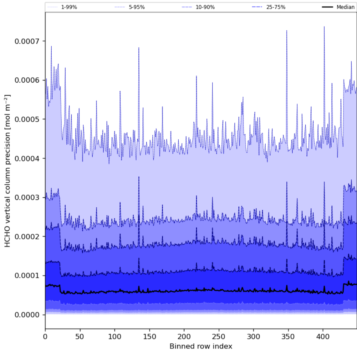
Figure 50: Along track statistics of “HCHO vertical column precision” for 2024-01-11 to 2024-01-13
