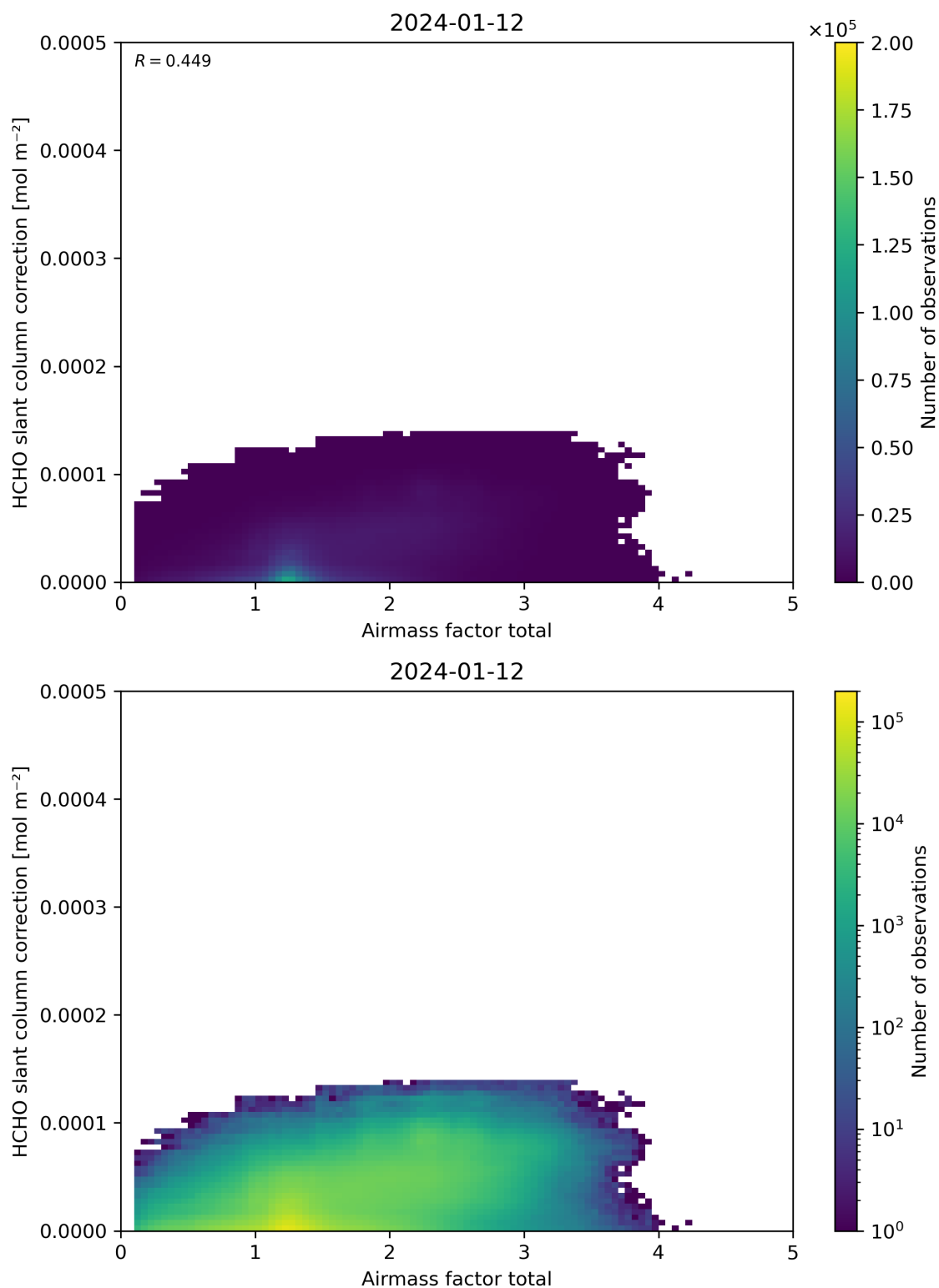
Figure 102: Scatter density plot of “Airmass factor total” against “HCHO slant column correction” for 2024-01-11 to 2024-01-13.
