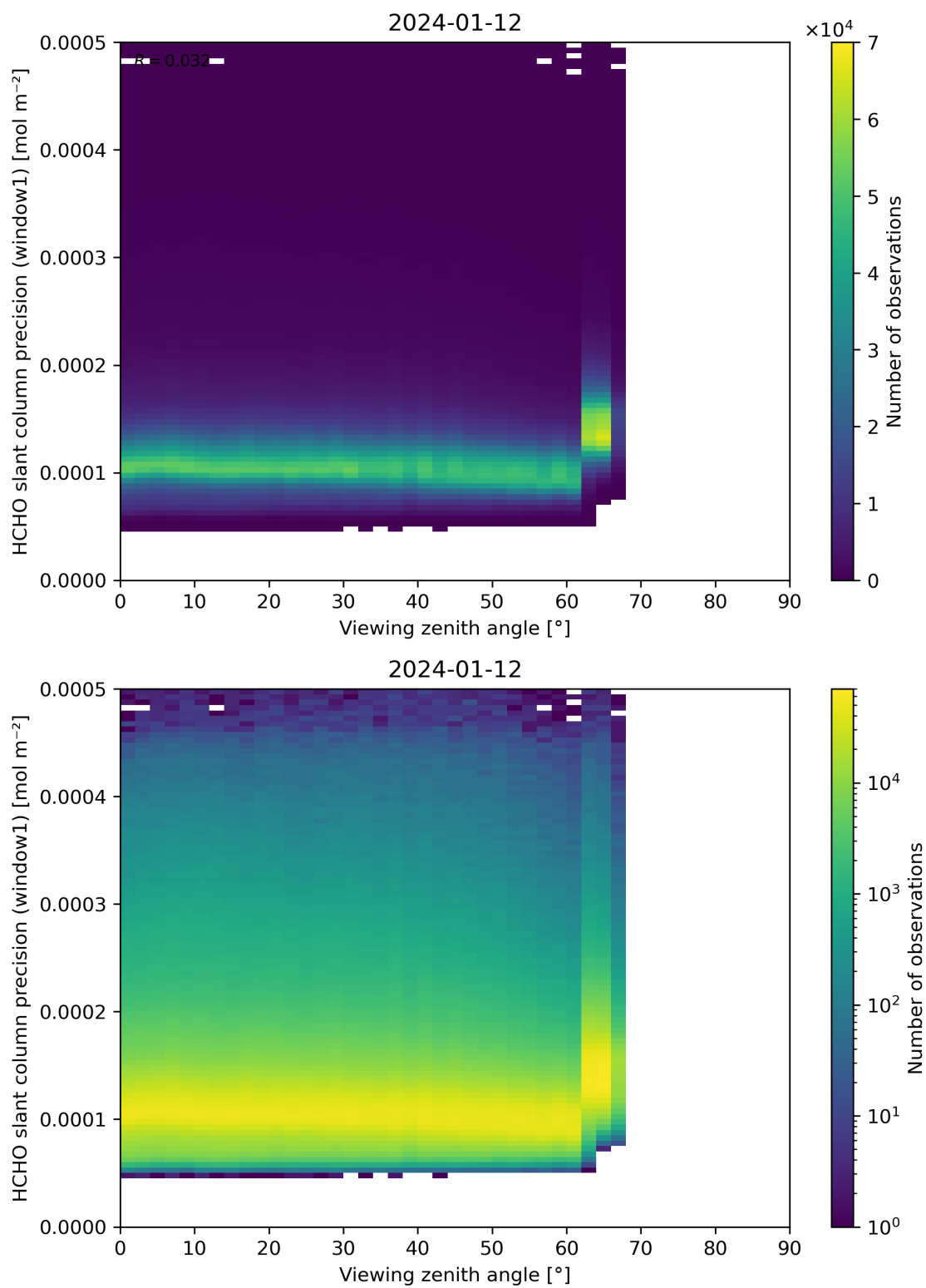
Figure 189: Scatter density plot of “Viewing zenith angle” against “HCHO slant column precision (window1)” for 2024-01-11 to 2024-01-13.
