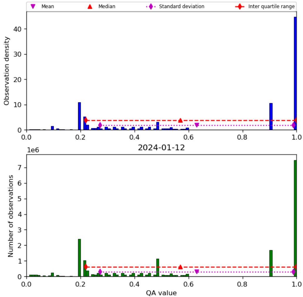
Figure 34: Histogram of “QA value” for 2024-01-11 to 2024-01-13
