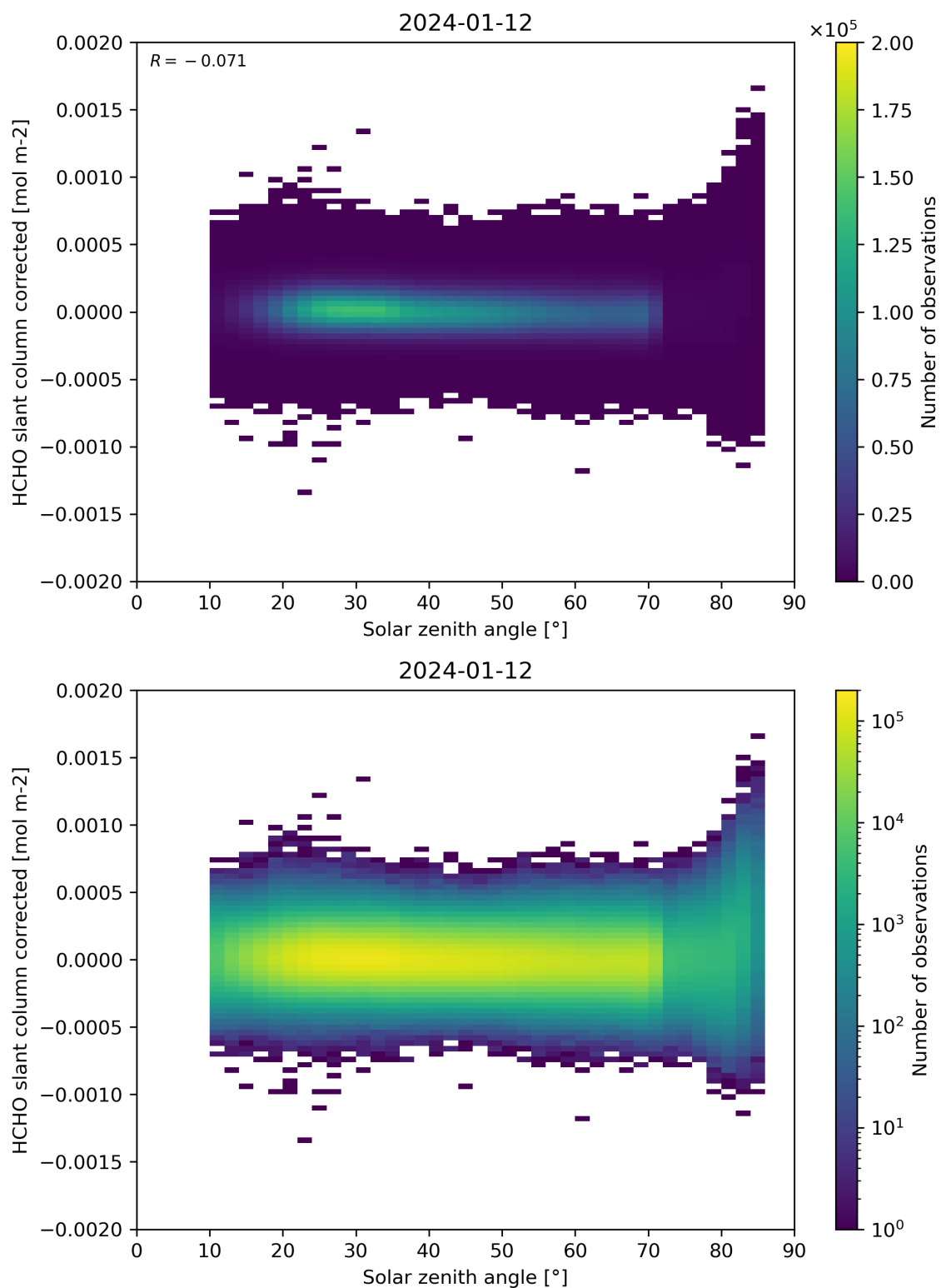
Figure 171: Scatter density plot of “Solar zenith angle” against “HCHO slant column corrected” for 2024-01-11 to 2024-01-13.
