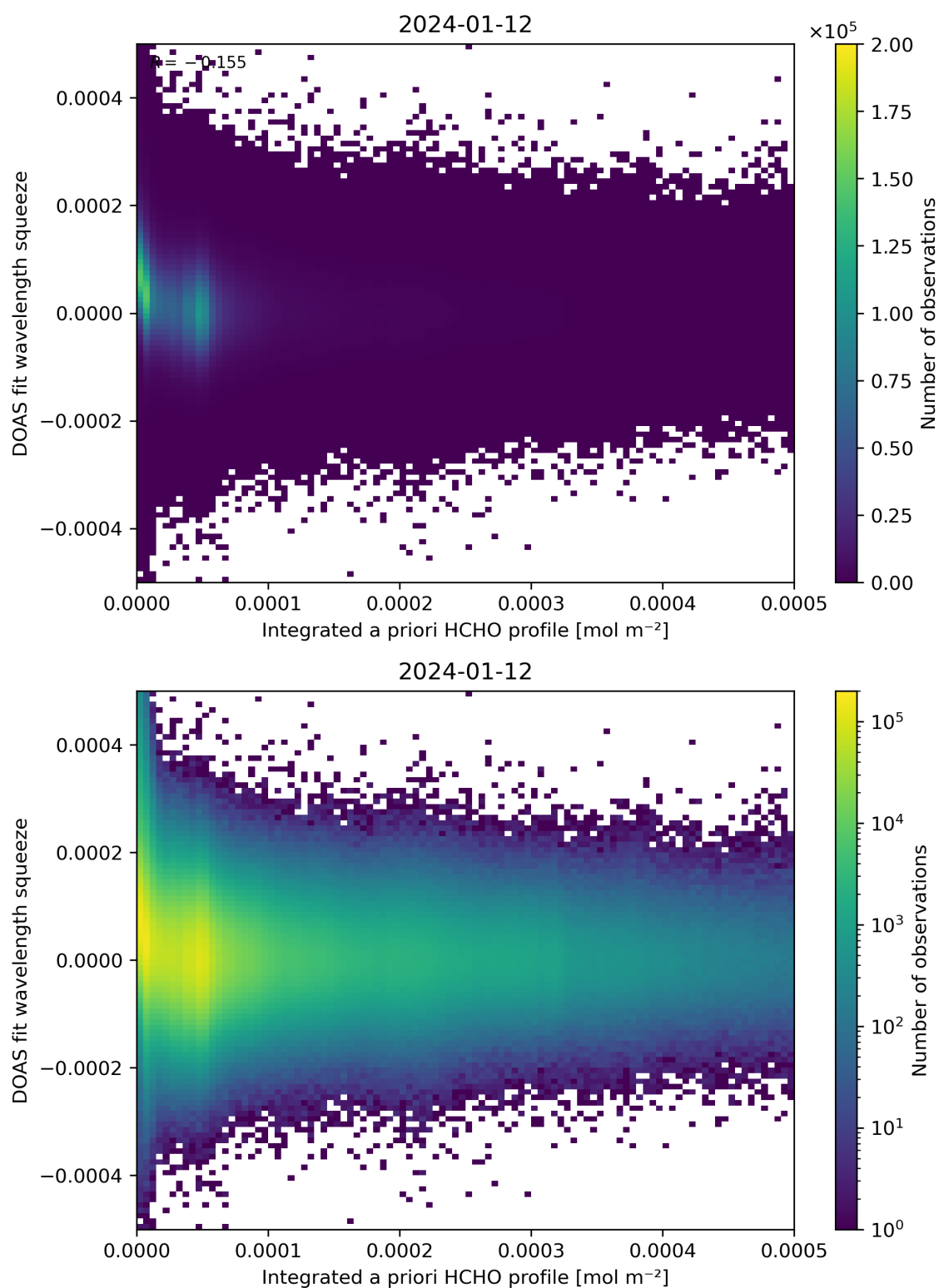
Figure 150: Scatter density plot of “Integrated a priori HCHO profile” against “DOAS fit wavelength squeeze” for 2024-01-11 to 2024-01-13.
