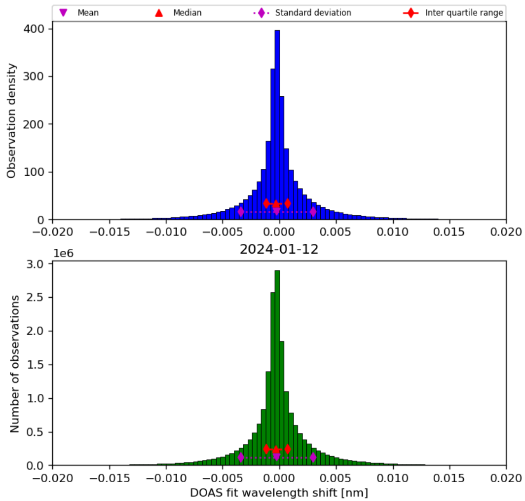
Figure 44: Histogram of “DOAS fit wavelength shift” for 2024-01-11 to 2024-01-13
