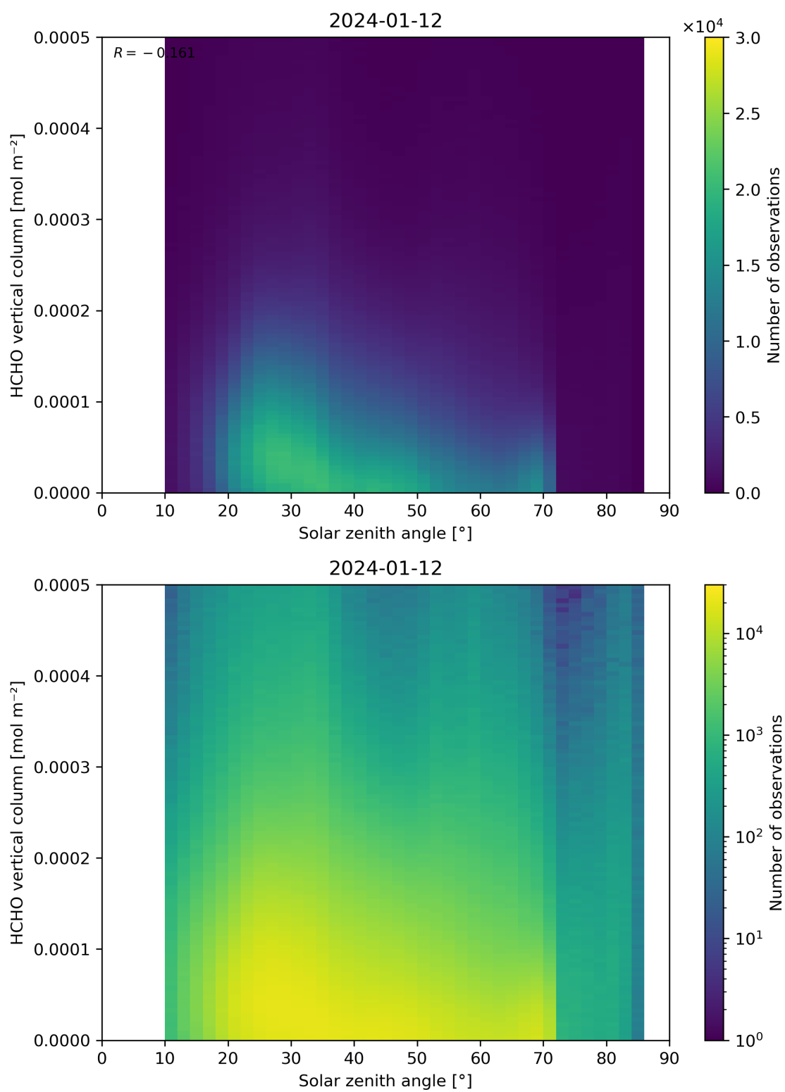
Figure 177: Scatter density plot of “Solar zenith angle” against “HCHO vertical column” for 2024-01-11 to 2024-01-13.
