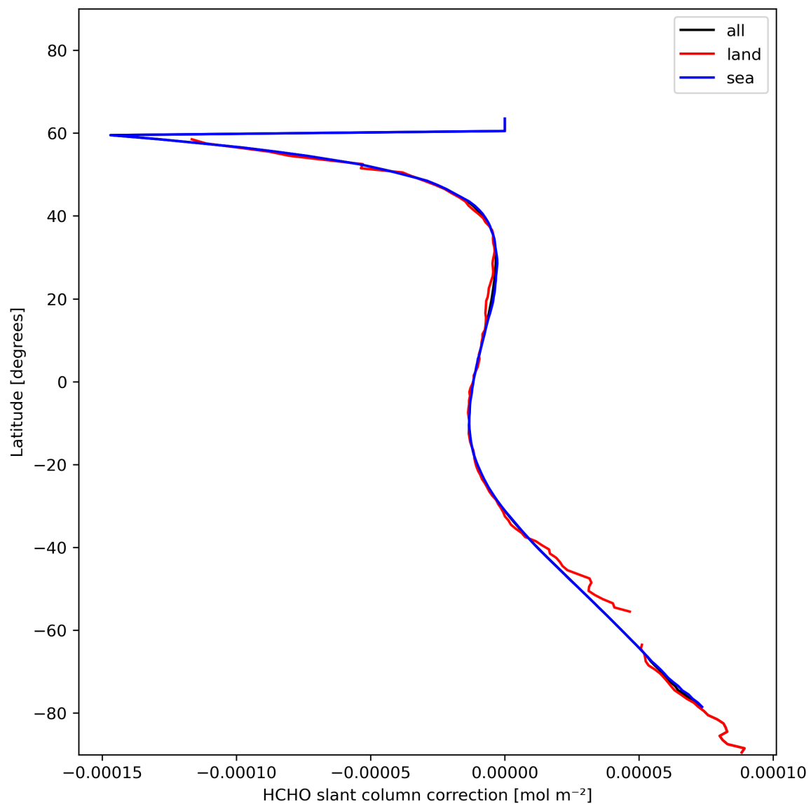
Figure 33: Zonal average of “HCHO slant column correction” for 2024-01-11 to 2024-01-13.
