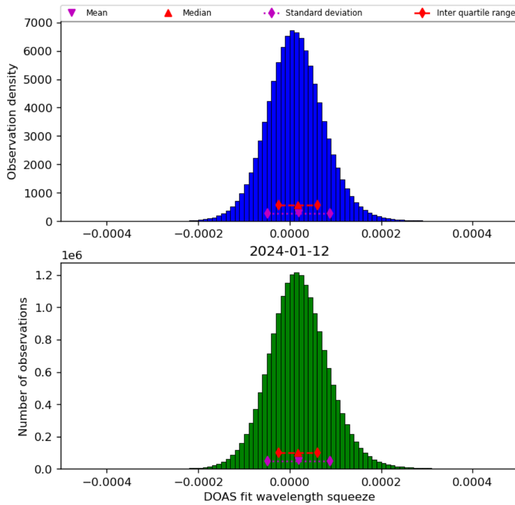
Figure 45: Histogram of “DOAS fit wavelength squeeze” for 2024-01-11 to 2024-01-13
