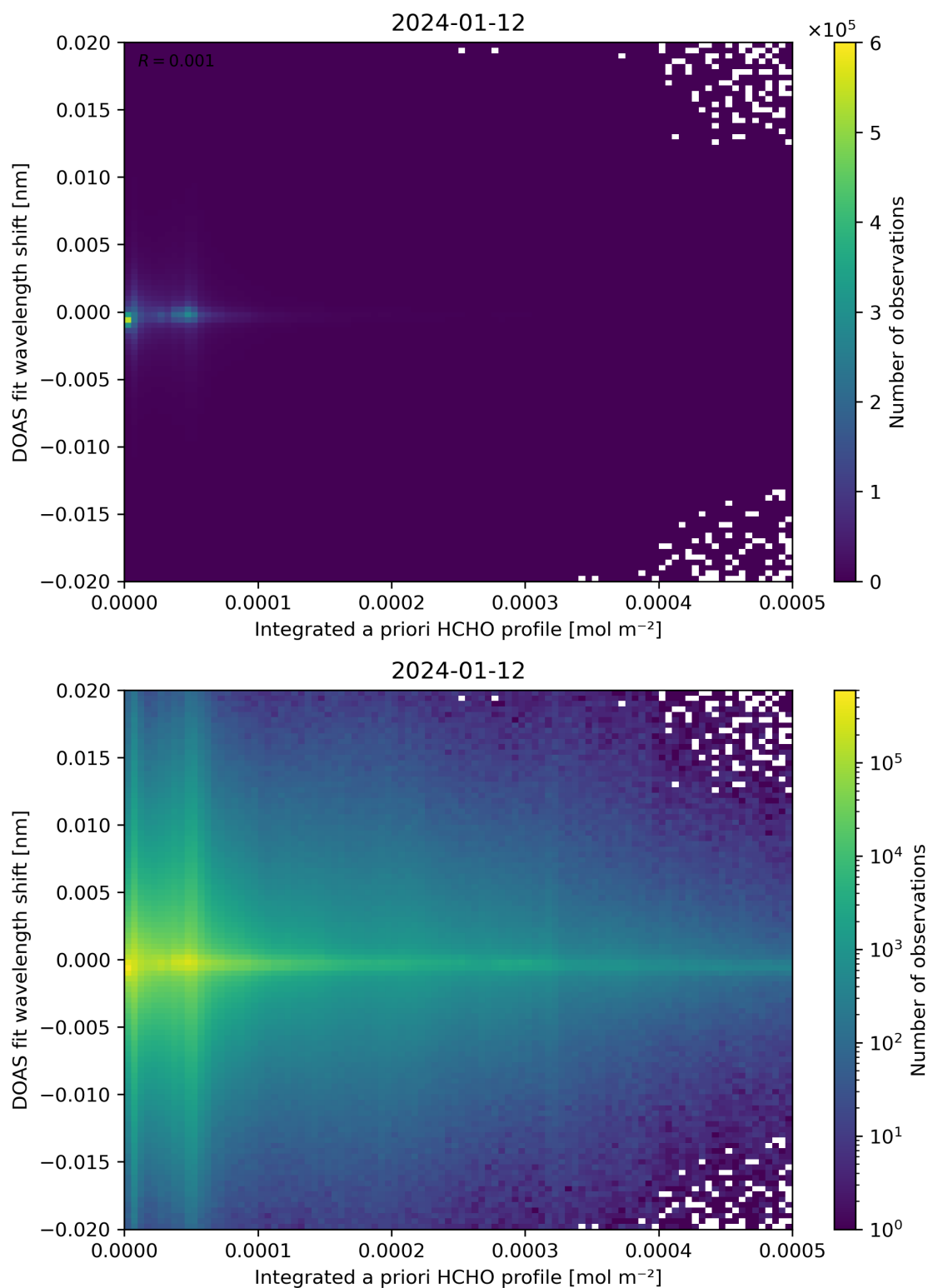
Figure 149: Scatter density plot of “Integrated a priori HCHO profile” against “DOAS fit wavelength shift” for 2024-01-11 to 2024-01-13.
