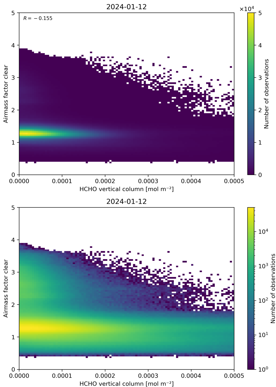
Figure 126: Scatter density plot of “HCHO vertical column” against “Airmass factor clear” for 2024-01-11 to 2024-01-13.
