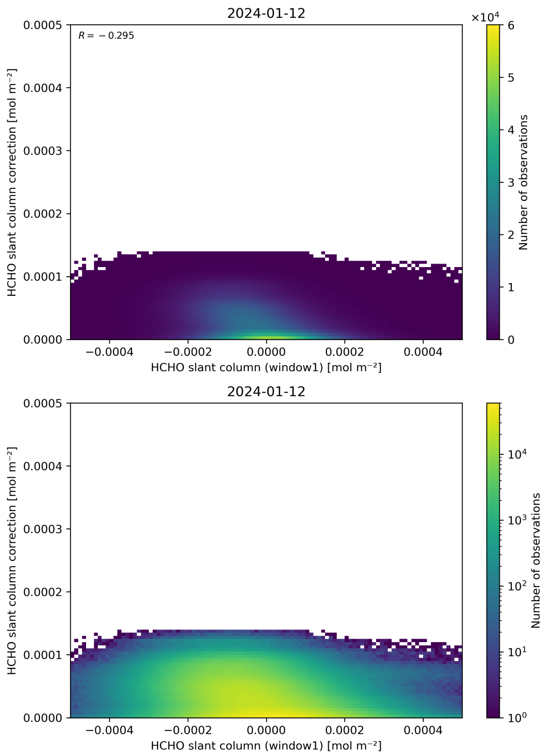
Figure 83: Scatter density plot of “HCHO slant column (window1)” against “HCHO slant column correction” for 2024-01-11 to 2024-01-13.
