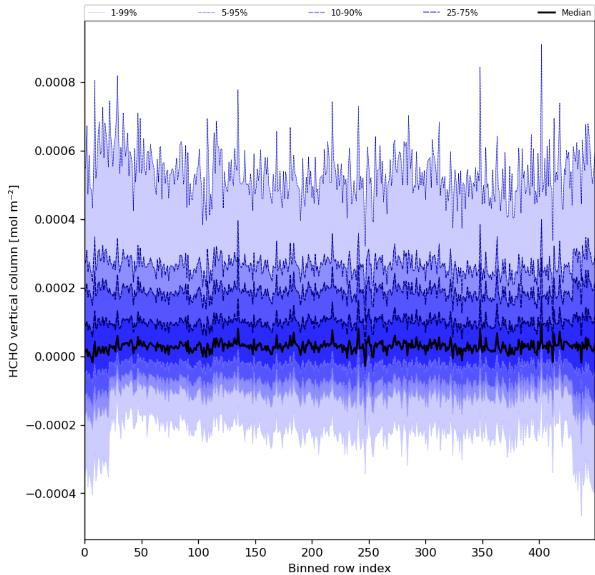
Figure 49: Along track statistics of “HCHO vertical column” for 2024-01-11 to 2024-01-13
