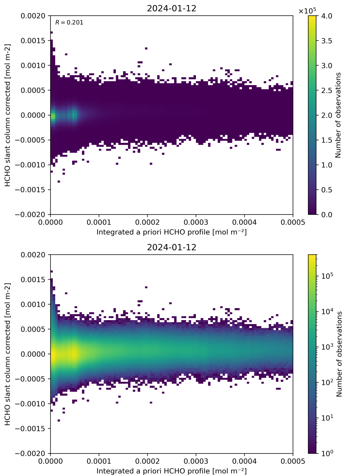
Figure 151: Scatter density plot of “Integrated a priori HCHO profile” against “HCHO slant column corrected” for 2024-01-11 to 2024-01-13.
