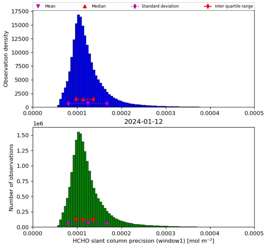
Figure 39: Histogram of “HCHO slant column precision (window1)” for 2024-01-11 to 2024-01-13
