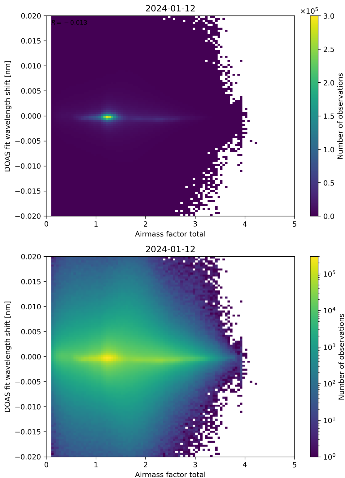
Figure 98: Scatter density plot of “Airmass factor total” against “DOAS fit wavelength shift” for 2024-01-11 to 2024-01-13.
