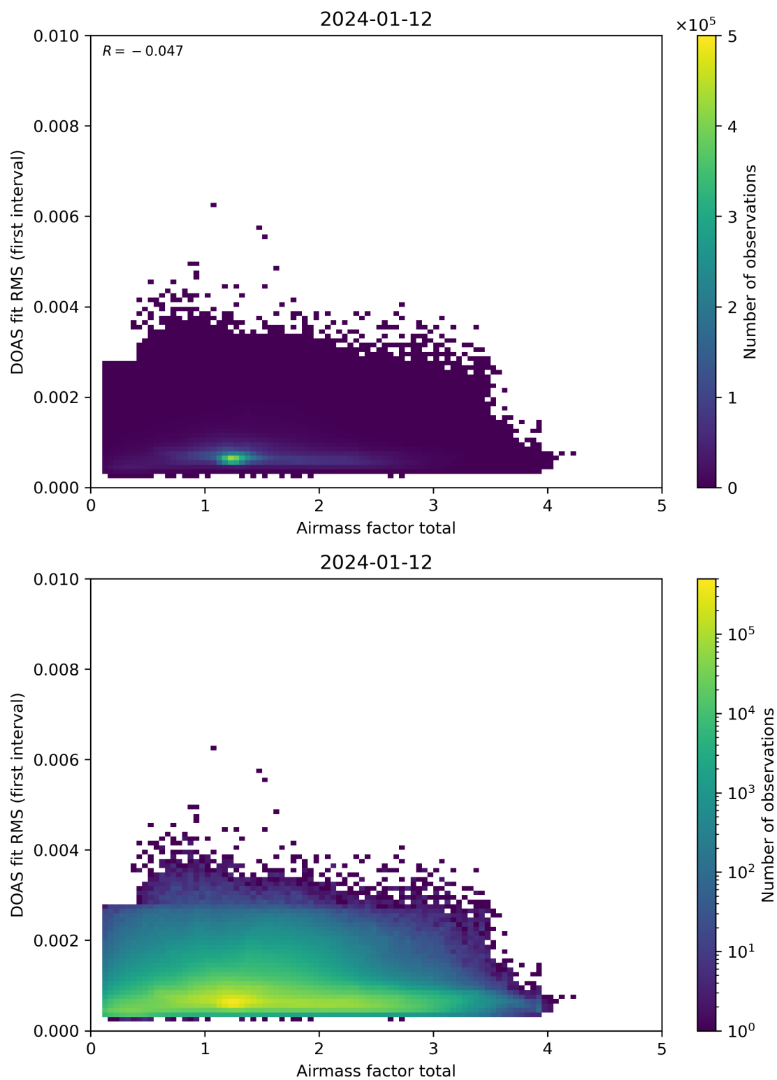
Figure 97: Scatter density plot of “Airmass factor total” against “DOAS fit RMS (first interval)” for 2024-01-11 to 2024-01-13.
