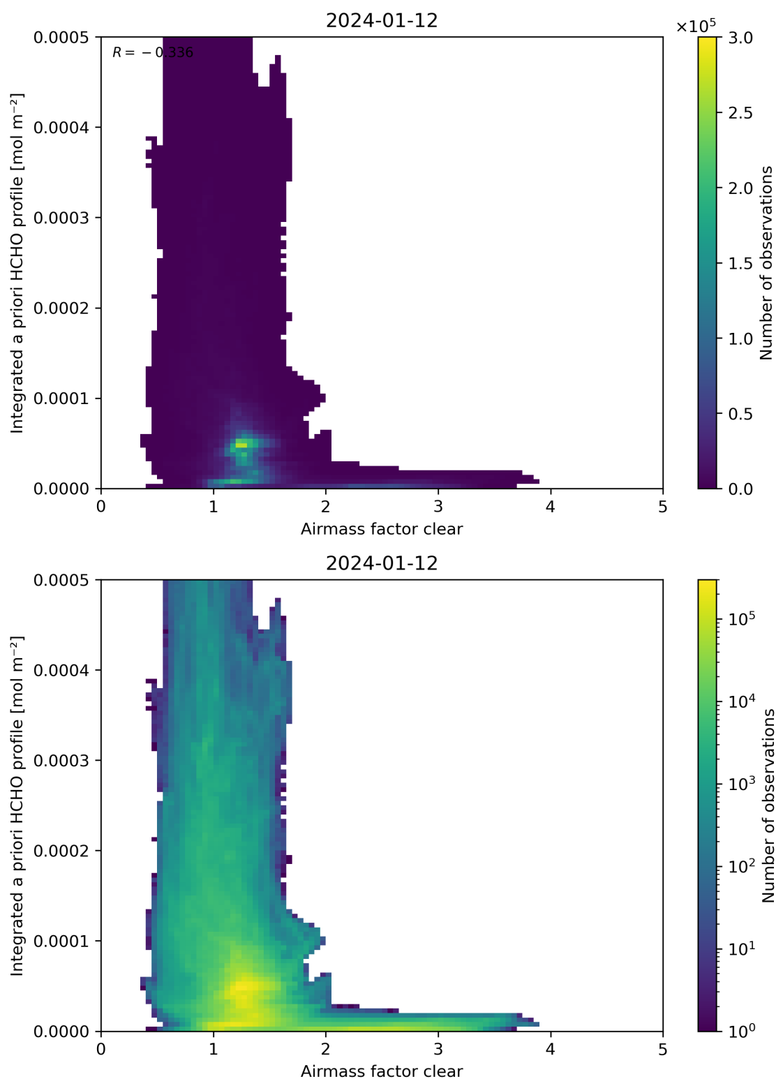
Figure 76: Scatter density plot of “Airmass factor clear” against “Integrated a priori HCHO profile” for 2024-01-11 to 2024-01-13.
