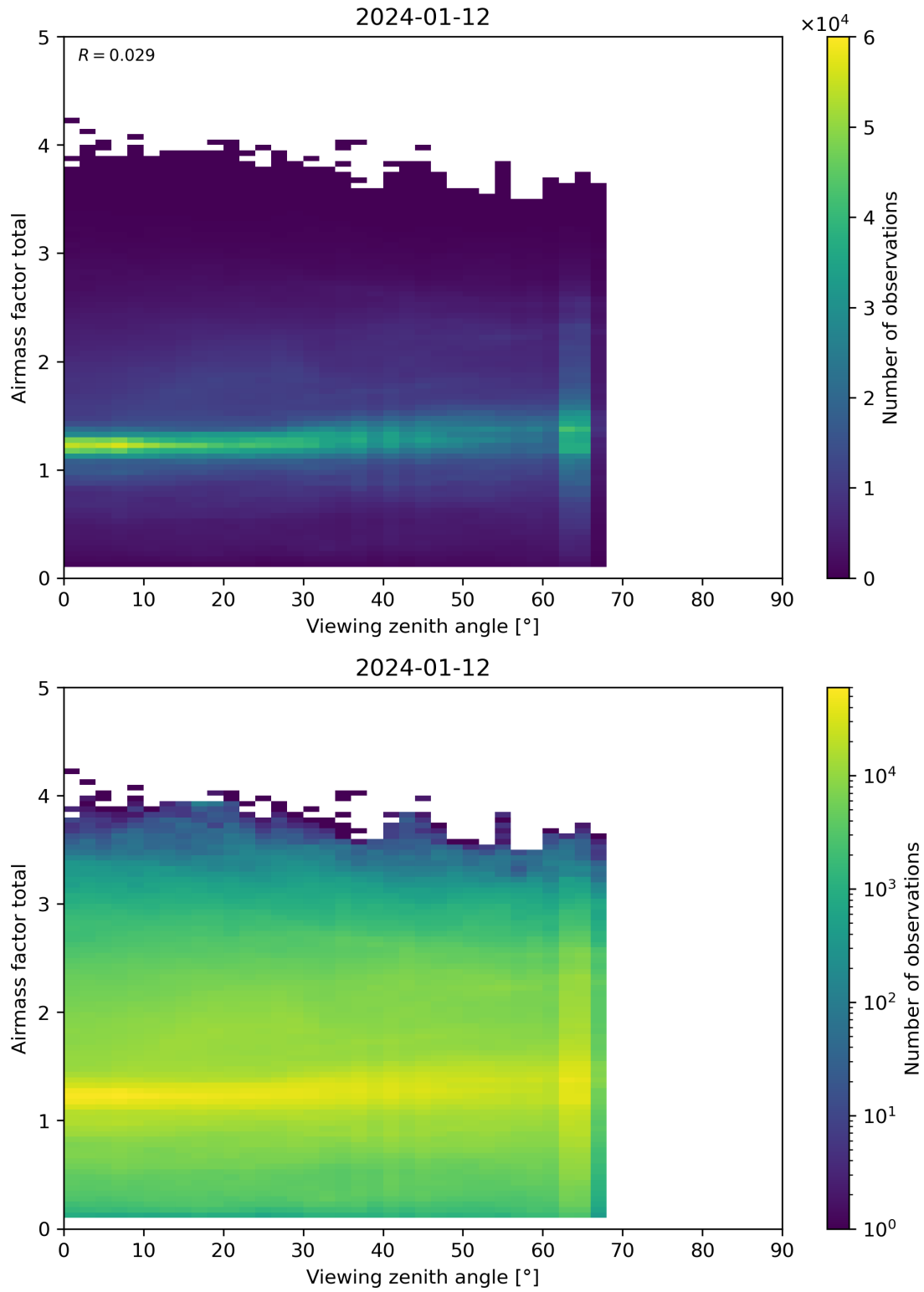
Figure 190: Scatter density plot of “Viewing zenith angle” against “Airmass factor total” for 2024-01-11 to 2024-01-13.
