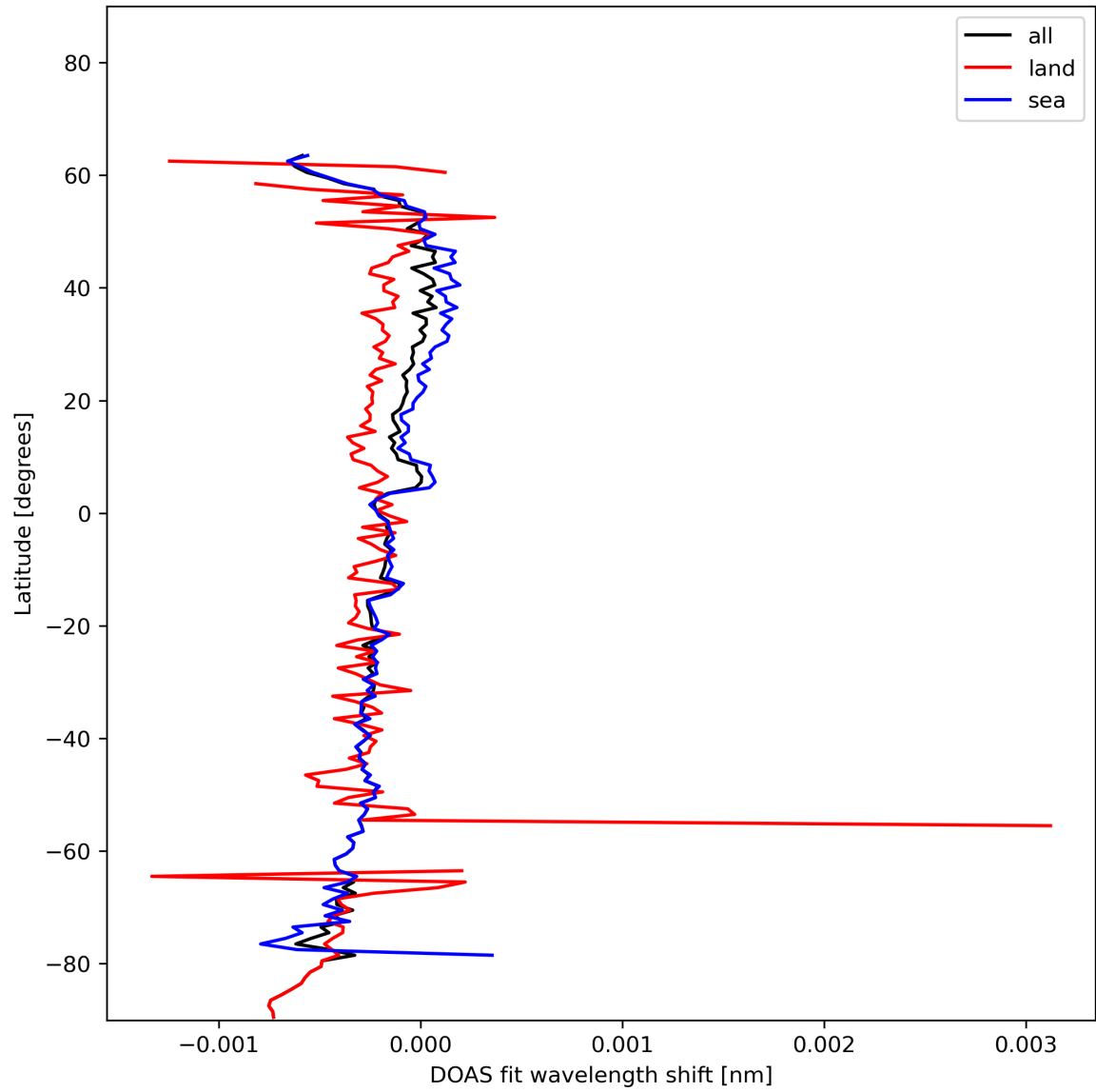
Figure 30: Zonal average of “DOAS fit wavelength shift” for 2024-01-11 to 2024-01-13.
