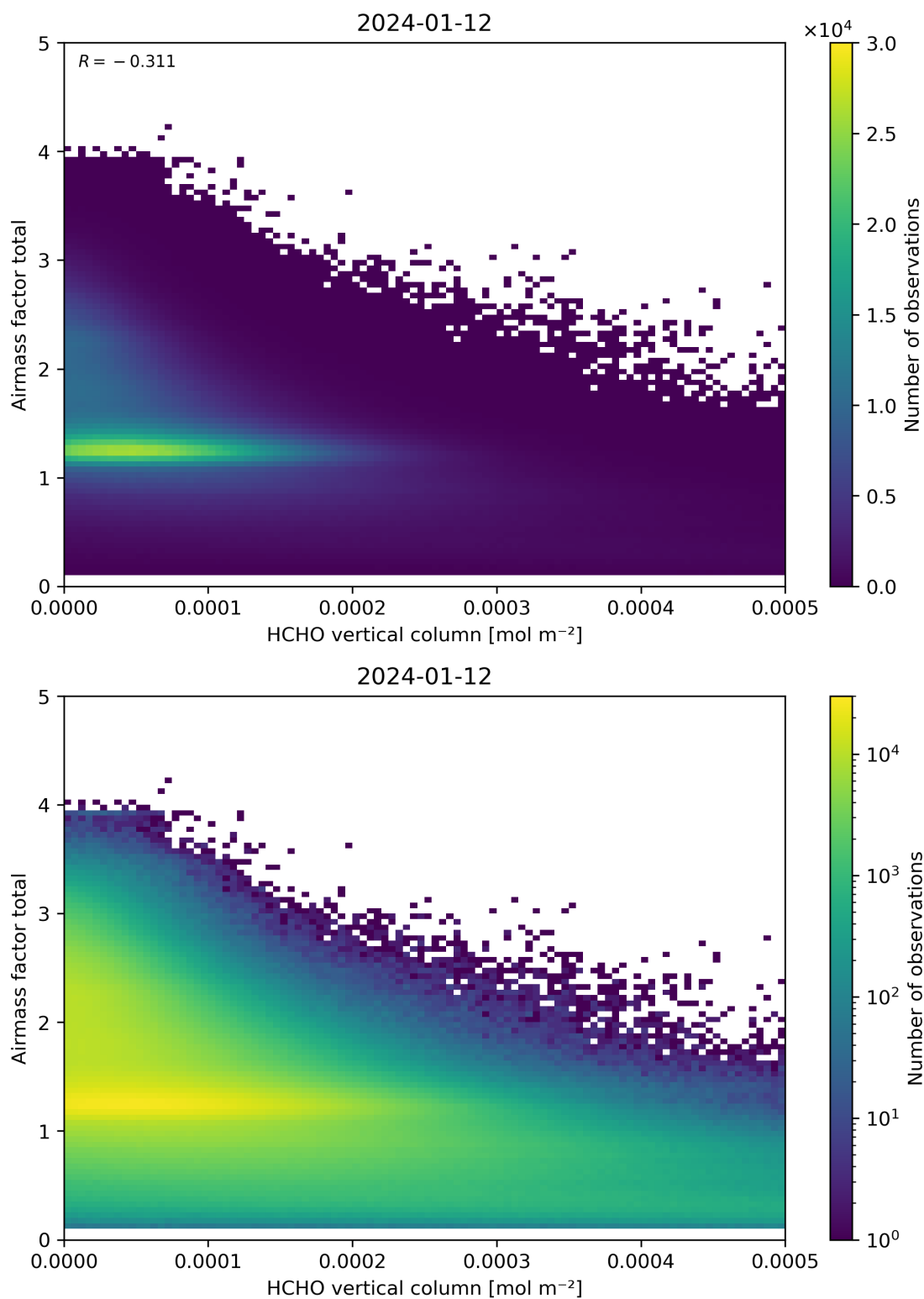
Figure 131: Scatter density plot of “HCHO vertical column” against “Airmass factor total” for 2024-01-11 to 2024-01-13.
