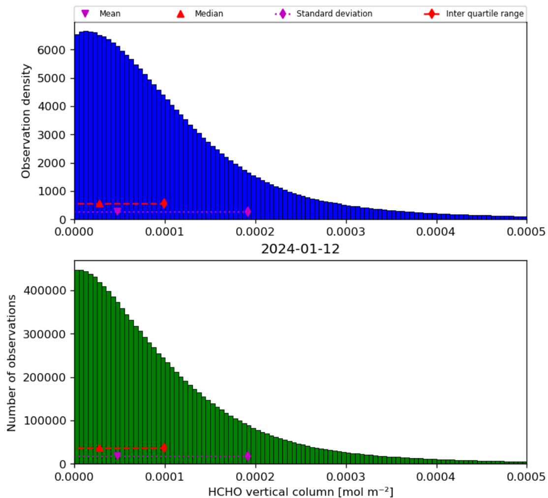
Figure 35: Histogram of “HCHO vertical column” for 2024-01-11 to 2024-01-13
