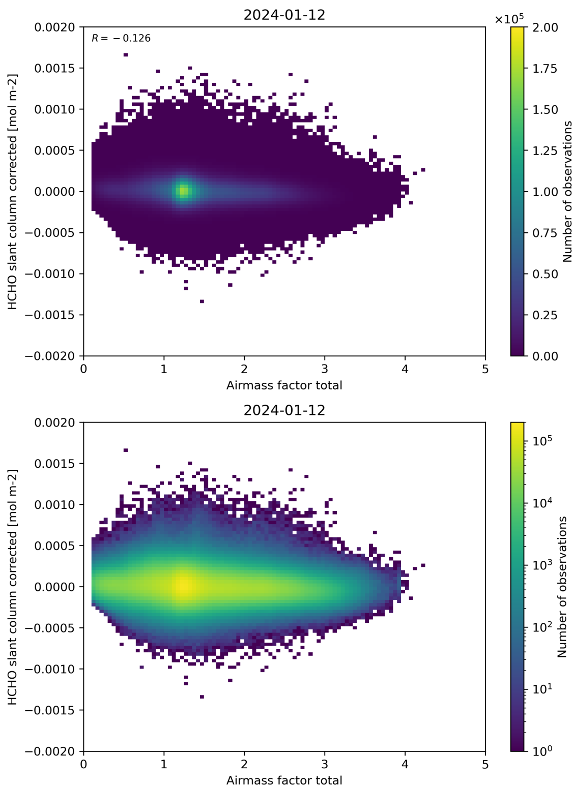
Figure 101: Scatter density plot of “Airmass factor total” against “HCHO slant column corrected” for 2024-01-11 to 2024-01-13.
