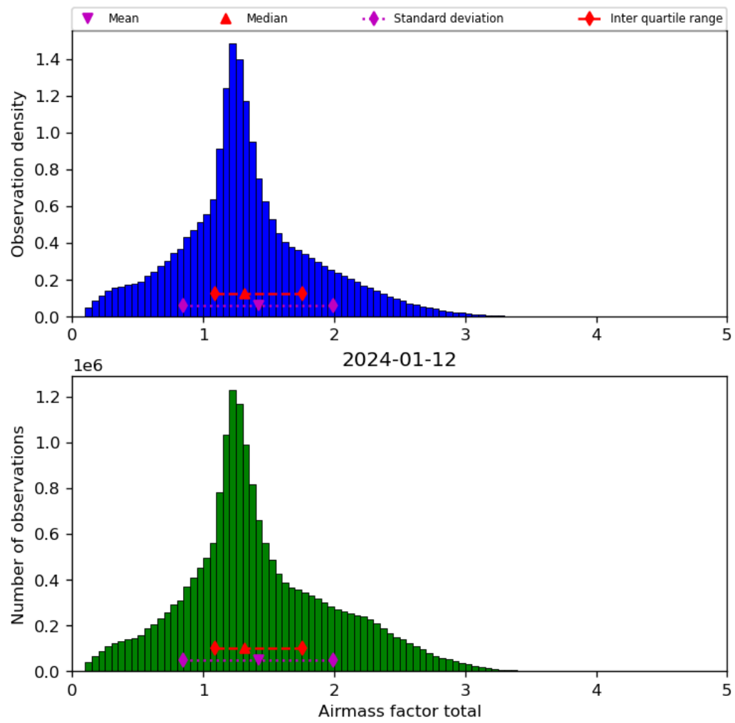
Figure 40: Histogram of “Airmass factor total” for 2024-01-11 to 2024-01-13
