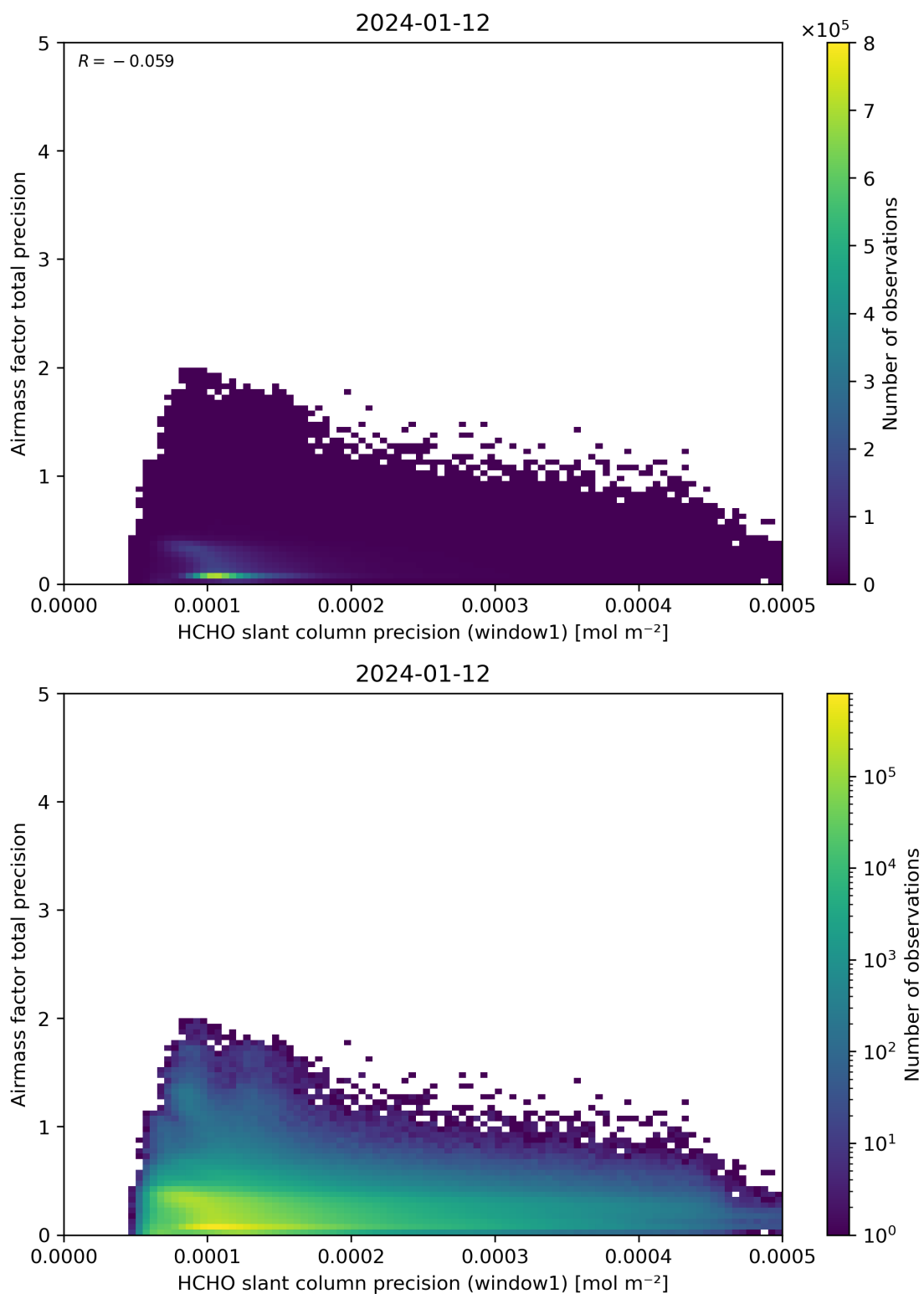
Figure 95: Scatter density plot of “HCHO slant column precision (window1)” against “Airmass factor total precision” for 2024-01-11 to 2024-01-13.
