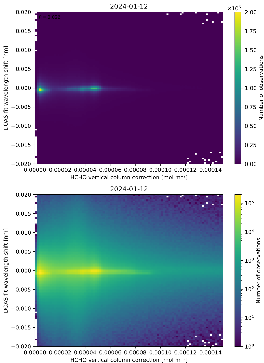
Figure 113: Scatter density plot of “HCHO vertical column correction” against “DOAS fit wavelength shift” for 2024-01-11 to 2024-01-13.
