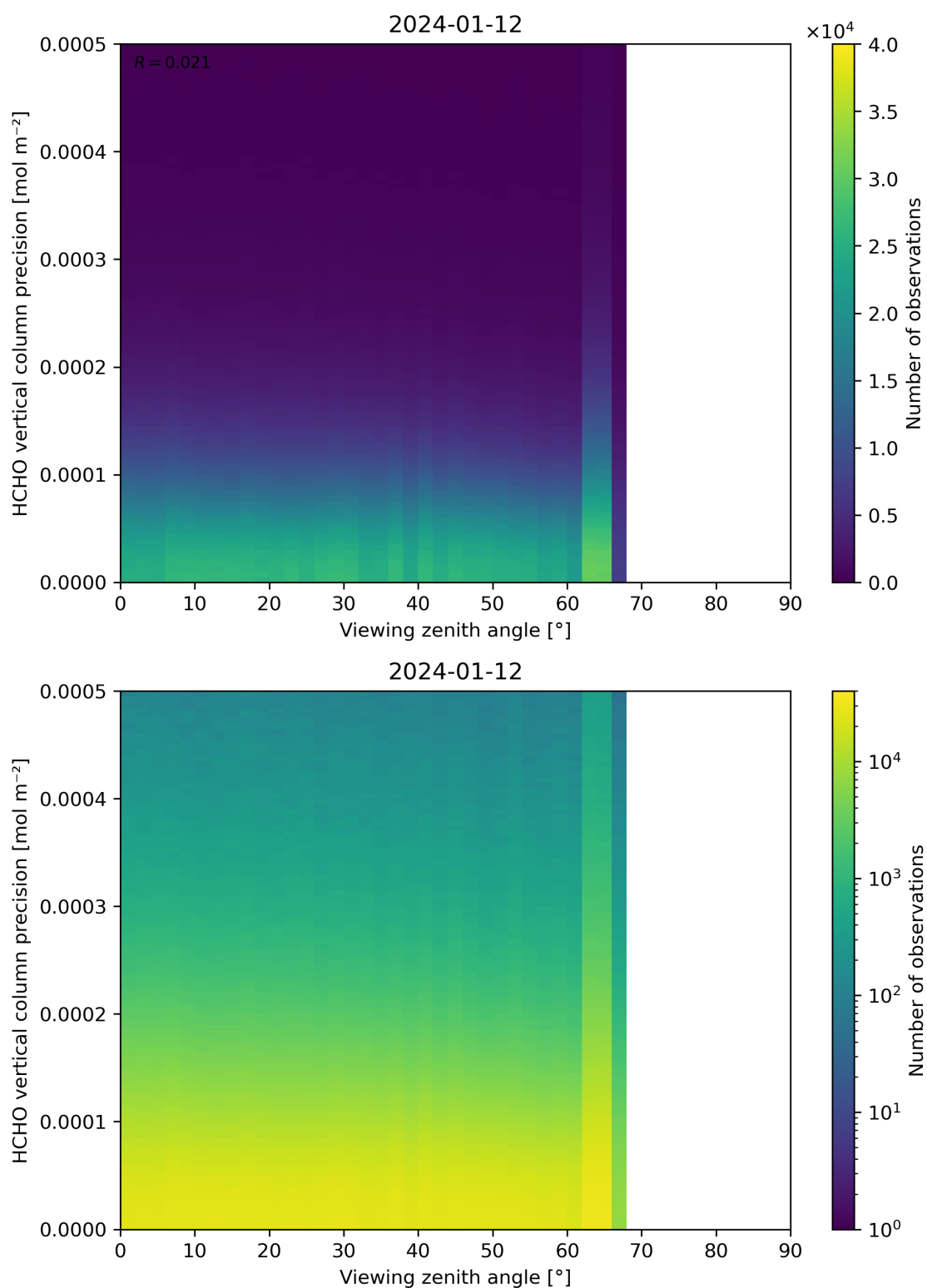
Figure 194: Scatter density plot of “Viewing zenith angle” against “HCHO vertical column precision” for 2024-01-11 to 2024-01-13.
