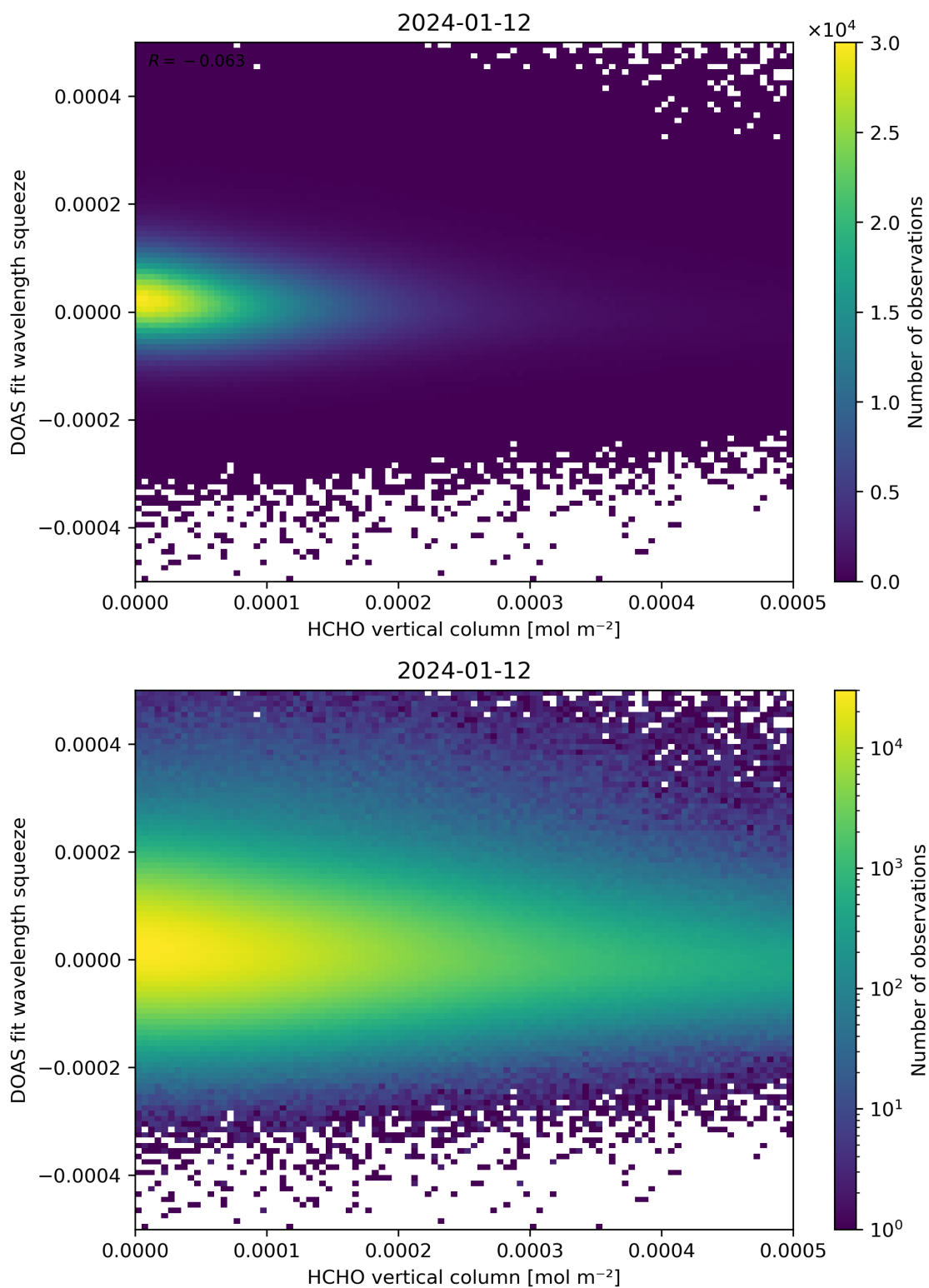
Figure 125: Scatter density plot of “HCHO vertical column” against “DOAS fit wavelength squeeze” for 2024-01-11 to 2024-01-13.
