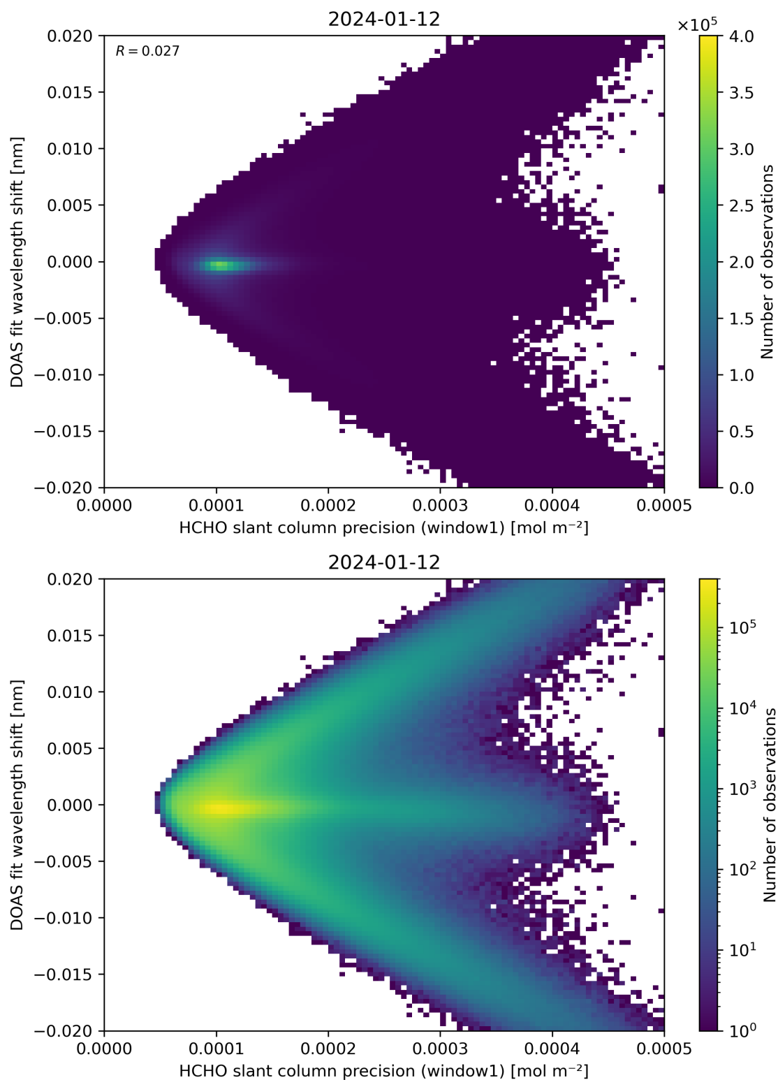
Figure 89: Scatter density plot of “HCHO slant column precision (window1)” against “DOAS fit wavelength shift” for 2024-01-11 to 2024-01-13.
