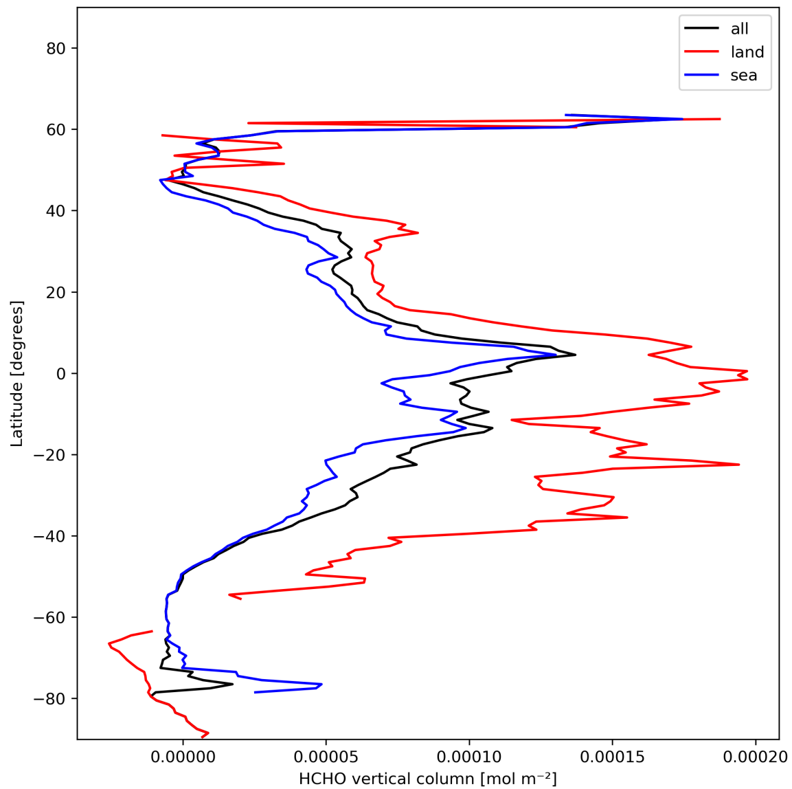
Figure 21: Zonal average of “HCHO vertical column” for 2024-01-11 to 2024-01-13.
