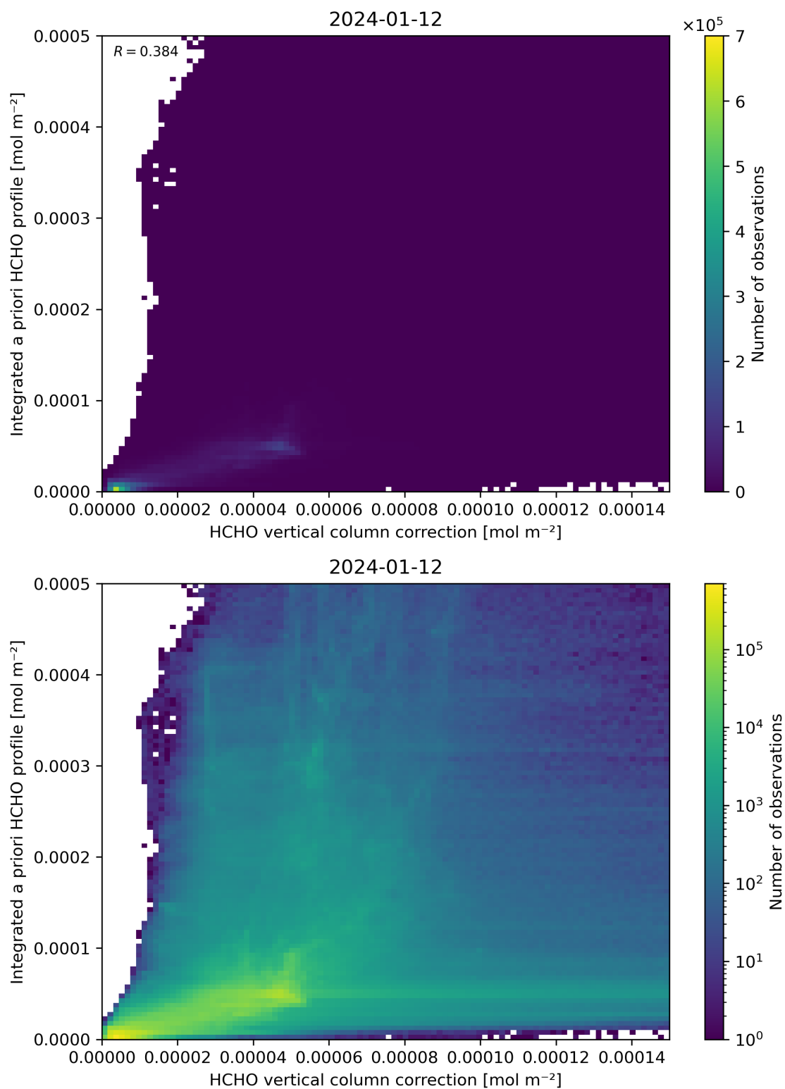
Figure 122: Scatter density plot of “HCHO vertical column correction” against “Integrated a priori HCHO profile” for 2024-01-11 to 2024-01-13.
