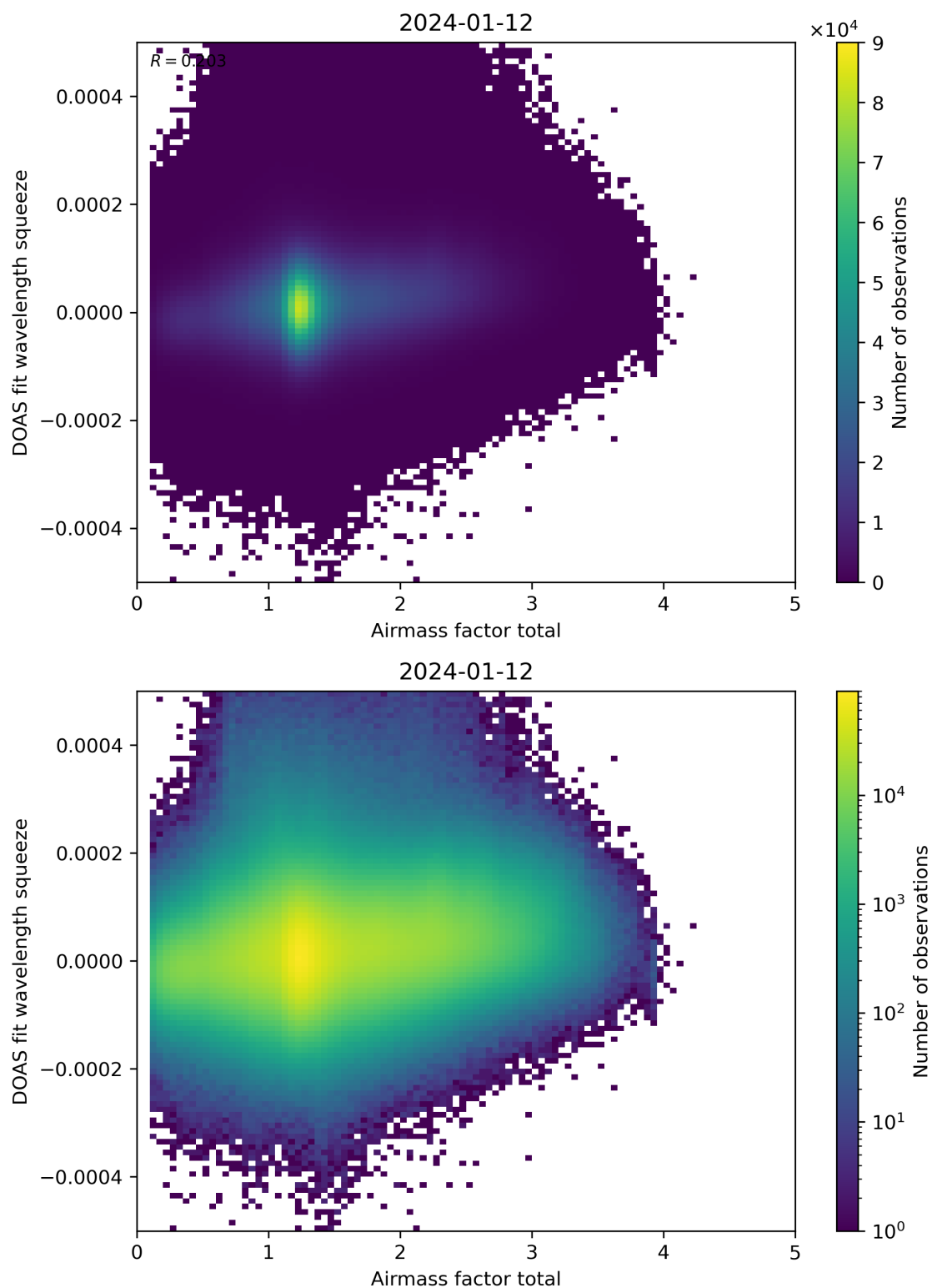
Figure 99: Scatter density plot of “Airmass factor total” against “DOAS fit wavelength squeeze” for 2024-01-11 to 2024-01-13.
