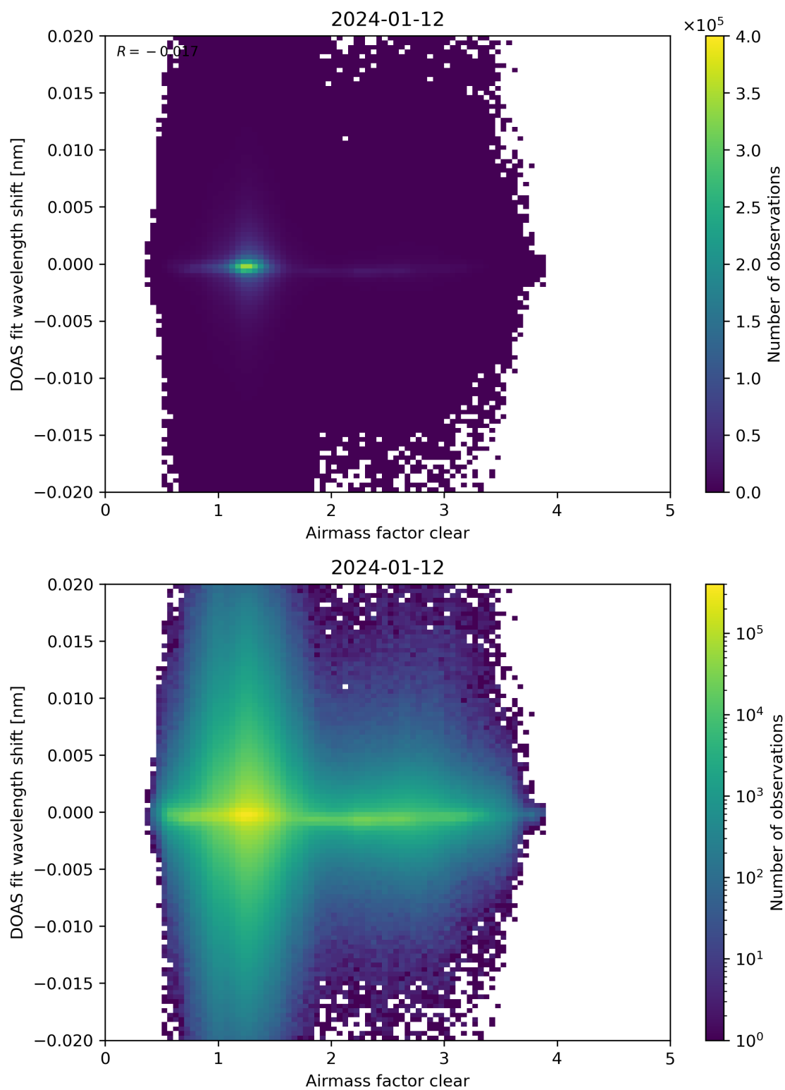
Figure 72: Scatter density plot of “Airmass factor clear” against “DOAS fit wavelength shift” for 2024-01-11 to 2024-01-13.
