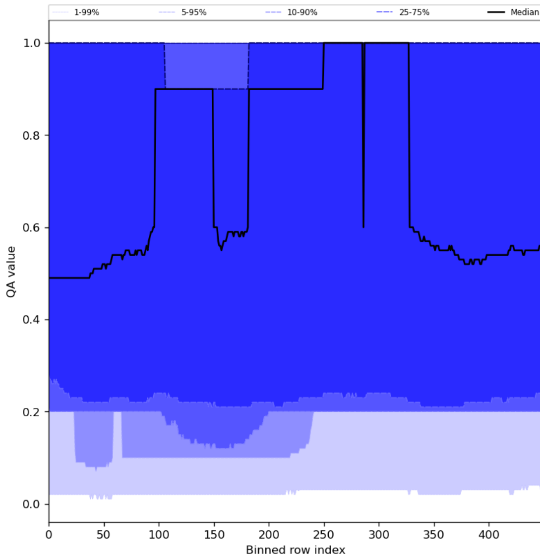
Figure 48: Along track statistics of “QA value” for 2024-01-11 to 2024-01-13
