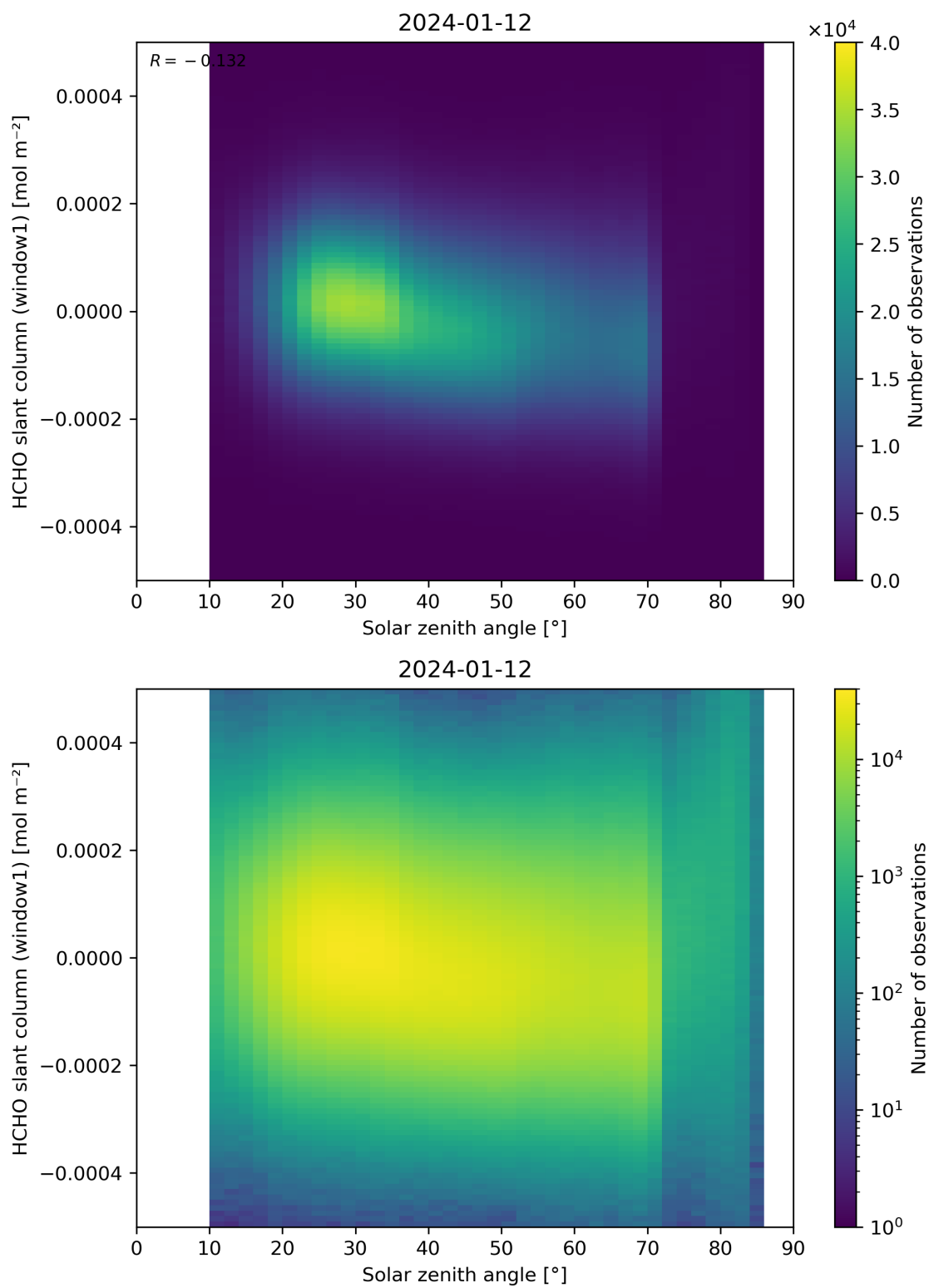
Figure 173: Scatter density plot of “Solar zenith angle” against “HCHO slant column (window1)” for 2024-01-11 to 2024-01-13.
