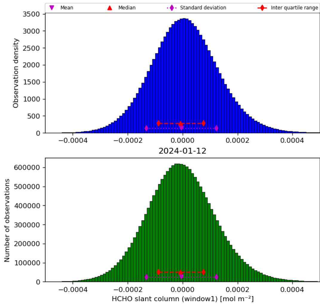
Figure 38: Histogram of “HCHO slant column (window1)” for 2024-01-11 to 2024-01-13
