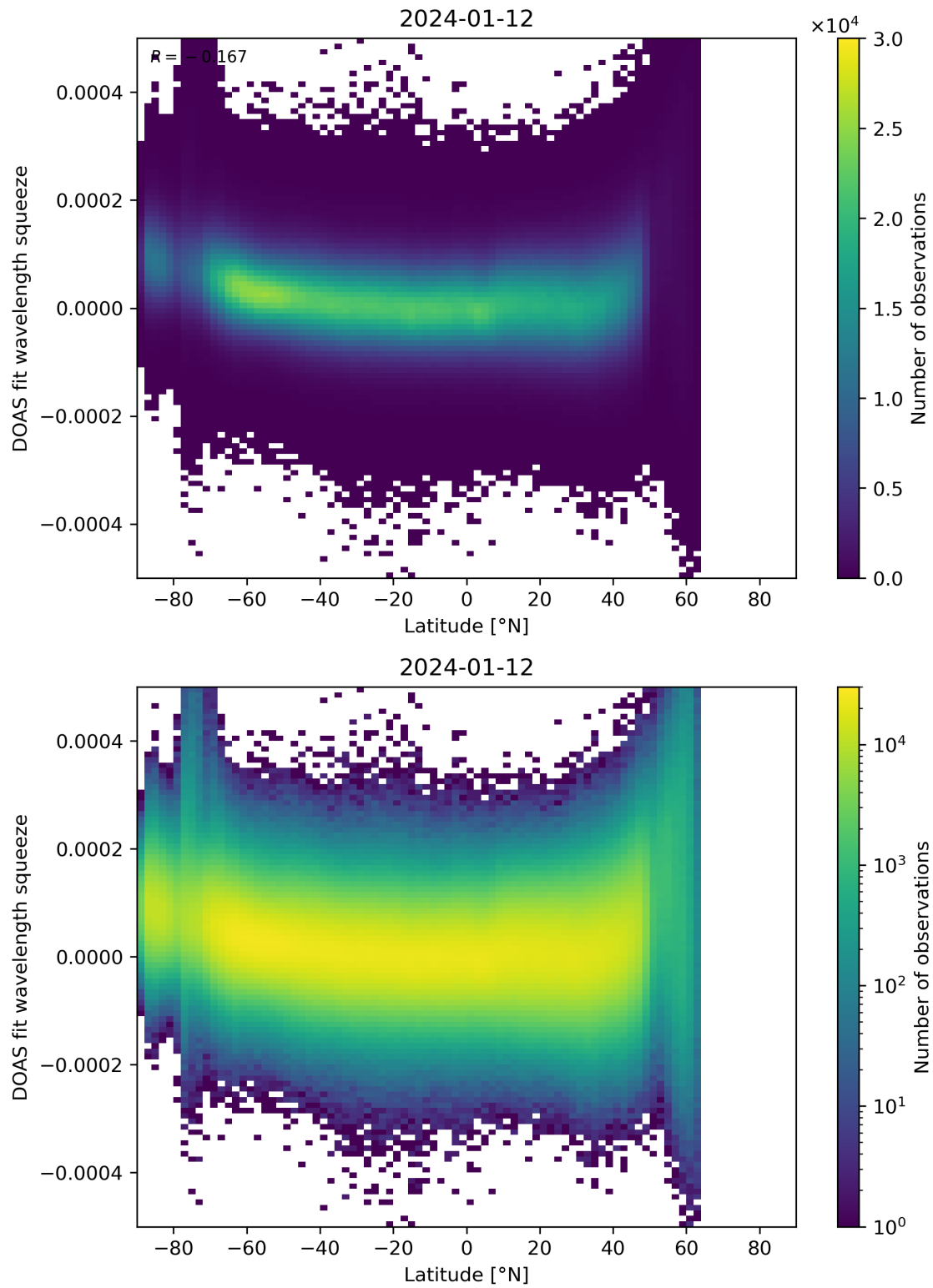
Figure 155: Scatter density plot of “Latitude” against “DOAS fit wavelength squeeze” for 2024-01-11 to 2024-01-13.
