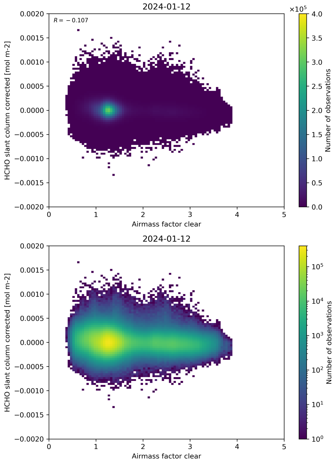
Figure 74: Scatter density plot of “Airmass factor clear” against “HCHO slant column corrected” for 2024-01-11 to 2024-01-13.
