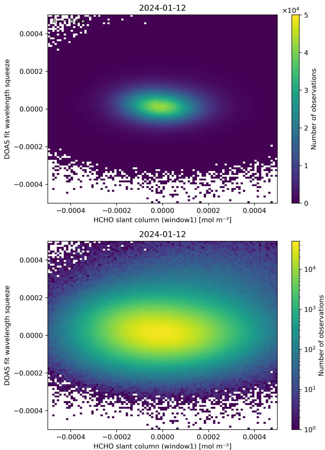
Figure 80: Scatter density plot of “HCHO slant column (window1)” against “DOAS fit wavelength squeeze” for 2024-01-11 to 2024-01-13.
