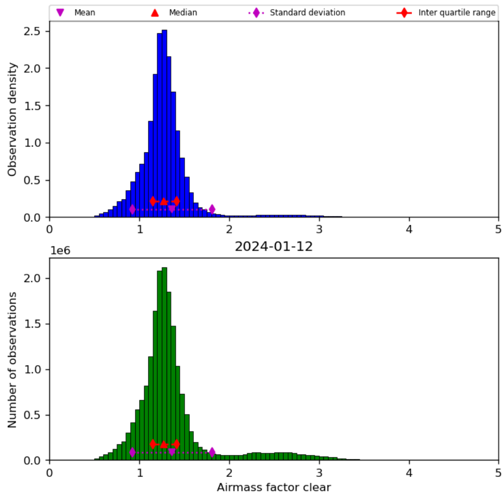
Figure 42: Histogram of “Airmass factor clear” for 2024-01-11 to 2024-01-13
