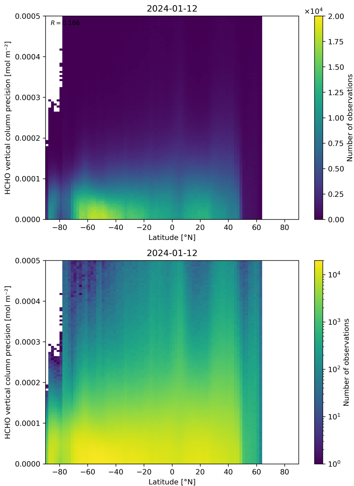
Figure 165: Scatter density plot of “Latitude” against “HCHO vertical column precision” for 2024-01-11 to 2024-01-13.
