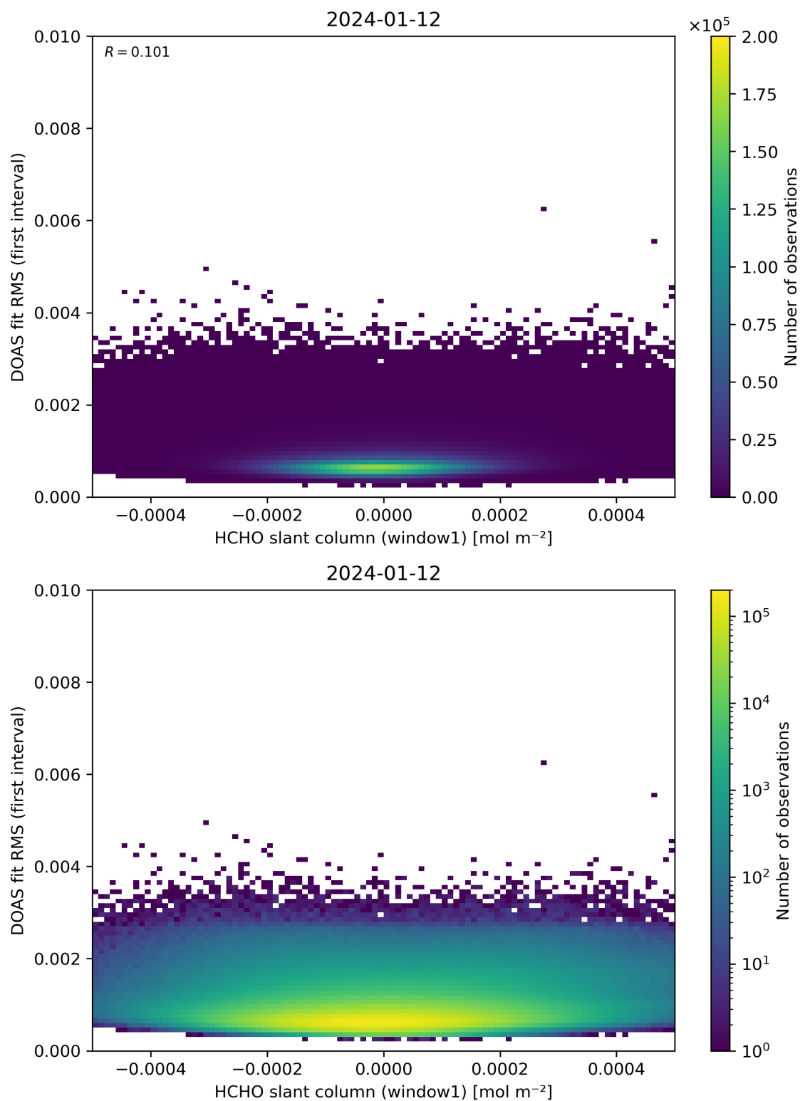
Figure 78: Scatter density plot of “HCHO slant column (window1)” against “DOAS fit RMS (first interval)” for 2024-01-11 to 2024-01-13.
