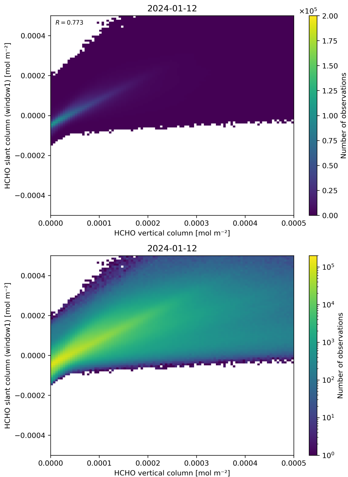
Figure 129: Scatter density plot of “HCHO vertical column” against “HCHO slant column (window1)” for 2024-01-11 to 2024-01-13.
