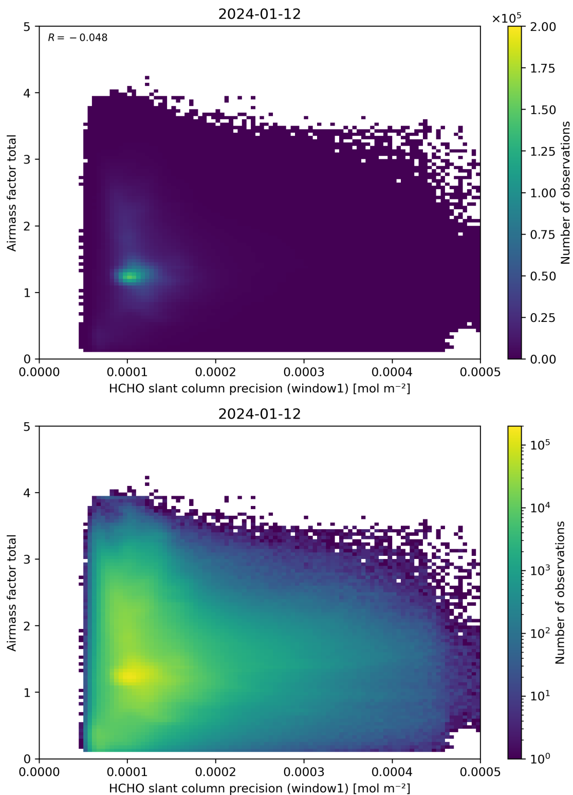
Figure 94: Scatter density plot of “HCHO slant column precision (window1)” against “Airmass factor total” for 2024-01-11 to 2024-01-13.
