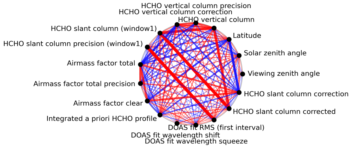
Figure 1: Map of correlation graph for 2024-01-11 to 2024-01-13.
