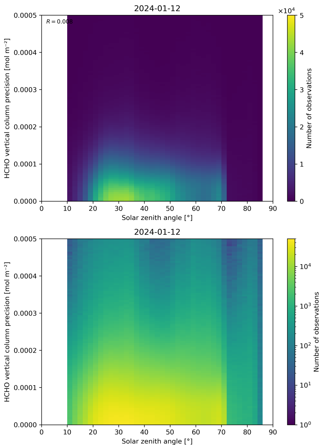
Figure 179: Scatter density plot of “Solar zenith angle” against “HCHO vertical column precision” for 2024-01-11 to 2024-01-13.
