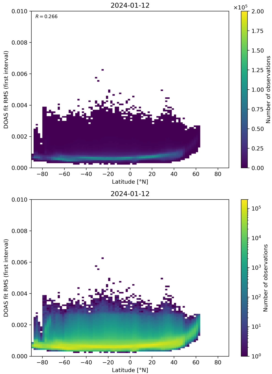
Figure 153: Scatter density plot of “Latitude” against “DOAS fit RMS (first interval)” for 2024-01-11 to 2024-01-13.
