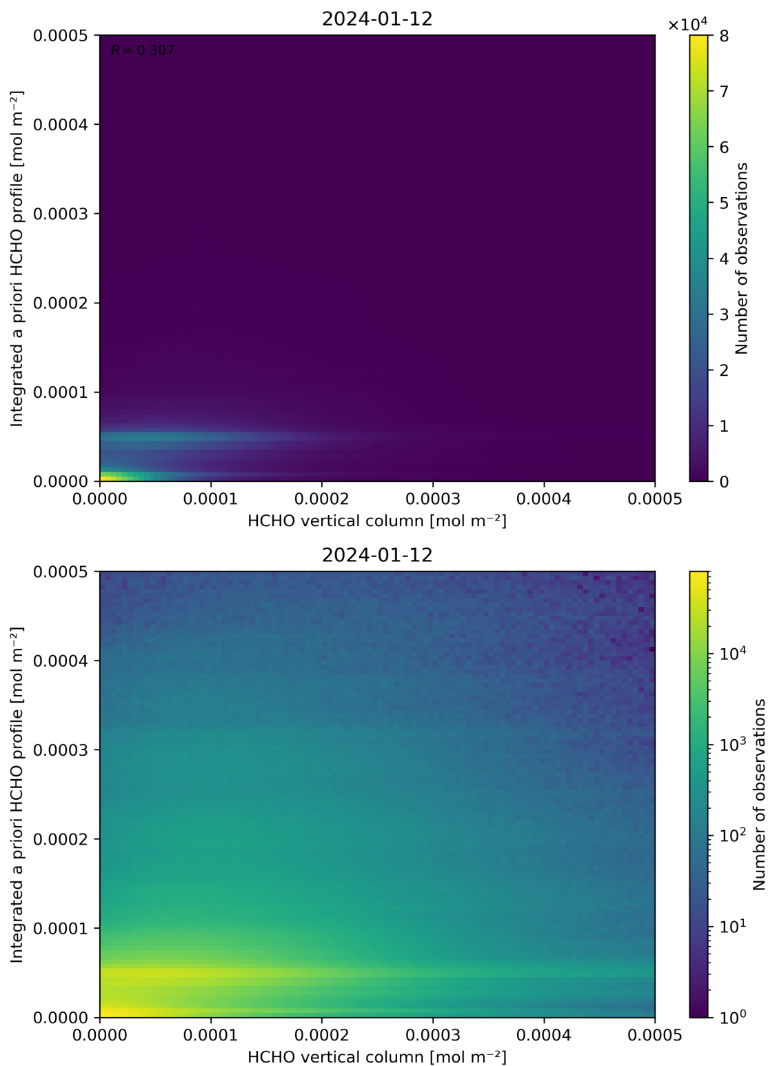
Figure 135: Scatter density plot of “HCHO vertical column” against “Integrated a priori HCHO profile” for 2024-01-11 to 2024-01-13.
