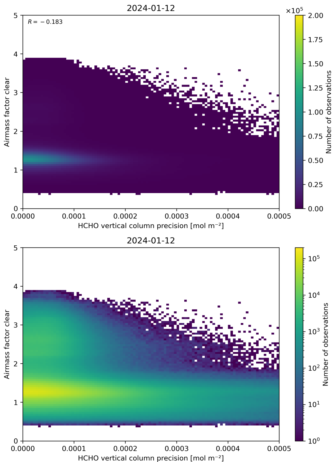
Figure 139: Scatter density plot of “HCHO vertical column precision” against “Airmass factor clear” for 2024-01-11 to 2024-01-13.
