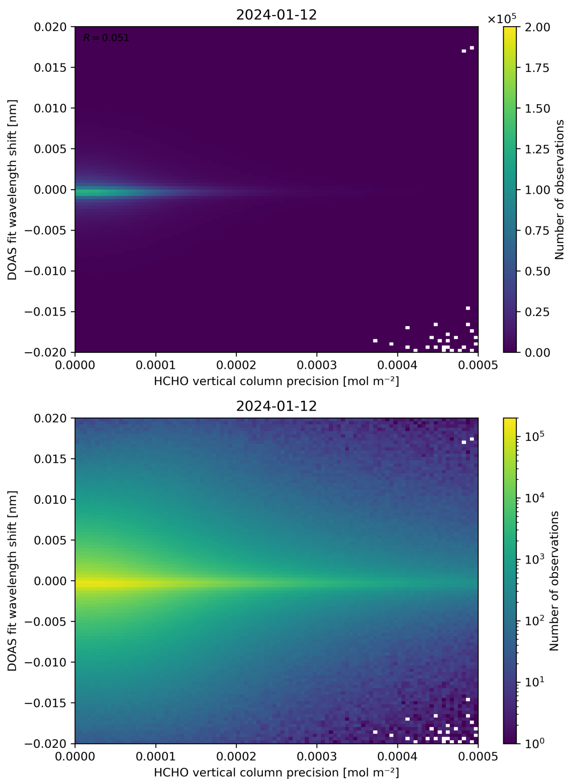
Figure 137: Scatter density plot of “HCHO vertical column precision” against “DOAS fit wavelength shift” for 2024-01-11 to 2024-01-13.
