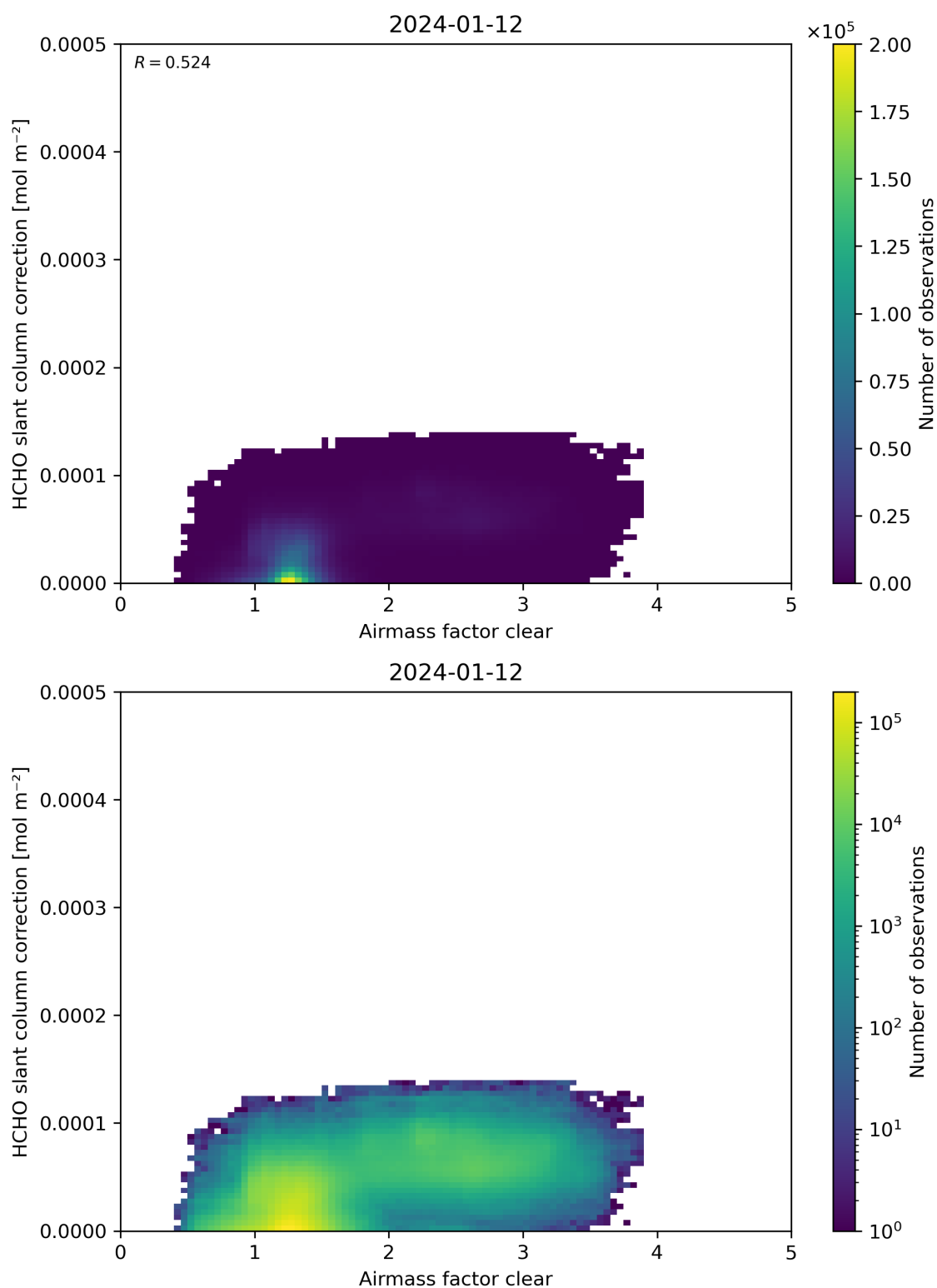
Figure 75: Scatter density plot of “Airmass factor clear” against “HCHO slant column correction” for 2024-01-11 to 2024-01-13.
