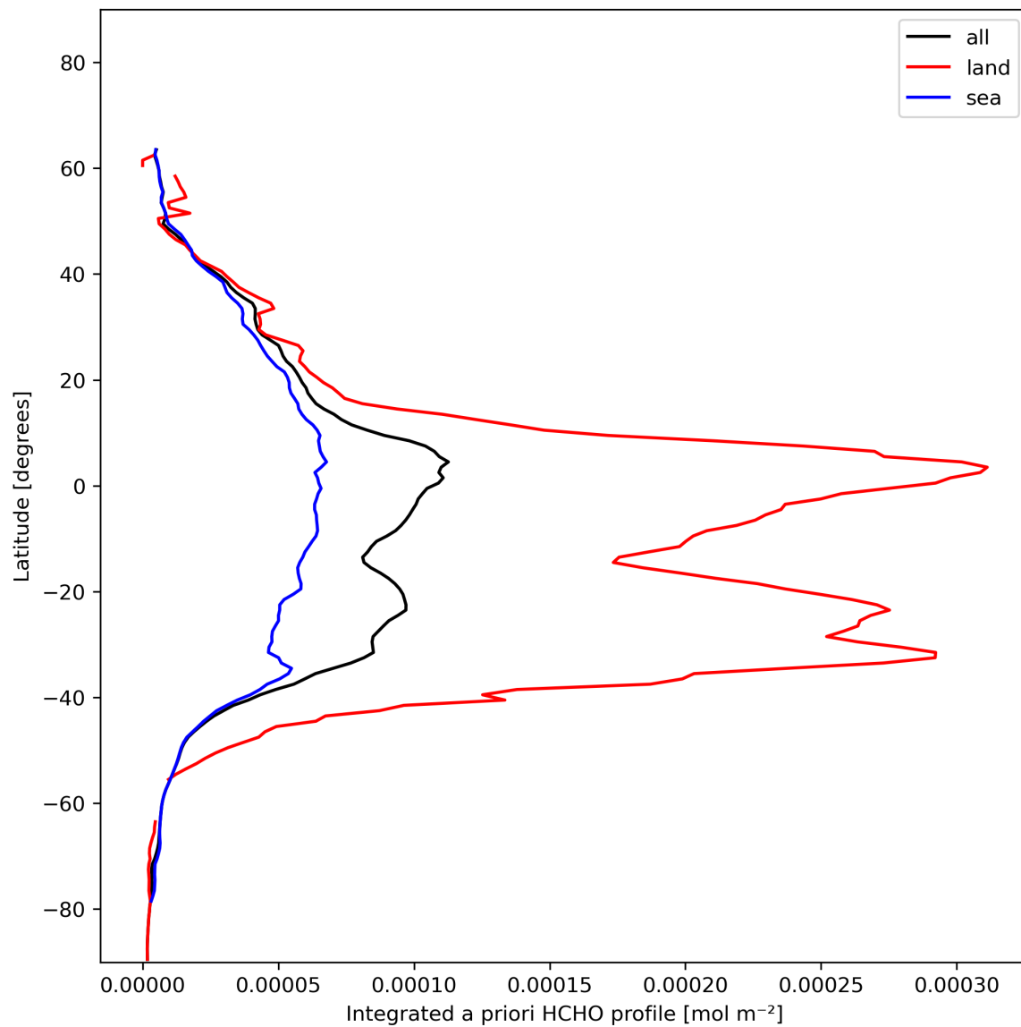
Figure 29: Zonal average of “Integrated a priori HCHO profile” for 2024-01-11 to 2024-01-13.
