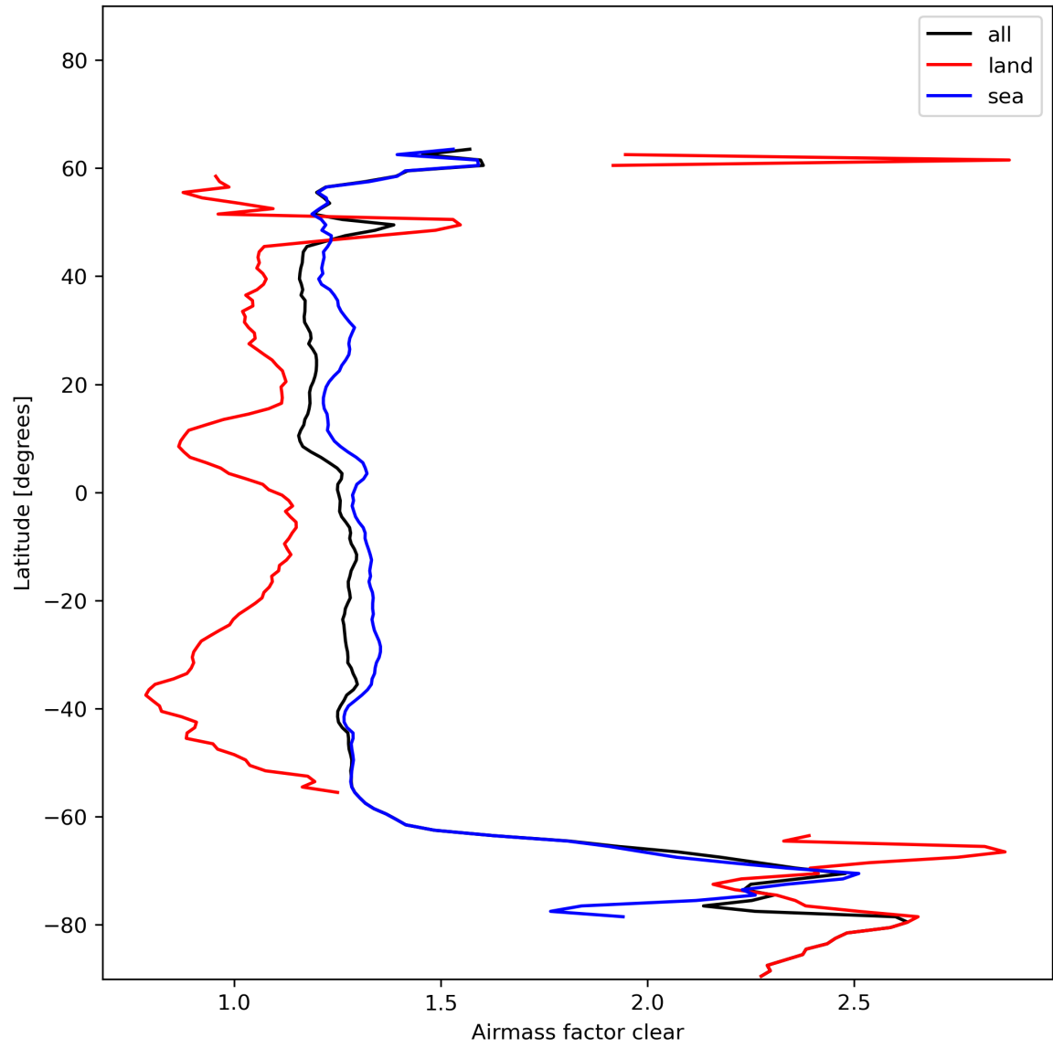
Figure 28: Zonal average of “Airmass factor clear” for 2024-01-11 to 2024-01-13.
