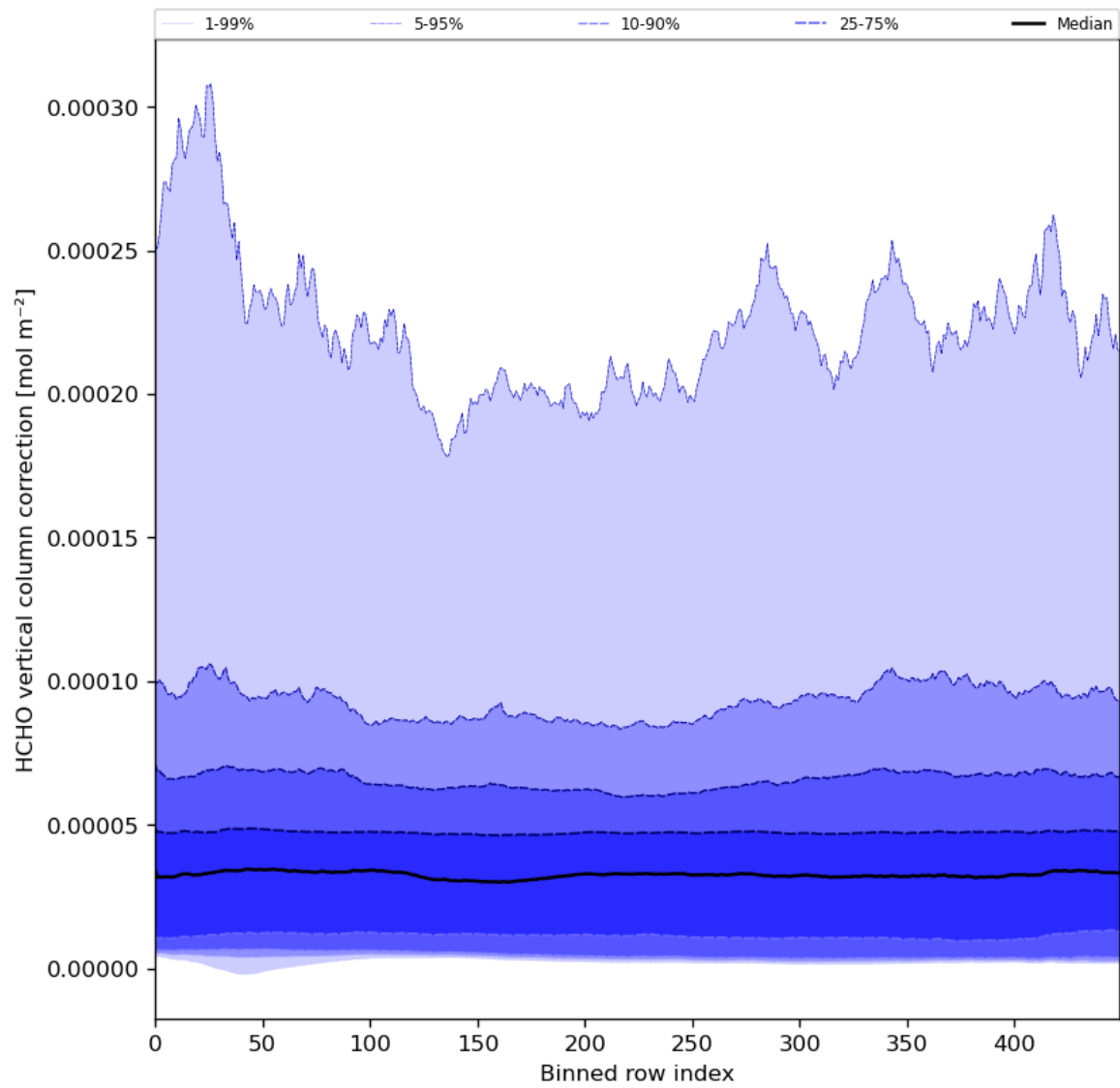
Figure 51: Along track statistics of “HCHO vertical column correction” for 2024-01-11 to 2024-01-13
