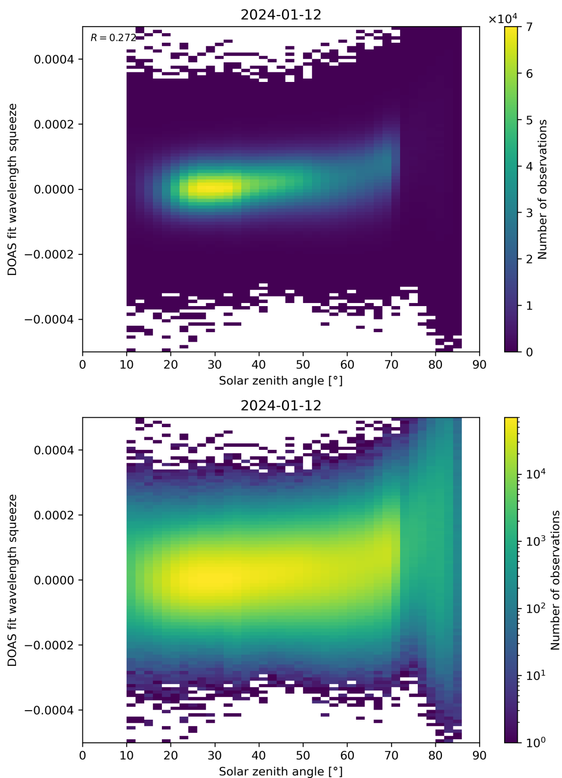
Figure 169: Scatter density plot of “Solar zenith angle” against “DOAS fit wavelength squeeze” for 2024-01-11 to 2024-01-13.
