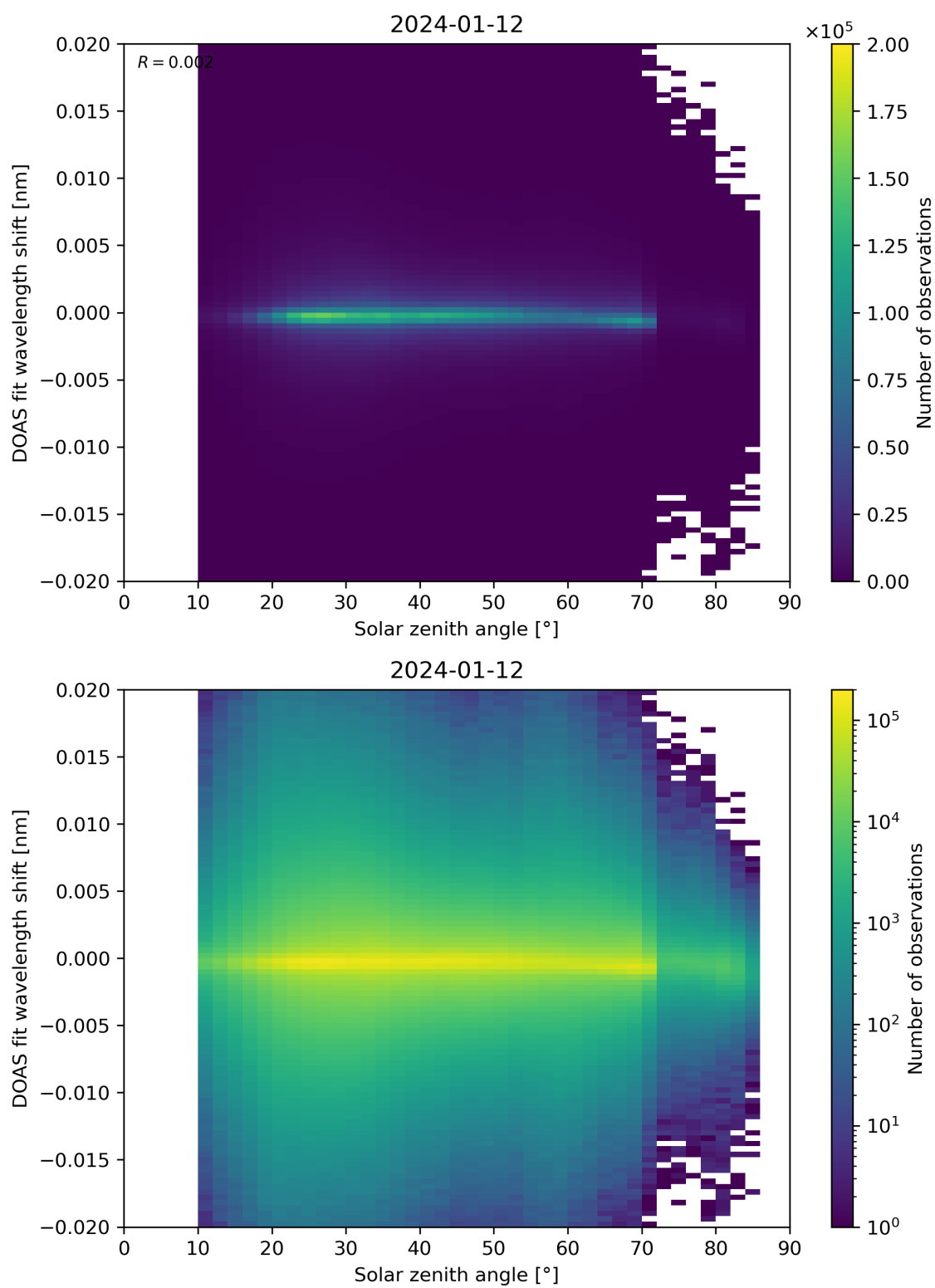
Figure 168: Scatter density plot of “Solar zenith angle” against “DOAS fit wavelength shift” for 2024-01-11 to 2024-01-13.
