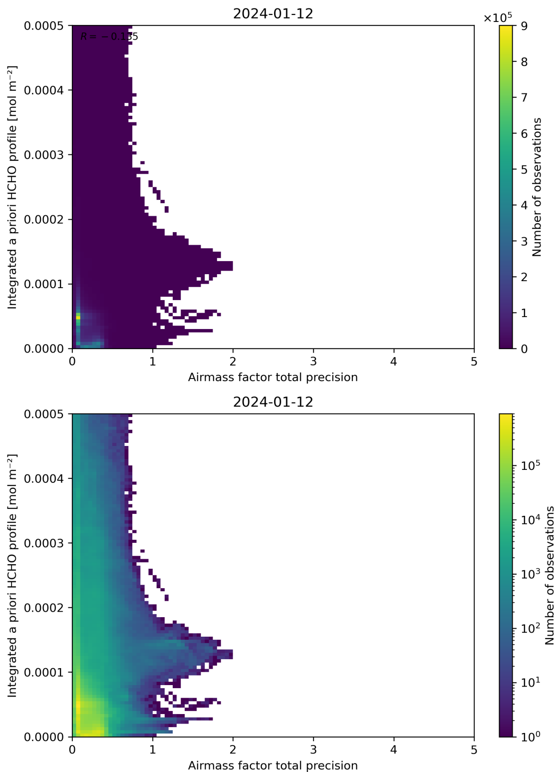
Figure 111: Scatter density plot of “Airmass factor total precision” against “Integrated a priori HCHO profile” for 2024-01-11 to 2024-01-13.
