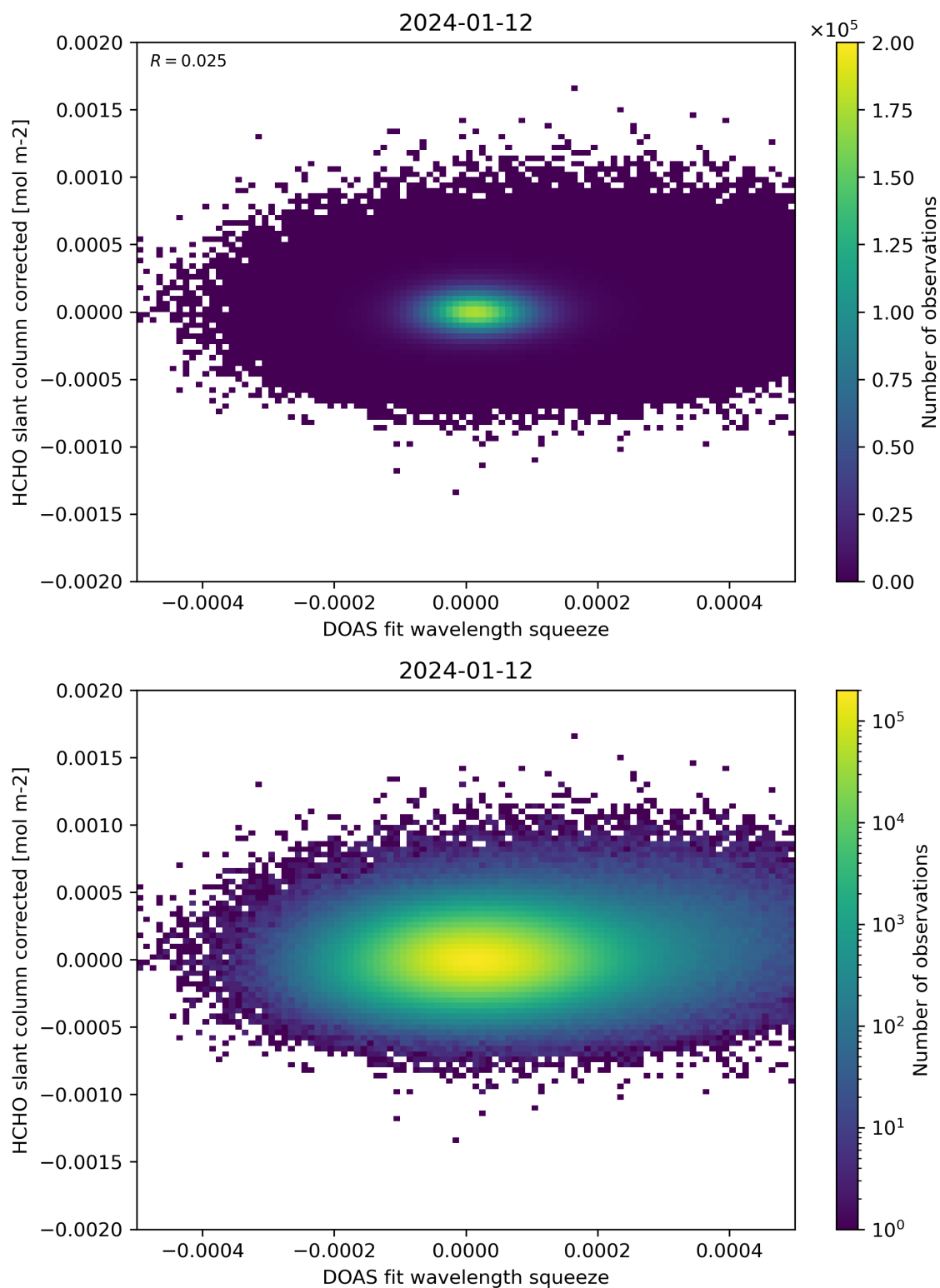
Figure 69: Scatter density plot of “DOAS fit wavelength squeeze” against “HCHO slant column corrected” for 2024-01-11 to 2024-01-13.
