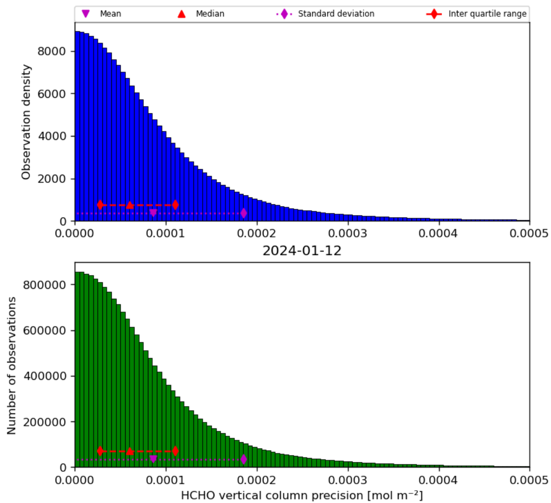
Figure 36: Histogram of “HCHO vertical column precision” for 2024-01-11 to 2024-01-13
