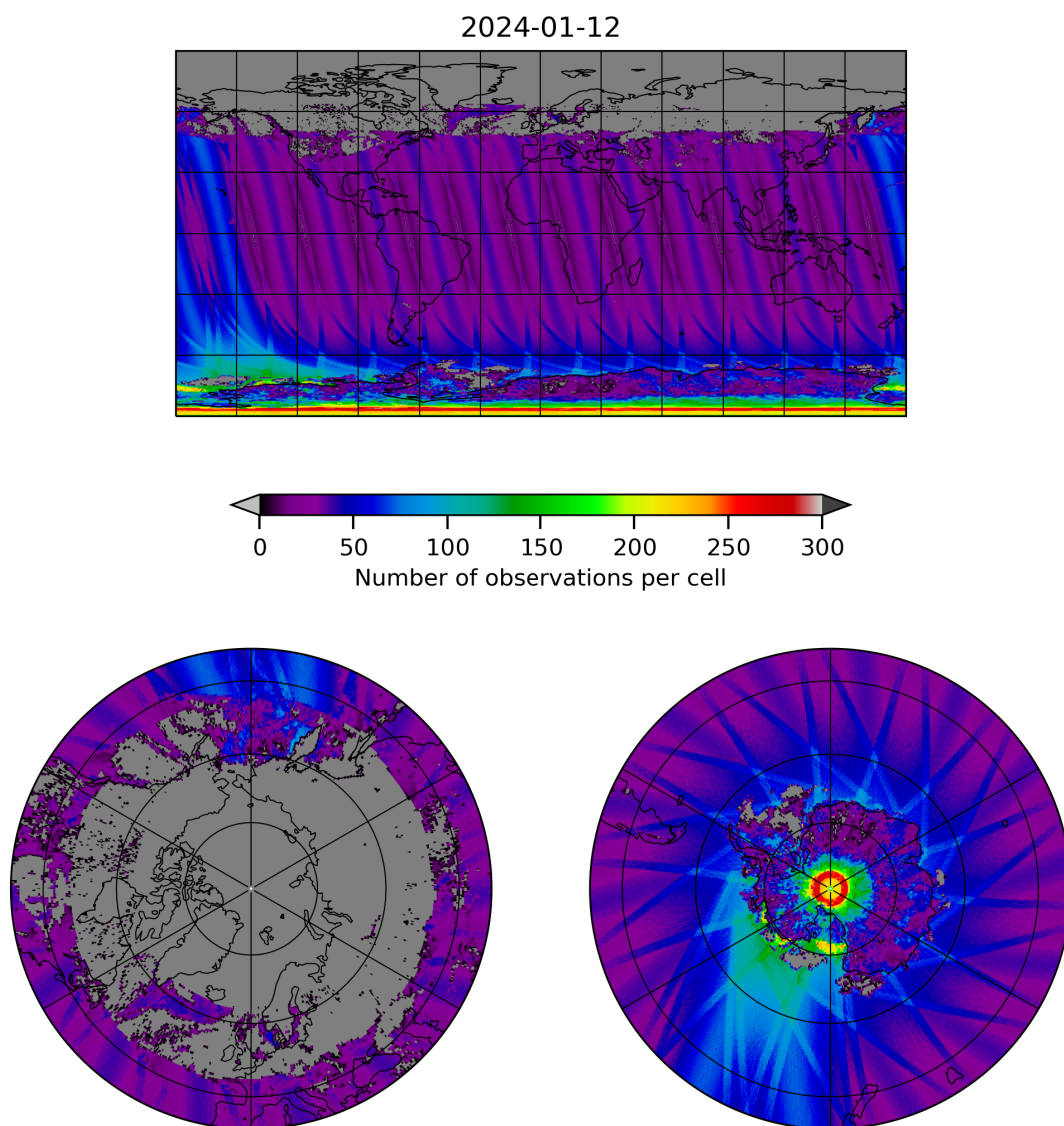
Figure 19: Map of the number of observations for 2024-01-11 to 2024-01-13
