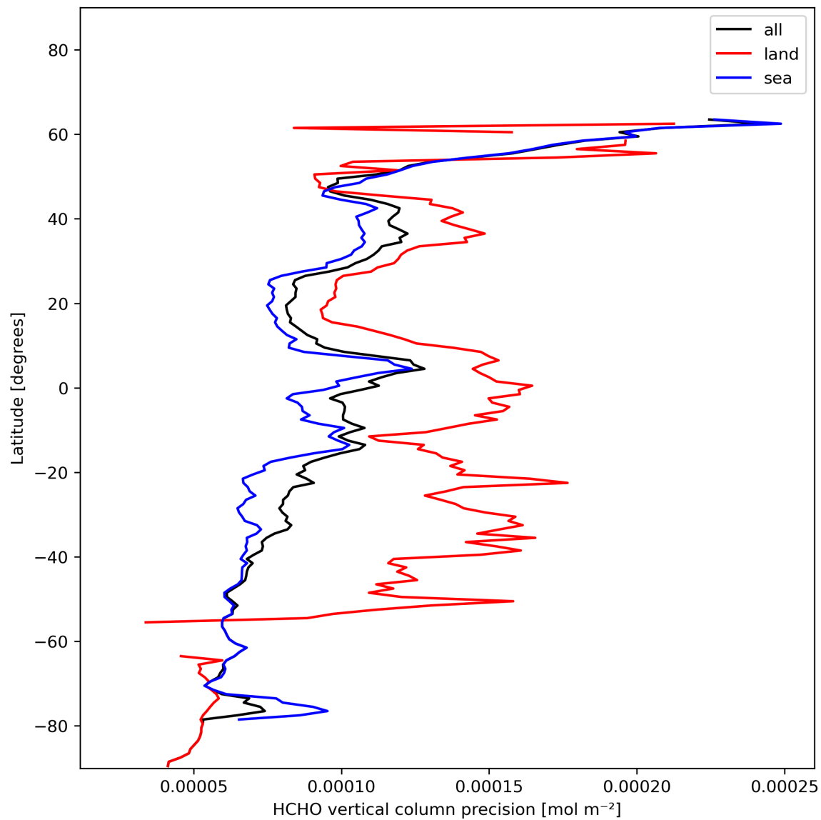
Figure 22: Zonal average of “HCHO vertical column precision” for 2024-01-11 to 2024-01-13.
