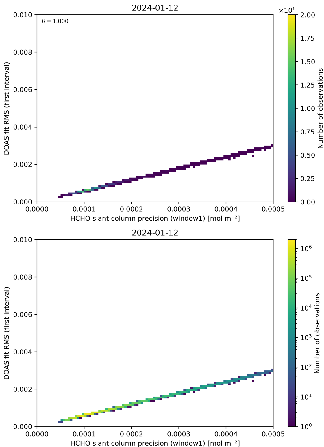
Figure 88: Scatter density plot of “HCHO slant column precision (window1)” against “DOAS fit RMS (first interval)” for 2024-01-11 to 2024-01-13.
