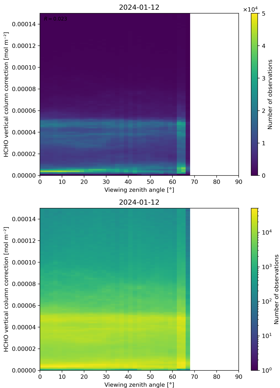
Figure 193: Scatter density plot of “Viewing zenith angle” against “HCHO vertical column correction” for 2024-01-11 to 2024-01-13.
