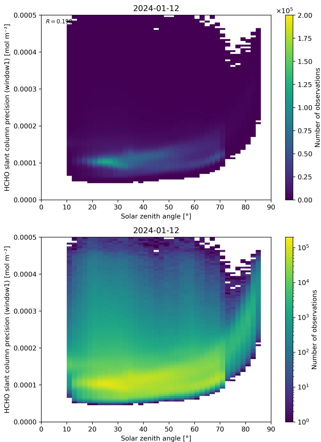
Figure 174: Scatter density plot of “Solar zenith angle” against “HCHO slant column precision (window1)” for 2024-01-11 to 2024-01-13.
