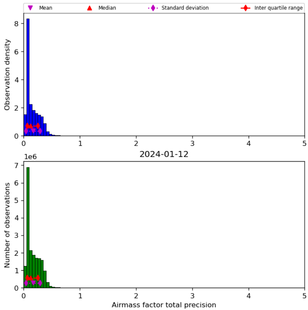
Figure 41: Histogram of “Airmass factor total precision” for 2024-01-11 to 2024-01-13
