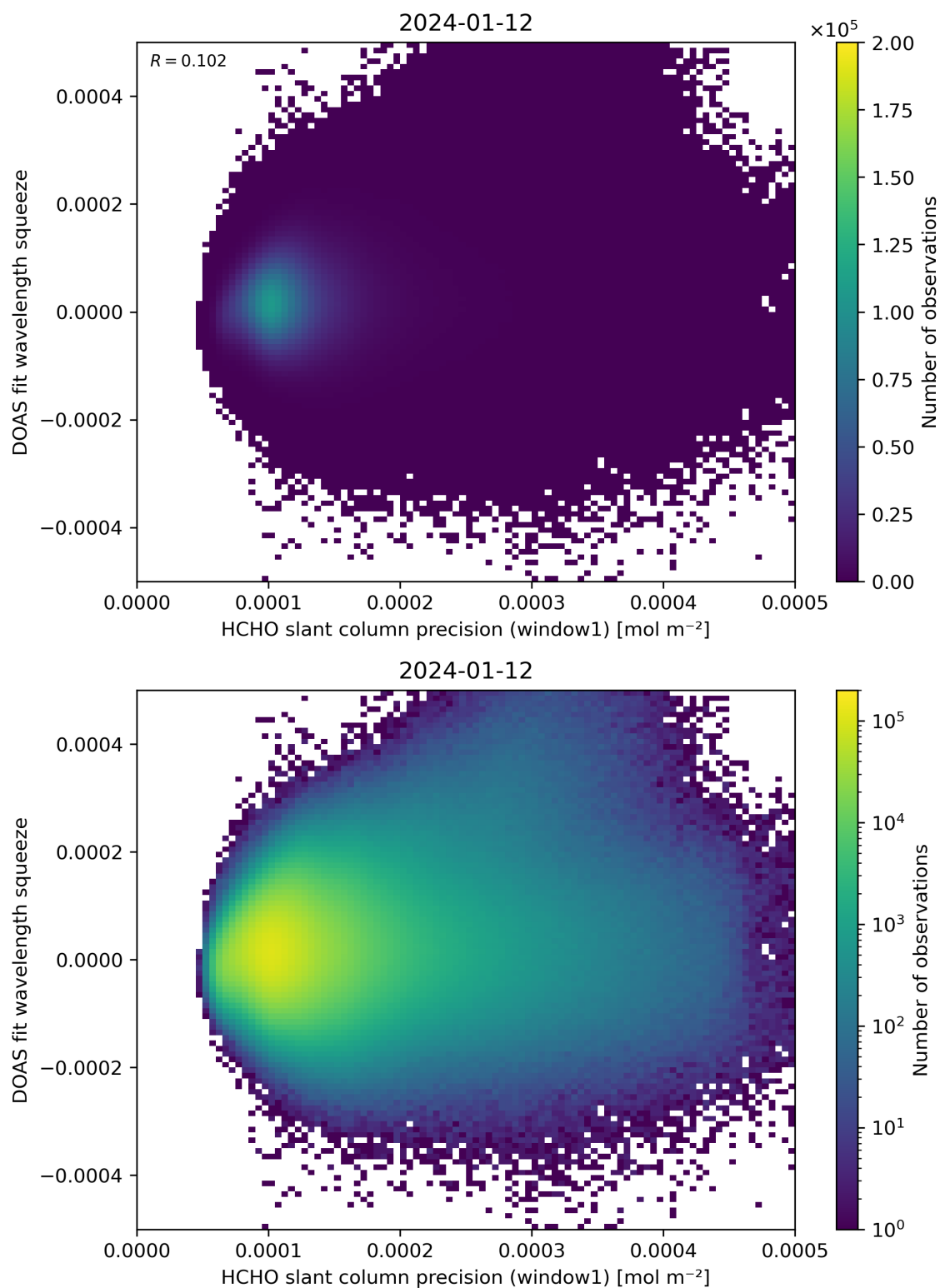
Figure 90: Scatter density plot of “HCHO slant column precision (window1)” against “DOAS fit wavelength squeeze” for 2024-01-11 to 2024-01-13.
