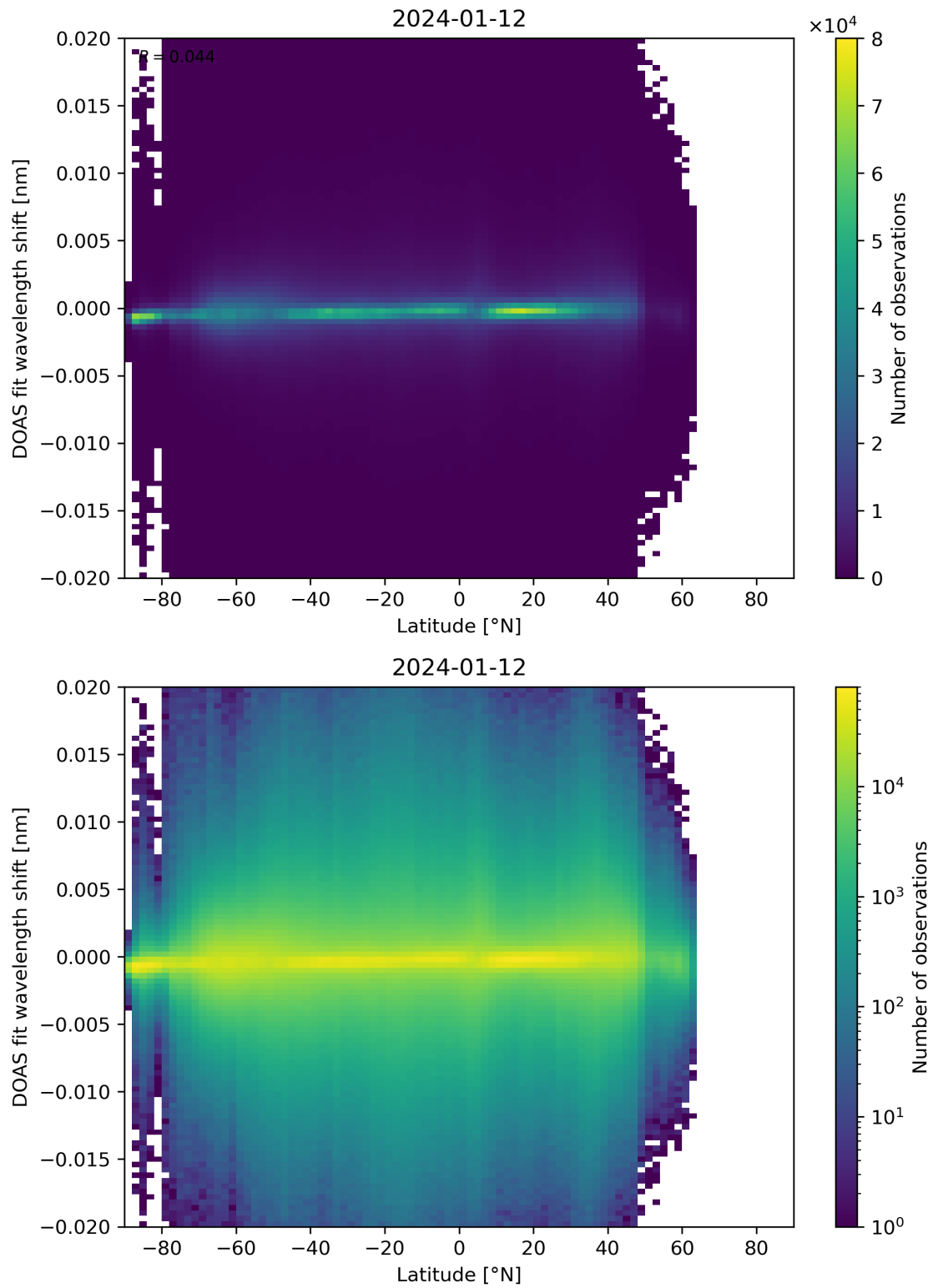
Figure 154: Scatter density plot of “Latitude” against “DOAS fit wavelength shift” for 2024-01-11 to 2024-01-13.
