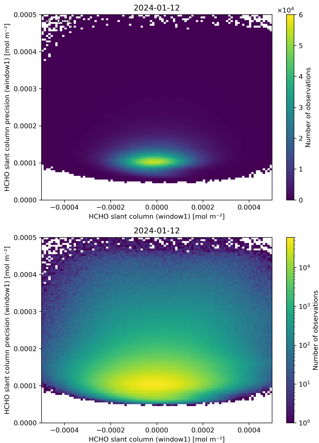
Figure 84: Scatter density plot of “HCHO slant column (window1)” against “HCHO slant column precision (window1)” for 2024-01-11 to 2024-01-13.
