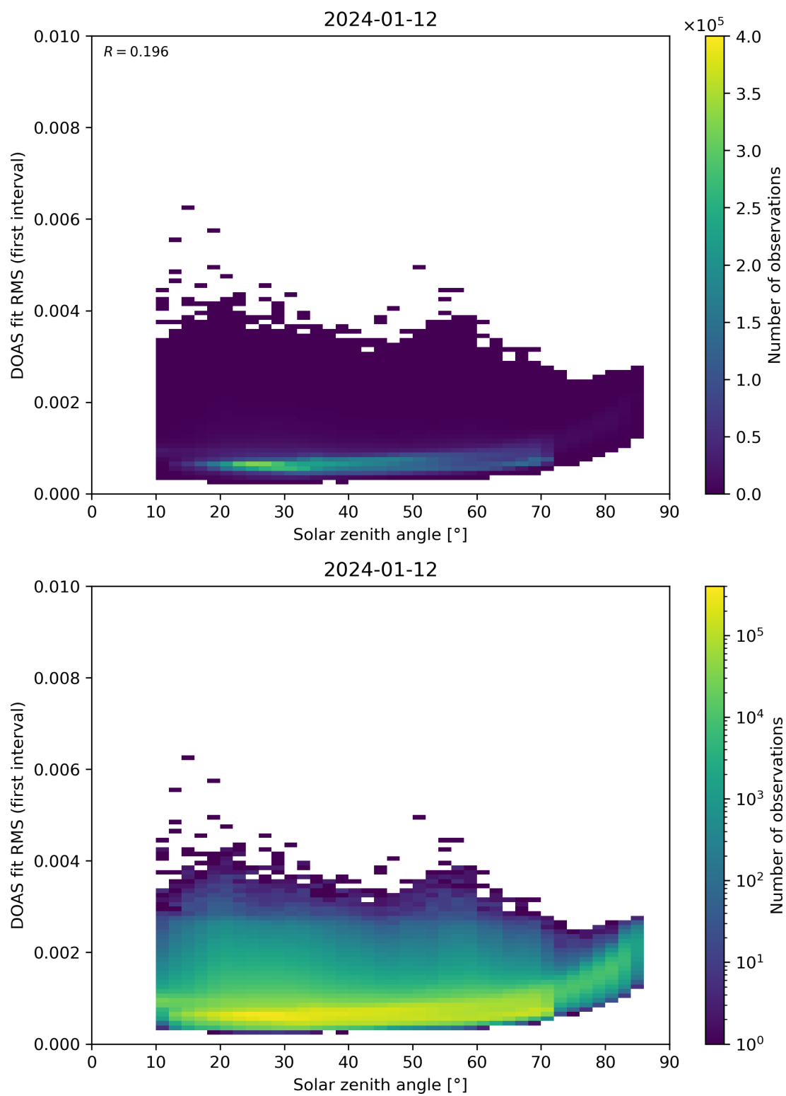
Figure 167: Scatter density plot of “Solar zenith angle” against “DOAS fit RMS (first interval)” for 2024-01-11 to 2024-01-13.
