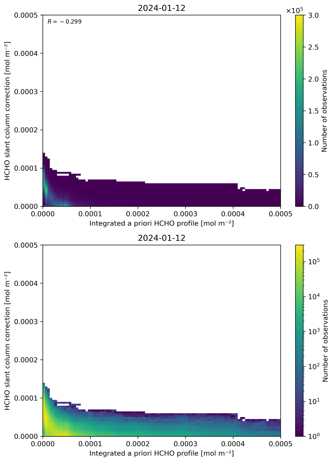
Figure 152: Scatter density plot of “Integrated a priori HCHO profile” against “HCHO slant column correction” for 2024-01-11 to 2024-01-13.
