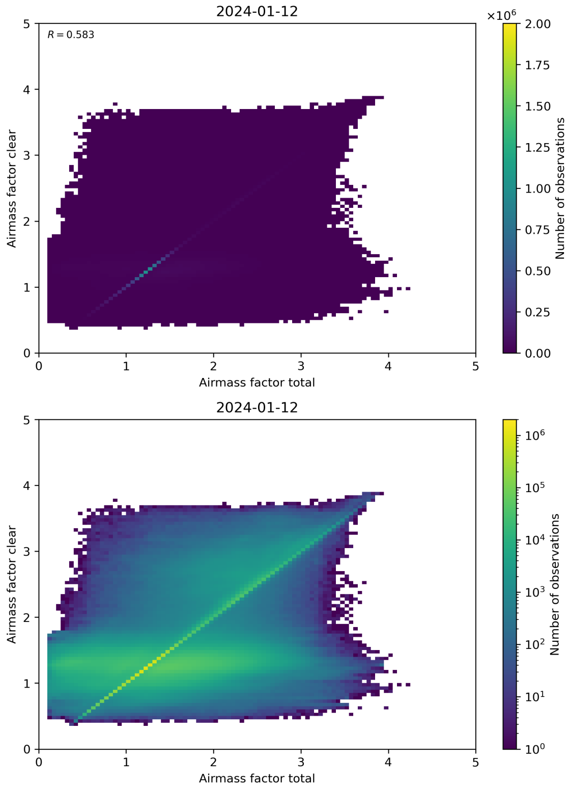
Figure 100: Scatter density plot of “Airmass factor total” against “Airmass factor clear” for 2024-01-11 to 2024-01-13.
