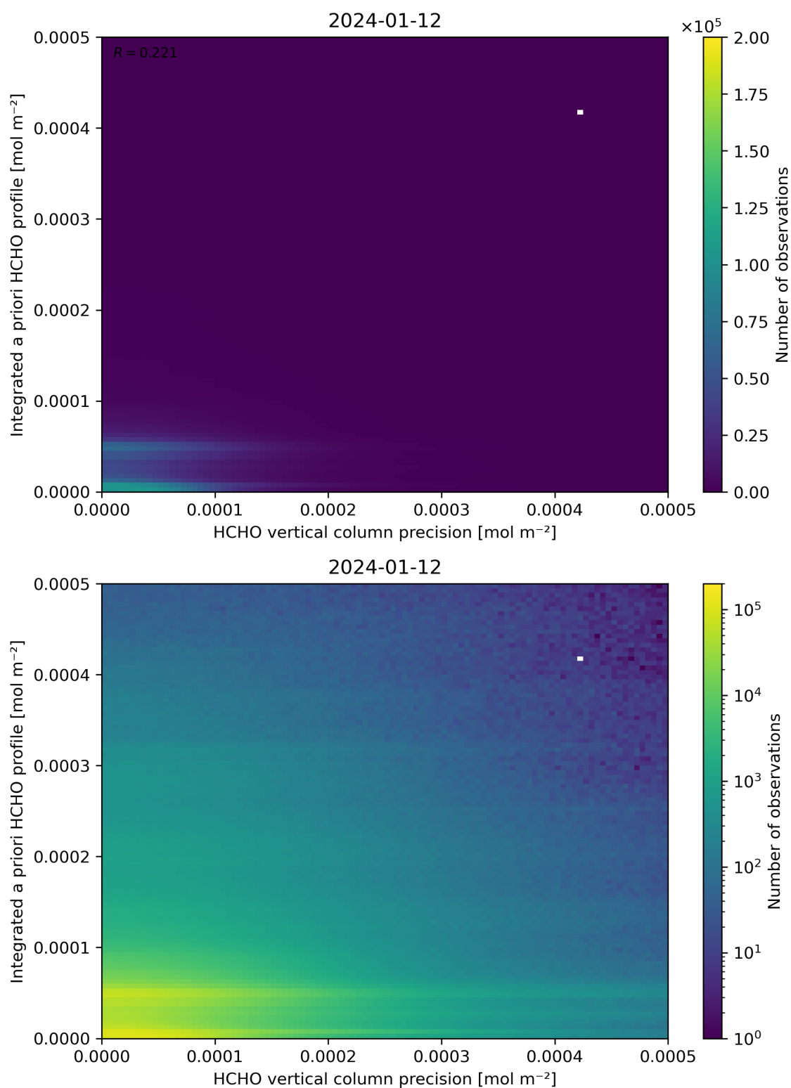
Figure 147: Scatter density plot of “HCHO vertical column precision” against “Integrated a priori HCHO profile” for 2024-01-11 to 2024-01-13.
