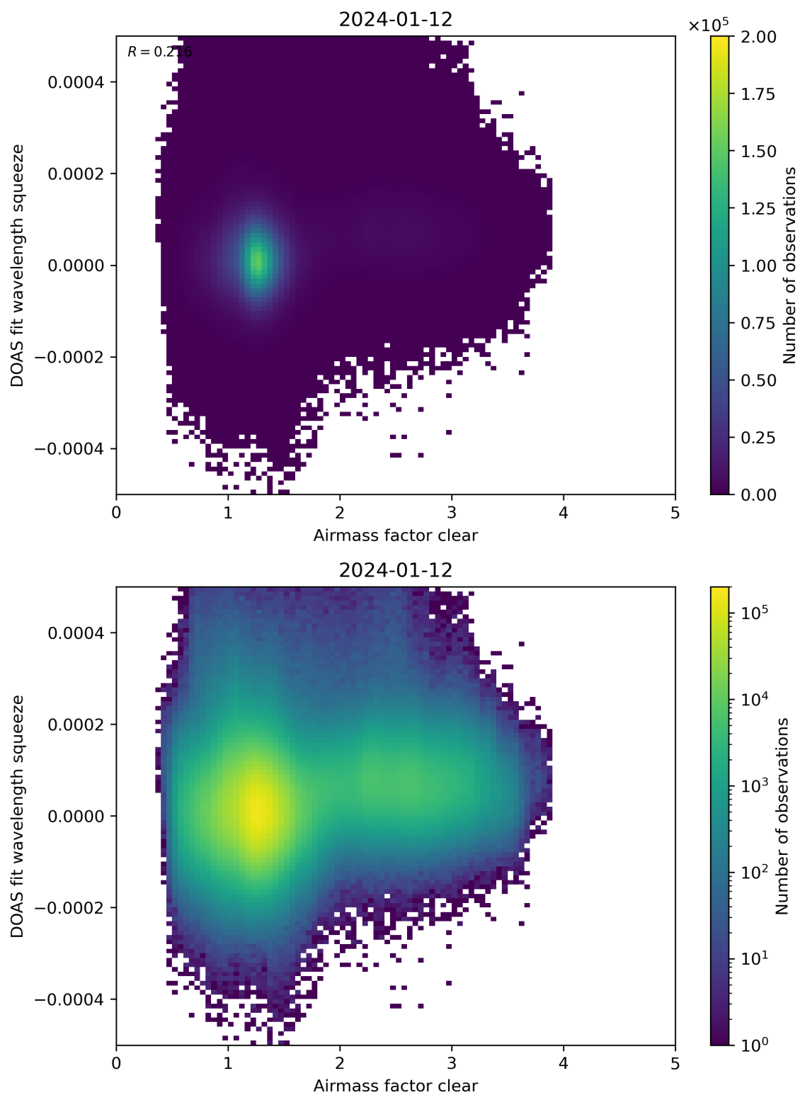
Figure 73: Scatter density plot of “Airmass factor clear” against “DOAS fit wavelength squeeze” for 2024-01-11 to 2024-01-13.
