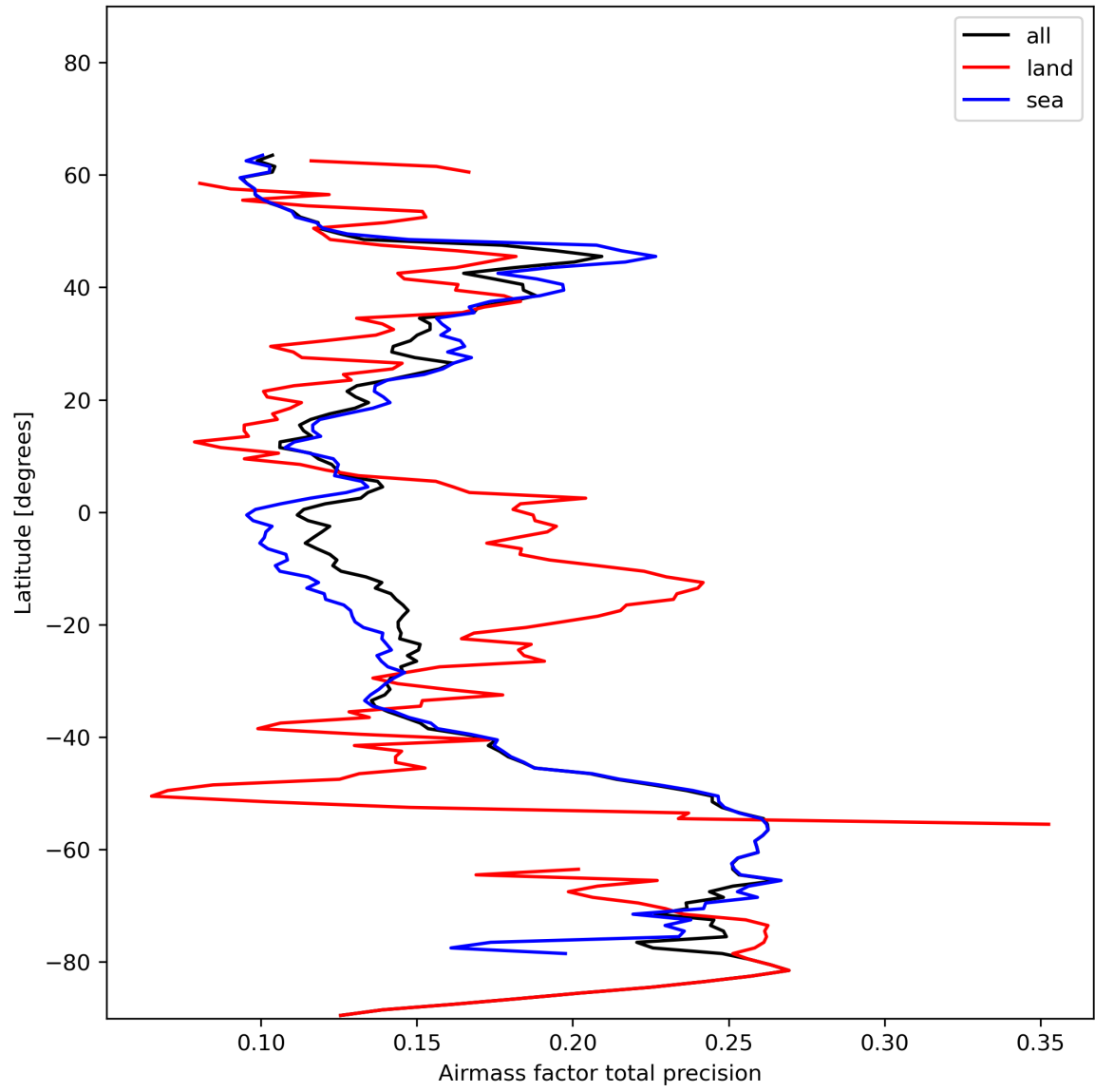
Figure 27: Zonal average of “Airmass factor total precision” for 2024-01-11 to 2024-01-13.
