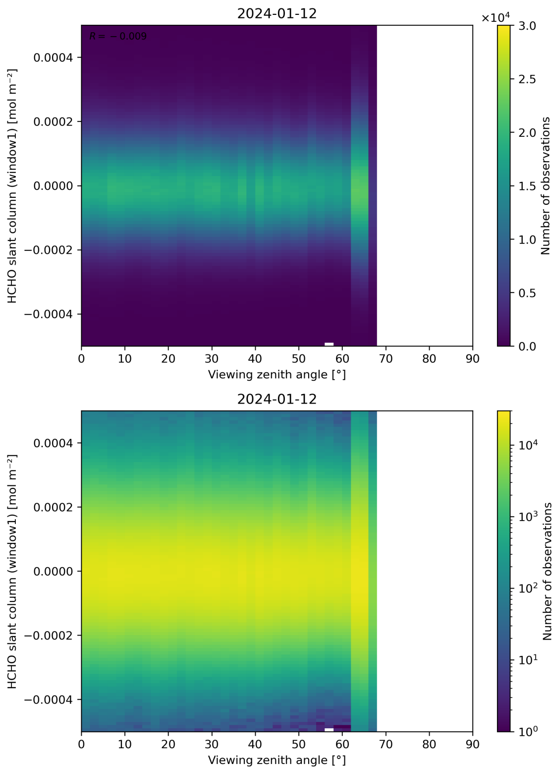
Figure 188: Scatter density plot of “Viewing zenith angle” against “HCHO slant column (window1)” for 2024-01-11 to 2024-01-13.
