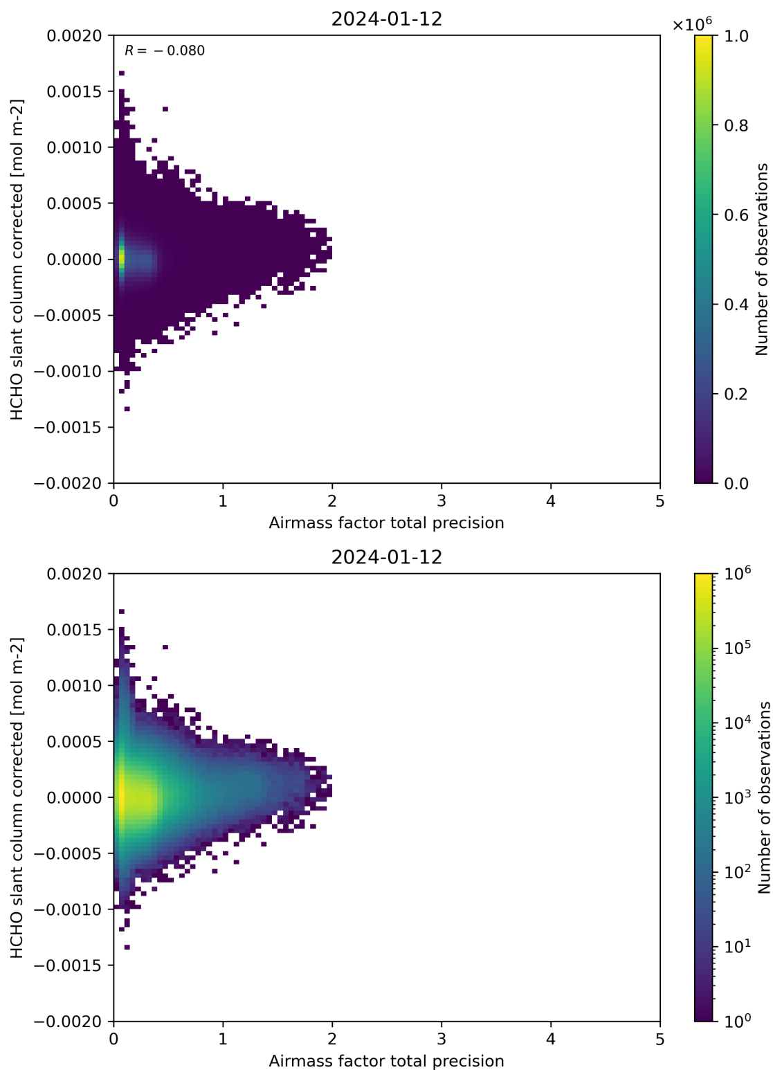
Figure 109: Scatter density plot of “Airmass factor total precision” against “HCHO slant column corrected” for 2024-01-11 to 2024-01-13.
