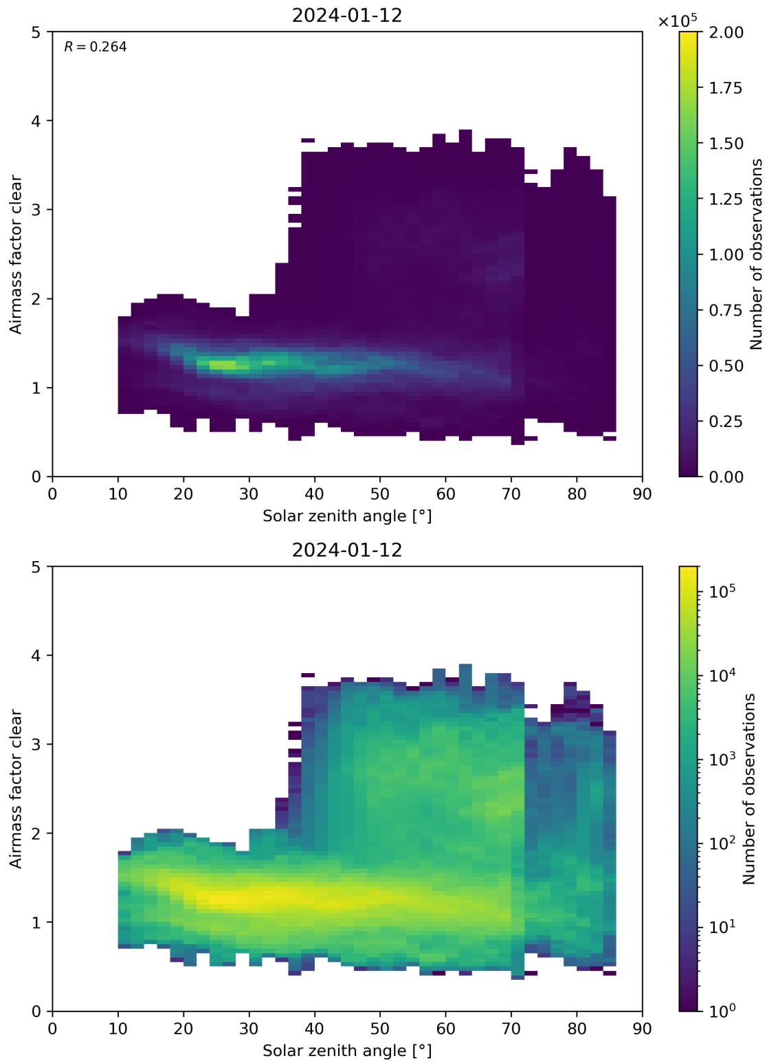
Figure 170: Scatter density plot of “Solar zenith angle” against “Airmass factor clear” for 2024-01-11 to 2024-01-13.
