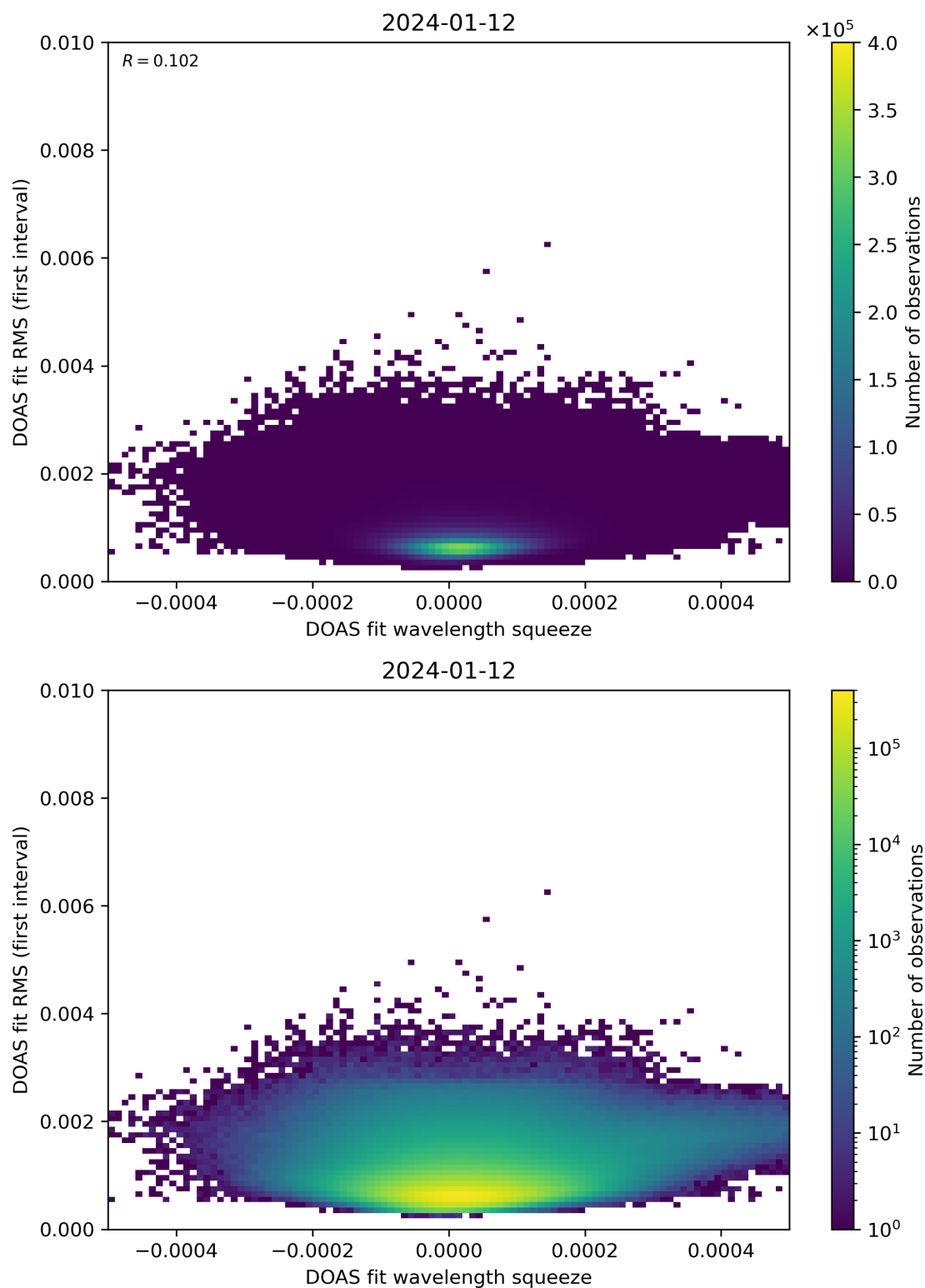
Figure 68: Scatter density plot of “DOAS fit wavelength squeeze” against “DOAS fit RMS (first interval)” for 2024-01-11 to 2024-01-13.
