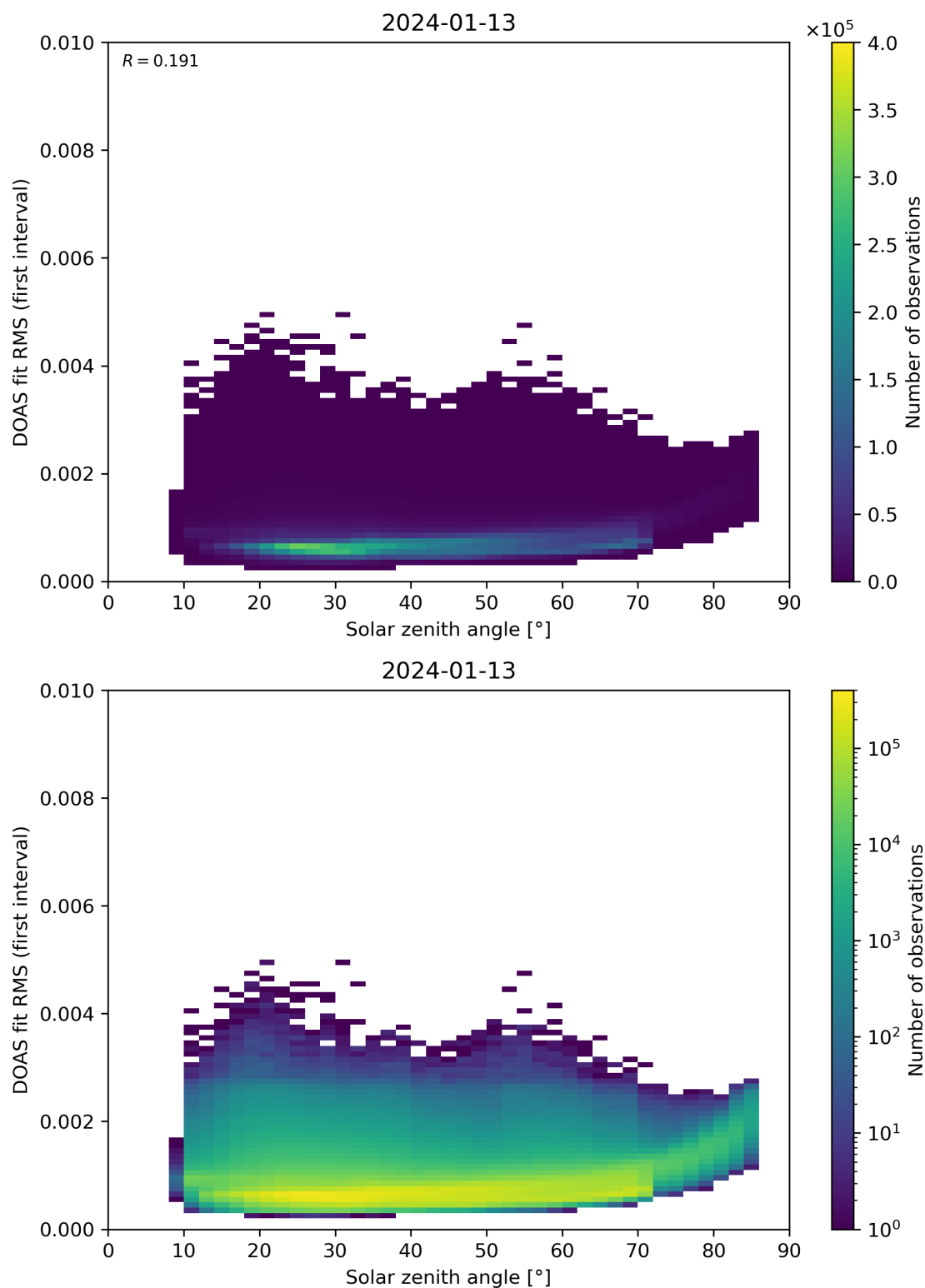
Figure 167: Scatter density plot of “Solar zenith angle” against “DOAS fit RMS (first interval)” for 2024-01-12 to 2024-01-14.
