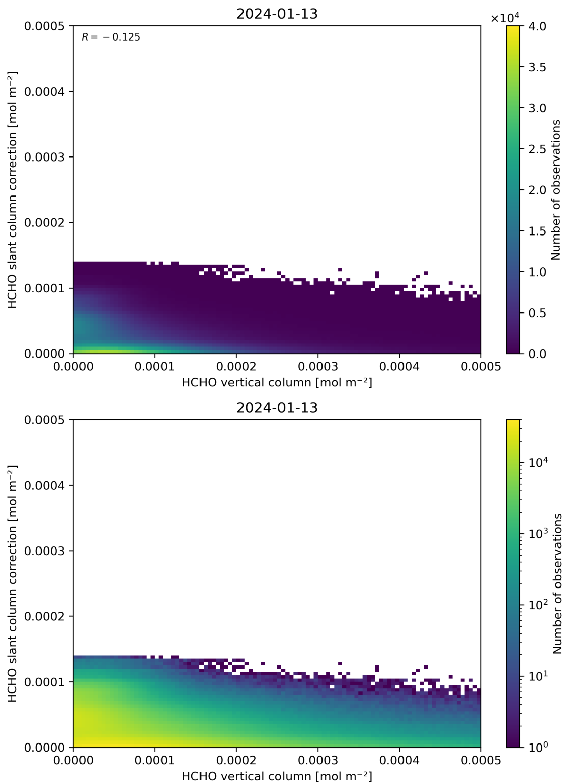
Figure 128: Scatter density plot of “HCHO vertical column” against “HCHO slant column correction” for 2024-01-12 to 2024-01-14.
