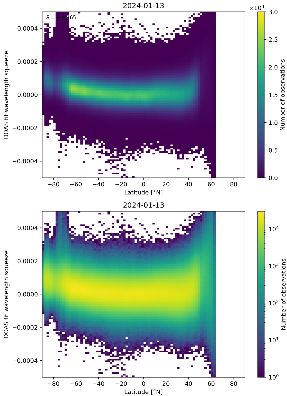
Figure 155: Scatter density plot of “Latitude” against “DOAS fit wavelength squeeze” for 2024-01-12 to 2024-01-14.
