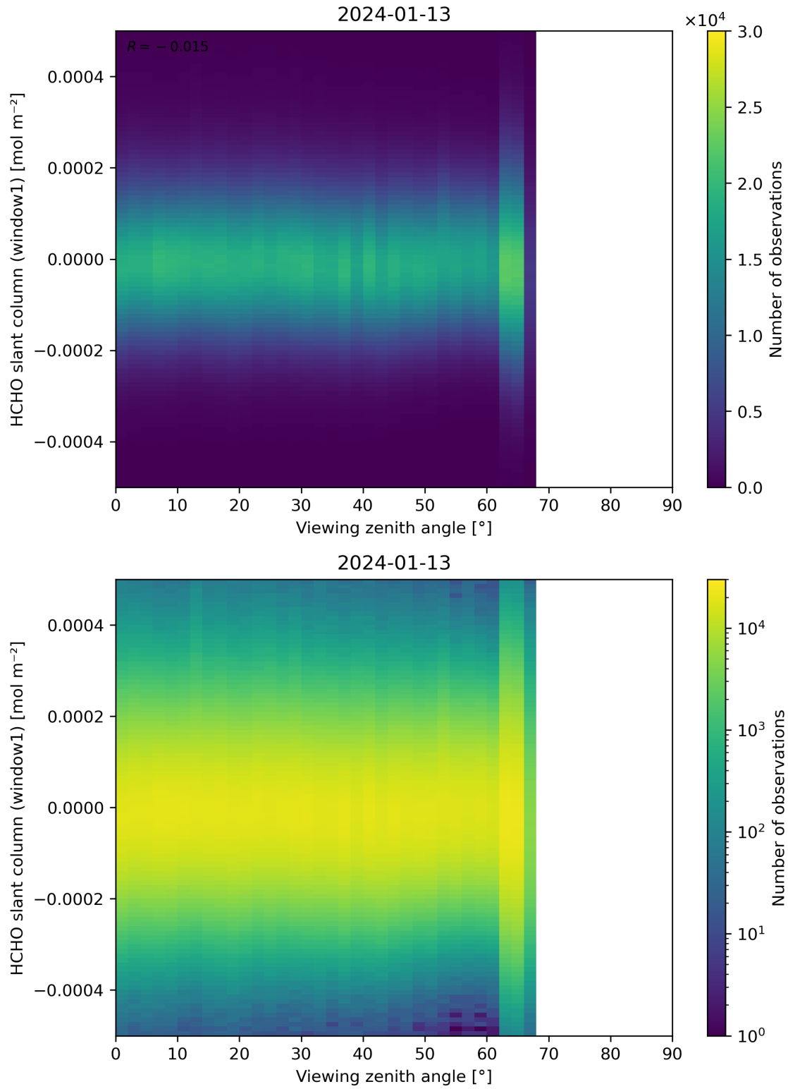
Figure 188: Scatter density plot of “Viewing zenith angle” against “HCHO slant column (window1)” for 2024-01-12 to 2024-01-14.
