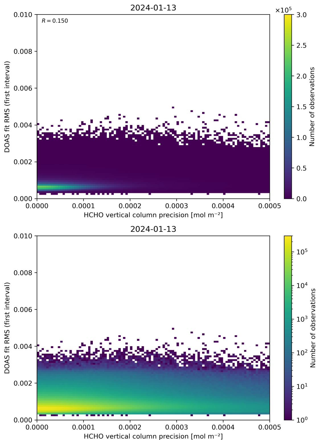
Figure 136: Scatter density plot of “HCHO vertical column precision” against “DOAS fit RMS (first interval)” for 2024-01-12 to 2024-01-14.
