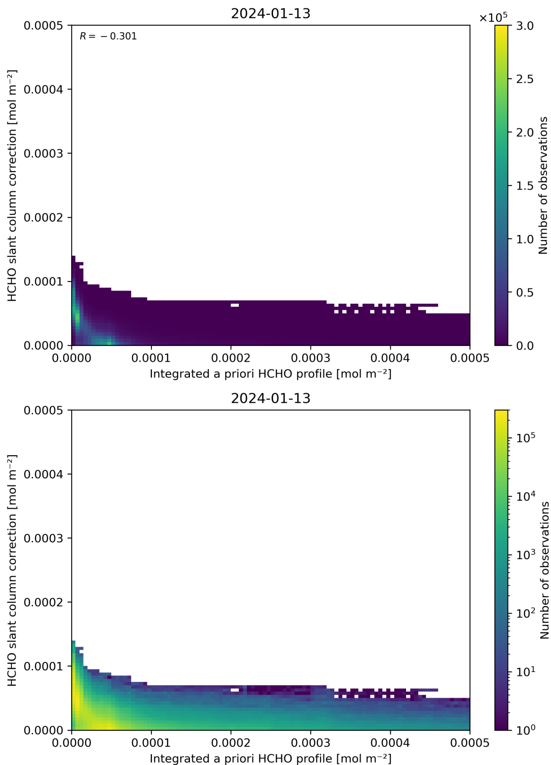
Figure 152: Scatter density plot of “Integrated a priori HCHO profile” against “HCHO slant column correction” for 2024-01-12 to 2024-01-14.
