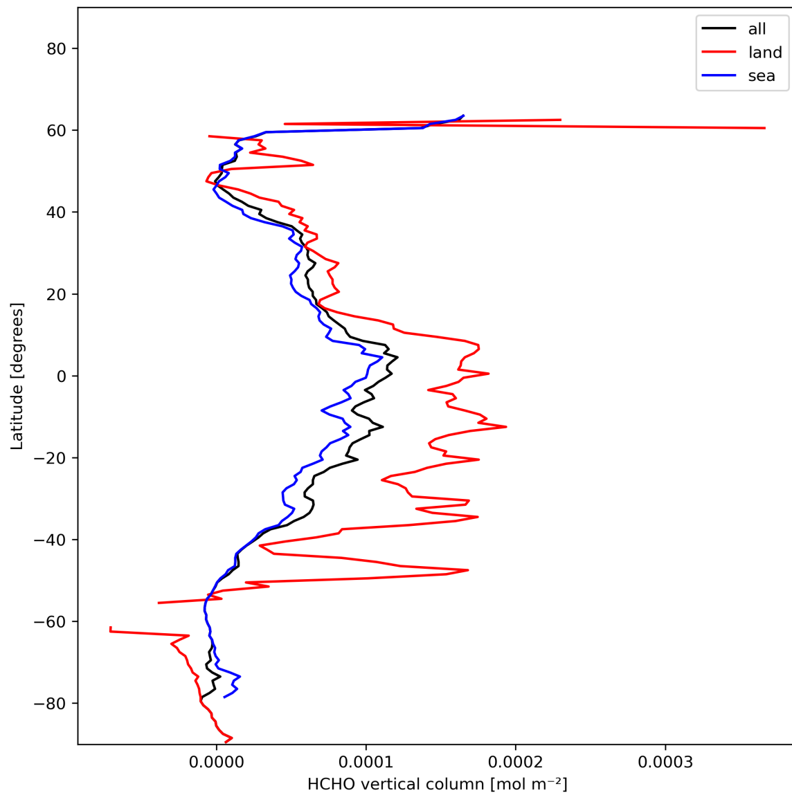
Figure 21: Zonal average of “HCHO vertical column” for 2024-01-12 to 2024-01-14.
