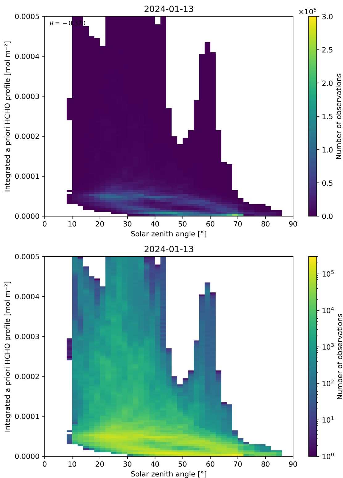
Figure 180: Scatter density plot of “Solar zenith angle” against “Integrated a priori HCHO profile” for 2024-01-12 to 2024-01-14.
