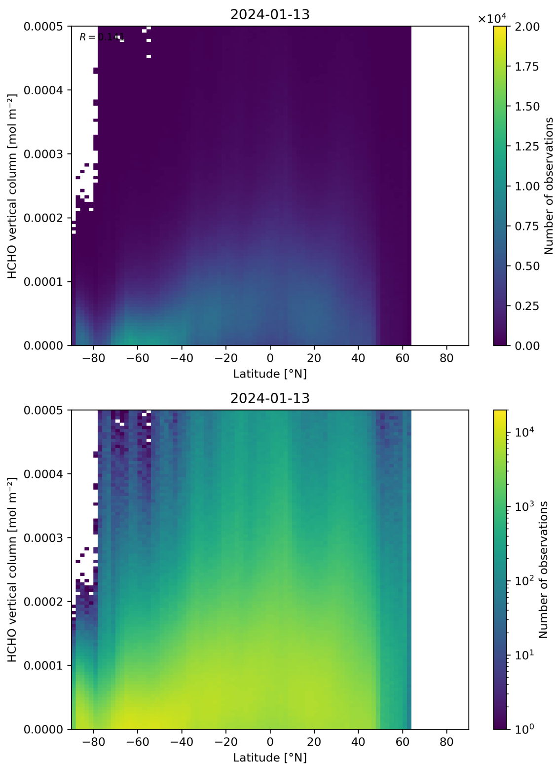
Figure 163: Scatter density plot of “Latitude” against “HCHO vertical column” for 2024-01-12 to 2024-01-14.
