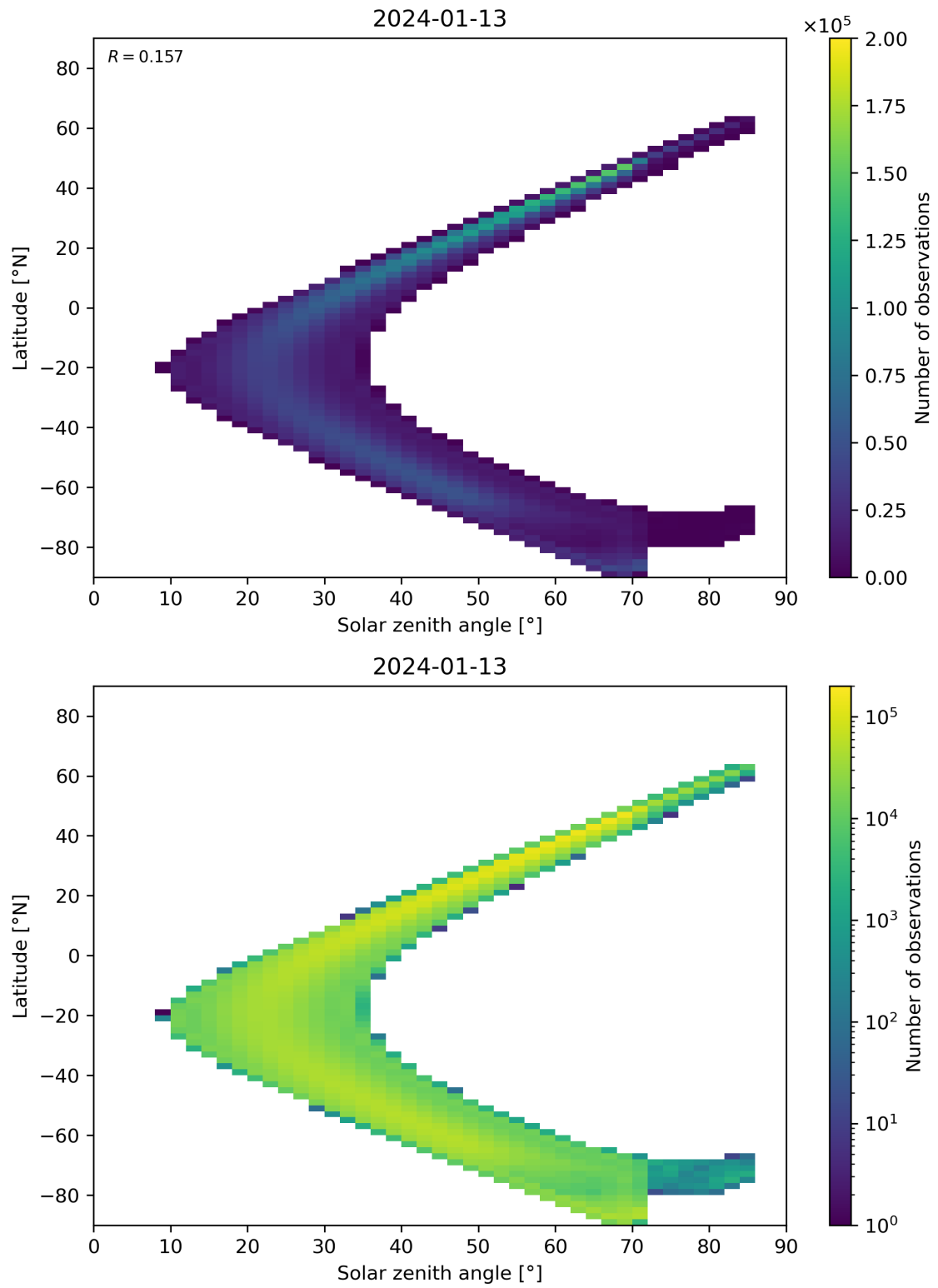
Figure 181: Scatter density plot of “Solar zenith angle” against “Latitude” for 2024-01-12 to 2024-01-14.
