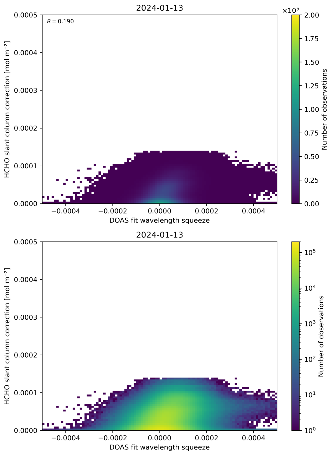
Figure 70: Scatter density plot of “DOAS fit wavelength squeeze” against “HCHO slant column correction” for 2024-01-12 to 2024-01-14.
