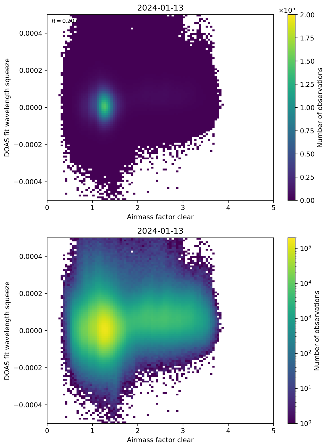
Figure 73: Scatter density plot of “Airmass factor clear” against “DOAS fit wavelength squeeze” for 2024-01-12 to 2024-01-14.
