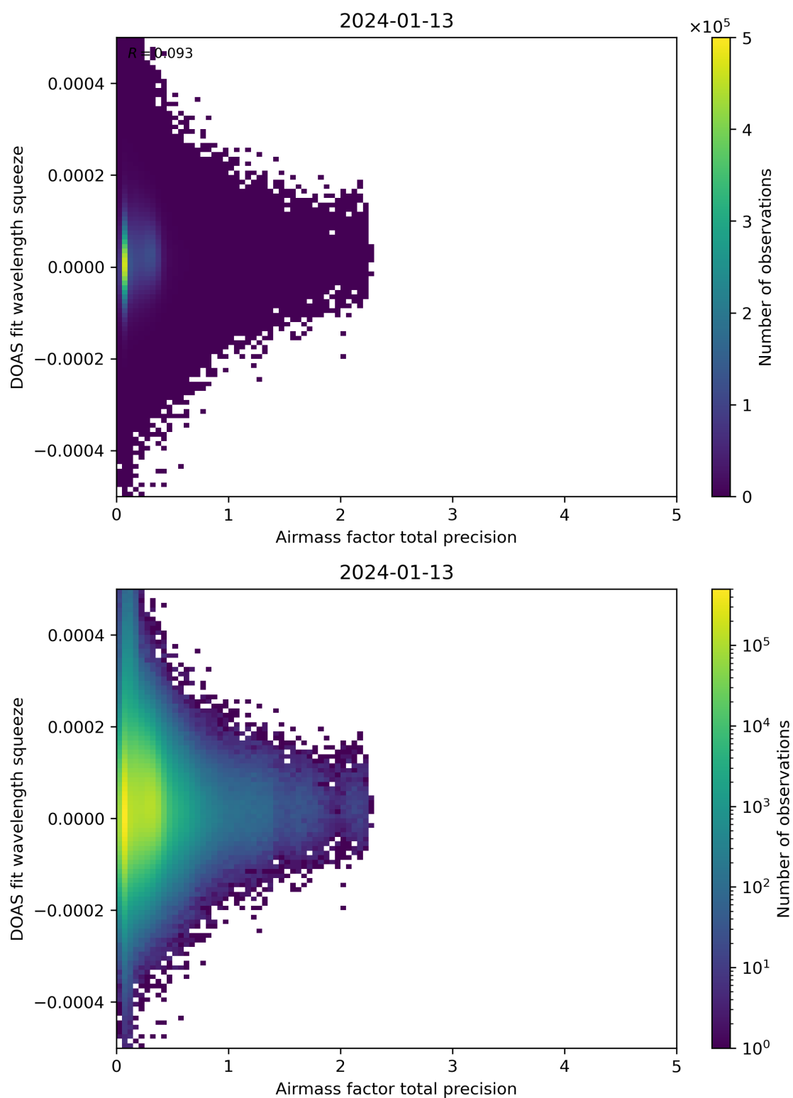
Figure 107: Scatter density plot of “Airmass factor total precision” against “DOAS fit wavelength squeeze” for 2024-01-12 to 2024-01-14.
