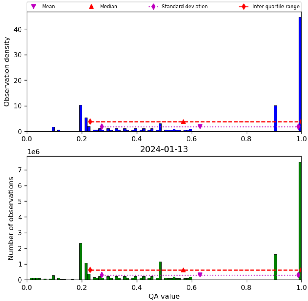
Figure 34: Histogram of “QA value” for 2024-01-12 to 2024-01-14
