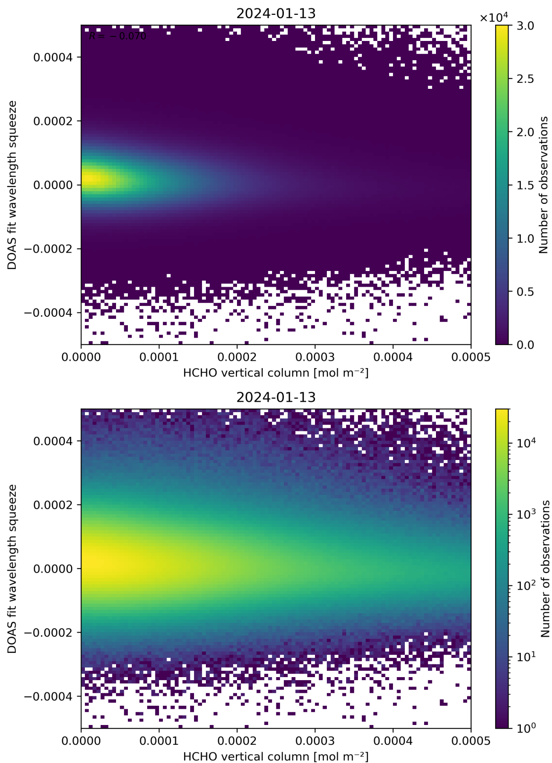
Figure 125: Scatter density plot of “HCHO vertical column” against “DOAS fit wavelength squeeze” for 2024-01-12 to 2024-01-14.
