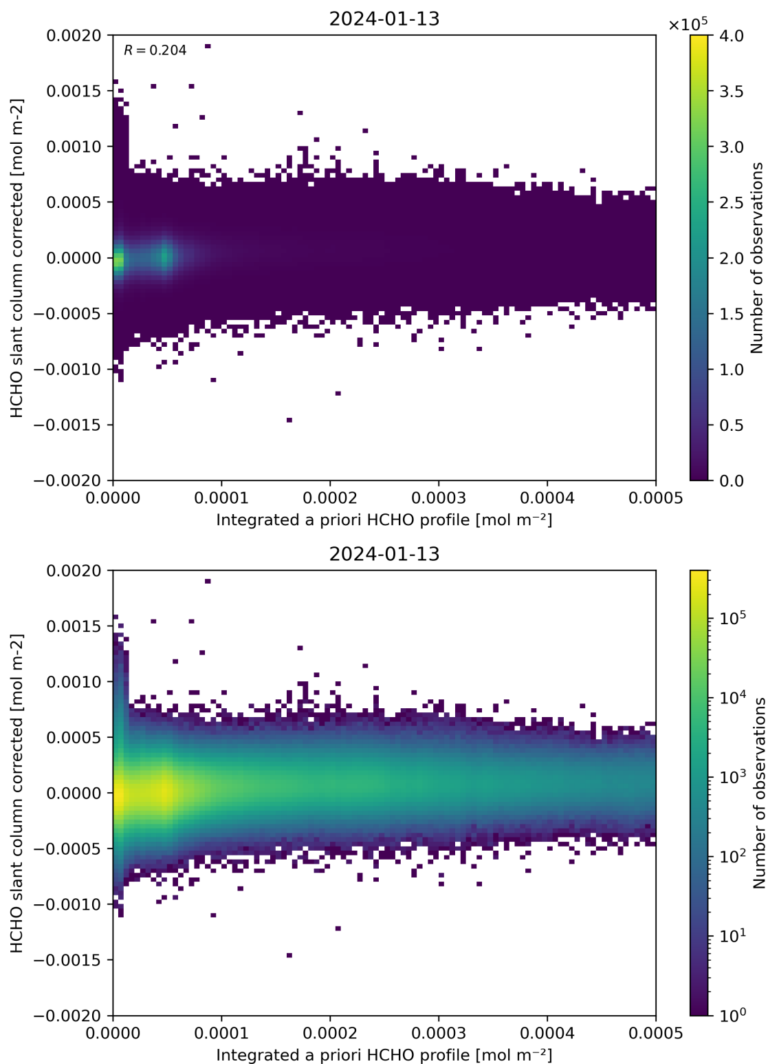
Figure 151: Scatter density plot of “Integrated a priori HCHO profile” against “HCHO slant column corrected” for 2024-01-12 to 2024-01-14.
