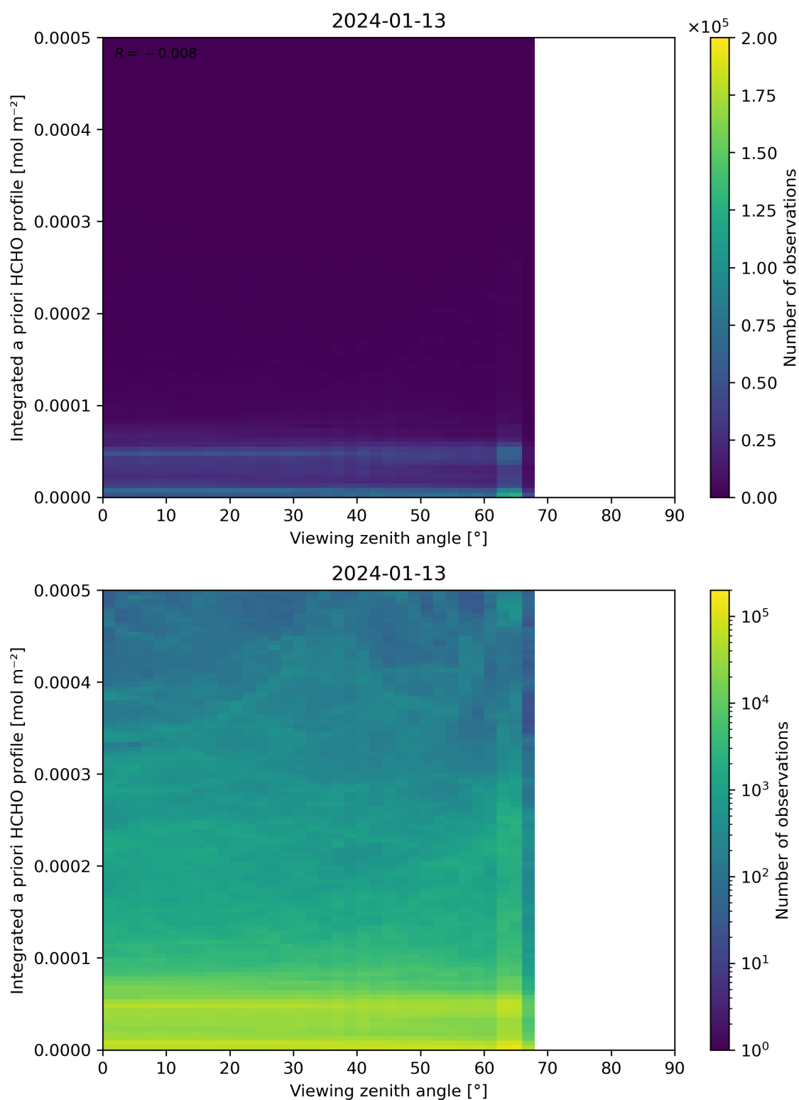
Figure 195: Scatter density plot of “Viewing zenith angle” against “Integrated a priori HCHO profile” for 2024-01-12 to 2024-01-14.
