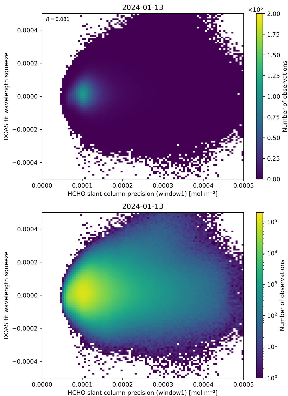
Figure 90: Scatter density plot of “HCHO slant column precision (window1)” against “DOAS fit wavelength squeeze” for 2024-01-12 to 2024-01-14.
