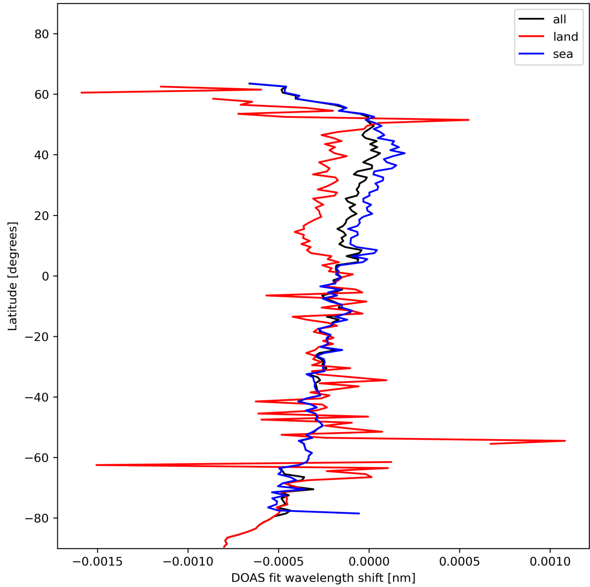
Figure 30: Zonal average of “DOAS fit wavelength shift” for 2024-01-12 to 2024-01-14.
