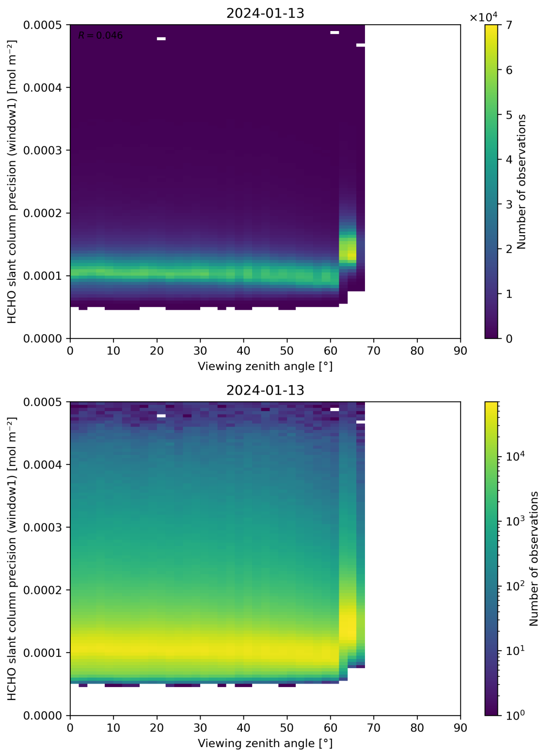
Figure 189: Scatter density plot of “Viewing zenith angle” against “HCHO slant column precision (window1)” for 2024-01-12 to 2024-01-14.
