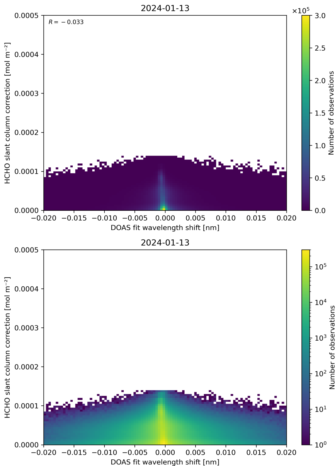
Figure 67: Scatter density plot of “DOAS fit wavelength shift” against “HCHO slant column correction” for 2024-01-12 to 2024-01-14.
