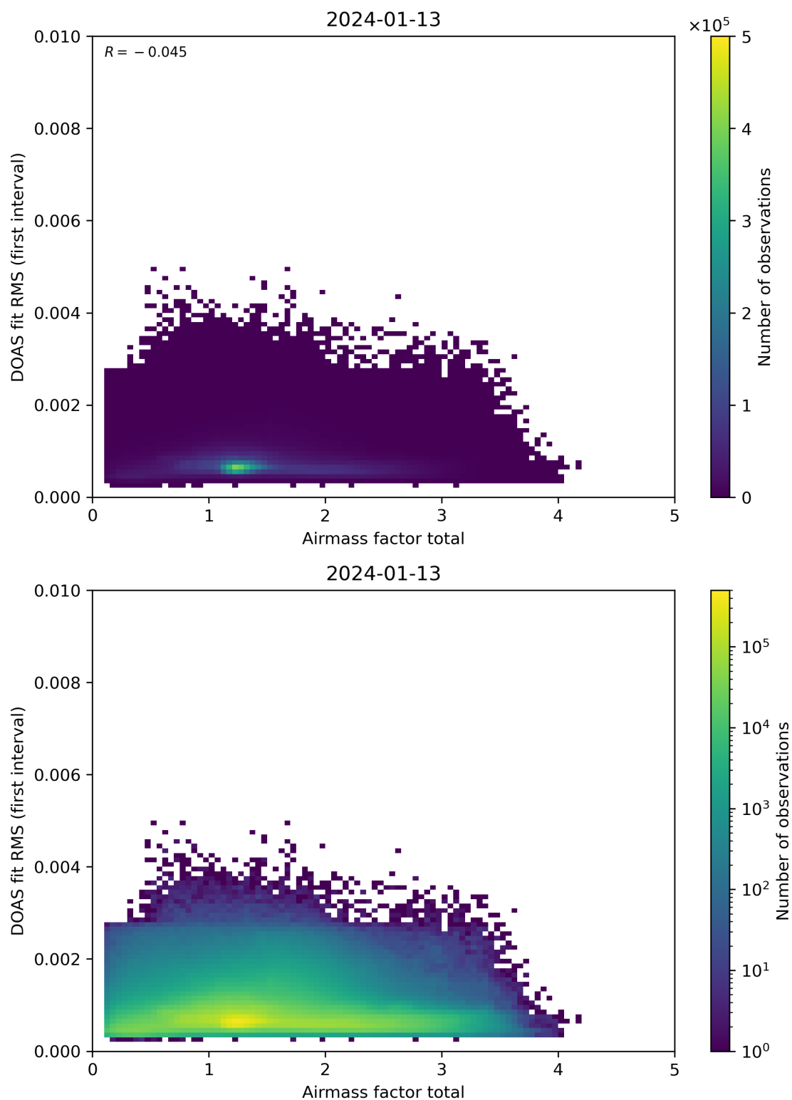
Figure 97: Scatter density plot of “Airmass factor total” against “DOAS fit RMS (first interval)” for 2024-01-12 to 2024-01-14.
