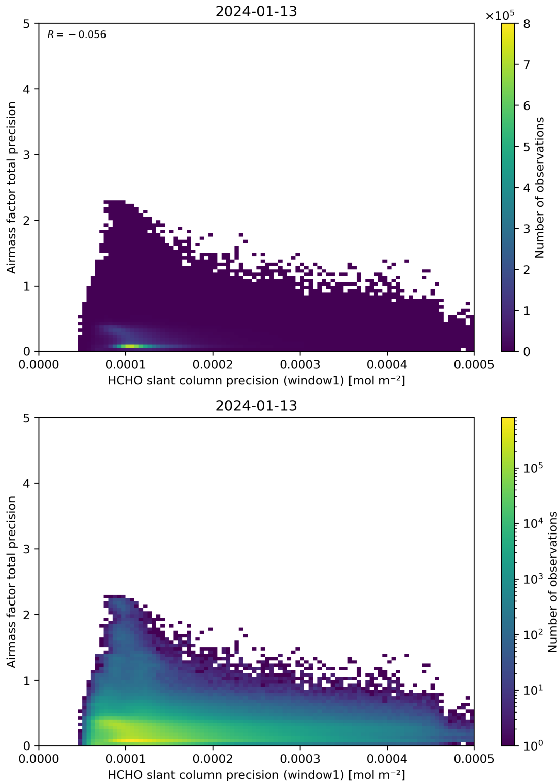
Figure 95: Scatter density plot of “HCHO slant column precision (window1)” against “Airmass factor total precision” for 2024-01-12 to 2024-01-14.
