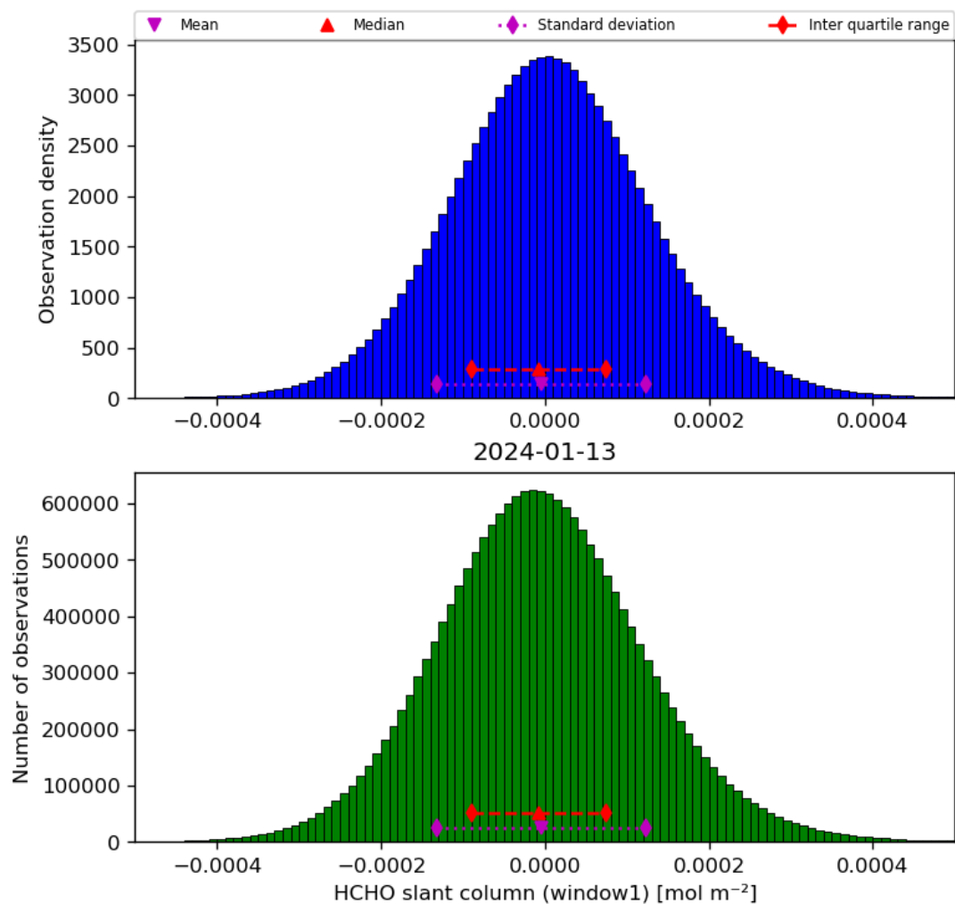
Figure 38: Histogram of “HCHO slant column (window1)” for 2024-01-12 to 2024-01-14
