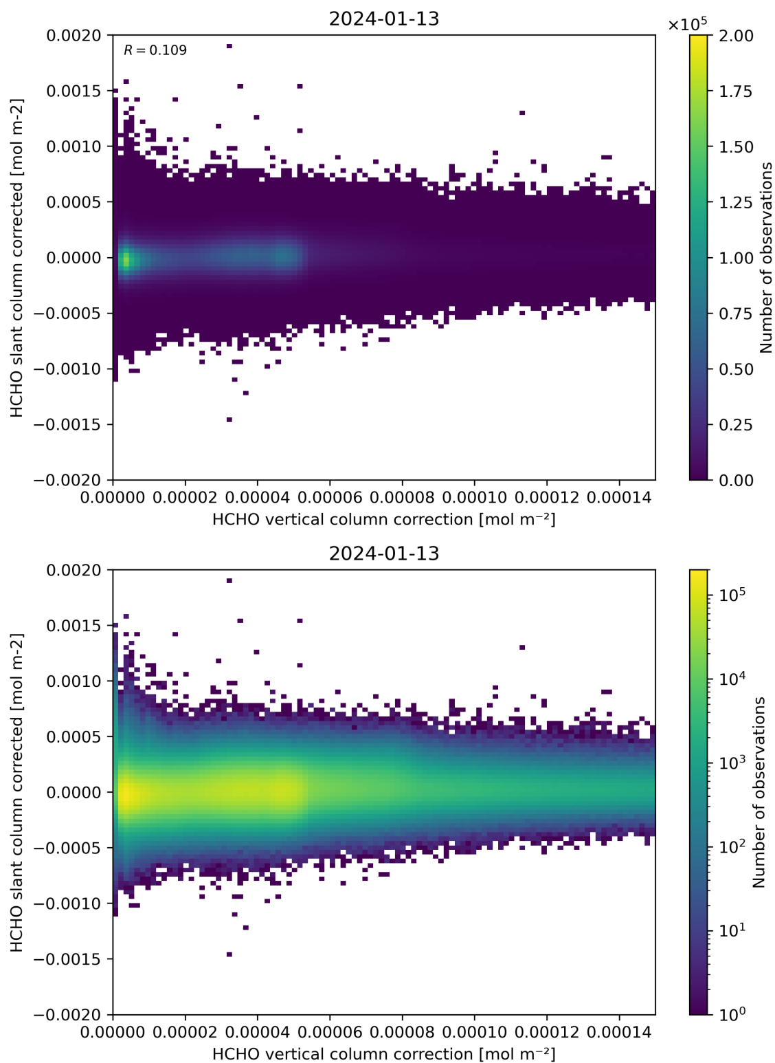
Figure 116: Scatter density plot of “HCHO vertical column correction” against “HCHO slant column corrected” for 2024-01-12 to 2024-01-14.
