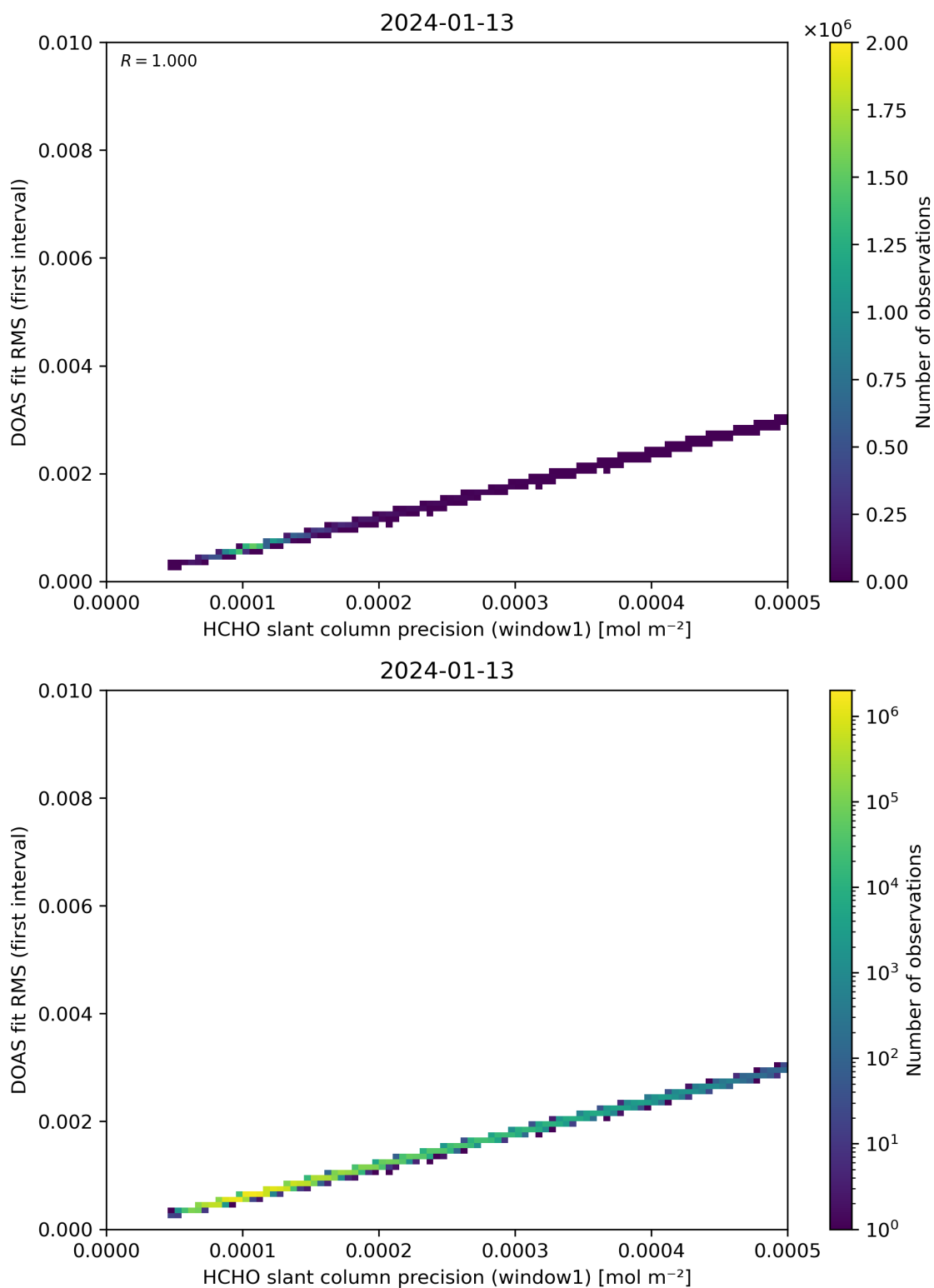
Figure 88: Scatter density plot of “HCHO slant column precision (window1)” against “DOAS fit RMS (first interval)” for 2024-01-12 to 2024-01-14.
