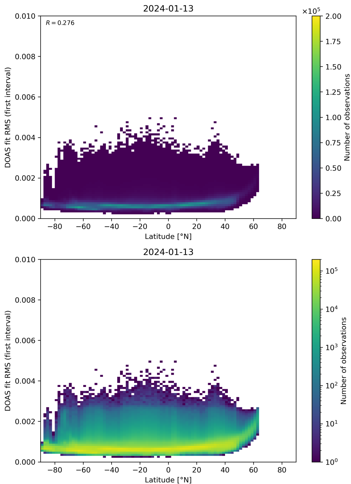
Figure 153: Scatter density plot of “Latitude” against “DOAS fit RMS (first interval)” for 2024-01-12 to 2024-01-14.
