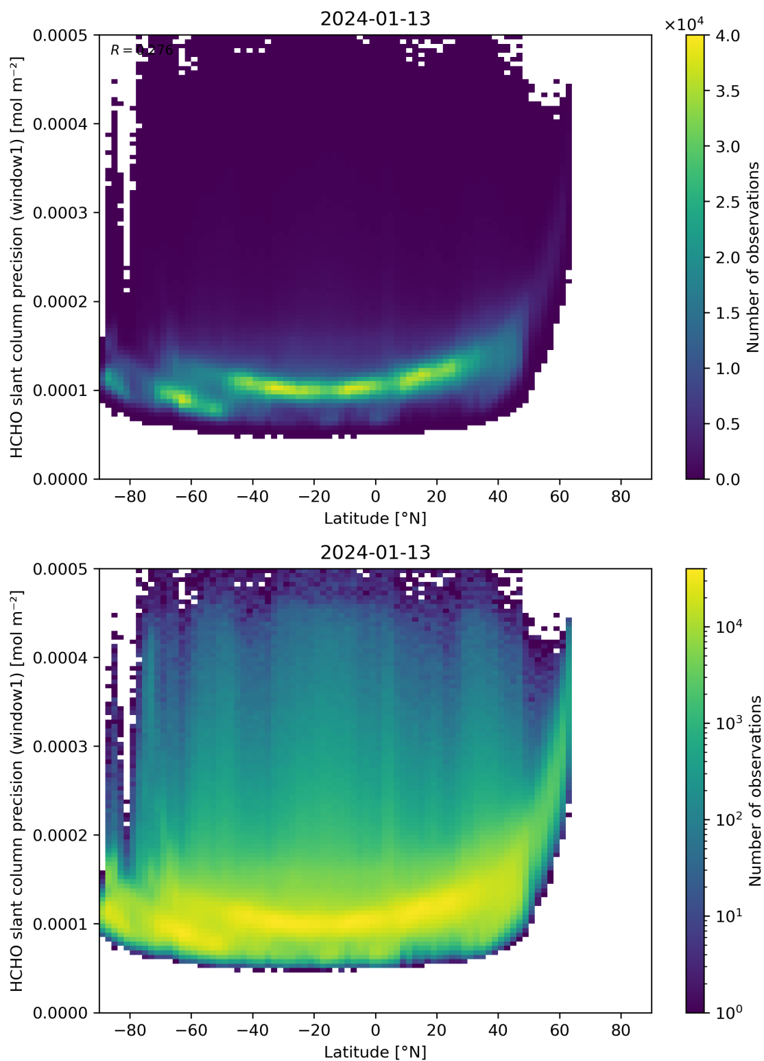
Figure 160: Scatter density plot of “Latitude” against “HCHO slant column precision (window1)” for 2024-01-12 to 2024-01-14.
