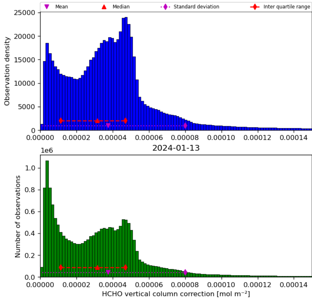
Figure 37: Histogram of “HCHO vertical column correction” for 2024-01-12 to 2024-01-14
