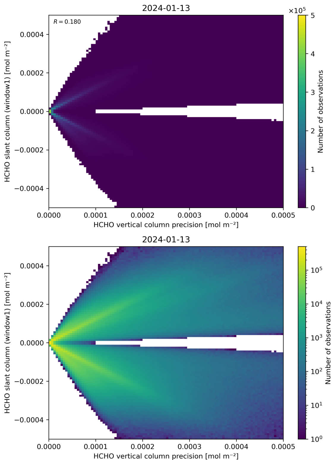
Figure 142: Scatter density plot of “HCHO vertical column precision” against “HCHO slant column (window1)” for 2024-01-12 to 2024-01-14.
