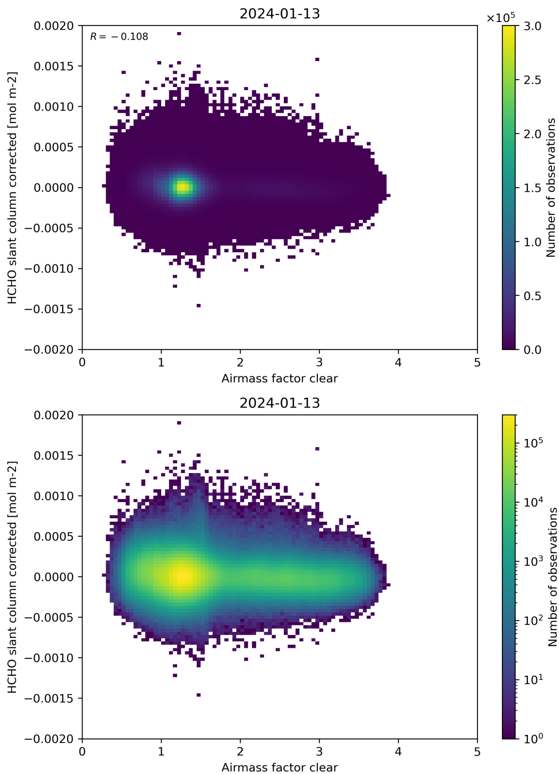
Figure 74: Scatter density plot of “Airmass factor clear” against “HCHO slant column corrected” for 2024-01-12 to 2024-01-14.
