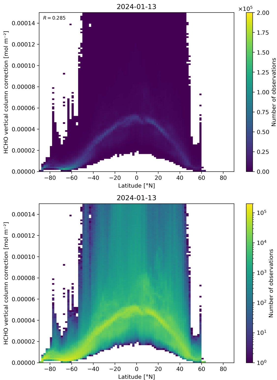
Figure 164: Scatter density plot of “Latitude” against “HCHO vertical column correction” for 2024-01-12 to 2024-01-14.
