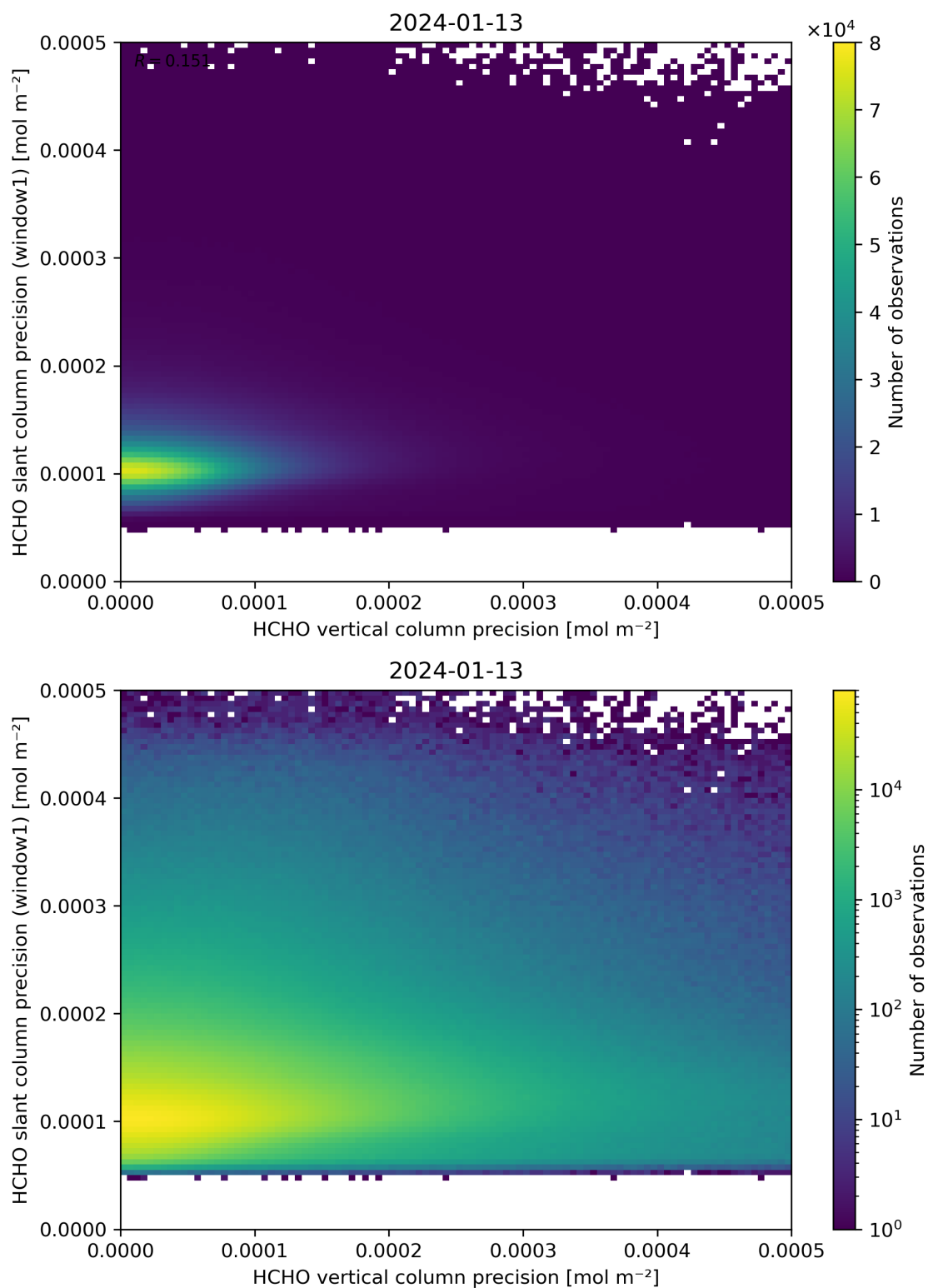
Figure 143: Scatter density plot of “HCHO vertical column precision” against “HCHO slant column precision (window1)” for 2024-01-12 to 2024-01-14.
