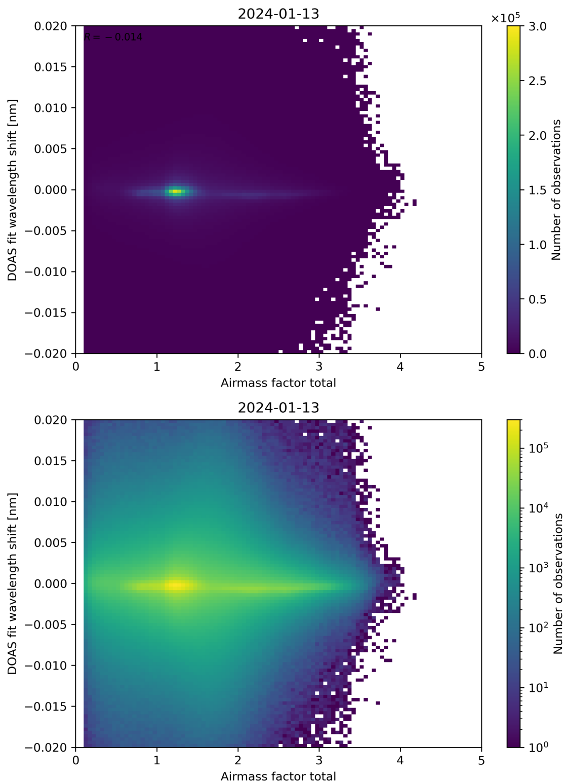
Figure 98: Scatter density plot of “Airmass factor total” against “DOAS fit wavelength shift” for 2024-01-12 to 2024-01-14.
