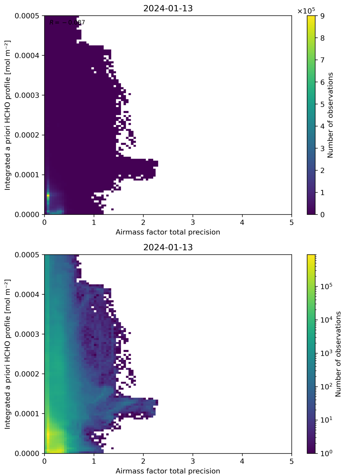
Figure 111: Scatter density plot of “Airmass factor total precision” against “Integrated a priori HCHO profile” for 2024-01-12 to 2024-01-14.
