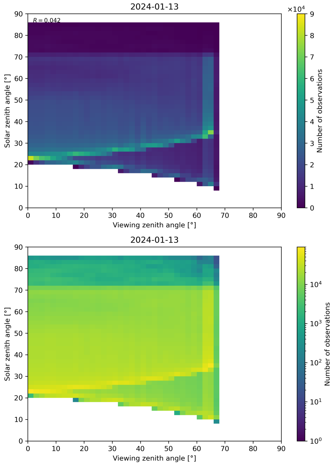
Figure 197: Scatter density plot of “Viewing zenith angle” against “Solar zenith angle” for 2024-01-12 to 2024-01-14.
