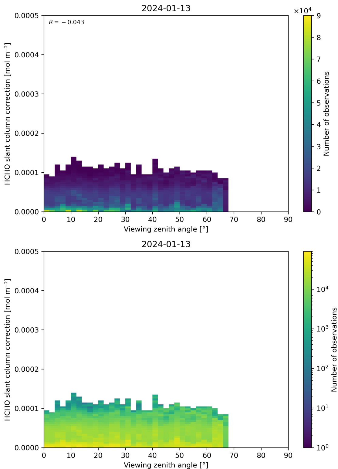
Figure 187: Scatter density plot of “Viewing zenith angle” against “HCHO slant column correction” for 2024-01-12 to 2024-01-14.
