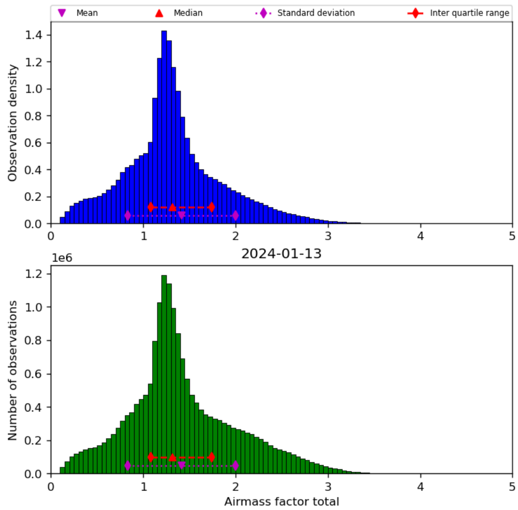
Figure 40: Histogram of “Airmass factor total” for 2024-01-12 to 2024-01-14
