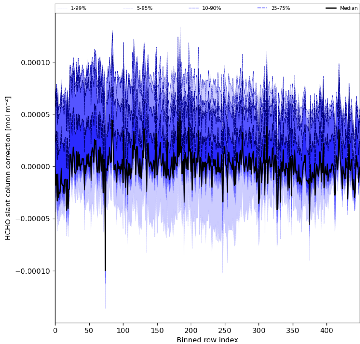
Figure 61: Along track statistics of “HCHO slant column correction” for 2024-01-12 to 2024-01-14
