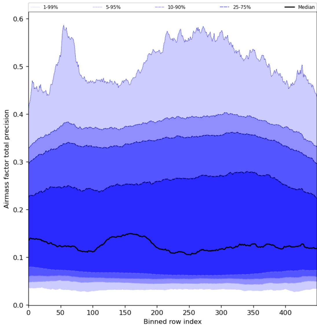
Figure 55: Along track statistics of “Airmass factor total precision” for 2024-01-12 to 2024-01-14
