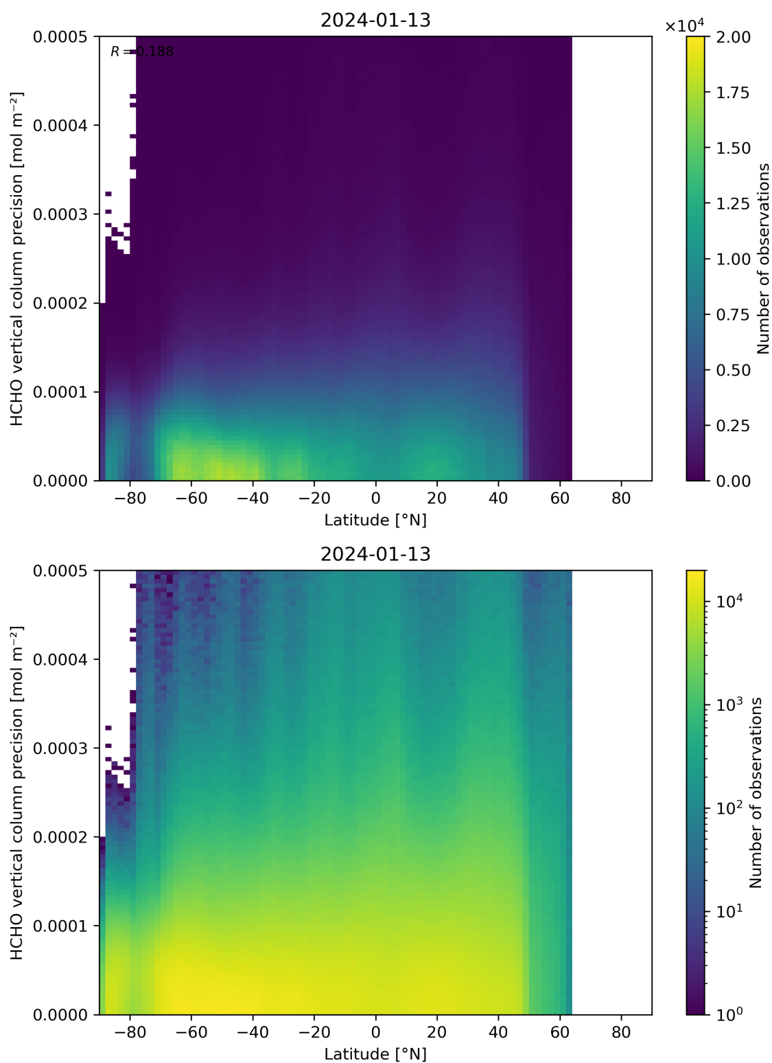
Figure 165: Scatter density plot of “Latitude” against “HCHO vertical column precision” for 2024-01-12 to 2024-01-14.
