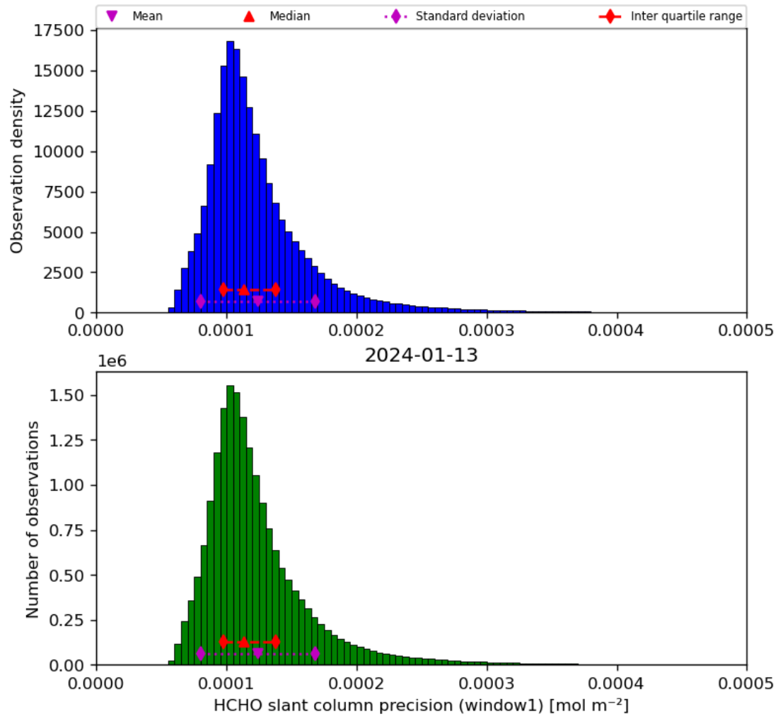
Figure 39: Histogram of “HCHO slant column precision (window1)” for 2024-01-12 to 2024-01-14
