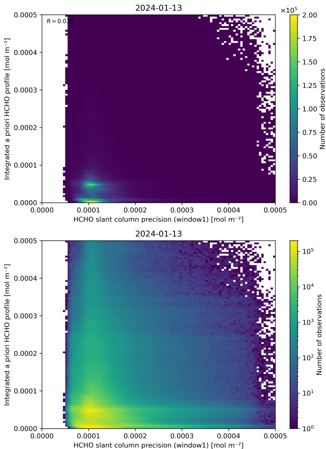
Figure 96: Scatter density plot of “HCHO slant column precision (window1)” against “Integrated a priori HCHO profile” for 2024-01-12 to 2024-01-14.
