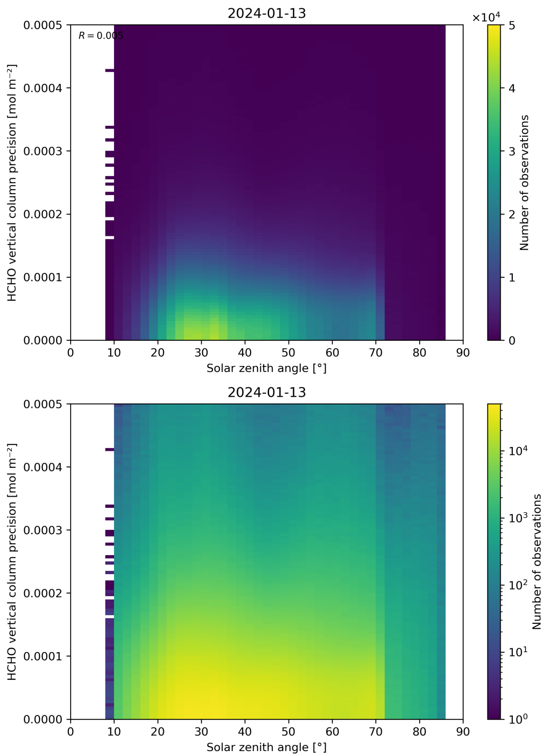
Figure 179: Scatter density plot of “Solar zenith angle” against “HCHO vertical column precision” for 2024-01-12 to 2024-01-14.
