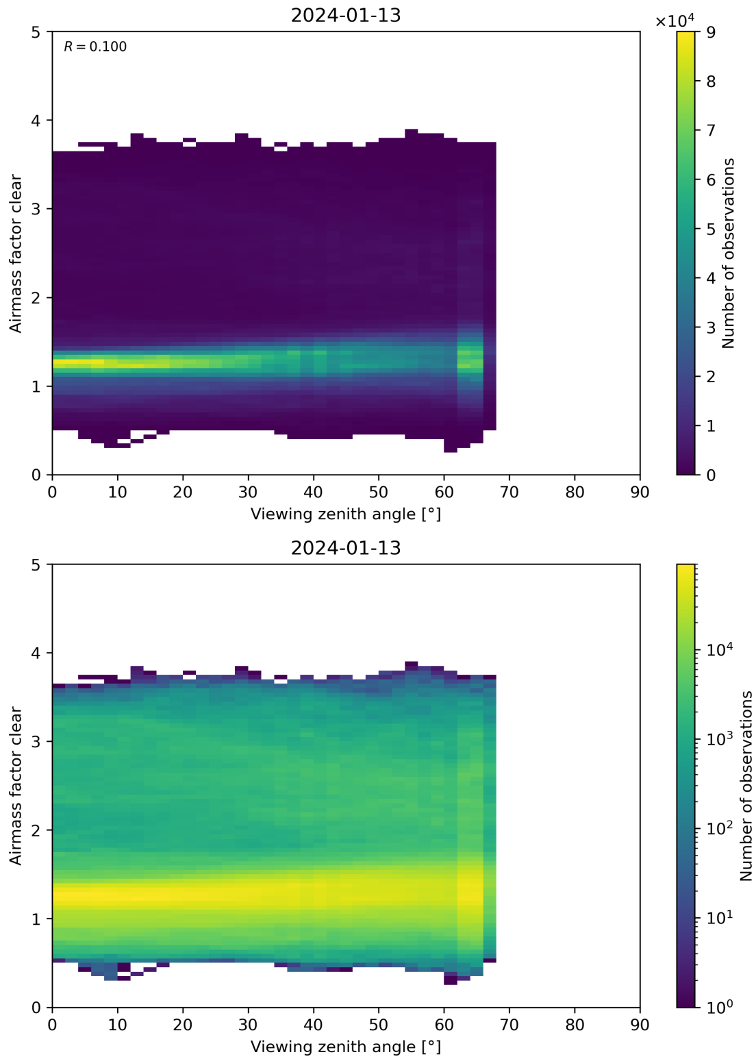
Figure 185: Scatter density plot of “Viewing zenith angle” against “Airmass factor clear” for 2024-01-12 to 2024-01-14.
