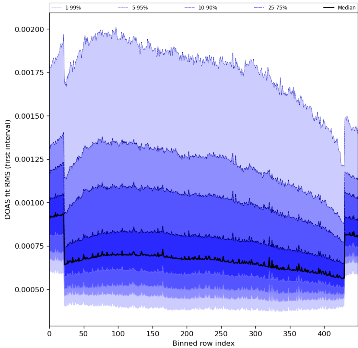
Figure 60: Along track statistics of “DOAS fit RMS (first interval)” for 2024-01-12 to 2024-01-14
