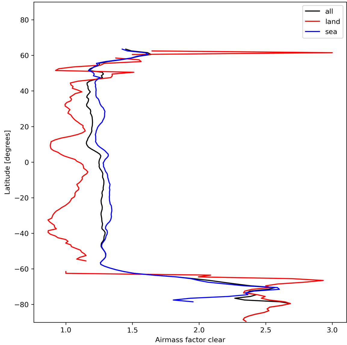
Figure 28: Zonal average of “Airmass factor clear” for 2024-01-12 to 2024-01-14.
