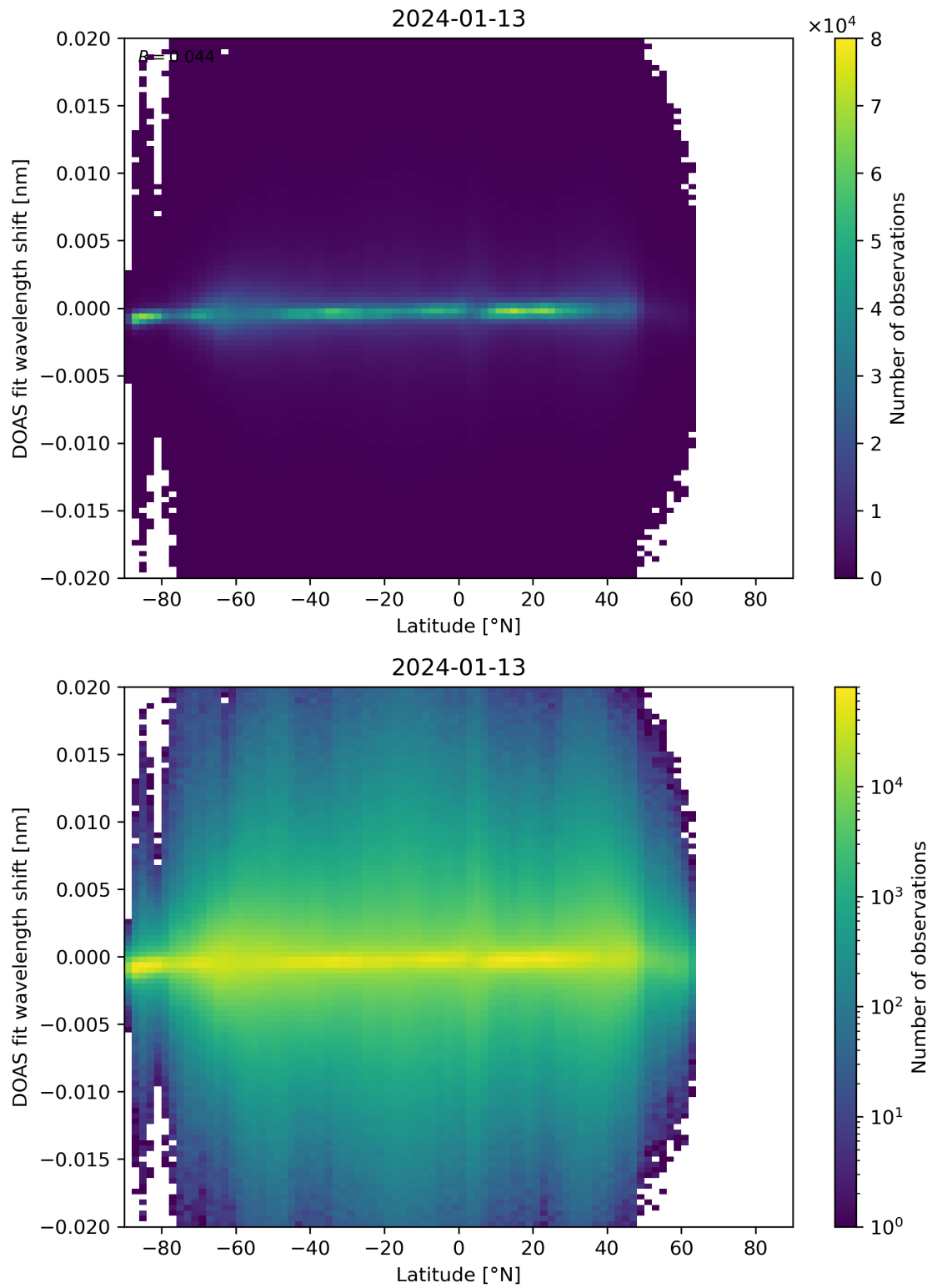
Figure 154: Scatter density plot of “Latitude” against “DOAS fit wavelength shift” for 2024-01-12 to 2024-01-14.
