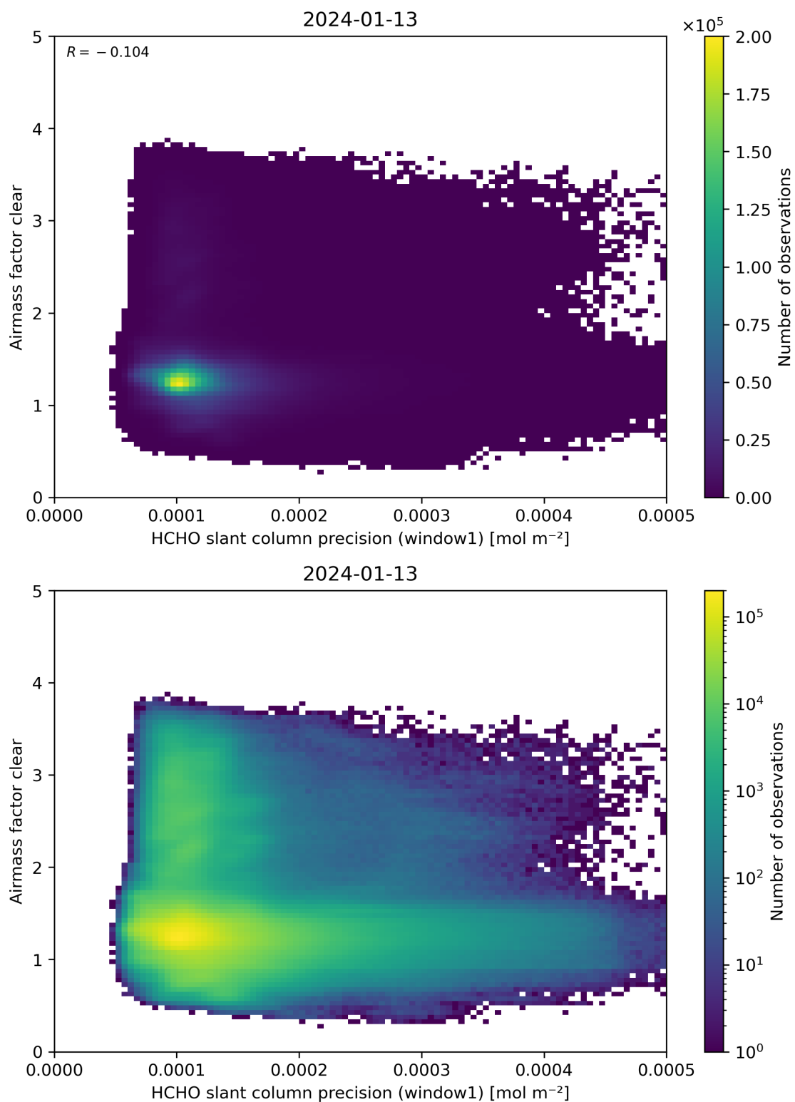
Figure 91: Scatter density plot of “HCHO slant column precision (window1)” against “Airmass factor clear” for 2024-01-12 to 2024-01-14.
