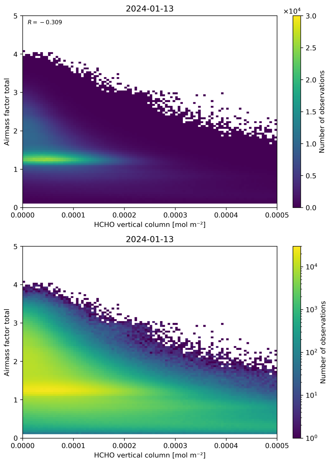
Figure 131: Scatter density plot of “HCHO vertical column” against “Airmass factor total” for 2024-01-12 to 2024-01-14.
