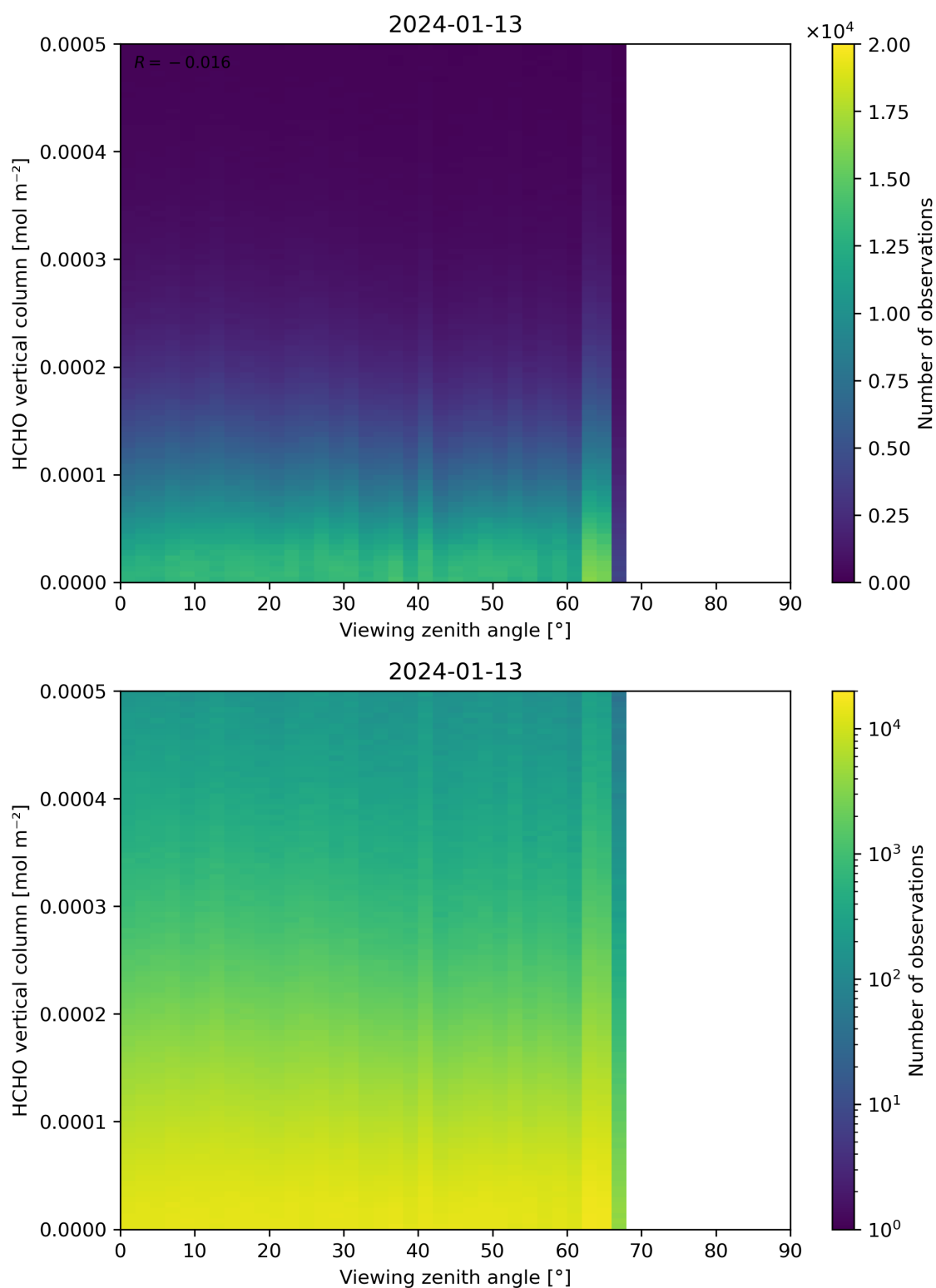
Figure 192: Scatter density plot of “Viewing zenith angle” against “HCHO vertical column” for 2024-01-12 to 2024-01-14.
