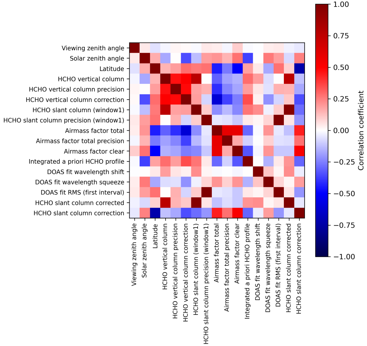
Figure 2: Map of correlation matrix for 2024-01-12 to 2024-01-14.
