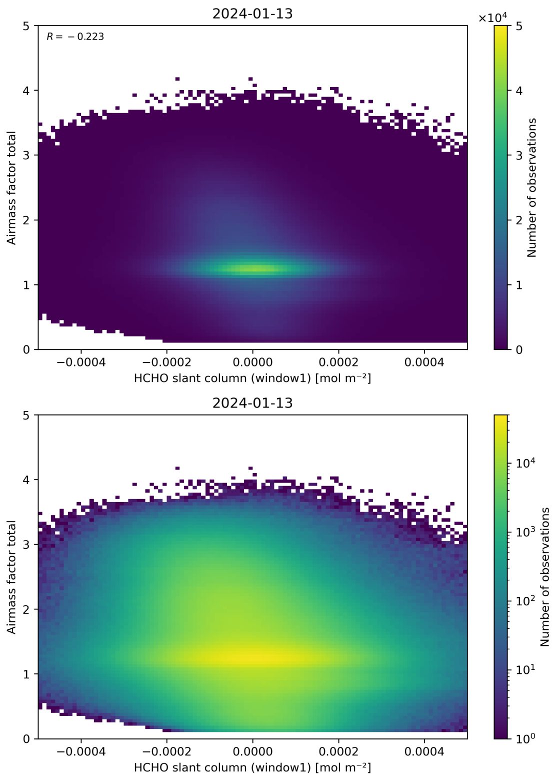
Figure 85: Scatter density plot of “HCHO slant column (window1)” against “Airmass factor total” for 2024-01-12 to 2024-01-14.
