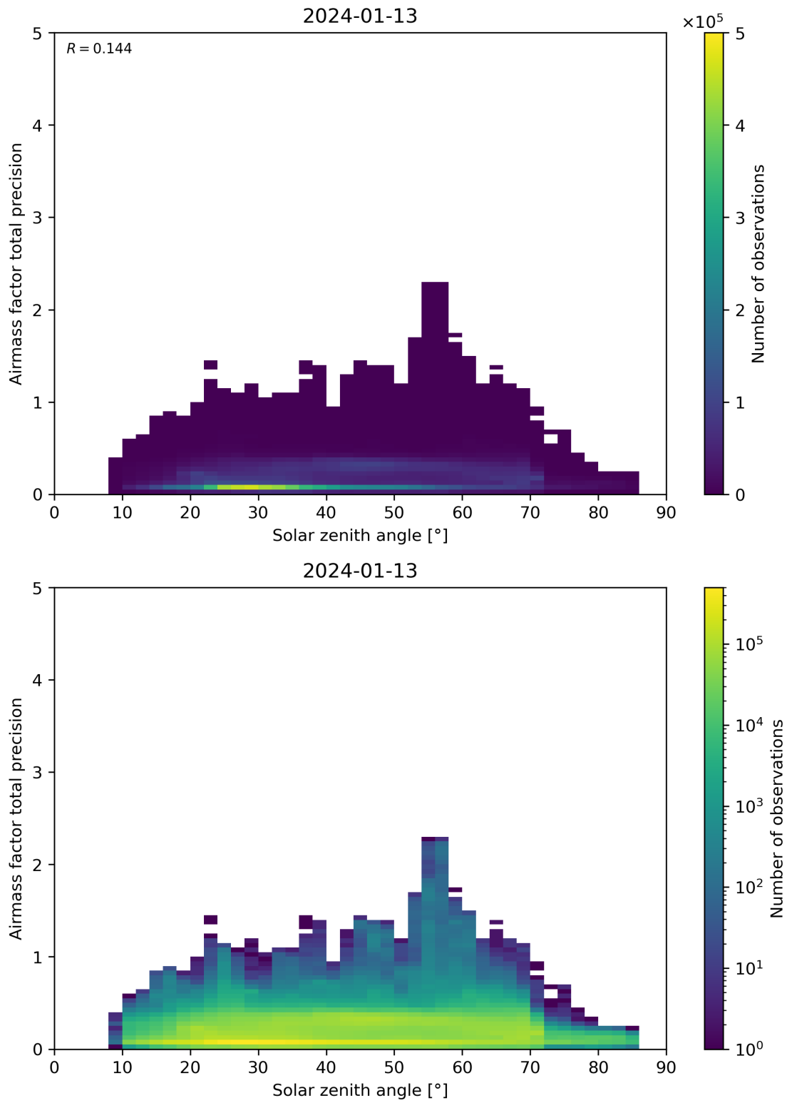
Figure 176: Scatter density plot of “Solar zenith angle” against “Airmass factor total precision” for 2024-01-12 to 2024-01-14.
