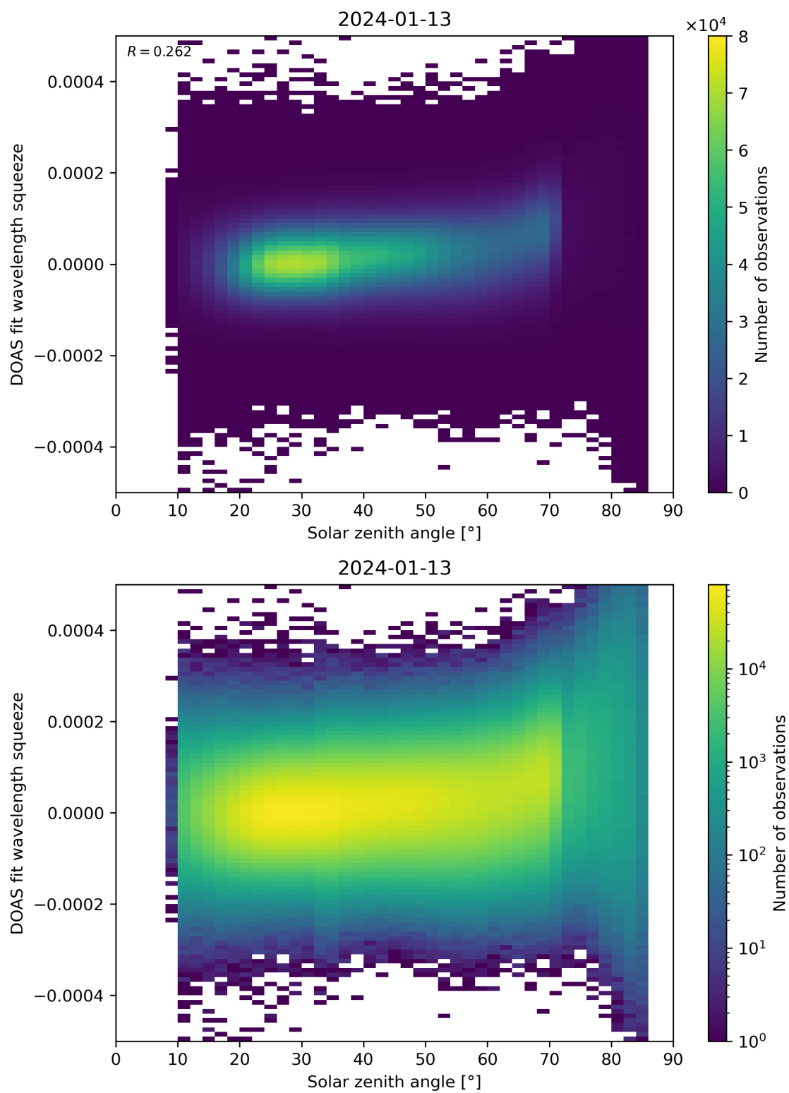
Figure 169: Scatter density plot of “Solar zenith angle” against “DOAS fit wavelength squeeze” for 2024-01-12 to 2024-01-14.
