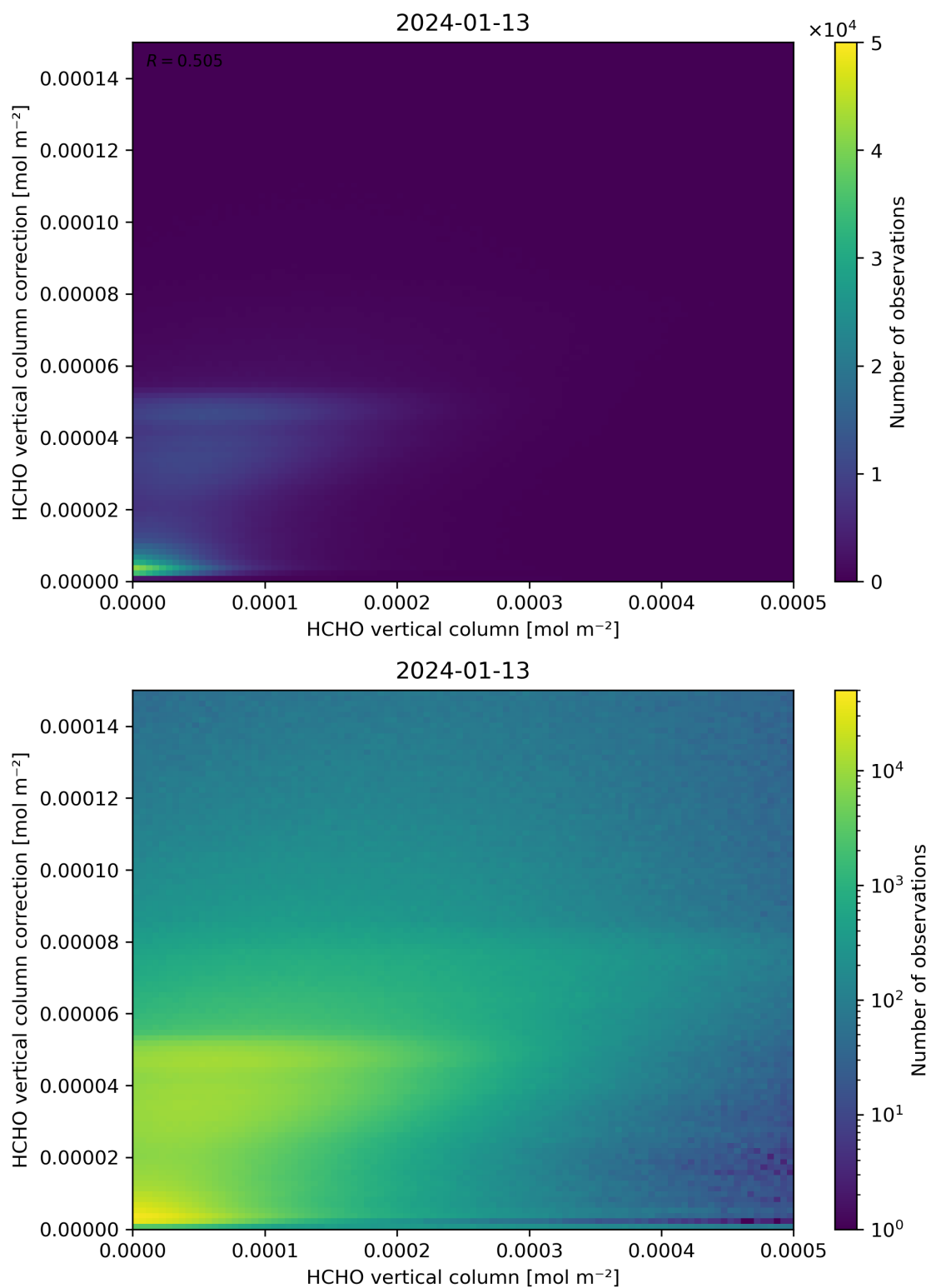
Figure 133: Scatter density plot of “HCHO vertical column” against “HCHO vertical column correction” for 2024-01-12 to 2024-01-14.
