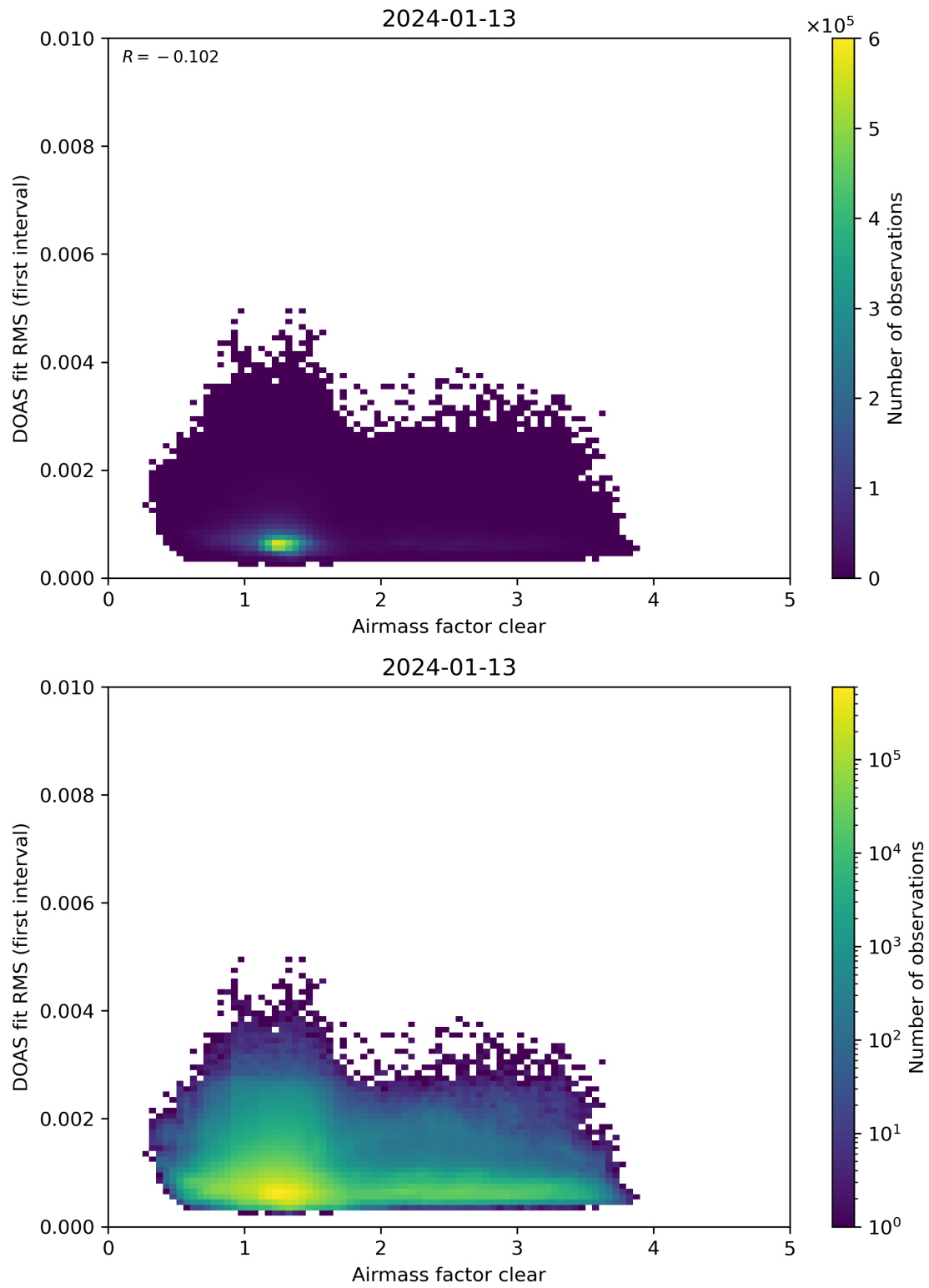
Figure 71: Scatter density plot of “Airmass factor clear” against “DOAS fit RMS (first interval)” for 2024-01-12 to 2024-01-14.
