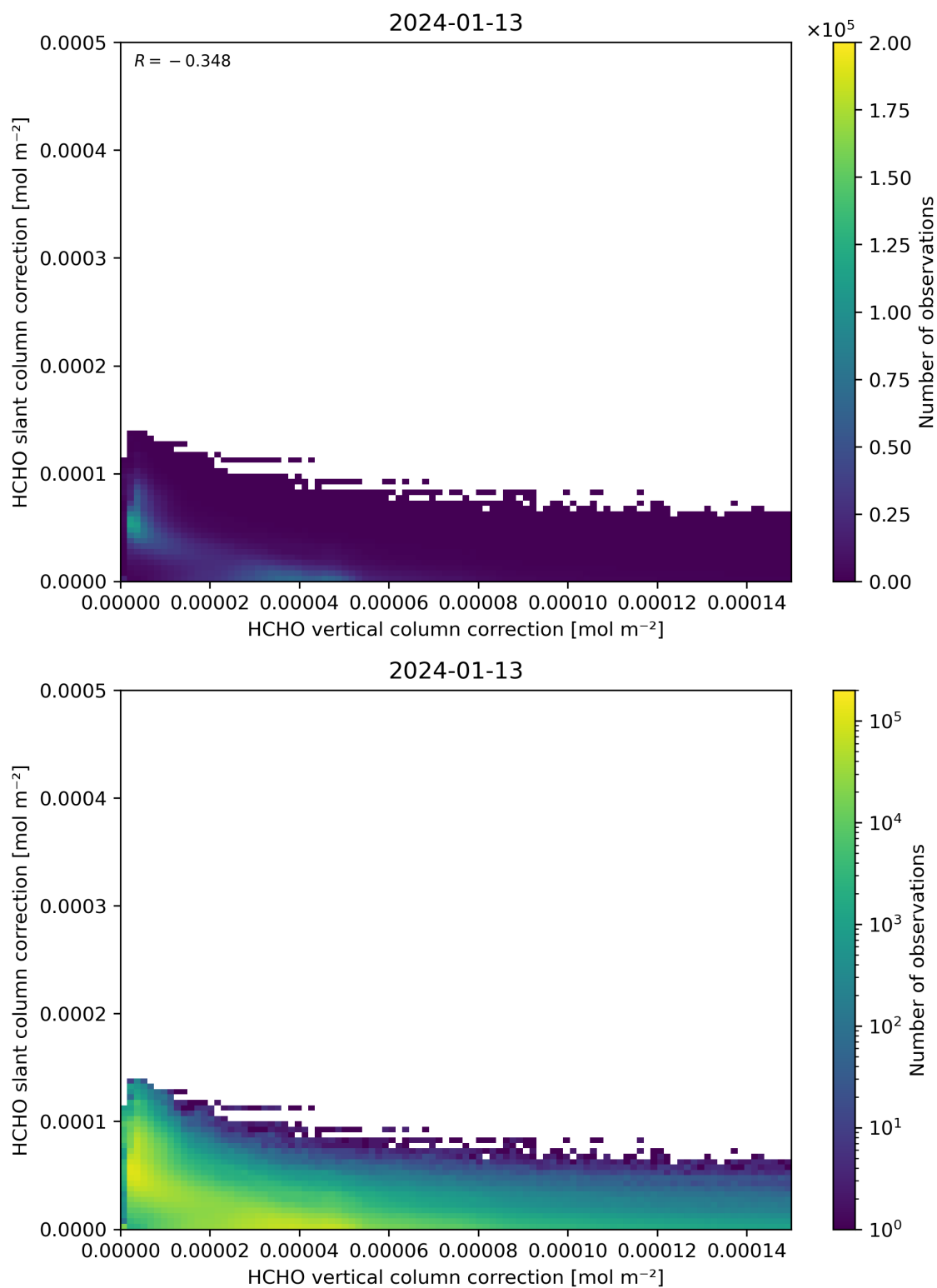
Figure 117: Scatter density plot of “HCHO vertical column correction” against “HCHO slant column correction” for 2024-01-12 to 2024-01-14.
