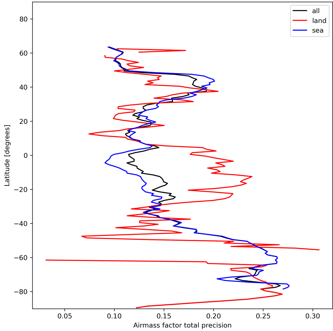
Figure 27: Zonal average of “Airmass factor total precision” for 2024-01-12 to 2024-01-14.
