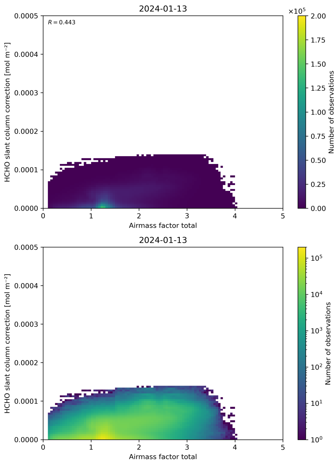
Figure 102: Scatter density plot of “Airmass factor total” against “HCHO slant column correction” for 2024-01-12 to 2024-01-14.
