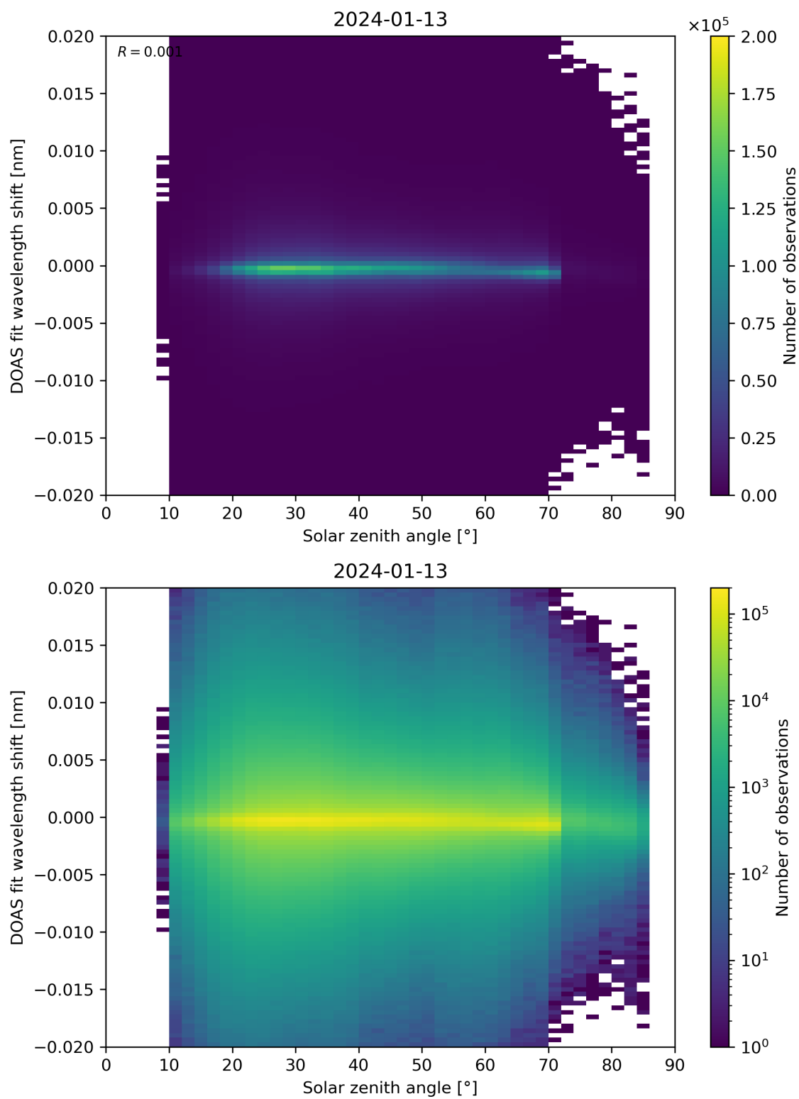
Figure 168: Scatter density plot of “Solar zenith angle” against “DOAS fit wavelength shift” for 2024-01-12 to 2024-01-14.
