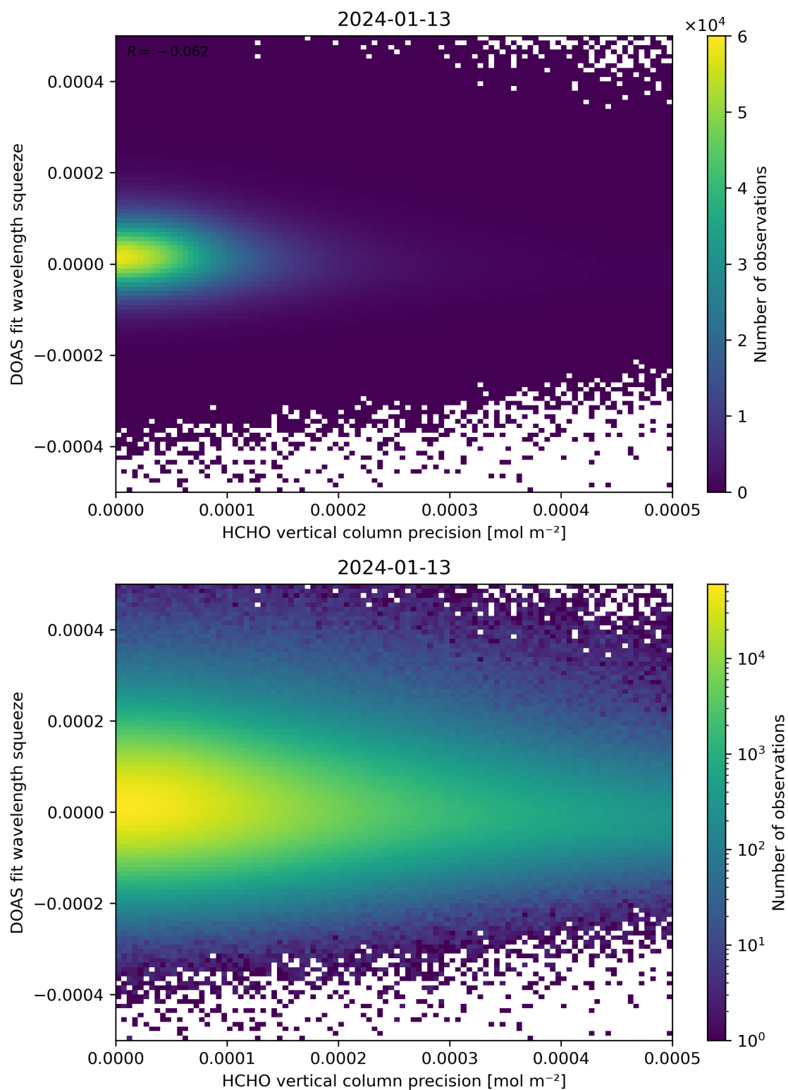
Figure 138: Scatter density plot of “HCHO vertical column precision” against “DOAS fit wavelength squeeze” for 2024-01-12 to 2024-01-14.
