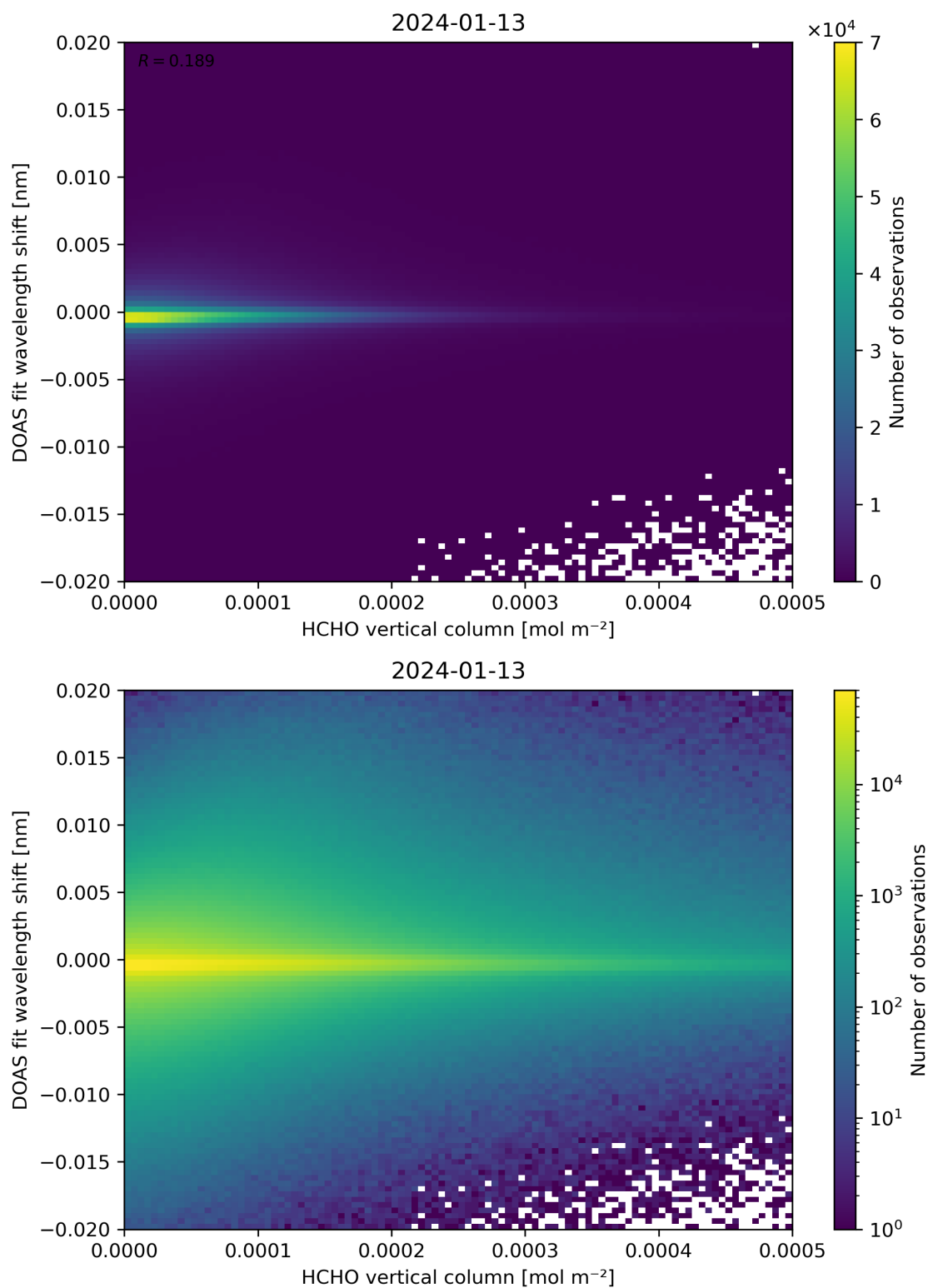
Figure 124: Scatter density plot of “HCHO vertical column” against “DOAS fit wavelength shift” for 2024-01-12 to 2024-01-14.
