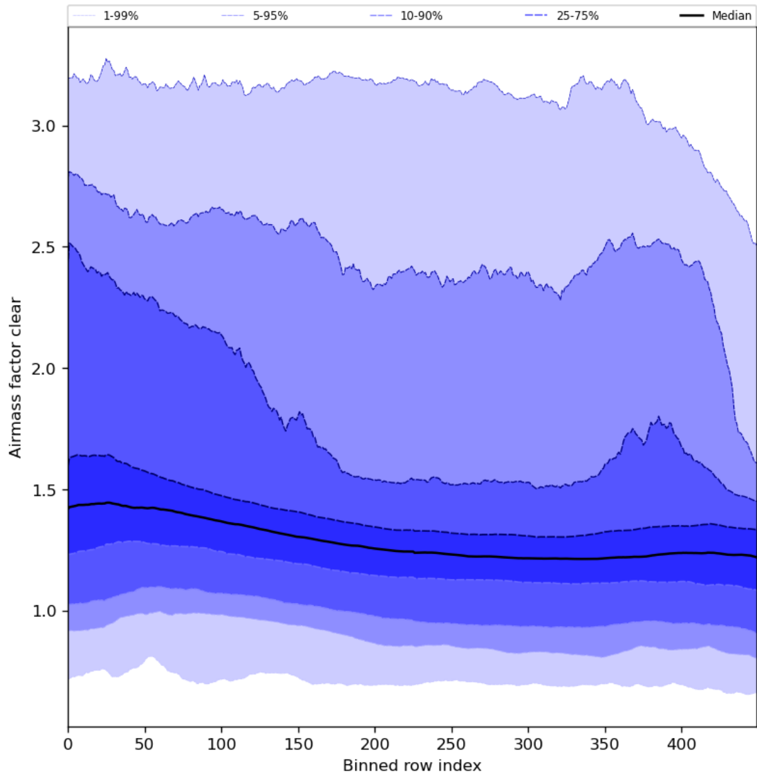
Figure 56: Along track statistics of “Air mass factor clear” for 2024-01-12 to 2024-01-14
