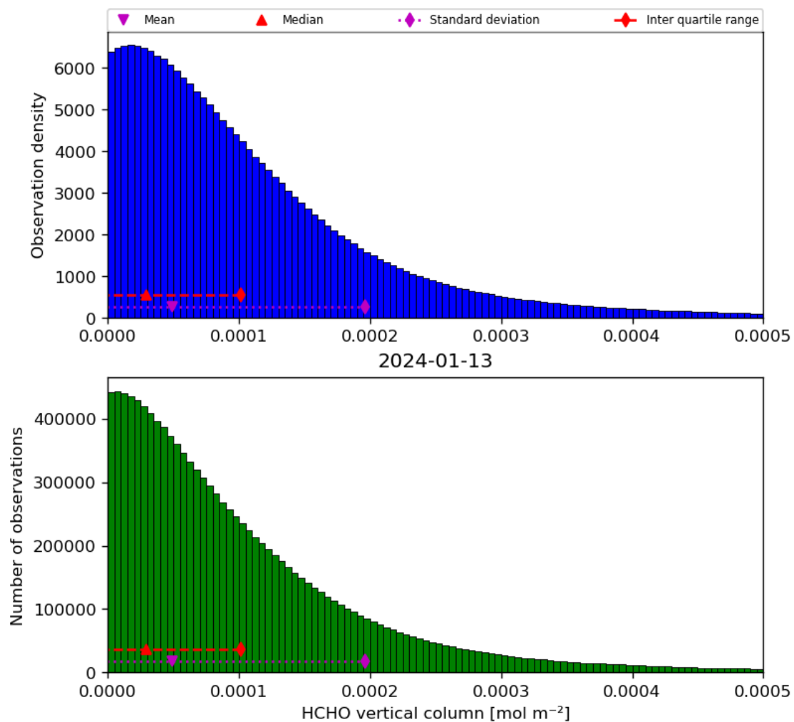
Figure 35: Histogram of “HCHO vertical column” for 2024-01-12 to 2024-01-14
