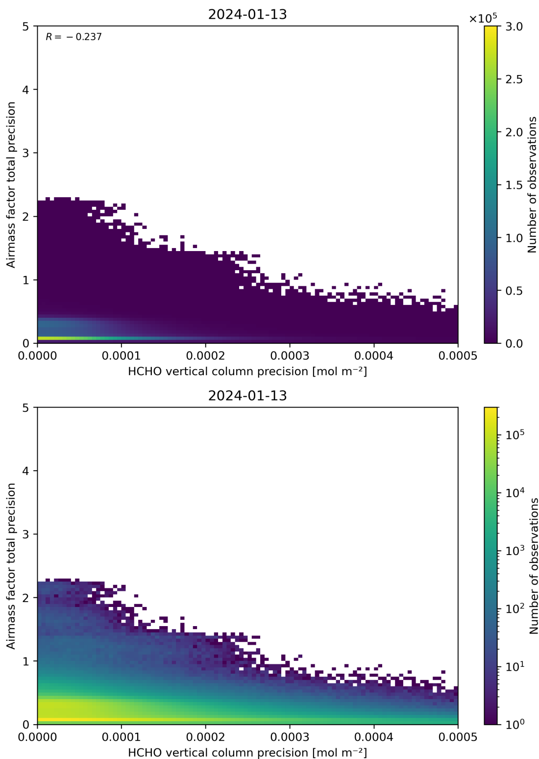
Figure 145: Scatter density plot of “HCHO vertical column precision” against “Airmass factor total precision” for 2024-01-12 to 2024-01-14.
