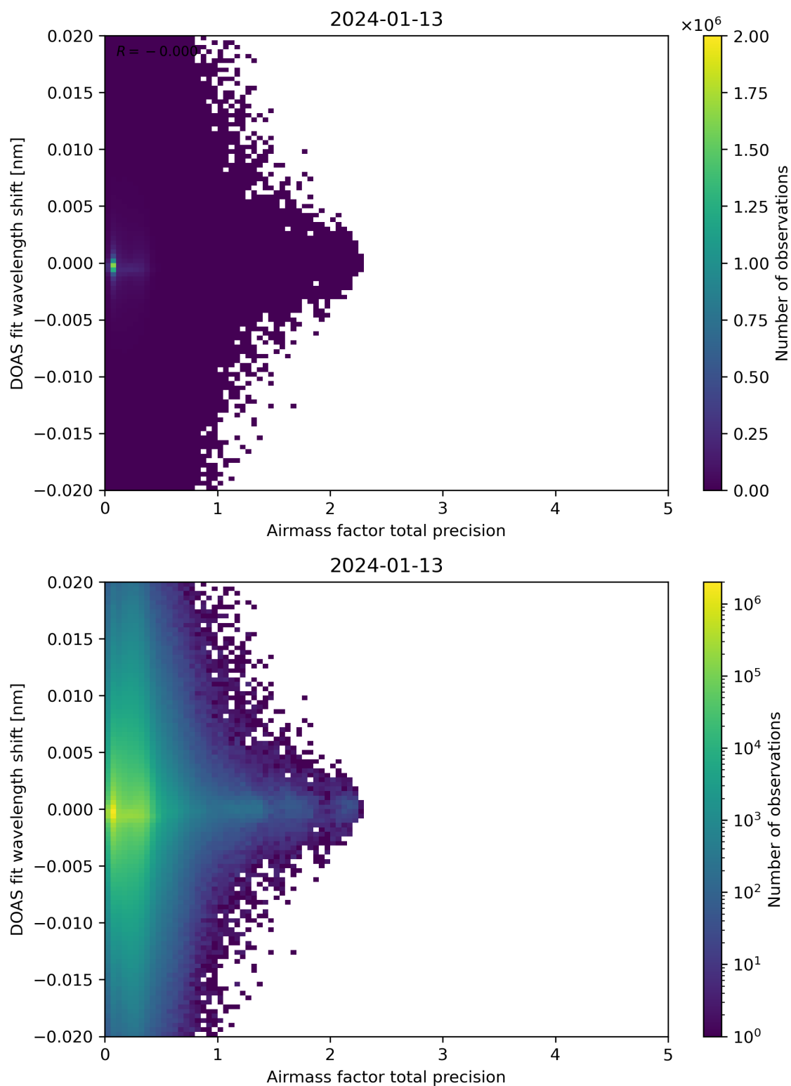
Figure 106: Scatter density plot of “Airmass factor total precision” against “DOAS fit wavelength shift” for 2024-01-12 to 2024-01-14.
