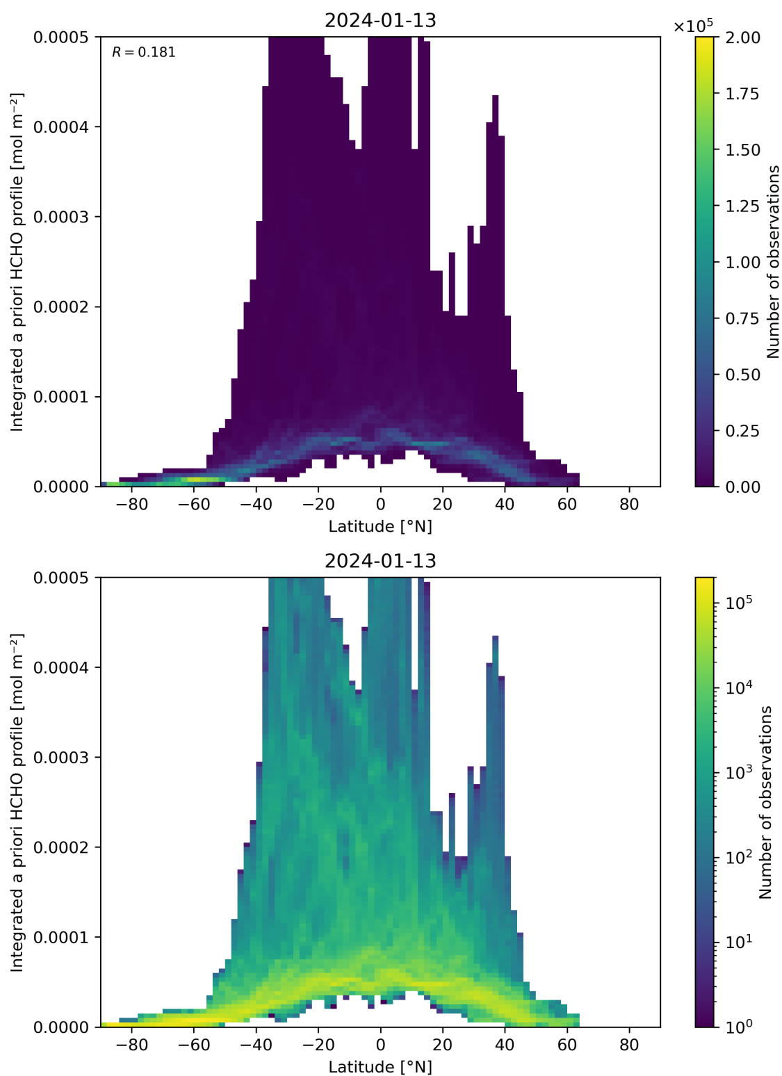
Figure 166: Scatter density plot of “Latitude” against “Integrated a priori HCHO profile” for 2024-01-12 to 2024-01-14.
