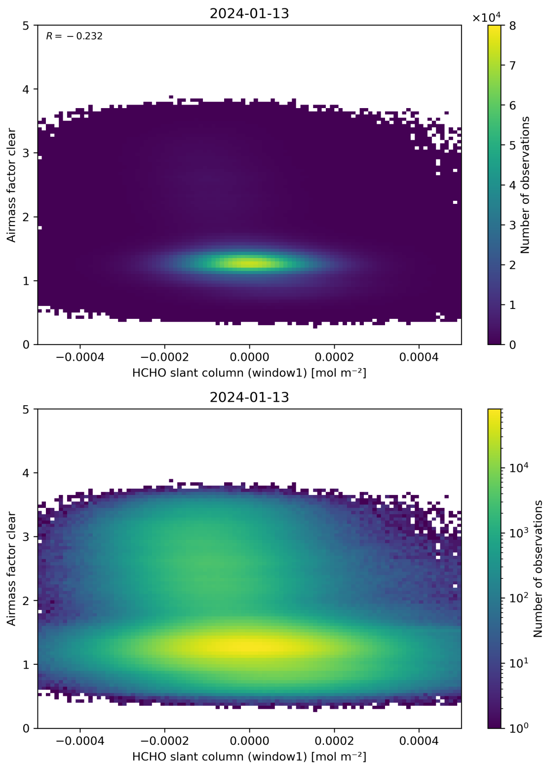
Figure 81: Scatter density plot of “HCHO slant column (window1)” against “Airmass factor clear” for 2024-01-12 to 2024-01-14.
