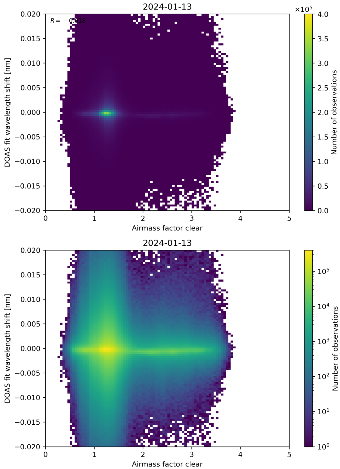
Figure 72: Scatter density plot of “Airmass factor clear” against “DOAS fit wavelength shift” for 2024-01-12 to 2024-01-14.
