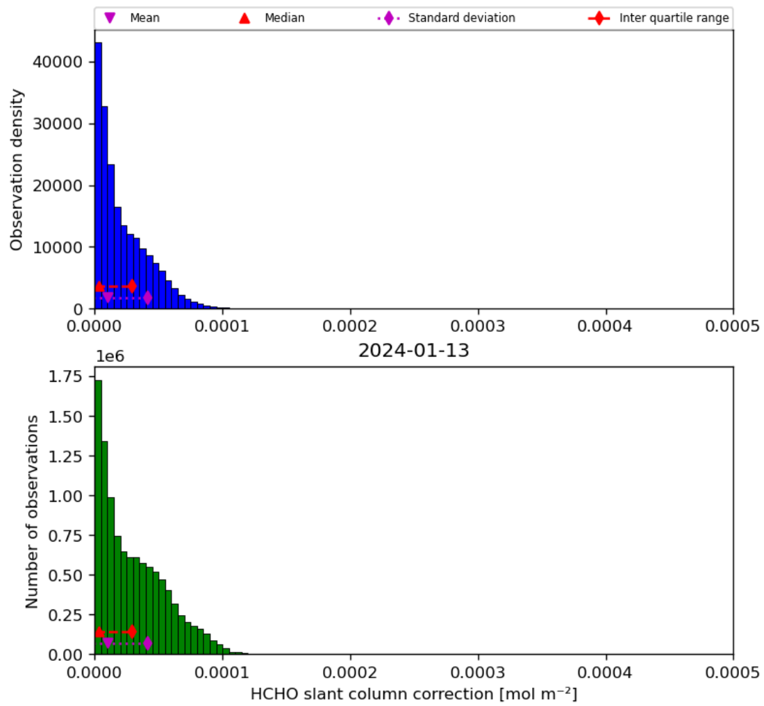
Figure 47: Histogram of “HCHO slant column correction” for 2024-01-12 to 2024-01-14
