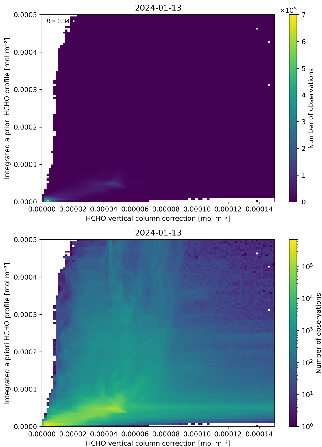
Figure 122: Scatter density plot of “HCHO vertical column correction” against “Integrated a priori HCHO profile” for 2024-01-12 to 2024-01-14.
