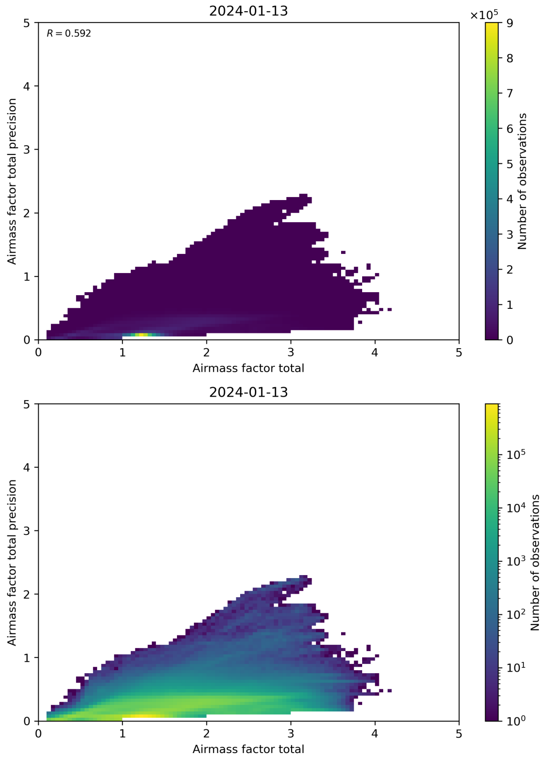
Figure 103: Scatter density plot of “Airmass factor total” against “Airmass factor total precision” for 2024-01-12 to 2024-01-14.
