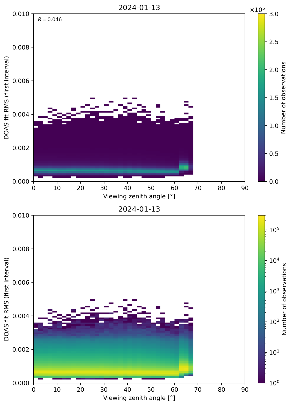
Figure 182: Scatter density plot of “Viewing zenith angle” against “DOAS fit RMS (first interval)” for 2024-01-12 to 2024-01-14.
