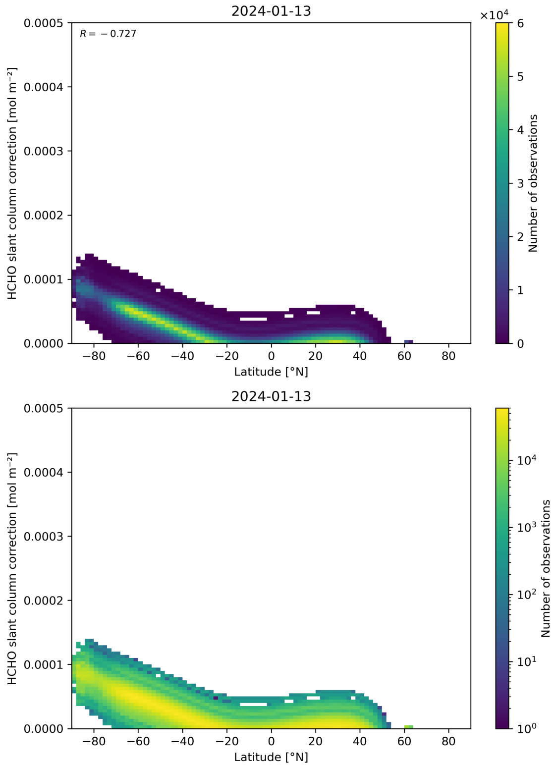
Figure 158: Scatter density plot of “Latitude” against “HCHO slant column correction” for 2024-01-12 to 2024-01-14.
