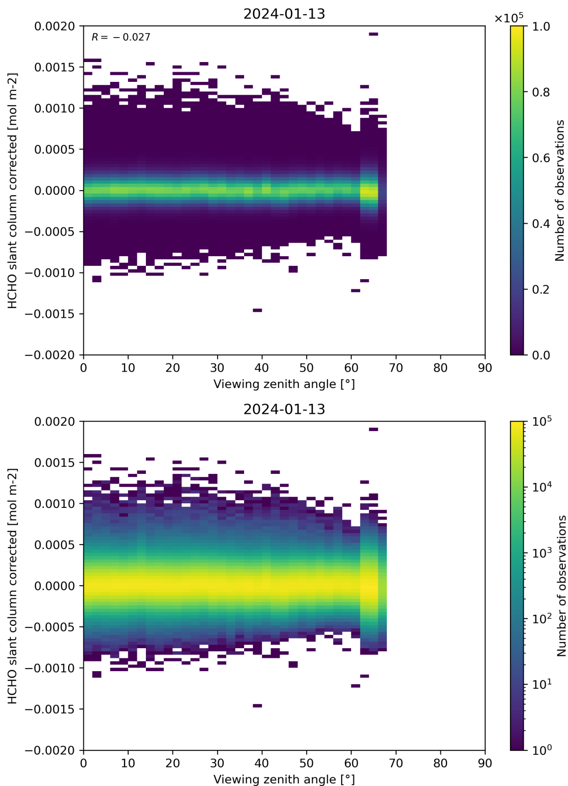
Figure 186: Scatter density plot of “Viewing zenith angle” against “HCHO slant column corrected” for 2024-01-12 to 2024-01-14.
