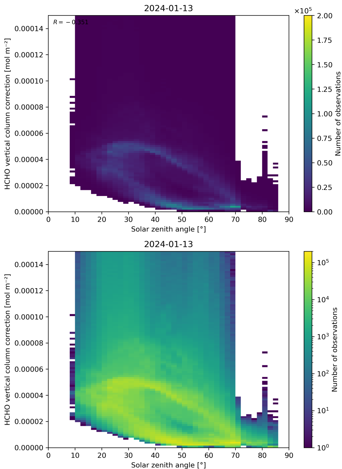
Figure 178: Scatter density plot of “Solar zenith angle” against “HCHO vertical column correction” for 2024-01-12 to 2024-01-14.
