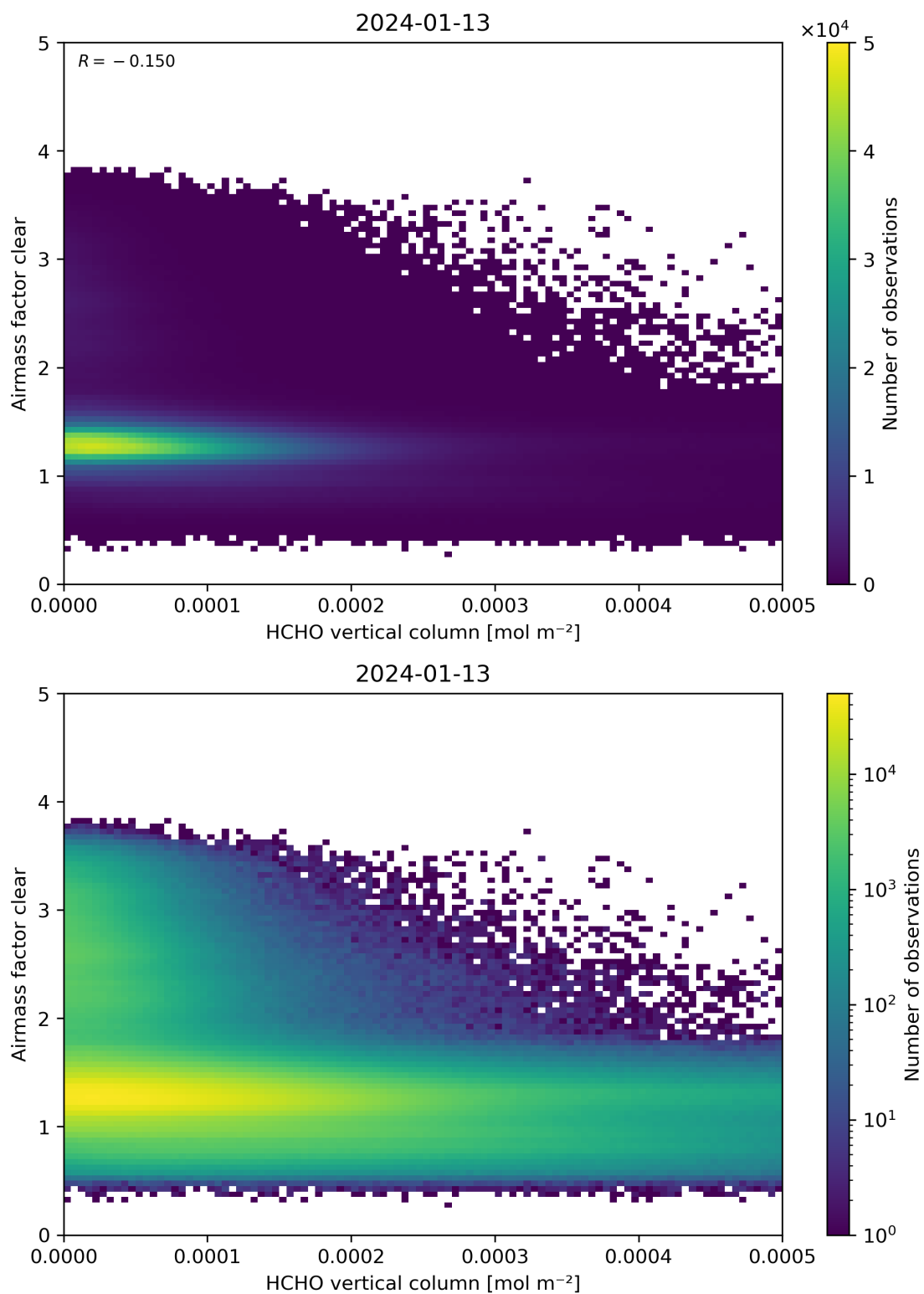
Figure 126: Scatter density plot of “HCHO vertical column” against “Airmass factor clear” for 2024-01-12 to 2024-01-14.
