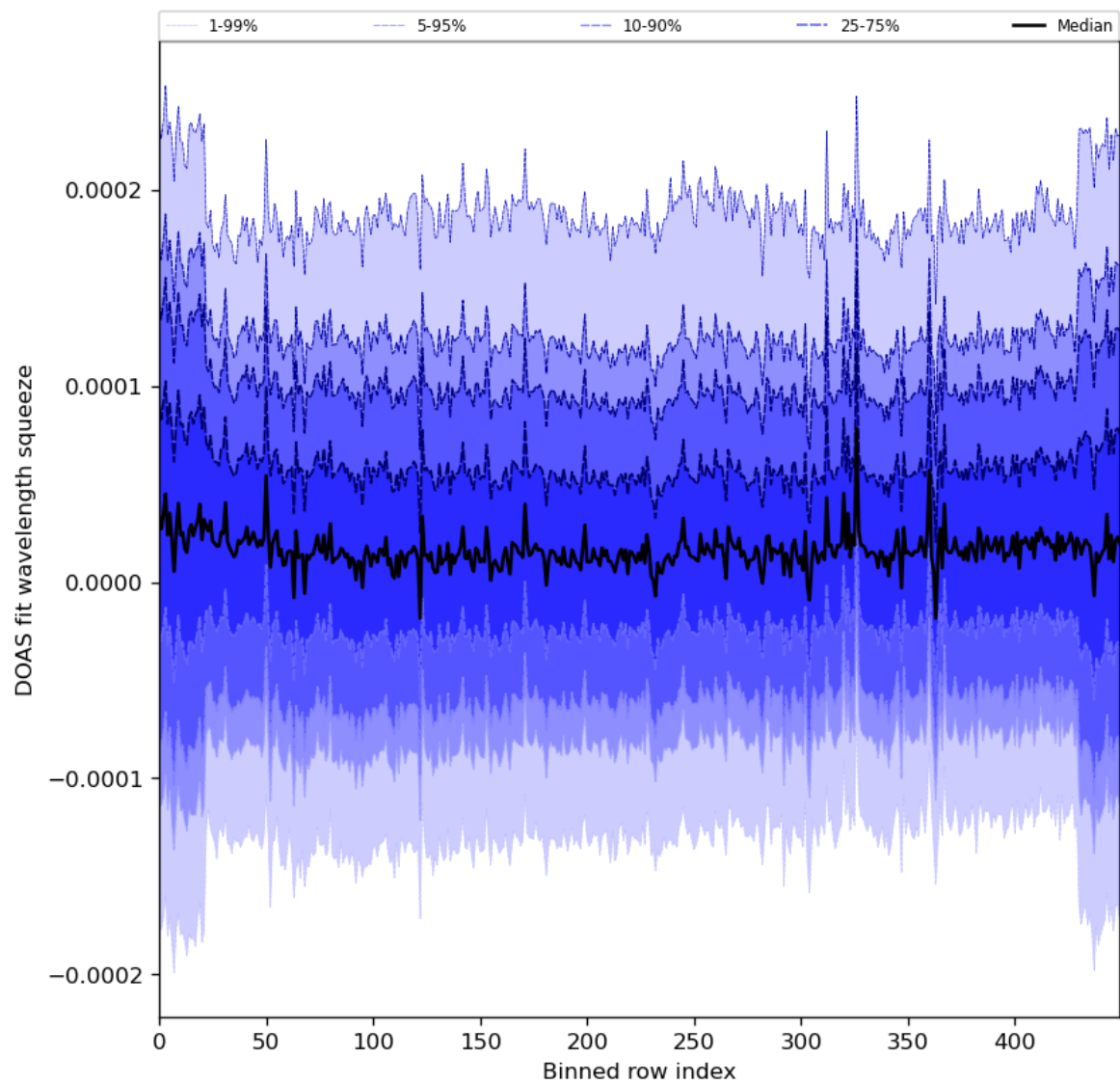
Figure 59: Along track statistics of “DOAS fit wavelength squeeze” for 2024-01-12 to 2024-01-14
