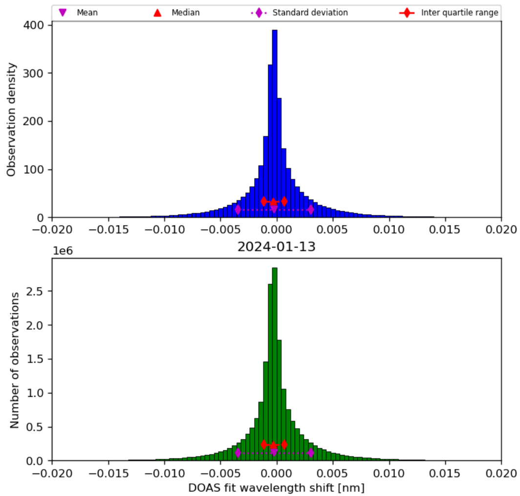
Figure 44: Histogram of “DOAS fit wavelength shift” for 2024-01-12 to 2024-01-14
