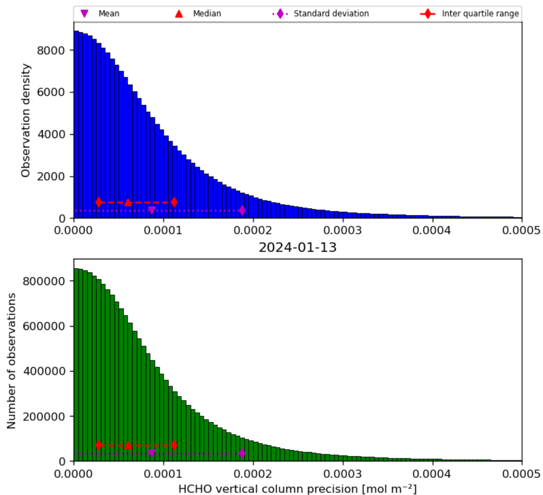
Figure 36: Histogram of “HCHO vertical column precision” for 2024-01-12 to 2024-01-14
