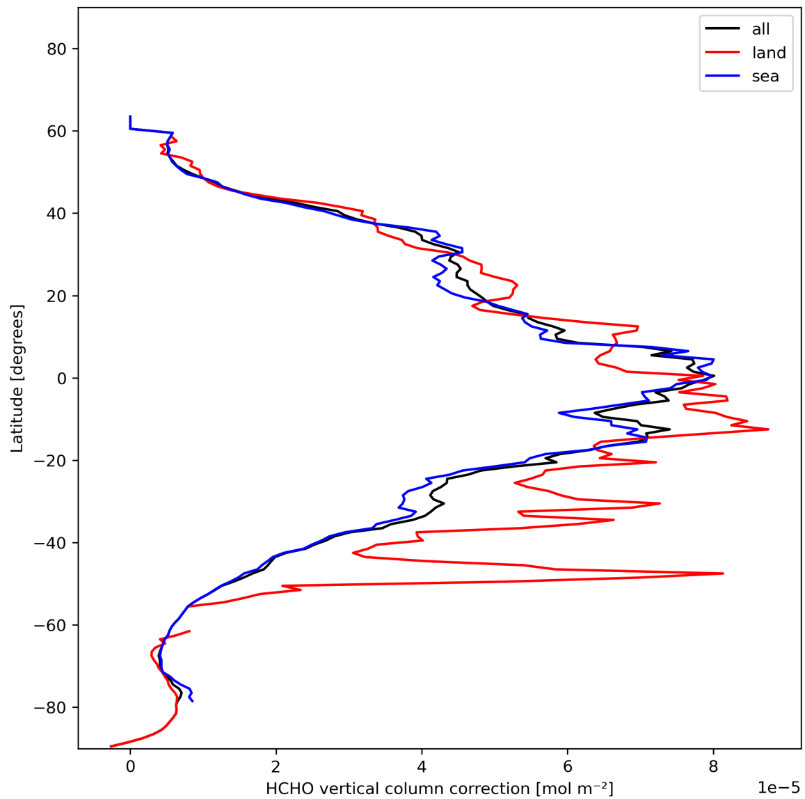
Figure 23: Zonal average of “HCHO vertical column correction” for 2024-01-12 to 2024-01-14.
