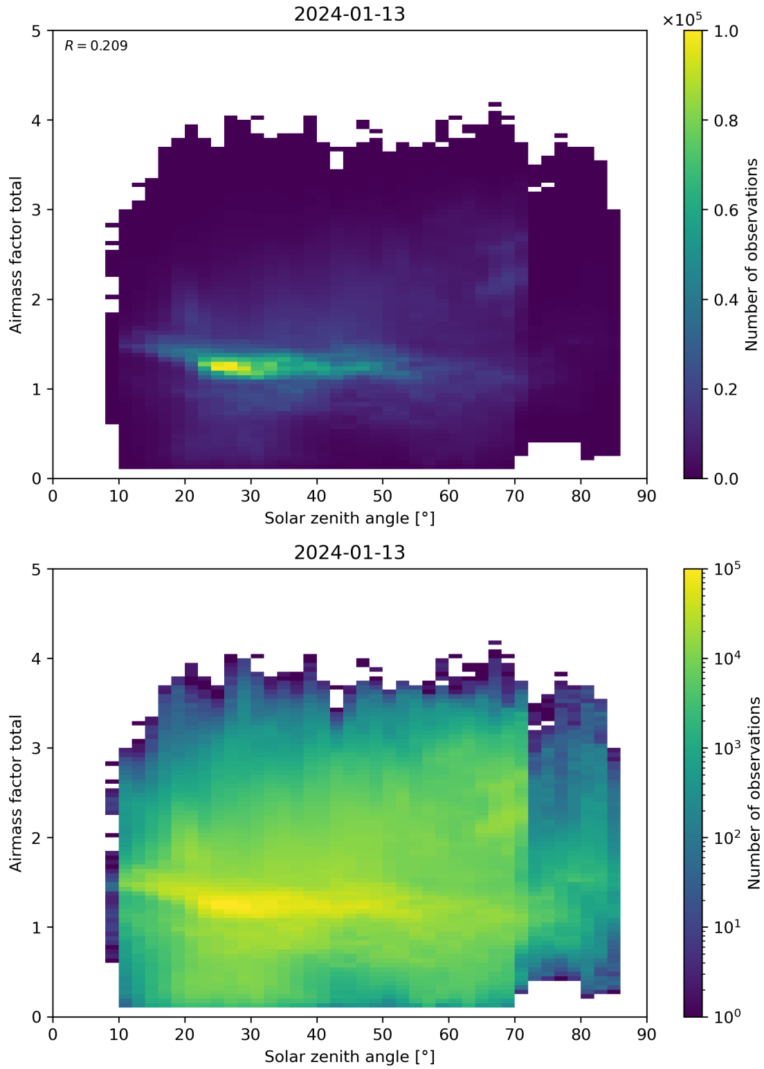
Figure 175: Scatter density plot of “Solar zenith angle” against “Airmass factor total” for 2024-01-12 to 2024-01-14.
