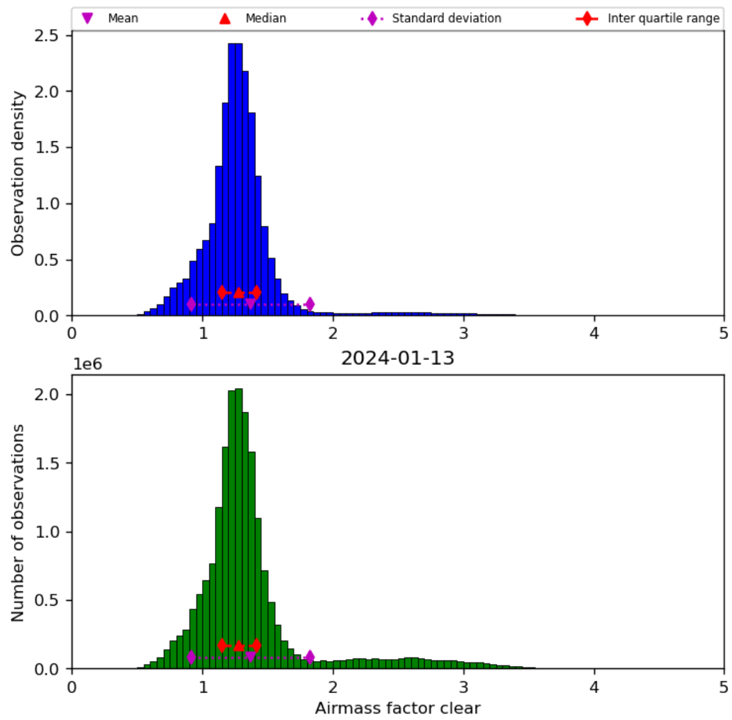
Figure 42: Histogram of “Airmass factor clear” for 2024-01-12 to 2024-01-14
