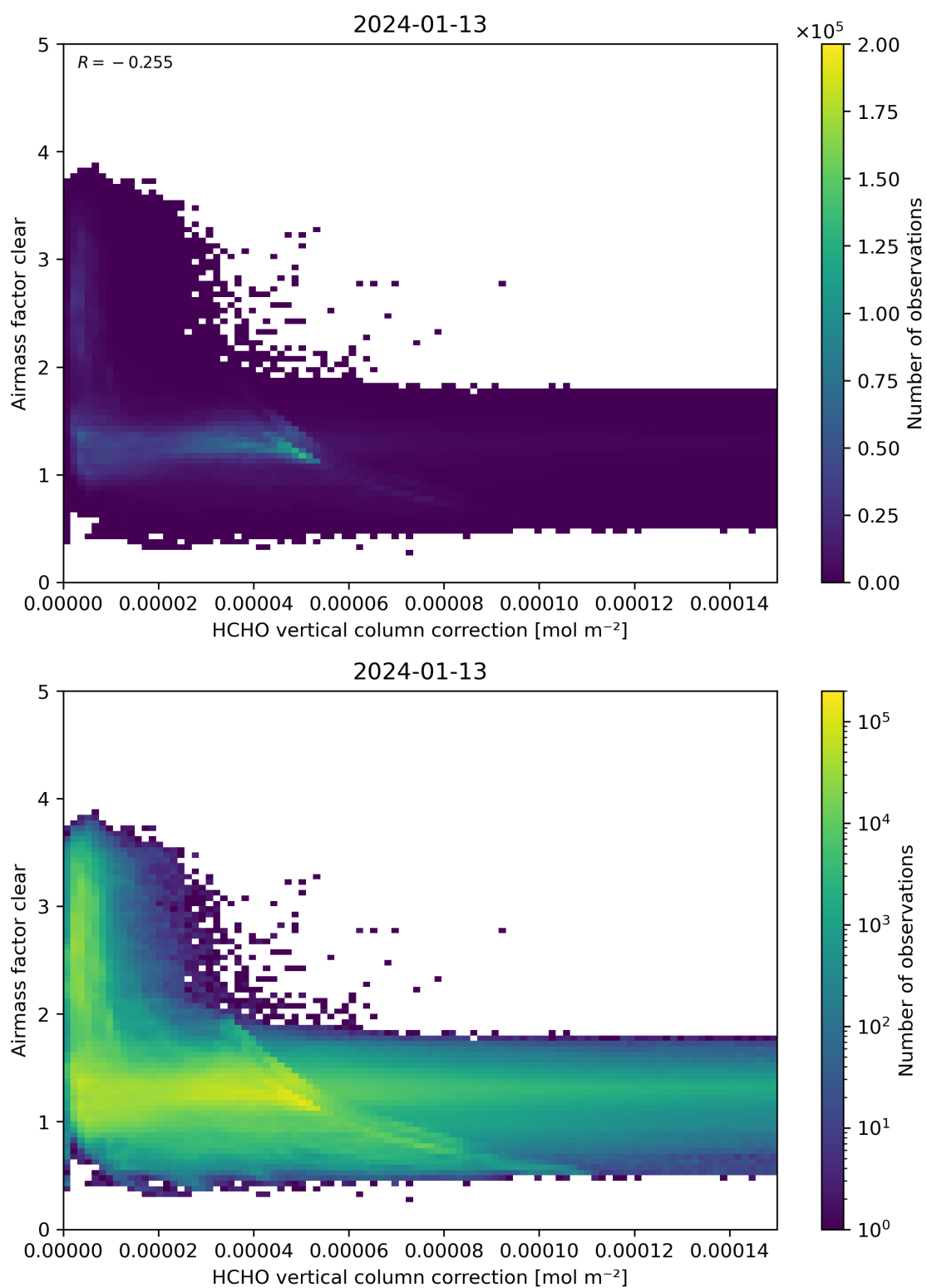
Figure 115: Scatter density plot of “HCHO vertical column correction” against “Airmass factor clear” for 2024-01-12 to 2024-01-14.
