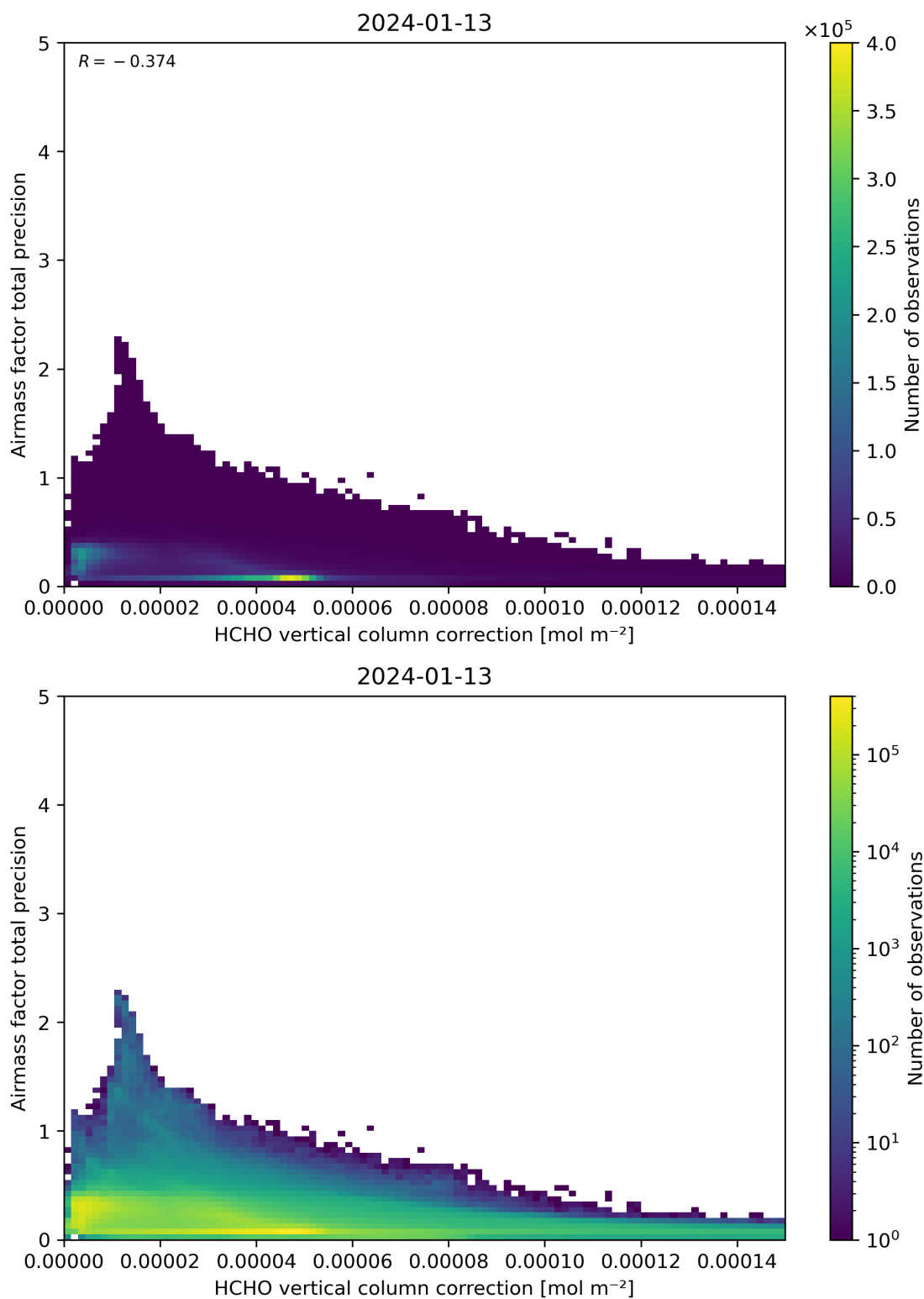
Figure 121: Scatter density plot of “HCHO vertical column correction” against “Airmass factor total precision” for 2024-01-12 to 2024-01-14.
