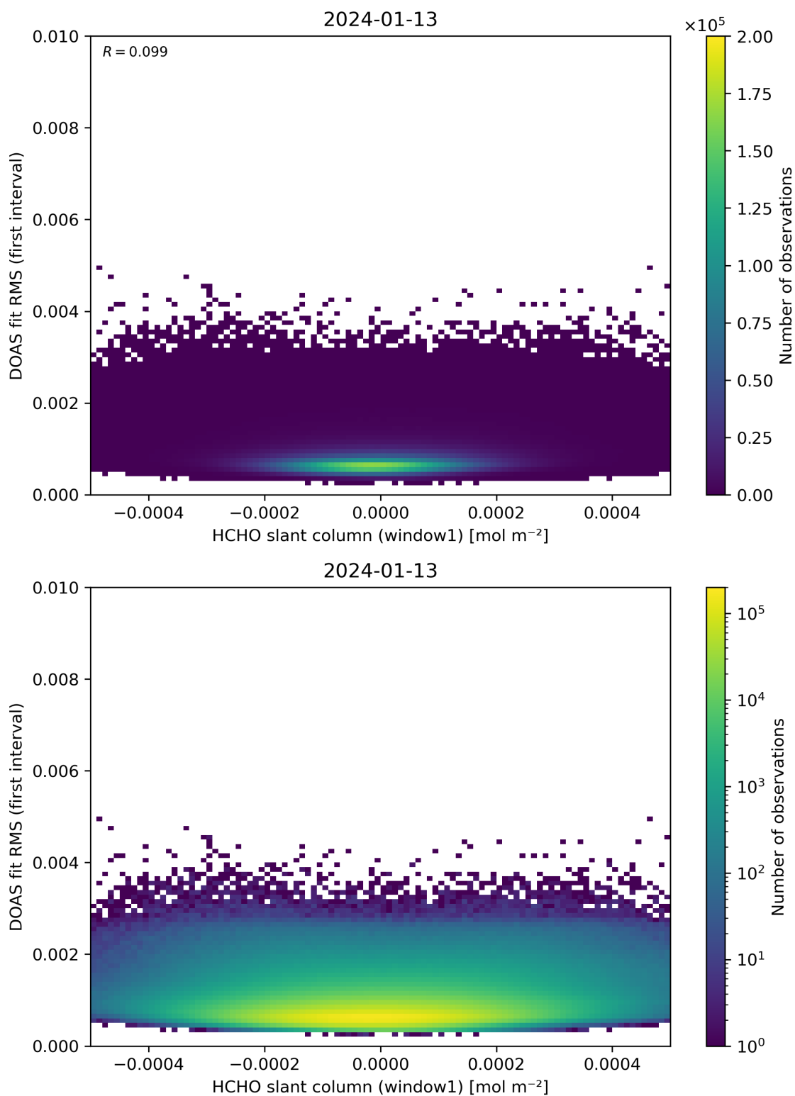
Figure 78: Scatter density plot of “HCHO slant column (window1)” against “DOAS fit RMS (first interval)” for 2024-01-12 to 2024-01-14.
