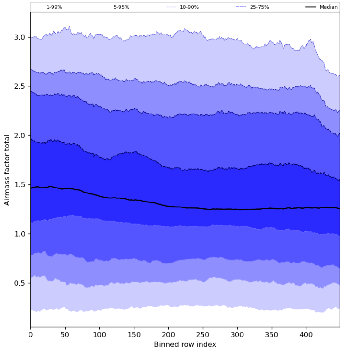
Figure 54: Along track statistics of “Airmass factor total” for 2024-01-12 to 2024-01-14
