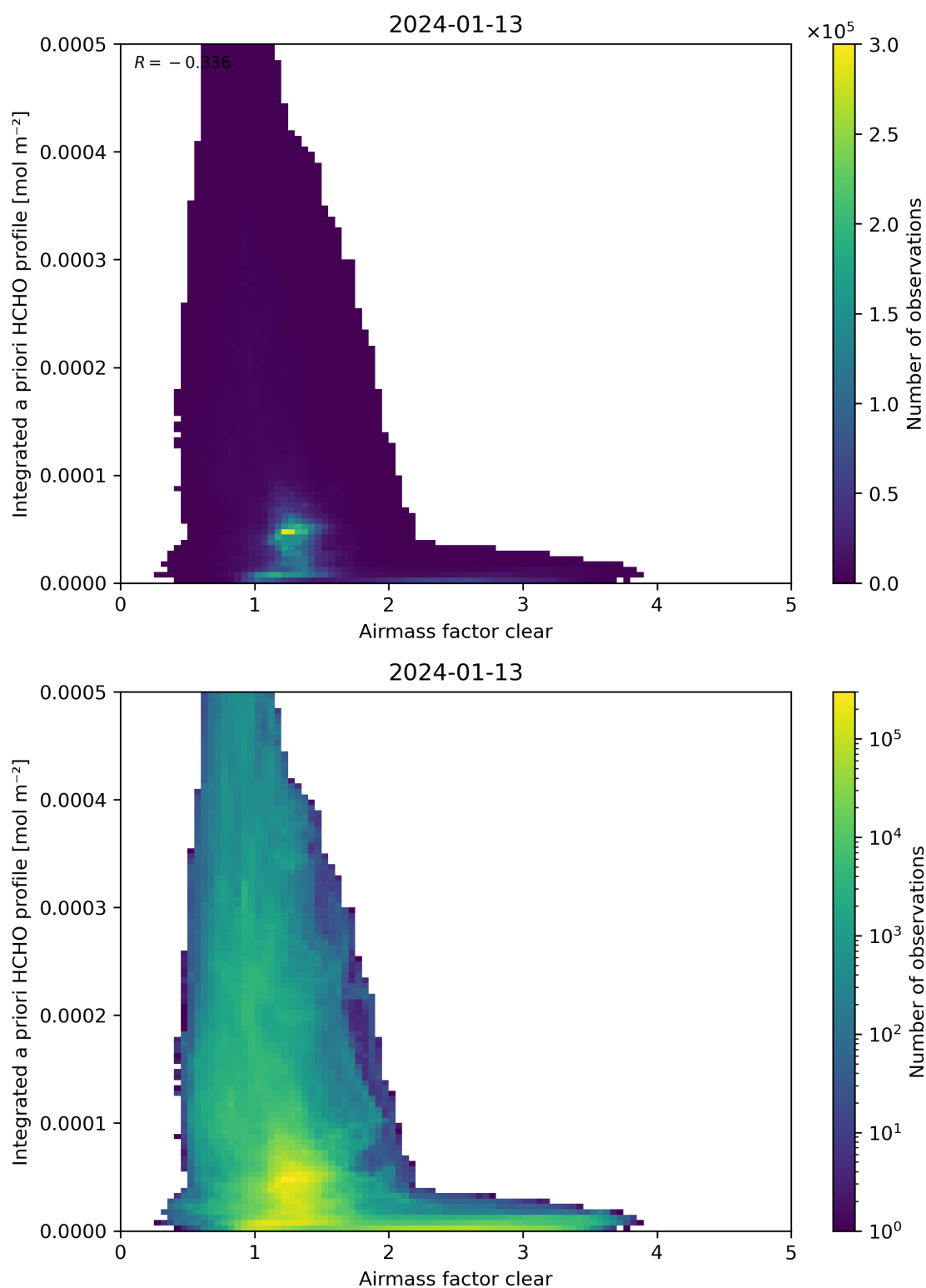
Figure 76: Scatter density plot of “Airmass factor clear” against “Integrated a priori HCHO profile” for 2024-01-12 to 2024-01-14.
