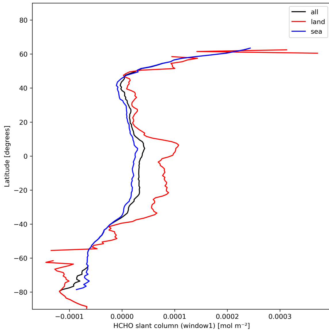
Figure 24: Zonal average of “HCHO slant column (window1)” for 2024-01-12 to 2024-01-14.
