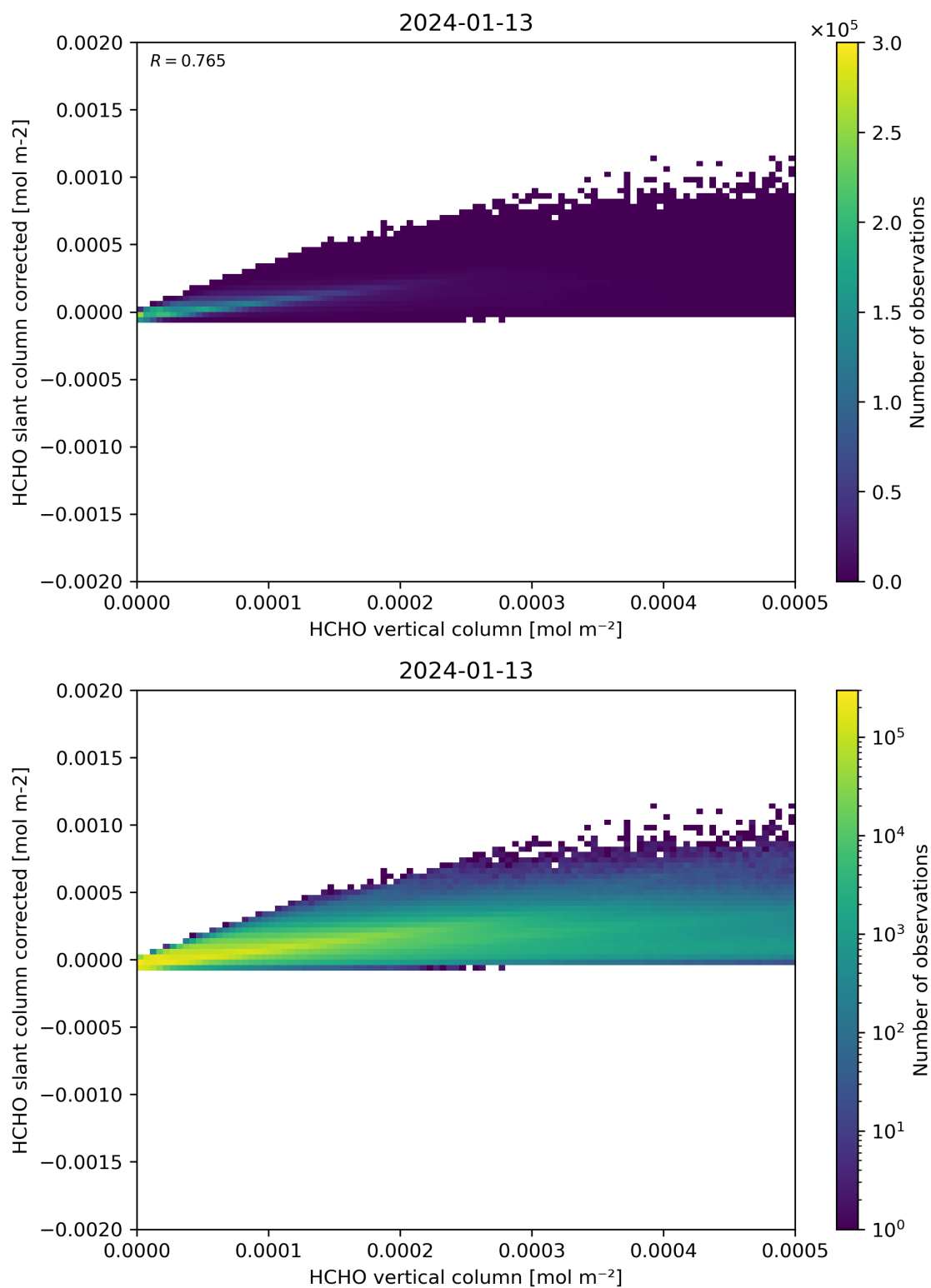
Figure 127: Scatter density plot of “HCHO vertical column” against “HCHO slant column corrected” for 2024-01-12 to 2024-01-14.
