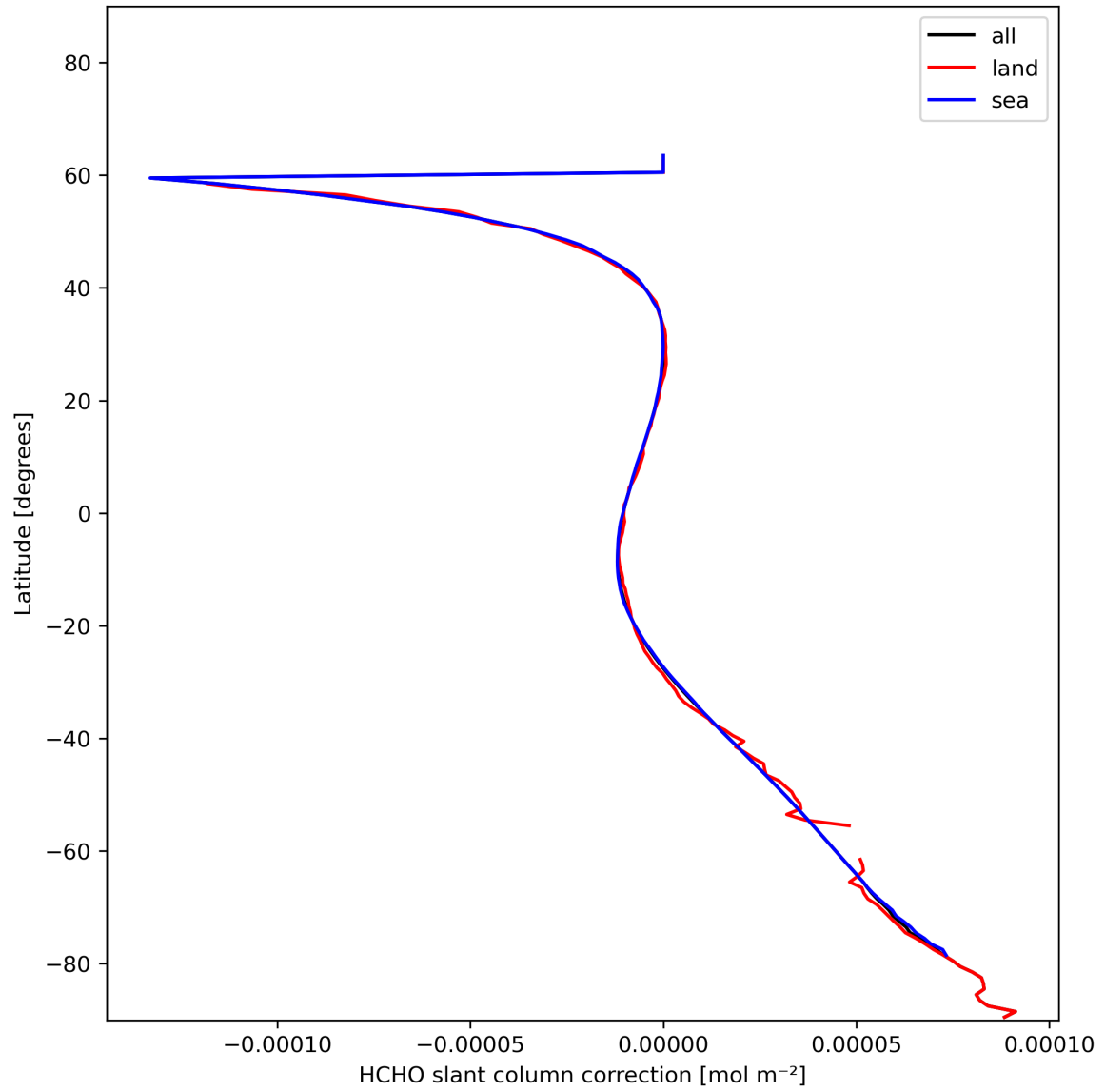
Figure 33: Zonal average of “HCHO slant column correction” for 2024-01-12 to 2024-01-14.
