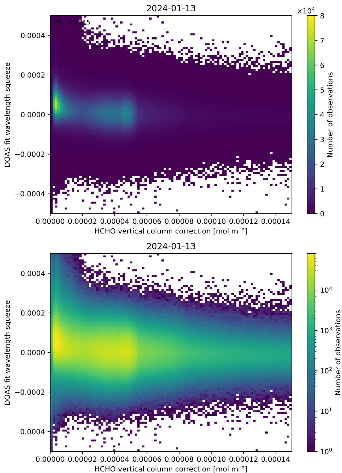
Figure 114: Scatter density plot of “HCHO vertical column correction” against “DOAS fit wavelength squeeze” for 2024-01-12 to 2024-01-14.
