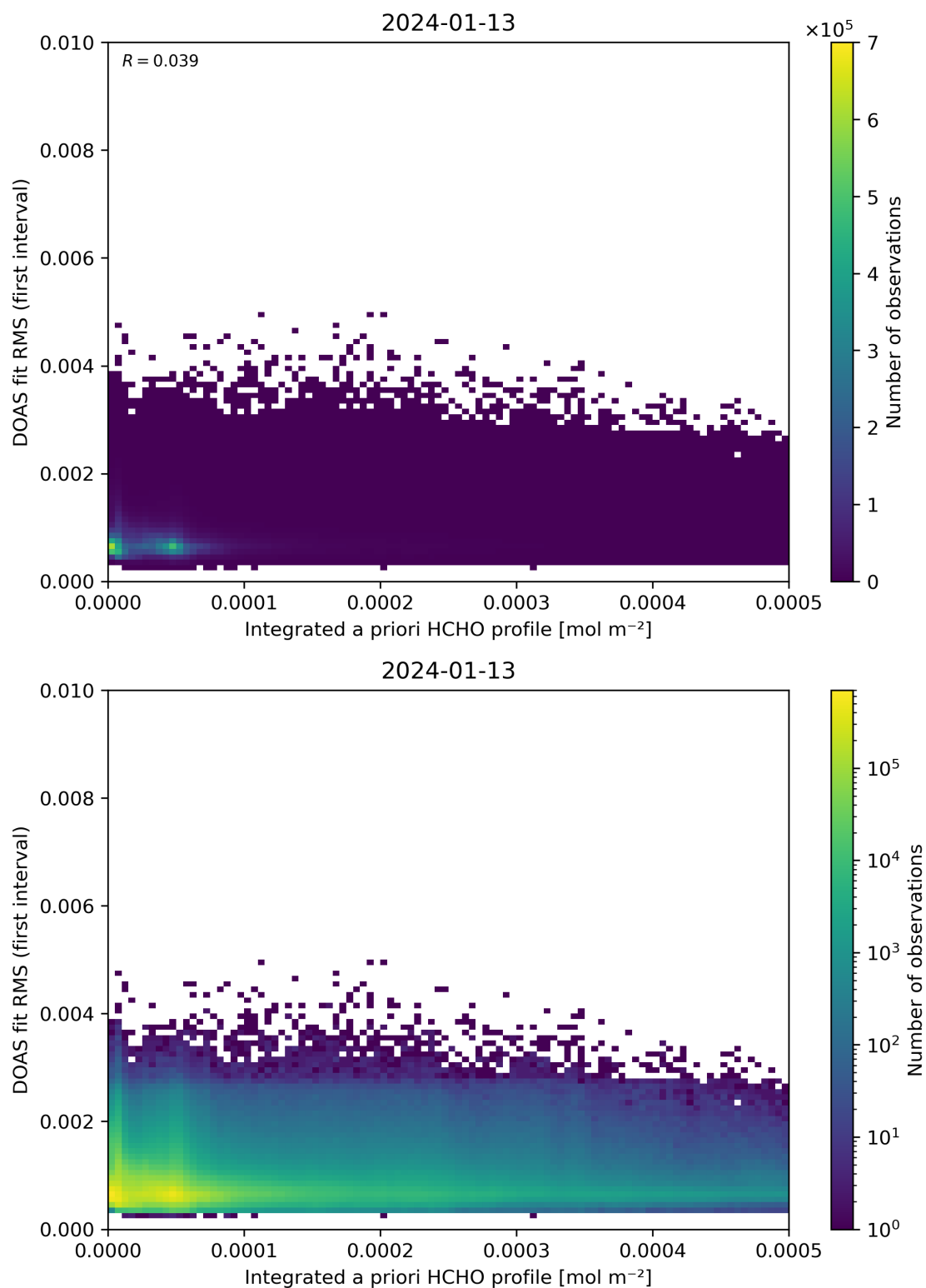
Figure 148: Scatter density plot of “Integrated a priori HCHO profile” against “DOAS fit RMS (first interval)” for 2024-01-12 to 2024-01-14.
