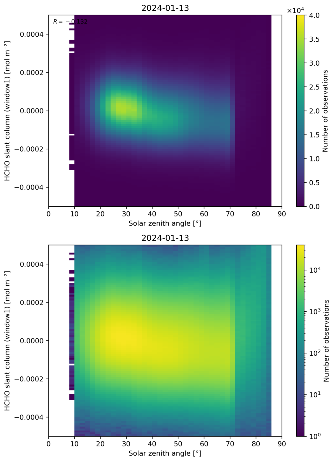
Figure 173: Scatter density plot of “Solar zenith angle” against “HCHO slant column (window1)” for 2024-01-12 to 2024-01-14.
