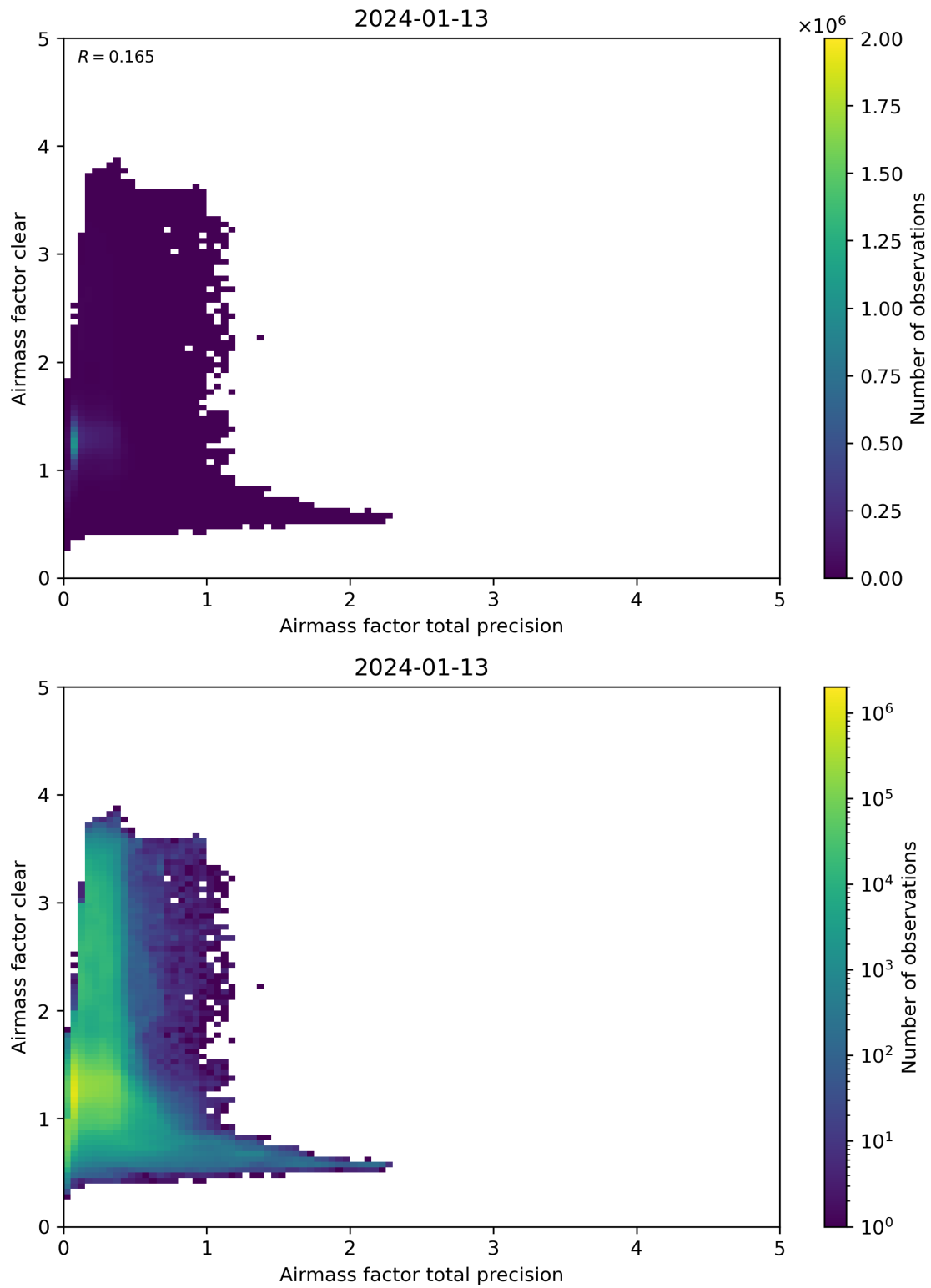
Figure 108: Scatter density plot of “Airmass factor total precision” against “Airmass factor clear” for 2024-01-12 to 2024-01-14.
