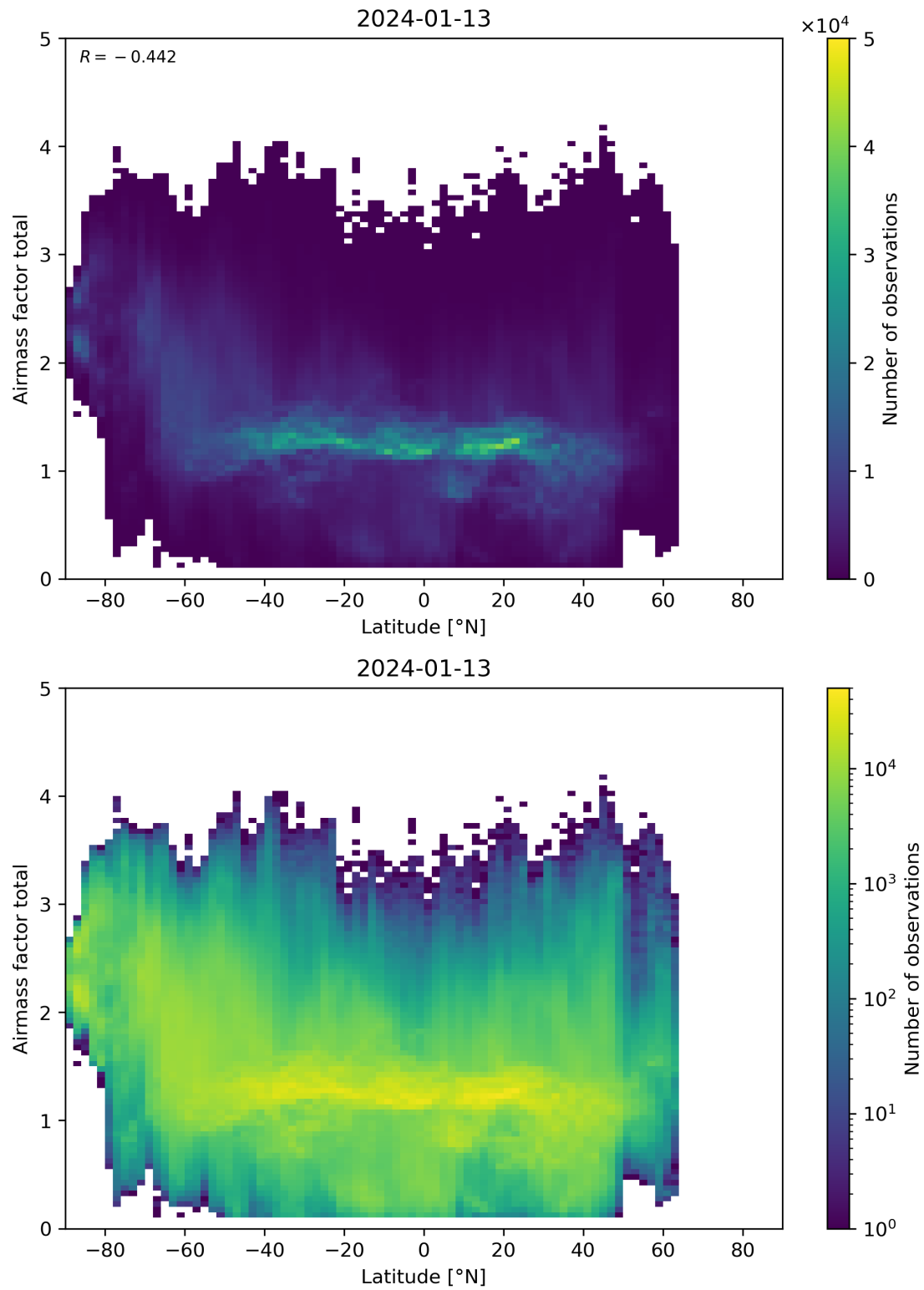
Figure 161: Scatter density plot of “Latitude” against “Airmass factor total” for 2024-01-12 to 2024-01-14.
