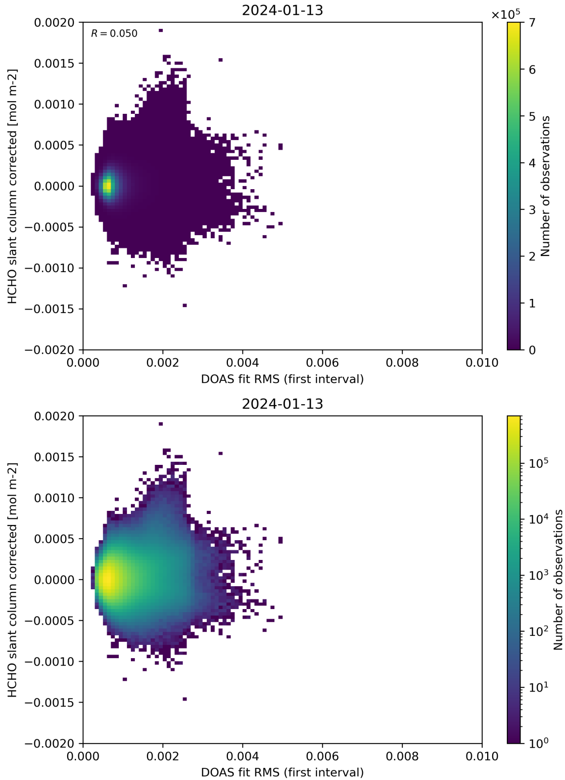
Figure 62: Scatter density plot of “DOAS fit RMS (first interval)” against “HCHO slant column corrected” for 2024-01-12 to 2024-01-14.
