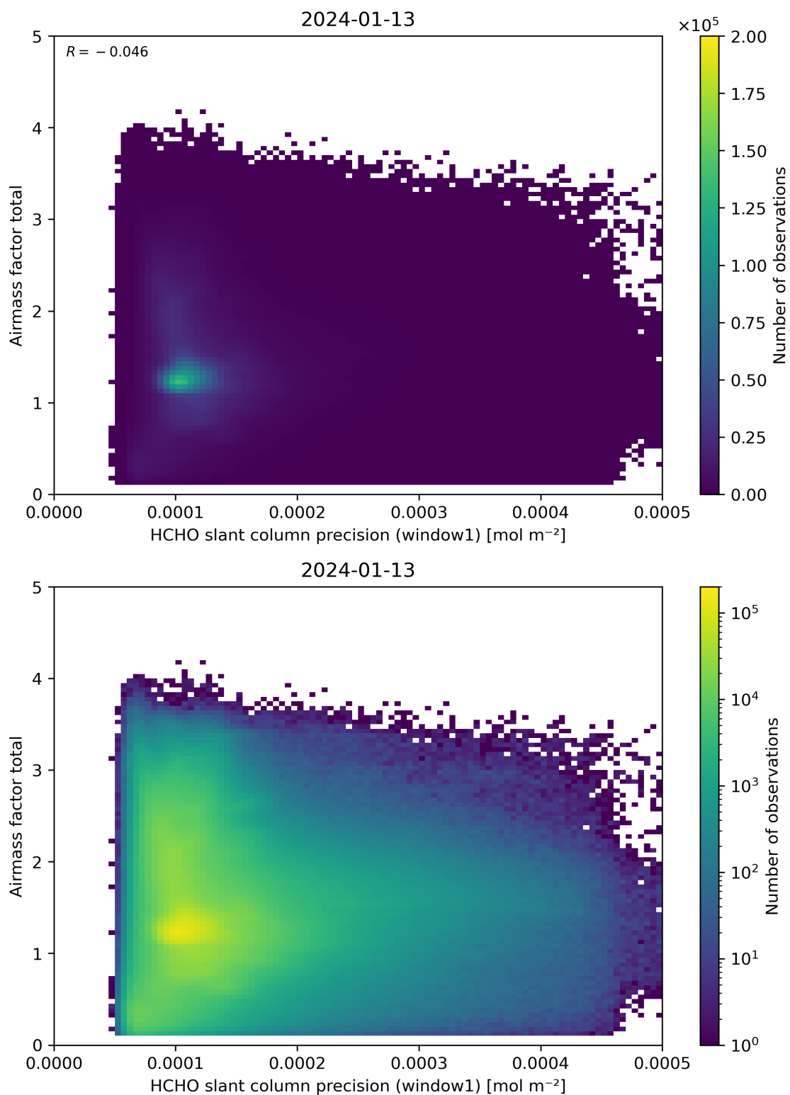
Figure 94: Scatter density plot of “HCHO slant column precision (window1)” against “Airmass factor total” for 2024-01-12 to 2024-01-14.
