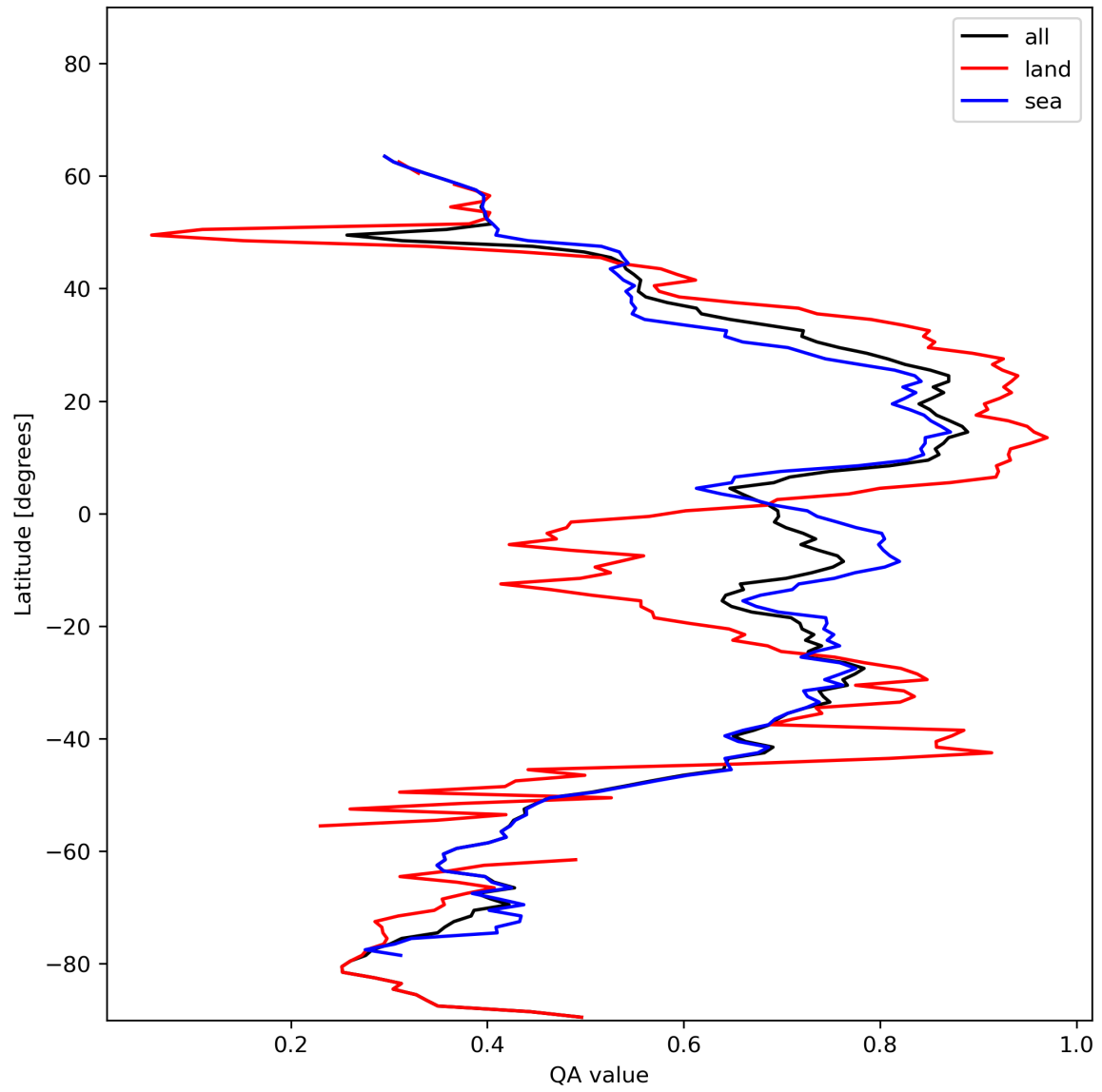
Figure 20: Zonal average of “QA value” for 2024-01-12 to 2024-01-14.
