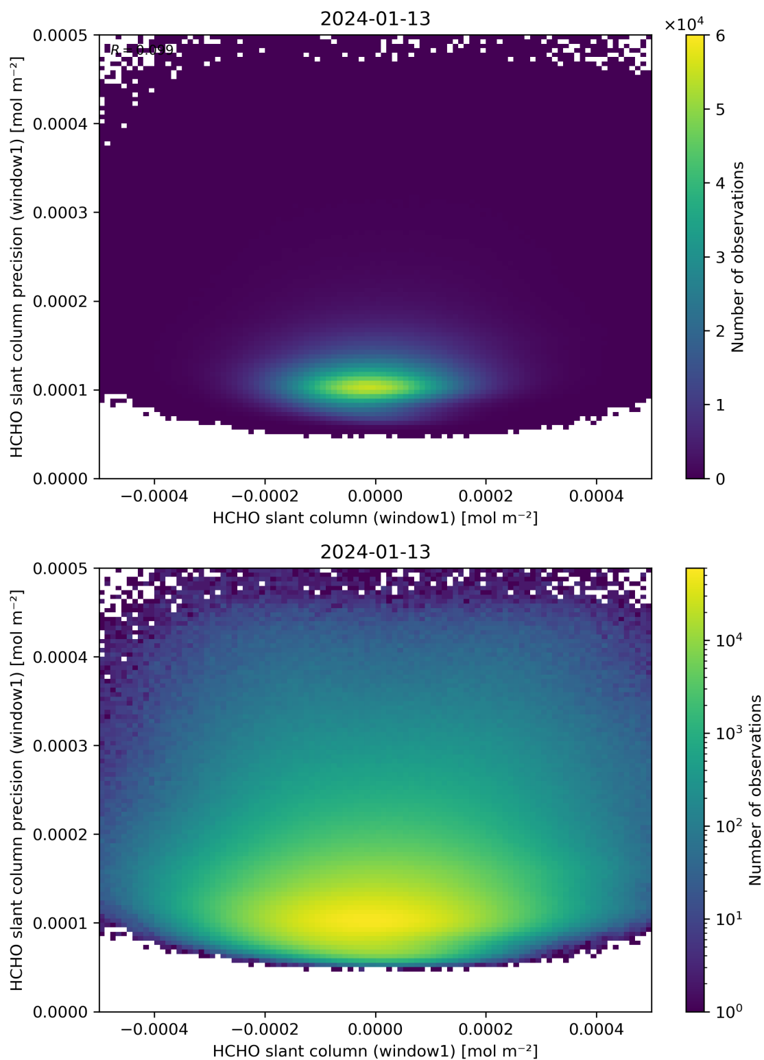
Figure 84: Scatter density plot of “HCHO slant column (window1)” against “HCHO slant column precision (window1)” for 2024-01-12 to 2024-01-14.
