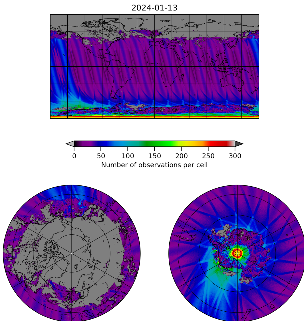
Figure 19: Map of the number of observations for 2024-01-12 to 2024-01-14
