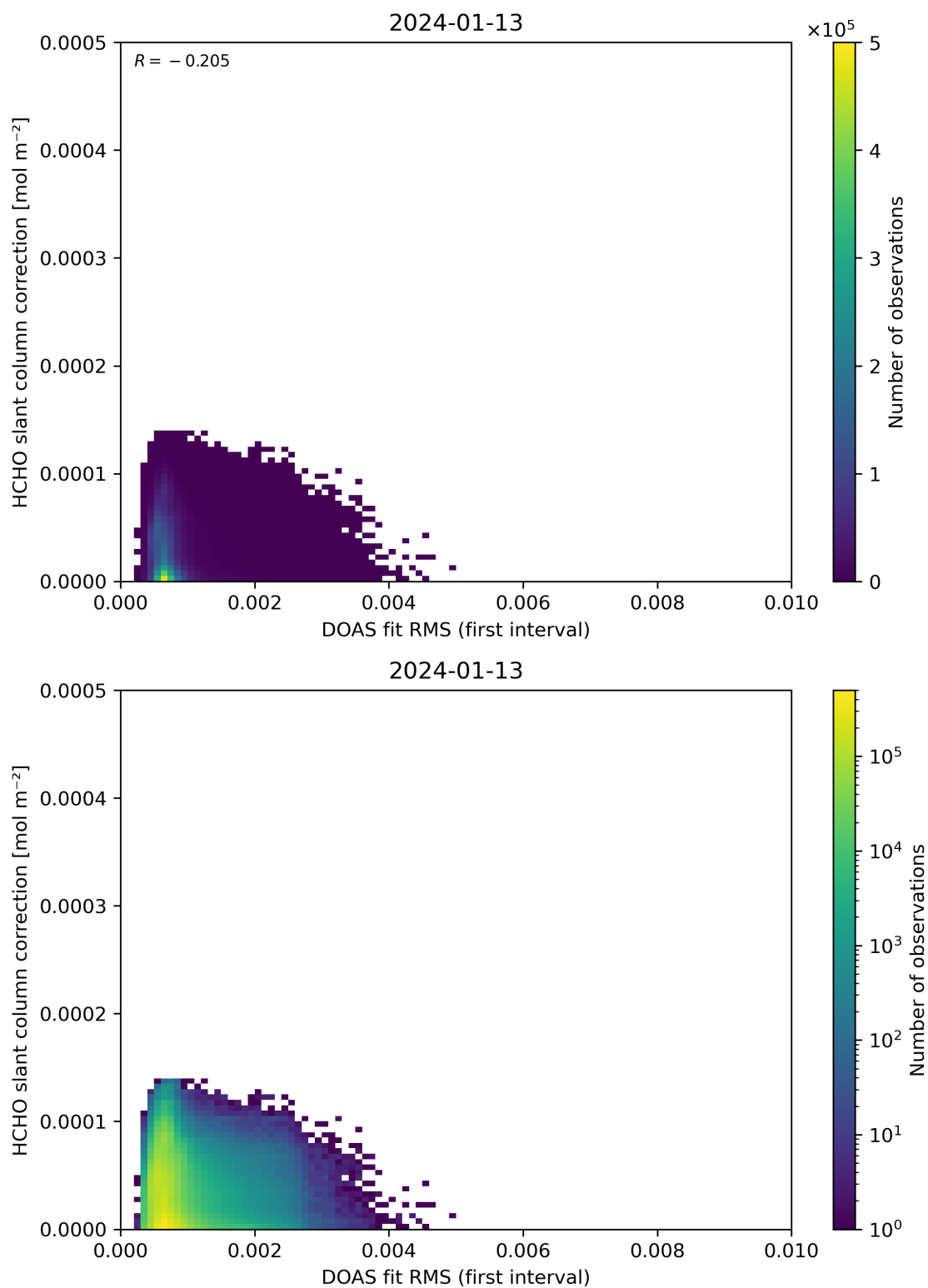
Figure 63: Scatter density plot of “DOAS fit RMS (first interval)” against “HCHO slant column correction” for 2024-01-12 to 2024-01-14.
