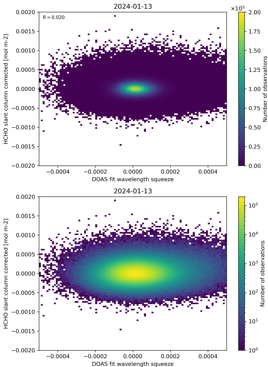
Figure 69: Scatter density plot of “DOAS fit wavelength squeeze” against “HCHO slant column corrected” for 2024-01-12 to 2024-01-14.
