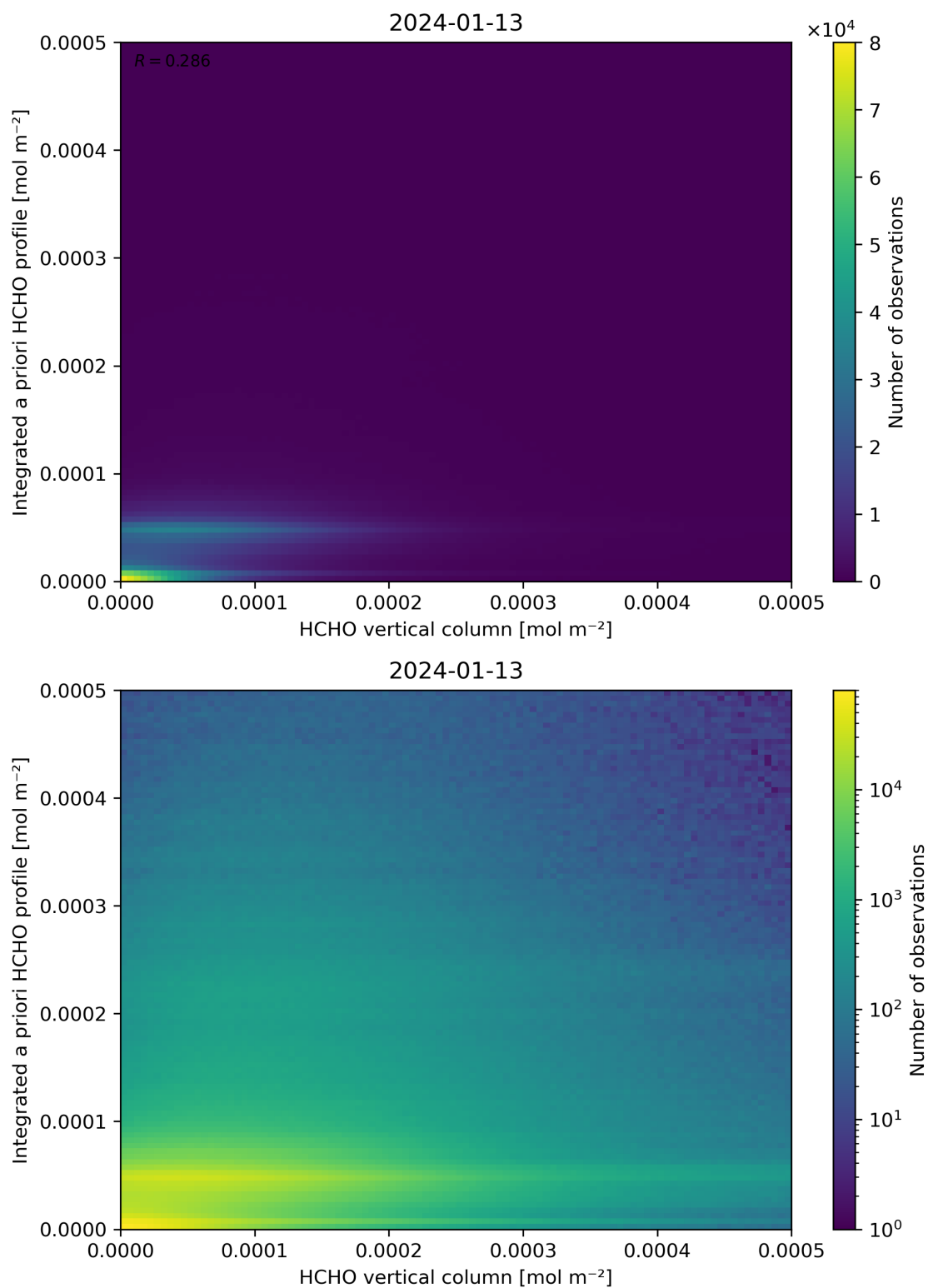
Figure 135: Scatter density plot of “HCHO vertical column” against “Integrated a priori HCHO profile” for 2024-01-12 to 2024-01-14.
