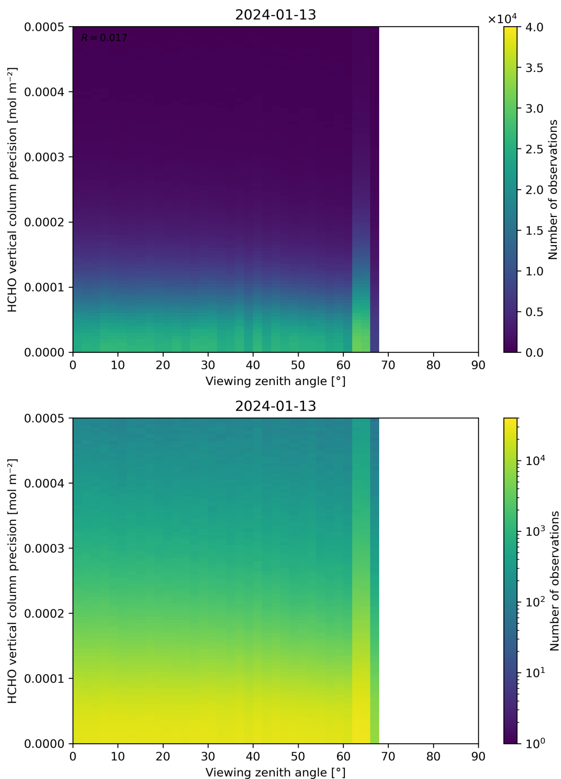
Figure 194: Scatter density plot of “Viewing zenith angle” against “HCHO vertical column precision” for 2024-01-12 to 2024-01-14.
