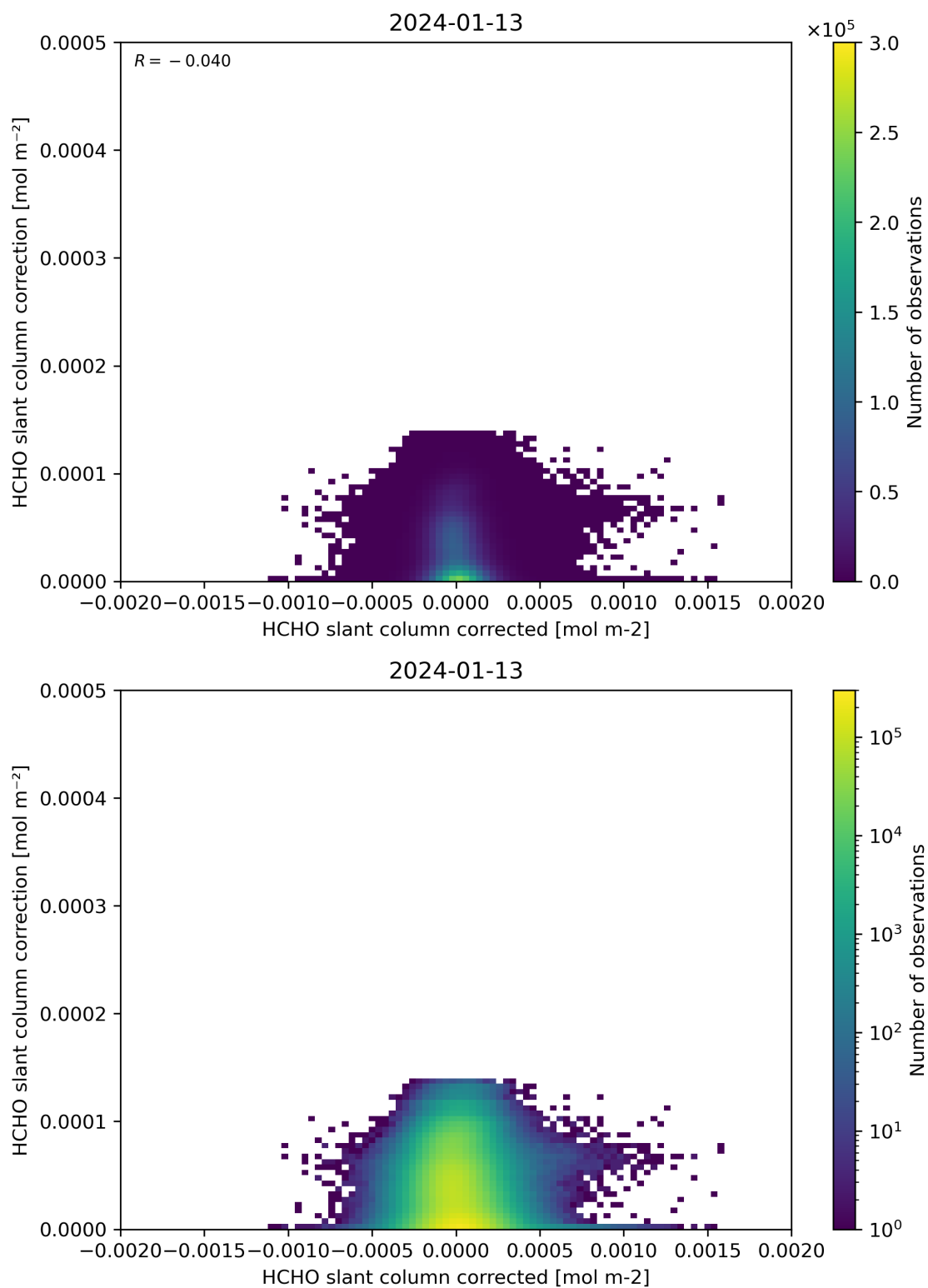
Figure 77: Scatter density plot of “HCHO slant column corrected” against “HCHO slant column correction” for 2024-01-12 to 2024-01-14.
