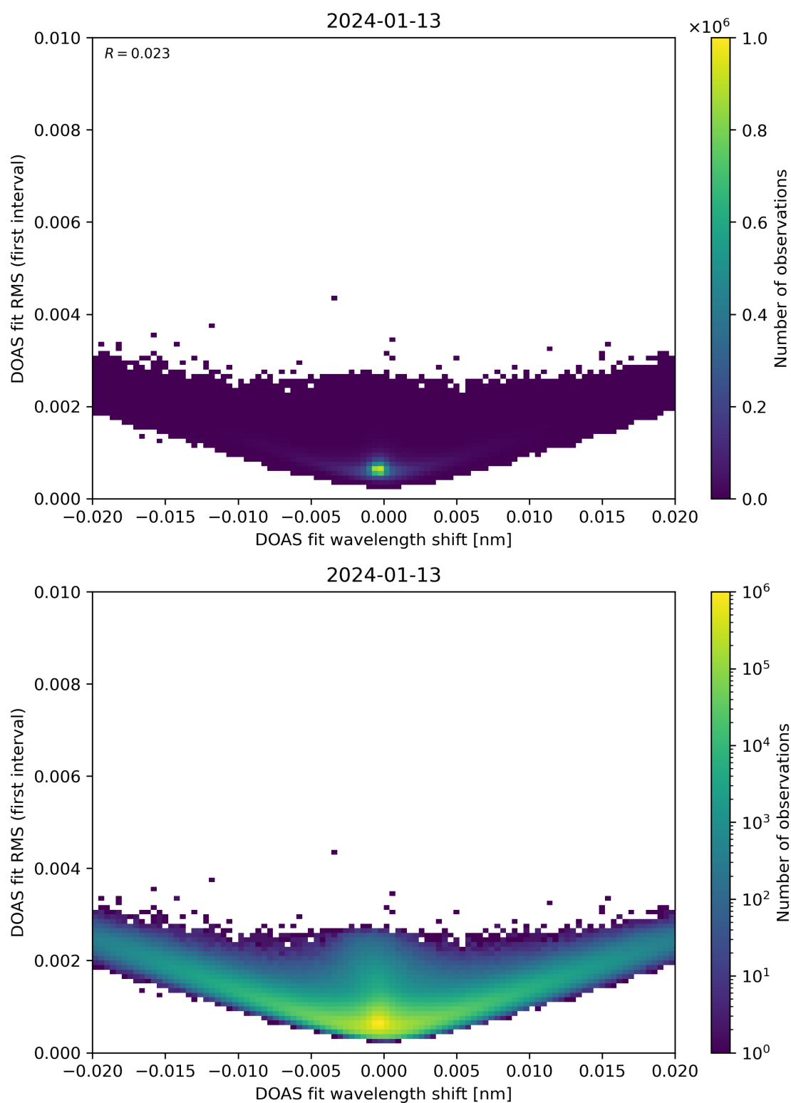
Figure 64: Scatter density plot of “DOAS fit wavelength shift” against “DOAS fit RMS (first interval)” for 2024-01-12 to 2024-01-14.
