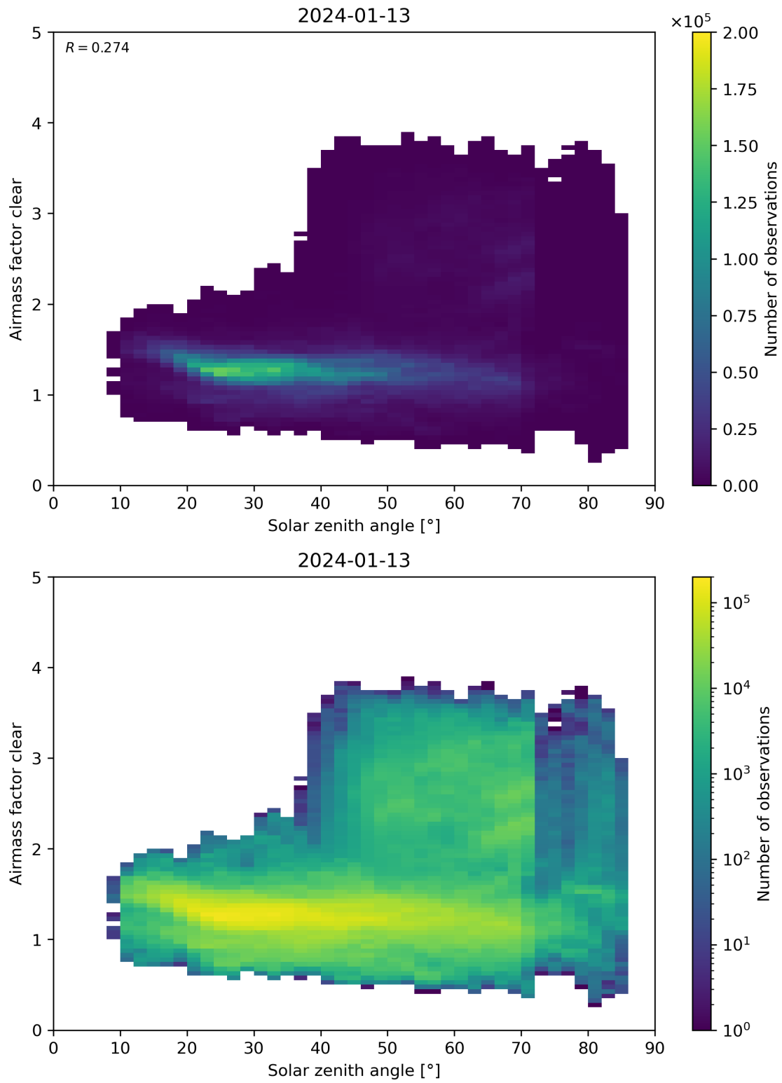
Figure 170: Scatter density plot of “Solar zenith angle” against “Airmass factor clear” for 2024-01-12 to 2024-01-14.
