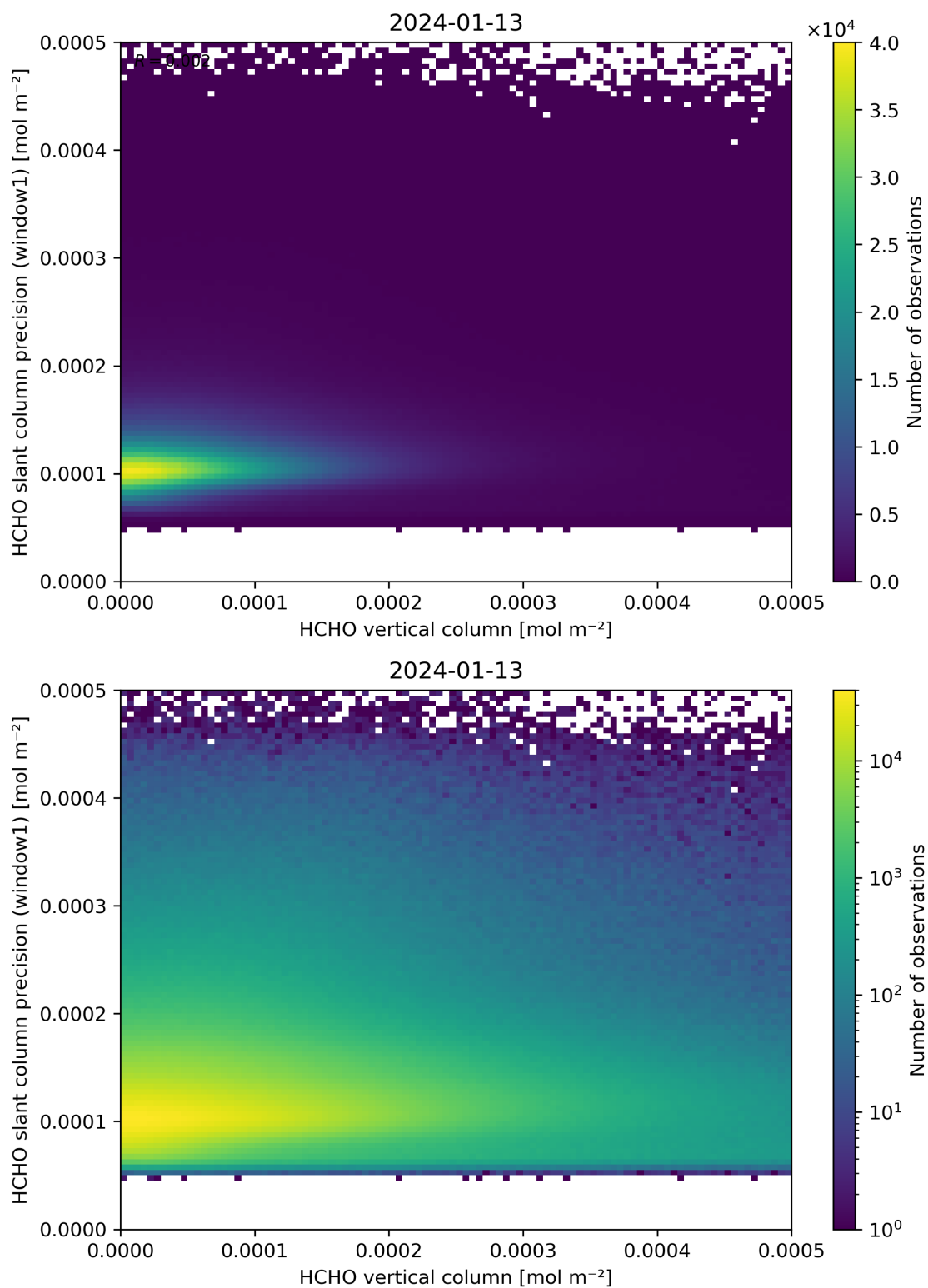
Figure 130: Scatter density plot of “HCHO vertical column” against “HCHO slant column precision (window1)” for 2024-01-12 to 2024-01-14.
