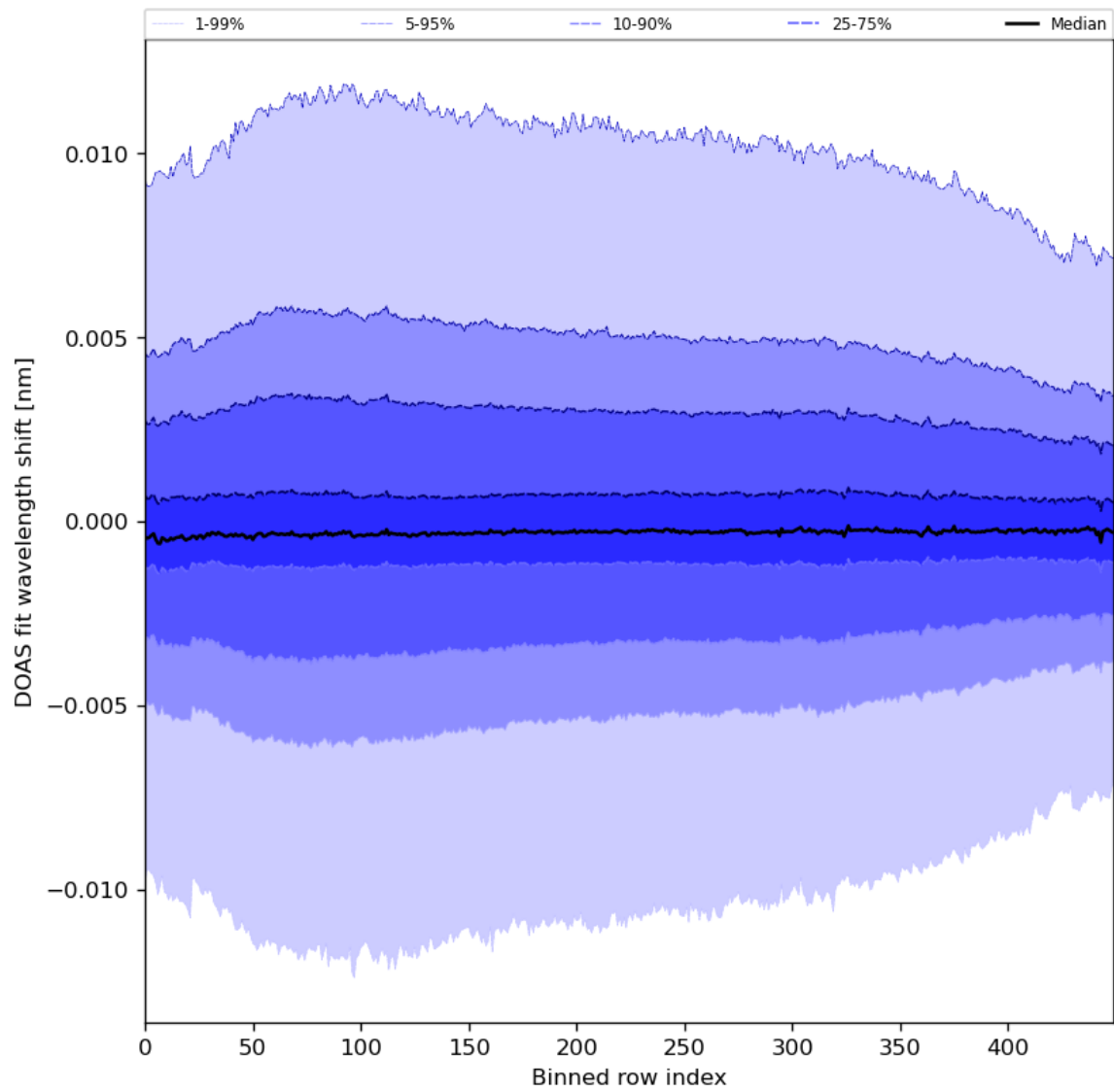
Figure 58: Along track statistics of “DOAS fit wavelength shift” for 2024-01-12 to 2024-01-14
