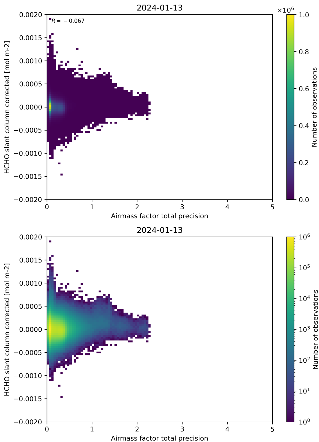
Figure 109: Scatter density plot of “Airmass factor total precision” against “HCHO slant column corrected” for 2024-01-12 to 2024-01-14.
