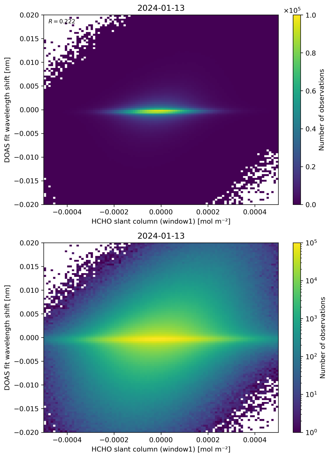
Figure 79: Scatter density plot of “HCHO slant column (window1)” against “DOAS fit wavelength shift” for 2024-01-12 to 2024-01-14.
