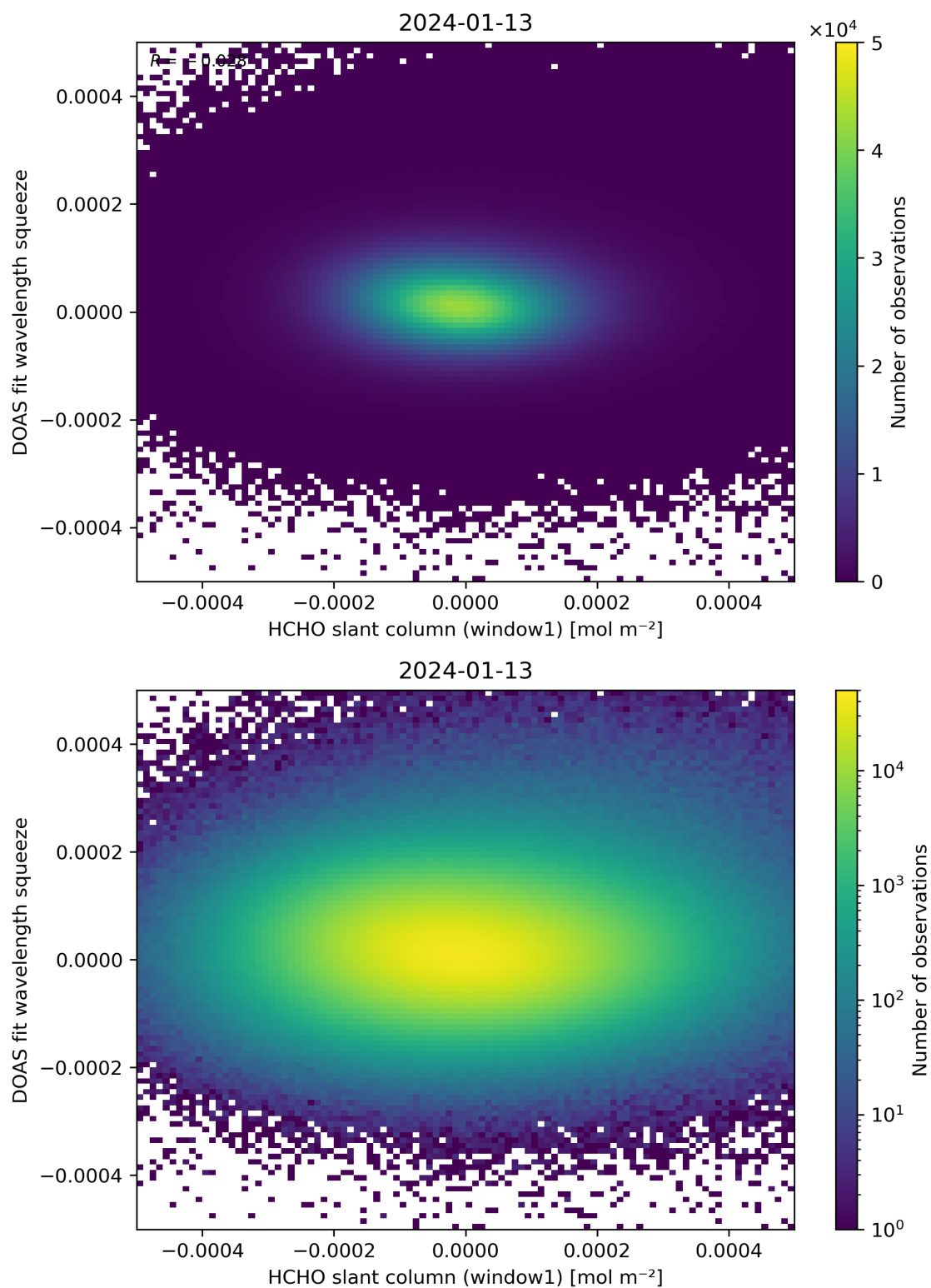
Figure 80: Scatter density plot of “HCHO slant column (window1)” against “DOAS fit wavelength squeeze” for 2024-01-12 to 2024-01-14.
