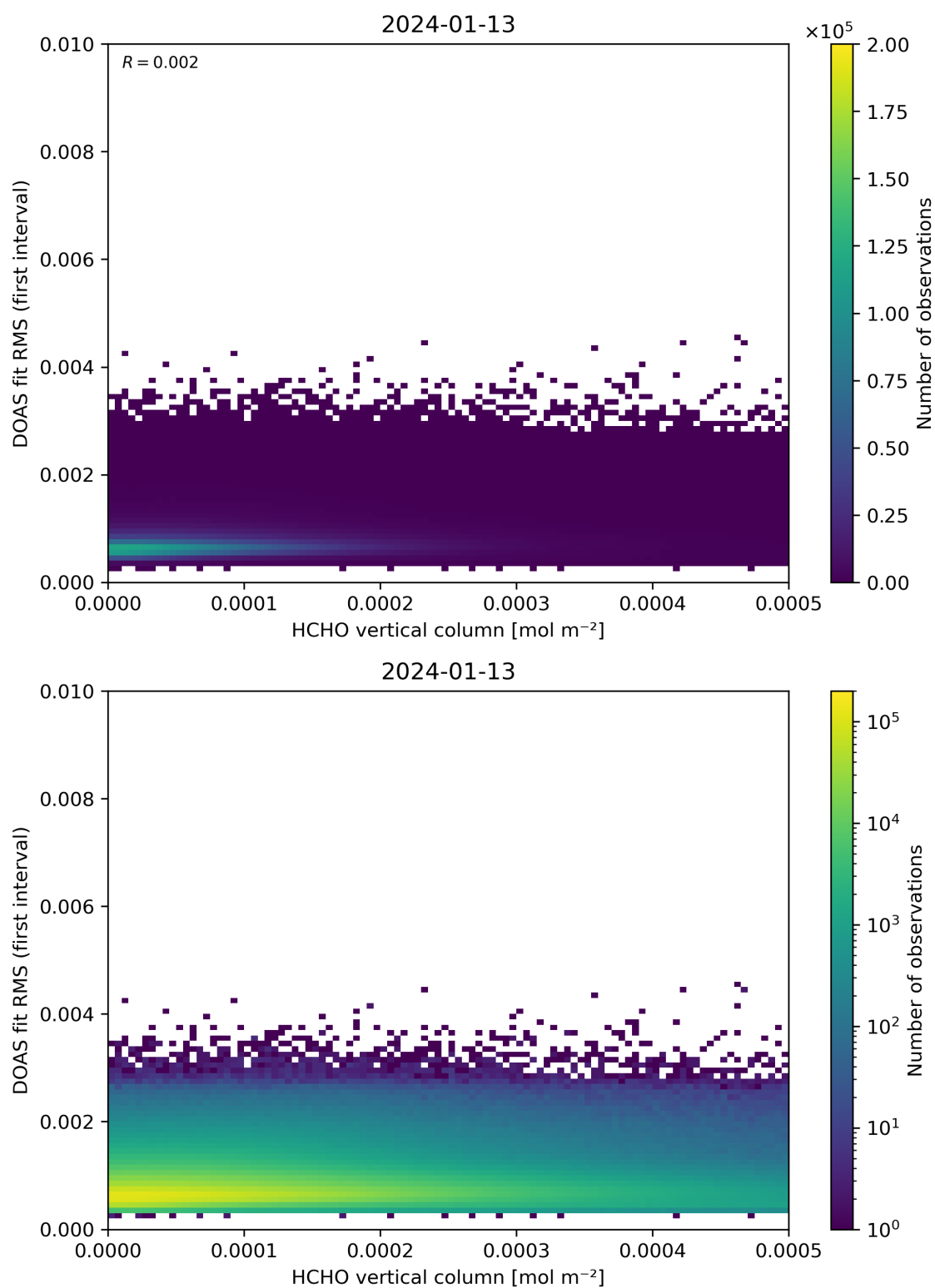
Figure 123: Scatter density plot of “HCHO vertical column” against “DOAS fit RMS (first interval)” for 2024-01-12 to 2024-01-14.
