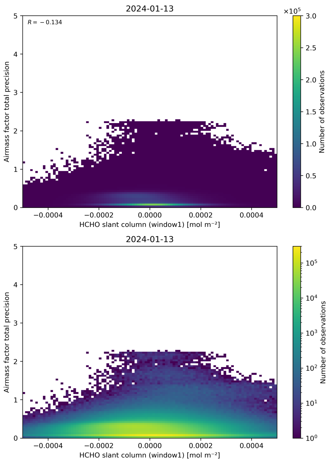
Figure 86: Scatter density plot of “HCHO slant column (window1)” against “Airmass factor total precision” for 2024-01-12 to 2024-01-14.
