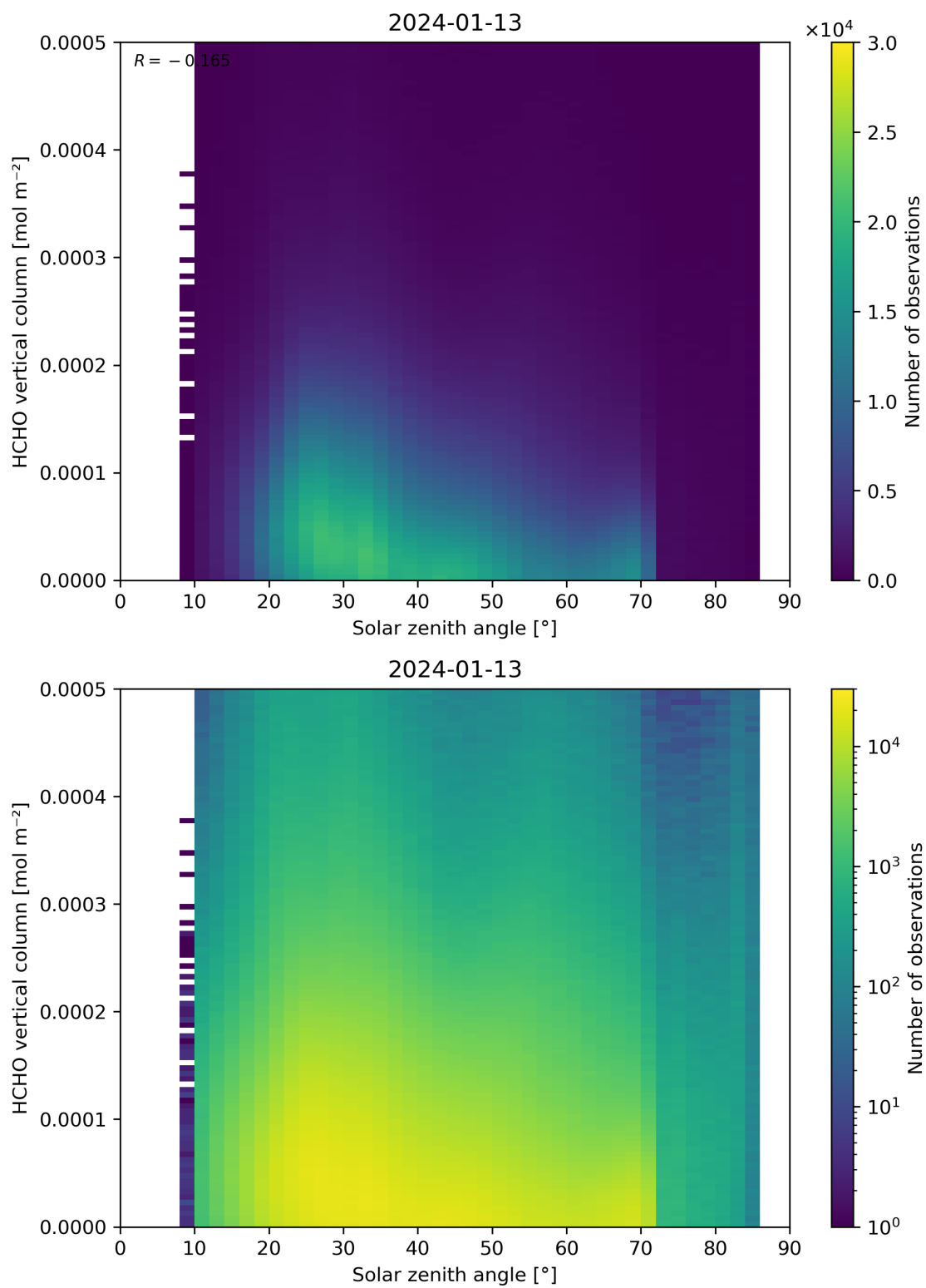
Figure 177: Scatter density plot of “Solar zenith angle” against “HCHO vertical column” for 2024-01-12 to 2024-01-14.
