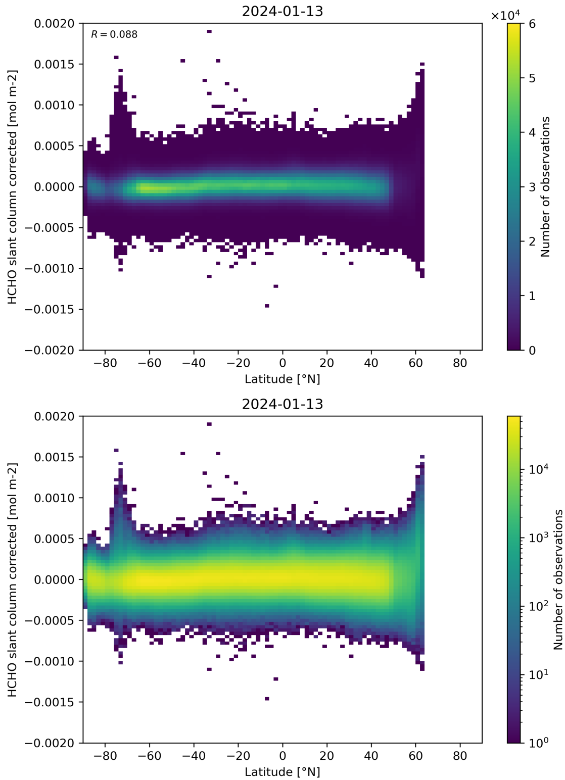
Figure 157: Scatter density plot of “Latitude” against “HCHO slant column corrected” for 2024-01-12 to 2024-01-14.
