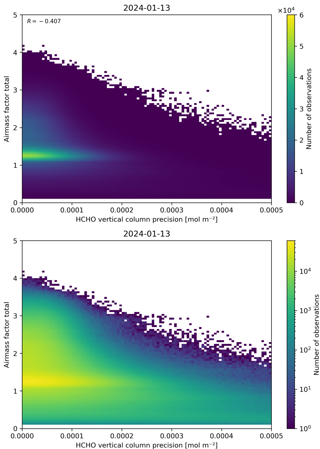
Figure 144: Scatter density plot of “HCHO vertical column precision” against “Airmass factor total” for 2024-01-12 to 2024-01-14.
