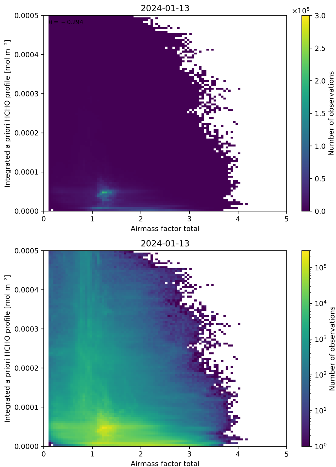
Figure 104: Scatter density plot of “Air mass factor total” against “Integrated a priori HCHO profile” for 2024-01-12 to 2024-01-14.
