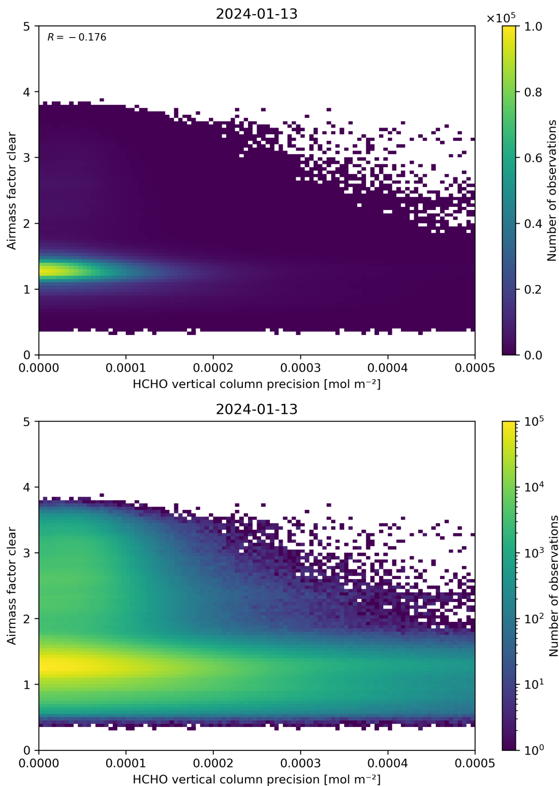
Figure 139: Scatter density plot of “HCHO vertical column precision” against “Airmass factor clear” for 2024-01-12 to 2024-01-14.
