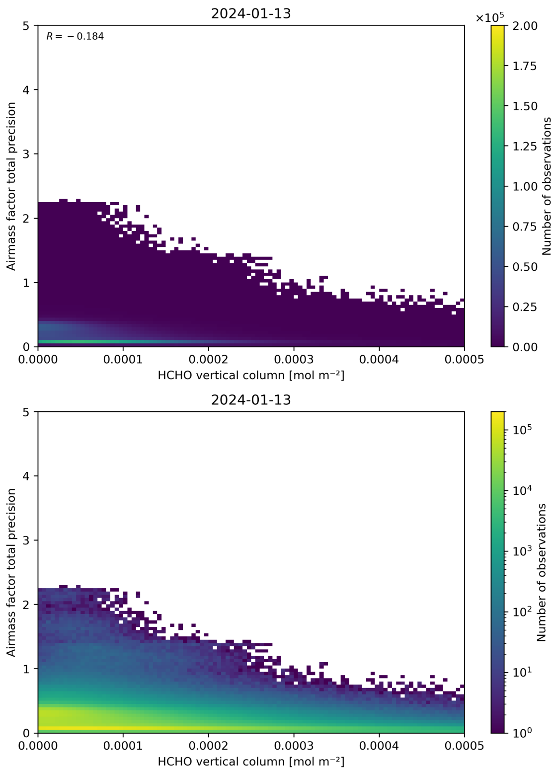
Figure 132: Scatter density plot of “HCHO vertical column” against “Airmass factor total precision” for 2024-01-12 to 2024-01-14.
