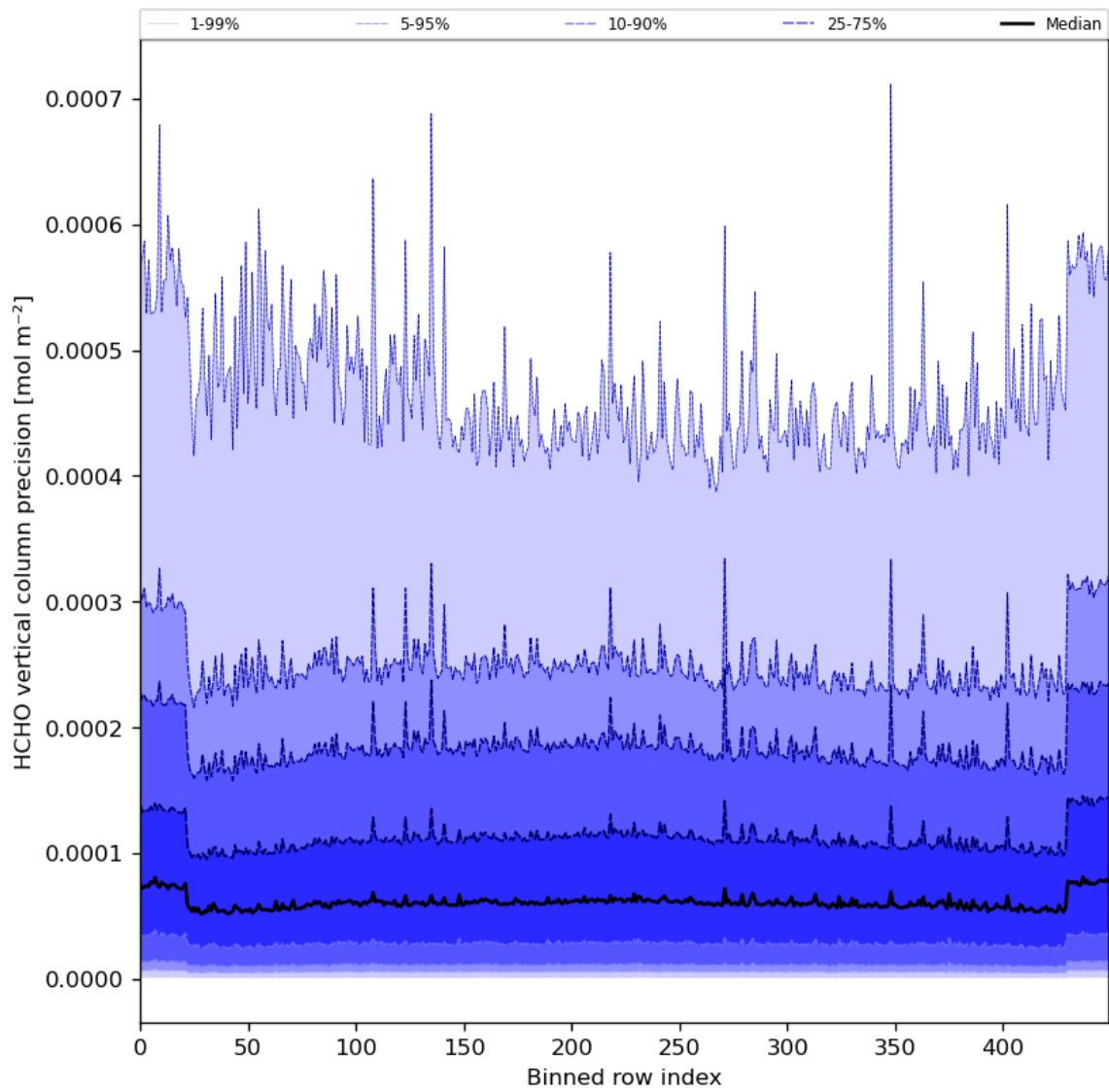
Figure 50: Along track statistics of “HCHO vertical column precision” for 2024-01-12 to 2024-01-14
