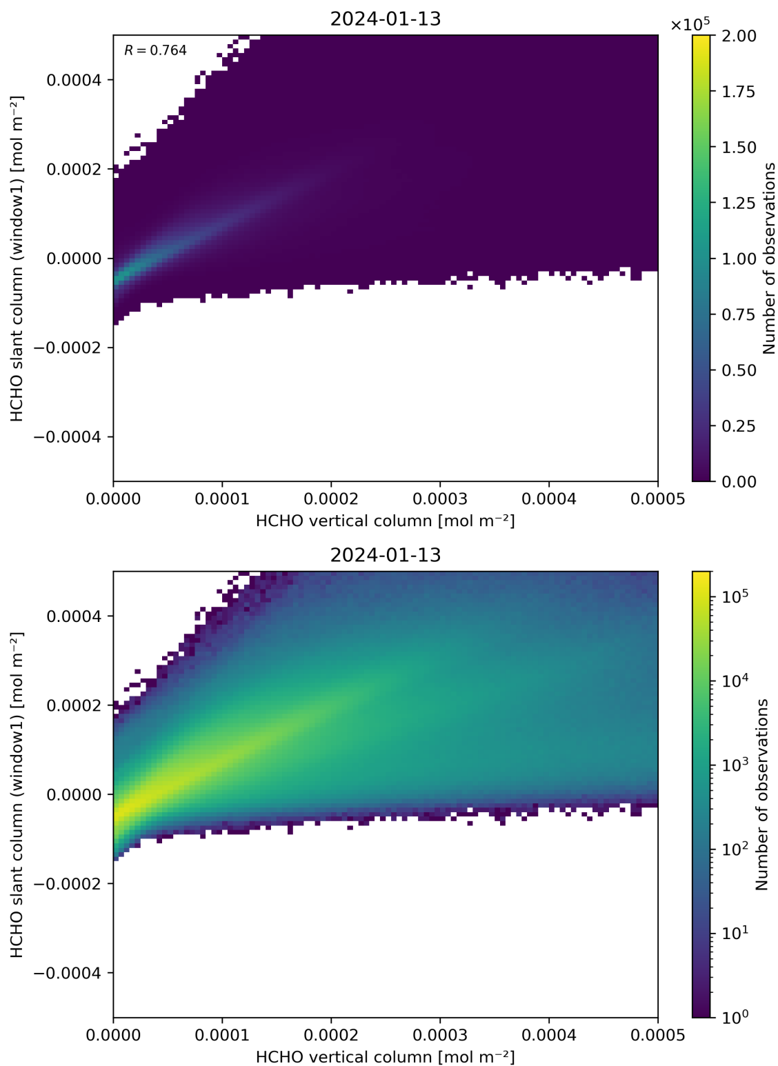
Figure 129: Scatter density plot of “HCHO vertical column” against “HCHO slant column (window1)” for 2024-01-12 to 2024-01-14.
