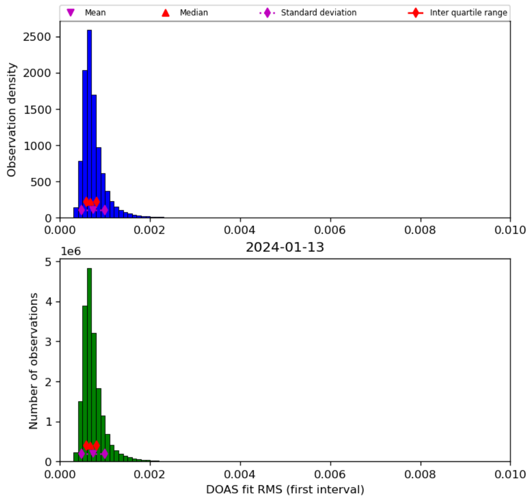
Figure 46: Histogram of “DOAS fit RMS (first interval)” for 2024-01-12 to 2024-01-14
