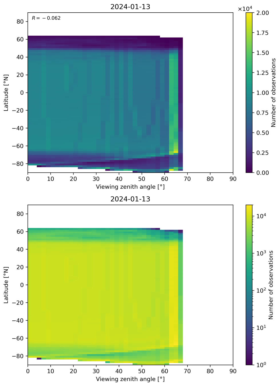
Figure 196: Scatter density plot of “Viewing zenith angle” against “Latitude” for 2024-01-12 to 2024-01-14.
