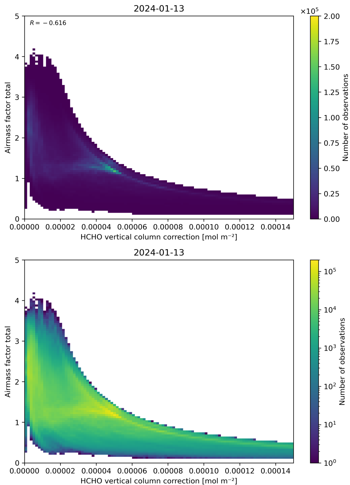
Figure 120: Scatter density plot of “HCHO vertical column correction” against “Airmass factor total” for 2024-01-12 to 2024-01-14.
