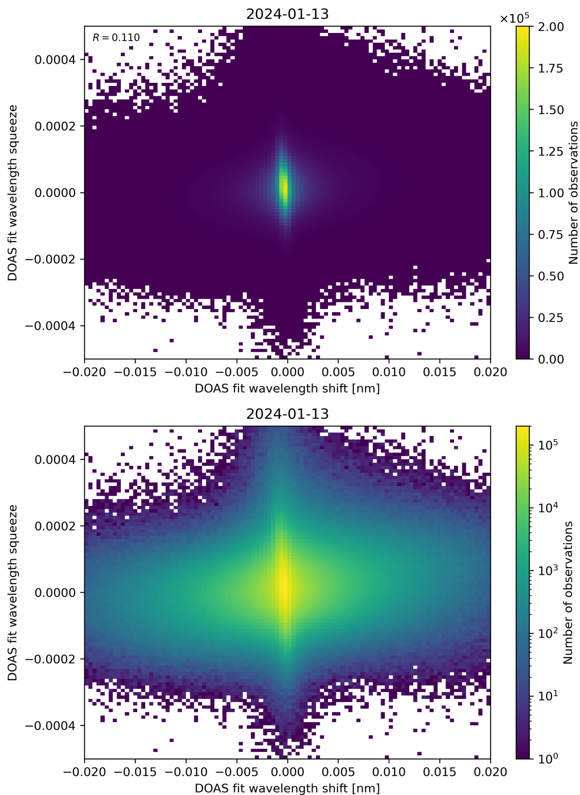
Figure 65: Scatter density plot of “DOAS fit wavelength shift” against “DOAS fit wavelength squeeze” for 2024-01-12 to 2024-01-14.
