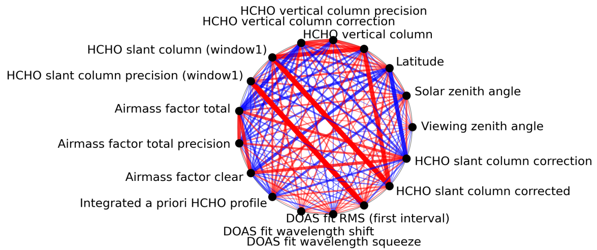
Figure 1: Map of correlation graph for 2024-01-12 to 2024-01-14.
