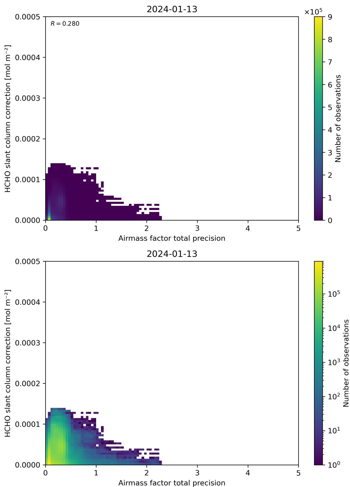
Figure 110: Scatter density plot of “Airmass factor total precision” against “HCHO slant column correction” for 2024-01-12 to 2024-01-14.
