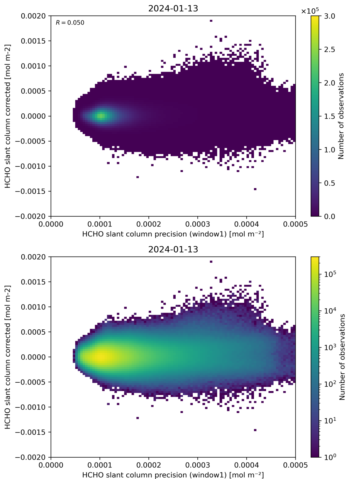
Figure 92: Scatter density plot of “HCHO slant column precision (window1)” against “HCHO slant column corrected” for 2024-01-12 to 2024-01-14.
