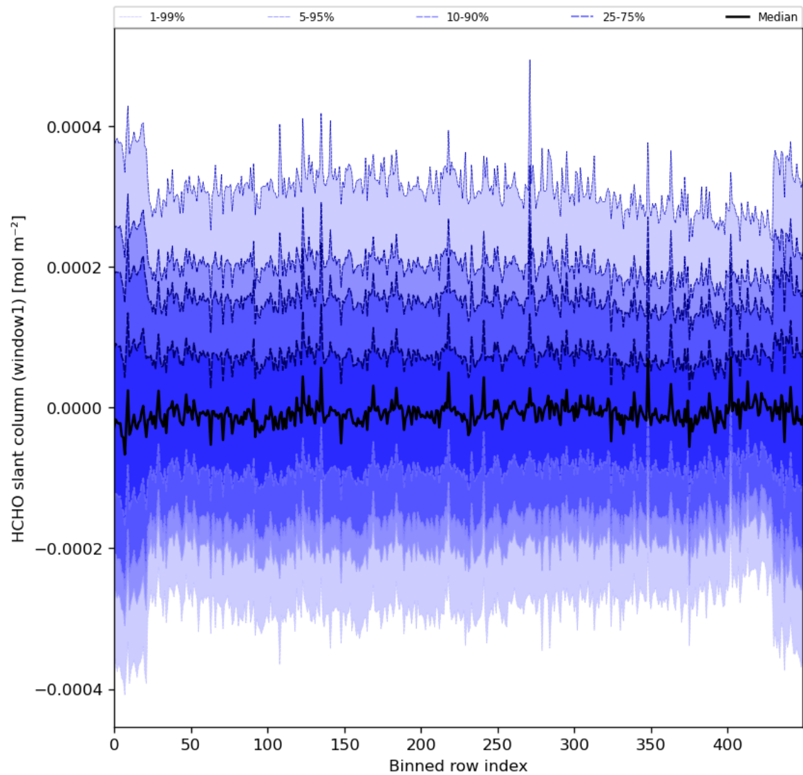
Figure 52: Along track statistics of “HCHO slant column (window1)” for 2024-01-12 to 2024-01-14
