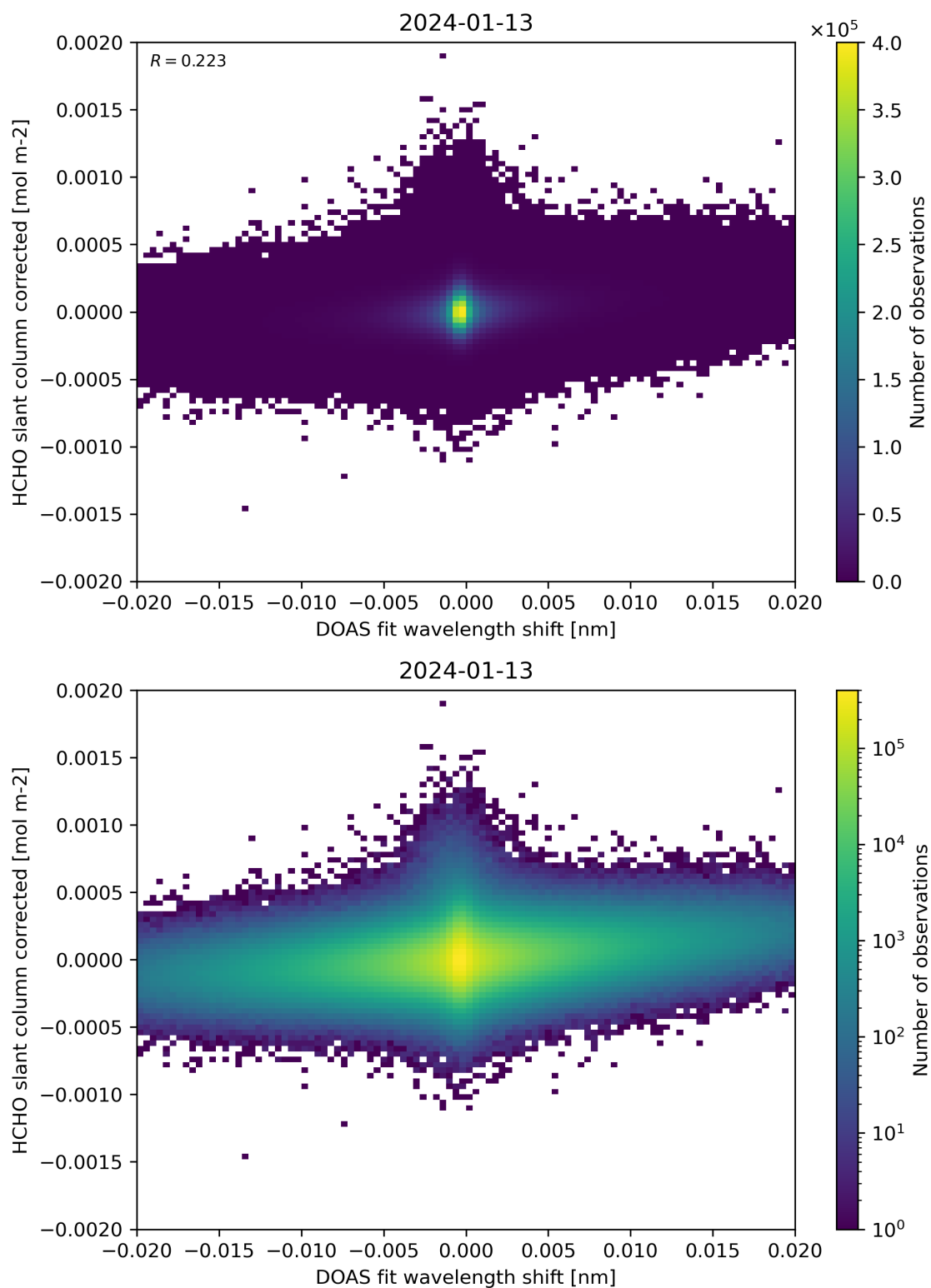
Figure 66: Scatter density plot of “DOAS fit wavelength shift” against “HCHO slant column corrected” for 2024-01-12 to 2024-01-14.
