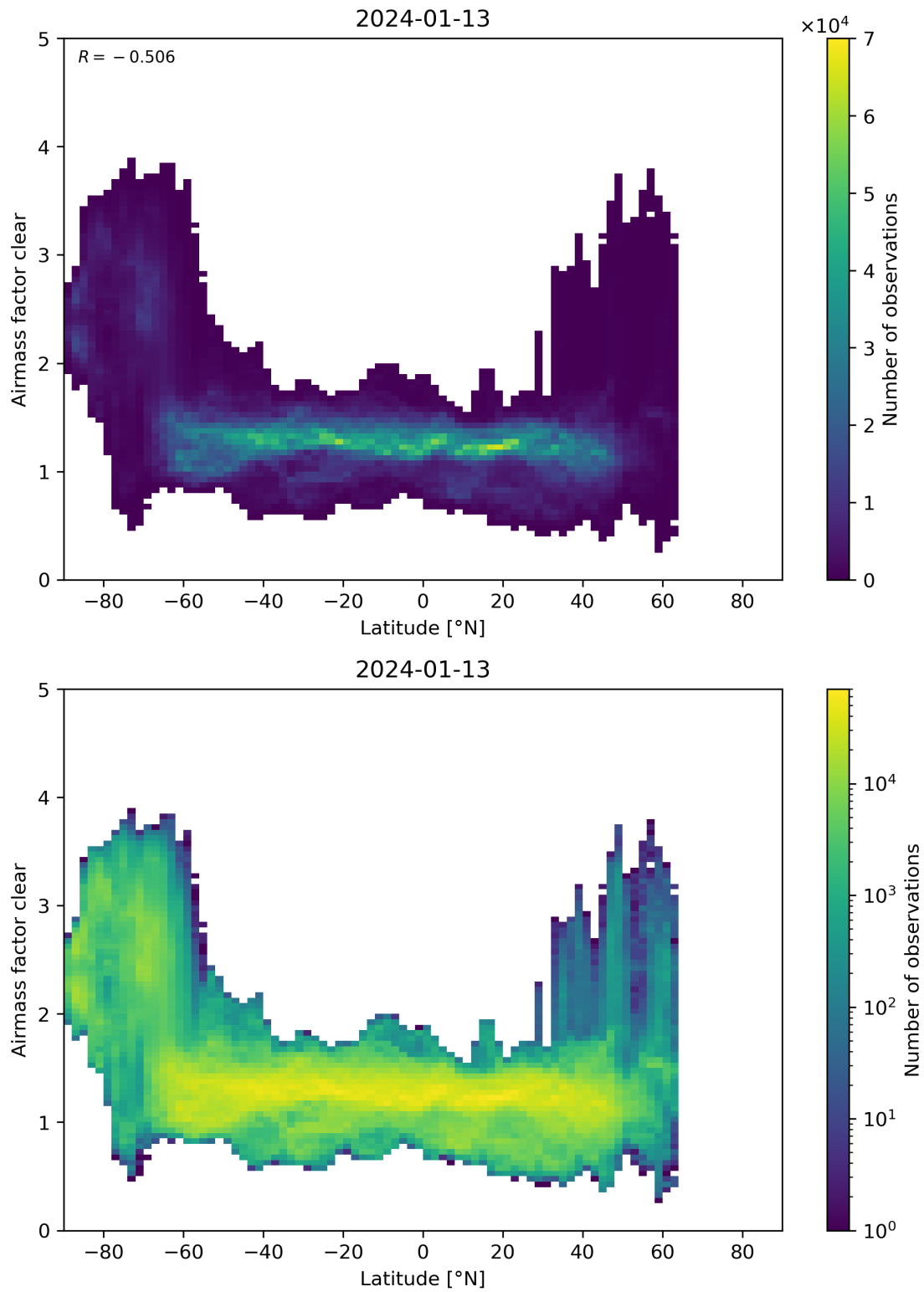
Figure 156: Scatter density plot of “Latitude” against “Airmass factor clear” for 2024-01-12 to 2024-01-14.
