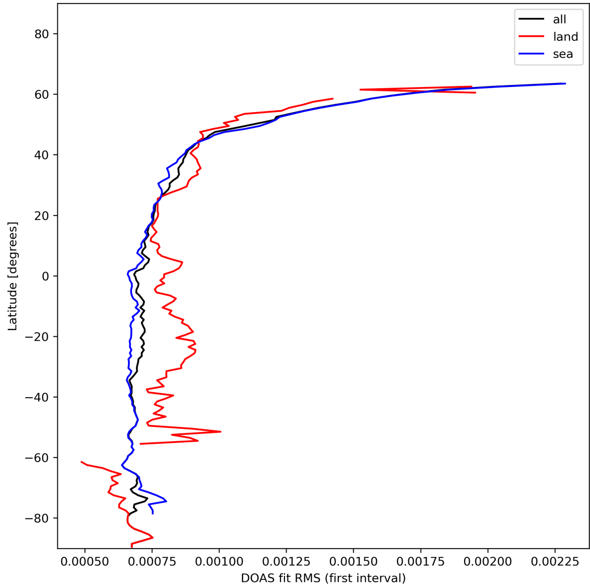
Figure 32: Zonal average of “DOAS fit RMS (first interval)” for 2024-01-12 to 2024-01-14.
