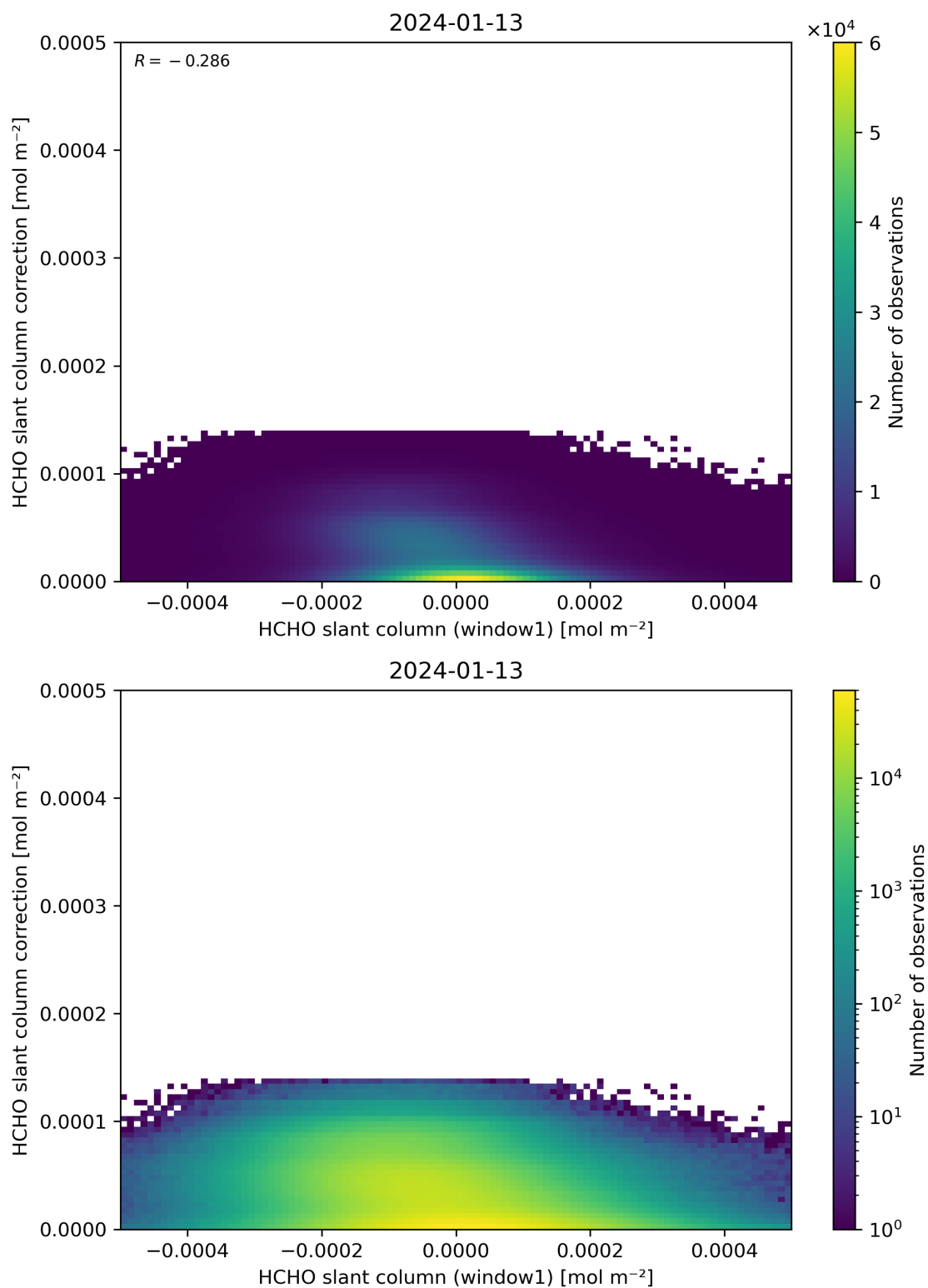
Figure 83: Scatter density plot of “HCHO slant column (window1)” against “HCHO slant column correction” for 2024-01-12 to 2024-01-14.
