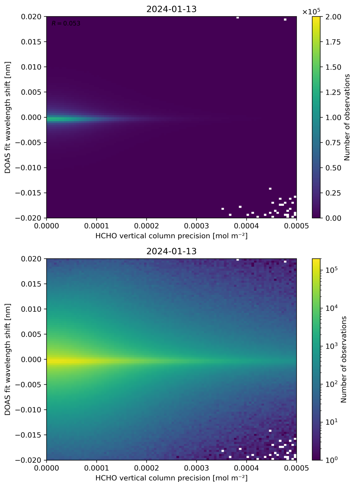
Figure 137: Scatter density plot of “HCHO vertical column precision” against “DOAS fit wavelength shift” for 2024-01-12 to 2024-01-14.
