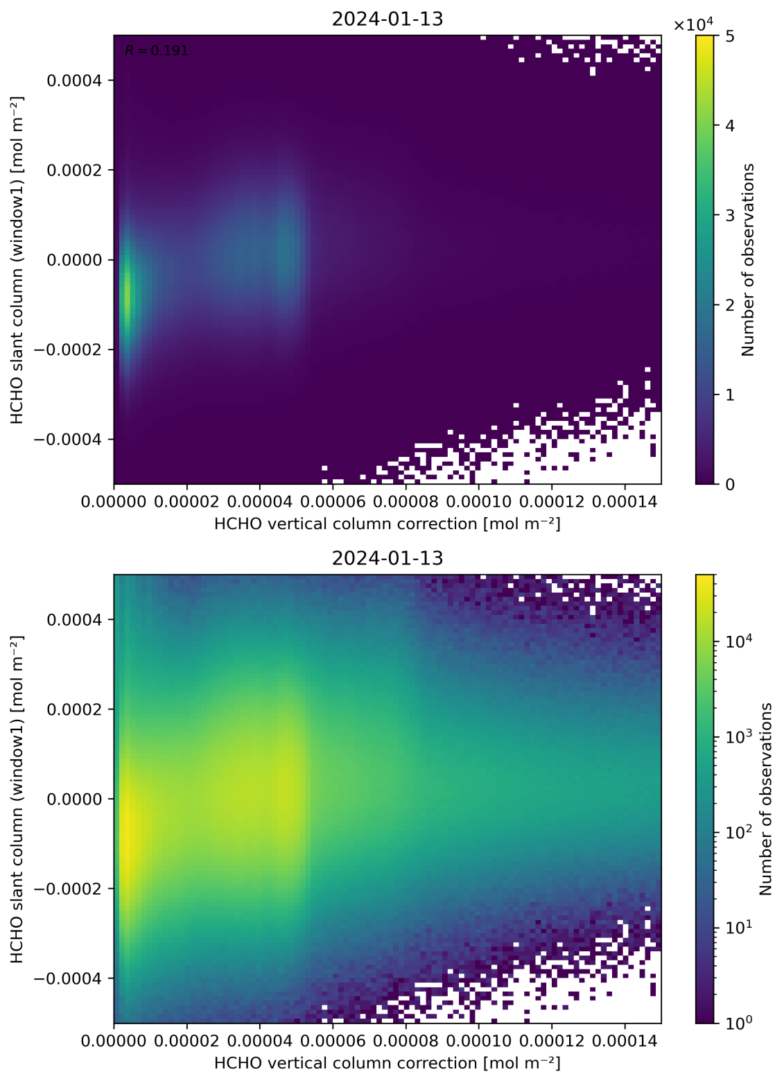
Figure 118: Scatter density plot of “HCHO vertical column correction” against “HCHO slant column (window1)” for 2024-01-12 to 2024-01-14.
