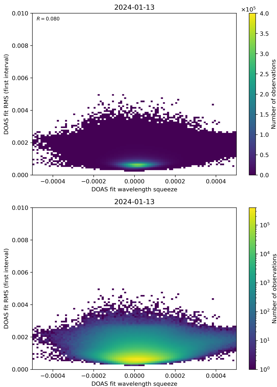
Figure 68: Scatter density plot of “DOAS fit wavelength squeeze” against “DOAS fit RMS (first interval)” for 2024-01-12 to 2024-01-14.
