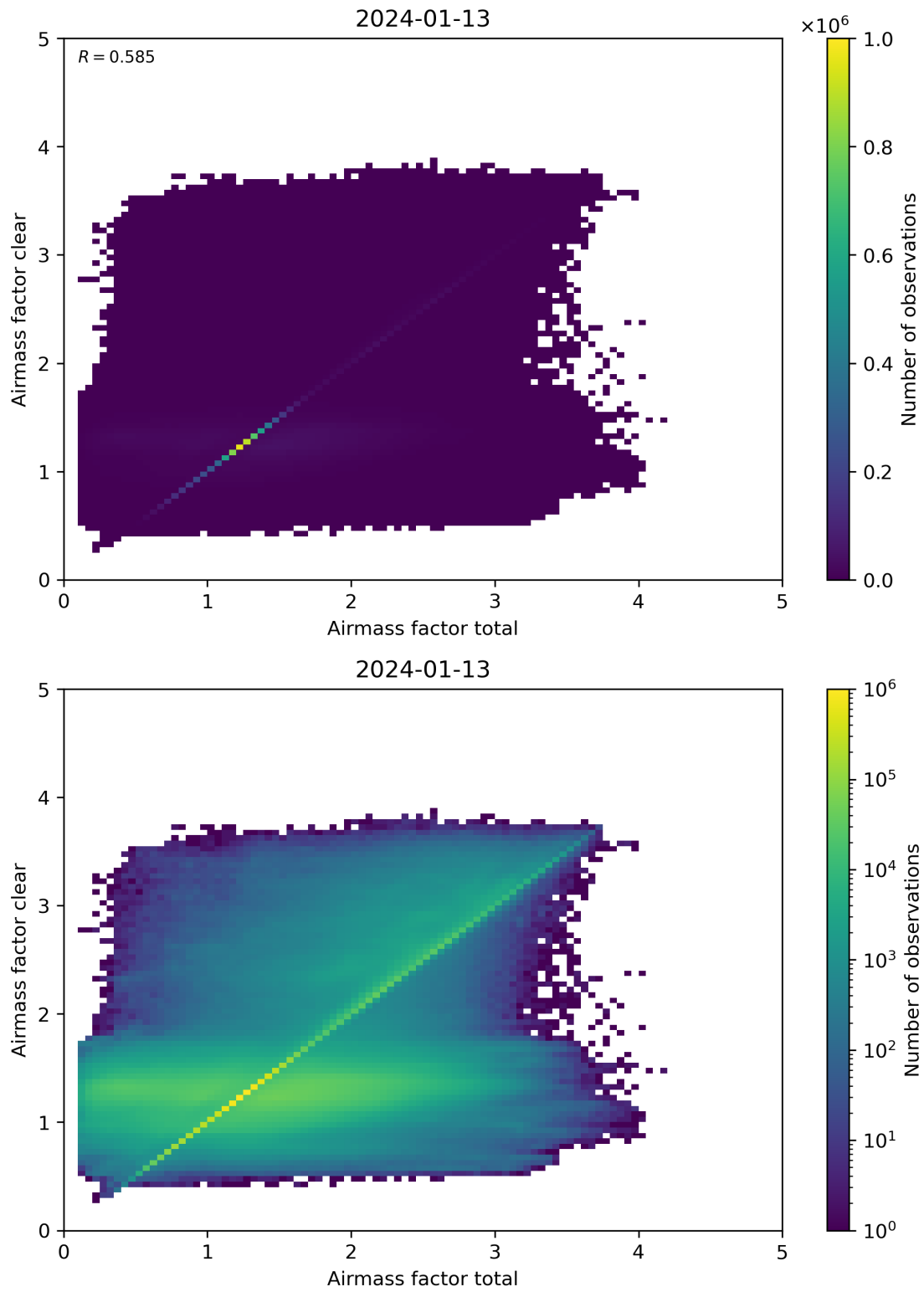
Figure 100: Scatter density plot of “Airmass factor total” against “Airmass factor clear” for 2024-01-12 to 2024-01-14.
