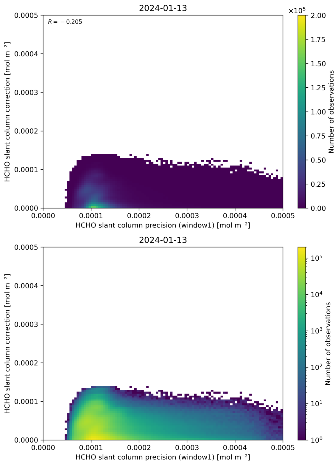
Figure 93: Scatter density plot of “HCHO slant column precision (window1)” against “HCHO slant column correction” for 2024-01-12 to 2024-01-14.
