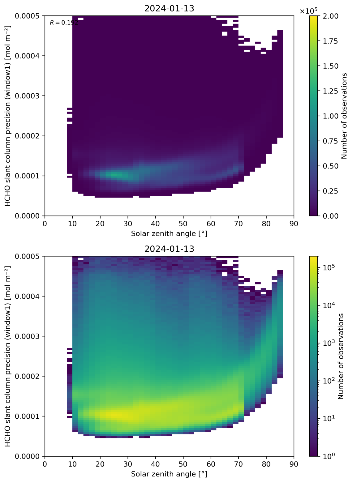
Figure 174: Scatter density plot of “Solar zenith angle” against “HCHO slant column precision (window1)” for 2024-01-12 to 2024-01-14.
