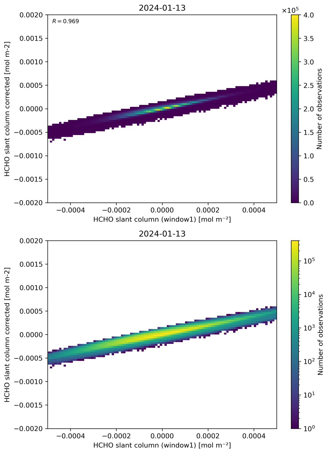
Figure 82: Scatter density plot of “HCHO slant column (window1)” against “HCHO slant column corrected” for 2024-01-12 to 2024-01-14.
