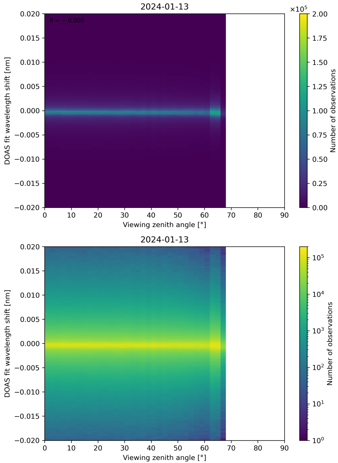
Figure 183: Scatter density plot of “Viewing zenith angle” against “DOAS fit wavelength shift” for 2024-01-12 to 2024-01-14.
