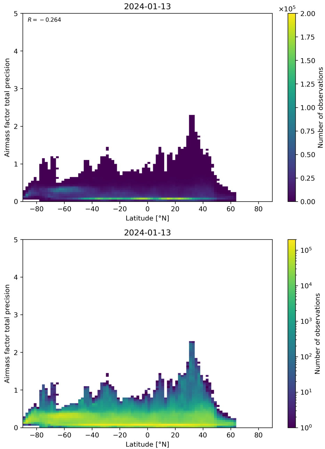
Figure 162: Scatter density plot of “Latitude” against “Airmass factor total precision” for 2024-01-12 to 2024-01-14.
