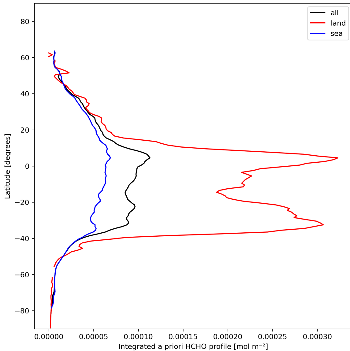
Figure 29: Zonal average of “Integrated a priori HCHO profile” for 2024-01-12 to 2024-01-14.
