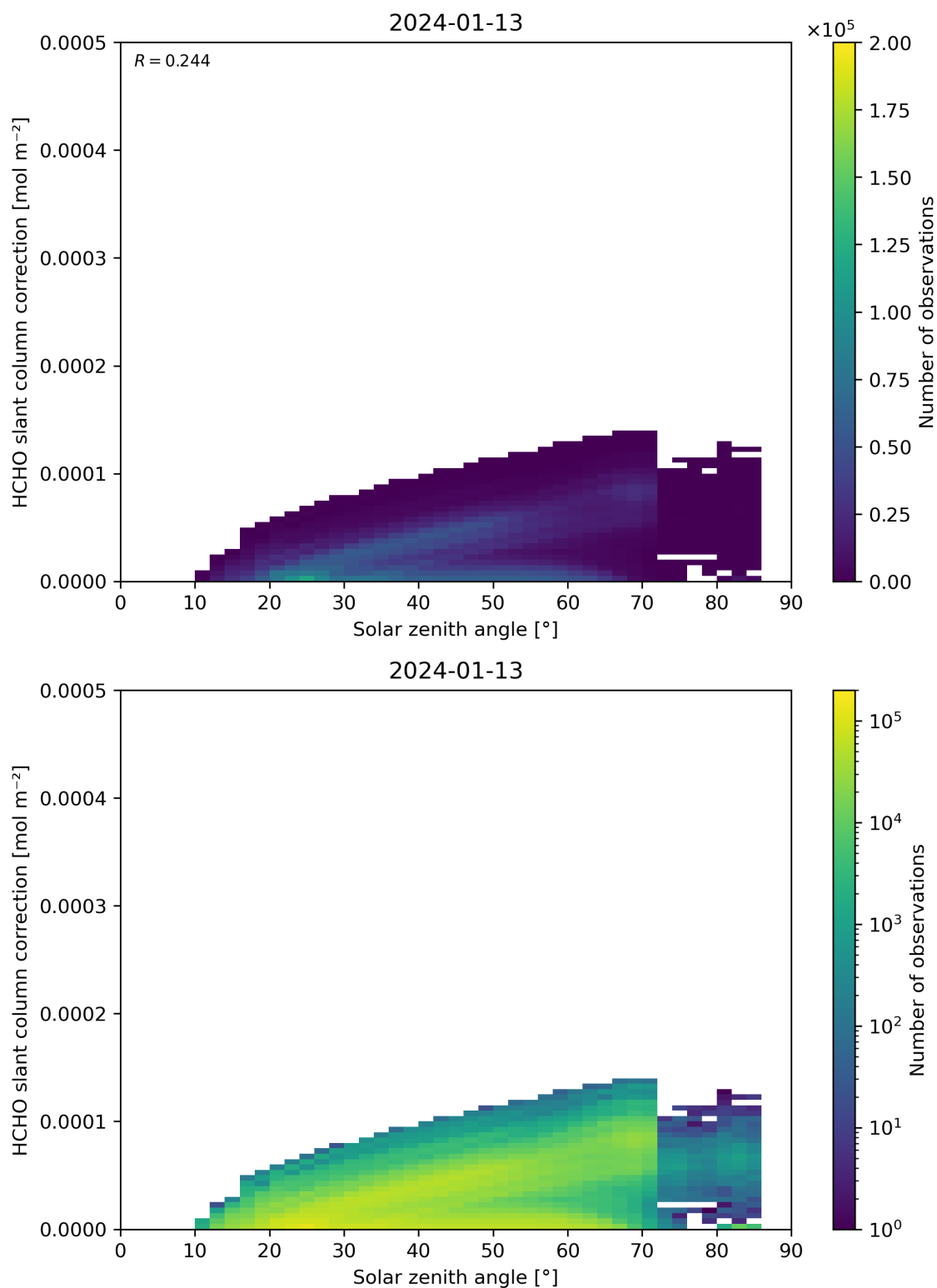
Figure 172: Scatter density plot of “Solar zenith angle” against “HCHO slant column correction” for 2024-01-12 to 2024-01-14.
