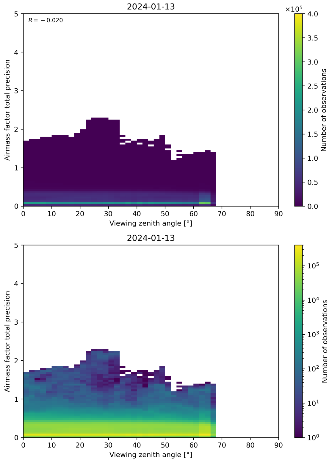
Figure 191: Scatter density plot of “Viewing zenith angle” against “Airmass factor total precision” for 2024-01-12 to 2024-01-14.
