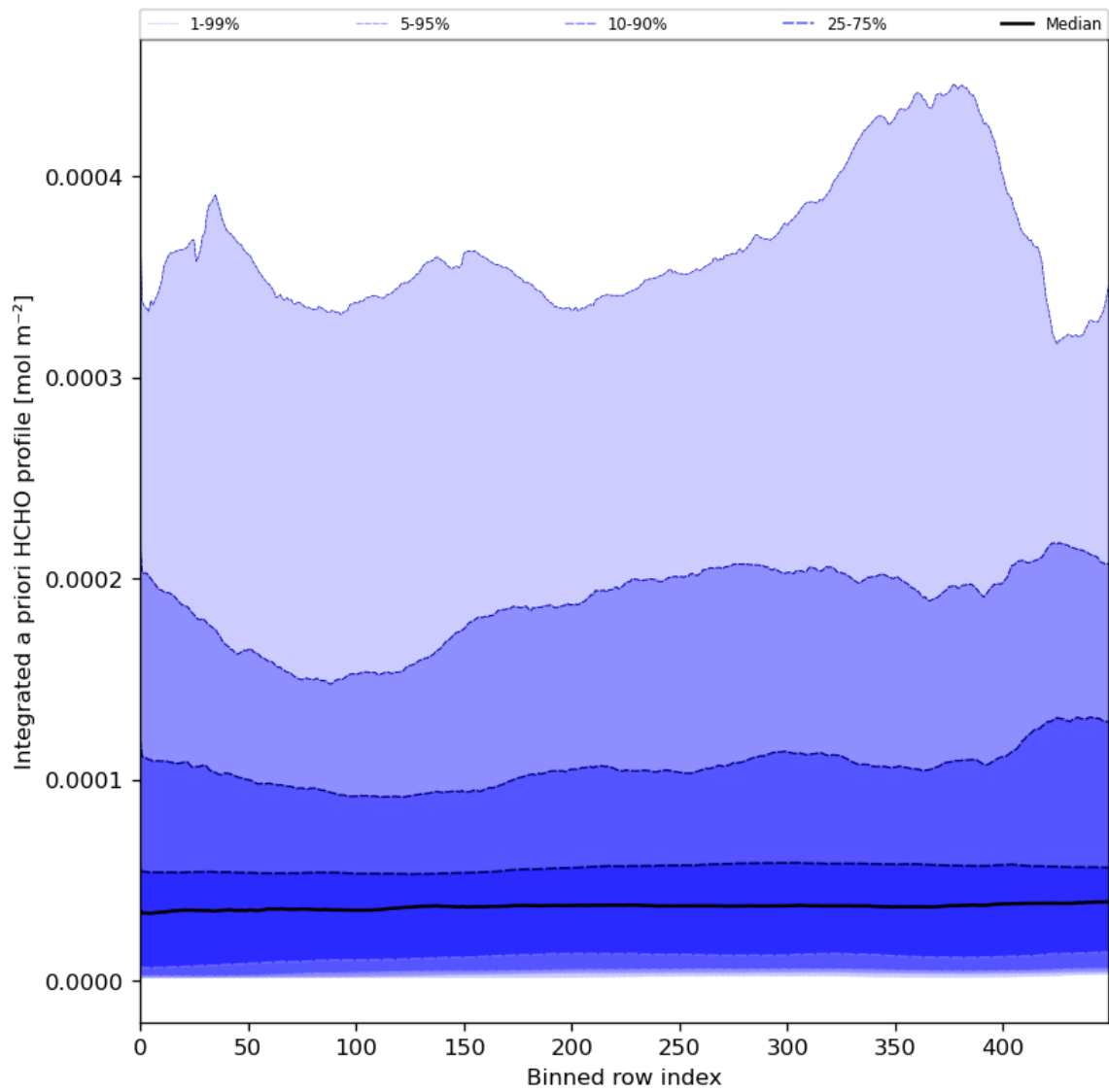
Figure 57: Along track statistics of “Integrated a priori HCHO profile” for 2024-01-12 to 2024-01-14
