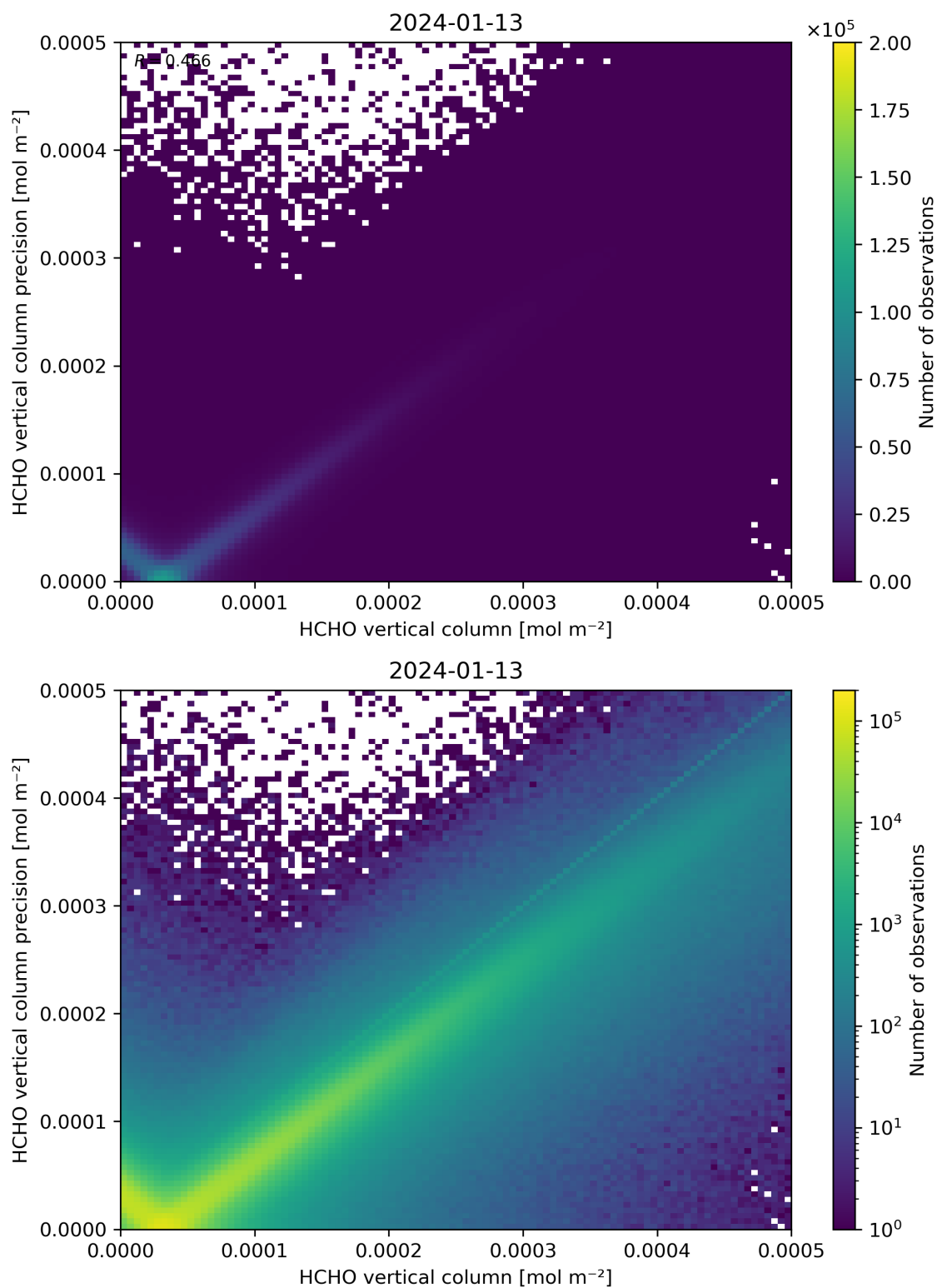
Figure 134: Scatter density plot of “HCHO vertical column” against “HCHO vertical column precision” for 2024-01-12 to 2024-01-14.
