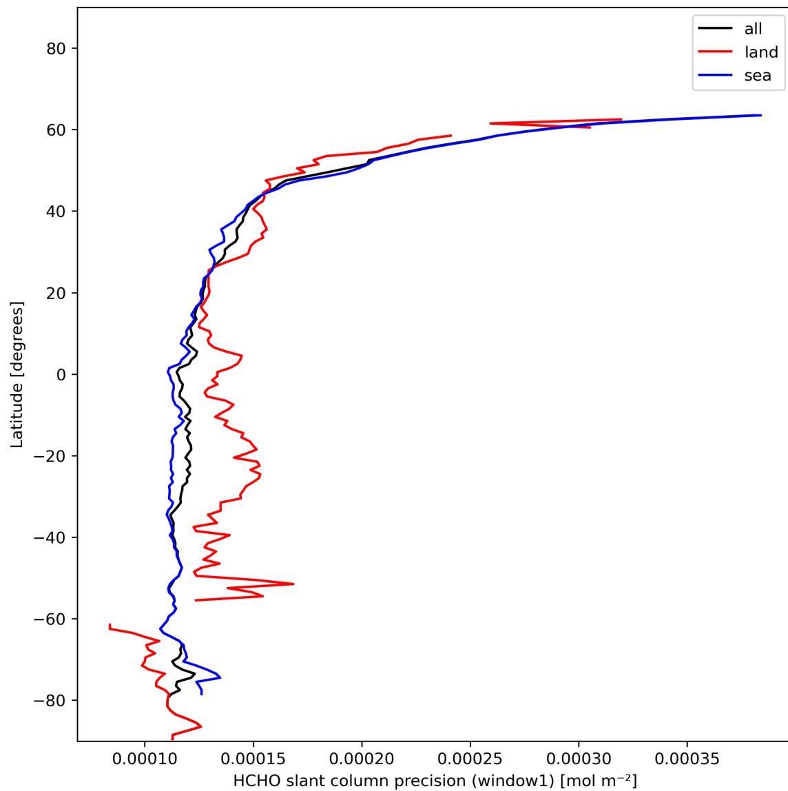
Figure 25: Zonal average of “HCHO slant column precision (window1)” for 2024-01-12 to 2024-01-14.
