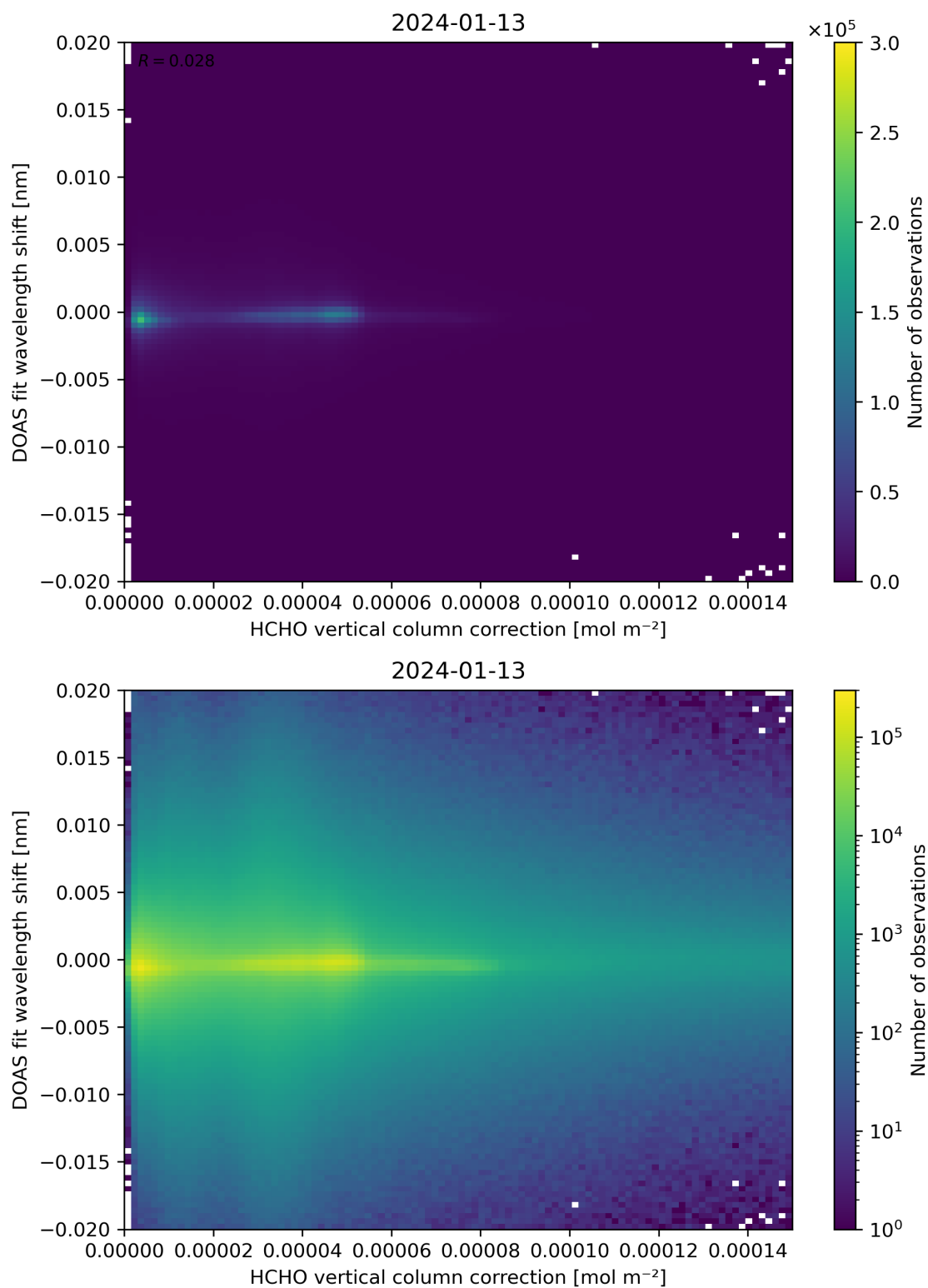
Figure 113: Scatter density plot of “HCHO vertical column correction” against “DOAS fit wavelength shift” for 2024-01-12 to 2024-01-14.
