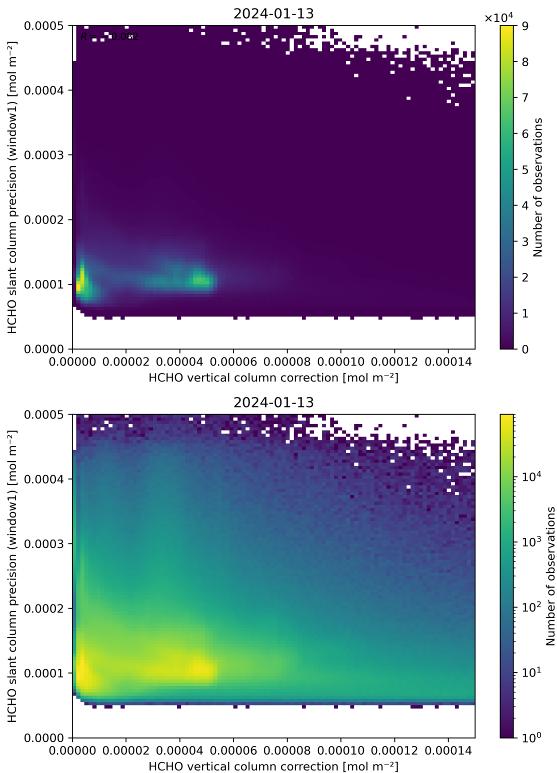
Figure 119: Scatter density plot of “HCHO vertical column correction” against “HCHO slant column precision (window1)” for 2024-01-12 to 2024-01-14.
