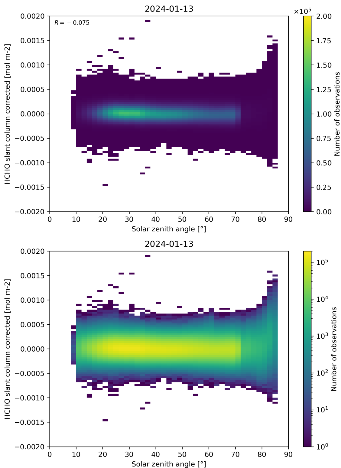
Figure 171: Scatter density plot of “Solar zenith angle” against “HCHO slant column corrected” for 2024-01-12 to 2024-01-14.
