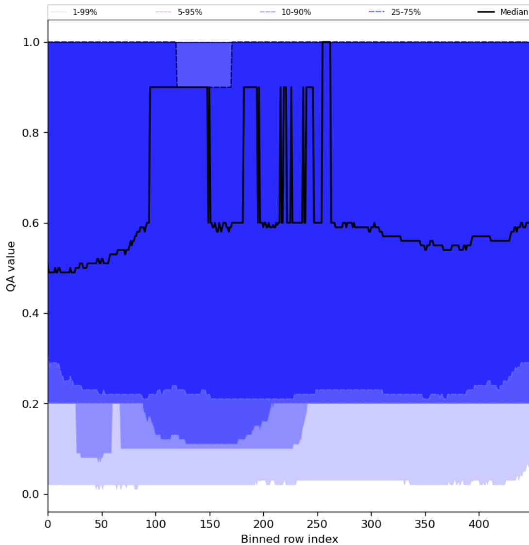
Figure 48: Along track statistics of “QA value” for 2024-01-12 to 2024-01-14
