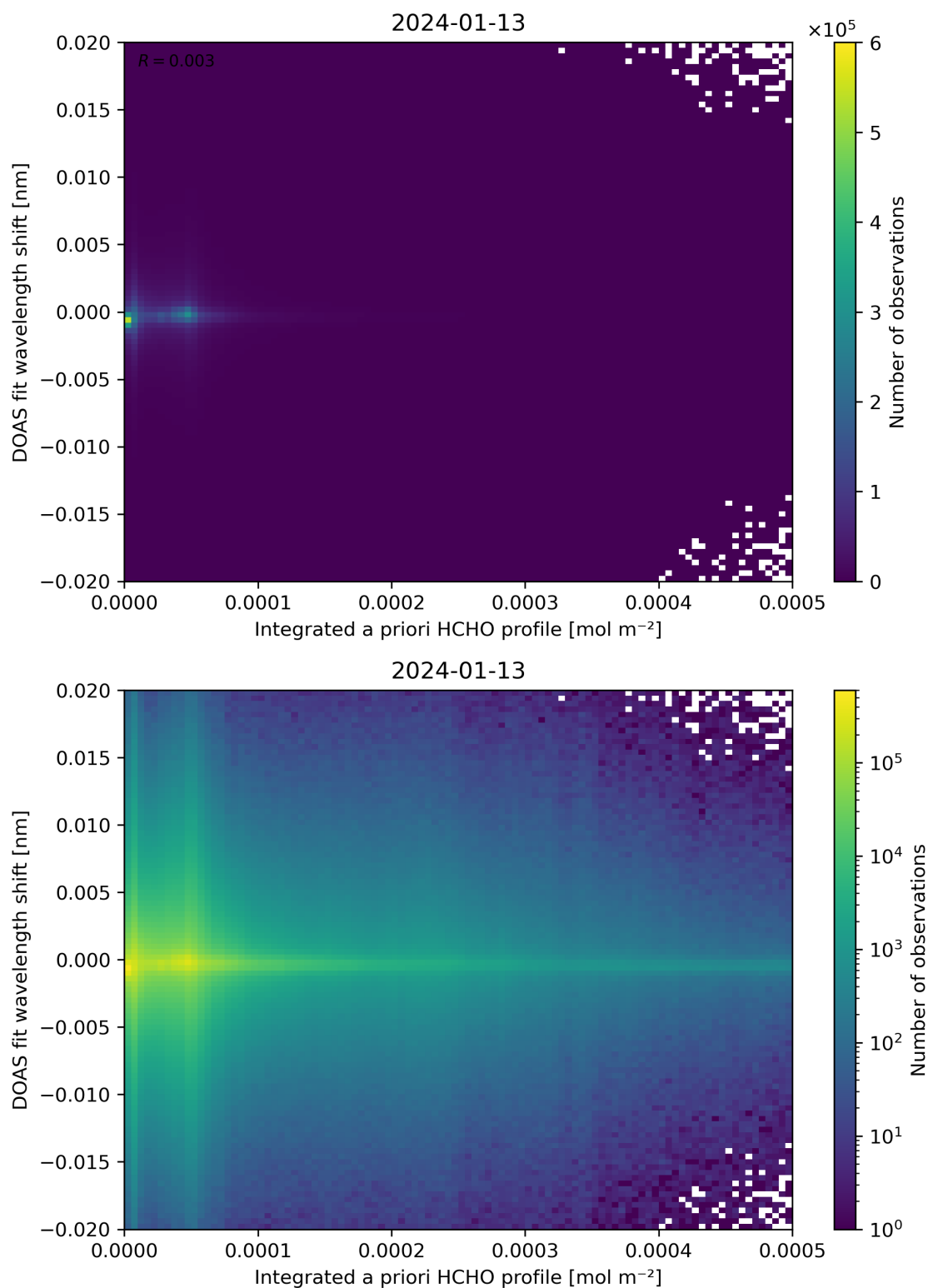
Figure 149: Scatter density plot of “Integrated a priori HCHO profile” against “DOAS fit wavelength shift” for 2024-01-12 to 2024-01-14.
