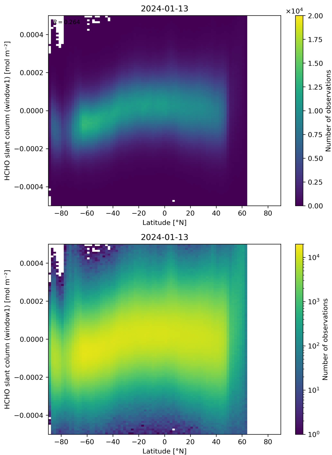
Figure 159: Scatter density plot of “Latitude” against “HCHO slant column (window1)” for 2024-01-12 to 2024-01-14.
