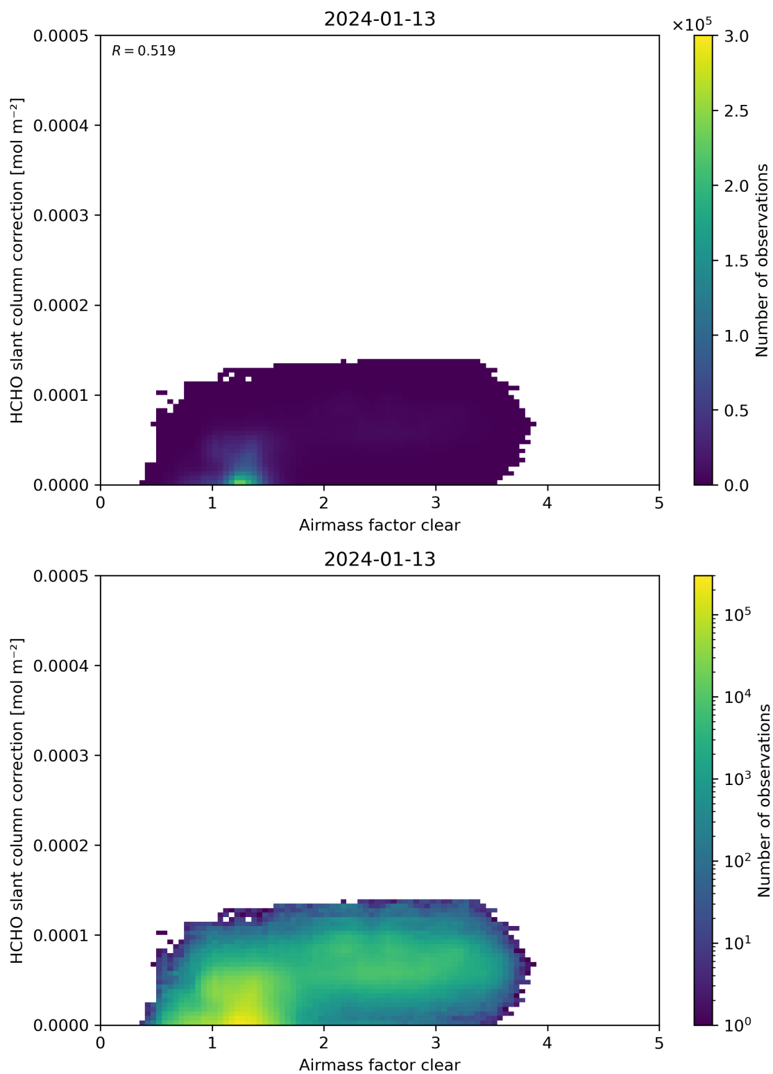
Figure 75: Scatter density plot of “Airmass factor clear” against “HCHO slant column correction” for 2024-01-12 to 2024-01-14.
