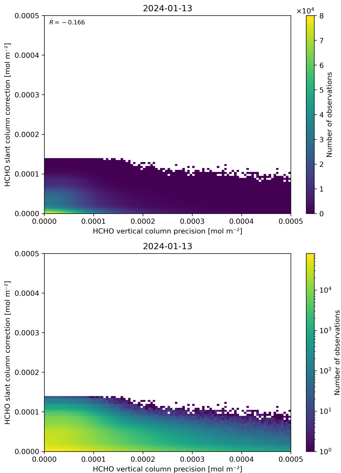
Figure 141: Scatter density plot of “HCHO vertical column precision” against “HCHO slant column correction” for 2024-01-12 to 2024-01-14.
