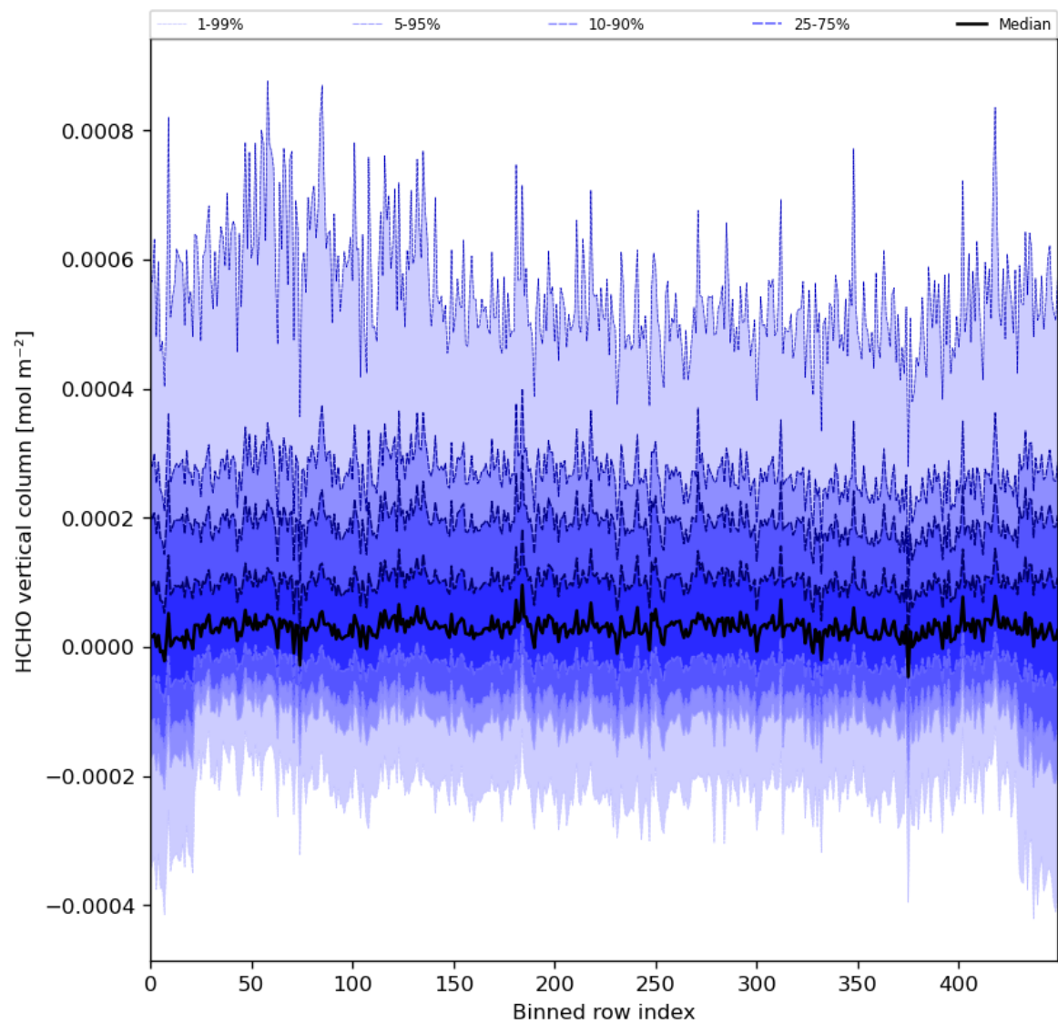
Figure 49: Along track statistics of “HCHO vertical column” for 2024-01-12 to 2024-01-14
