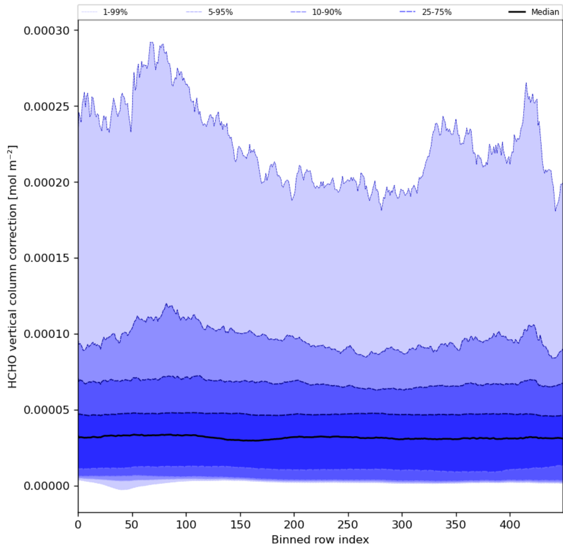
Figure 51: Along track statistics of “HCHO vertical column correction” for 2024-01-12 to 2024-01-14
