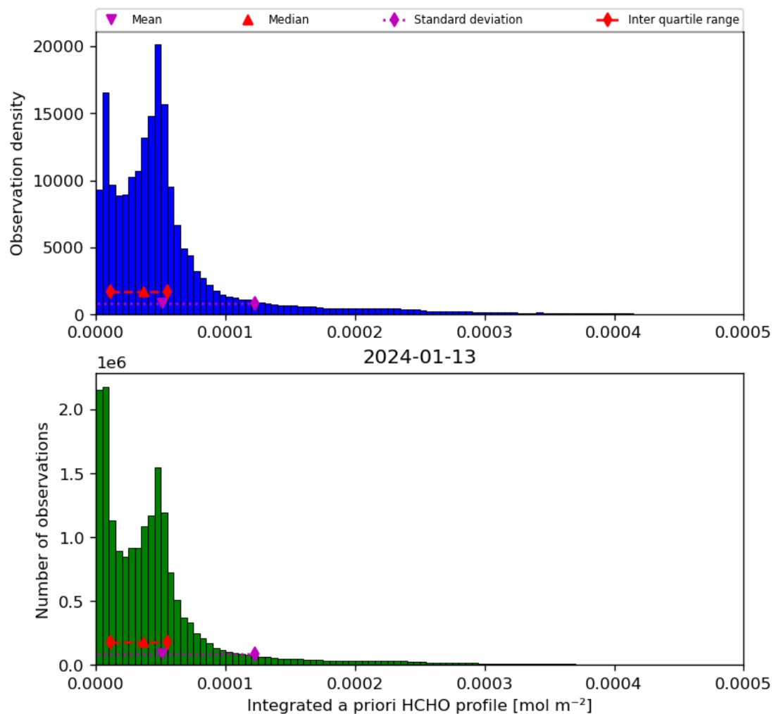
Figure 43: Histogram of “Integrated a priori HCHO profile” for 2024-01-12 to 2024-01-14
