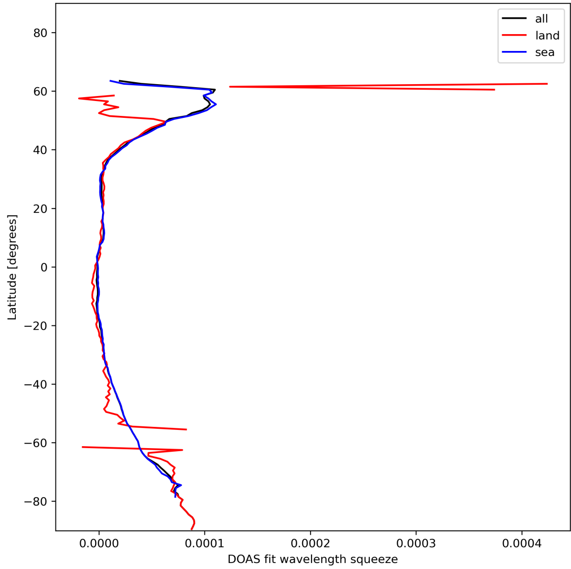
Figure 31: Zonal average of “DOAS fit wavelength squeeze” for 2024-01-12 to 2024-01-14.
