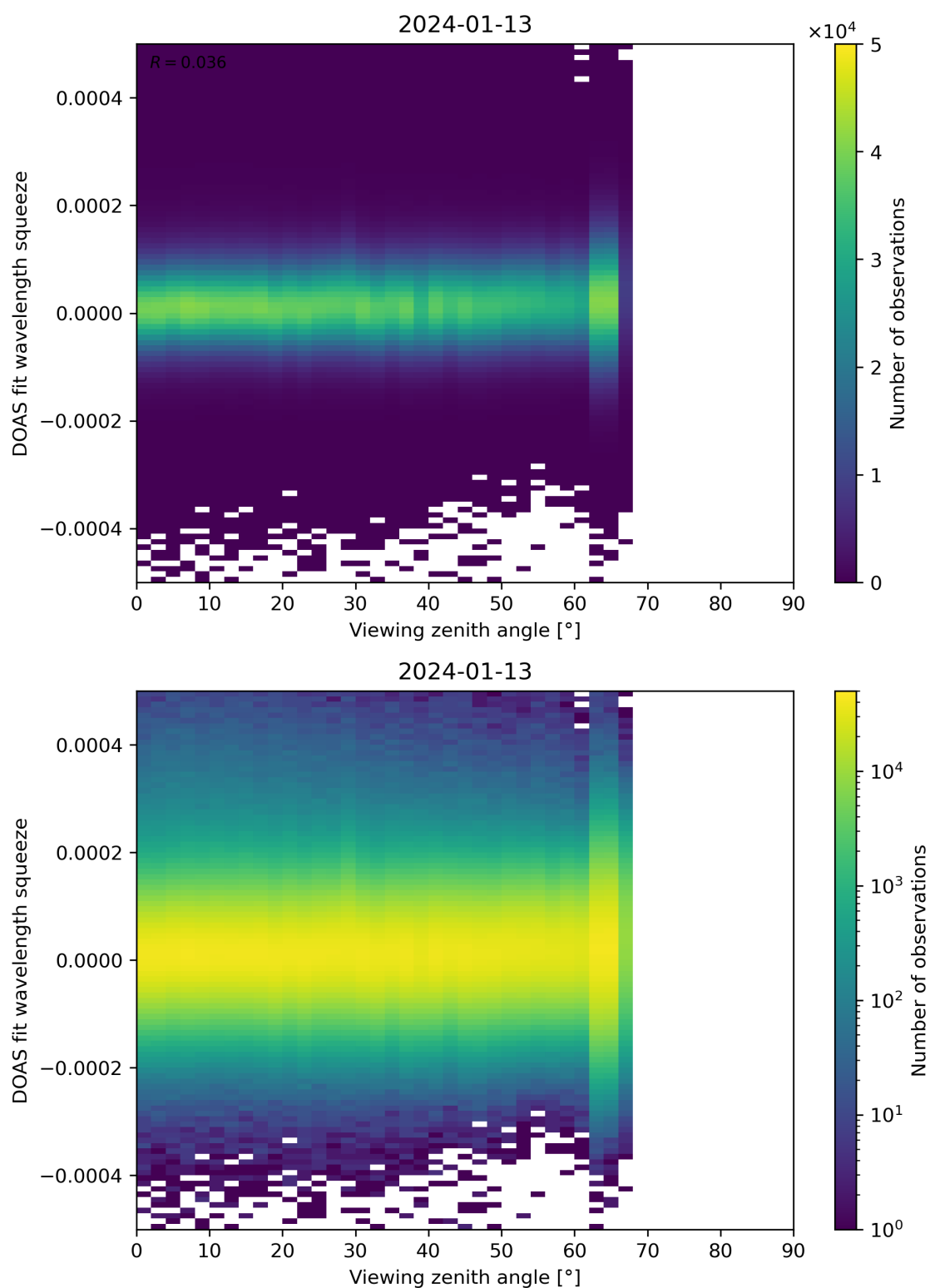
Figure 184: Scatter density plot of “Viewing zenith angle” against “DOAS fit wavelength squeeze” for 2024-01-12 to 2024-01-14.
