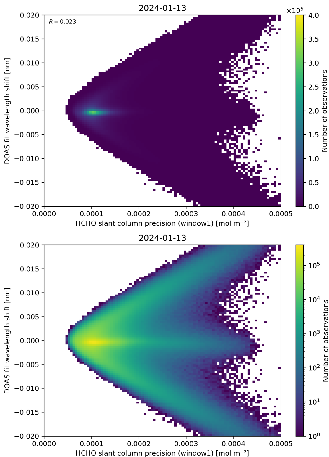
Figure 89: Scatter density plot of “HCHO slant column precision (window1)” against “DOAS fit wavelength shift” for 2024-01-12 to 2024-01-14.
