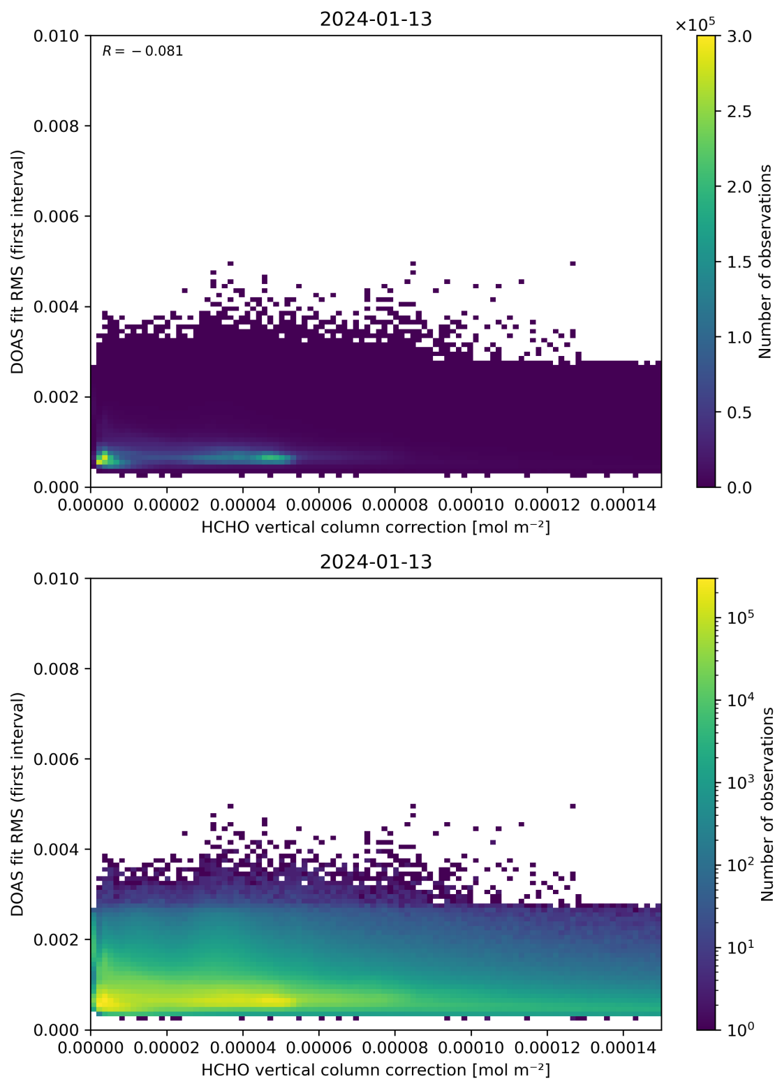
Figure 112: Scatter density plot of “HCHO vertical column correction” against “DOAS fit RMS (first interval)” for 2024-01-12 to 2024-01-14.
