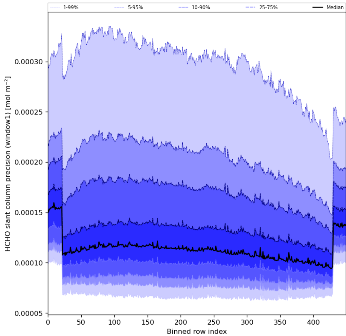
Figure 53: Along track statistics of “HCHO slant column precision (window1)” for 2024-01-12 to 2024-01-14
