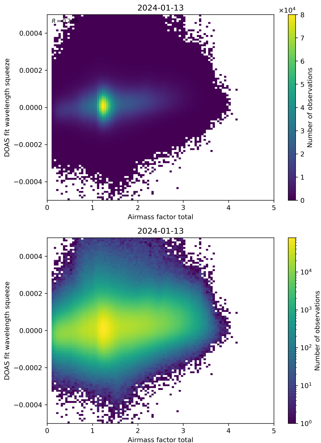
Figure 99: Scatter density plot of “Airmass factor total” against “DOAS fit wavelength squeeze” for 2024-01-12 to 2024-01-14.
