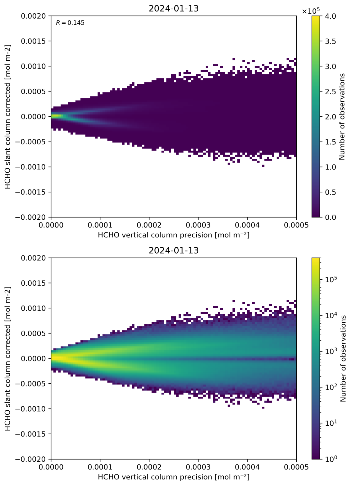
Figure 140: Scatter density plot of “HCHO vertical column precision” against “HCHO slant column corrected” for 2024-01-12 to 2024-01-14.
