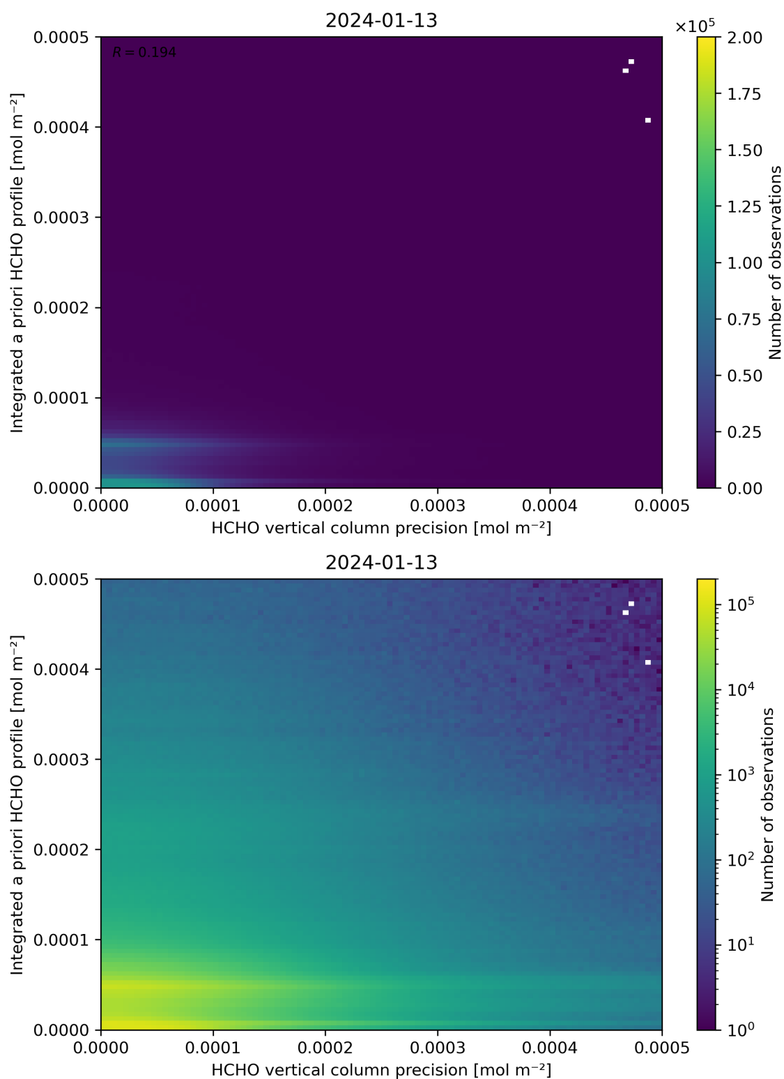
Figure 147: Scatter density plot of “HCHO vertical column precision” against “Integrated a priori HCHO profile” for 2024-01-12 to 2024-01-14.
