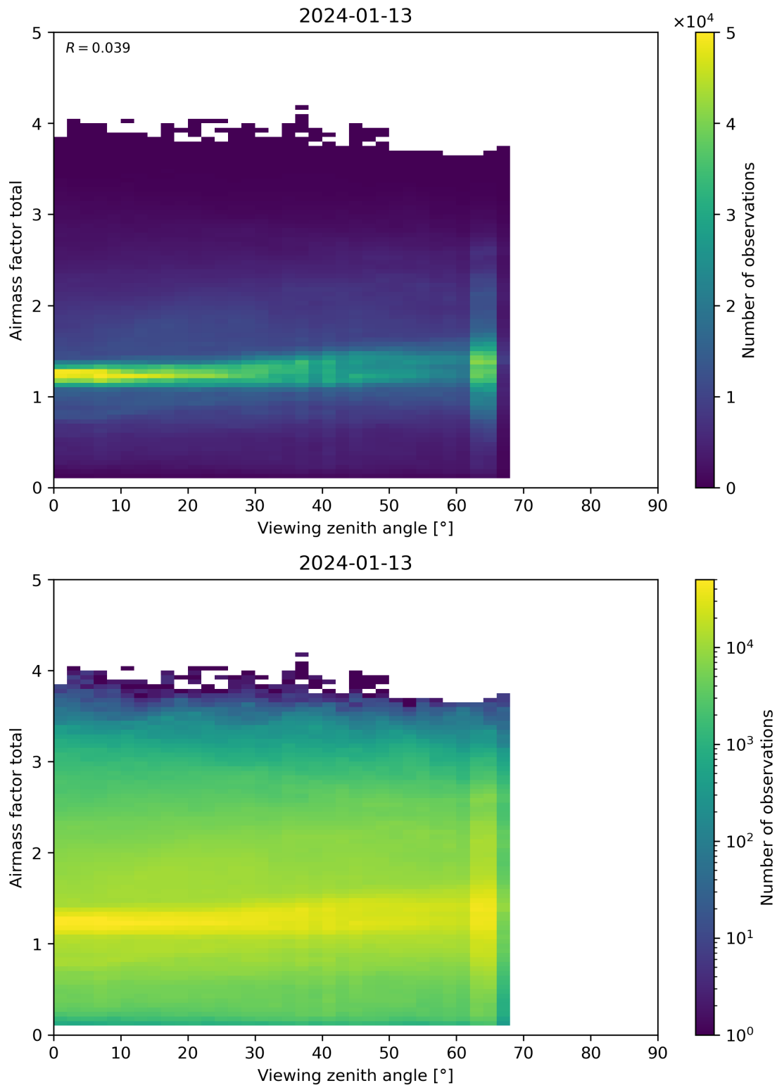
Figure 190: Scatter density plot of “Viewing zenith angle” against “Airmass factor total” for 2024-01-12 to 2024-01-14.
