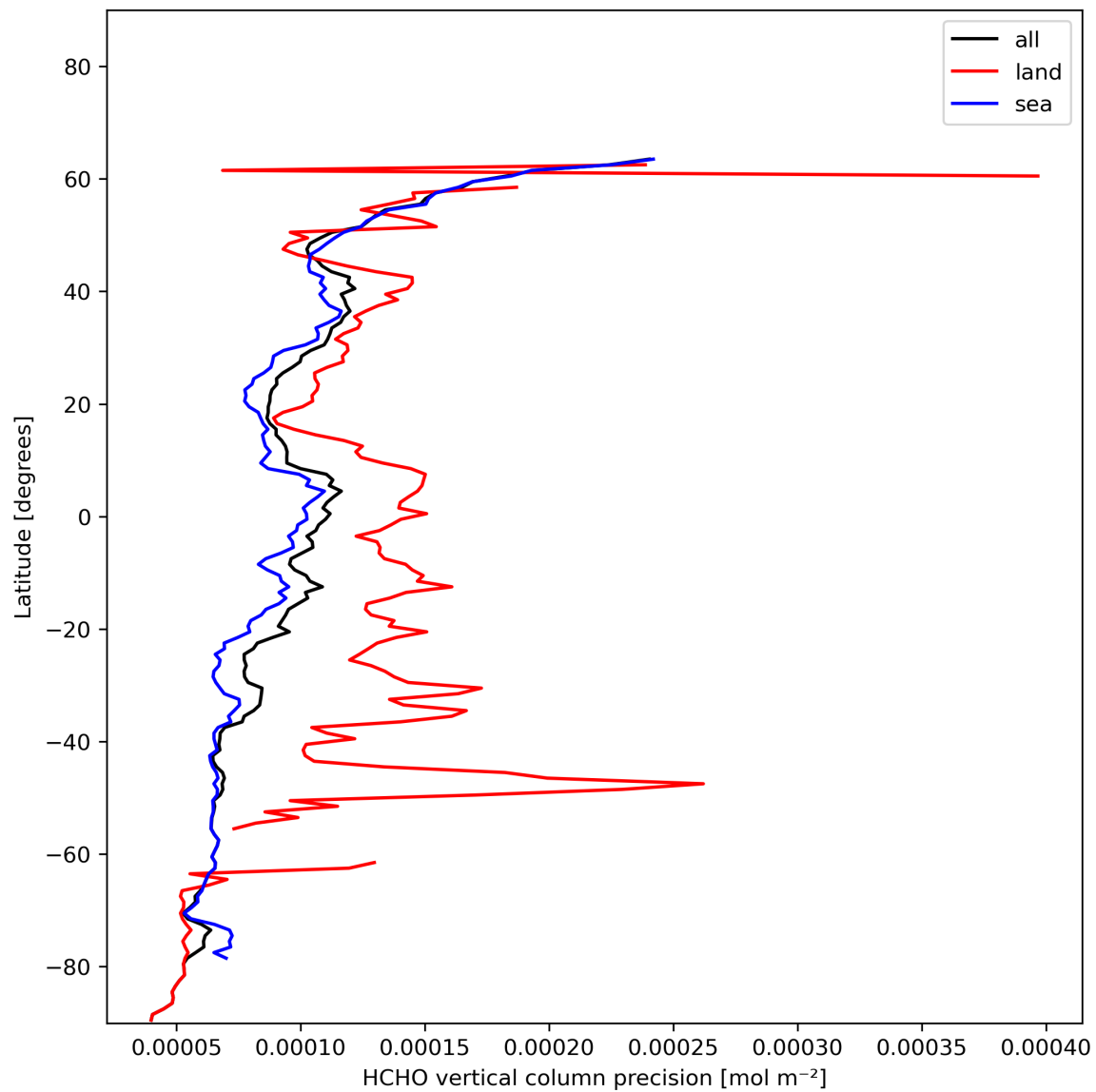
Figure 22: Zonal average of “HCHO vertical column precision” for 2024-01-12 to 2024-01-14.
