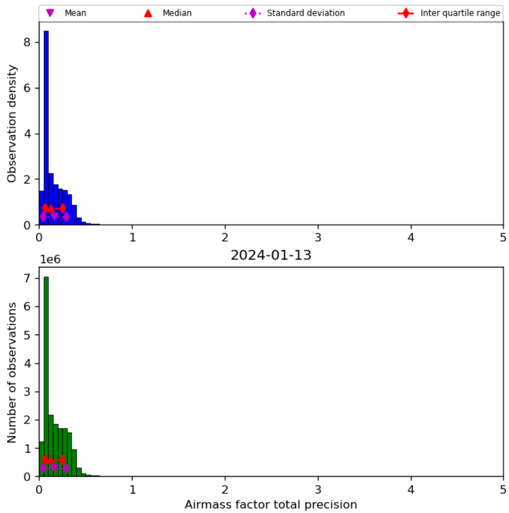
Figure 41: Histogram of “Airmass factor total precision” for 2024-01-12 to 2024-01-14
