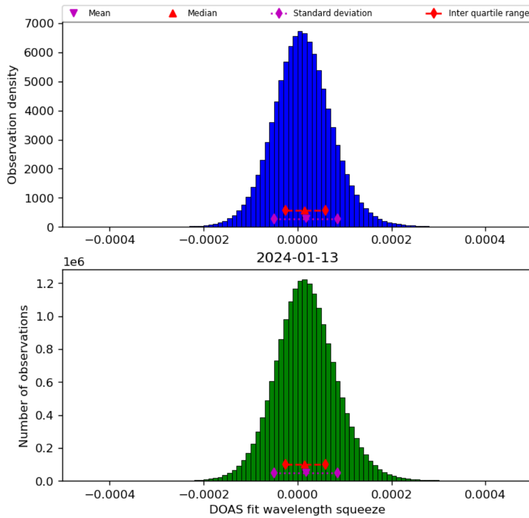
Figure 45: Histogram of “DOAS fit wavelength squeeze” for 2024-01-12 to 2024-01-14
