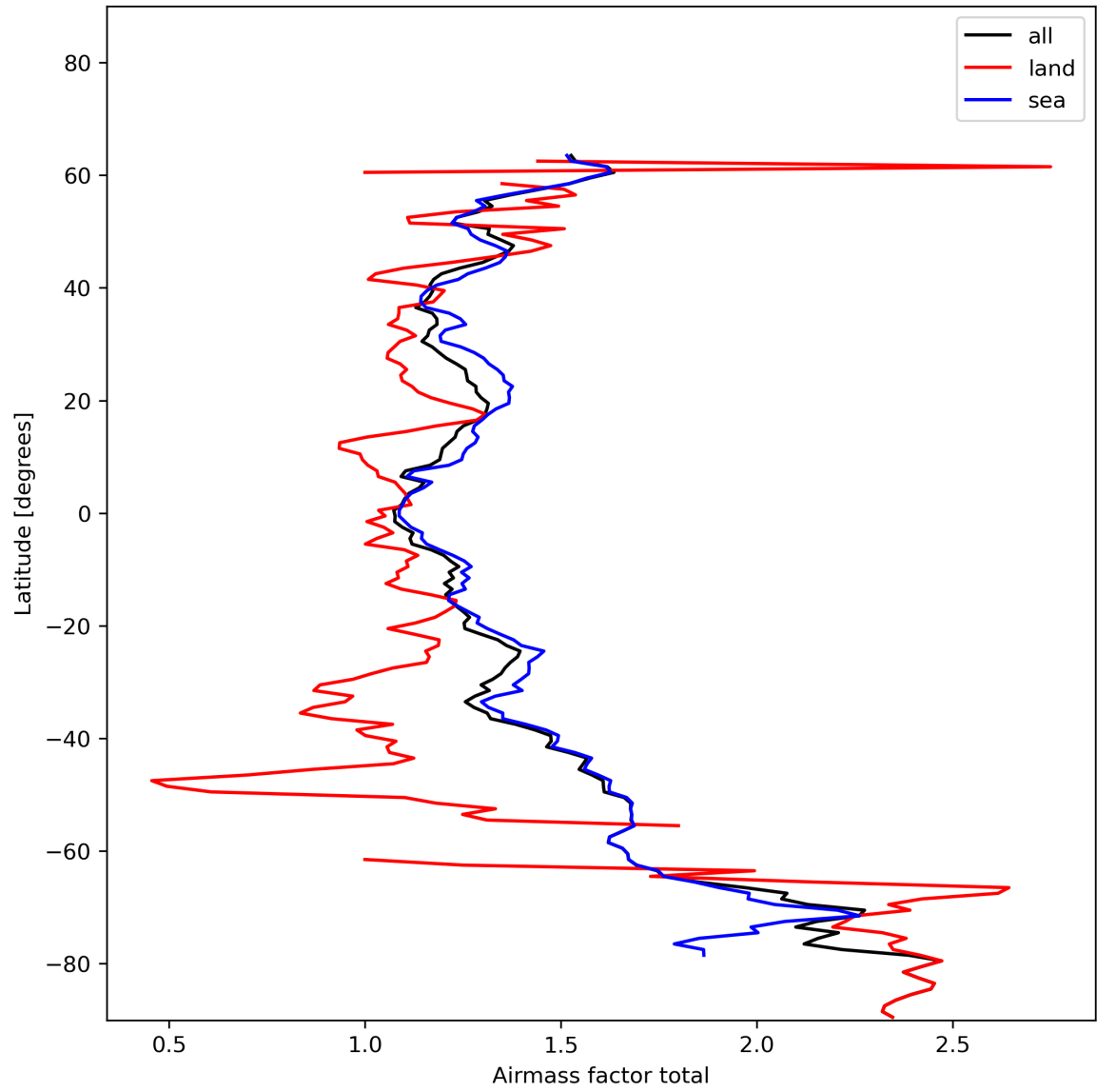
Figure 26: Zonal average of “Airmass factor total” for 2024-01-12 to 2024-01-14.
