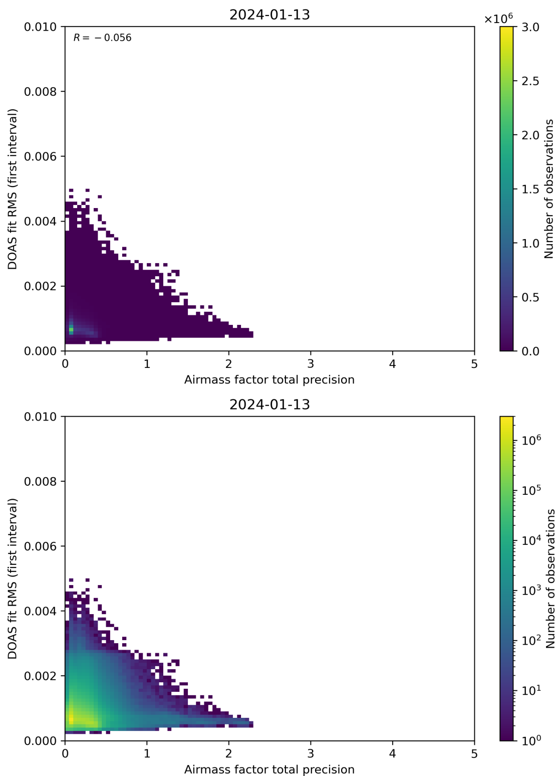
Figure 105: Scatter density plot of “Airmass factor total precision” against “DOAS fit RMS (first interval)” for 2024-01-12 to 2024-01-14.
