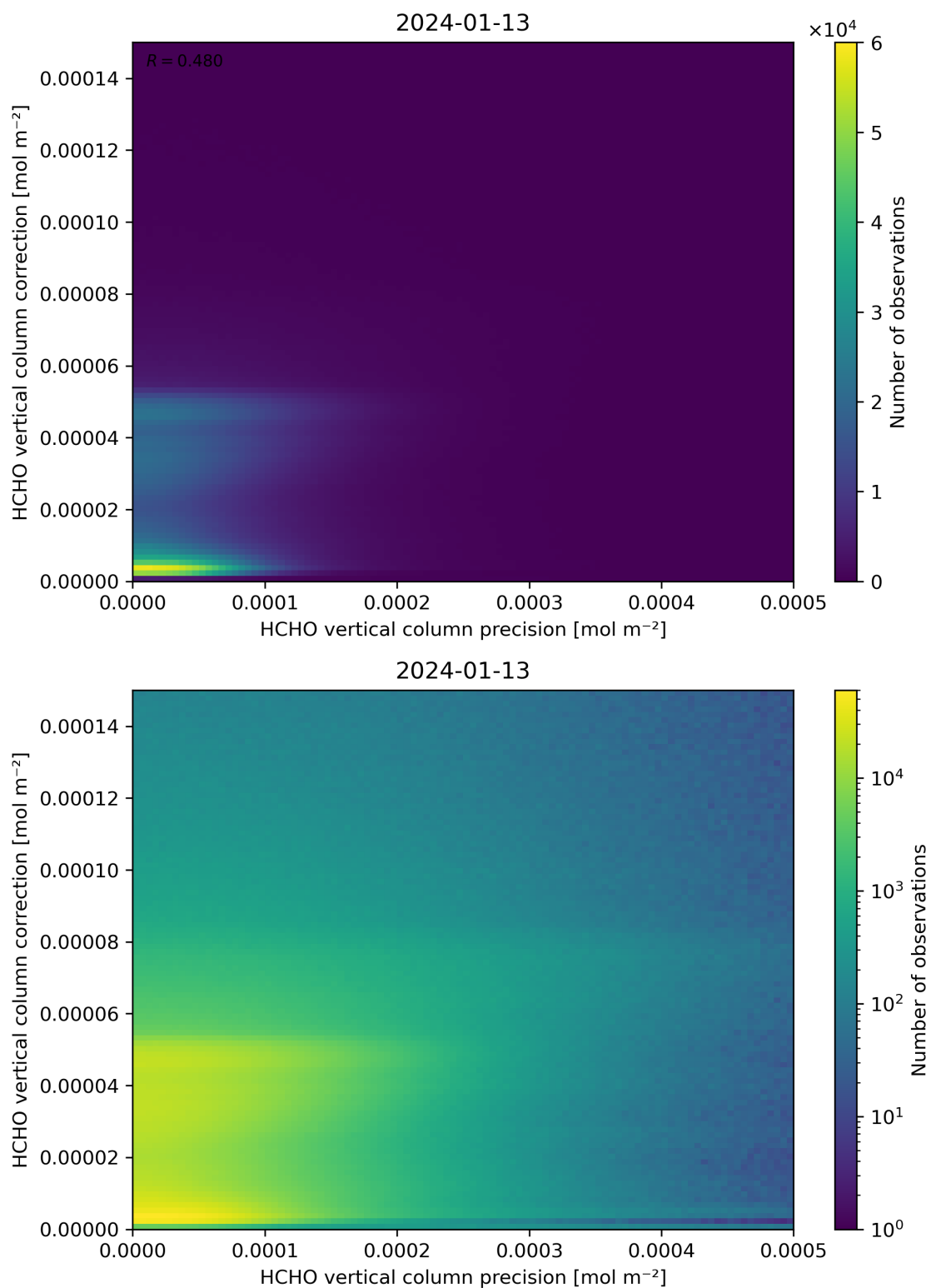
Figure 146: Scatter density plot of “HCHO vertical column precision” against “HCHO vertical column correction” for 2024-01-12 to 2024-01-14.
