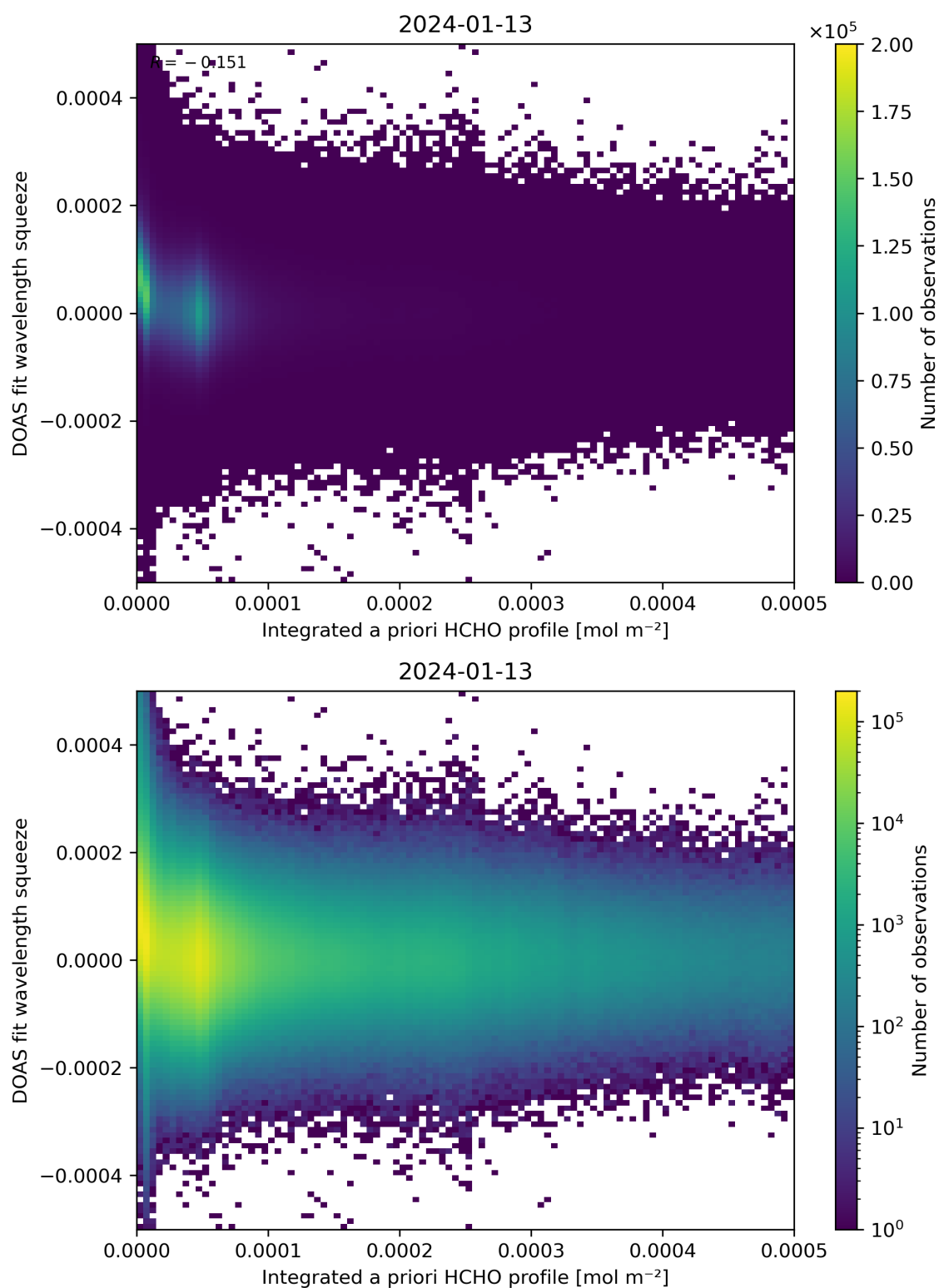
Figure 150: Scatter density plot of “Integrated a priori HCHO profile” against “DOAS fit wavelength squeeze” for 2024-01-12 to 2024-01-14.
