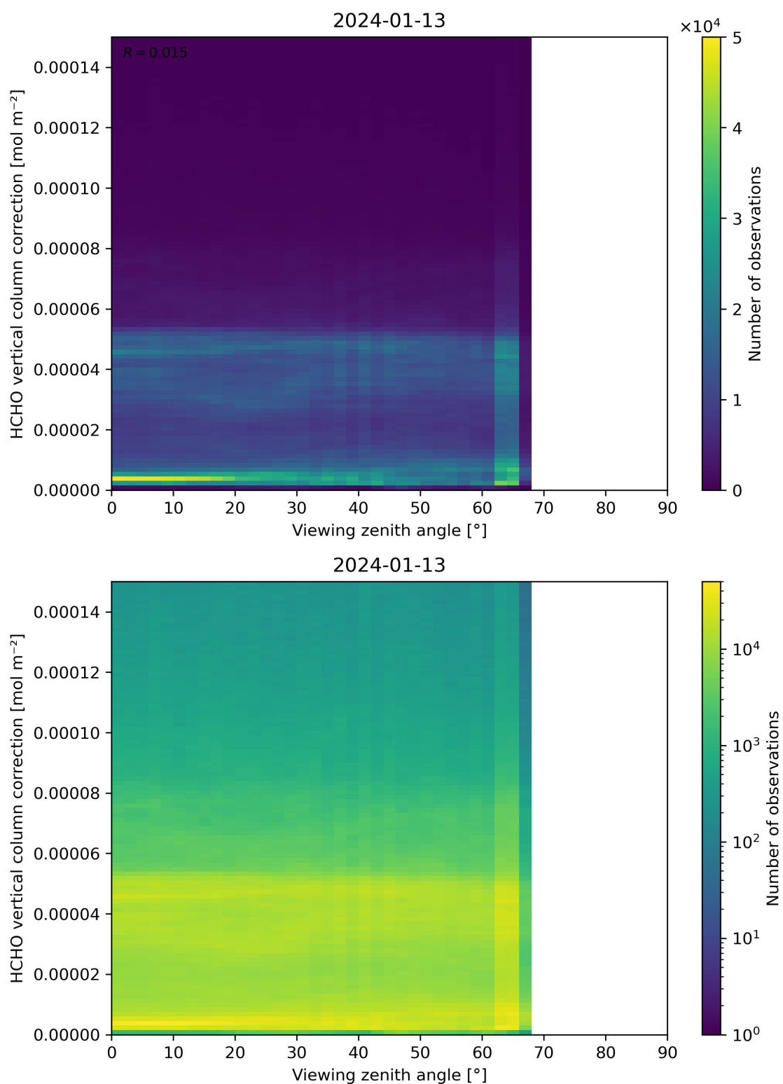
Figure 193: Scatter density plot of “Viewing zenith angle” against “HCHO vertical column correction” for 2024-01-12 to 2024-01-14.
