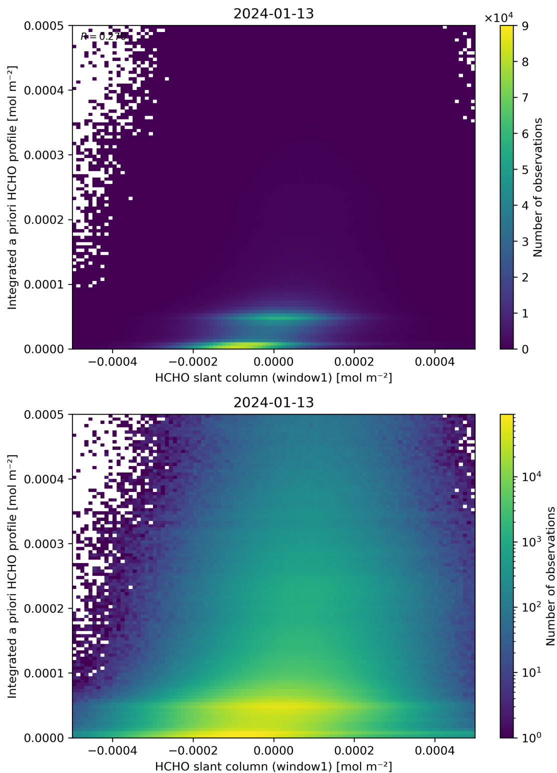
Figure 87: Scatter density plot of “HCHO slant column (window1)” against “Integrated a priori HCHO profile” for 2024-01-12 to 2024-01-14.
