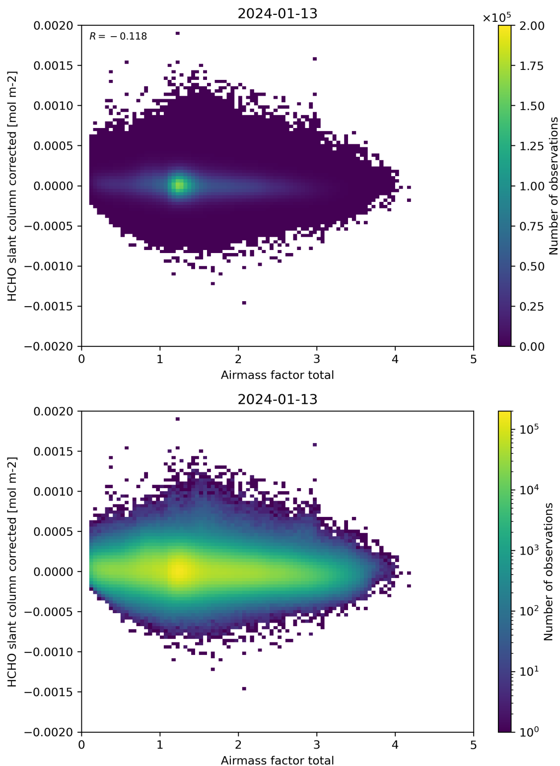
Figure 101: Scatter density plot of “Airmass factor total” against “HCHO slant column corrected” for 2024-01-12 to 2024-01-14.
