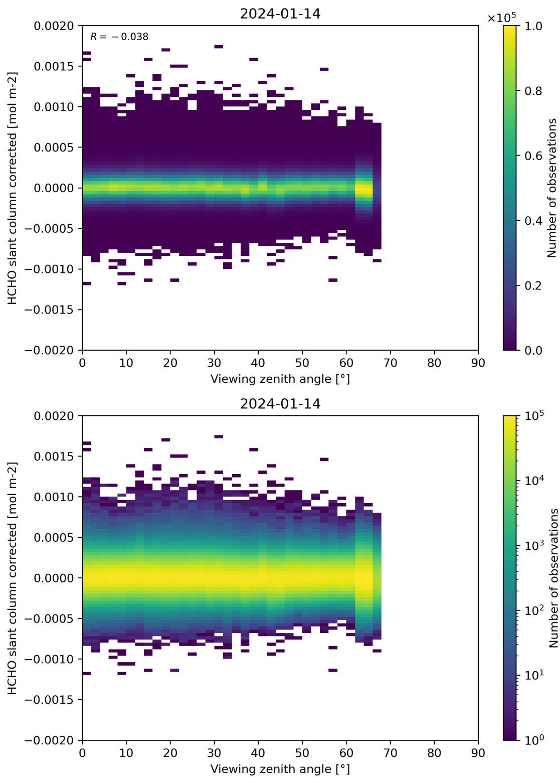
Figure 186: Scatter density plot of “Viewing zenith angle” against “HCHO slant column corrected” for 2024-01-13 to 2024-01-15.
