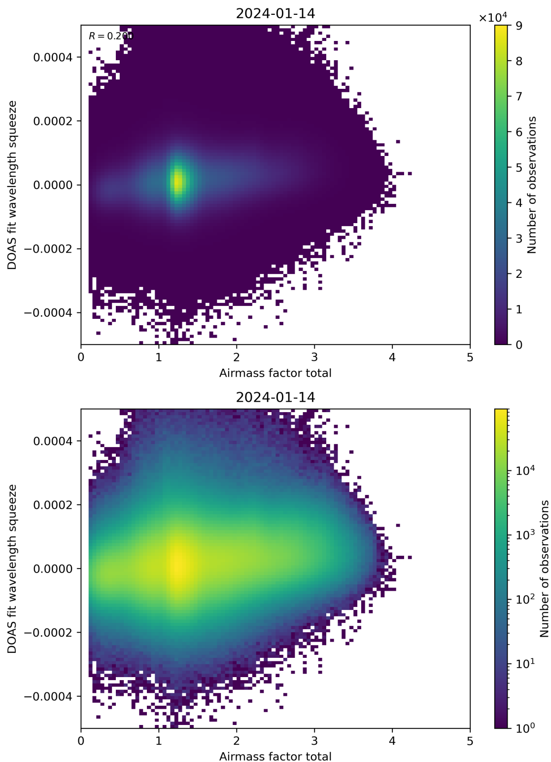
Figure 99: Scatter density plot of “Airmass factor total” against “DOAS fit wavelength squeeze” for 2024-01-13 to 2024-01-15.
