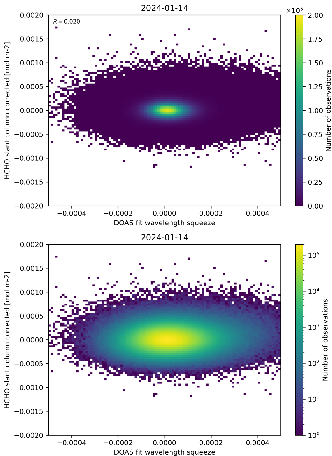
Figure 69: Scatter density plot of “DOAS fit wavelength squeeze” against “HCHO slant column corrected” for 2024-01-13 to 2024-01-15.
