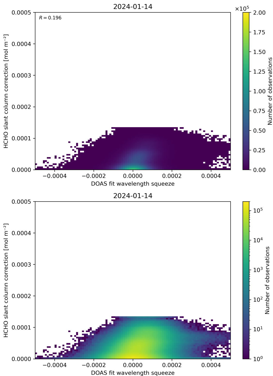
Figure 70: Scatter density plot of “DOAS fit wavelength squeeze” against “HCHO slant column correction” for 2024-01-13 to 2024-01-15.
