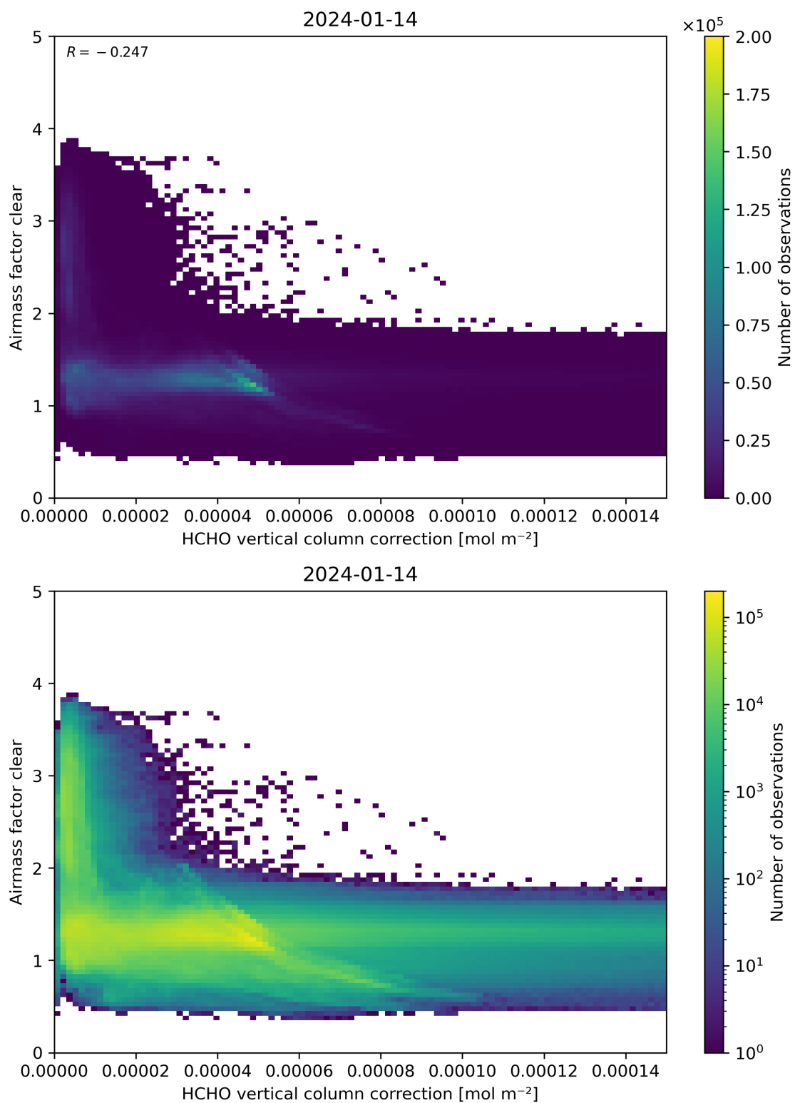
Figure 115: Scatter density plot of “HCHO vertical column correction” against “Airmass factor clear” for 2024-01-13 to 2024-01-15.
