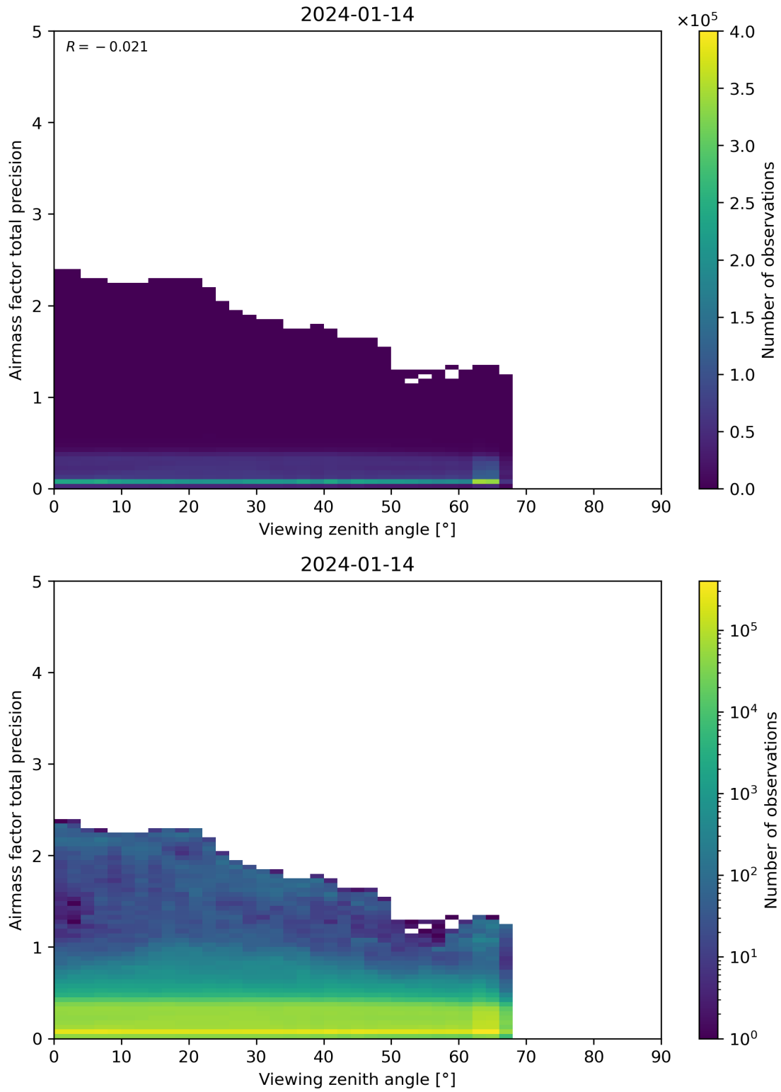
Figure 191: Scatter density plot of “Viewing zenith angle” against “Airmass factor total precision” for 2024-01-13 to 2024-01-15.
