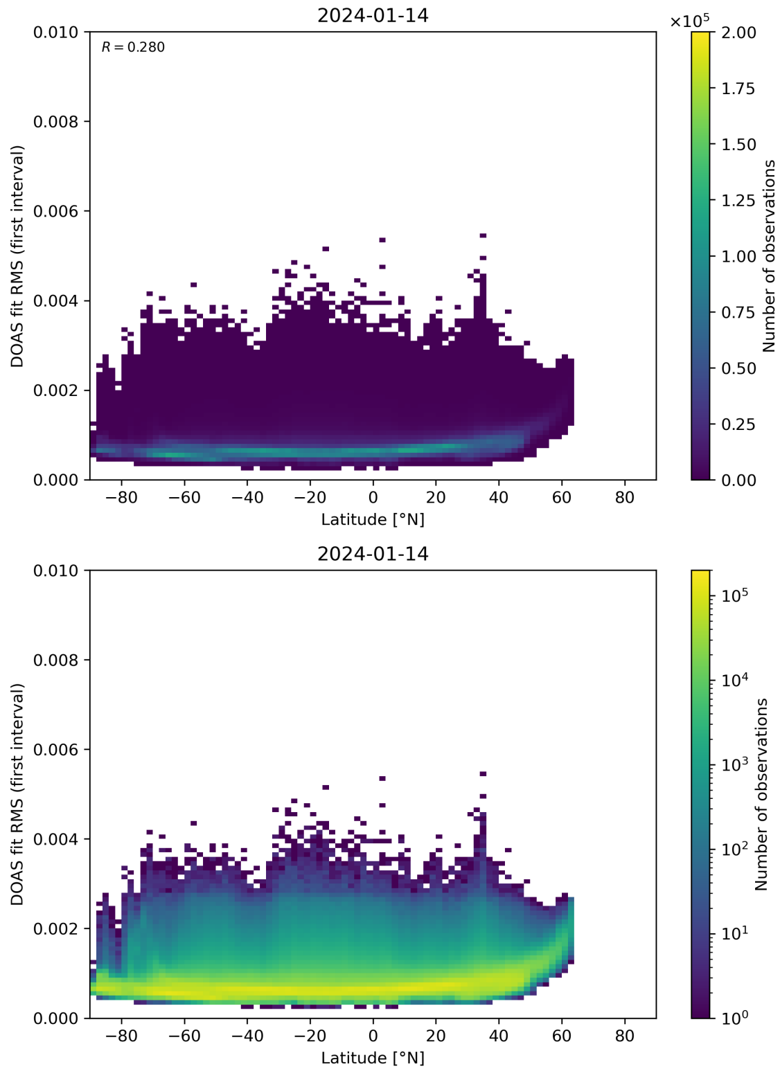
Figure 153: Scatter density plot of “Latitude” against “DOAS fit RMS (first interval)” for 2024-01-13 to 2024-01-15.
