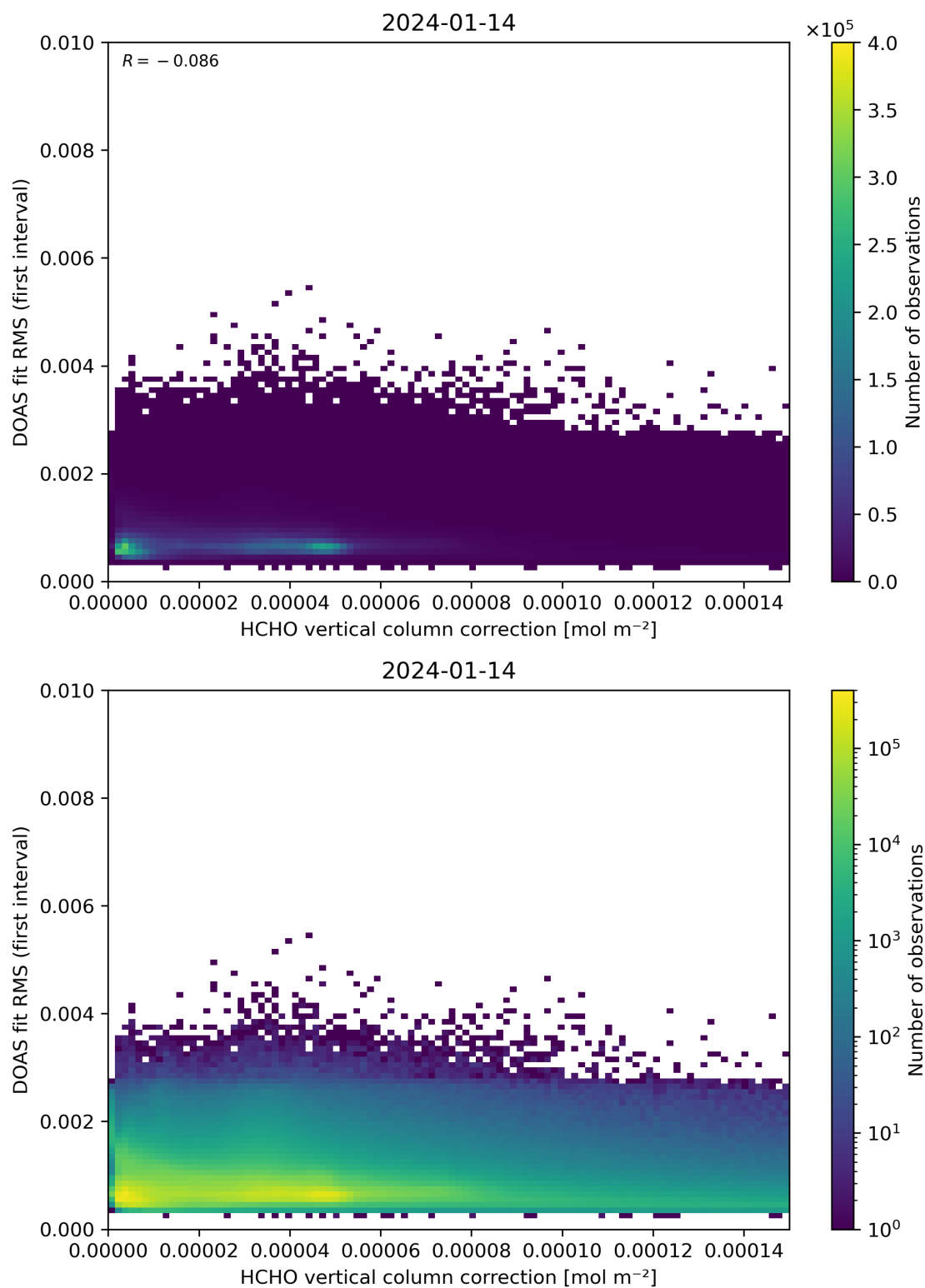
Figure 112: Scatter density plot of “HCHO vertical column correction” against “DOAS fit RMS (first interval)” for 2024-01-13 to 2024-01-15.
