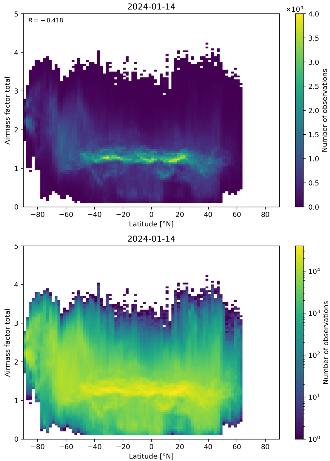
Figure 161: Scatter density plot of “Latitude” against “Airmass factor total” for 2024-01-13 to 2024-01-15.
