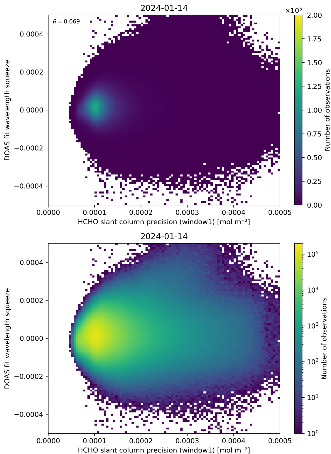
Figure 90: Scatter density plot of “HCHO slant column precision (window1)” against “DOAS fit wavelength squeeze” for 2024-01-13 to 2024-01-15.
