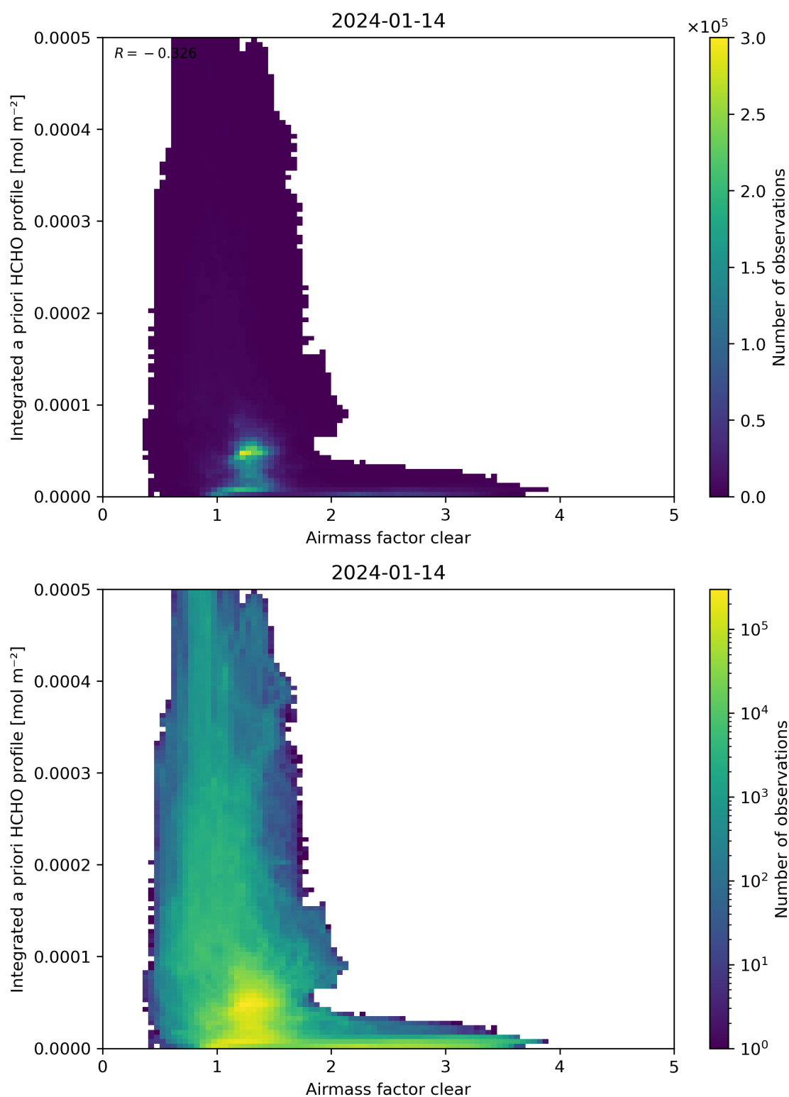
Figure 76: Scatter density plot of “Airmass factor clear” against “Integrated a priori HCHO profile” for 2024-01-13 to 2024-01-15.
