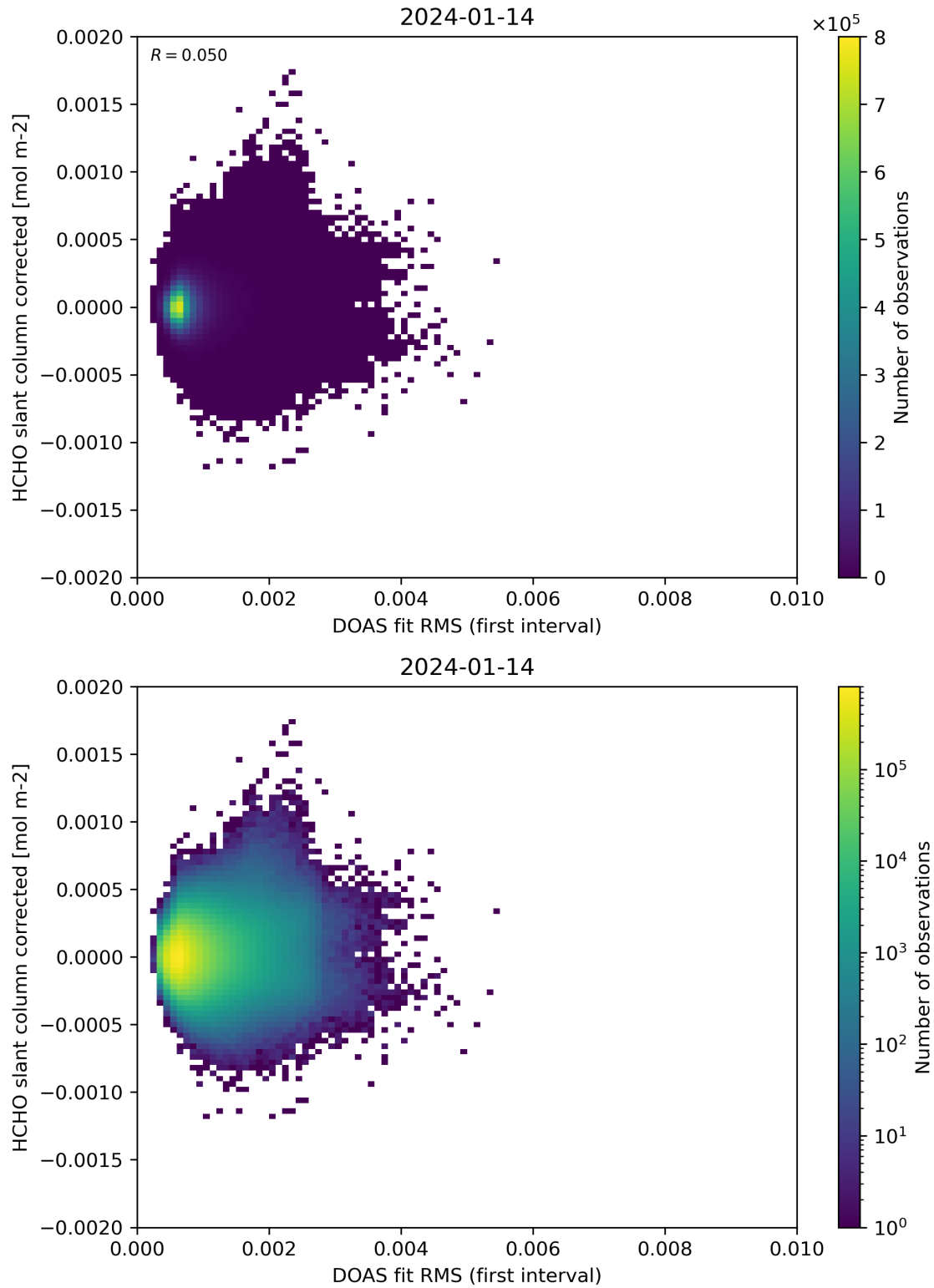
Figure 62: Scatter density plot of “DOAS fit RMS (first interval)” against “HCHO slant column corrected” for 2024-01-13 to 2024-01-15.
