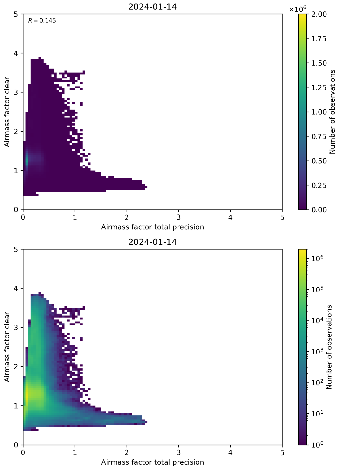
Figure 108: Scatter density plot of “Airmass factor total precision” against “Airmass factor clear” for 2024-01-13 to 2024-01-15.
