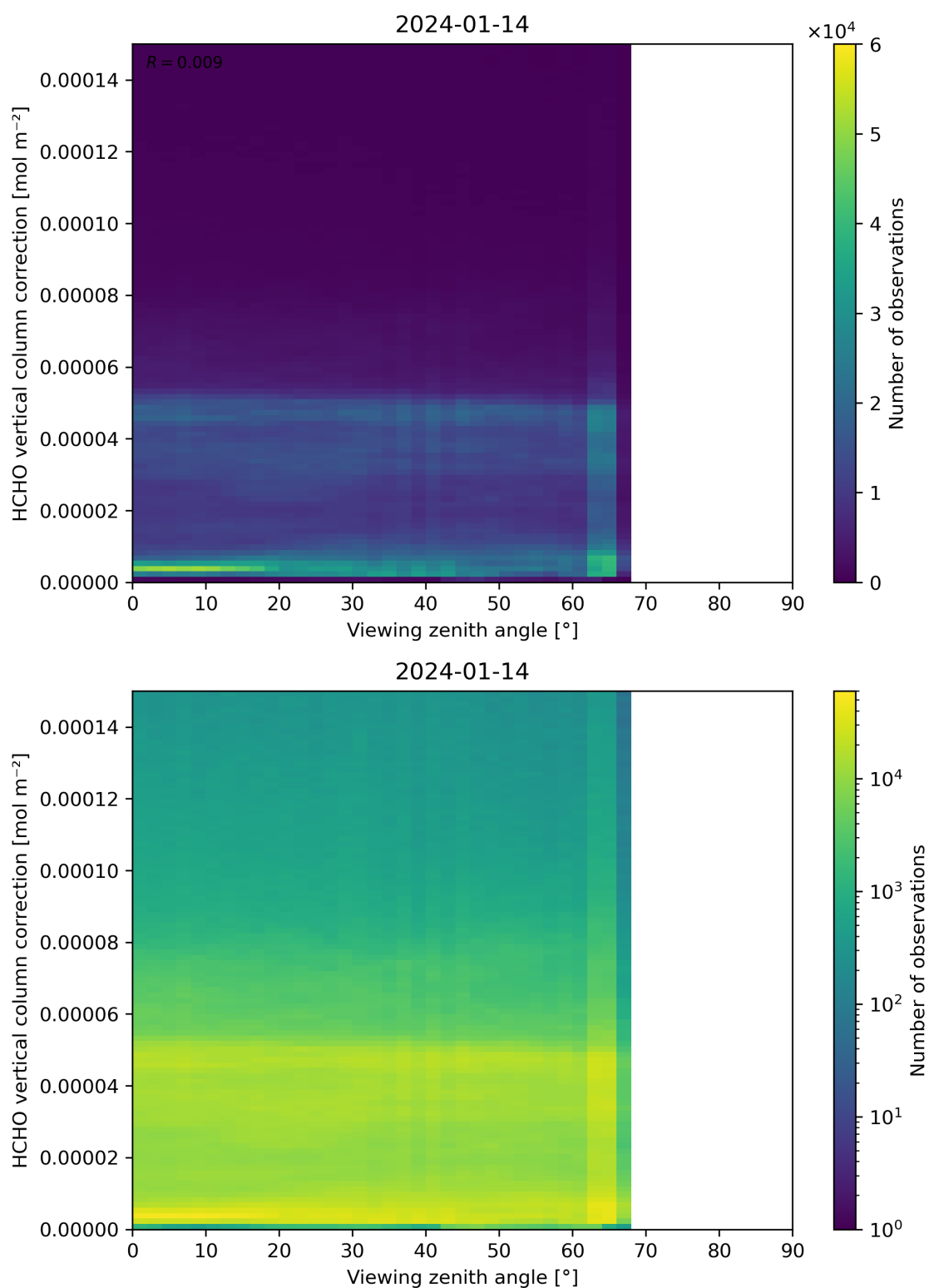
Figure 193: Scatter density plot of “Viewing zenith angle” against “HCHO vertical column correction” for 2024-01-13 to 2024-01-15.
