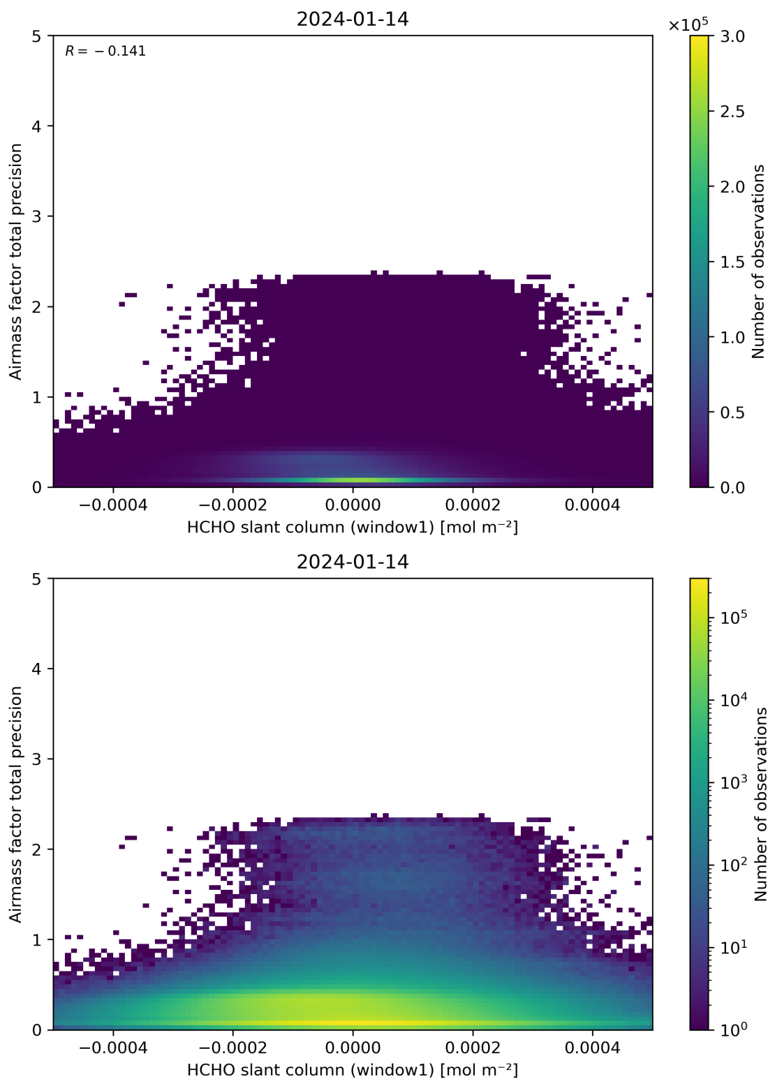
Figure 86: Scatter density plot of “HCHO slant column (window1)” against “Airmass factor total precision” for 2024-01-13 to 2024-01-15.
