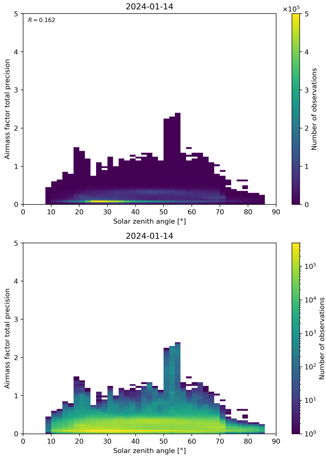
Figure 176: Scatter density plot of “Solar zenith angle” against “Airmass factor total precision” for 2024-01-13 to 2024-01-15.
