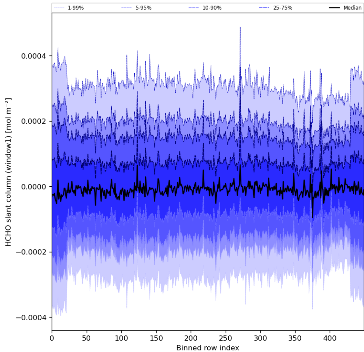
Figure 52: Along track statistics of “HCHO slant column (window1)” for 2024-01-13 to 2024-01-15
