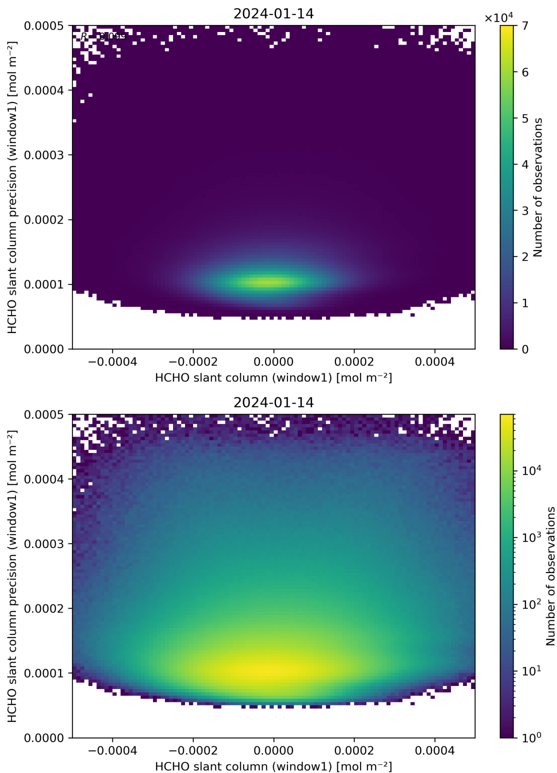
Figure 84: Scatter density plot of “HCHO slant column (window1)” against “HCHO slant column precision (window1)” for 2024-01-13 to 2024-01-15.
