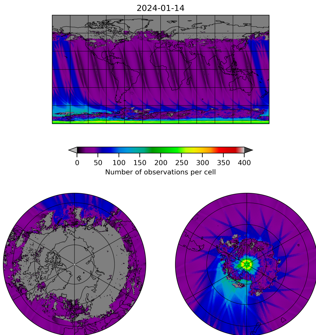
Figure 19: Map of the number of observations for 2024-01-13 to 2024-01-15
