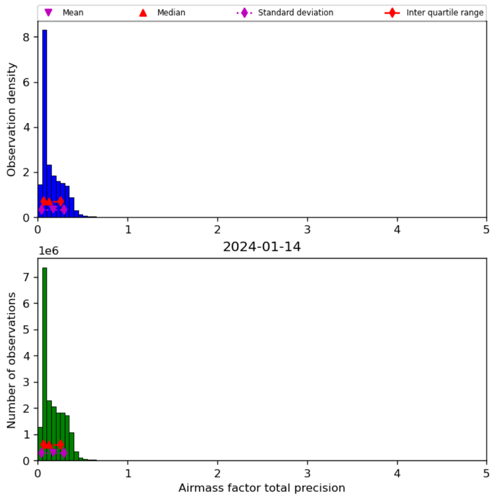
Figure 41: Histogram of “Airmass factor total precision” for 2024-01-13 to 2024-01-15
