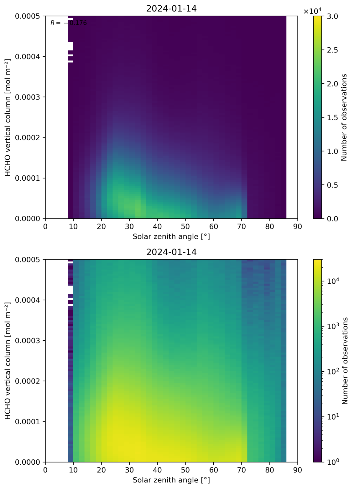
Figure 177: Scatter density plot of “Solar zenith angle” against “HCHO vertical column” for 2024-01-13 to 2024-01-15.
