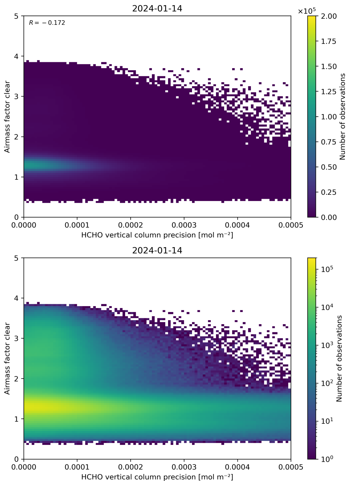
Figure 139: Scatter density plot of “HCHO vertical column precision” against “Airmass factor clear” for 2024-01-13 to 2024-01-15.
