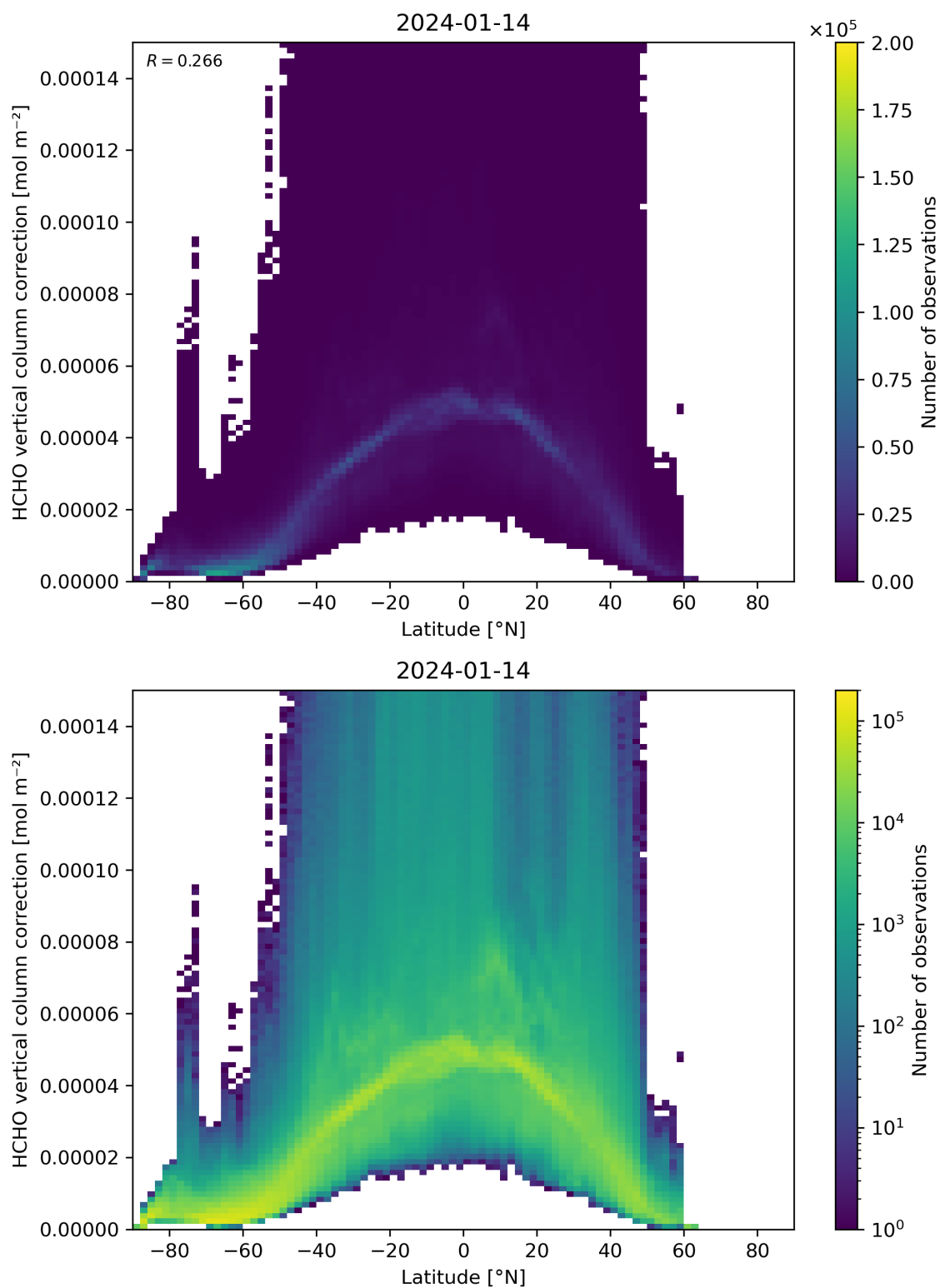
Figure 164: Scatter density plot of “Latitude” against “HCHO vertical column correction” for 2024-01-13 to 2024-01-15.
