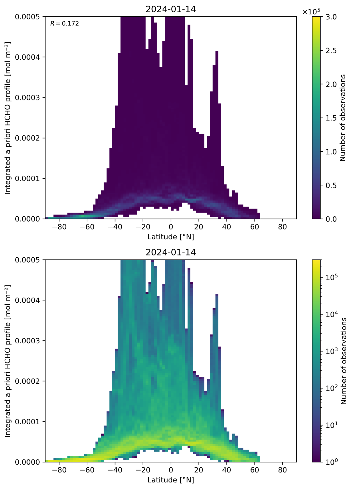
Figure 166: Scatter density plot of “Latitude” against “Integrated a priori HCHO profile” for 2024-01-13 to 2024-01-15.
