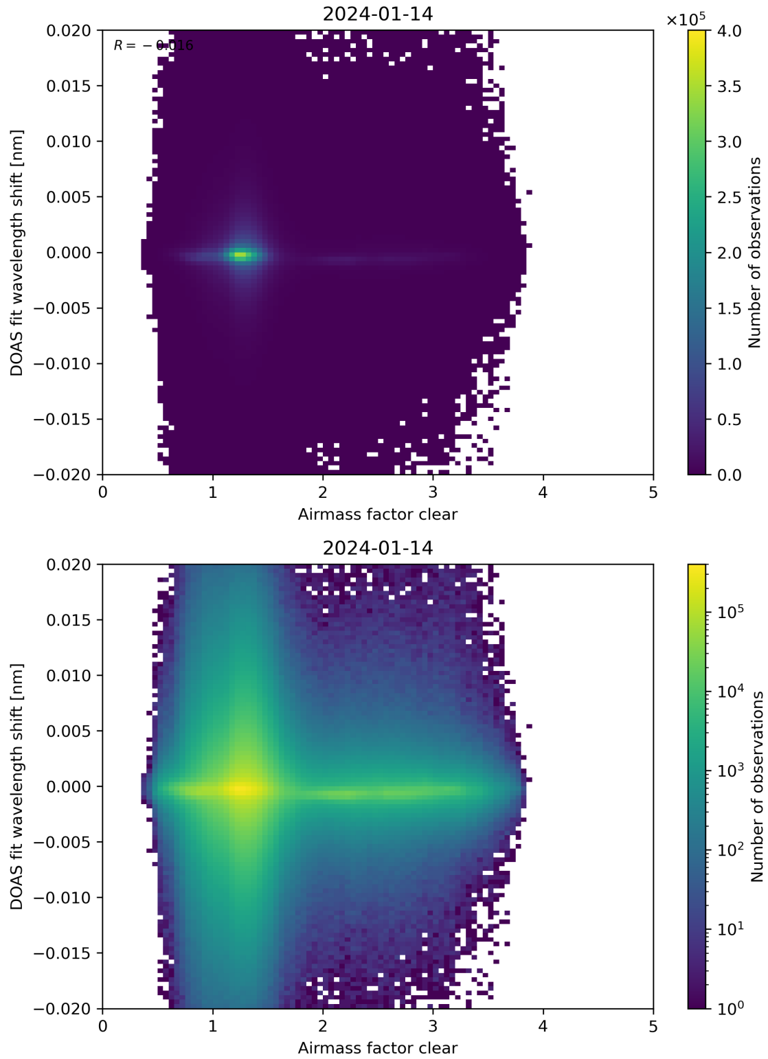
Figure 72: Scatter density plot of “Airmass factor clear” against “DOAS fit wavelength shift” for 2024-01-13 to 2024-01-15.
