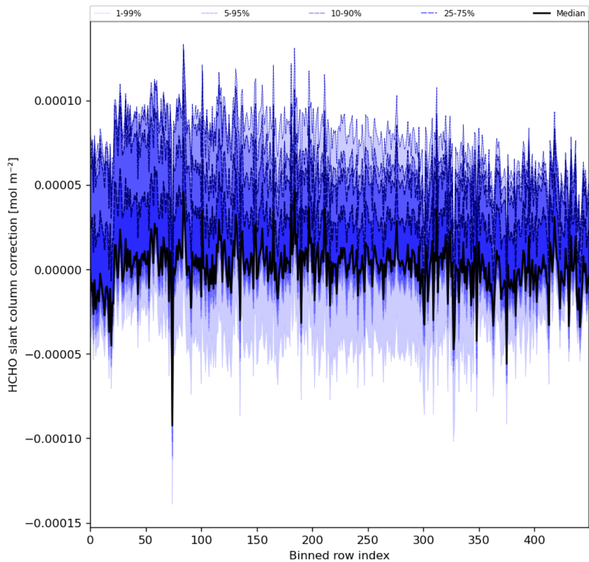
Figure 61: Along track statistics of “HCHO slant column correction” for 2024-01-13 to 2024-01-15
