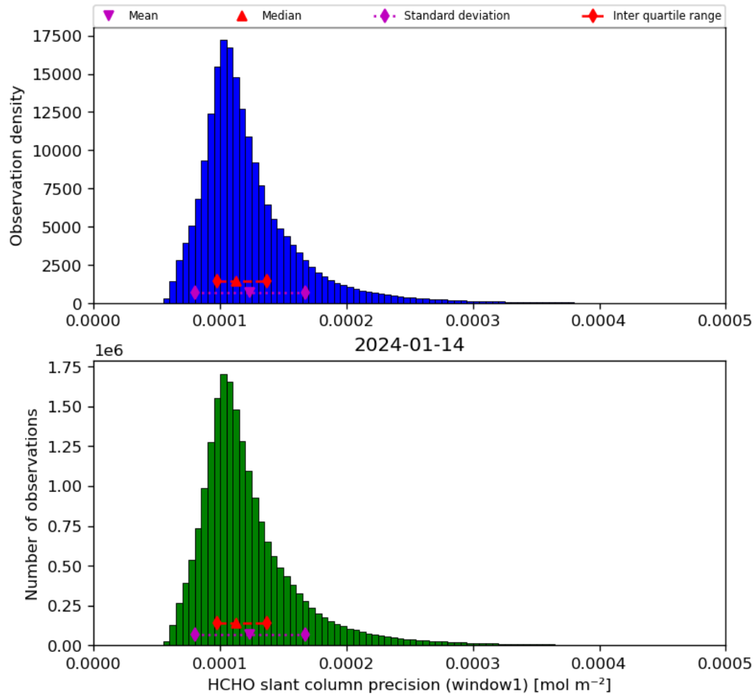
Figure 39: Histogram of “HCHO slant column precision (window1)” for 2024-01-13 to 2024-01-15
