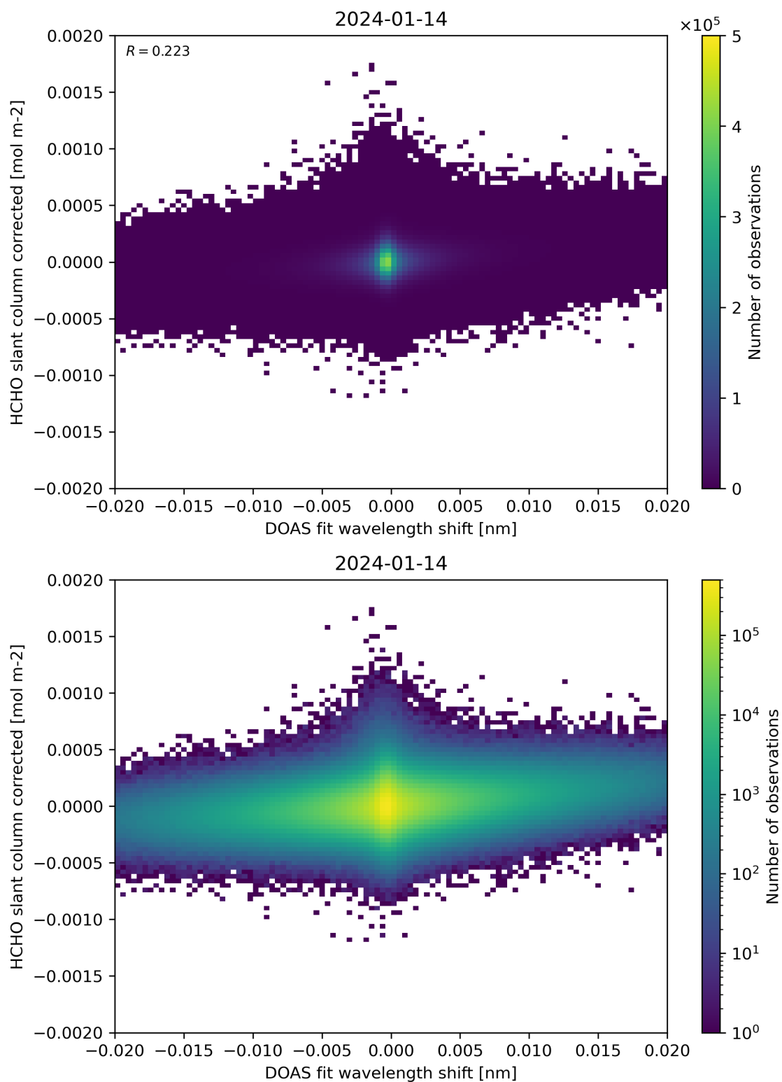
Figure 66: Scatter density plot of “DOAS fit wavelength shift” against “HCHO slant column corrected” for 2024-01-13 to 2024-01-15.
