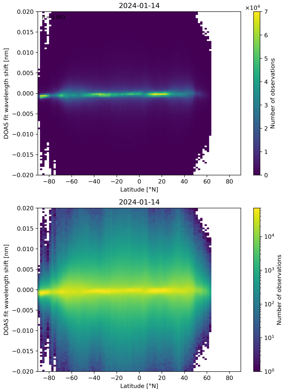
Figure 154: Scatter density plot of “Latitude” against “DOAS fit wavelength shift” for 2024-01-13 to 2024-01-15.
