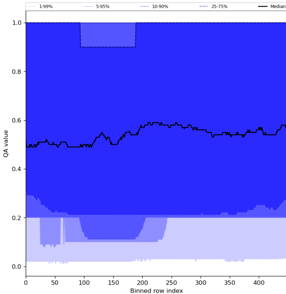
Figure 48: Along track statistics of “QA value” for 2024-01-13 to 2024-01-15
