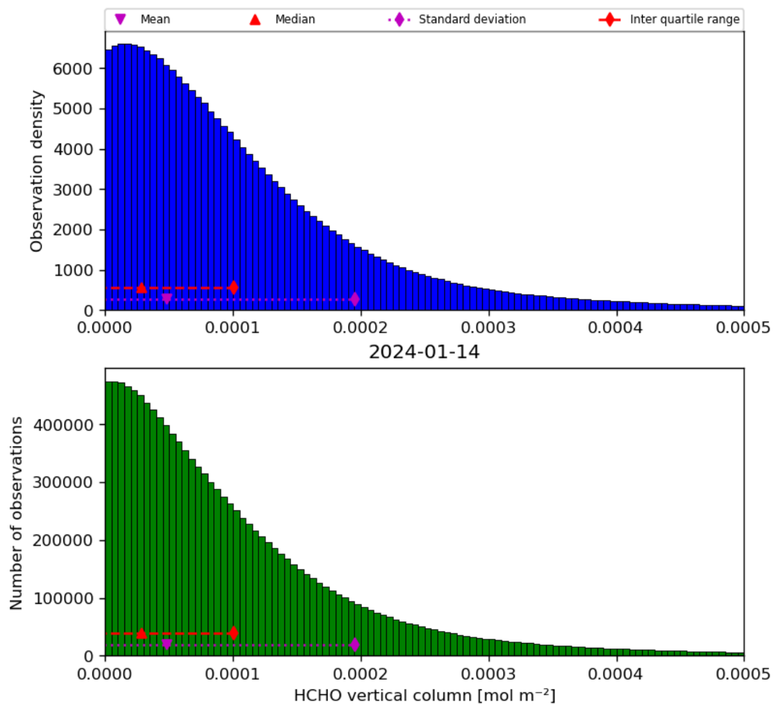
Figure 35: Histogram of “HCHO vertical column” for 2024-01-13 to 2024-01-15
