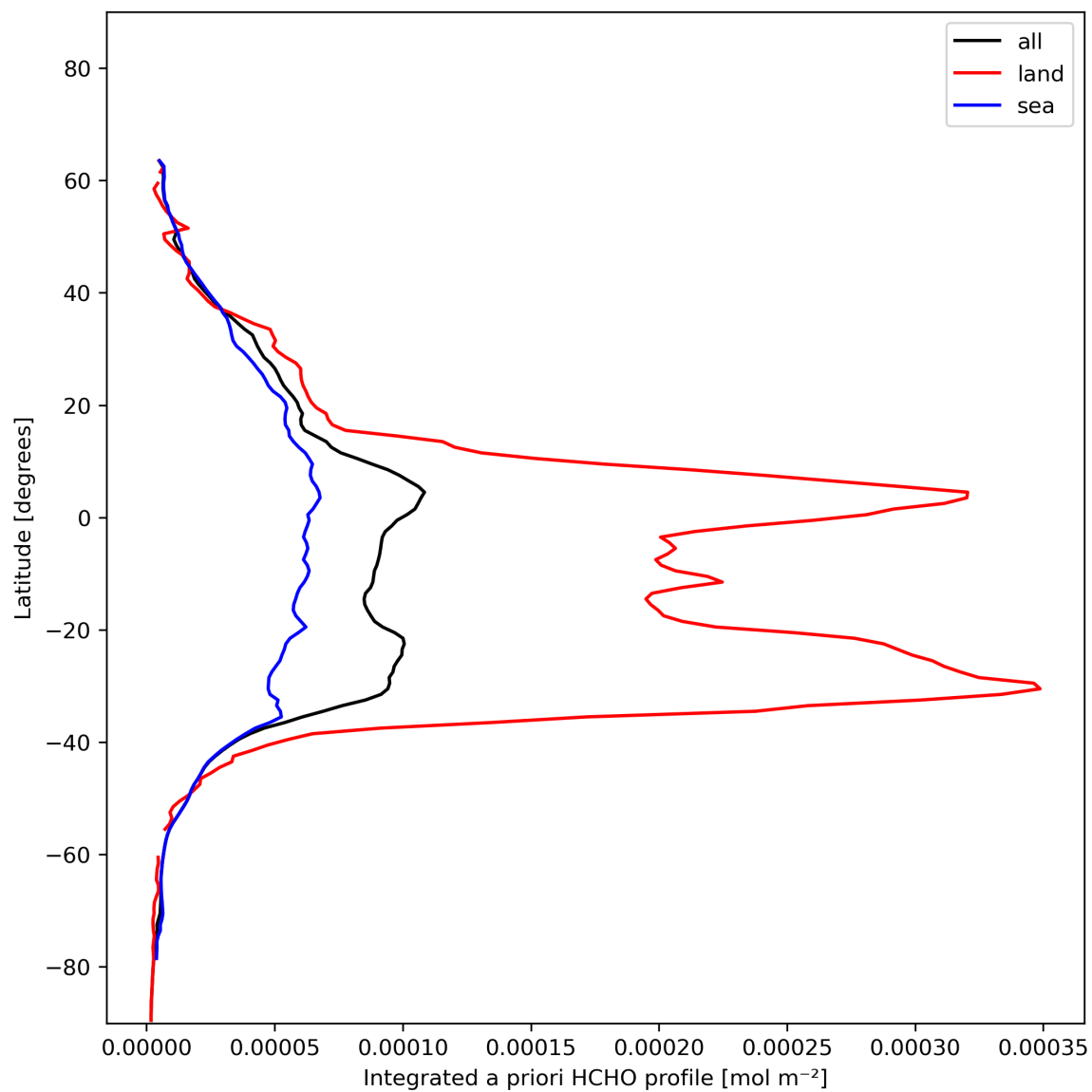
Figure 29: Zonal average of “Integrated a priori HCHO profile” for 2024-01-13 to 2024-01-15.
