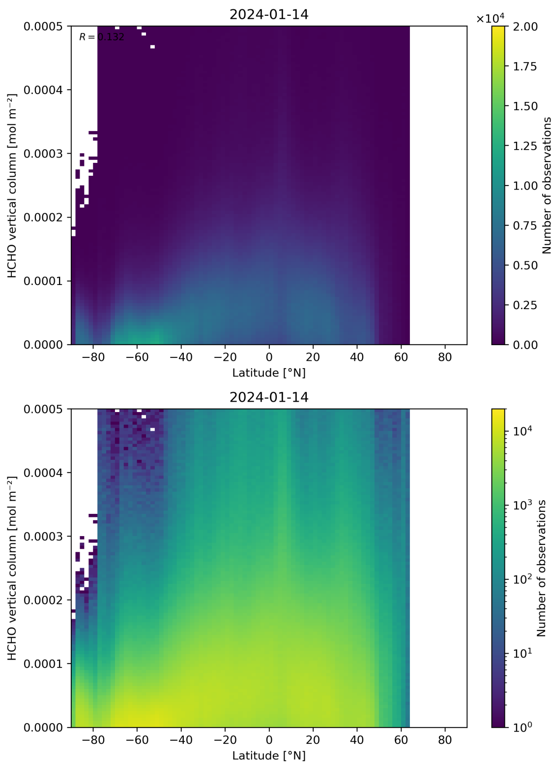
Figure 163: Scatter density plot of “Latitude” against “HCHO vertical column” for 2024-01-13 to 2024-01-15.
