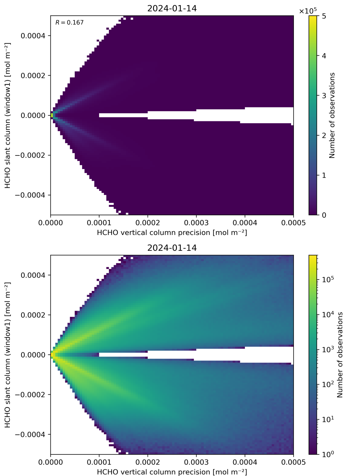
Figure 142: Scatter density plot of “HCHO vertical column precision” against “HCHO slant column (window1)” for 2024-01-13 to 2024-01-15.
