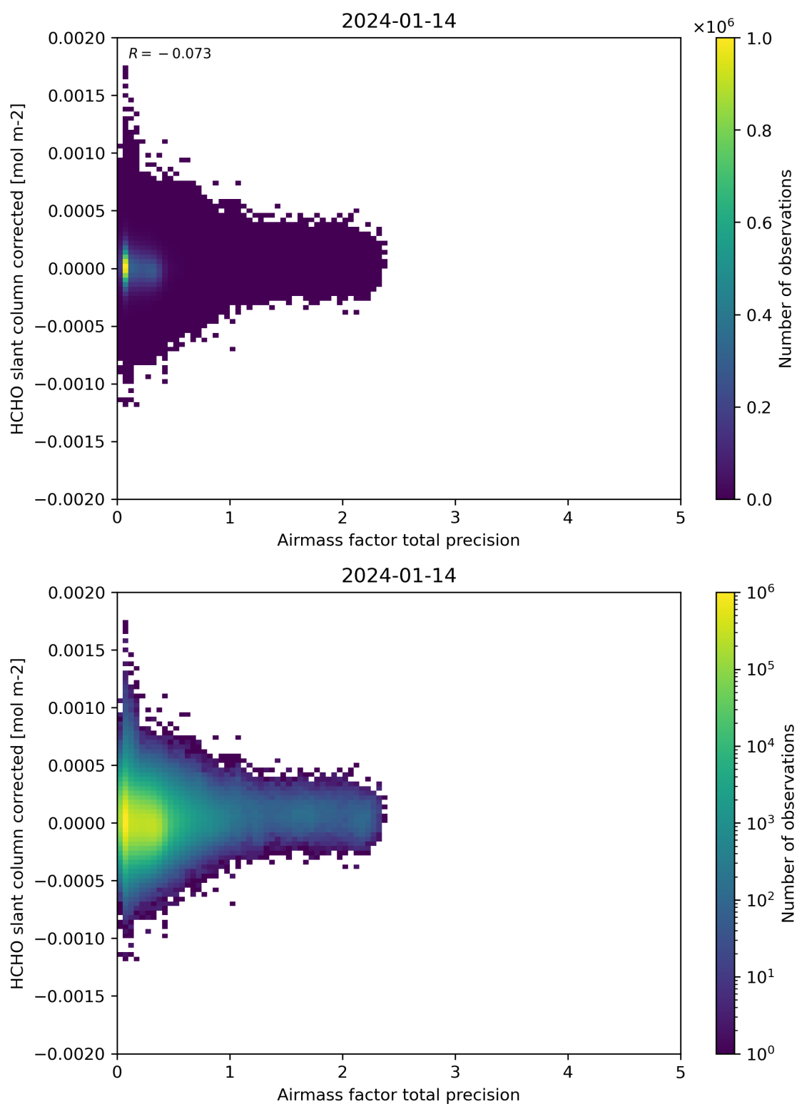
Figure 109: Scatter density plot of “Airmass factor total precision” against “HCHO slant column corrected” for 2024-01-13 to 2024-01-15.
