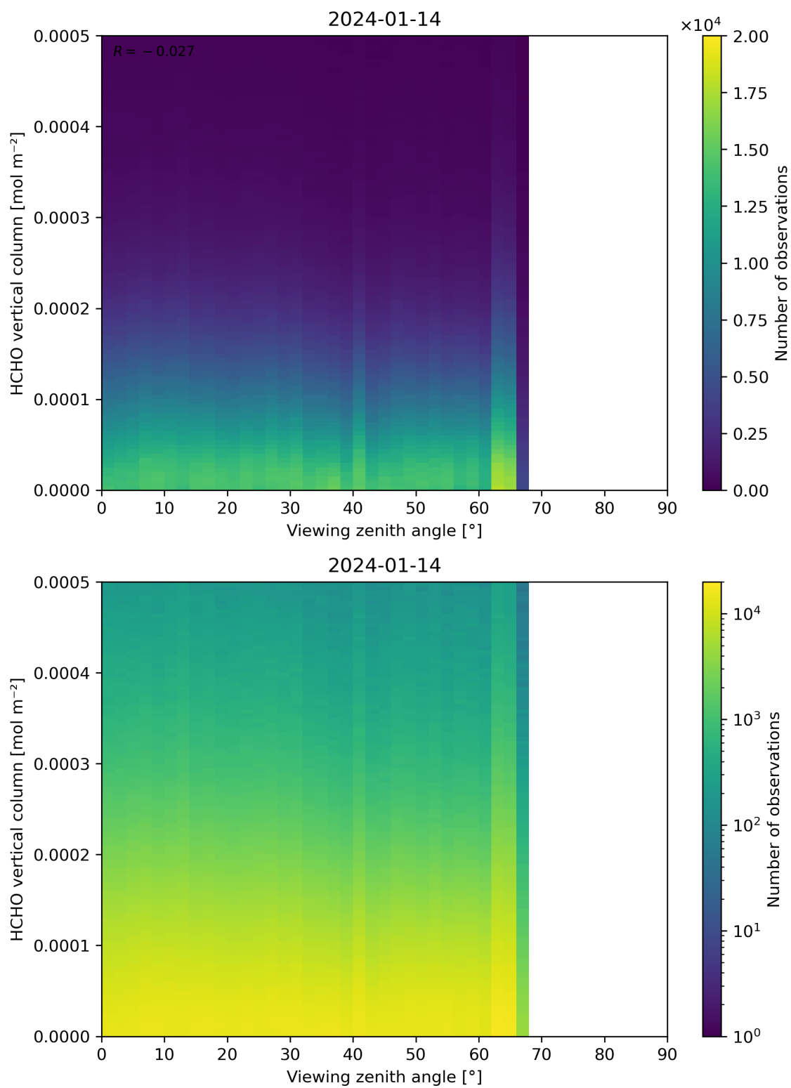
Figure 192: Scatter density plot of “Viewing zenith angle” against “HCHO vertical column” for 2024-01-13 to 2024-01-15.
