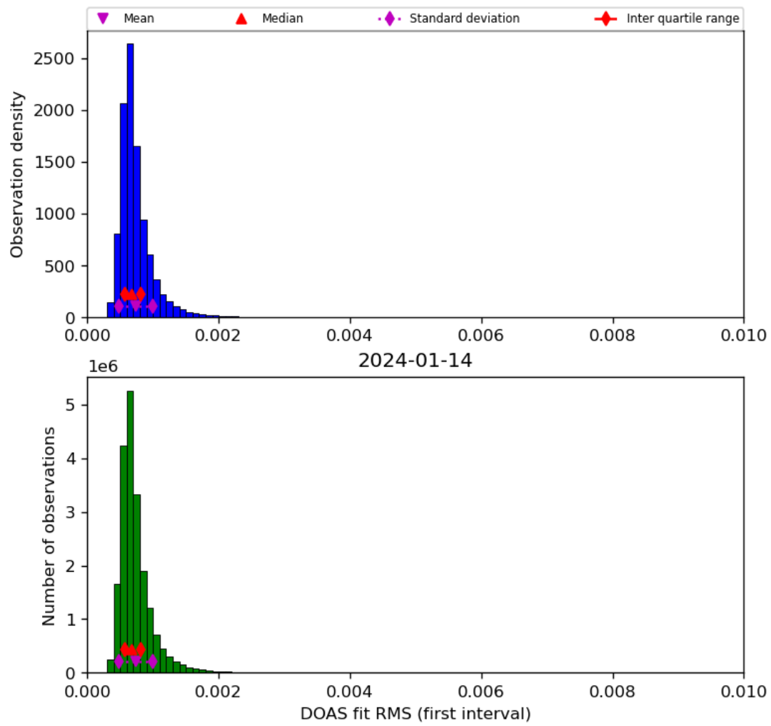
Figure 46: Histogram of “DOAS fit RMS (first interval)” for 2024-01-13 to 2024-01-15
