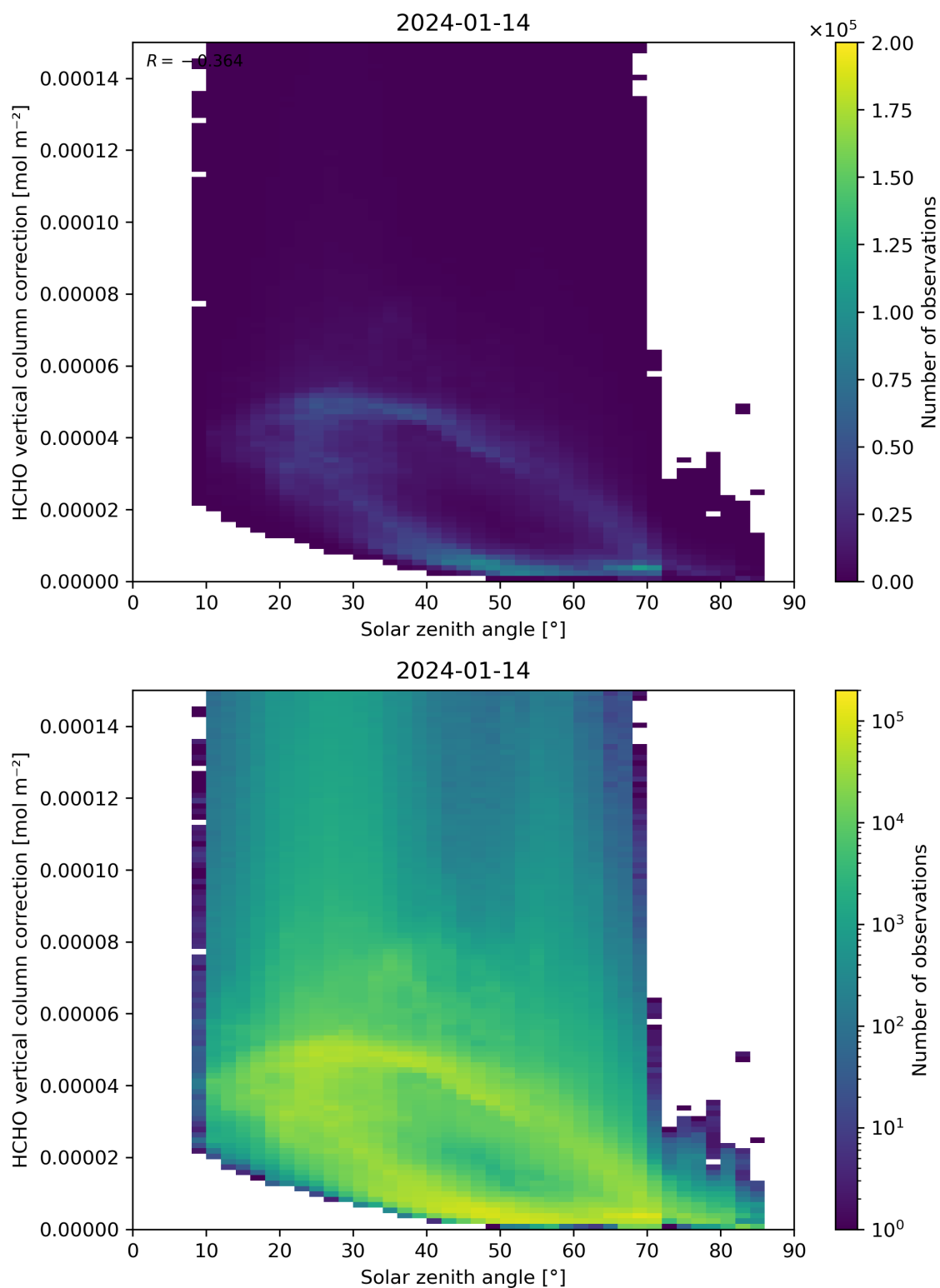
Figure 178: Scatter density plot of “Solar zenith angle” against “HCHO vertical column correction” for 2024-01-13 to 2024-01-15.
