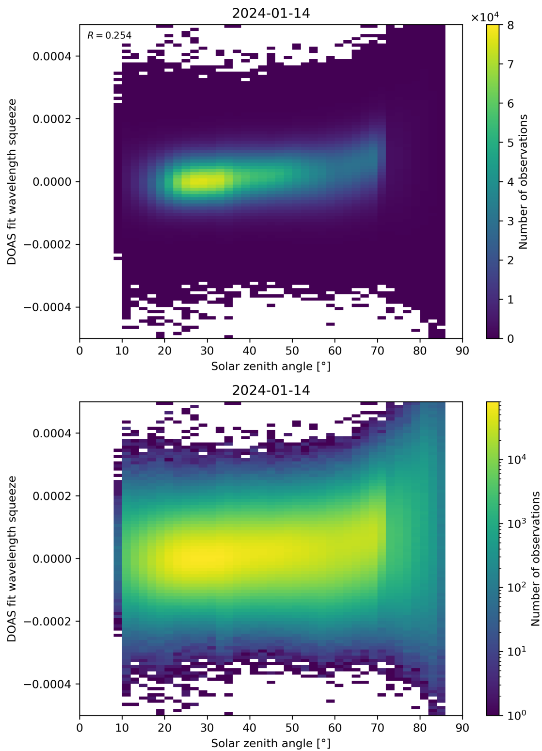
Figure 169: Scatter density plot of “Solar zenith angle” against “DOAS fit wavelength squeeze” for 2024-01-13 to 2024-01-15.
