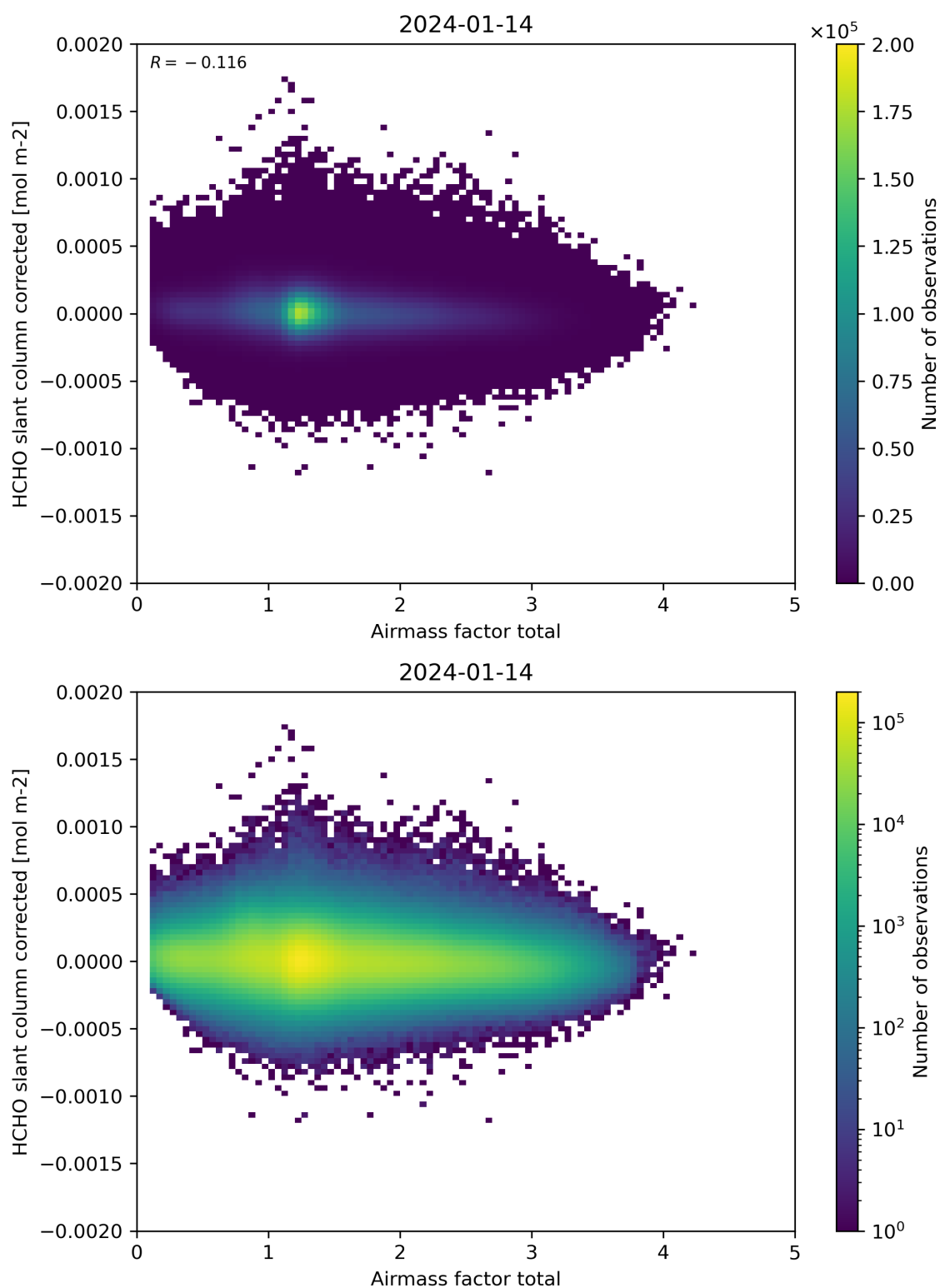
Figure 101: Scatter density plot of “Airmass factor total” against “HCHO slant column corrected” for 2024-01-13 to 2024-01-15.
