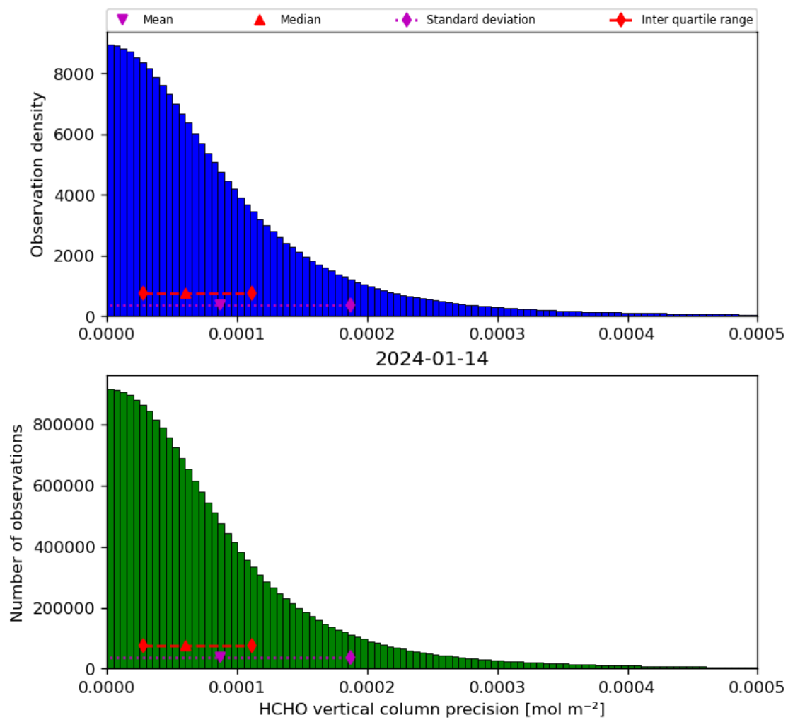
Figure 36: Histogram of “HCHO vertical column precision” for 2024-01-13 to 2024-01-15
