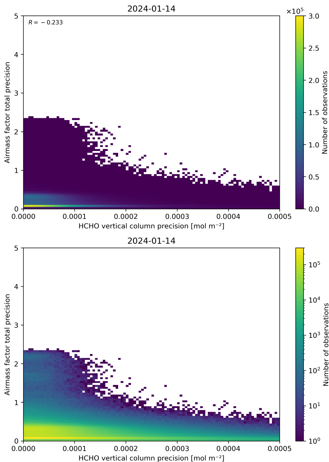
Figure 145: Scatter density plot of “HCHO vertical column precision” against “Airmass factor total precision” for 2024-01-13 to 2024-01-15.
