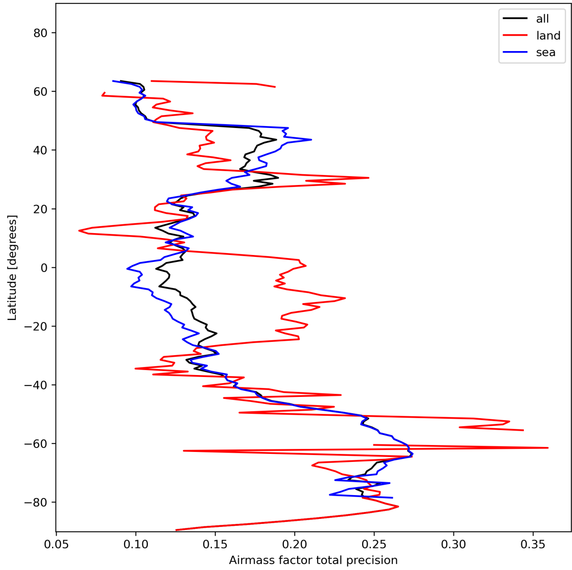
Figure 27: Zonal average of “Airmass factor total precision” for 2024-01-13 to 2024-01-15.
