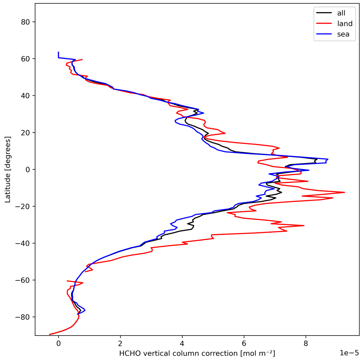
Figure 23: Zonal average of “HCHO vertical column correction” for 2024-01-13 to 2024-01-15.
