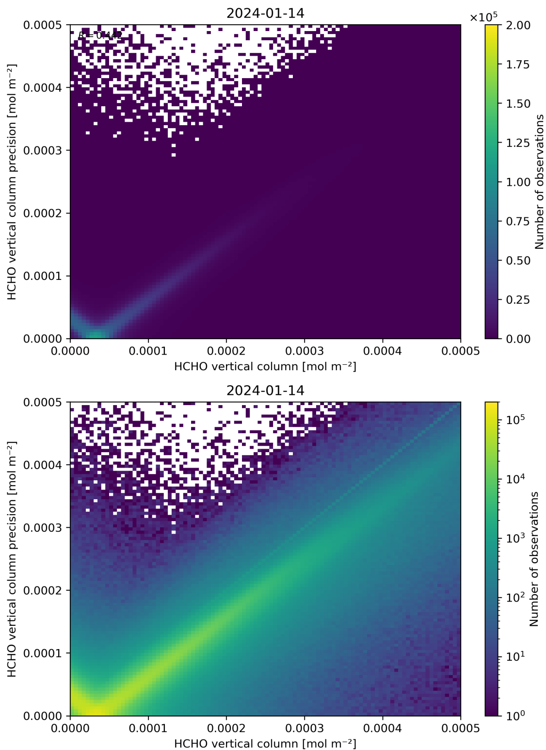
Figure 134: Scatter density plot of “HCHO vertical column” against “HCHO vertical column precision” for 2024-01-13 to 2024-01-15.
