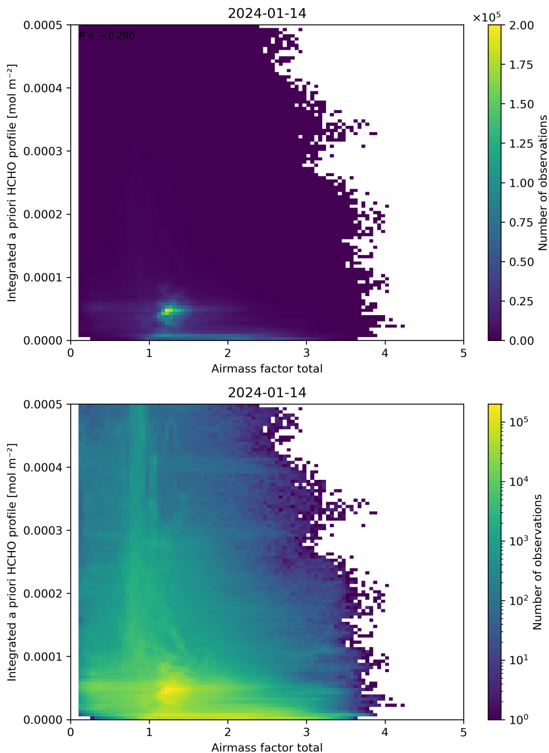
Figure 104: Scatter density plot of “Air mass factor total” against “Integrated a priori HCHO profile” for 2024-01-13 to 2024-01-15.
