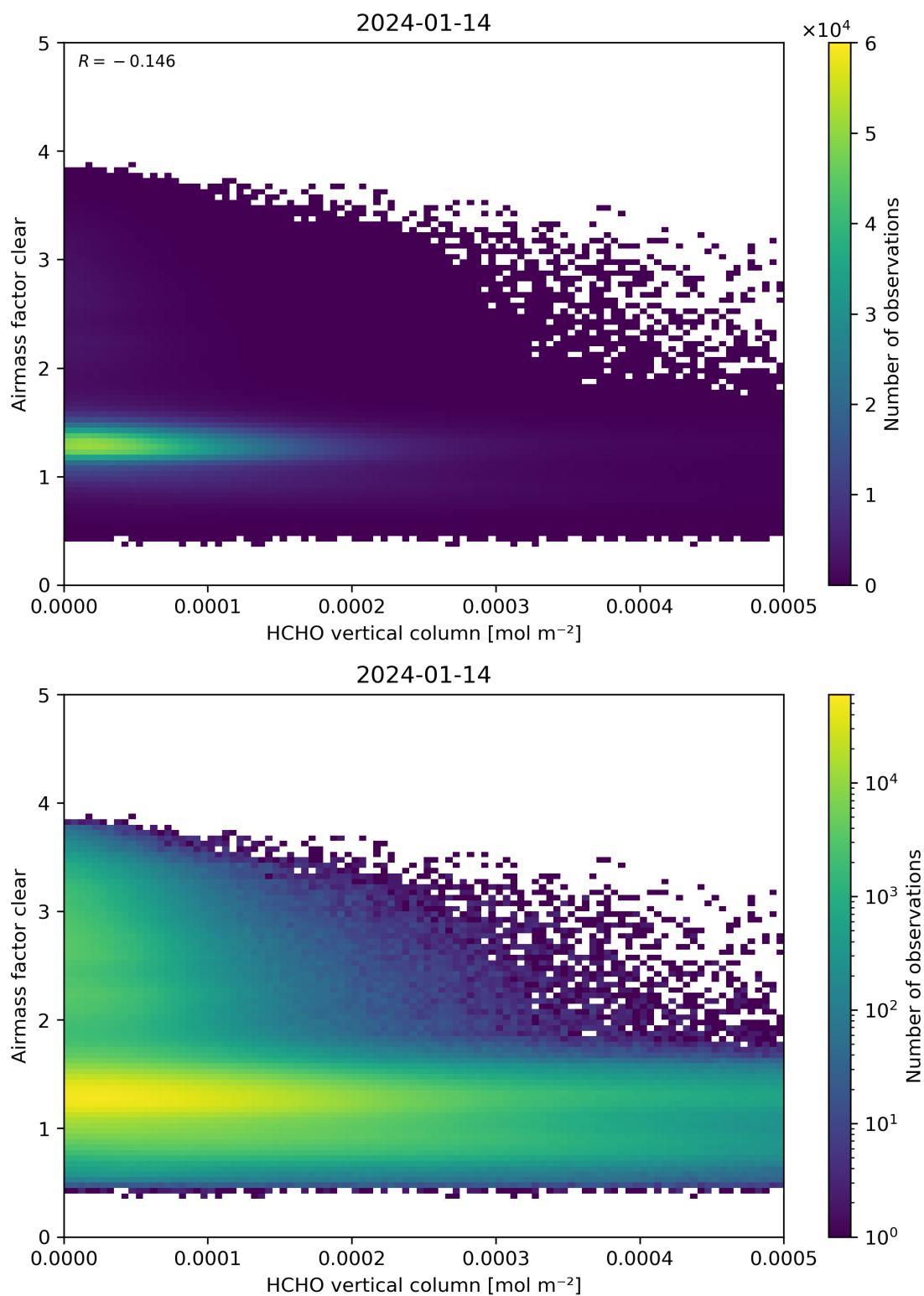
Figure 126: Scatter density plot of “HCHO vertical column” against “Airmass factor clear” for 2024-01-13 to 2024-01-15.
