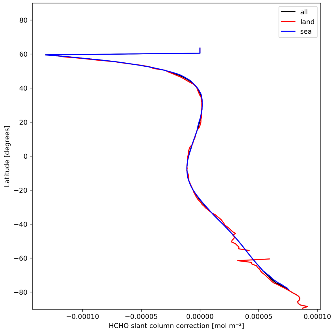
Figure 33: Zonal average of “HCHO slant column correction” for 2024-01-13 to 2024-01-15.
