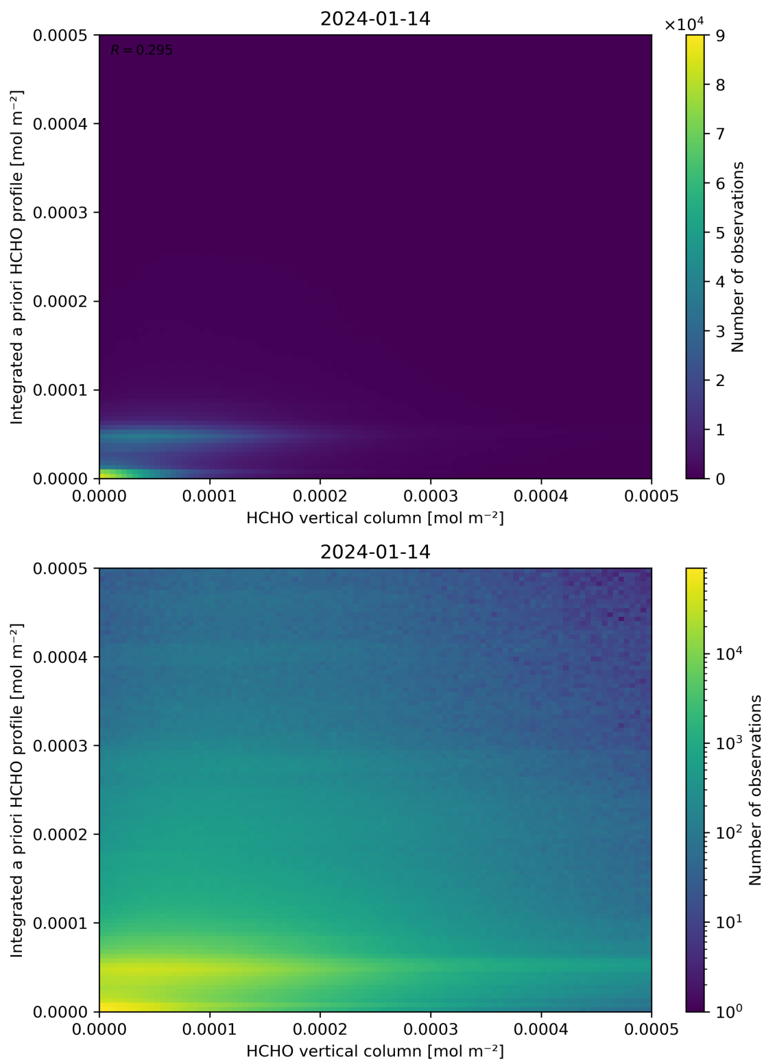
Figure 135: Scatter density plot of “HCHO vertical column” against “Integrated a priori HCHO profile” for 2024-01-13 to 2024-01-15.
