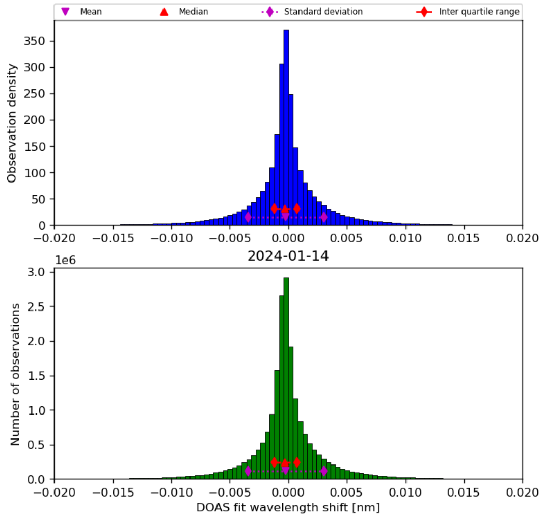
Figure 44: Histogram of “DOAS fit wavelength shift” for 2024-01-13 to 2024-01-15
