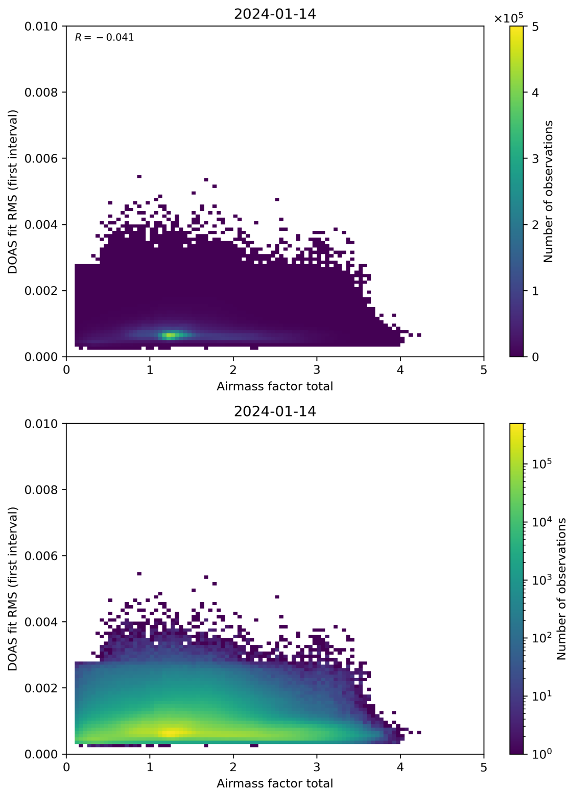
Figure 97: Scatter density plot of “Airmass factor total” against “DOAS fit RMS (first interval)” for 2024-01-13 to 2024-01-15.
