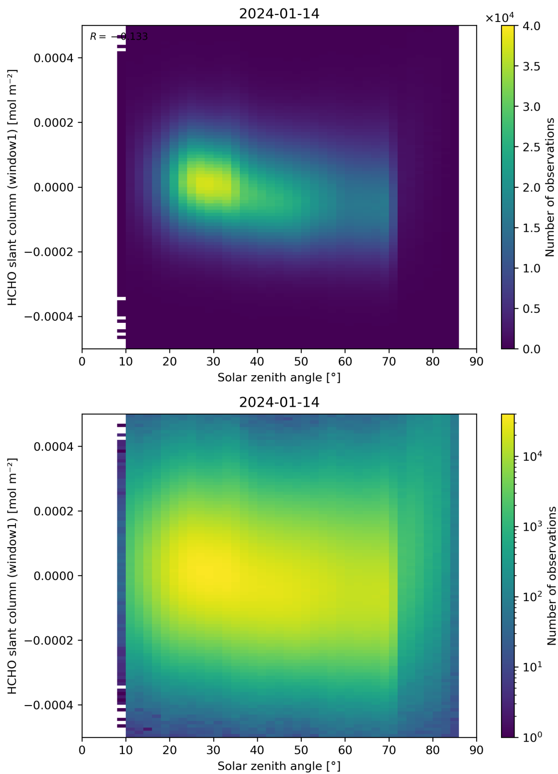
Figure 173: Scatter density plot of “Solar zenith angle” against “HCHO slant column (window1)” for 2024-01-13 to 2024-01-15.
