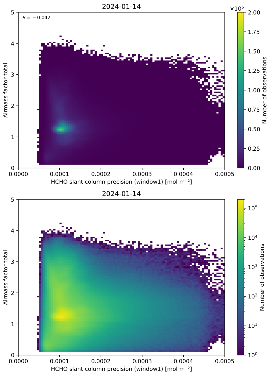
Figure 94: Scatter density plot of “HCHO slant column precision (window1)” against “Airmass factor total” for 2024-01-13 to 2024-01-15.
