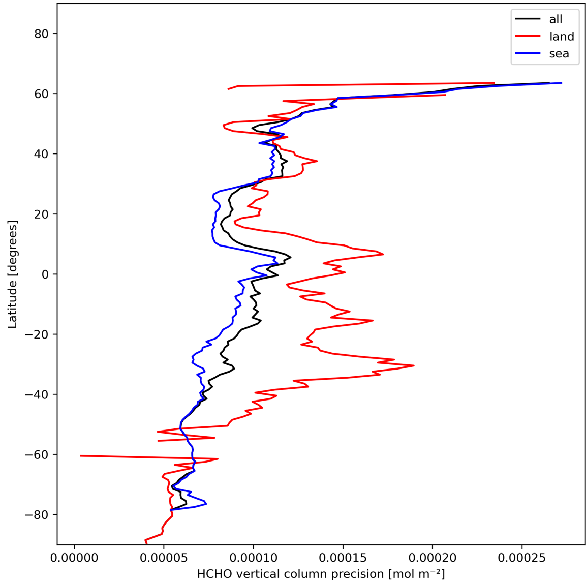
Figure 22: Zonal average of “HCHO vertical column precision” for 2024-01-13 to 2024-01-15.
