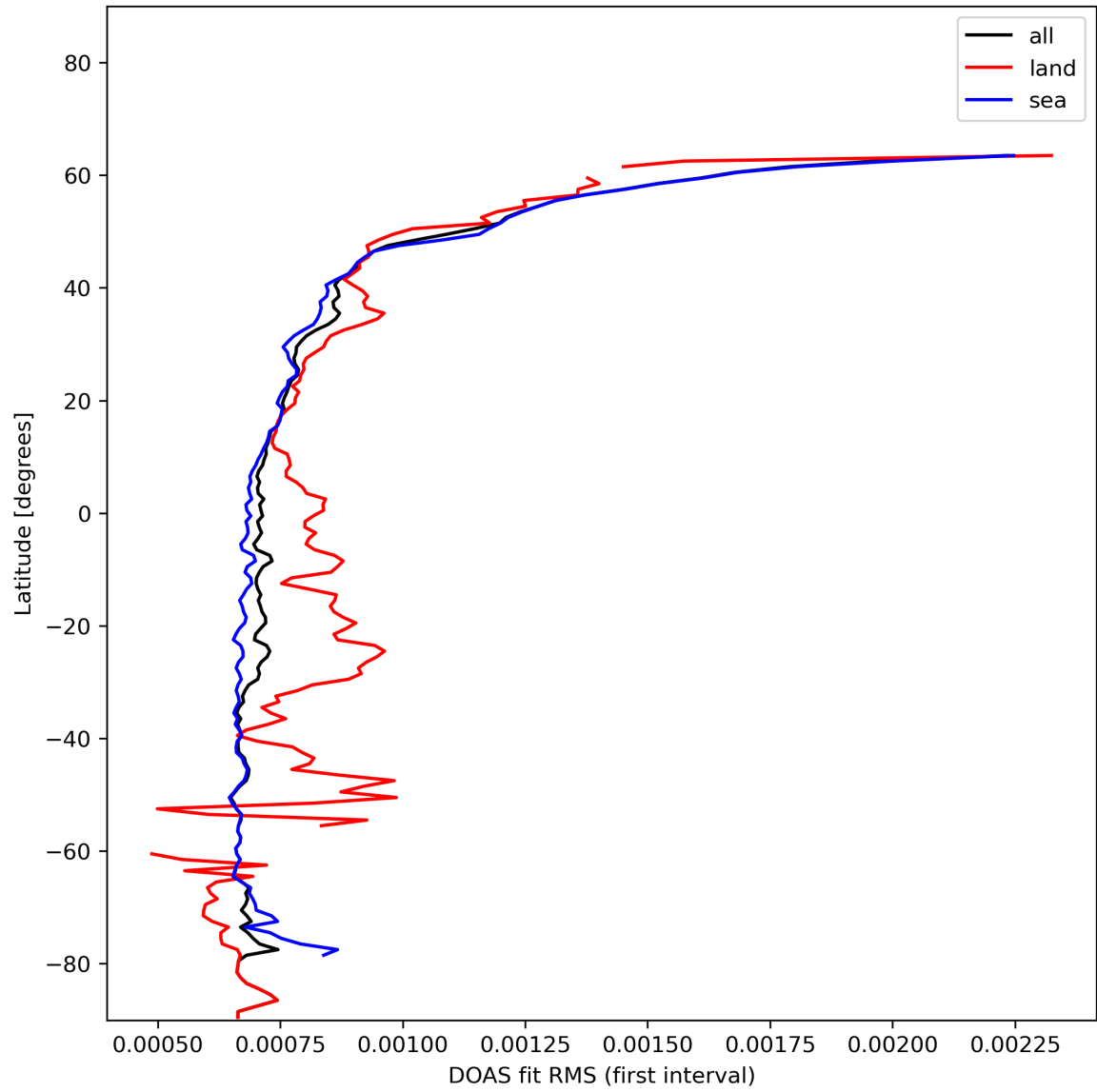
Figure 32: Zonal average of “DOAS fit RMS (first interval)” for 2024-01-13 to 2024-01-15.
