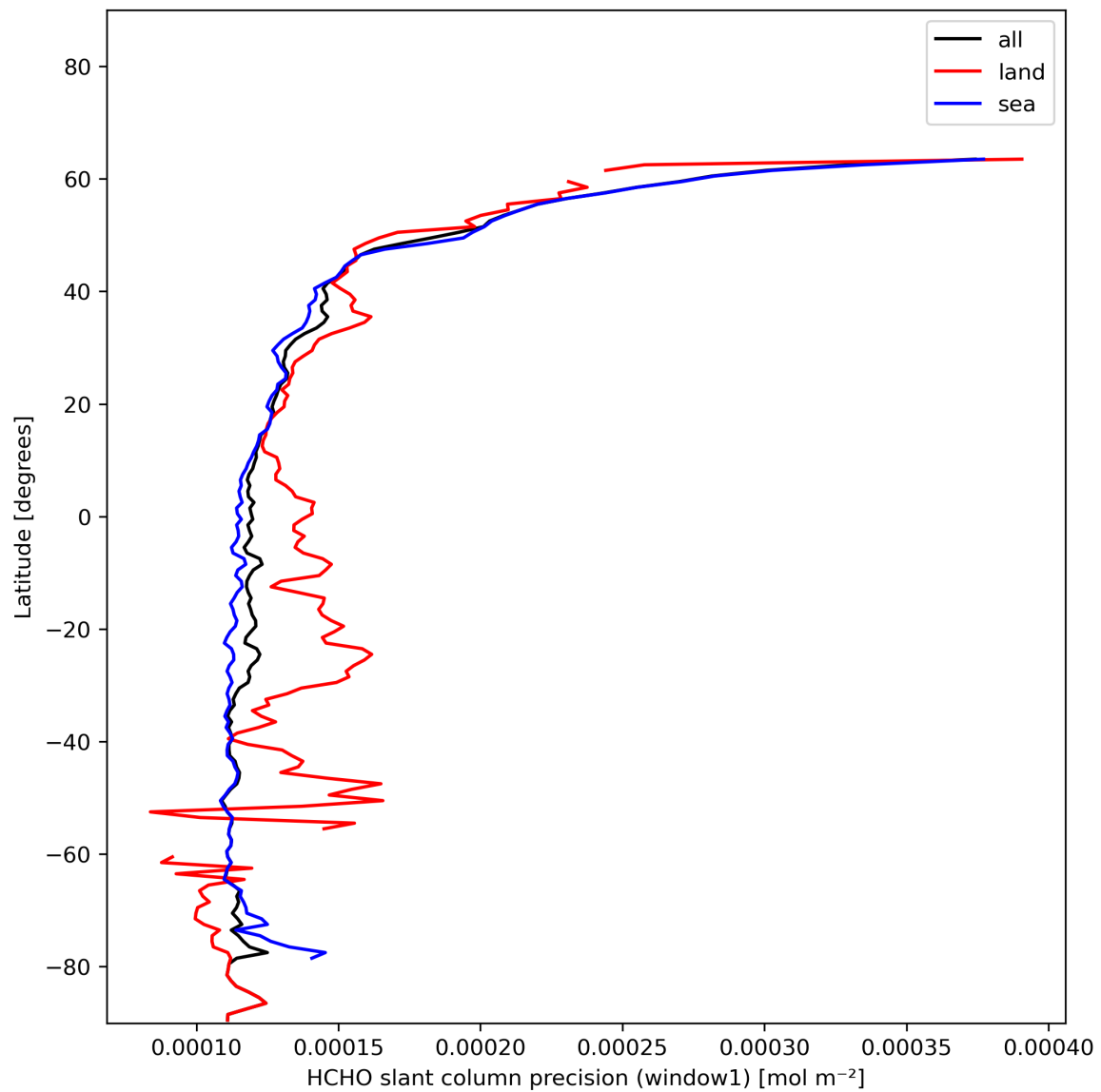
Figure 25: Zonal average of “HCHO slant column precision (window1)” for 2024-01-13 to 2024-01-15.
