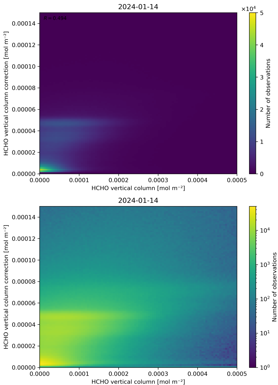
Figure 133: Scatter density plot of “HCHO vertical column” against “HCHO vertical column correction” for 2024-01-13 to 2024-01-15.
