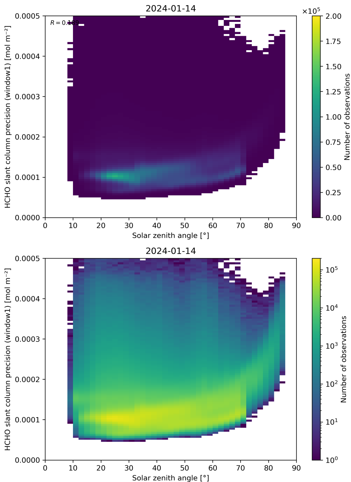
Figure 174: Scatter density plot of “Solar zenith angle” against “HCHO slant column precision (window1)” for 2024-01-13 to 2024-01-15.
