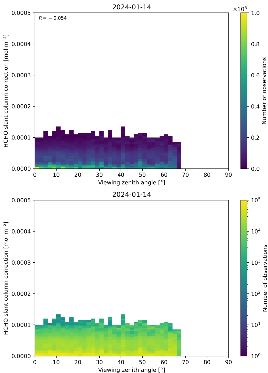
Figure 187: Scatter density plot of “Viewing zenith angle” against “HCHO slant column correction” for 2024-01-13 to 2024-01-15.
