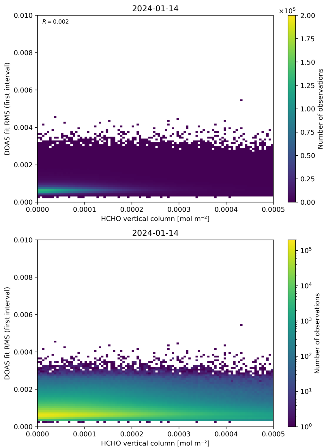
Figure 123: Scatter density plot of “HCHO vertical column” against “DOAS fit RMS (first interval)” for 2024-01-13 to 2024-01-15.
