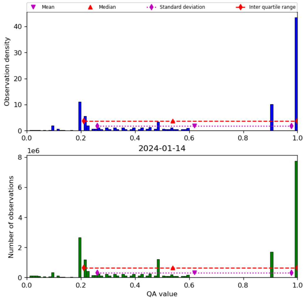
Figure 34: Histogram of “QA value” for 2024-01-13 to 2024-01-15
