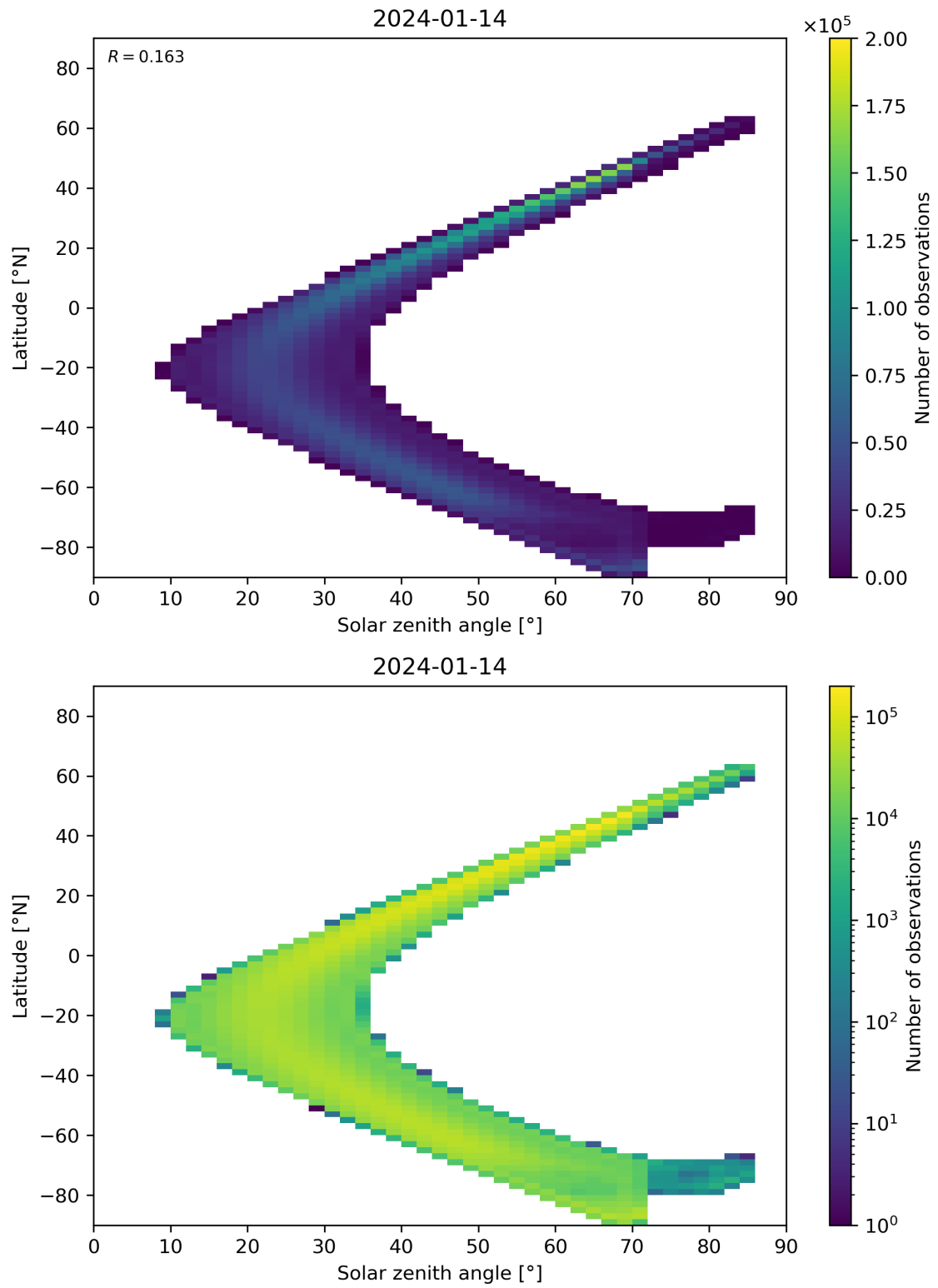
Figure 181: Scatter density plot of “Solar zenith angle” against “Latitude” for 2024-01-13 to 2024-01-15.
