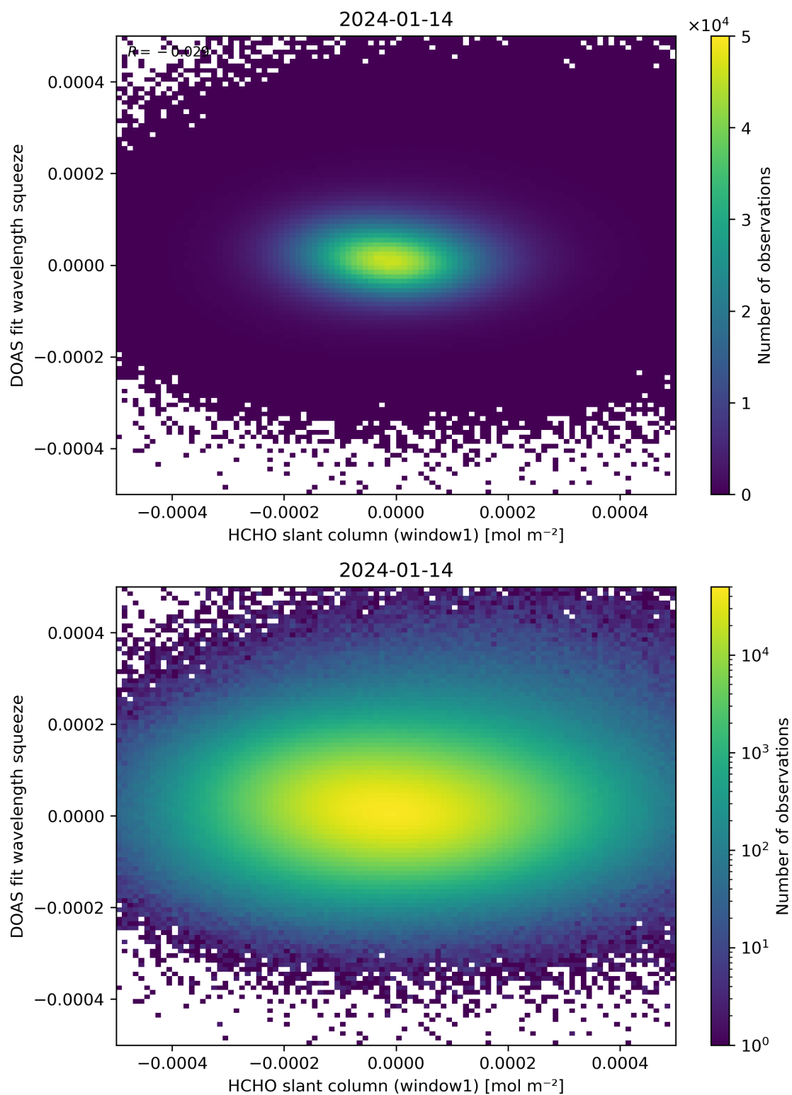
Figure 80: Scatter density plot of “HCHO slant column (window1)” against “DOAS fit wavelength squeeze” for 2024-01-13 to 2024-01-15.
