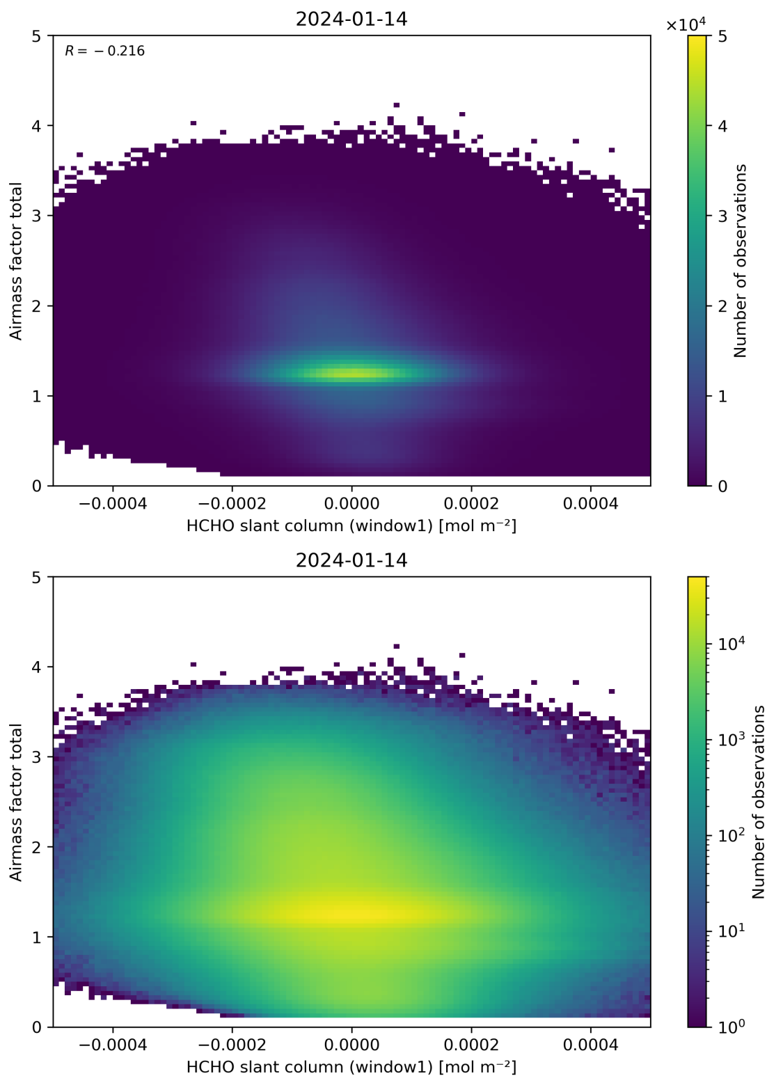
Figure 85: Scatter density plot of “HCHO slant column (window1)” against “Airmass factor total” for 2024-01-13 to 2024-01-15.
