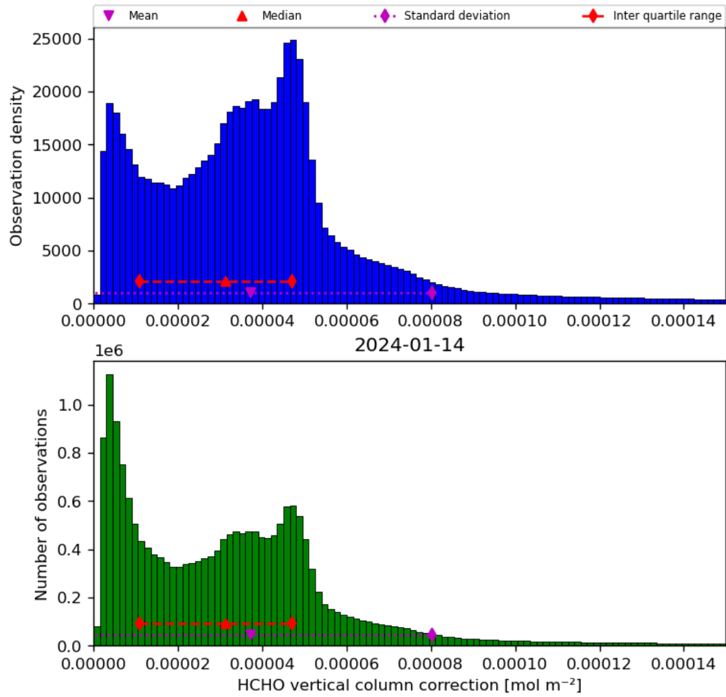
Figure 37: Histogram of “HCHO vertical column correction” for 2024-01-13 to 2024-01-15
