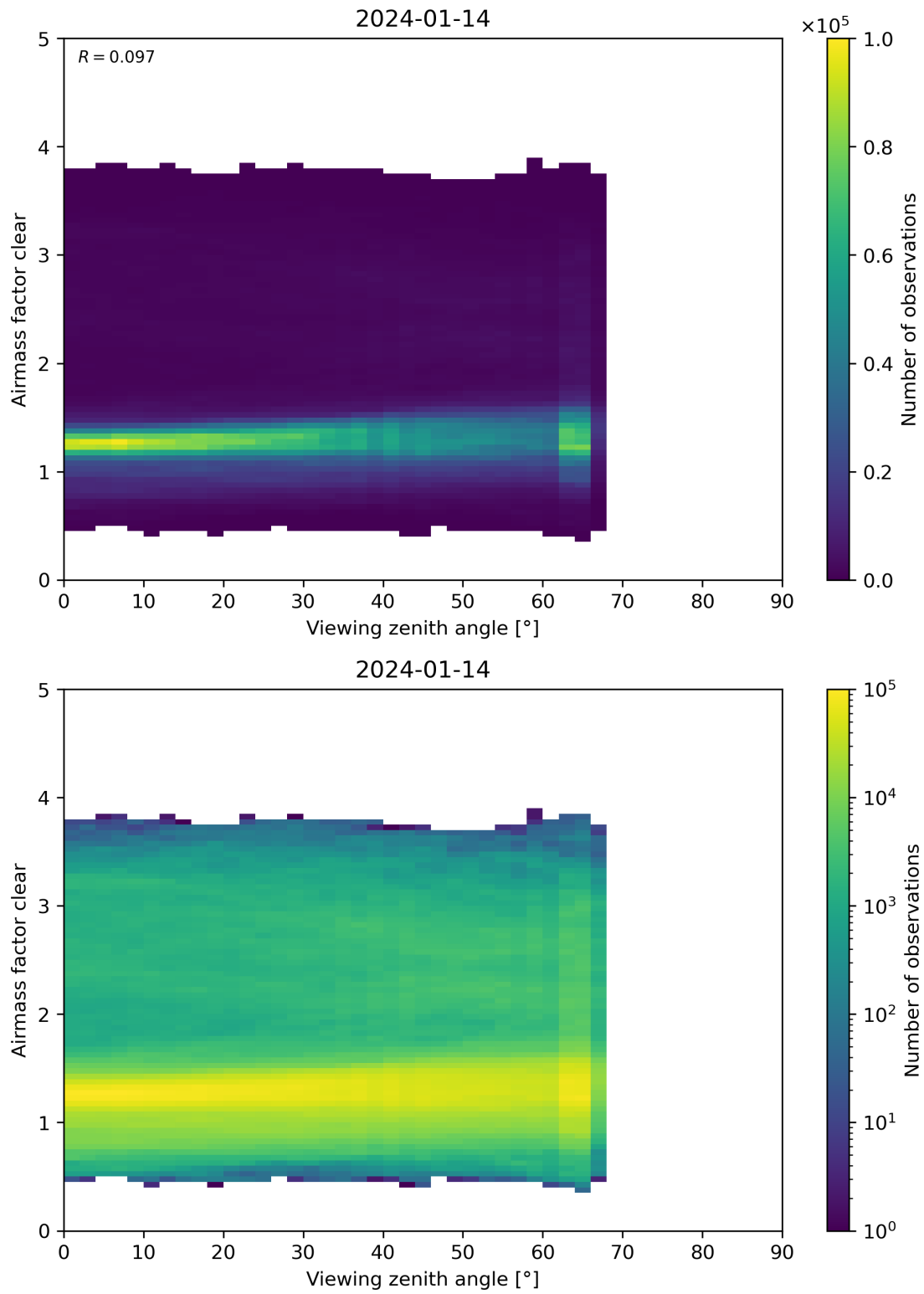
Figure 185: Scatter density plot of “Viewing zenith angle” against “Airmass factor clear” for 2024-01-13 to 2024-01-15.
