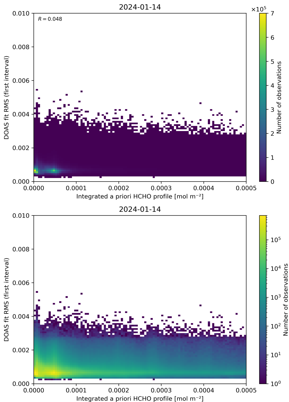
Figure 148: Scatter density plot of “Integrated a priori HCHO profile” against “DOAS fit RMS (first interval)” for 2024-01-13 to 2024-01-15.
