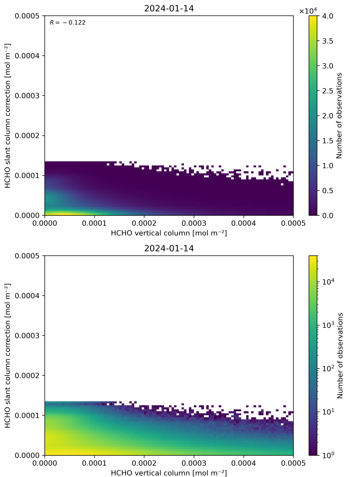
Figure 128: Scatter density plot of “HCHO vertical column” against “HCHO slant column correction” for 2024-01-13 to 2024-01-15.
