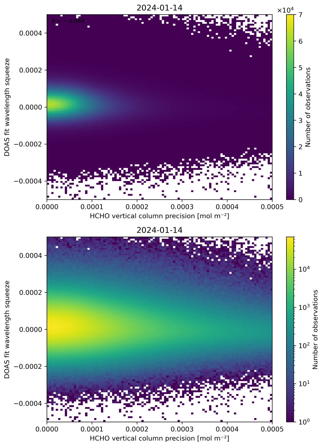
Figure 138: Scatter density plot of “HCHO vertical column precision” against “DOAS fit wavelength squeeze” for 2024-01-13 to 2024-01-15.
