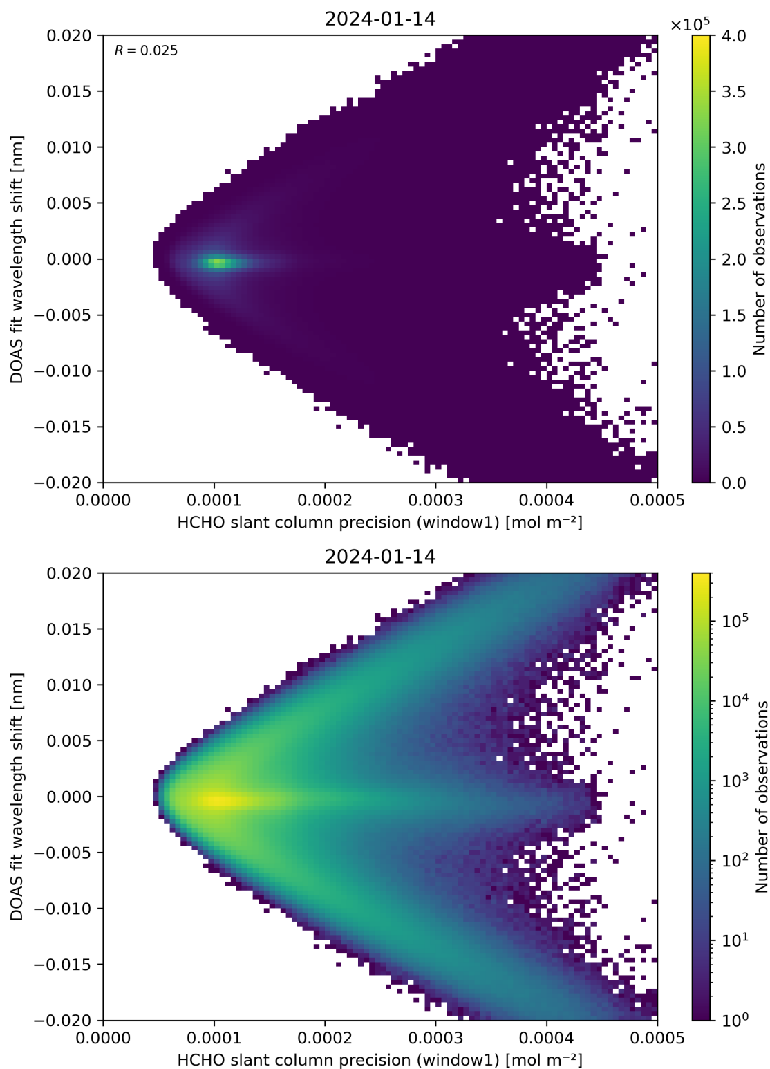
Figure 89: Scatter density plot of “HCHO slant column precision (window1)” against “DOAS fit wavelength shift” for 2024-01-13 to 2024-01-15.
