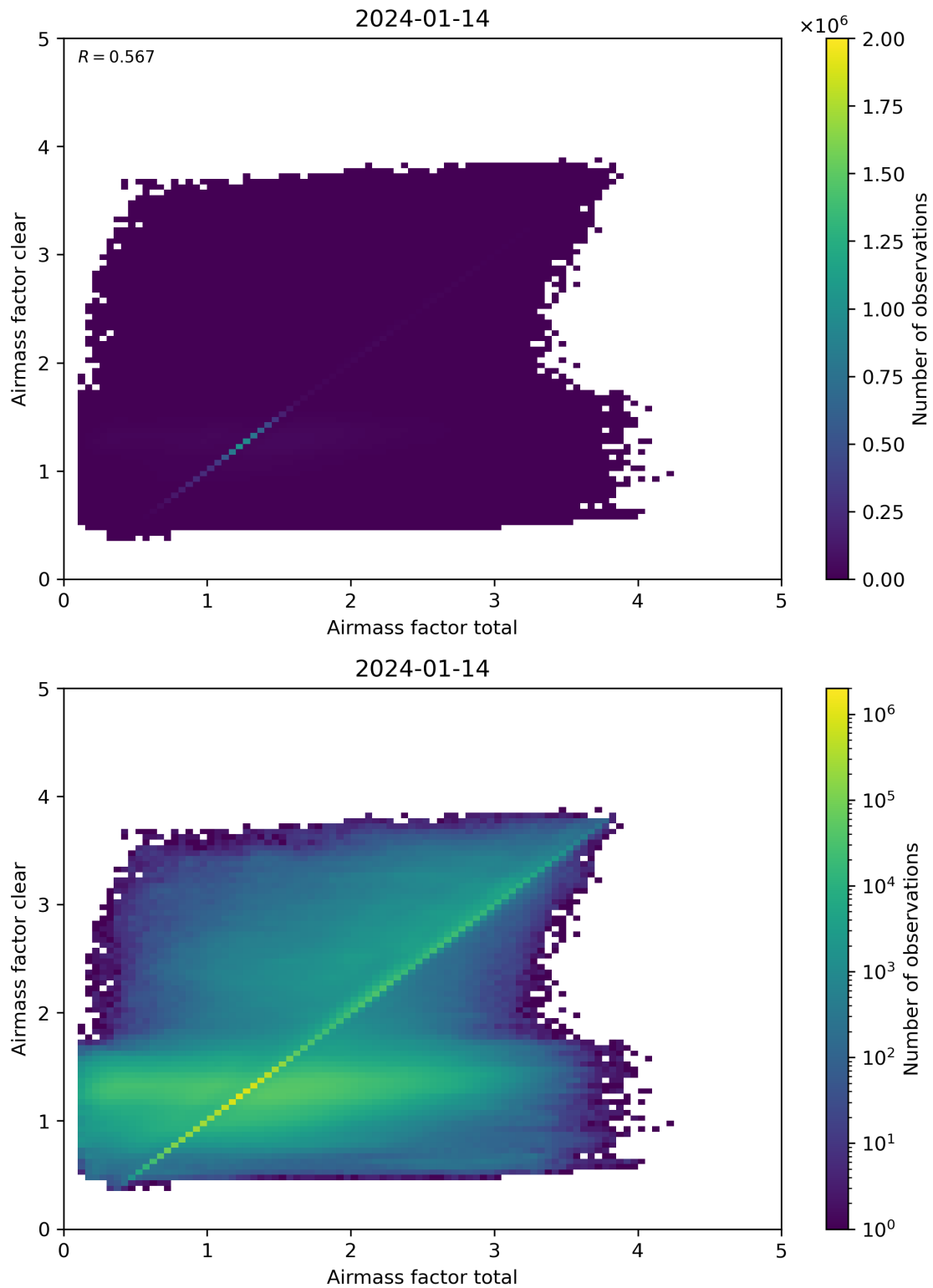
Figure 100: Scatter density plot of “Airmass factor total” against “Airmass factor clear” for 2024-01-13 to 2024-01-15.
