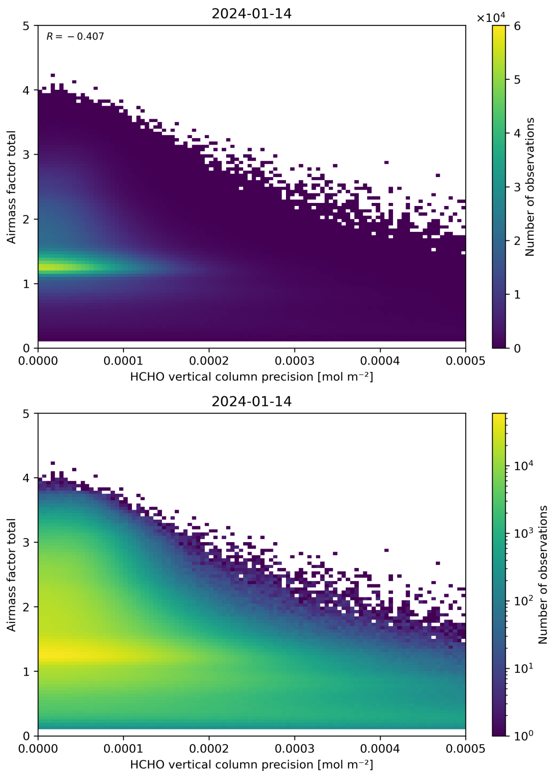
Figure 144: Scatter density plot of “HCHO vertical column precision” against “Airmass factor total” for 2024-01-13 to 2024-01-15.
