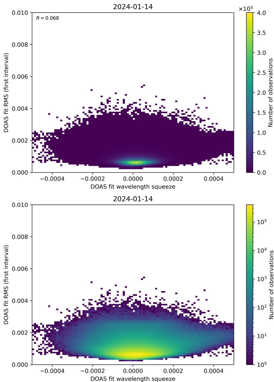
Figure 68: Scatter density plot of “DOAS fit wavelength squeeze” against “DOAS fit RMS (first interval)” for 2024-01-13 to 2024-01-15.
