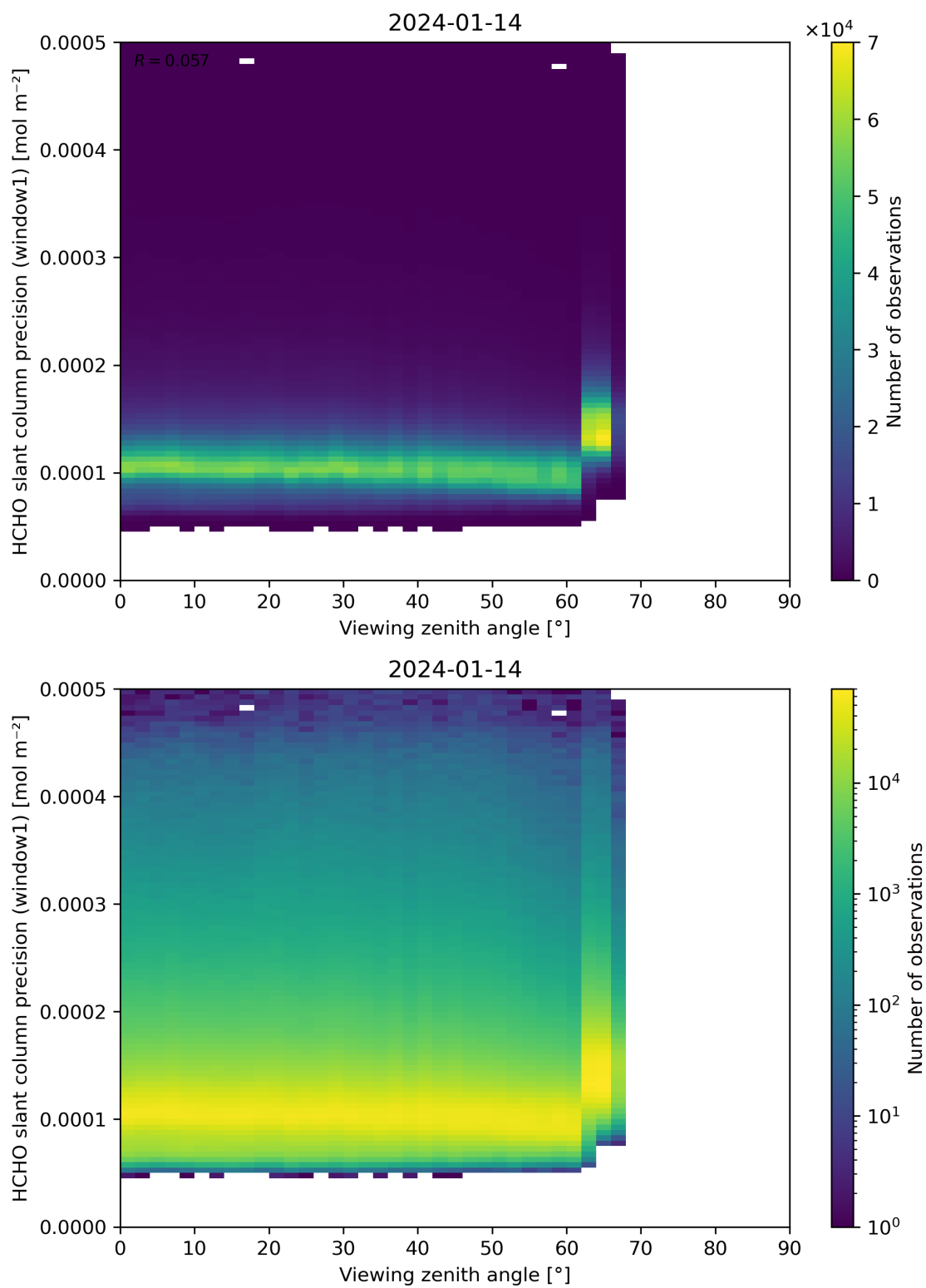
Figure 189: Scatter density plot of “Viewing zenith angle” against “HCHO slant column precision (window1)” for 2024-01-13 to 2024-01-15.
