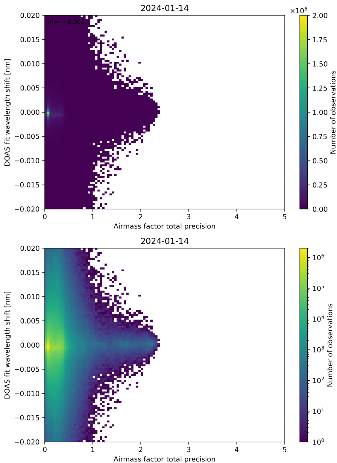
Figure 106: Scatter density plot of “Airmass factor total precision” against “DOAS fit wavelength shift” for 2024-01-13 to 2024-01-15.
