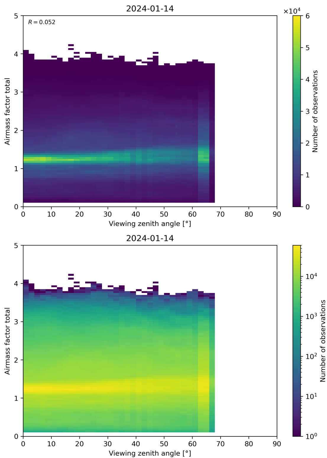
Figure 190: Scatter density plot of “Viewing zenith angle” against “Airmass factor total” for 2024-01-13 to 2024-01-15.
