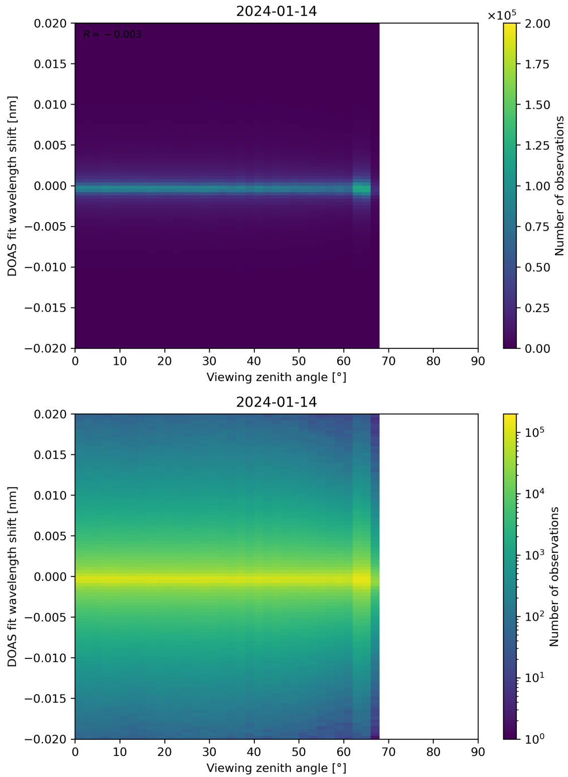
Figure 183: Scatter density plot of “Viewing zenith angle” against “DOAS fit wavelength shift” for 2024-01-13 to 2024-01-15.
