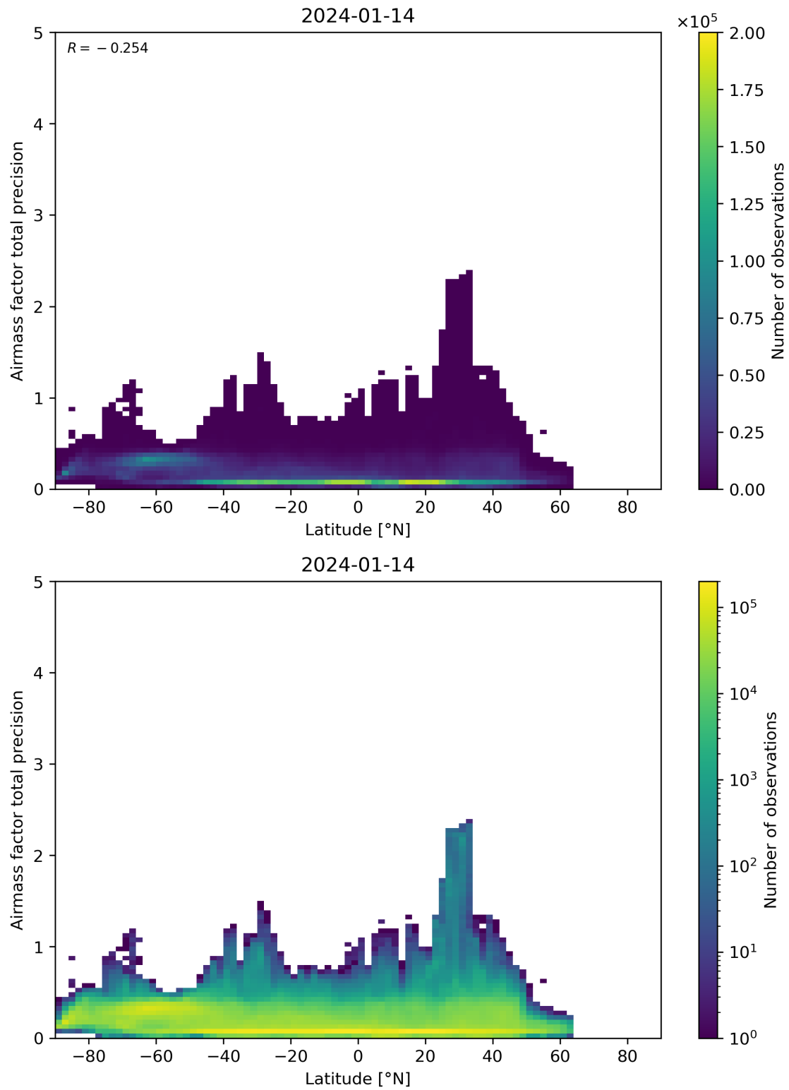
Figure 162: Scatter density plot of “Latitude” against “Airmass factor total precision” for 2024-01-13 to 2024-01-15.
