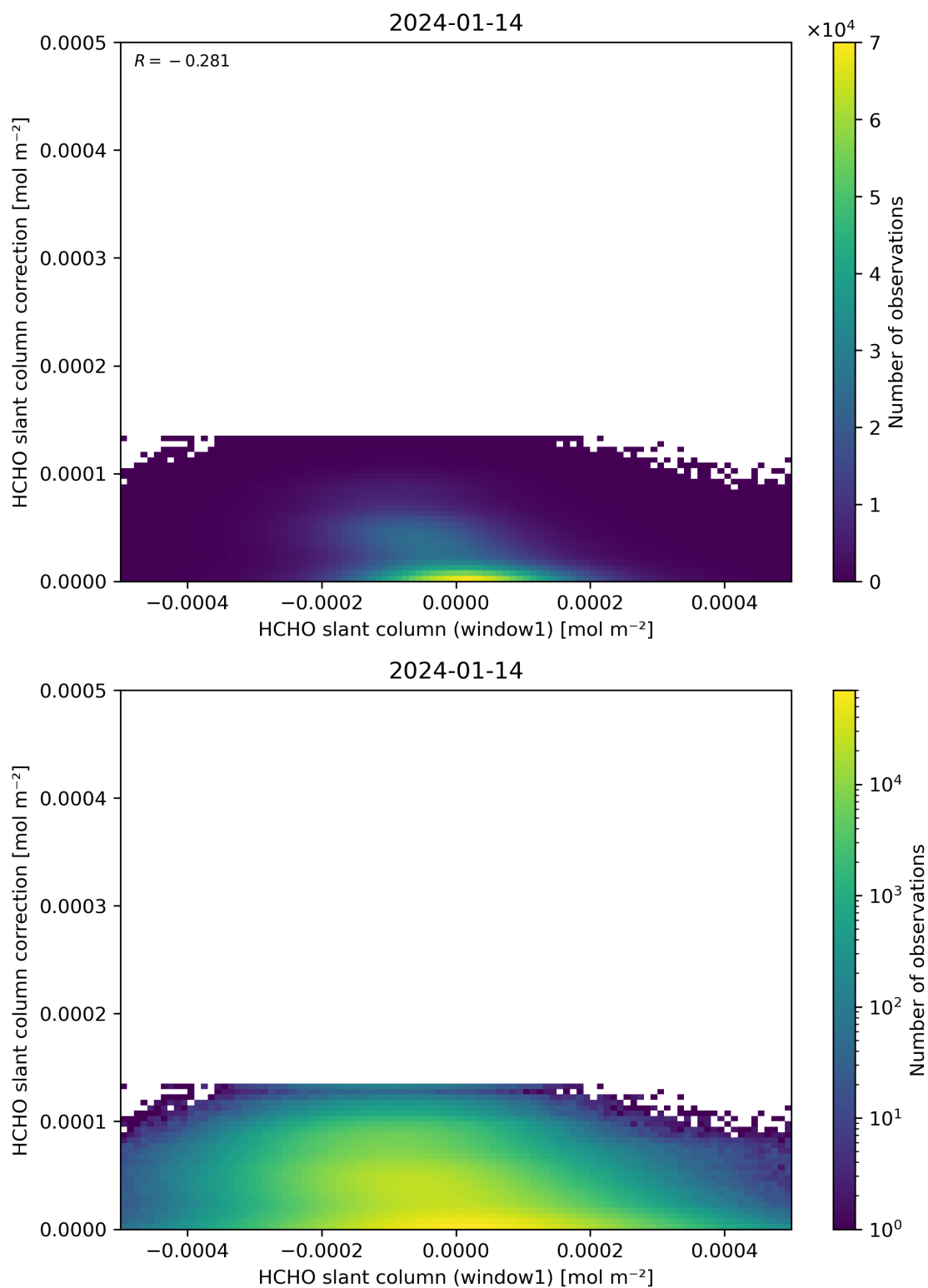
Figure 83: Scatter density plot of “HCHO slant column (window1)” against “HCHO slant column correction” for 2024-01-13 to 2024-01-15.
