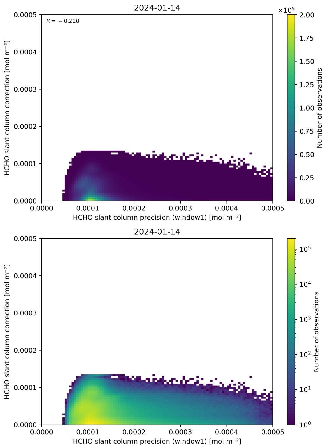
Figure 93: Scatter density plot of “HCHO slant column precision (window1)” against “HCHO slant column correction” for 2024-01-13 to 2024-01-15.
