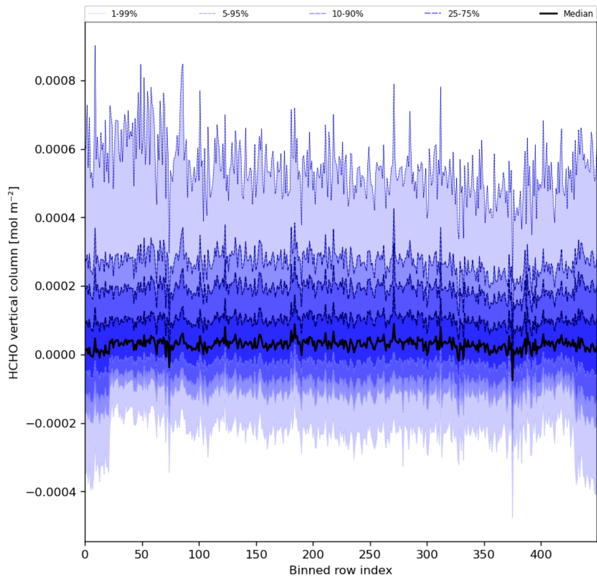
Figure 49: Along track statistics of “HCHO vertical column” for 2024-01-13 to 2024-01-15
