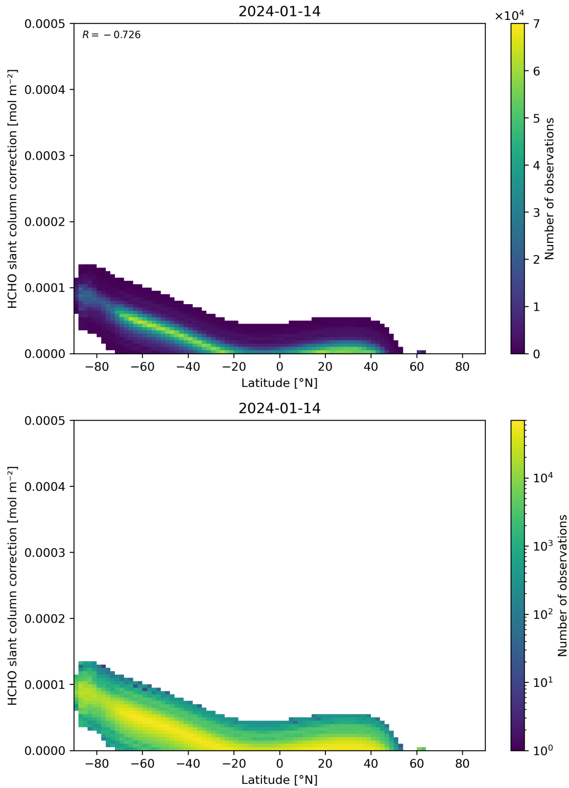
Figure 158: Scatter density plot of “Latitude” against “HCHO slant column correction” for 2024-01-13 to 2024-01-15.
