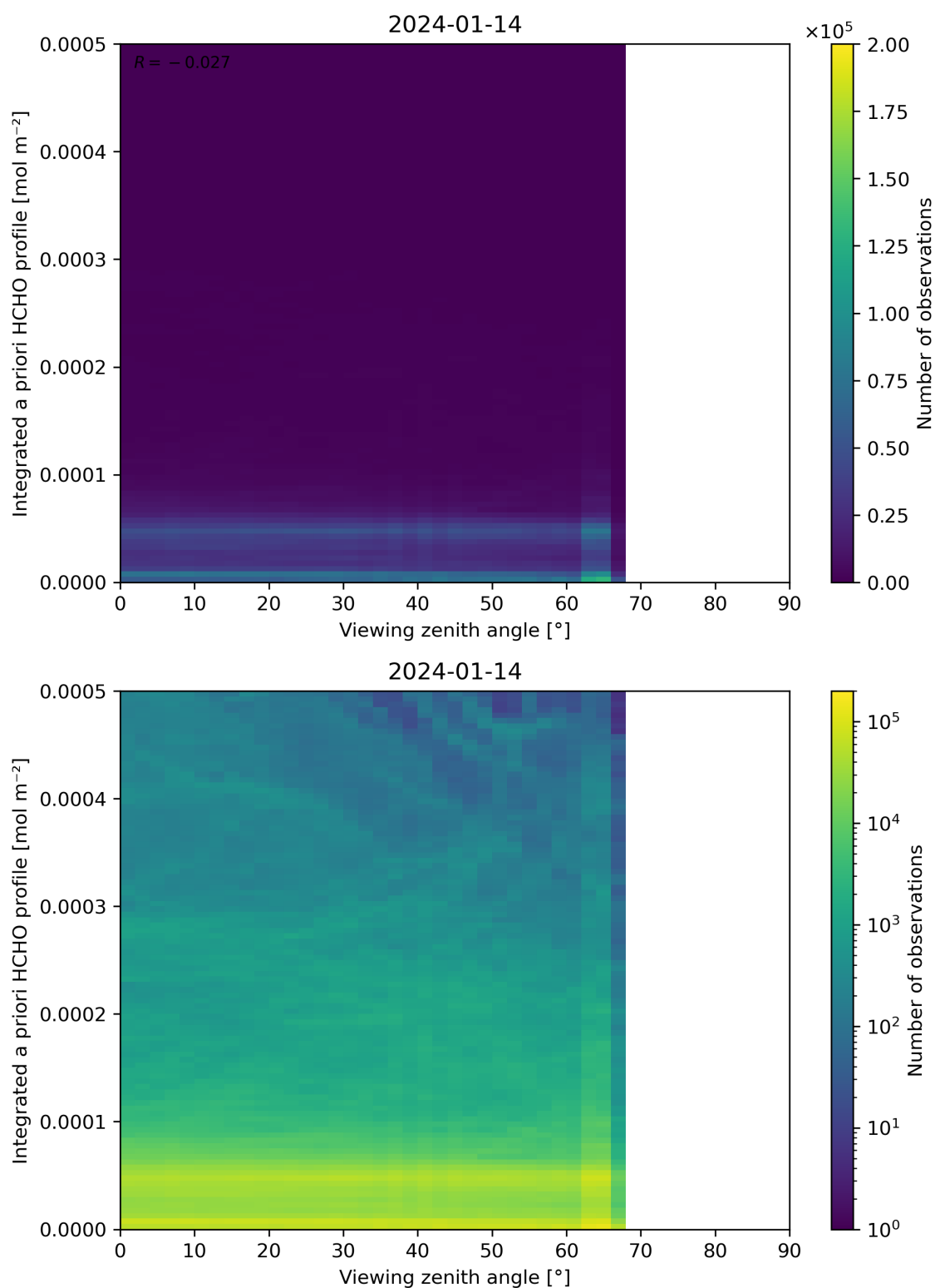
Figure 195: Scatter density plot of “Viewing zenith angle” against “Integrated a priori HCHO profile” for 2024-01-13 to 2024-01-15.
