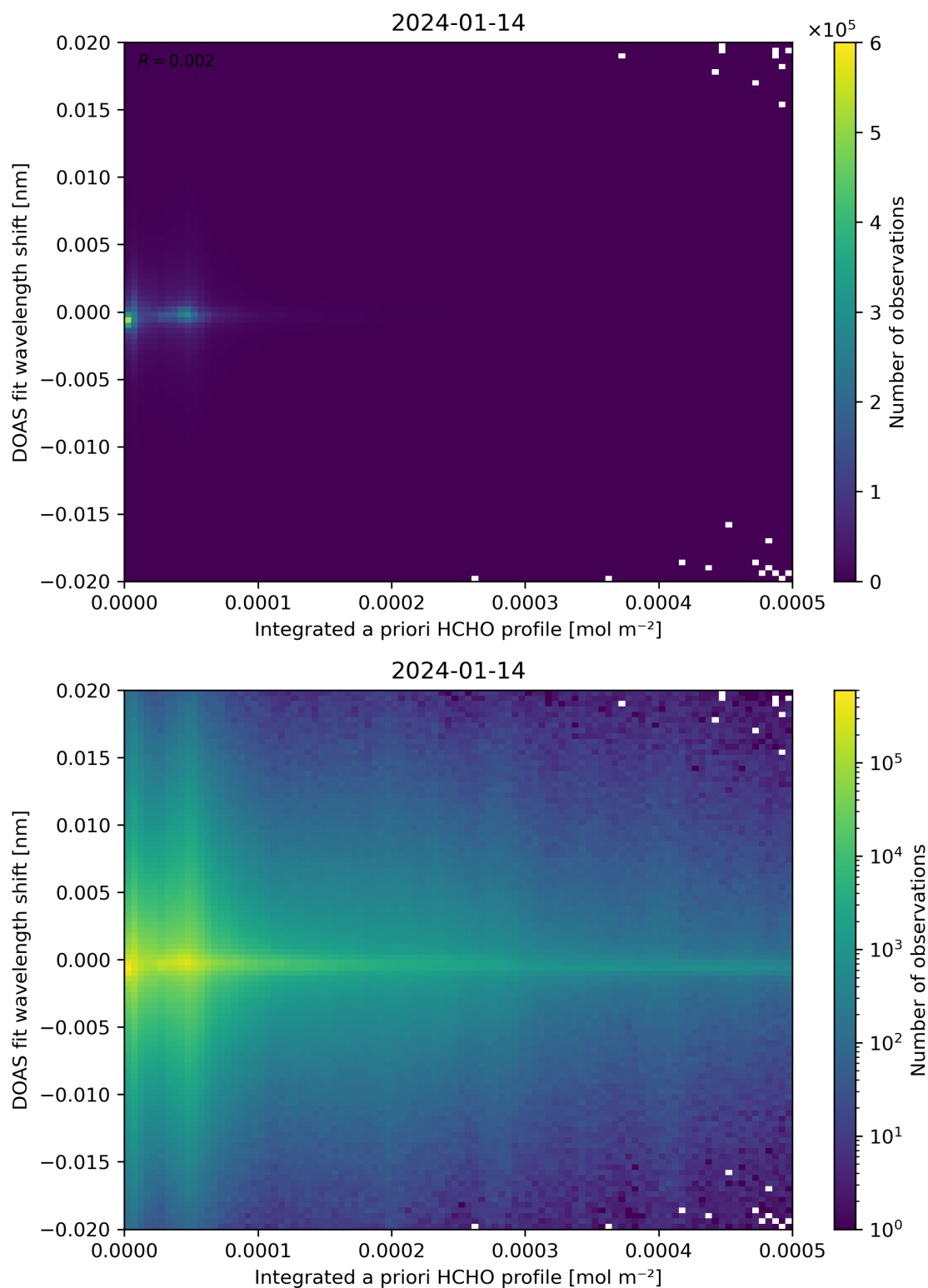
Figure 149: Scatter density plot of “Integrated a priori HCHO profile” against “DOAS fit wavelength shift” for 2024-01-13 to 2024-01-15.
