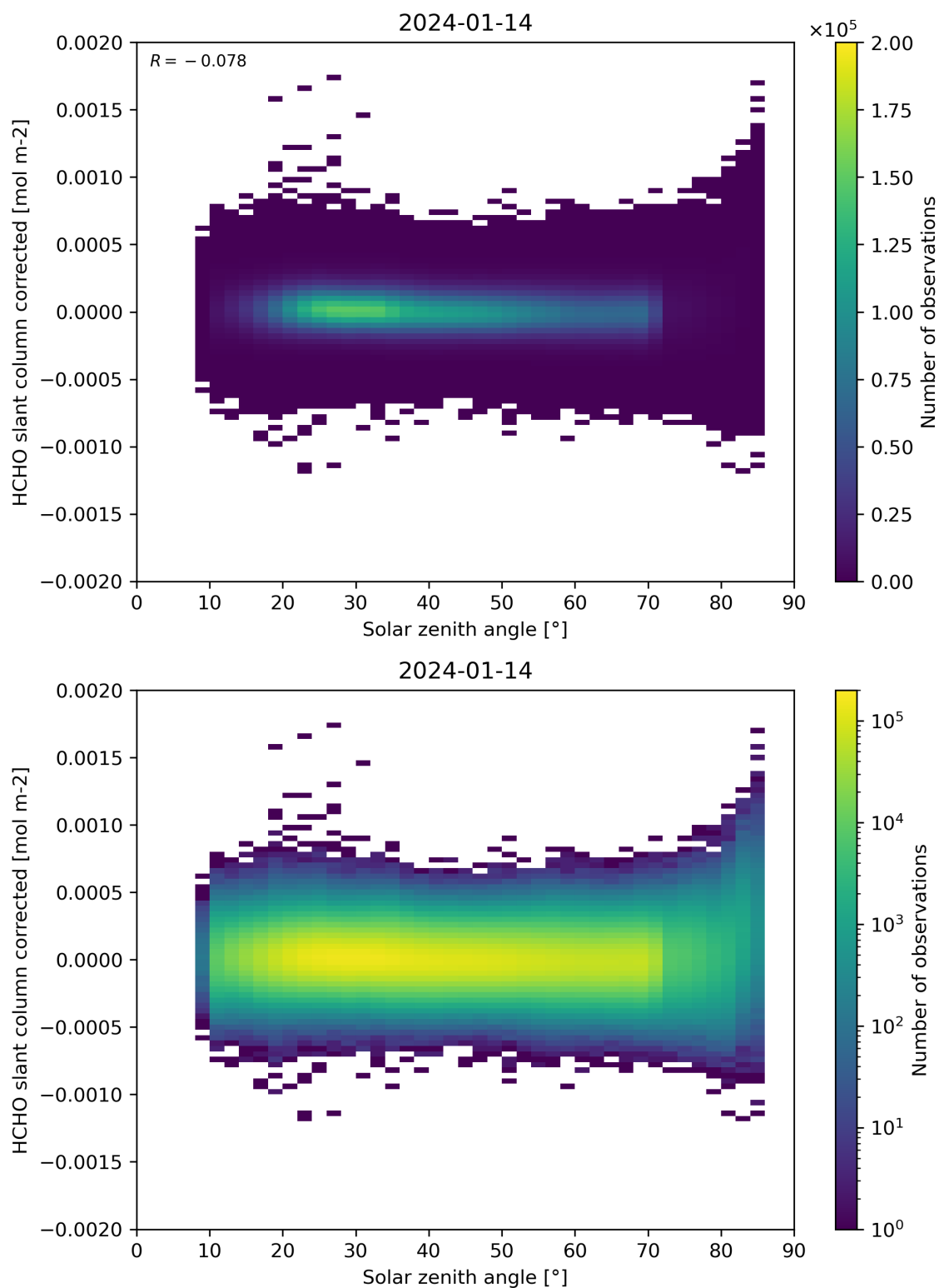
Figure 171: Scatter density plot of “Solar zenith angle” against “HCHO slant column corrected” for 2024-01-13 to 2024-01-15.
