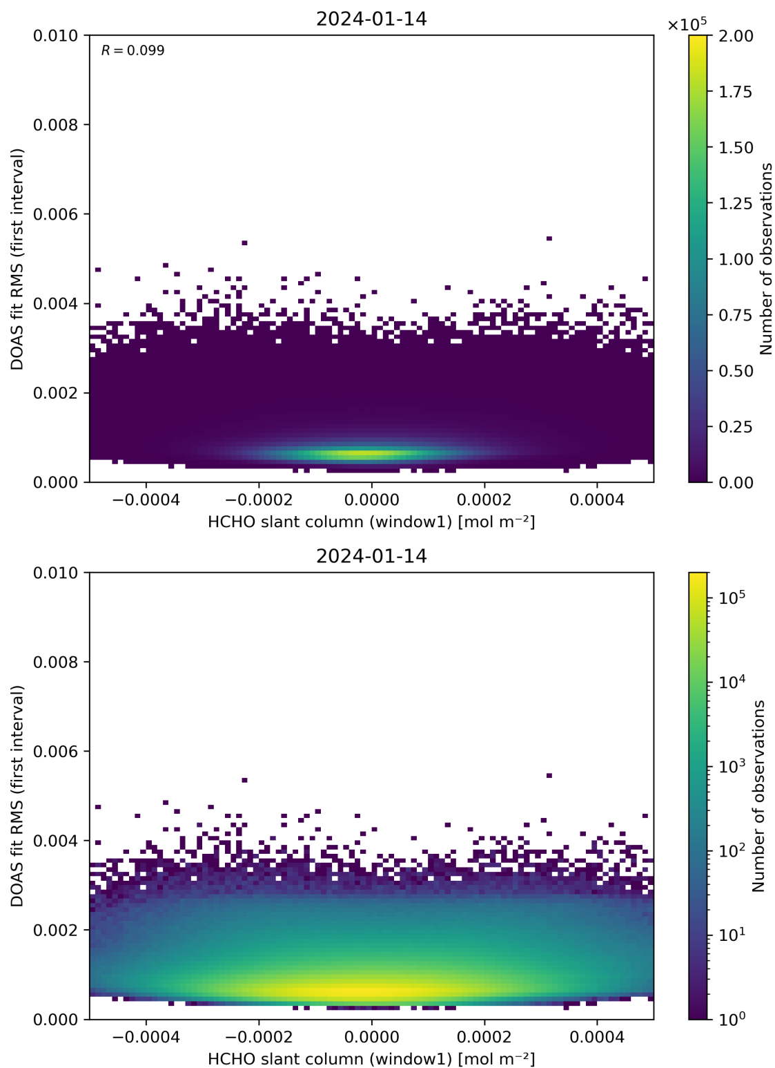
Figure 78: Scatter density plot of “HCHO slant column (window1)” against “DOAS fit RMS (first interval)” for 2024-01-13 to 2024-01-15.
