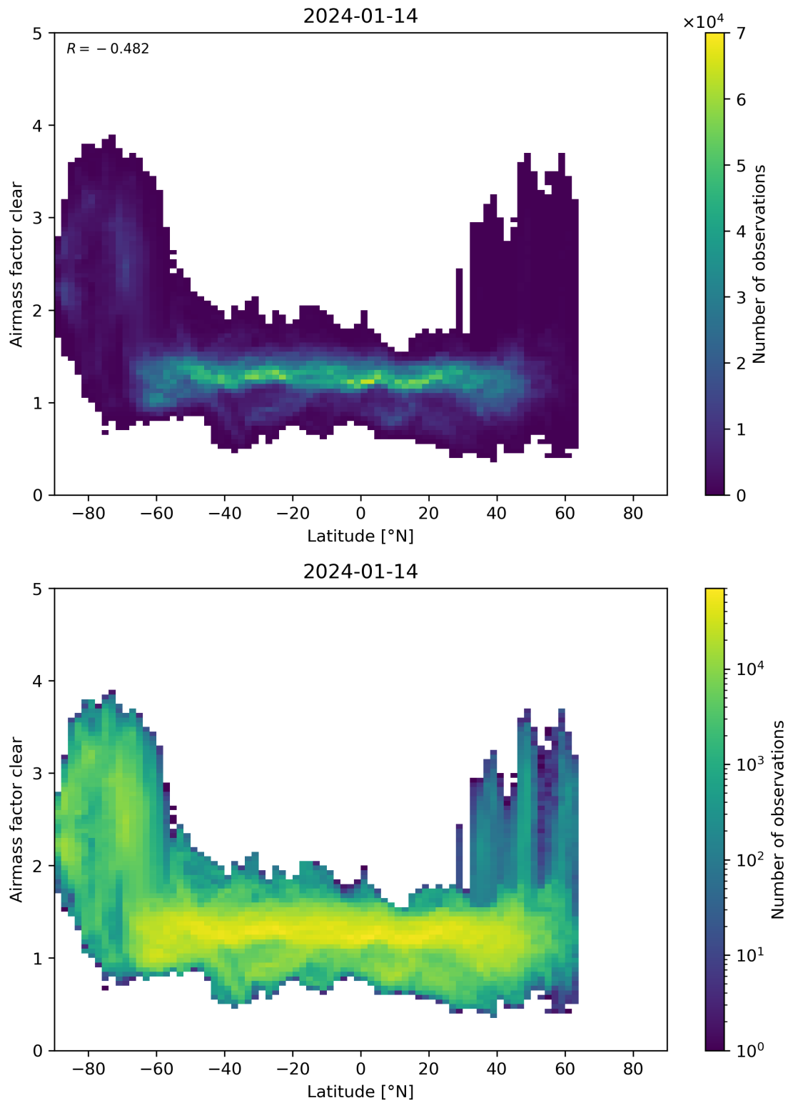
Figure 156: Scatter density plot of “Latitude” against “Airmass factor clear” for 2024-01-13 to 2024-01-15.
