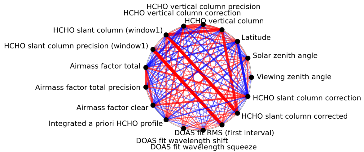
Figure 1: Map of correlation graph for 2024-01-13 to 2024-01-15.
