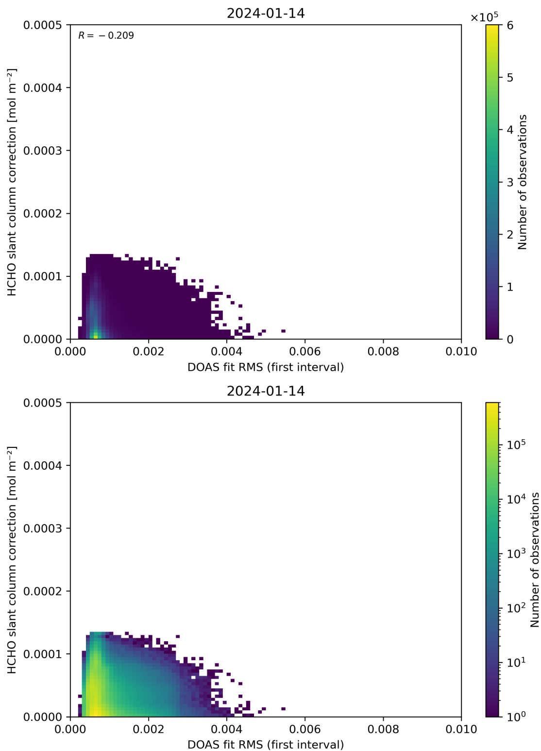
Figure 63: Scatter density plot of “DOAS fit RMS (first interval)” against “HCHO slant column correction” for 2024-01-13 to 2024-01-15.
