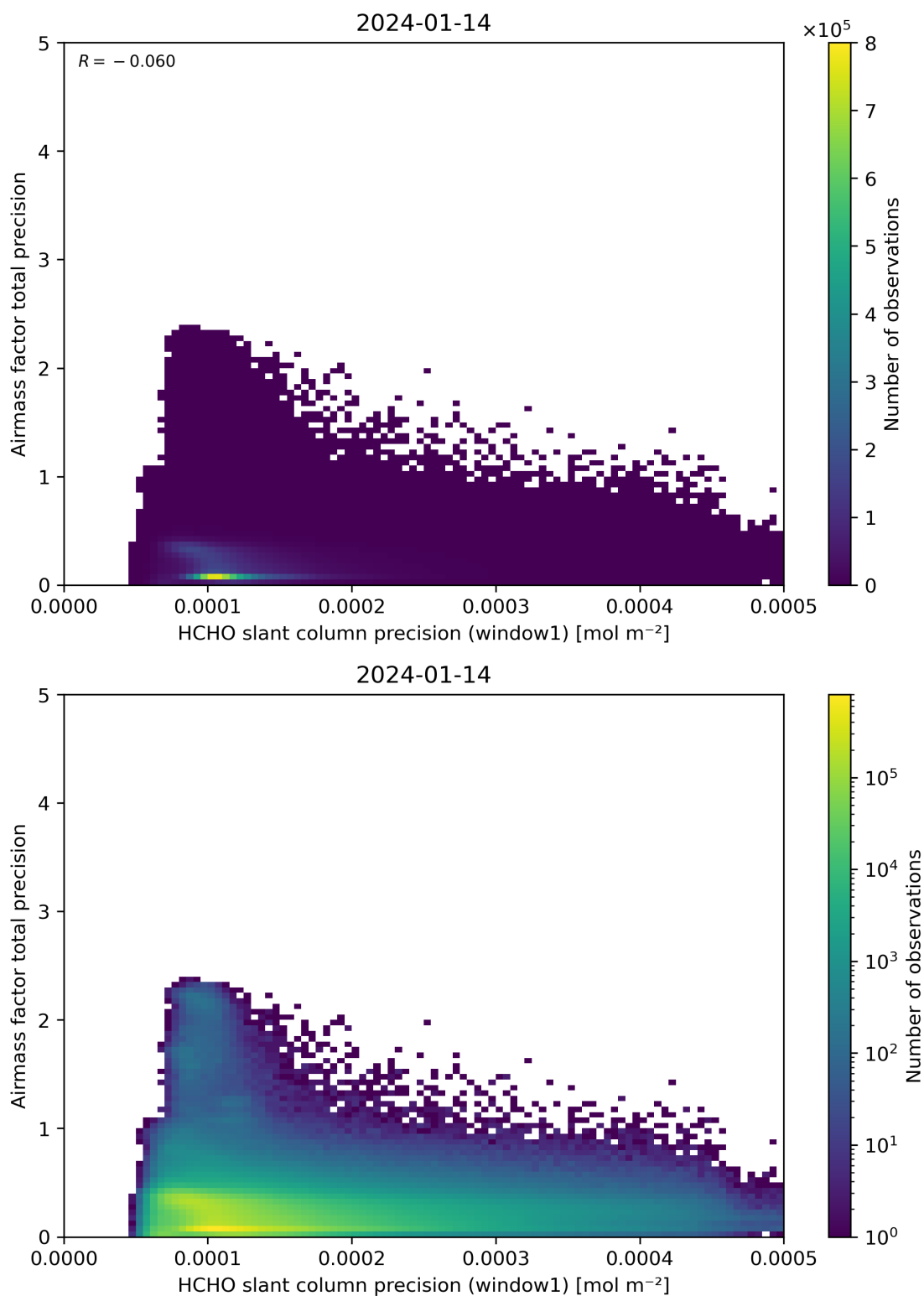
Figure 95: Scatter density plot of “HCHO slant column precision (window1)” against “Airmass factor total precision” for 2024-01-13 to 2024-01-15.
