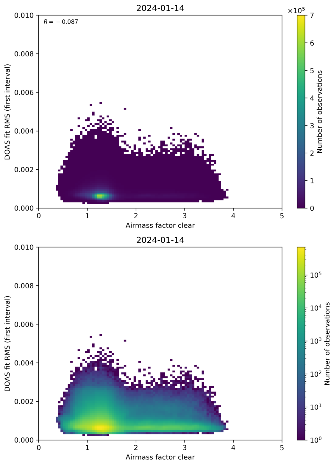
Figure 71: Scatter density plot of “Airmass factor clear” against “DOAS fit RMS (first interval)” for 2024-01-13 to 2024-01-15.
