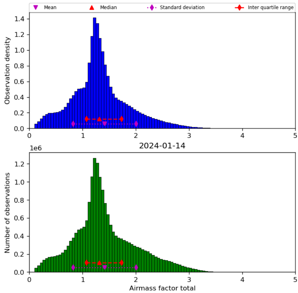
Figure 40: Histogram of “Airmass factor total” for 2024-01-13 to 2024-01-15
