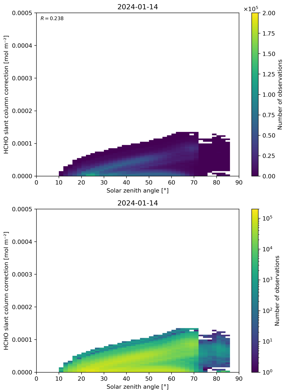
Figure 172: Scatter density plot of “Solar zenith angle” against “HCHO slant column correction” for 2024-01-13 to 2024-01-15.
