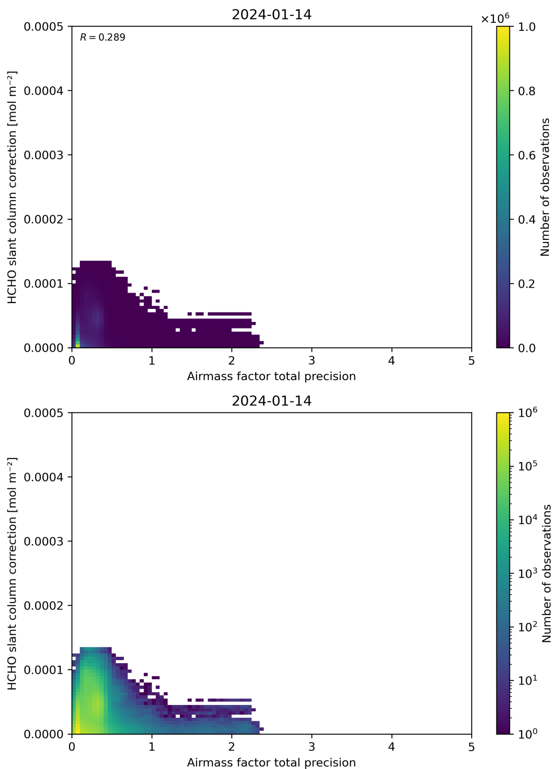
Figure 110: Scatter density plot of “Airmass factor total precision” against “HCHO slant column correction” for 2024-01-13 to 2024-01-15.
