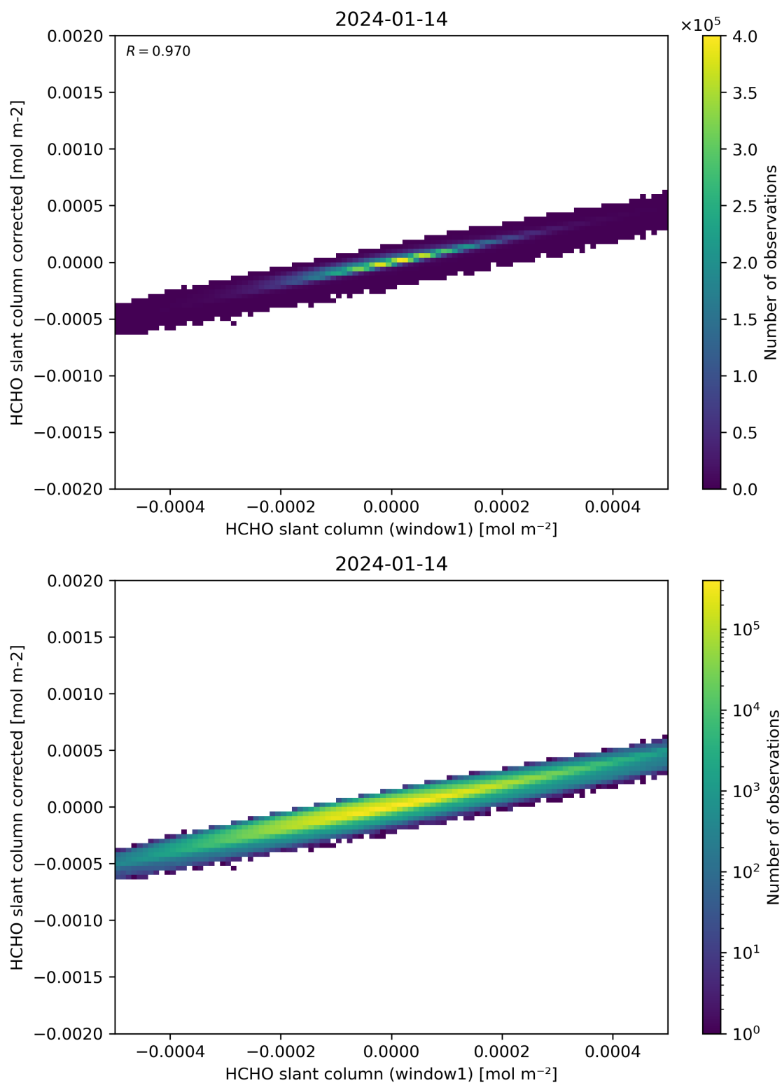
Figure 82: Scatter density plot of “HCHO slant column (window1)” against “HCHO slant column corrected” for 2024-01-13 to 2024-01-15.
