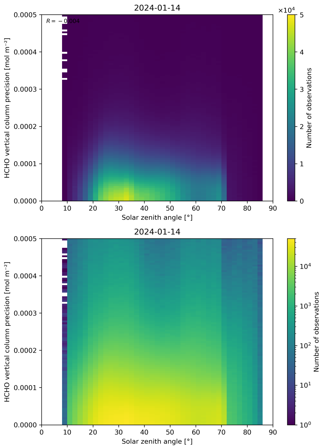
Figure 179: Scatter density plot of “Solar zenith angle” against “HCHO vertical column precision” for 2024-01-13 to 2024-01-15.
