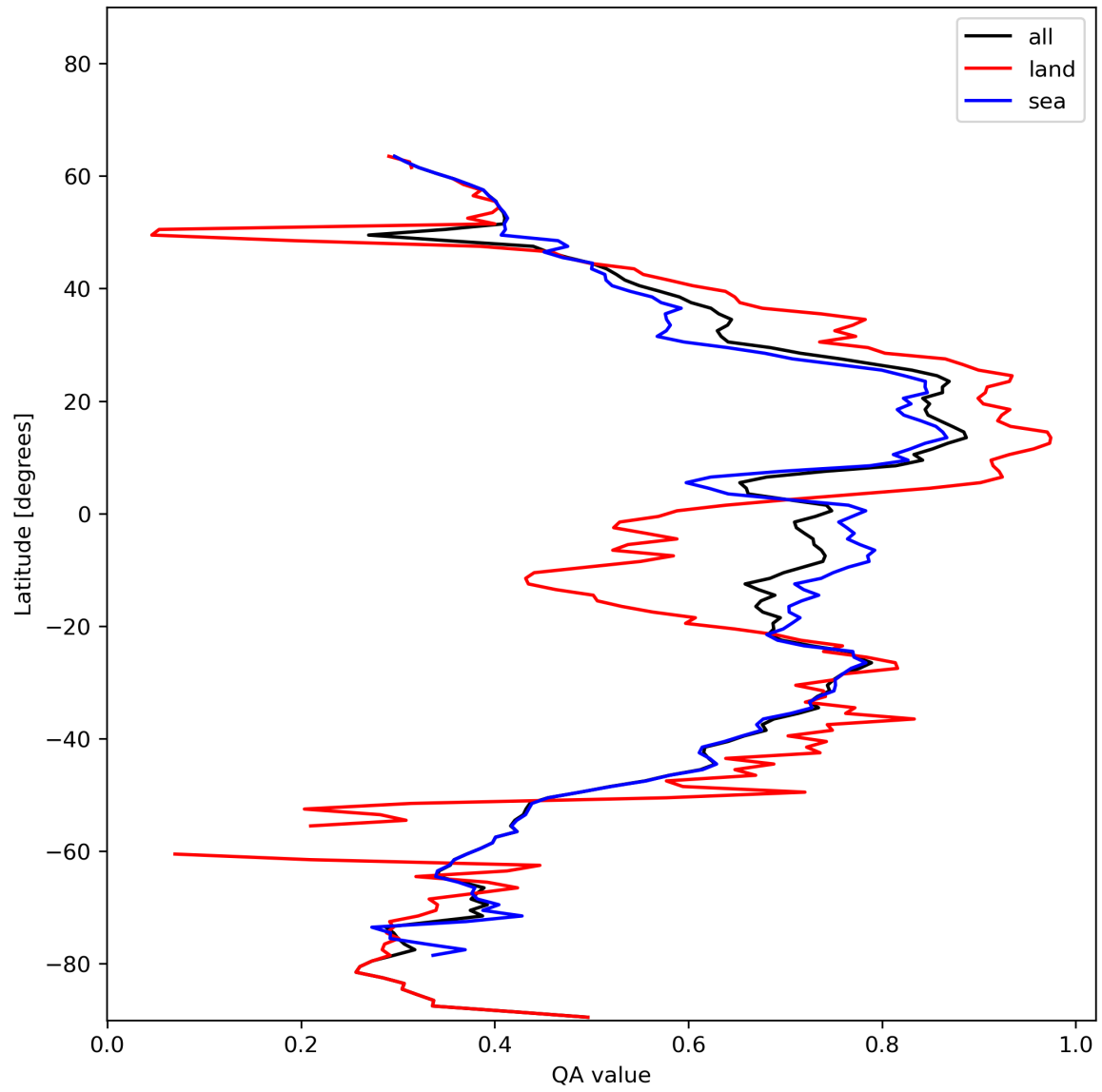
Figure 20: Zonal average of “QA value” for 2024-01-13 to 2024-01-15.
