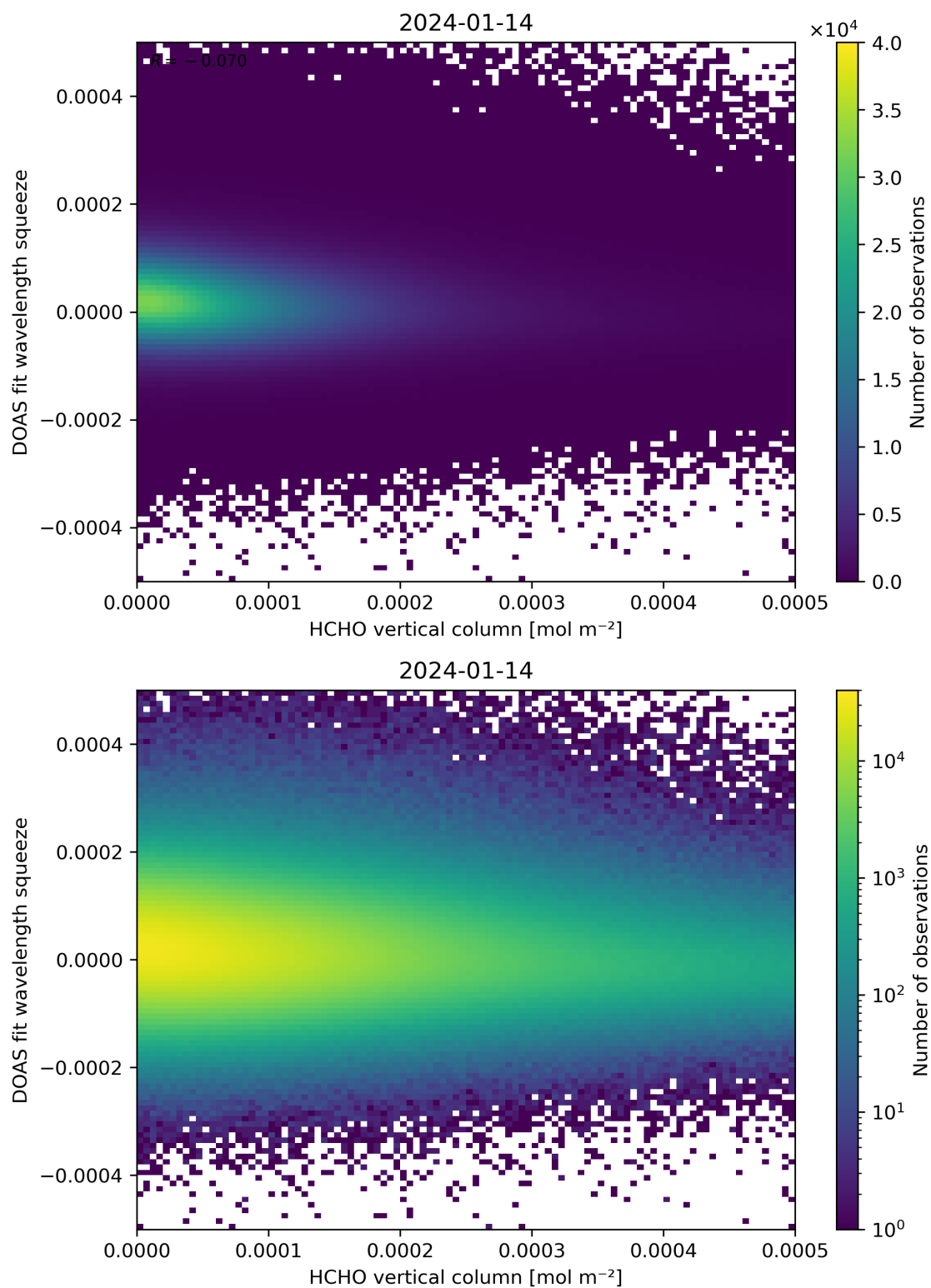
Figure 125: Scatter density plot of “HCHO vertical column” against “DOAS fit wavelength squeeze” for 2024-01-13 to 2024-01-15.
