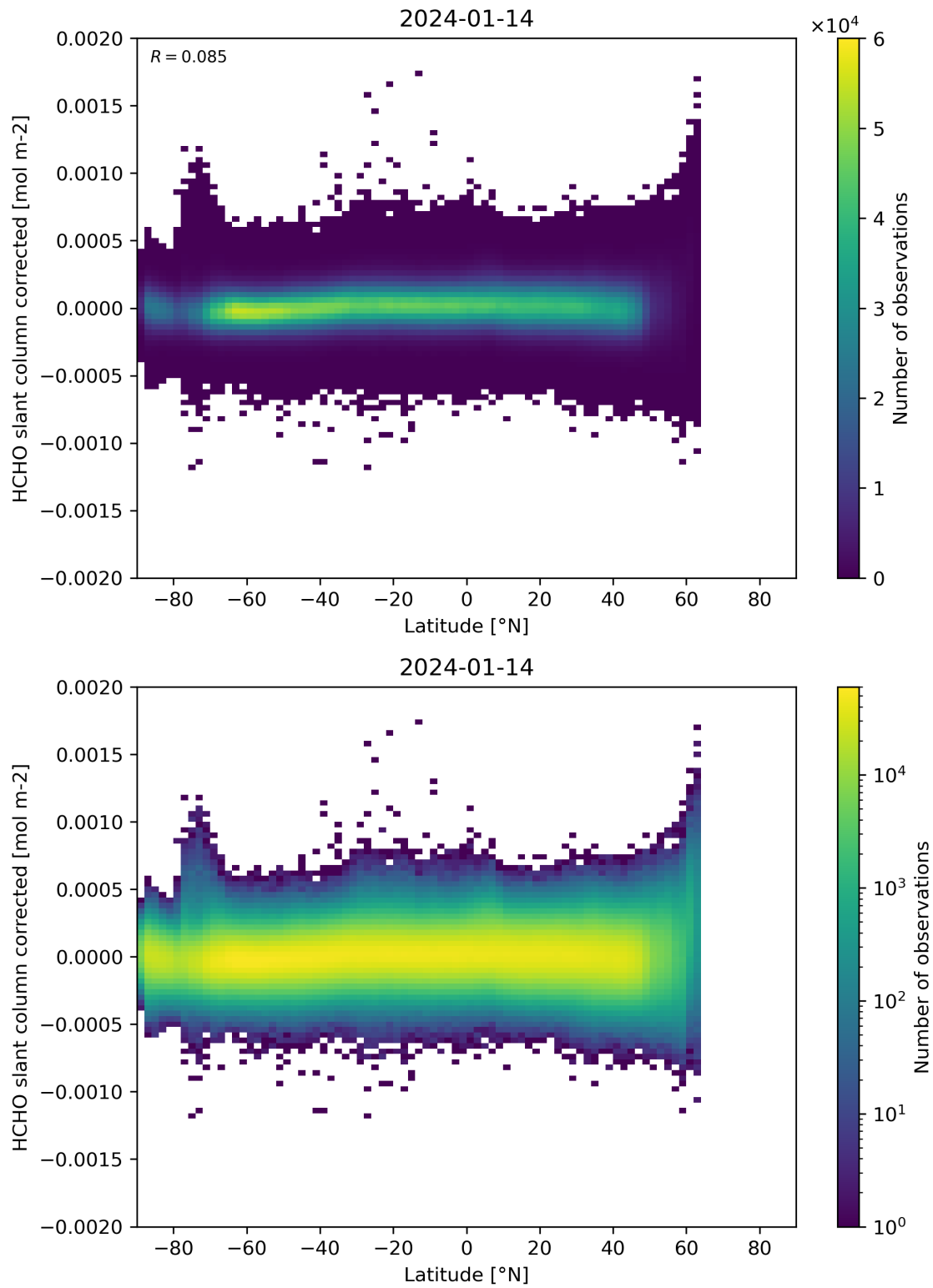
Figure 157: Scatter density plot of “Latitude” against “HCHO slant column corrected” for 2024-01-13 to 2024-01-15.
