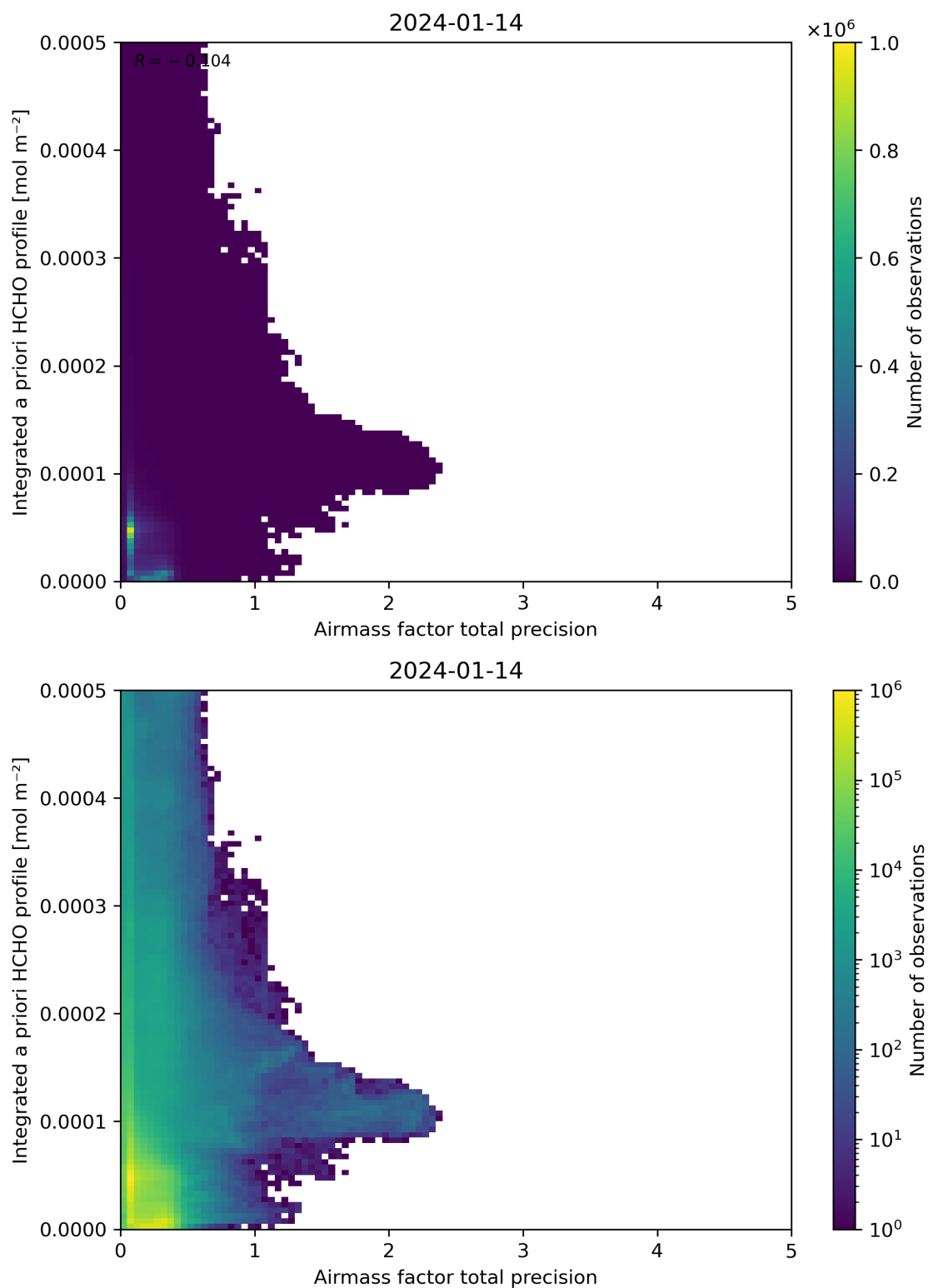
Figure 111: Scatter density plot of “Airmass factor total precision” against “Integrated a priori HCHO profile” for 2024-01-13 to 2024-01-15.
