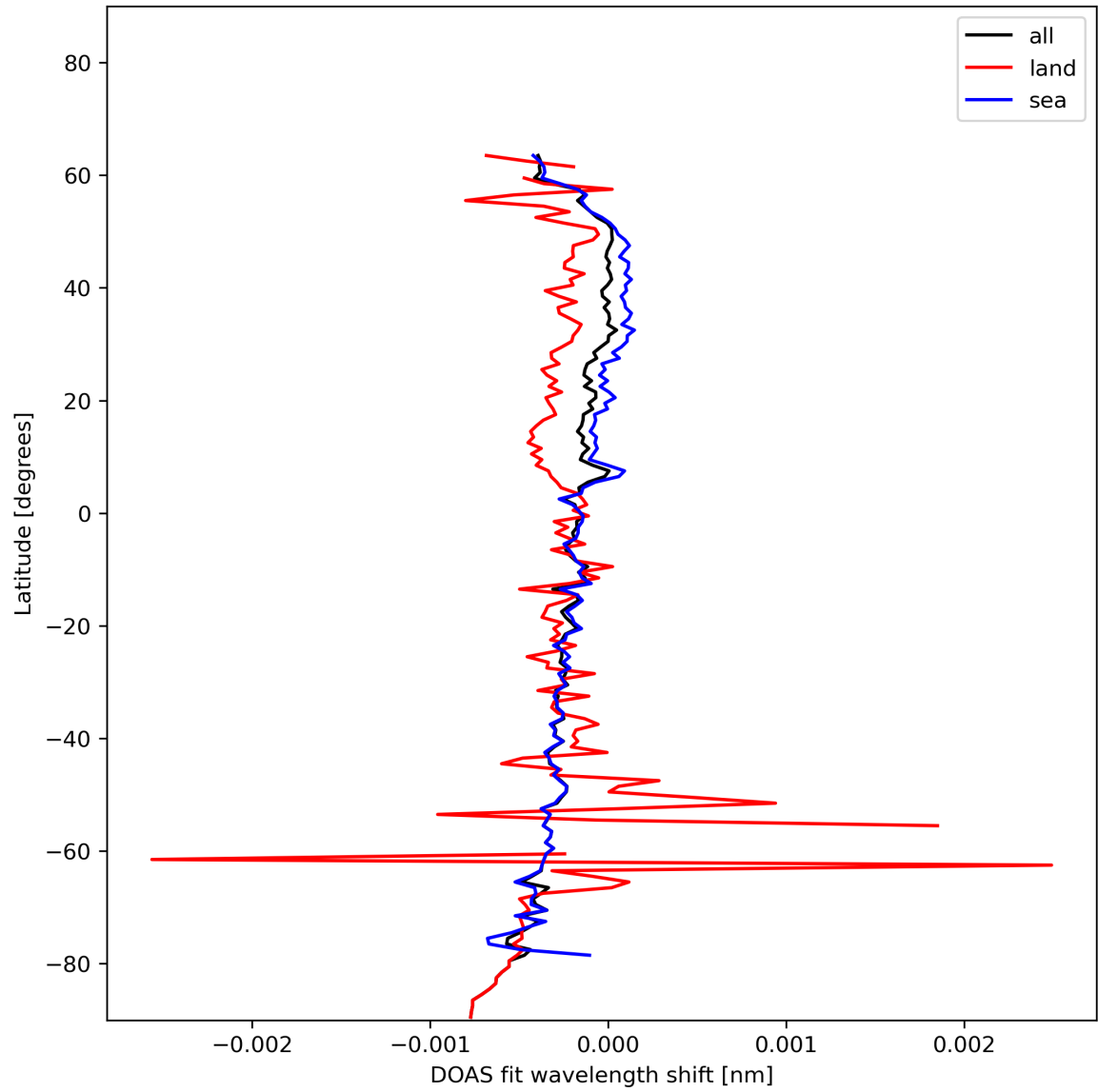
Figure 30: Zonal average of “DOAS fit wavelength shift” for 2024-01-13 to 2024-01-15.
