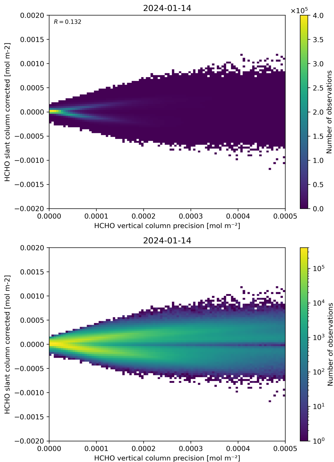
Figure 140: Scatter density plot of “HCHO vertical column precision” against “HCHO slant column corrected” for 2024-01-13 to 2024-01-15.
