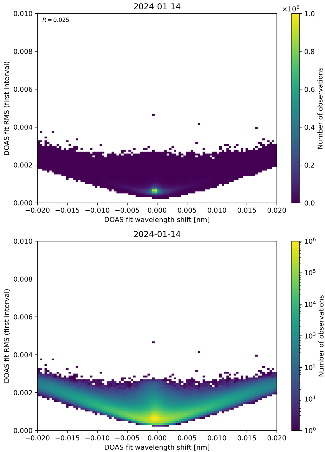
Figure 64: Scatter density plot of “DOAS fit wavelength shift” against “DOAS fit RMS (first interval)” for 2024-01-13 to 2024-01-15.
