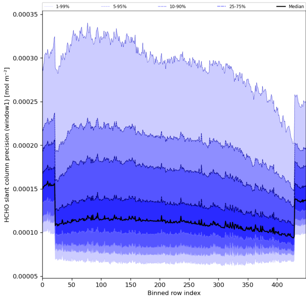
Figure 53: Along track statistics of “HCHO slant column precision (window1)” for 2024-01-13 to 2024-01-15
