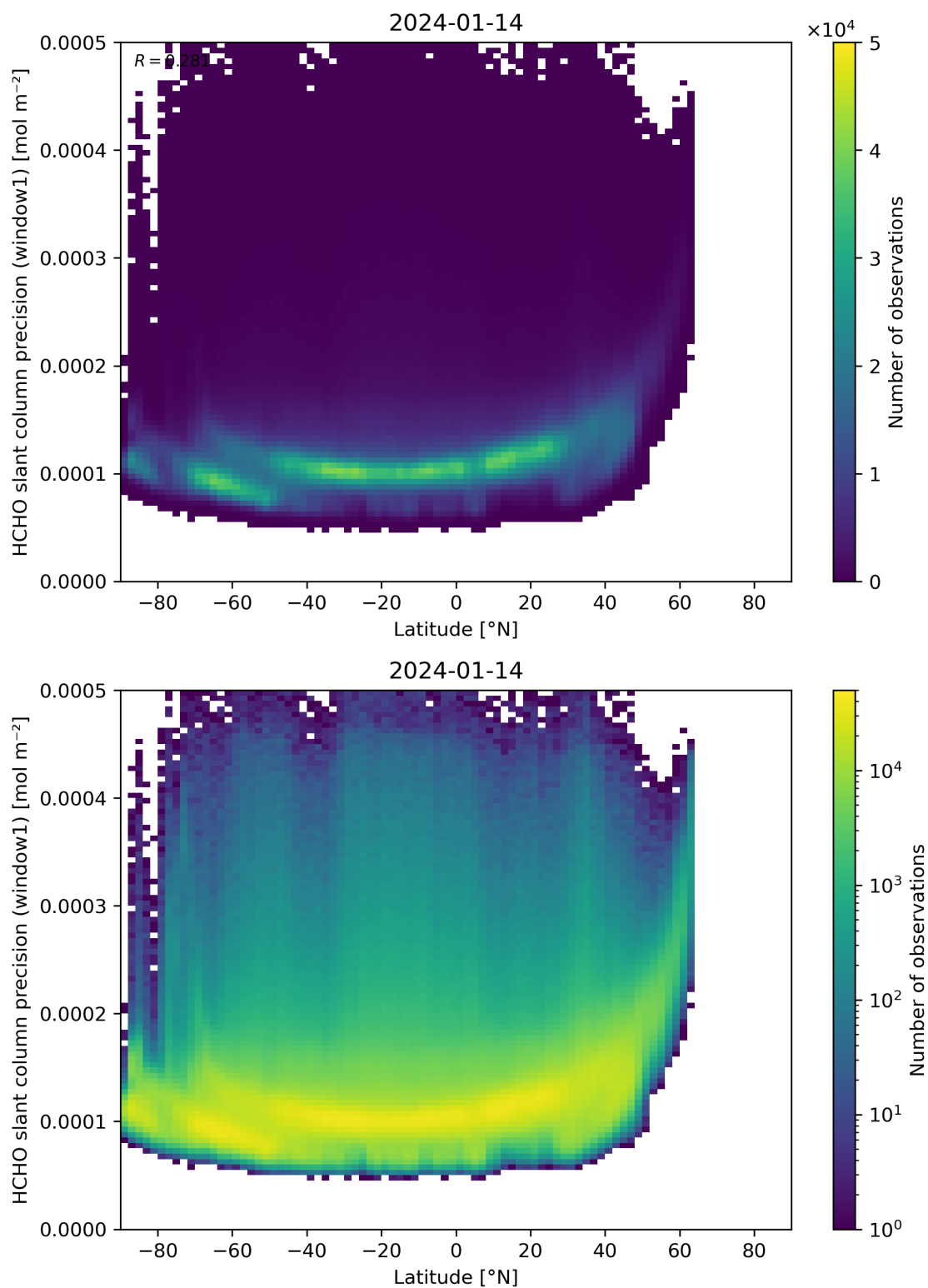
Figure 160: Scatter density plot of “Latitude” against “HCHO slant column precision (window1)” for 2024-01-13 to 2024-01-15.
