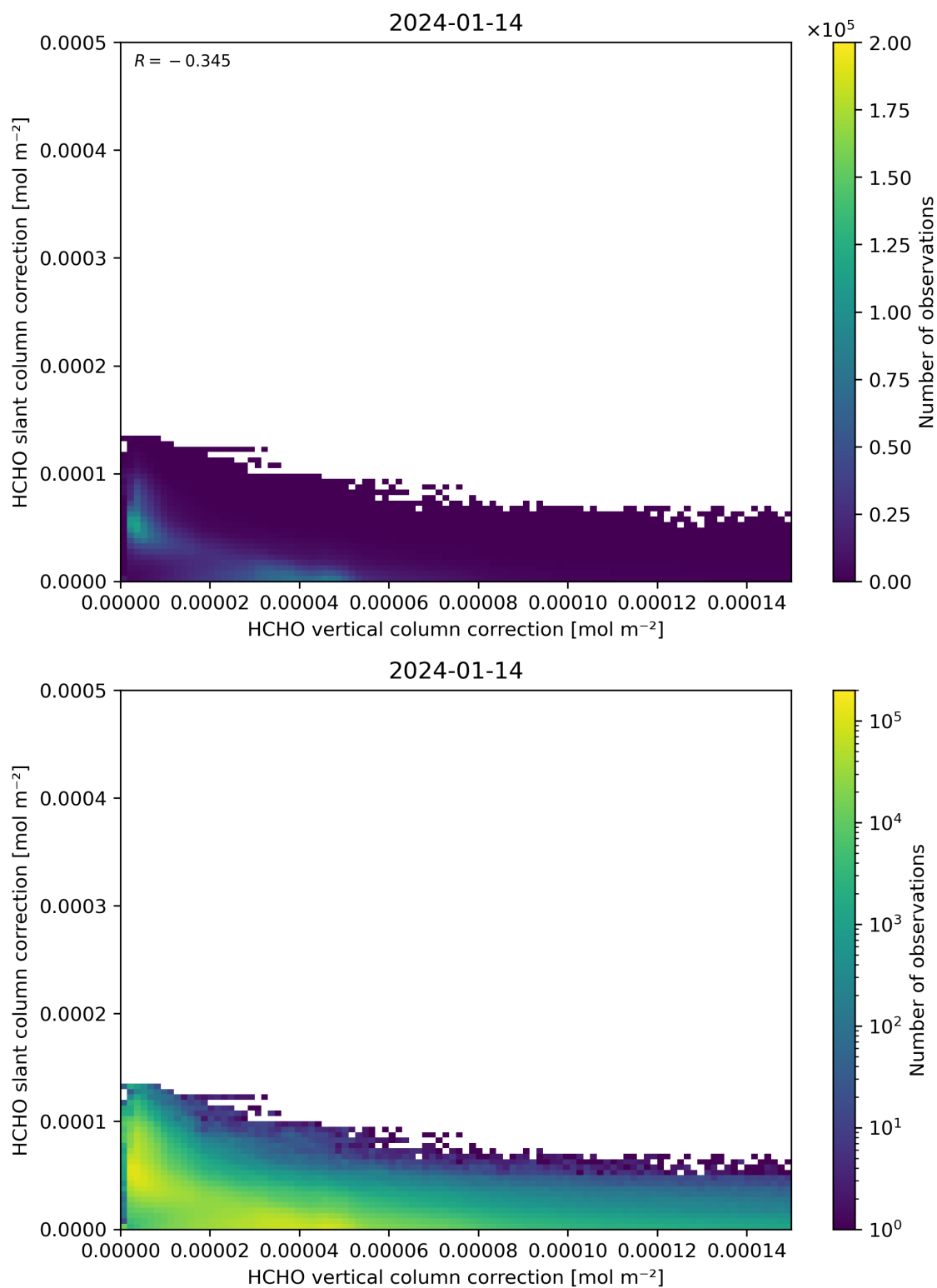
Figure 117: Scatter density plot of “HCHO vertical column correction” against “HCHO slant column correction” for 2024-01-13 to 2024-01-15.
