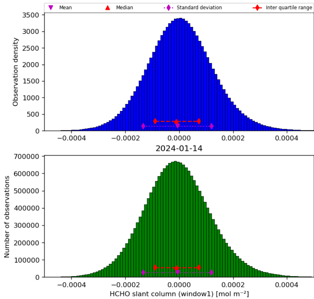
Figure 38: Histogram of “HCHO slant column (window1)” for 2024-01-13 to 2024-01-15
