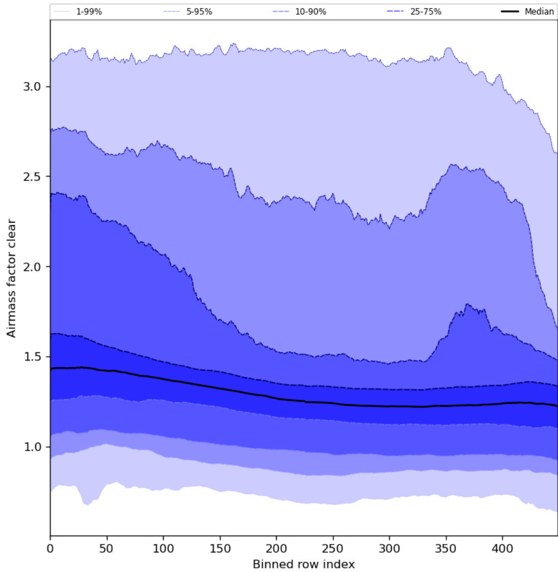
Figure 56: Along track statistics of “Airmass factor clear” for 2024-01-13 to 2024-01-15
