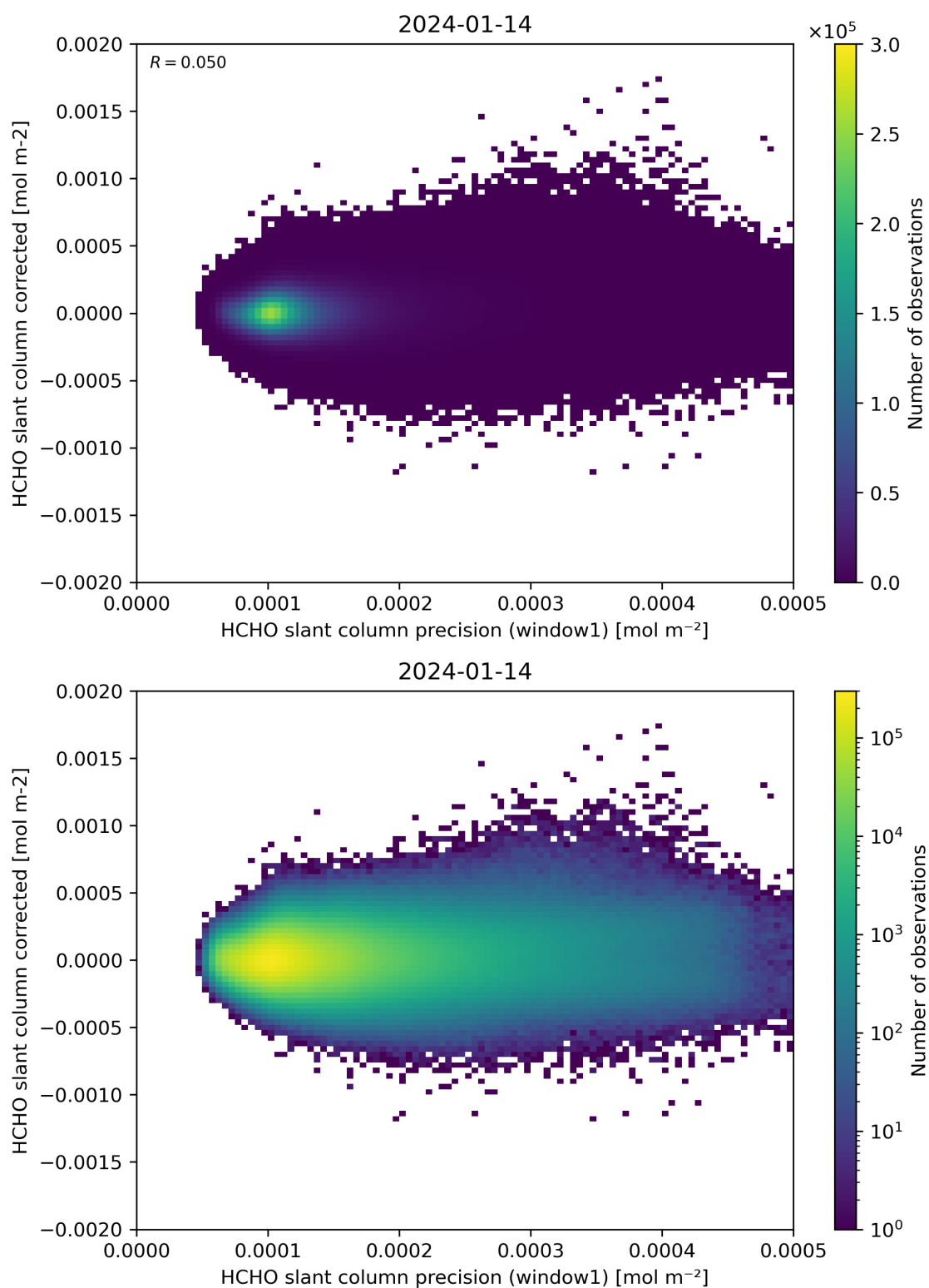
Figure 92: Scatter density plot of “HCHO slant column precision (window1)” against “HCHO slant column corrected” for 2024-01-13 to 2024-01-15.
