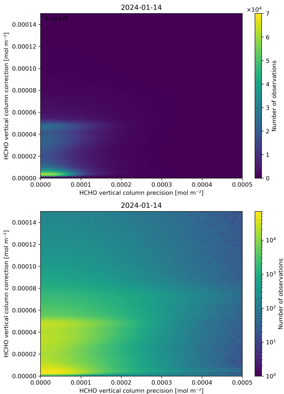
Figure 146: Scatter density plot of “HCHO vertical column precision” against “HCHO vertical column correction” for 2024-01-13 to 2024-01-15.
