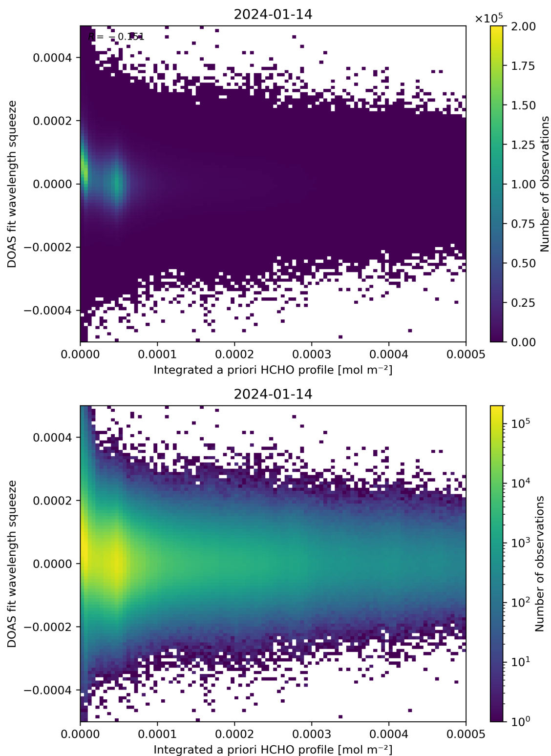
Figure 150: Scatter density plot of “Integrated a priori HCHO profile” against “DOAS fit wavelength squeeze” for 2024-01-13 to 2024-01-15.
