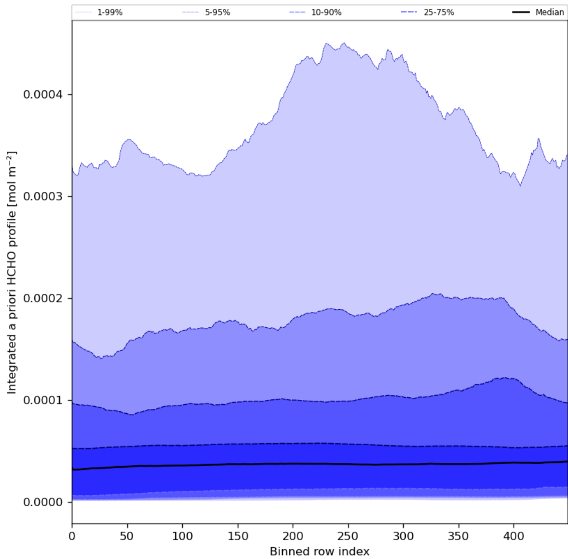
Figure 57: Along track statistics of “Integrated a priori HCHO profile” for 2024-01-13 to 2024-01-15
