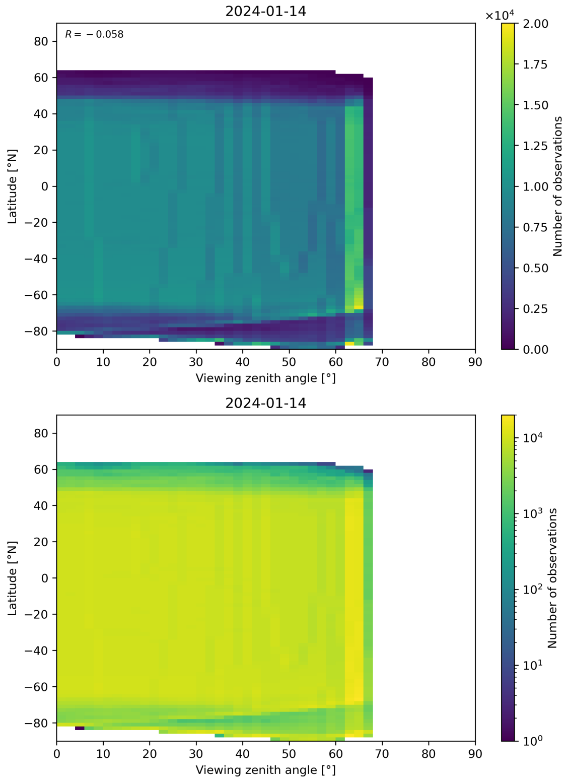
Figure 196: Scatter density plot of “Viewing zenith angle” against “Latitude” for 2024-01-13 to 2024-01-15.
