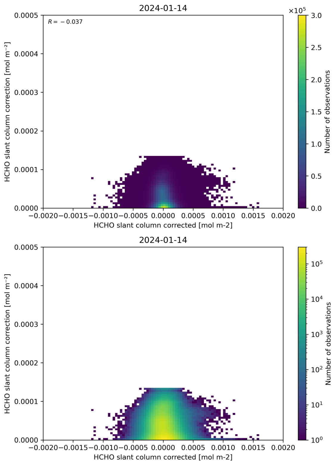
Figure 77: Scatter density plot of “HCHO slant column corrected” against “HCHO slant column correction” for 2024-01-13 to 2024-01-15.
