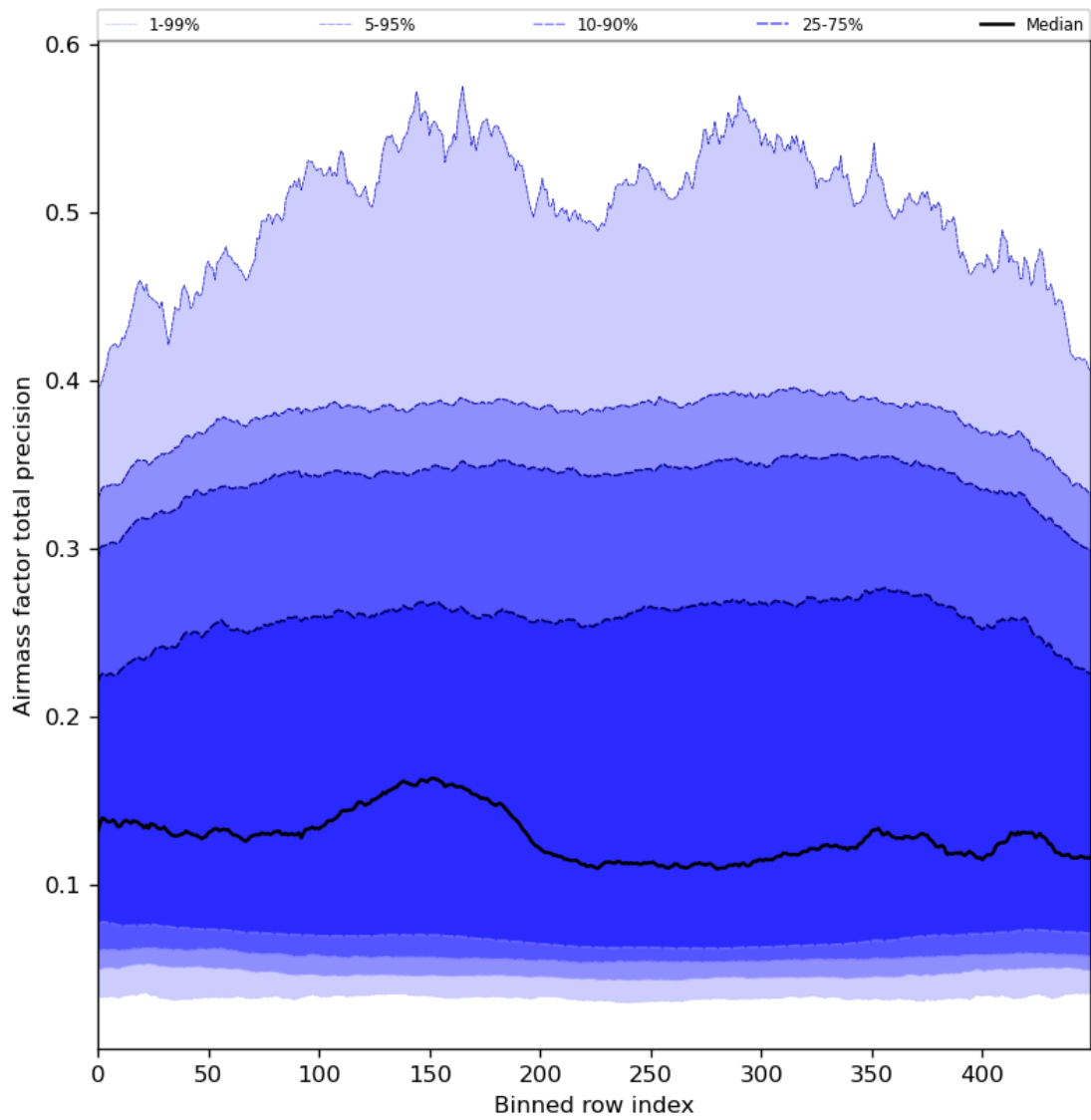
Figure 55: Along track statistics of “Airmass factor total precision” for 2024-01-13 to 2024-01-15
