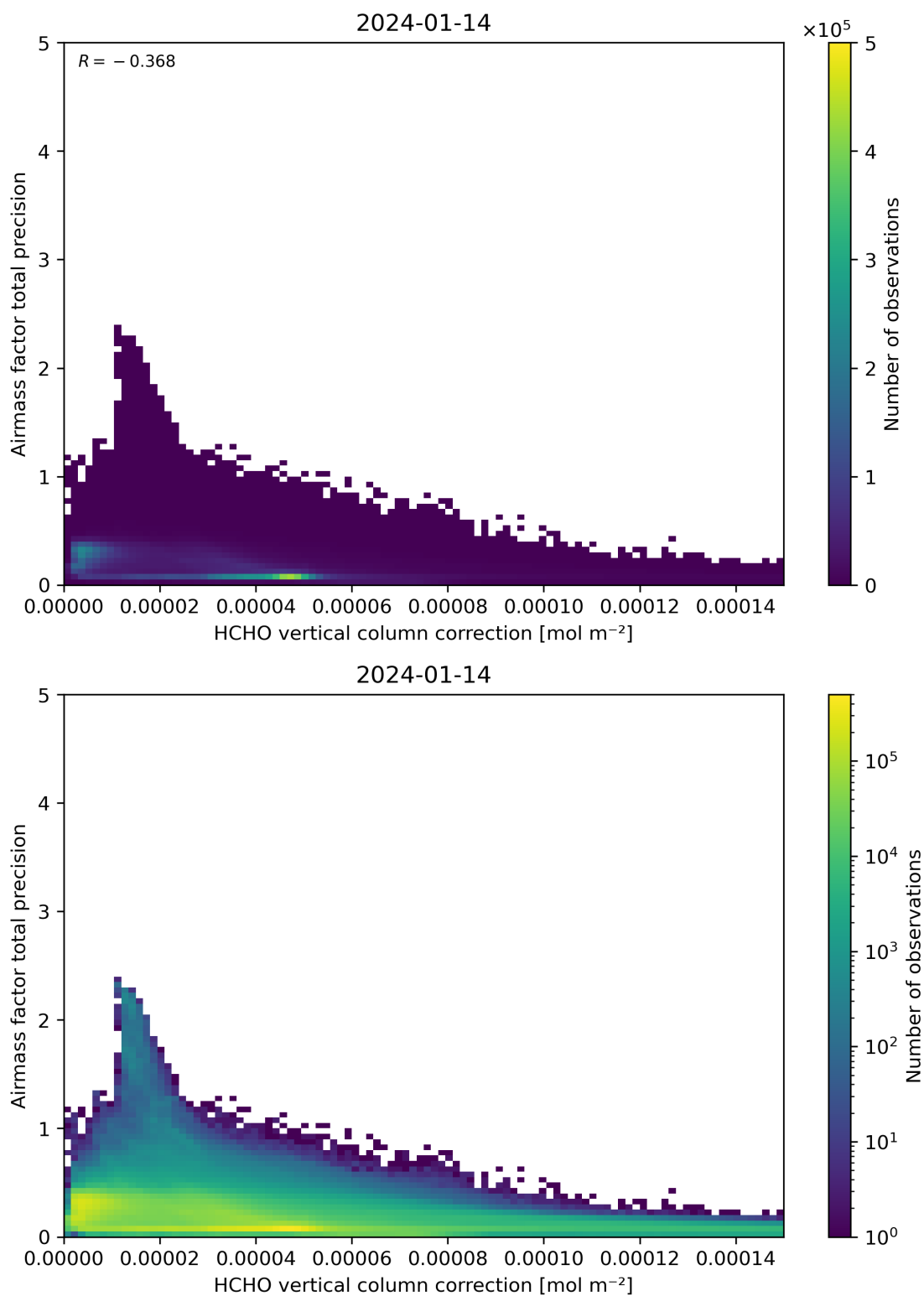
Figure 121: Scatter density plot of “HCHO vertical column correction” against “Airmass factor total precision” for 2024-01-13 to 2024-01-15.
