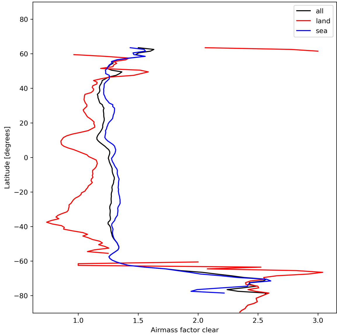
Figure 28: Zonal average of “Airmass factor clear” for 2024-01-13 to 2024-01-15.
