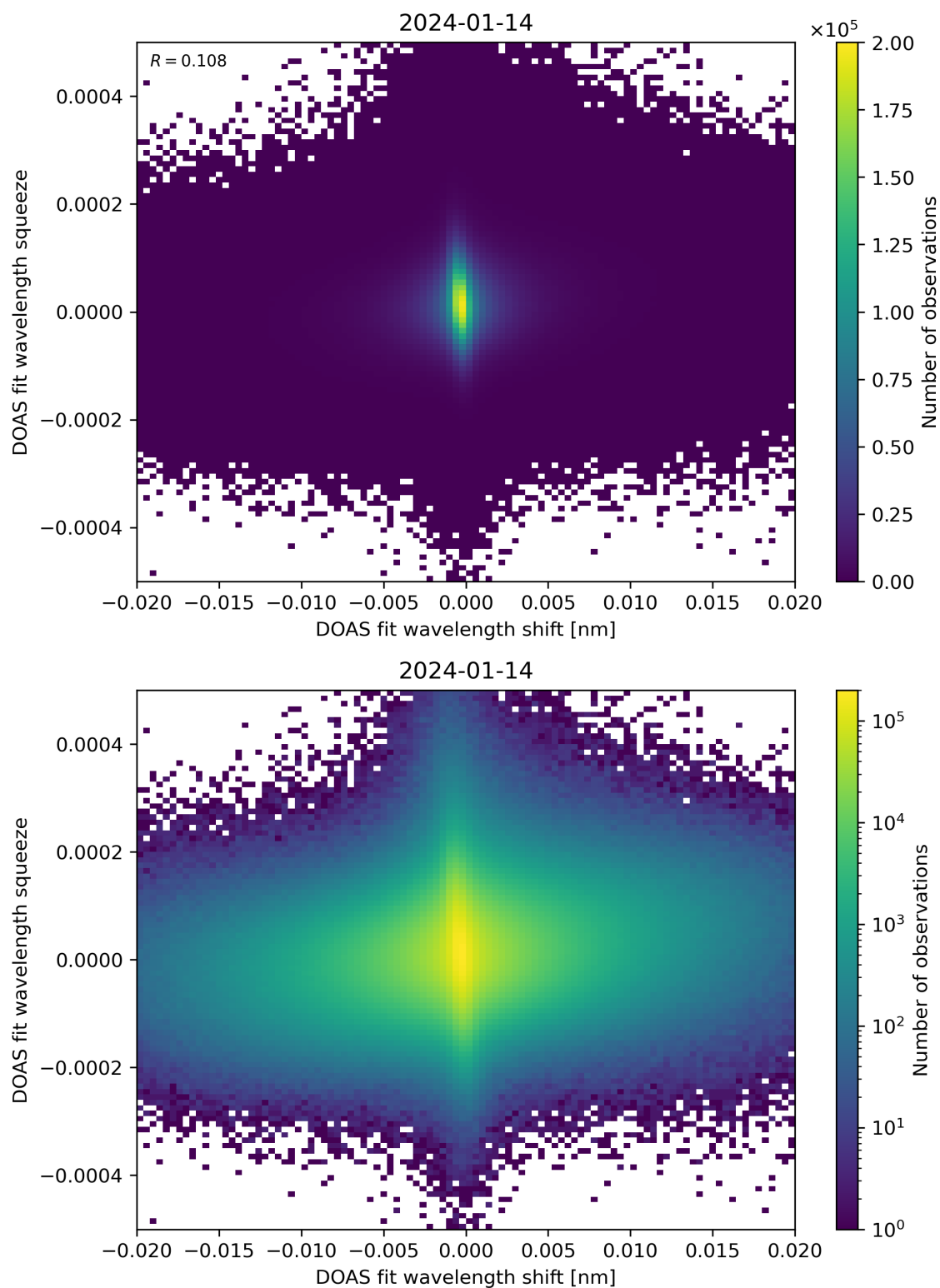
Figure 65: Scatter density plot of “DOAS fit wavelength shift” against “DOAS fit wavelength squeeze” for 2024-01-13 to 2024-01-15.
