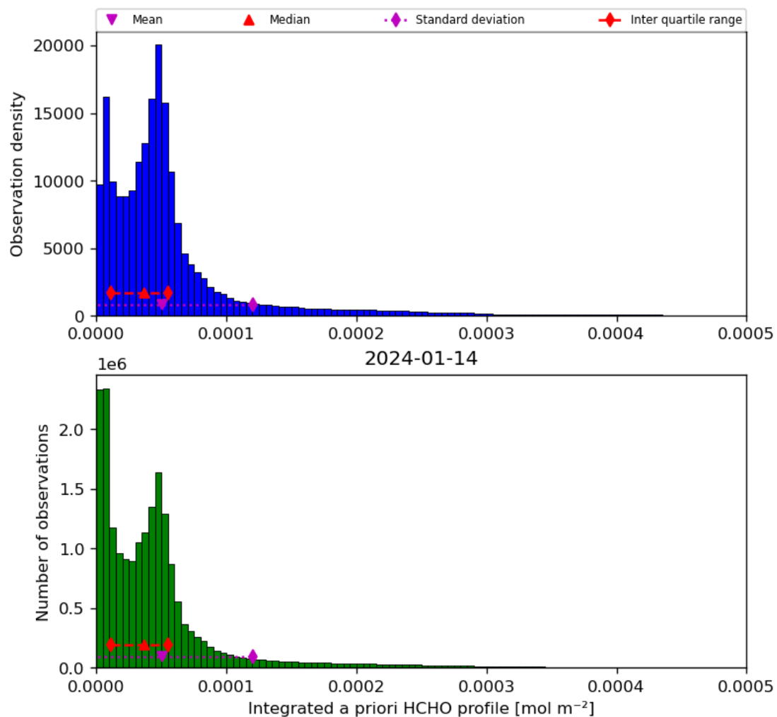
Figure 43: Histogram of “Integrated a priori HCHO profile” for 2024-01-13 to 2024-01-15
