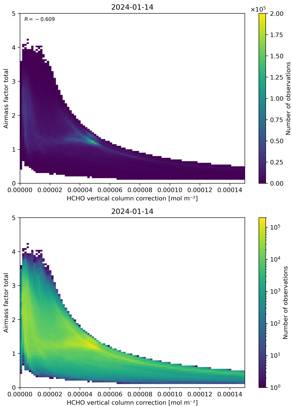
Figure 120: Scatter density plot of “HCHO vertical column correction” against “Airmass factor total” for 2024-01-13 to 2024-01-15.
