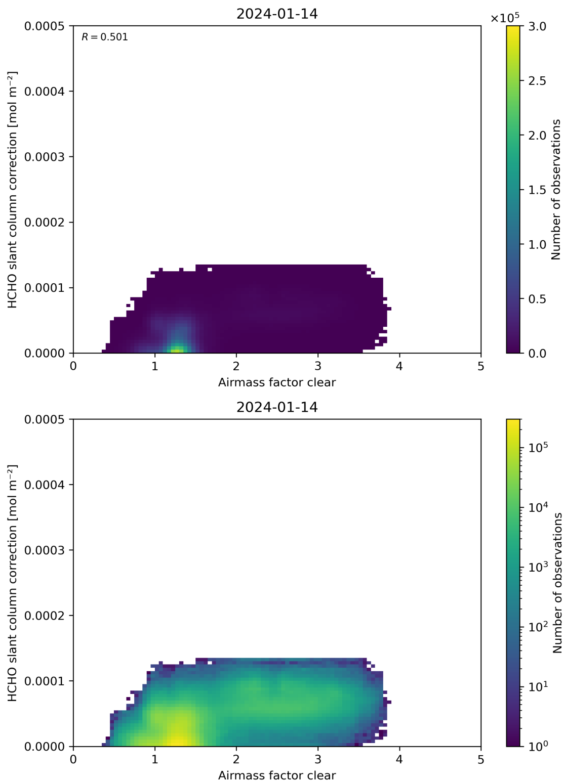
Figure 75: Scatter density plot of “Airmass factor clear” against “HCHO slant column correction” for 2024-01-13 to 2024-01-15.
