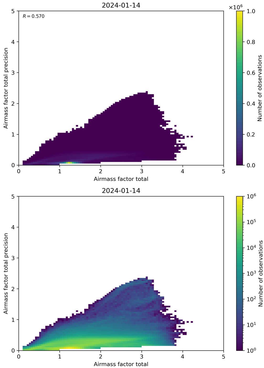
Figure 103: Scatter density plot of “Airmass factor total” against “Airmass factor total precision” for 2024-01-13 to 2024-01-15.
