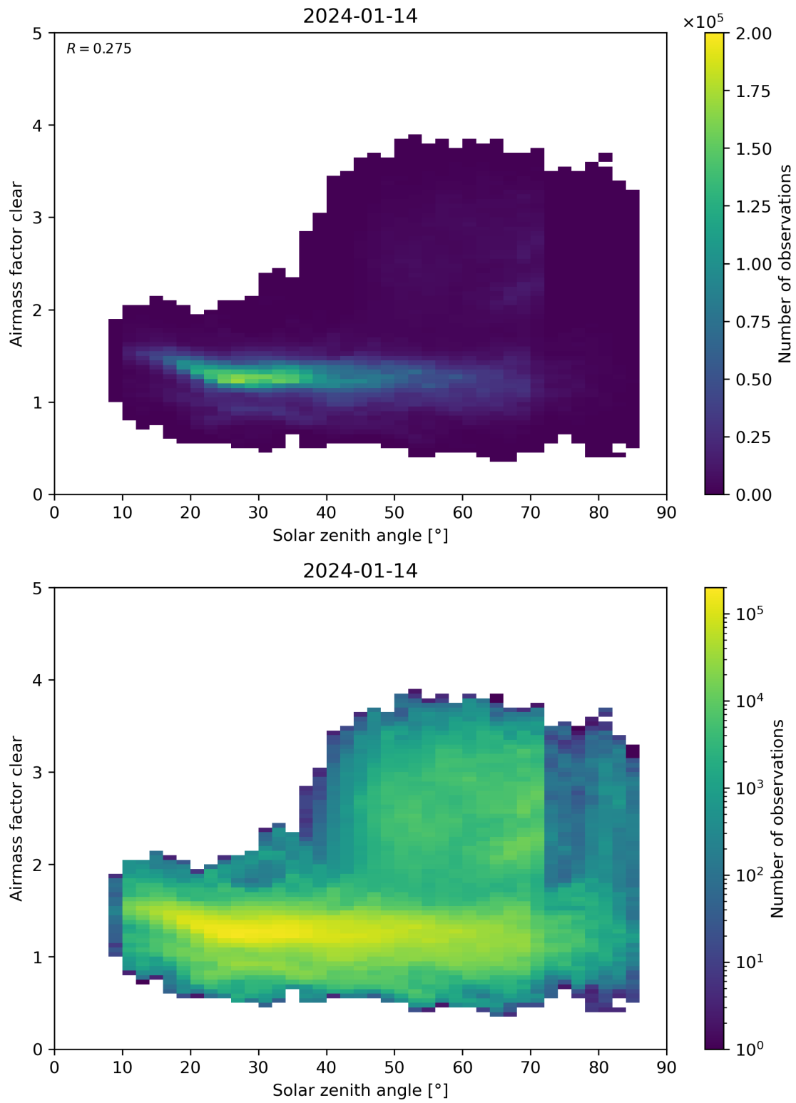
Figure 170: Scatter density plot of “Solar zenith angle” against “Airmass factor clear” for 2024-01-13 to 2024-01-15.
