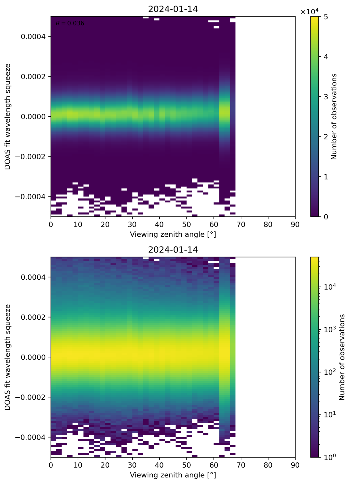
Figure 184: Scatter density plot of “Viewing zenith angle” against “DOAS fit wavelength squeeze” for 2024-01-13 to 2024-01-15.
