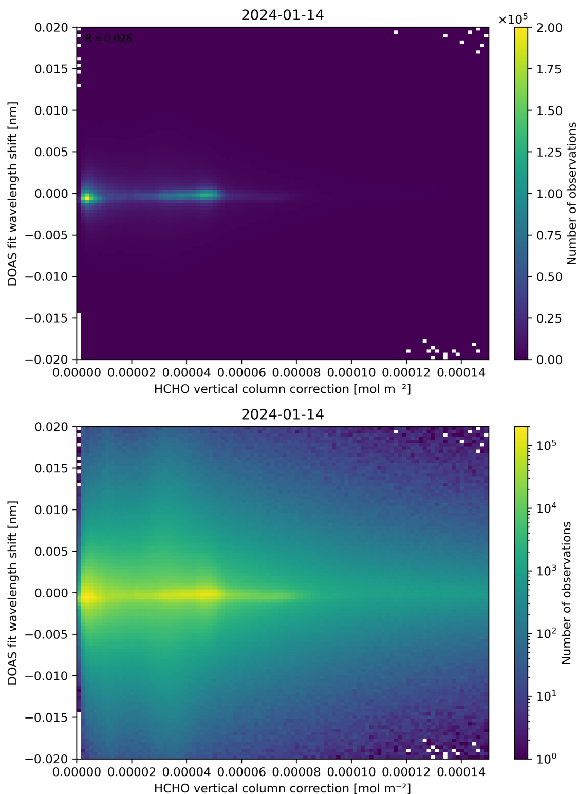
Figure 113: Scatter density plot of “HCHO vertical column correction” against “DOAS fit wavelength shift” for 2024-01-13 to 2024-01-15.
