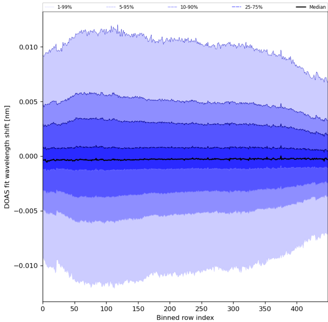
Figure 58: Along track statistics of “DOAS fit wavelength shift” for 2024-01-13 to 2024-01-15
