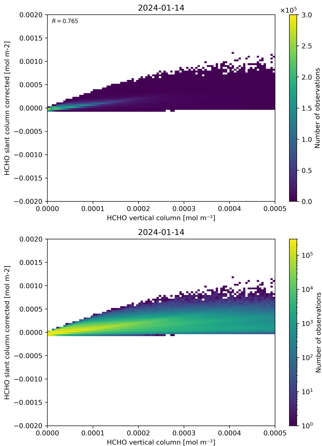
Figure 127: Scatter density plot of “HCHO vertical column” against “HCHO slant column corrected” for 2024-01-13 to 2024-01-15.
