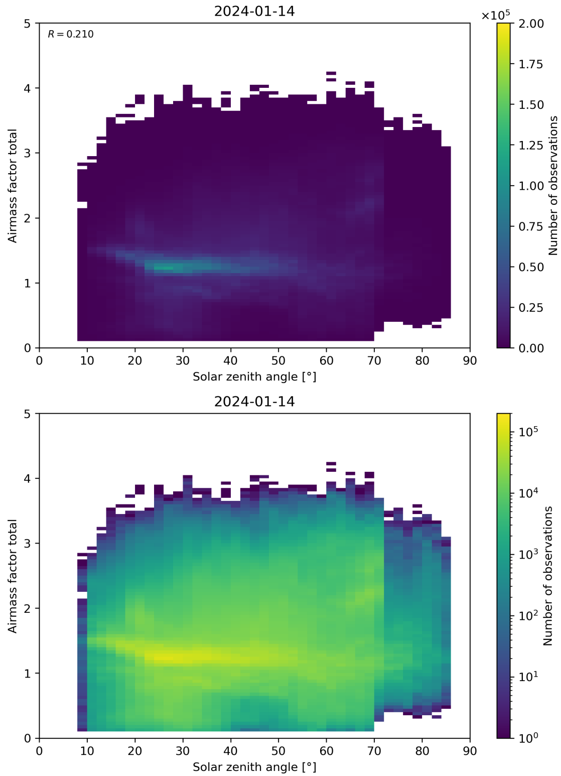
Figure 175: Scatter density plot of “Solar zenith angle” against “Airmass factor total” for 2024-01-13 to 2024-01-15.
