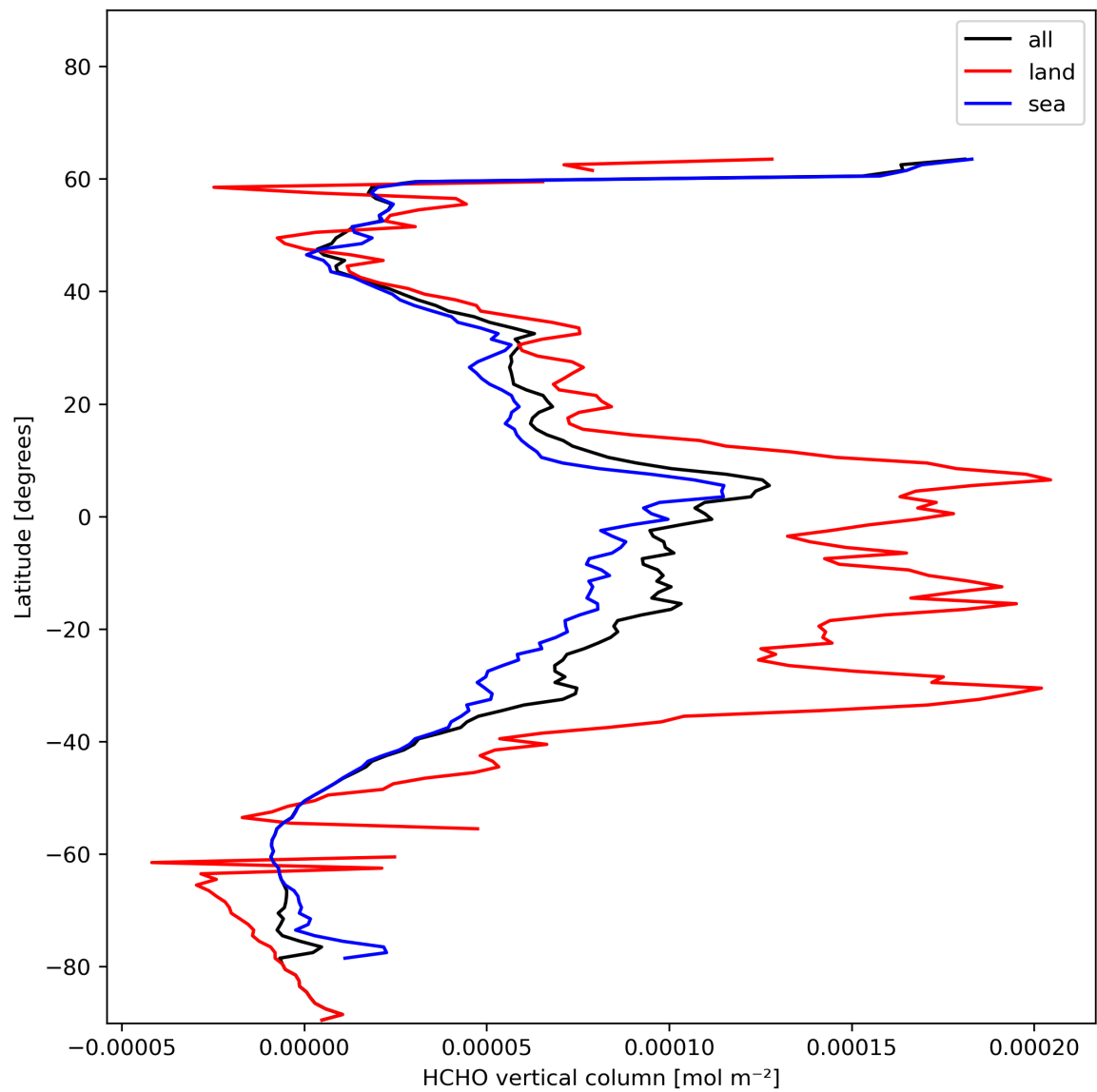
Figure 21: Zonal average of “HCHO vertical column” for 2024-01-13 to 2024-01-15.
