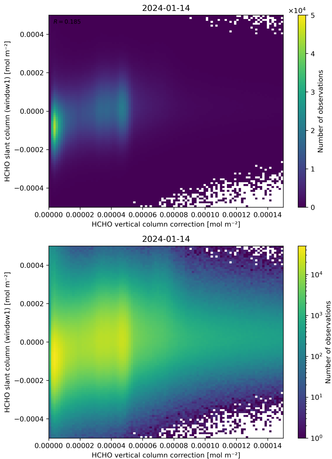
Figure 118: Scatter density plot of “HCHO vertical column correction” against “HCHO slant column (window1)” for 2024-01-13 to 2024-01-15.
