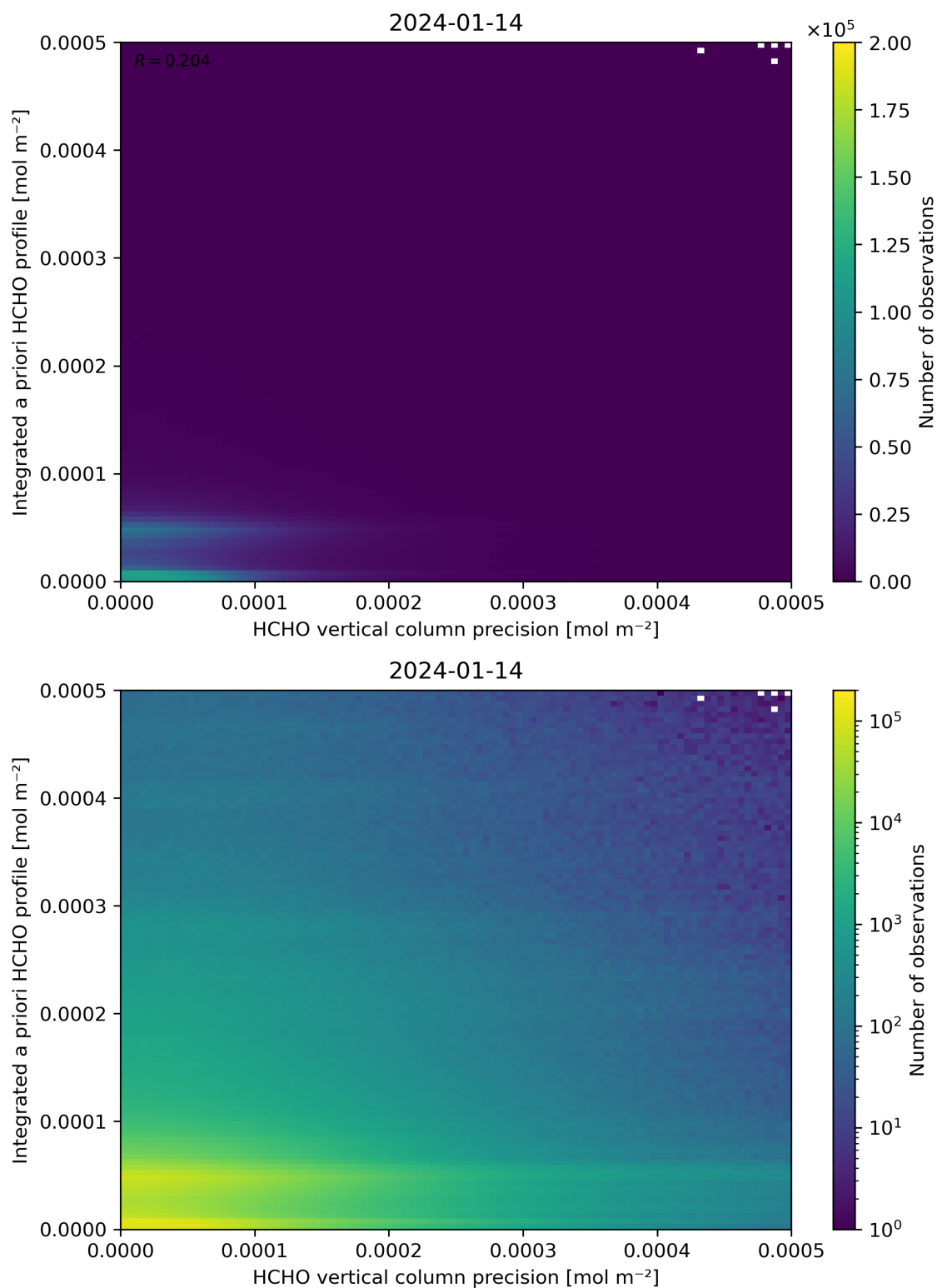
Figure 147: Scatter density plot of “HCHO vertical column precision” against “Integrated a priori HCHO profile” for 2024-01-13 to 2024-01-15.
