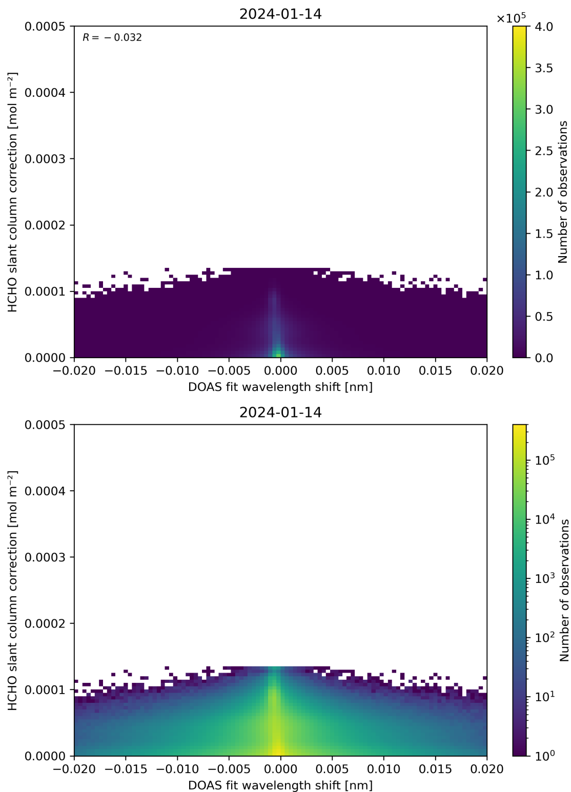
Figure 67: Scatter density plot of “DOAS fit wavelength shift” against “HCHO slant column correction” for 2024-01-13 to 2024-01-15.
