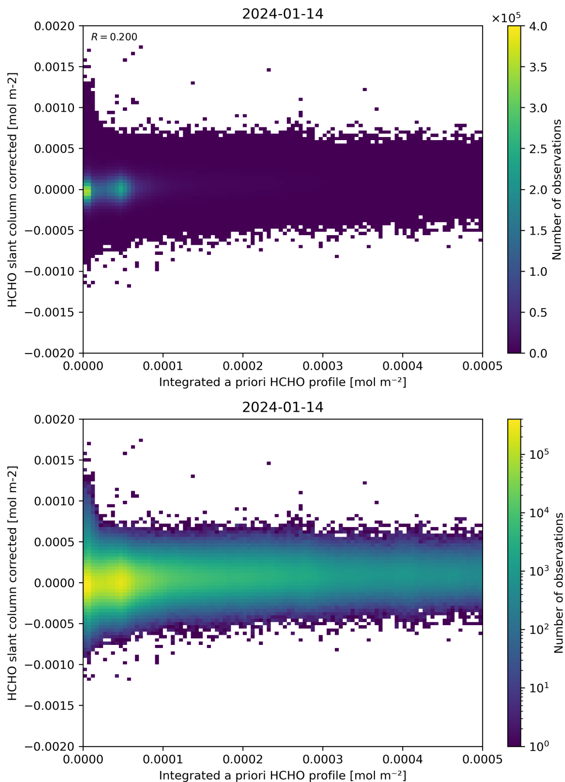
Figure 151: Scatter density plot of “Integrated a priori HCHO profile” against “HCHO slant column corrected” for 2024-01-13 to 2024-01-15.
