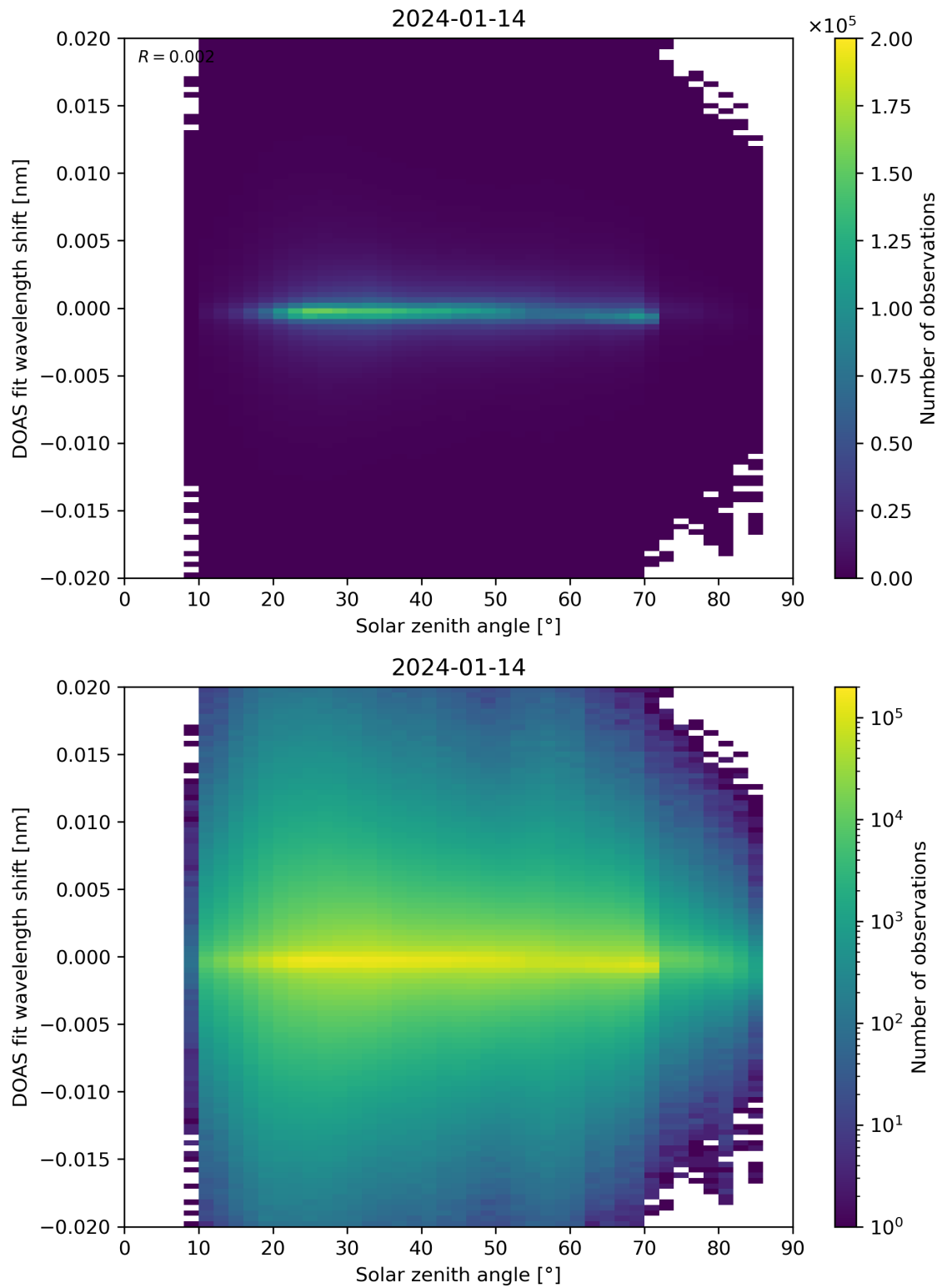
Figure 168: Scatter density plot of “Solar zenith angle” against “DOAS fit wavelength shift” for 2024-01-13 to 2024-01-15.
