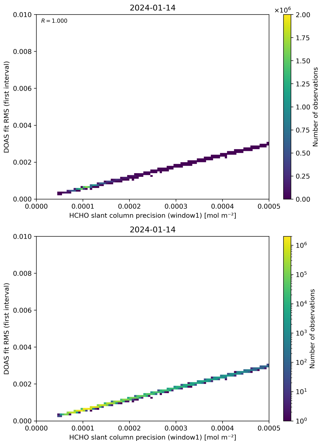
Figure 88: Scatter density plot of “HCHO slant column precision (window1)” against “DOAS fit RMS (first interval)” for 2024-01-13 to 2024-01-15.
