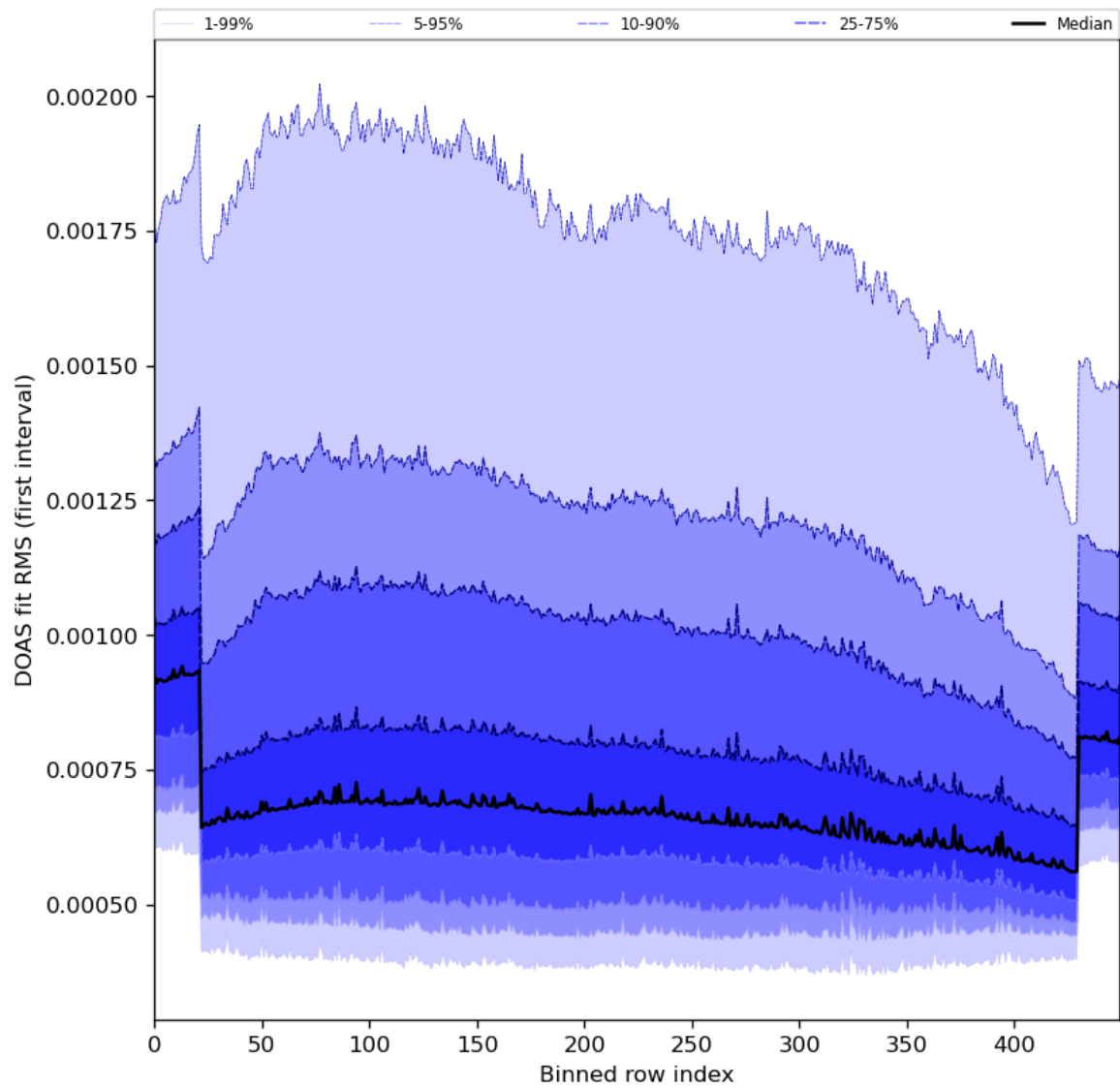
Figure 60: Along track statistics of “DOAS fit RMS (first interval)” for 2024-01-13 to 2024-01-15
