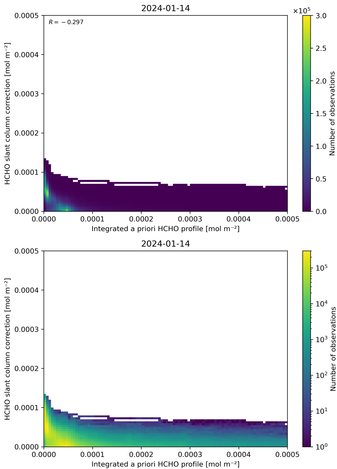
Figure 152: Scatter density plot of “Integrated a priori HCHO profile” against “HCHO slant column correction” for 2024-01-13 to 2024-01-15.
