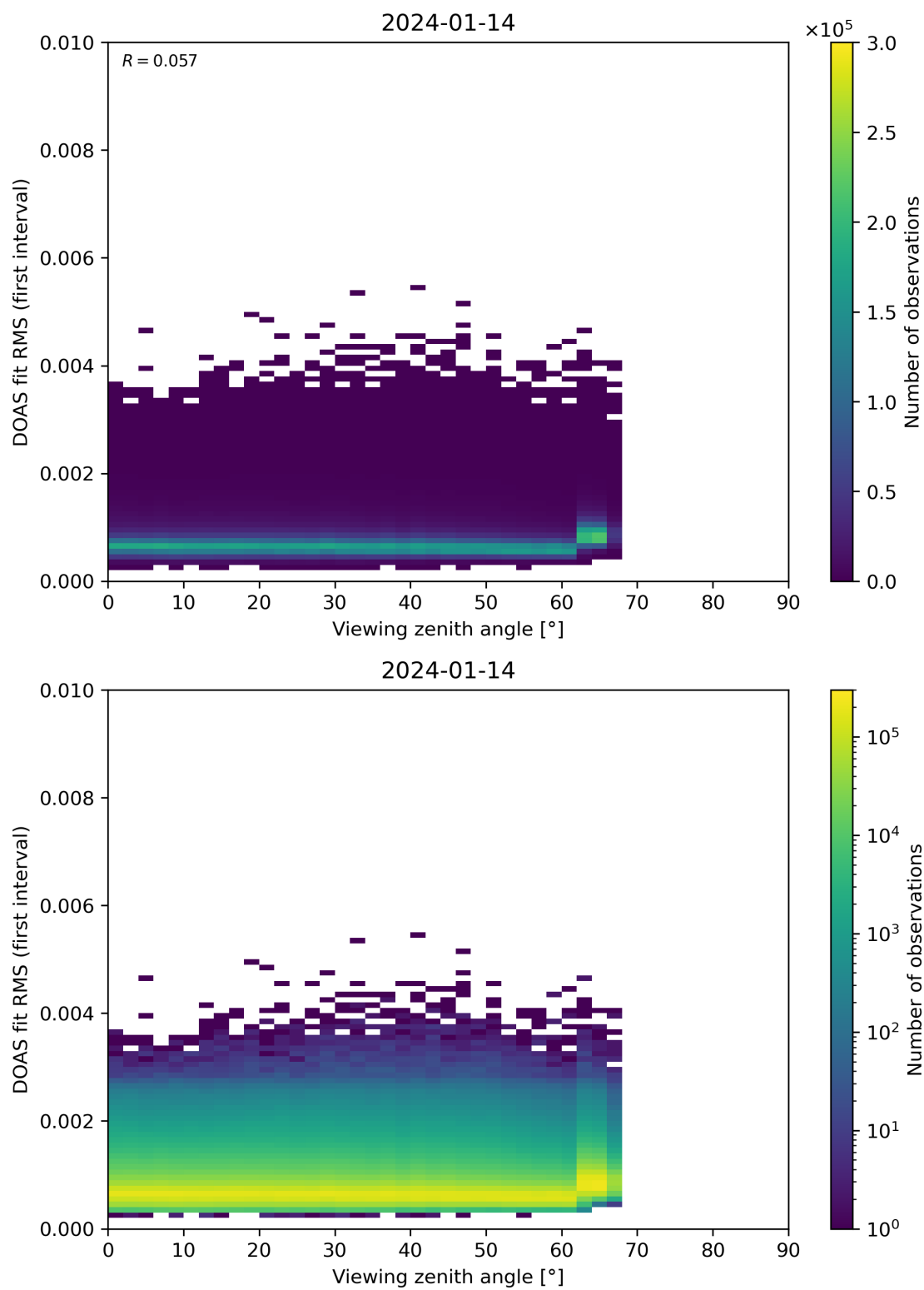
Figure 182: Scatter density plot of “Viewing zenith angle” against “DOAS fit RMS (first interval)” for 2024-01-13 to 2024-01-15.
