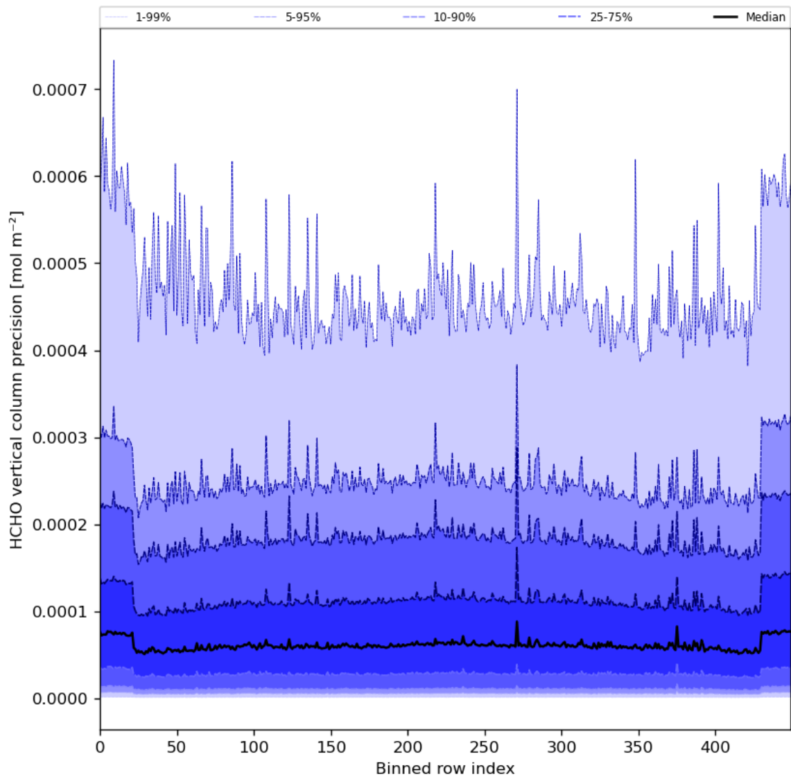
Figure 50: Along track statistics of “HCHO vertical column precision” for 2024-01-13 to 2024-01-15
