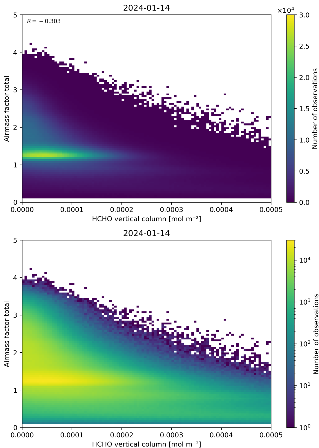
Figure 131: Scatter density plot of “HCHO vertical column” against “Airmass factor total” for 2024-01-13 to 2024-01-15.
