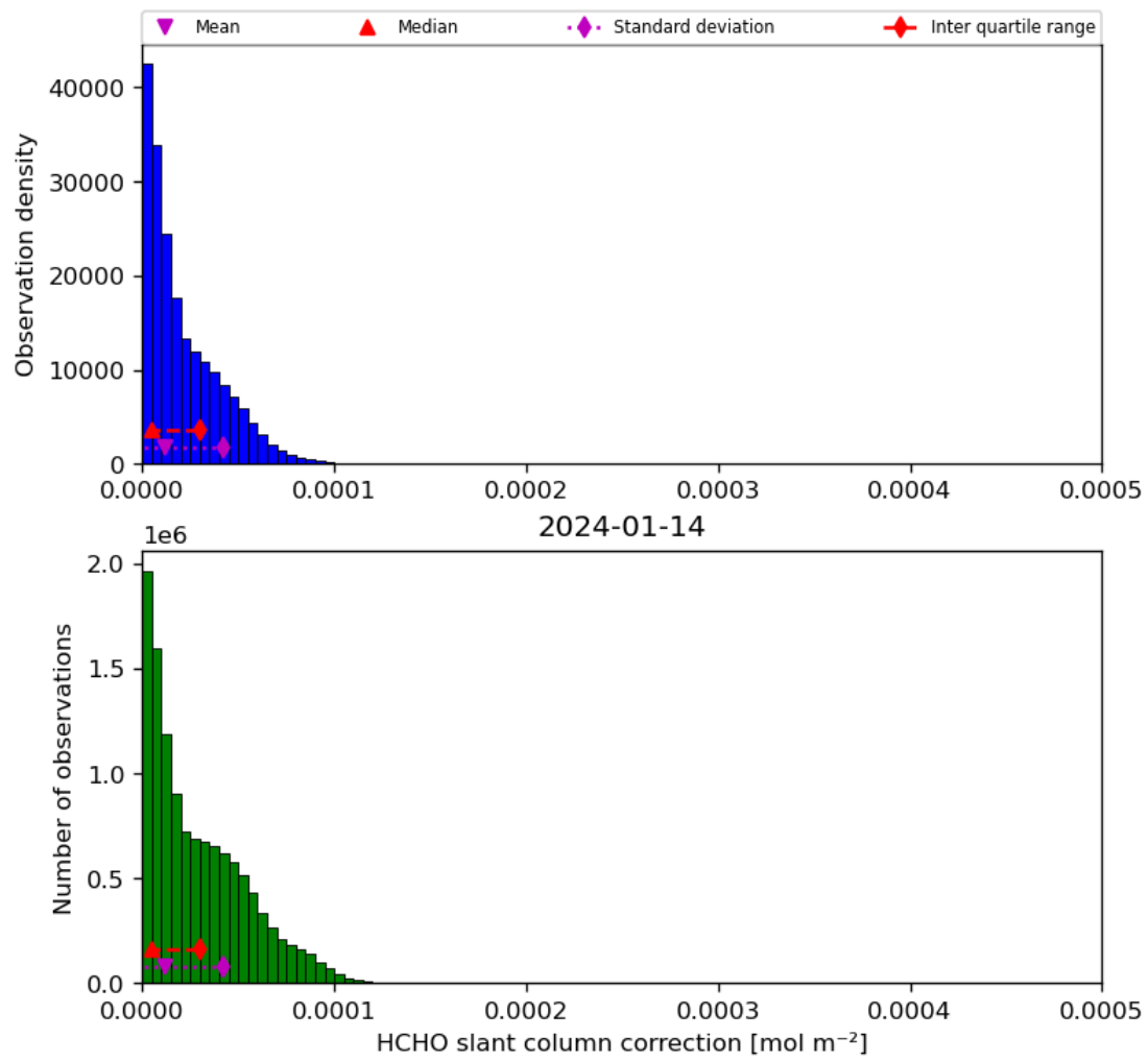
Figure 47: Histogram of “HCHO slant column correction” for 2024-01-13 to 2024-01-15
