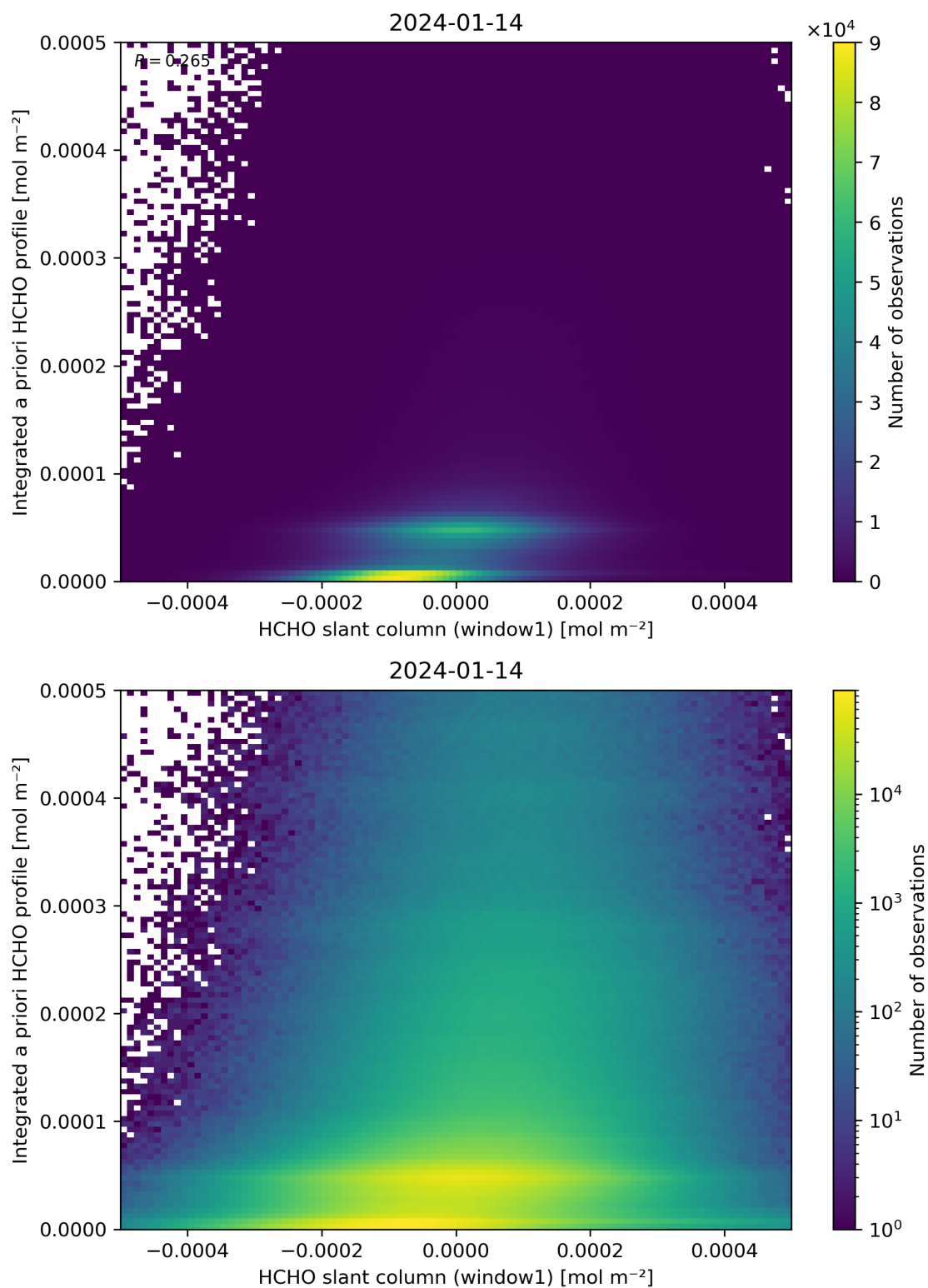
Figure 87: Scatter density plot of “HCHO slant column (window1)” against “Integrated a priori HCHO profile” for 2024-01-13 to 2024-01-15.
