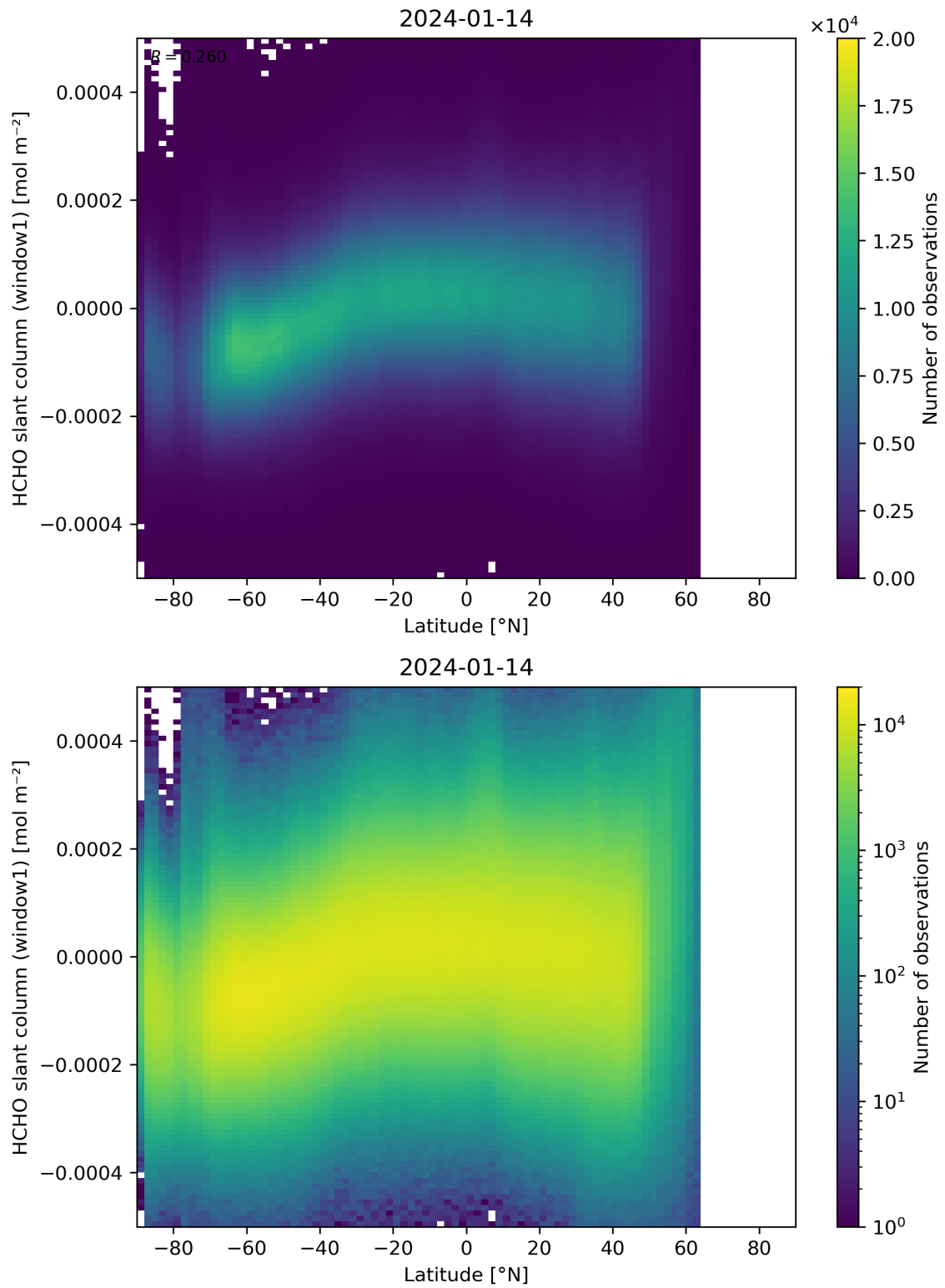
Figure 159: Scatter density plot of “Latitude” against “HCHO slant column (window1)” for 2024-01-13 to 2024-01-15.
