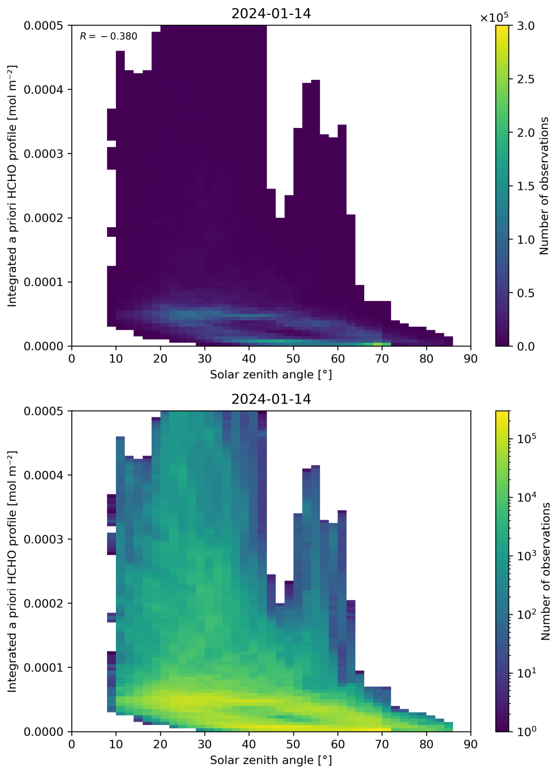
Figure 180: Scatter density plot of “Solar zenith angle” against “Integrated a priori HCHO profile” for 2024-01-13 to 2024-01-15.
