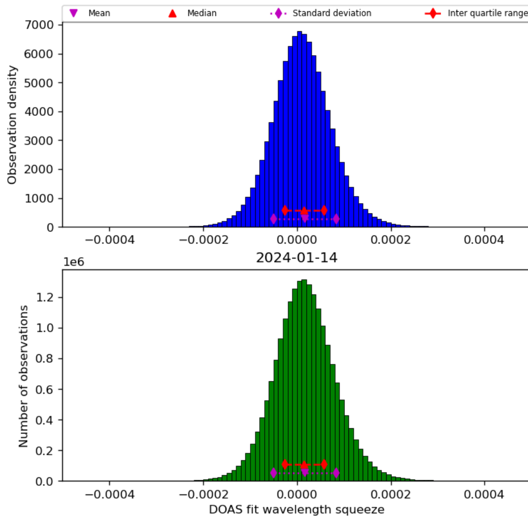
Figure 45: Histogram of “DOAS fit wavelength squeeze” for 2024-01-13 to 2024-01-15
