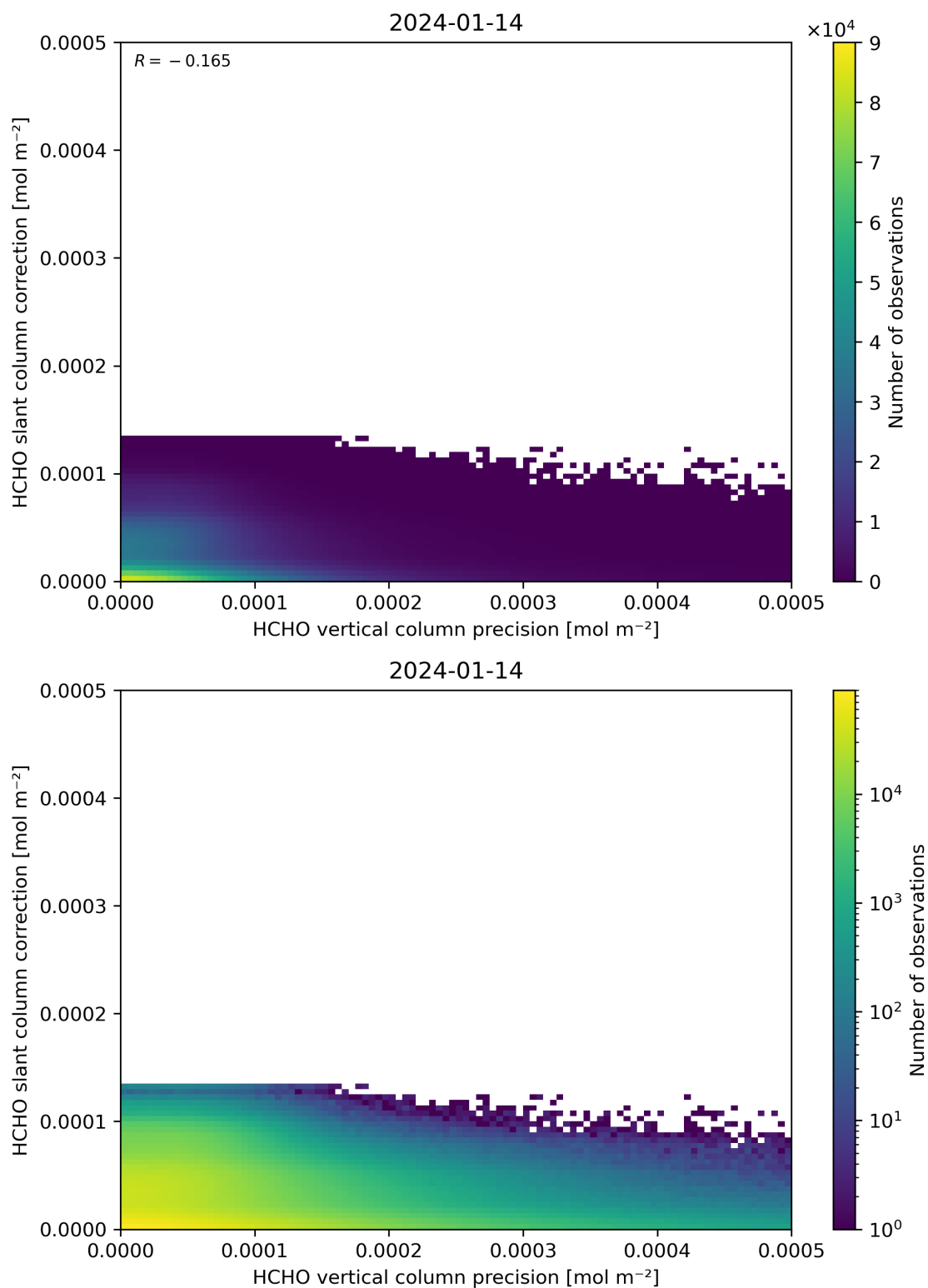
Figure 141: Scatter density plot of “HCHO vertical column precision” against “HCHO slant column correction” for 2024-01-13 to 2024-01-15.
