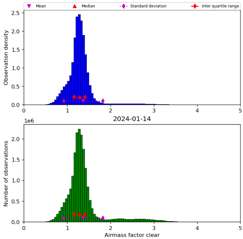
Figure 42: Histogram of “Airmass factor clear” for 2024-01-13 to 2024-01-15
