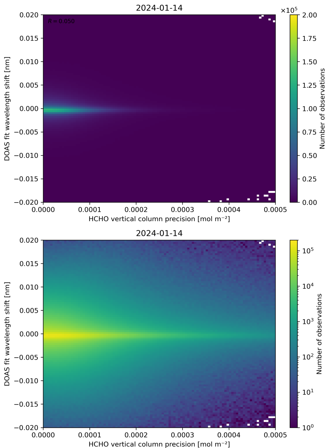
Figure 137: Scatter density plot of “HCHO vertical column precision” against “DOAS fit wavelength shift” for 2024-01-13 to 2024-01-15.
