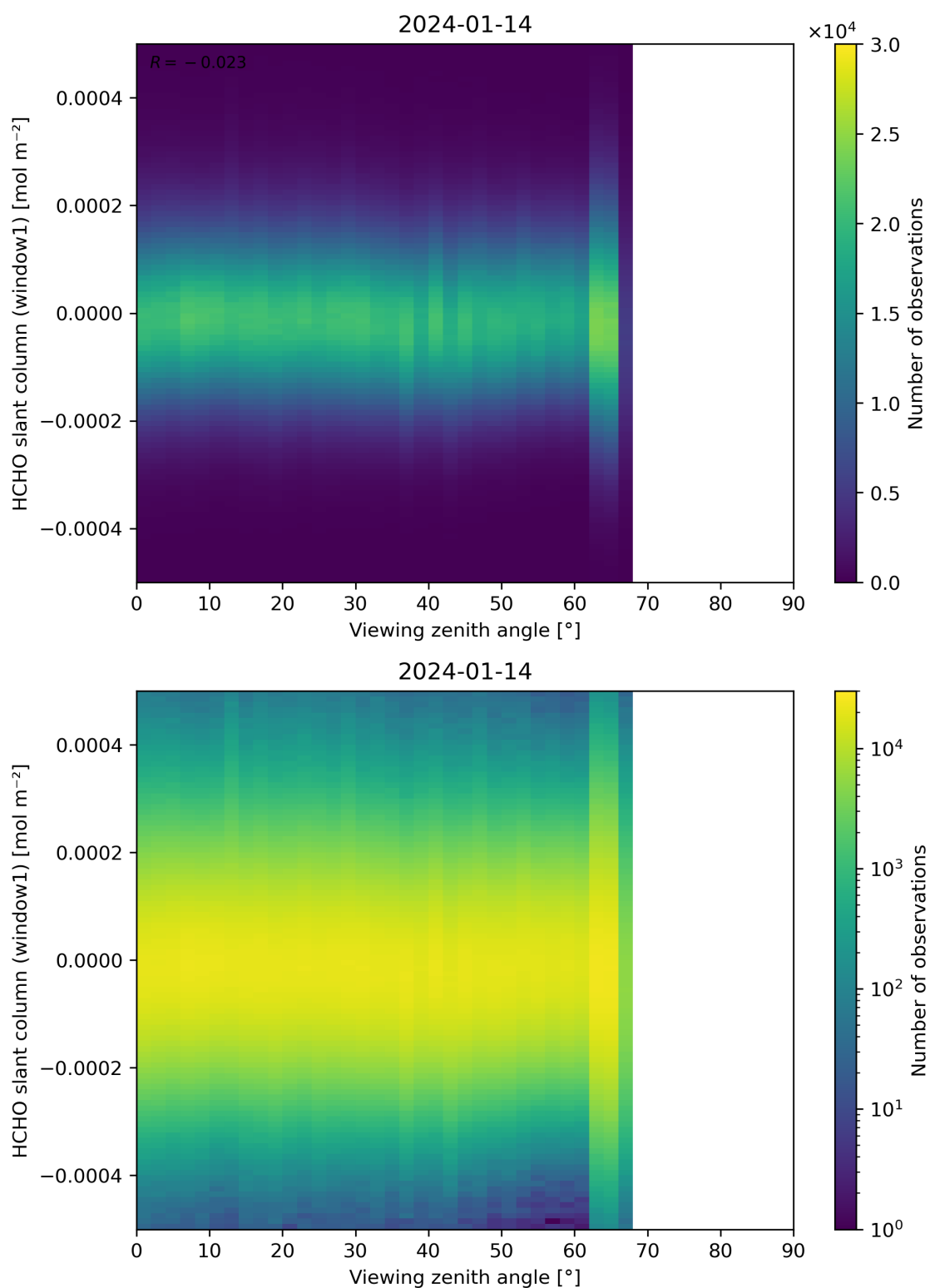
Figure 188: Scatter density plot of “Viewing zenith angle” against “HCHO slant column (window1)” for 2024-01-13 to 2024-01-15.
