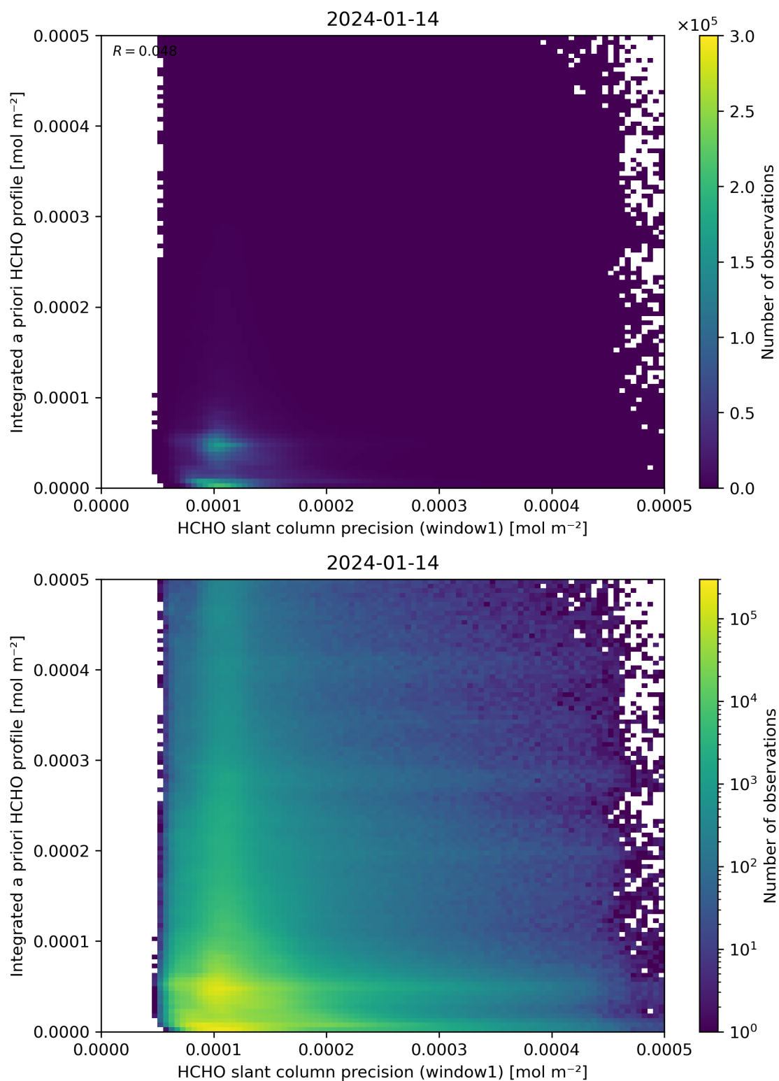
Figure 96: Scatter density plot of “HCHO slant column precision (window1)” against “Integrated a priori HCHO profile” for 2024-01-13 to 2024-01-15.
