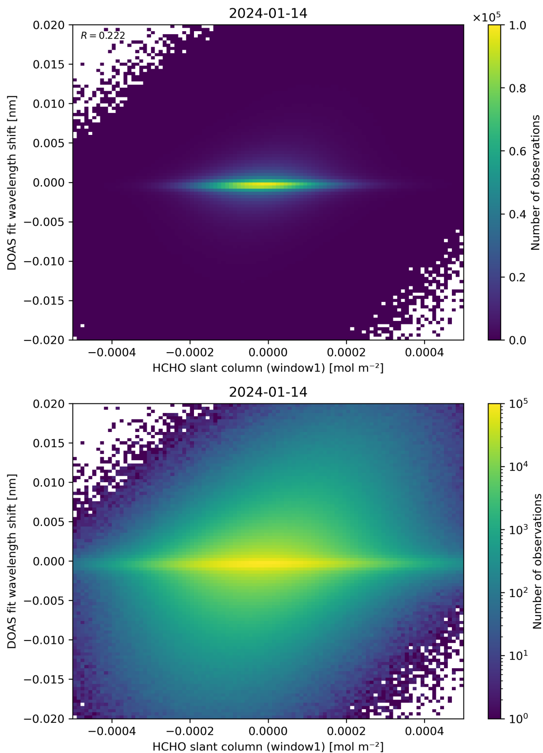
Figure 79: Scatter density plot of “HCHO slant column (window1)” against “DOAS fit wavelength shift” for 2024-01-13 to 2024-01-15.
