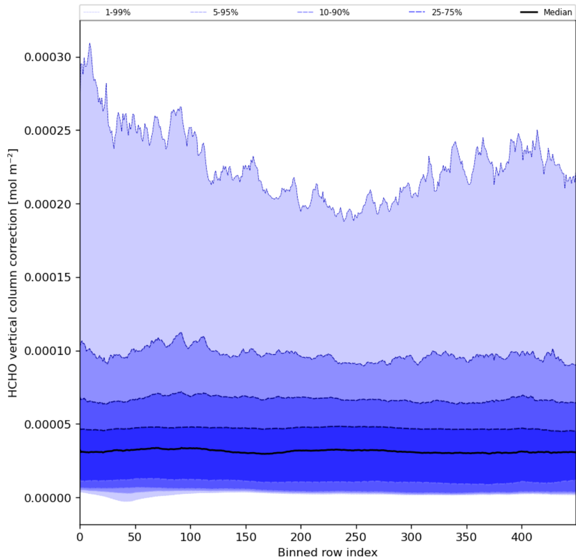
Figure 51: Along track statistics of “HCHO vertical column correction” for 2024-01-13 to 2024-01-15
