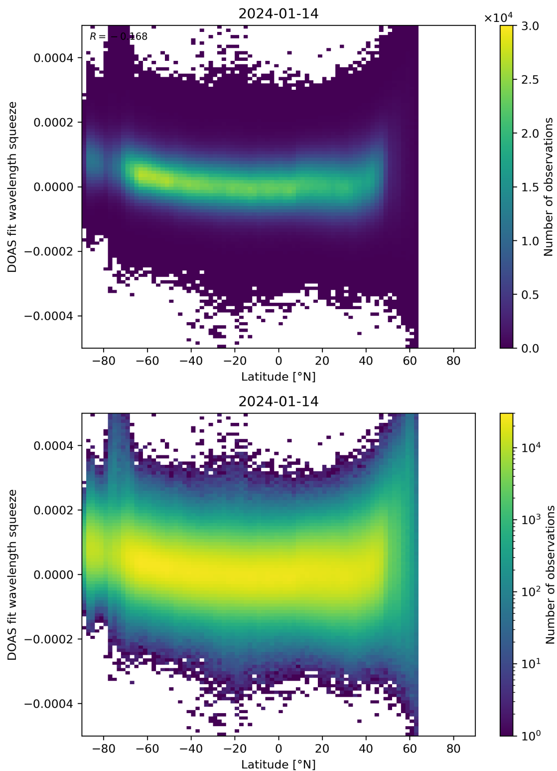
Figure 155: Scatter density plot of “Latitude” against “DOAS fit wavelength squeeze” for 2024-01-13 to 2024-01-15.
