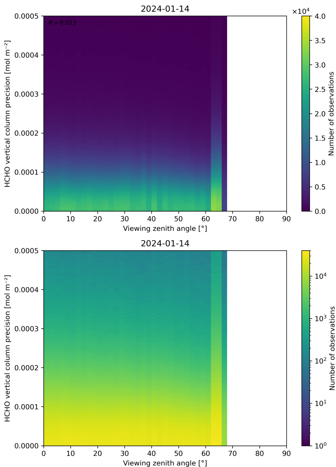
Figure 194: Scatter density plot of “Viewing zenith angle” against “HCHO vertical column precision” for 2024-01-13 to 2024-01-15.
