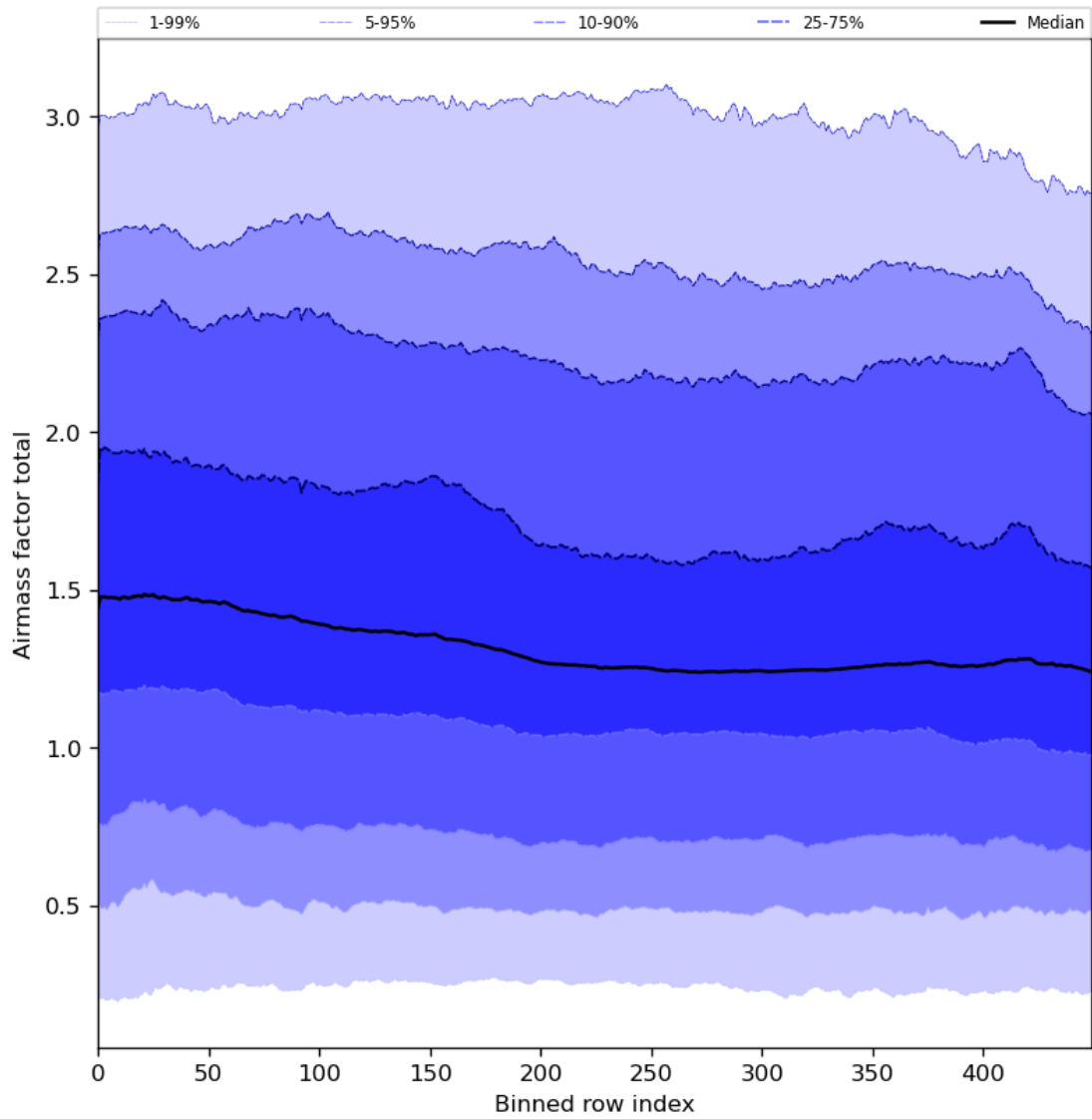
Figure 54: Along track statistics of “Airmass factor total” for 2024-01-13 to 2024-01-15
