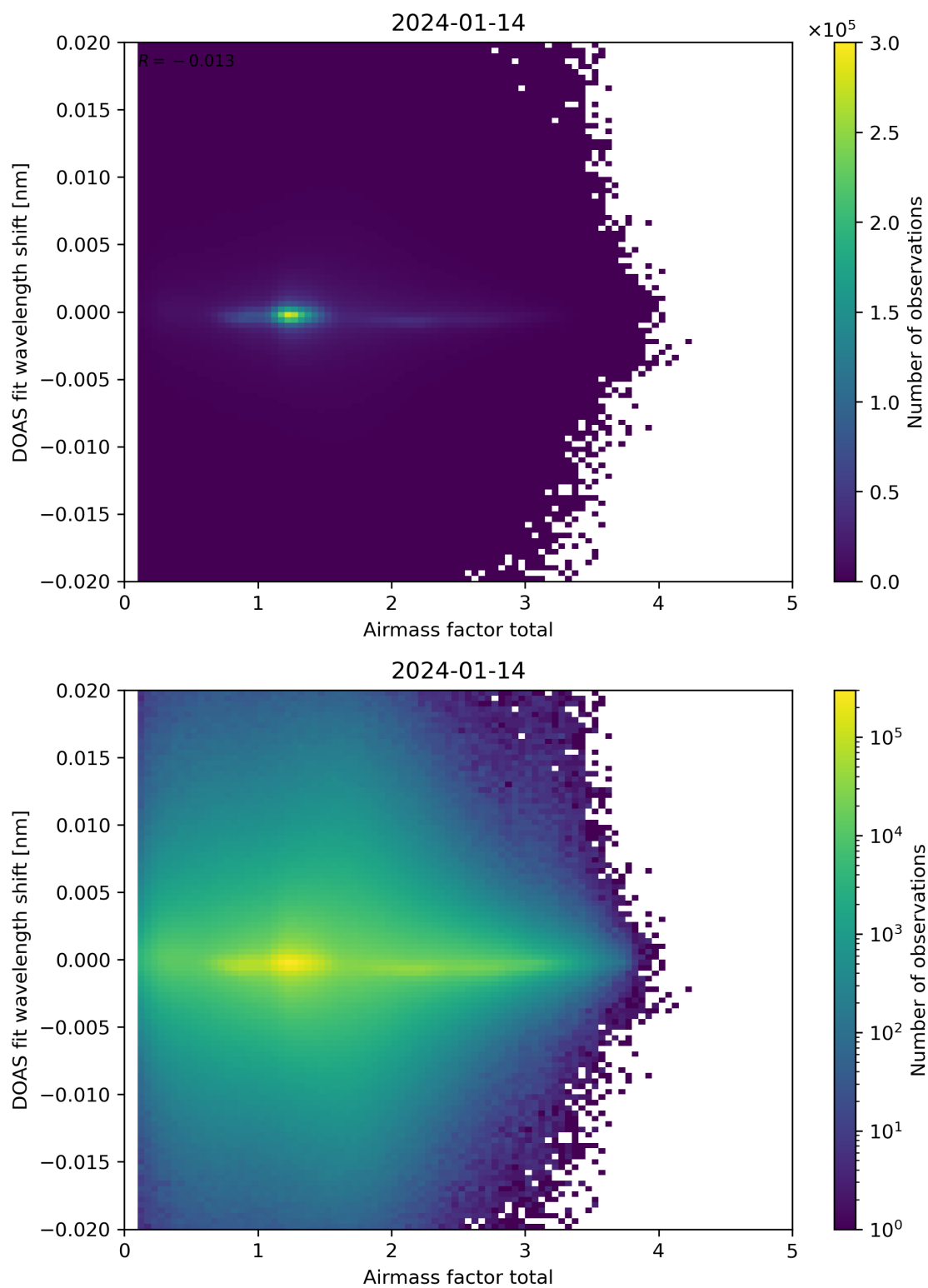
Figure 98: Scatter density plot of “Airmass factor total” against “DOAS fit wavelength shift” for 2024-01-13 to 2024-01-15.
