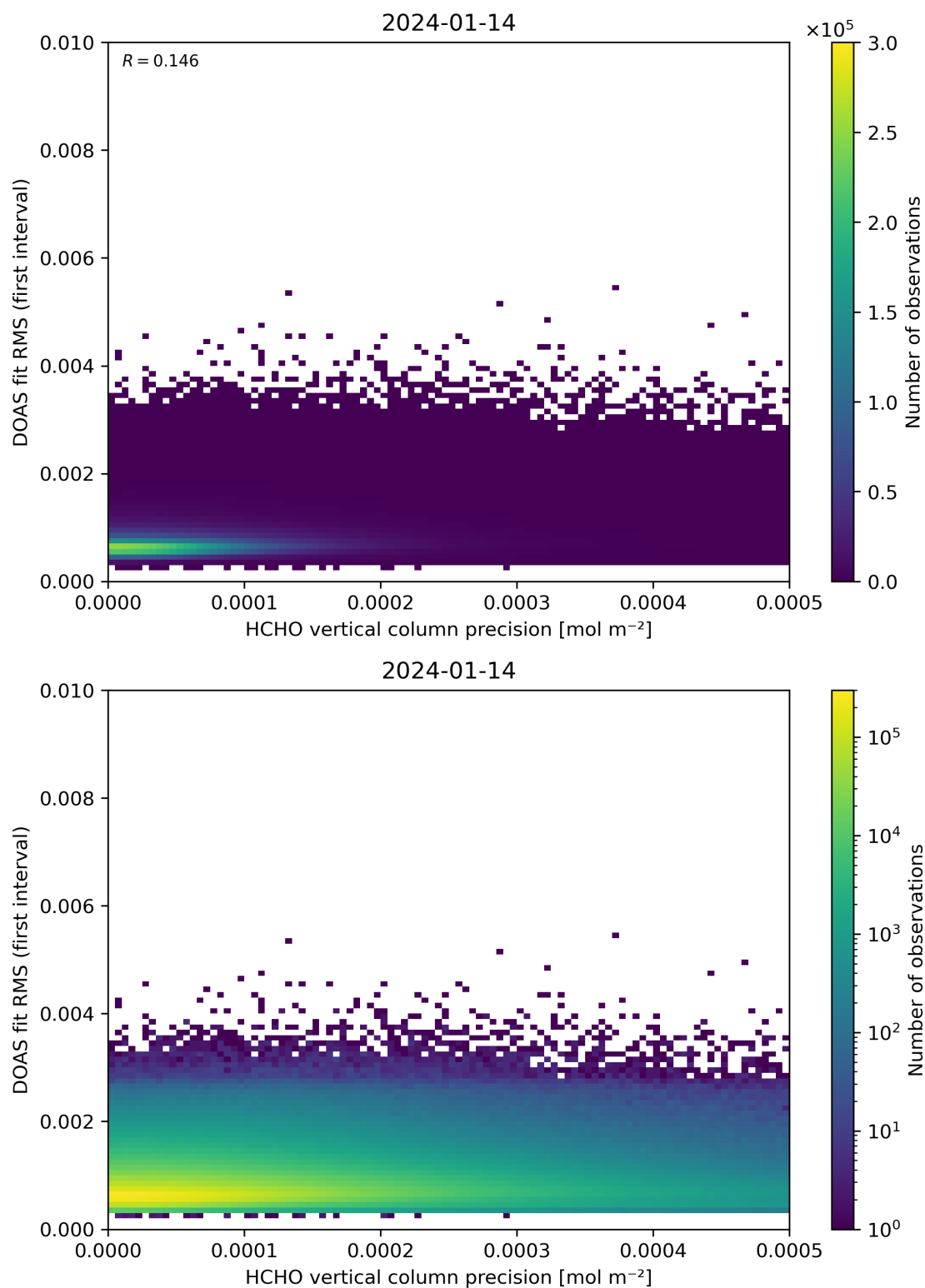
Figure 136: Scatter density plot of “HCHO vertical column precision” against “DOAS fit RMS (first interval)” for 2024-01-13 to 2024-01-15.
