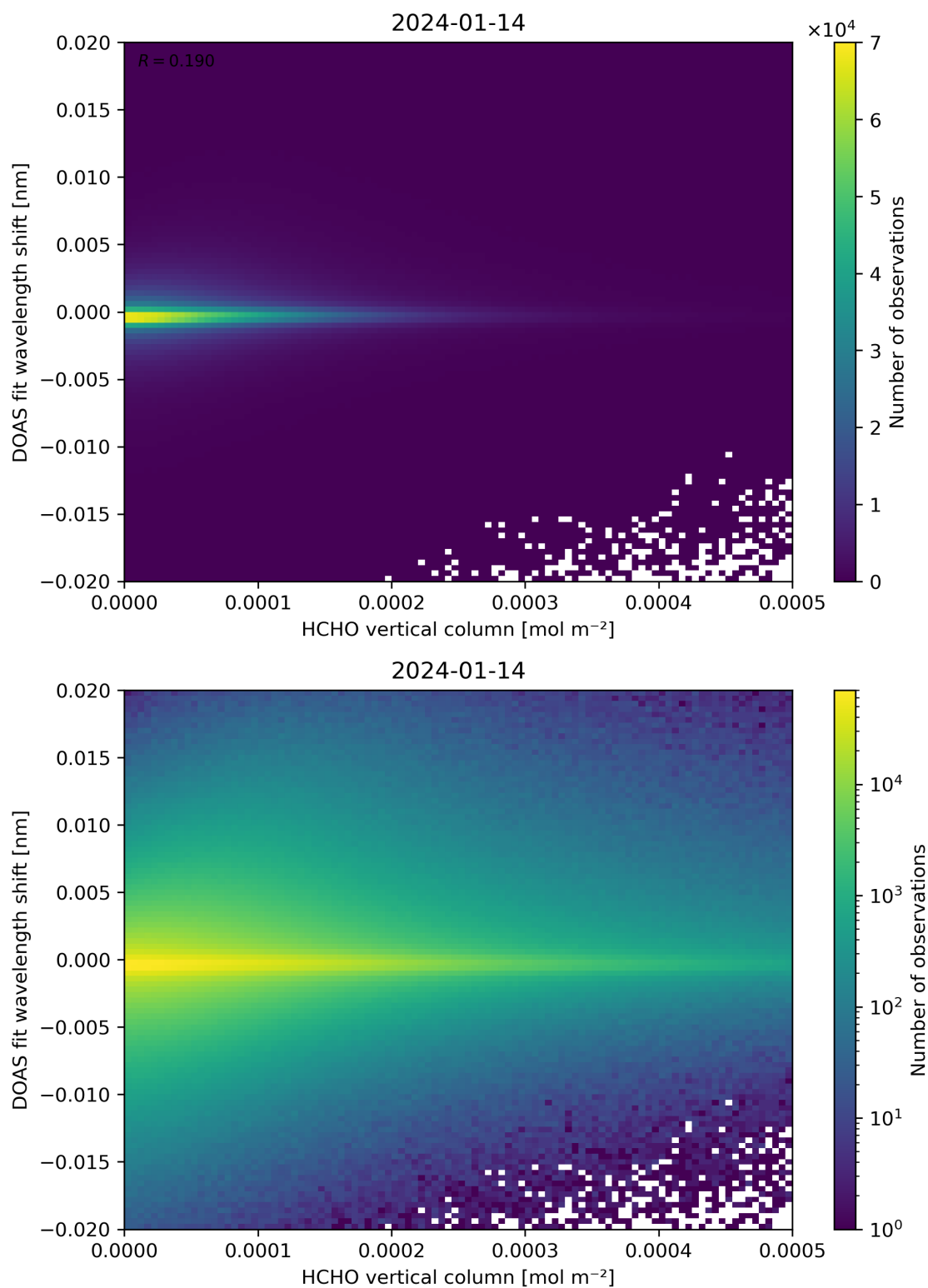
Figure 124: Scatter density plot of “HCHO vertical column” against “DOAS fit wavelength shift” for 2024-01-13 to 2024-01-15.
