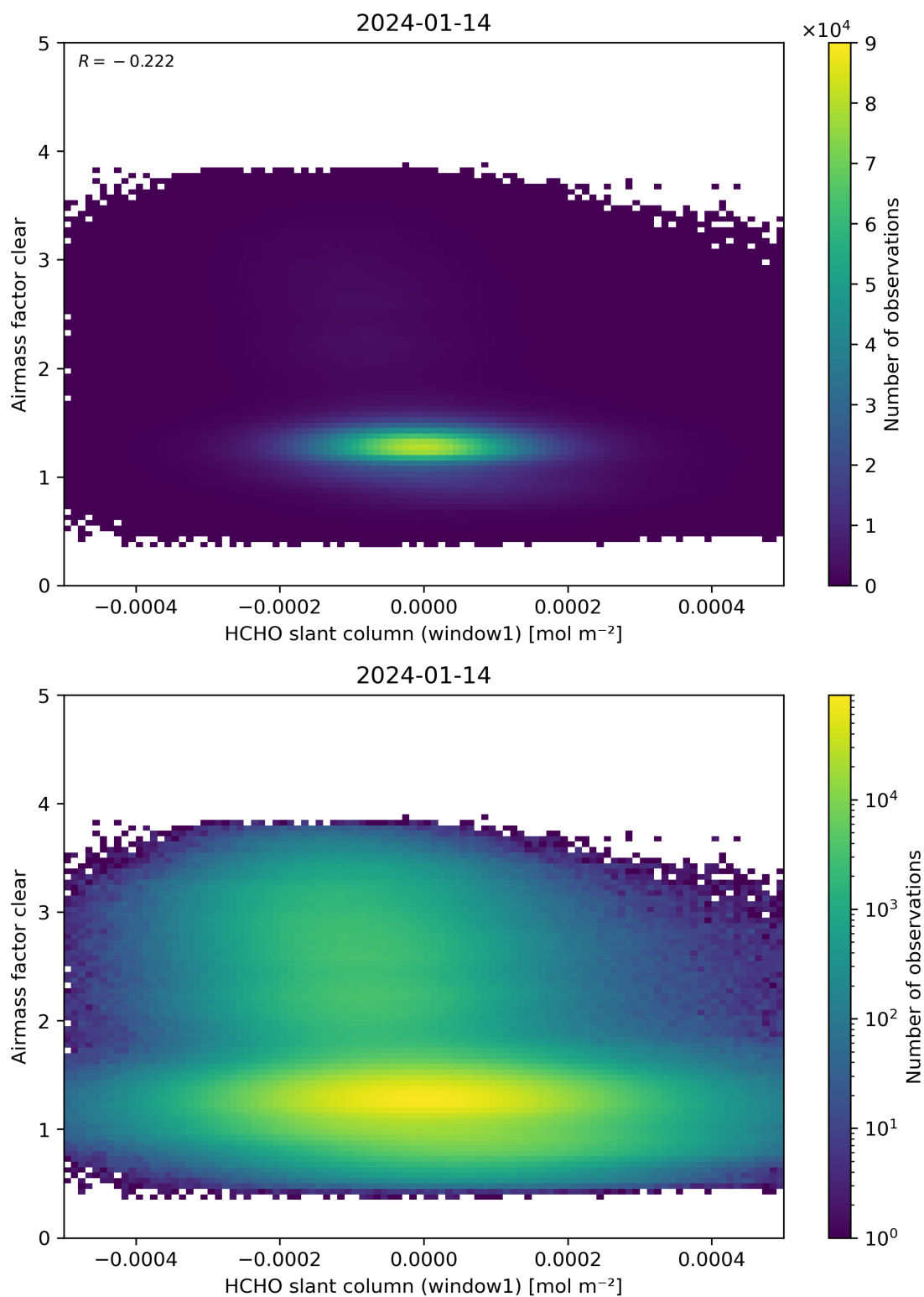
Figure 81: Scatter density plot of “HCHO slant column (window1)” against “Airmass factor clear” for 2024-01-13 to 2024-01-15.
