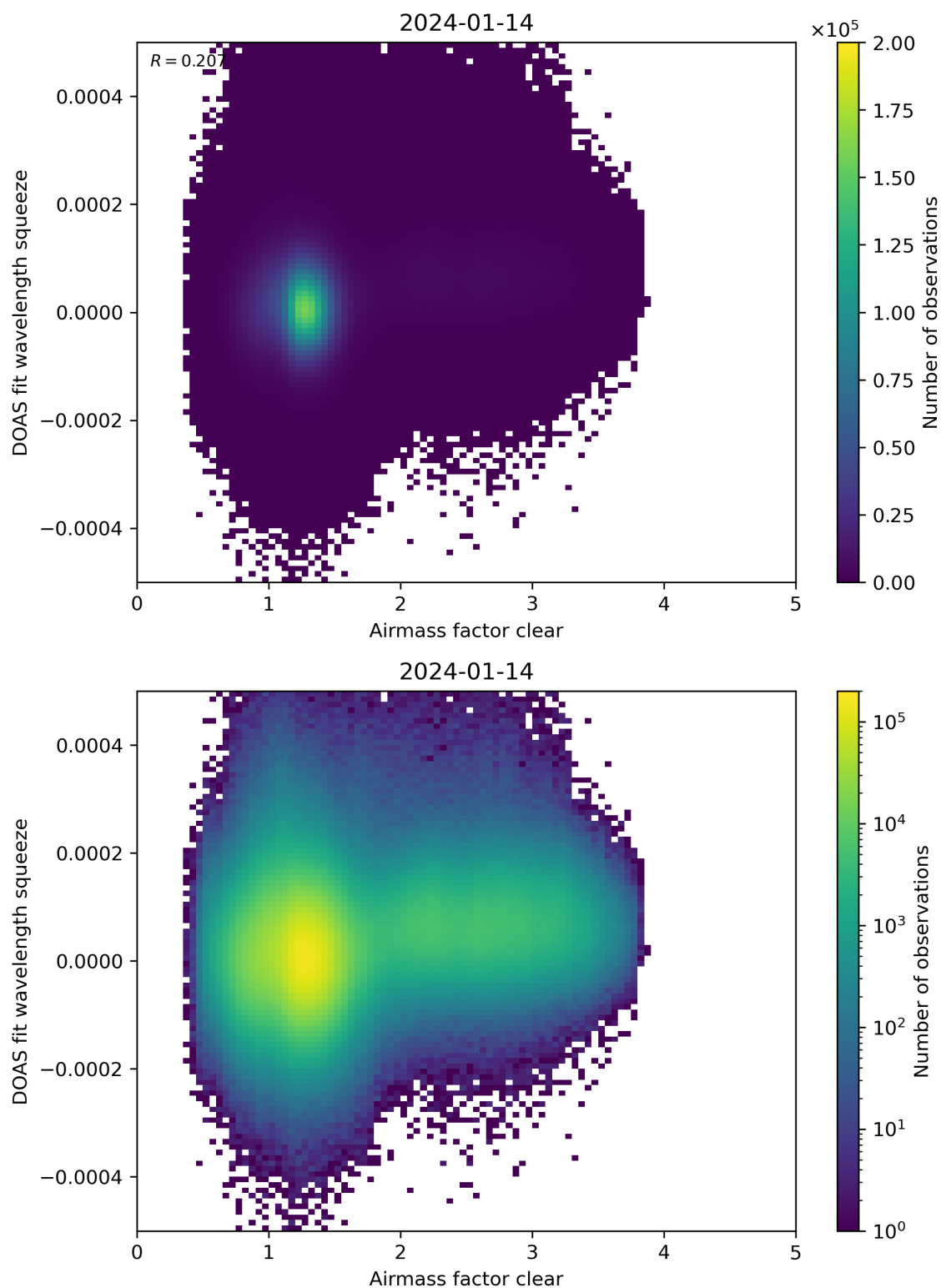
Figure 73: Scatter density plot of “Airmass factor clear” against “DOAS fit wavelength squeeze” for 2024-01-13 to 2024-01-15.
