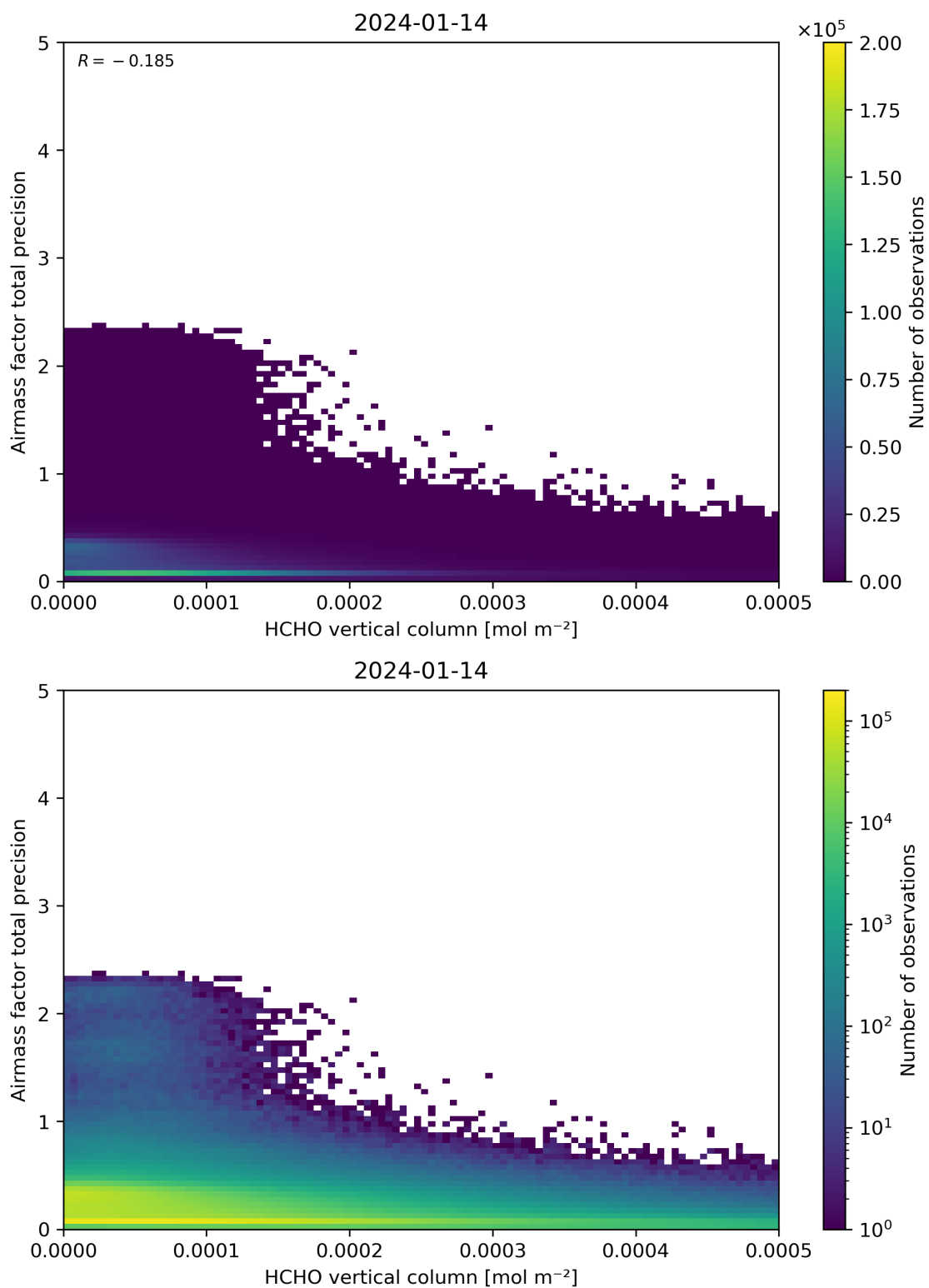
Figure 132: Scatter density plot of “HCHO vertical column” against “Airmass factor total precision” for 2024-01-13 to 2024-01-15.
