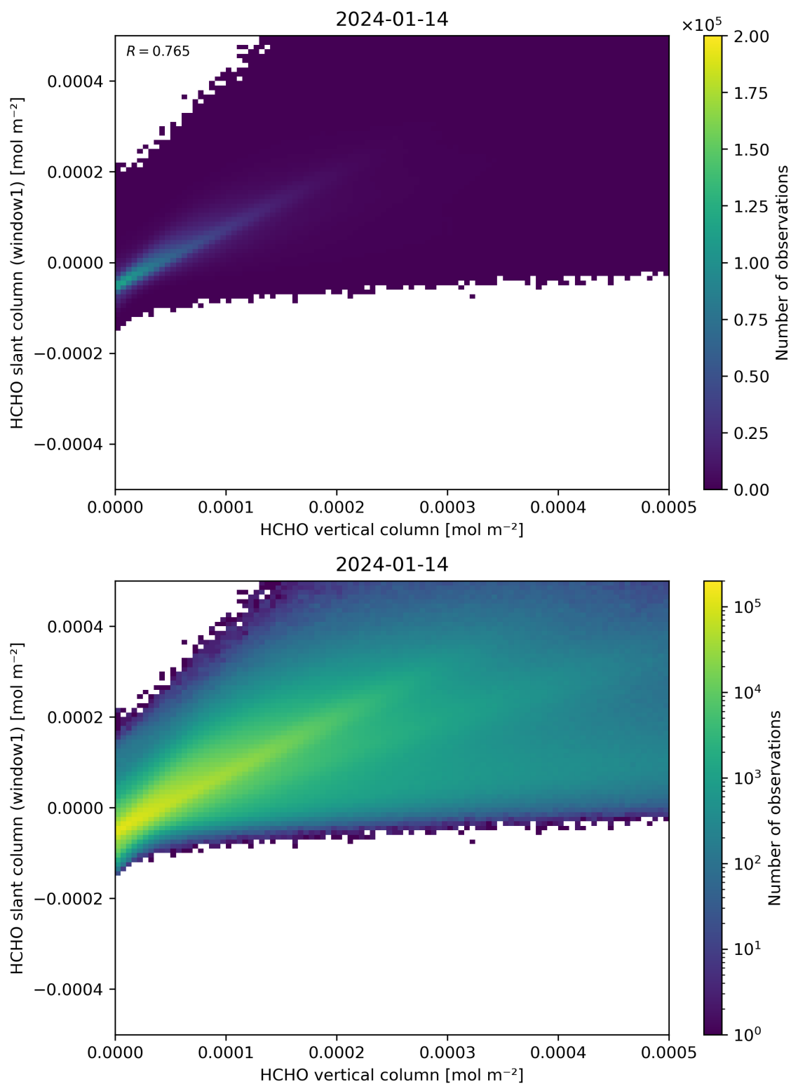
Figure 129: Scatter density plot of “HCHO vertical column” against “HCHO slant column (window1)” for 2024-01-13 to 2024-01-15.
