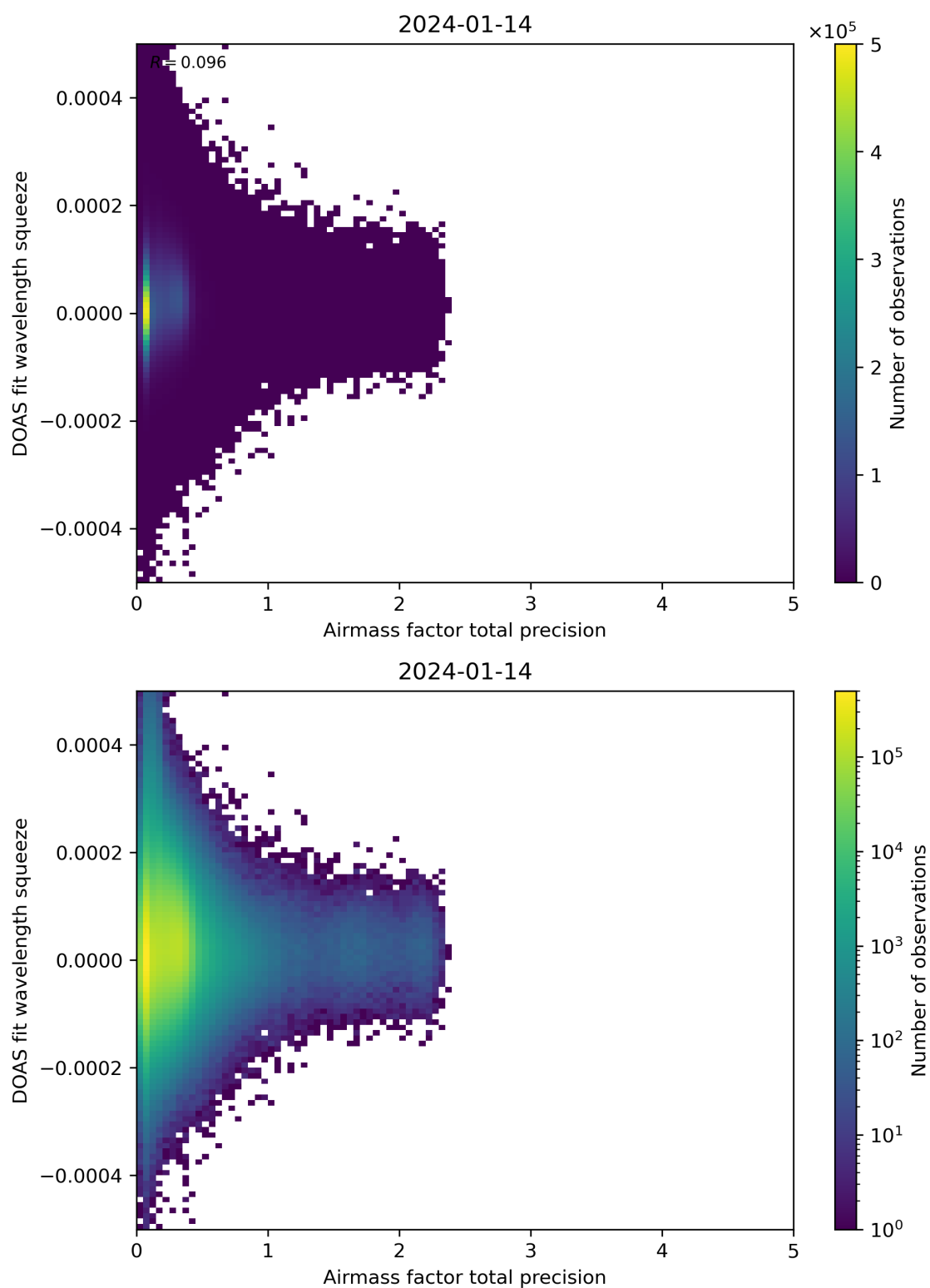
Figure 107: Scatter density plot of “Airmass factor total precision” against “DOAS fit wavelength squeeze” for 2024-01-13 to 2024-01-15.
