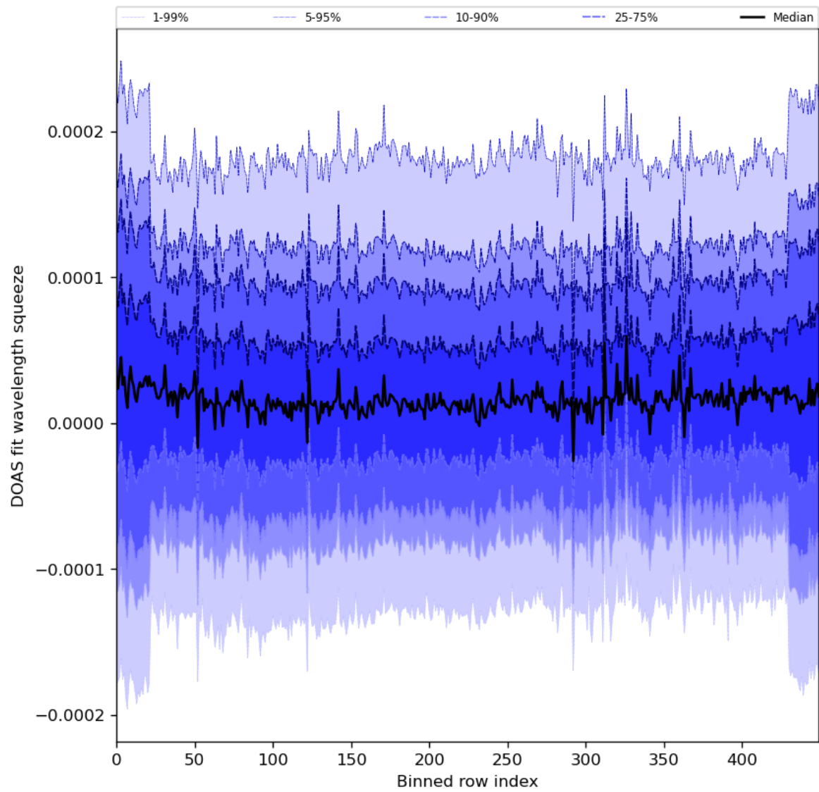
Figure 59: Along track statistics of “DOAS fit wavelength squeeze” for 2024-01-13 to 2024-01-15
