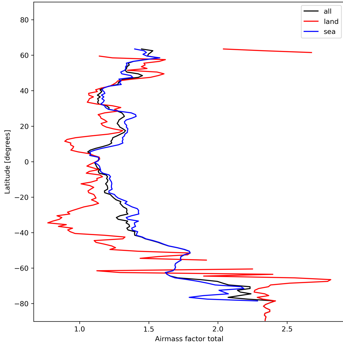
Figure 26: Zonal average of “Airmass factor total” for 2024-01-13 to 2024-01-15.
