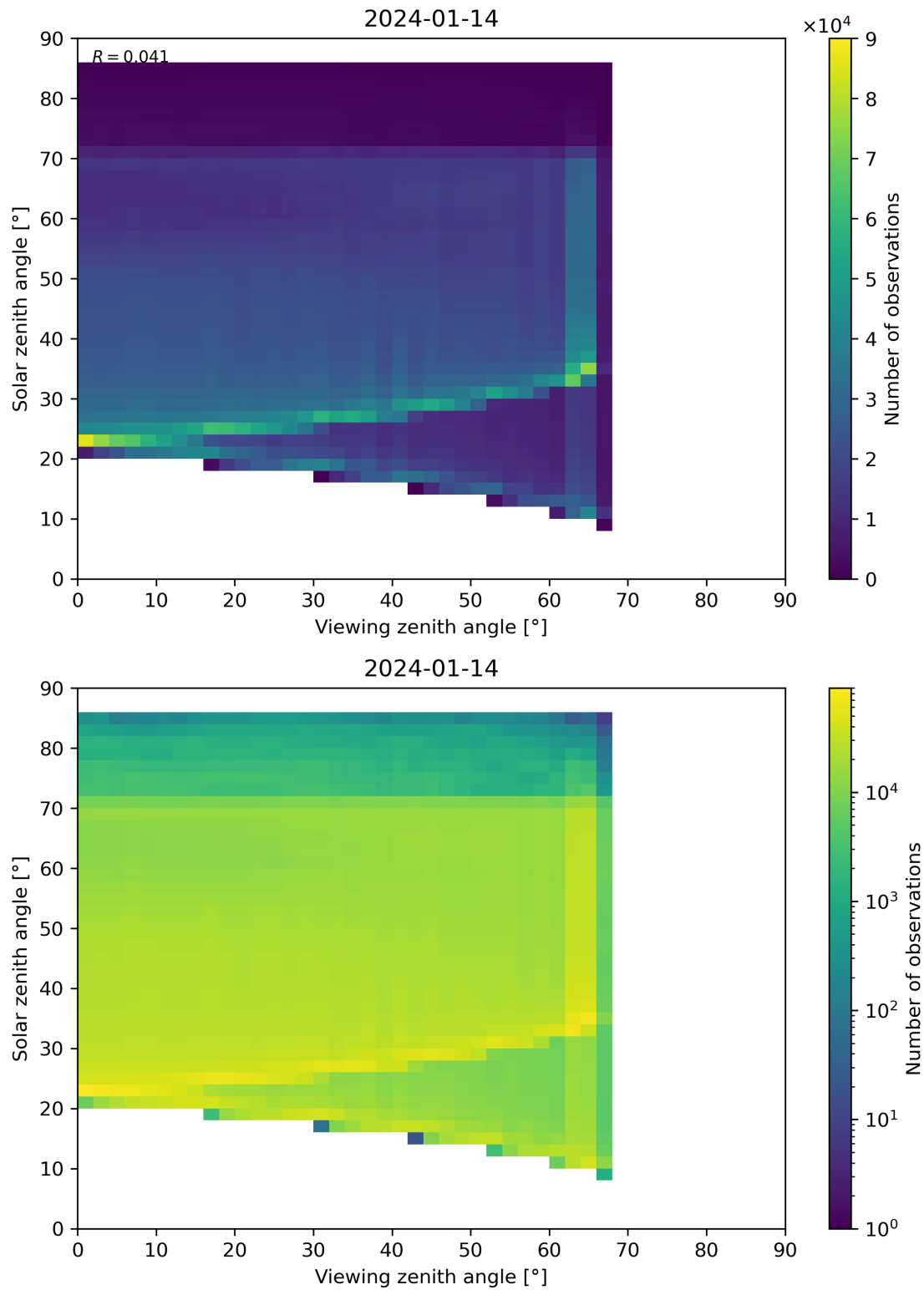
Figure 197: Scatter density plot of “Viewing zenith angle” against “Solar zenith angle” for 2024-01-13 to 2024-01-15.
