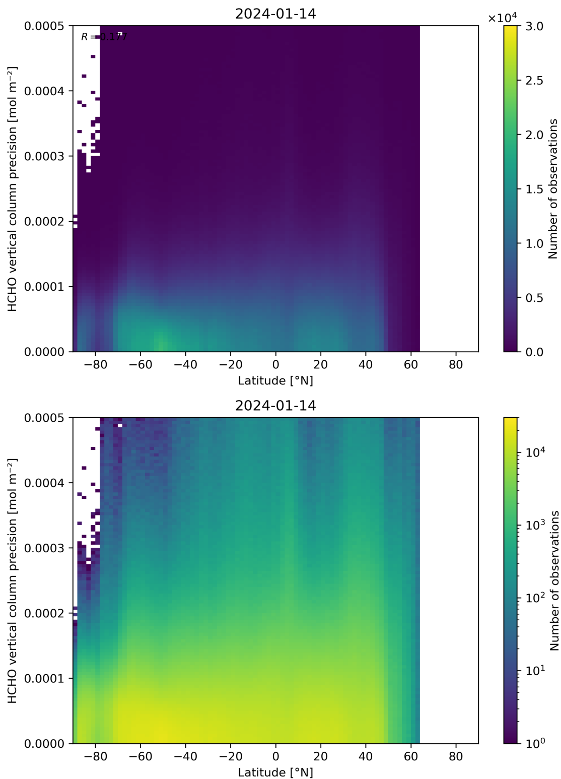
Figure 165: Scatter density plot of “Latitude” against “HCHO vertical column precision” for 2024-01-13 to 2024-01-15.
