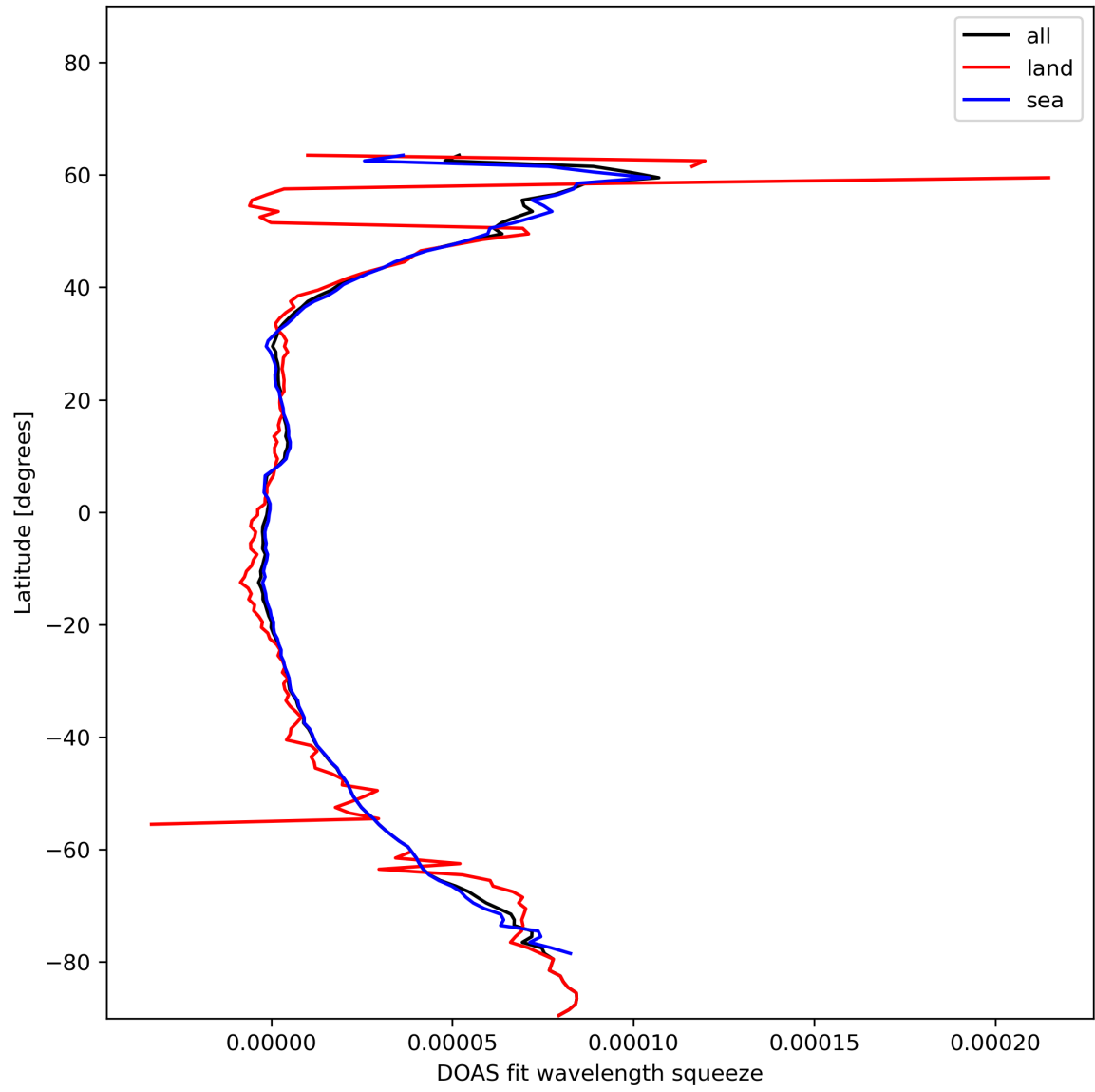
Figure 31: Zonal average of “DOAS fit wavelength squeeze” for 2024-01-13 to 2024-01-15.
