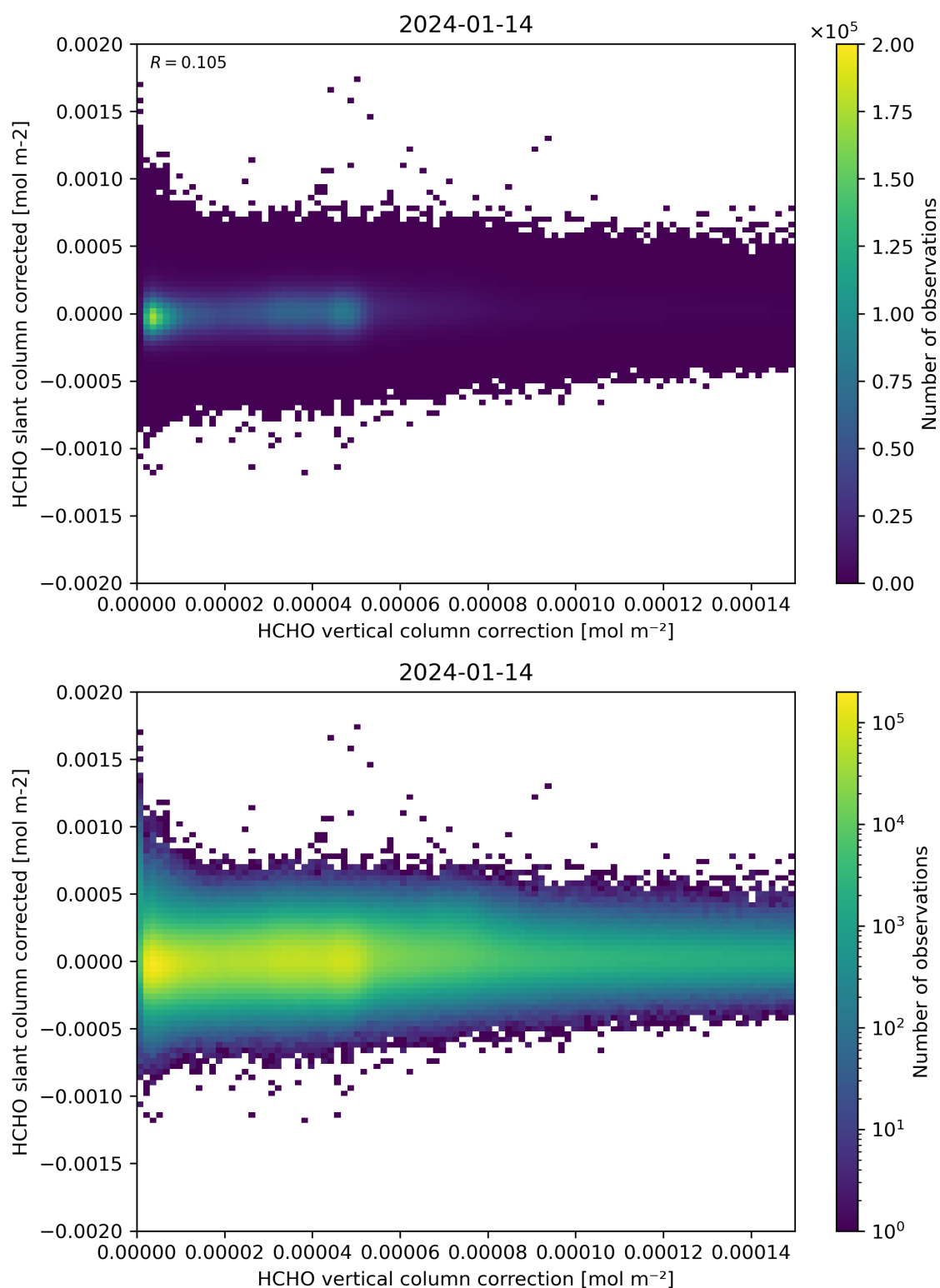
Figure 116: Scatter density plot of “HCHO vertical column correction” against “HCHO slant column corrected” for 2024-01-13 to 2024-01-15.
