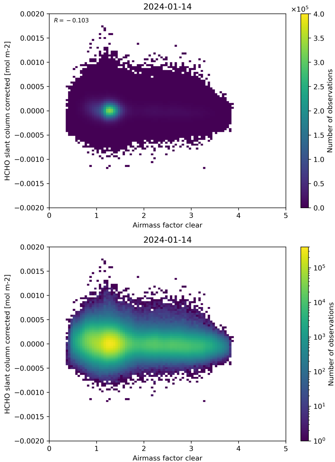
Figure 74: Scatter density plot of “Airmass factor clear” against “HCHO slant column corrected” for 2024-01-13 to 2024-01-15.
