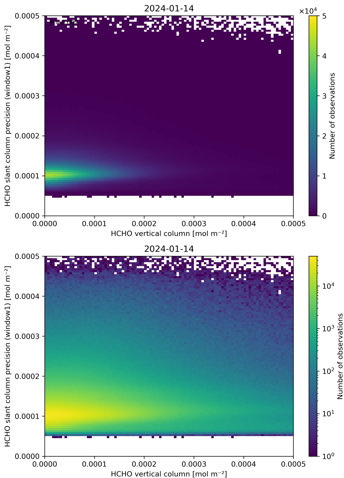
Figure 130: Scatter density plot of “HCHO vertical column” against “HCHO slant column precision (window1)” for 2024-01-13 to 2024-01-15.
