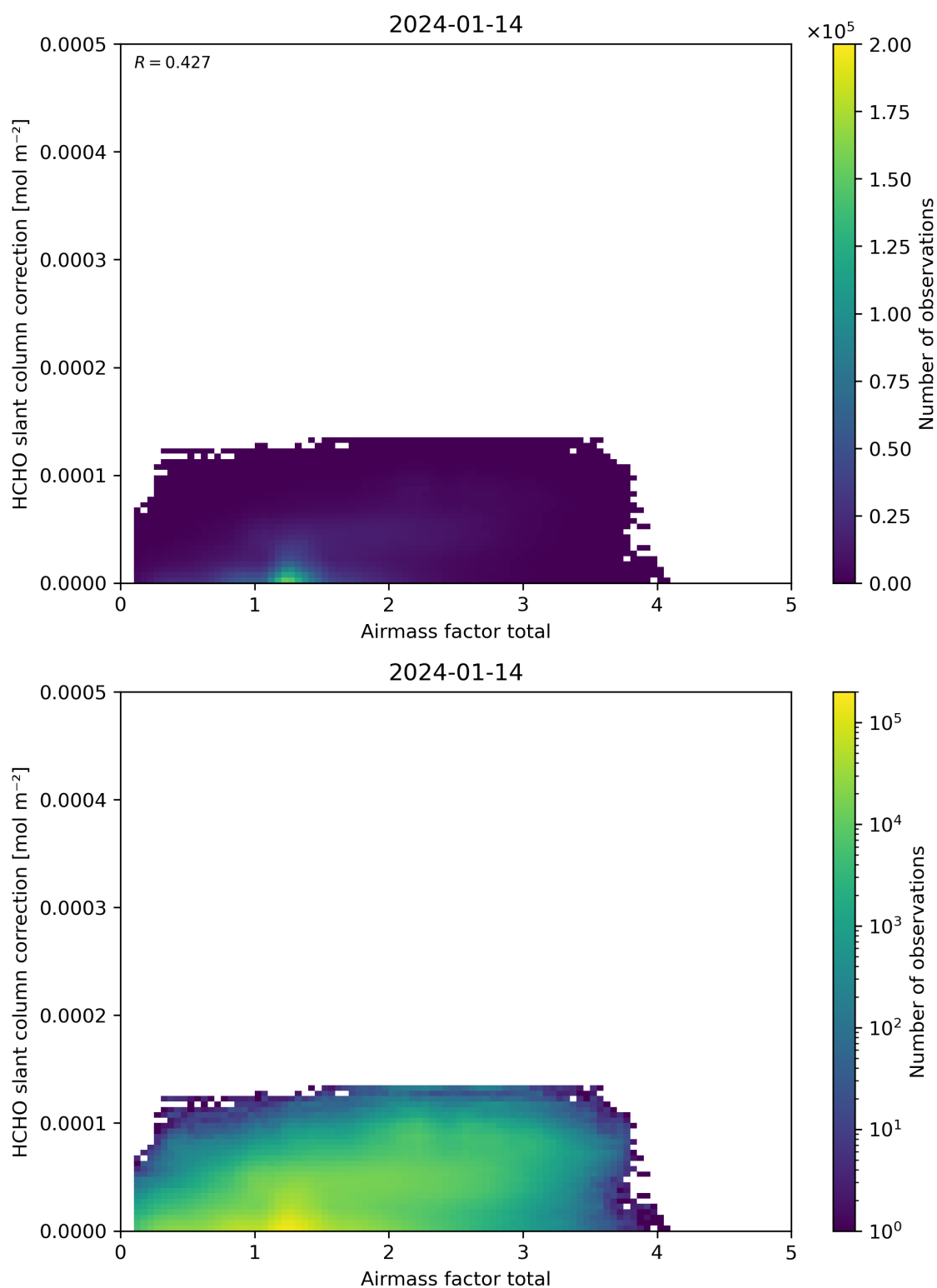
Figure 102: Scatter density plot of “Airmass factor total” against “HCHO slant column correction” for 2024-01-13 to 2024-01-15.
