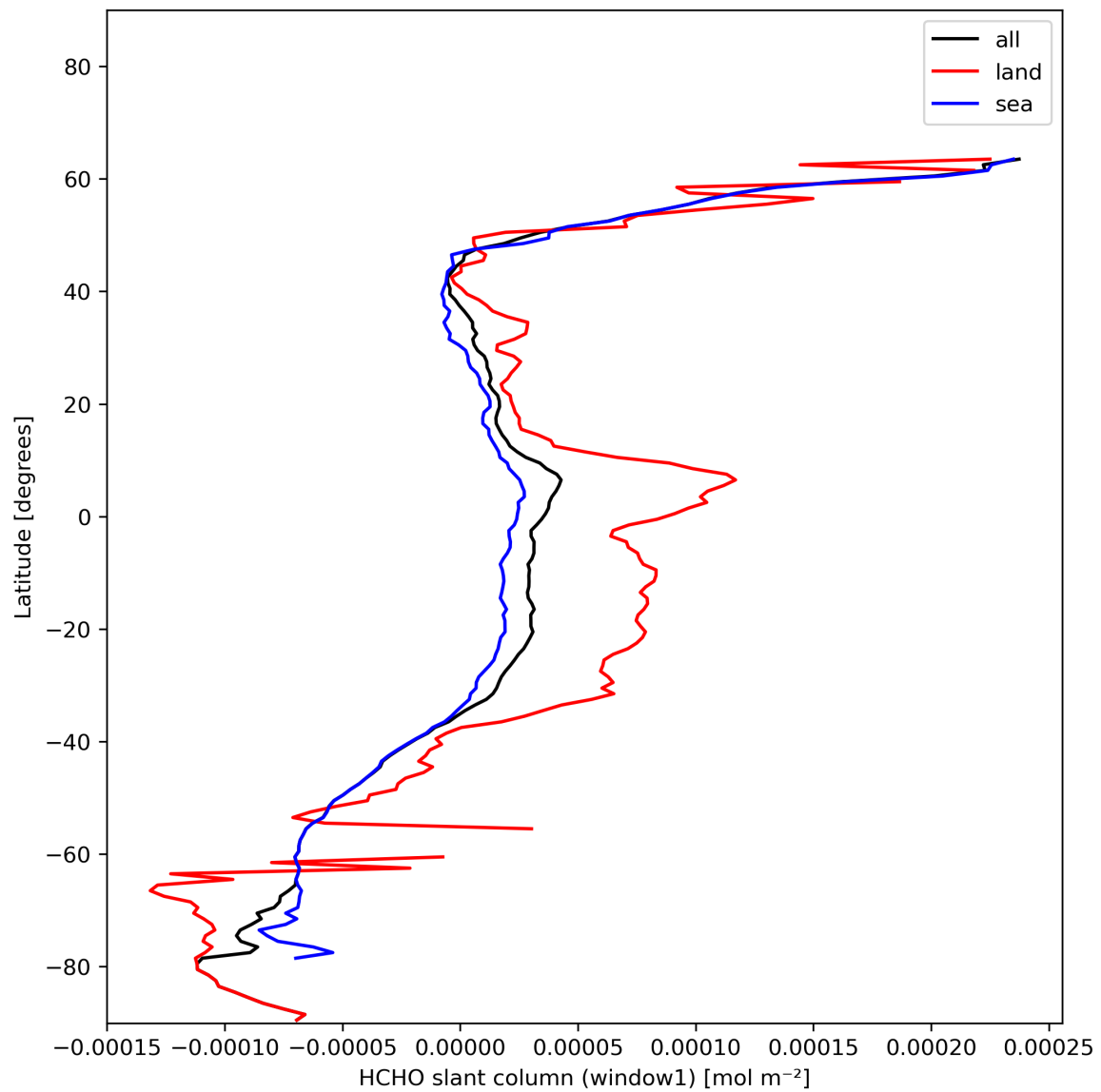
Figure 24: Zonal average of “HCHO slant column (window1)” for 2024-01-13 to 2024-01-15.
