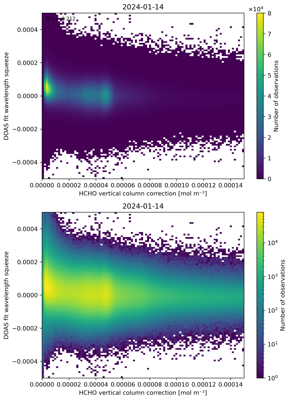
Figure 114: Scatter density plot of “HCHO vertical column correction” against “DOAS fit wavelength squeeze” for 2024-01-13 to 2024-01-15.
