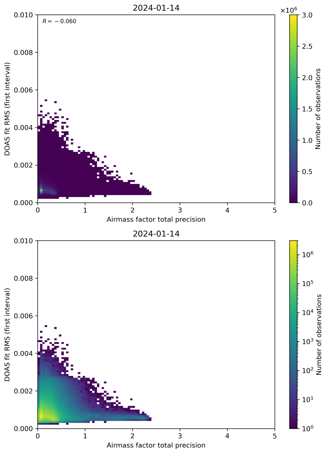
Figure 105: Scatter density plot of “Airmass factor total precision” against “DOAS fit RMS (first interval)” for 2024-01-13 to 2024-01-15.
