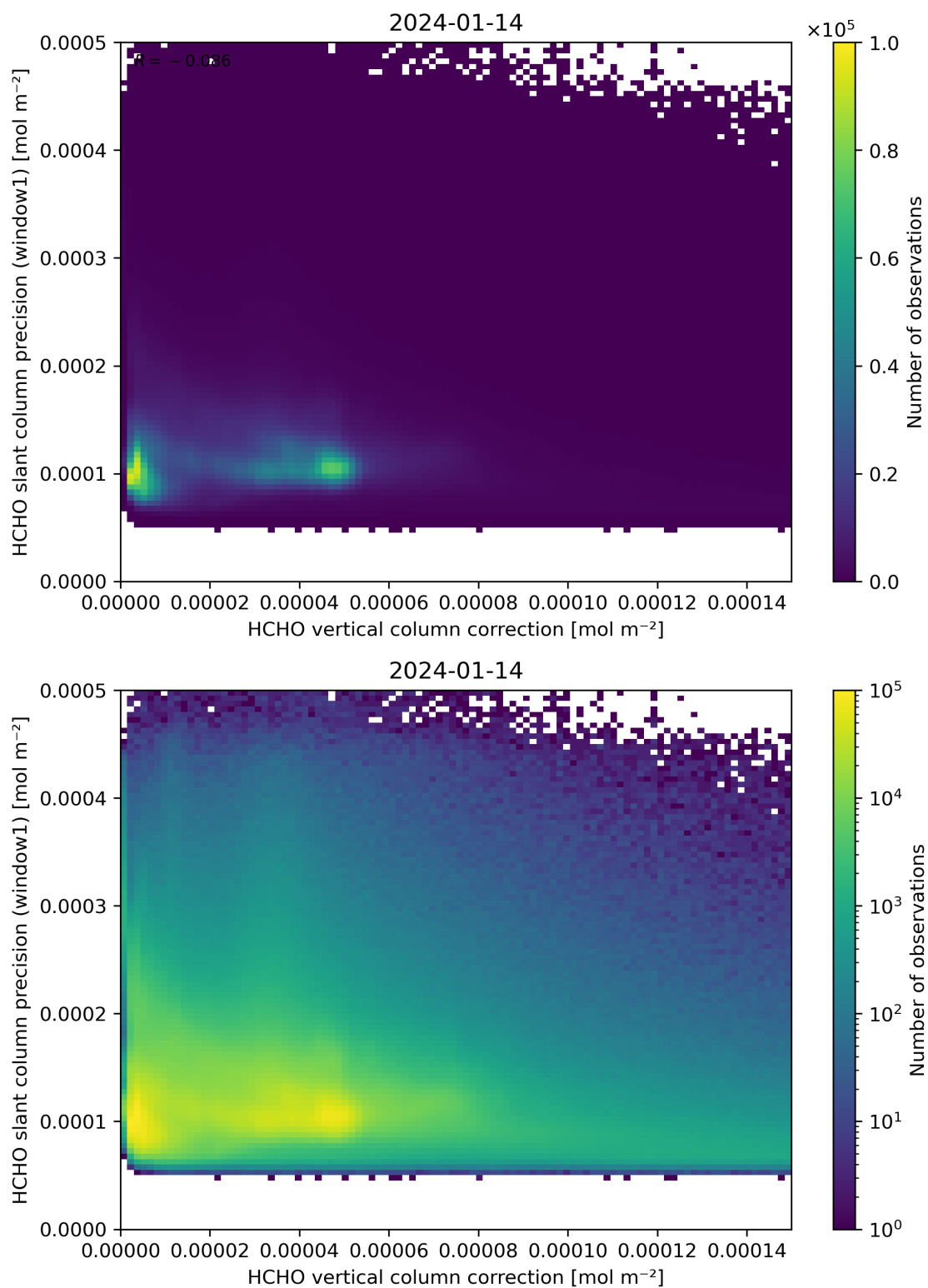
Figure 119: Scatter density plot of “HCHO vertical column correction” against “HCHO slant column precision (window1)” for 2024-01-13 to 2024-01-15.
