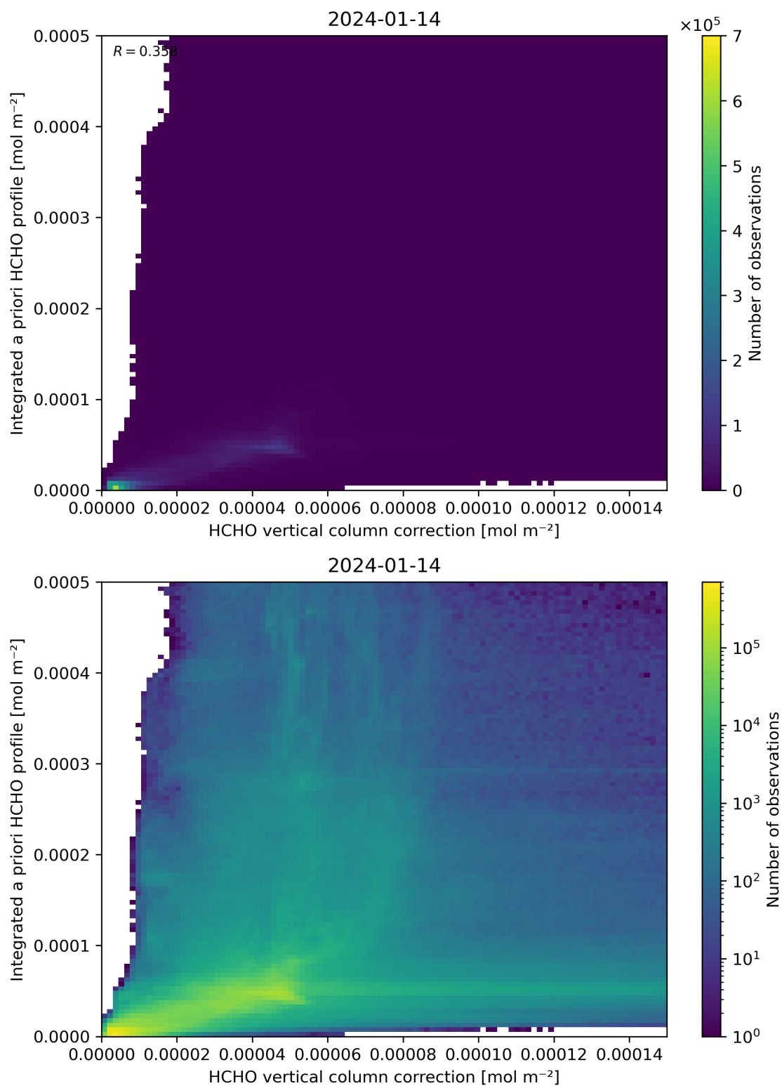
Figure 122: Scatter density plot of “HCHO vertical column correction” against “Integrated a priori HCHO profile” for 2024-01-13 to 2024-01-15.
