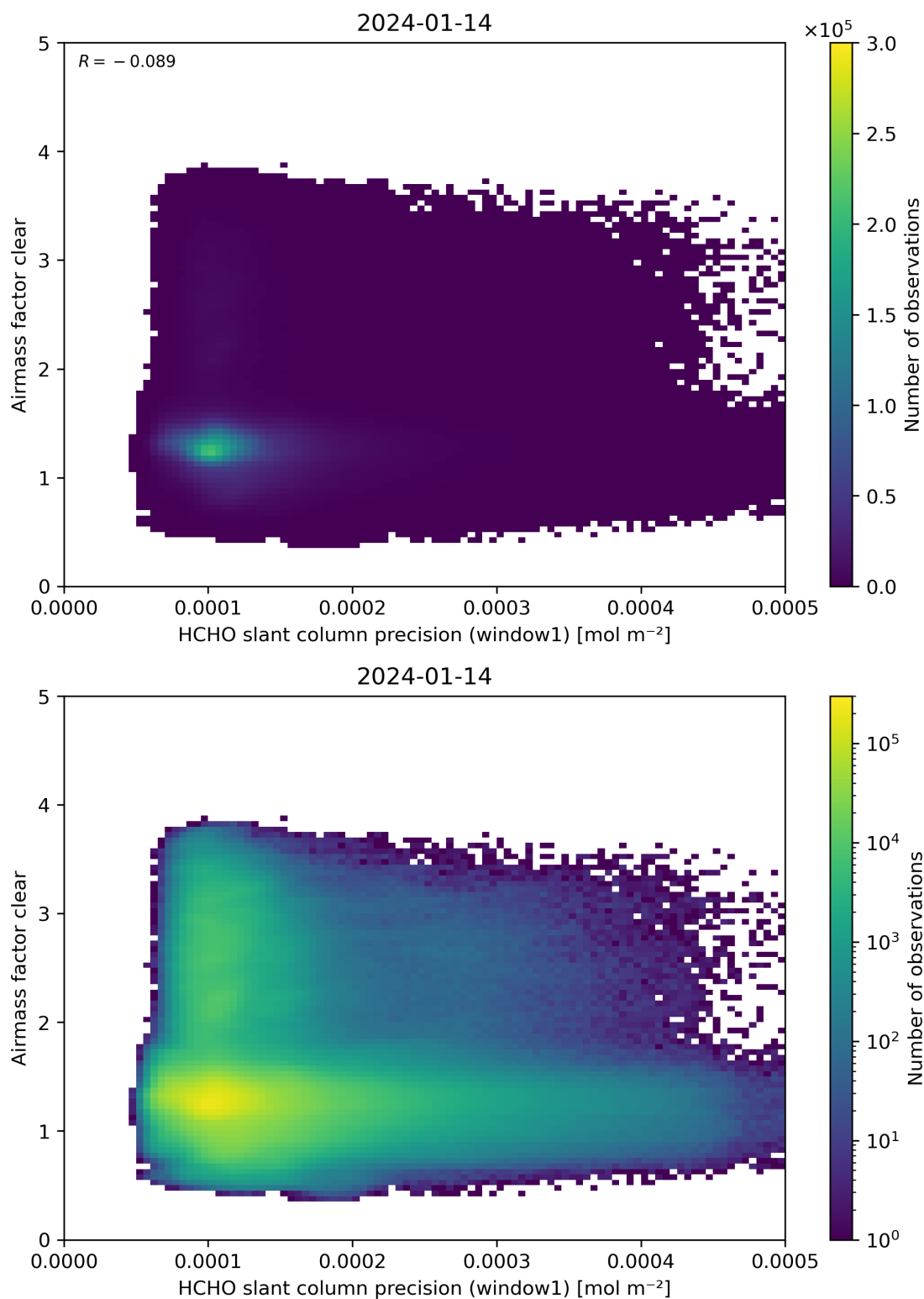
Figure 91: Scatter density plot of “HCHO slant column precision (window1)” against “Airmass factor clear” for 2024-01-13 to 2024-01-15.
