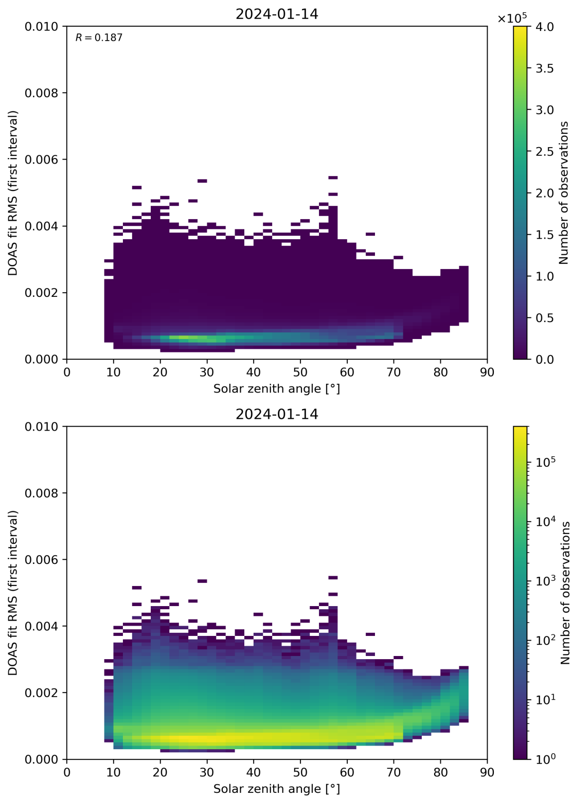
Figure 167: Scatter density plot of “Solar zenith angle” against “DOAS fit RMS (first interval)” for 2024-01-13 to 2024-01-15.
