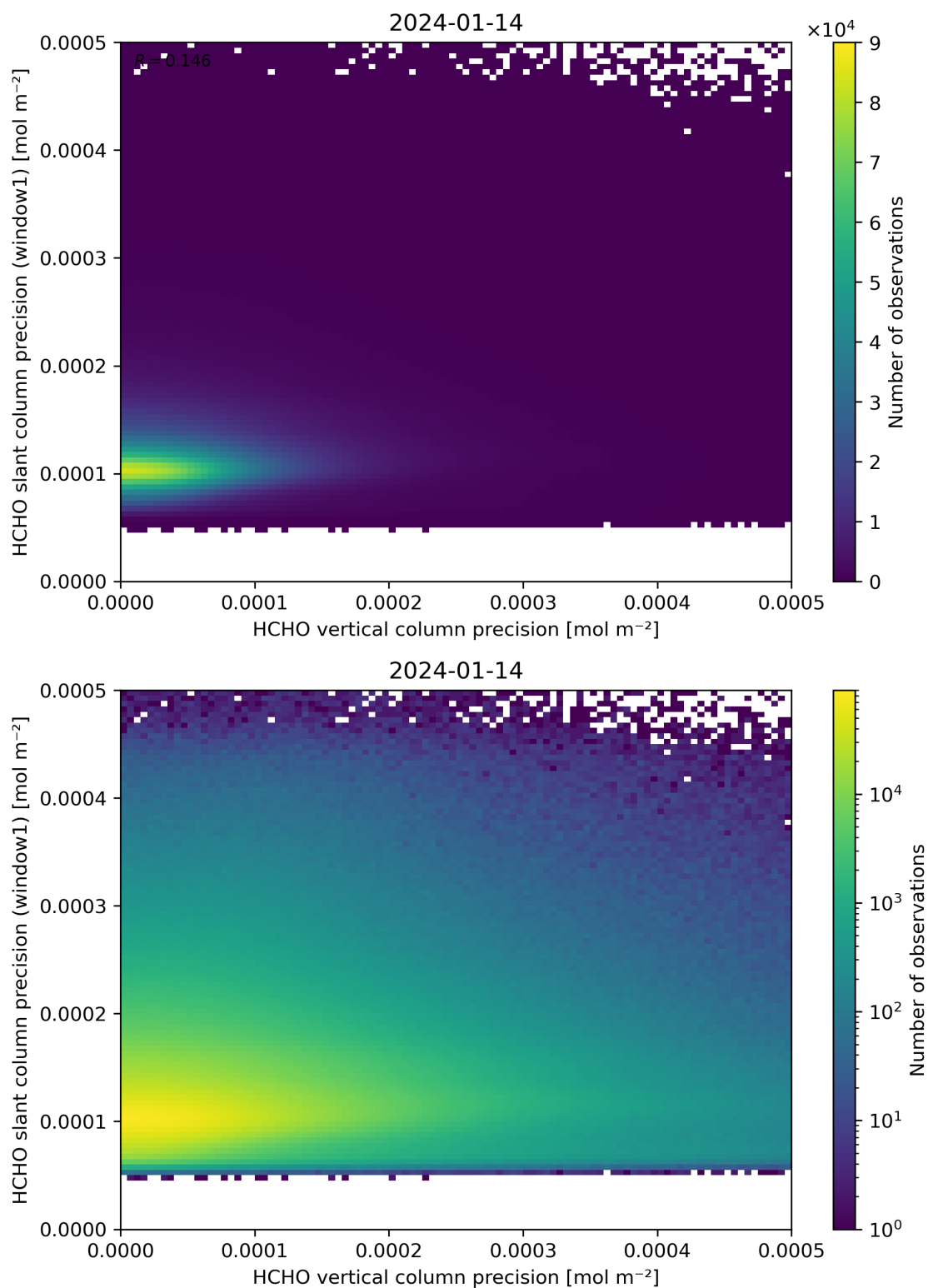
Figure 143: Scatter density plot of “HCHO vertical column precision” against “HCHO slant column precision (window1)” for 2024-01-13 to 2024-01-15.
