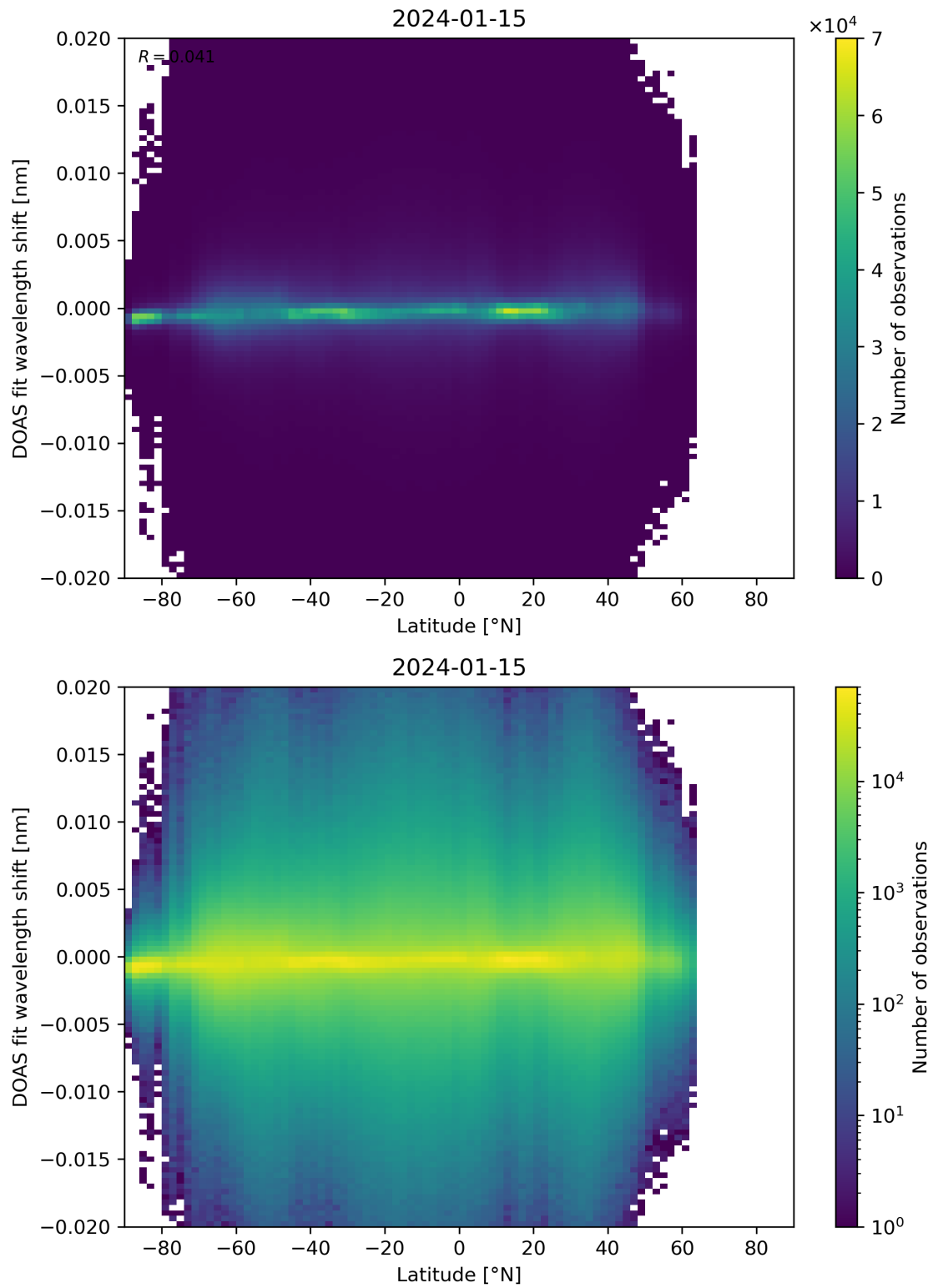
Figure 154: Scatter density plot of “Latitude” against “DOAS fit wavelength shift” for 2024-01-15 to 2024-01-16.
