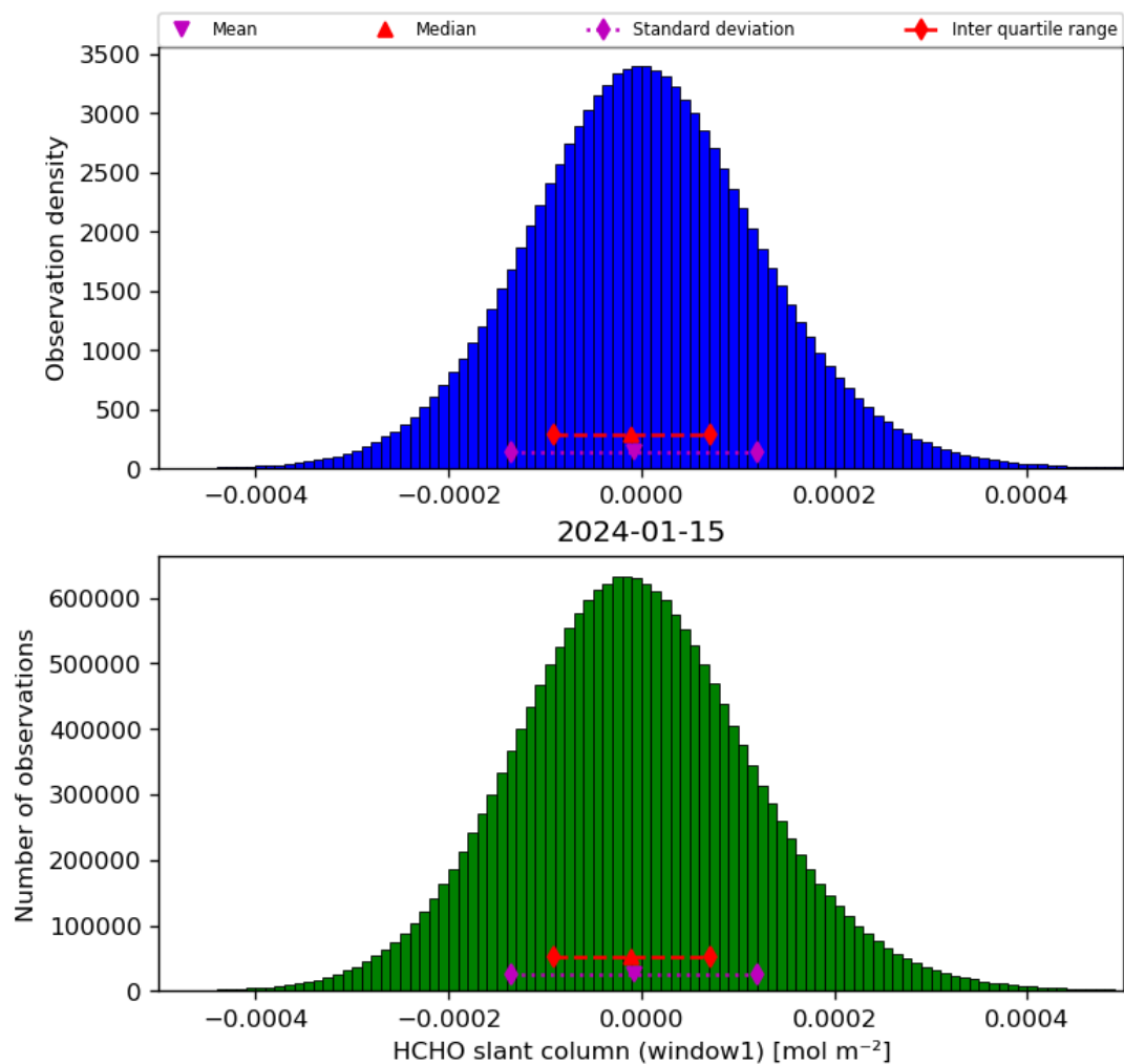
Figure 38: Histogram of “HCHO slant column (window1)” for 2024-01-15 to 2024-01-16
