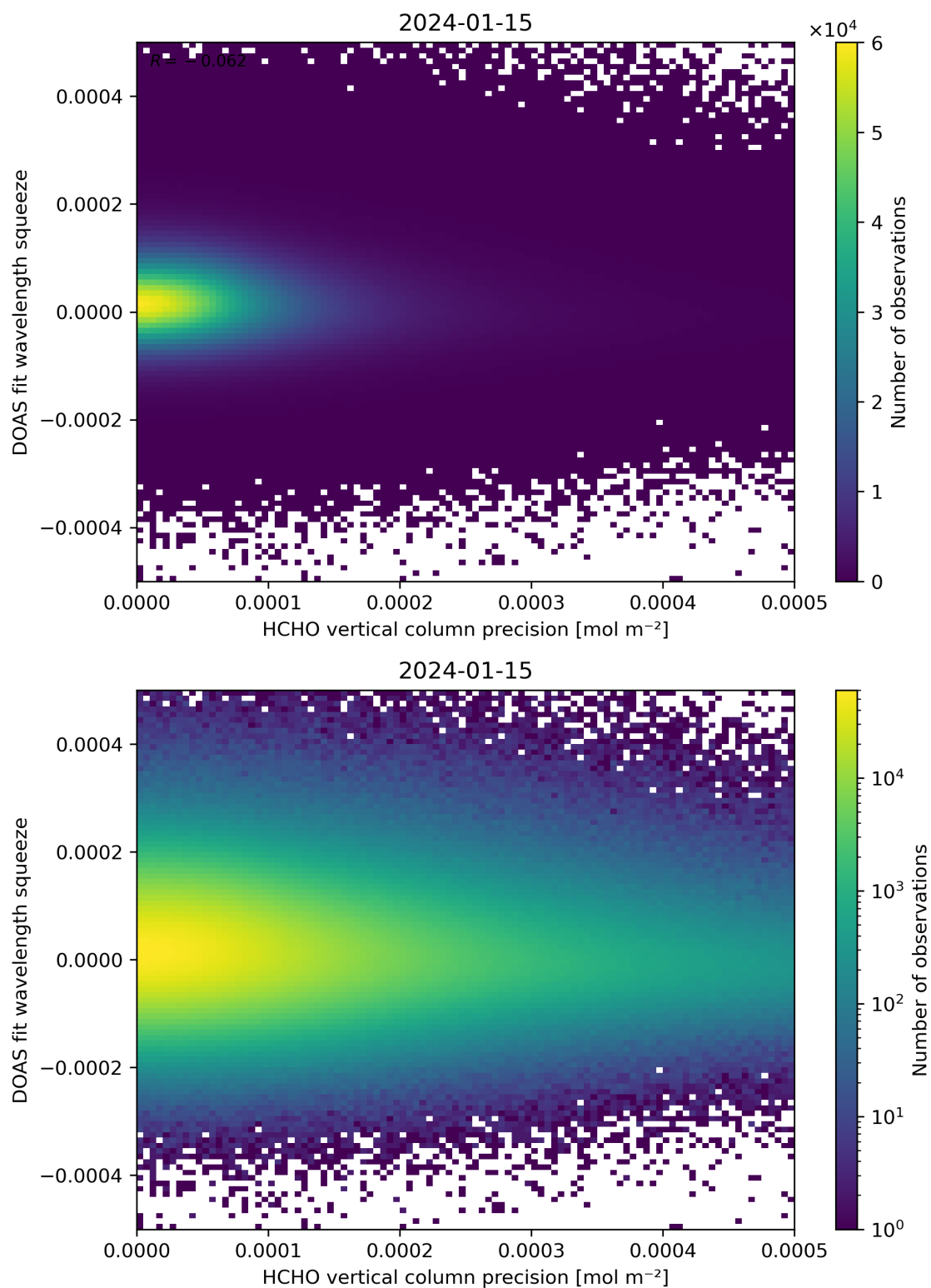
Figure 138: Scatter density plot of “HCHO vertical column precision” against “DOAS fit wavelength squeeze” for 2024-01-15 to 2024-01-16.
