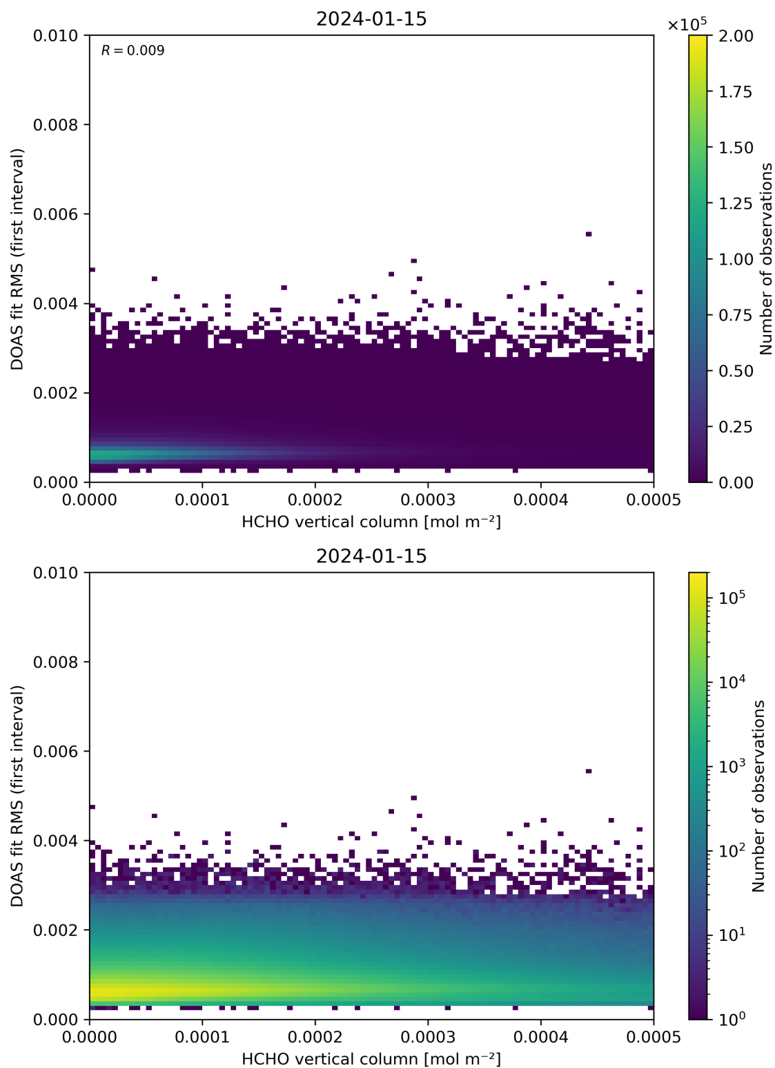
Figure 123: Scatter density plot of “HCHO vertical column” against “DOAS fit RMS (first interval)” for 2024-01-15 to 2024-01-16.
