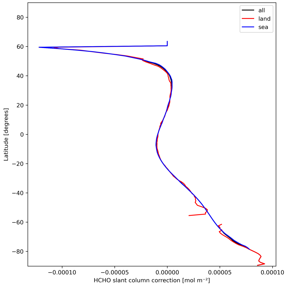
Figure 33: Zonal average of “HCHO slant column correction” for 2024-01-15 to 2024-01-16.
