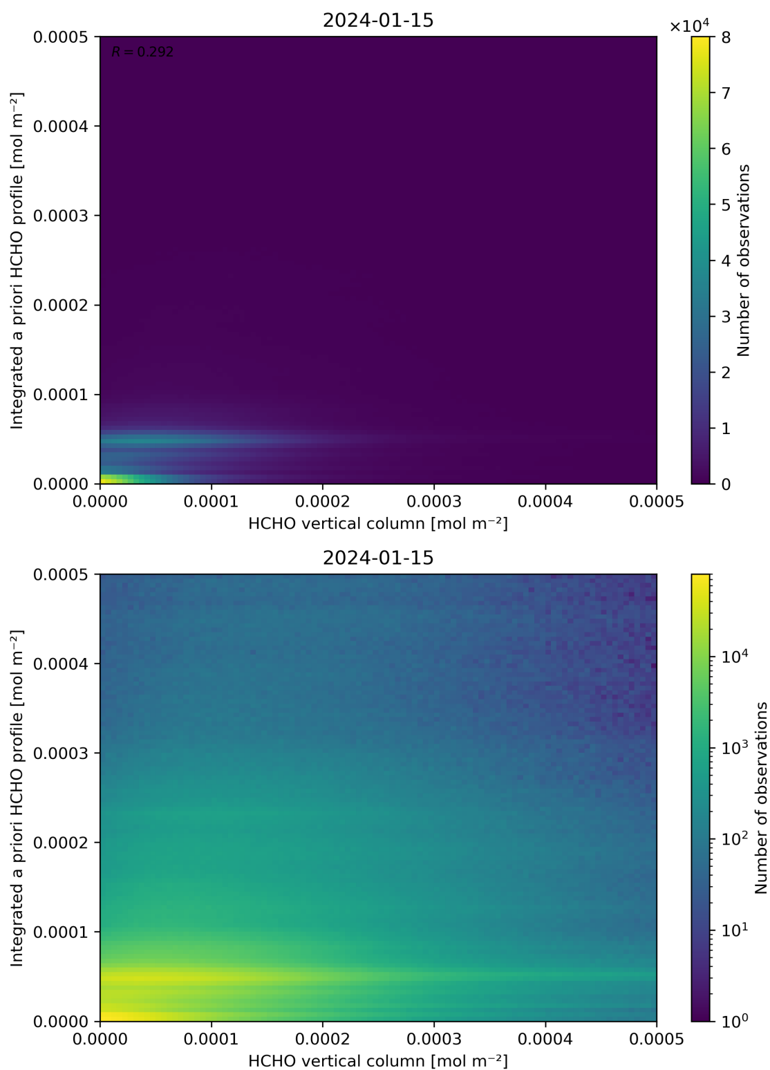
Figure 135: Scatter density plot of “HCHO vertical column” against “Integrated a priori HCHO profile” for 2024-01-15 to 2024-01-16.
