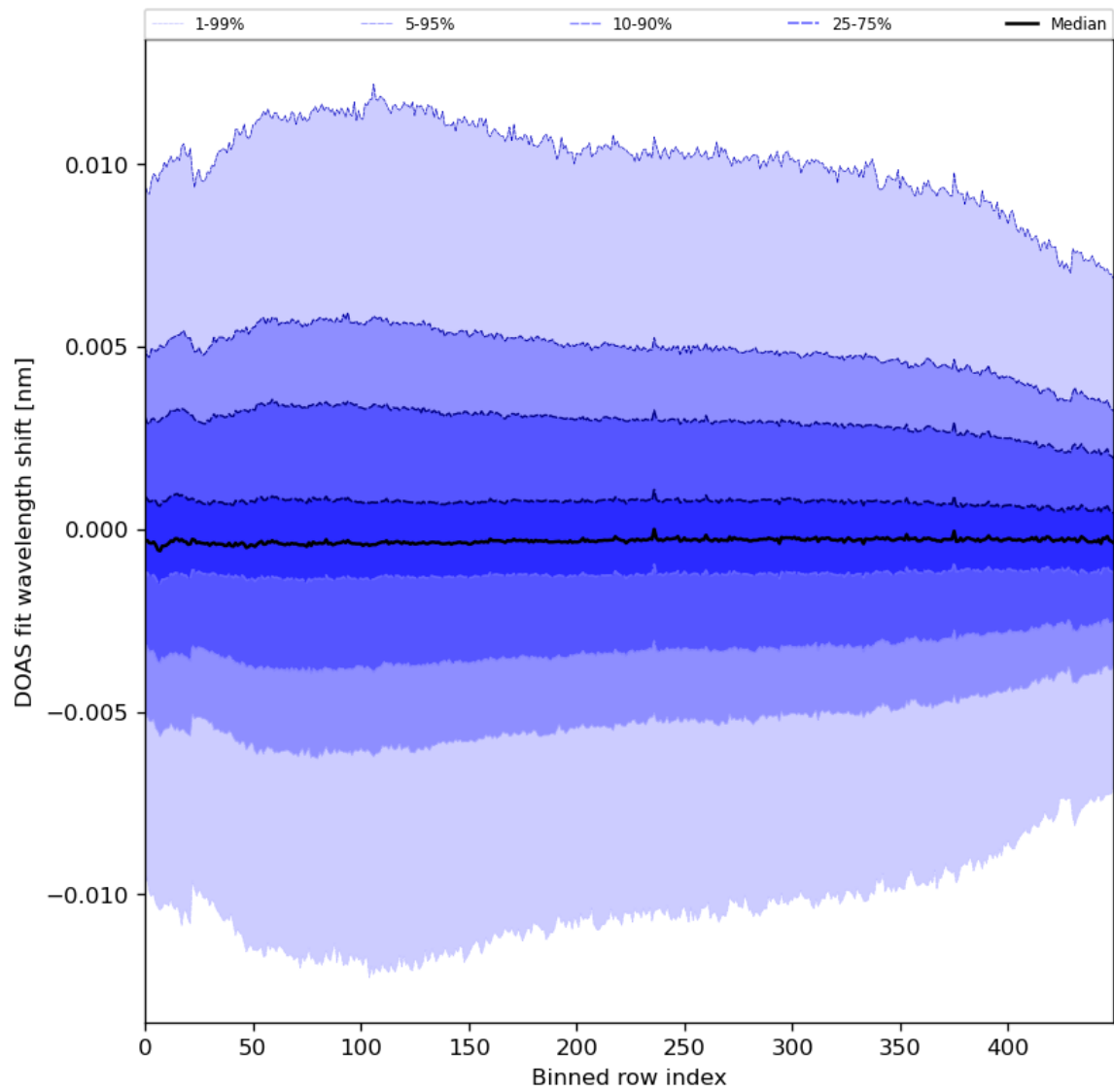
Figure 58: Along track statistics of “DOAS fit wavelength shift” for 2024-01-15 to 2024-01-16
