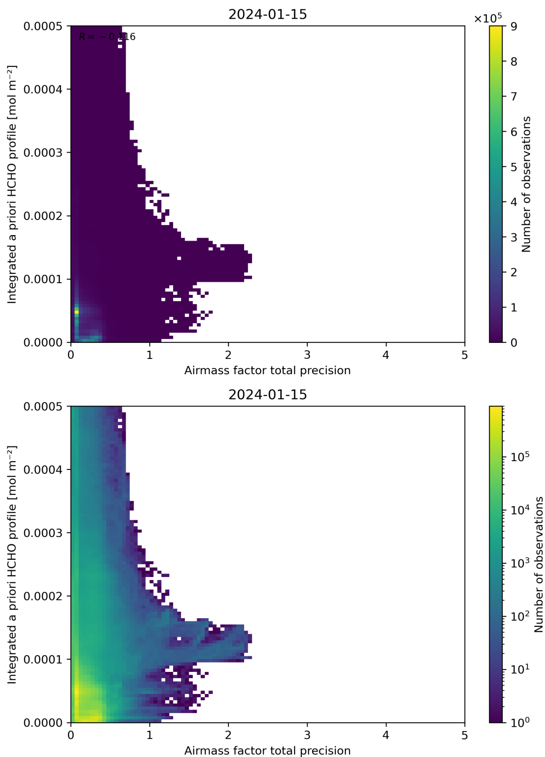
Figure 111: Scatter density plot of “Airmass factor total precision” against “Integrated a priori HCHO profile” for 2024-01-15 to 2024-01-16.
