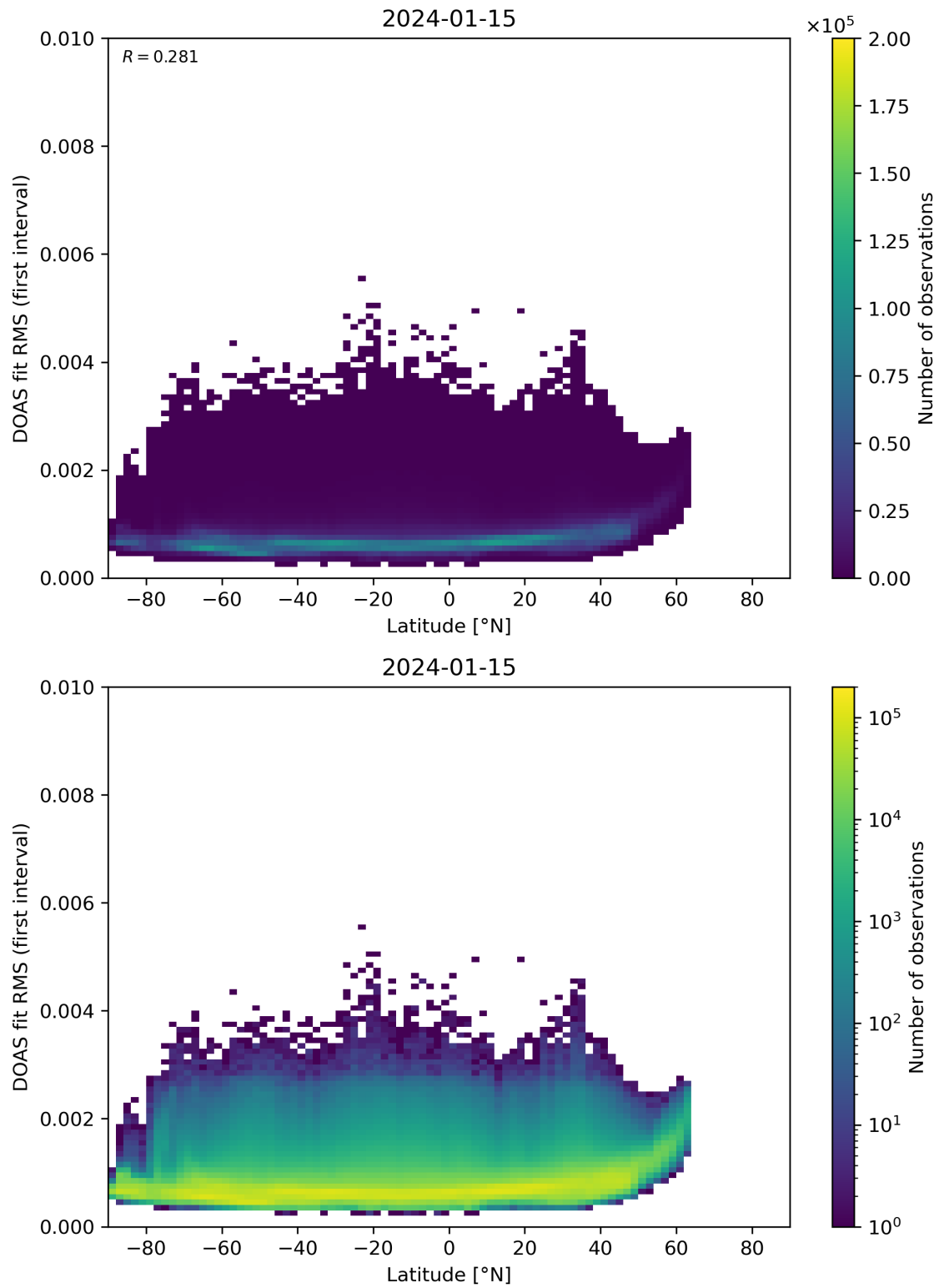
Figure 153: Scatter density plot of “Latitude” against “DOAS fit RMS (first interval)” for 2024-01-15 to 2024-01-16.
