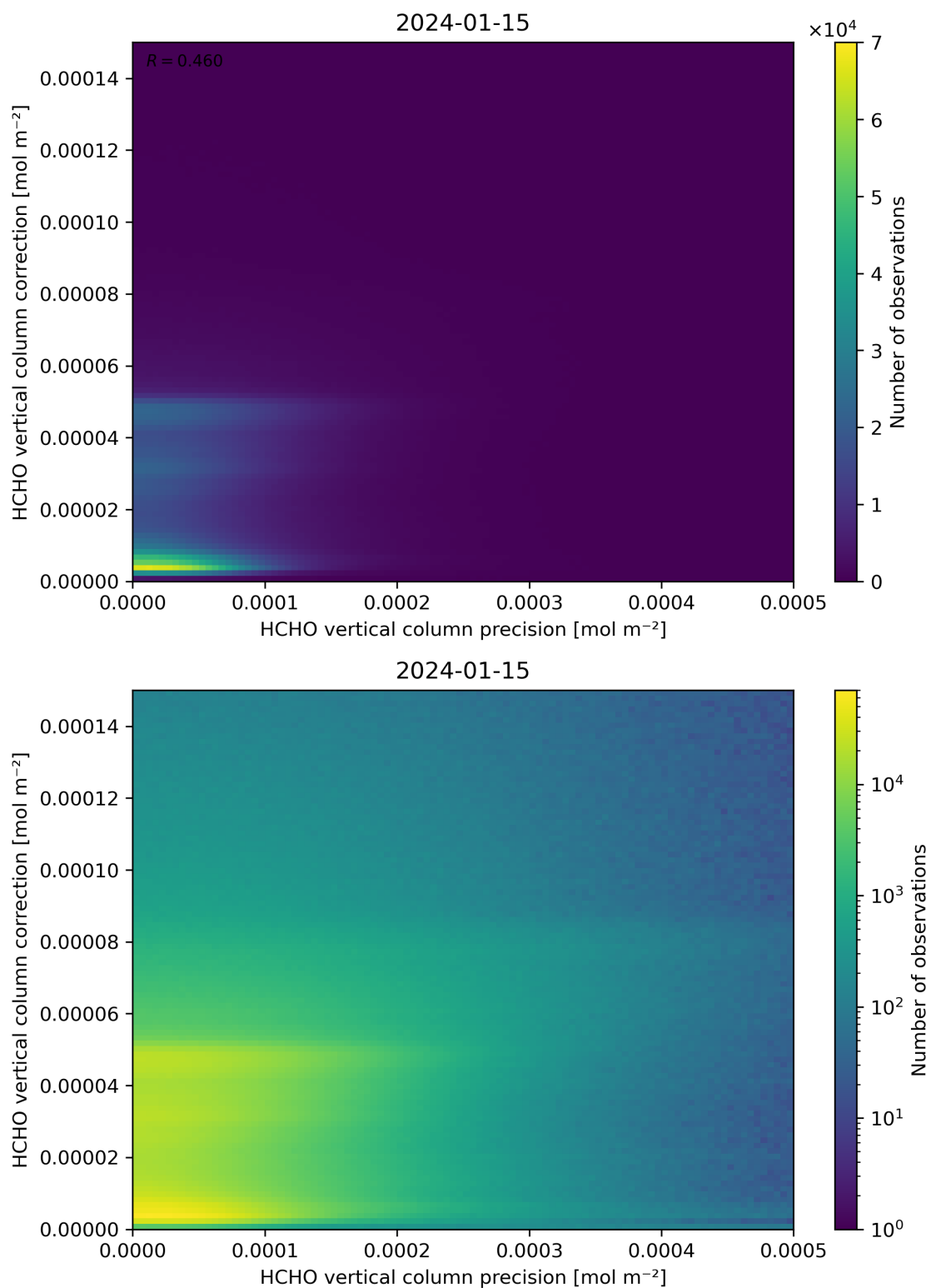
Figure 146: Scatter density plot of “HCHO vertical column precision” against “HCHO vertical column correction” for 2024-01-15 to 2024-01-16.
