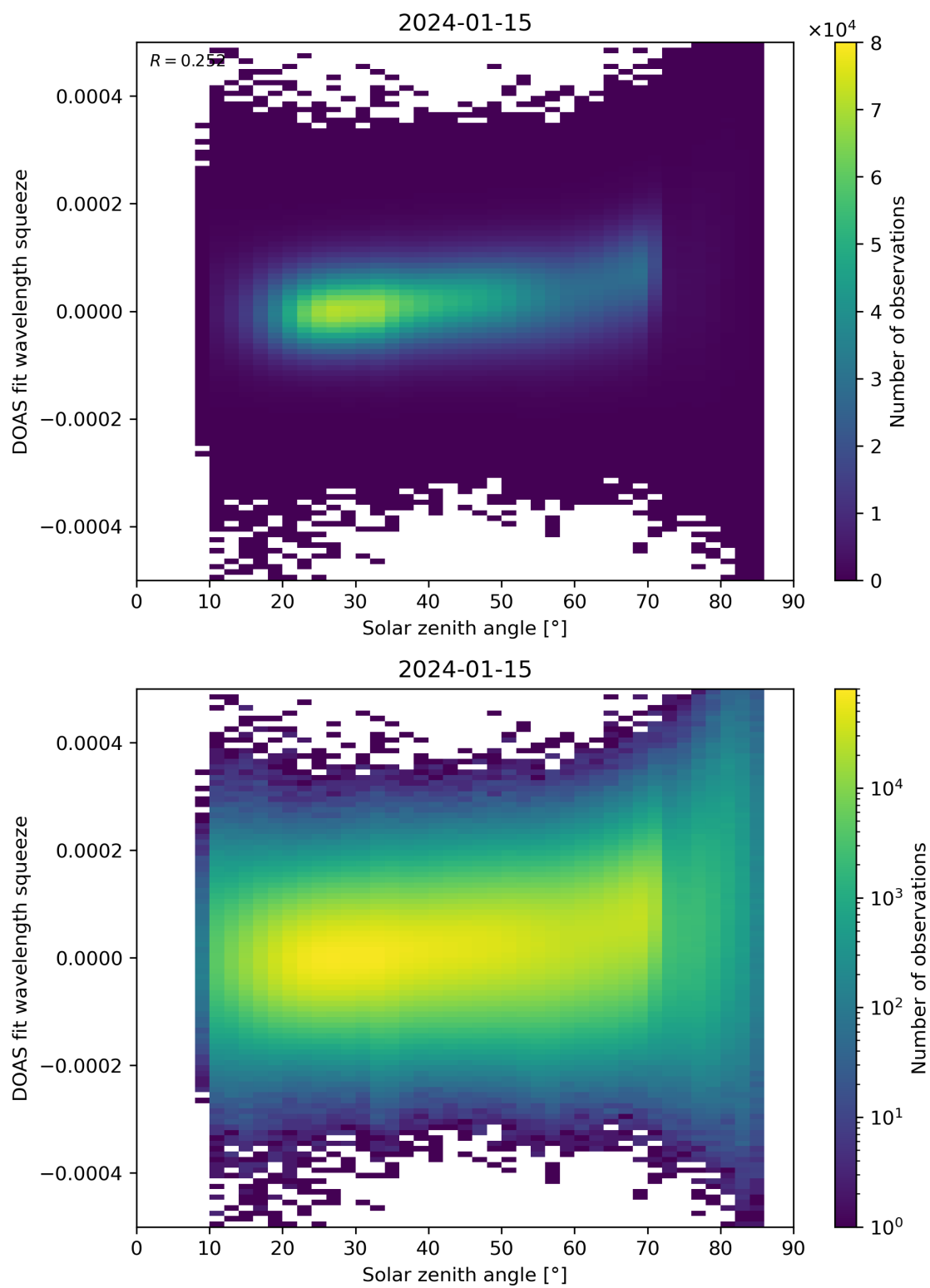
Figure 169: Scatter density plot of “Solar zenith angle” against “DOAS fit wavelength squeeze” for 2024-01-15 to 2024-01-16.
