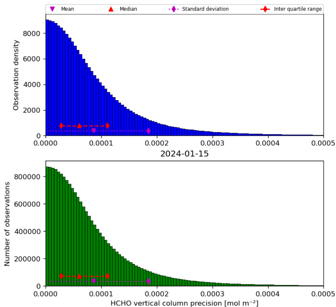
Figure 36: Histogram of “HCHO vertical column precision” for 2024-01-15 to 2024-01-16
