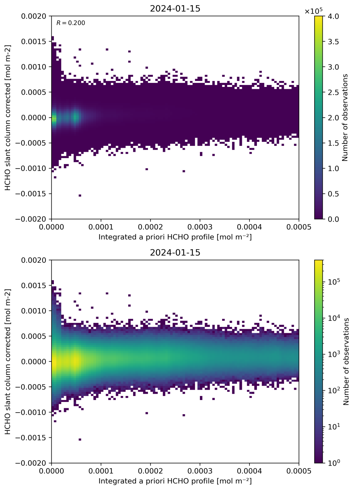
Figure 151: Scatter density plot of “Integrated a priori HCHO profile” against “HCHO slant column corrected” for 2024-01-15 to 2024-01-16.
