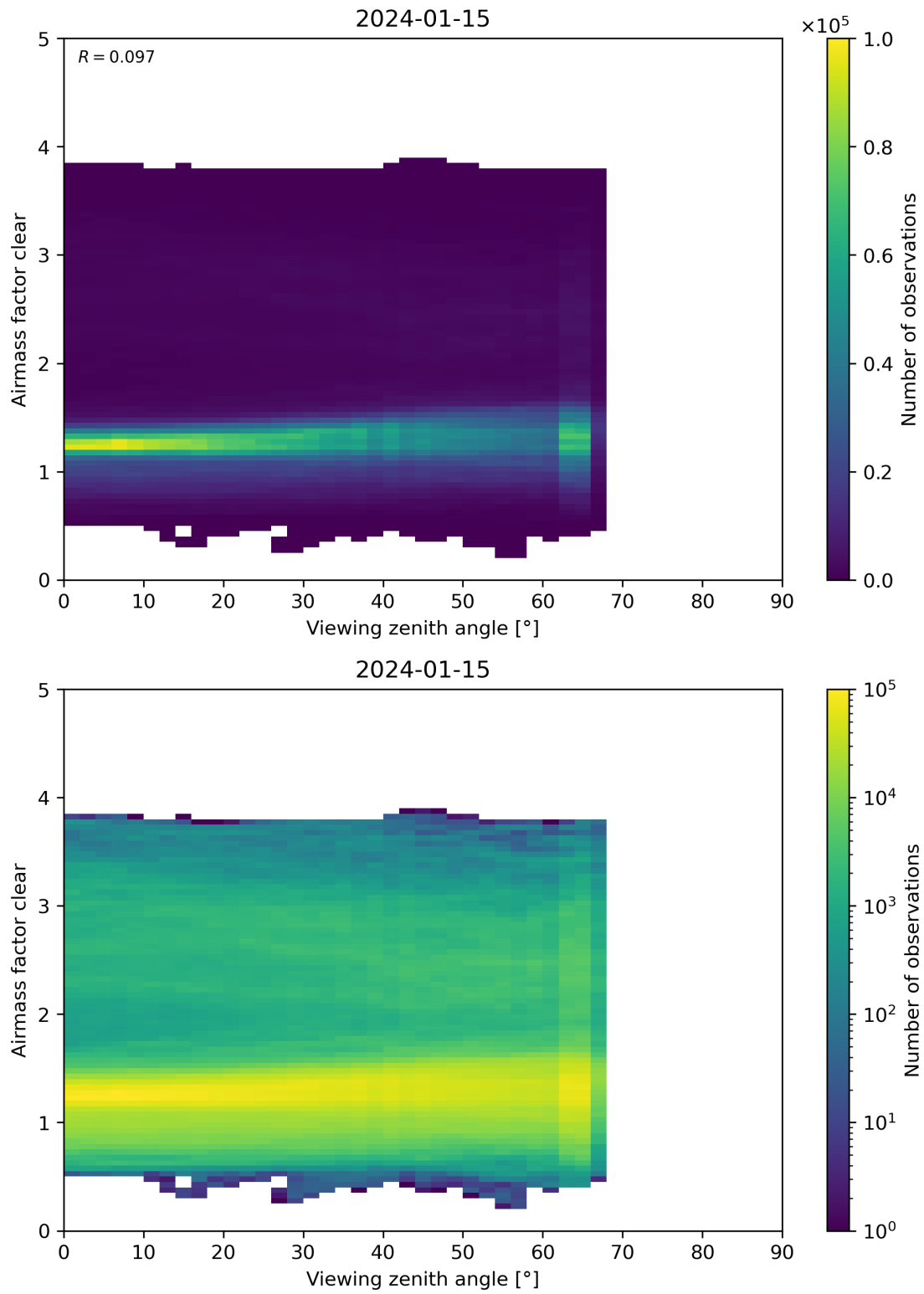
Figure 185: Scatter density plot of “Viewing zenith angle” against “Airmass factor clear” for 2024-01-15 to 2024-01-16.
