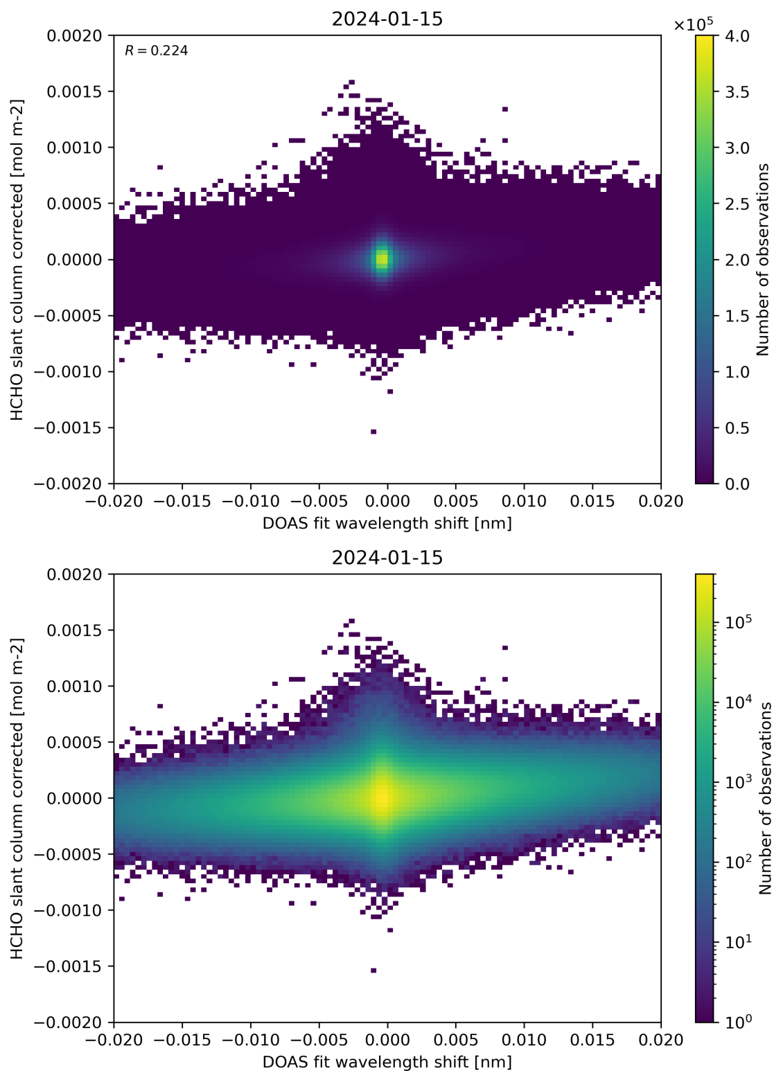
Figure 66: Scatter density plot of “DOAS fit wavelength shift” against “HCHO slant column corrected” for 2024-01-15 to 2024-01-16.
