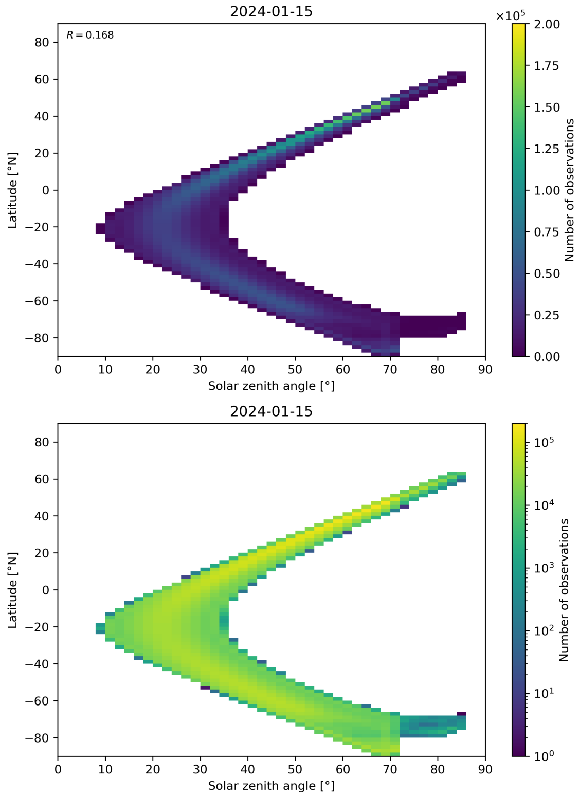
Figure 181: Scatter density plot of “Solar zenith angle” against “Latitude” for 2024-01-15 to 2024-01-16.
