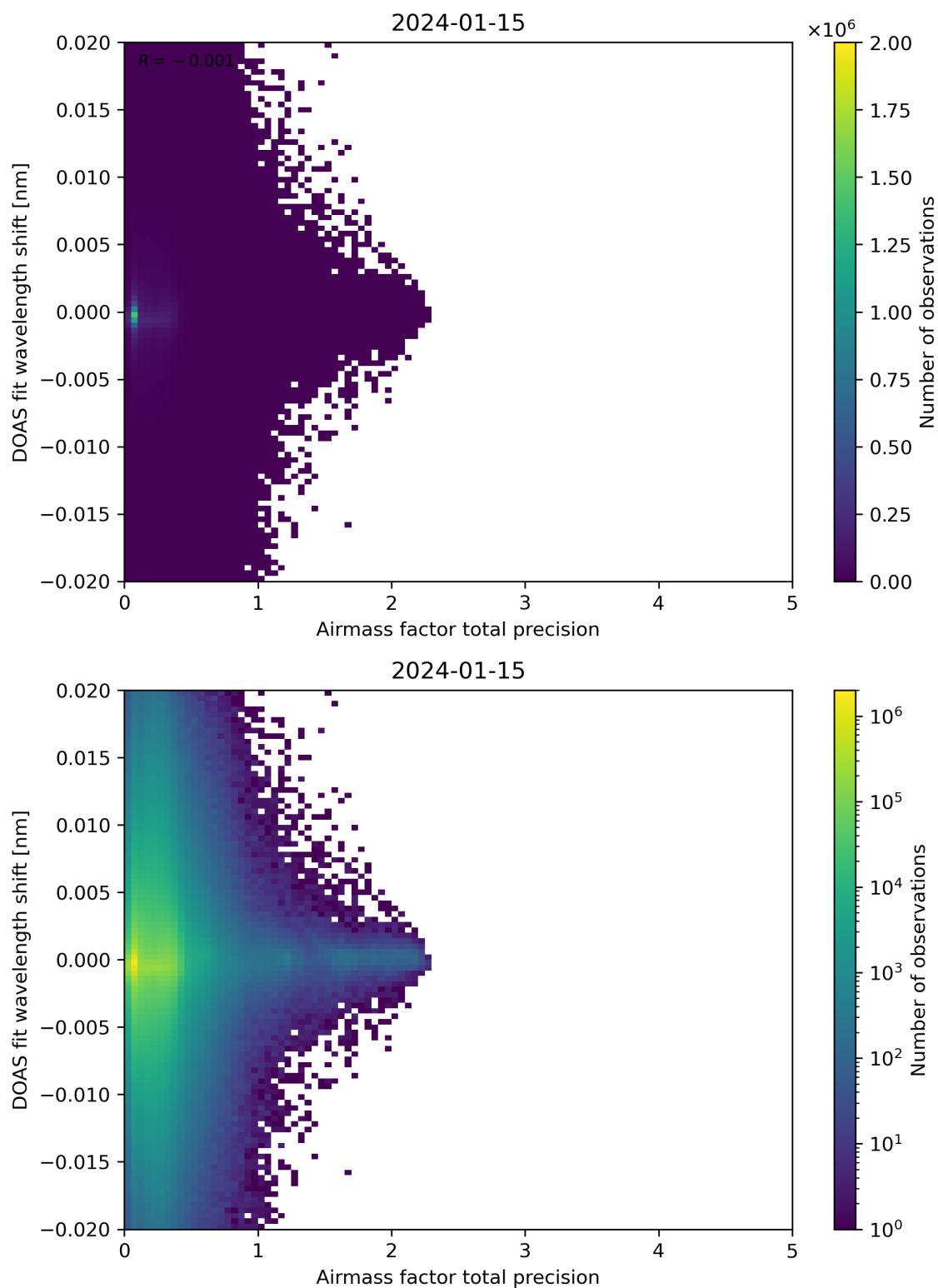
Figure 106: Scatter density plot of “Airmass factor total precision” against “DOAS fit wavelength shift” for 2024-01-15 to 2024-01-16.
