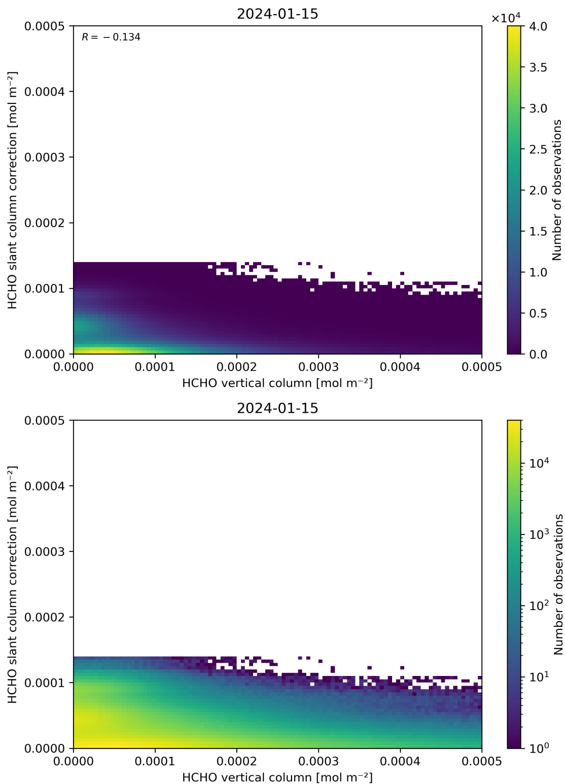
Figure 128: Scatter density plot of “HCHO vertical column” against “HCHO slant column correction” for 2024-01-15 to 2024-01-16.
