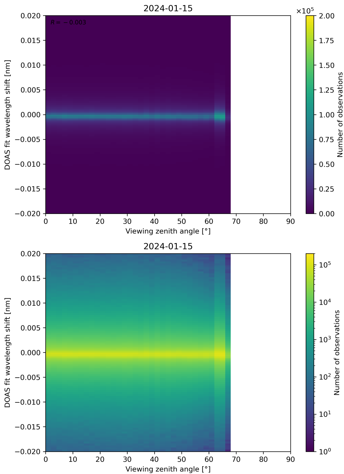
Figure 183: Scatter density plot of “Viewing zenith angle” against “DOAS fit wavelength shift” for 2024-01-15 to 2024-01-16.
