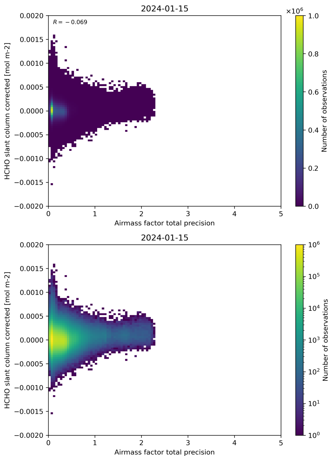
Figure 109: Scatter density plot of “Airmass factor total precision” against “HCHO slant column corrected” for 2024-01-15 to 2024-01-16.
