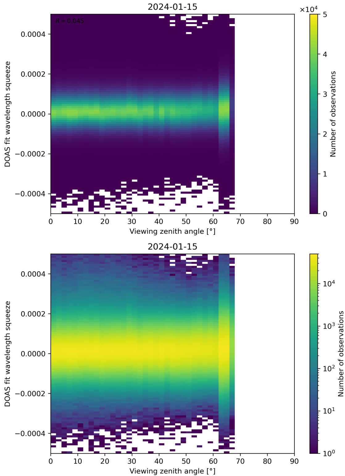
Figure 184: Scatter density plot of “Viewing zenith angle” against “DOAS fit wavelength squeeze” for 2024-01-15 to 2024-01-16.
