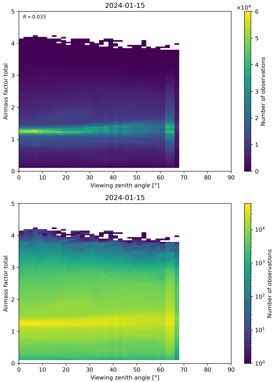
Figure 190: Scatter density plot of “Viewing zenith angle” against “Airmass factor total” for 2024-01-15 to 2024-01-16.
