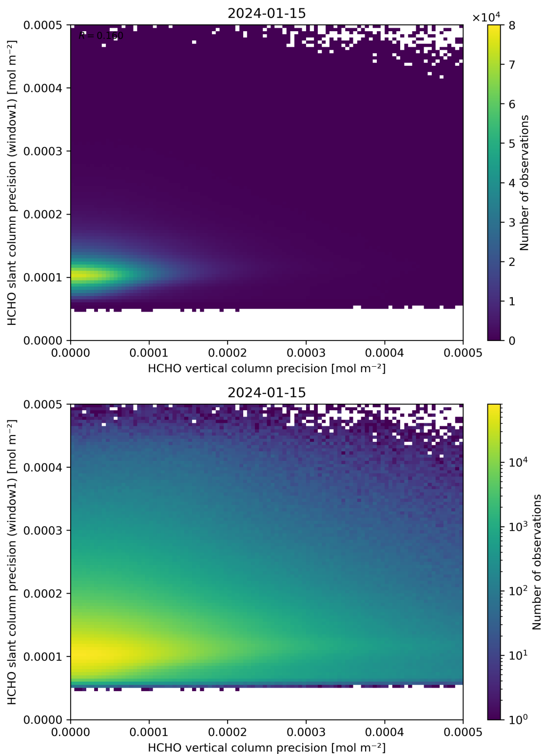
Figure 143: Scatter density plot of “HCHO vertical column precision” against “HCHO slant column precision (window1)” for 2024-01-15 to 2024-01-16.
