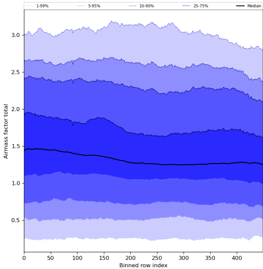
Figure 54: Along track statistics of “Airmass factor total” for 2024-01-15 to 2024-01-16
