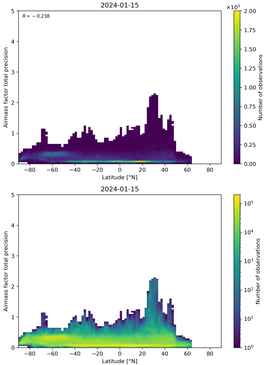
Figure 162: Scatter density plot of “Latitude” against “Airmass factor total precision” for 2024-01-15 to 2024-01-16.
