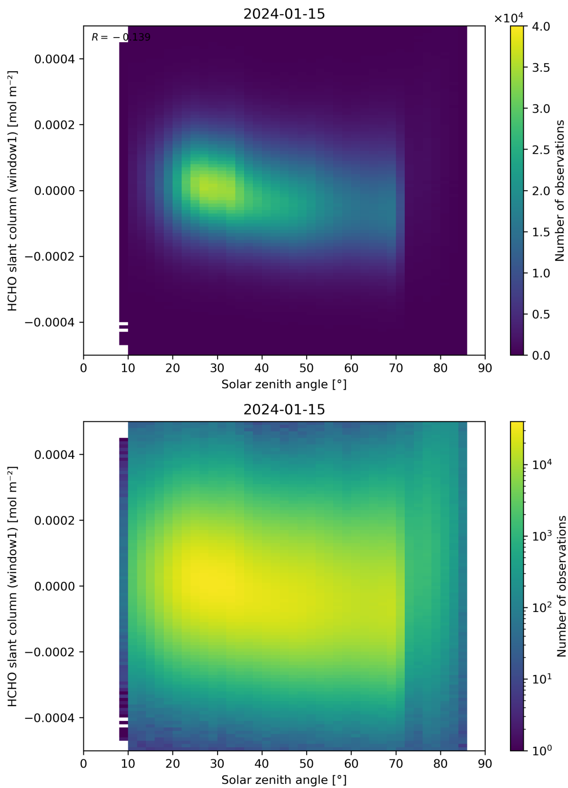
Figure 173: Scatter density plot of “Solar zenith angle” against “HCHO slant column (window1)” for 2024-01-15 to 2024-01-16.
