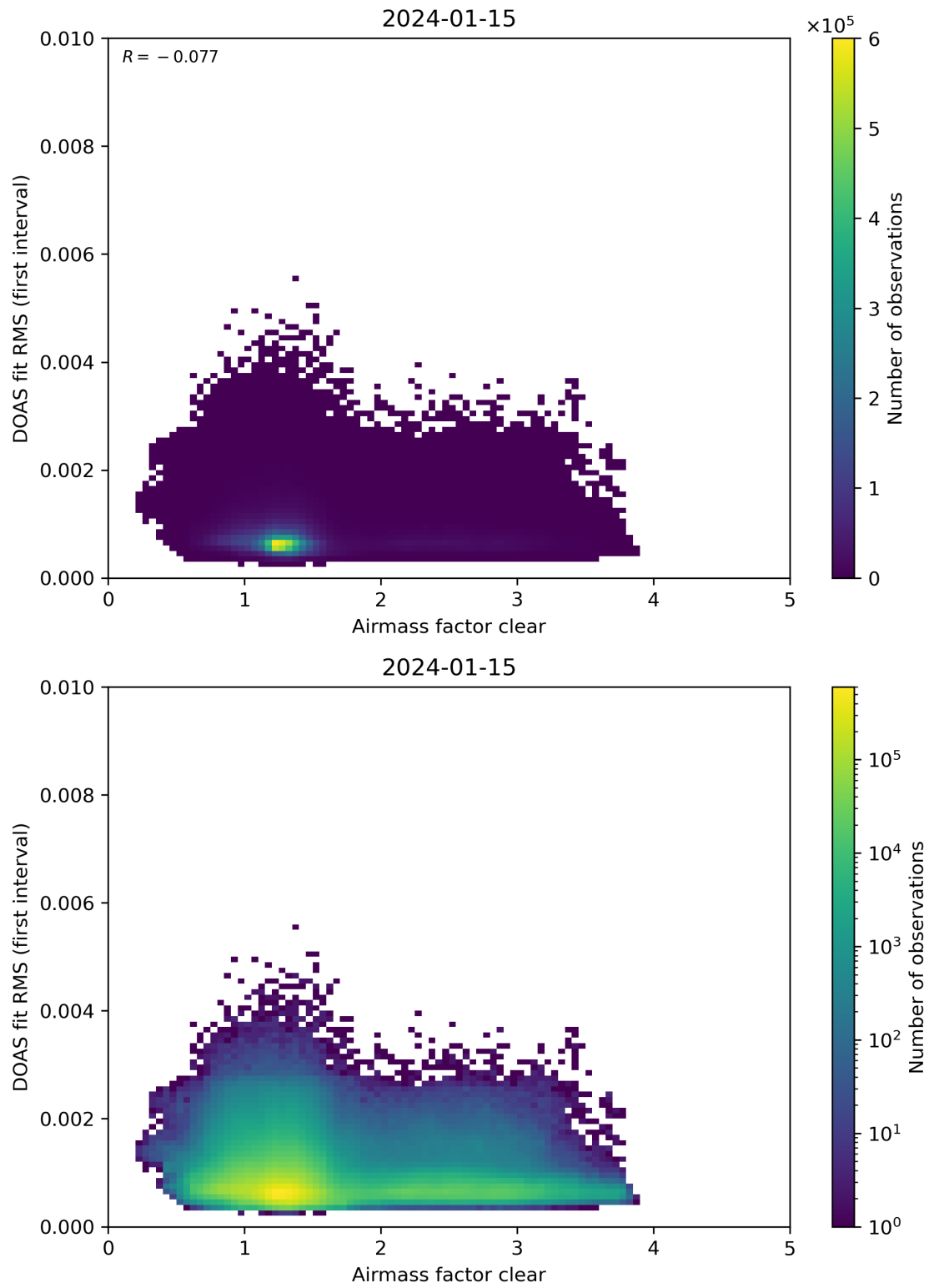
Figure 71: Scatter density plot of “Airmass factor clear” against “DOAS fit RMS (first interval)” for 2024-01-15 to 2024-01-16.
