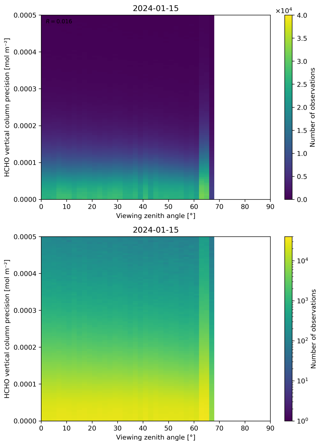
Figure 194: Scatter density plot of “Viewing zenith angle” against “HCHO vertical column precision” for 2024-01-15 to 2024-01-16.
