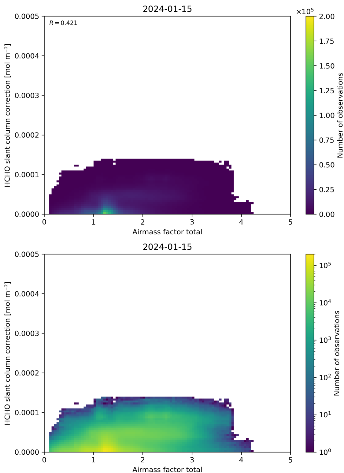
Figure 102: Scatter density plot of “Airmass factor total” against “HCHO slant column correction” for 2024-01-15 to 2024-01-16.
