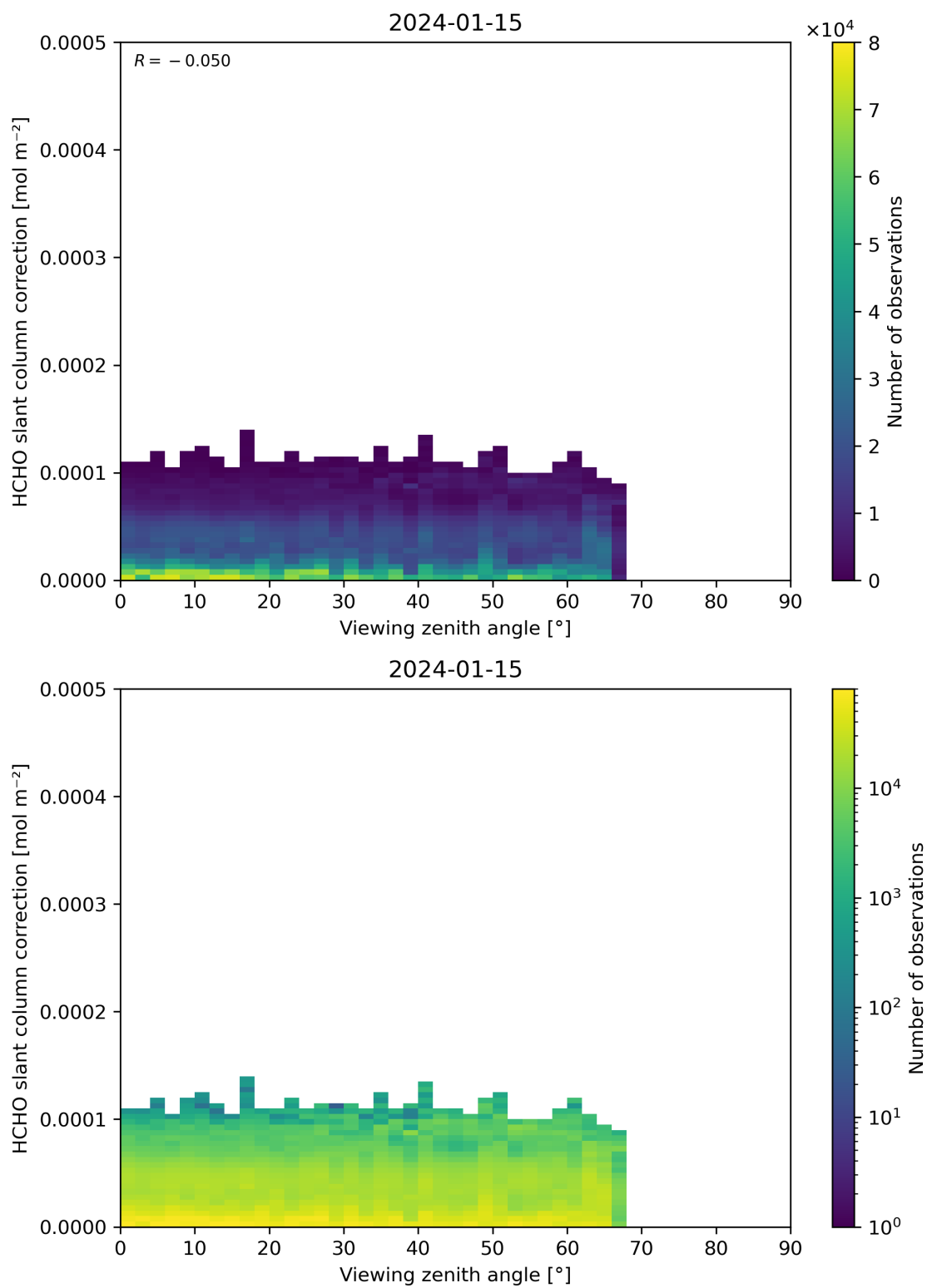
Figure 187: Scatter density plot of “Viewing zenith angle” against “HCHO slant column correction” for 2024-01-15 to 2024-01-16.
