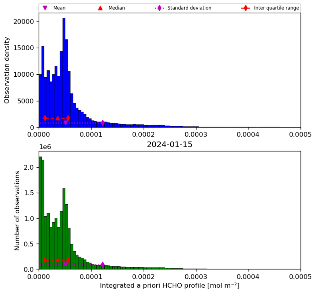
Figure 43: Histogram of “Integrated a priori HCHO profile” for 2024-01-15 to 2024-01-16
