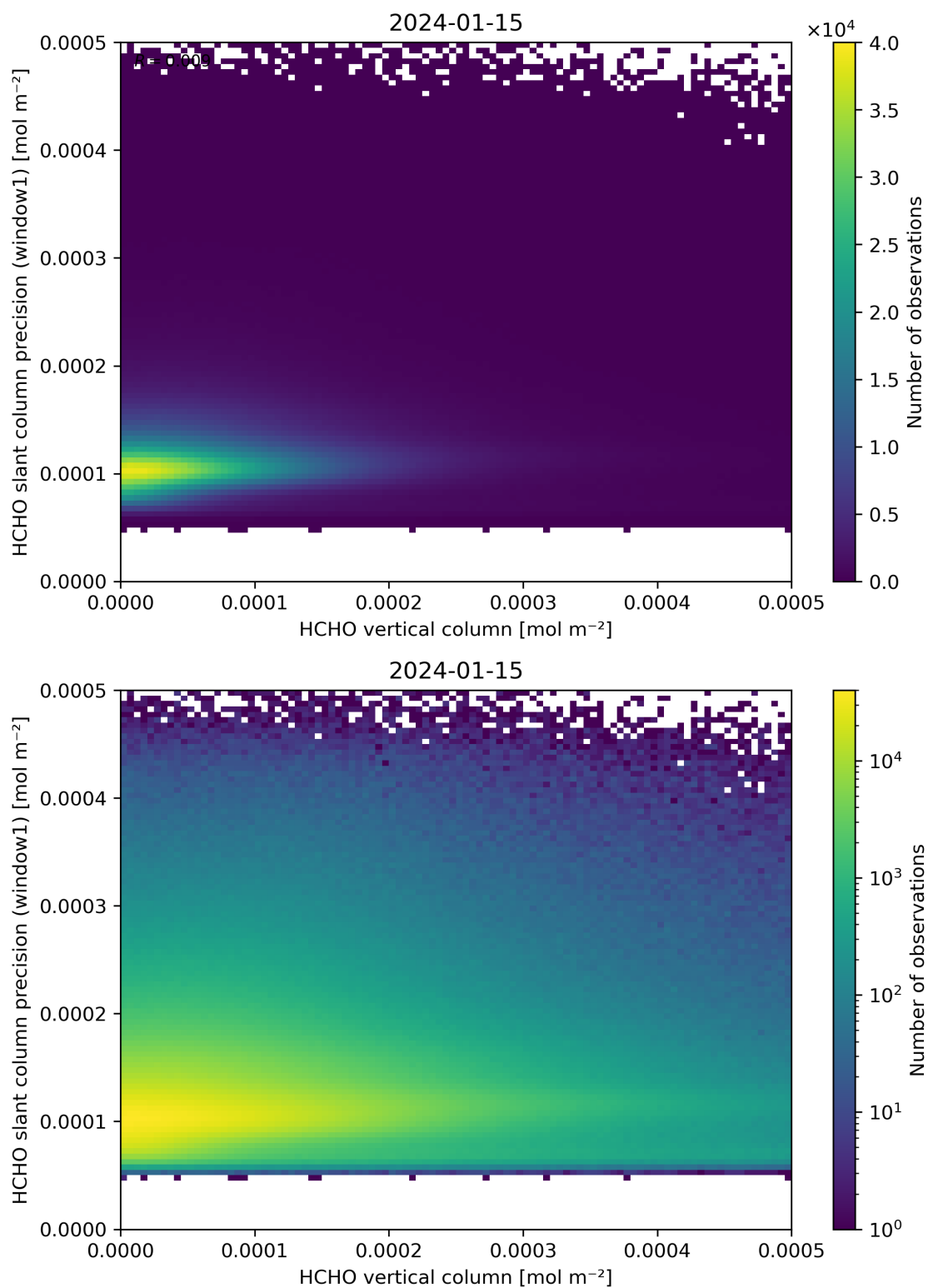
Figure 130: Scatter density plot of “HCHO vertical column” against “HCHO slant column precision (window1)” for 2024-01-15 to 2024-01-16.
