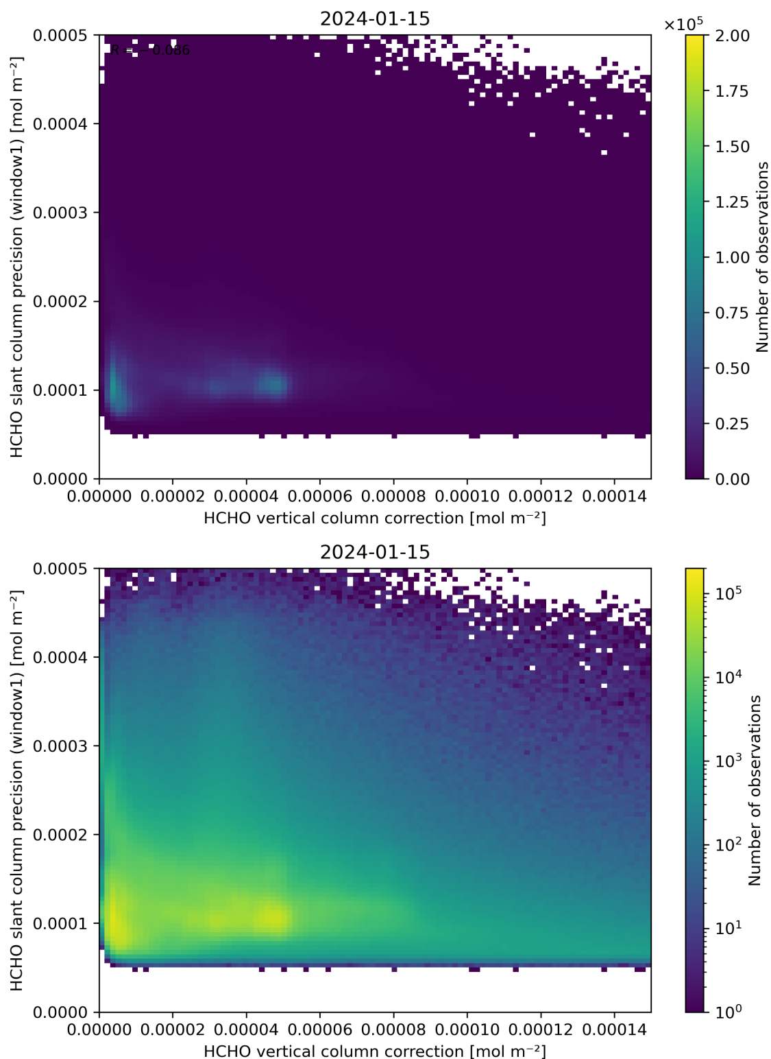
Figure 119: Scatter density plot of “HCHO vertical column correction” against “HCHO slant column precision (window1)” for 2024-01-15 to 2024-01-16.
