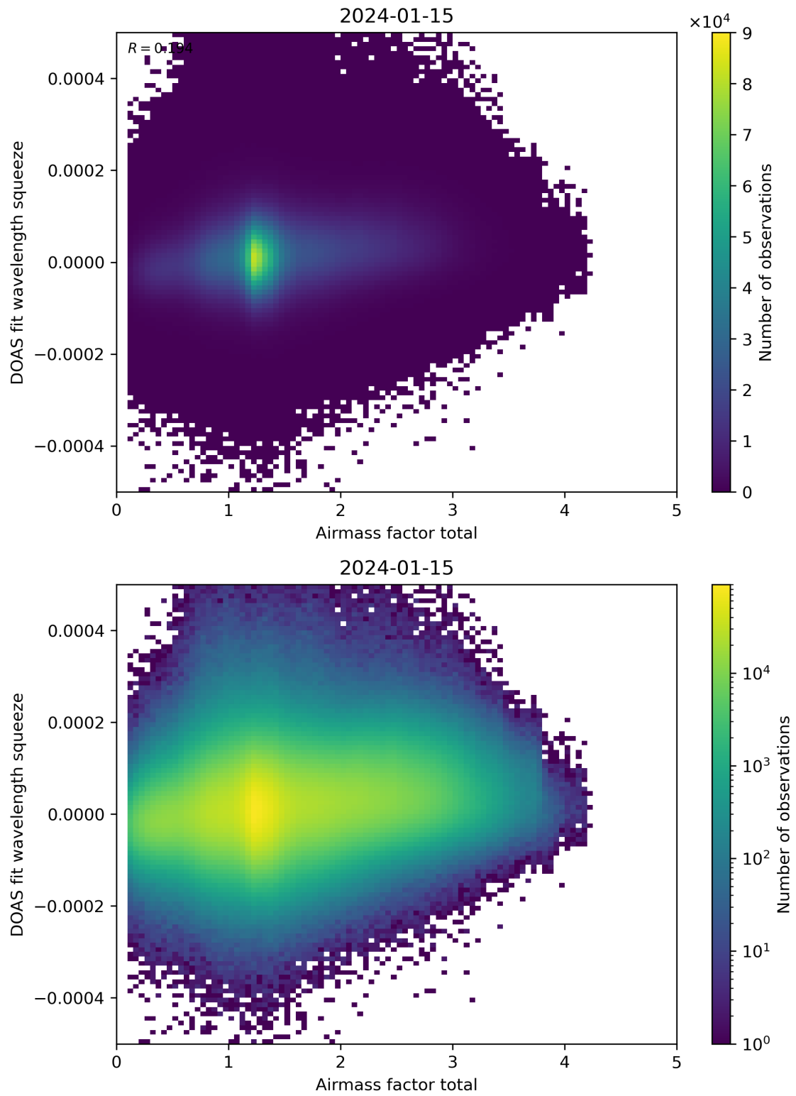
Figure 99: Scatter density plot of “Airmass factor total” against “DOAS fit wavelength squeeze” for 2024-01-15 to 2024-01-16.
