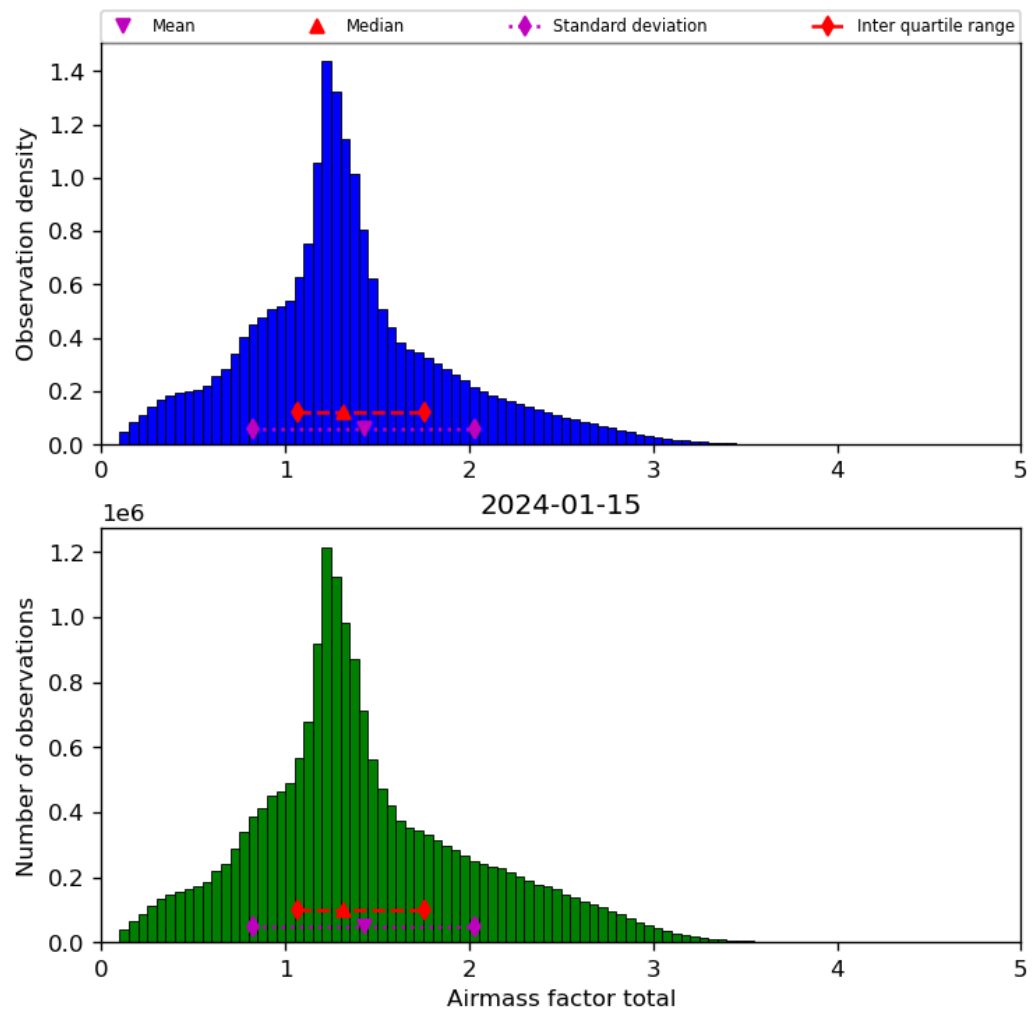
Figure 40: Histogram of “Airmass factor total” for 2024-01-15 to 2024-01-16
