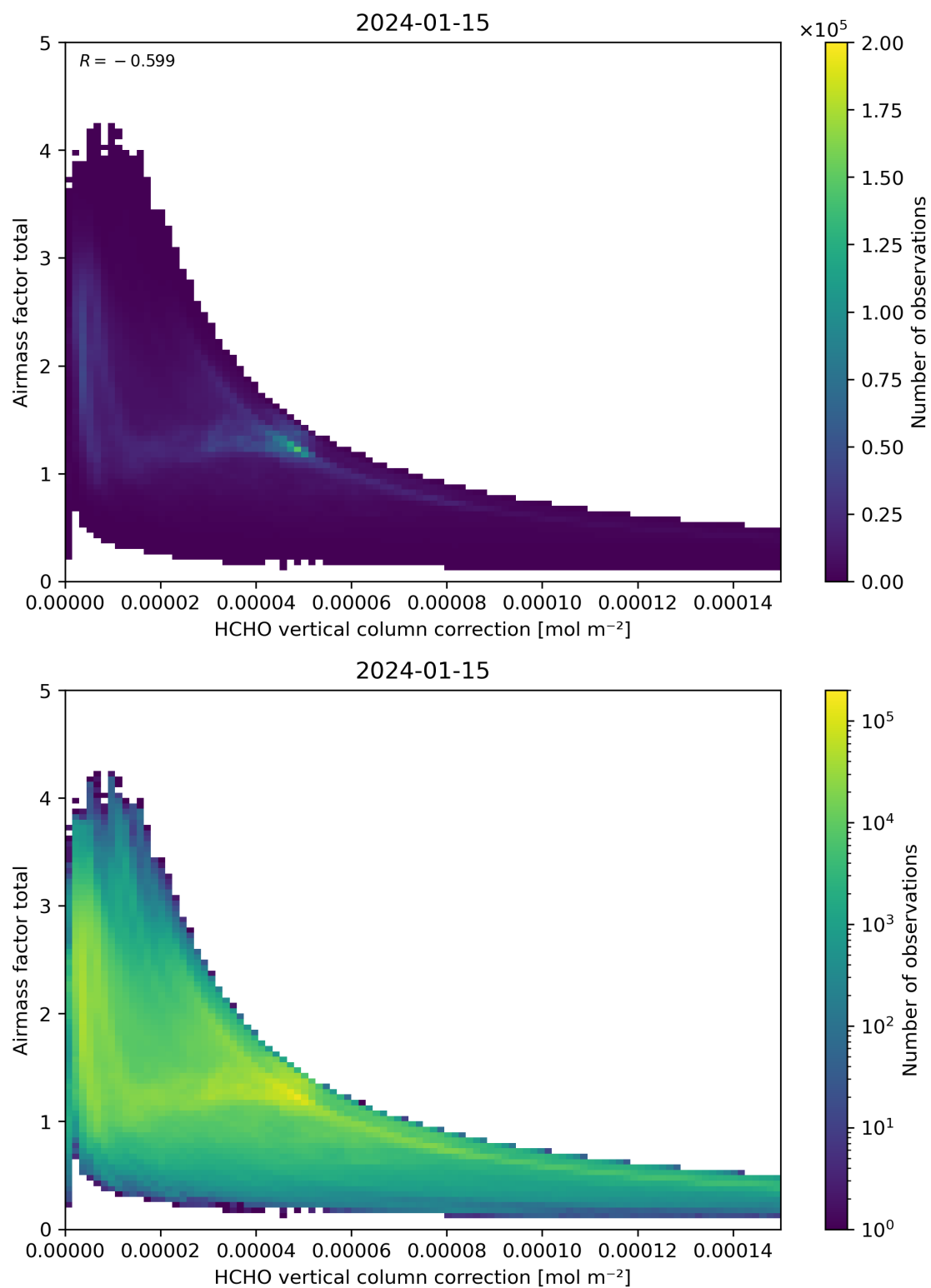
Figure 120: Scatter density plot of “HCHO vertical column correction” against “Airmass factor total” for 2024-01-15 to 2024-01-16.
