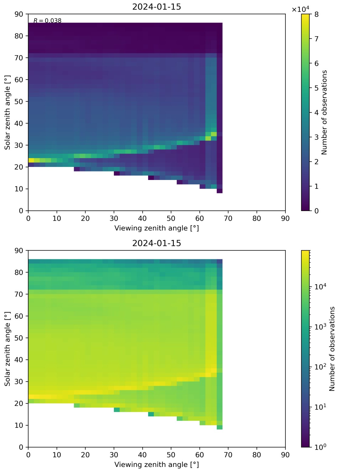
Figure 197: Scatter density plot of “Viewing zenith angle” against “Solar zenith angle” for 2024-01-15 to 2024-01-16.
