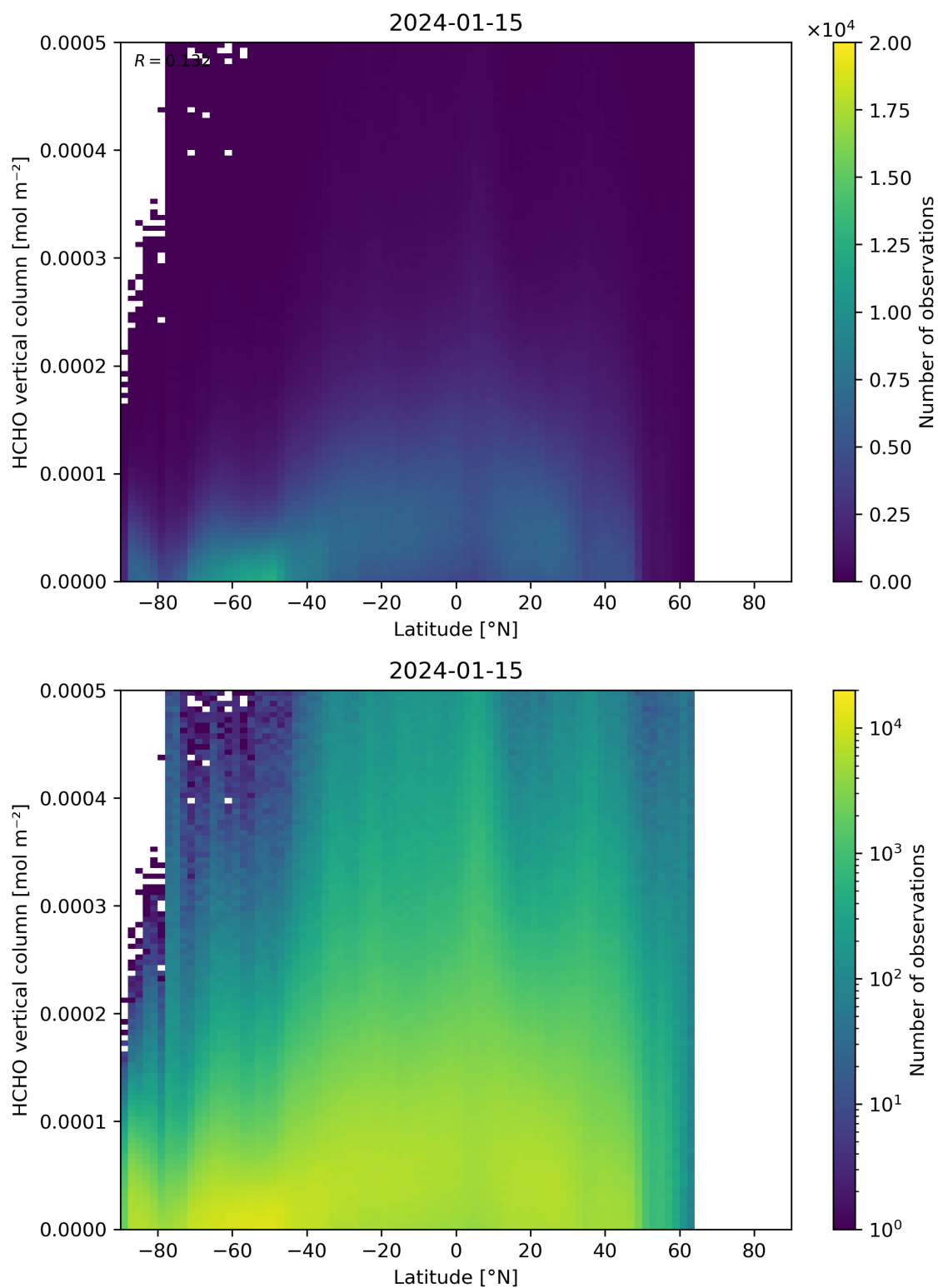
Figure 163: Scatter density plot of “Latitude” against “HCHO vertical column” for 2024-01-15 to 2024-01-16.
