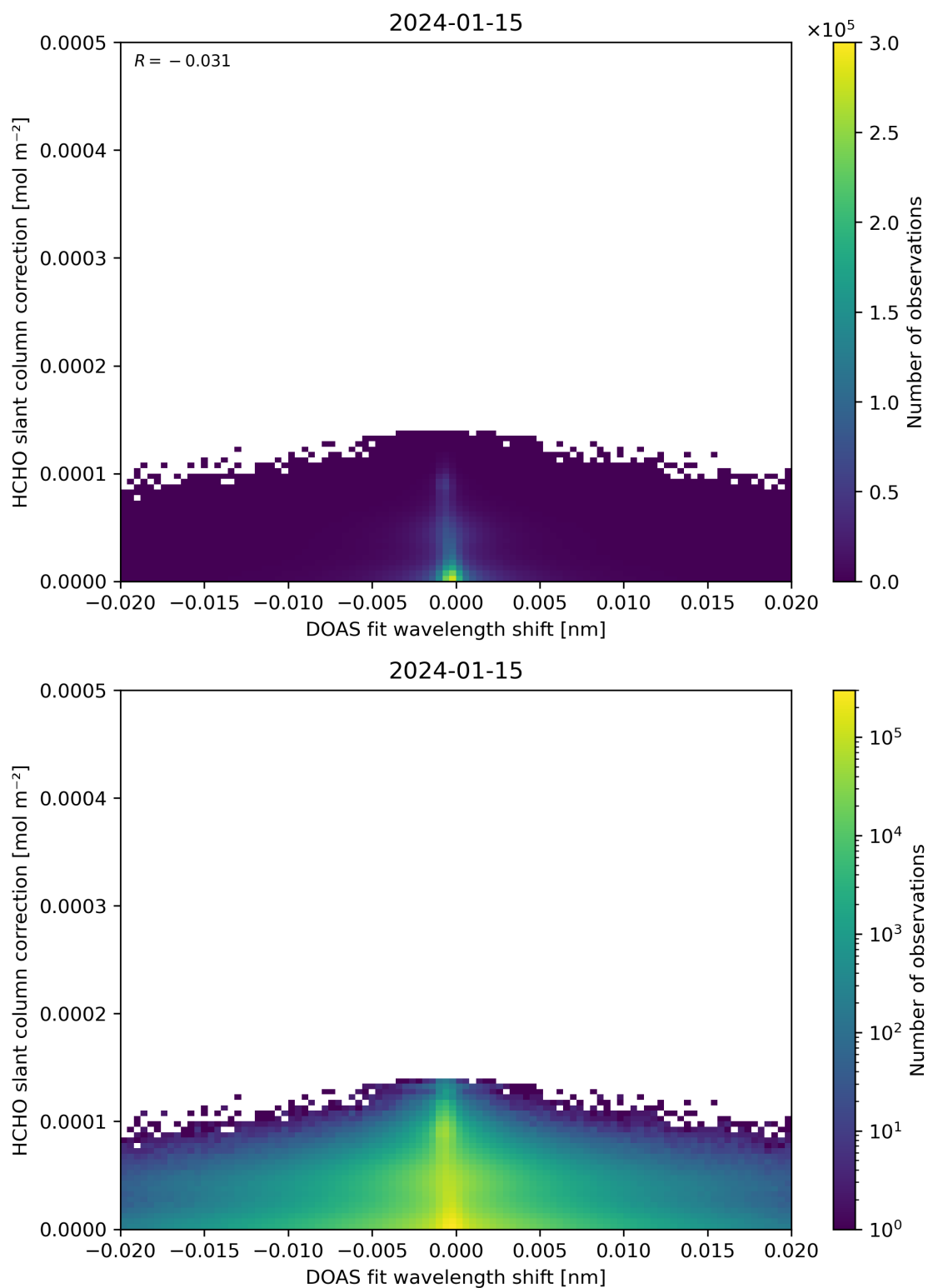
Figure 67: Scatter density plot of “DOAS fit wavelength shift” against “HCHO slant column correction” for 2024-01-15 to 2024-01-16.
