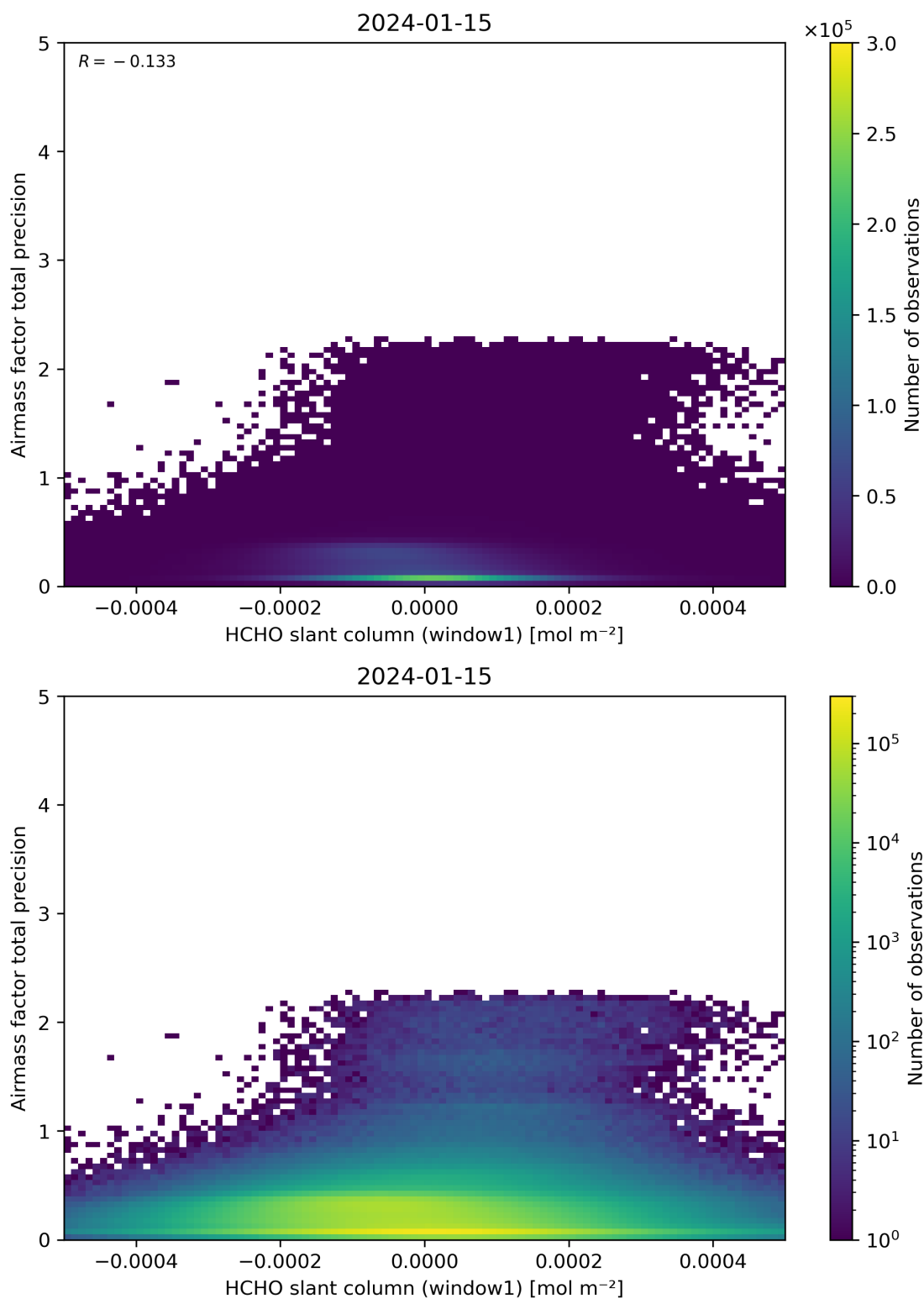
Figure 86: Scatter density plot of “HCHO slant column (window1)” against “Airmass factor total precision” for 2024-01-15 to 2024-01-16.
