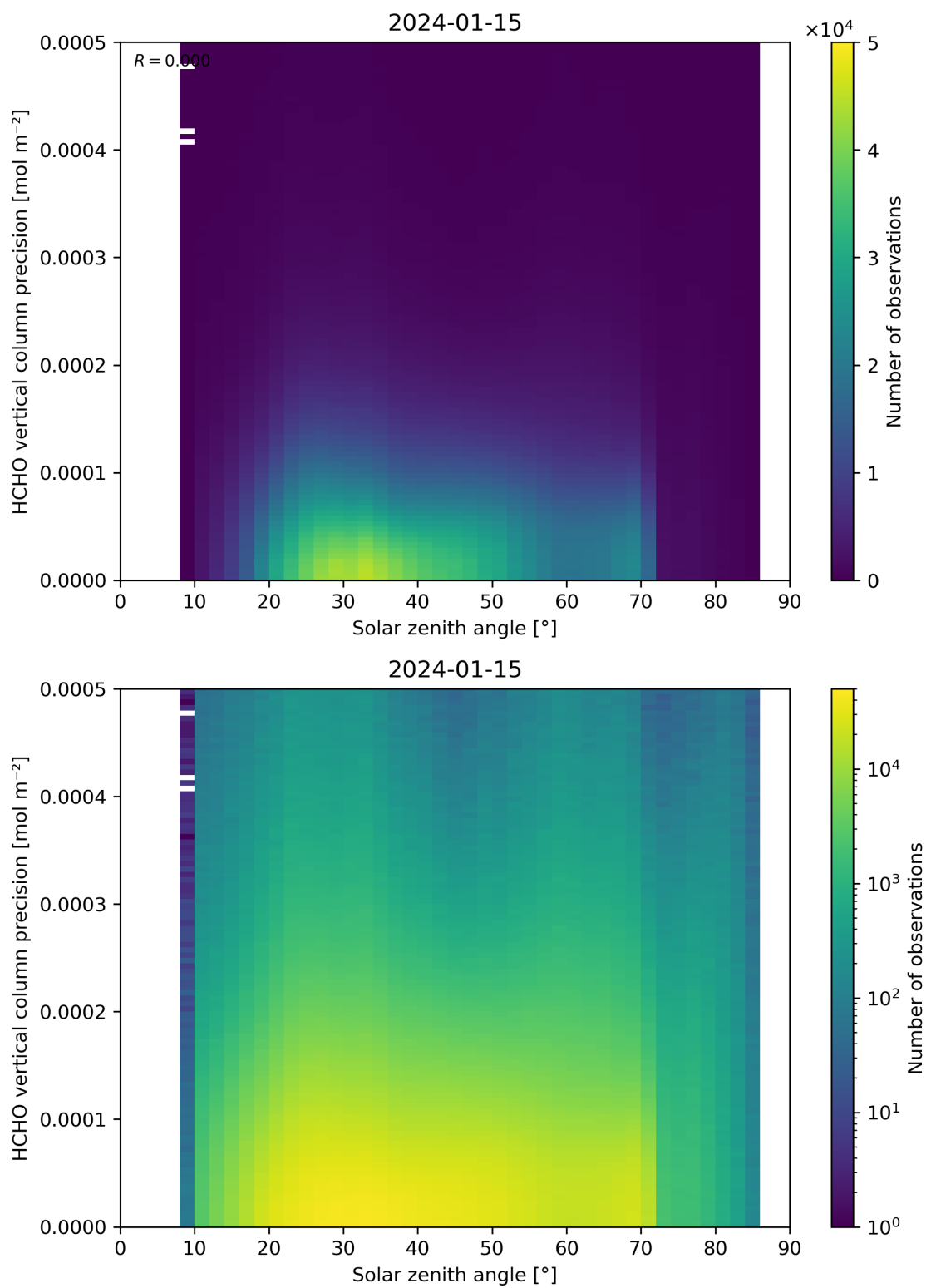
Figure 179: Scatter density plot of “Solar zenith angle” against “HCHO vertical column precision” for 2024-01-15 to 2024-01-16.
