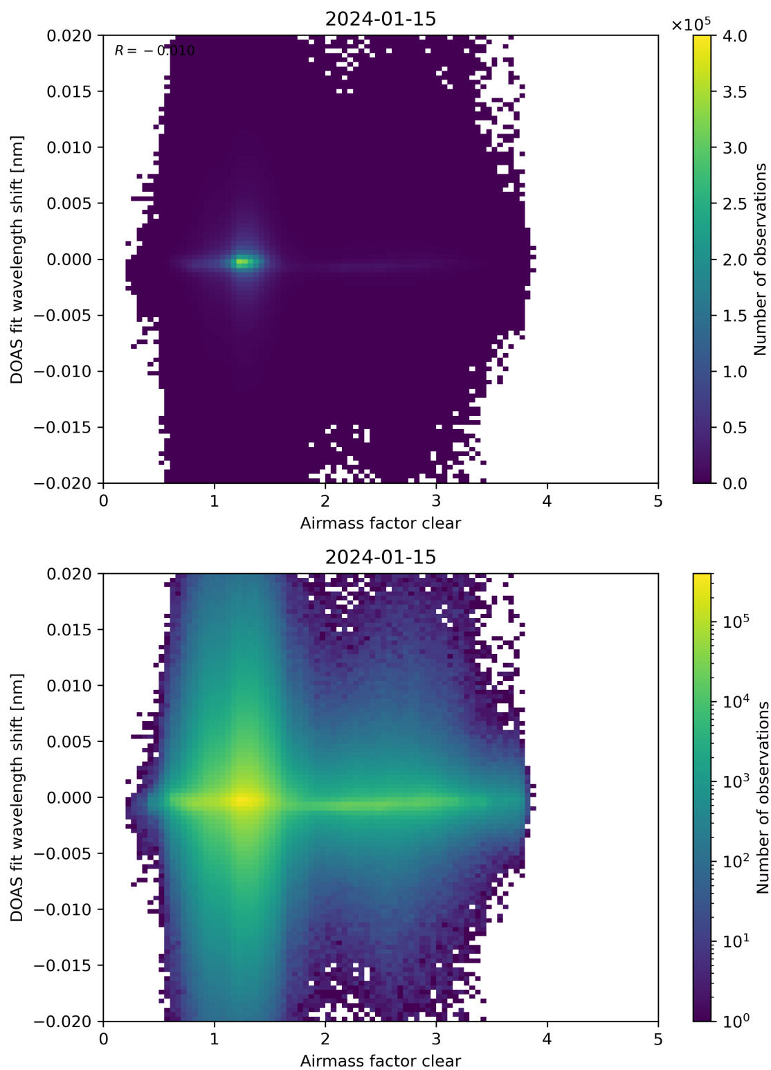
Figure 72: Scatter density plot of “Airmass factor clear” against “DOAS fit wavelength shift” for 2024-01-15 to 2024-01-16.
