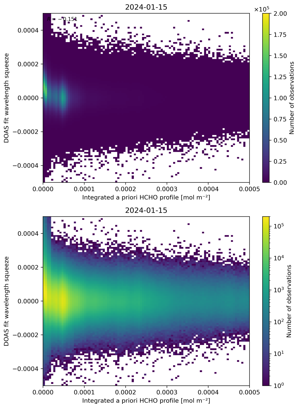
Figure 150: Scatter density plot of “Integrated a priori HCHO profile” against “DOAS fit wavelength squeeze” for 2024-01-15 to 2024-01-16.
