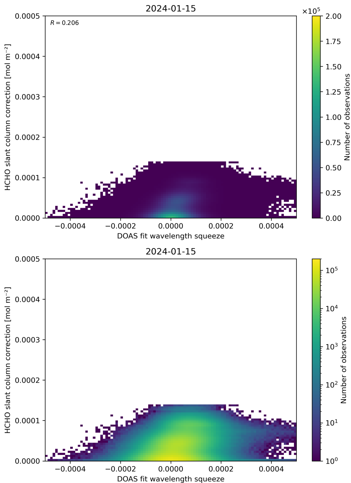
Figure 70: Scatter density plot of “DOAS fit wavelength squeeze” against “HCHO slant column correction” for 2024-01-15 to 2024-01-16.
