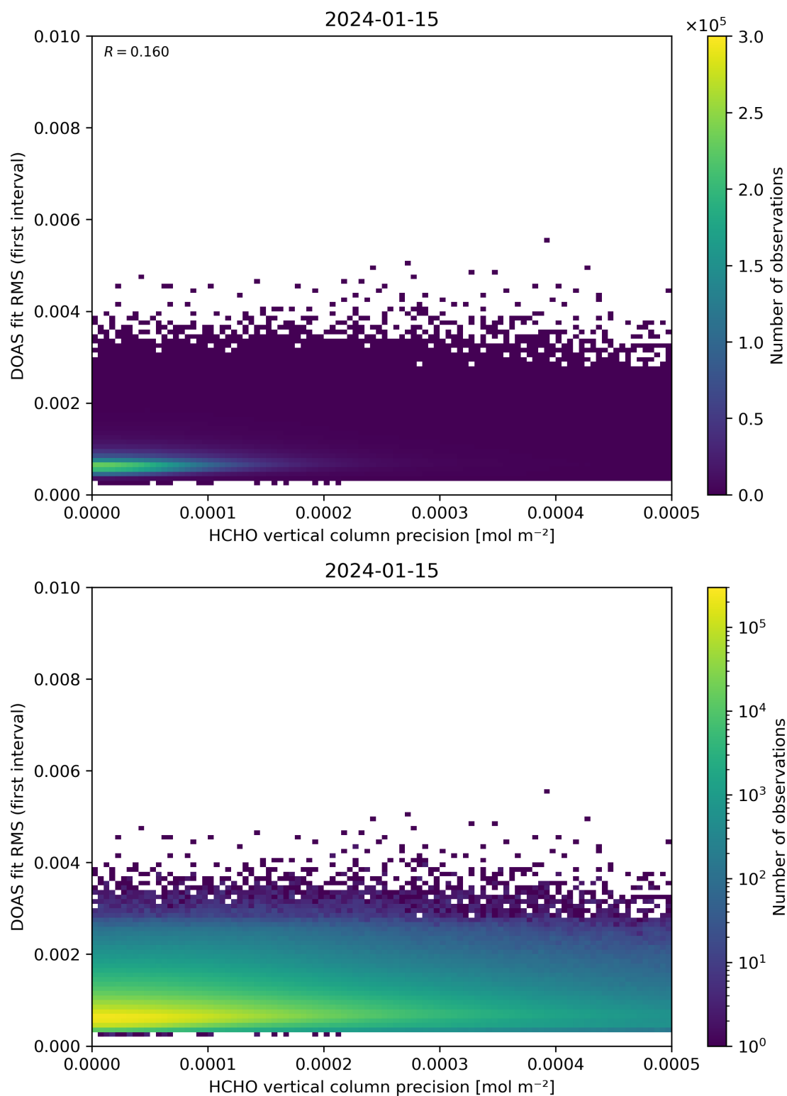
Figure 136: Scatter density plot of “HCHO vertical column precision” against “DOAS fit RMS (first interval)” for 2024-01-15 to 2024-01-16.
