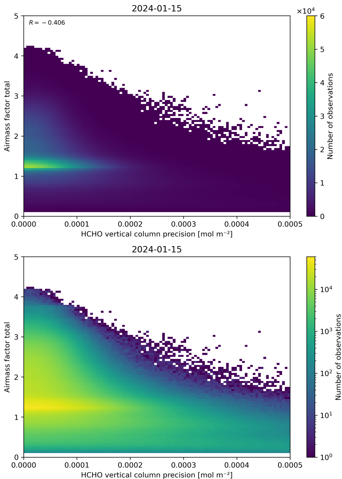
Figure 144: Scatter density plot of “HCHO vertical column precision” against “Airmass factor total” for 2024-01-15 to 2024-01-16.
