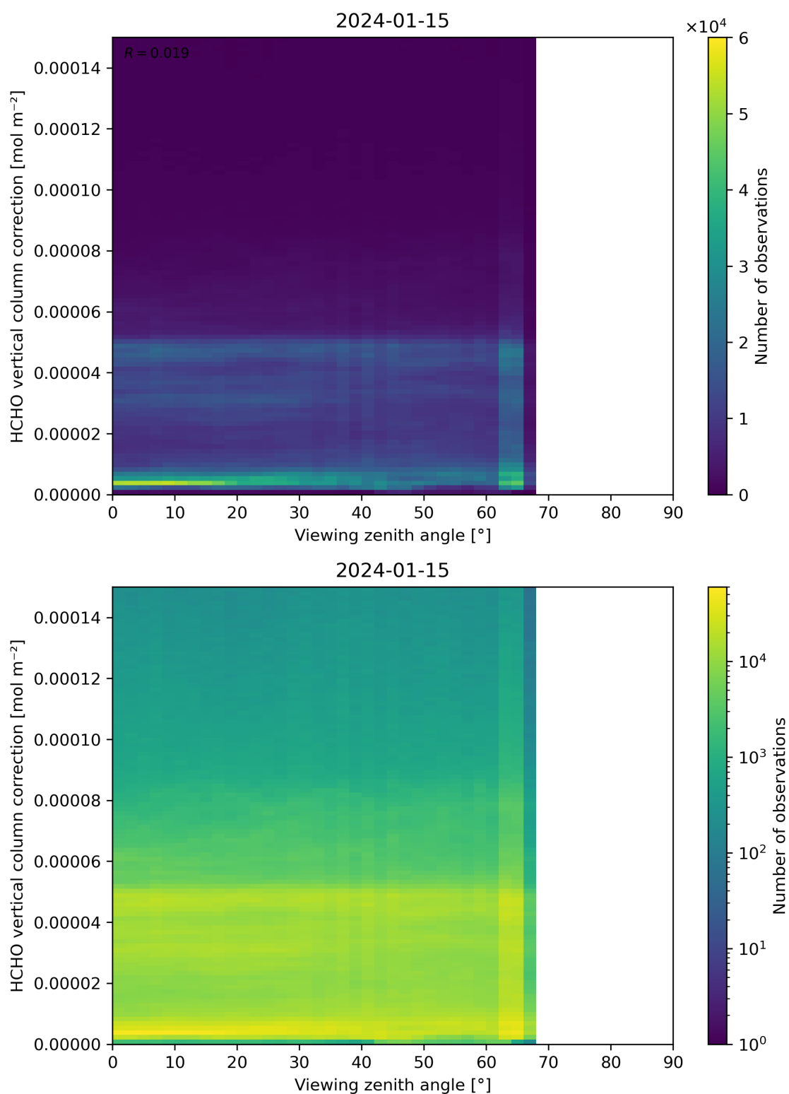
Figure 193: Scatter density plot of “Viewing zenith angle” against “HCHO vertical column correction” for 2024-01-15 to 2024-01-16.
