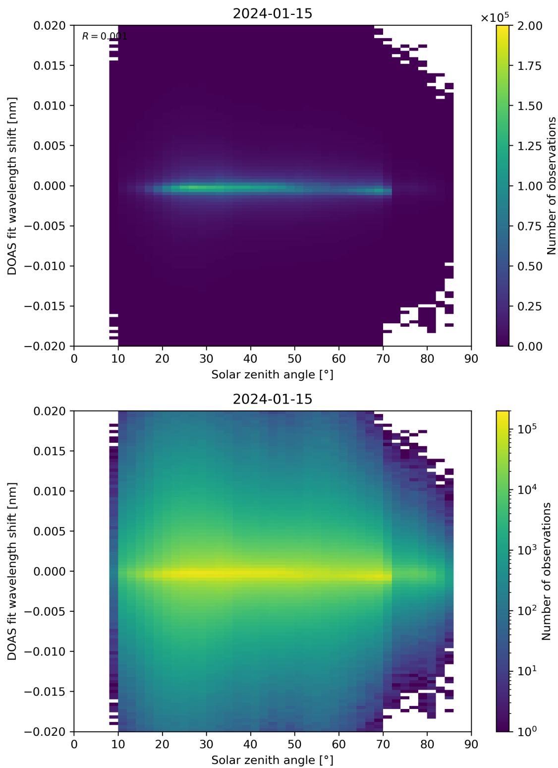
Figure 168: Scatter density plot of “Solar zenith angle” against “DOAS fit wavelength shift” for 2024-01-15 to 2024-01-16.
