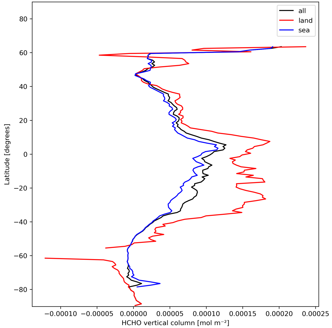
Figure 21: Zonal average of “HCHO vertical column” for 2024-01-15 to 2024-01-16.
