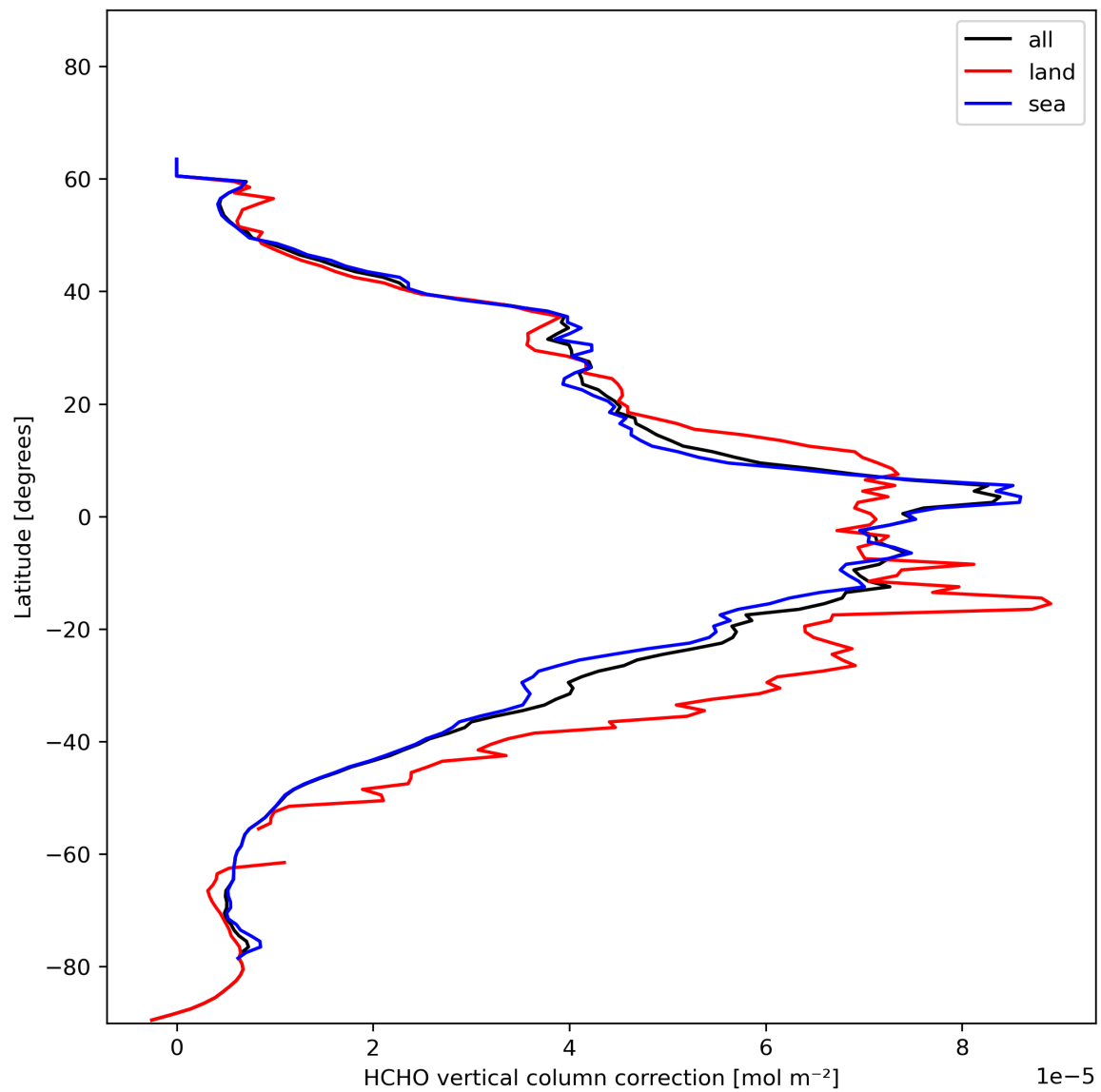
Figure 23: Zonal average of “HCHO vertical column correction” for 2024-01-15 to 2024-01-16.
