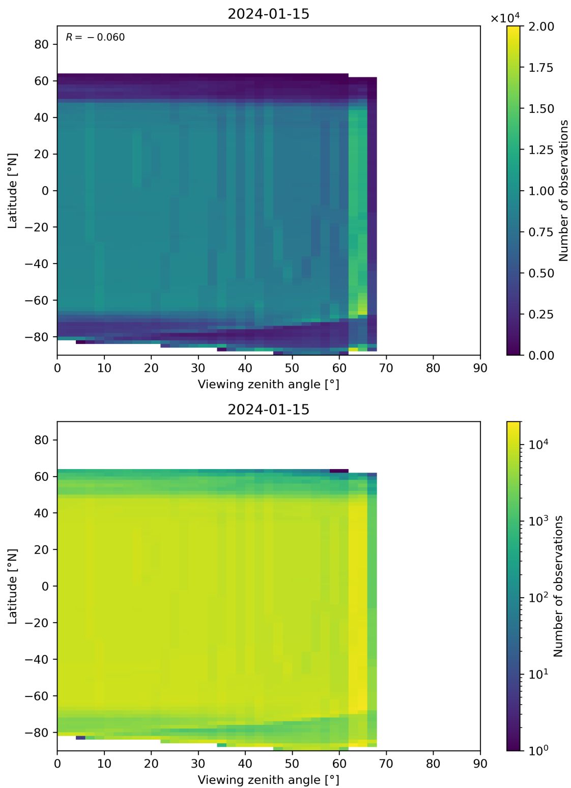
Figure 196: Scatter density plot of “Viewing zenith angle” against “Latitude” for 2024-01-15 to 2024-01-16.
