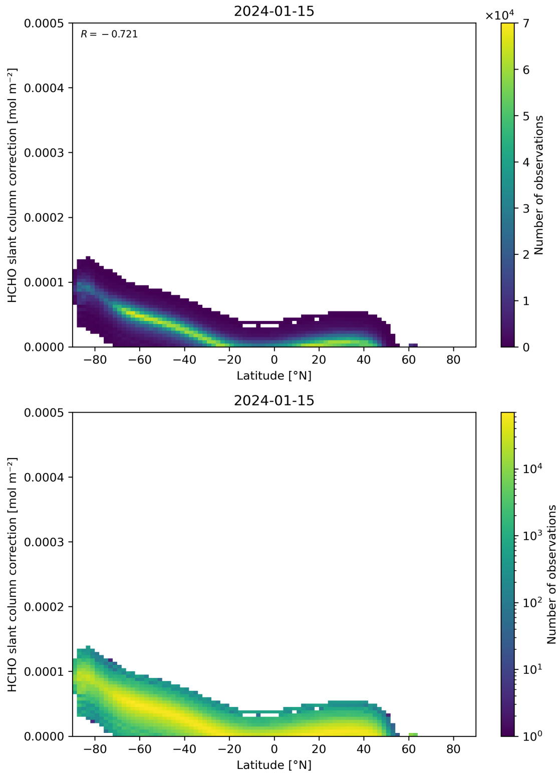
Figure 158: Scatter density plot of “Latitude” against “HCHO slant column correction” for 2024-01-15 to 2024-01-16.
