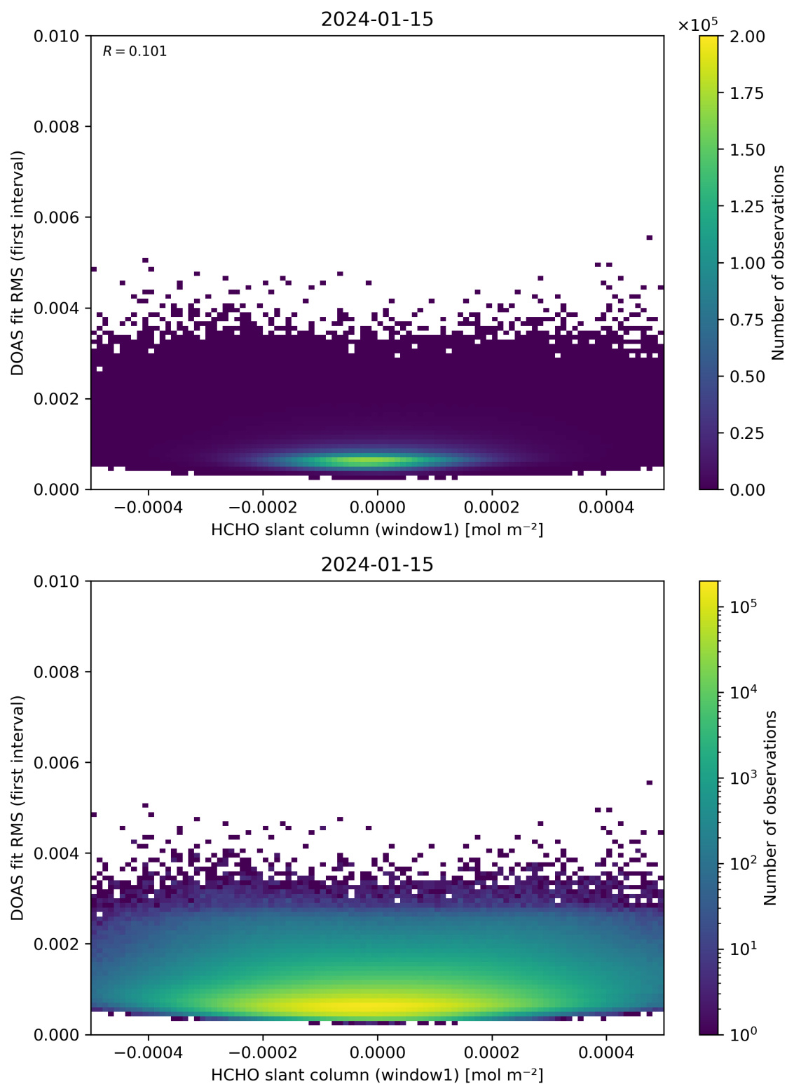
Figure 78: Scatter density plot of “HCHO slant column (window1)” against “DOAS fit RMS (first interval)” for 2024-01-15 to 2024-01-16.
