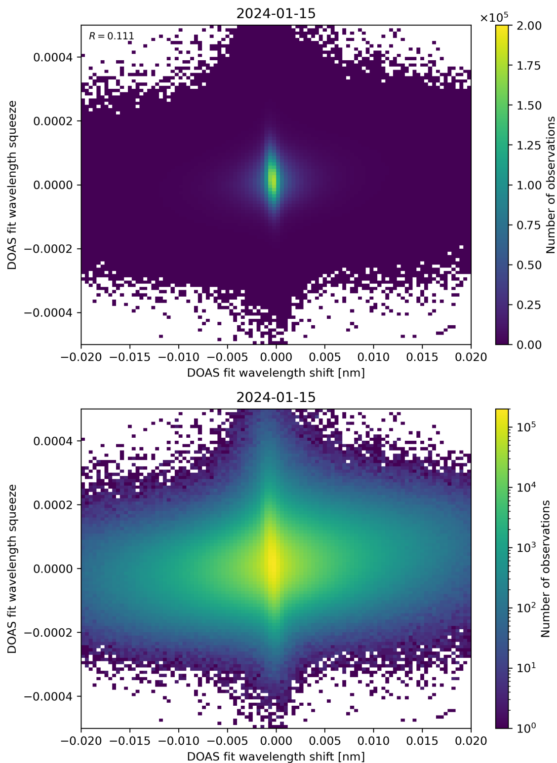
Figure 65: Scatter density plot of “DOAS fit wavelength shift” against “DOAS fit wavelength squeeze” for 2024-01-15 to 2024-01-16.
