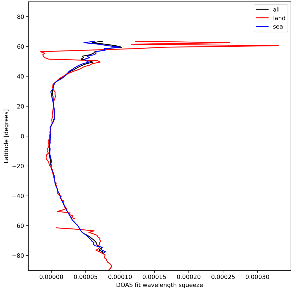
Figure 31: Zonal average of “DOAS fit wavelength squeeze” for 2024-01-15 to 2024-01-16.
