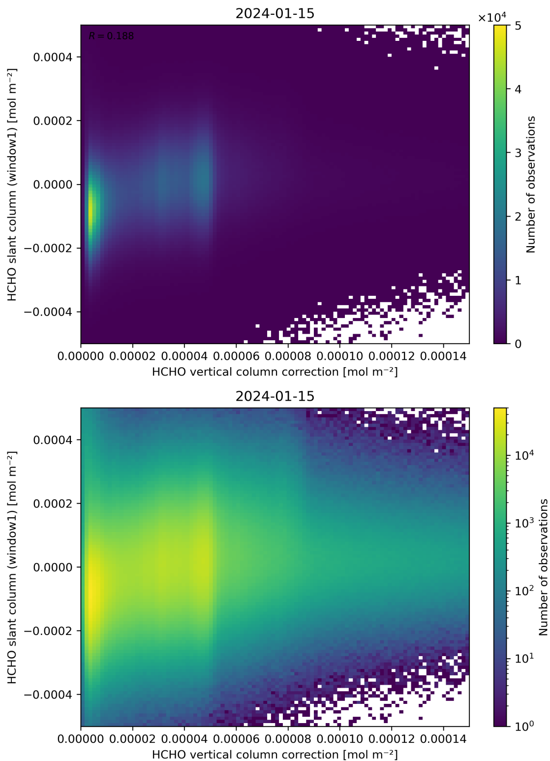
Figure 118: Scatter density plot of “HCHO vertical column correction” against “HCHO slant column (window1)” for 2024-01-15 to 2024-01-16.
