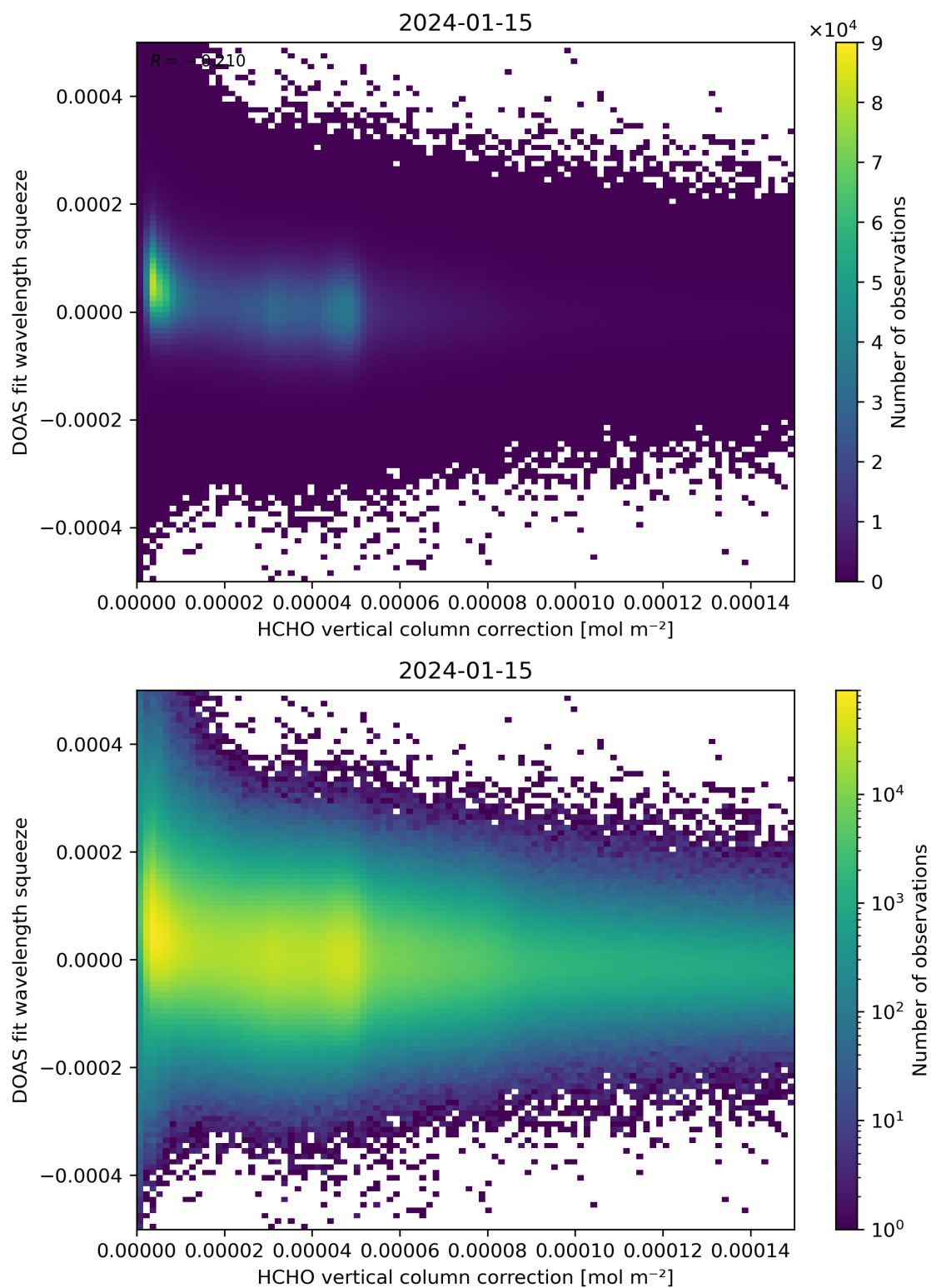
Figure 114: Scatter density plot of “HCHO vertical column correction” against “DOAS fit wavelength squeeze” for 2024-01-15 to 2024-01-16.
