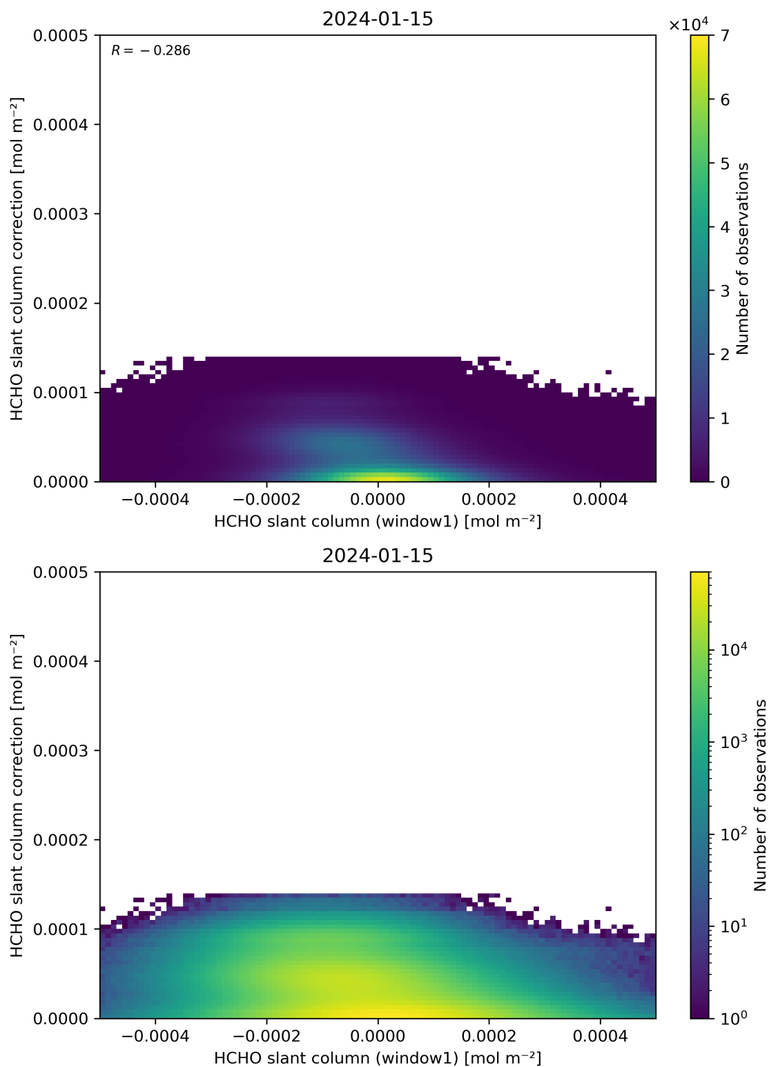
Figure 83: Scatter density plot of “HCHO slant column (window1)” against “HCHO slant column correction” for 2024-01-15 to 2024-01-16.
