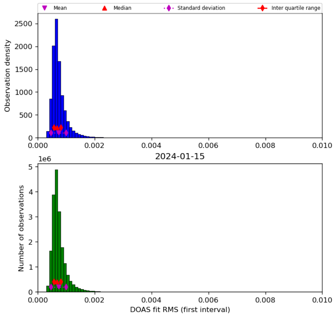
Figure 46: Histogram of “DOAS fit RMS (first interval)” for 2024-01-15 to 2024-01-16
