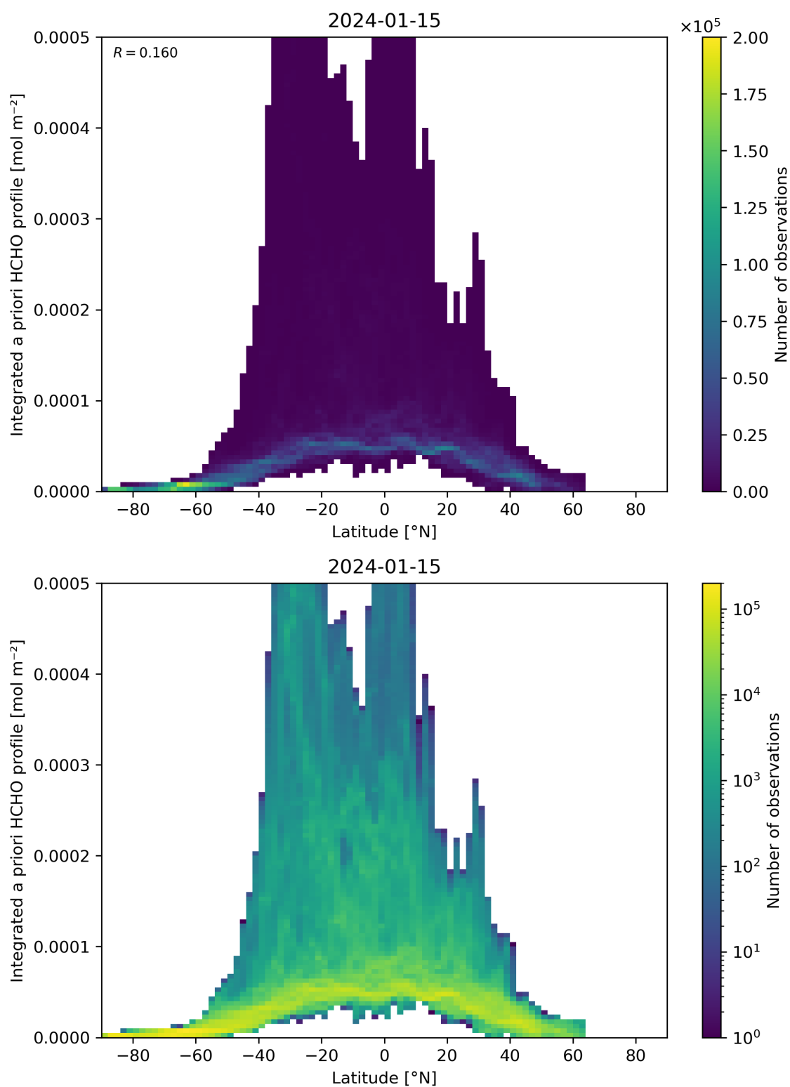
Figure 166: Scatter density plot of “Latitude” against “Integrated a priori HCHO profile” for 2024-01-15 to 2024-01-16.
