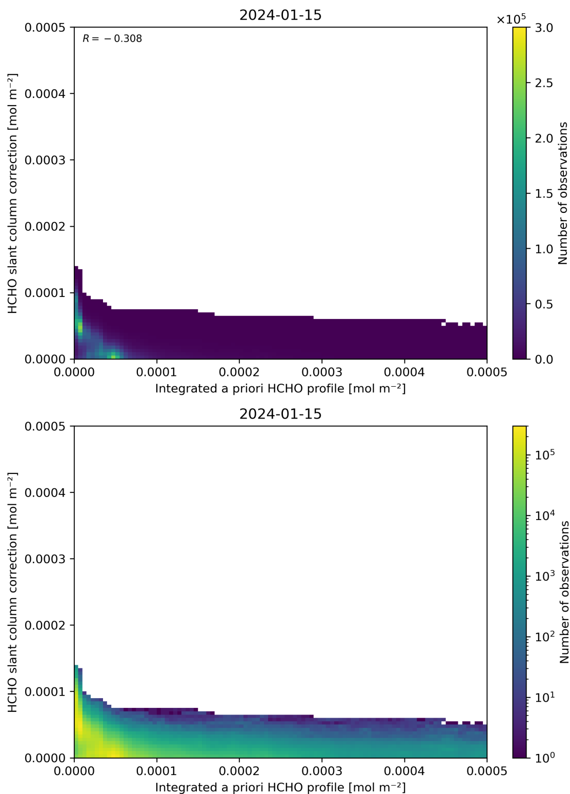
Figure 152: Scatter density plot of “Integrated a priori HCHO profile” against “HCHO slant column correction” for 2024-01-15 to 2024-01-16.
