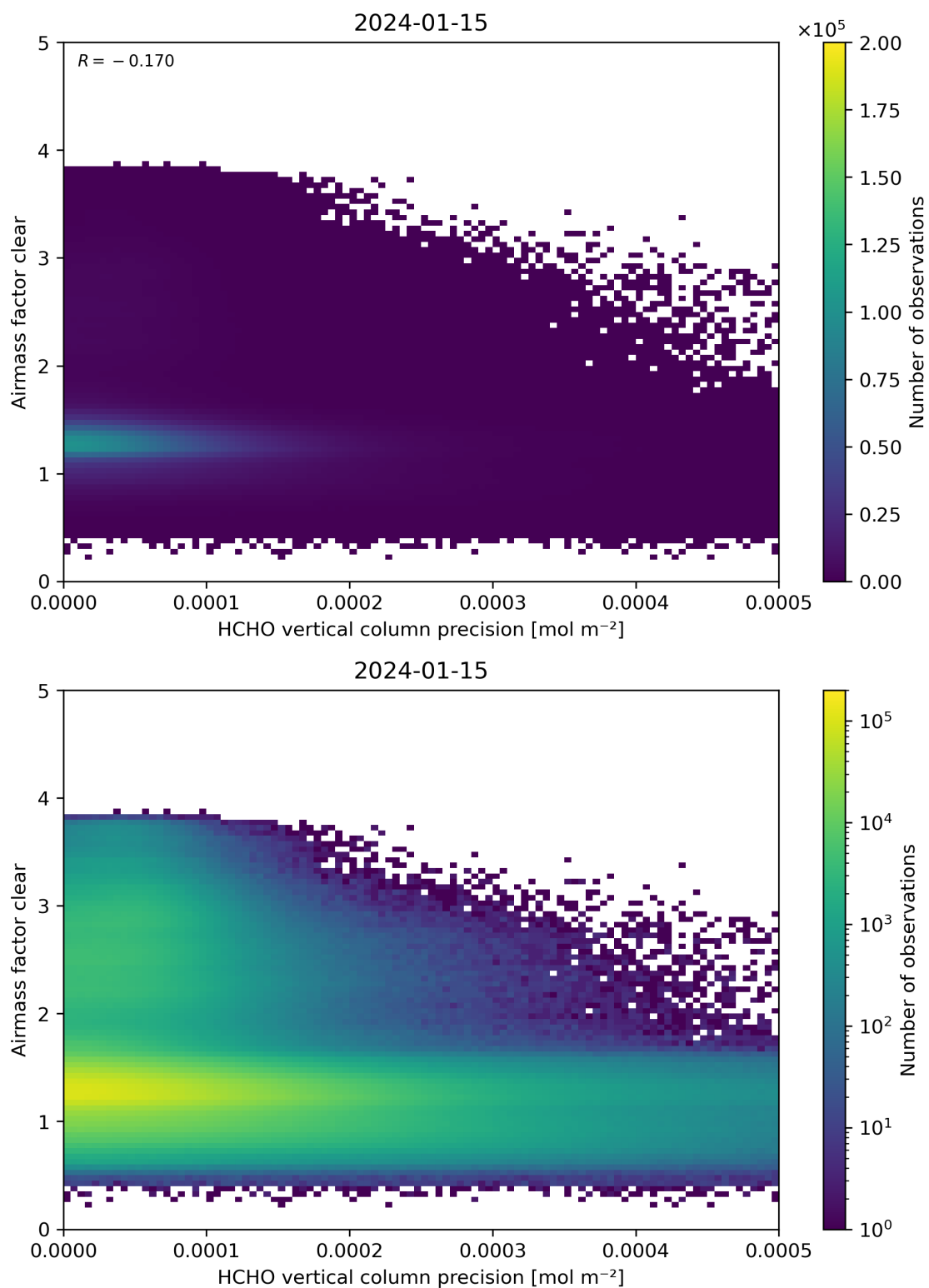
Figure 139: Scatter density plot of “HCHO vertical column precision” against “Airmass factor clear” for 2024-01-15 to 2024-01-16.
