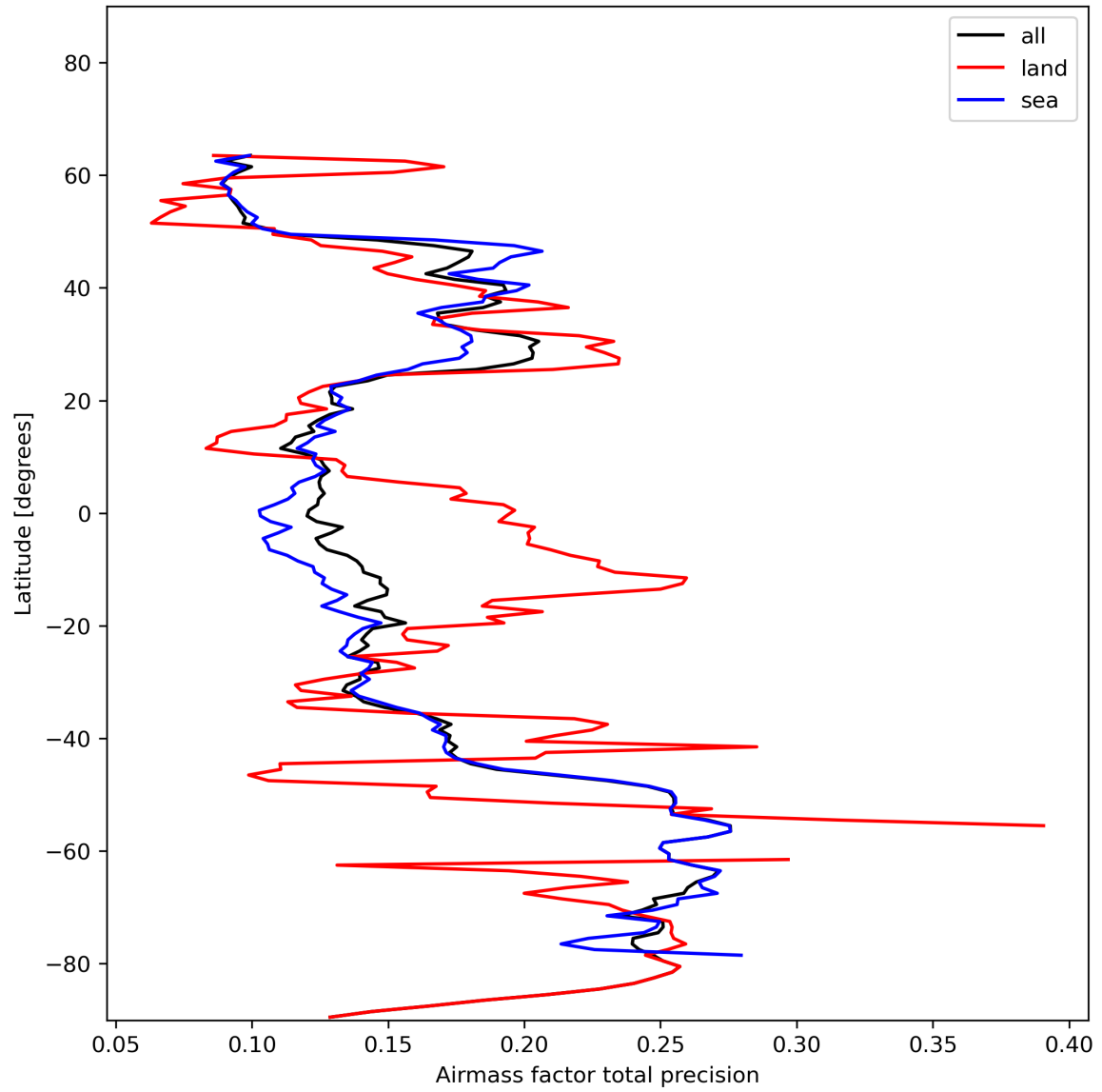
Figure 27: Zonal average of “Airmass factor total precision” for 2024-01-15 to 2024-01-16.
