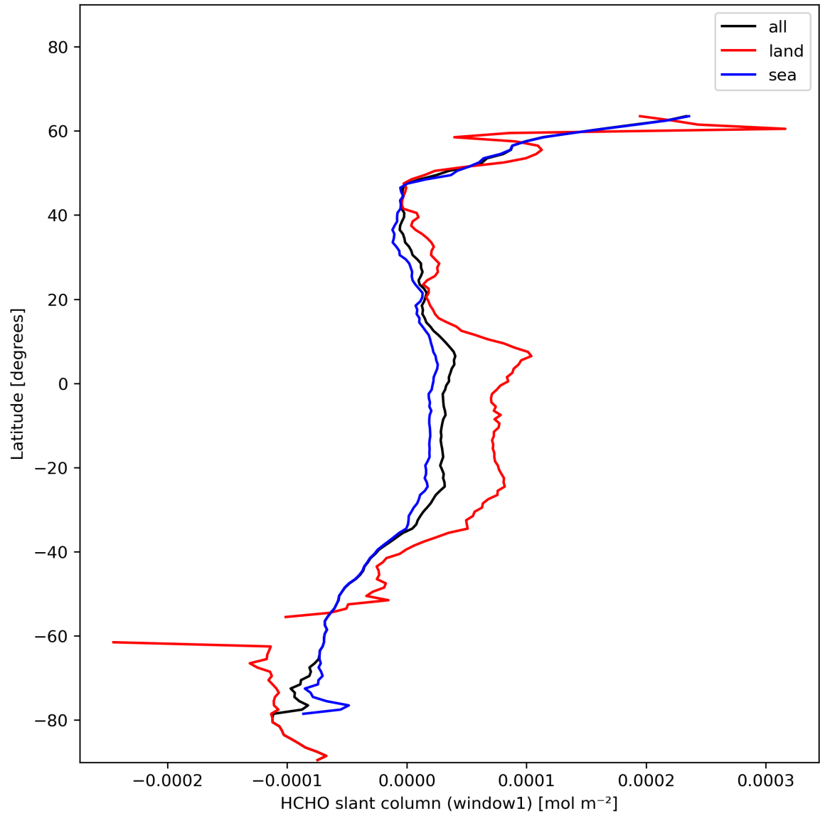
Figure 24: Zonal average of “HCHO slant column (window1)” for 2024-01-15 to 2024-01-16.
