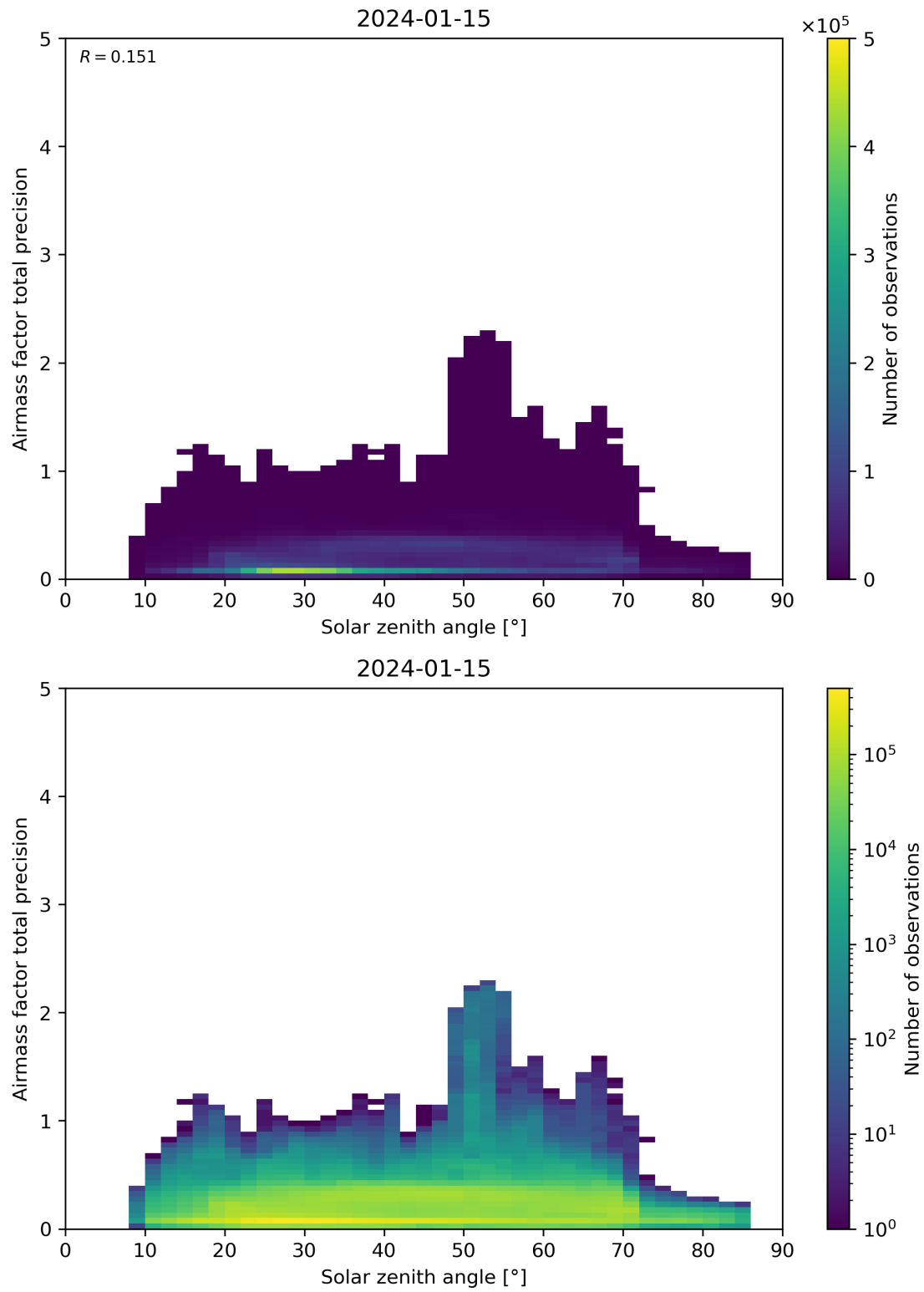
Figure 176: Scatter density plot of “Solar zenith angle” against “Airmass factor total precision” for 2024-01-15 to 2024-01-16.
