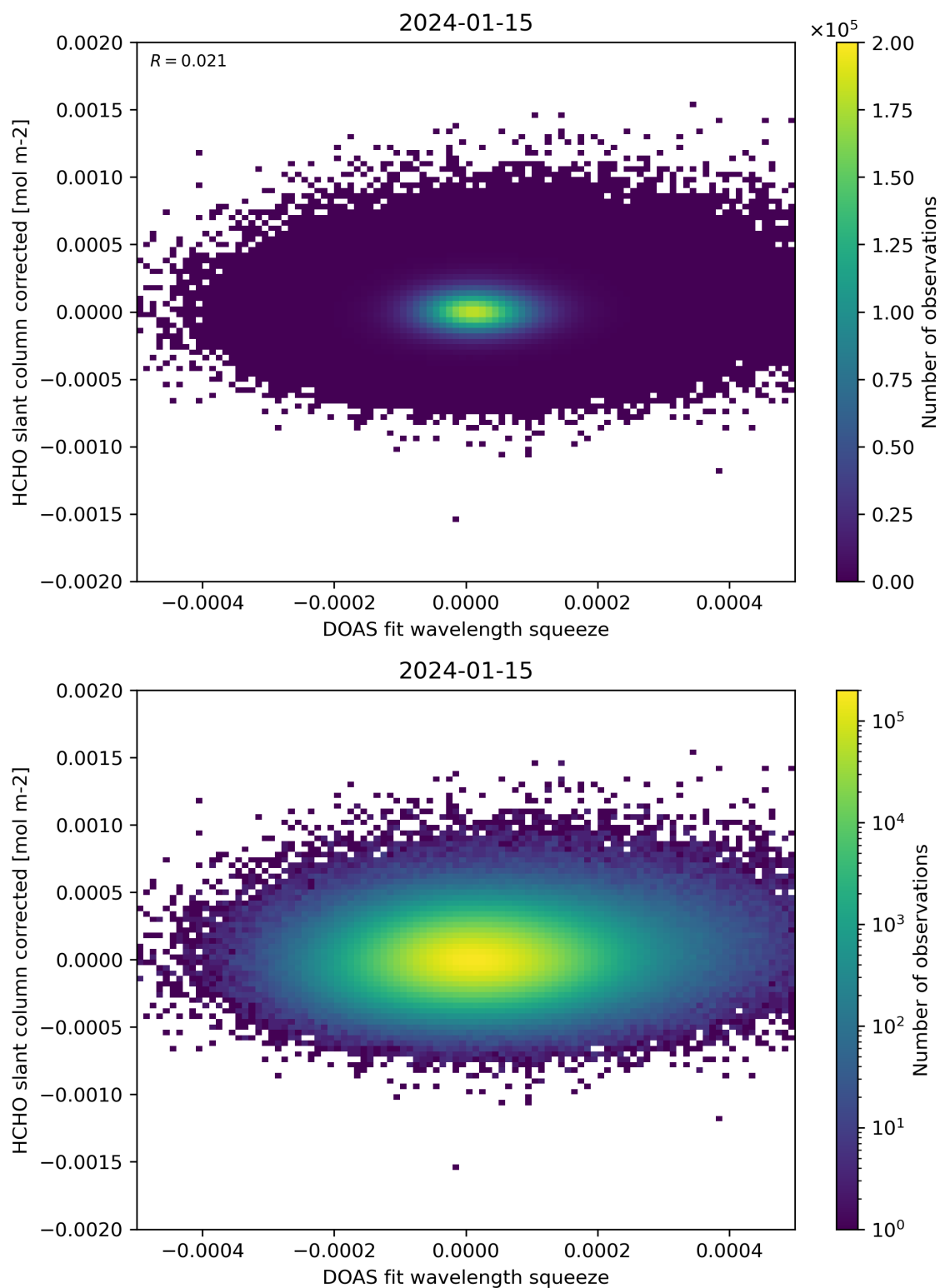
Figure 69: Scatter density plot of “DOAS fit wavelength squeeze” against “HCHO slant column corrected” for 2024-01-15 to 2024-01-16.
