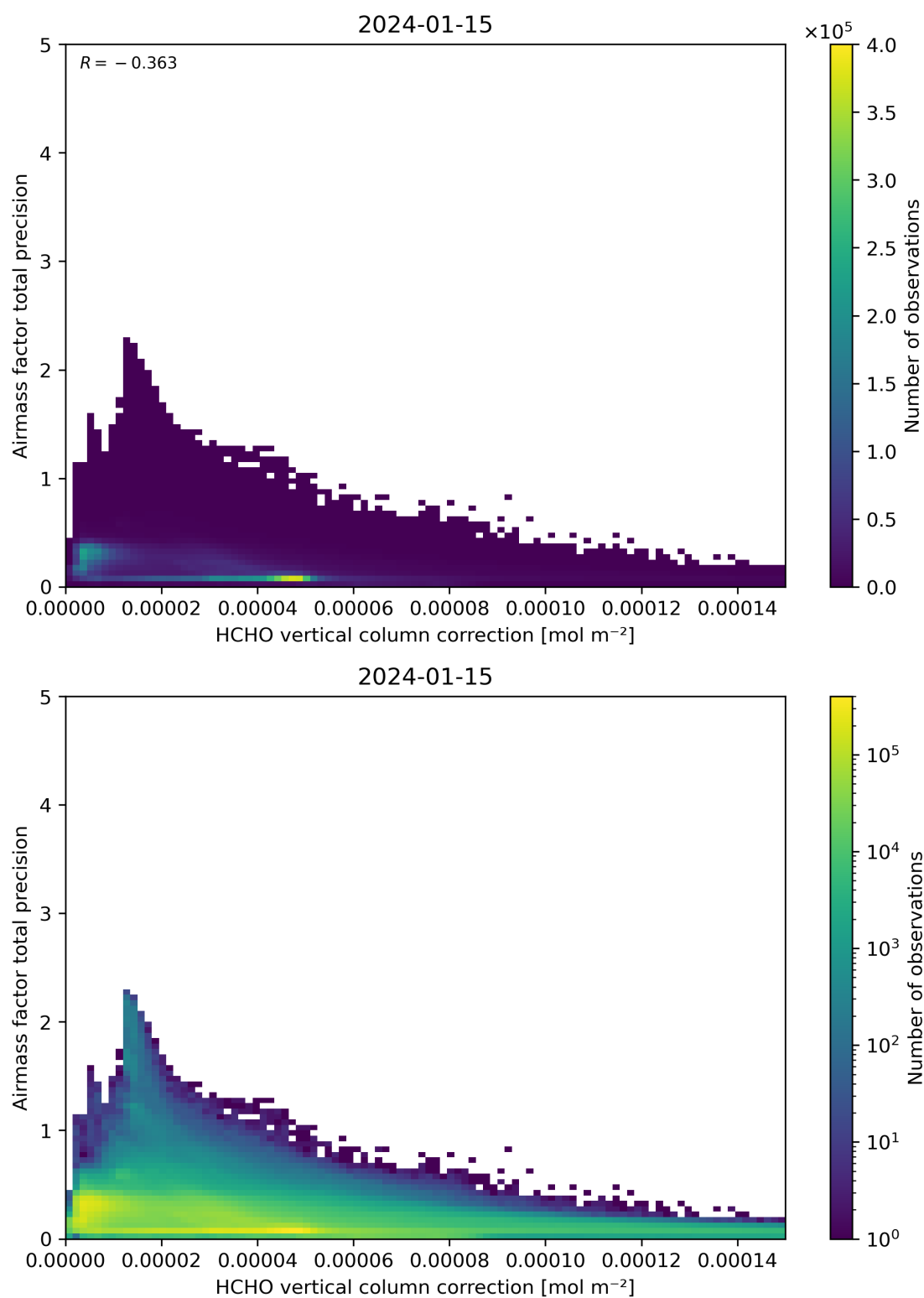
Figure 121: Scatter density plot of “HCHO vertical column correction” against “Airmass factor total precision” for 2024-01-15 to 2024-01-16.
