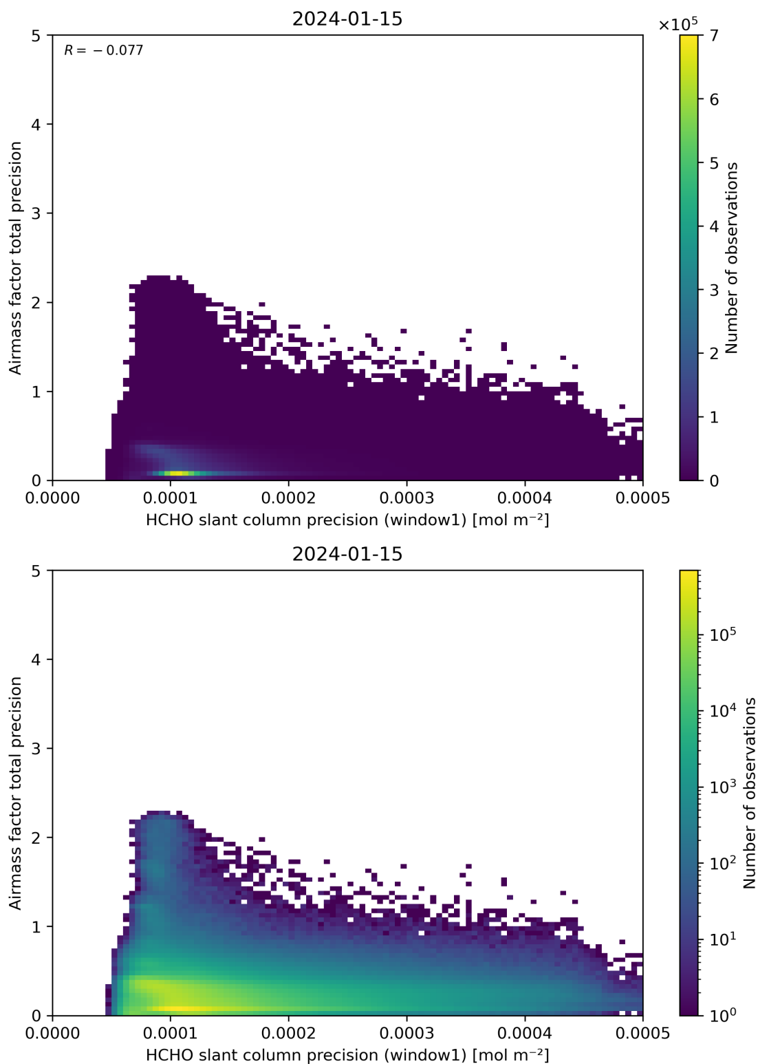
Figure 95: Scatter density plot of “HCHO slant column precision (window1)” against “Airmass factor total precision” for 2024-01-15 to 2024-01-16.
