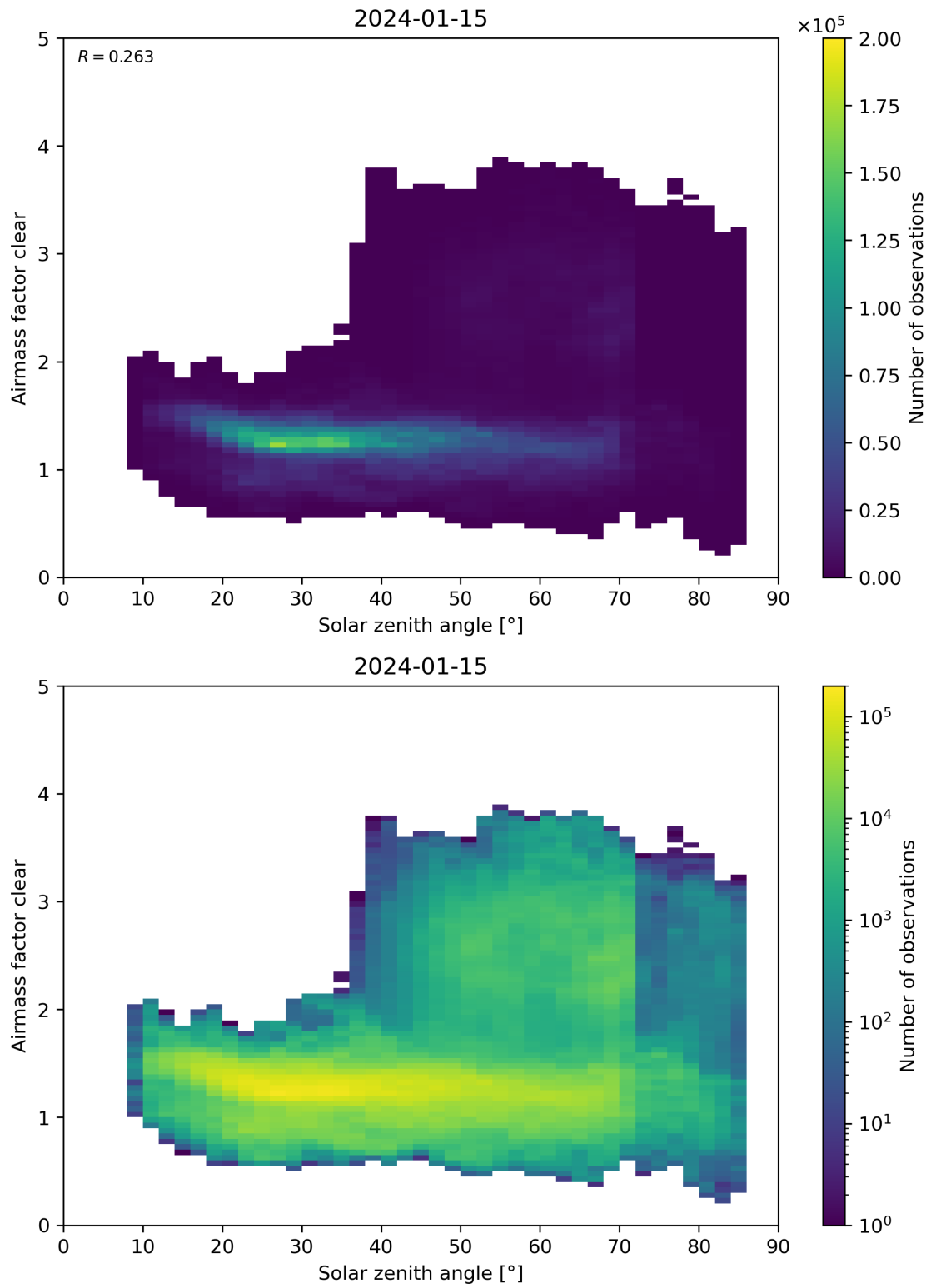
Figure 170: Scatter density plot of “Solar zenith angle” against “Airmass factor clear” for 2024-01-15 to 2024-01-16.
