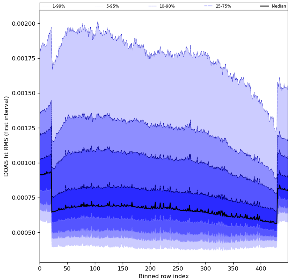
Figure 60: Along track statistics of “DOAS fit RMS (first interval)” for 2024-01-15 to 2024-01-16
