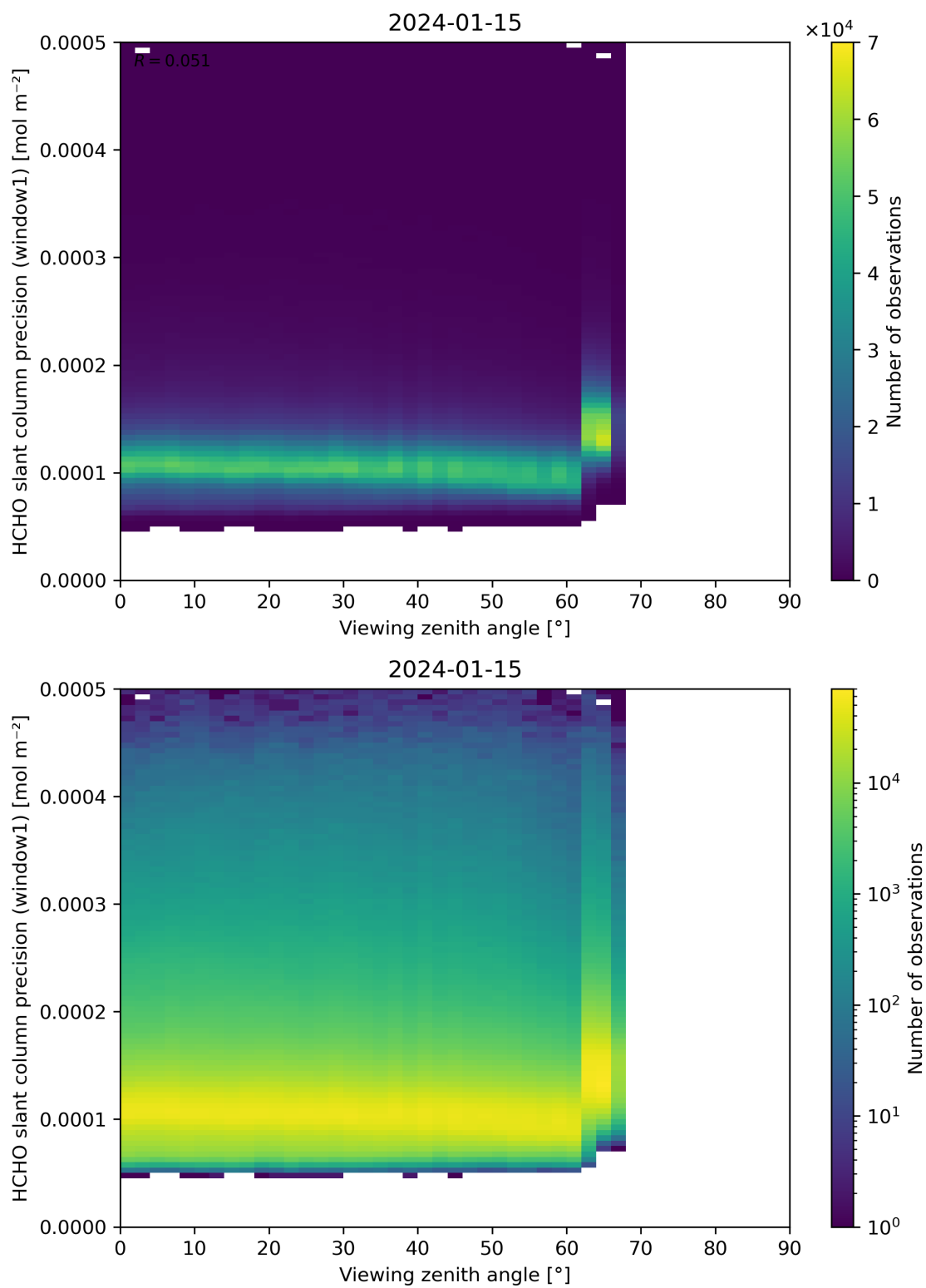
Figure 189: Scatter density plot of “Viewing zenith angle” against “HCHO slant column precision (window1)” for 2024-01-15 to 2024-01-16.
