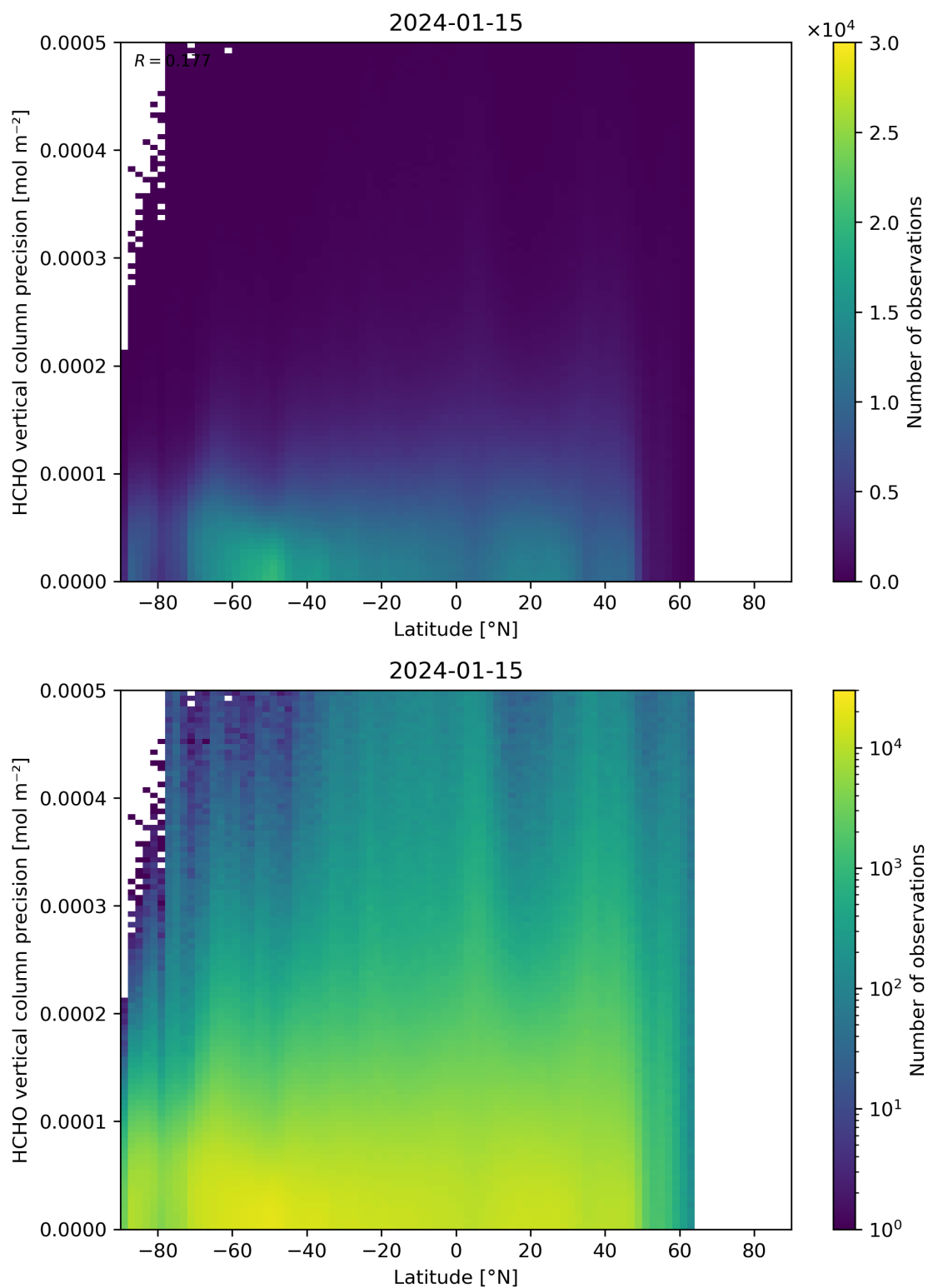
Figure 165: Scatter density plot of “Latitude” against “HCHO vertical column precision” for 2024-01-15 to 2024-01-16.
