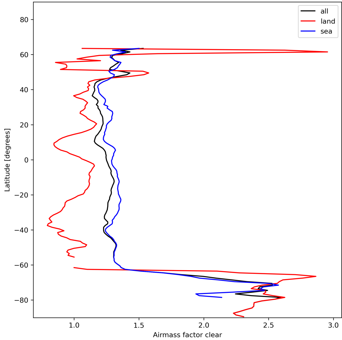
Figure 28: Zonal average of “Airmass factor clear” for 2024-01-15 to 2024-01-16.
