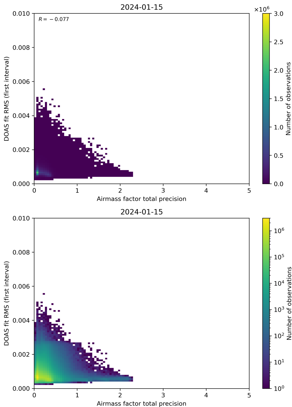
Figure 105: Scatter density plot of “Airmass factor total precision” against “DOAS fit RMS (first interval)” for 2024-01-15 to 2024-01-16.
