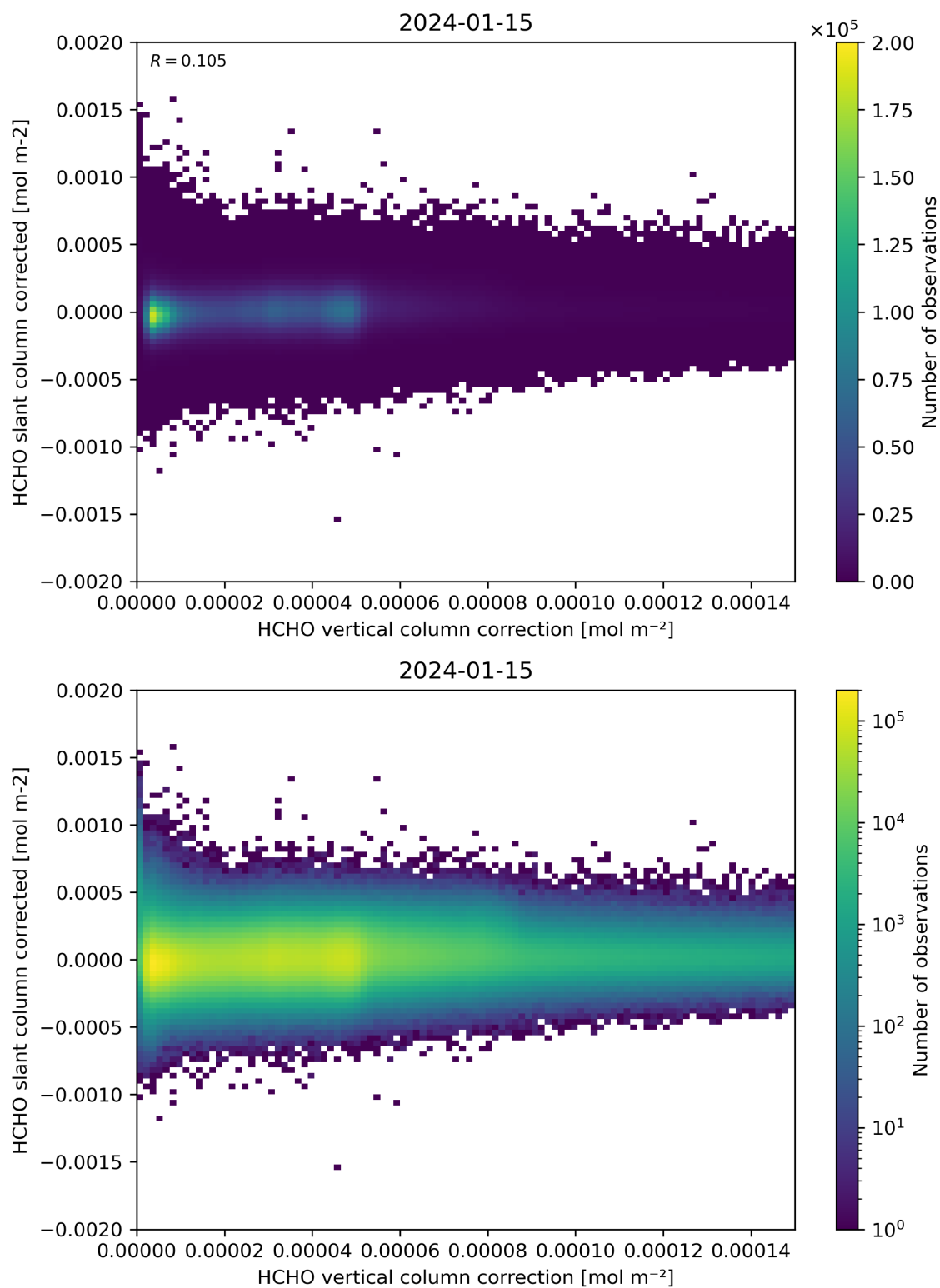
Figure 116: Scatter density plot of “HCHO vertical column correction” against “HCHO slant column corrected” for 2024-01-15 to 2024-01-16.
