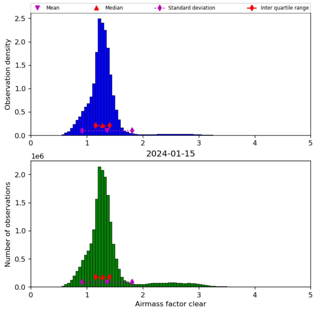
Figure 42: Histogram of “Airmass factor clear” for 2024-01-15 to 2024-01-16
