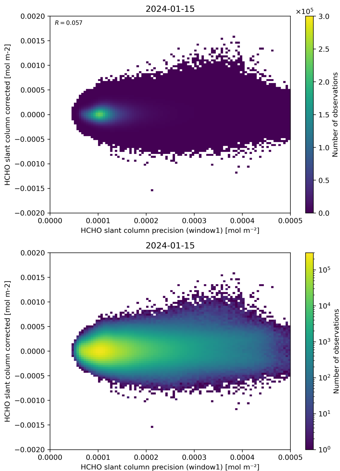
Figure 92: Scatter density plot of “HCHO slant column precision (window1)” against “HCHO slant column corrected” for 2024-01-15 to 2024-01-16.
