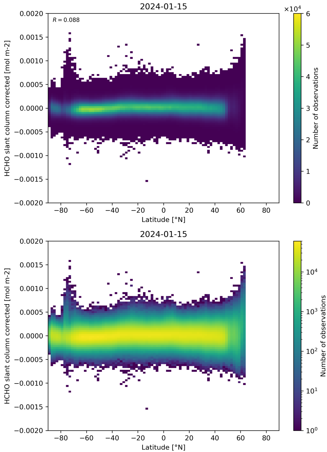
Figure 157: Scatter density plot of “Latitude” against “HCHO slant column corrected” for 2024-01-15 to 2024-01-16.
