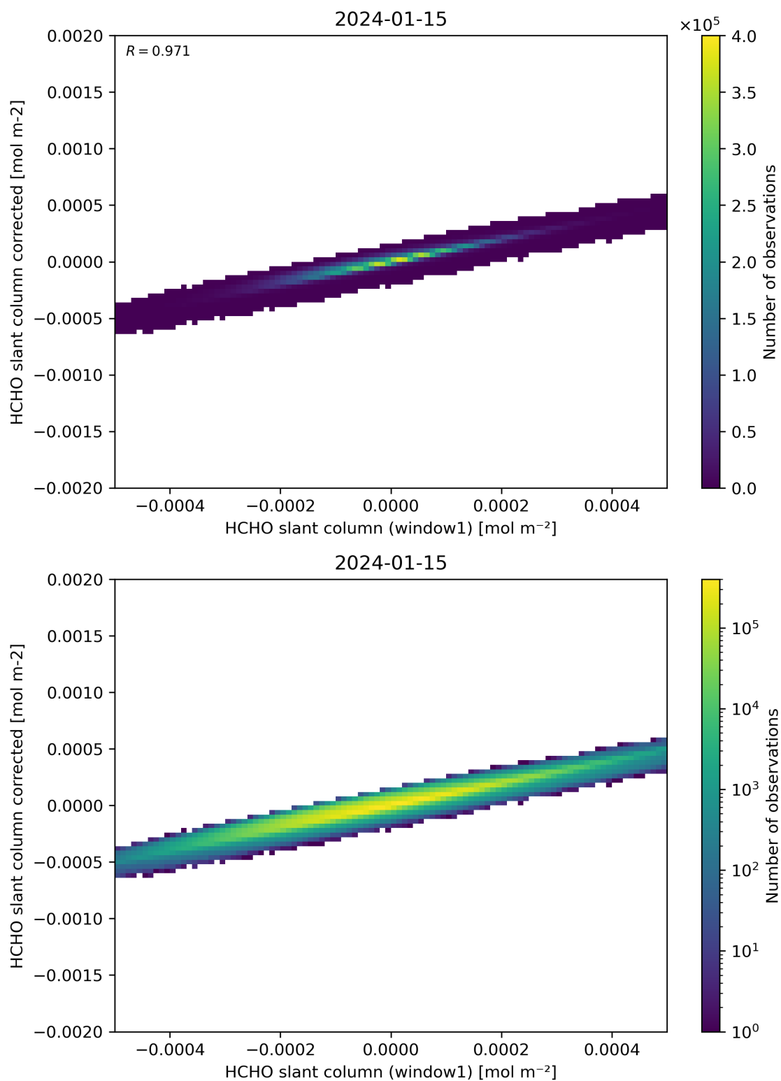
Figure 82: Scatter density plot of “HCHO slant column (window1)” against “HCHO slant column corrected” for 2024-01-15 to 2024-01-16.
