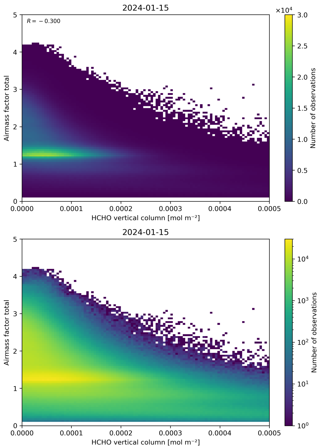
Figure 131: Scatter density plot of “HCHO vertical column” against “Airmass factor total” for 2024-01-15 to 2024-01-16.
