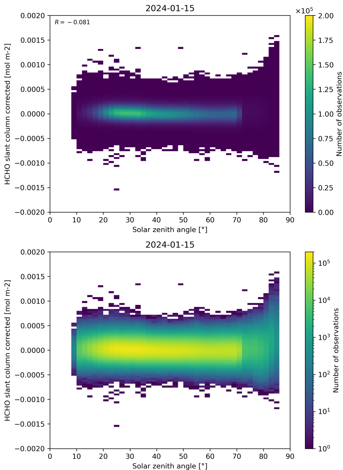
Figure 171: Scatter density plot of “Solar zenith angle” against “HCHO slant column corrected” for 2024-01-15 to 2024-01-16.
