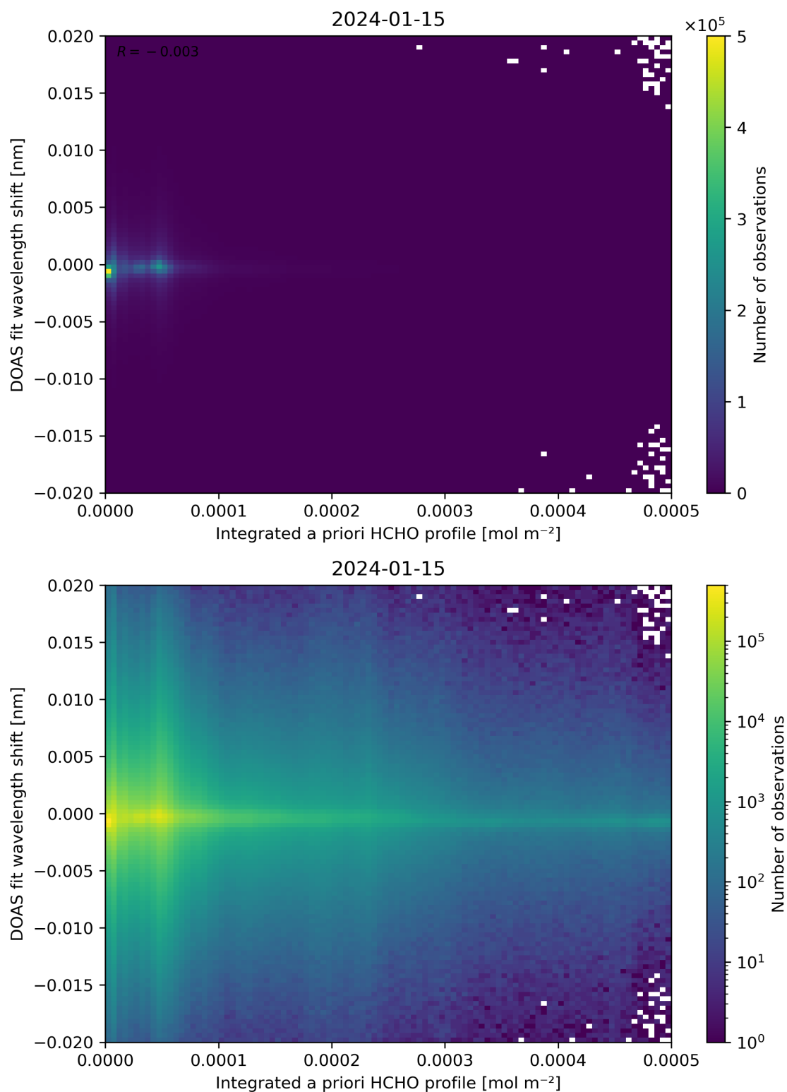
Figure 149: Scatter density plot of “Integrated a priori HCHO profile” against “DOAS fit wavelength shift” for 2024-01-15 to 2024-01-16.
