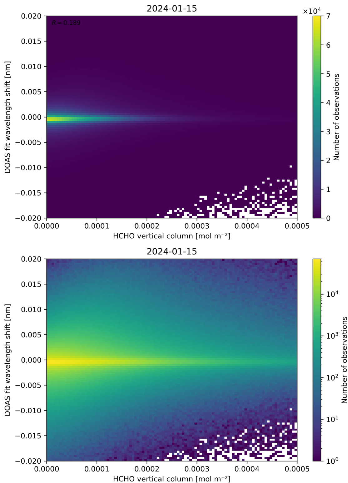
Figure 124: Scatter density plot of “HCHO vertical column” against “DOAS fit wavelength shift” for 2024-01-15 to 2024-01-16.
