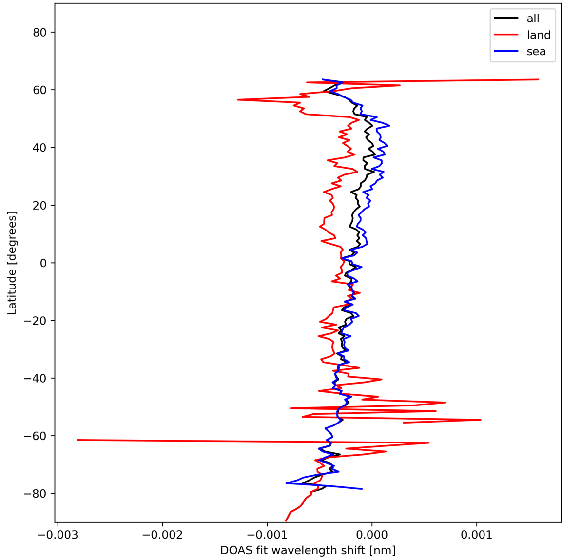
Figure 30: Zonal average of "DOAS fit wavelength shift" for 2024-01-15 to 2024-01-16.
