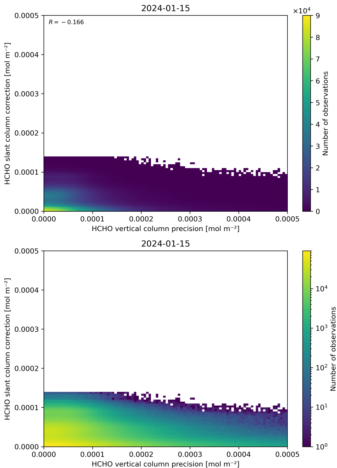
Figure 141: Scatter density plot of “HCHO vertical column precision” against “HCHO slant column correction” for 2024-01-15 to 2024-01-16.
