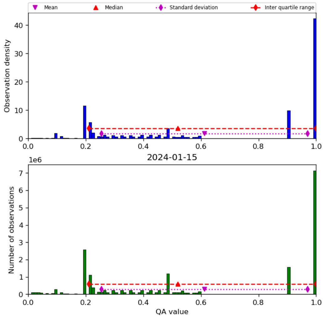
Figure 34: Histogram of “QA value” for 2024-01-15 to 2024-01-16
