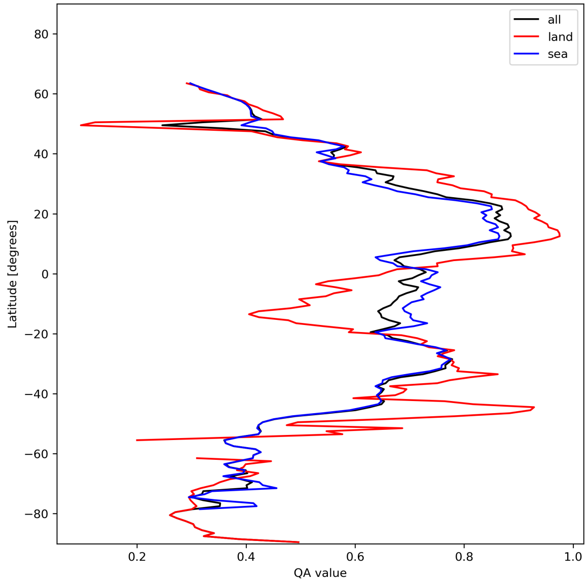
Figure 20: Zonal average of “QA value” for 2024-01-15 to 2024-01-16.
