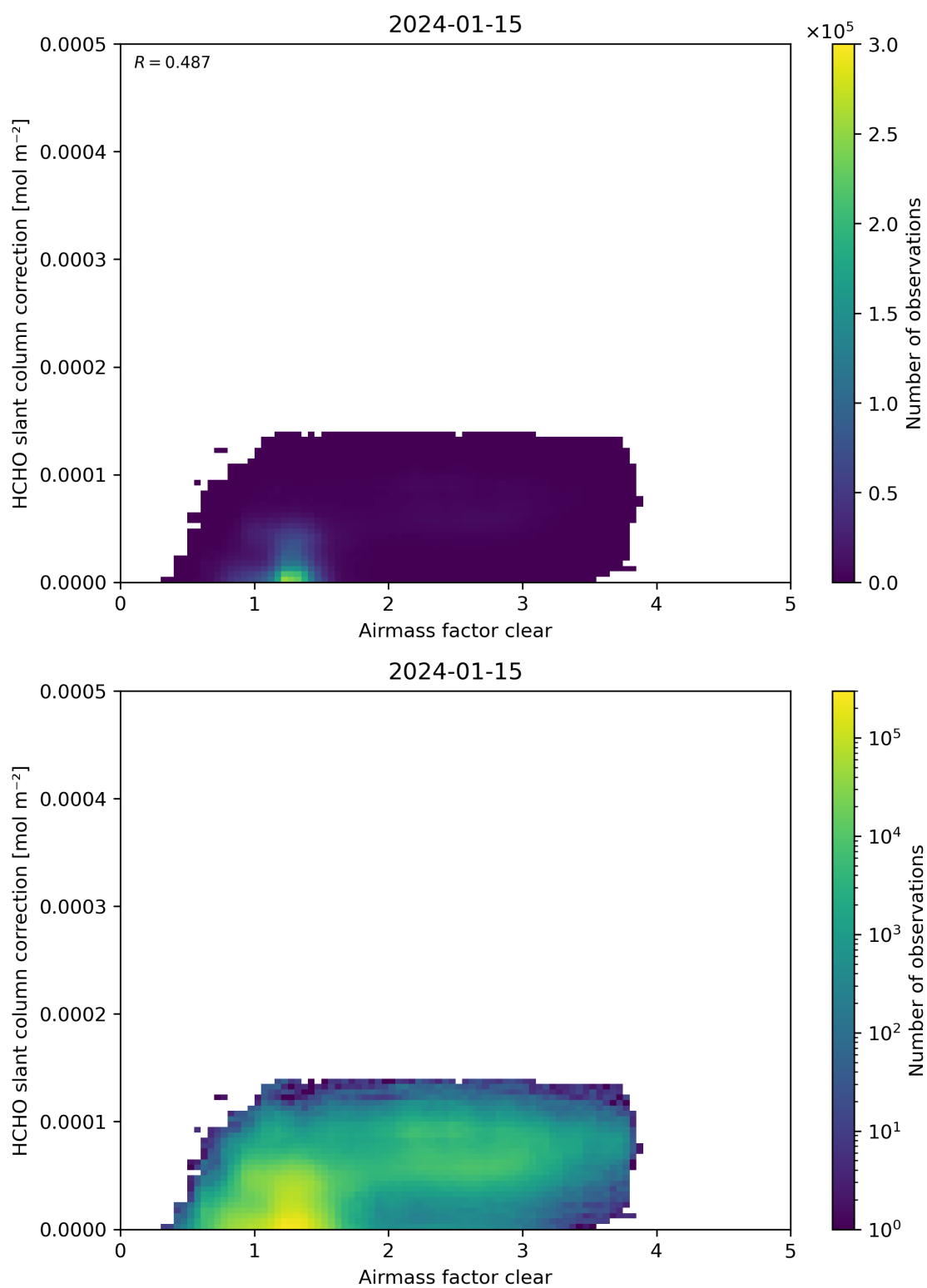
Figure 75: Scatter density plot of “Airmass factor clear” against “HCHO slant column correction” for 2024-01-15 to 2024-01-16.
