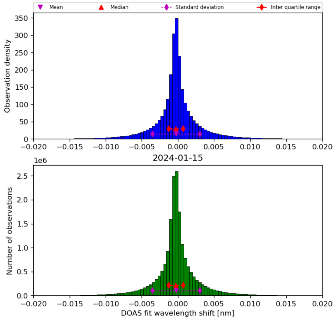
Figure 44: Histogram of “DOAS fit wavelength shift” for 2024-01-15 to 2024-01-16
