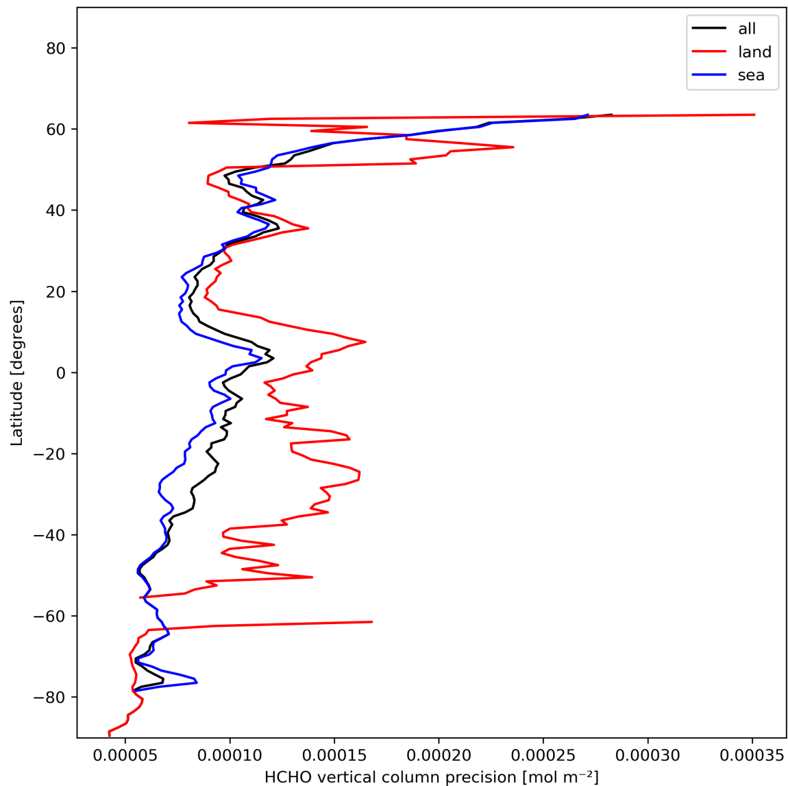
Figure 22: Zonal average of “HCHO vertical column precision” for 2024-01-15 to 2024-01-16.
