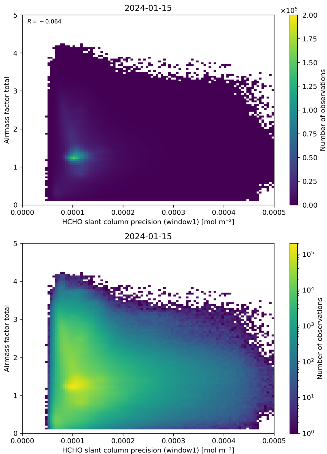
Figure 94: Scatter density plot of “HCHO slant column precision (window1)” against “Airmass factor total” for 2024-01-15 to 2024-01-16.
