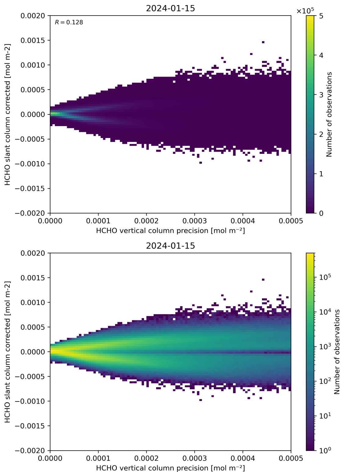
Figure 140: Scatter density plot of “HCHO vertical column precision” against “HCHO slant column corrected” for 2024-01-15 to 2024-01-16.
