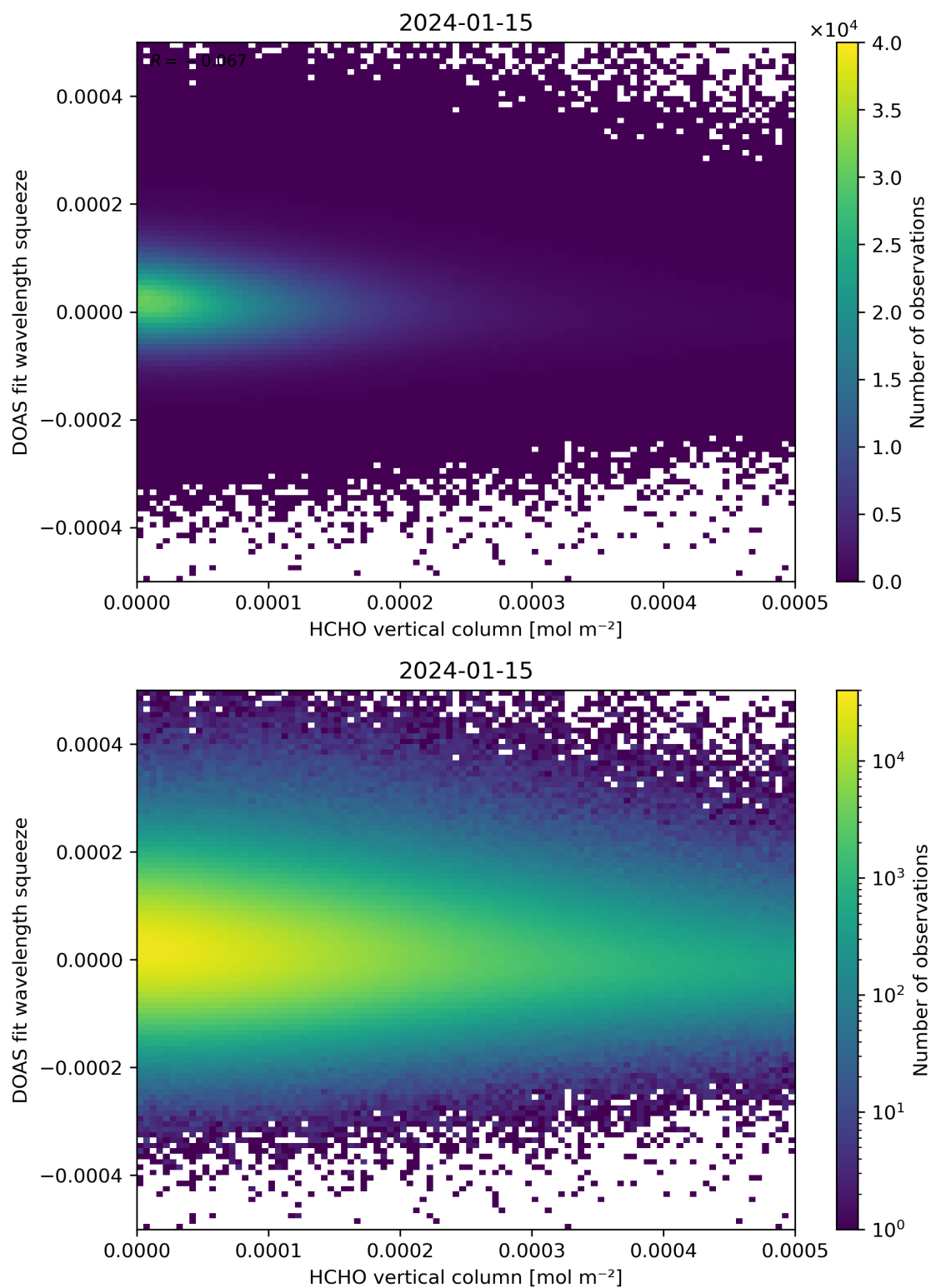
Figure 125: Scatter density plot of “HCHO vertical column” against “DOAS fit wavelength squeeze” for 2024-01-15 to 2024-01-16.
