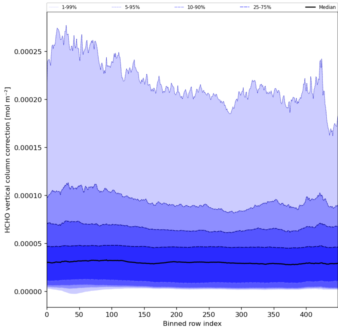
Figure 51: Along track statistics of “HCHO vertical column correction” for 2024-01-15 to 2024-01-16
