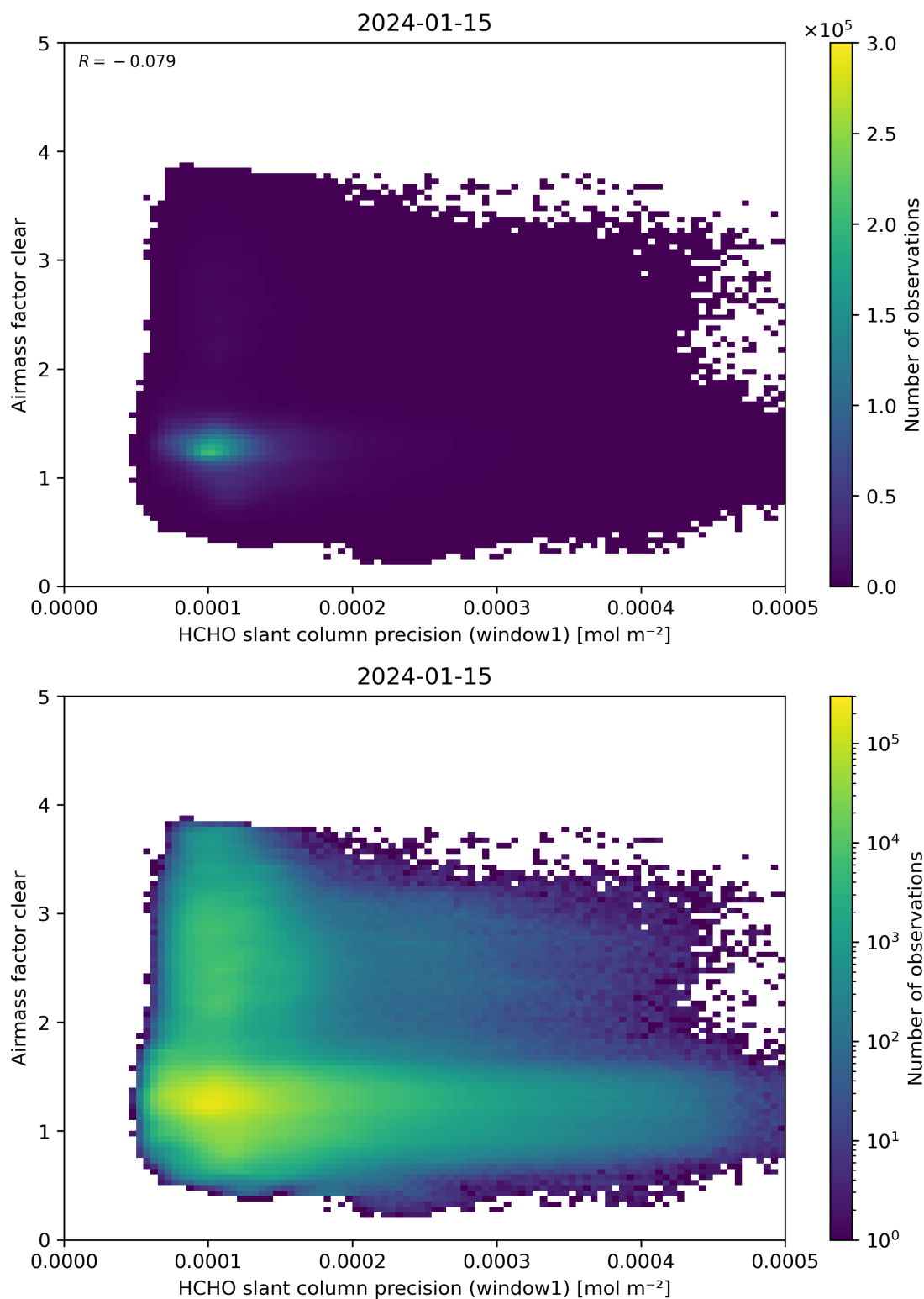
Figure 91: Scatter density plot of “HCHO slant column precision (window1)” against “Airmass factor clear” for 2024-01-15 to 2024-01-16.
