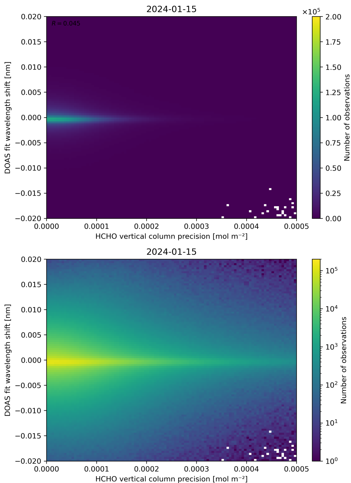
Figure 137: Scatter density plot of “HCHO vertical column precision” against “DOAS fit wavelength shift” for 2024-01-15 to 2024-01-16.
