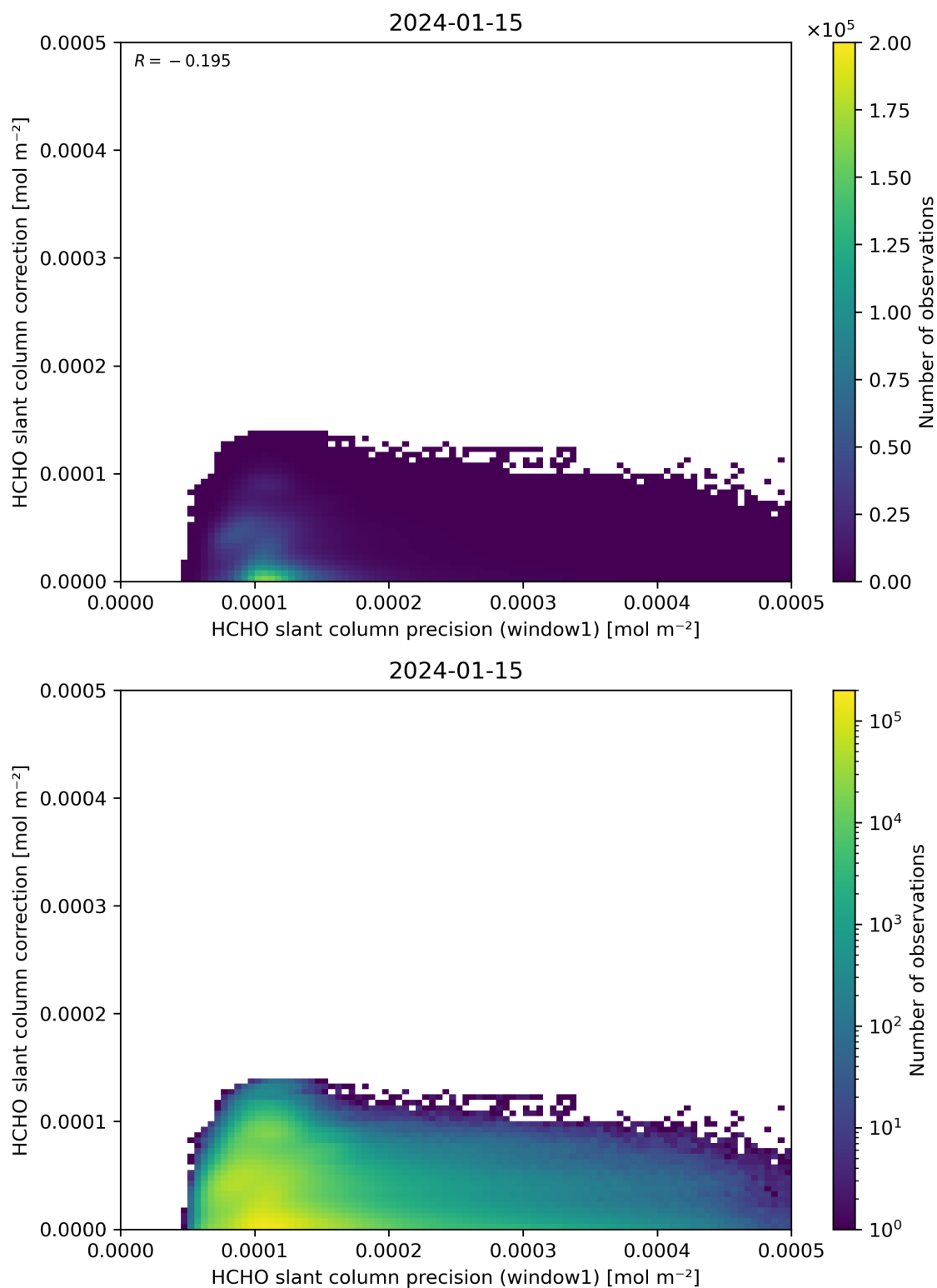
Figure 93: Scatter density plot of “HCHO slant column precision (window1)” against “HCHO slant column correction” for 2024-01-15 to 2024-01-16.
