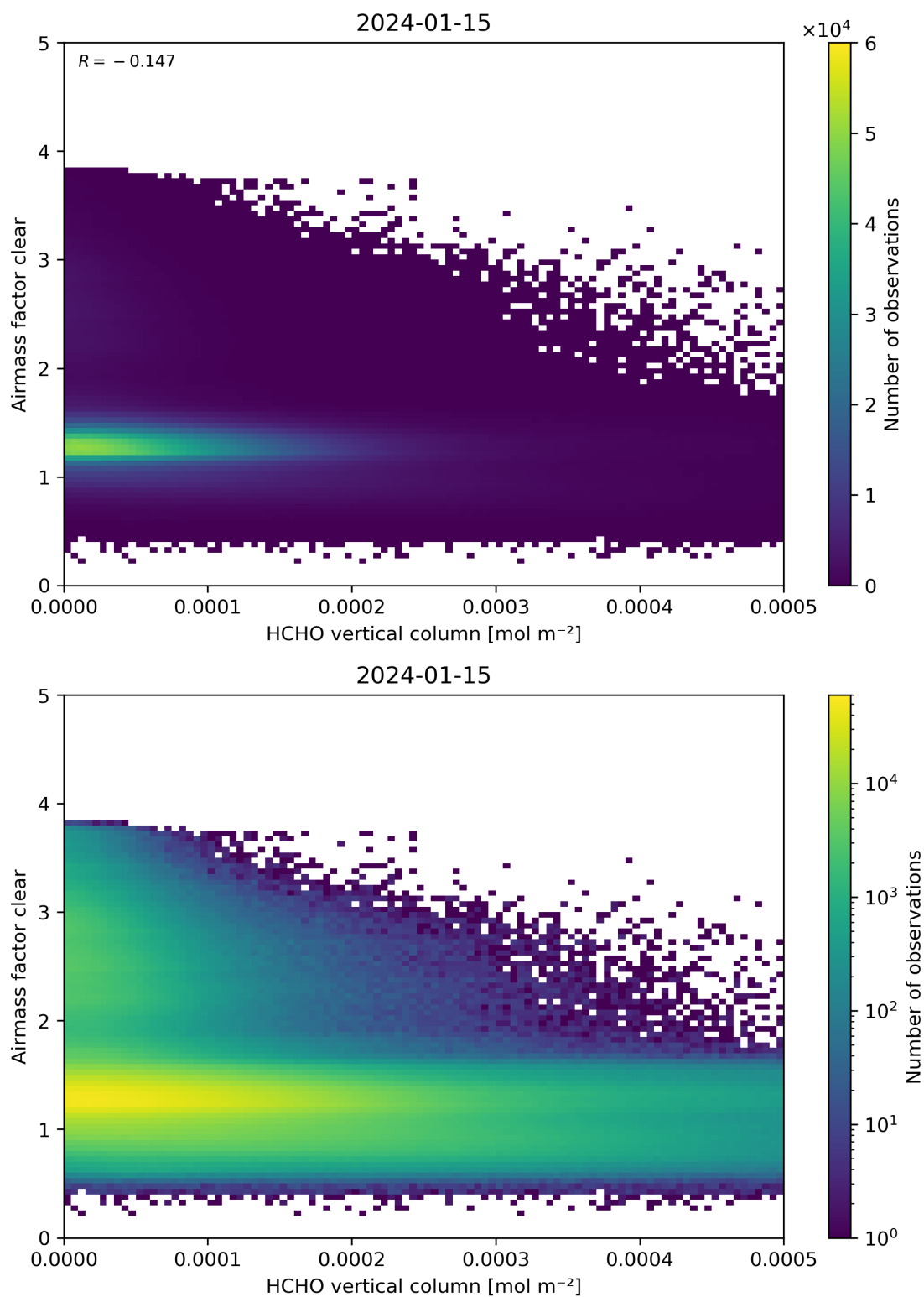
Figure 126: Scatter density plot of “HCHO vertical column” against “Airmass factor clear” for 2024-01-15 to 2024-01-16.
