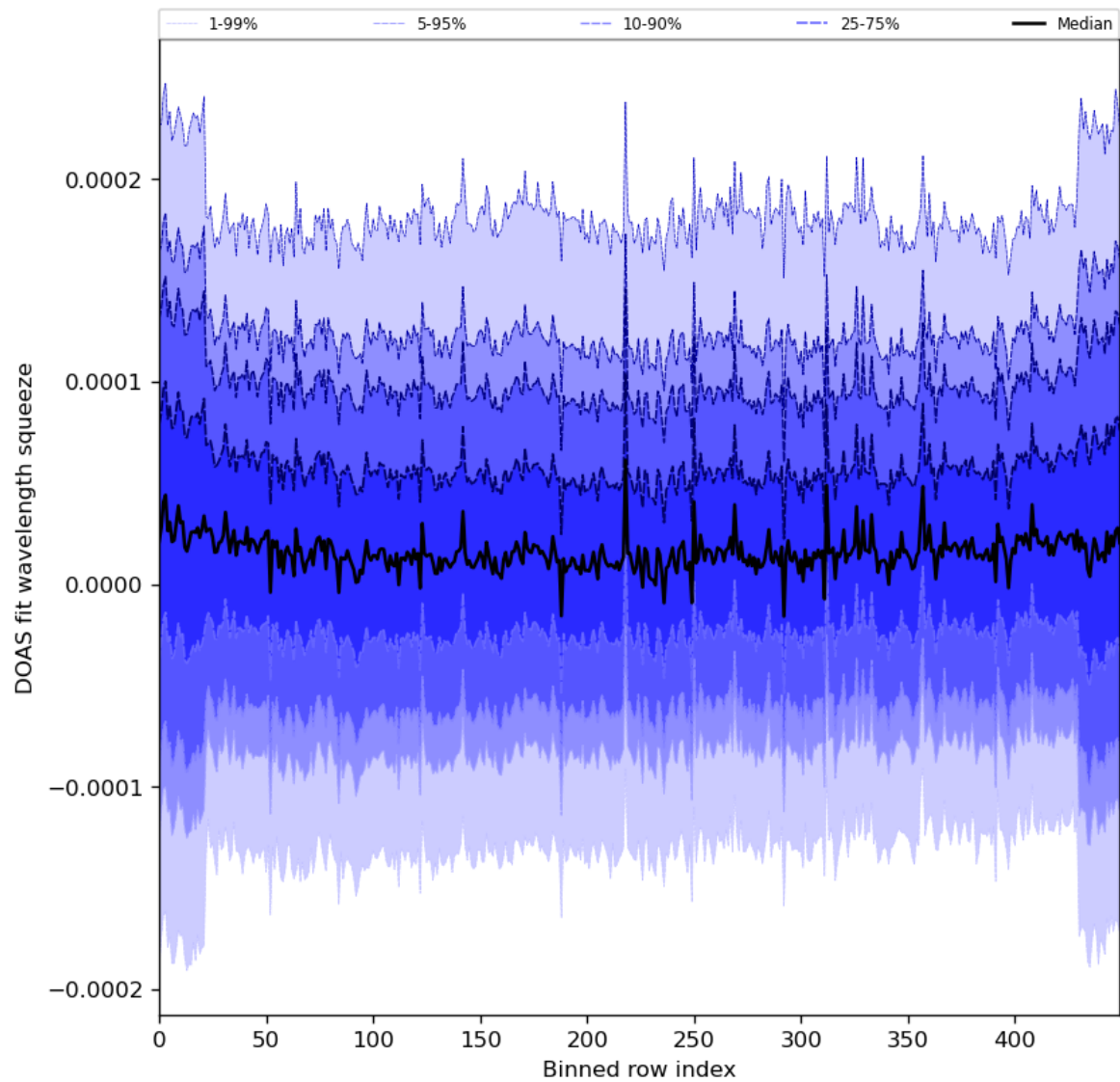
Figure 59: Along track statistics of “DOAS fit wavelength squeeze” for 2024-01-15 to 2024-01-16
