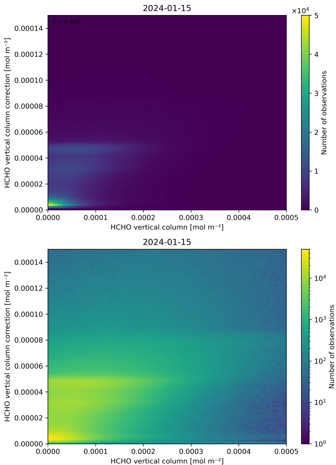
Figure 133: Scatter density plot of “HCHO vertical column” against “HCHO vertical column correction” for 2024-01-15 to 2024-01-16.
