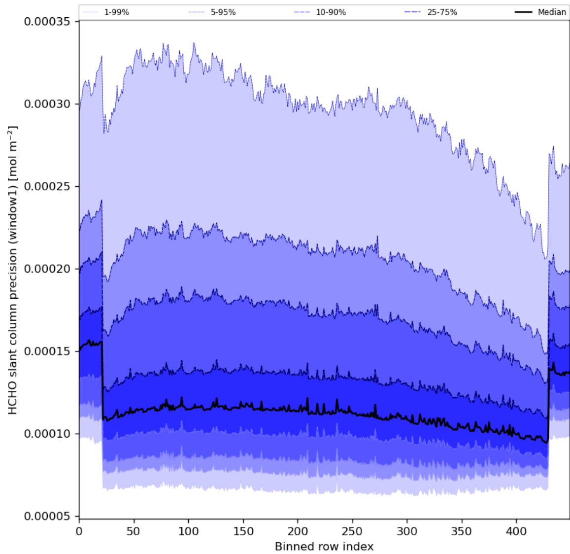
Figure 53: Along track statistics of “HCHO slant column precision (window1)” for 2024-01-15 to 2024-01-16
