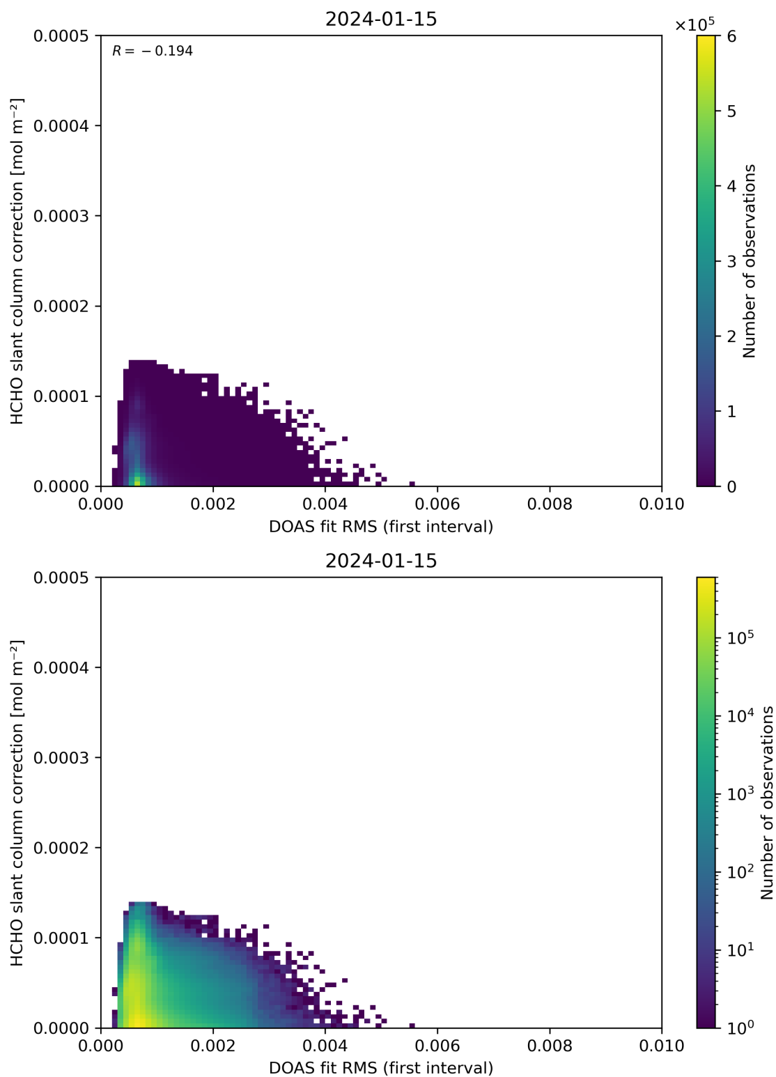
Figure 63: Scatter density plot of “DOAS fit RMS (first interval)” against “HCHO slant column correction” for 2024-01-15 to 2024-01-16.
