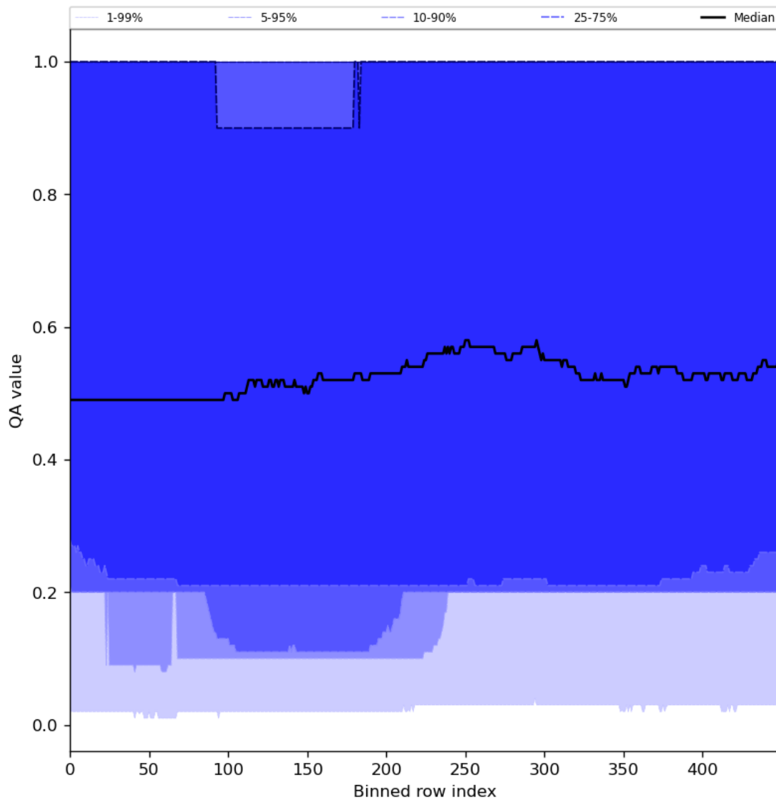
Figure 48: Along track statistics of “QA value” for 2024-01-15 to 2024-01-16
