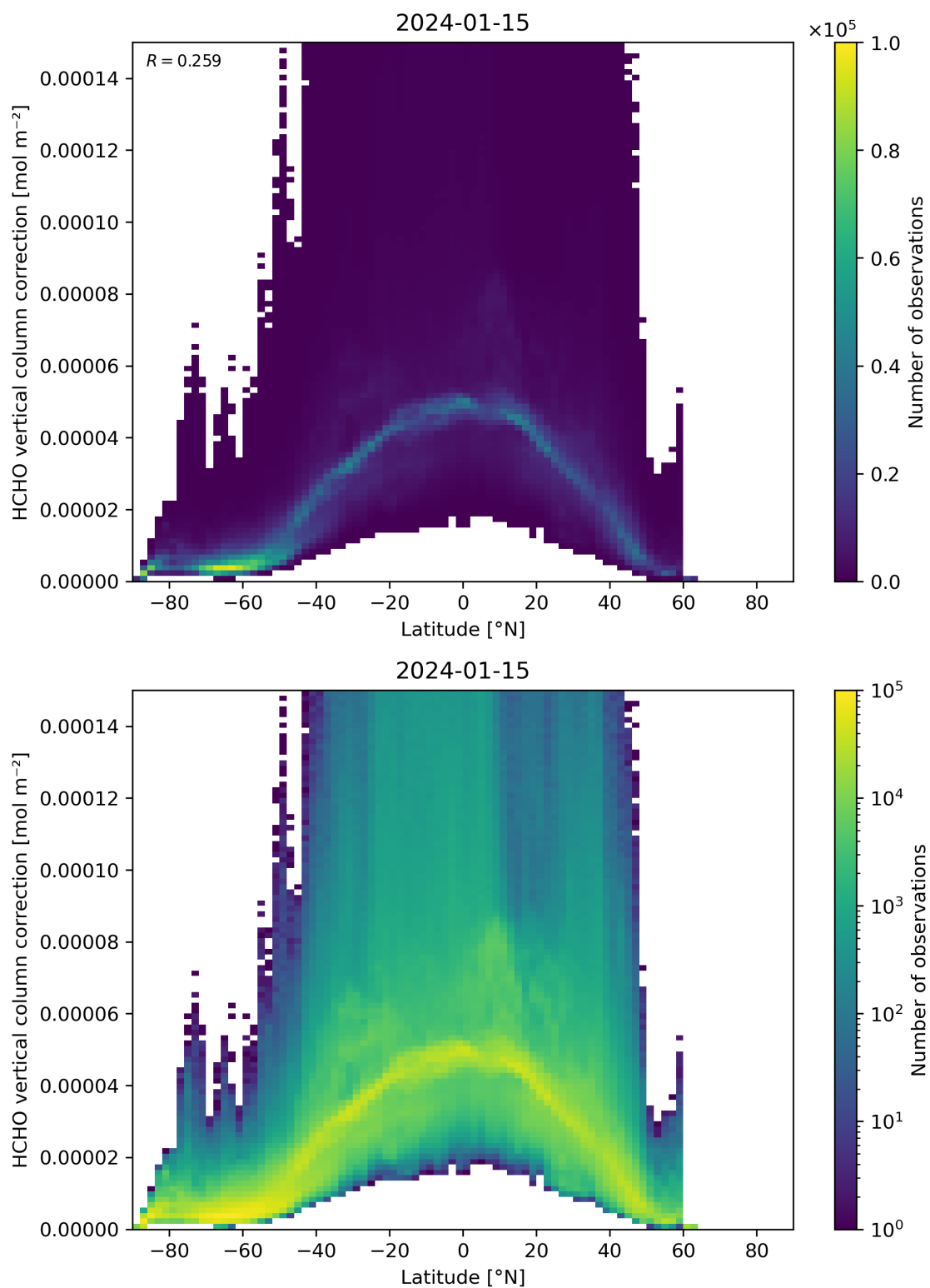
Figure 164: Scatter density plot of “Latitude” against “HCHO vertical column correction” for 2024-01-15 to 2024-01-16.
