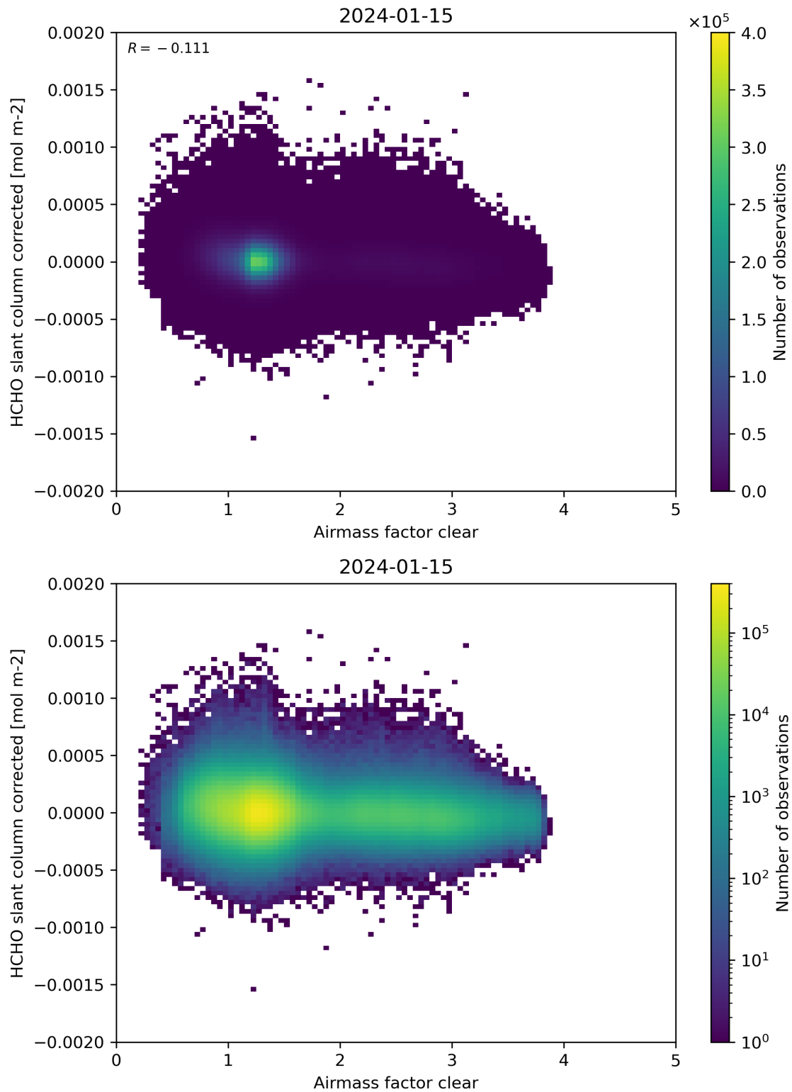
Figure 74: Scatter density plot of “Airmass factor clear” against “HCHO slant column corrected” for 2024-01-15 to 2024-01-16.
