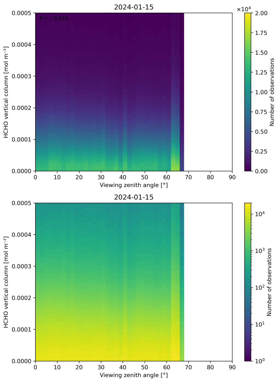
Figure 192: Scatter density plot of “Viewing zenith angle” against “HCHO vertical column” for 2024-01-15 to 2024-01-16.
