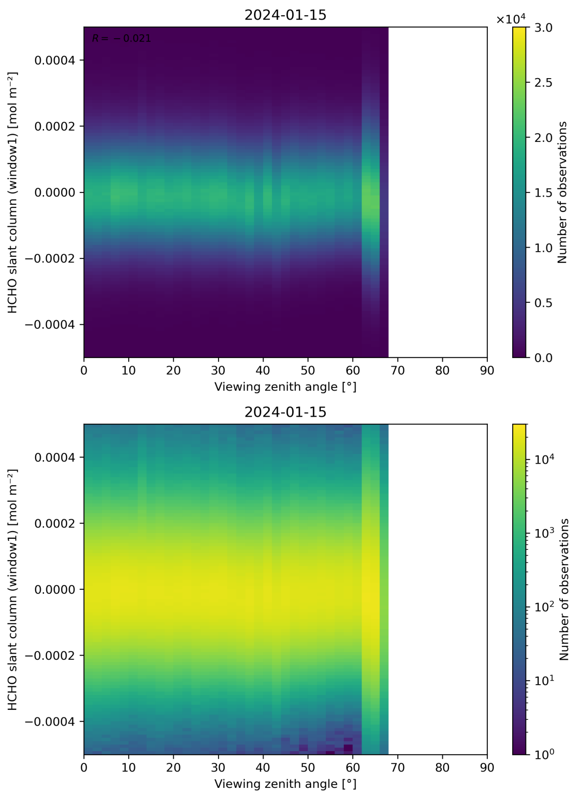
Figure 188: Scatter density plot of “Viewing zenith angle” against “HCHO slant column (window1)” for 2024-01-15 to 2024-01-16.
