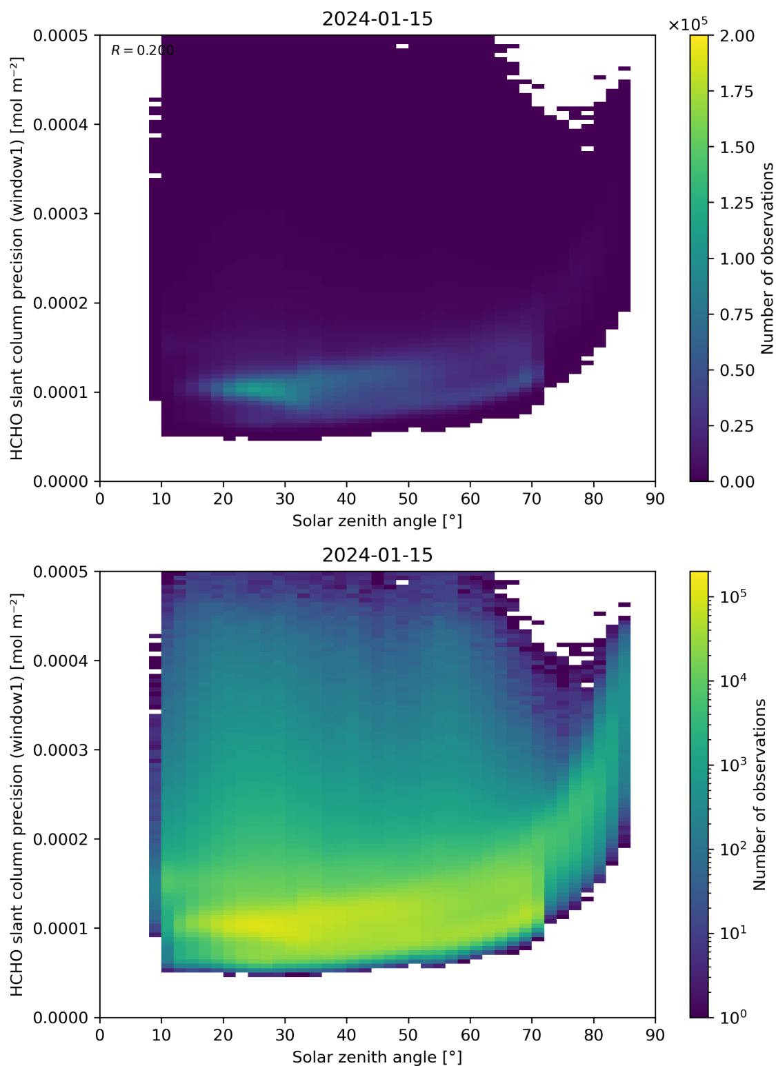
Figure 174: Scatter density plot of “Solar zenith angle” against “HCHO slant column precision (window1)” for 2024-01-15 to 2024-01-16.
