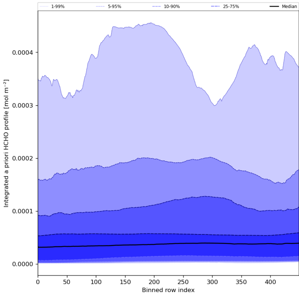
Figure 57: Along track statistics of “Integrated a priori HCHO profile” for 2024-01-15 to 2024-01-16
