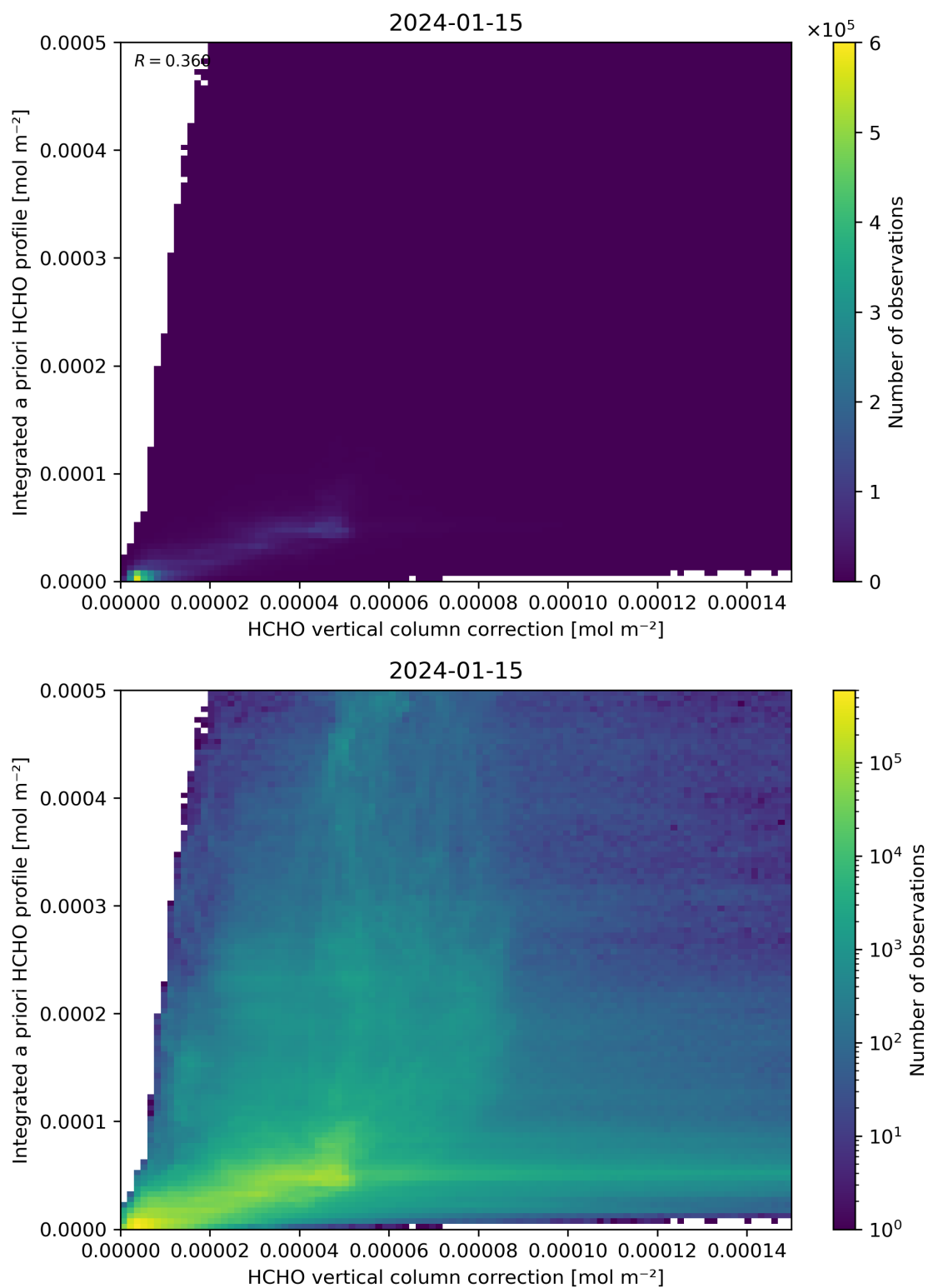
Figure 122: Scatter density plot of “HCHO vertical column correction” against “Integrated a priori HCHO profile” for 2024-01-15 to 2024-01-16.
