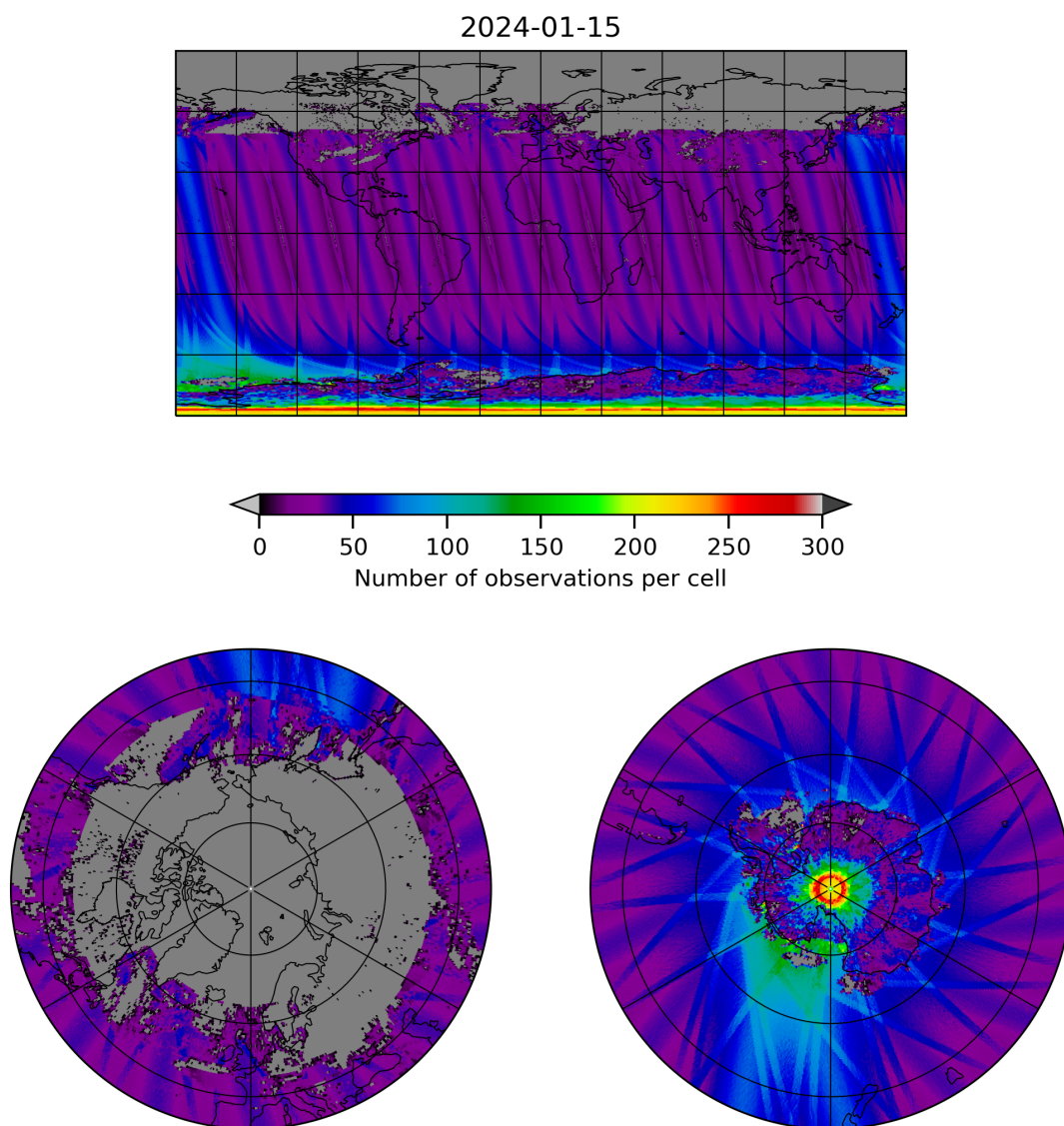
Figure 19: Map of the number of observations for 2024-01-15 to 2024-01-16
