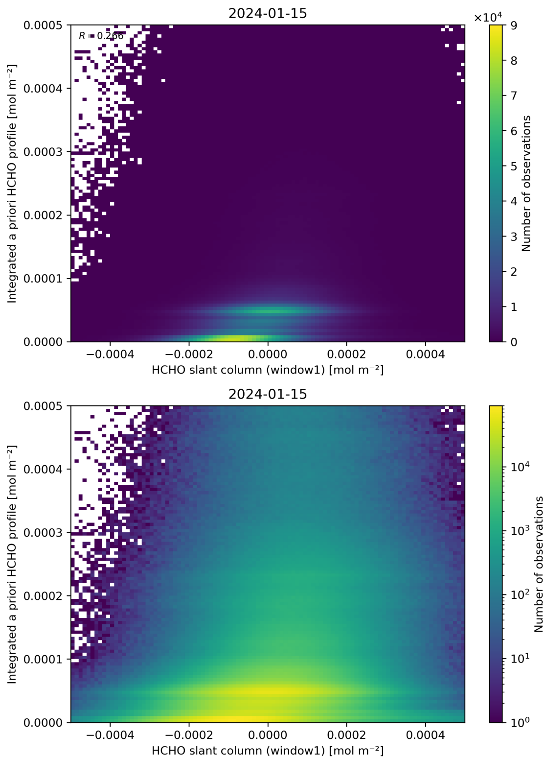
Figure 87: Scatter density plot of “HCHO slant column (window1)” against “Integrated a priori HCHO profile” for 2024-01-15 to 2024-01-16.
