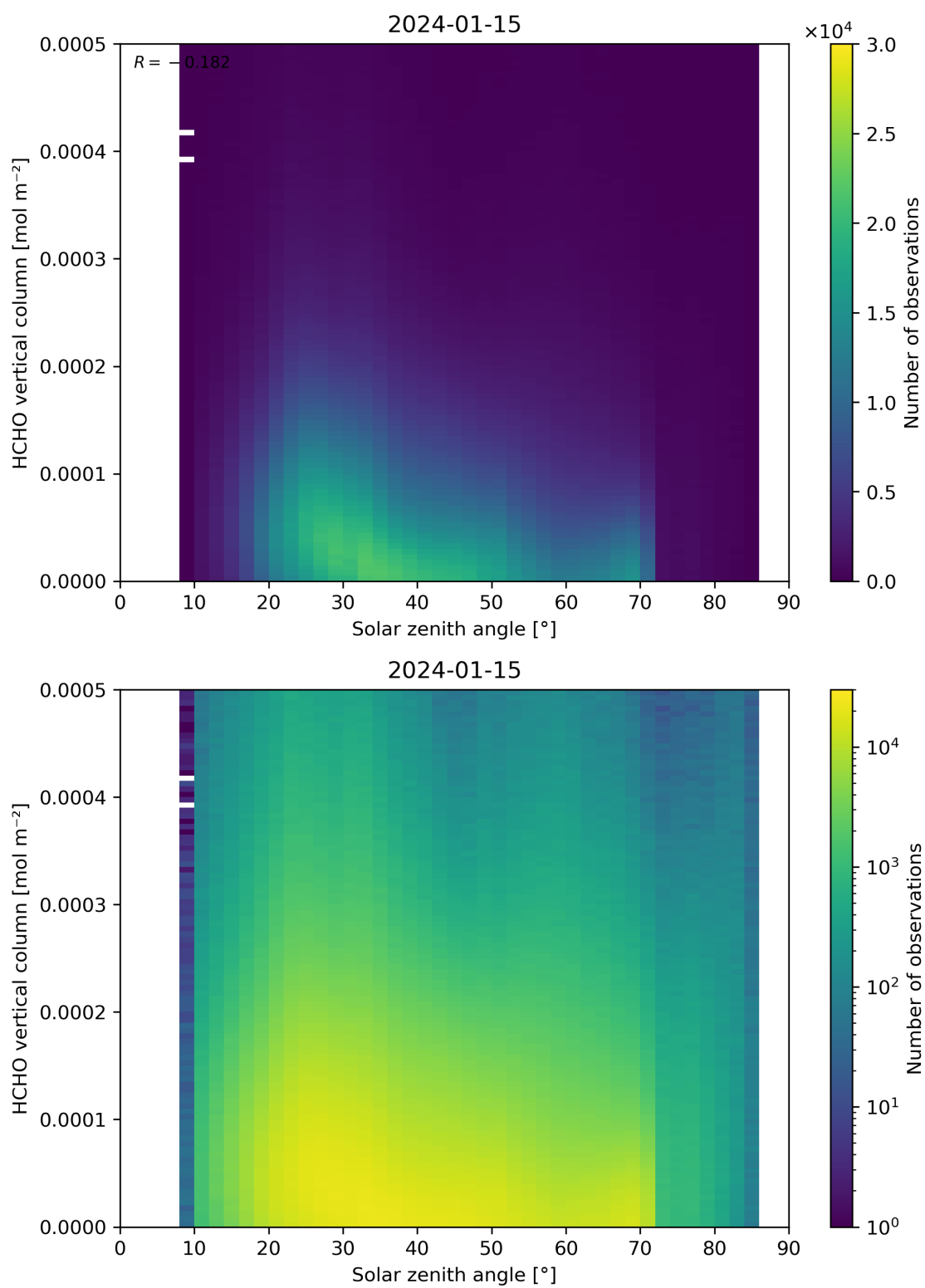
Figure 177: Scatter density plot of “Solar zenith angle” against “HCHO vertical column” for 2024-01-15 to 2024-01-16.
