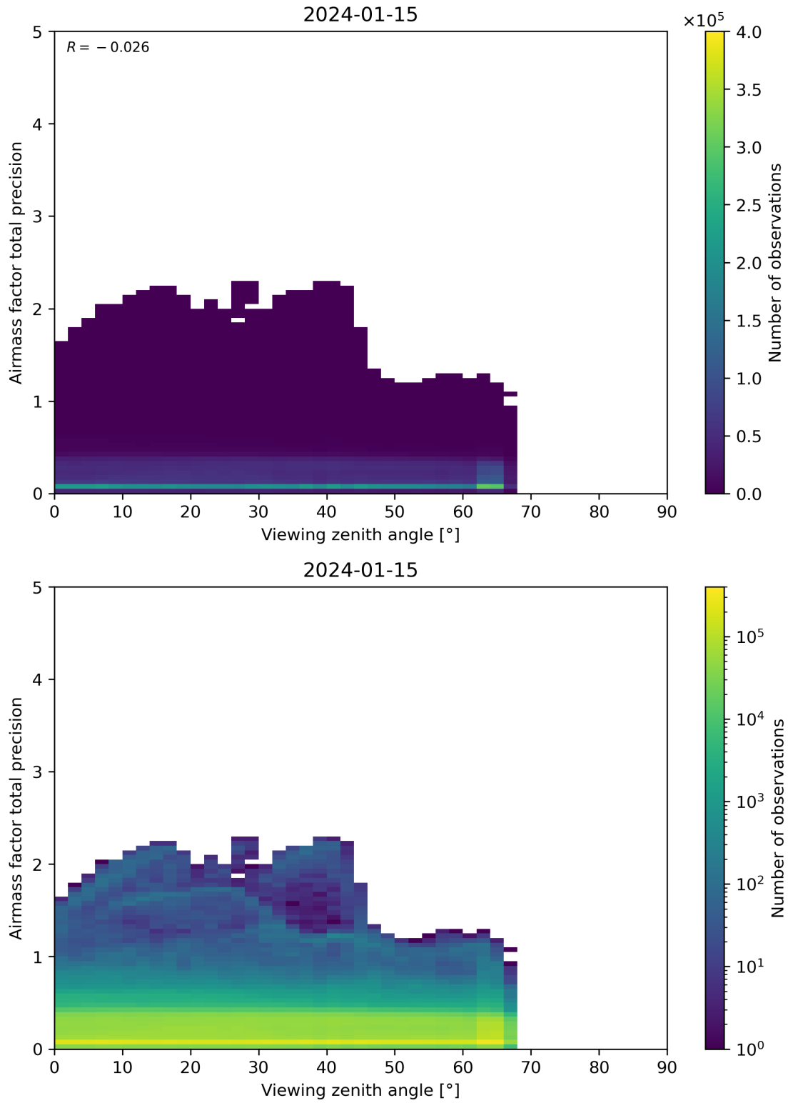
Figure 191: Scatter density plot of “Viewing zenith angle” against “Airmass factor total precision” for 2024-01-15 to 2024-01-16.
