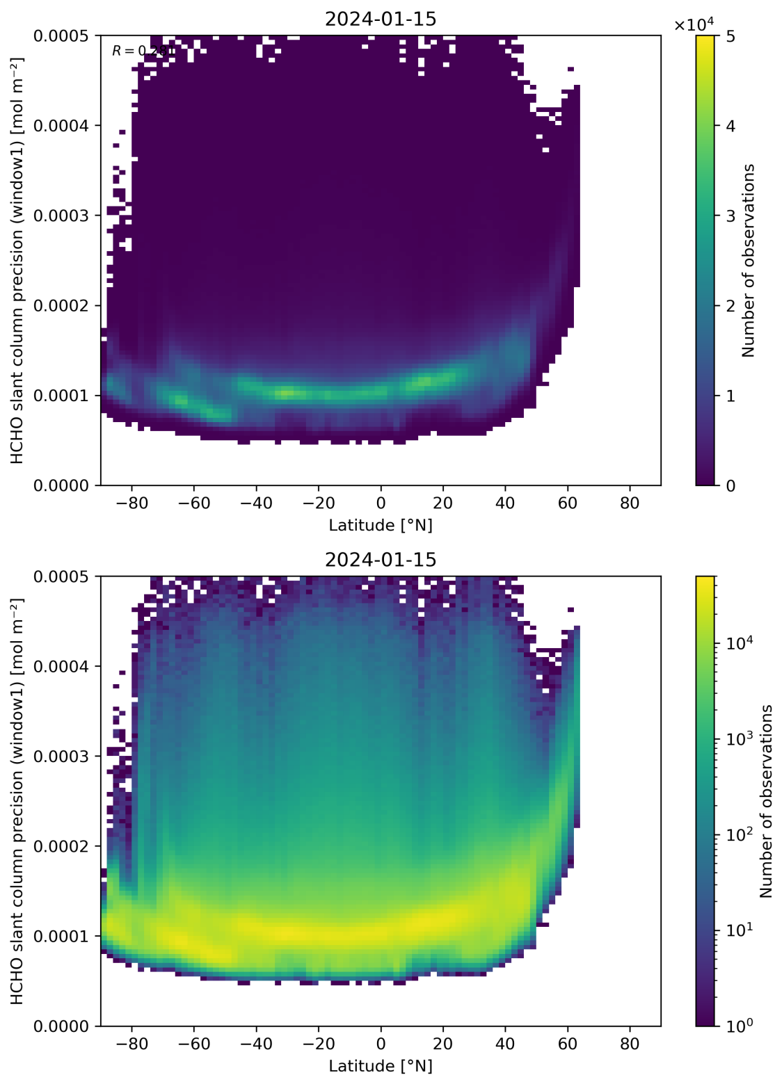
Figure 160: Scatter density plot of “Latitude” against “HCHO slant column precision (window1)” for 2024-01-15 to 2024-01-16.
