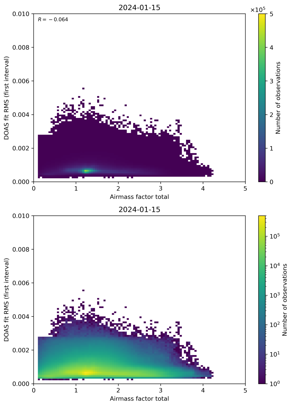
Figure 97: Scatter density plot of “Airmass factor total” against “DOAS fit RMS (first interval)” for 2024-01-15 to 2024-01-16.
