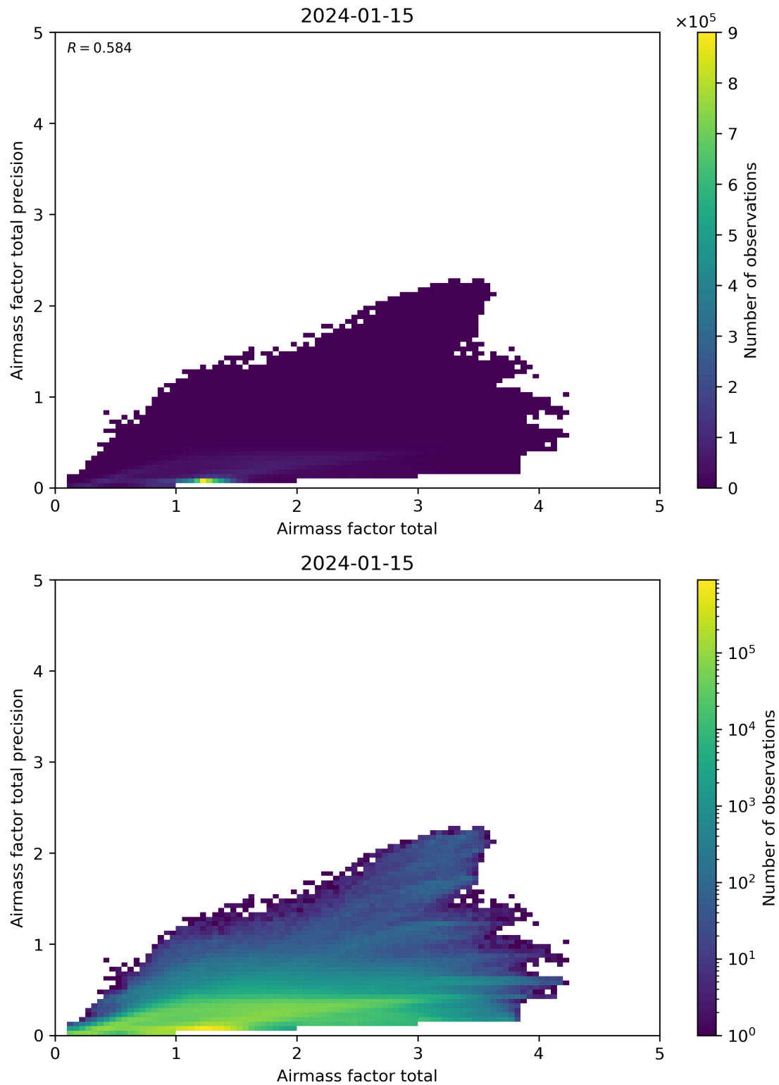
Figure 103: Scatter density plot of “Airmass factor total” against “Airmass factor total precision” for 2024-01-15 to 2024-01-16.
