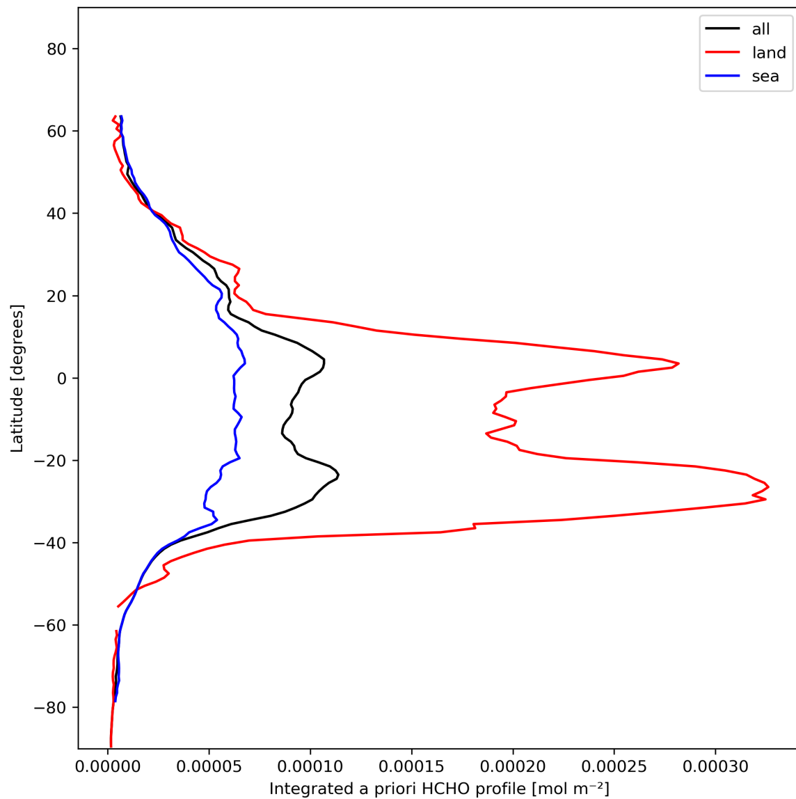
Figure 29: Zonal average of “Integrated a priori HCHO profile” for 2024-01-15 to 2024-01-16.
