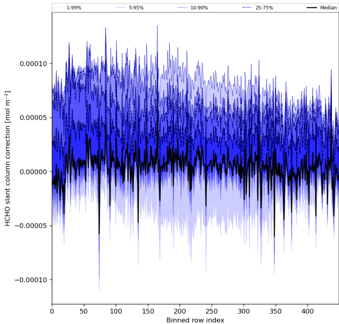
Figure 61: Along track statistics of “HCHO slant column correction” for 2024-01-15 to 2024-01-16
