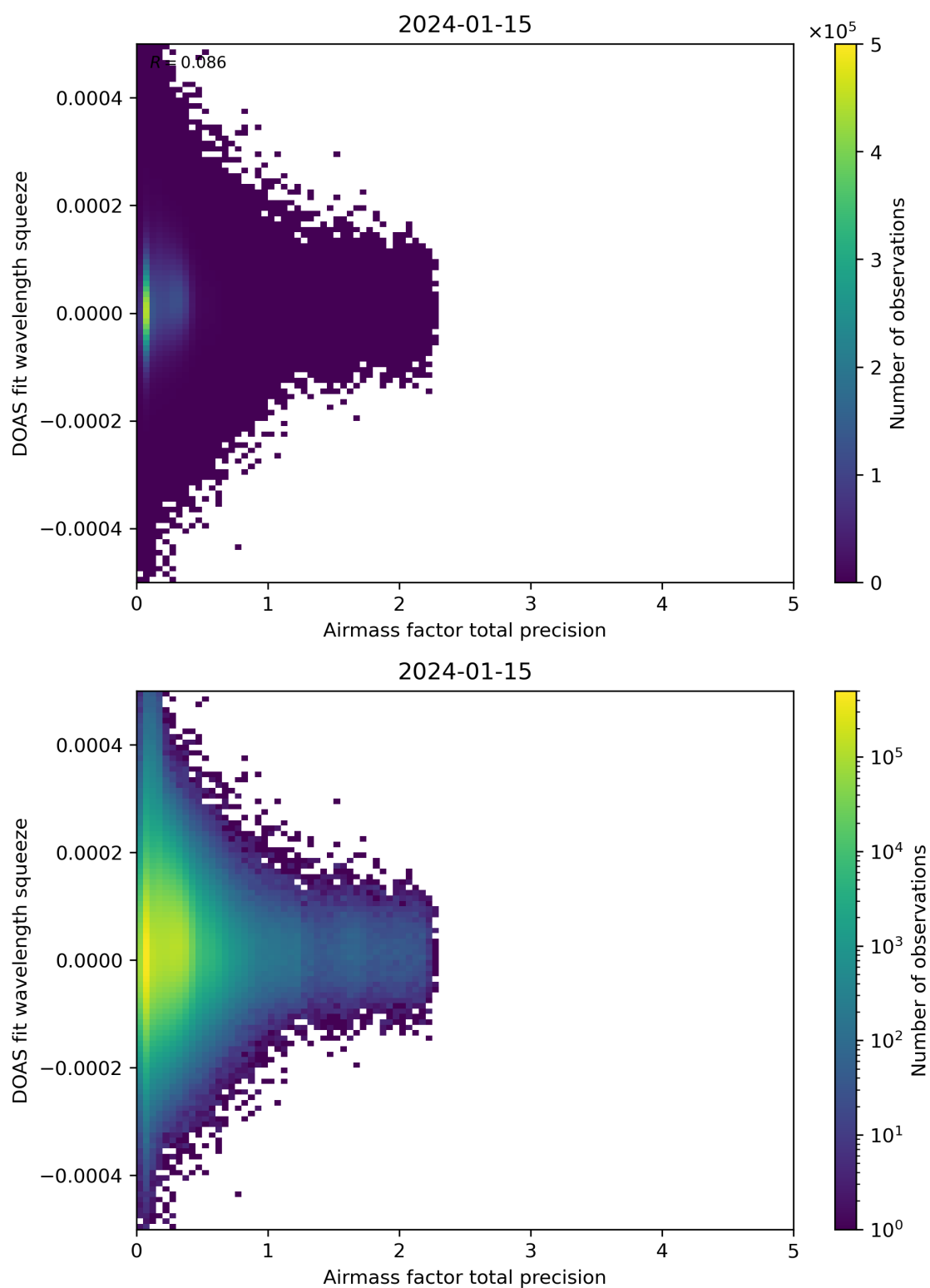
Figure 107: Scatter density plot of “Airmass factor total precision” against “DOAS fit wavelength squeeze” for 2024-01-15 to 2024-01-16.
