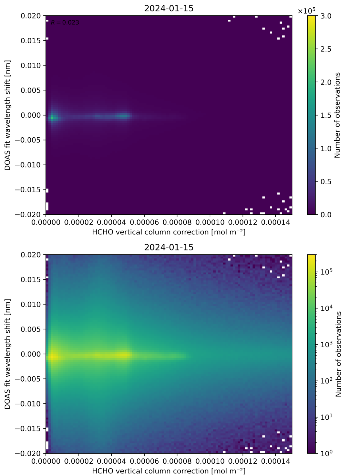
Figure 113: Scatter density plot of “HCHO vertical column correction” against “DOAS fit wavelength shift” for 2024-01-15 to 2024-01-16.
