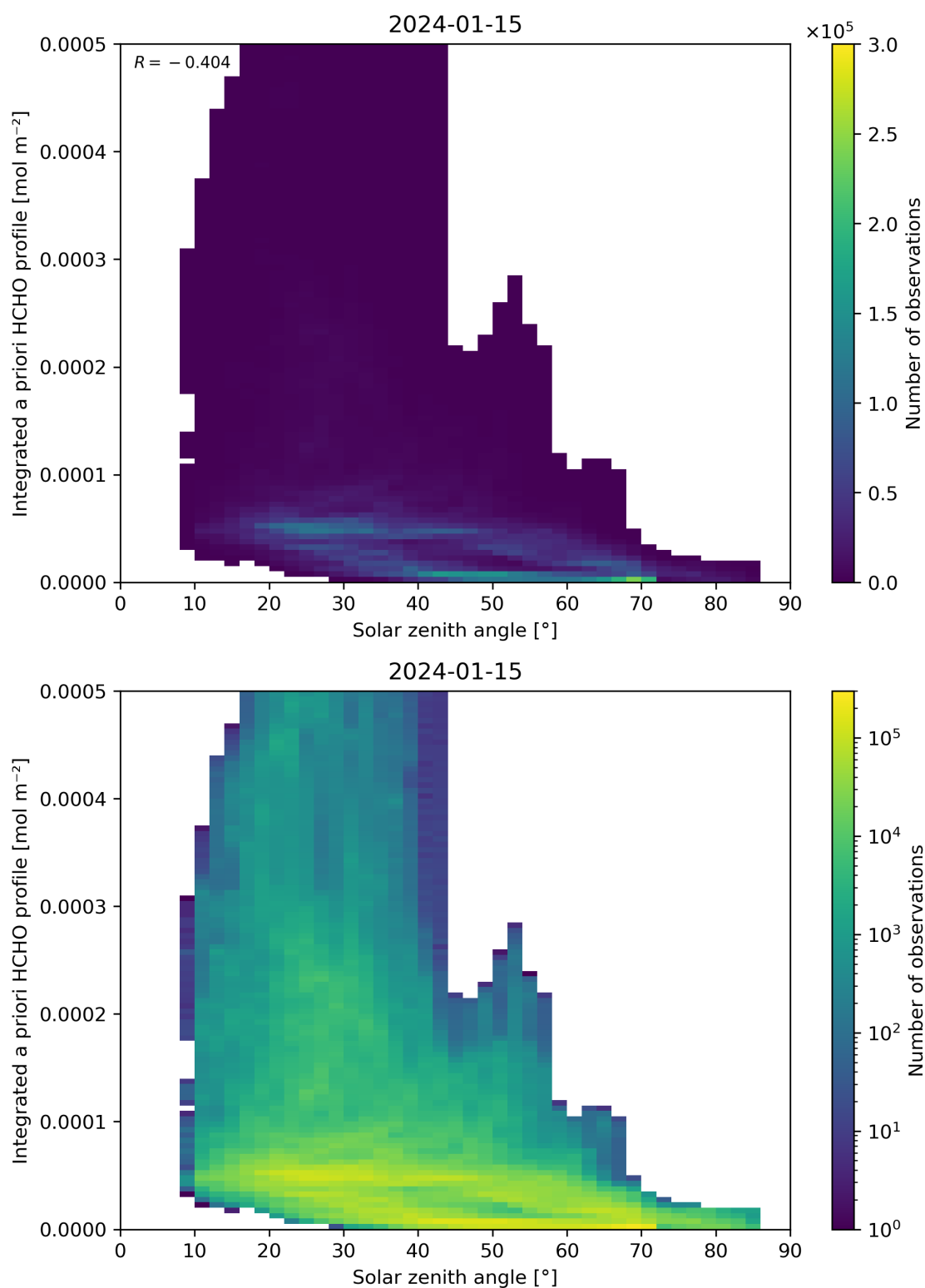
Figure 180: Scatter density plot of “Solar zenith angle” against “Integrated a priori HCHO profile” for 2024-01-15 to 2024-01-16.
