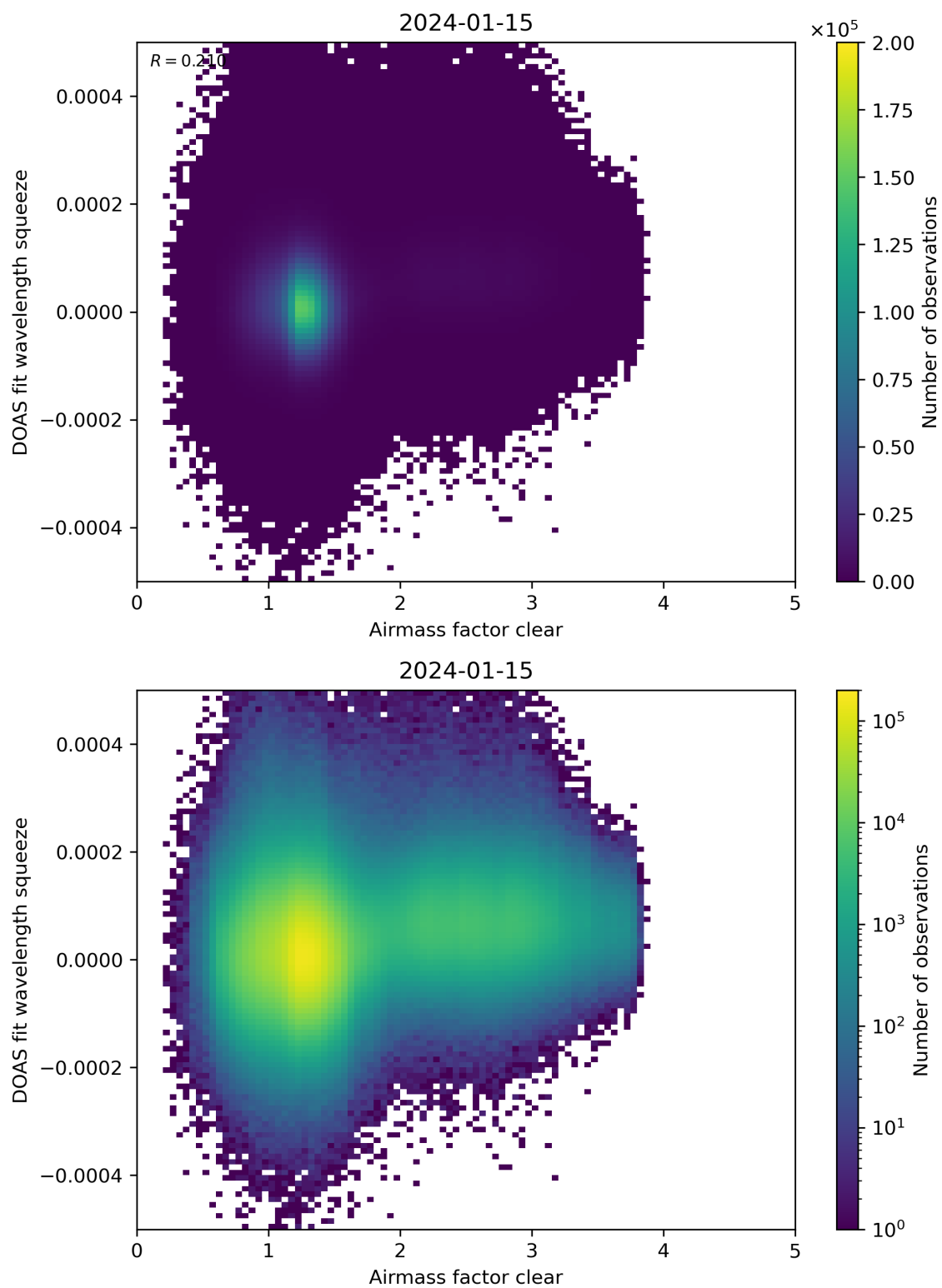
Figure 73: Scatter density plot of “Airmass factor clear” against “DOAS fit wavelength squeeze” for 2024-01-15 to 2024-01-16.
