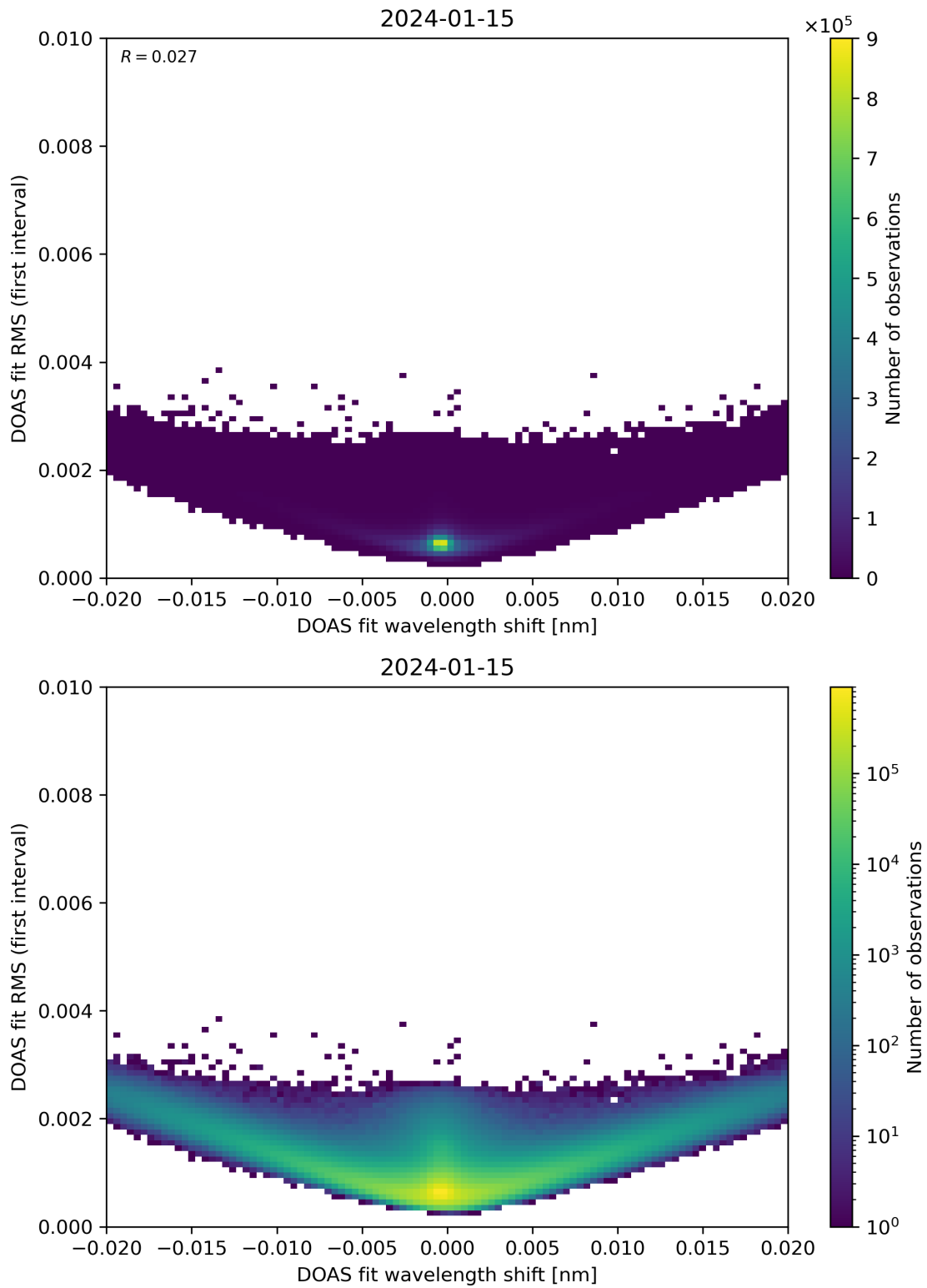
Figure 64: Scatter density plot of “DOAS fit wavelength shift” against “DOAS fit RMS (first interval)” for 2024-01-15 to 2024-01-16.
