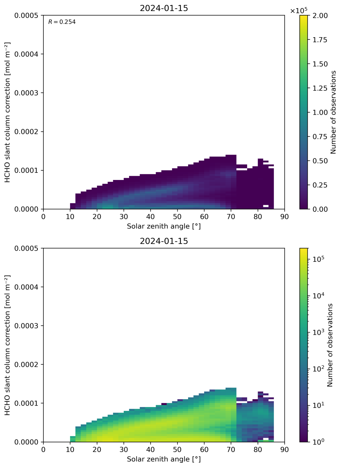
Figure 172: Scatter density plot of “Solar zenith angle” against “HCHO slant column correction” for 2024-01-15 to 2024-01-16.
