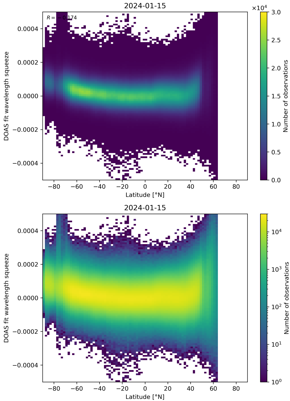
Figure 155: Scatter density plot of “Latitude” against “DOAS fit wavelength squeeze” for 2024-01-15 to 2024-01-16.
