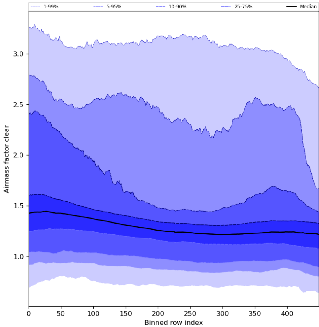
Figure 56: Along track statistics of “Airmass factor clear” for 2024-01-15 to 2024-01-16
