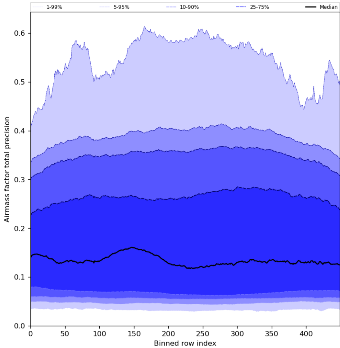
Figure 55: Along track statistics of “Airmass factor total precision” for 2024-01-15 to 2024-01-16
