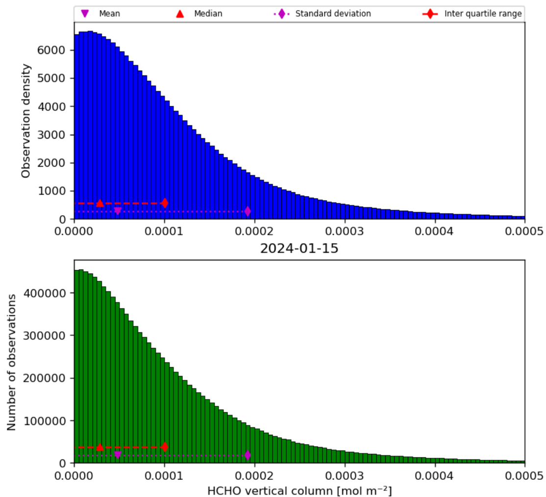
Figure 35: Histogram of “HCHO vertical column” for 2024-01-15 to 2024-01-16
