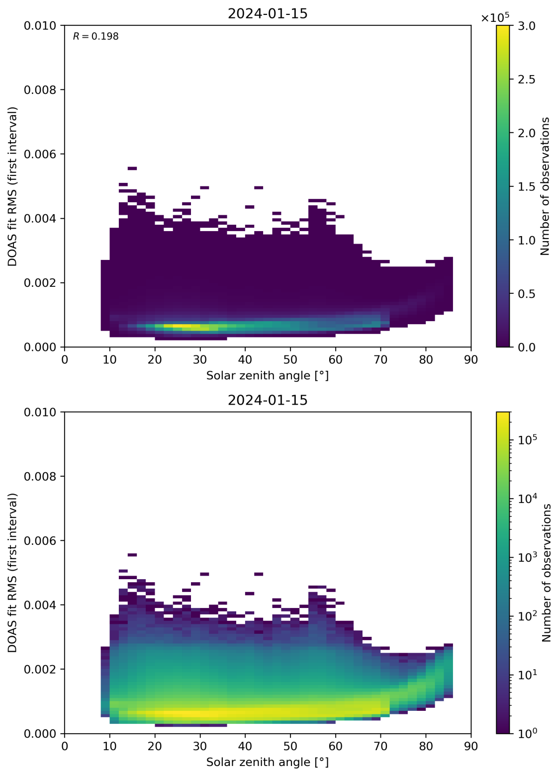
Figure 167: Scatter density plot of “Solar zenith angle” against “DOAS fit RMS (first interval)” for 2024-01-15 to 2024-01-16.
