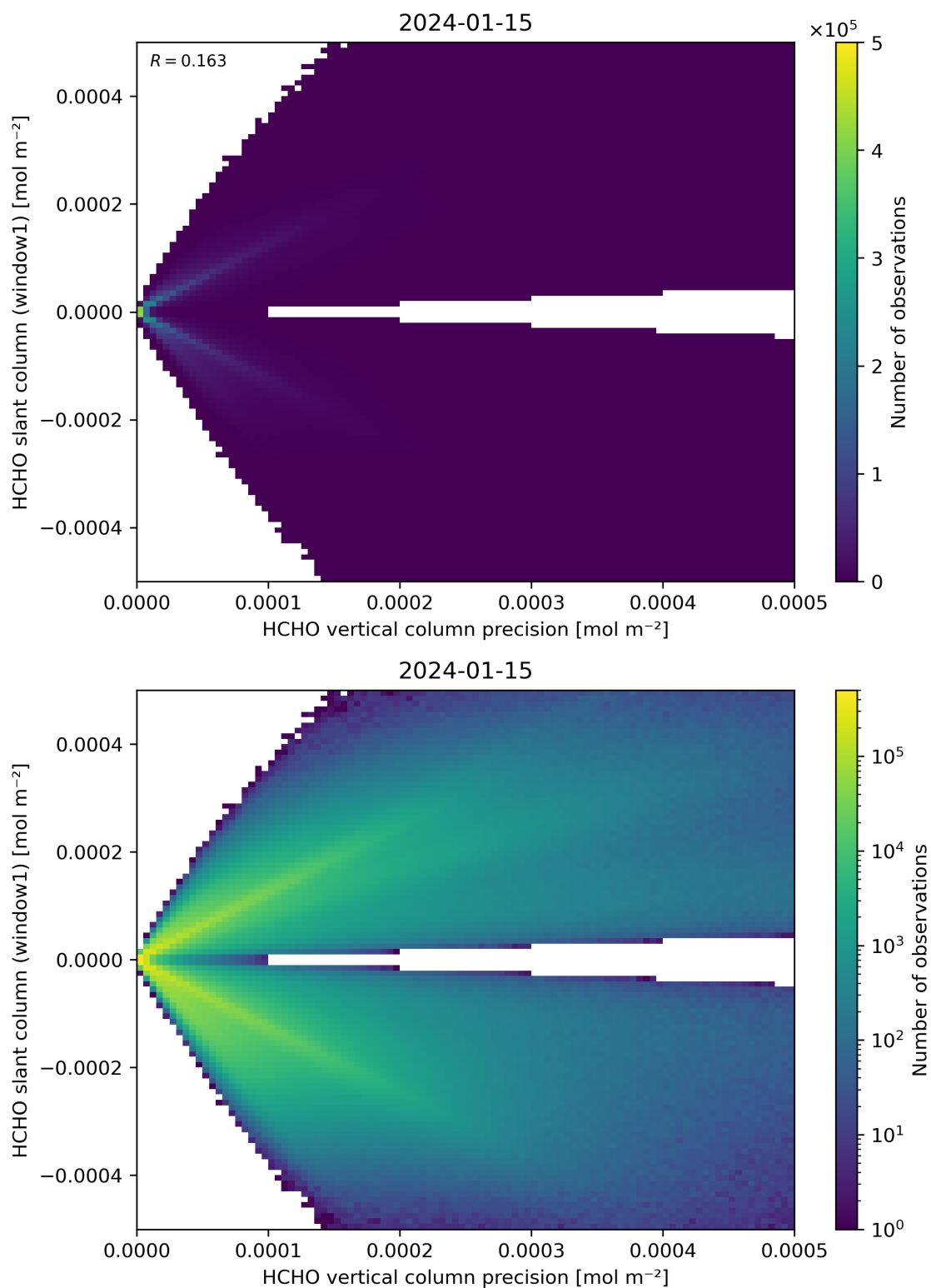
Figure 142: Scatter density plot of “HCHO vertical column precision” against “HCHO slant column (window1)” for 2024-01-15 to 2024-01-16.
