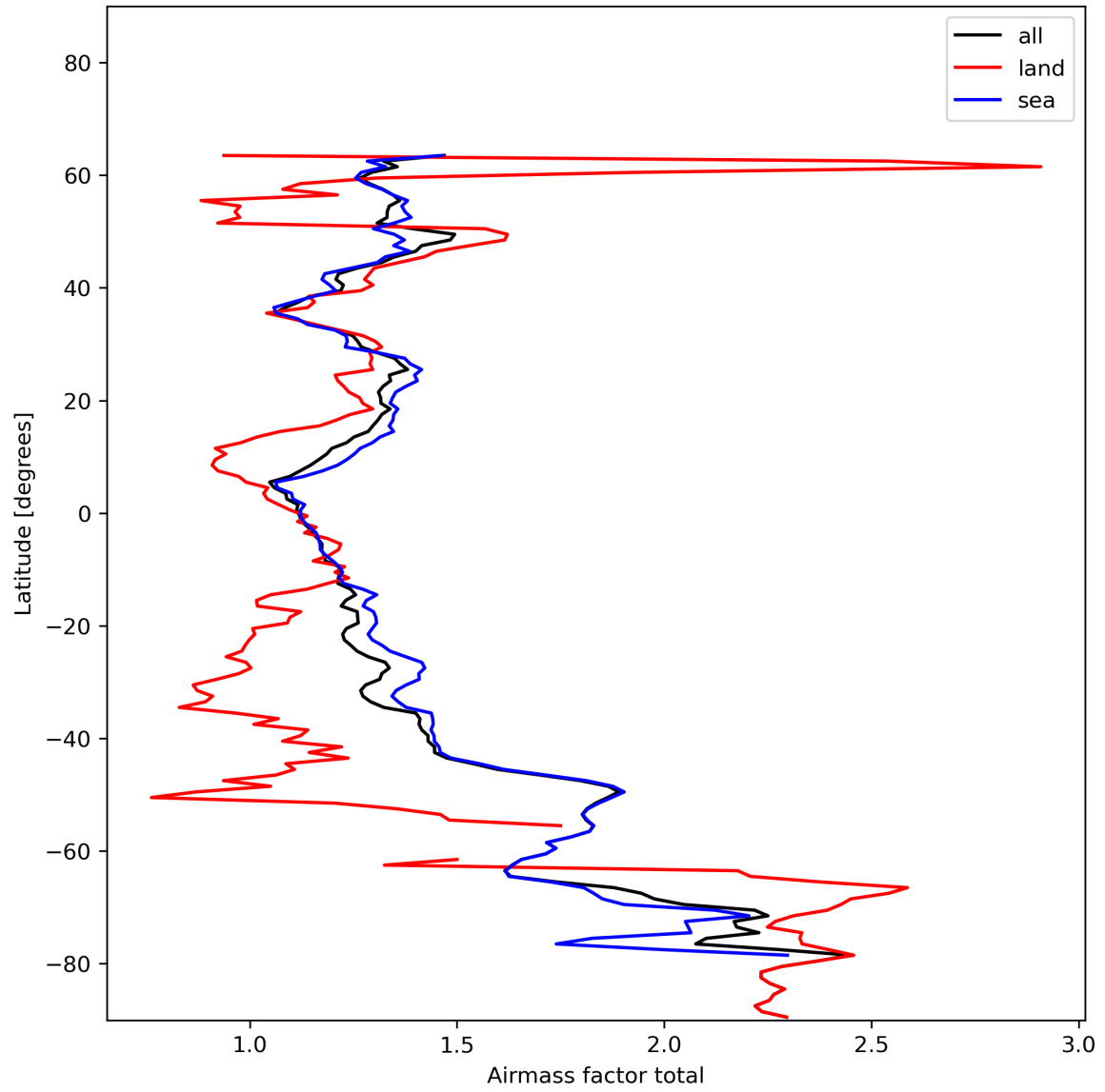
Figure 26: Zonal average of “Airmass factor total” for 2024-01-15 to 2024-01-16.
