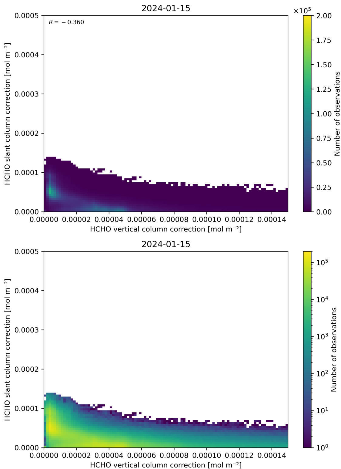
Figure 117: Scatter density plot of “HCHO vertical column correction” against “HCHO slant column correction” for 2024-01-15 to 2024-01-16.
