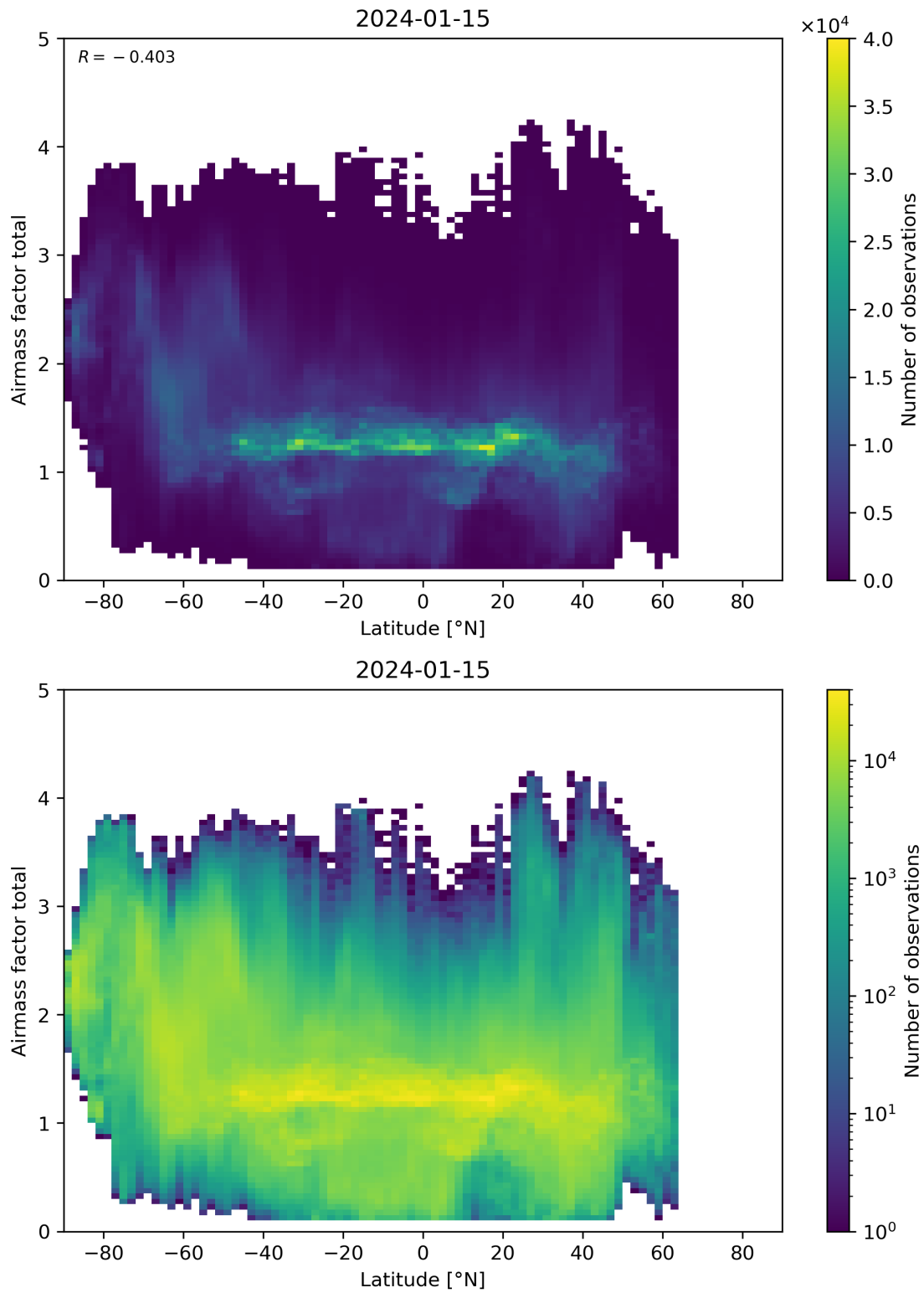
Figure 161: Scatter density plot of “Latitude” against “Airmass factor total” for 2024-01-15 to 2024-01-16.
