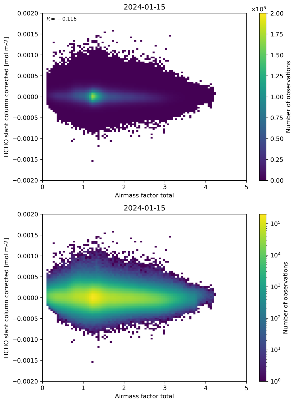
Figure 101: Scatter density plot of “Airmass factor total” against “HCHO slant column corrected” for 2024-01-15 to 2024-01-16.
