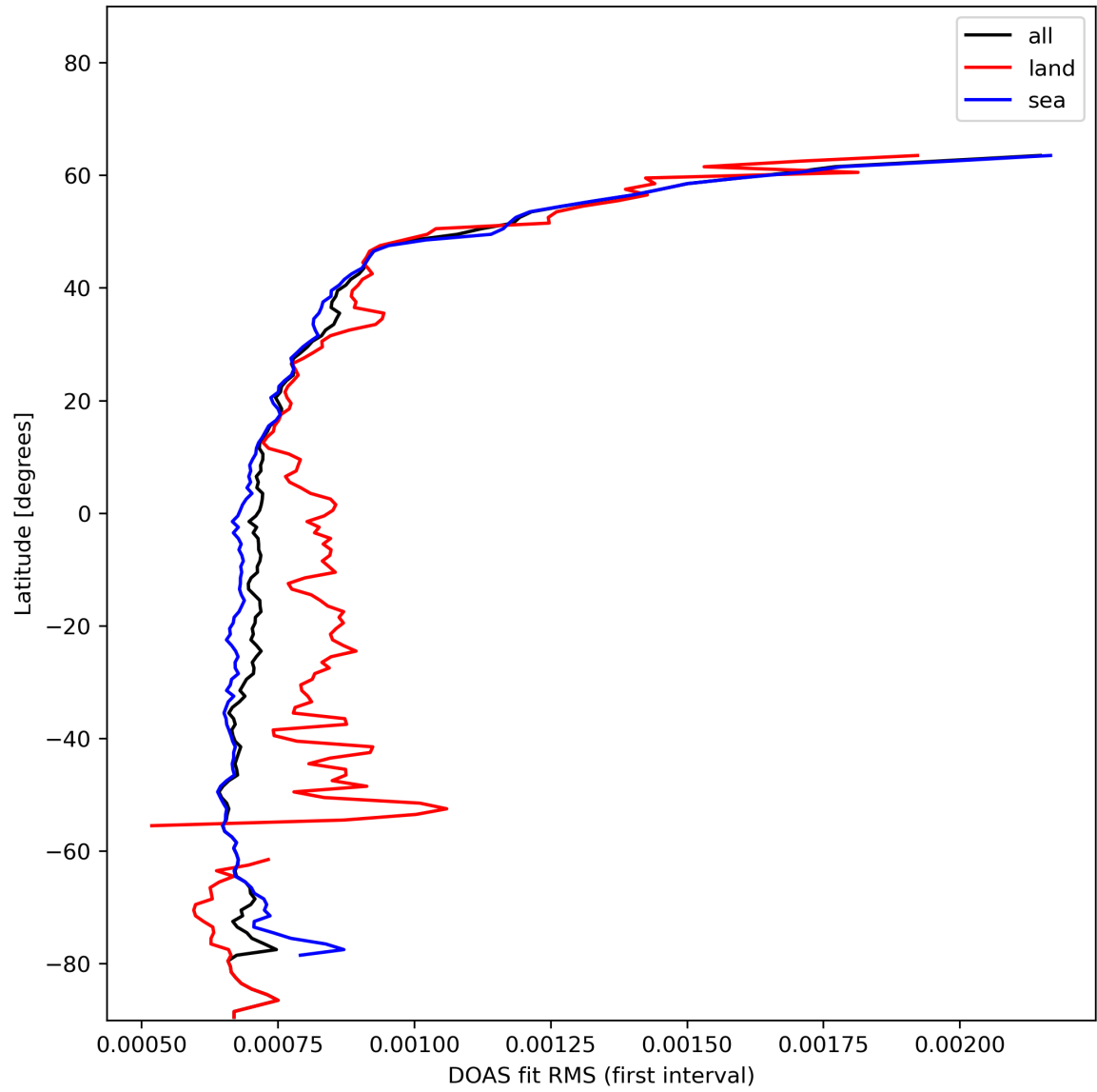
Figure 32: Zonal average of “DOAS fit RMS (first interval)” for 2024-01-15 to 2024-01-16.
