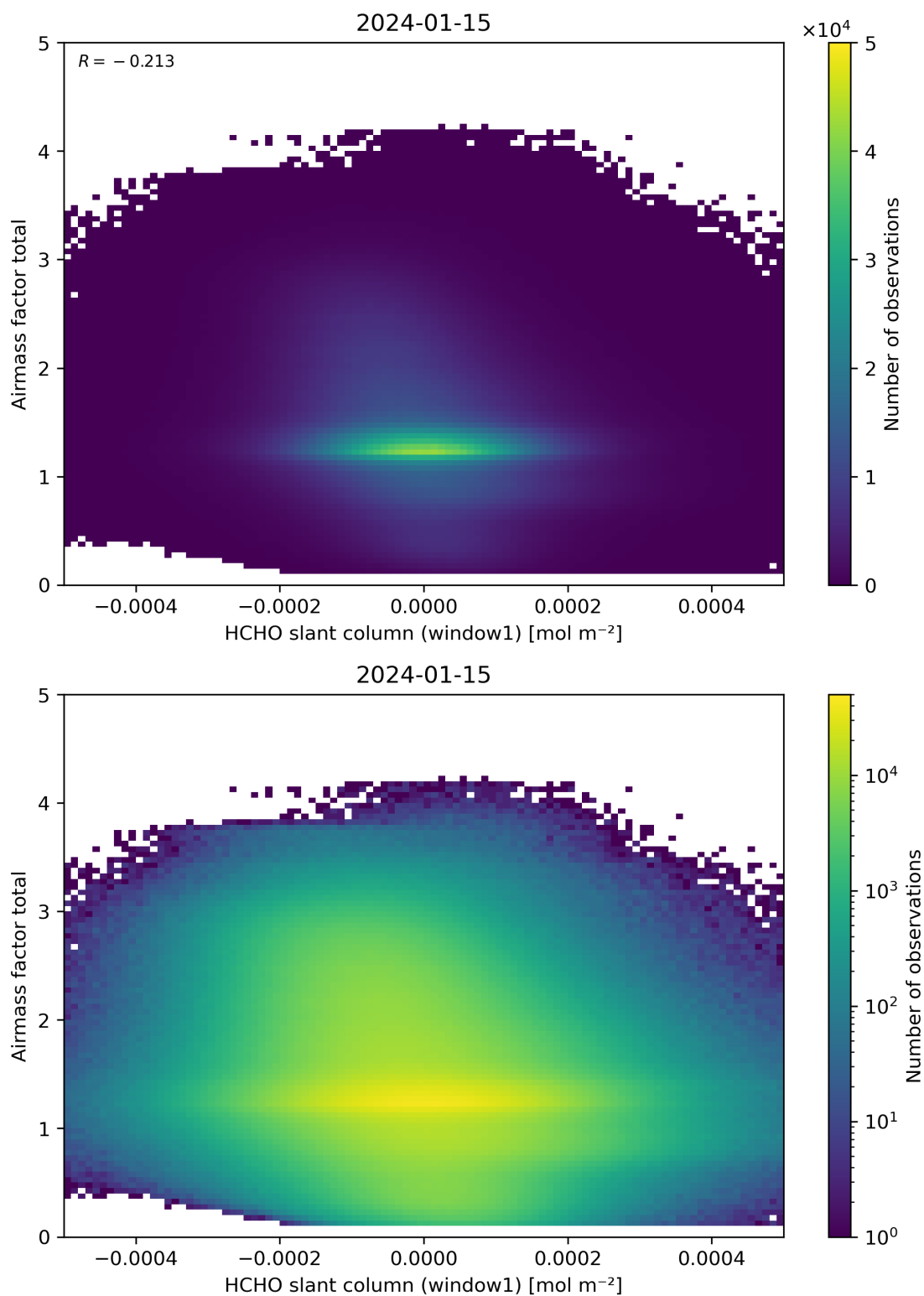
Figure 85: Scatter density plot of “HCHO slant column (window1)” against “Airmass factor total” for 2024-01-15 to 2024-01-16.
