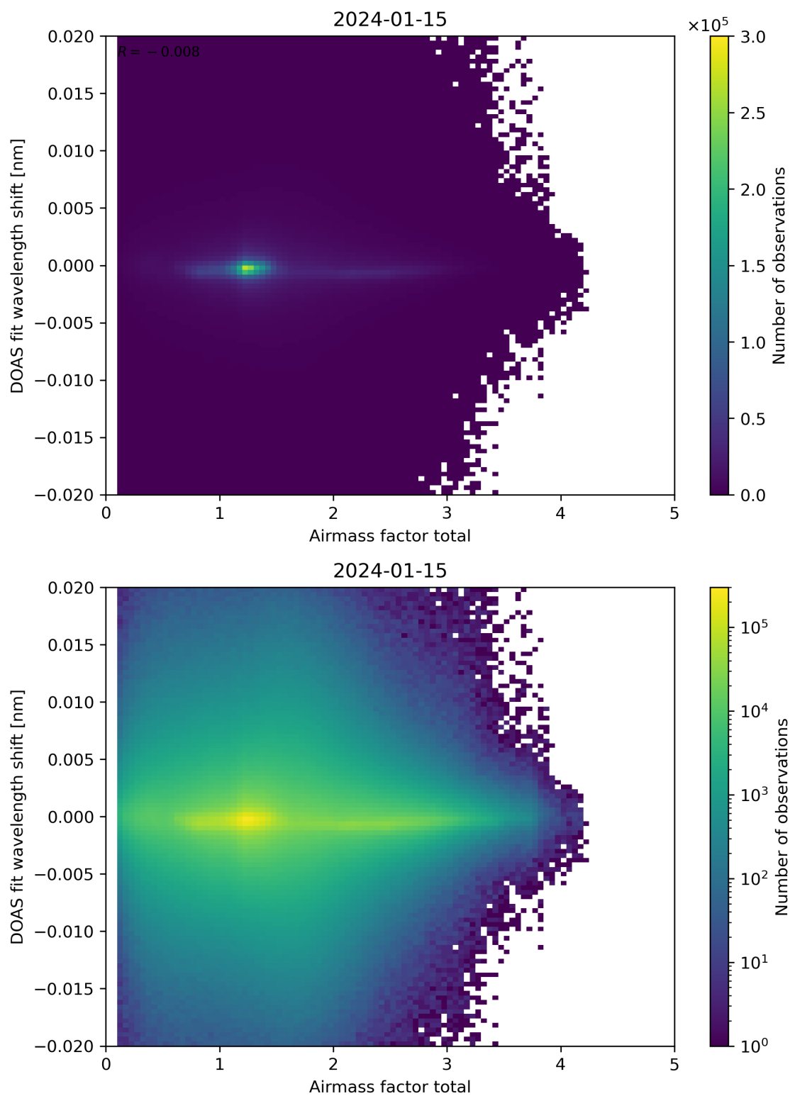
Figure 98: Scatter density plot of “Airmass factor total” against “DOAS fit wavelength shift” for 2024-01-15 to 2024-01-16.
