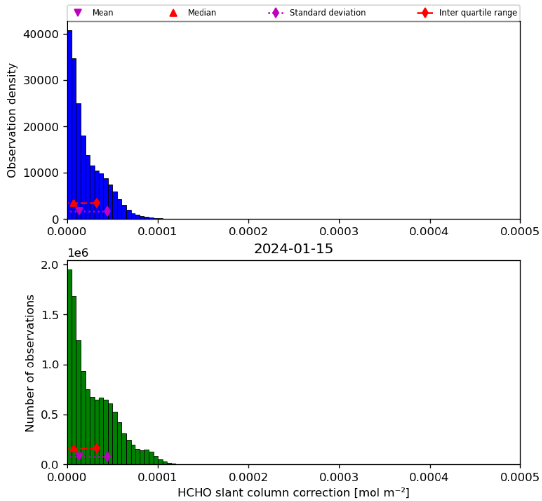
Figure 47: Histogram of “HCHO slant column correction” for 2024-01-15 to 2024-01-16
