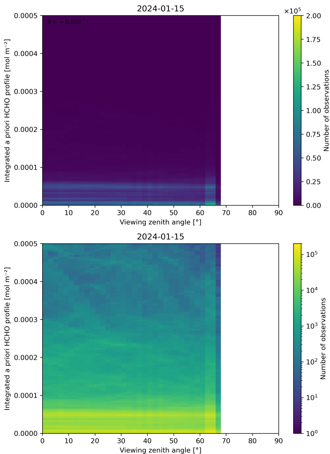
Figure 195: Scatter density plot of “Viewing zenith angle” against “Integrated a priori HCHO profile” for 2024-01-15 to 2024-01-16.
