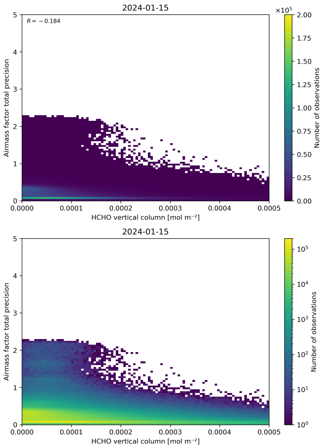
Figure 132: Scatter density plot of “HCHO vertical column” against “Airmass factor total precision” for 2024-01-15 to 2024-01-16.
