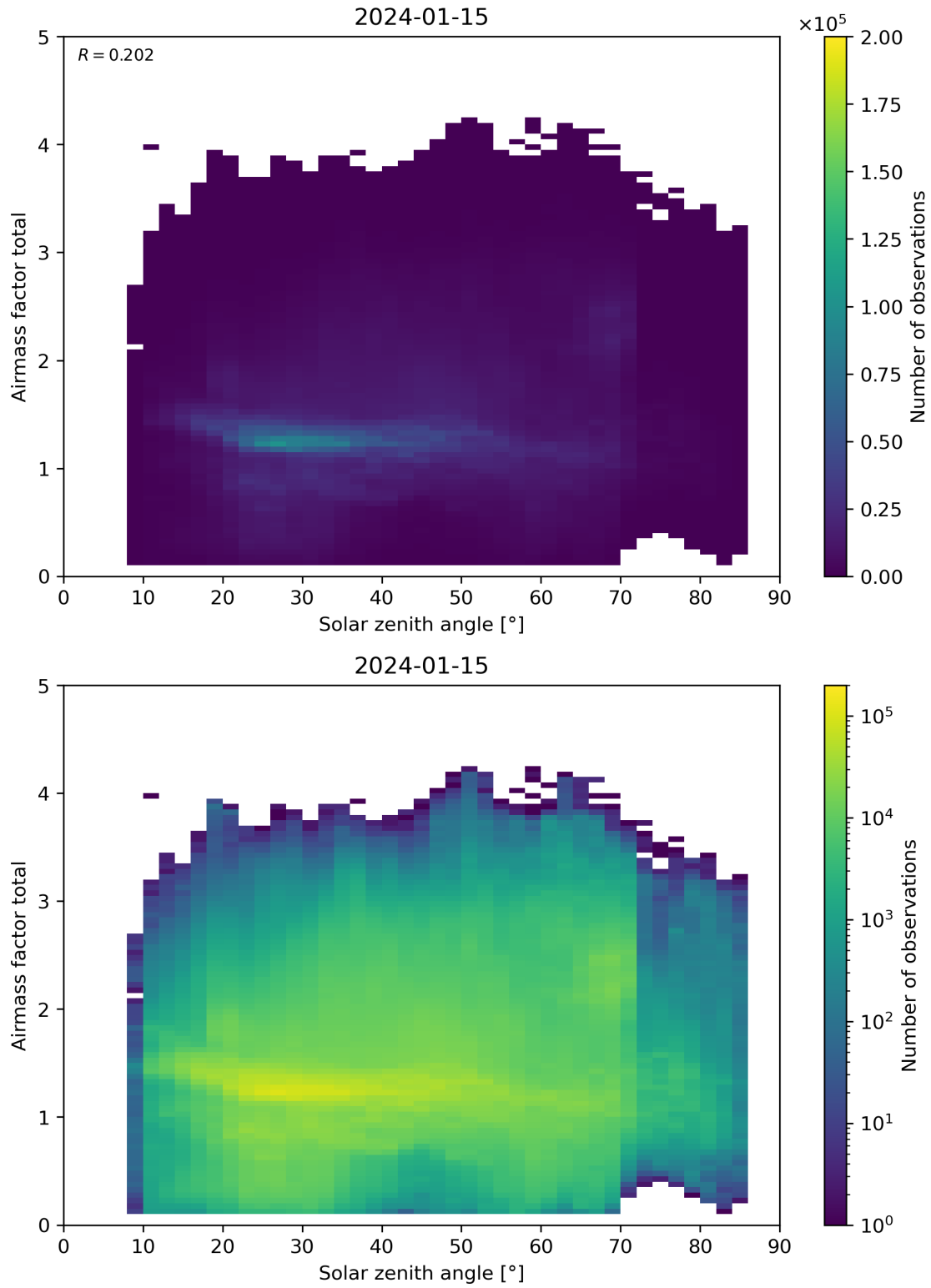
Figure 175: Scatter density plot of “Solar zenith angle” against “Airmass factor total” for 2024-01-15 to 2024-01-16.
