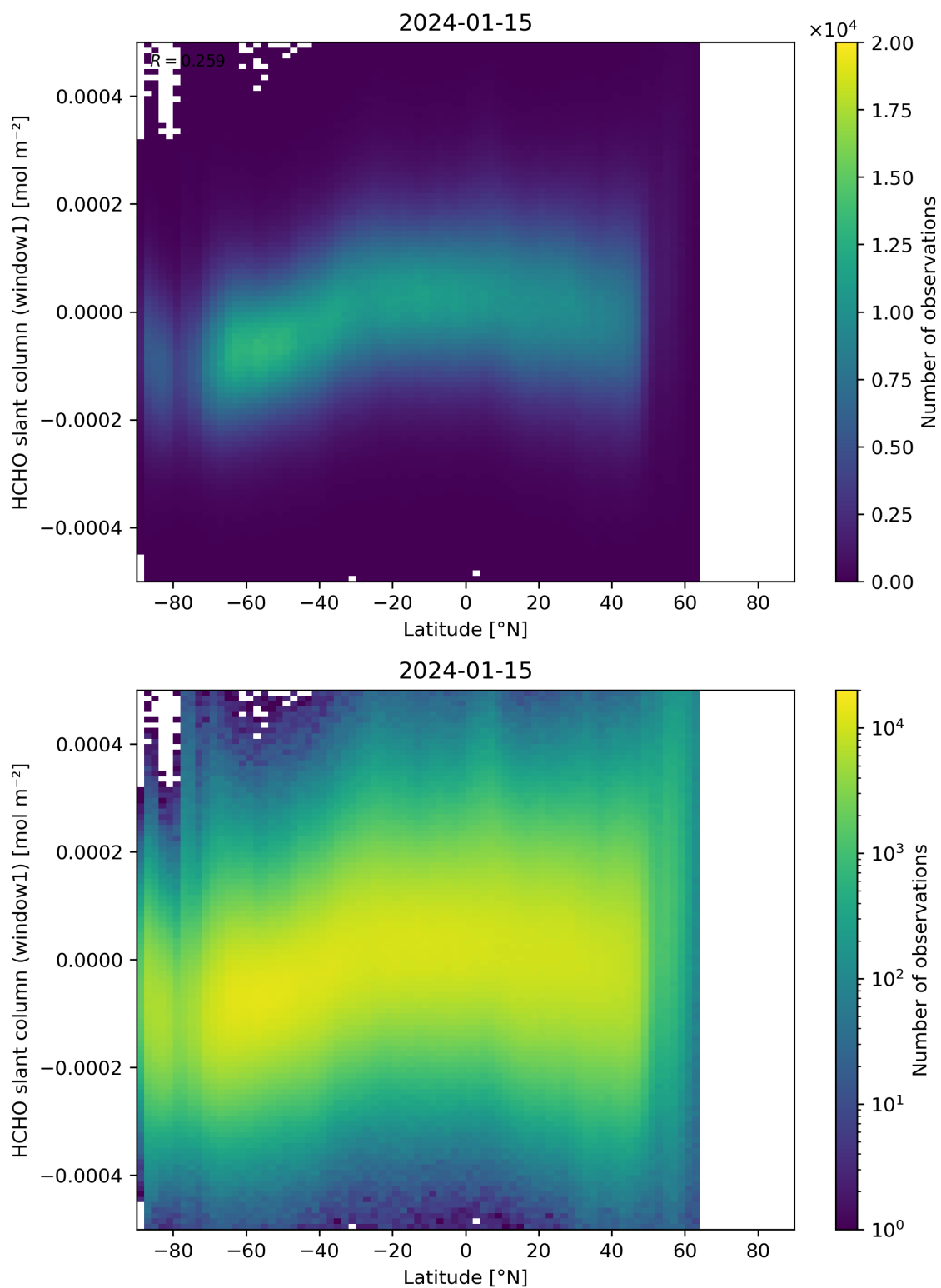
Figure 159: Scatter density plot of “Latitude” against “HCHO slant column (window1)” for 2024-01-15 to 2024-01-16.
