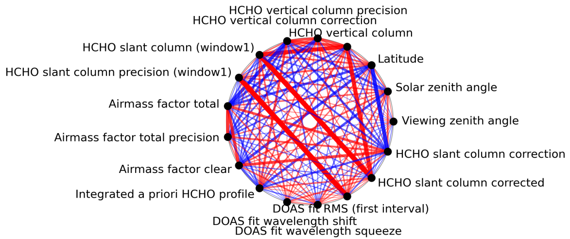
Figure 1: Map of correlation graph for 2024-01-15 to 2024-01-16.
