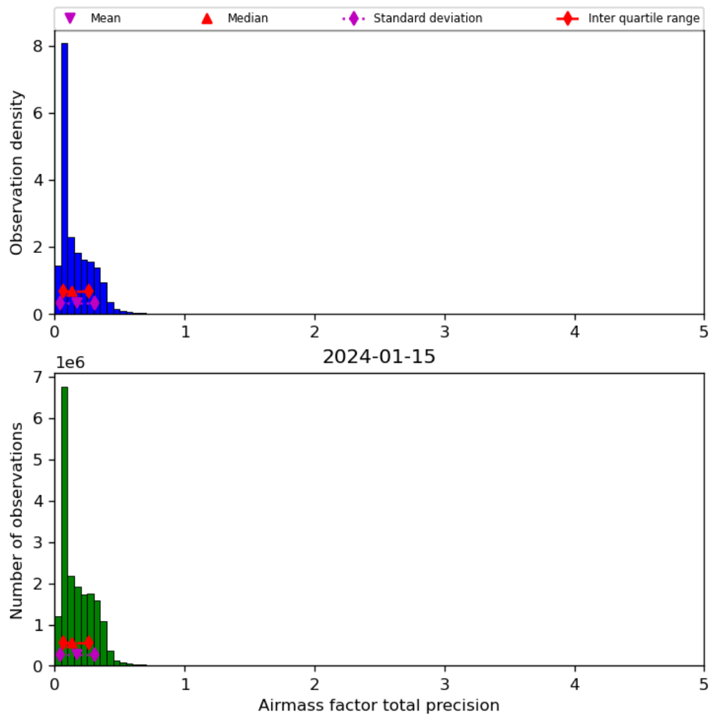
Figure 41: Histogram of “Airmass factor total precision” for 2024-01-15 to 2024-01-16
