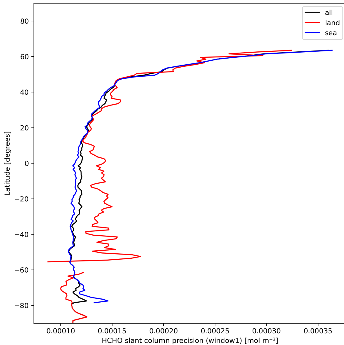
Figure 25: Zonal average of “HCHO slant column precision (window1)” for 2024-01-15 to 2024-01-16.
