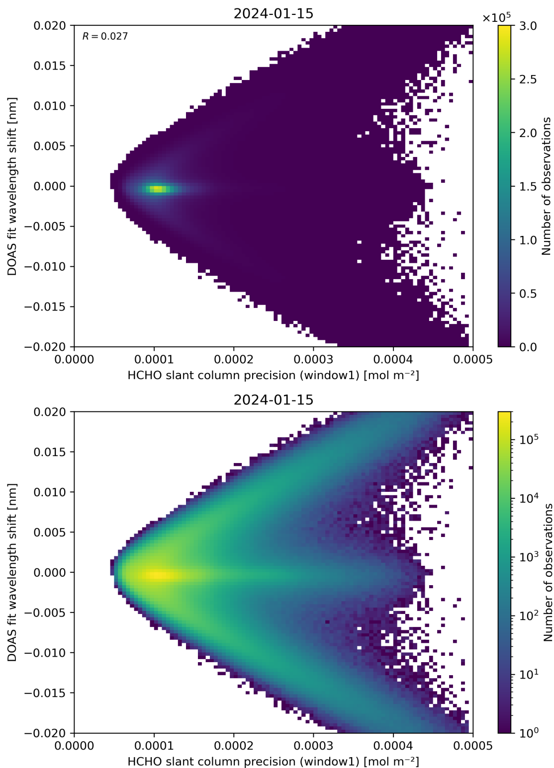
Figure 89: Scatter density plot of “HCHO slant column precision (window1)” against “DOAS fit wavelength shift” for 2024-01-15 to 2024-01-16.
