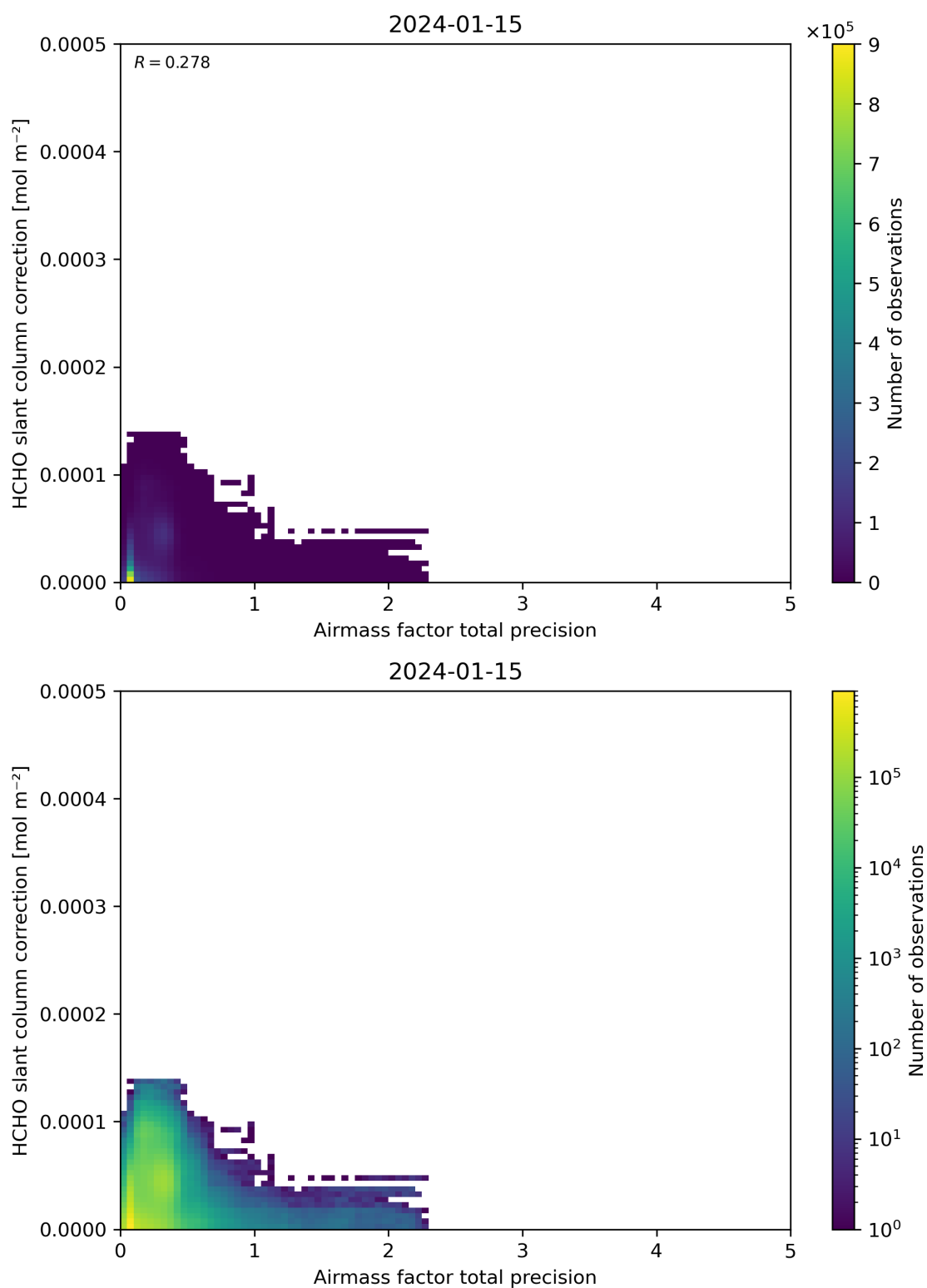
Figure 110: Scatter density plot of “Airmass factor total precision” against “HCHO slant column correction” for 2024-01-15 to 2024-01-16.
