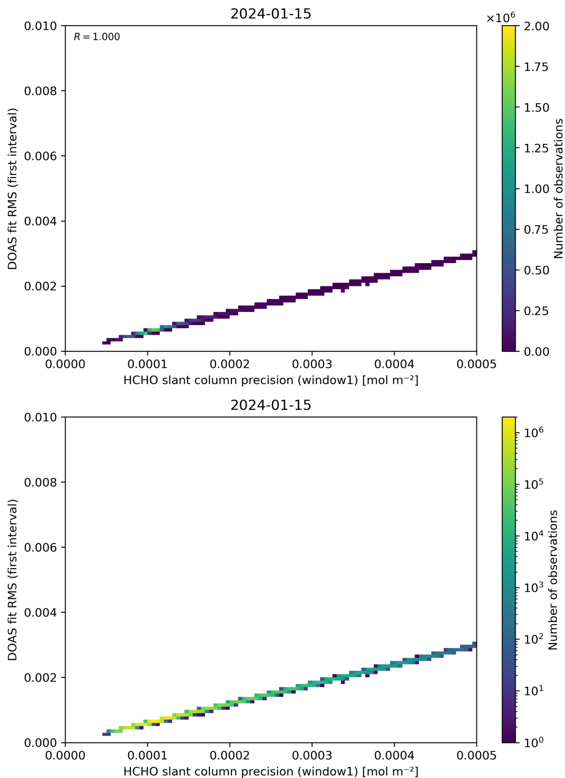
Figure 88: Scatter density plot of “HCHO slant column precision (window1)” against “DOAS fit RMS (first interval)” for 2024-01-15 to 2024-01-16.
