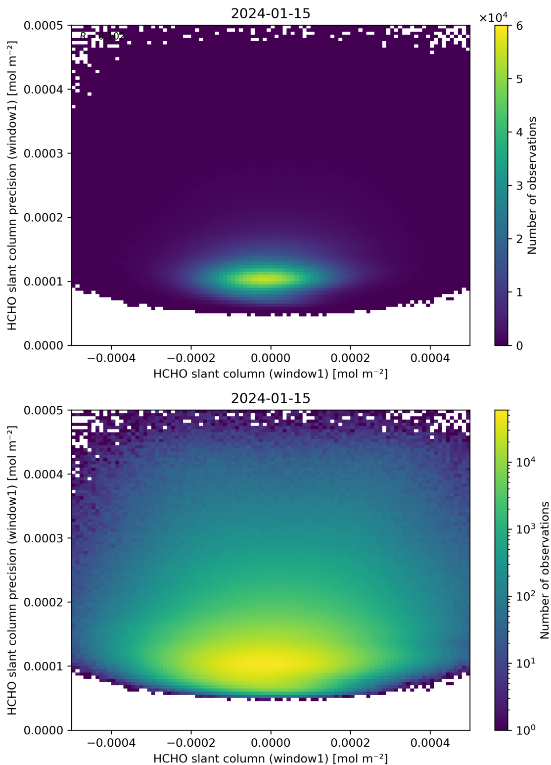
Figure 84: Scatter density plot of “HCHO slant column (window1)” against “HCHO slant column precision (window1)” for 2024-01-15 to 2024-01-16.
