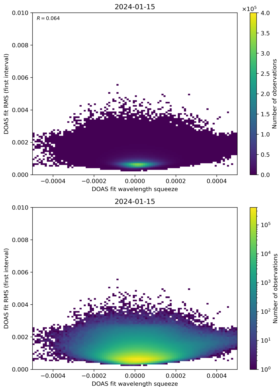
Figure 68: Scatter density plot of “DOAS fit wavelength squeeze” against “DOAS fit RMS (first interval)” for 2024-01-15 to 2024-01-16.
