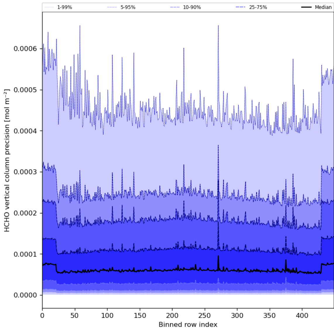
Figure 50: Along track statistics of “HCHO vertical column precision” for 2024-01-15 to 2024-01-16
