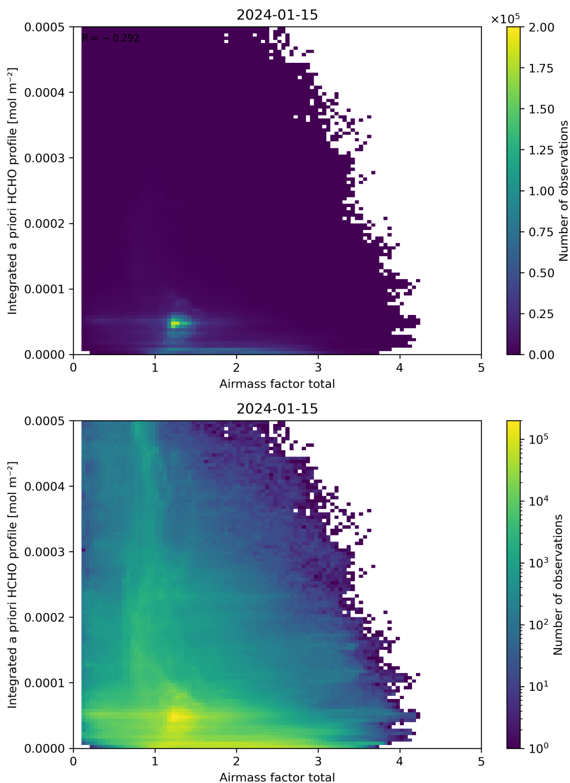
Figure 104: Scatter density plot of “Airmass factor total” against “Integrated a priori HCHO profile” for 2024-01-15 to 2024-01-16.
