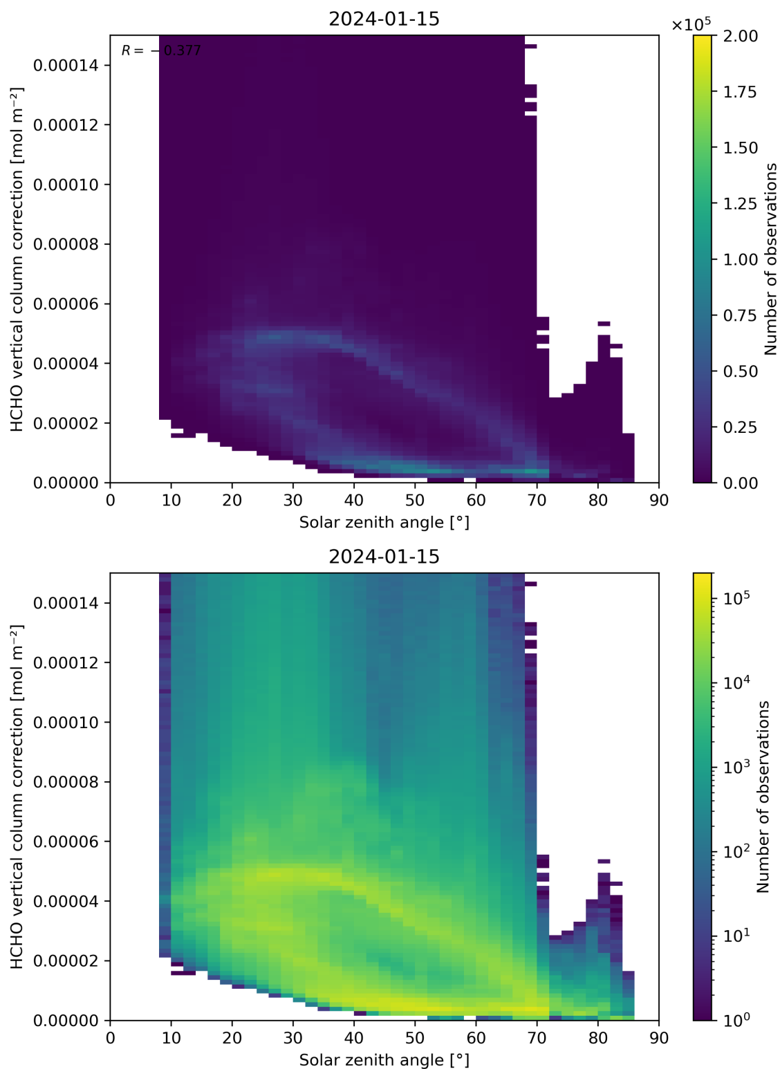
Figure 178: Scatter density plot of “Solar zenith angle” against “HCHO vertical column correction” for 2024-01-15 to 2024-01-16.
