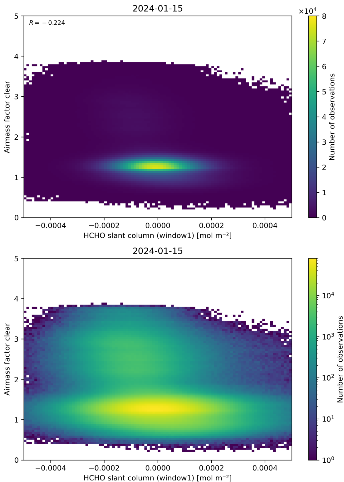
Figure 81: Scatter density plot of “HCHO slant column (window1)” against “Airmass factor clear” for 2024-01-15 to 2024-01-16.
