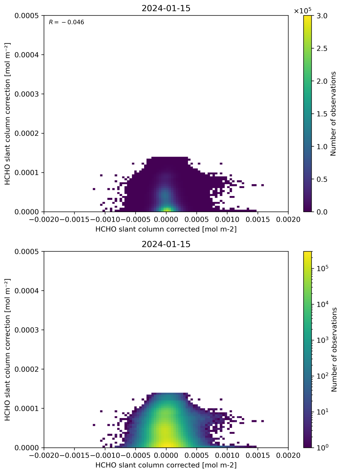
Figure 77: Scatter density plot of “HCHO slant column corrected” against “HCHO slant column correction” for 2024-01-15 to 2024-01-16.
