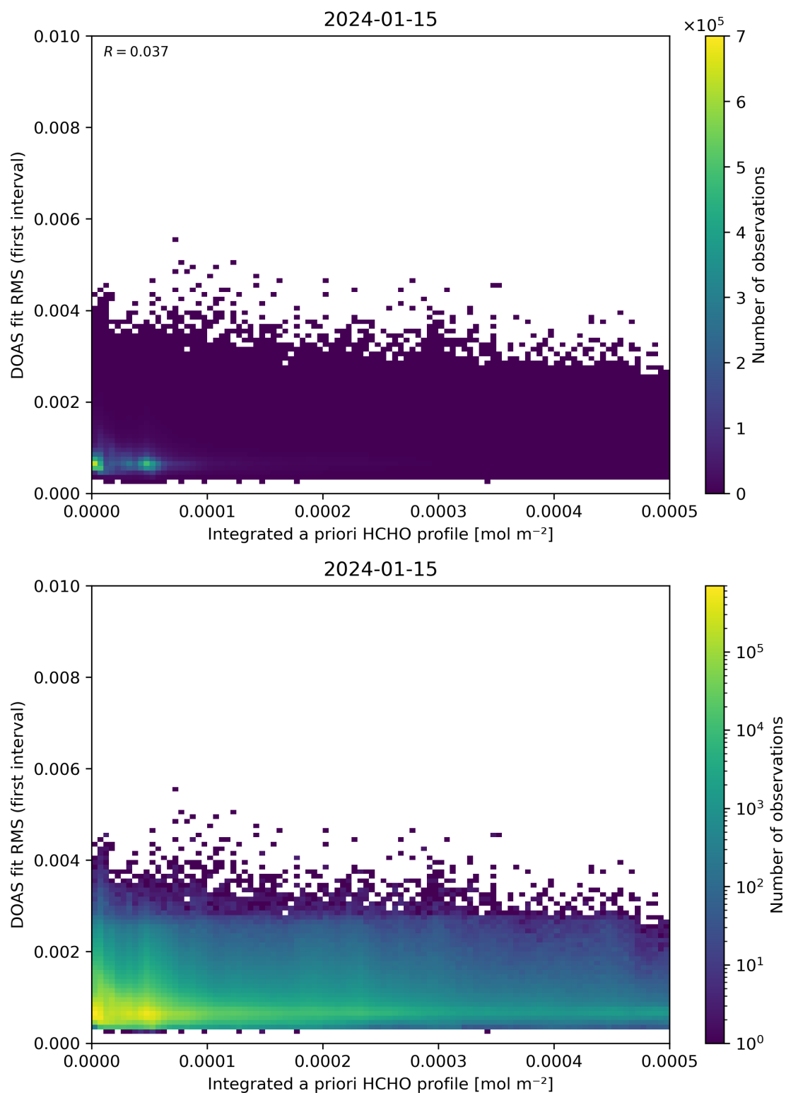
Figure 148: Scatter density plot of “Integrated a priori HCHO profile” against “DOAS fit RMS (first interval)” for 2024-01-15 to 2024-01-16.
