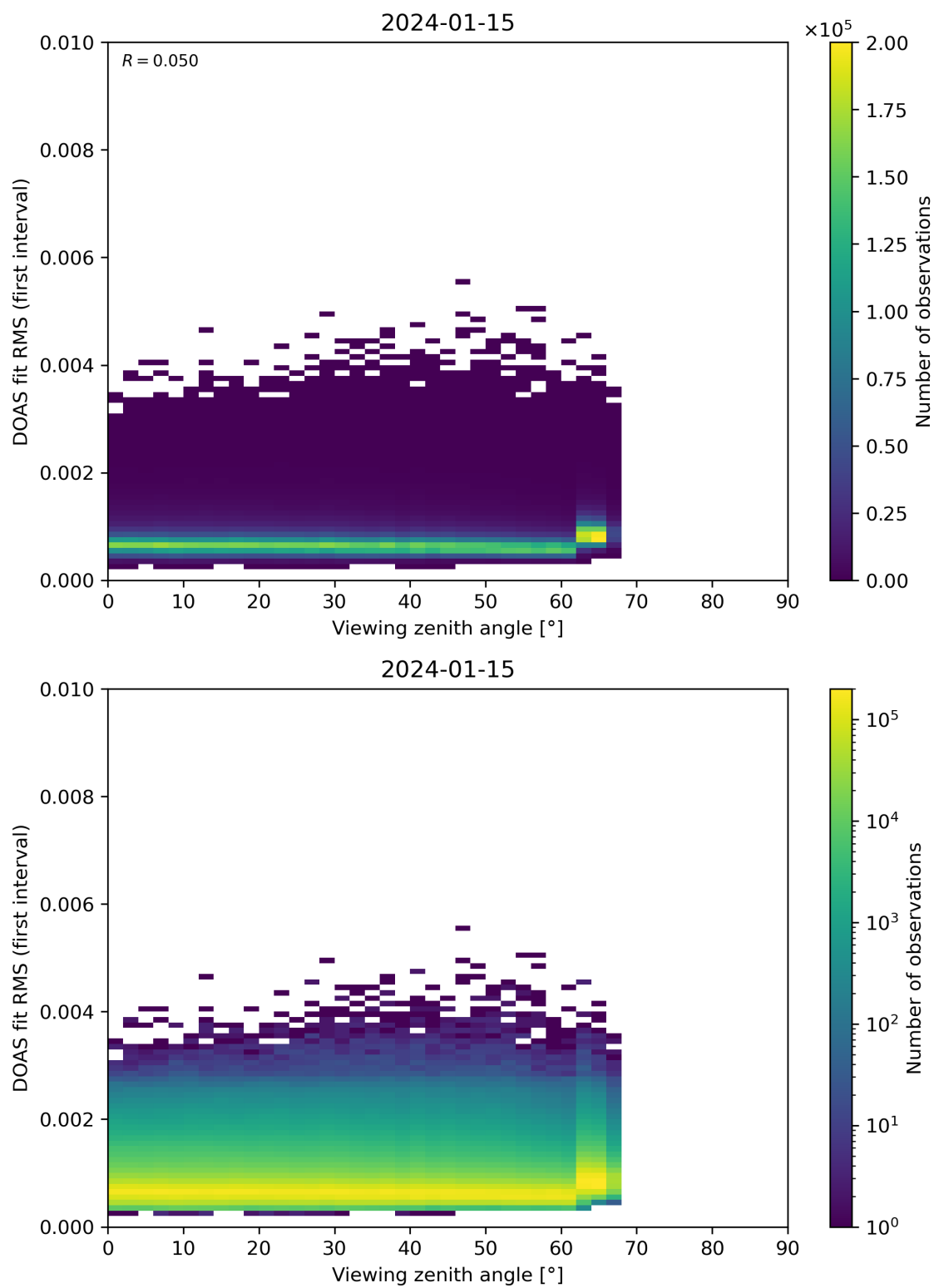
Figure 182: Scatter density plot of “Viewing zenith angle” against “DOAS fit RMS (first interval)” for 2024-01-15 to 2024-01-16.
