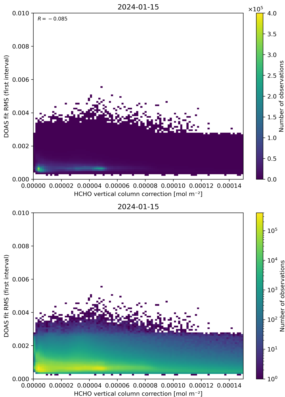
Figure 112: Scatter density plot of “HCHO vertical column correction” against “DOAS fit RMS (first interval)” for 2024-01-15 to 2024-01-16.
