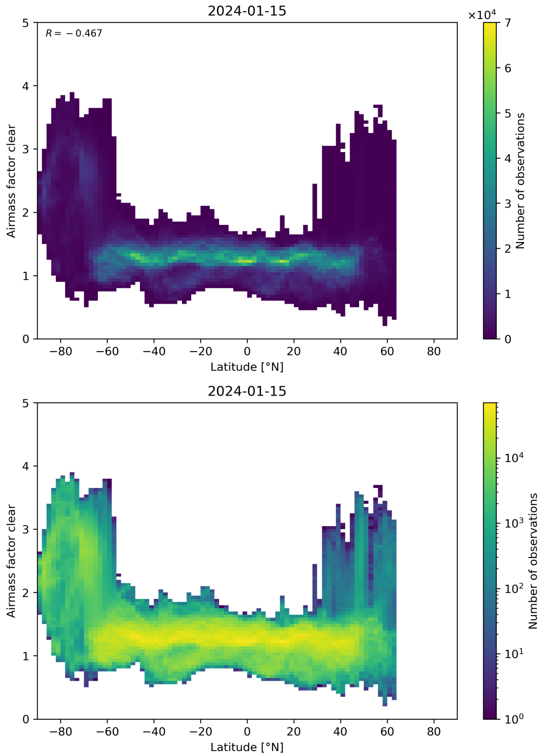
Figure 156: Scatter density plot of “Latitude” against “Airmass factor clear” for 2024-01-15 to 2024-01-16.
