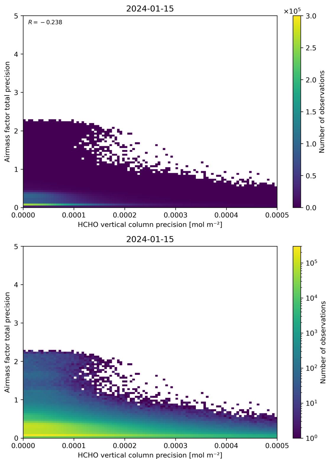
Figure 145: Scatter density plot of “HCHO vertical column precision” against “Airmass factor total precision” for 2024-01-15 to 2024-01-16.
