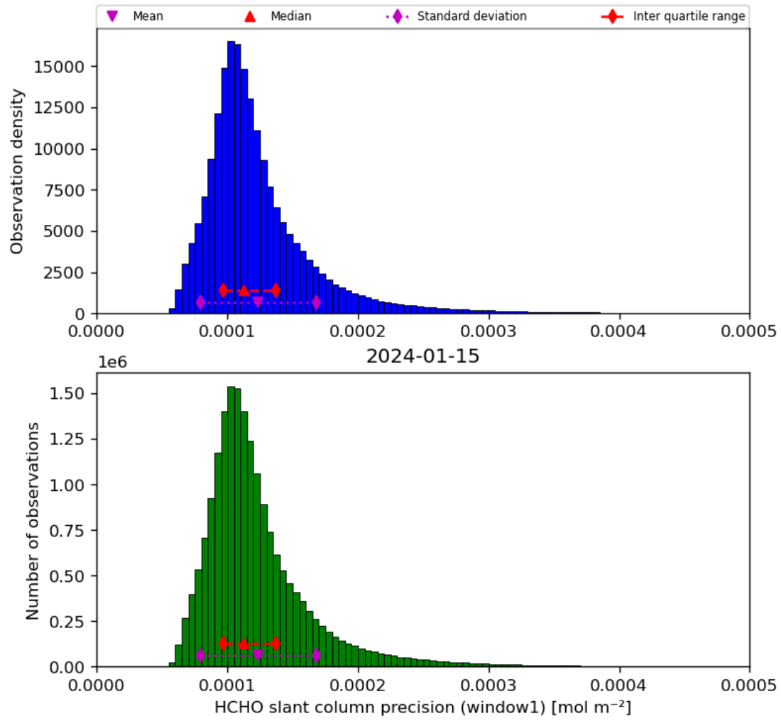
Figure 39: Histogram of “HCHO slant column precision (window1)” for 2024-01-15 to 2024-01-16
