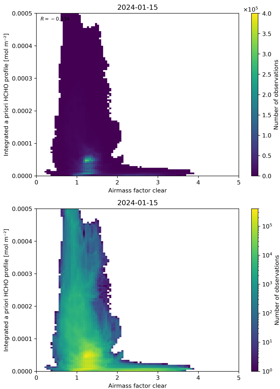
Figure 76: Scatter density plot of “Airmass factor clear” against “Integrated a priori HCHO profile” for 2024-01-15 to 2024-01-16.
