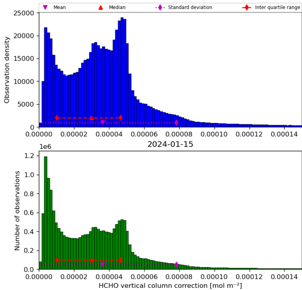
Figure 37: Histogram of “HCHO vertical column correction” for 2024-01-15 to 2024-01-16
