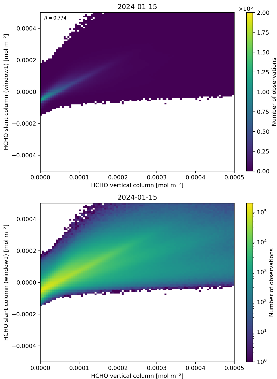
Figure 129: Scatter density plot of “HCHO vertical column” against “HCHO slant column (window1)” for 2024-01-15 to 2024-01-16.
