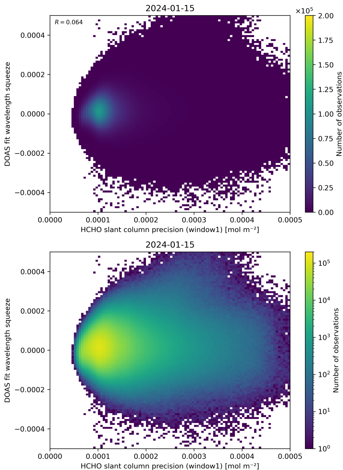
Figure 90: Scatter density plot of “HCHO slant column precision (window1)” against “DOAS fit wavelength squeeze” for 2024-01-15 to 2024-01-16.
