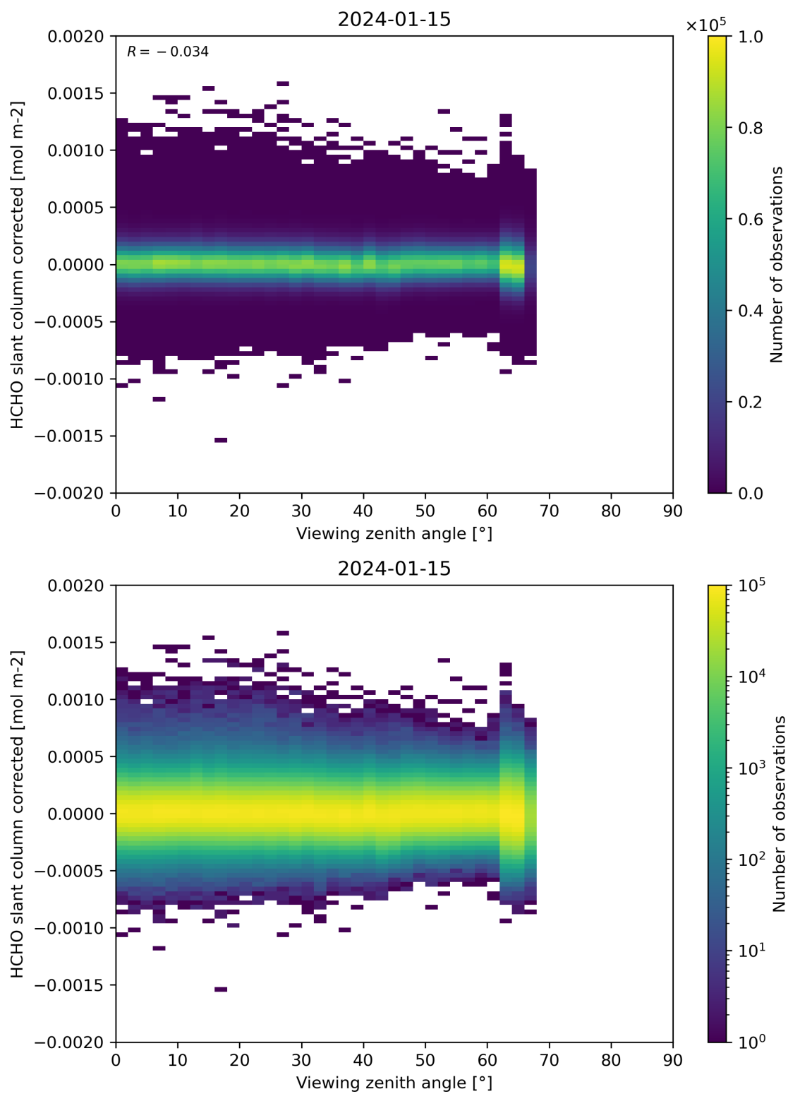
Figure 186: Scatter density plot of “Viewing zenith angle” against “HCHO slant column corrected” for 2024-01-15 to 2024-01-16.
