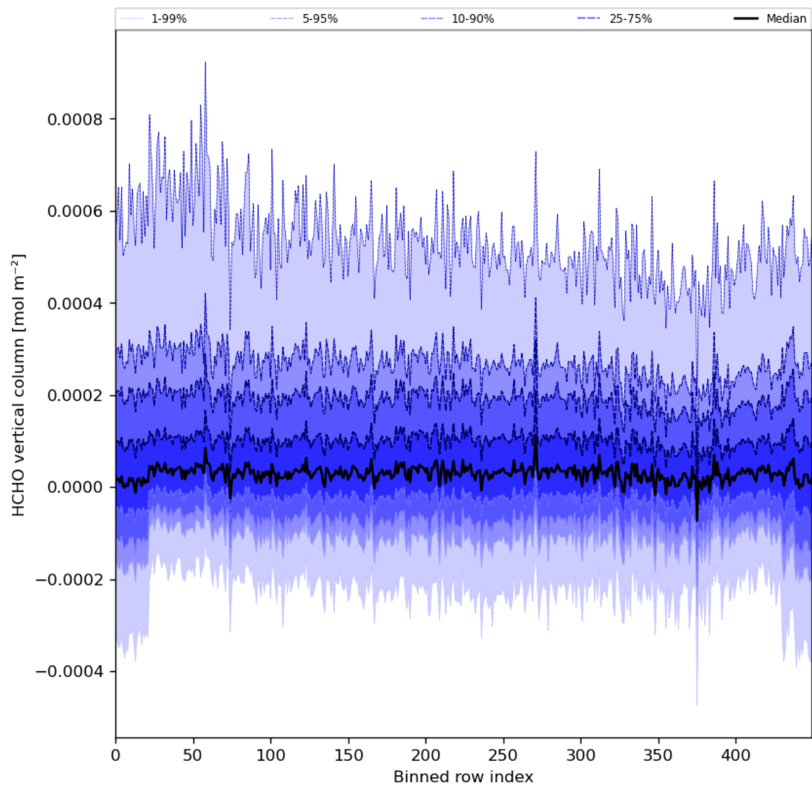
Figure 49: Along track statistics of “HCHO vertical column” for 2024-01-15 to 2024-01-16
