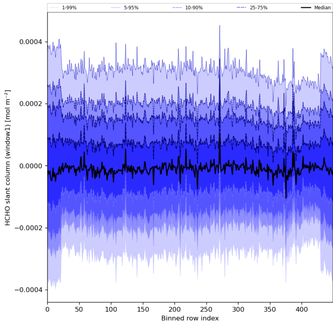
Figure 52: Along track statistics of “HCHO slant column (window1)” for 2024-01-15 to 2024-01-16
