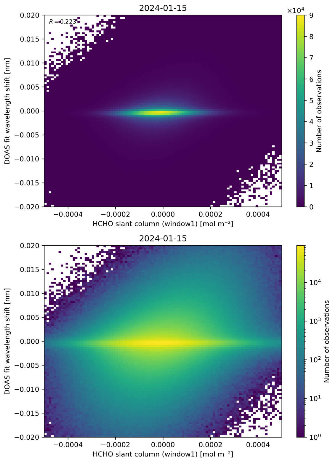
Figure 79: Scatter density plot of “HCHO slant column (window1)” against “DOAS fit wavelength shift” for 2024-01-15 to 2024-01-16.
