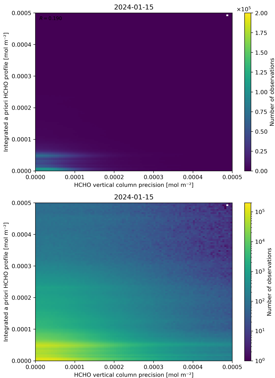
Figure 147: Scatter density plot of “HCHO vertical column precision” against “Integrated a priori HCHO profile” for 2024-01-15 to 2024-01-16.
