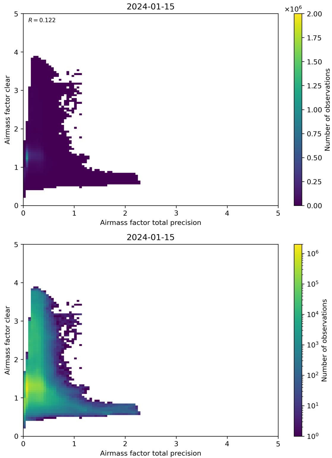
Figure 108: Scatter density plot of “Airmass factor total precision” against “Airmass factor clear” for 2024-01-15 to 2024-01-16.
