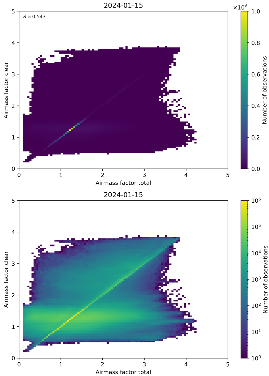
Figure 100: Scatter density plot of “Airmass factor total” against “Airmass factor clear” for 2024-01-15 to 2024-01-16.
