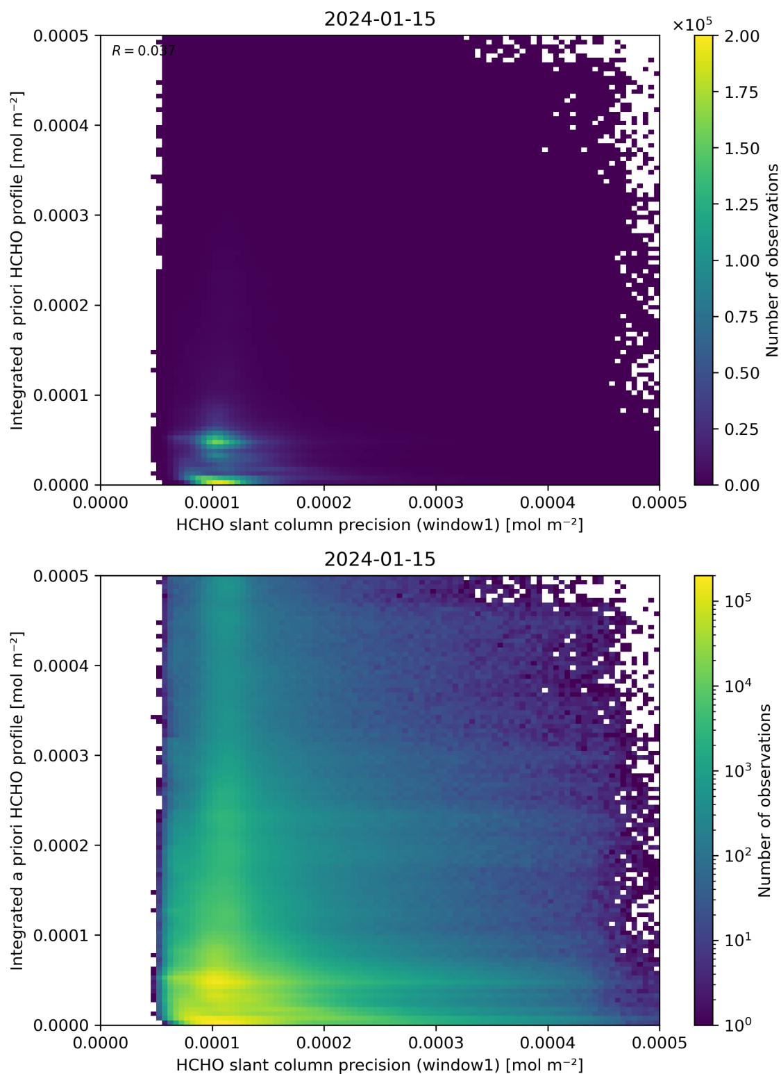
Figure 96: Scatter density plot of “HCHO slant column precision (window1)” against “Integrated a priori HCHO profile” for 2024-01-15 to 2024-01-16.
