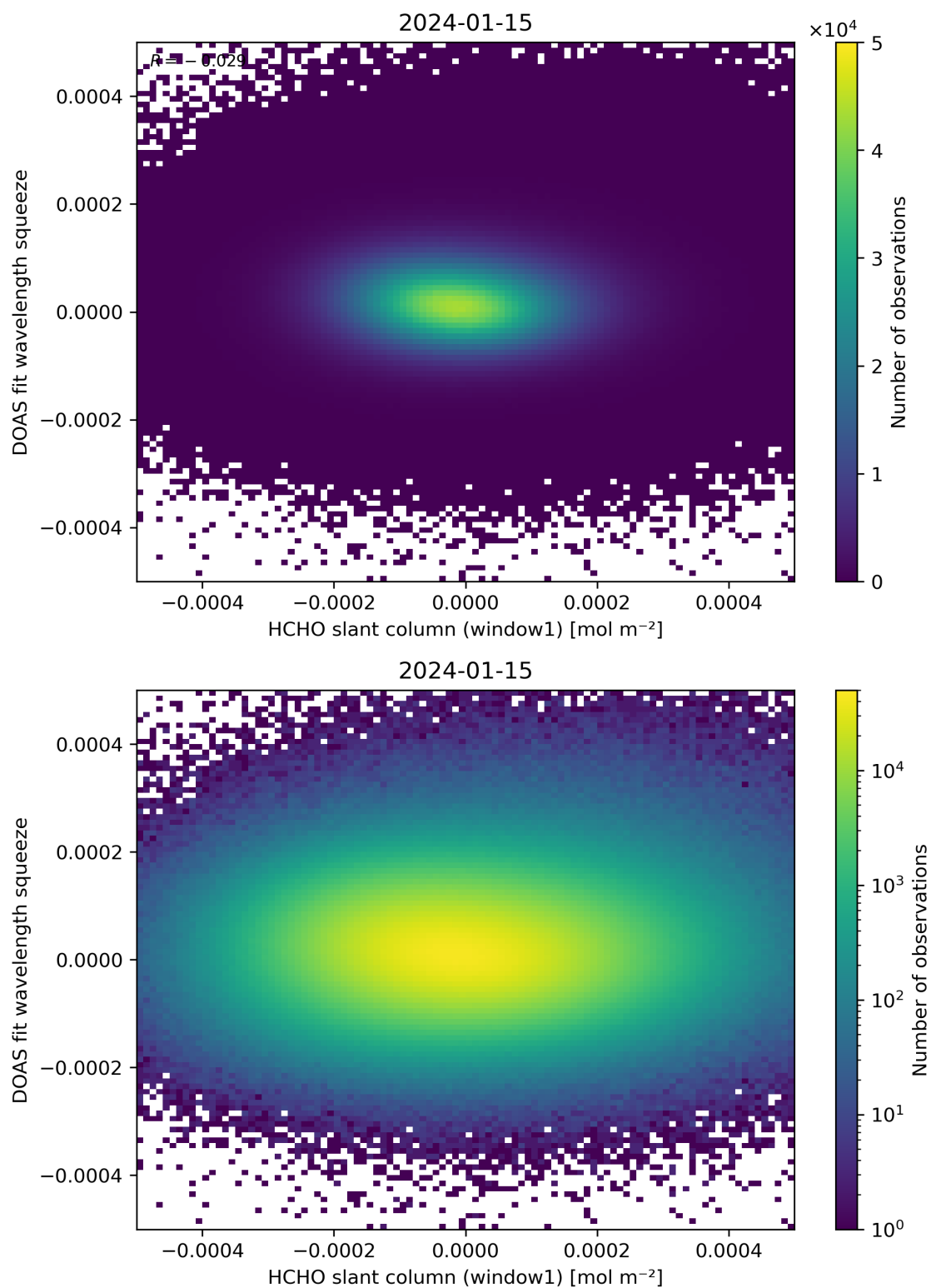
Figure 80: Scatter density plot of “HCHO slant column (window1)” against “DOAS fit wavelength squeeze” for 2024-01-15 to 2024-01-16.
