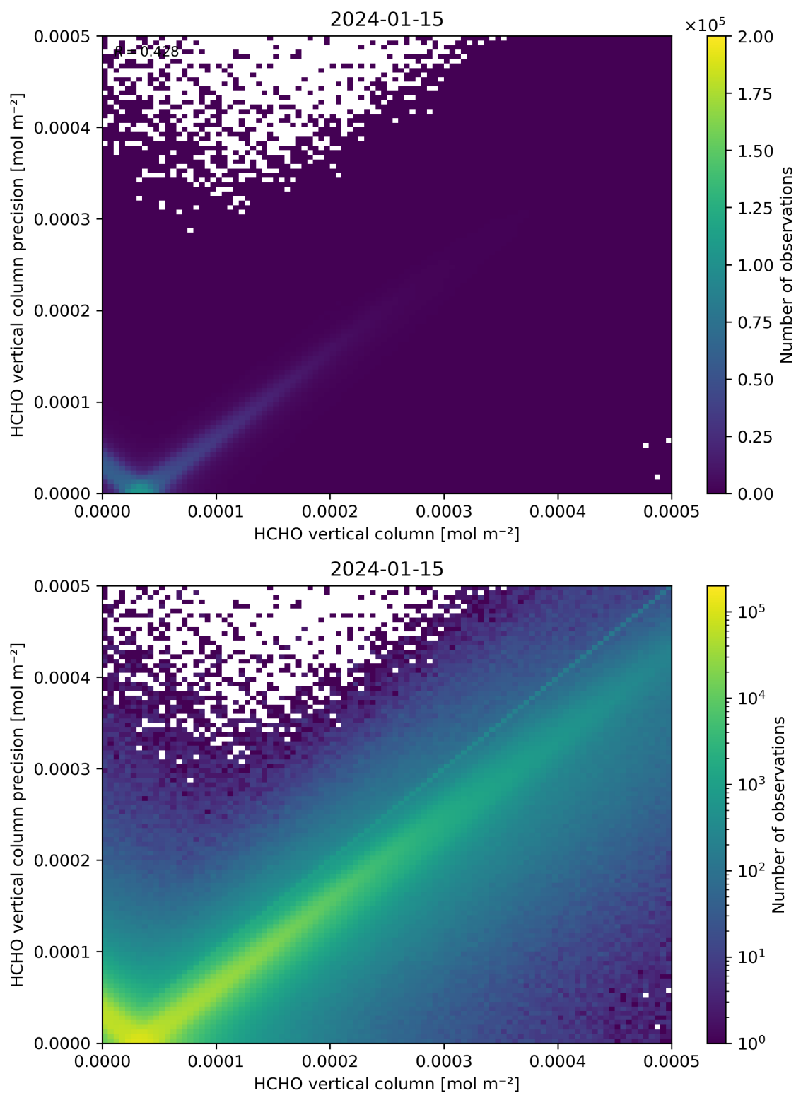
Figure 134: Scatter density plot of “HCHO vertical column” against “HCHO vertical column precision” for 2024-01-15 to 2024-01-16.
