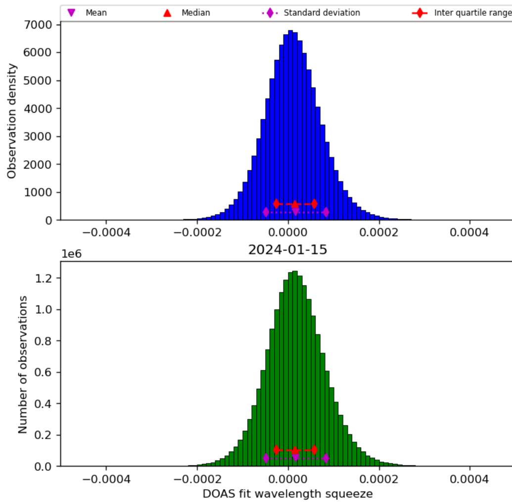
Figure 45: Histogram of “DOAS fit wavelength squeeze” for 2024-01-15 to 2024-01-16
