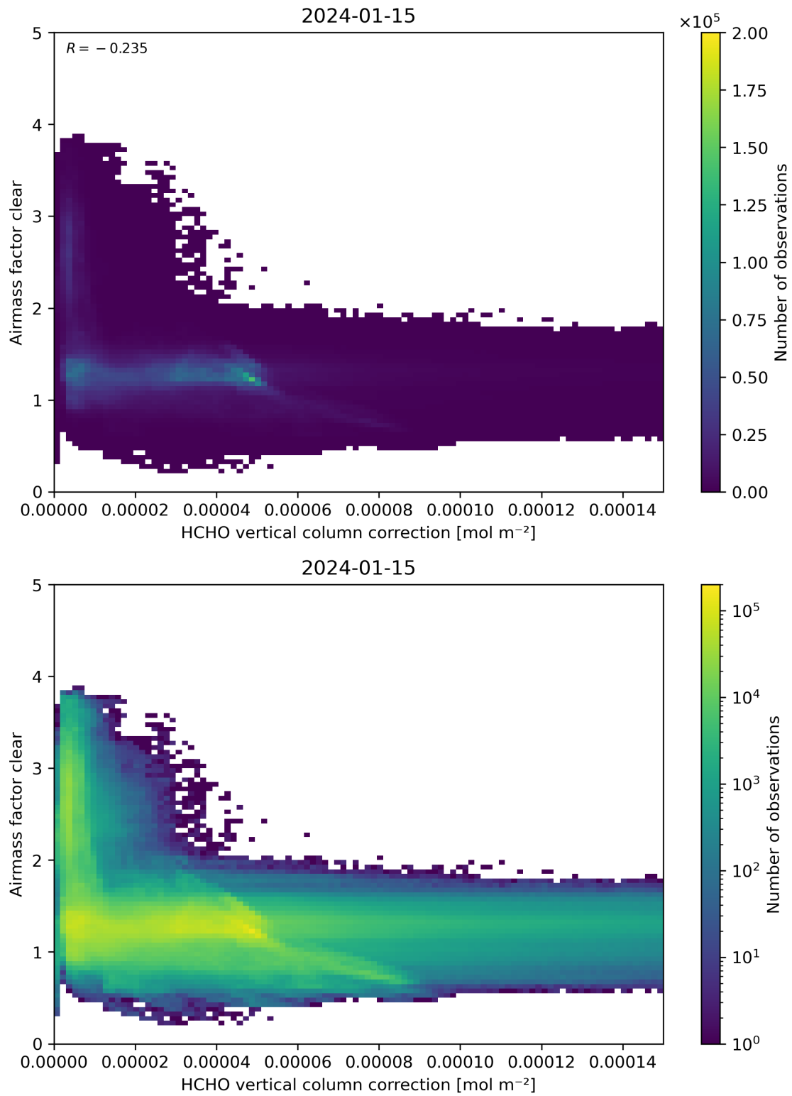
Figure 115: Scatter density plot of “HCHO vertical column correction” against “Airmass factor clear” for 2024-01-15 to 2024-01-16.
