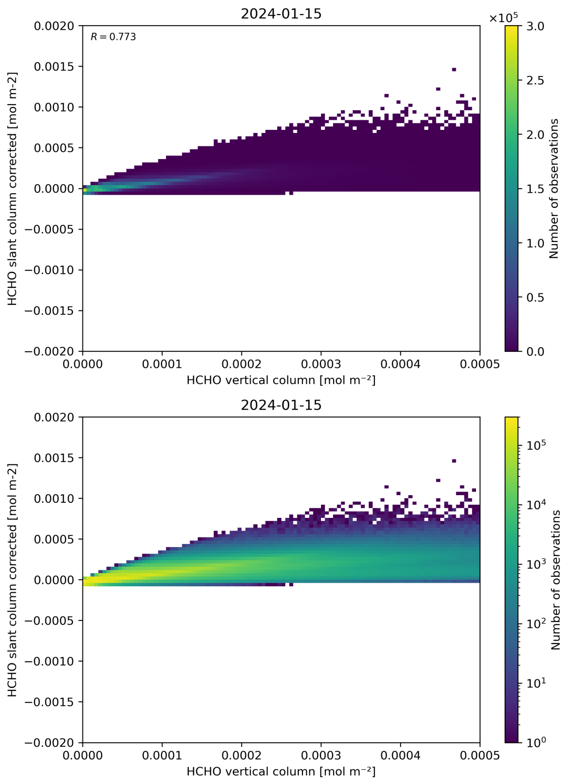
Figure 127: Scatter density plot of “HCHO vertical column” against “HCHO slant column corrected” for 2024-01-15 to 2024-01-16.
