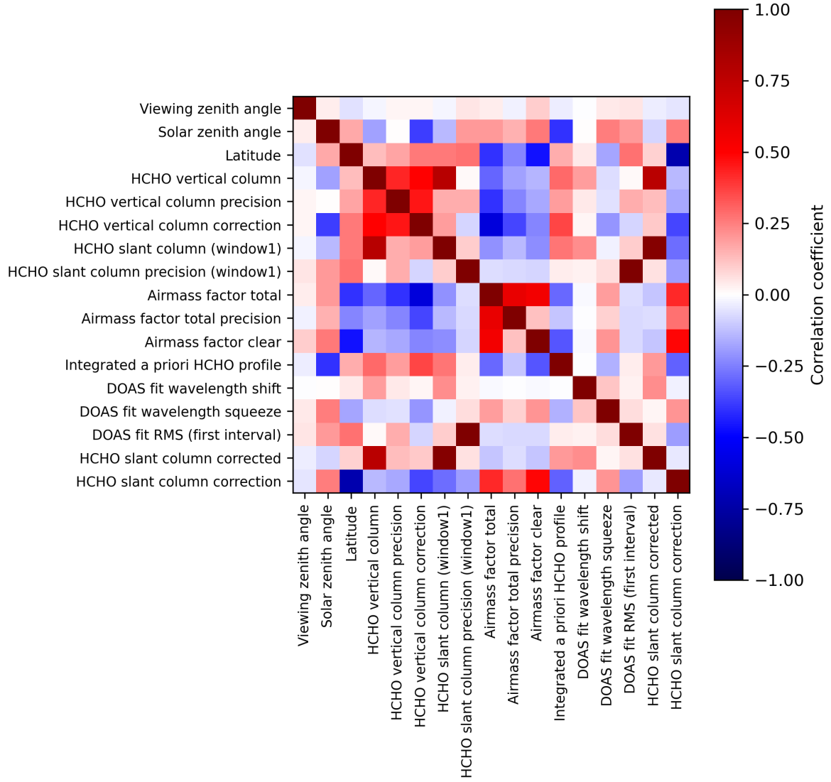
Figure 2: Map of correlation matrix for 2024-01-15 to 2024-01-16.
