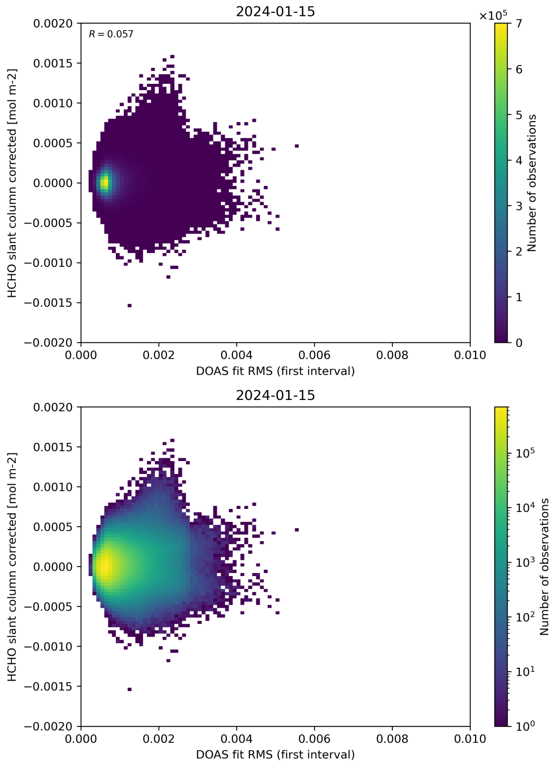
Figure 62: Scatter density plot of “DOAS fit RMS (first interval)” against “HCHO slant column corrected” for 2024-01-15 to 2024-01-16.
