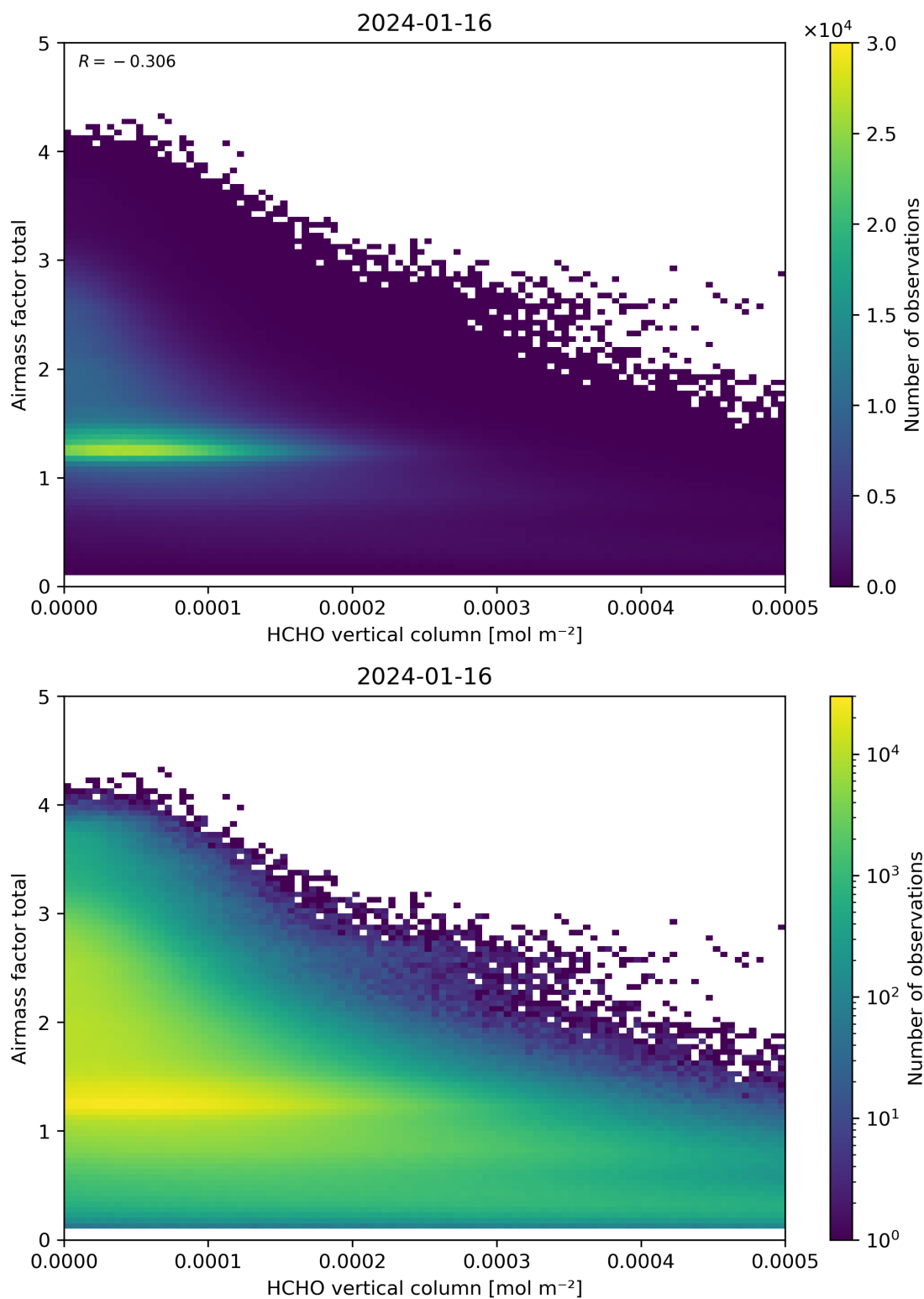
Figure 131: Scatter density plot of “HCHO vertical column” against “Airmass factor total” for 2024-01-15 to 2024-01-17.
