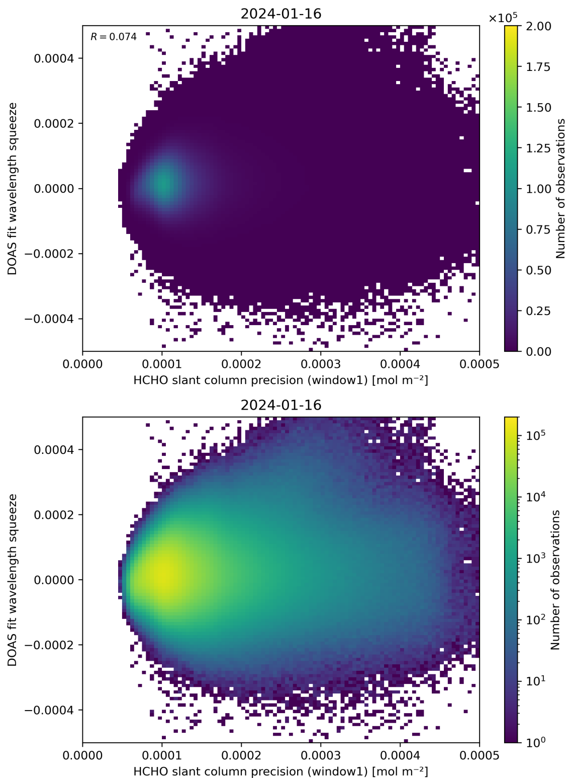
Figure 90: Scatter density plot of “HCHO slant column precision (window1)” against “DOAS fit wavelength squeeze” for 2024-01-15 to 2024-01-17.
