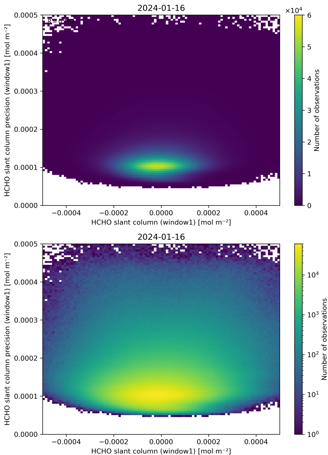
Figure 84: Scatter density plot of “HCHO slant column (window1)” against “HCHO slant column precision (window1)” for 2024-01-15 to 2024-01-17.
