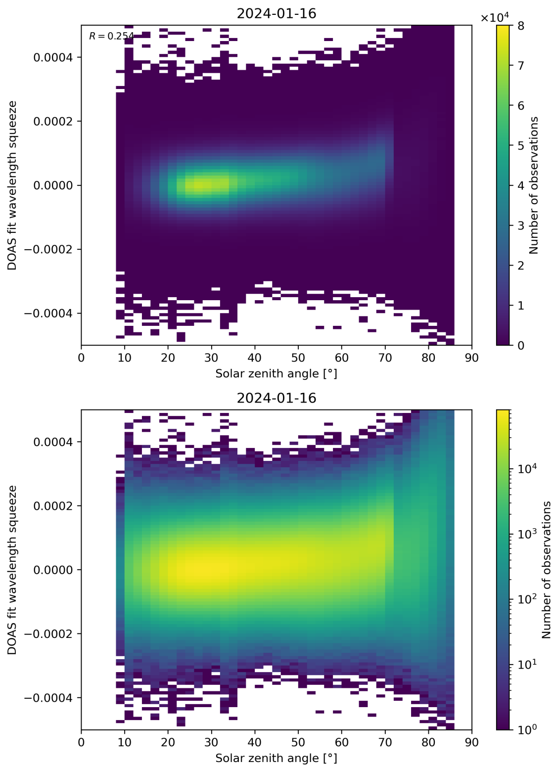
Figure 169: Scatter density plot of “Solar zenith angle” against “DOAS fit wavelength squeeze” for 2024-01-15 to 2024-01-17.
