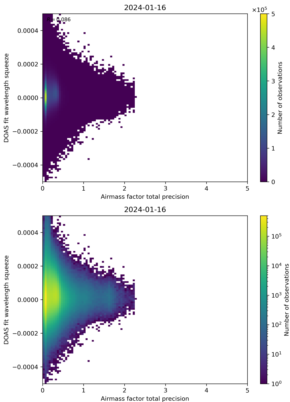
Figure 107: Scatter density plot of “Airmass factor total precision” against “DOAS fit wavelength squeeze” for 2024-01-15 to 2024-01-17.
