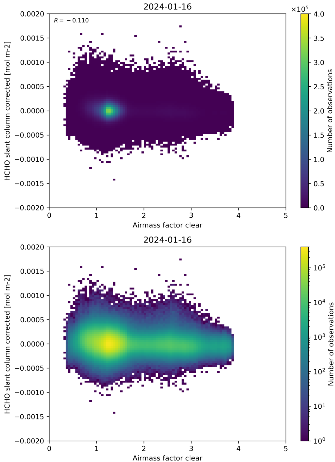
Figure 74: Scatter density plot of “Airmass factor clear” against “HCHO slant column corrected” for 2024-01-15 to 2024-01-17.
