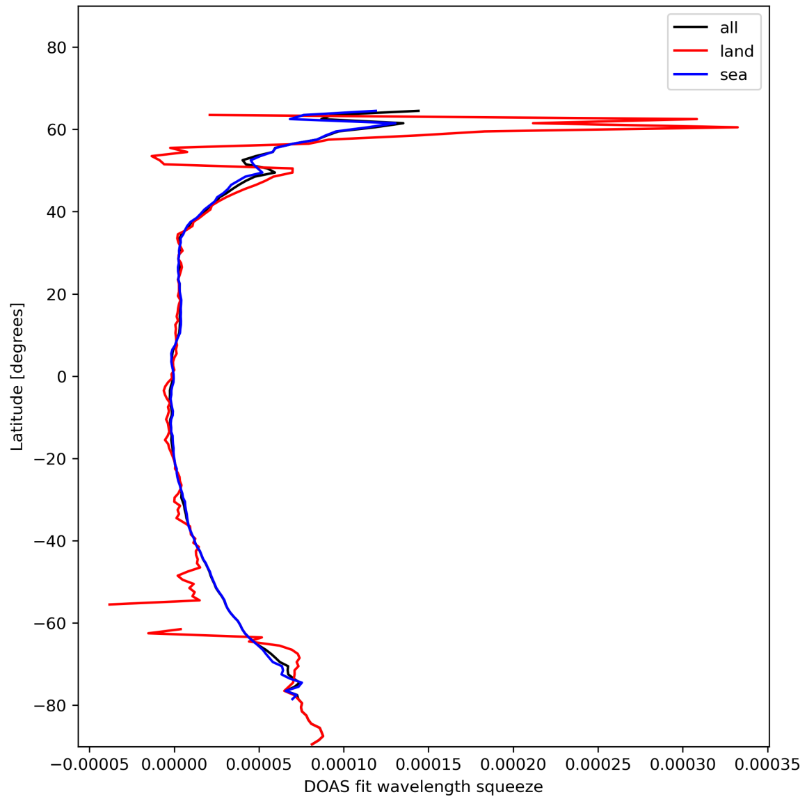
Figure 31: Zonal average of “DOAS fit wavelength squeeze” for 2024-01-15 to 2024-01-17.
