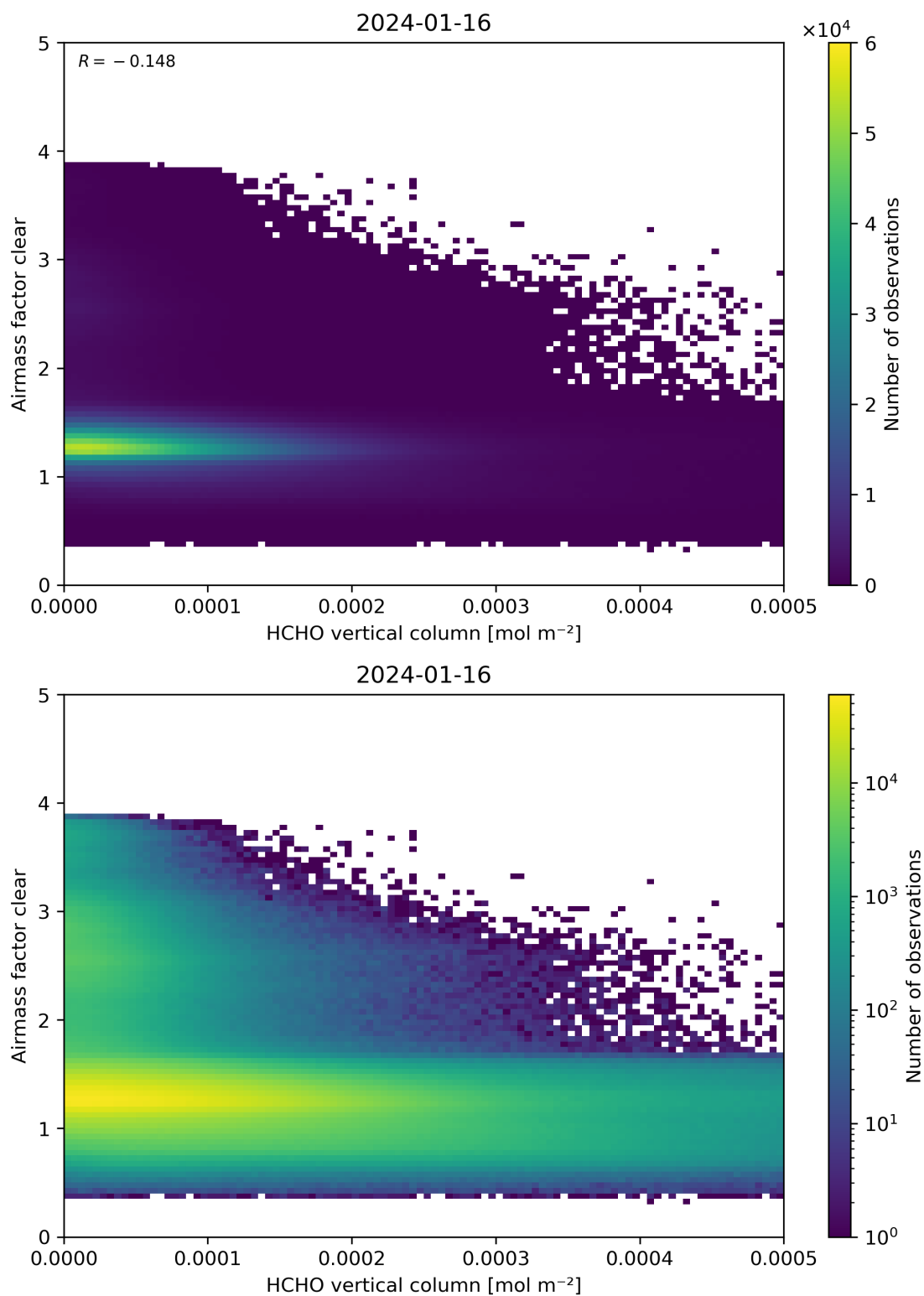
Figure 126: Scatter density plot of “HCHO vertical column” against “Airmass factor clear” for 2024-01-15 to 2024-01-17.
