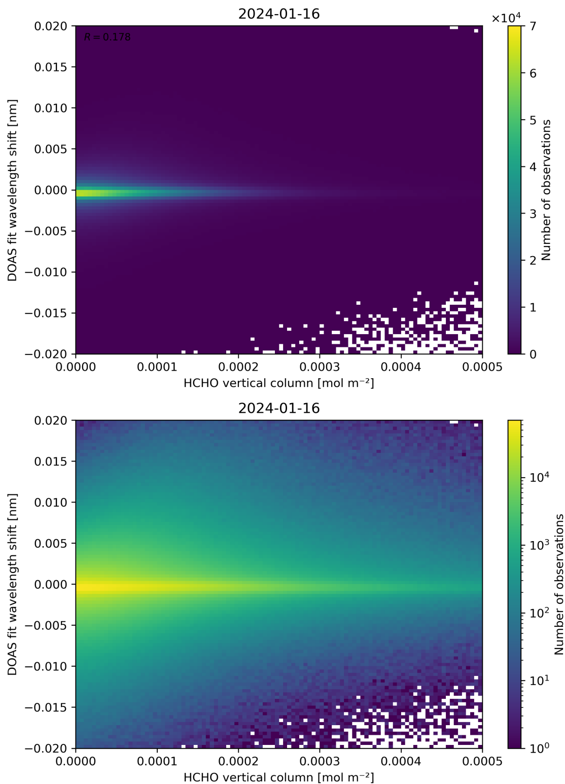
Figure 124: Scatter density plot of “HCHO vertical column” against “DOAS fit wavelength shift” for 2024-01-15 to 2024-01-17.
