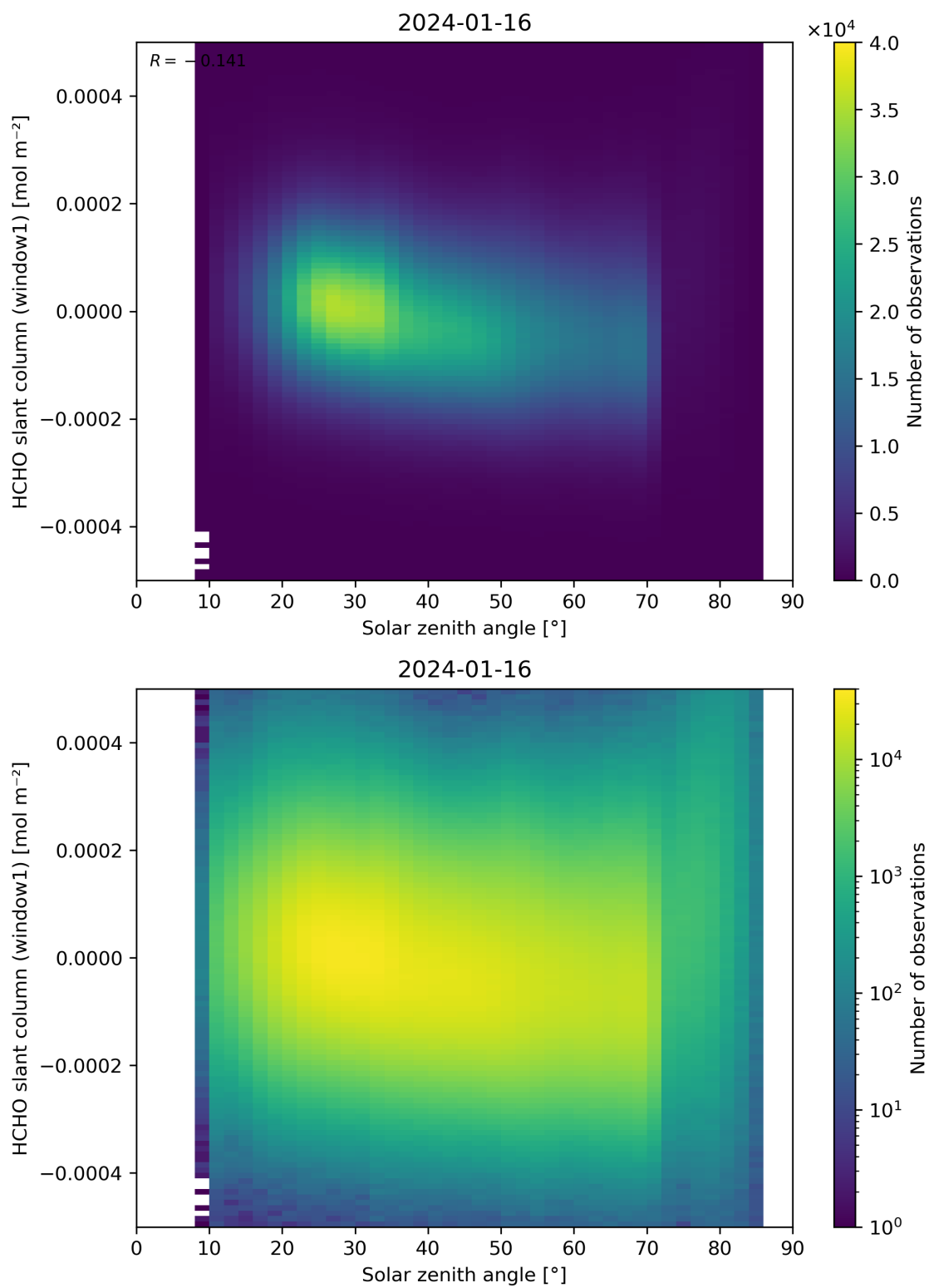
Figure 173: Scatter density plot of “Solar zenith angle” against “HCHO slant column (window1)” for 2024-01-15 to 2024-01-17.
