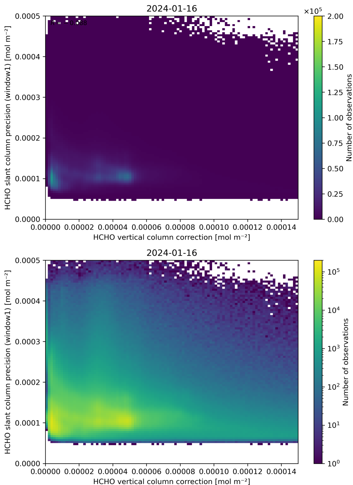
Figure 119: Scatter density plot of “HCHO vertical column correction” against “HCHO slant column precision (window1)” for 2024-01-15 to 2024-01-17.
