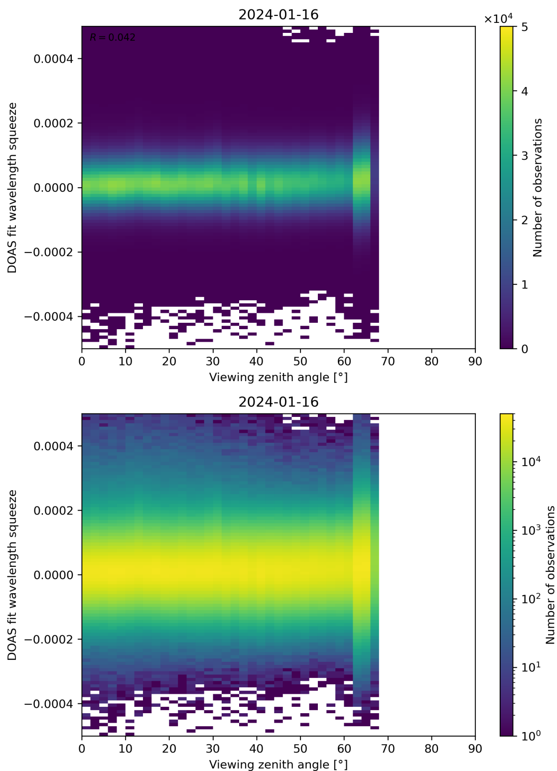
Figure 184: Scatter density plot of “Viewing zenith angle” against “DOAS fit wavelength squeeze” for 2024-01-15 to 2024-01-17.
