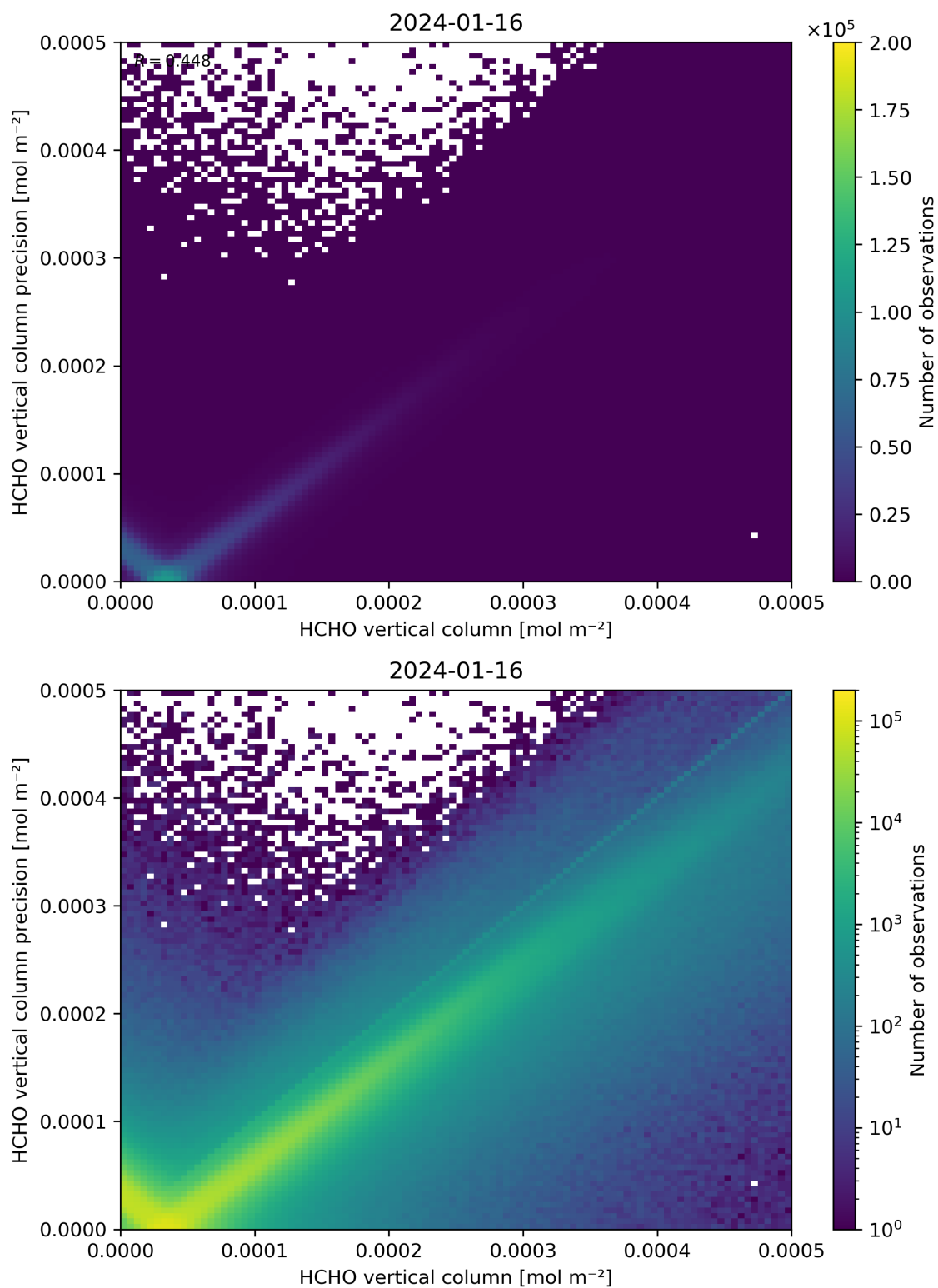
Figure 134: Scatter density plot of “HCHO vertical column” against “HCHO vertical column precision” for 2024-01-15 to 2024-01-17.
