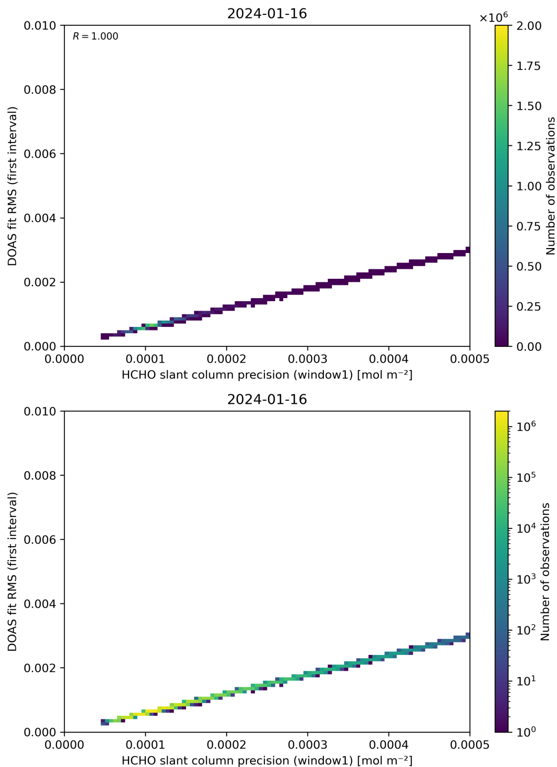
Figure 88: Scatter density plot of “HCHO slant column precision (window1)” against “DOAS fit RMS (first interval)” for 2024-01-15 to 2024-01-17.
