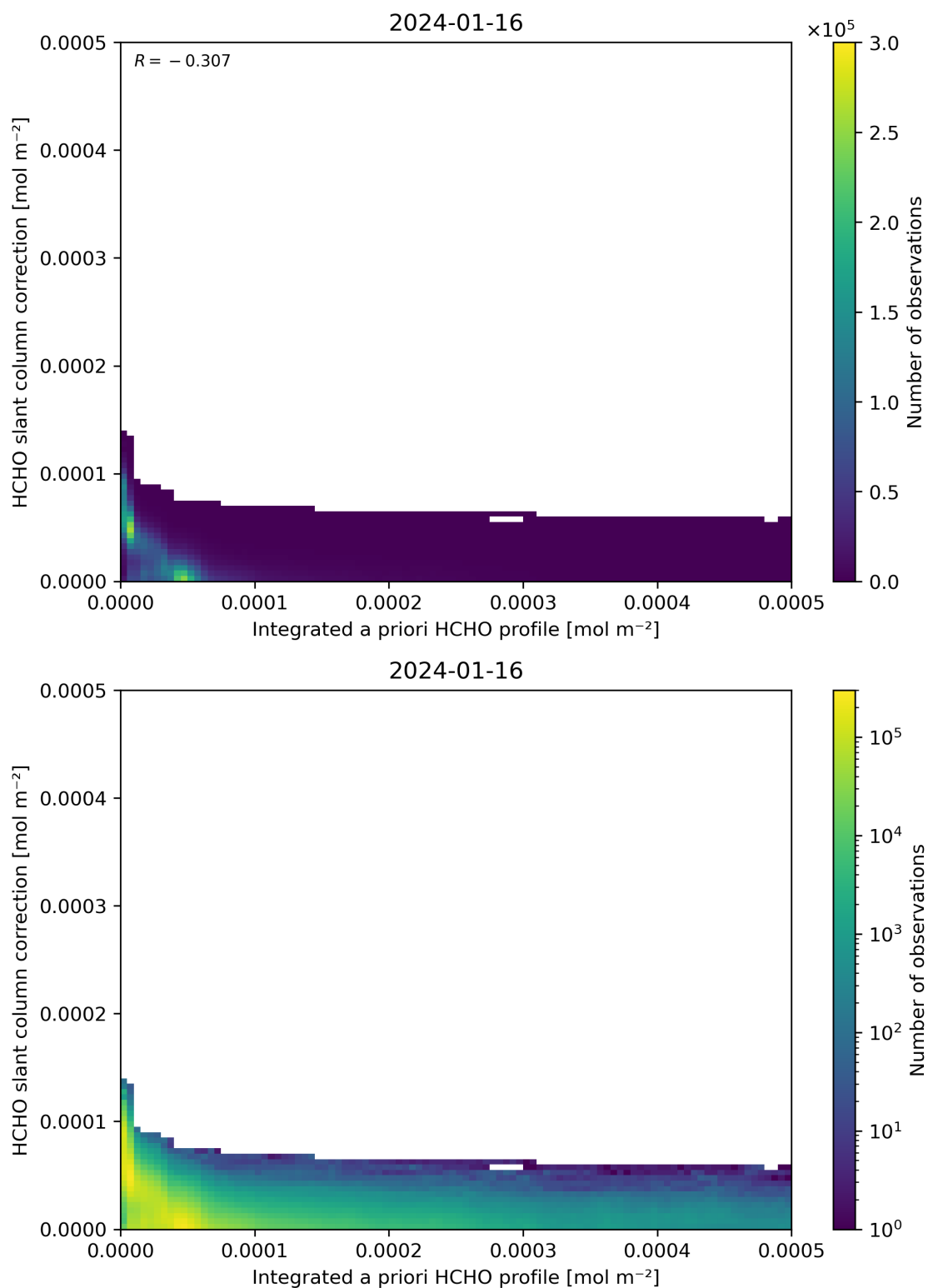
Figure 152: Scatter density plot of “Integrated a priori HCHO profile” against “HCHO slant column correction” for 2024-01-15 to 2024-01-17.
