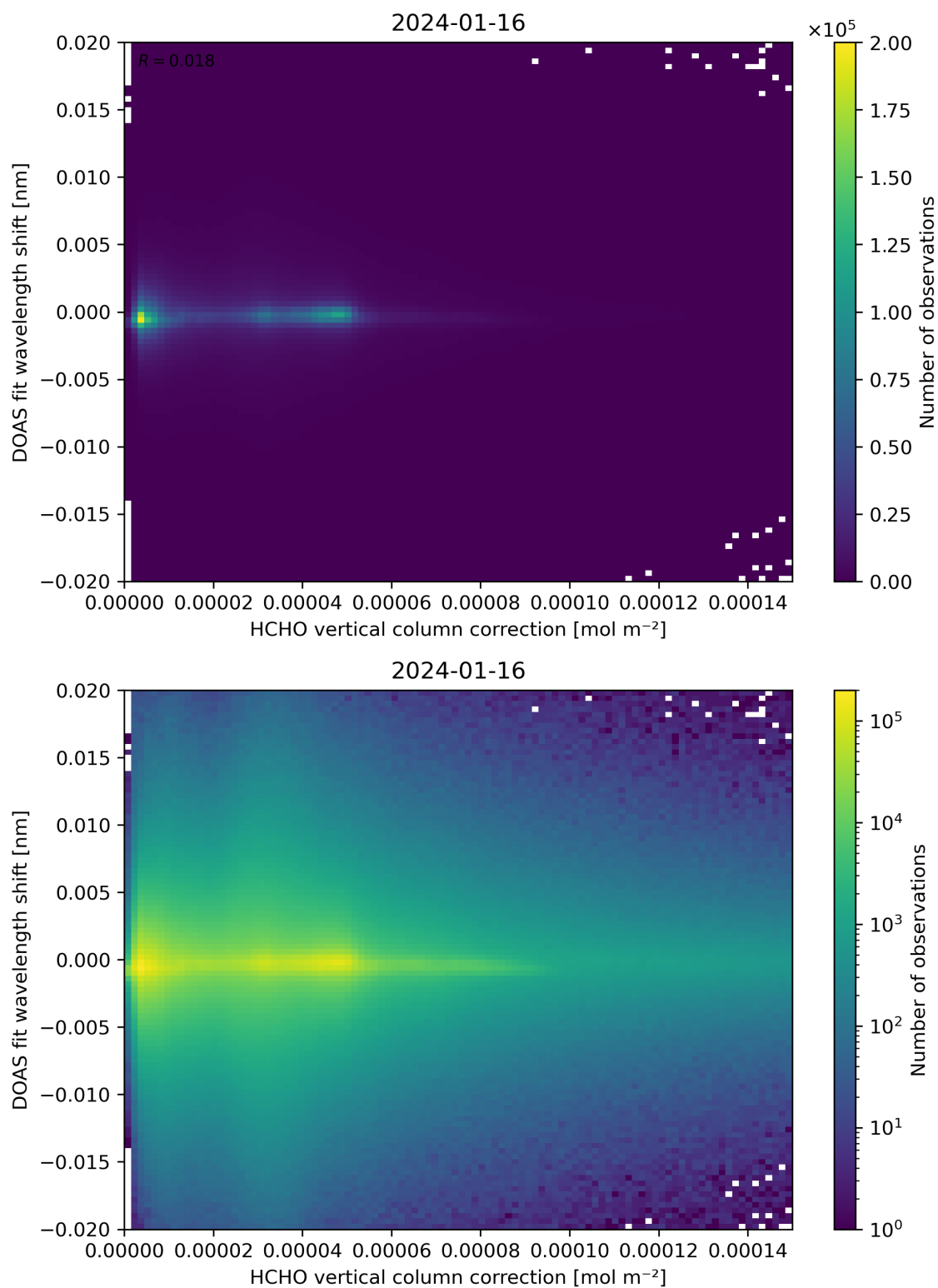
Figure 113: Scatter density plot of “HCHO vertical column correction” against “DOAS fit wavelength shift” for 2024-01-15 to 2024-01-17.
