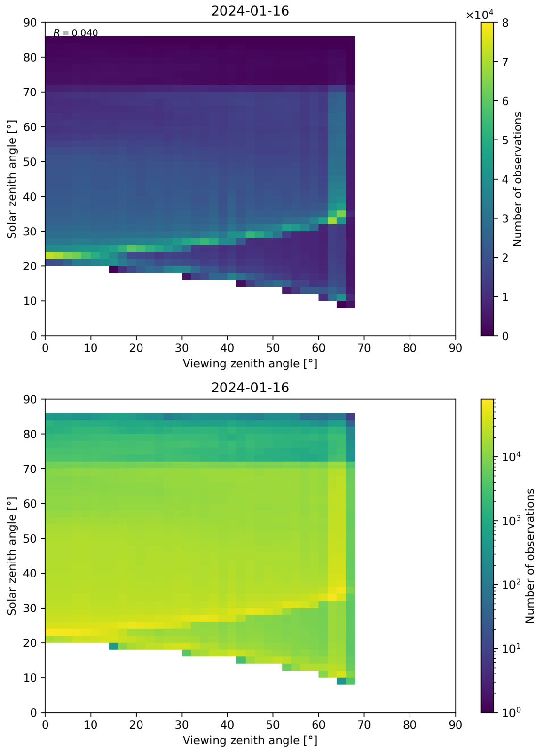
Figure 197: Scatter density plot of “Viewing zenith angle” against “Solar zenith angle” for 2024-01-15 to 2024-01-17.
