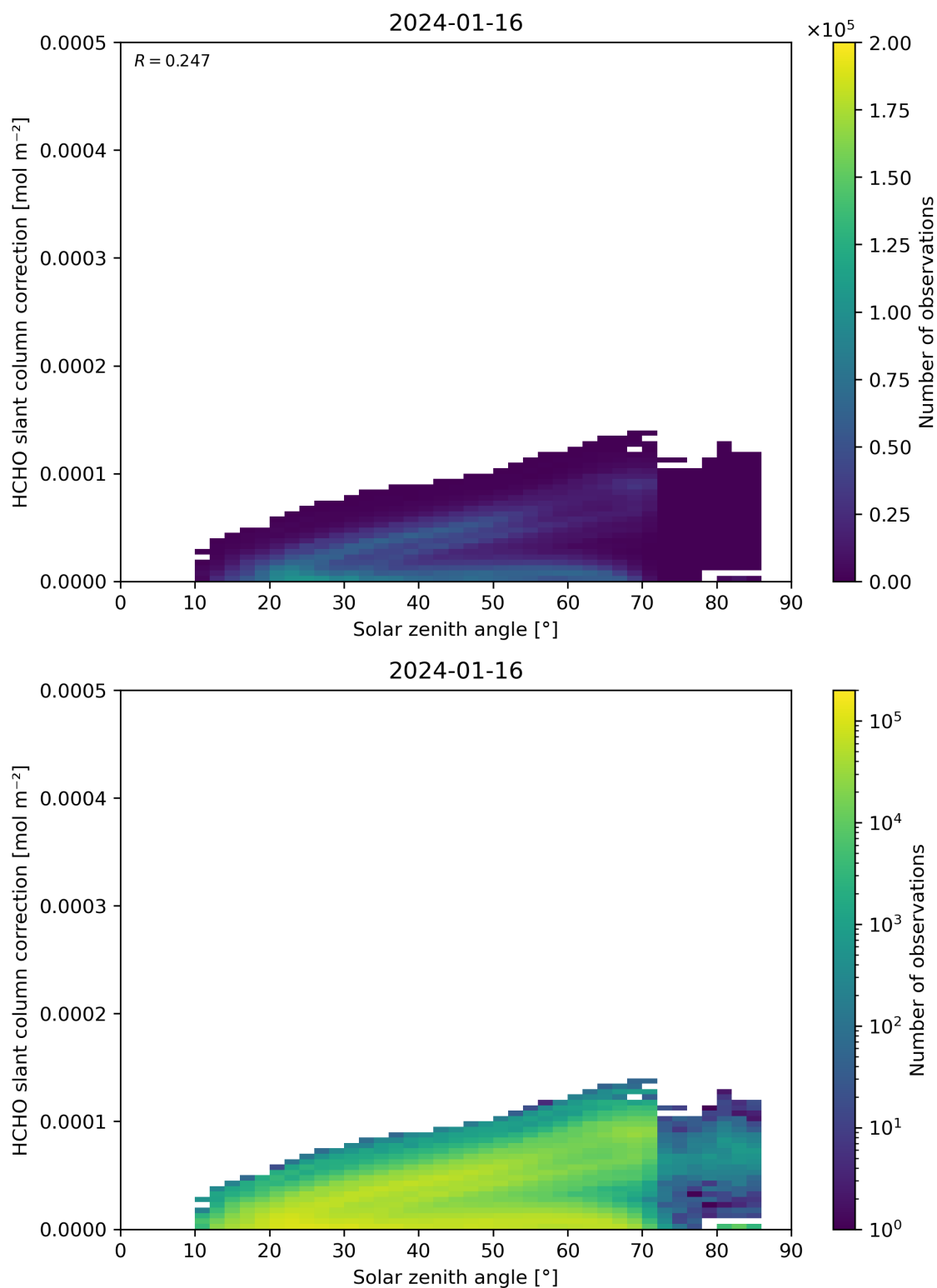
Figure 172: Scatter density plot of “Solar zenith angle” against “HCHO slant column correction” for 2024-01-15 to 2024-01-17.
