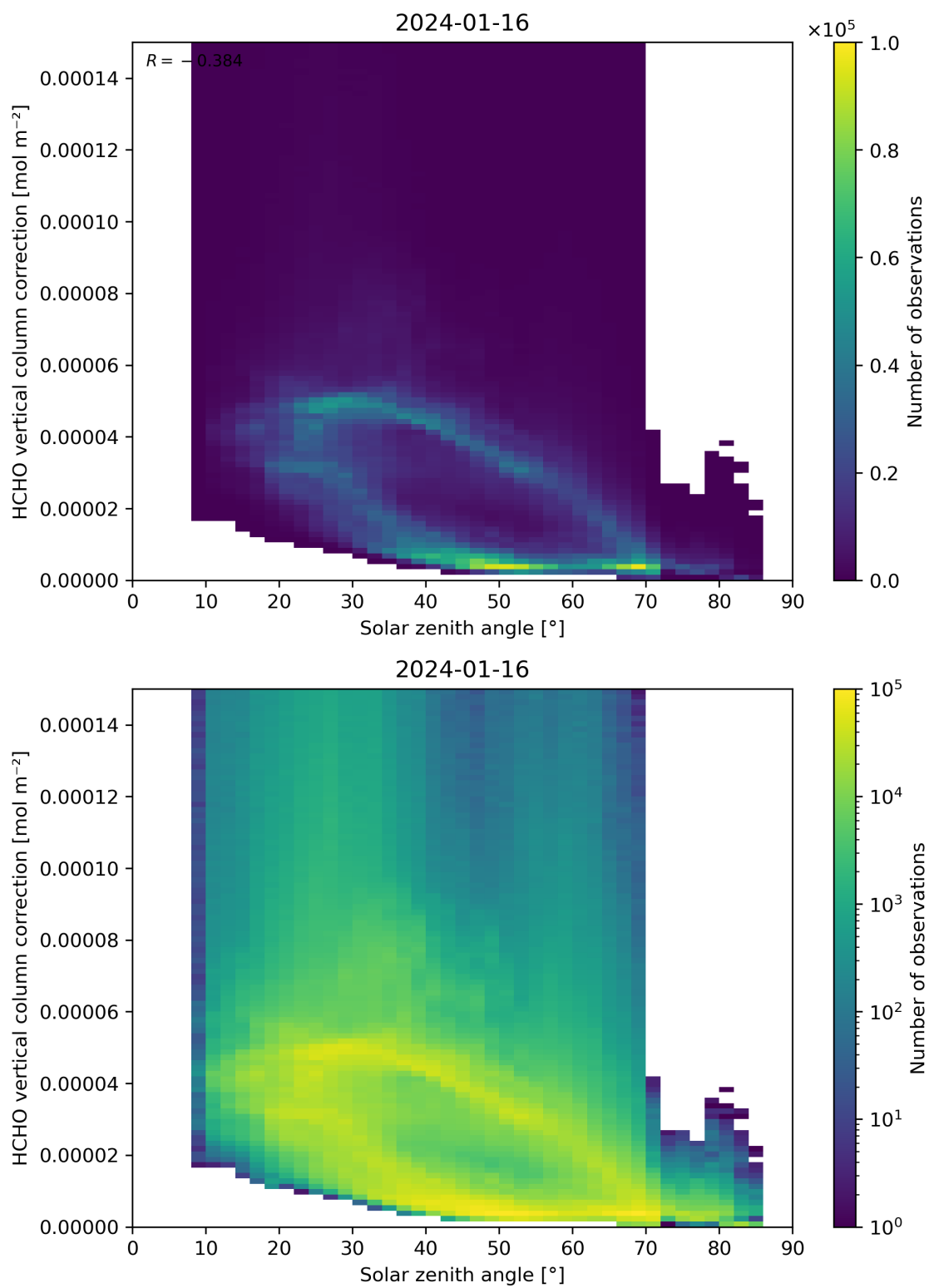
Figure 178: Scatter density plot of “Solar zenith angle” against “HCHO vertical column correction” for 2024-01-15 to 2024-01-17.
