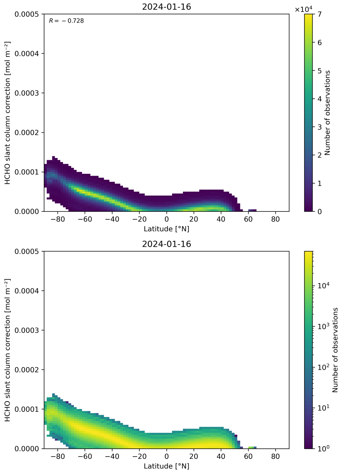
Figure 158: Scatter density plot of “Latitude” against “HCHO slant column correction” for 2024-01-15 to 2024-01-17.
