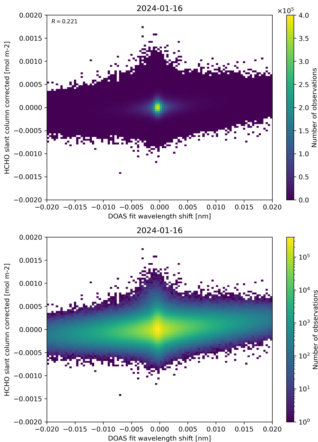
Figure 66: Scatter density plot of “DOAS fit wavelength shift” against “HCHO slant column corrected” for 2024-01-15 to 2024-01-17.
