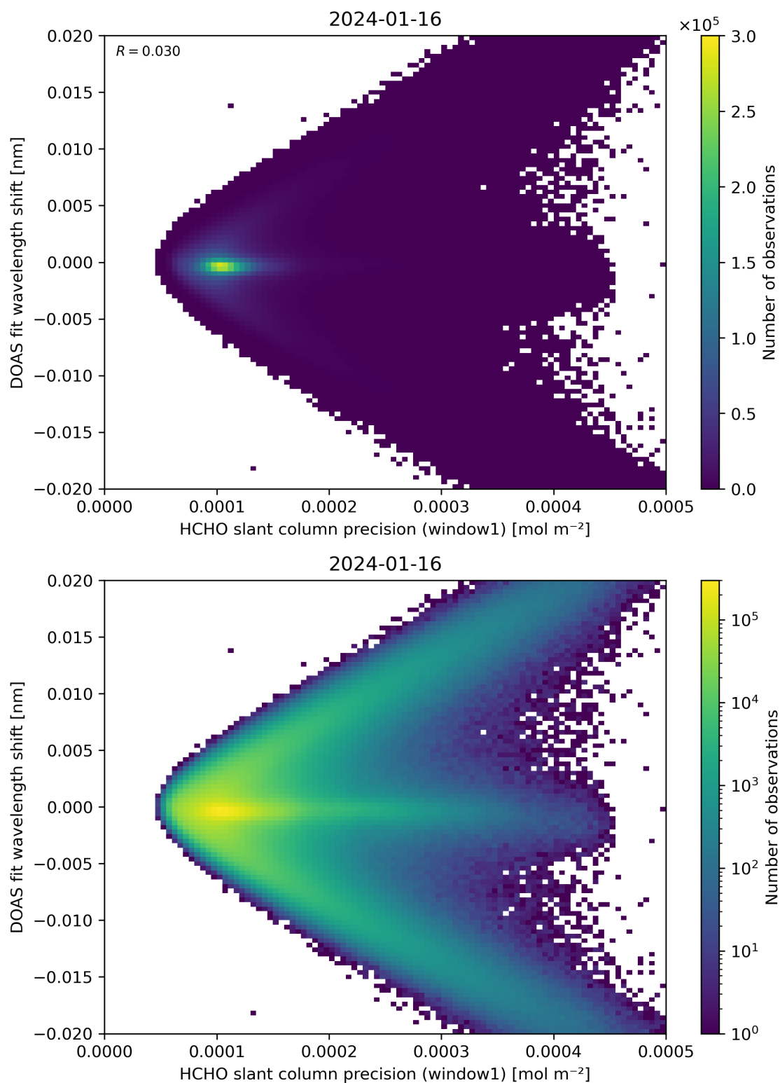
Figure 89: Scatter density plot of “HCHO slant column precision (window1)” against “DOAS fit wavelength shift” for 2024-01-15 to 2024-01-17.
