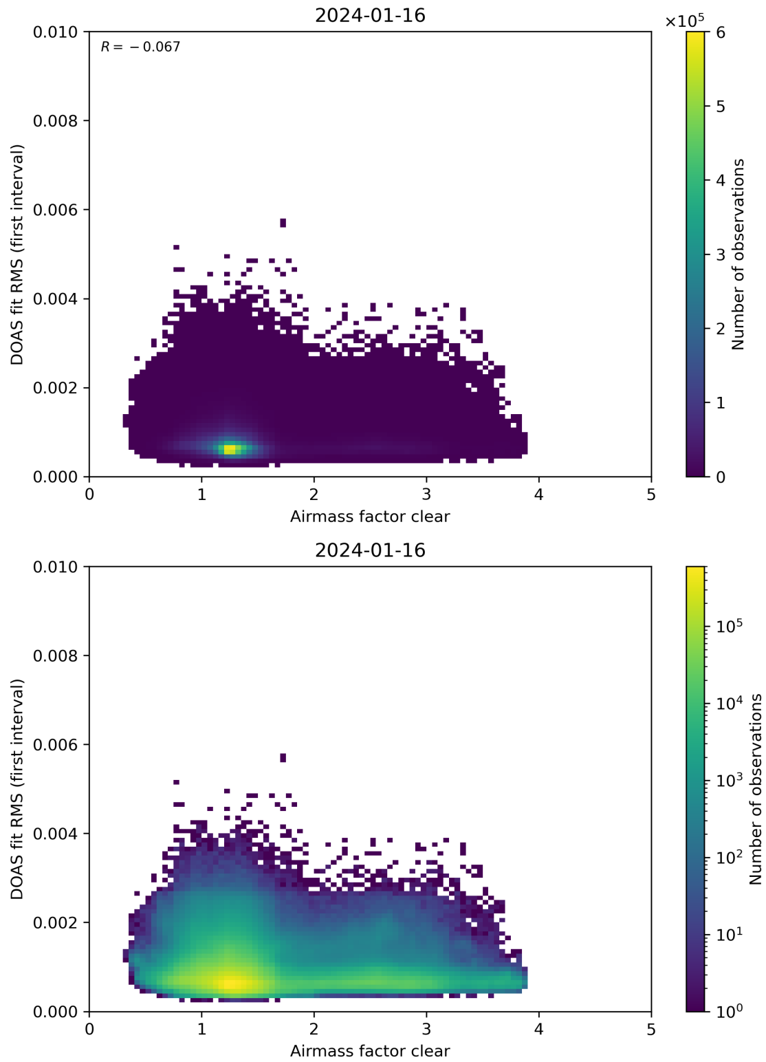
Figure 71: Scatter density plot of “Airmass factor clear” against “DOAS fit RMS (first interval)” for 2024-01-15 to 2024-01-17.
