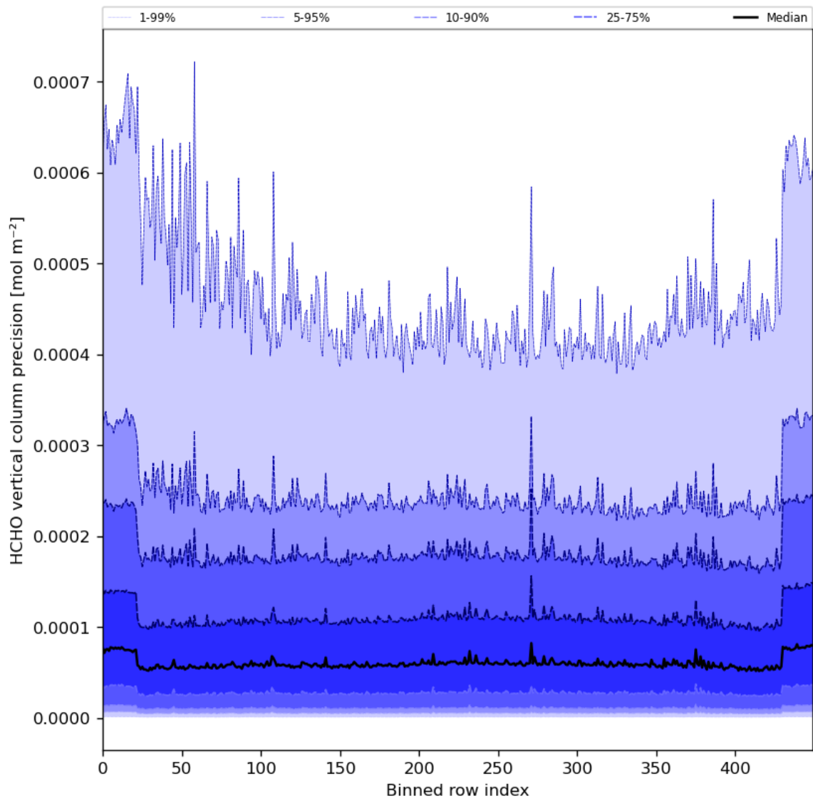
Figure 50: Along track statistics of “HCHO vertical column precision” for 2024-01-15 to 2024-01-17
