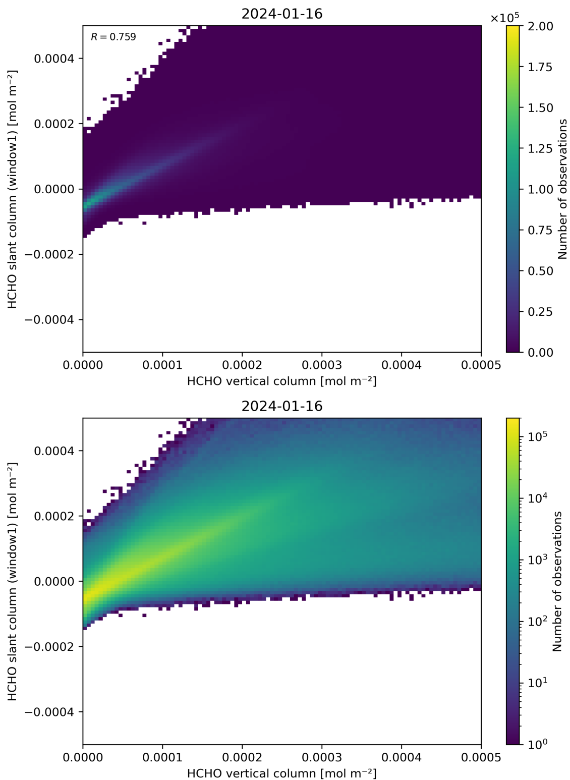
Figure 129: Scatter density plot of “HCHO vertical column” against “HCHO slant column (window1)” for 2024-01-15 to 2024-01-17.
