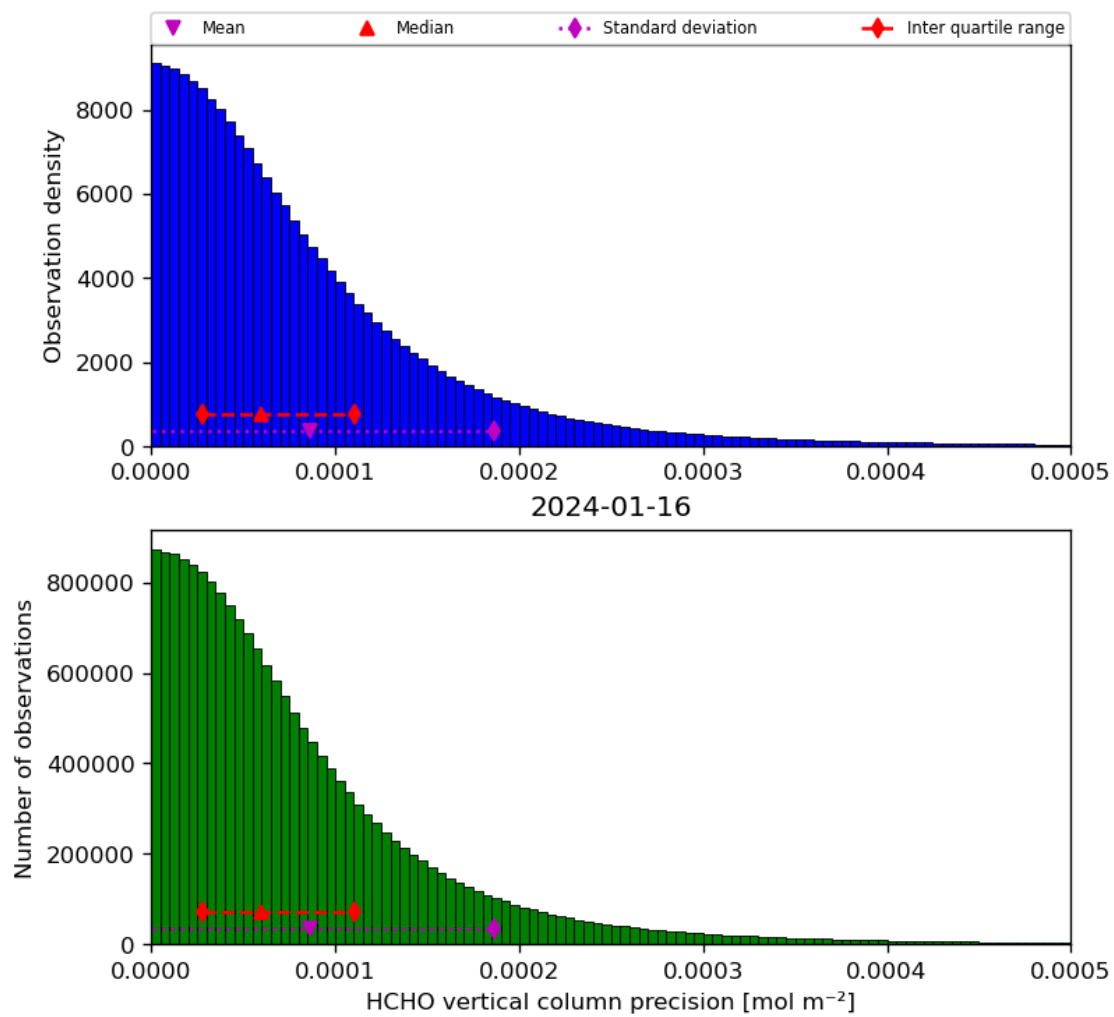
Figure 36: Histogram of “HCHO vertical column precision” for 2024-01-15 to 2024-01-17
