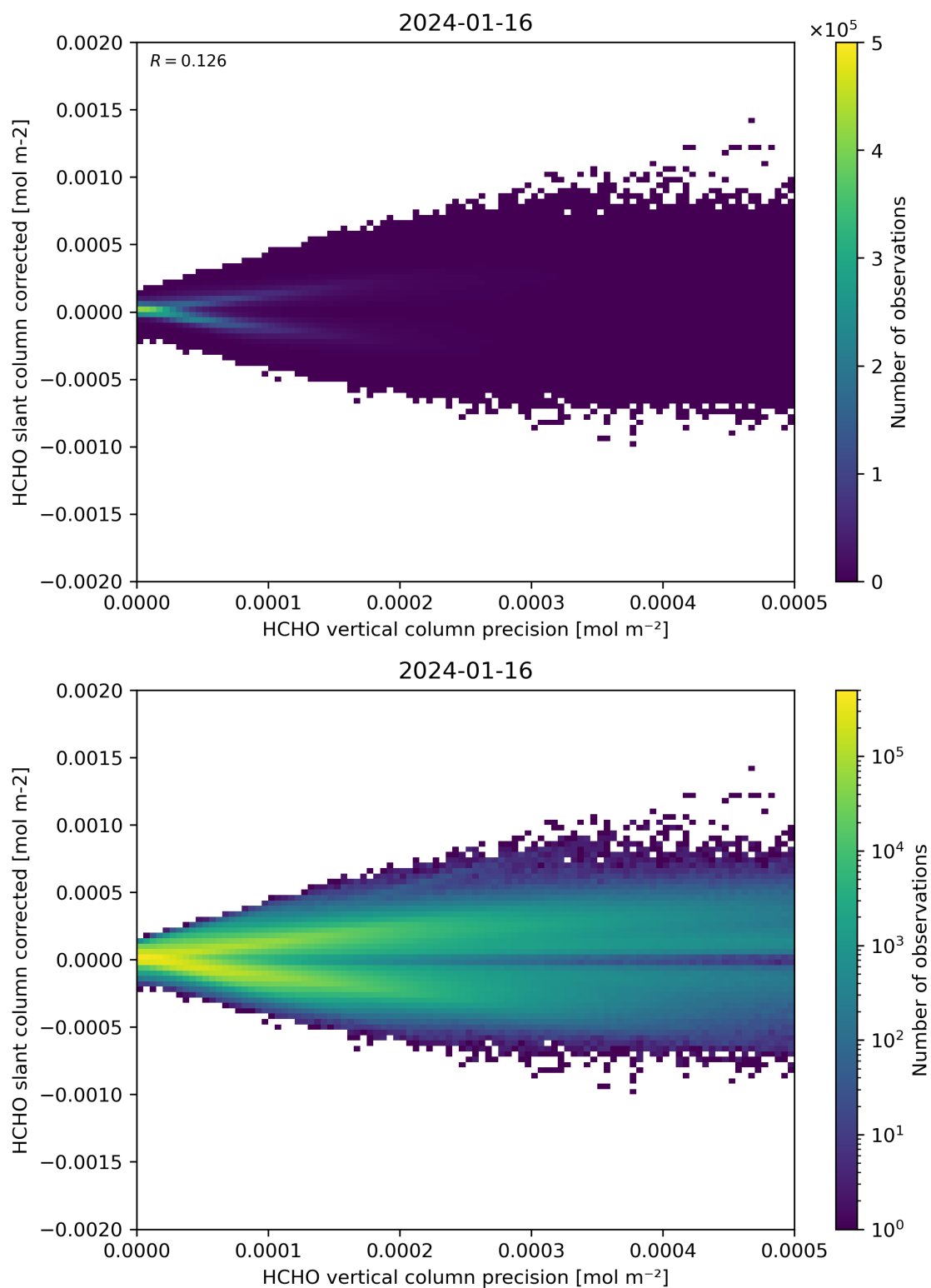
Figure 140: Scatter density plot of “HCHO vertical column precision” against “HCHO slant column corrected” for 2024-01-15 to 2024-01-17.
