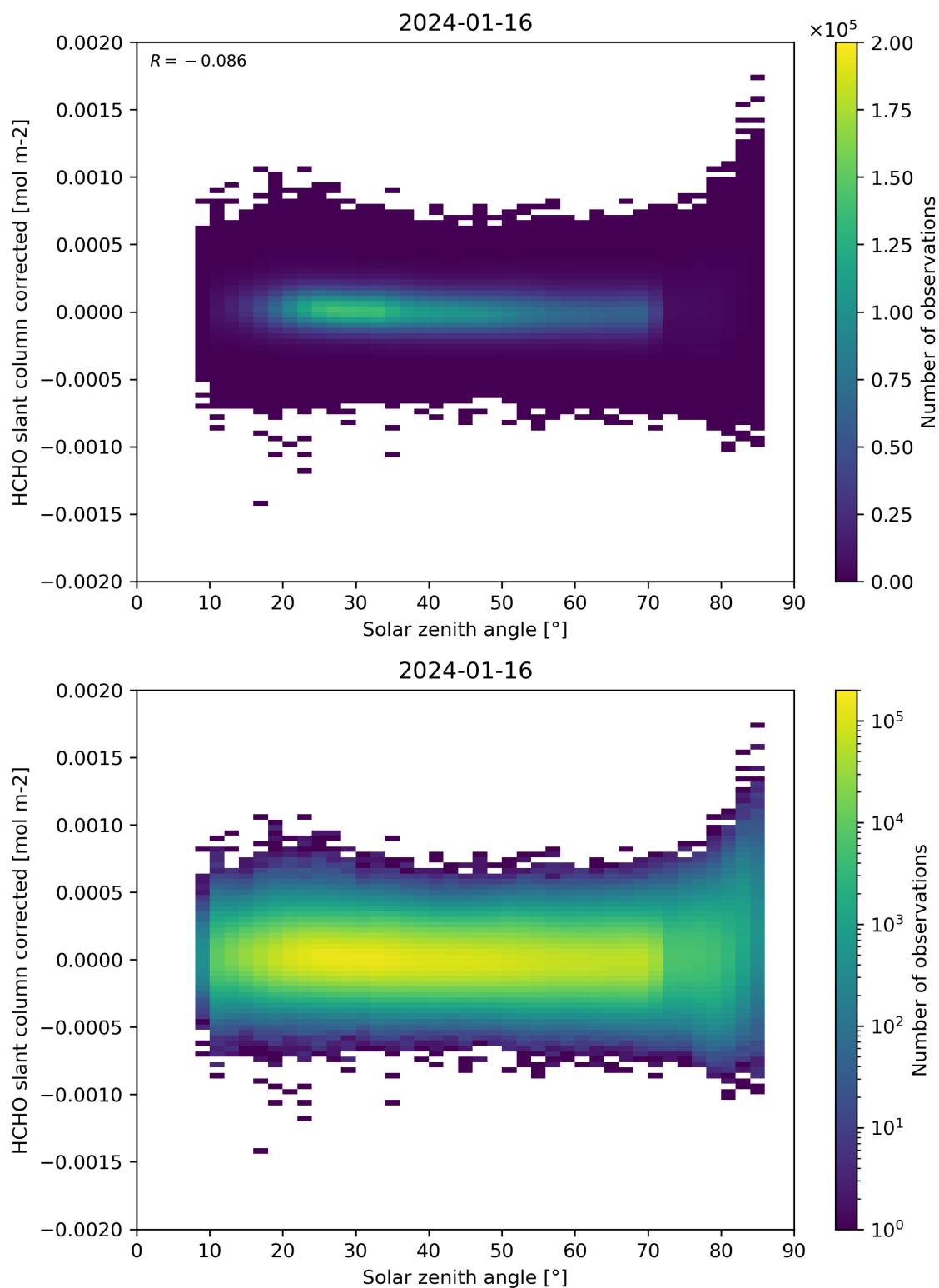
Figure 171: Scatter density plot of “Solar zenith angle” against “HCHO slant column corrected” for 2024-01-15 to 2024-01-17.
