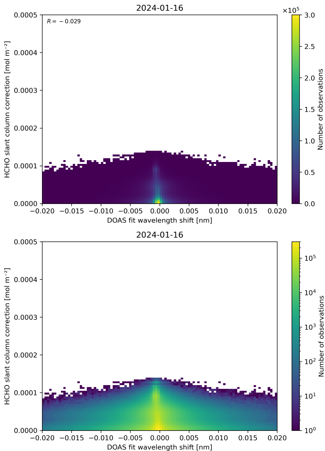
Figure 67: Scatter density plot of “DOAS fit wavelength shift” against “HCHO slant column correction” for 2024-01-15 to 2024-01-17.
