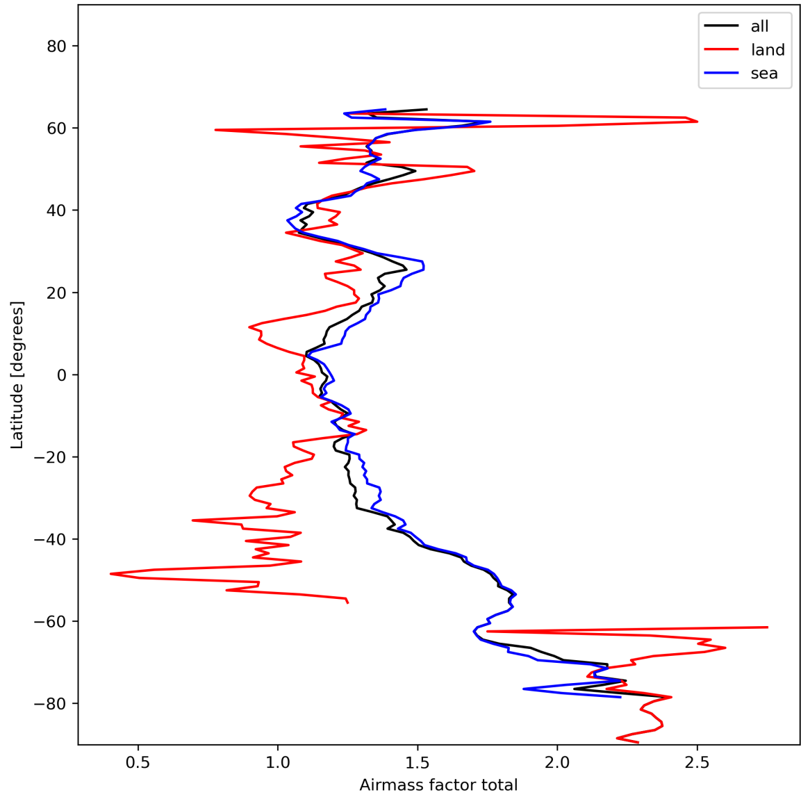
Figure 26: Zonal average of “Airmass factor total” for 2024-01-15 to 2024-01-17.
