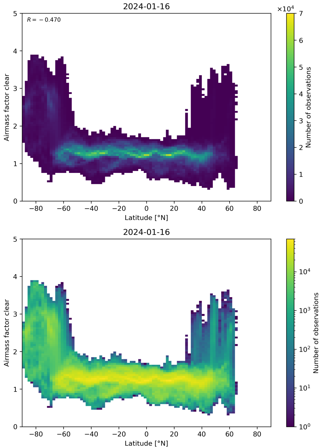
Figure 156: Scatter density plot of “Latitude” against “Airmass factor clear” for 2024-01-15 to 2024-01-17.
