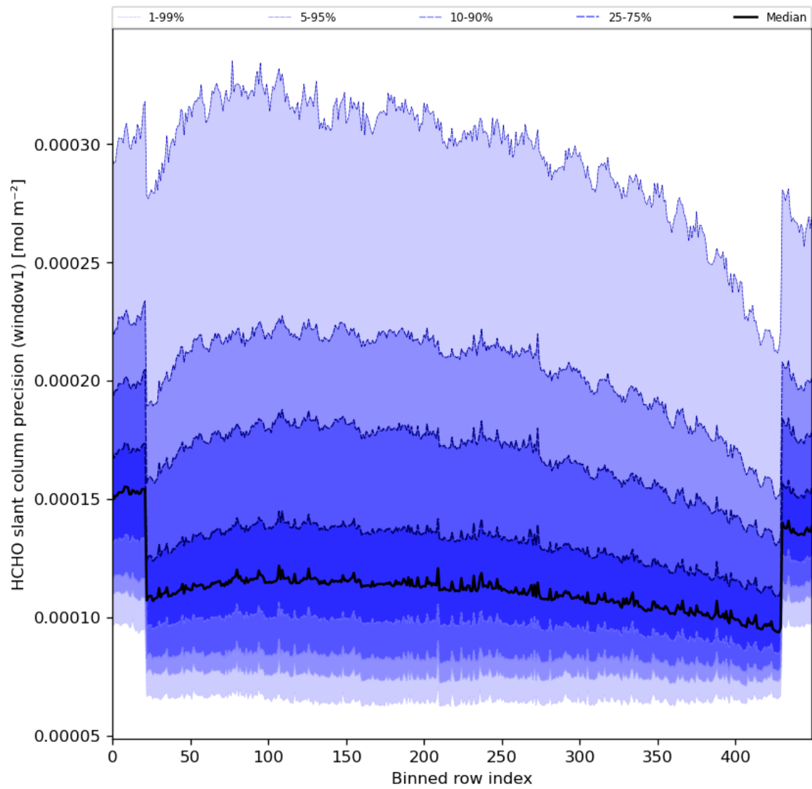
Figure 53: Along track statistics of “HCHO slant column precision (window1)” for 2024-01-15 to 2024-01-17
