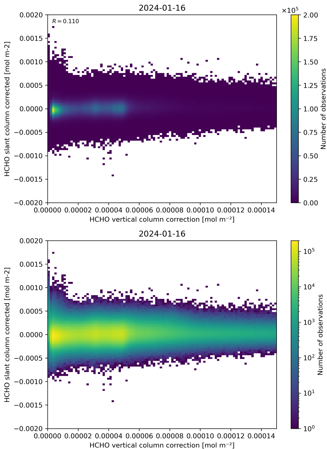
Figure 116: Scatter density plot of “HCHO vertical column correction” against “HCHO slant column corrected” for 2024-01-15 to 2024-01-17.
