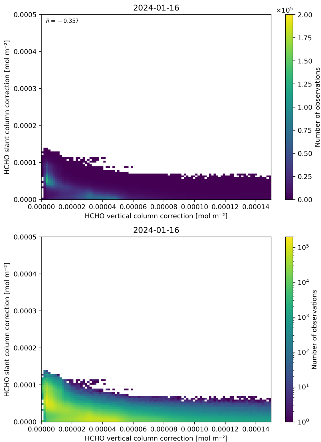
Figure 117: Scatter density plot of “HCHO vertical column correction” against “HCHO slant column correction” for 2024-01-15 to 2024-01-17.
