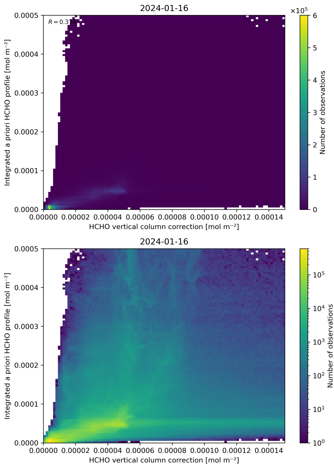
Figure 122: Scatter density plot of “HCHO vertical column correction” against “Integrated a priori HCHO profile” for 2024-01-15 to 2024-01-17.
