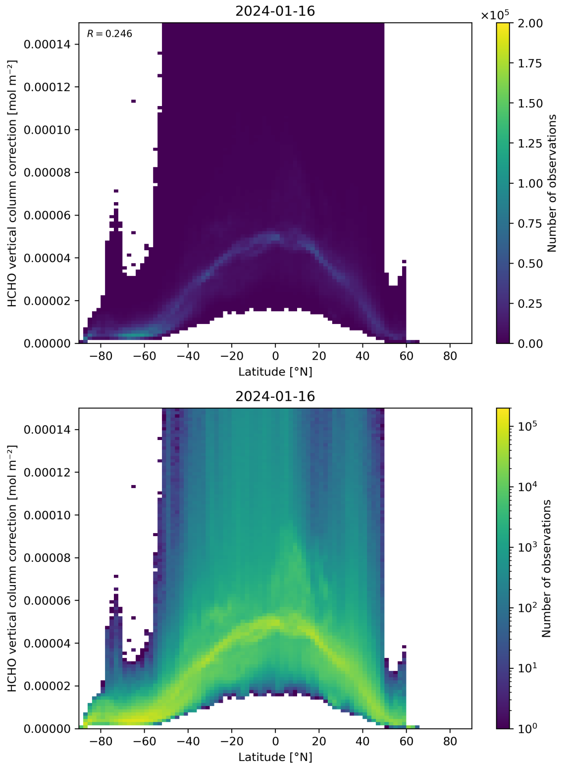
Figure 164: Scatter density plot of “Latitude” against “HCHO vertical column correction” for 2024-01-15 to 2024-01-17.
