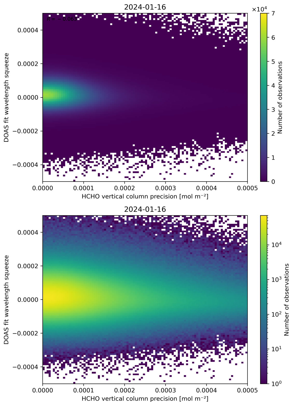
Figure 138: Scatter density plot of “HCHO vertical column precision” against “DOAS fit wavelength squeeze” for 2024-01-15 to 2024-01-17.
