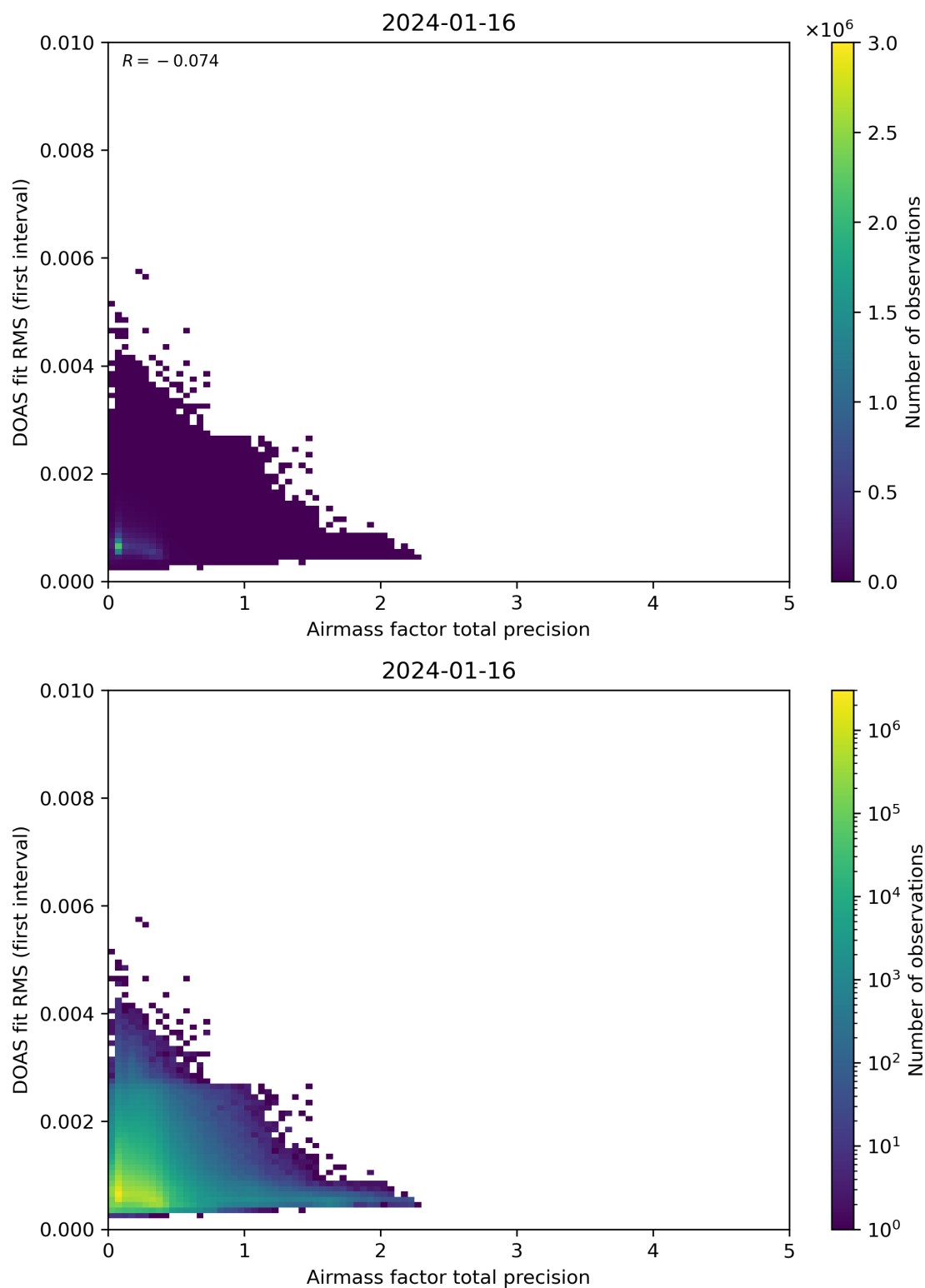
Figure 105: Scatter density plot of “Airmass factor total precision” against “DOAS fit RMS (first interval)” for 2024-01-15 to 2024-01-17.
