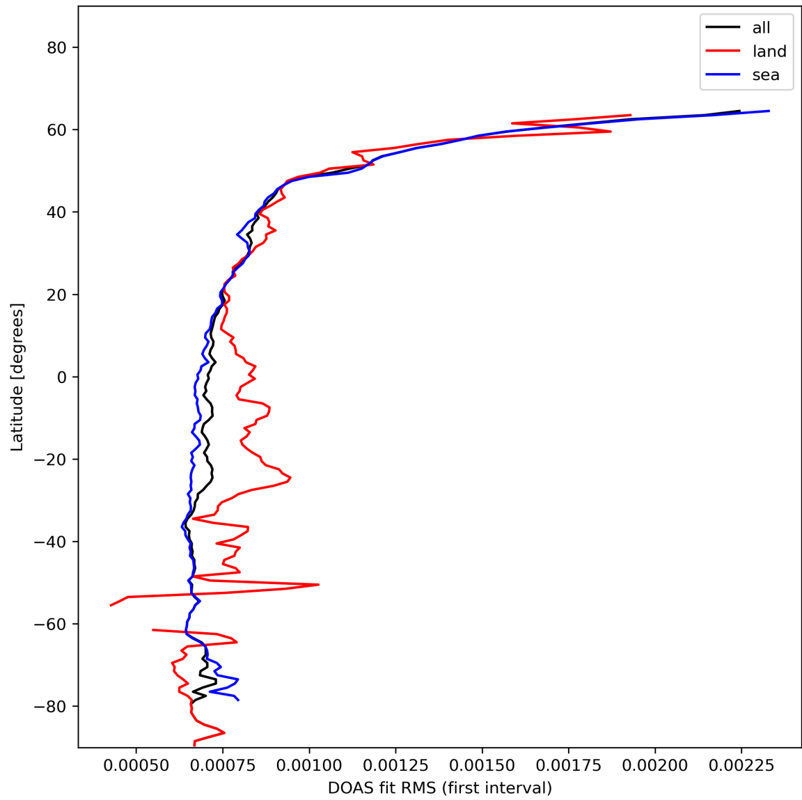
Figure 32: Zonal average of “DOAS fit RMS (first interval)” for 2024-01-15 to 2024-01-17.
