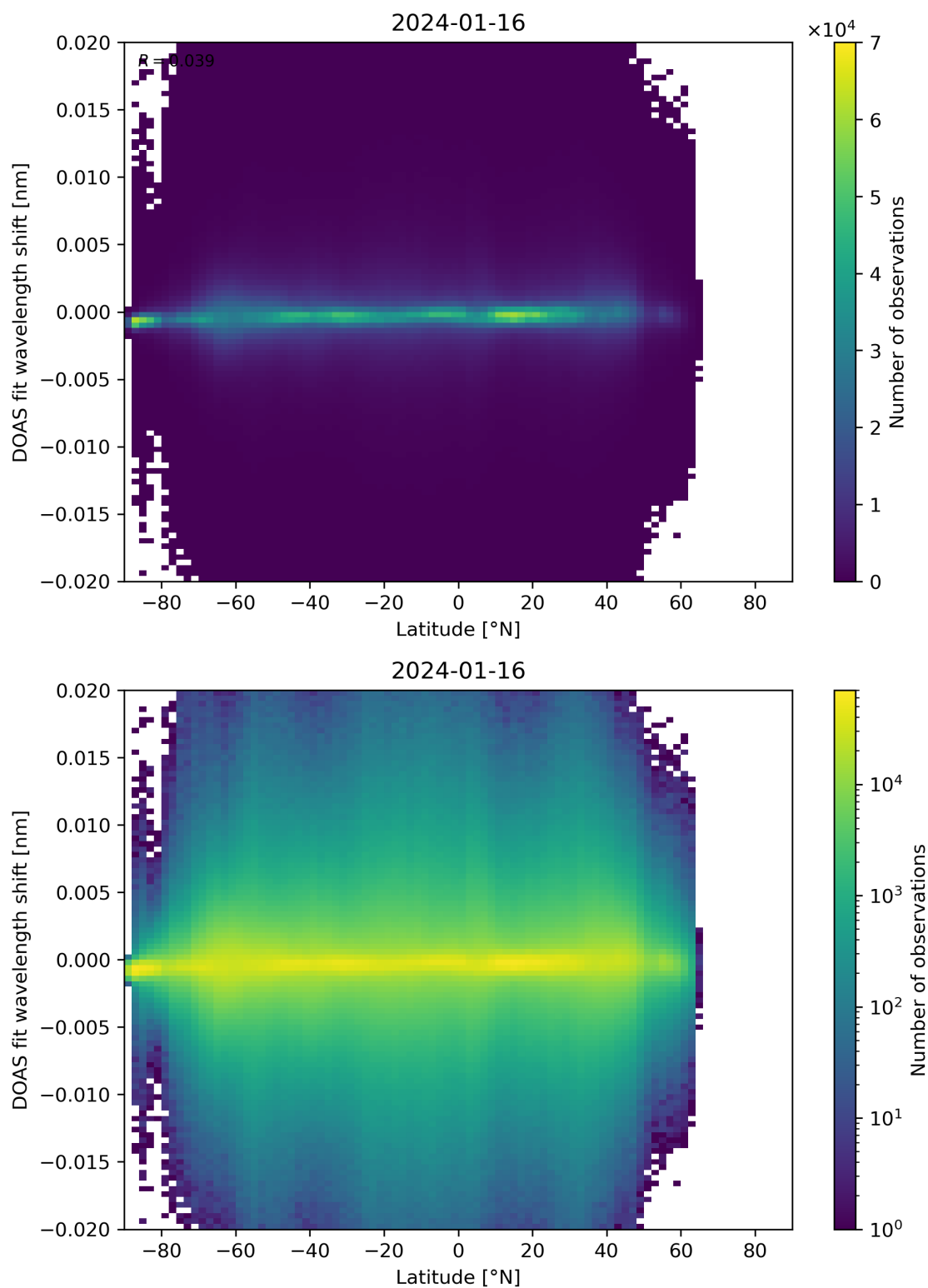
Figure 154: Scatter density plot of “Latitude” against “DOAS fit wavelength shift” for 2024-01-15 to 2024-01-17.
