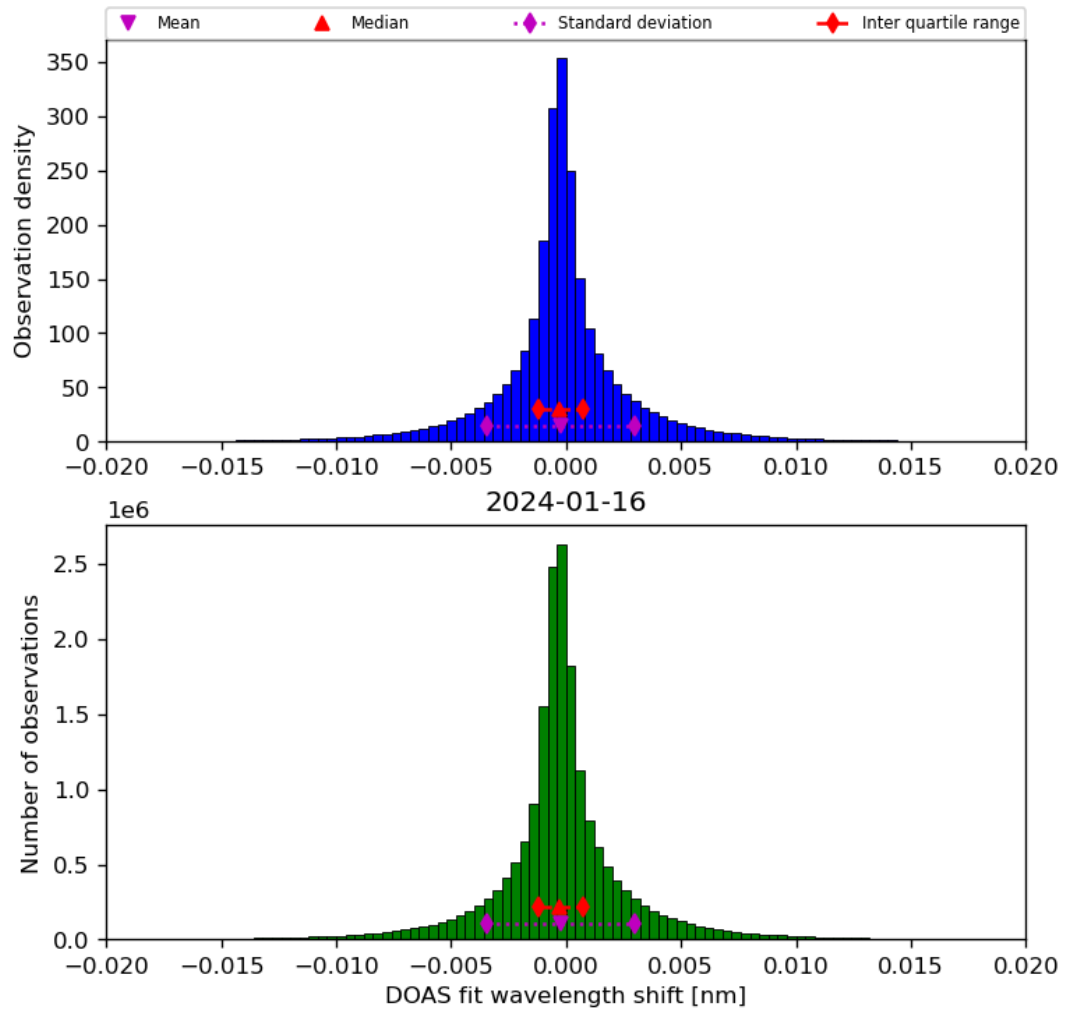
Figure 44: Histogram of “DOAS fit wavelength shift” for 2024-01-15 to 2024-01-17
