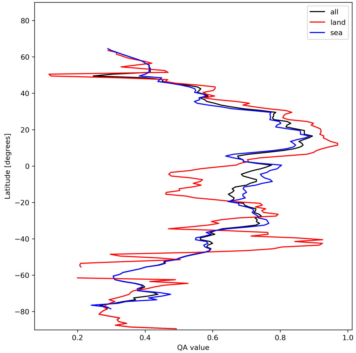
Figure 20: Zonal average of “QA value” for 2024-01-15 to 2024-01-17.
