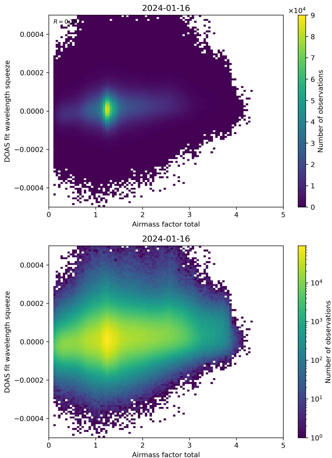
Figure 99: Scatter density plot of “Airmass factor total” against “DOAS fit wavelength squeeze” for 2024-01-15 to 2024-01-17.
