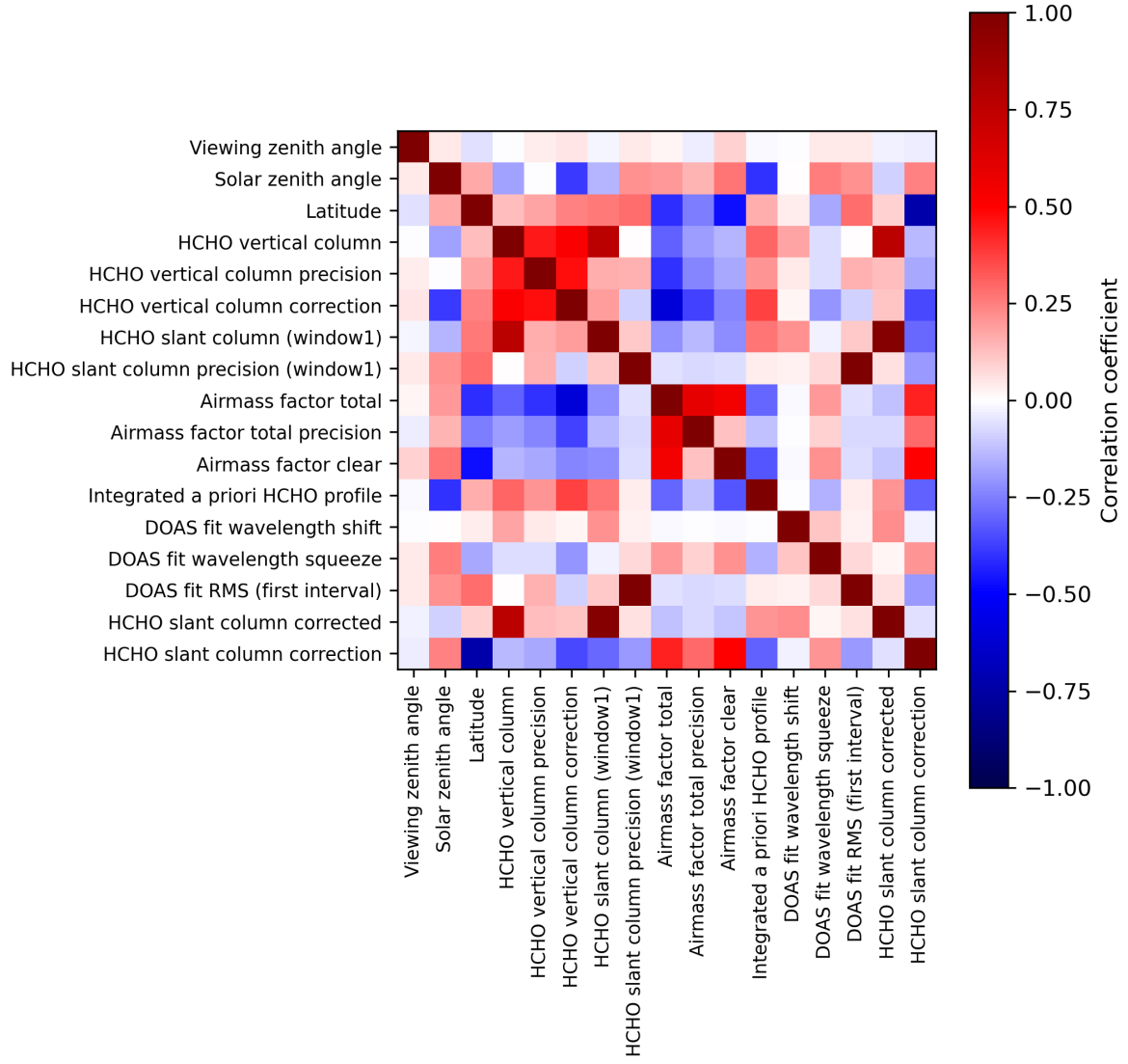
Figure 2: Map of correlation matrix for 2024-01-15 to 2024-01-17.
