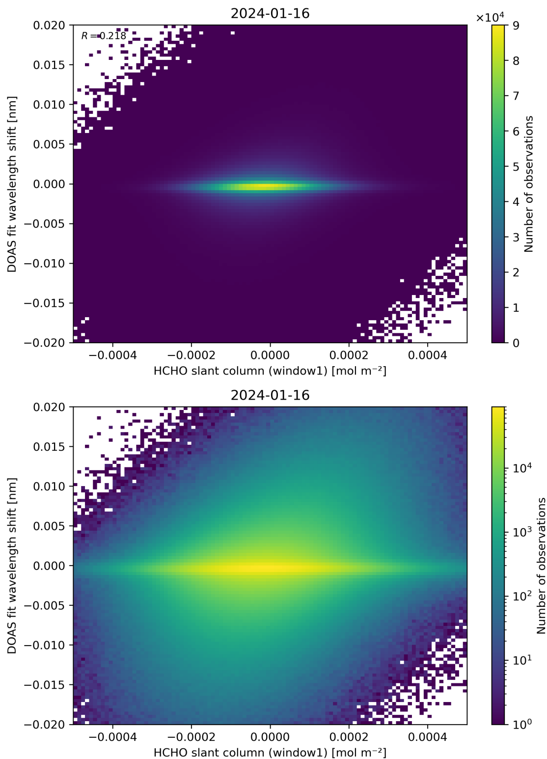
Figure 79: Scatter density plot of “HCHO slant column (window1)” against “DOAS fit wavelength shift” for 2024-01-15 to 2024-01-17.
