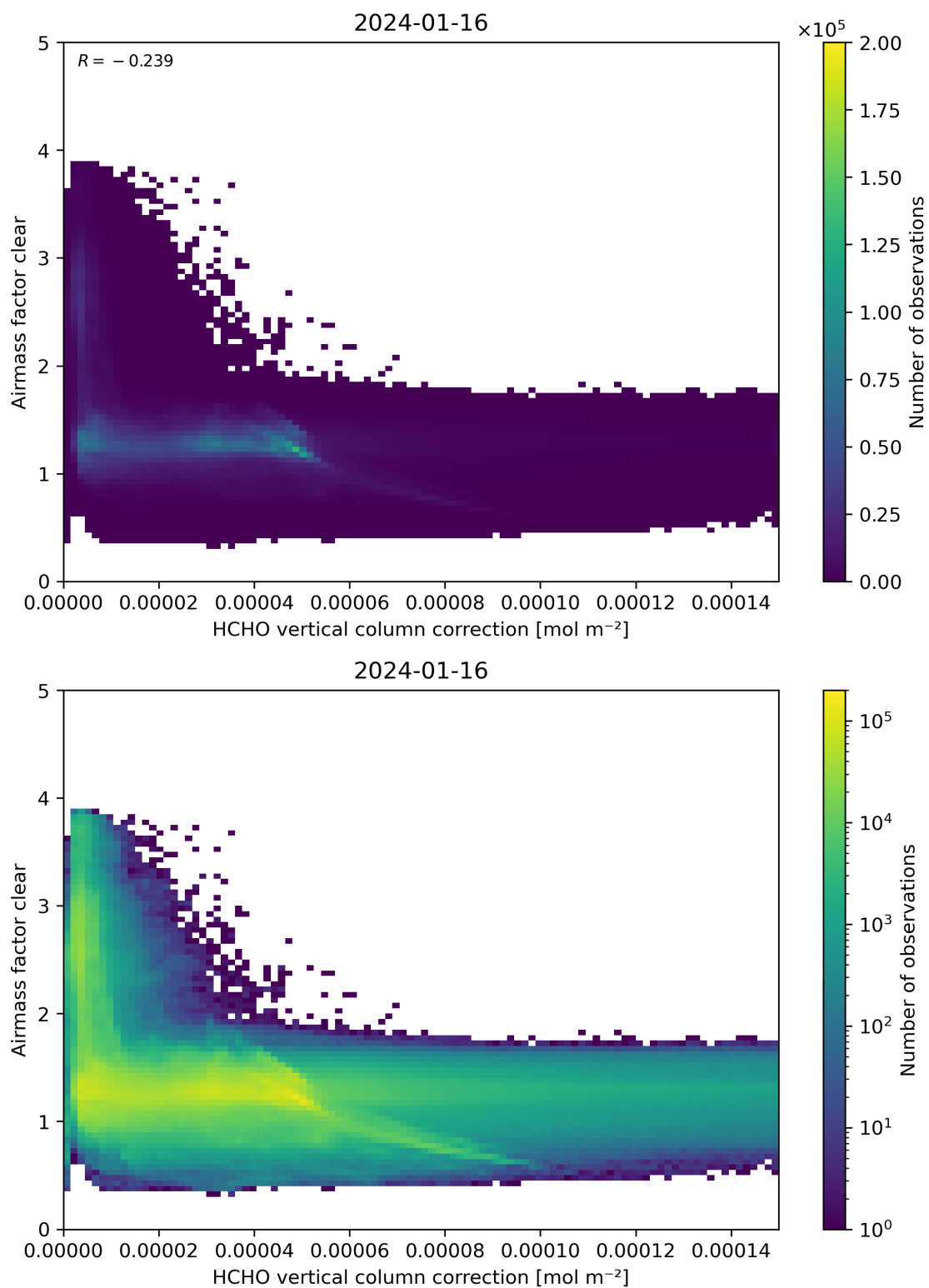
Figure 115: Scatter density plot of “HCHO vertical column correction” against “Airmass factor clear” for 2024-01-15 to 2024-01-17.
