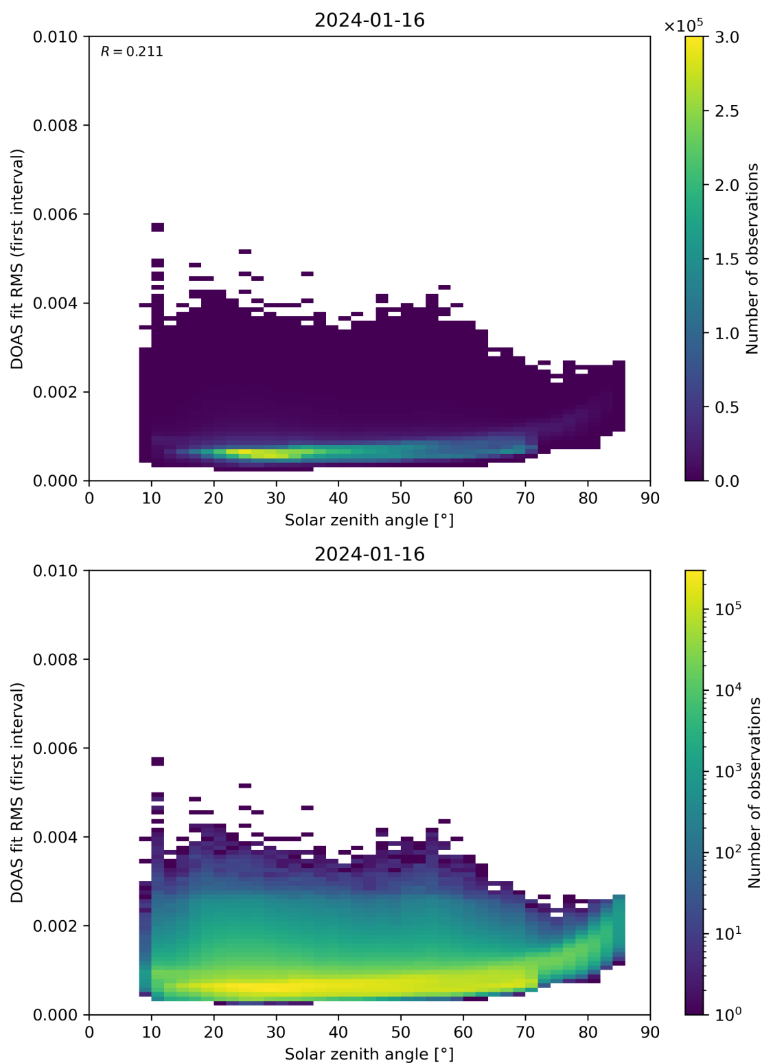
Figure 167: Scatter density plot of “Solar zenith angle” against “DOAS fit RMS (first interval)” for 2024-01-15 to 2024-01-17.
