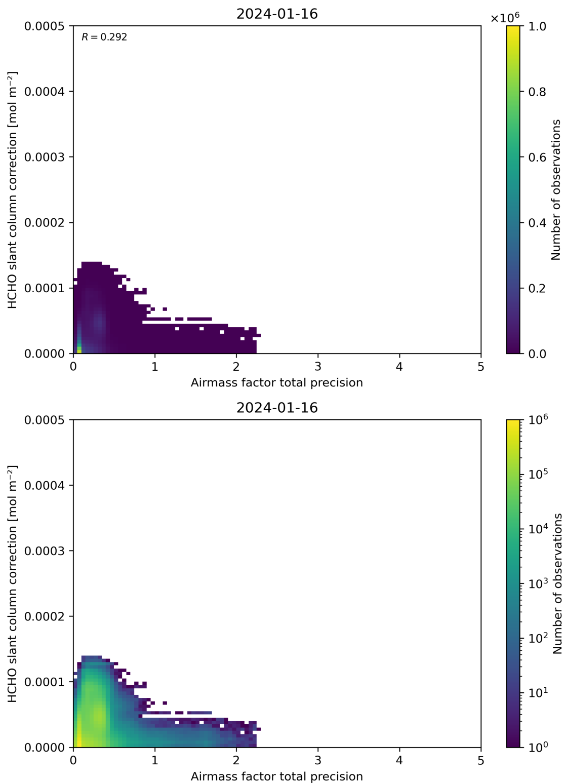
Figure 110: Scatter density plot of “Airmass factor total precision” against “HCHO slant column correction” for 2024-01-15 to 2024-01-17.
