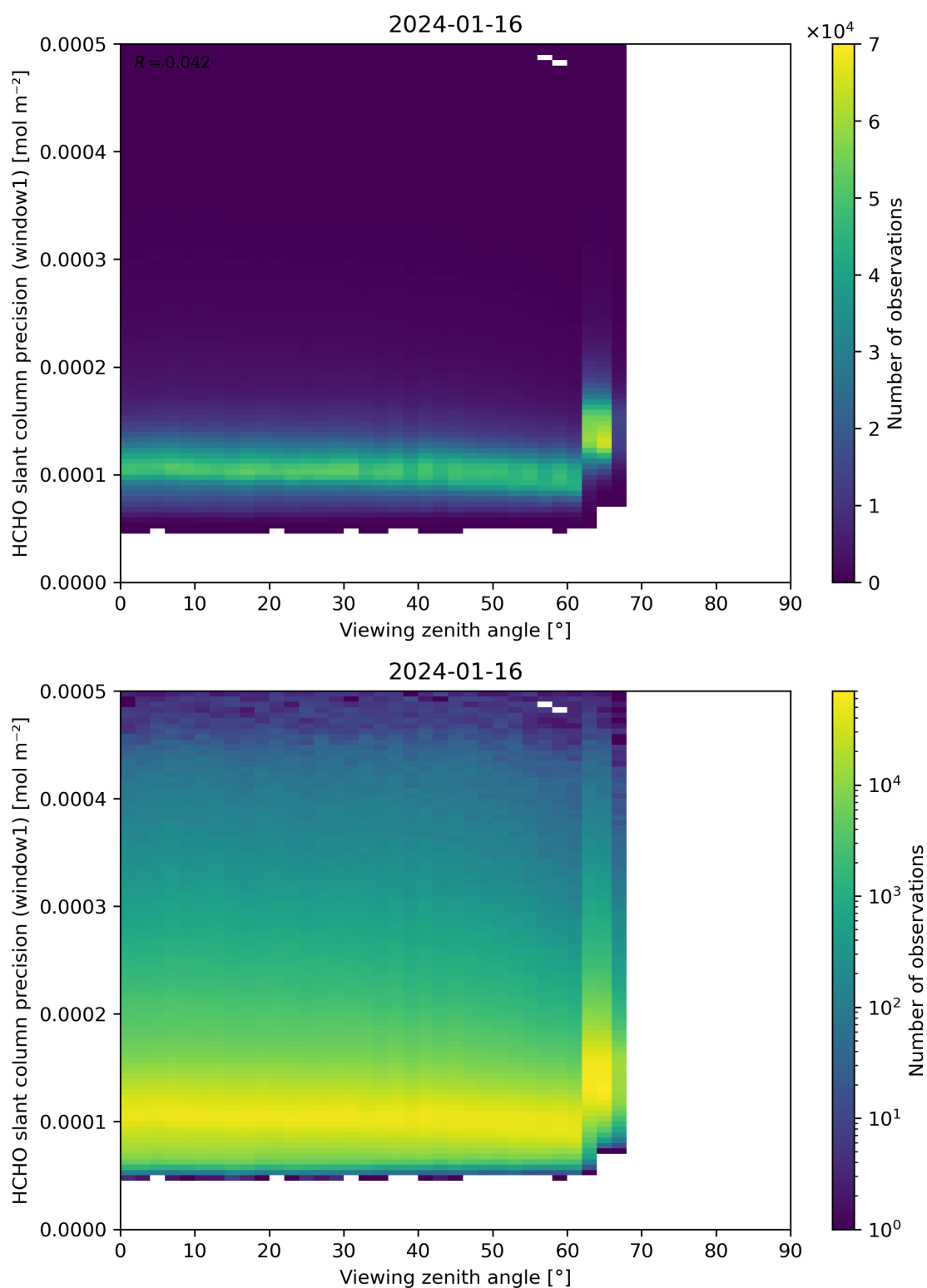
Figure 189: Scatter density plot of “Viewing zenith angle” against “HCHO slant column precision (window1)” for 2024-01-15 to 2024-01-17.
