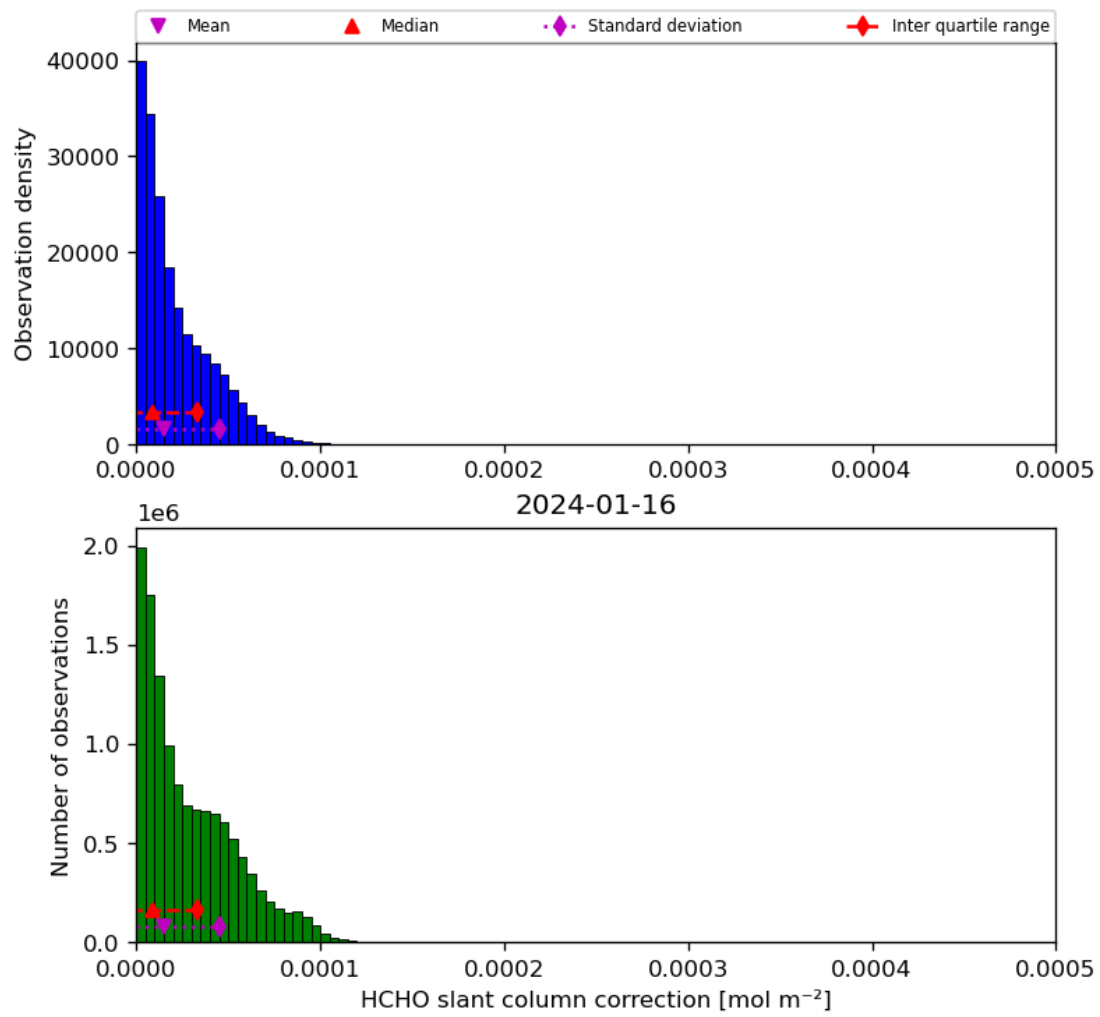
Figure 47: Histogram of “HCHO slant column correction” for 2024-01-15 to 2024-01-17
