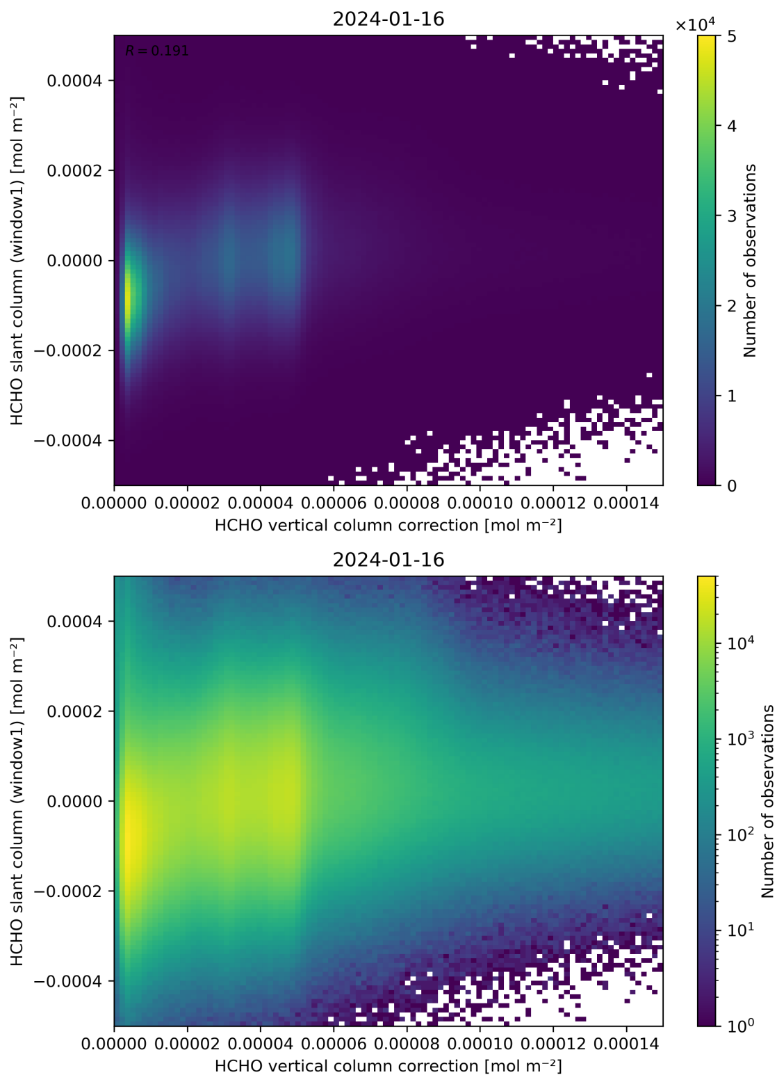
Figure 118: Scatter density plot of “HCHO vertical column correction” against “HCHO slant column (window1)” for 2024-01-15 to 2024-01-17.
