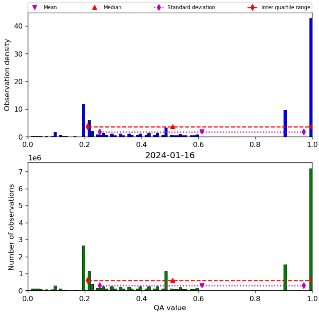
Figure 34: Histogram of “QA value” for 2024-01-15 to 2024-01-17
