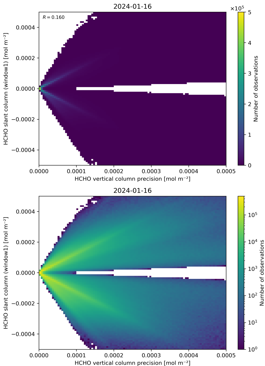
Figure 142: Scatter density plot of “HCHO vertical column precision” against “HCHO slant column (window1)” for 2024-01-15 to 2024-01-17.
