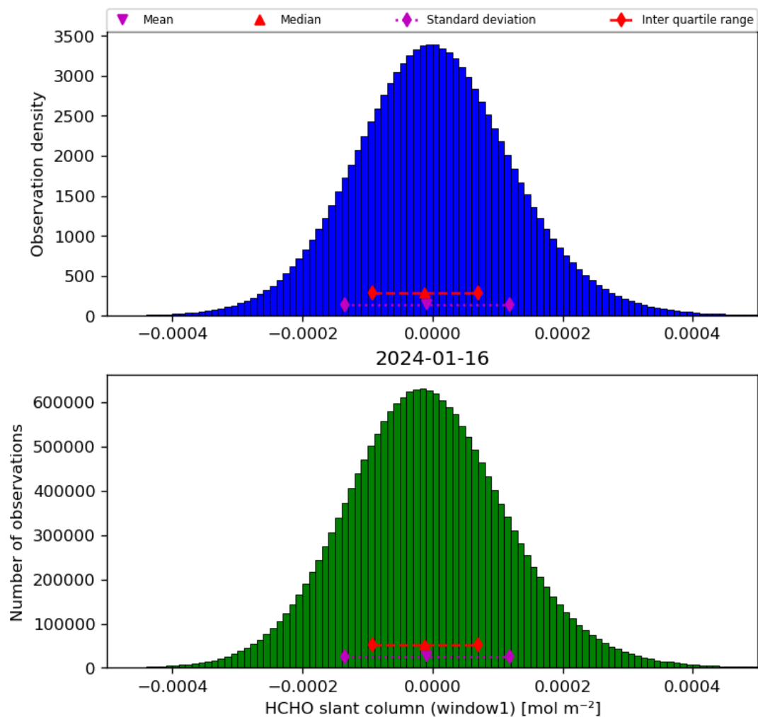
Figure 38: Histogram of “HCHO slant column (window1)” for 2024-01-15 to 2024-01-17
