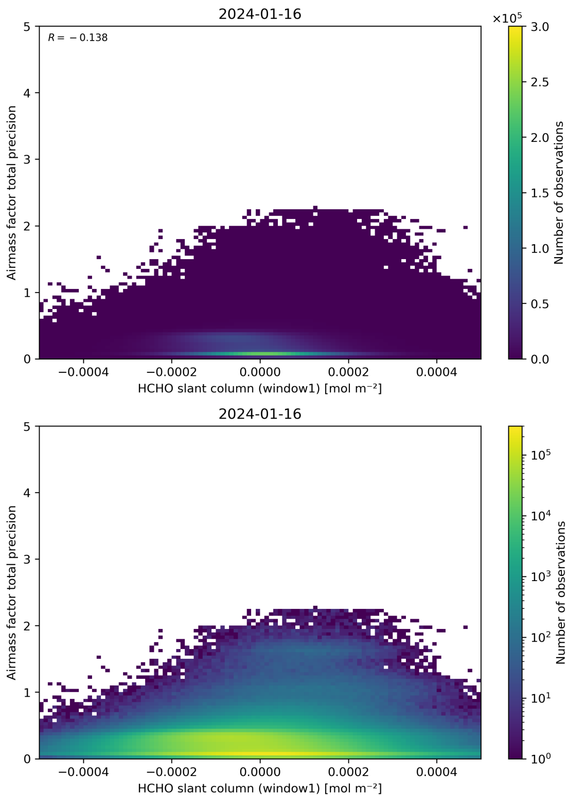
Figure 86: Scatter density plot of “HCHO slant column (window1)” against “Airmass factor total precision” for 2024-01-15 to 2024-01-17.
