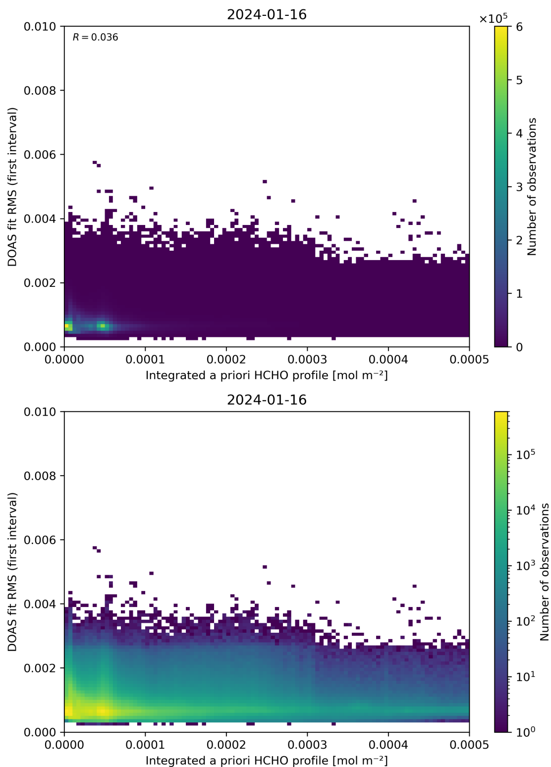
Figure 148: Scatter density plot of “Integrated a priori HCHO profile” against “DOAS fit RMS (first interval)” for 2024-01-15 to 2024-01-17.
