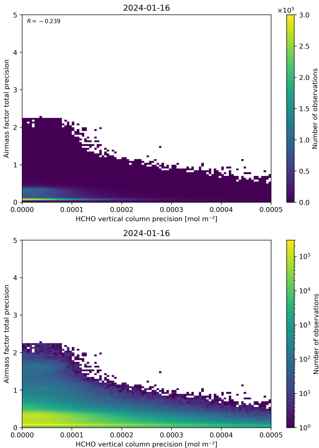
Figure 145: Scatter density plot of “HCHO vertical column precision” against “Airmass factor total precision” for 2024-01-15 to 2024-01-17.
