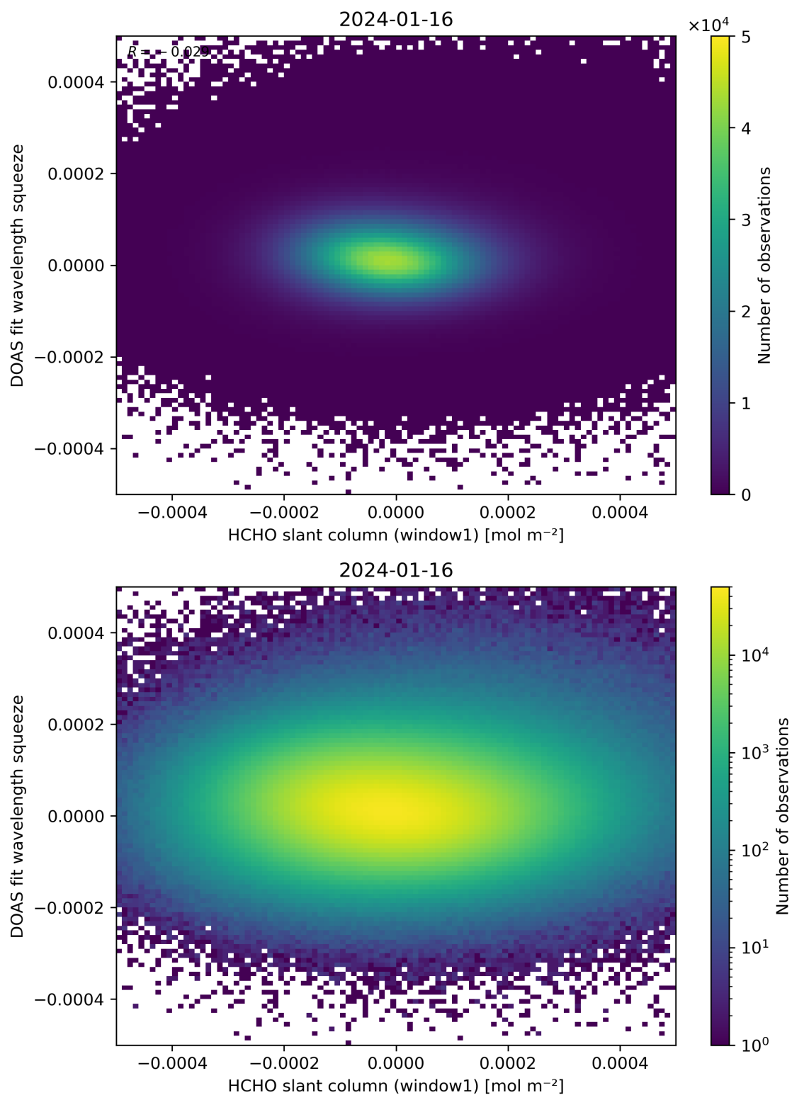
Figure 80: Scatter density plot of “HCHO slant column (window1)” against “DOAS fit wavelength squeeze” for 2024-01-15 to 2024-01-17.
