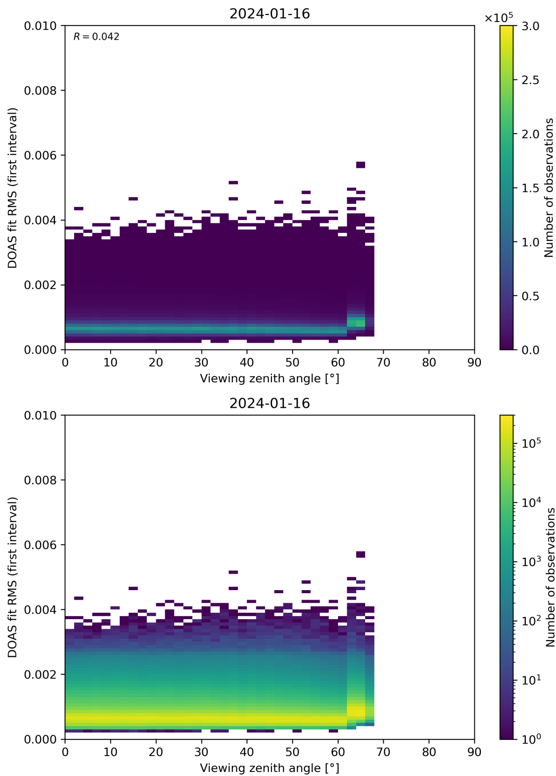
Figure 182: Scatter density plot of “Viewing zenith angle” against “DOAS fit RMS (first interval)” for 2024-01-15 to 2024-01-17.
