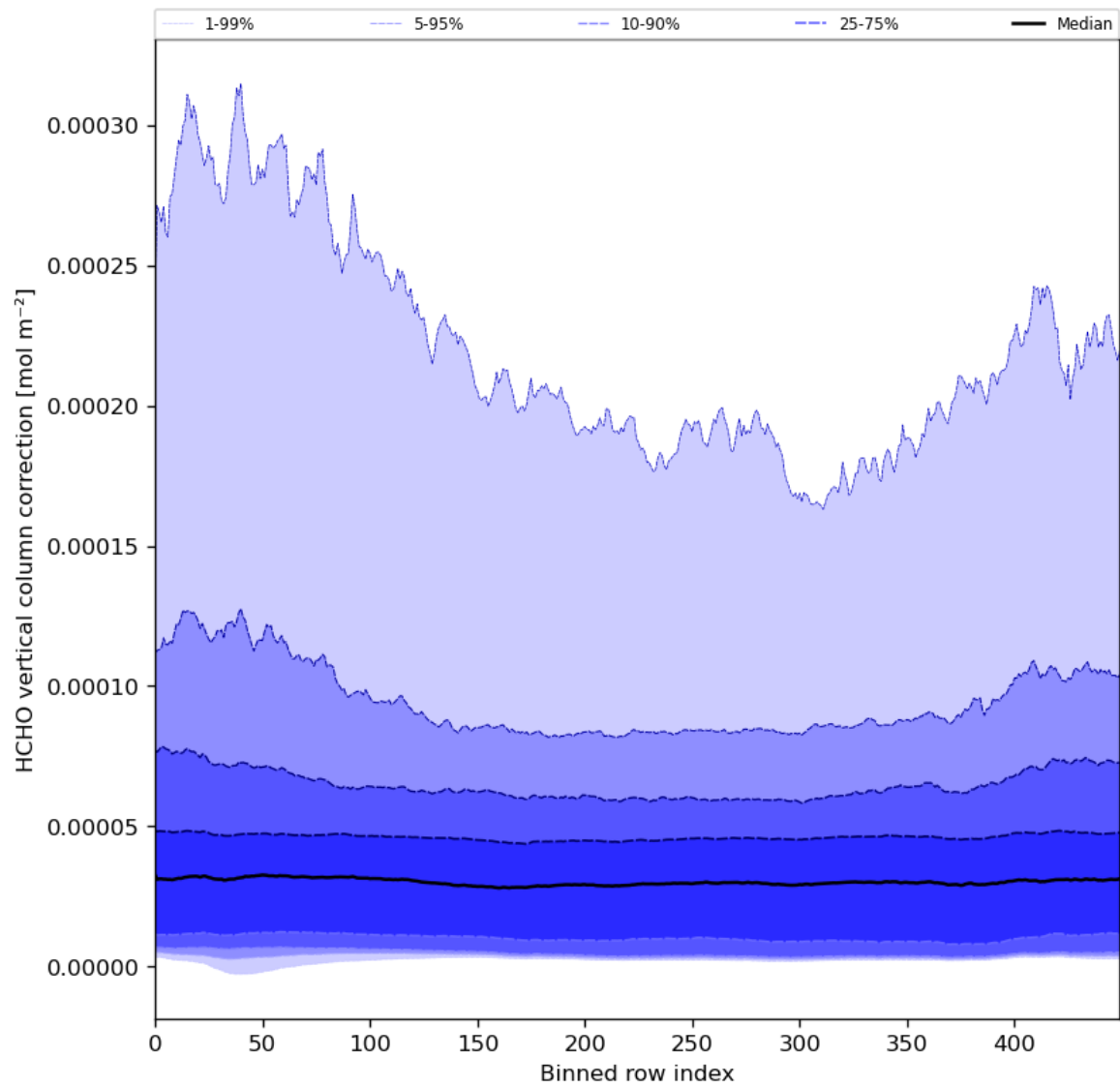
Figure 51: Along track statistics of “HCHO vertical column correction” for 2024-01-15 to 2024-01-17
