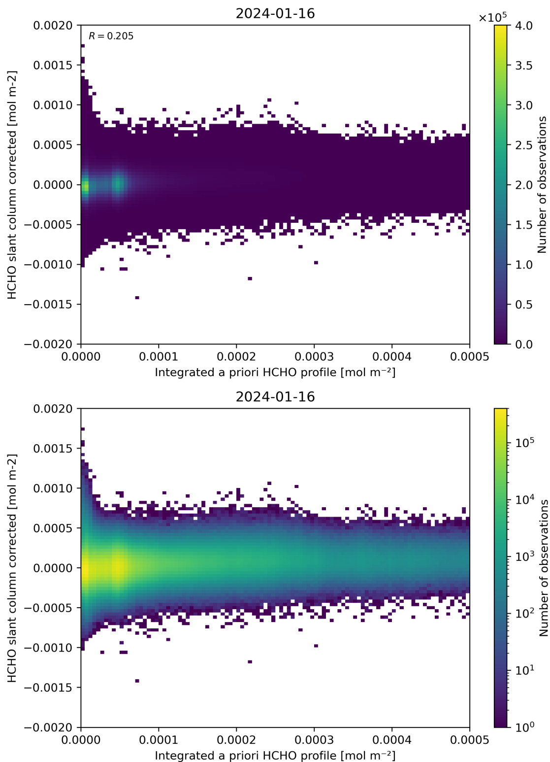
Figure 151: Scatter density plot of “Integrated a priori HCHO profile” against “HCHO slant column corrected” for 2024-01-15 to 2024-01-17.
