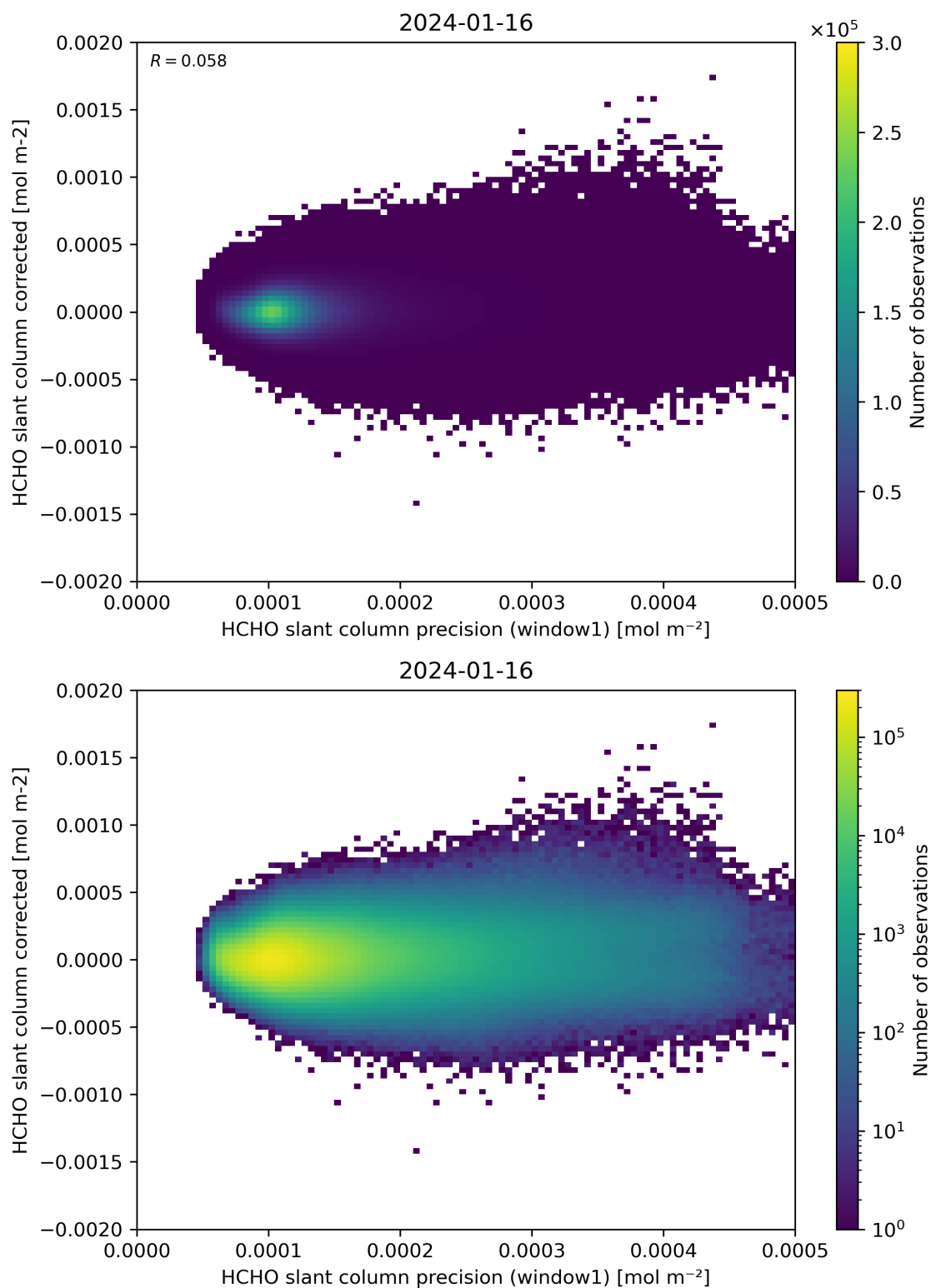
Figure 92: Scatter density plot of “HCHO slant column precision (window1)” against “HCHO slant column corrected” for 2024-01-15 to 2024-01-17.
