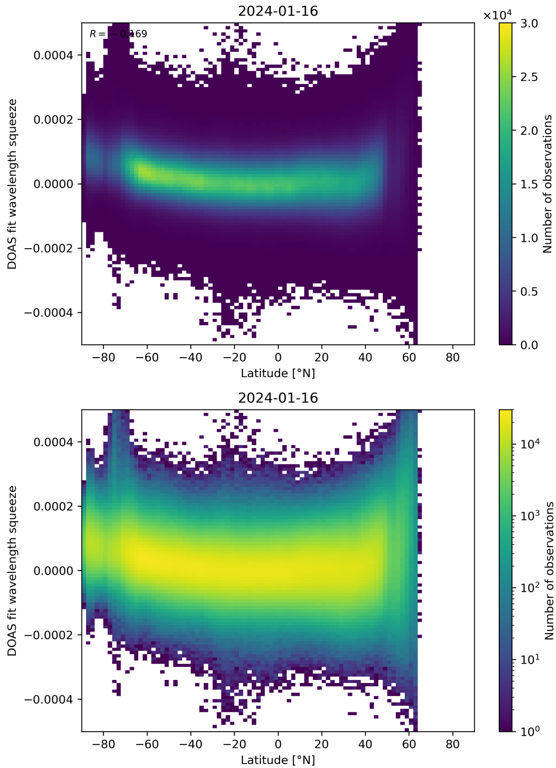
Figure 155: Scatter density plot of “Latitude” against “DOAS fit wavelength squeeze” for 2024-01-15 to 2024-01-17.
