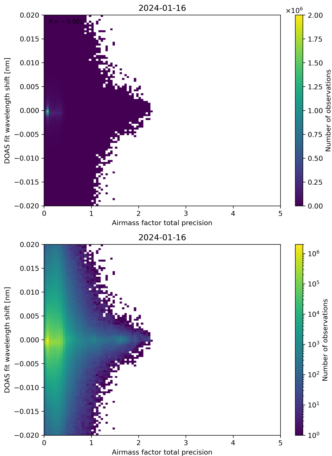
Figure 106: Scatter density plot of “Airmass factor total precision” against “DOAS fit wavelength shift” for 2024-01-15 to 2024-01-17.
