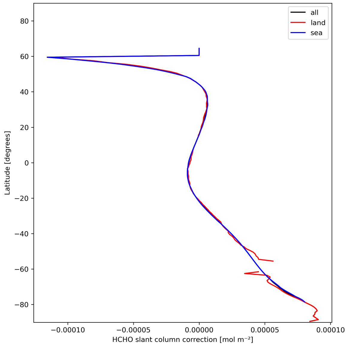
Figure 33: Zonal average of “HCHO slant column correction” for 2024-01-15 to 2024-01-17.
