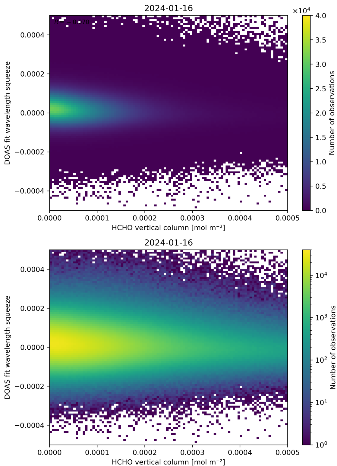
Figure 125: Scatter density plot of “HCHO vertical column” against “DOAS fit wavelength squeeze” for 2024-01-15 to 2024-01-17.
