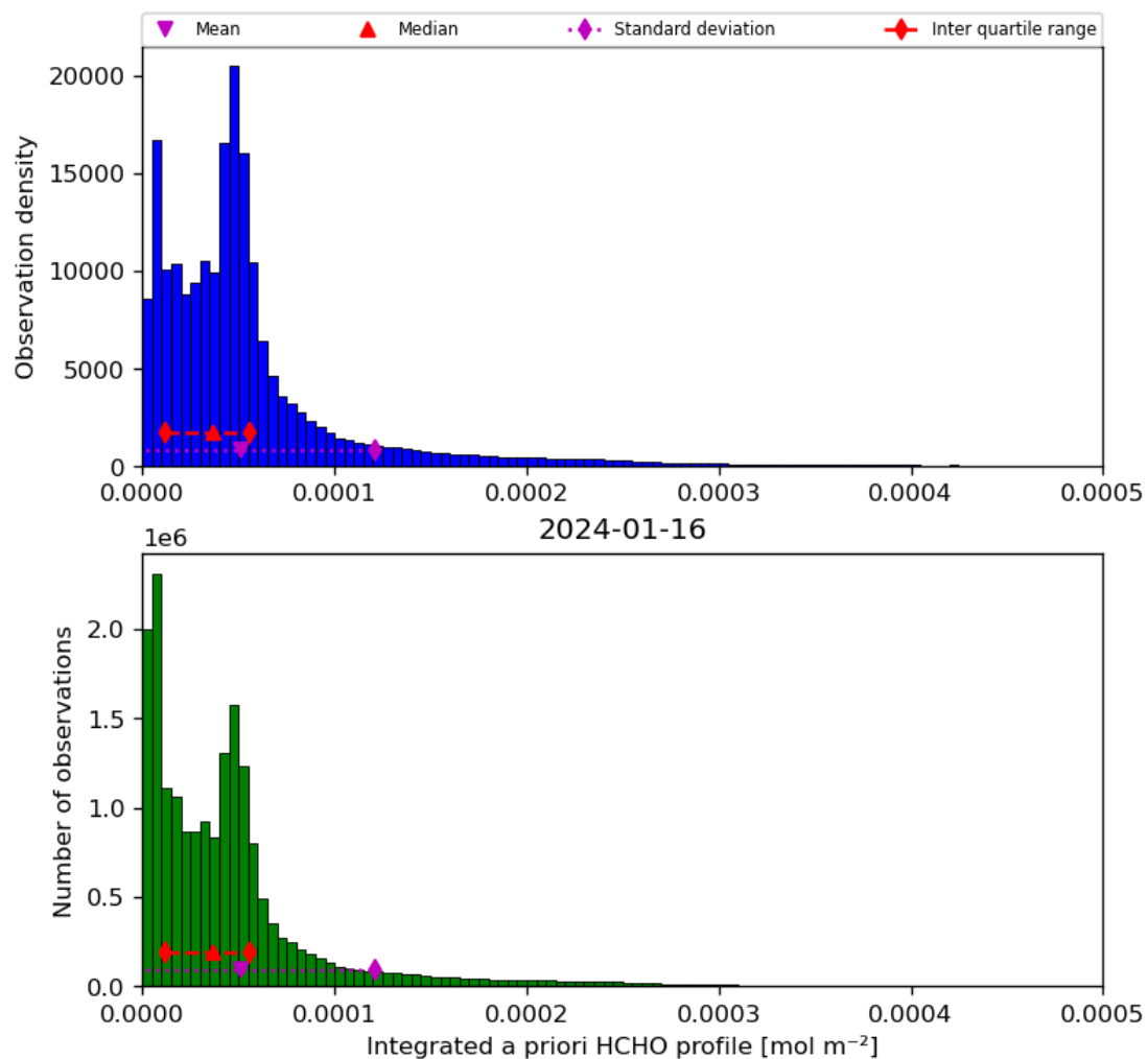
Figure 43: Histogram of “Integrated a priori HCHO profile” for 2024-01-15 to 2024-01-17
