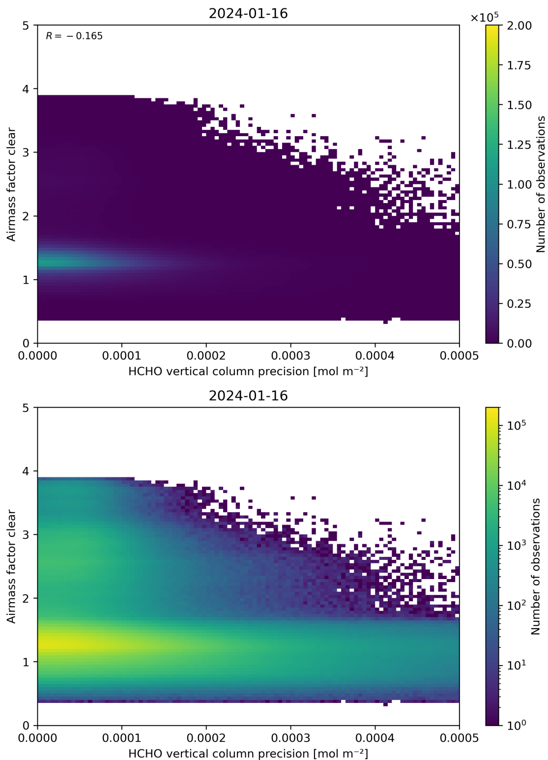
Figure 139: Scatter density plot of “HCHO vertical column precision” against “Airmass factor clear” for 2024-01-15 to 2024-01-17.
