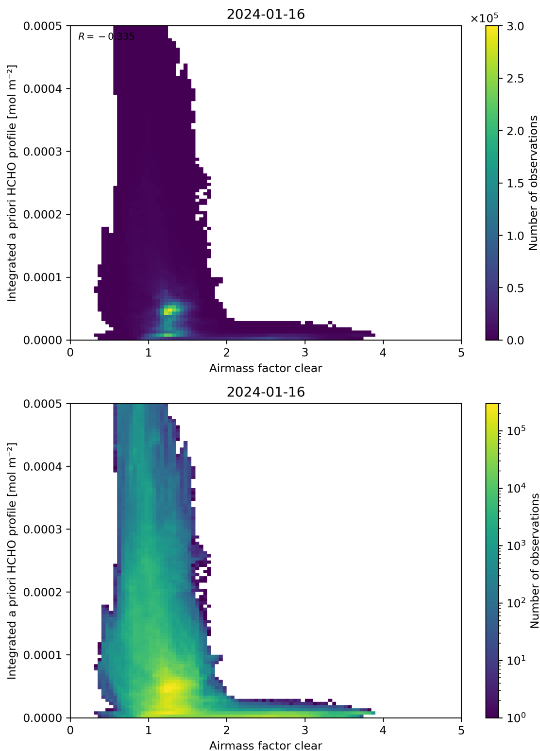
Figure 76: Scatter density plot of “Airmass factor clear” against “Integrated a priori HCHO profile” for 2024-01-15 to 2024-01-17.
