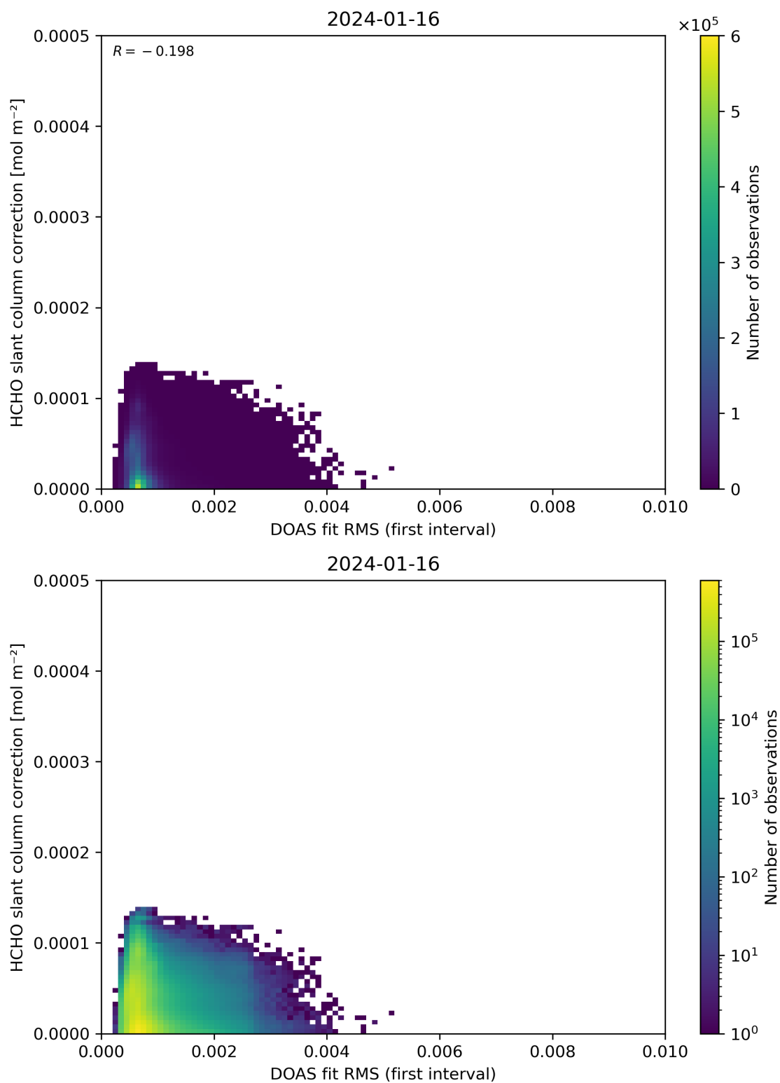
Figure 63: Scatter density plot of “DOAS fit RMS (first interval)” against “HCHO slant column correction” for 2024-01-15 to 2024-01-17.
