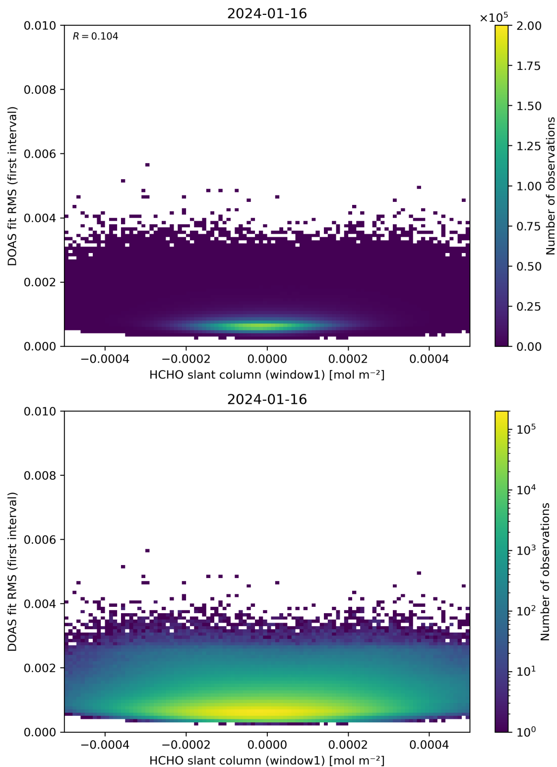
Figure 78: Scatter density plot of “HCHO slant column (window1)” against “DOAS fit RMS (first interval)” for 2024-01-15 to 2024-01-17.
