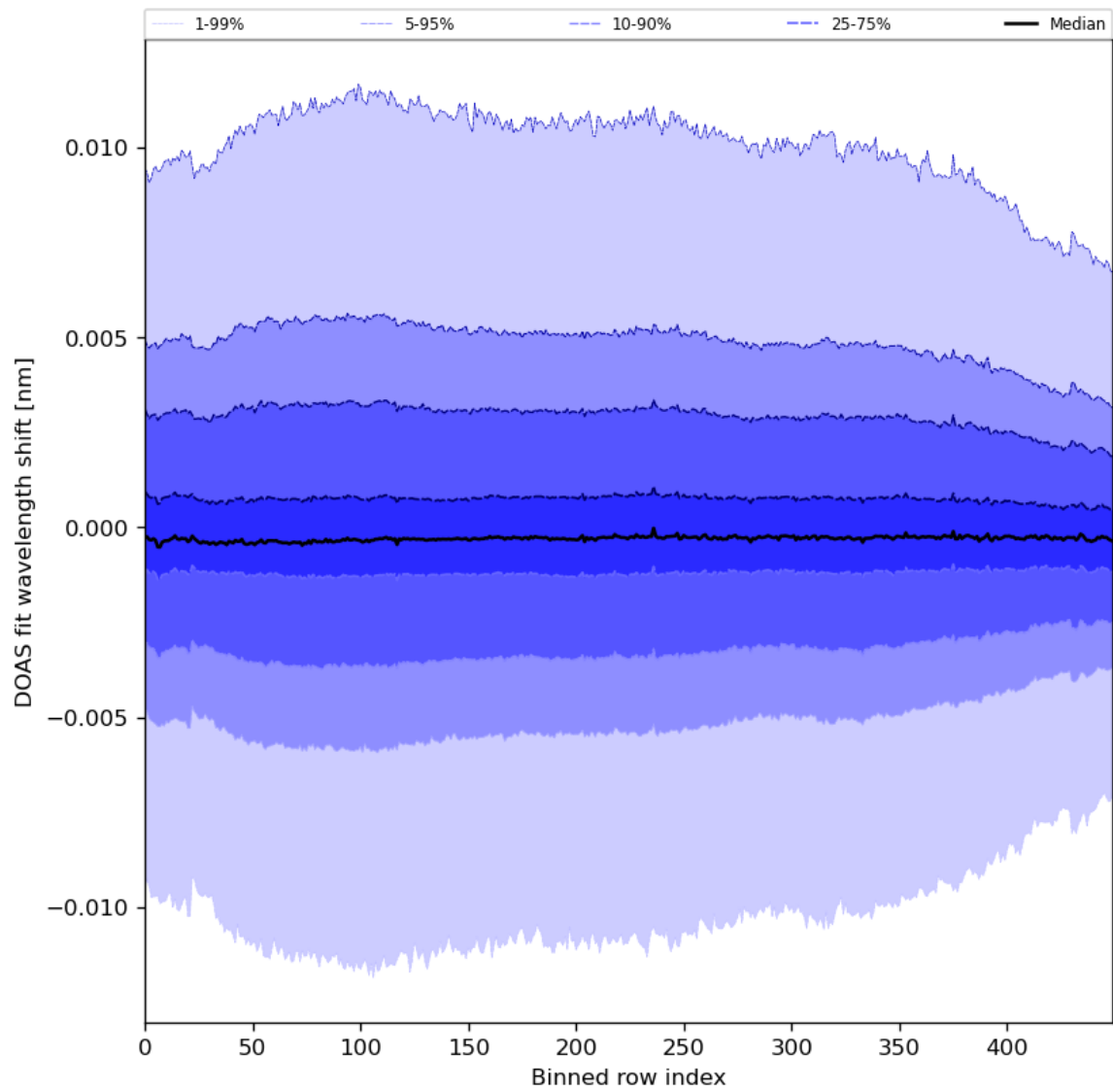
Figure 58: Along track statistics of “DOAS fit wavelength shift” for 2024-01-15 to 2024-01-17
