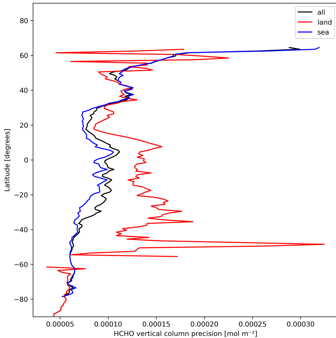
Figure 22: Zonal average of “HCHO vertical column precision” for 2024-01-15 to 2024-01-17.
