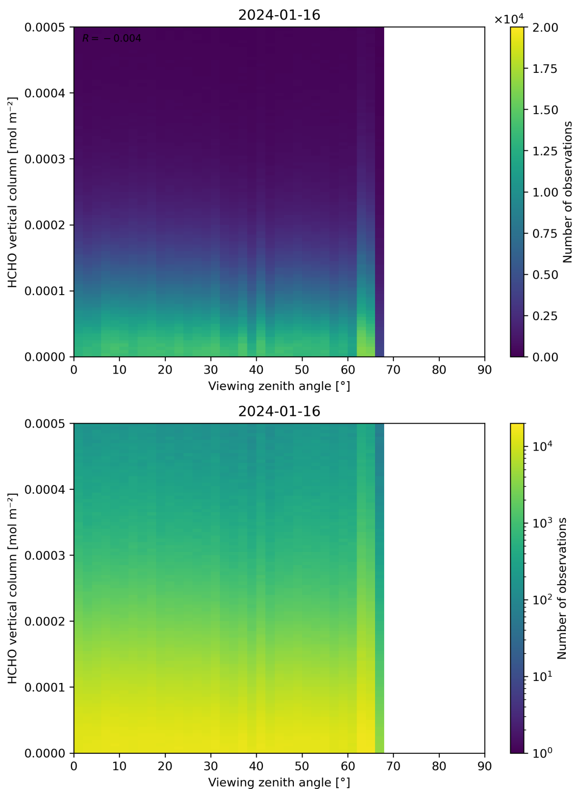
Figure 192: Scatter density plot of “Viewing zenith angle” against “HCHO vertical column” for 2024-01-15 to 2024-01-17.
