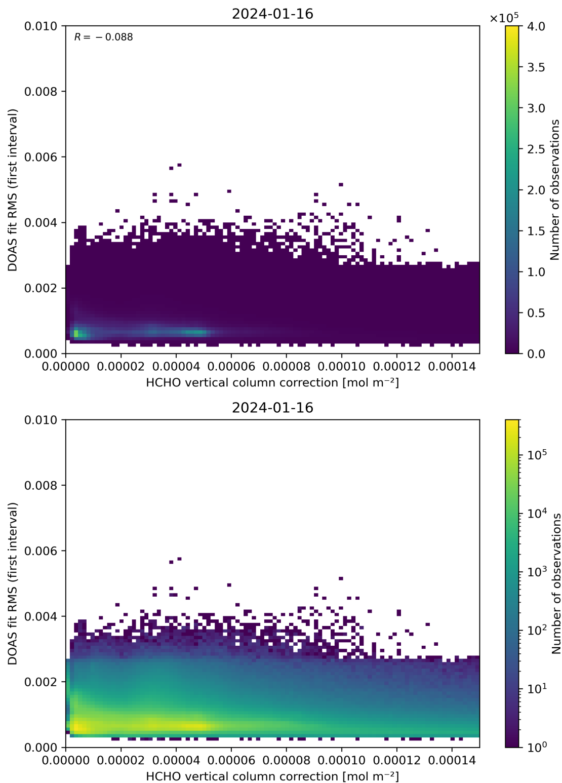
Figure 112: Scatter density plot of “HCHO vertical column correction” against “DOAS fit RMS (first interval)” for 2024-01-15 to 2024-01-17.
