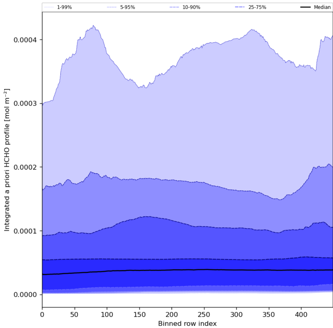
Figure 57: Along track statistics of "Integrated a priori HCHO profile" for 2024-01-15 to 2024-01-17
