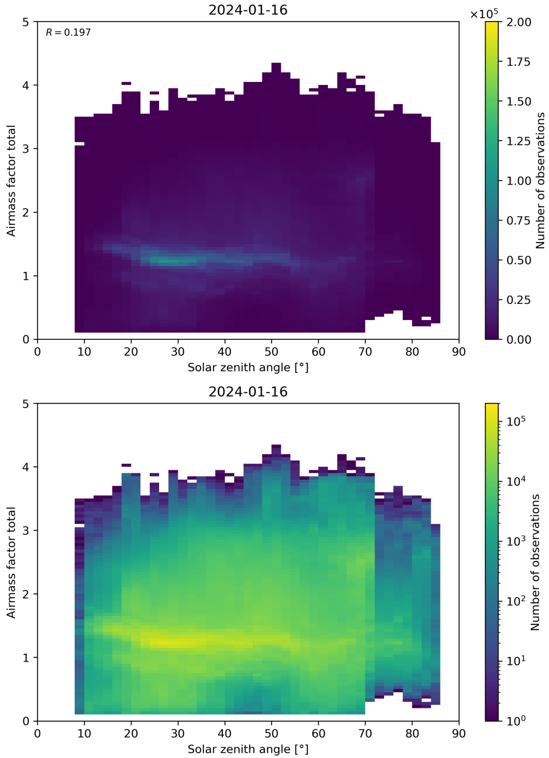
Figure 175: Scatter density plot of “Solar zenith angle” against “Airmass factor total” for 2024-01-15 to 2024-01-17.
