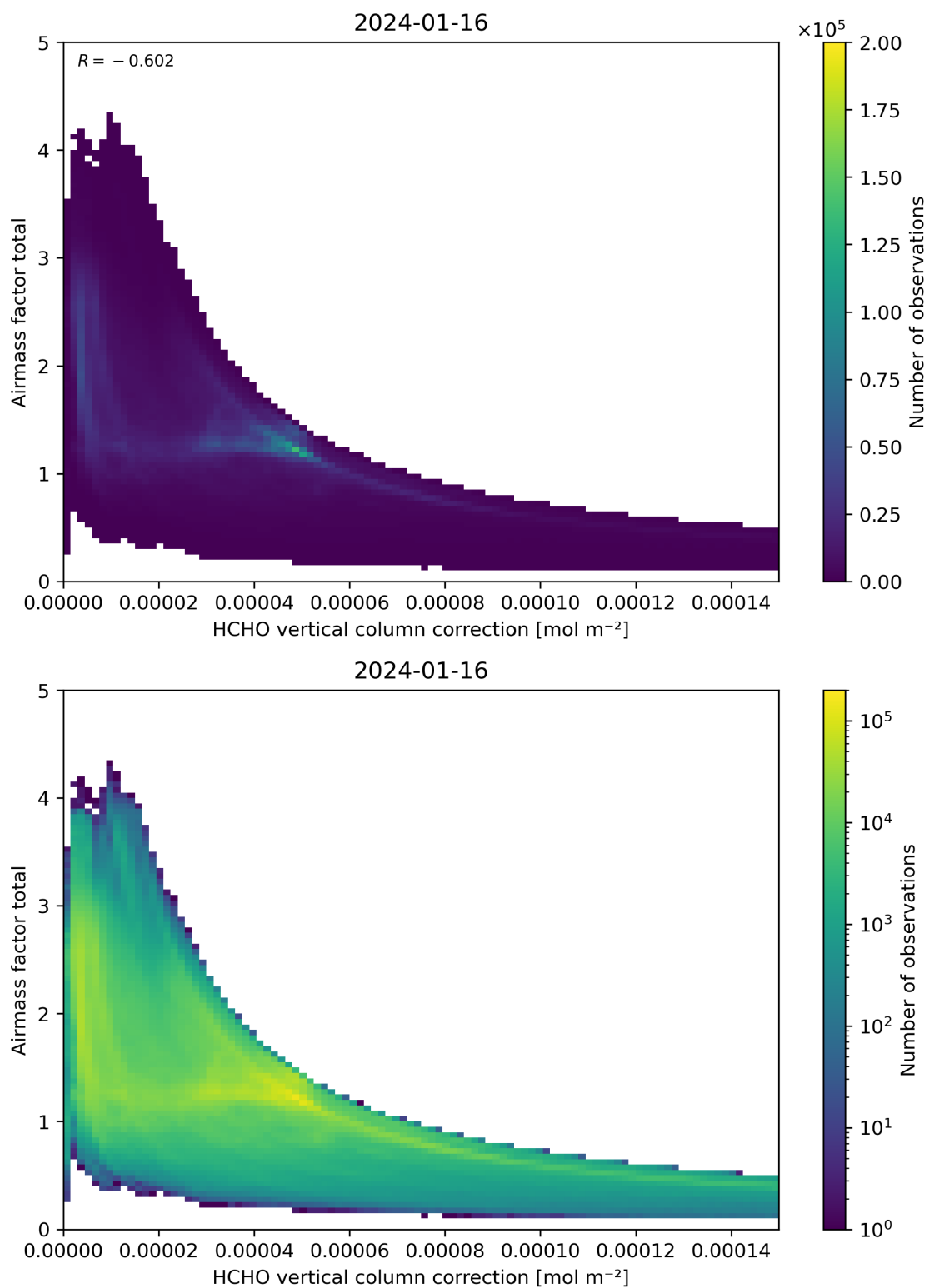
Figure 120: Scatter density plot of “HCHO vertical column correction” against “Airmass factor total” for 2024-01-15 to 2024-01-17.
