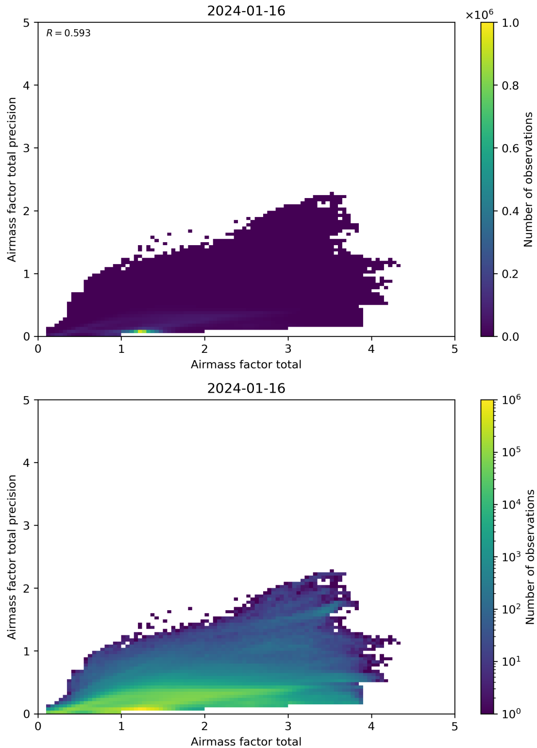
Figure 103: Scatter density plot of “Airmass factor total” against “Airmass factor total precision” for 2024-01-15 to 2024-01-17.
