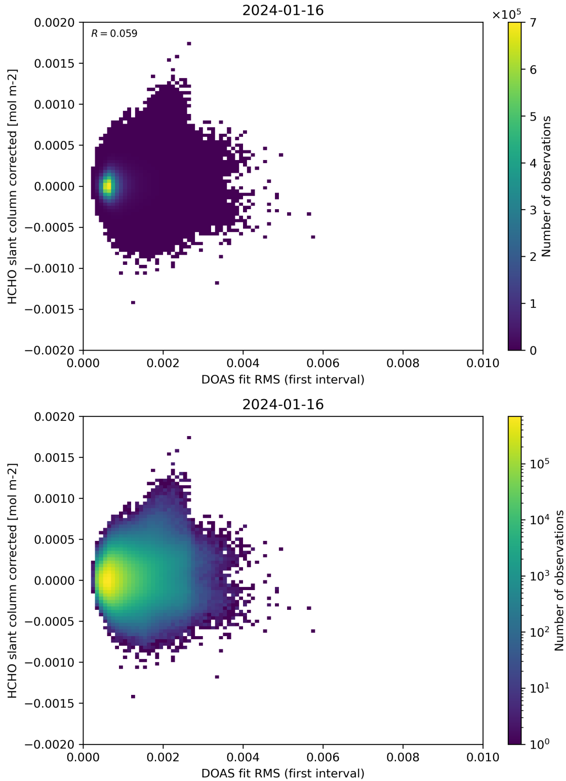
Figure 62: Scatter density plot of “DOAS fit RMS (first interval)” against “HCHO slant column corrected” for 2024-01-15 to 2024-01-17.
