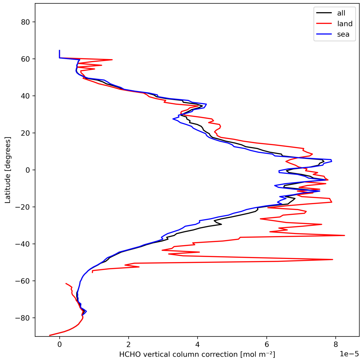
Figure 23: Zonal average of “HCHO vertical column correction” for 2024-01-15 to 2024-01-17.
