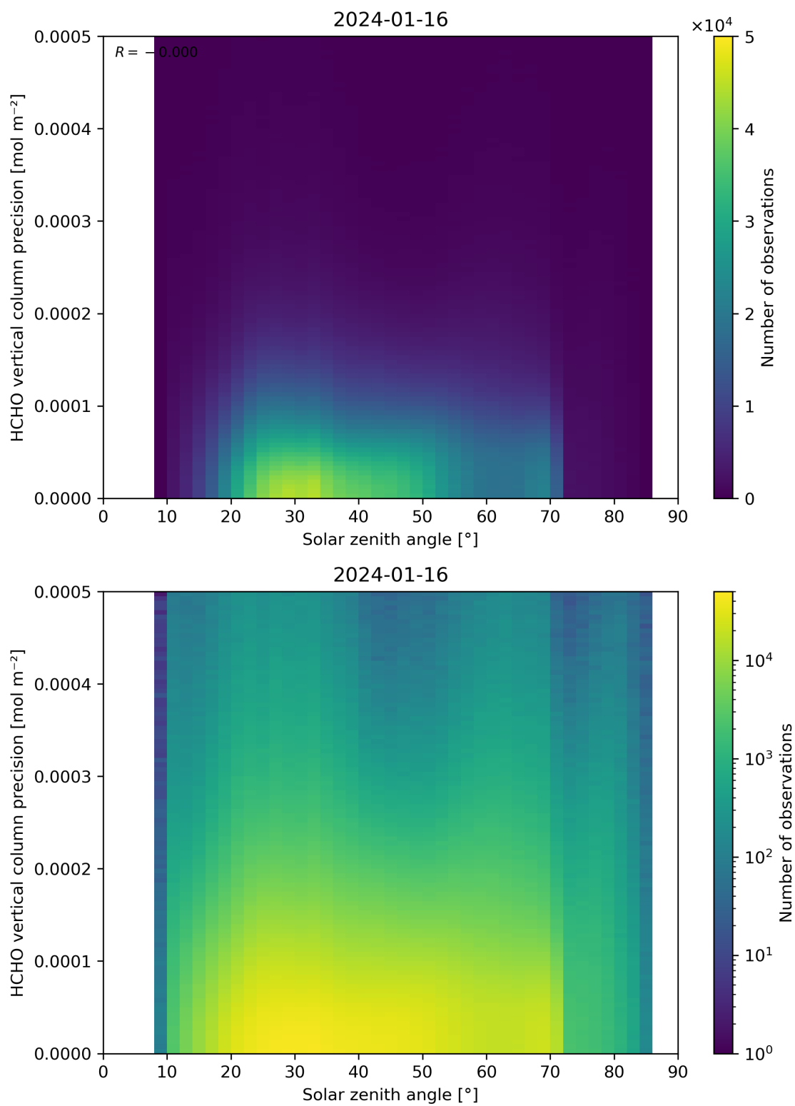
Figure 179: Scatter density plot of “Solar zenith angle” against “HCHO vertical column precision” for 2024-01-15 to 2024-01-17.
