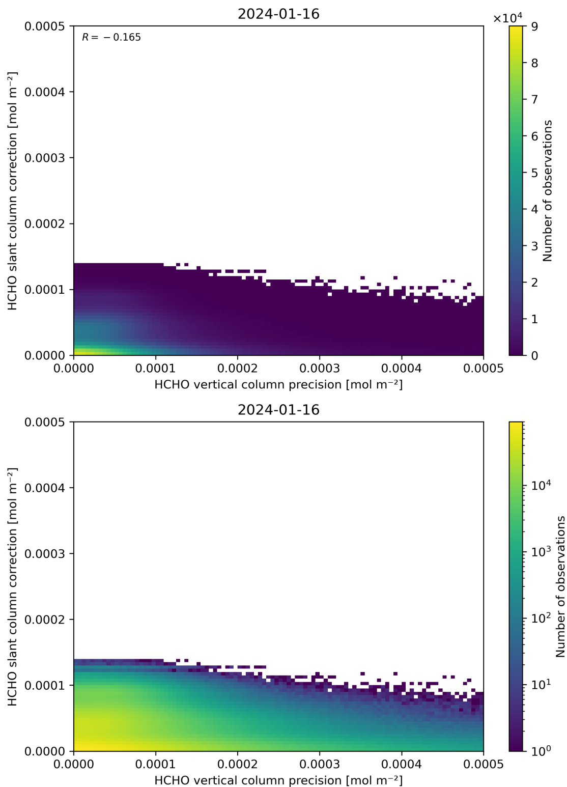
Figure 141: Scatter density plot of “HCHO vertical column precision” against “HCHO slant column correction” for 2024-01-15 to 2024-01-17.
