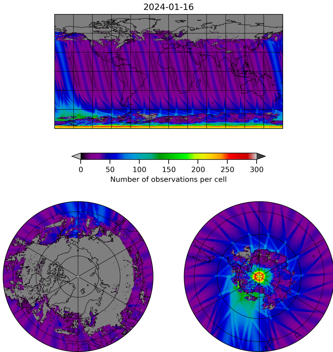
Figure 19: Map of the number of observations for 2024-01-15 to 2024-01-17
