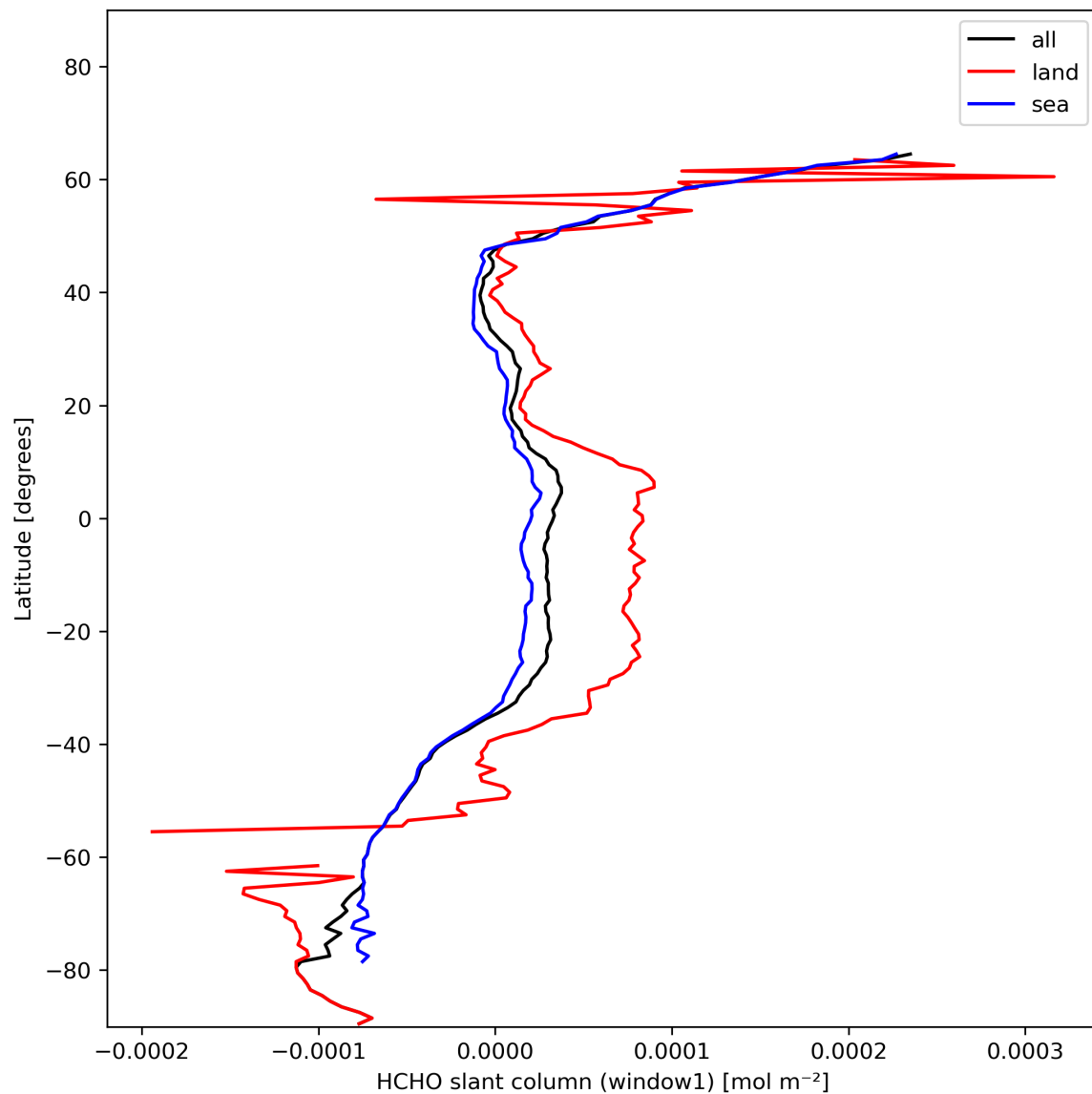
Figure 24: Zonal average of “HCHO slant column (window1)” for 2024-01-15 to 2024-01-17.
