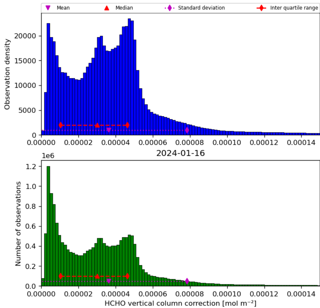
Figure 37: Histogram of “HCHO vertical column correction” for 2024-01-15 to 2024-01-17
