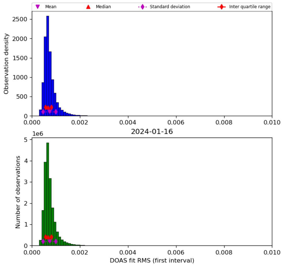
Figure 46: Histogram of “DOAS fit RMS (first interval)” for 2024-01-15 to 2024-01-17
