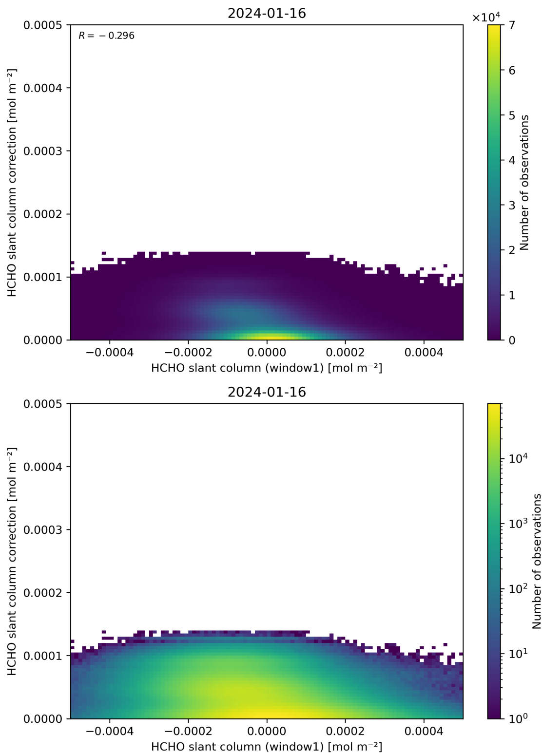
Figure 83: Scatter density plot of “HCHO slant column (window1)” against “HCHO slant column correction” for 2024-01-15 to 2024-01-17.
