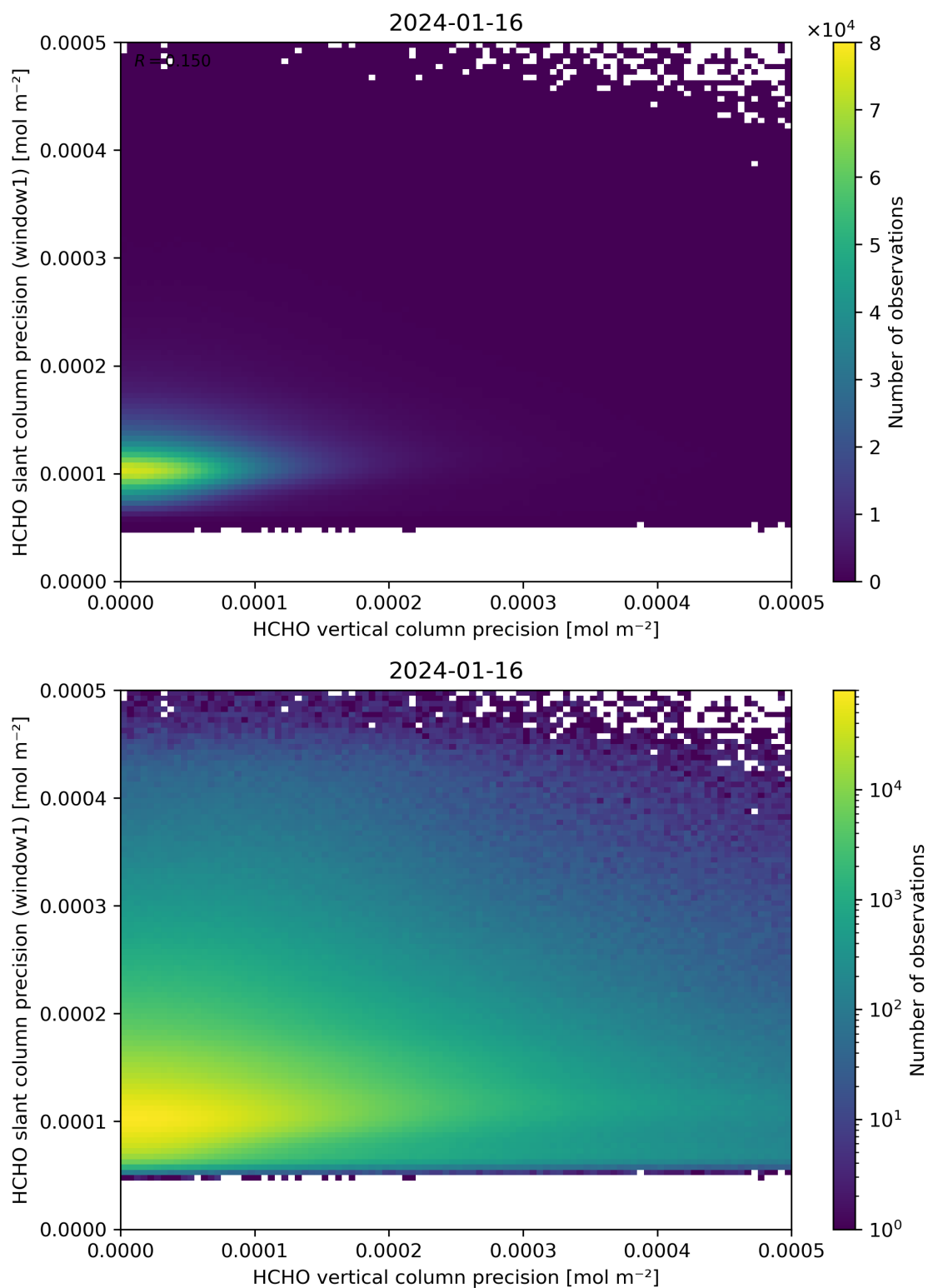
Figure 143: Scatter density plot of “HCHO vertical column precision” against “HCHO slant column precision (window1)” for 2024-01-15 to 2024-01-17.
