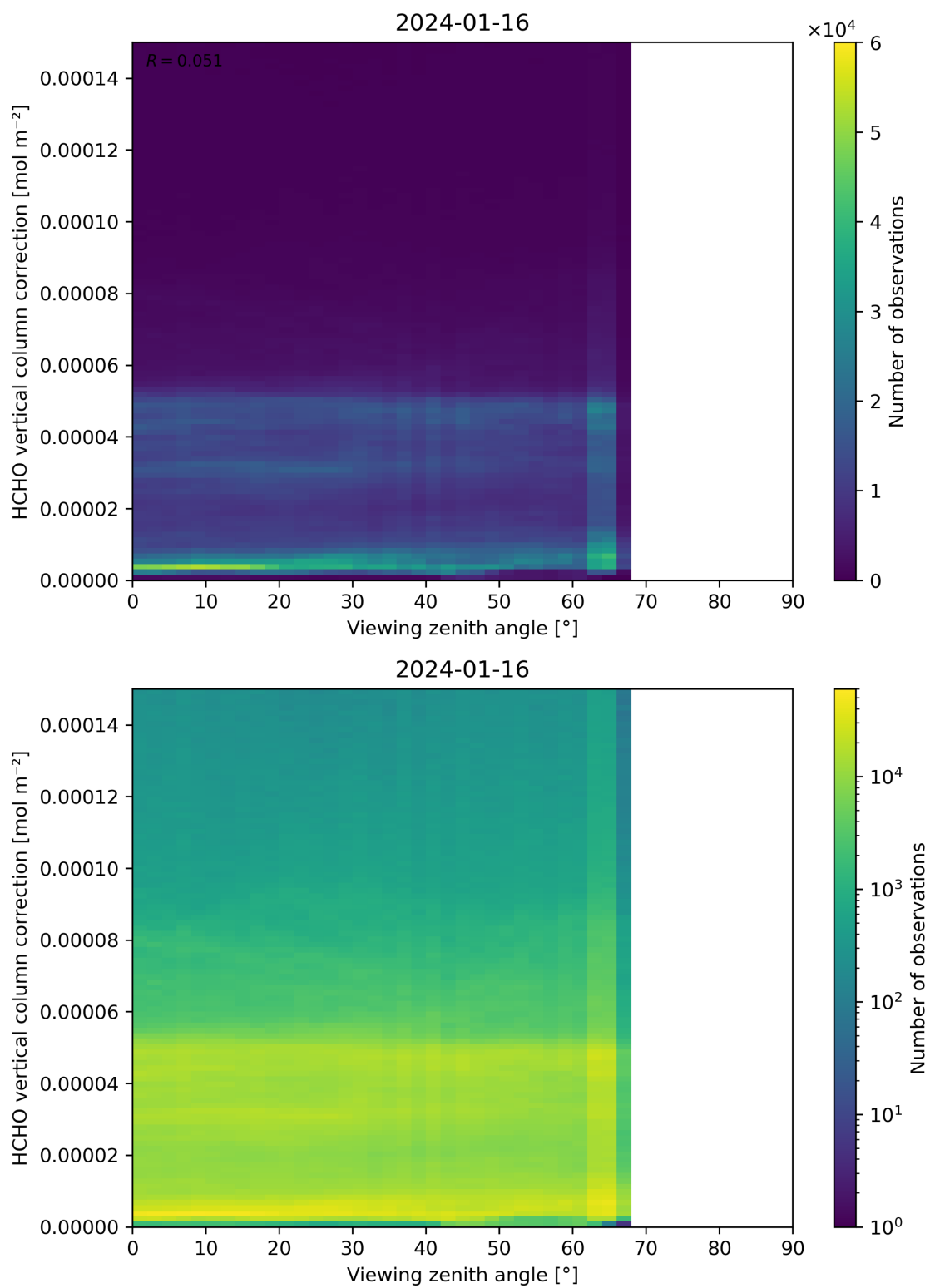
Figure 193: Scatter density plot of “Viewing zenith angle” against “HCHO vertical column correction” for 2024-01-15 to 2024-01-17.
