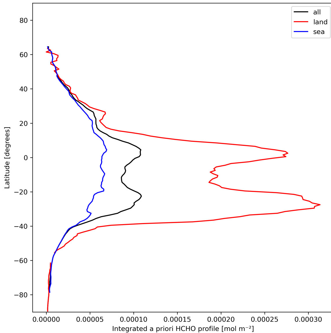
Figure 29: Zonal average of “Integrated a priori HCHO profile” for 2024-01-15 to 2024-01-17.
