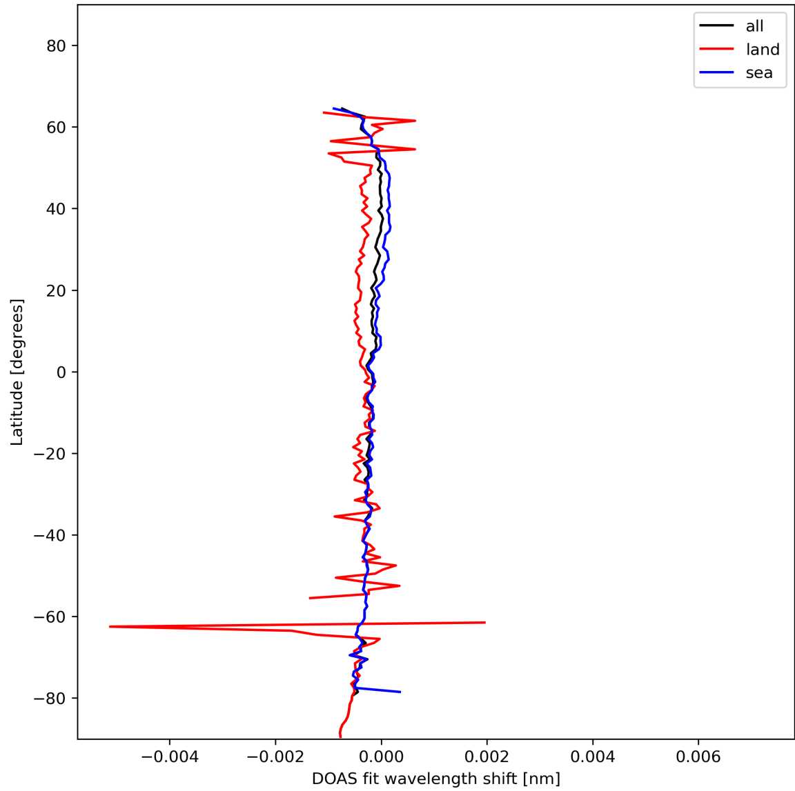
Figure 30: Zonal average of “DOAS fit wavelength shift” for 2024-01-15 to 2024-01-17.
