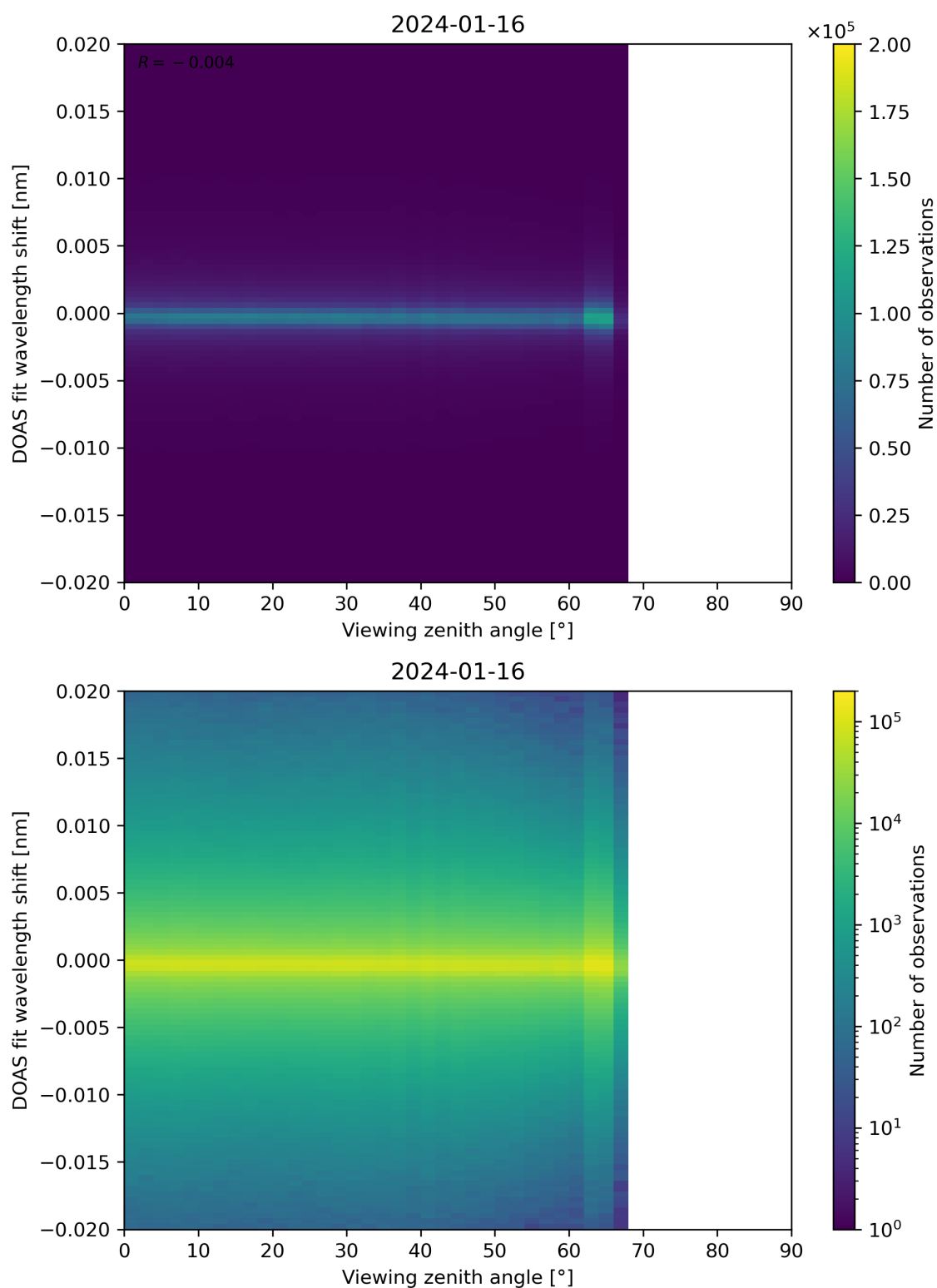
Figure 183: Scatter density plot of “Viewing zenith angle” against “DOAS fit wavelength shift” for 2024-01-15 to 2024-01-17.
