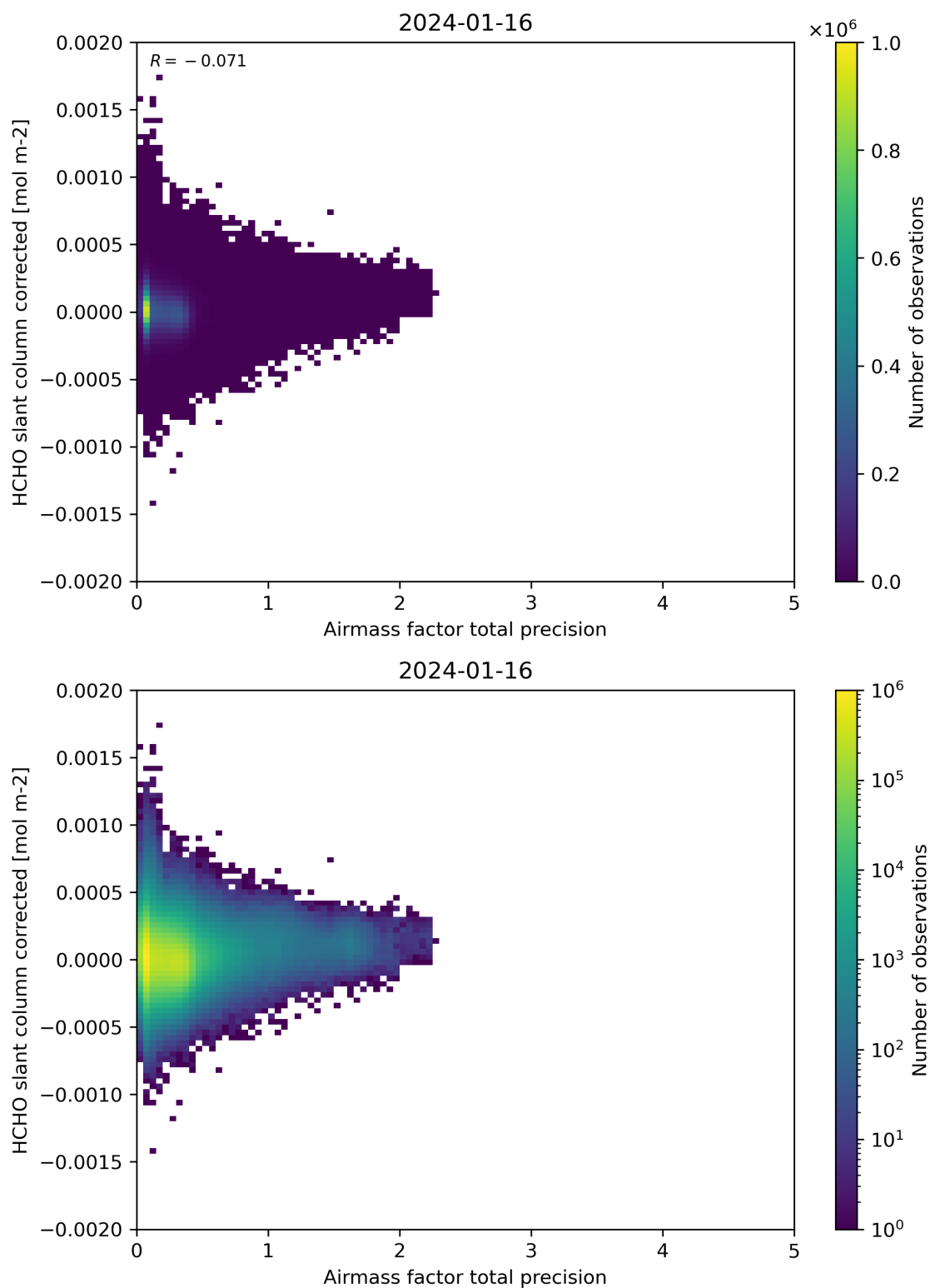
Figure 109: Scatter density plot of “Airmass factor total precision” against “HCHO slant column corrected” for 2024-01-15 to 2024-01-17.
