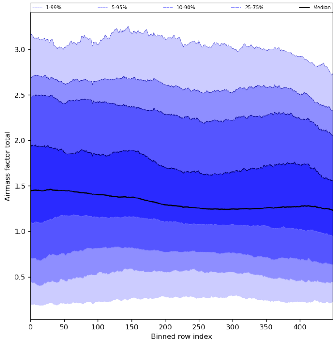
Figure 54: Along track statistics of “Airmass factor total” for 2024-01-15 to 2024-01-17
