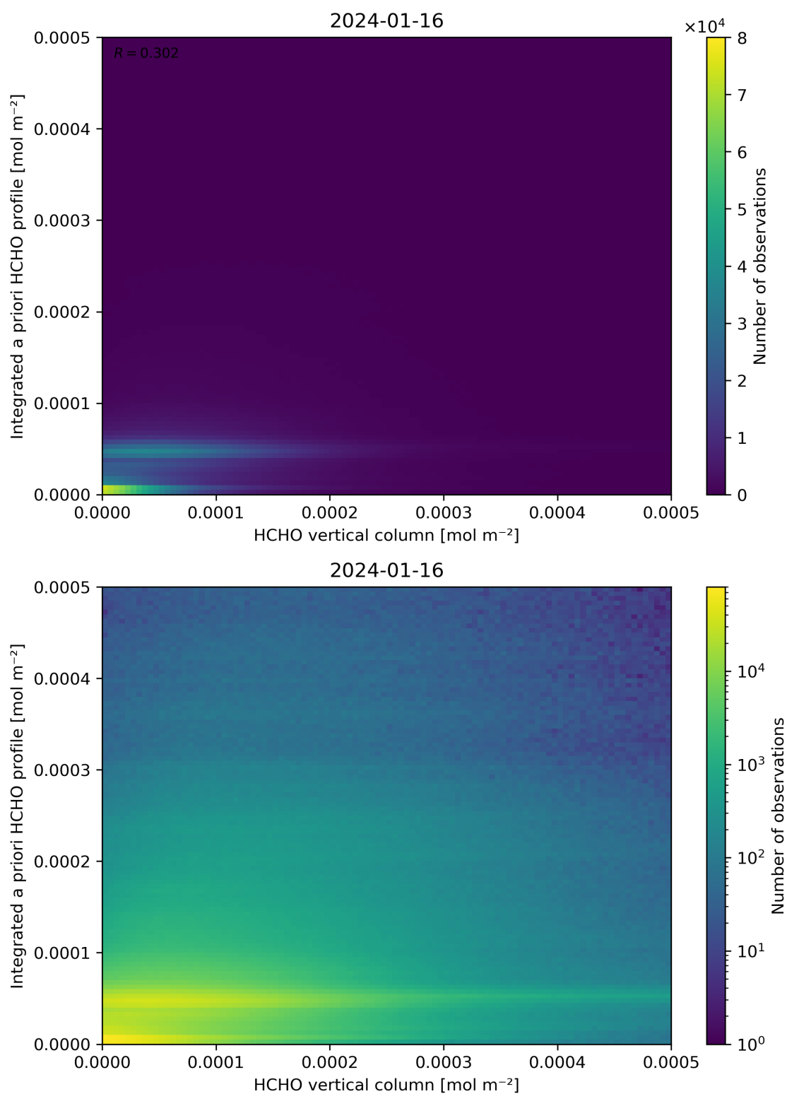
Figure 135: Scatter density plot of “HCHO vertical column” against “Integrated a priori HCHO profile” for 2024-01-15 to 2024-01-17.
