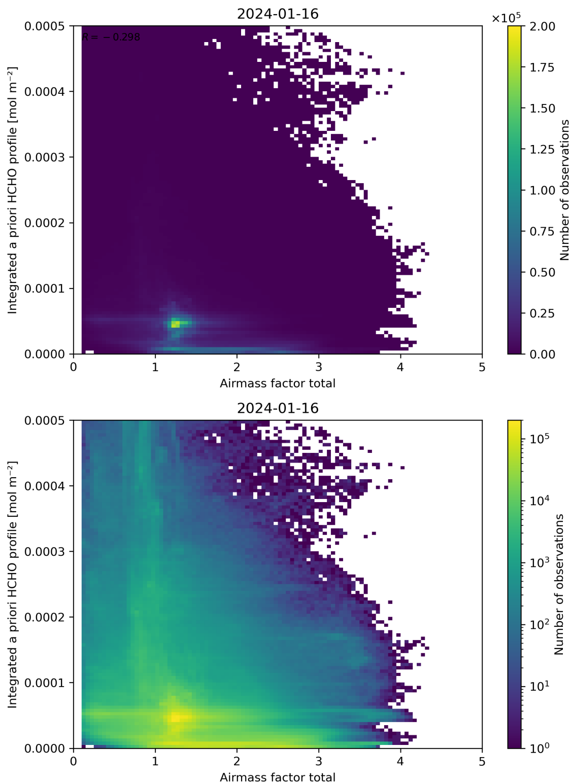
Figure 104: Scatter density plot of “Air mass factor total” against “Integrated a priori HCHO profile” for 2024-01-15 to 2024-01-17.
