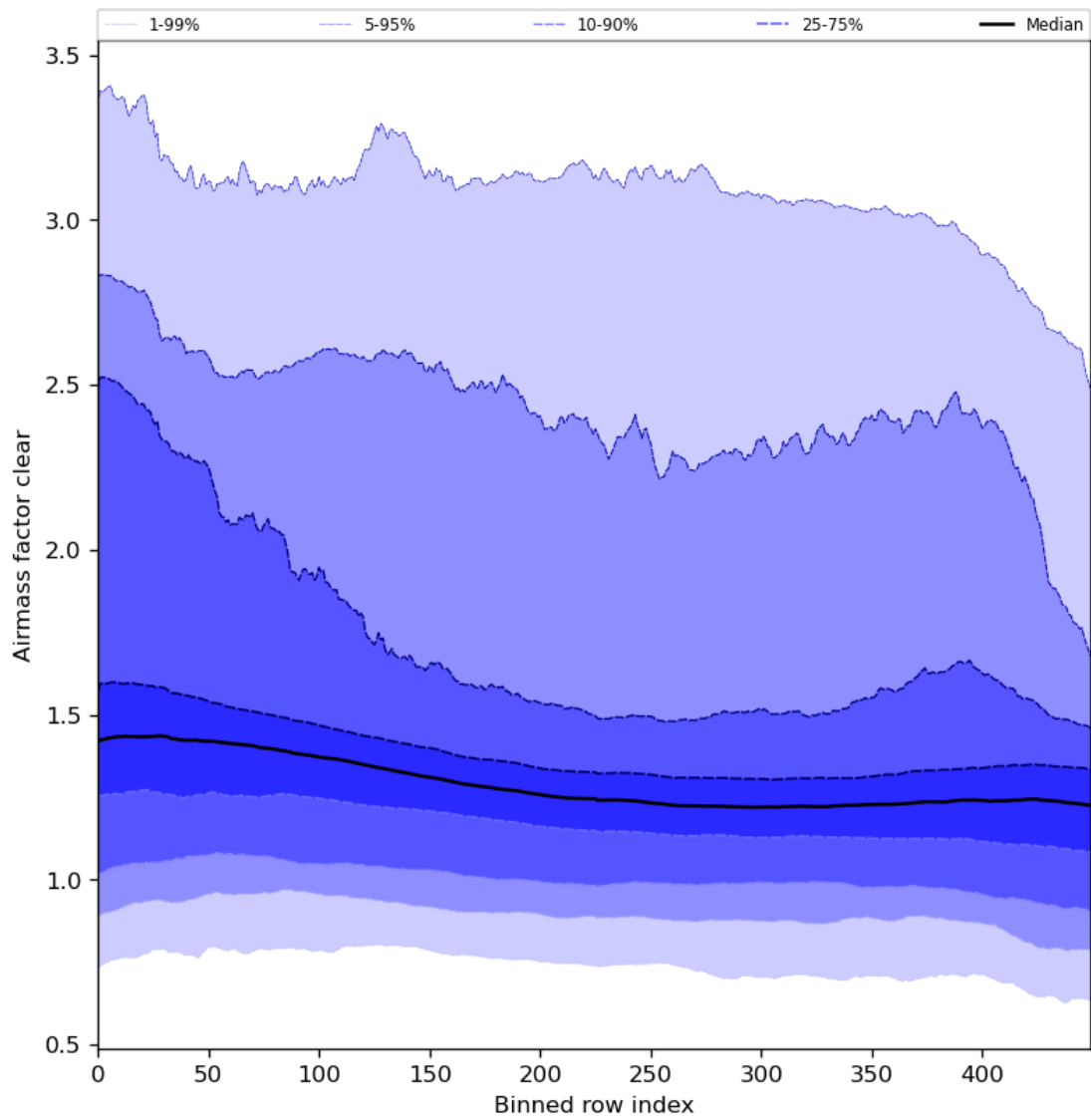
Figure 56: Along track statistics of “Airmass factor clear” for 2024-01-15 to 2024-01-17
