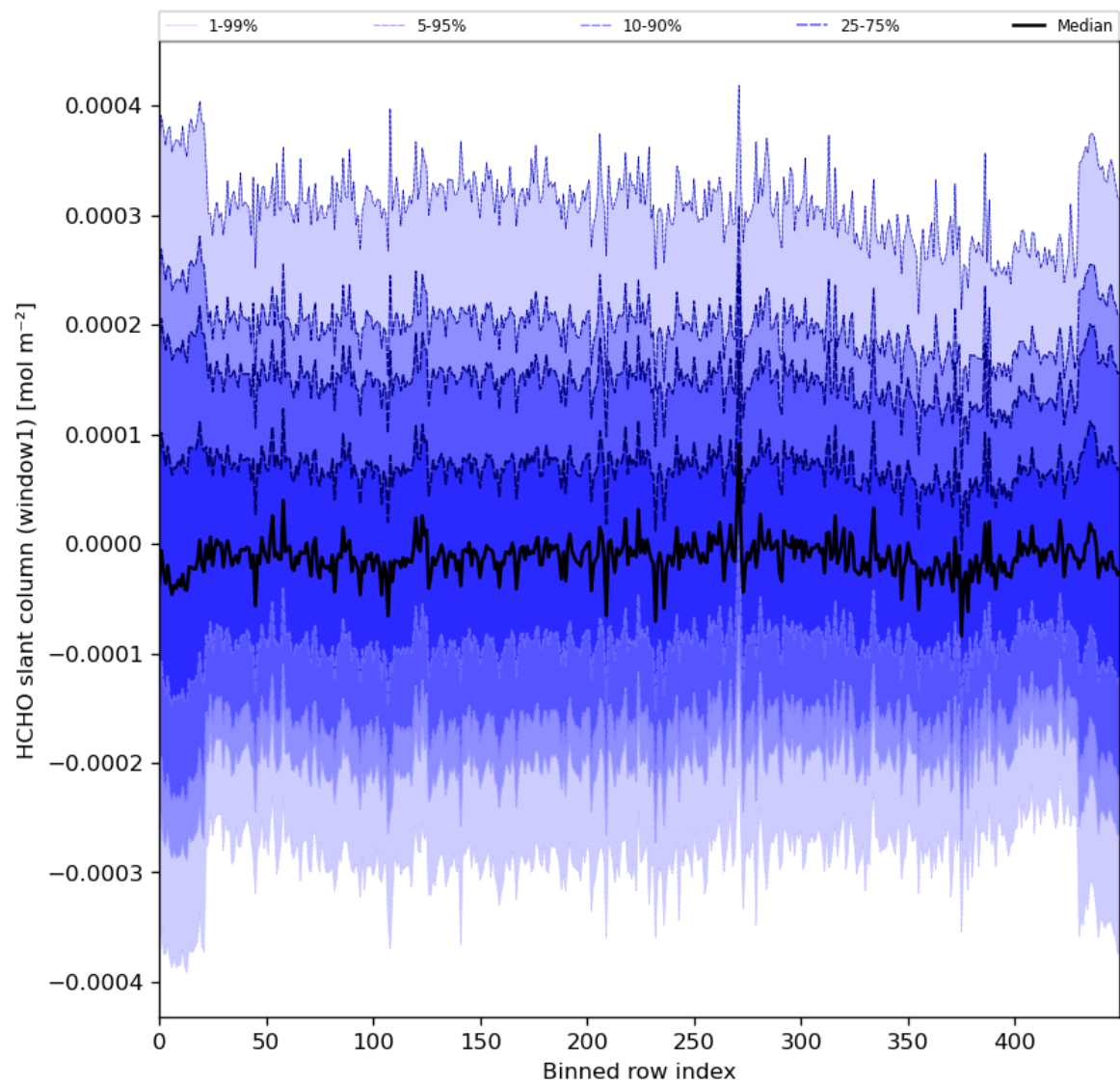
Figure 52: Along track statistics of “HCHO slant column (window1)” for 2024-01-15 to 2024-01-17
