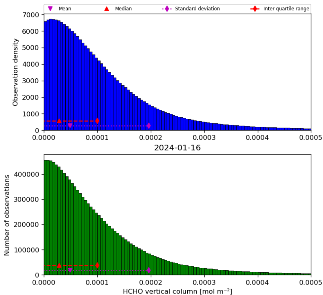
Figure 35: Histogram of “HCHO vertical column” for 2024-01-15 to 2024-01-17
