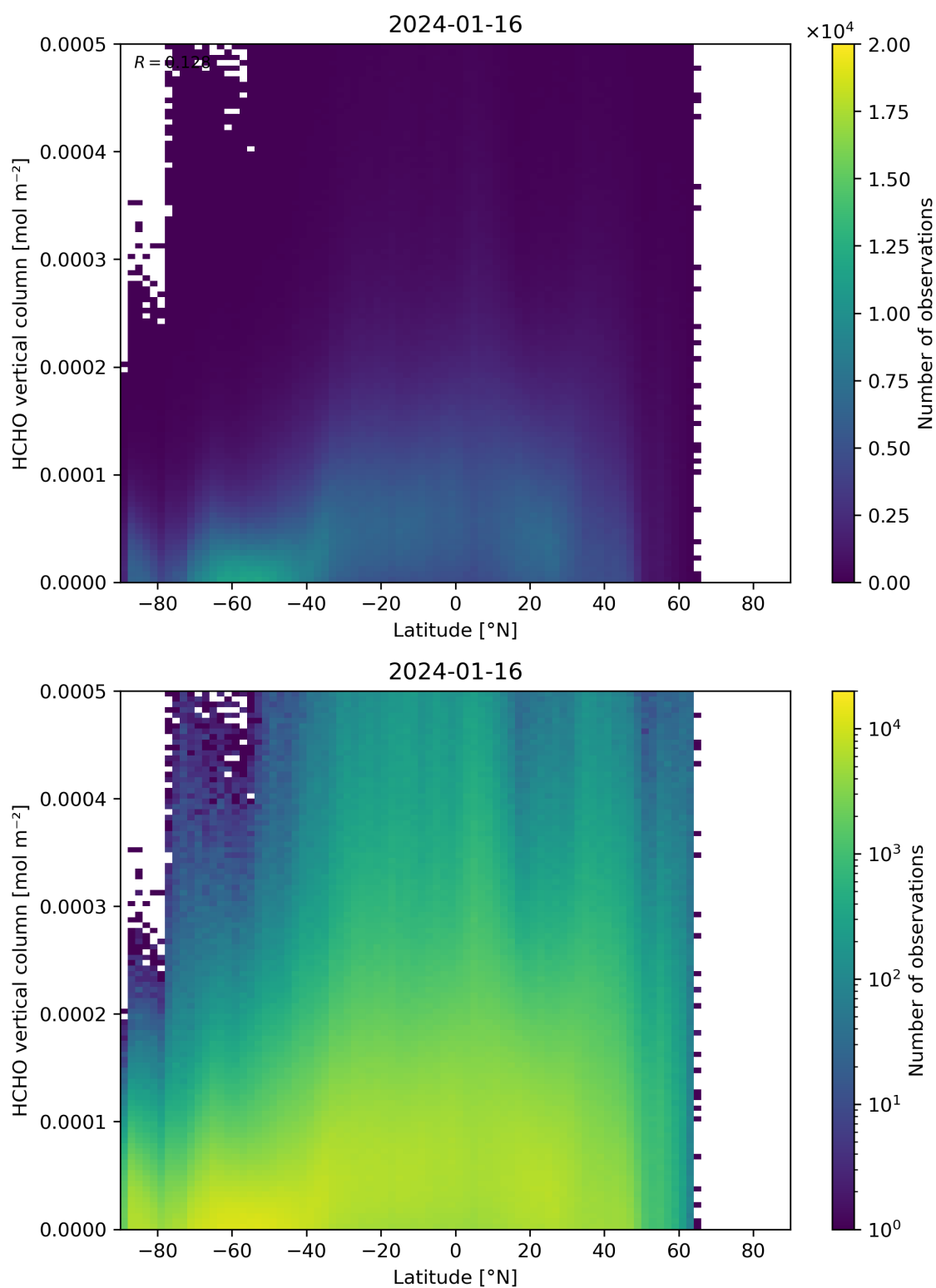
Figure 163: Scatter density plot of “Latitude” against “HCHO vertical column” for 2024-01-15 to 2024-01-17.
