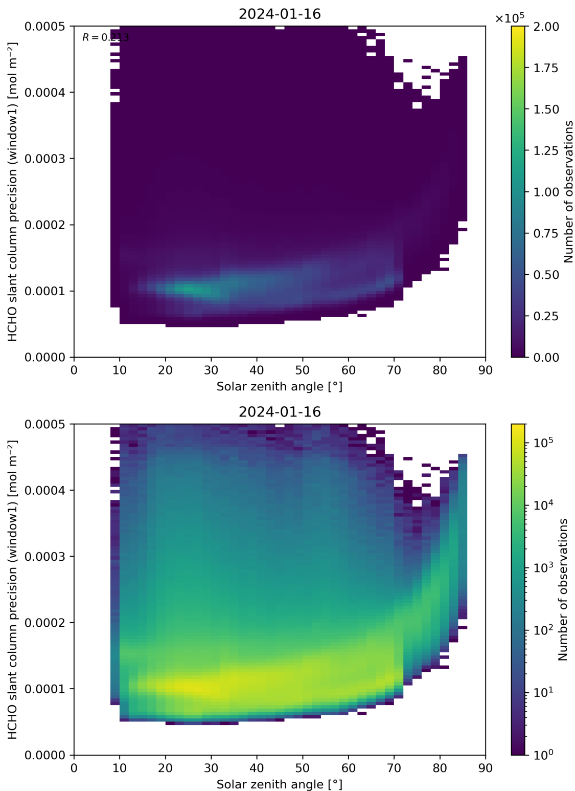
Figure 174: Scatter density plot of “Solar zenith angle” against “HCHO slant column precision (window1)” for 2024-01-15 to 2024-01-17.
