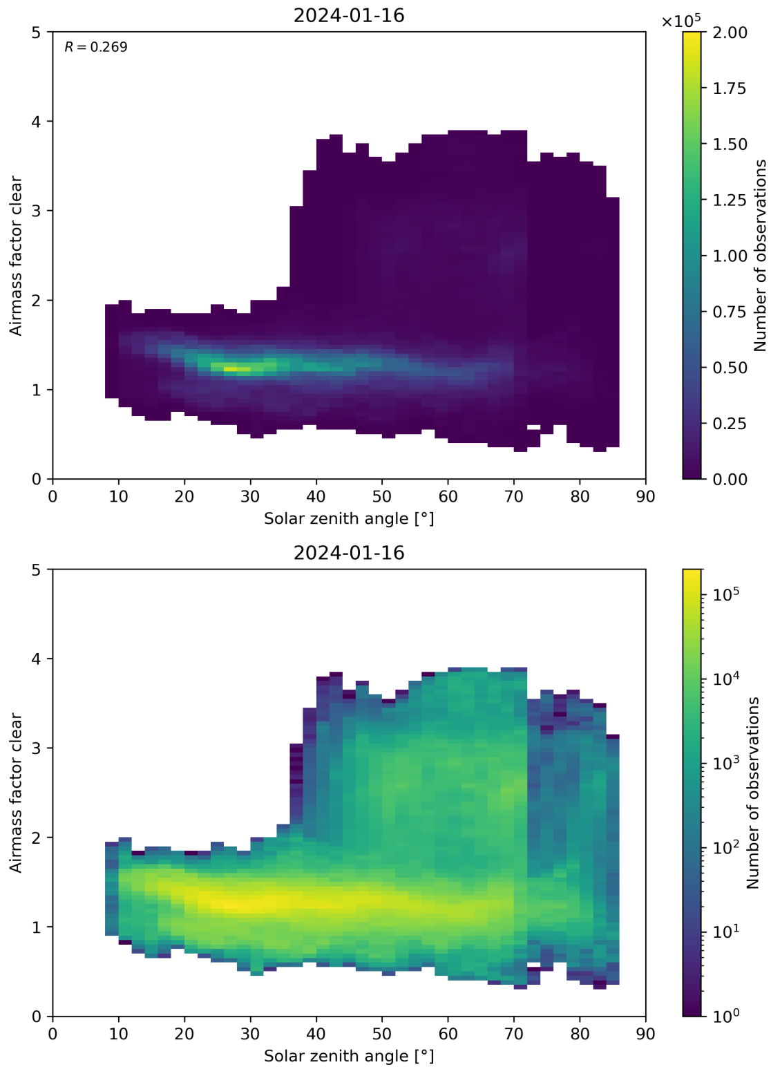
Figure 170: Scatter density plot of “Solar zenith angle” against “Airmass factor clear” for 2024-01-15 to 2024-01-17.
