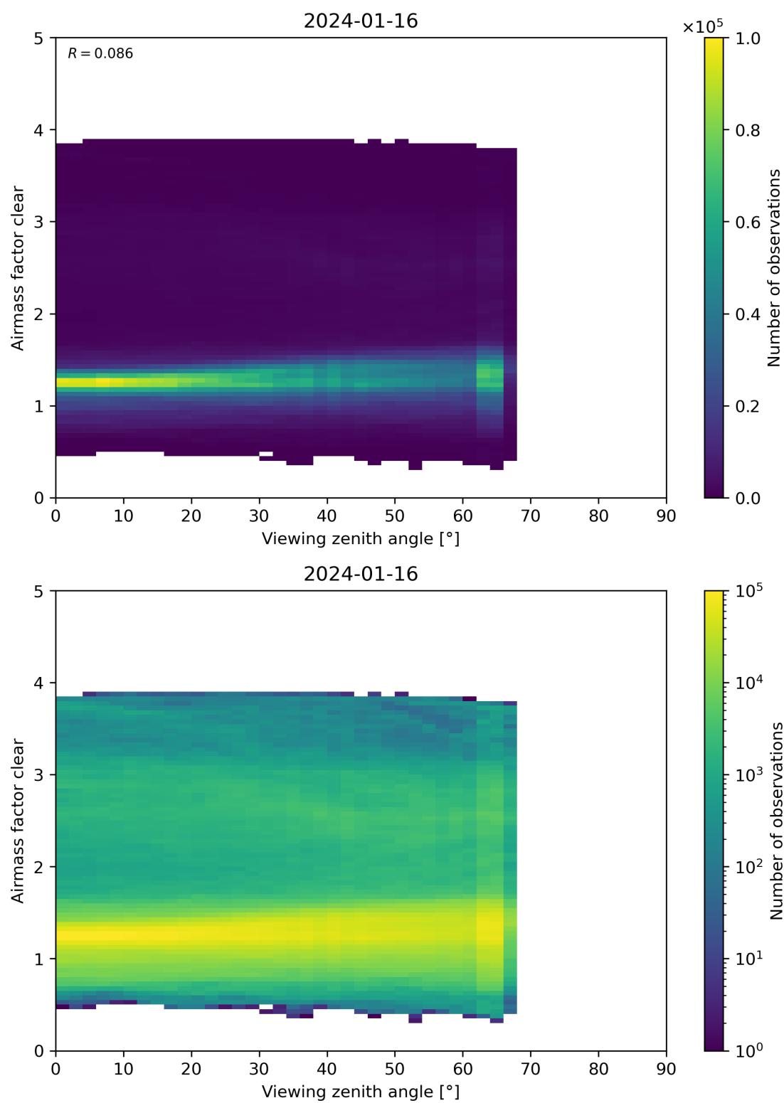
Figure 185: Scatter density plot of “Viewing zenith angle” against “Airmass factor clear” for 2024-01-15 to 2024-01-17.
