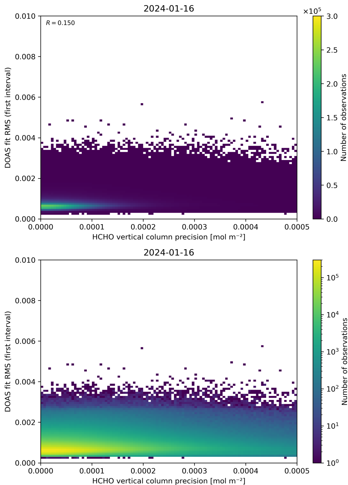
Figure 136: Scatter density plot of “HCHO vertical column precision” against “DOAS fit RMS (first interval)” for 2024-01-15 to 2024-01-17.
