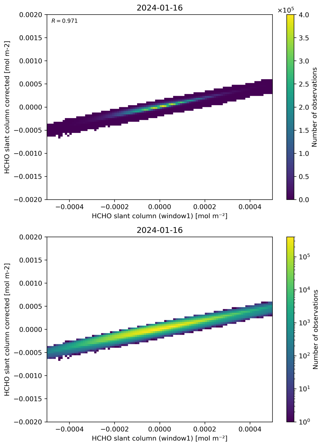
Figure 82: Scatter density plot of “HCHO slant column (window1)” against “HCHO slant column corrected” for 2024-01-15 to 2024-01-17.
