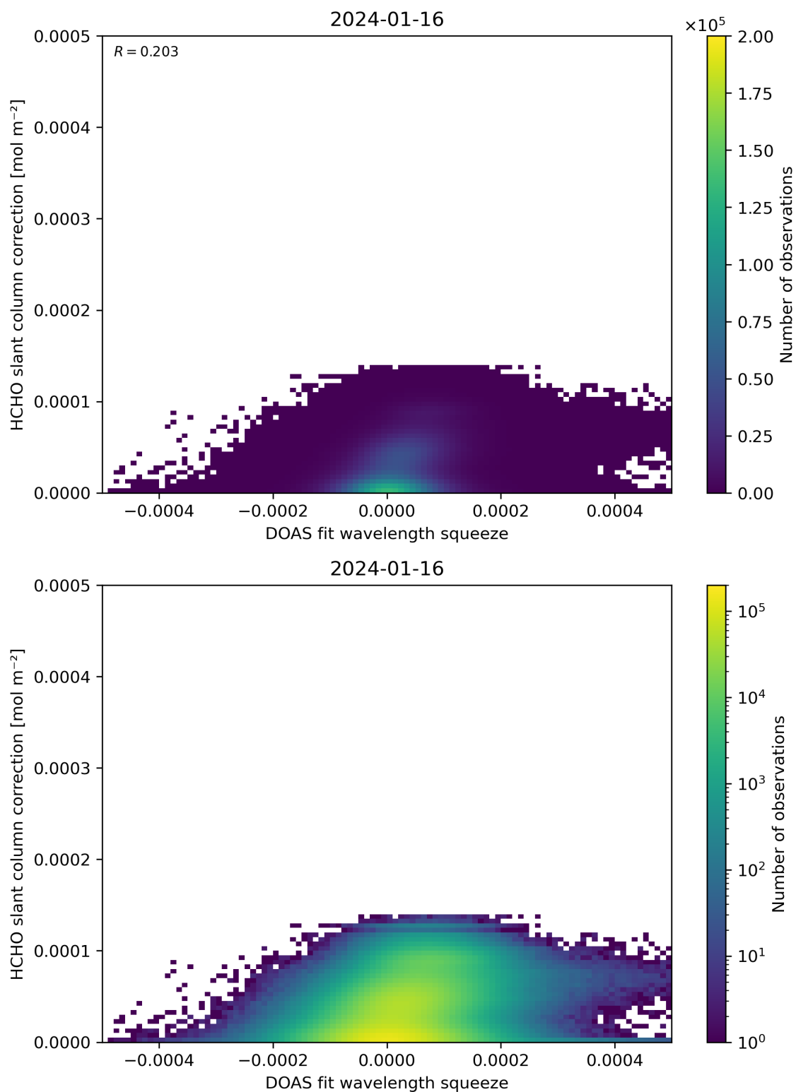
Figure 70: Scatter density plot of “DOAS fit wavelength squeeze” against “HCHO slant column correction” for 2024-01-15 to 2024-01-17.
