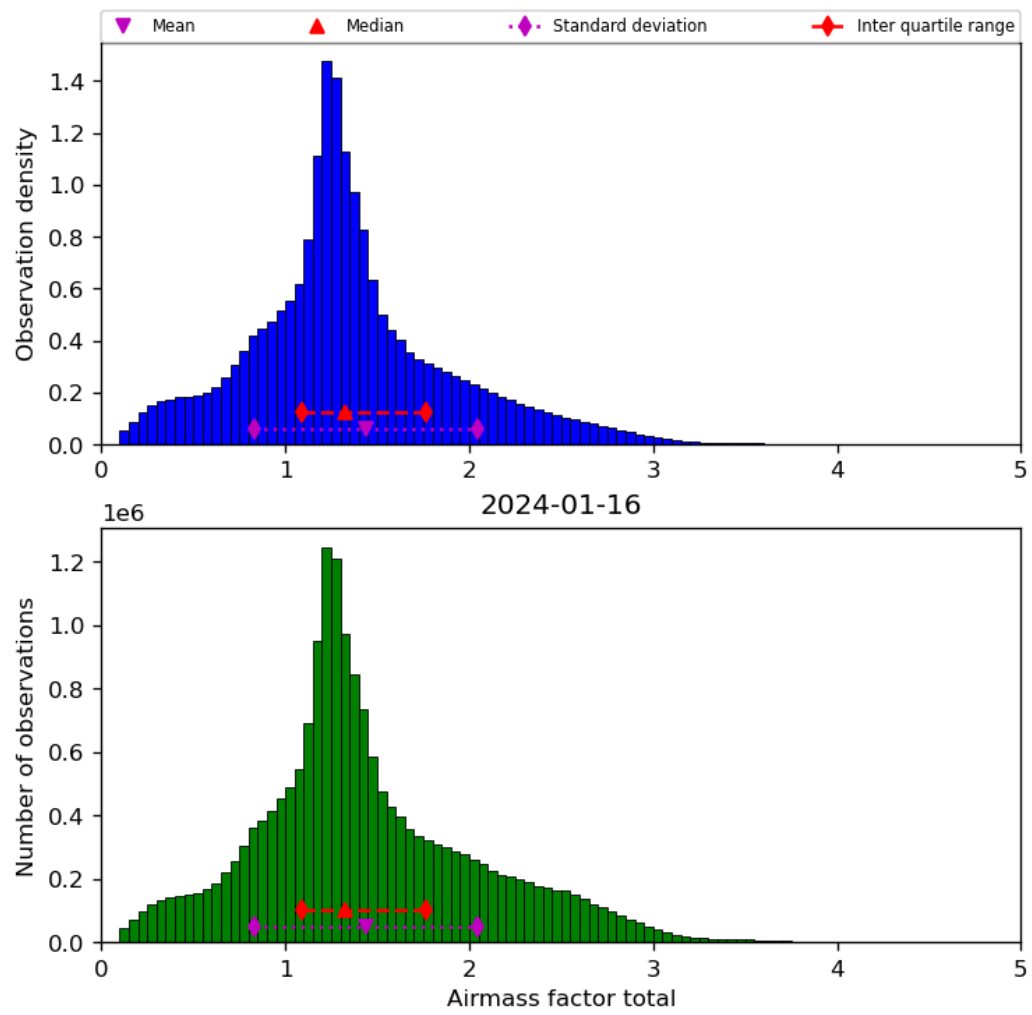
Figure 40: Histogram of “Airmass factor total” for 2024-01-15 to 2024-01-17
