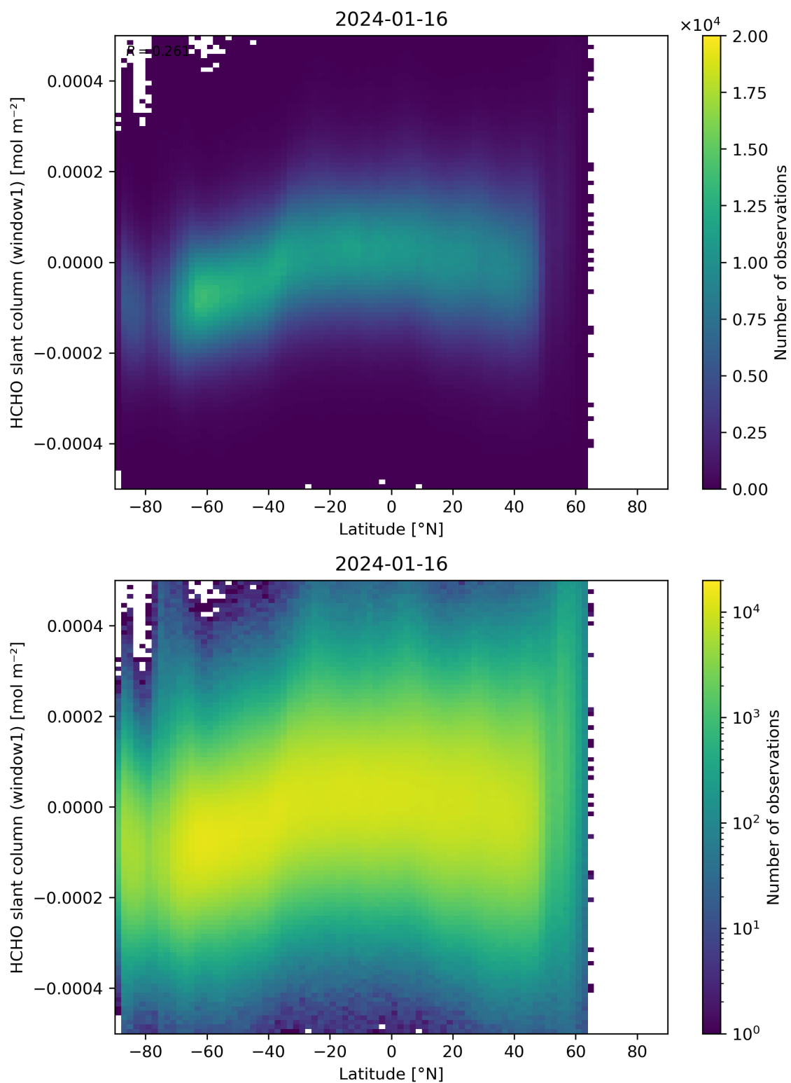
Figure 159: Scatter density plot of “Latitude” against “HCHO slant column (window1)” for 2024-01-15 to 2024-01-17.
