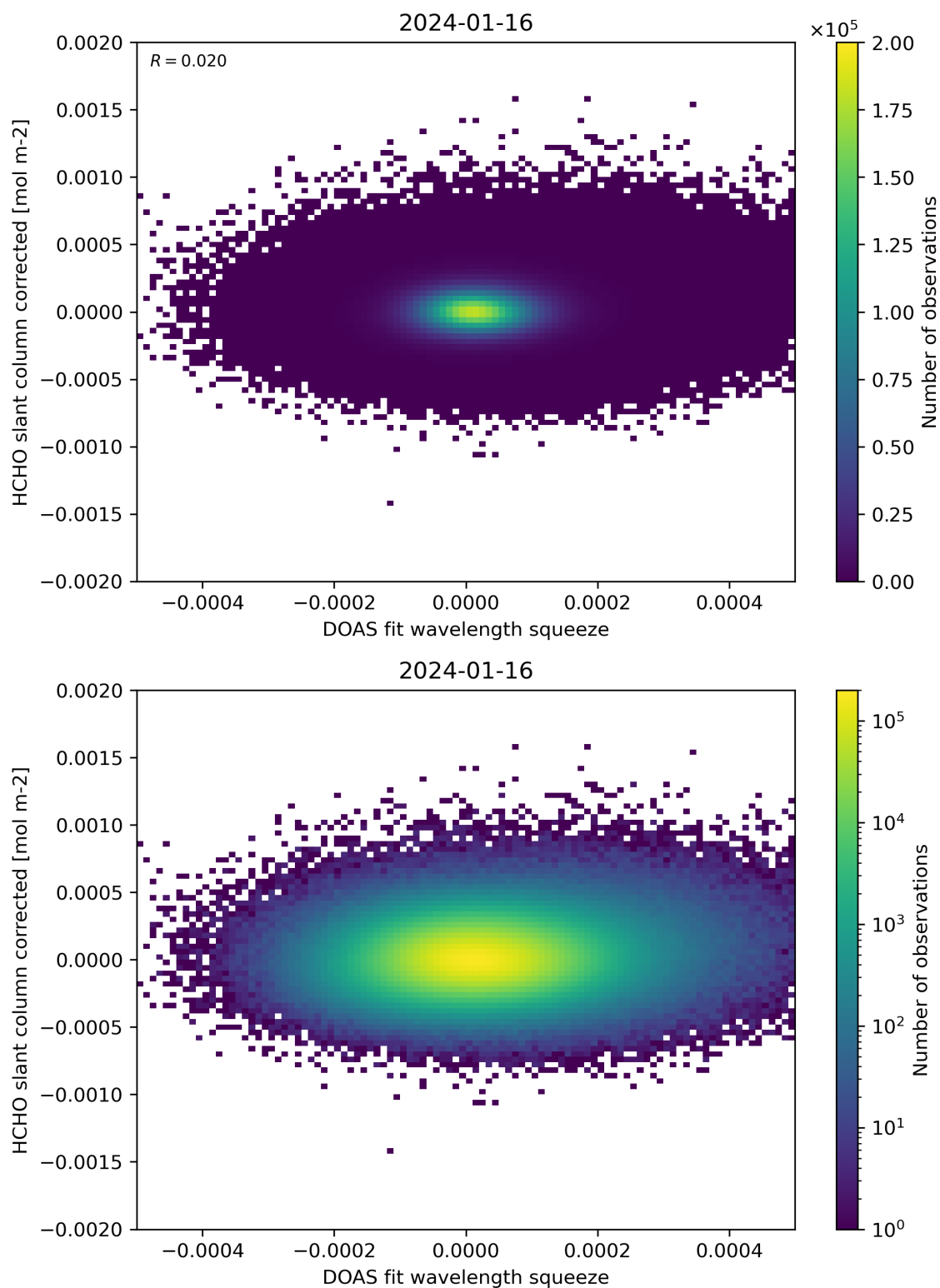
Figure 69: Scatter density plot of “DOAS fit wavelength squeeze” against “HCHO slant column corrected” for 2024-01-15 to 2024-01-17.
