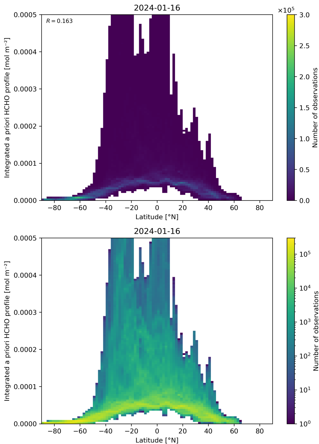
Figure 166: Scatter density plot of “Latitude” against “Integrated a priori HCHO profile” for 2024-01-15 to 2024-01-17.
