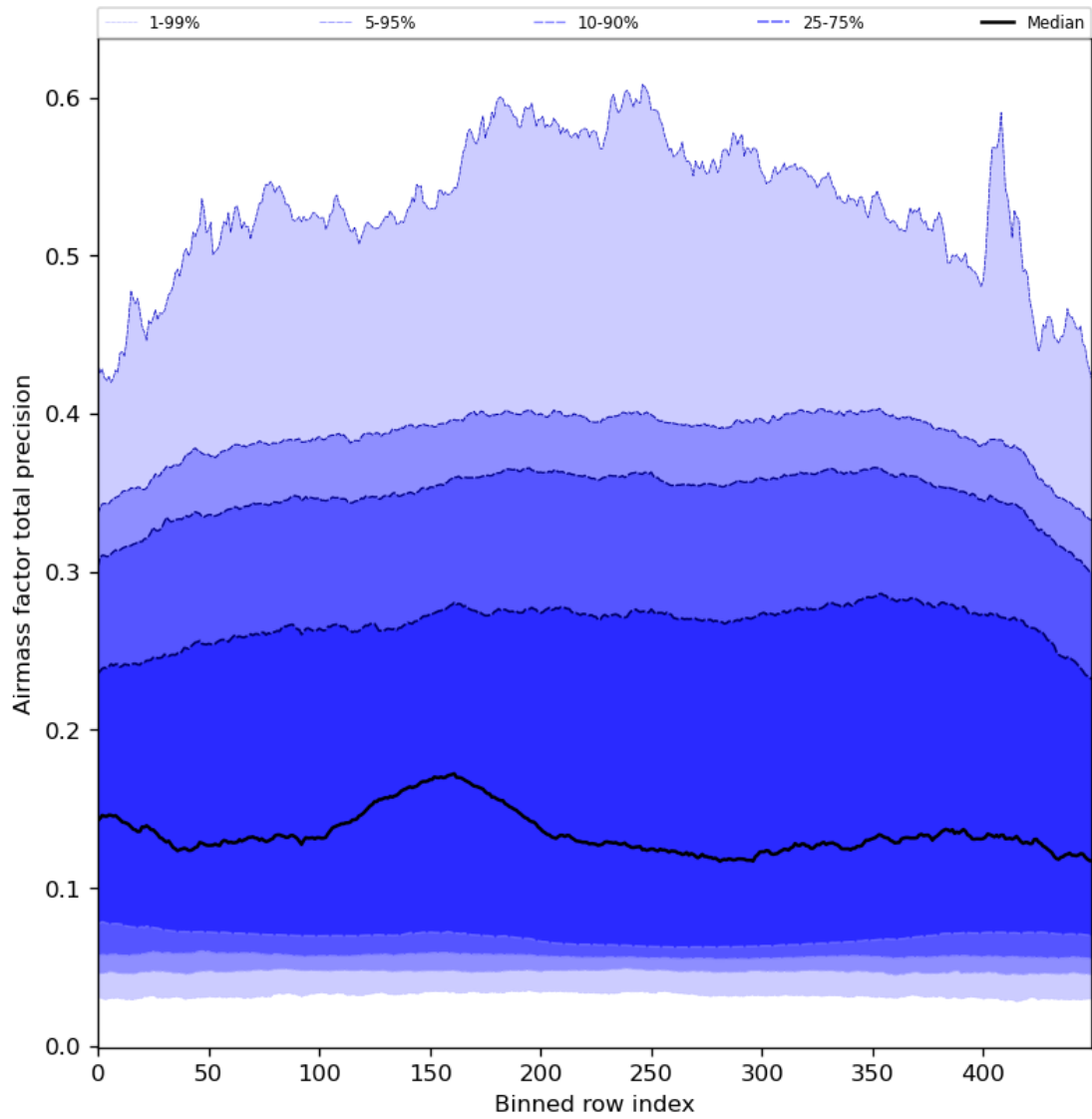
Figure 55: Along track statistics of “Airmass factor total precision” for 2024-01-15 to 2024-01-17
