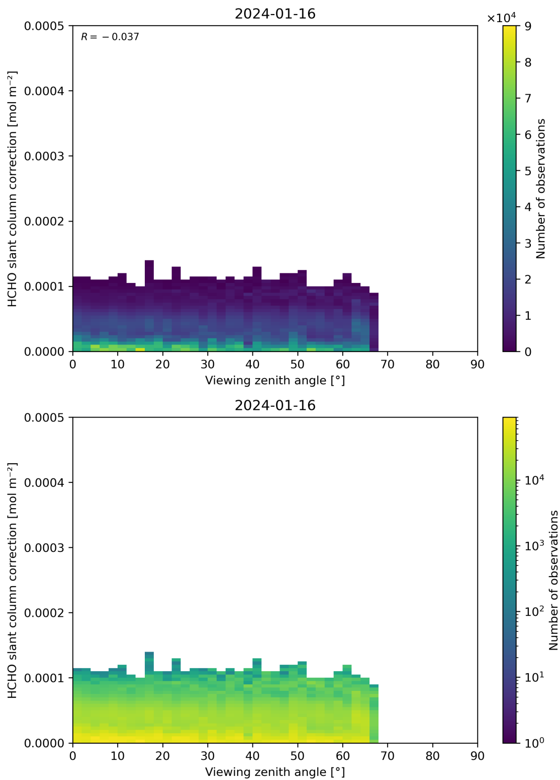
Figure 187: Scatter density plot of “Viewing zenith angle” against “HCHO slant column correction” for 2024-01-15 to 2024-01-17.
