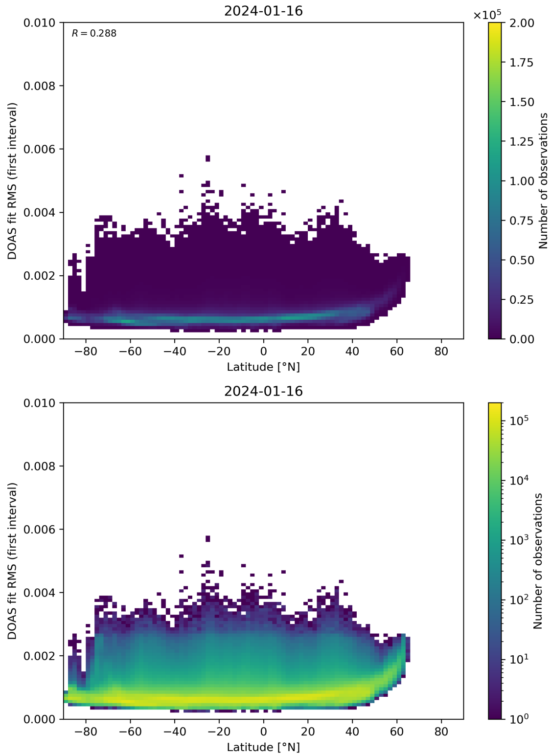
Figure 153: Scatter density plot of “Latitude” against “DOAS fit RMS (first interval)” for 2024-01-15 to 2024-01-17.
