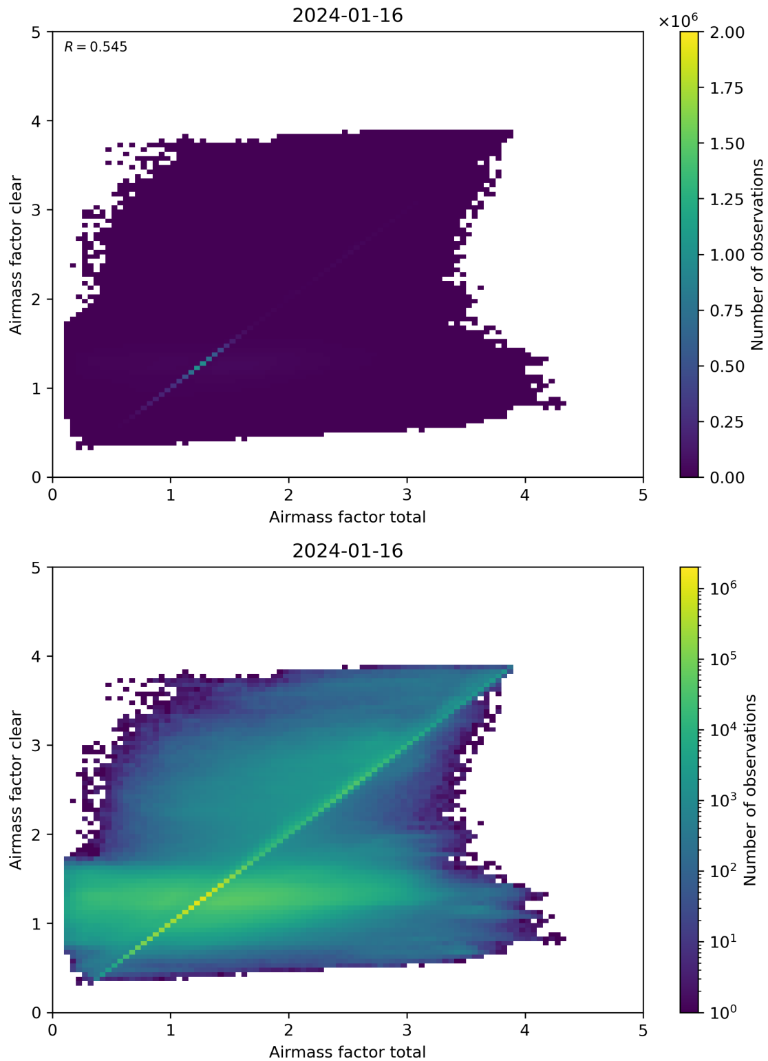
Figure 100: Scatter density plot of “Airmass factor total” against “Airmass factor clear” for 2024-01-15 to 2024-01-17.
