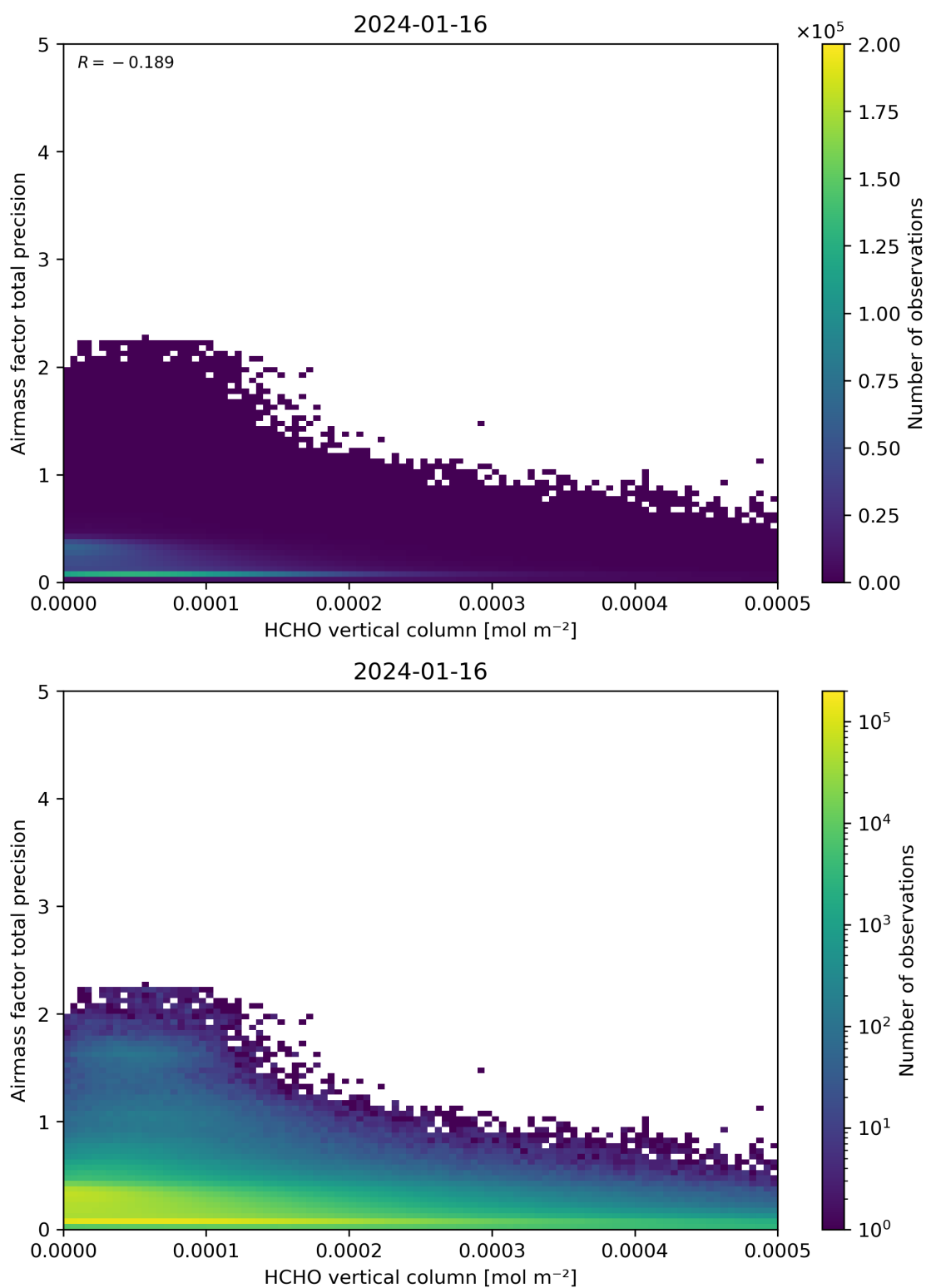
Figure 132: Scatter density plot of “HCHO vertical column” against “Airmass factor total precision” for 2024-01-15 to 2024-01-17.
