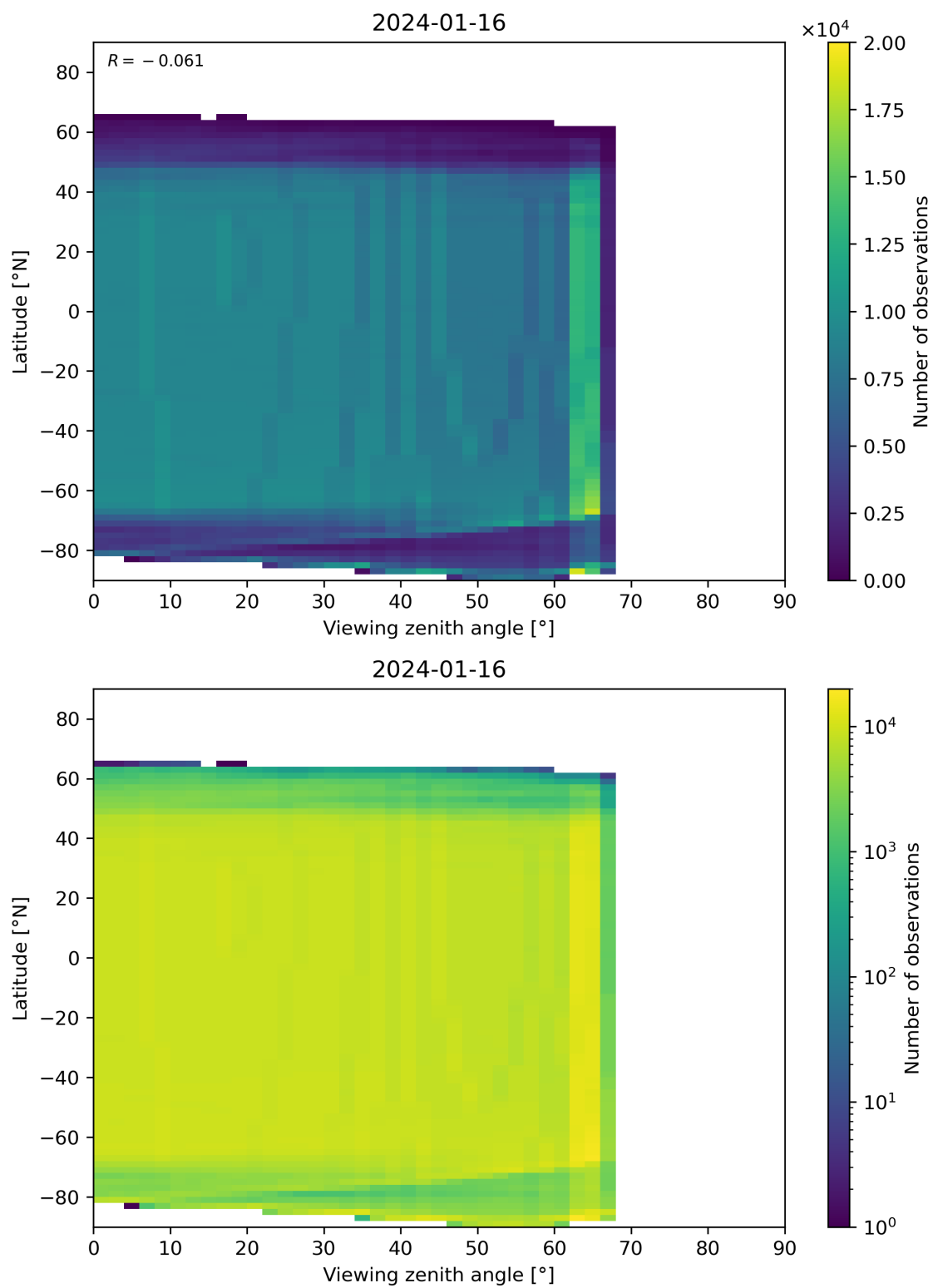
Figure 196: Scatter density plot of “Viewing zenith angle” against “Latitude” for 2024-01-15 to 2024-01-17.
