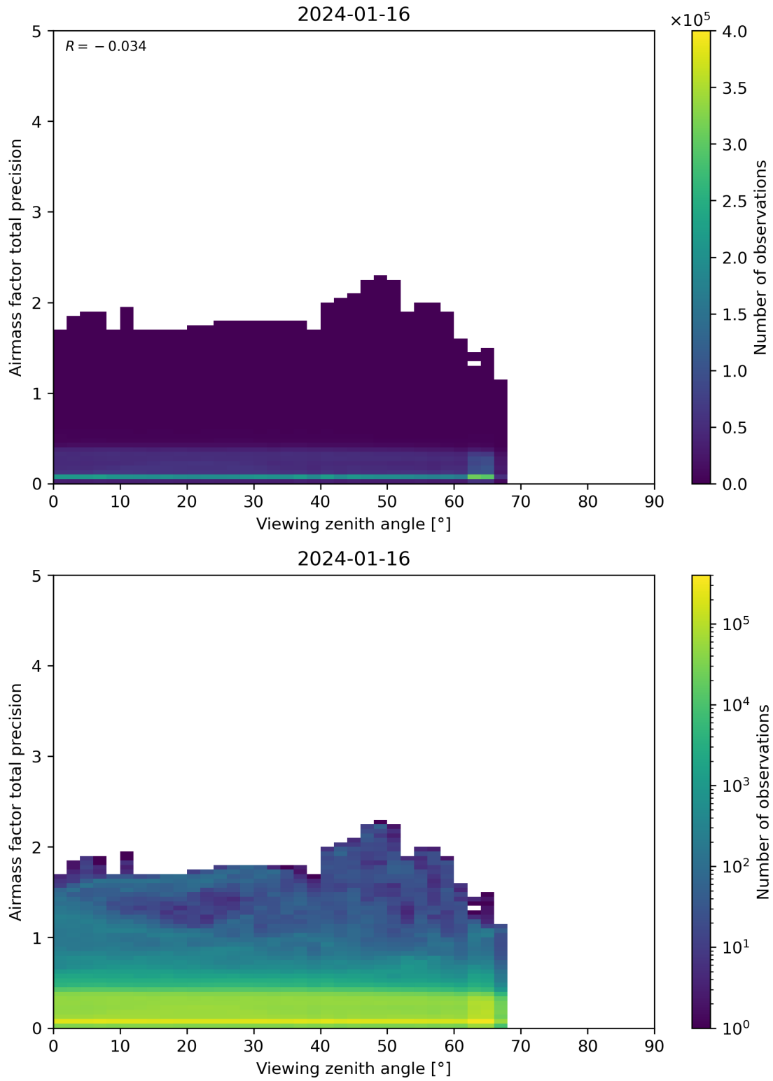
Figure 191: Scatter density plot of “Viewing zenith angle” against “Airmass factor total precision” for 2024-01-15 to 2024-01-17.
