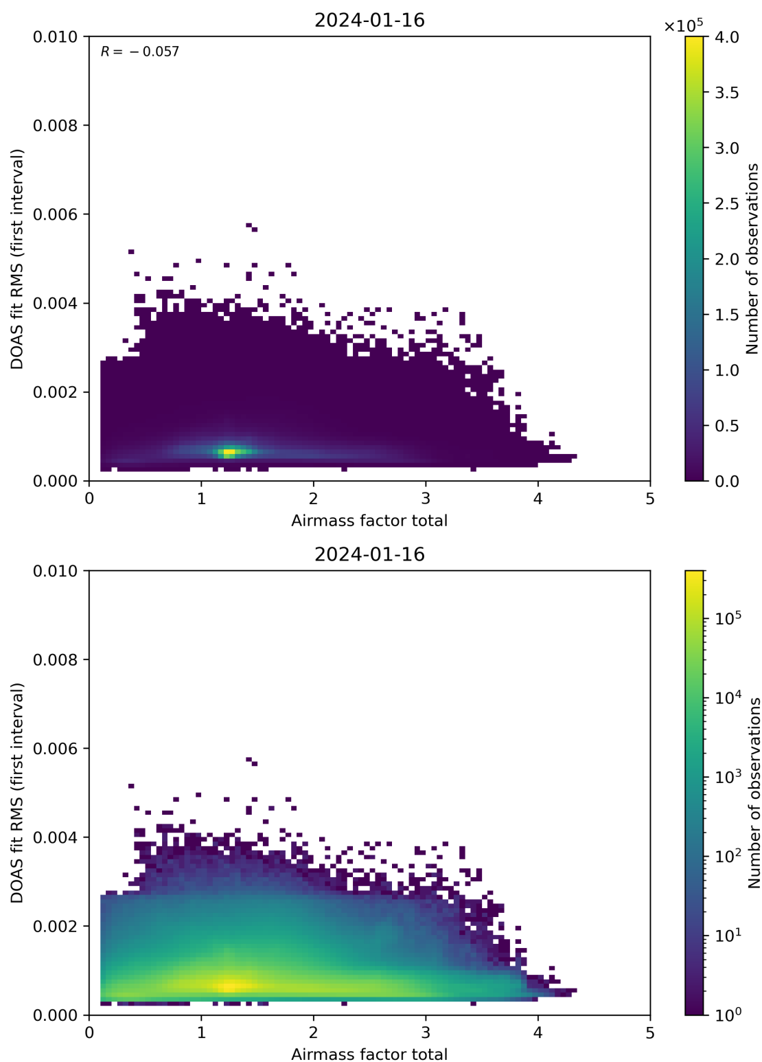
Figure 97: Scatter density plot of “Airmass factor total” against “DOAS fit RMS (first interval)” for 2024-01-15 to 2024-01-17.
