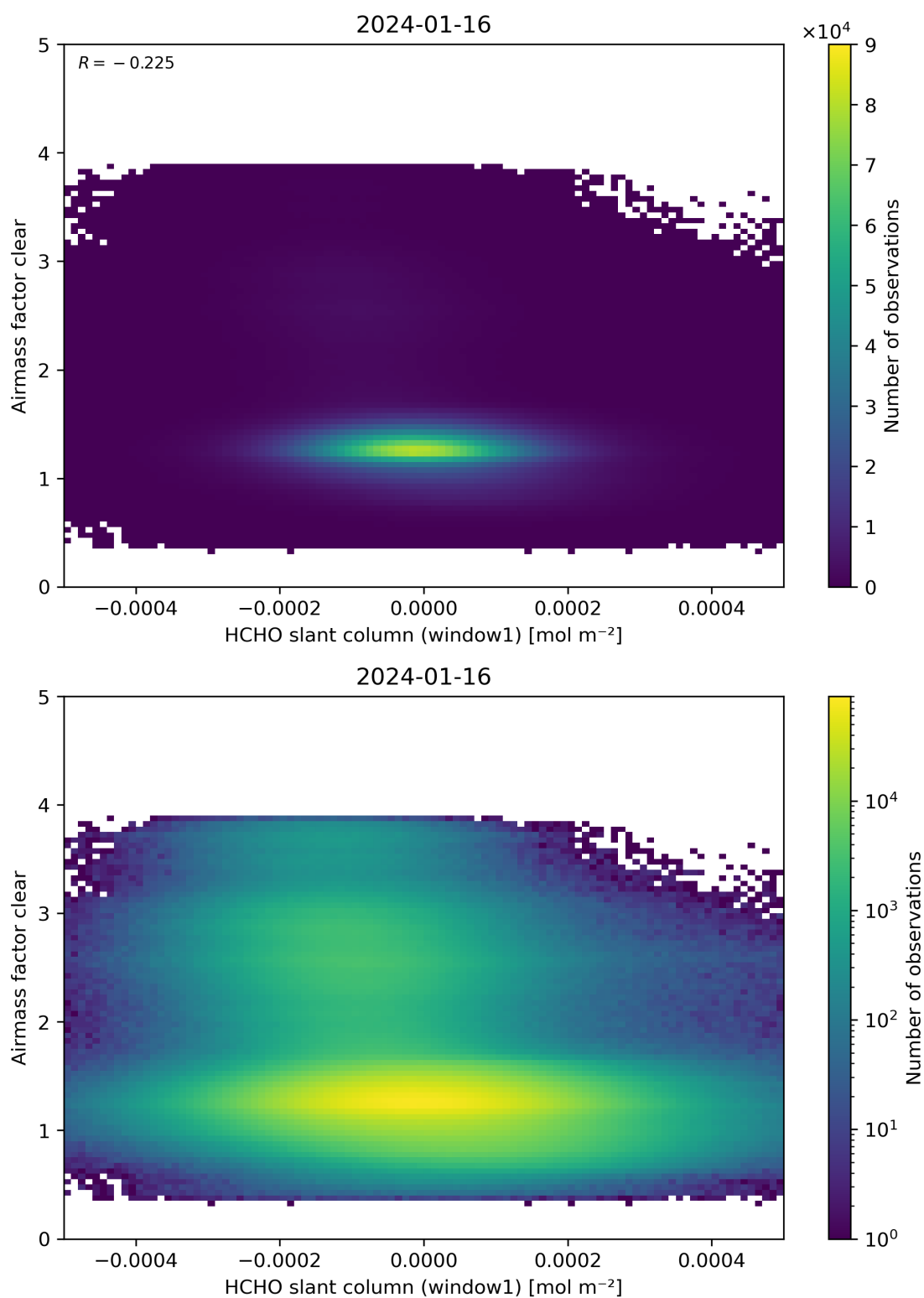
Figure 81: Scatter density plot of “HCHO slant column (window1)” against “Airmass factor clear” for 2024-01-15 to 2024-01-17.
