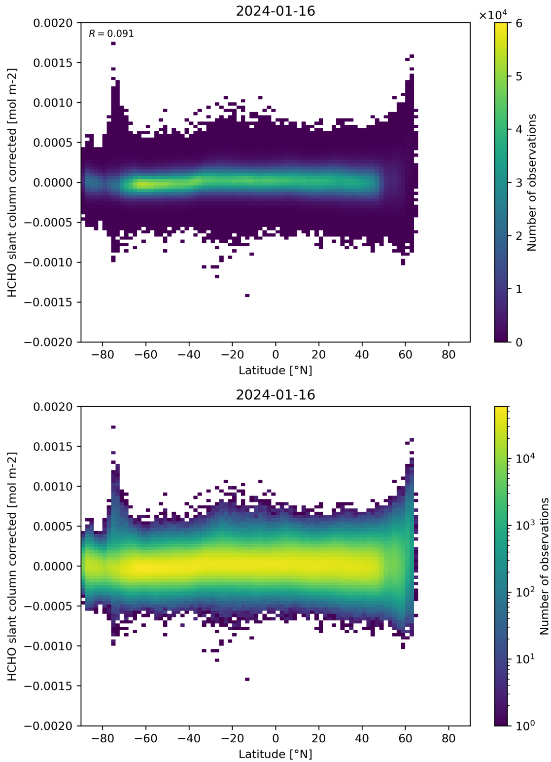
Figure 157: Scatter density plot of “Latitude” against “HCHO slant column corrected” for 2024-01-15 to 2024-01-17.
