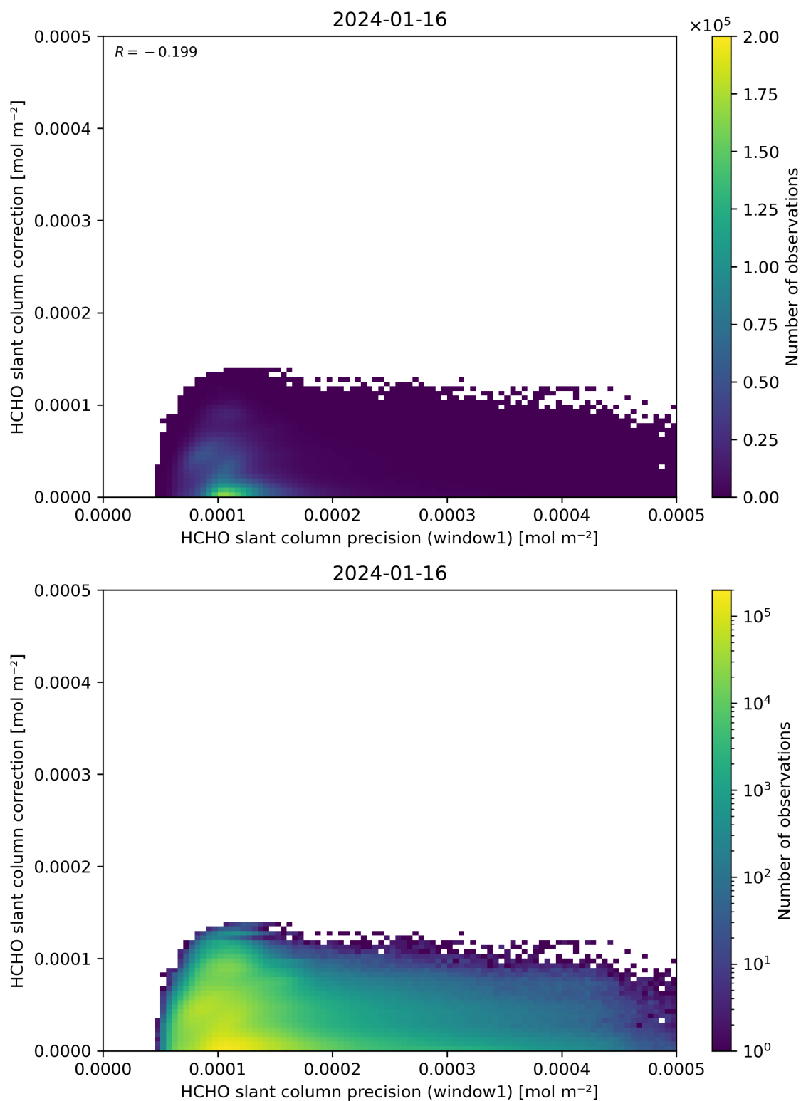
Figure 93: Scatter density plot of “HCHO slant column precision (window1)” against “HCHO slant column correction” for 2024-01-15 to 2024-01-17.
