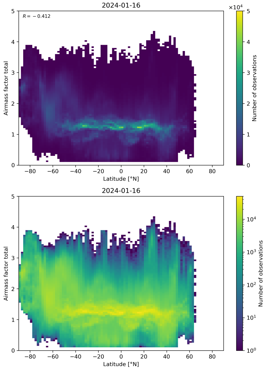
Figure 161: Scatter density plot of “Latitude” against “Airmass factor total” for 2024-01-15 to 2024-01-17.
