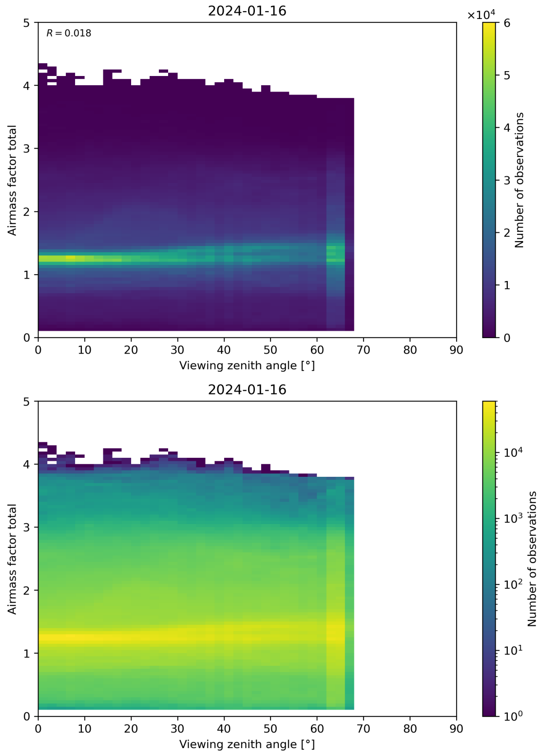
Figure 190: Scatter density plot of “Viewing zenith angle” against “Airmass factor total” for 2024-01-15 to 2024-01-17.
