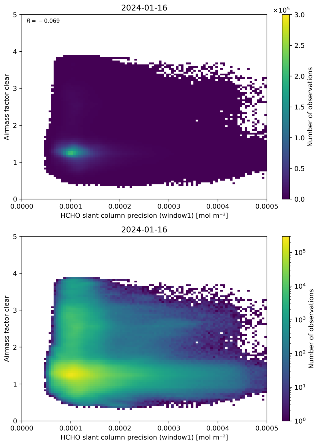
Figure 91: Scatter density plot of “HCHO slant column precision (window1)” against “Airmass factor clear” for 2024-01-15 to 2024-01-17.
