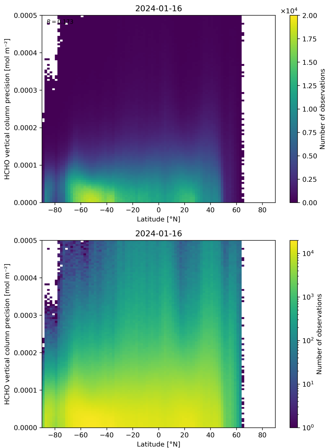
Figure 165: Scatter density plot of “Latitude” against “HCHO vertical column precision” for 2024-01-15 to 2024-01-17.
