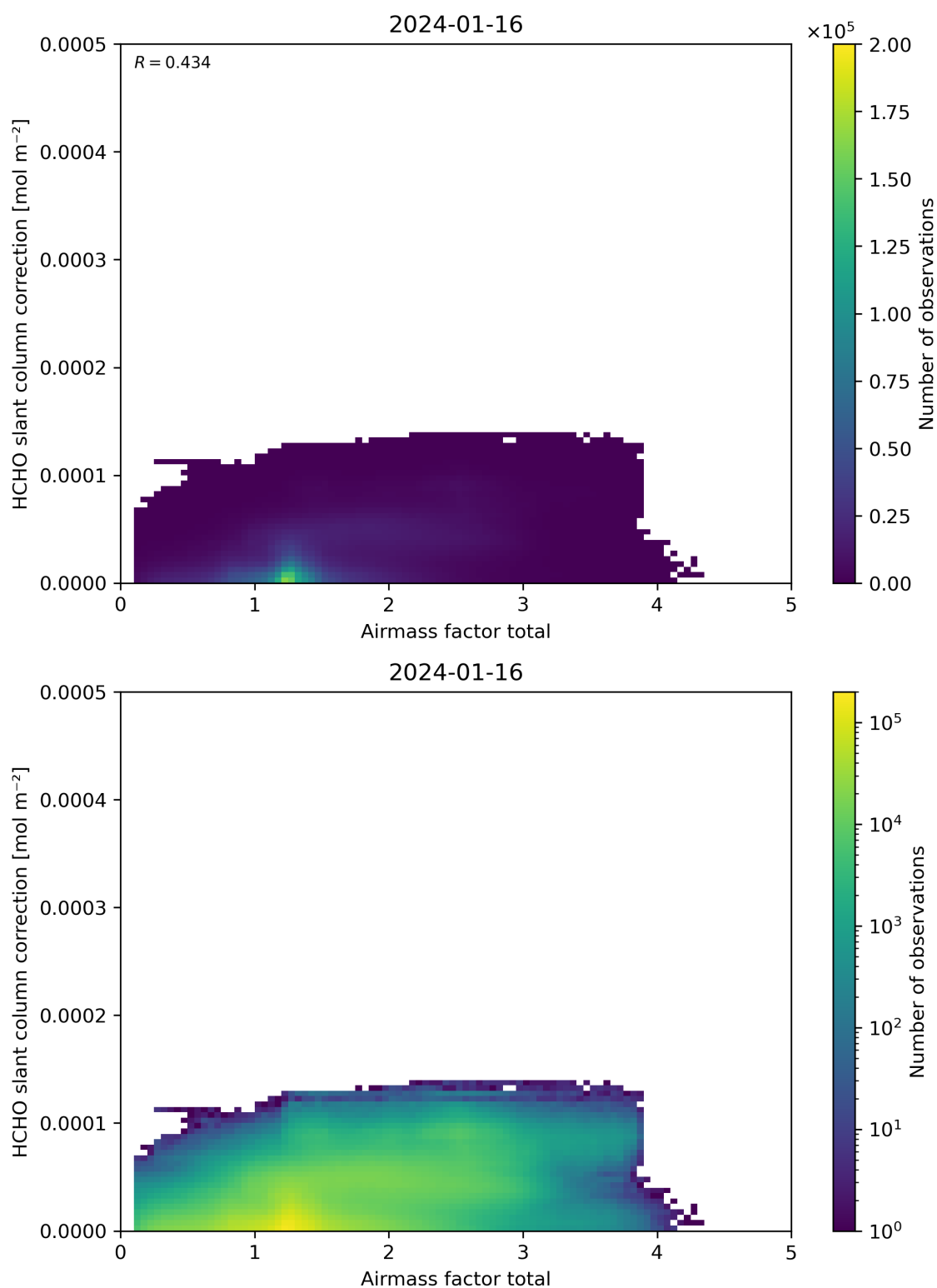
Figure 102: Scatter density plot of “Airmass factor total” against “HCHO slant column correction” for 2024-01-15 to 2024-01-17.
