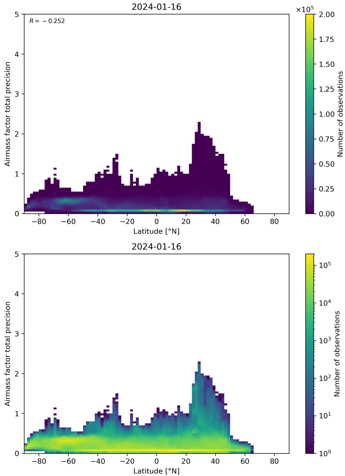
Figure 162: Scatter density plot of “Latitude” against “Airmass factor total precision” for 2024-01-15 to 2024-01-17.
