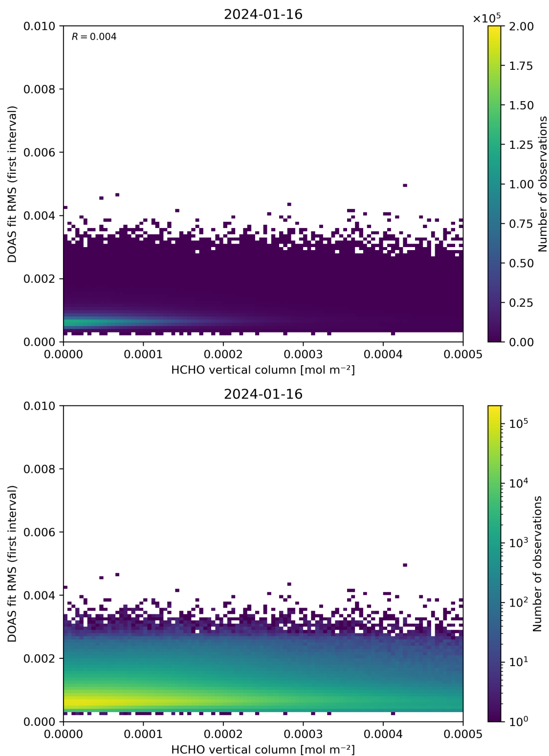
Figure 123: Scatter density plot of “HCHO vertical column” against “DOAS fit RMS (first interval)” for 2024-01-15 to 2024-01-17.
