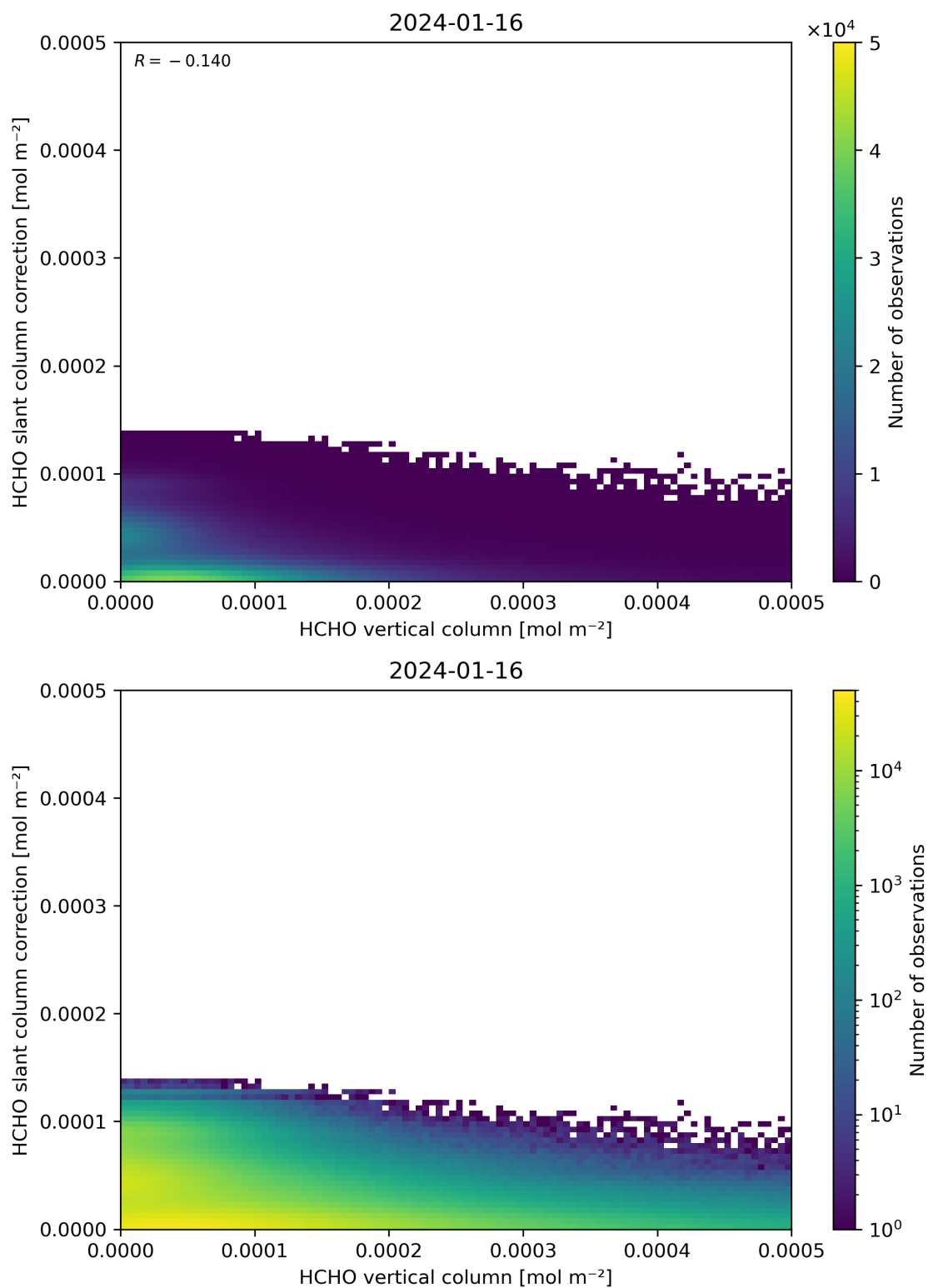
Figure 128: Scatter density plot of “HCHO vertical column” against “HCHO slant column correction” for 2024-01-15 to 2024-01-17.
