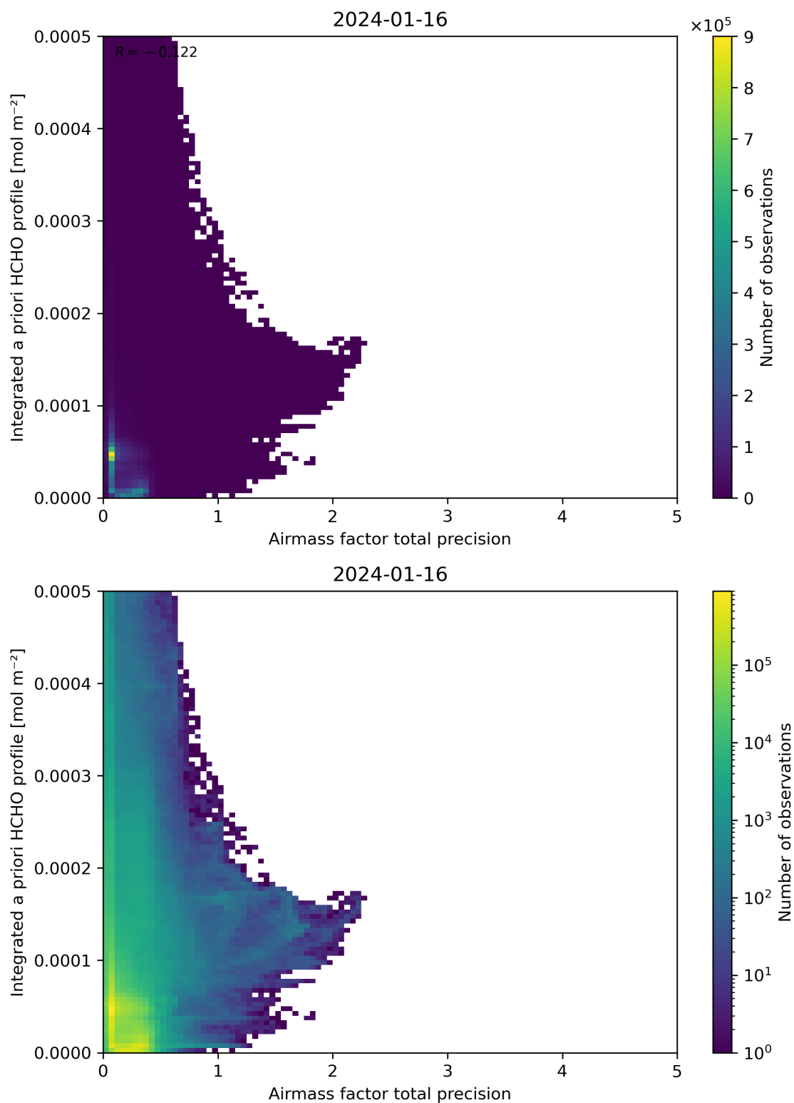
Figure 111: Scatter density plot of “Airmass factor total precision” against “Integrated a priori HCHO profile” for 2024-01-15 to 2024-01-17.
