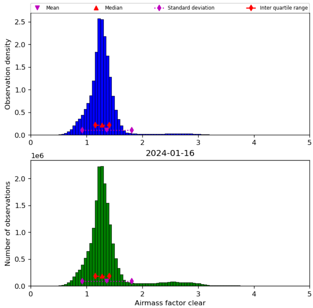
Figure 42: Histogram of “Airmass factor clear” for 2024-01-15 to 2024-01-17
