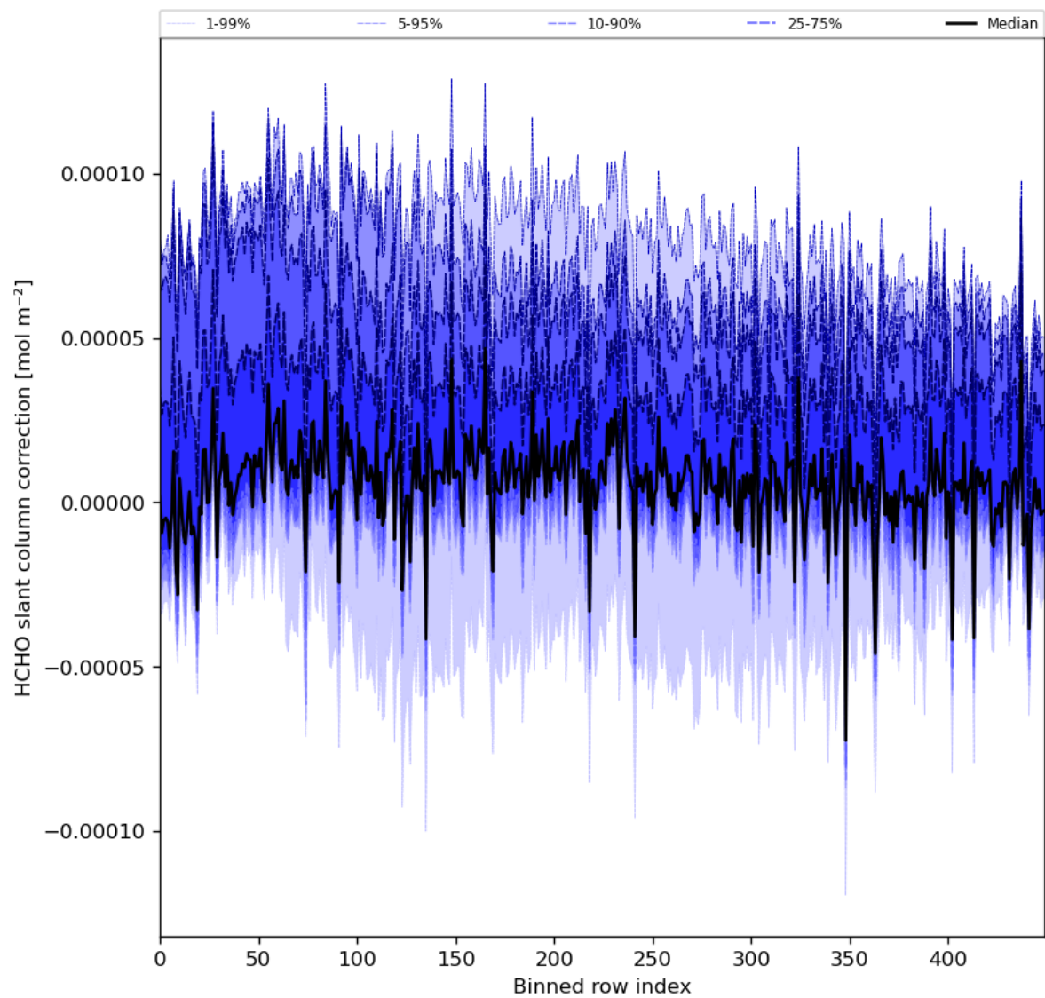
Figure 61: Along track statistics of “HCHO slant column correction” for 2024-01-15 to 2024-01-17
