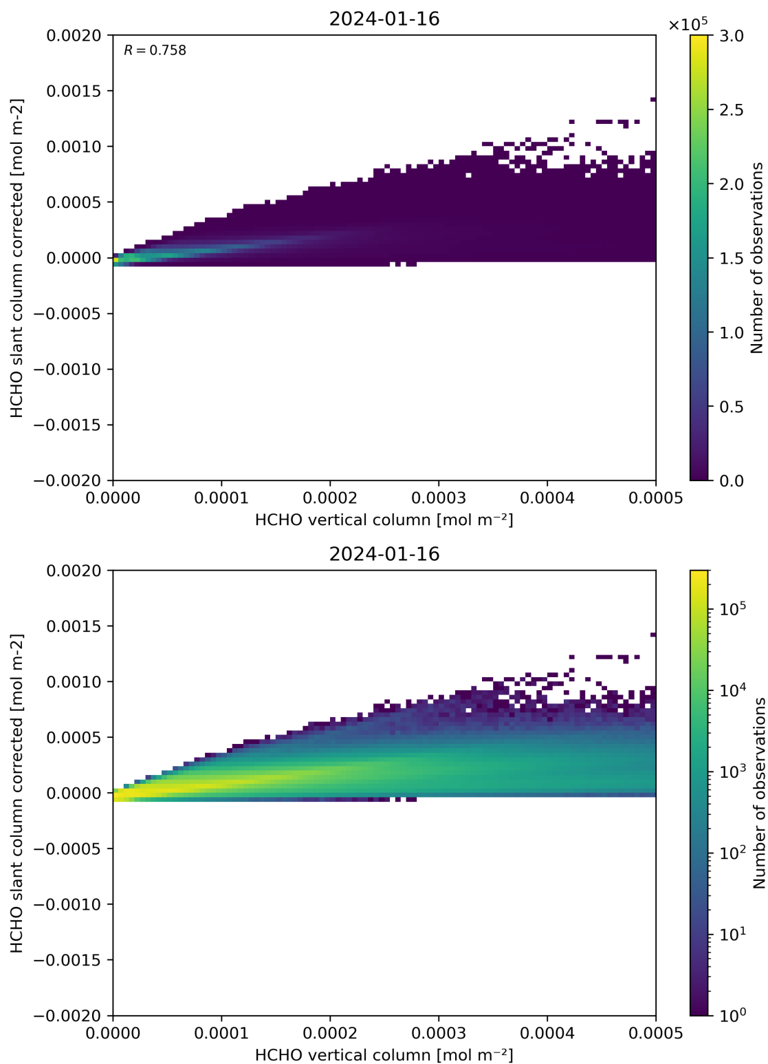
Figure 127: Scatter density plot of “HCHO vertical column” against “HCHO slant column corrected” for 2024-01-15 to 2024-01-17.
