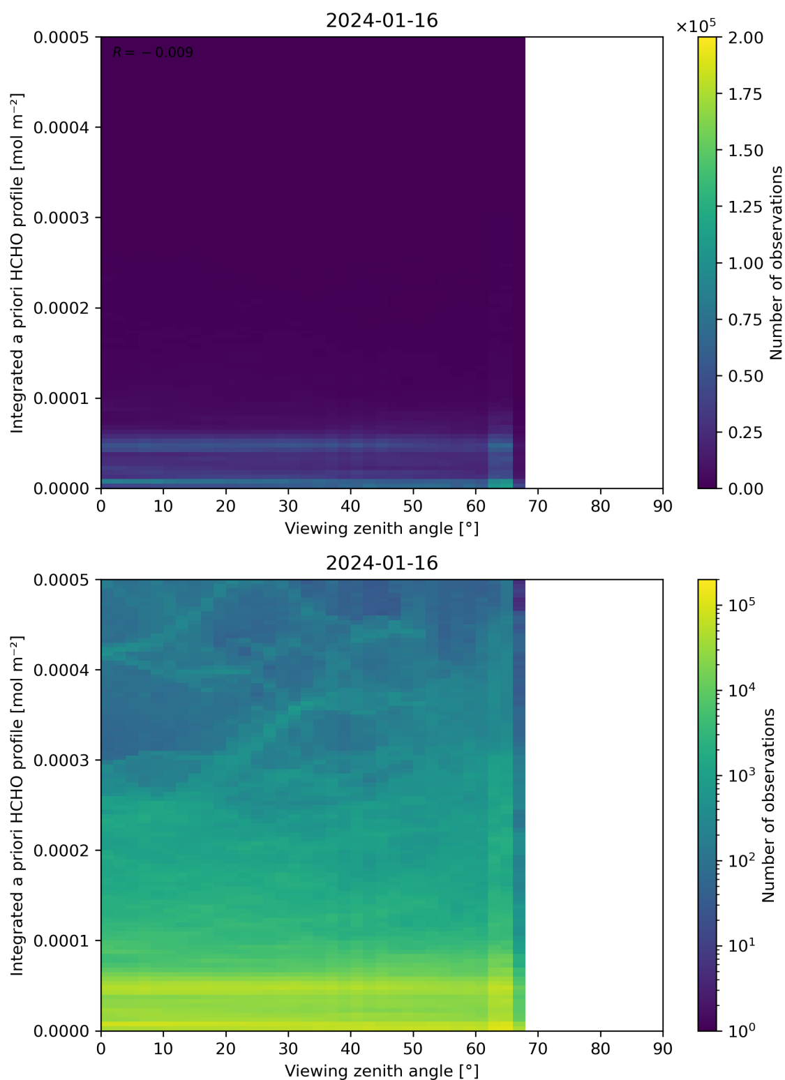
Figure 195: Scatter density plot of “Viewing zenith angle” against “Integrated a priori HCHO profile” for 2024-01-15 to 2024-01-17.
