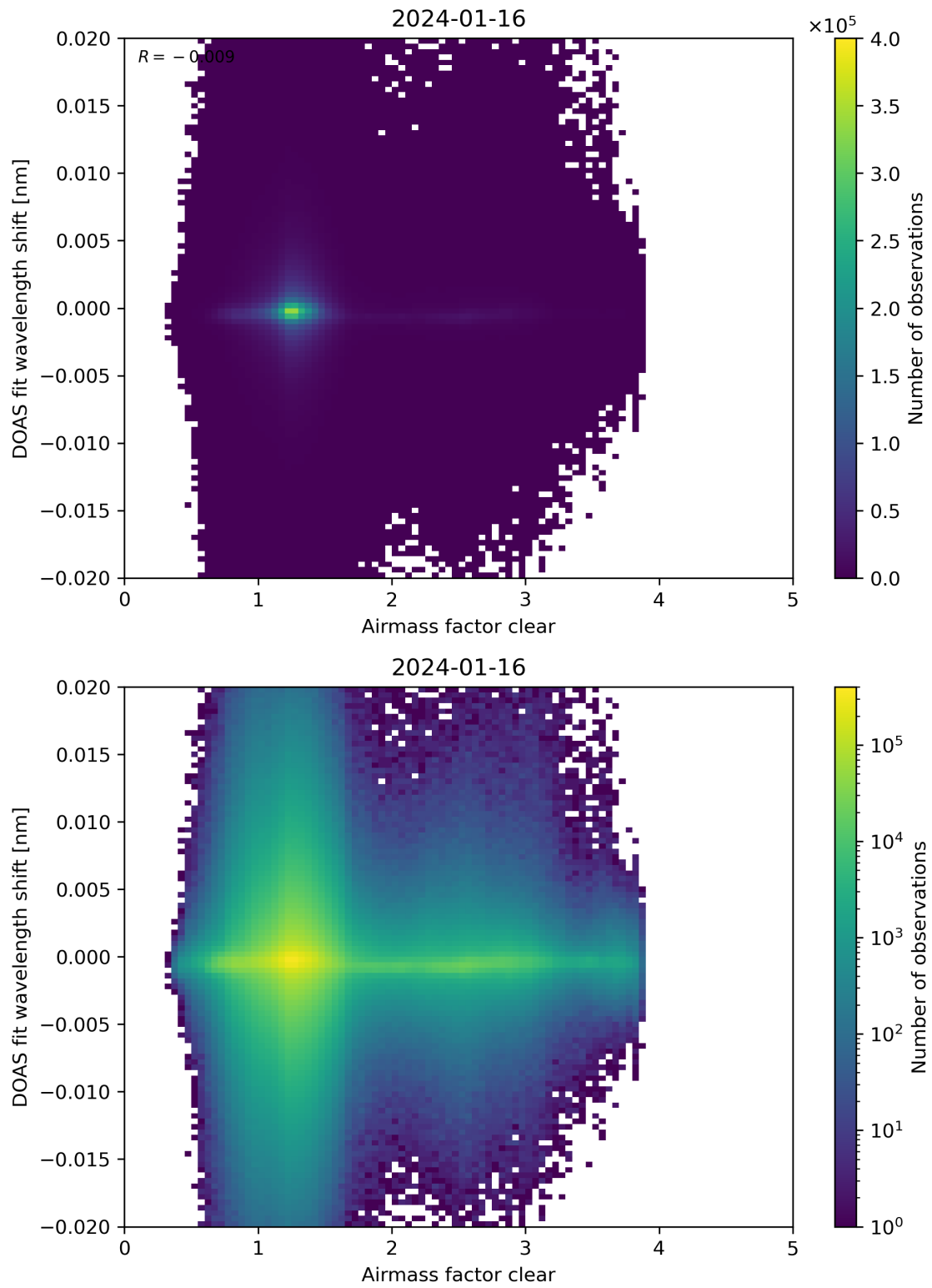
Figure 72: Scatter density plot of “Airmass factor clear” against “DOAS fit wavelength shift” for 2024-01-15 to 2024-01-17.
