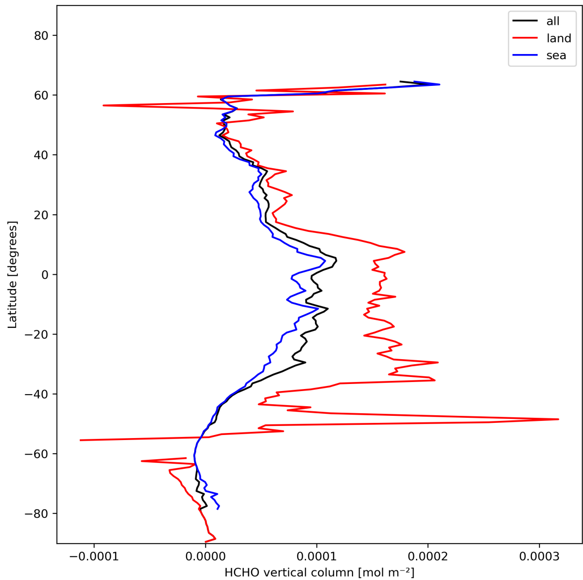
Figure 21: Zonal average of “HCHO vertical column” for 2024-01-15 to 2024-01-17.
