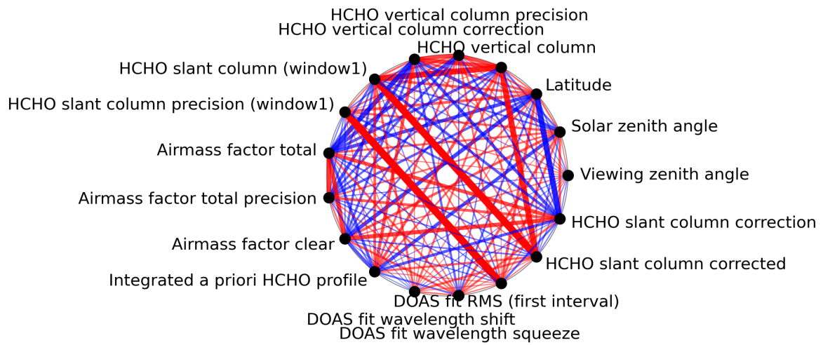
Figure 1: Map of correlation graph for 2024-01-15 to 2024-01-17.
