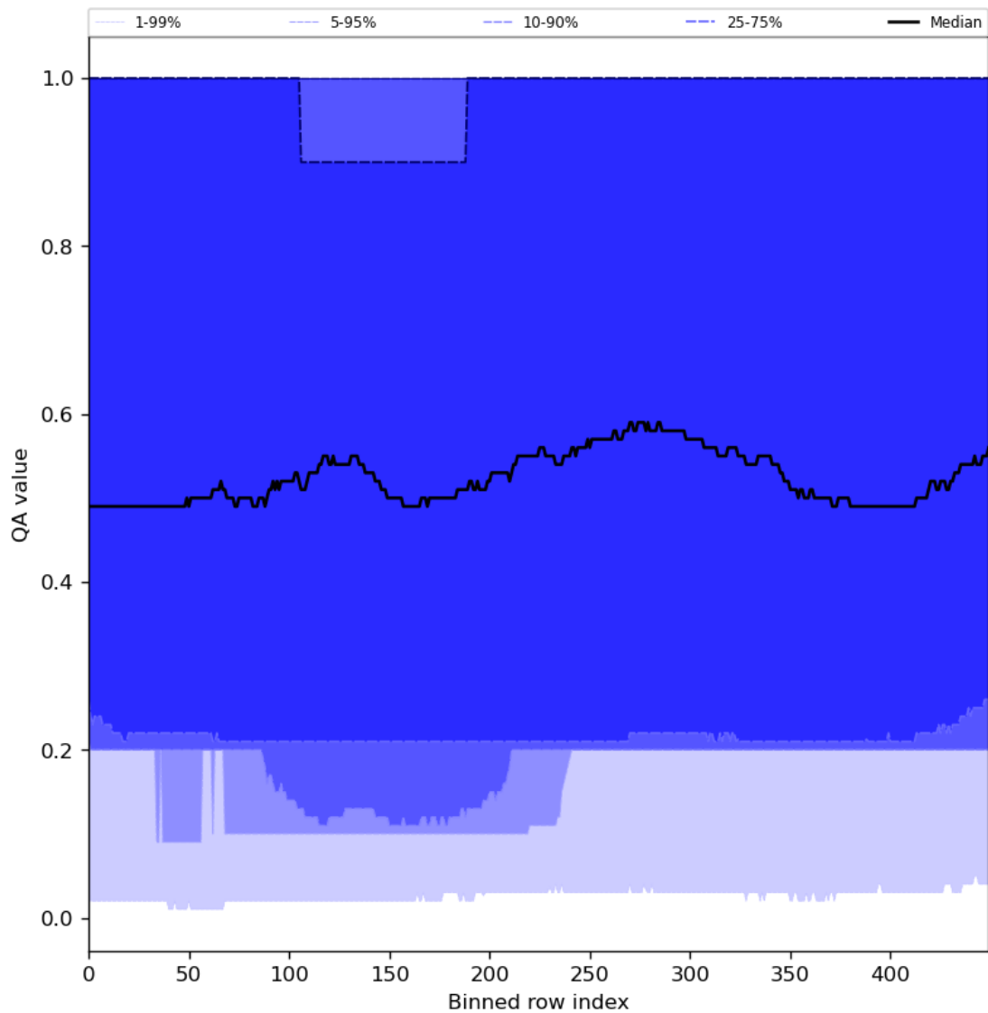
Figure 48: Along track statistics of “QA value” for 2024-01-15 to 2024-01-17
