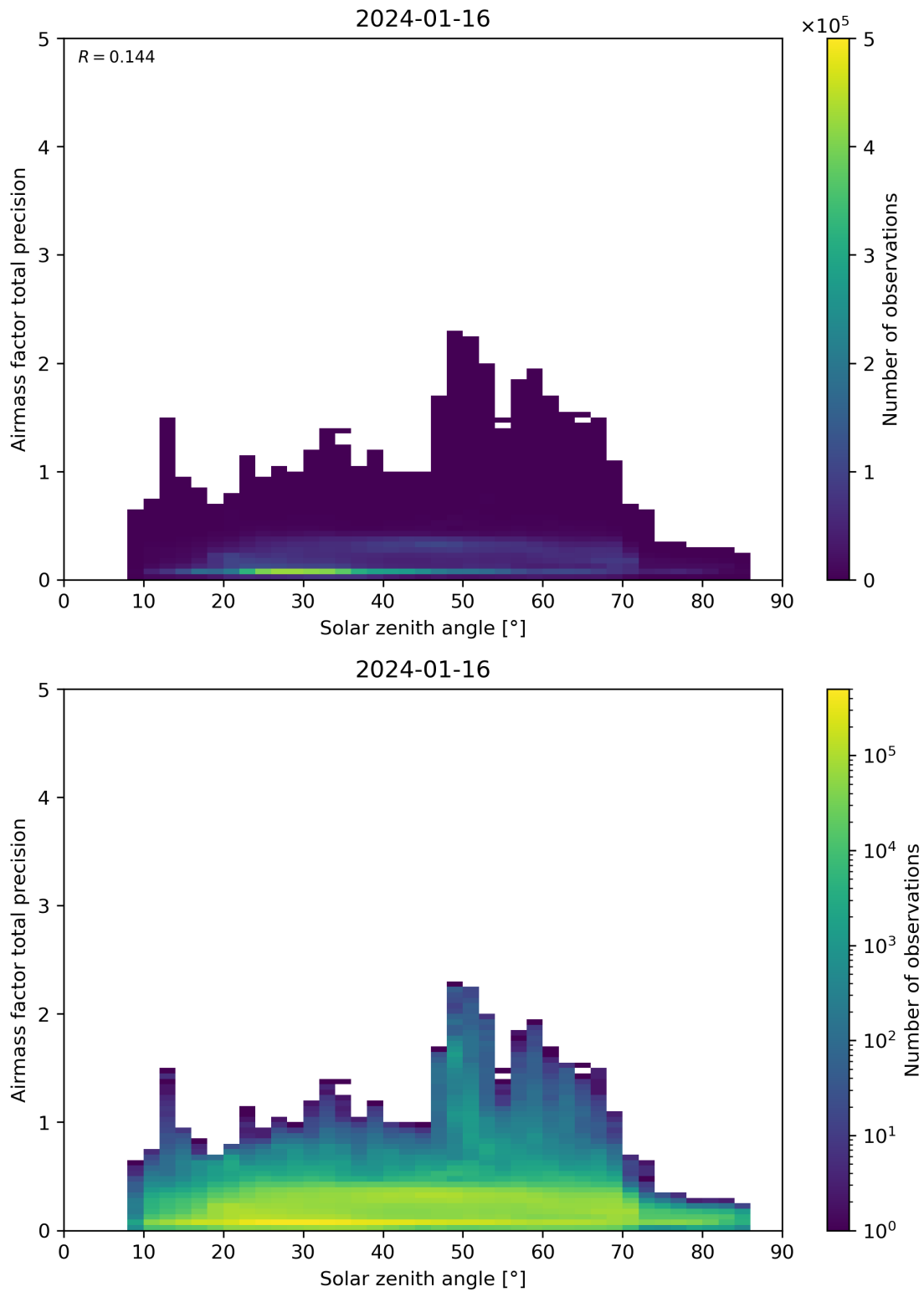
Figure 176: Scatter density plot of “Solar zenith angle” against “Airmass factor total precision” for 2024-01-15 to 2024-01-17.
