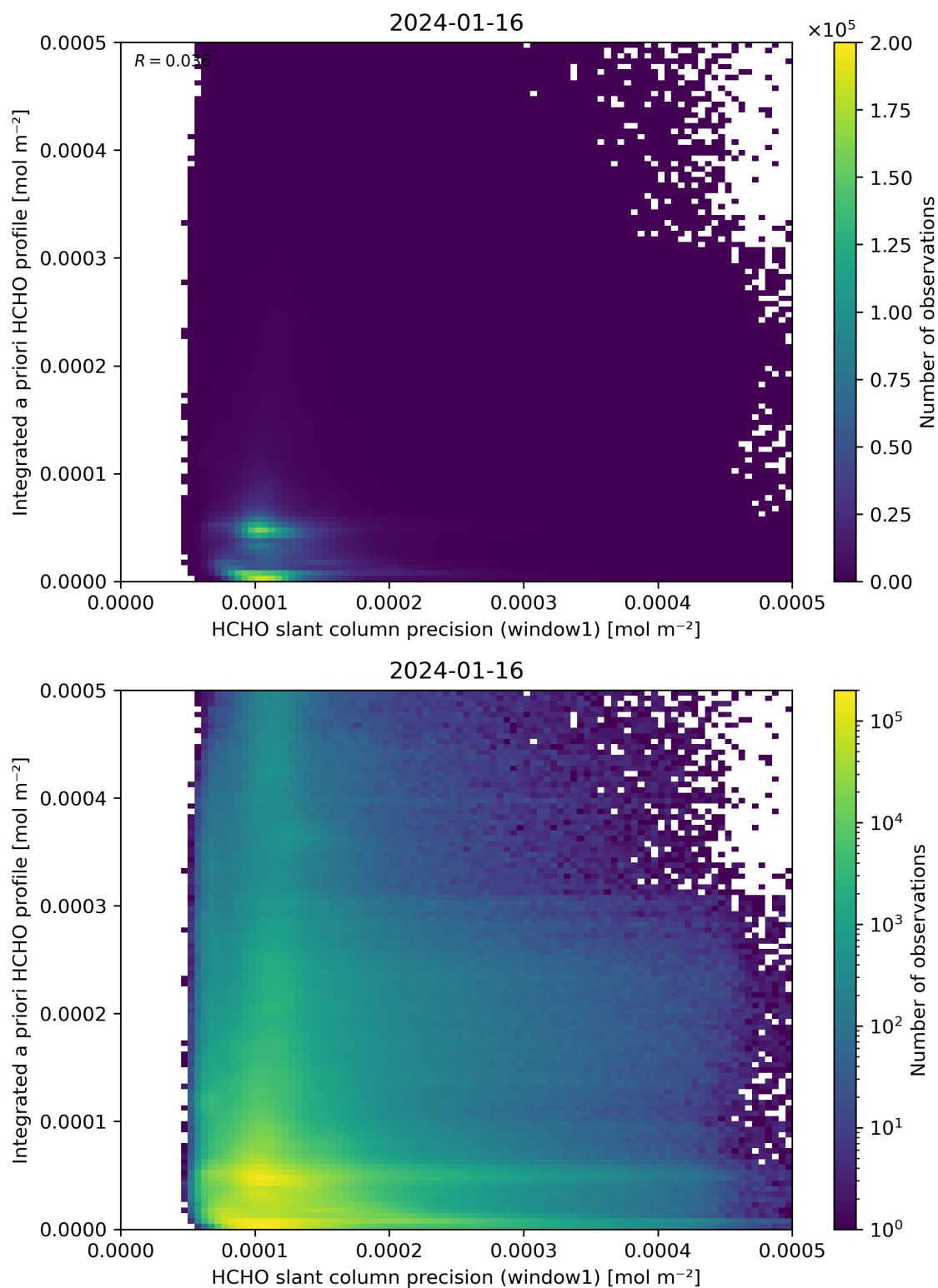
Figure 96: Scatter density plot of “HCHO slant column precision (window1)” against “Integrated a priori HCHO profile” for 2024-01-15 to 2024-01-17.
