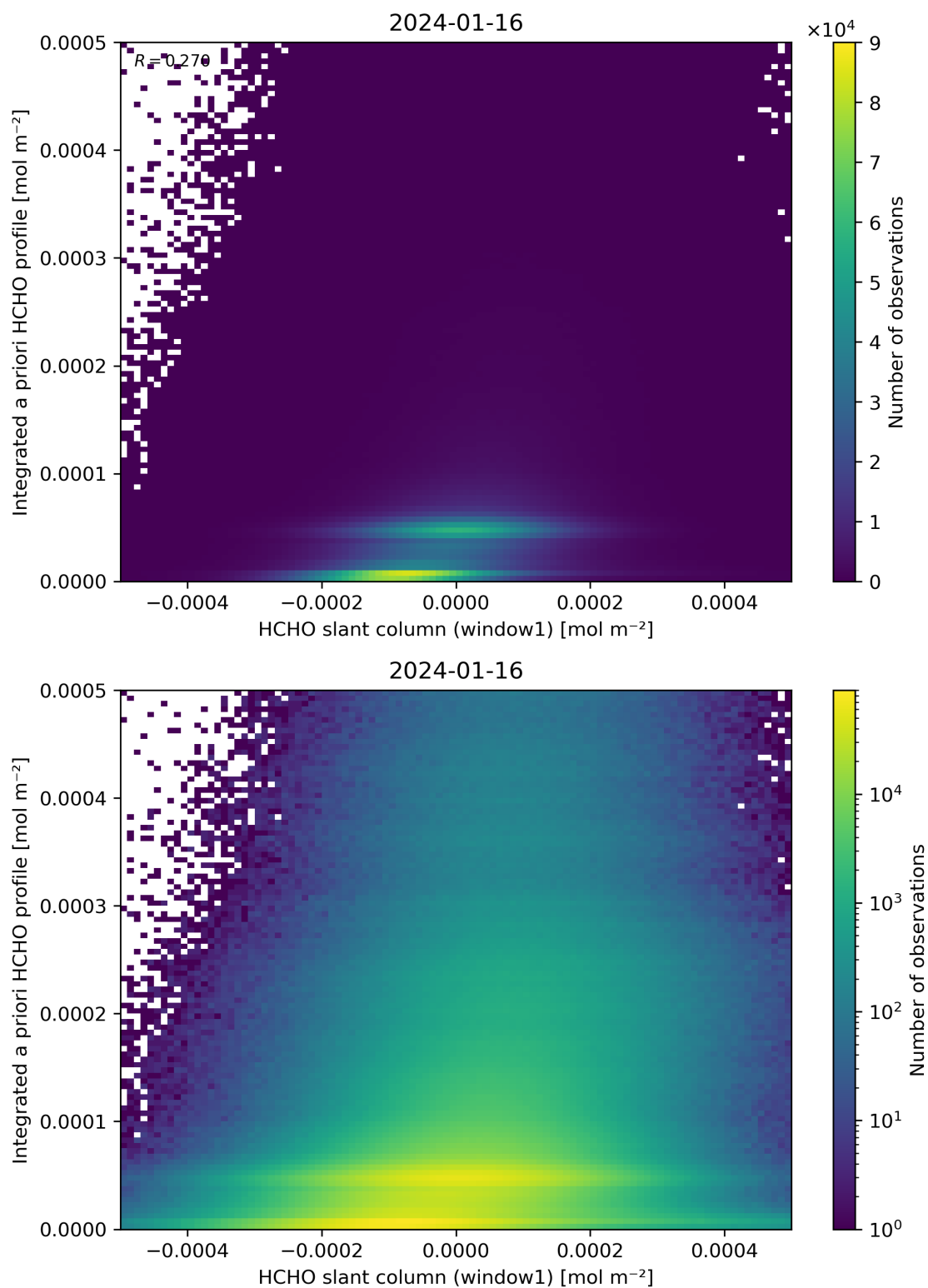
Figure 87: Scatter density plot of “HCHO slant column (window1)” against “Integrated a priori HCHO profile” for 2024-01-15 to 2024-01-17.
