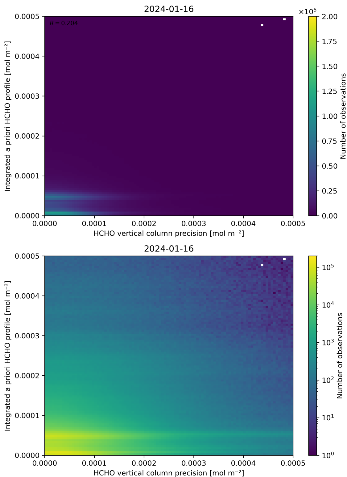
Figure 147: Scatter density plot of “HCHO vertical column precision” against “Integrated a priori HCHO profile” for 2024-01-15 to 2024-01-17.
