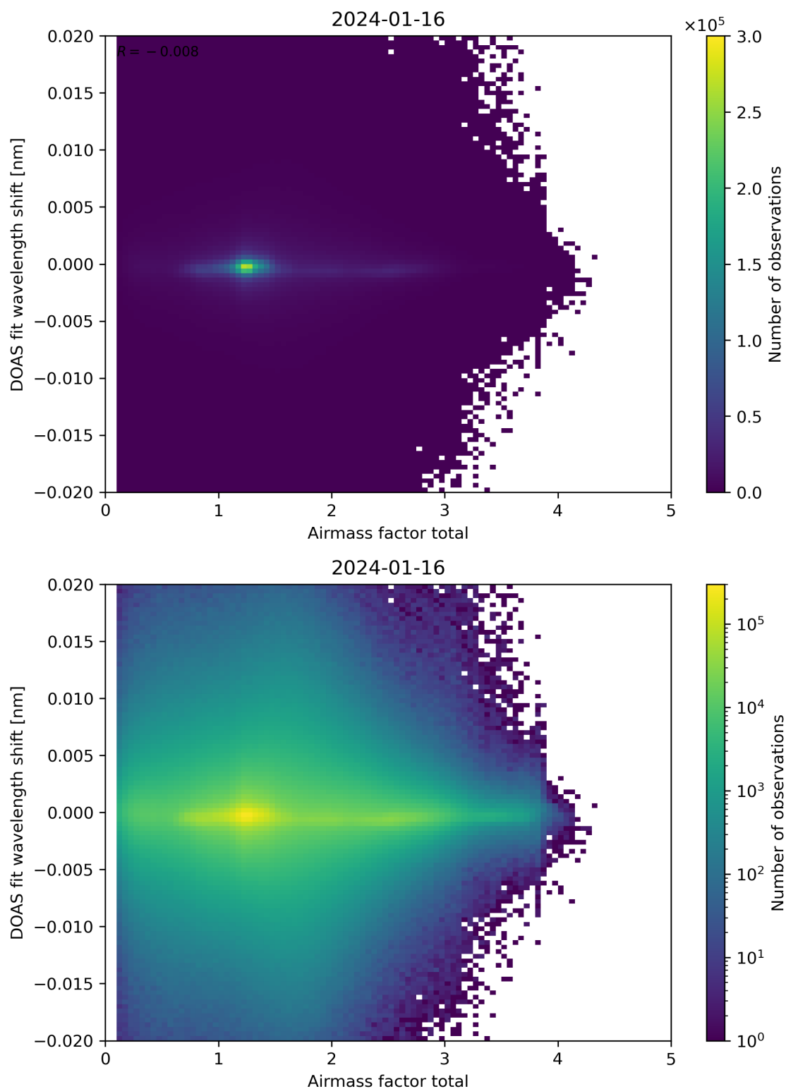
Figure 98: Scatter density plot of “Airmass factor total” against “DOAS fit wavelength shift” for 2024-01-15 to 2024-01-17.
