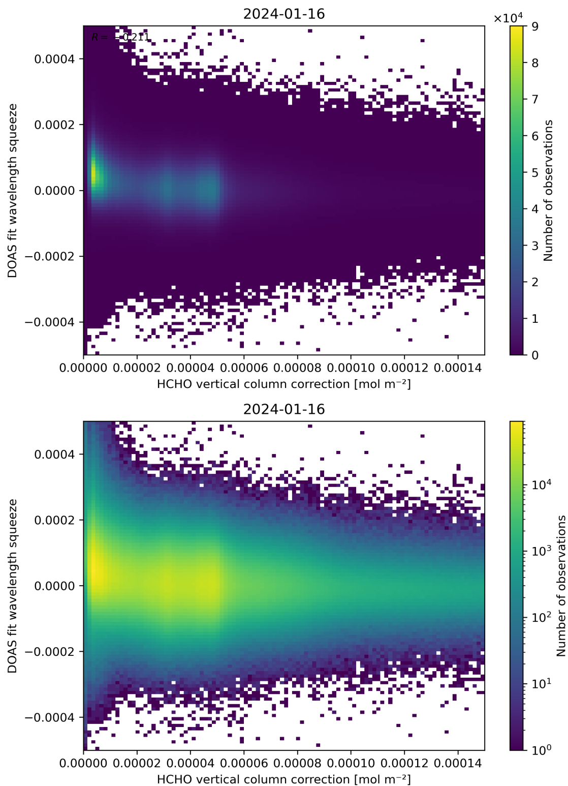
Figure 114: Scatter density plot of “HCHO vertical column correction” against “DOAS fit wavelength squeeze” for 2024-01-15 to 2024-01-17.
