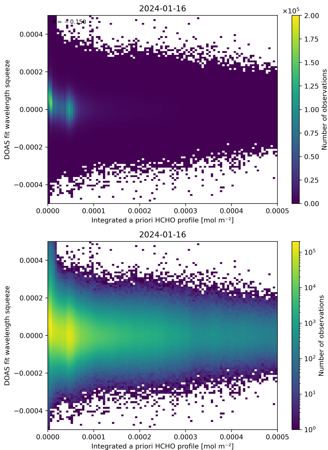
Figure 150: Scatter density plot of “Integrated a priori HCHO profile” against “DOAS fit wavelength squeeze” for 2024-01-15 to 2024-01-17.
