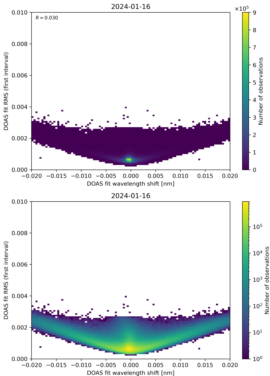
Figure 64: Scatter density plot of “DOAS fit wavelength shift” against “DOAS fit RMS (first interval)” for 2024-01-15 to 2024-01-17.
