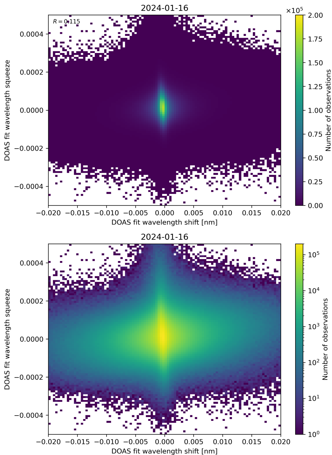
Figure 65: Scatter density plot of “DOAS fit wavelength shift” against “DOAS fit wavelength squeeze” for 2024-01-15 to 2024-01-17.
