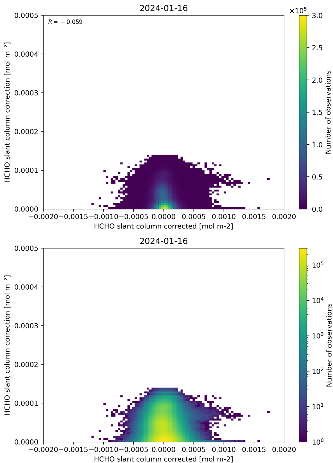
Figure 77: Scatter density plot of “HCHO slant column corrected” against “HCHO slant column correction” for 2024-01-15 to 2024-01-17.
