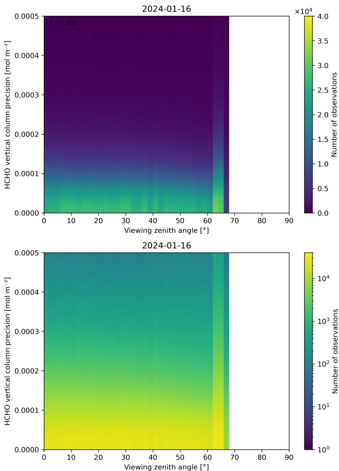
Figure 194: Scatter density plot of “Viewing zenith angle” against “HCHO vertical column precision” for 2024-01-15 to 2024-01-17.
