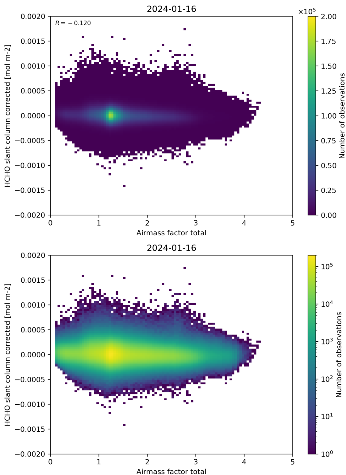
Figure 101: Scatter density plot of “Airmass factor total” against “HCHO slant column corrected” for 2024-01-15 to 2024-01-17.
