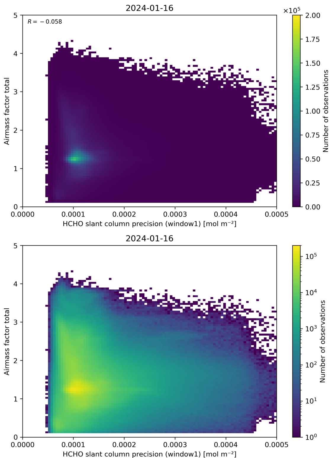
Figure 94: Scatter density plot of “HCHO slant column precision (window1)” against “Airmass factor total” for 2024-01-15 to 2024-01-17.
