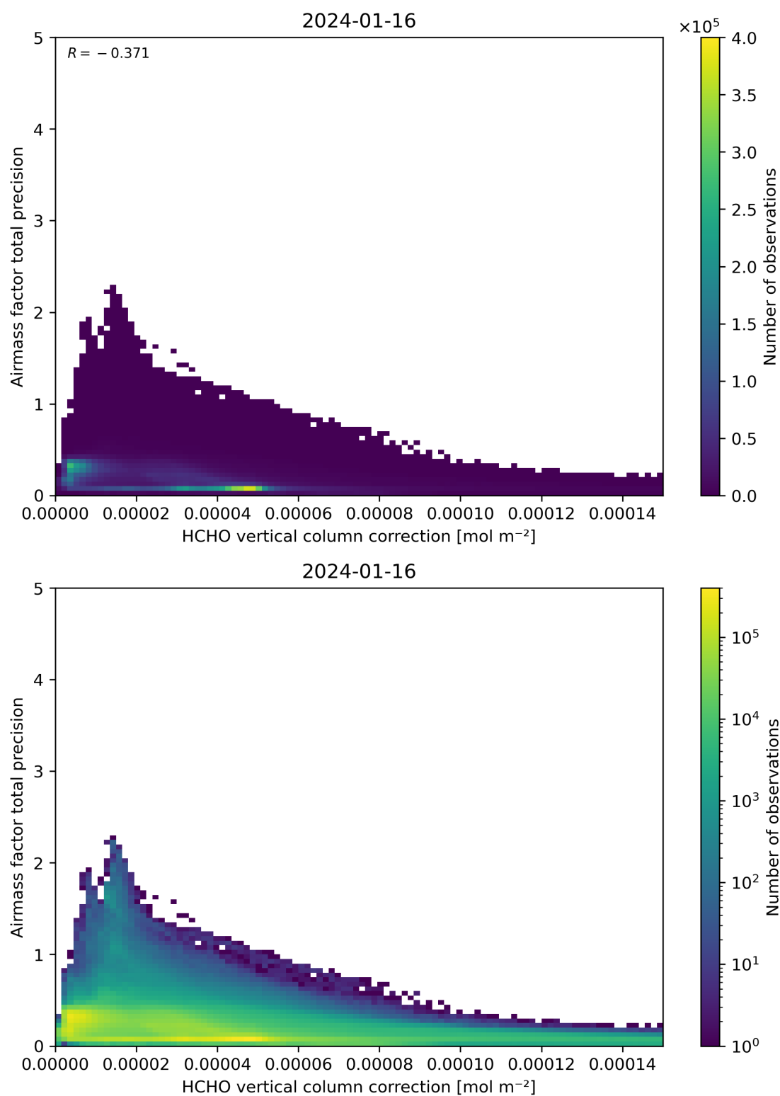
Figure 121: Scatter density plot of “HCHO vertical column correction” against “Airmass factor total precision” for 2024-01-15 to 2024-01-17.
