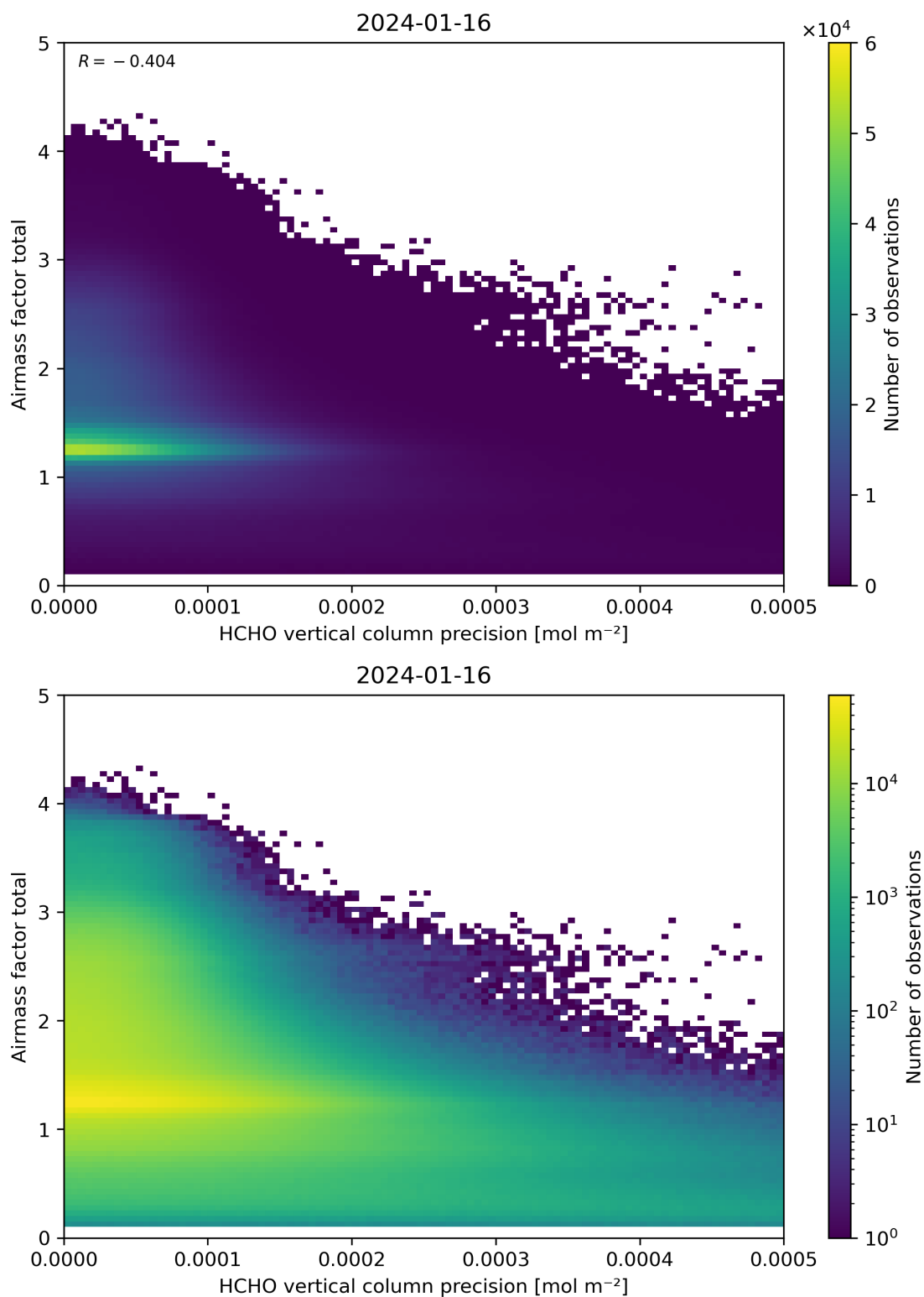
Figure 144: Scatter density plot of “HCHO vertical column precision” against “Airmass factor total” for 2024-01-15 to 2024-01-17.
