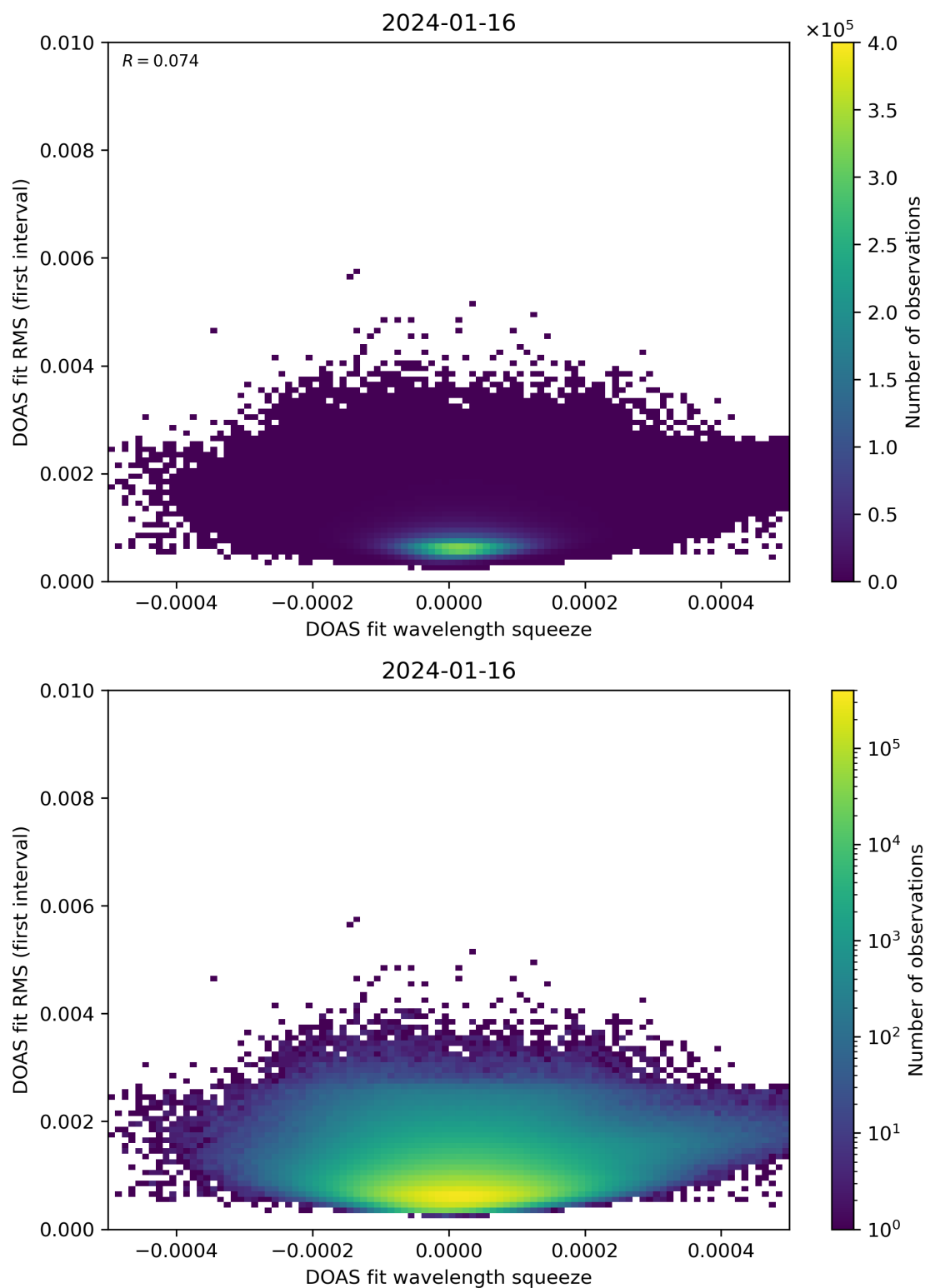
Figure 68: Scatter density plot of “DOAS fit wavelength squeeze” against “DOAS fit RMS (first interval)” for 2024-01-15 to 2024-01-17.
