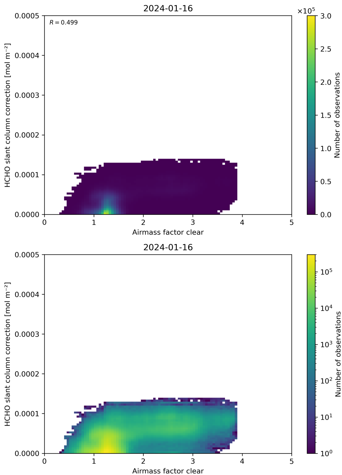
Figure 75: Scatter density plot of “Airmass factor clear” against “HCHO slant column correction” for 2024-01-15 to 2024-01-17.
