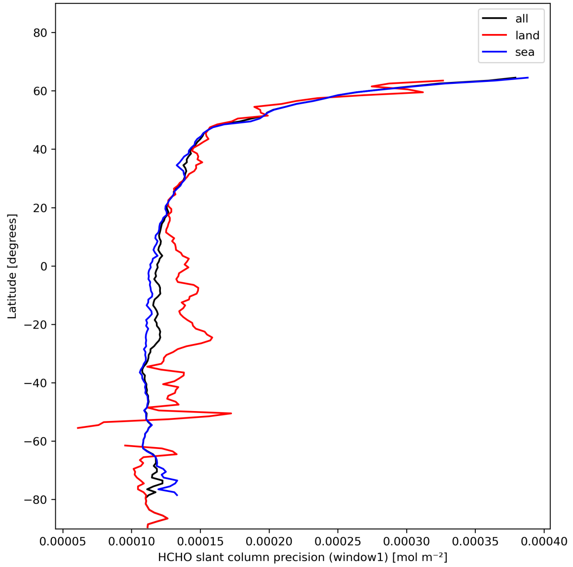
Figure 25: Zonal average of “HCHO slant column precision (window1)” for 2024-01-15 to 2024-01-17.
