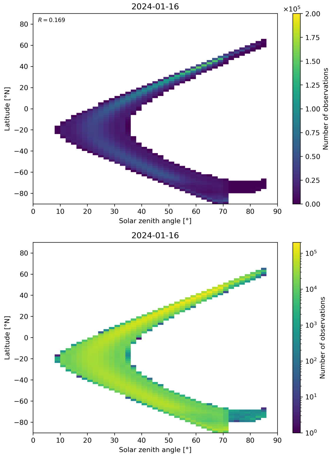
Figure 181: Scatter density plot of “Solar zenith angle” against “Latitude” for 2024-01-15 to 2024-01-17.
