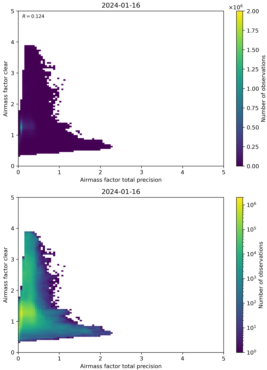
Figure 108: Scatter density plot of “Airmass factor total precision” against “Airmass factor clear” for 2024-01-15 to 2024-01-17.
