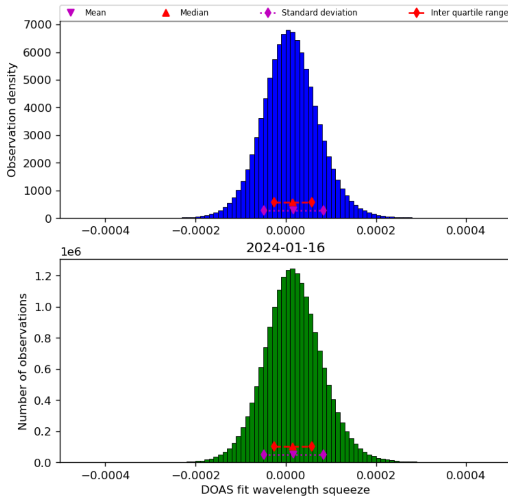
Figure 45: Histogram of “DOAS fit wavelength squeeze” for 2024-01-15 to 2024-01-17
