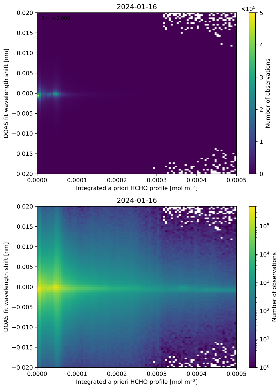
Figure 149: Scatter density plot of “Integrated a priori HCHO profile” against “DOAS fit wavelength shift” for 2024-01-15 to 2024-01-17.
