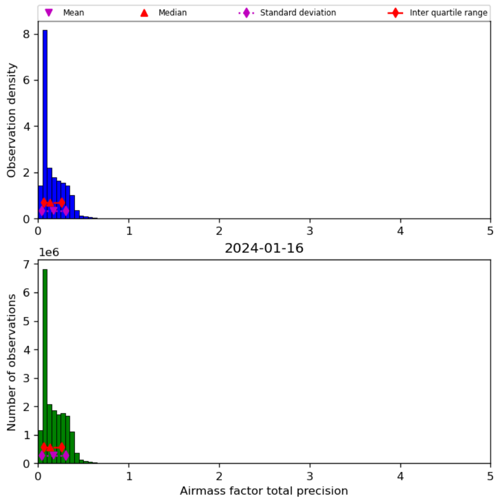
Figure 41: Histogram of “Airmass factor total precision” for 2024-01-15 to 2024-01-17
