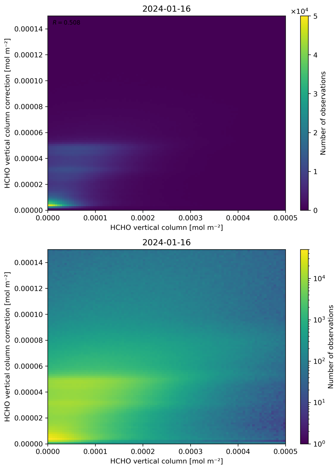
Figure 133: Scatter density plot of “HCHO vertical column” against “HCHO vertical column correction” for 2024-01-15 to 2024-01-17.
