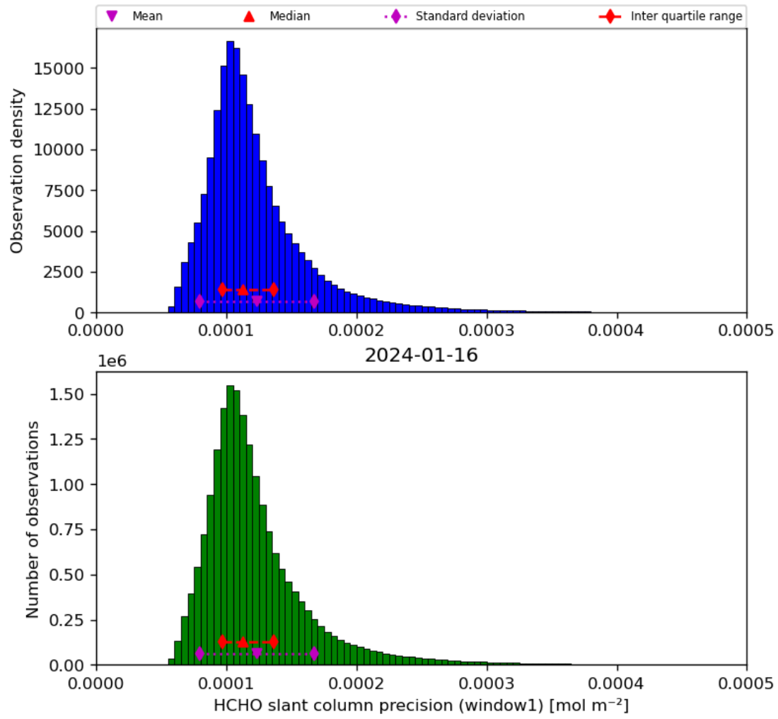
Figure 39: Histogram of “HCHO slant column precision (window1)” for 2024-01-15 to 2024-01-17
