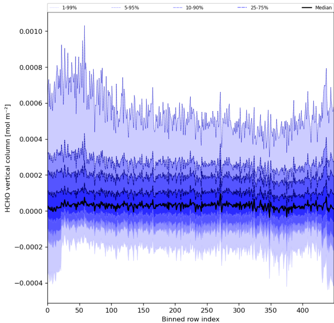
Figure 49: Along track statistics of “HCHO vertical column” for 2024-01-15 to 2024-01-17
