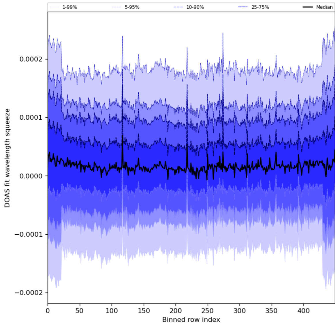
Figure 59: Along track statistics of “DOAS fit wavelength squeeze” for 2024-01-15 to 2024-01-17
