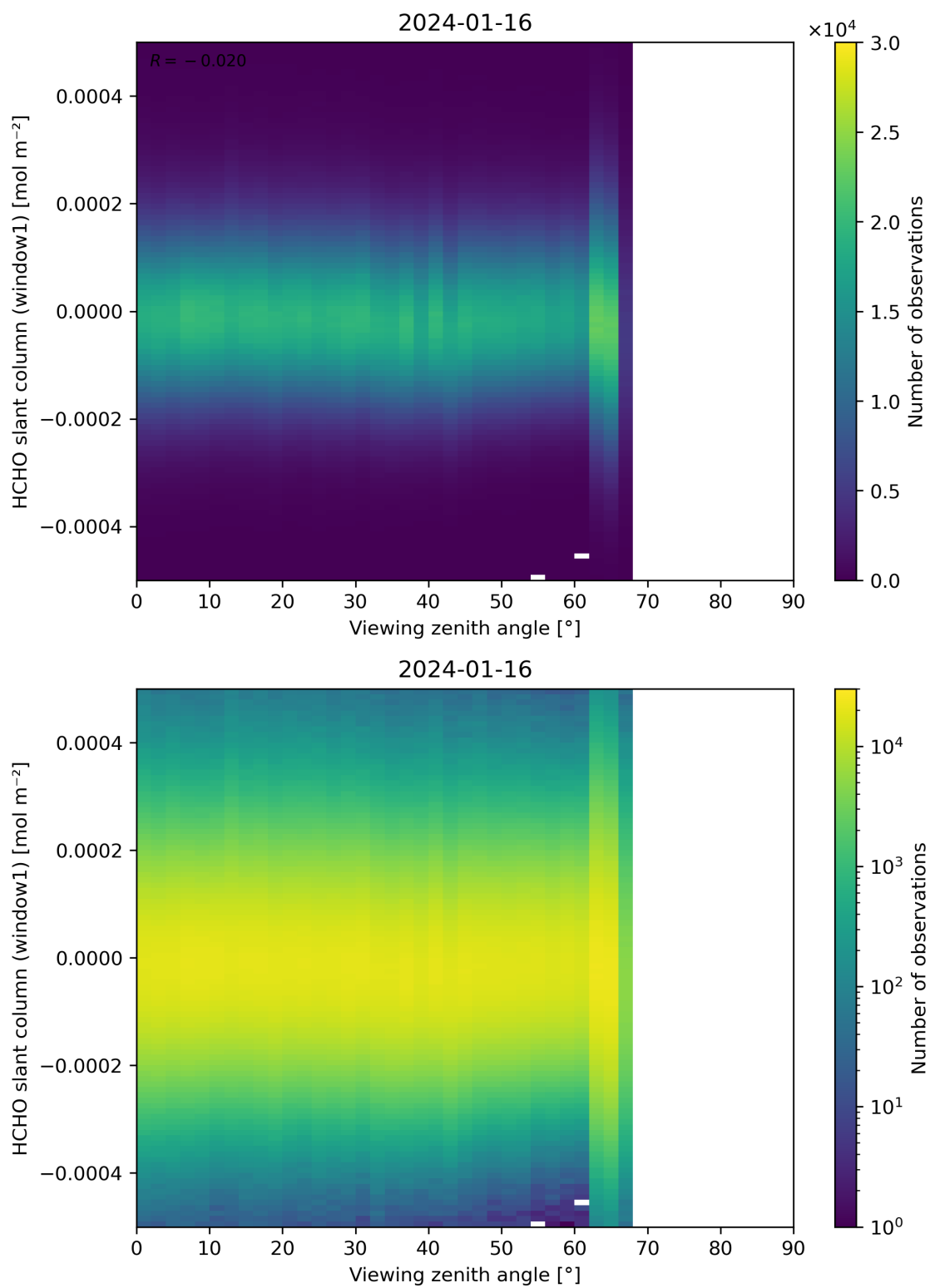
Figure 188: Scatter density plot of “Viewing zenith angle” against “HCHO slant column (window1)” for 2024-01-15 to 2024-01-17.
