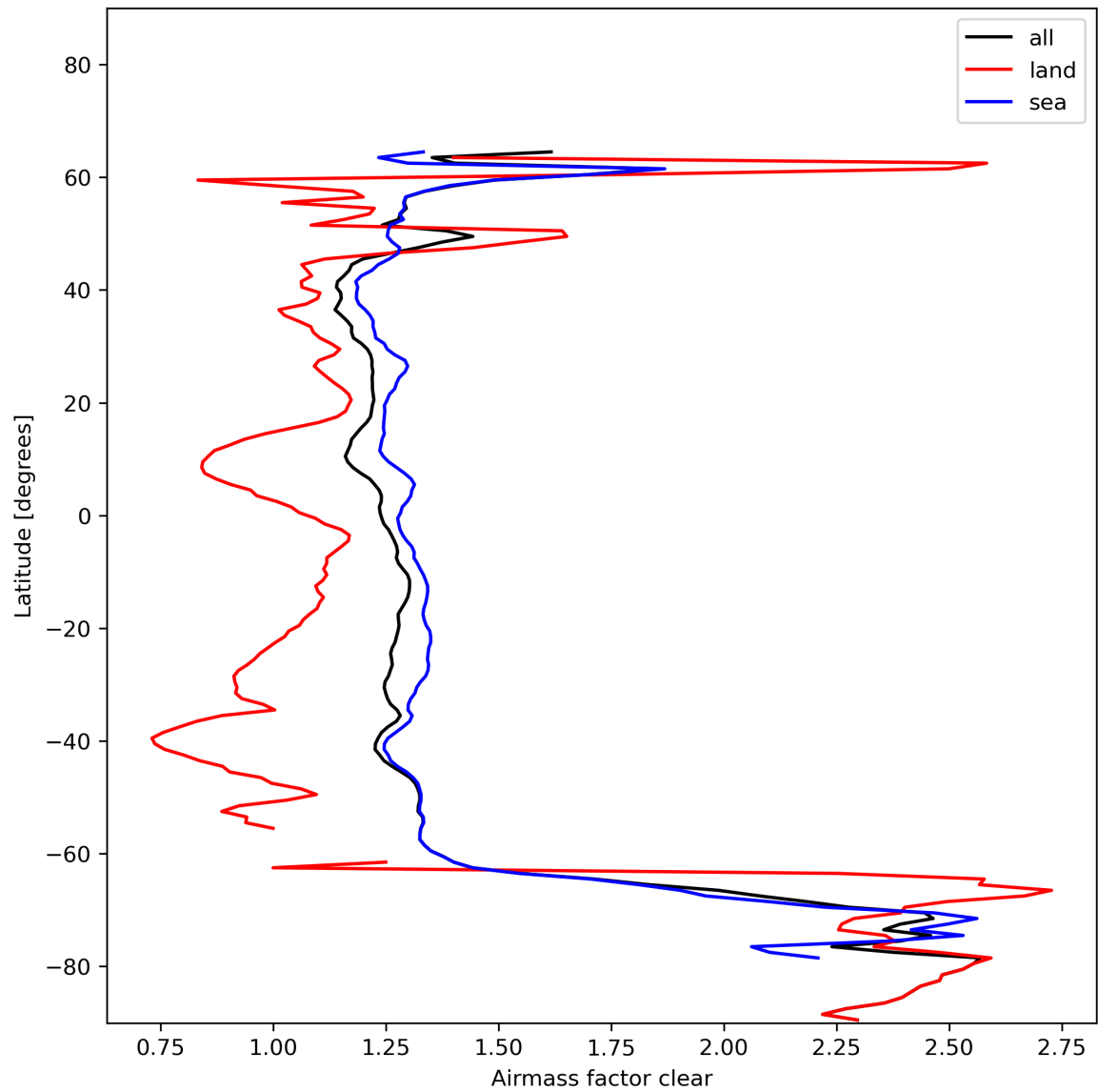
Figure 28: Zonal average of “Airmass factor clear” for 2024-01-15 to 2024-01-17.
