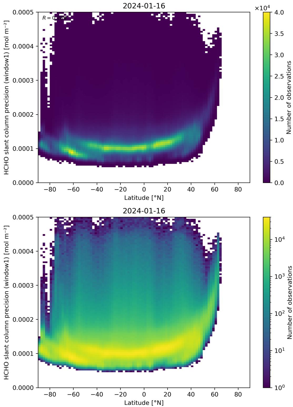
Figure 160: Scatter density plot of “Latitude” against “HCHO slant column precision (window1)” for 2024-01-15 to 2024-01-17.
