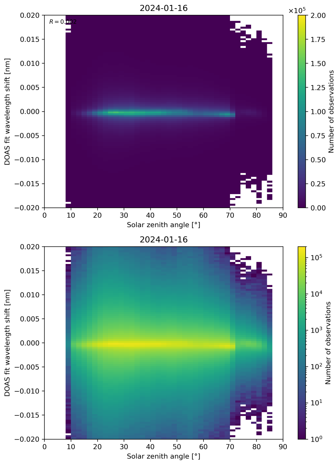
Figure 168: Scatter density plot of “Solar zenith angle” against “DOAS fit wavelength shift” for 2024-01-15 to 2024-01-17.
