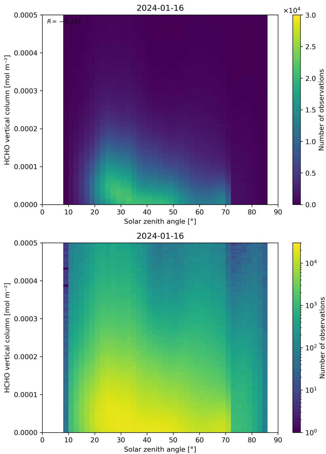
Figure 177: Scatter density plot of “Solar zenith angle” against “HCHO vertical column” for 2024-01-15 to 2024-01-17.
