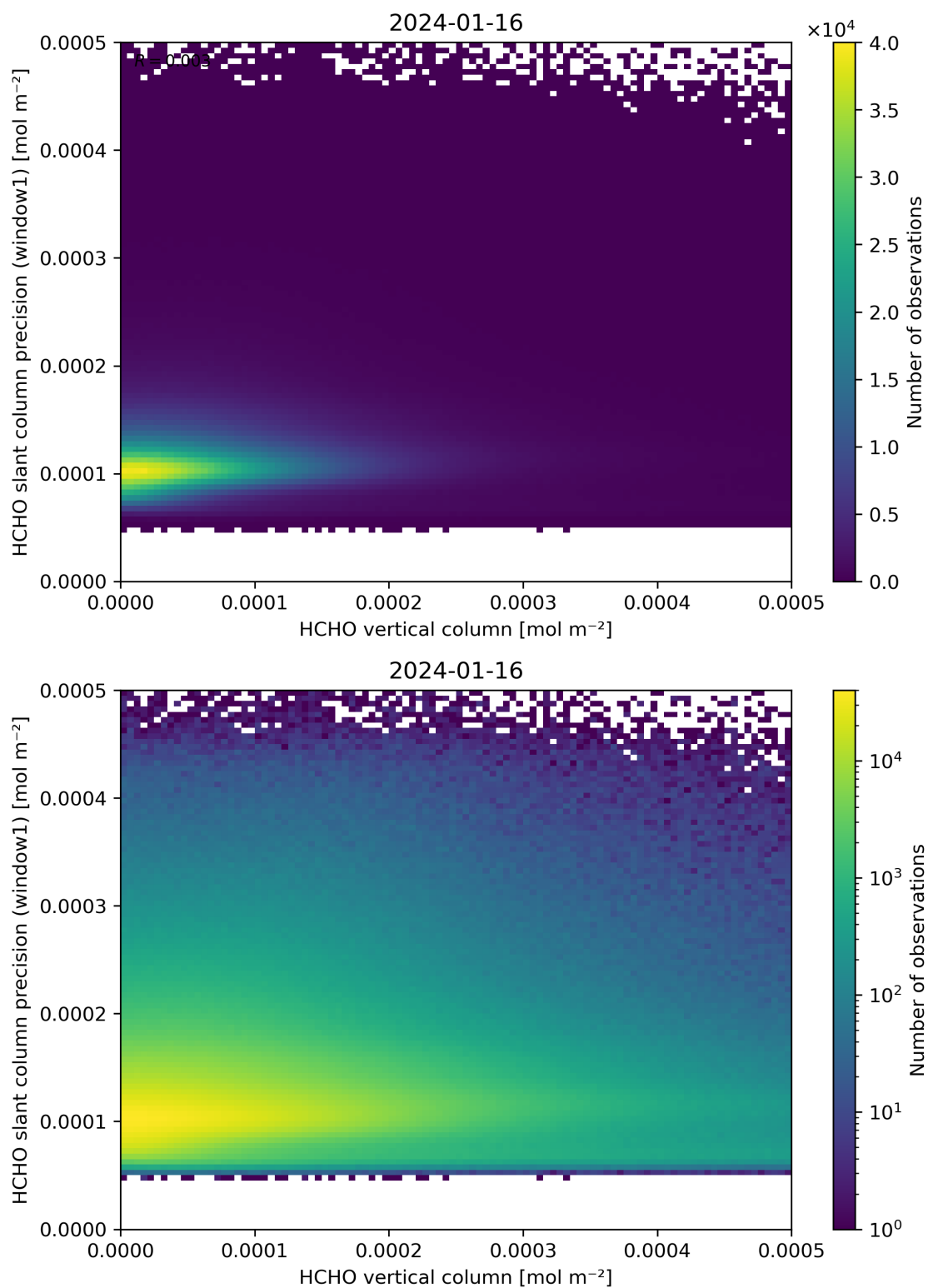
Figure 130: Scatter density plot of “HCHO vertical column” against “HCHO slant column precision (window1)” for 2024-01-15 to 2024-01-17.
