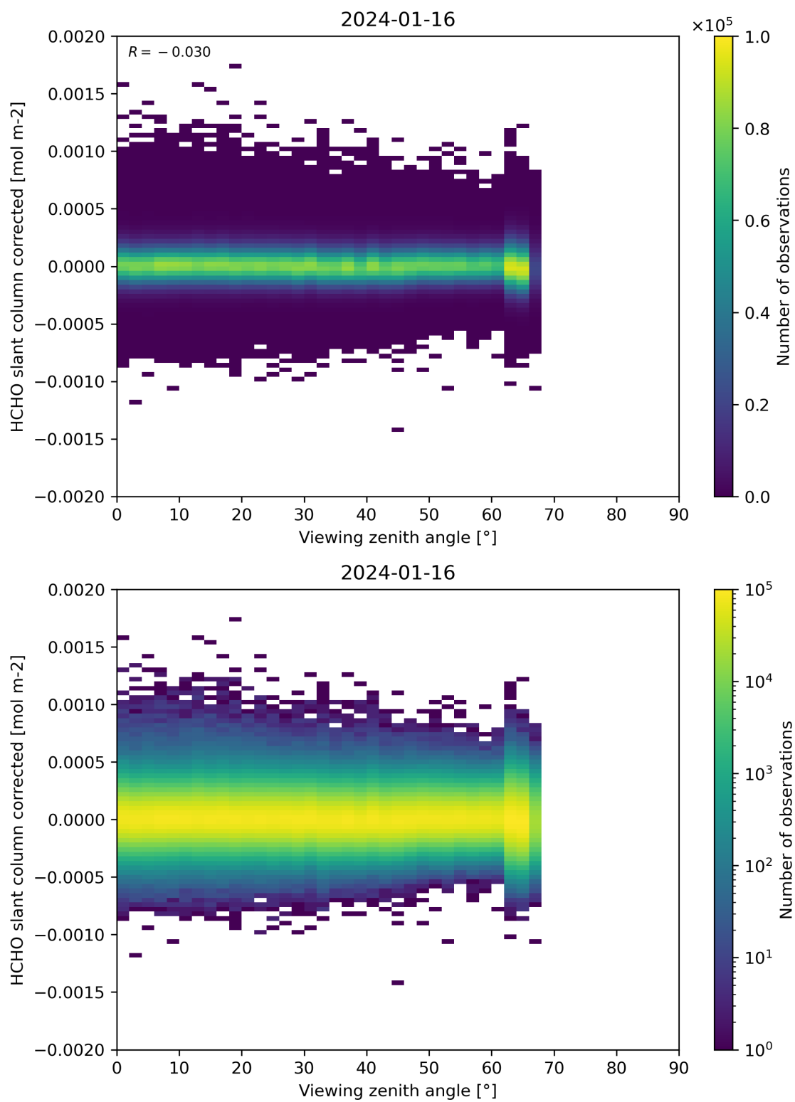
Figure 186: Scatter density plot of “Viewing zenith angle” against “HCHO slant column corrected” for 2024-01-15 to 2024-01-17.
