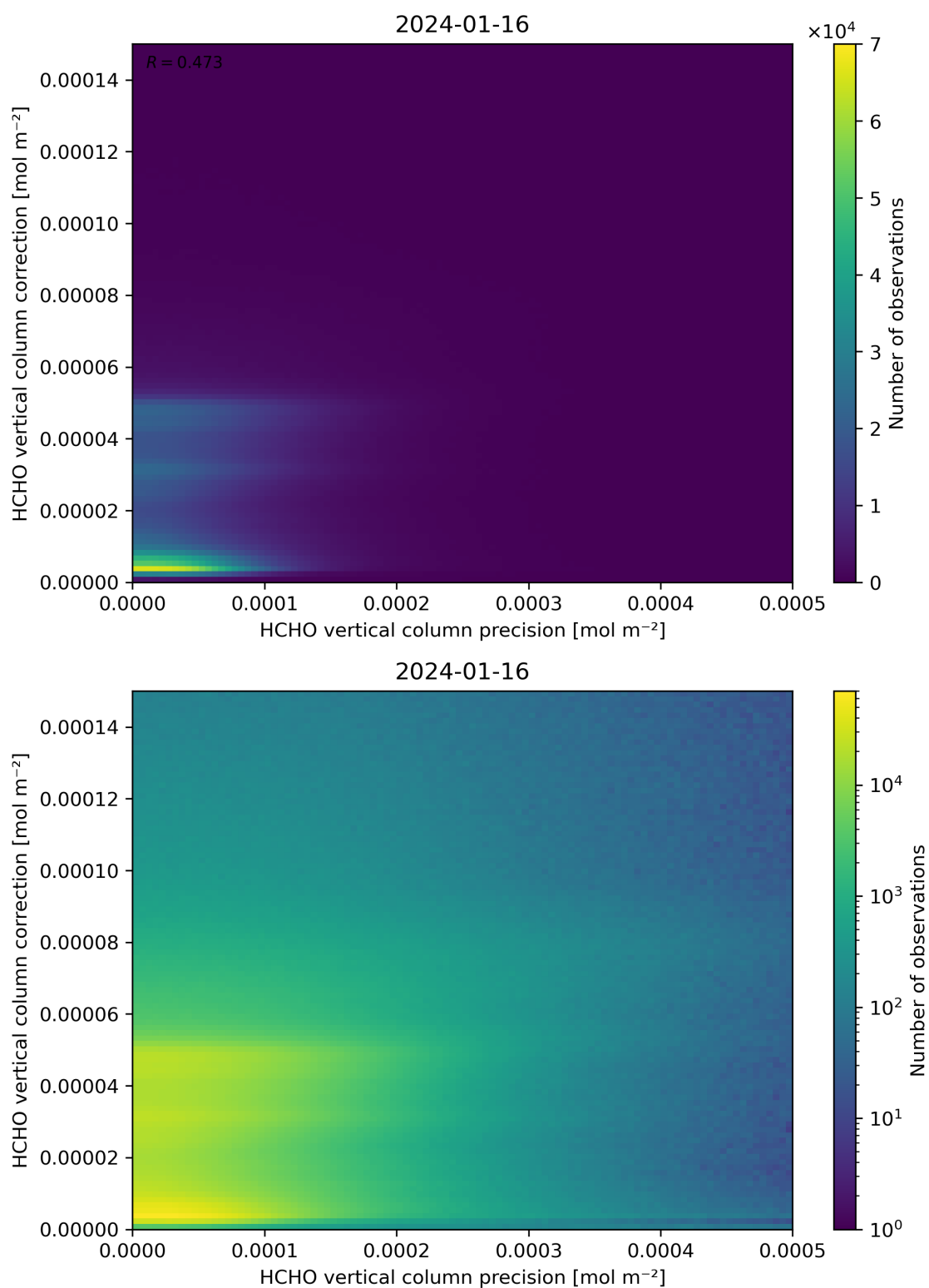
Figure 146: Scatter density plot of “HCHO vertical column precision” against “HCHO vertical column correction” for 2024-01-15 to 2024-01-17.
