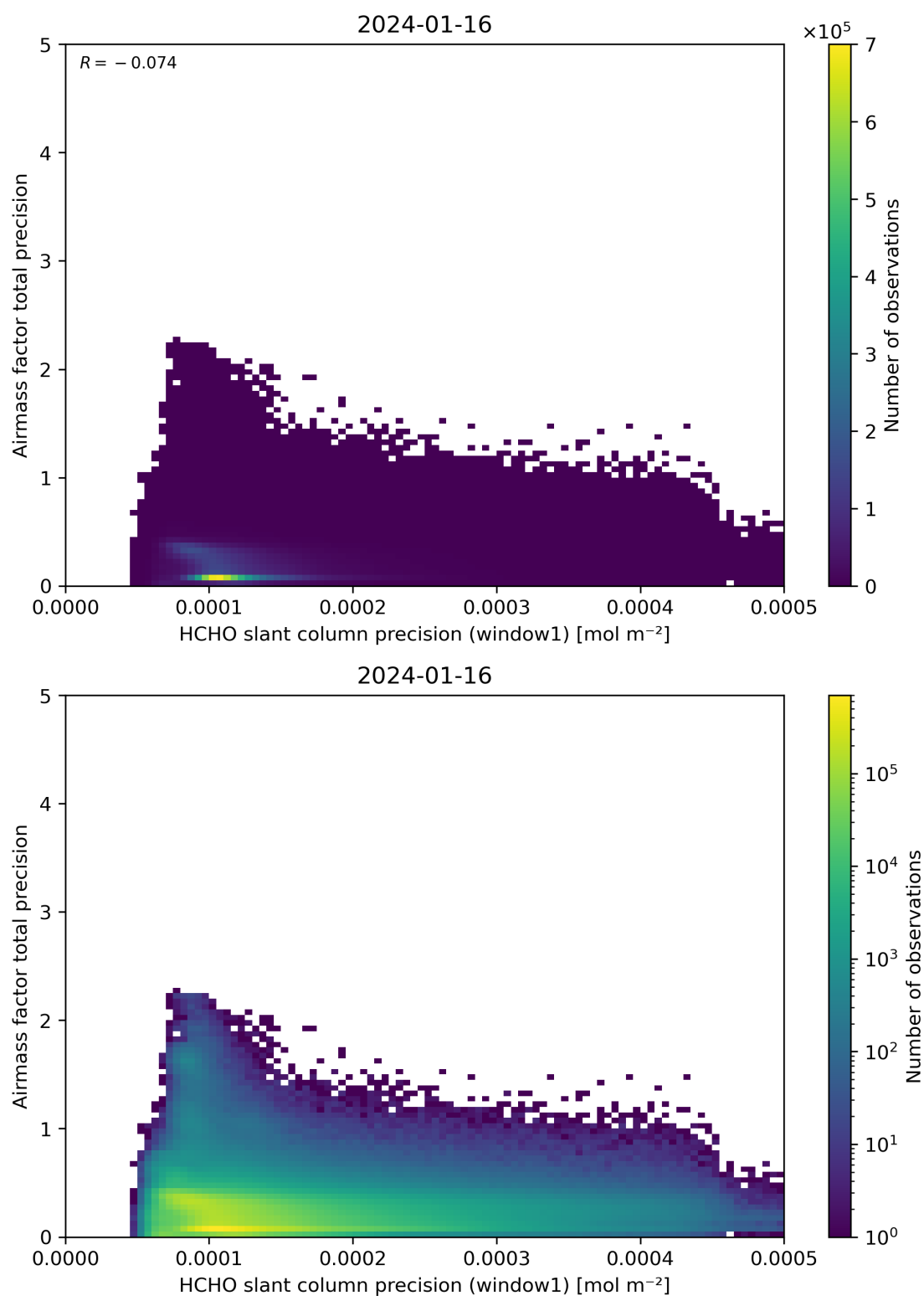
Figure 95: Scatter density plot of “HCHO slant column precision (window1)” against “Airmass factor total precision” for 2024-01-15 to 2024-01-17.
