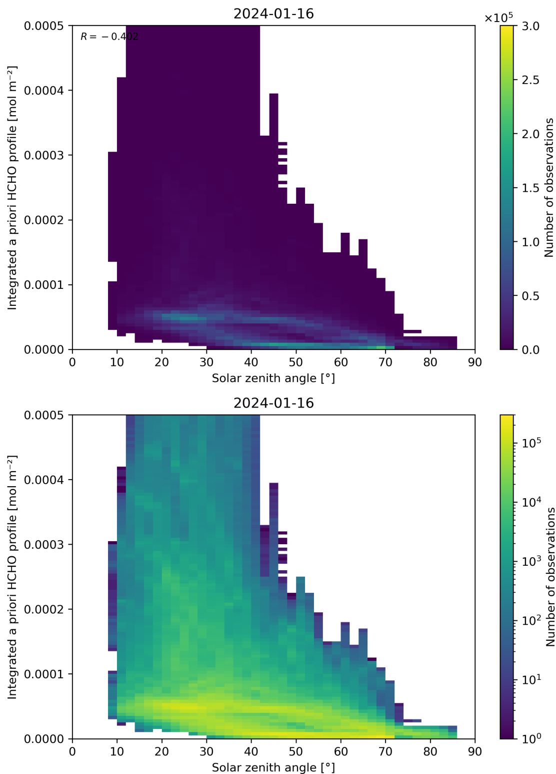
Figure 180: Scatter density plot of “Solar zenith angle” against “Integrated a priori HCHO profile” for 2024-01-15 to 2024-01-17.
