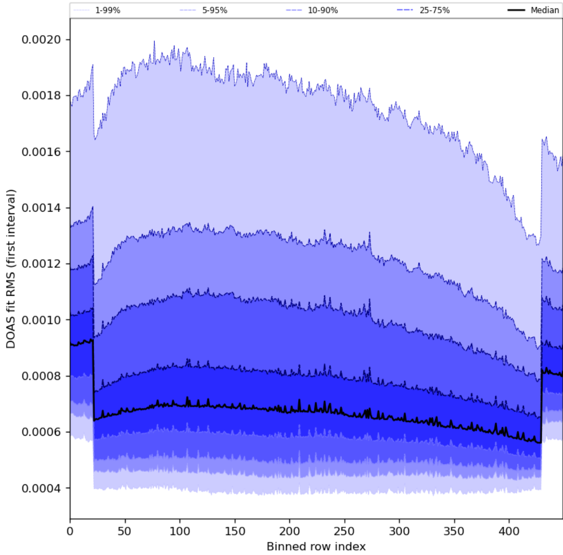
Figure 60: Along track statistics of “DOAS fit RMS (first interval)” for 2024-01-15 to 2024-01-17
