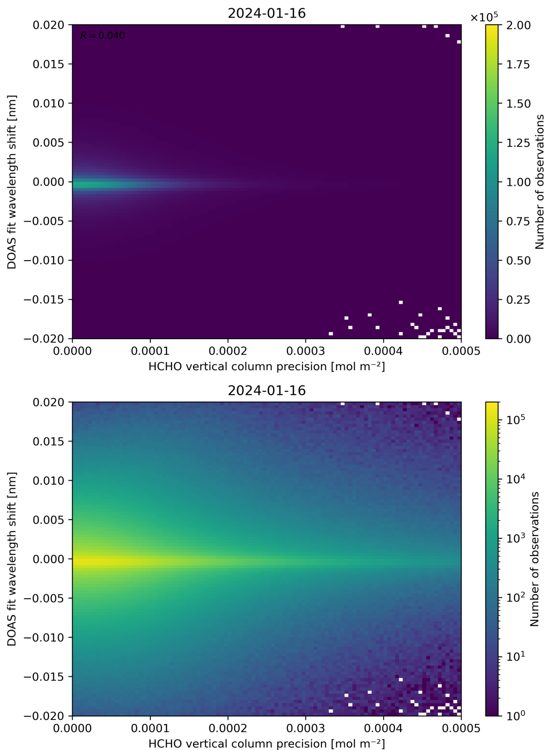
Figure 137: Scatter density plot of “HCHO vertical column precision” against “DOAS fit wavelength shift” for 2024-01-15 to 2024-01-17.
