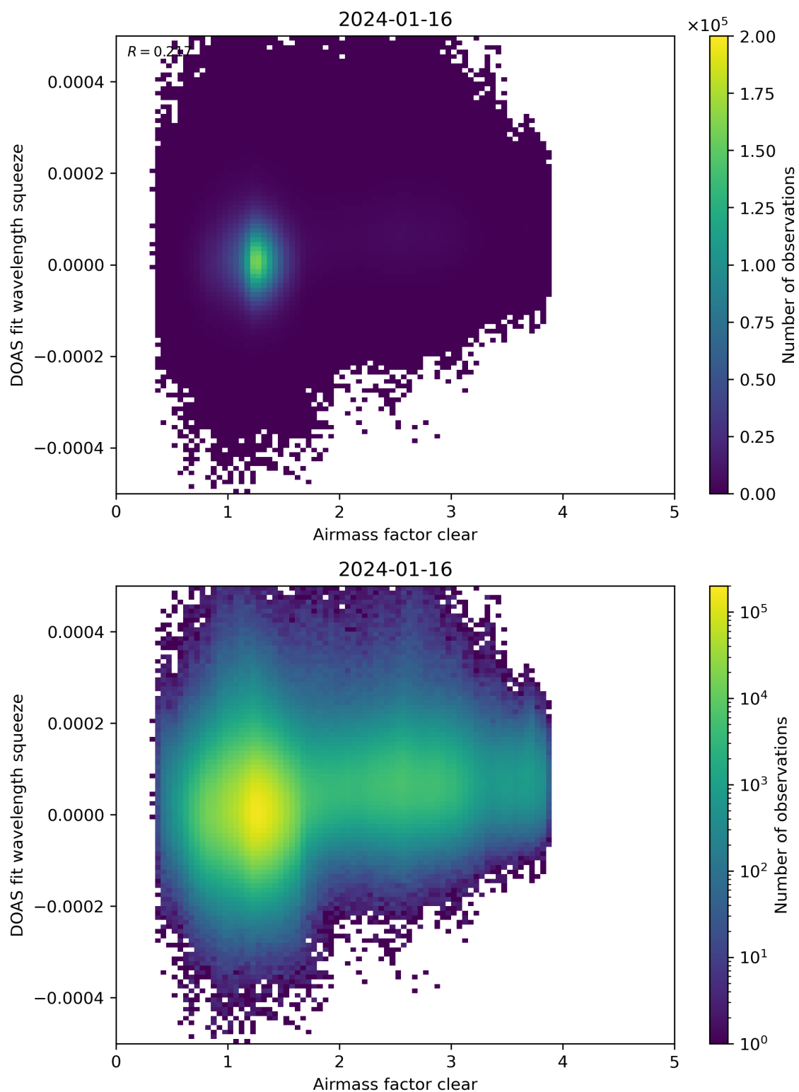
Figure 73: Scatter density plot of “Airmass factor clear” against “DOAS fit wavelength squeeze” for 2024-01-15 to 2024-01-17.
