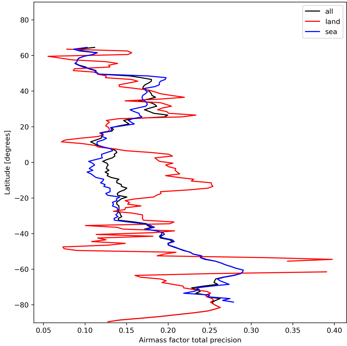
Figure 27: Zonal average of “Airmass factor total precision” for 2024-01-15 to 2024-01-17.
