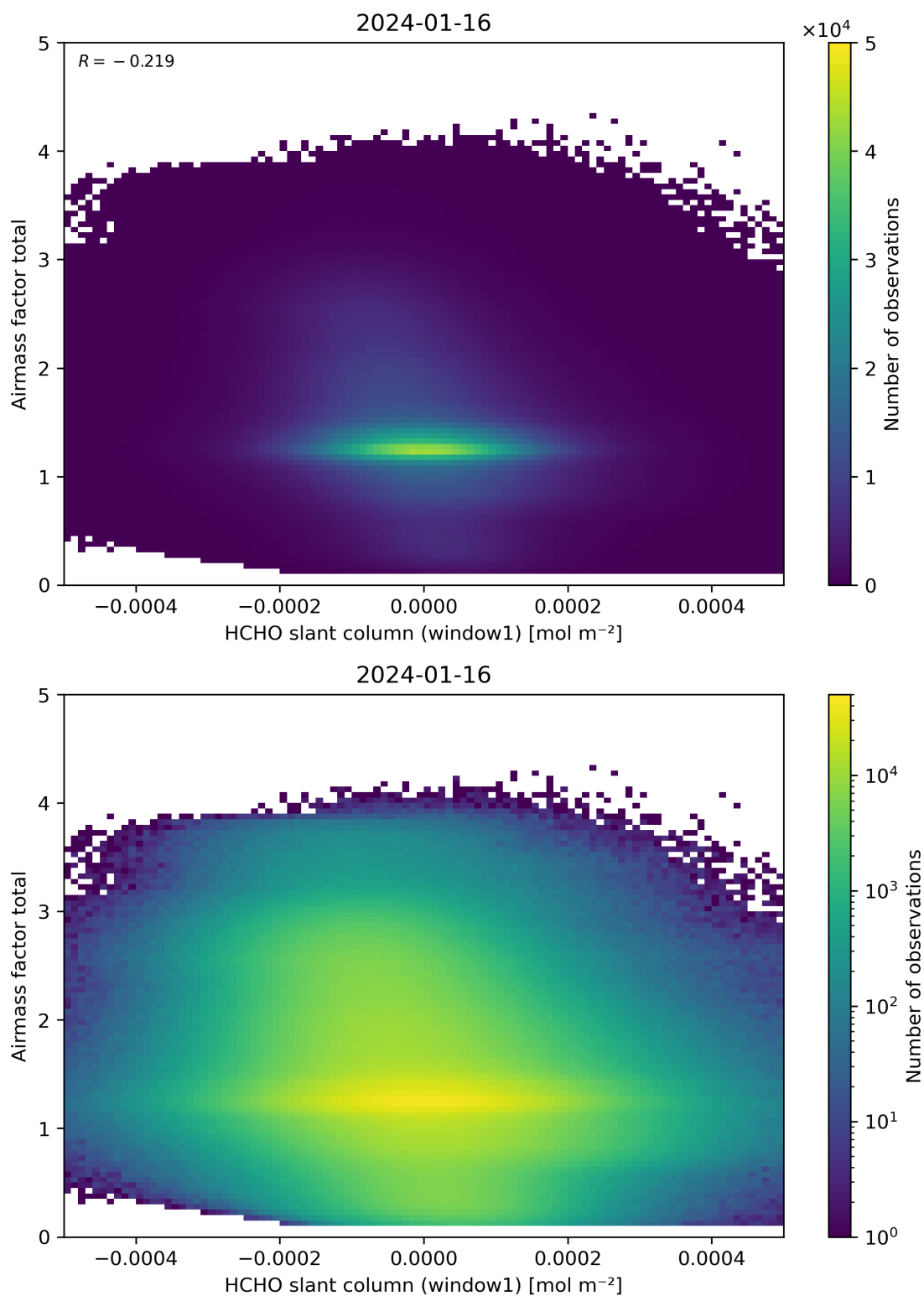
Figure 85: Scatter density plot of “HCHO slant column (window1)” against “Airmass factor total” for 2024-01-15 to 2024-01-17.
