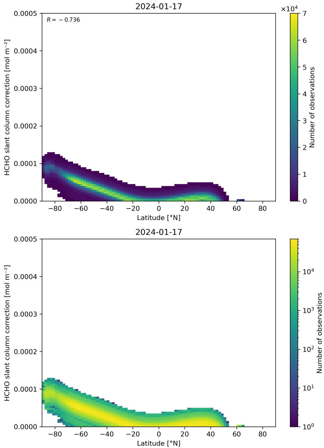
Figure 158: Scatter density plot of “Latitude” against “HCHO slant column correction” for 2024-01-16 to 2024-01-18.
