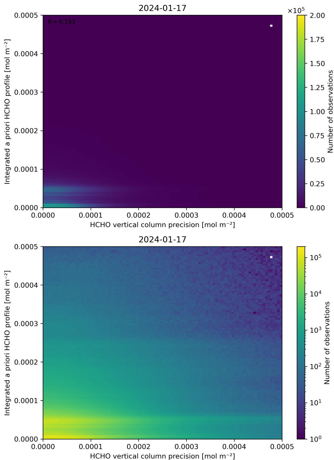
Figure 147: Scatter density plot of “HCHO vertical column precision” against “Integrated a priori HCHO profile” for 2024-01-16 to 2024-01-18.
