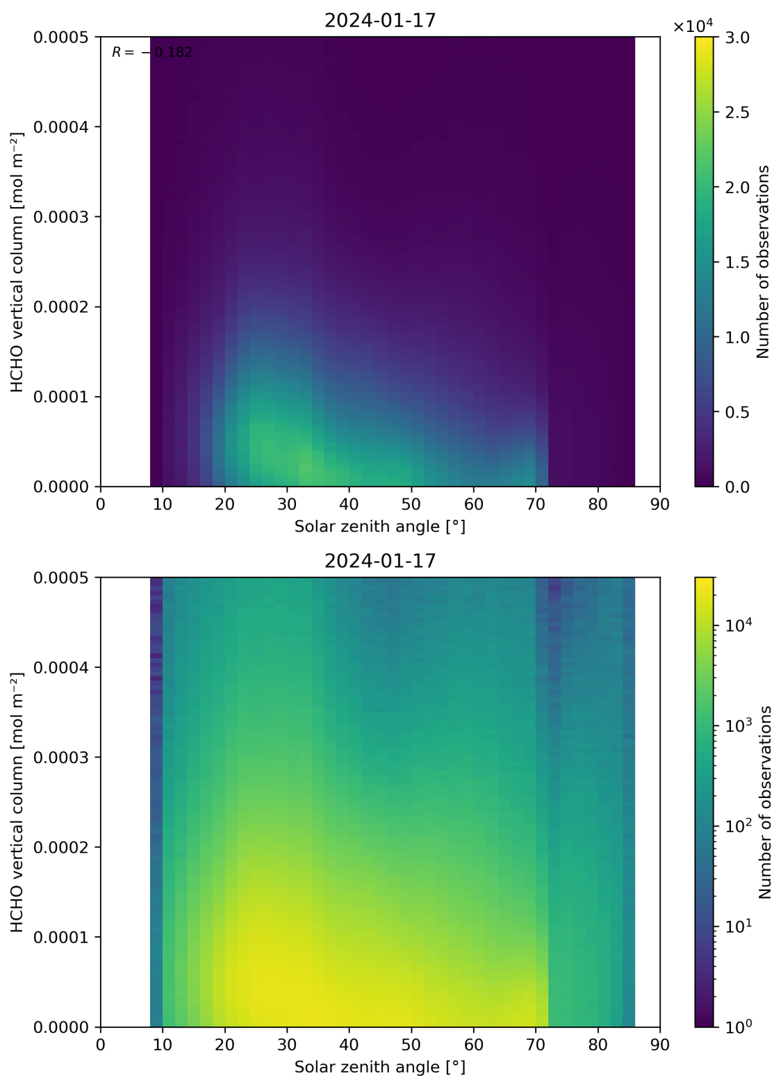
Figure 177: Scatter density plot of “Solar zenith angle” against “HCHO vertical column” for 2024-01-16 to 2024-01-18.
