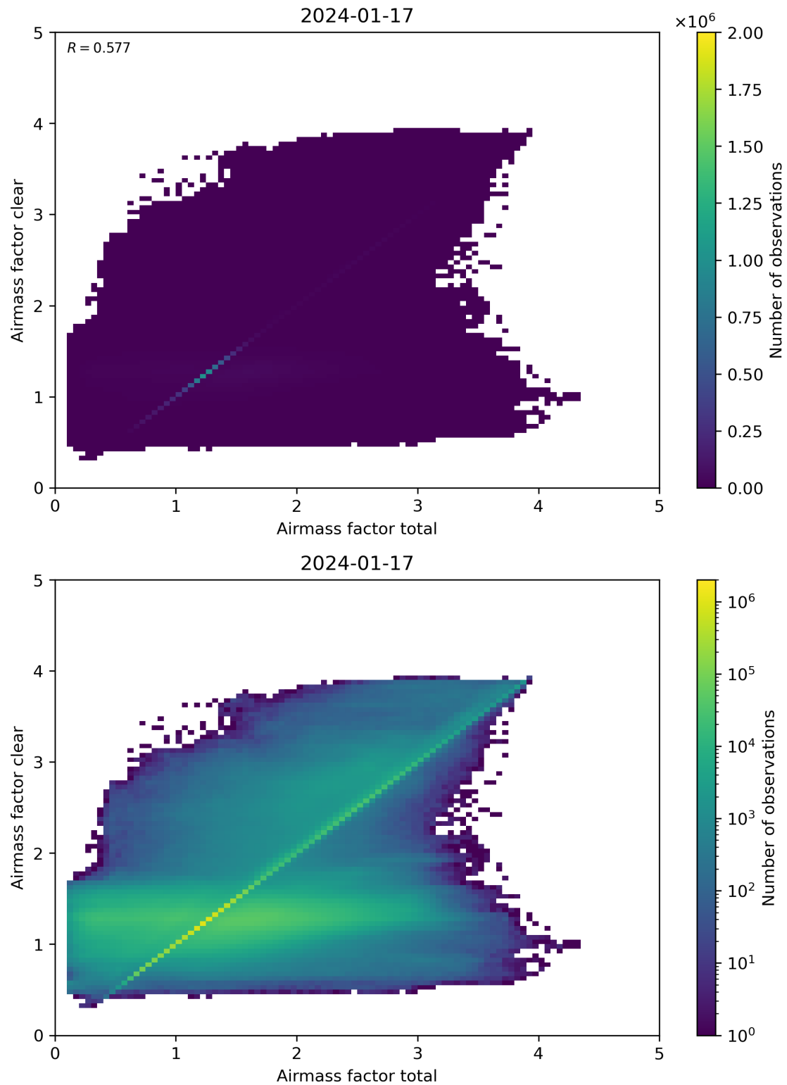
Figure 100: Scatter density plot of “Airmass factor total” against “Airmass factor clear” for 2024-01-16 to 2024-01-18.
