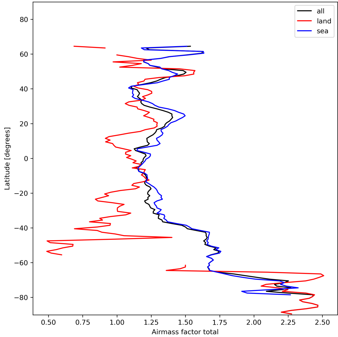
Figure 26: Zonal average of “Airmass factor total” for 2024-01-16 to 2024-01-18.
