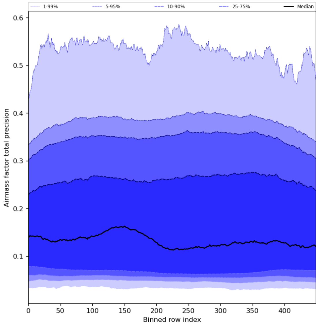
Figure 55: Along track statistics of “Airmass factor total precision” for 2024-01-16 to 2024-01-18
