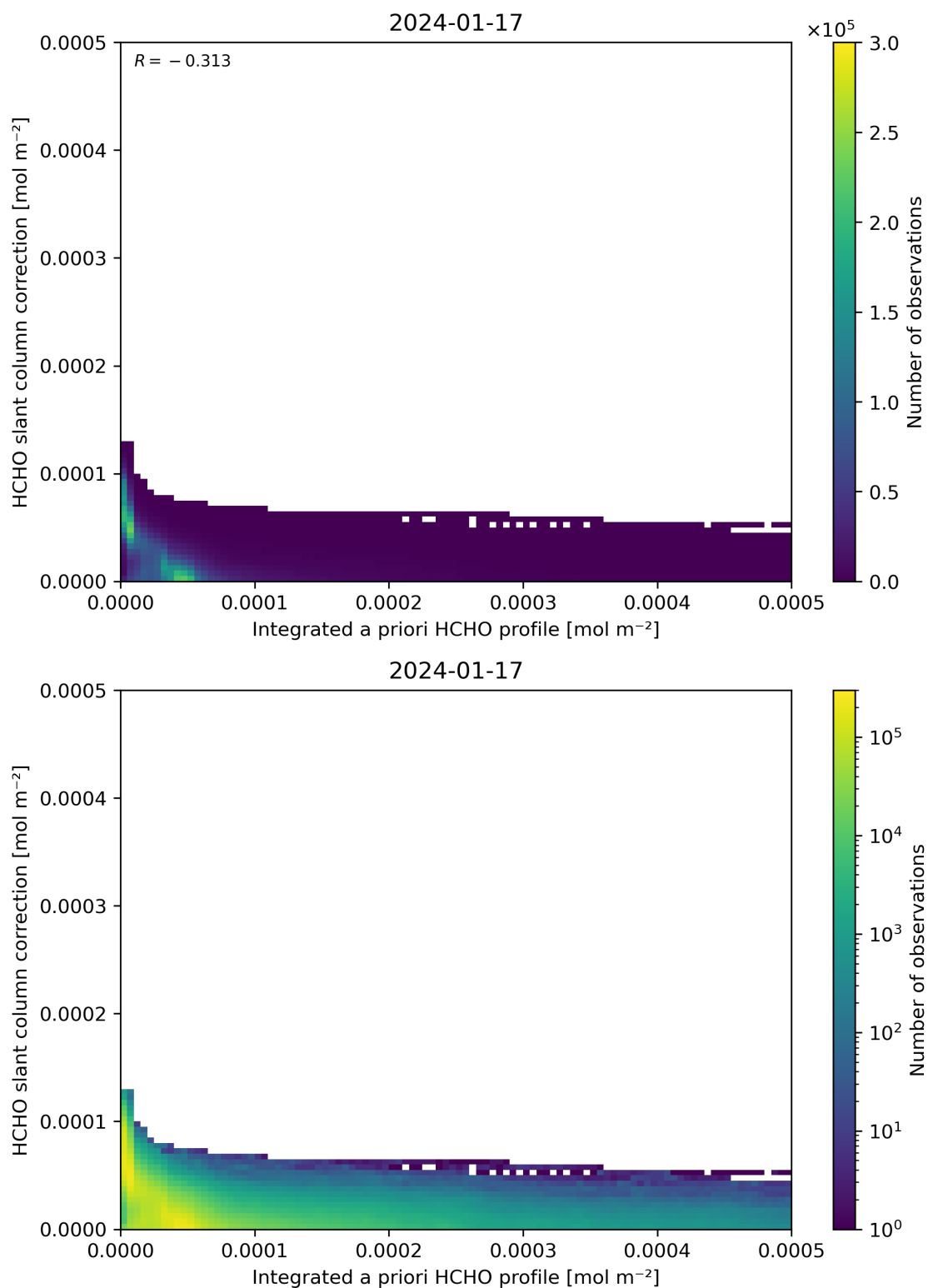
Figure 152: Scatter density plot of “Integrated a priori HCHO profile” against “HCHO slant column correction” for 2024-01-16 to 2024-01-18.
