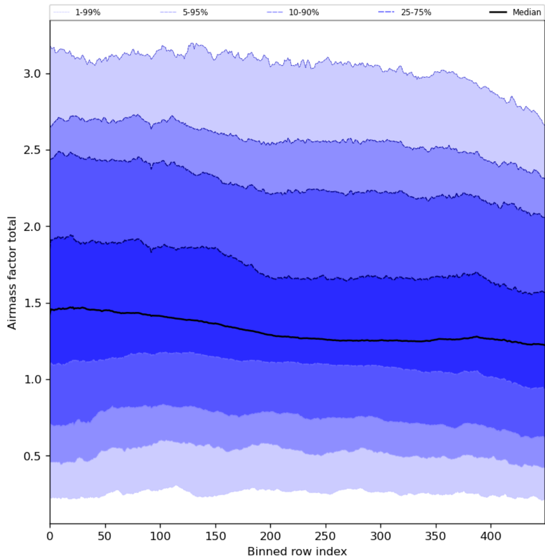
Figure 54: Along track statistics of “Airmass factor total” for 2024-01-16 to 2024-01-18
