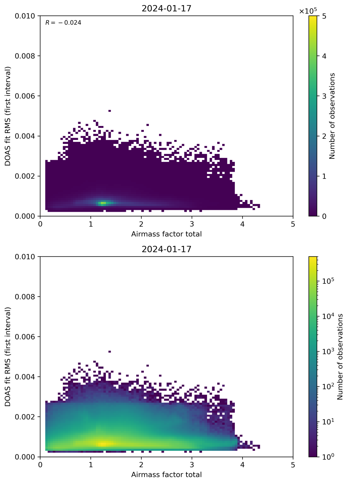
Figure 97: Scatter density plot of “Airmass factor total” against “DOAS fit RMS (first interval)” for 2024-01-16 to 2024-01-18.
