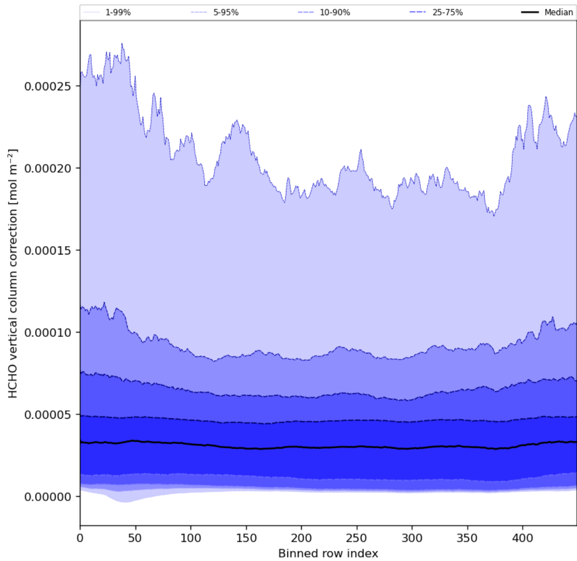
Figure 51: Along track statistics of “HCHO vertical column correction” for 2024-01-16 to 2024-01-18
