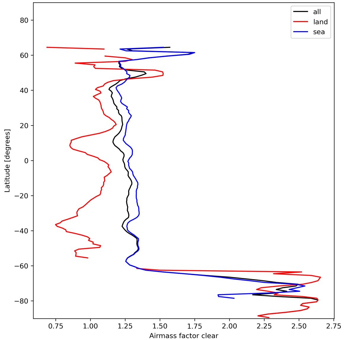
Figure 28: Zonal average of “Airmass factor clear” for 2024-01-16 to 2024-01-18.
