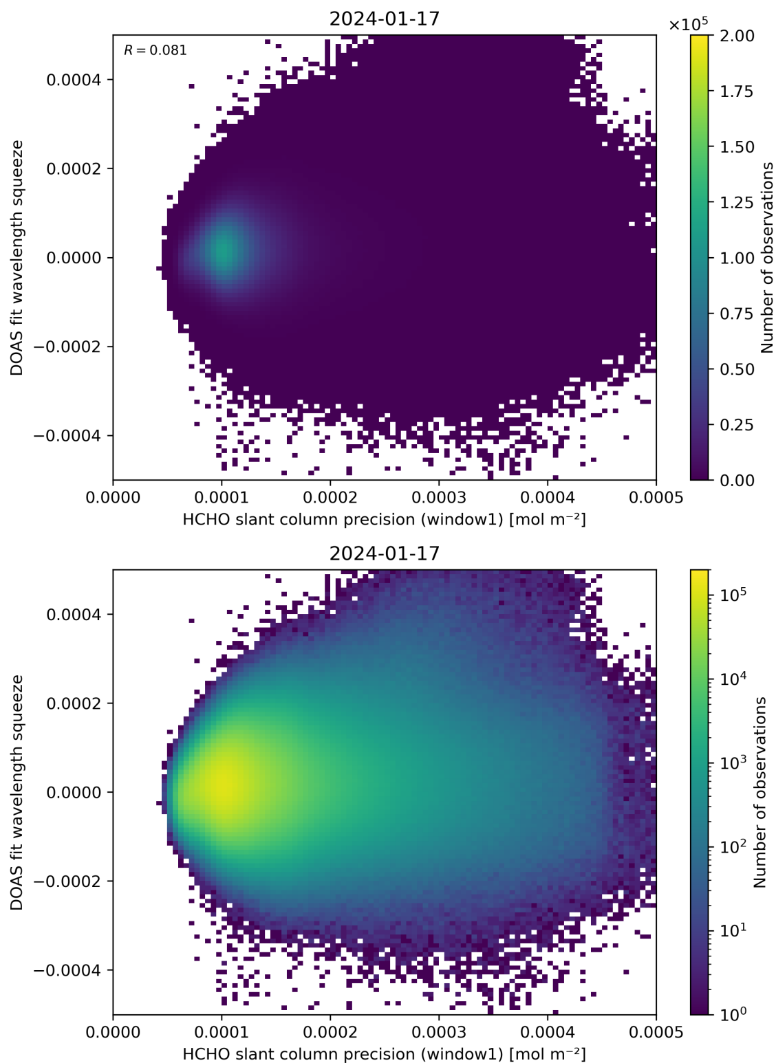
Figure 90: Scatter density plot of “HCHO slant column precision (window1)” against “DOAS fit wavelength squeeze” for 2024-01-16 to 2024-01-18.
