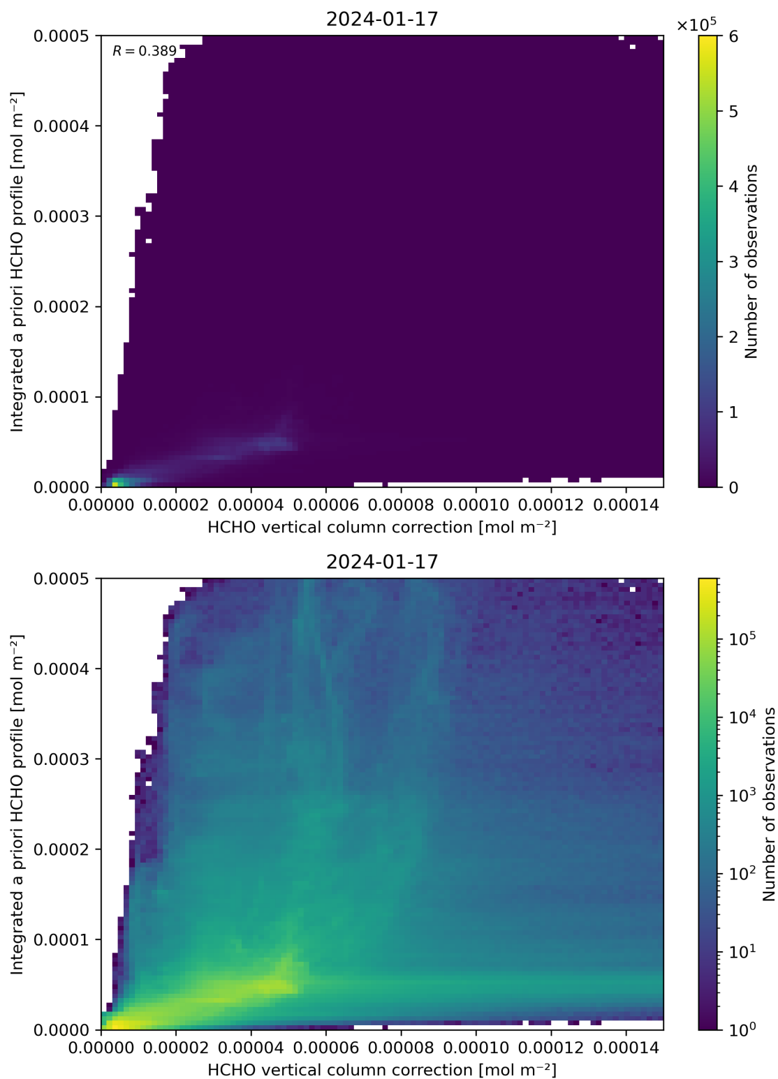
Figure 122: Scatter density plot of “HCHO vertical column correction” against “Integrated a priori HCHO profile” for 2024-01-16 to 2024-01-18.
