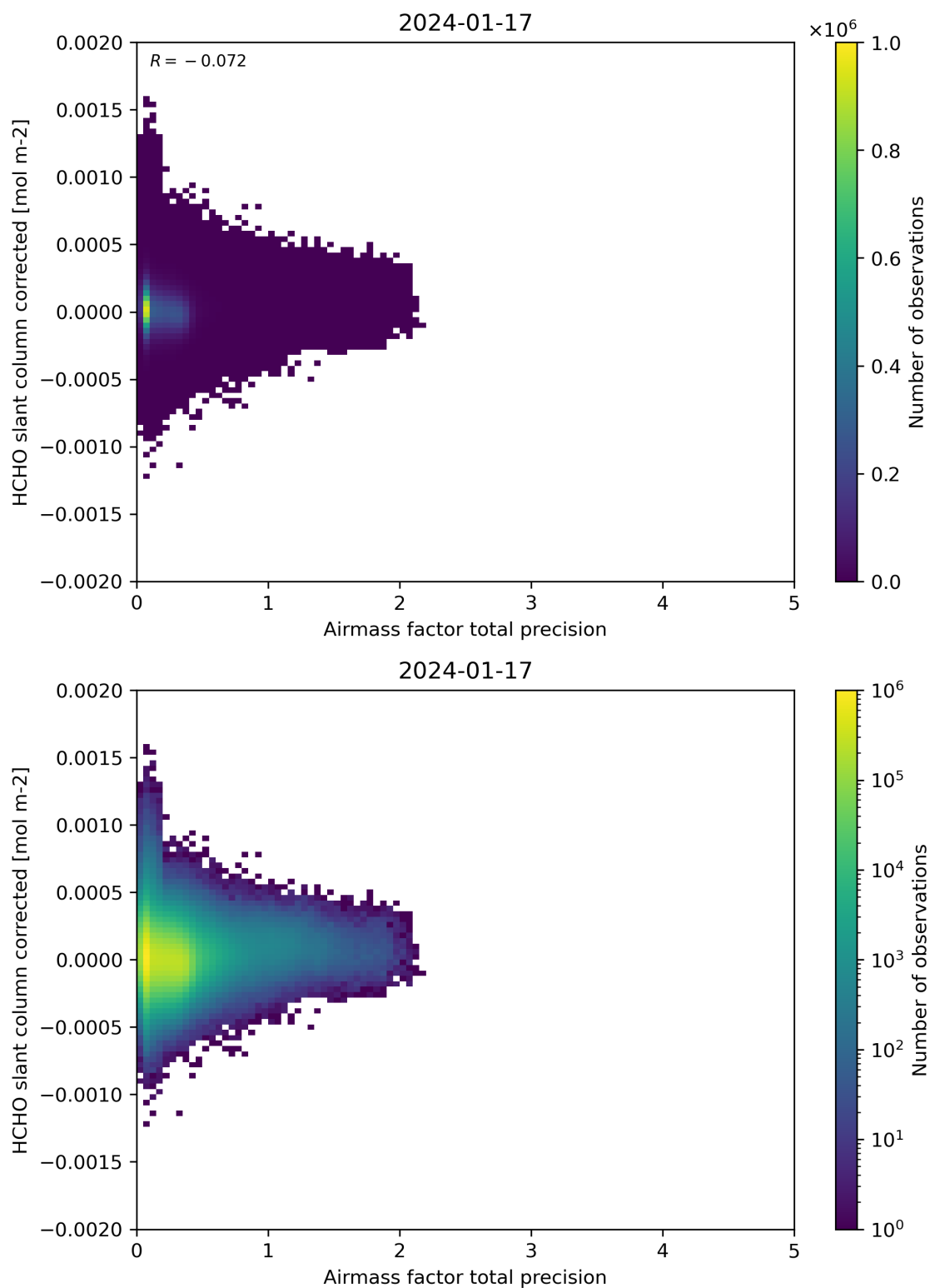
Figure 109: Scatter density plot of “Airmass factor total precision” against “HCHO slant column corrected” for 2024-01-16 to 2024-01-18.
