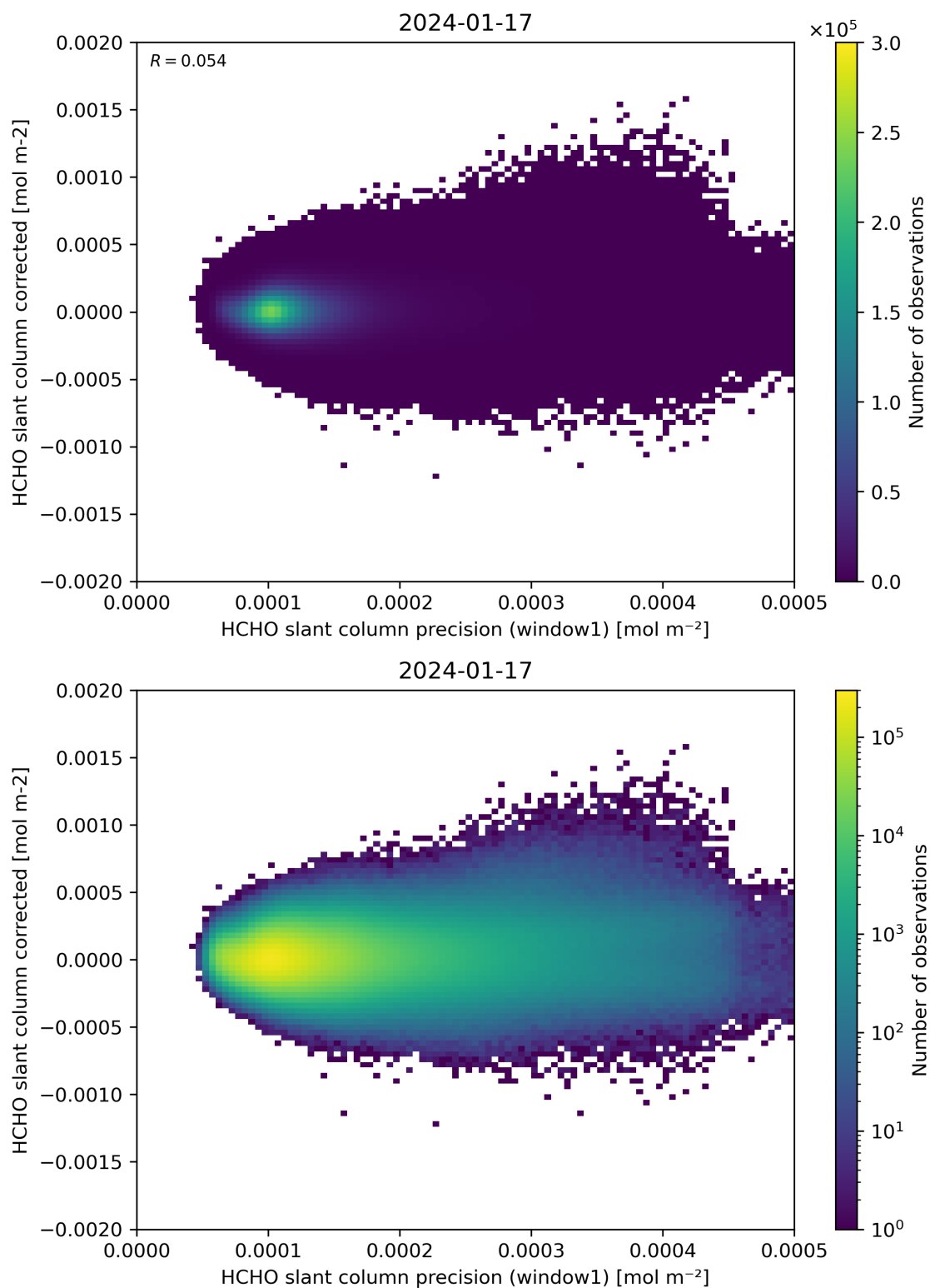
Figure 92: Scatter density plot of “HCHO slant column precision (window1)” against “HCHO slant column corrected” for 2024-01-16 to 2024-01-18.
