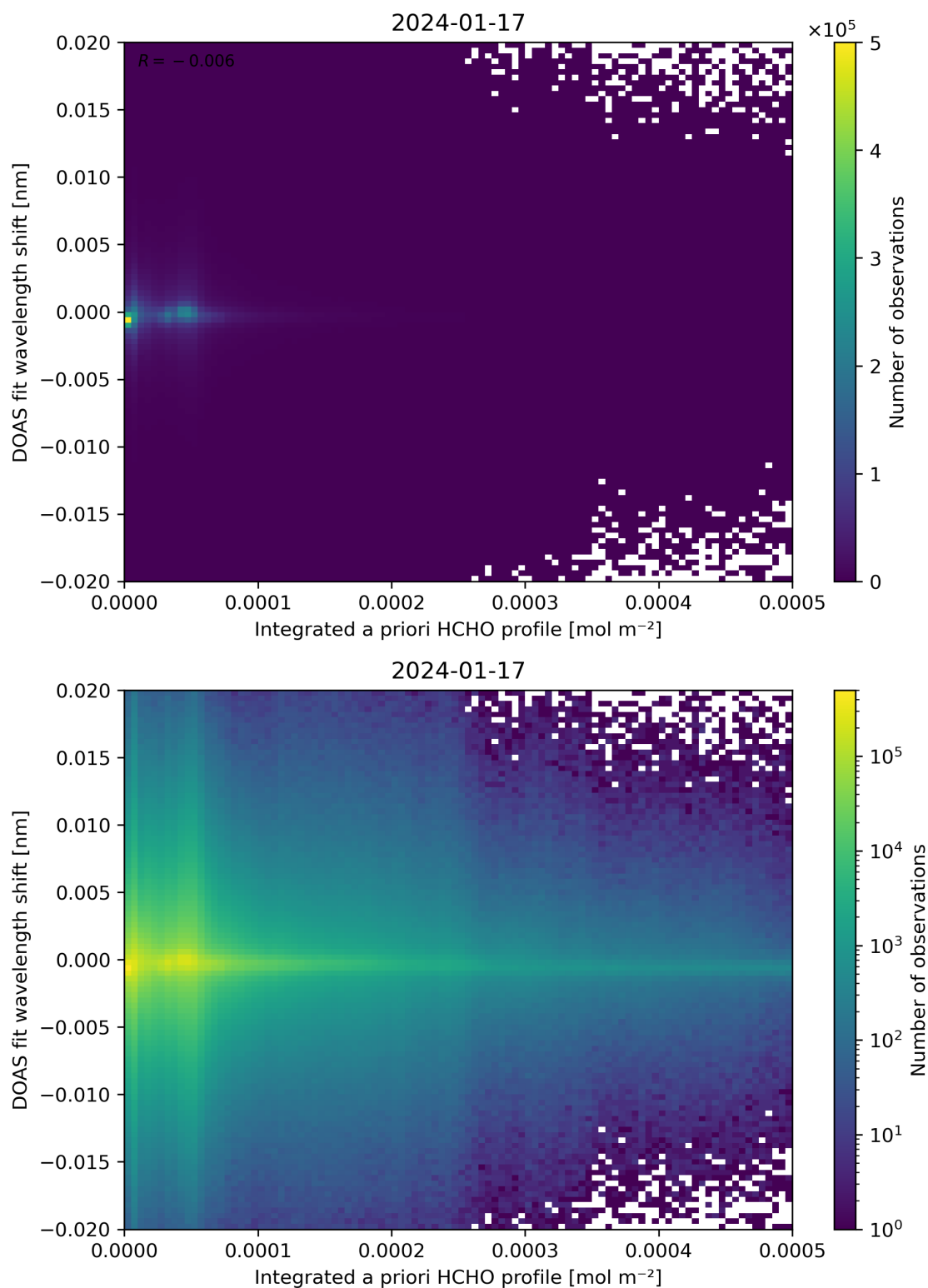
Figure 149: Scatter density plot of “Integrated a priori HCHO profile” against “DOAS fit wavelength shift” for 2024-01-16 to 2024-01-18.
