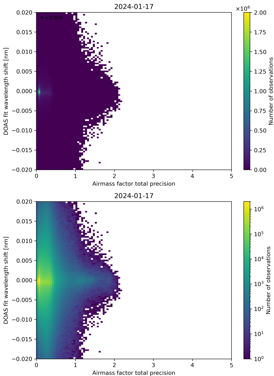
Figure 106: Scatter density plot of “Airmass factor total precision” against “DOAS fit wavelength shift” for 2024-01-16 to 2024-01-18.
