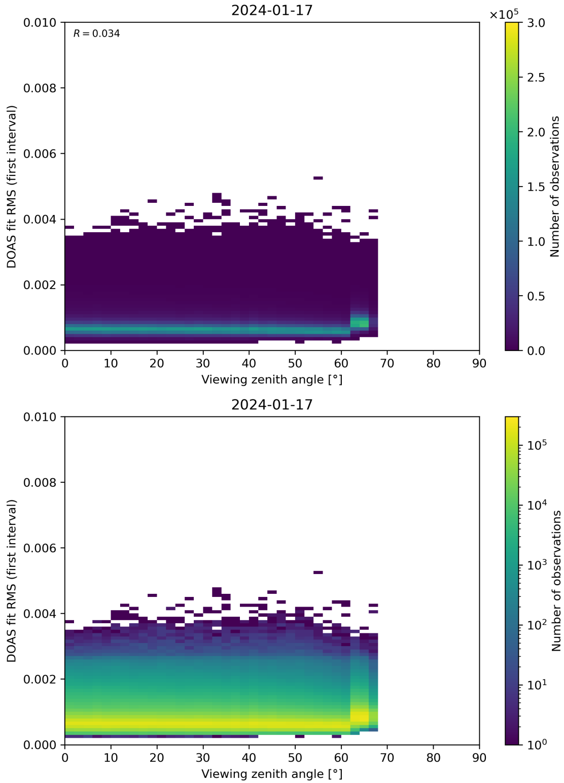
Figure 182: Scatter density plot of “Viewing zenith angle” against “DOAS fit RMS (first interval)” for 2024-01-16 to 2024-01-18.
