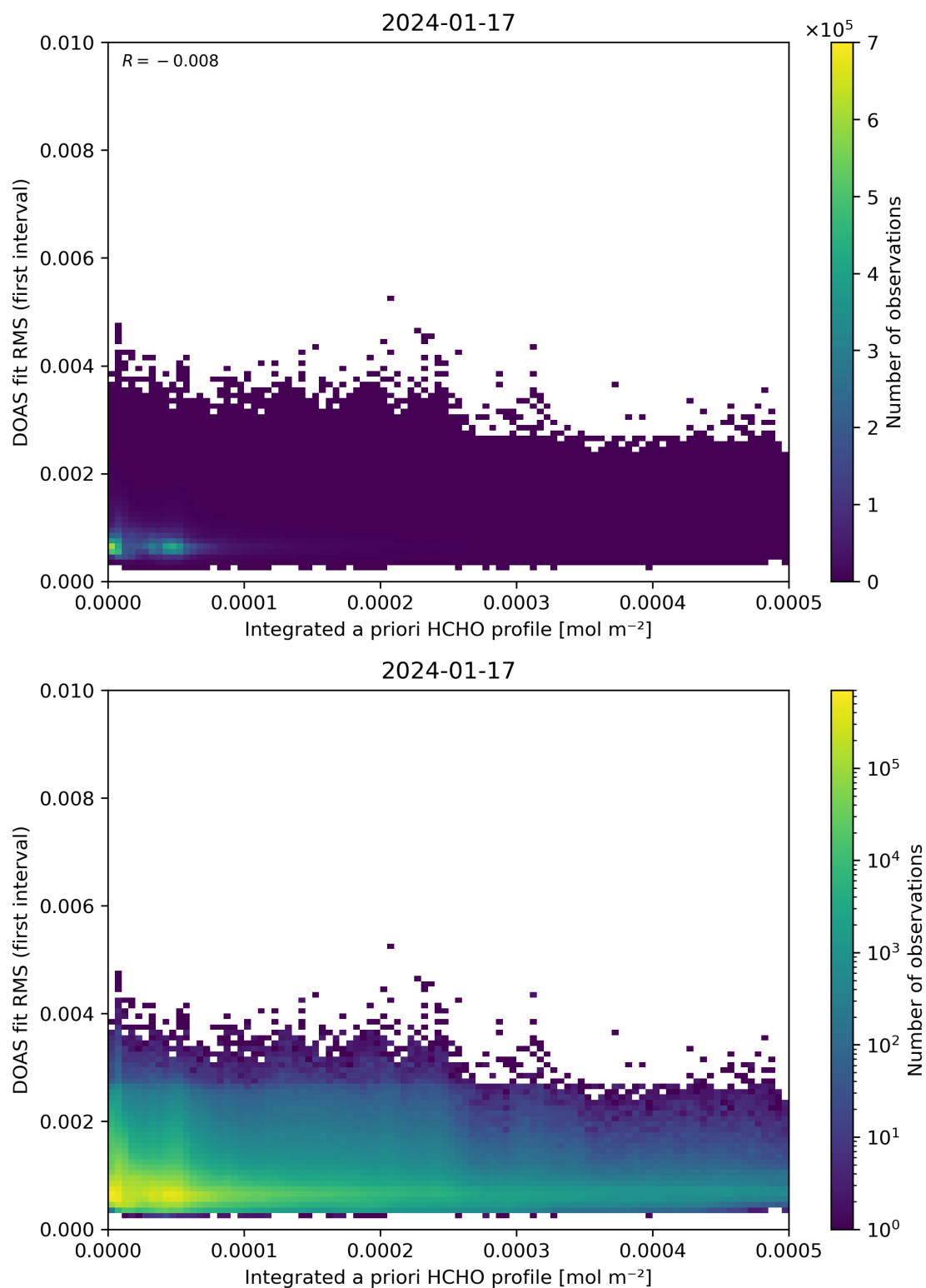
Figure 148: Scatter density plot of “Integrated a priori HCHO profile” against “DOAS fit RMS (first interval)” for 2024-01-16 to 2024-01-18.
