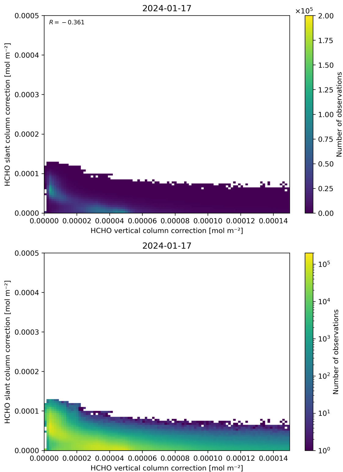
Figure 117: Scatter density plot of “HCHO vertical column correction” against “HCHO slant column correction” for 2024-01-16 to 2024-01-18.
