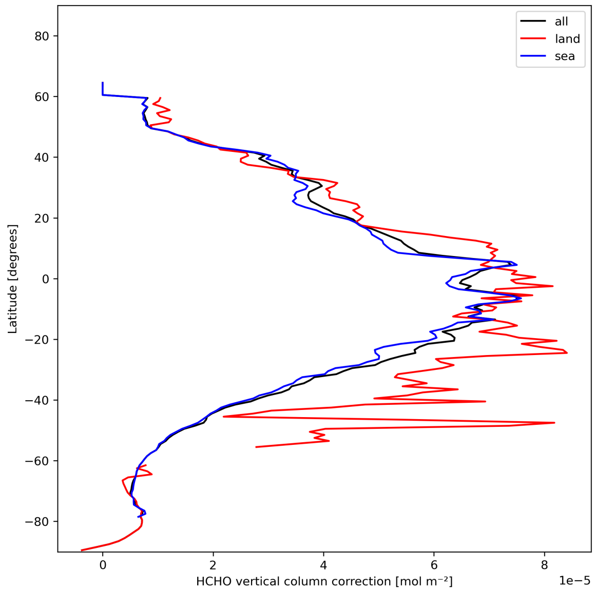
Figure 23: Zonal average of “HCHO vertical column correction” for 2024-01-16 to 2024-01-18.
