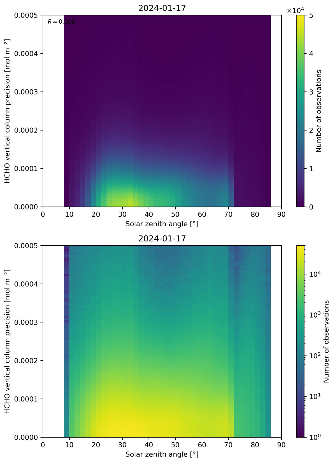
Figure 179: Scatter density plot of “Solar zenith angle” against “HCHO vertical column precision” for 2024-01-16 to 2024-01-18.
