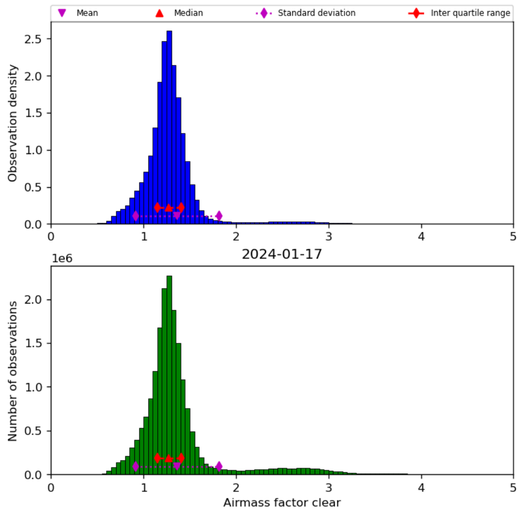
Figure 42: Histogram of “Airmass factor clear” for 2024-01-16 to 2024-01-18
