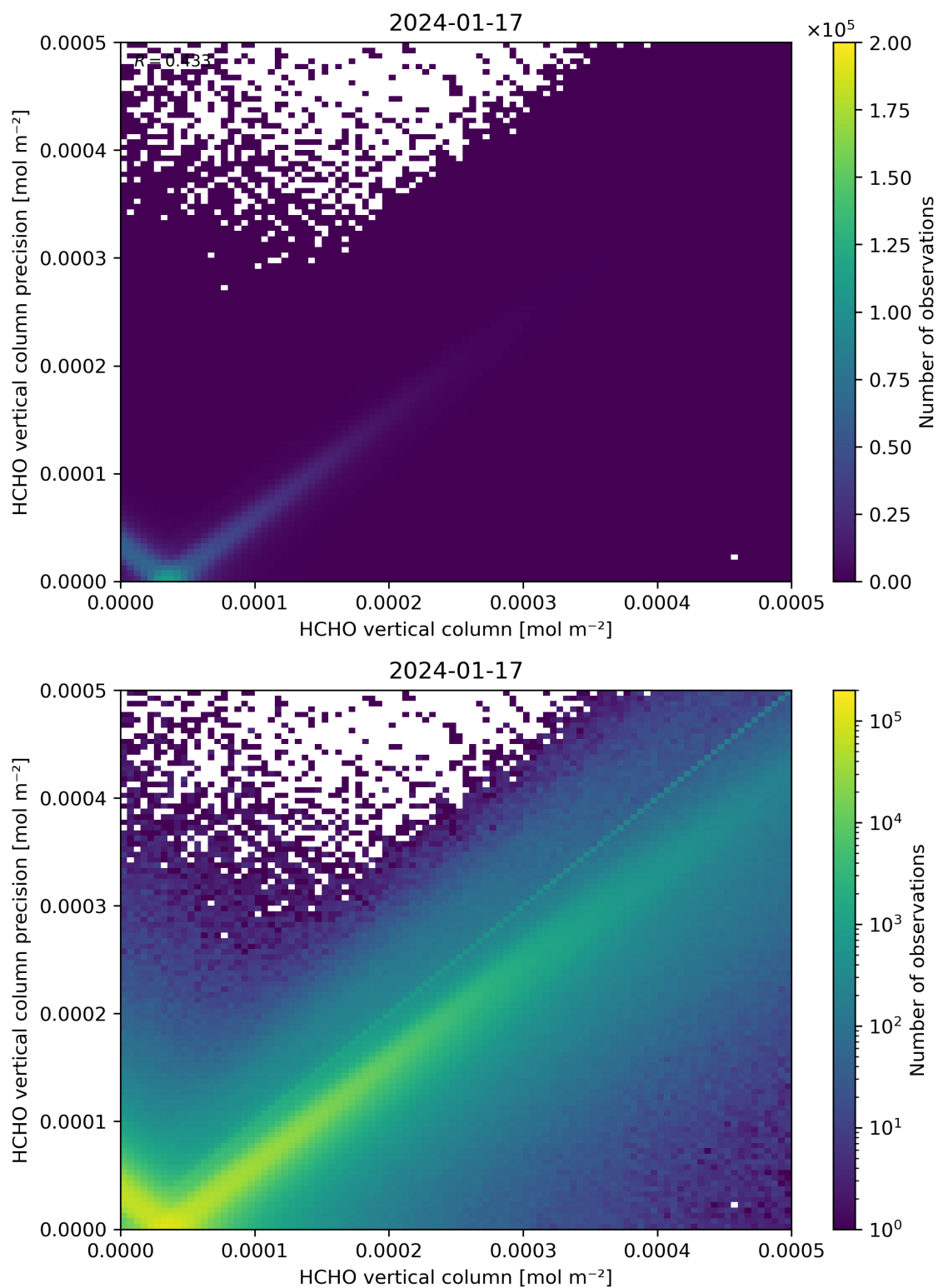
Figure 134: Scatter density plot of “HCHO vertical column” against “HCHO vertical column precision” for 2024-01-16 to 2024-01-18.
