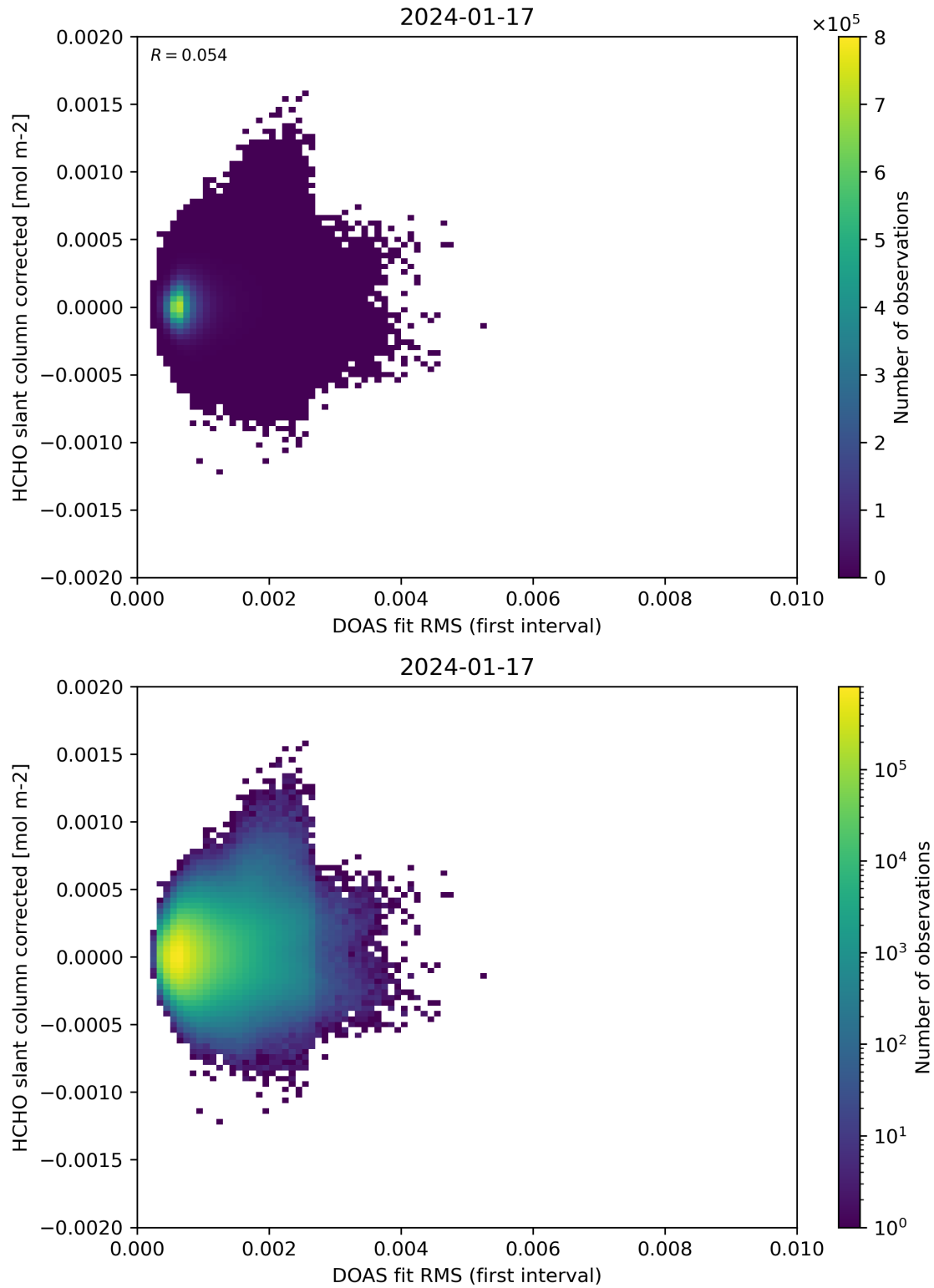
Figure 62: Scatter density plot of “DOAS fit RMS (first interval)” against “HCHO slant column corrected” for 2024-01-16 to 2024-01-18.
