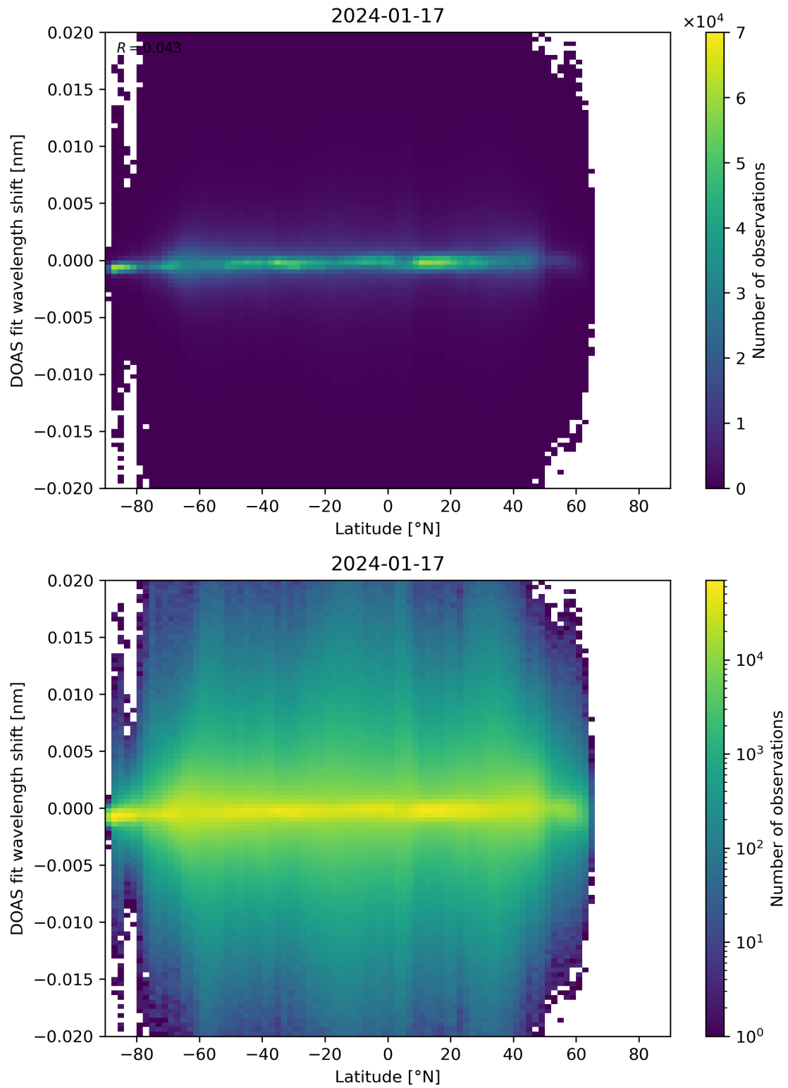
Figure 154: Scatter density plot of “Latitude” against “DOAS fit wavelength shift” for 2024-01-16 to 2024-01-18.
