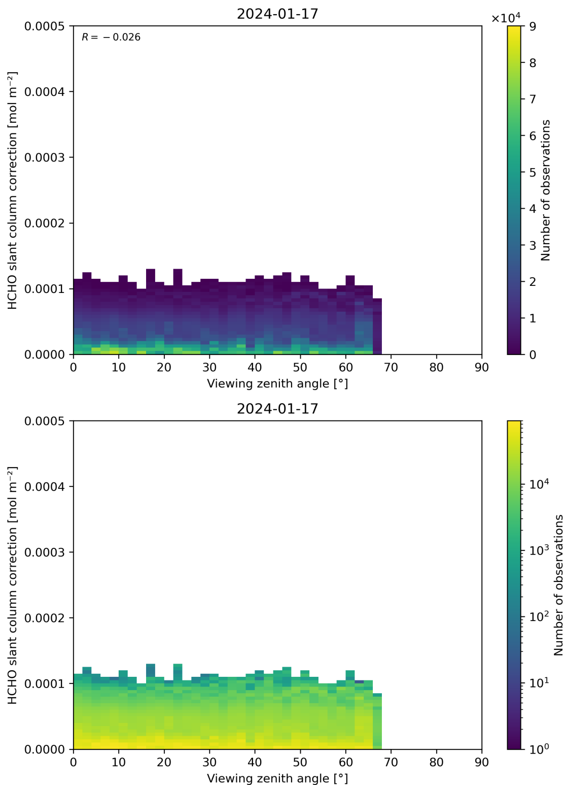
Figure 187: Scatter density plot of “Viewing zenith angle” against “HCHO slant column correction” for 2024-01-16 to 2024-01-18.
