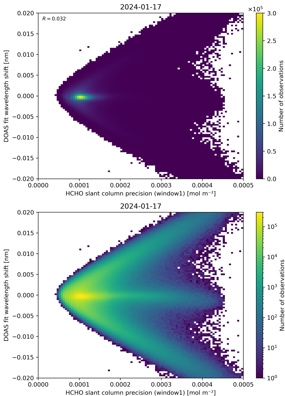
Figure 89: Scatter density plot of “HCHO slant column precision (window1)” against “DOAS fit wavelength shift” for 2024-01-16 to 2024-01-18.
