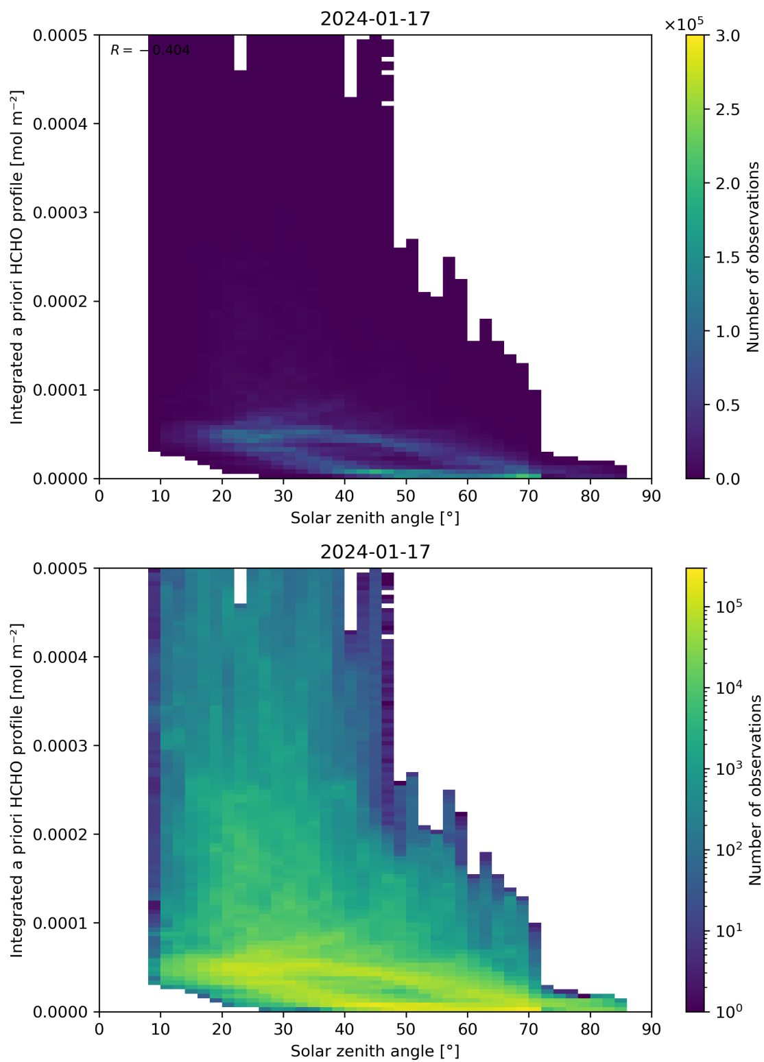
Figure 180: Scatter density plot of “Solar zenith angle” against “Integrated a priori HCHO profile” for 2024-01-16 to 2024-01-18.
