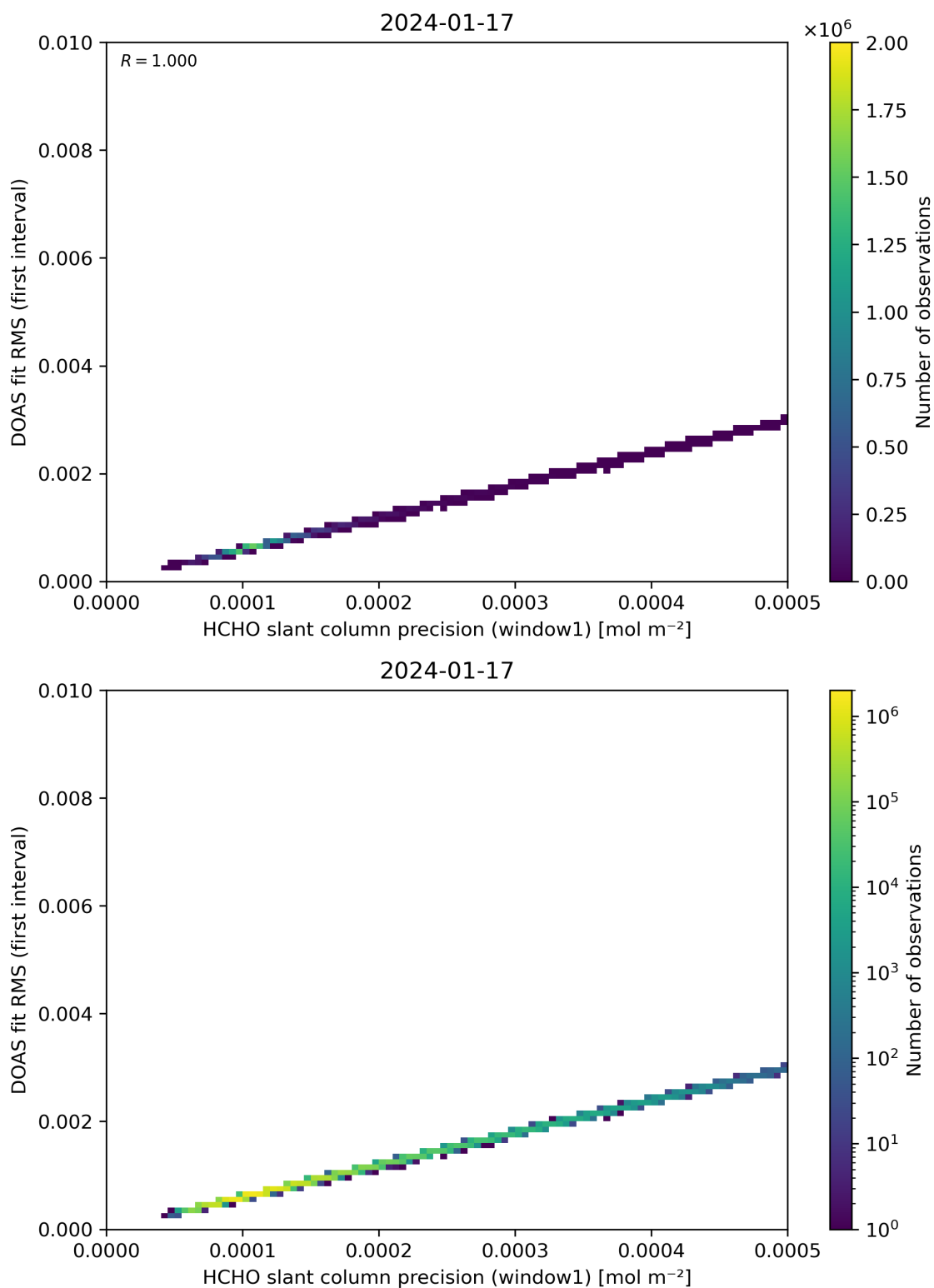
Figure 88: Scatter density plot of “HCHO slant column precision (window1)” against “DOAS fit RMS (first interval)” for 2024-01-16 to 2024-01-18.
