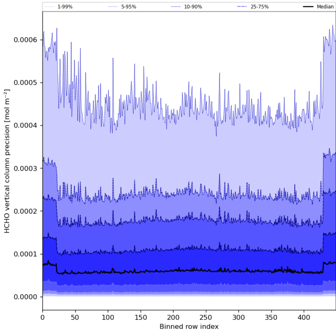
Figure 50: Along track statistics of “HCHO vertical column precision” for 2024-01-16 to 2024-01-18
