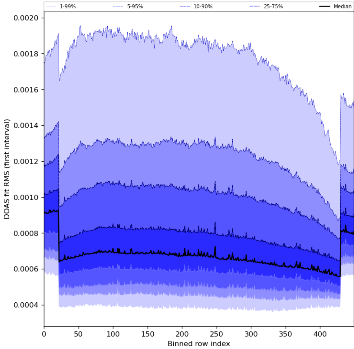
Figure 60: Along track statistics of “DOAS fit RMS (first interval)” for 2024-01-16 to 2024-01-18
