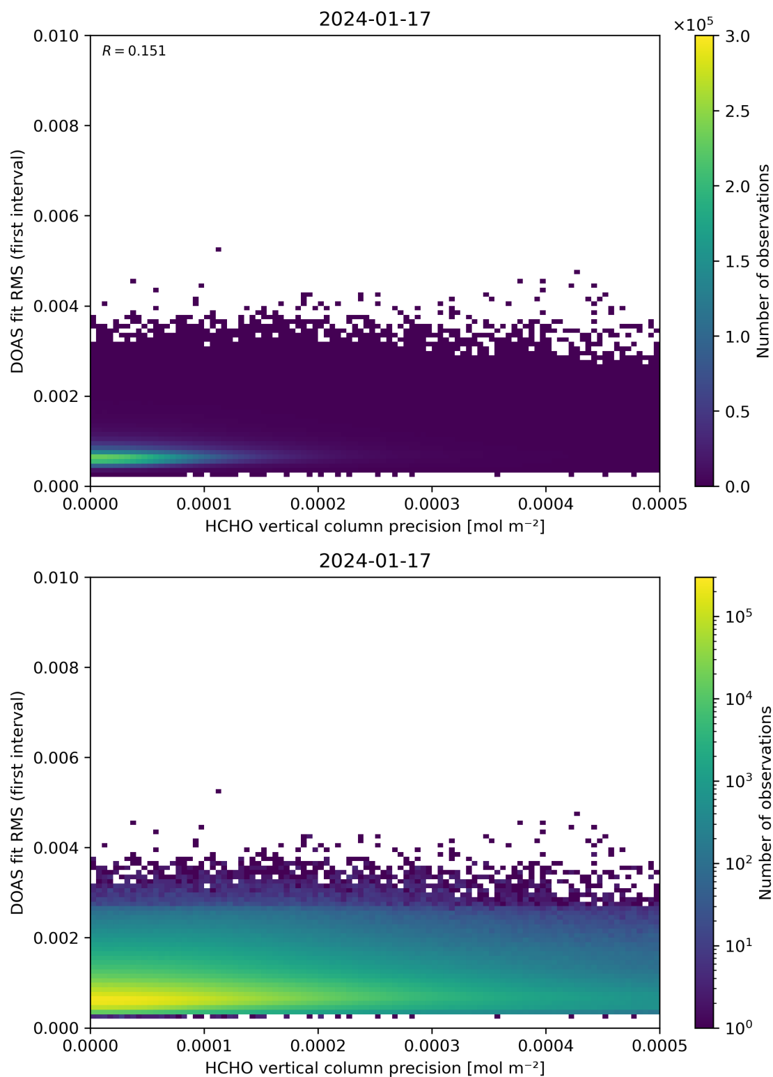
Figure 136: Scatter density plot of “HCHO vertical column precision” against “DOAS fit RMS (first interval)” for 2024-01-16 to 2024-01-18.
