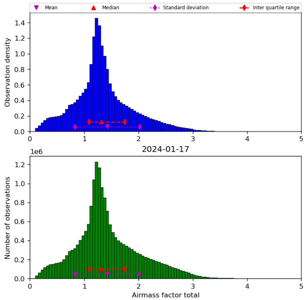
Figure 40: Histogram of “Airmass factor total” for 2024-01-16 to 2024-01-18
