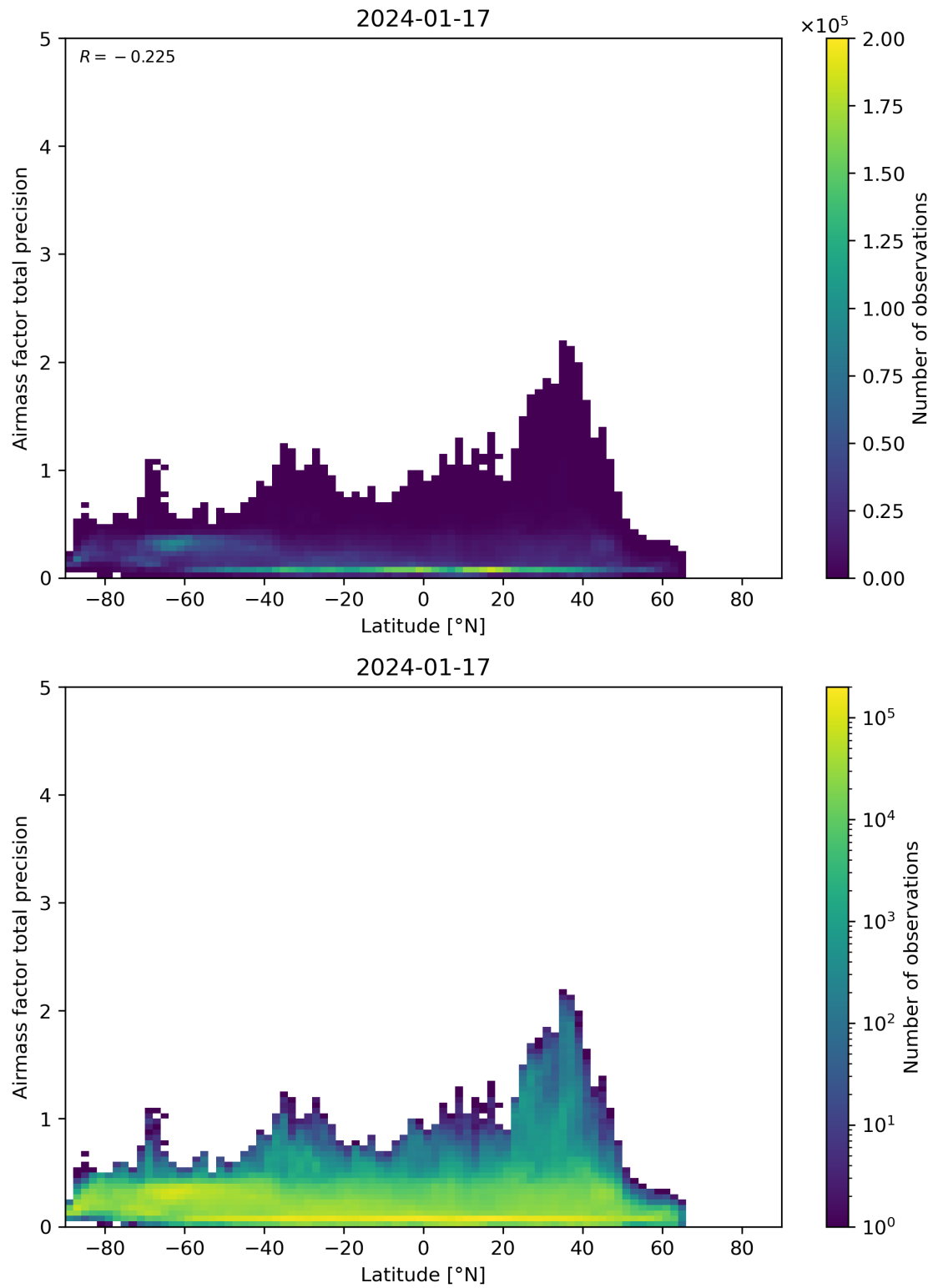
Figure 162: Scatter density plot of “Latitude” against “Airmass factor total precision” for 2024-01-16 to 2024-01-18.
