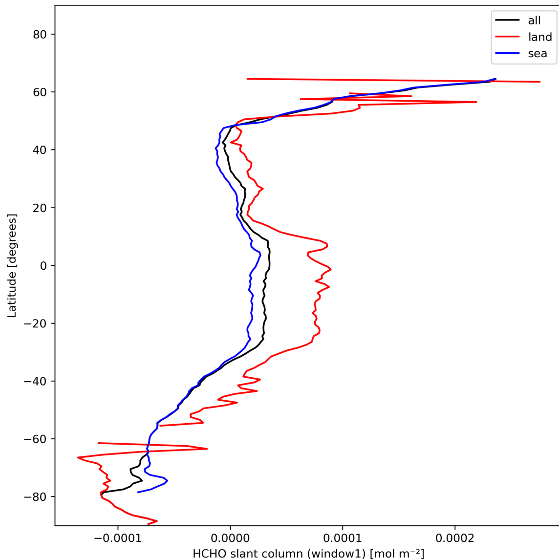
Figure 24: Zonal average of “HCHO slant column (window1)” for 2024-01-16 to 2024-01-18.
