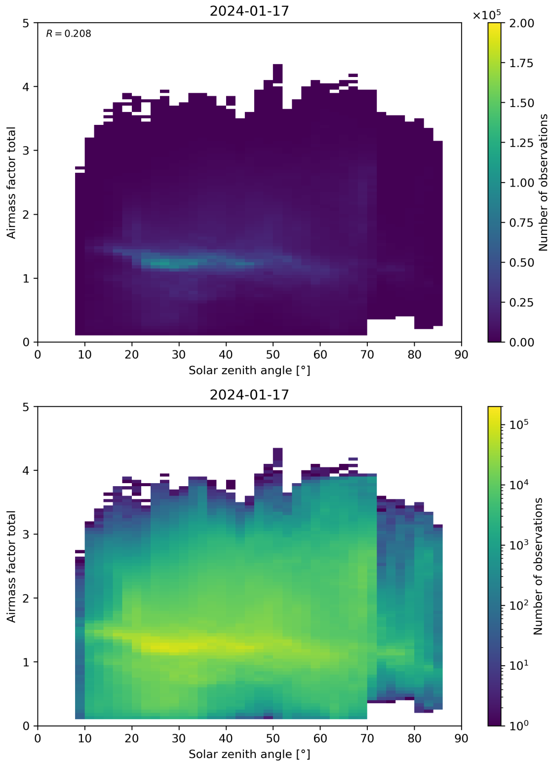
Figure 175: Scatter density plot of “Solar zenith angle” against “Airmass factor total” for 2024-01-16 to 2024-01-18.
