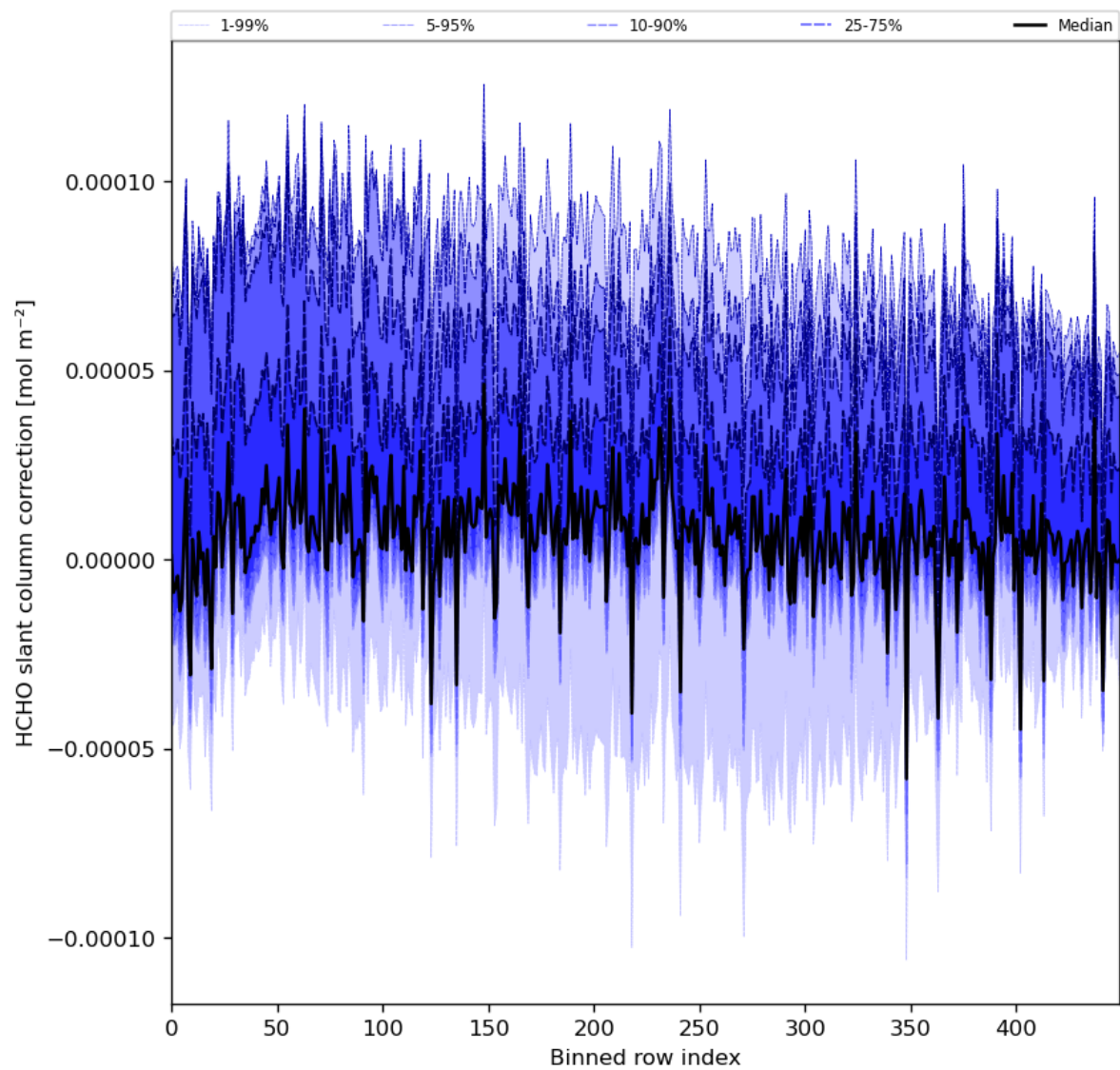
Figure 61: Along track statistics of “HCHO slant column correction” for 2024-01-16 to 2024-01-18
