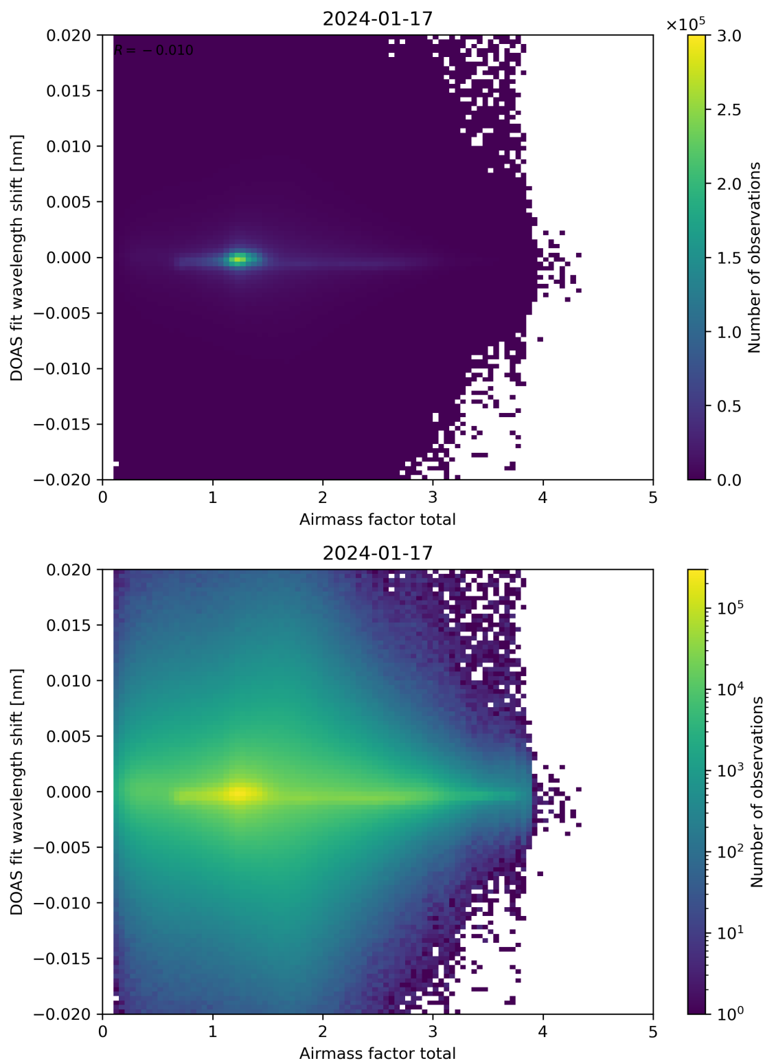
Figure 98: Scatter density plot of “Airmass factor total” against “DOAS fit wavelength shift” for 2024-01-16 to 2024-01-18.
