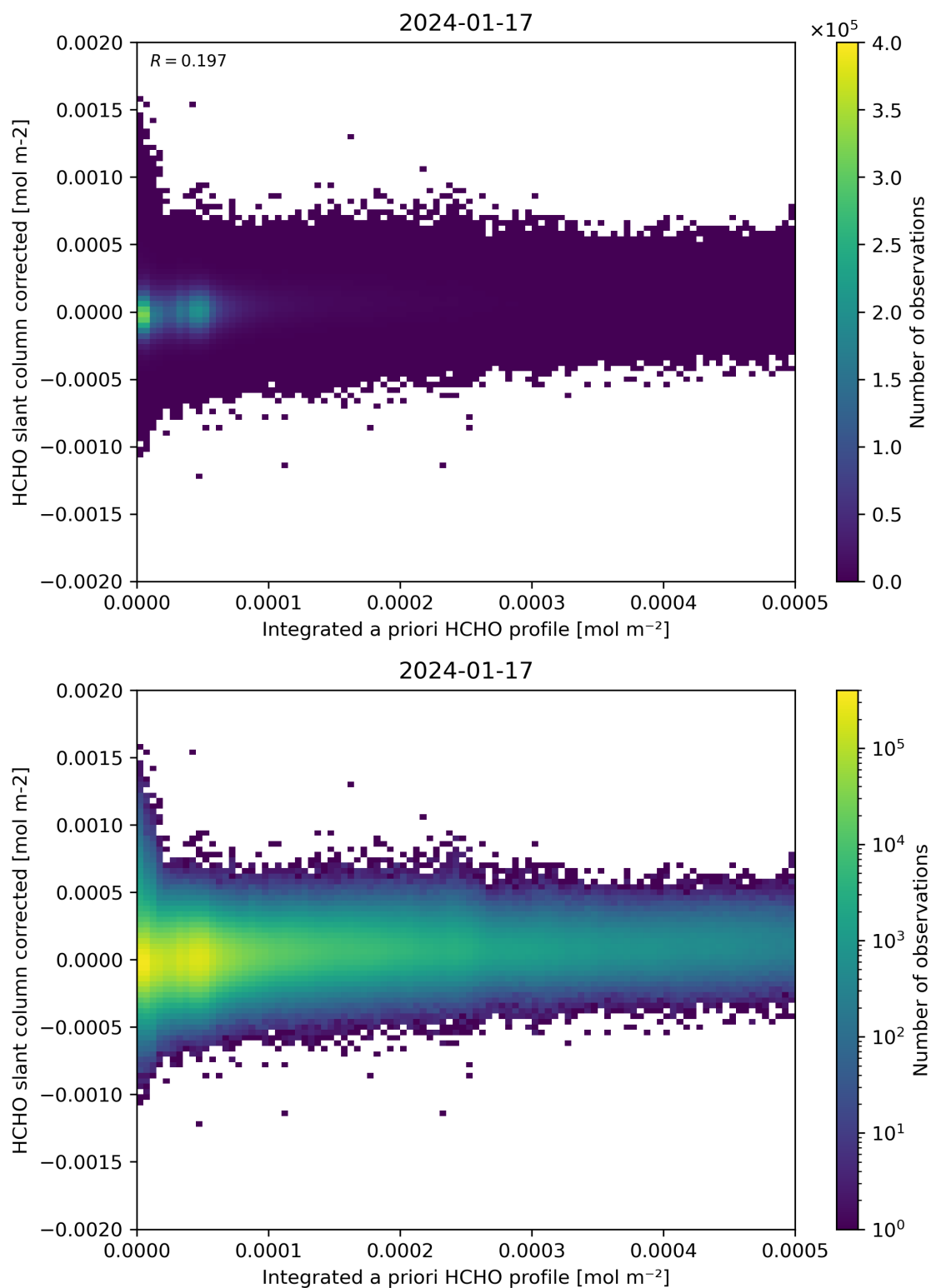
Figure 151: Scatter density plot of “Integrated a priori HCHO profile” against “HCHO slant column corrected” for 2024-01-16 to 2024-01-18.
