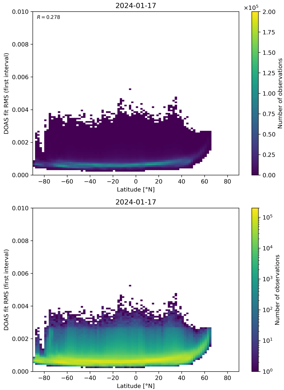
Figure 153: Scatter density plot of “Latitude” against “DOAS fit RMS (first interval)” for 2024-01-16 to 2024-01-18.
