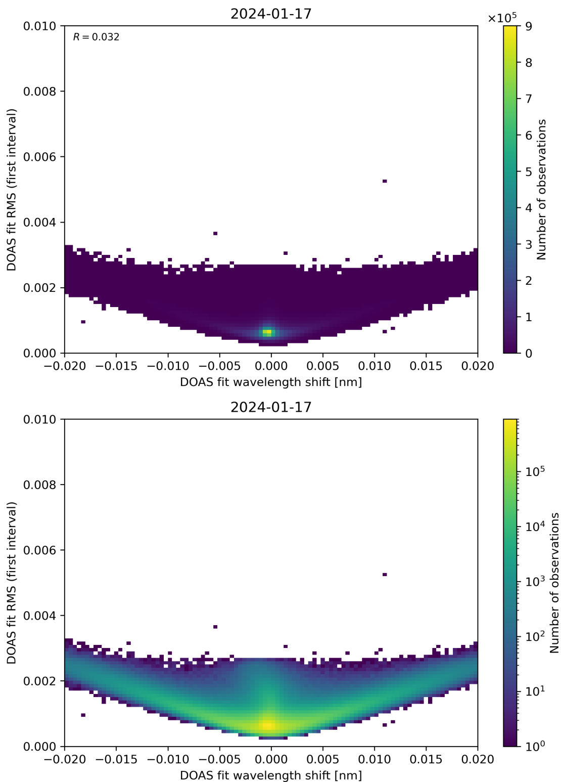
Figure 64: Scatter density plot of “DOAS fit wavelength shift” against “DOAS fit RMS (first interval)” for 2024-01-16 to 2024-01-18.
