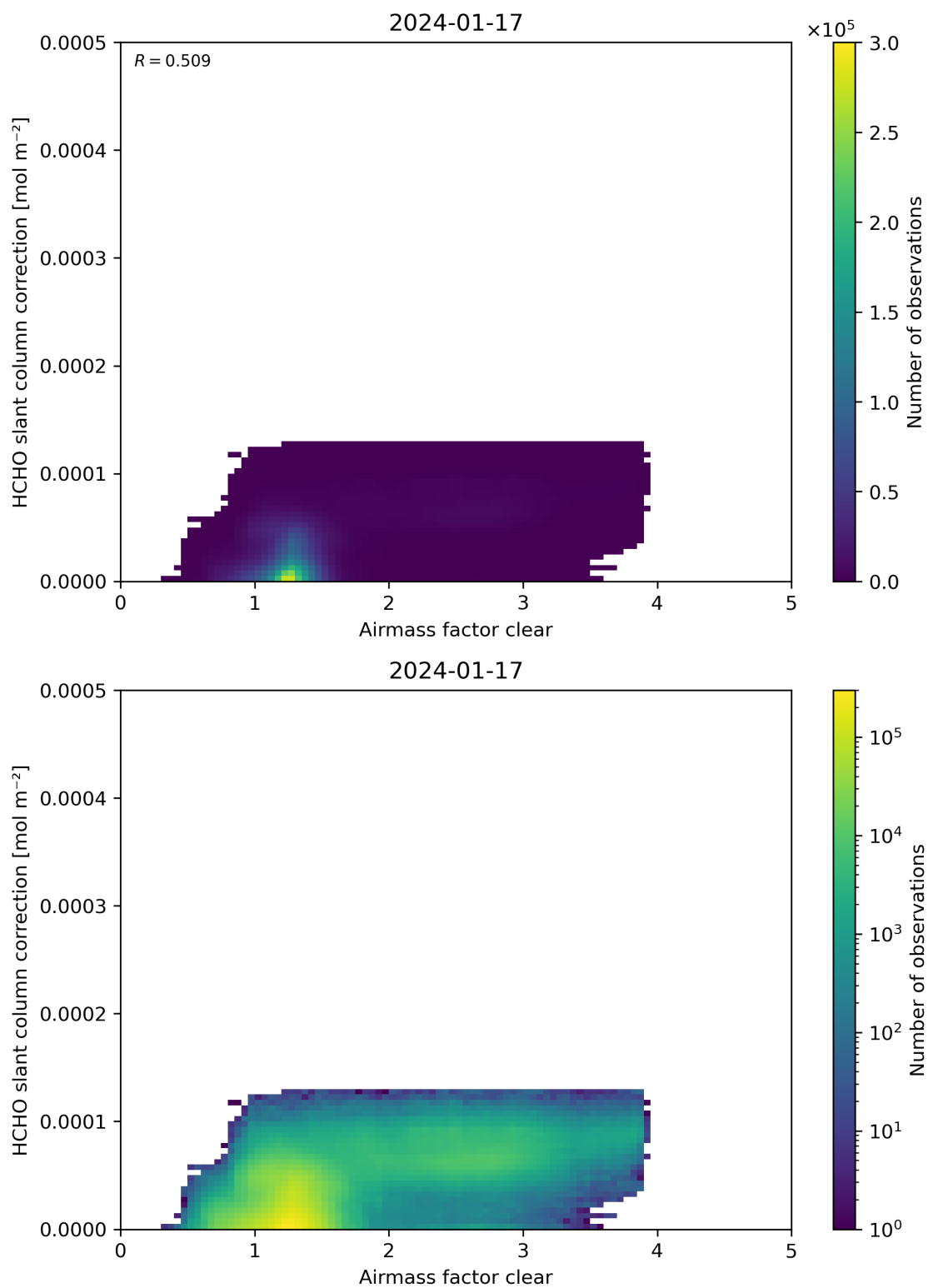
Figure 75: Scatter density plot of “Airmass factor clear” against “HCHO slant column correction” for 2024-01-16 to 2024-01-18.
