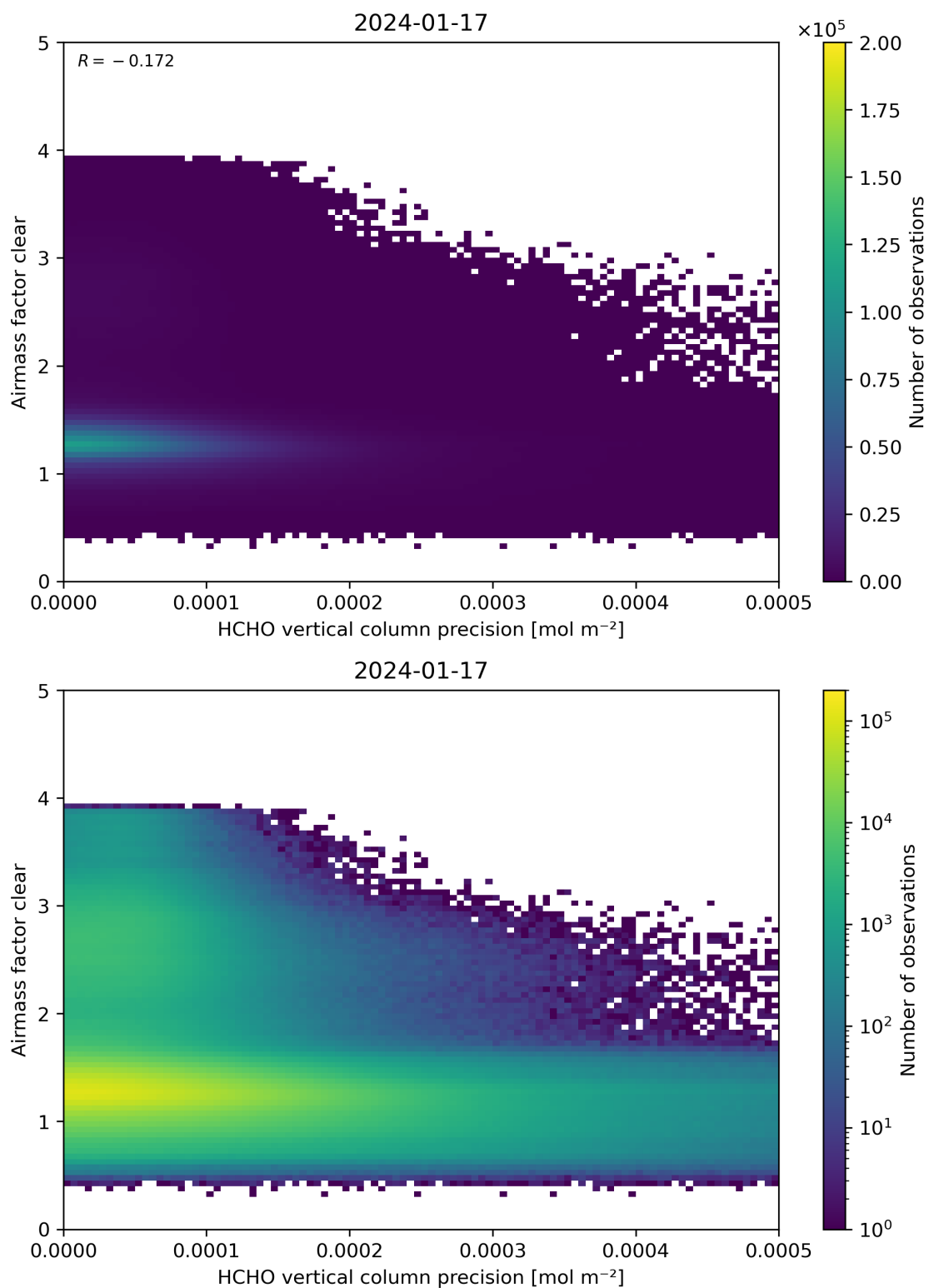
Figure 139: Scatter density plot of “HCHO vertical column precision” against “Airmass factor clear” for 2024-01-16 to 2024-01-18.
