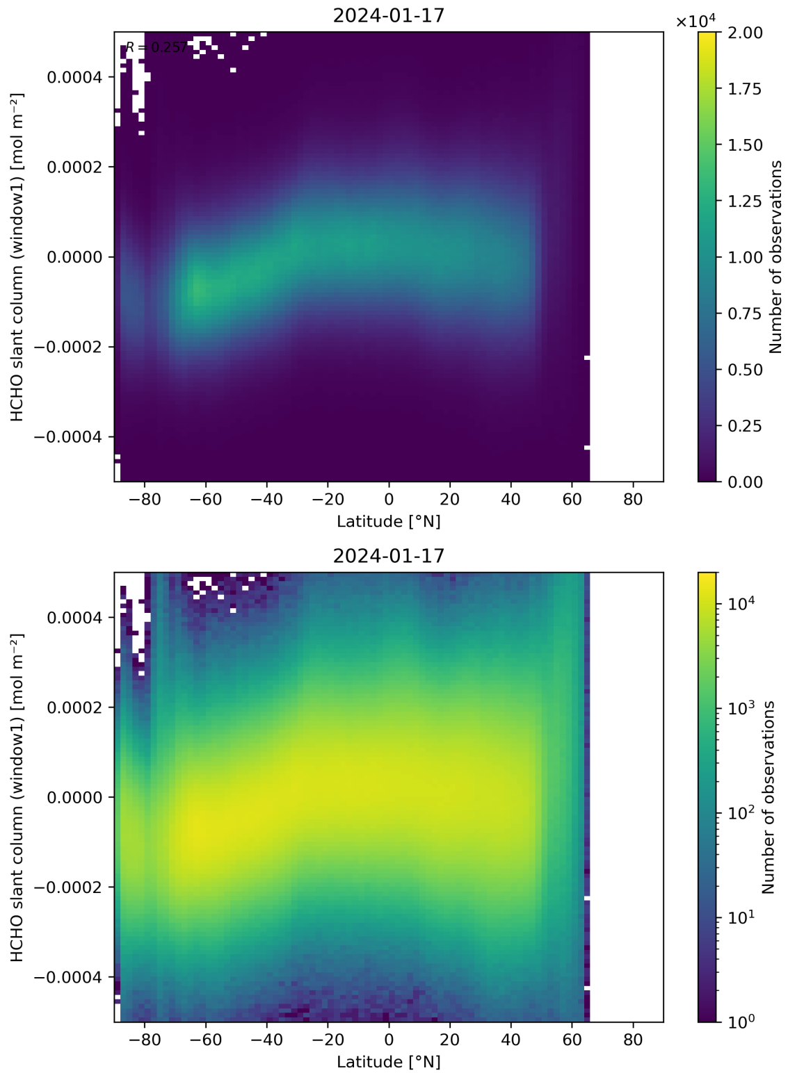
Figure 159: Scatter density plot of “Latitude” against “HCHO slant column (window1)” for 2024-01-16 to 2024-01-18.
