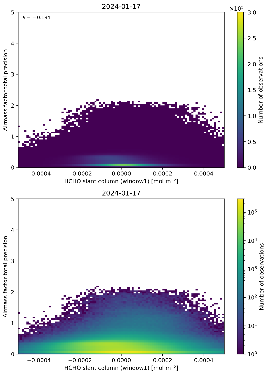
Figure 86: Scatter density plot of “HCHO slant column (window1)” against “Airmass factor total precision” for 2024-01-16 to 2024-01-18.
