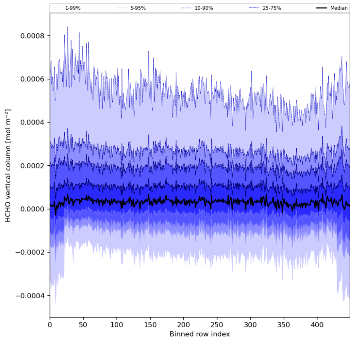
Figure 49: Along track statistics of “HCHO vertical column” for 2024-01-16 to 2024-01-18
