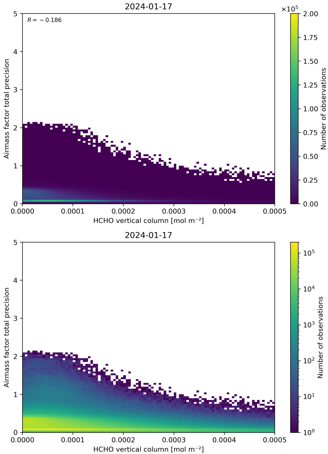
Figure 132: Scatter density plot of “HCHO vertical column” against “Airmass factor total precision” for 2024-01-16 to 2024-01-18.
