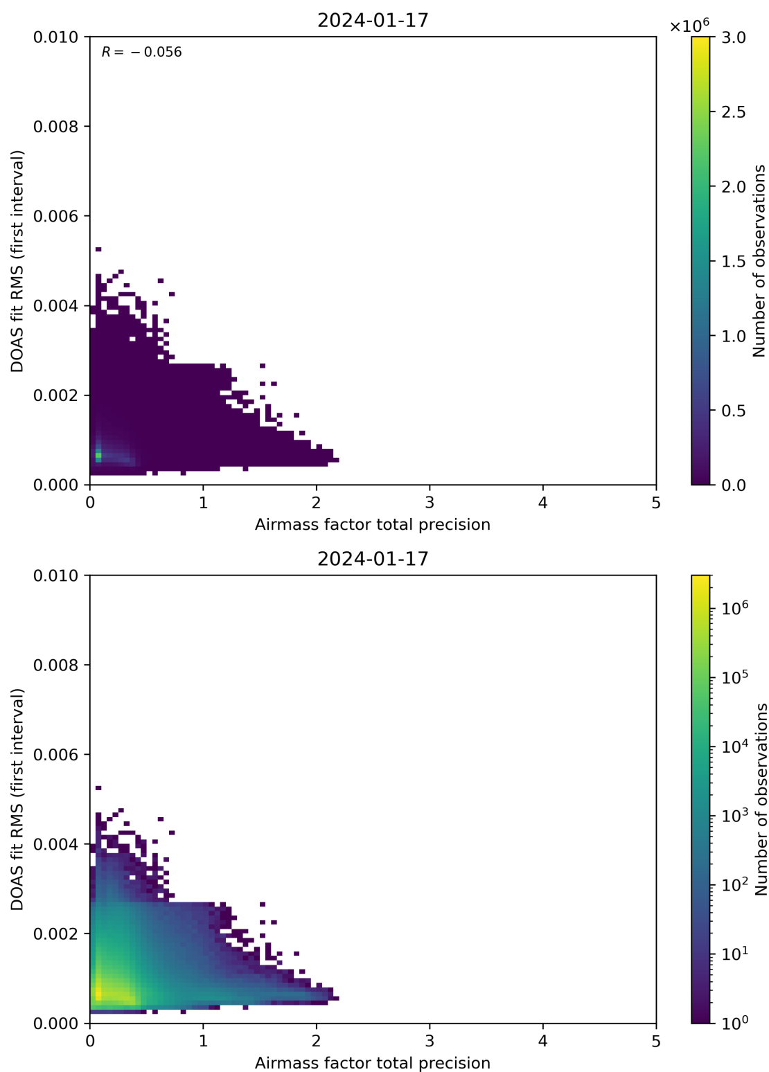
Figure 105: Scatter density plot of “Airmass factor total precision” against “DOAS fit RMS (first interval)” for 2024-01-16 to 2024-01-18.
