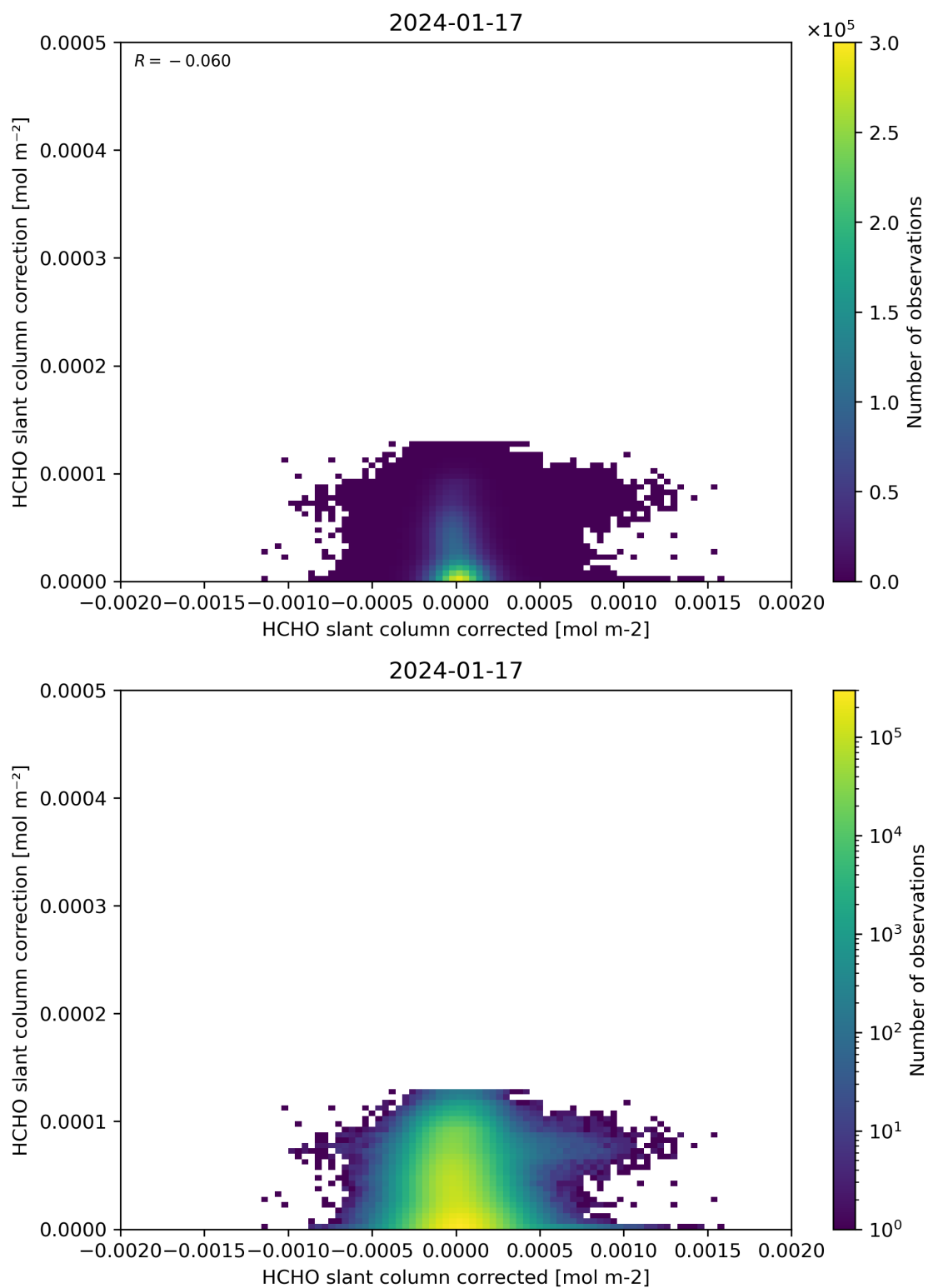
Figure 77: Scatter density plot of “HCHO slant column corrected” against “HCHO slant column correction” for 2024-01-16 to 2024-01-18.
