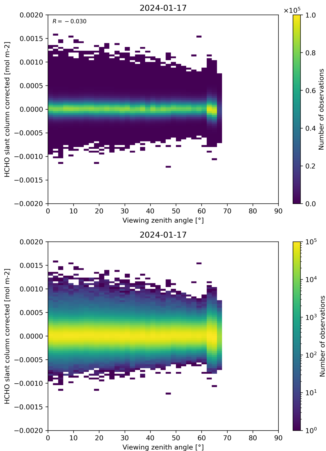
Figure 186: Scatter density plot of “Viewing zenith angle” against “HCHO slant column corrected” for 2024-01-16 to 2024-01-18.
