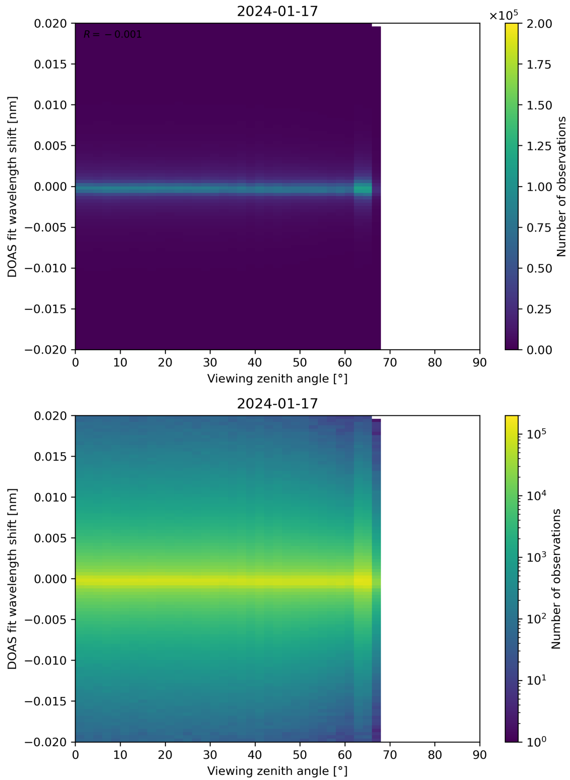
Figure 183: Scatter density plot of “Viewing zenith angle” against “DOAS fit wavelength shift” for 2024-01-16 to 2024-01-18.
