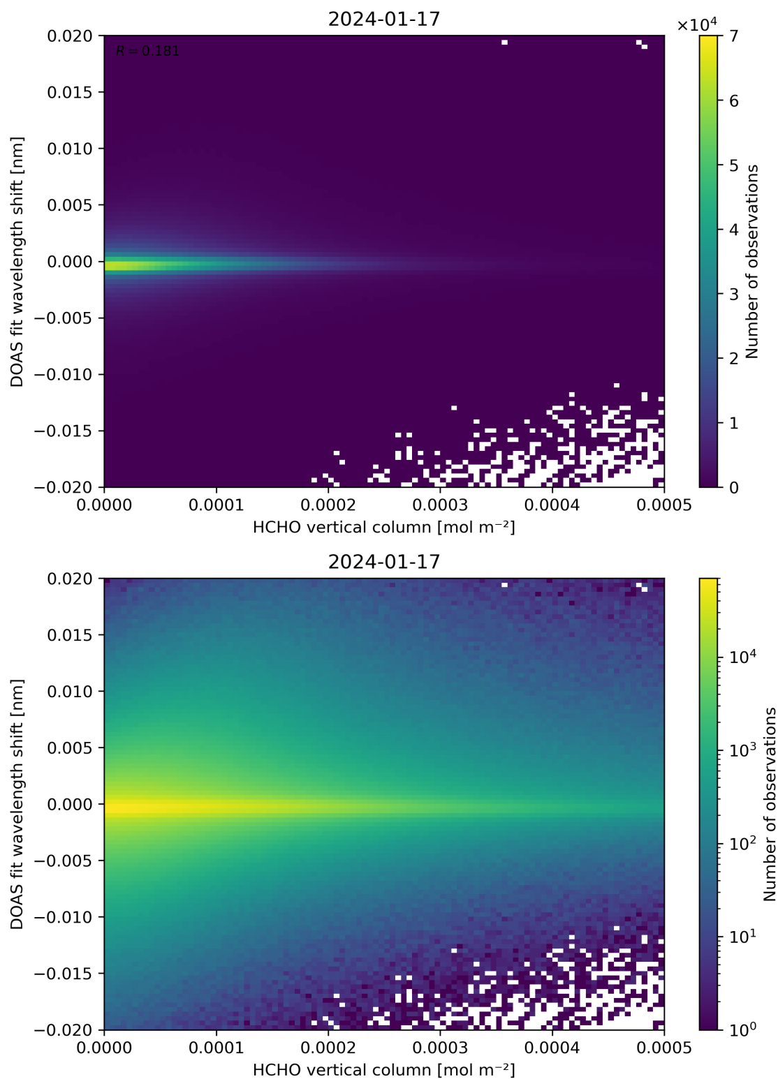
Figure 124: Scatter density plot of “HCHO vertical column” against “DOAS fit wavelength shift” for 2024-01-16 to 2024-01-18.
