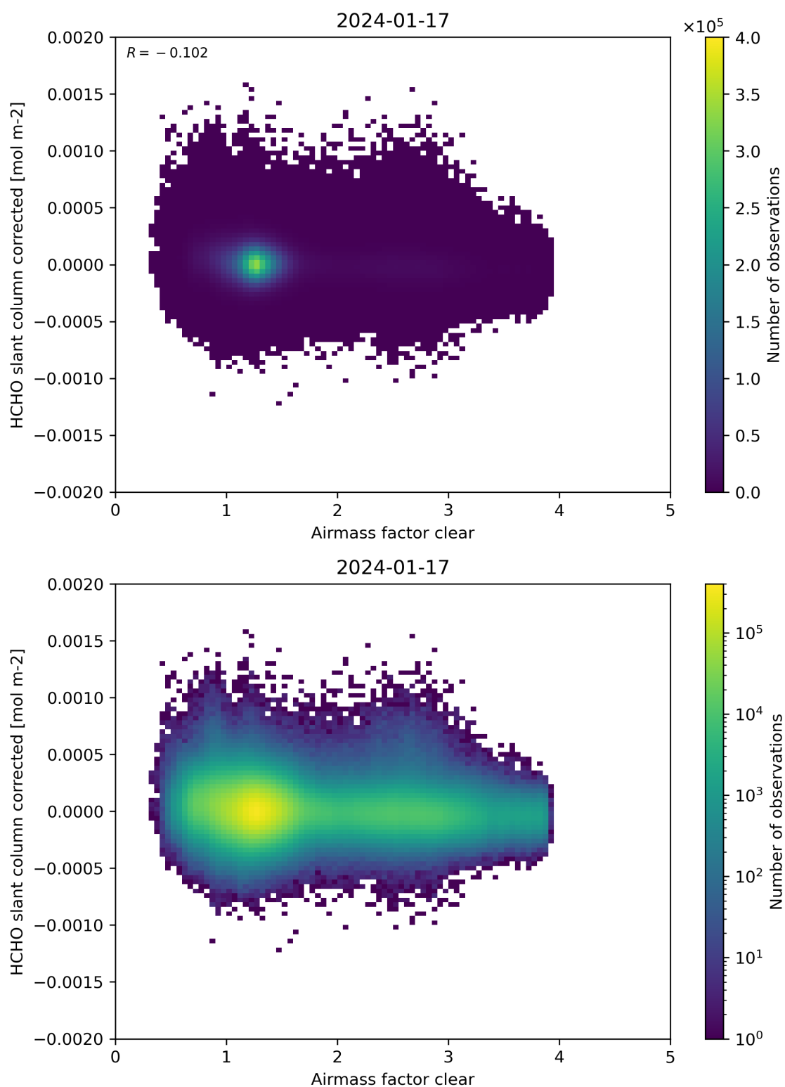
Figure 74: Scatter density plot of “Airmass factor clear” against “HCHO slant column corrected” for 2024-01-16 to 2024-01-18.
