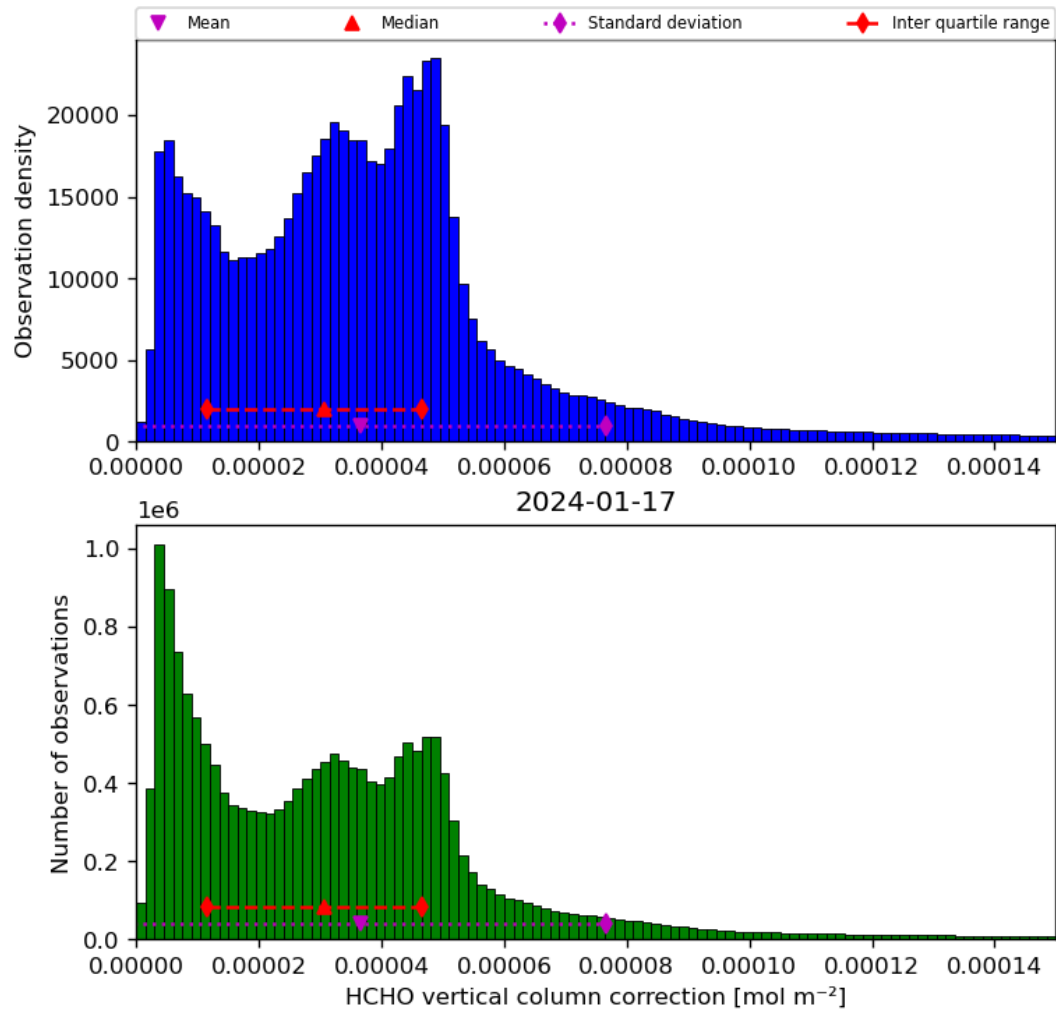
Figure 37: Histogram of “HCHO vertical column correction” for 2024-01-16 to 2024-01-18
