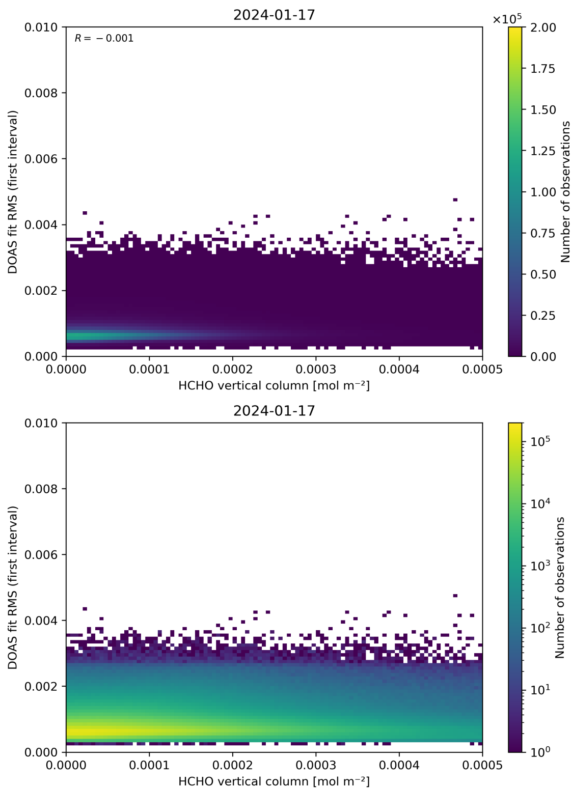
Figure 123: Scatter density plot of “HCHO vertical column” against “DOAS fit RMS (first interval)” for 2024-01-16 to 2024-01-18.
