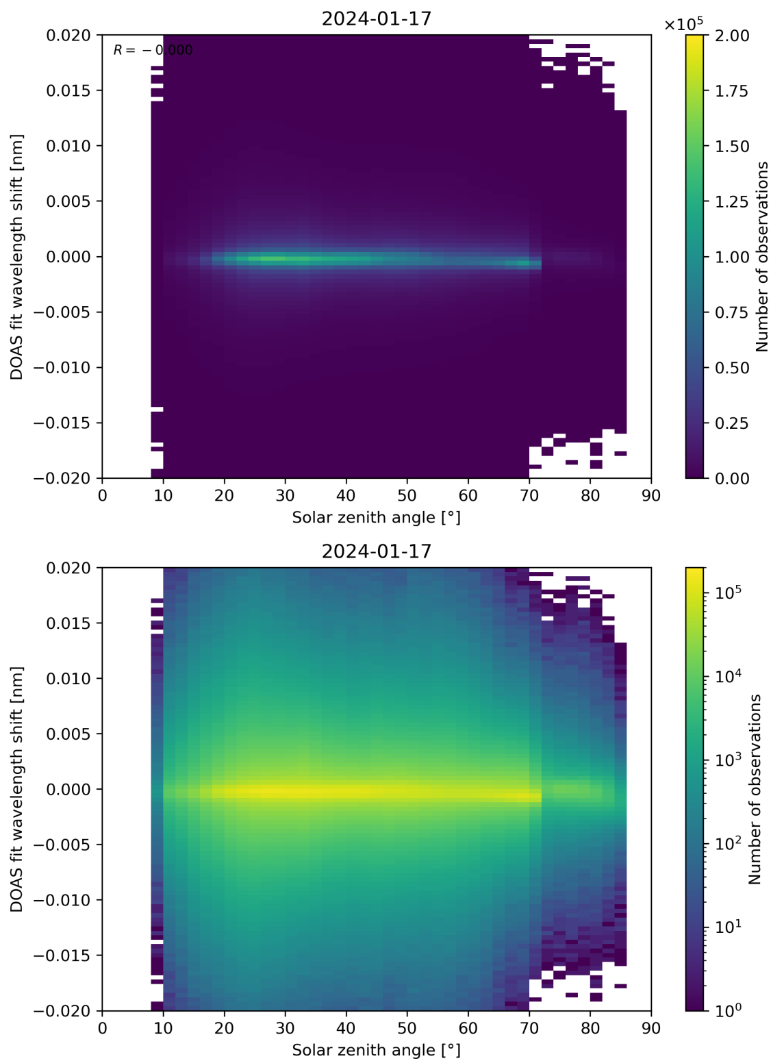
Figure 168: Scatter density plot of “Solar zenith angle” against “DOAS fit wavelength shift” for 2024-01-16 to 2024-01-18.
