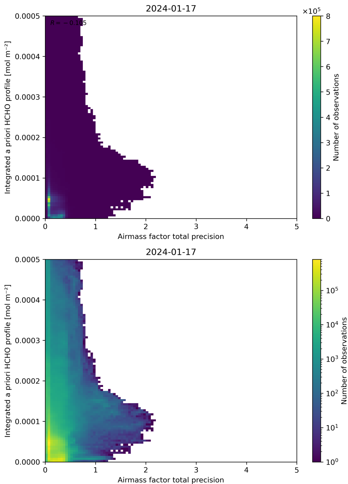
Figure 111: Scatter density plot of “Airmass factor total precision” against “Integrated a priori HCHO profile” for 2024-01-16 to 2024-01-18.
