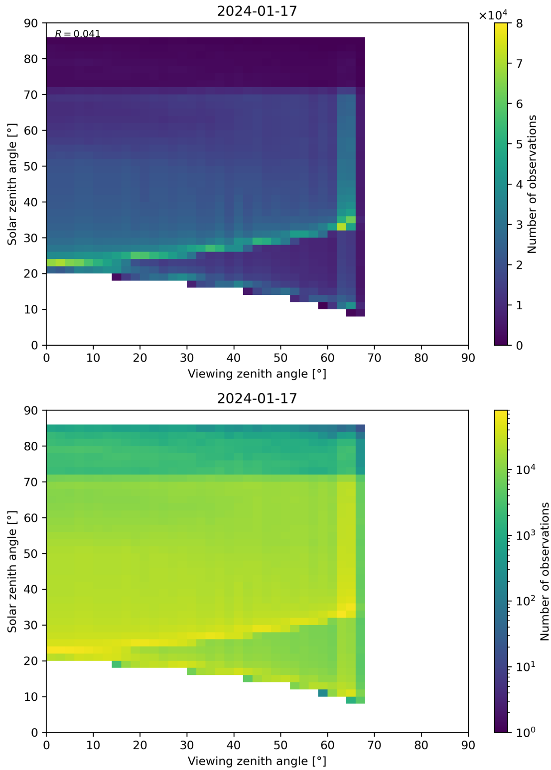
Figure 197: Scatter density plot of “Viewing zenith angle” against “Solar zenith angle” for 2024-01-16 to 2024-01-18.
