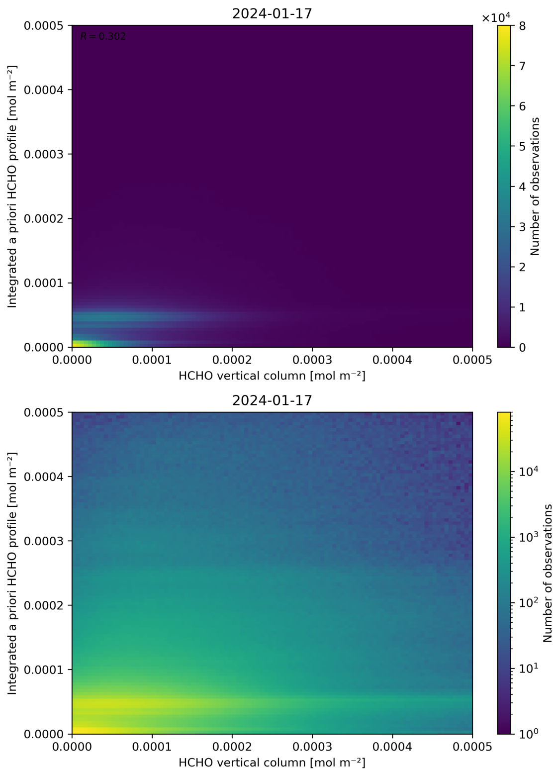
Figure 135: Scatter density plot of “HCHO vertical column” against “Integrated a priori HCHO profile” for 2024-01-16 to 2024-01-18.
