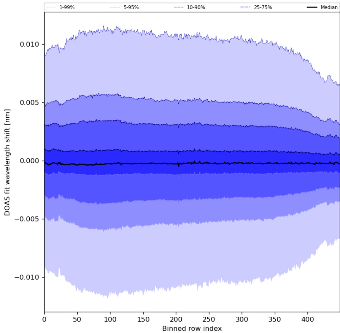
Figure 58: Along track statistics of “DOAS fit wavelength shift” for 2024-01-16 to 2024-01-18
