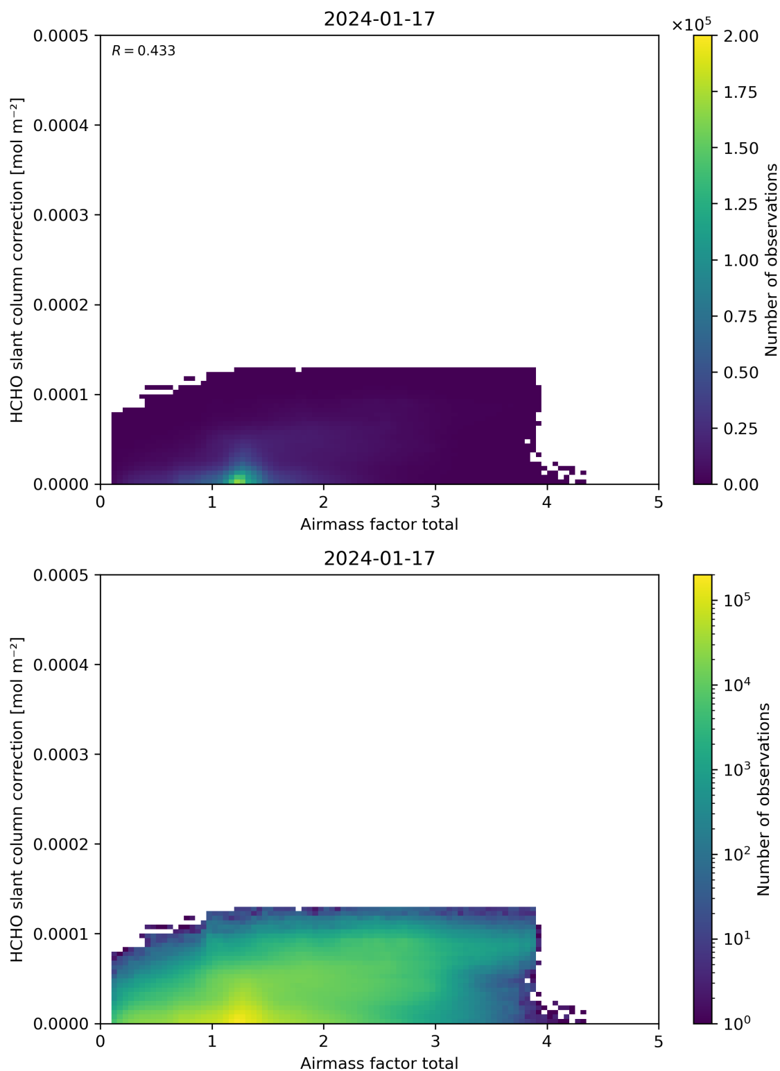
Figure 102: Scatter density plot of “Airmass factor total” against “HCHO slant column correction” for 2024-01-16 to 2024-01-18.
