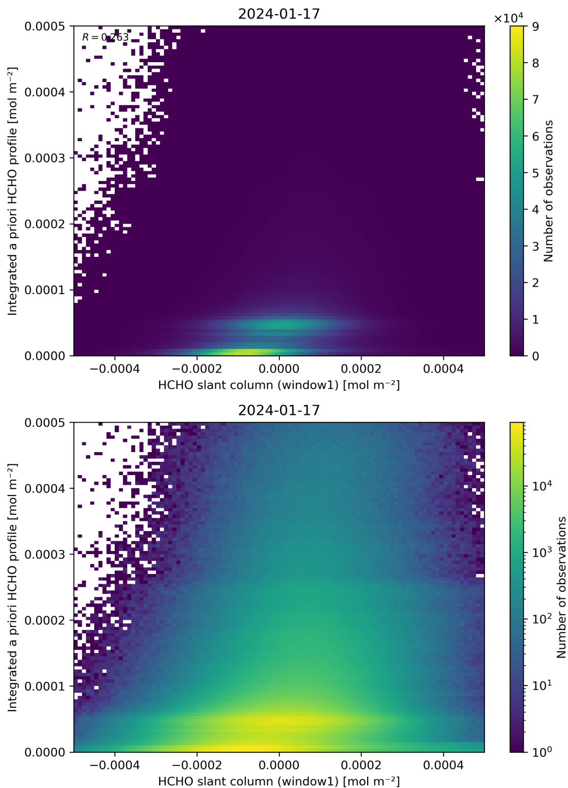
Figure 87: Scatter density plot of “HCHO slant column (window1)” against “Integrated a priori HCHO profile” for 2024-01-16 to 2024-01-18.
