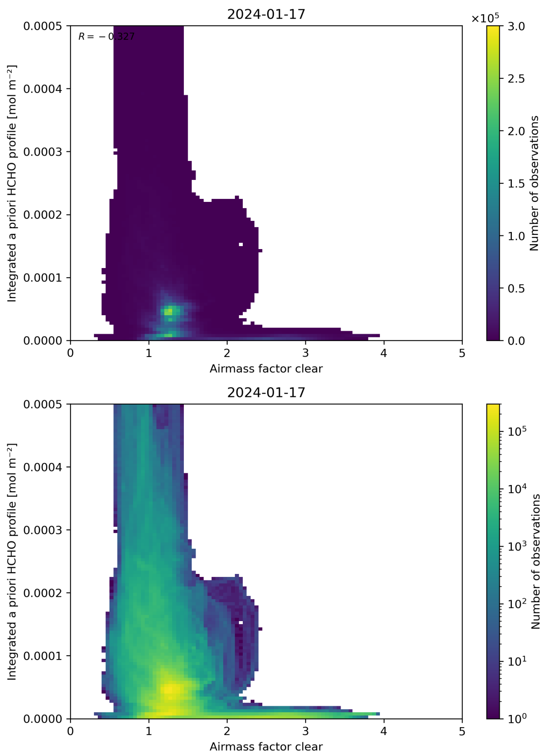
Figure 76: Scatter density plot of “Airmass factor clear” against “Integrated a priori HCHO profile” for 2024-01-16 to 2024-01-18.
