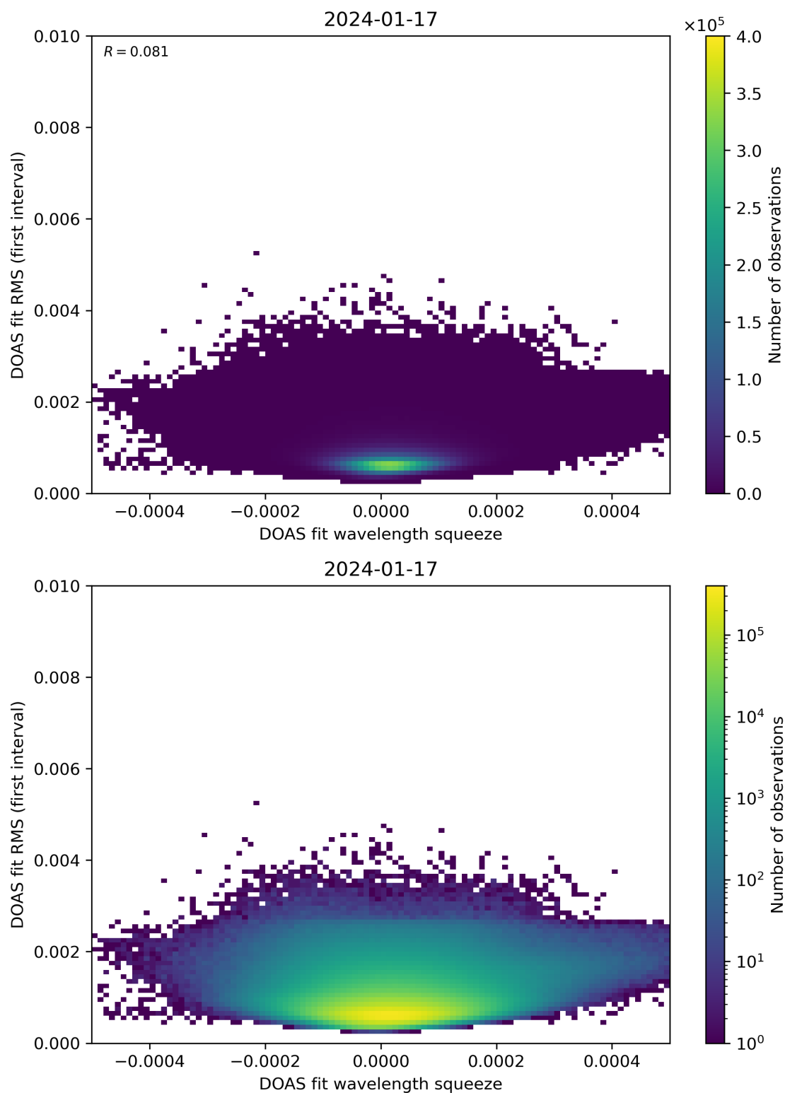
Figure 68: Scatter density plot of “DOAS fit wavelength squeeze” against “DOAS fit RMS (first interval)” for 2024-01-16 to 2024-01-18.
