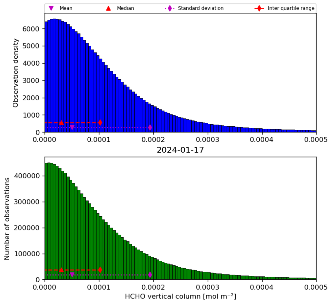
Figure 35: Histogram of “HCHO vertical column” for 2024-01-16 to 2024-01-18
