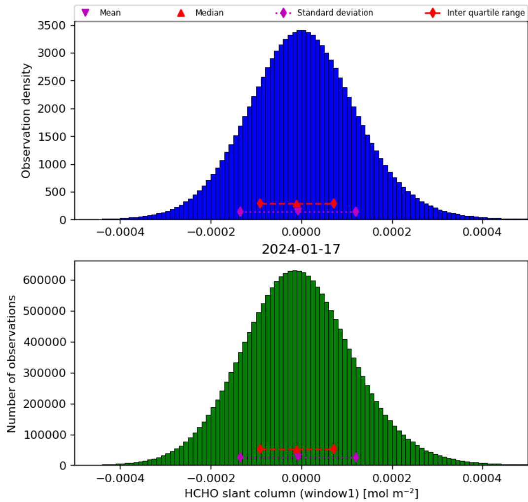
Figure 38: Histogram of “HCHO slant column (window1)” for 2024-01-16 to 2024-01-18
