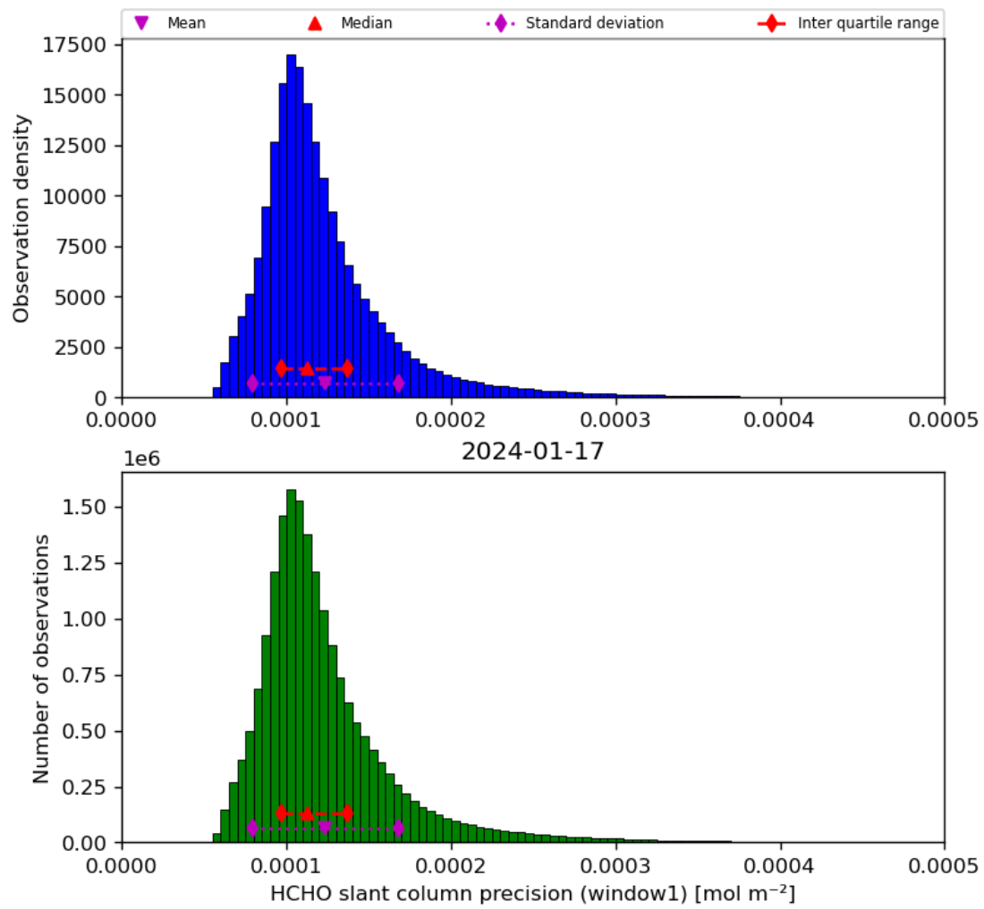
Figure 39: Histogram of “HCHO slant column precision (window1)” for 2024-01-16 to 2024-01-18
