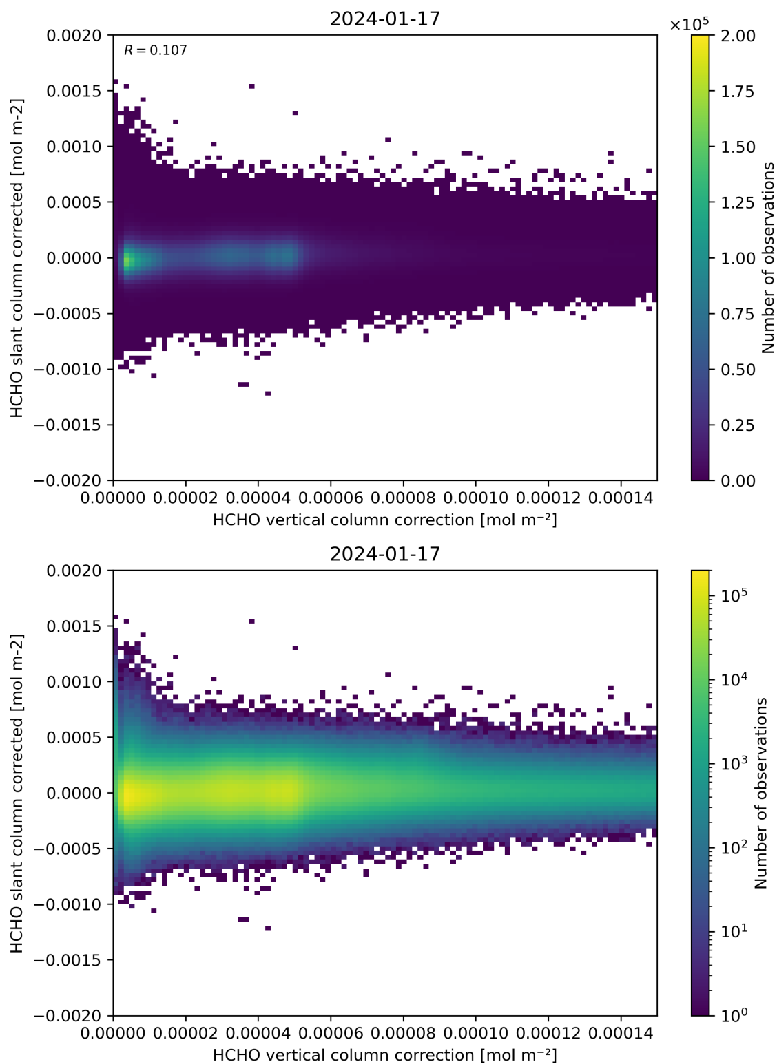
Figure 116: Scatter density plot of “HCHO vertical column correction” against “HCHO slant column corrected” for 2024-01-16 to 2024-01-18.
