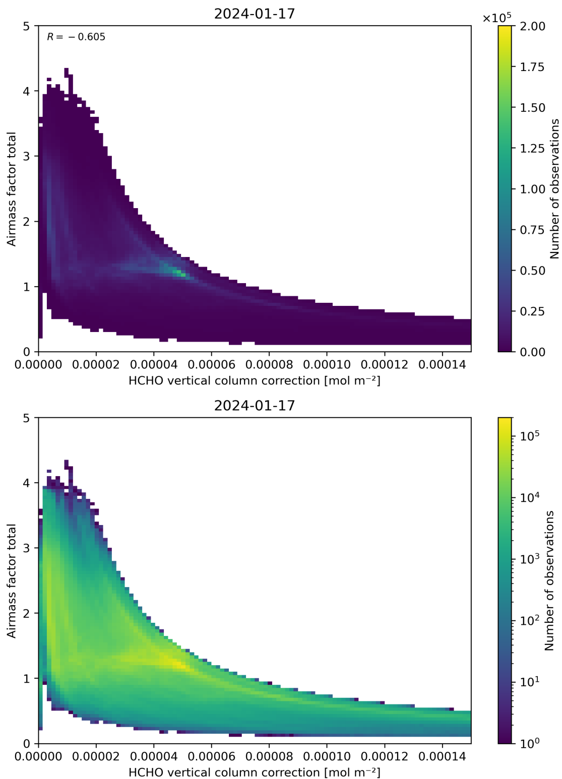
Figure 120: Scatter density plot of “HCHO vertical column correction” against “Airmass factor total” for 2024-01-16 to 2024-01-18.
