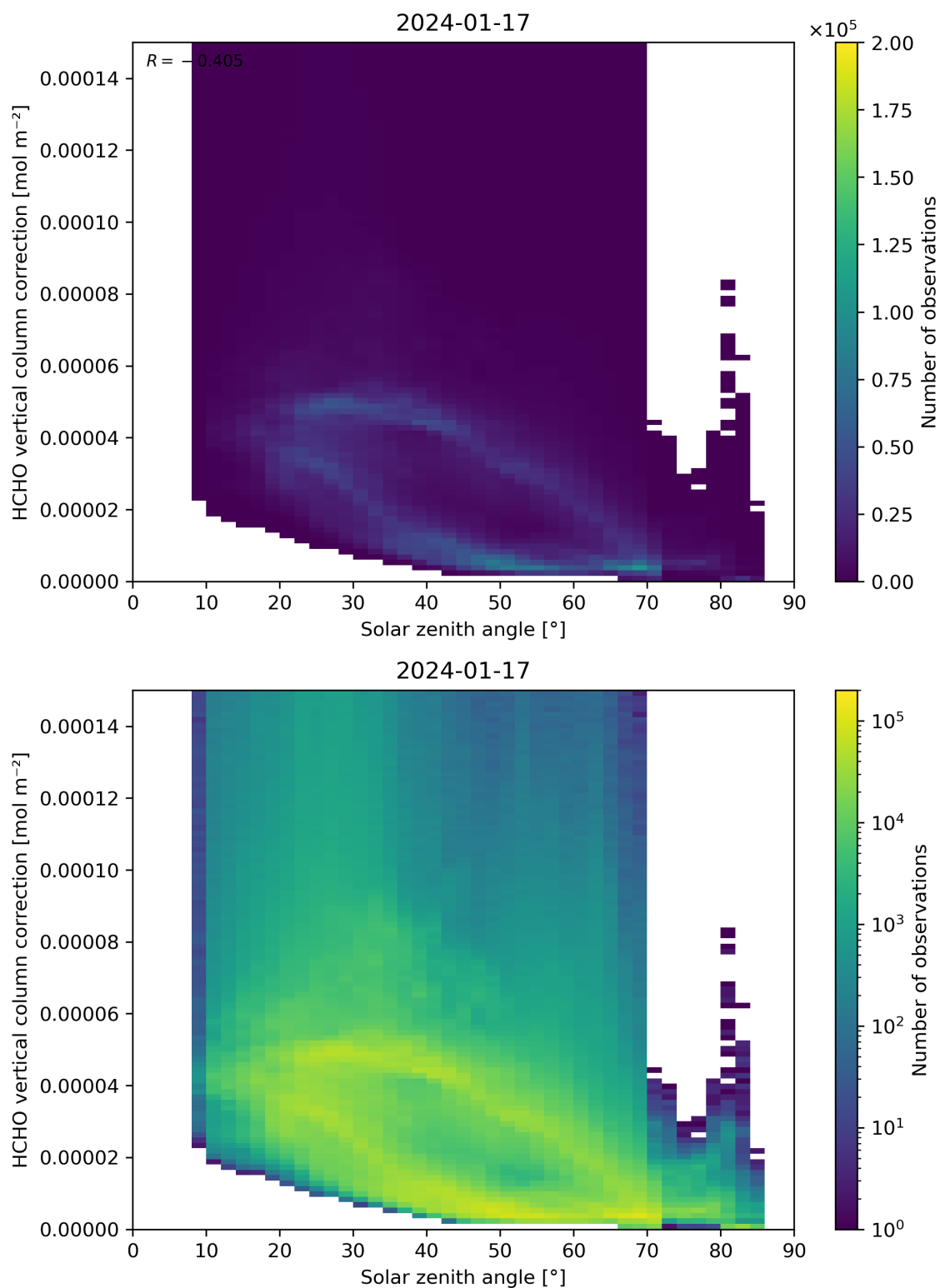
Figure 178: Scatter density plot of “Solar zenith angle” against “HCHO vertical column correction” for 2024-01-16 to 2024-01-18.
