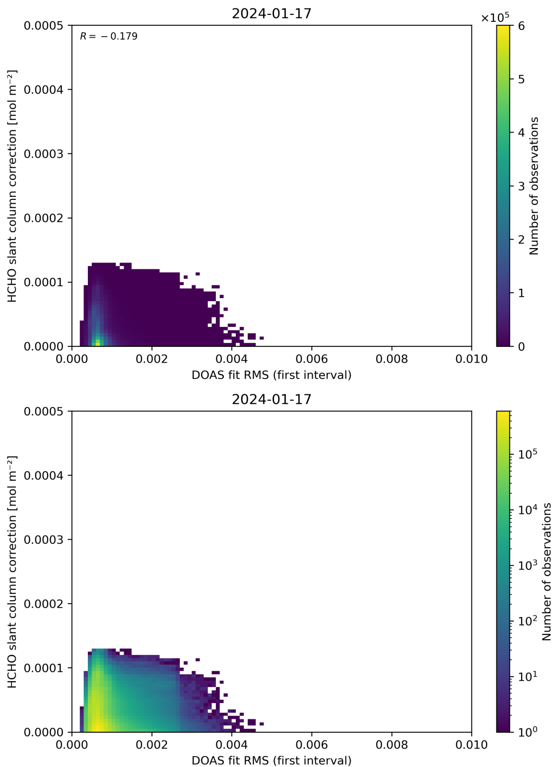
Figure 63: Scatter density plot of “DOAS fit RMS (first interval)” against “HCHO slant column correction” for 2024-01-16 to 2024-01-18.
