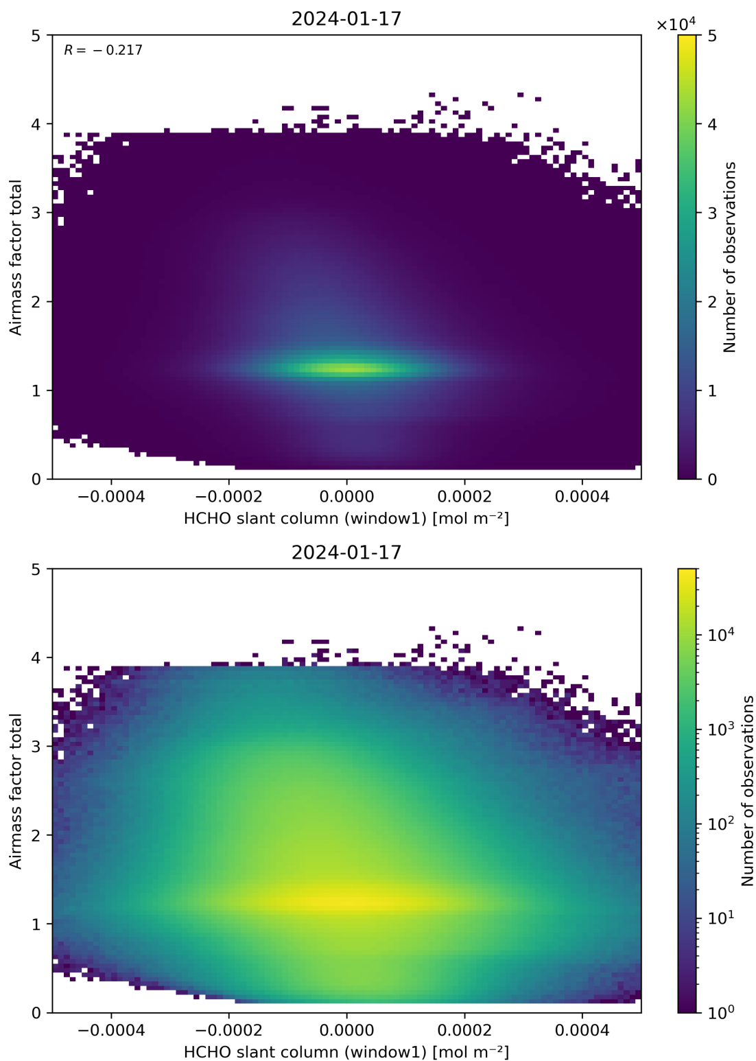
Figure 85: Scatter density plot of “HCHO slant column (window1)” against “Airmass factor total” for 2024-01-16 to 2024-01-18.
