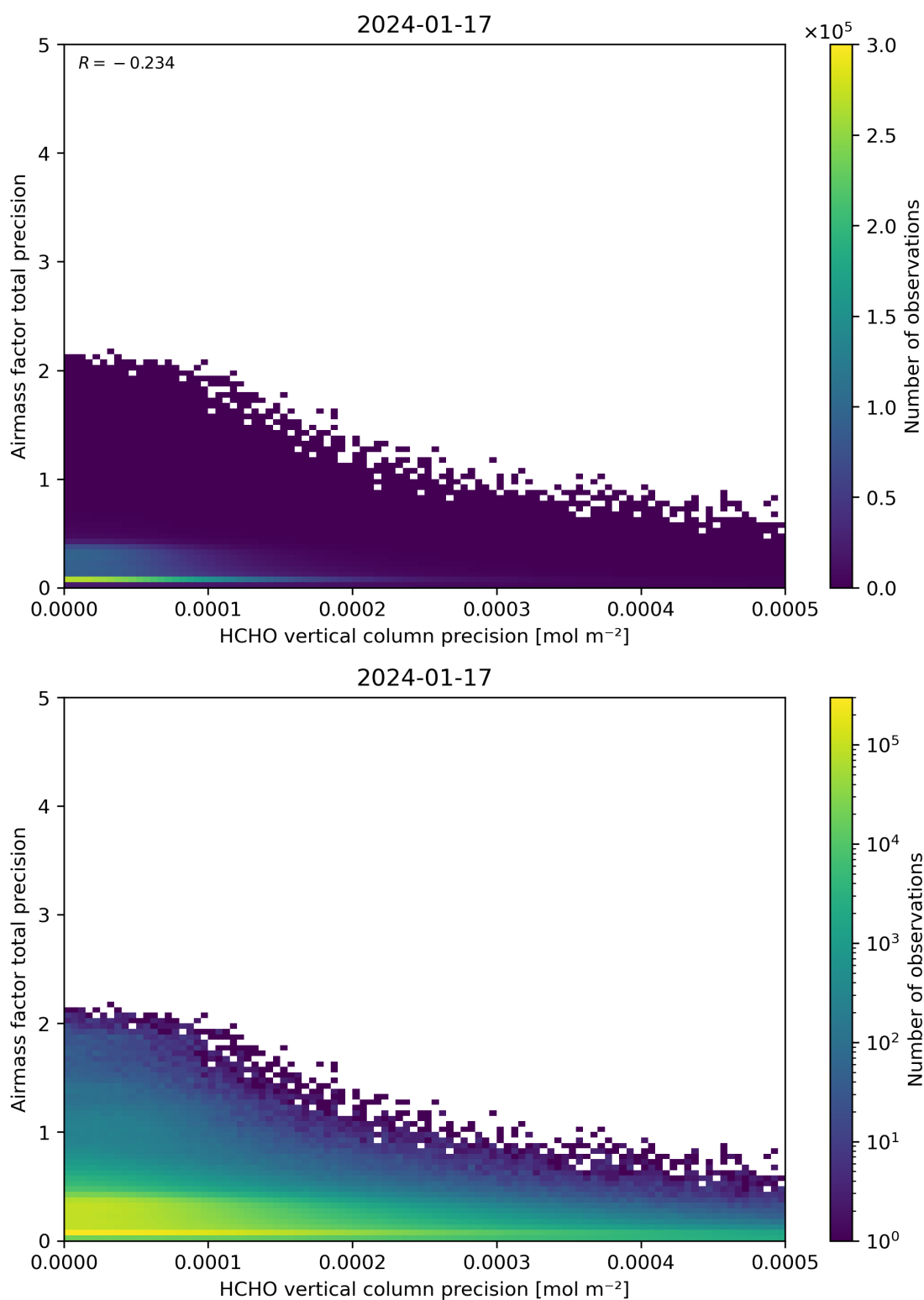
Figure 145: Scatter density plot of “HCHO vertical column precision” against “Airmass factor total precision” for 2024-01-16 to 2024-01-18.
