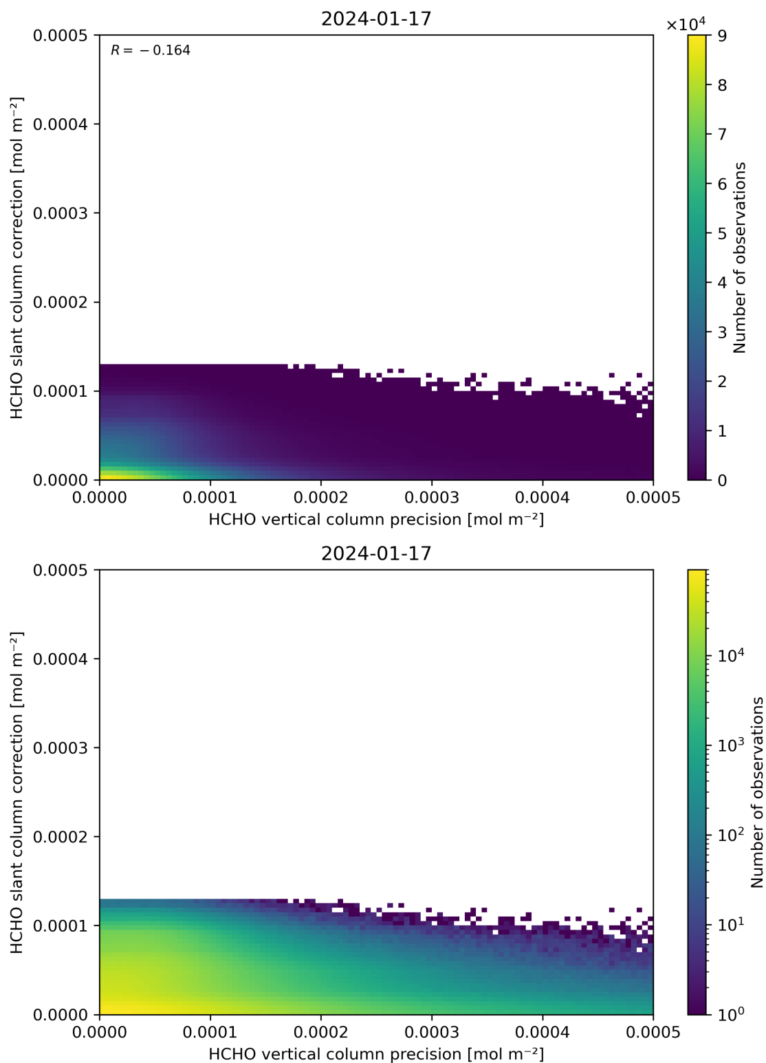
Figure 141: Scatter density plot of “HCHO vertical column precision” against “HCHO slant column correction” for 2024-01-16 to 2024-01-18.
