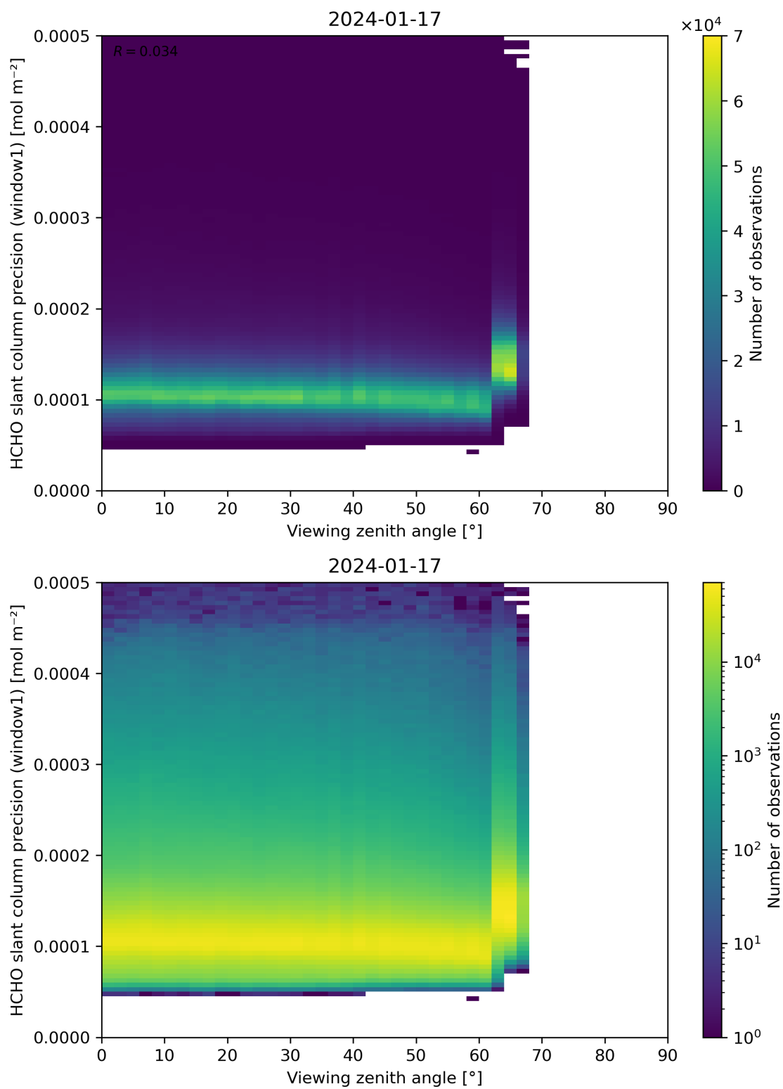
Figure 189: Scatter density plot of “Viewing zenith angle” against “HCHO slant column precision (window1)” for 2024-01-16 to 2024-01-18.
