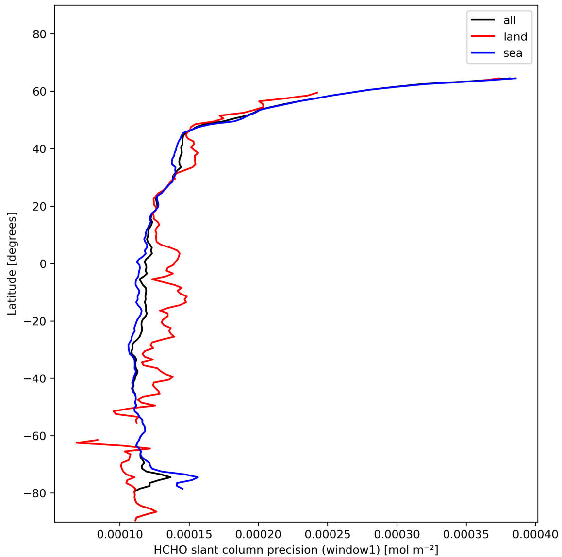
Figure 25: Zonal average of “HCHO slant column precision (window1)” for 2024-01-16 to 2024-01-18.
