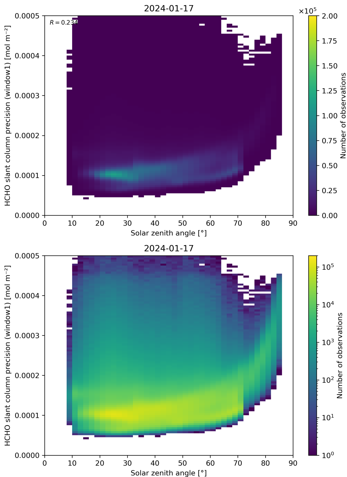
Figure 174: Scatter density plot of “Solar zenith angle” against “HCHO slant column precision (window1)” for 2024-01-16 to 2024-01-18.
