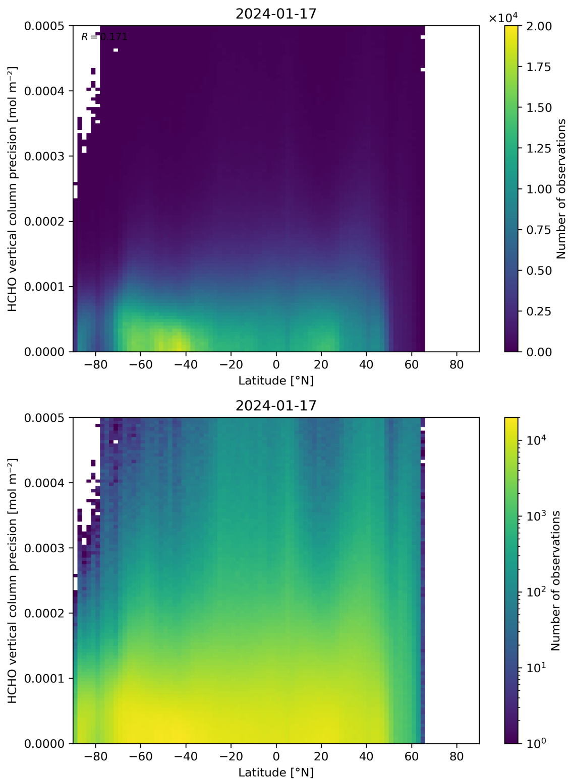
Figure 165: Scatter density plot of “Latitude” against “HCHO vertical column precision” for 2024-01-16 to 2024-01-18.
