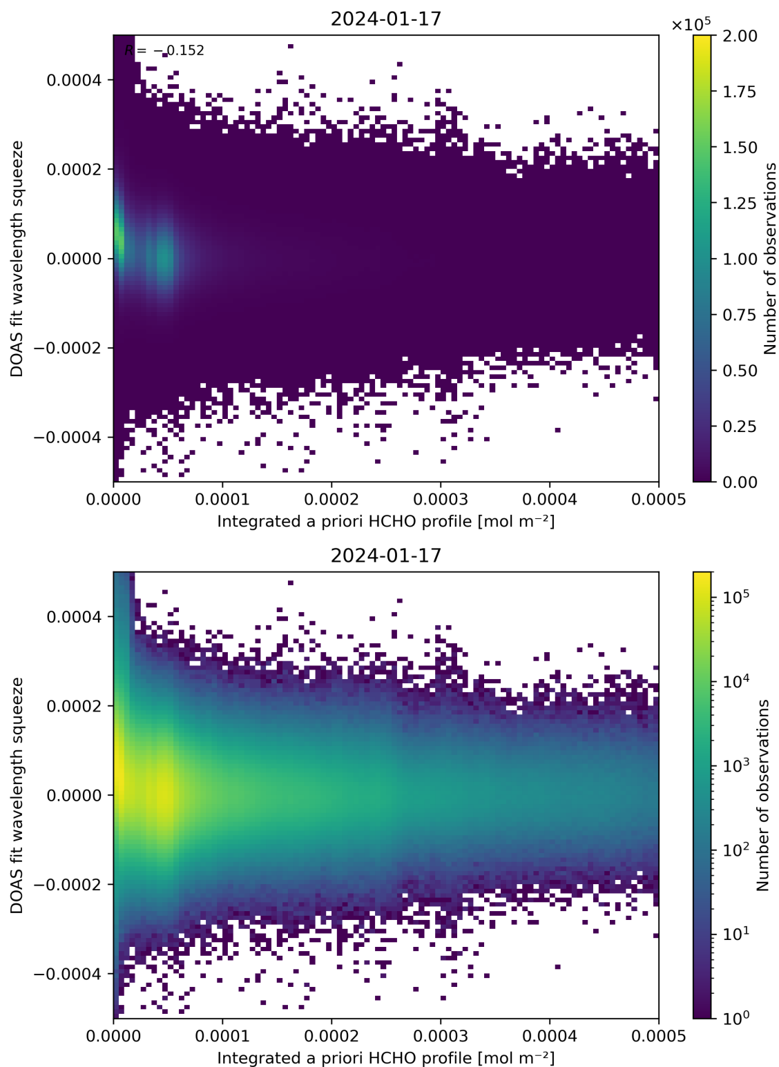
Figure 150: Scatter density plot of “Integrated a priori HCHO profile” against “DOAS fit wavelength squeeze” for 2024-01-16 to 2024-01-18.
