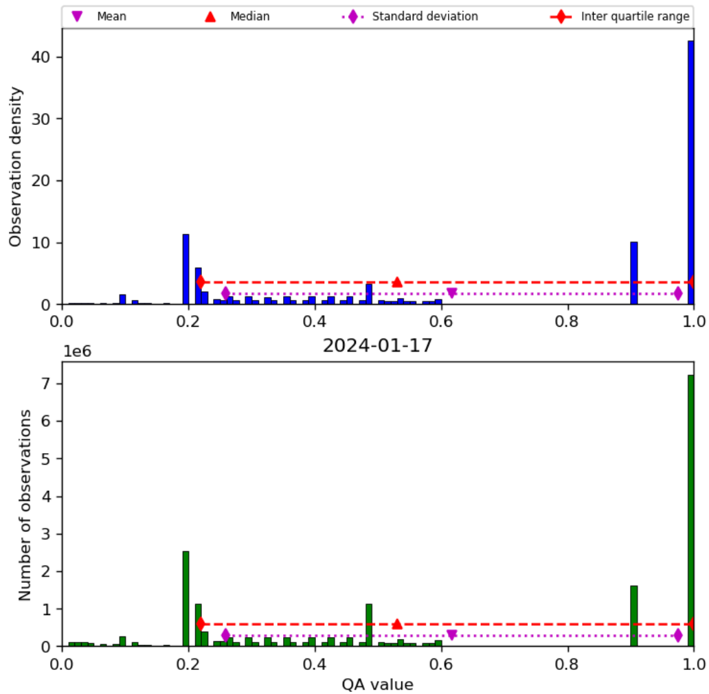
Figure 34: Histogram of “QA value” for 2024-01-16 to 2024-01-18
