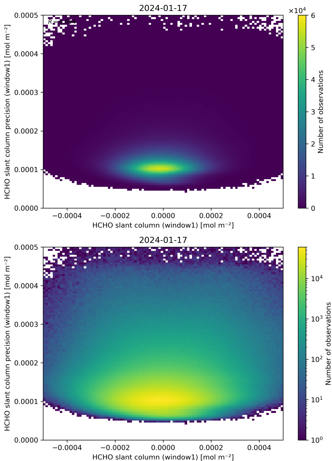
Figure 84: Scatter density plot of “HCHO slant column (window1)” against “HCHO slant column precision (window1)” for 2024-01-16 to 2024-01-18.
