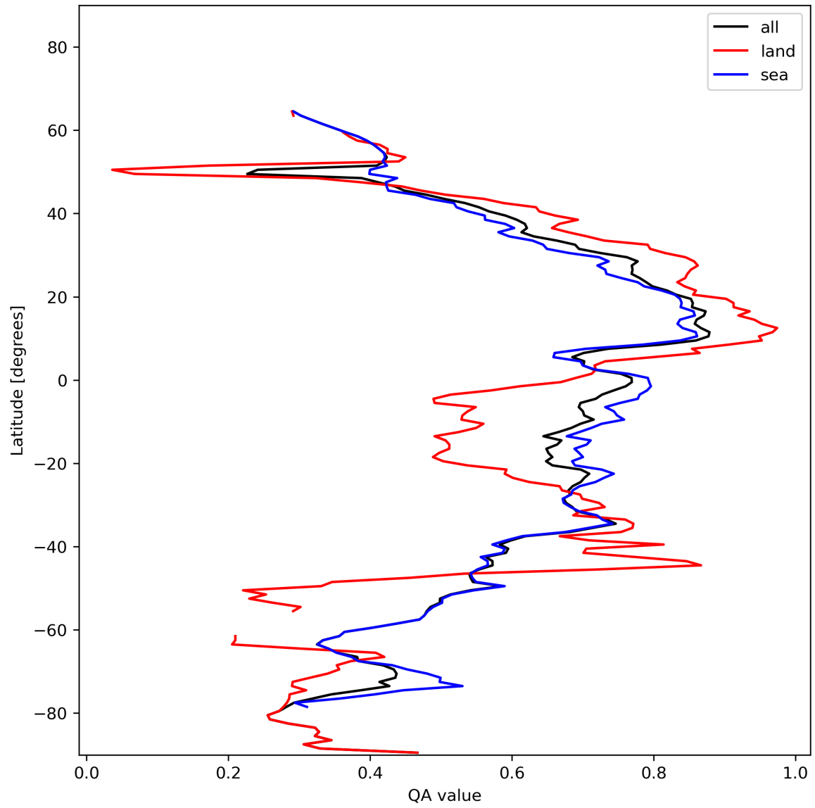
Figure 20: Zonal average of “QA value” for 2024-01-16 to 2024-01-18.
