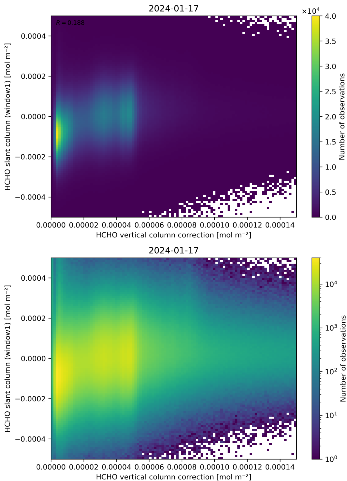
Figure 118: Scatter density plot of “HCHO vertical column correction” against “HCHO slant column (window1)” for 2024-01-16 to 2024-01-18.
