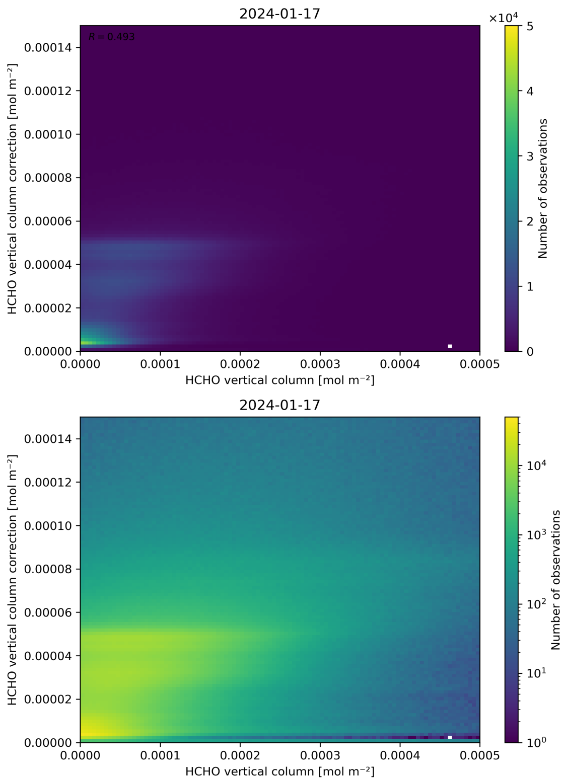
Figure 133: Scatter density plot of “HCHO vertical column” against “HCHO vertical column correction” for 2024-01-16 to 2024-01-18.
