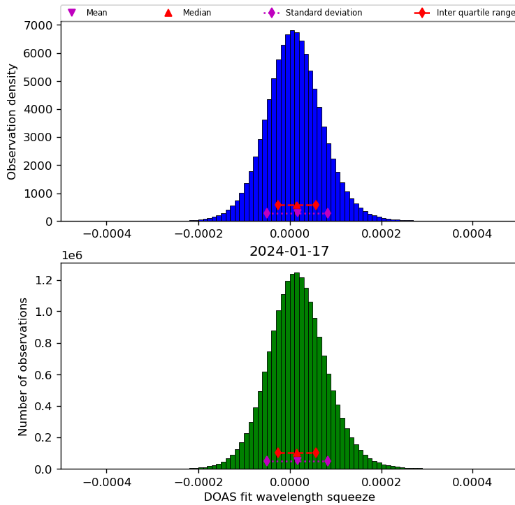
Figure 45: Histogram of “DOAS fit wavelength squeeze” for 2024-01-16 to 2024-01-18
