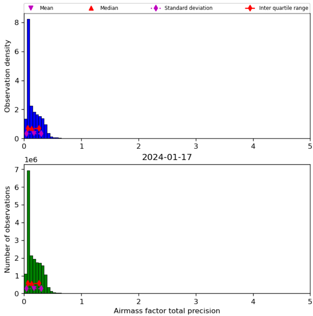
Figure 41: Histogram of “Airmass factor total precision” for 2024-01-16 to 2024-01-18
