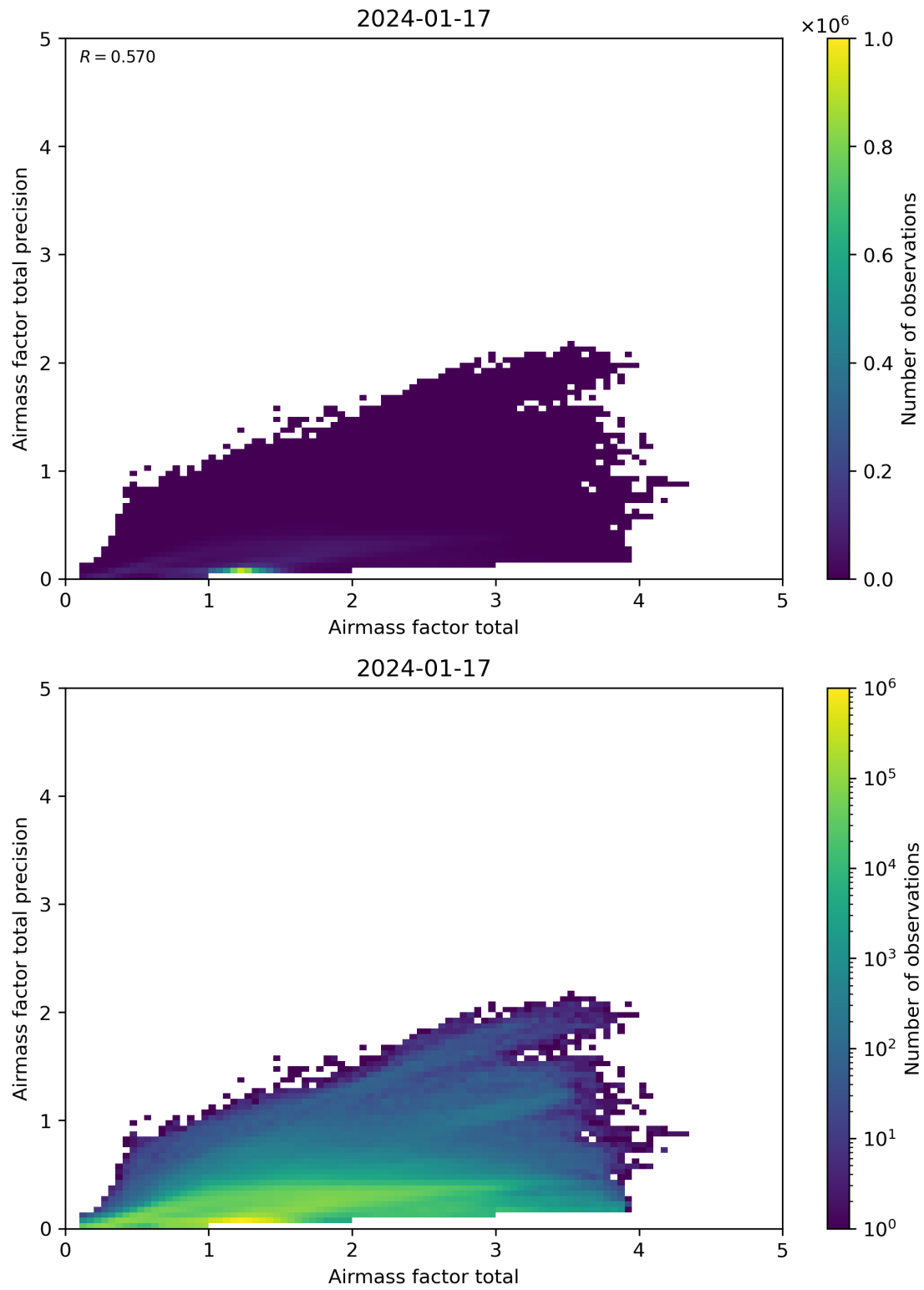
Figure 103: Scatter density plot of “Airmass factor total” against “Airmass factor total precision” for 2024-01-16 to 2024-01-18.
