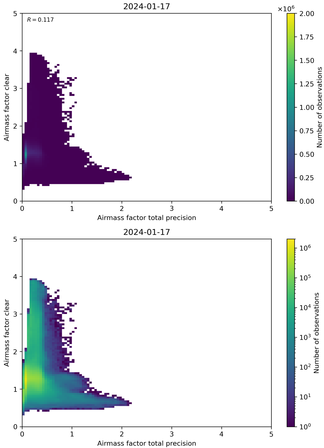
Figure 108: Scatter density plot of “Airmass factor total precision” against “Airmass factor clear” for 2024-01-16 to 2024-01-18.
