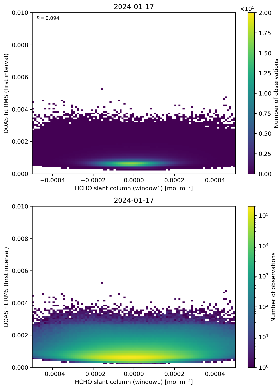
Figure 78: Scatter density plot of “HCHO slant column (window1)” against “DOAS fit RMS (first interval)” for 2024-01-16 to 2024-01-18.
