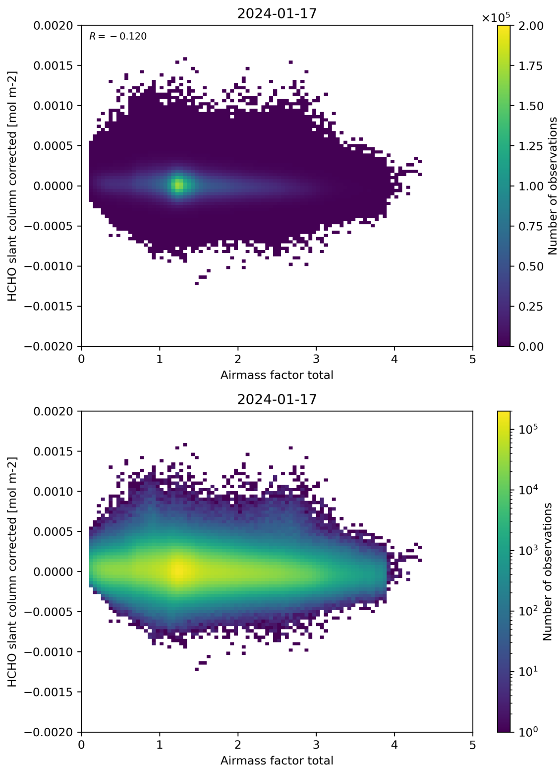
Figure 101: Scatter density plot of “Airmass factor total” against “HCHO slant column corrected” for 2024-01-16 to 2024-01-18.
