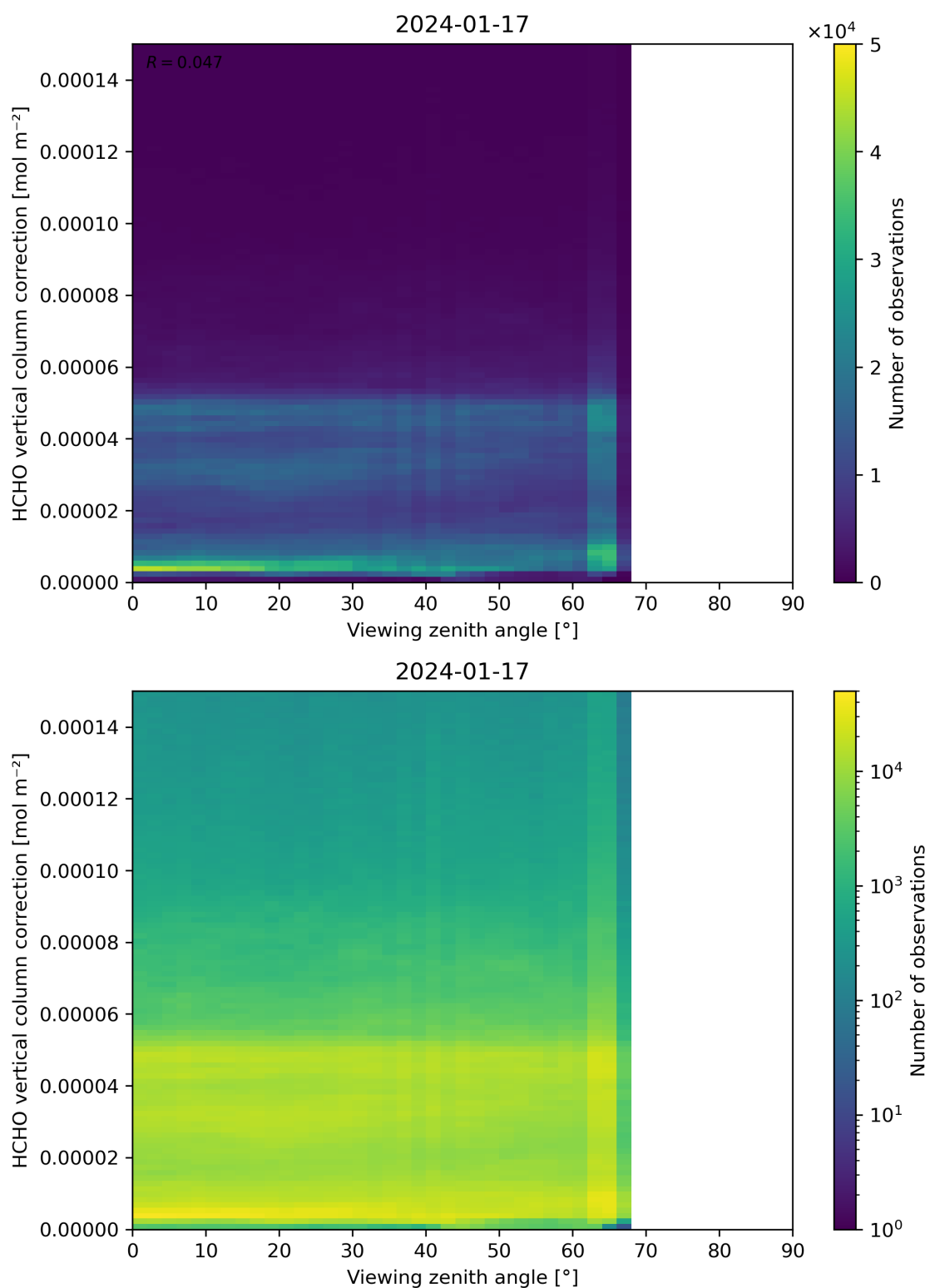
Figure 193: Scatter density plot of “Viewing zenith angle” against “HCHO vertical column correction” for 2024-01-16 to 2024-01-18.
