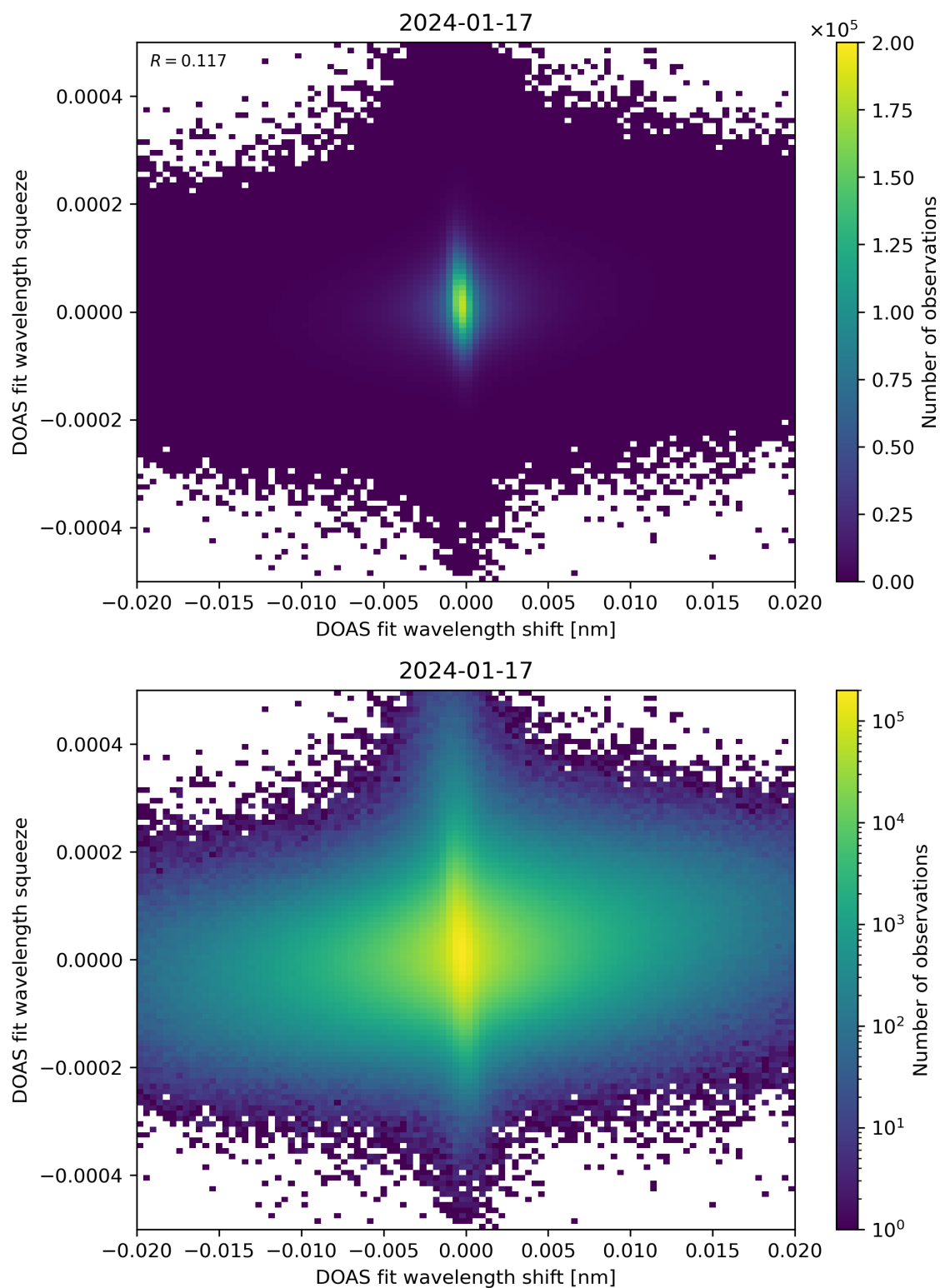
Figure 65: Scatter density plot of “DOAS fit wavelength shift” against “DOAS fit wavelength squeeze” for 2024-01-16 to 2024-01-18.
