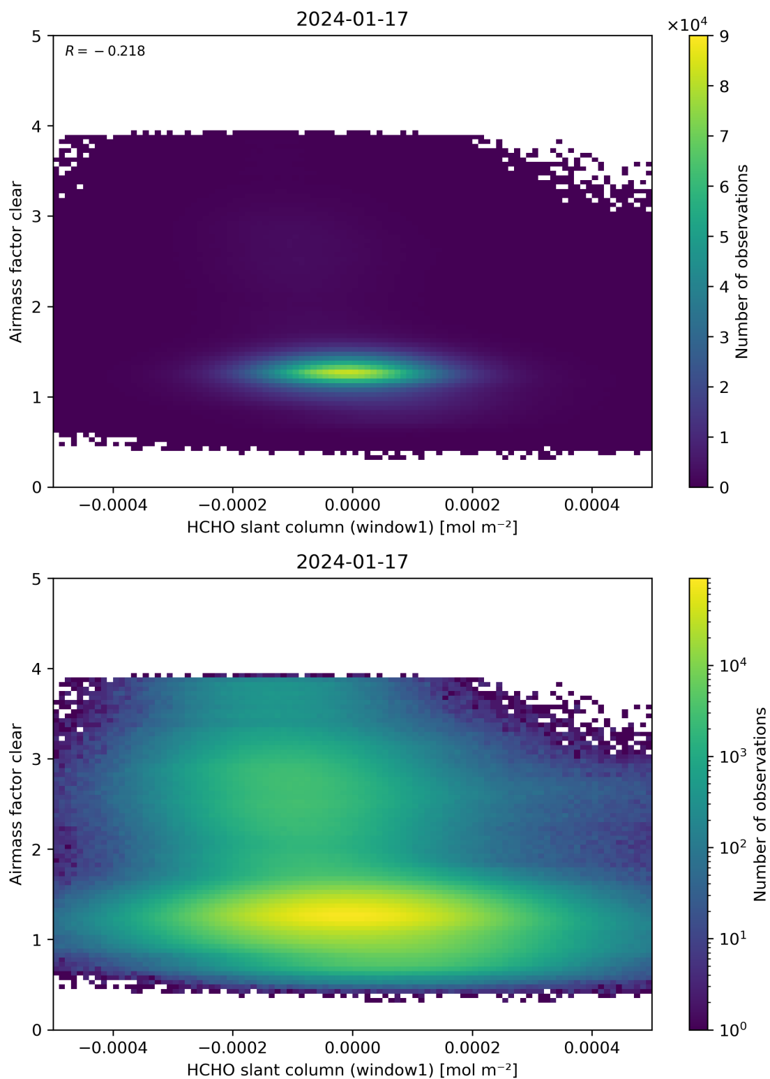
Figure 81: Scatter density plot of “HCHO slant column (window1)” against “Airmass factor clear” for 2024-01-16 to 2024-01-18.
