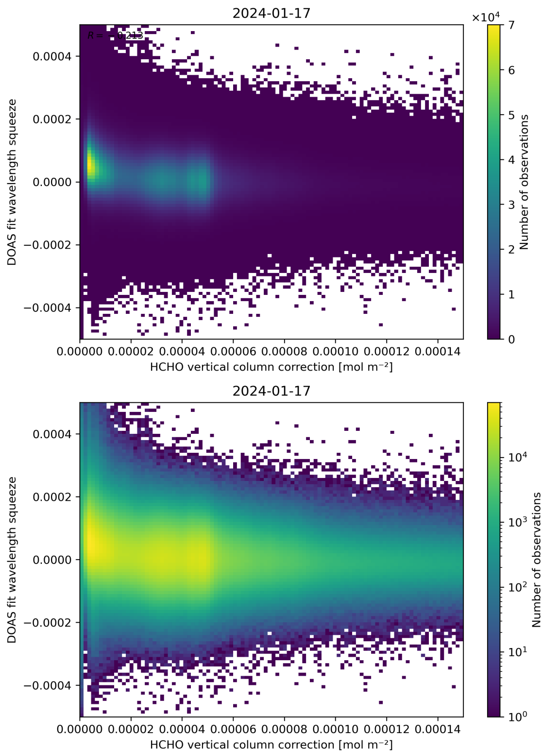
Figure 114: Scatter density plot of “HCHO vertical column correction” against “DOAS fit wavelength squeeze” for 2024-01-16 to 2024-01-18.
