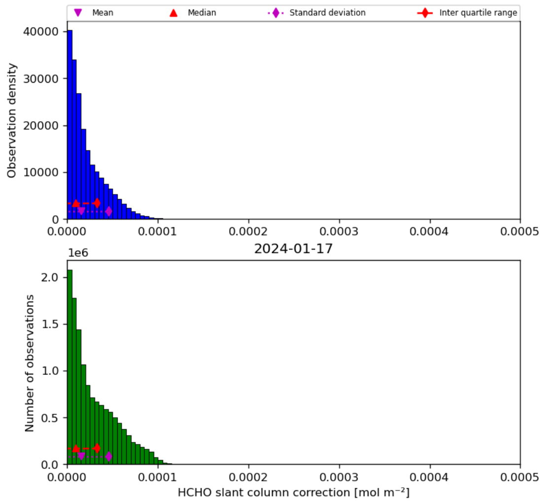
Figure 47: Histogram of “HCHO slant column correction” for 2024-01-16 to 2024-01-18
