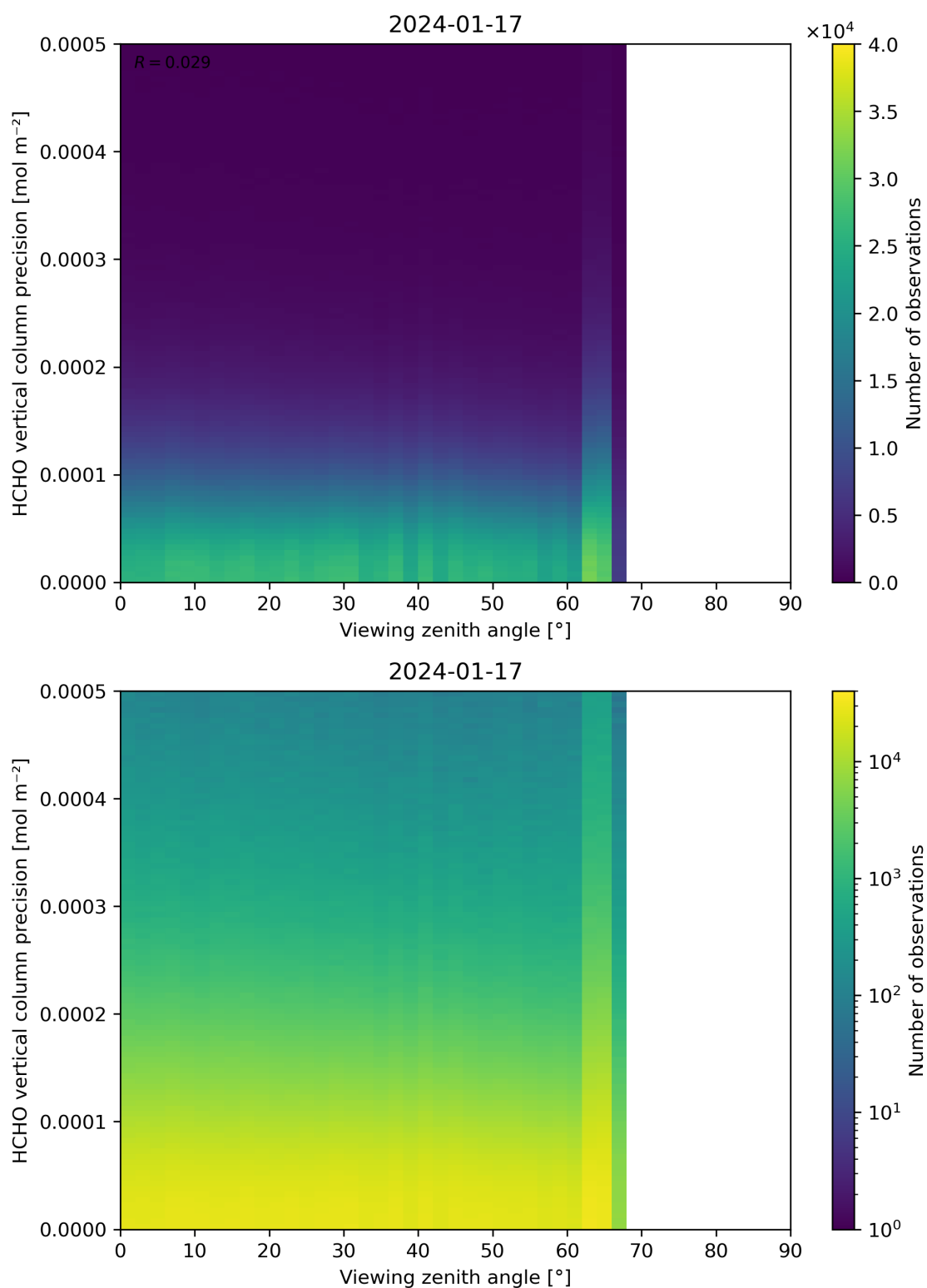
Figure 194: Scatter density plot of “Viewing zenith angle” against “HCHO vertical column precision” for 2024-01-16 to 2024-01-18.
