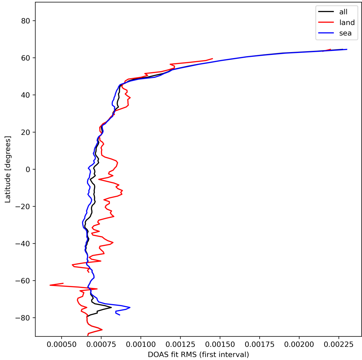
Figure 32: Zonal average of "DOAS fit RMS (first interval)" for 2024-01-16 to 2024-01-18.
