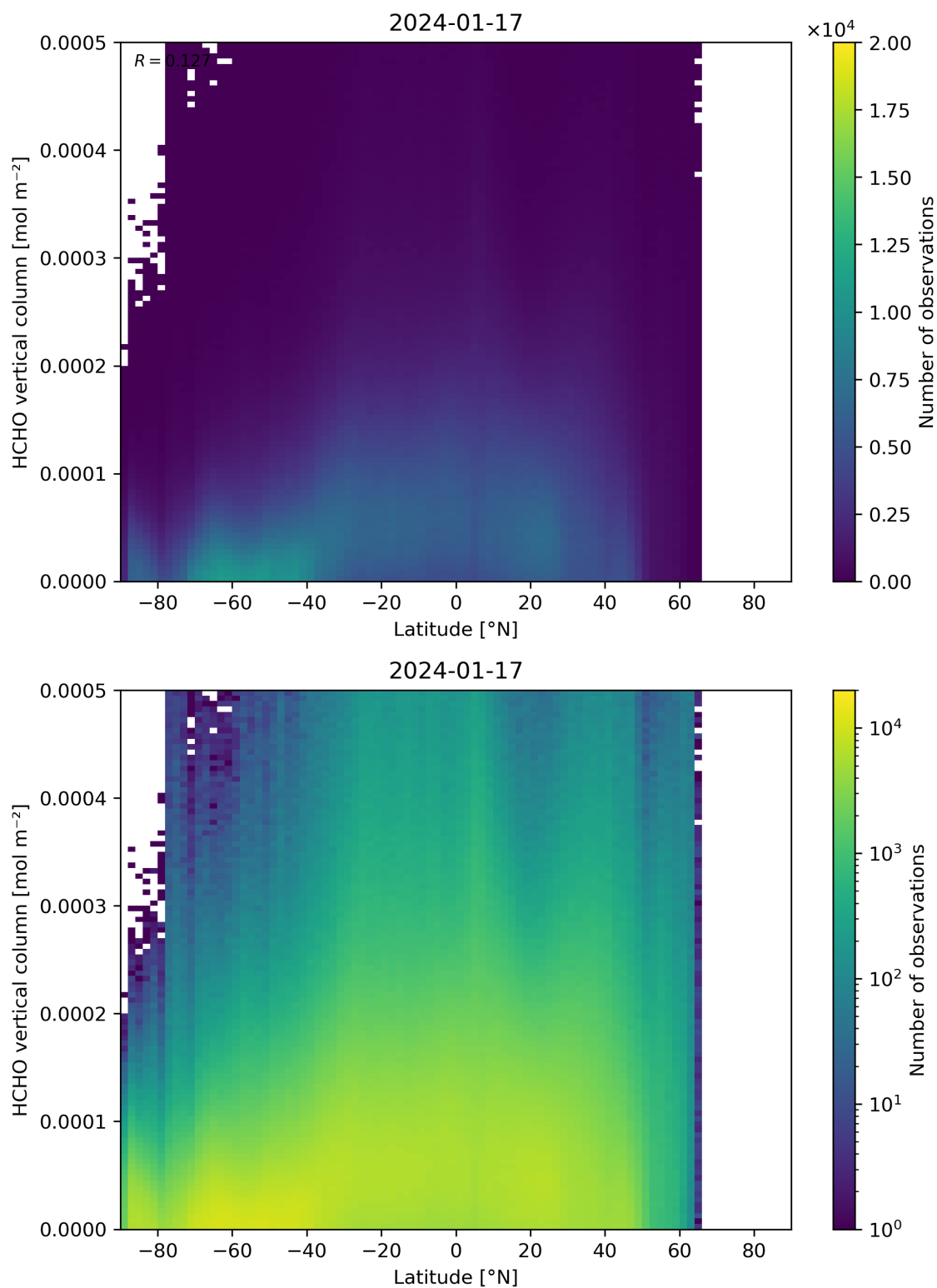
Figure 163: Scatter density plot of “Latitude” against “HCHO vertical column” for 2024-01-16 to 2024-01-18.
