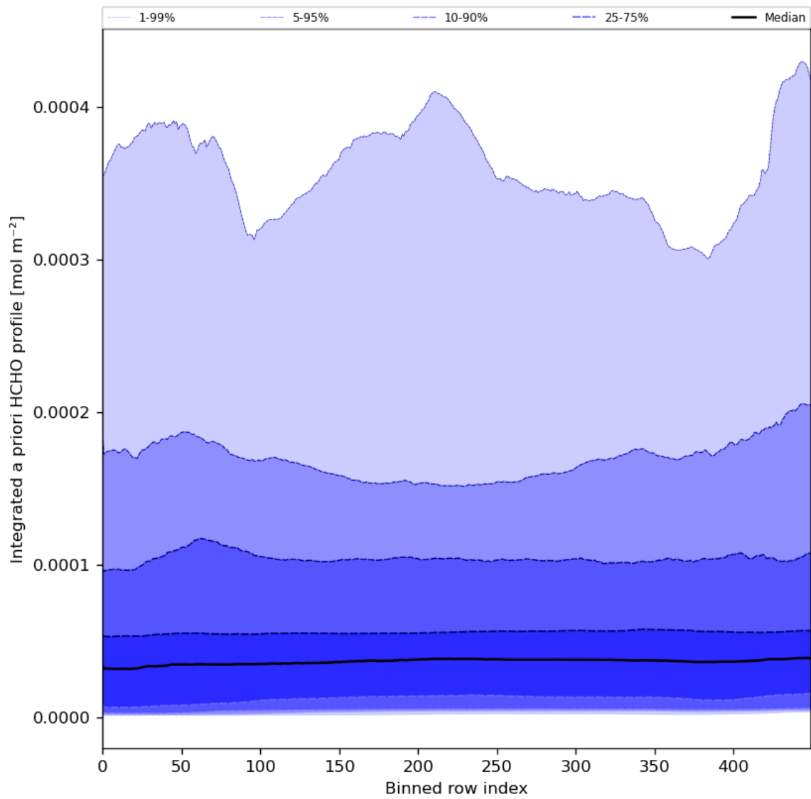
Figure 57: Along track statistics of “Integrated a priori HCHO profile” for 2024-01-16 to 2024-01-18
