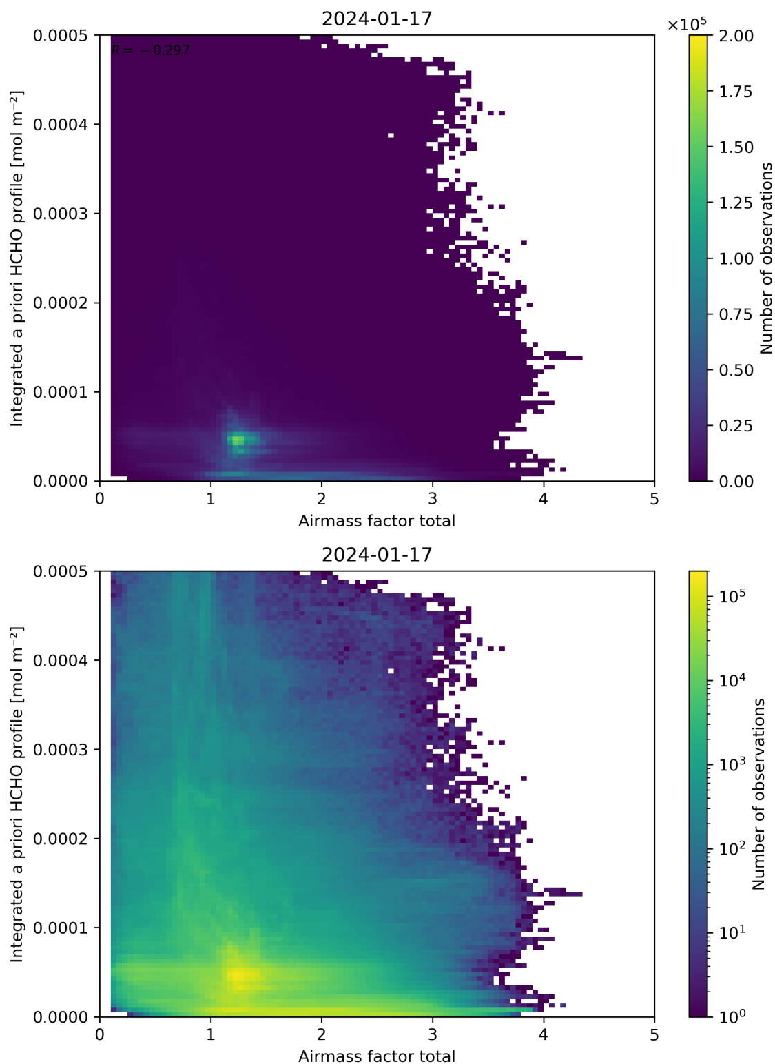
Figure 104: Scatter density plot of “Airmass factor total” against “Integrated a priori HCHO profile” for 2024-01-16 to 2024-01-18.
