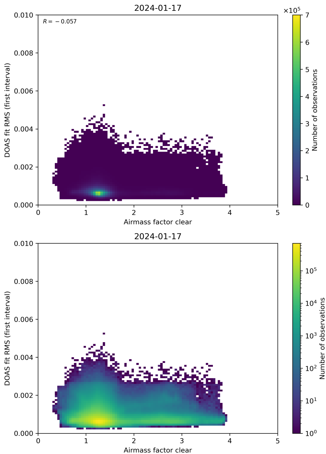
Figure 71: Scatter density plot of “Airmass factor clear” against “DOAS fit RMS (first interval)” for 2024-01-16 to 2024-01-18.
