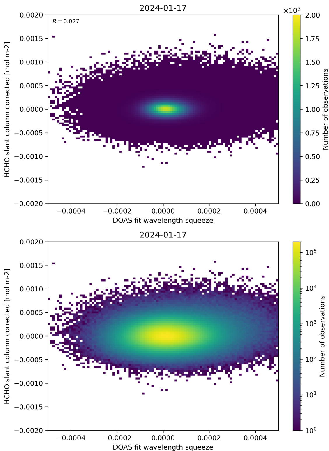
Figure 69: Scatter density plot of “DOAS fit wavelength squeeze” against “HCHO slant column corrected” for 2024-01-16 to 2024-01-18.
