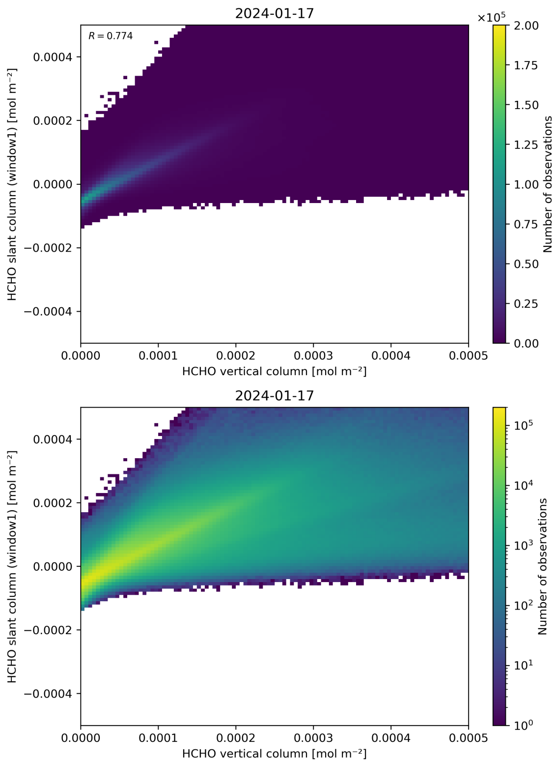
Figure 129: Scatter density plot of “HCHO vertical column” against “HCHO slant column (window1)” for 2024-01-16 to 2024-01-18.
