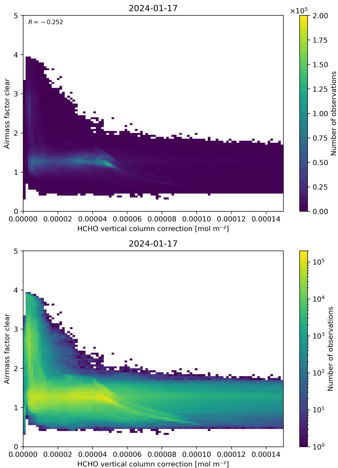
Figure 115: Scatter density plot of “HCHO vertical column correction” against “Airmass factor clear” for 2024-01-16 to 2024-01-18.
