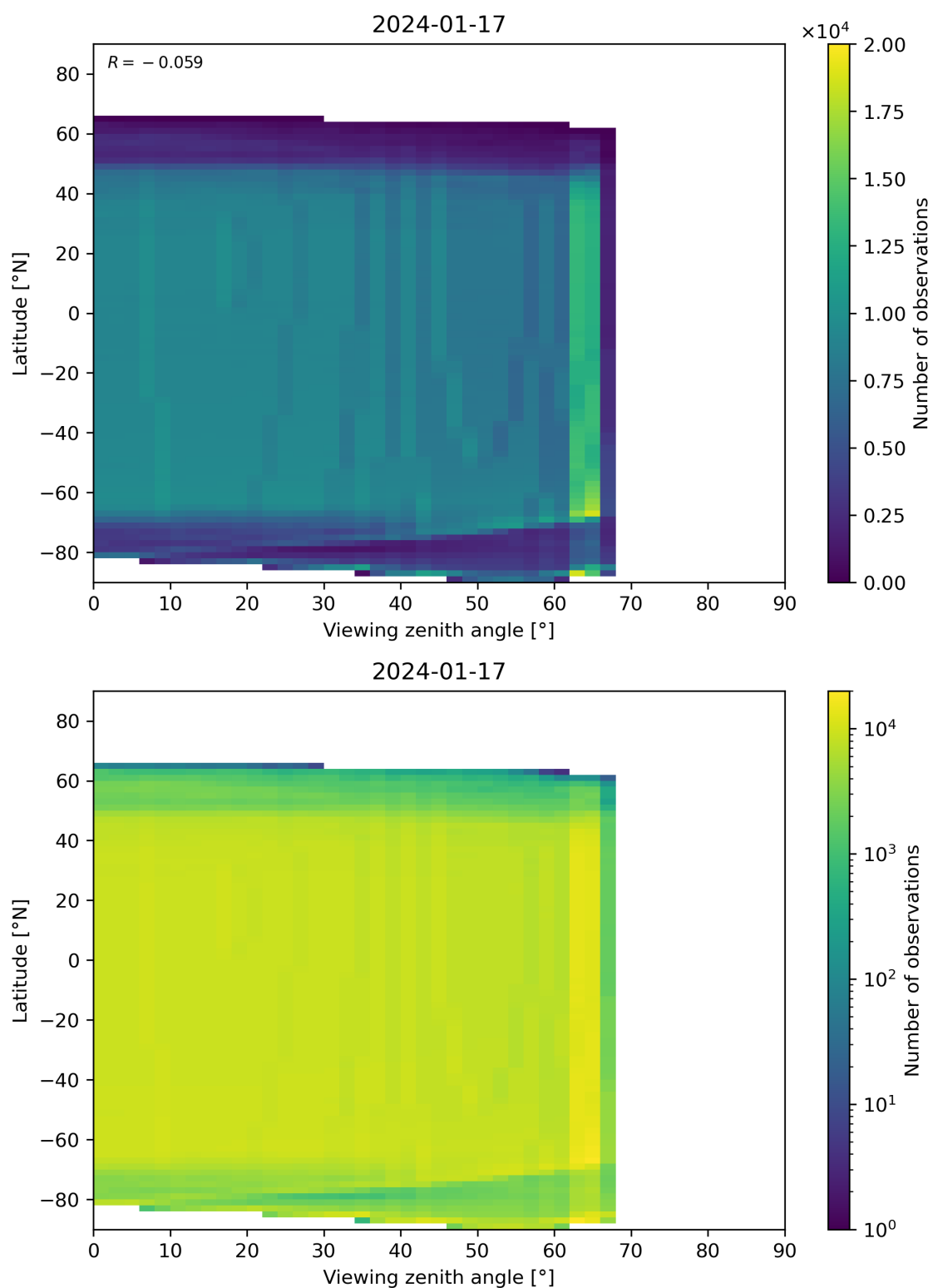
Figure 196: Scatter density plot of “Viewing zenith angle” against “Latitude” for 2024-01-16 to 2024-01-18.
