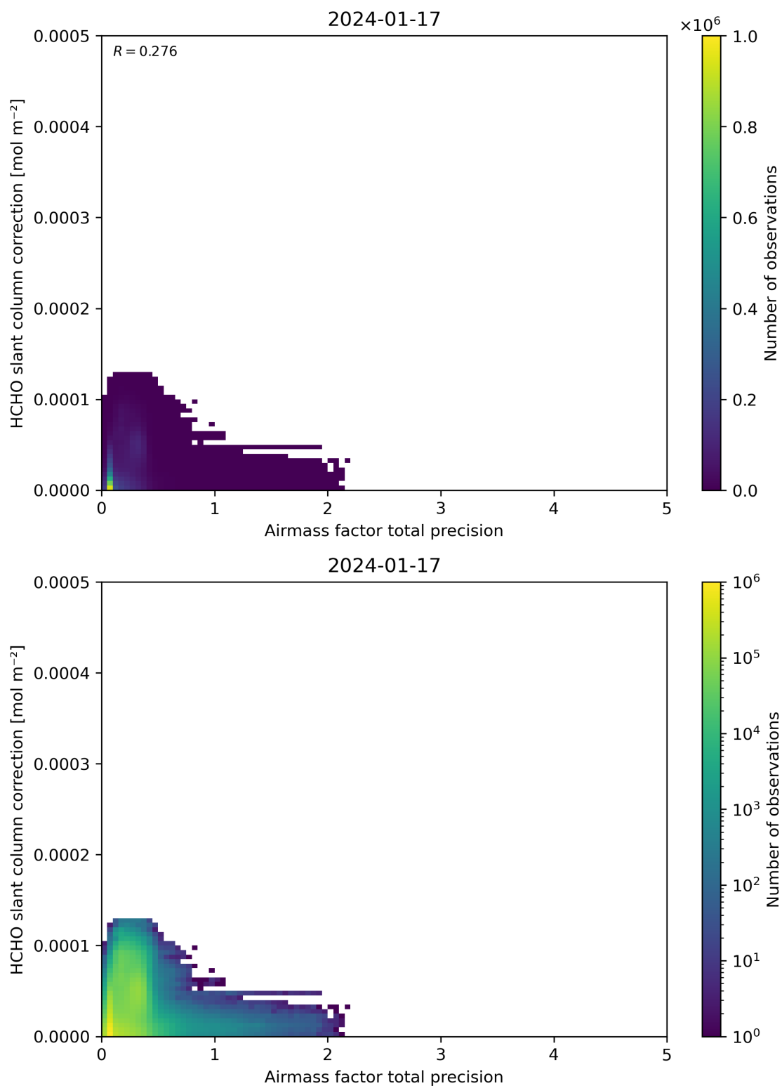
Figure 110: Scatter density plot of “Airmass factor total precision” against “HCHO slant column correction” for 2024-01-16 to 2024-01-18.
