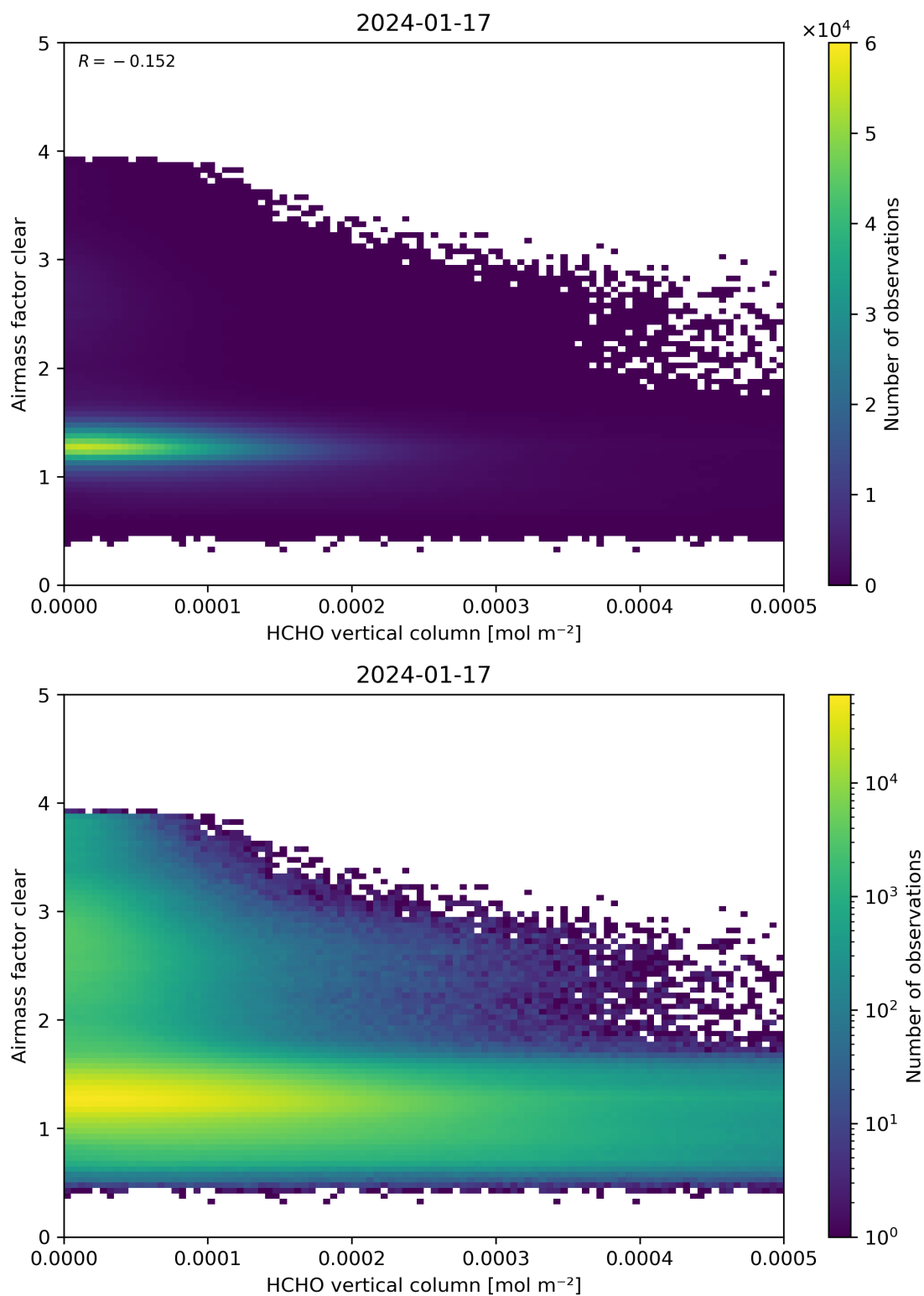
Figure 126: Scatter density plot of “HCHO vertical column” against “Airmass factor clear” for 2024-01-16 to 2024-01-18.
