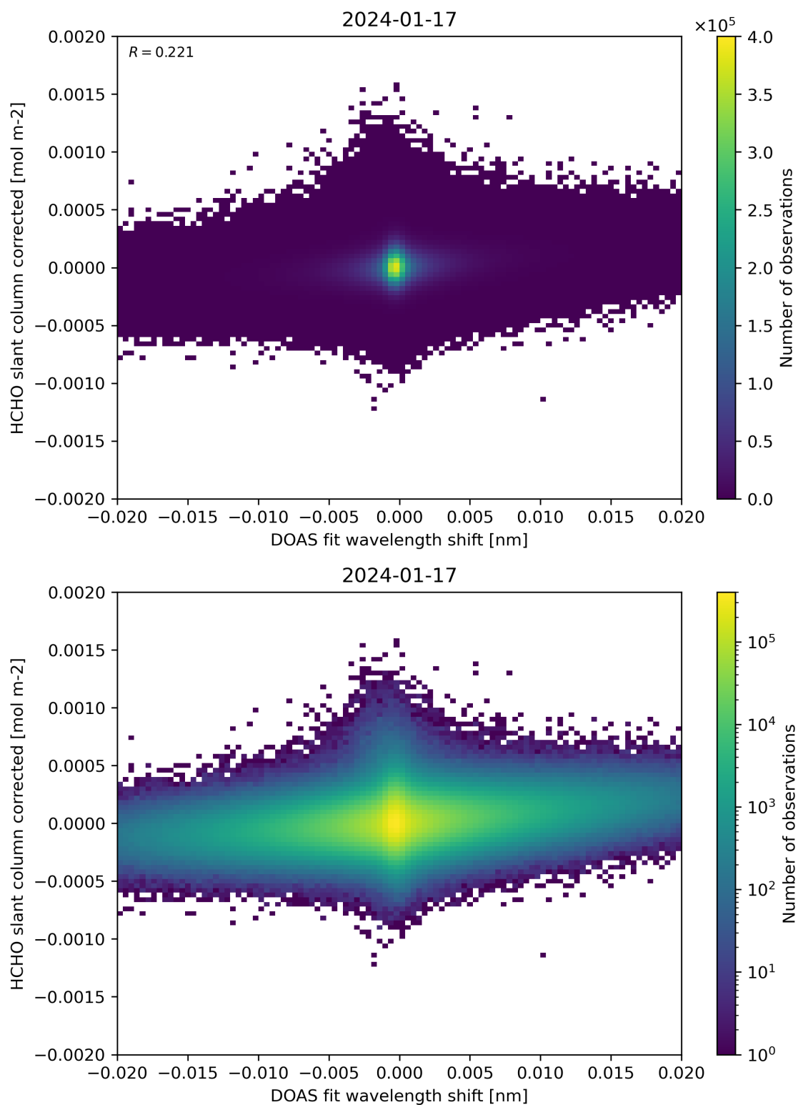
Figure 66: Scatter density plot of “DOAS fit wavelength shift” against “HCHO slant column corrected” for 2024-01-16 to 2024-01-18.
