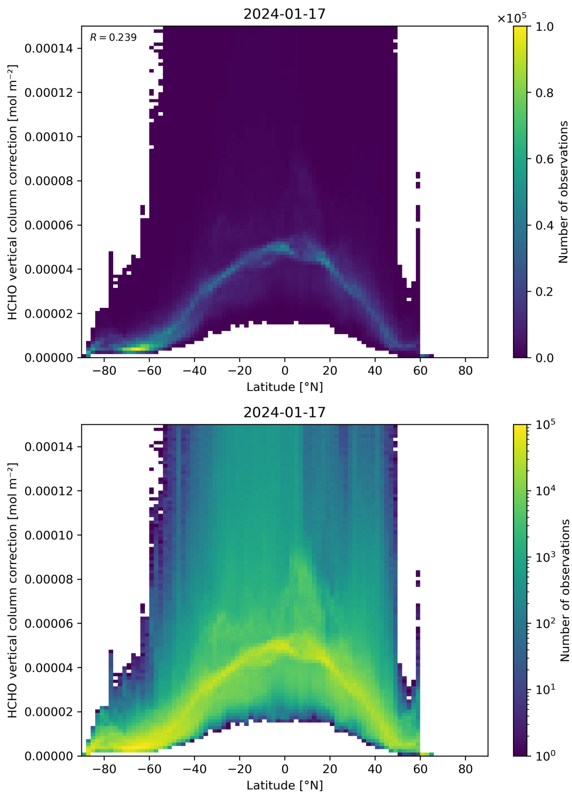
Figure 164: Scatter density plot of “Latitude” against “HCHO vertical column correction” for 2024-01-16 to 2024-01-18.
