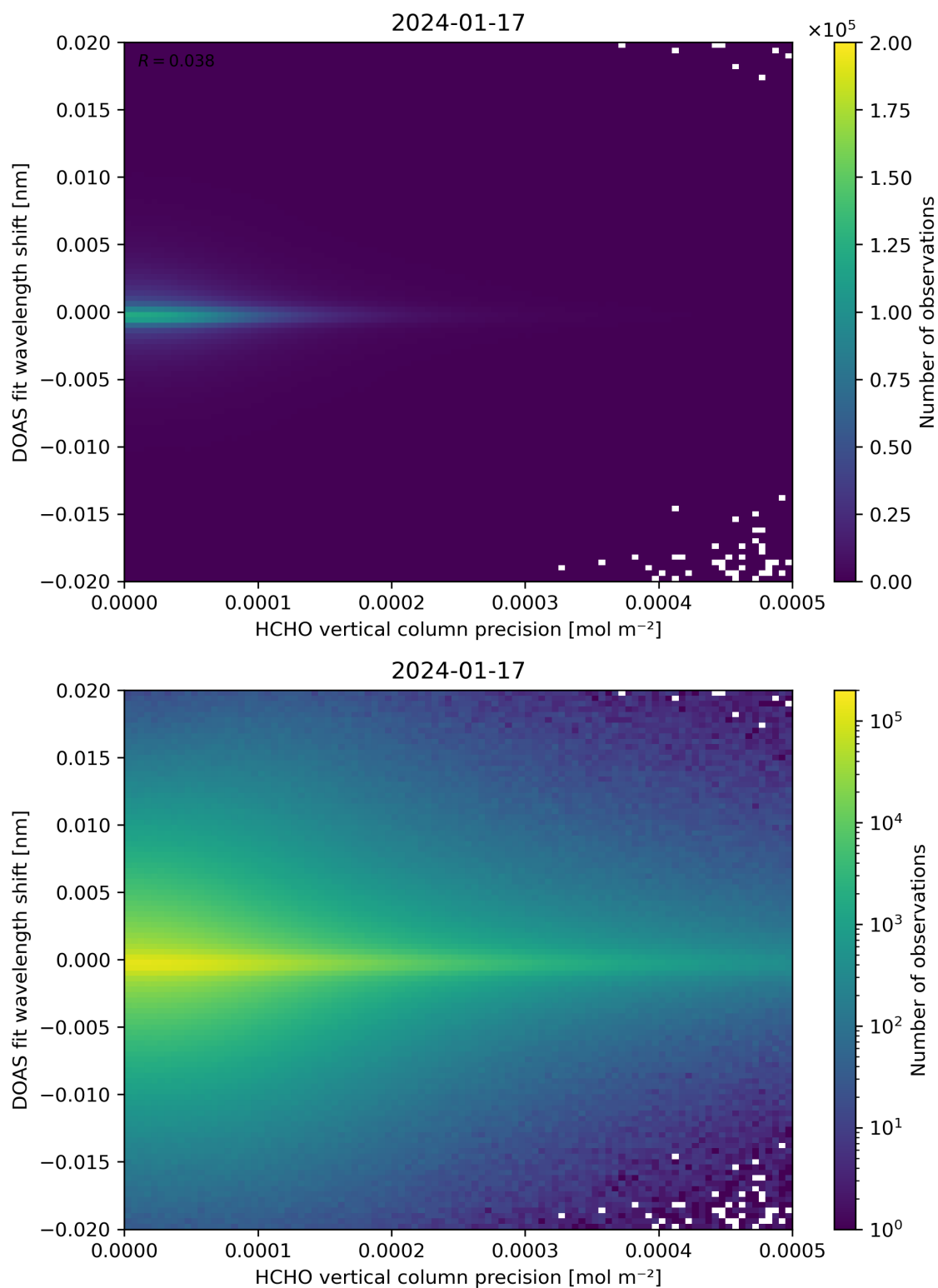
Figure 137: Scatter density plot of “HCHO vertical column precision” against “DOAS fit wavelength shift” for 2024-01-16 to 2024-01-18.
