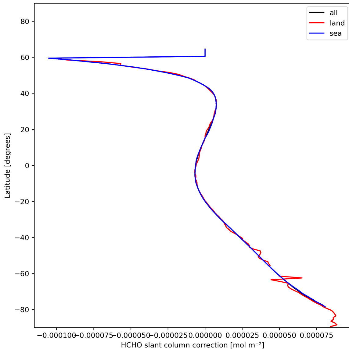
Figure 33: Zonal average of “HCHO slant column correction” for 2024-01-16 to 2024-01-18.
