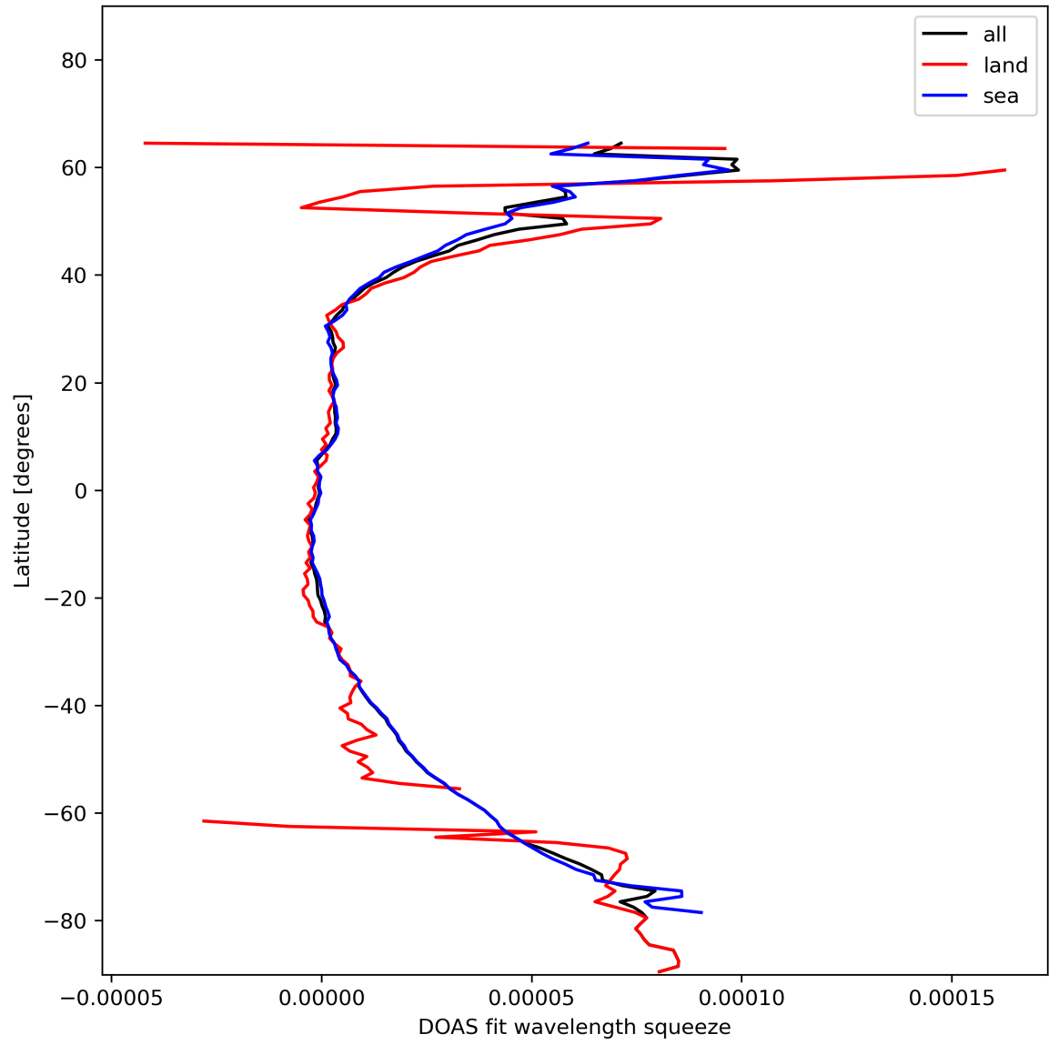
Figure 31: Zonal average of “DOAS fit wavelength squeeze” for 2024-01-16 to 2024-01-18.
