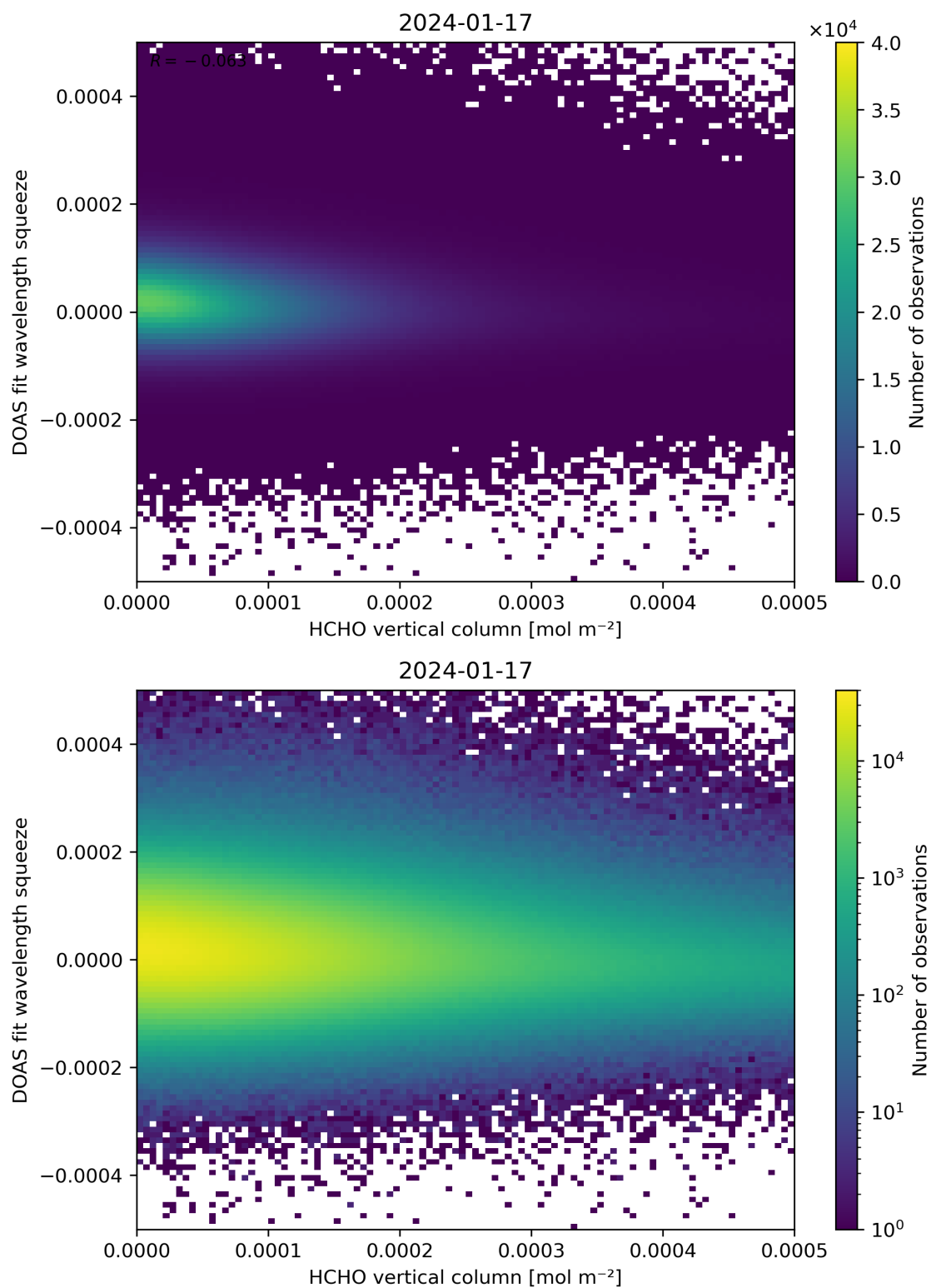
Figure 125: Scatter density plot of “HCHO vertical column” against “DOAS fit wavelength squeeze” for 2024-01-16 to 2024-01-18.
