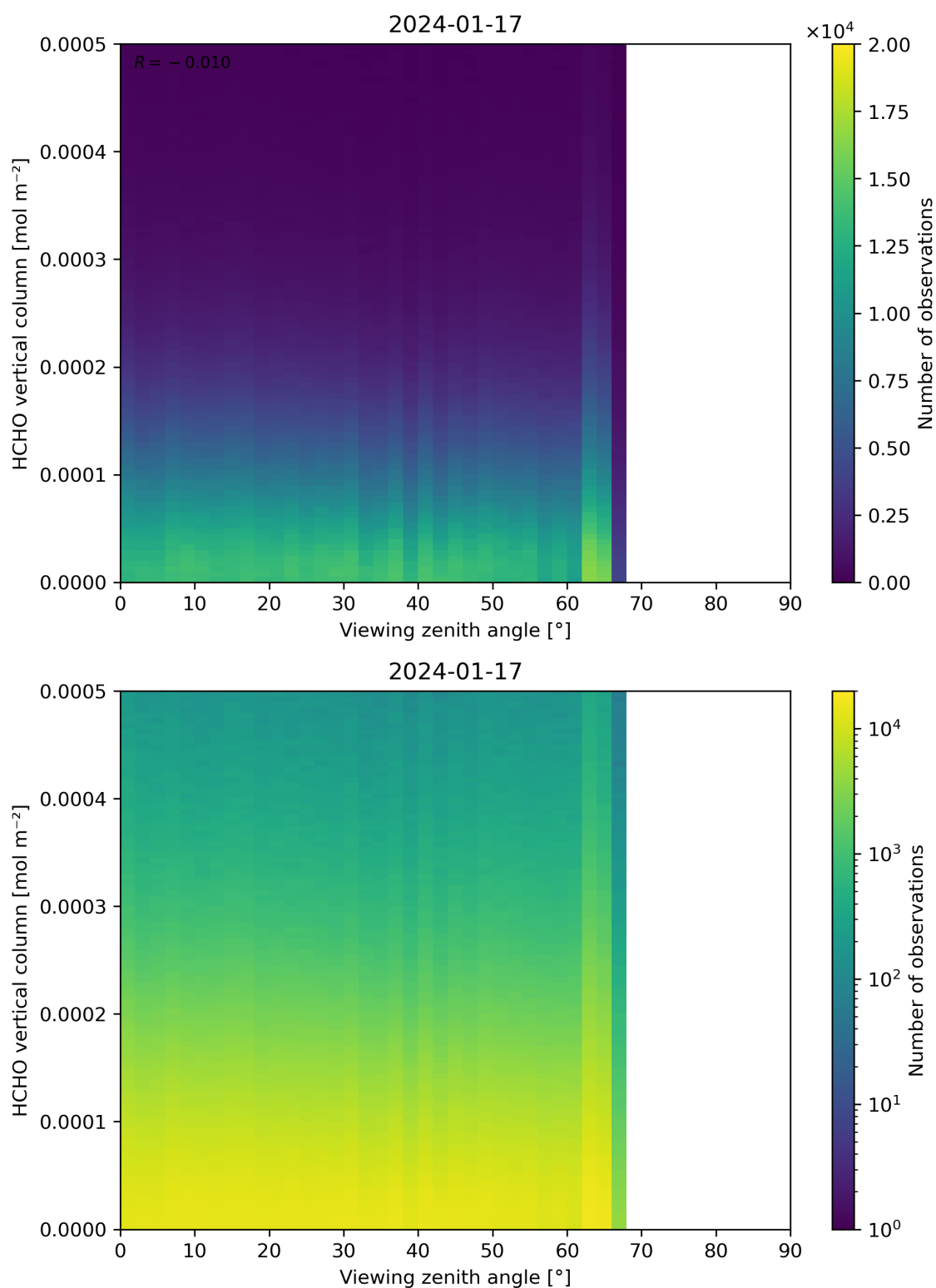
Figure 192: Scatter density plot of “Viewing zenith angle” against “HCHO vertical column” for 2024-01-16 to 2024-01-18.
