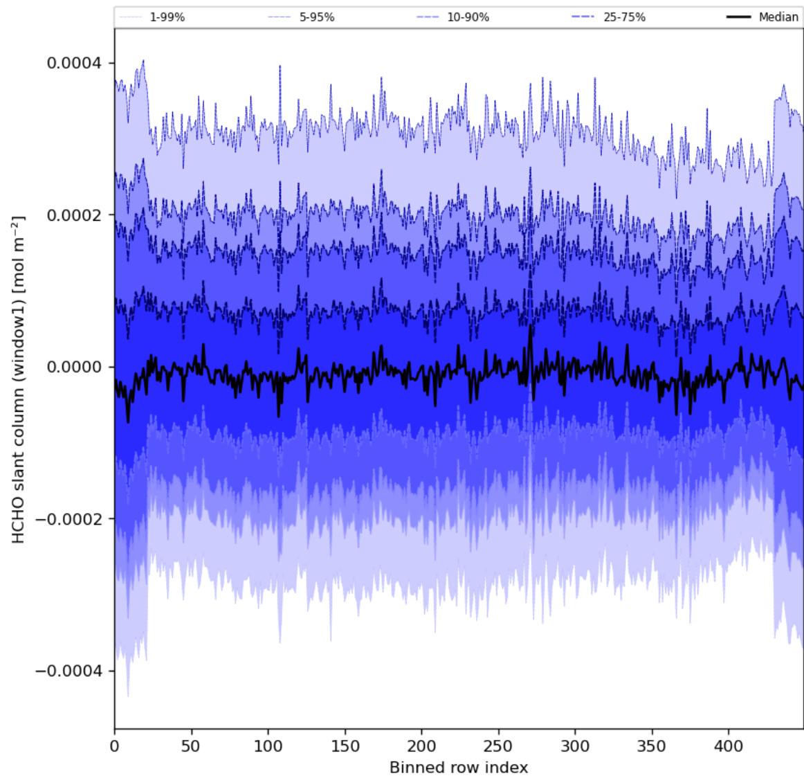
Figure 52: Along track statistics of “HCHO slant column (window1)” for 2024-01-16 to 2024-01-18
