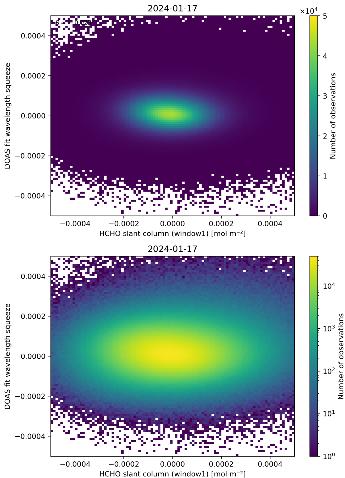
Figure 80: Scatter density plot of “HCHO slant column (window1)” against “DOAS fit wavelength squeeze” for 2024-01-16 to 2024-01-18.
