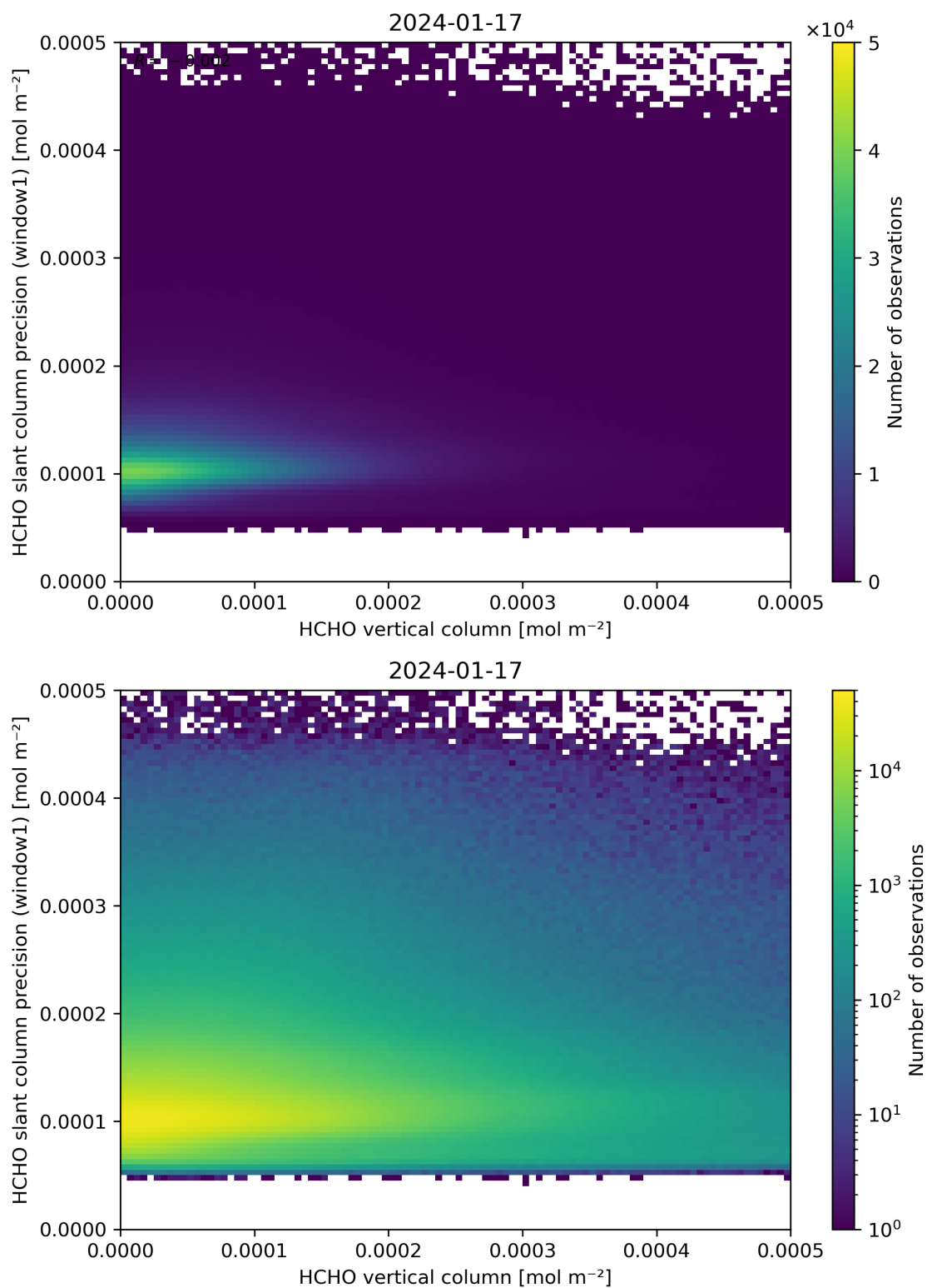
Figure 130: Scatter density plot of “HCHO vertical column” against “HCHO slant column precision (window1)” for 2024-01-16 to 2024-01-18.
