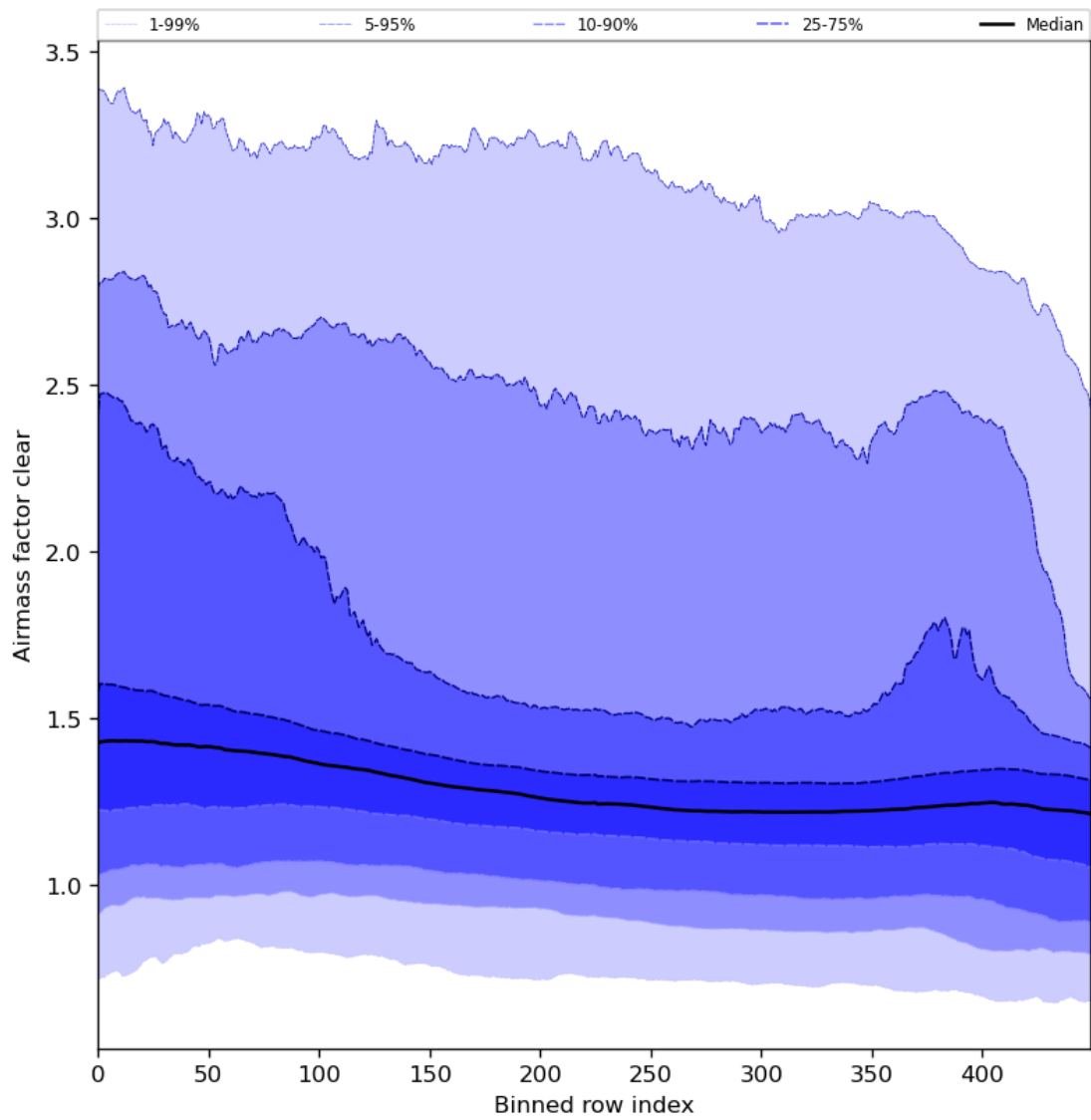
Figure 56: Along track statistics of “Air mass factor clear” for 2024-01-16 to 2024-01-18
