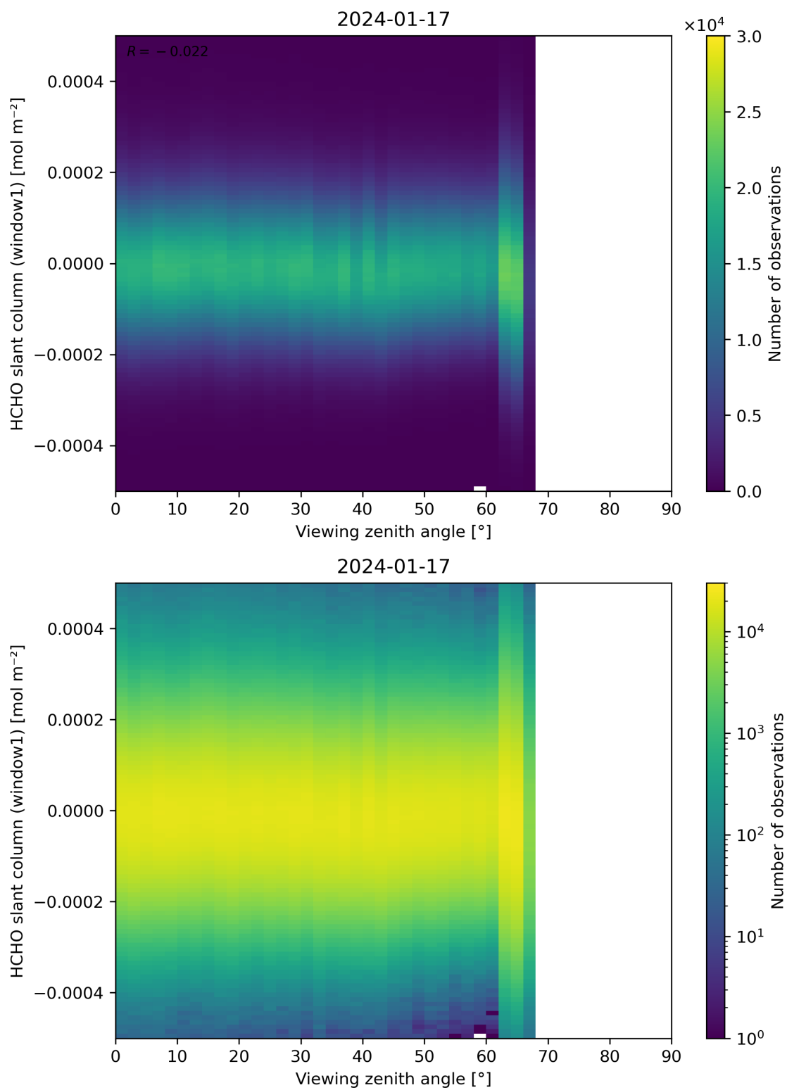
Figure 188: Scatter density plot of “Viewing zenith angle” against “HCHO slant column (window1)” for 2024-01-16 to 2024-01-18.
