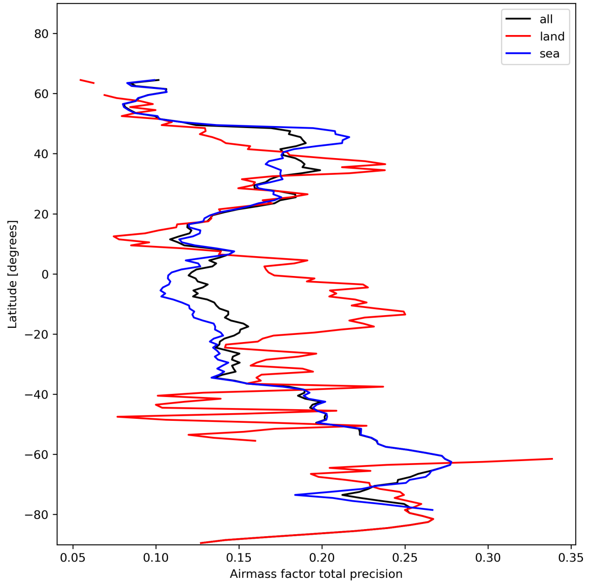
Figure 27: Zonal average of “Airmass factor total precision” for 2024-01-16 to 2024-01-18.
