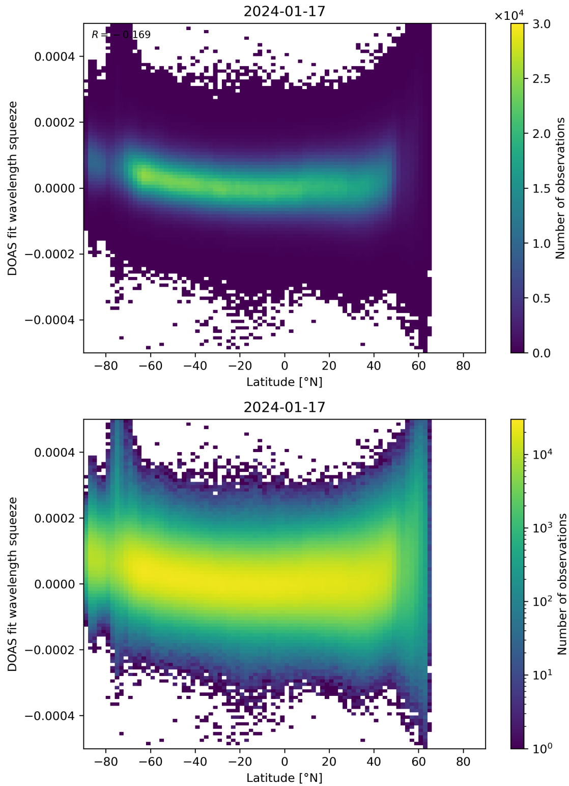
Figure 155: Scatter density plot of “Latitude” against “DOAS fit wavelength squeeze” for 2024-01-16 to 2024-01-18.
