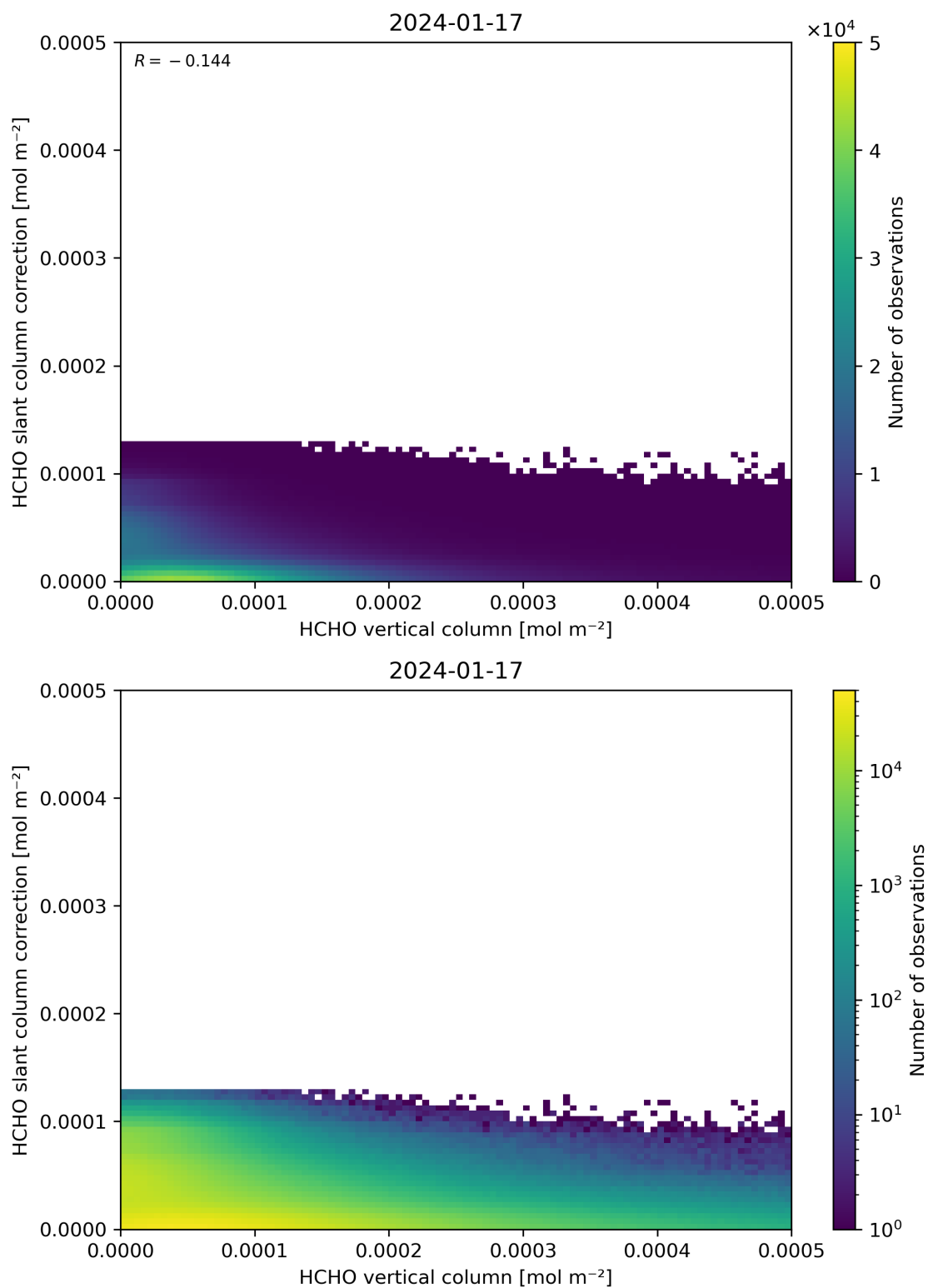
Figure 128: Scatter density plot of “HCHO vertical column” against “HCHO slant column correction” for 2024-01-16 to 2024-01-18.
