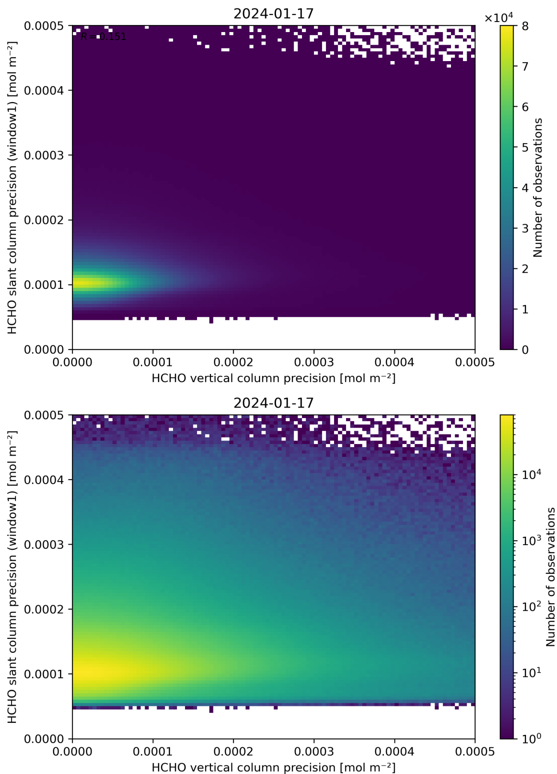
Figure 143: Scatter density plot of “HCHO vertical column precision” against “HCHO slant column precision (window1)” for 2024-01-16 to 2024-01-18.
