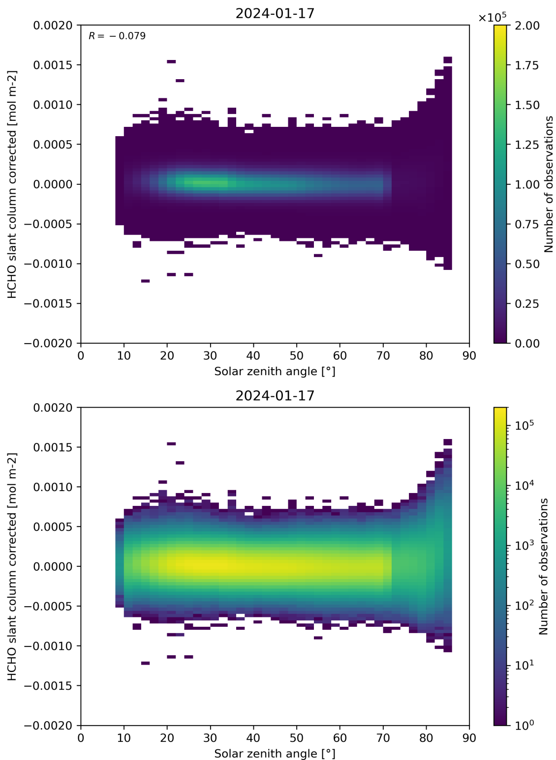
Figure 171: Scatter density plot of “Solar zenith angle” against “HCHO slant column corrected” for 2024-01-16 to 2024-01-18.
