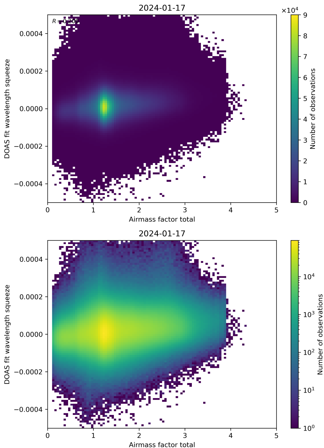
Figure 99: Scatter density plot of “Airmass factor total” against “DOAS fit wavelength squeeze” for 2024-01-16 to 2024-01-18.
