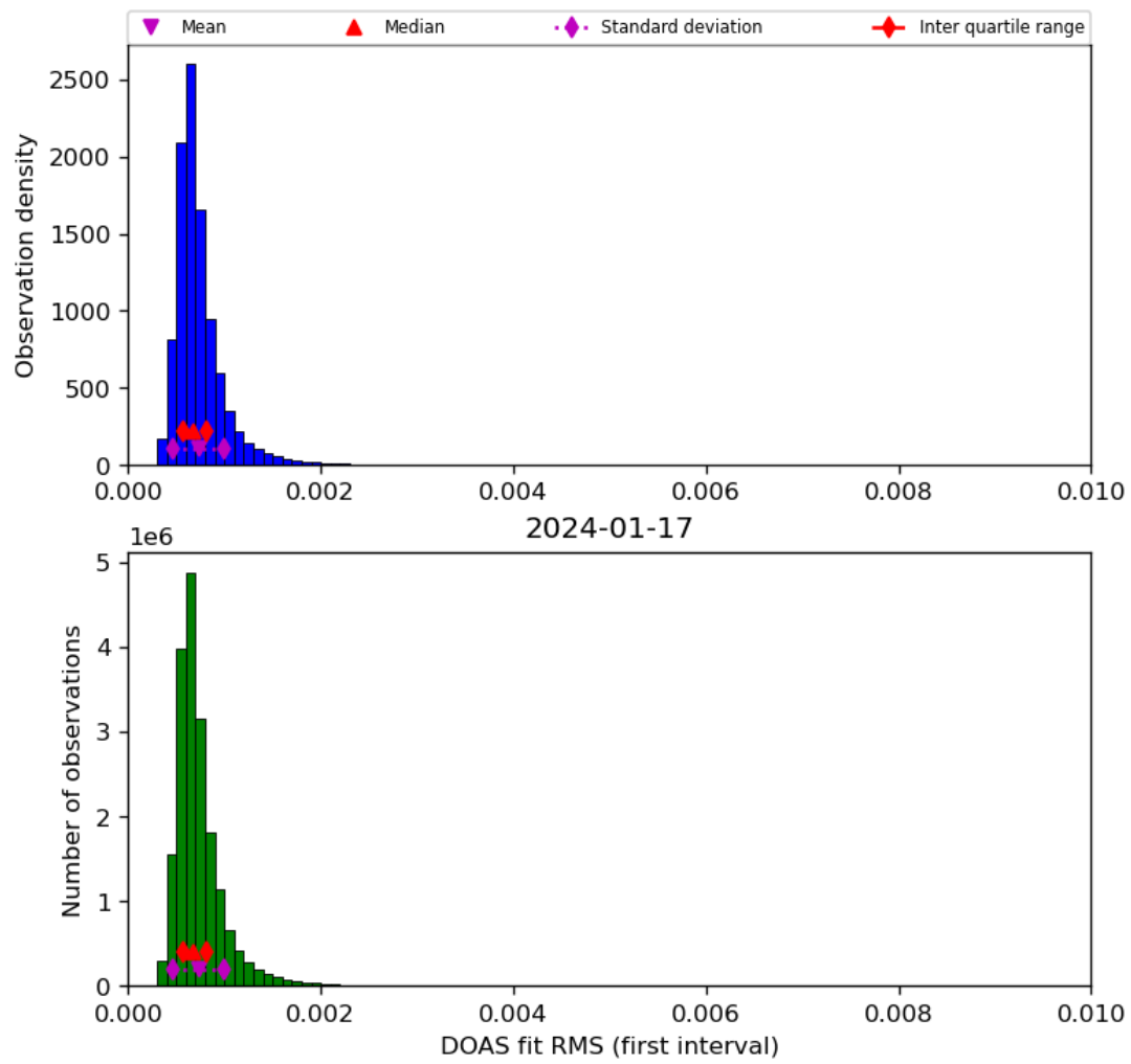
Figure 46: Histogram of “DOAS fit RMS (first interval)” for 2024-01-16 to 2024-01-18
