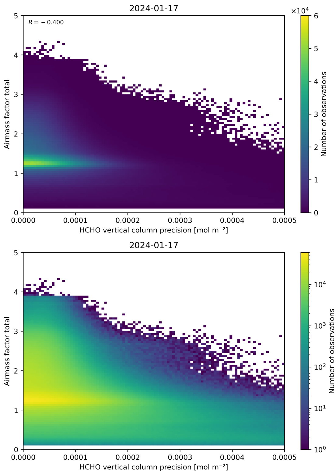
Figure 144: Scatter density plot of “HCHO vertical column precision” against “Airmass factor total” for 2024-01-16 to 2024-01-18.
