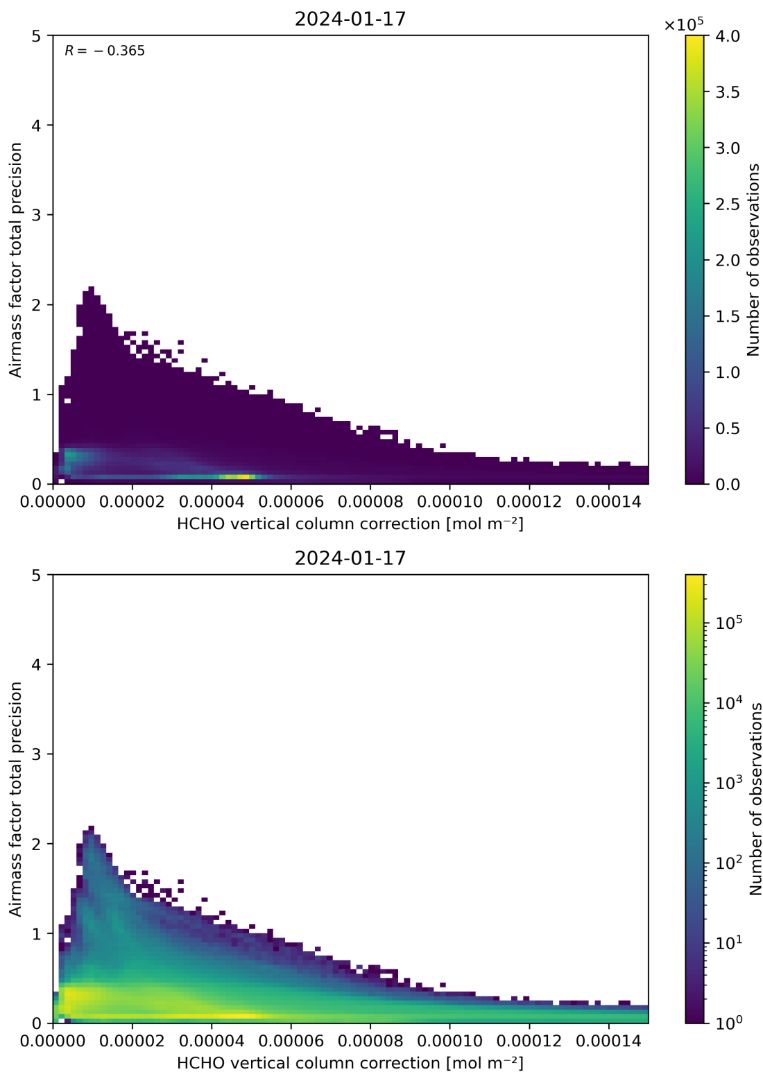
Figure 121: Scatter density plot of “HCHO vertical column correction” against “Airmass factor total precision” for 2024-01-16 to 2024-01-18.
