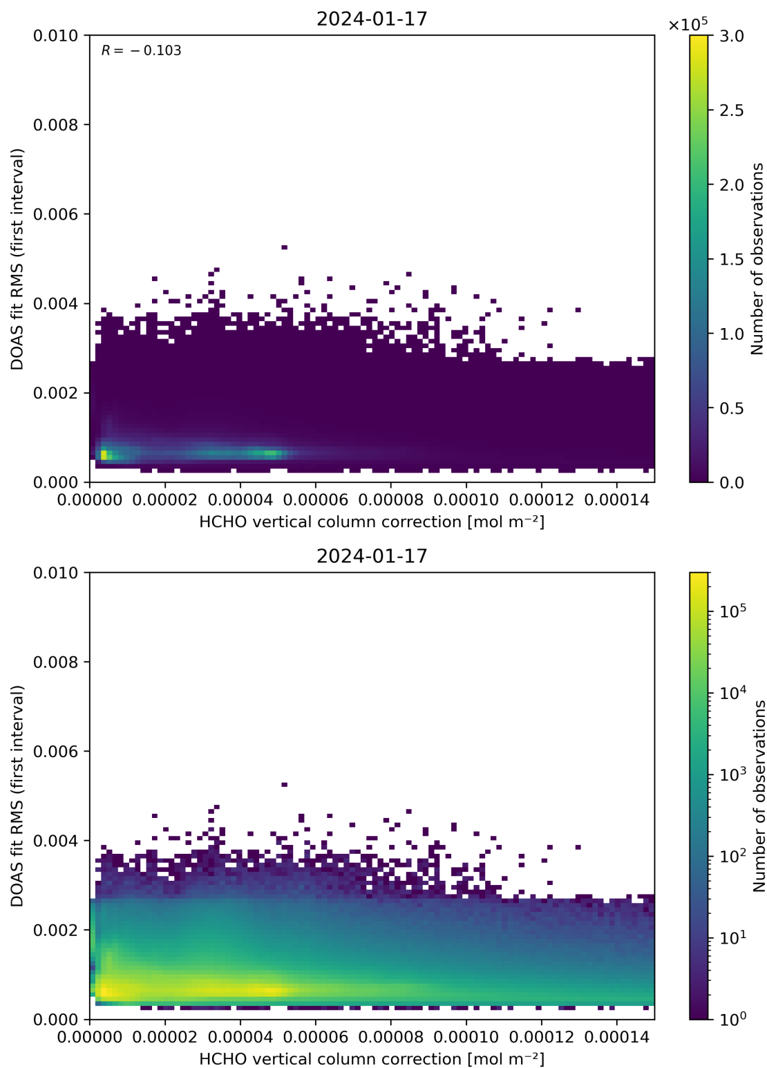
Figure 112: Scatter density plot of “HCHO vertical column correction” against “DOAS fit RMS (first interval)” for 2024-01-16 to 2024-01-18.
