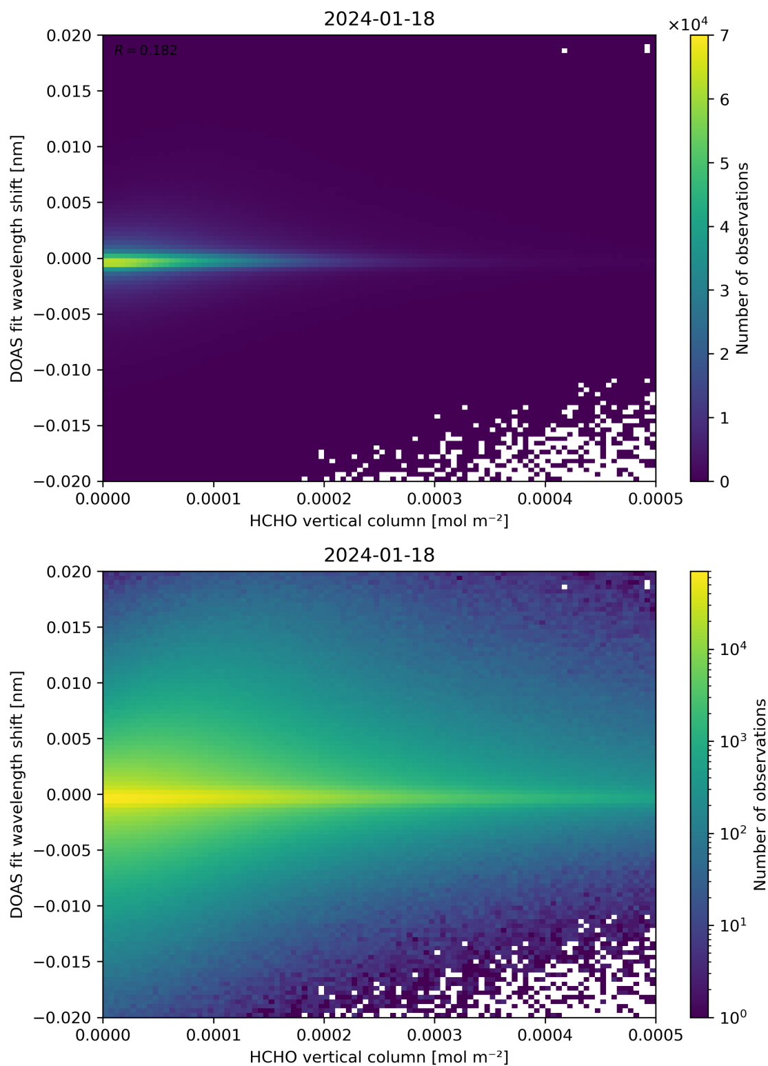
Figure 124: Scatter density plot of “HCHO vertical column” against “DOAS fit wavelength shift” for 2024-01-17 to 2024-01-19.
