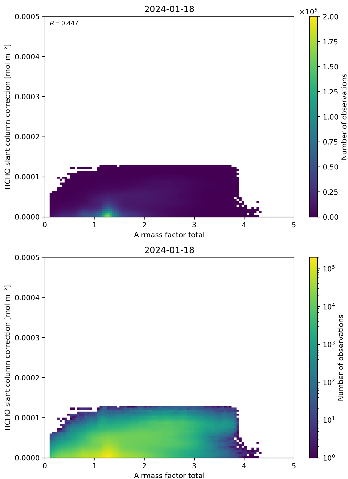
Figure 102: Scatter density plot of “Airmass factor total” against “HCHO slant column correction” for 2024-01-17 to 2024-01-19.
