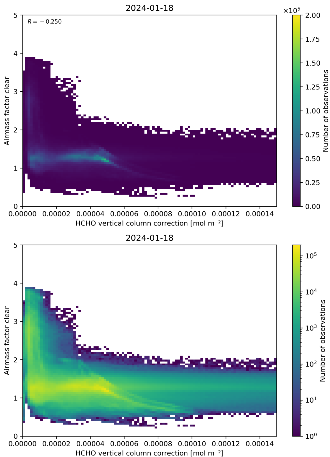
Figure 115: Scatter density plot of “HCHO vertical column correction” against “Airmass factor clear” for 2024-01-17 to 2024-01-19.
