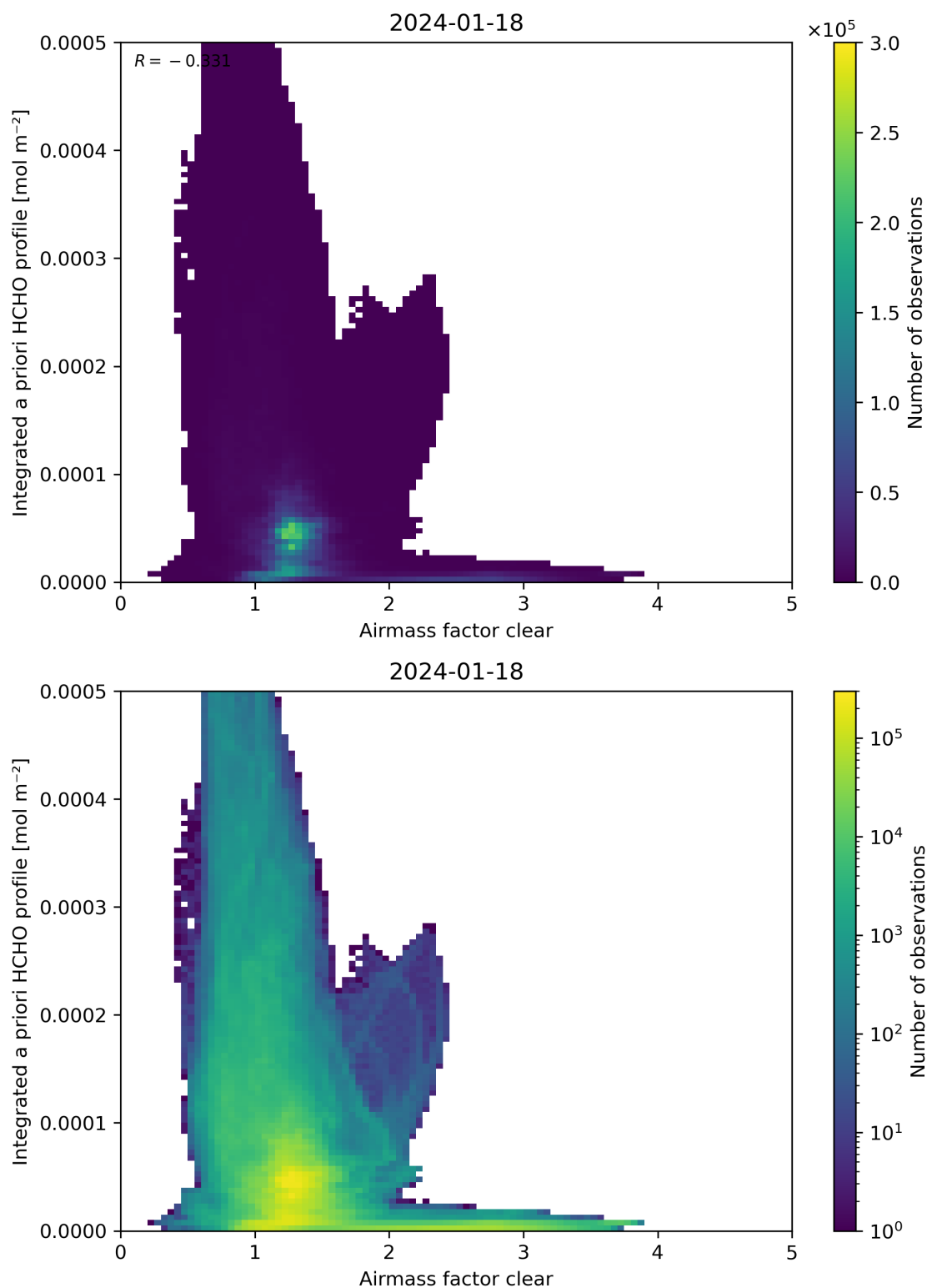
Figure 76: Scatter density plot of “Airmass factor clear” against “Integrated a priori HCHO profile” for 2024-01-17 to 2024-01-19.
