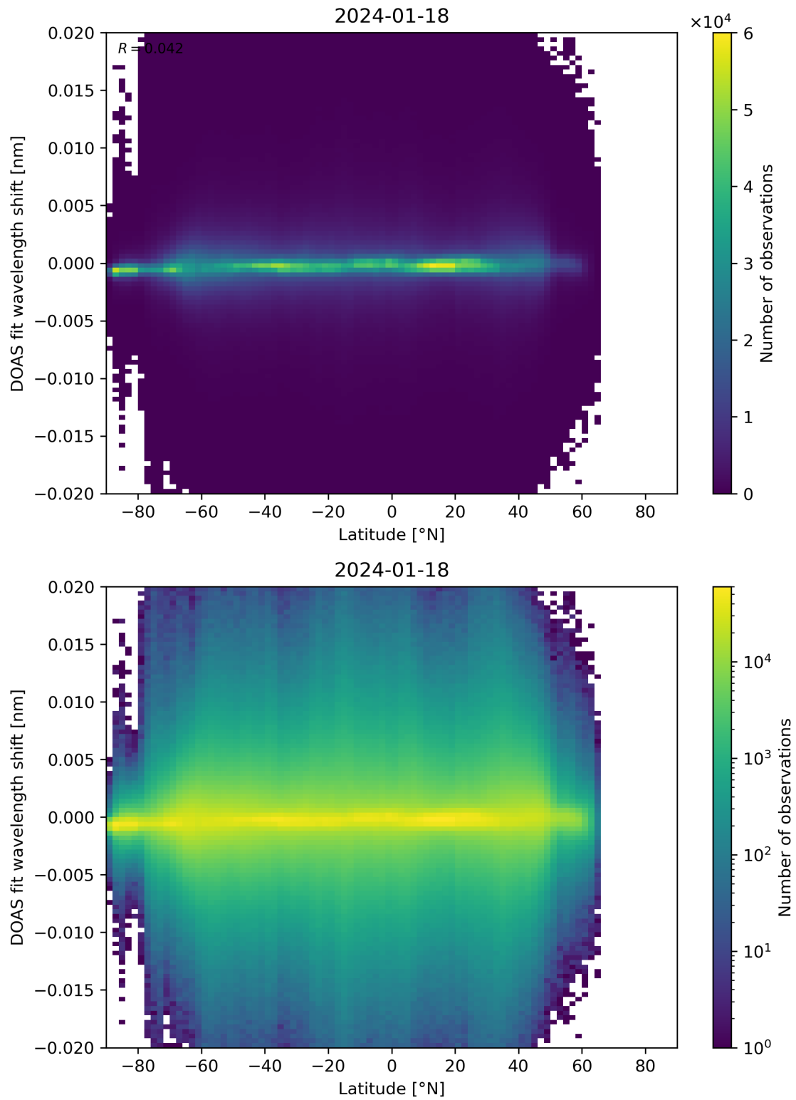
Figure 154: Scatter density plot of “Latitude” against “DOAS fit wavelength shift” for 2024-01-17 to 2024-01-19.
