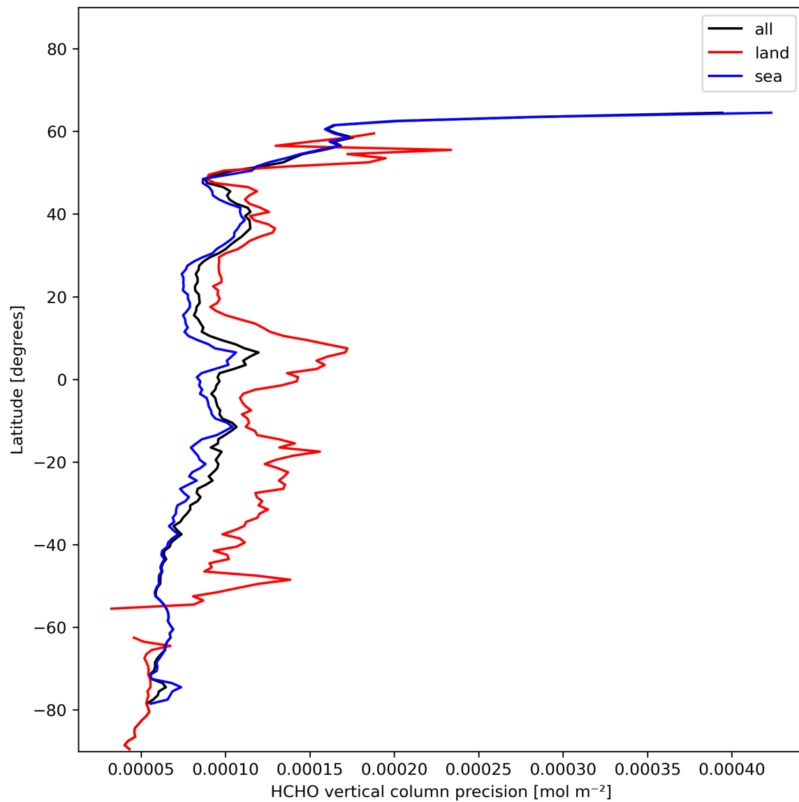
Figure 22: Zonal average of “HCHO vertical column precision” for 2024-01-17 to 2024-01-19.
