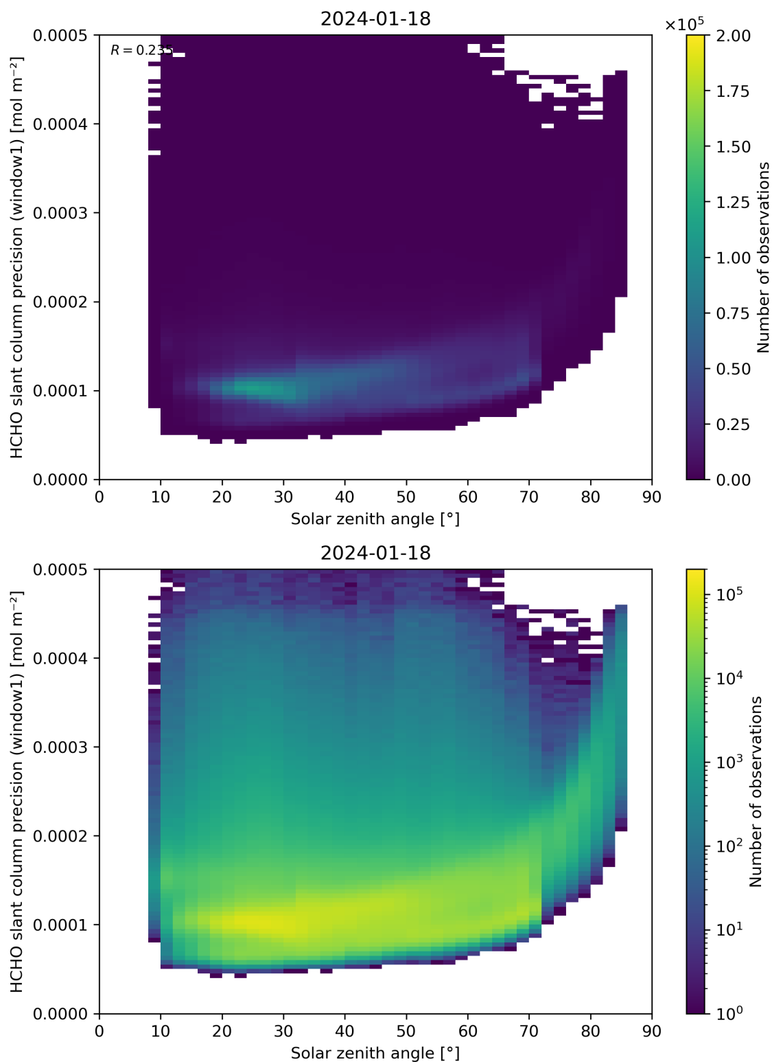
Figure 174: Scatter density plot of “Solar zenith angle” against “HCHO slant column precision (window1)” for 2024-01-17 to 2024-01-19.
