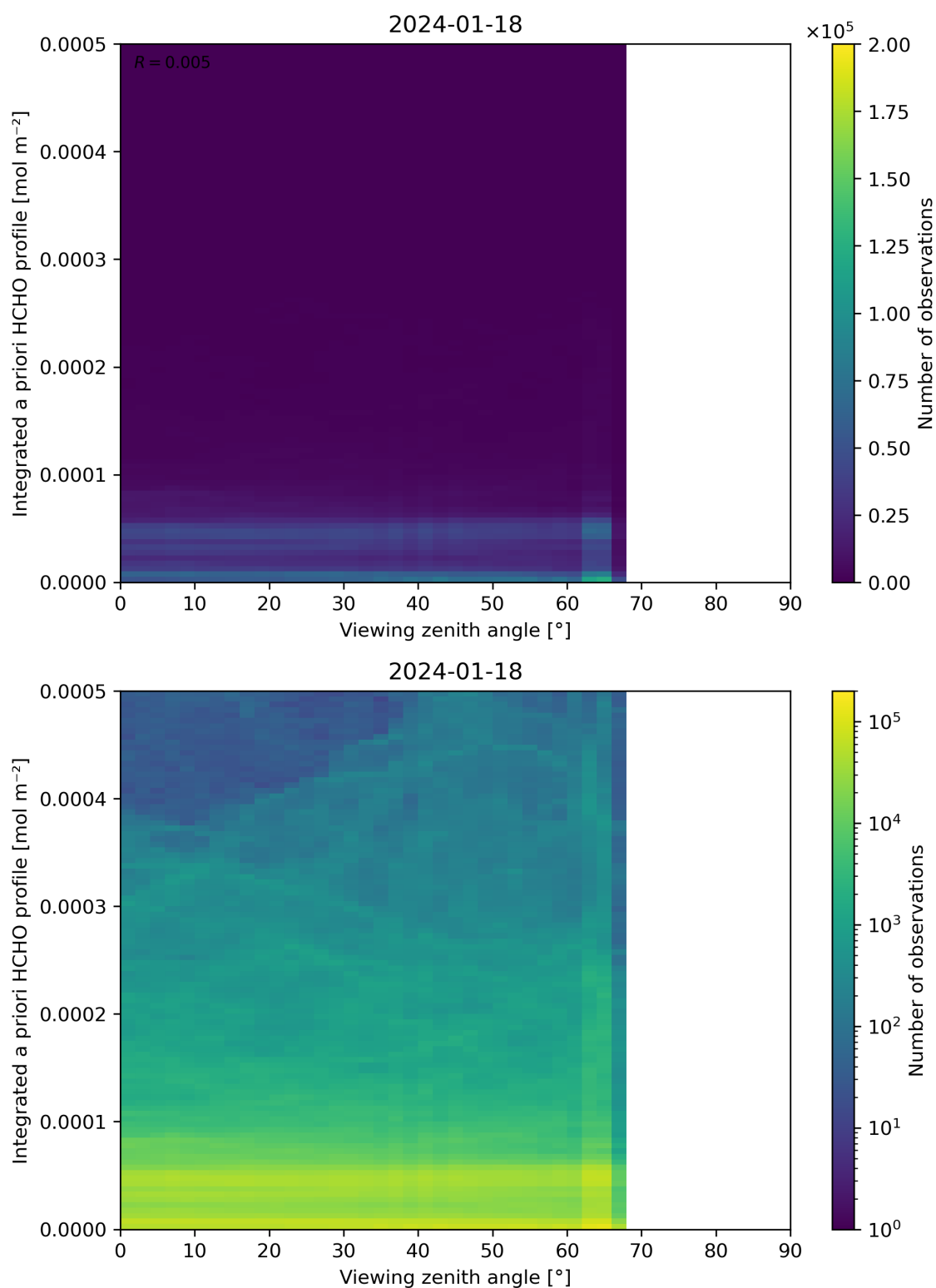
Figure 195: Scatter density plot of “Viewing zenith angle” against “Integrated a priori HCHO profile” for 2024-01-17 to 2024-01-19.
