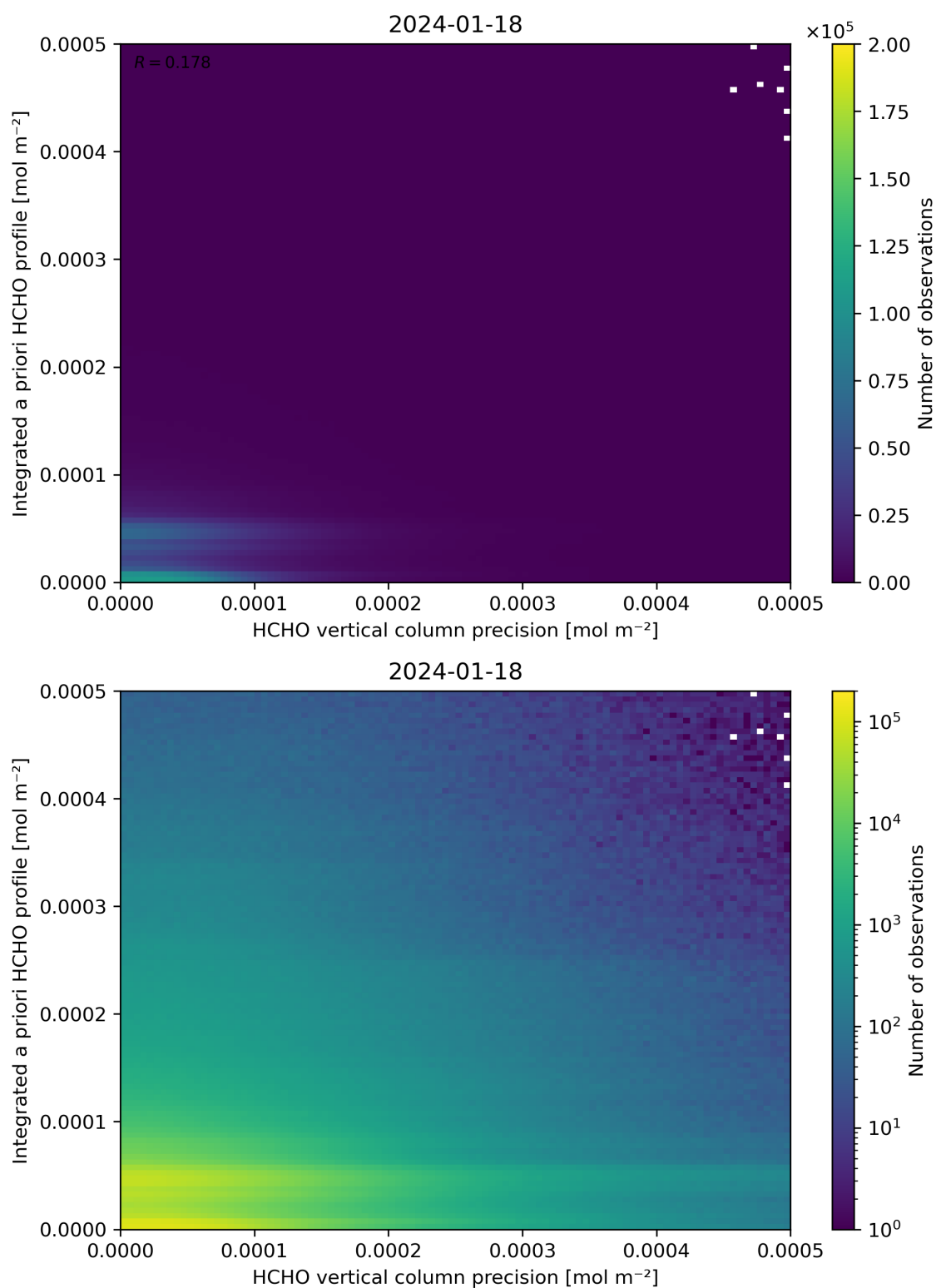
Figure 147: Scatter density plot of “HCHO vertical column precision” against “Integrated a priori HCHO profile” for 2024-01-17 to 2024-01-19.
