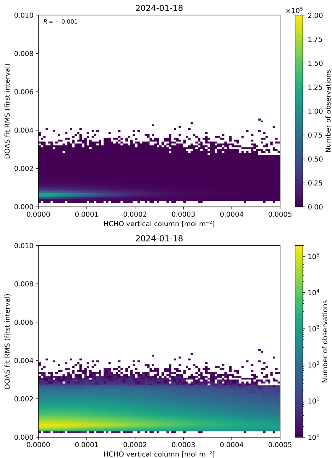
Figure 123: Scatter density plot of “HCHO vertical column” against “DOAS fit RMS (first interval)” for 2024-01-17 to 2024-01-19.
