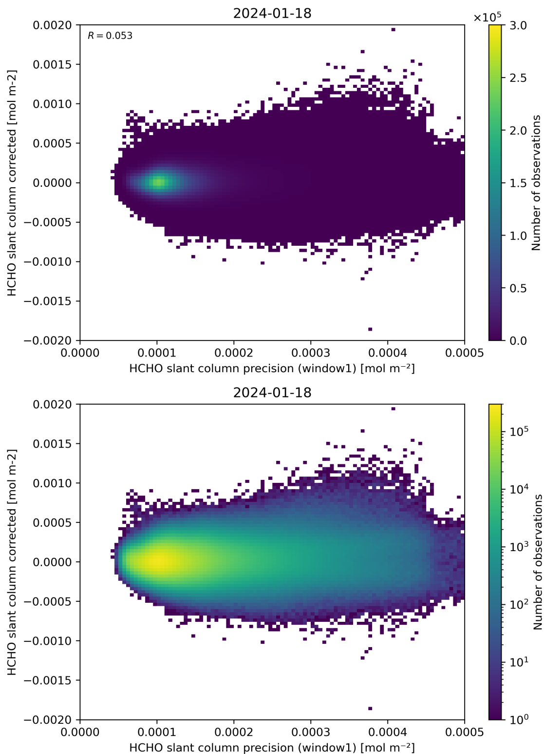
Figure 92: Scatter density plot of “HCHO slant column precision (window1)” against “HCHO slant column corrected” for 2024-01-17 to 2024-01-19.
