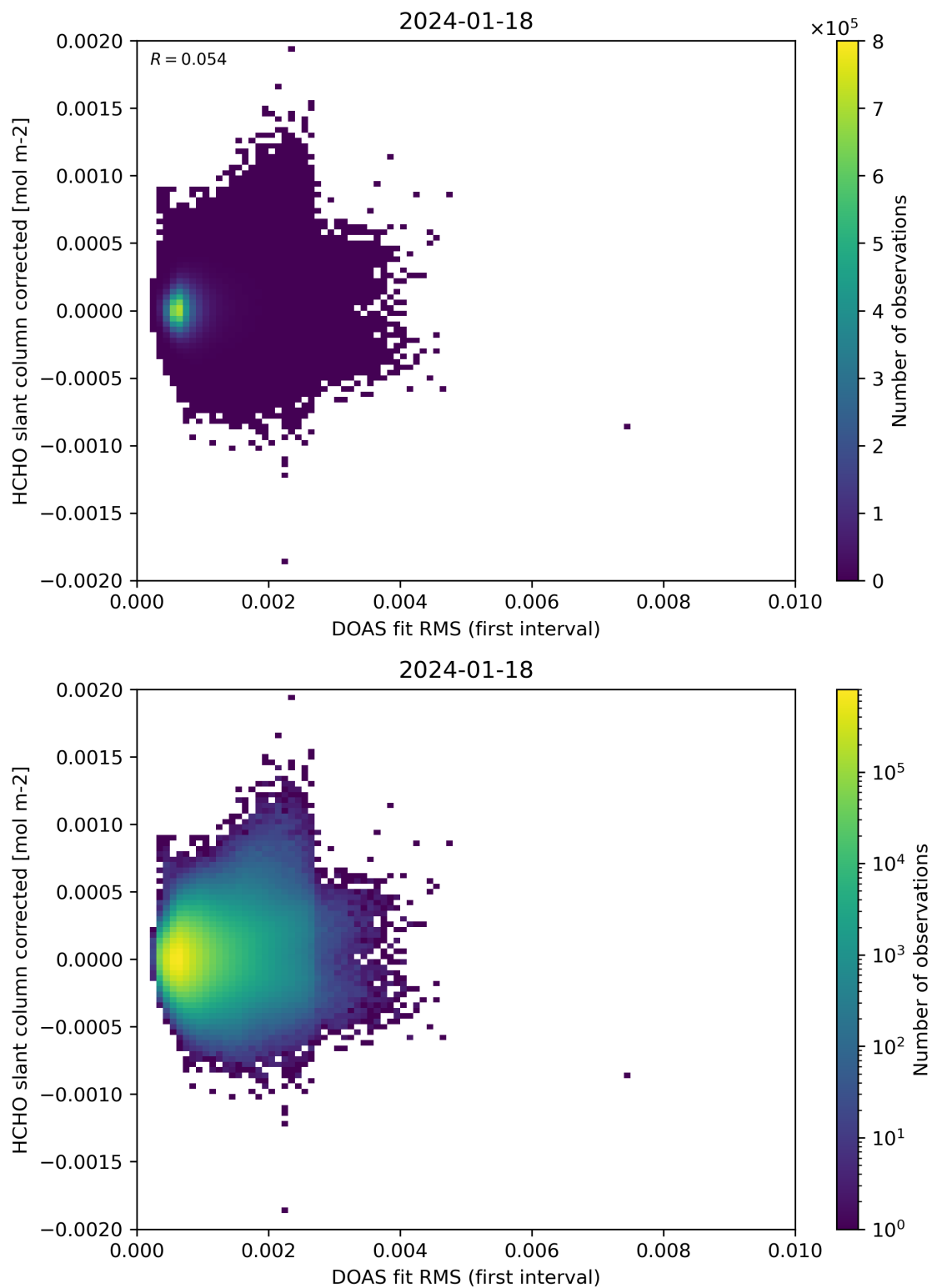
Figure 62: Scatter density plot of “DOAS fit RMS (first interval)” against “HCHO slant column corrected” for 2024-01-17 to 2024-01-19.
