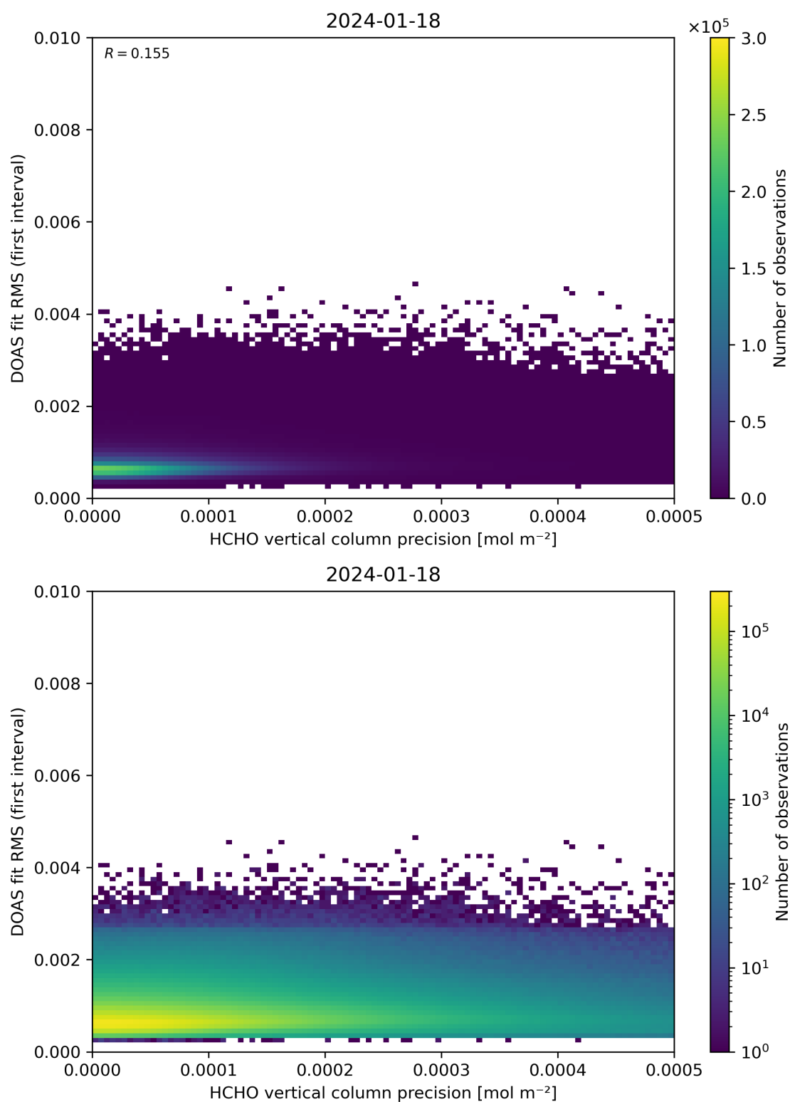
Figure 136: Scatter density plot of “HCHO vertical column precision” against “DOAS fit RMS (first interval)” for 2024-01-17 to 2024-01-19.
