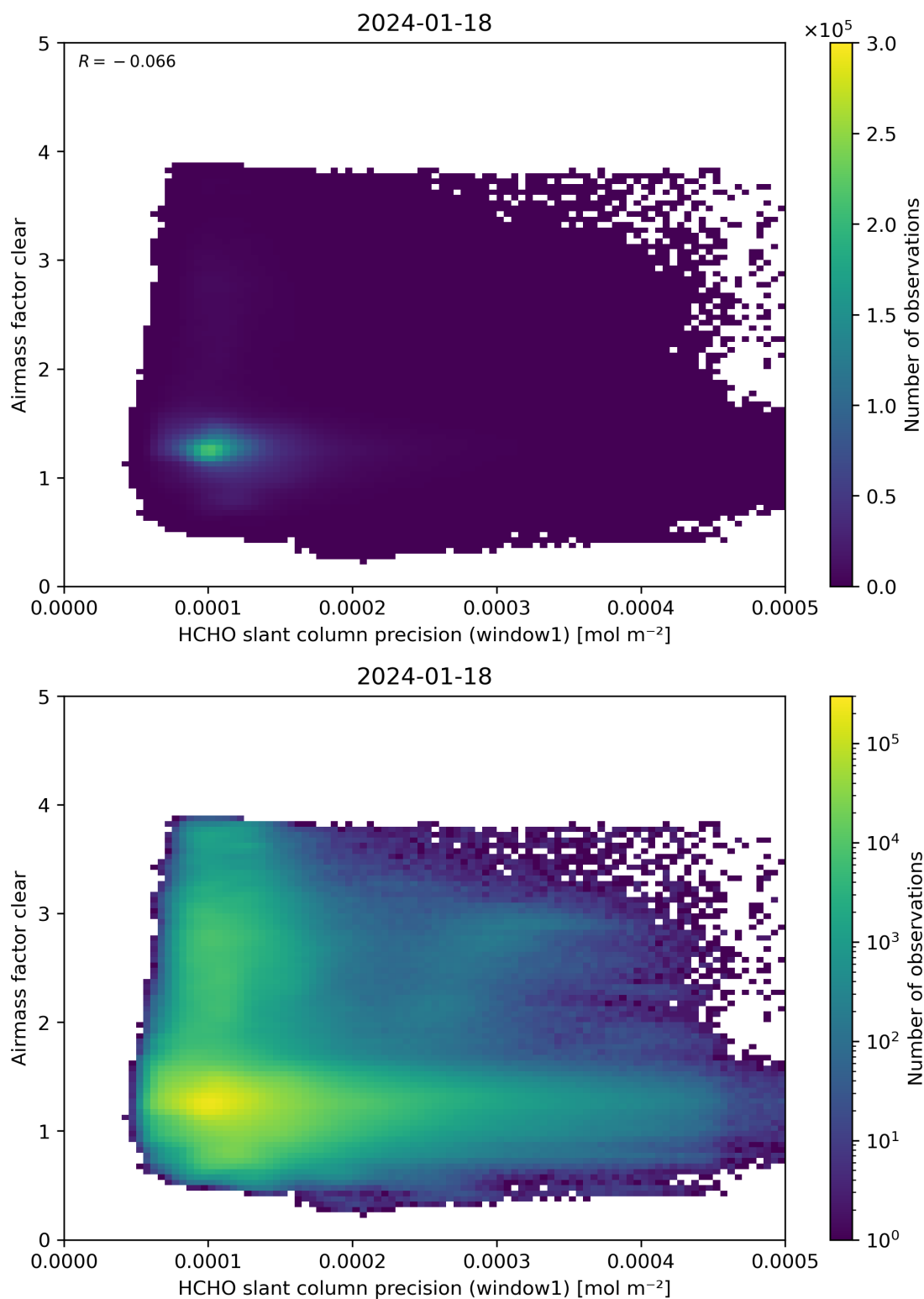
Figure 91: Scatter density plot of “HCHO slant column precision (window1)” against “Airmass factor clear” for 2024-01-17 to 2024-01-19.
