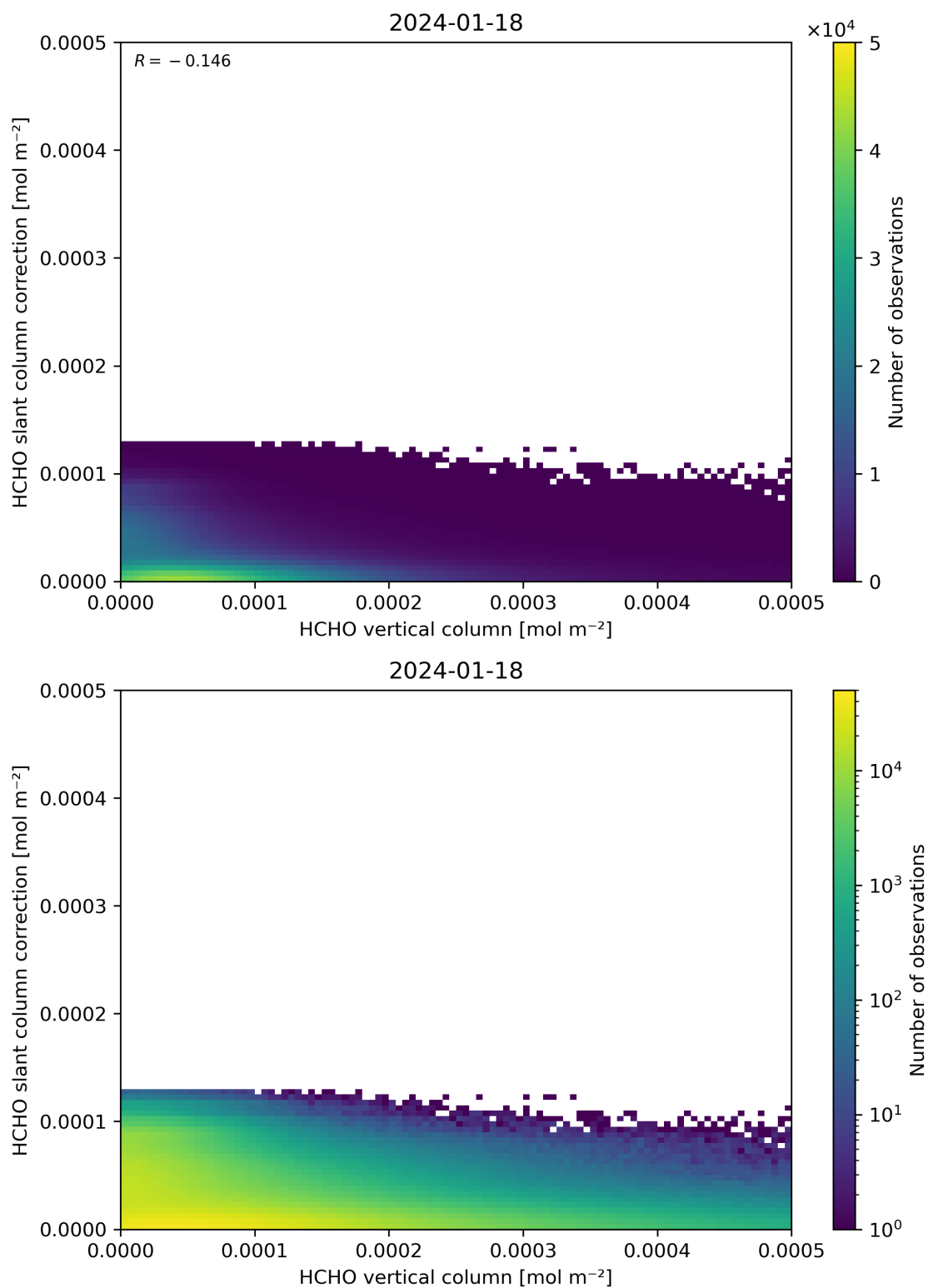
Figure 128: Scatter density plot of “HCHO vertical column” against “HCHO slant column correction” for 2024-01-17 to 2024-01-19.
