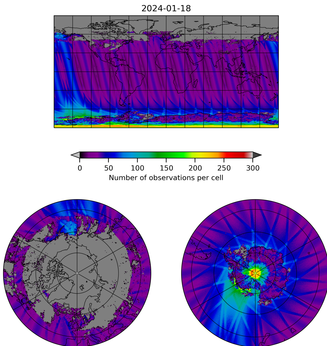
Figure 19: Map of the number of observations for 2024-01-17 to 2024-01-19
