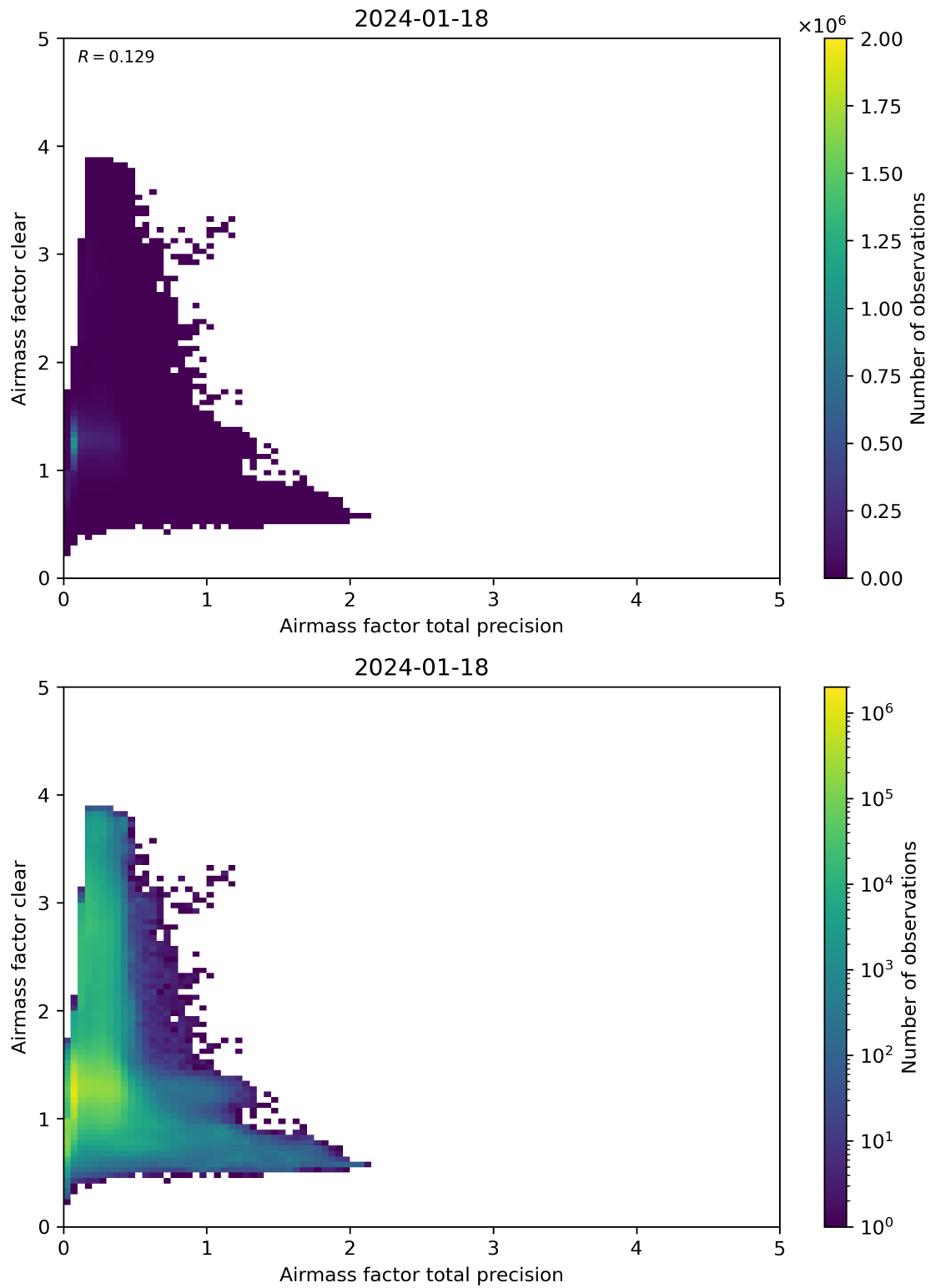
Figure 108: Scatter density plot of “Airmass factor total precision” against “Airmass factor clear” for 2024-01-17 to 2024-01-19.
