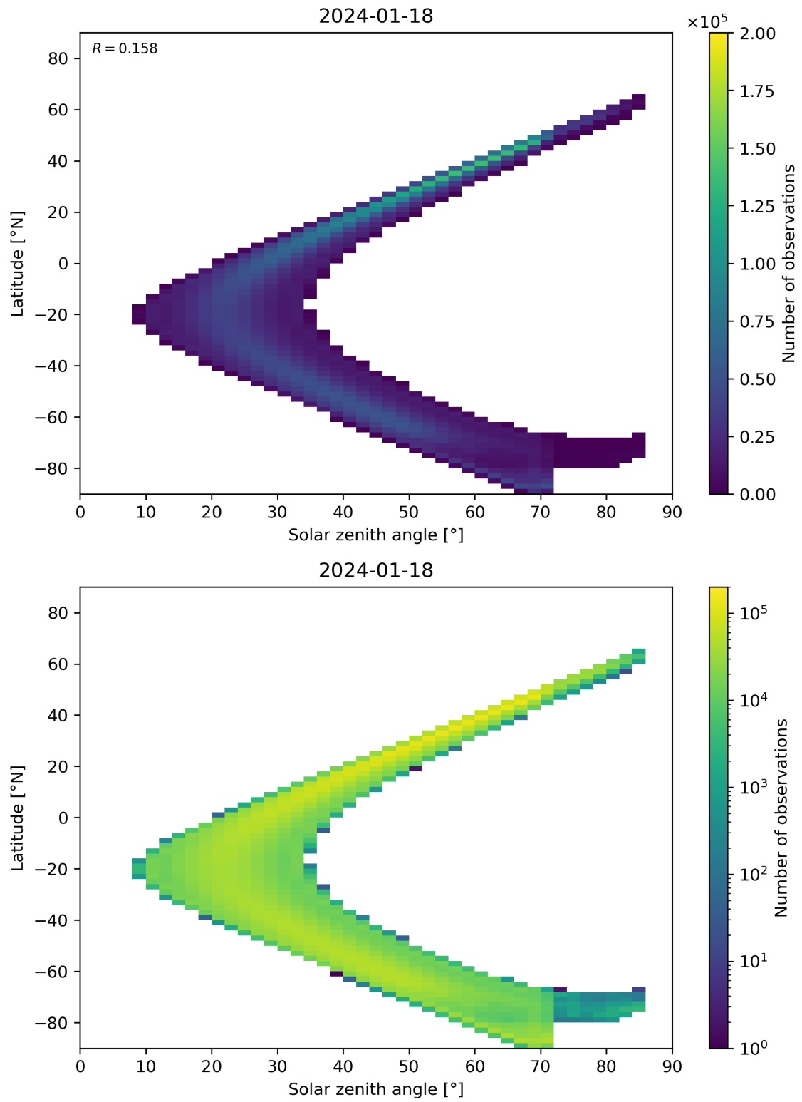
Figure 181: Scatter density plot of “Solar zenith angle” against “Latitude” for 2024-01-17 to 2024-01-19.
