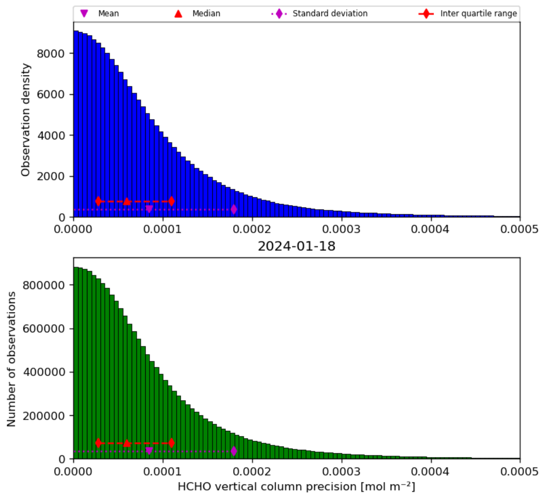
Figure 36: Histogram of “HCHO vertical column precision” for 2024-01-17 to 2024-01-19
