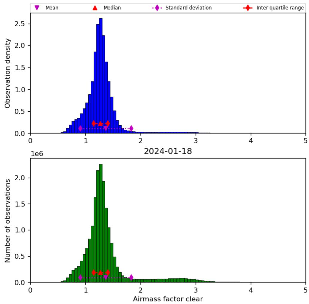
Figure 42: Histogram of “Airmass factor clear” for 2024-01-17 to 2024-01-19
