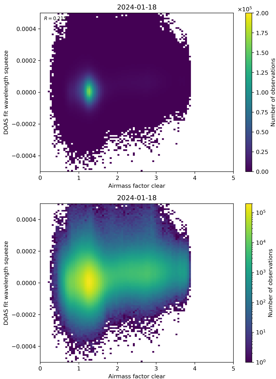
Figure 73: Scatter density plot of “Airmass factor clear” against “DOAS fit wavelength squeeze” for 2024-01-17 to 2024-01-19.
