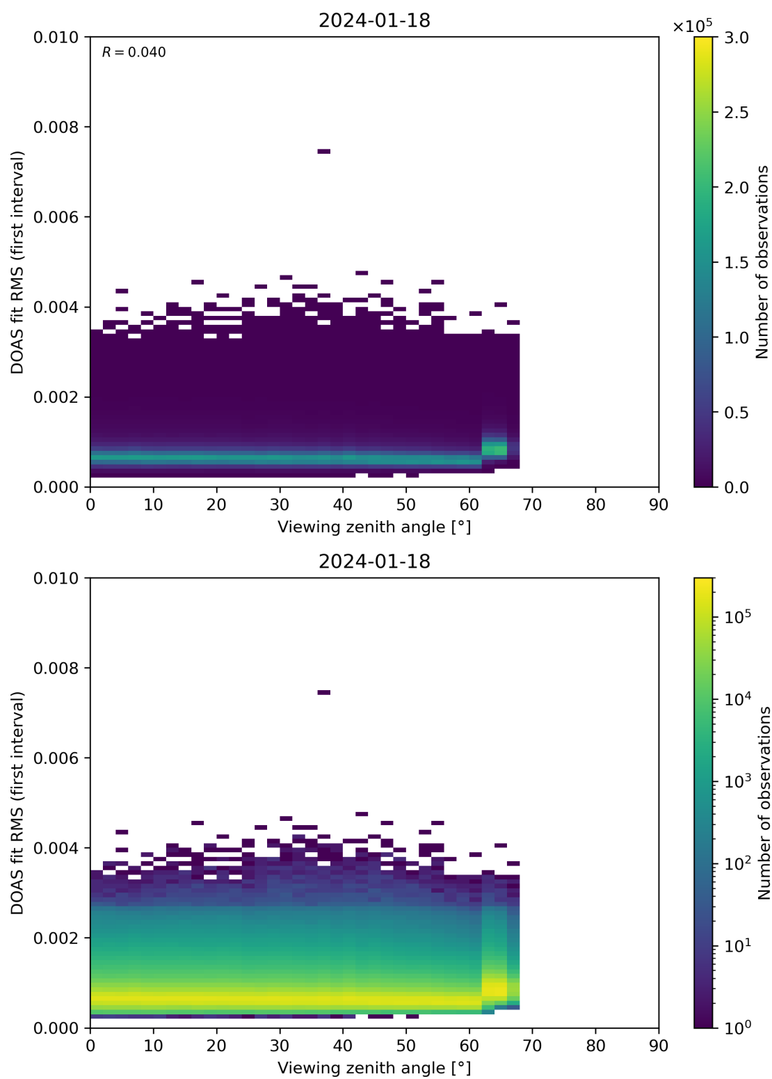
Figure 182: Scatter density plot of “Viewing zenith angle” against “DOAS fit RMS (first interval)” for 2024-01-17 to 2024-01-19.
