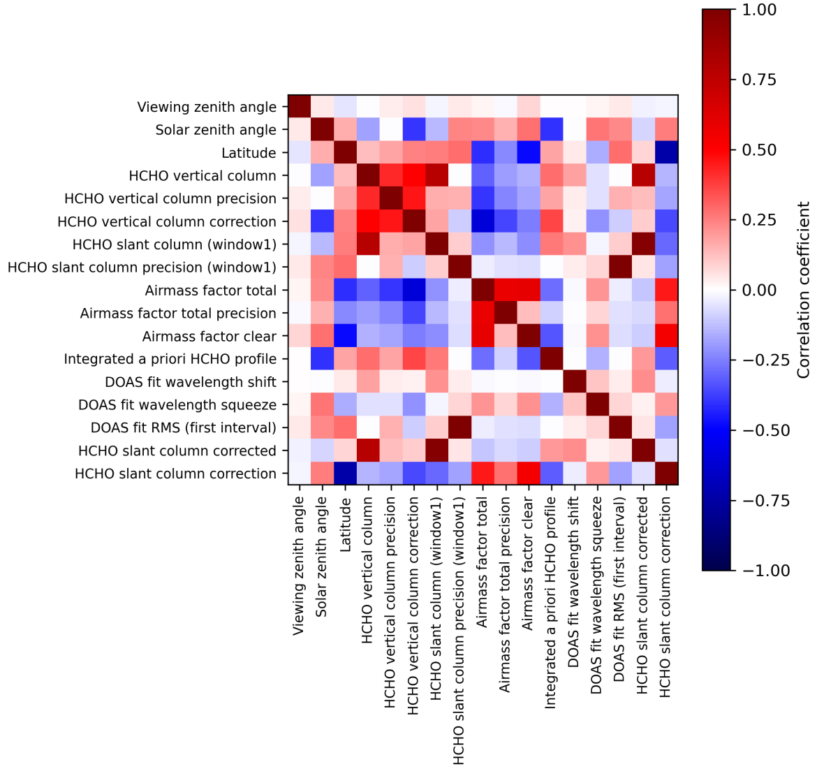
Figure 2: Map of correlation matrix for 2024-01-17 to 2024-01-19.
