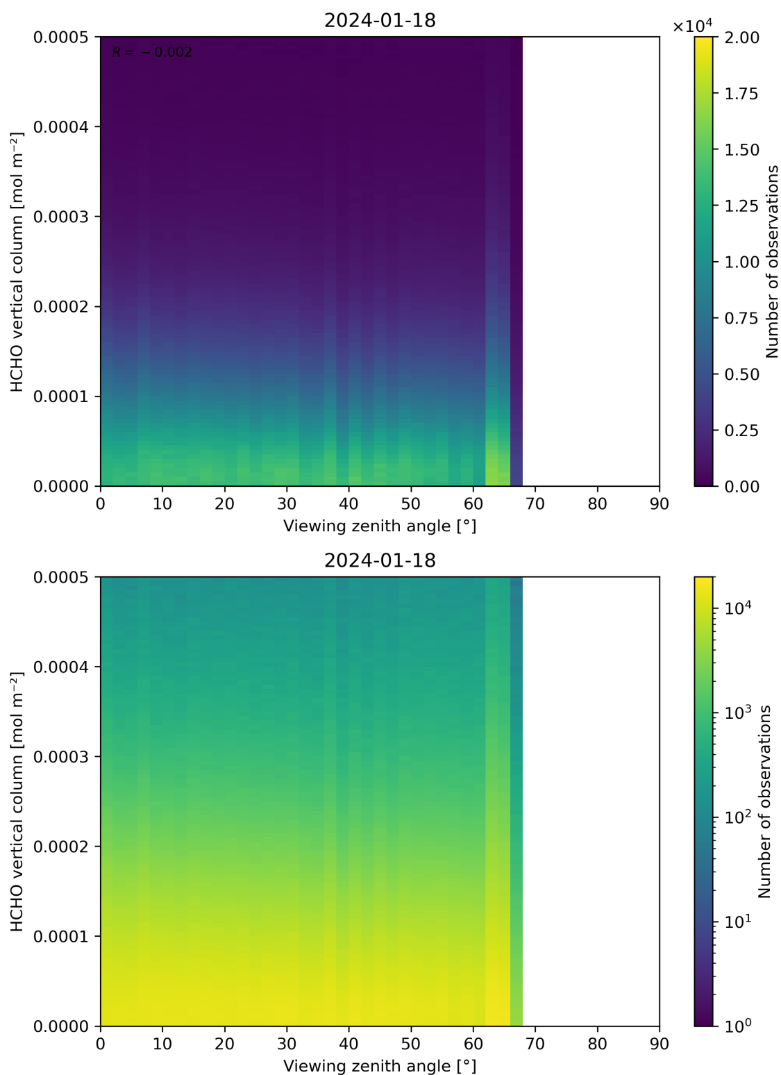
Figure 192: Scatter density plot of “Viewing zenith angle” against “HCHO vertical column” for 2024-01-17 to 2024-01-19.
