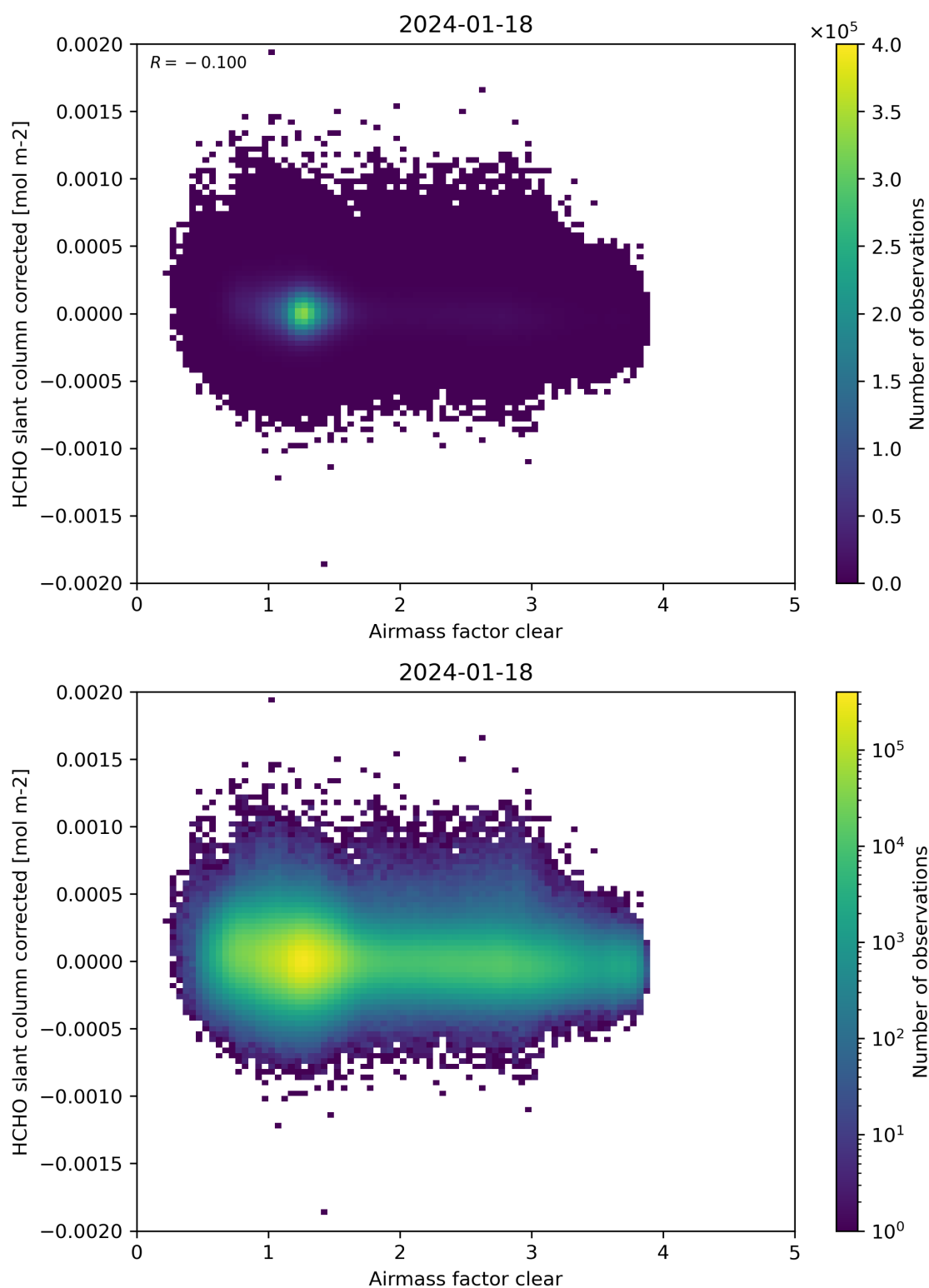
Figure 74: Scatter density plot of “Airmass factor clear” against “HCHO slant column corrected” for 2024-01-17 to 2024-01-19.
