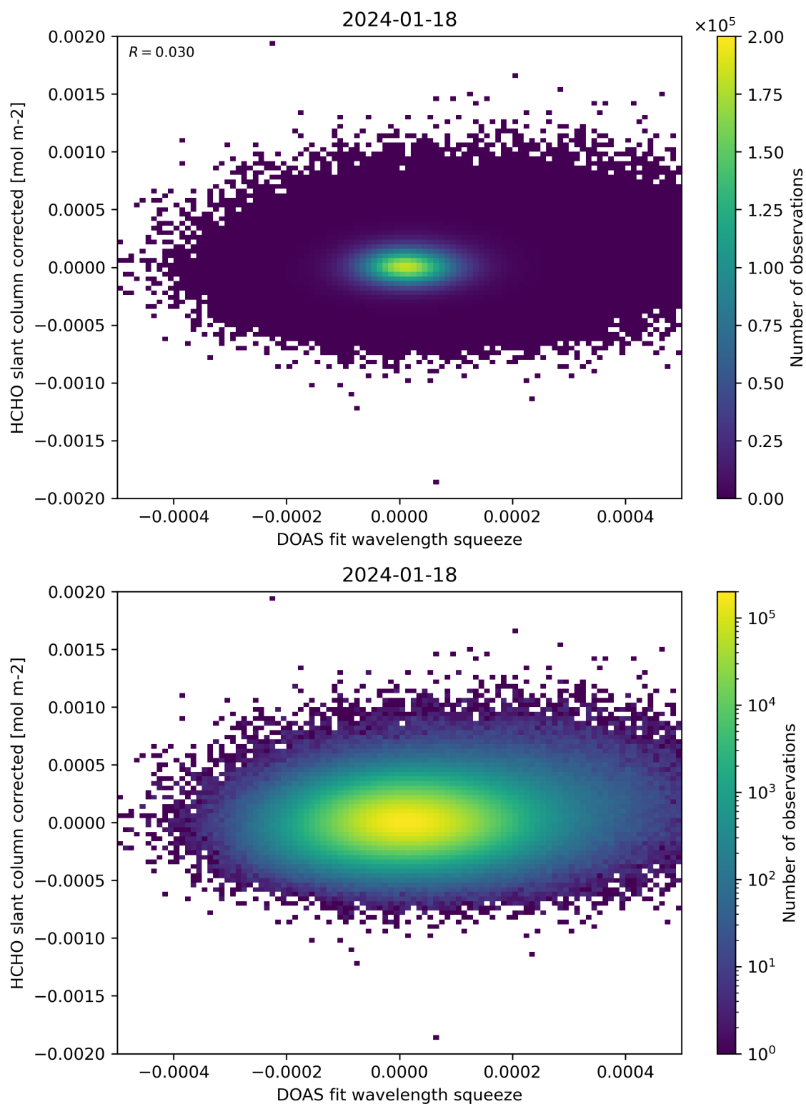
Figure 69: Scatter density plot of “DOAS fit wavelength squeeze” against “HCHO slant column corrected” for 2024-01-17 to 2024-01-19.
