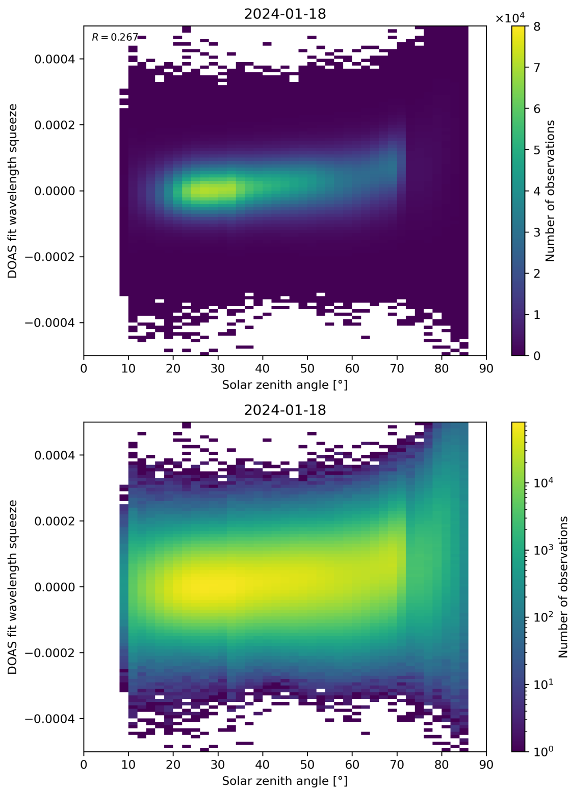
Figure 169: Scatter density plot of “Solar zenith angle” against “DOAS fit wavelength squeeze” for 2024-01-17 to 2024-01-19.
