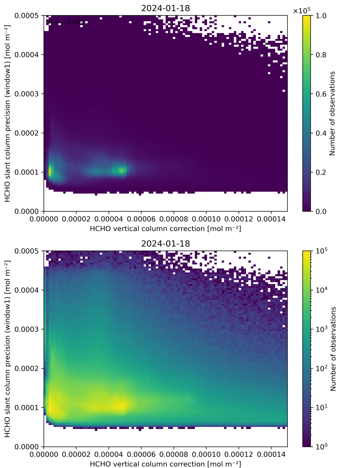
Figure 119: Scatter density plot of “HCHO vertical column correction” against “HCHO slant column precision (window1)” for 2024-01-17 to 2024-01-19.
