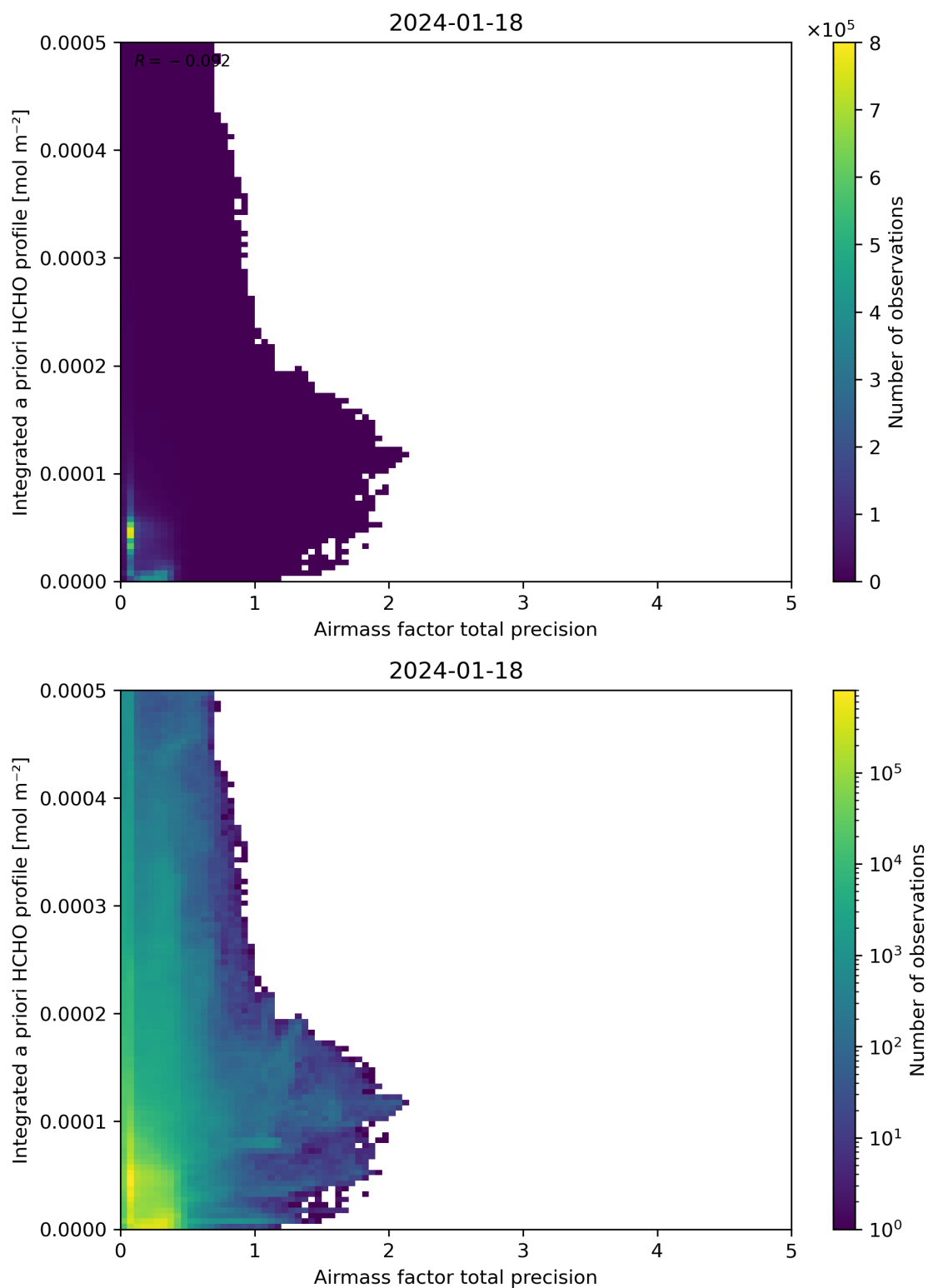
Figure 111: Scatter density plot of “Airmass factor total precision” against “Integrated a priori HCHO profile” for 2024-01-17 to 2024-01-19.
