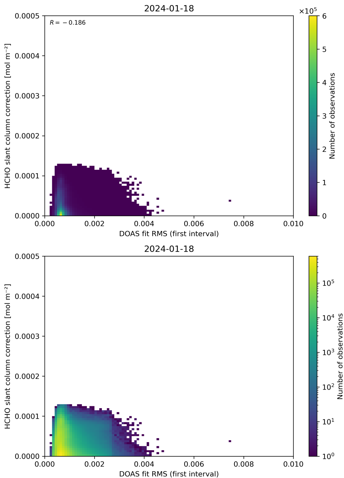
Figure 63: Scatter density plot of “DOAS fit RMS (first interval)” against “HCHO slant column correction” for 2024-01-17 to 2024-01-19.
