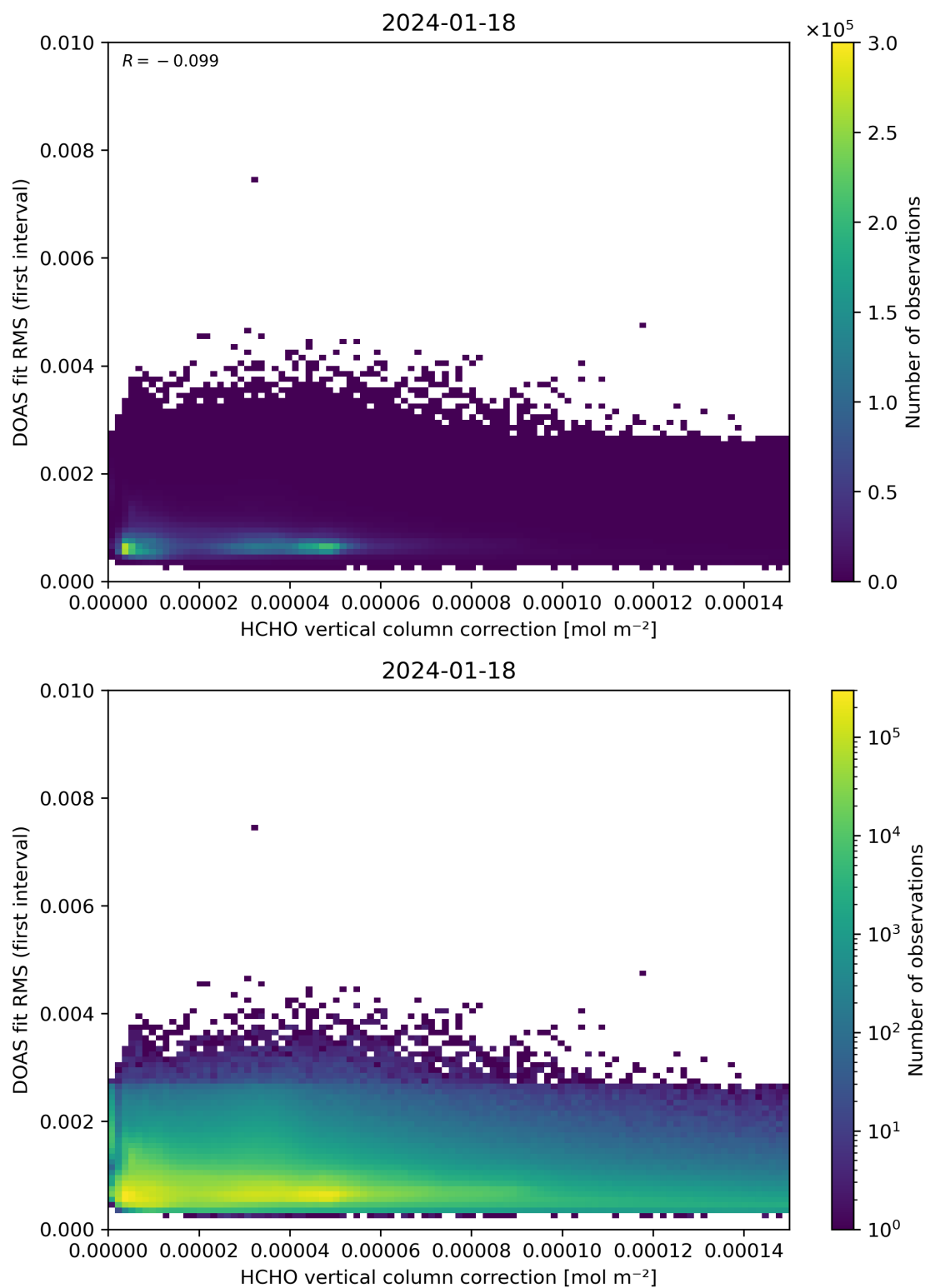
Figure 112: Scatter density plot of “HCHO vertical column correction” against “DOAS fit RMS (first interval)” for 2024-01-17 to 2024-01-19.
