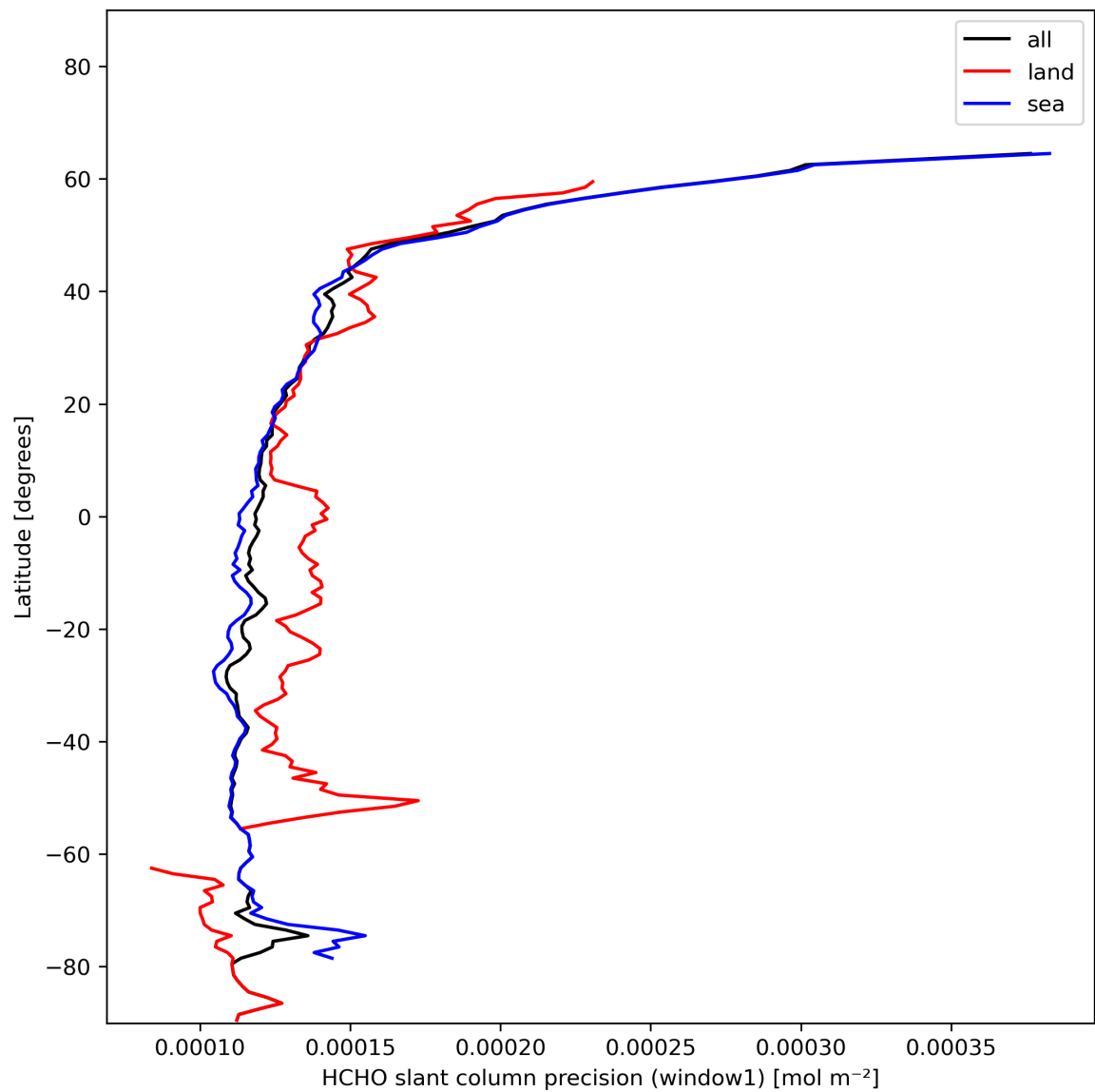
Figure 25: Zonal average of “HCHO slant column precision (window1)” for 2024-01-17 to 2024-01-19.
