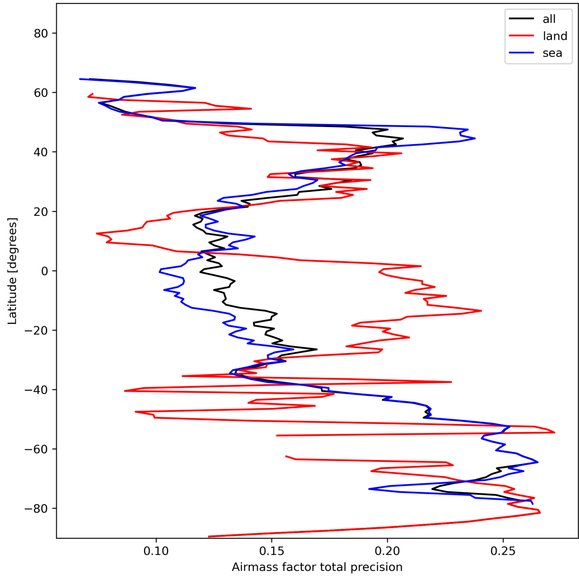
Figure 27: Zonal average of “Airmass factor total precision” for 2024-01-17 to 2024-01-19.
