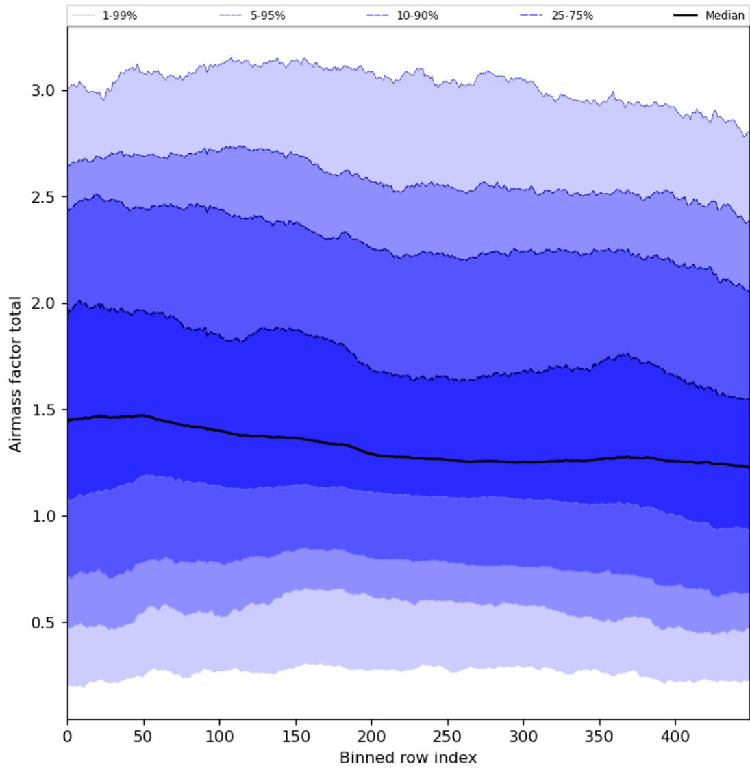
Figure 54: Along track statistics of “Airmass factor total” for 2024-01-17 to 2024-01-19
