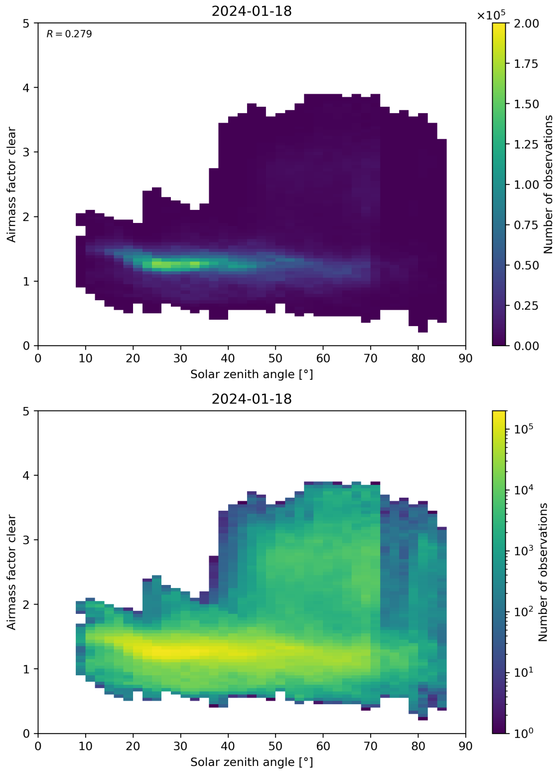
Figure 170: Scatter density plot of “Solar zenith angle” against “Airmass factor clear” for 2024-01-17 to 2024-01-19.
