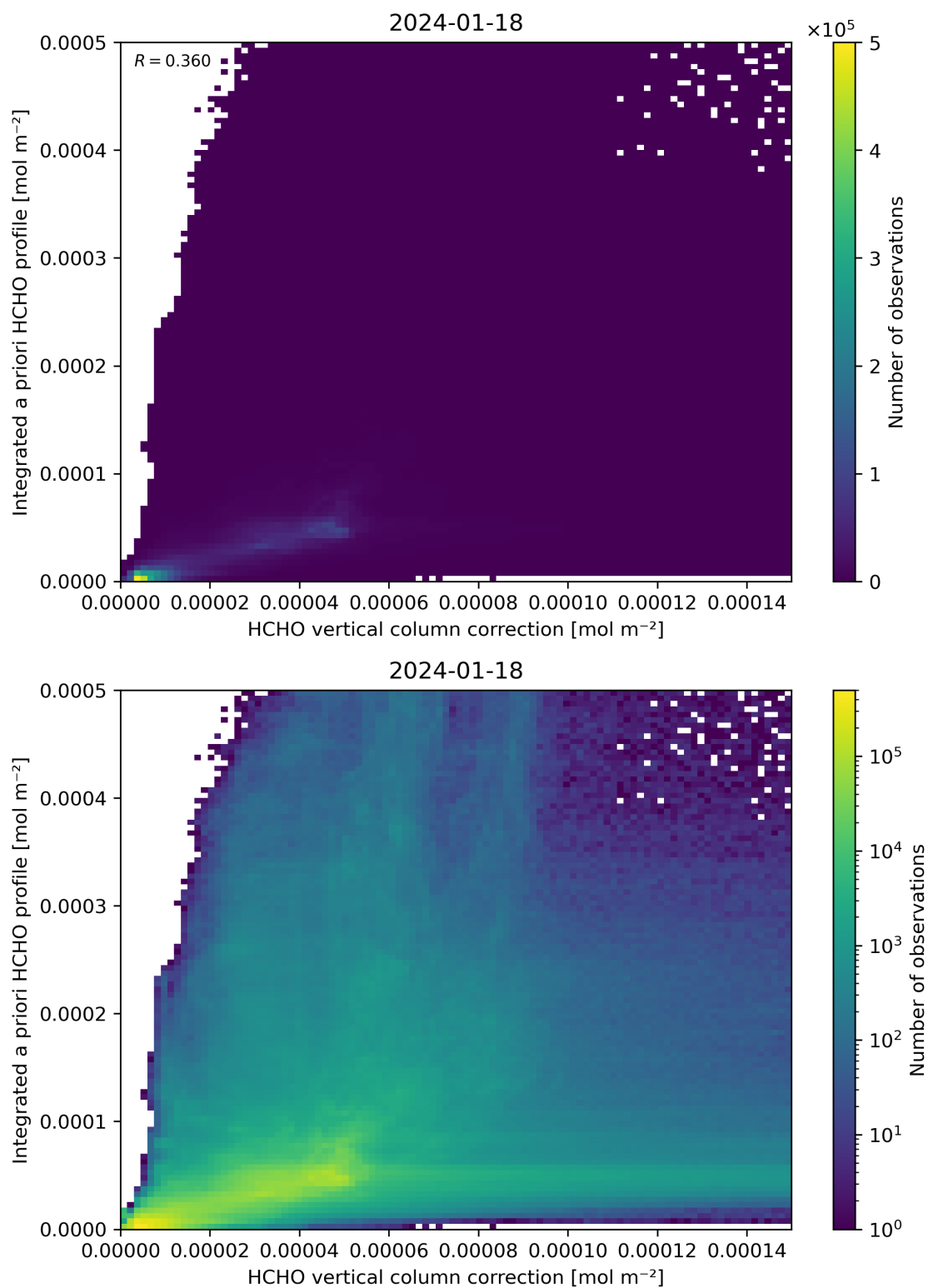
Figure 122: Scatter density plot of “HCHO vertical column correction” against “Integrated a priori HCHO profile” for 2024-01-17 to 2024-01-19.
