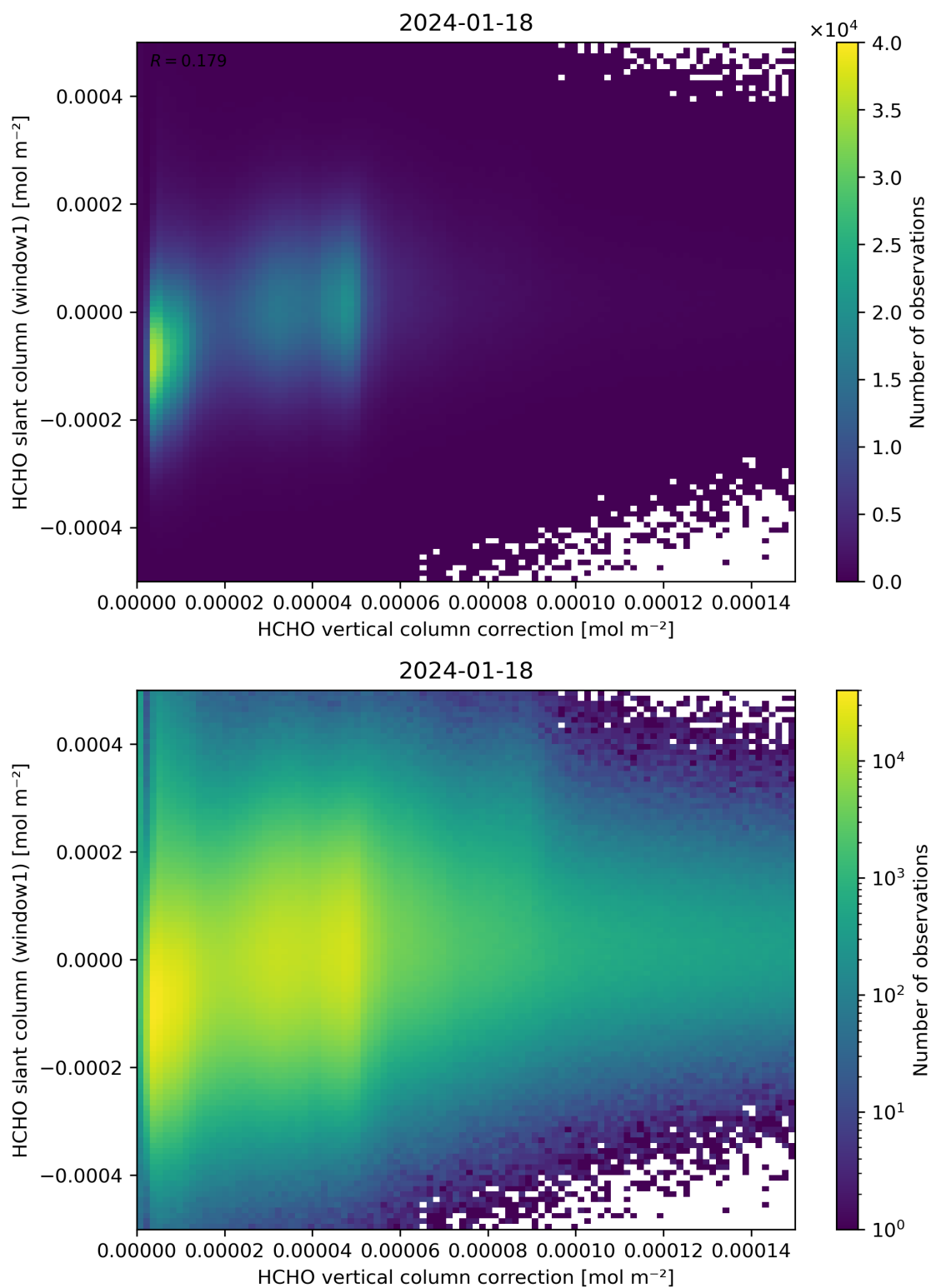
Figure 118: Scatter density plot of “HCHO vertical column correction” against “HCHO slant column (window1)” for 2024-01-17 to 2024-01-19.
