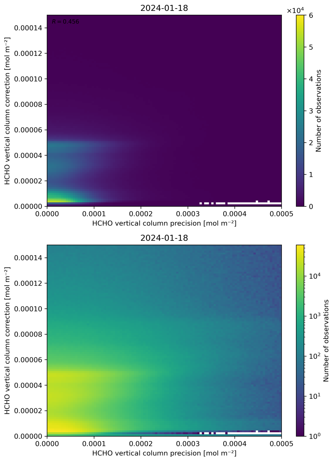
Figure 146: Scatter density plot of “HCHO vertical column precision” against “HCHO vertical column correction” for 2024-01-17 to 2024-01-19.
