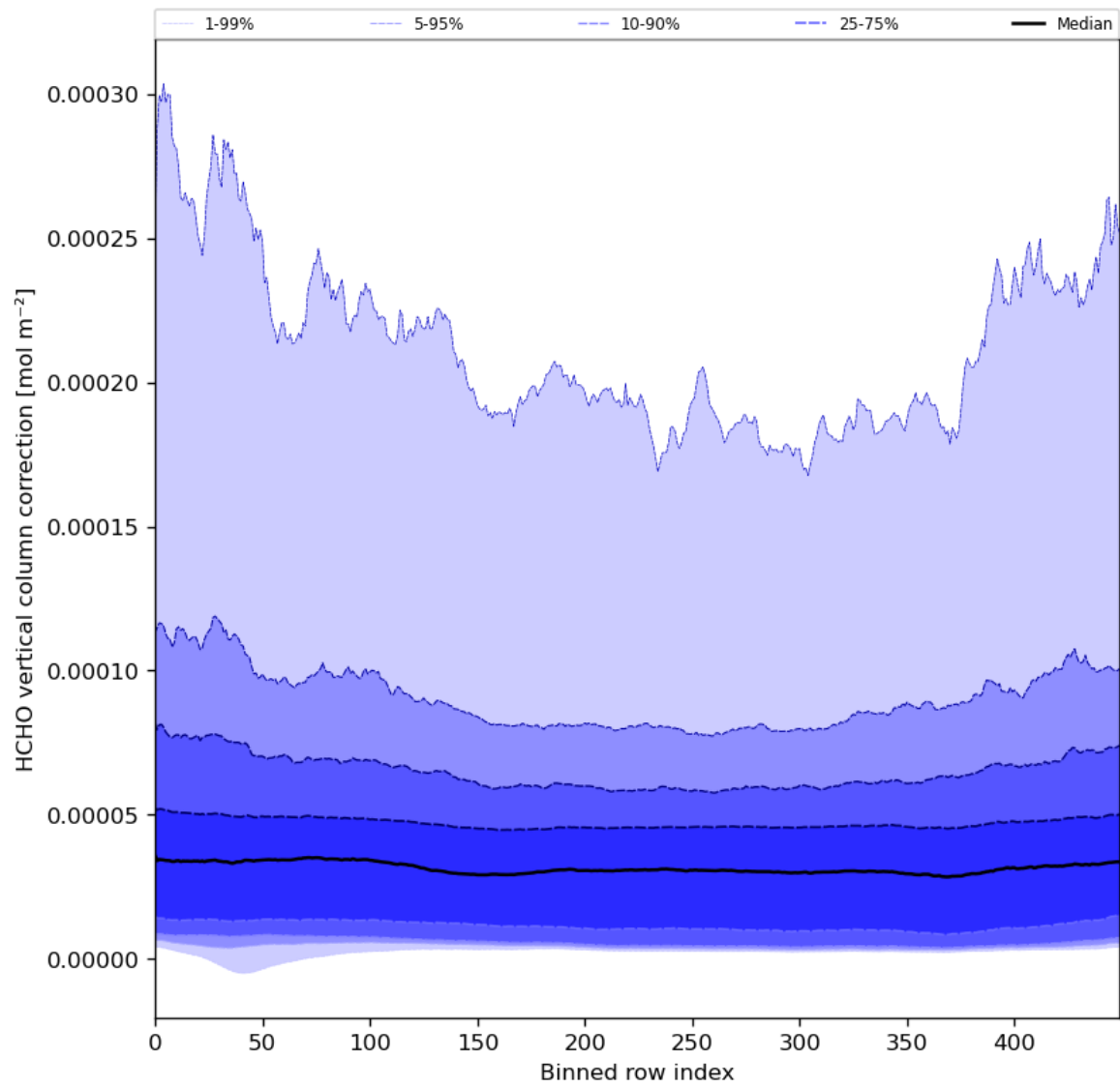
Figure 51: Along track statistics of “HCHO vertical column correction” for 2024-01-17 to 2024-01-19
