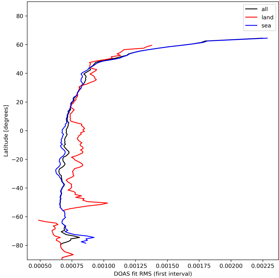
Figure 32: Zonal average of “DOAS fit RMS (first interval)” for 2024-01-17 to 2024-01-19.
