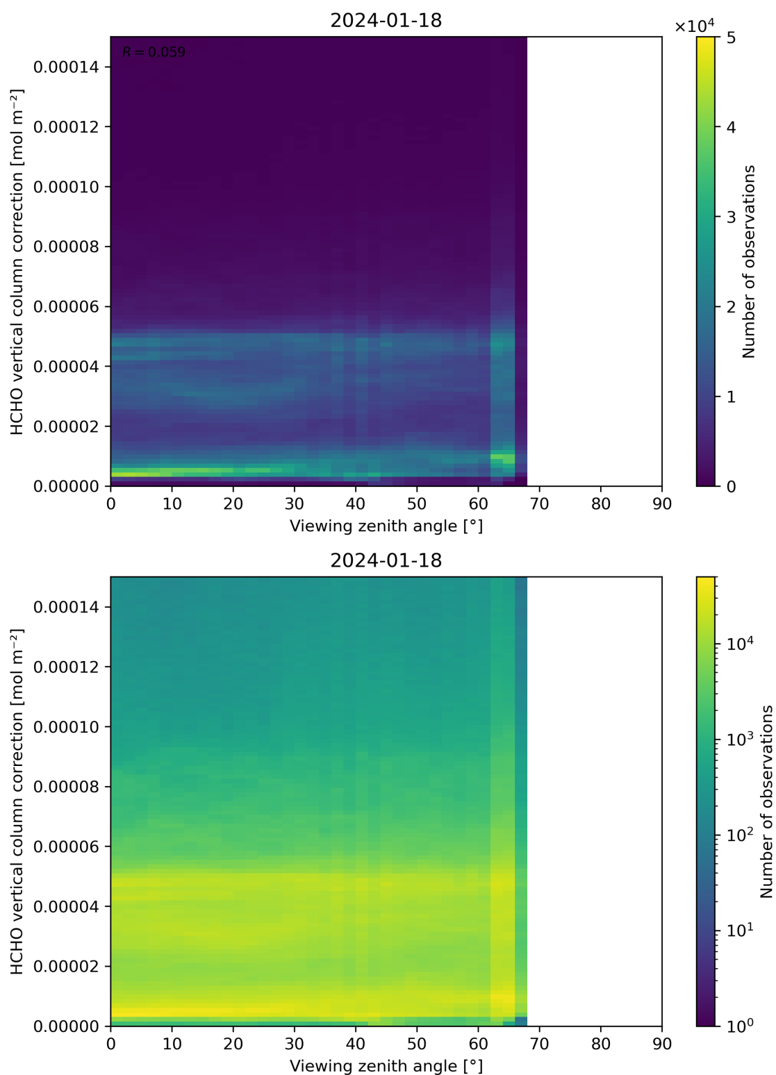
Figure 193: Scatter density plot of “Viewing zenith angle” against “HCHO vertical column correction” for 2024-01-17 to 2024-01-19.
