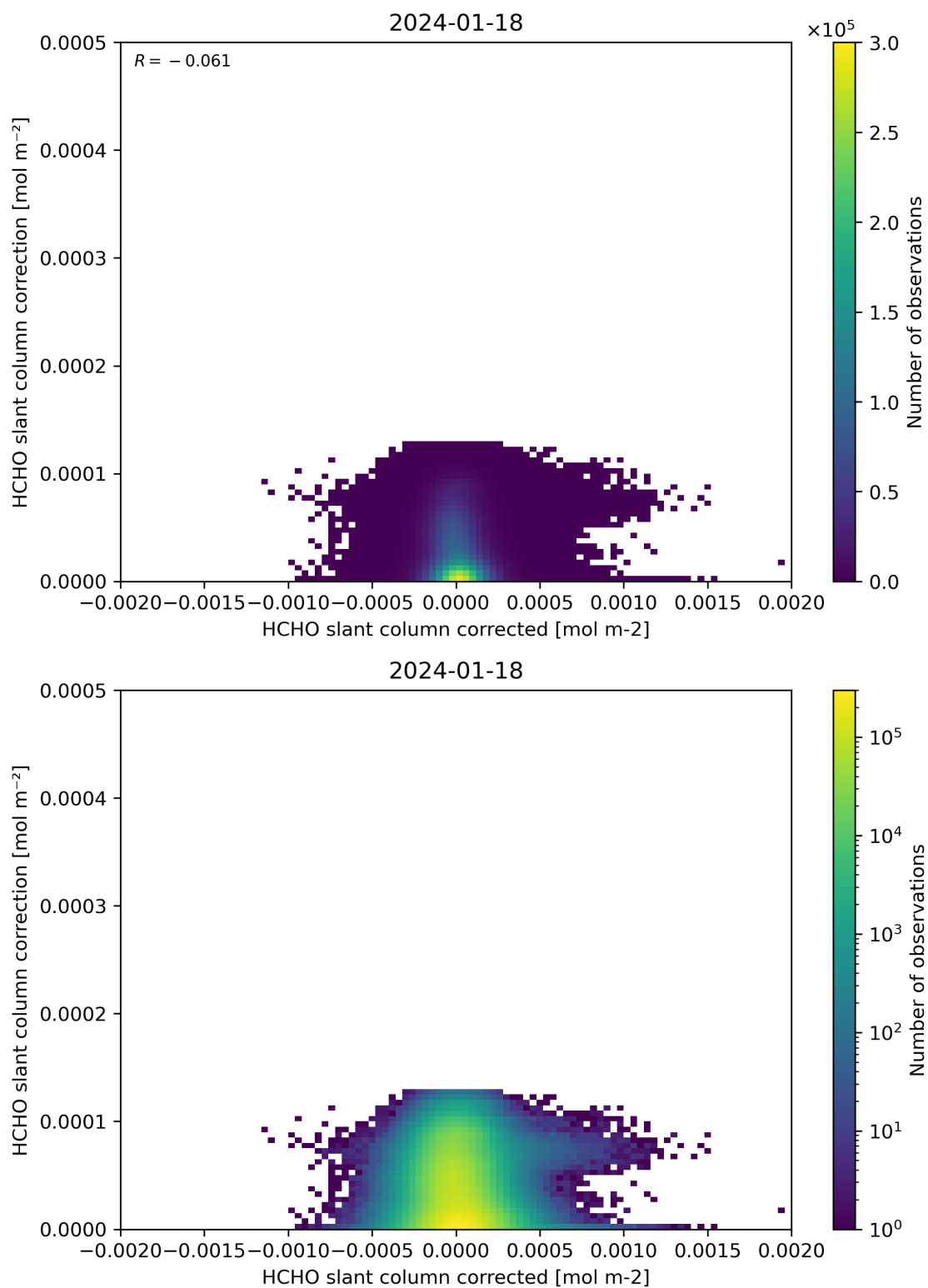
Figure 77: Scatter density plot of “HCHO slant column corrected” against “HCHO slant column correction” for 2024-01-17 to 2024-01-19.
