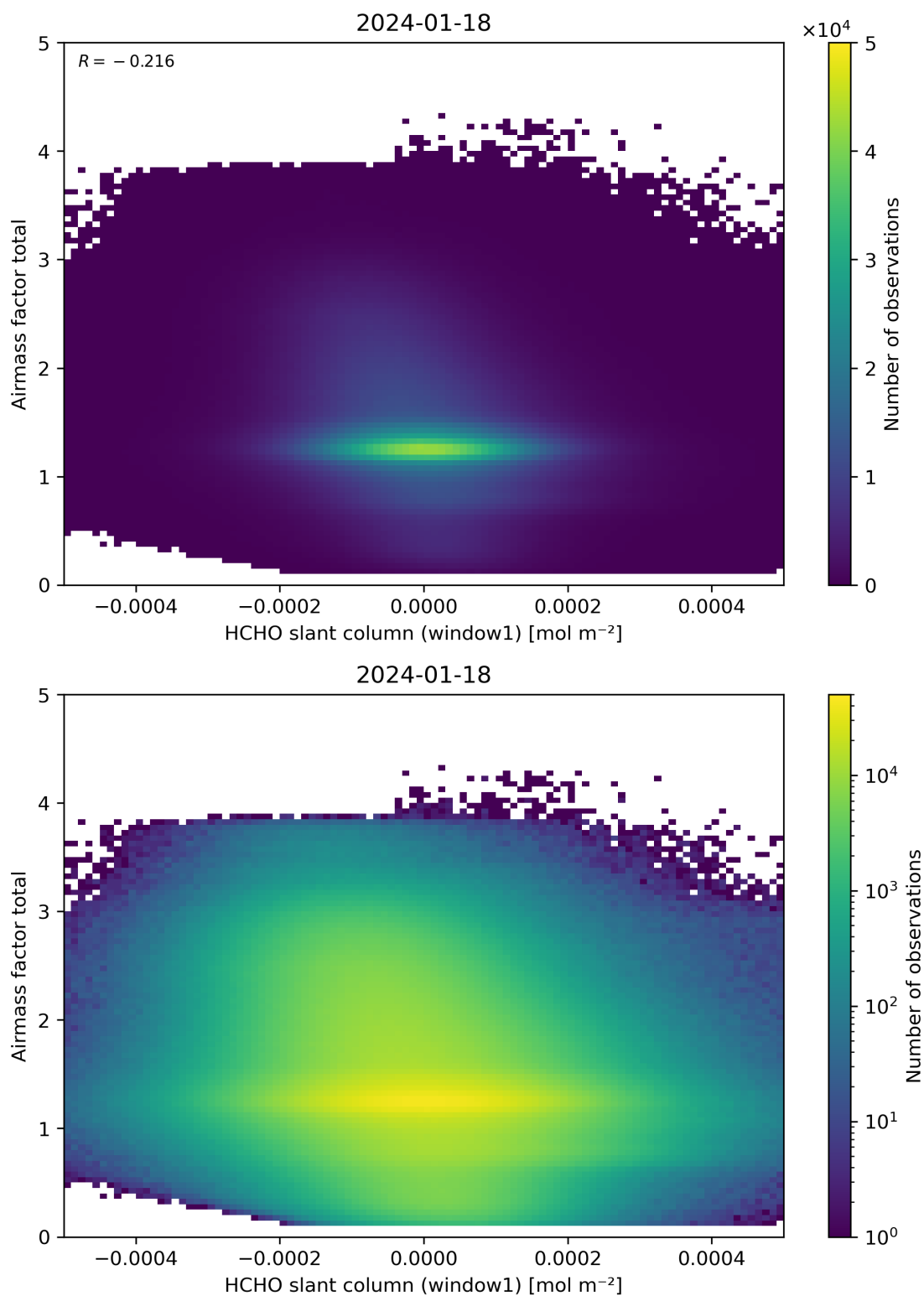
Figure 85: Scatter density plot of “HCHO slant column (window1)” against “Airmass factor total” for 2024-01-17 to 2024-01-19.
