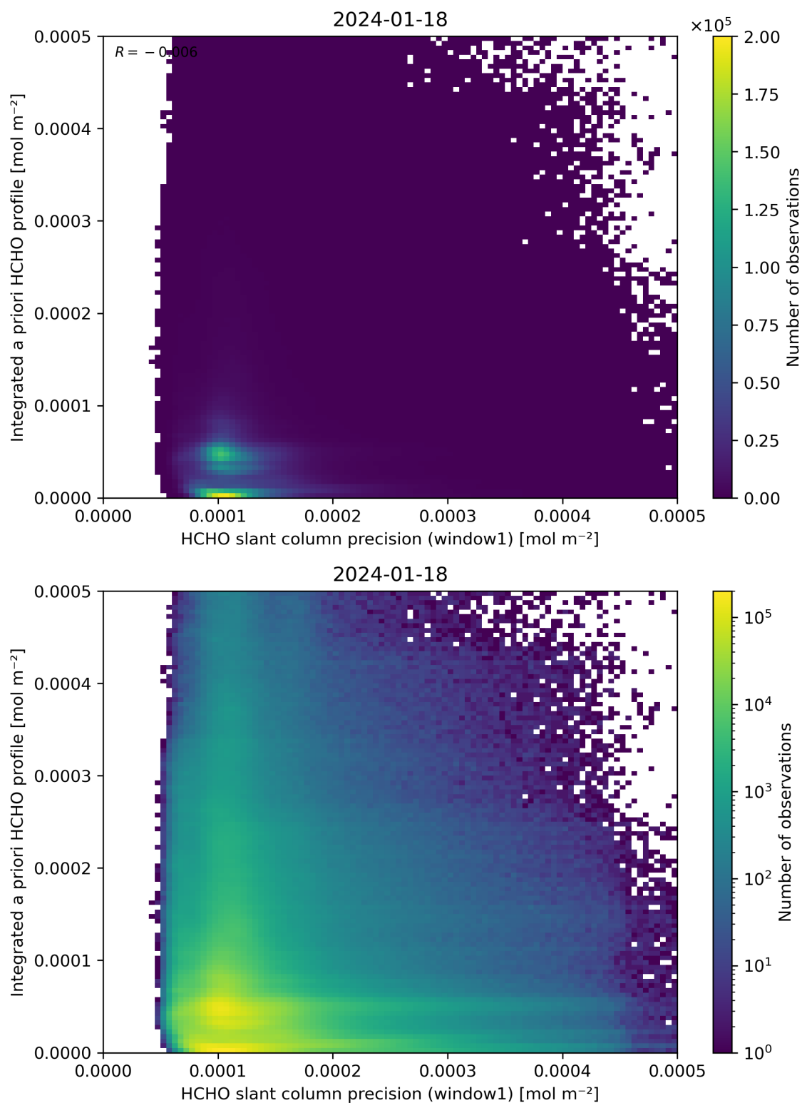
Figure 96: Scatter density plot of “HCHO slant column precision (window1)” against “Integrated a priori HCHO profile” for 2024-01-17 to 2024-01-19.
