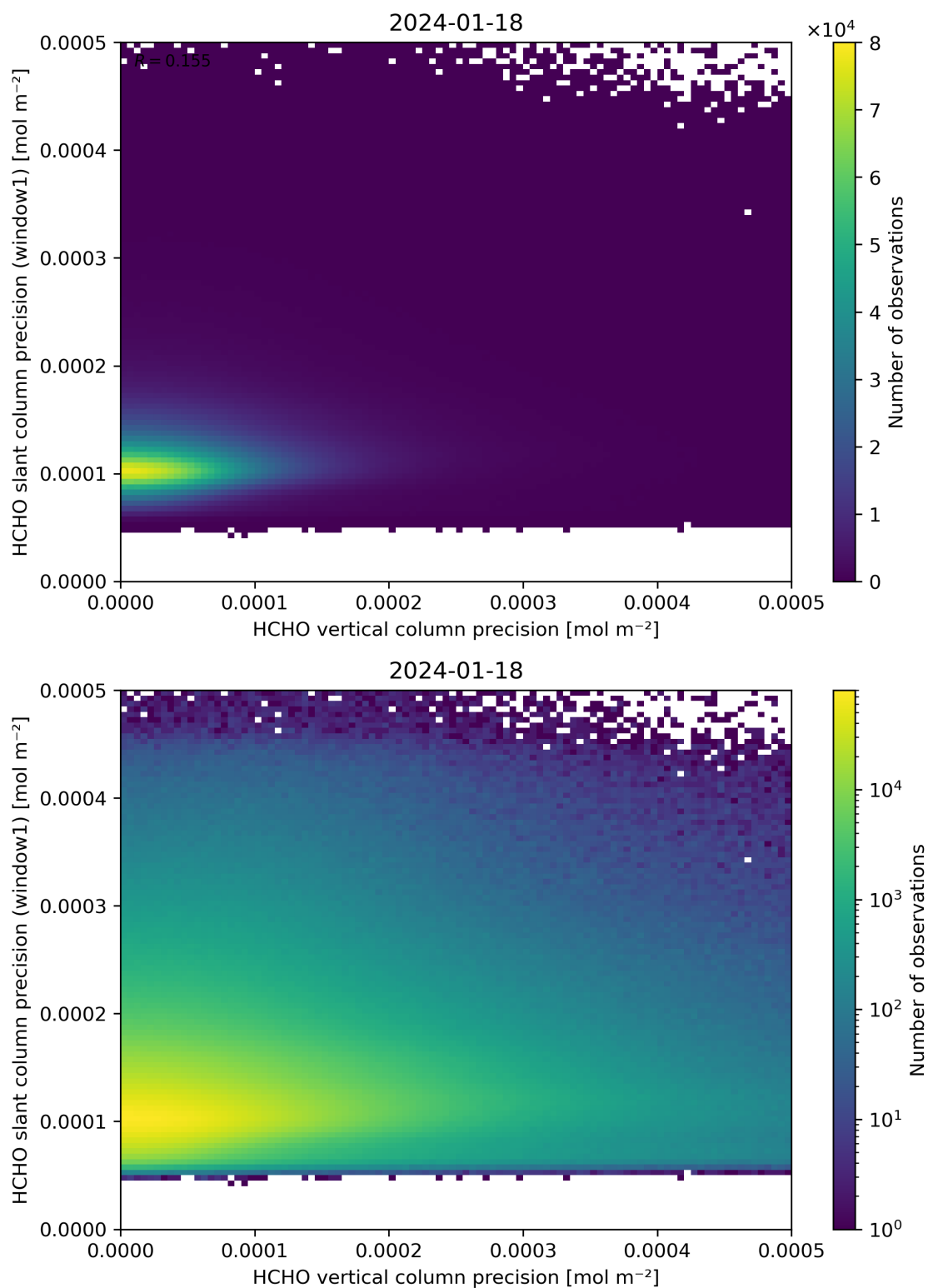
Figure 143: Scatter density plot of “HCHO vertical column precision” against “HCHO slant column precision (window1)” for 2024-01-17 to 2024-01-19.
