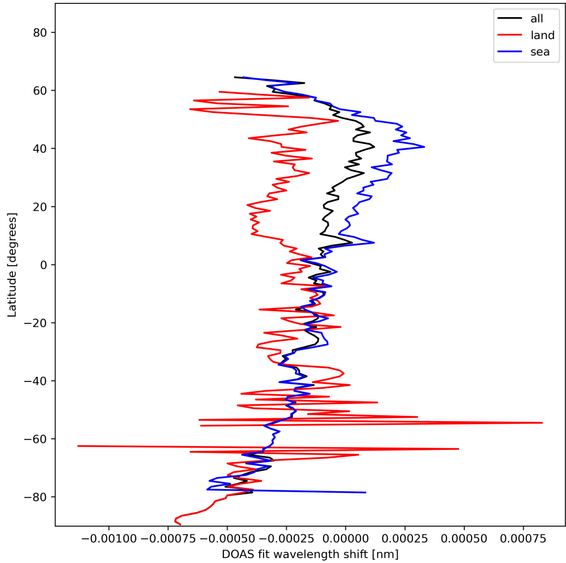
Figure 30: Zonal average of “DOAS fit wavelength shift” for 2024-01-17 to 2024-01-19.
