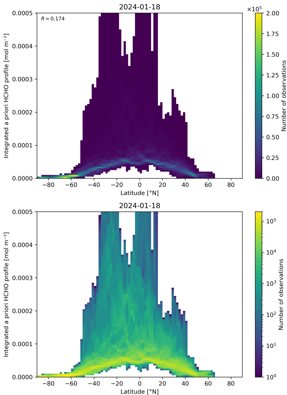
Figure 166: Scatter density plot of “Latitude” against “Integrated a priori HCHO profile” for 2024-01-17 to 2024-01-19.
