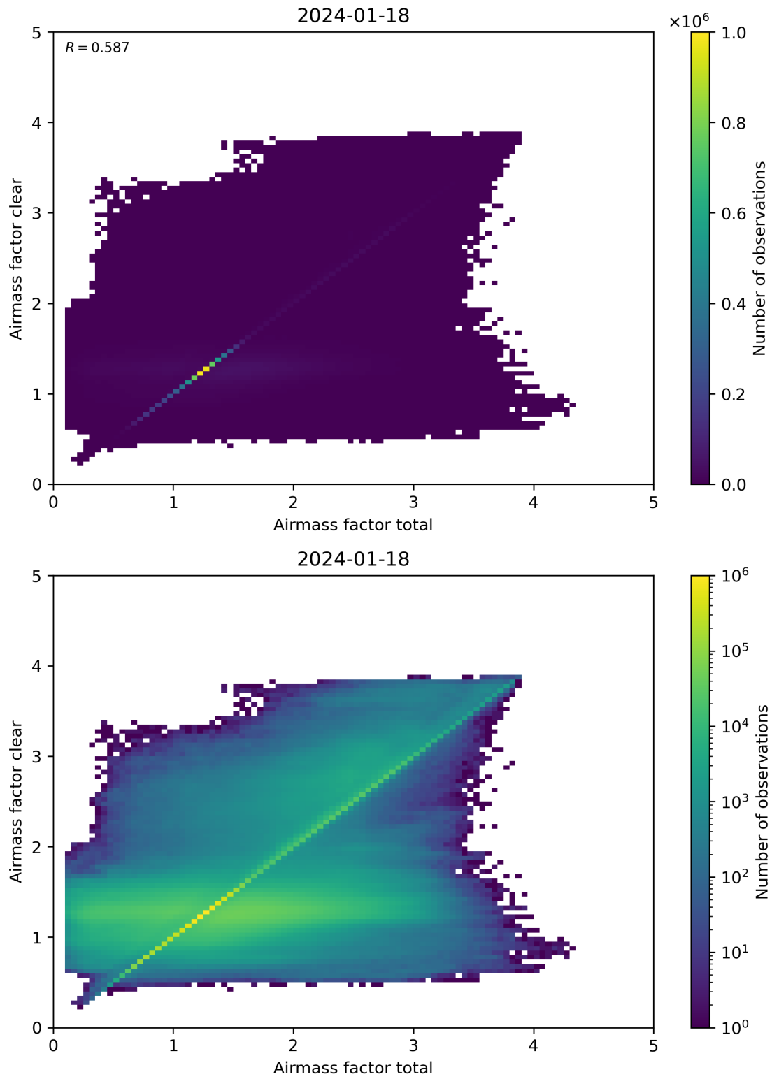
Figure 100: Scatter density plot of “Airmass factor total” against “Airmass factor clear” for 2024-01-17 to 2024-01-19.
