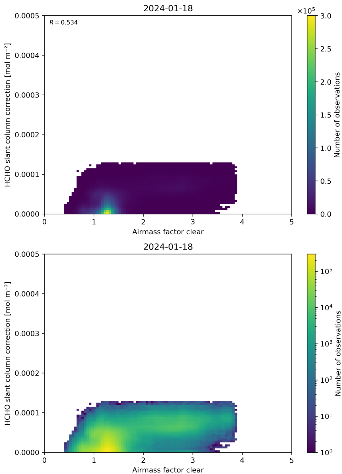
Figure 75: Scatter density plot of “Airmass factor clear” against “HCHO slant column correction” for 2024-01-17 to 2024-01-19.
