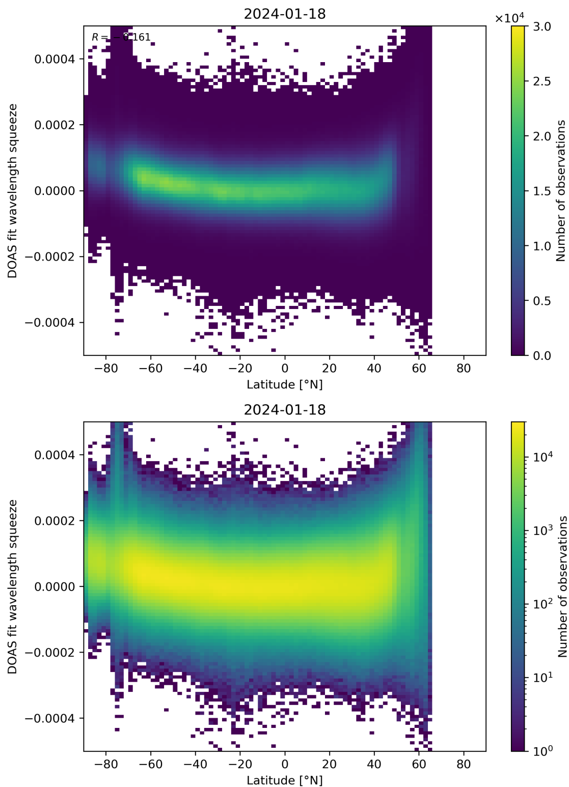
Figure 155: Scatter density plot of “Latitude” against “DOAS fit wavelength squeeze” for 2024-01-17 to 2024-01-19.
