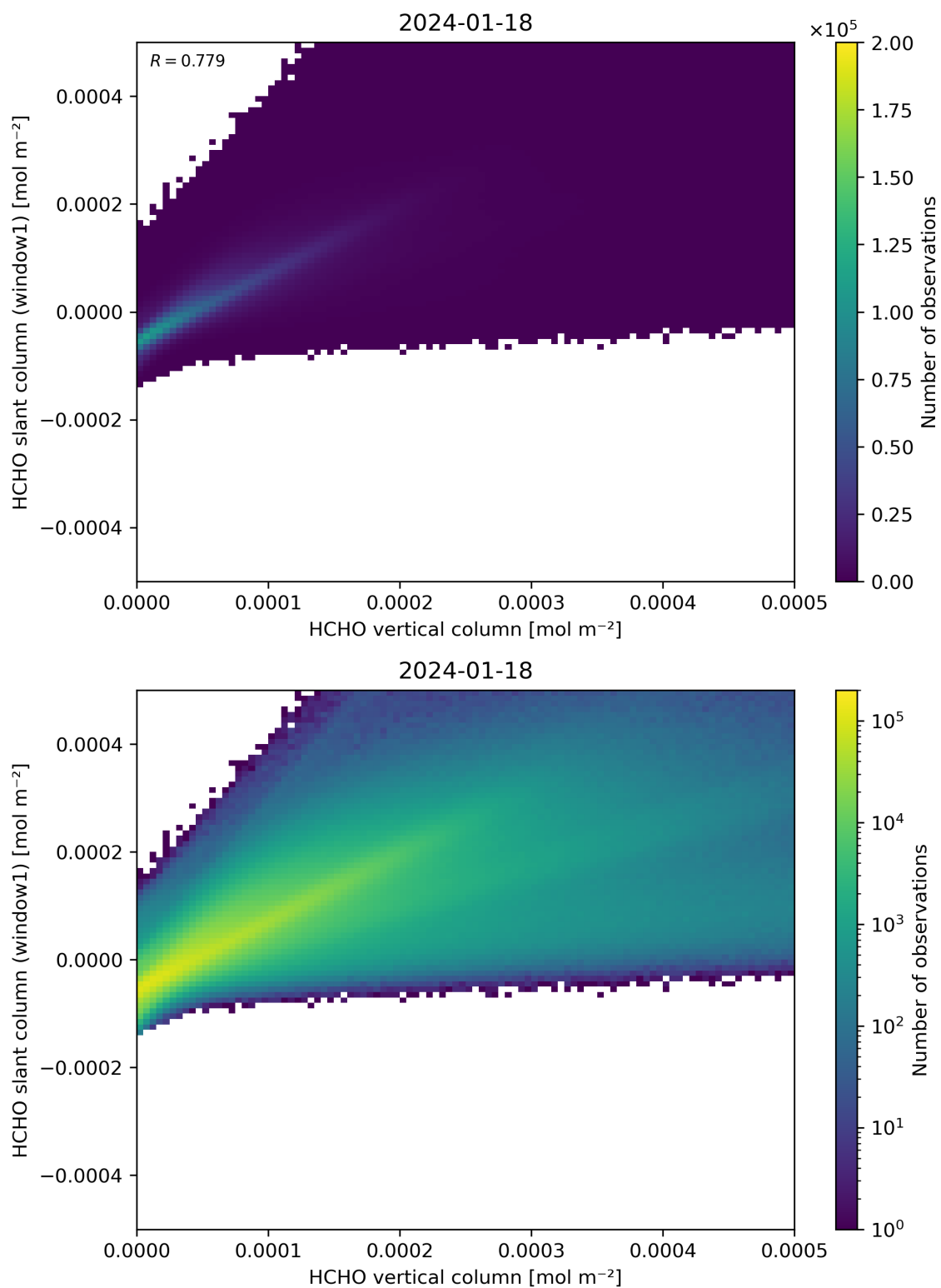
Figure 129: Scatter density plot of “HCHO vertical column” against “HCHO slant column (window1)” for 2024-01-17 to 2024-01-19.
