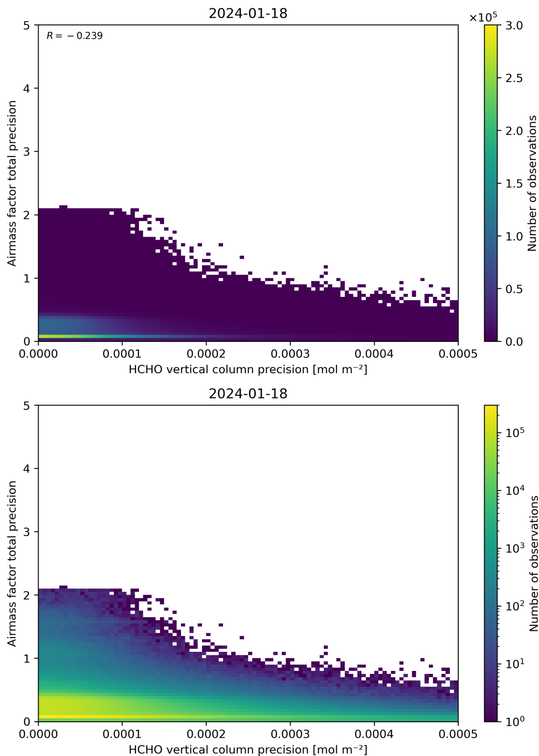
Figure 145: Scatter density plot of “HCHO vertical column precision” against “Airmass factor total precision” for 2024-01-17 to 2024-01-19.
