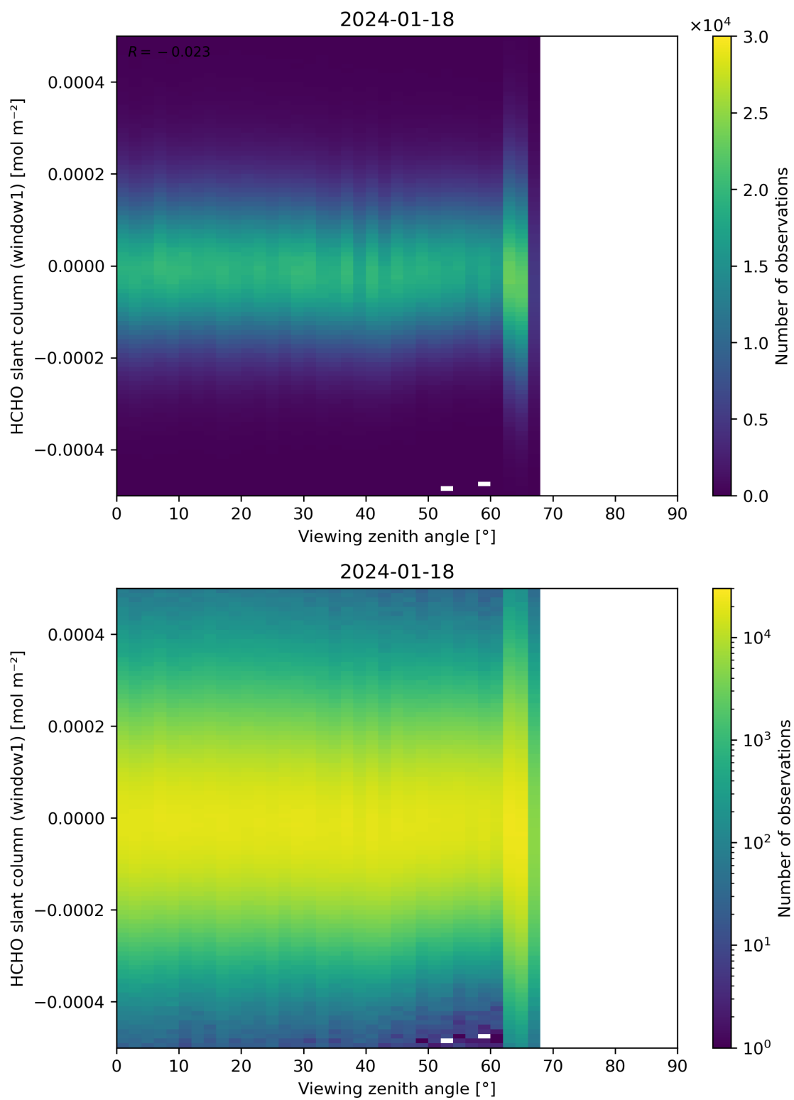
Figure 188: Scatter density plot of “Viewing zenith angle” against “HCHO slant column (window1)” for 2024-01-17 to 2024-01-19.
