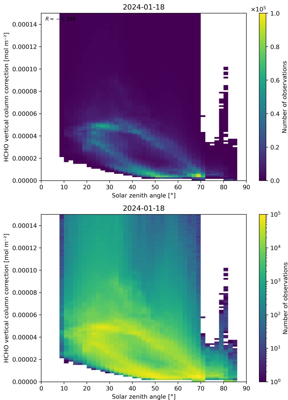
Figure 178: Scatter density plot of “Solar zenith angle” against “HCHO vertical column correction” for 2024-01-17 to 2024-01-19.
