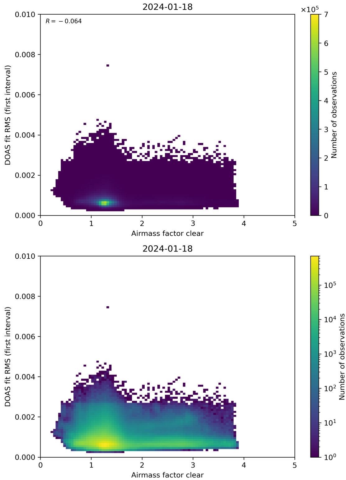
Figure 71: Scatter density plot of “Airmass factor clear” against “DOAS fit RMS (first interval)” for 2024-01-17 to 2024-01-19.
