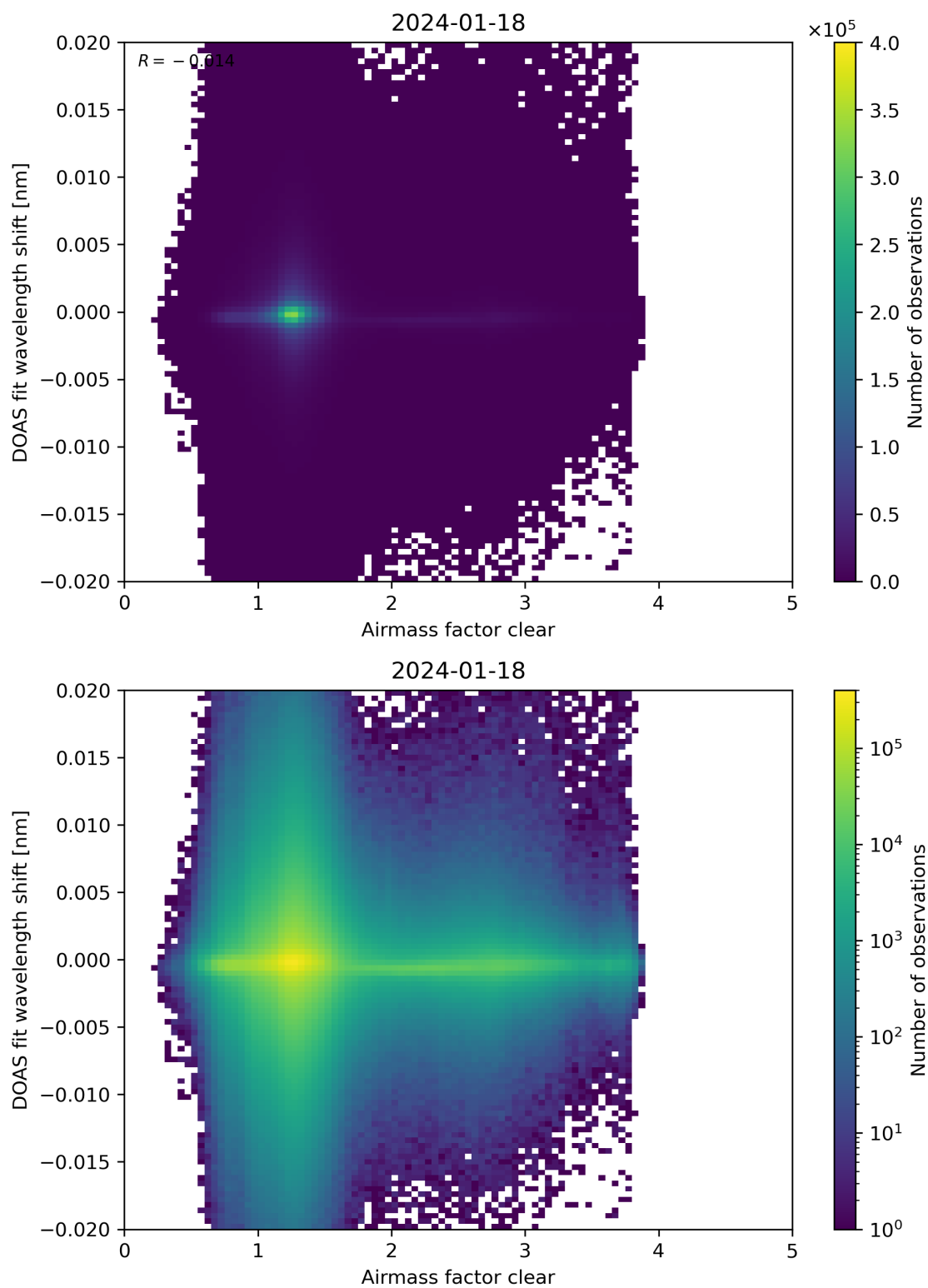
Figure 72: Scatter density plot of “Airmass factor clear” against “DOAS fit wavelength shift” for 2024-01-17 to 2024-01-19.
