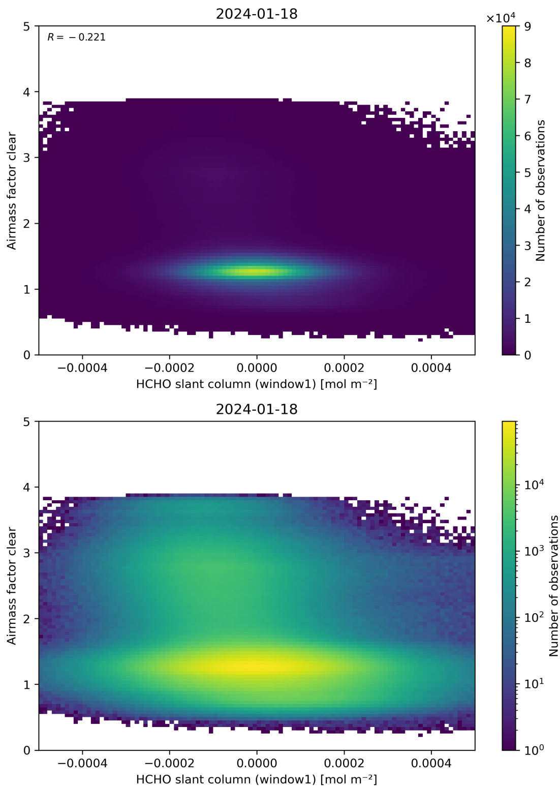
Figure 81: Scatter density plot of “HCHO slant column (window1)” against “Airmass factor clear” for 2024-01-17 to 2024-01-19.
