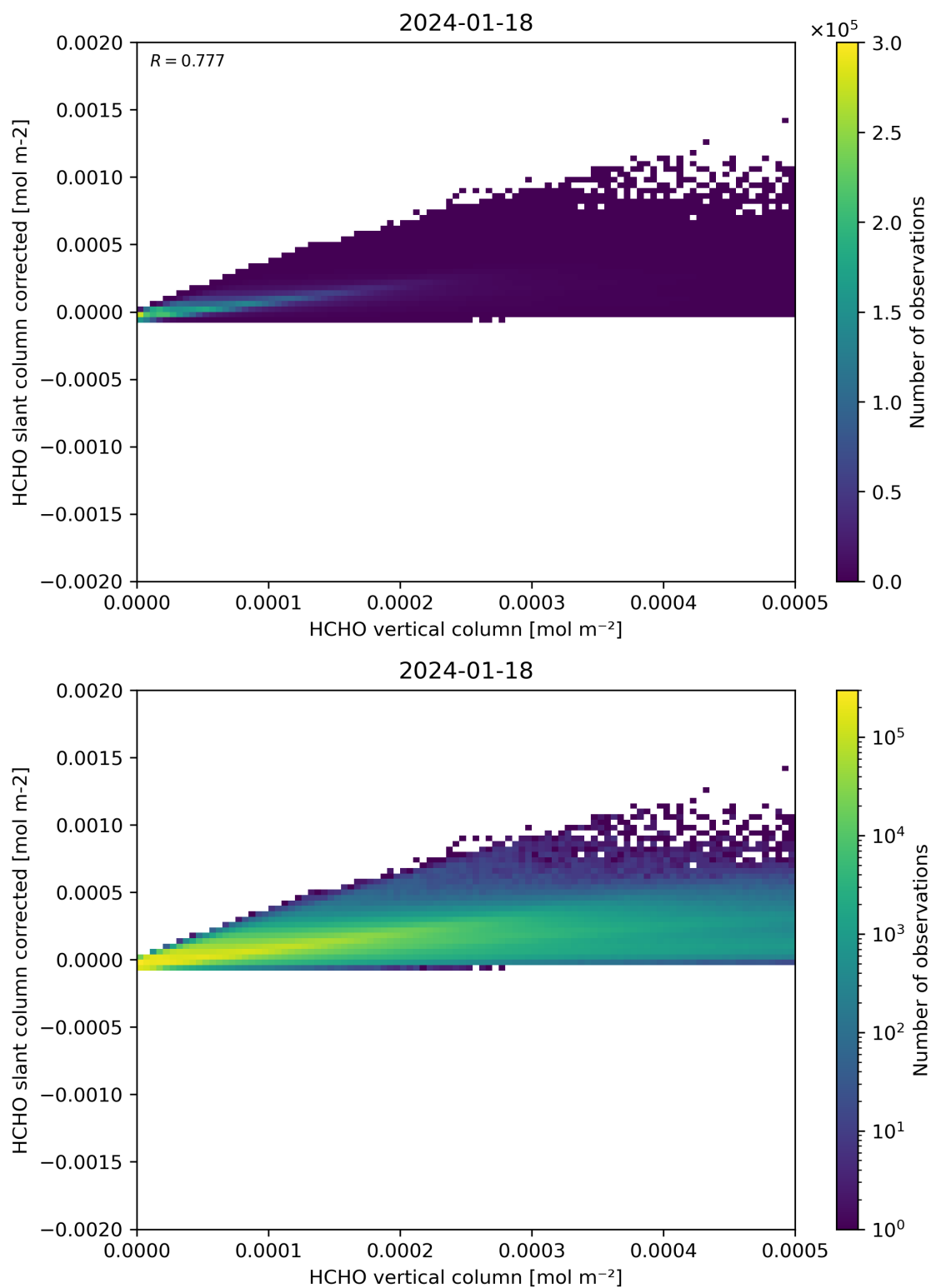
Figure 127: Scatter density plot of “HCHO vertical column” against “HCHO slant column corrected” for 2024-01-17 to 2024-01-19.
