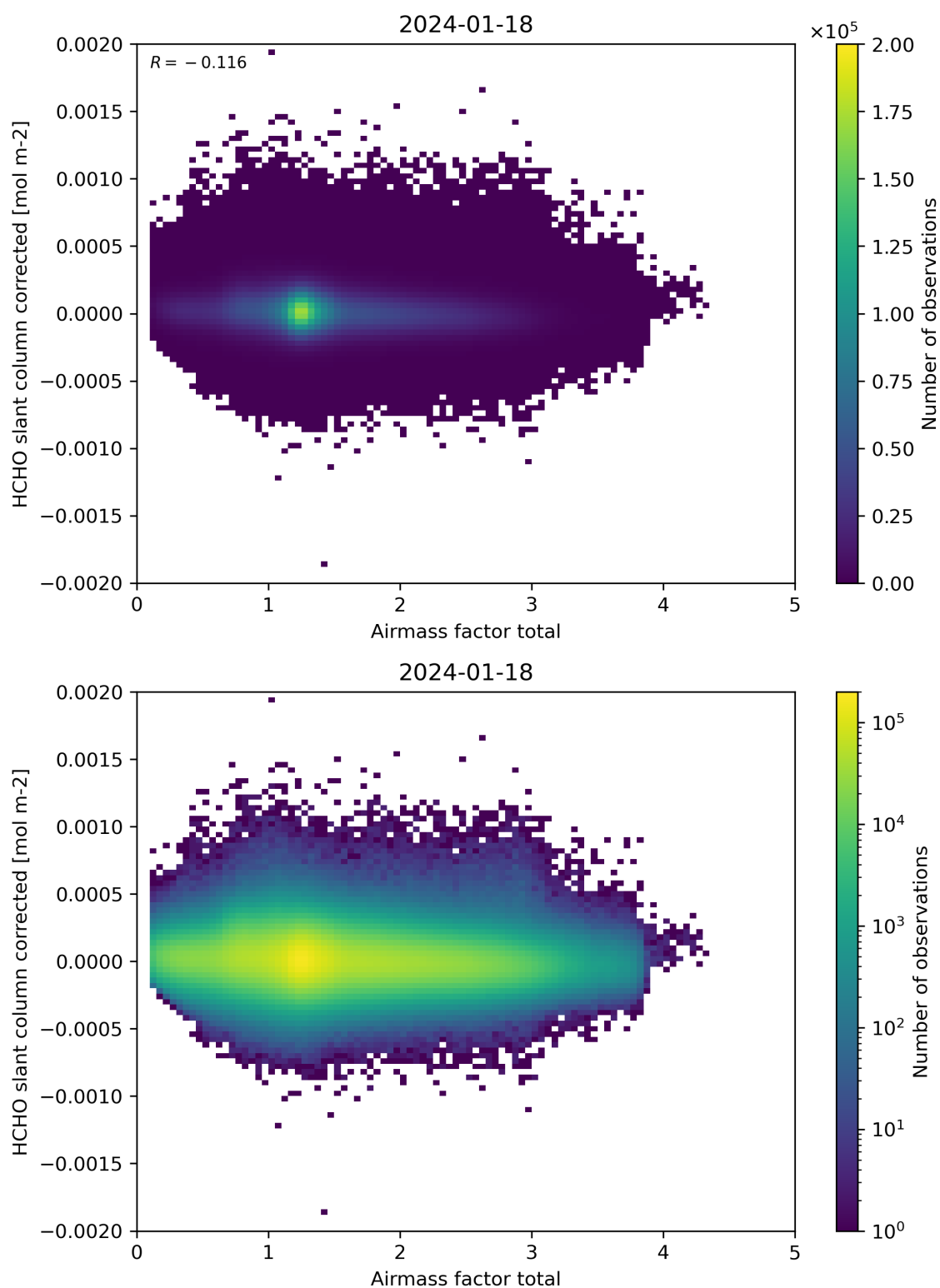
Figure 101: Scatter density plot of “Airmass factor total” against “HCHO slant column corrected” for 2024-01-17 to 2024-01-19.
