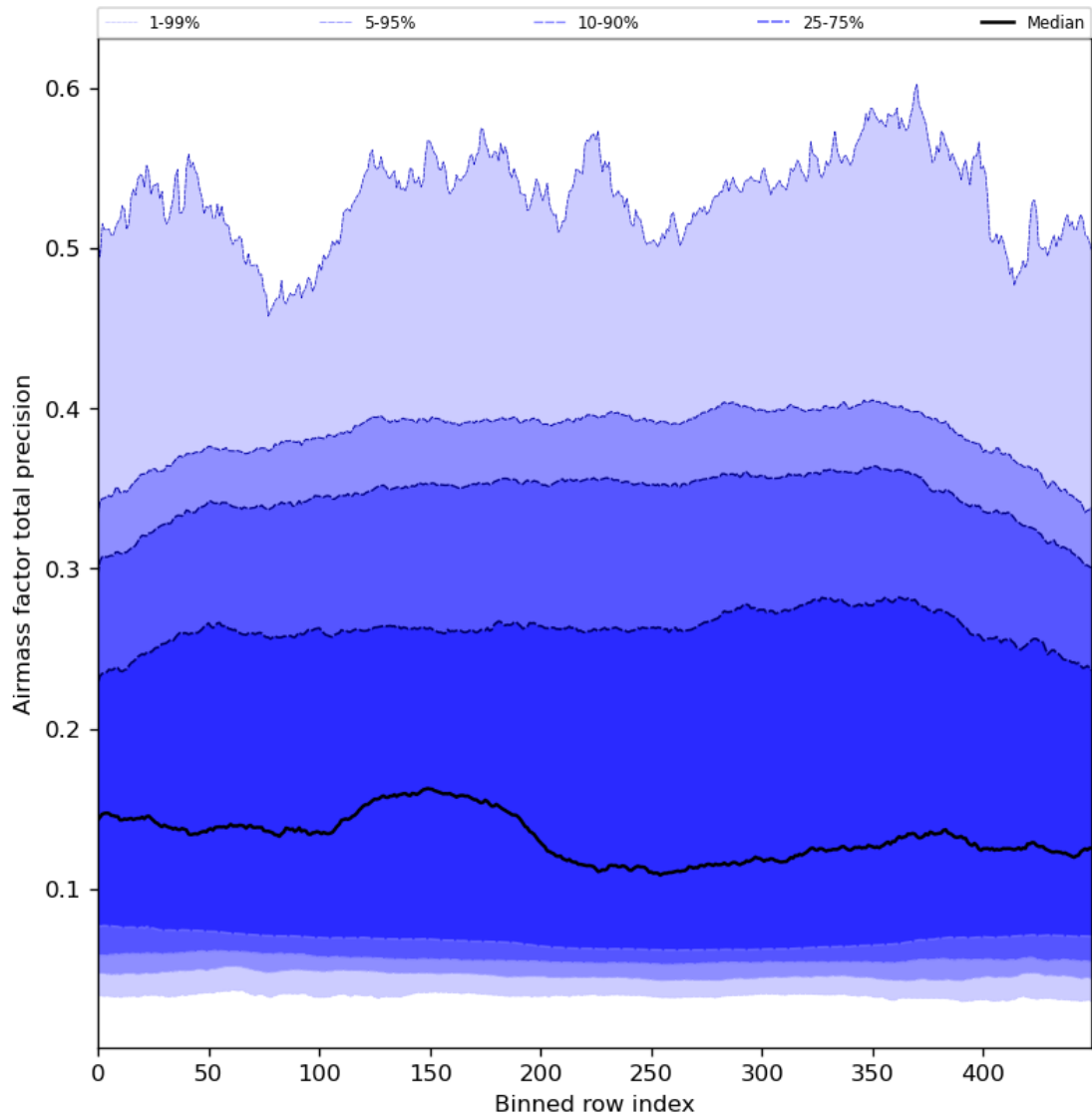
Figure 55: Along track statistics of “Airmass factor total precision” for 2024-01-17 to 2024-01-19
