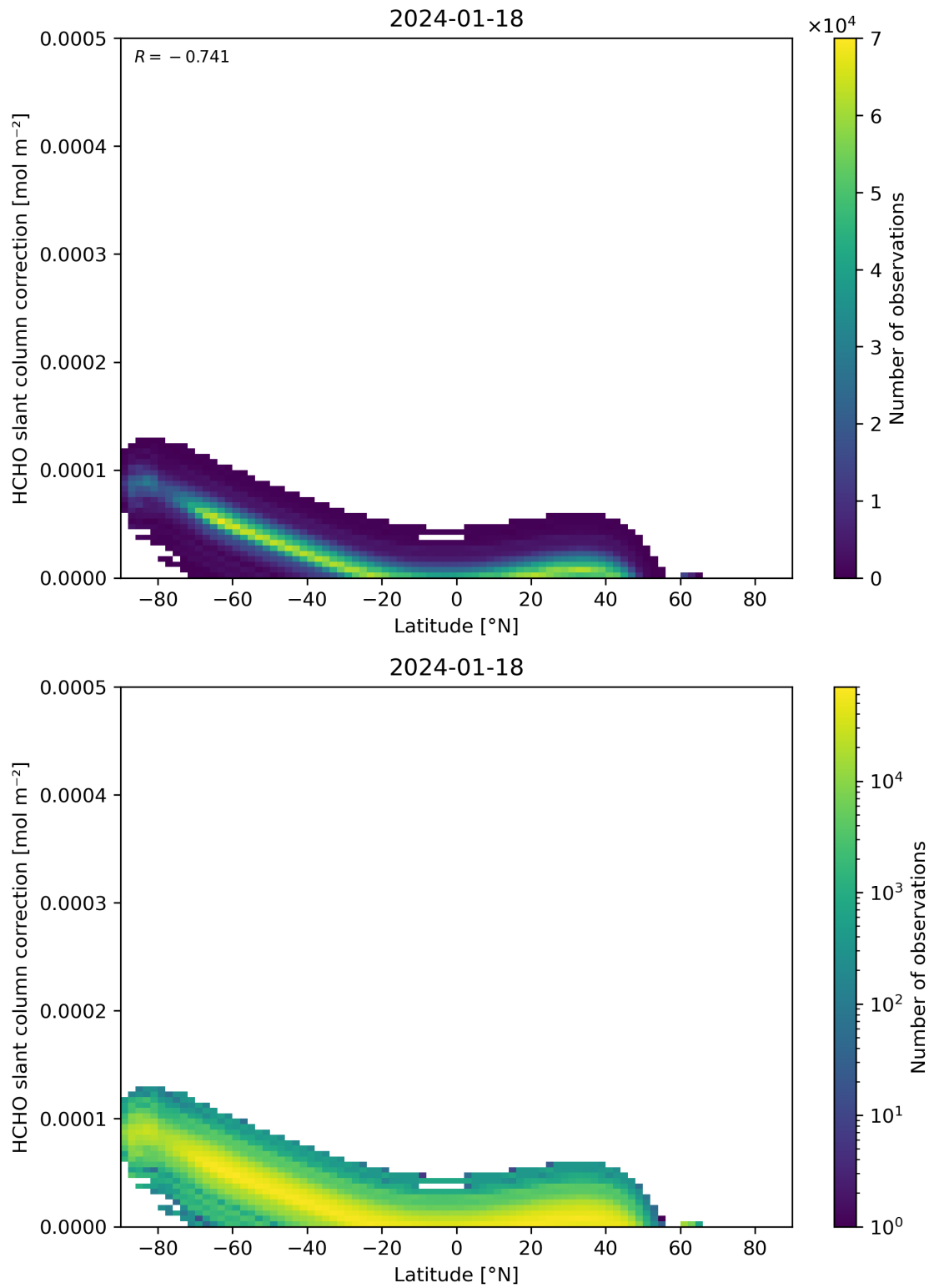
Figure 158: Scatter density plot of “Latitude” against “HCHO slant column correction” for 2024-01-17 to 2024-01-19.
