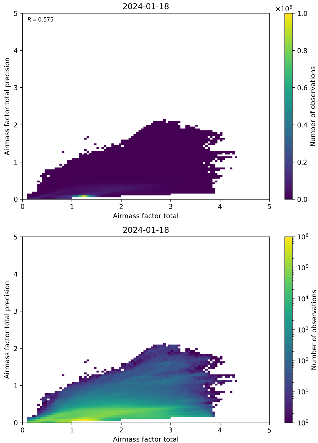
Figure 103: Scatter density plot of “Airmass factor total” against “Airmass factor total precision” for 2024-01-17 to 2024-01-19.
