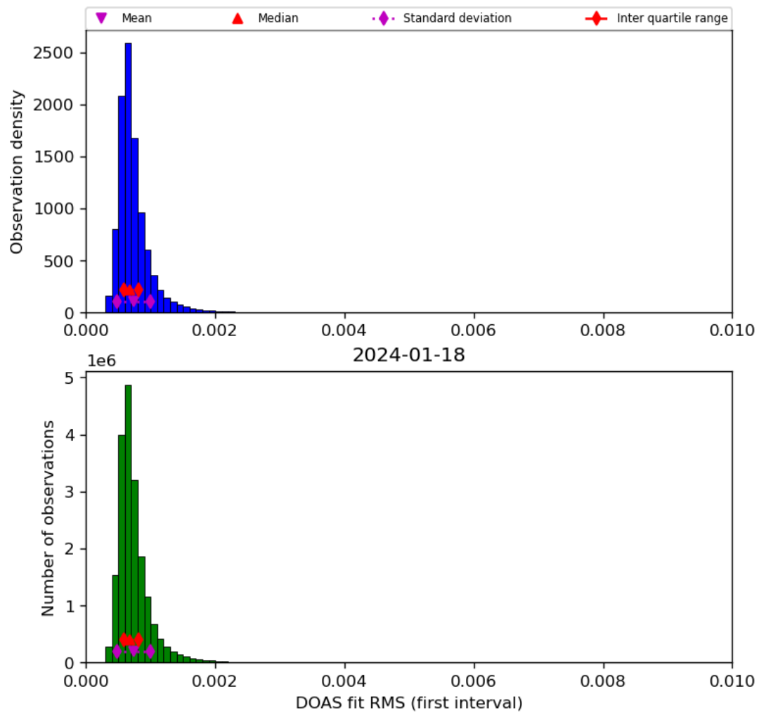
Figure 46: Histogram of “DOAS fit RMS (first interval)” for 2024-01-17 to 2024-01-19
