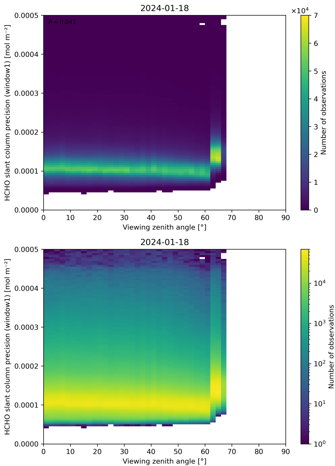
Figure 189: Scatter density plot of “Viewing zenith angle” against “HCHO slant column precision (window1)” for 2024-01-17 to 2024-01-19.
