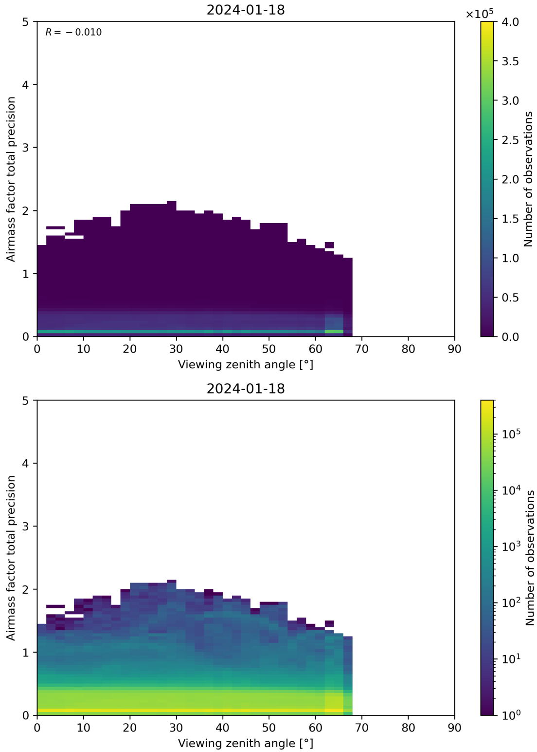
Figure 191: Scatter density plot of “Viewing zenith angle” against “Airmass factor total precision” for 2024-01-17 to 2024-01-19.
