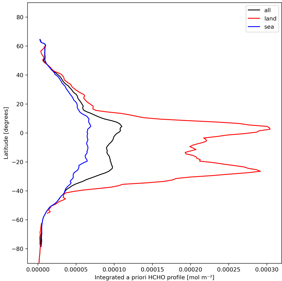
Figure 29: Zonal average of “Integrated a priori HCHO profile” for 2024-01-17 to 2024-01-19.
