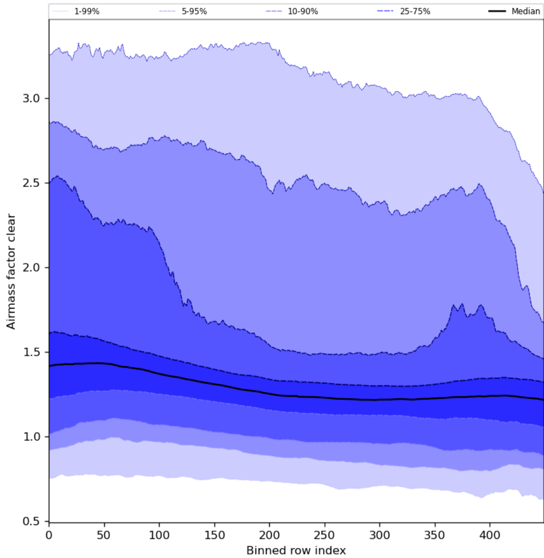
Figure 56: Along track statistics of “Airmass factor clear” for 2024-01-17 to 2024-01-19
