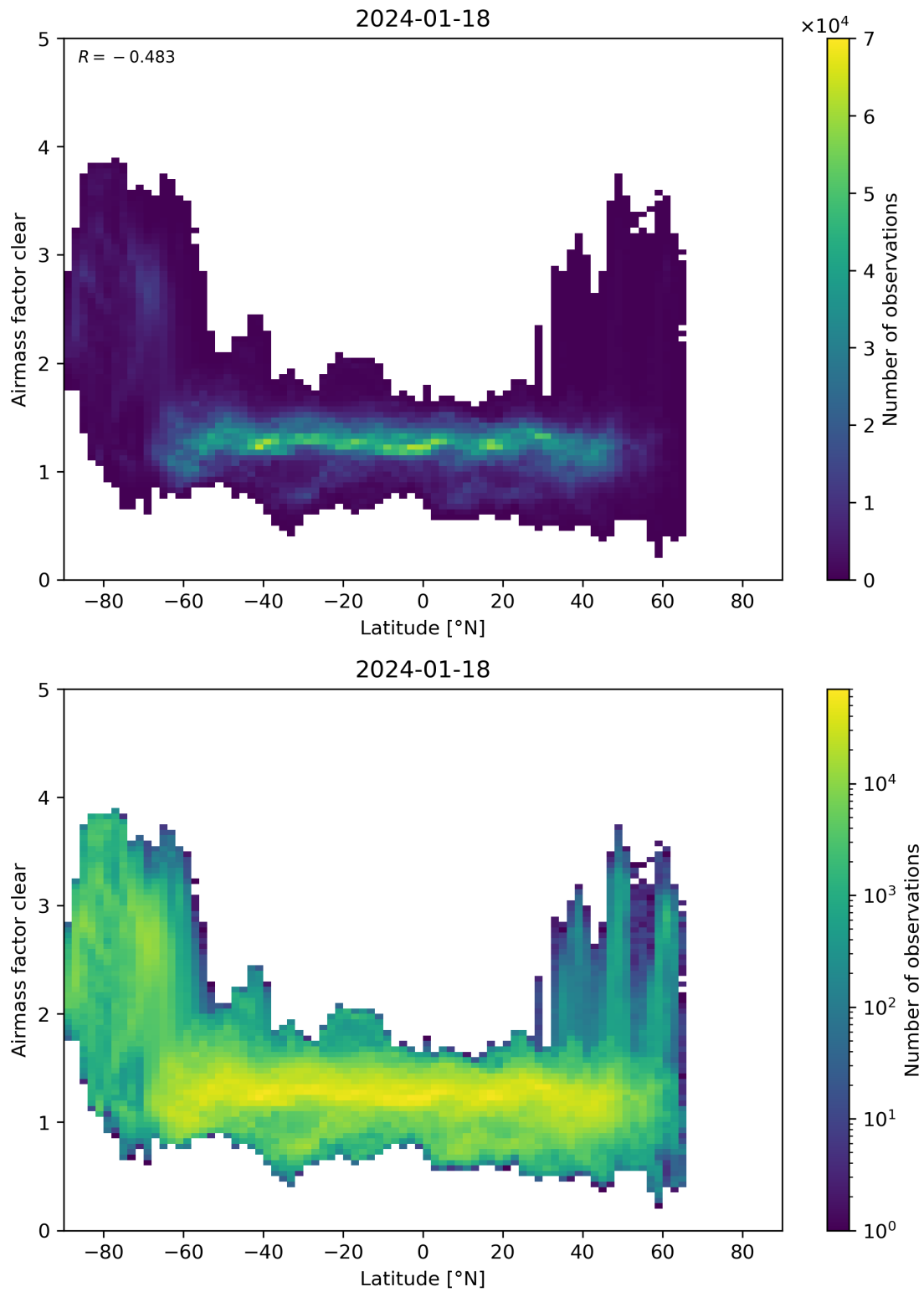
Figure 156: Scatter density plot of “Latitude” against “Airmass factor clear” for 2024-01-17 to 2024-01-19.
