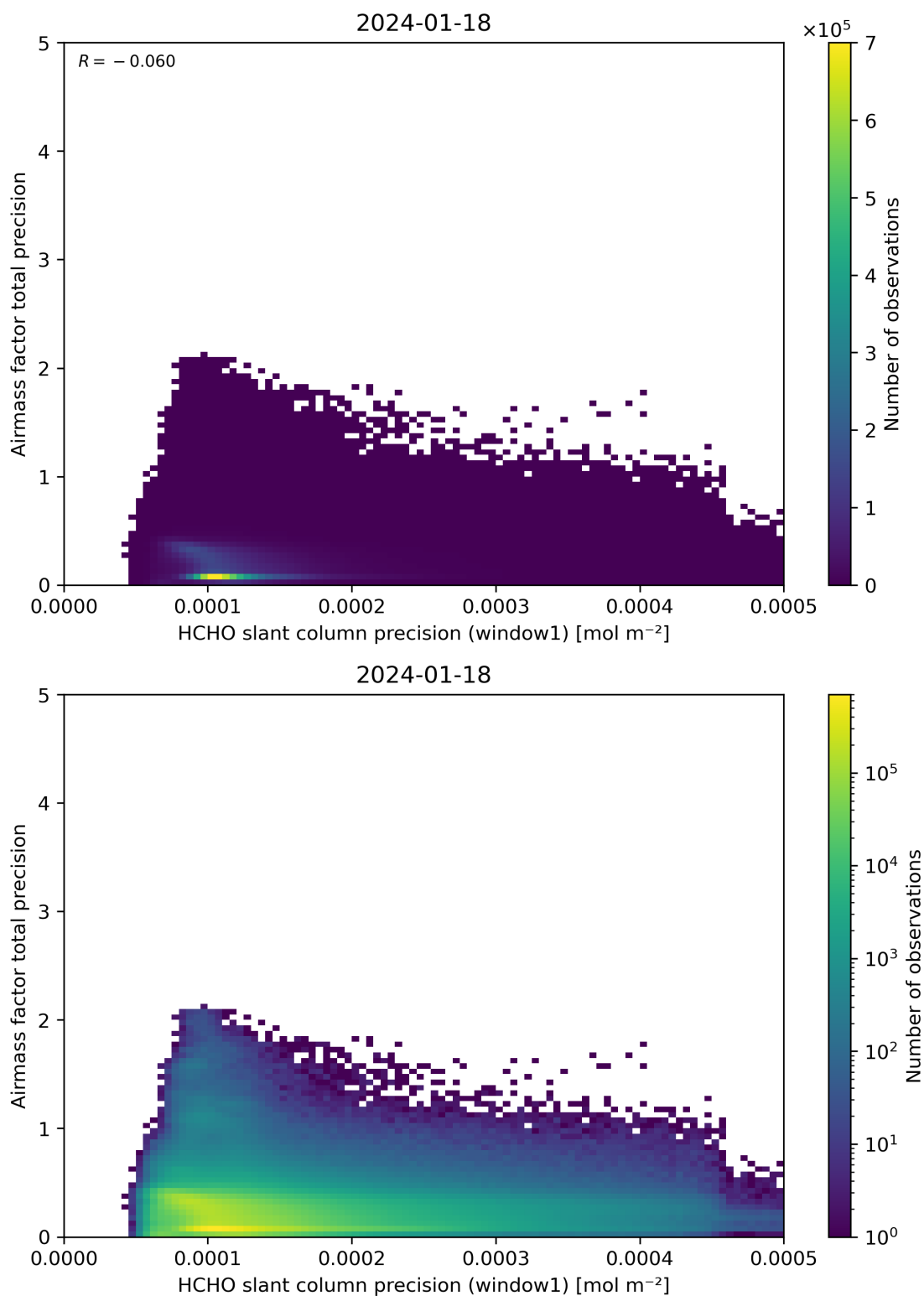
Figure 95: Scatter density plot of “HCHO slant column precision (window1)” against “Airmass factor total precision” for 2024-01-17 to 2024-01-19.
