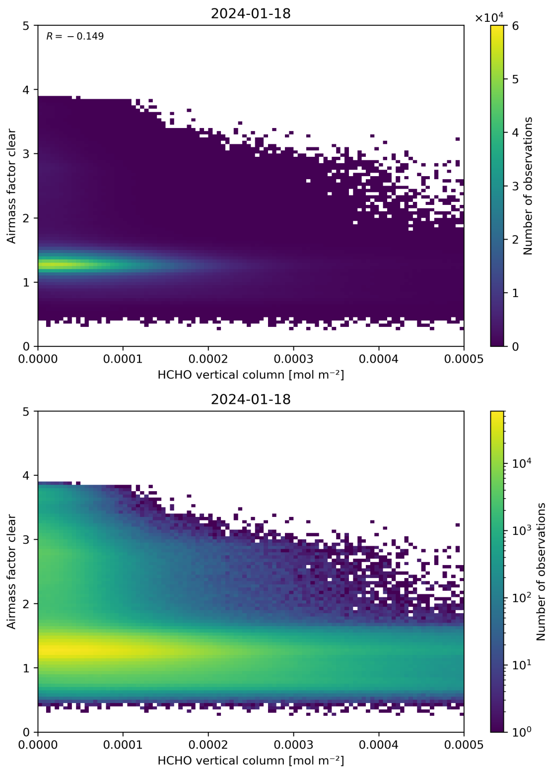
Figure 126: Scatter density plot of “HCHO vertical column” against “Airmass factor clear” for 2024-01-17 to 2024-01-19.
