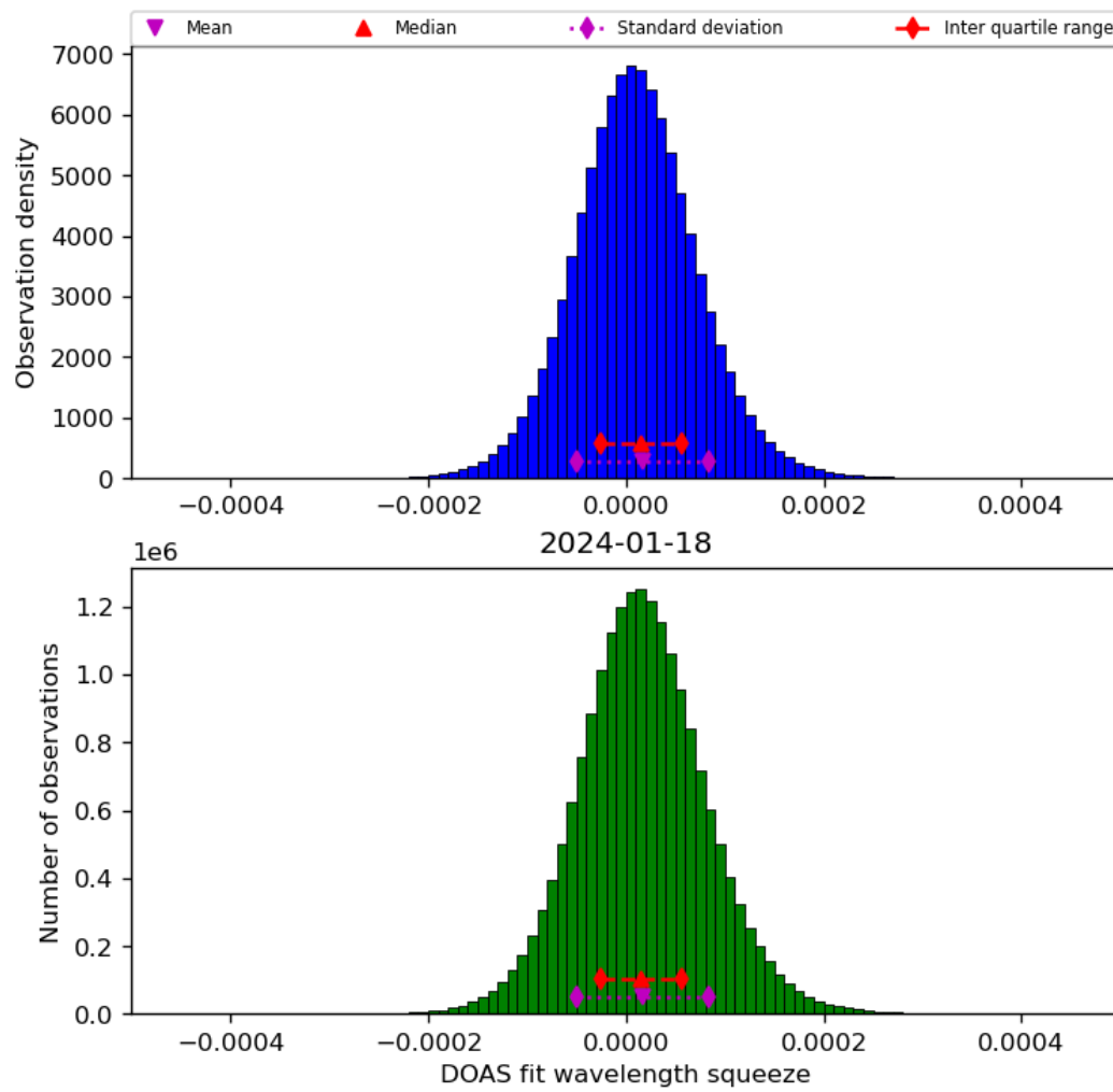
Figure 45: Histogram of “DOAS fit wavelength squeeze” for 2024-01-17 to 2024-01-19
