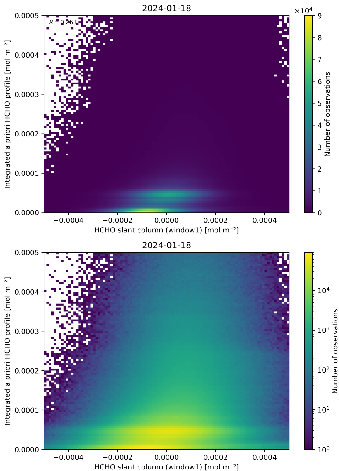
Figure 87: Scatter density plot of “HCHO slant column (window1)” against “Integrated a priori HCHO profile” for 2024-01-17 to 2024-01-19.
