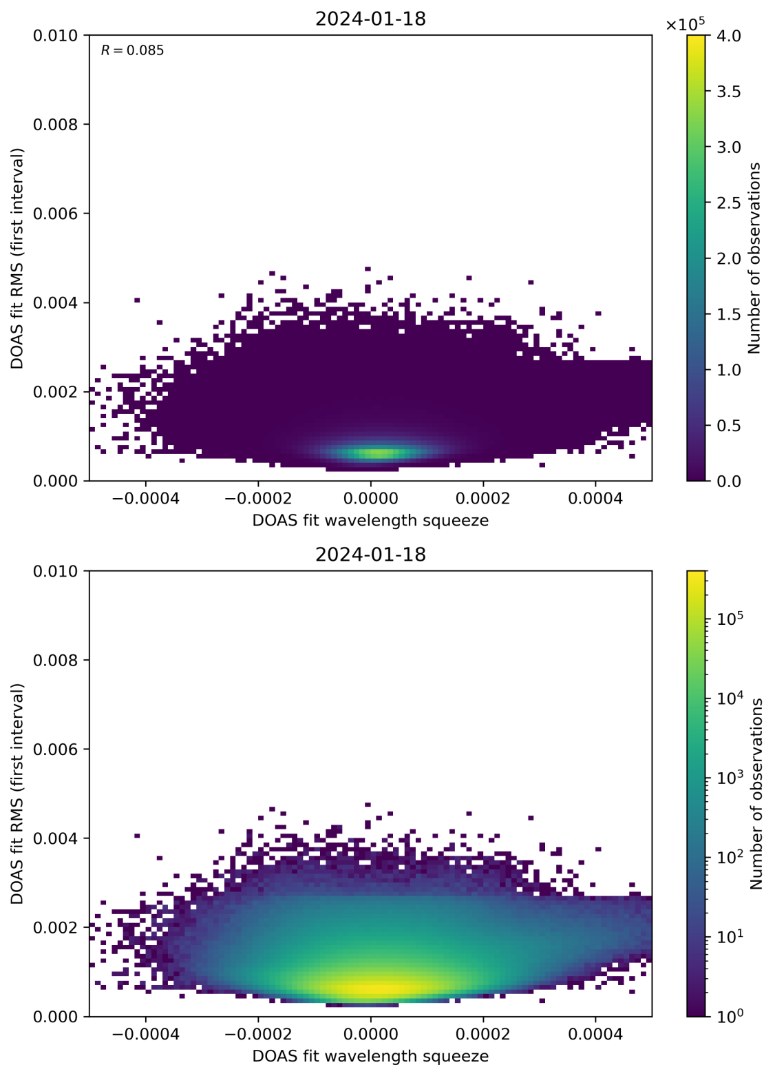
Figure 68: Scatter density plot of “DOAS fit wavelength squeeze” against “DOAS fit RMS (first interval)” for 2024-01-17 to 2024-01-19.
