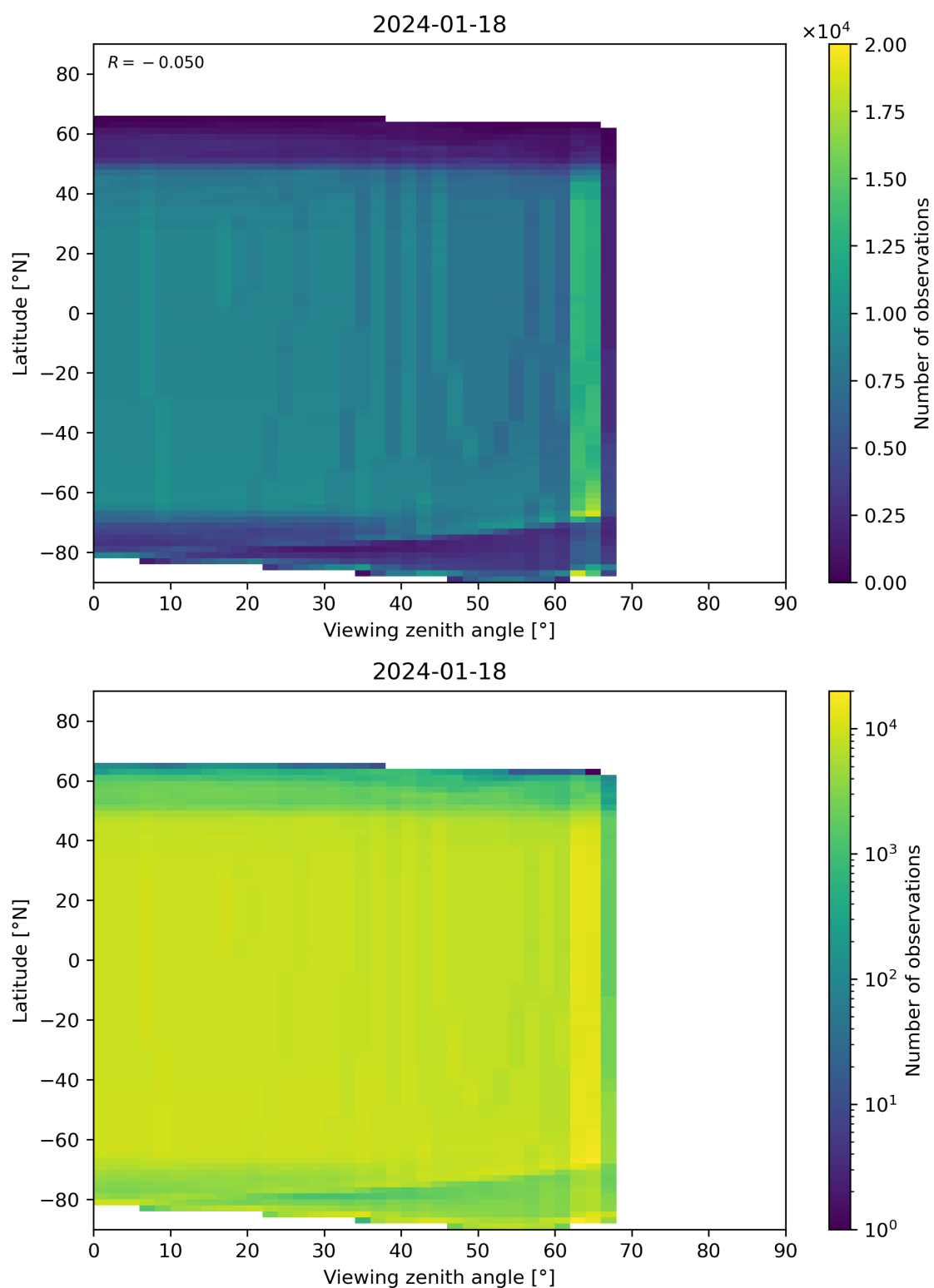
Figure 196: Scatter density plot of “Viewing zenith angle” against “Latitude” for 2024-01-17 to 2024-01-19.
