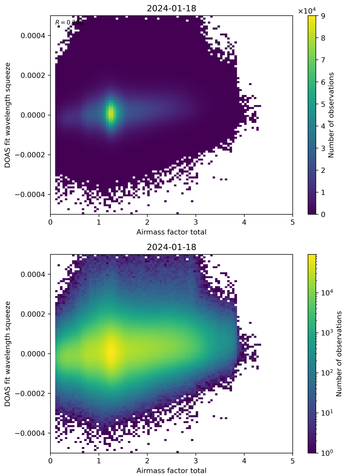
Figure 99: Scatter density plot of “Airmass factor total” against “DOAS fit wavelength squeeze” for 2024-01-17 to 2024-01-19.
