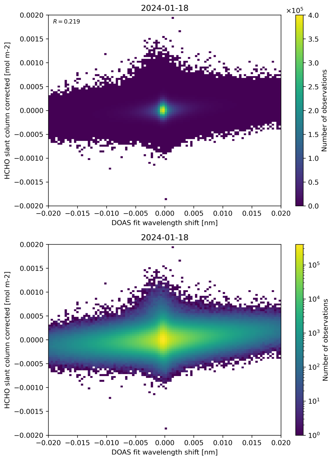
Figure 66: Scatter density plot of “DOAS fit wavelength shift” against “HCHO slant column corrected” for 2024-01-17 to 2024-01-19.
