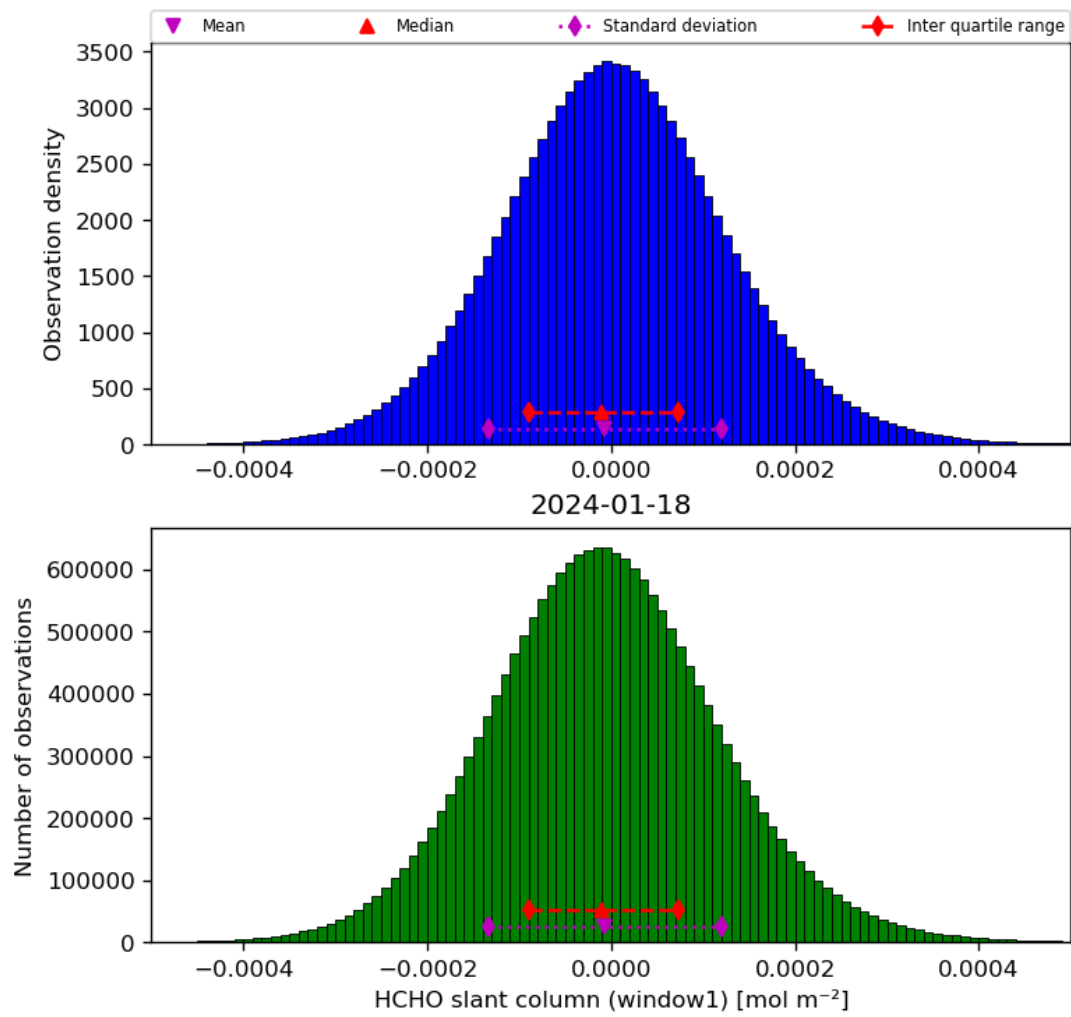
Figure 38: Histogram of “HCHO slant column (window1)” for 2024-01-17 to 2024-01-19
