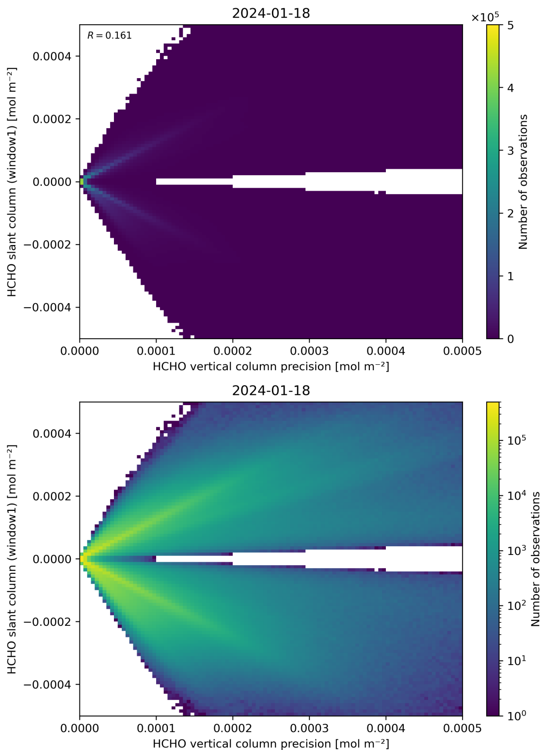
Figure 142: Scatter density plot of “HCHO vertical column precision” against “HCHO slant column (window1)” for 2024-01-17 to 2024-01-19.
