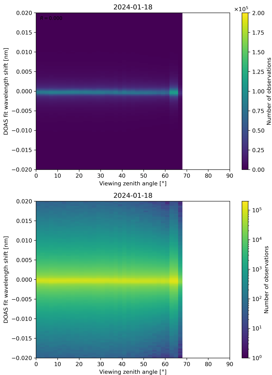
Figure 183: Scatter density plot of “Viewing zenith angle” against “DOAS fit wavelength shift” for 2024-01-17 to 2024-01-19.
