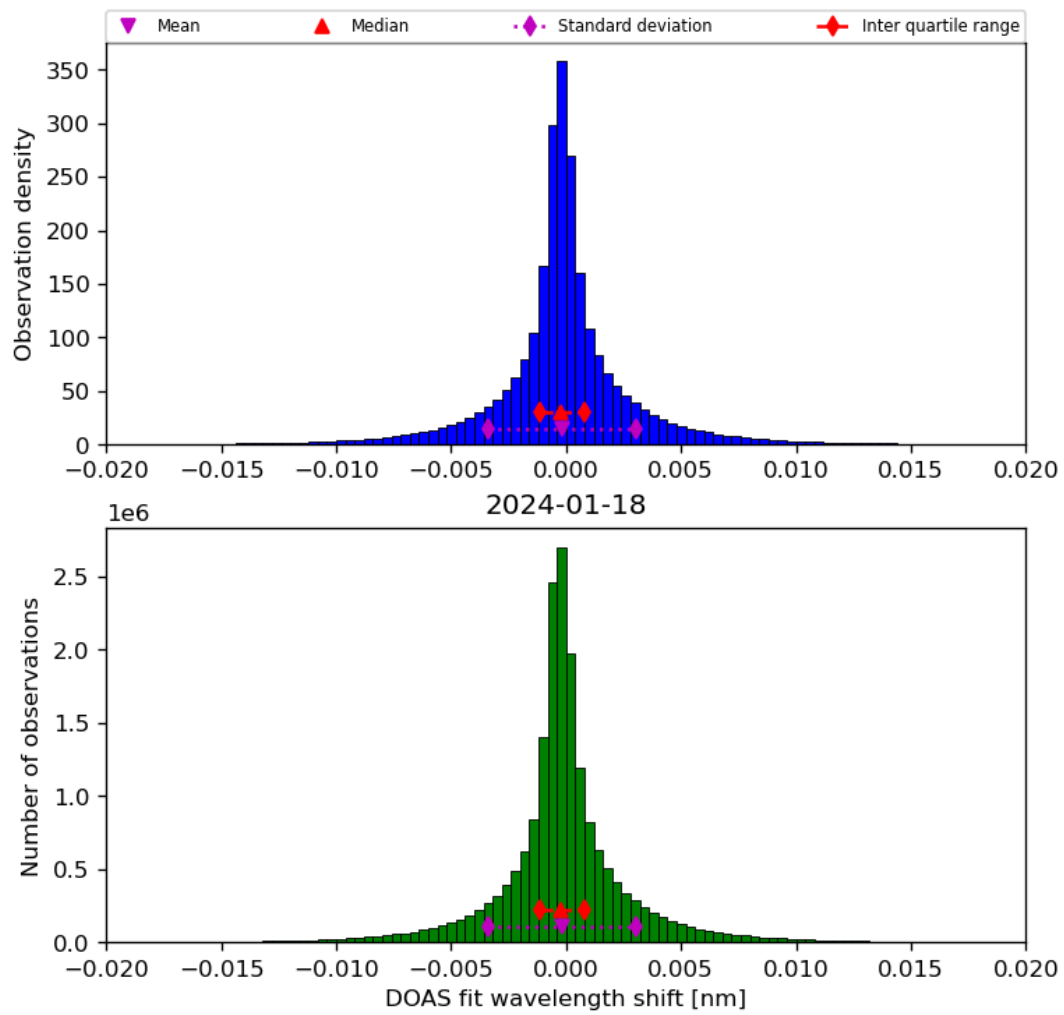
Figure 44: Histogram of “DOAS fit wavelength shift” for 2024-01-17 to 2024-01-19
