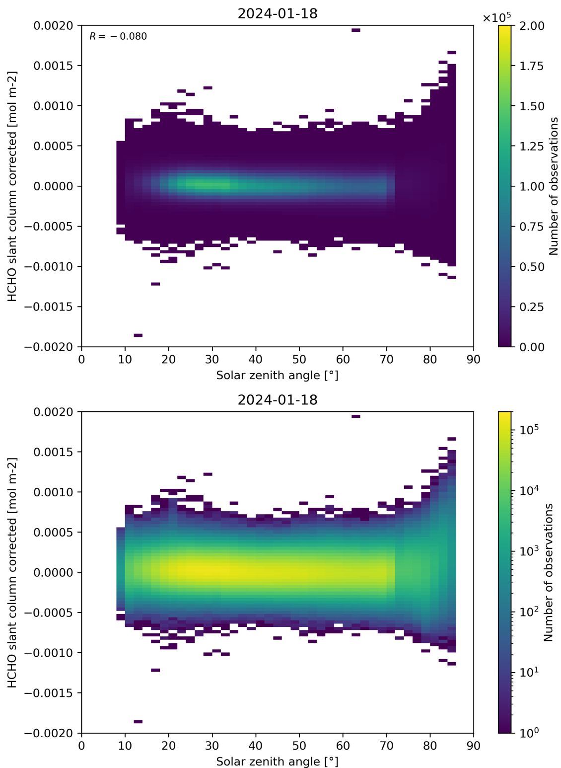
Figure 171: Scatter density plot of “Solar zenith angle” against “HCHO slant column corrected” for 2024-01-17 to 2024-01-19.
