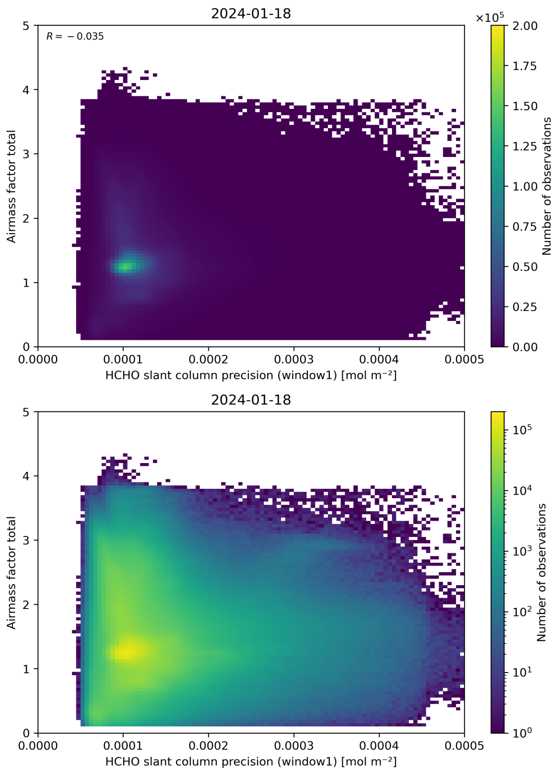
Figure 94: Scatter density plot of “HCHO slant column precision (window1)” against “Airmass factor total” for 2024-01-17 to 2024-01-19.
