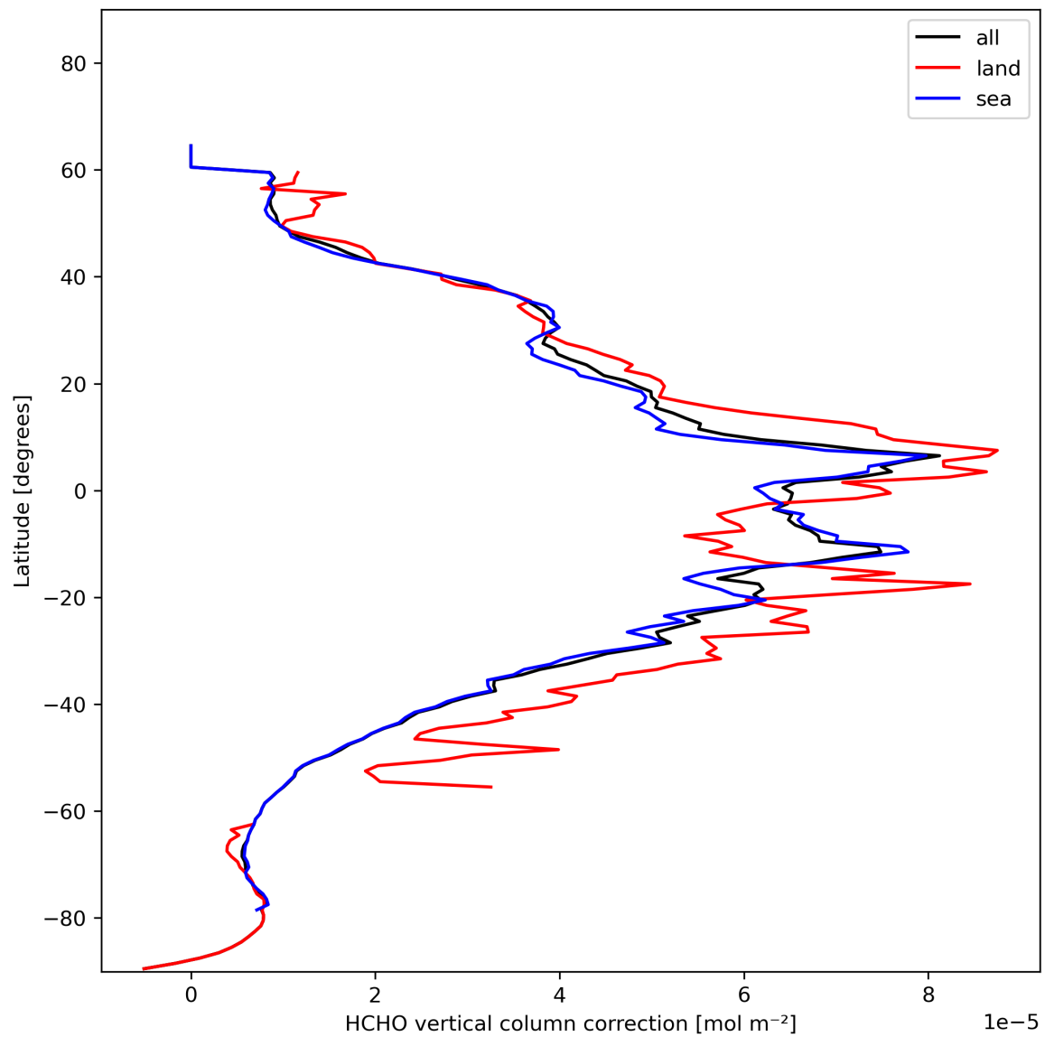
Figure 23: Zonal average of “HCHO vertical column correction” for 2024-01-17 to 2024-01-19.
