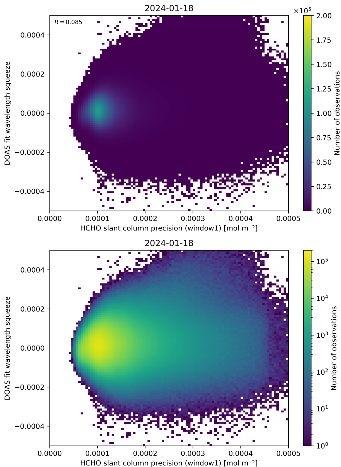
Figure 90: Scatter density plot of “HCHO slant column precision (window1)” against “DOAS fit wavelength squeeze” for 2024-01-17 to 2024-01-19.
