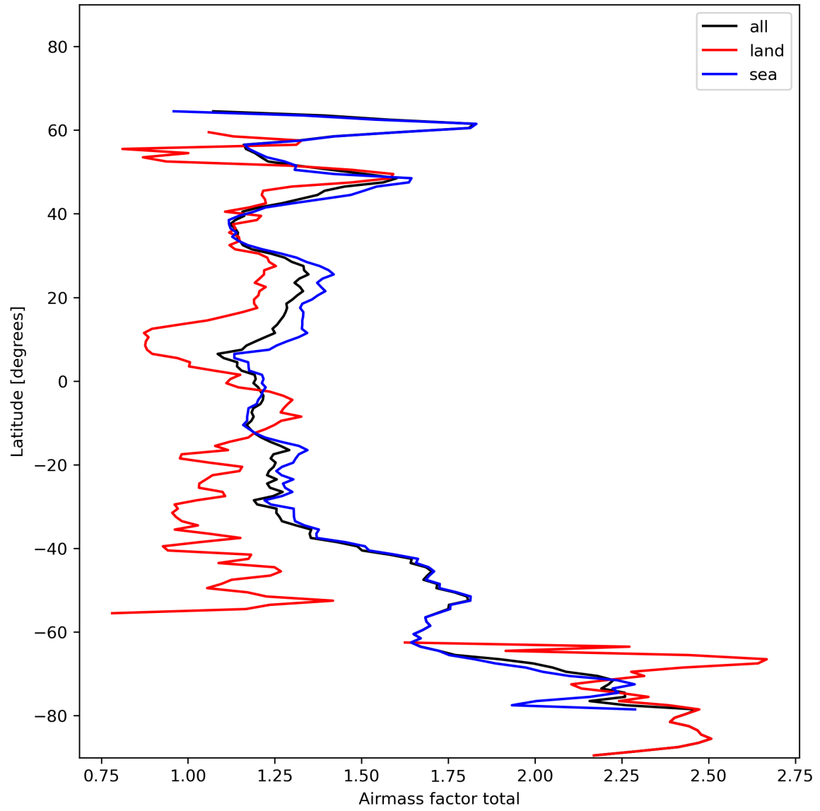
Figure 26: Zonal average of “Airmass factor total” for 2024-01-17 to 2024-01-19.
