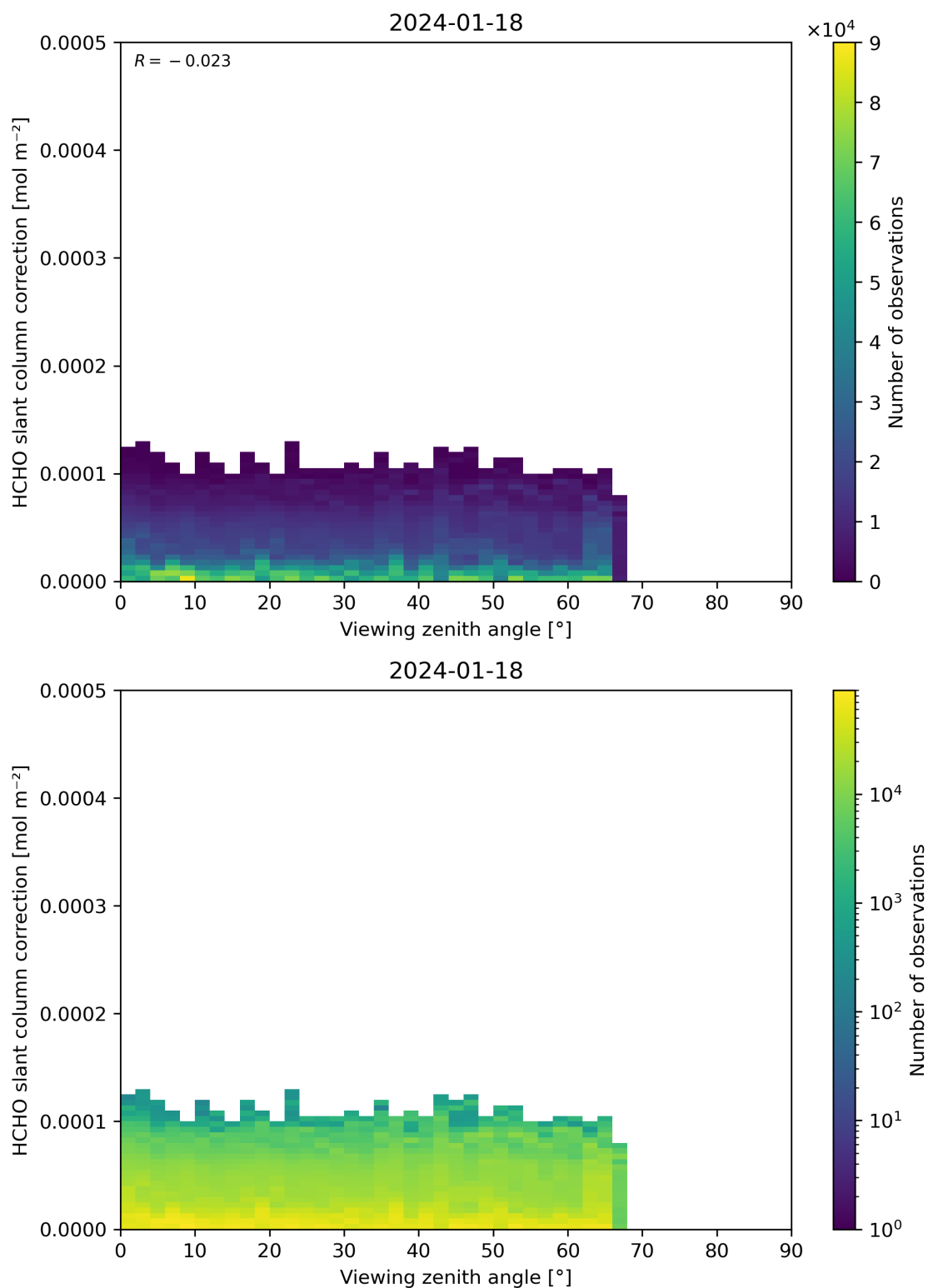
Figure 187: Scatter density plot of “Viewing zenith angle” against “HCHO slant column correction” for 2024-01-17 to 2024-01-19.
