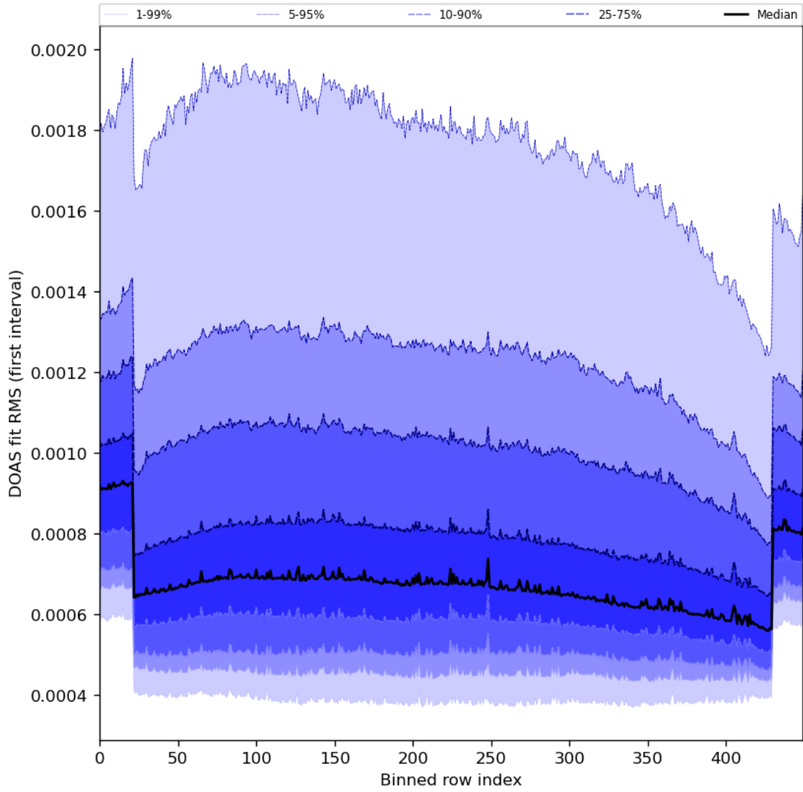
Figure 60: Along track statistics of “DOAS fit RMS (first interval)” for 2024-01-17 to 2024-01-19
