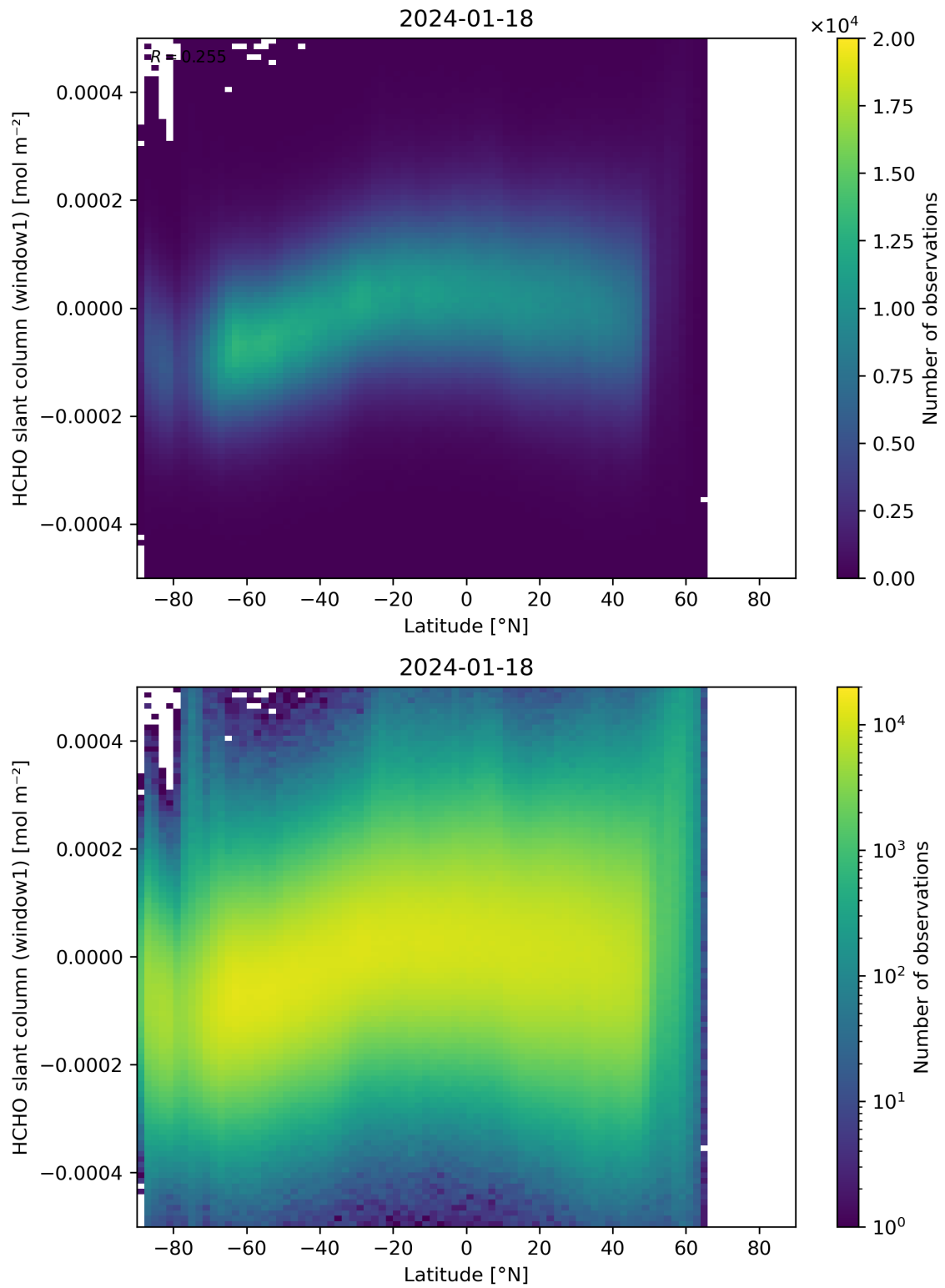
Figure 159: Scatter density plot of “Latitude” against “HCHO slant column (window1)” for 2024-01-17 to 2024-01-19.
