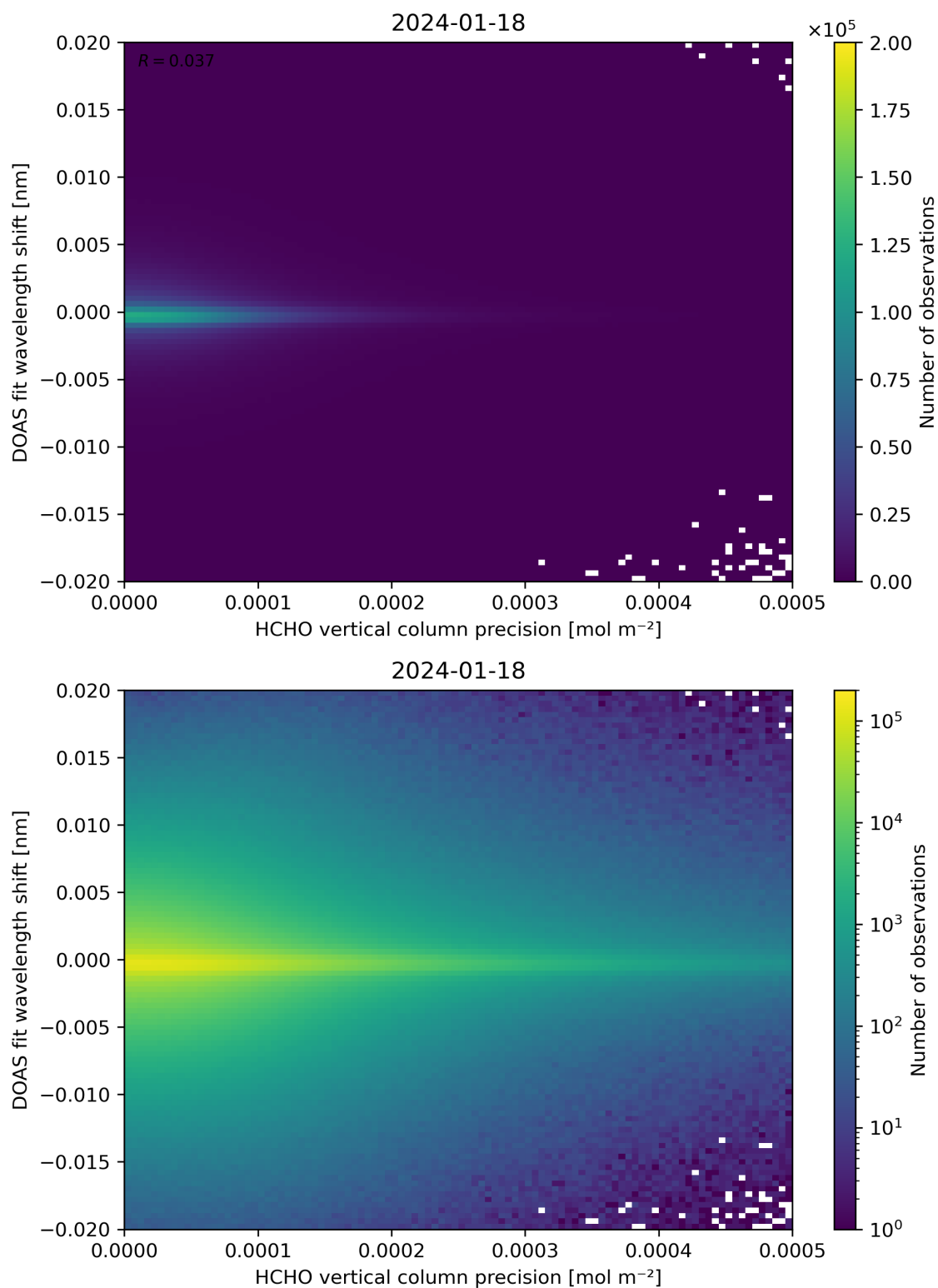
Figure 137: Scatter density plot of “HCHO vertical column precision” against “DOAS fit wavelength shift” for 2024-01-17 to 2024-01-19.
