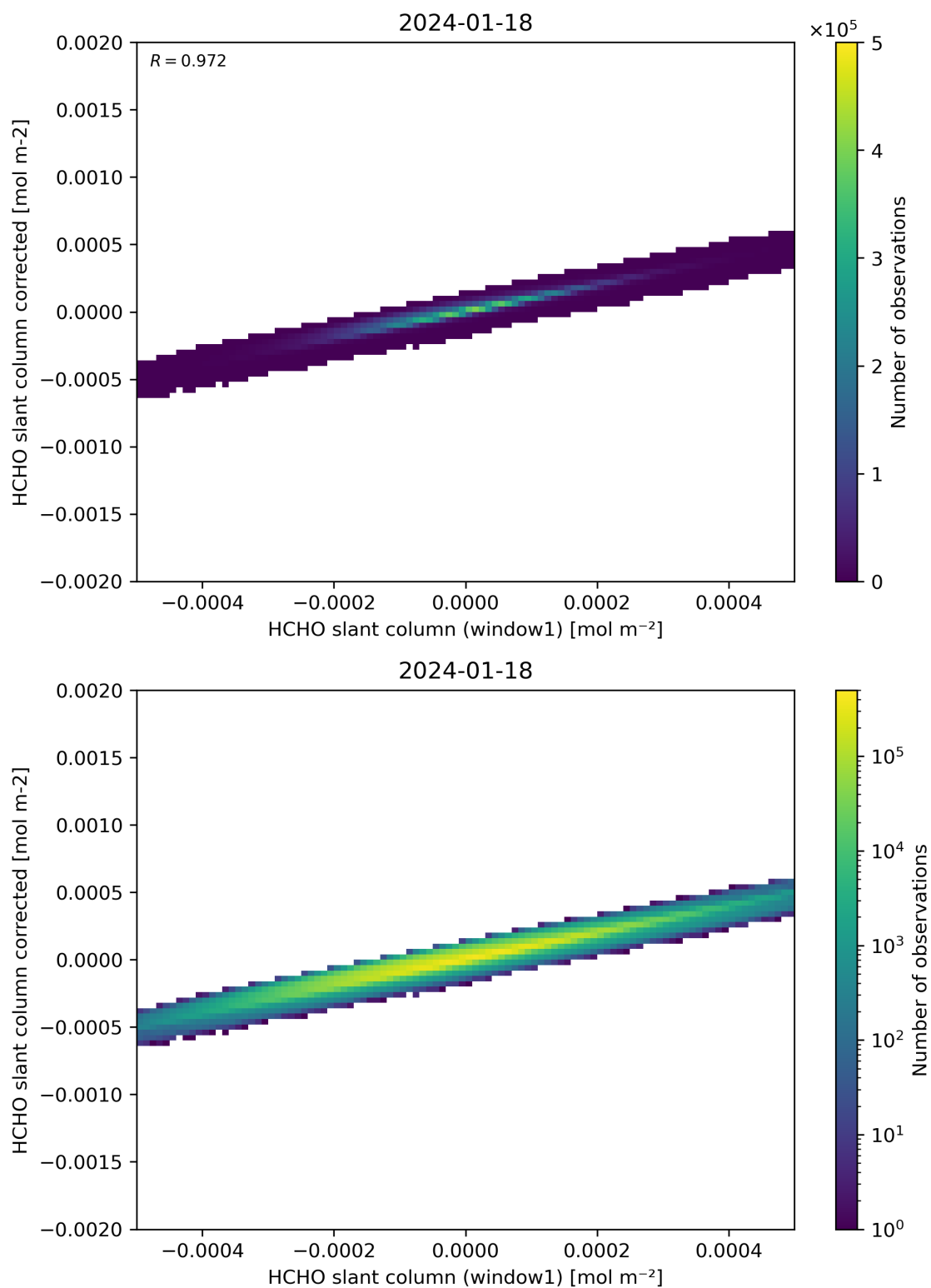
Figure 82: Scatter density plot of “HCHO slant column (window1)” against “HCHO slant column corrected” for 2024-01-17 to 2024-01-19.
