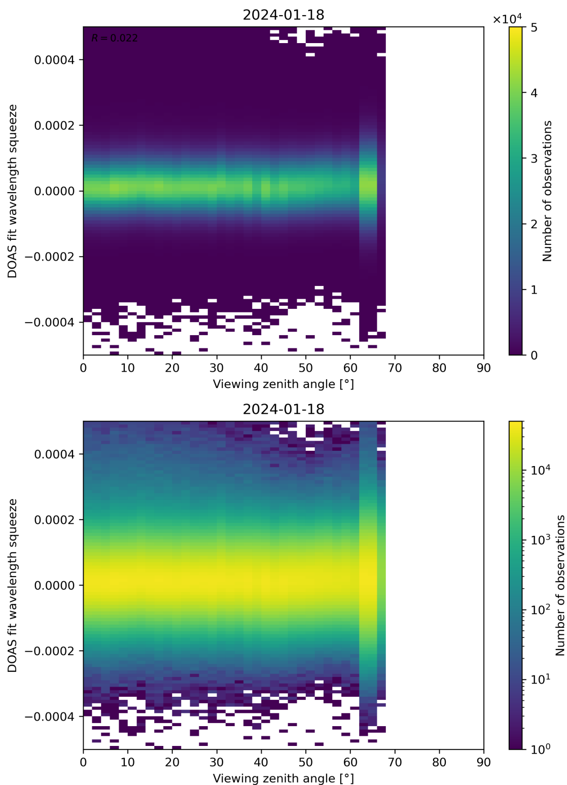
Figure 184: Scatter density plot of “Viewing zenith angle” against “DOAS fit wavelength squeeze” for 2024-01-17 to 2024-01-19.
