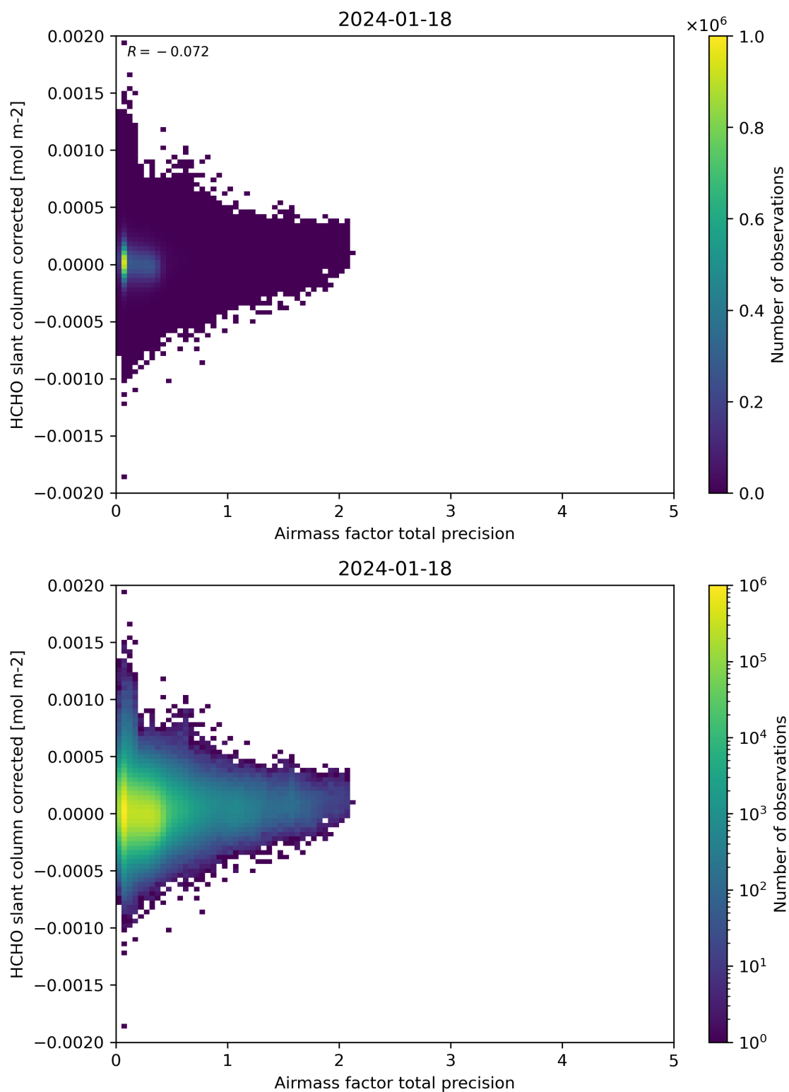
Figure 109: Scatter density plot of “Airmass factor total precision” against “HCHO slant column corrected” for 2024-01-17 to 2024-01-19.
