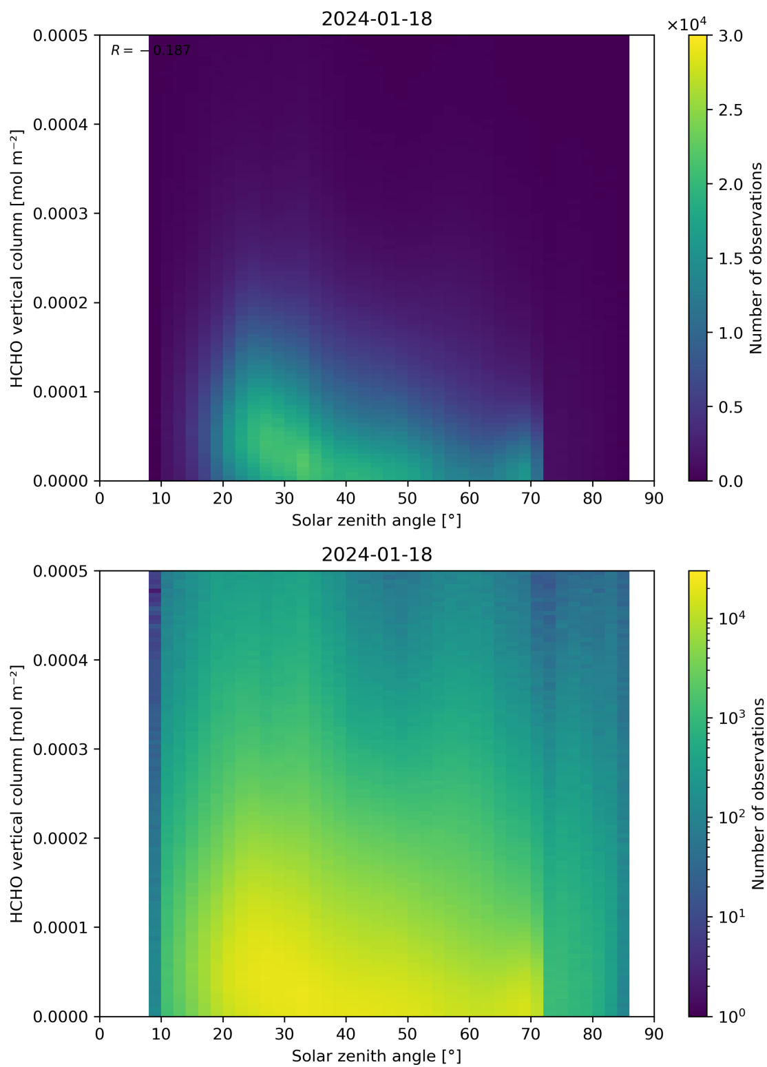
Figure 177: Scatter density plot of “Solar zenith angle” against “HCHO vertical column” for 2024-01-17 to 2024-01-19.
