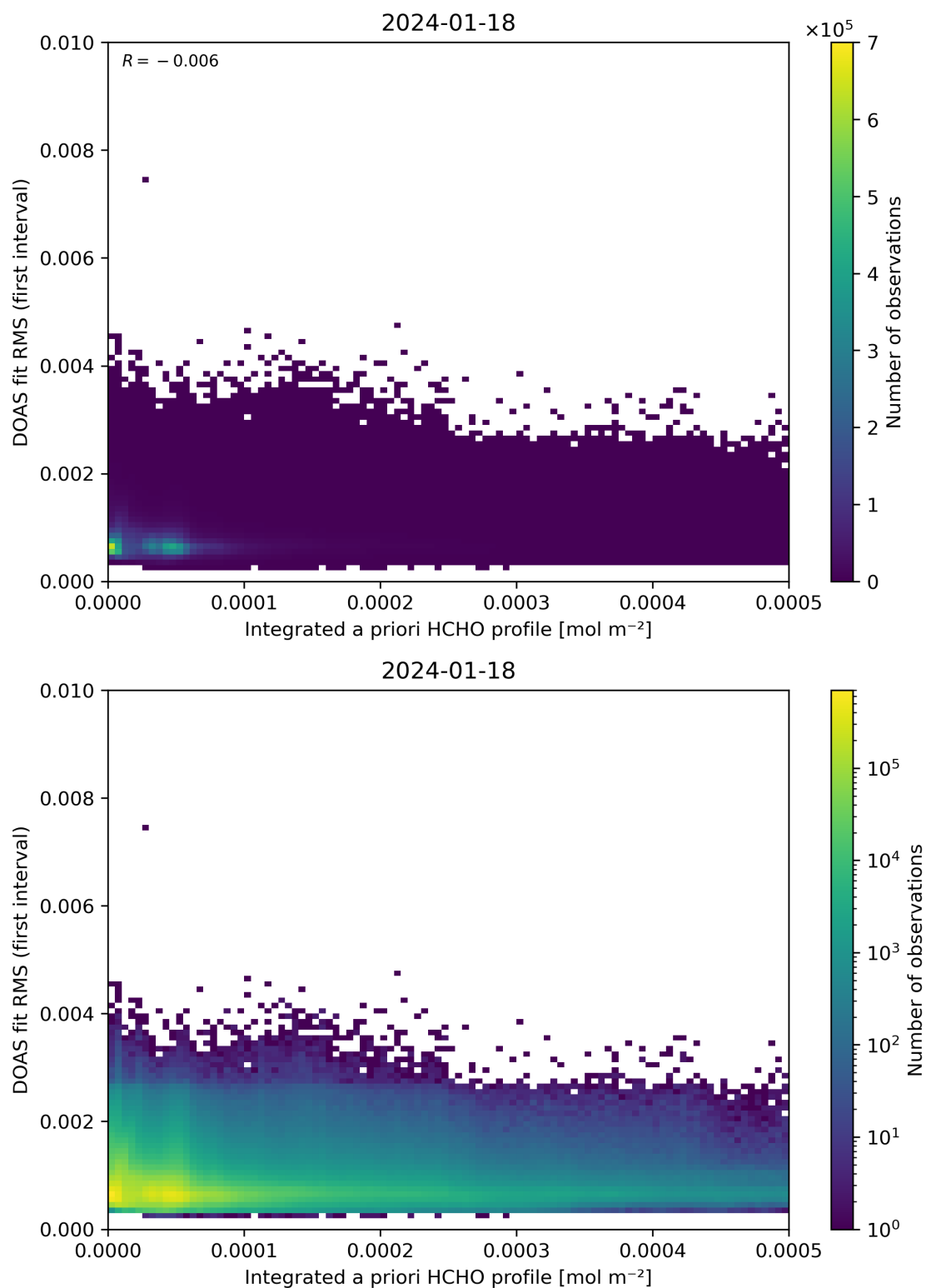
Figure 148: Scatter density plot of “Integrated a priori HCHO profile” against “DOAS fit RMS (first interval)” for 2024-01-17 to 2024-01-19.
