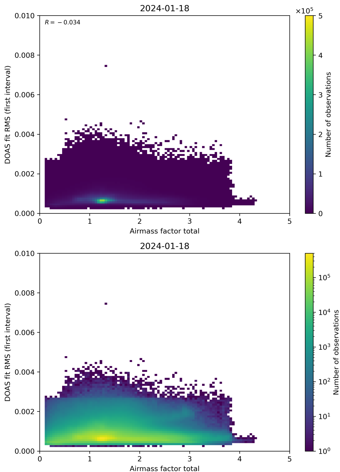
Figure 97: Scatter density plot of “Airmass factor total” against “DOAS fit RMS (first interval)” for 2024-01-17 to 2024-01-19.
