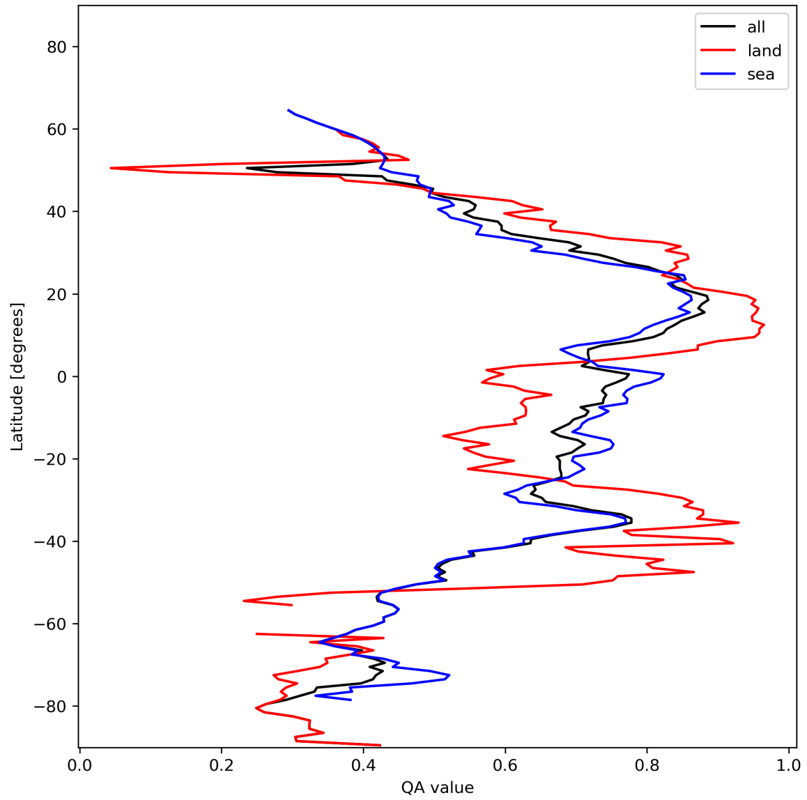
Figure 20: Zonal average of “QA value” for 2024-01-17 to 2024-01-19.
