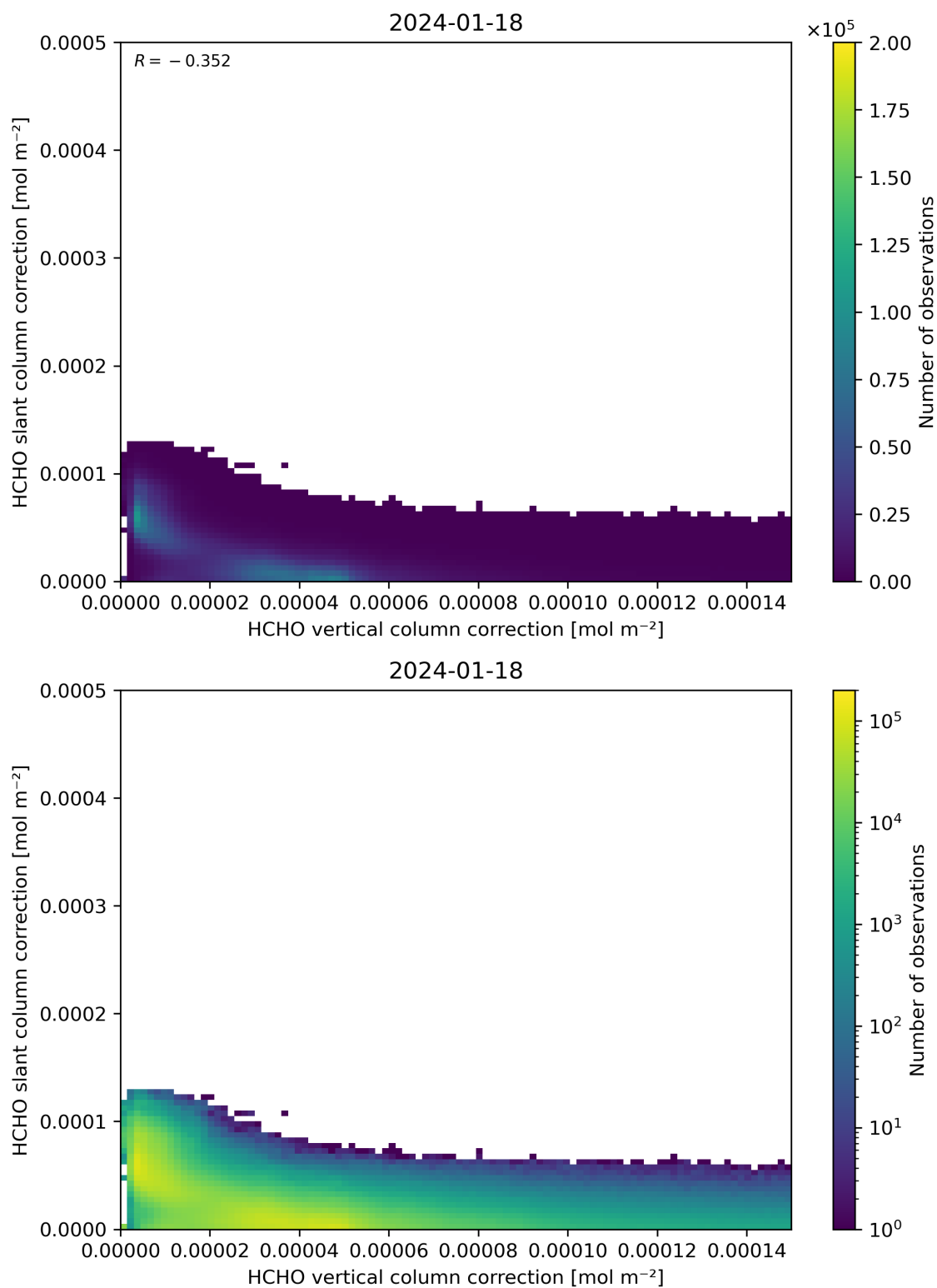
Figure 117: Scatter density plot of “HCHO vertical column correction” against “HCHO slant column correction” for 2024-01-17 to 2024-01-19.
