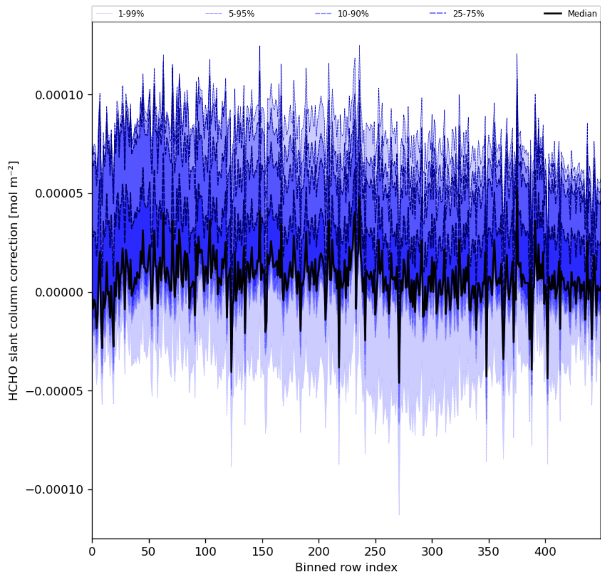
Figure 61: Along track statistics of “HCHO slant column correction” for 2024-01-17 to 2024-01-19
