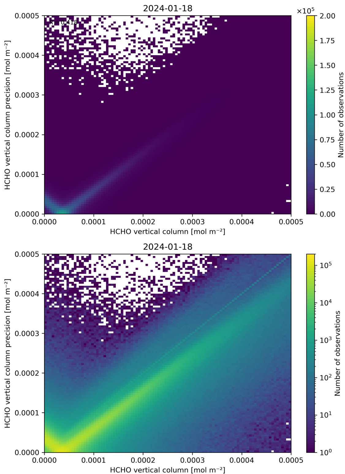
Figure 134: Scatter density plot of “HCHO vertical column” against “HCHO vertical column precision” for 2024-01-17 to 2024-01-19.
