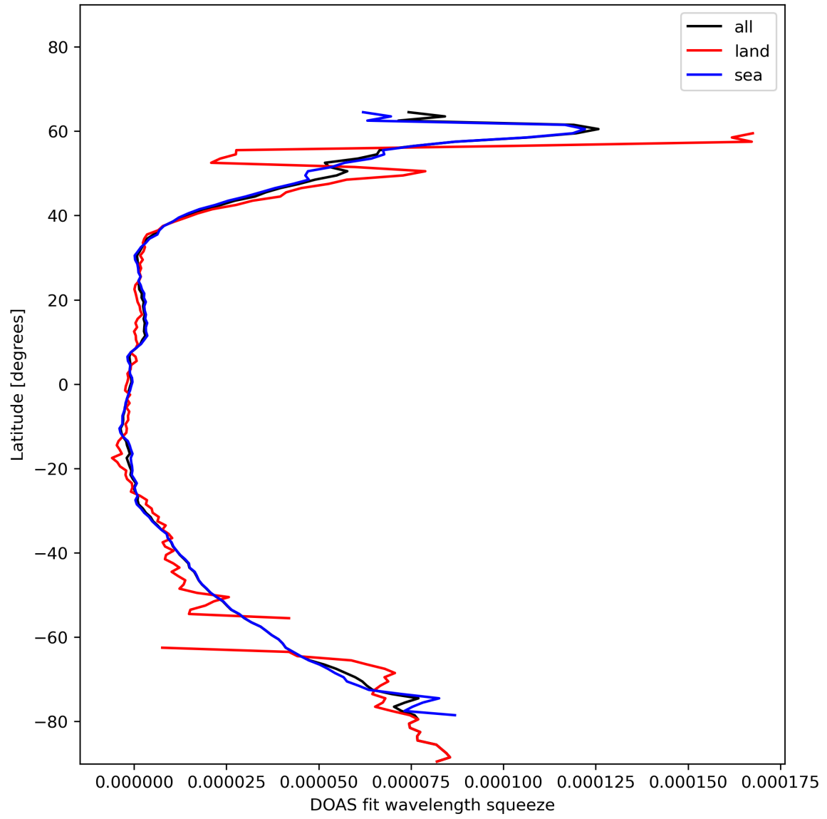
Figure 31: Zonal average of “DOAS fit wavelength squeeze” for 2024-01-17 to 2024-01-19.
