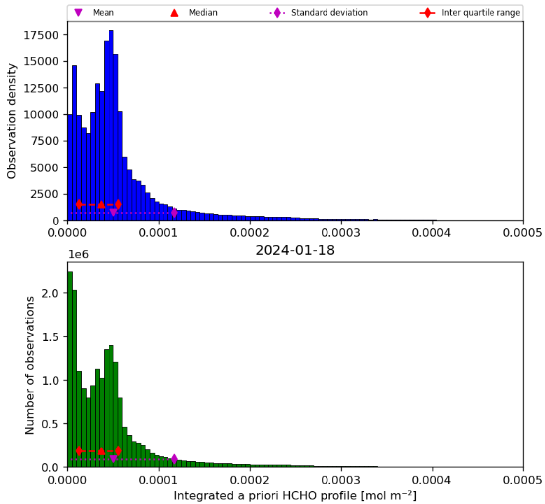
Figure 43: Histogram of “Integrated a priori HCHO profile” for 2024-01-17 to 2024-01-19
