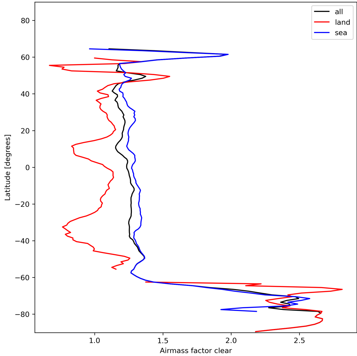
Figure 28: Zonal average of “Airmass factor clear” for 2024-01-17 to 2024-01-19.
