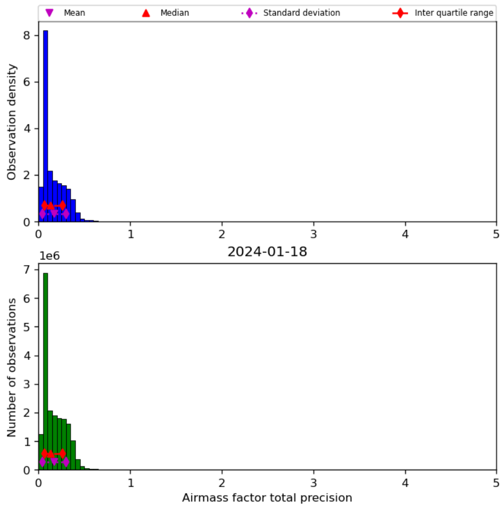
Figure 41: Histogram of “Airmass factor total precision” for 2024-01-17 to 2024-01-19
