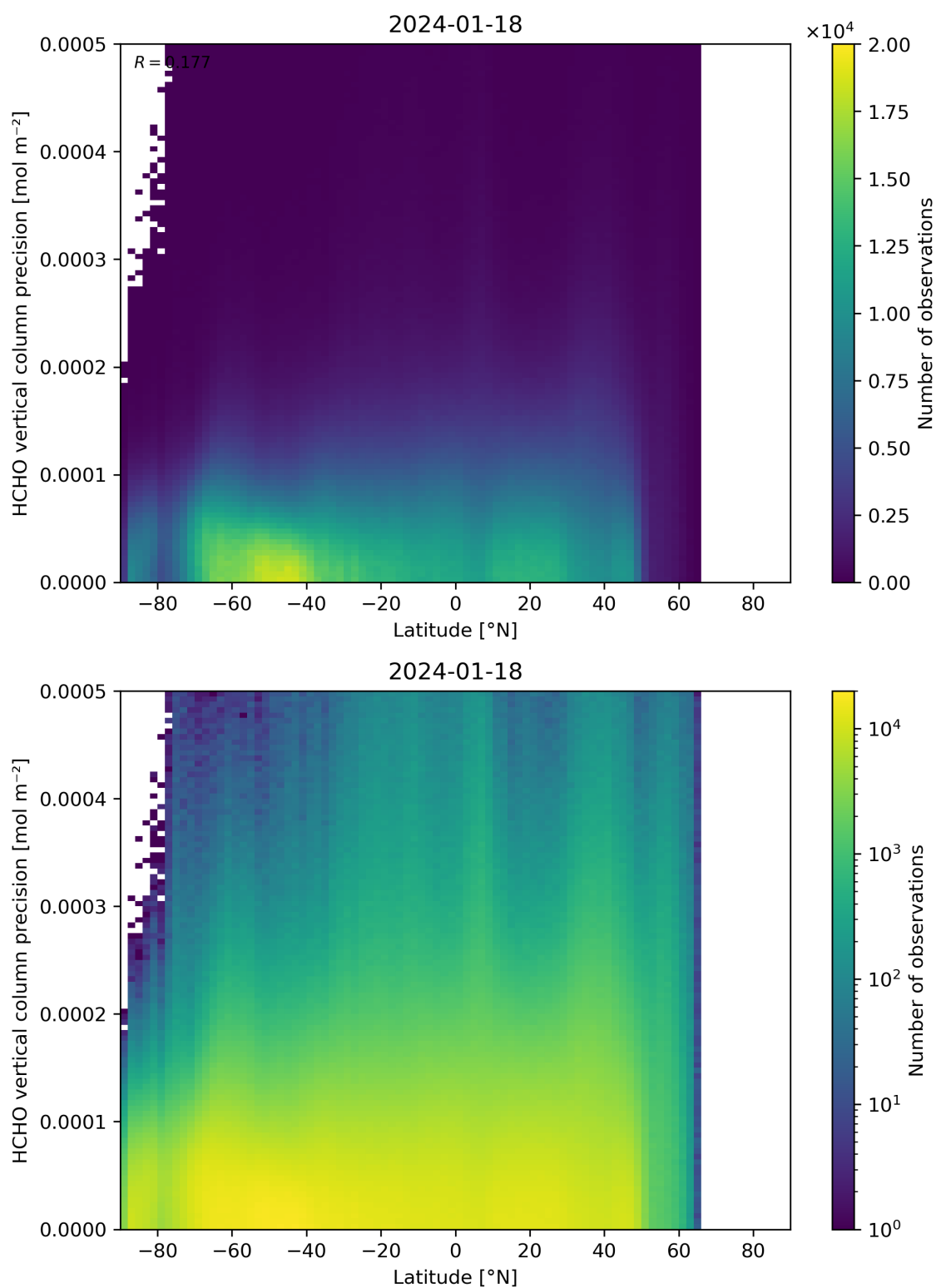
Figure 165: Scatter density plot of “Latitude” against “HCHO vertical column precision” for 2024-01-17 to 2024-01-19.
