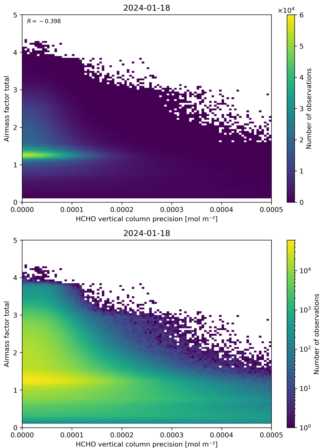
Figure 144: Scatter density plot of “HCHO vertical column precision” against “Airmass factor total” for 2024-01-17 to 2024-01-19.
