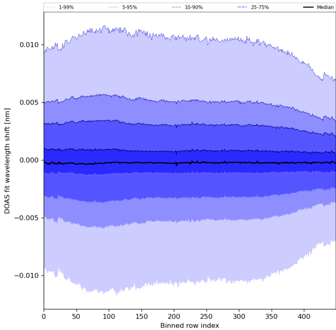
Figure 58: Along track statistics of “DOAS fit wavelength shift” for 2024-01-17 to 2024-01-19
