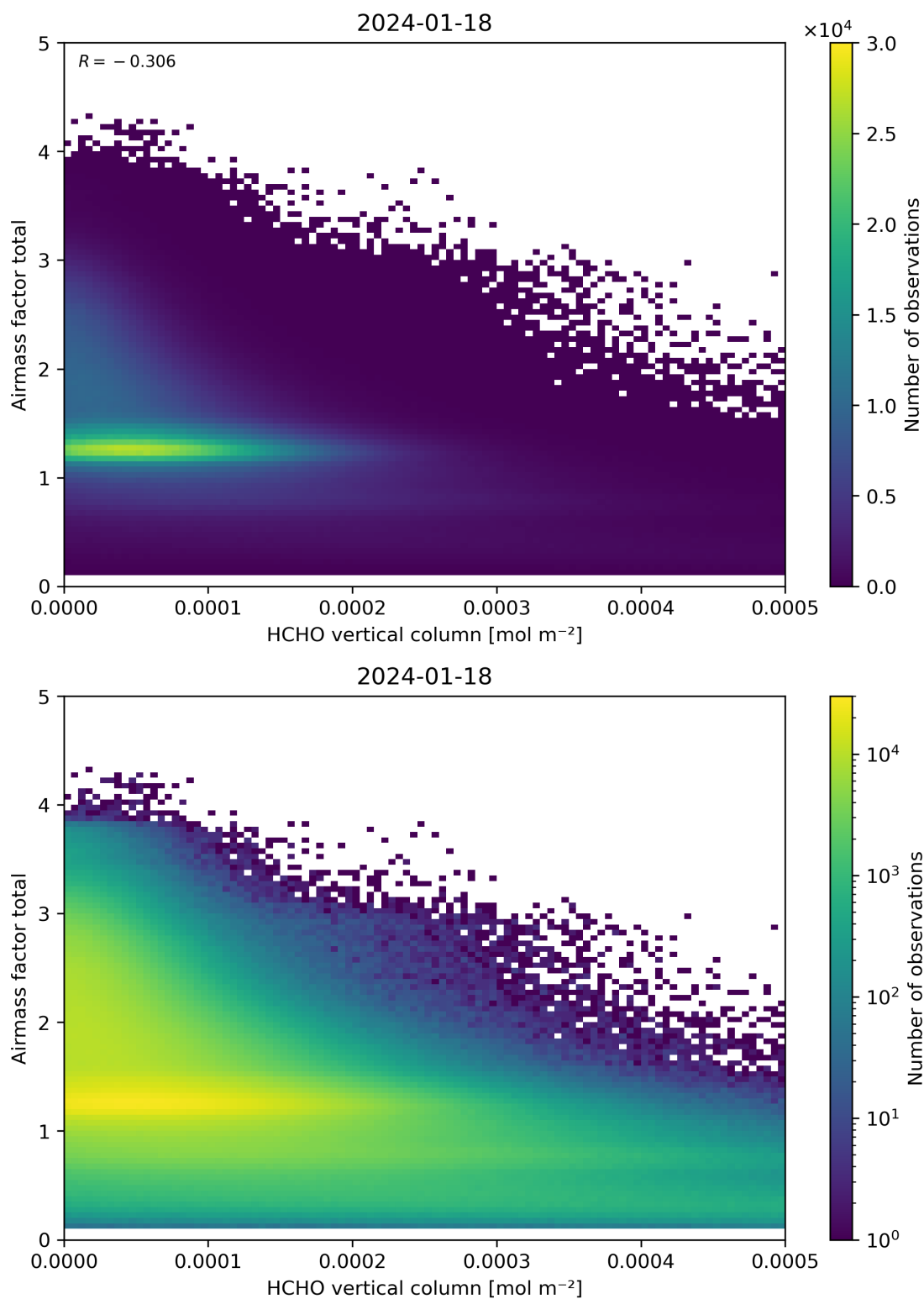
Figure 131: Scatter density plot of “HCHO vertical column” against “Airmass factor total” for 2024-01-17 to 2024-01-19.
