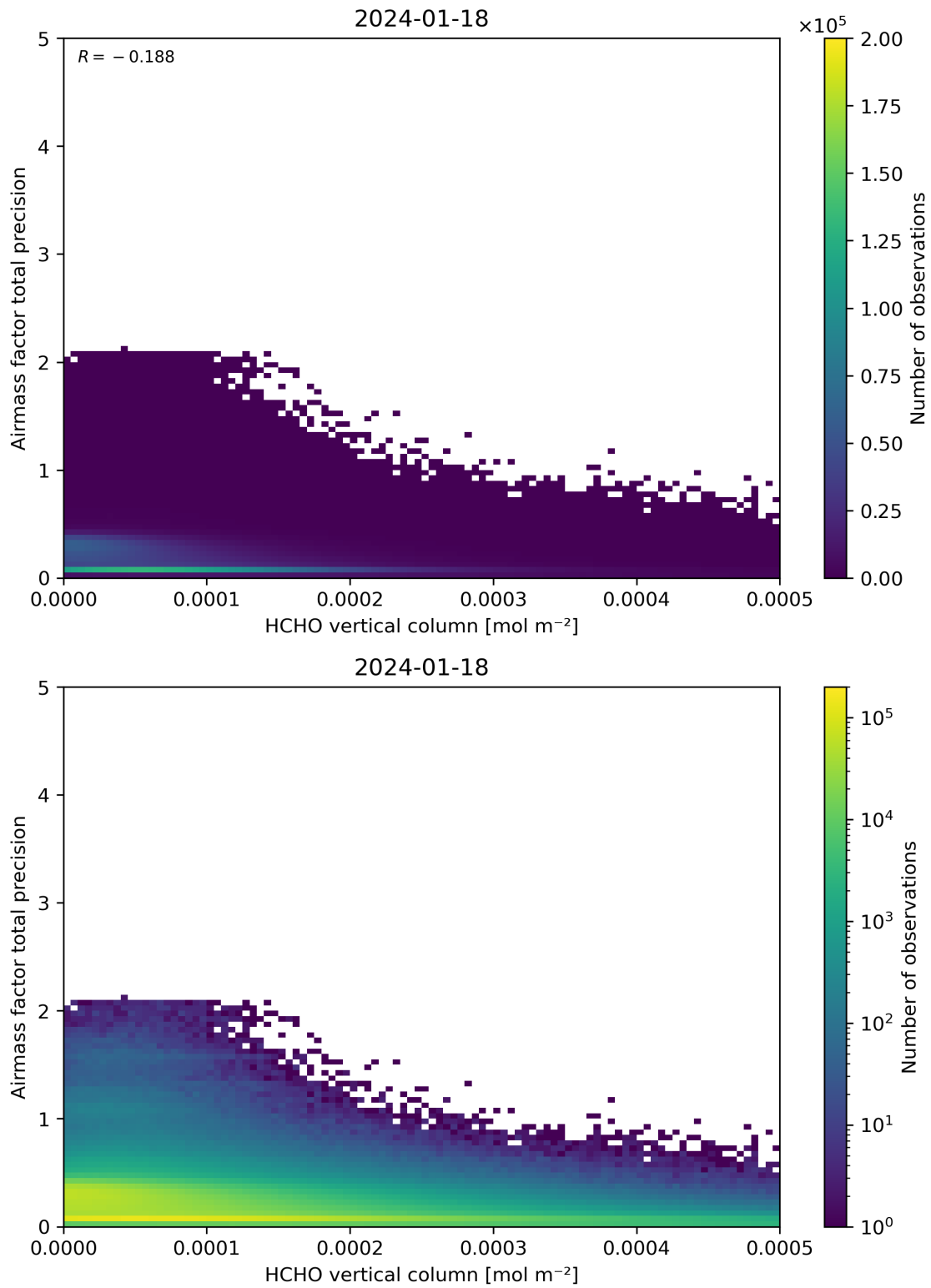
Figure 132: Scatter density plot of “HCHO vertical column” against “Airmass factor total precision” for 2024-01-17 to 2024-01-19.
