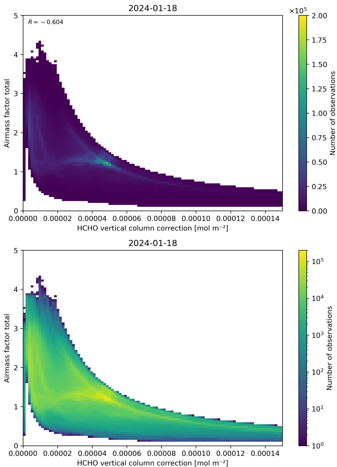
Figure 120: Scatter density plot of “HCHO vertical column correction” against “Airmass factor total” for 2024-01-17 to 2024-01-19.
