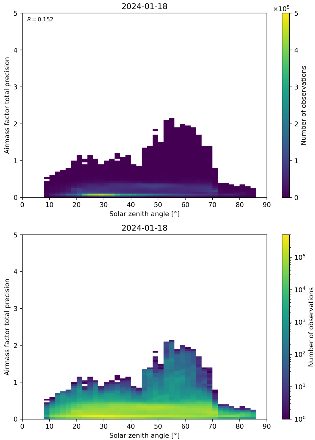
Figure 176: Scatter density plot of “Solar zenith angle” against “Airmass factor total precision” for 2024-01-17 to 2024-01-19.
