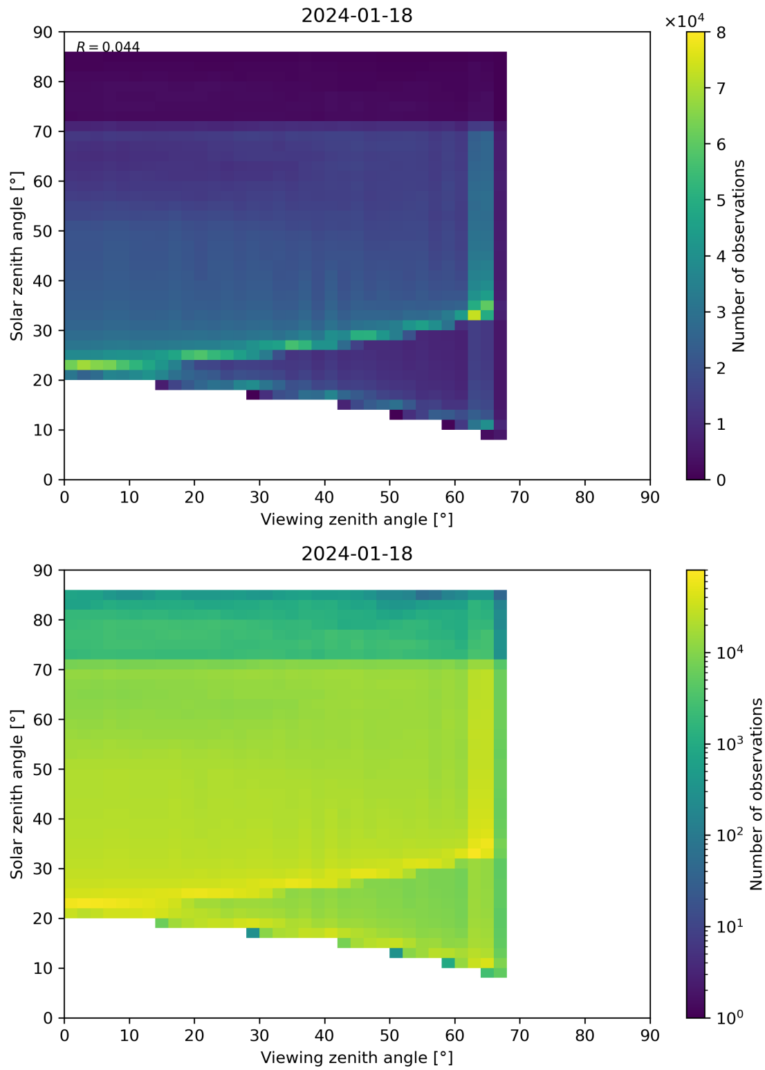
Figure 197: Scatter density plot of “Viewing zenith angle” against “Solar zenith angle” for 2024-01-17 to 2024-01-19.
