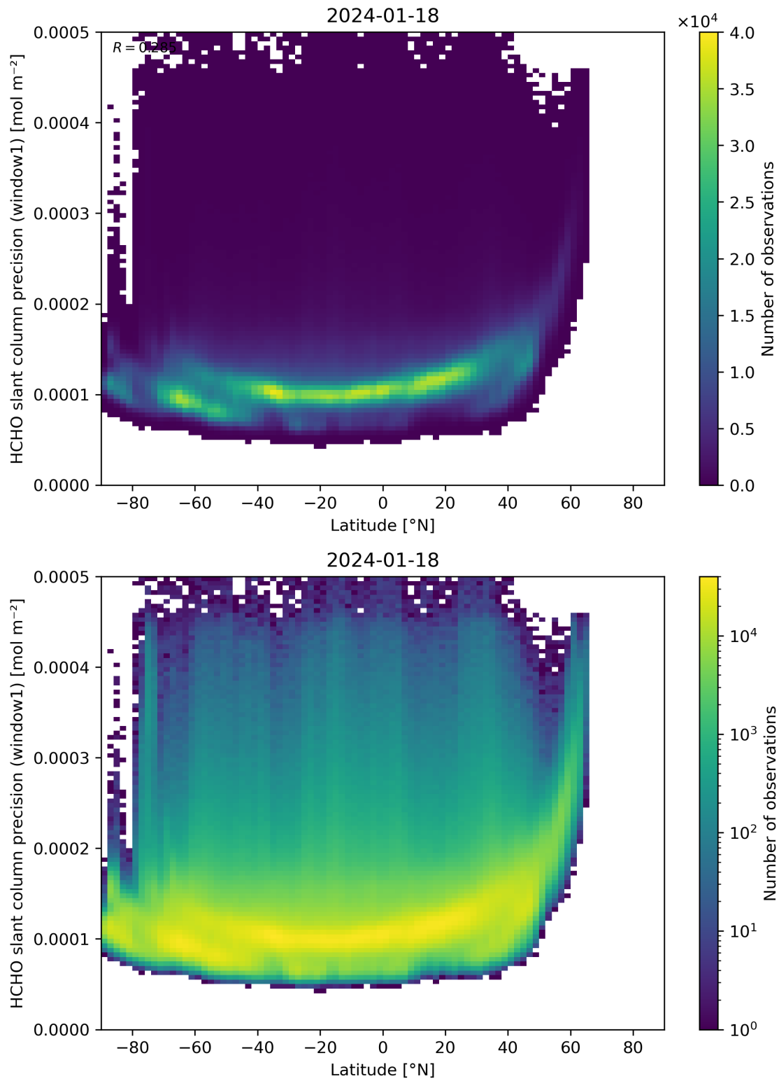
Figure 160: Scatter density plot of “Latitude” against “HCHO slant column precision (window1)” for 2024-01-17 to 2024-01-19.
