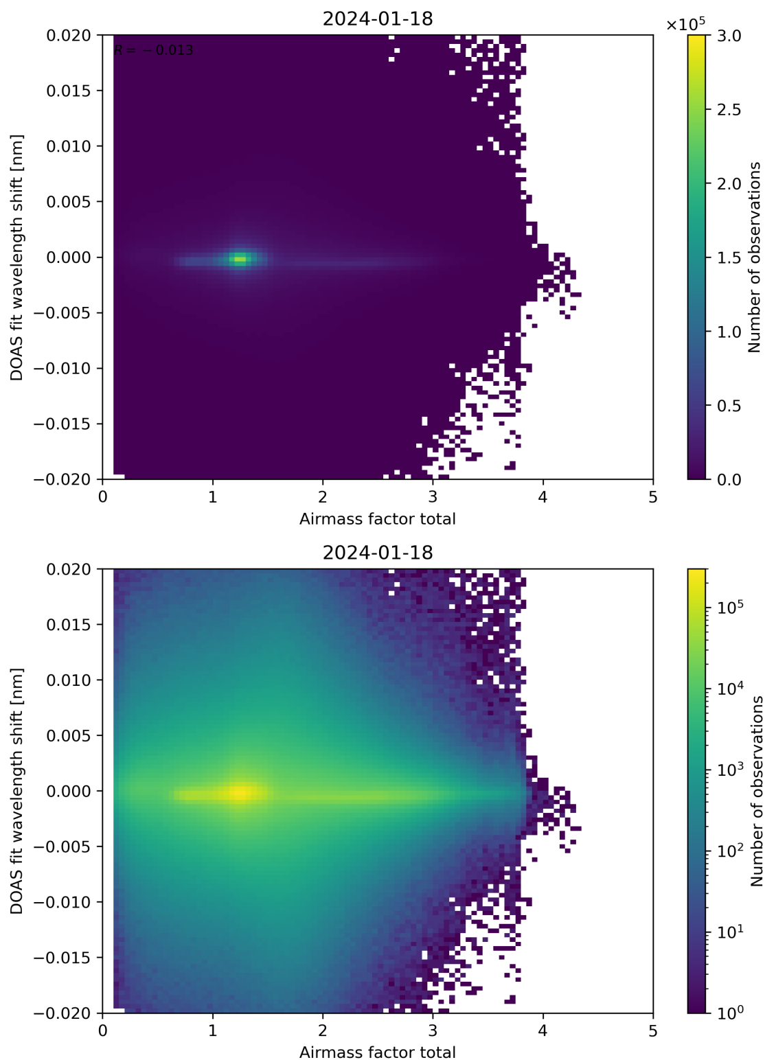
Figure 98: Scatter density plot of “Airmass factor total” against “DOAS fit wavelength shift” for 2024-01-17 to 2024-01-19.
