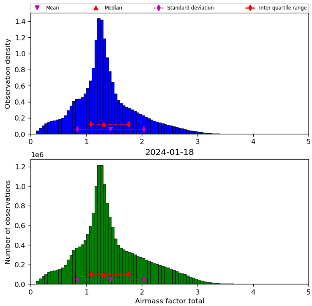
Figure 40: Histogram of “Airmass factor total” for 2024-01-17 to 2024-01-19
