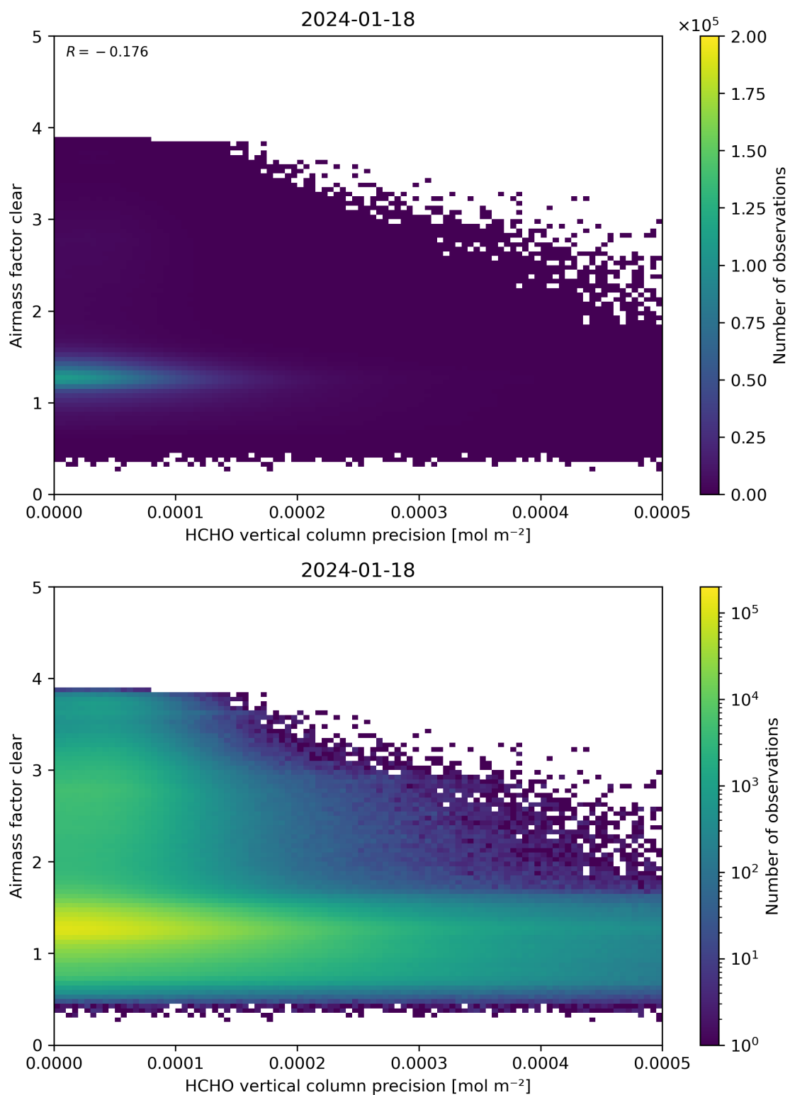
Figure 139: Scatter density plot of “HCHO vertical column precision” against “Airmass factor clear” for 2024-01-17 to 2024-01-19.
