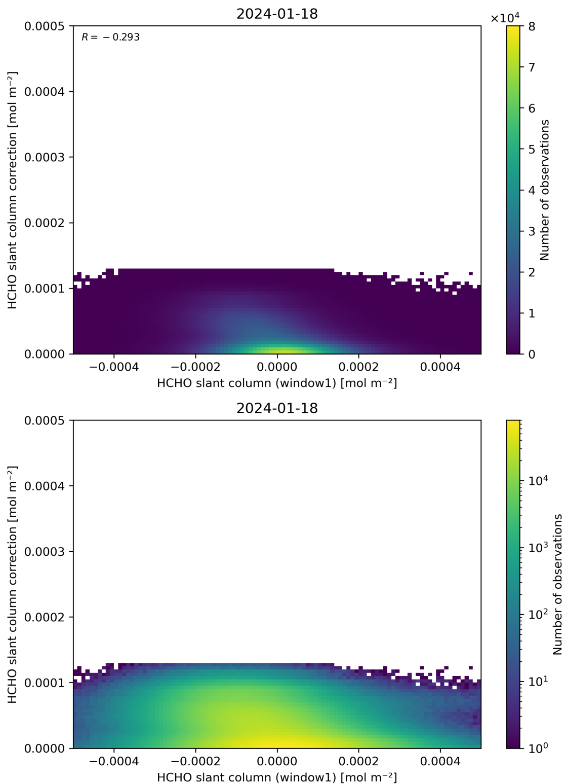
Figure 83: Scatter density plot of “HCHO slant column (window1)” against “HCHO slant column correction” for 2024-01-17 to 2024-01-19.
