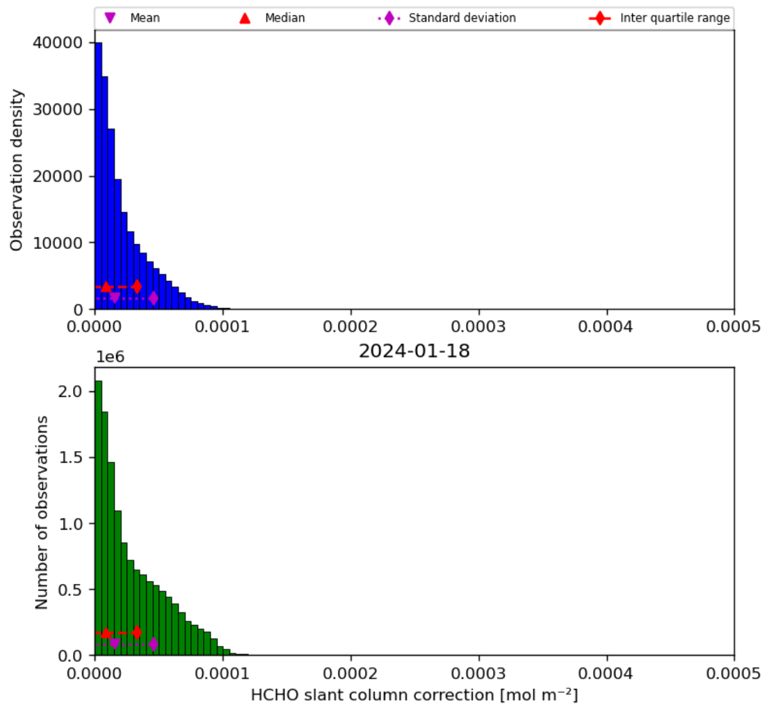
Figure 47: Histogram of “HCHO slant column correction” for 2024-01-17 to 2024-01-19
