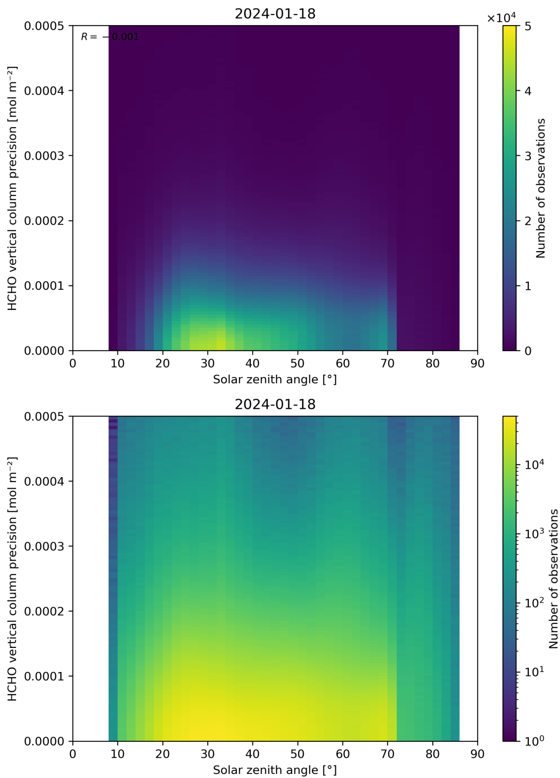
Figure 179: Scatter density plot of “Solar zenith angle” against “HCHO vertical column precision” for 2024-01-17 to 2024-01-19.
