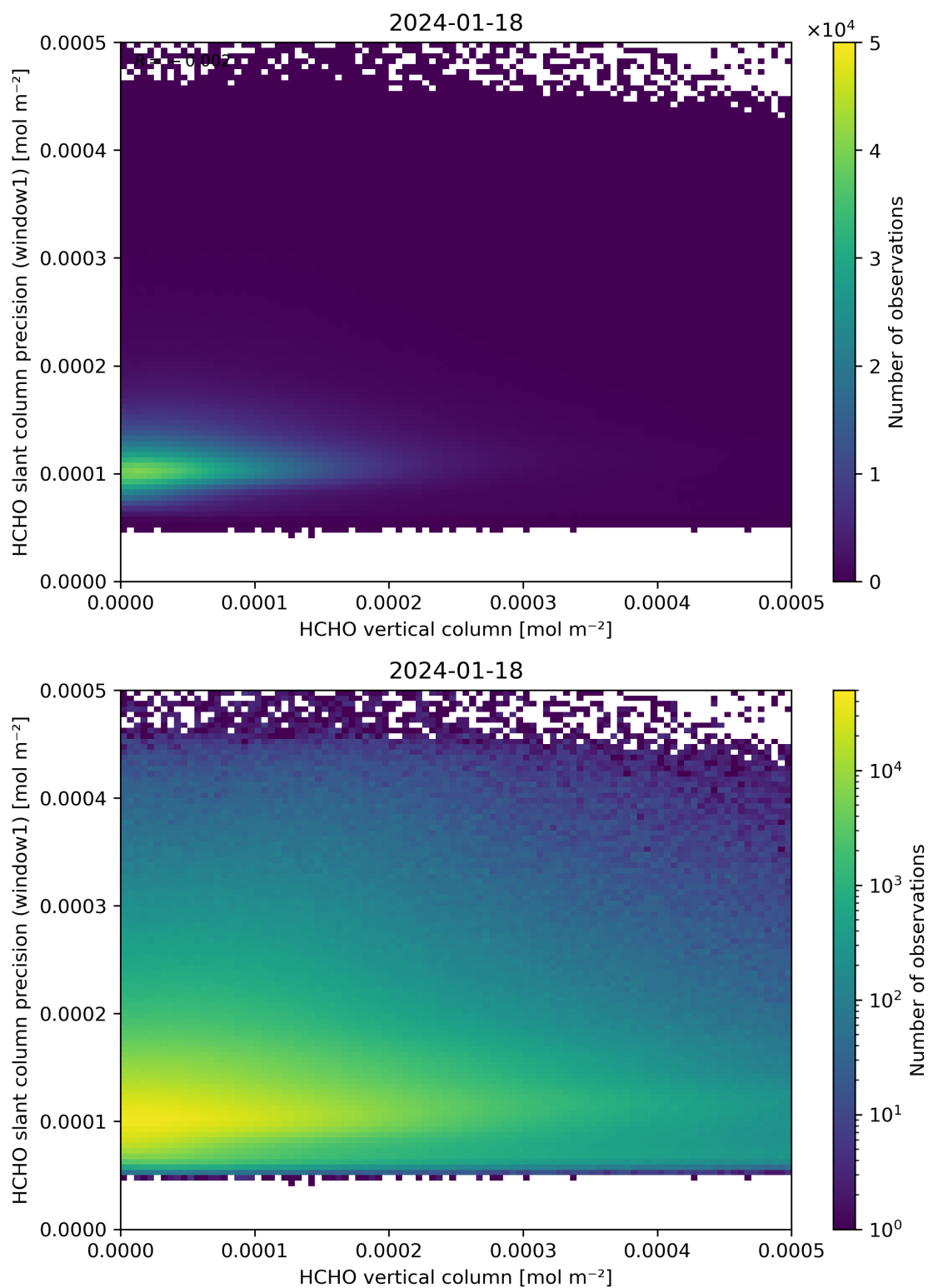
Figure 130: Scatter density plot of “HCHO vertical column” against “HCHO slant column precision (window1)” for 2024-01-17 to 2024-01-19.
