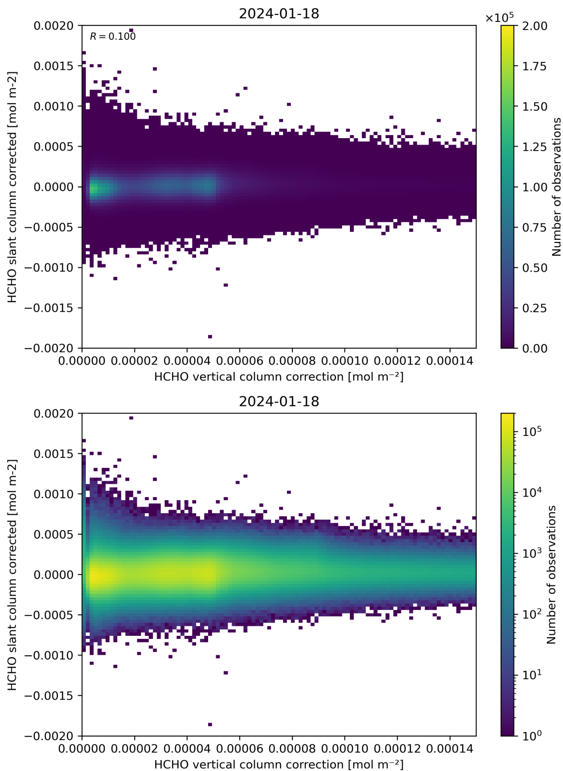
Figure 116: Scatter density plot of “HCHO vertical column correction” against “HCHO slant column corrected” for 2024-01-17 to 2024-01-19.
