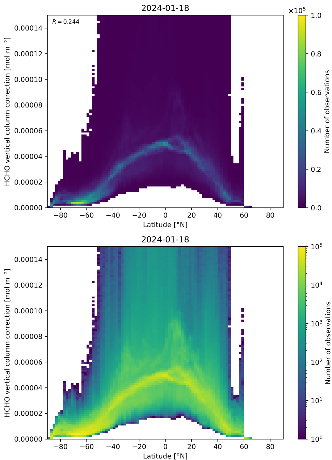
Figure 164: Scatter density plot of “Latitude” against “HCHO vertical column correction” for 2024-01-17 to 2024-01-19.
