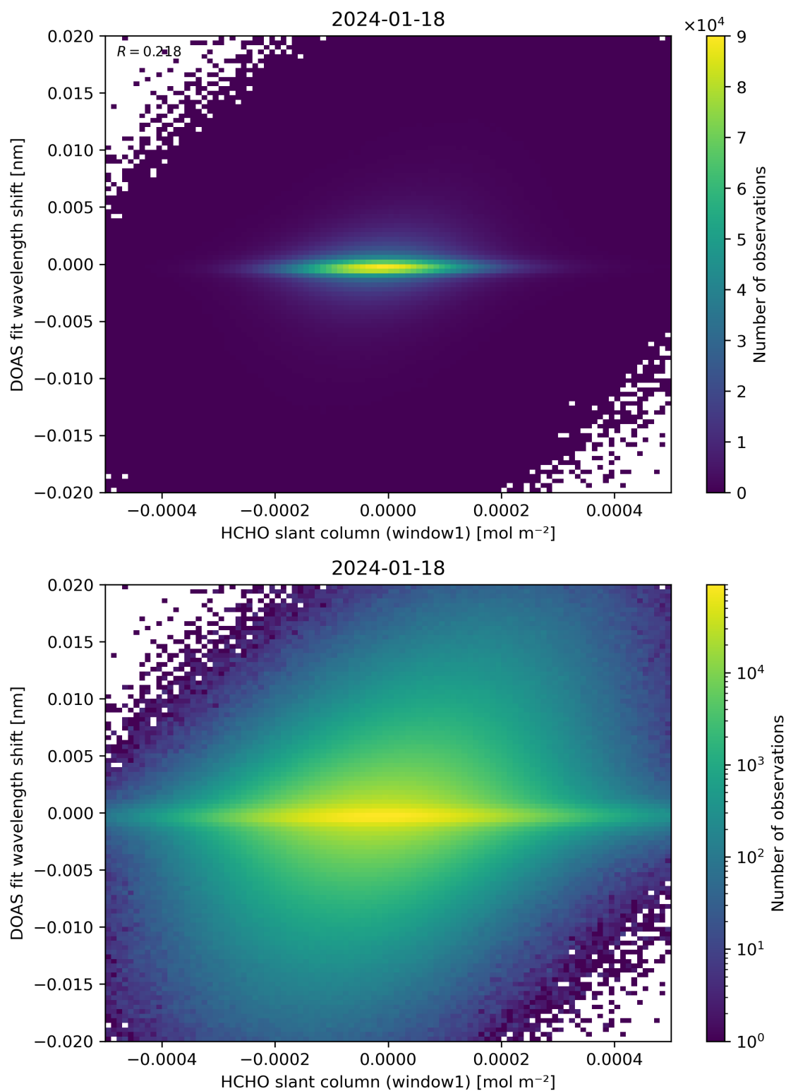
Figure 79: Scatter density plot of “HCHO slant column (window1)” against “DOAS fit wavelength shift” for 2024-01-17 to 2024-01-19.
