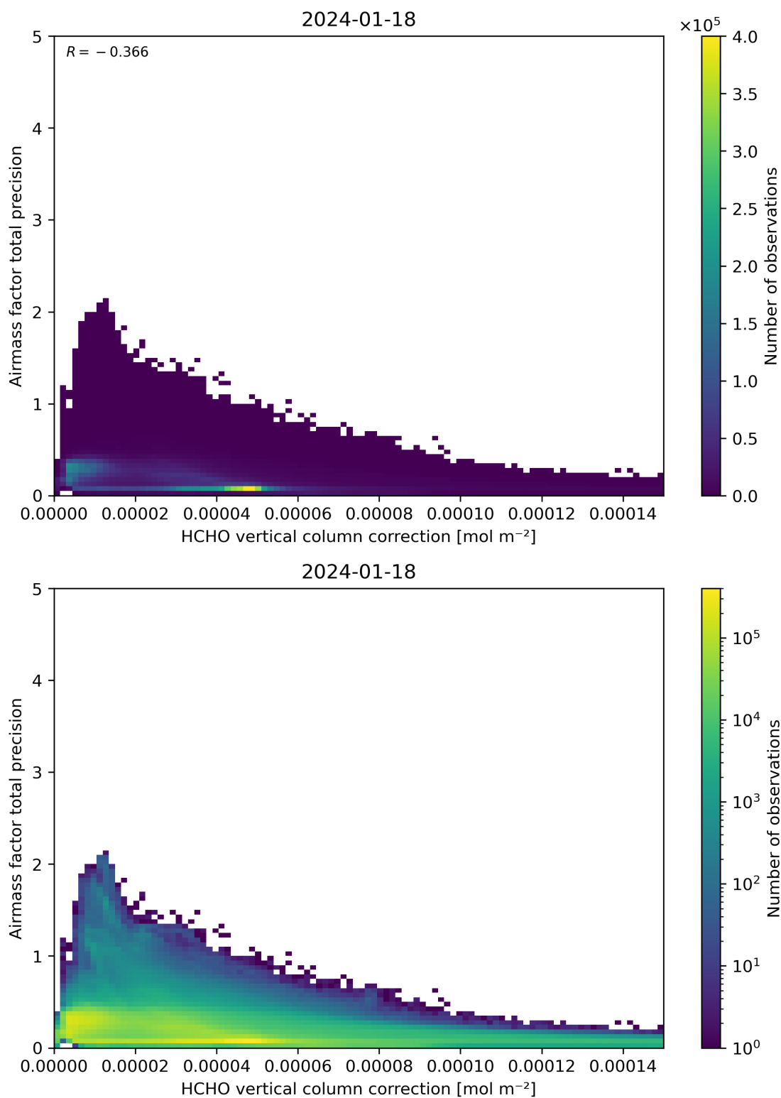
Figure 121: Scatter density plot of “HCHO vertical column correction” against “Airmass factor total precision” for 2024-01-17 to 2024-01-19.
