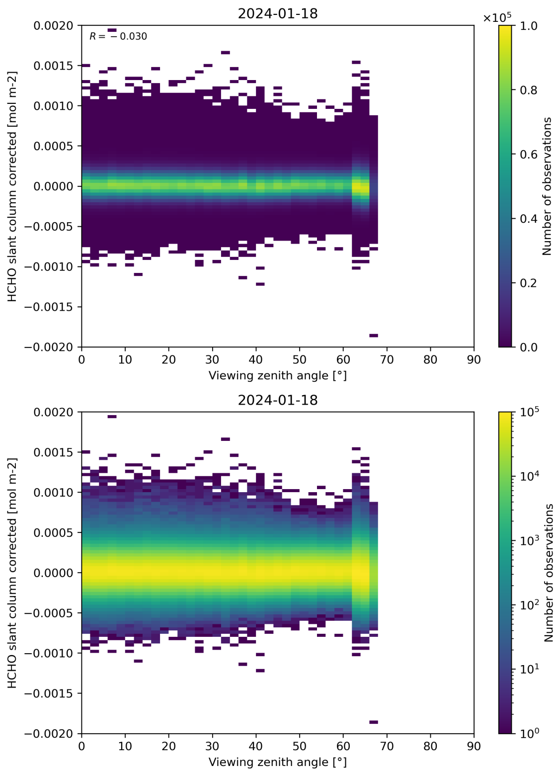
Figure 186: Scatter density plot of “Viewing zenith angle” against “HCHO slant column corrected” for 2024-01-17 to 2024-01-19.
