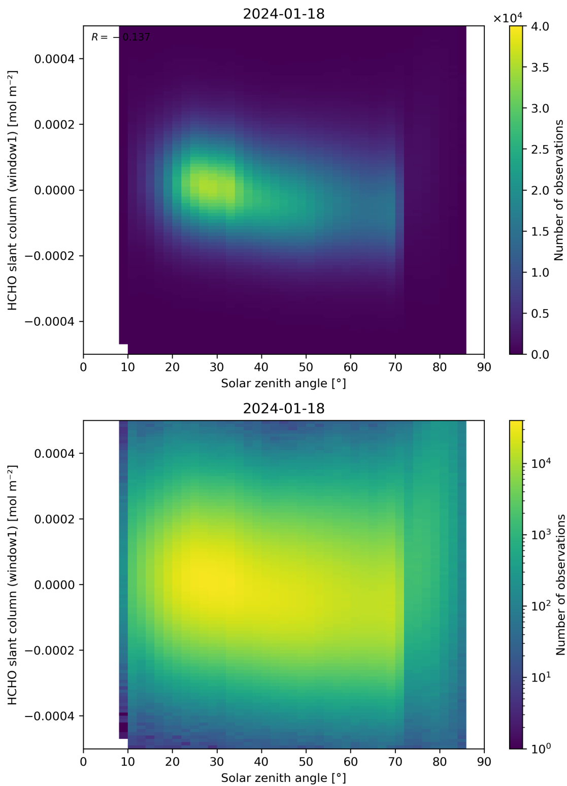
Figure 173: Scatter density plot of “Solar zenith angle” against “HCHO slant column (window1)” for 2024-01-17 to 2024-01-19.
