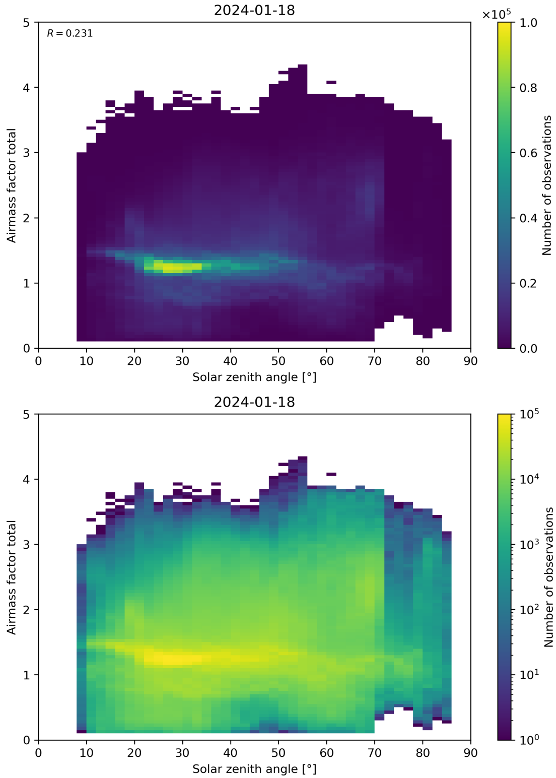
Figure 175: Scatter density plot of “Solar zenith angle” against “Airmass factor total” for 2024-01-17 to 2024-01-19.
