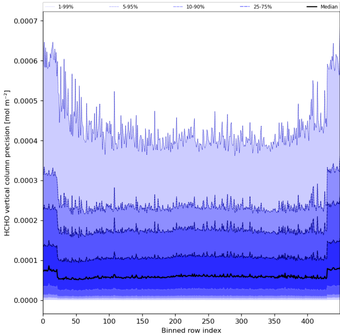
Figure 50: Along track statistics of “HCHO vertical column precision” for 2024-01-17 to 2024-01-19
