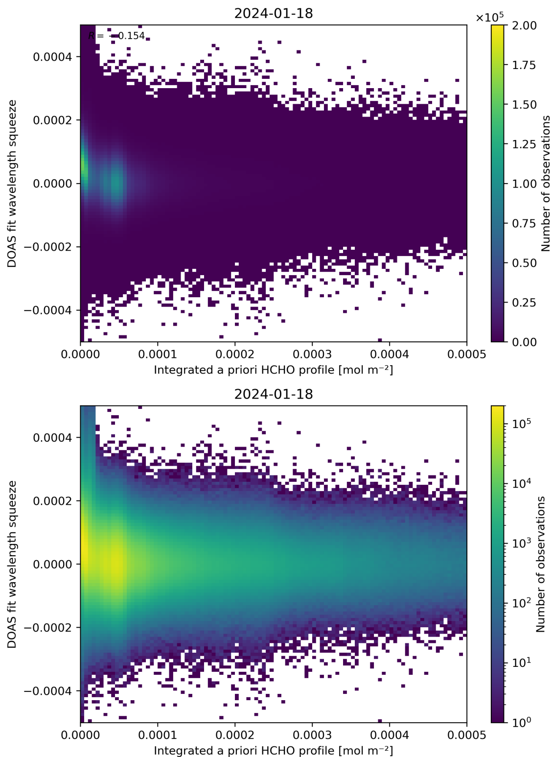
Figure 150: Scatter density plot of “Integrated a priori HCHO profile” against “DOAS fit wavelength squeeze” for 2024-01-17 to 2024-01-19.
