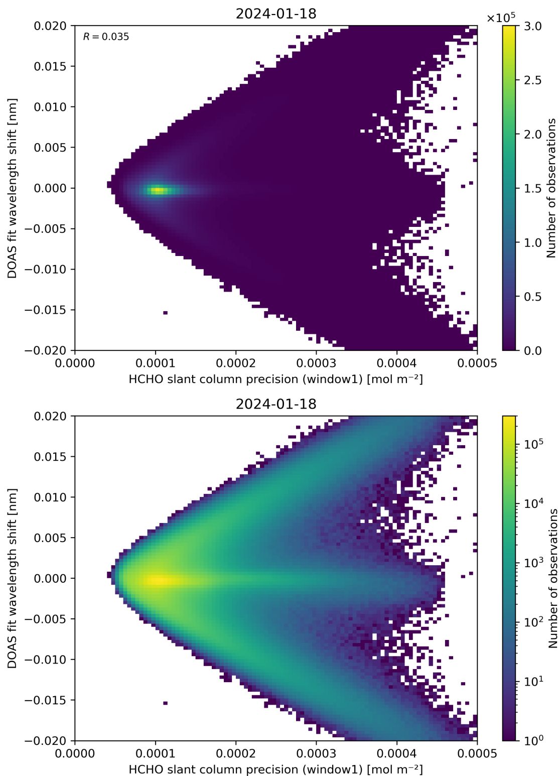
Figure 89: Scatter density plot of “HCHO slant column precision (window1)” against “DOAS fit wavelength shift” for 2024-01-17 to 2024-01-19.
