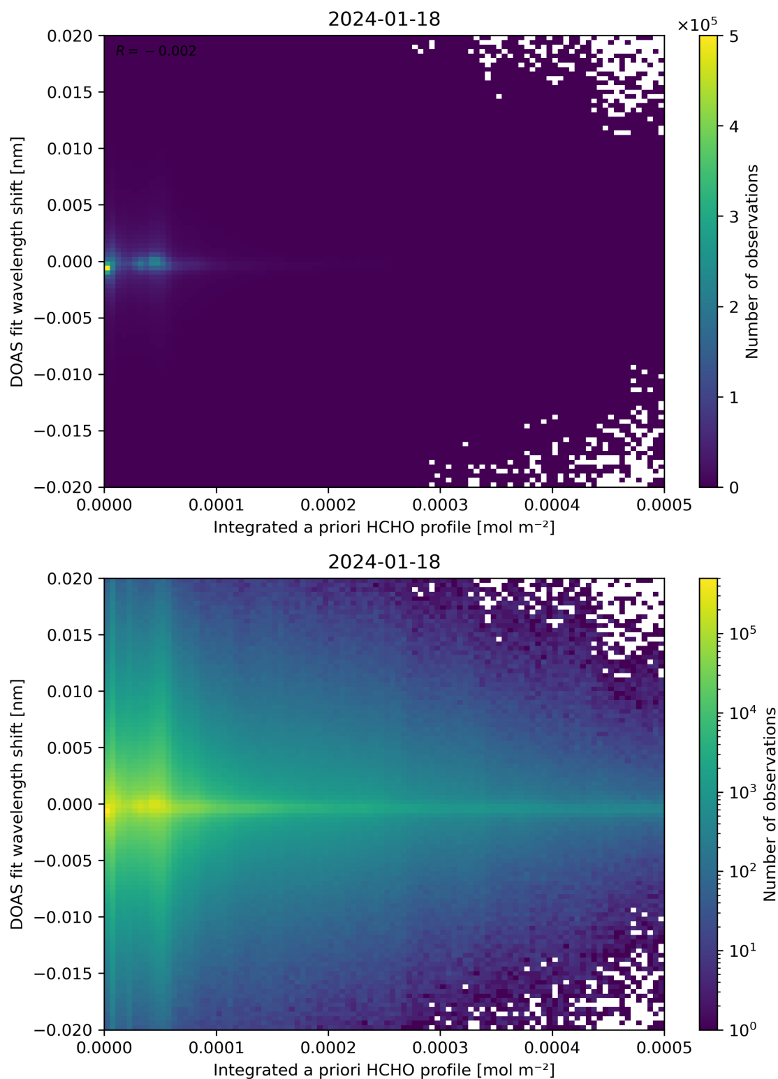
Figure 149: Scatter density plot of “Integrated a priori HCHO profile” against “DOAS fit wavelength shift” for 2024-01-17 to 2024-01-19.
