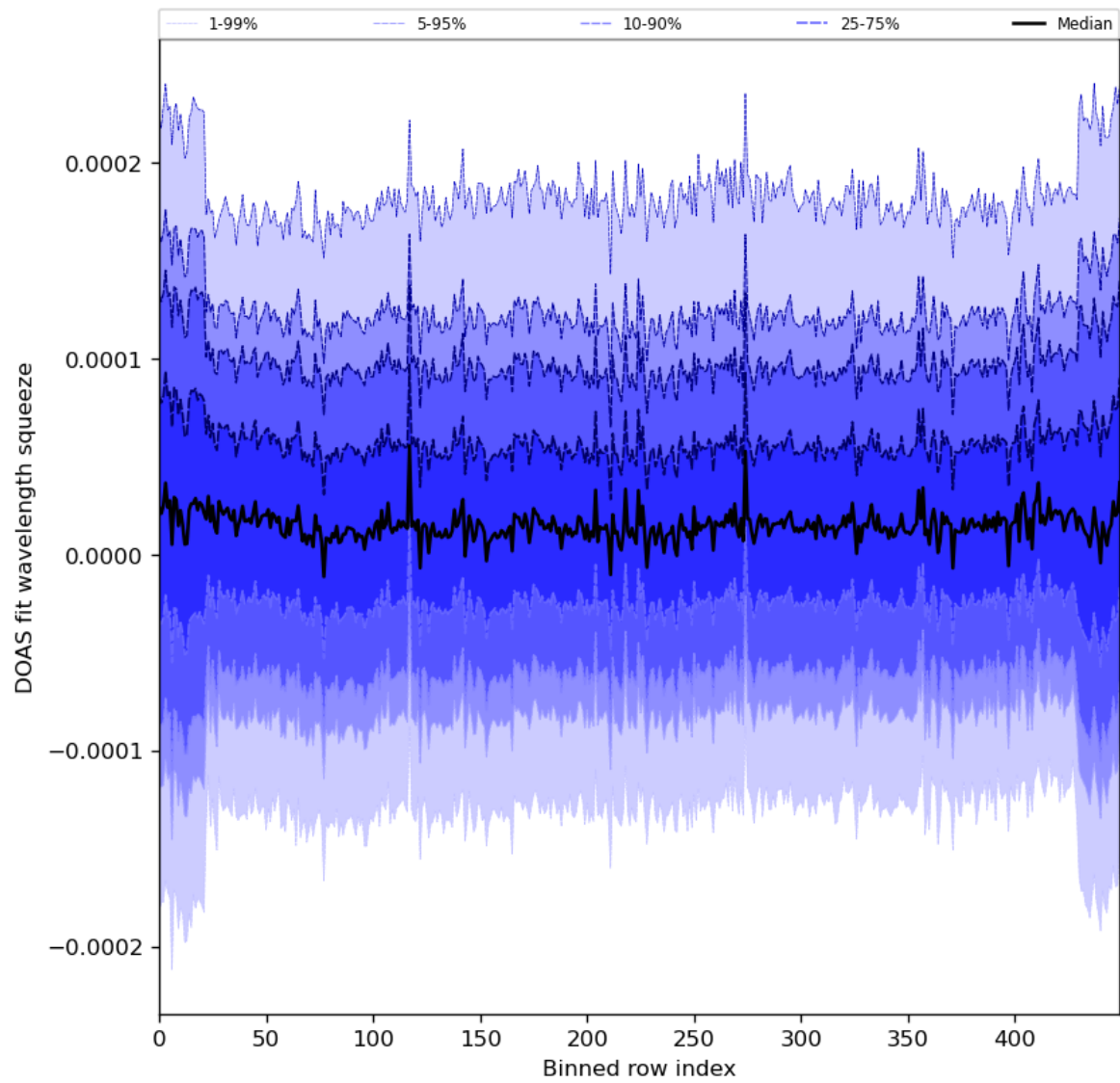
Figure 59: Along track statistics of “DOAS fit wavelength squeeze” for 2024-01-17 to 2024-01-19
