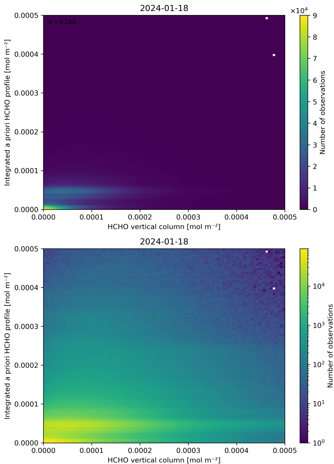
Figure 135: Scatter density plot of “HCHO vertical column” against “Integrated a priori HCHO profile” for 2024-01-17 to 2024-01-19.
