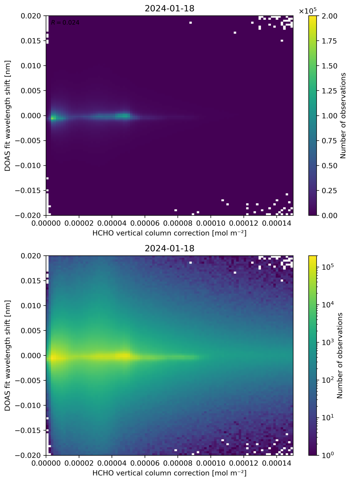
Figure 113: Scatter density plot of “HCHO vertical column correction” against “DOAS fit wavelength shift” for 2024-01-17 to 2024-01-19.
