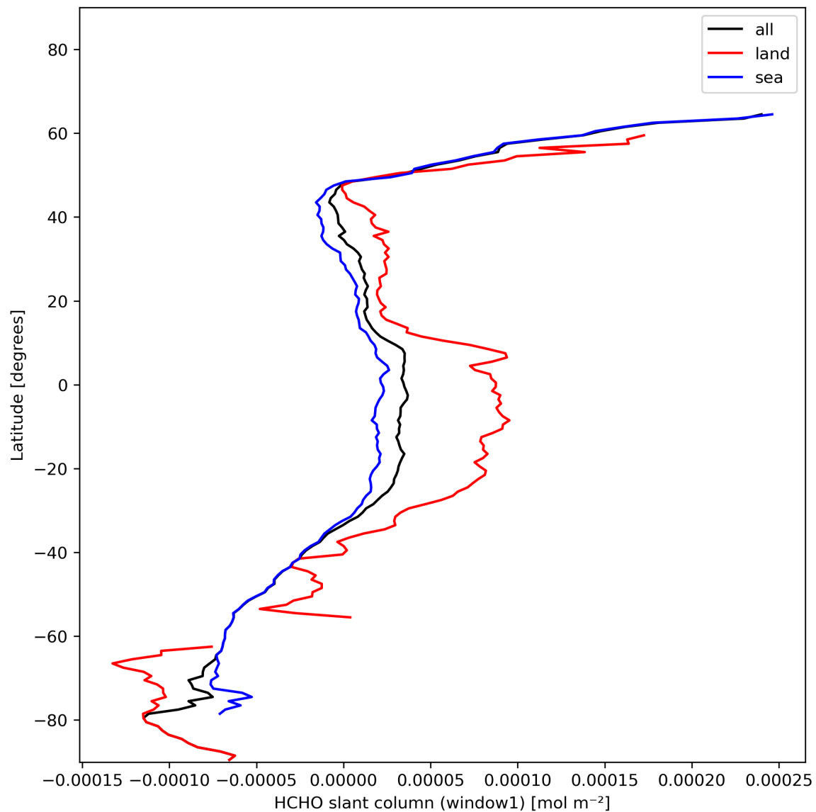
Figure 24: Zonal average of “HCHO slant column (window1)” for 2024-01-17 to 2024-01-19.
