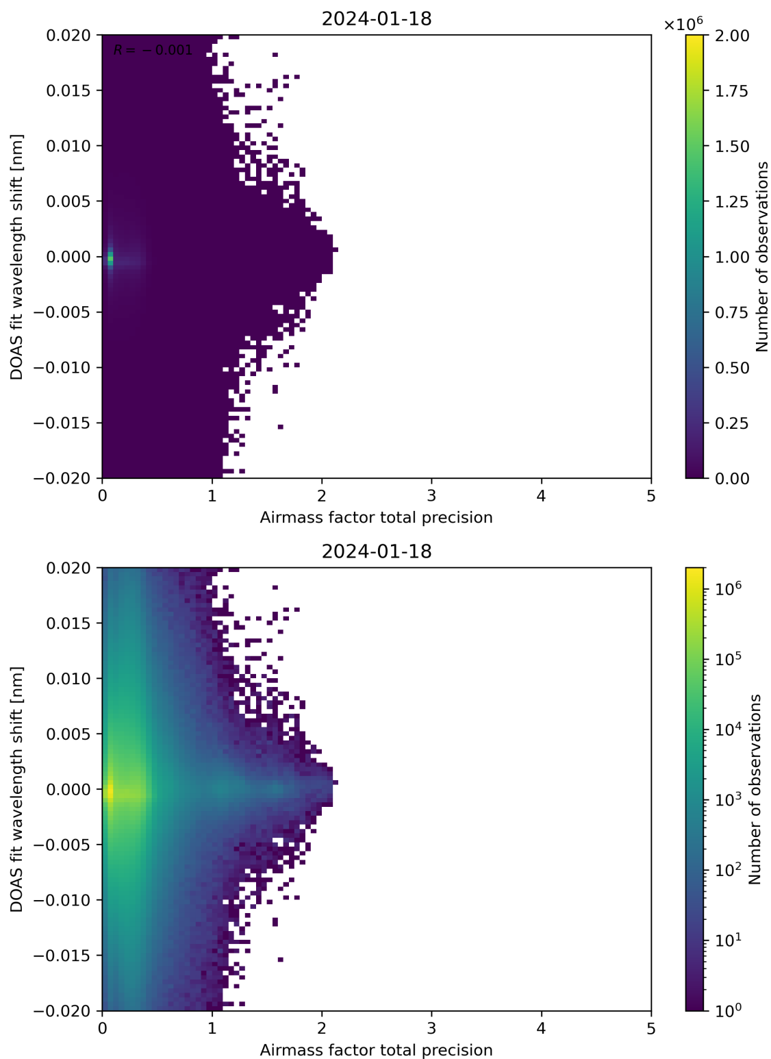
Figure 106: Scatter density plot of “Airmass factor total precision” against “DOAS fit wavelength shift” for 2024-01-17 to 2024-01-19.
