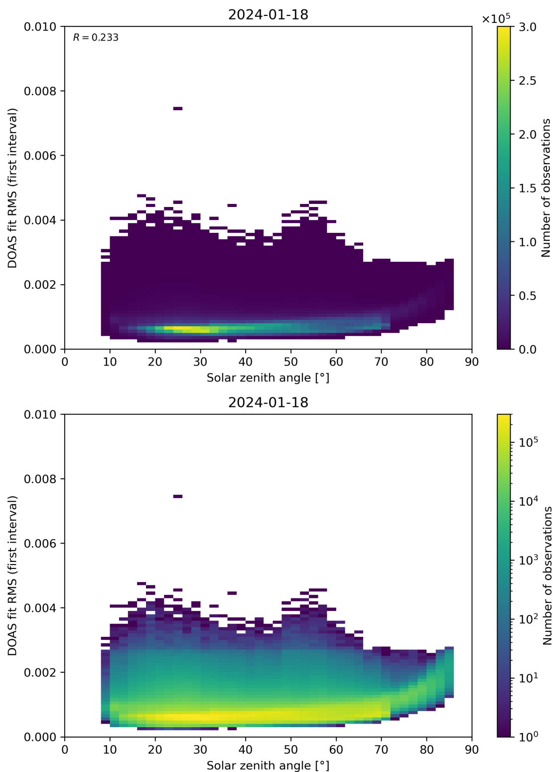
Figure 167: Scatter density plot of “Solar zenith angle” against “DOAS fit RMS (first interval)” for 2024-01-17 to 2024-01-19.
