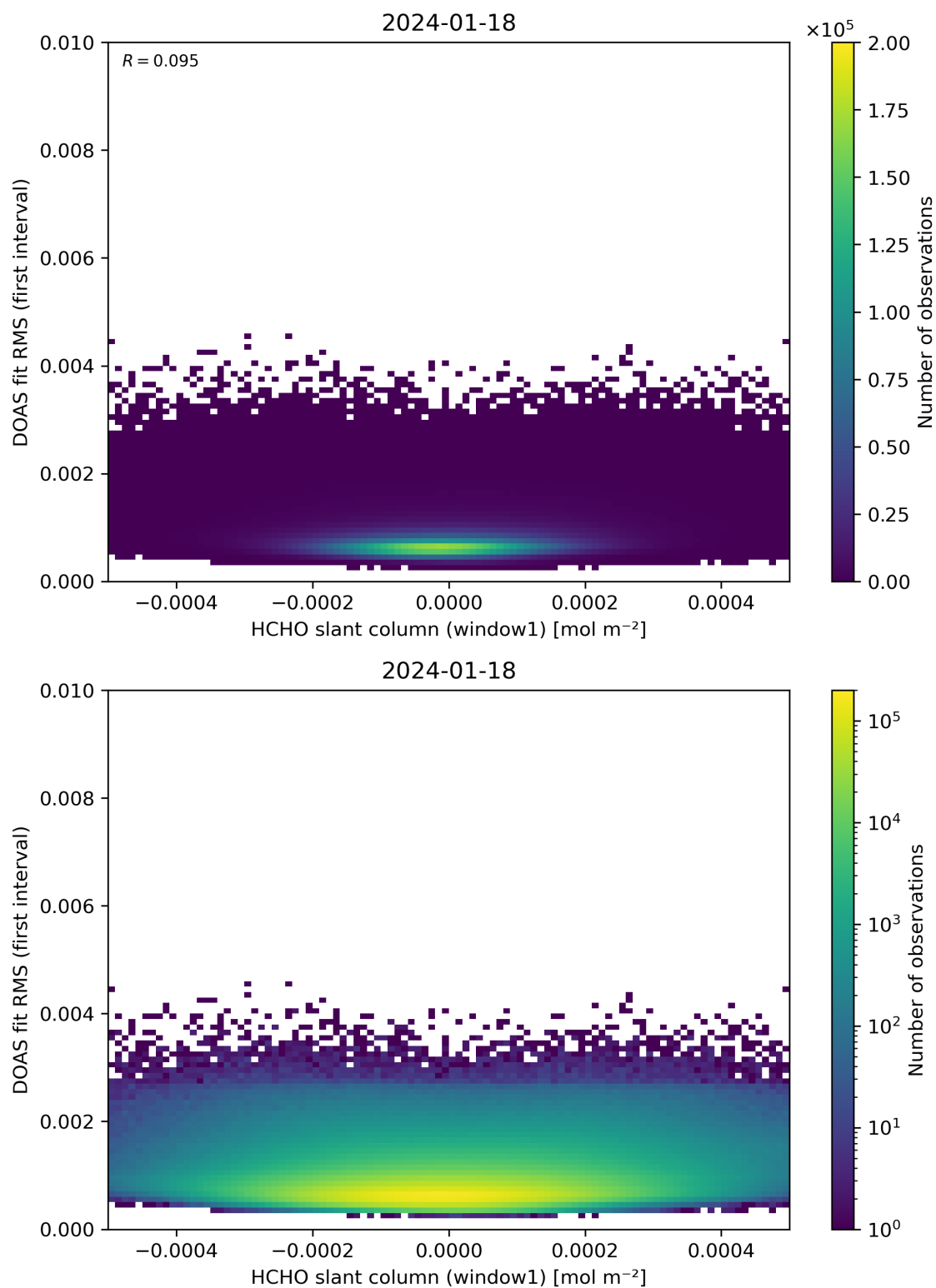
Figure 78: Scatter density plot of “HCHO slant column (window1)” against “DOAS fit RMS (first interval)” for 2024-01-17 to 2024-01-19.
