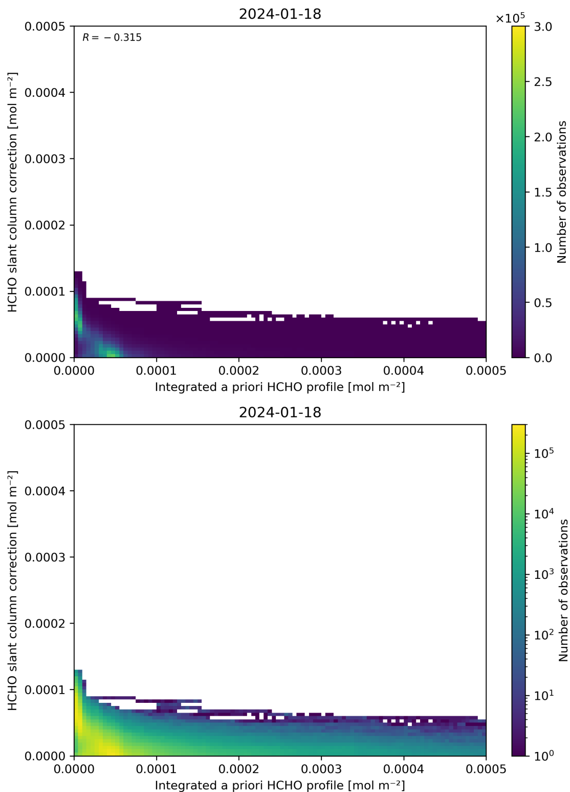
Figure 152: Scatter density plot of “Integrated a priori HCHO profile” against “HCHO slant column correction” for 2024-01-17 to 2024-01-19.
