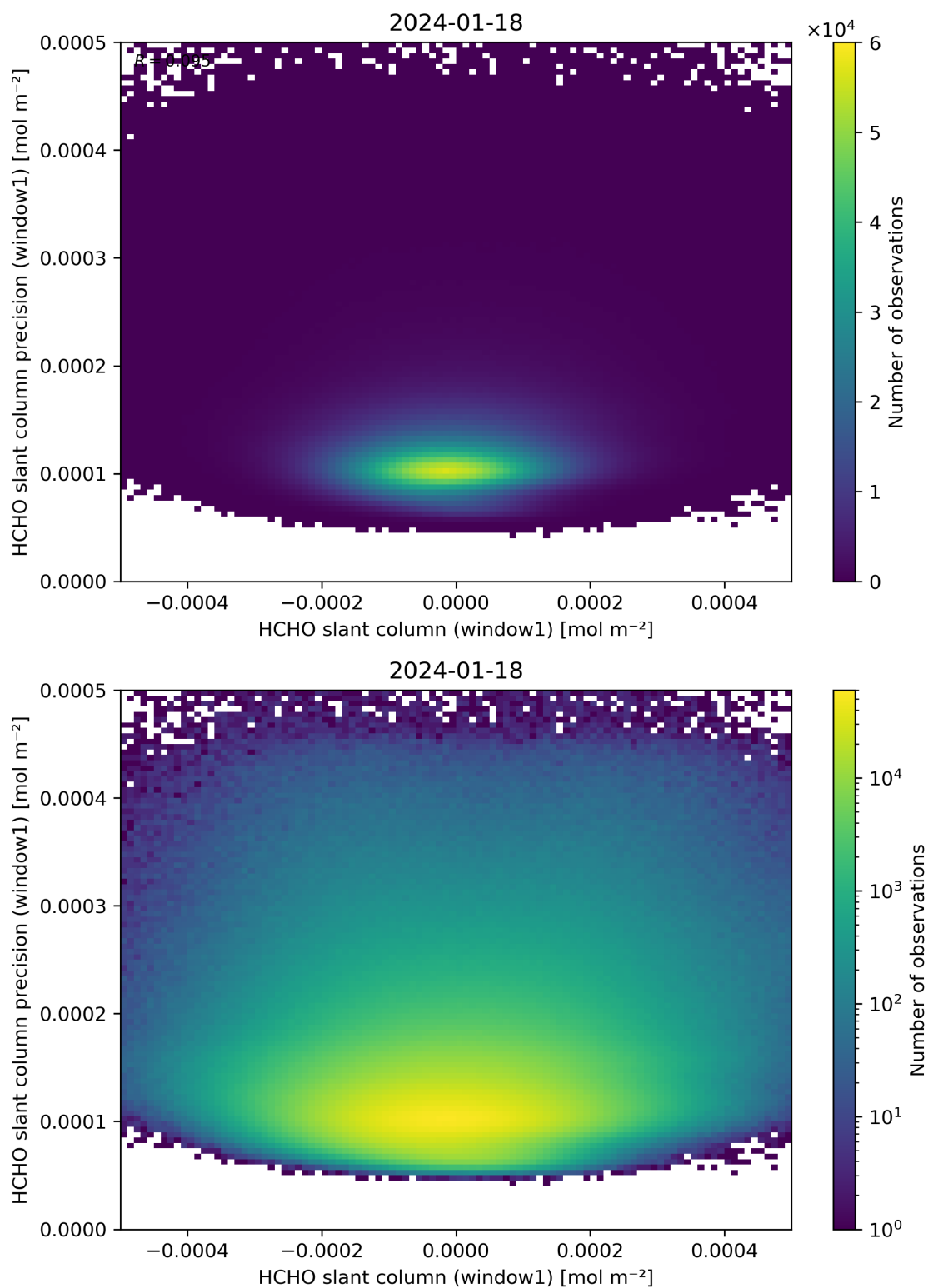
Figure 84: Scatter density plot of “HCHO slant column (window1)” against “HCHO slant column precision (window1)” for 2024-01-17 to 2024-01-19.
