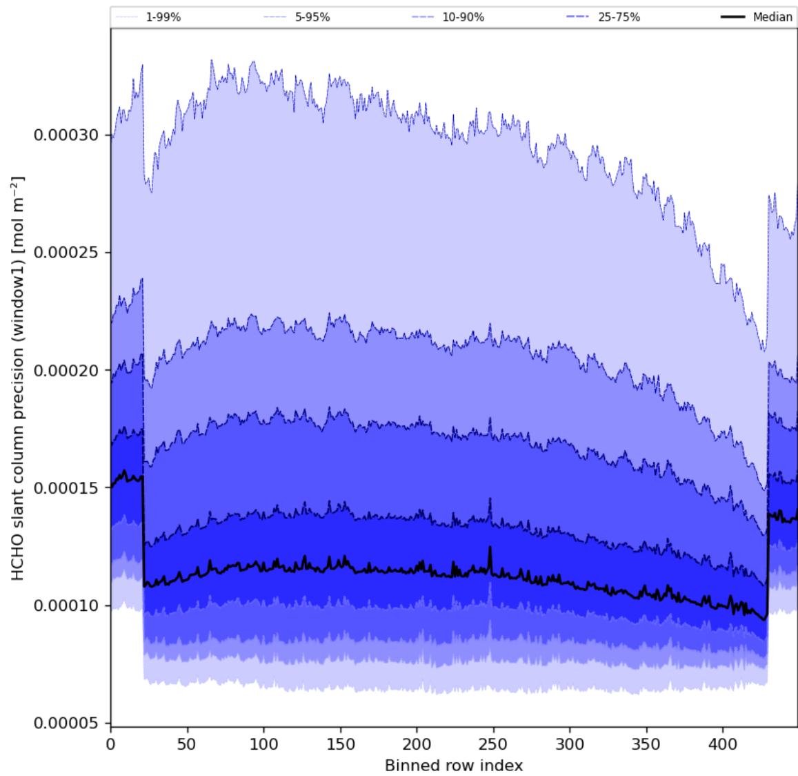
Figure 53: Along track statistics of “HCHO slant column precision (window1)” for 2024-01-17 to 2024-01-19
