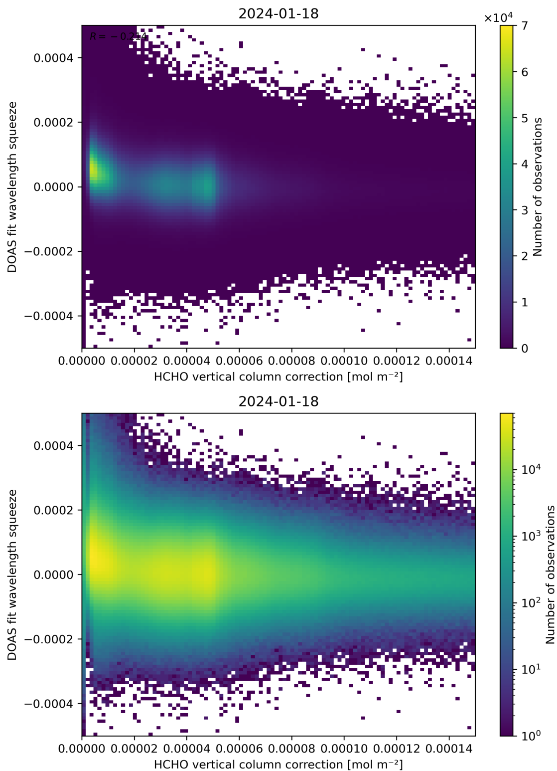
Figure 114: Scatter density plot of “HCHO vertical column correction” against “DOAS fit wavelength squeeze” for 2024-01-17 to 2024-01-19.
