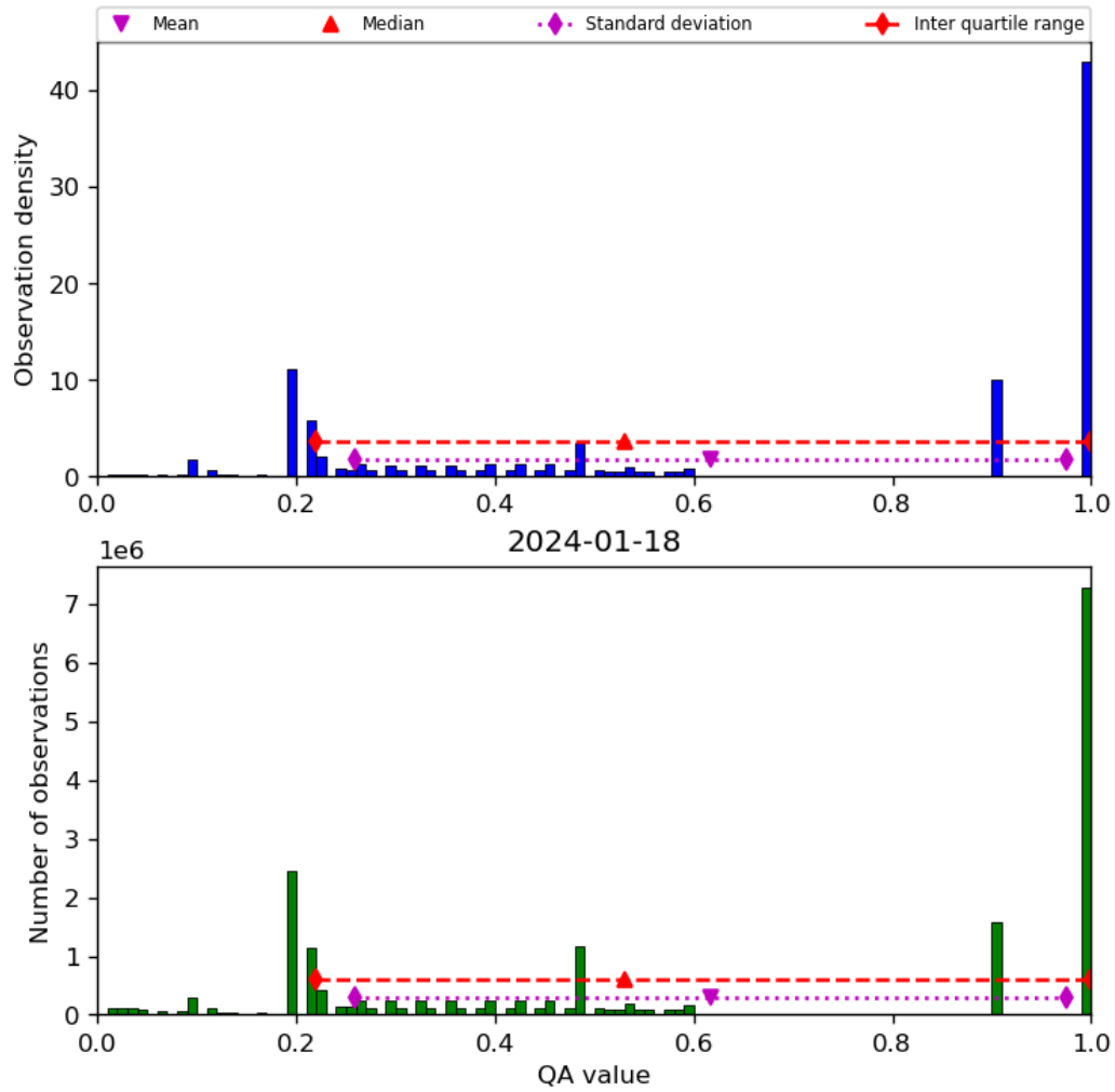
Figure 34: Histogram of “QA value” for 2024-01-17 to 2024-01-19
