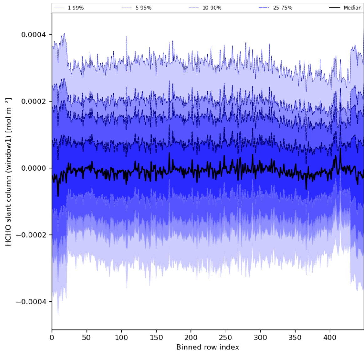
Figure 52: Along track statistics of “HCHO slant column (window1)” for 2024-01-17 to 2024-01-19
