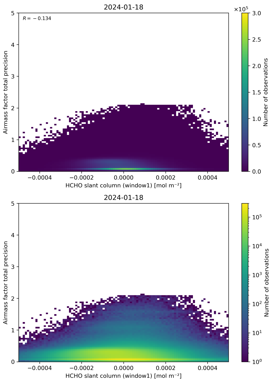
Figure 86: Scatter density plot of “HCHO slant column (window1)” against “Airmass factor total precision” for 2024-01-17 to 2024-01-19.
