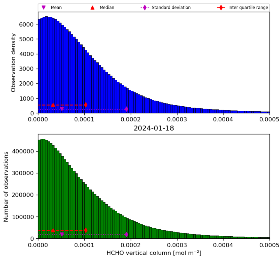
Figure 35: Histogram of “HCHO vertical column” for 2024-01-17 to 2024-01-19
