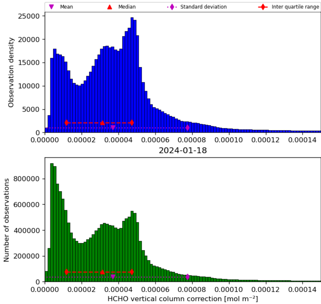
Figure 37: Histogram of “HCHO vertical column correction” for 2024-01-17 to 2024-01-19
