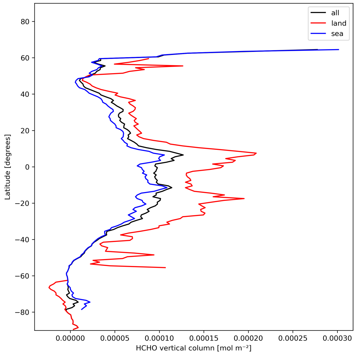
Figure 21: Zonal average of “HCHO vertical column” for 2024-01-17 to 2024-01-19.
