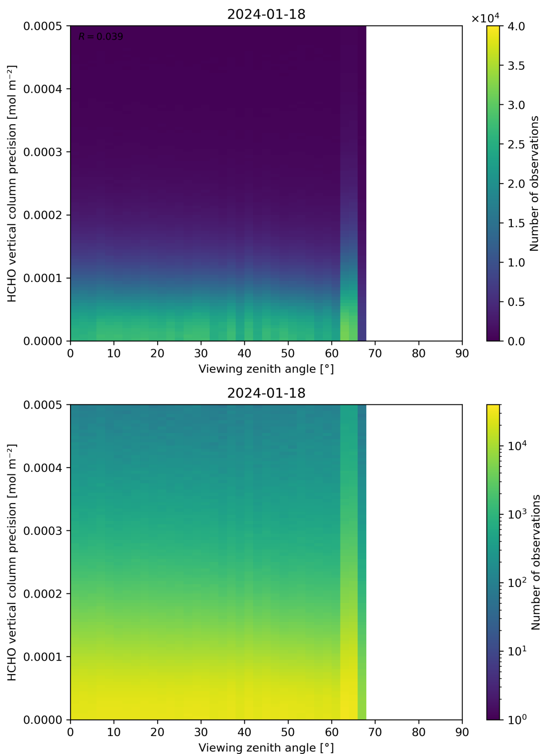
Figure 194: Scatter density plot of “Viewing zenith angle” against “HCHO vertical column precision” for 2024-01-17 to 2024-01-19.
