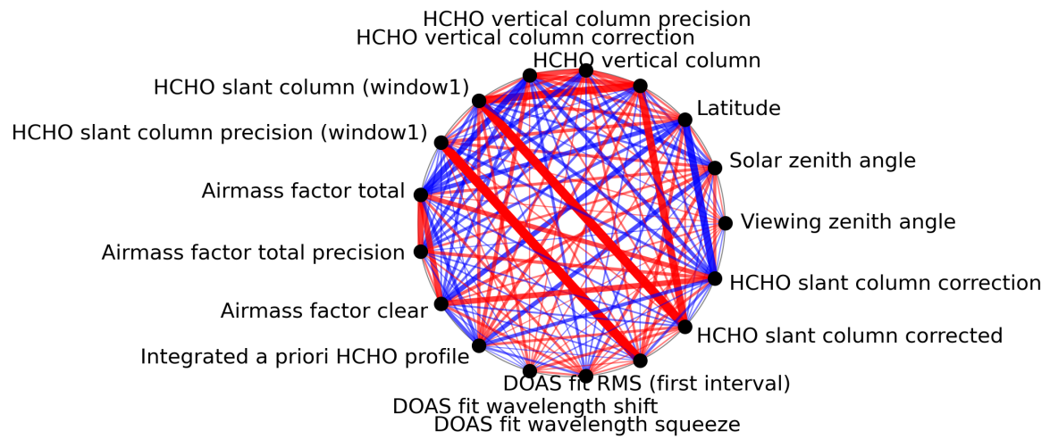
Figure 1: Map of correlation graph for 2024-01-17 to 2024-01-19.
