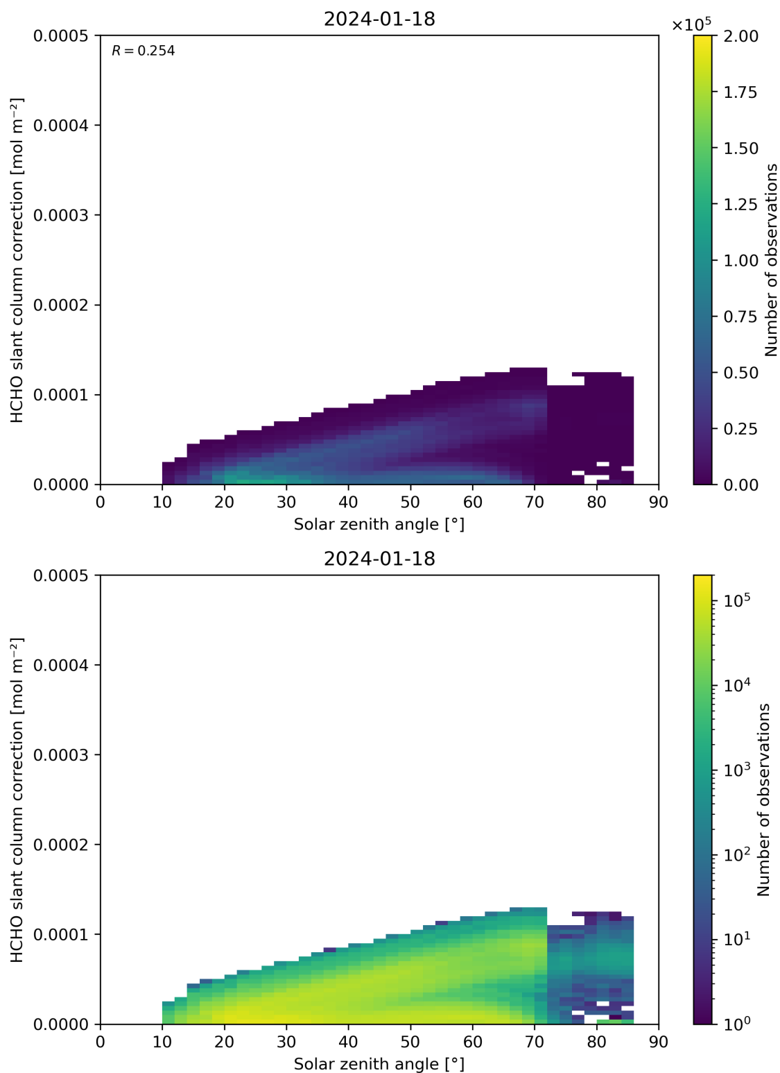
Figure 172: Scatter density plot of “Solar zenith angle” against “HCHO slant column correction” for 2024-01-17 to 2024-01-19.
