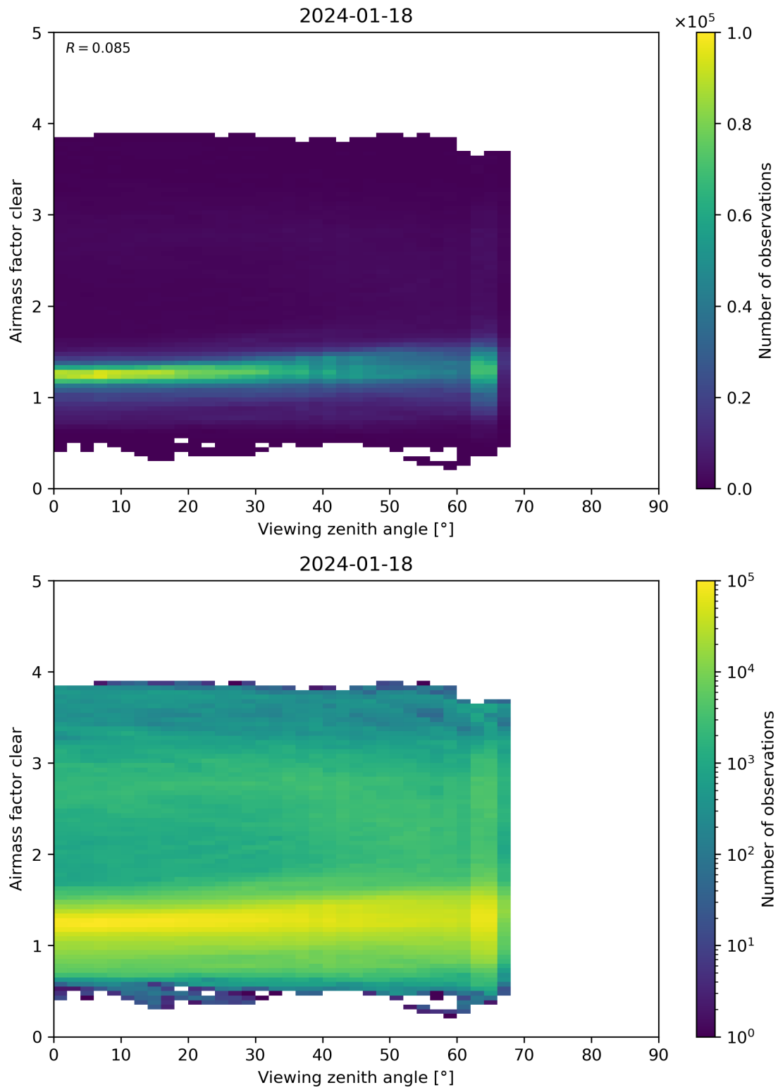
Figure 185: Scatter density plot of “Viewing zenith angle” against “Airmass factor clear” for 2024-01-17 to 2024-01-19.
