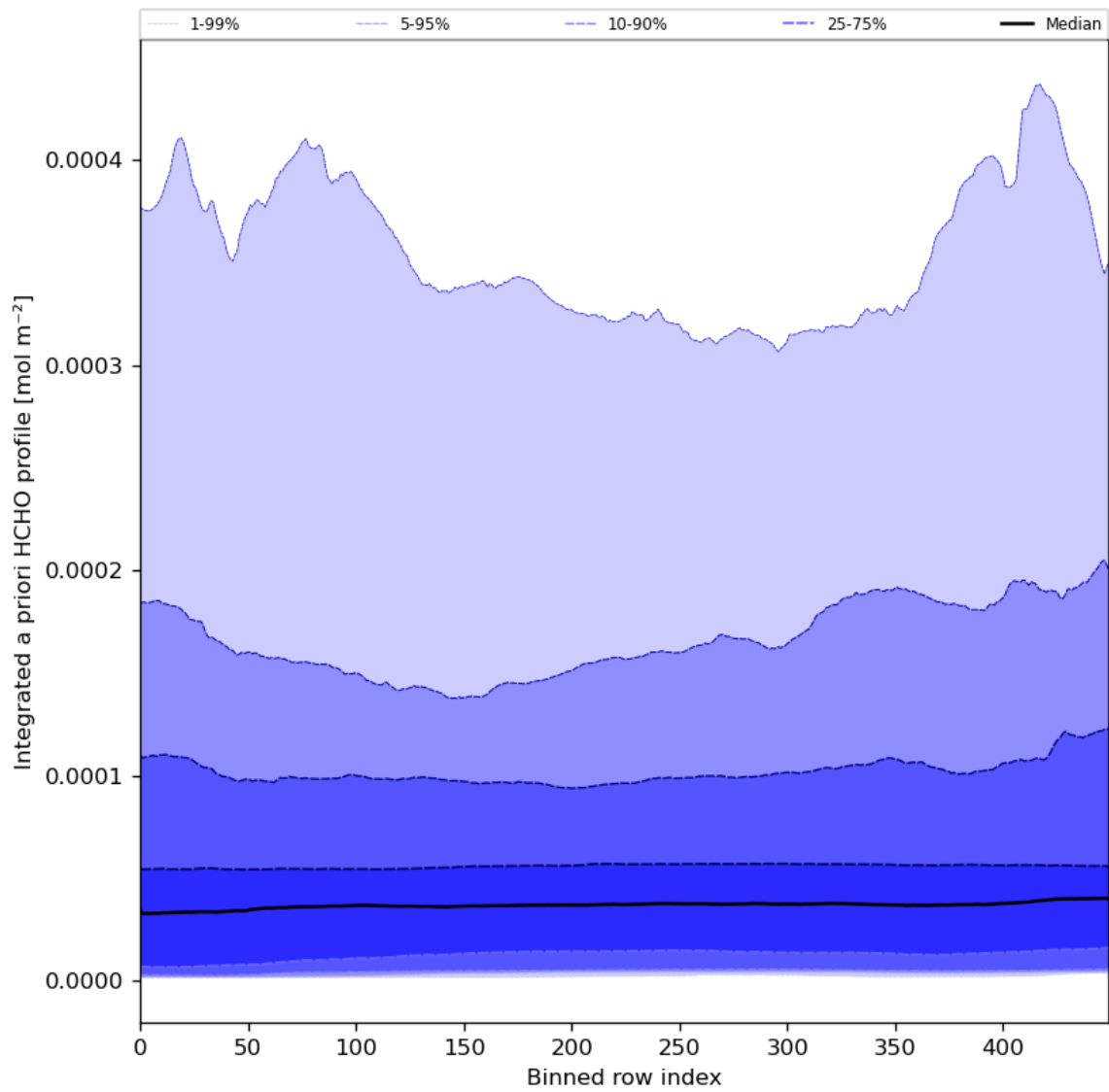
Figure 57: Along track statistics of “Integrated a priori HCHO profile” for 2024-01-17 to 2024-01-19
