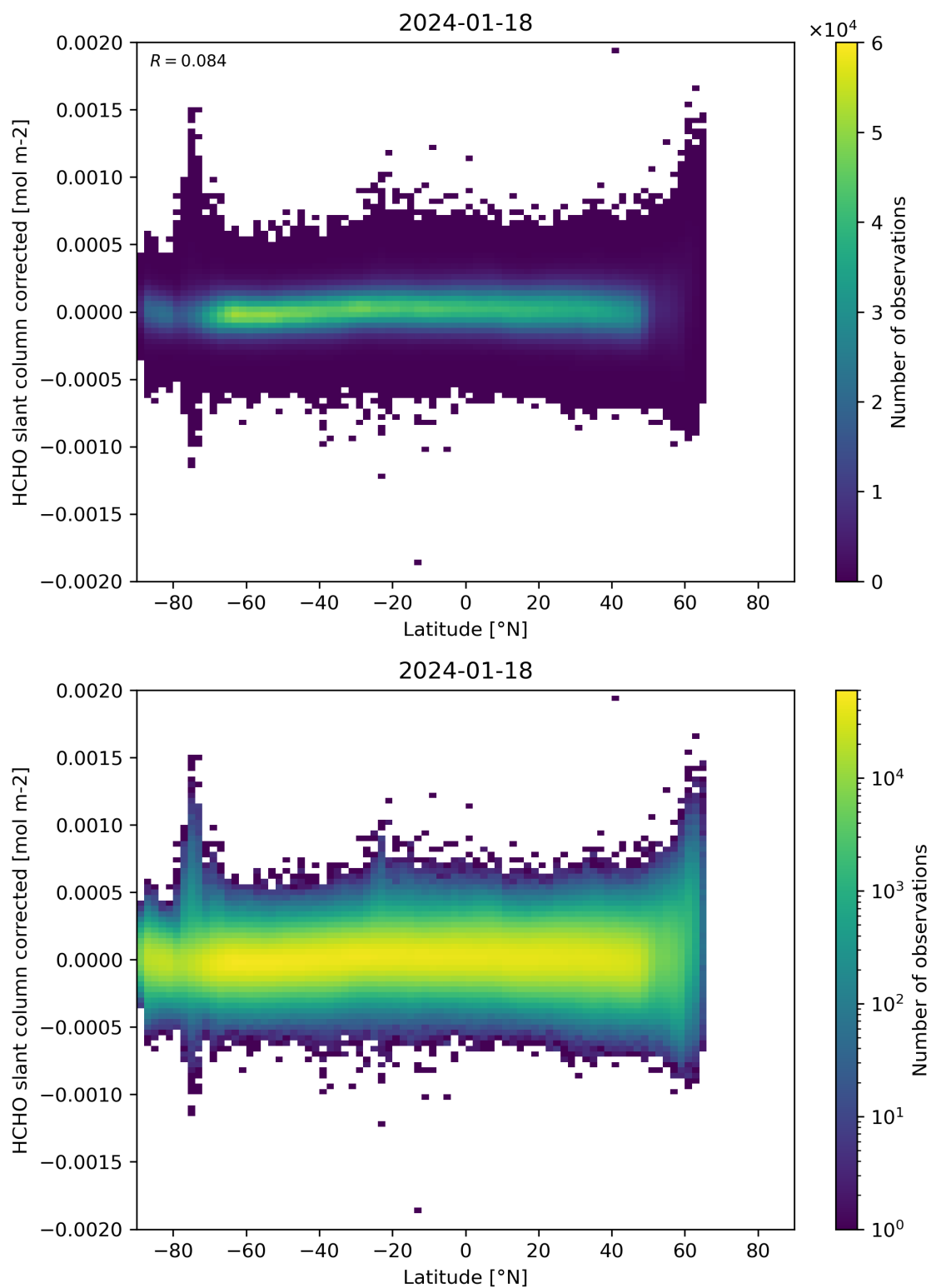
Figure 157: Scatter density plot of “Latitude” against “HCHO slant column corrected” for 2024-01-17 to 2024-01-19.
