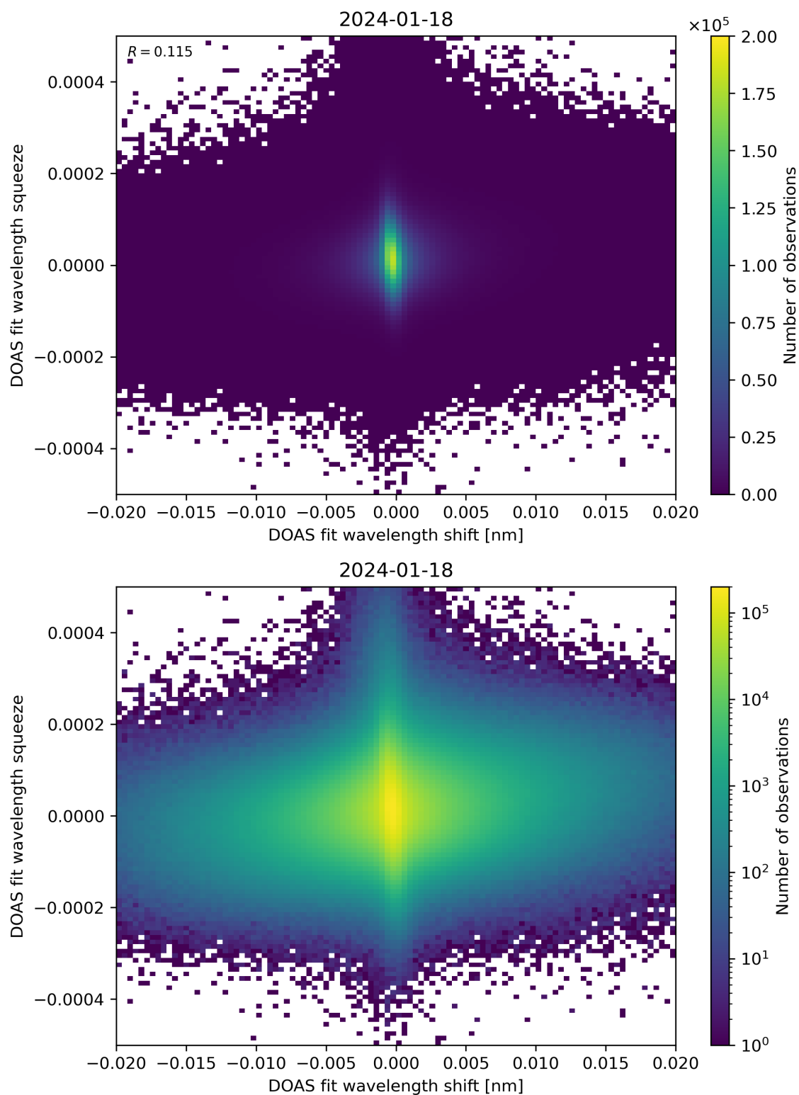
Figure 65: Scatter density plot of “DOAS fit wavelength shift” against “DOAS fit wavelength squeeze” for 2024-01-17 to 2024-01-19.
