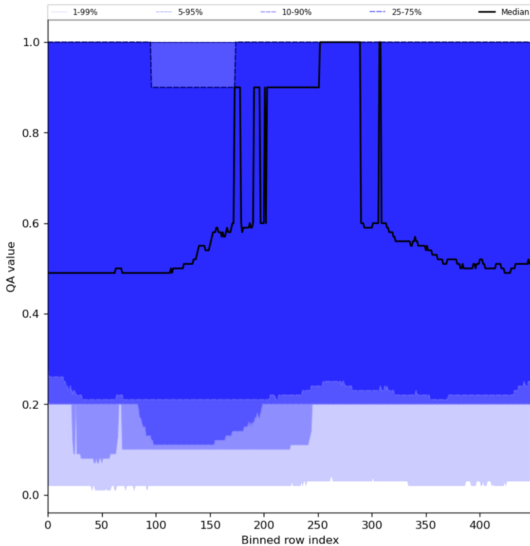
Figure 48: Along track statistics of “QA value” for 2024-01-17 to 2024-01-19
