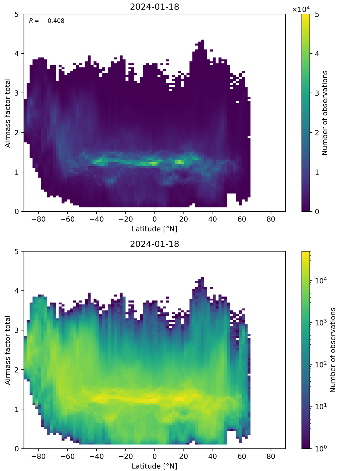
Figure 161: Scatter density plot of “Latitude” against “Airmass factor total” for 2024-01-17 to 2024-01-19.
