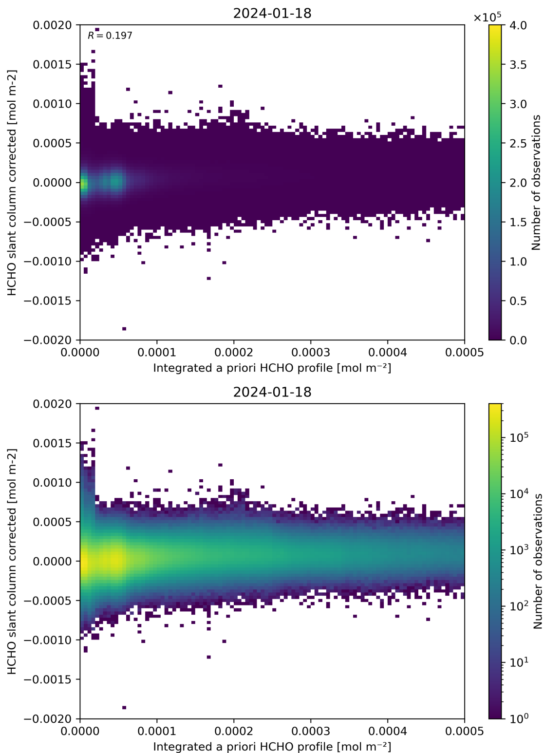
Figure 151: Scatter density plot of “Integrated a priori HCHO profile” against “HCHO slant column corrected” for 2024-01-17 to 2024-01-19.
