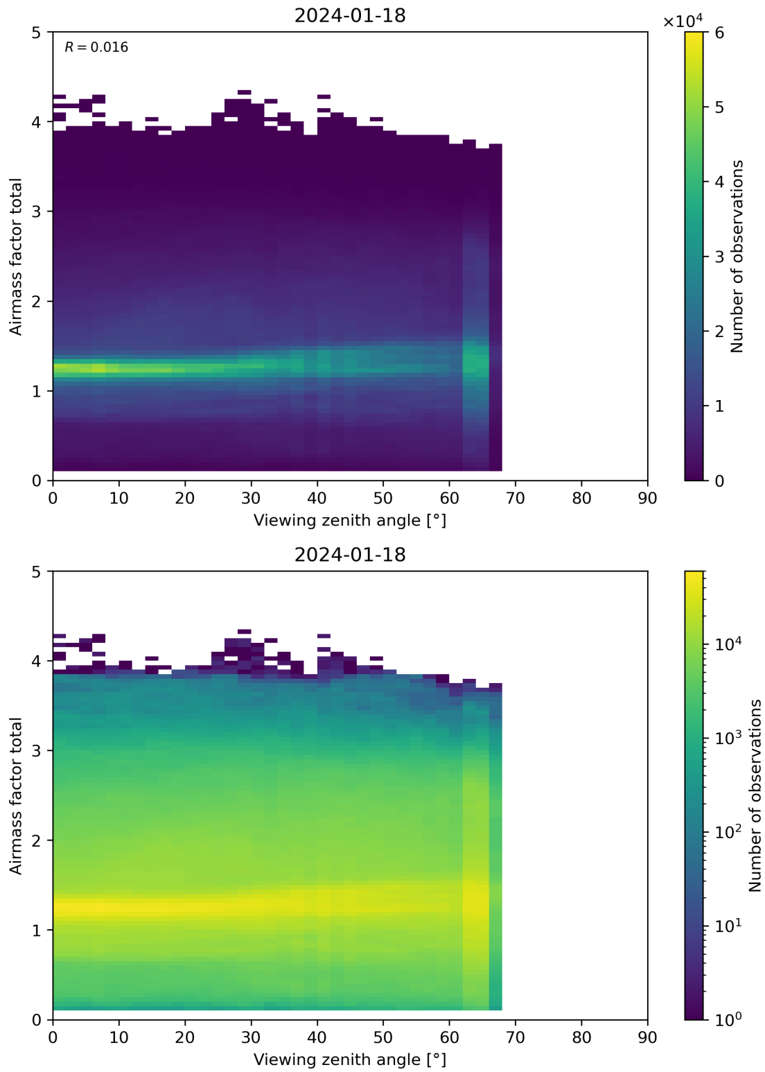
Figure 190: Scatter density plot of “Viewing zenith angle” against “Airmass factor total” for 2024-01-17 to 2024-01-19.
