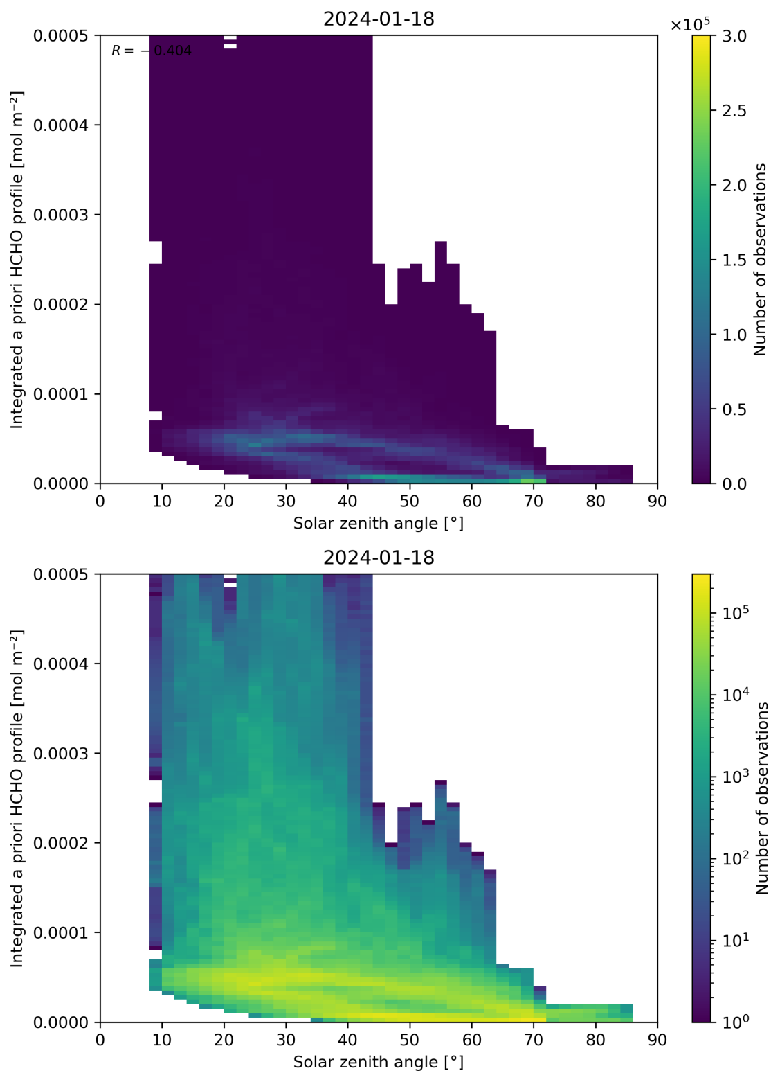
Figure 180: Scatter density plot of “Solar zenith angle” against “Integrated a priori HCHO profile” for 2024-01-17 to 2024-01-19.
