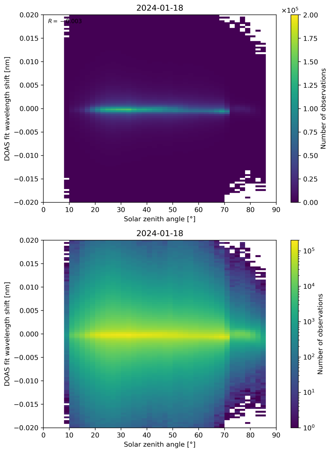
Figure 168: Scatter density plot of “Solar zenith angle” against “DOAS fit wavelength shift” for 2024-01-17 to 2024-01-19.
