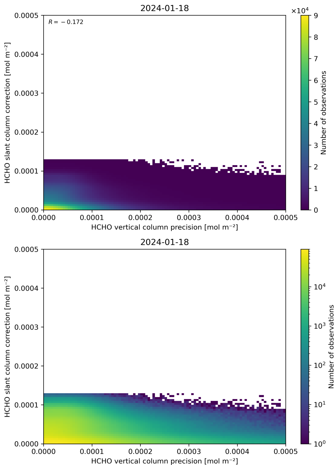
Figure 141: Scatter density plot of “HCHO vertical column precision” against “HCHO slant column correction” for 2024-01-17 to 2024-01-19.
