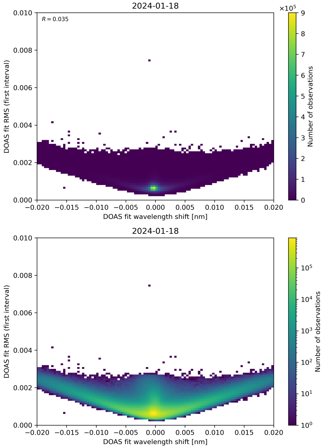
Figure 64: Scatter density plot of “DOAS fit wavelength shift” against “DOAS fit RMS (first interval)” for 2024-01-17 to 2024-01-19.
