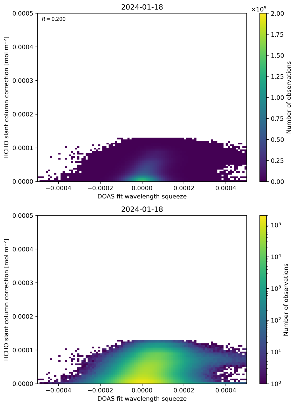
Figure 70: Scatter density plot of “DOAS fit wavelength squeeze” against “HCHO slant column correction” for 2024-01-17 to 2024-01-19.
