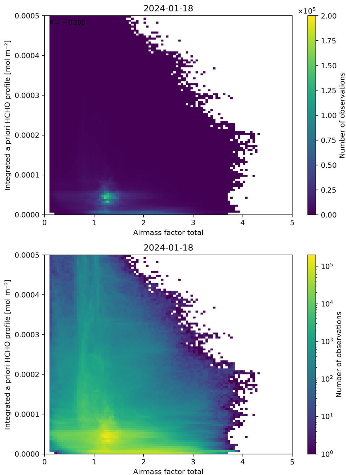
Figure 104: Scatter density plot of “Airmass factor total” against “Integrated a priori HCHO profile” for 2024-01-17 to 2024-01-19.
