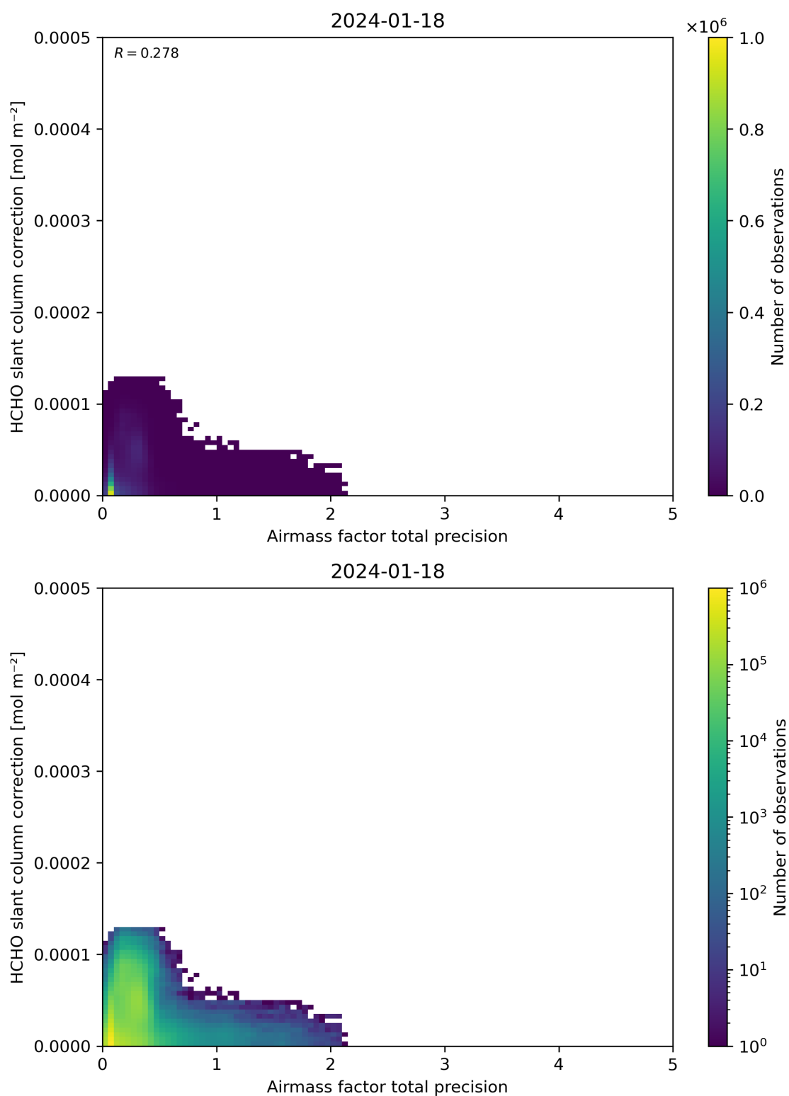
Figure 110: Scatter density plot of “Airmass factor total precision” against “HCHO slant column correction” for 2024-01-17 to 2024-01-19.
