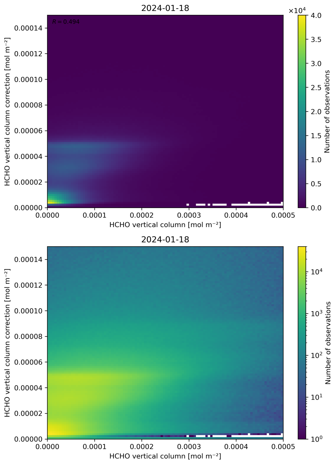
Figure 133: Scatter density plot of “HCHO vertical column” against “HCHO vertical column correction” for 2024-01-17 to 2024-01-19.
