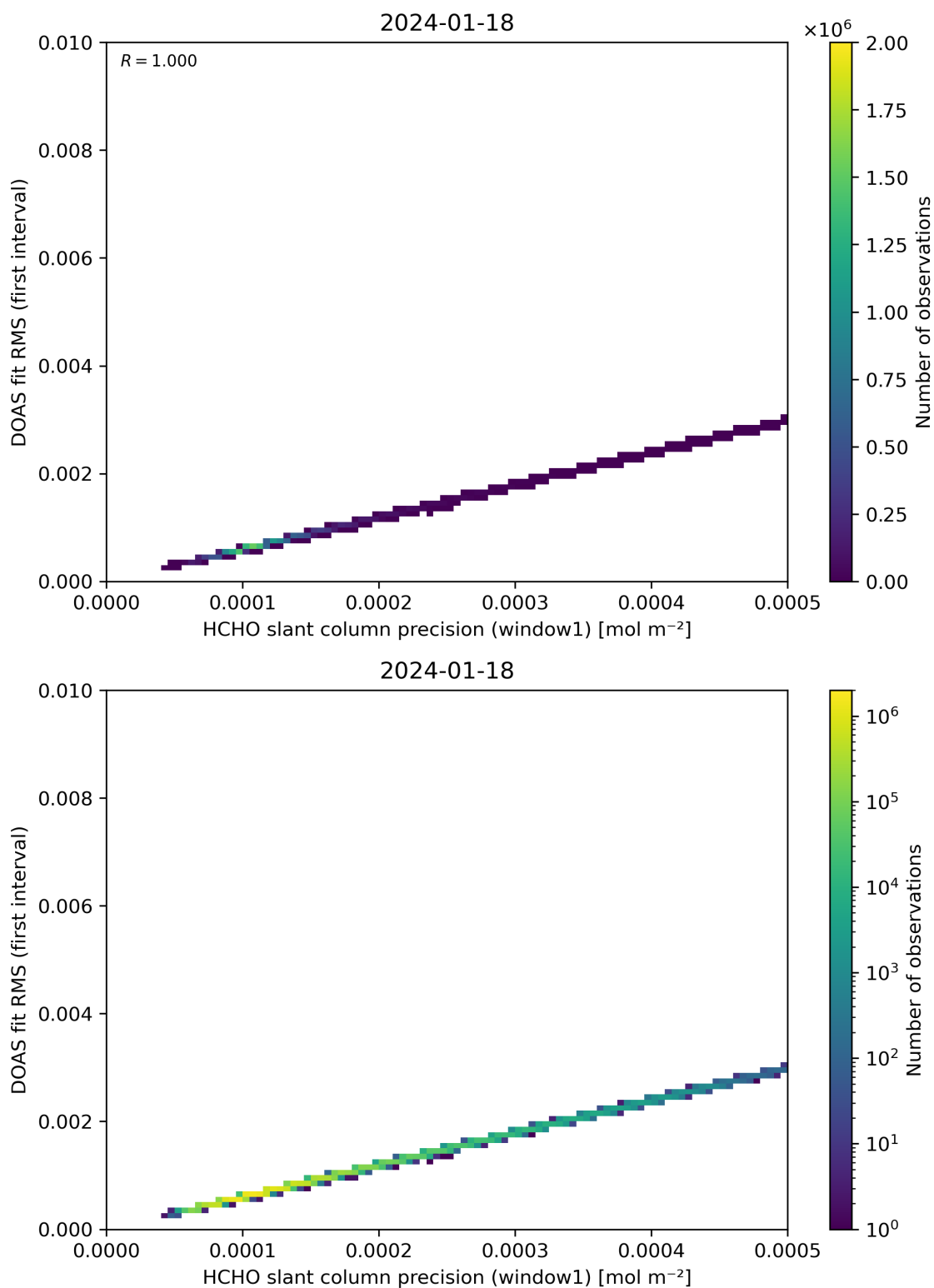
Figure 88: Scatter density plot of “HCHO slant column precision (window1)” against “DOAS fit RMS (first interval)” for 2024-01-17 to 2024-01-19.
