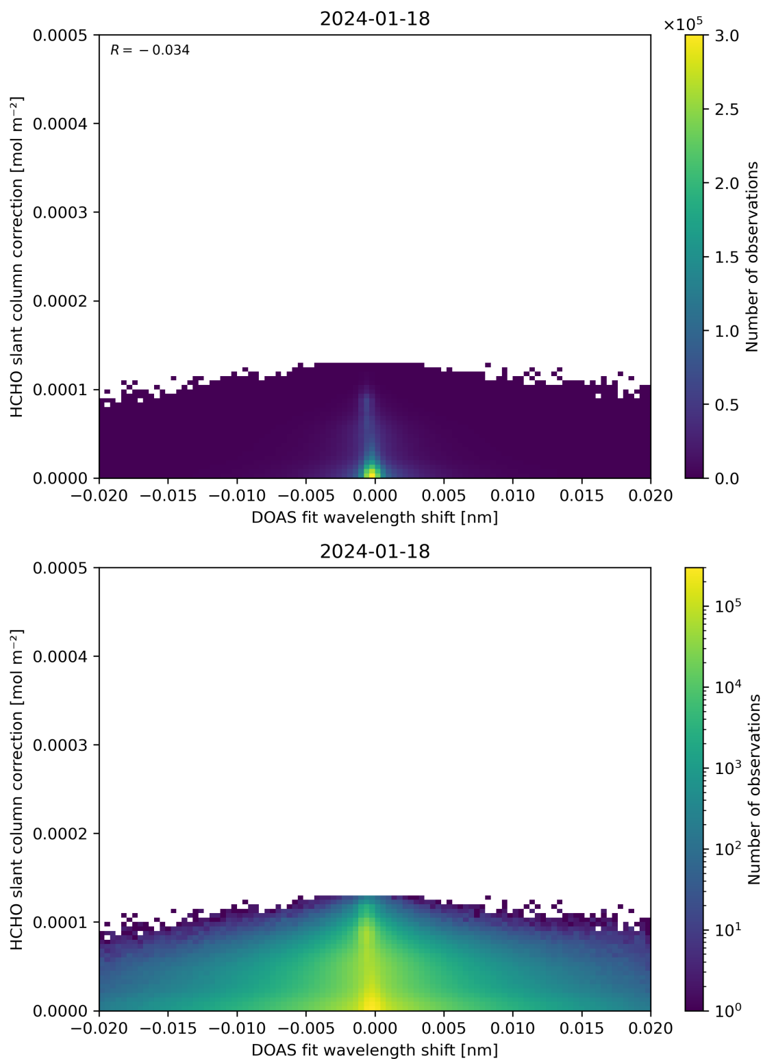
Figure 67: Scatter density plot of “DOAS fit wavelength shift” against “HCHO slant column correction” for 2024-01-17 to 2024-01-19.
