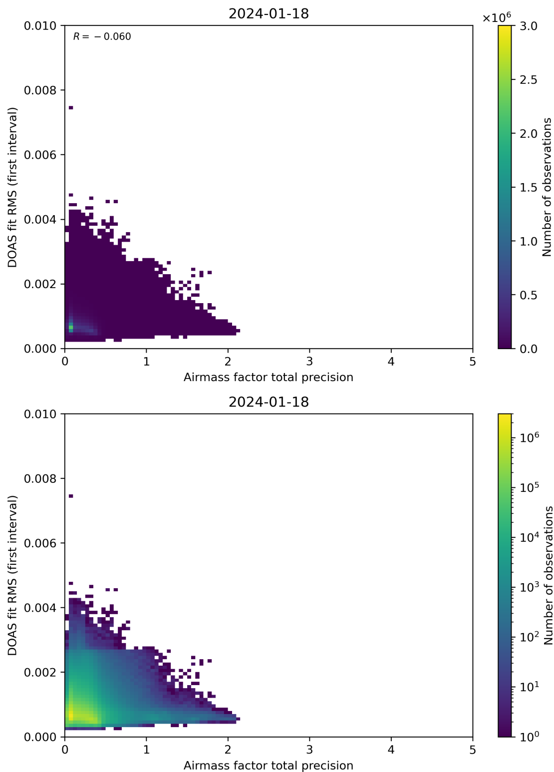
Figure 105: Scatter density plot of “Airmass factor total precision” against “DOAS fit RMS (first interval)” for 2024-01-17 to 2024-01-19.
