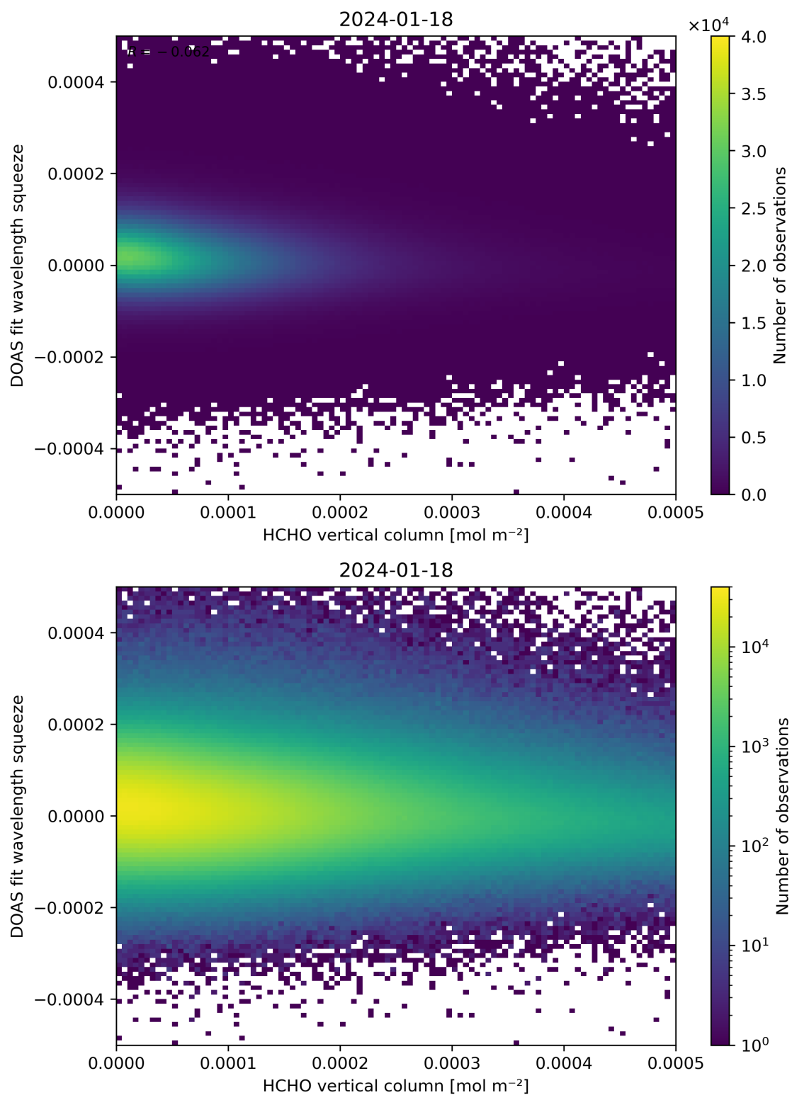
Figure 125: Scatter density plot of “HCHO vertical column” against “DOAS fit wavelength squeeze” for 2024-01-17 to 2024-01-19.
