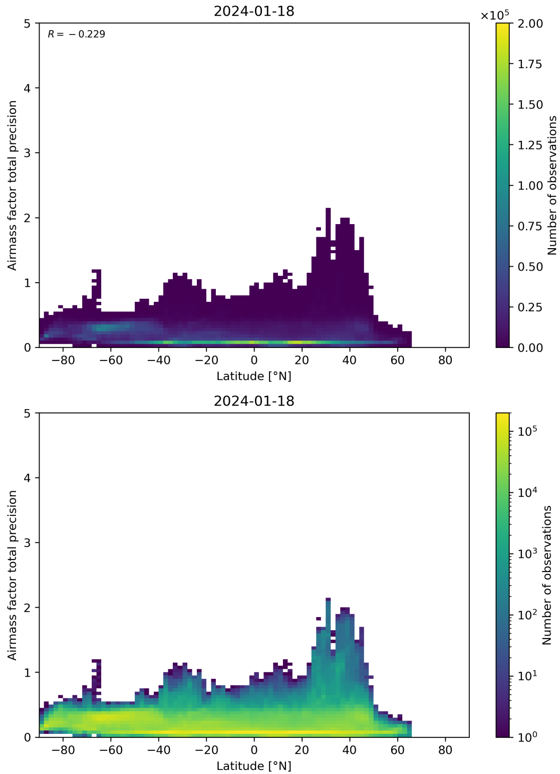
Figure 162: Scatter density plot of “Latitude” against “Airmass factor total precision” for 2024-01-17 to 2024-01-19.
