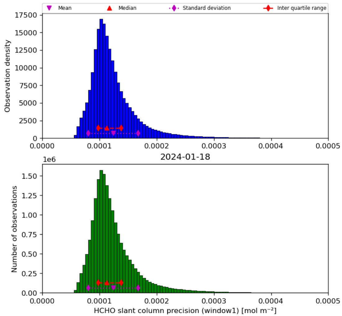
Figure 39: Histogram of “HCHO slant column precision (window1)” for 2024-01-17 to 2024-01-19
