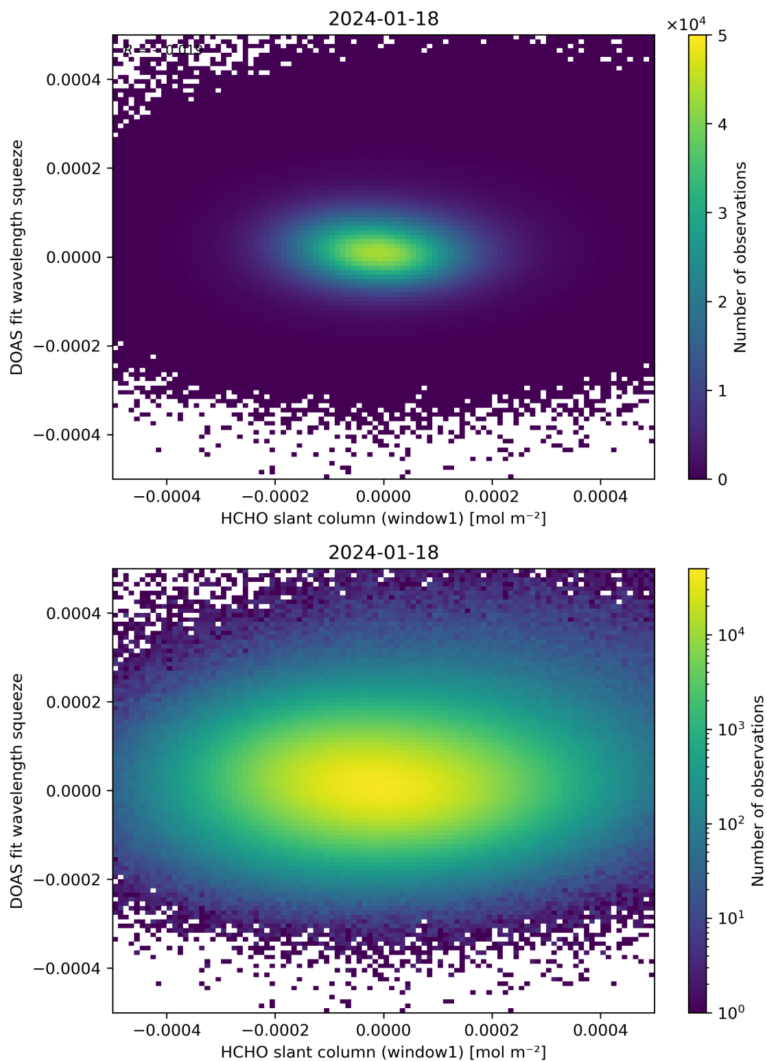
Figure 80: Scatter density plot of “HCHO slant column (window1)” against “DOAS fit wavelength squeeze” for 2024-01-17 to 2024-01-19.
