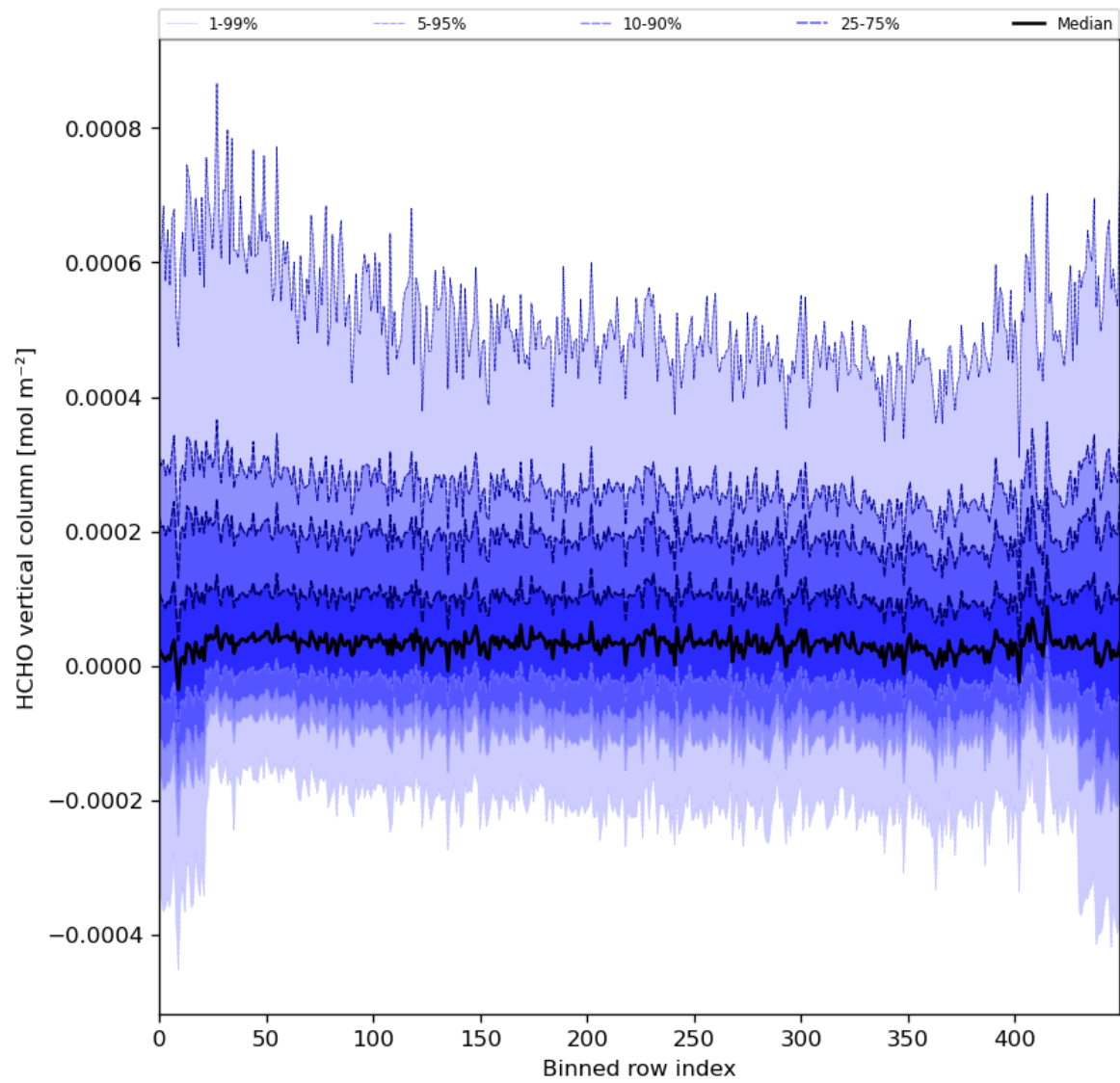
Figure 49: Along track statistics of “HCHO vertical column” for 2024-01-17 to 2024-01-19
