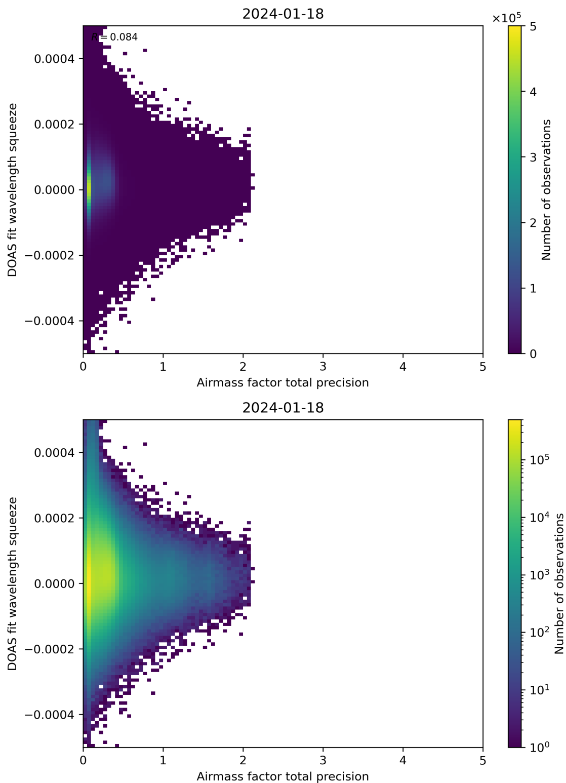
Figure 107: Scatter density plot of “Airmass factor total precision” against “DOAS fit wavelength squeeze” for 2024-01-17 to 2024-01-19.
