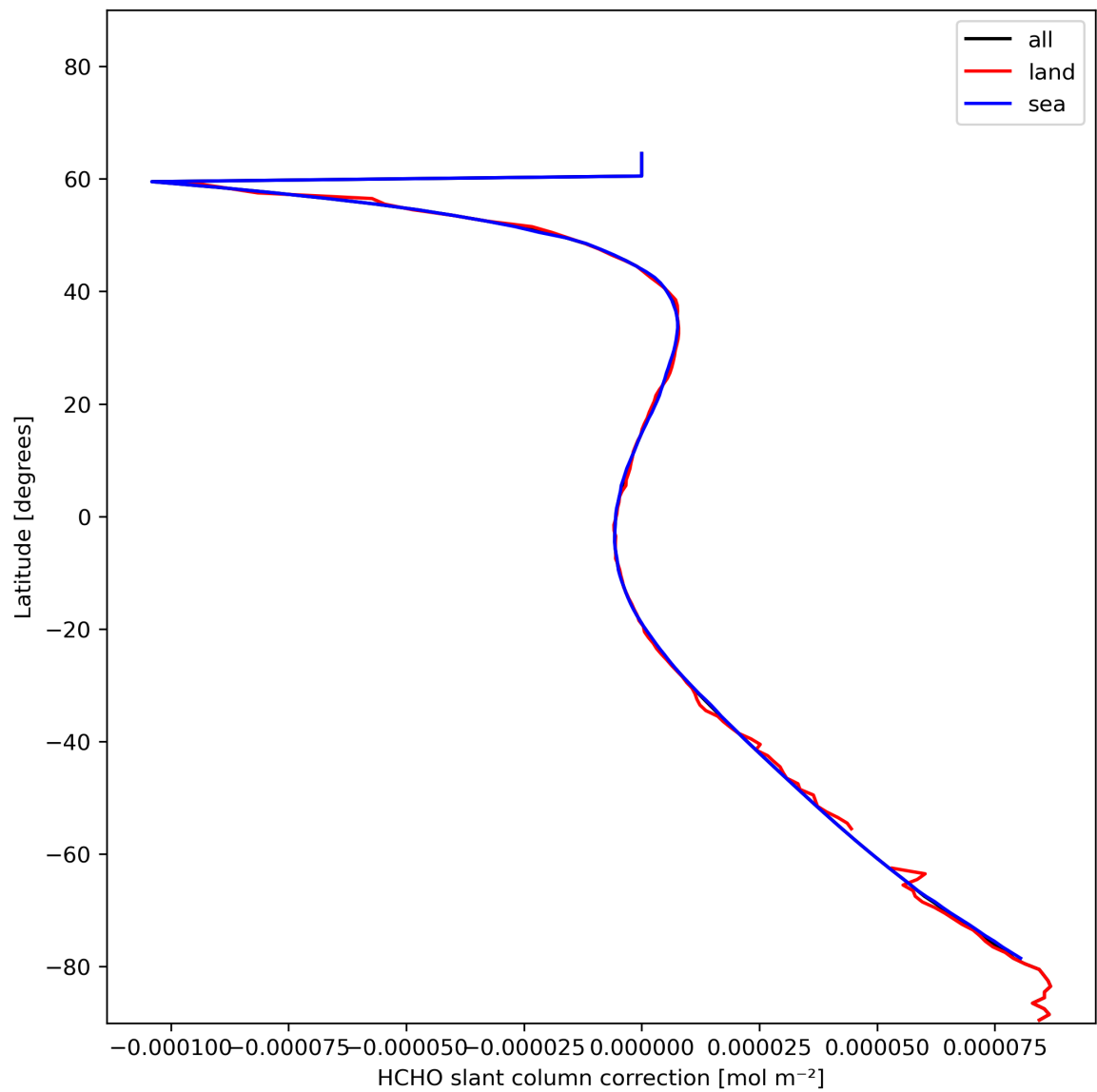
Figure 33: Zonal average of “HCHO slant column correction” for 2024-01-17 to 2024-01-19.
