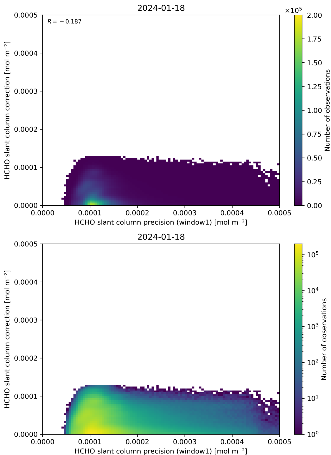
Figure 93: Scatter density plot of “HCHO slant column precision (window1)” against “HCHO slant column correction” for 2024-01-17 to 2024-01-19.
