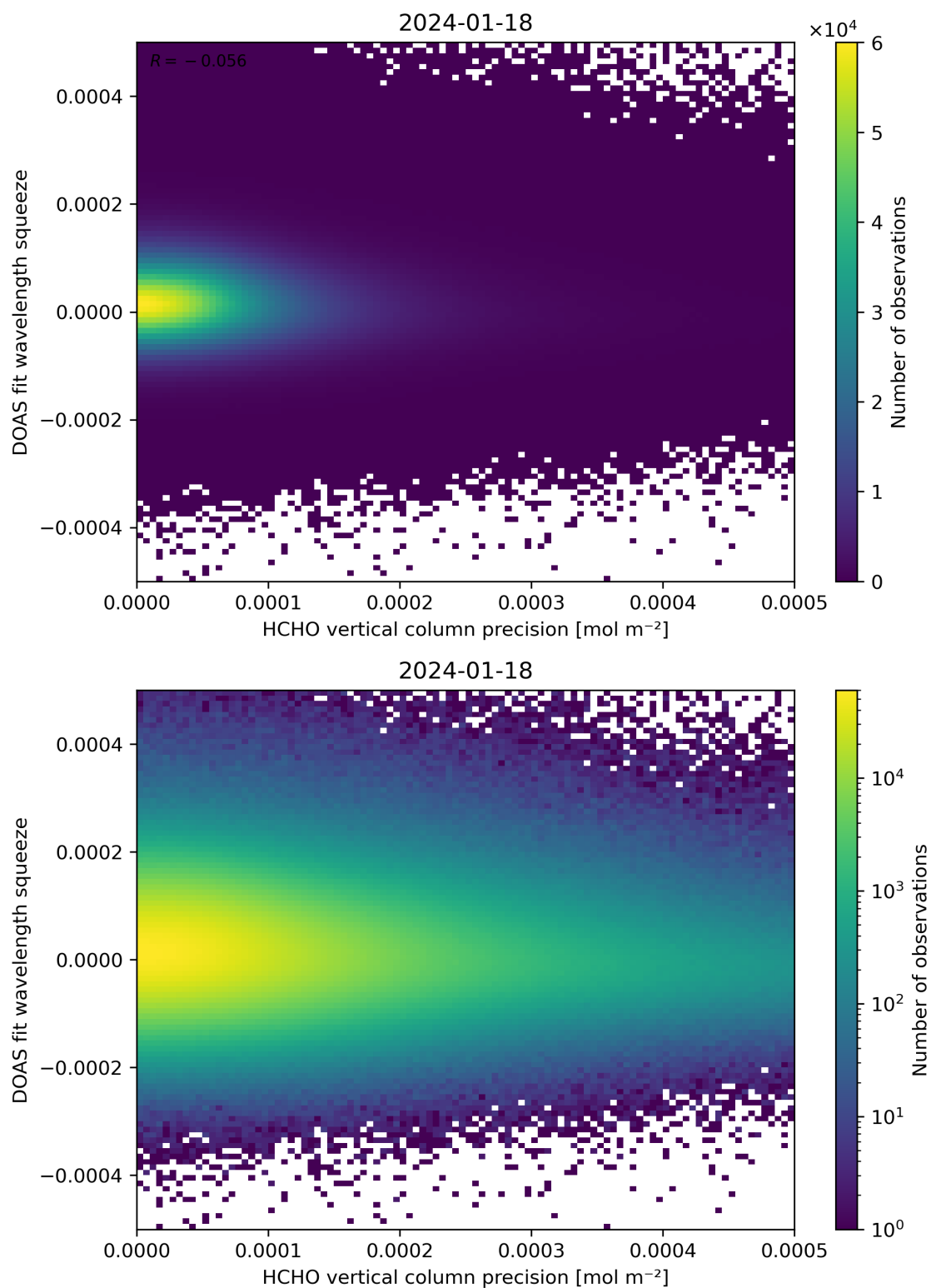
Figure 138: Scatter density plot of “HCHO vertical column precision” against “DOAS fit wavelength squeeze” for 2024-01-17 to 2024-01-19.
