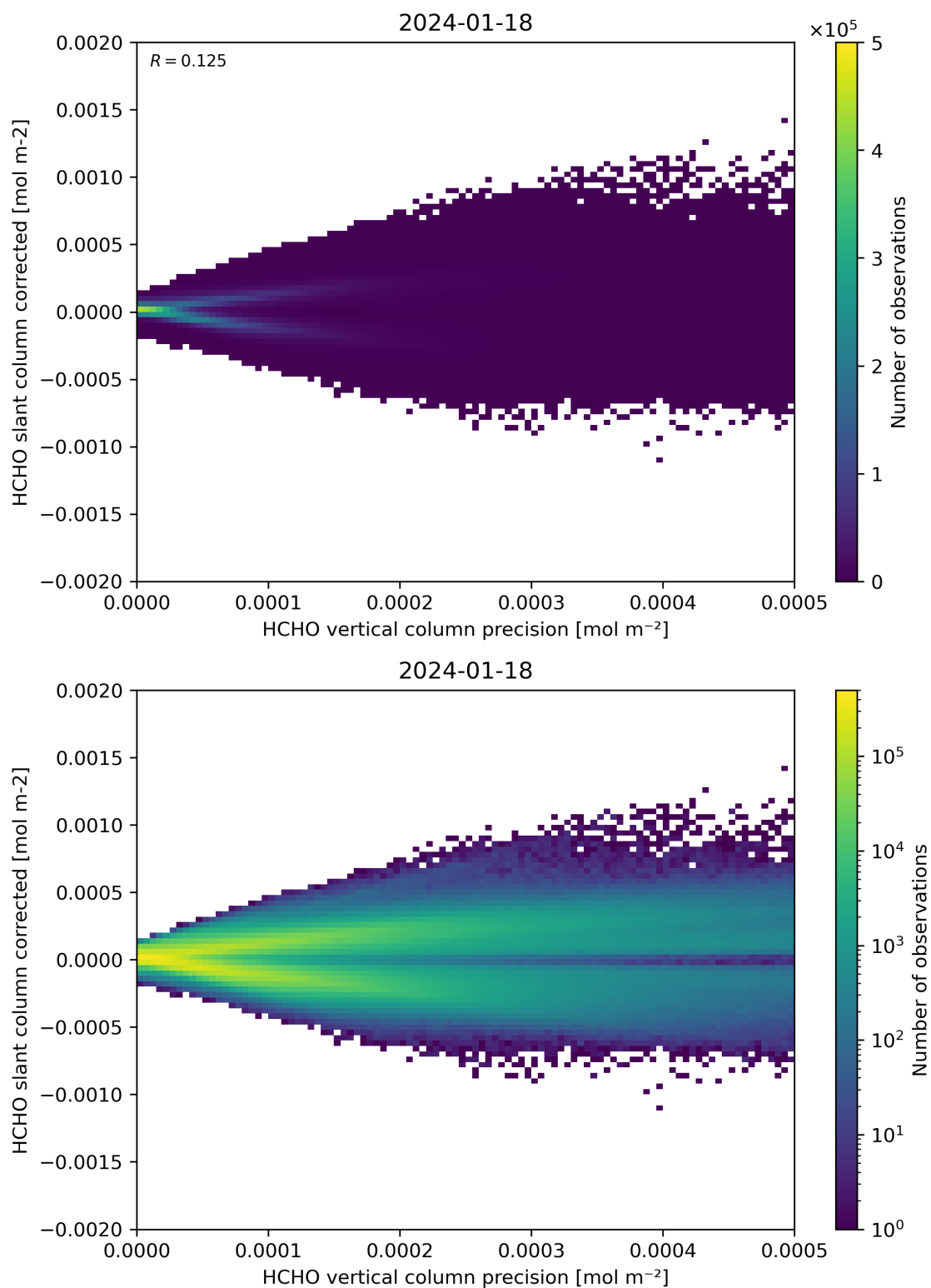
Figure 140: Scatter density plot of “HCHO vertical column precision” against “HCHO slant column corrected” for 2024-01-17 to 2024-01-19.
