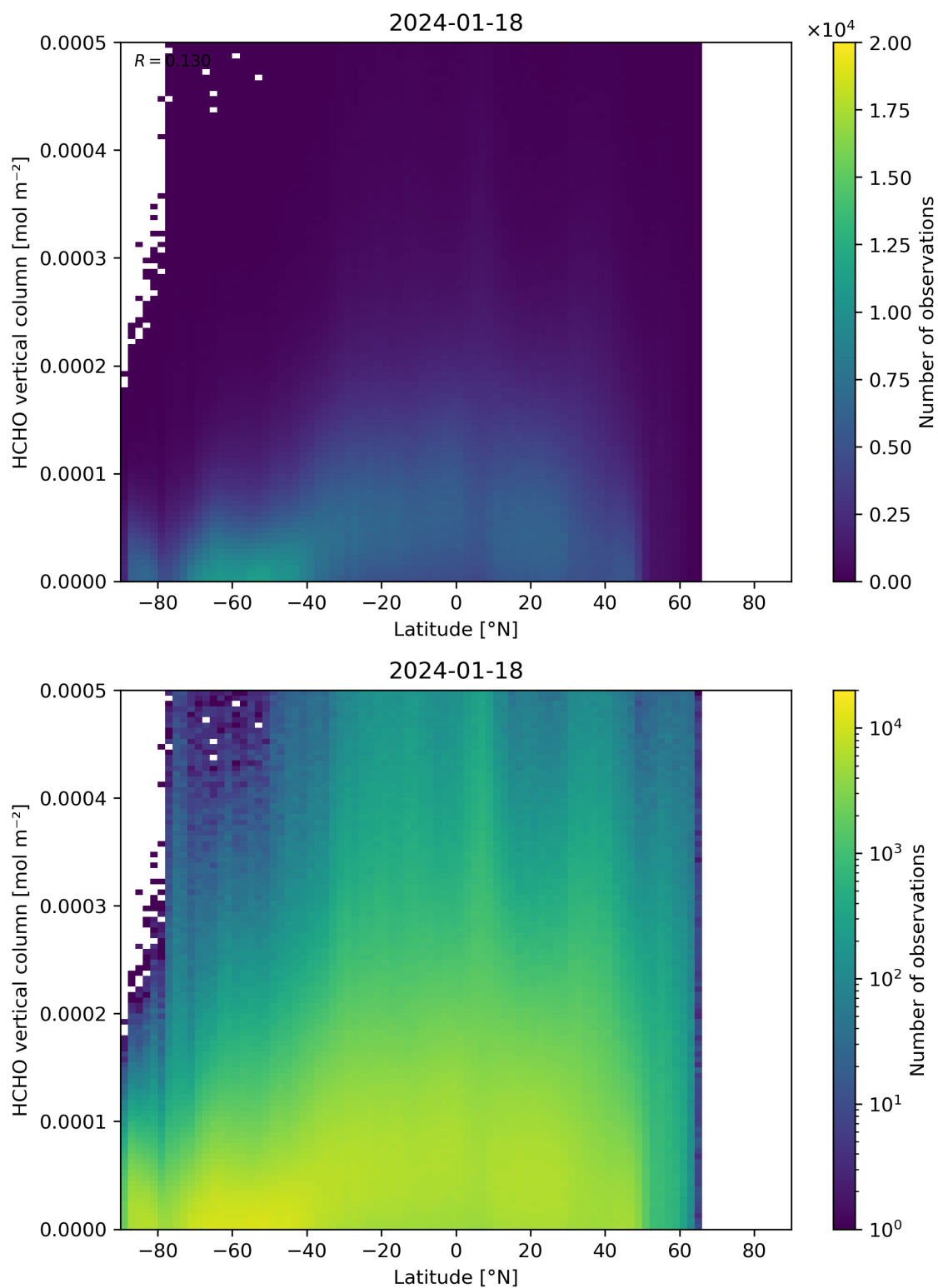
Figure 163: Scatter density plot of “Latitude” against “HCHO vertical column” for 2024-01-17 to 2024-01-19.
