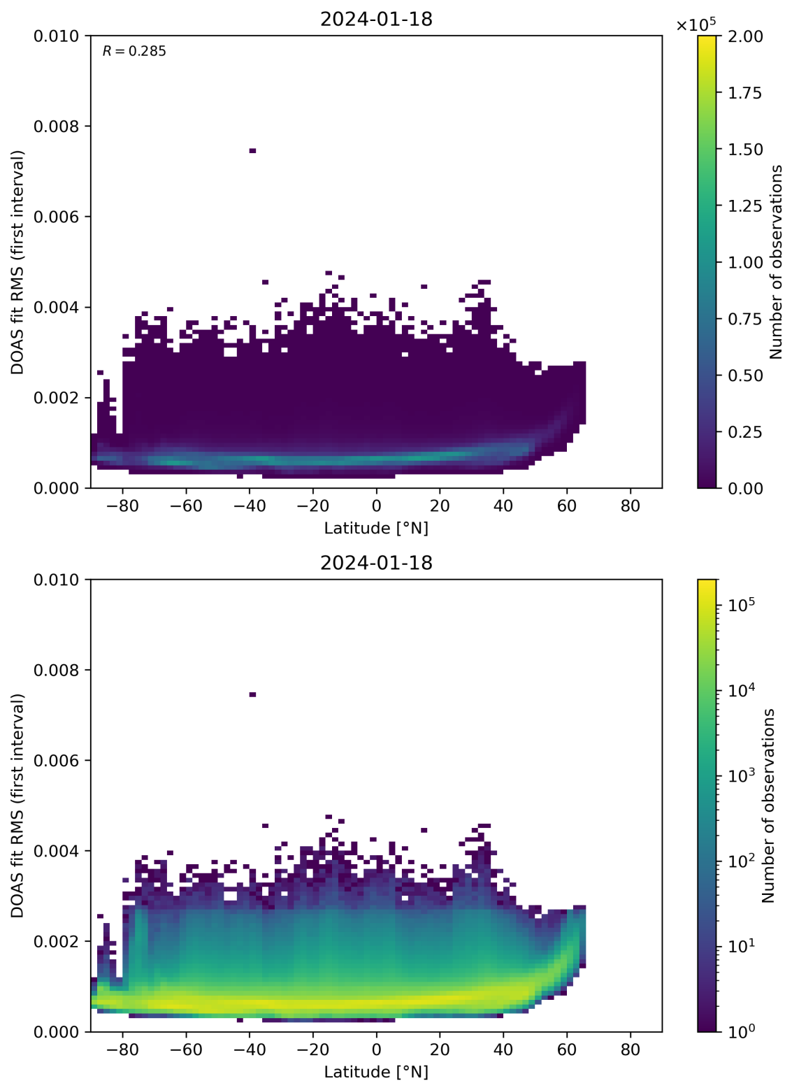
Figure 153: Scatter density plot of “Latitude” against “DOAS fit RMS (first interval)” for 2024-01-17 to 2024-01-19.
