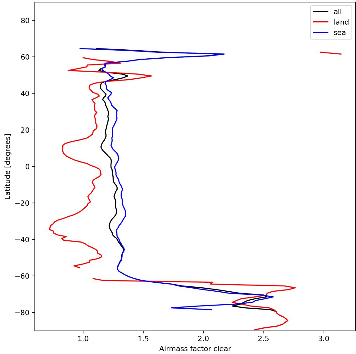
Figure 28: Zonal average of “Airmass factor clear” for 2024-01-18 to 2024-01-20.
