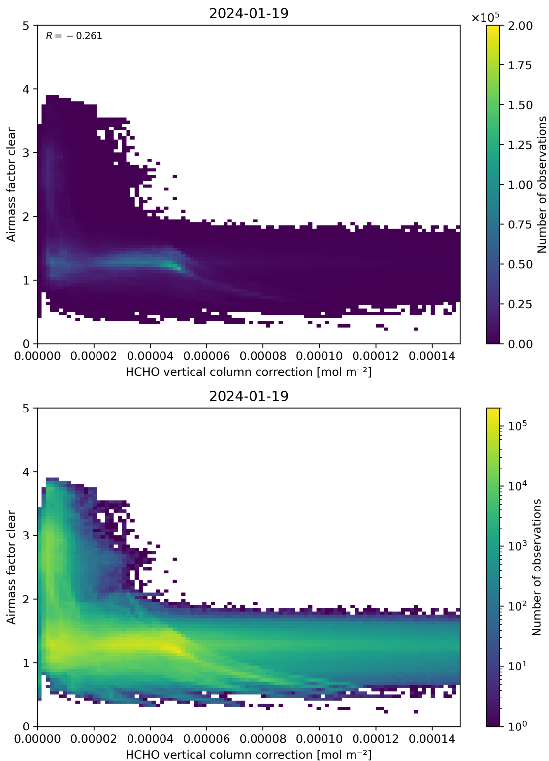
Figure 115: Scatter density plot of “HCHO vertical column correction” against “Airmass factor clear” for 2024-01-18 to 2024-01-20.
