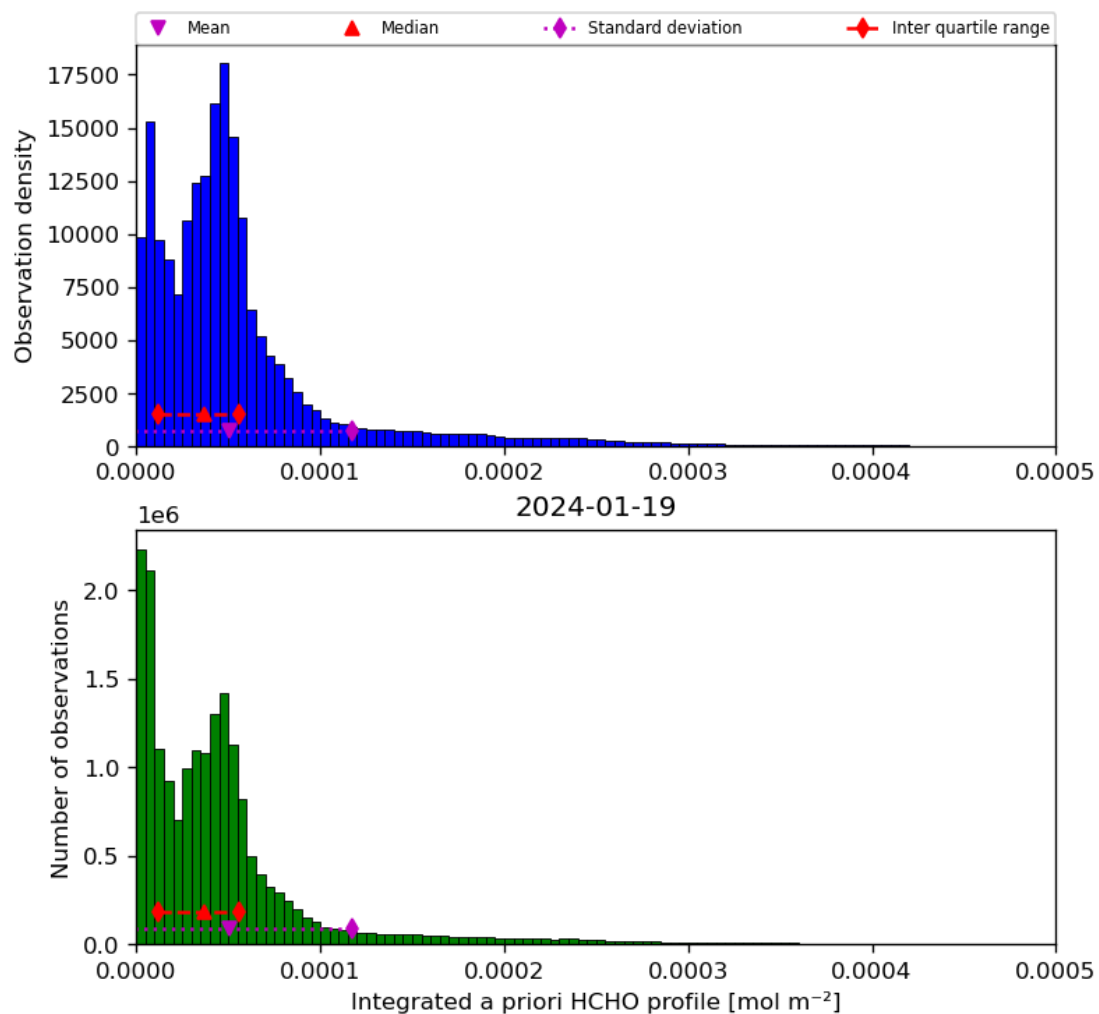
Figure 43: Histogram of “Integrated a priori HCHO profile” for 2024-01-18 to 2024-01-20
