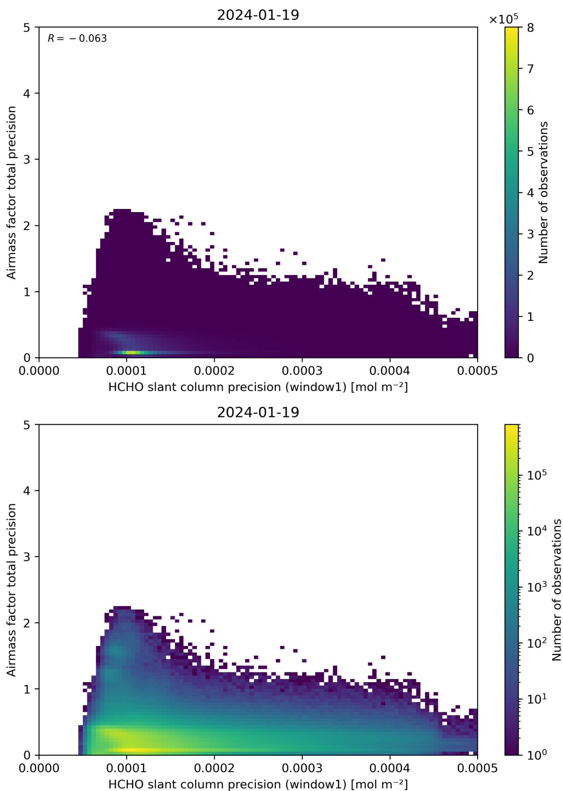
Figure 95: Scatter density plot of “HCHO slant column precision (window1)” against “Airmass factor total precision” for 2024-01-18 to 2024-01-20.
