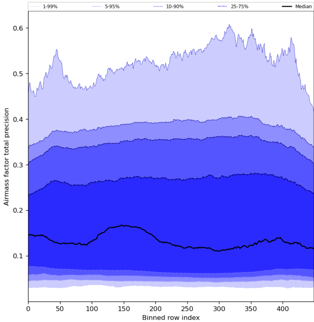
Figure 55: Along track statistics of “Airmass factor total precision” for 2024-01-18 to 2024-01-20
