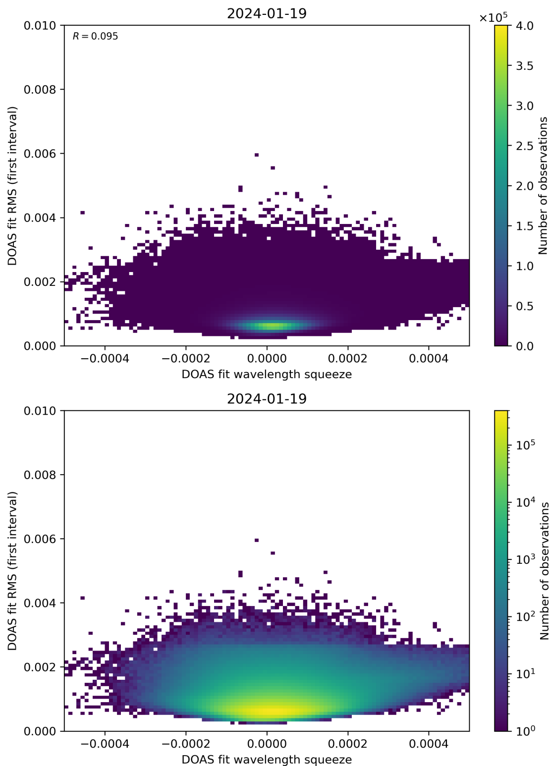
Figure 68: Scatter density plot of “DOAS fit wavelength squeeze” against “DOAS fit RMS (first interval)” for 2024-01-18 to 2024-01-20.
