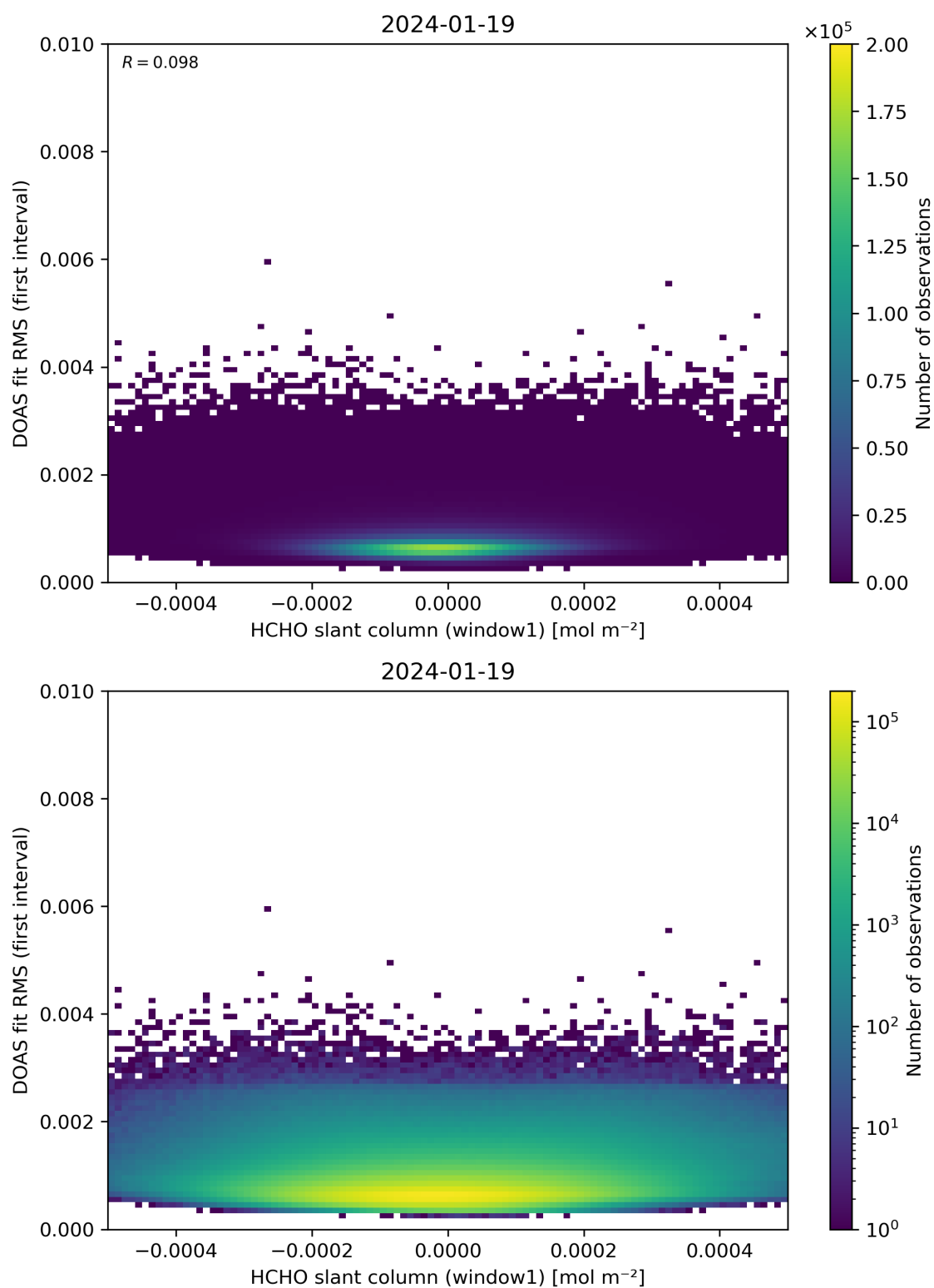
Figure 78: Scatter density plot of “HCHO slant column (window1)” against “DOAS fit RMS (first interval)” for 2024-01-18 to 2024-01-20.
