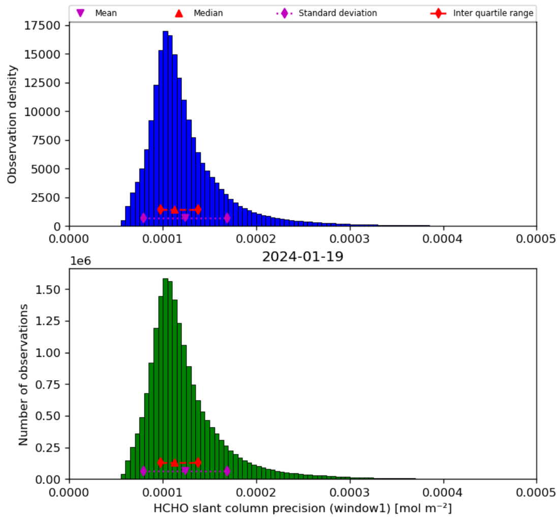
Figure 39: Histogram of “HCHO slant column precision (window1)” for 2024-01-18 to 2024-01-20
