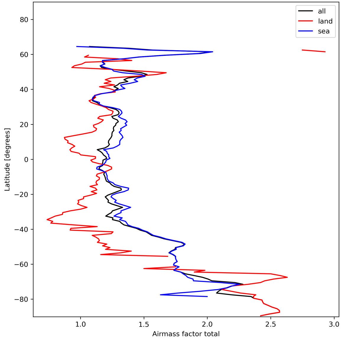
Figure 26: Zonal average of “Airmass factor total” for 2024-01-18 to 2024-01-20.
