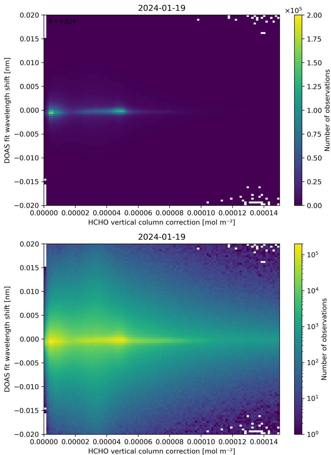
Figure 113: Scatter density plot of “HCHO vertical column correction” against “DOAS fit wavelength shift” for 2024-01-18 to 2024-01-20.
