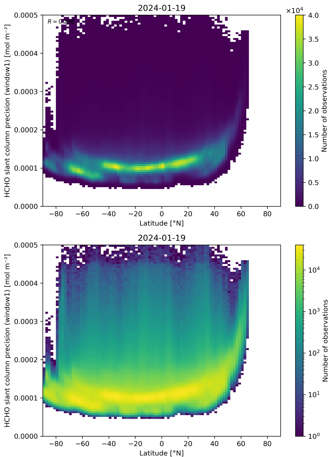
Figure 160: Scatter density plot of “Latitude” against “HCHO slant column precision (window1)” for 2024-01-18 to 2024-01-20.
