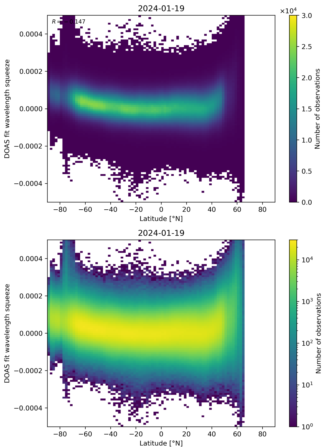
Figure 155: Scatter density plot of “Latitude” against “DOAS fit wavelength squeeze” for 2024-01-18 to 2024-01-20.
