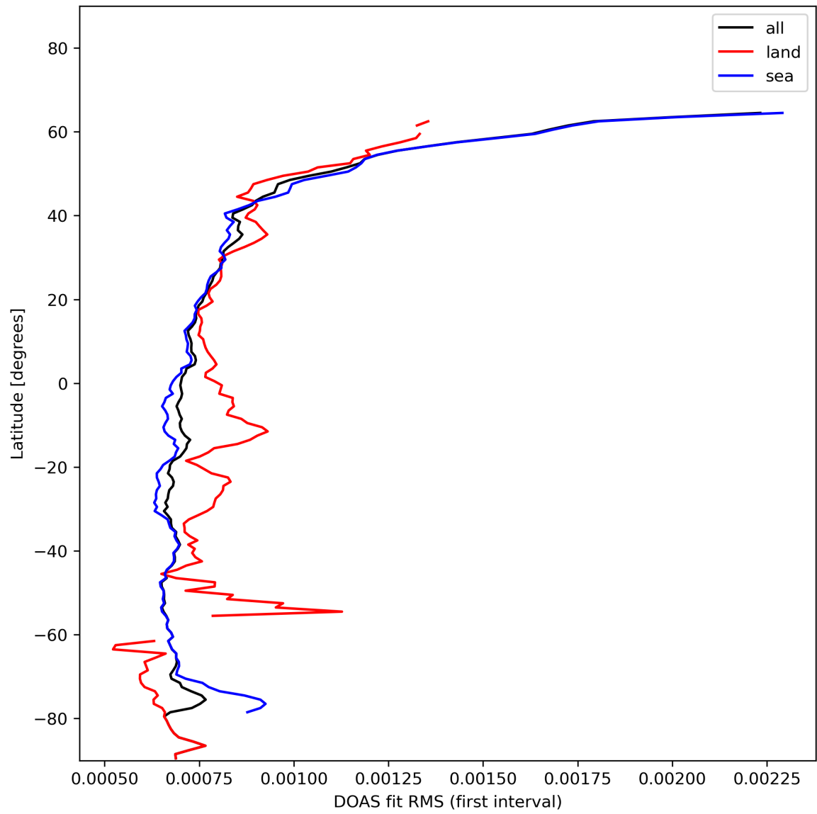
Figure 32: Zonal average of "DOAS fit RMS (first interval)" for 2024-01-18 to 2024-01-20.
