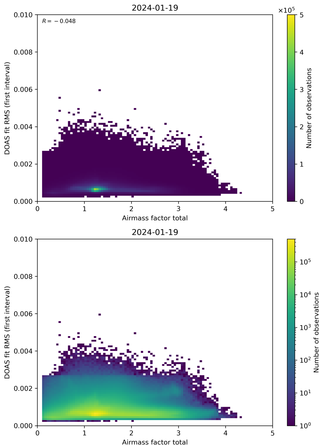
Figure 97: Scatter density plot of “Airmass factor total” against “DOAS fit RMS (first interval)” for 2024-01-18 to 2024-01-20.
