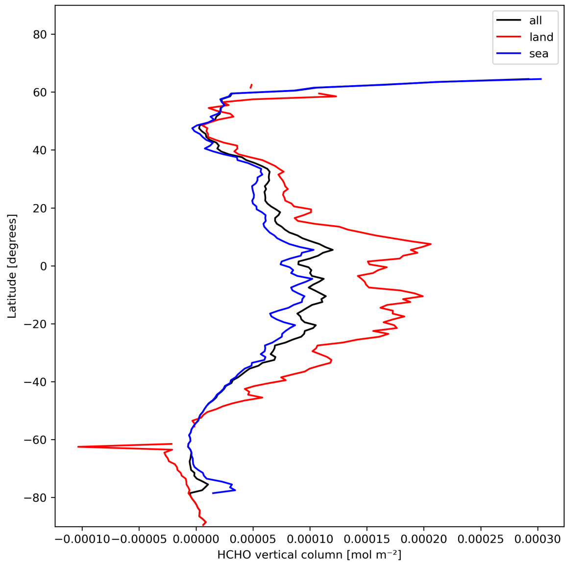
Figure 21: Zonal average of “HCHO vertical column” for 2024-01-18 to 2024-01-20.
