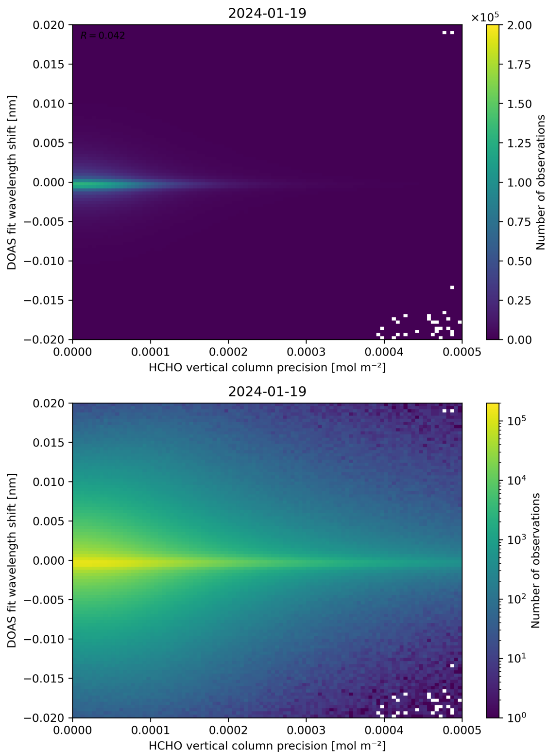
Figure 137: Scatter density plot of “HCHO vertical column precision” against “DOAS fit wavelength shift” for 2024-01-18 to 2024-01-20.
