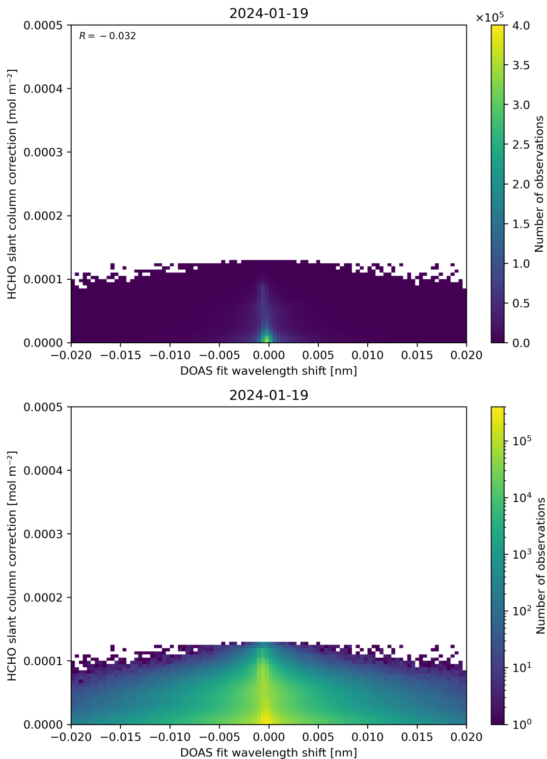
Figure 67: Scatter density plot of “DOAS fit wavelength shift” against “HCHO slant column correction” for 2024-01-18 to 2024-01-20.
