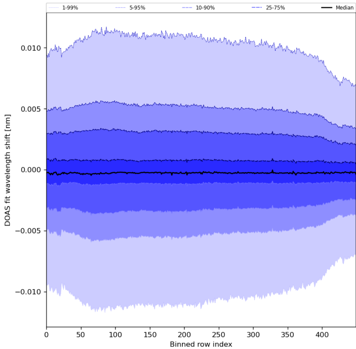
Figure 58: Along track statistics of “DOAS fit wavelength shift” for 2024-01-18 to 2024-01-20
