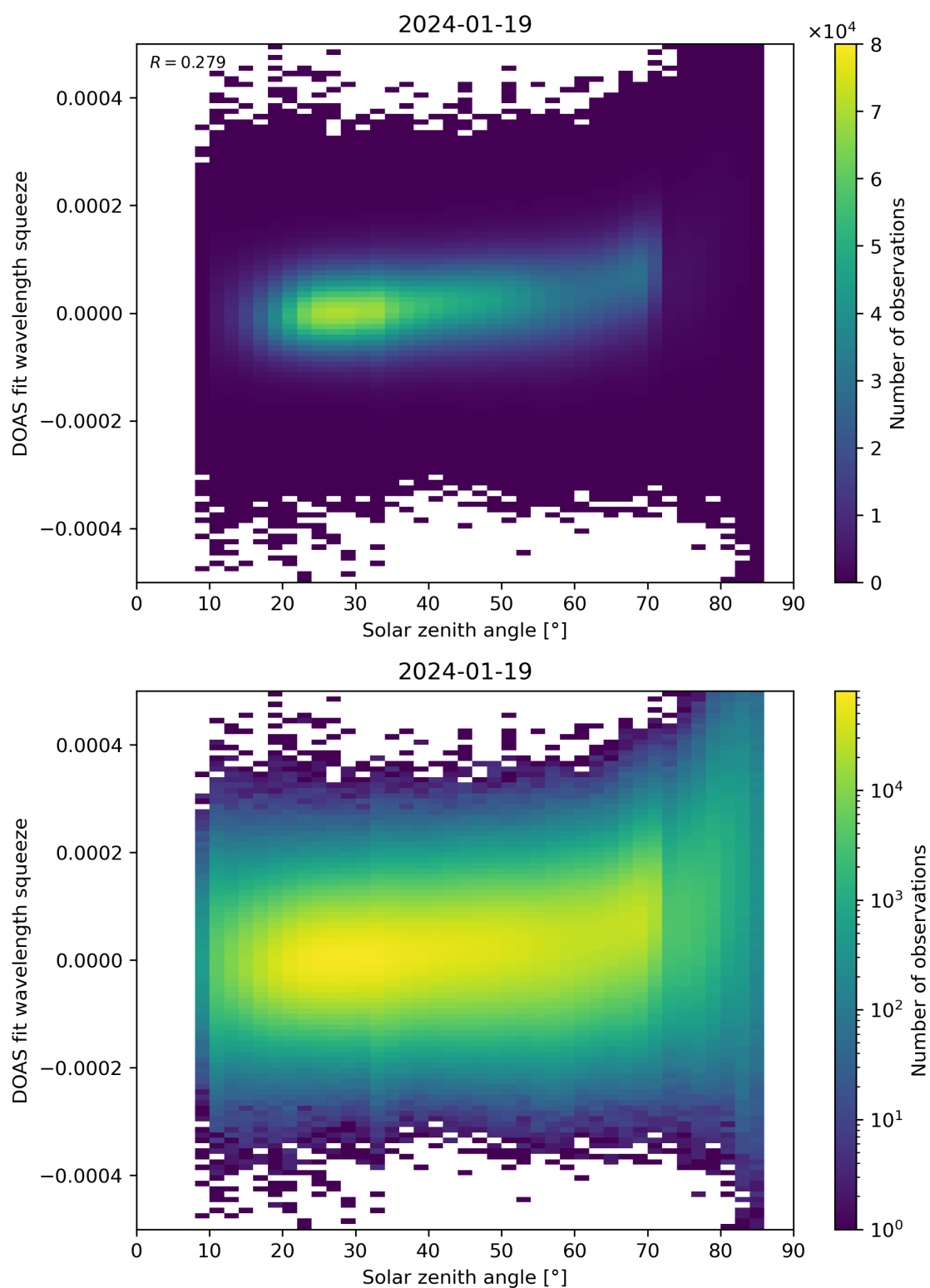
Figure 169: Scatter density plot of “Solar zenith angle” against “DOAS fit wavelength squeeze” for 2024-01-18 to 2024-01-20.
