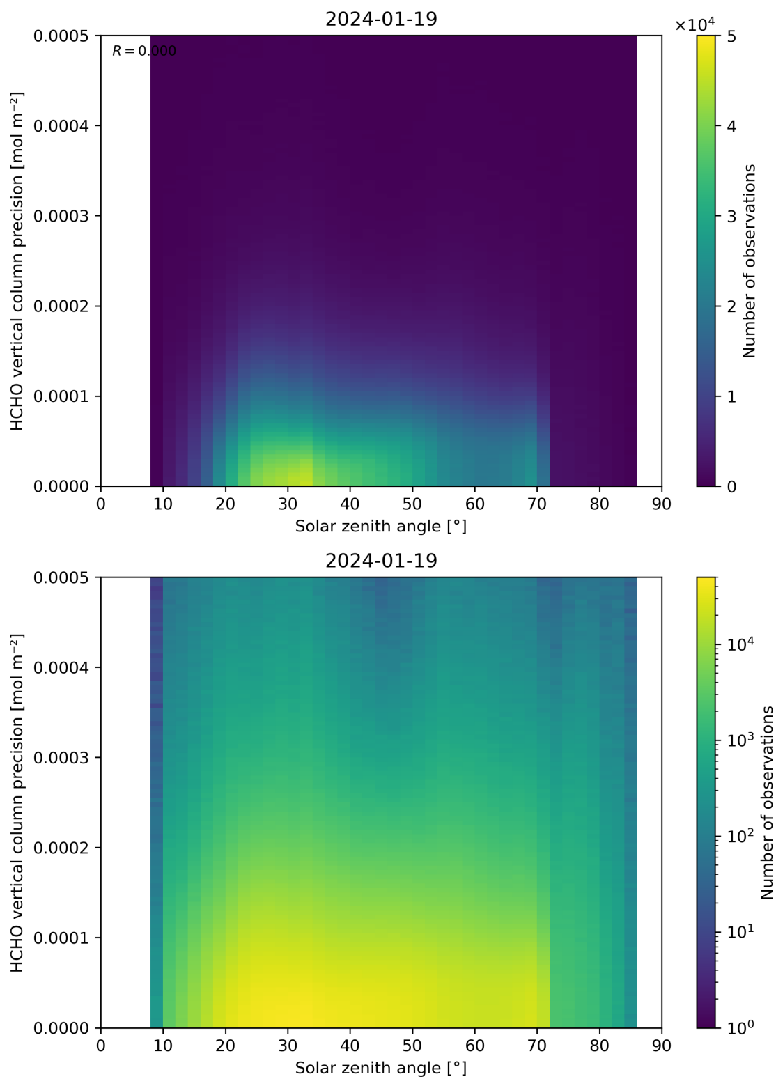
Figure 179: Scatter density plot of “Solar zenith angle” against “HCHO vertical column precision” for 2024-01-18 to 2024-01-20.
