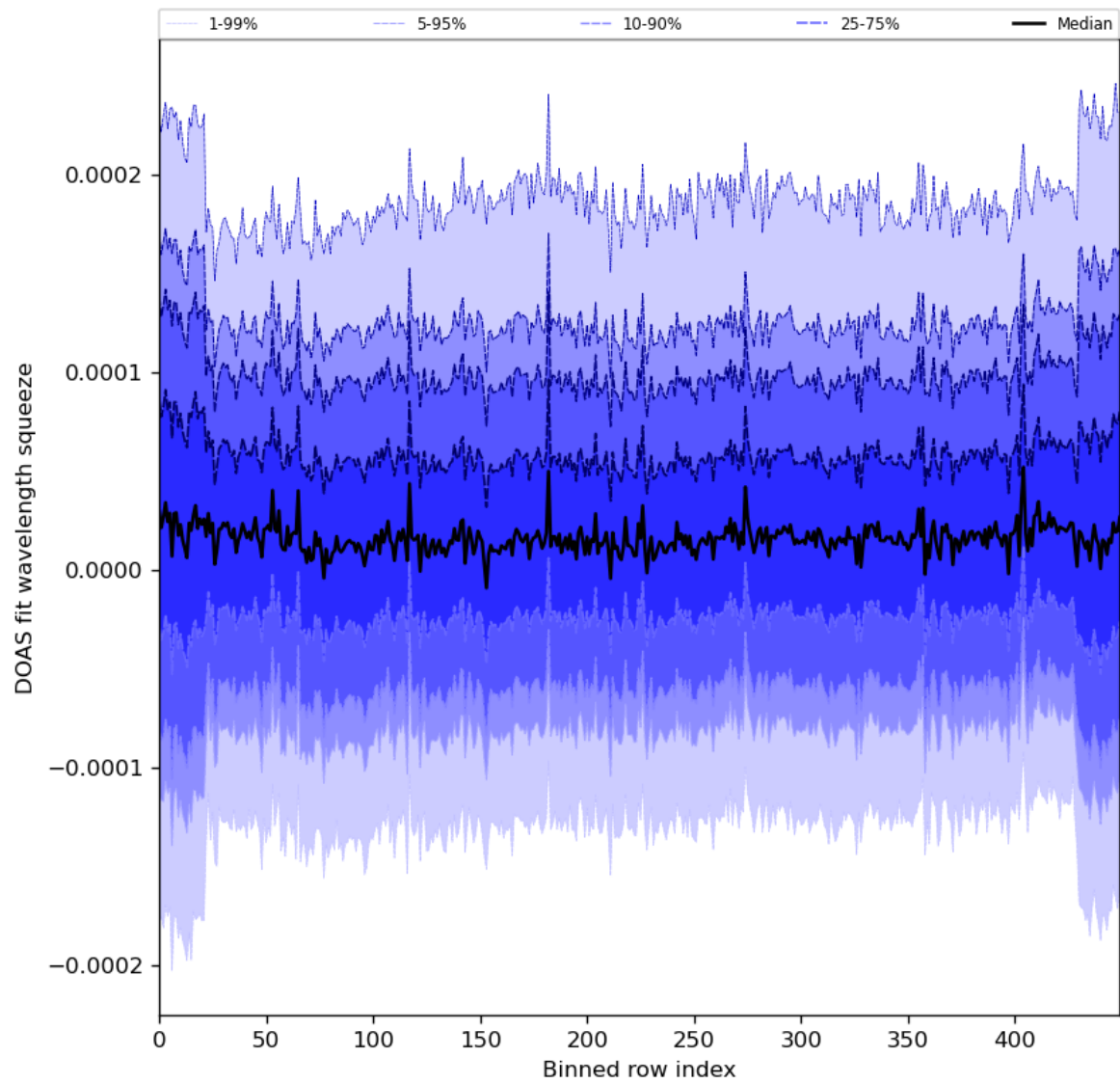
Figure 59: Along track statistics of “DOAS fit wavelength squeeze” for 2024-01-18 to 2024-01-20
