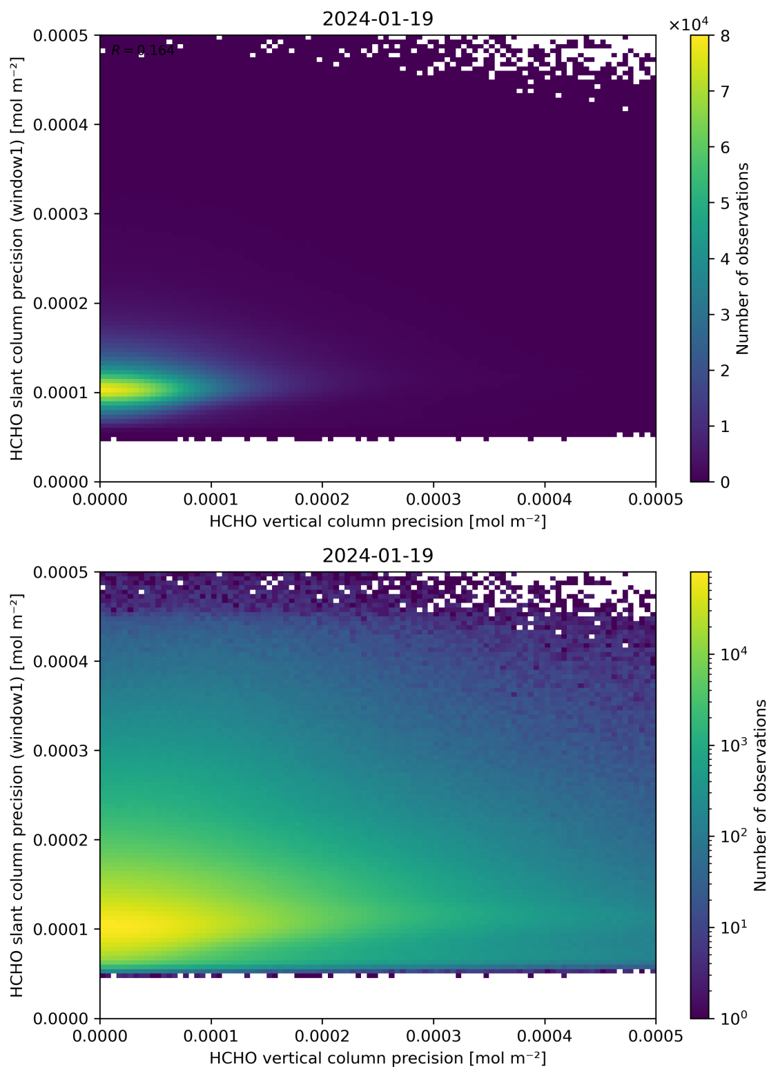
Figure 143: Scatter density plot of “HCHO vertical column precision” against “HCHO slant column precision (window1)” for 2024-01-18 to 2024-01-20.
