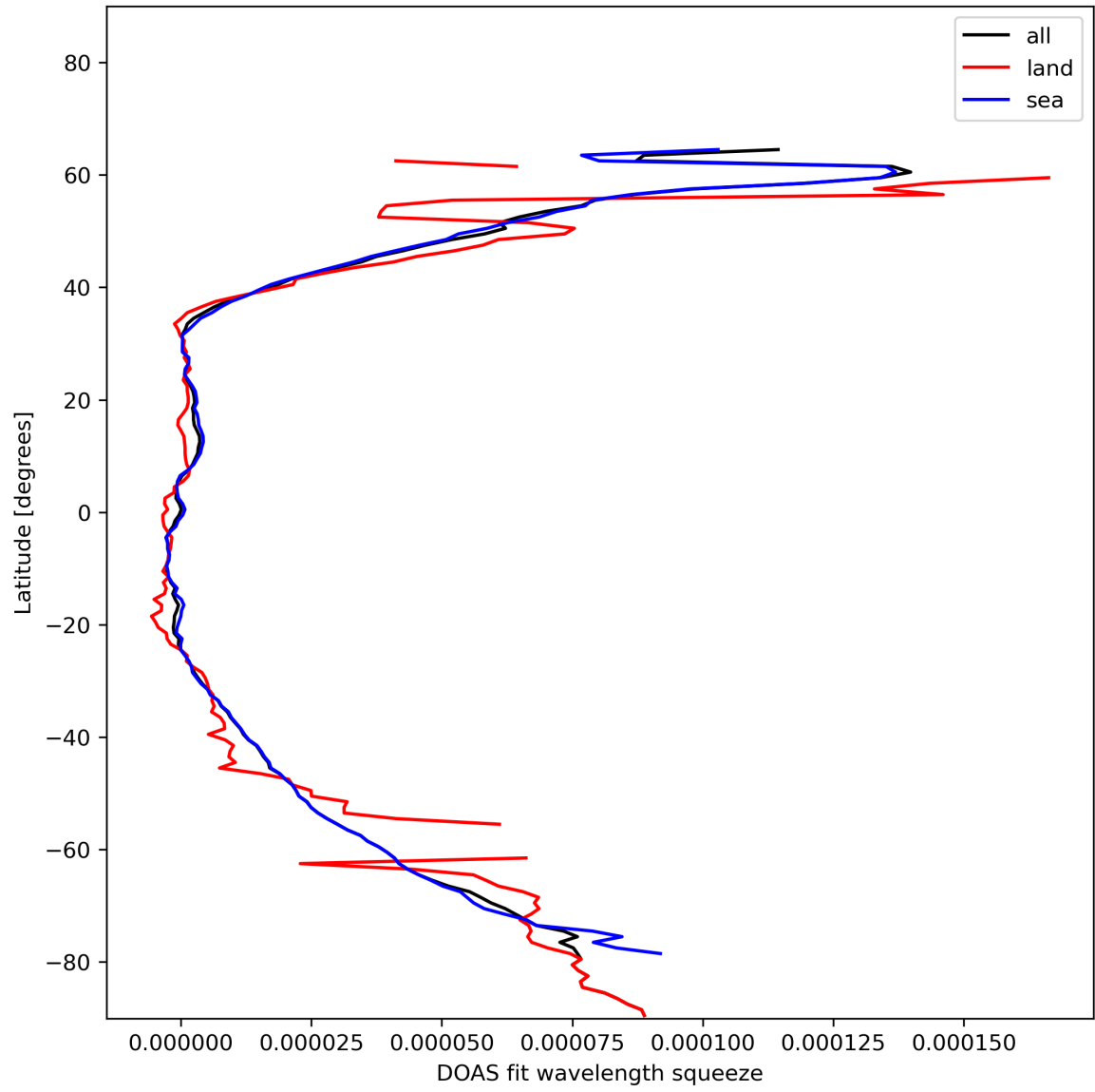
Figure 31: Zonal average of “DOAS fit wavelength squeeze” for 2024-01-18 to 2024-01-20.
