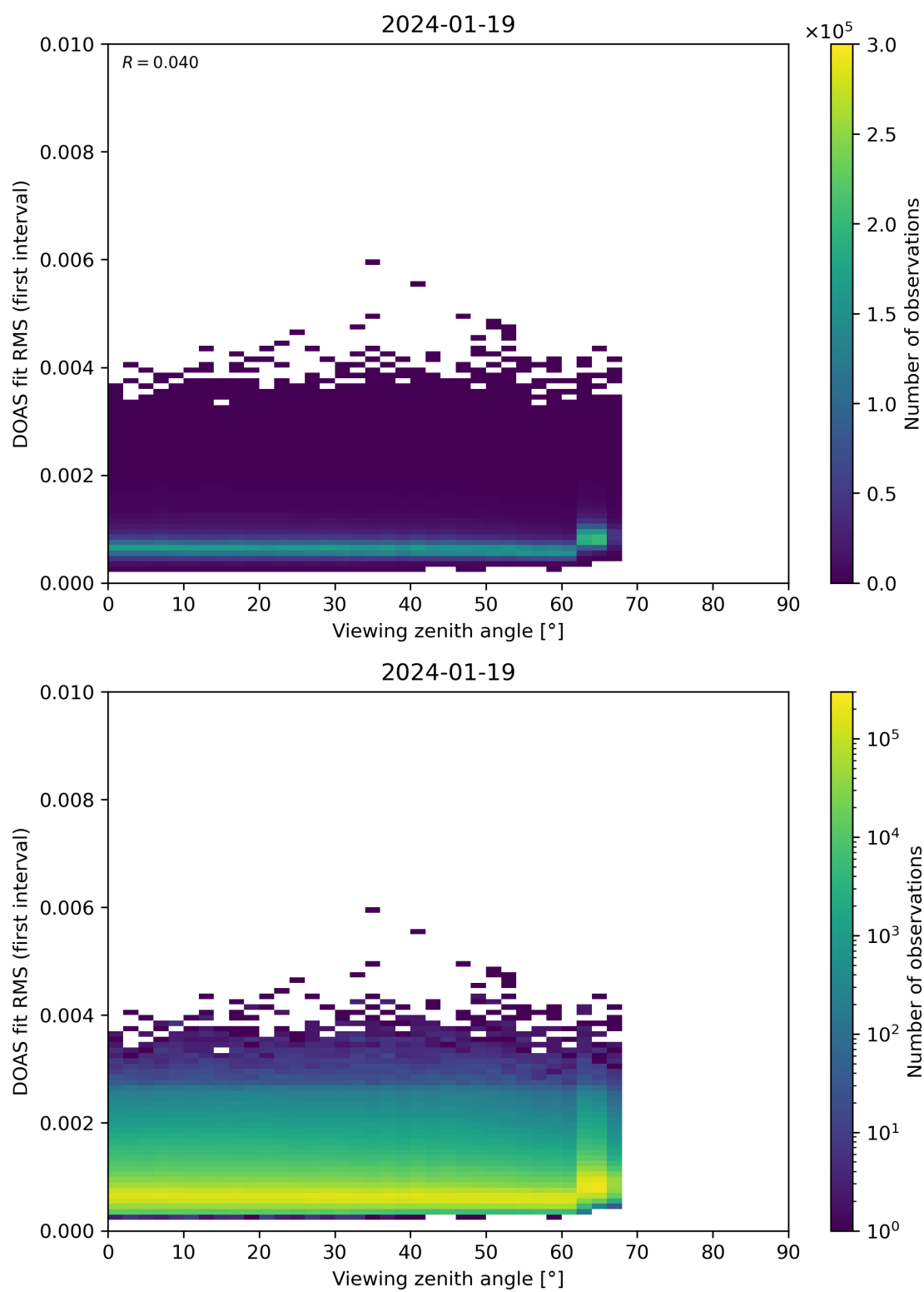
Figure 182: Scatter density plot of “Viewing zenith angle” against “DOAS fit RMS (first interval)” for 2024-01-18 to 2024-01-20.
