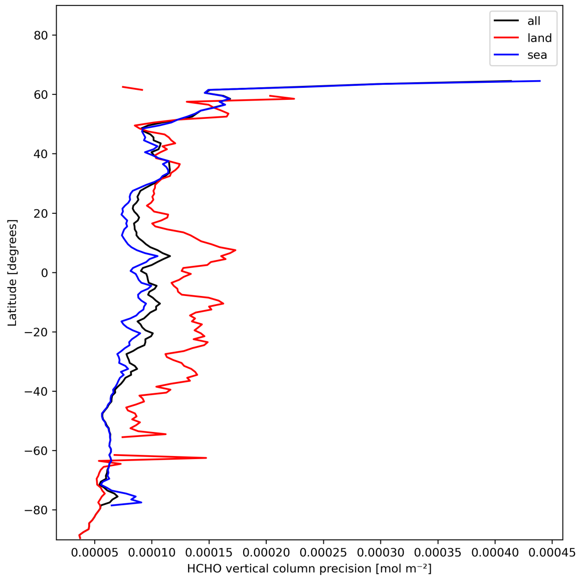
Figure 22: Zonal average of “HCHO vertical column precision” for 2024-01-18 to 2024-01-20.
