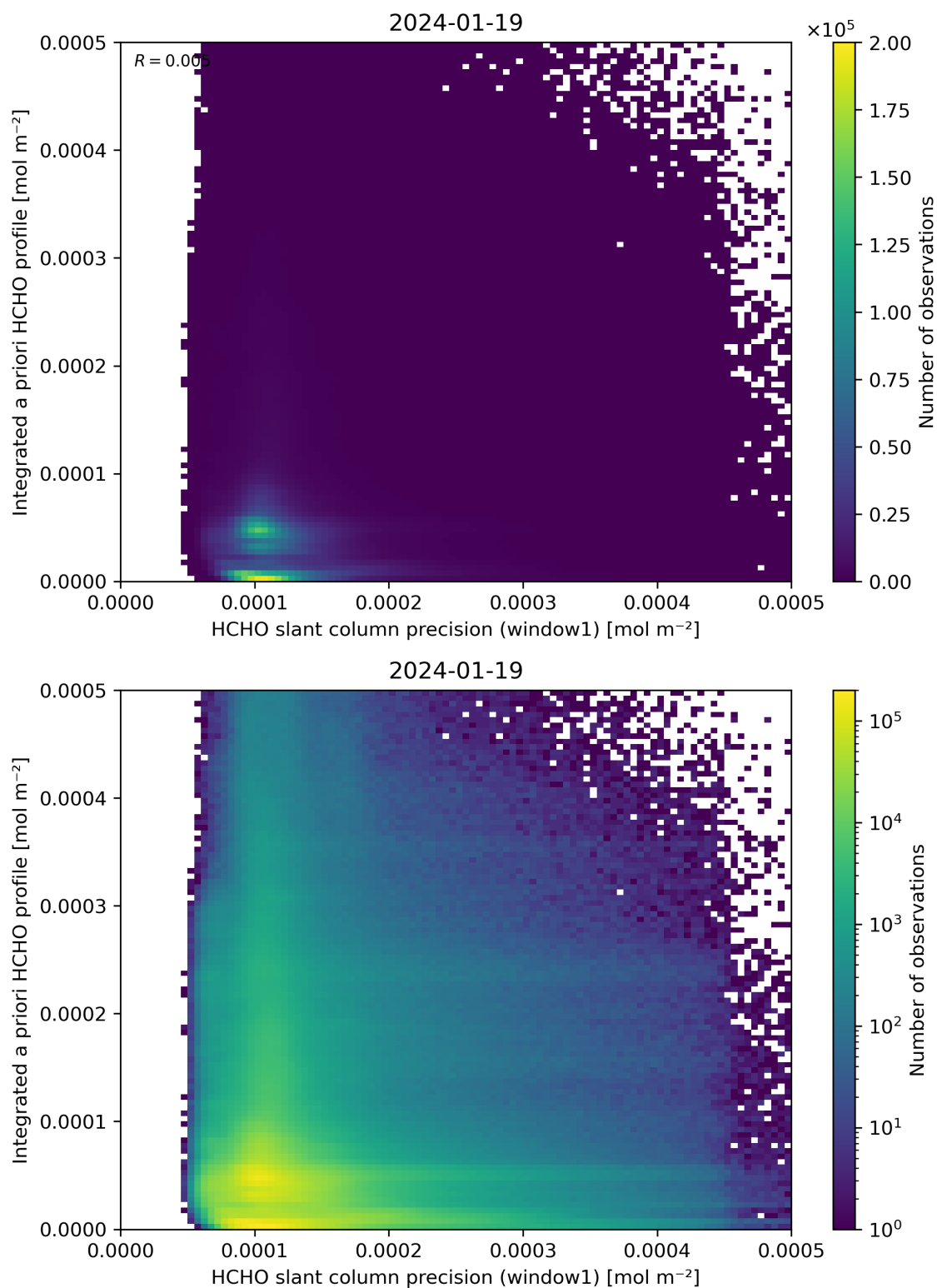
Figure 96: Scatter density plot of “HCHO slant column precision (window1)” against “Integrated a priori HCHO profile” for 2024-01-18 to 2024-01-20.
