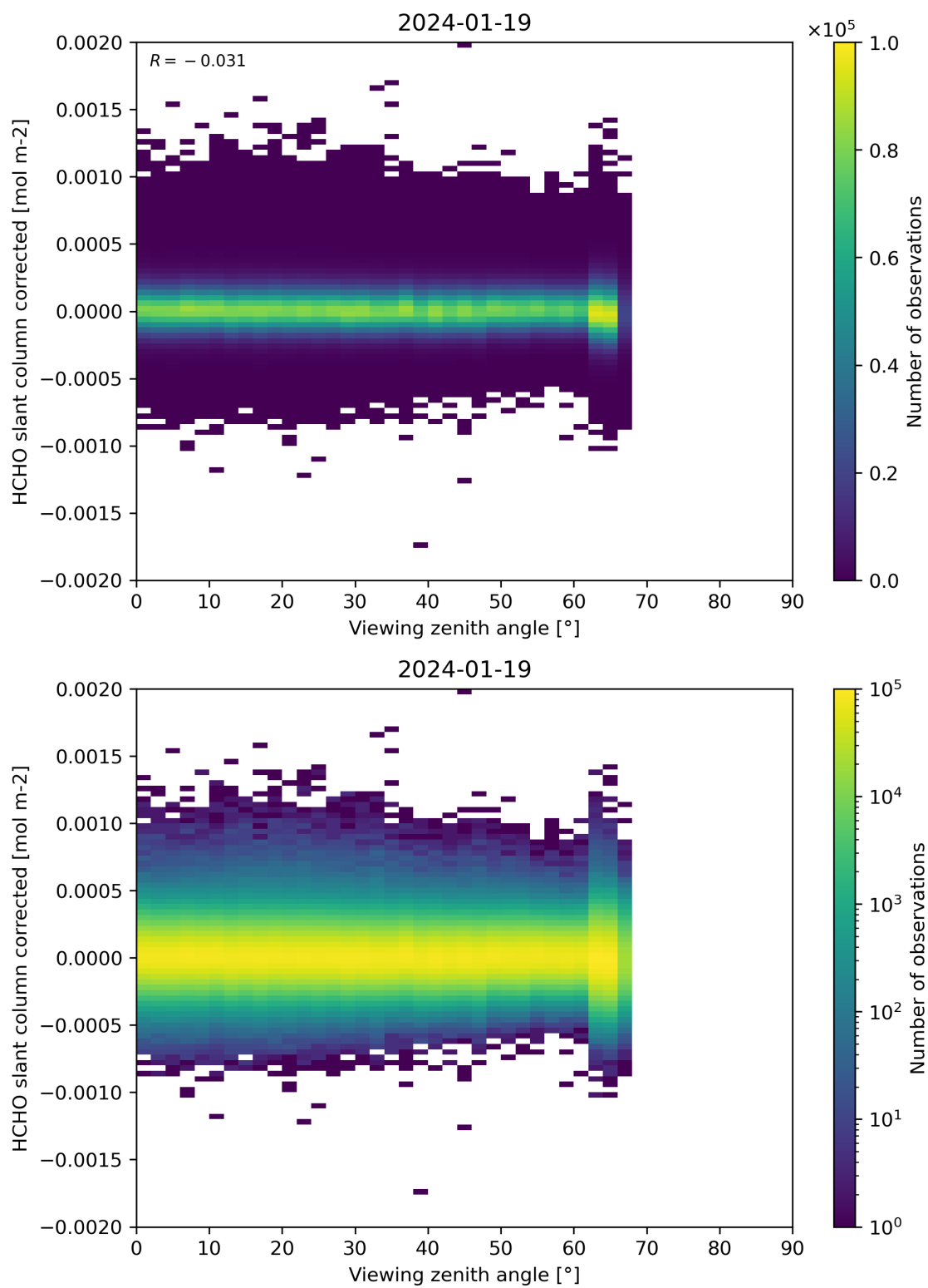
Figure 186: Scatter density plot of “Viewing zenith angle” against “HCHO slant column corrected” for 2024-01-18 to 2024-01-20.
