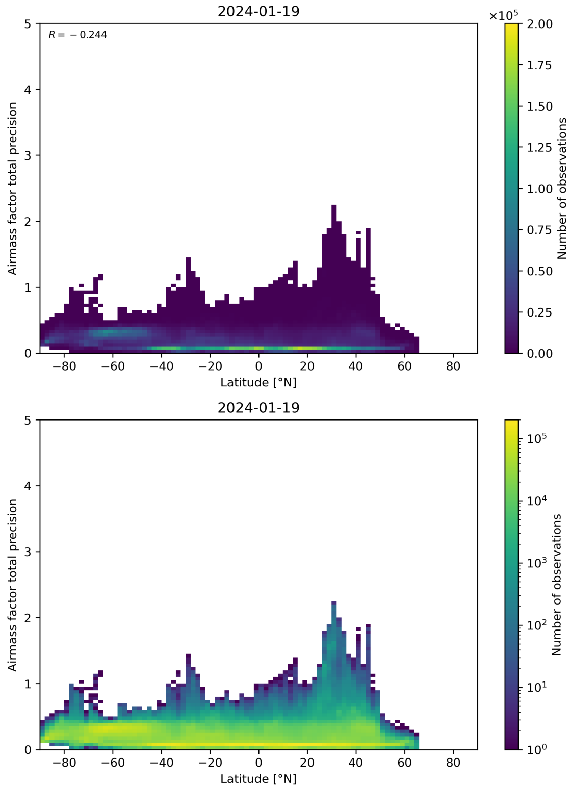
Figure 162: Scatter density plot of “Latitude” against “Airmass factor total precision” for 2024-01-18 to 2024-01-20.
