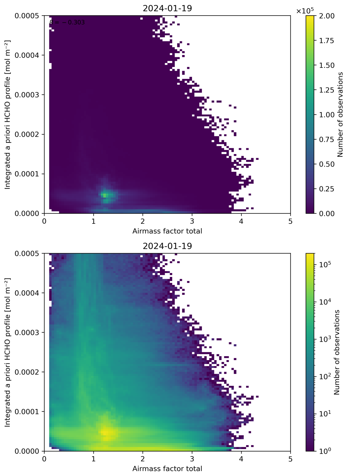
Figure 104: Scatter density plot of “Airmass factor total” against “Integrated a priori HCHO profile” for 2024-01-18 to 2024-01-20.
