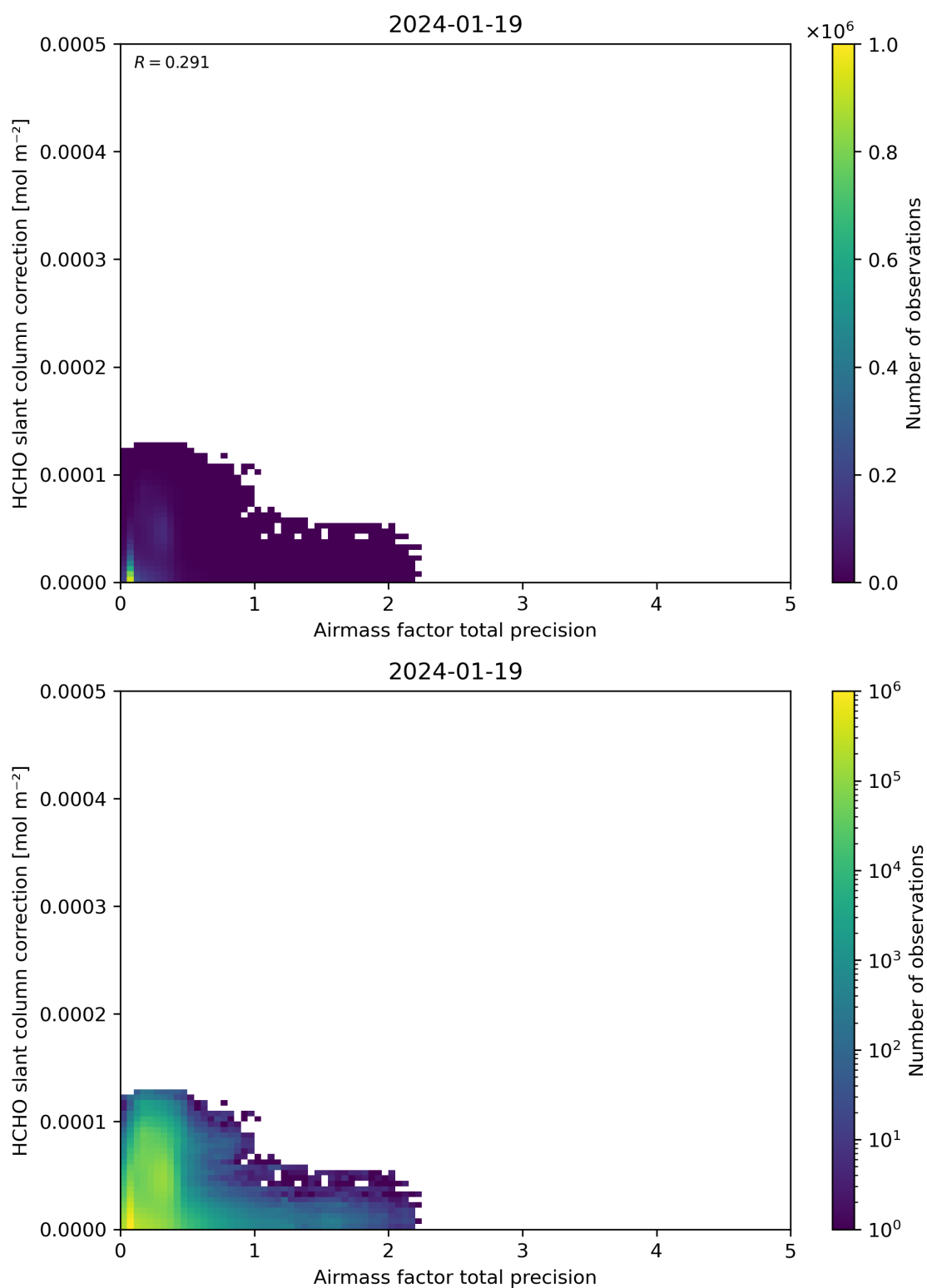
Figure 110: Scatter density plot of “Airmass factor total precision” against “HCHO slant column correction” for 2024-01-18 to 2024-01-20.
