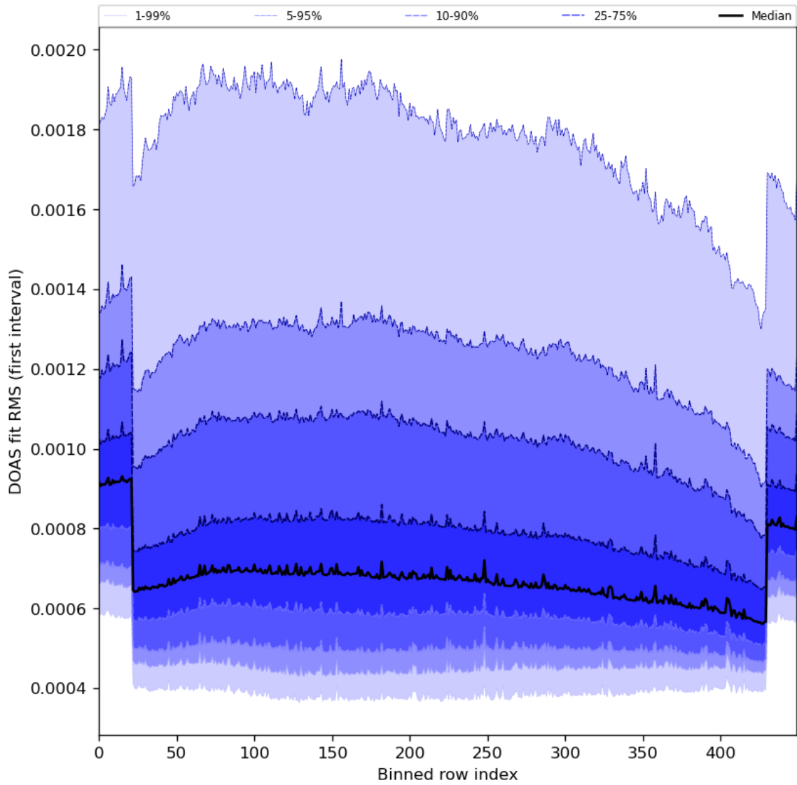
Figure 60: Along track statistics of “DOAS fit RMS (first interval)” for 2024-01-18 to 2024-01-20
