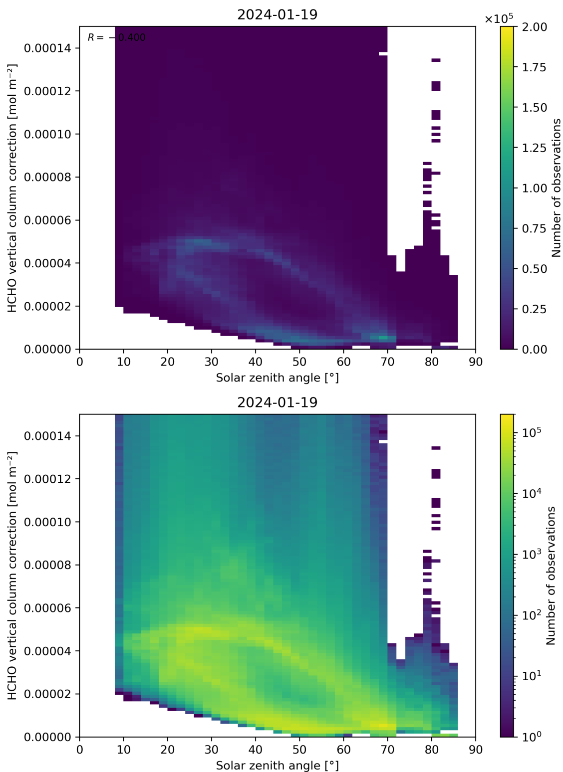
Figure 178: Scatter density plot of “Solar zenith angle” against “HCHO vertical column correction” for 2024-01-18 to 2024-01-20.
