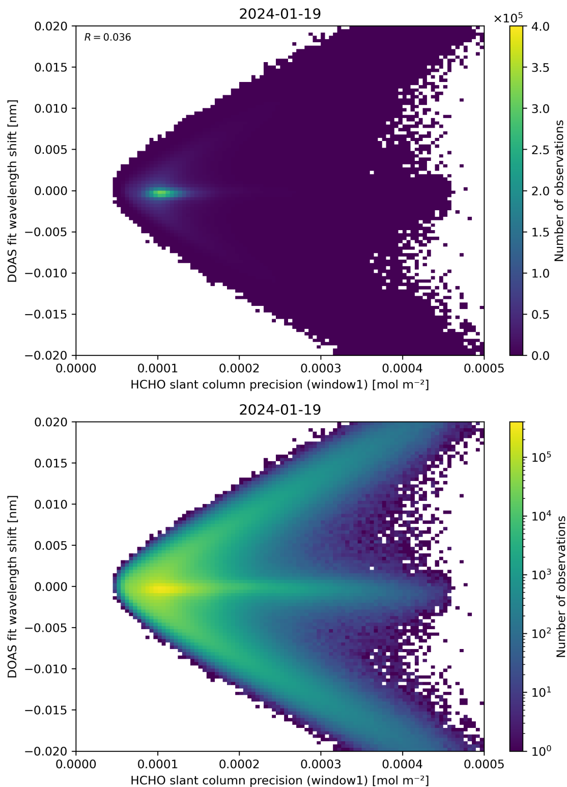
Figure 89: Scatter density plot of “HCHO slant column precision (window1)” against “DOAS fit wavelength shift” for 2024-01-18 to 2024-01-20.
