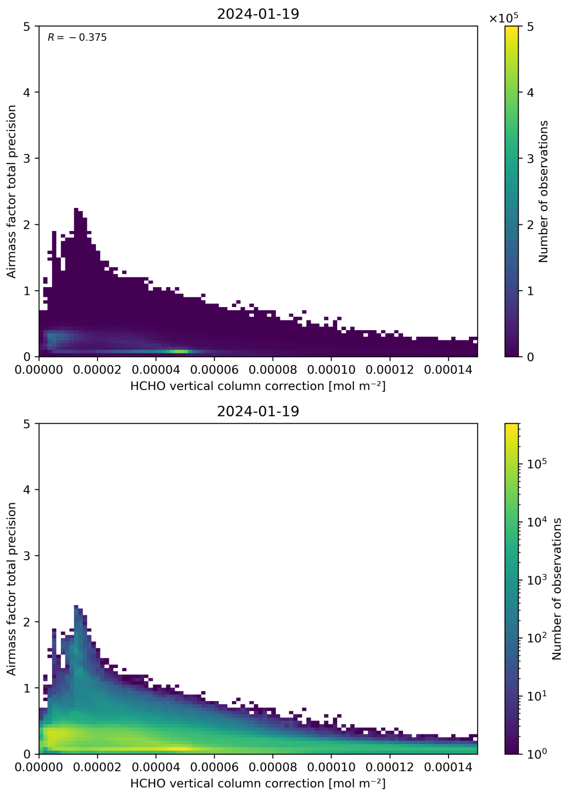
Figure 121: Scatter density plot of “HCHO vertical column correction” against “Airmass factor total precision” for 2024-01-18 to 2024-01-20.
