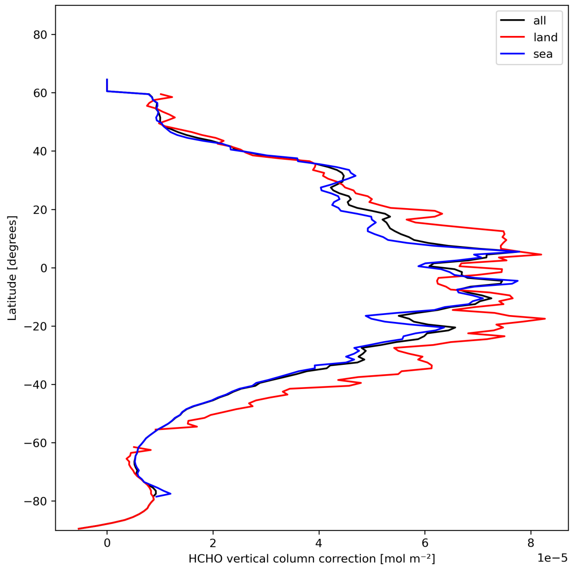
Figure 23: Zonal average of “HCHO vertical column correction” for 2024-01-18 to 2024-01-20.
