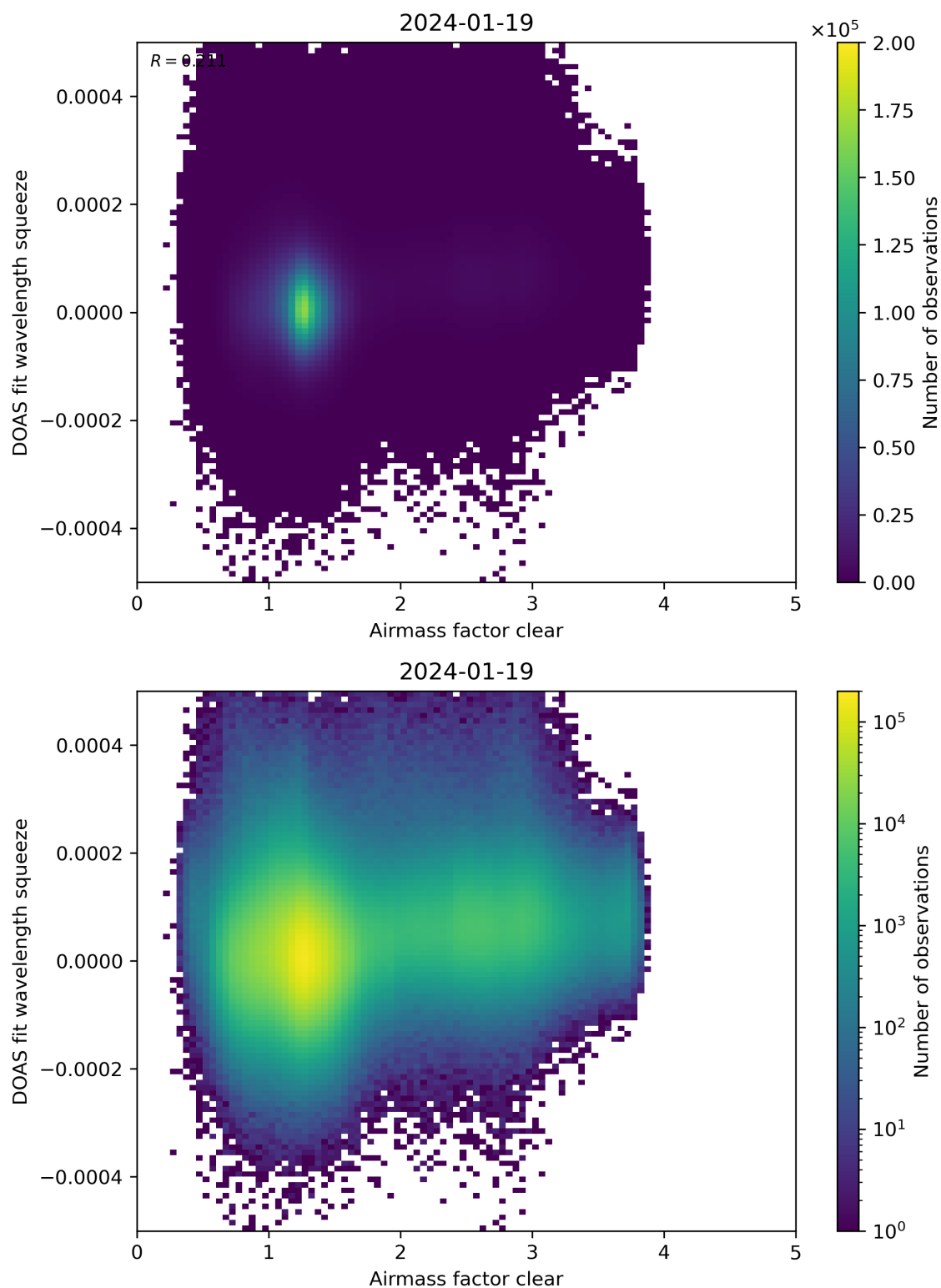
Figure 73: Scatter density plot of “Airmass factor clear” against “DOAS fit wavelength squeeze” for 2024-01-18 to 2024-01-20.
