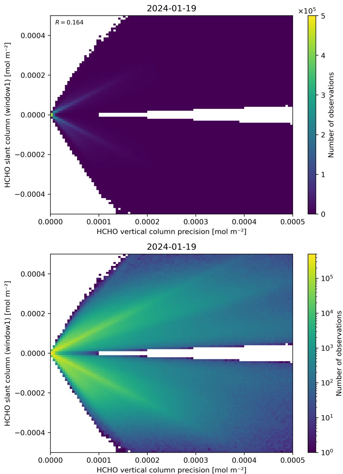
Figure 142: Scatter density plot of “HCHO vertical column precision” against “HCHO slant column (window1)” for 2024-01-18 to 2024-01-20.
