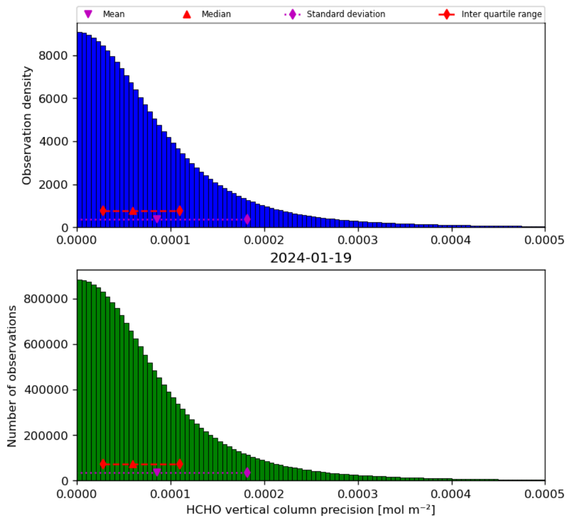
Figure 36: Histogram of “HCHO vertical column precision” for 2024-01-18 to 2024-01-20
