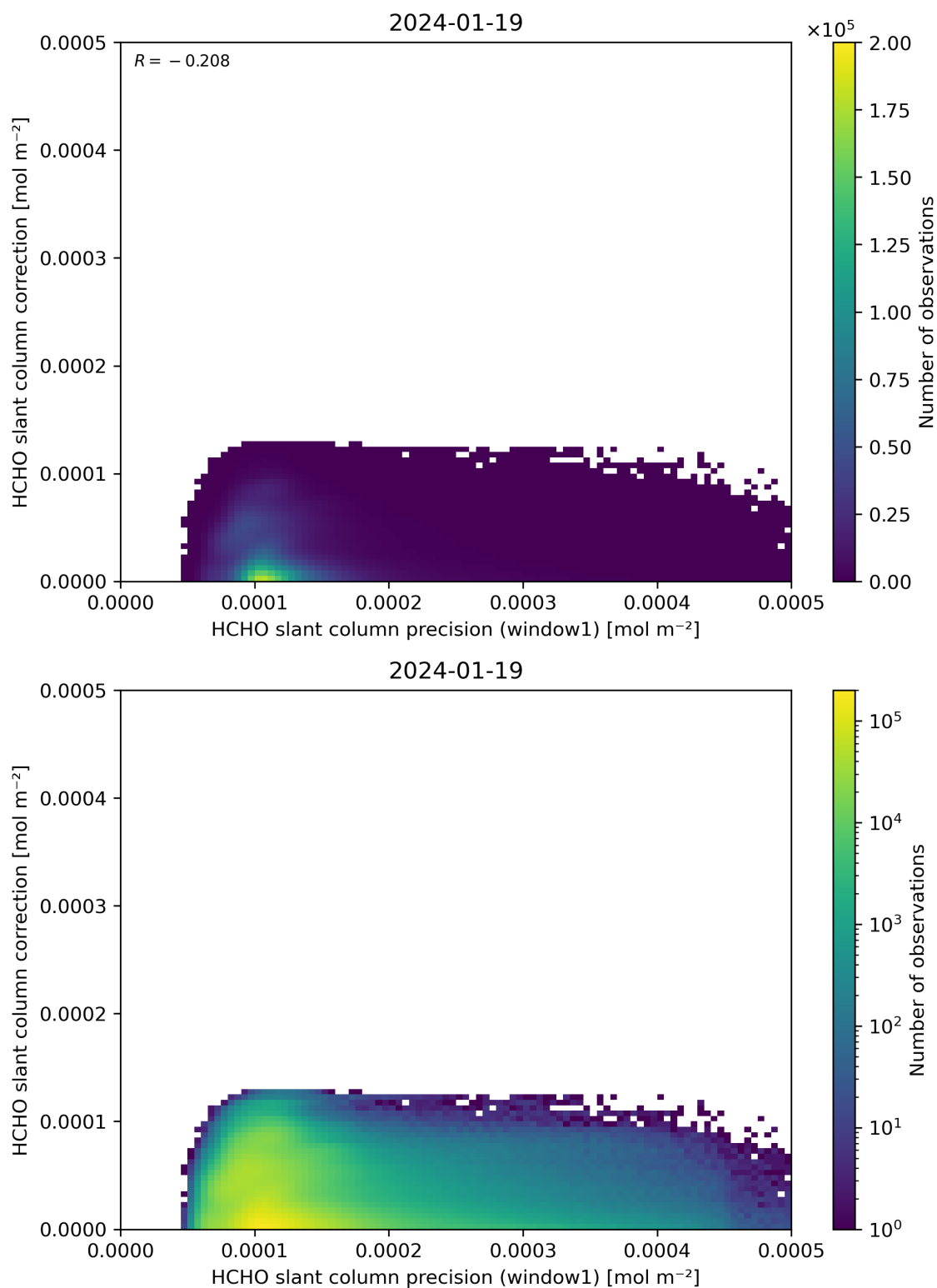
Figure 93: Scatter density plot of “HCHO slant column precision (window1)” against “HCHO slant column correction” for 2024-01-18 to 2024-01-20.
