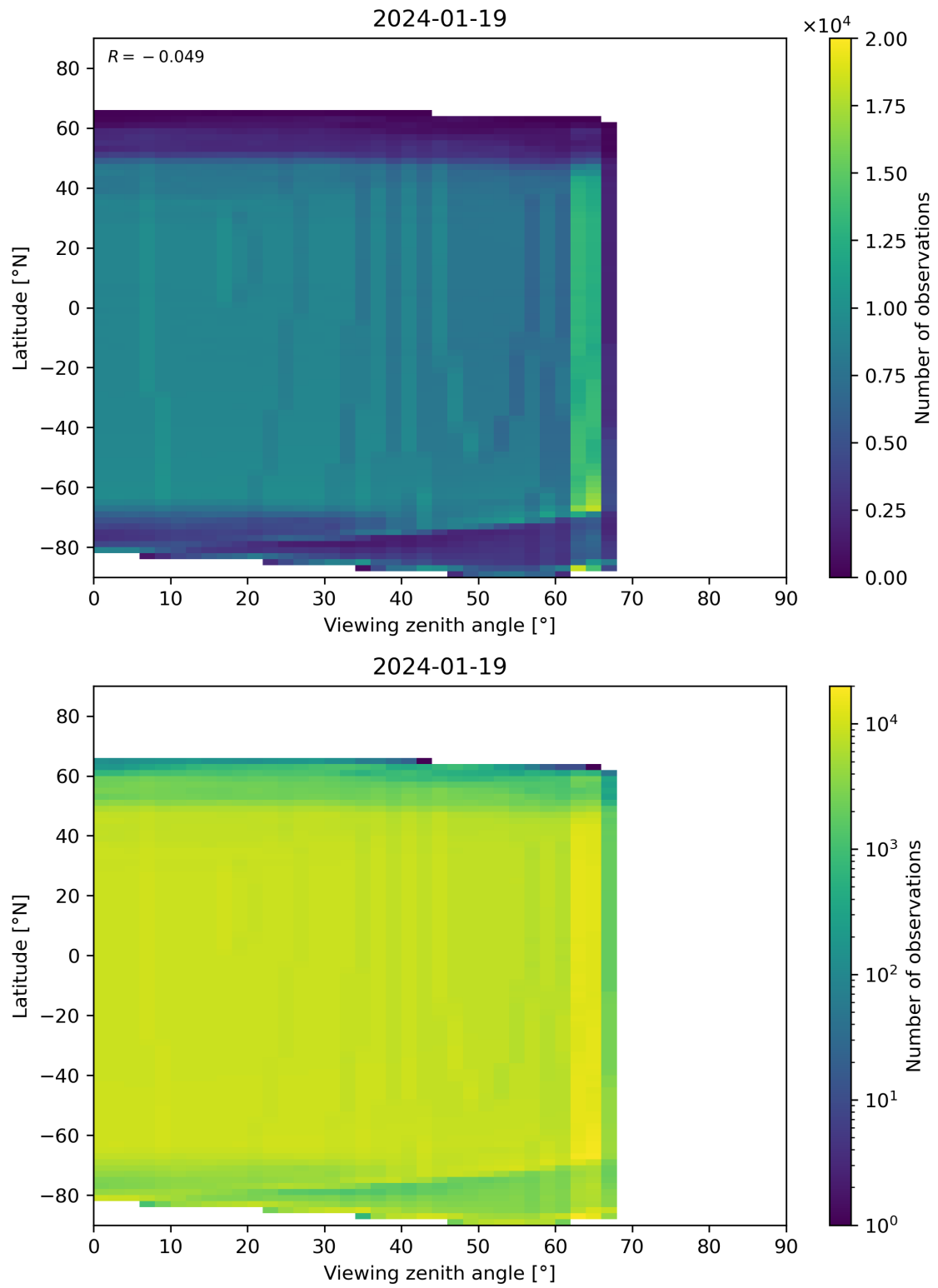
Figure 196: Scatter density plot of “Viewing zenith angle” against “Latitude” for 2024-01-18 to 2024-01-20.
