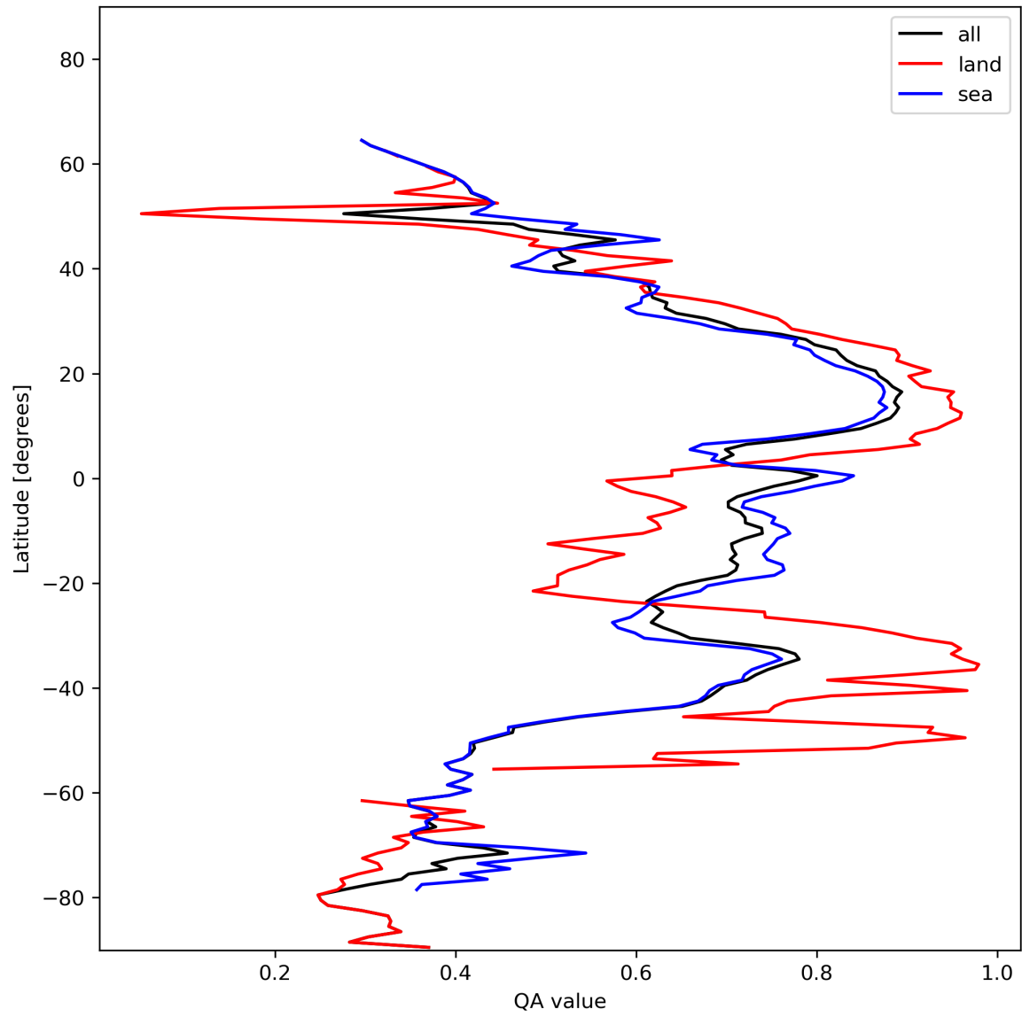
Figure 20: Zonal average of “QA value” for 2024-01-18 to 2024-01-20.
