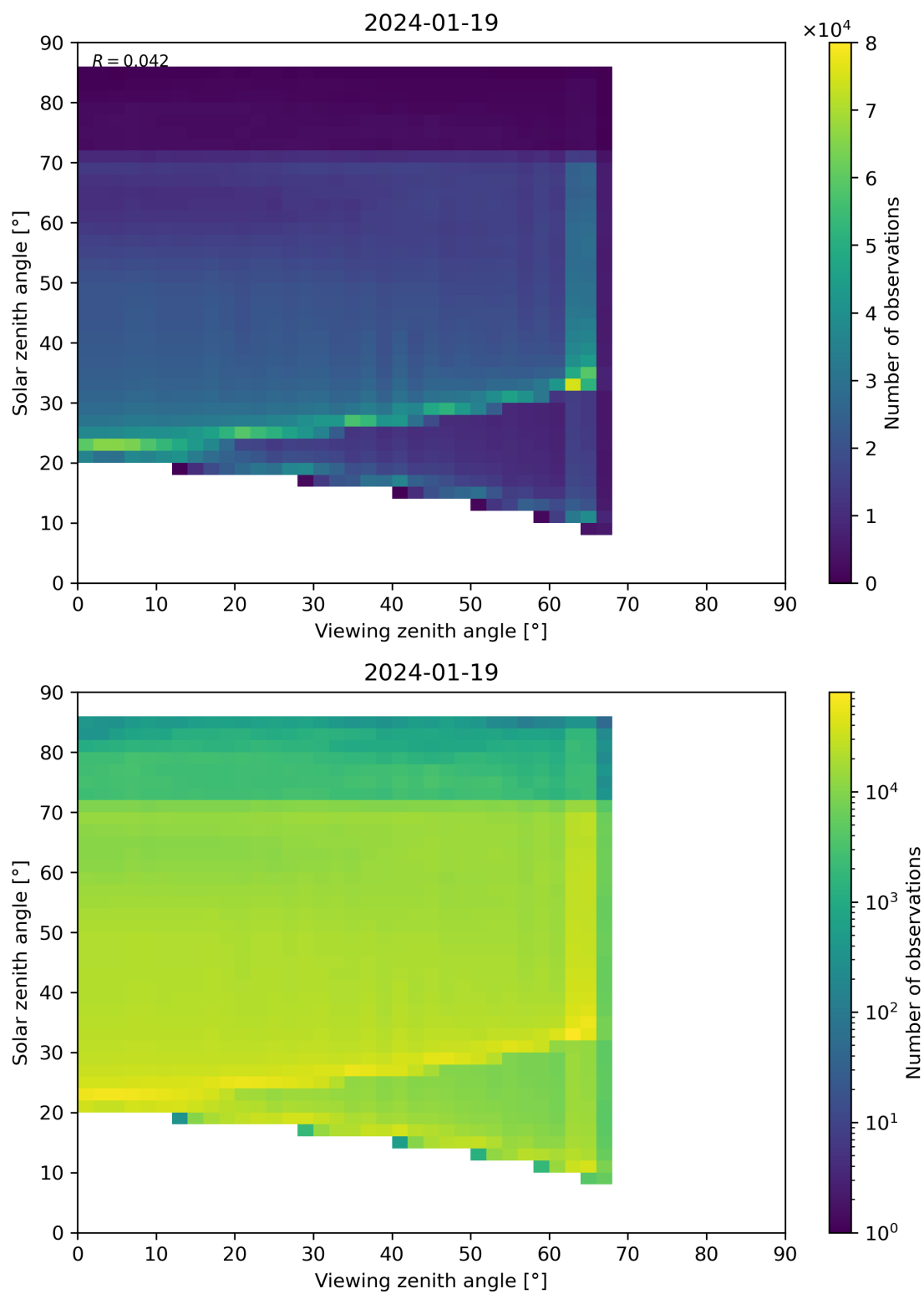
Figure 197: Scatter density plot of “Viewing zenith angle” against “Solar zenith angle” for 2024-01-18 to 2024-01-20.
