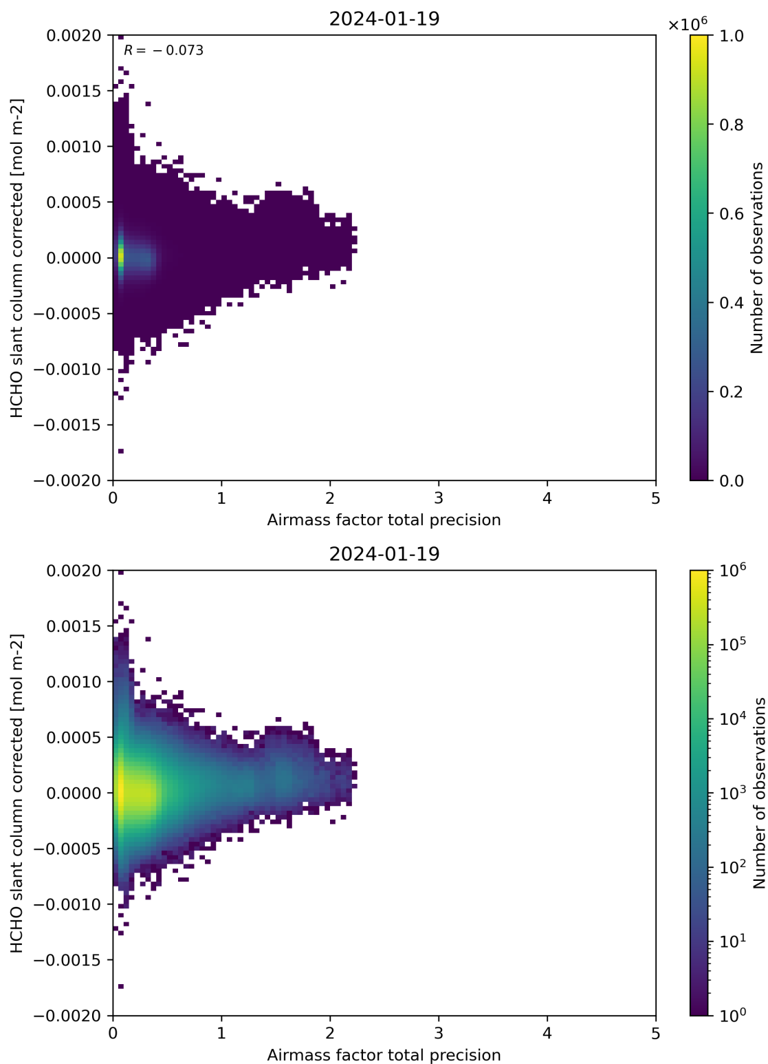
Figure 109: Scatter density plot of “Airmass factor total precision” against “HCHO slant column corrected” for 2024-01-18 to 2024-01-20.
