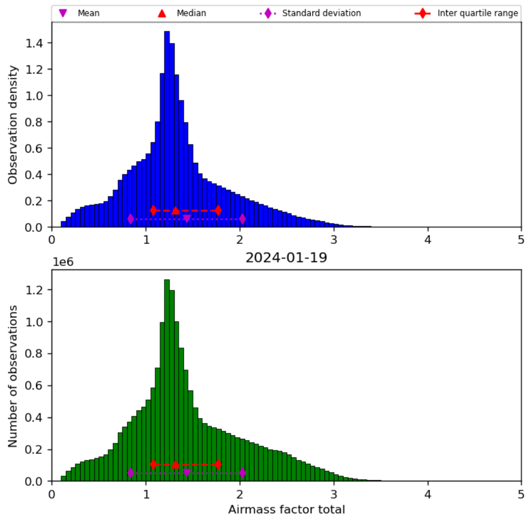
Figure 40: Histogram of “Airmass factor total” for 2024-01-18 to 2024-01-20
