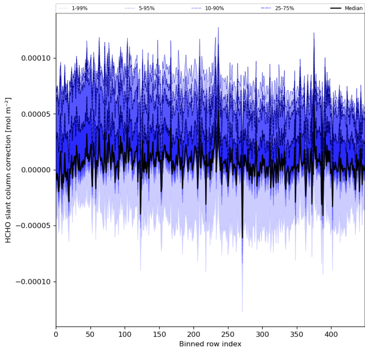
Figure 61: Along track statistics of “HCHO slant column correction” for 2024-01-18 to 2024-01-20
