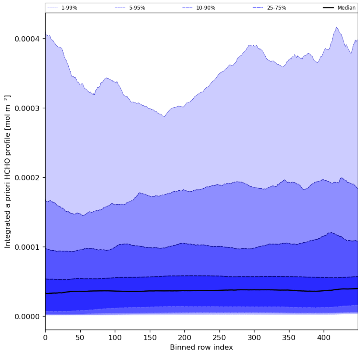
Figure 57: Along track statistics of “Integrated a priori HCHO profile” for 2024-01-18 to 2024-01-20
