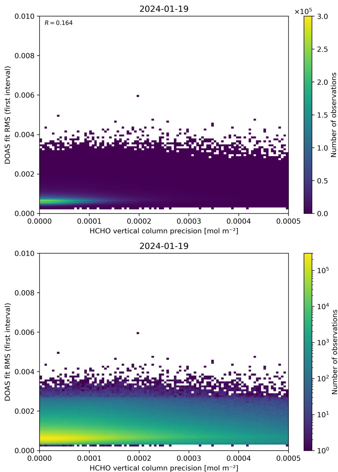
Figure 136: Scatter density plot of “HCHO vertical column precision” against “DOAS fit RMS (first interval)” for 2024-01-18 to 2024-01-20.
