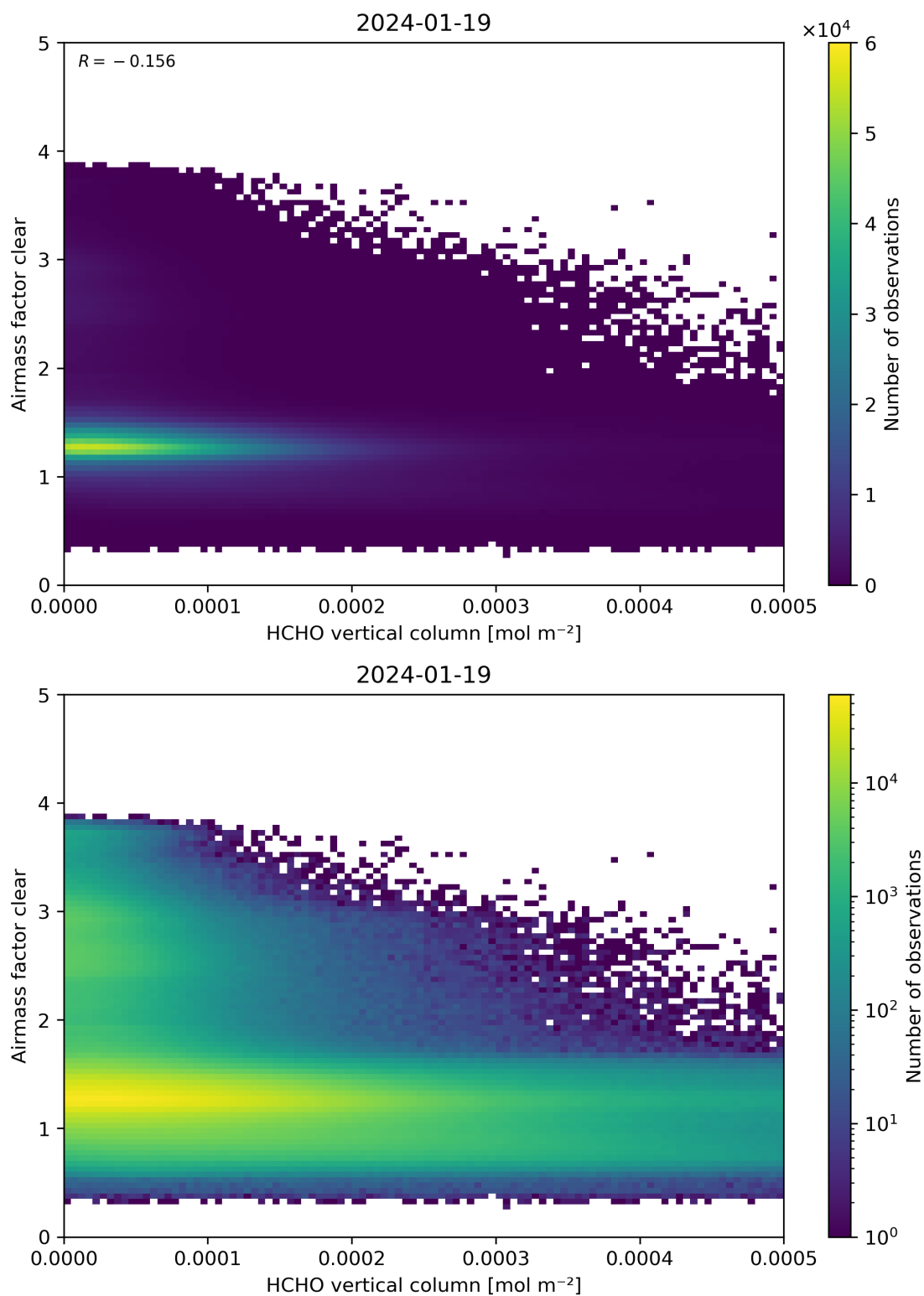
Figure 126: Scatter density plot of “HCHO vertical column” against “Airmass factor clear” for 2024-01-18 to 2024-01-20.
