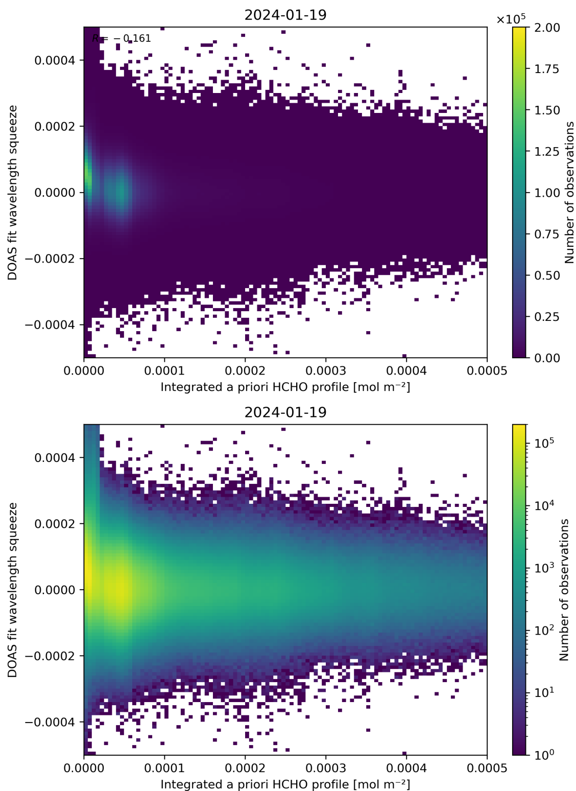
Figure 150: Scatter density plot of “Integrated a priori HCHO profile” against “DOAS fit wavelength squeeze” for 2024-01-18 to 2024-01-20.
