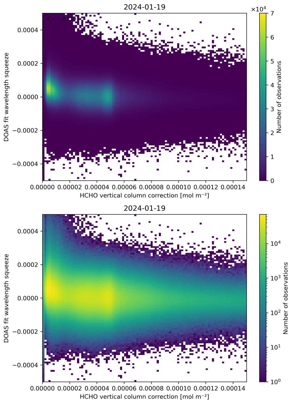
Figure 114: Scatter density plot of “HCHO vertical column correction” against “DOAS fit wavelength squeeze” for 2024-01-18 to 2024-01-20.
