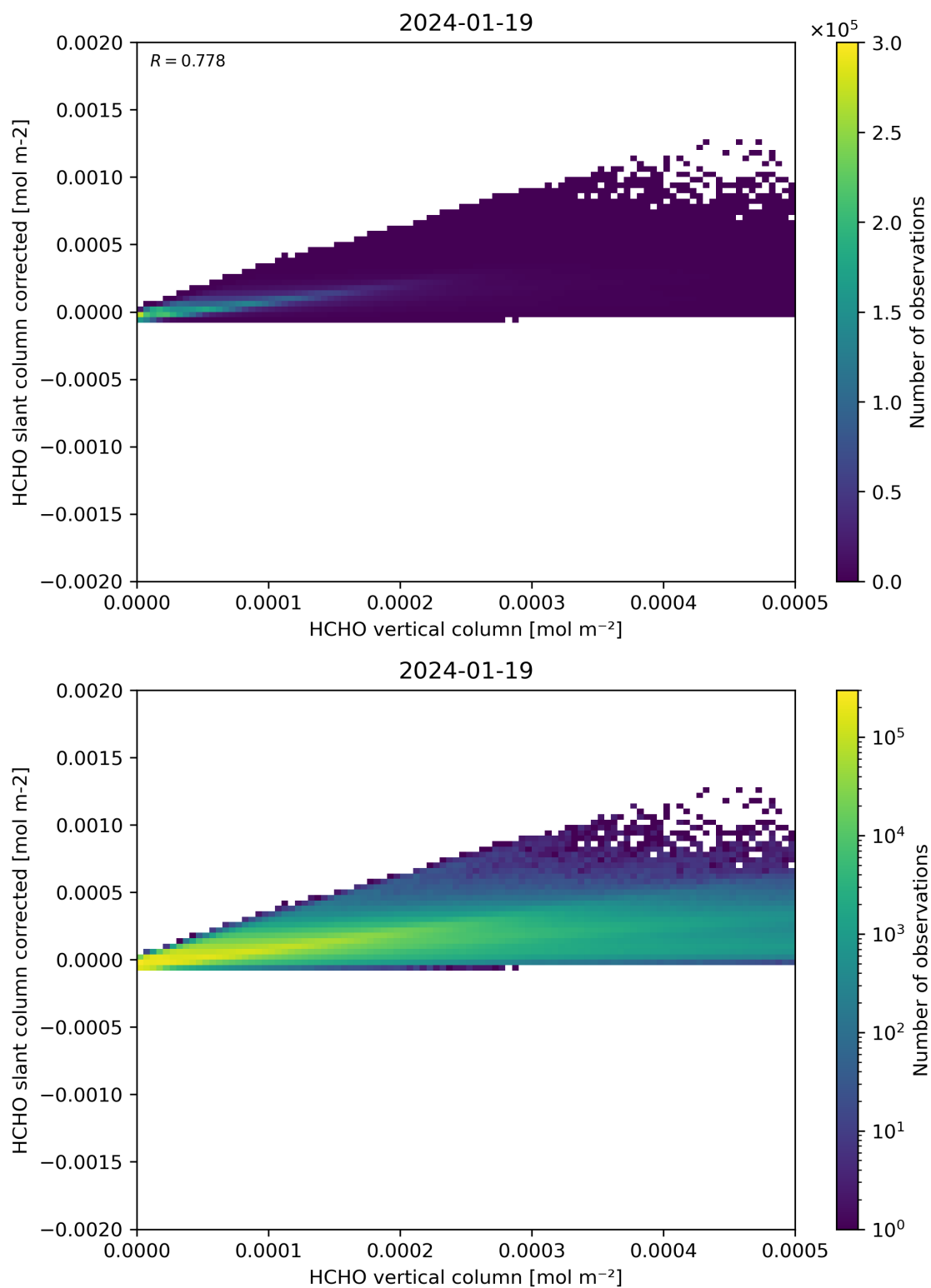
Figure 127: Scatter density plot of “HCHO vertical column” against “HCHO slant column corrected” for 2024-01-18 to 2024-01-20.
