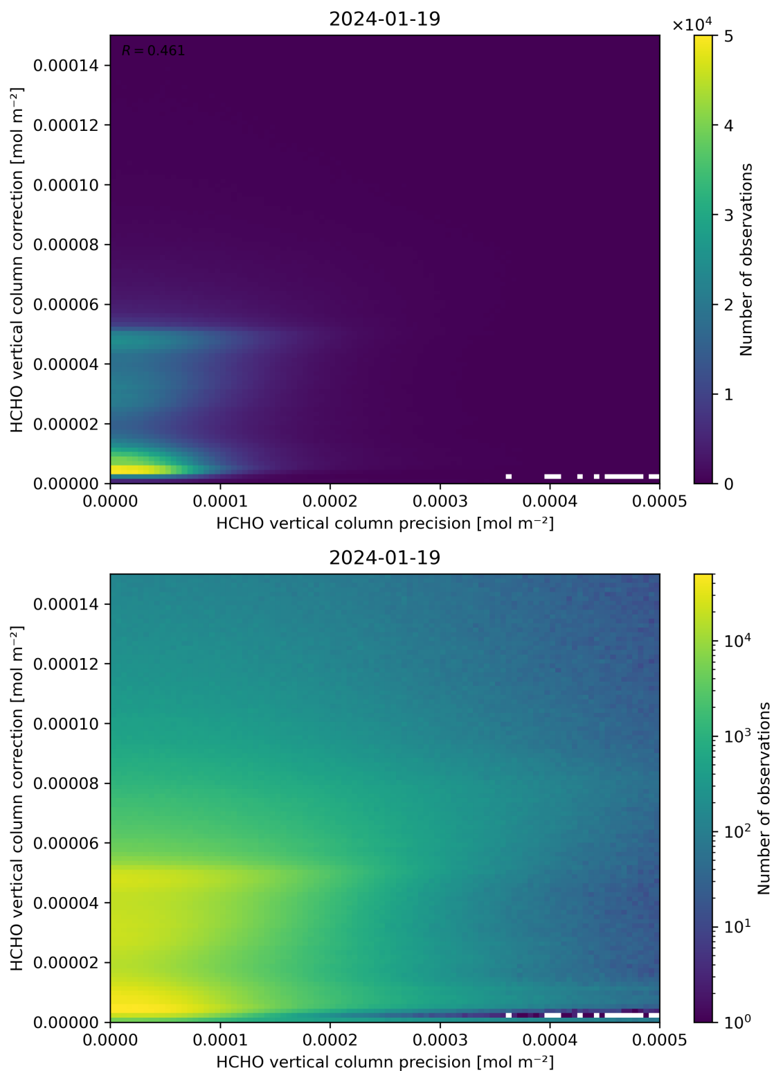
Figure 146: Scatter density plot of “HCHO vertical column precision” against “HCHO vertical column correction” for 2024-01-18 to 2024-01-20.
