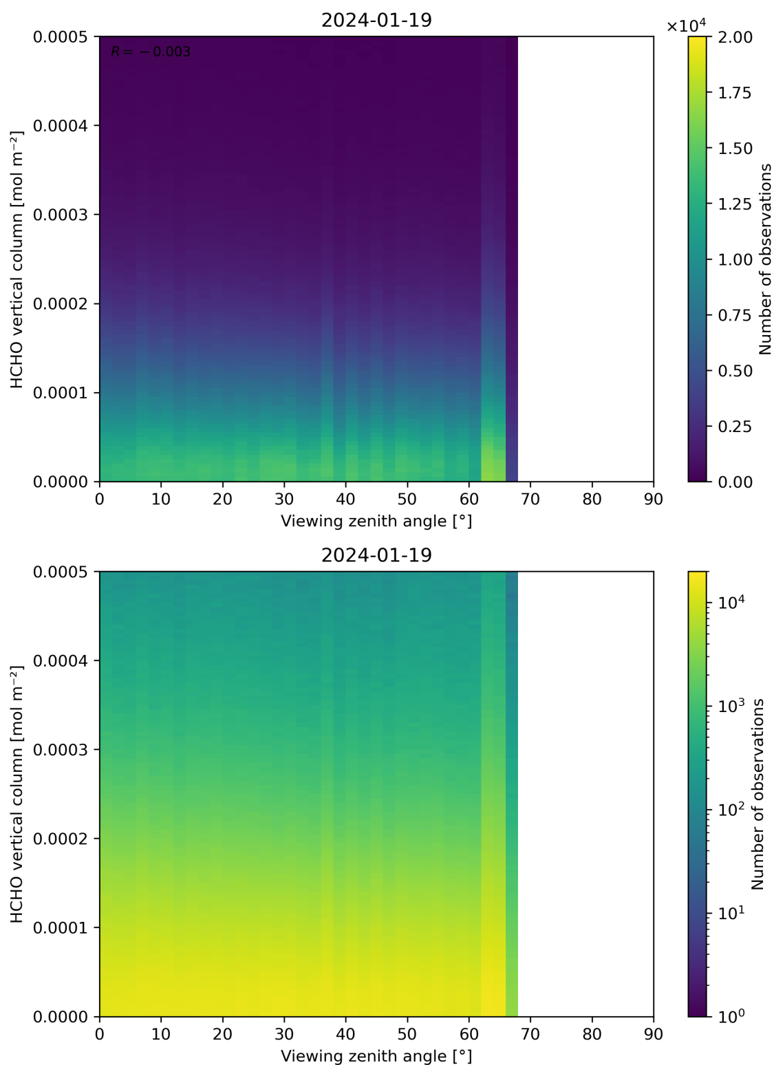
Figure 192: Scatter density plot of “Viewing zenith angle” against “HCHO vertical column” for 2024-01-18 to 2024-01-20.
