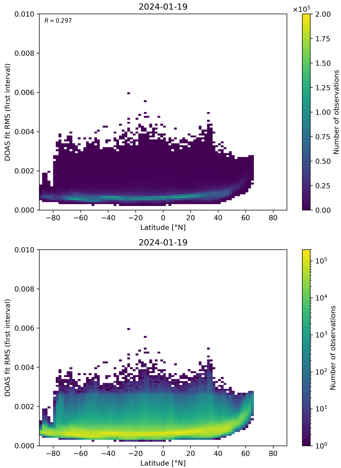
Figure 153: Scatter density plot of “Latitude” against “DOAS fit RMS (first interval)” for 2024-01-18 to 2024-01-20.
