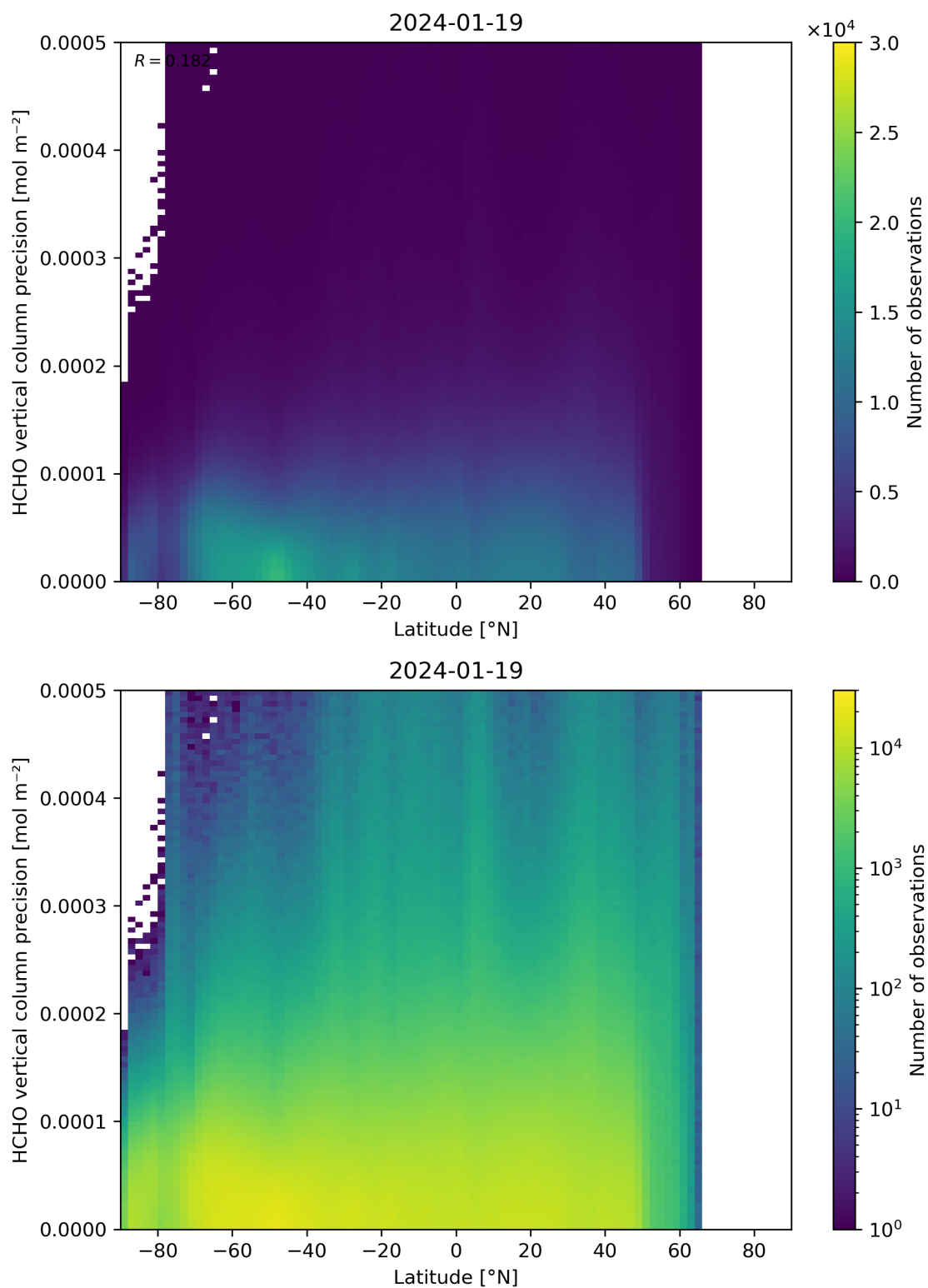
Figure 165: Scatter density plot of “Latitude” against “HCHO vertical column precision” for 2024-01-18 to 2024-01-20.
