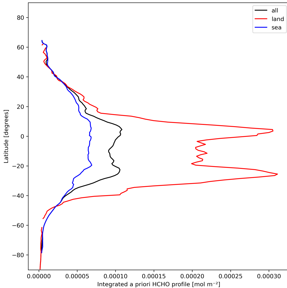
Figure 29: Zonal average of “Integrated a priori HCHO profile” for 2024-01-18 to 2024-01-20.
