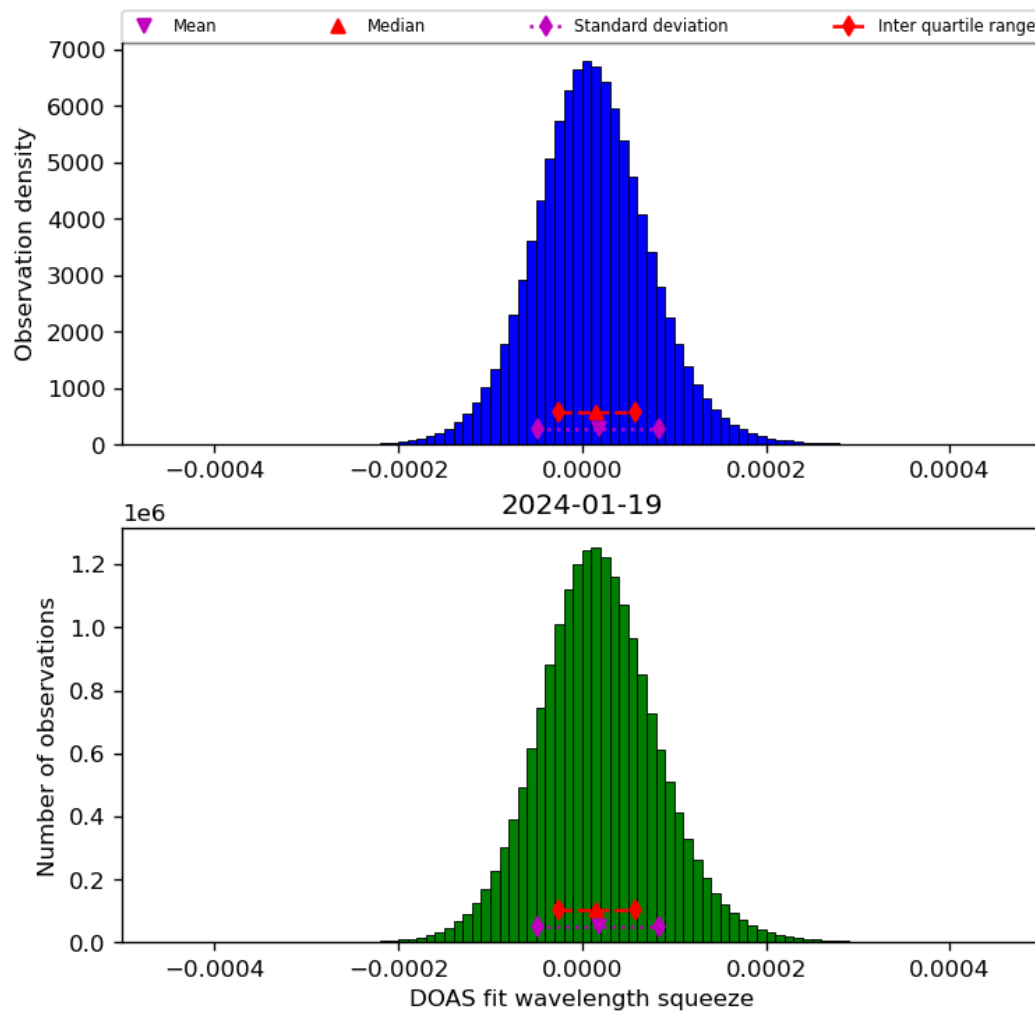
Figure 45: Histogram of “DOAS fit wavelength squeeze” for 2024-01-18 to 2024-01-20
