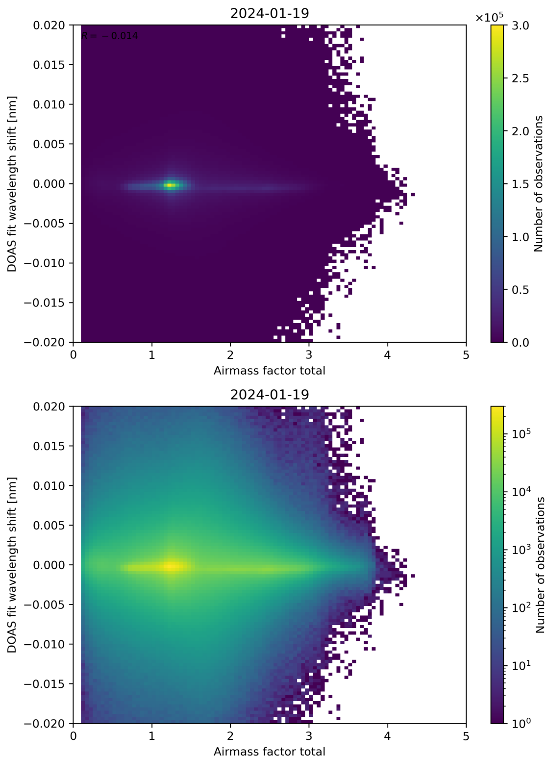
Figure 98: Scatter density plot of “Airmass factor total” against “DOAS fit wavelength shift” for 2024-01-18 to 2024-01-20.
