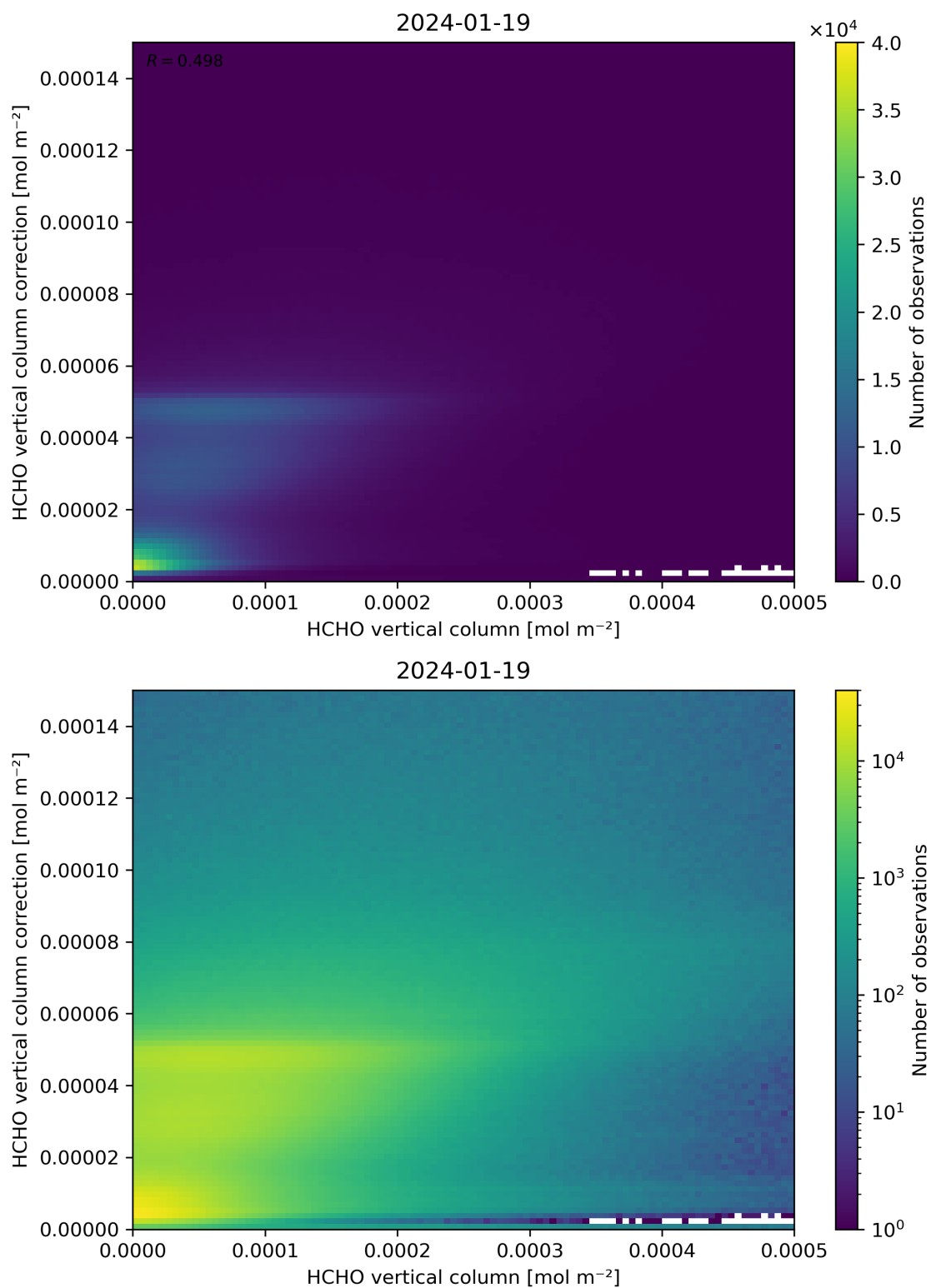
Figure 133: Scatter density plot of “HCHO vertical column” against “HCHO vertical column correction” for 2024-01-18 to 2024-01-20.
