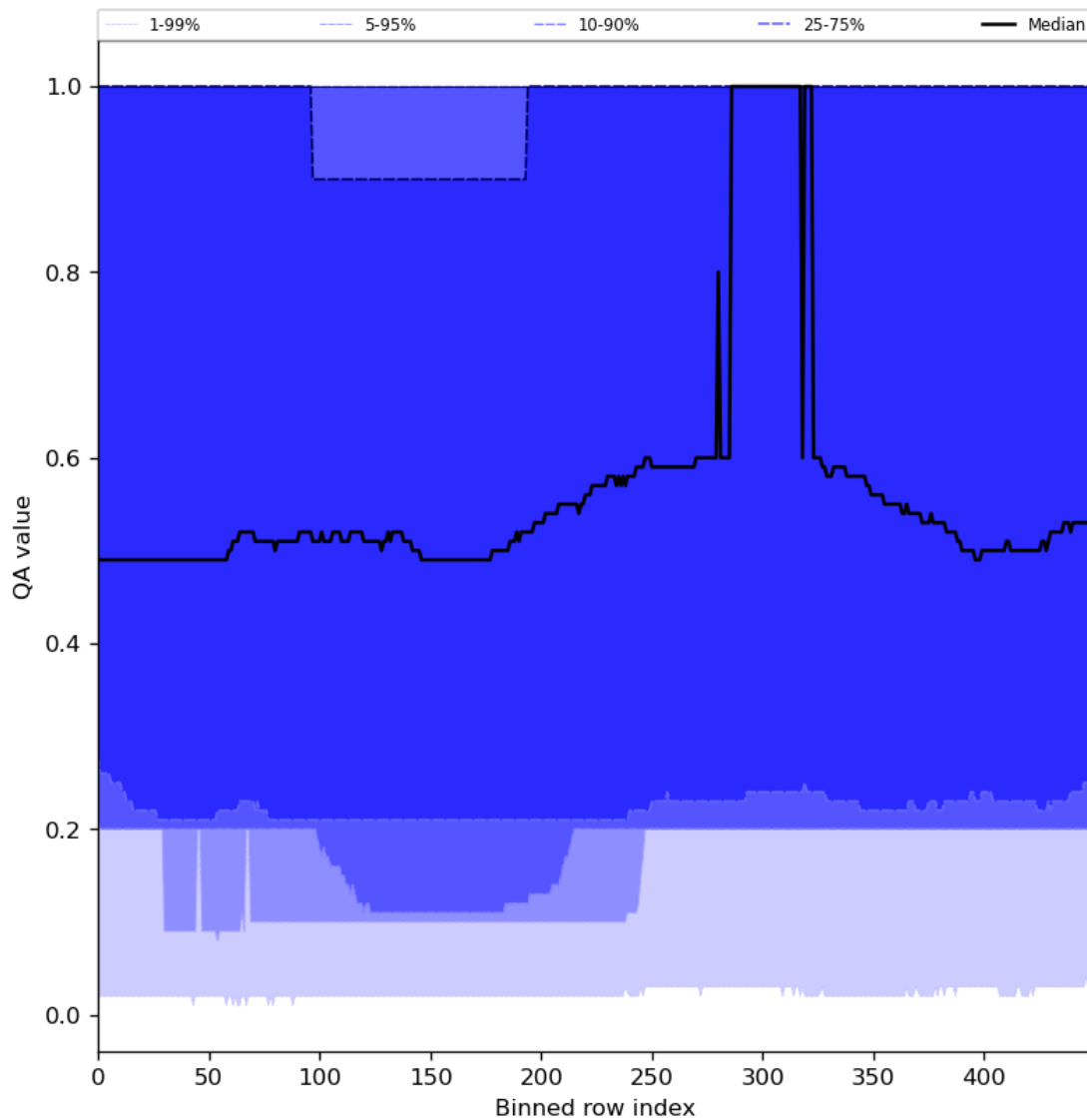
Figure 48: Along track statistics of “QA value” for 2024-01-18 to 2024-01-20
