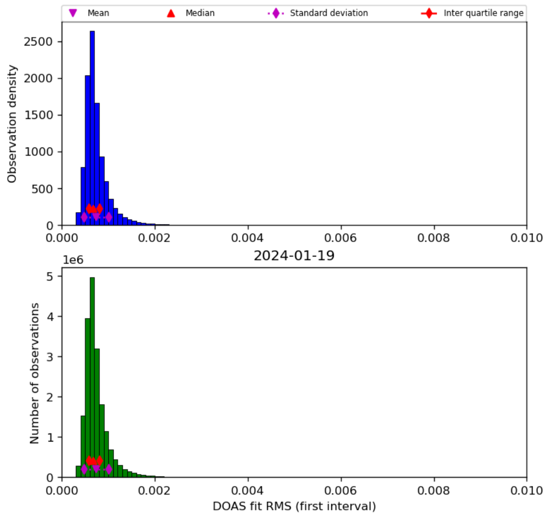
Figure 46: Histogram of “DOAS fit RMS (first interval)” for 2024-01-18 to 2024-01-20
