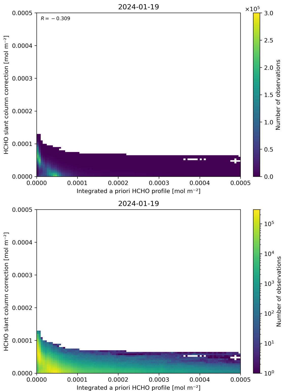
Figure 152: Scatter density plot of “Integrated a priori HCHO profile” against “HCHO slant column correction” for 2024-01-18 to 2024-01-20.
