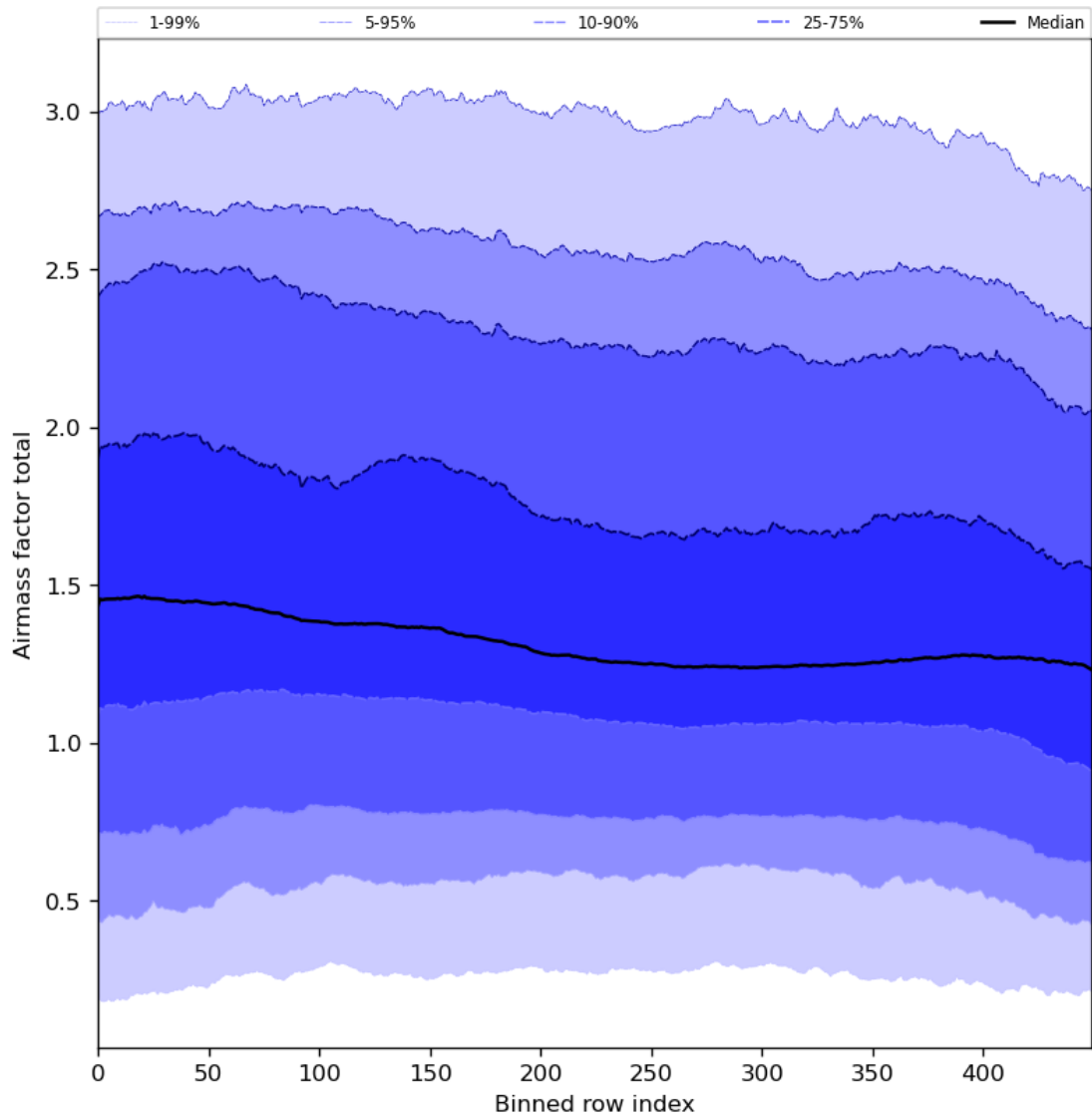
Figure 54: Along track statistics of “Airmass factor total” for 2024-01-18 to 2024-01-20
