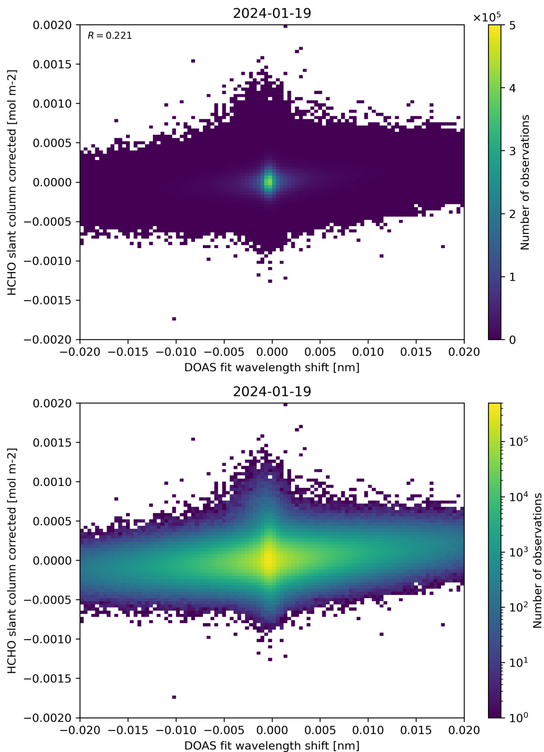
Figure 66: Scatter density plot of “DOAS fit wavelength shift” against “HCHO slant column corrected” for 2024-01-18 to 2024-01-20.
