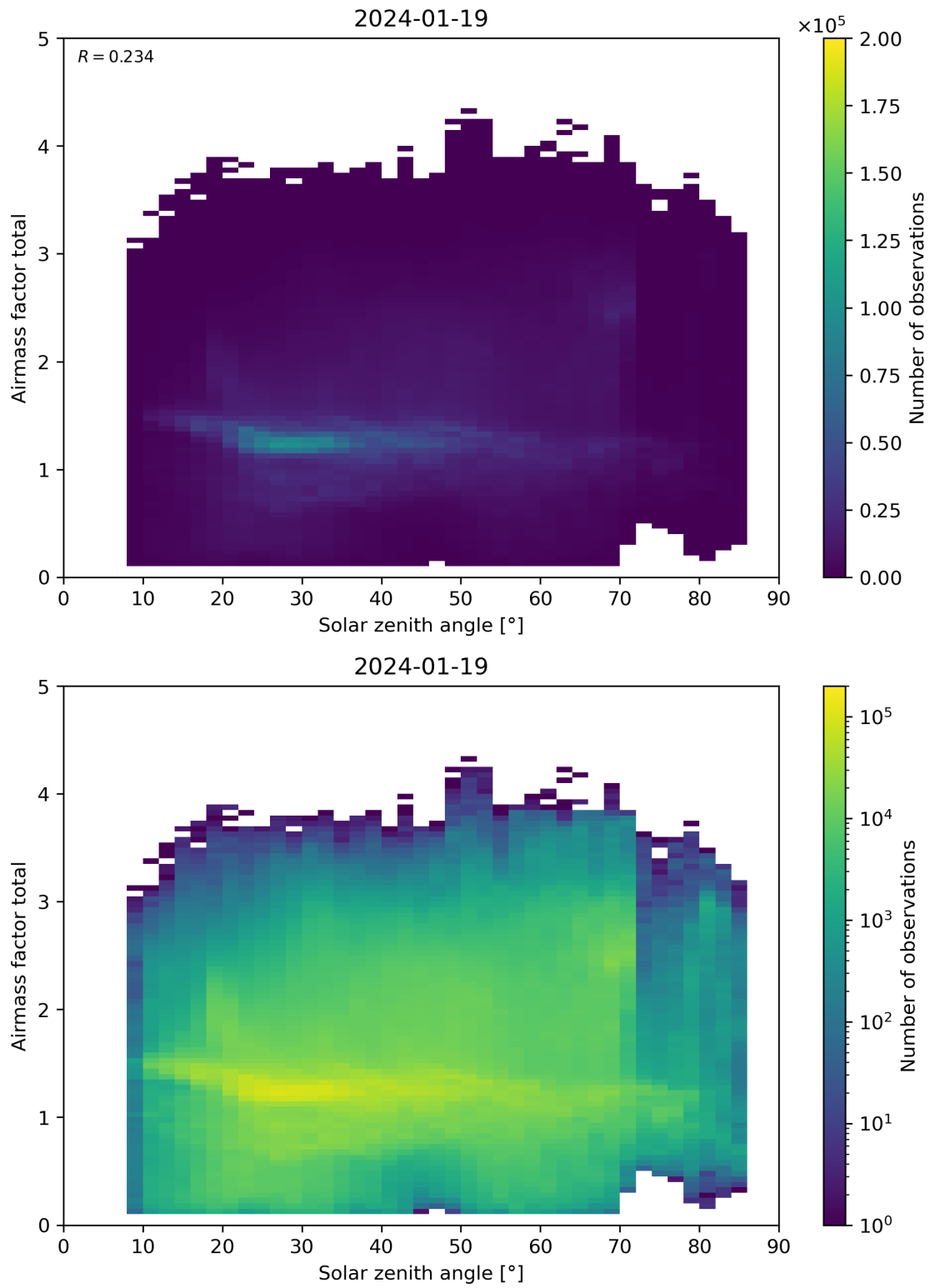
Figure 175: Scatter density plot of “Solar zenith angle” against “Airmass factor total” for 2024-01-18 to 2024-01-20.
