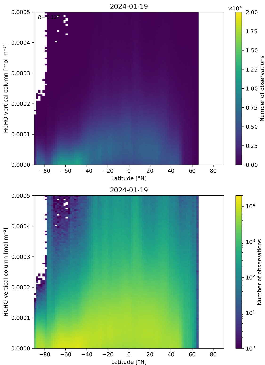
Figure 163: Scatter density plot of “Latitude” against “HCHO vertical column” for 2024-01-18 to 2024-01-20.
