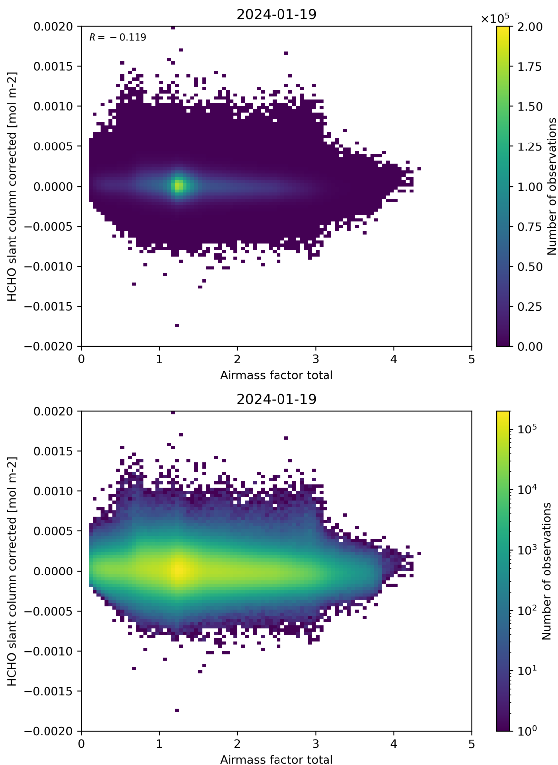
Figure 101: Scatter density plot of “Airmass factor total” against “HCHO slant column corrected” for 2024-01-18 to 2024-01-20.
