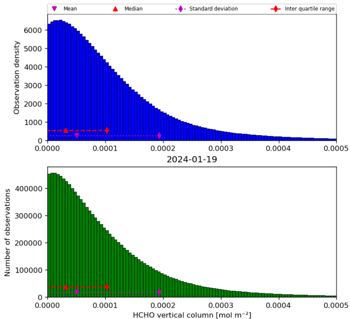
Figure 35: Histogram of “HCHO vertical column” for 2024-01-18 to 2024-01-20
