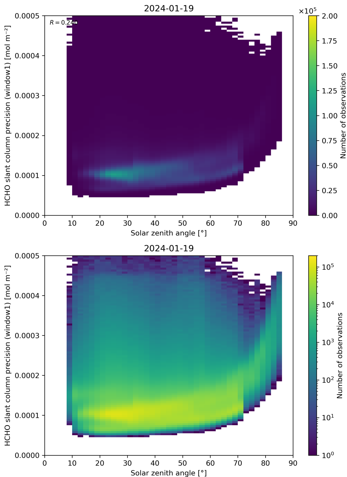
Figure 174: Scatter density plot of “Solar zenith angle” against “HCHO slant column precision (window1)” for 2024-01-18 to 2024-01-20.
