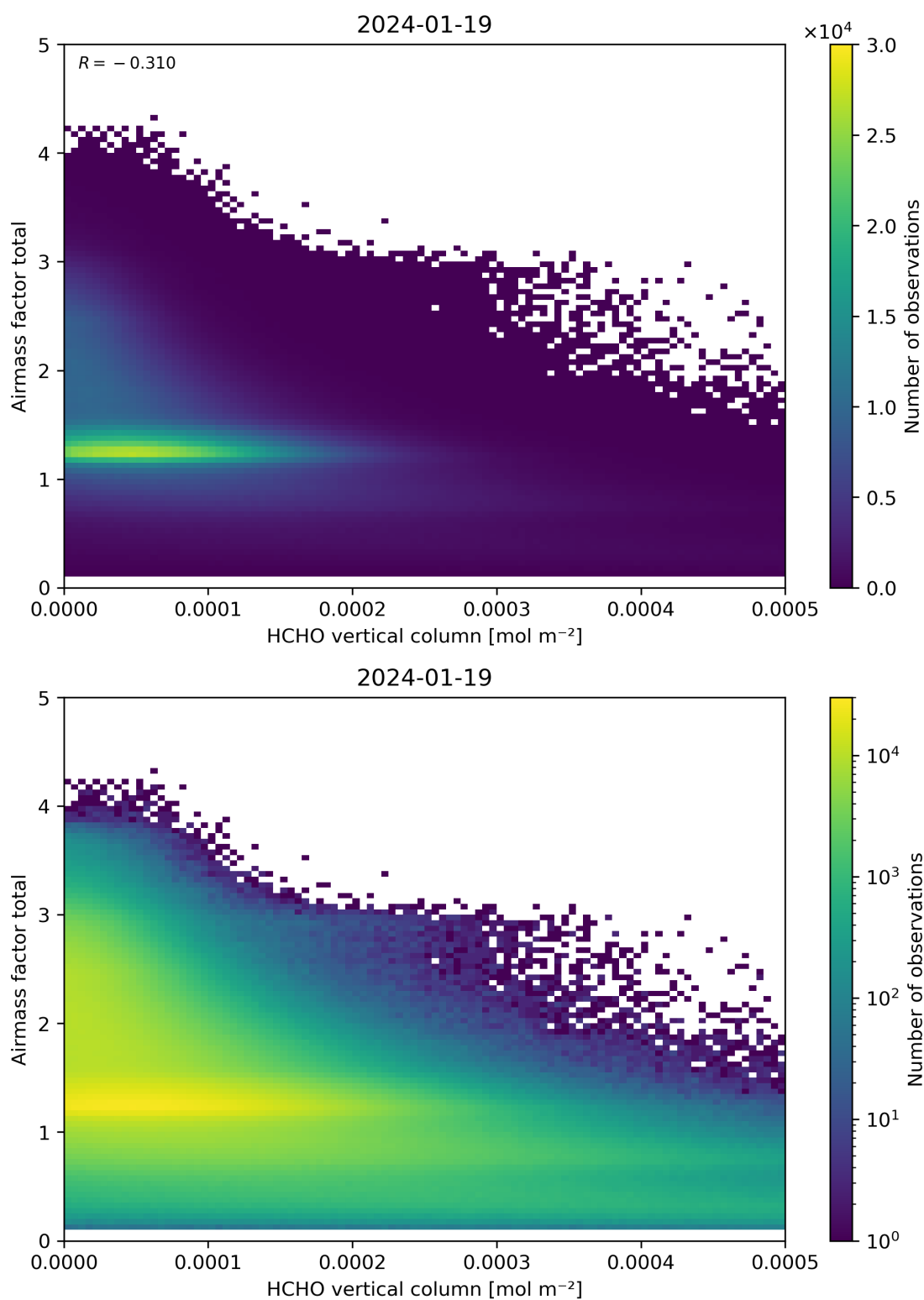
Figure 131: Scatter density plot of “HCHO vertical column” against “Airmass factor total” for 2024-01-18 to 2024-01-20.
