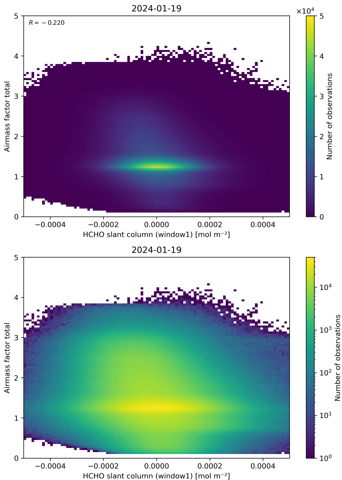
Figure 85: Scatter density plot of “HCHO slant column (window1)” against “Airmass factor total” for 2024-01-18 to 2024-01-20.
