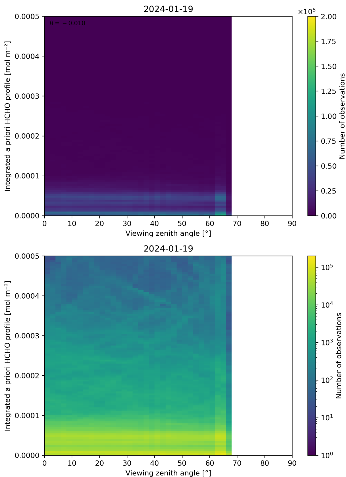
Figure 195: Scatter density plot of “Viewing zenith angle” against “Integrated a priori HCHO profile” for 2024-01-18 to 2024-01-20.
