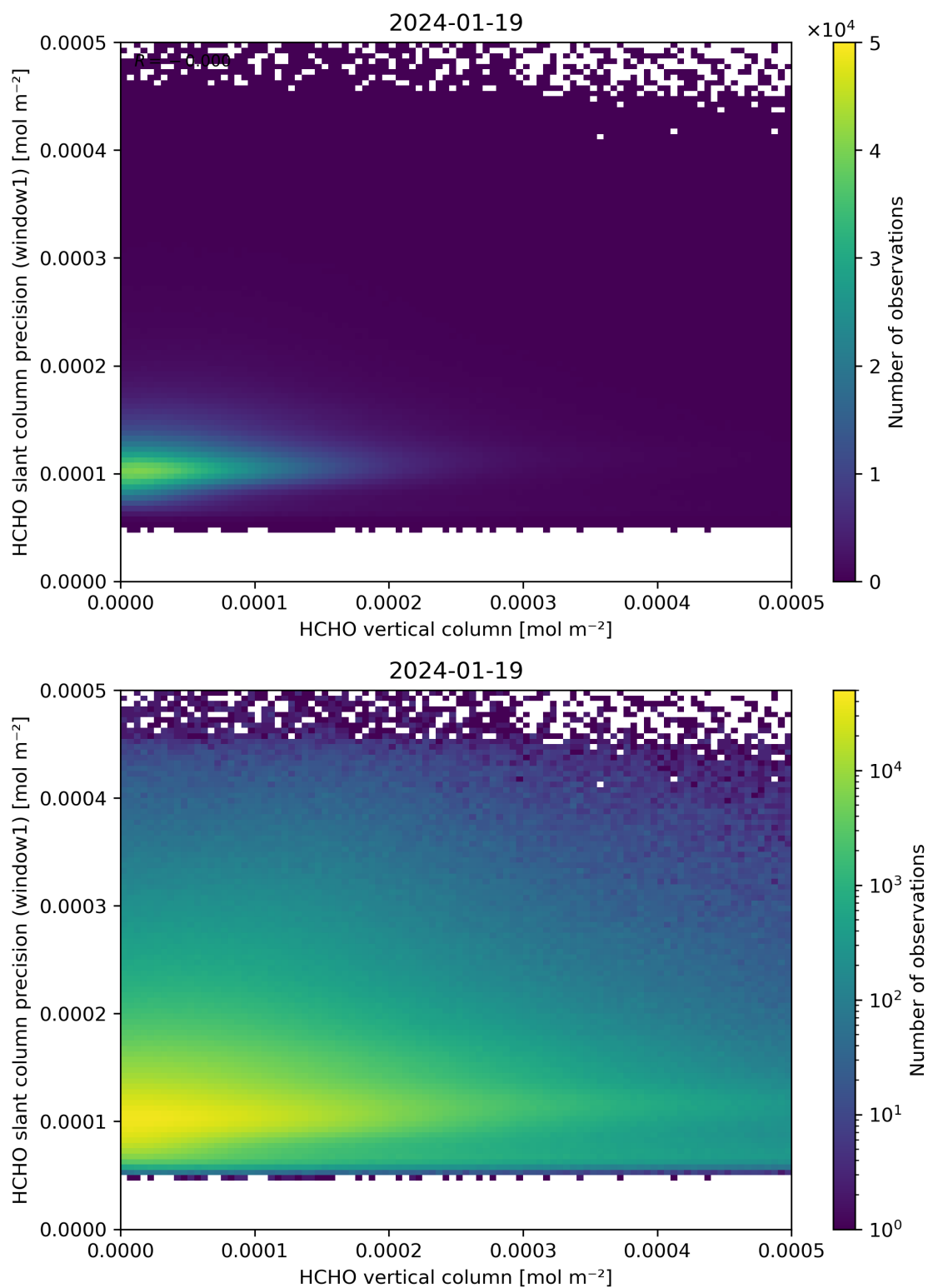
Figure 130: Scatter density plot of “HCHO vertical column” against “HCHO slant column precision (window1)” for 2024-01-18 to 2024-01-20.
