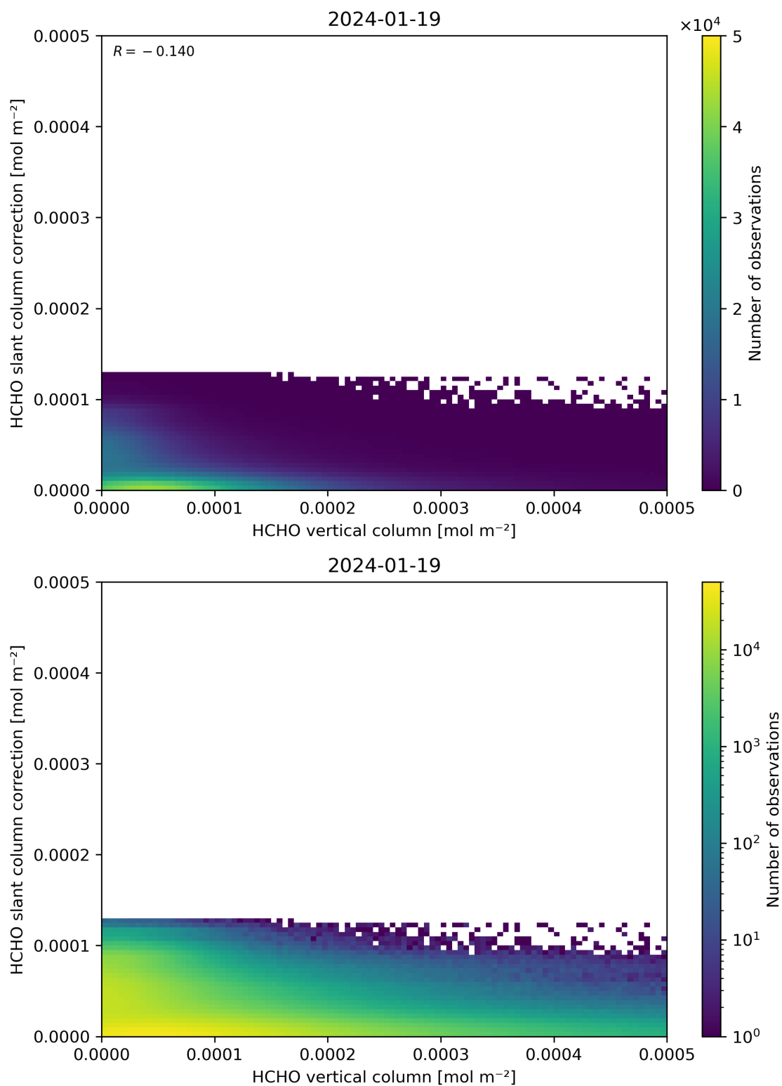
Figure 128: Scatter density plot of “HCHO vertical column” against “HCHO slant column correction” for 2024-01-18 to 2024-01-20.
