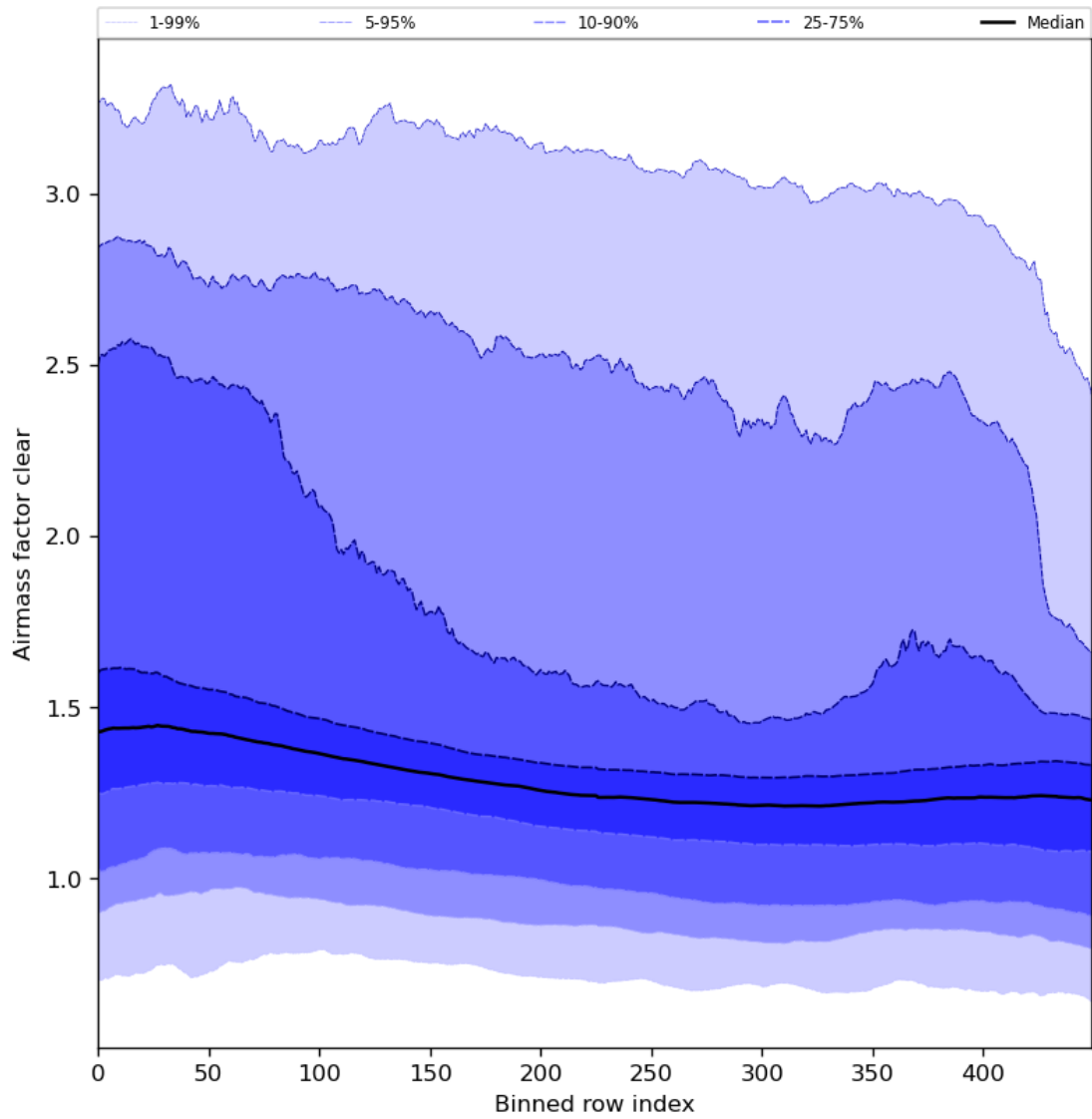
Figure 56: Along track statistics of “Airmass factor clear” for 2024-01-18 to 2024-01-20
