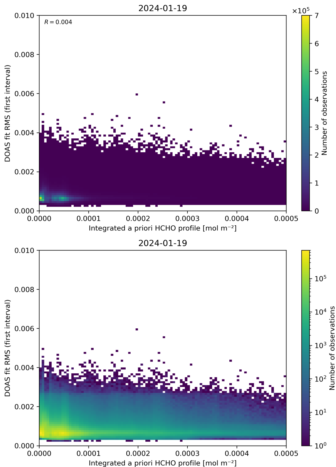
Figure 148: Scatter density plot of “Integrated a priori HCHO profile” against “DOAS fit RMS (first interval)” for 2024-01-18 to 2024-01-20.
