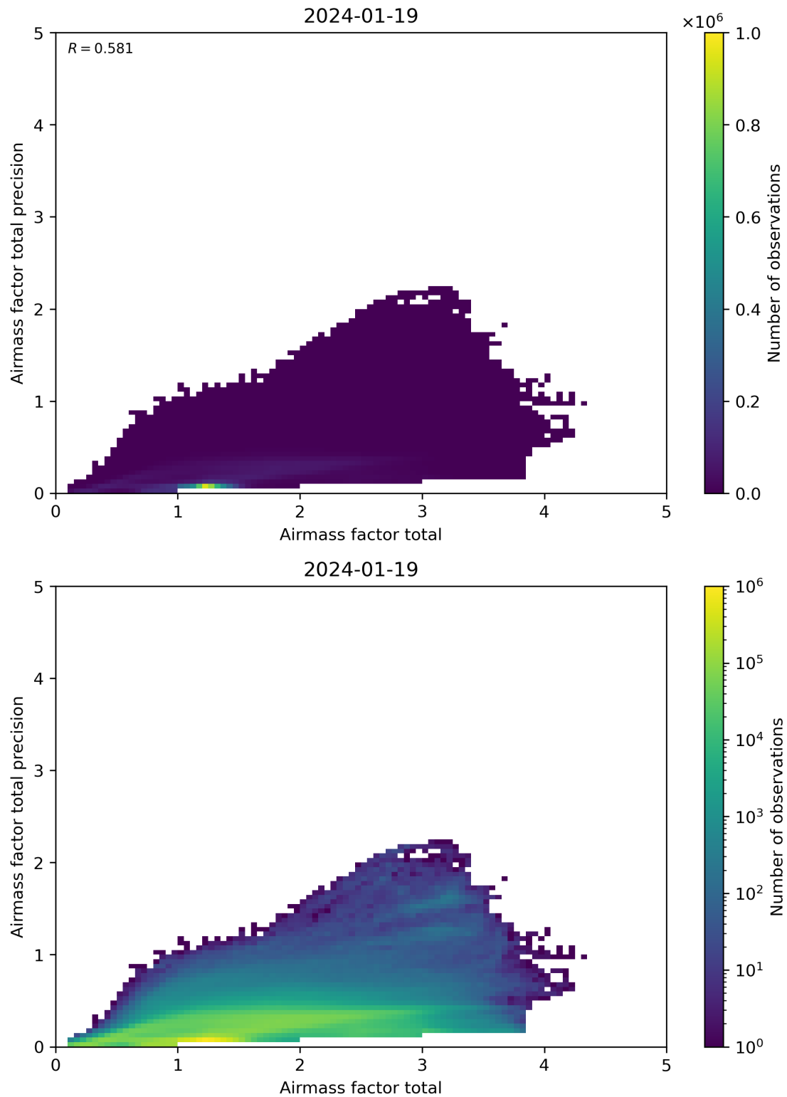
Figure 103: Scatter density plot of “Airmass factor total” against “Airmass factor total precision” for 2024-01-18 to 2024-01-20.
