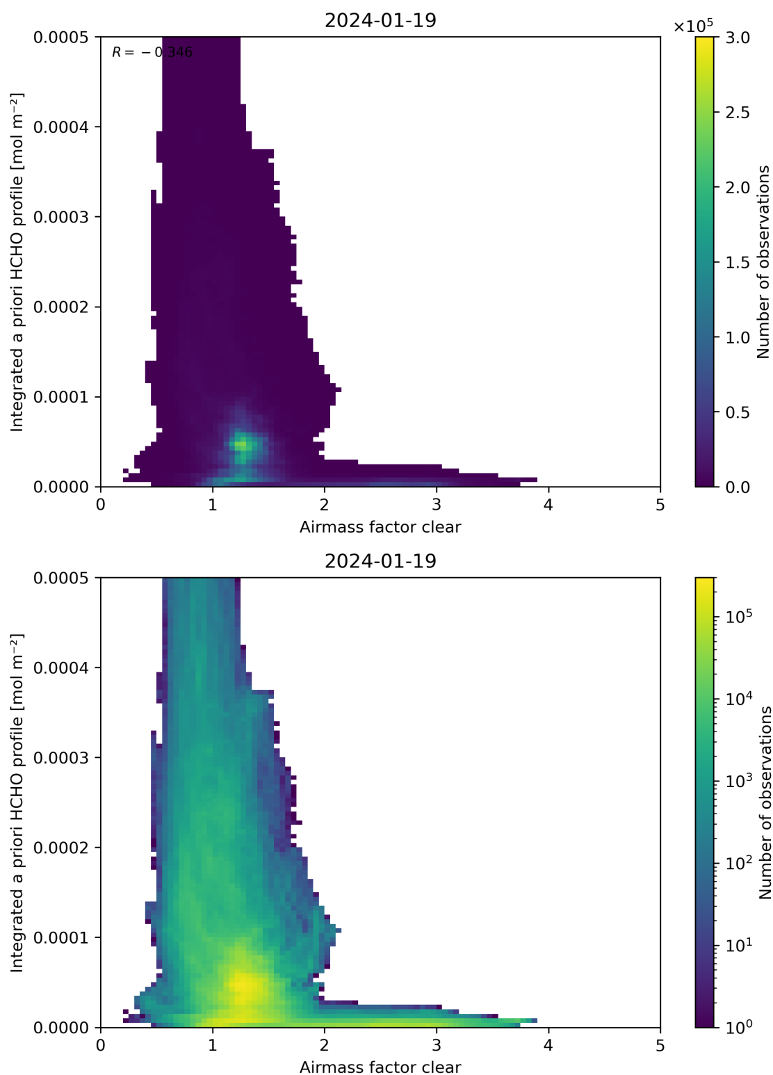
Figure 76: Scatter density plot of “Airmass factor clear” against “Integrated a priori HCHO profile” for 2024-01-18 to 2024-01-20.
