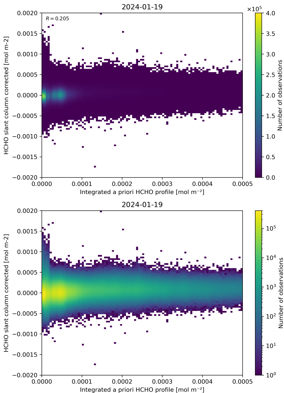
Figure 151: Scatter density plot of “Integrated a priori HCHO profile” against “HCHO slant column corrected” for 2024-01-18 to 2024-01-20.
