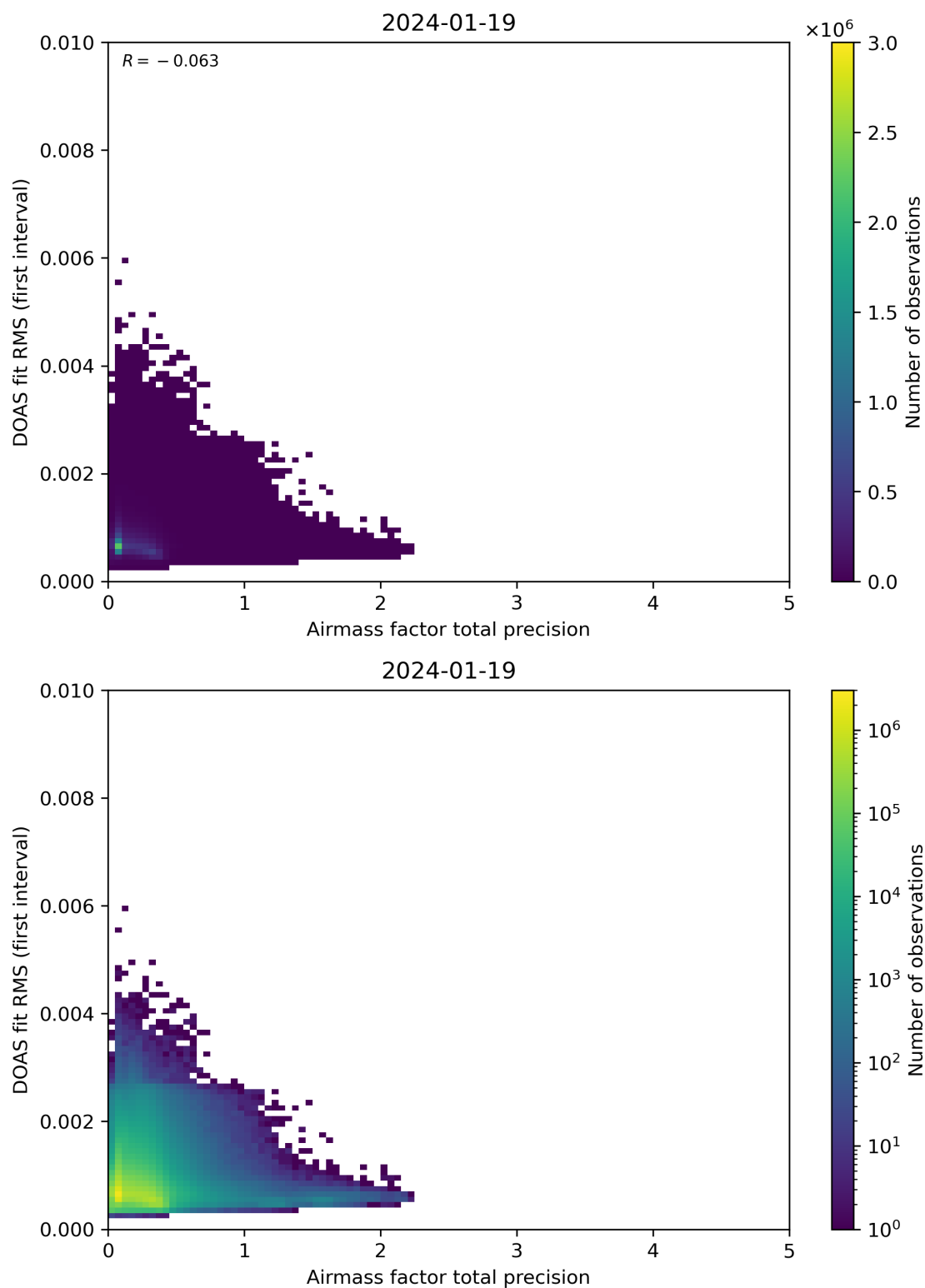
Figure 105: Scatter density plot of “Airmass factor total precision” against “DOAS fit RMS (first interval)” for 2024-01-18 to 2024-01-20.
