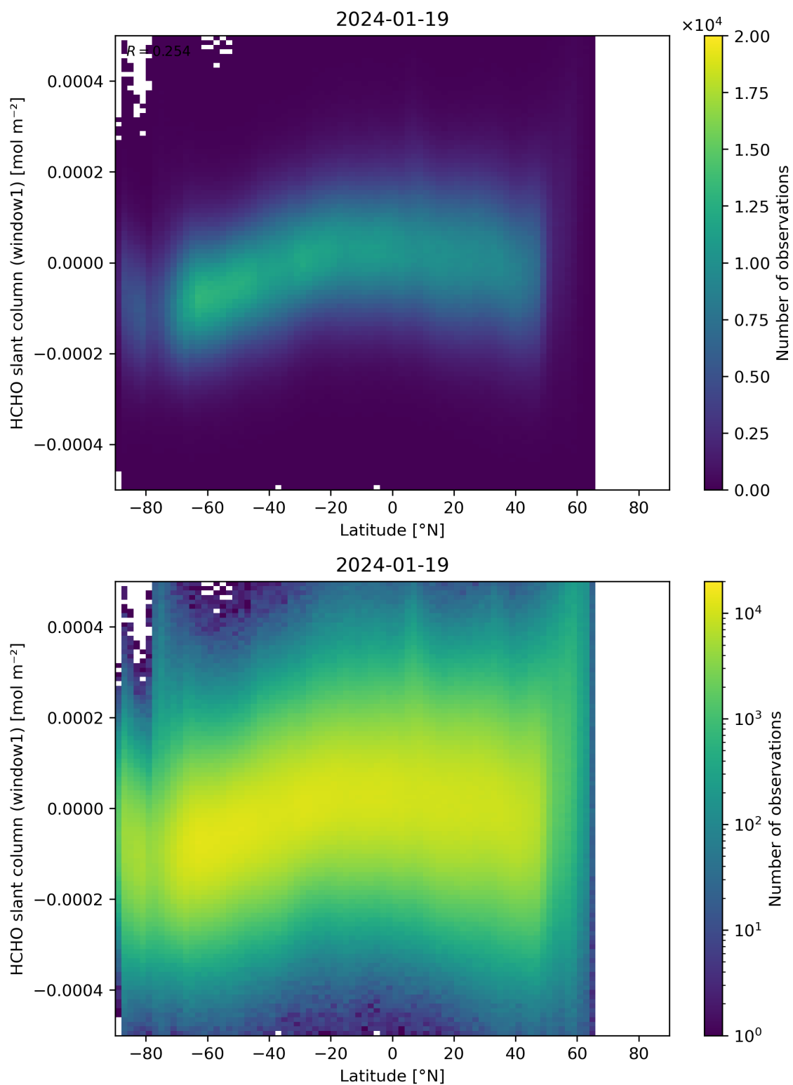
Figure 159: Scatter density plot of “Latitude” against “HCHO slant column (window1)” for 2024-01-18 to 2024-01-20.
