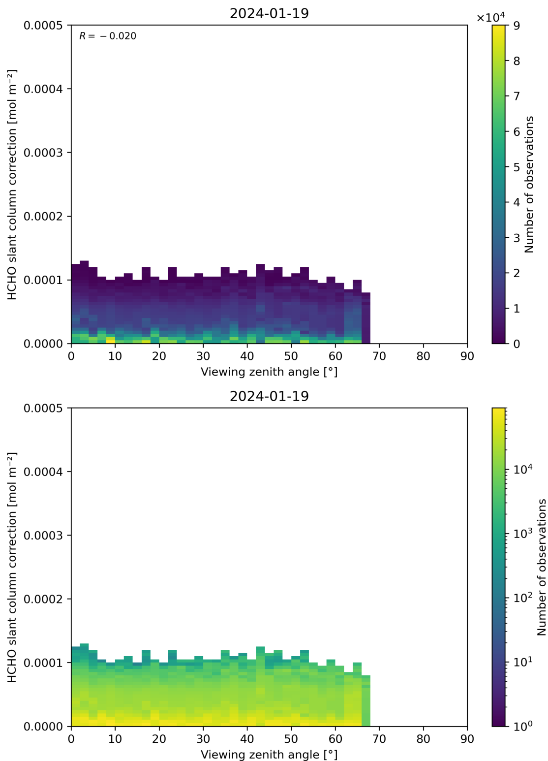
Figure 187: Scatter density plot of “Viewing zenith angle” against “HCHO slant column correction” for 2024-01-18 to 2024-01-20.
