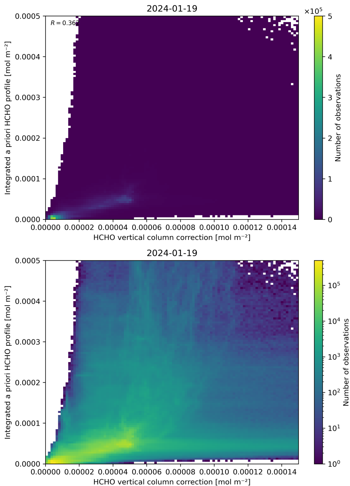
Figure 122: Scatter density plot of “HCHO vertical column correction” against “Integrated a priori HCHO profile” for 2024-01-18 to 2024-01-20.
