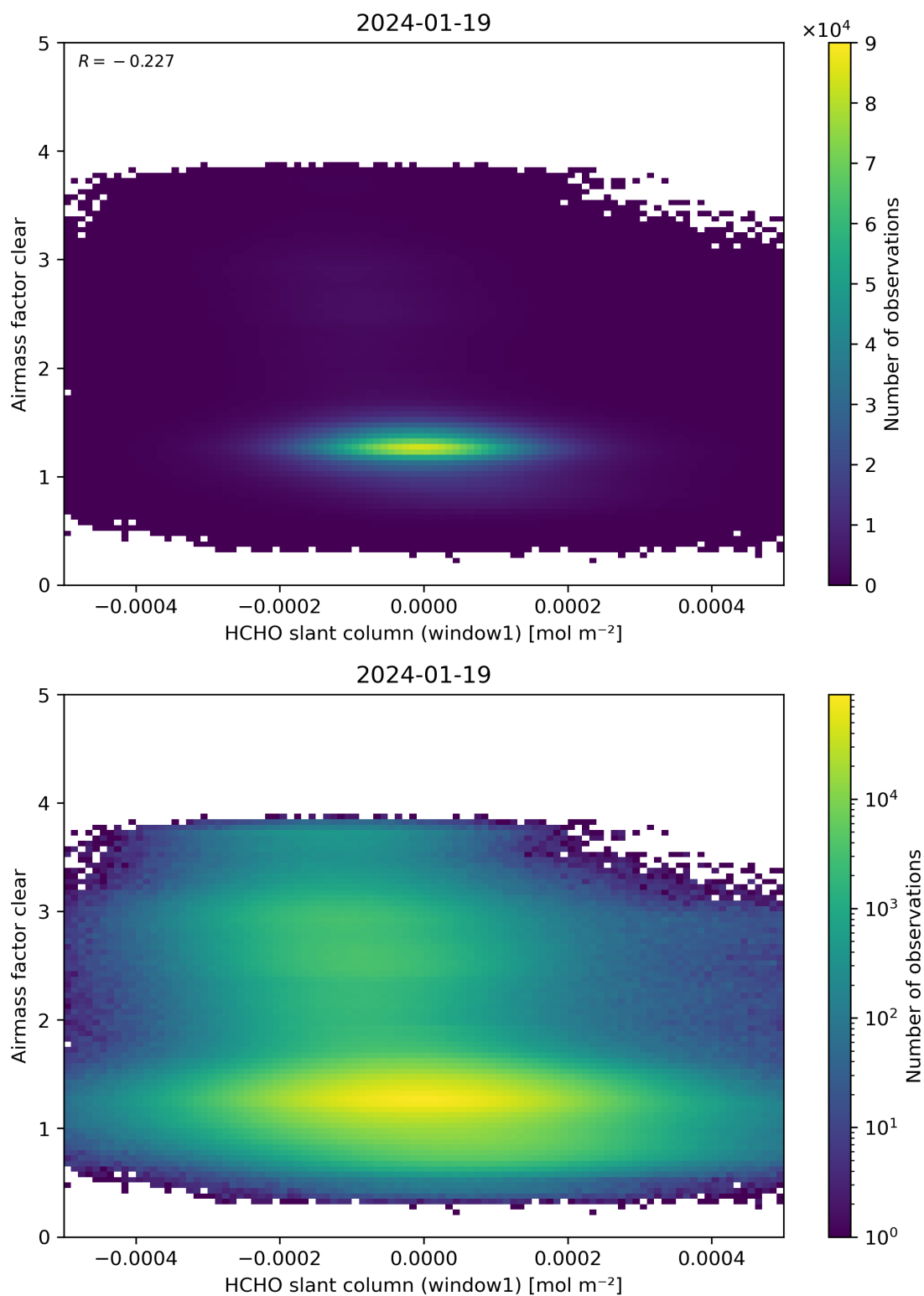
Figure 81: Scatter density plot of “HCHO slant column (window1)” against “Airmass factor clear” for 2024-01-18 to 2024-01-20.
