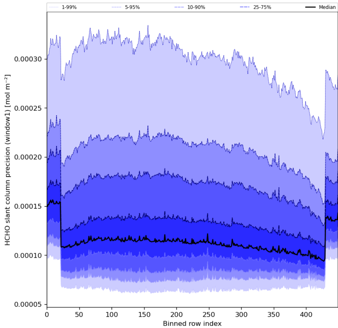
Figure 53: Along track statistics of “HCHO slant column precision (window1)” for 2024-01-18 to 2024-01-20
