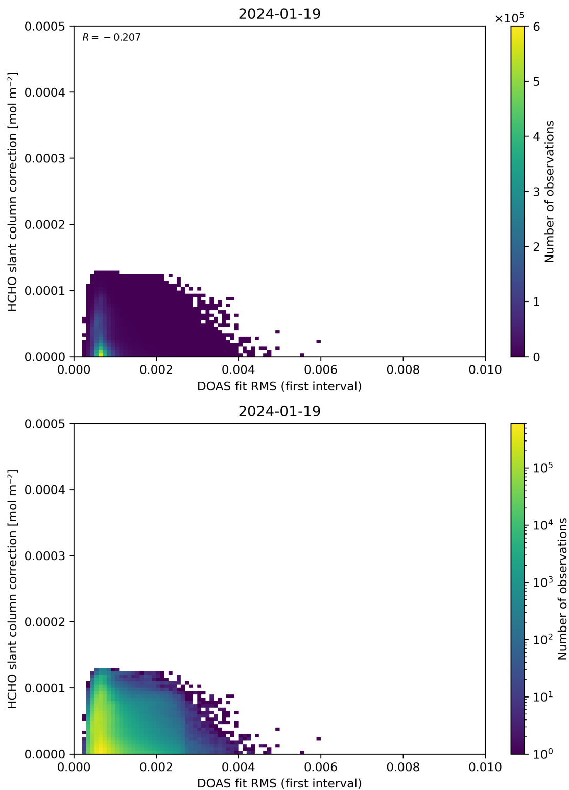
Figure 63: Scatter density plot of “DOAS fit RMS (first interval)” against “HCHO slant column correction” for 2024-01-18 to 2024-01-20.
