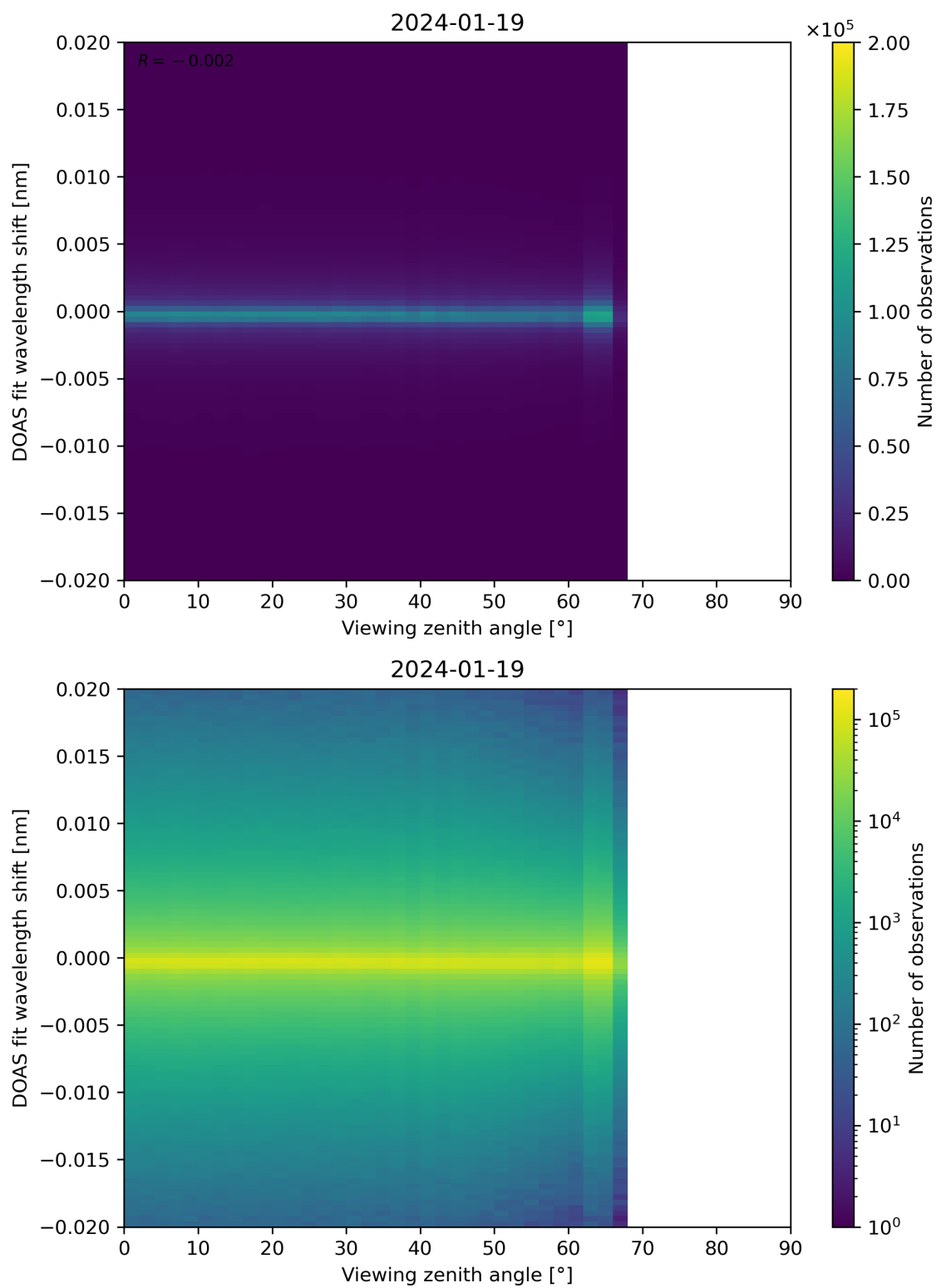
Figure 183: Scatter density plot of “Viewing zenith angle” against “DOAS fit wavelength shift” for 2024-01-18 to 2024-01-20.
