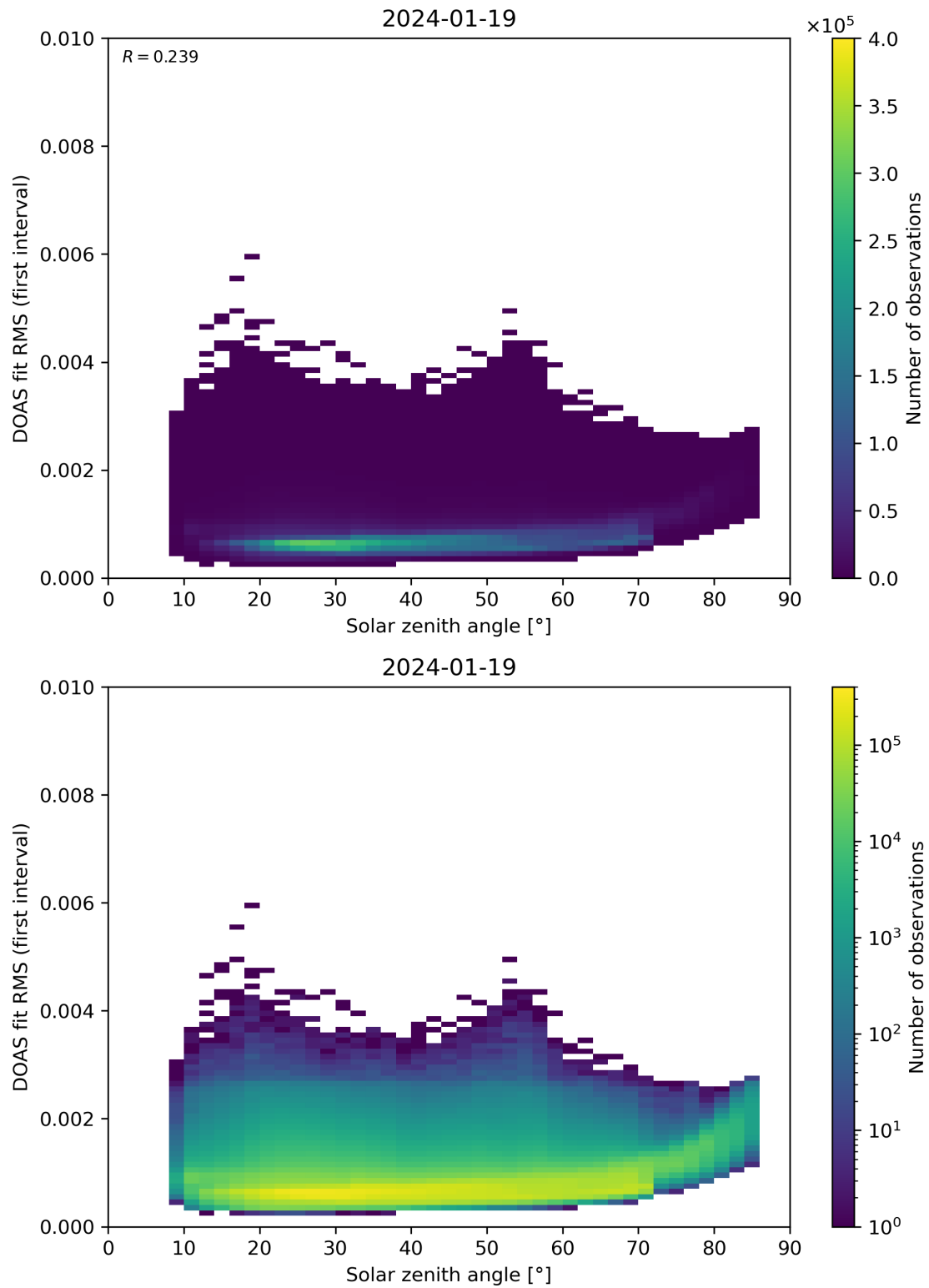
Figure 167: Scatter density plot of “Solar zenith angle” against “DOAS fit RMS (first interval)” for 2024-01-18 to 2024-01-20.
