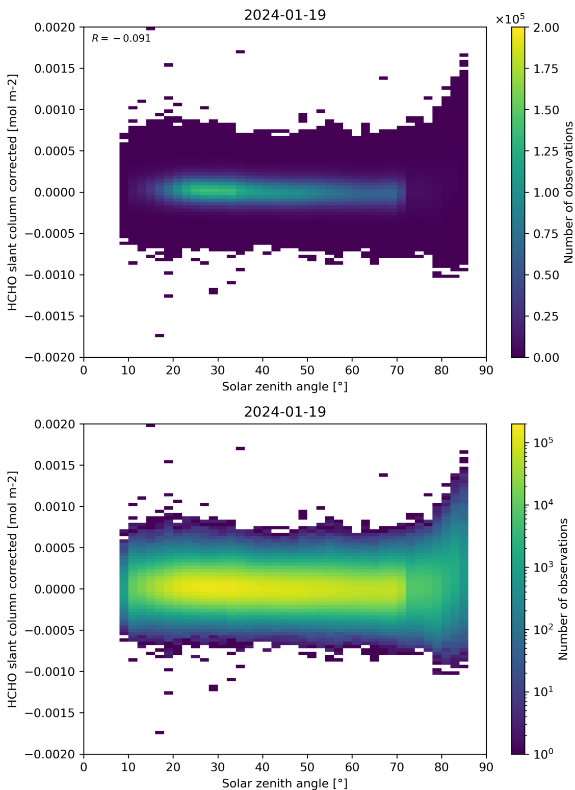
Figure 171: Scatter density plot of “Solar zenith angle” against “HCHO slant column corrected” for 2024-01-18 to 2024-01-20.
