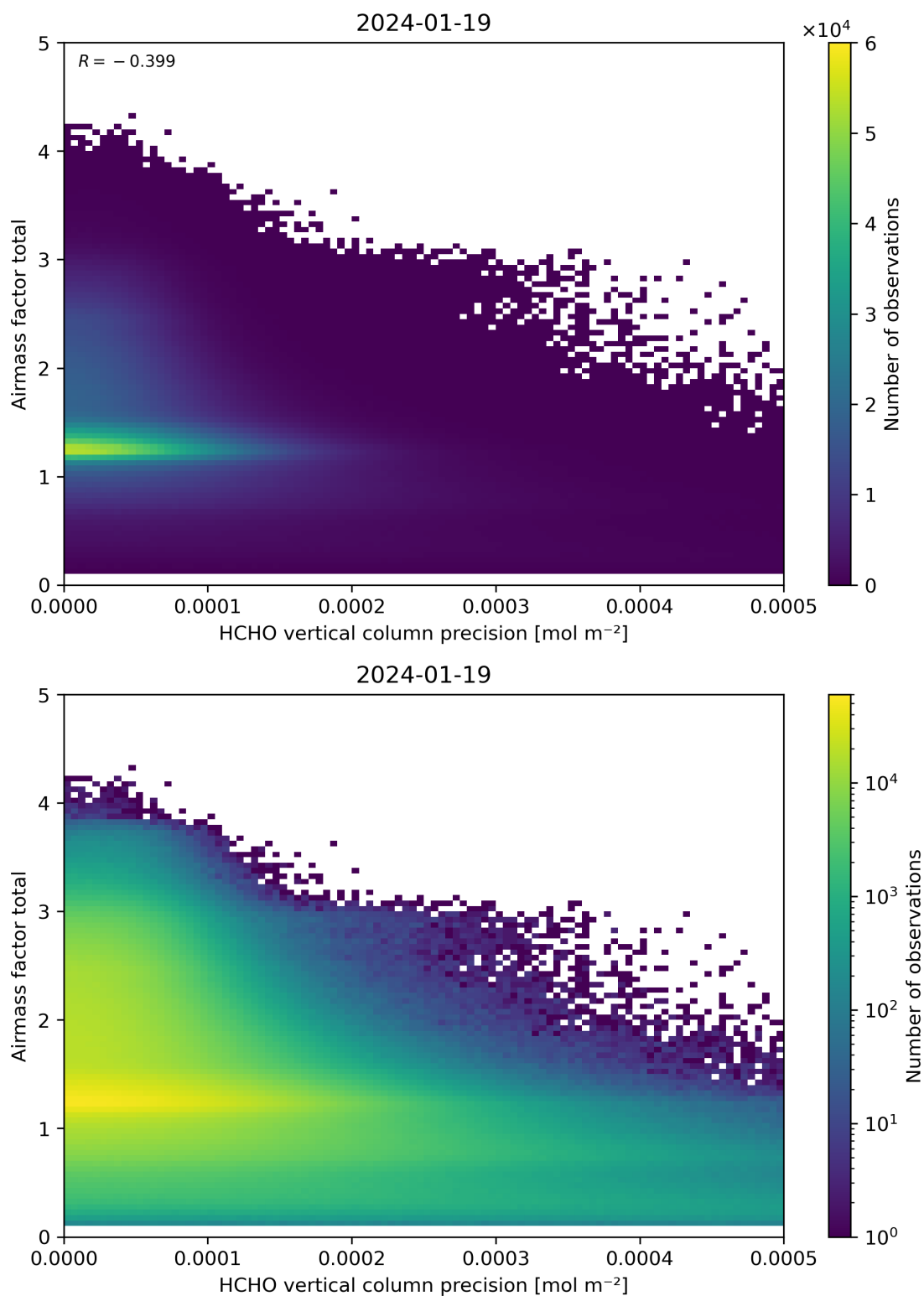
Figure 144: Scatter density plot of “HCHO vertical column precision” against “Airmass factor total” for 2024-01-18 to 2024-01-20.
