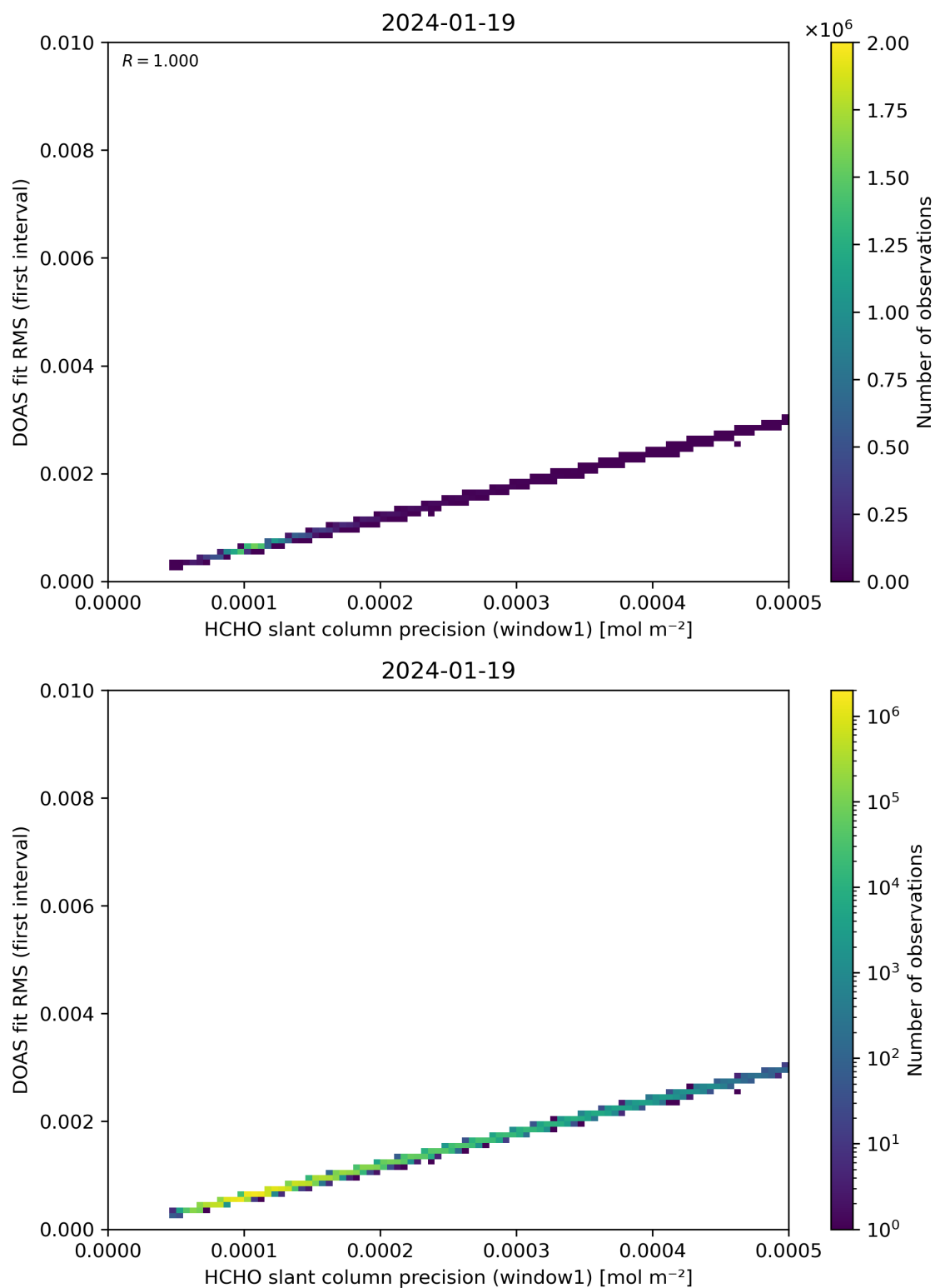
Figure 88: Scatter density plot of “HCHO slant column precision (window1)” against “DOAS fit RMS (first interval)” for 2024-01-18 to 2024-01-20.
