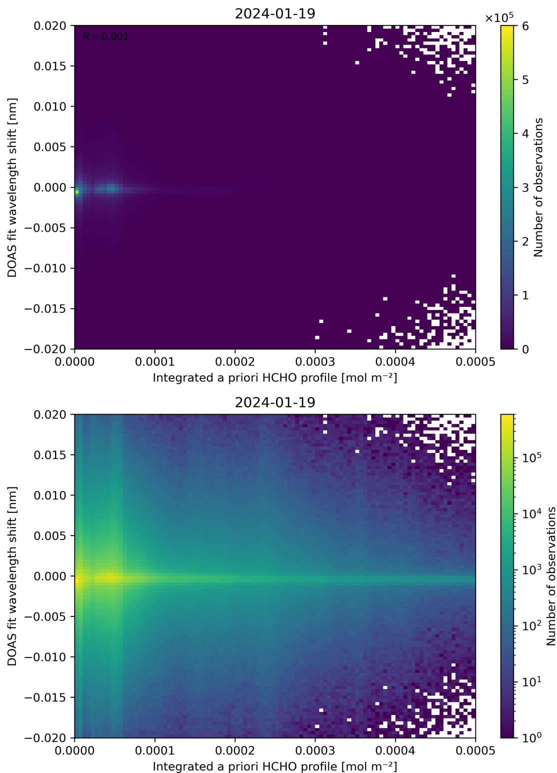
Figure 149: Scatter density plot of “Integrated a priori HCHO profile” against “DOAS fit wavelength shift” for 2024-01-18 to 2024-01-20.
