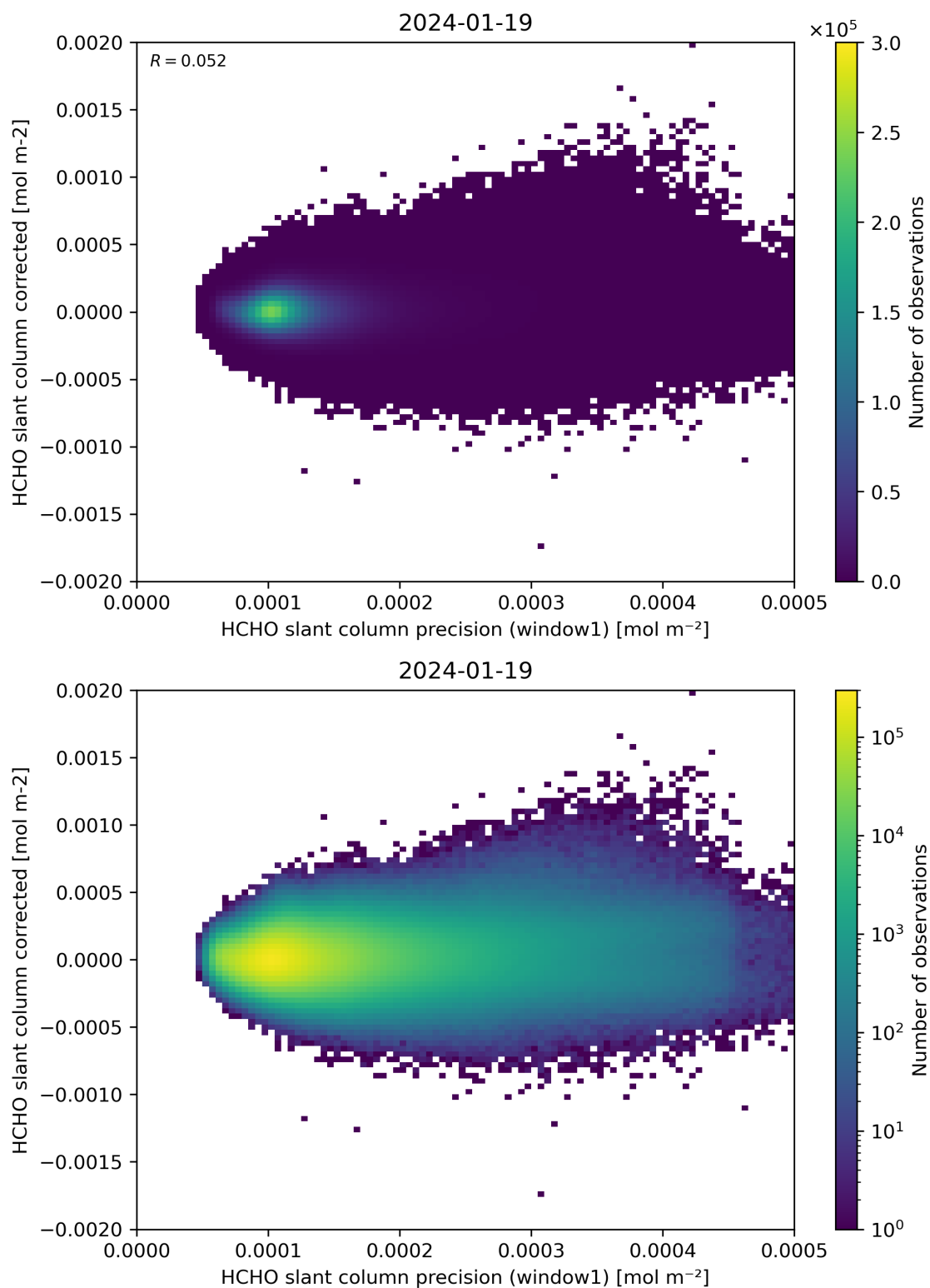
Figure 92: Scatter density plot of “HCHO slant column precision (window1)” against “HCHO slant column corrected” for 2024-01-18 to 2024-01-20.
