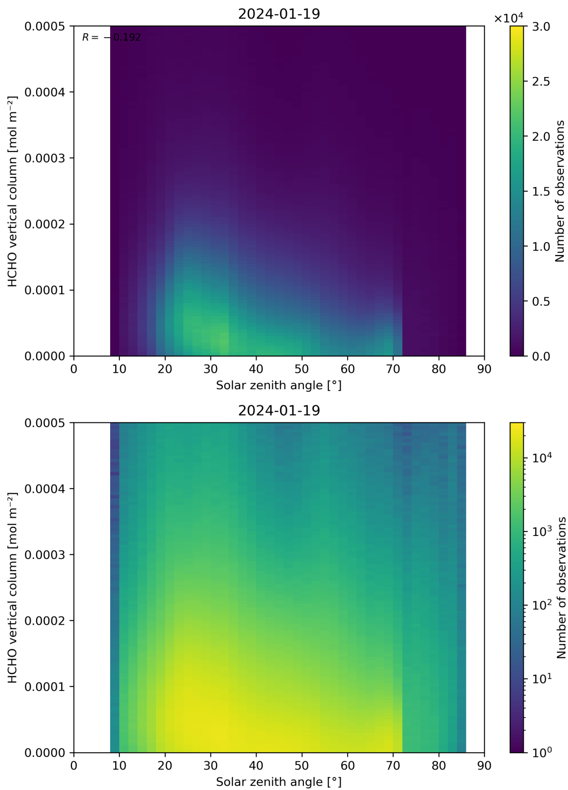
Figure 177: Scatter density plot of “Solar zenith angle” against “HCHO vertical column” for 2024-01-18 to 2024-01-20.
