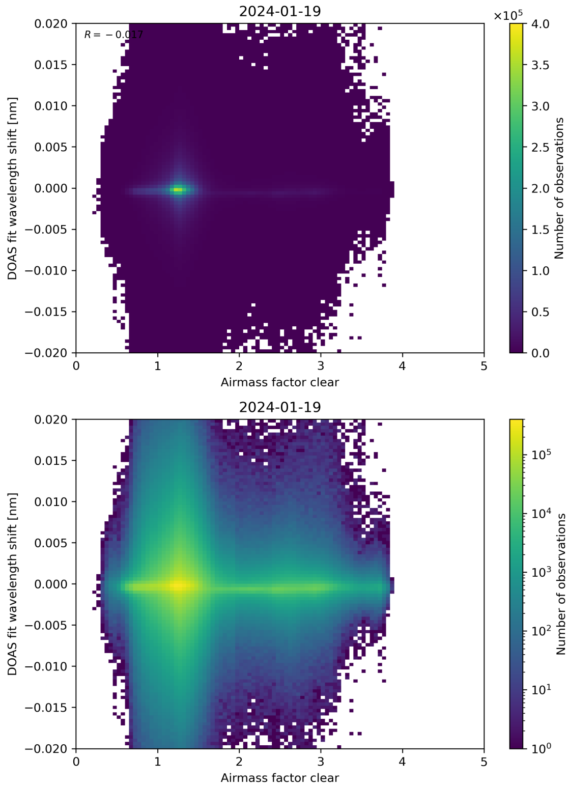
Figure 72: Scatter density plot of “Airmass factor clear” against “DOAS fit wavelength shift” for 2024-01-18 to 2024-01-20.
