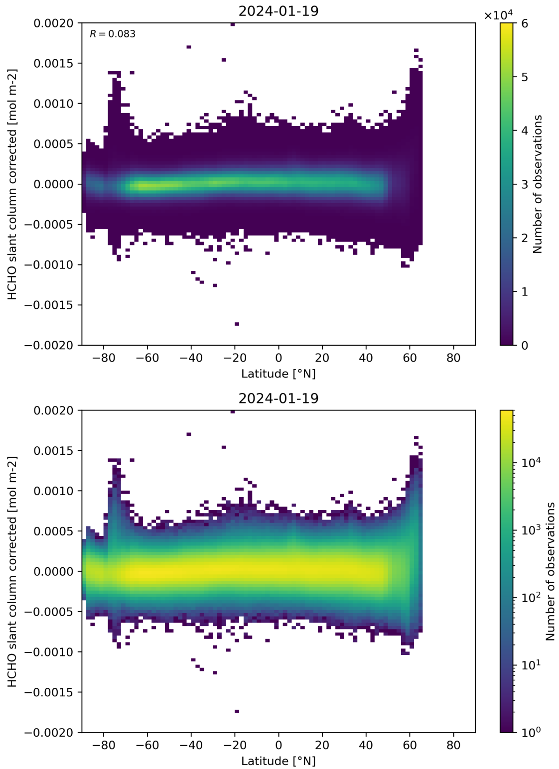
Figure 157: Scatter density plot of “Latitude” against “HCHO slant column corrected” for 2024-01-18 to 2024-01-20.
