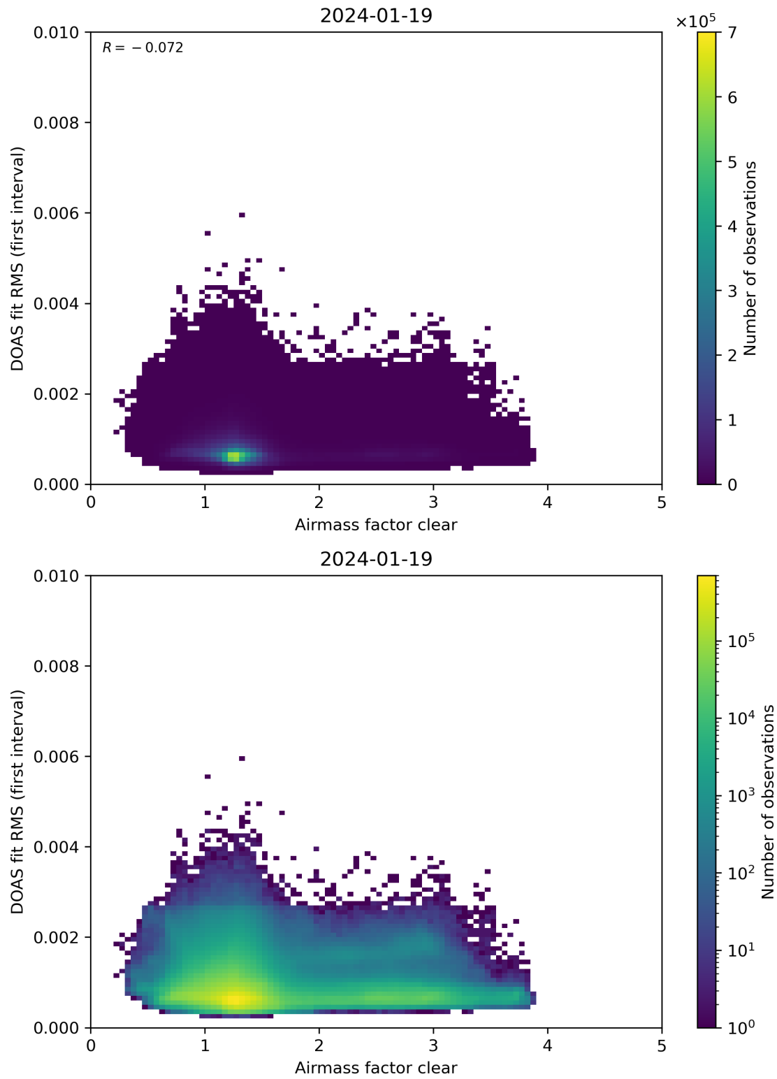
Figure 71: Scatter density plot of “Airmass factor clear” against “DOAS fit RMS (first interval)” for 2024-01-18 to 2024-01-20.
