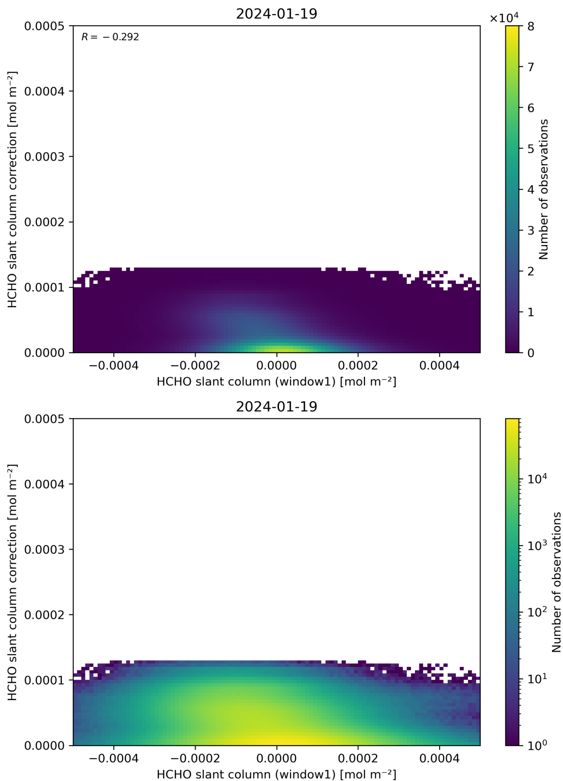
Figure 83: Scatter density plot of “HCHO slant column (window1)” against “HCHO slant column correction” for 2024-01-18 to 2024-01-20.
