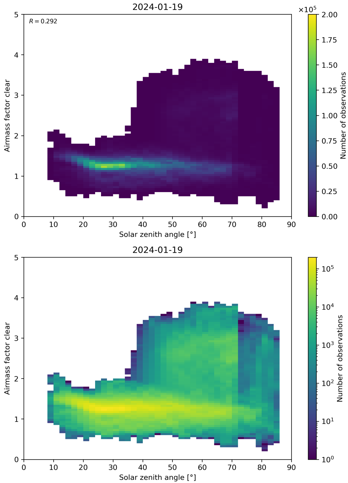
Figure 170: Scatter density plot of “Solar zenith angle” against “Airmass factor clear” for 2024-01-18 to 2024-01-20.
