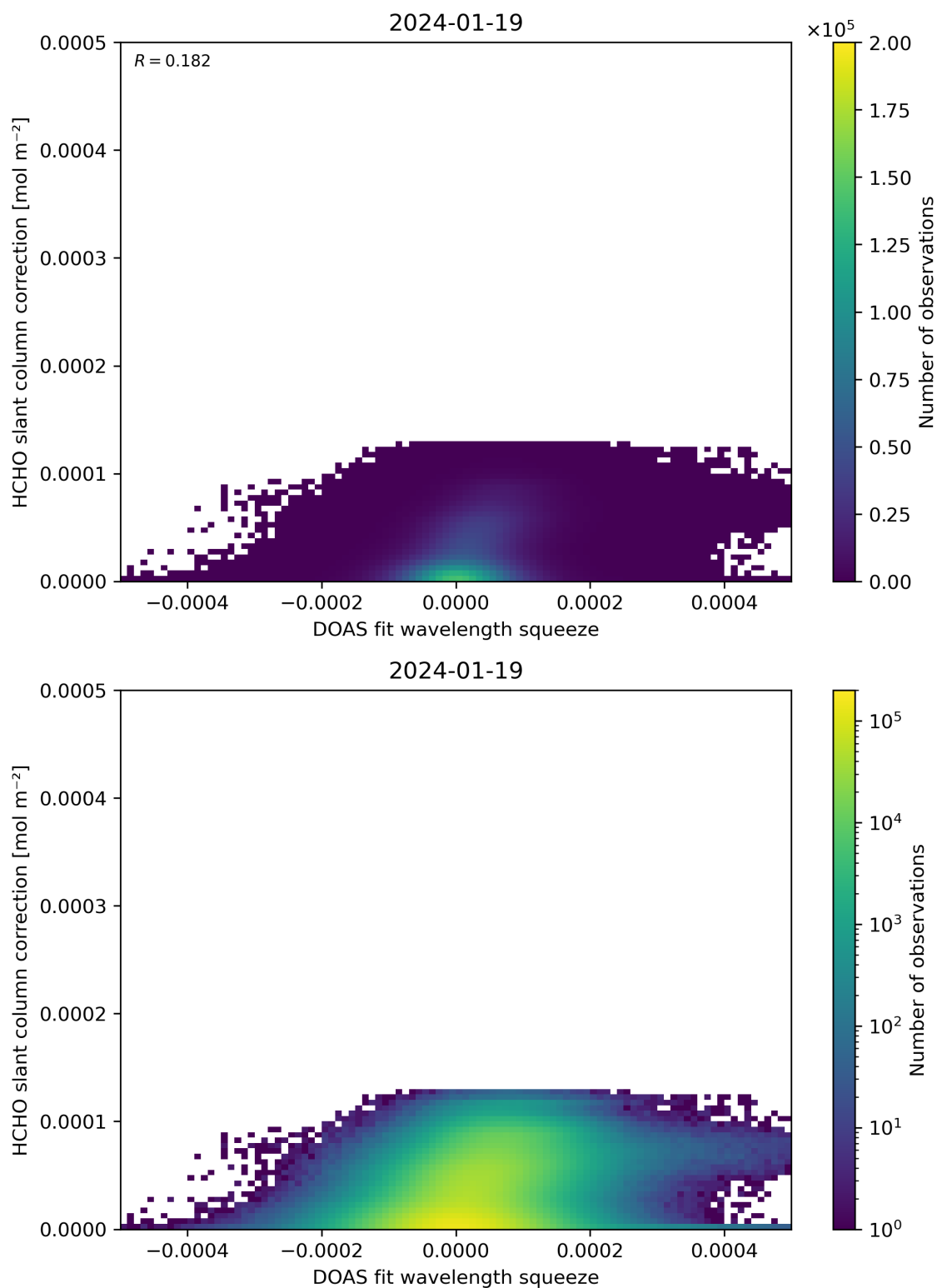
Figure 70: Scatter density plot of “DOAS fit wavelength squeeze” against “HCHO slant column correction” for 2024-01-18 to 2024-01-20.
