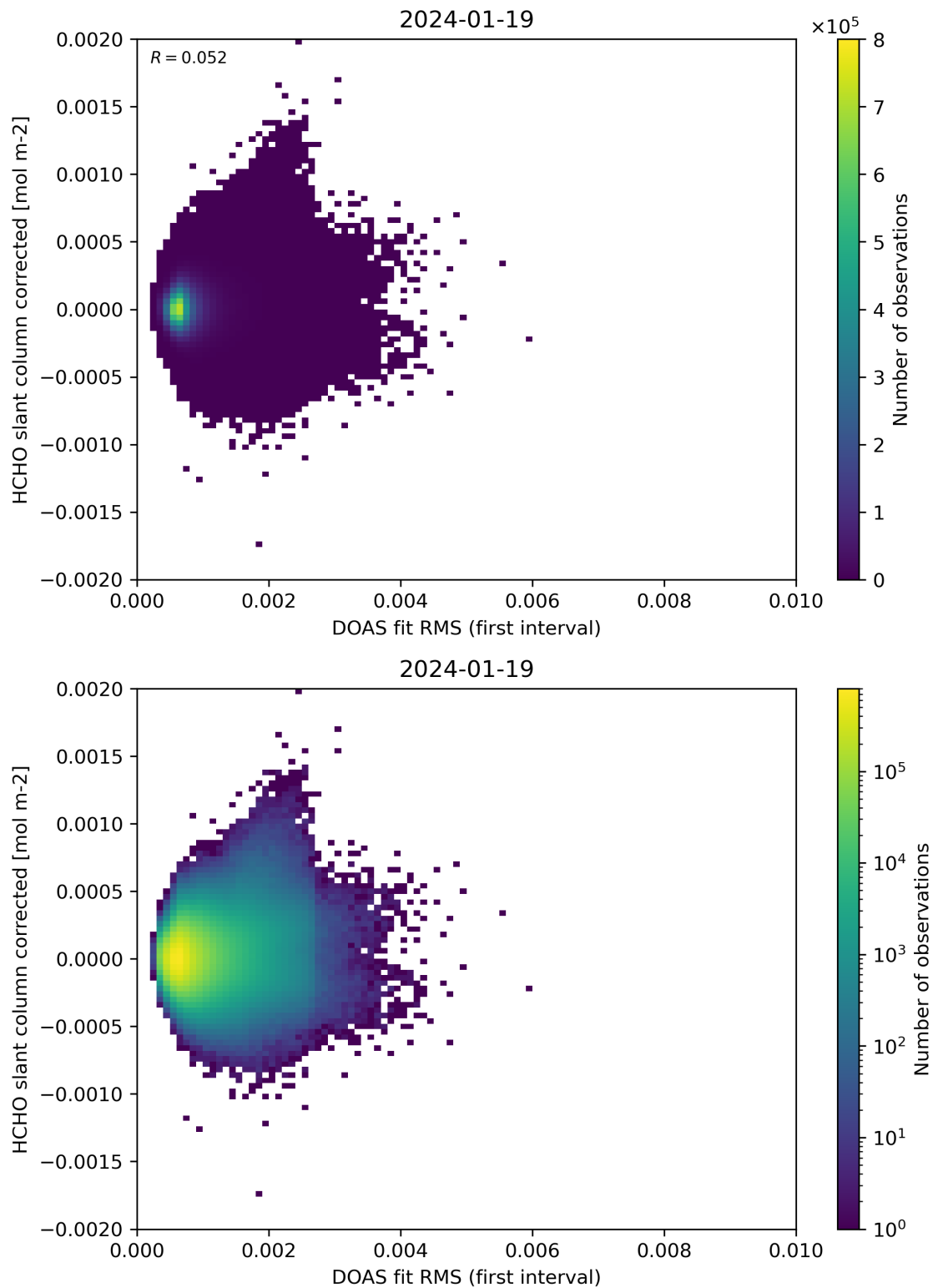
Figure 62: Scatter density plot of “DOAS fit RMS (first interval)” against “HCHO slant column corrected” for 2024-01-18 to 2024-01-20.
