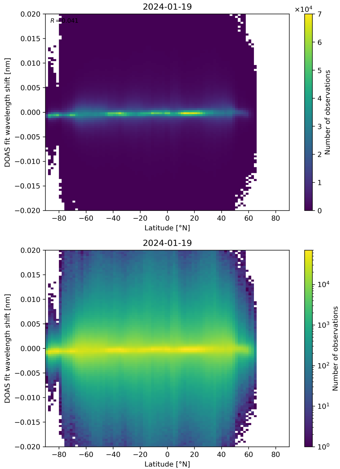
Figure 154: Scatter density plot of “Latitude” against “DOAS fit wavelength shift” for 2024-01-18 to 2024-01-20.
