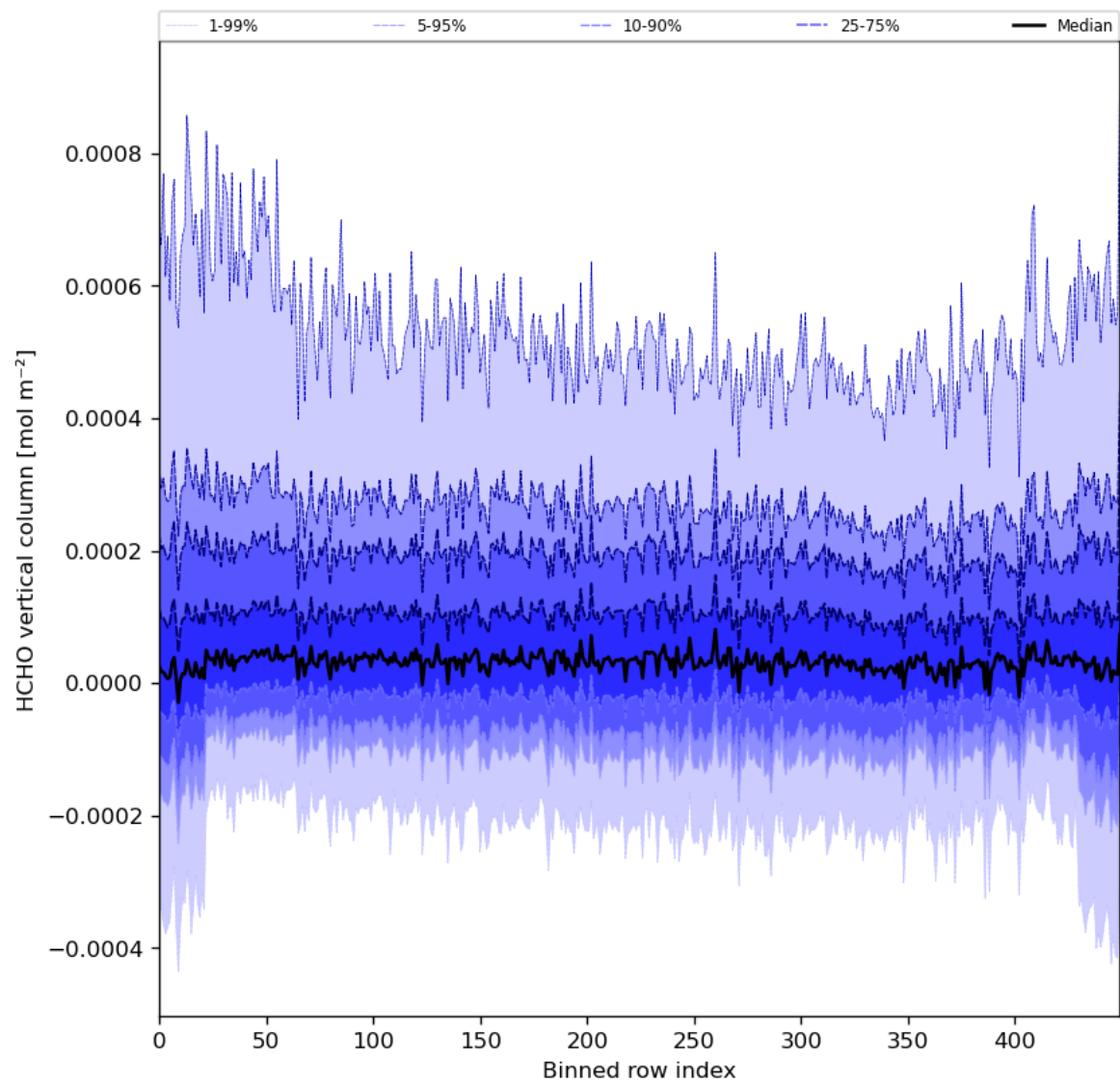
Figure 49: Along track statistics of “HCHO vertical column” for 2024-01-18 to 2024-01-20
