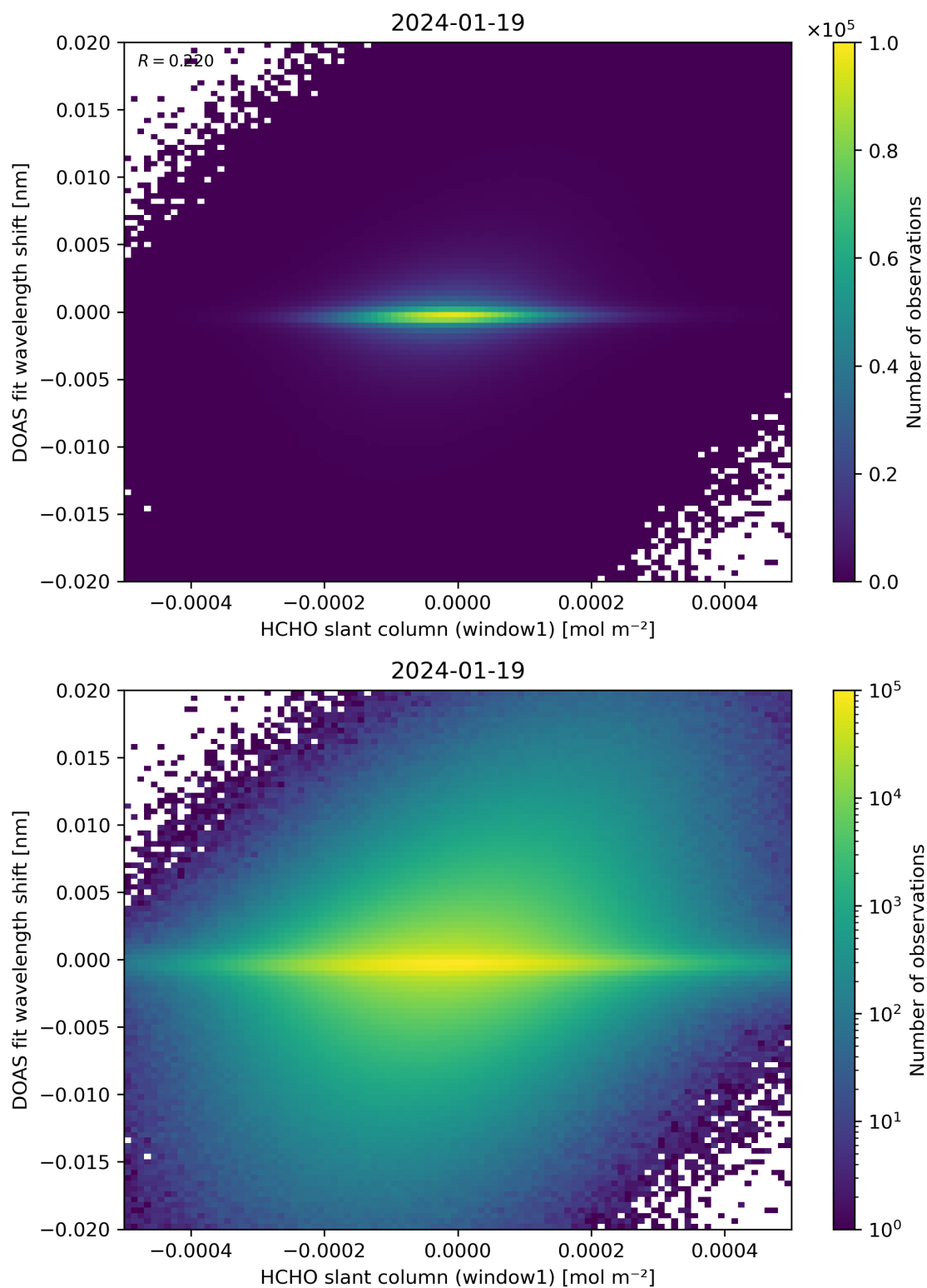
Figure 79: Scatter density plot of “HCHO slant column (window1)” against “DOAS fit wavelength shift” for 2024-01-18 to 2024-01-20.
