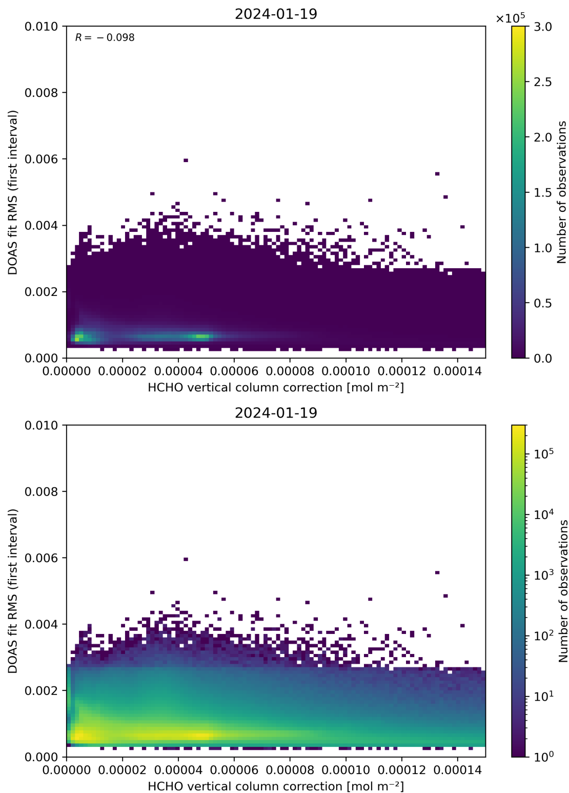
Figure 112: Scatter density plot of “HCHO vertical column correction” against “DOAS fit RMS (first interval)” for 2024-01-18 to 2024-01-20.
