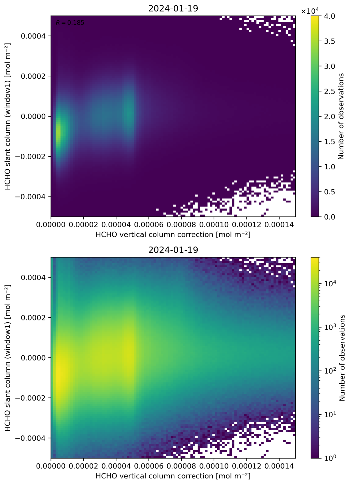
Figure 118: Scatter density plot of “HCHO vertical column correction” against “HCHO slant column (window1)” for 2024-01-18 to 2024-01-20.
