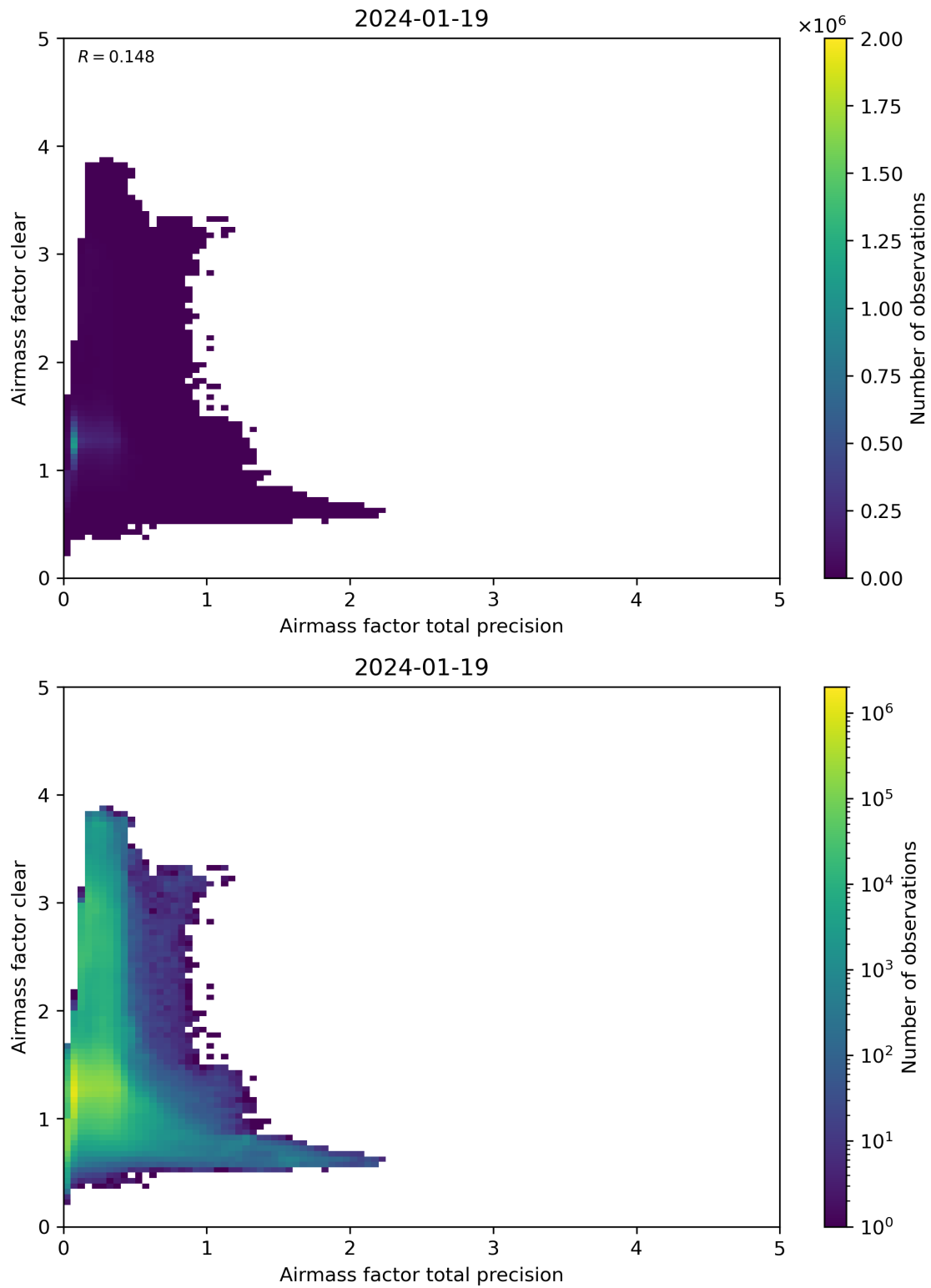
Figure 108: Scatter density plot of “Airmass factor total precision” against “Airmass factor clear” for 2024-01-18 to 2024-01-20.
