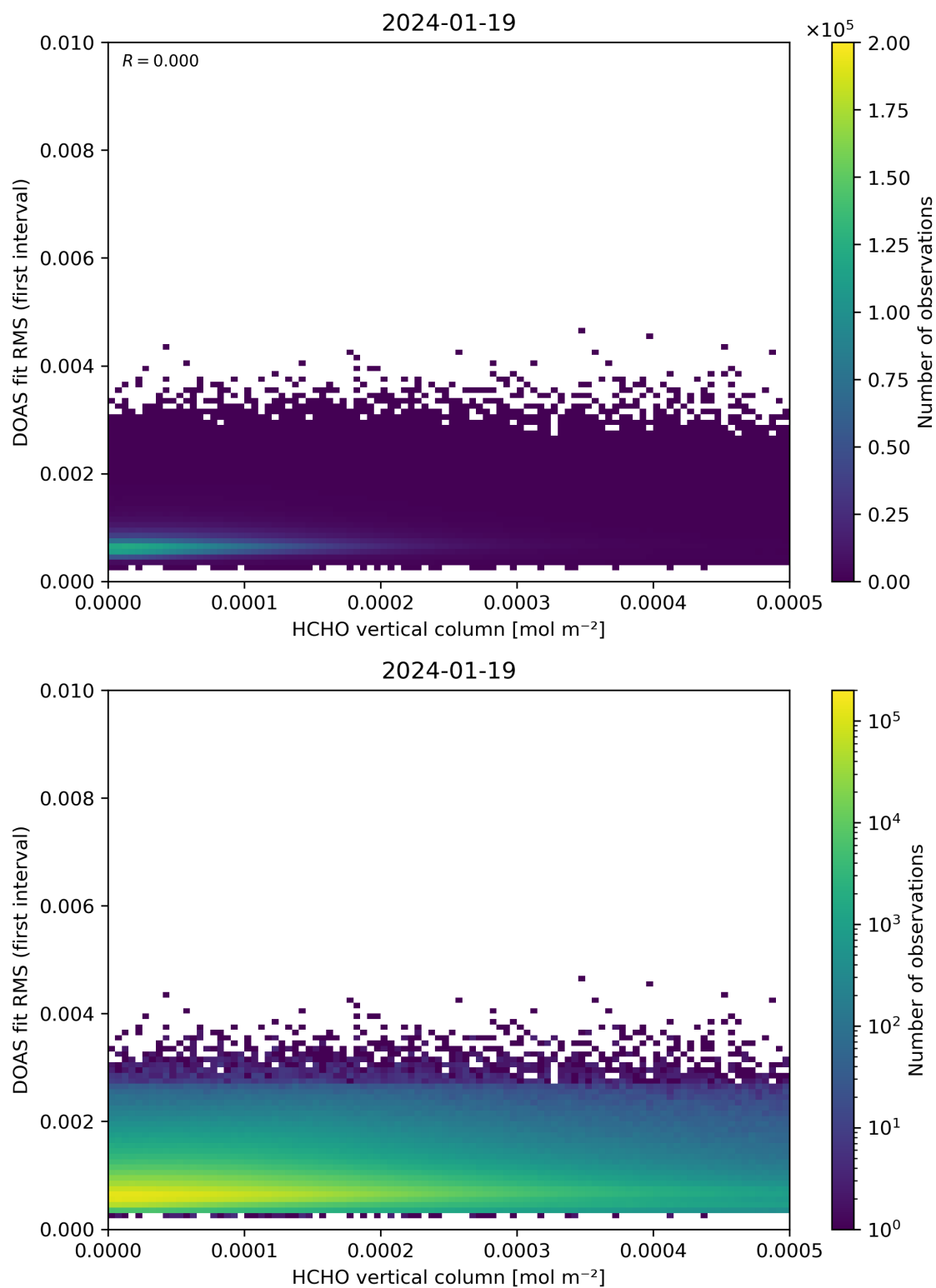
Figure 123: Scatter density plot of “HCHO vertical column” against “DOAS fit RMS (first interval)” for 2024-01-18 to 2024-01-20.
