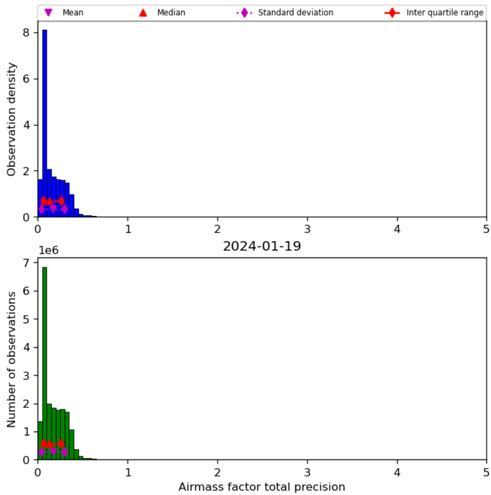
Figure 41: Histogram of “Airmass factor total precision” for 2024-01-18 to 2024-01-20
