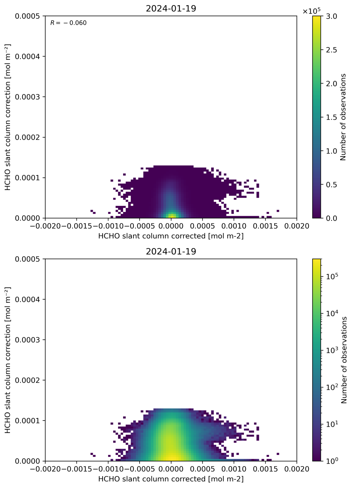
Figure 77: Scatter density plot of “HCHO slant column corrected” against “HCHO slant column correction” for 2024-01-18 to 2024-01-20.
