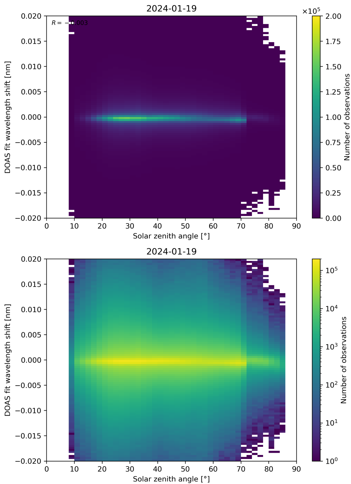
Figure 168: Scatter density plot of “Solar zenith angle” against “DOAS fit wavelength shift” for 2024-01-18 to 2024-01-20.
