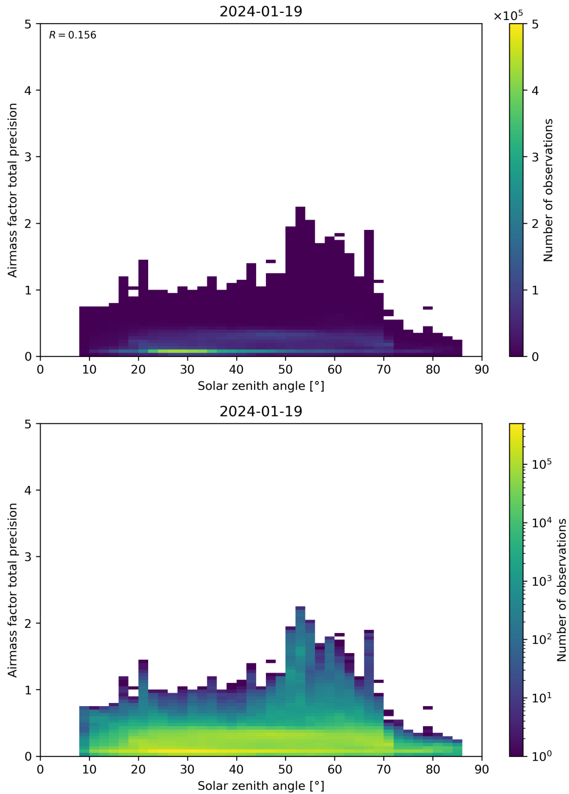
Figure 176: Scatter density plot of “Solar zenith angle” against “Airmass factor total precision” for 2024-01-18 to 2024-01-20.
