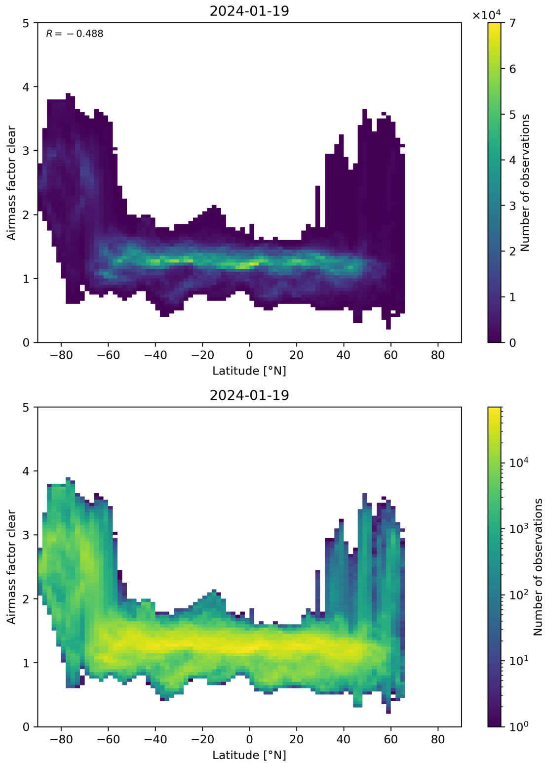
Figure 156: Scatter density plot of “Latitude” against “Airmass factor clear” for 2024-01-18 to 2024-01-20.
