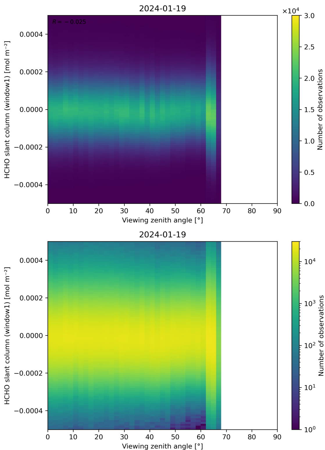
Figure 188: Scatter density plot of “Viewing zenith angle” against “HCHO slant column (window1)” for 2024-01-18 to 2024-01-20.
