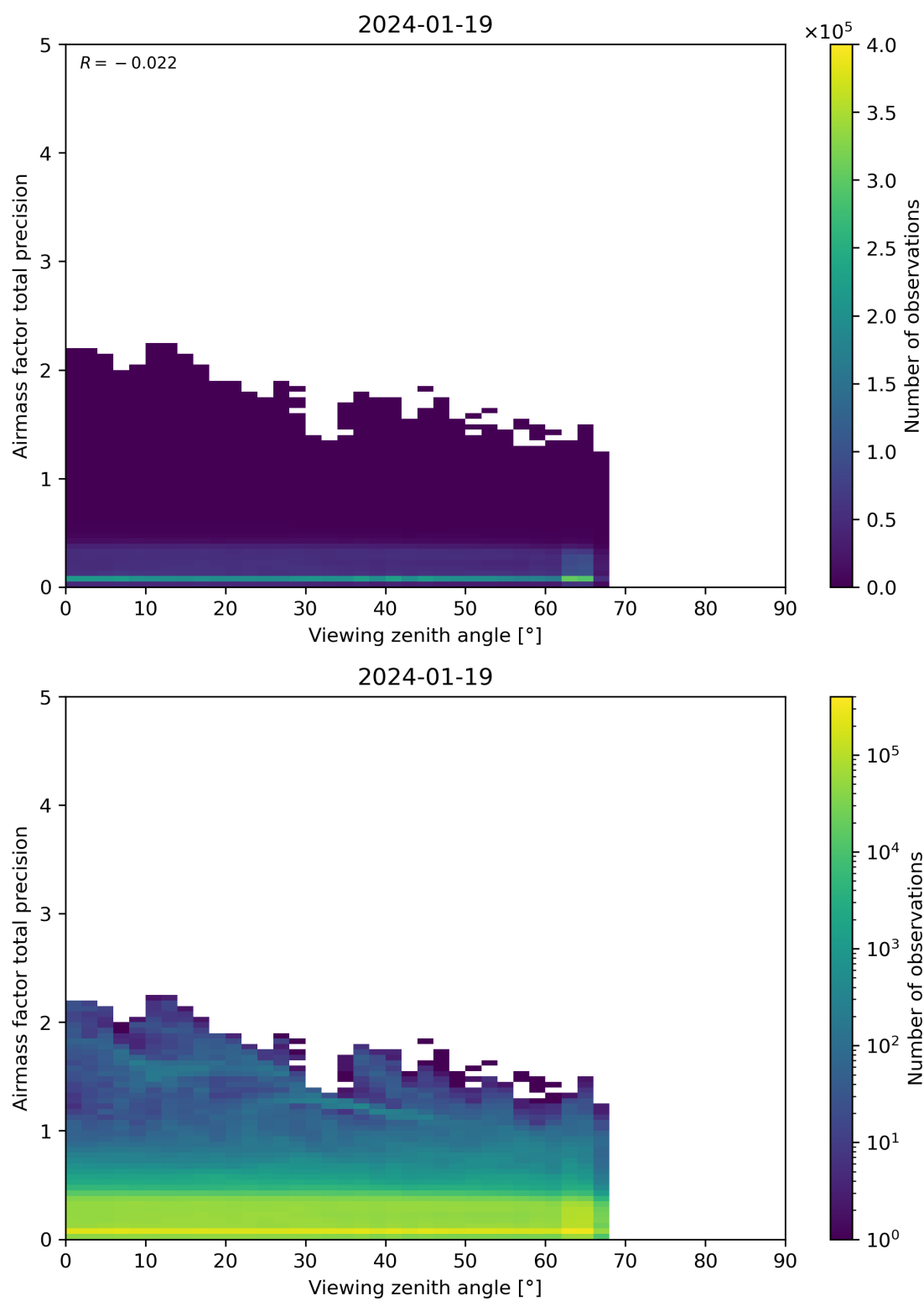
Figure 191: Scatter density plot of “Viewing zenith angle” against “Airmass factor total precision” for 2024-01-18 to 2024-01-20.
