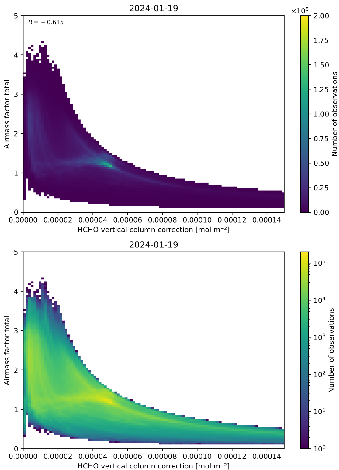
Figure 120: Scatter density plot of “HCHO vertical column correction” against “Airmass factor total” for 2024-01-18 to 2024-01-20.
