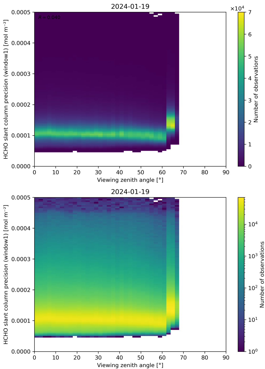
Figure 189: Scatter density plot of “Viewing zenith angle” against “HCHO slant column precision (window1)” for 2024-01-18 to 2024-01-20.
