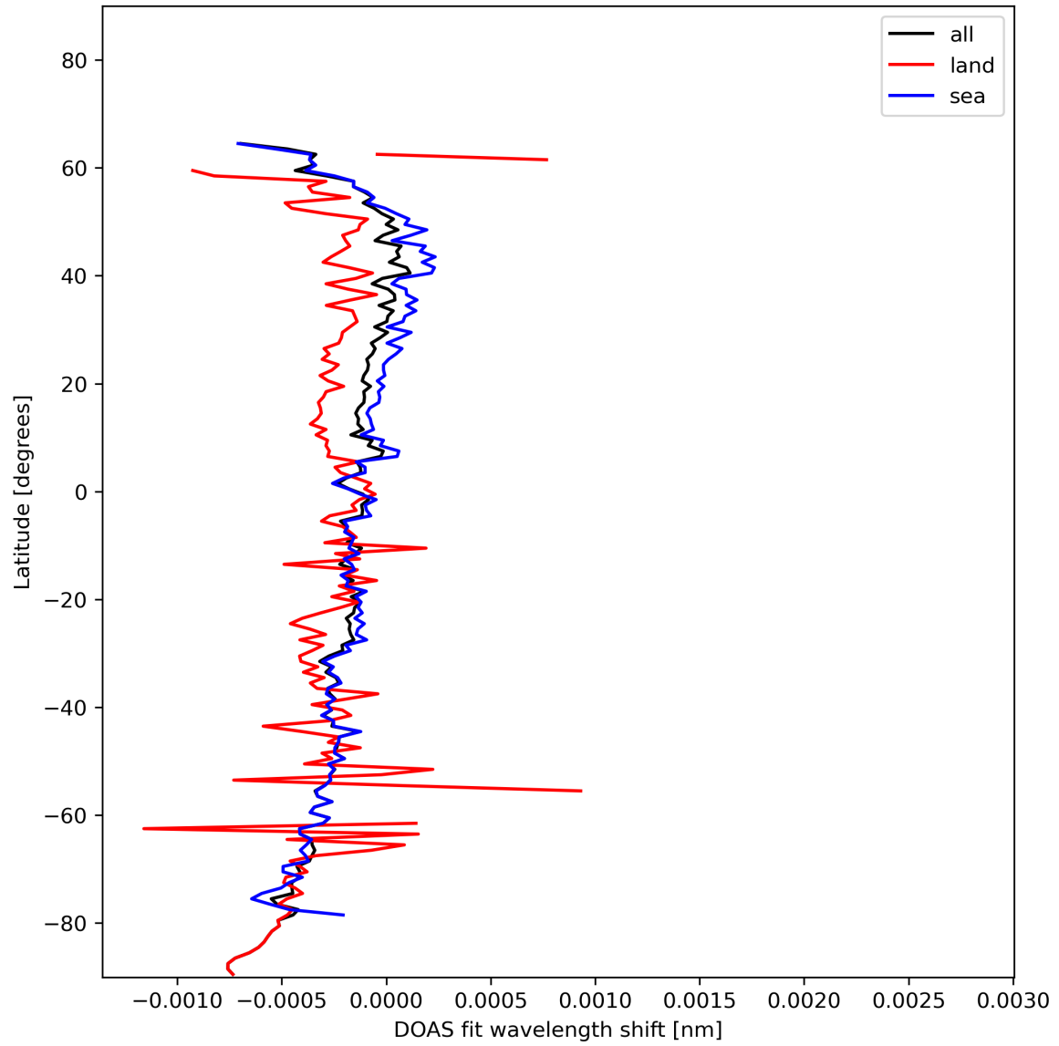
Figure 30: Zonal average of “DOAS fit wavelength shift” for 2024-01-18 to 2024-01-20.
