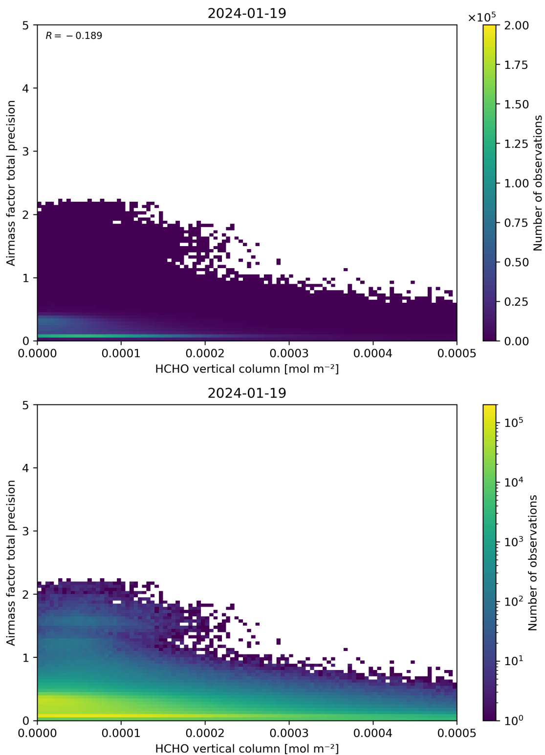
Figure 132: Scatter density plot of “HCHO vertical column” against “Airmass factor total precision” for 2024-01-18 to 2024-01-20.
