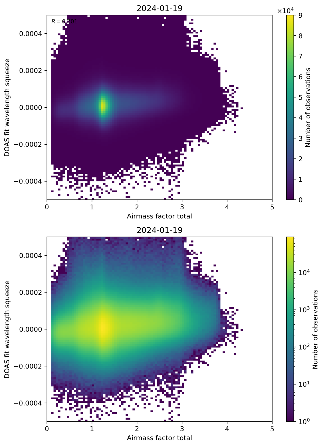
Figure 99: Scatter density plot of “Airmass factor total” against “DOAS fit wavelength squeeze” for 2024-01-18 to 2024-01-20.
