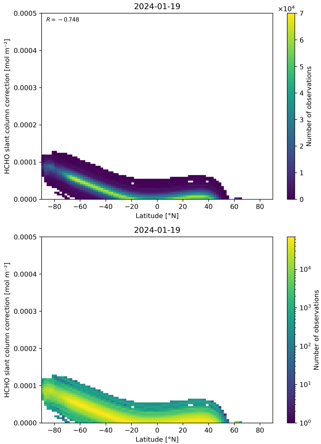
Figure 158: Scatter density plot of “Latitude” against “HCHO slant column correction” for 2024-01-18 to 2024-01-20.
