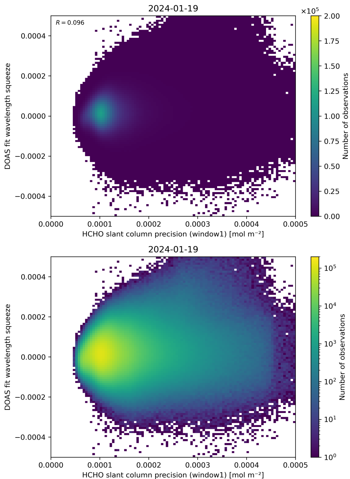
Figure 90: Scatter density plot of “HCHO slant column precision (window1)” against “DOAS fit wavelength squeeze” for 2024-01-18 to 2024-01-20.
