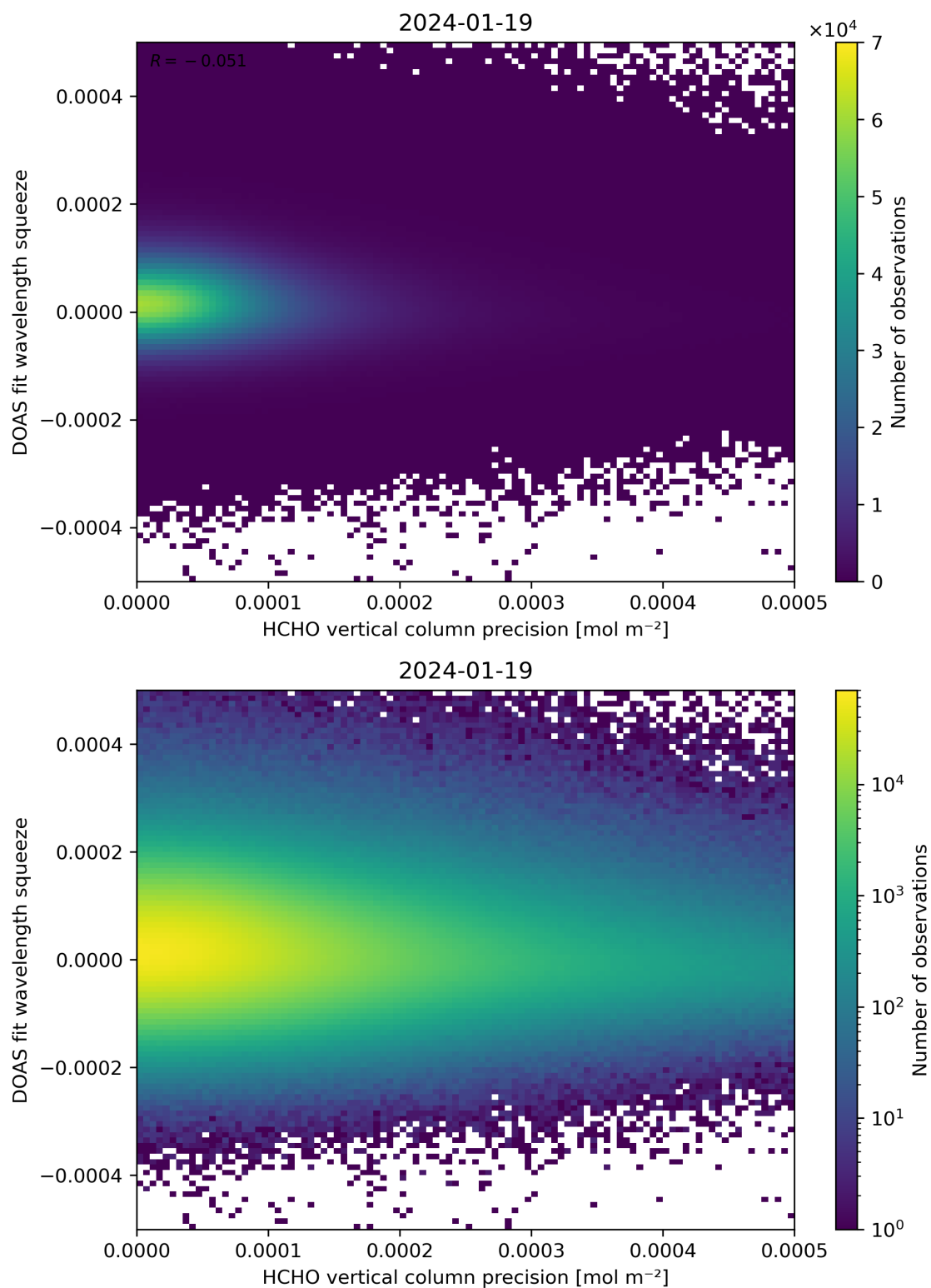
Figure 138: Scatter density plot of “HCHO vertical column precision” against “DOAS fit wavelength squeeze” for 2024-01-18 to 2024-01-20.
