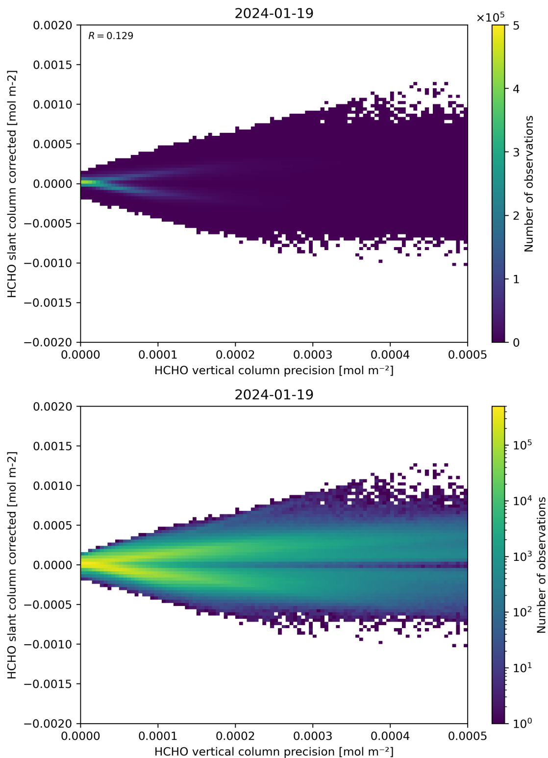
Figure 140: Scatter density plot of “HCHO vertical column precision” against “HCHO slant column corrected” for 2024-01-18 to 2024-01-20.
