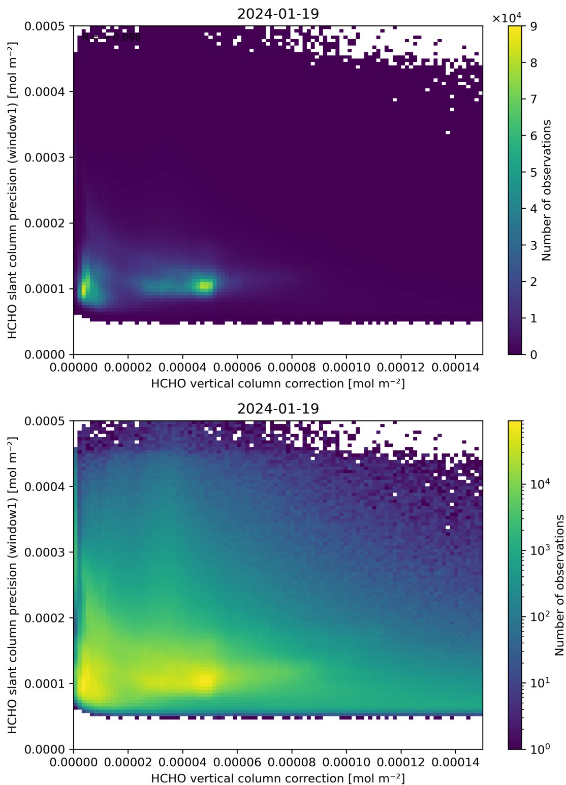
Figure 119: Scatter density plot of “HCHO vertical column correction” against “HCHO slant column precision (window1)” for 2024-01-18 to 2024-01-20.
