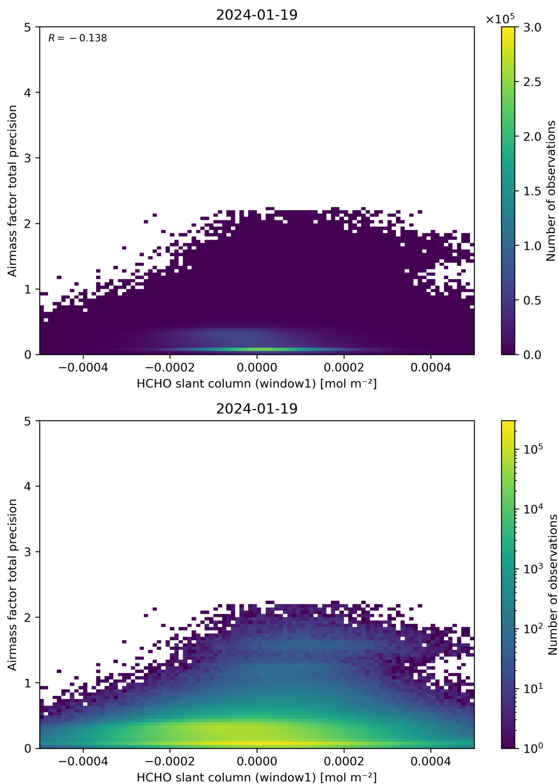
Figure 86: Scatter density plot of “HCHO slant column (window1)” against “Airmass factor total precision” for 2024-01-18 to 2024-01-20.
