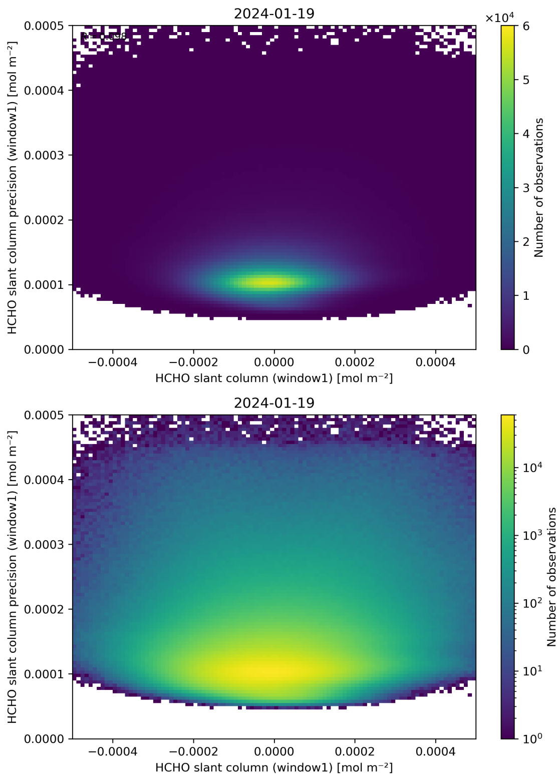
Figure 84: Scatter density plot of “HCHO slant column (window1)” against “HCHO slant column precision (window1)” for 2024-01-18 to 2024-01-20.
