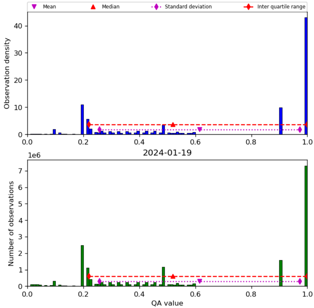
Figure 34: Histogram of “QA value” for 2024-01-18 to 2024-01-20
