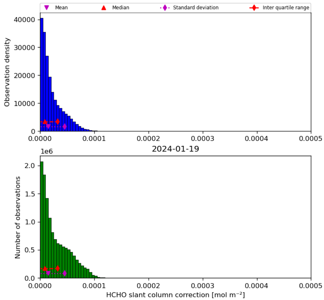
Figure 47: Histogram of “HCHO slant column correction” for 2024-01-18 to 2024-01-20
