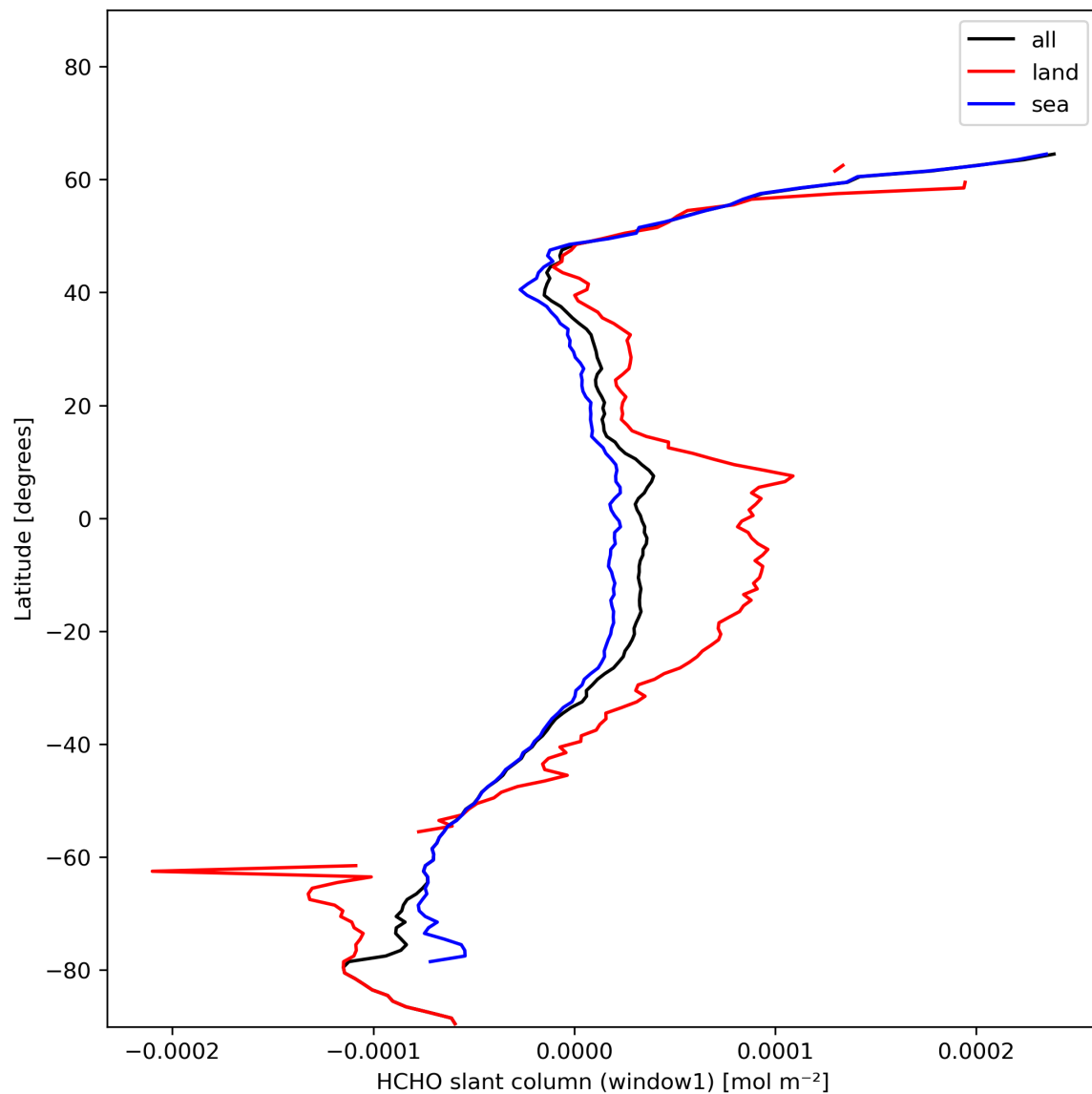
Figure 24: Zonal average of “HCHO slant column (window1)” for 2024-01-18 to 2024-01-20.
