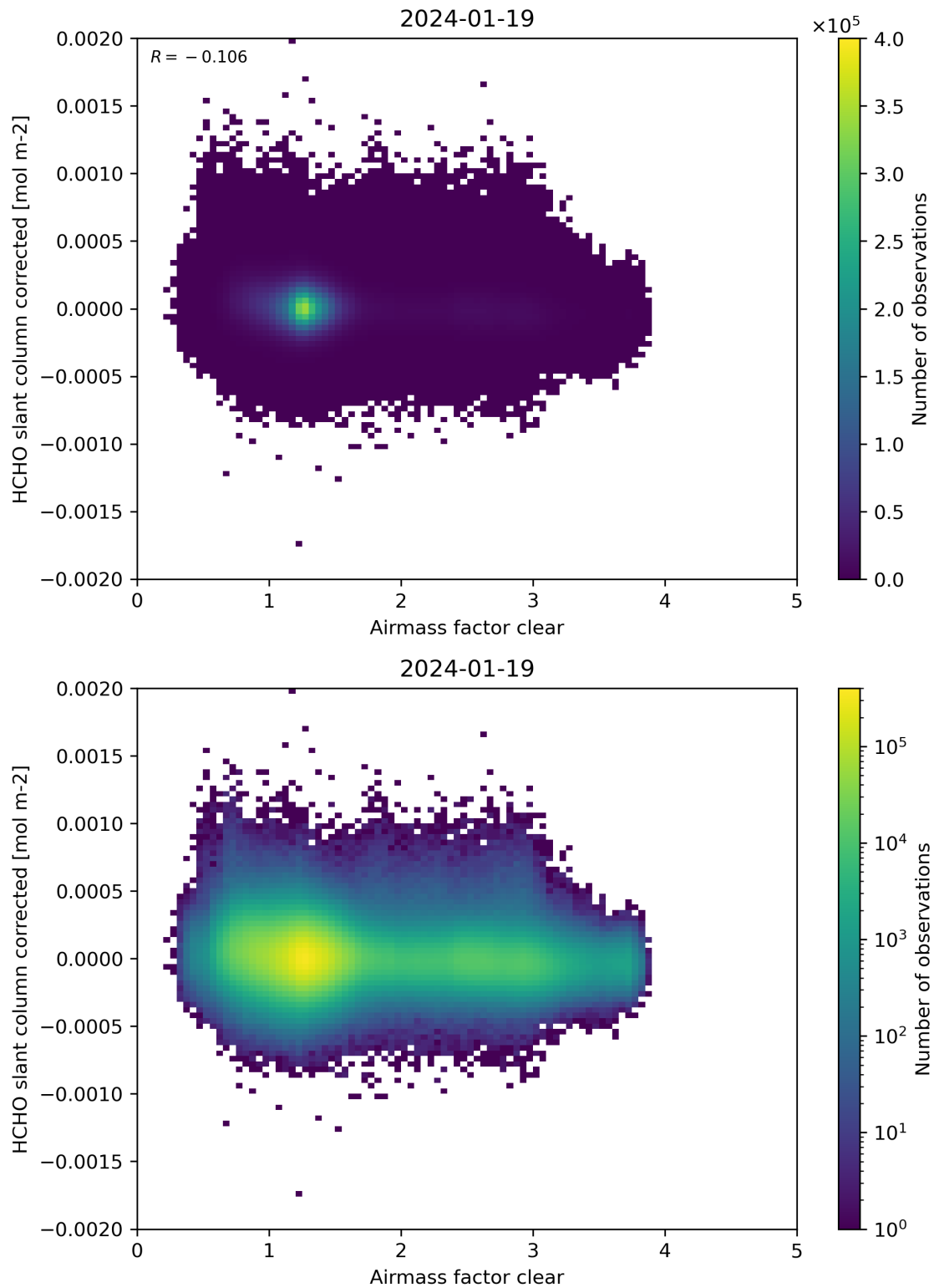
Figure 74: Scatter density plot of “Airmass factor clear” against “HCHO slant column corrected” for 2024-01-18 to 2024-01-20.
