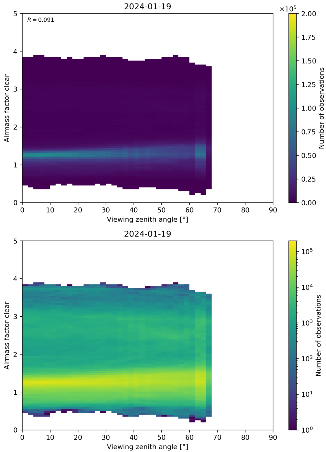
Figure 185: Scatter density plot of “Viewing zenith angle” against “Airmass factor clear” for 2024-01-18 to 2024-01-20.
