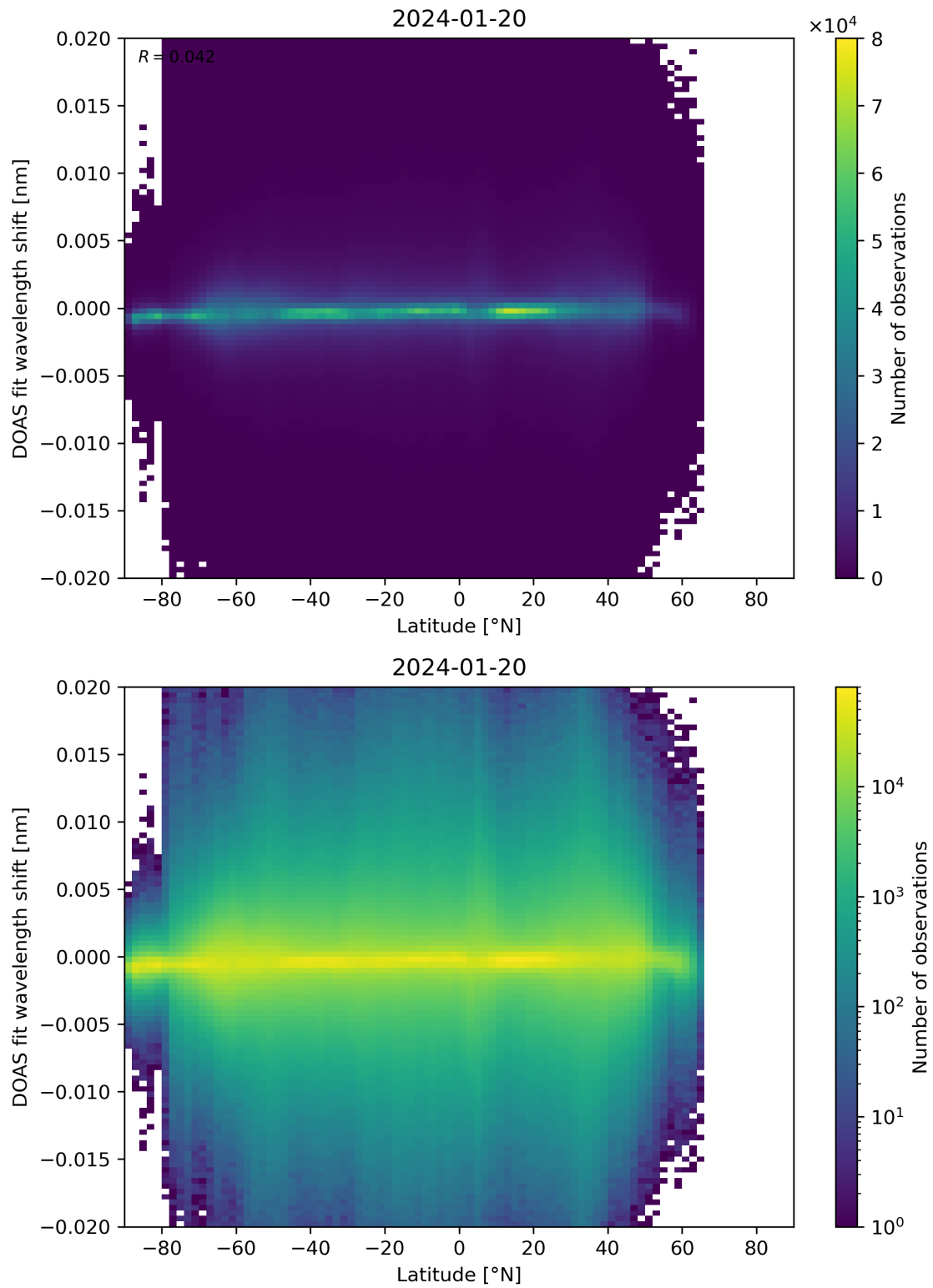
Figure 154: Scatter density plot of “Latitude” against “DOAS fit wavelength shift” for 2024-01-19 to 2024-01-21.
