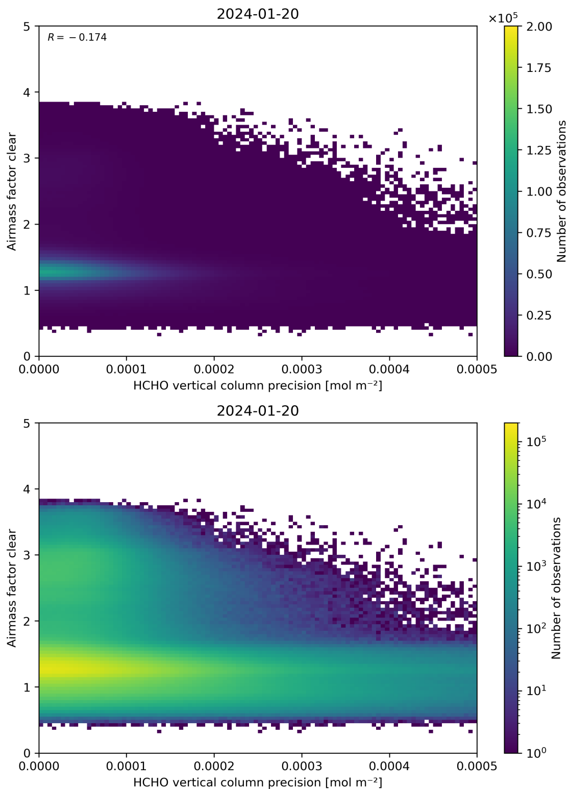
Figure 139: Scatter density plot of “HCHO vertical column precision” against “Airmass factor clear” for 2024-01-19 to 2024-01-21.
