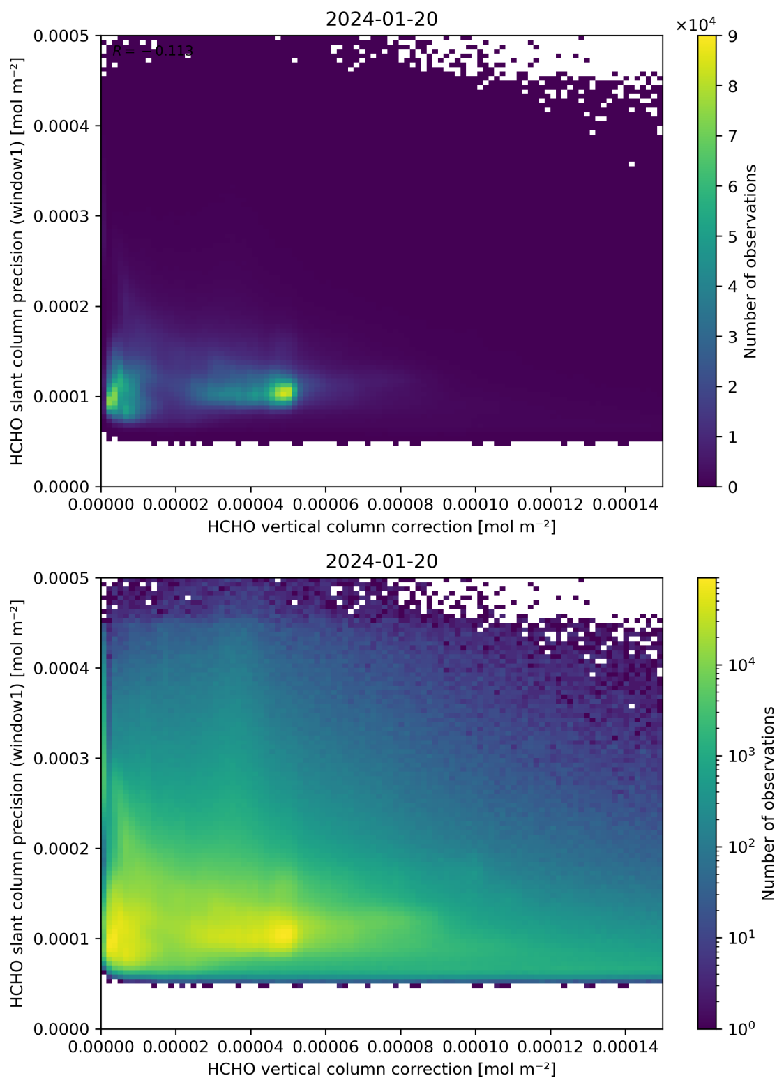
Figure 119: Scatter density plot of “HCHO vertical column correction” against “HCHO slant column precision (window1)” for 2024-01-19 to 2024-01-21.
