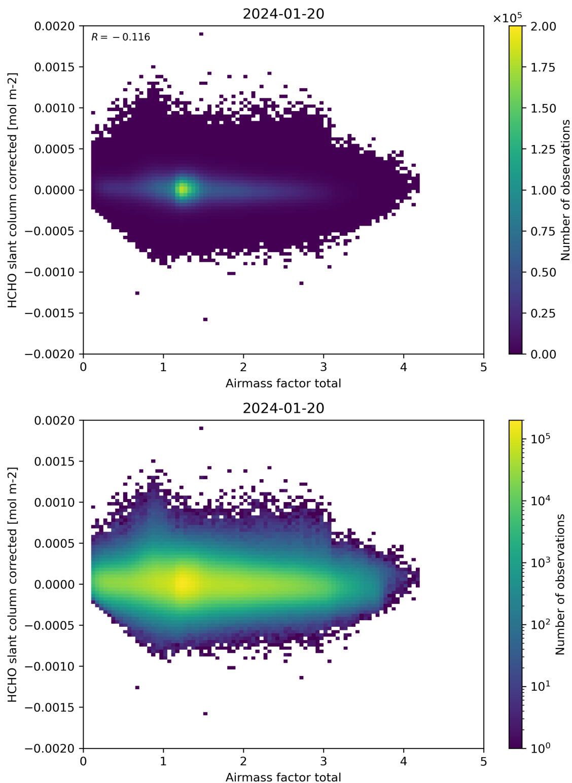
Figure 101: Scatter density plot of “Airmass factor total” against “HCHO slant column corrected” for 2024-01-19 to 2024-01-21.
