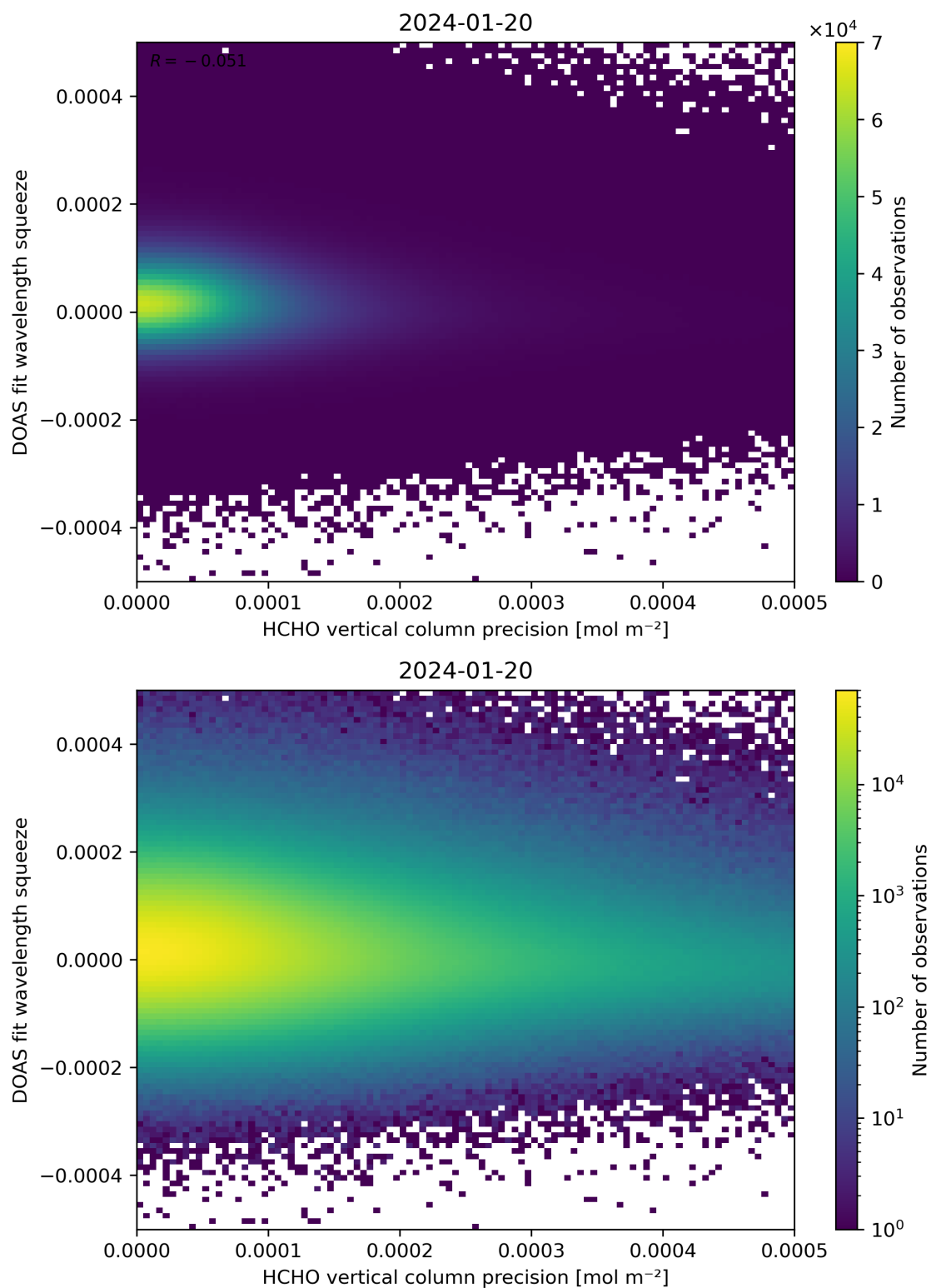
Figure 138: Scatter density plot of “HCHO vertical column precision” against “DOAS fit wavelength squeeze” for 2024-01-19 to 2024-01-21.
