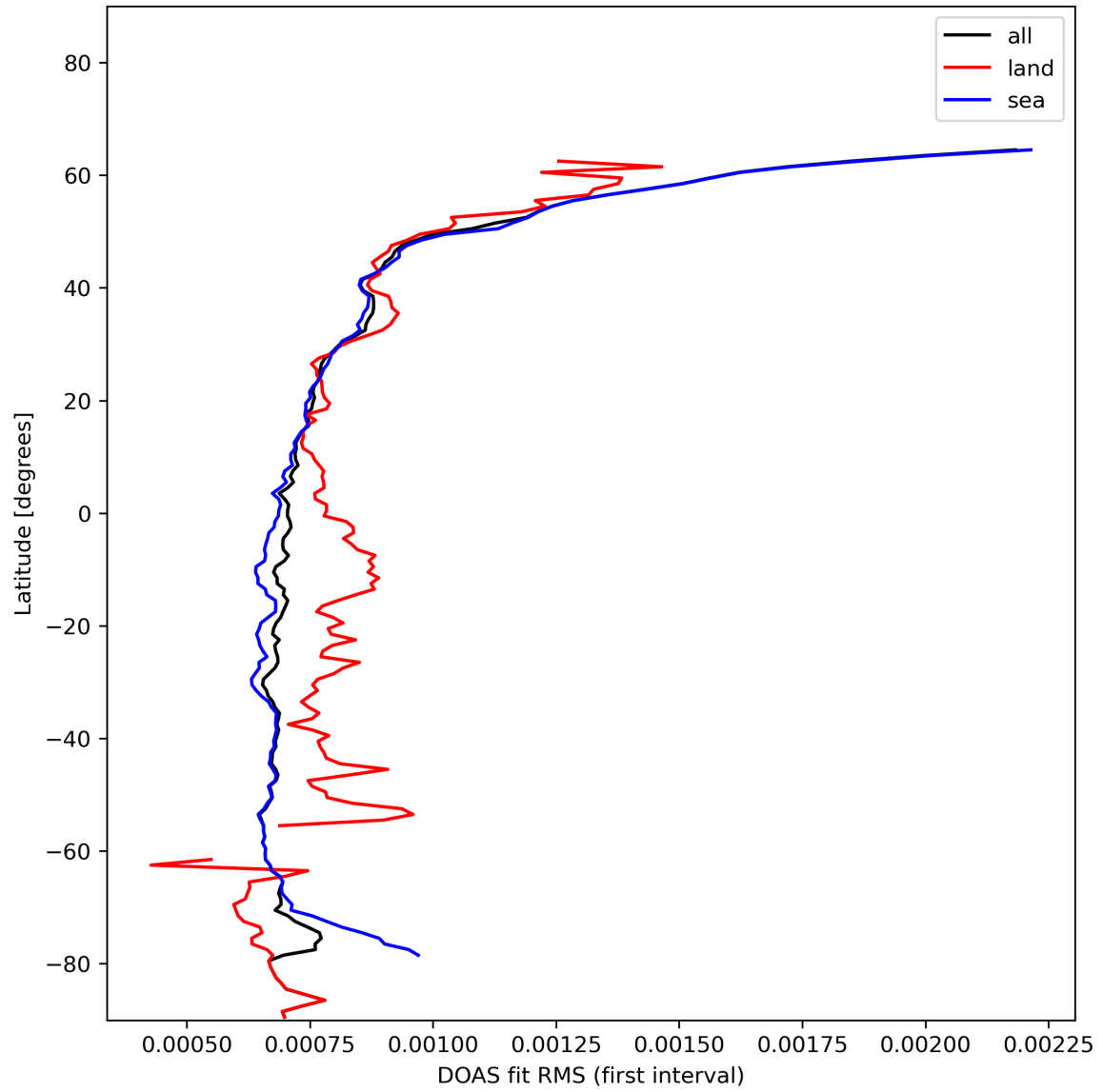
Figure 32: Zonal average of “DOAS fit RMS (first interval)” for 2024-01-19 to 2024-01-21.
