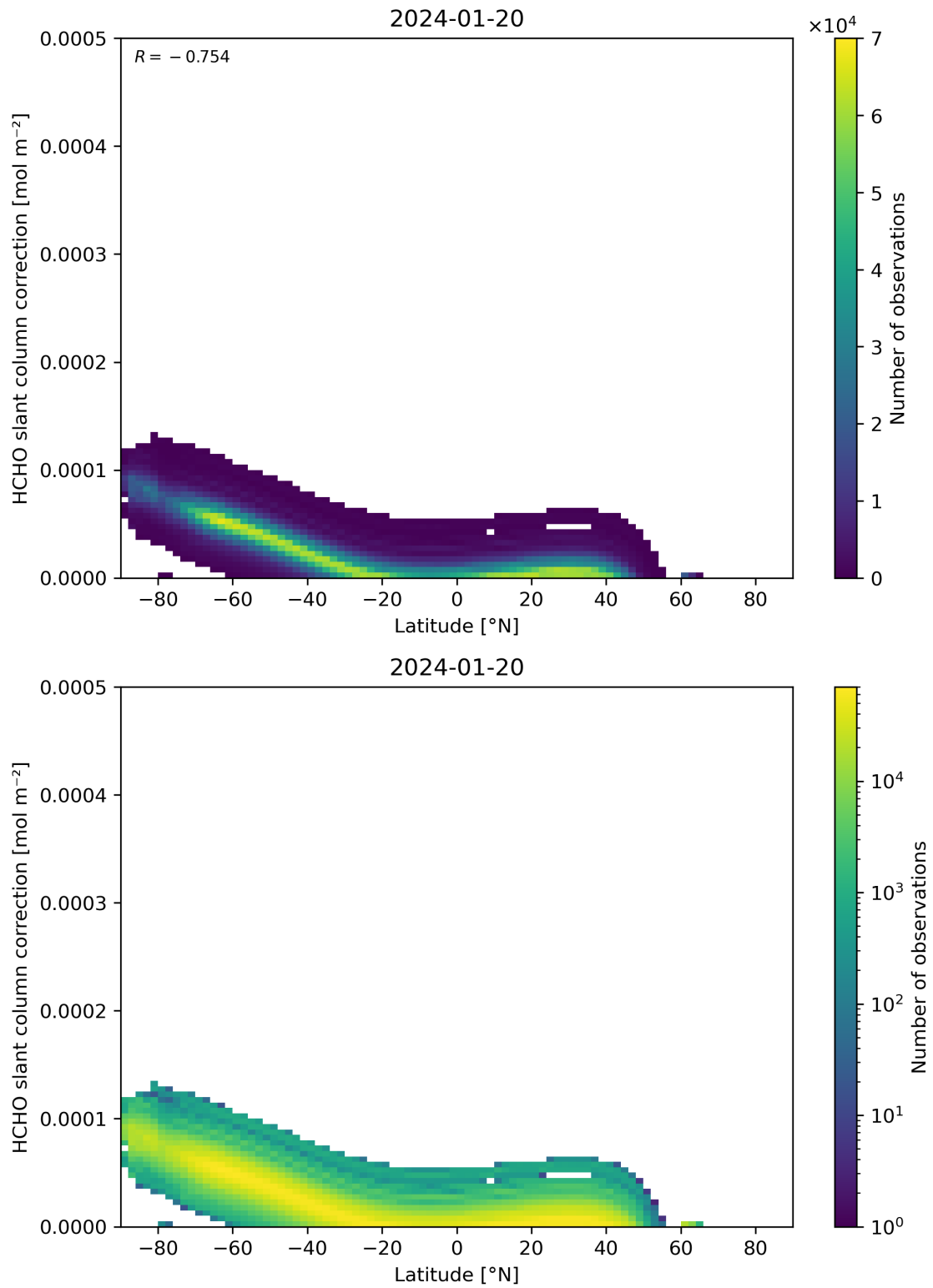
Figure 158: Scatter density plot of “Latitude” against “HCHO slant column correction” for 2024-01-19 to 2024-01-21.
