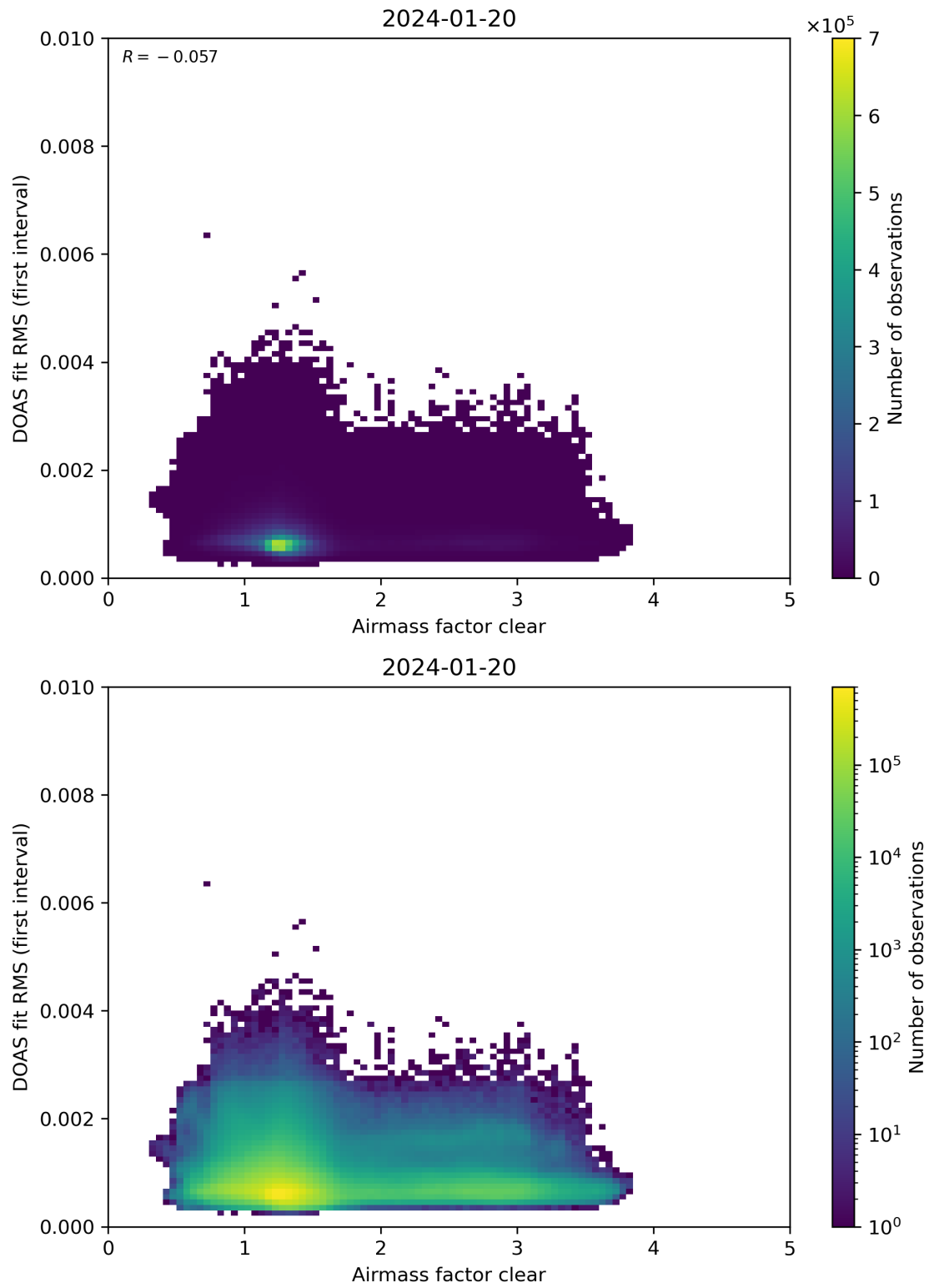
Figure 71: Scatter density plot of “Airmass factor clear” against “DOAS fit RMS (first interval)” for 2024-01-19 to 2024-01-21.
