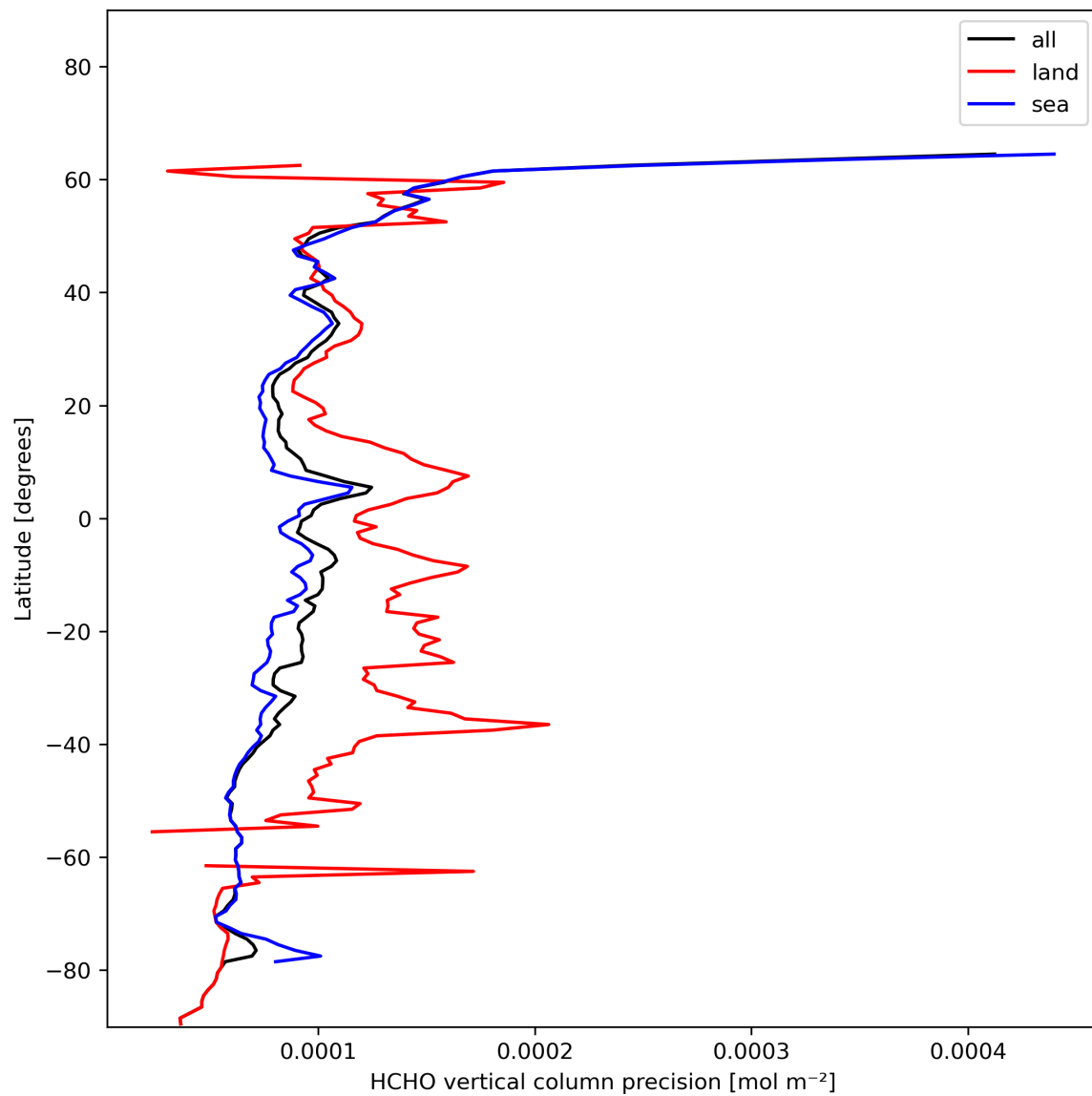
Figure 22: Zonal average of “HCHO vertical column precision” for 2024-01-19 to 2024-01-21.
