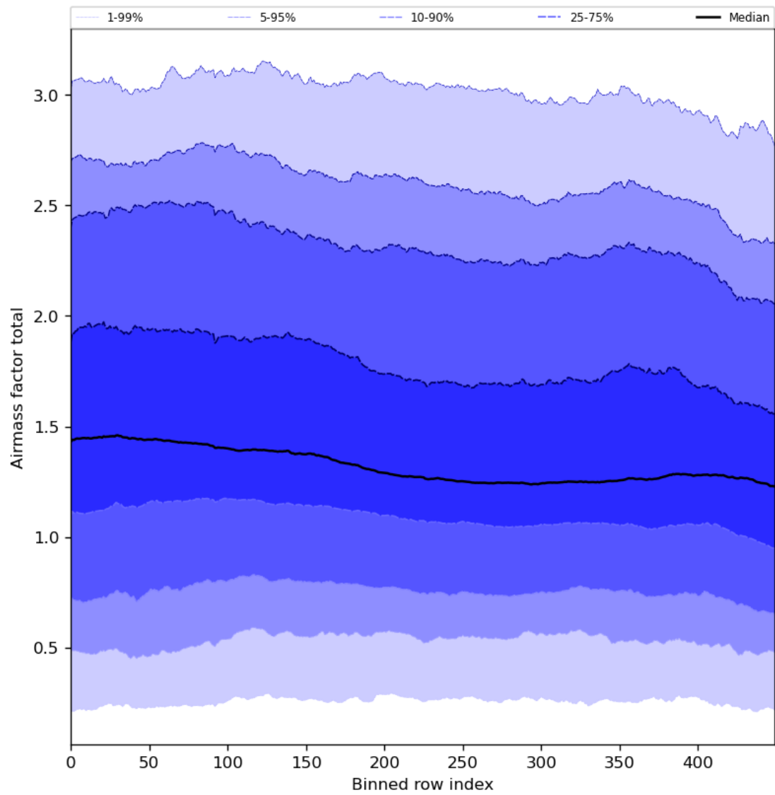
Figure 54: Along track statistics of “Airmass factor total” for 2024-01-19 to 2024-01-21
