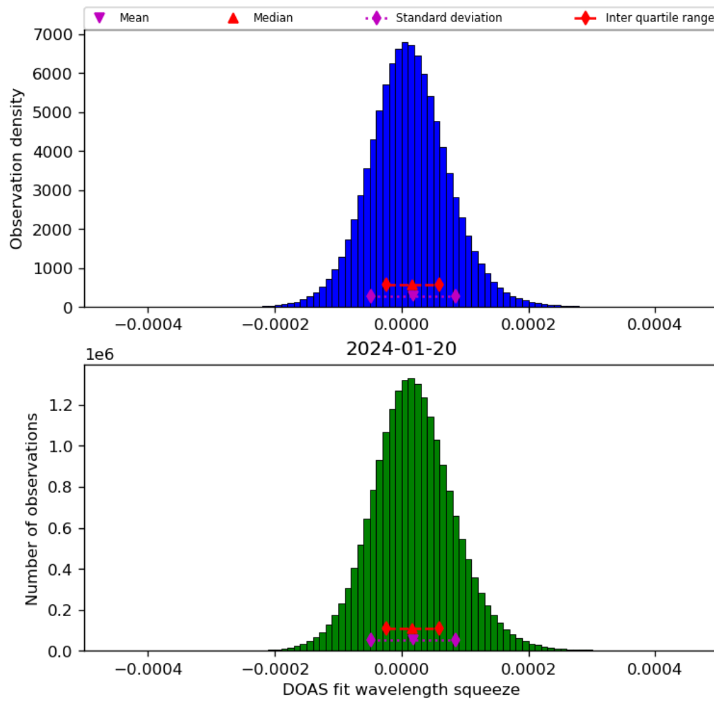
Figure 45: Histogram of “DOAS fit wavelength squeeze” for 2024-01-19 to 2024-01-21
