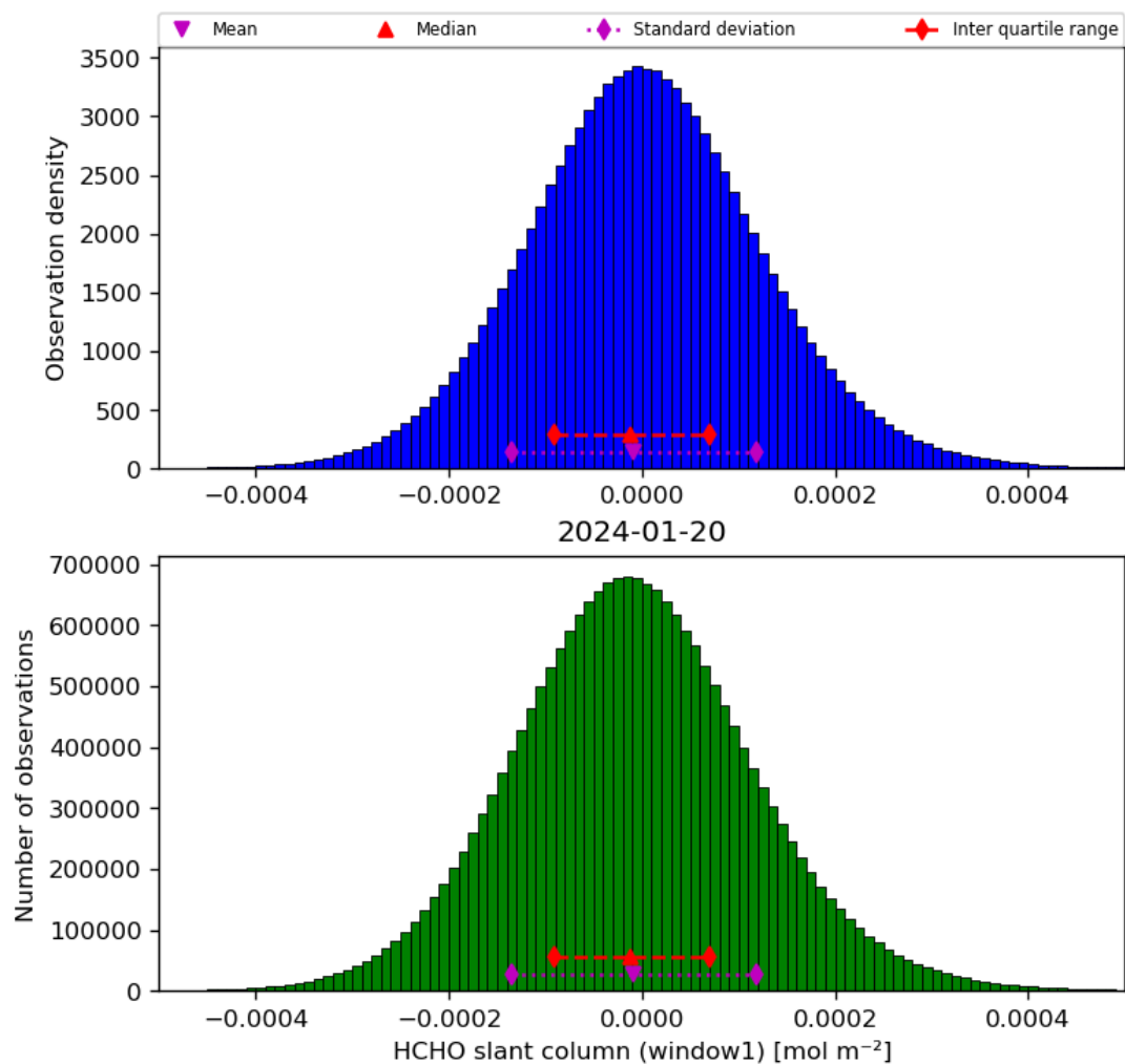
Figure 38: Histogram of “HCHO slant column (window1)” for 2024-01-19 to 2024-01-21
