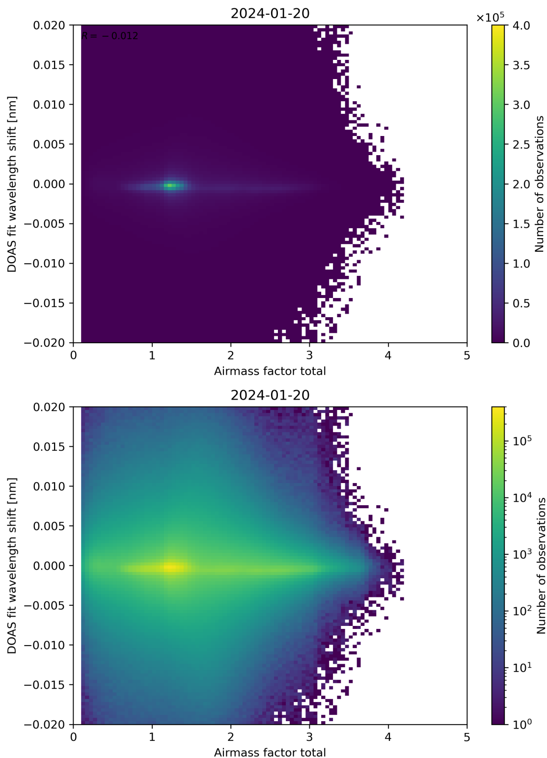
Figure 98: Scatter density plot of “Airmass factor total” against “DOAS fit wavelength shift” for 2024-01-19 to 2024-01-21.
