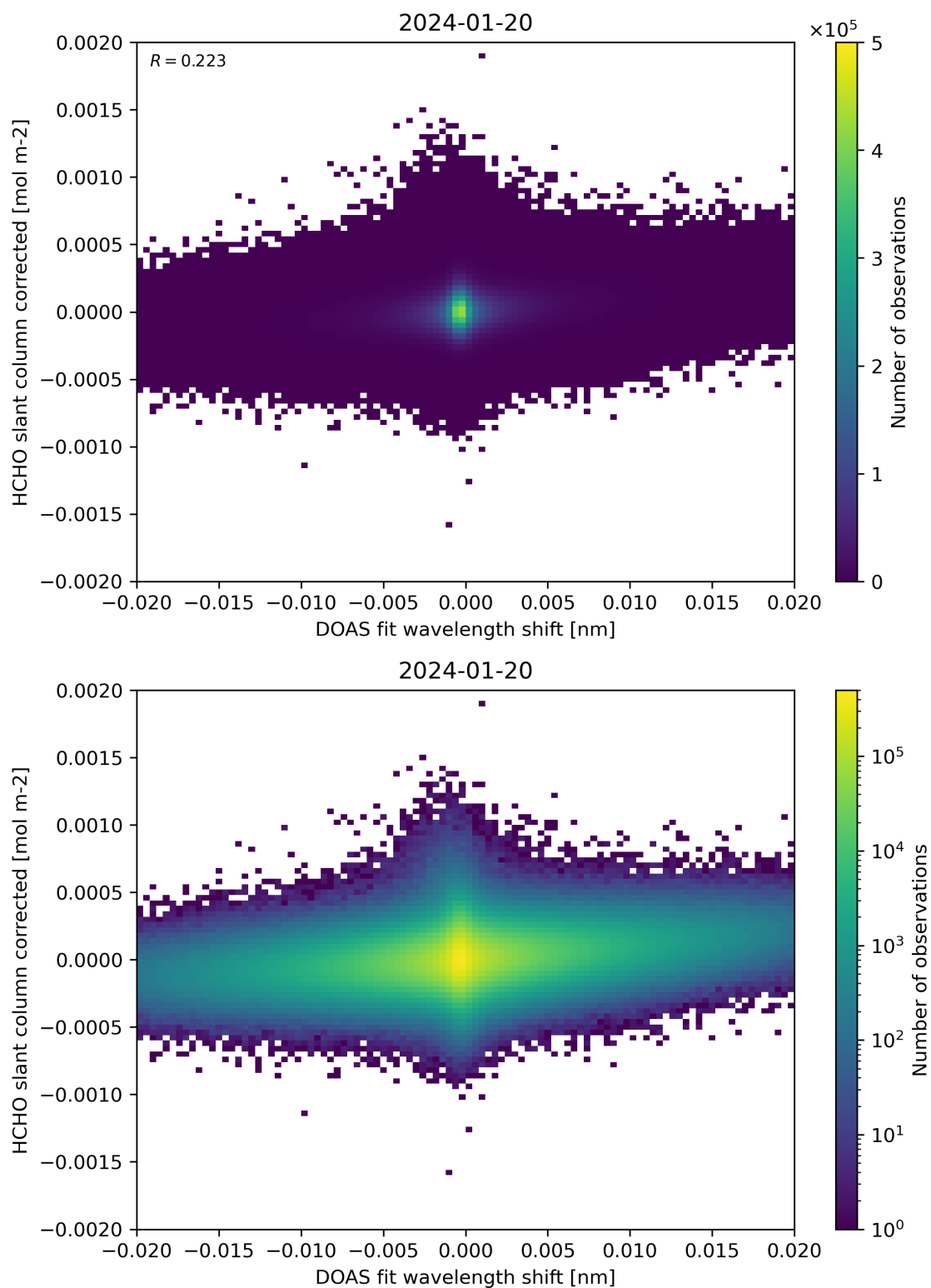
Figure 66: Scatter density plot of “DOAS fit wavelength shift” against “HCHO slant column corrected” for 2024-01-19 to 2024-01-21.
