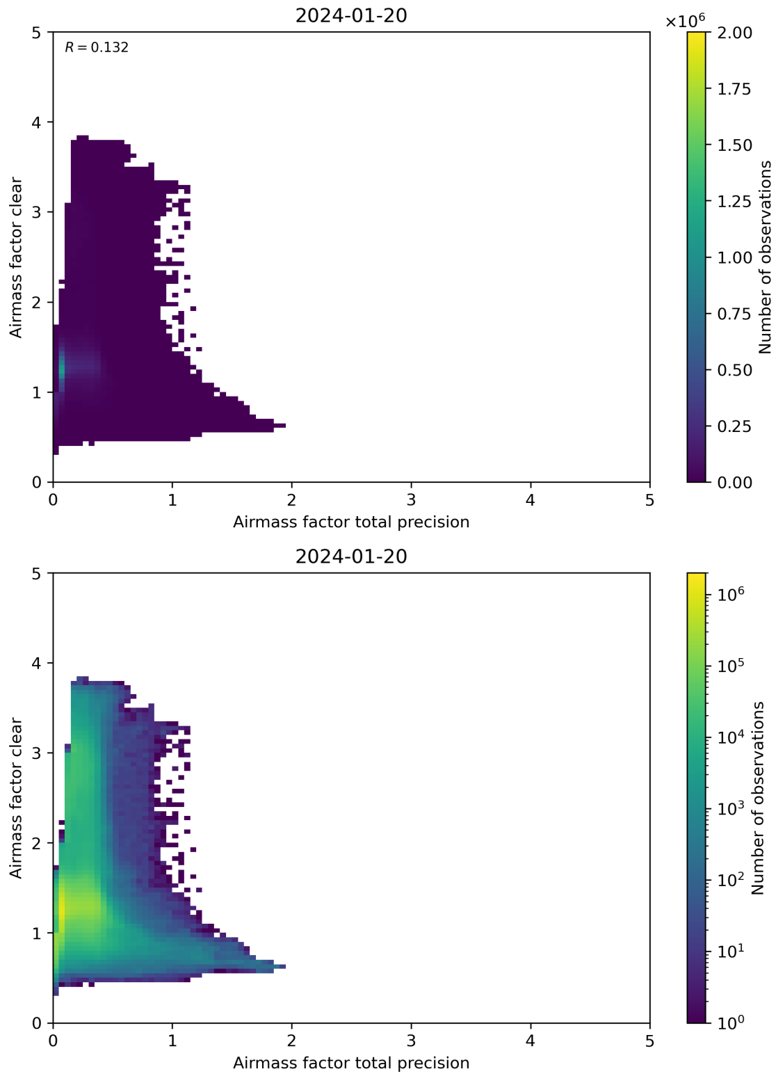
Figure 108: Scatter density plot of “Airmass factor total precision” against “Airmass factor clear” for 2024-01-19 to 2024-01-21.
