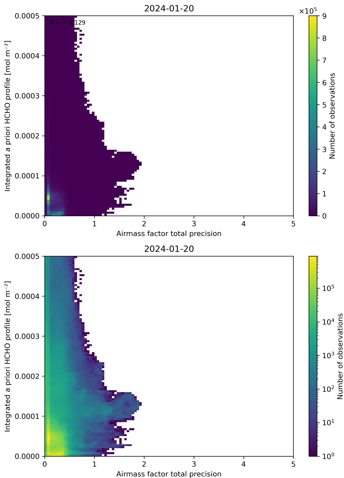
Figure 111: Scatter density plot of “Airmass factor total precision” against “Integrated a priori HCHO profile” for 2024-01-19 to 2024-01-21.
