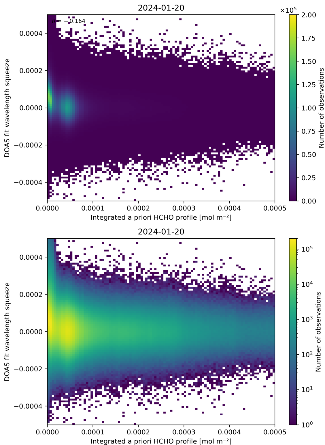
Figure 150: Scatter density plot of “Integrated a priori HCHO profile” against “DOAS fit wavelength squeeze” for 2024-01-19 to 2024-01-21.
