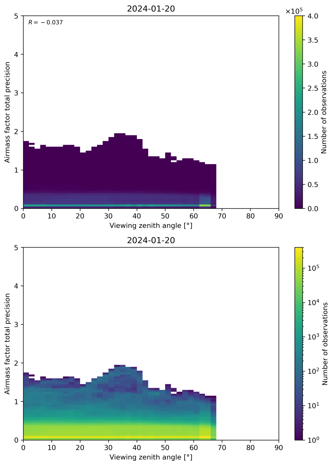
Figure 191: Scatter density plot of “Viewing zenith angle” against “Airmass factor total precision” for 2024-01-19 to 2024-01-21.
