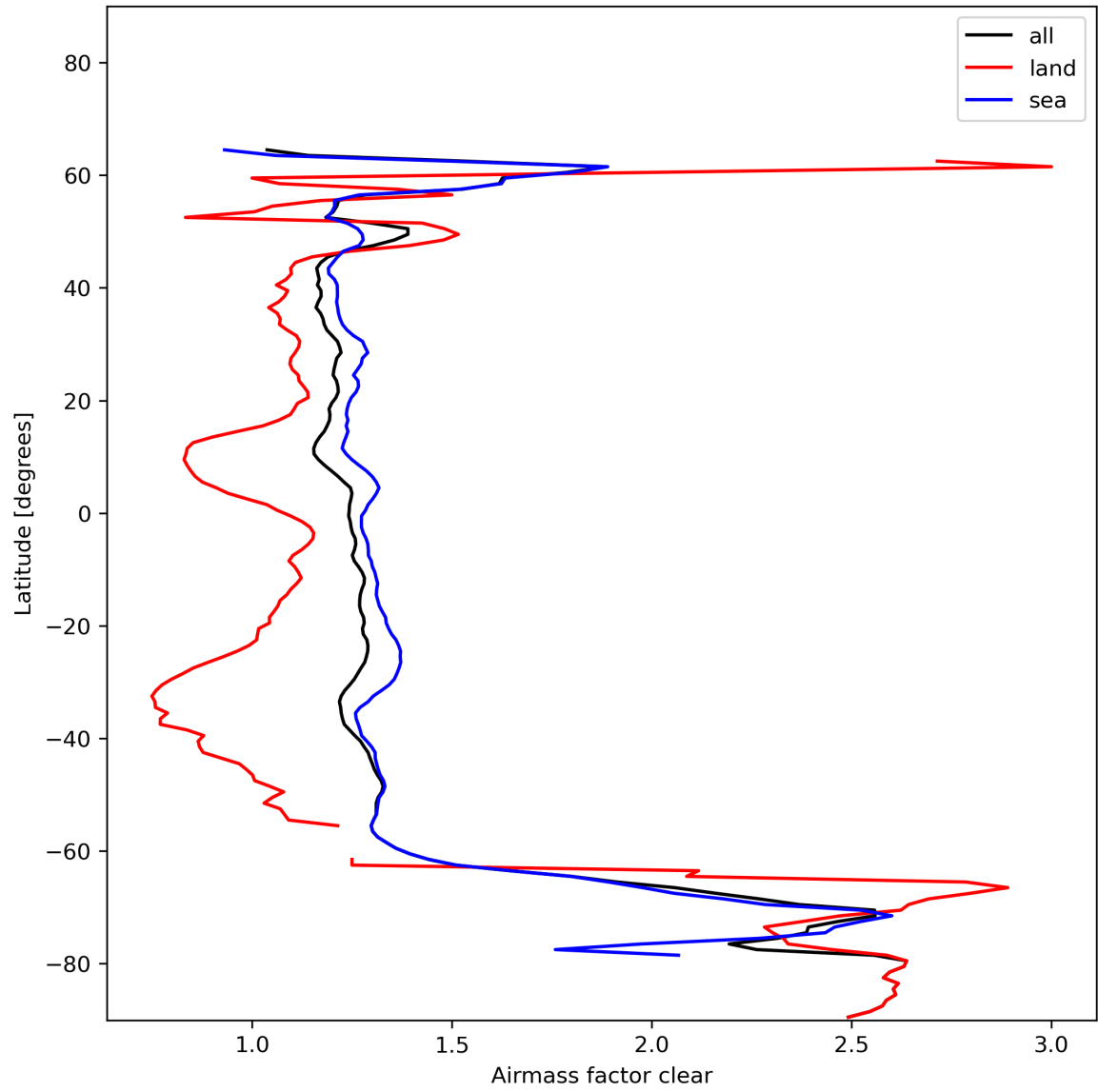
Figure 28: Zonal average of “Airmass factor clear” for 2024-01-19 to 2024-01-21.
