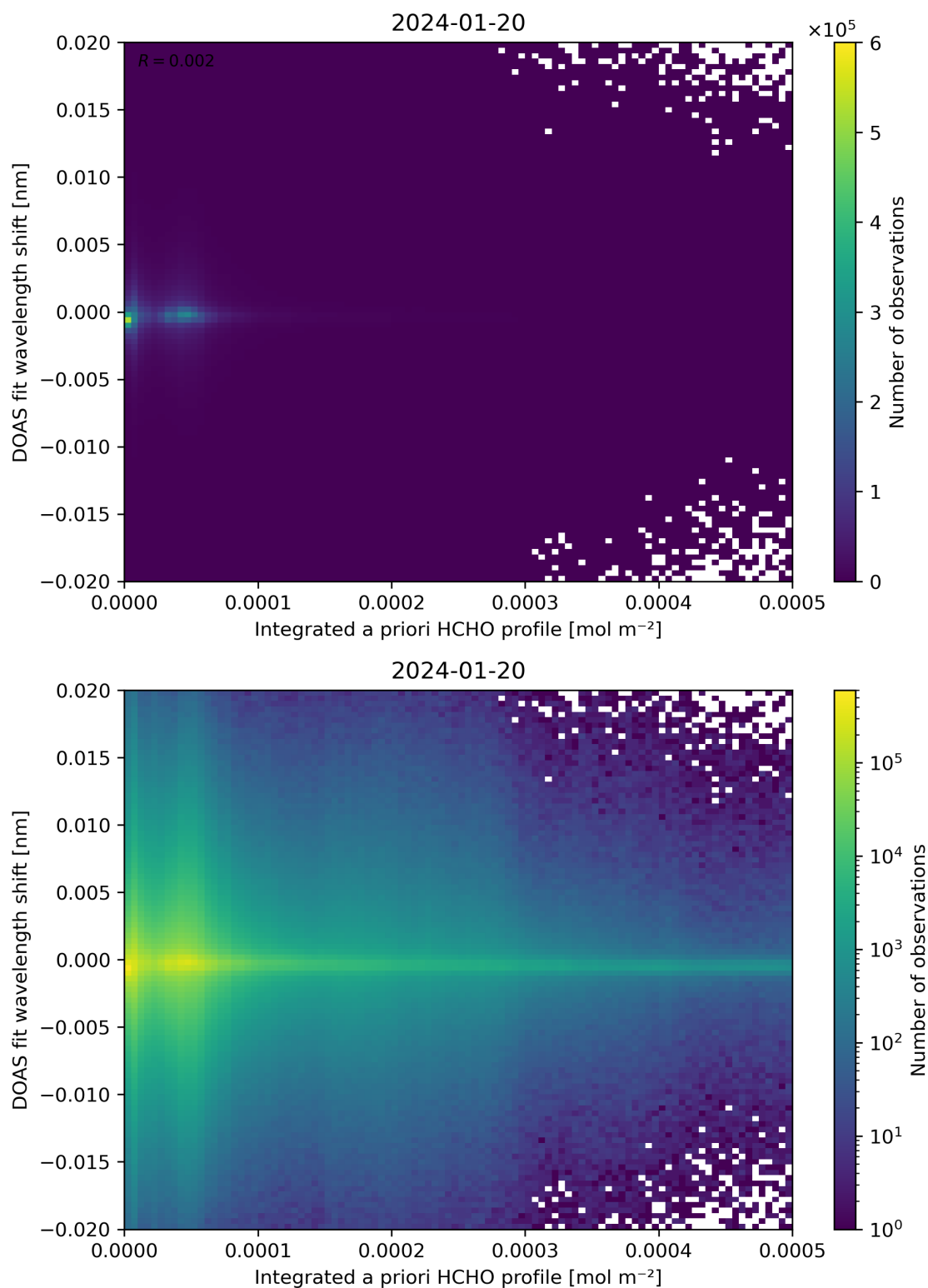
Figure 149: Scatter density plot of “Integrated a priori HCHO profile” against “DOAS fit wavelength shift” for 2024-01-19 to 2024-01-21.
