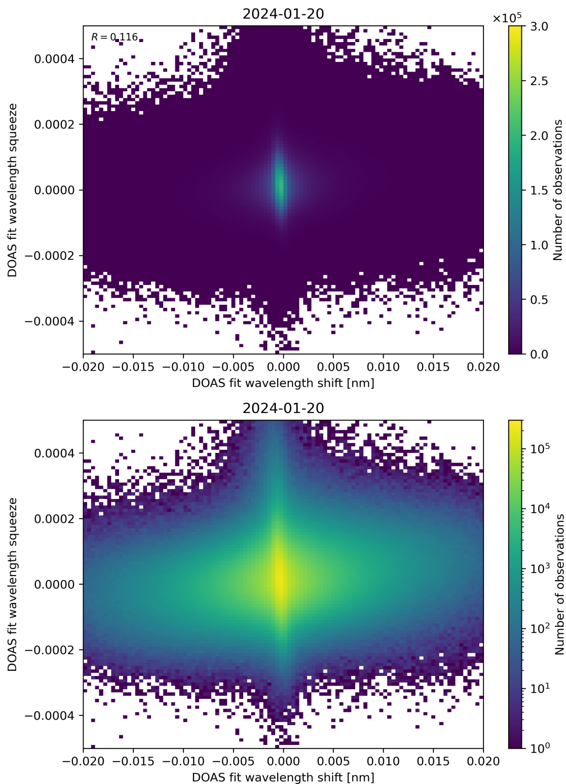
Figure 65: Scatter density plot of “DOAS fit wavelength shift” against “DOAS fit wavelength squeeze” for 2024-01-19 to 2024-01-21.
