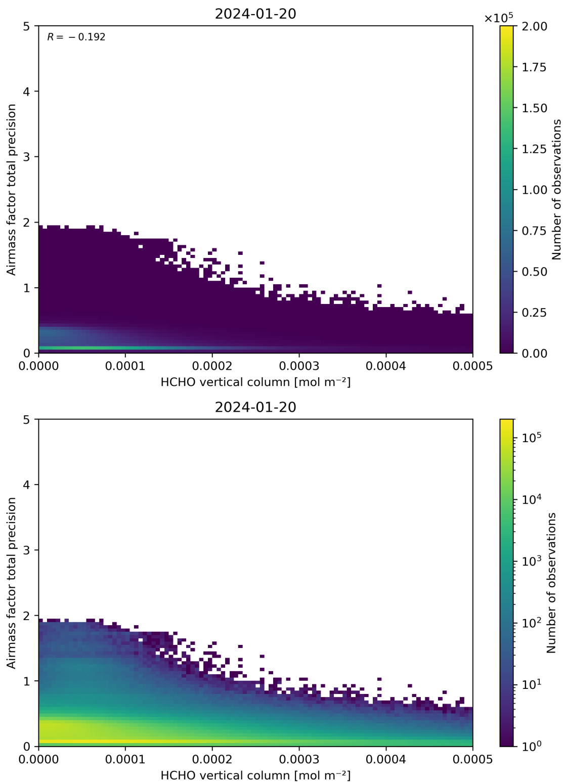
Figure 132: Scatter density plot of “HCHO vertical column” against “Airmass factor total precision” for 2024-01-19 to 2024-01-21.
