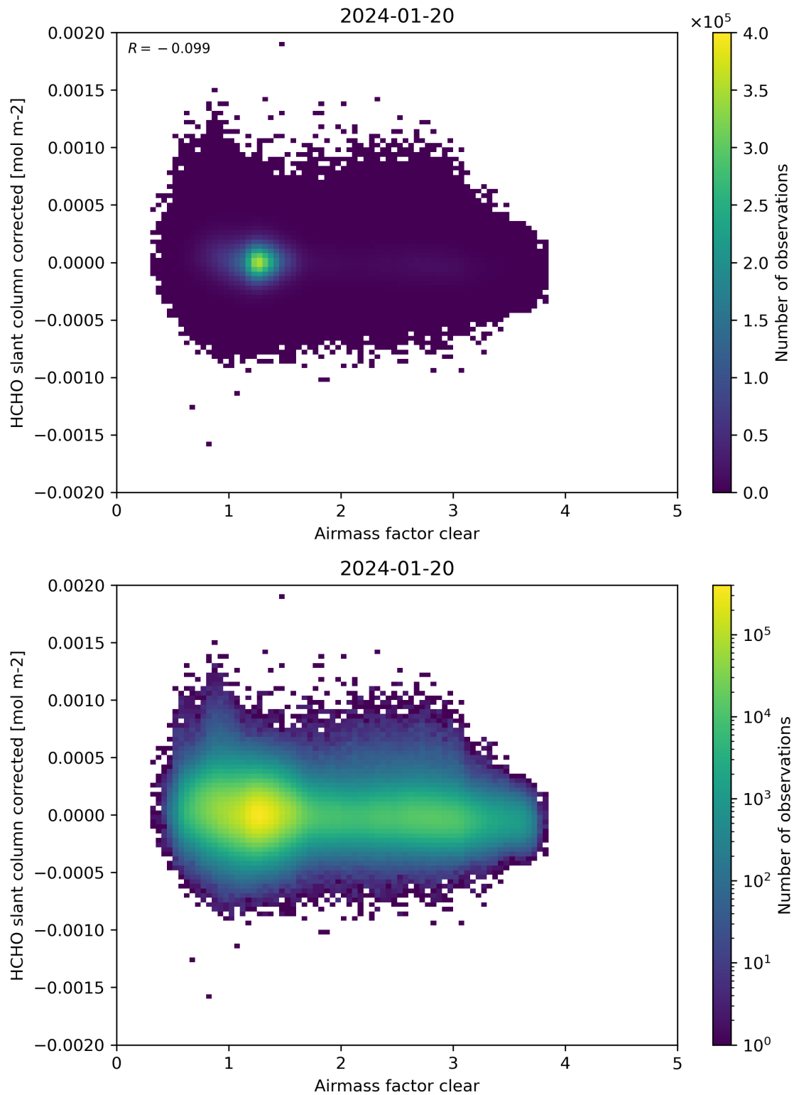
Figure 74: Scatter density plot of “Airmass factor clear” against “HCHO slant column corrected” for 2024-01-19 to 2024-01-21.
