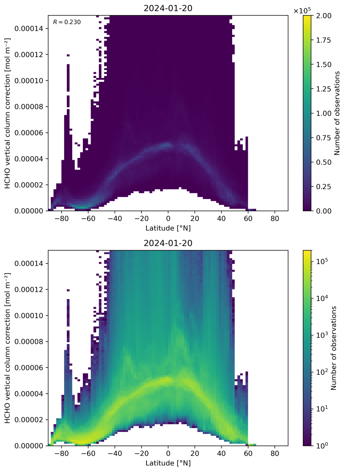
Figure 164: Scatter density plot of “Latitude” against “HCHO vertical column correction” for 2024-01-19 to 2024-01-21.
