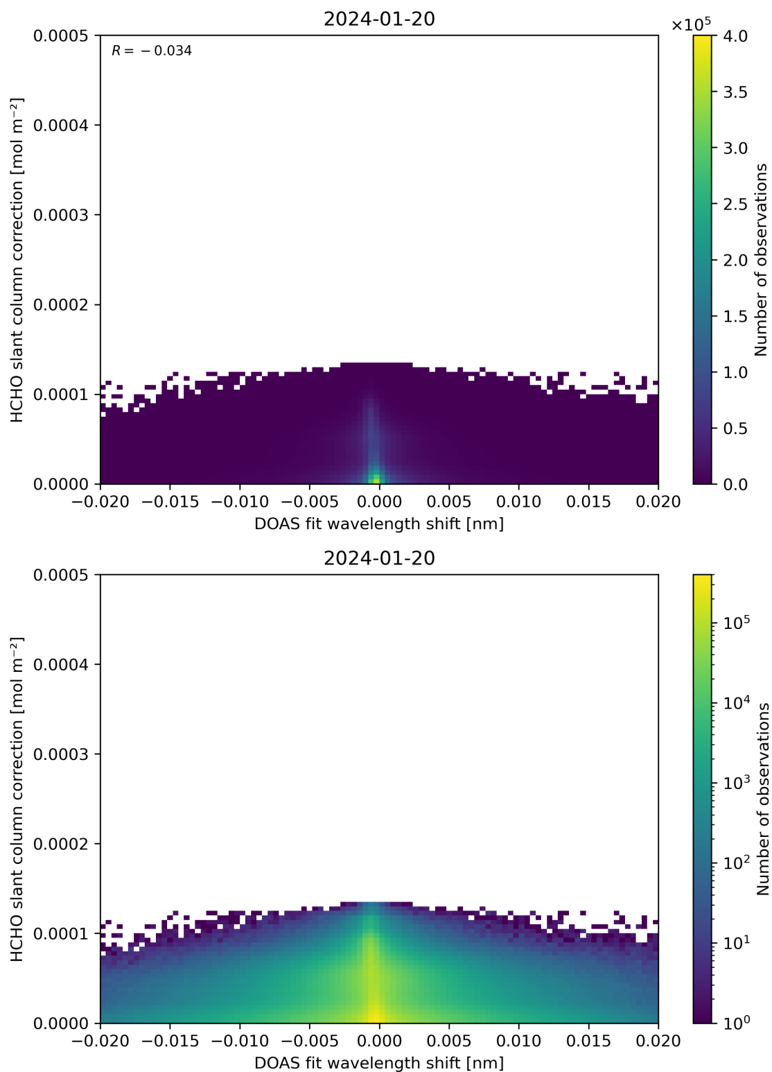
Figure 67: Scatter density plot of “DOAS fit wavelength shift” against “HCHO slant column correction” for 2024-01-19 to 2024-01-21.
