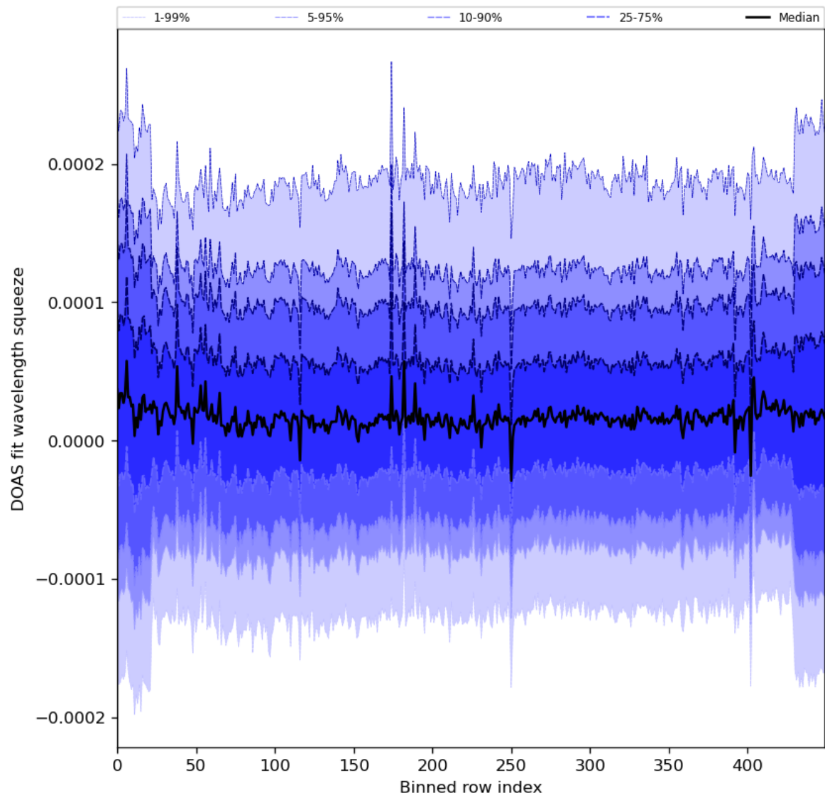
Figure 59: Along track statistics of “DOAS fit wavelength squeeze” for 2024-01-19 to 2024-01-21
