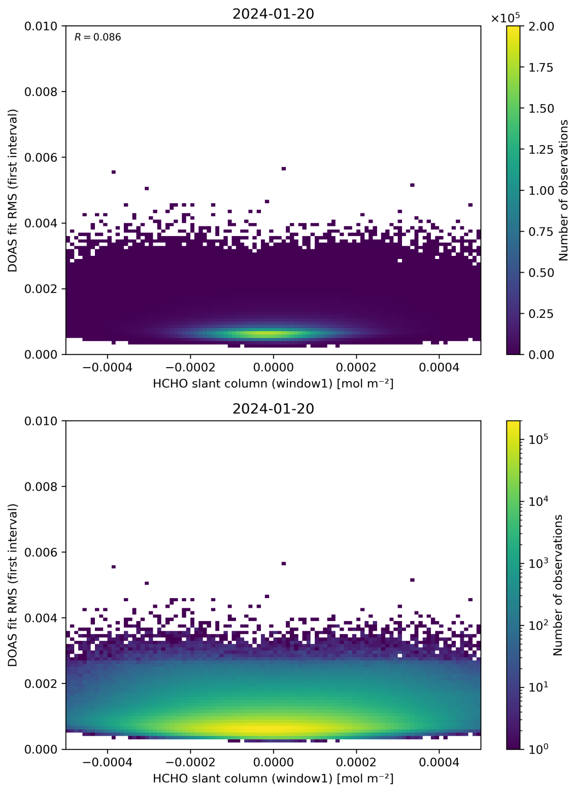
Figure 78: Scatter density plot of “HCHO slant column (window1)” against “DOAS fit RMS (first interval)” for 2024-01-19 to 2024-01-21.
