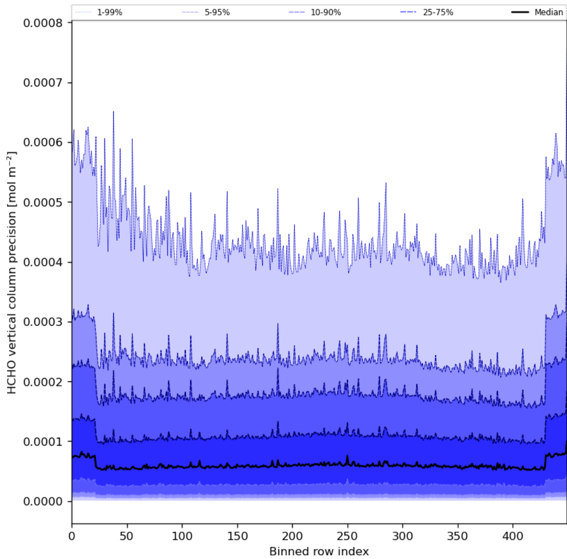
Figure 50: Along track statistics of “HCHO vertical column precision” for 2024-01-19 to 2024-01-21
