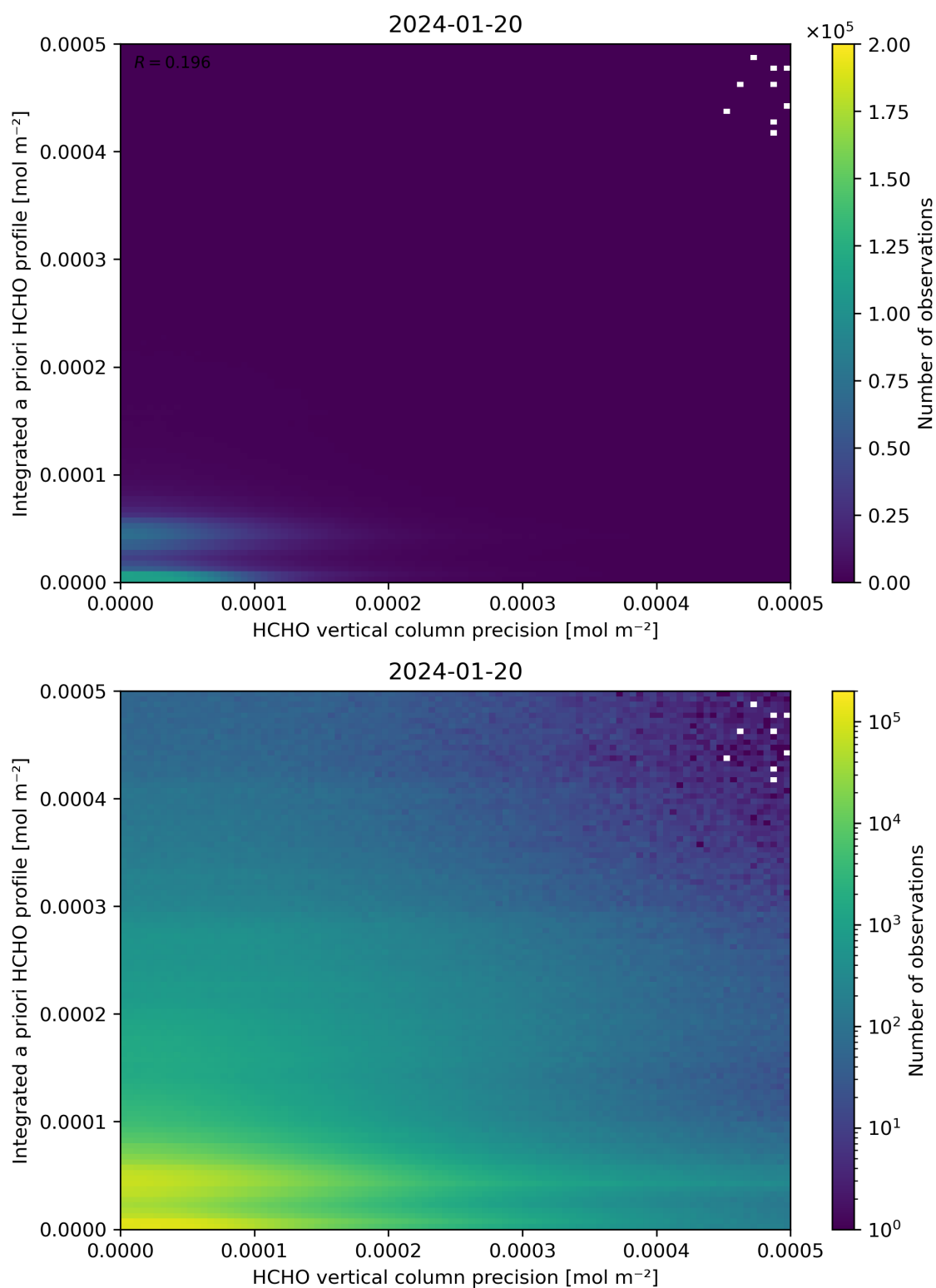
Figure 147: Scatter density plot of “HCHO vertical column precision” against “Integrated a priori HCHO profile” for 2024-01-19 to 2024-01-21.
