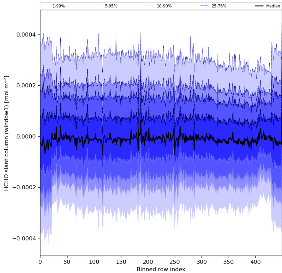
Figure 52: Along track statistics of “HCHO slant column (window1)” for 2024-01-19 to 2024-01-21
