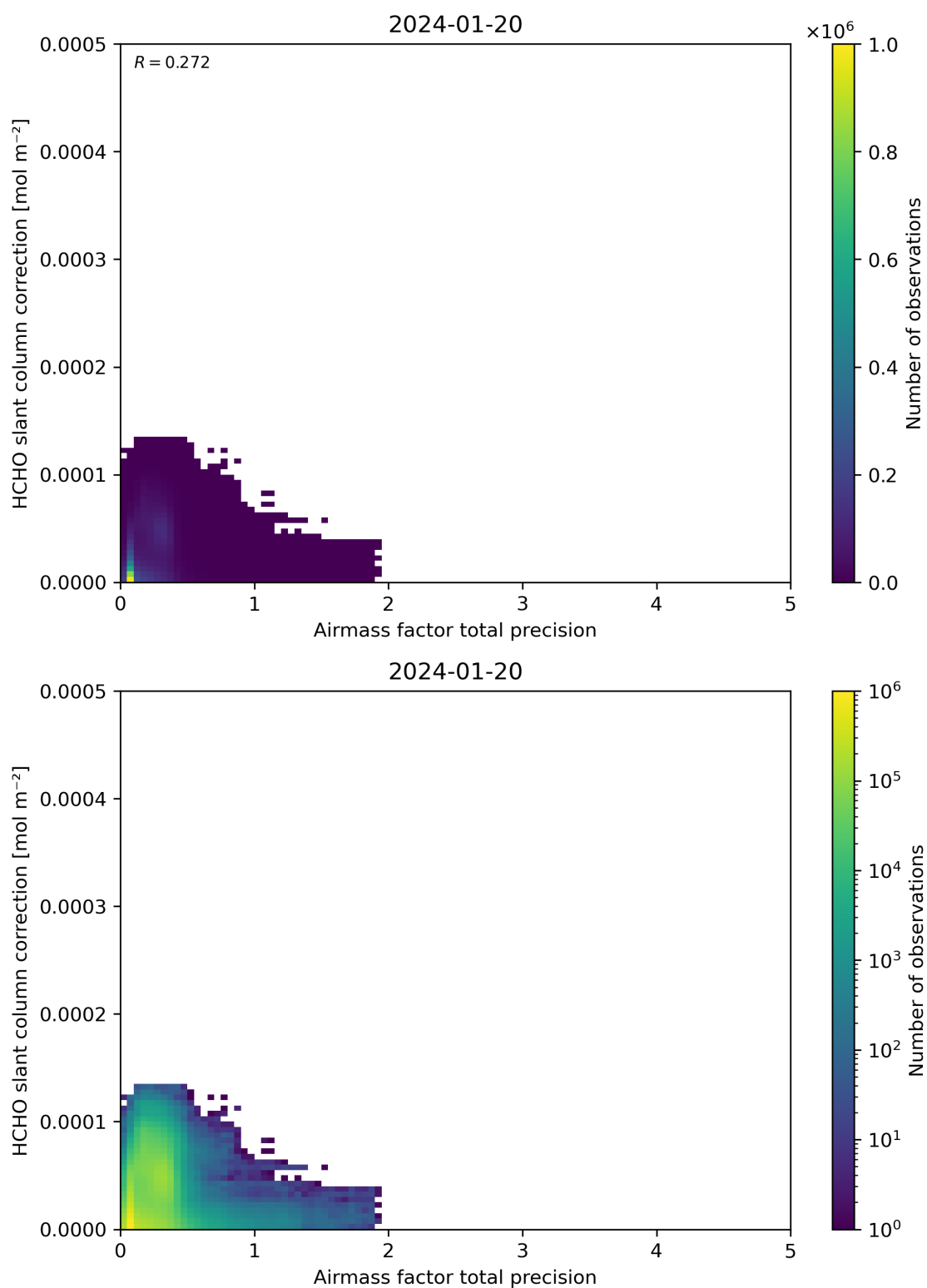
Figure 110: Scatter density plot of “Airmass factor total precision” against “HCHO slant column correction” for 2024-01-19 to 2024-01-21.
