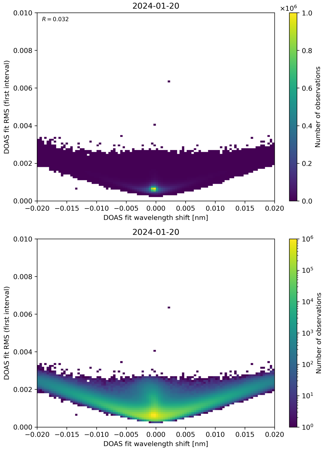
Figure 64: Scatter density plot of “DOAS fit wavelength shift” against “DOAS fit RMS (first interval)” for 2024-01-19 to 2024-01-21.
