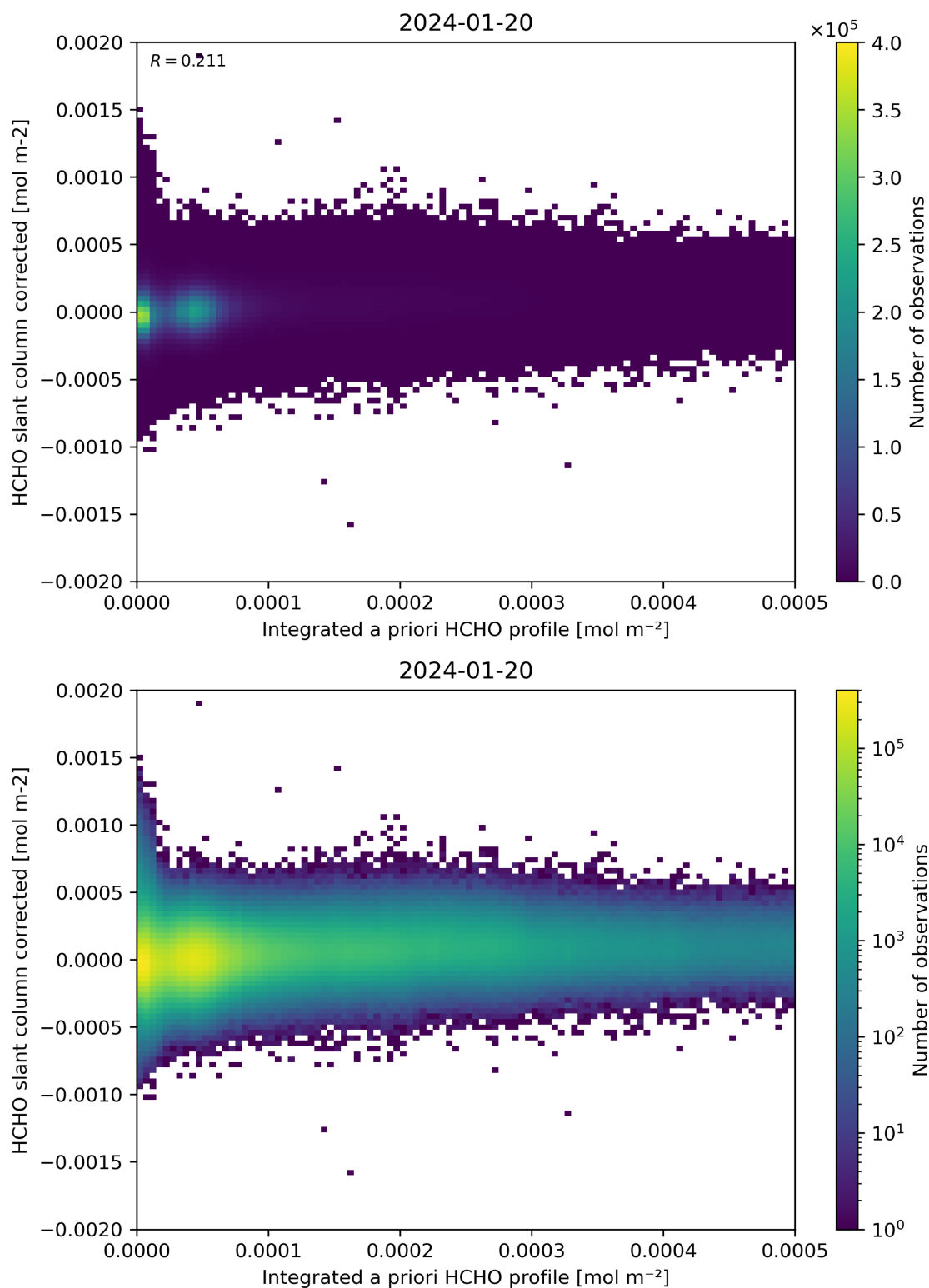
Figure 151: Scatter density plot of “Integrated a priori HCHO profile” against “HCHO slant column corrected” for 2024-01-19 to 2024-01-21.
