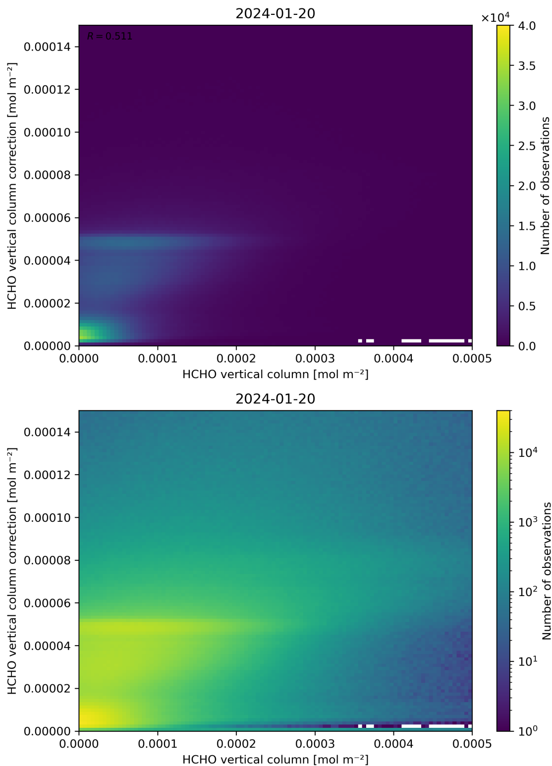
Figure 133: Scatter density plot of “HCHO vertical column” against “HCHO vertical column correction” for 2024-01-19 to 2024-01-21.
