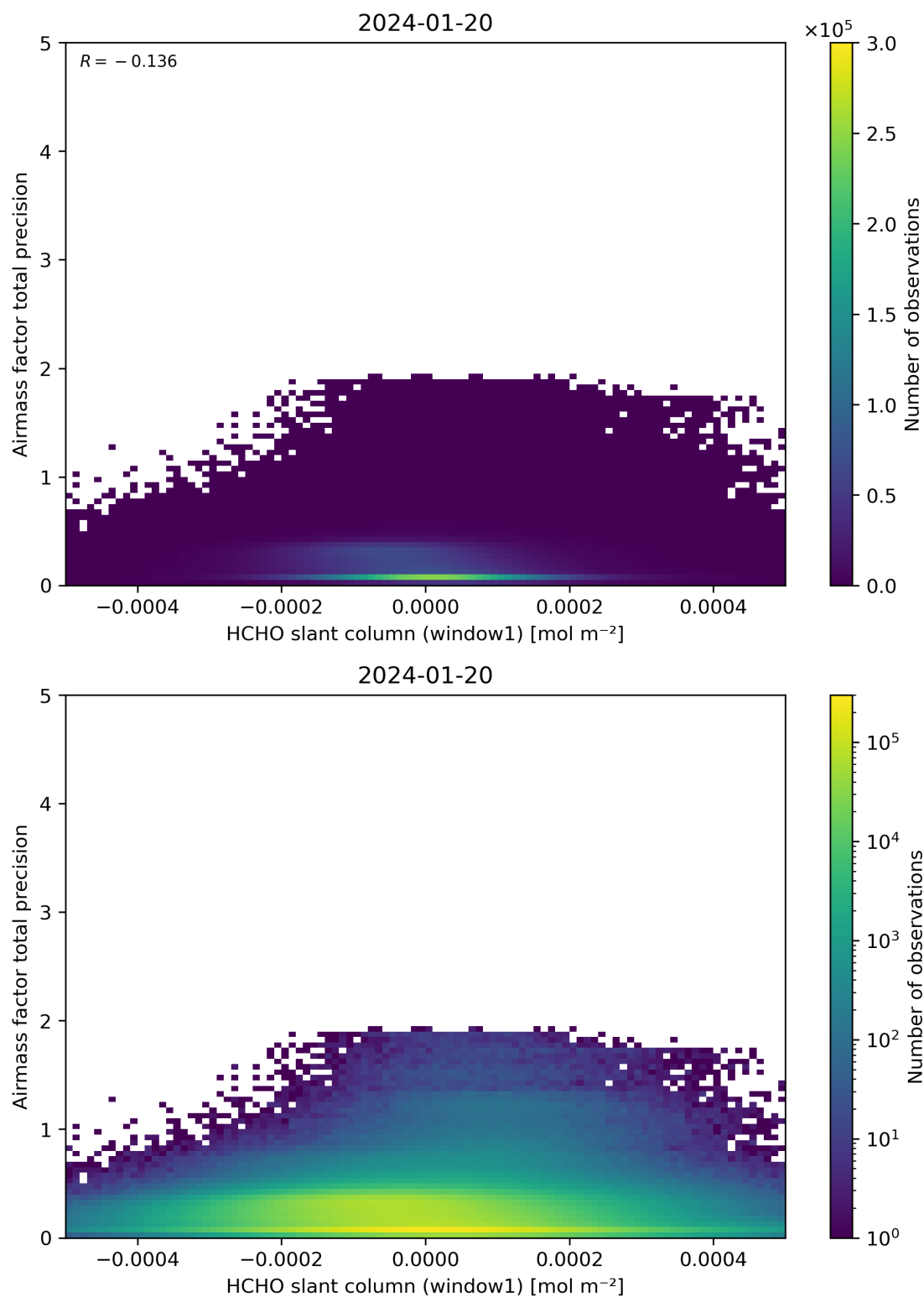
Figure 86: Scatter density plot of “HCHO slant column (window1)” against “Airmass factor total precision” for 2024-01-19 to 2024-01-21.
