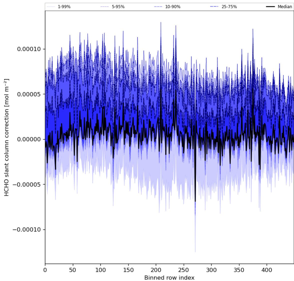
Figure 61: Along track statistics of “HCHO slant column correction” for 2024-01-19 to 2024-01-21
