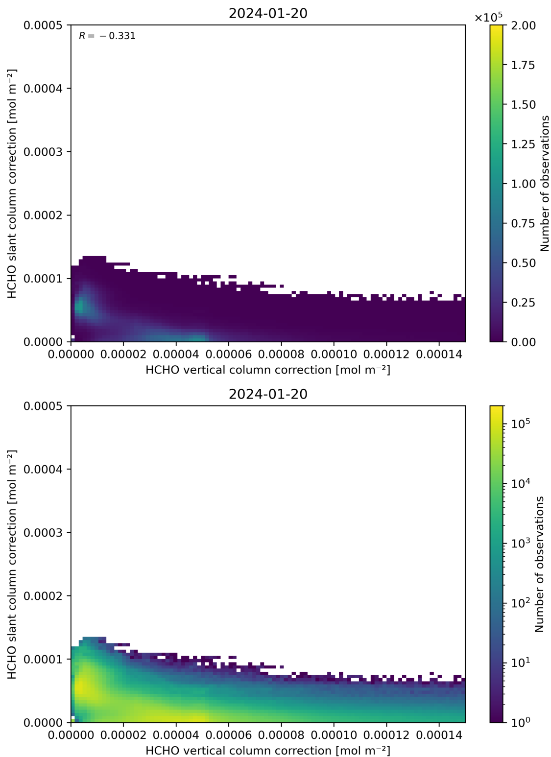
Figure 117: Scatter density plot of “HCHO vertical column correction” against “HCHO slant column correction” for 2024-01-19 to 2024-01-21.
