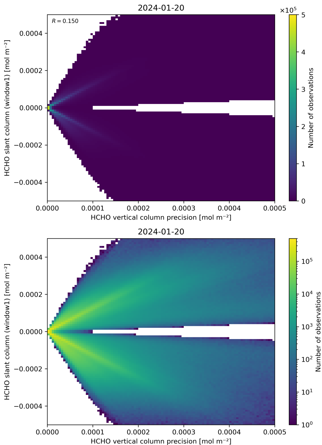
Figure 142: Scatter density plot of “HCHO vertical column precision” against “HCHO slant column (window1)” for 2024-01-19 to 2024-01-21.
