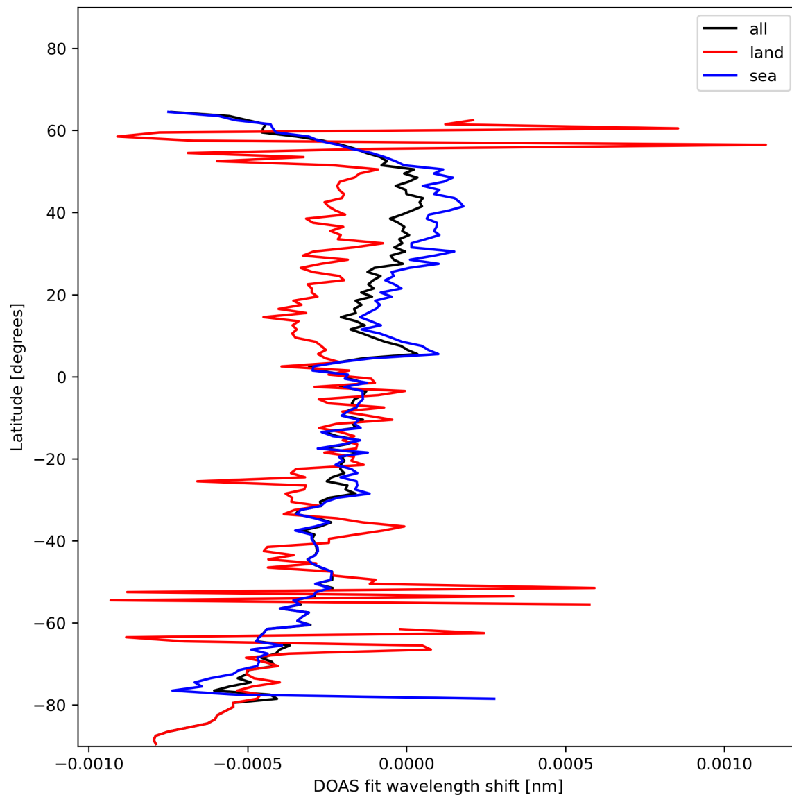
Figure 30: Zonal average of “DOAS fit wavelength shift” for 2024-01-19 to 2024-01-21.
