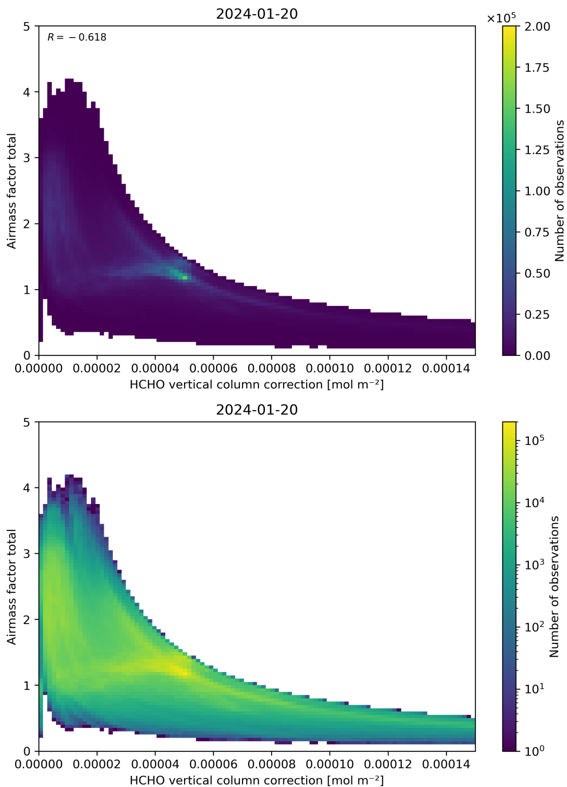
Figure 120: Scatter density plot of “HCHO vertical column correction” against “Airmass factor total” for 2024-01-19 to 2024-01-21.
