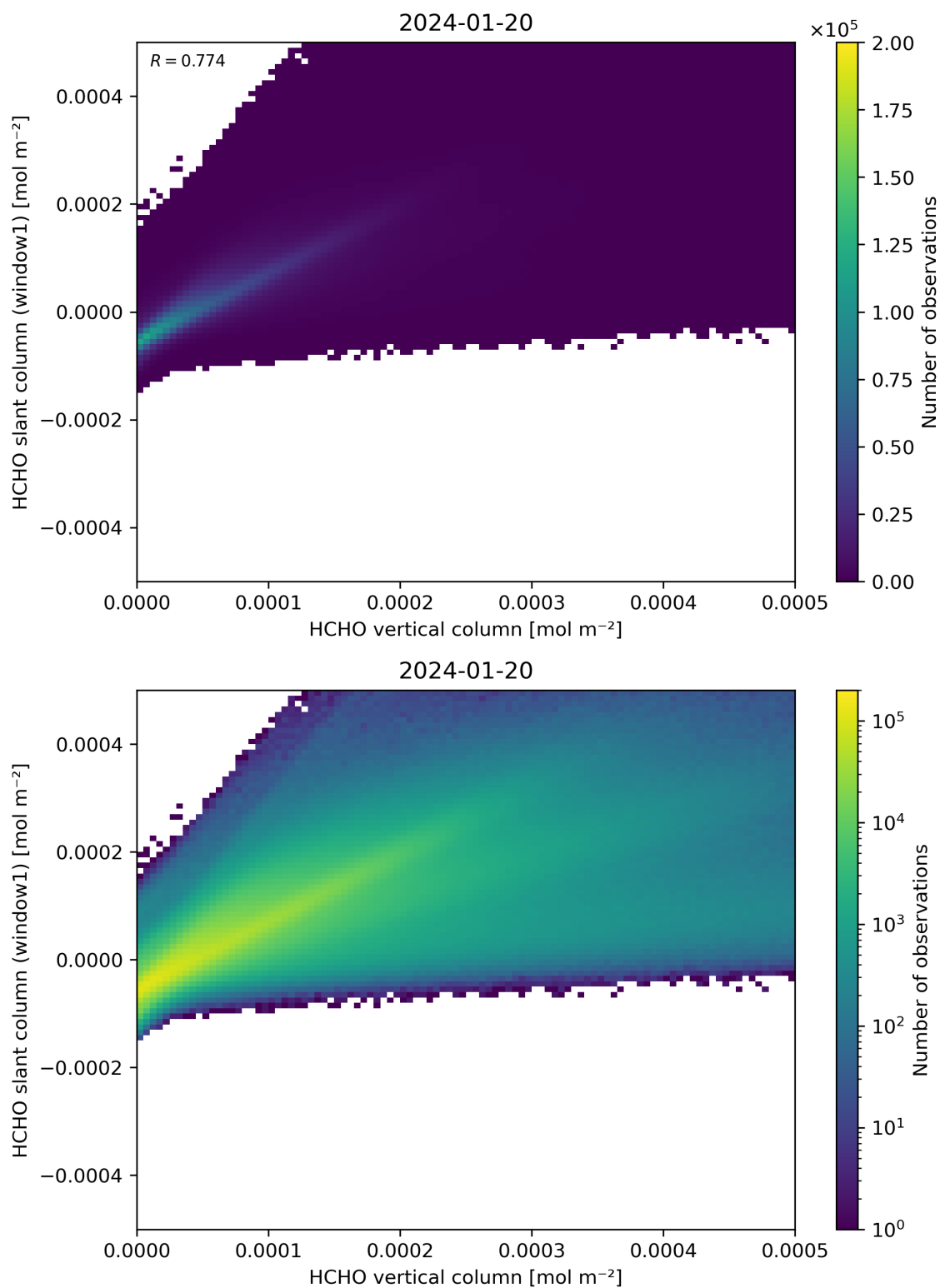
Figure 129: Scatter density plot of “HCHO vertical column” against “HCHO slant column (window1)” for 2024-01-19 to 2024-01-21.
