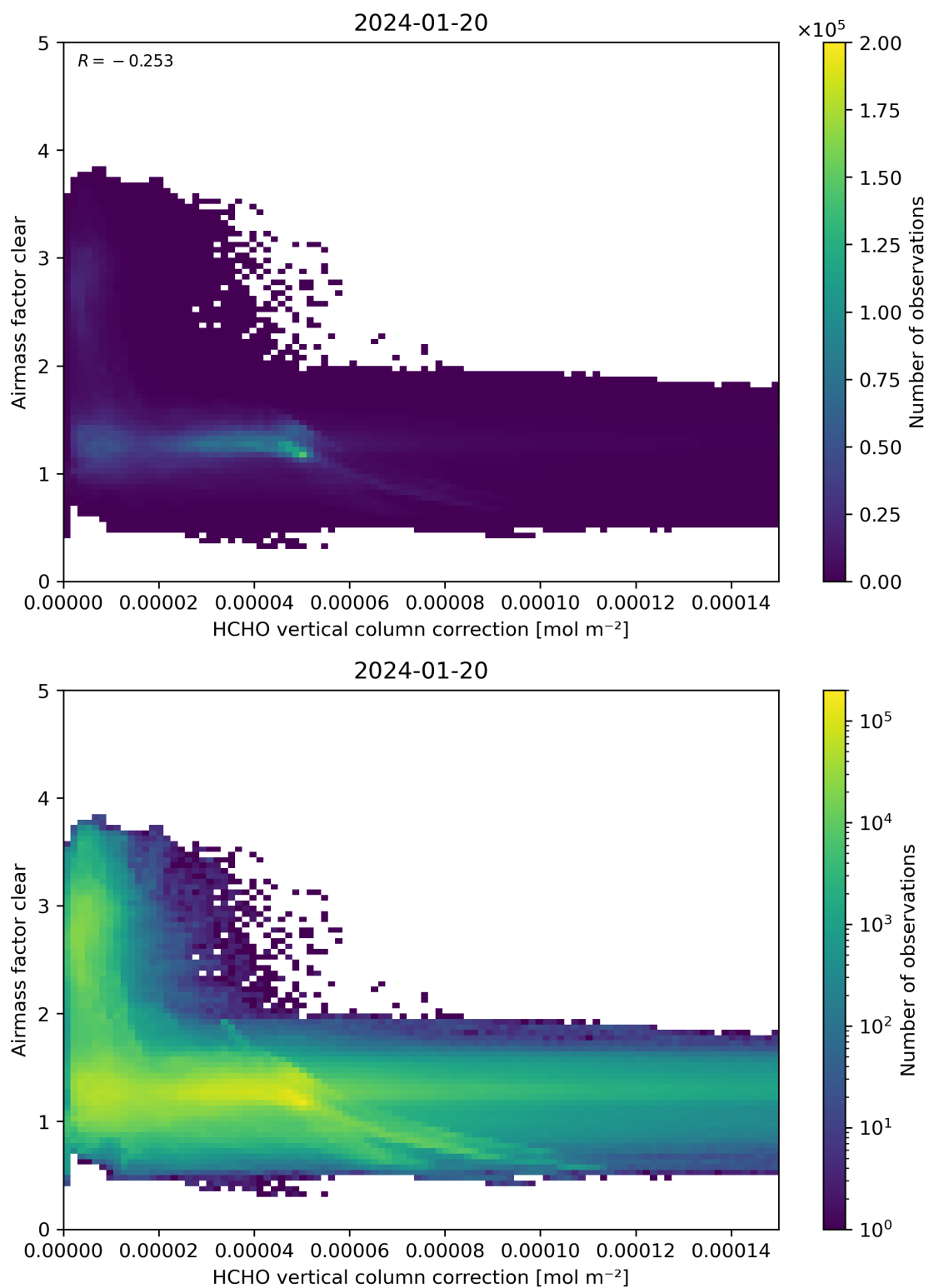
Figure 115: Scatter density plot of “HCHO vertical column correction” against “Airmass factor clear” for 2024-01-19 to 2024-01-21.
