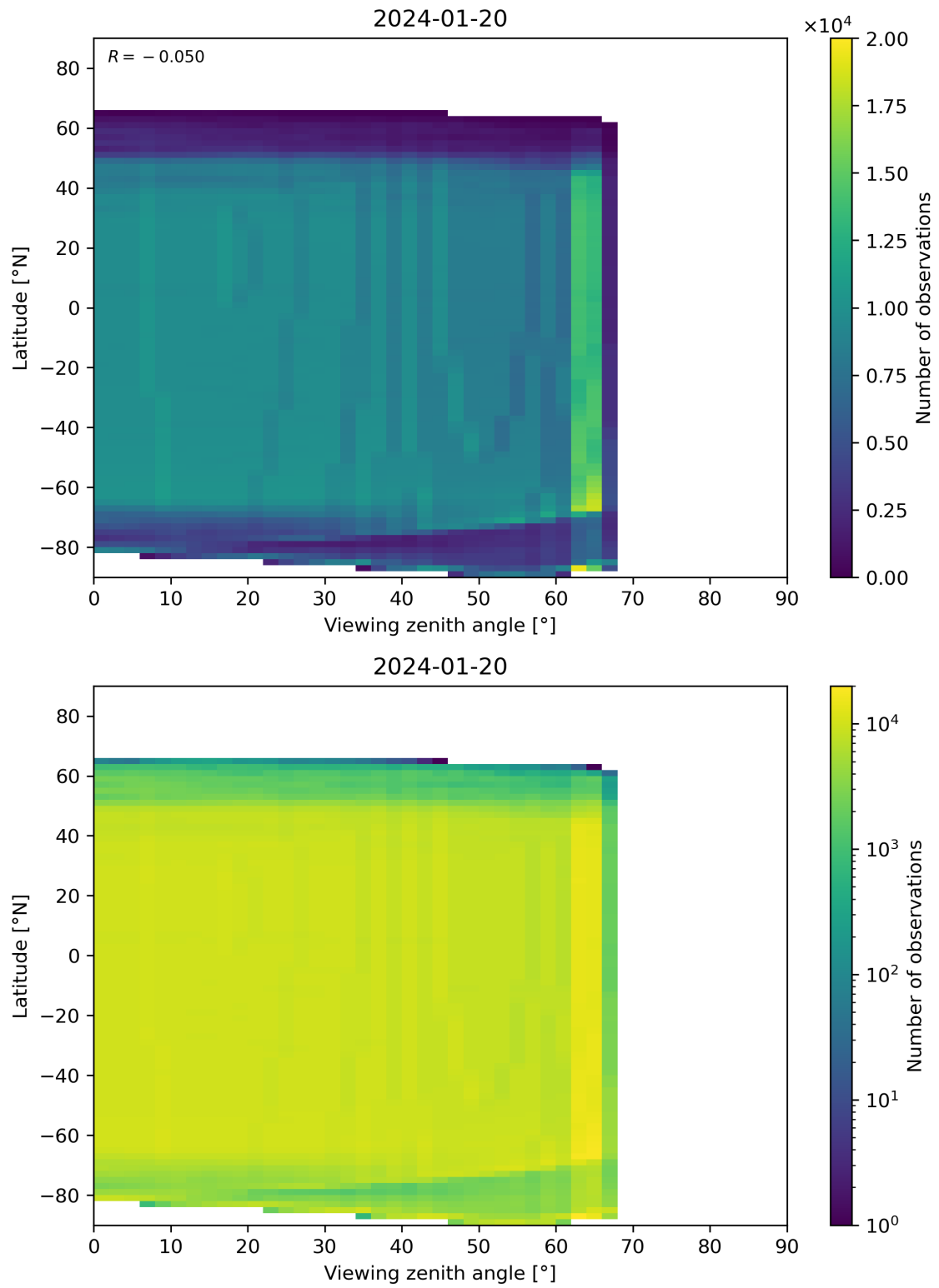
Figure 196: Scatter density plot of “Viewing zenith angle” against “Latitude” for 2024-01-19 to 2024-01-21.
