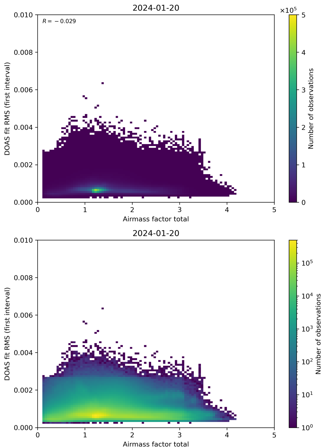
Figure 97: Scatter density plot of “Airmass factor total” against “DOAS fit RMS (first interval)” for 2024-01-19 to 2024-01-21.
