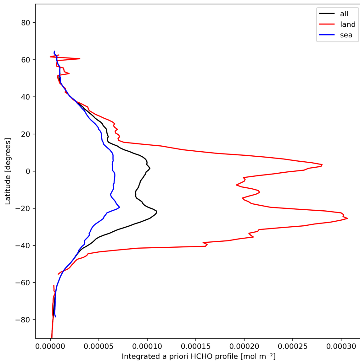
Figure 29: Zonal average of “Integrated a priori HCHO profile” for 2024-01-19 to 2024-01-21.
