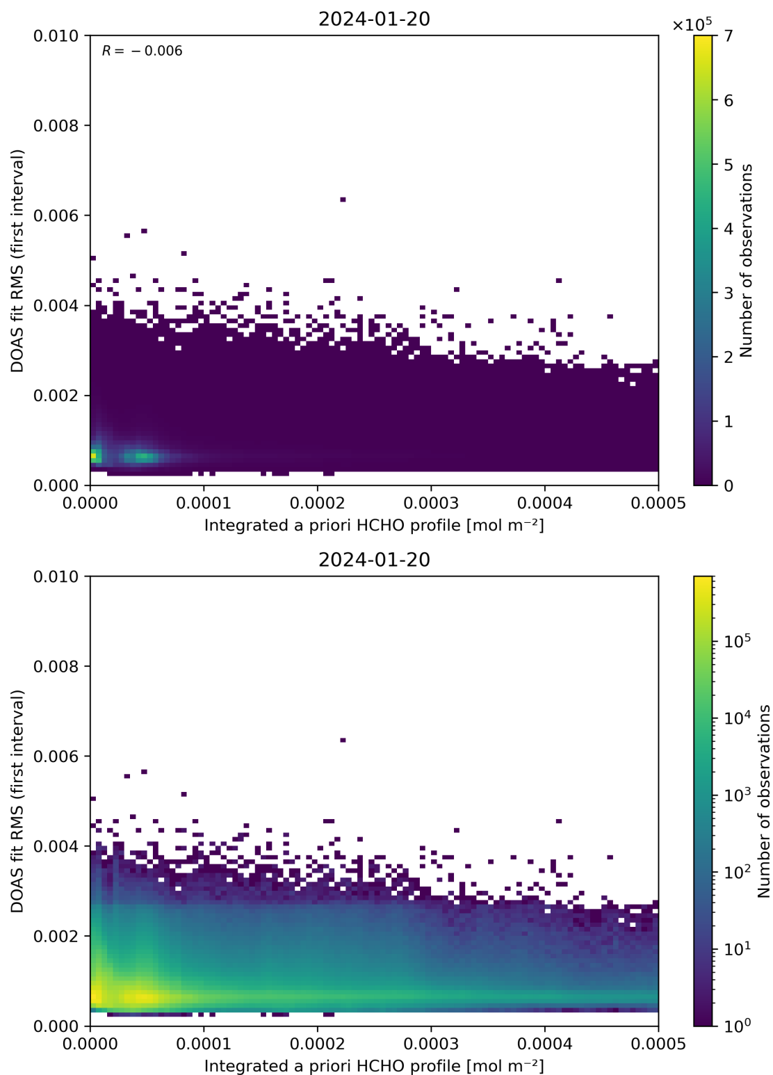
Figure 148: Scatter density plot of “Integrated a priori HCHO profile” against “DOAS fit RMS (first interval)” for 2024-01-19 to 2024-01-21.
