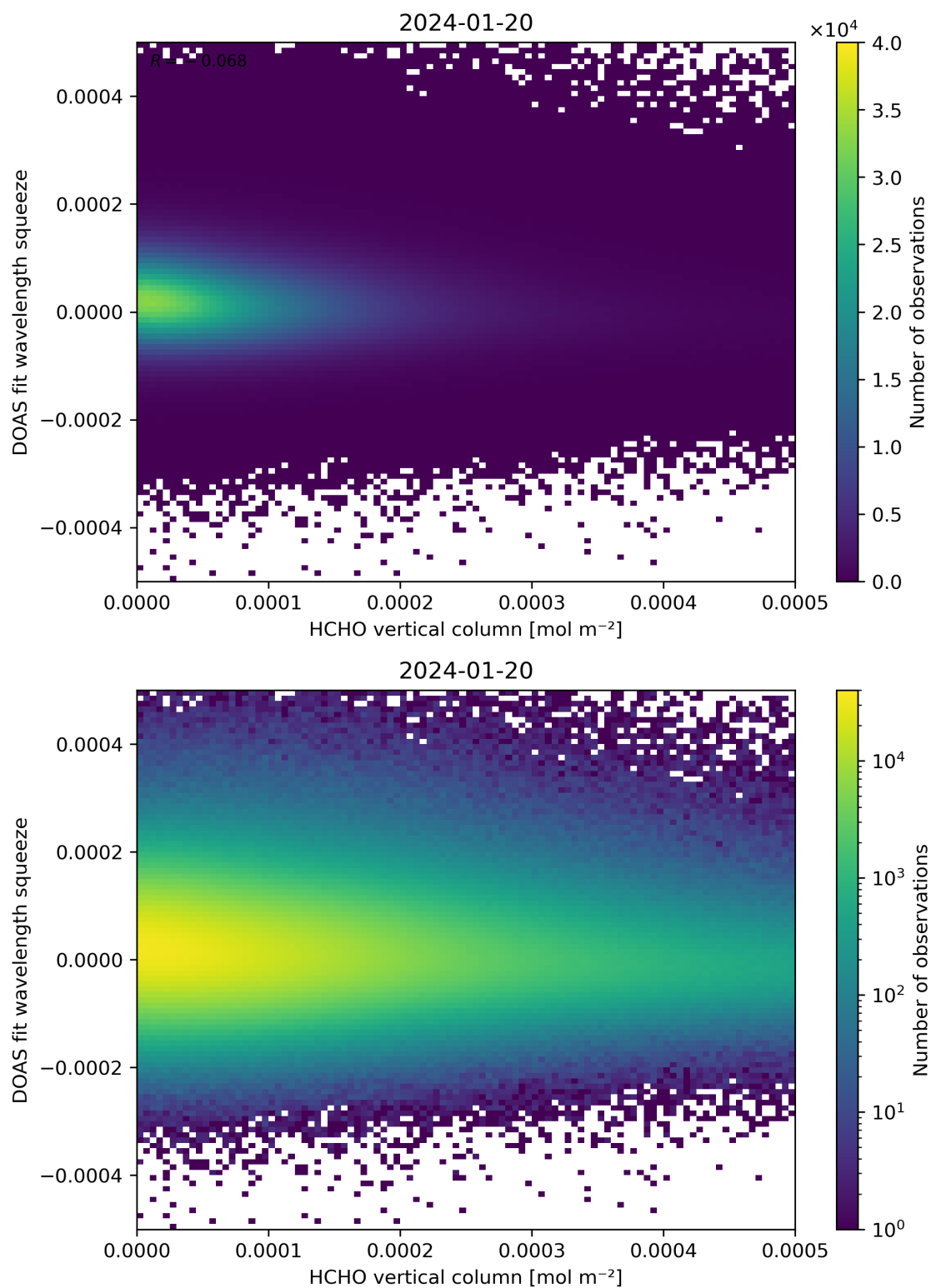
Figure 125: Scatter density plot of “HCHO vertical column” against “DOAS fit wavelength squeeze” for 2024-01-19 to 2024-01-21.
