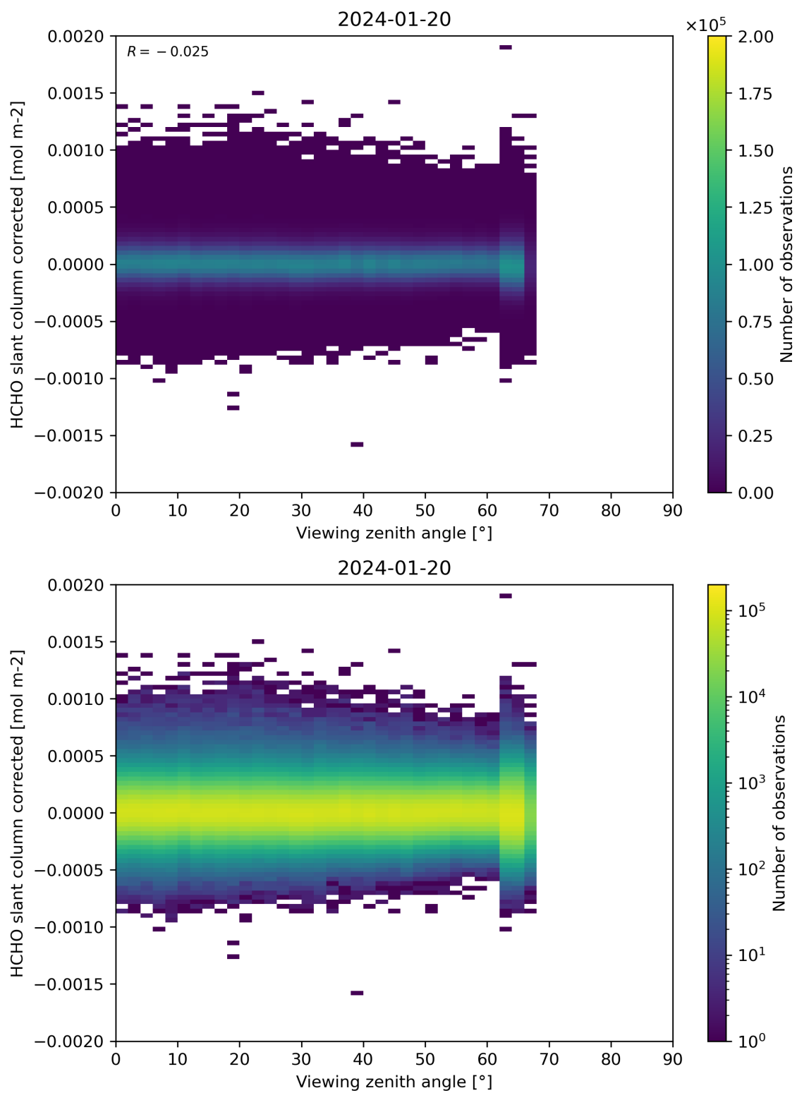
Figure 186: Scatter density plot of “Viewing zenith angle” against “HCHO slant column corrected” for 2024-01-19 to 2024-01-21.
