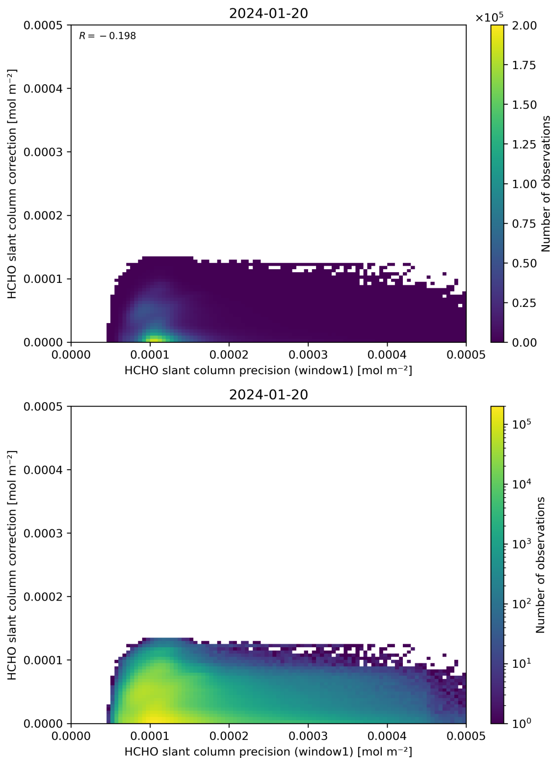
Figure 93: Scatter density plot of “HCHO slant column precision (window1)” against “HCHO slant column correction” for 2024-01-19 to 2024-01-21.
