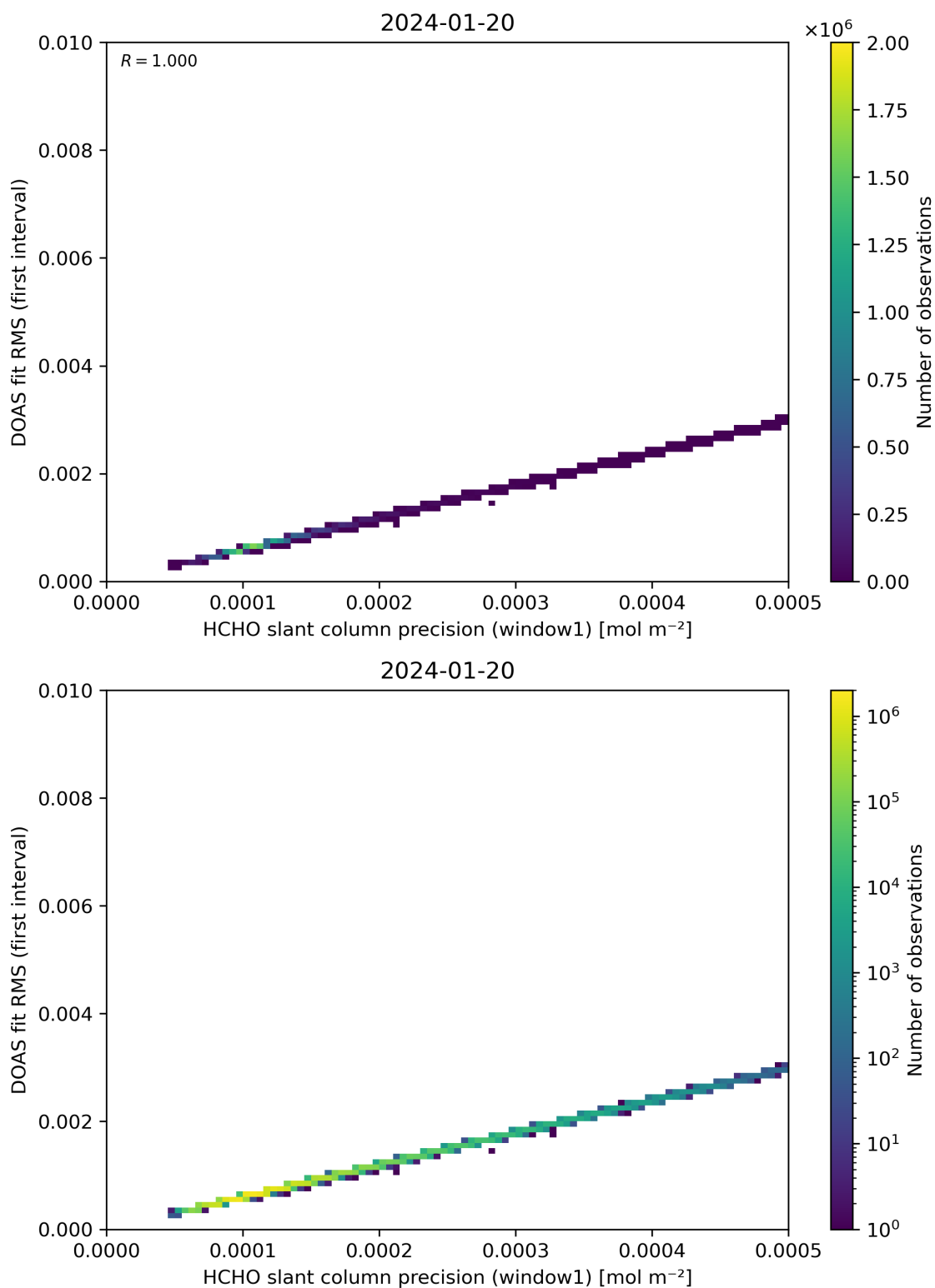
Figure 88: Scatter density plot of “HCHO slant column precision (window1)” against “DOAS fit RMS (first interval)” for 2024-01-19 to 2024-01-21.
