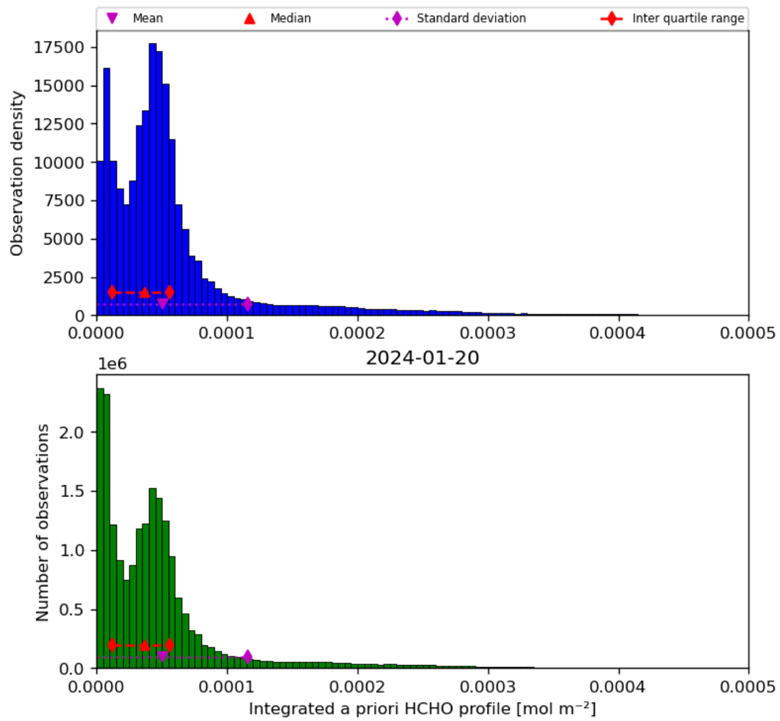
Figure 43: Histogram of “Integrated a priori HCHO profile” for 2024-01-19 to 2024-01-21
