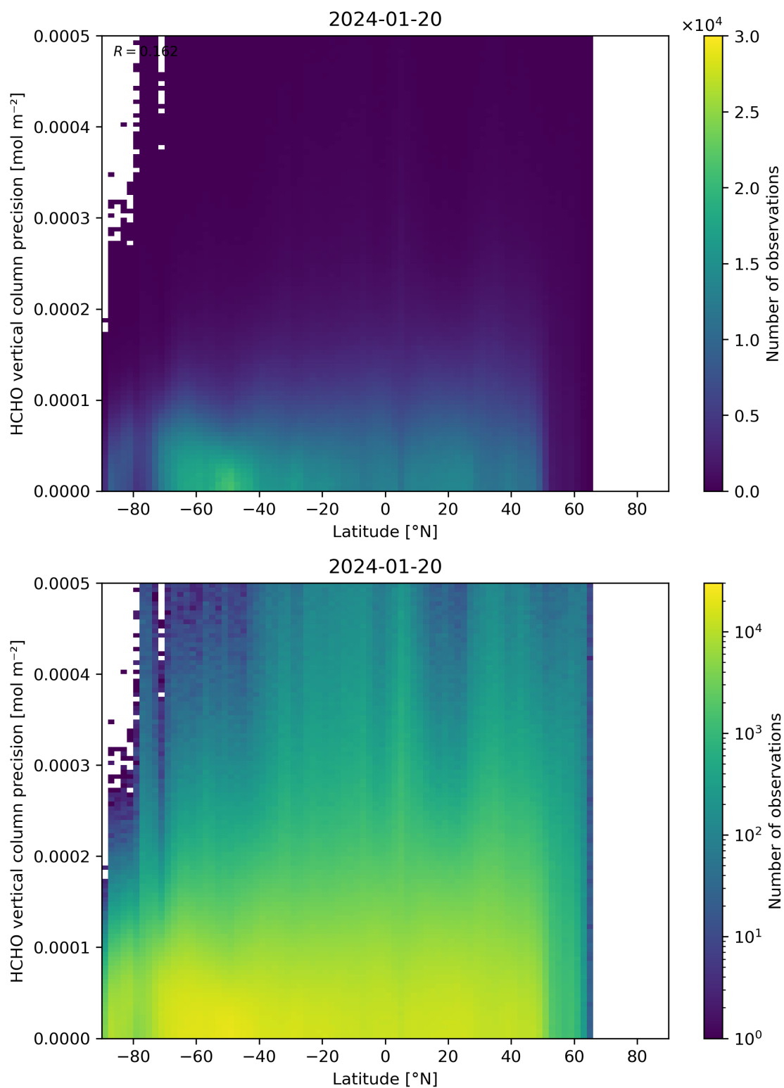
Figure 165: Scatter density plot of “Latitude” against “HCHO vertical column precision” for 2024-01-19 to 2024-01-21.
