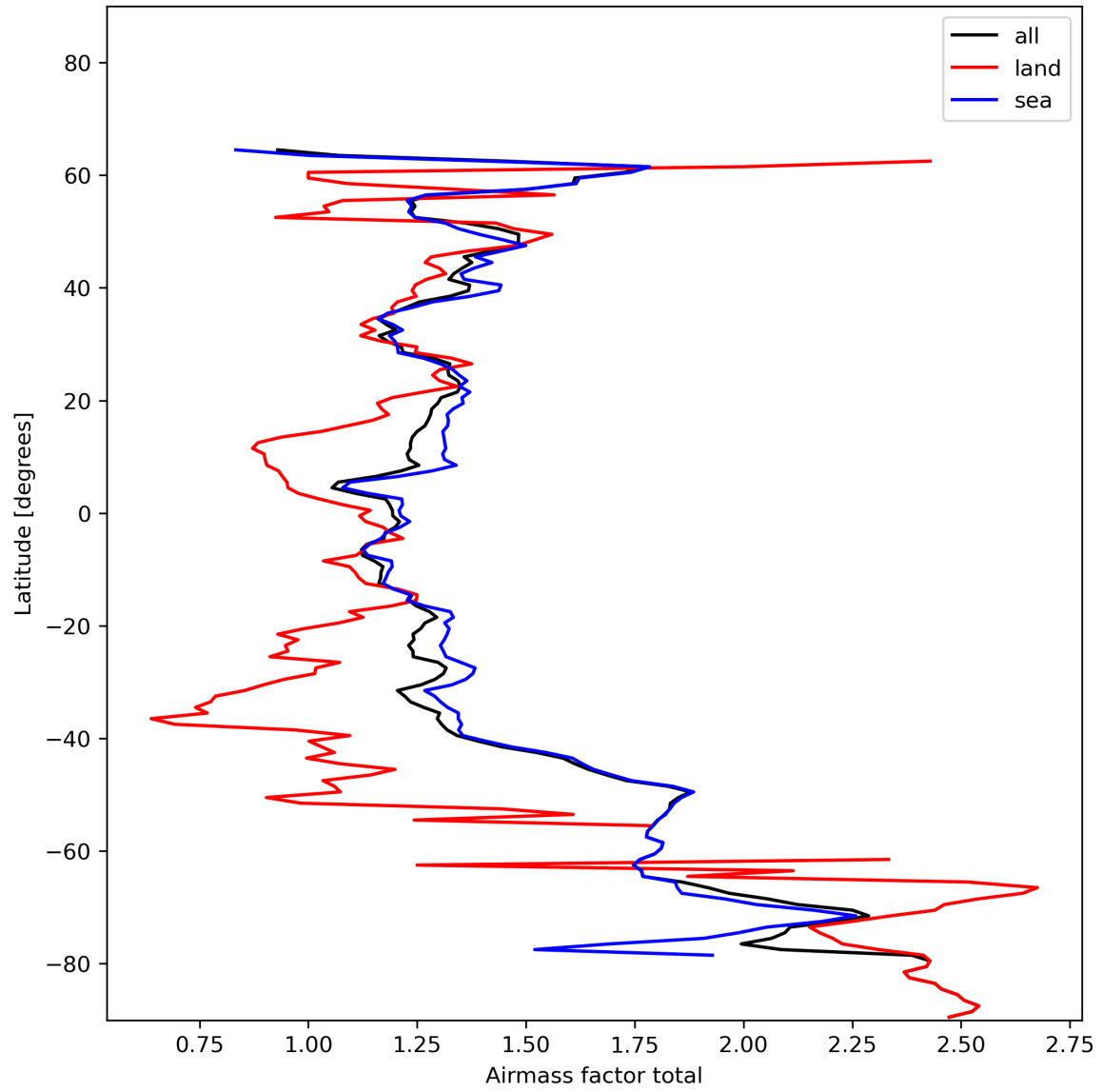
Figure 26: Zonal average of “Airmass factor total” for 2024-01-19 to 2024-01-21.
