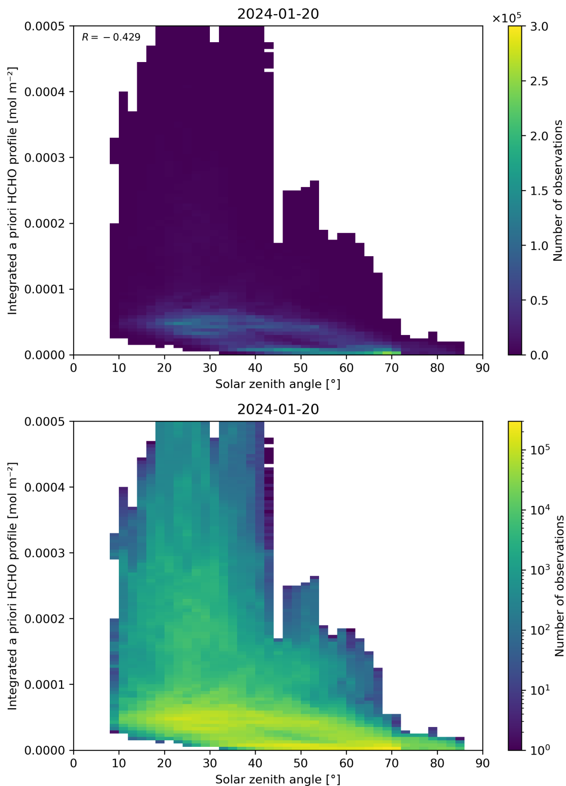
Figure 180: Scatter density plot of “Solar zenith angle” against “Integrated a priori HCHO profile” for 2024-01-19 to 2024-01-21.
