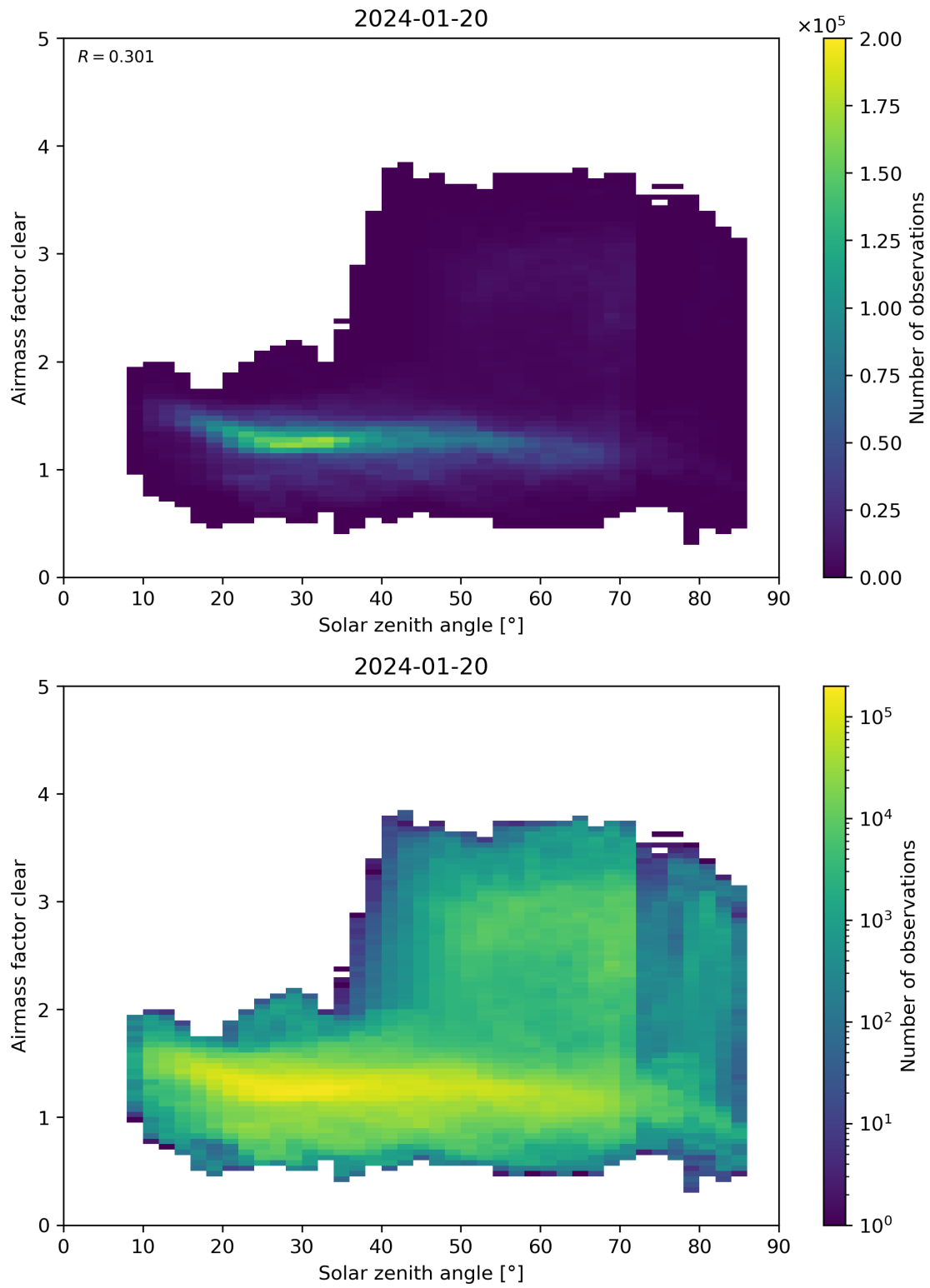
Figure 170: Scatter density plot of “Solar zenith angle” against “Airmass factor clear” for 2024-01-19 to 2024-01-21.
