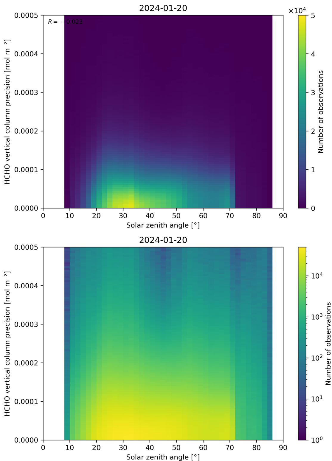
Figure 179: Scatter density plot of “Solar zenith angle” against “HCHO vertical column precision” for 2024-01-19 to 2024-01-21.
