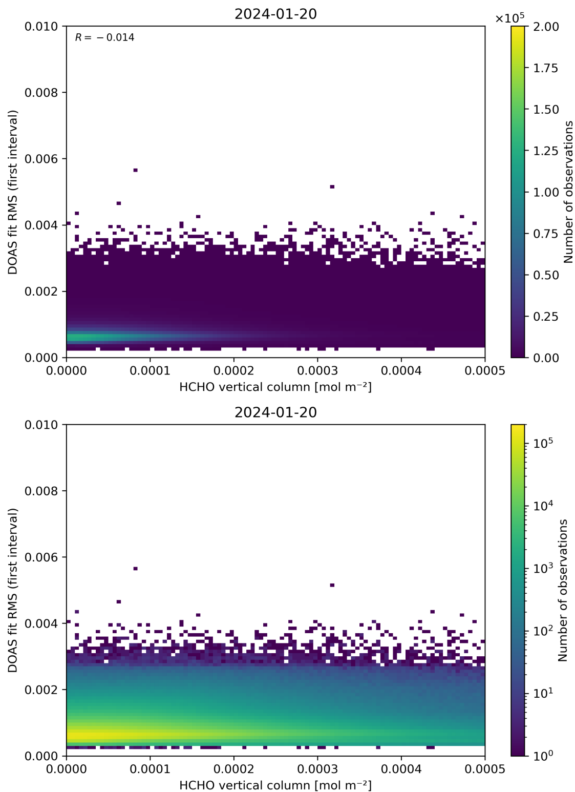
Figure 123: Scatter density plot of “HCHO vertical column” against “DOAS fit RMS (first interval)” for 2024-01-19 to 2024-01-21.
