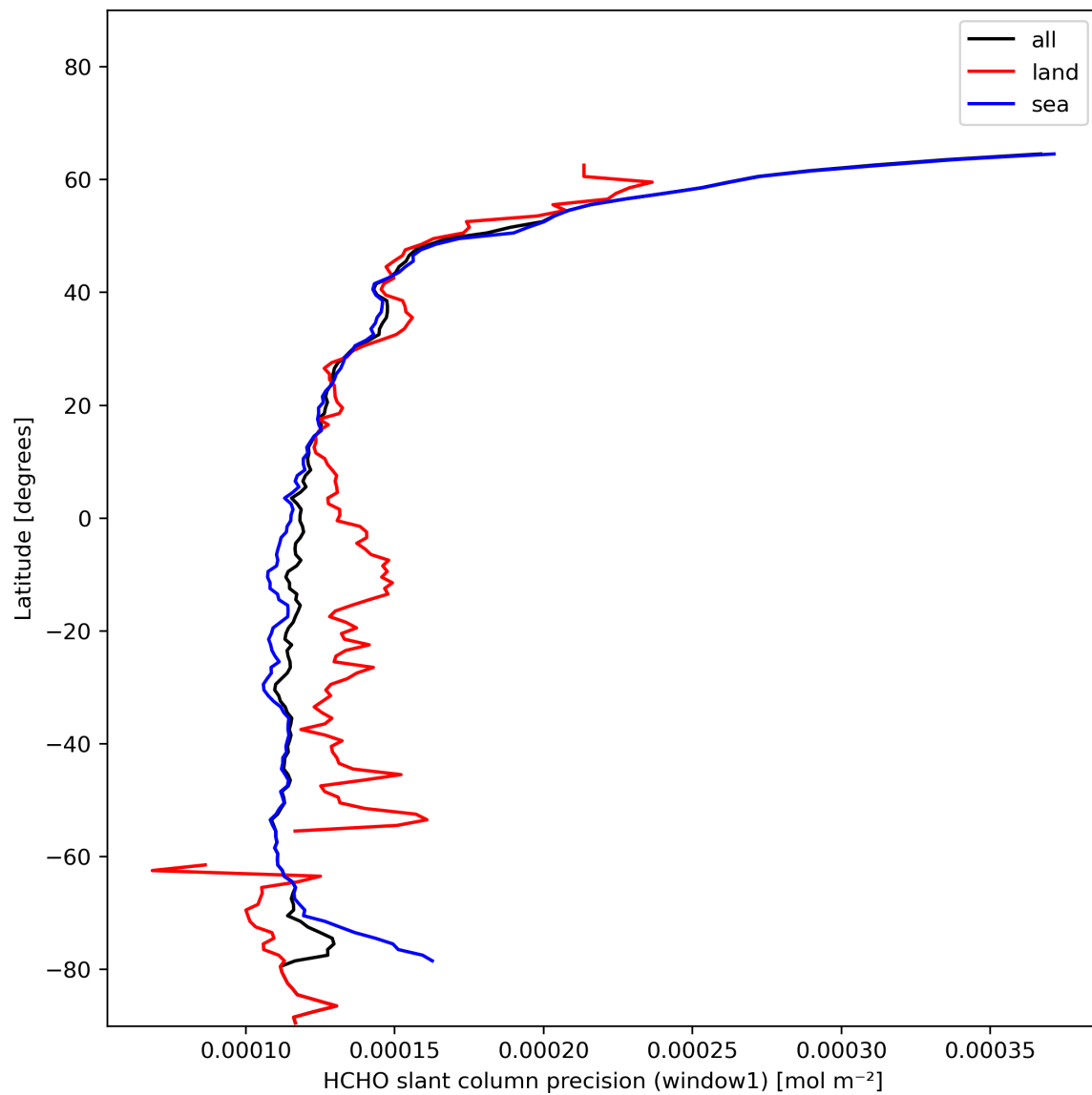
Figure 25: Zonal average of “HCHO slant column precision (window1)” for 2024-01-19 to 2024-01-21.
