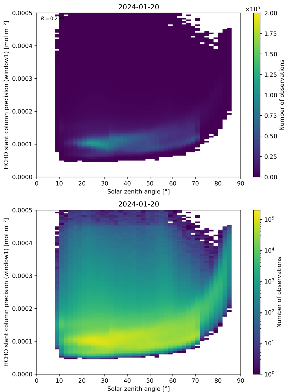
Figure 174: Scatter density plot of “Solar zenith angle” against “HCHO slant column precision (window1)” for 2024-01-19 to 2024-01-21.
