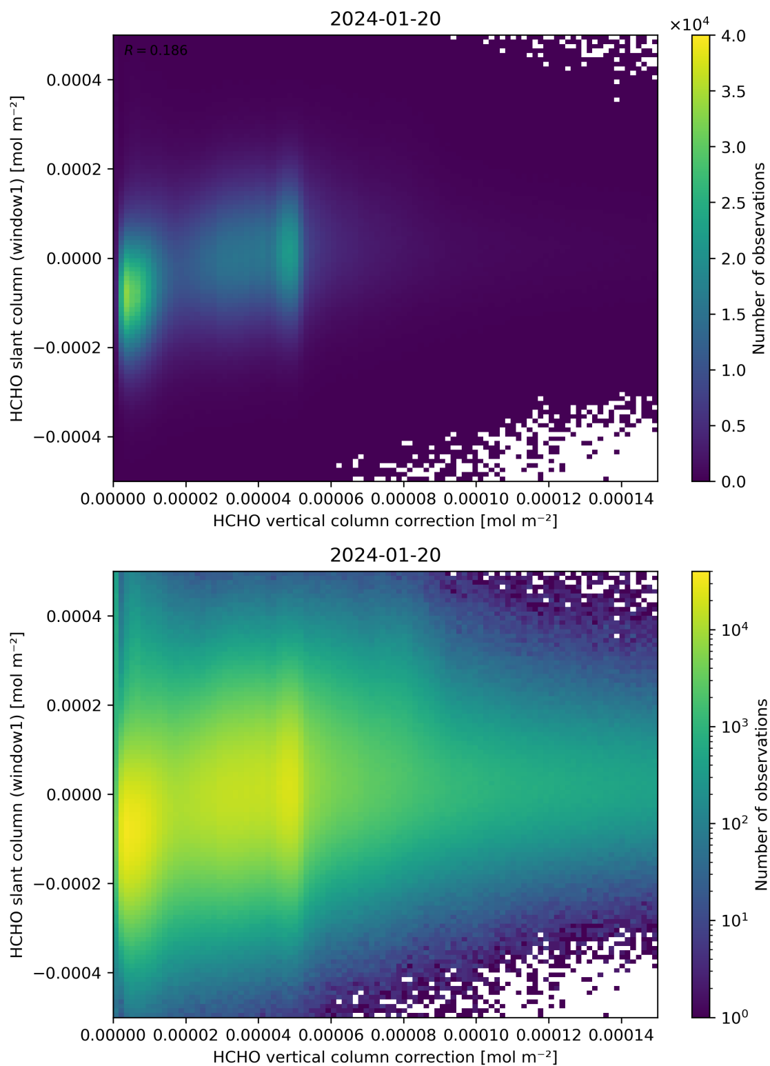
Figure 118: Scatter density plot of “HCHO vertical column correction” against “HCHO slant column (window1)” for 2024-01-19 to 2024-01-21.
