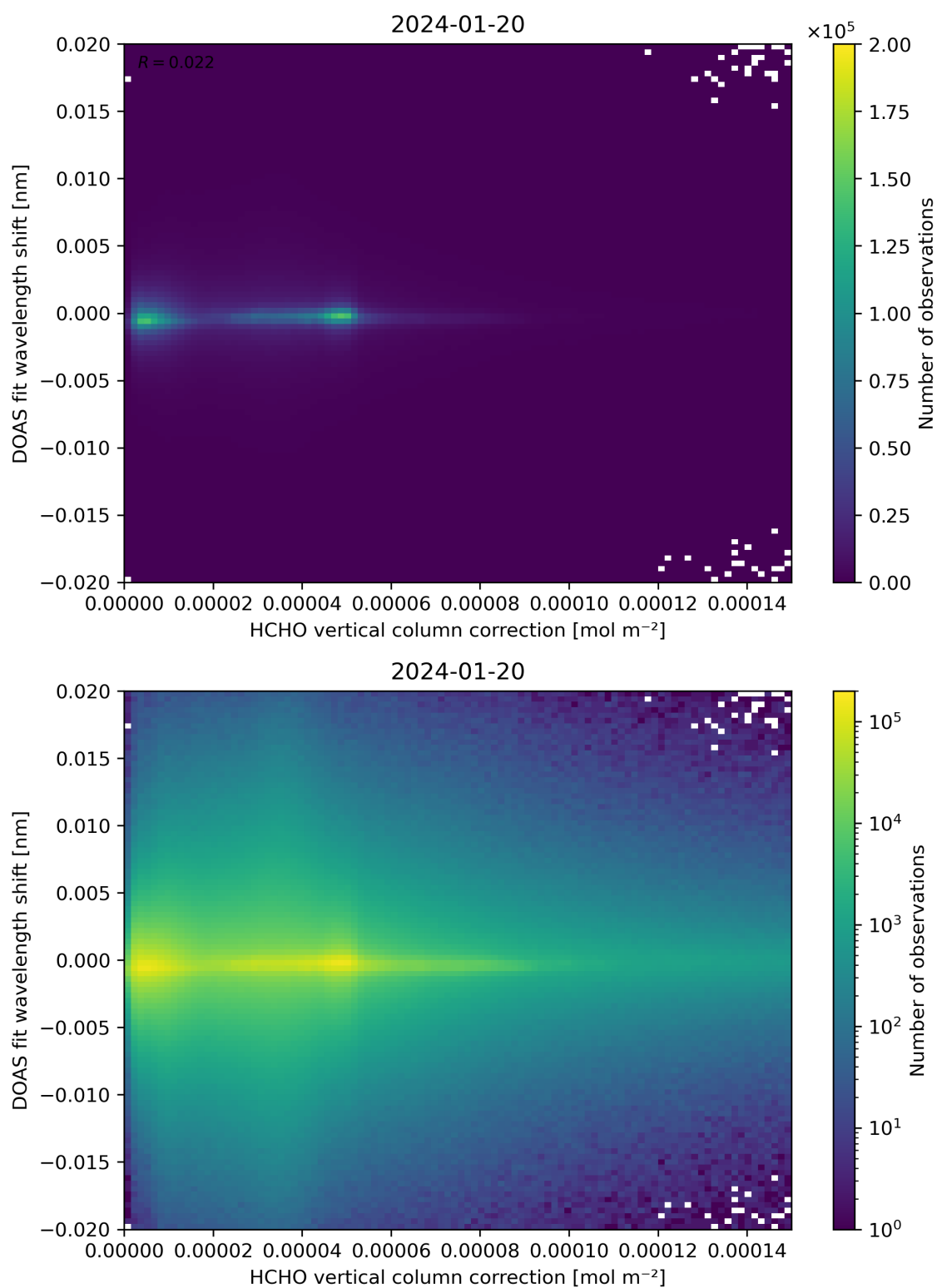
Figure 113: Scatter density plot of “HCHO vertical column correction” against “DOAS fit wavelength shift” for 2024-01-19 to 2024-01-21.
