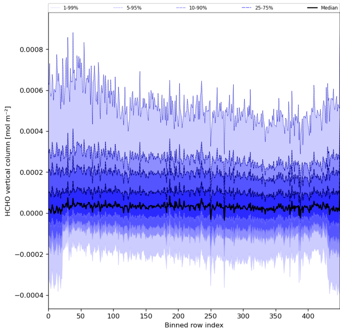
Figure 49: Along track statistics of “HCHO vertical column” for 2024-01-19 to 2024-01-21
