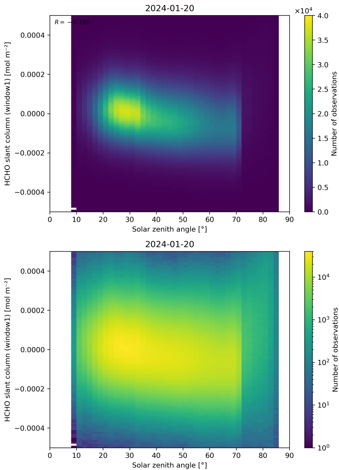
Figure 173: Scatter density plot of “Solar zenith angle” against “HCHO slant column (window1)” for 2024-01-19 to 2024-01-21.
