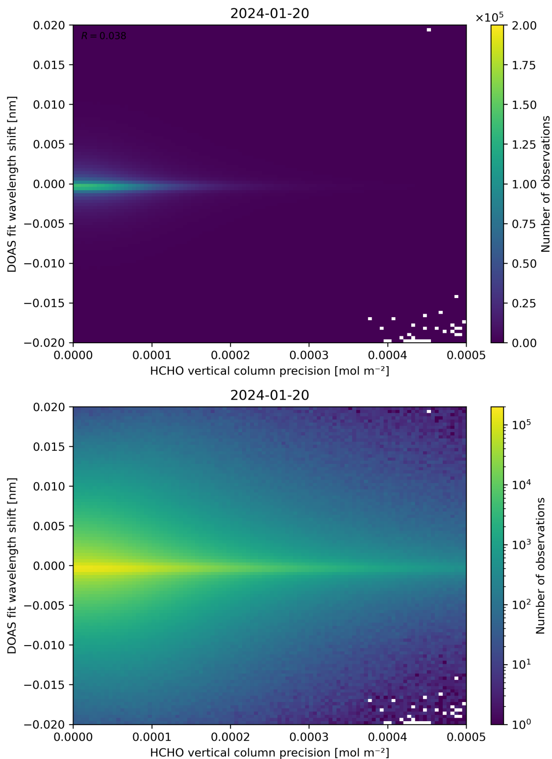
Figure 137: Scatter density plot of “HCHO vertical column precision” against “DOAS fit wavelength shift” for 2024-01-19 to 2024-01-21.
