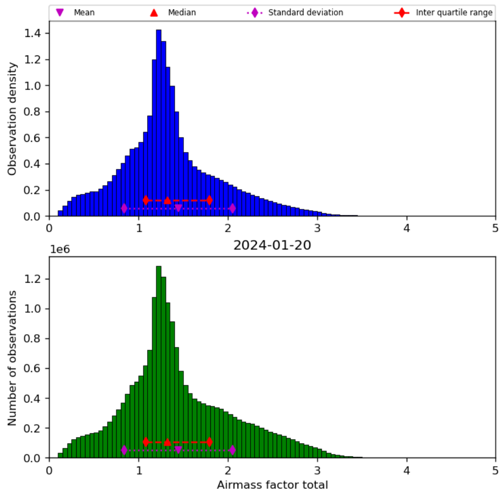
Figure 40: Histogram of “Airmass factor total” for 2024-01-19 to 2024-01-21
