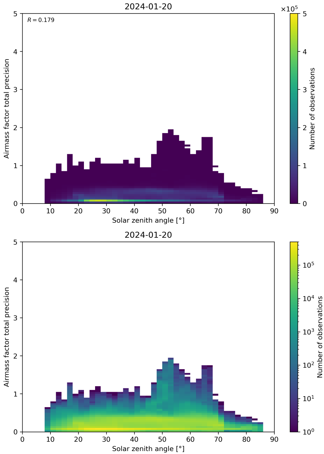
Figure 176: Scatter density plot of “Solar zenith angle” against “Airmass factor total precision” for 2024-01-19 to 2024-01-21.
