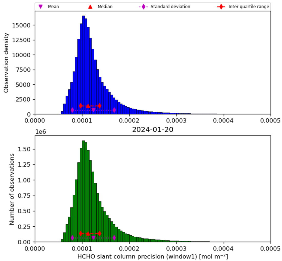
Figure 39: Histogram of “HCHO slant column precision (window1)” for 2024-01-19 to 2024-01-21
