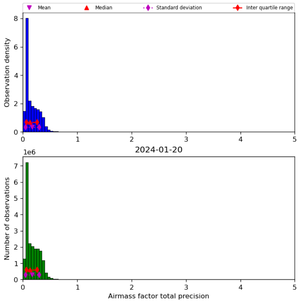
Figure 41: Histogram of “Airmass factor total precision” for 2024-01-19 to 2024-01-21
