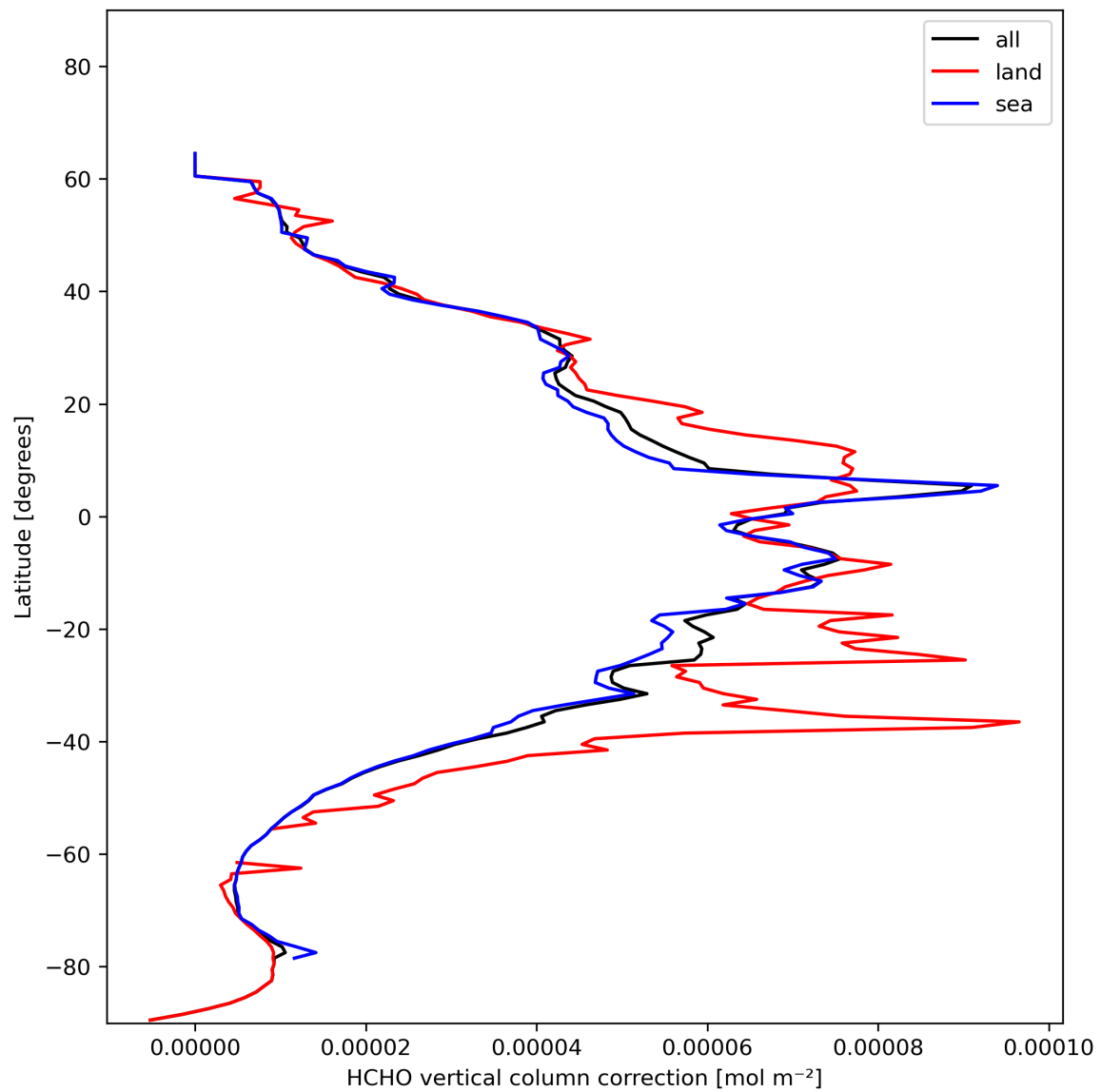
Figure 23: Zonal average of “HCHO vertical column correction” for 2024-01-19 to 2024-01-21.
