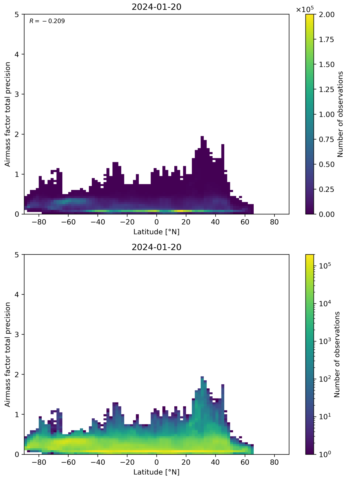
Figure 162: Scatter density plot of “Latitude” against “Airmass factor total precision” for 2024-01-19 to 2024-01-21.
