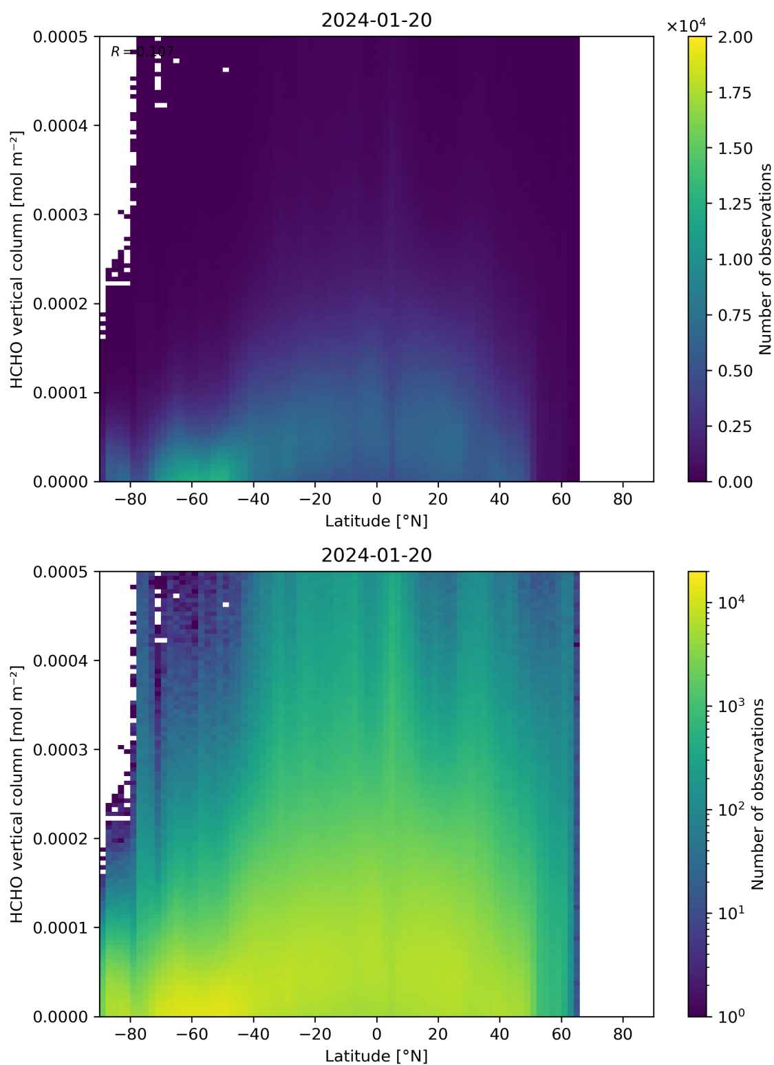
Figure 163: Scatter density plot of “Latitude” against “HCHO vertical column” for 2024-01-19 to 2024-01-21.
