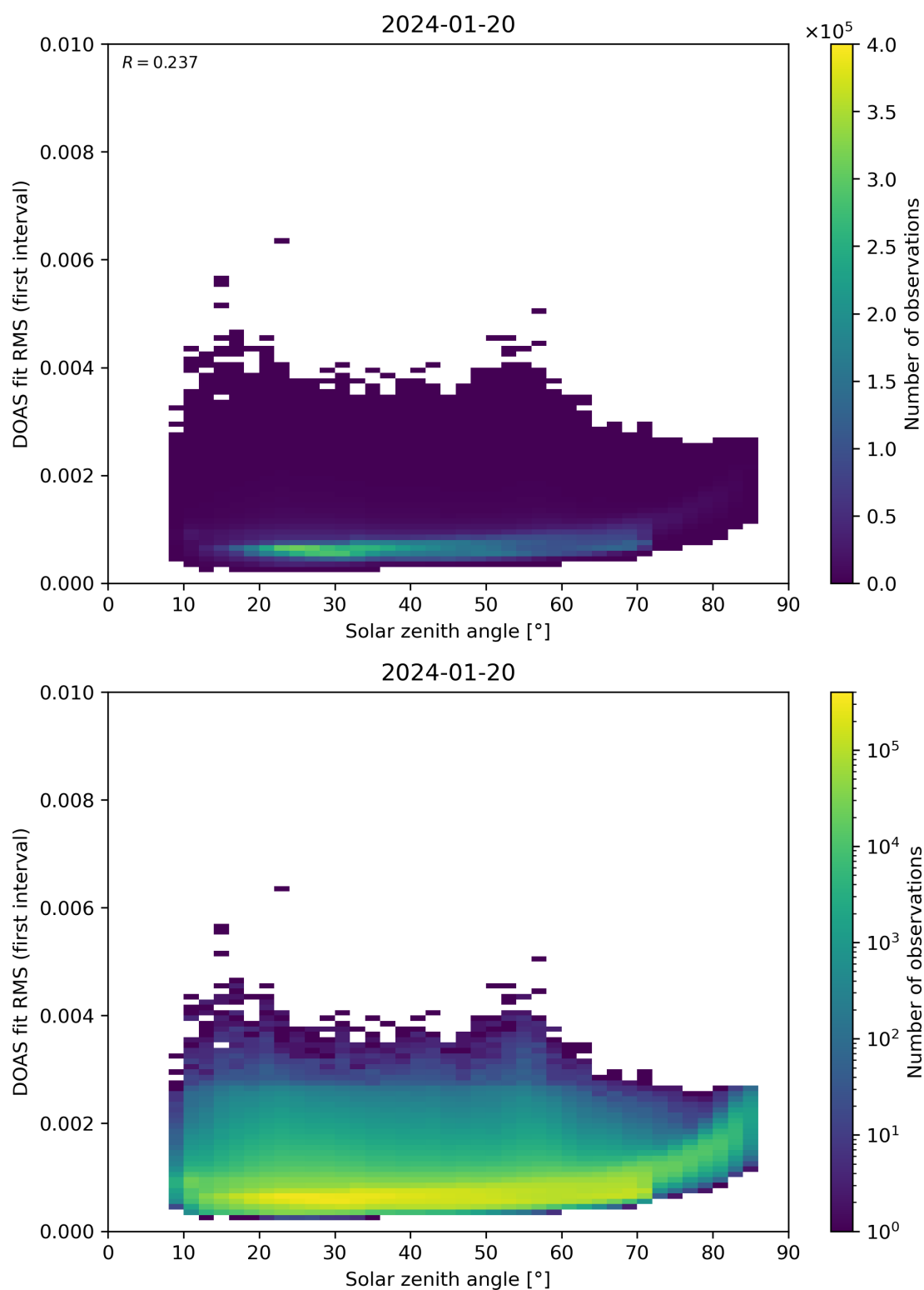
Figure 167: Scatter density plot of “Solar zenith angle” against “DOAS fit RMS (first interval)” for 2024-01-19 to 2024-01-21.
