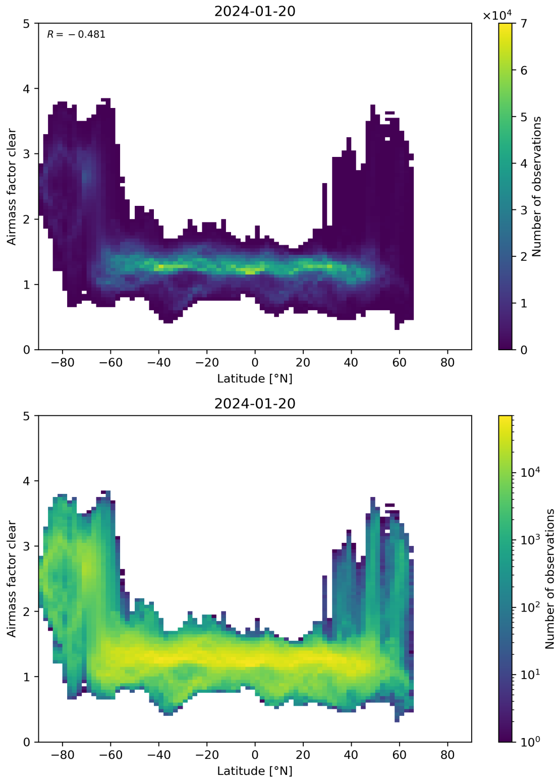
Figure 156: Scatter density plot of “Latitude” against “Airmass factor clear” for 2024-01-19 to 2024-01-21.
