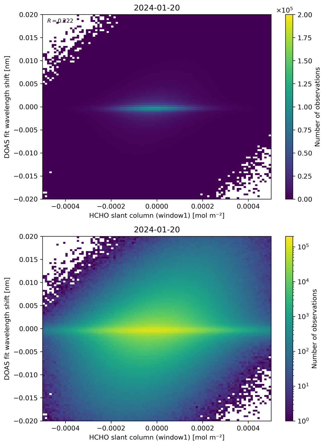
Figure 79: Scatter density plot of “HCHO slant column (window1)” against “DOAS fit wavelength shift” for 2024-01-19 to 2024-01-21.
