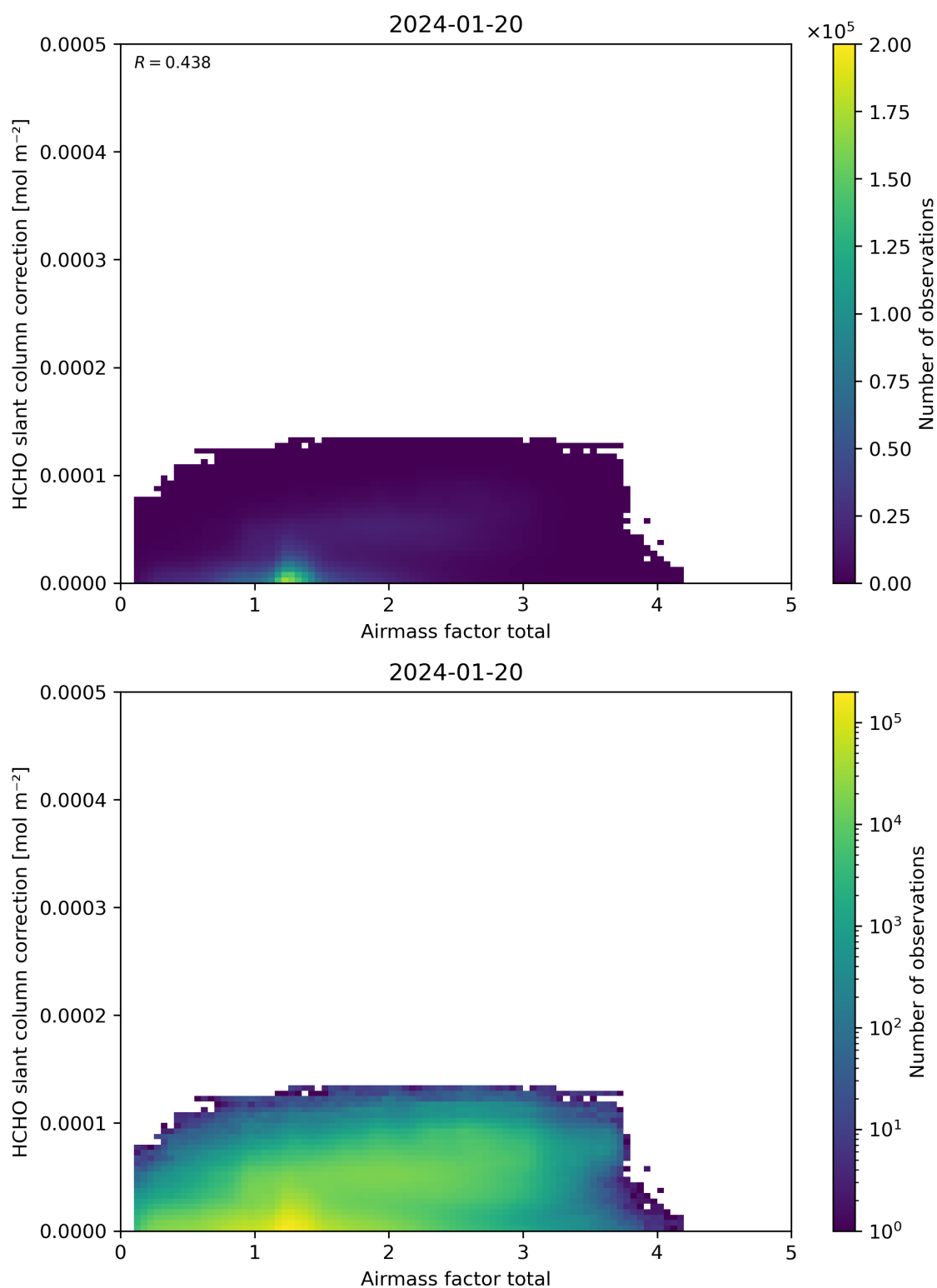
Figure 102: Scatter density plot of “Airmass factor total” against “HCHO slant column correction” for 2024-01-19 to 2024-01-21.
