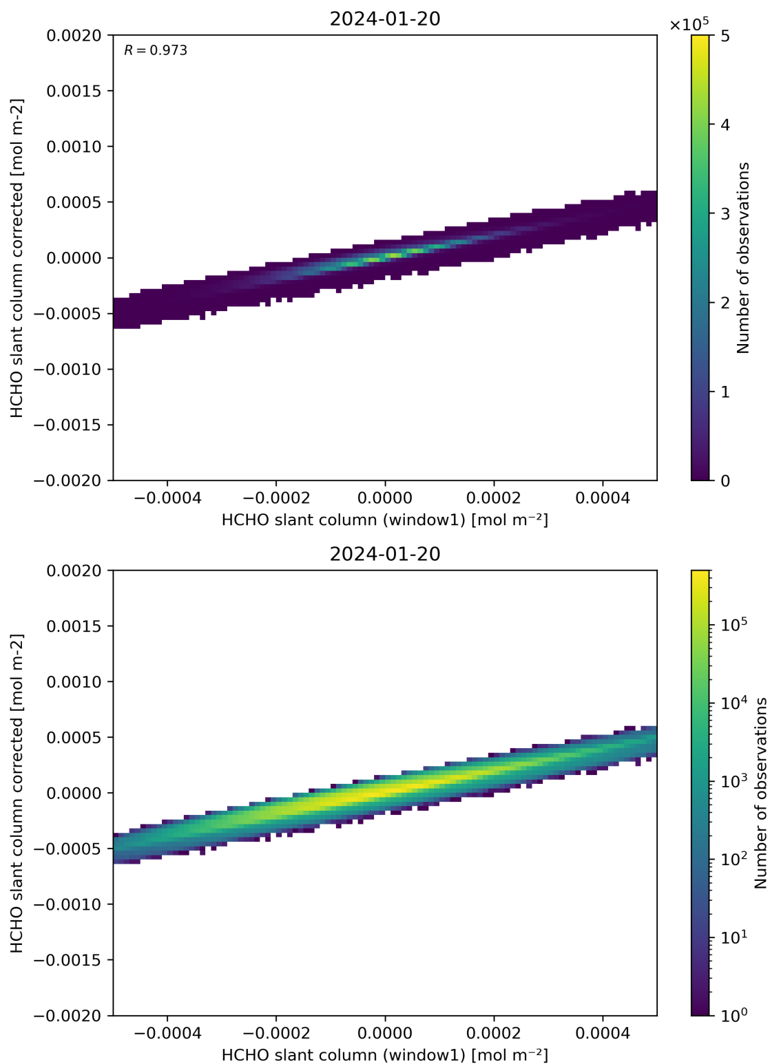
Figure 82: Scatter density plot of “HCHO slant column (window1)” against “HCHO slant column corrected” for 2024-01-19 to 2024-01-21.
