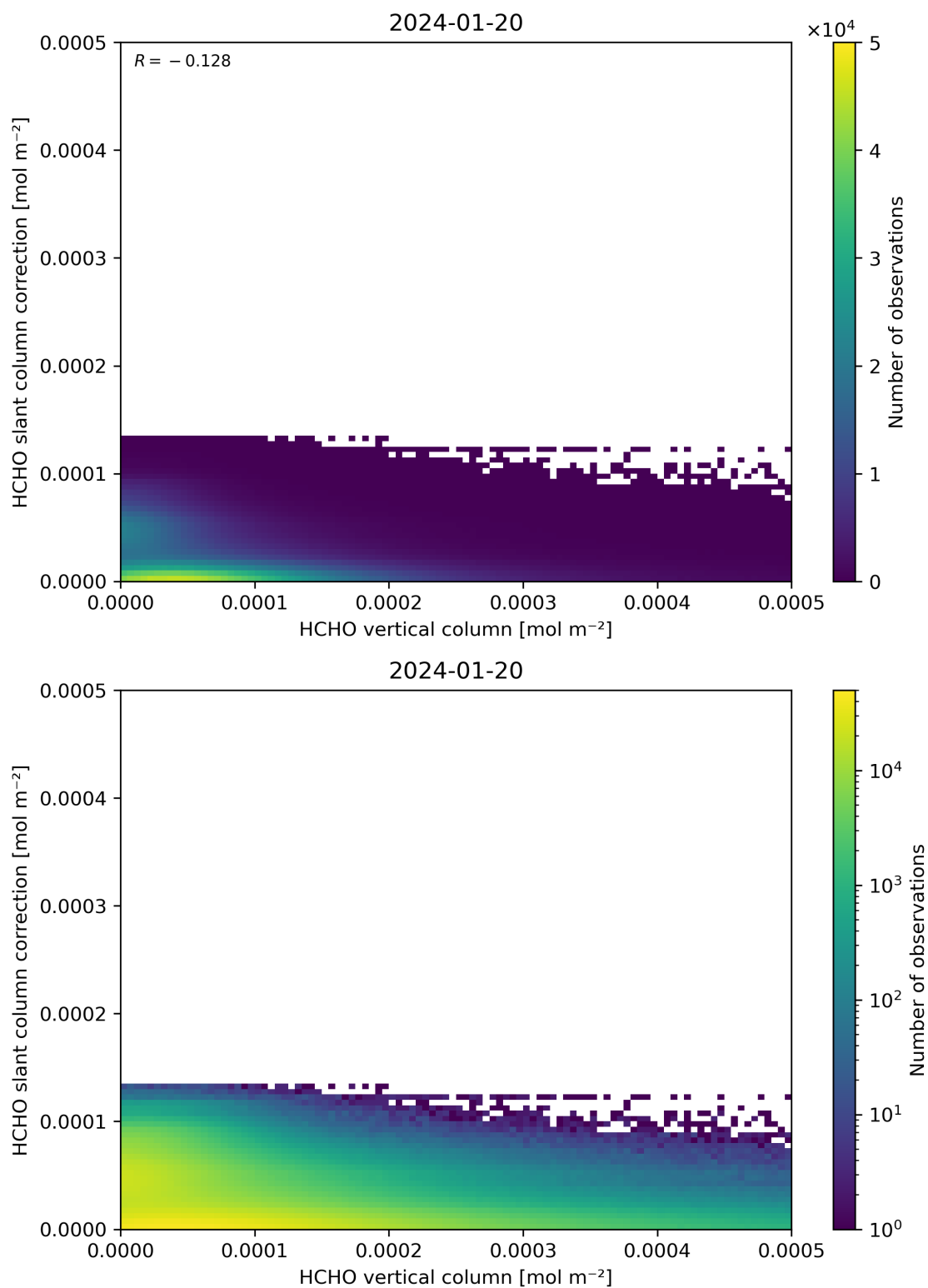
Figure 128: Scatter density plot of “HCHO vertical column” against “HCHO slant column correction” for 2024-01-19 to 2024-01-21.
