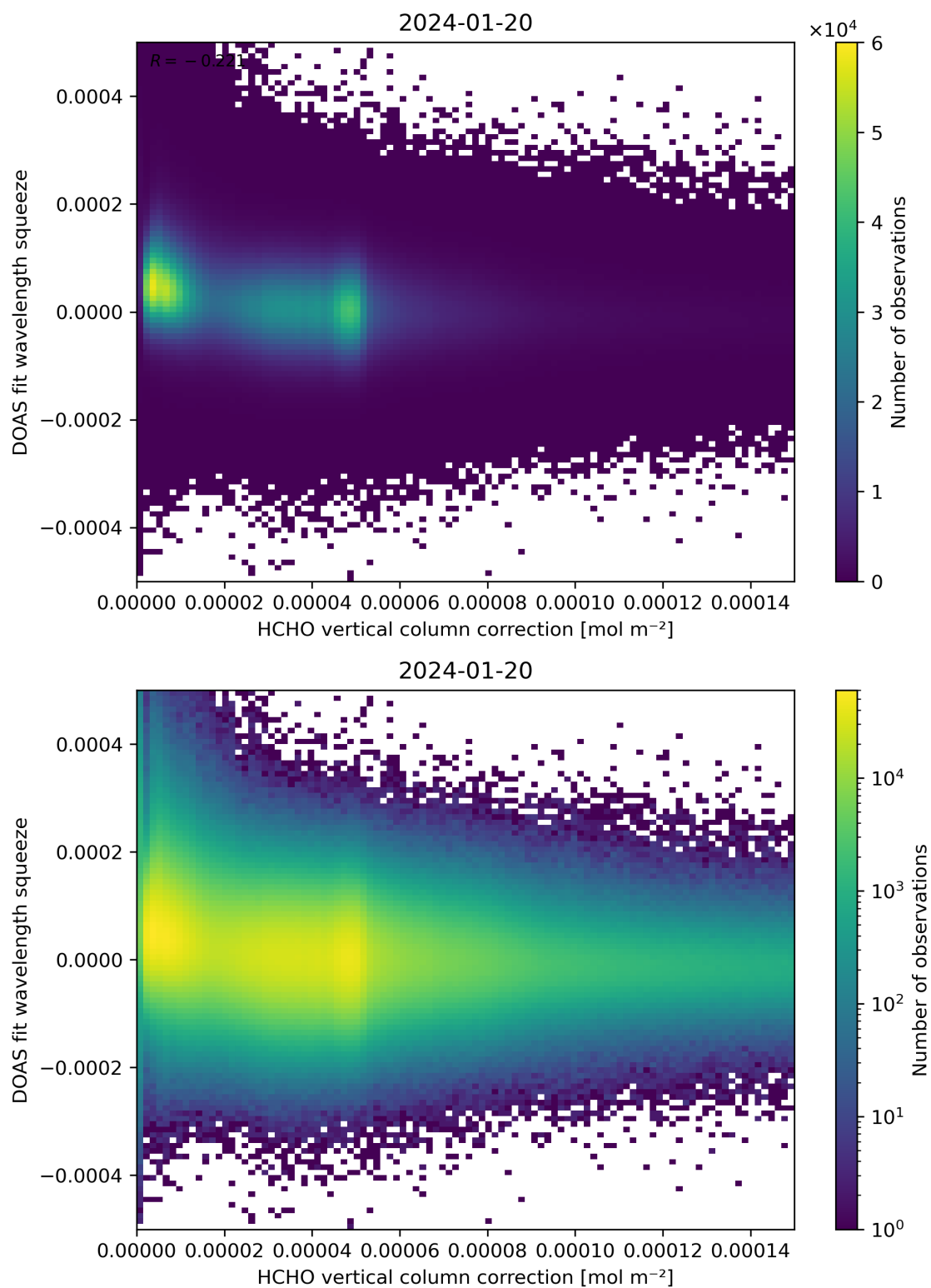
Figure 114: Scatter density plot of “HCHO vertical column correction” against “DOAS fit wavelength squeeze” for 2024-01-19 to 2024-01-21.
