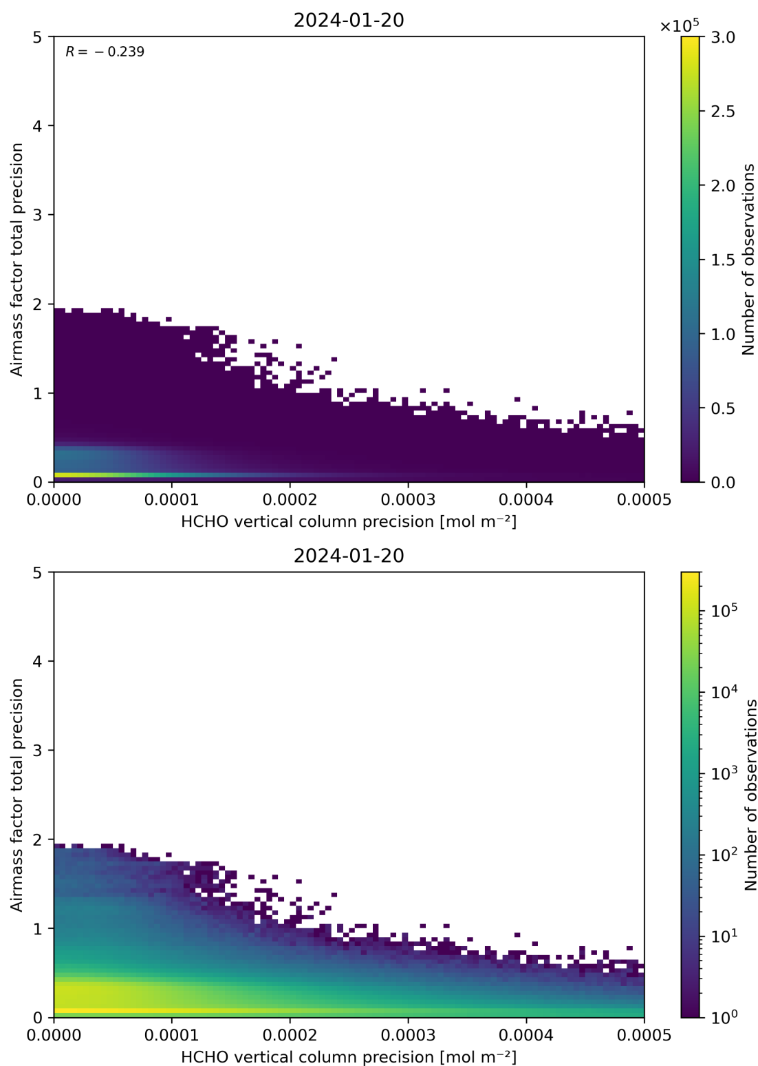
Figure 145: Scatter density plot of “HCHO vertical column precision” against “Airmass factor total precision” for 2024-01-19 to 2024-01-21.
