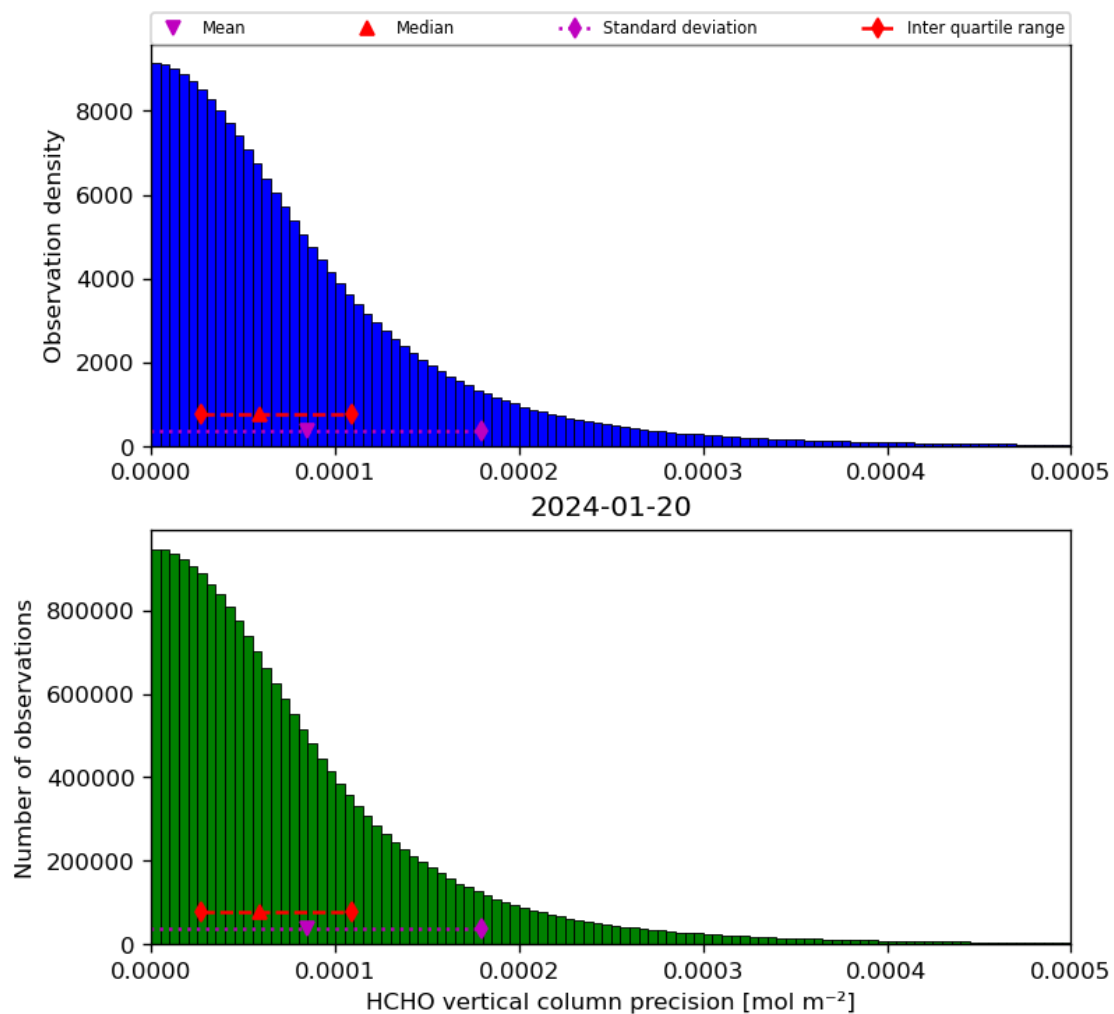
Figure 36: Histogram of “HCHO vertical column precision” for 2024-01-19 to 2024-01-21
