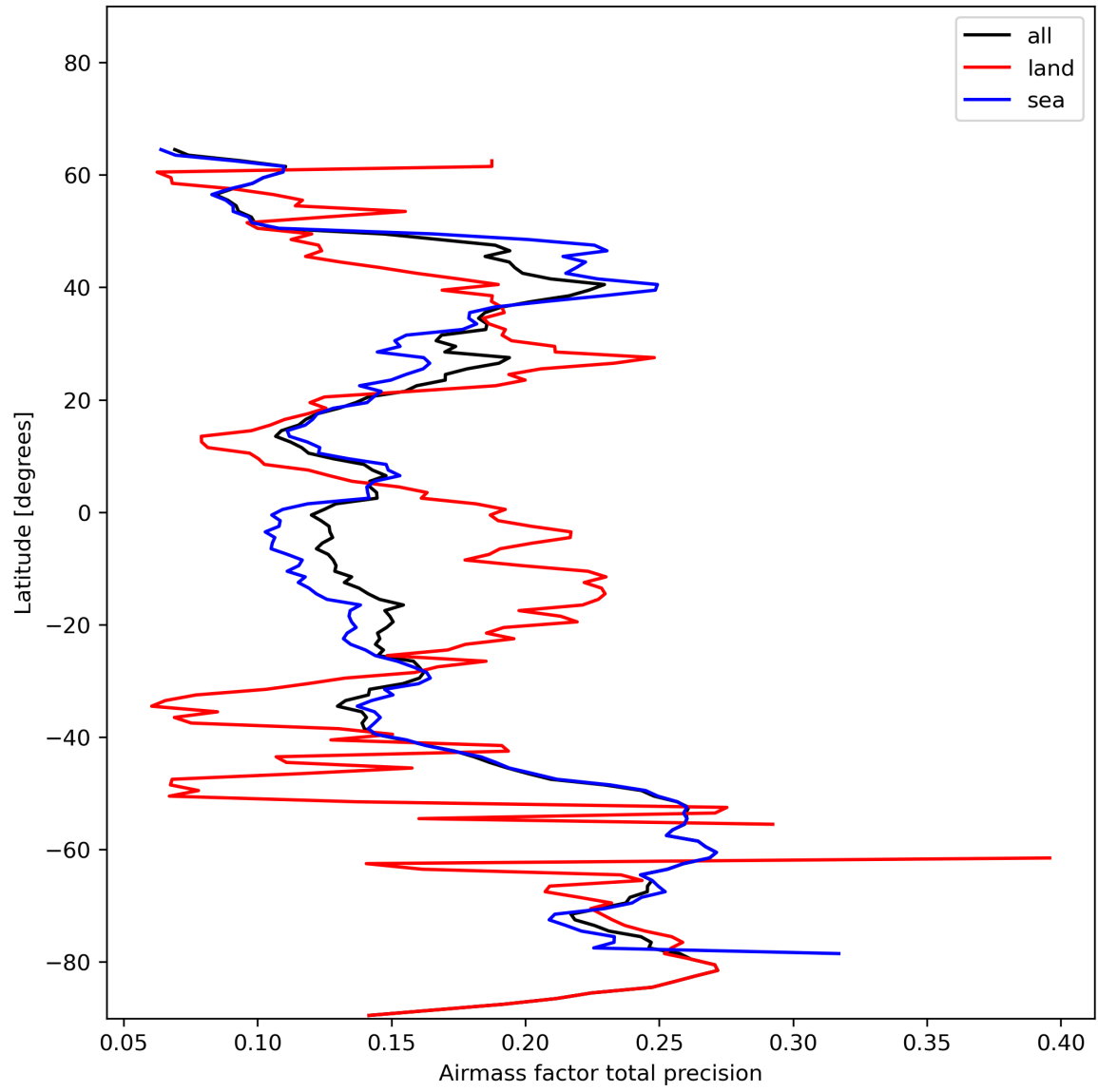
Figure 27: Zonal average of “Airmass factor total precision” for 2024-01-19 to 2024-01-21.
