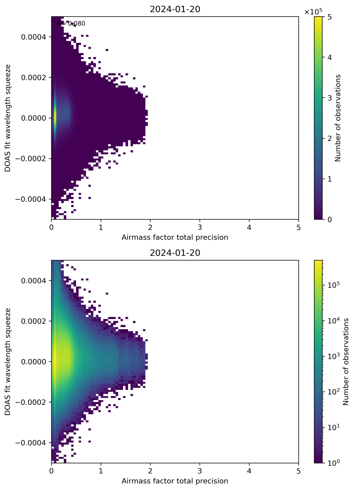
Figure 107: Scatter density plot of “Airmass factor total precision” against “DOAS fit wavelength squeeze” for 2024-01-19 to 2024-01-21.
