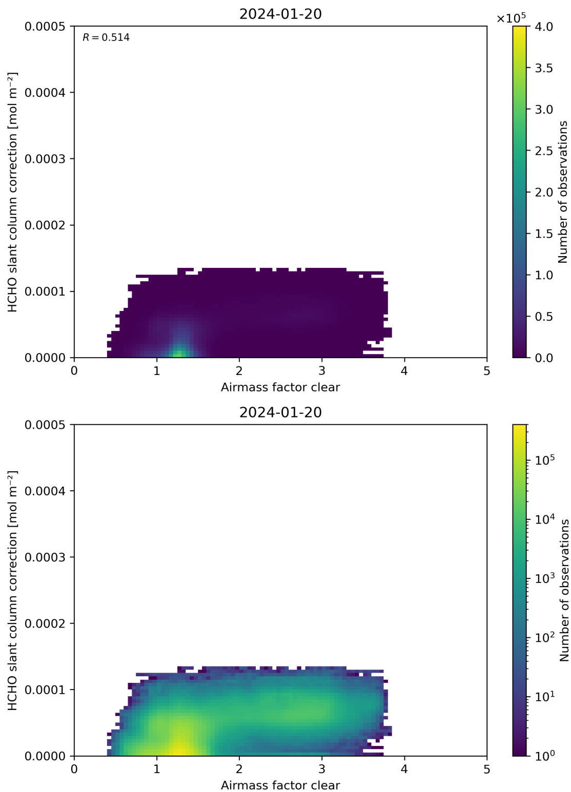
Figure 75: Scatter density plot of “Airmass factor clear” against “HCHO slant column correction” for 2024-01-19 to 2024-01-21.
