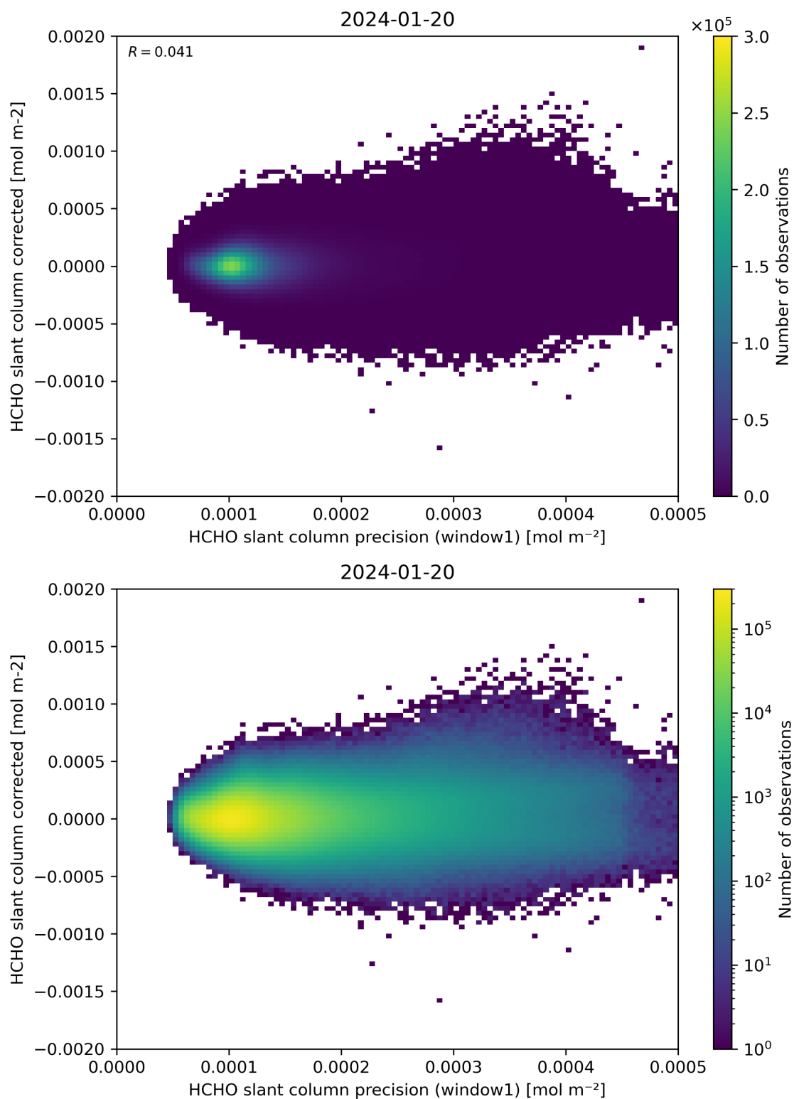
Figure 92: Scatter density plot of “HCHO slant column precision (window1)” against “HCHO slant column corrected” for 2024-01-19 to 2024-01-21.
