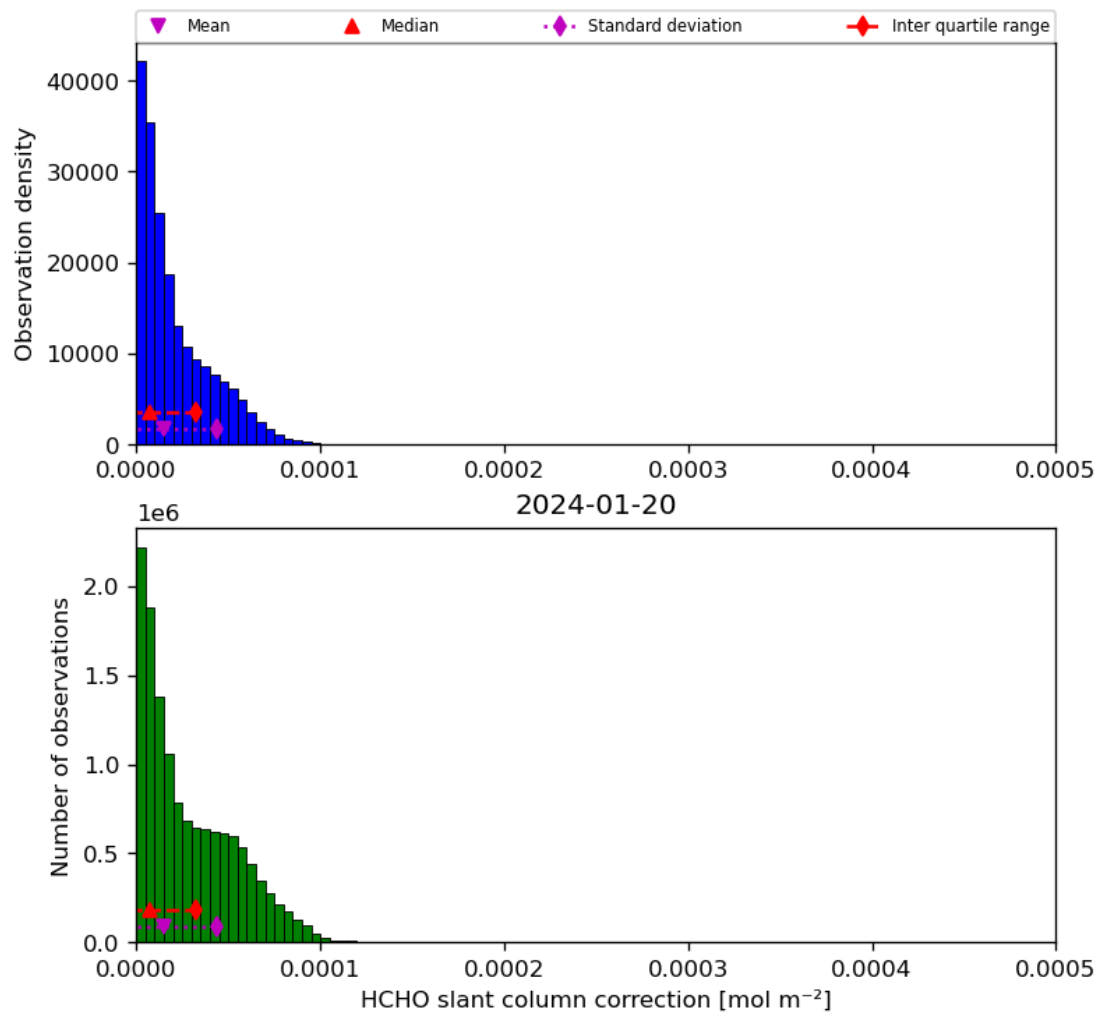
Figure 47: Histogram of “HCHO slant column correction” for 2024-01-19 to 2024-01-21
