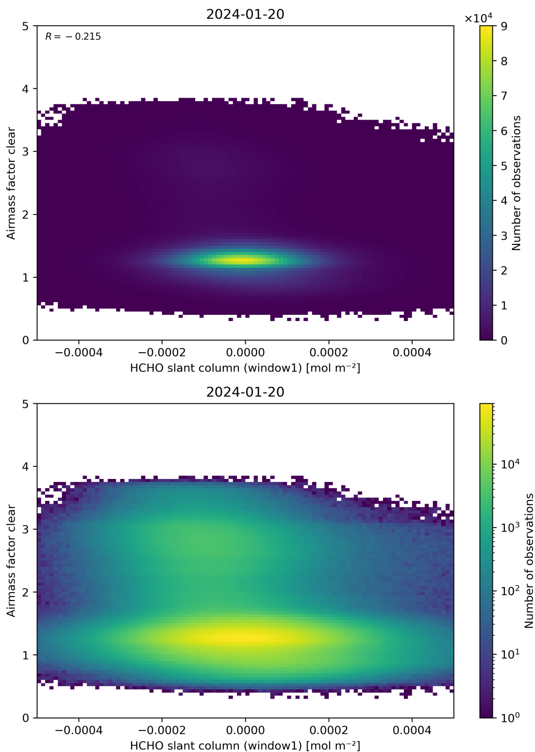
Figure 81: Scatter density plot of “HCHO slant column (window1)” against “Airmass factor clear” for 2024-01-19 to 2024-01-21.
