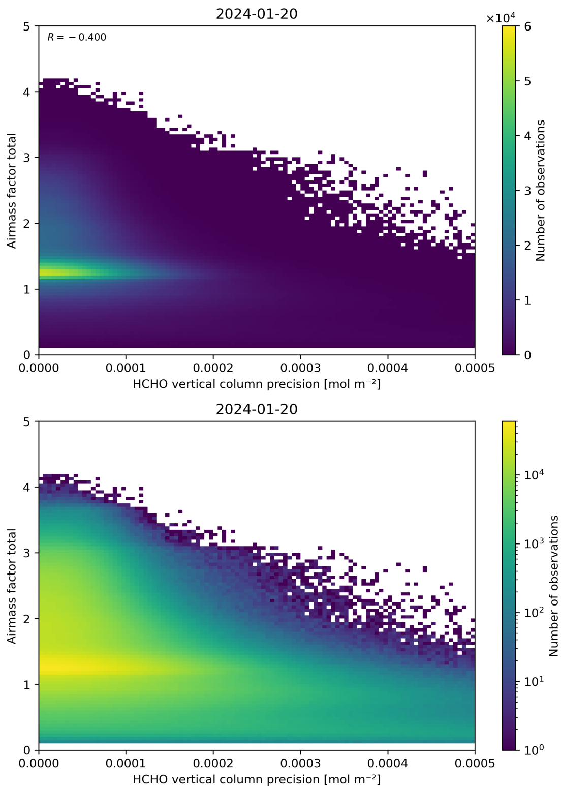
Figure 144: Scatter density plot of “HCHO vertical column precision” against “Airmass factor total” for 2024-01-19 to 2024-01-21.
