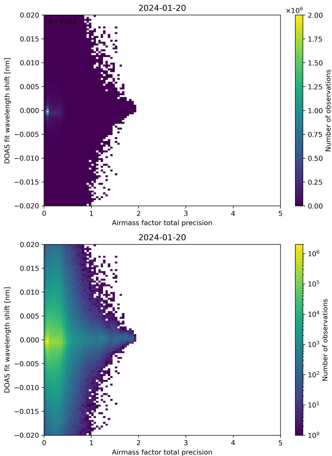
Figure 106: Scatter density plot of “Airmass factor total precision” against “DOAS fit wavelength shift” for 2024-01-19 to 2024-01-21.
