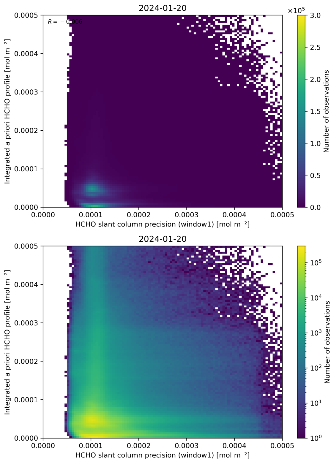
Figure 96: Scatter density plot of “HCHO slant column precision (window1)” against “Integrated a priori HCHO profile” for 2024-01-19 to 2024-01-21.
