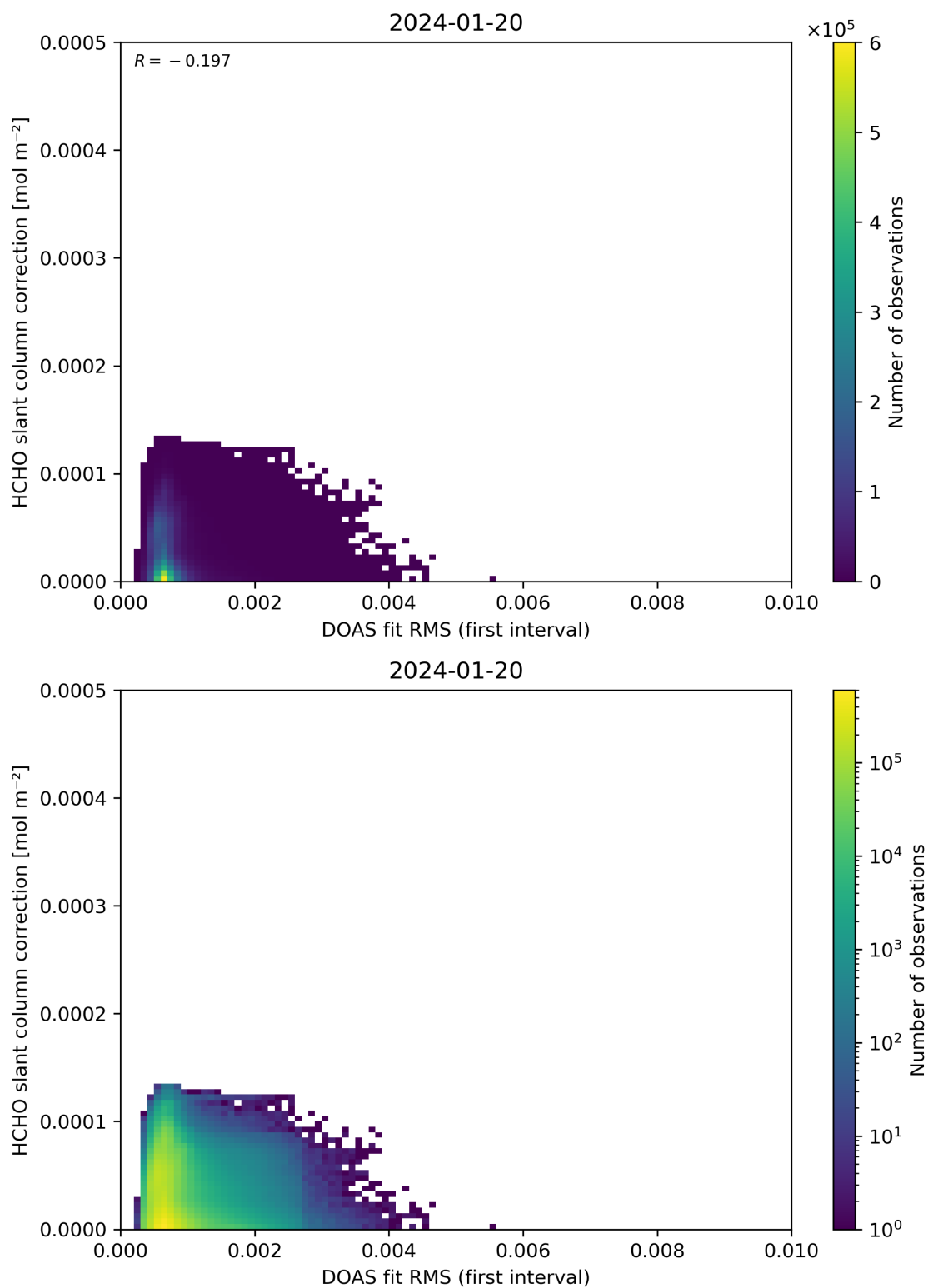
Figure 63: Scatter density plot of “DOAS fit RMS (first interval)” against “HCHO slant column correction” for 2024-01-19 to 2024-01-21.
