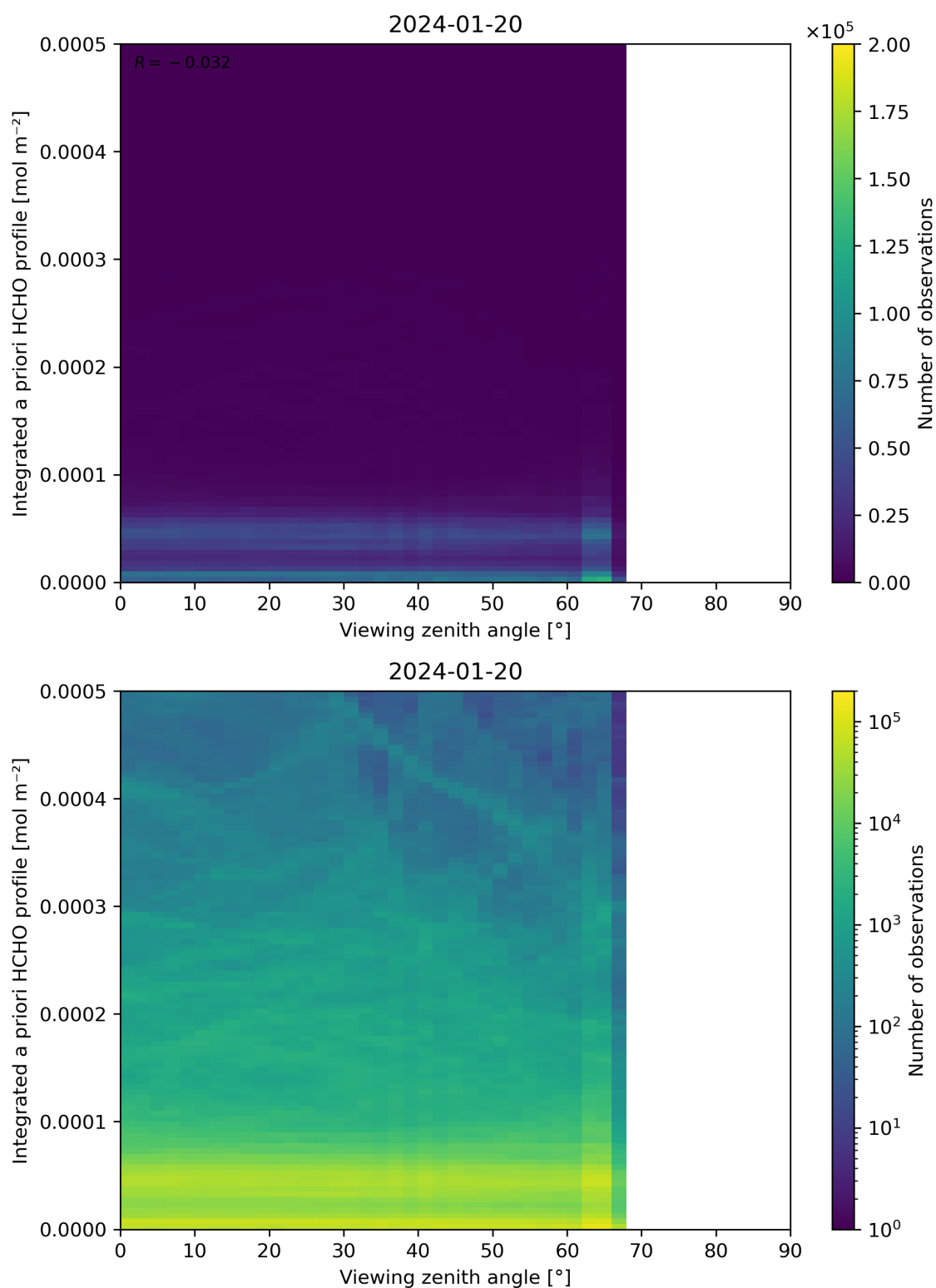
Figure 195: Scatter density plot of “Viewing zenith angle” against “Integrated a priori HCHO profile” for 2024-01-19 to 2024-01-21.
