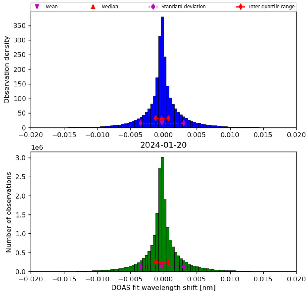
Figure 44: Histogram of “DOAS fit wavelength shift” for 2024-01-19 to 2024-01-21
