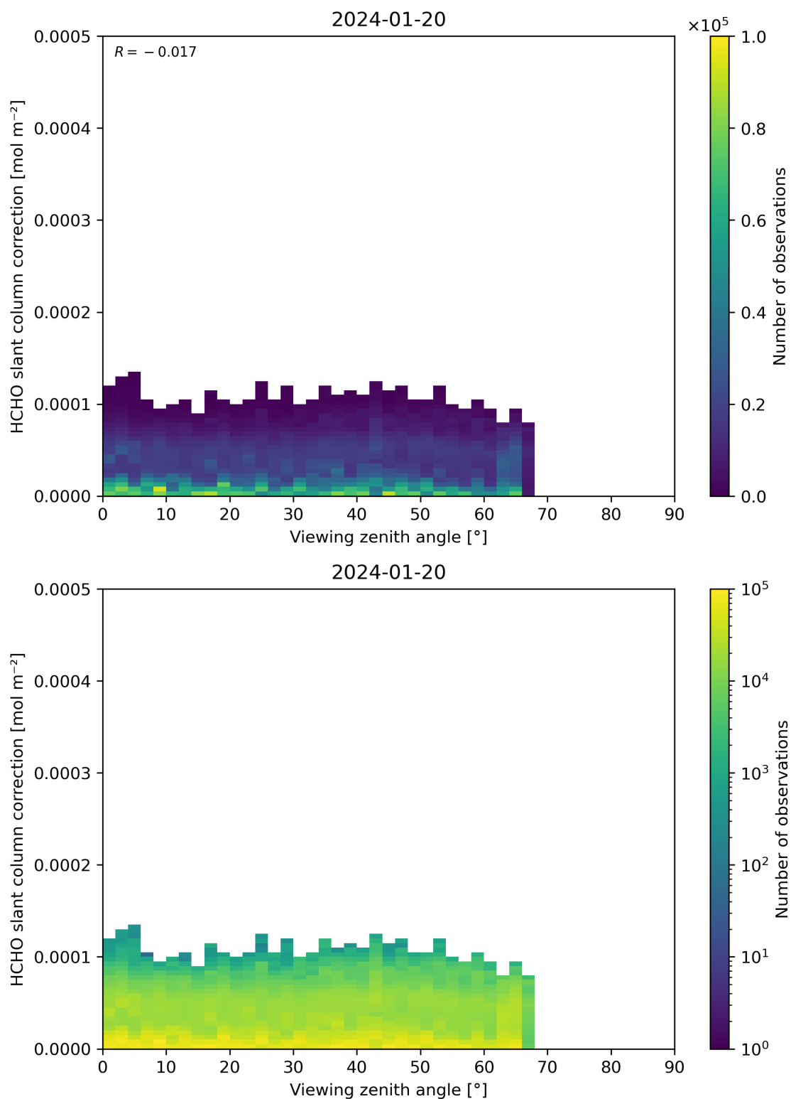
Figure 187: Scatter density plot of “Viewing zenith angle” against “HCHO slant column correction” for 2024-01-19 to 2024-01-21.
