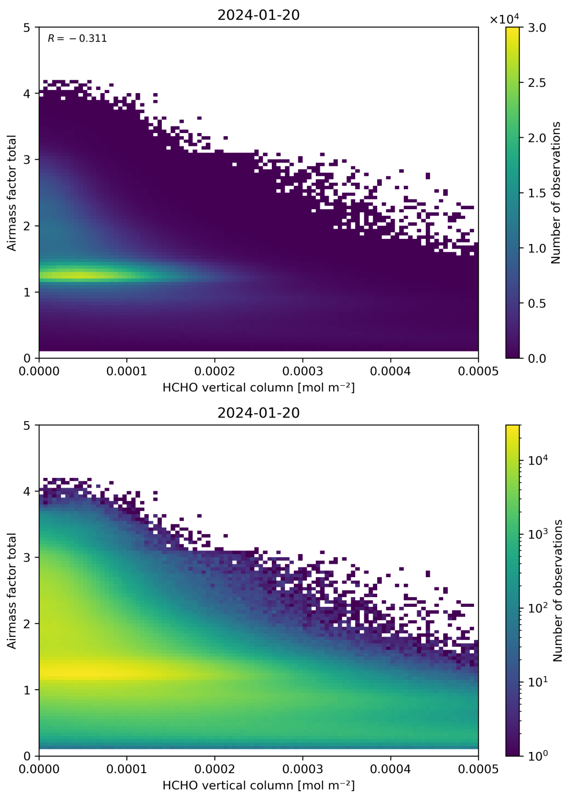
Figure 131: Scatter density plot of “HCHO vertical column” against “Airmass factor total” for 2024-01-19 to 2024-01-21.
