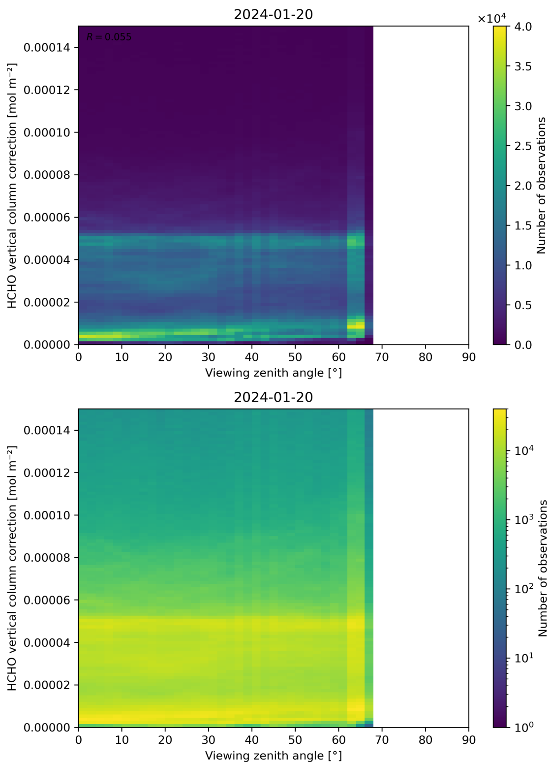
Figure 193: Scatter density plot of “Viewing zenith angle” against “HCHO vertical column correction” for 2024-01-19 to 2024-01-21.
