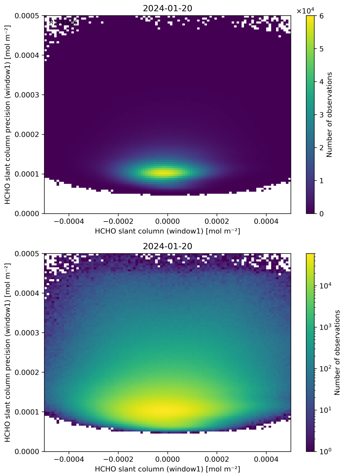
Figure 84: Scatter density plot of “HCHO slant column (window1)” against “HCHO slant column precision (window1)” for 2024-01-19 to 2024-01-21.
