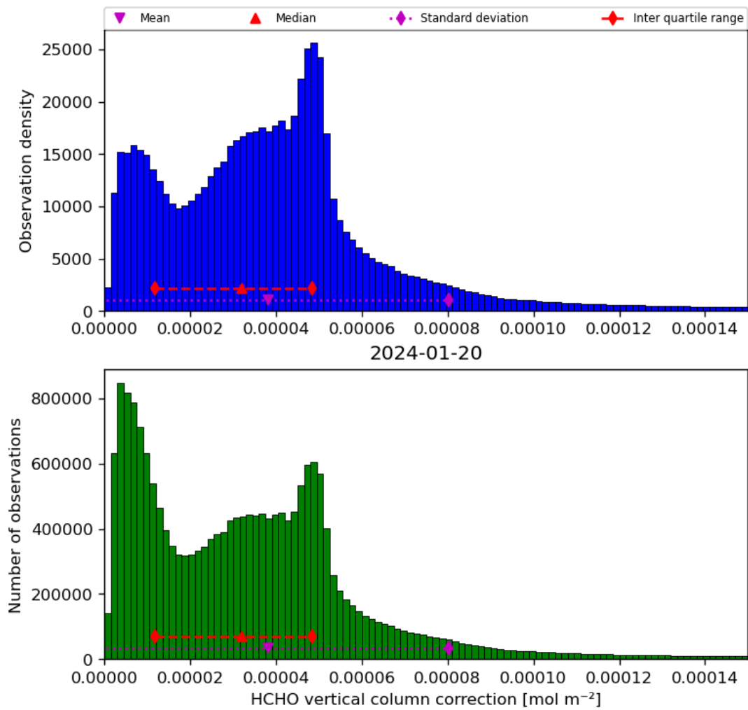
Figure 37: Histogram of “HCHO vertical column correction” for 2024-01-19 to 2024-01-21
