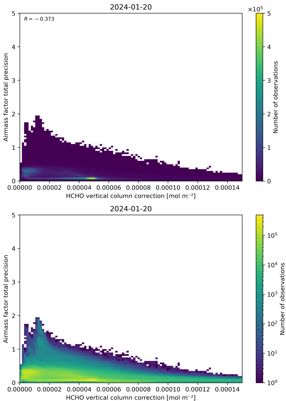
Figure 121: Scatter density plot of “HCHO vertical column correction” against “Airmass factor total precision” for 2024-01-19 to 2024-01-21.
