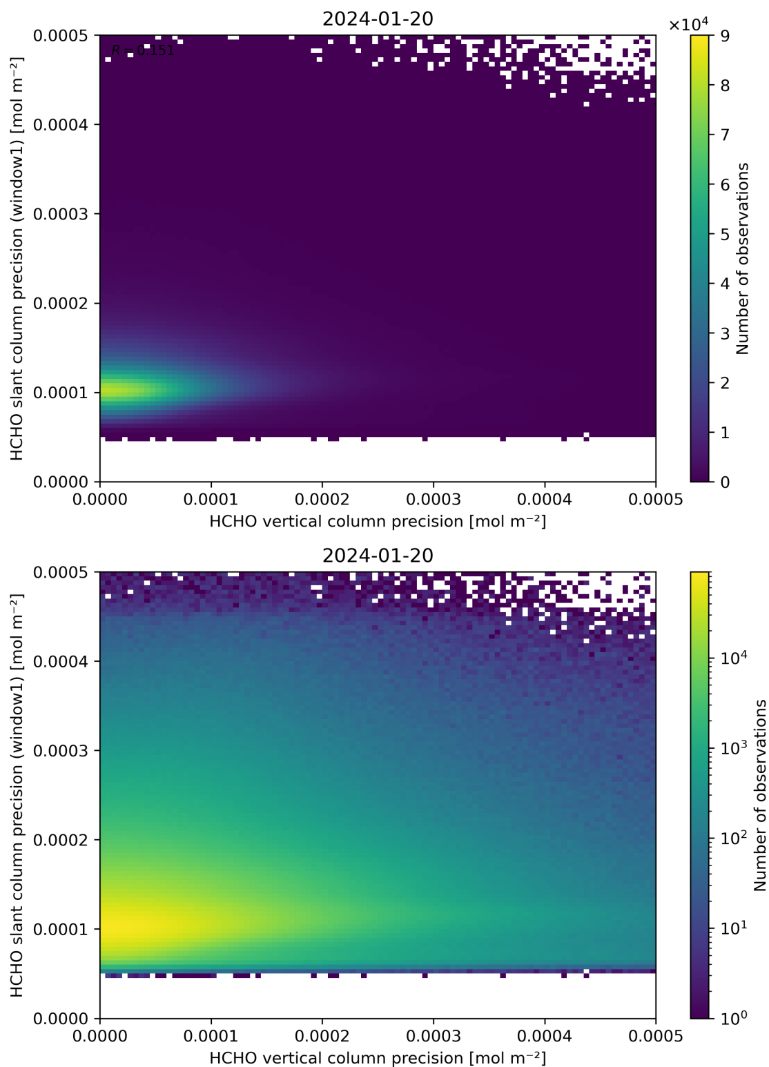
Figure 143: Scatter density plot of “HCHO vertical column precision” against “HCHO slant column precision (window1)” for 2024-01-19 to 2024-01-21.
