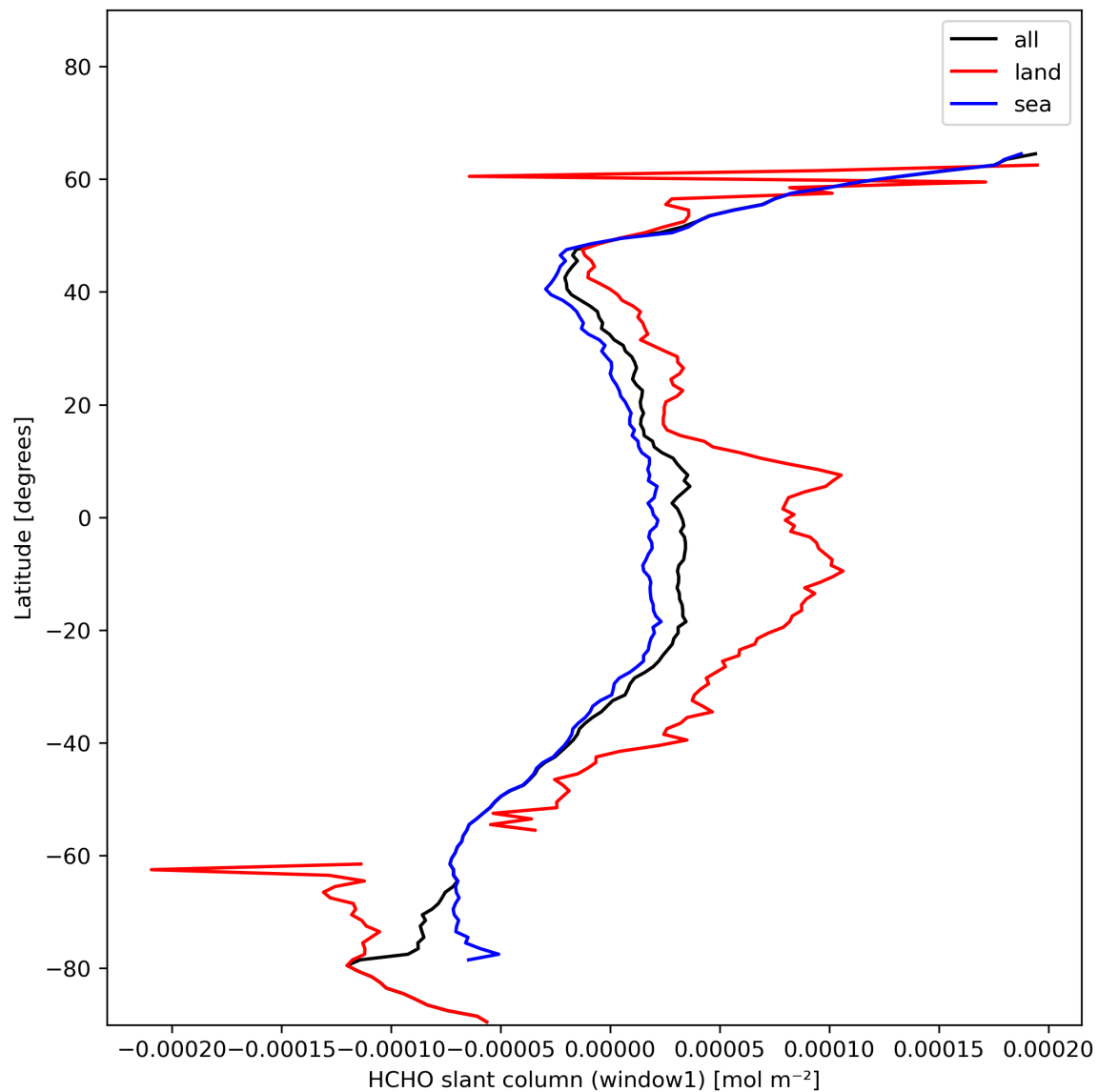
Figure 24: Zonal average of “HCHO slant column (window1)” for 2024-01-19 to 2024-01-21.
