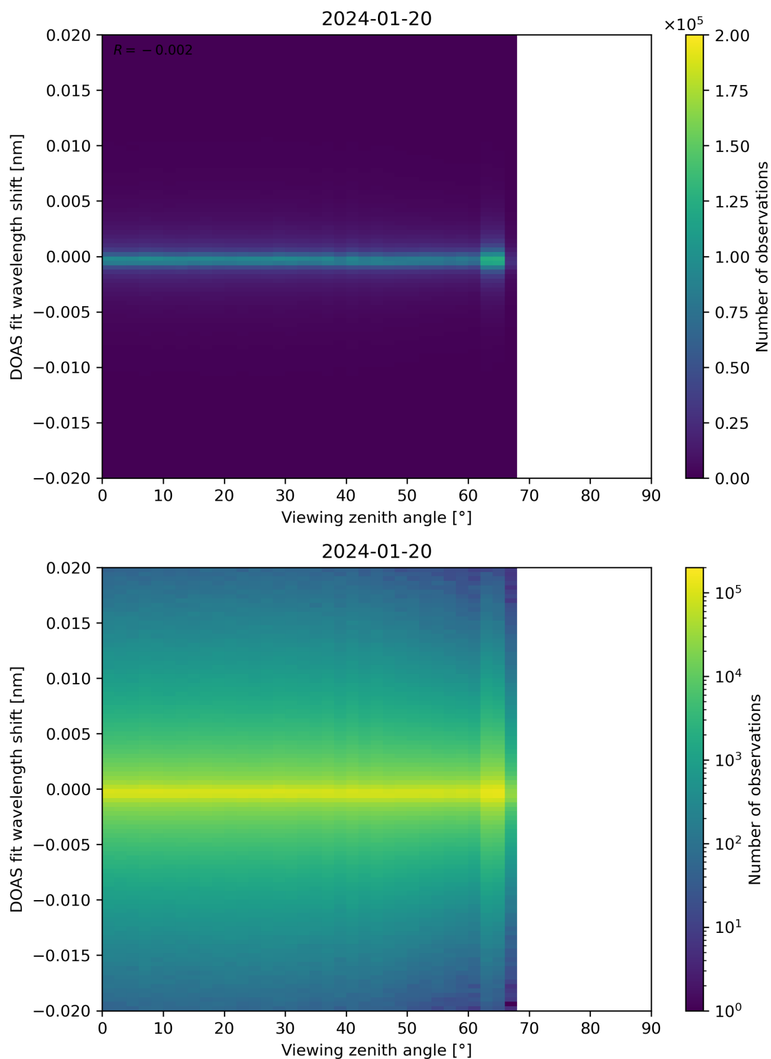
Figure 183: Scatter density plot of “Viewing zenith angle” against “DOAS fit wavelength shift” for 2024-01-19 to 2024-01-21.
