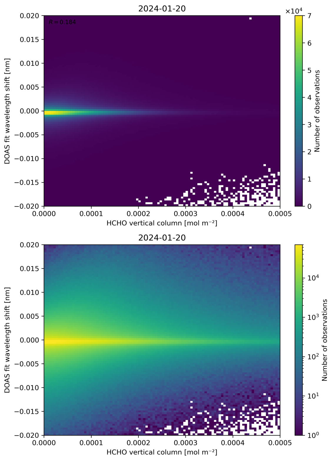
Figure 124: Scatter density plot of “HCHO vertical column” against “DOAS fit wavelength shift” for 2024-01-19 to 2024-01-21.
