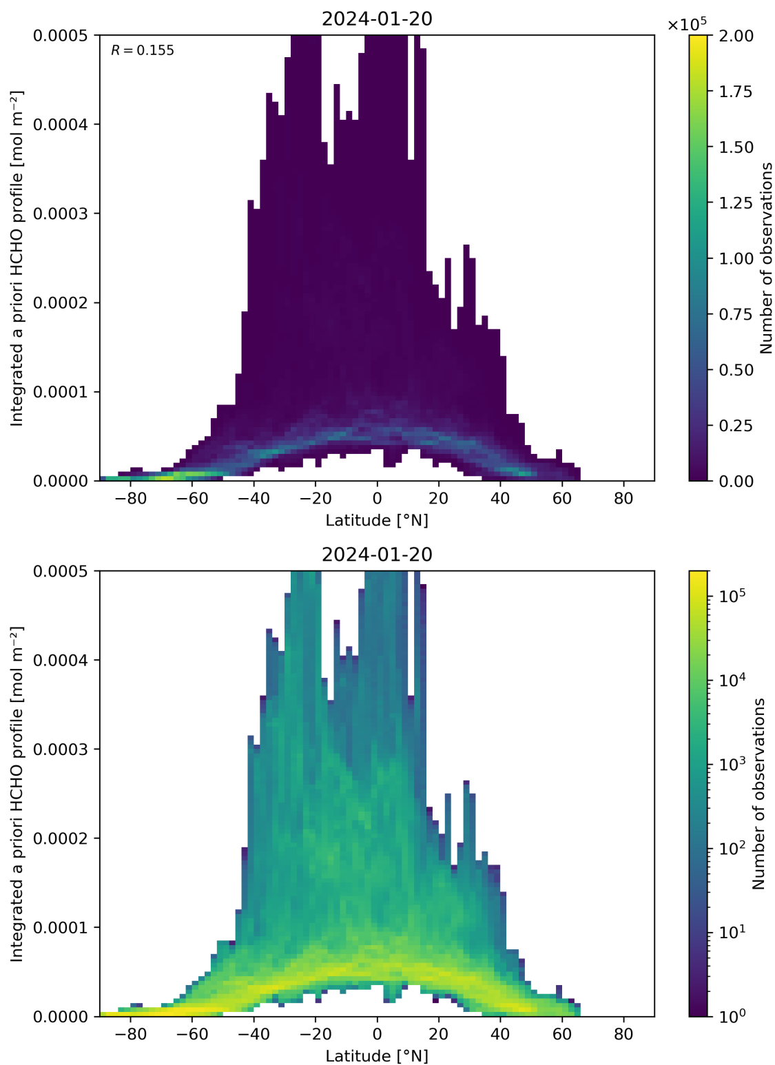
Figure 166: Scatter density plot of “Latitude” against “Integrated a priori HCHO profile” for 2024-01-19 to 2024-01-21.
