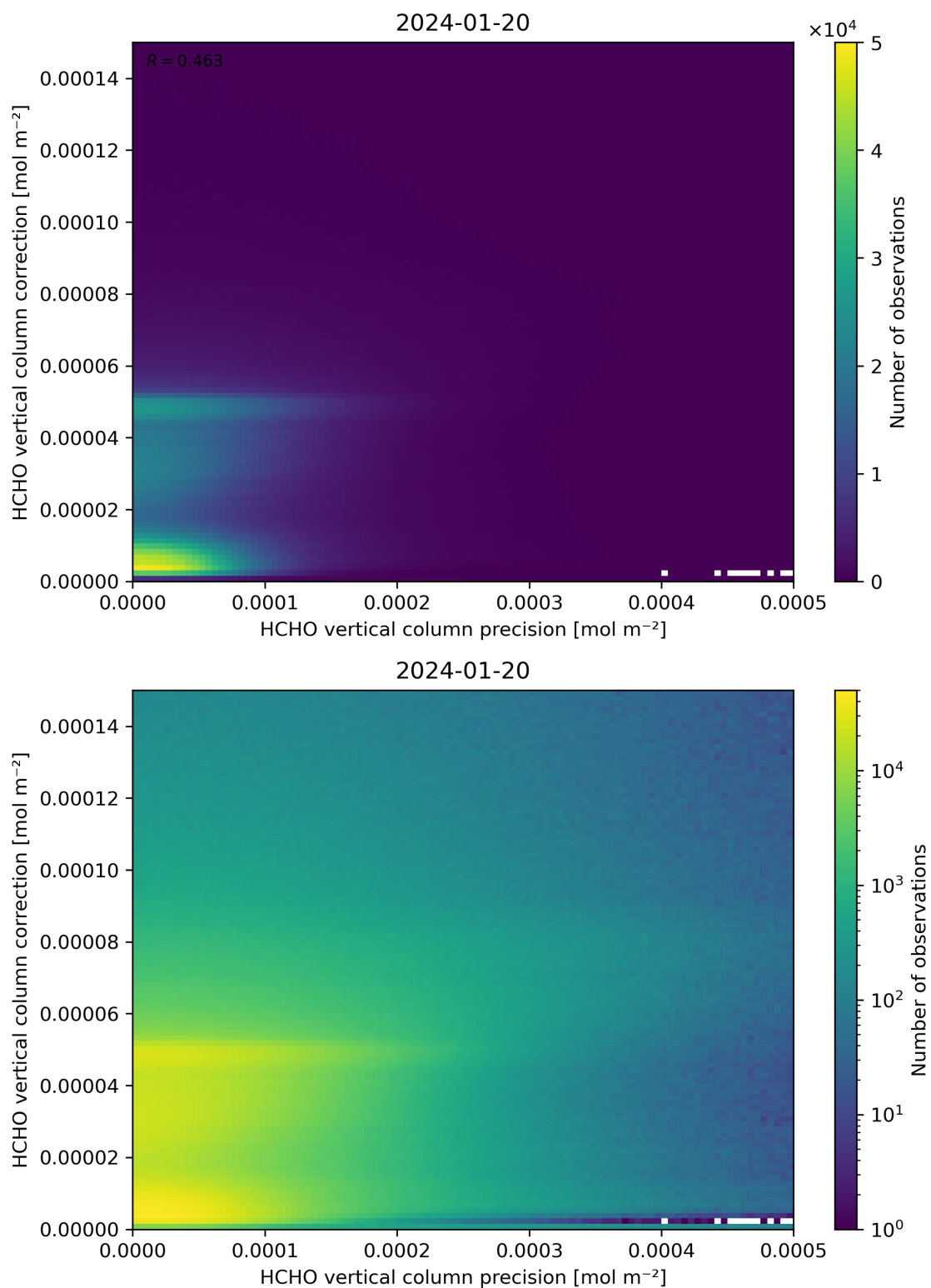
Figure 146: Scatter density plot of “HCHO vertical column precision” against “HCHO vertical column correction” for 2024-01-19 to 2024-01-21.
