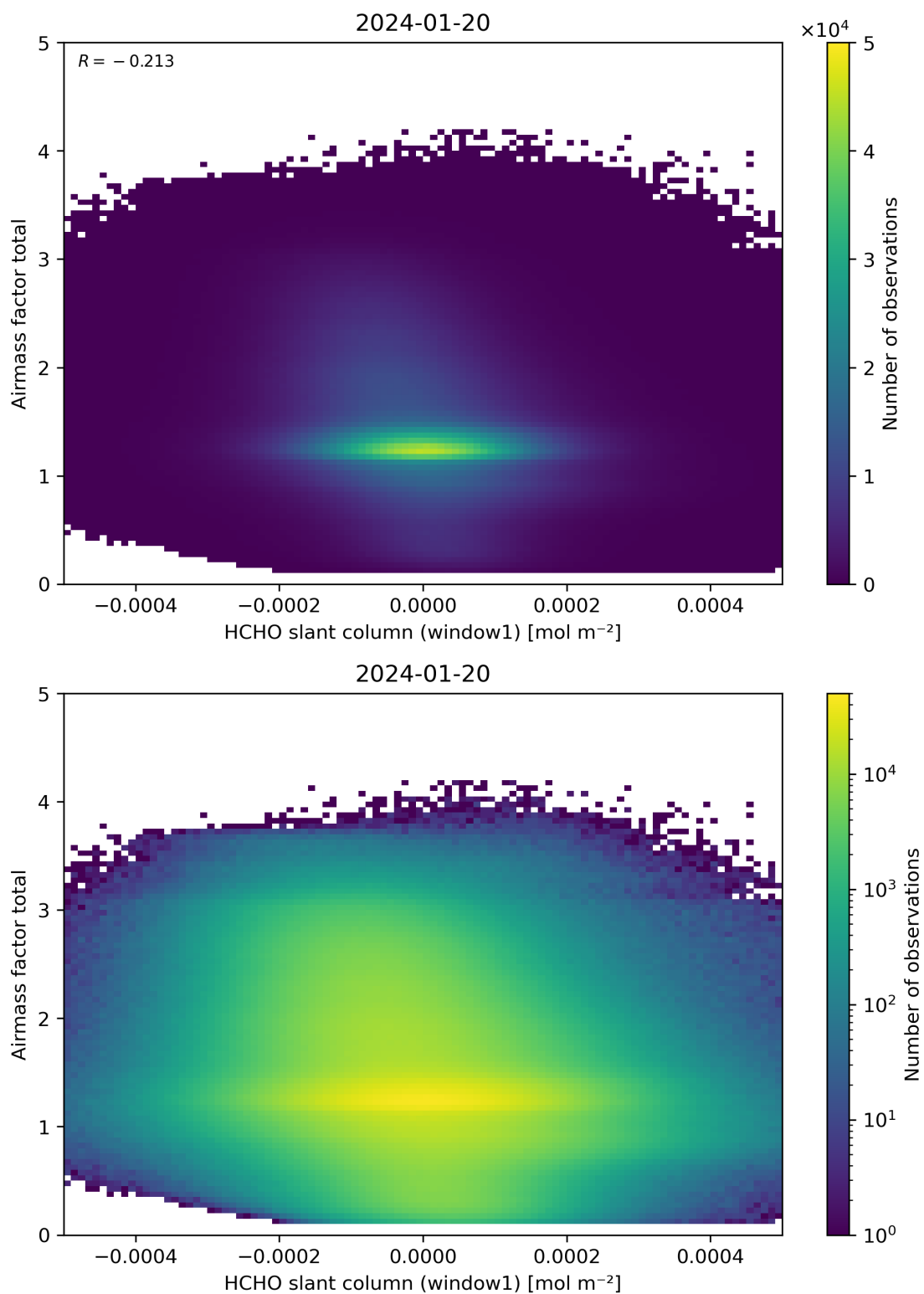
Figure 85: Scatter density plot of “HCHO slant column (window1)” against “Airmass factor total” for 2024-01-19 to 2024-01-21.
