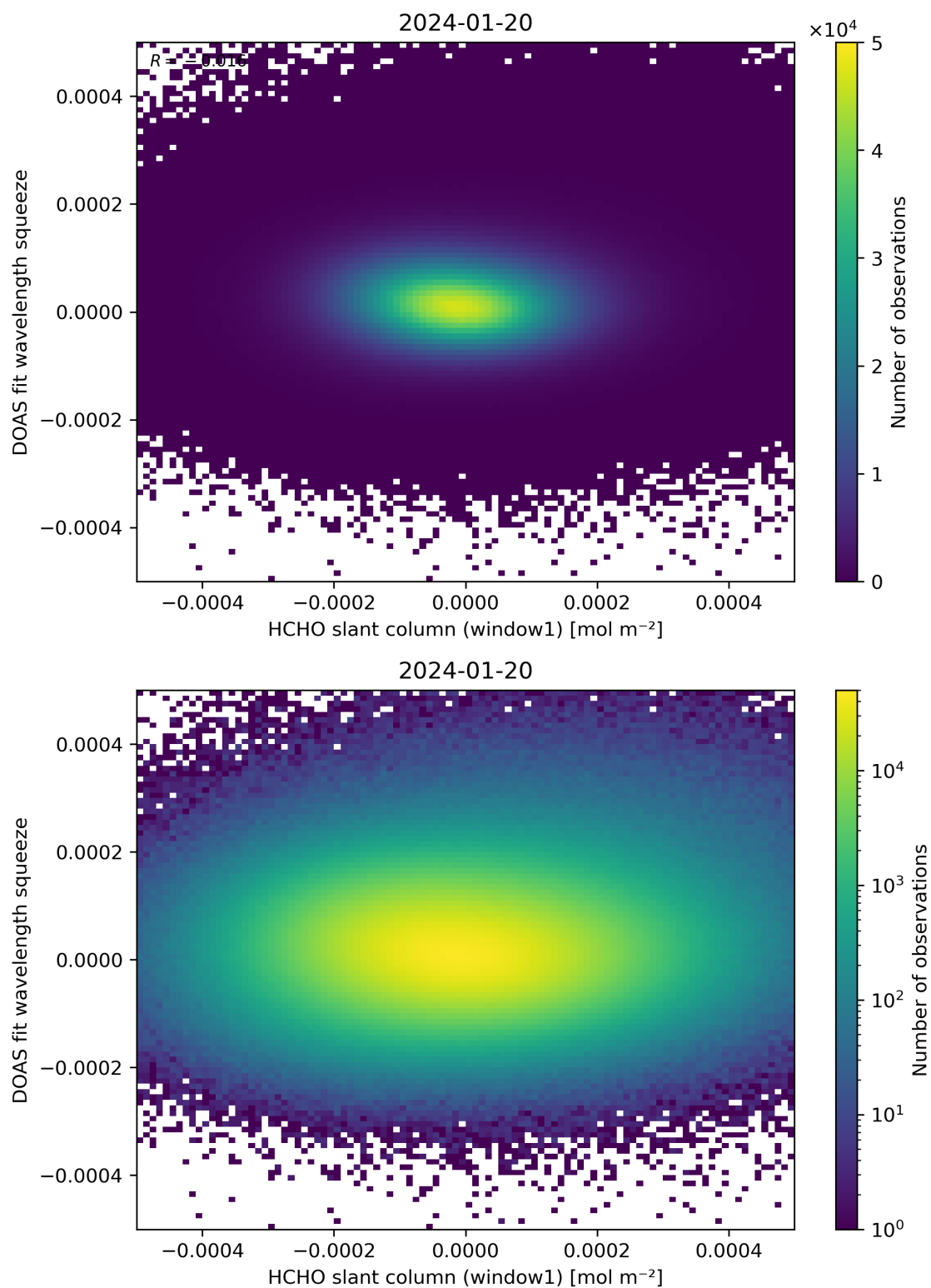
Figure 80: Scatter density plot of “HCHO slant column (window1)” against “DOAS fit wavelength squeeze” for 2024-01-19 to 2024-01-21.
