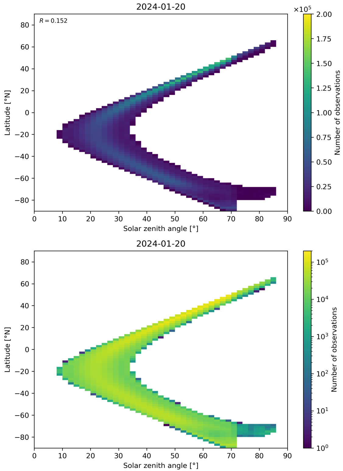
Figure 181: Scatter density plot of “Solar zenith angle” against “Latitude” for 2024-01-19 to 2024-01-21.
