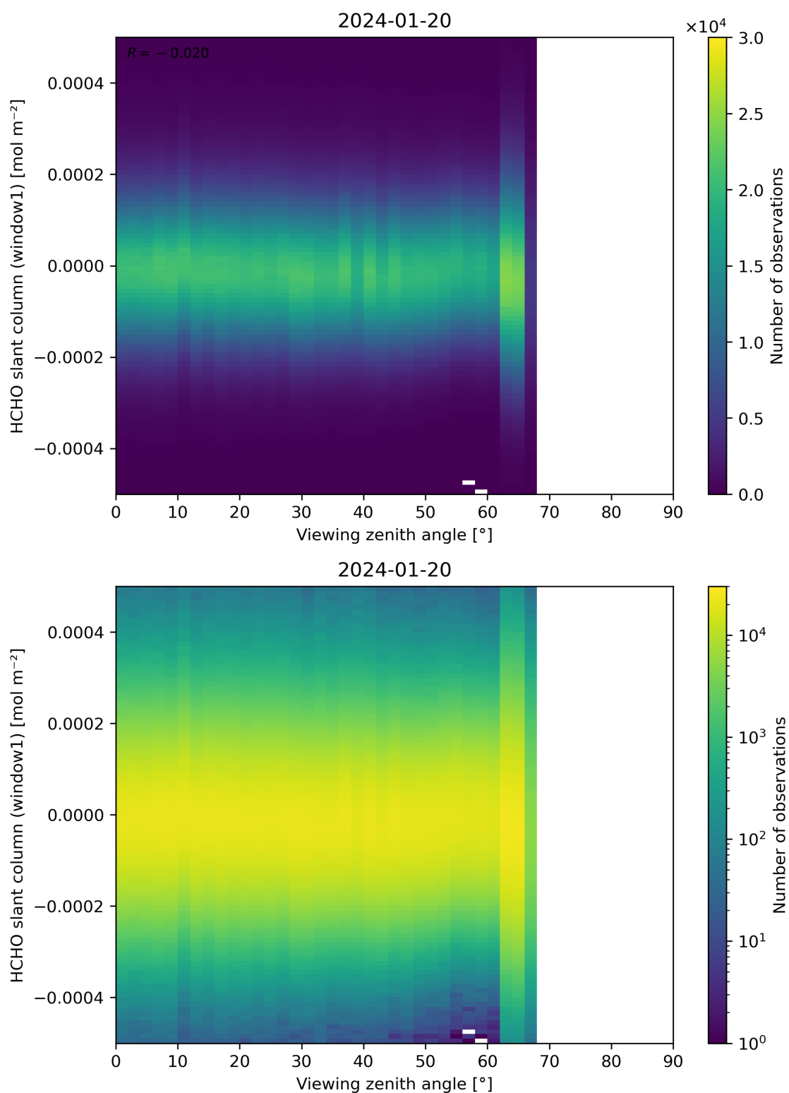
Figure 188: Scatter density plot of “Viewing zenith angle” against “HCHO slant column (window1)” for 2024-01-19 to 2024-01-21.
