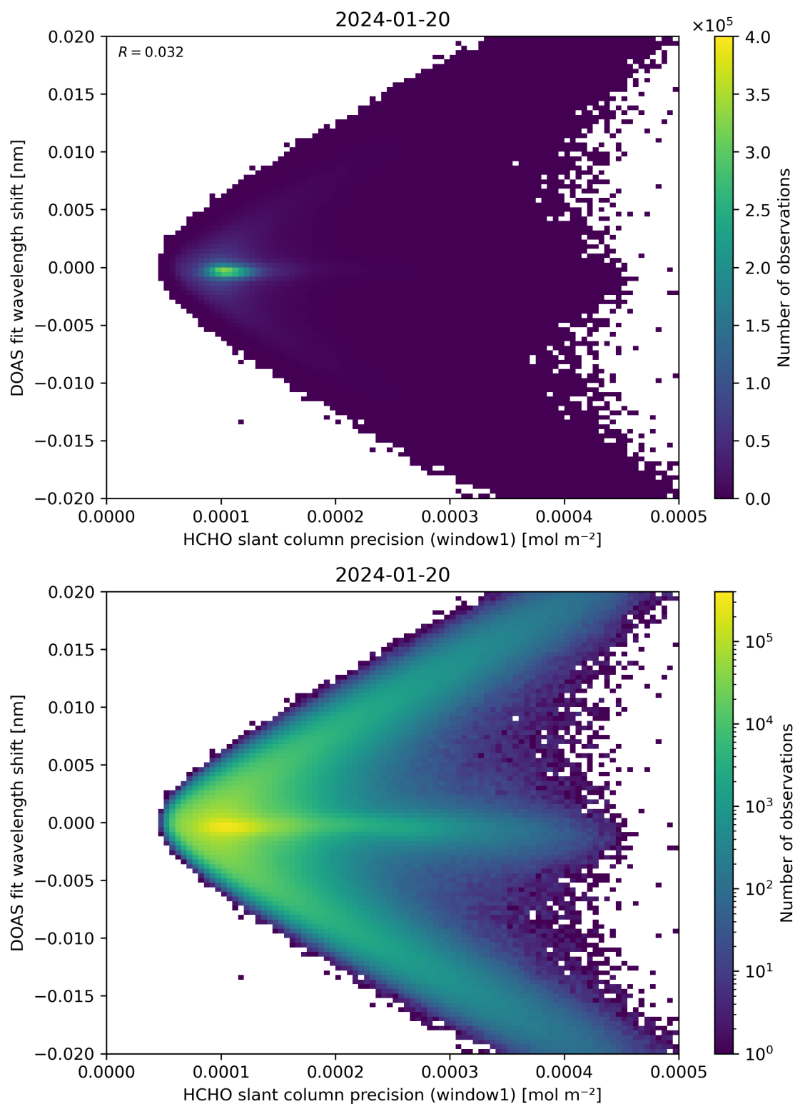
Figure 89: Scatter density plot of “HCHO slant column precision (window1)” against “DOAS fit wavelength shift” for 2024-01-19 to 2024-01-21.
