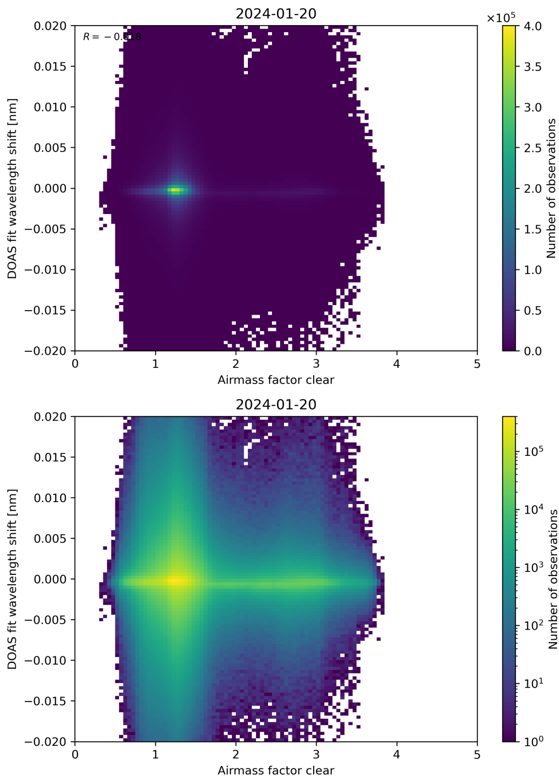
Figure 72: Scatter density plot of “Airmass factor clear” against “DOAS fit wavelength shift” for 2024-01-19 to 2024-01-21.
