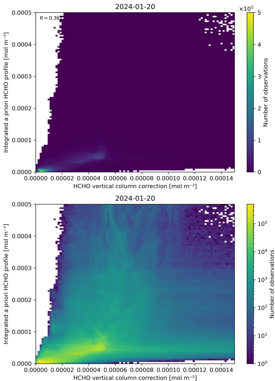
Figure 122: Scatter density plot of “HCHO vertical column correction” against “Integrated a priori HCHO profile” for 2024-01-19 to 2024-01-21.
