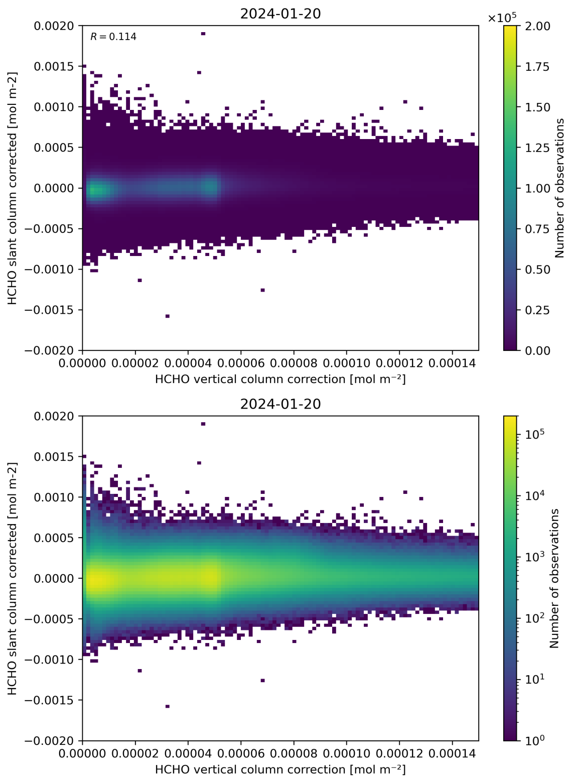
Figure 116: Scatter density plot of “HCHO vertical column correction” against “HCHO slant column corrected” for 2024-01-19 to 2024-01-21.
