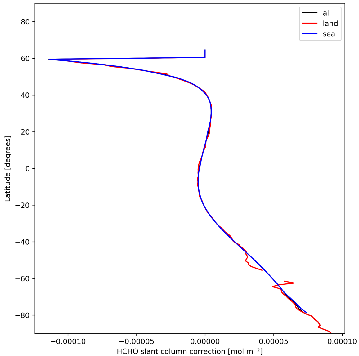
Figure 33: Zonal average of “HCHO slant column correction” for 2024-01-19 to 2024-01-21.
