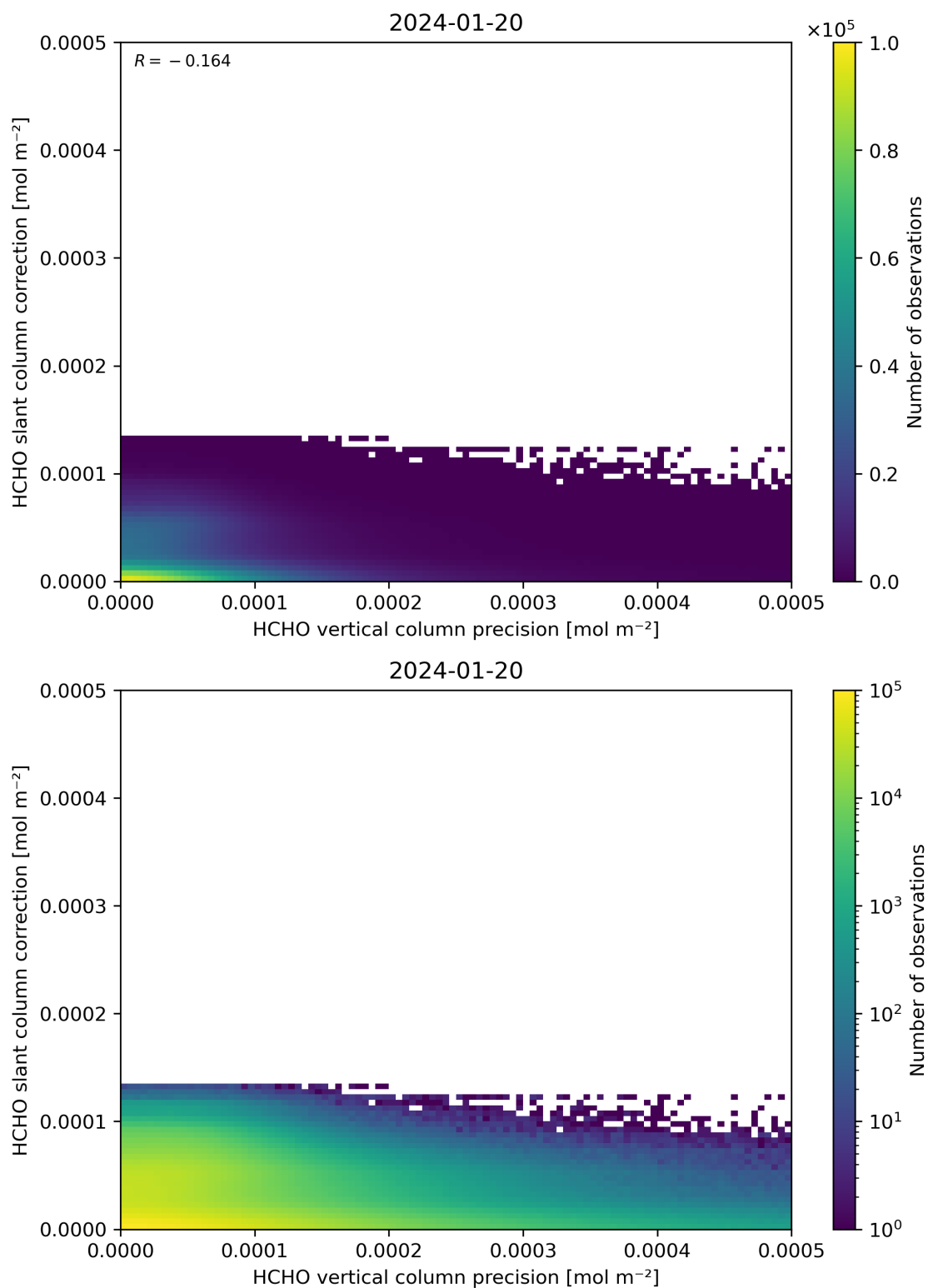
Figure 141: Scatter density plot of “HCHO vertical column precision” against “HCHO slant column correction” for 2024-01-19 to 2024-01-21.
