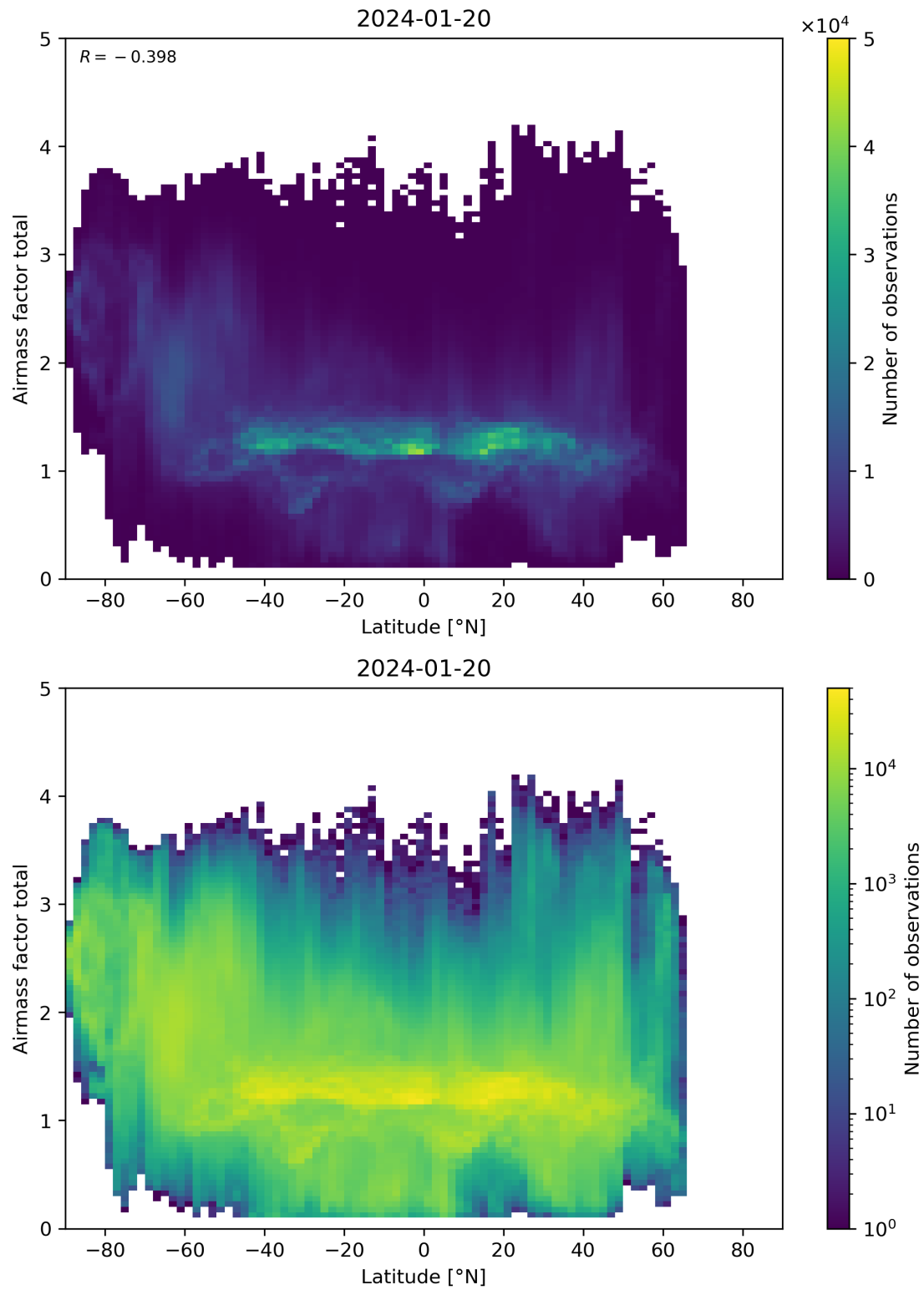
Figure 161: Scatter density plot of “Latitude” against “Airmass factor total” for 2024-01-19 to 2024-01-21.
