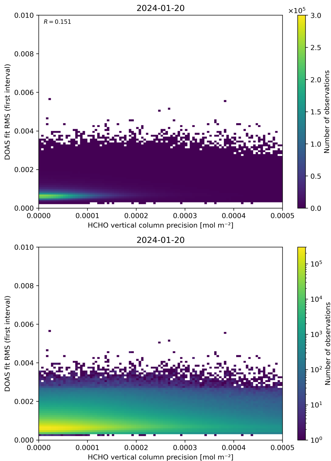
Figure 136: Scatter density plot of “HCHO vertical column precision” against “DOAS fit RMS (first interval)” for 2024-01-19 to 2024-01-21.
