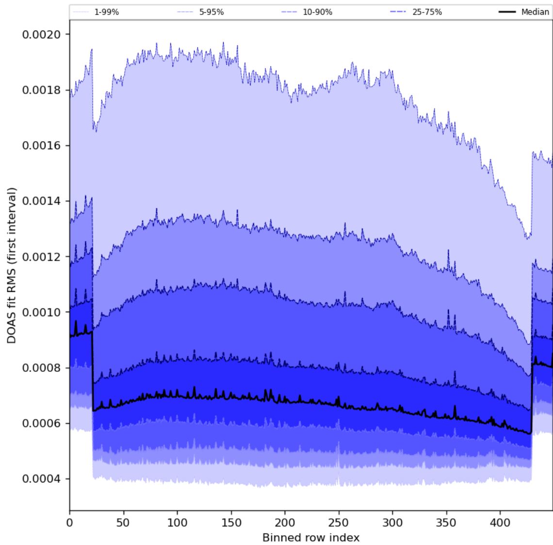
Figure 60: Along track statistics of “DOAS fit RMS (first interval)” for 2024-01-19 to 2024-01-21
