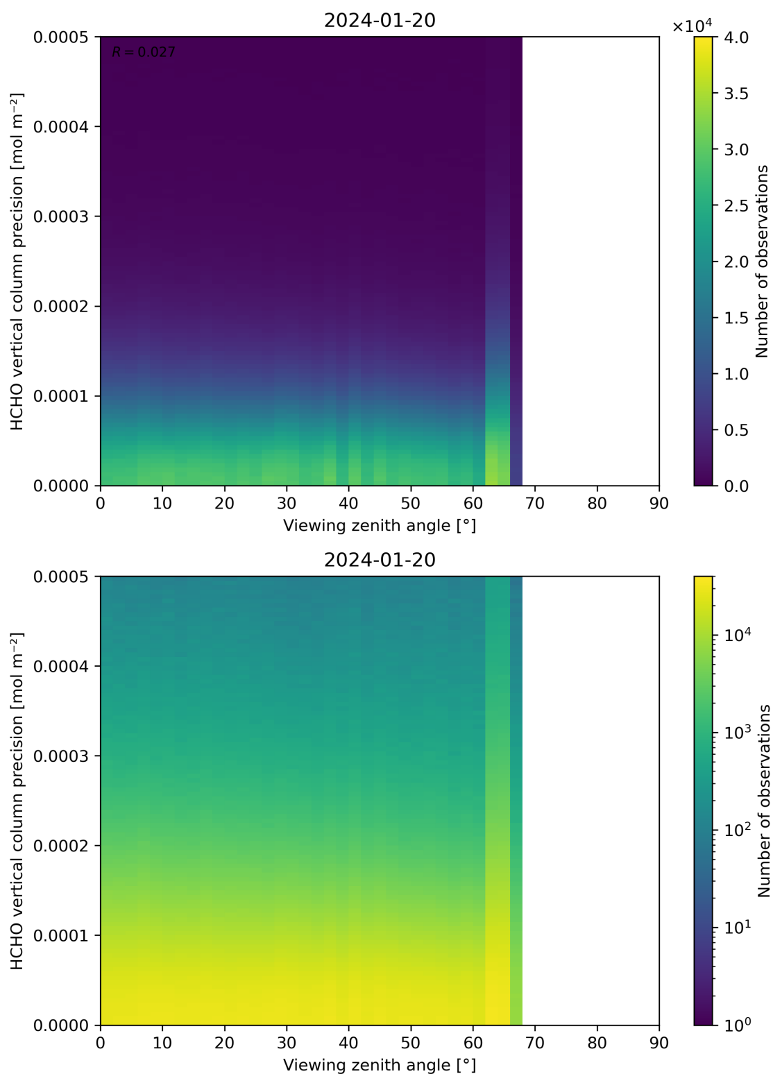
Figure 194: Scatter density plot of “Viewing zenith angle” against “HCHO vertical column precision” for 2024-01-19 to 2024-01-21.
