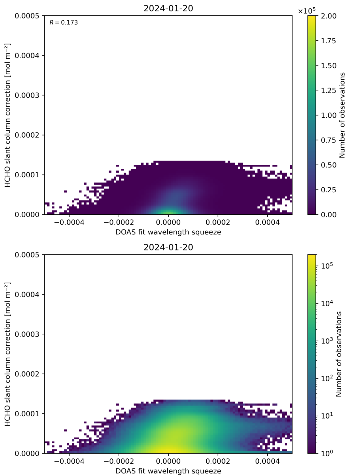
Figure 70: Scatter density plot of “DOAS fit wavelength squeeze” against “HCHO slant column correction” for 2024-01-19 to 2024-01-21.
