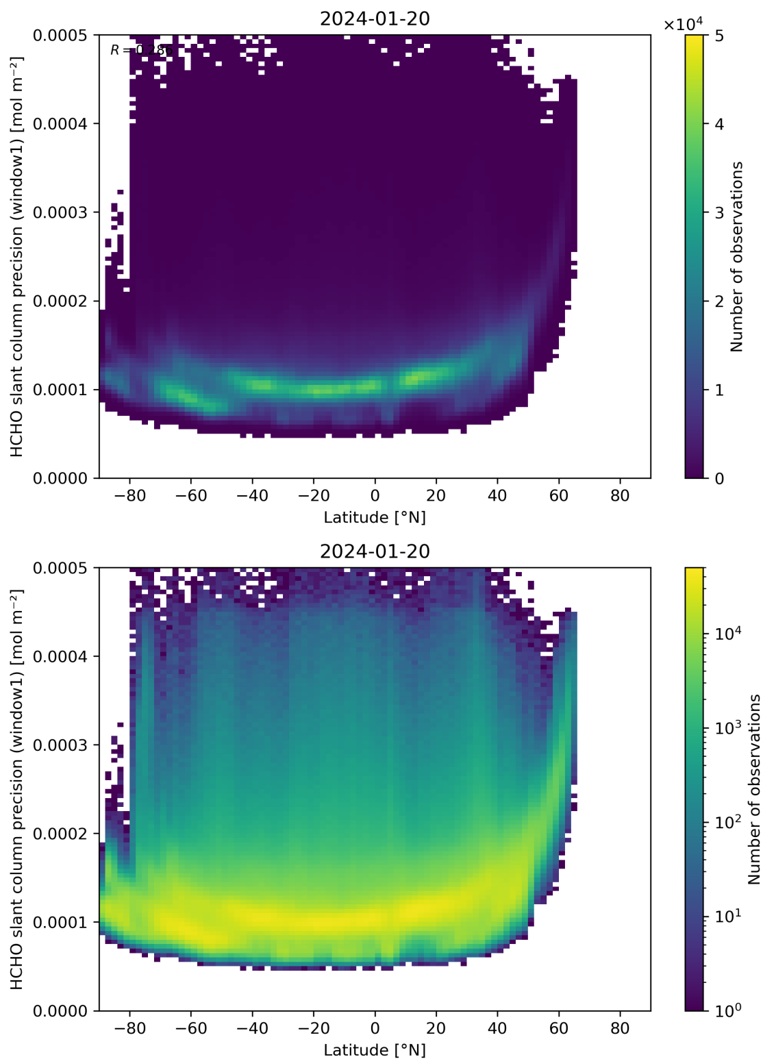
Figure 160: Scatter density plot of “Latitude” against “HCHO slant column precision (window1)” for 2024-01-19 to 2024-01-21.
