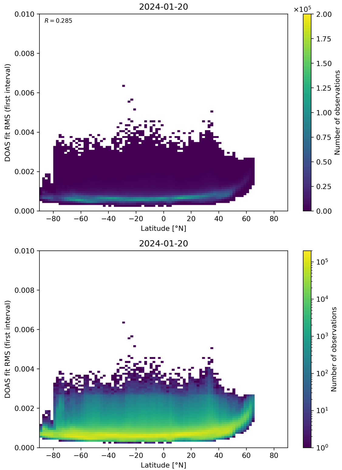
Figure 153: Scatter density plot of “Latitude” against “DOAS fit RMS (first interval)” for 2024-01-19 to 2024-01-21.
