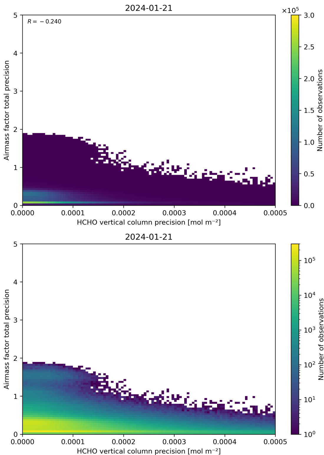
Figure 145: Scatter density plot of “HCHO vertical column precision” against “Airmass factor total precision” for 2024-01-21 to 2024-01-22.
