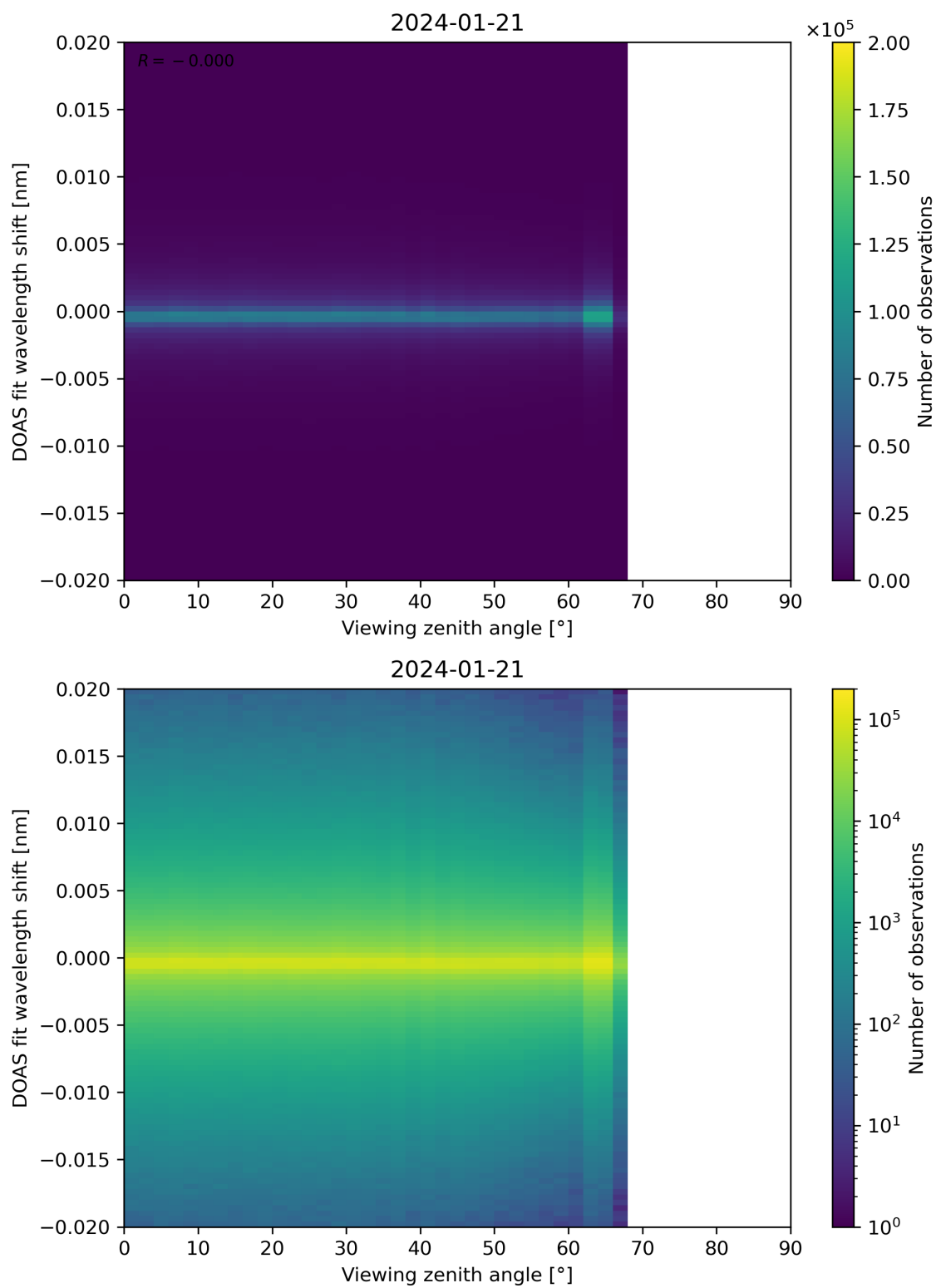
Figure 183: Scatter density plot of “Viewing zenith angle” against “DOAS fit wavelength shift” for 2024-01-21 to 2024-01-22.
