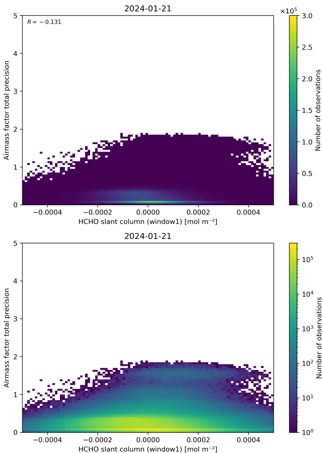
Figure 86: Scatter density plot of “HCHO slant column (window1)” against “Airmass factor total precision” for 2024-01-21 to 2024-01-22.
