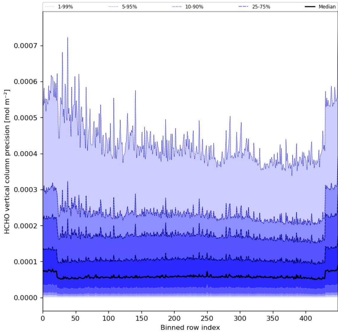
Figure 50: Along track statistics of “HCHO vertical column precision” for 2024-01-21 to 2024-01-22
