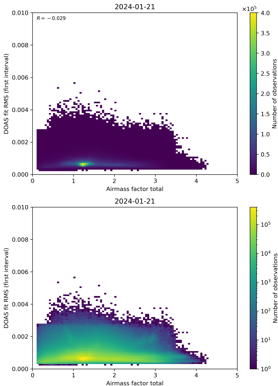
Figure 97: Scatter density plot of “Airmass factor total” against “DOAS fit RMS (first interval)” for 2024-01-21 to 2024-01-22.
