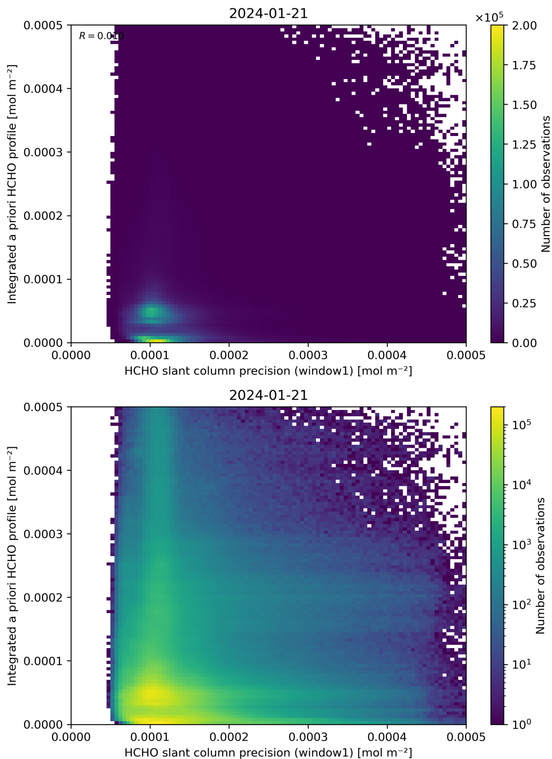
Figure 96: Scatter density plot of “HCHO slant column precision (window1)” against “Integrated a priori HCHO profile” for 2024-01-21 to 2024-01-22.
