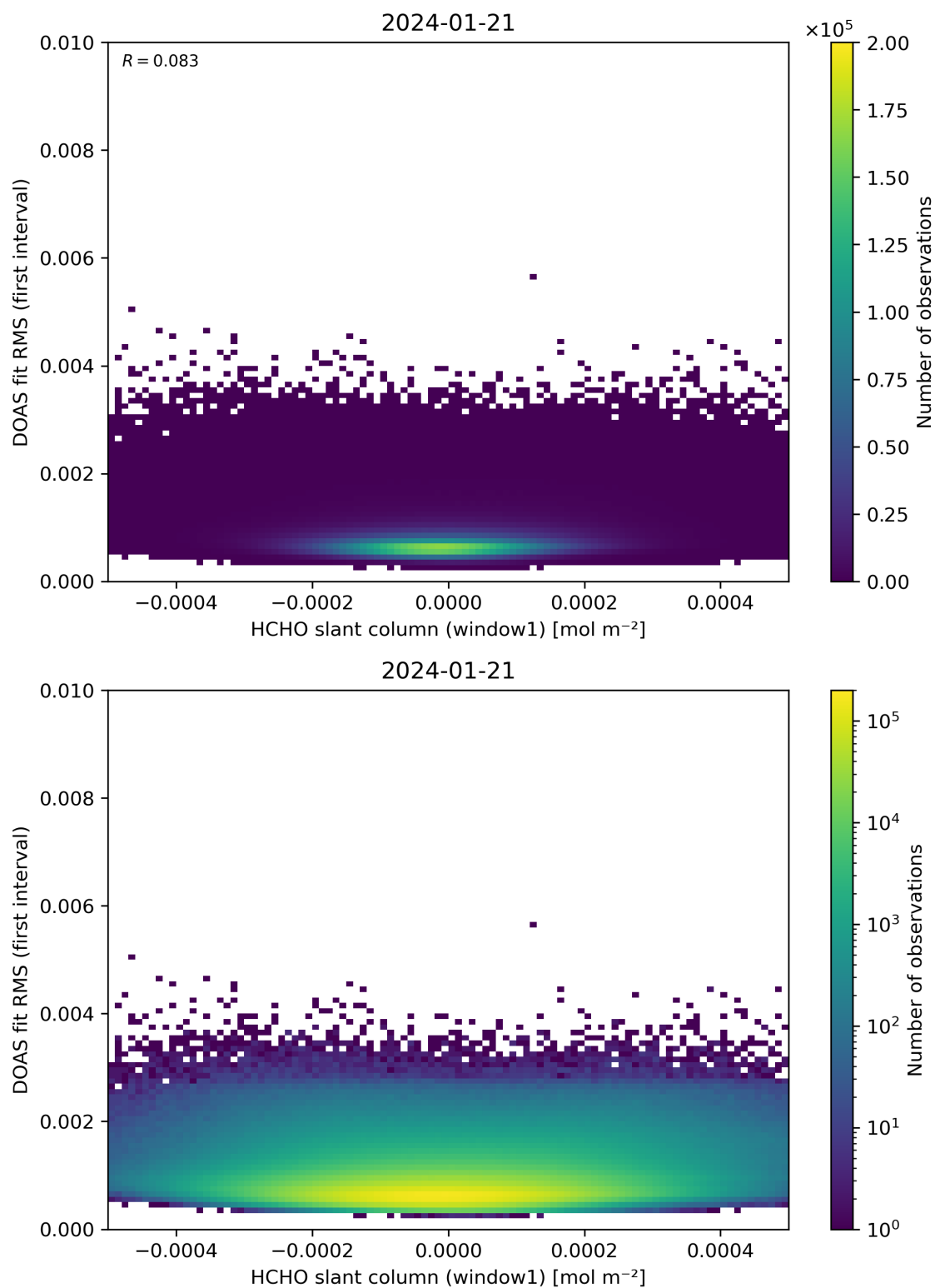
Figure 78: Scatter density plot of “HCHO slant column (window1)” against “DOAS fit RMS (first interval)” for 2024-01-21 to 2024-01-22.
