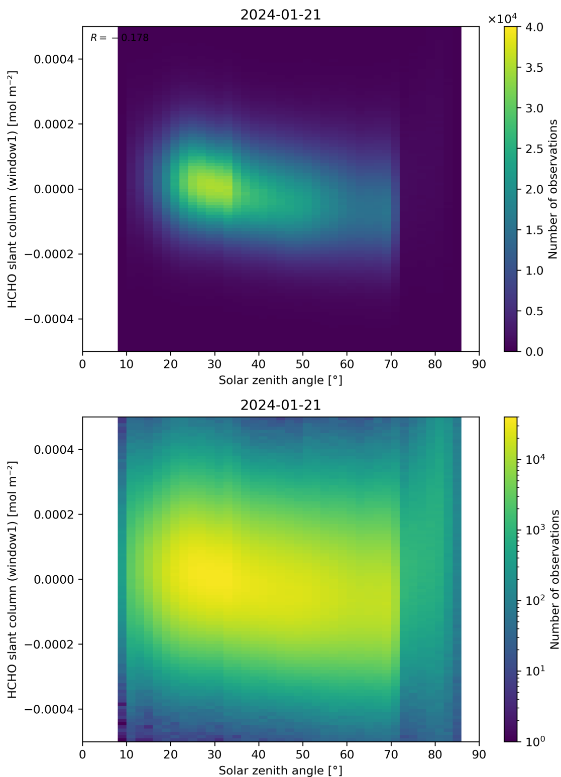
Figure 173: Scatter density plot of “Solar zenith angle” against “HCHO slant column (window1)” for 2024-01-21 to 2024-01-22.
