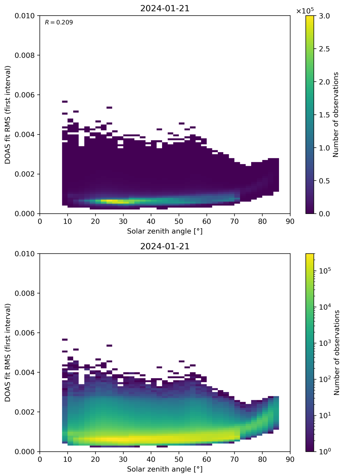
Figure 167: Scatter density plot of “Solar zenith angle” against “DOAS fit RMS (first interval)” for 2024-01-21 to 2024-01-22.
