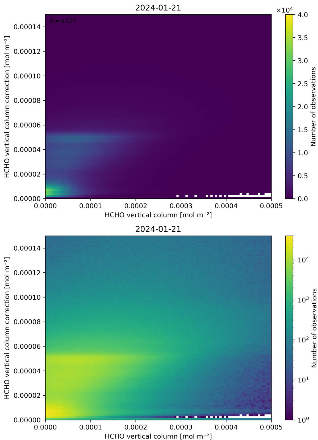
Figure 133: Scatter density plot of “HCHO vertical column” against “HCHO vertical column correction” for 2024-01-21 to 2024-01-22.
