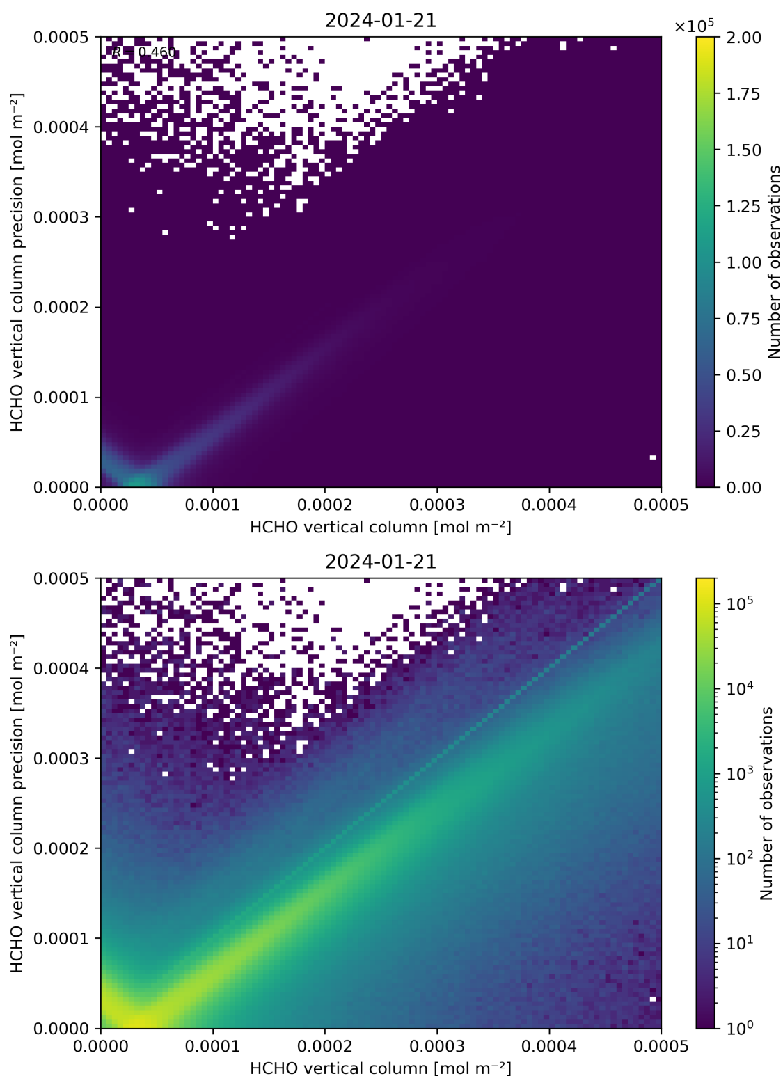
Figure 134: Scatter density plot of “HCHO vertical column” against “HCHO vertical column precision” for 2024-01-21 to 2024-01-22.
