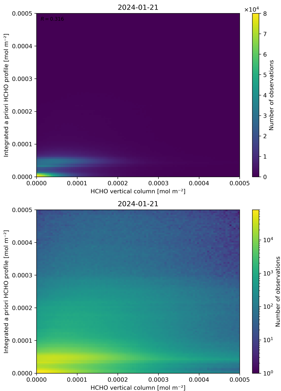
Figure 135: Scatter density plot of “HCHO vertical column” against “Integrated a priori HCHO profile” for 2024-01-21 to 2024-01-22.
