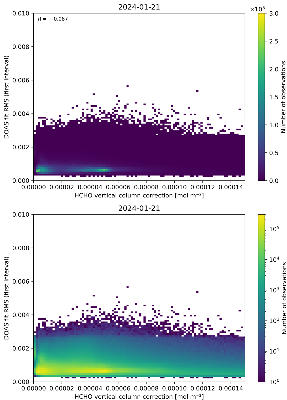
Figure 112: Scatter density plot of “HCHO vertical column correction” against “DOAS fit RMS (first interval)” for 2024-01-21 to 2024-01-22.
