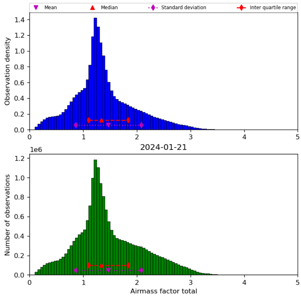
Figure 40: Histogram of “Airmass factor total” for 2024-01-21 to 2024-01-22
