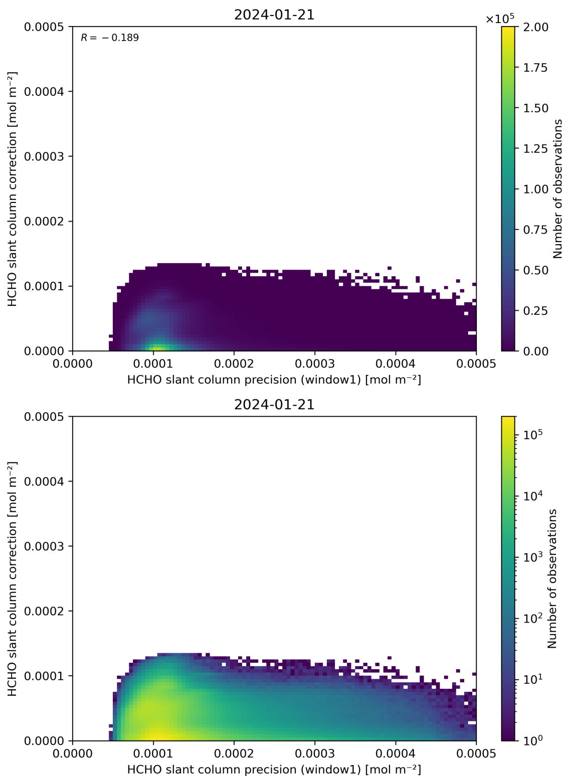
Figure 93: Scatter density plot of “HCHO slant column precision (window1)” against “HCHO slant column correction” for 2024-01-21 to 2024-01-22.
