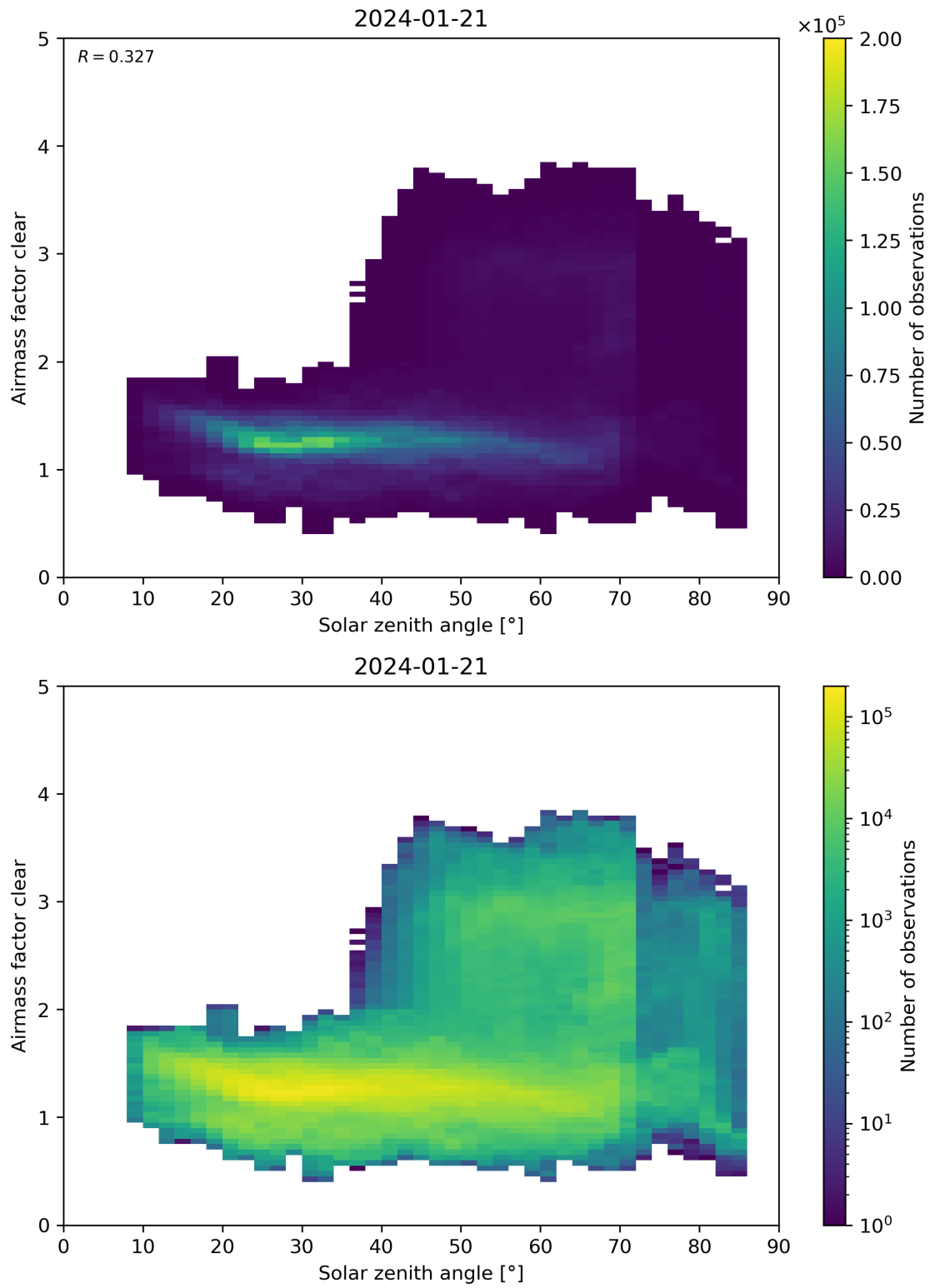
Figure 170: Scatter density plot of “Solar zenith angle” against “Airmass factor clear” for 2024-01-21 to 2024-01-22.
