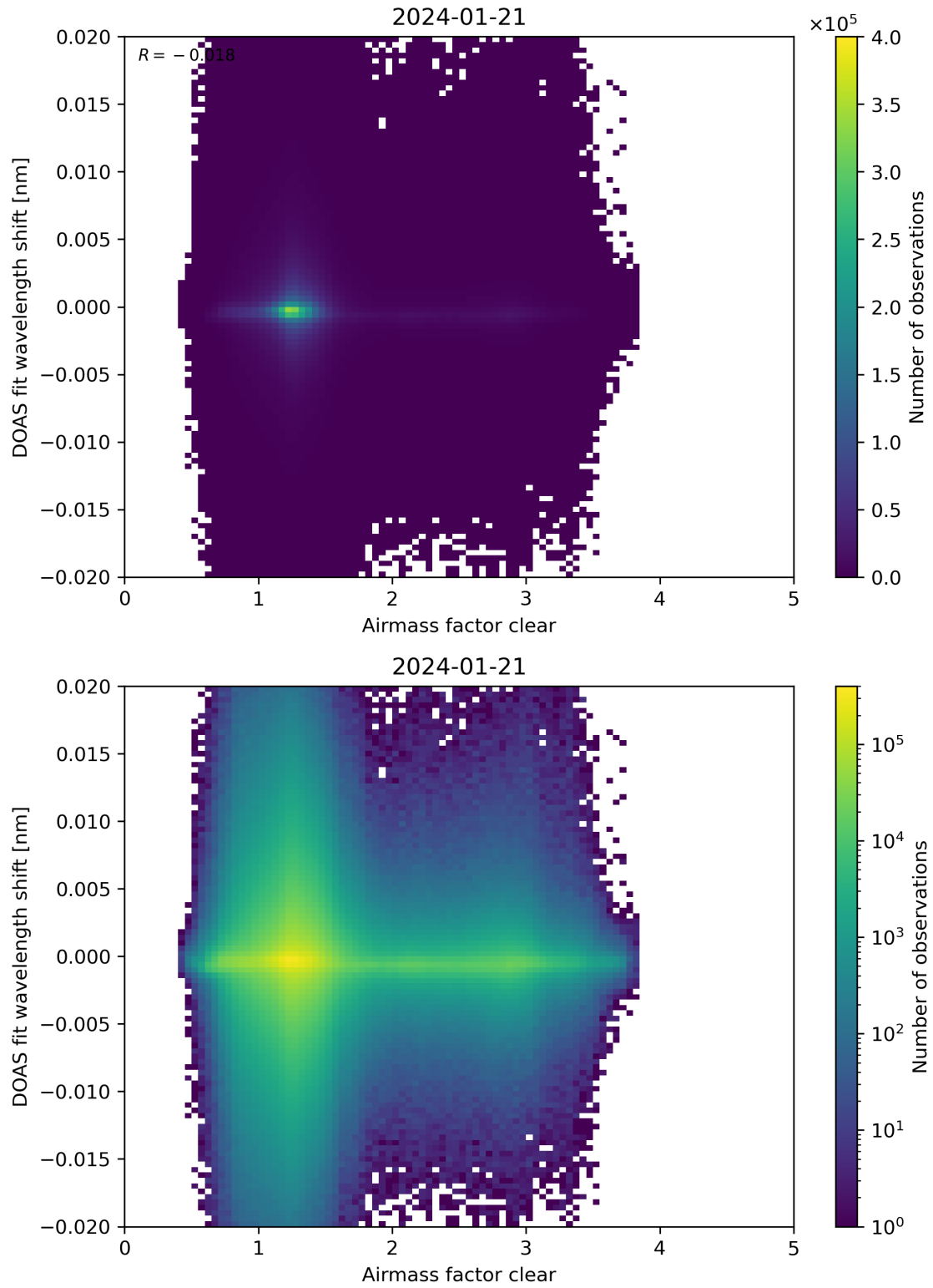
Figure 72: Scatter density plot of “Airmass factor clear” against “DOAS fit wavelength shift” for 2024-01-21 to 2024-01-22.
