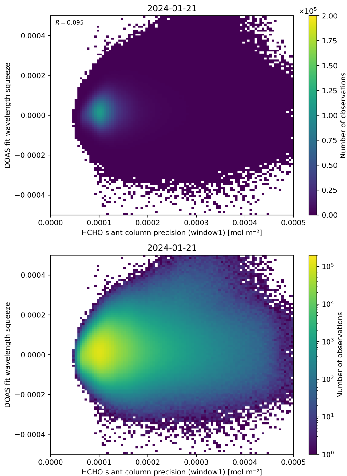
Figure 90: Scatter density plot of “HCHO slant column precision (window1)” against “DOAS fit wavelength squeeze” for 2024-01-21 to 2024-01-22.
