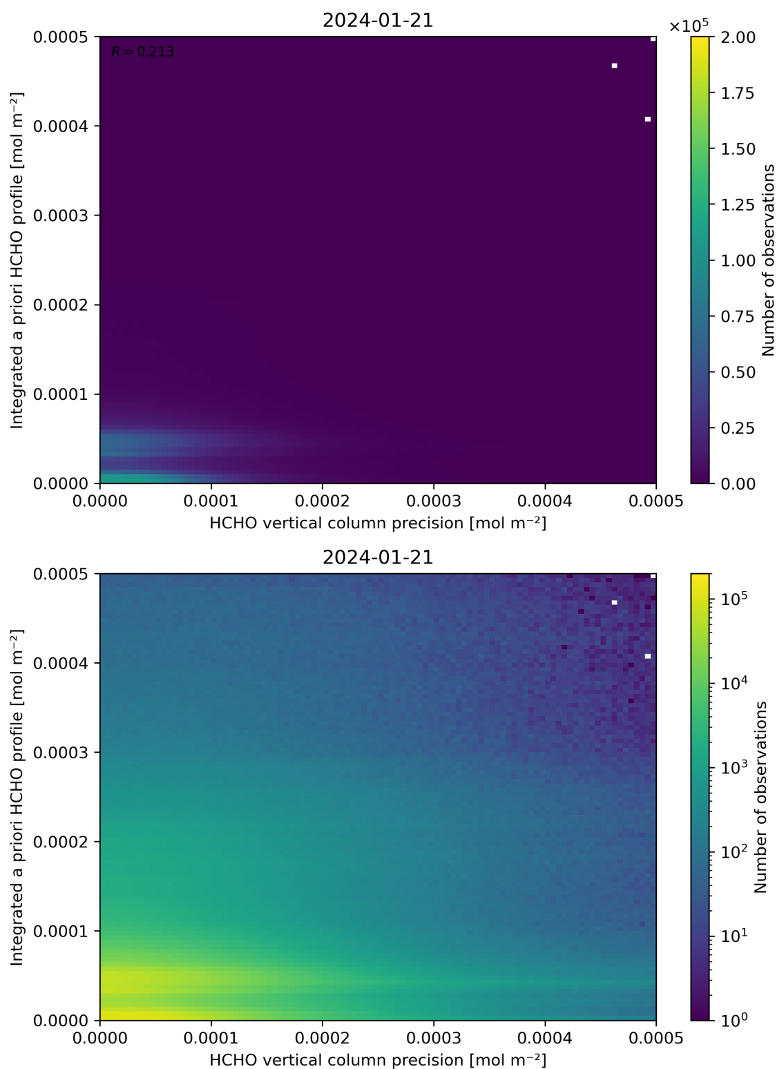
Figure 147: Scatter density plot of “HCHO vertical column precision” against “Integrated a priori HCHO profile” for 2024-01-21 to 2024-01-22.
