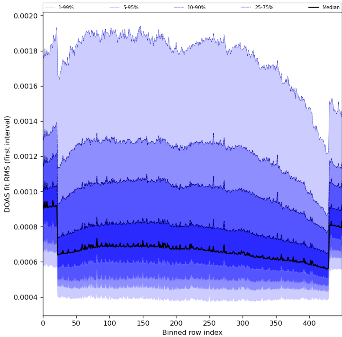
Figure 60: Along track statistics of “DOAS fit RMS (first interval)” for 2024-01-21 to 2024-01-22
