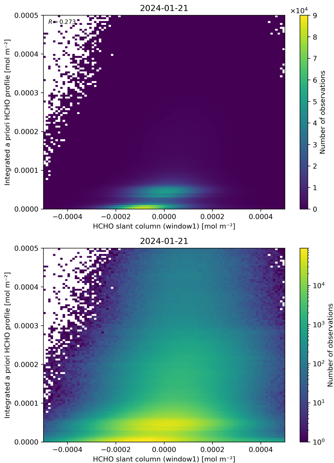
Figure 87: Scatter density plot of “HCHO slant column (window1)” against “Integrated a priori HCHO profile” for 2024-01-21 to 2024-01-22.
