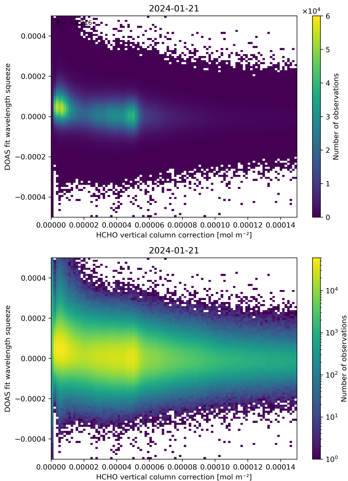
Figure 114: Scatter density plot of “HCHO vertical column correction” against “DOAS fit wavelength squeeze” for 2024-01-21 to 2024-01-22.
