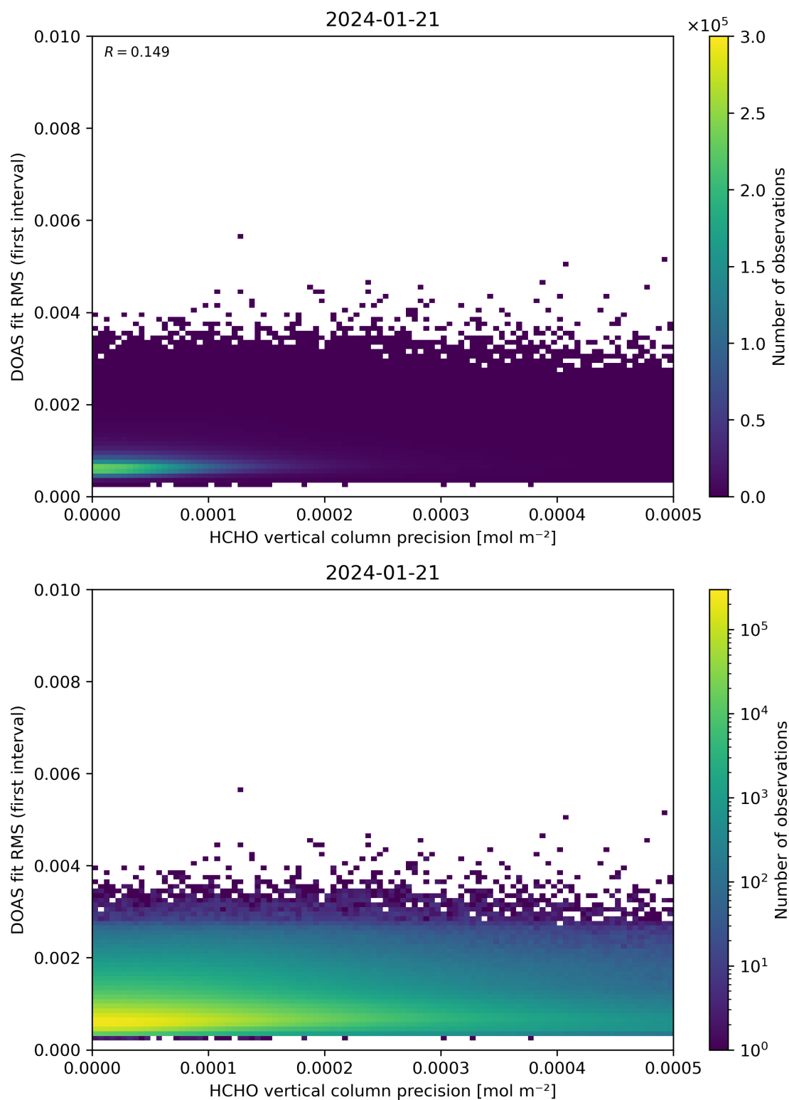
Figure 136: Scatter density plot of “HCHO vertical column precision” against “DOAS fit RMS (first interval)” for 2024-01-21 to 2024-01-22.
