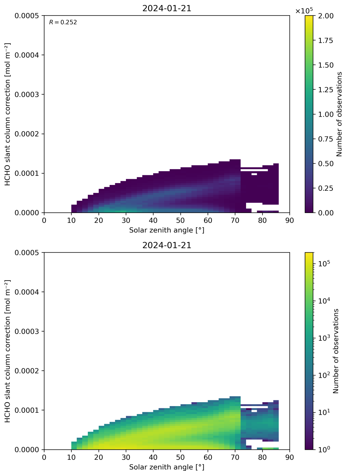
Figure 172: Scatter density plot of “Solar zenith angle” against “HCHO slant column correction” for 2024-01-21 to 2024-01-22.
