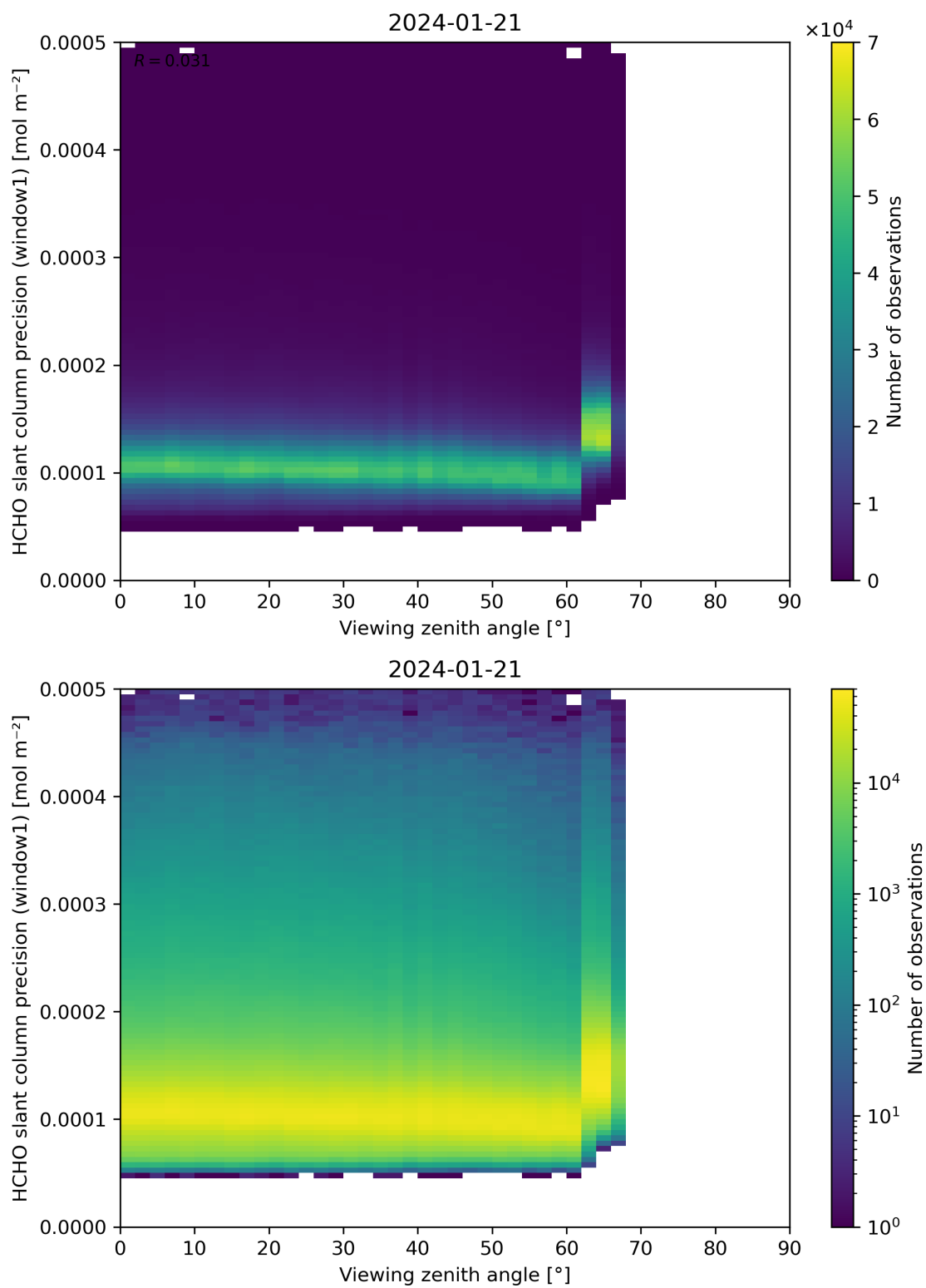
Figure 189: Scatter density plot of “Viewing zenith angle” against “HCHO slant column precision (window1)” for 2024-01-21 to 2024-01-22.
