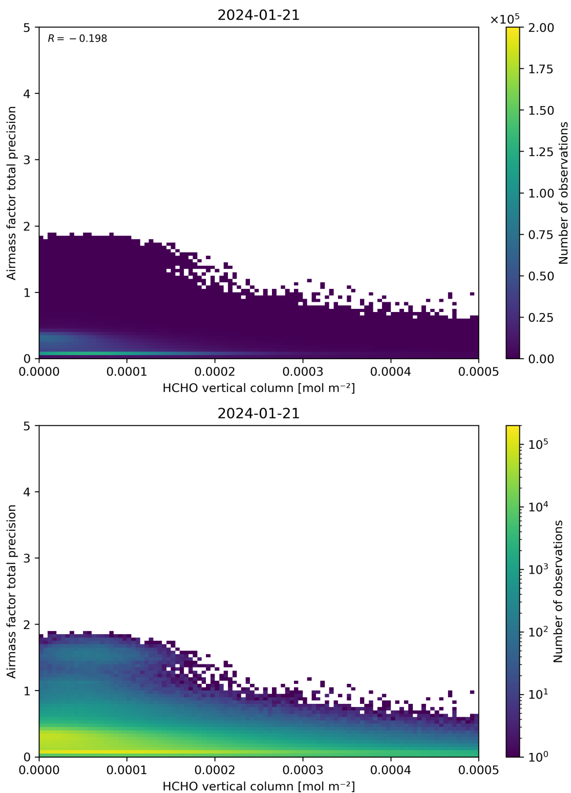
Figure 132: Scatter density plot of “HCHO vertical column” against “Airmass factor total precision” for 2024-01-21 to 2024-01-22.
