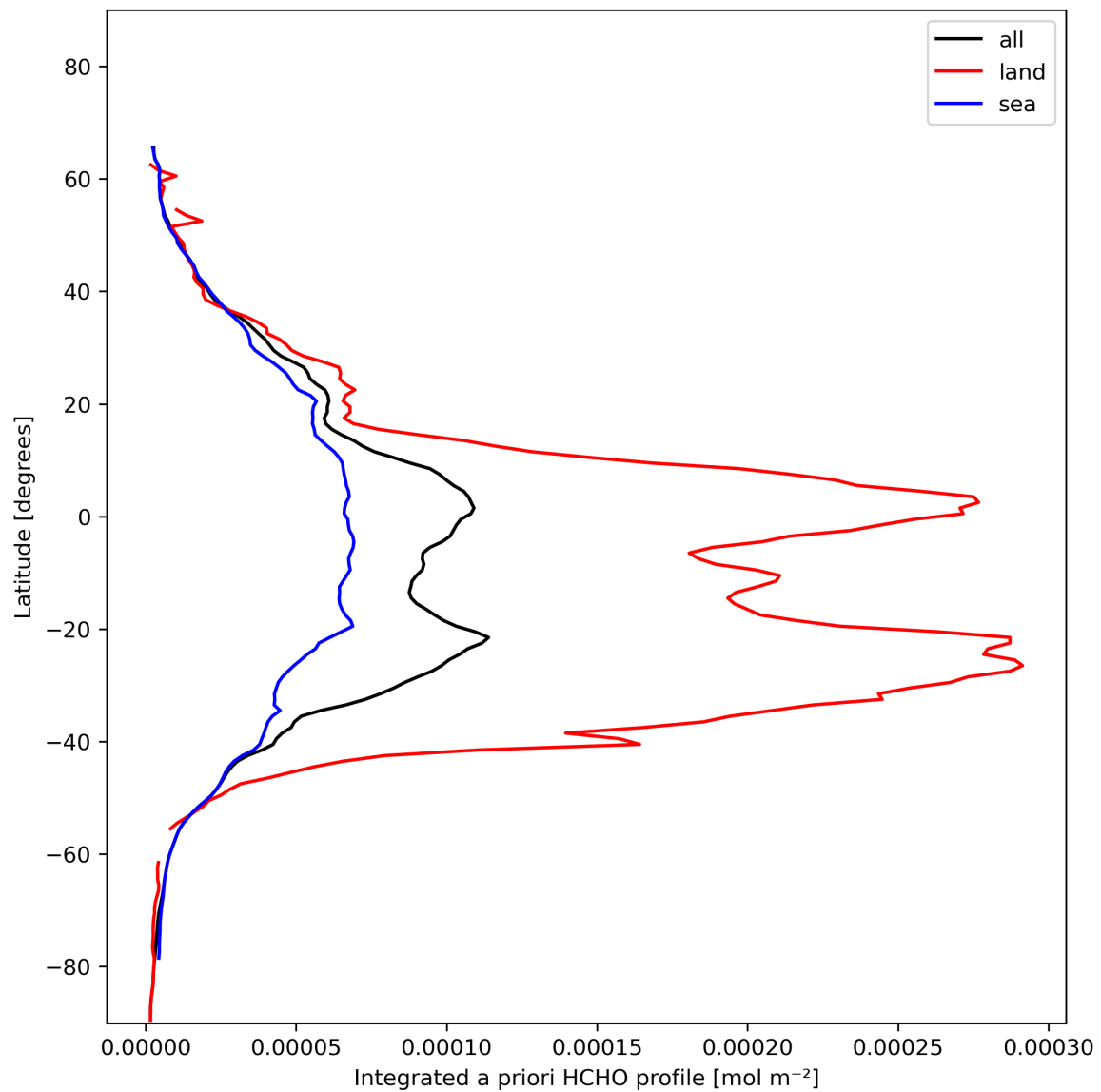
Figure 29: Zonal average of “Integrated a priori HCHO profile” for 2024-01-21 to 2024-01-22.
