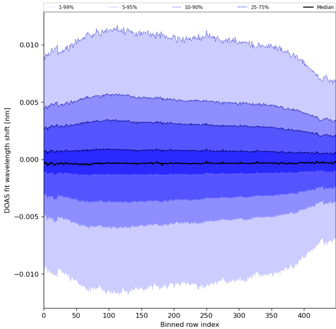
Figure 58: Along track statistics of “DOAS fit wavelength shift” for 2024-01-21 to 2024-01-22
