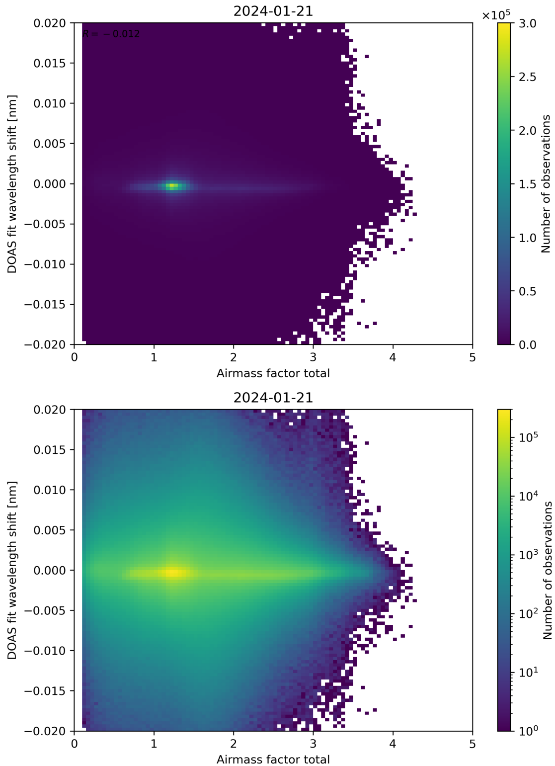
Figure 98: Scatter density plot of “Airmass factor total” against “DOAS fit wavelength shift” for 2024-01-21 to 2024-01-22.
