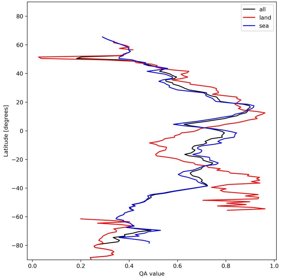
Figure 20: Zonal average of “QA value” for 2024-01-21 to 2024-01-22.
