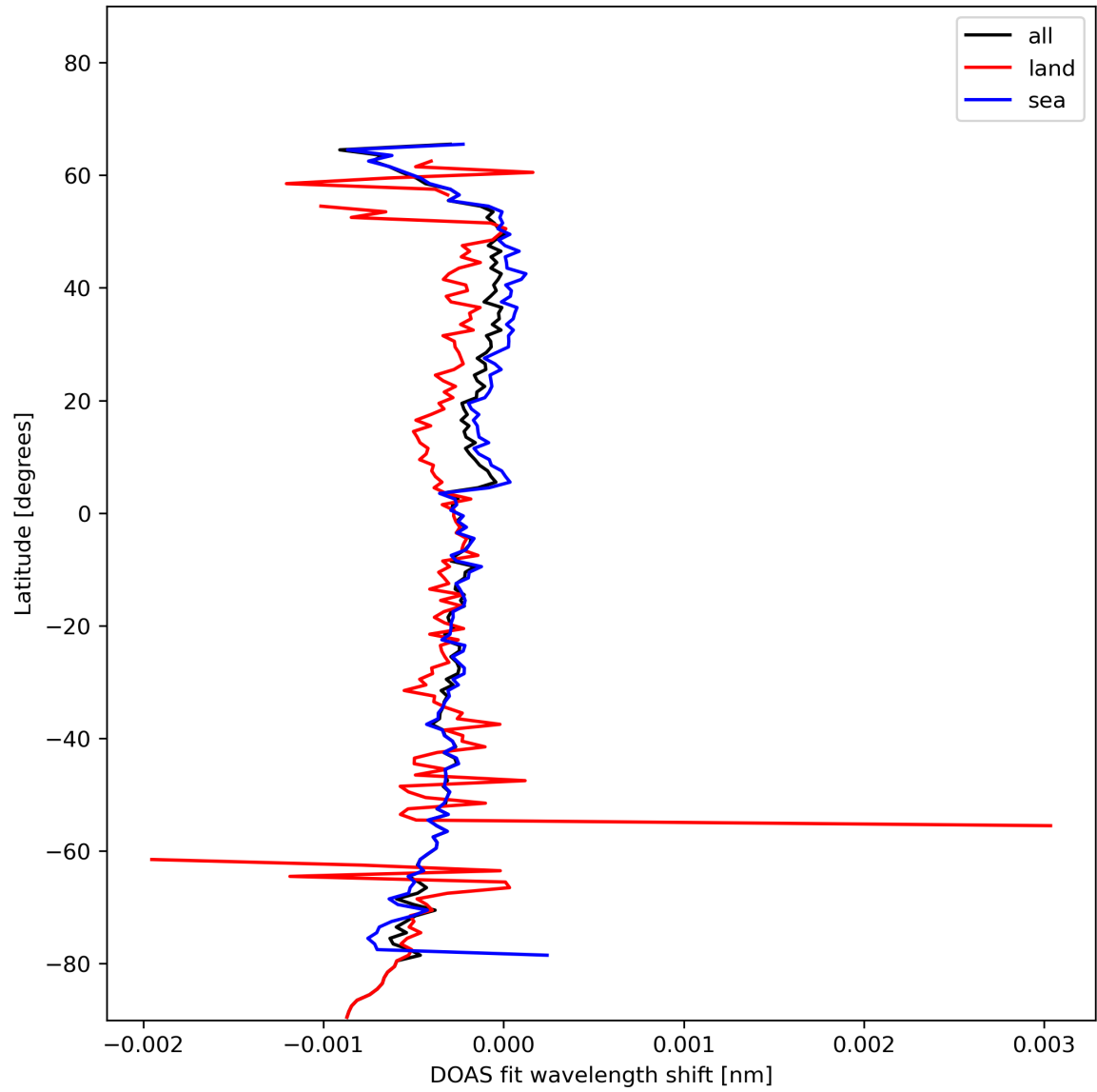
Figure 30: Zonal average of “DOAS fit wavelength shift” for 2024-01-21 to 2024-01-22.
