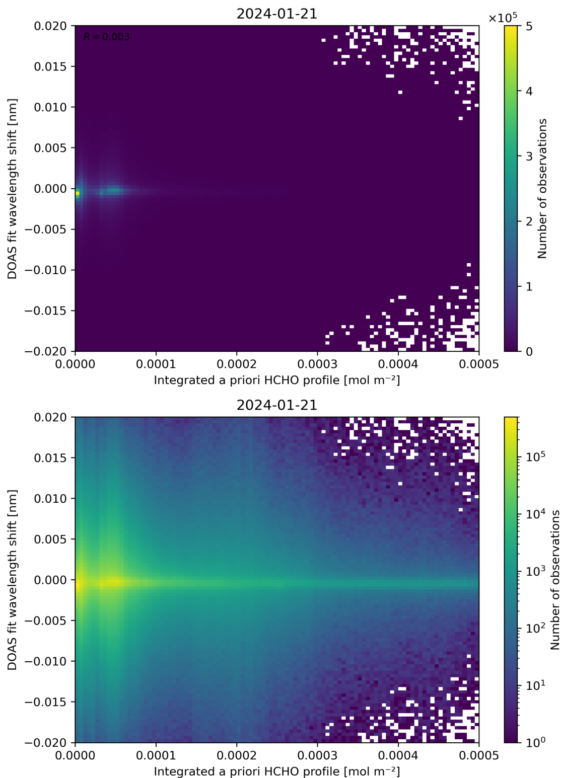
Figure 149: Scatter density plot of “Integrated a priori HCHO profile” against “DOAS fit wavelength shift” for 2024-01-21 to 2024-01-22.
