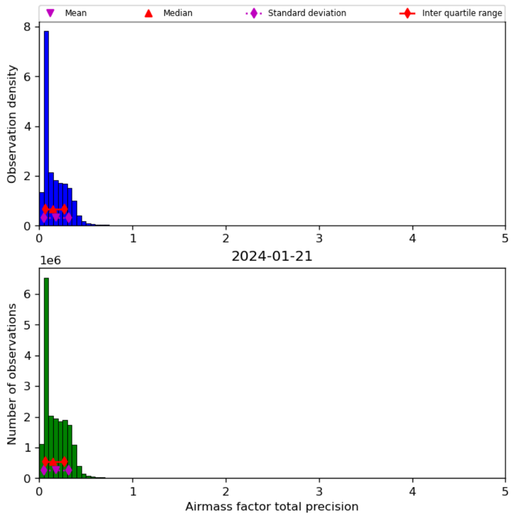
Figure 41: Histogram of “Airmass factor total precision” for 2024-01-21 to 2024-01-22
