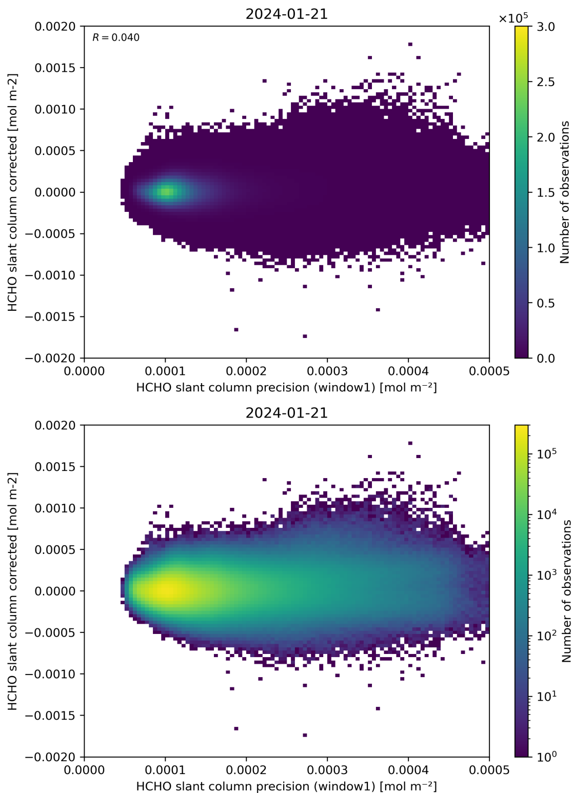
Figure 92: Scatter density plot of “HCHO slant column precision (window1)” against “HCHO slant column corrected” for 2024-01-21 to 2024-01-22.
