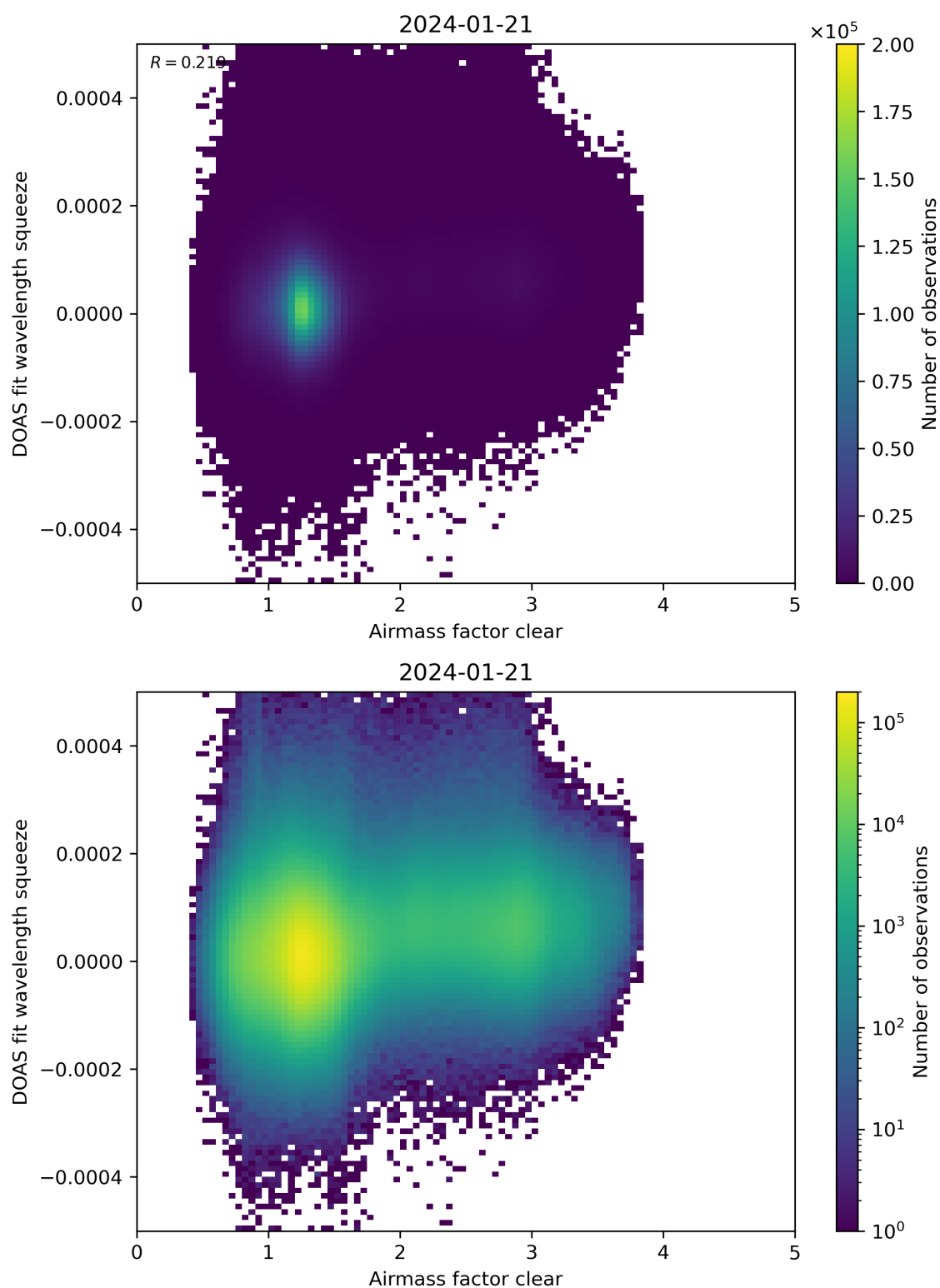
Figure 73: Scatter density plot of “Airmass factor clear” against “DOAS fit wavelength squeeze” for 2024-01-21 to 2024-01-22.
