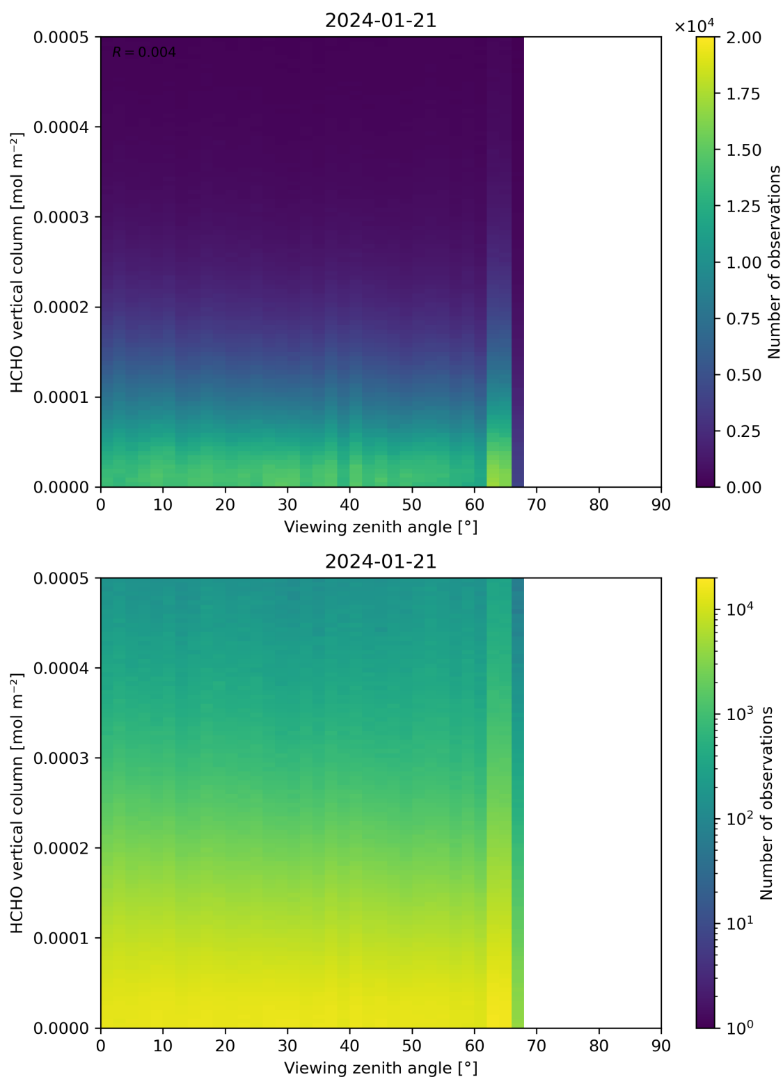
Figure 192: Scatter density plot of “Viewing zenith angle” against “HCHO vertical column” for 2024-01-21 to 2024-01-22.
