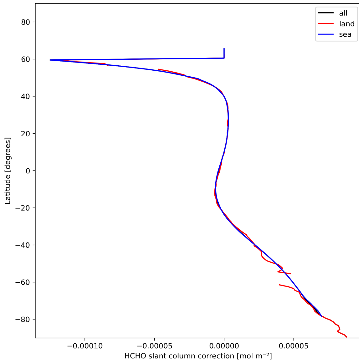
Figure 33: Zonal average of “HCHO slant column correction” for 2024-01-21 to 2024-01-22.
