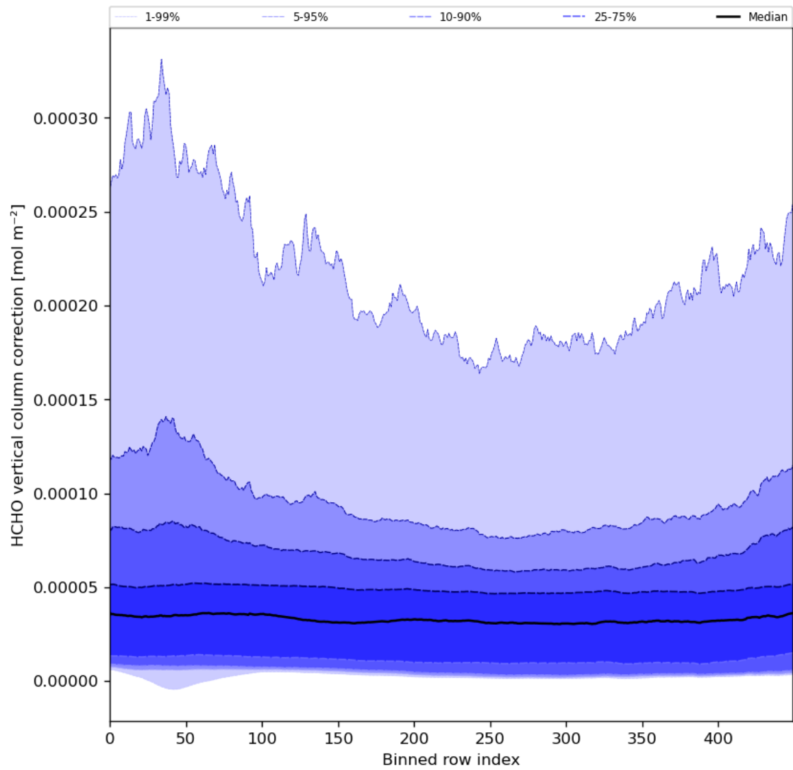
Figure 51: Along track statistics of “HCHO vertical column correction” for 2024-01-21 to 2024-01-22
