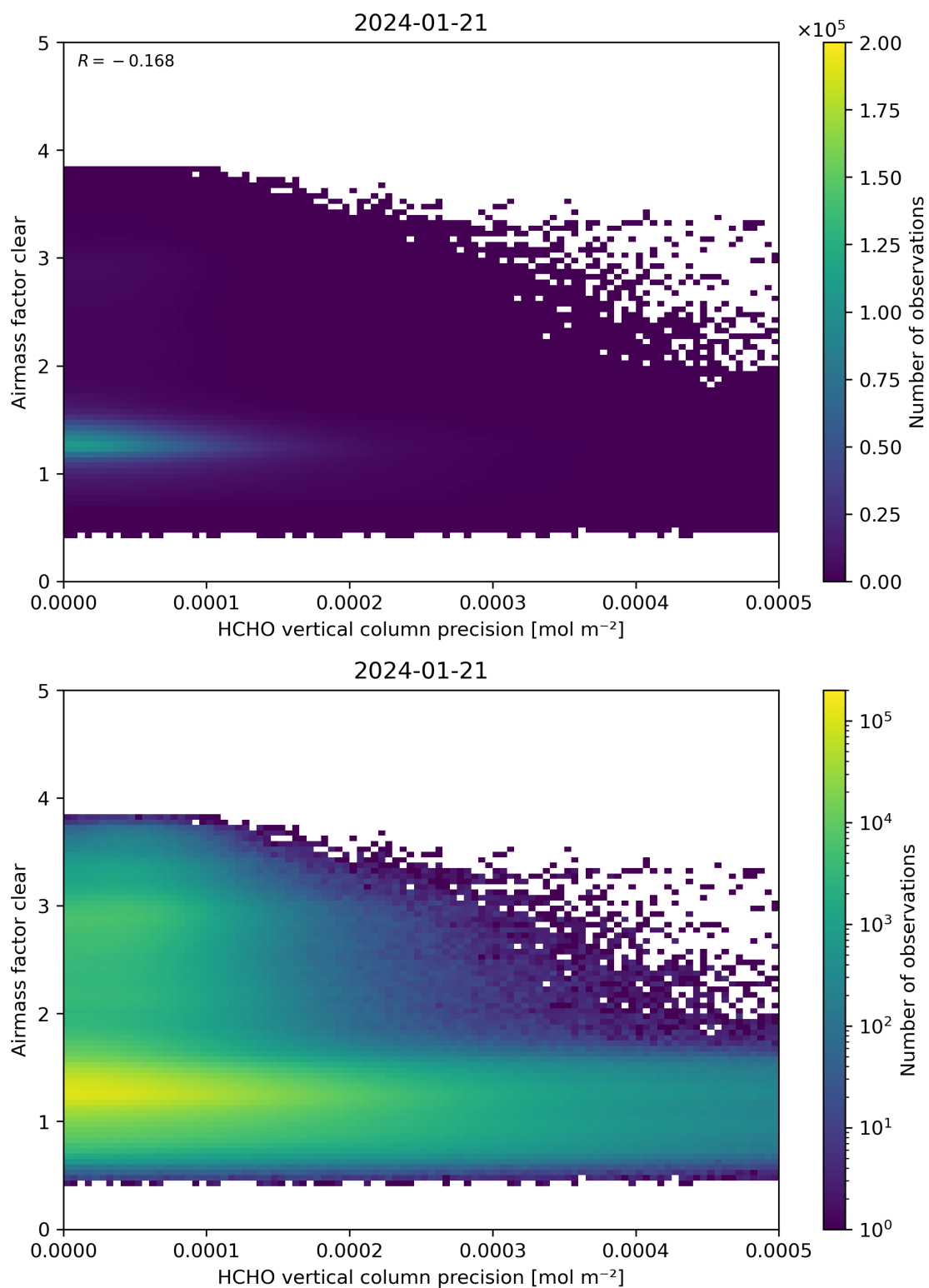
Figure 139: Scatter density plot of “HCHO vertical column precision” against “Airmass factor clear” for 2024-01-21 to 2024-01-22.
