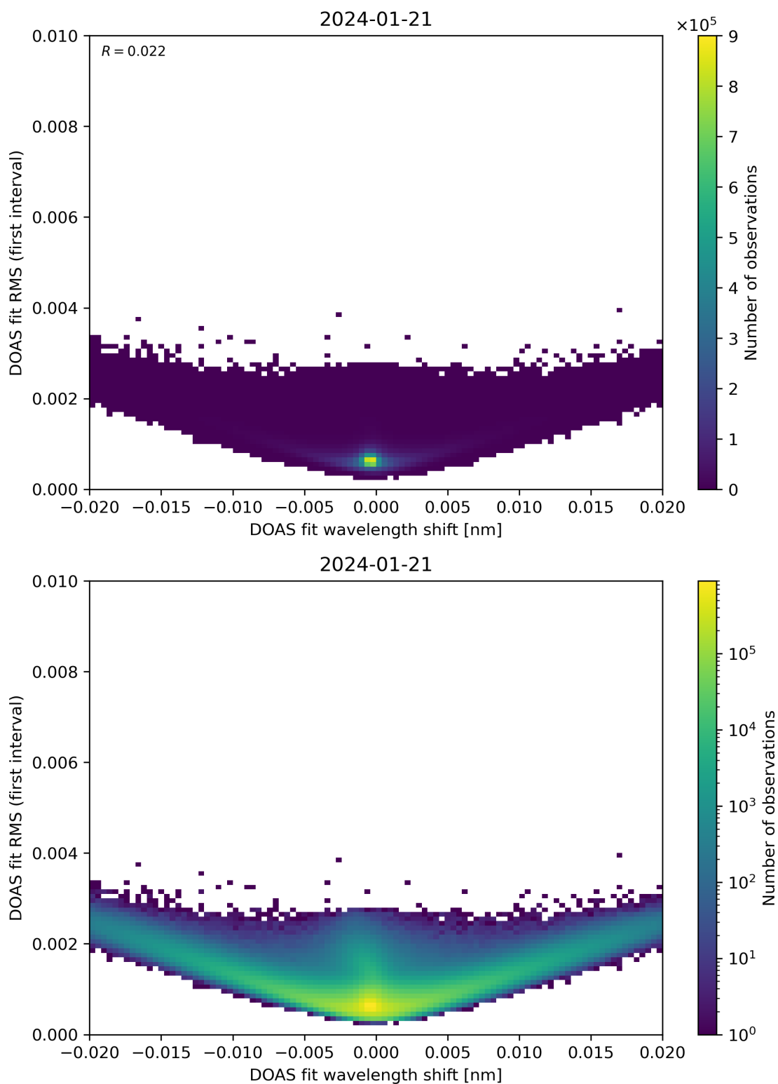
Figure 64: Scatter density plot of “DOAS fit wavelength shift” against “DOAS fit RMS (first interval)” for 2024-01-21 to 2024-01-22.
