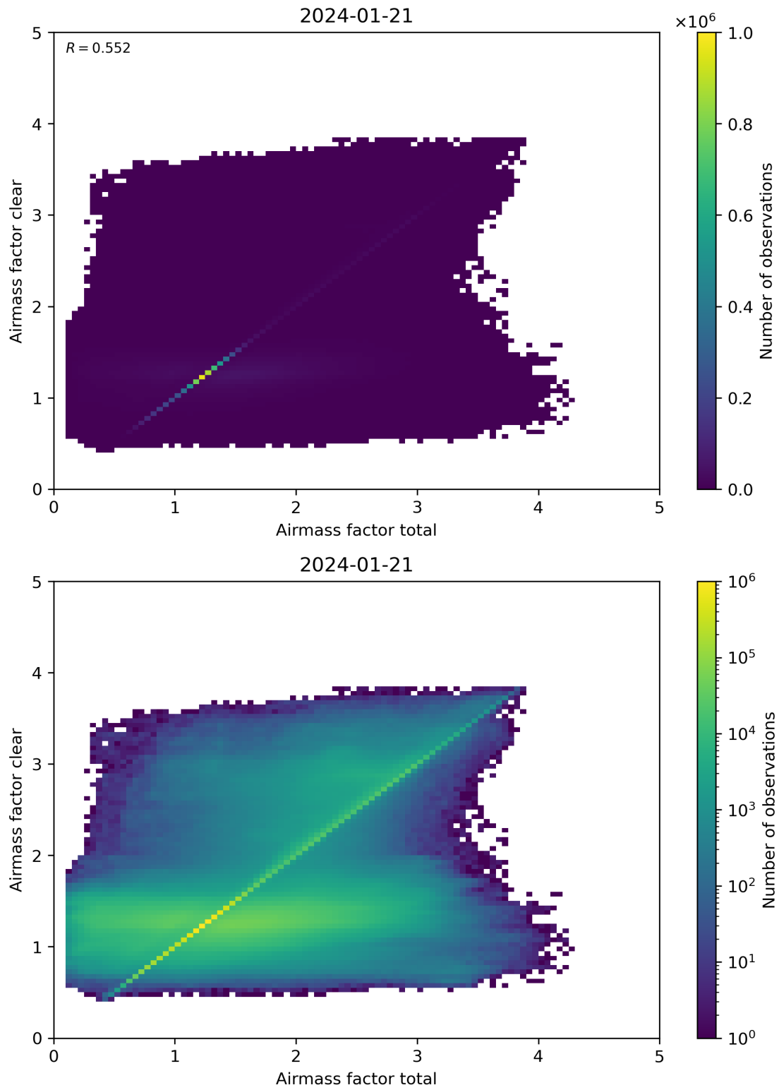
Figure 100: Scatter density plot of “Airmass factor total” against “Airmass factor clear” for 2024-01-21 to 2024-01-22.
