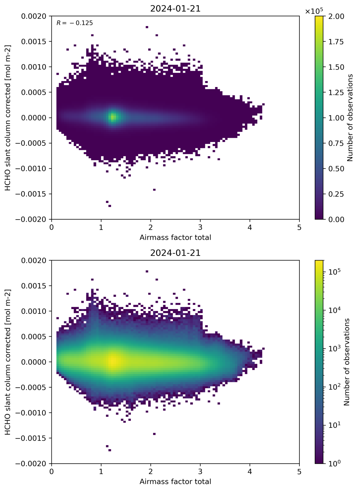
Figure 101: Scatter density plot of “Airmass factor total” against “HCHO slant column corrected” for 2024-01-21 to 2024-01-22.
