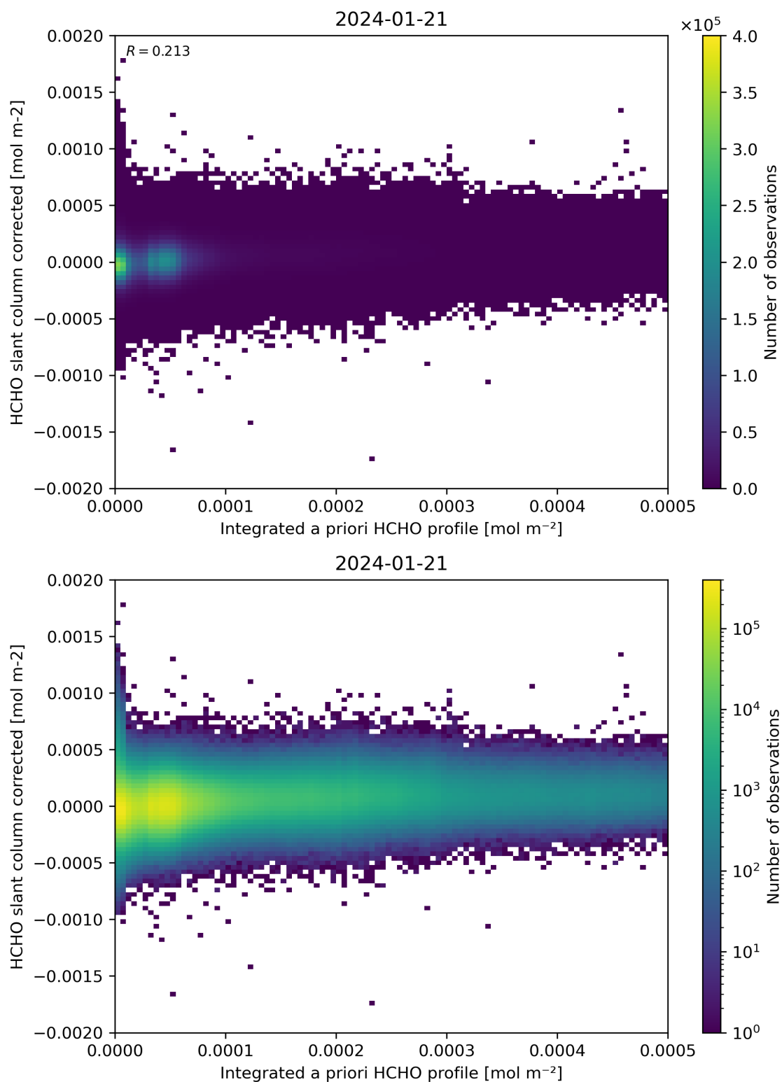
Figure 151: Scatter density plot of “Integrated a priori HCHO profile” against “HCHO slant column corrected” for 2024-01-21 to 2024-01-22.
