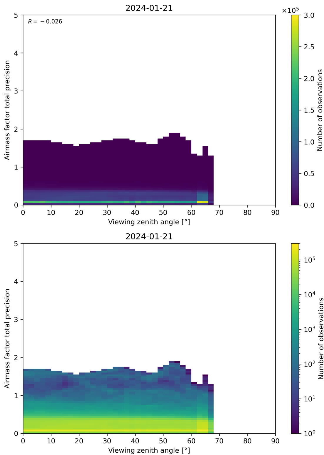
Figure 191: Scatter density plot of “Viewing zenith angle” against “Airmass factor total precision” for 2024-01-21 to 2024-01-22.
