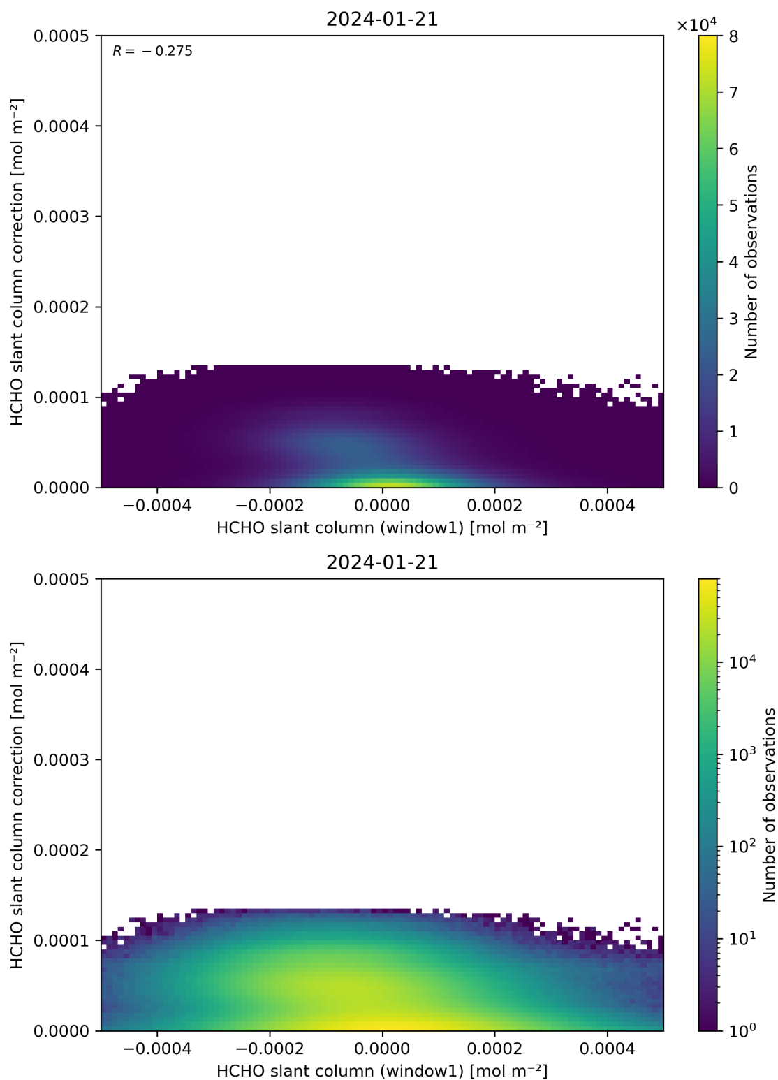
Figure 83: Scatter density plot of “HCHO slant column (window1)” against “HCHO slant column correction” for 2024-01-21 to 2024-01-22.
