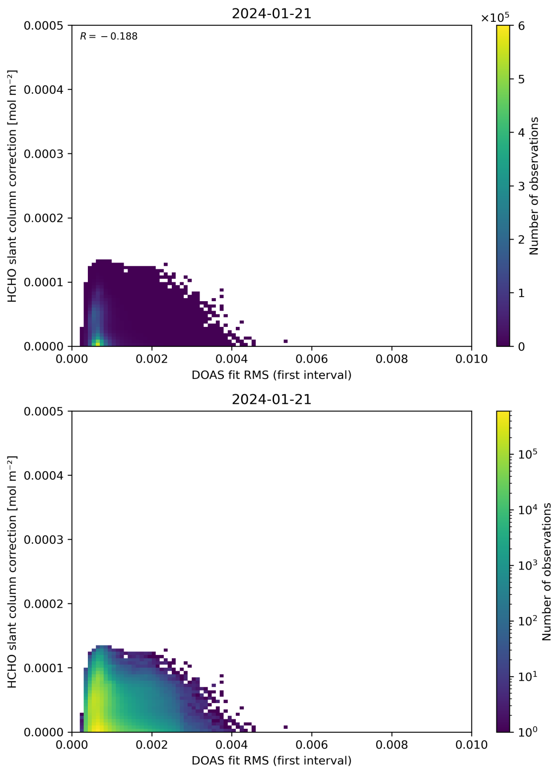
Figure 63: Scatter density plot of “DOAS fit RMS (first interval)” against “HCHO slant column correction” for 2024-01-21 to 2024-01-22.
