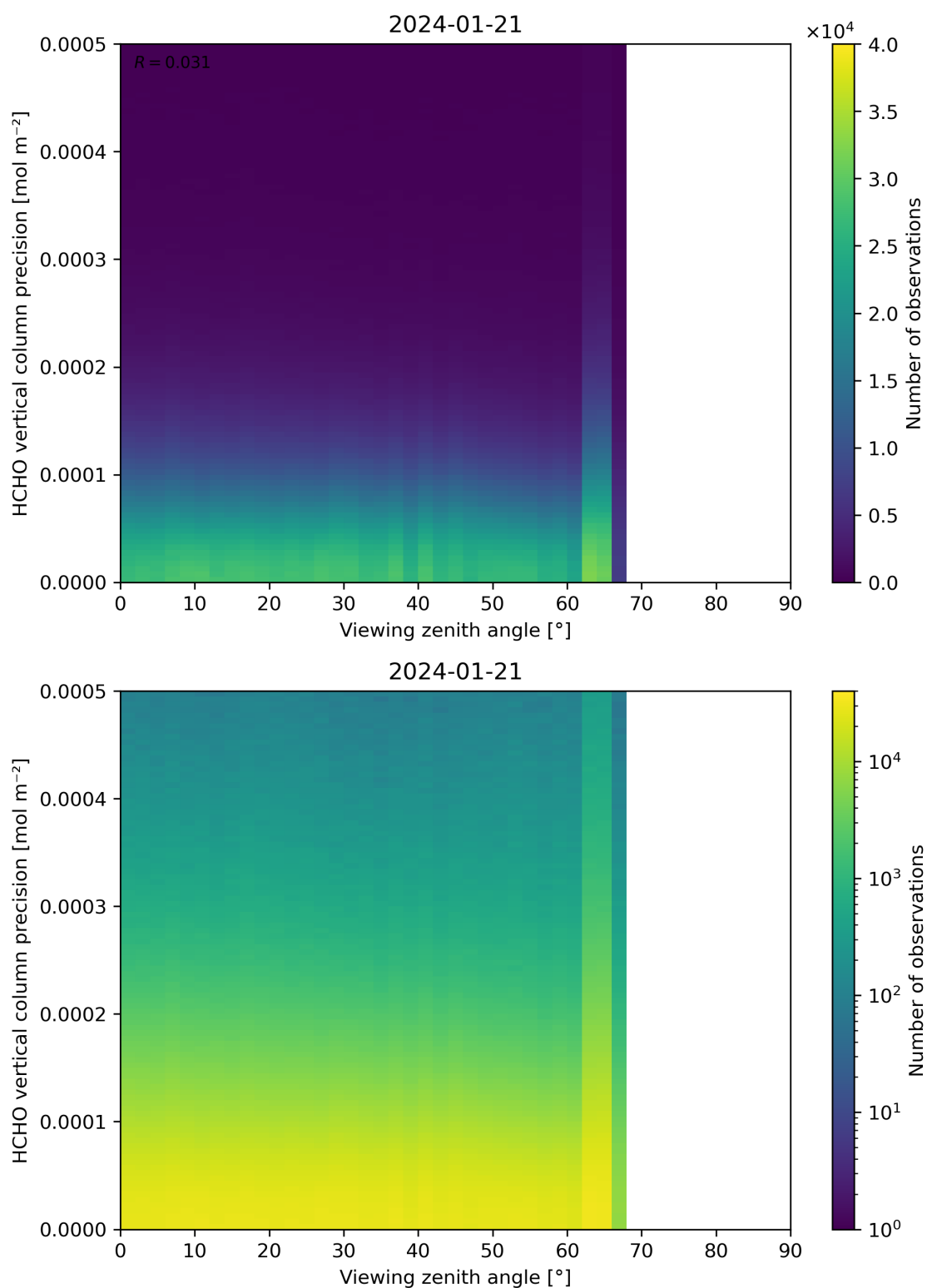
Figure 194: Scatter density plot of “Viewing zenith angle” against “HCHO vertical column precision” for 2024-01-21 to 2024-01-22.
