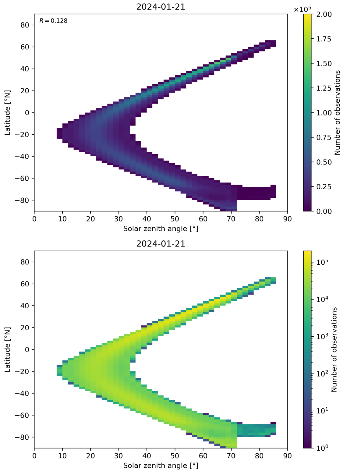
Figure 181: Scatter density plot of “Solar zenith angle” against “Latitude” for 2024-01-21 to 2024-01-22.
