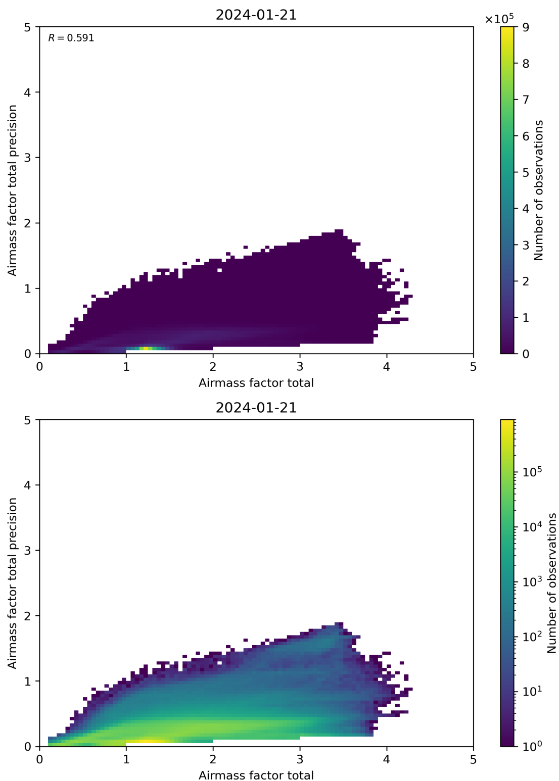
Figure 103: Scatter density plot of “Airmass factor total” against “Airmass factor total precision” for 2024-01-21 to 2024-01-22.
