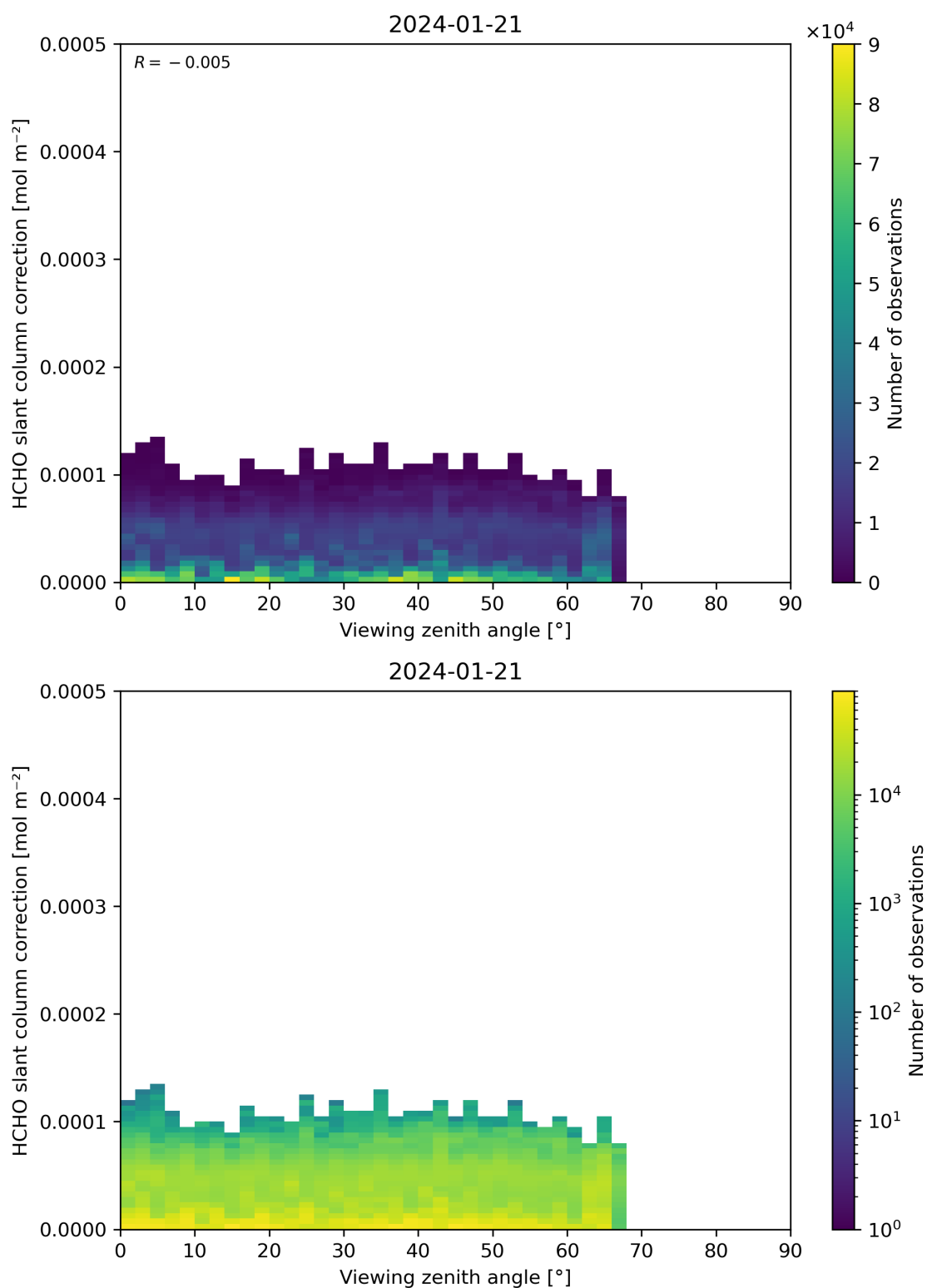
Figure 187: Scatter density plot of “Viewing zenith angle” against “HCHO slant column correction” for 2024-01-21 to 2024-01-22.
