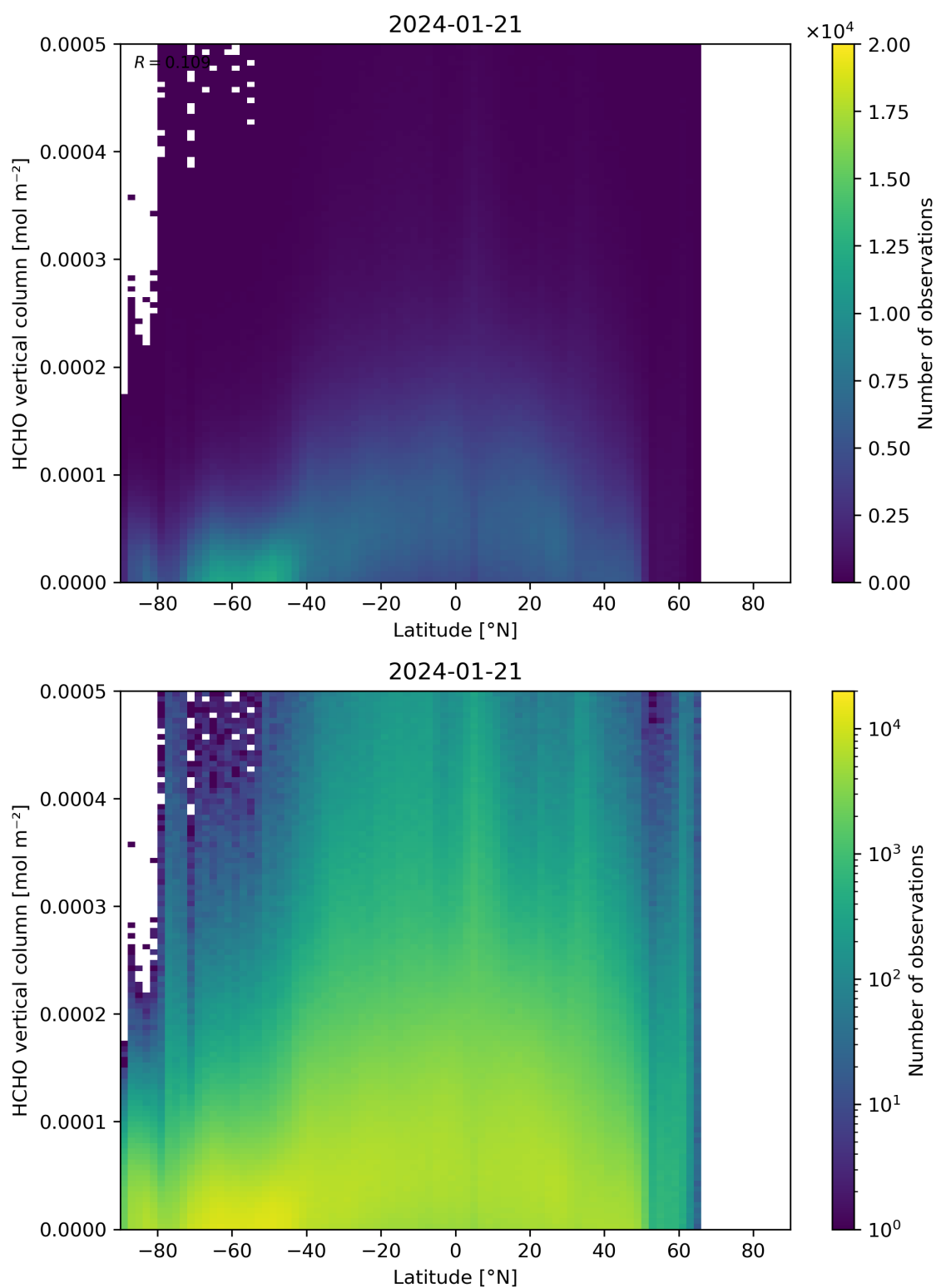
Figure 163: Scatter density plot of “Latitude” against “HCHO vertical column” for 2024-01-21 to 2024-01-22.
