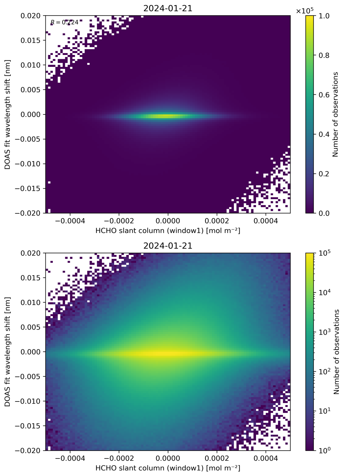
Figure 79: Scatter density plot of “HCHO slant column (window1)” against “DOAS fit wavelength shift” for 2024-01-21 to 2024-01-22.
