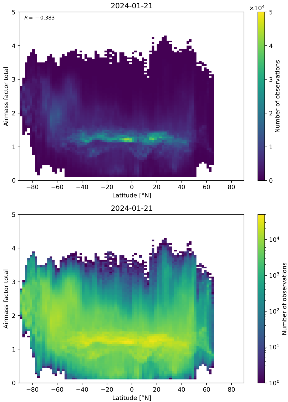
Figure 161: Scatter density plot of “Latitude” against “Airmass factor total” for 2024-01-21 to 2024-01-22.
