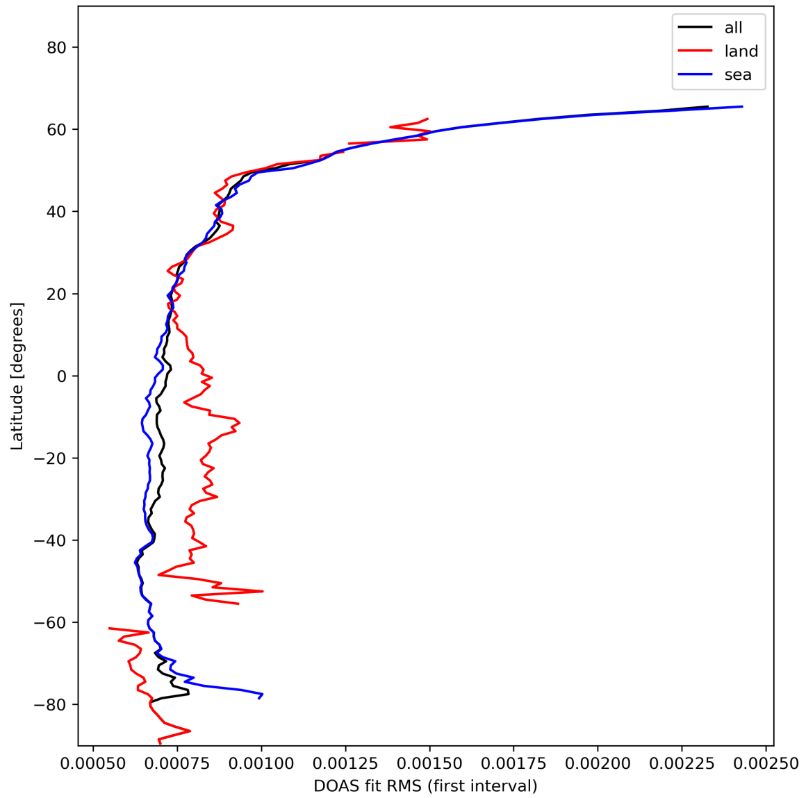
Figure 32: Zonal average of “DOAS fit RMS (first interval)” for 2024-01-21 to 2024-01-22.
