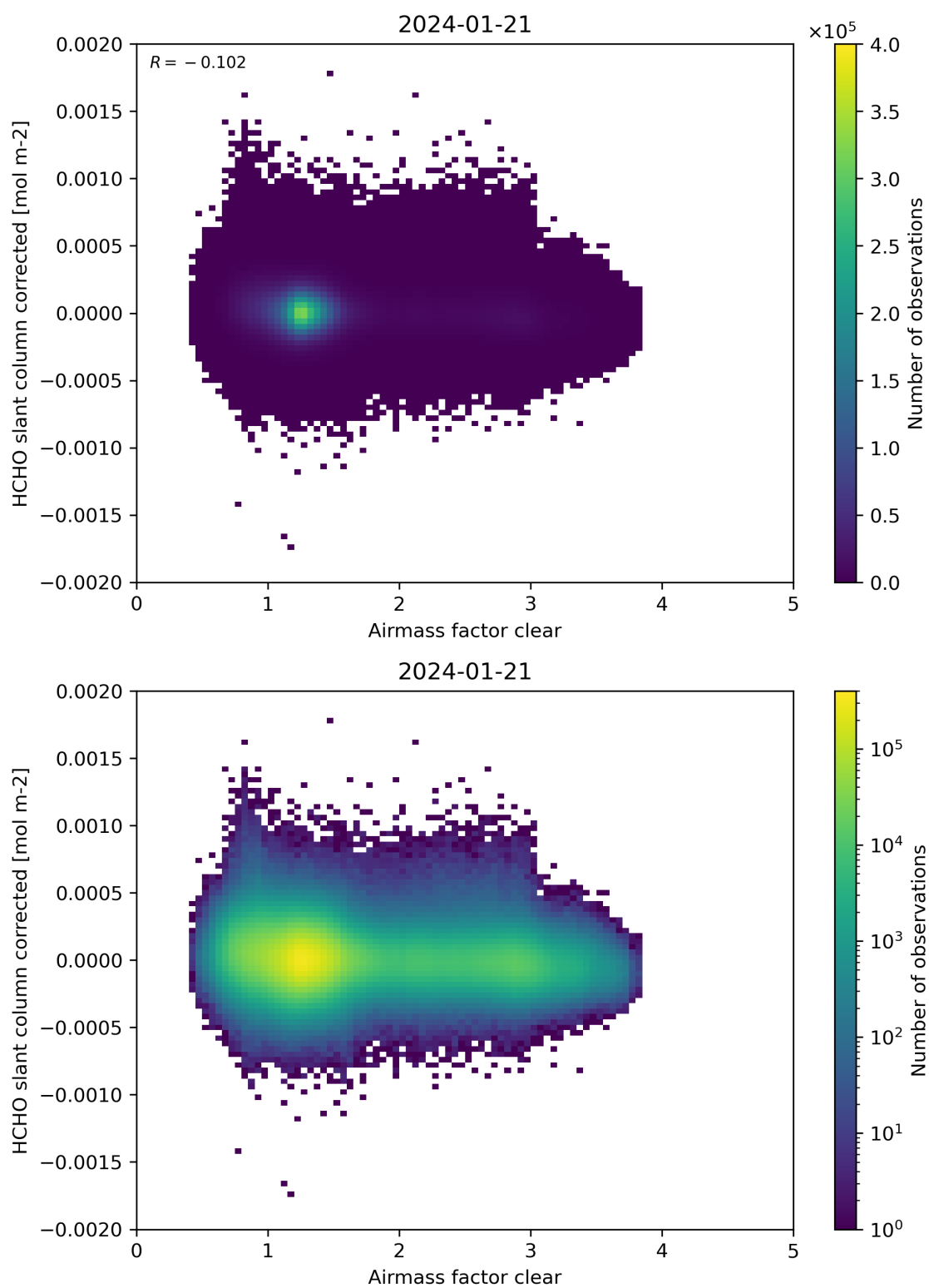
Figure 74: Scatter density plot of “Airmass factor clear” against “HCHO slant column corrected” for 2024-01-21 to 2024-01-22.
