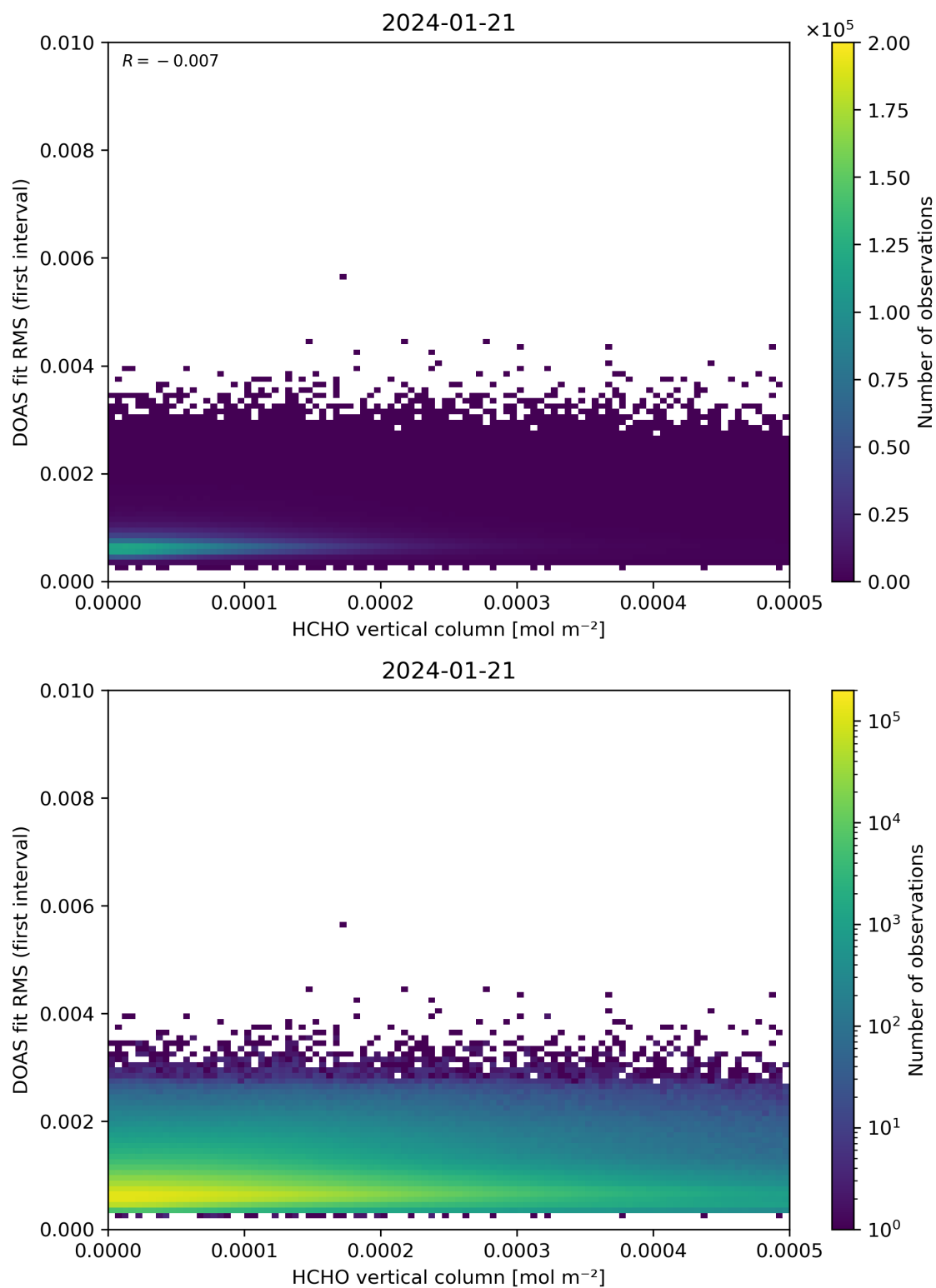
Figure 123: Scatter density plot of “HCHO vertical column” against “DOAS fit RMS (first interval)” for 2024-01-21 to 2024-01-22.
