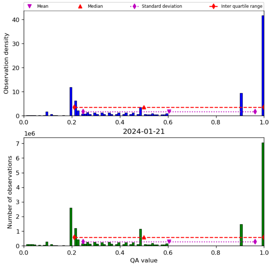
Figure 34: Histogram of “QA value” for 2024-01-21 to 2024-01-22
