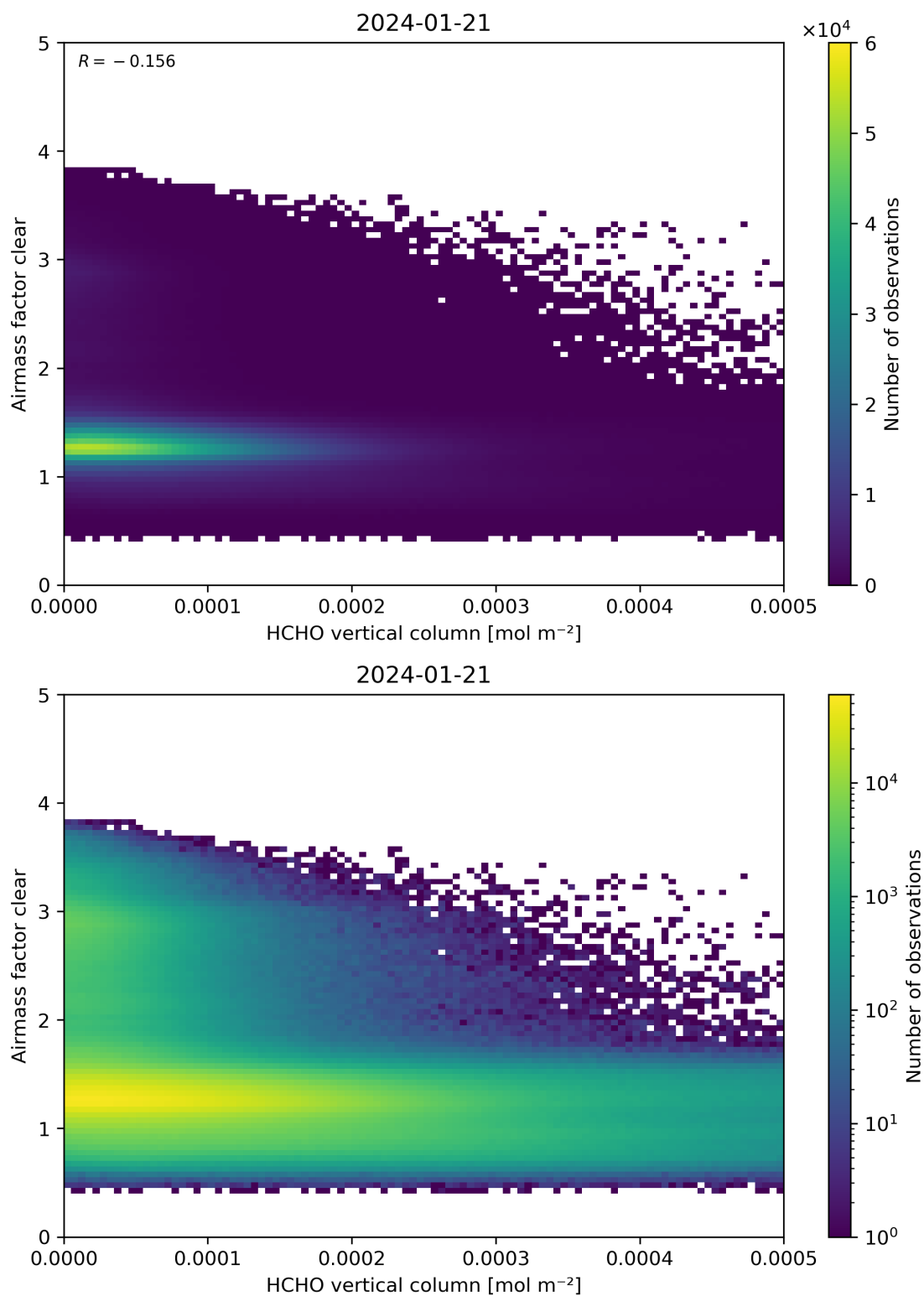
Figure 126: Scatter density plot of “HCHO vertical column” against “Airmass factor clear” for 2024-01-21 to 2024-01-22.
