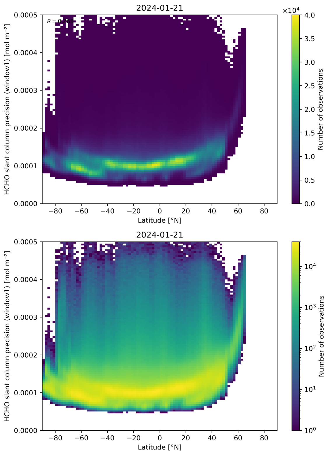
Figure 160: Scatter density plot of “Latitude” against “HCHO slant column precision (window1)” for 2024-01-21 to 2024-01-22.
