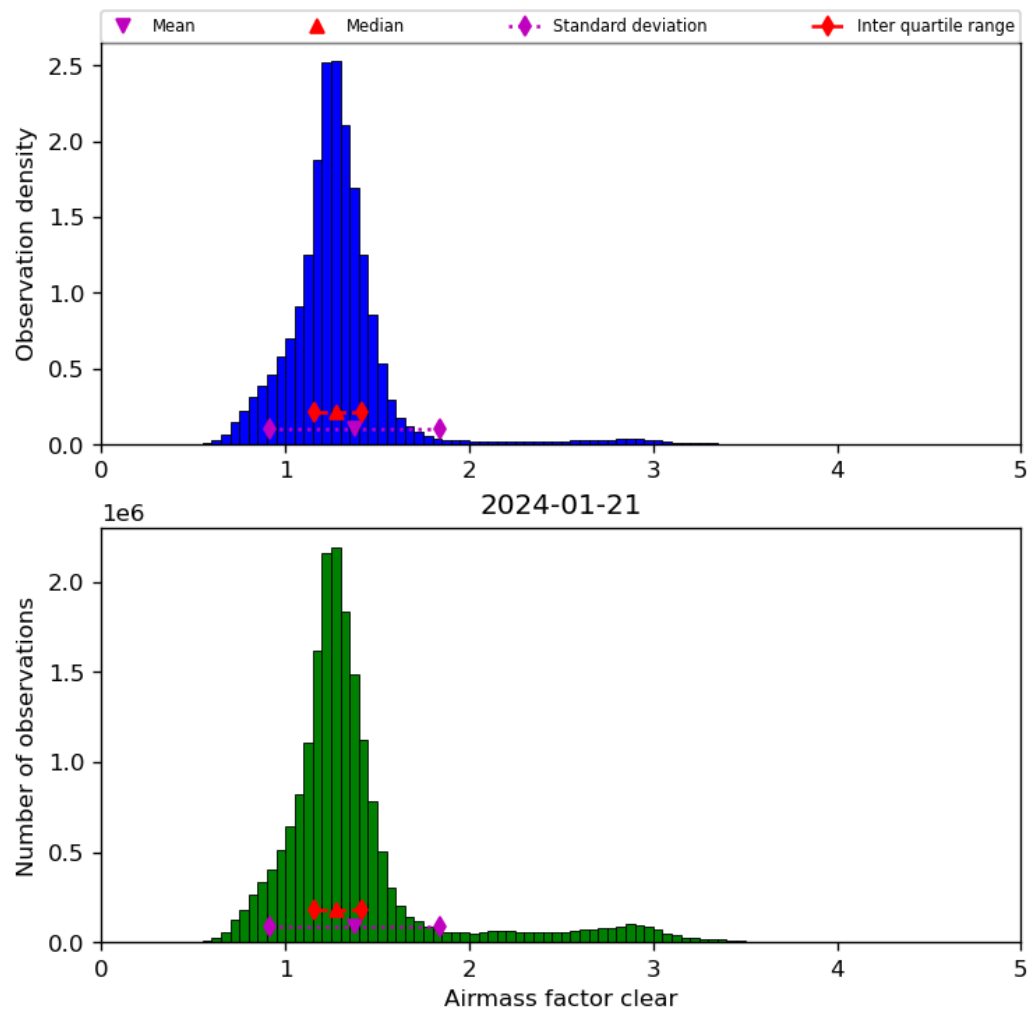
Figure 42: Histogram of “Airmass factor clear” for 2024-01-21 to 2024-01-22
