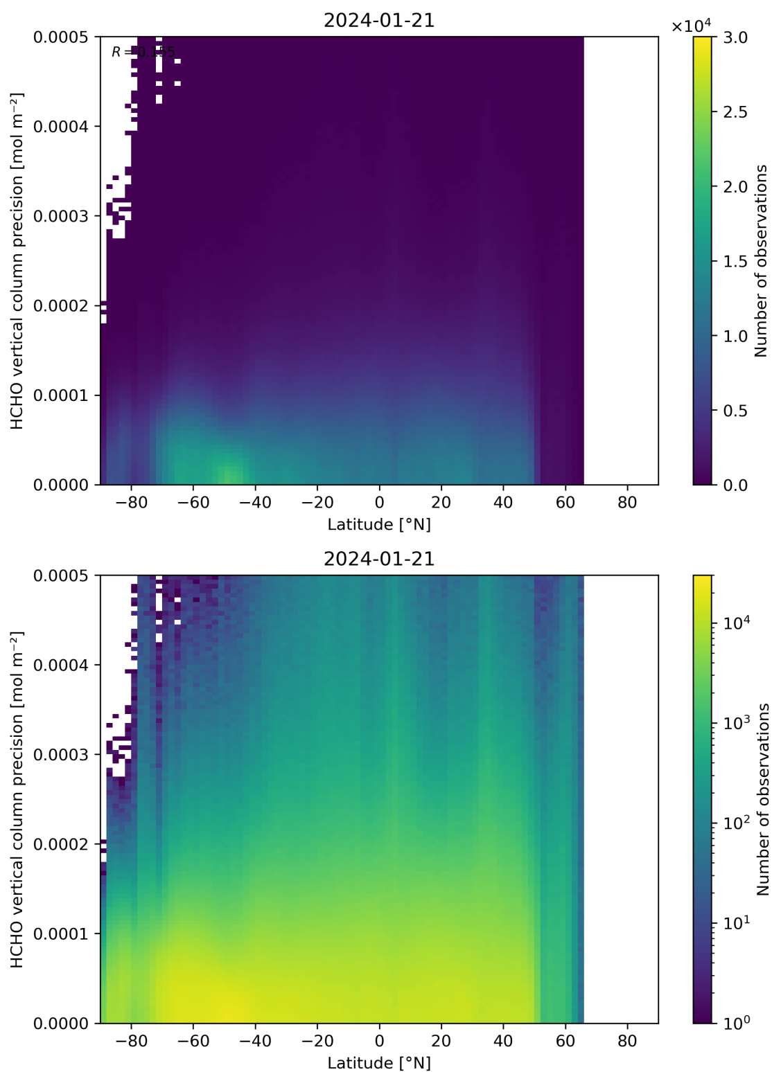
Figure 165: Scatter density plot of “Latitude” against “HCHO vertical column precision” for 2024-01-21 to 2024-01-22.
