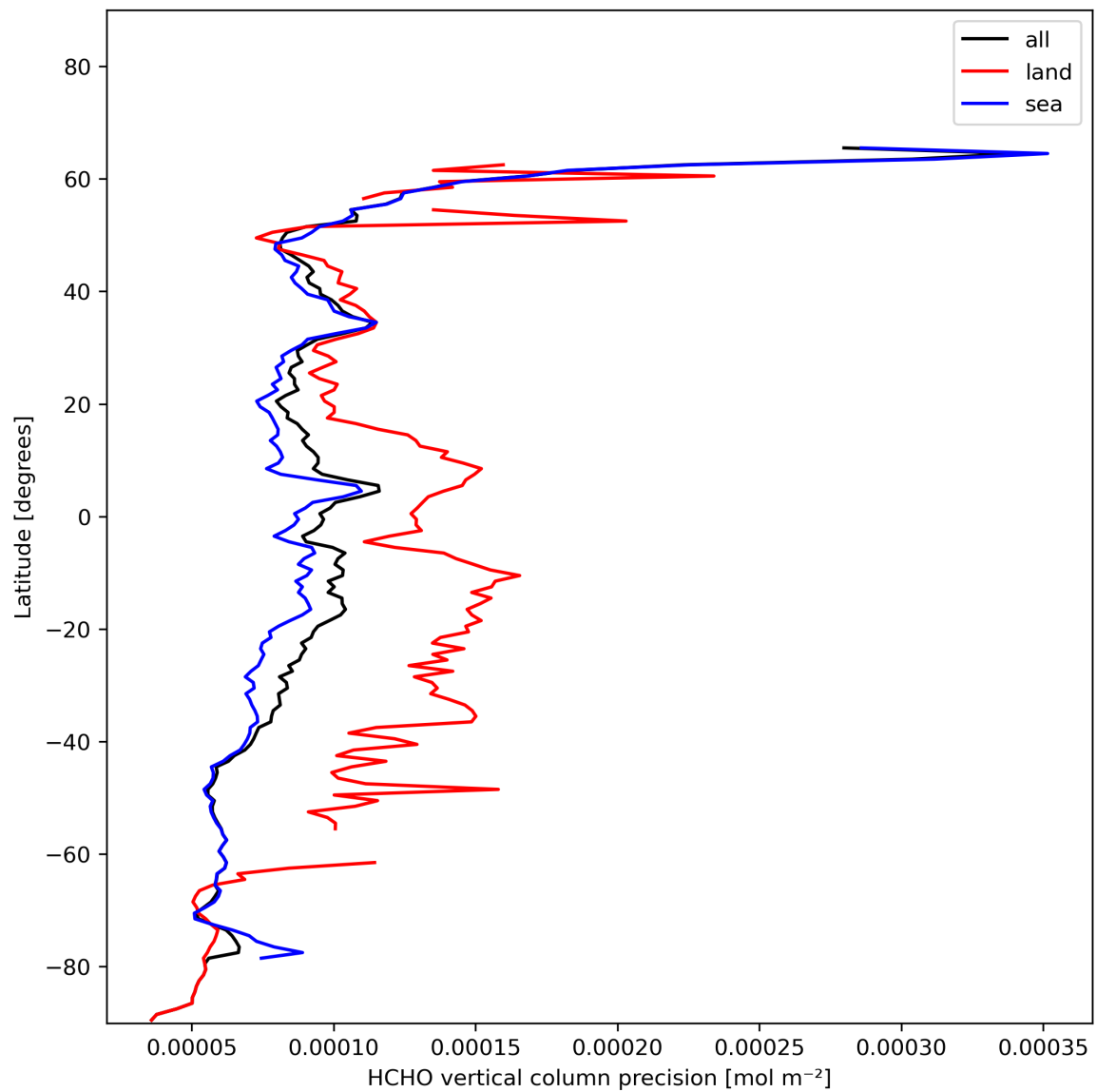
Figure 22: Zonal average of “HCHO vertical column precision” for 2024-01-21 to 2024-01-22.
