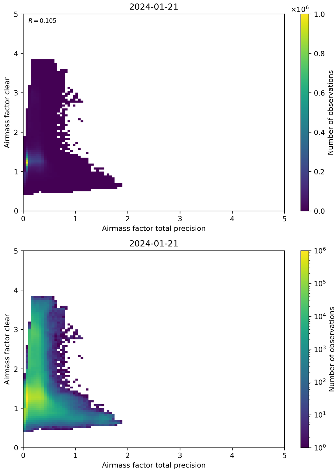
Figure 108: Scatter density plot of “Airmass factor total precision” against “Airmass factor clear” for 2024-01-21 to 2024-01-22.
