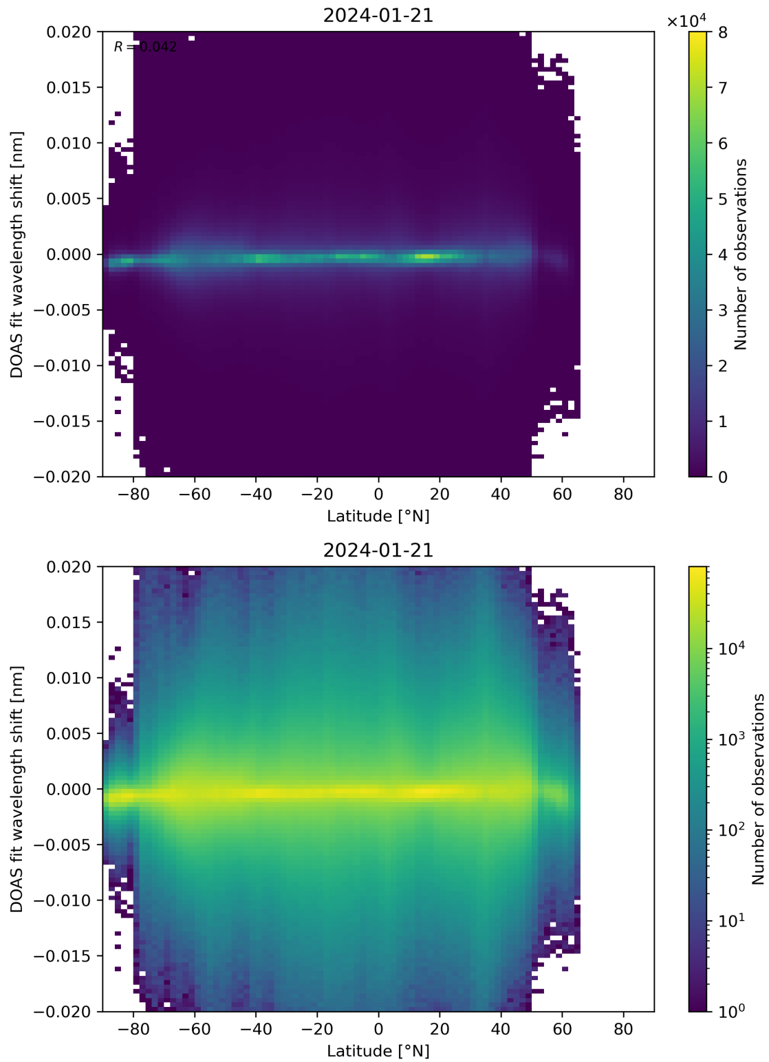
Figure 154: Scatter density plot of “Latitude” against “DOAS fit wavelength shift” for 2024-01-21 to 2024-01-22.
