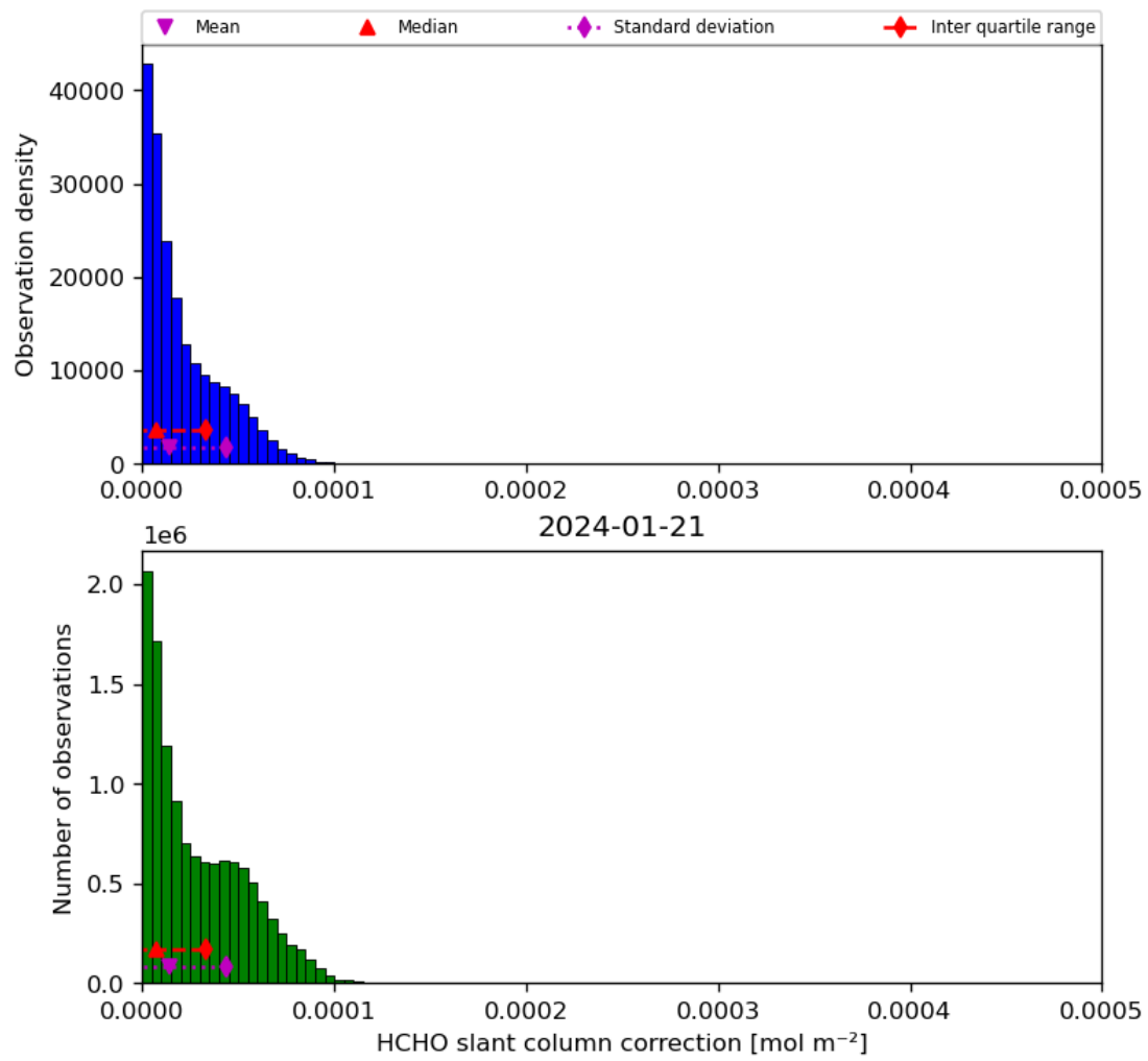
Figure 47: Histogram of “HCHO slant column correction” for 2024-01-21 to 2024-01-22
