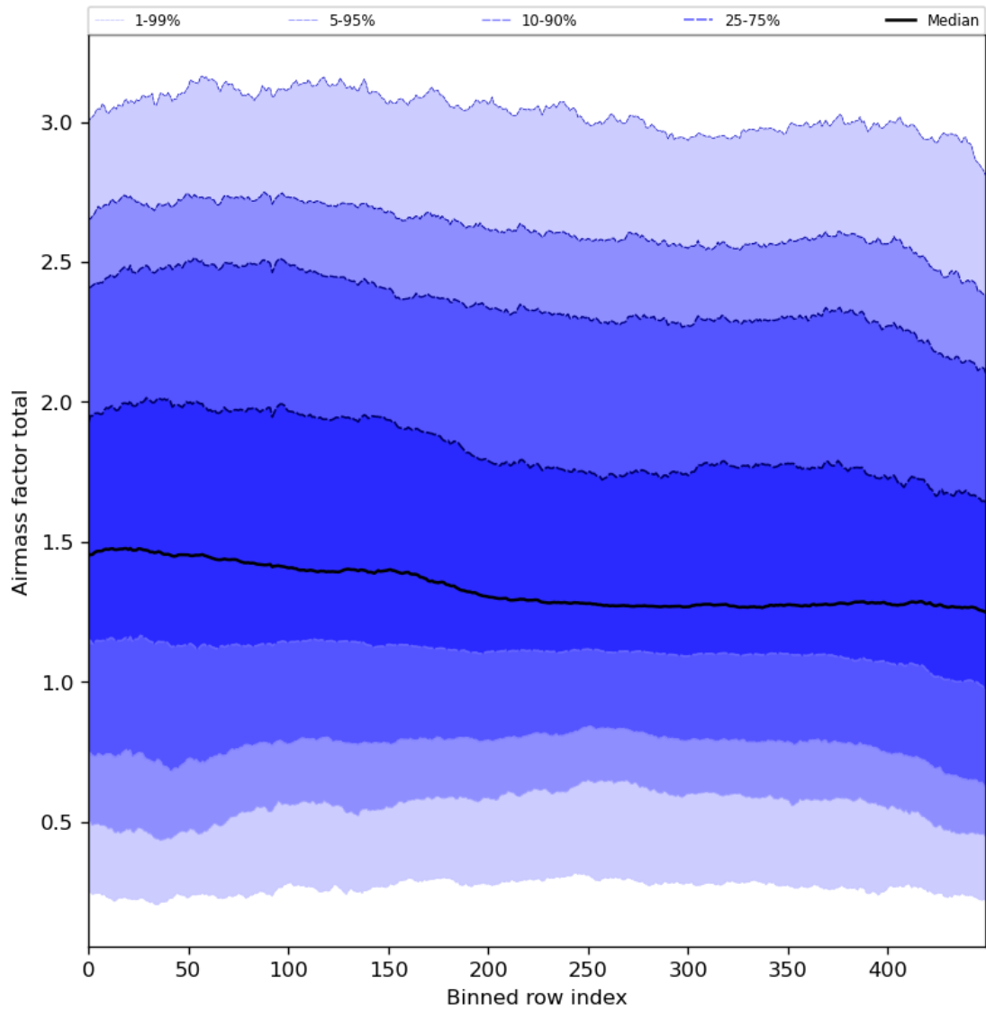
Figure 54: Along track statistics of “Airmass factor total” for 2024-01-21 to 2024-01-22
