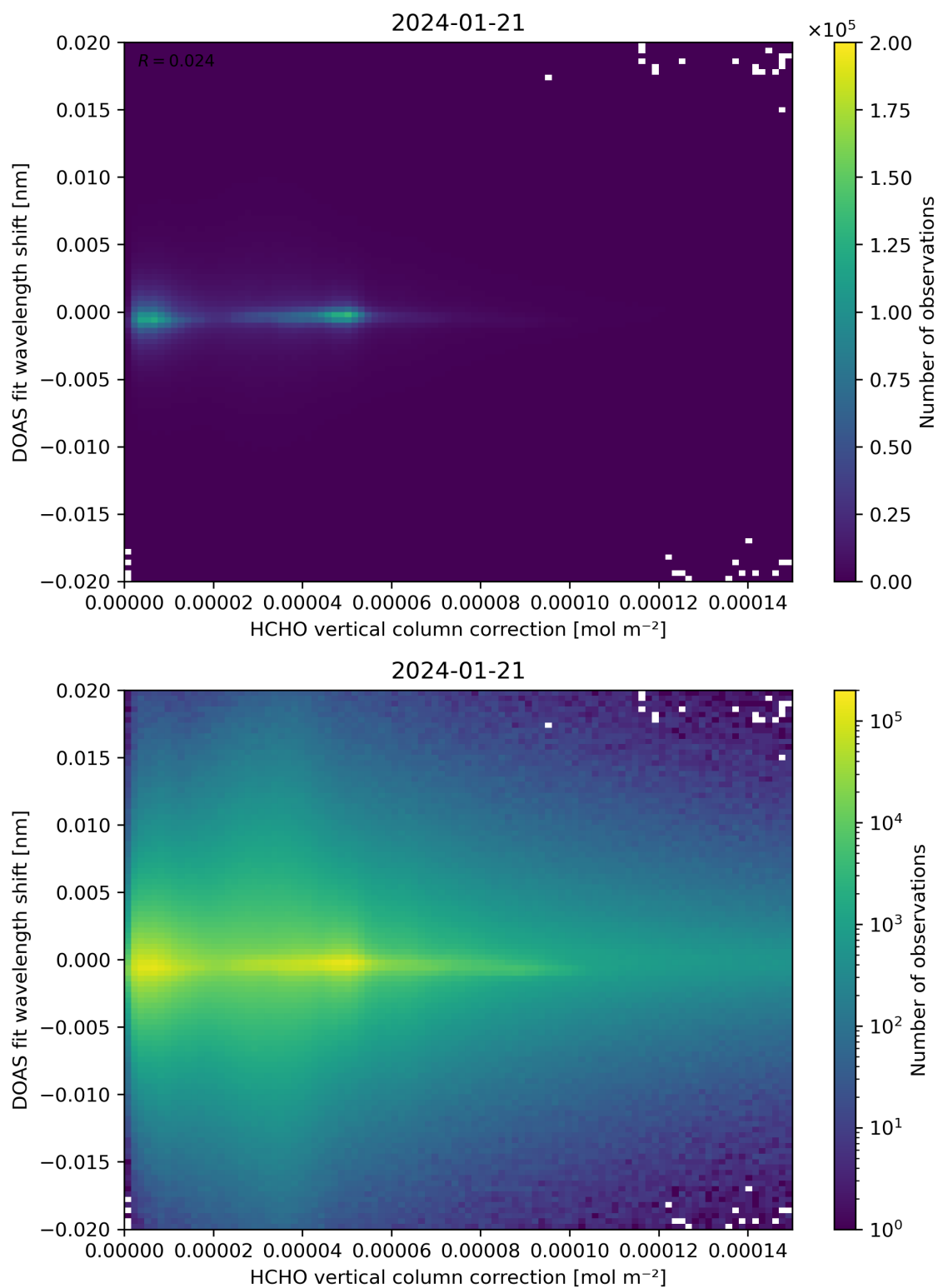
Figure 113: Scatter density plot of “HCHO vertical column correction” against “DOAS fit wavelength shift” for 2024-01-21 to 2024-01-22.
