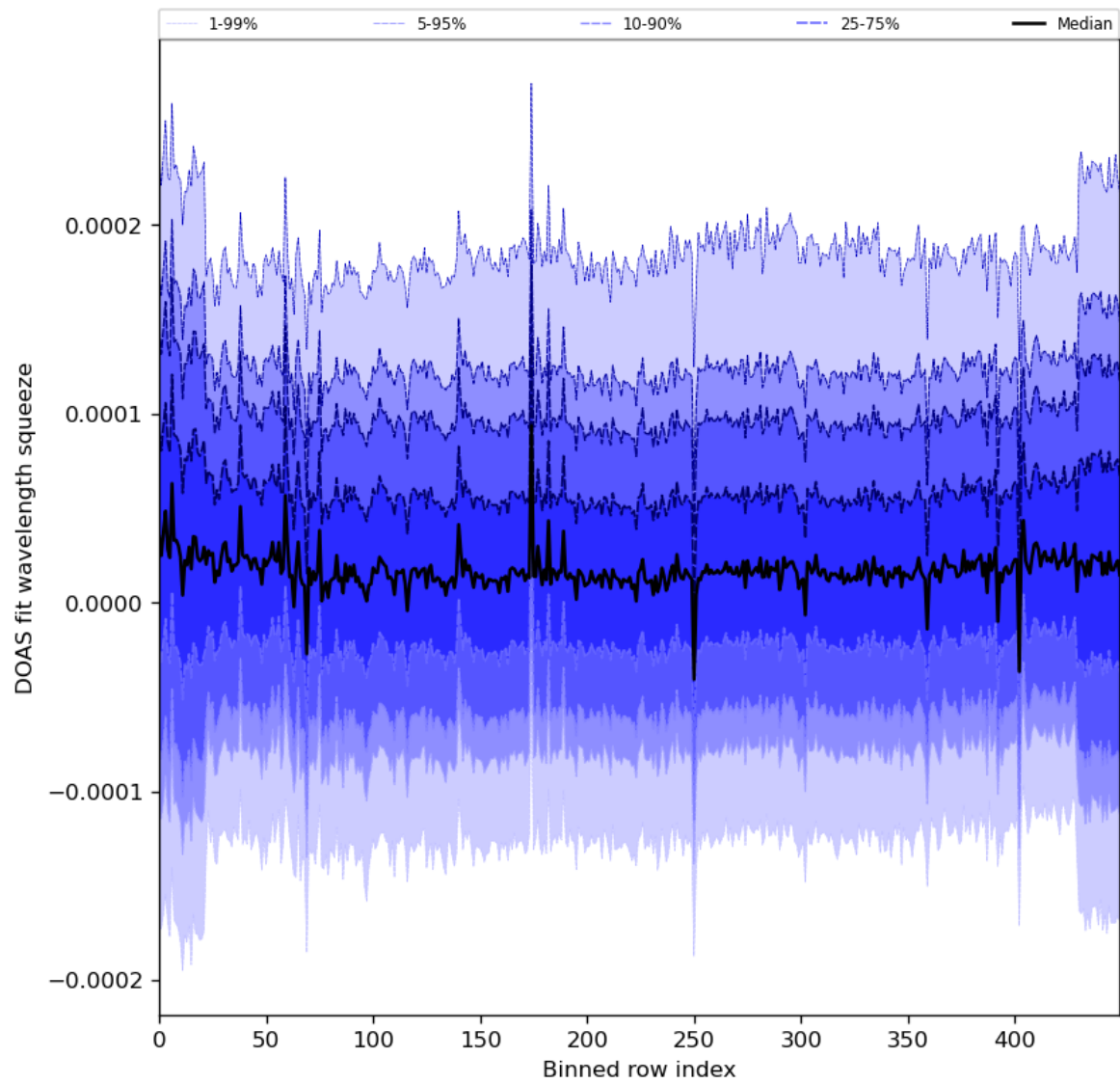
Figure 59: Along track statistics of “DOAS fit wavelength squeeze” for 2024-01-21 to 2024-01-22
