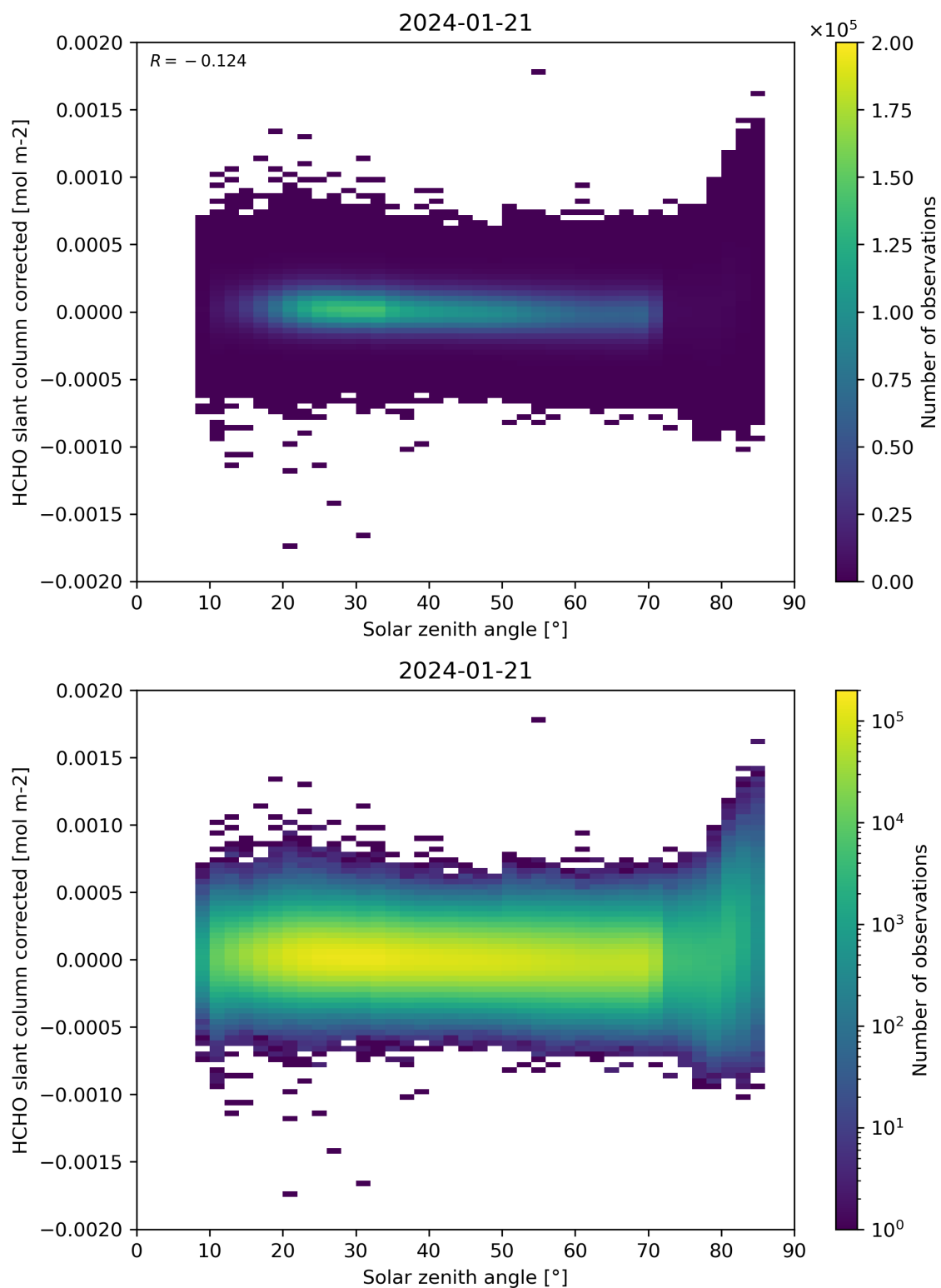
Figure 171: Scatter density plot of “Solar zenith angle” against “HCHO slant column corrected” for 2024-01-21 to 2024-01-22.
