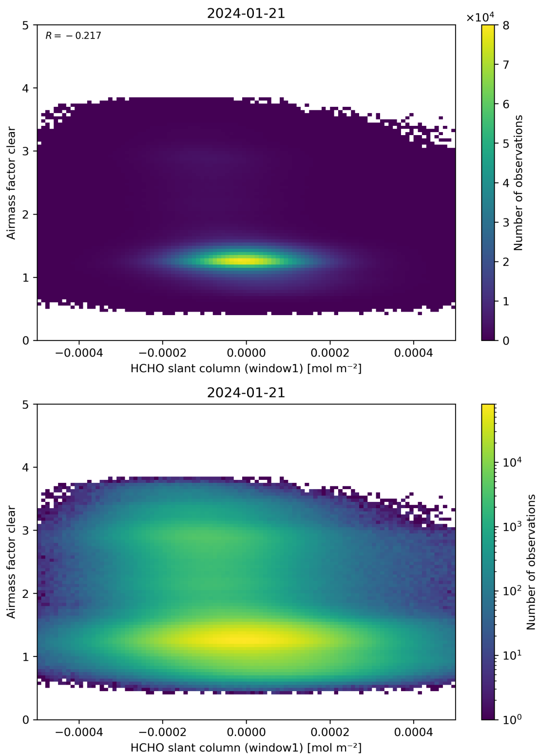
Figure 81: Scatter density plot of “HCHO slant column (window1)” against “Airmass factor clear” for 2024-01-21 to 2024-01-22.
