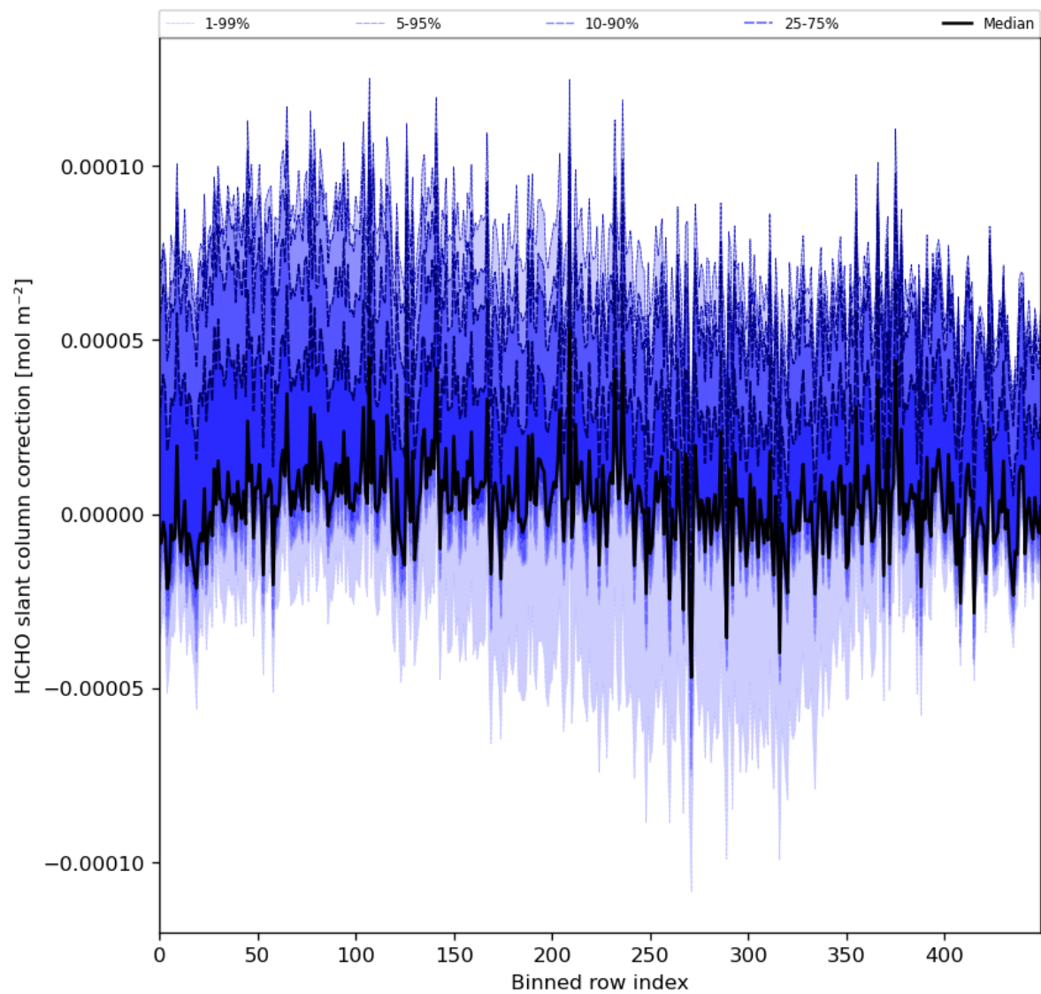
Figure 61: Along track statistics of “HCHO slant column correction” for 2024-01-21 to 2024-01-22
