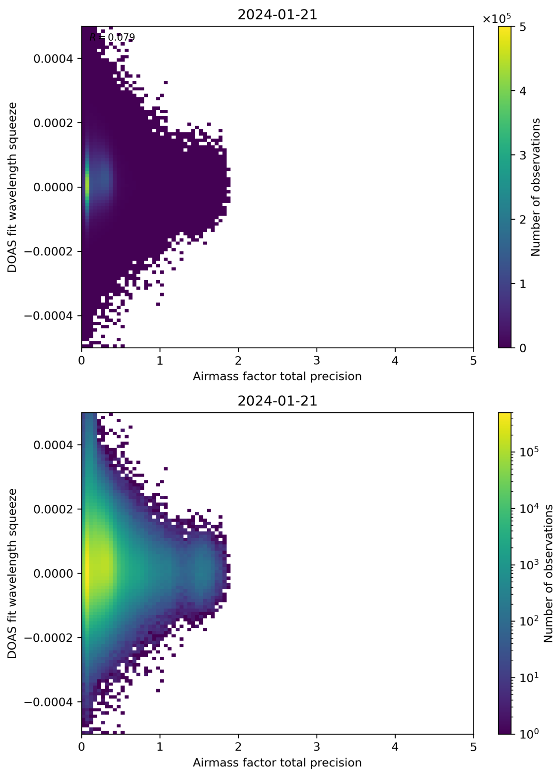
Figure 107: Scatter density plot of “Airmass factor total precision” against “DOAS fit wavelength squeeze” for 2024-01-21 to 2024-01-22.
