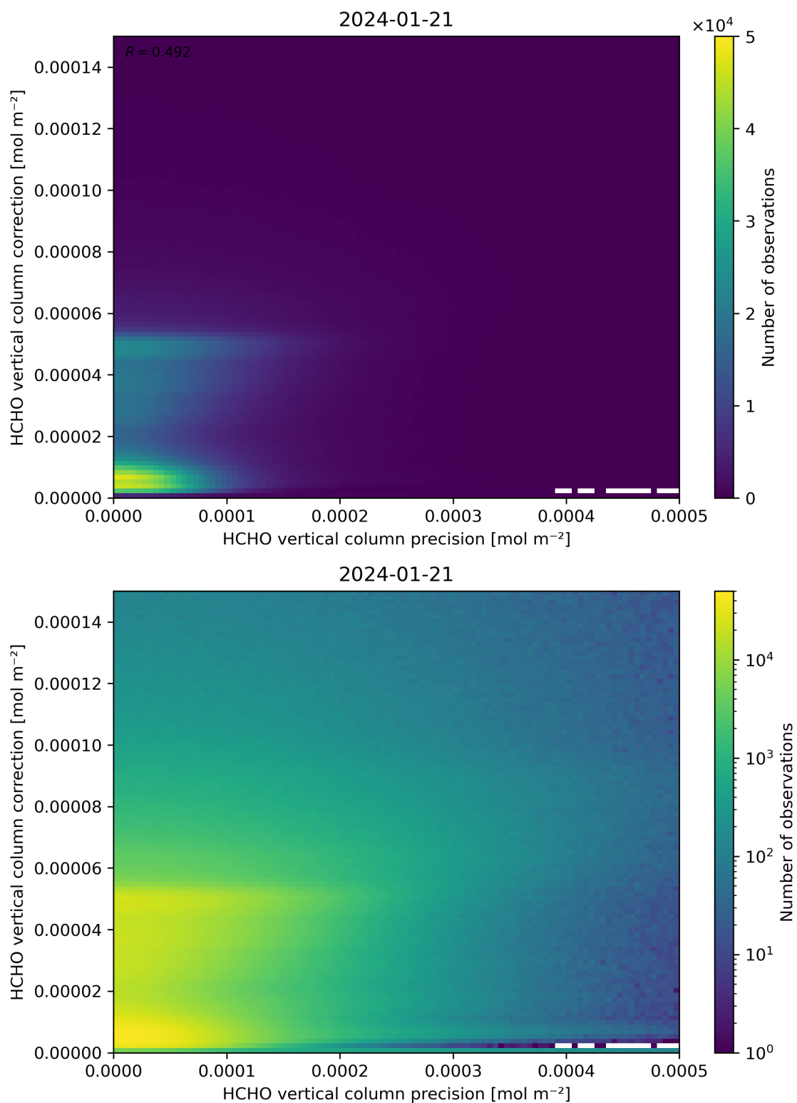
Figure 146: Scatter density plot of “HCHO vertical column precision” against “HCHO vertical column correction” for 2024-01-21 to 2024-01-22.
