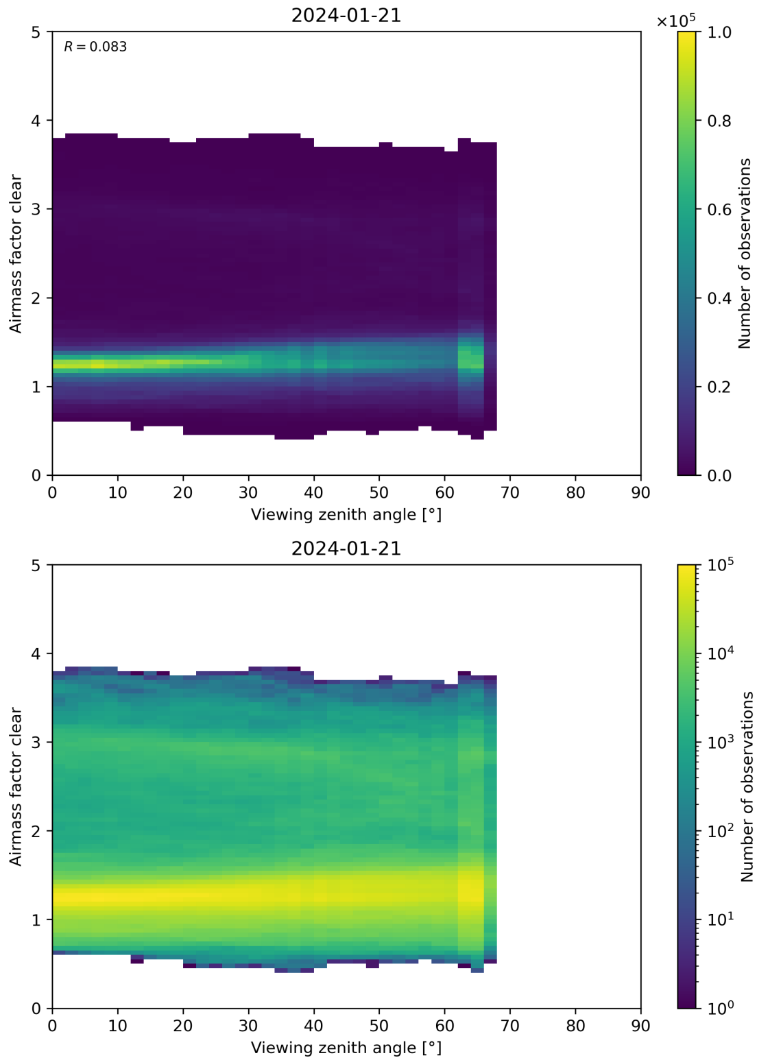
Figure 185: Scatter density plot of “Viewing zenith angle” against “Airmass factor clear” for 2024-01-21 to 2024-01-22.
