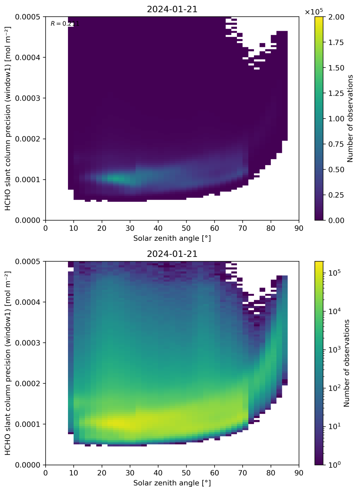
Figure 174: Scatter density plot of “Solar zenith angle” against “HCHO slant column precision (window1)” for 2024-01-21 to 2024-01-22.
