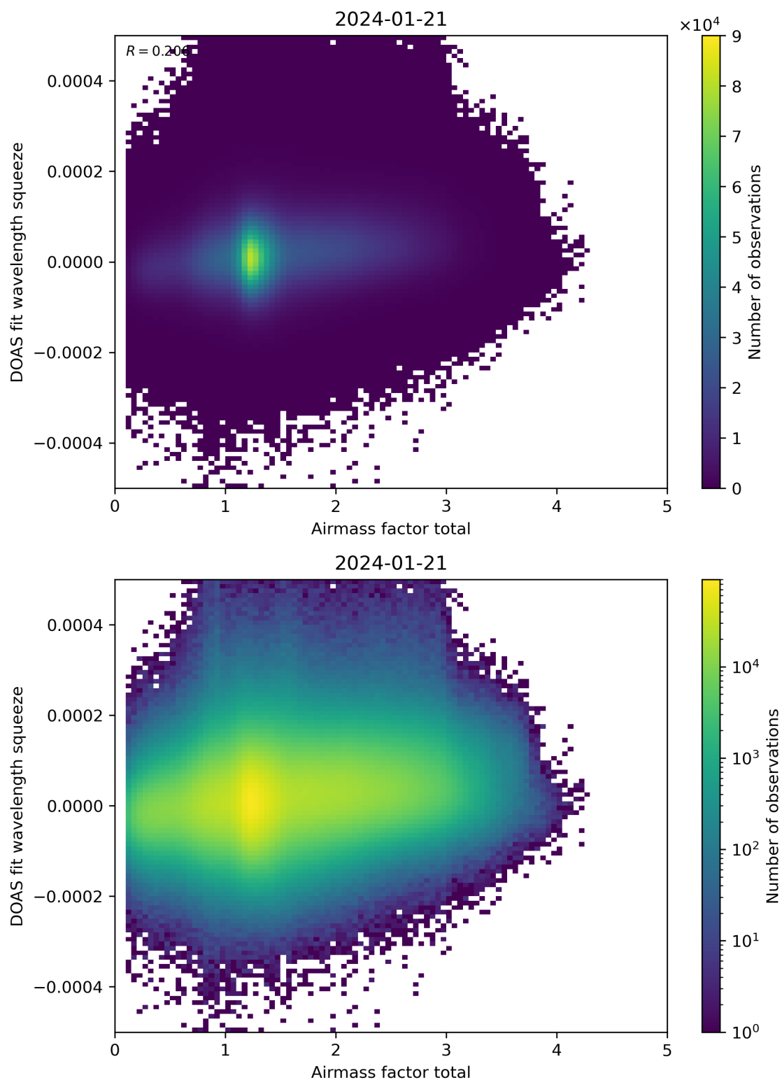
Figure 99: Scatter density plot of “Airmass factor total” against “DOAS fit wavelength squeeze” for 2024-01-21 to 2024-01-22.
