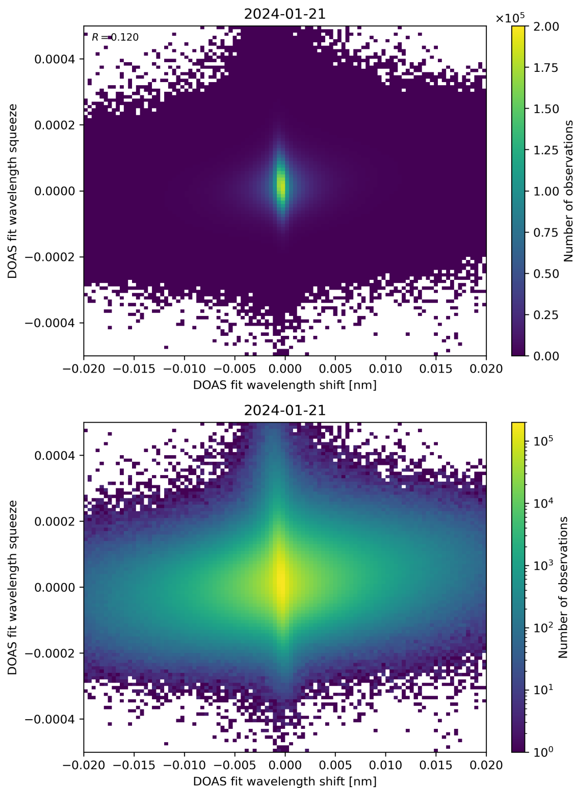
Figure 65: Scatter density plot of “DOAS fit wavelength shift” against “DOAS fit wavelength squeeze” for 2024-01-21 to 2024-01-22.
