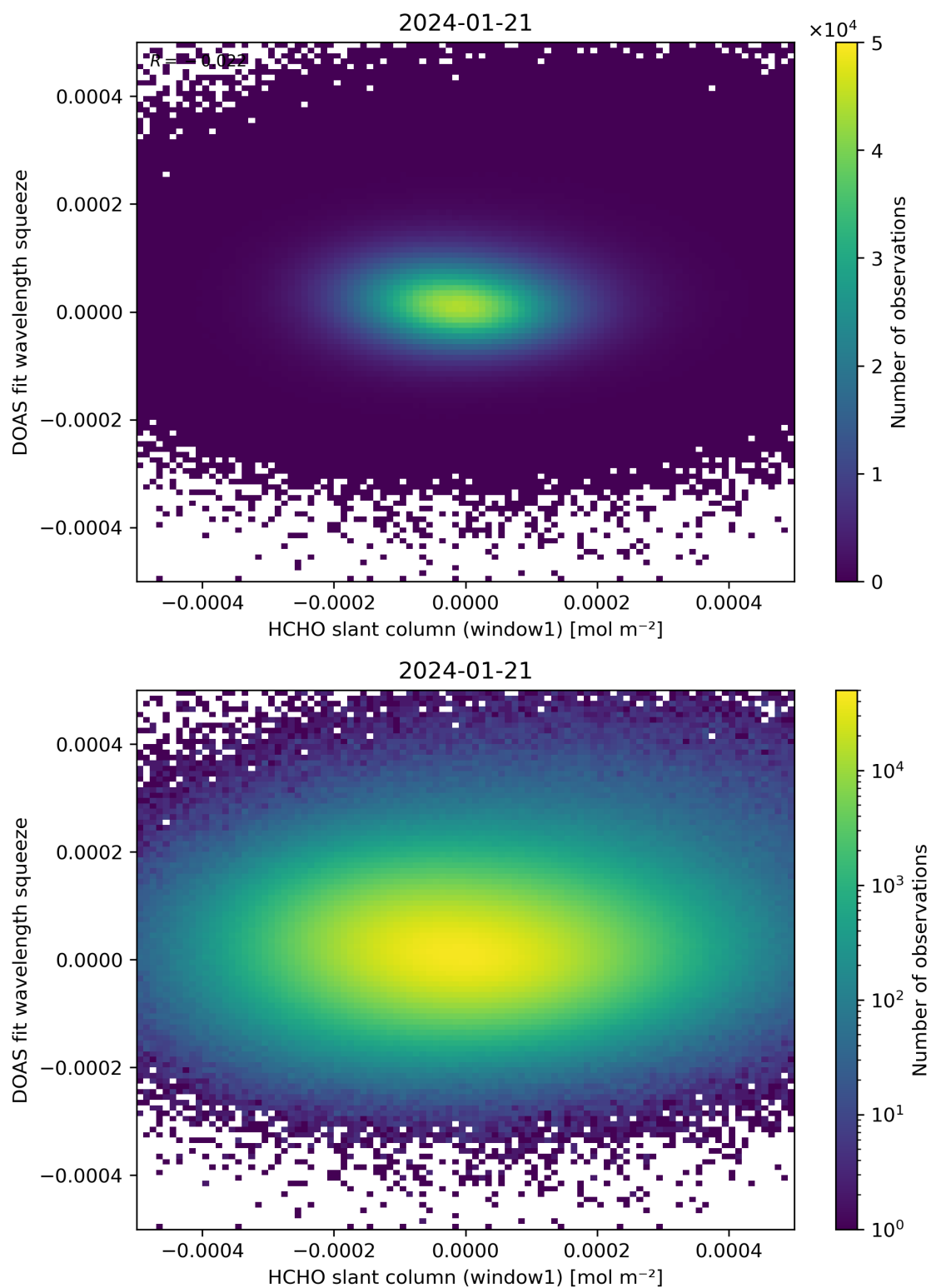
Figure 80: Scatter density plot of “HCHO slant column (window1)” against “DOAS fit wavelength squeeze” for 2024-01-21 to 2024-01-22.
