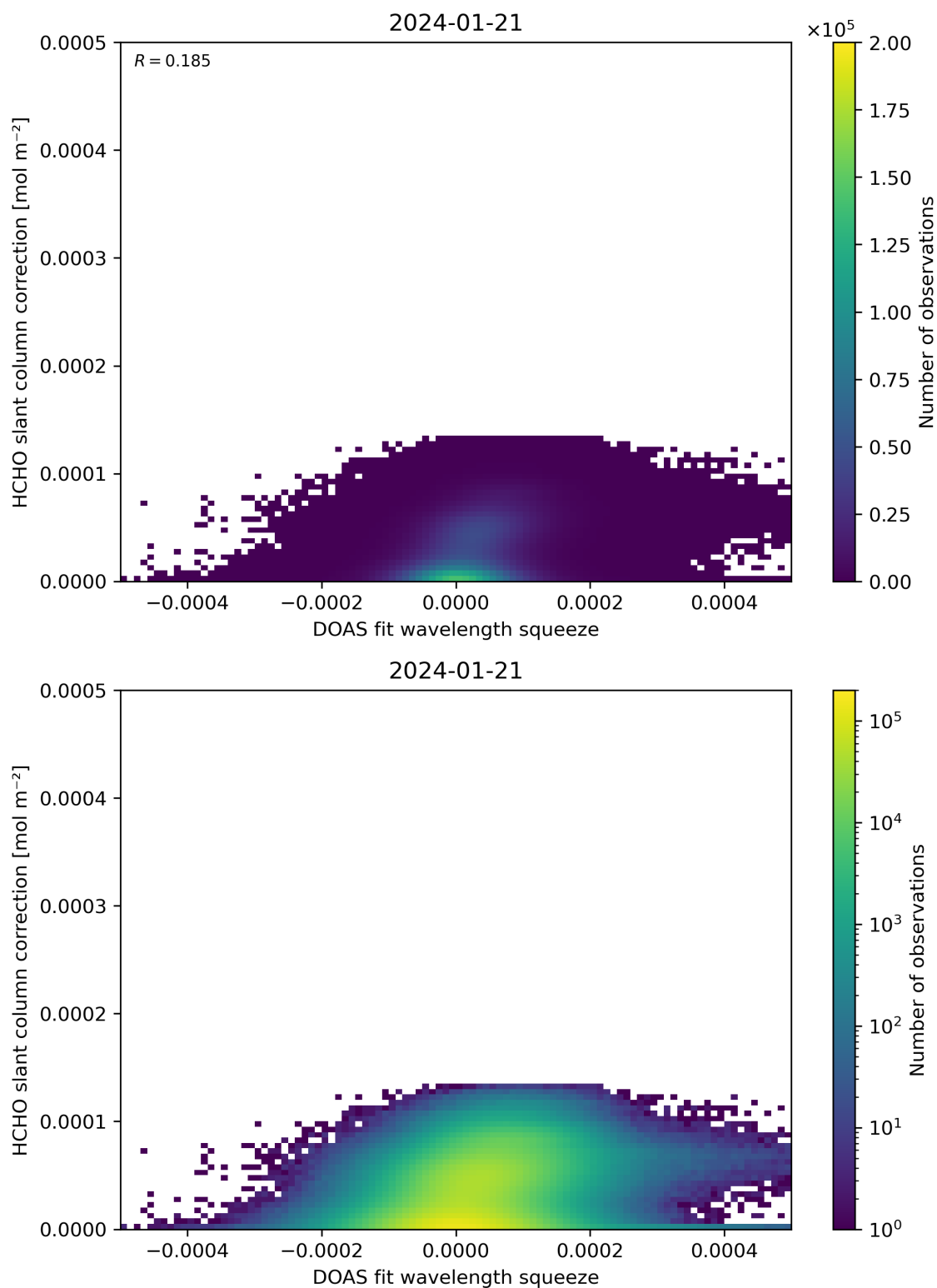
Figure 70: Scatter density plot of “DOAS fit wavelength squeeze” against “HCHO slant column correction” for 2024-01-21 to 2024-01-22.
