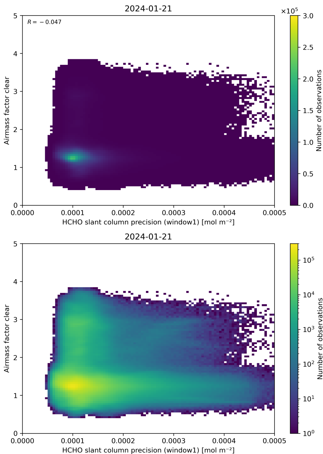
Figure 91: Scatter density plot of “HCHO slant column precision (window1)” against “Airmass factor clear” for 2024-01-21 to 2024-01-22.
