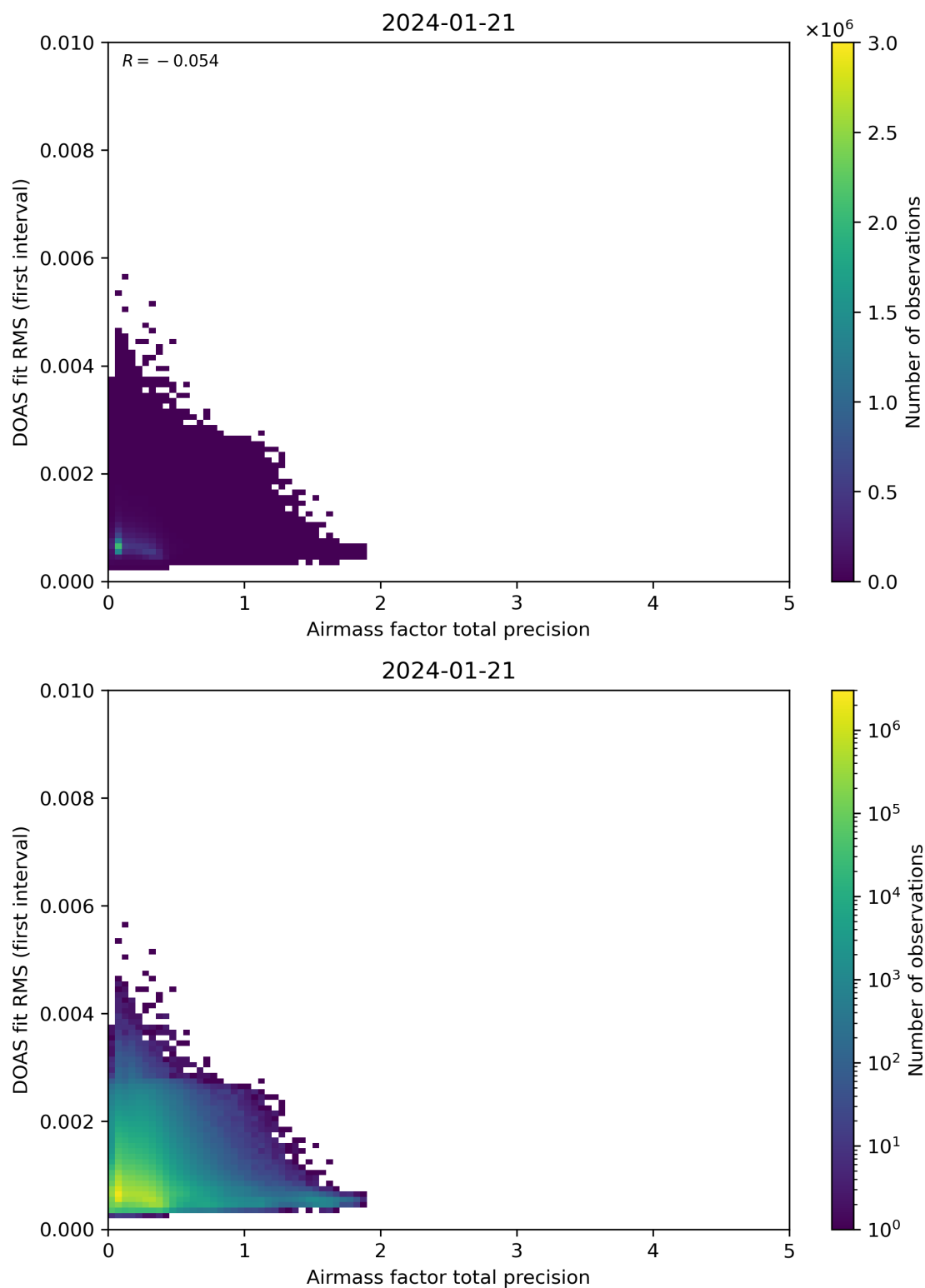
Figure 105: Scatter density plot of “Airmass factor total precision” against “DOAS fit RMS (first interval)” for 2024-01-21 to 2024-01-22.
