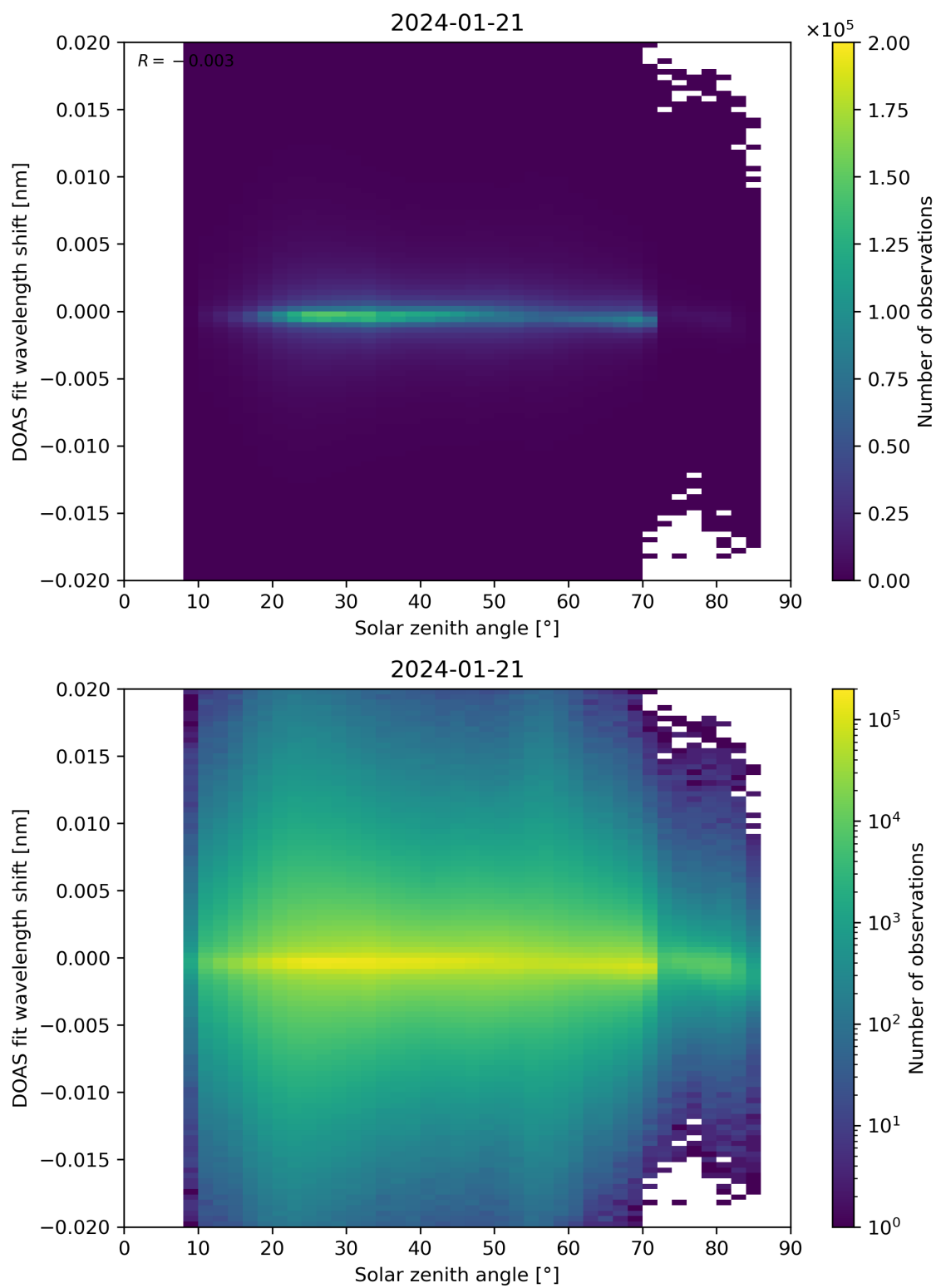
Figure 168: Scatter density plot of “Solar zenith angle” against “DOAS fit wavelength shift” for 2024-01-21 to 2024-01-22.
