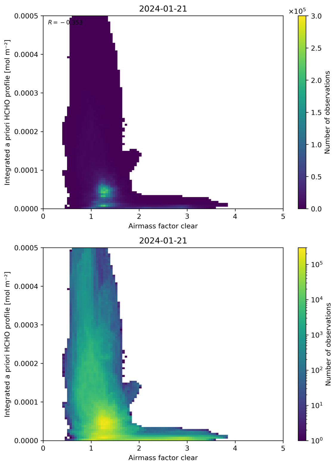
Figure 76: Scatter density plot of “Airmass factor clear” against “Integrated a priori HCHO profile” for 2024-01-21 to 2024-01-22.
