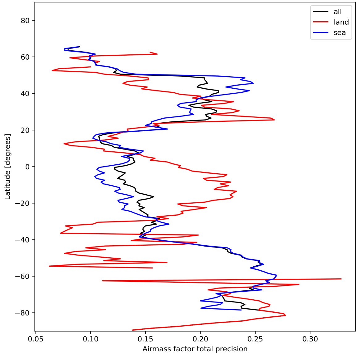
Figure 27: Zonal average of “Airmass factor total precision” for 2024-01-21 to 2024-01-22.
