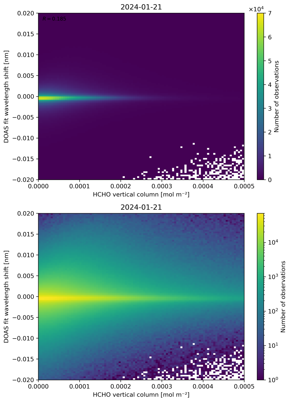
Figure 124: Scatter density plot of “HCHO vertical column” against “DOAS fit wavelength shift” for 2024-01-21 to 2024-01-22.
