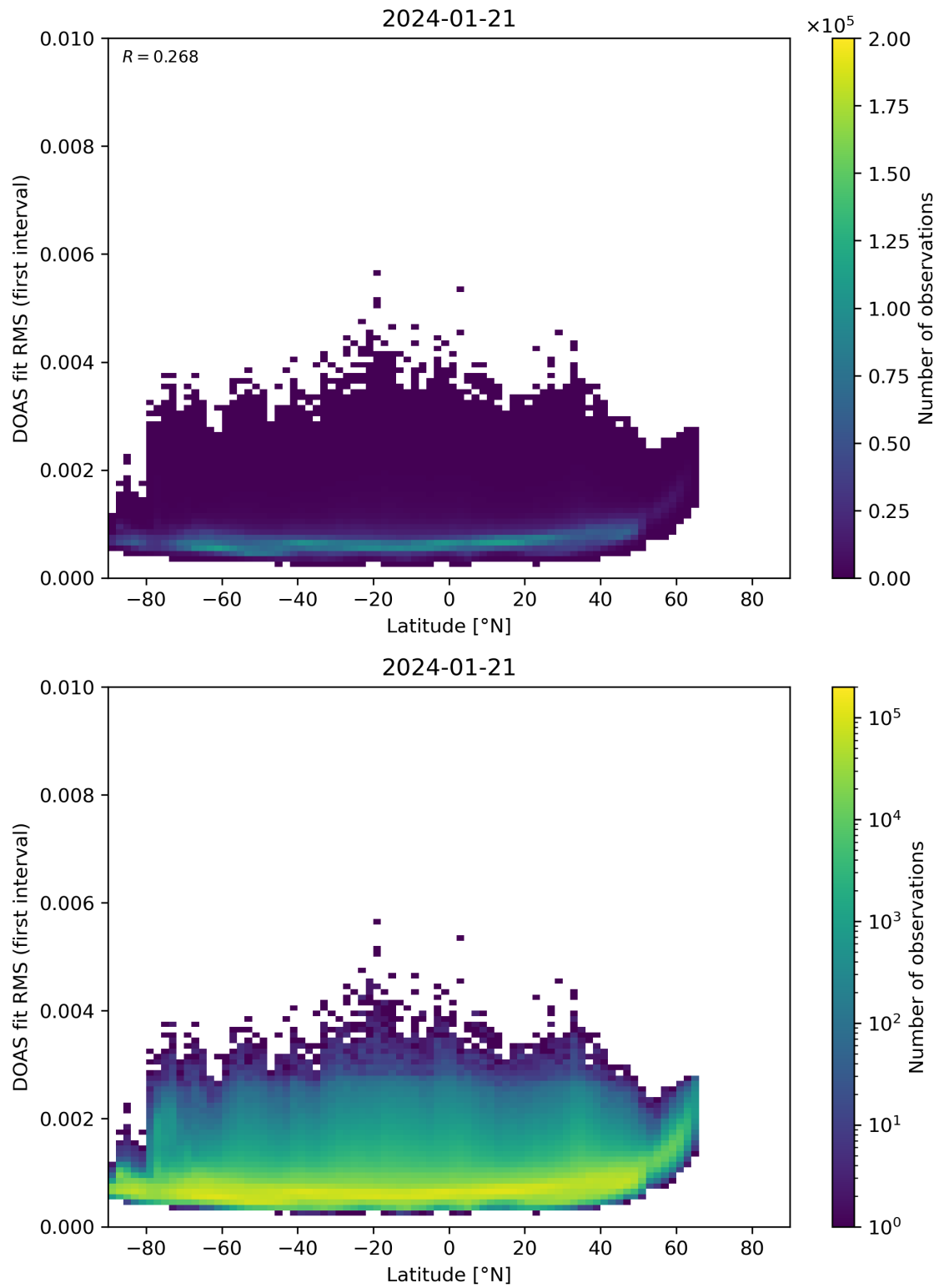
Figure 153: Scatter density plot of “Latitude” against “DOAS fit RMS (first interval)” for 2024-01-21 to 2024-01-22.
