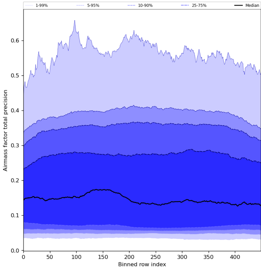
Figure 55: Along track statistics of “Airmass factor total precision” for 2024-01-21 to 2024-01-22
