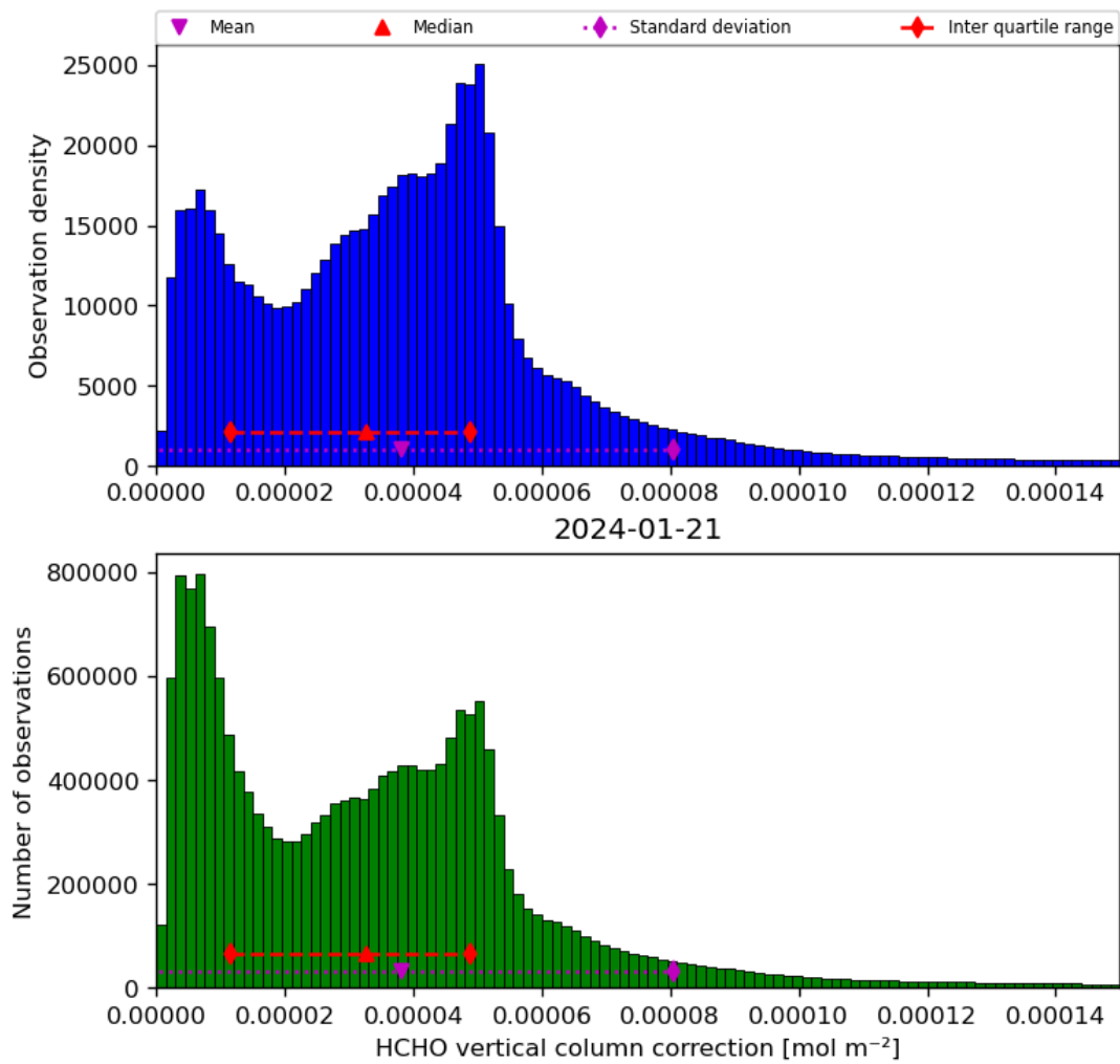
Figure 37: Histogram of “HCHO vertical column correction” for 2024-01-21 to 2024-01-22
