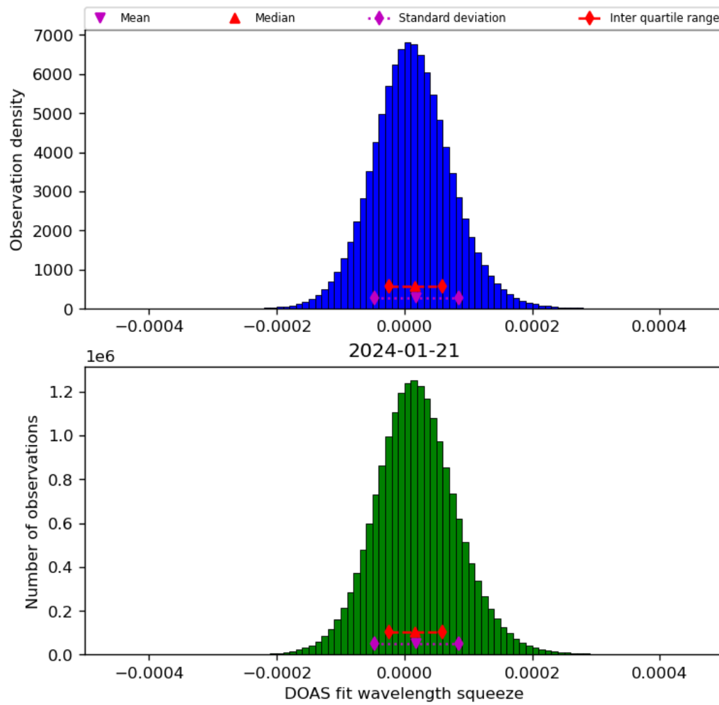
Figure 45: Histogram of “DOAS fit wavelength squeeze” for 2024-01-21 to 2024-01-22
