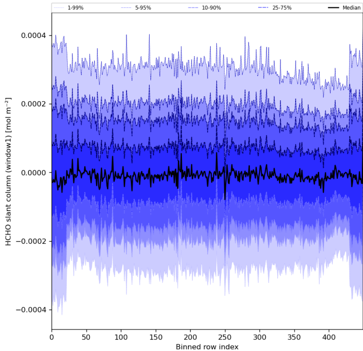
Figure 52: Along track statistics of “HCHO slant column (window1)” for 2024-01-21 to 2024-01-22
