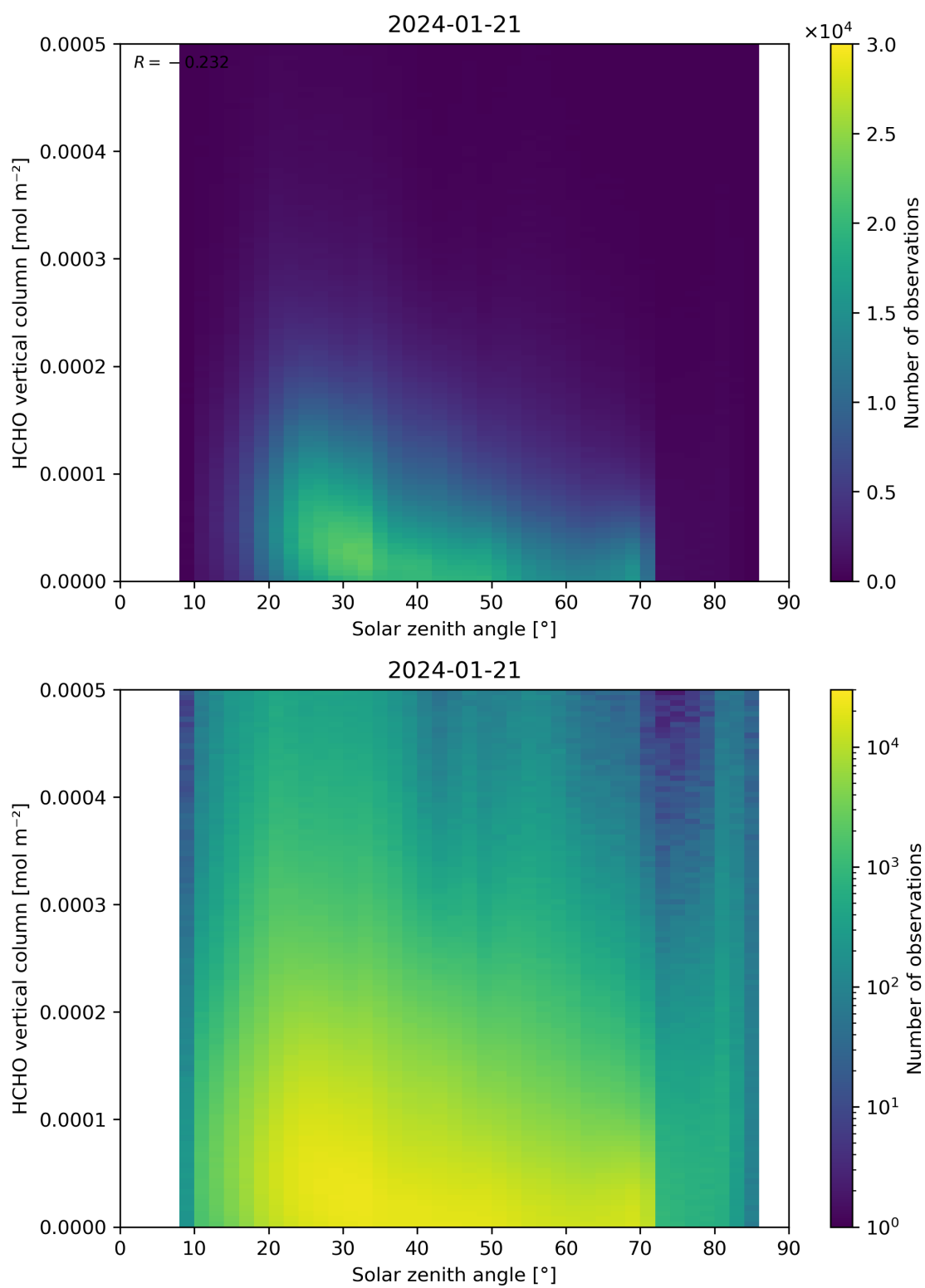
Figure 177: Scatter density plot of “Solar zenith angle” against “HCHO vertical column” for 2024-01-21 to 2024-01-22.
