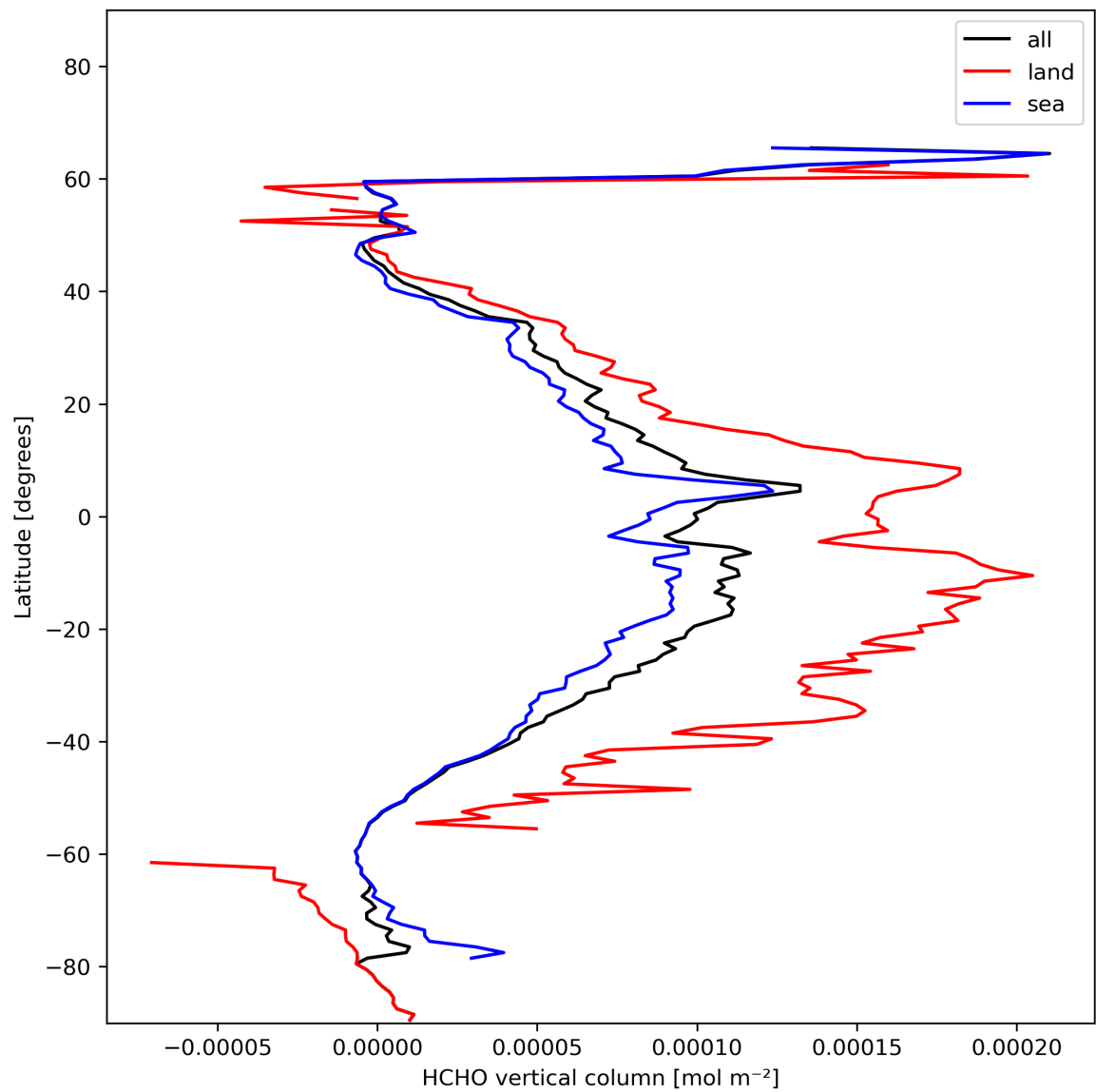
Figure 21: Zonal average of “HCHO vertical column” for 2024-01-21 to 2024-01-22.
