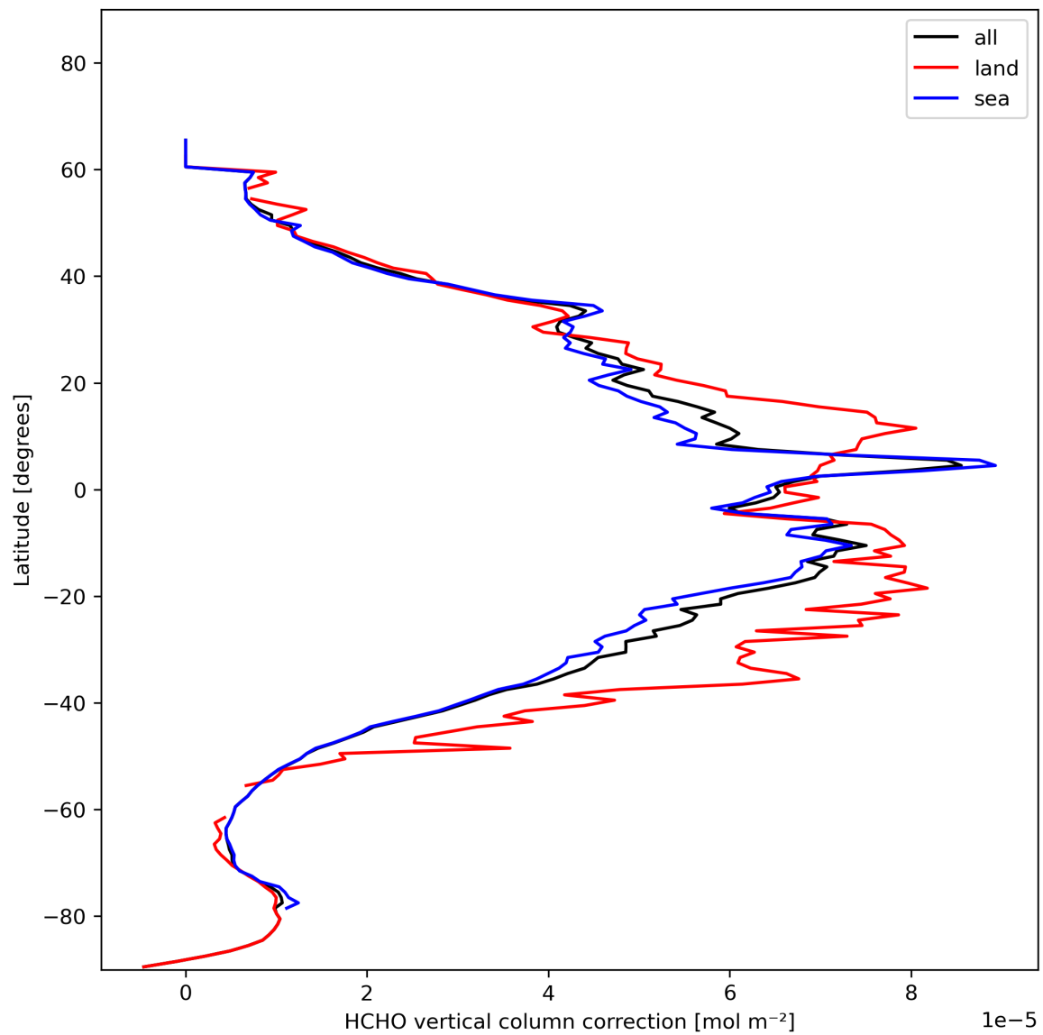
Figure 23: Zonal average of “HCHO vertical column correction” for 2024-01-21 to 2024-01-22.
