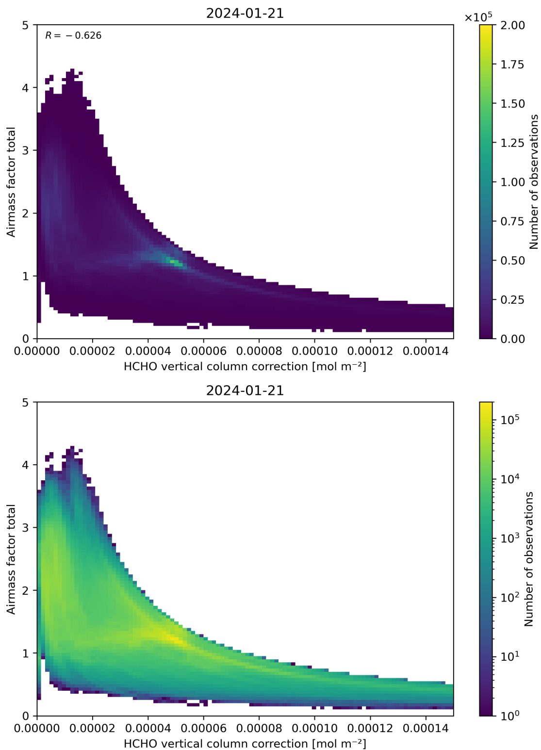
Figure 120: Scatter density plot of “HCHO vertical column correction” against “Airmass factor total” for 2024-01-21 to 2024-01-22.
