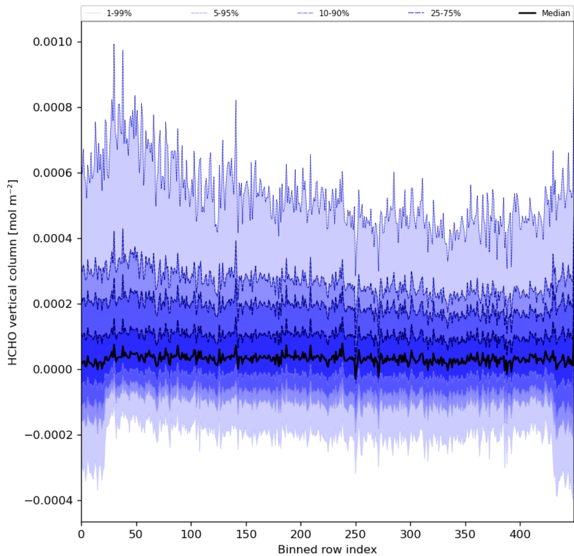
Figure 49: Along track statistics of “HCHO vertical column” for 2024-01-21 to 2024-01-22
