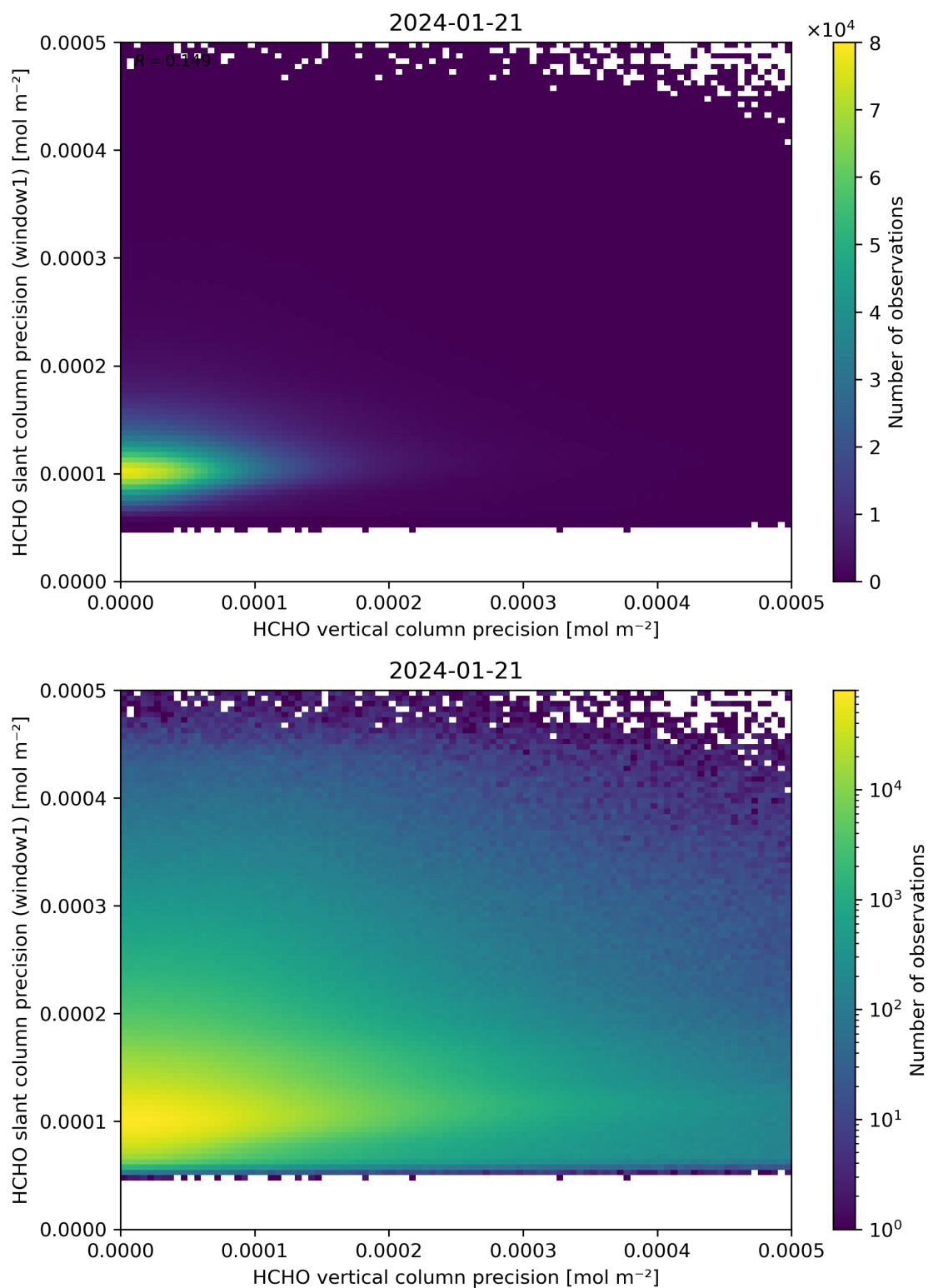
Figure 143: Scatter density plot of “HCHO vertical column precision” against “HCHO slant column precision (window1)” for 2024-01-21 to 2024-01-22.
