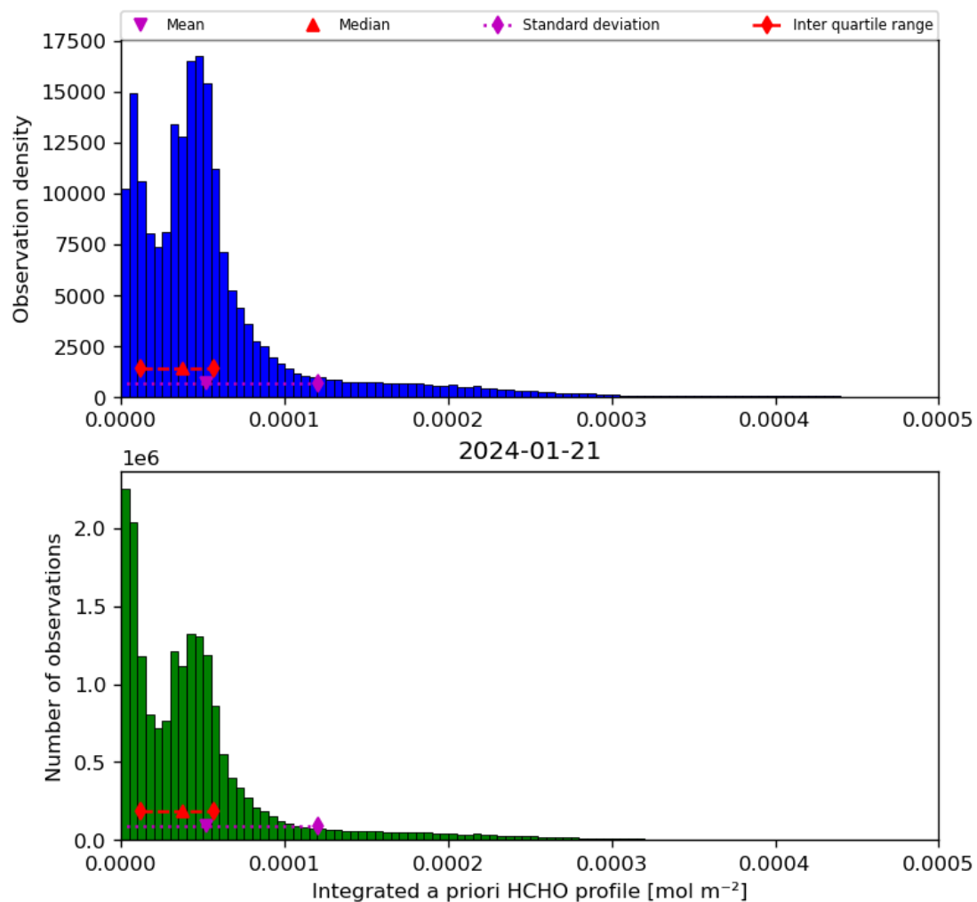
Figure 43: Histogram of “Integrated a priori HCHO profile” for 2024-01-21 to 2024-01-22
