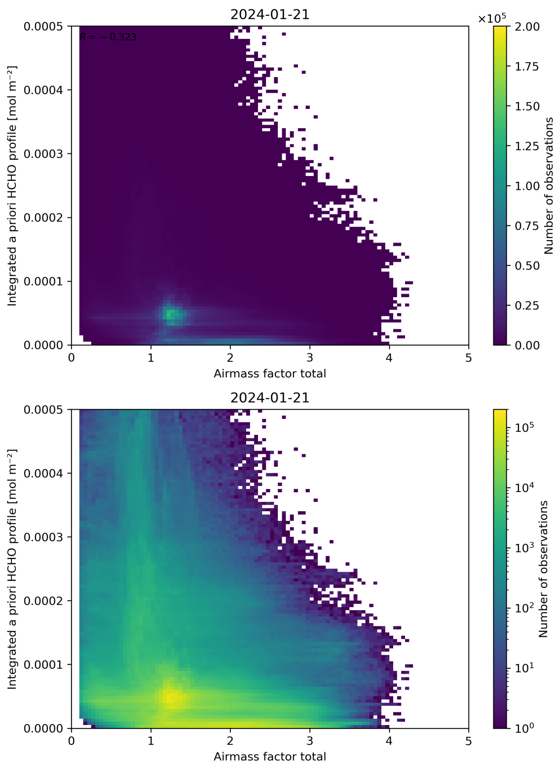
Figure 104: Scatter density plot of “Airmass factor total” against “Integrated a priori HCHO profile” for 2024-01-21 to 2024-01-22.
