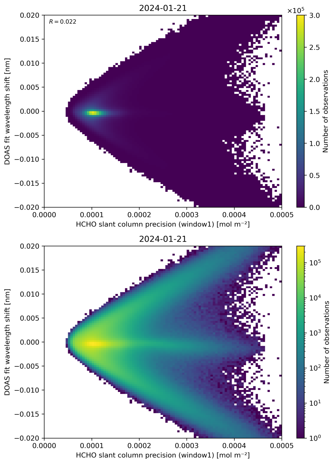
Figure 89: Scatter density plot of “HCHO slant column precision (window1)” against “DOAS fit wavelength shift” for 2024-01-21 to 2024-01-22.
