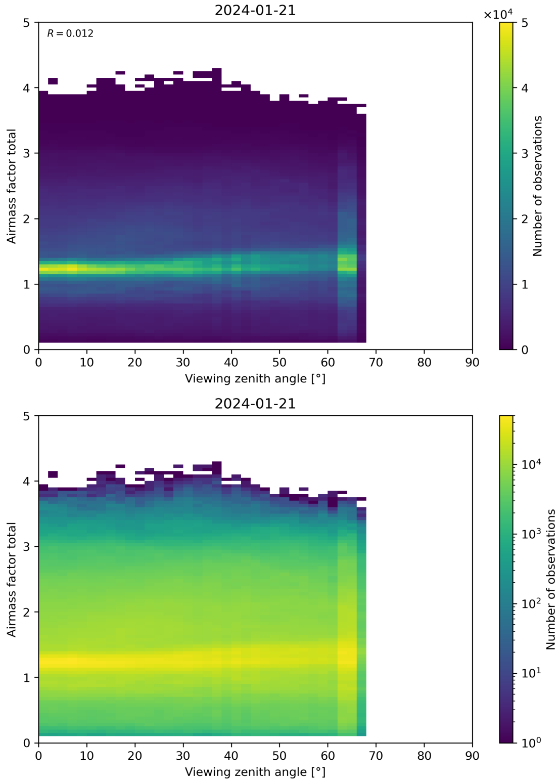
Figure 190: Scatter density plot of “Viewing zenith angle” against “Airmass factor total” for 2024-01-21 to 2024-01-22.
