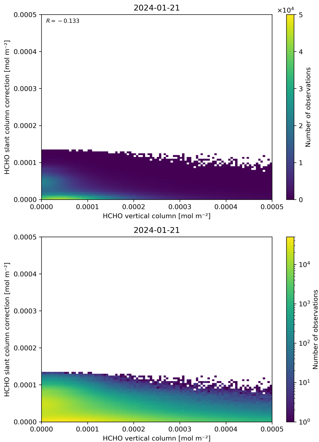
Figure 128: Scatter density plot of “HCHO vertical column” against “HCHO slant column correction” for 2024-01-21 to 2024-01-22.
