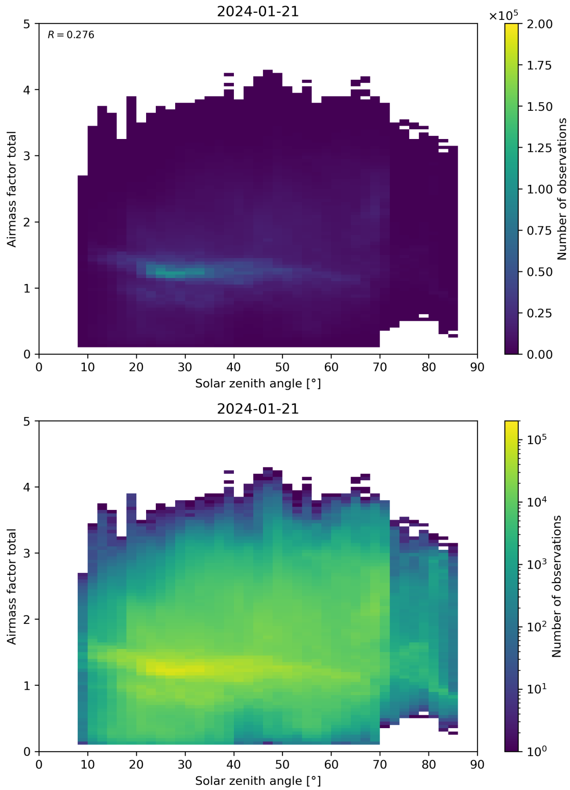
Figure 175: Scatter density plot of “Solar zenith angle” against “Airmass factor total” for 2024-01-21 to 2024-01-22.
