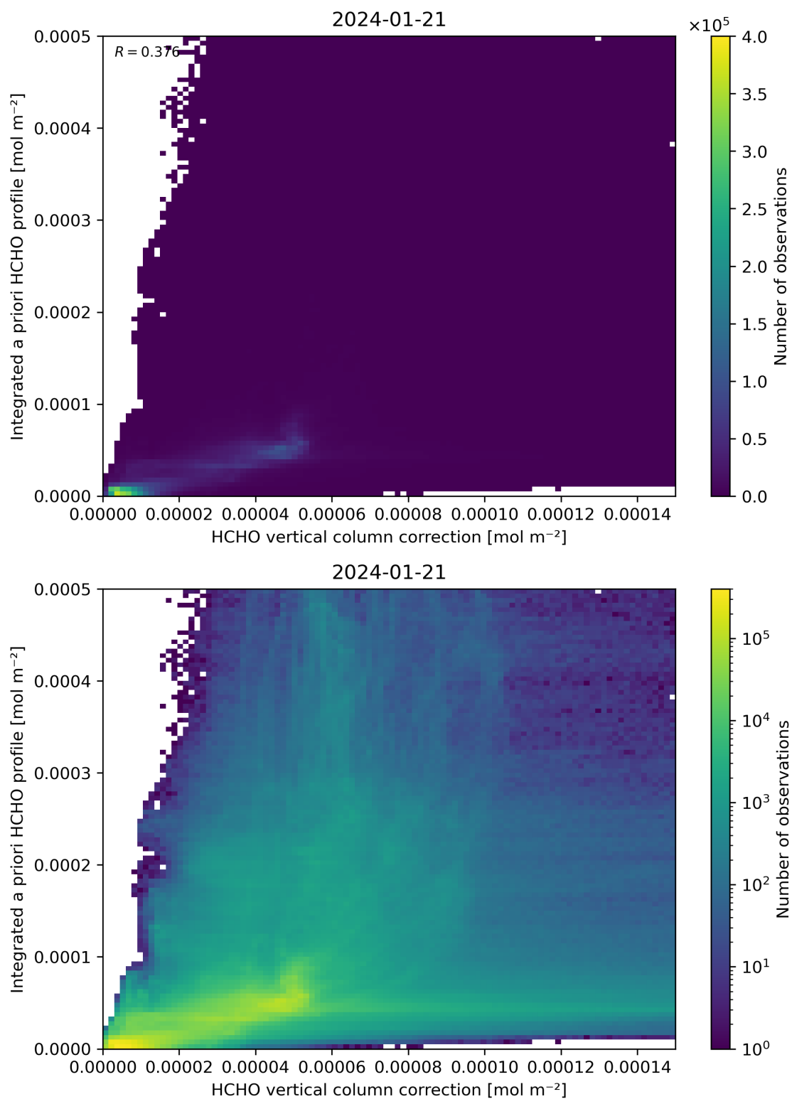
Figure 122: Scatter density plot of “HCHO vertical column correction” against “Integrated a priori HCHO profile” for 2024-01-21 to 2024-01-22.
