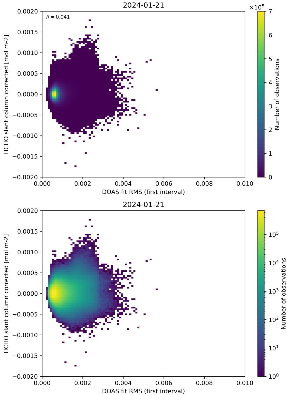
Figure 62: Scatter density plot of “DOAS fit RMS (first interval)” against “HCHO slant column corrected” for 2024-01-21 to 2024-01-22.
