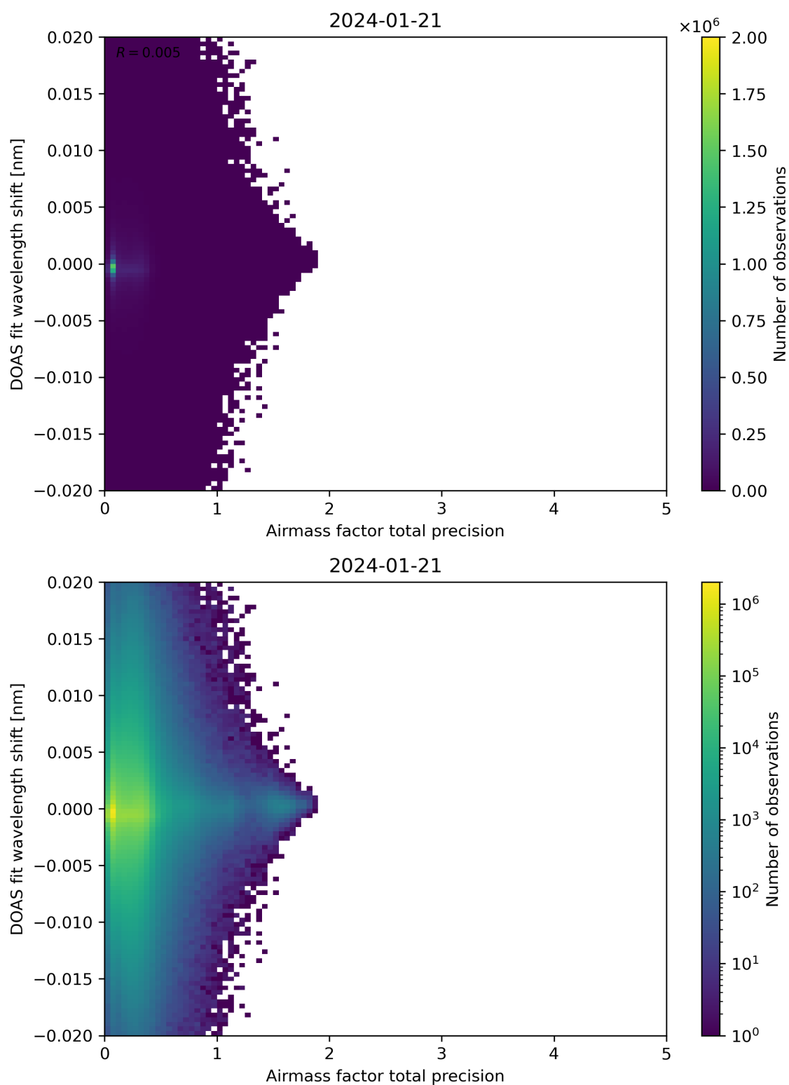
Figure 106: Scatter density plot of “Airmass factor total precision” against “DOAS fit wavelength shift” for 2024-01-21 to 2024-01-22.
