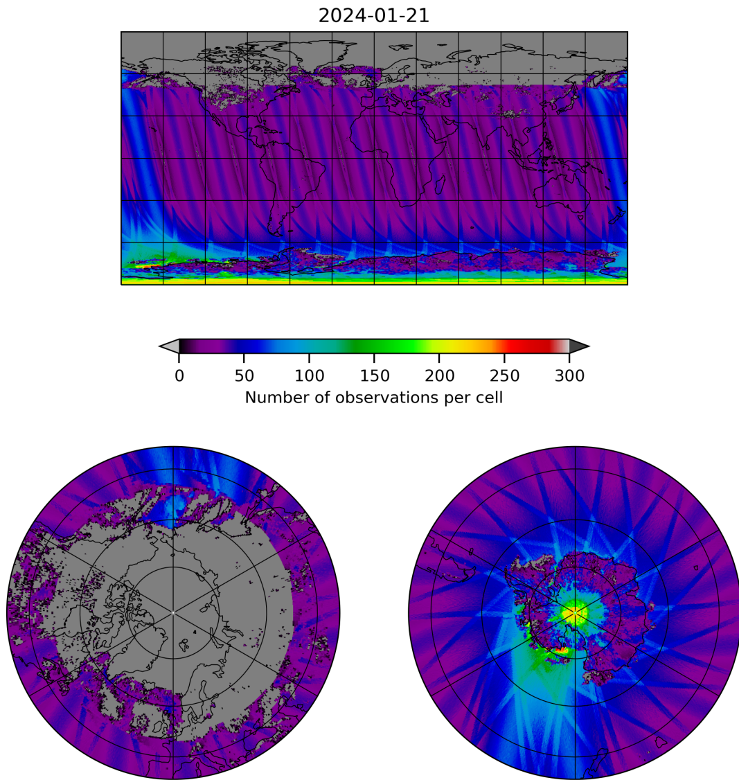
Figure 19: Map of the number of observations for 2024-01-21 to 2024-01-22
