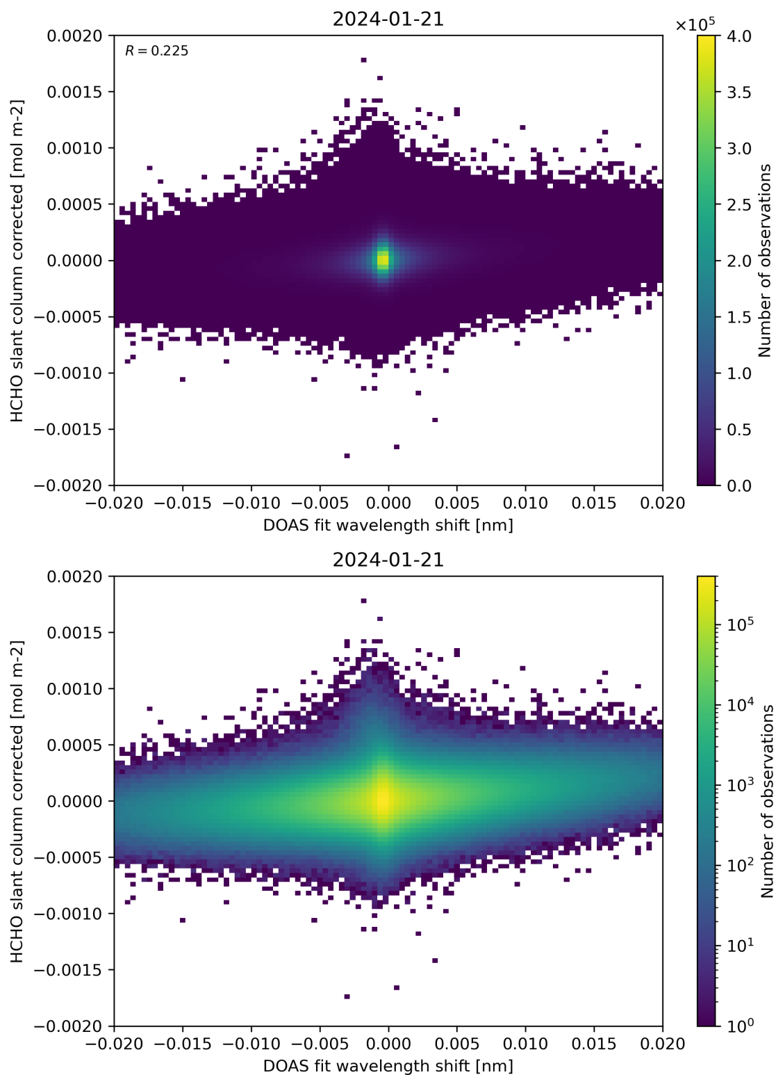
Figure 66: Scatter density plot of “DOAS fit wavelength shift” against “HCHO slant column corrected” for 2024-01-21 to 2024-01-22.
