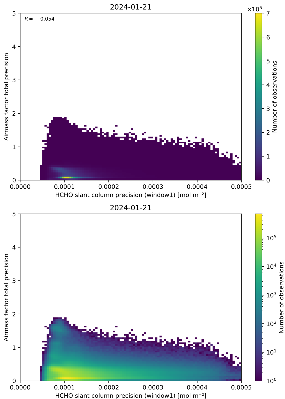
Figure 95: Scatter density plot of “HCHO slant column precision (window1)” against “Airmass factor total precision” for 2024-01-21 to 2024-01-22.
