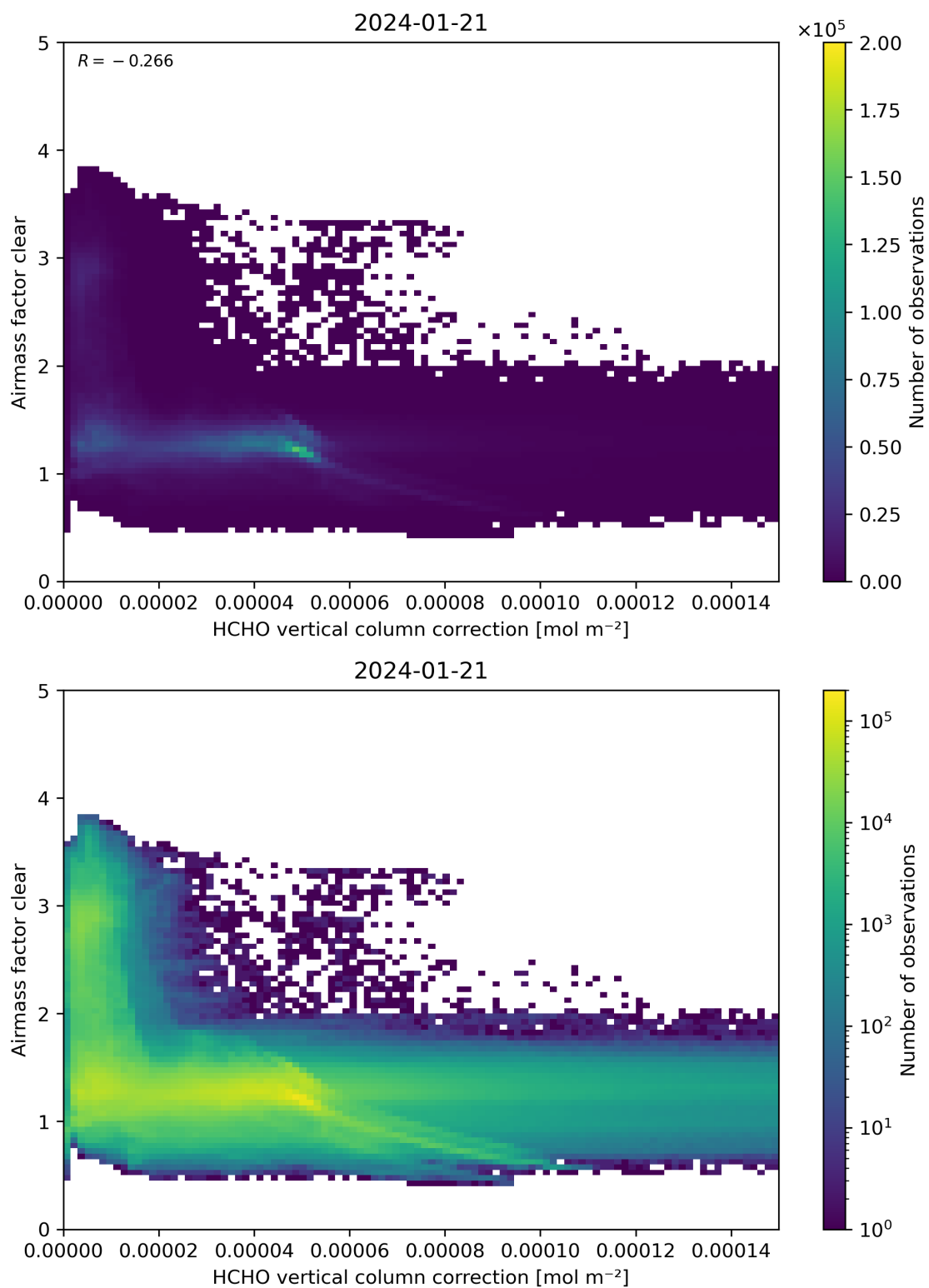
Figure 115: Scatter density plot of “HCHO vertical column correction” against “Airmass factor clear” for 2024-01-21 to 2024-01-22.
