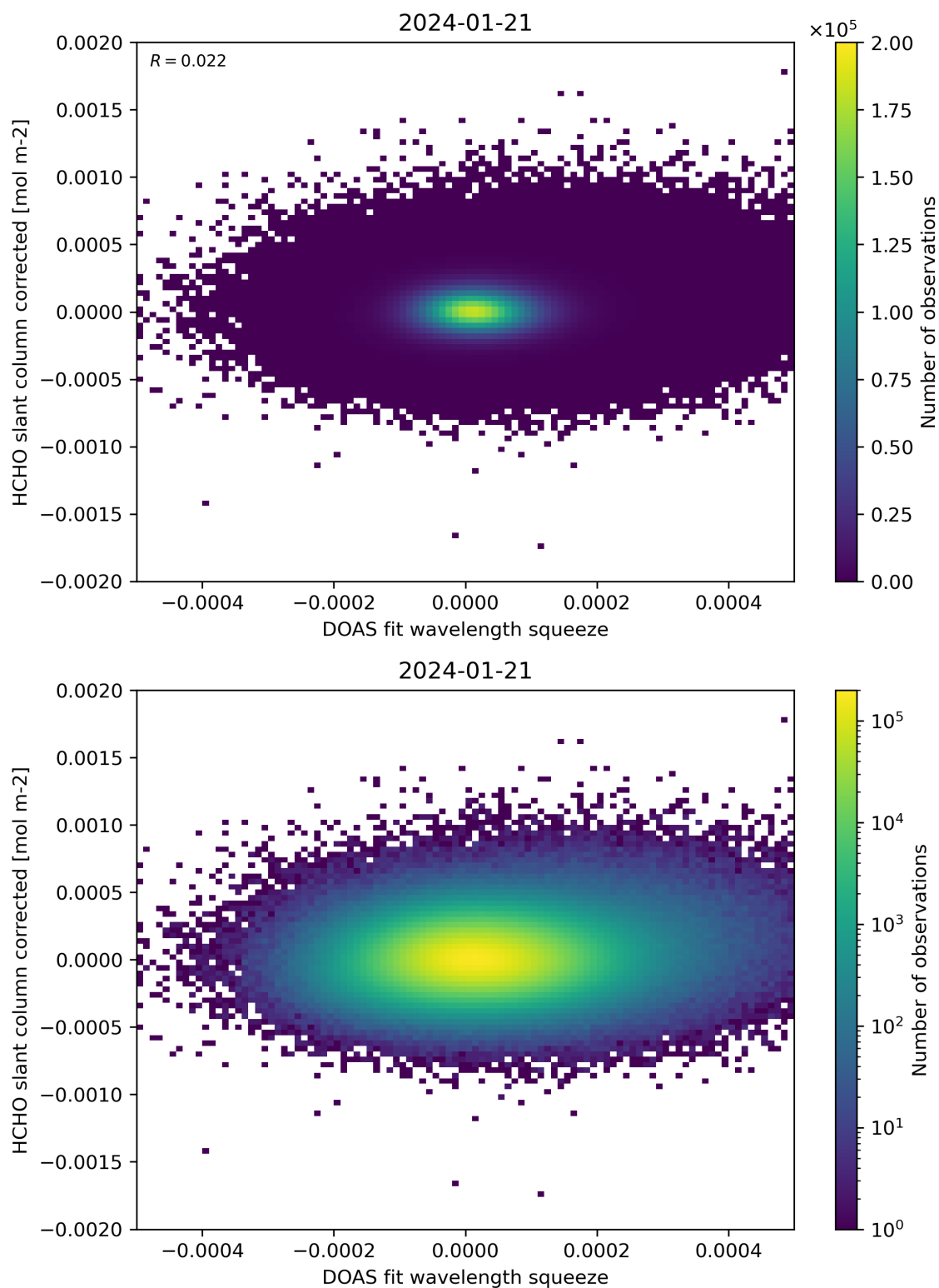
Figure 69: Scatter density plot of “DOAS fit wavelength squeeze” against “HCHO slant column corrected” for 2024-01-21 to 2024-01-22.
