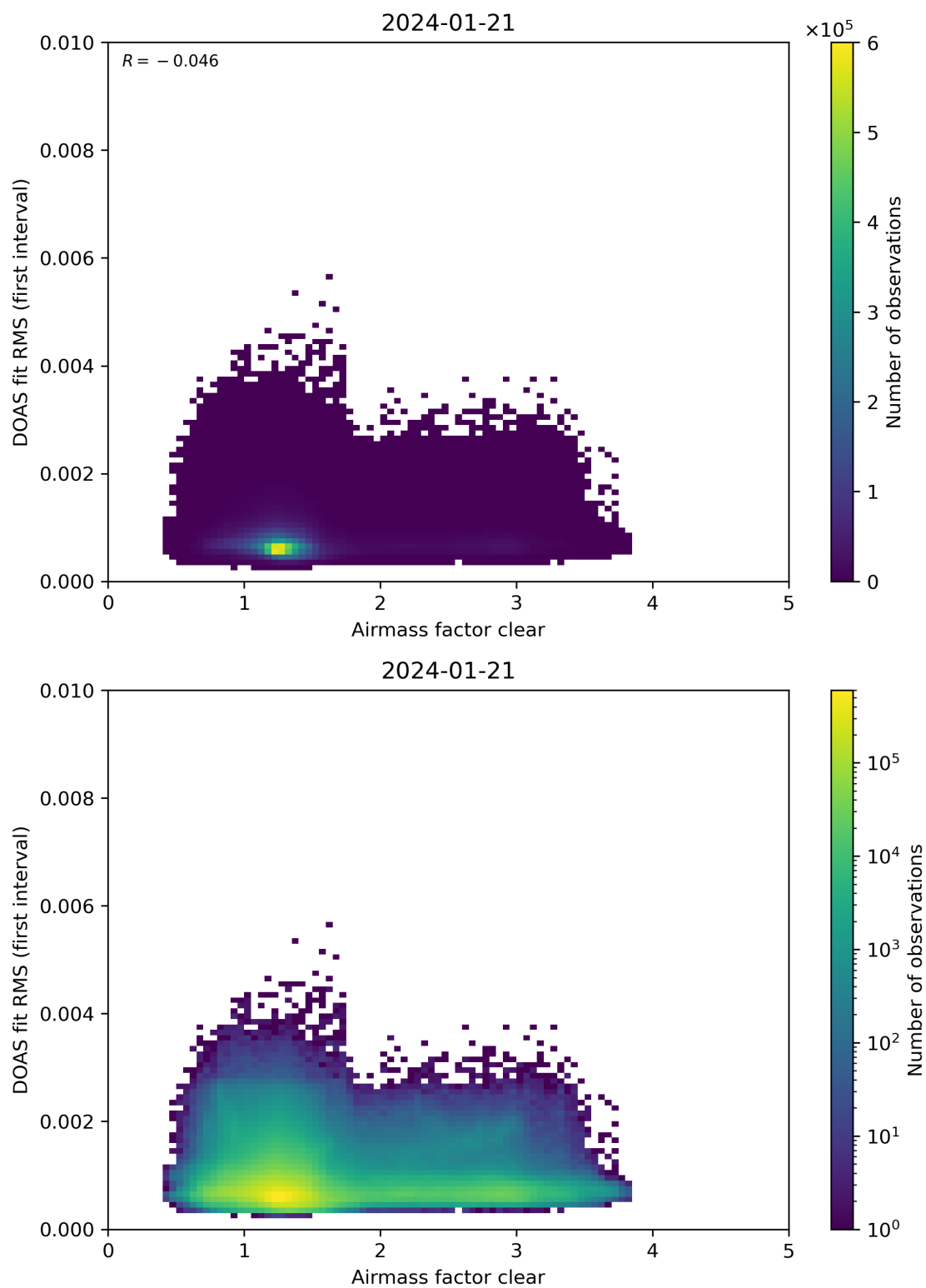
Figure 71: Scatter density plot of “Airmass factor clear” against “DOAS fit RMS (first interval)” for 2024-01-21 to 2024-01-22.
