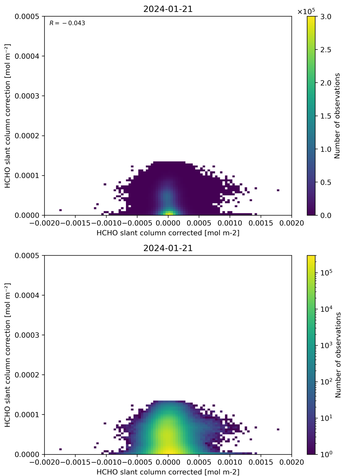
Figure 77: Scatter density plot of “HCHO slant column corrected” against “HCHO slant column correction” for 2024-01-21 to 2024-01-22.
