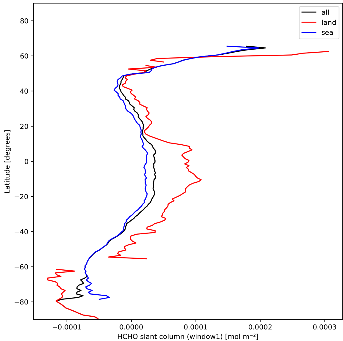
Figure 24: Zonal average of “HCHO slant column (window1)” for 2024-01-21 to 2024-01-22.
