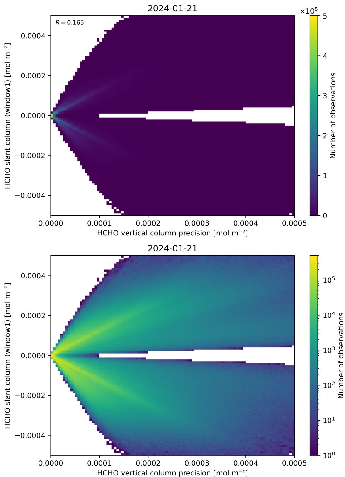
Figure 142: Scatter density plot of “HCHO vertical column precision” against “HCHO slant column (window1)” for 2024-01-21 to 2024-01-22.
