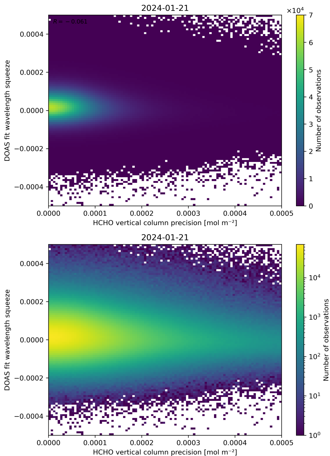
Figure 138: Scatter density plot of “HCHO vertical column precision” against “DOAS fit wavelength squeeze” for 2024-01-21 to 2024-01-22.
