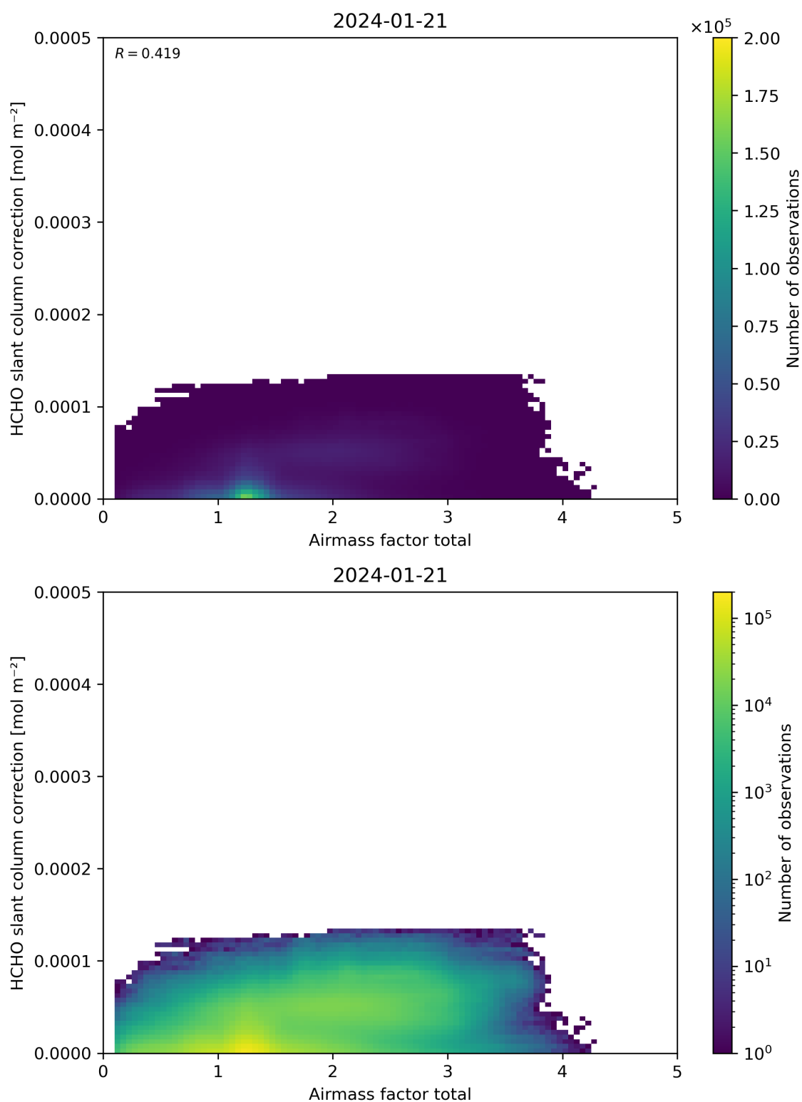
Figure 102: Scatter density plot of “Airmass factor total” against “HCHO slant column correction” for 2024-01-21 to 2024-01-22.
