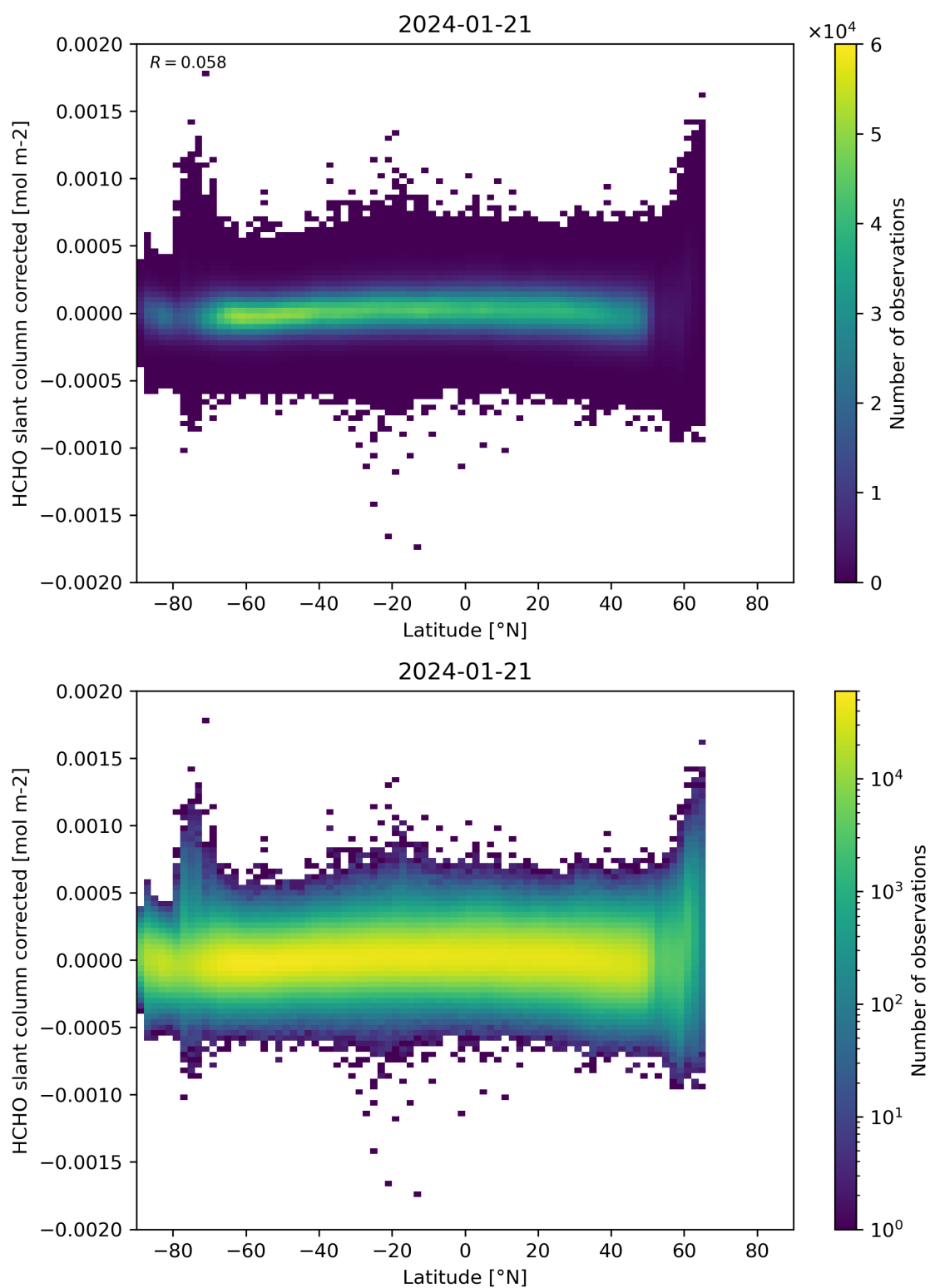
Figure 157: Scatter density plot of “Latitude” against “HCHO slant column corrected” for 2024-01-21 to 2024-01-22.
