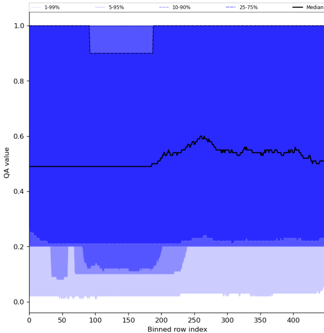
Figure 48: Along track statistics of “QA value” for 2024-01-21 to 2024-01-22
