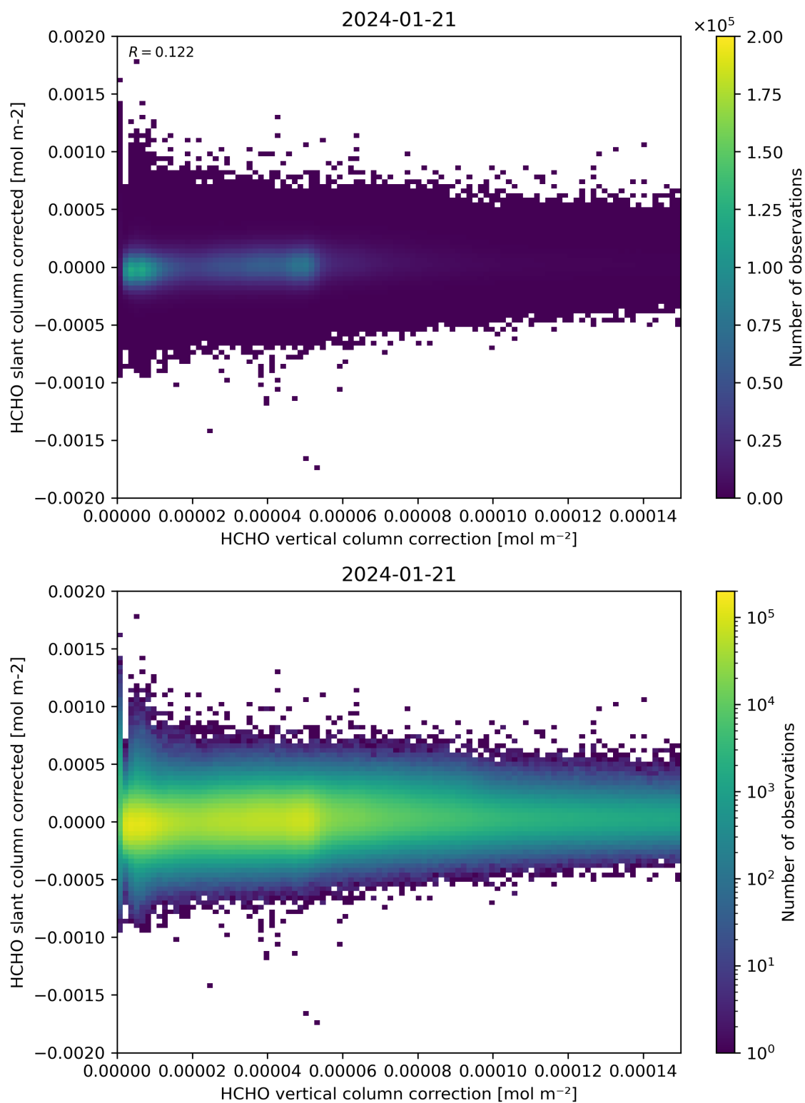
Figure 116: Scatter density plot of “HCHO vertical column correction” against “HCHO slant column corrected” for 2024-01-21 to 2024-01-22.
