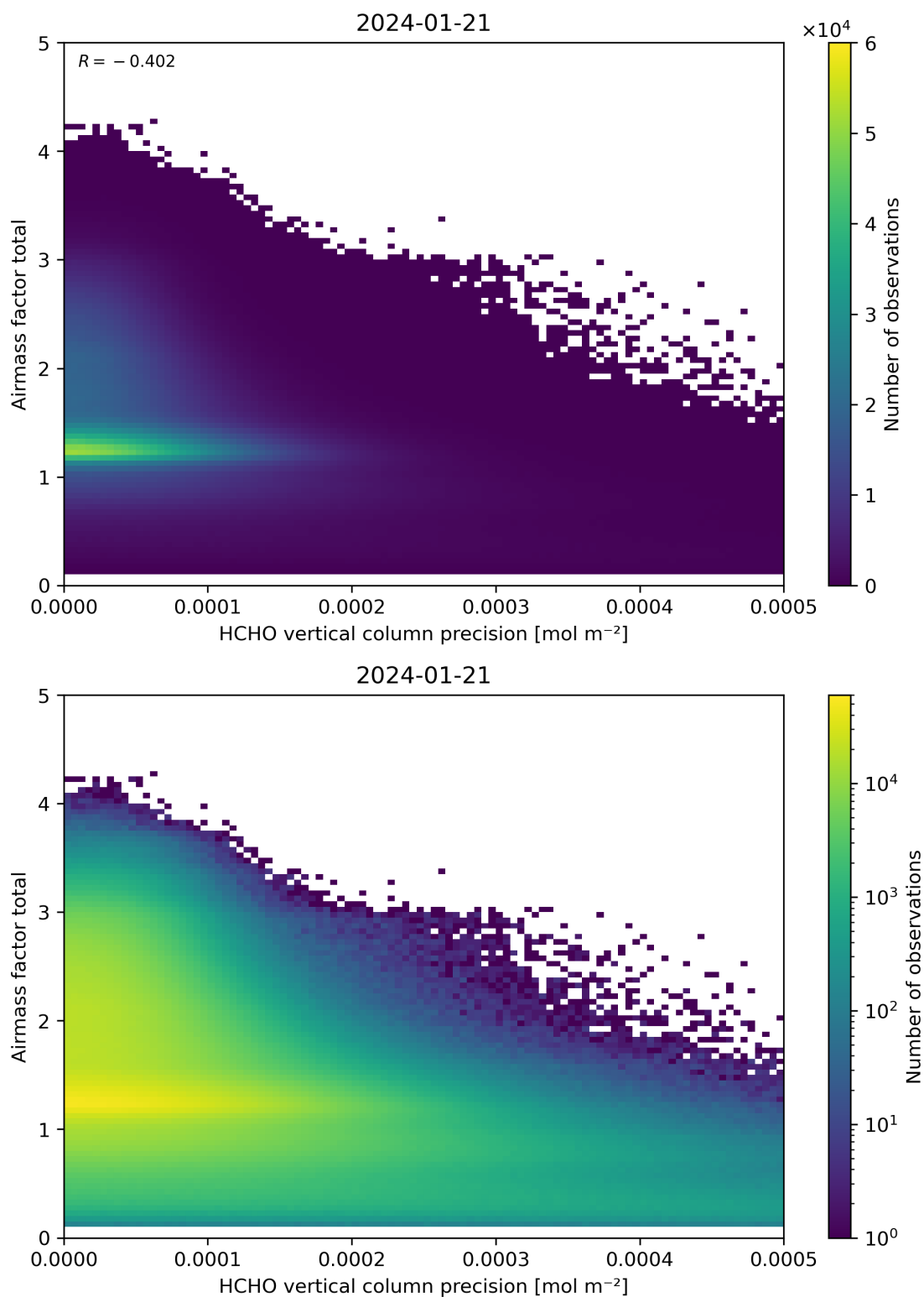
Figure 144: Scatter density plot of “HCHO vertical column precision” against “Airmass factor total” for 2024-01-21 to 2024-01-22.
