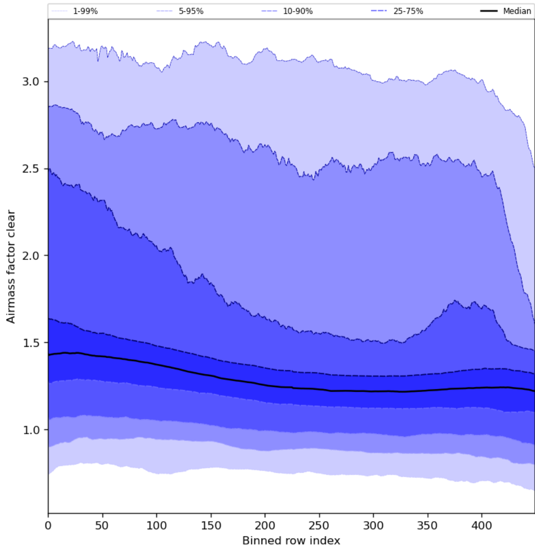
Figure 56: Along track statistics of “Airmass factor clear” for 2024-01-21 to 2024-01-22
