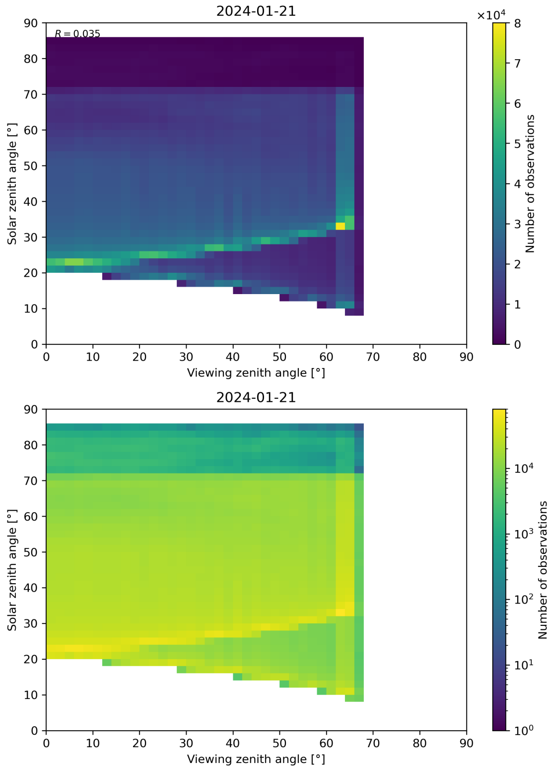
Figure 197: Scatter density plot of “Viewing zenith angle” against “Solar zenith angle” for 2024-01-21 to 2024-01-22.
