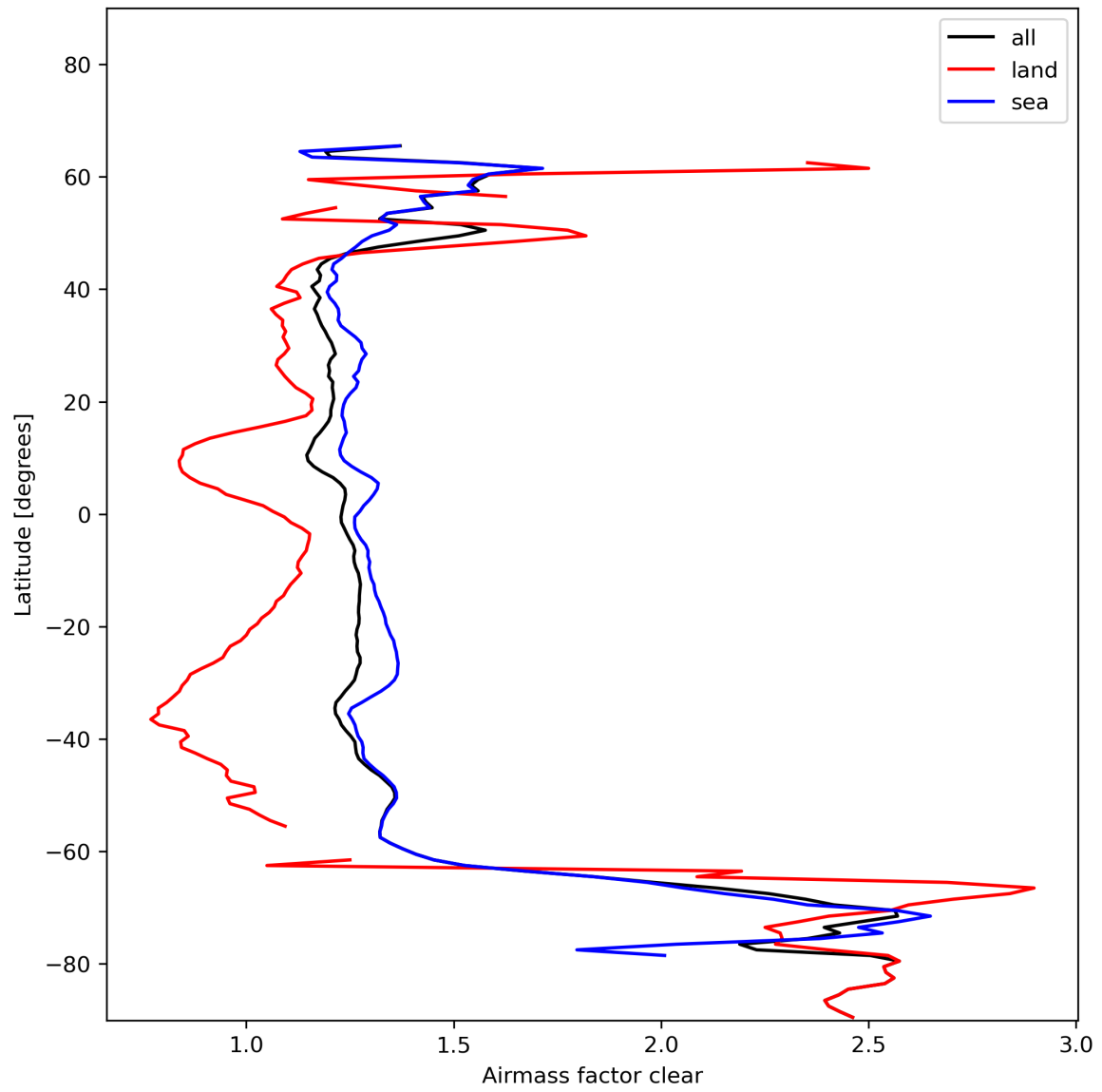
Figure 28: Zonal average of “Airmass factor clear” for 2024-01-21 to 2024-01-22.
