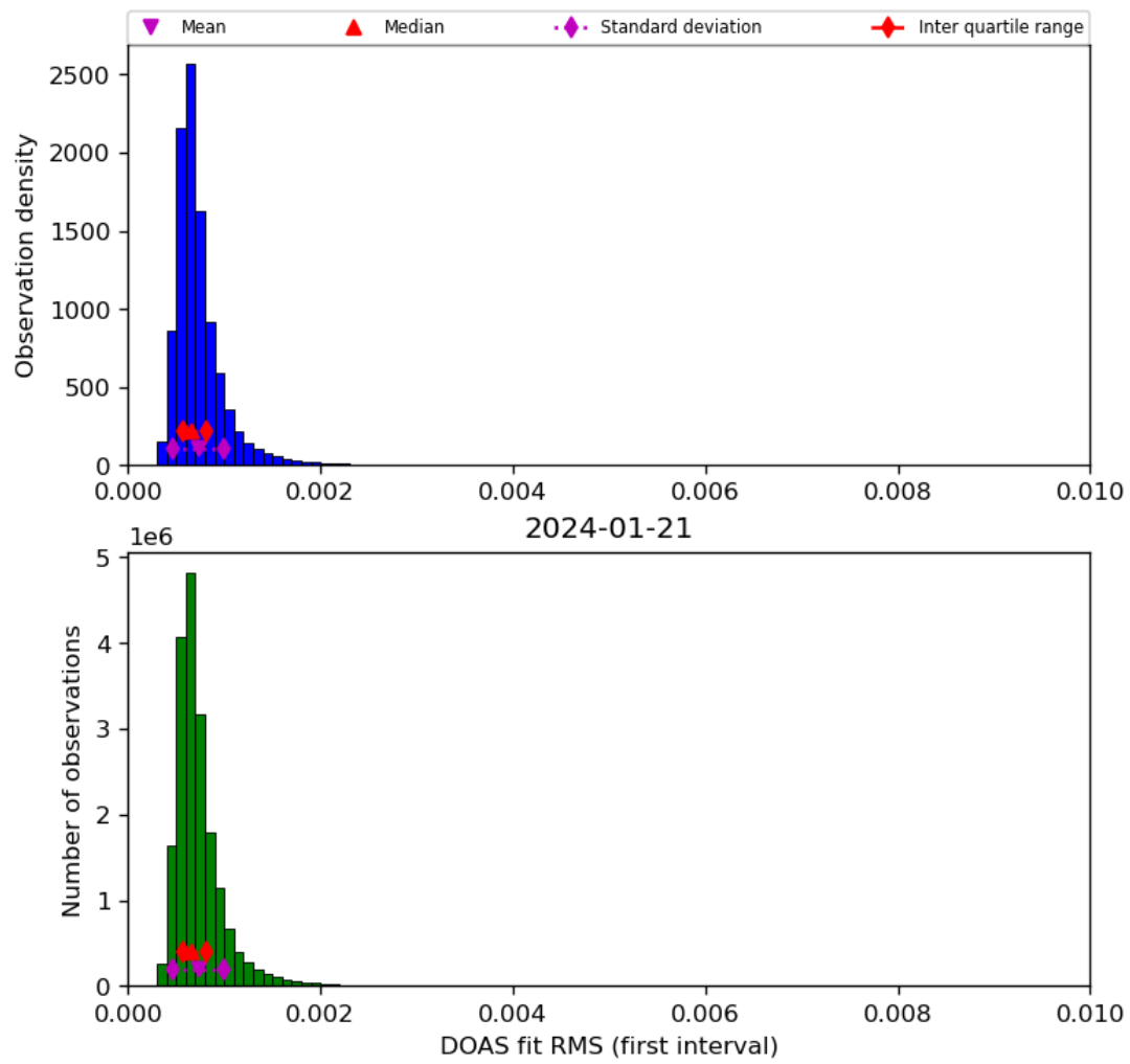
Figure 46: Histogram of “DOAS fit RMS (first interval)” for 2024-01-21 to 2024-01-22
