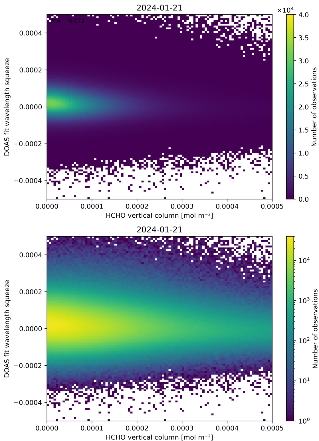
Figure 125: Scatter density plot of “HCHO vertical column” against “DOAS fit wavelength squeeze” for 2024-01-21 to 2024-01-22.
