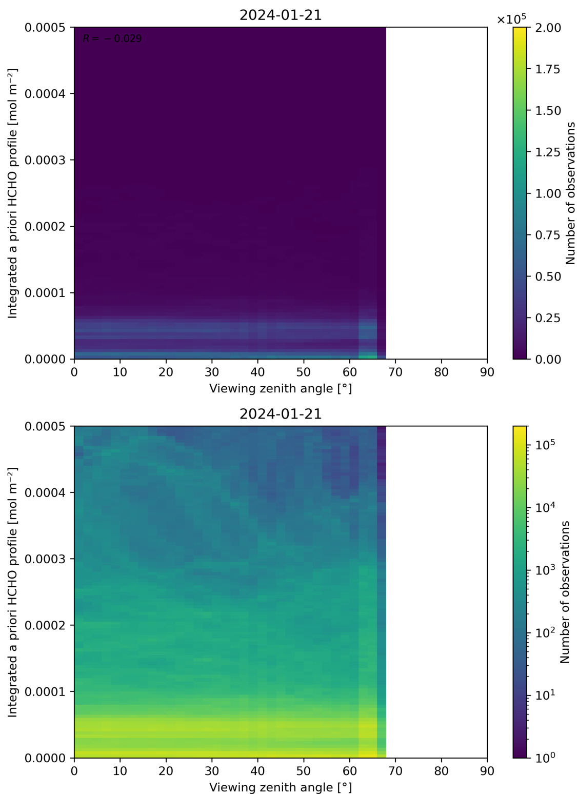
Figure 195: Scatter density plot of “Viewing zenith angle” against “Integrated a priori HCHO profile” for 2024-01-21 to 2024-01-22.
