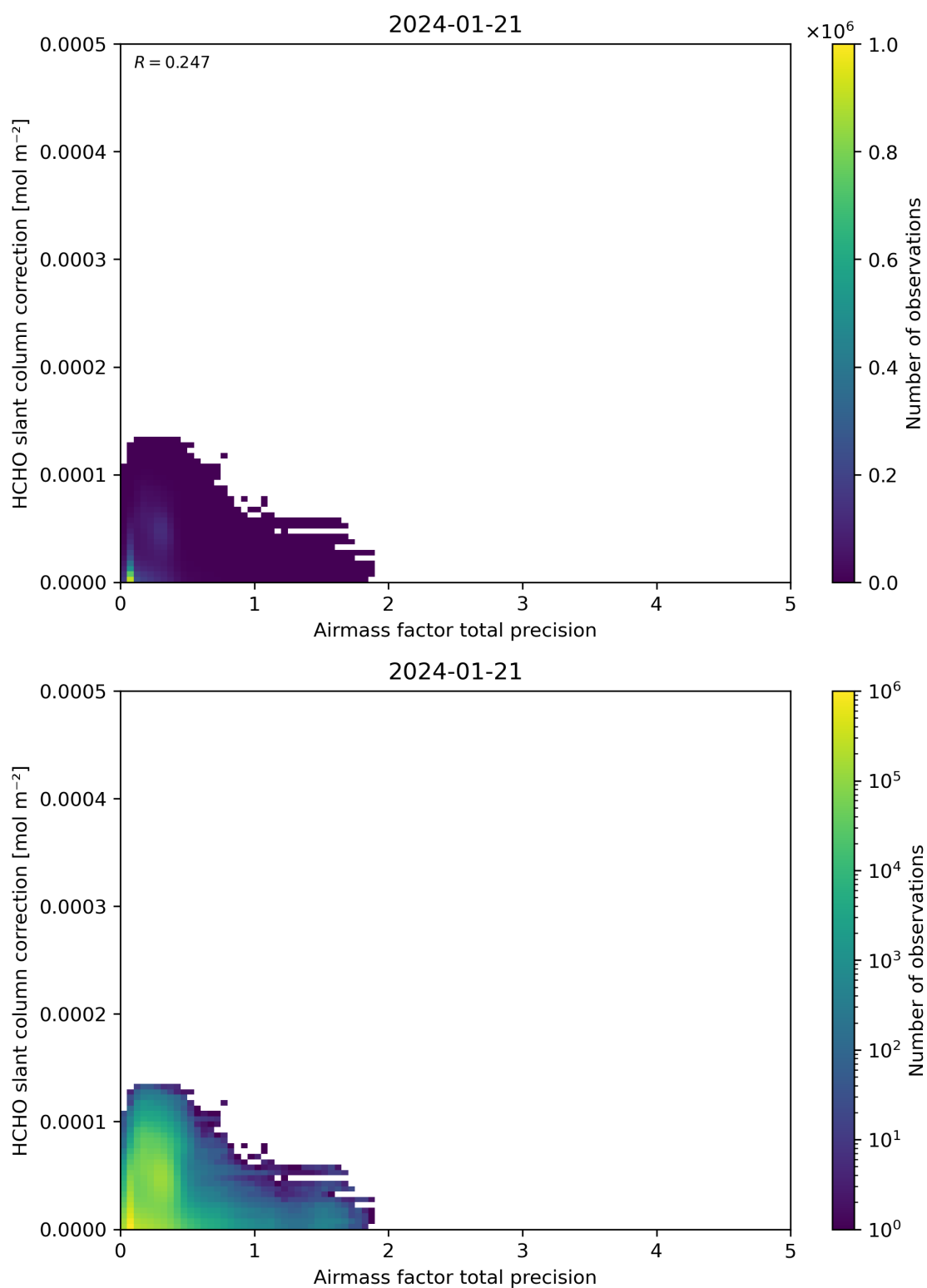
Figure 110: Scatter density plot of “Airmass factor total precision” against “HCHO slant column correction” for 2024-01-21 to 2024-01-22.
