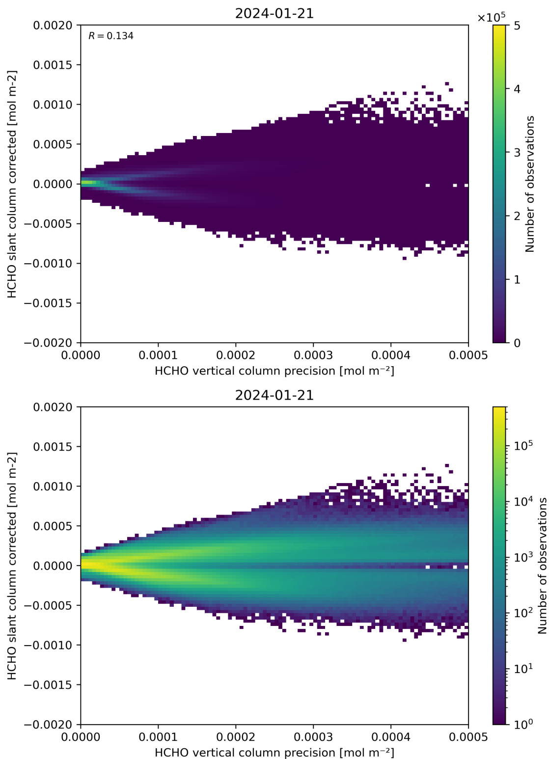
Figure 140: Scatter density plot of “HCHO vertical column precision” against “HCHO slant column corrected” for 2024-01-21 to 2024-01-22.
