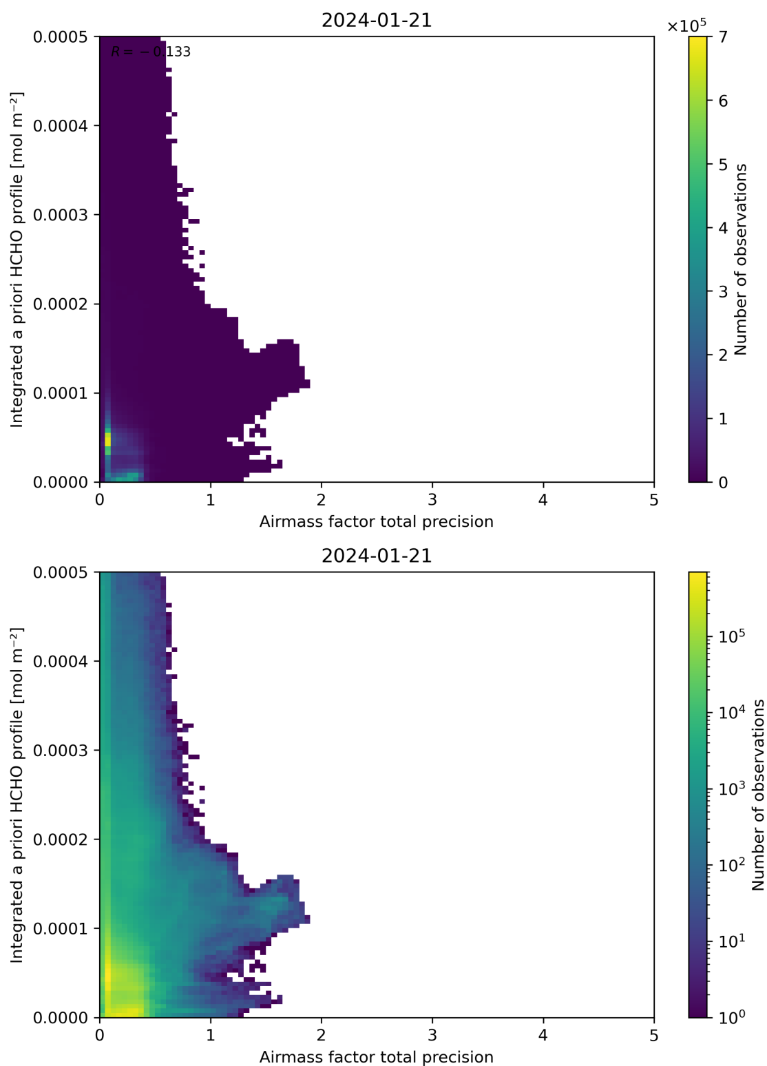
Figure 111: Scatter density plot of “Airmass factor total precision” against “Integrated a priori HCHO profile” for 2024-01-21 to 2024-01-22.
