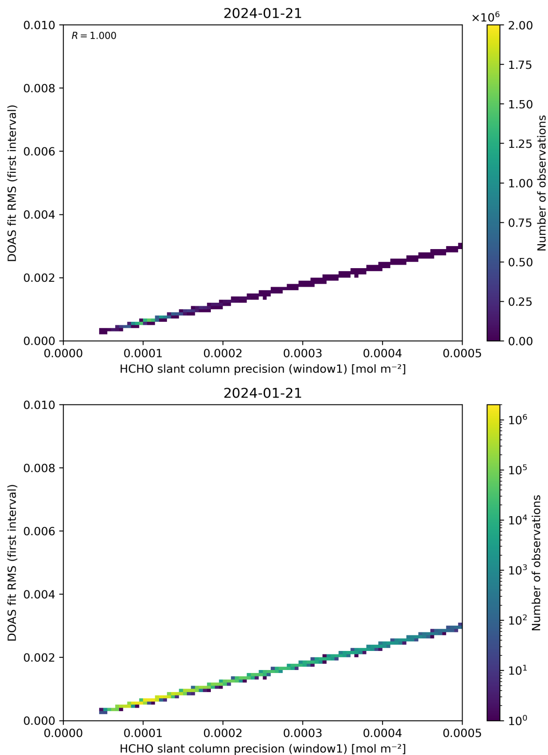
Figure 88: Scatter density plot of “HCHO slant column precision (window1)” against “DOAS fit RMS (first interval)” for 2024-01-21 to 2024-01-22.
