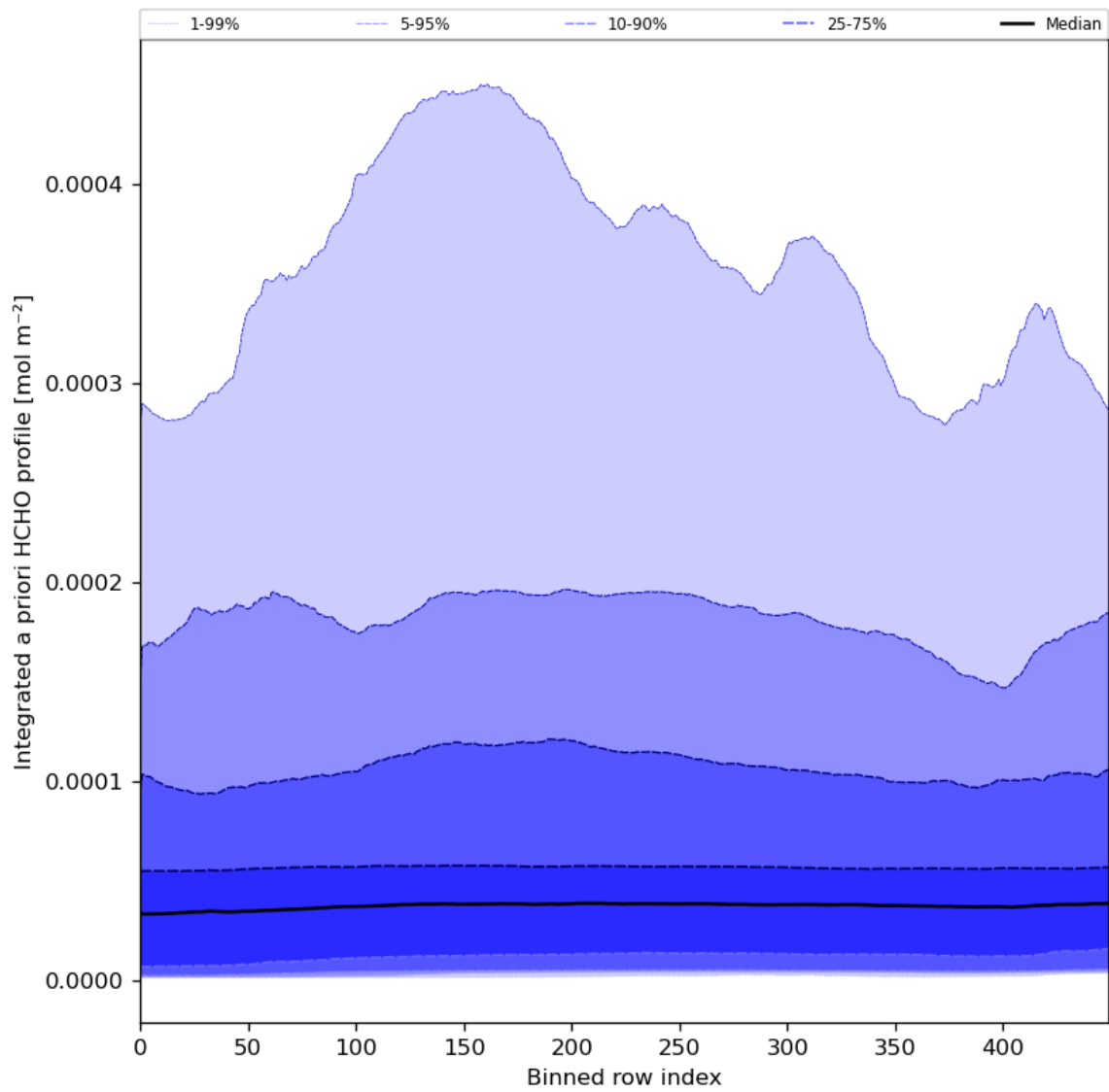
Figure 57: Along track statistics of "Integrated a priori HCHO profile" for 2024-01-21 to 2024-01-22
