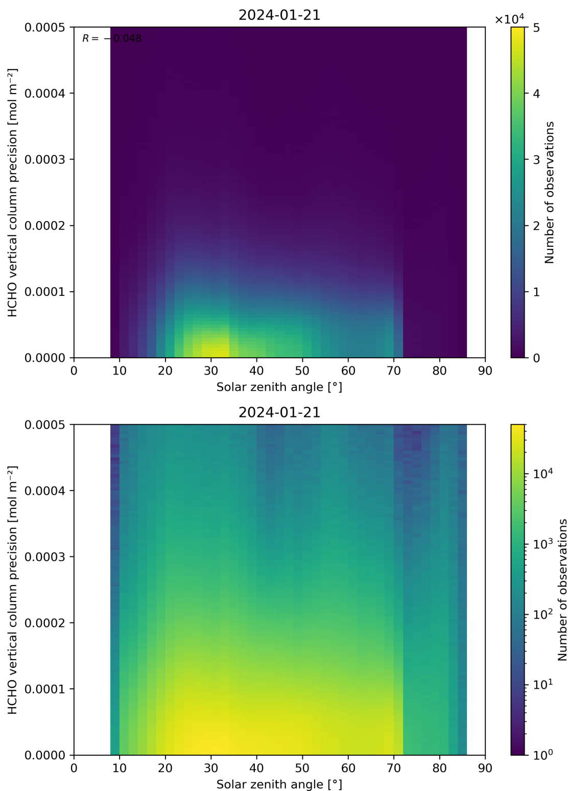
Figure 179: Scatter density plot of “Solar zenith angle” against “HCHO vertical column precision” for 2024-01-21 to 2024-01-22.
