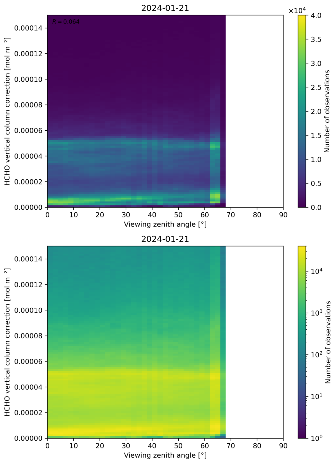
Figure 193: Scatter density plot of “Viewing zenith angle” against “HCHO vertical column correction” for 2024-01-21 to 2024-01-22.
