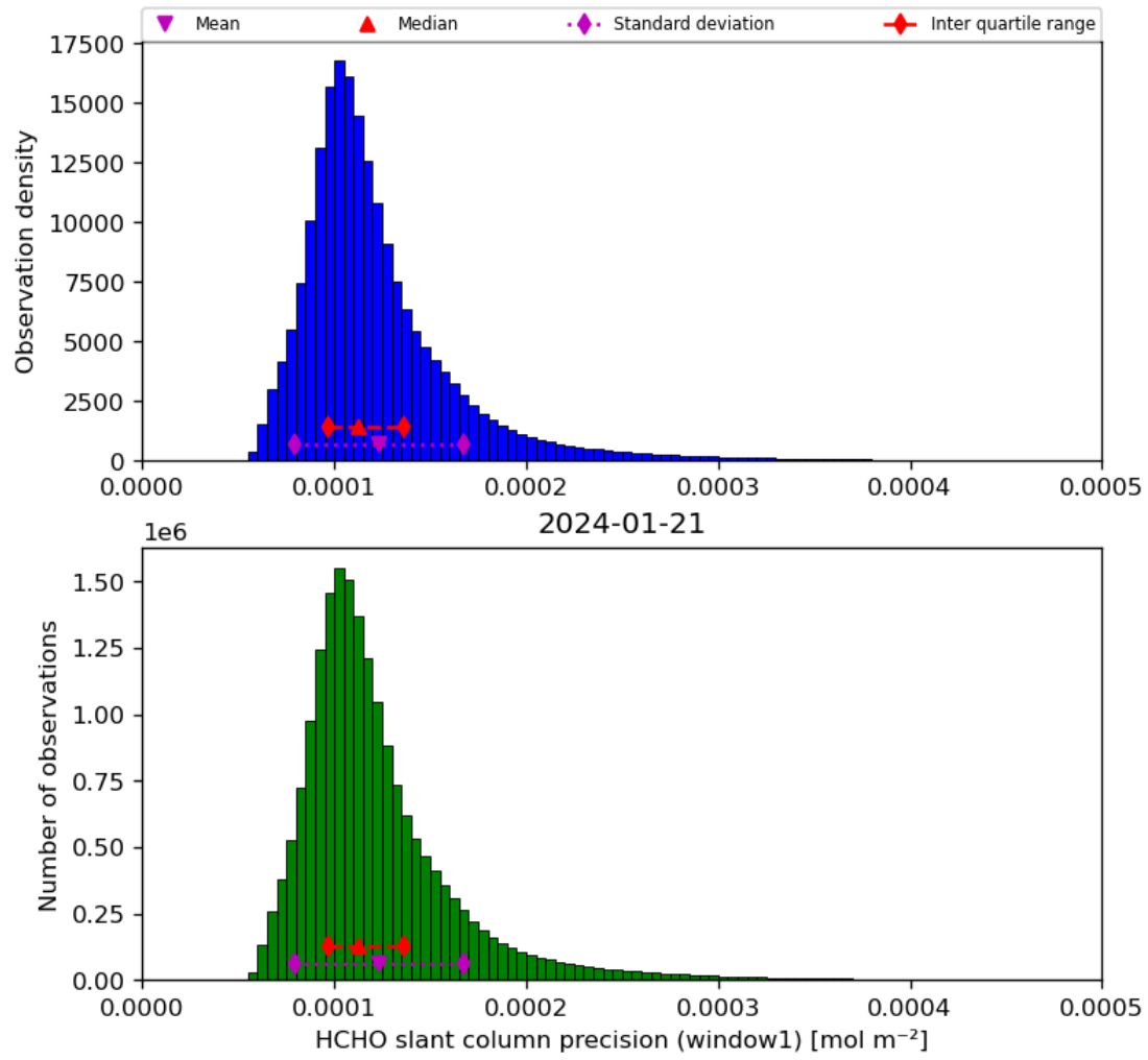
Figure 39: Histogram of “HCHO slant column precision (window1)” for 2024-01-21 to 2024-01-22
