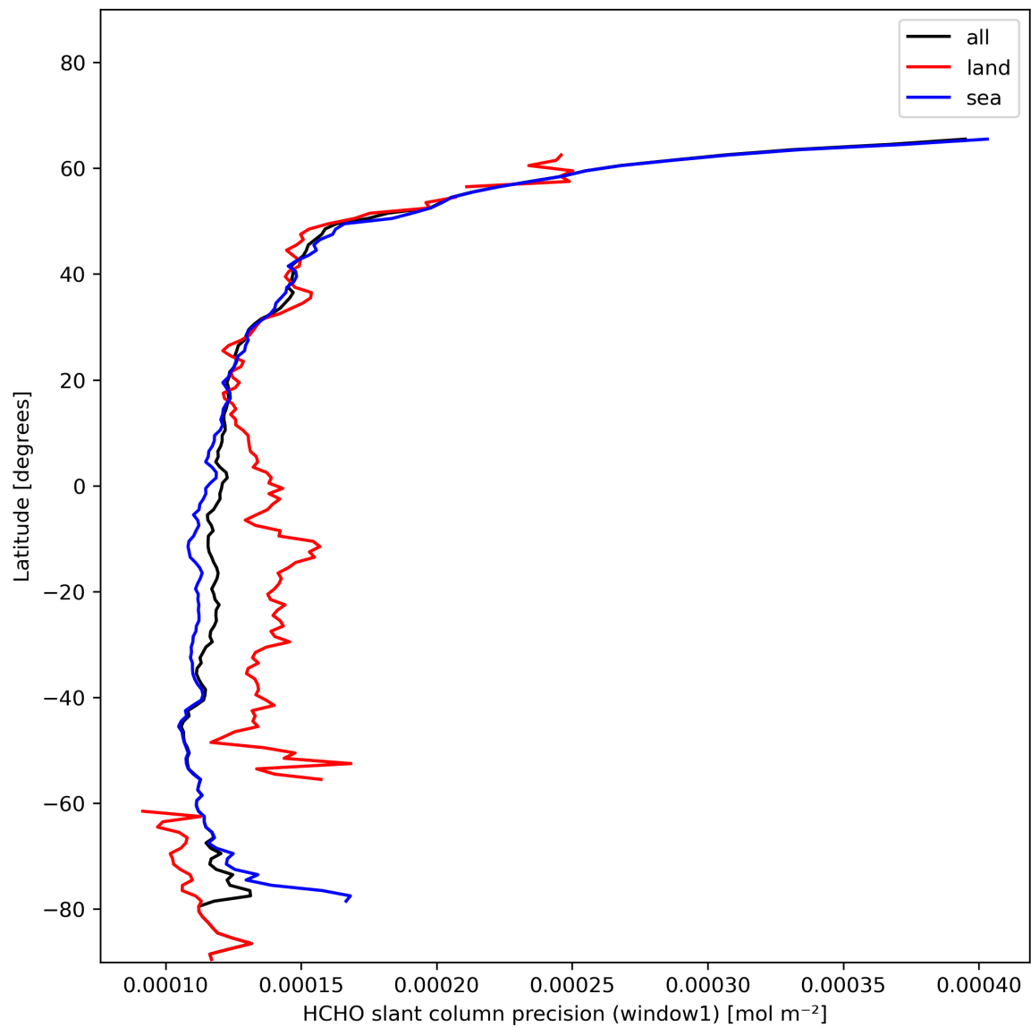
Figure 25: Zonal average of “HCHO slant column precision (window1)” for 2024-01-21 to 2024-01-22.
