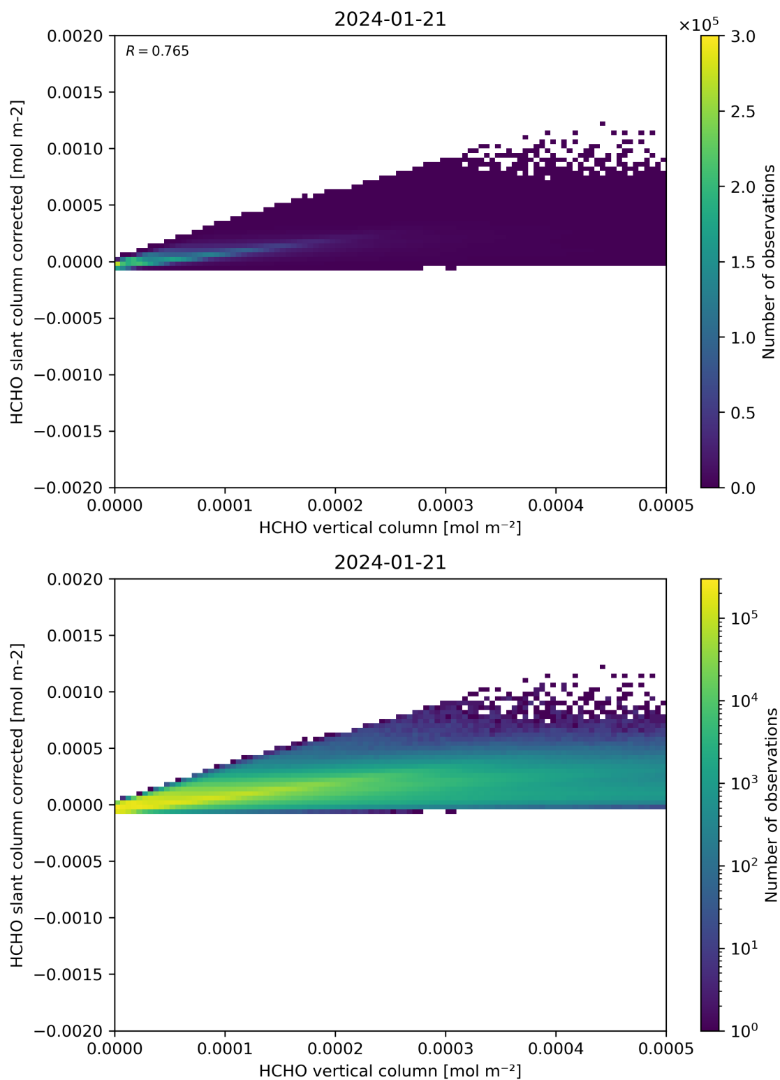
Figure 127: Scatter density plot of “HCHO vertical column” against “HCHO slant column corrected” for 2024-01-21 to 2024-01-22.
