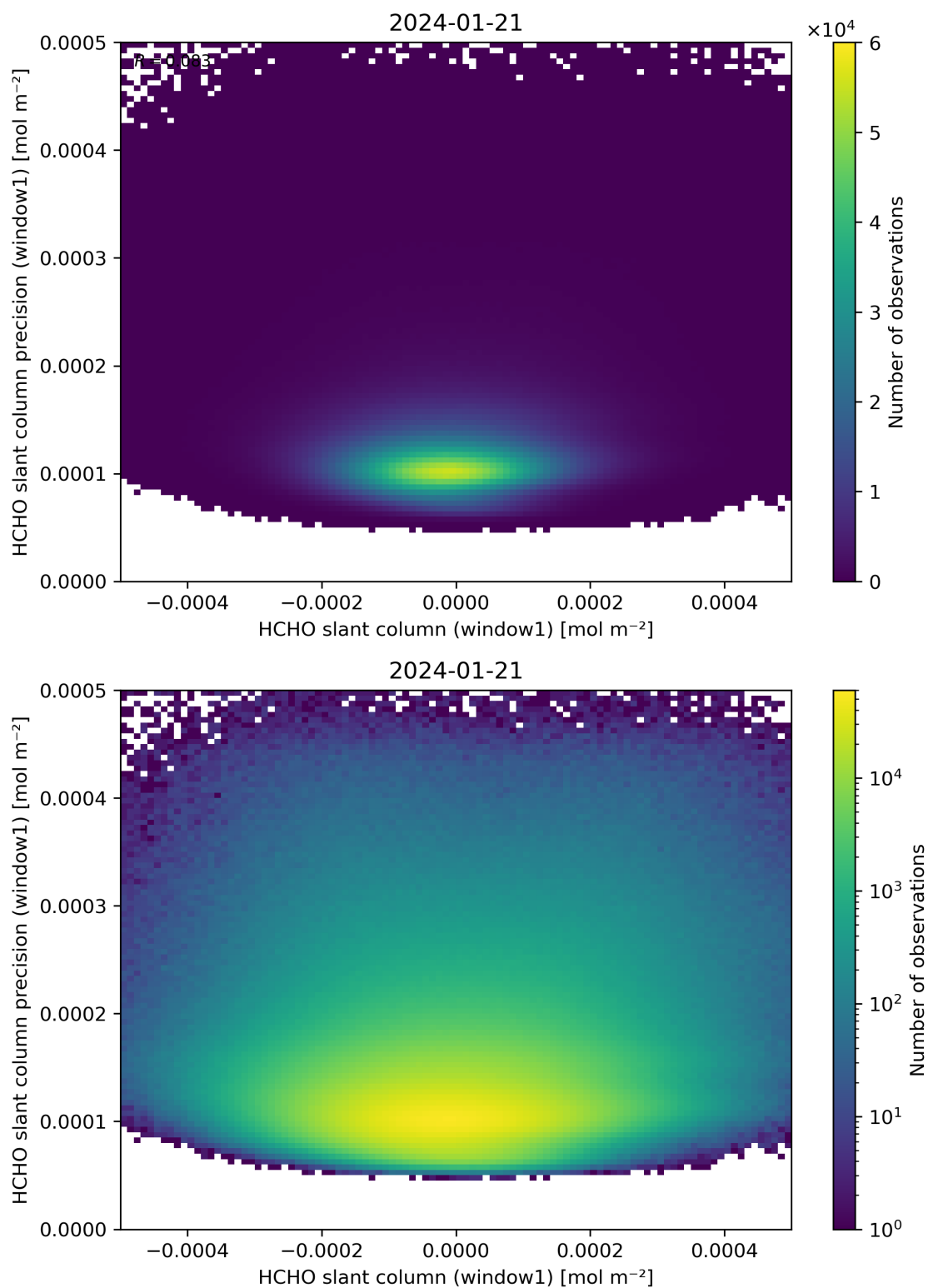
Figure 84: Scatter density plot of “HCHO slant column (window1)” against “HCHO slant column precision (window1)” for 2024-01-21 to 2024-01-22.
