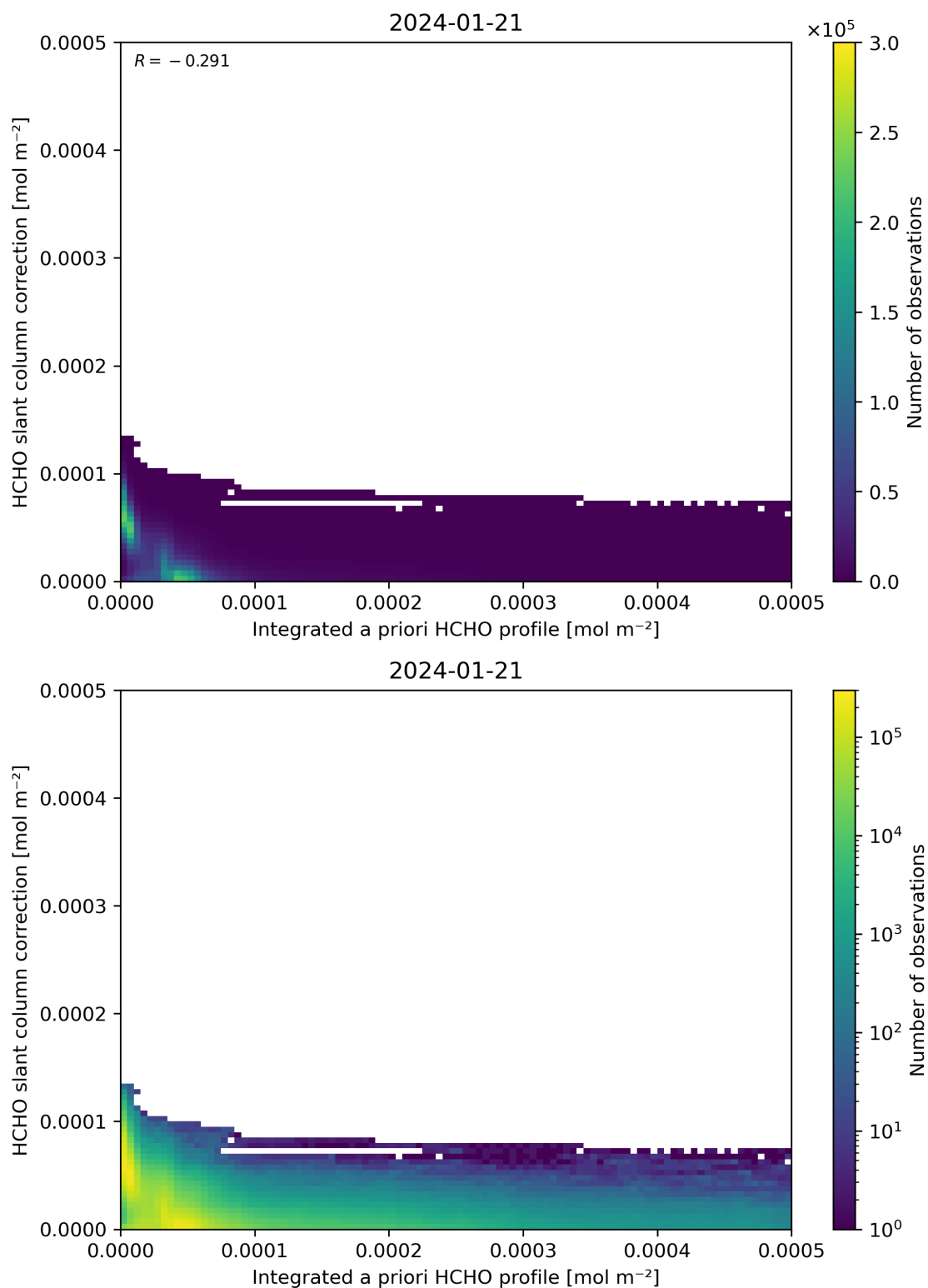
Figure 152: Scatter density plot of “Integrated a priori HCHO profile” against “HCHO slant column correction” for 2024-01-21 to 2024-01-22.
