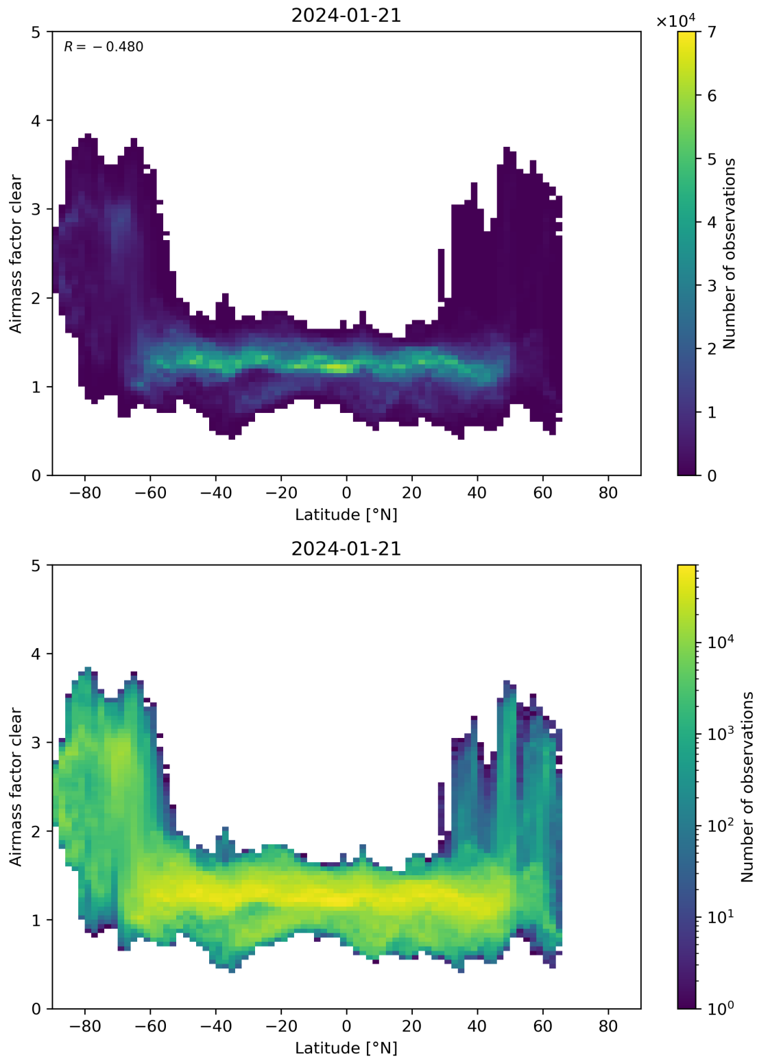
Figure 156: Scatter density plot of “Latitude” against “Airmass factor clear” for 2024-01-21 to 2024-01-22.
