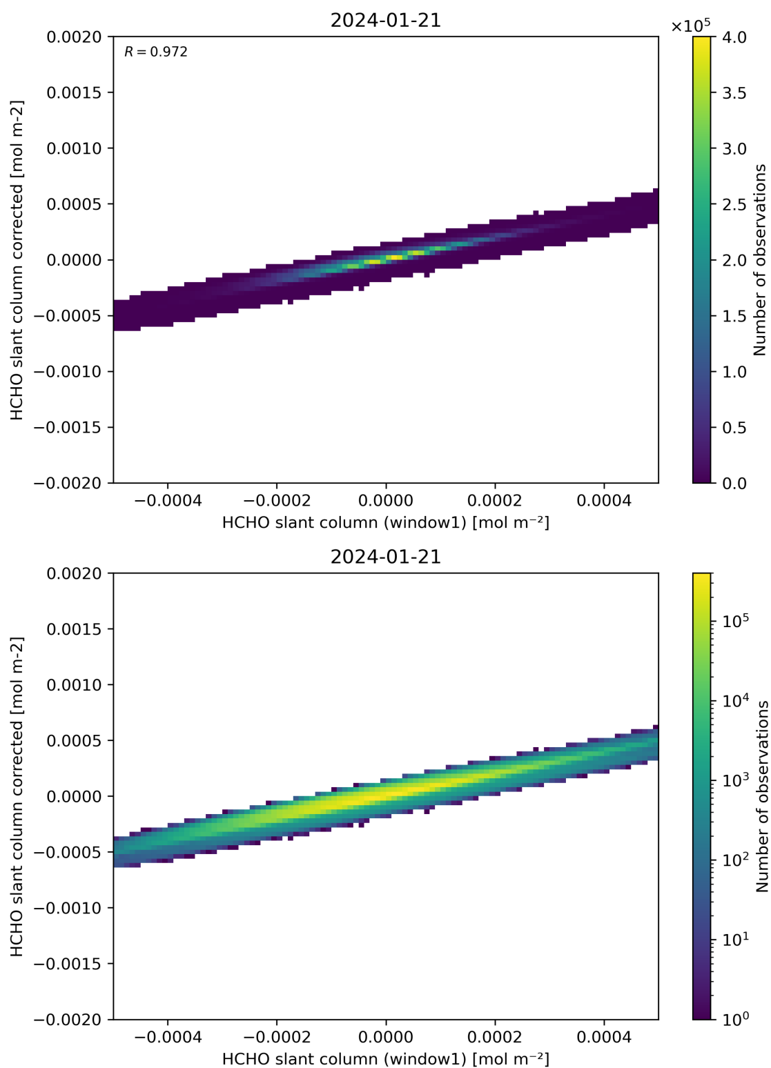
Figure 82: Scatter density plot of “HCHO slant column (window1)” against “HCHO slant column corrected” for 2024-01-21 to 2024-01-22.
