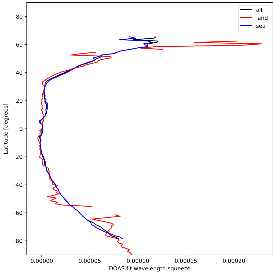
Figure 31: Zonal average of “DOAS fit wavelength squeeze” for 2024-01-21 to 2024-01-22.
