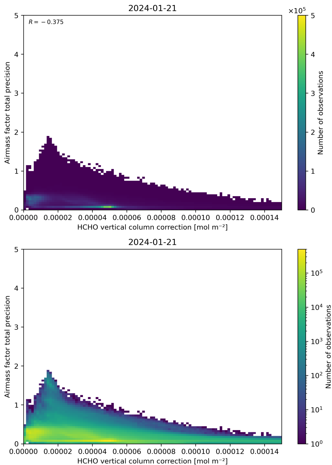
Figure 121: Scatter density plot of “HCHO vertical column correction” against “Airmass factor total precision” for 2024-01-21 to 2024-01-22.
