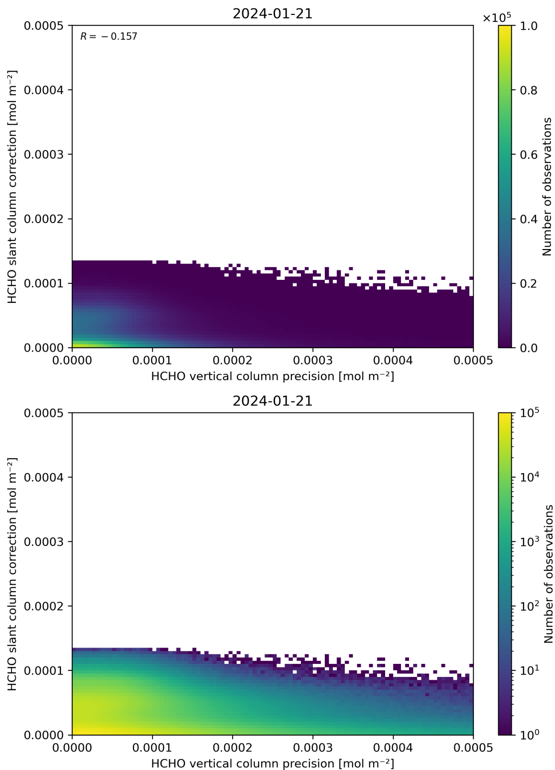
Figure 141: Scatter density plot of “HCHO vertical column precision” against “HCHO slant column correction” for 2024-01-21 to 2024-01-22.
