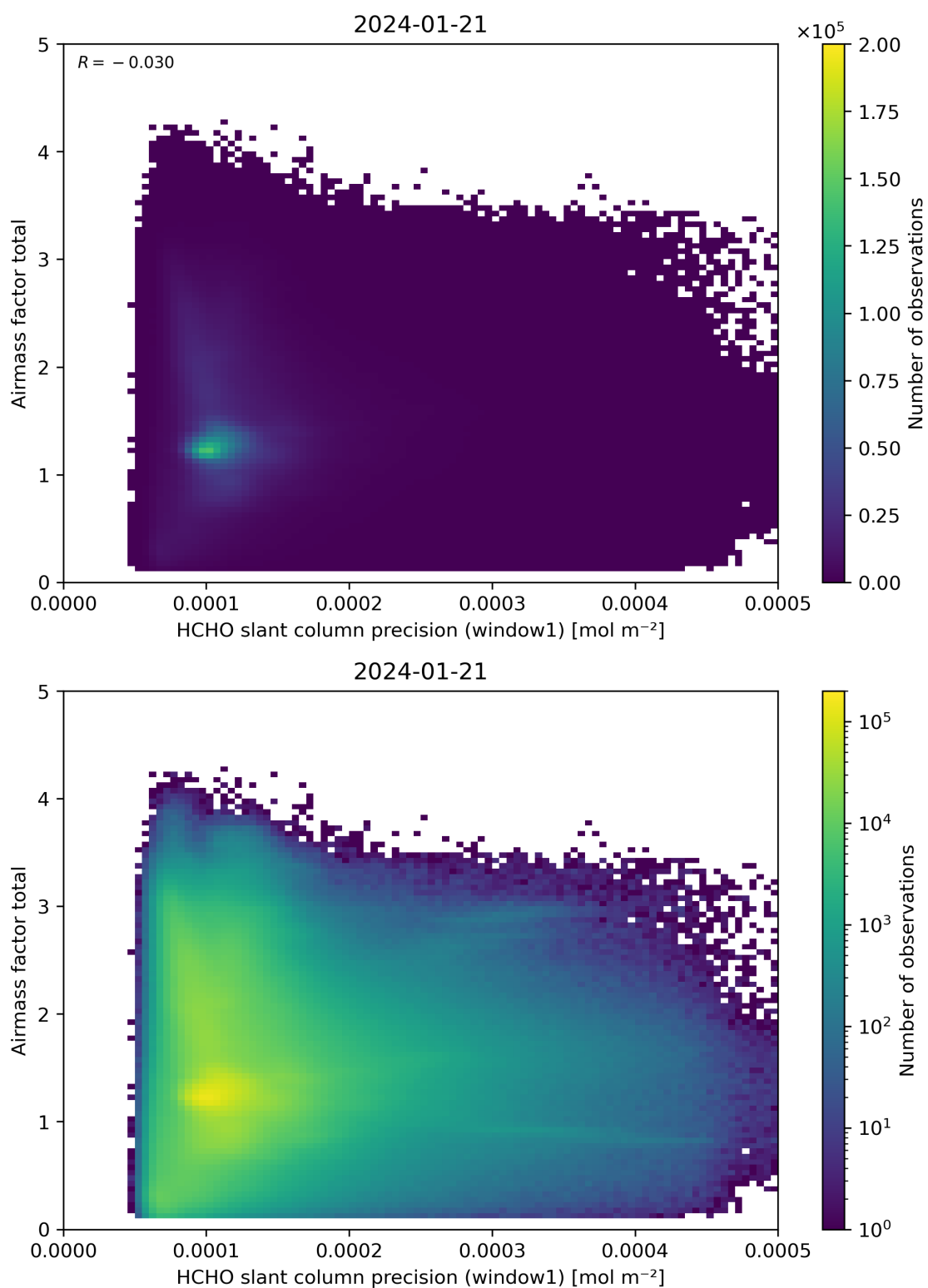
Figure 94: Scatter density plot of “HCHO slant column precision (window1)” against “Airmass factor total” for 2024-01-21 to 2024-01-22.
