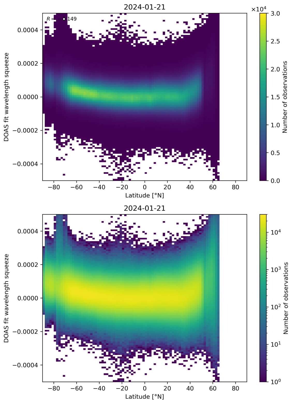
Figure 155: Scatter density plot of “Latitude” against “DOAS fit wavelength squeeze” for 2024-01-21 to 2024-01-22.
