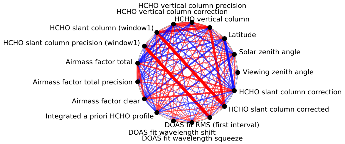
Figure 1: Map of correlation graph for 2024-01-21 to 2024-01-22.
