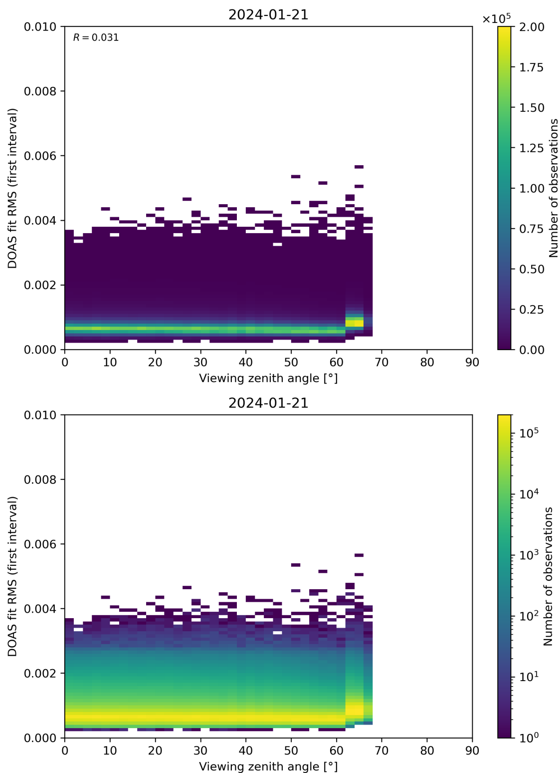
Figure 182: Scatter density plot of “Viewing zenith angle” against “DOAS fit RMS (first interval)” for 2024-01-21 to 2024-01-22.
