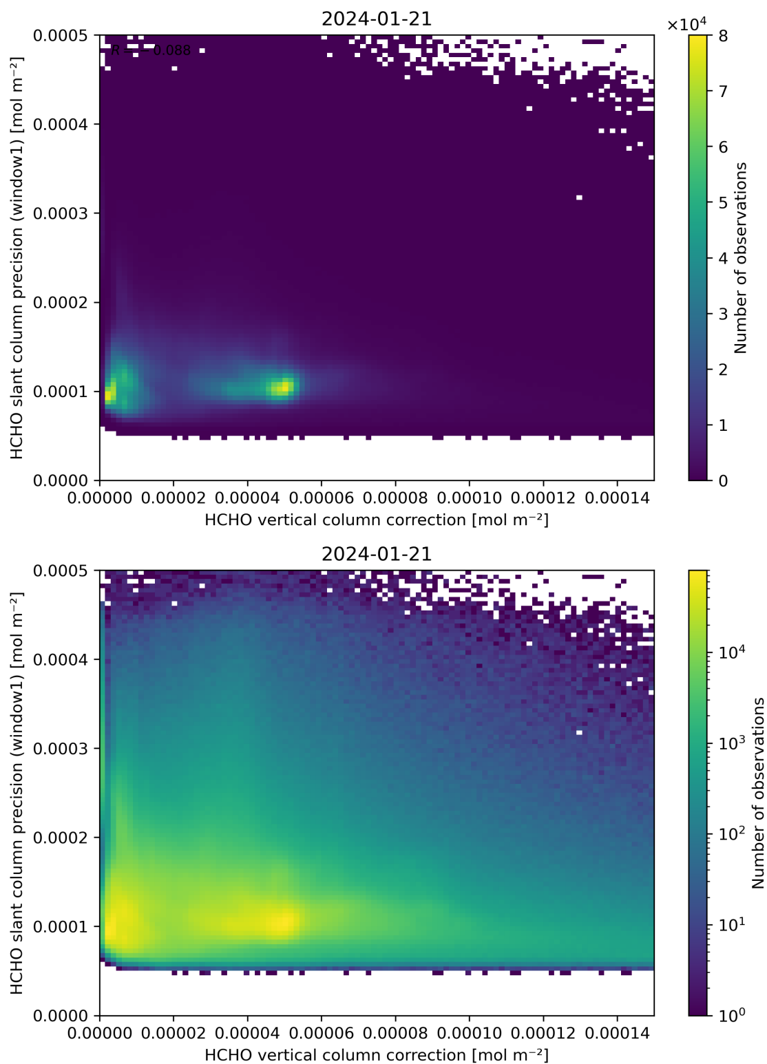
Figure 119: Scatter density plot of “HCHO vertical column correction” against “HCHO slant column precision (window1)” for 2024-01-21 to 2024-01-22.
