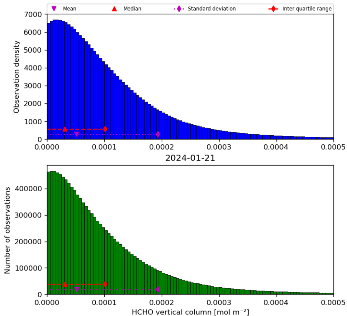
Figure 35: Histogram of “HCHO vertical column” for 2024-01-21 to 2024-01-22
