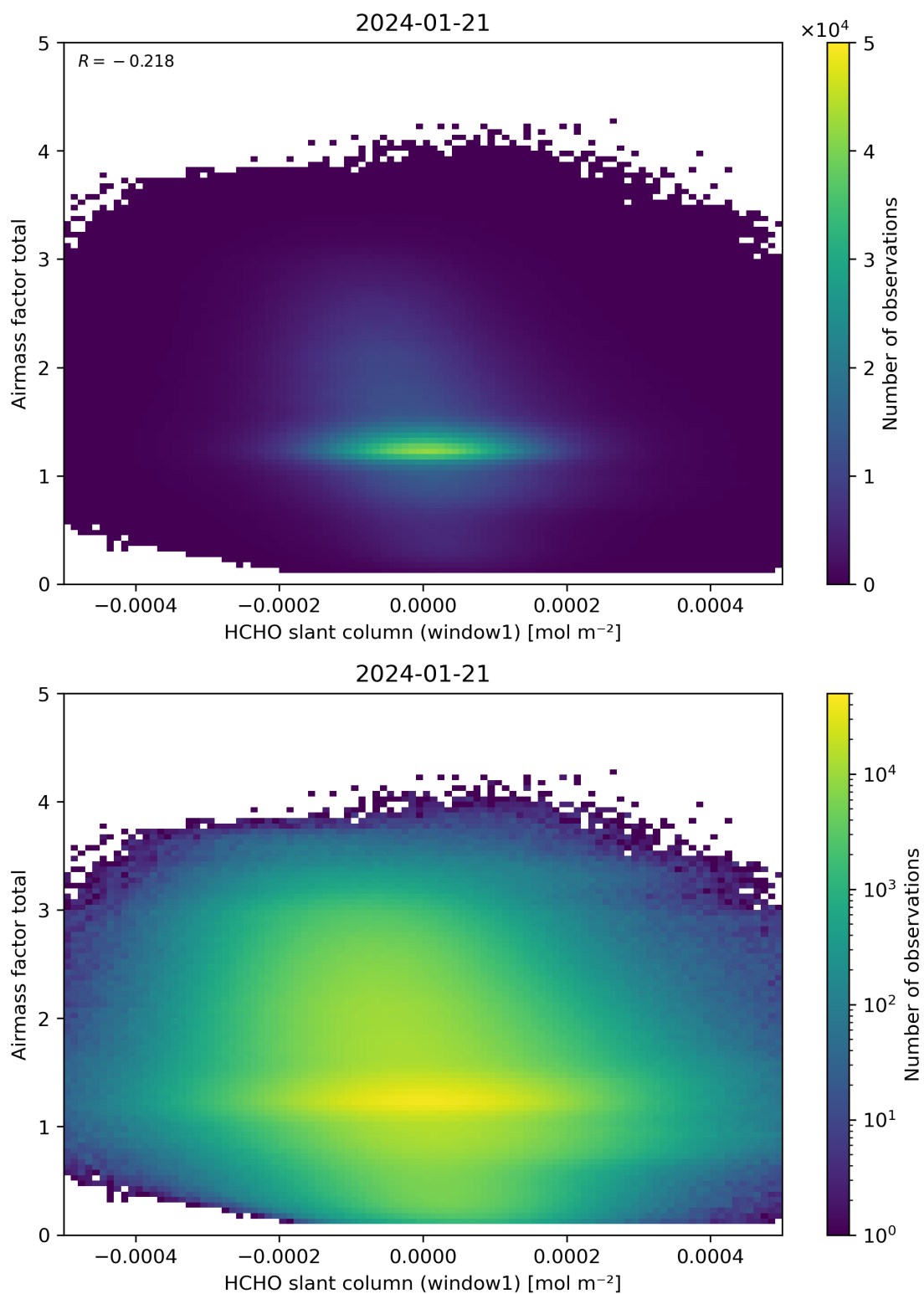
Figure 85: Scatter density plot of “HCHO slant column (window1)” against “Airmass factor total” for 2024-01-21 to 2024-01-22.
