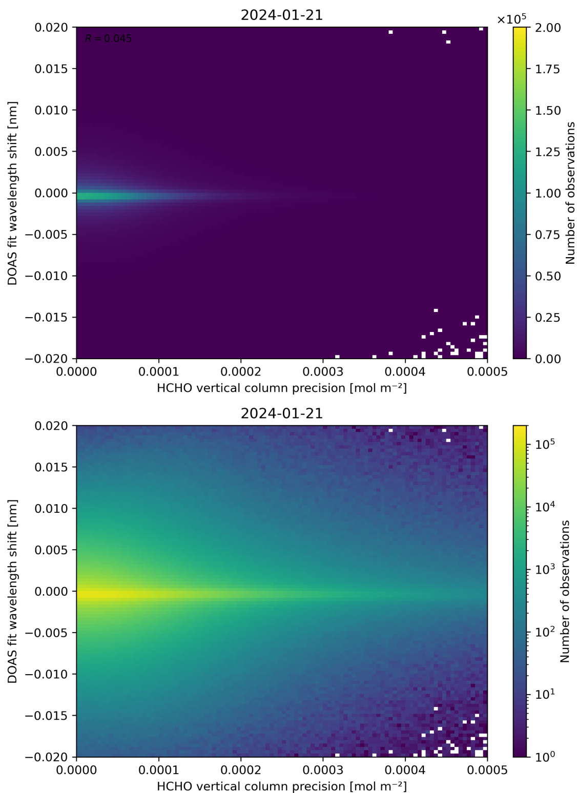
Figure 137: Scatter density plot of “HCHO vertical column precision” against “DOAS fit wavelength shift” for 2024-01-21 to 2024-01-22.
