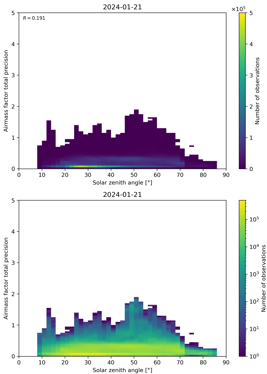
Figure 176: Scatter density plot of “Solar zenith angle” against “Airmass factor total precision” for 2024-01-21 to 2024-01-22.
