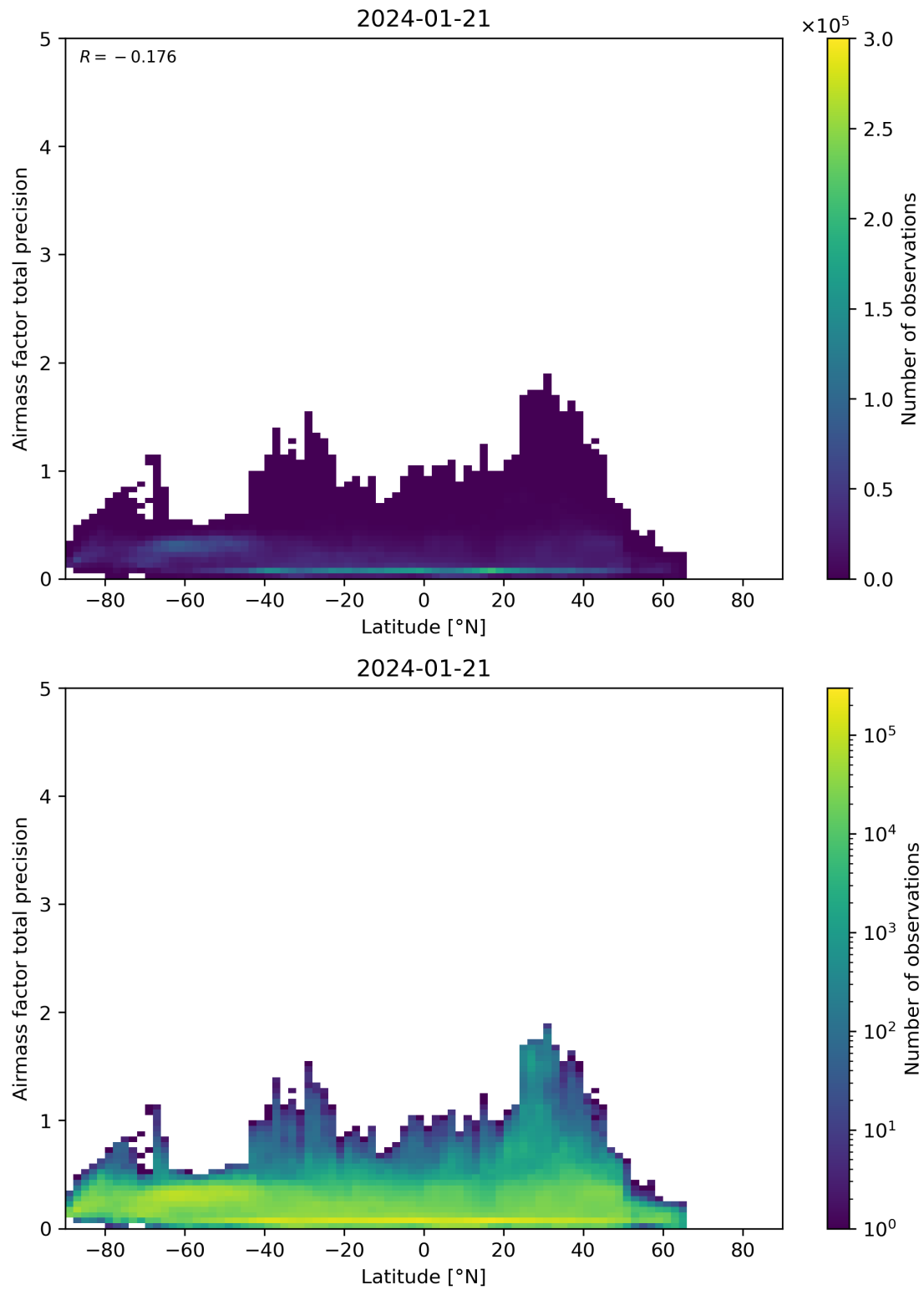
Figure 162: Scatter density plot of “Latitude” against “Airmass factor total precision” for 2024-01-21 to 2024-01-22.
