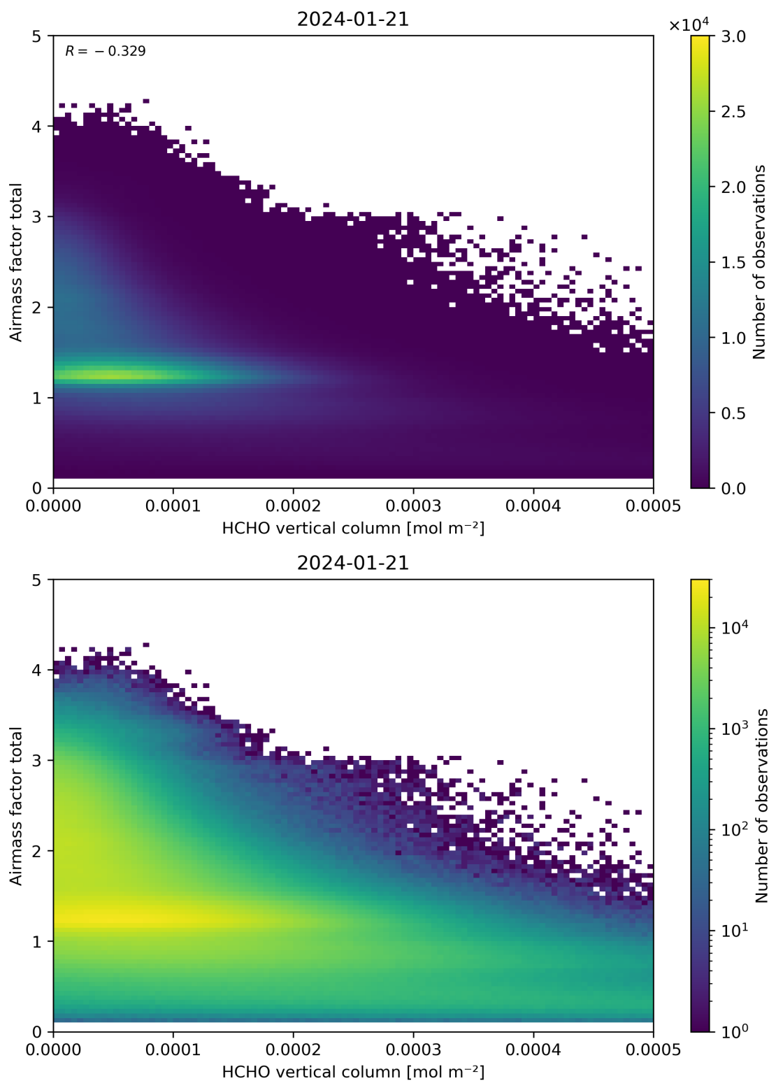
Figure 131: Scatter density plot of “HCHO vertical column” against “Airmass factor total” for 2024-01-21 to 2024-01-22.
