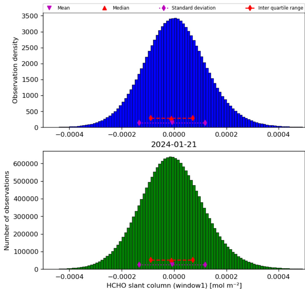
Figure 38: Histogram of “HCHO slant column (window1)” for 2024-01-21 to 2024-01-22
