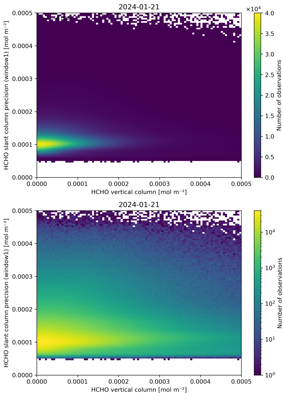
Figure 130: Scatter density plot of “HCHO vertical column” against “HCHO slant column precision (window1)” for 2024-01-21 to 2024-01-22.
