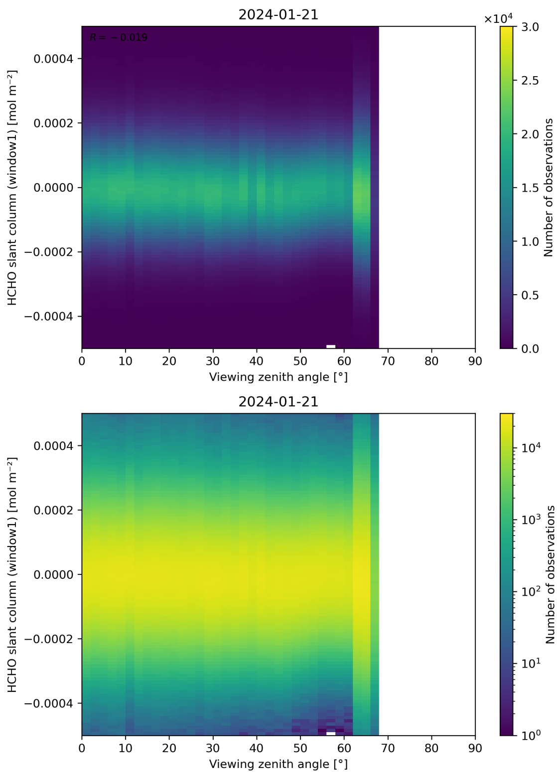
Figure 188: Scatter density plot of “Viewing zenith angle” against “HCHO slant column (window1)” for 2024-01-21 to 2024-01-22.
