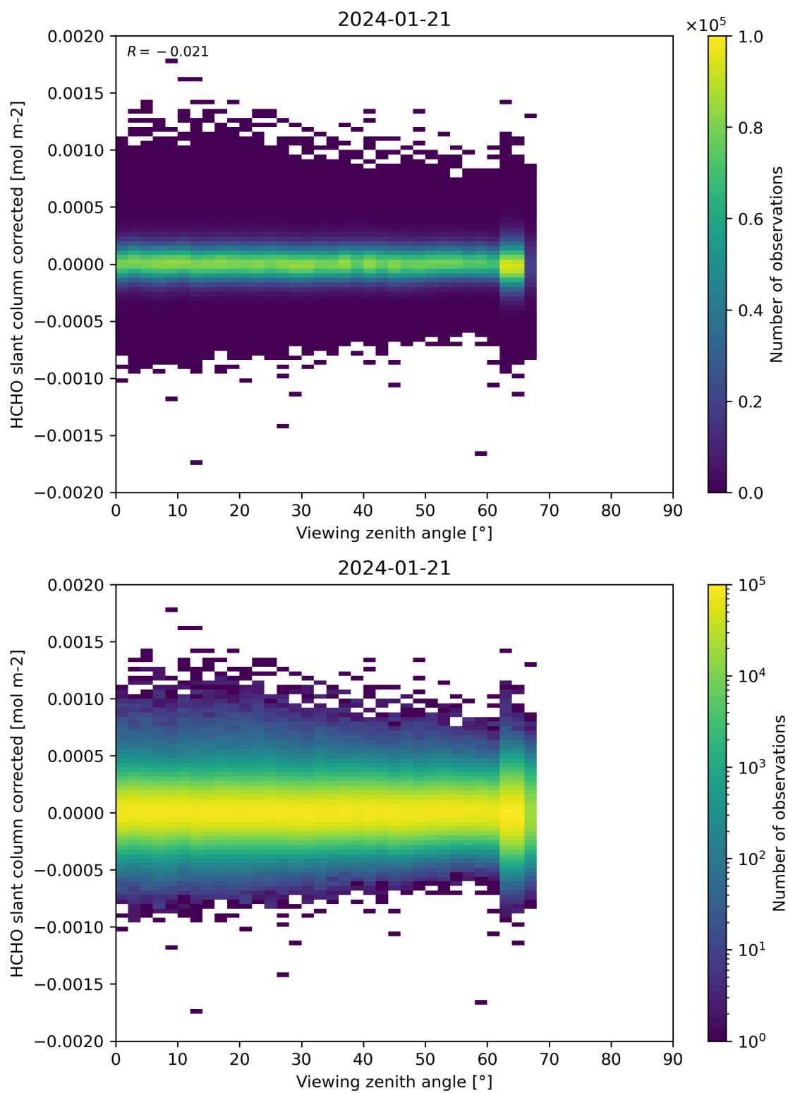
Figure 186: Scatter density plot of “Viewing zenith angle” against “HCHO slant column corrected” for 2024-01-21 to 2024-01-22.
