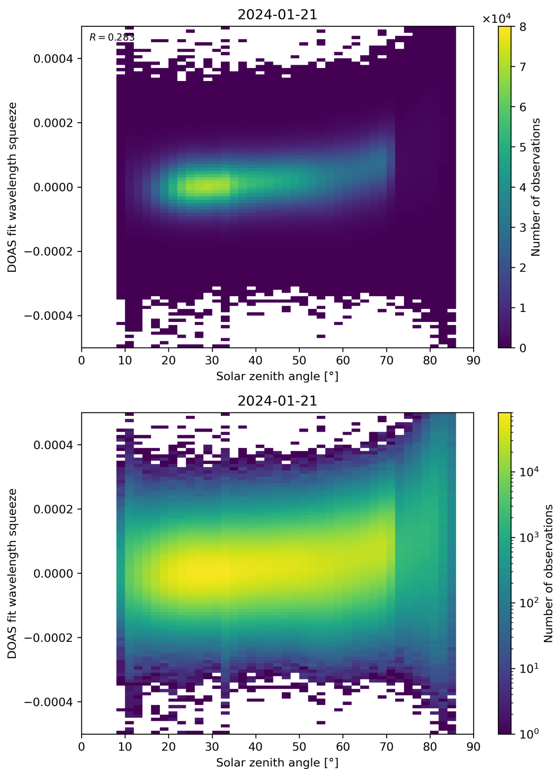
Figure 169: Scatter density plot of “Solar zenith angle” against “DOAS fit wavelength squeeze” for 2024-01-21 to 2024-01-22.
