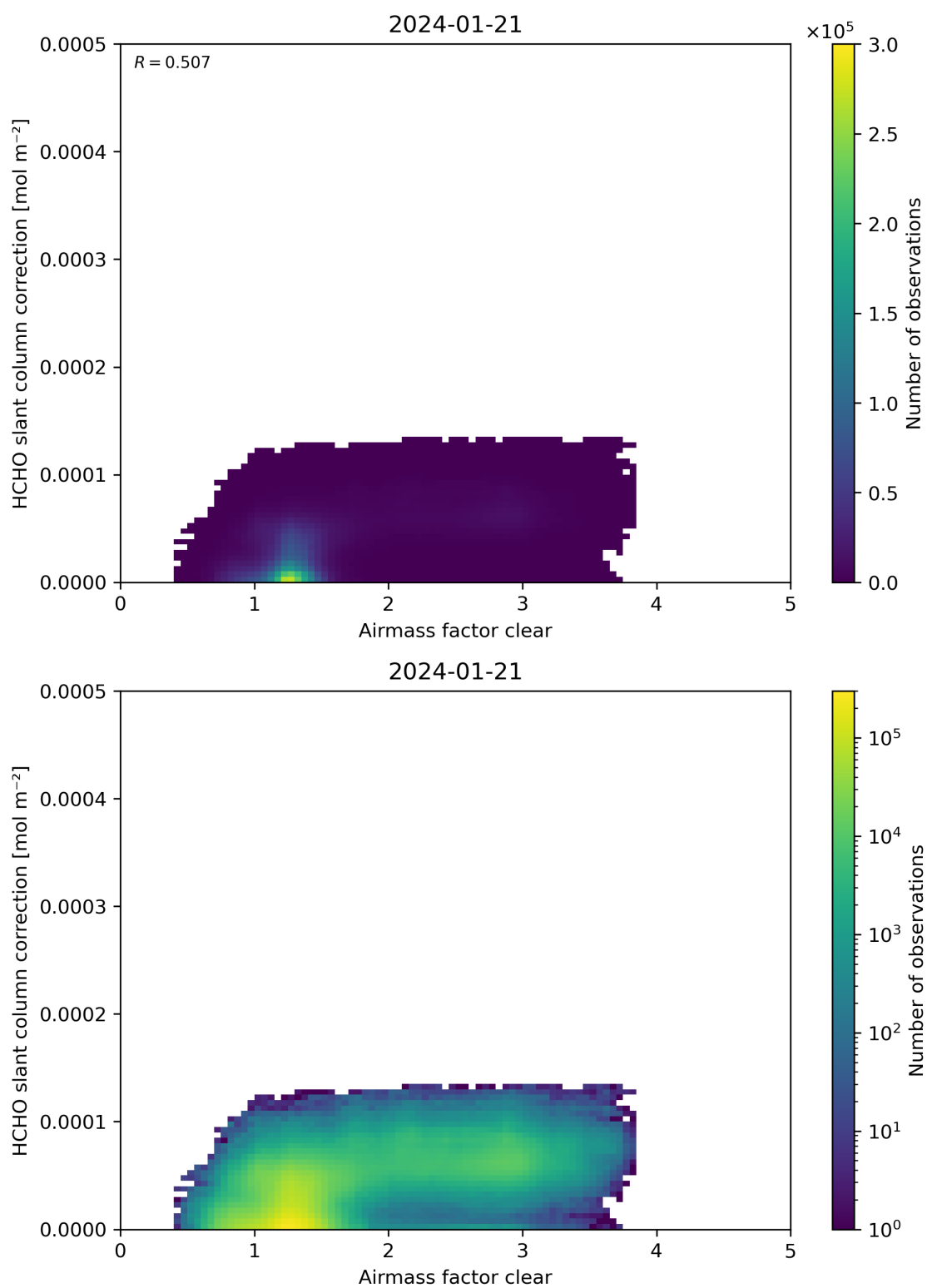
Figure 75: Scatter density plot of “Airmass factor clear” against “HCHO slant column correction” for 2024-01-21 to 2024-01-22.
