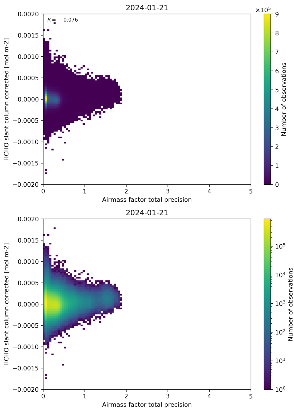
Figure 109: Scatter density plot of “Airmass factor total precision” against “HCHO slant column corrected” for 2024-01-21 to 2024-01-22.
