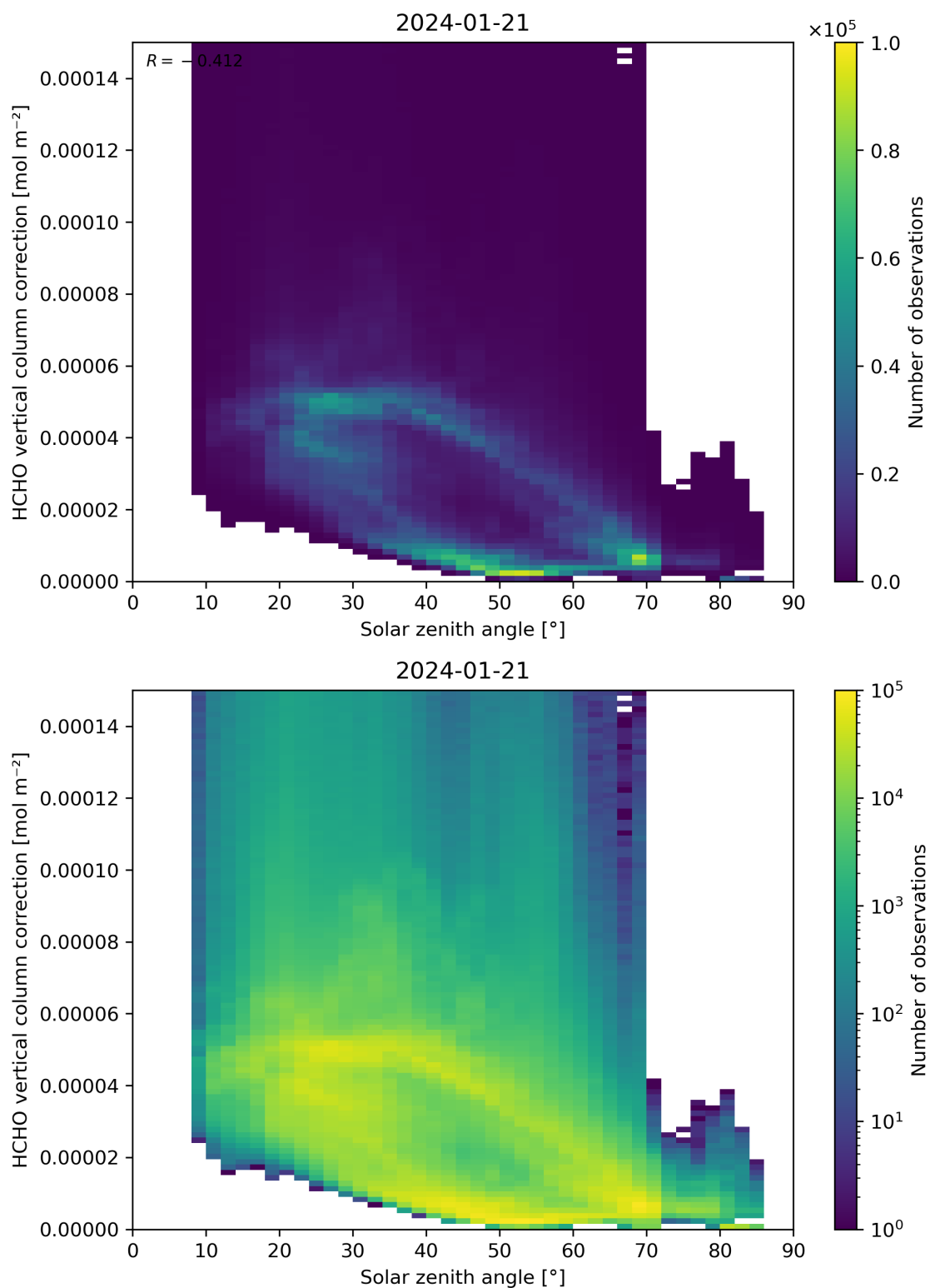
Figure 178: Scatter density plot of “Solar zenith angle” against “HCHO vertical column correction” for 2024-01-21 to 2024-01-22.
