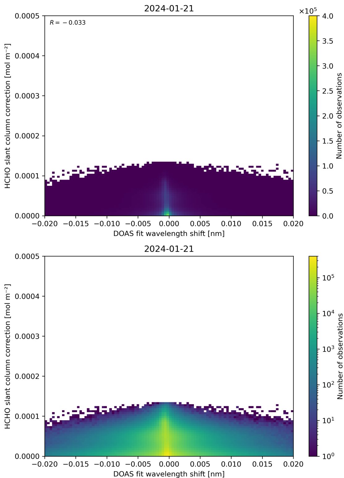
Figure 67: Scatter density plot of “DOAS fit wavelength shift” against “HCHO slant column correction” for 2024-01-21 to 2024-01-22.
