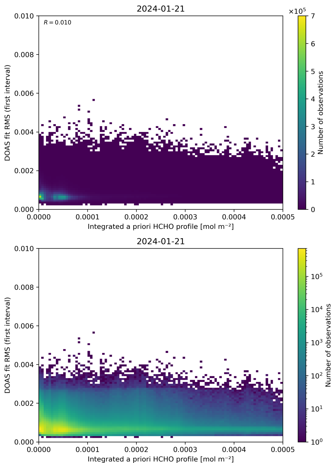
Figure 148: Scatter density plot of “Integrated a priori HCHO profile” against “DOAS fit RMS (first interval)” for 2024-01-21 to 2024-01-22.
