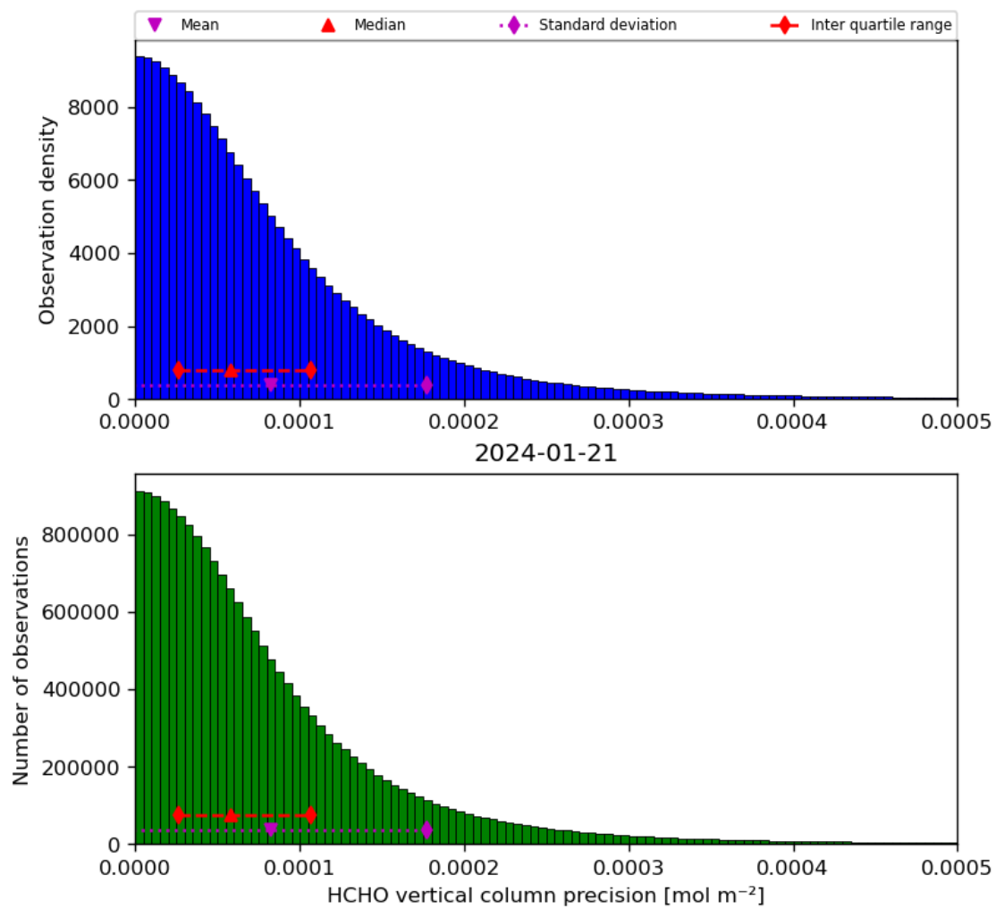
Figure 36: Histogram of “HCHO vertical column precision” for 2024-01-21 to 2024-01-22
