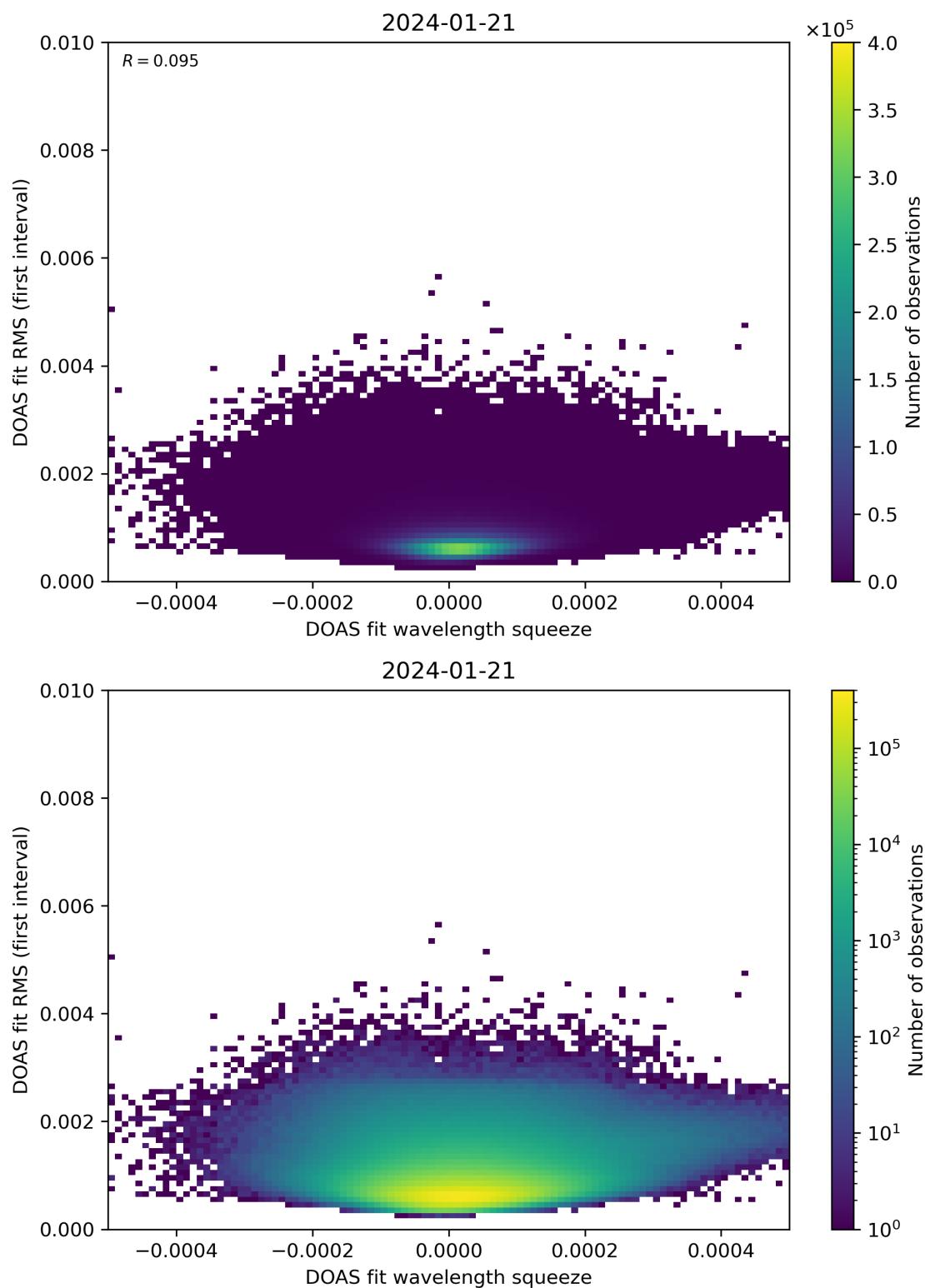
Figure 68: Scatter density plot of “DOAS fit wavelength squeeze” against “DOAS fit RMS (first interval)” for 2024-01-21 to 2024-01-22.
