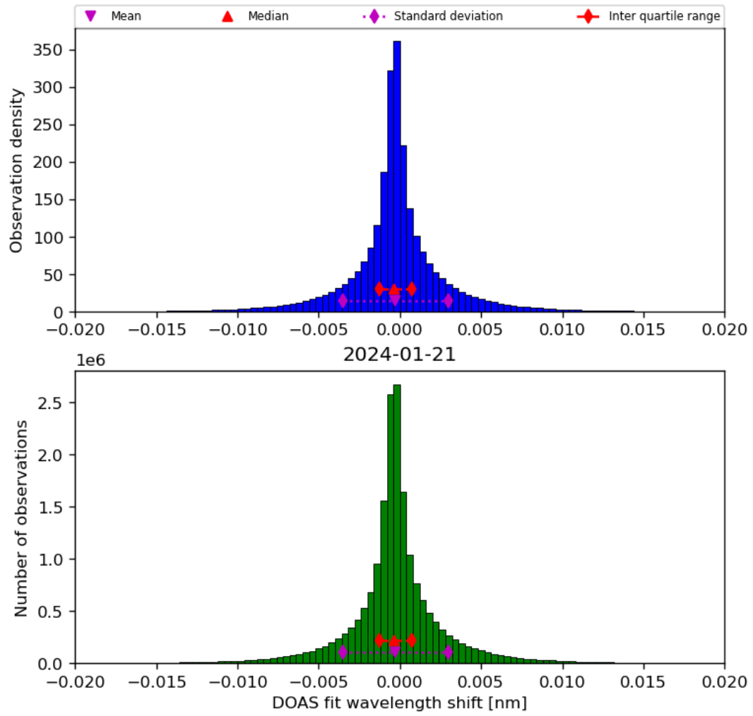
Figure 44: Histogram of “DOAS fit wavelength shift” for 2024-01-21 to 2024-01-22
