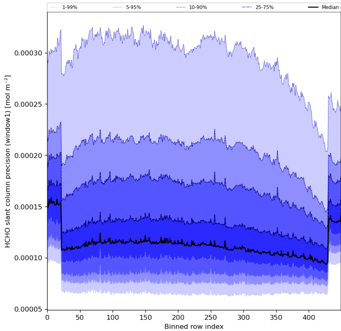
Figure 53: Along track statistics of “HCHO slant column precision (window1)” for 2024-01-21 to 2024-01-22
