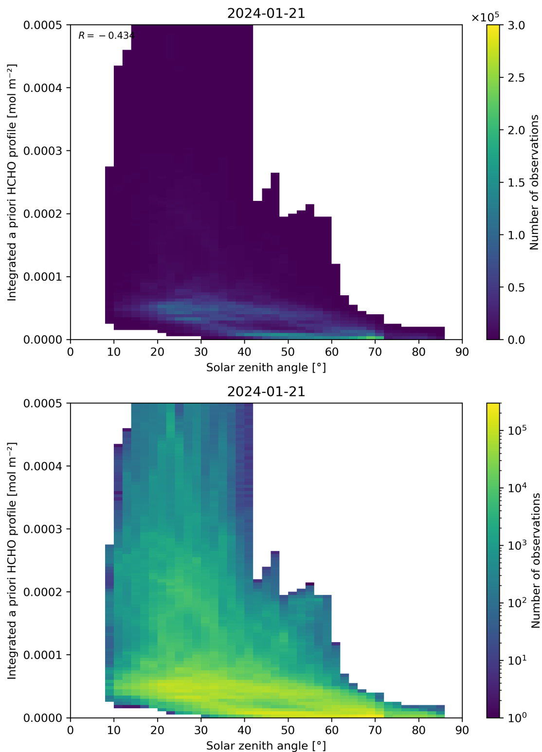
Figure 180: Scatter density plot of “Solar zenith angle” against “Integrated a priori HCHO profile” for 2024-01-21 to 2024-01-22.
