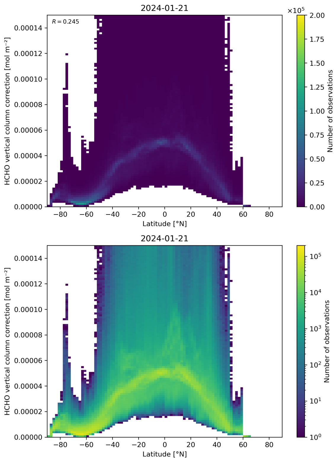
Figure 164: Scatter density plot of “Latitude” against “HCHO vertical column correction” for 2024-01-21 to 2024-01-22.
