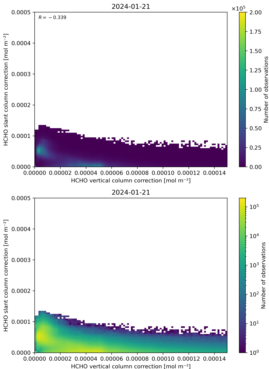
Figure 117: Scatter density plot of “HCHO vertical column correction” against “HCHO slant column correction” for 2024-01-21 to 2024-01-22.
