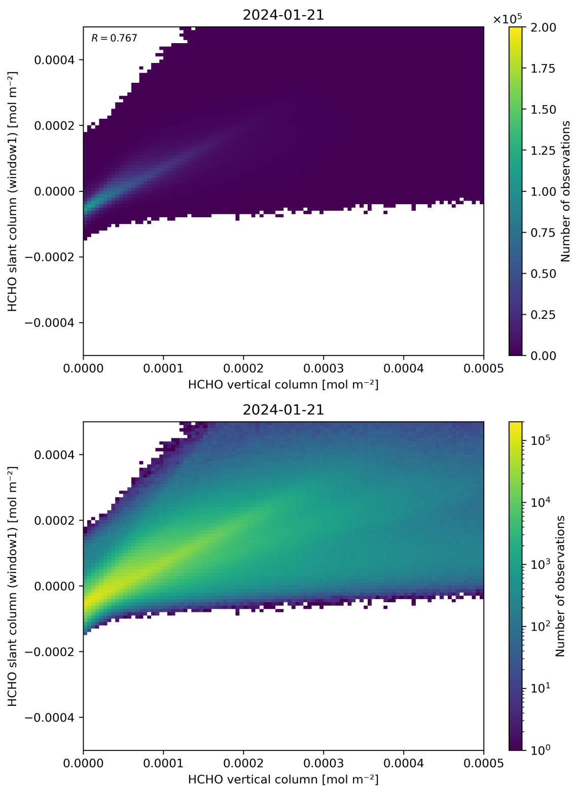
Figure 129: Scatter density plot of “HCHO vertical column” against “HCHO slant column (window1)” for 2024-01-21 to 2024-01-22.
