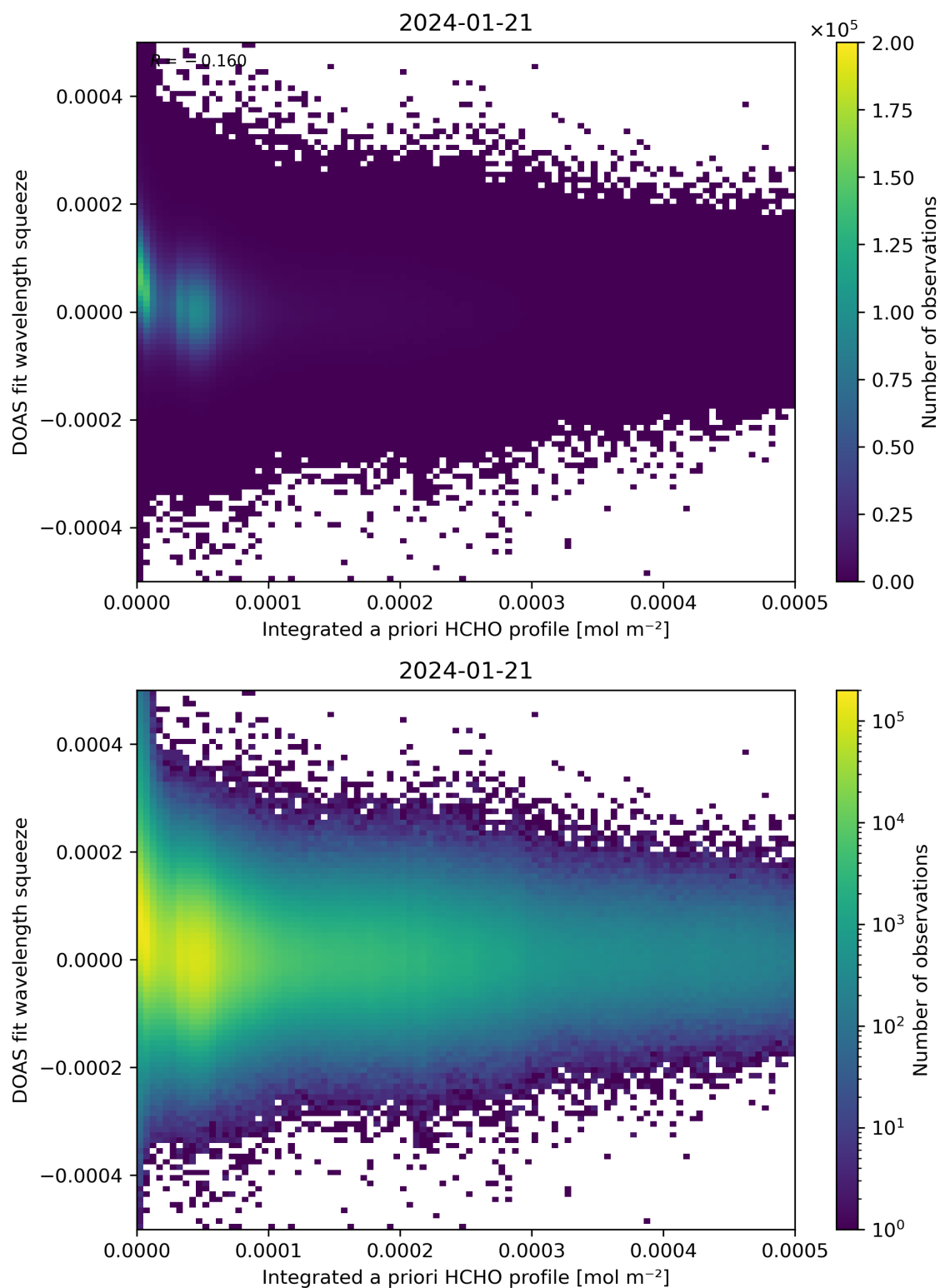
Figure 150: Scatter density plot of “Integrated a priori HCHO profile” against “DOAS fit wavelength squeeze” for 2024-01-21 to 2024-01-22.
