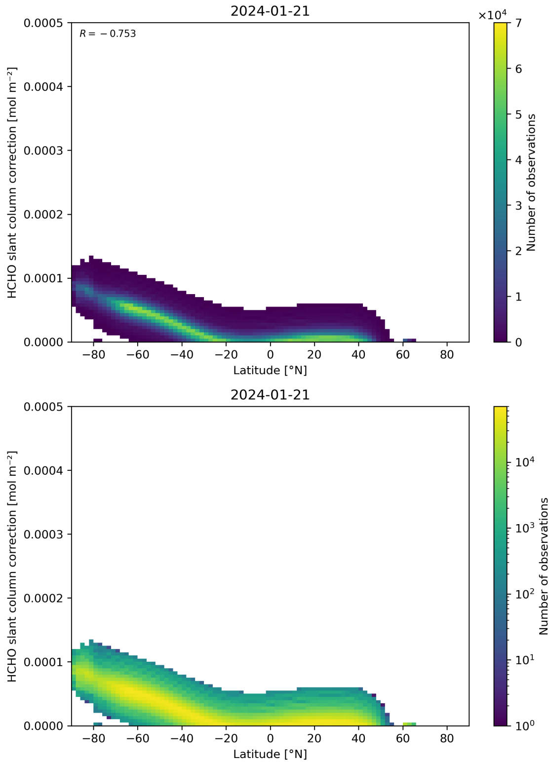
Figure 158: Scatter density plot of “Latitude” against “HCHO slant column correction” for 2024-01-21 to 2024-01-22.
