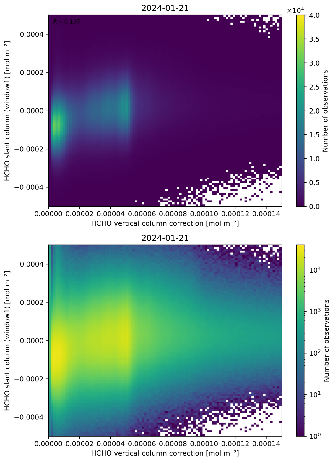
Figure 118: Scatter density plot of “HCHO vertical column correction” against “HCHO slant column (window1)” for 2024-01-21 to 2024-01-22.
