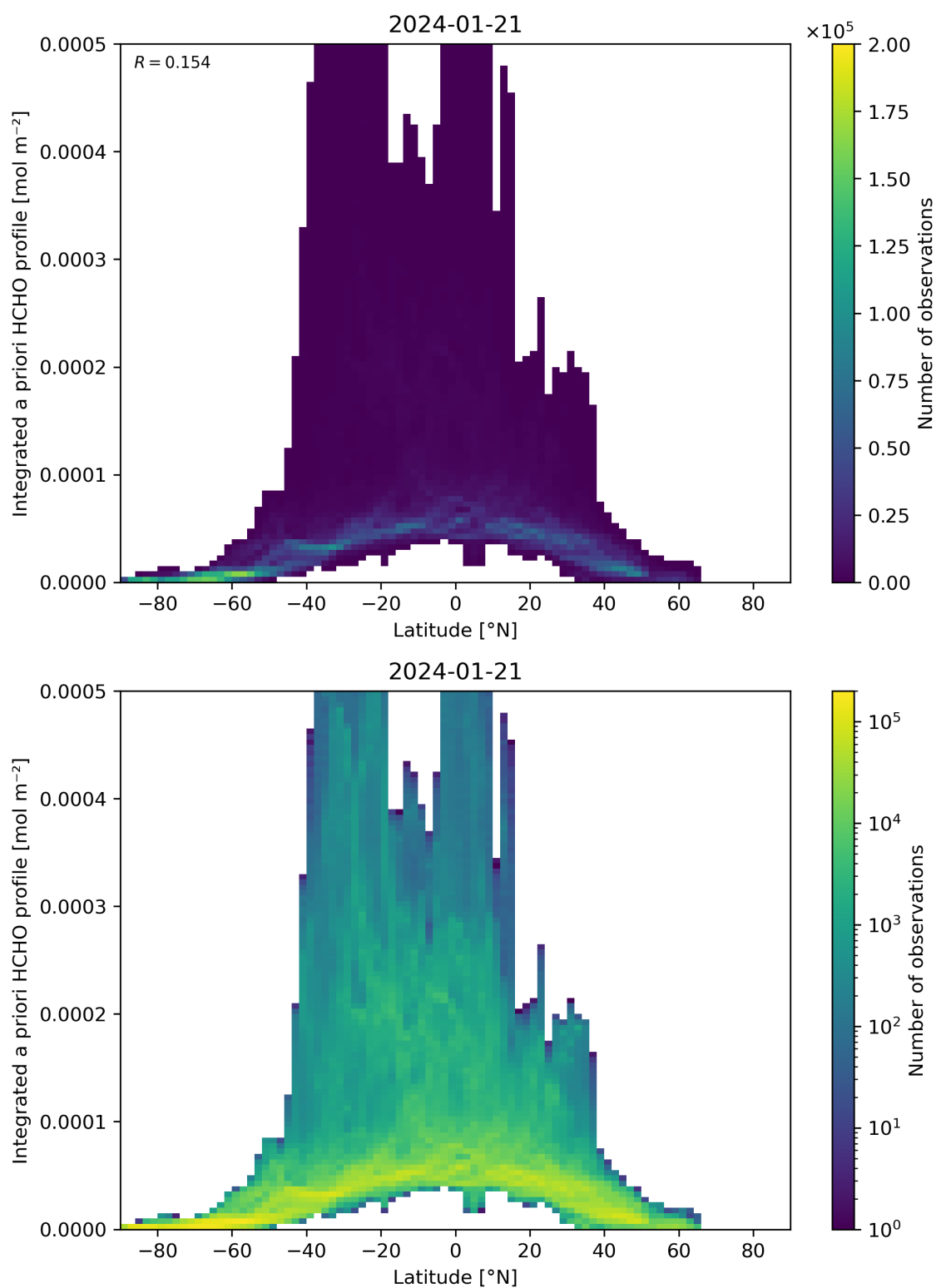
Figure 166: Scatter density plot of “Latitude” against “Integrated a priori HCHO profile” for 2024-01-21 to 2024-01-22.
