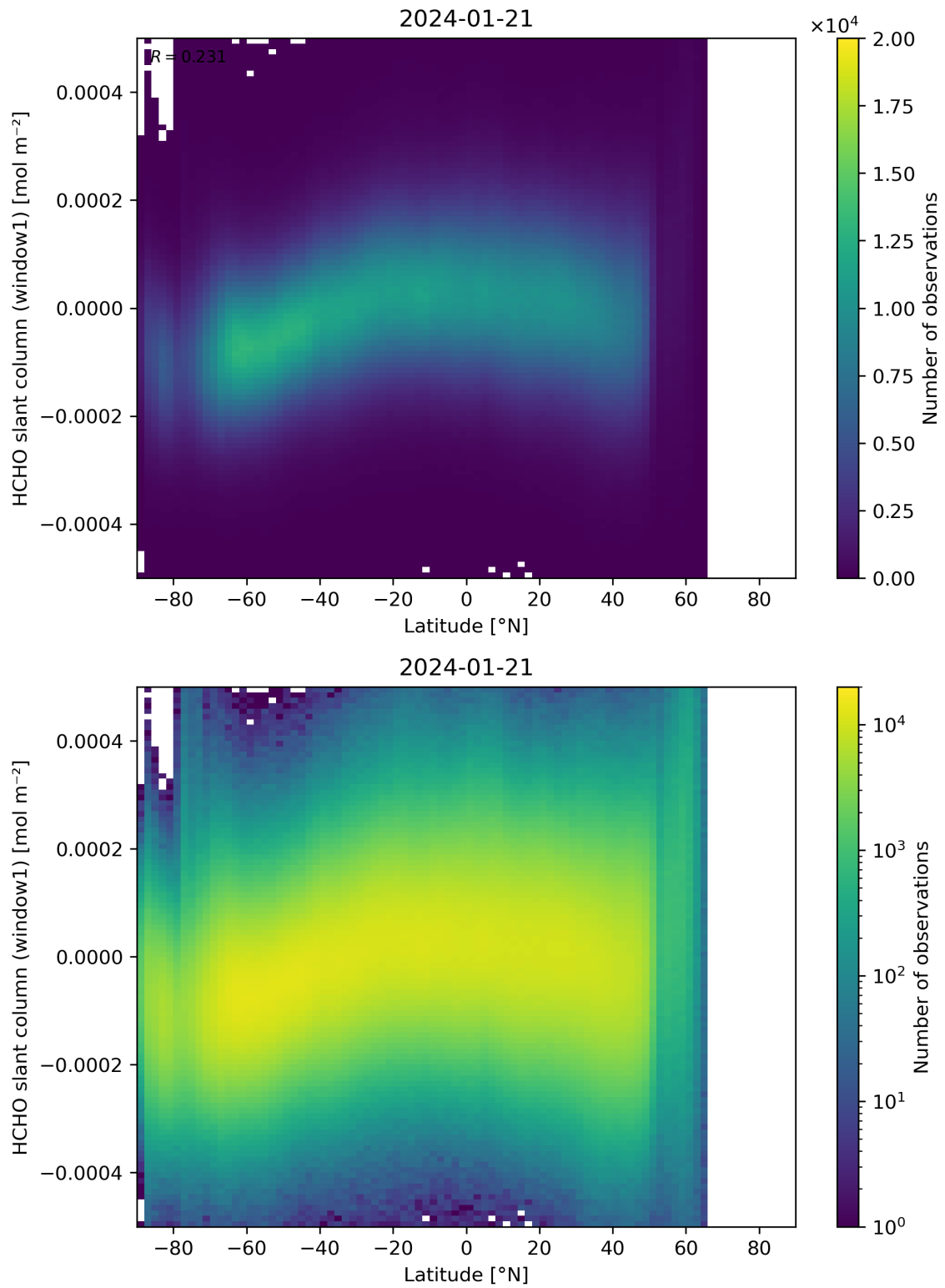
Figure 159: Scatter density plot of “Latitude” against “HCHO slant column (window1)” for 2024-01-21 to 2024-01-22.
