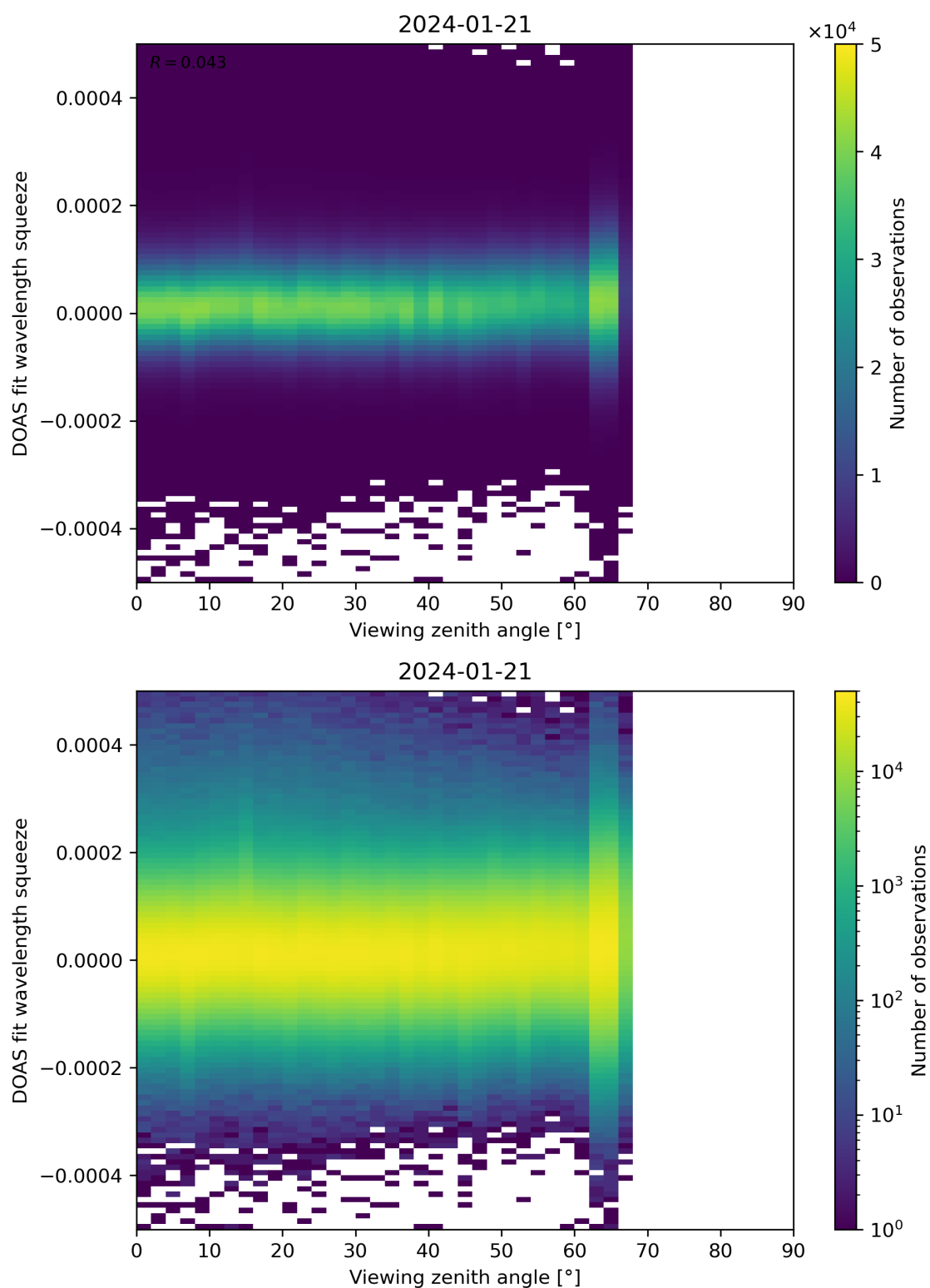
Figure 184: Scatter density plot of “Viewing zenith angle” against “DOAS fit wavelength squeeze” for 2024-01-21 to 2024-01-22.
