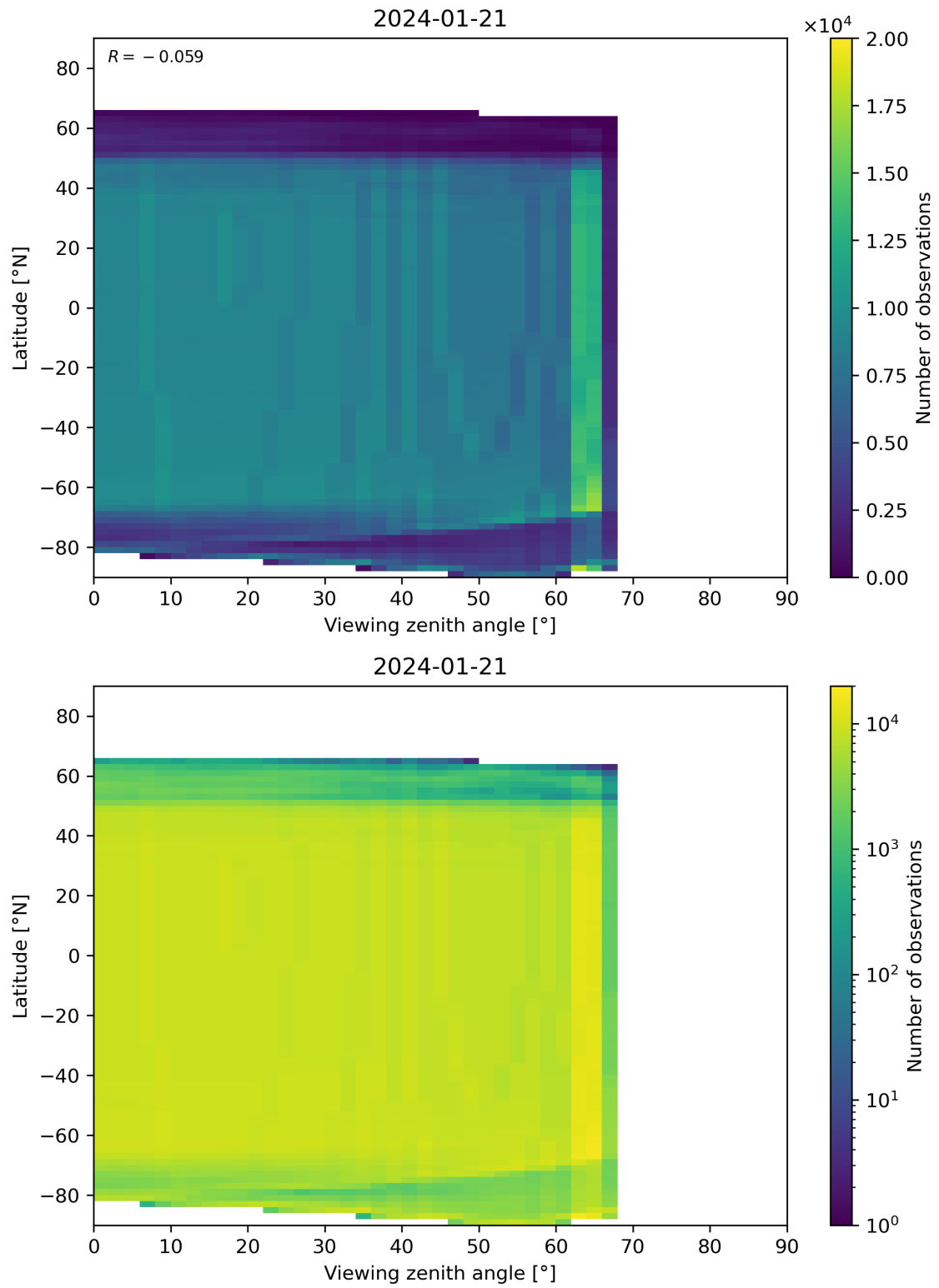
Figure 196: Scatter density plot of “Viewing zenith angle” against “Latitude” for 2024-01-21 to 2024-01-22.
