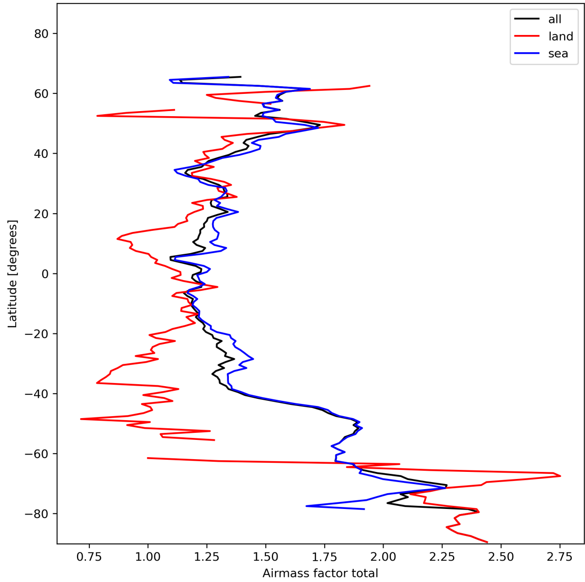
Figure 26: Zonal average of “Airmass factor total” for 2024-01-21 to 2024-01-22.
