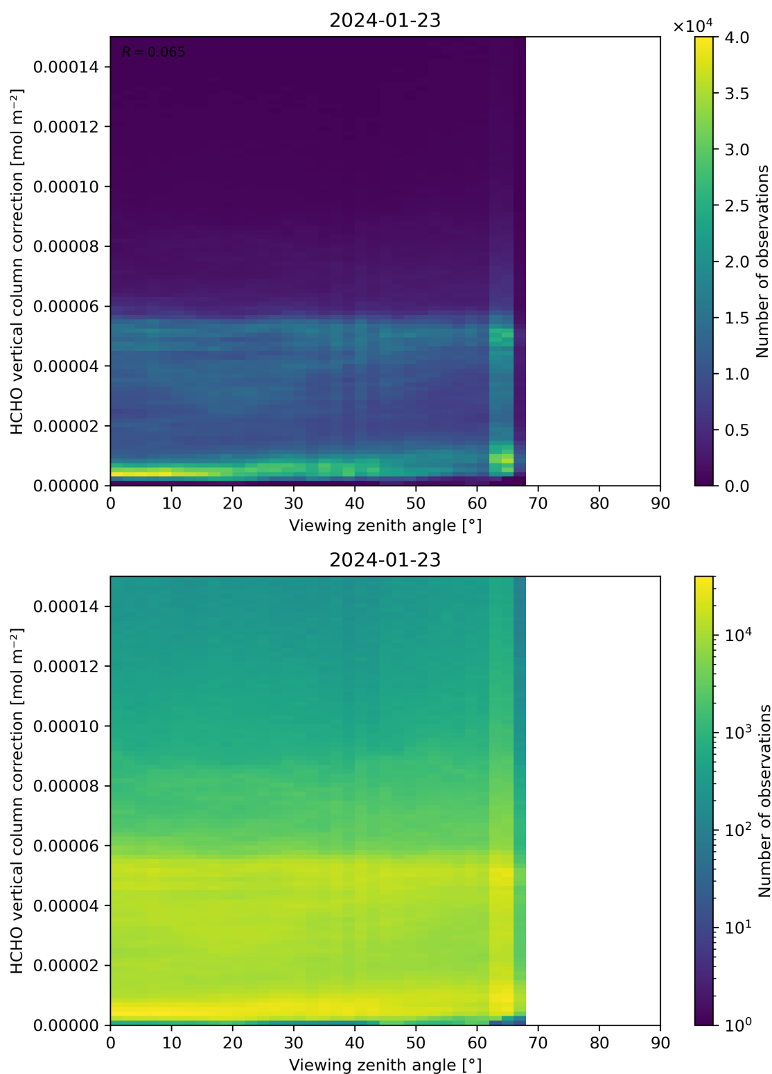
Figure 193: Scatter density plot of “Viewing zenith angle” against “HCHO vertical column correction” for 2024-01-22 to 2024-01-24.
