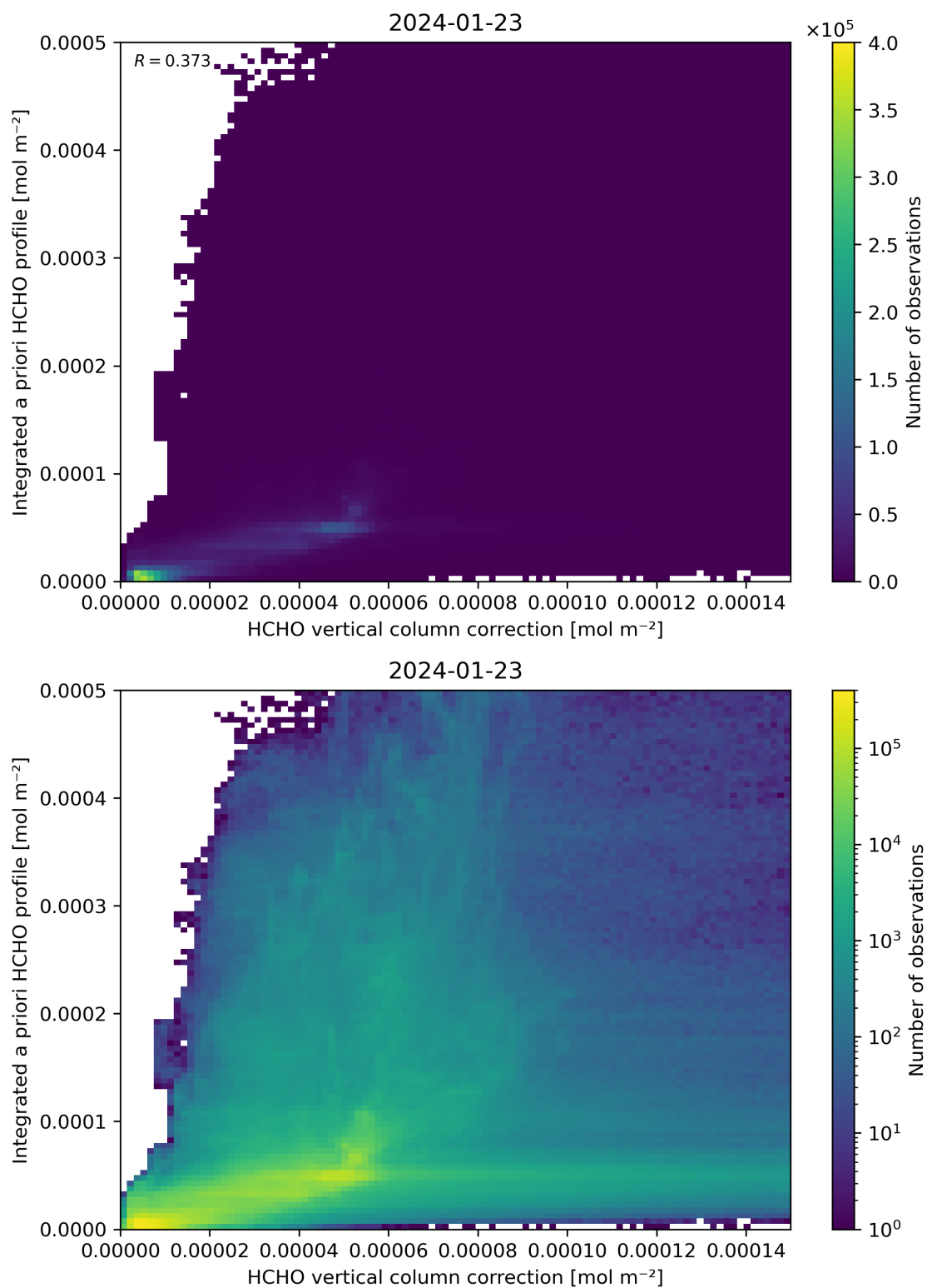
Figure 122: Scatter density plot of “HCHO vertical column correction” against “Integrated a priori HCHO profile” for 2024-01-22 to 2024-01-24.
