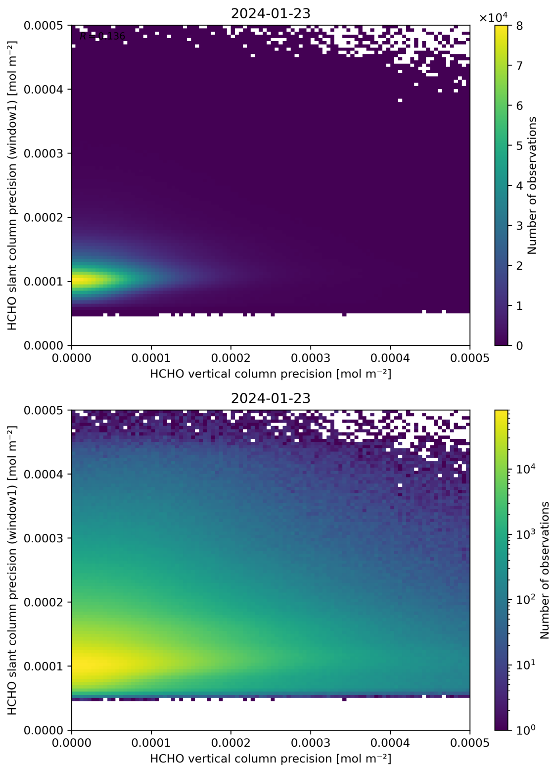
Figure 143: Scatter density plot of “HCHO vertical column precision” against “HCHO slant column precision (window1)” for 2024-01-22 to 2024-01-24.
