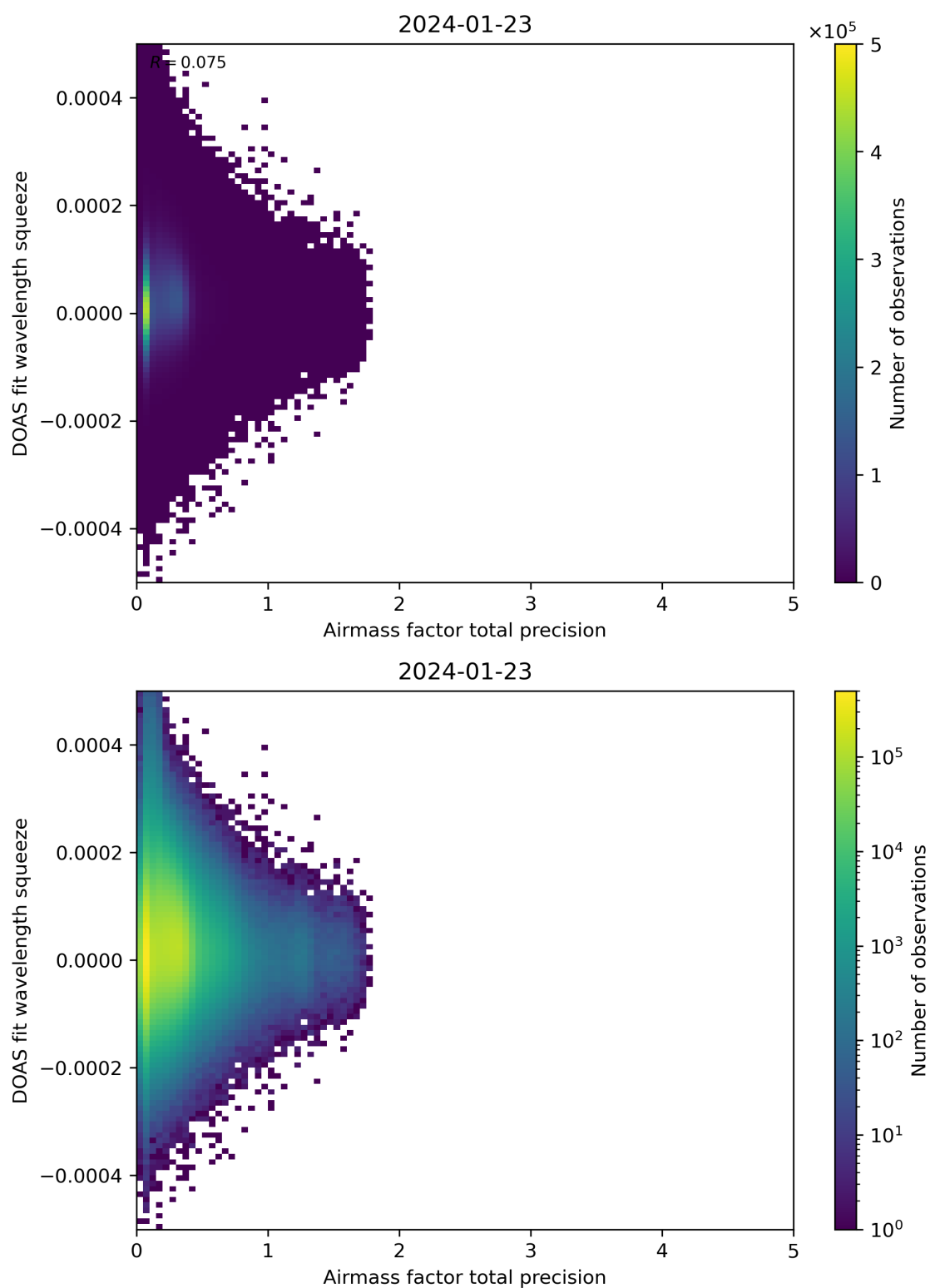
Figure 107: Scatter density plot of “Airmass factor total precision” against “DOAS fit wavelength squeeze” for 2024-01-22 to 2024-01-24.
