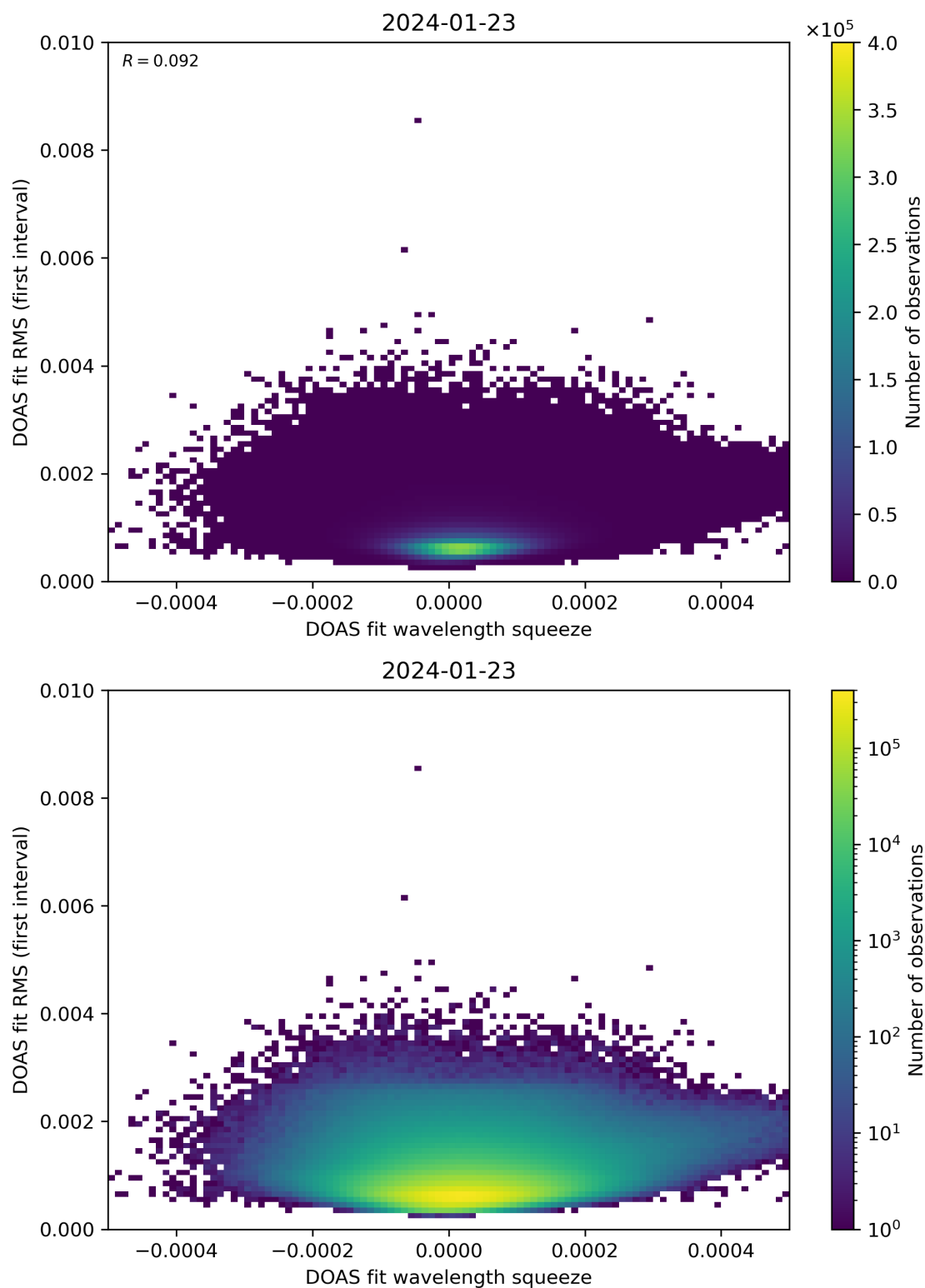
Figure 68: Scatter density plot of “DOAS fit wavelength squeeze” against “DOAS fit RMS (first interval)” for 2024-01-22 to 2024-01-24.
