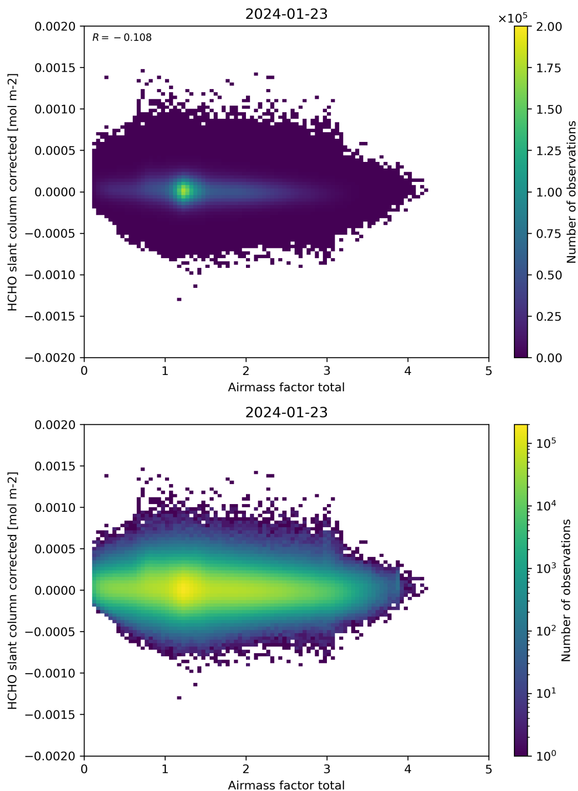
Figure 101: Scatter density plot of “Airmass factor total” against “HCHO slant column corrected” for 2024-01-22 to 2024-01-24.
