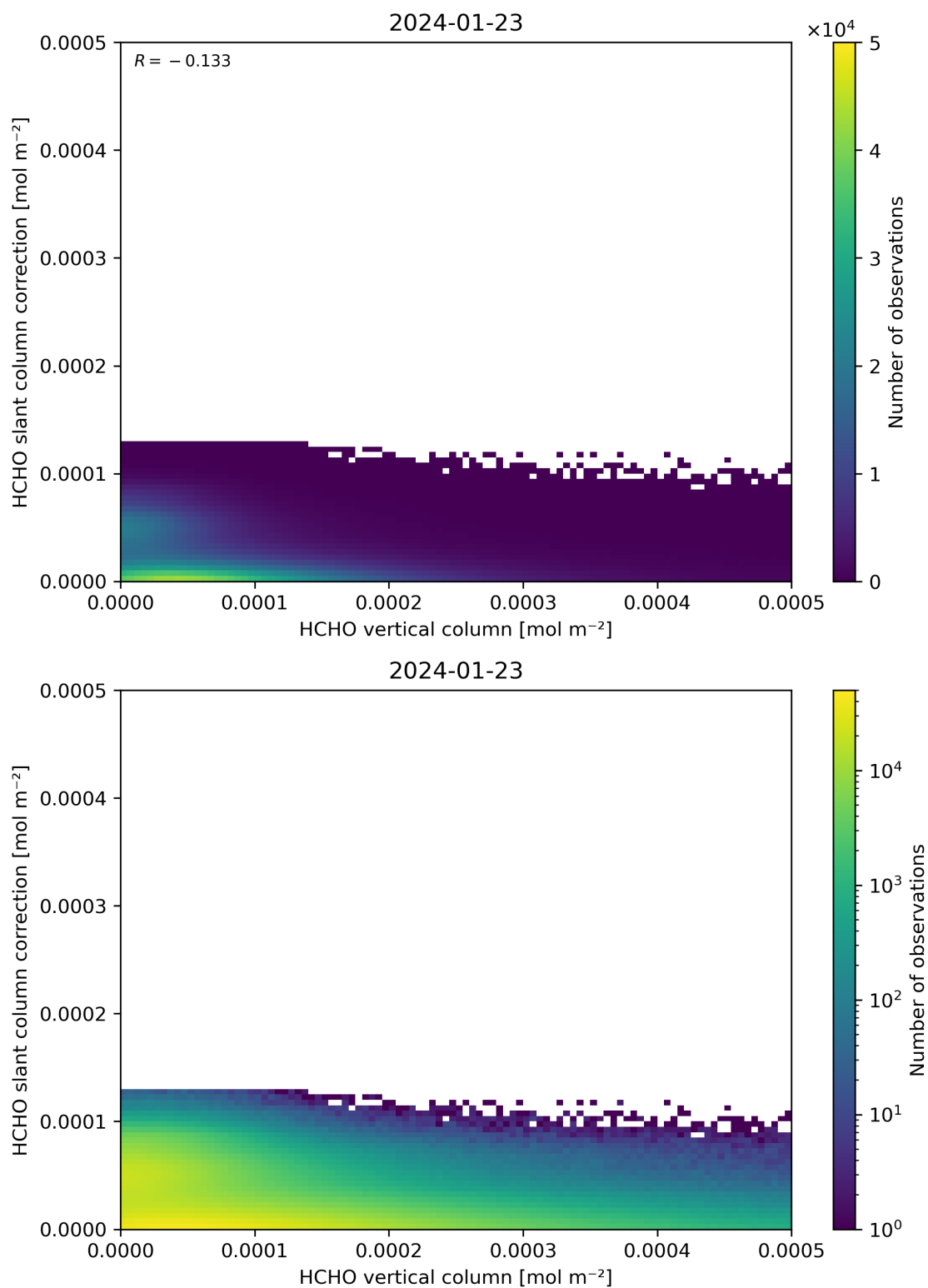
Figure 128: Scatter density plot of “HCHO vertical column” against “HCHO slant column correction” for 2024-01-22 to 2024-01-24.
