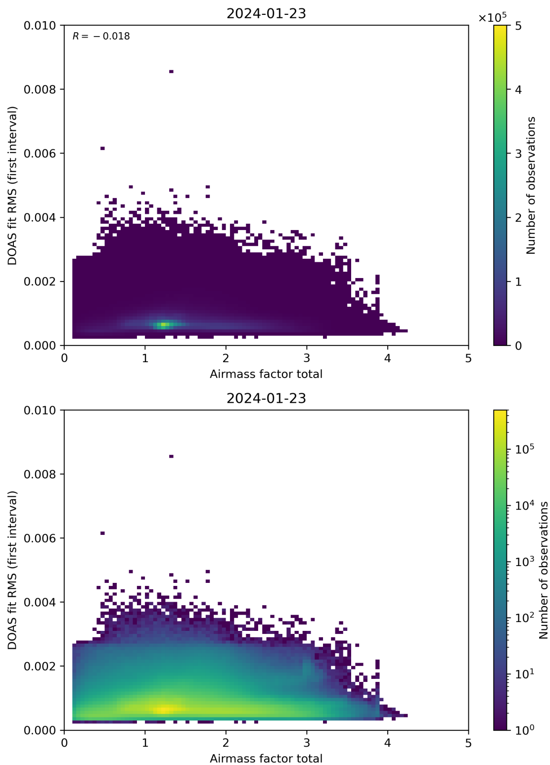
Figure 97: Scatter density plot of “Airmass factor total” against “DOAS fit RMS (first interval)” for 2024-01-22 to 2024-01-24.
