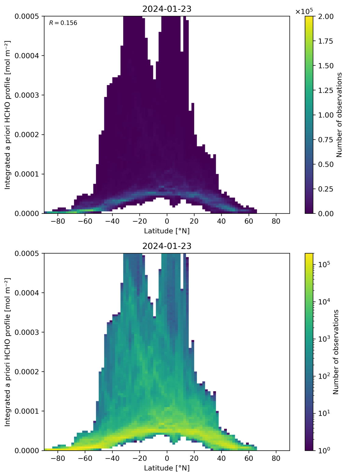
Figure 166: Scatter density plot of “Latitude” against “Integrated a priori HCHO profile” for 2024-01-22 to 2024-01-24.
