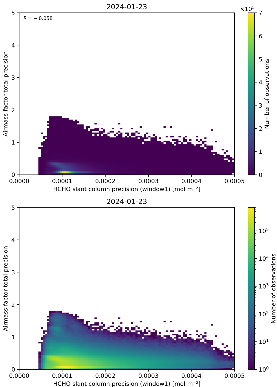
Figure 95: Scatter density plot of “HCHO slant column precision (window1)” against “Airmass factor total precision” for 2024-01-22 to 2024-01-24.
