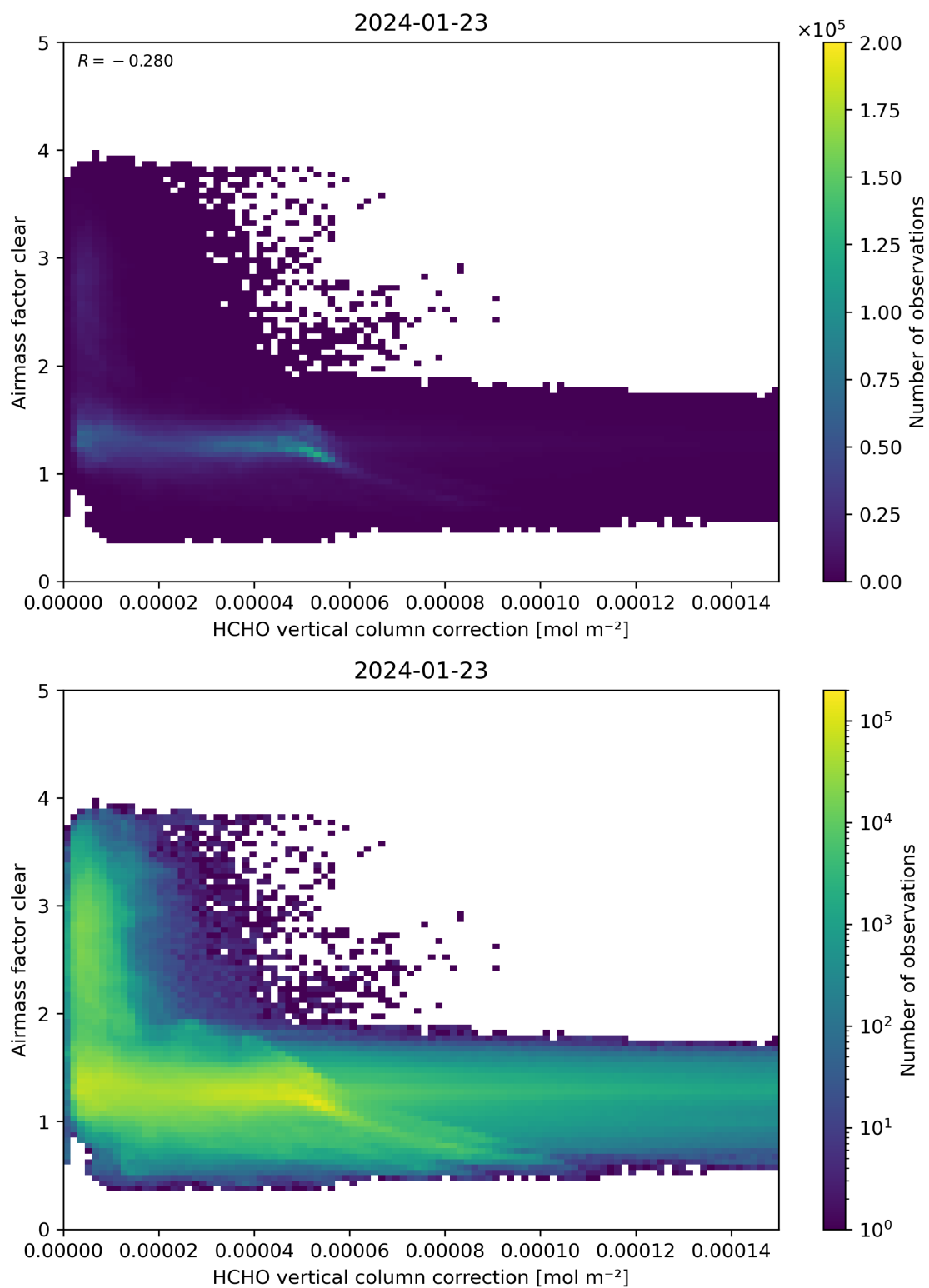
Figure 115: Scatter density plot of “HCHO vertical column correction” against “Airmass factor clear” for 2024-01-22 to 2024-01-24.
