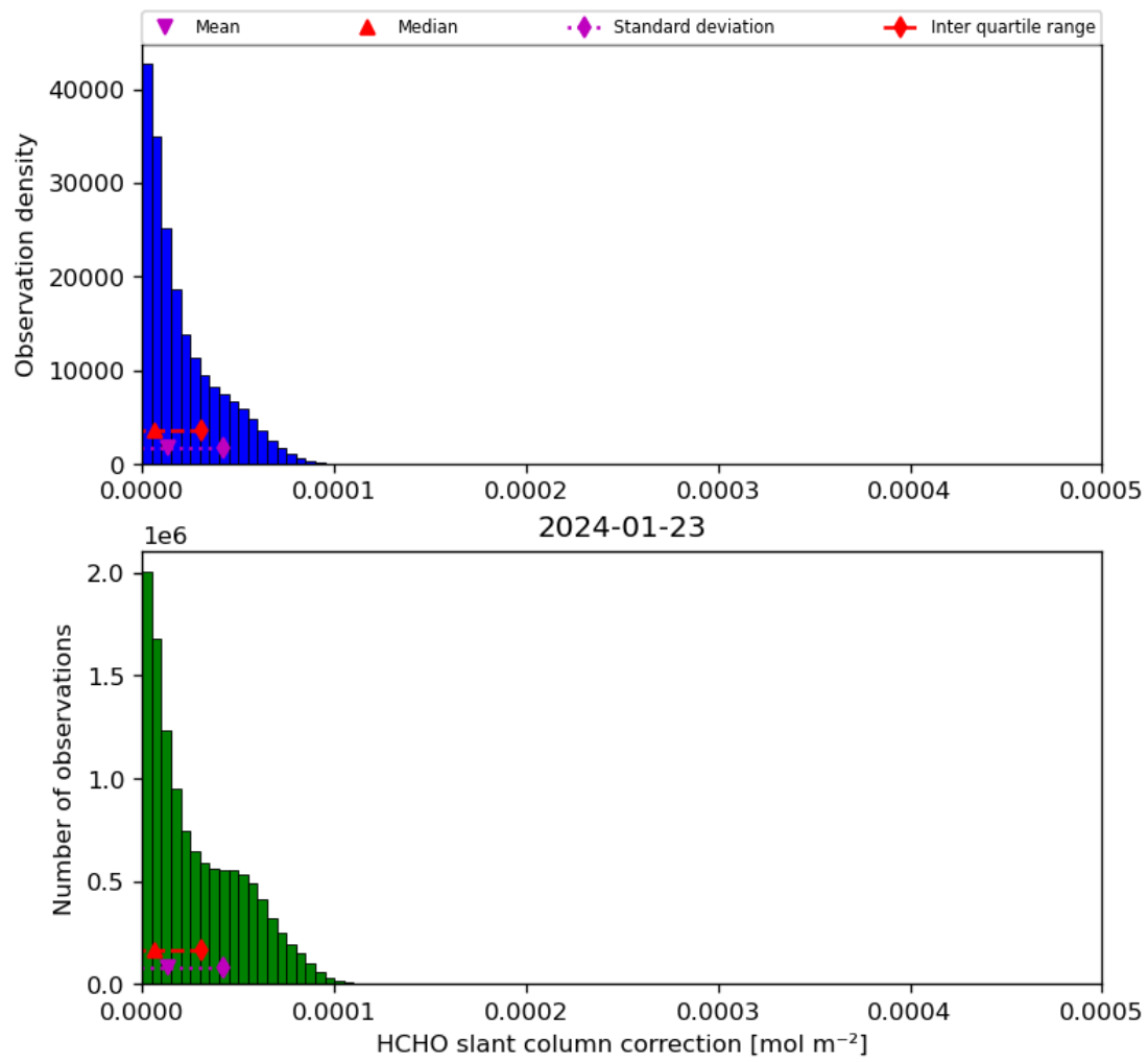
Figure 47: Histogram of “HCHO slant column correction” for 2024-01-22 to 2024-01-24
