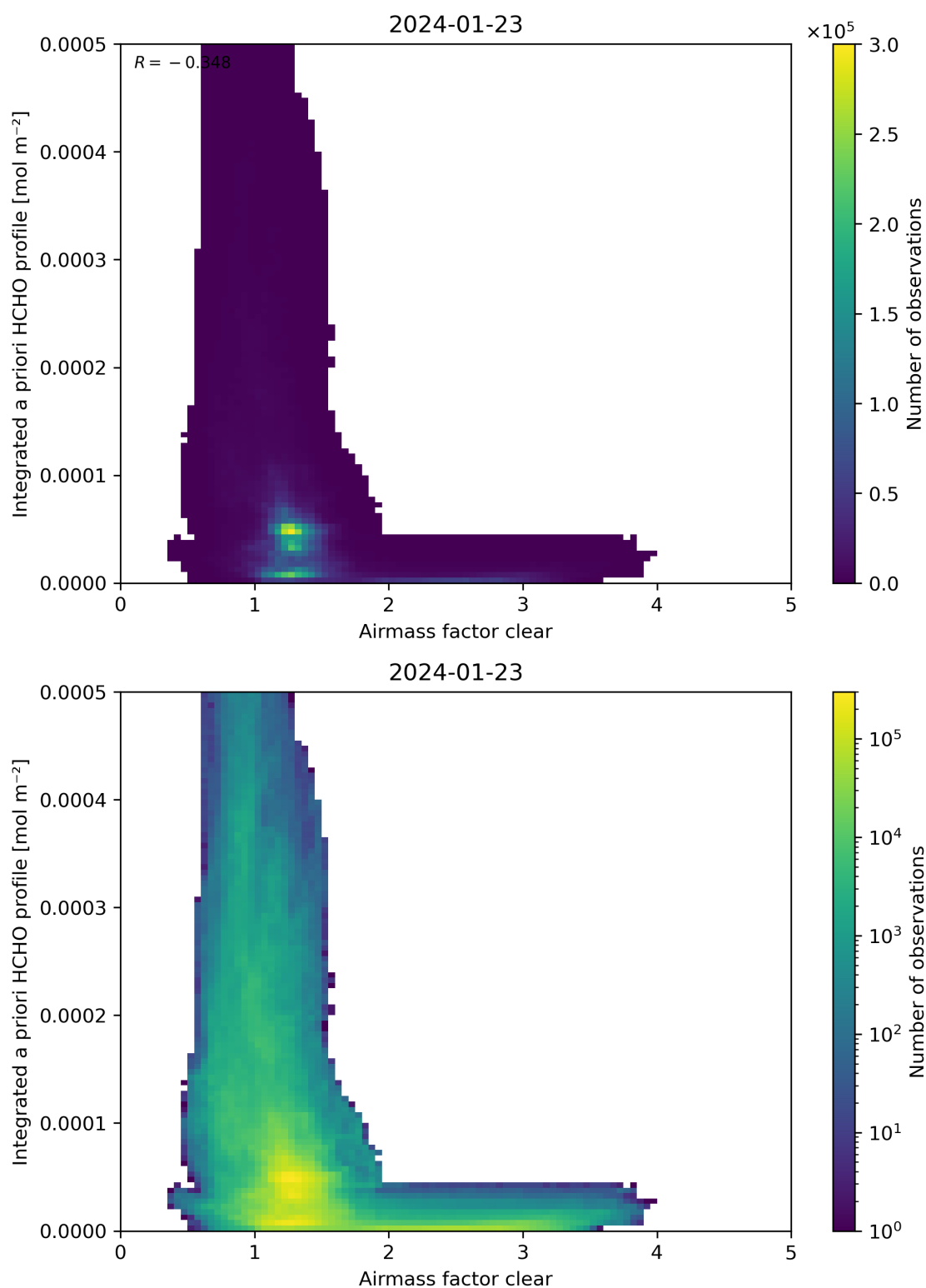
Figure 76: Scatter density plot of “Airmass factor clear” against “Integrated a priori HCHO profile” for 2024-01-22 to 2024-01-24.
