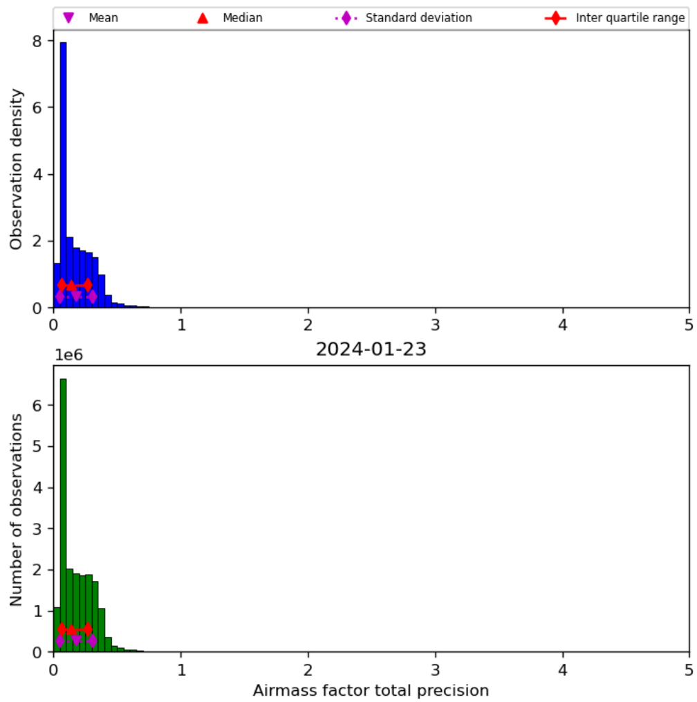
Figure 41: Histogram of “Airmass factor total precision” for 2024-01-22 to 2024-01-24
