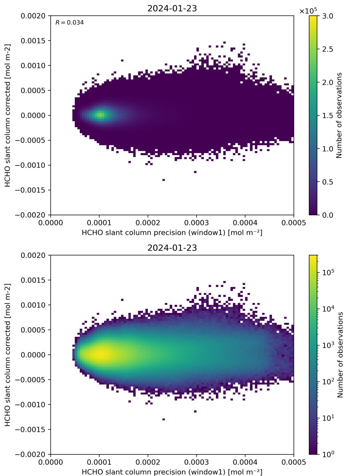
Figure 92: Scatter density plot of “HCHO slant column precision (window1)” against “HCHO slant column corrected” for 2024-01-22 to 2024-01-24.
