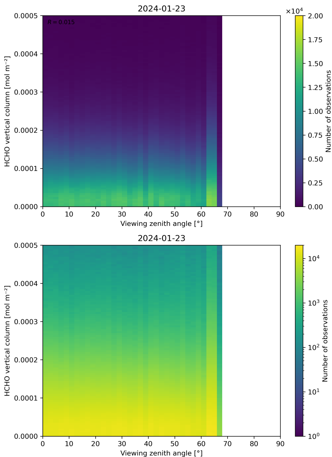
Figure 192: Scatter density plot of “Viewing zenith angle” against “HCHO vertical column” for 2024-01-22 to 2024-01-24.
