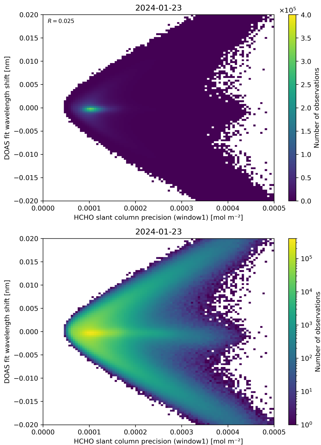
Figure 89: Scatter density plot of “HCHO slant column precision (window1)” against “DOAS fit wavelength shift” for 2024-01-22 to 2024-01-24.
