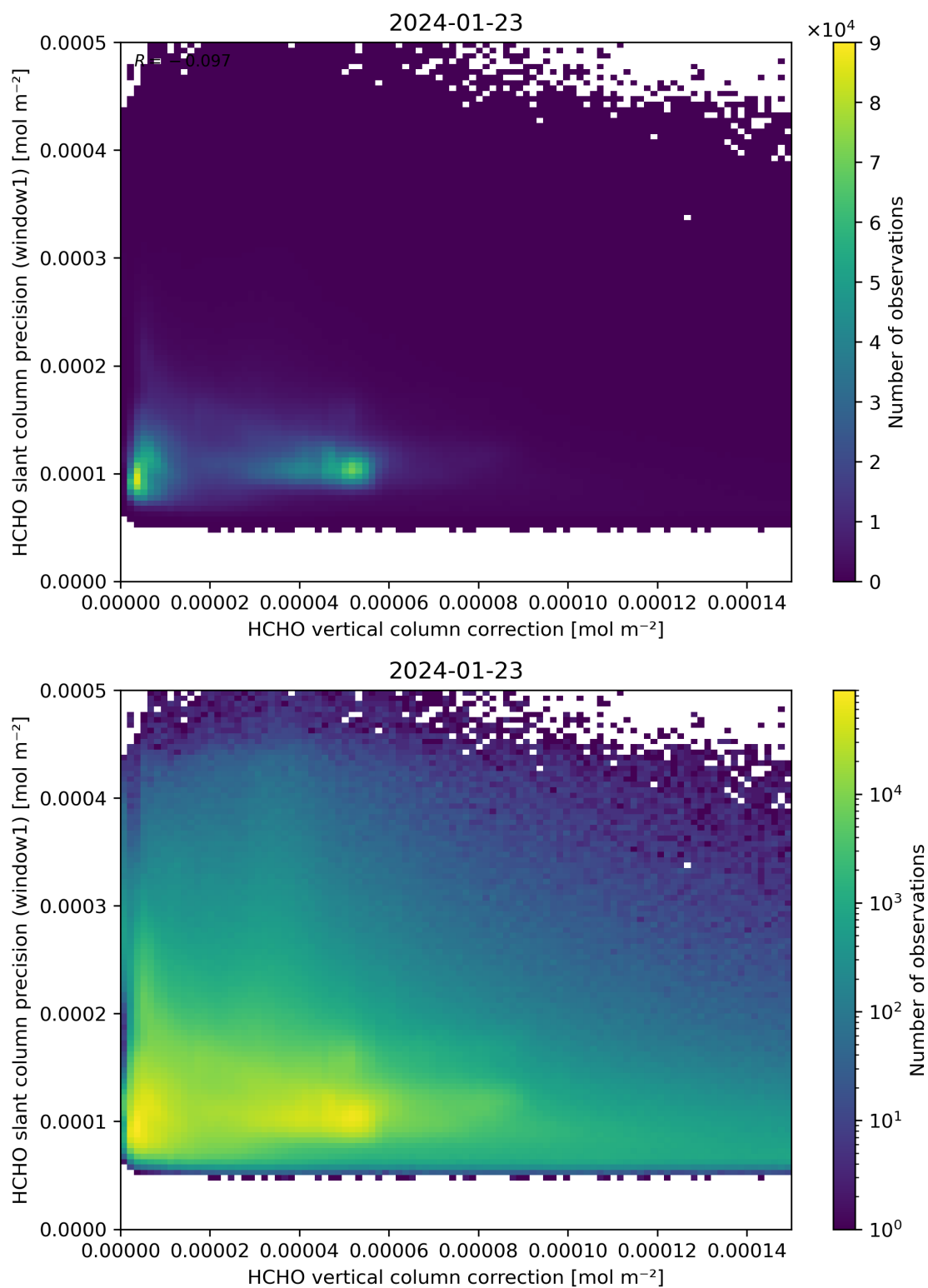
Figure 119: Scatter density plot of “HCHO vertical column correction” against “HCHO slant column precision (window1)” for 2024-01-22 to 2024-01-24.
