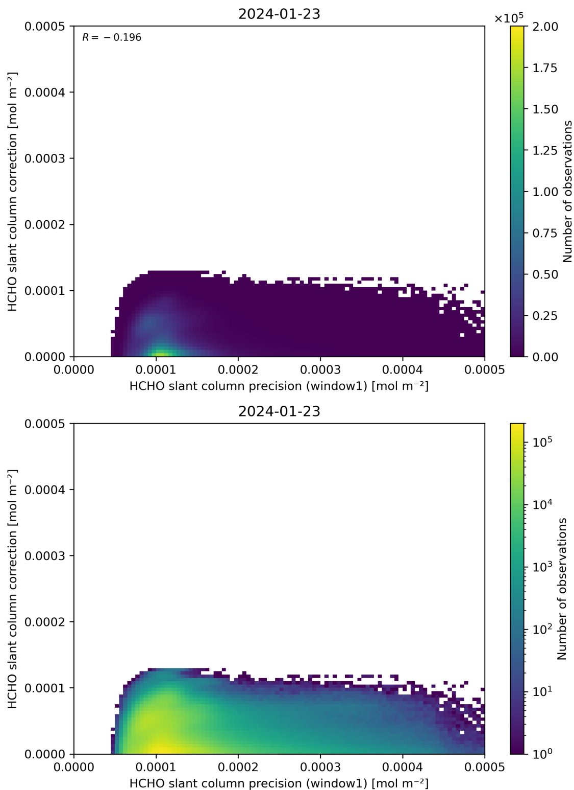
Figure 93: Scatter density plot of “HCHO slant column precision (window1)” against “HCHO slant column correction” for 2024-01-22 to 2024-01-24.
