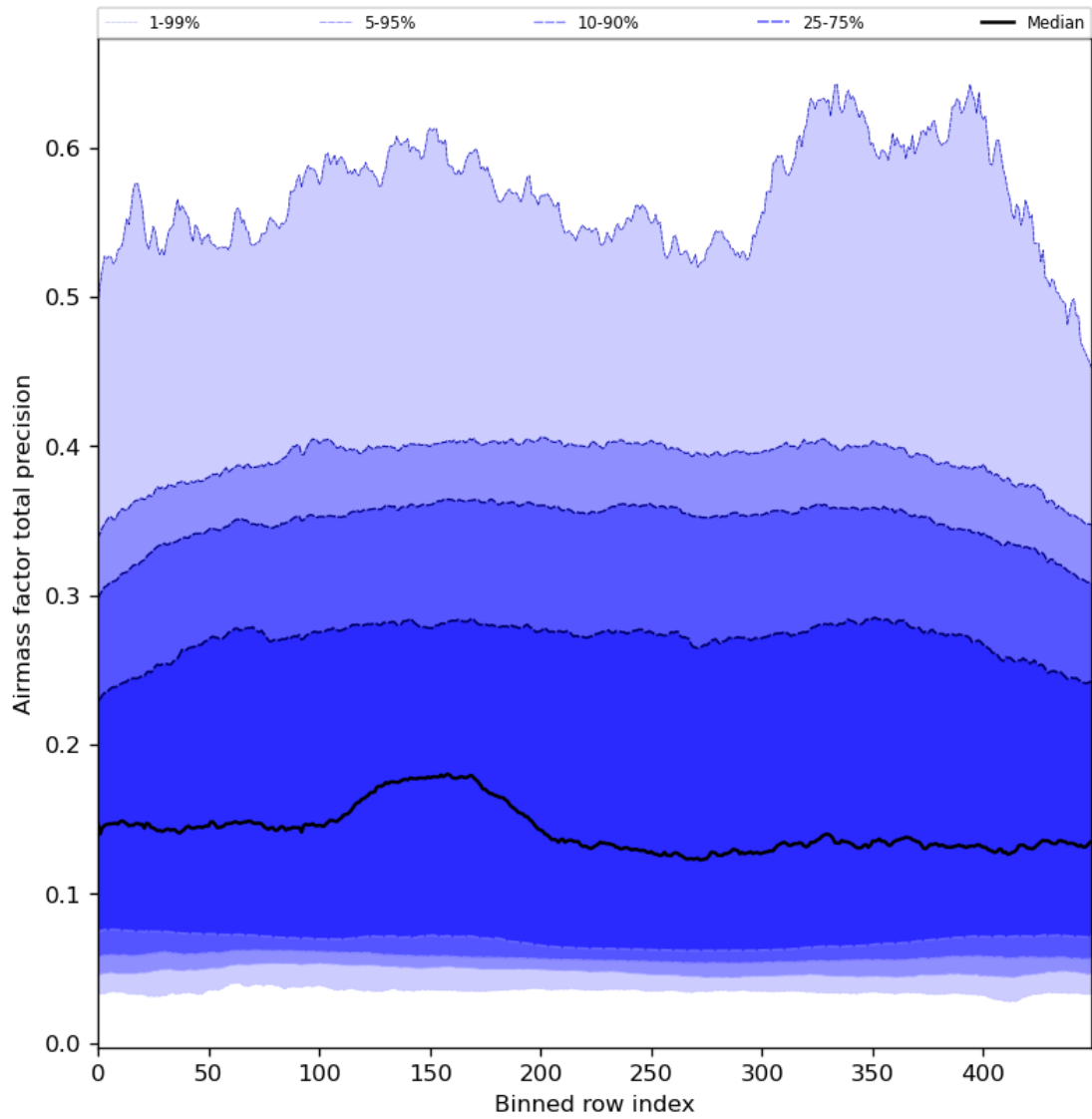
Figure 55: Along track statistics of “Airmass factor total precision” for 2024-01-22 to 2024-01-24
