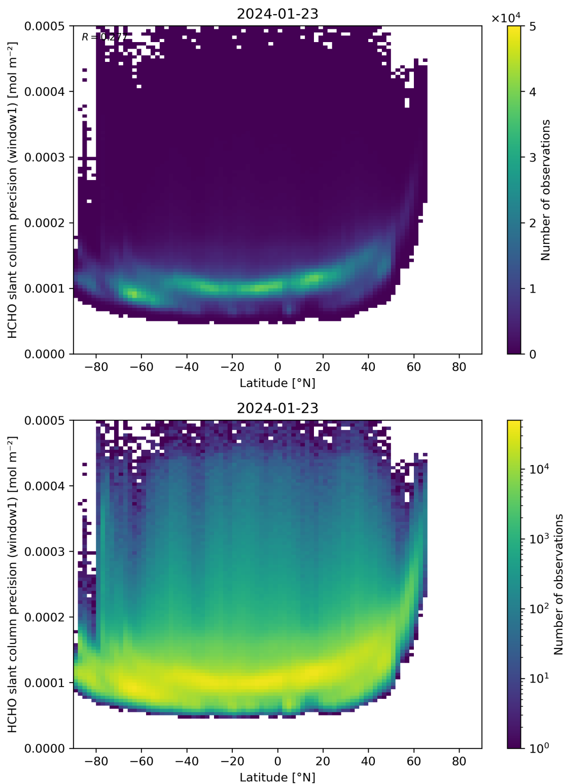
Figure 160: Scatter density plot of “Latitude” against “HCHO slant column precision (window1)” for 2024-01-22 to 2024-01-24.
