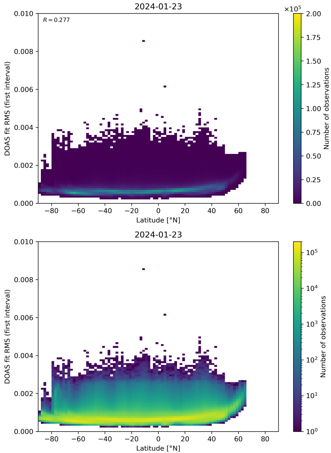
Figure 153: Scatter density plot of “Latitude” against “DOAS fit RMS (first interval)” for 2024-01-22 to 2024-01-24.
