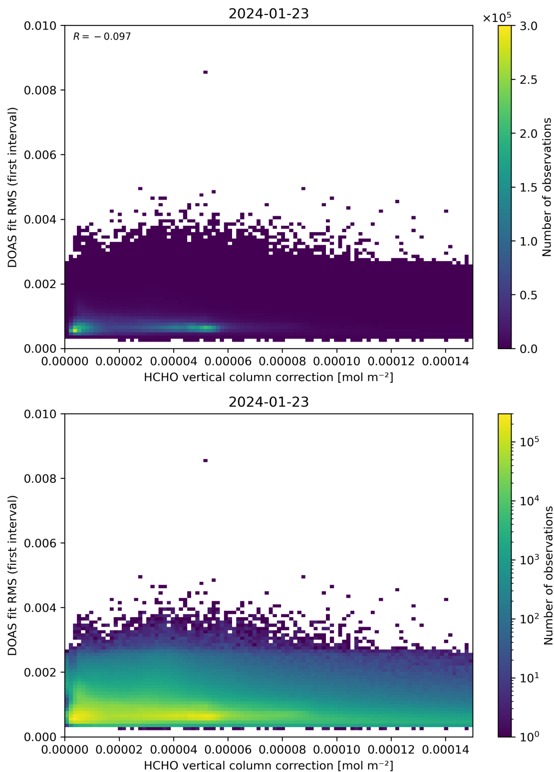
Figure 112: Scatter density plot of “HCHO vertical column correction” against “DOAS fit RMS (first interval)” for 2024-01-22 to 2024-01-24.
