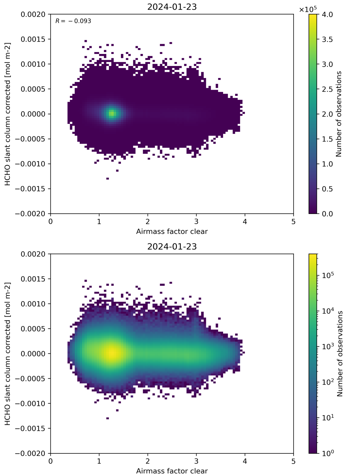
Figure 74: Scatter density plot of “Airmass factor clear” against “HCHO slant column corrected” for 2024-01-22 to 2024-01-24.
