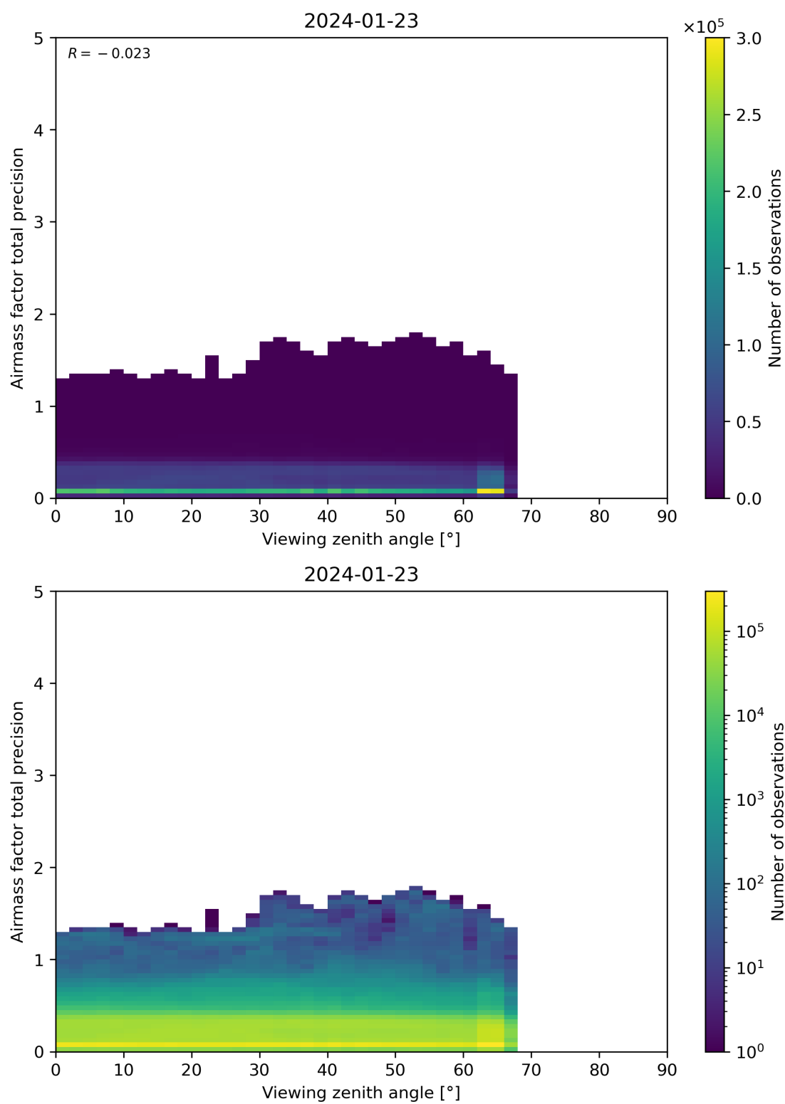
Figure 191: Scatter density plot of “Viewing zenith angle” against “Airmass factor total precision” for 2024-01-22 to 2024-01-24.
