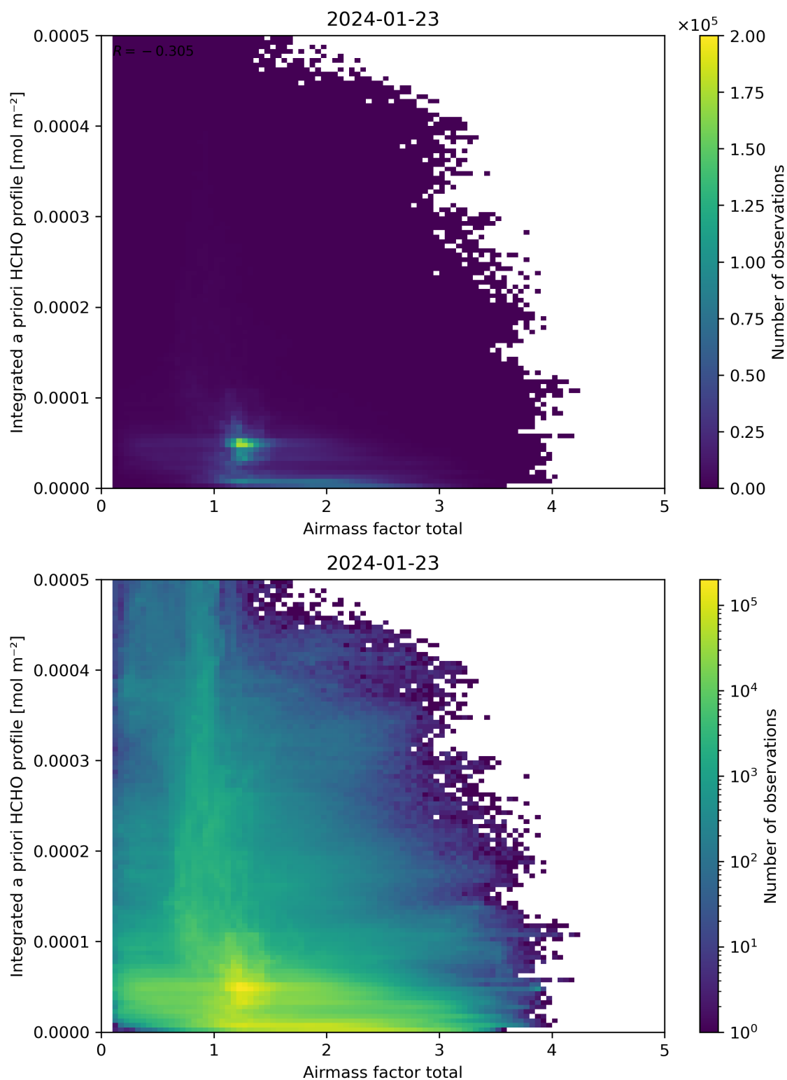
Figure 104: Scatter density plot of “Airmass factor total” against “Integrated a priori HCHO profile” for 2024-01-22 to 2024-01-24.
