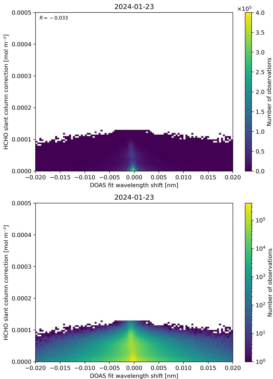
Figure 67: Scatter density plot of “DOAS fit wavelength shift” against “HCHO slant column correction” for 2024-01-22 to 2024-01-24.
