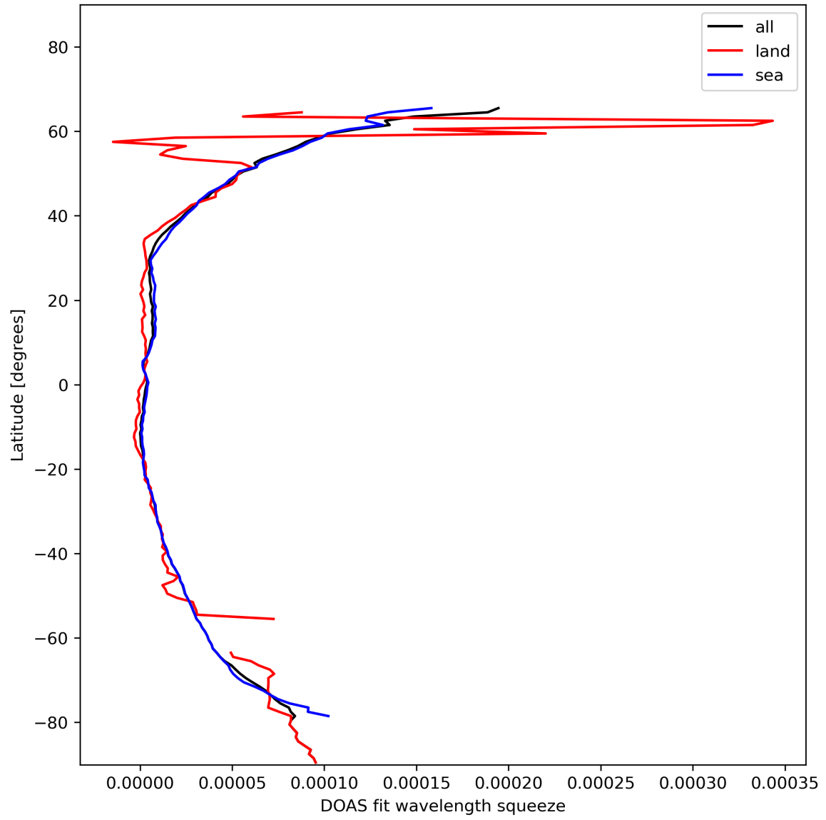
Figure 31: Zonal average of “DOAS fit wavelength squeeze” for 2024-01-22 to 2024-01-24.
