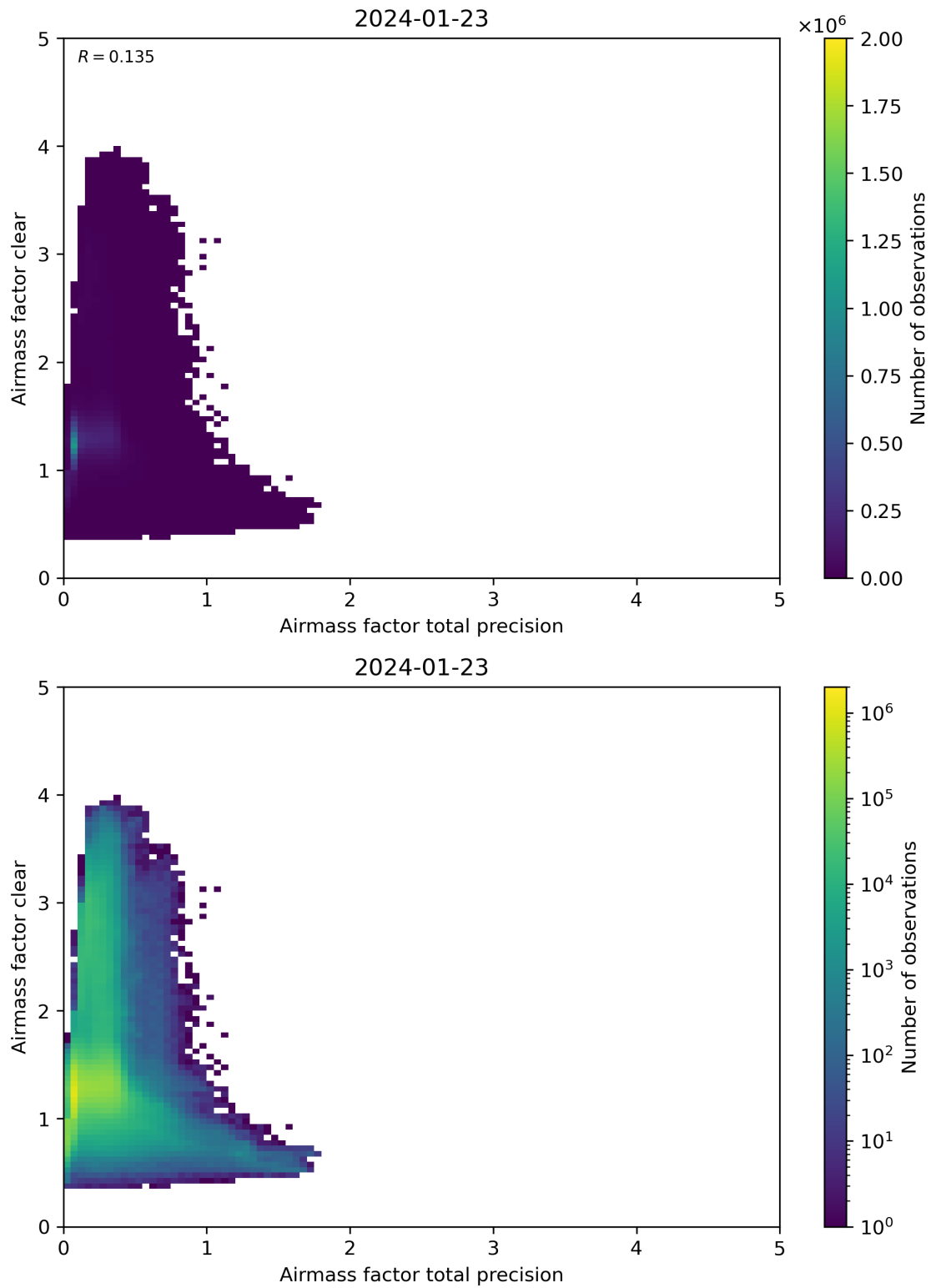
Figure 108: Scatter density plot of “Airmass factor total precision” against “Airmass factor clear” for 2024-01-22 to 2024-01-24.
