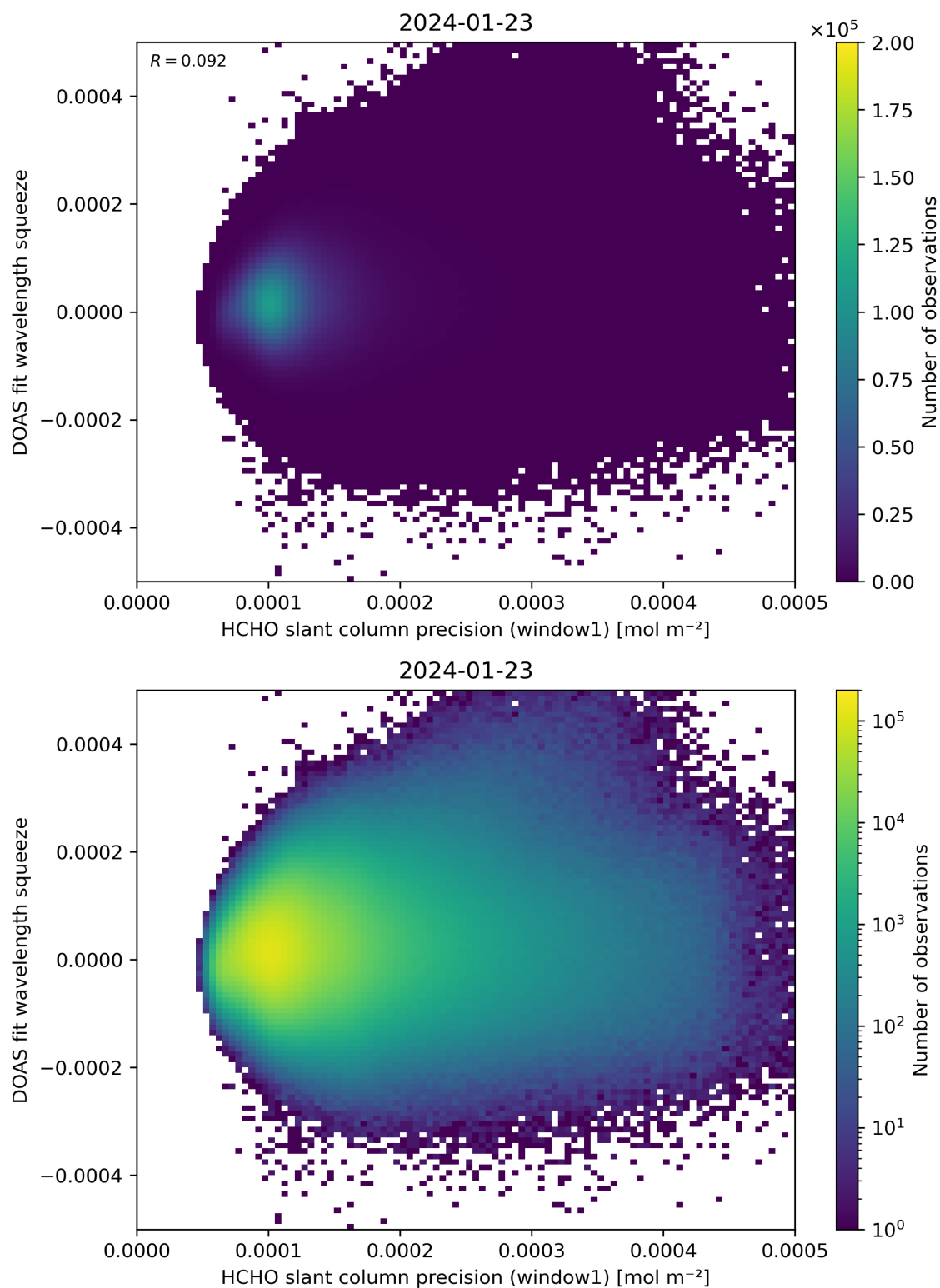
Figure 90: Scatter density plot of “HCHO slant column precision (window1)” against “DOAS fit wavelength squeeze” for 2024-01-22 to 2024-01-24.
