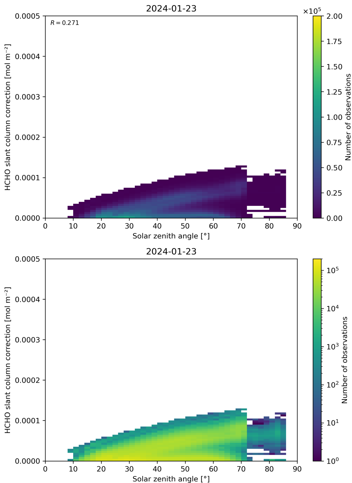
Figure 172: Scatter density plot of “Solar zenith angle” against “HCHO slant column correction” for 2024-01-22 to 2024-01-24.
