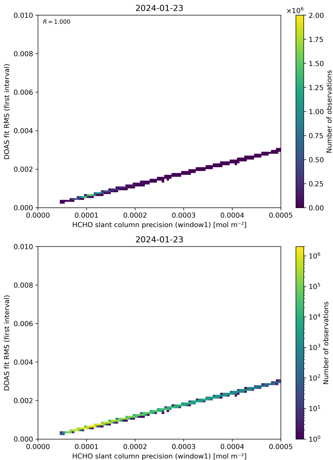
Figure 88: Scatter density plot of “HCHO slant column precision (window1)” against “DOAS fit RMS (first interval)” for 2024-01-22 to 2024-01-24.
