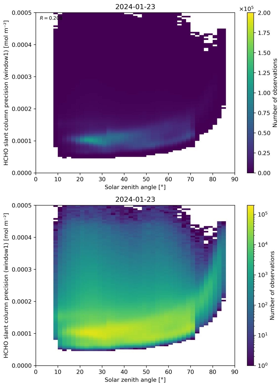
Figure 174: Scatter density plot of “Solar zenith angle” against “HCHO slant column precision (window1)” for 2024-01-22 to 2024-01-24.
