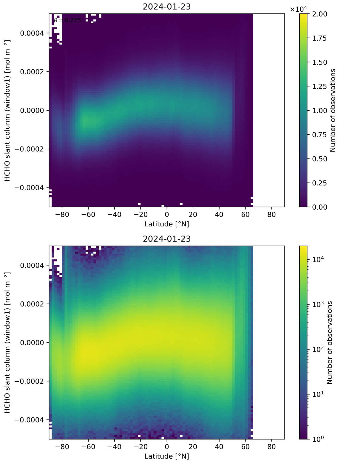
Figure 159: Scatter density plot of “Latitude” against “HCHO slant column (window1)” for 2024-01-22 to 2024-01-24.
