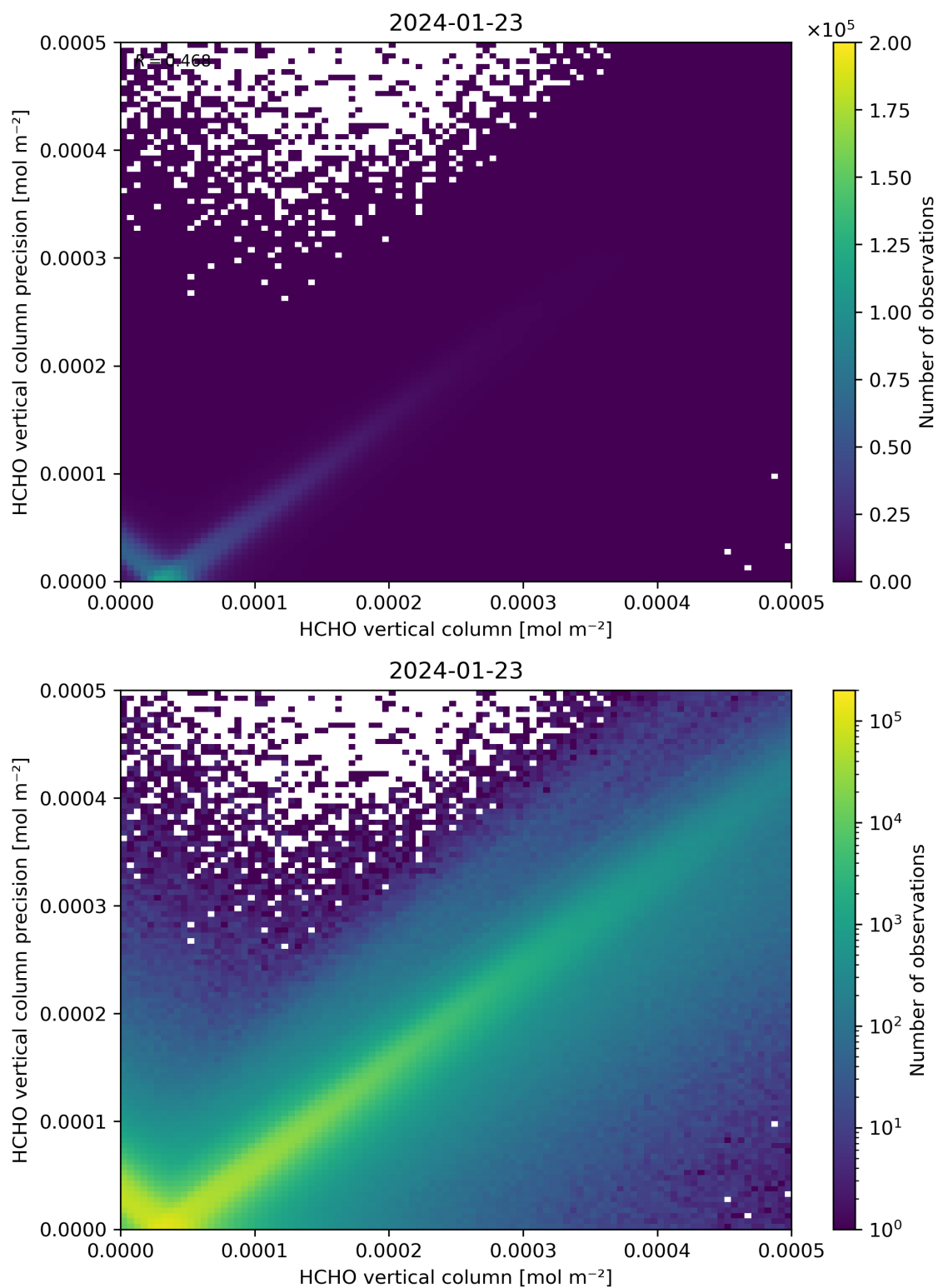
Figure 134: Scatter density plot of “HCHO vertical column” against “HCHO vertical column precision” for 2024-01-22 to 2024-01-24.
