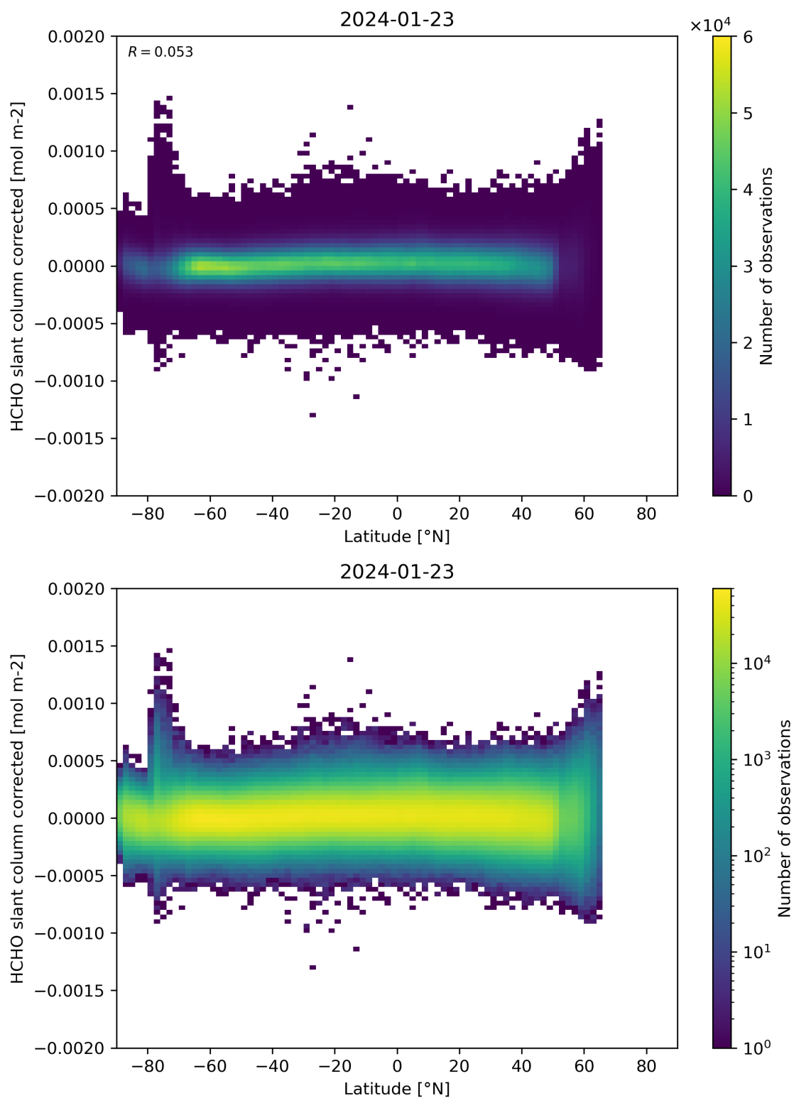
Figure 157: Scatter density plot of “Latitude” against “HCHO slant column corrected” for 2024-01-22 to 2024-01-24.
