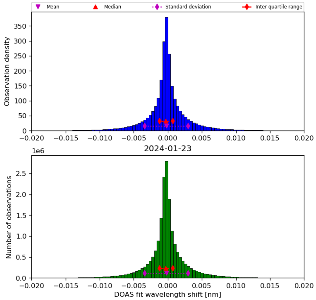
Figure 44: Histogram of “DOAS fit wavelength shift” for 2024-01-22 to 2024-01-24
