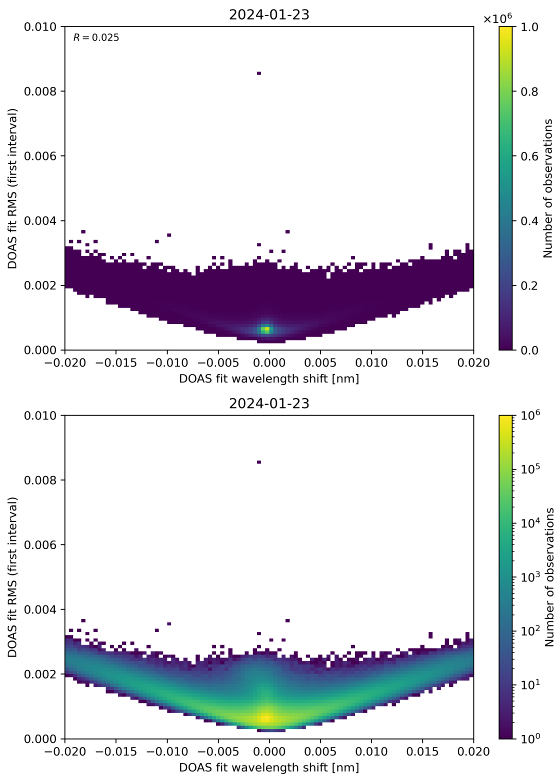
Figure 64: Scatter density plot of “DOAS fit wavelength shift” against “DOAS fit RMS (first interval)” for 2024-01-22 to 2024-01-24.
