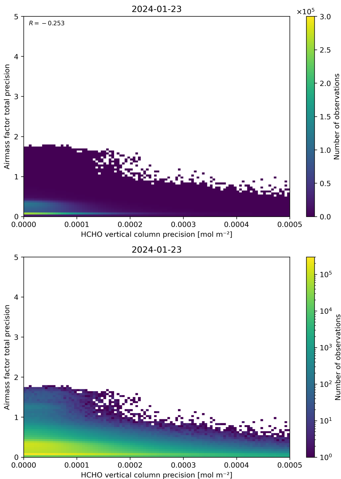
Figure 145: Scatter density plot of “HCHO vertical column precision” against “Airmass factor total precision” for 2024-01-22 to 2024-01-24.
