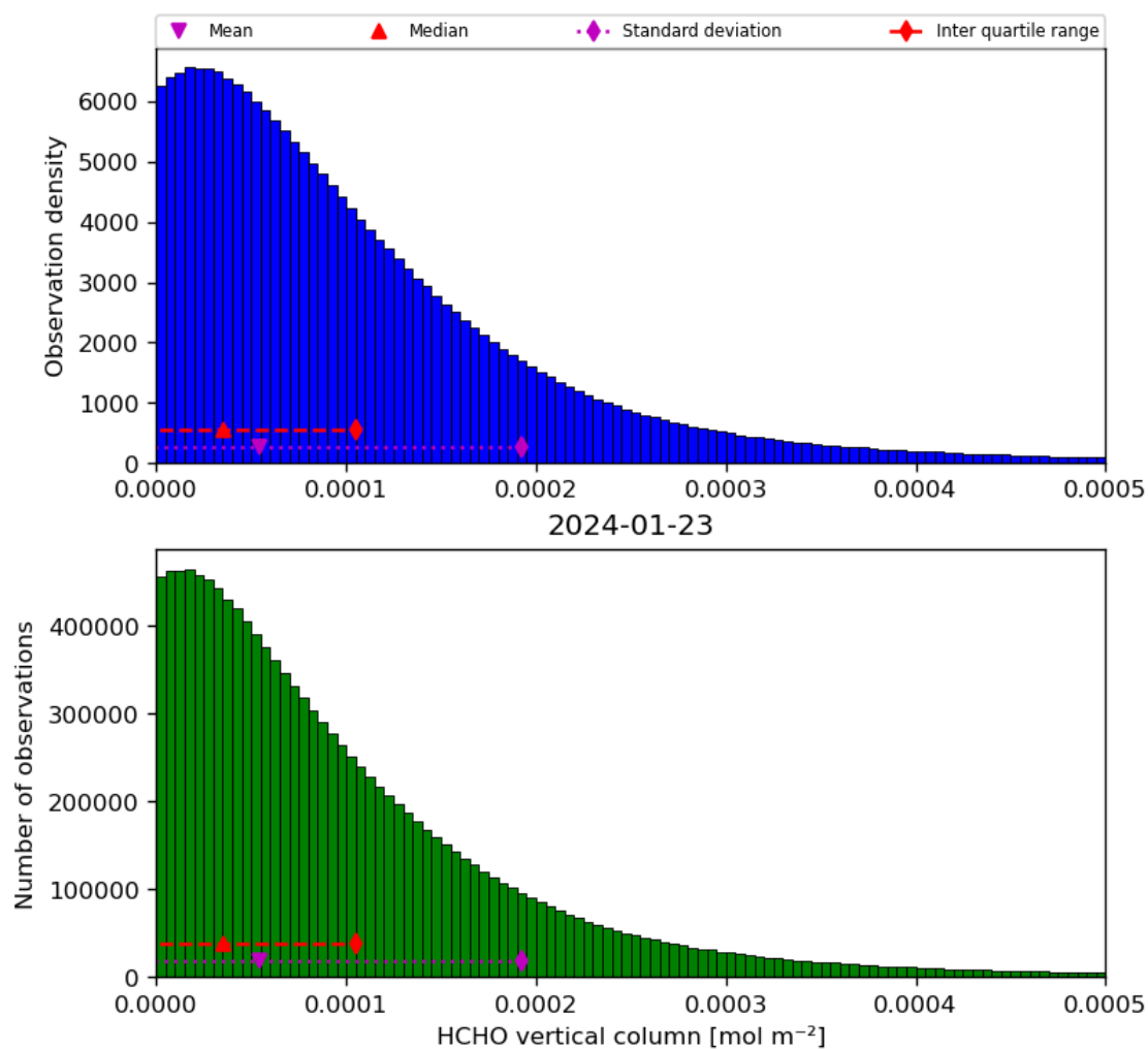
Figure 35: Histogram of “HCHO vertical column” for 2024-01-22 to 2024-01-24
