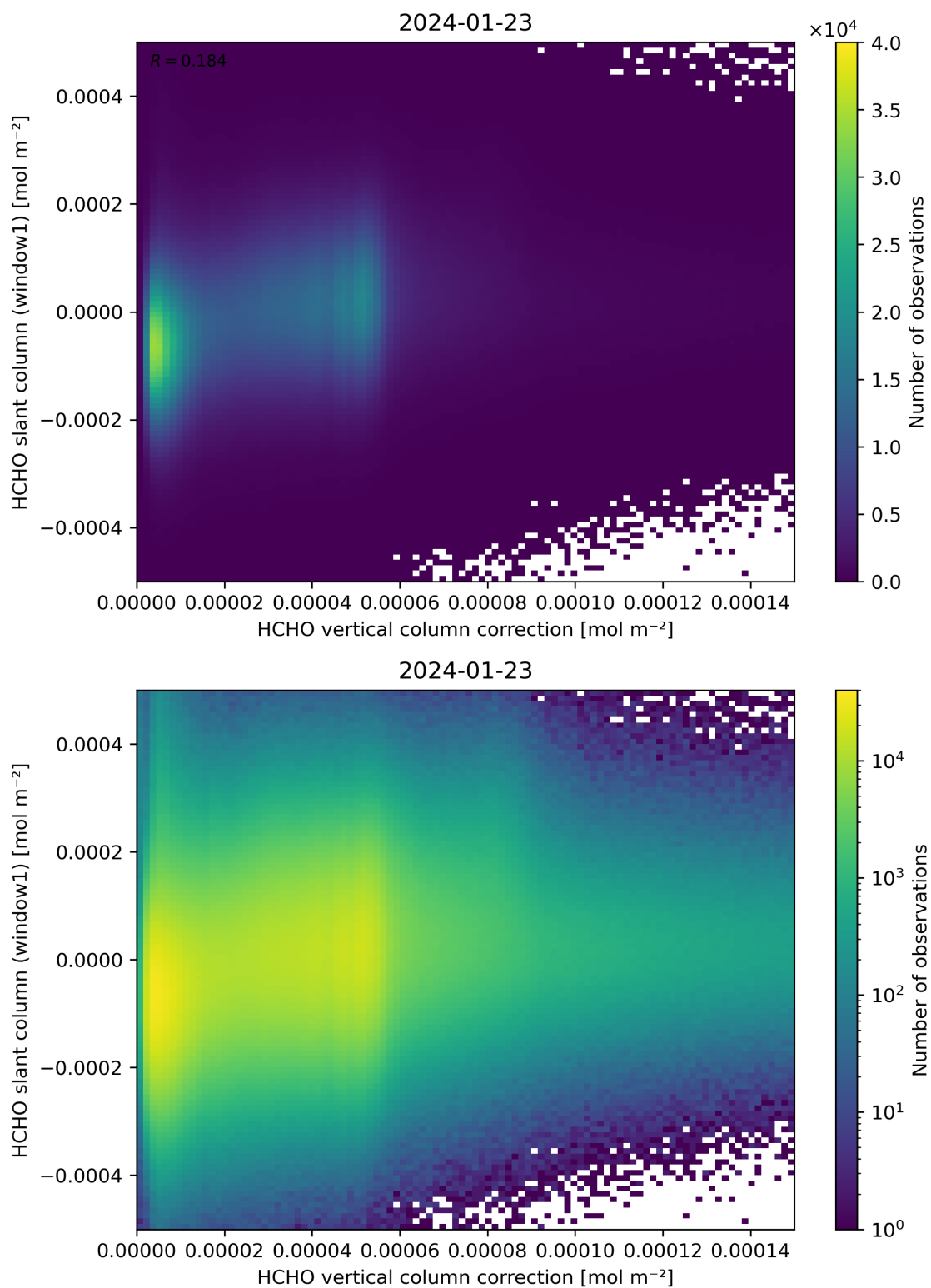
Figure 118: Scatter density plot of “HCHO vertical column correction” against “HCHO slant column (window1)” for 2024-01-22 to 2024-01-24.
