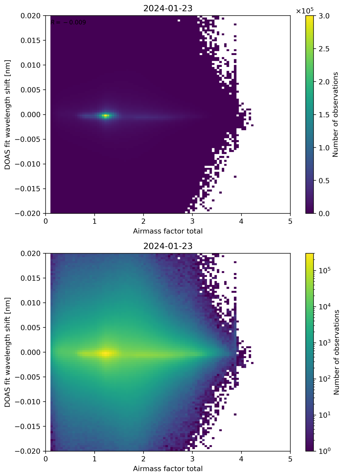
Figure 98: Scatter density plot of “Airmass factor total” against “DOAS fit wavelength shift” for 2024-01-22 to 2024-01-24.
