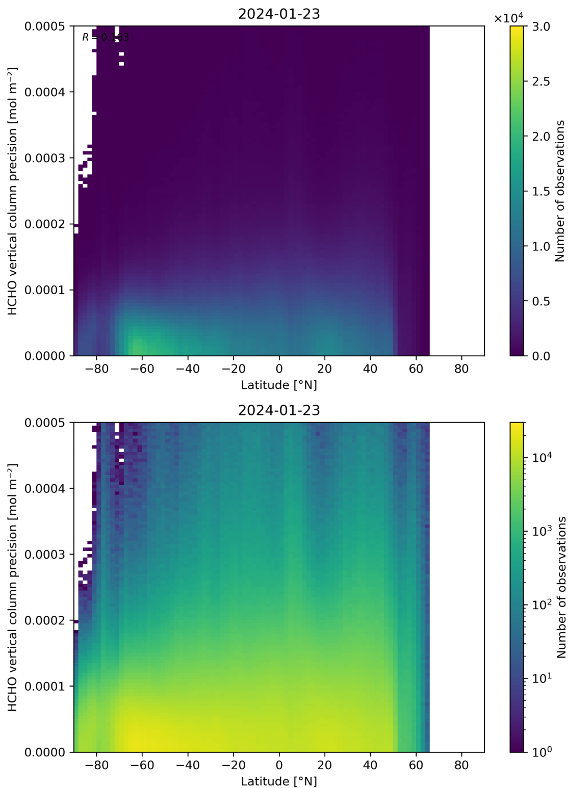
Figure 165: Scatter density plot of “Latitude” against “HCHO vertical column precision” for 2024-01-22 to 2024-01-24.
