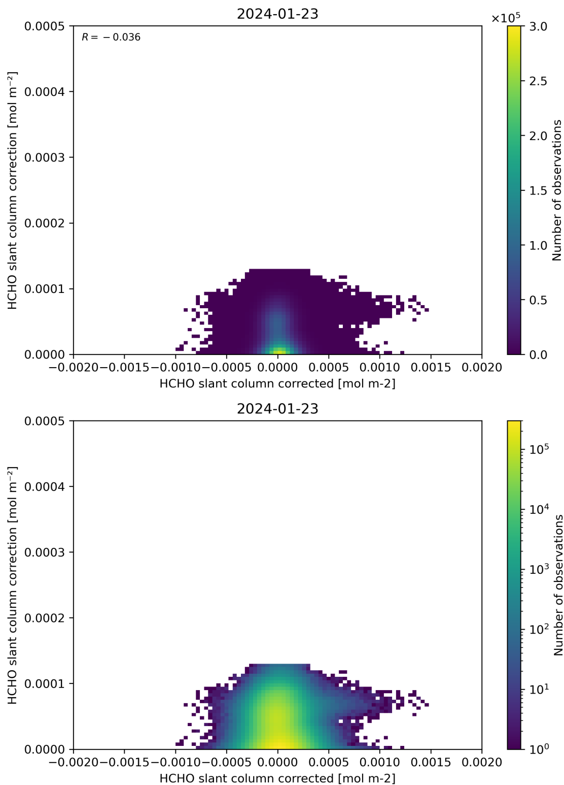
Figure 77: Scatter density plot of “HCHO slant column corrected” against “HCHO slant column correction” for 2024-01-22 to 2024-01-24.
