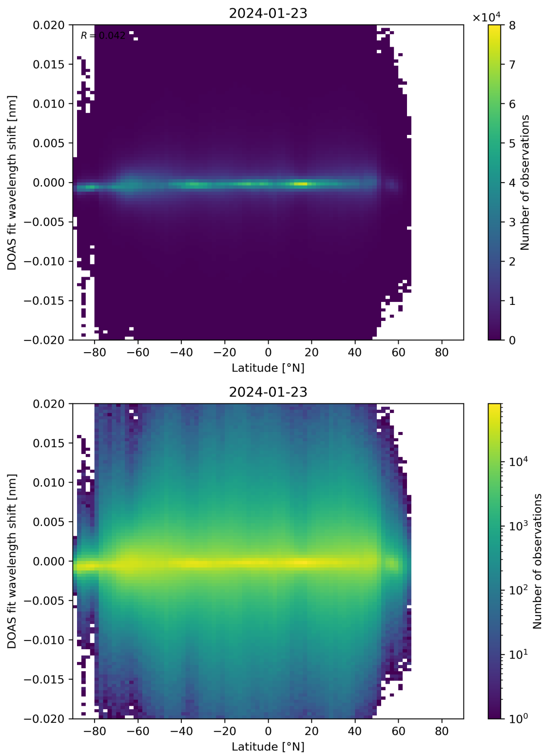
Figure 154: Scatter density plot of “Latitude” against “DOAS fit wavelength shift” for 2024-01-22 to 2024-01-24.
