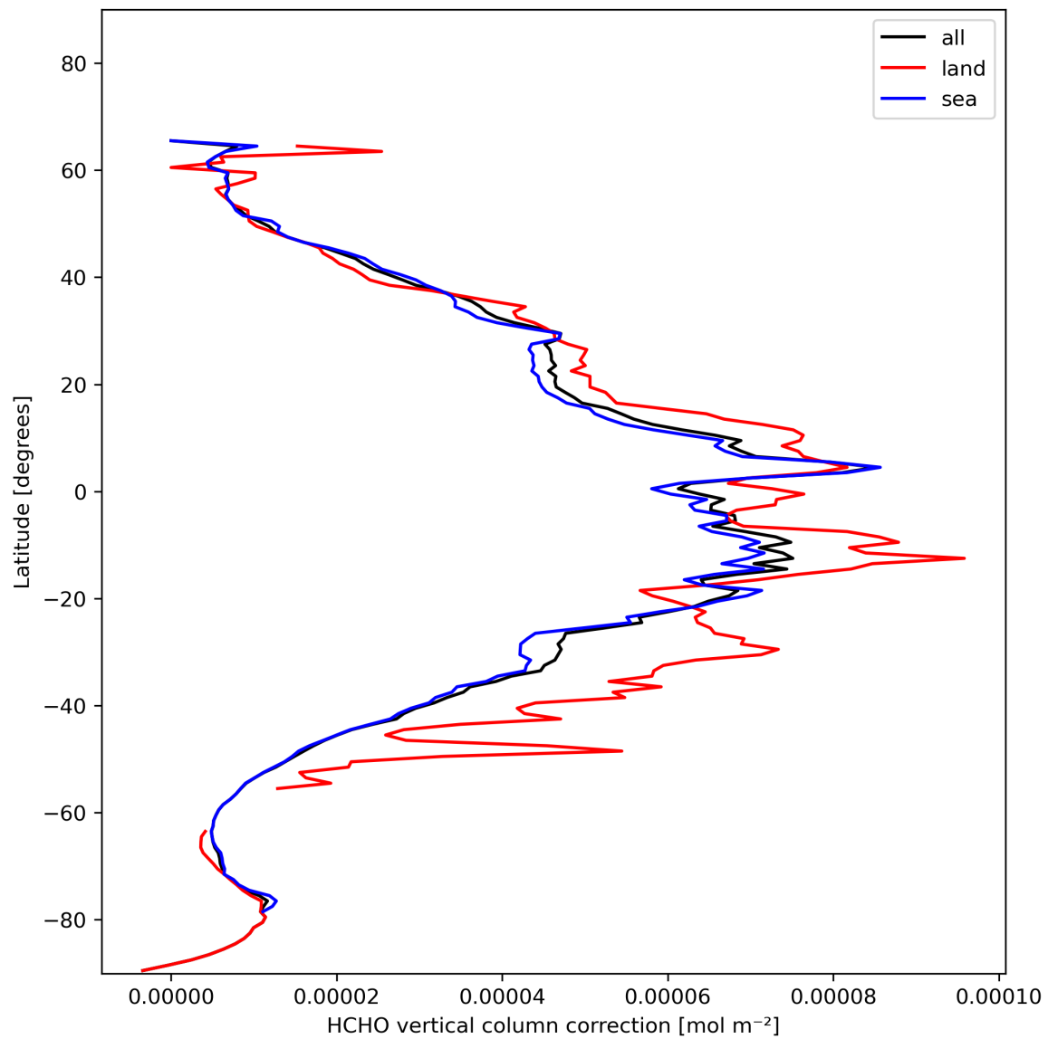
Figure 23: Zonal average of “HCHO vertical column correction” for 2024-01-22 to 2024-01-24.
