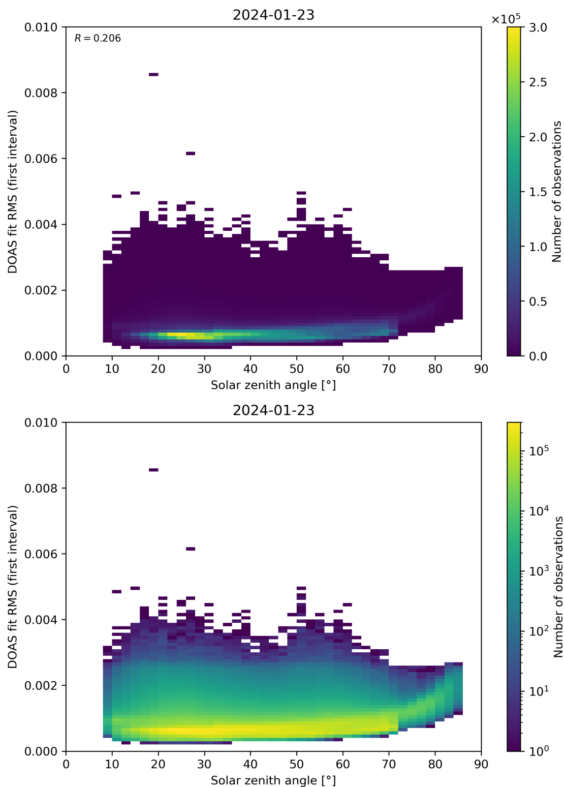
Figure 167: Scatter density plot of “Solar zenith angle” against “DOAS fit RMS (first interval)” for 2024-01-22 to 2024-01-24.
