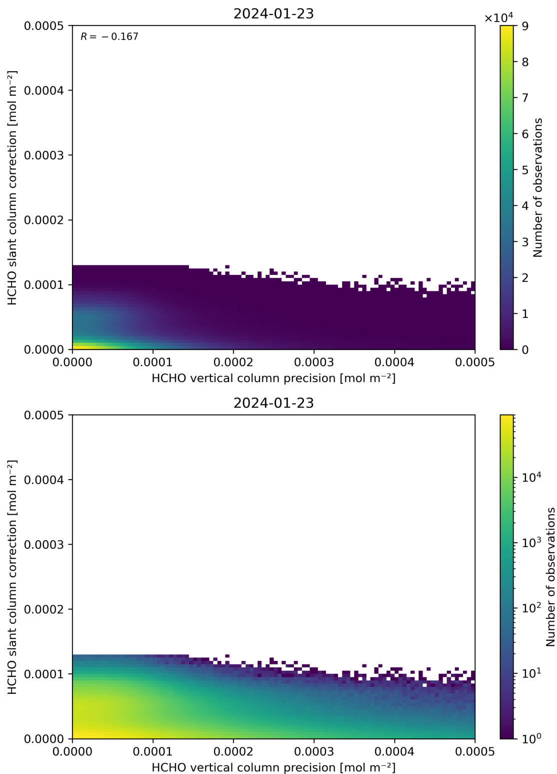
Figure 141: Scatter density plot of “HCHO vertical column precision” against “HCHO slant column correction” for 2024-01-22 to 2024-01-24.
