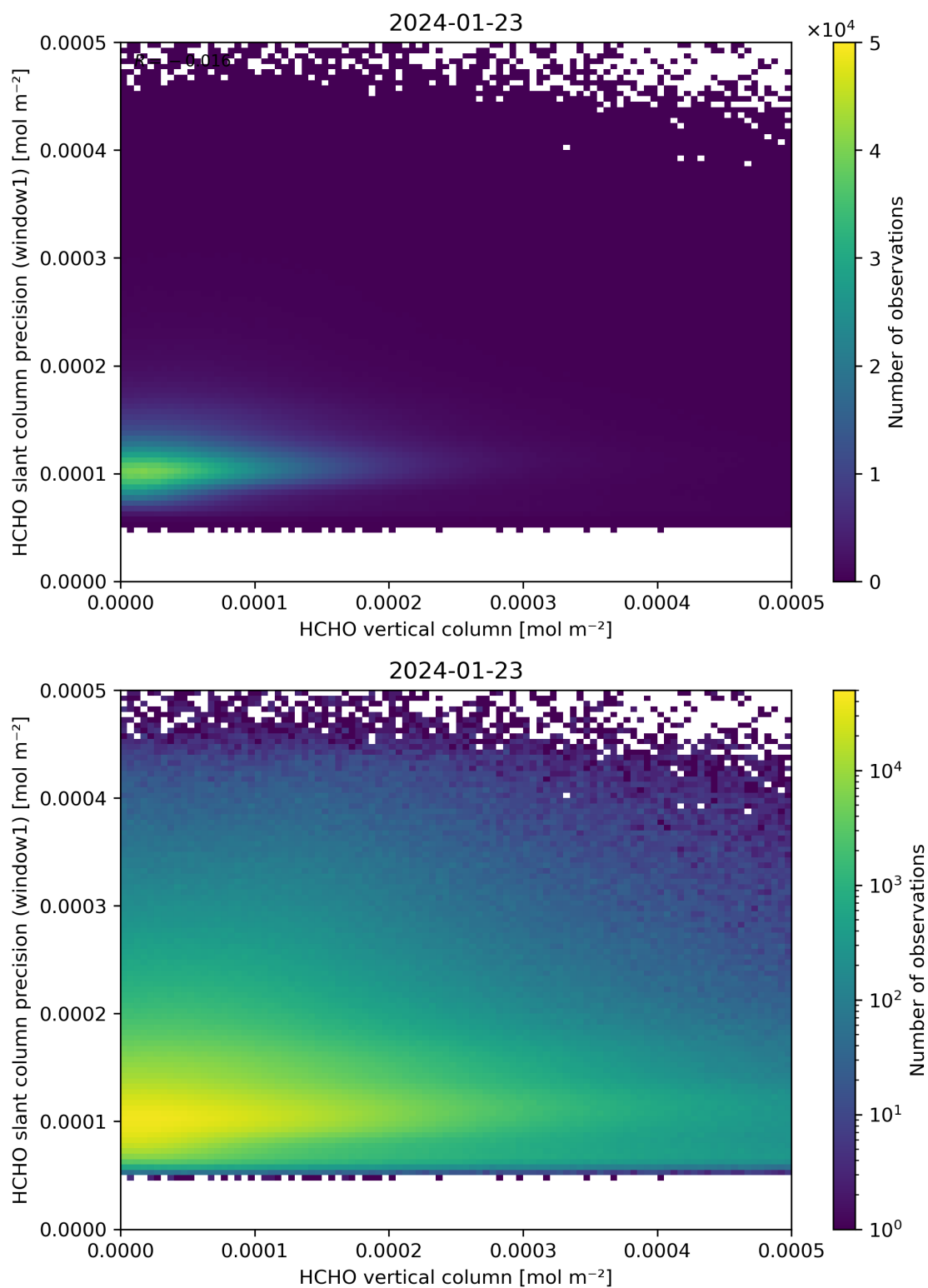
Figure 130: Scatter density plot of “HCHO vertical column” against “HCHO slant column precision (window1)” for 2024-01-22 to 2024-01-24.
