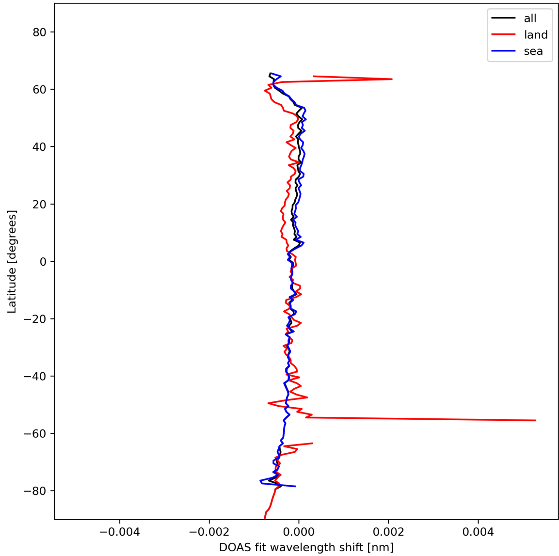
Figure 30: Zonal average of “DOAS fit wavelength shift” for 2024-01-22 to 2024-01-24.
