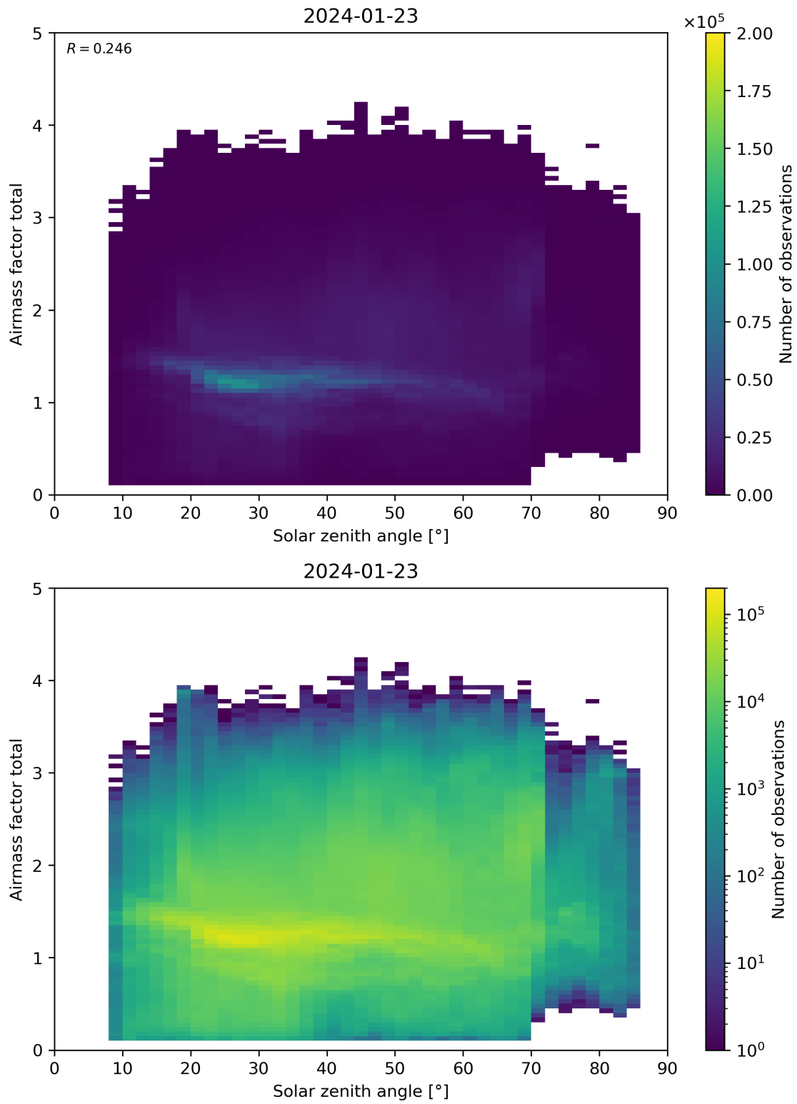
Figure 175: Scatter density plot of “Solar zenith angle” against “Airmass factor total” for 2024-01-22 to 2024-01-24.
