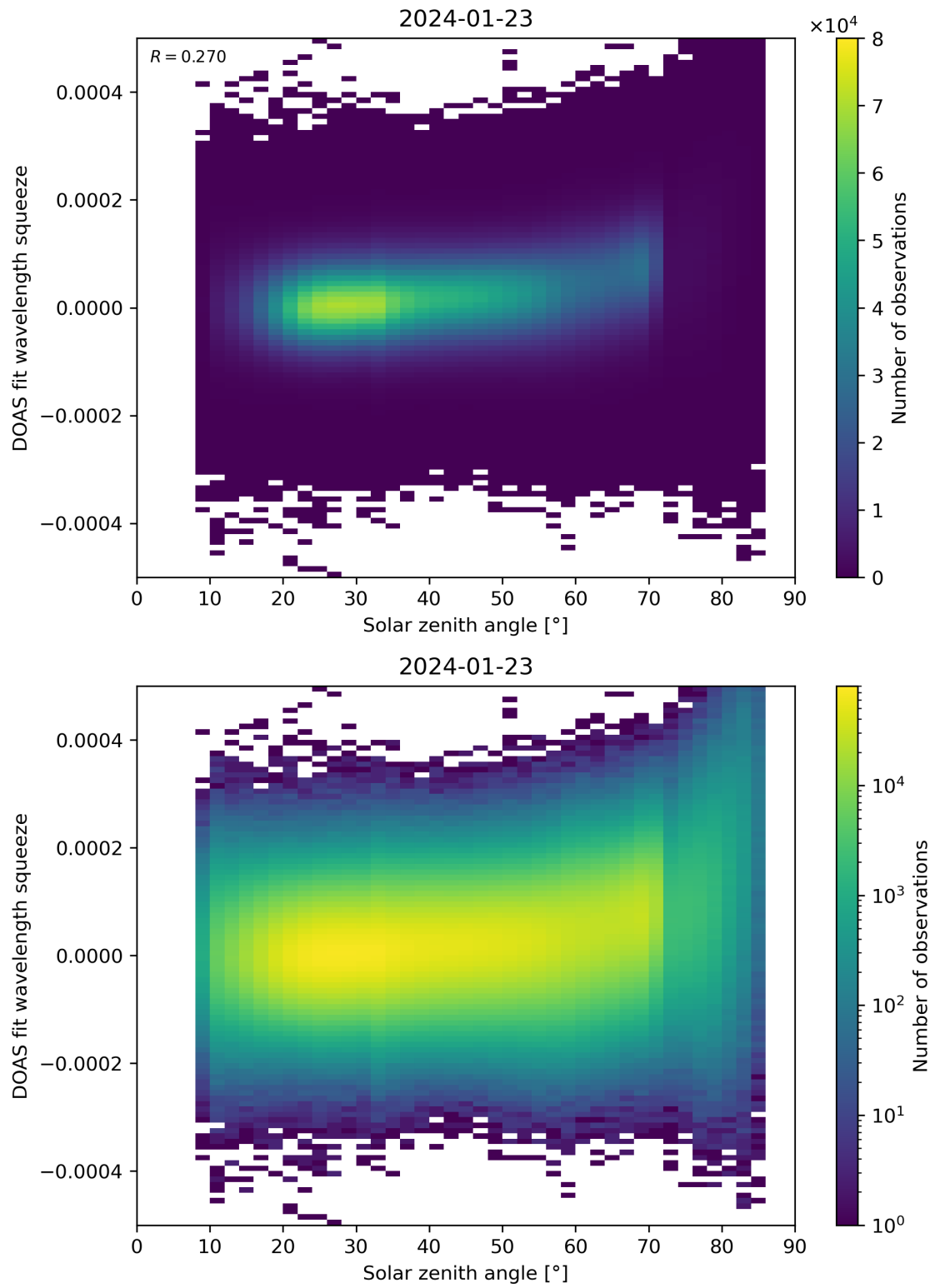
Figure 169: Scatter density plot of “Solar zenith angle” against “DOAS fit wavelength squeeze” for 2024-01-22 to 2024-01-24.
