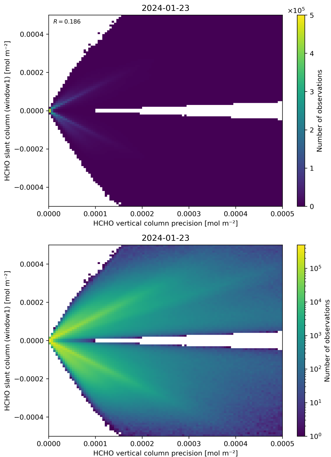
Figure 142: Scatter density plot of “HCHO vertical column precision” against “HCHO slant column (window1)” for 2024-01-22 to 2024-01-24.
