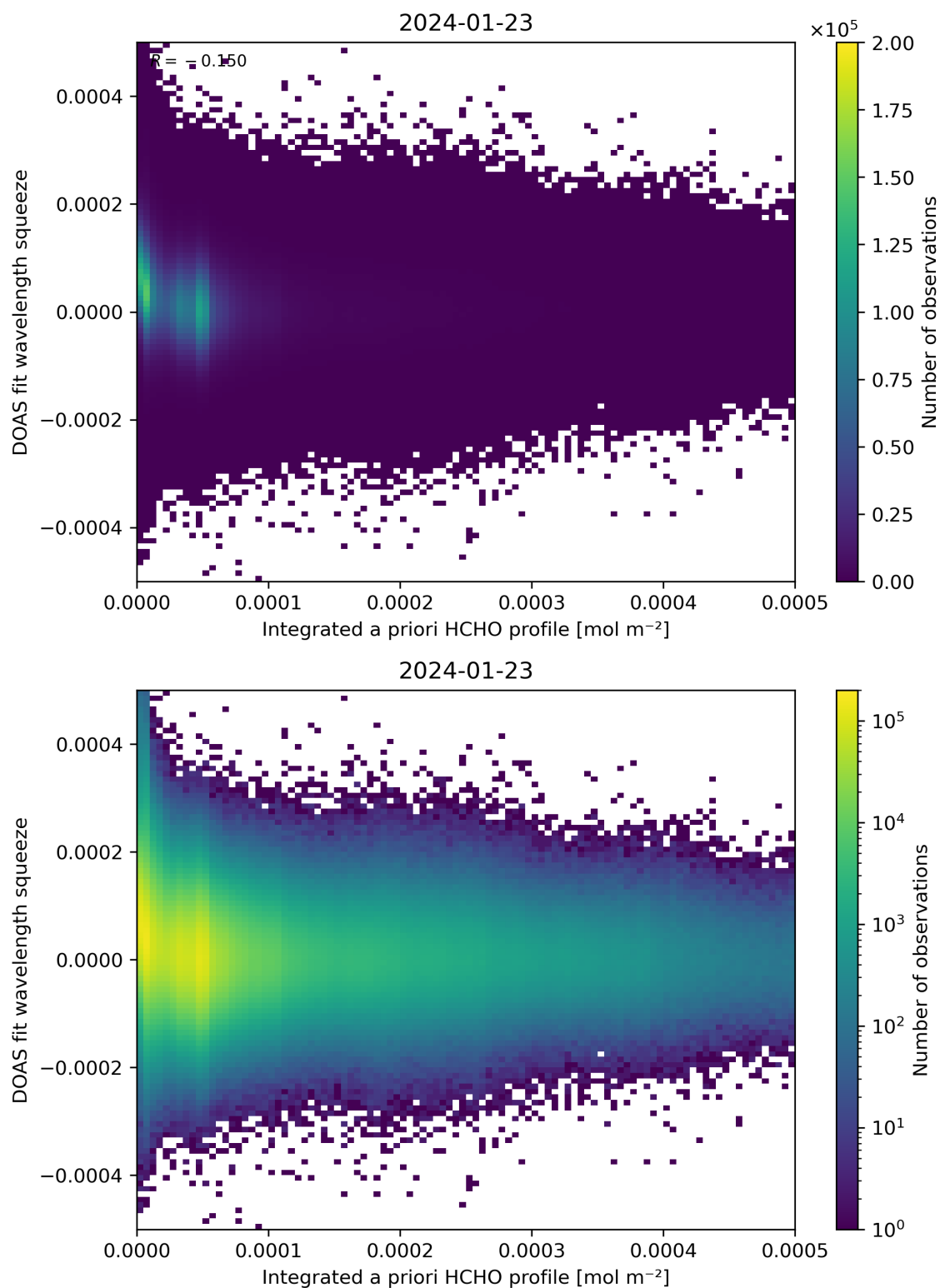
Figure 150: Scatter density plot of “Integrated a priori HCHO profile” against “DOAS fit wavelength squeeze” for 2024-01-22 to 2024-01-24.
