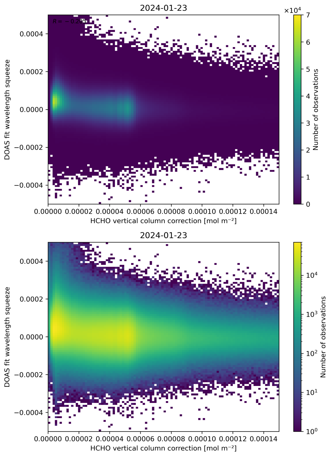
Figure 114: Scatter density plot of “HCHO vertical column correction” against “DOAS fit wavelength squeeze” for 2024-01-22 to 2024-01-24.
