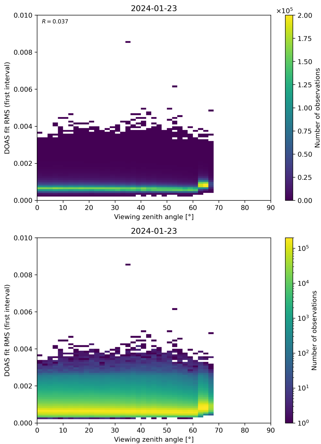
Figure 182: Scatter density plot of “Viewing zenith angle” against “DOAS fit RMS (first interval)” for 2024-01-22 to 2024-01-24.
