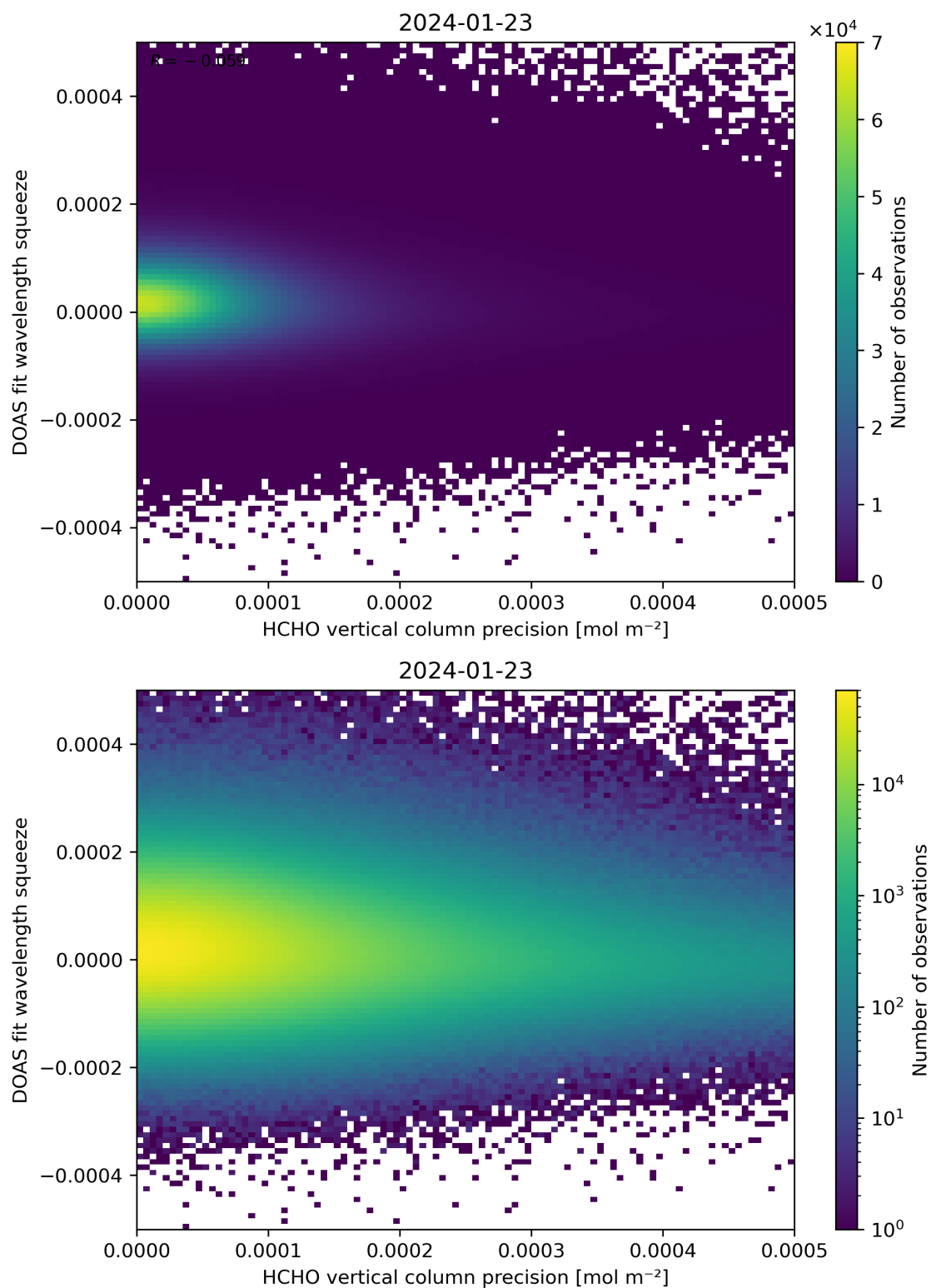
Figure 138: Scatter density plot of “HCHO vertical column precision” against “DOAS fit wavelength squeeze” for 2024-01-22 to 2024-01-24.
