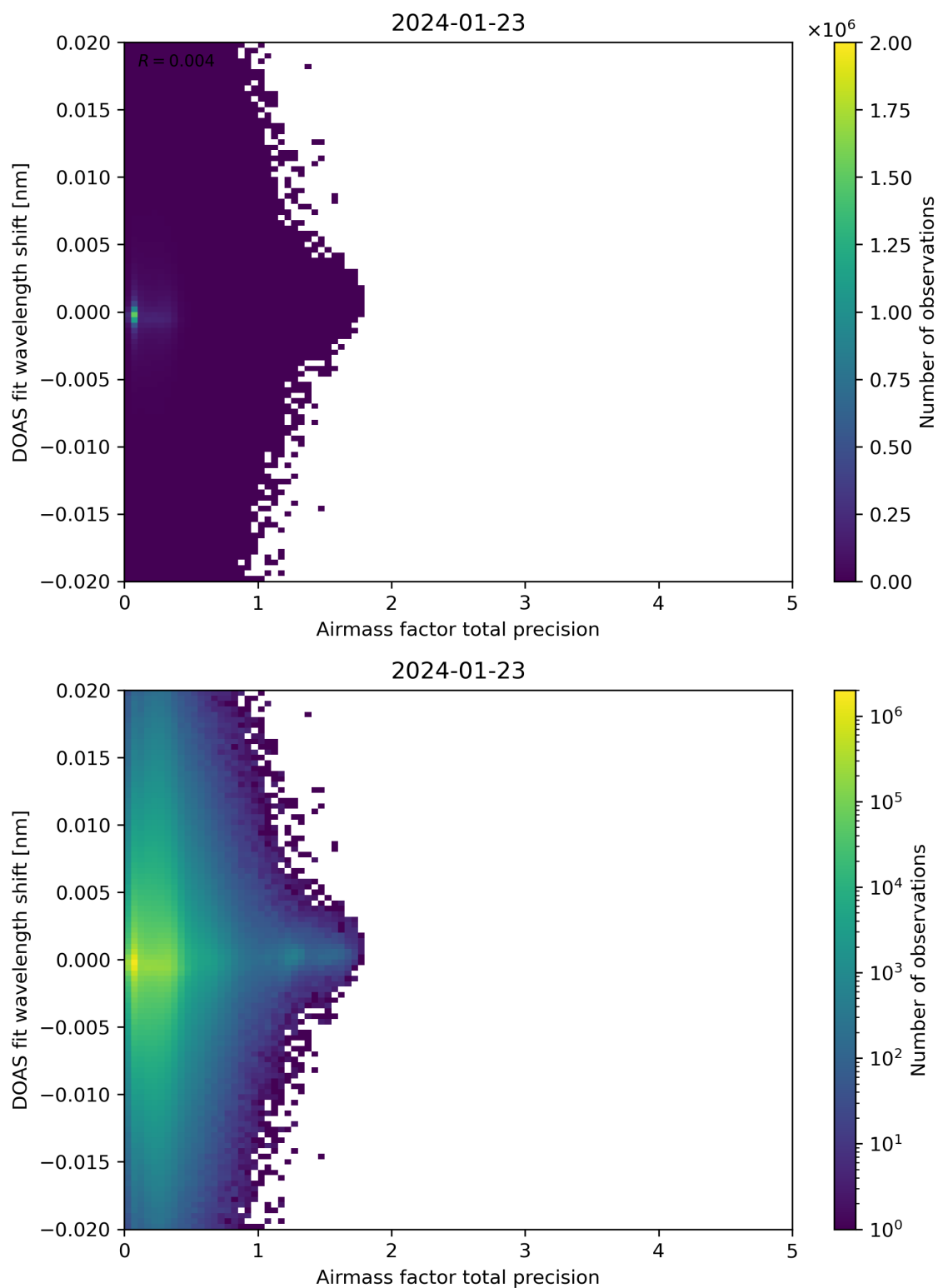
Figure 106: Scatter density plot of “Airmass factor total precision” against “DOAS fit wavelength shift” for 2024-01-22 to 2024-01-24.
