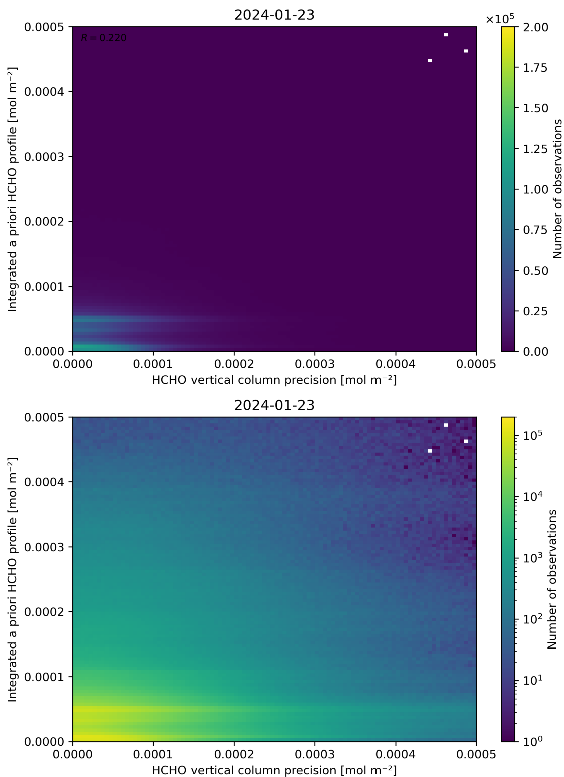
Figure 147: Scatter density plot of “HCHO vertical column precision” against “Integrated a priori HCHO profile” for 2024-01-22 to 2024-01-24.
