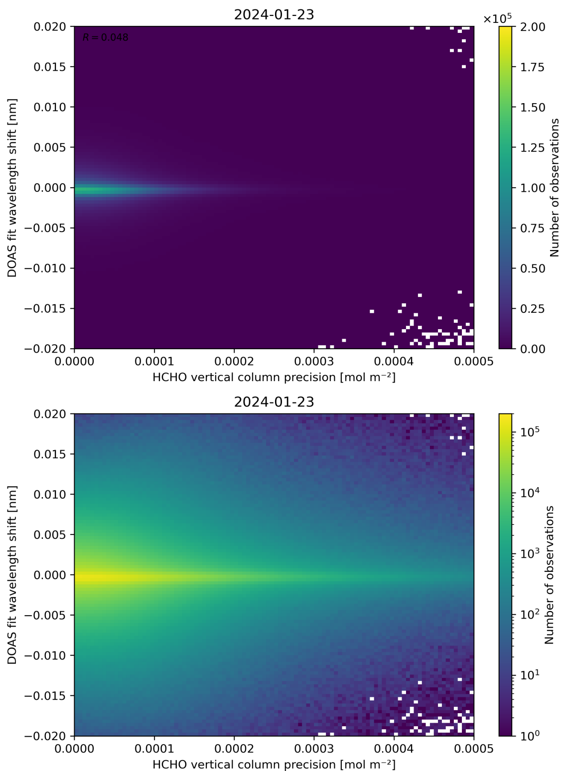
Figure 137: Scatter density plot of “HCHO vertical column precision” against “DOAS fit wavelength shift” for 2024-01-22 to 2024-01-24.
