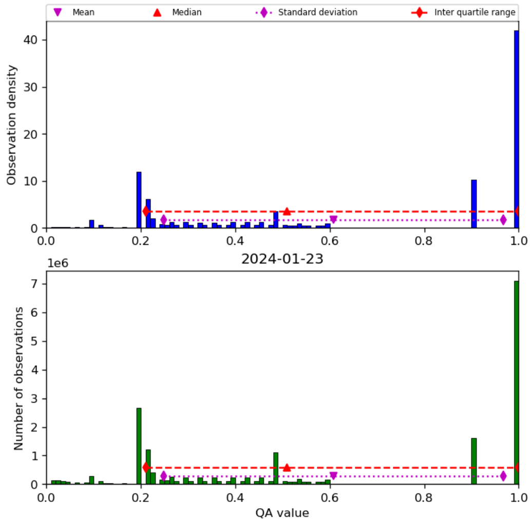
Figure 34: Histogram of “QA value” for 2024-01-22 to 2024-01-24
