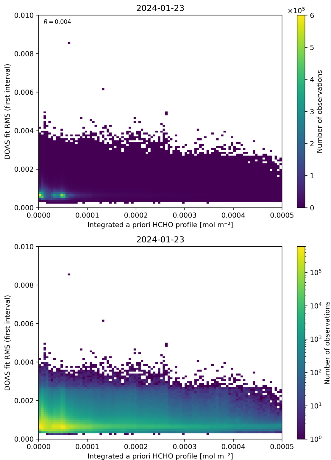
Figure 148: Scatter density plot of “Integrated a priori HCHO profile” against “DOAS fit RMS (first interval)” for 2024-01-22 to 2024-01-24.
