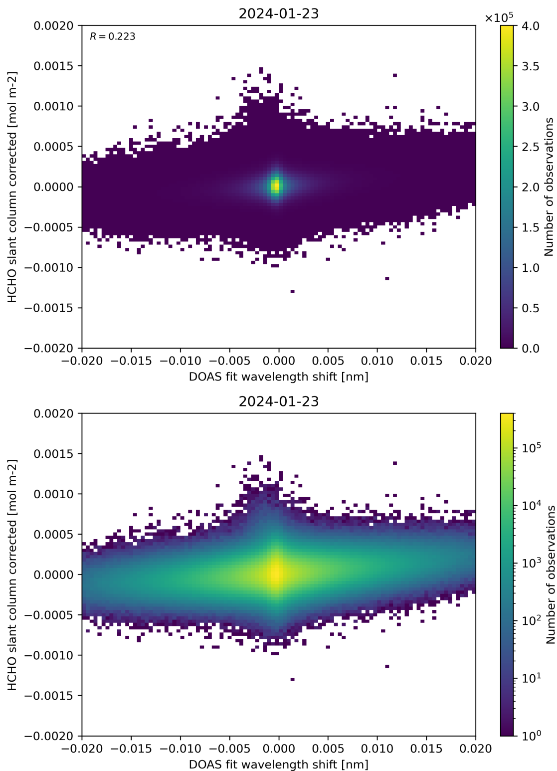
Figure 66: Scatter density plot of “DOAS fit wavelength shift” against “HCHO slant column corrected” for 2024-01-22 to 2024-01-24.
