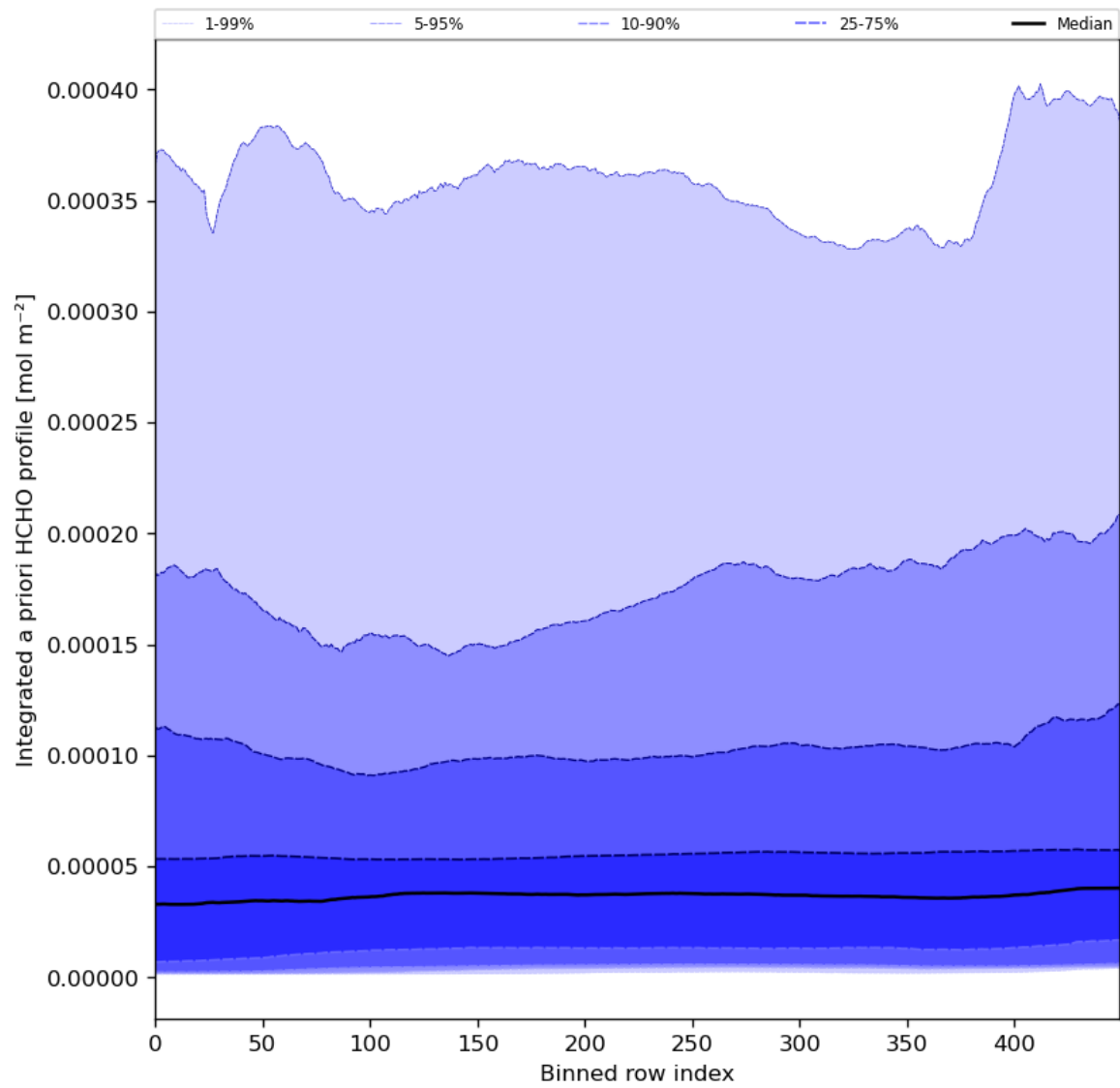
Figure 57: Along track statistics of "Integrated a priori HCHO profile" for 2024-01-22 to 2024-01-24
