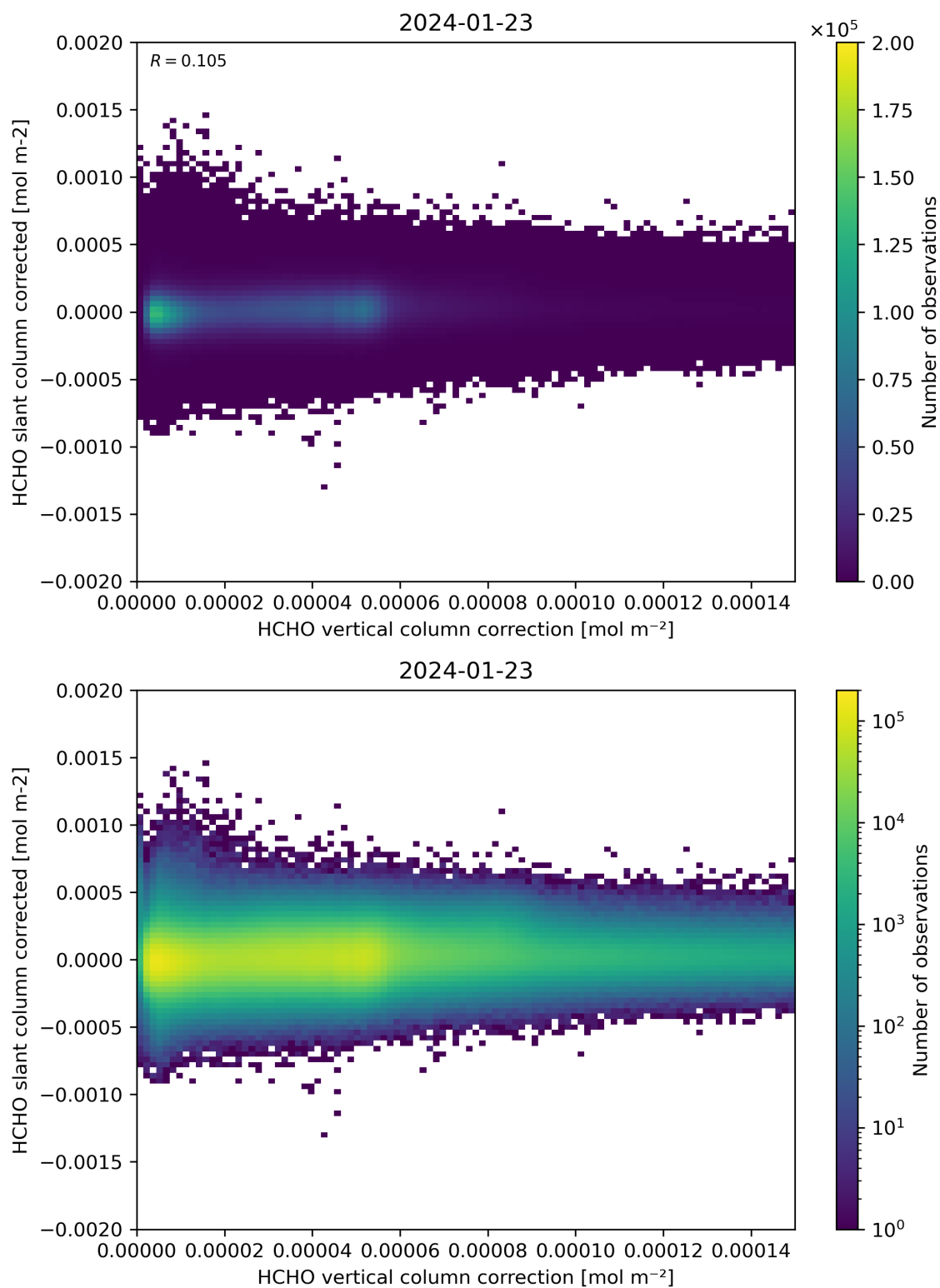
Figure 116: Scatter density plot of “HCHO vertical column correction” against “HCHO slant column corrected” for 2024-01-22 to 2024-01-24.
