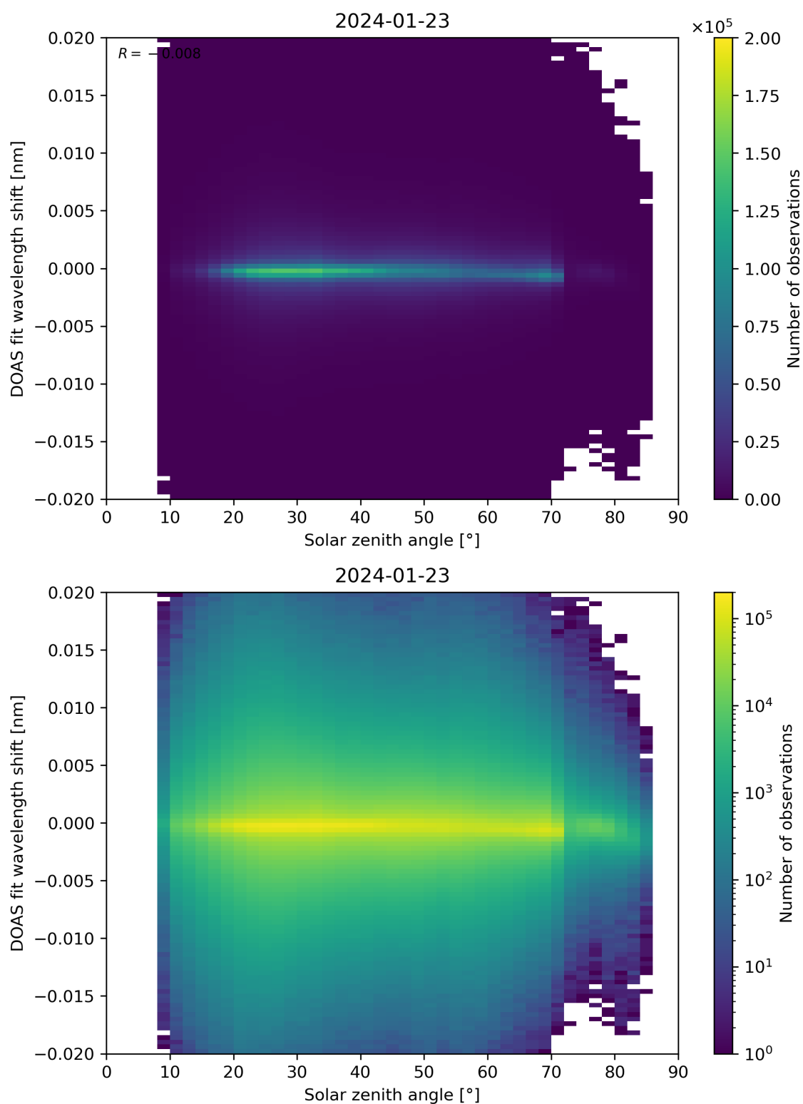
Figure 168: Scatter density plot of “Solar zenith angle” against “DOAS fit wavelength shift” for 2024-01-22 to 2024-01-24.
