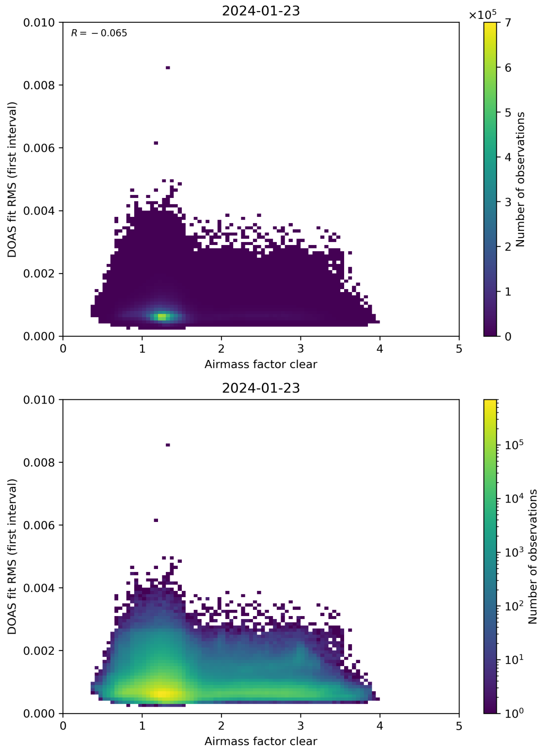
Figure 71: Scatter density plot of “Airmass factor clear” against “DOAS fit RMS (first interval)” for 2024-01-22 to 2024-01-24.
