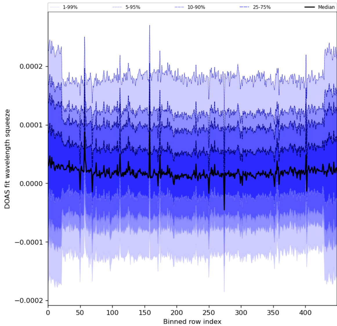
Figure 59: Along track statistics of “DOAS fit wavelength squeeze” for 2024-01-22 to 2024-01-24
