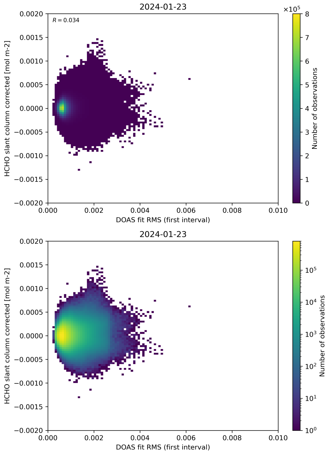
Figure 62: Scatter density plot of “DOAS fit RMS (first interval)” against “HCHO slant column corrected” for 2024-01-22 to 2024-01-24.
