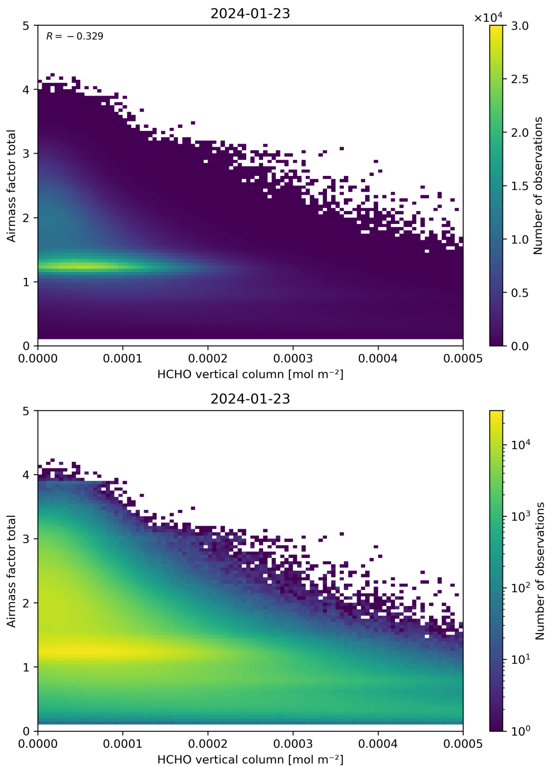
Figure 131: Scatter density plot of “HCHO vertical column” against “Airmass factor total” for 2024-01-22 to 2024-01-24.
