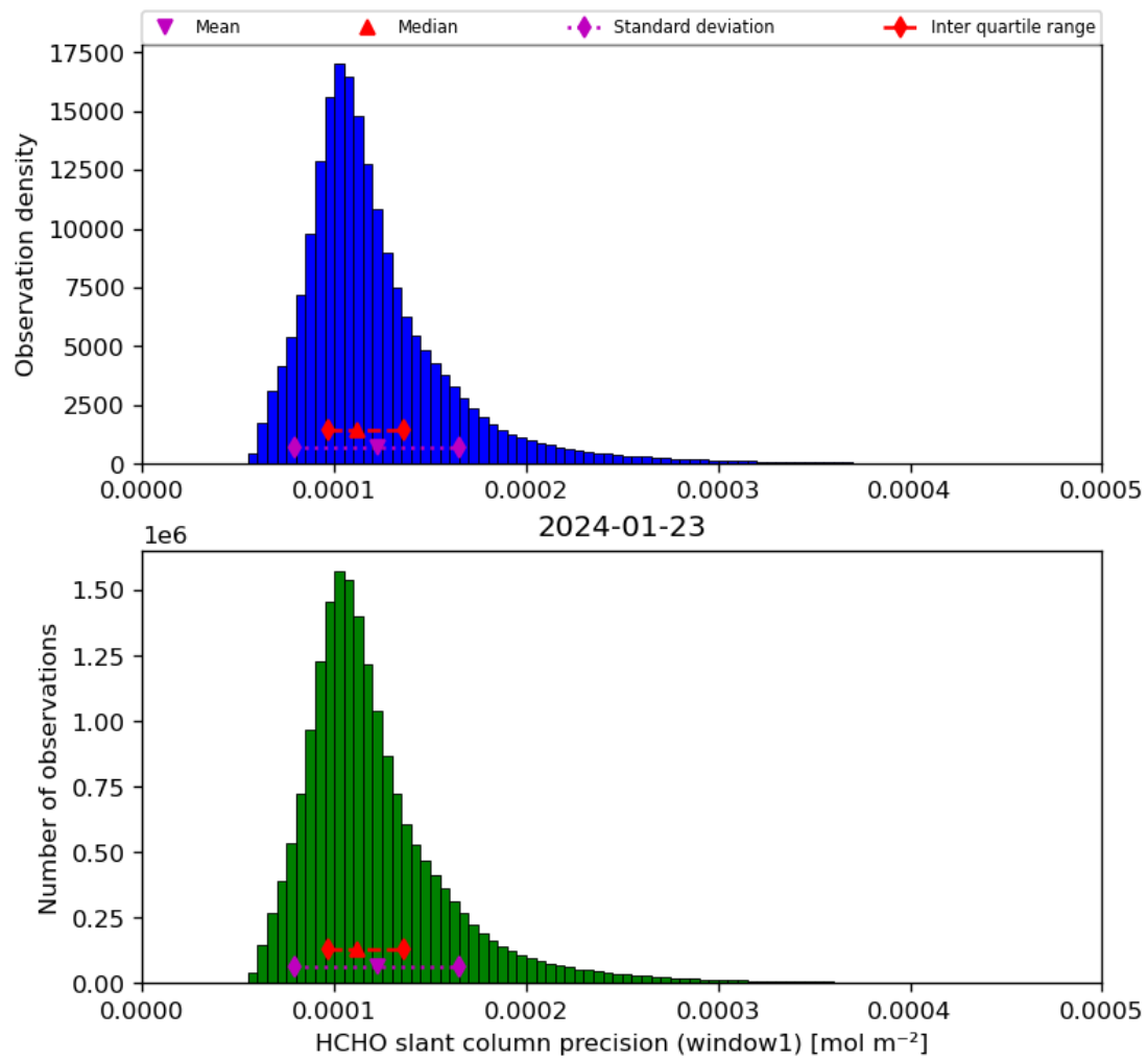
Figure 39: Histogram of “HCHO slant column precision (window1)” for 2024-01-22 to 2024-01-24
