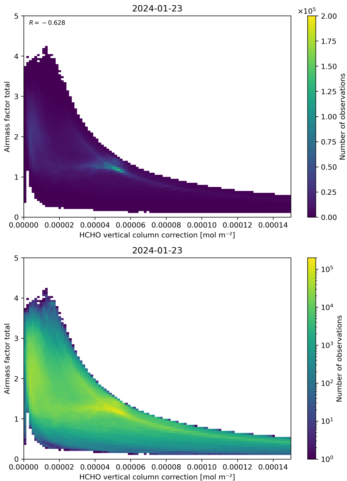
Figure 120: Scatter density plot of “HCHO vertical column correction” against “Airmass factor total” for 2024-01-22 to 2024-01-24.
