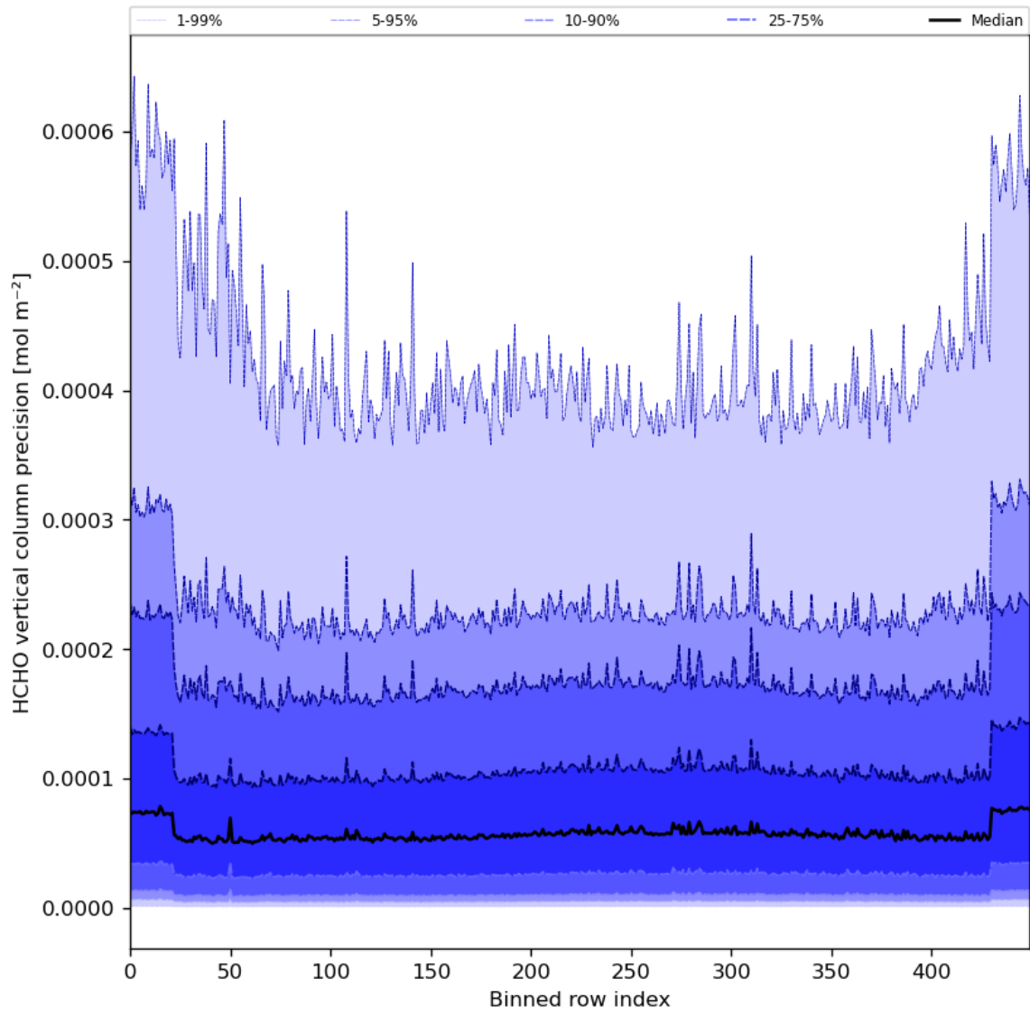
Figure 50: Along track statistics of “HCHO vertical column precision” for 2024-01-22 to 2024-01-24
