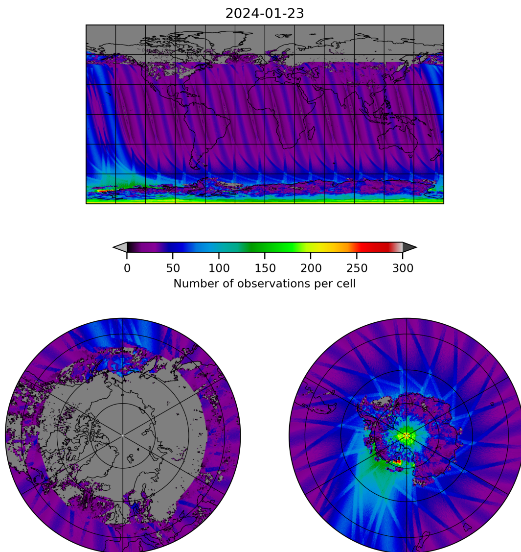
Figure 19: Map of the number of observations for 2024-01-22 to 2024-01-24
