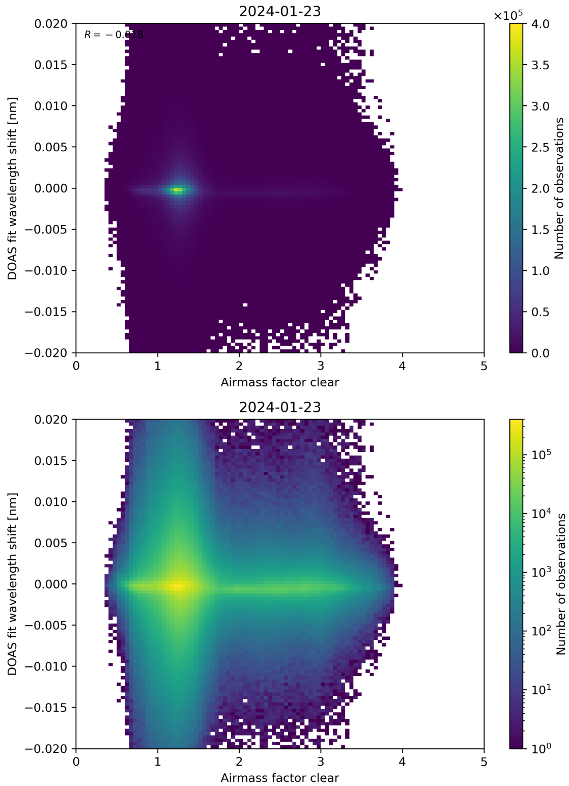
Figure 72: Scatter density plot of “Airmass factor clear” against “DOAS fit wavelength shift” for 2024-01-22 to 2024-01-24.
