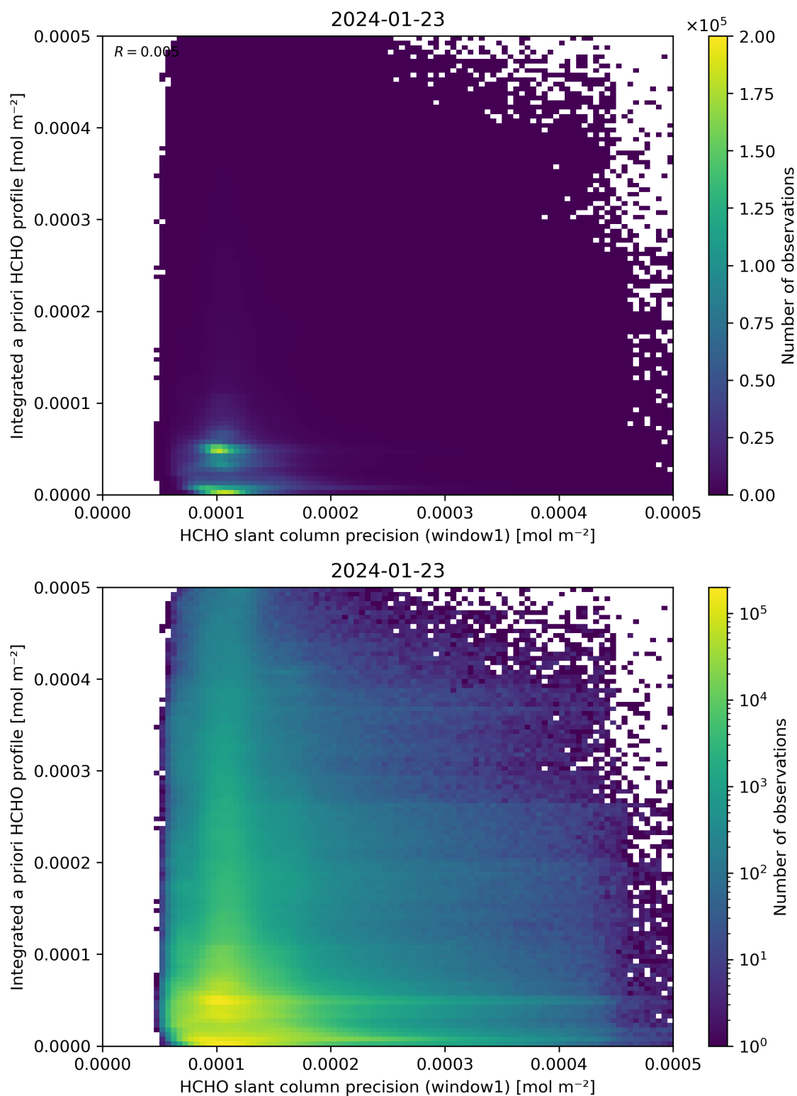
Figure 96: Scatter density plot of “HCHO slant column precision (window1)” against “Integrated a priori HCHO profile” for 2024-01-22 to 2024-01-24.
