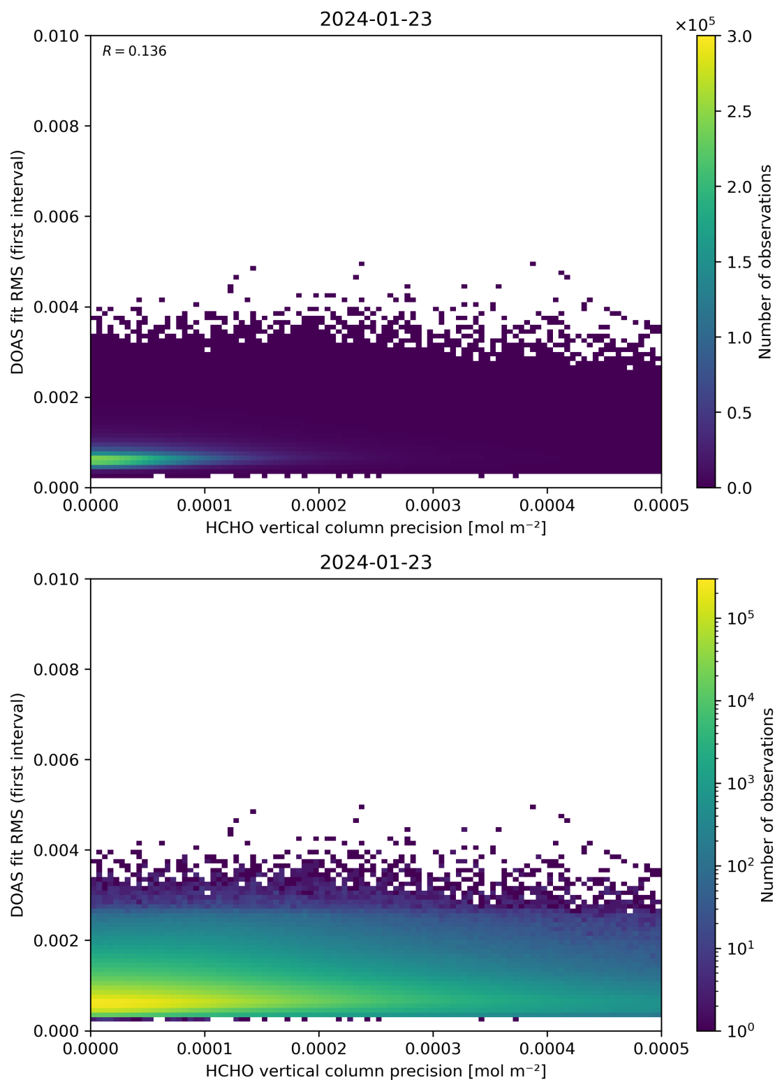
Figure 136: Scatter density plot of “HCHO vertical column precision” against “DOAS fit RMS (first interval)” for 2024-01-22 to 2024-01-24.
