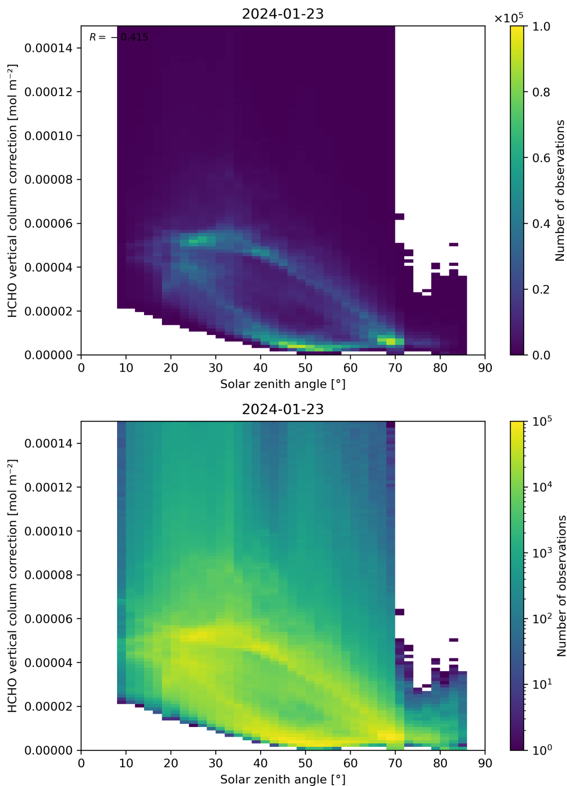
Figure 178: Scatter density plot of “Solar zenith angle” against “HCHO vertical column correction” for 2024-01-22 to 2024-01-24.
