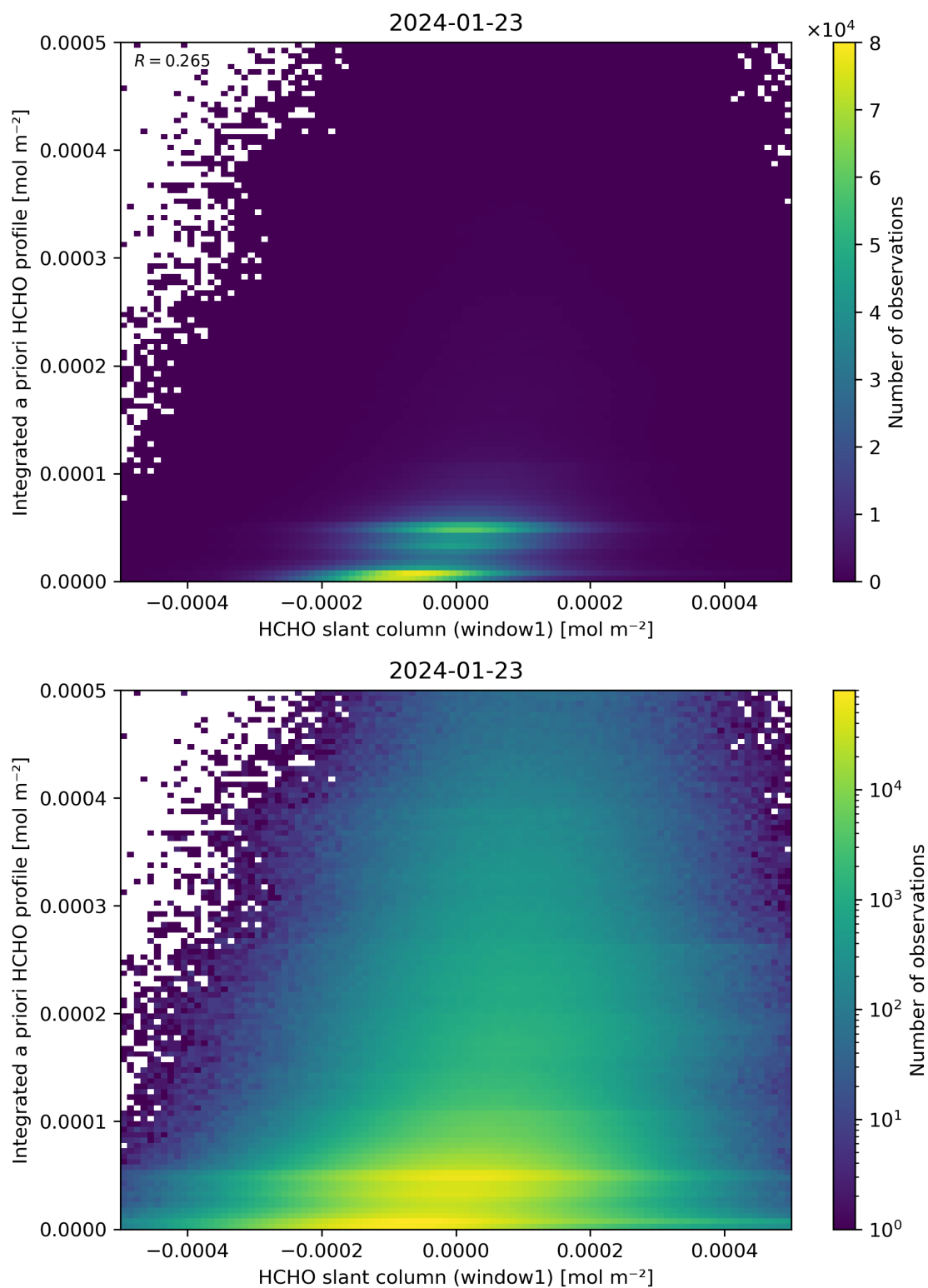
Figure 87: Scatter density plot of “HCHO slant column (window1)” against “Integrated a priori HCHO profile” for 2024-01-22 to 2024-01-24.
