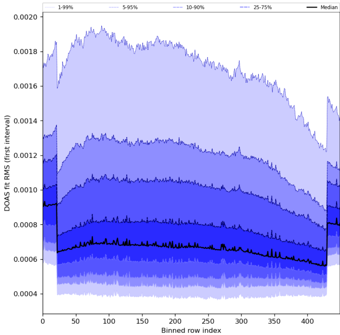
Figure 60: Along track statistics of “DOAS fit RMS (first interval)” for 2024-01-22 to 2024-01-24
