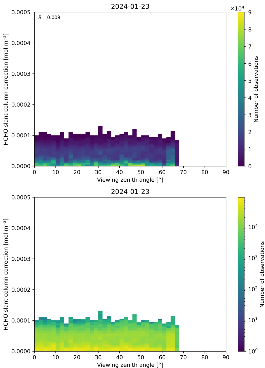
Figure 187: Scatter density plot of “Viewing zenith angle” against “HCHO slant column correction” for 2024-01-22 to 2024-01-24.
