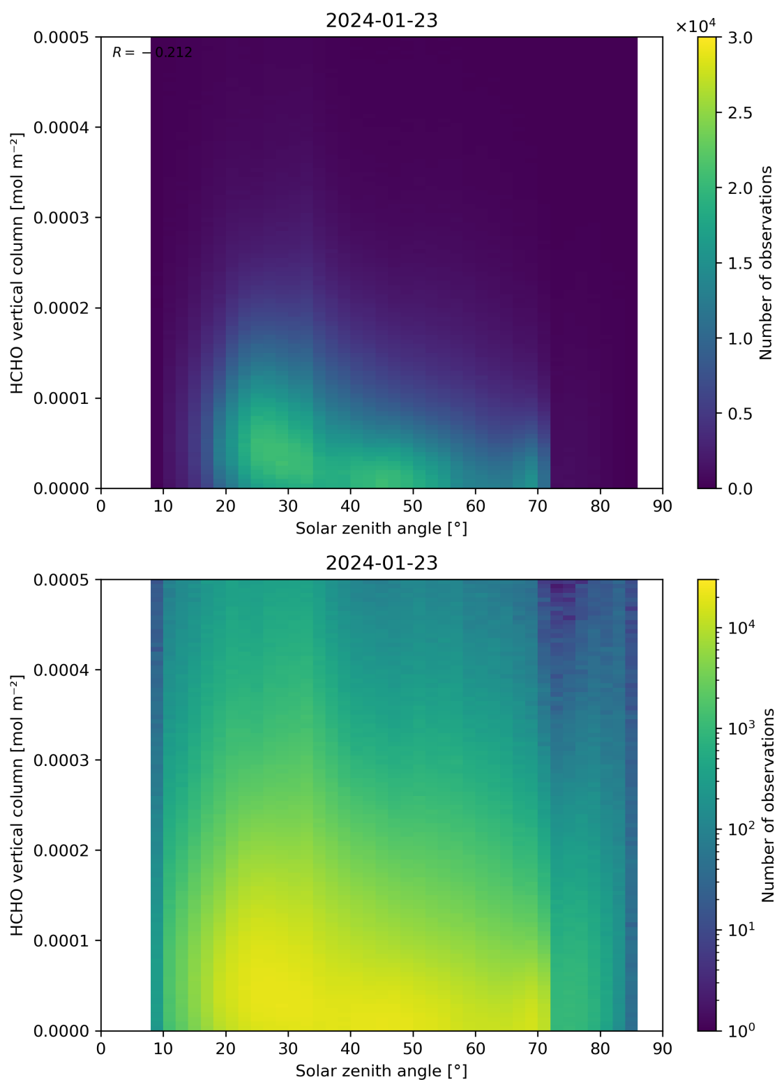
Figure 177: Scatter density plot of “Solar zenith angle” against “HCHO vertical column” for 2024-01-22 to 2024-01-24.
