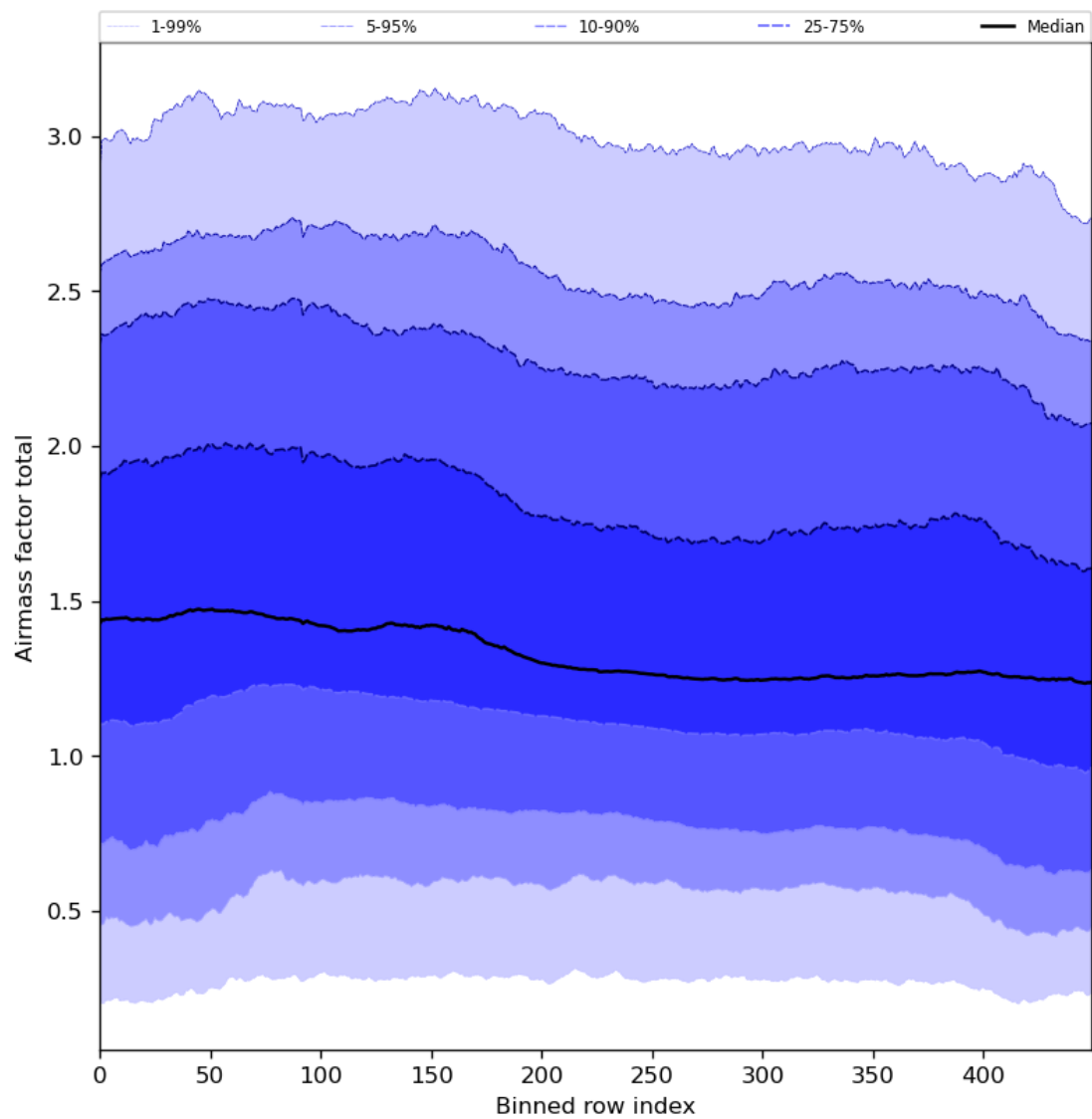
Figure 54: Along track statistics of “Airmass factor total” for 2024-01-22 to 2024-01-24
