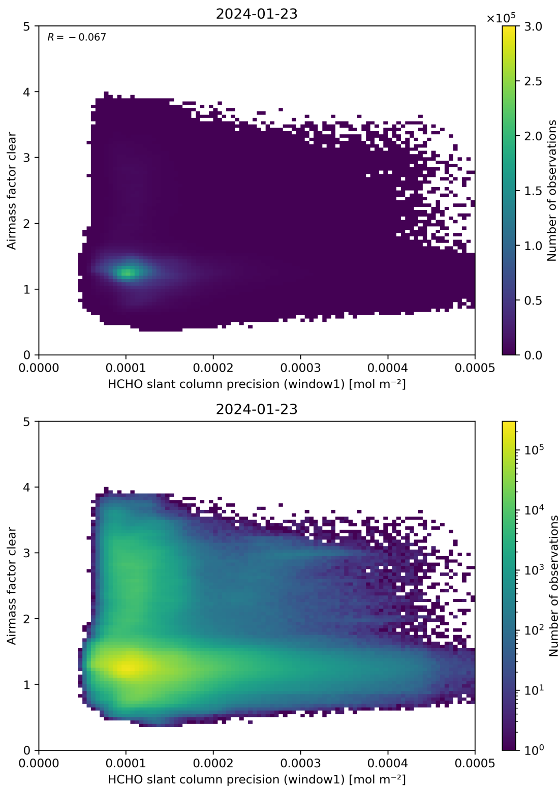
Figure 91: Scatter density plot of “HCHO slant column precision (window1)” against “Airmass factor clear” for 2024-01-22 to 2024-01-24.
