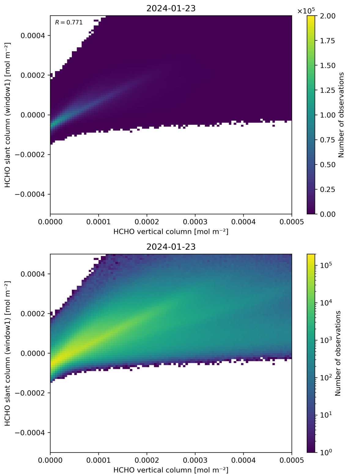
Figure 129: Scatter density plot of “HCHO vertical column” against “HCHO slant column (window1)” for 2024-01-22 to 2024-01-24.
