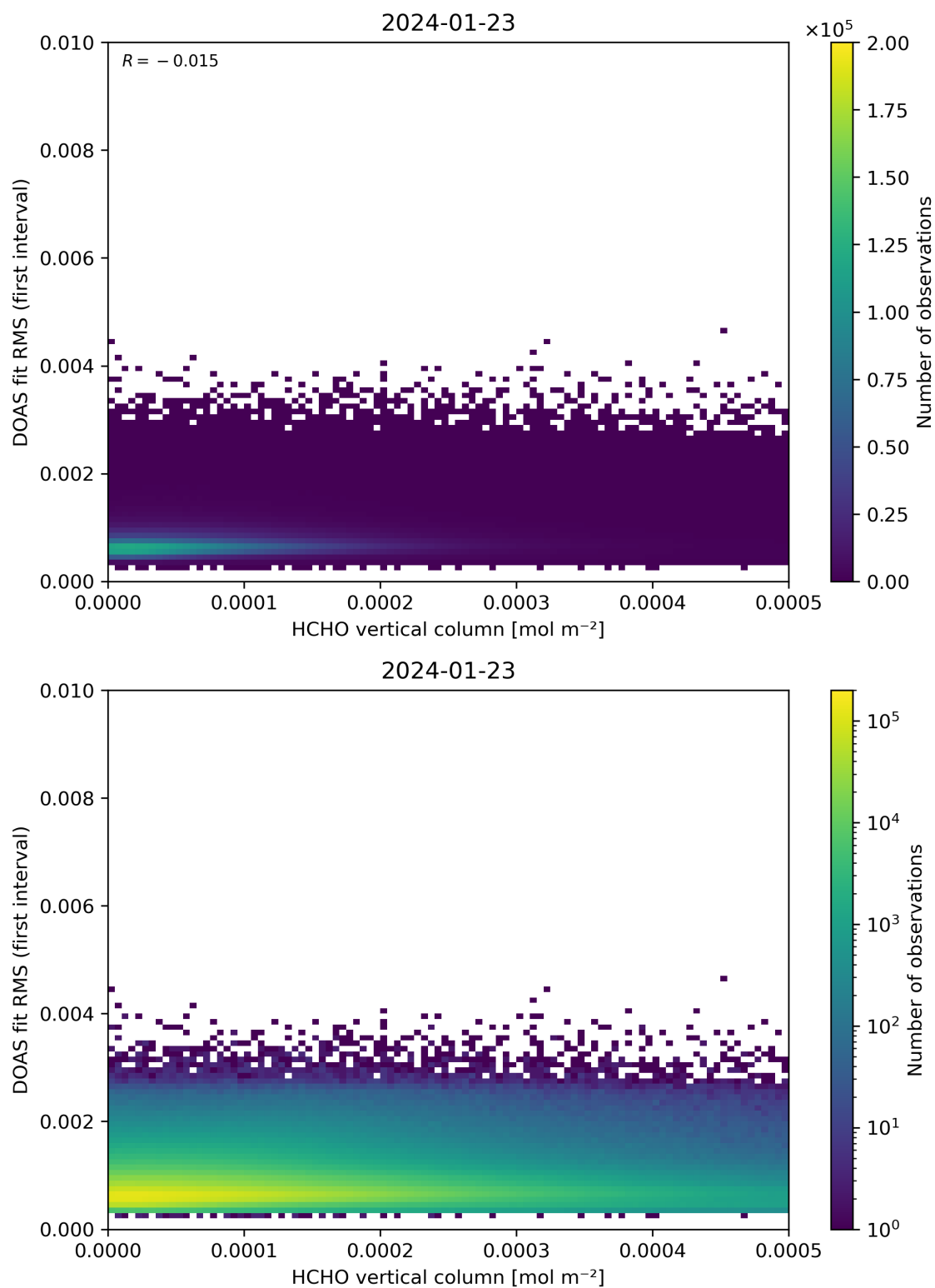
Figure 123: Scatter density plot of “HCHO vertical column” against “DOAS fit RMS (first interval)” for 2024-01-22 to 2024-01-24.
