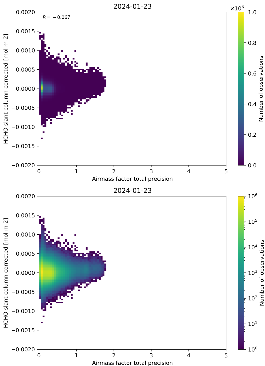
Figure 109: Scatter density plot of “Airmass factor total precision” against “HCHO slant column corrected” for 2024-01-22 to 2024-01-24.
