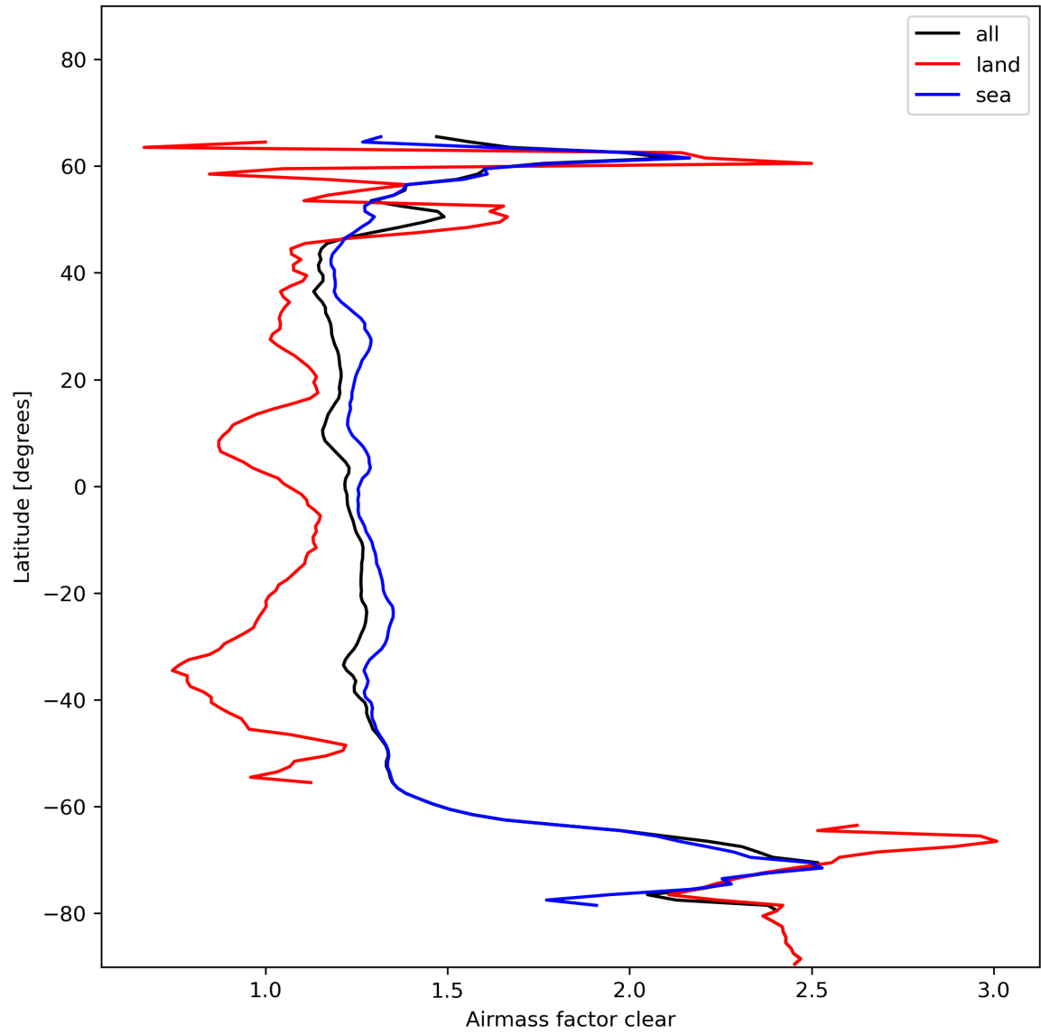
Figure 28: Zonal average of “Airmass factor clear” for 2024-01-22 to 2024-01-24.
