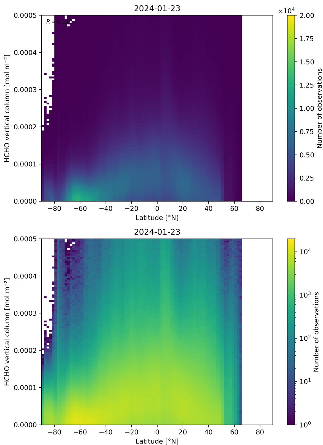
Figure 163: Scatter density plot of “Latitude” against “HCHO vertical column” for 2024-01-22 to 2024-01-24.
