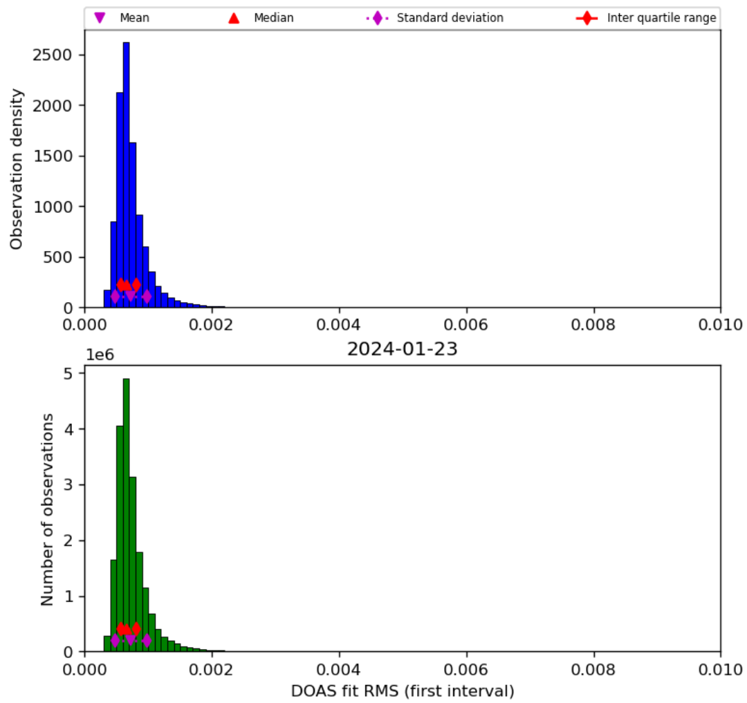
Figure 46: Histogram of “DOAS fit RMS (first interval)” for 2024-01-22 to 2024-01-24
