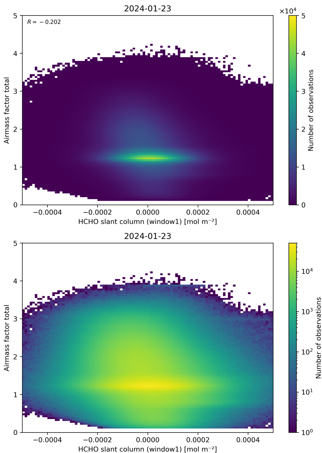
Figure 85: Scatter density plot of “HCHO slant column (window1)” against “Airmass factor total” for 2024-01-22 to 2024-01-24.
