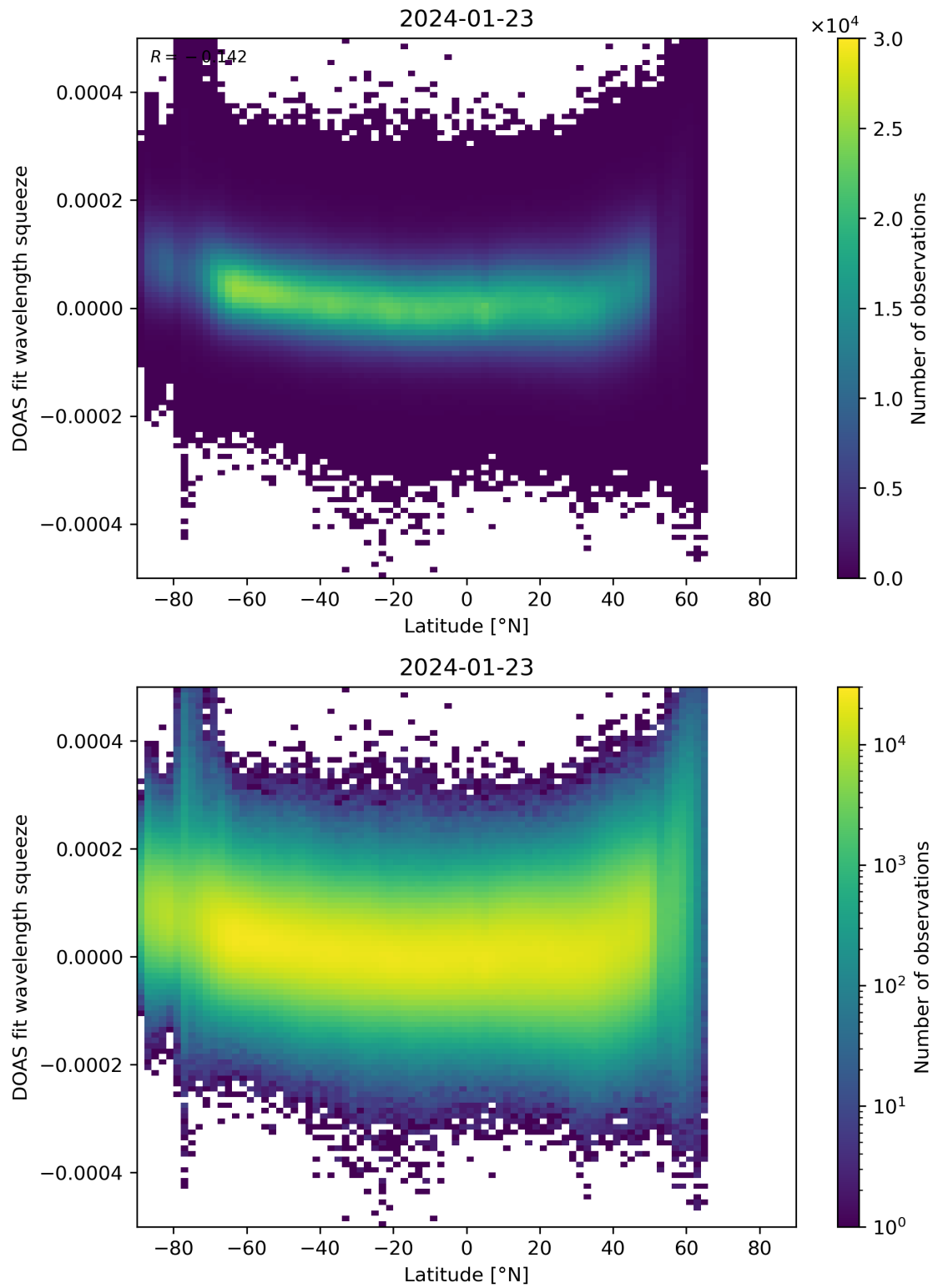
Figure 155: Scatter density plot of “Latitude” against “DOAS fit wavelength squeeze” for 2024-01-22 to 2024-01-24.
