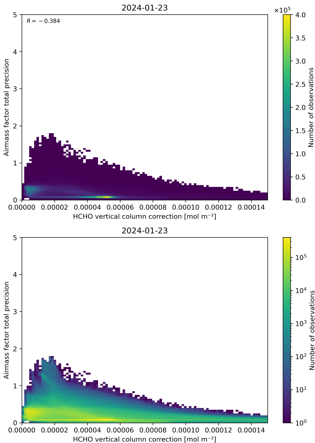
Figure 121: Scatter density plot of “HCHO vertical column correction” against “Airmass factor total precision” for 2024-01-22 to 2024-01-24.
