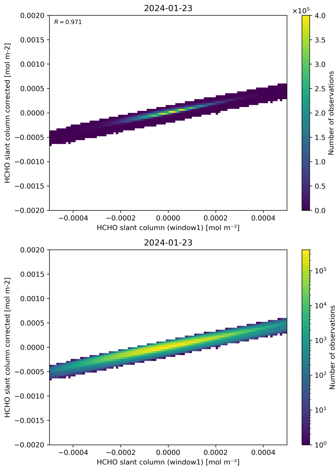
Figure 82: Scatter density plot of “HCHO slant column (window1)” against “HCHO slant column corrected” for 2024-01-22 to 2024-01-24.
