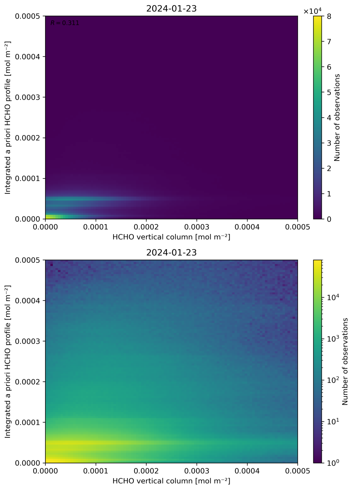
Figure 135: Scatter density plot of “HCHO vertical column” against “Integrated a priori HCHO profile” for 2024-01-22 to 2024-01-24.
