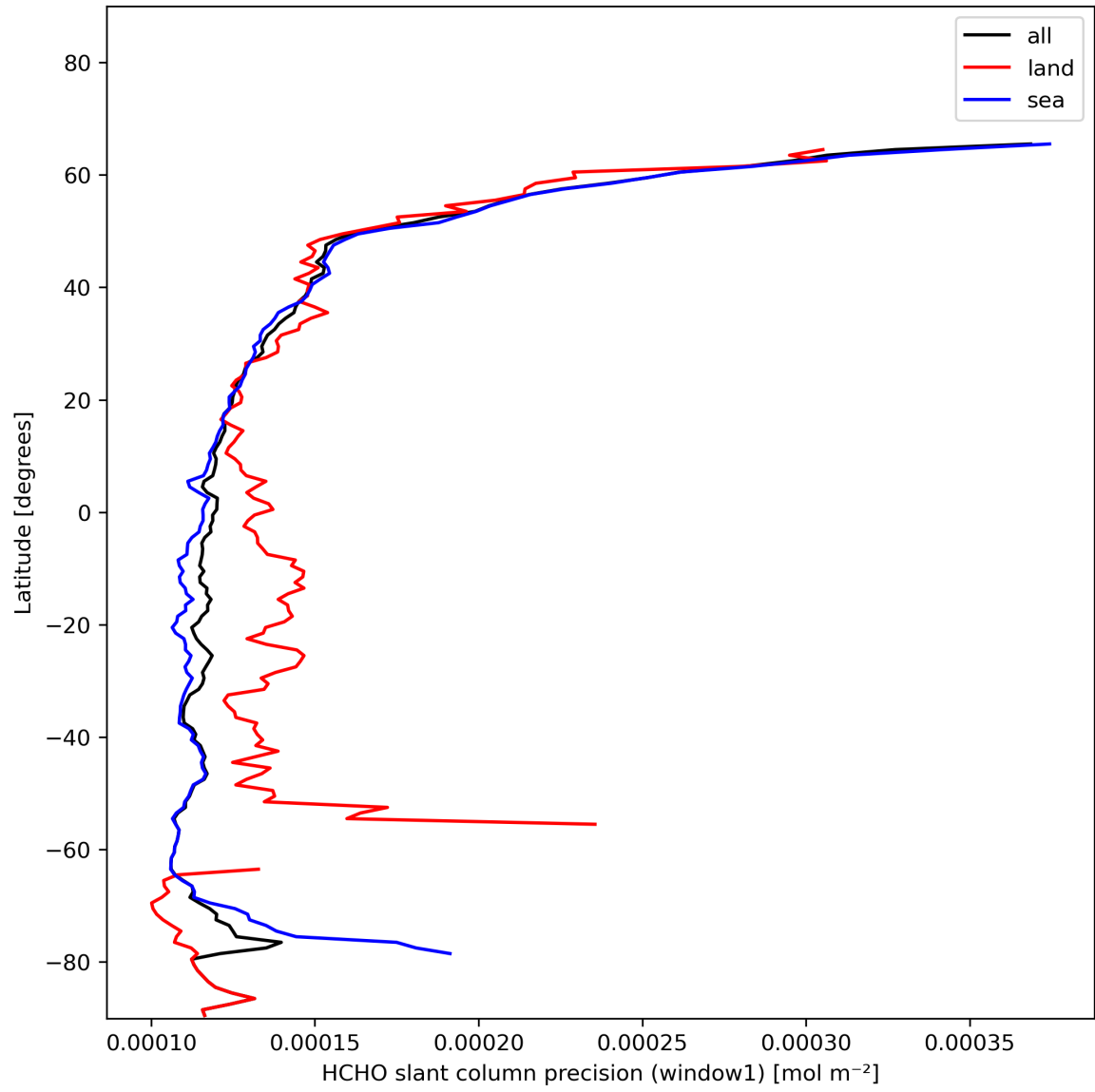
Figure 25: Zonal average of “HCHO slant column precision (window1)” for 2024-01-22 to 2024-01-24.
