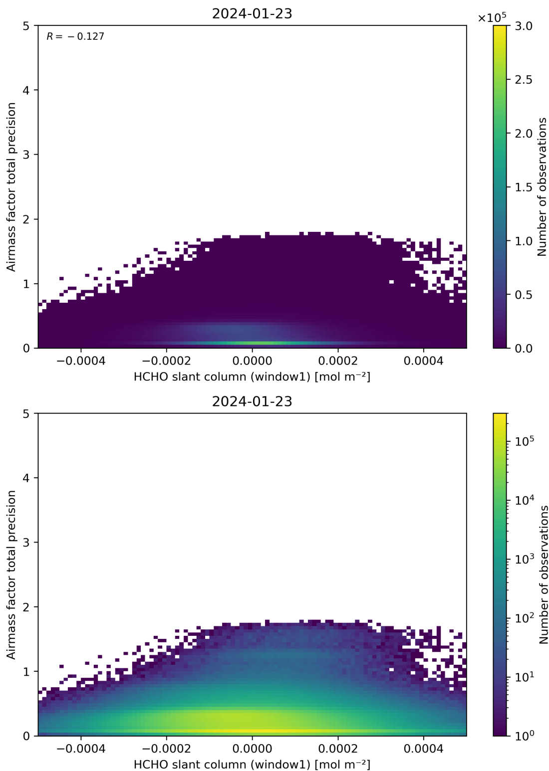
Figure 86: Scatter density plot of “HCHO slant column (window1)” against “Airmass factor total precision” for 2024-01-22 to 2024-01-24.
