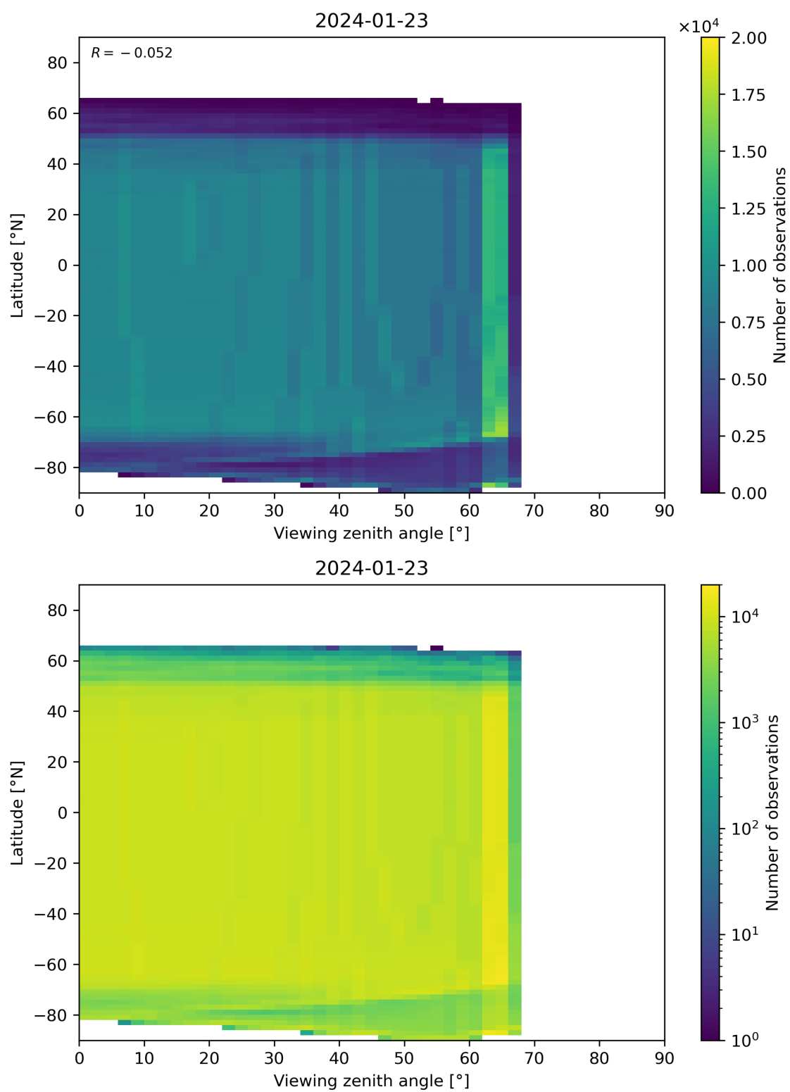
Figure 196: Scatter density plot of “Viewing zenith angle” against “Latitude” for 2024-01-22 to 2024-01-24.
