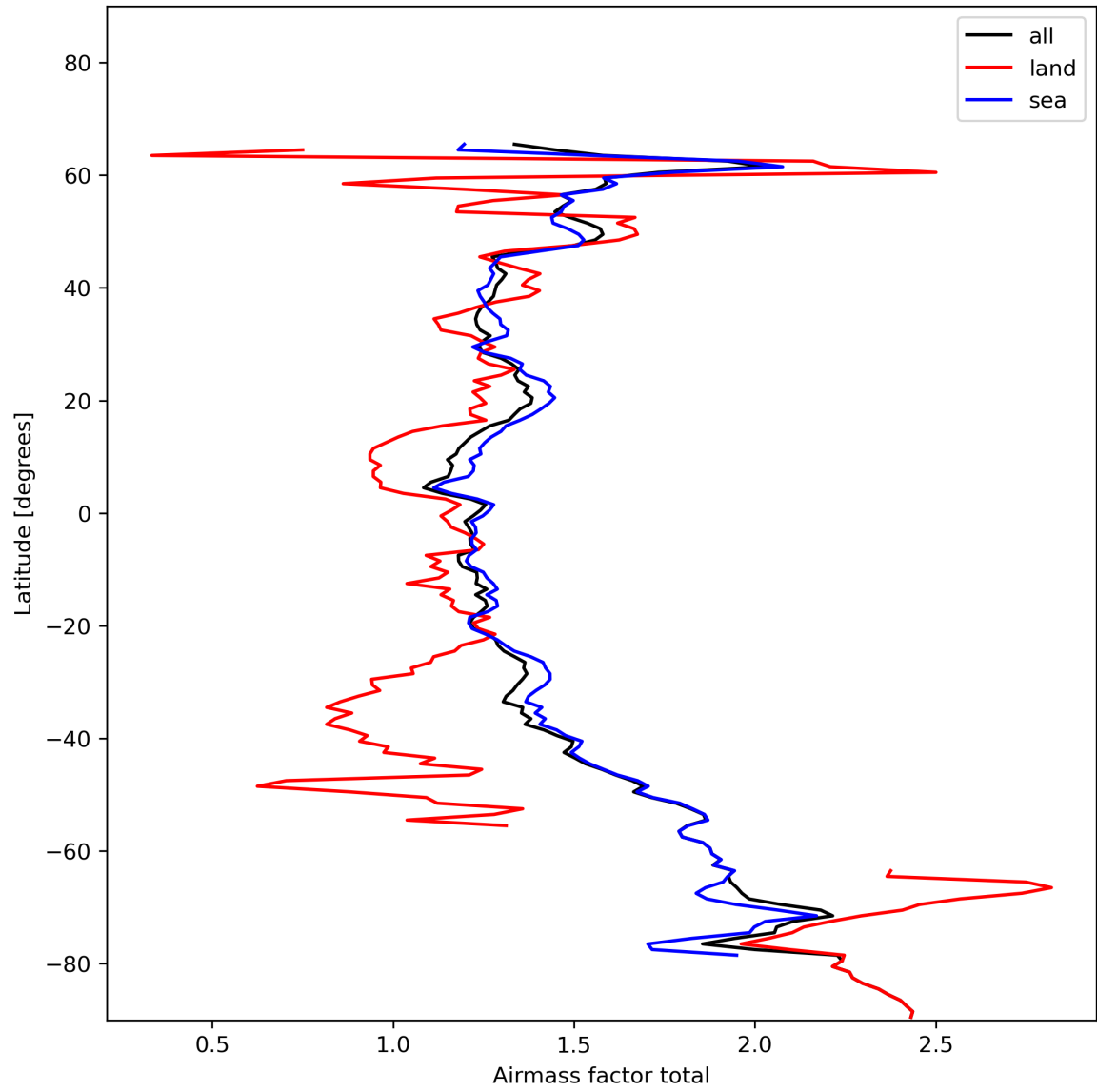
Figure 26: Zonal average of “Airmass factor total” for 2024-01-22 to 2024-01-24.
