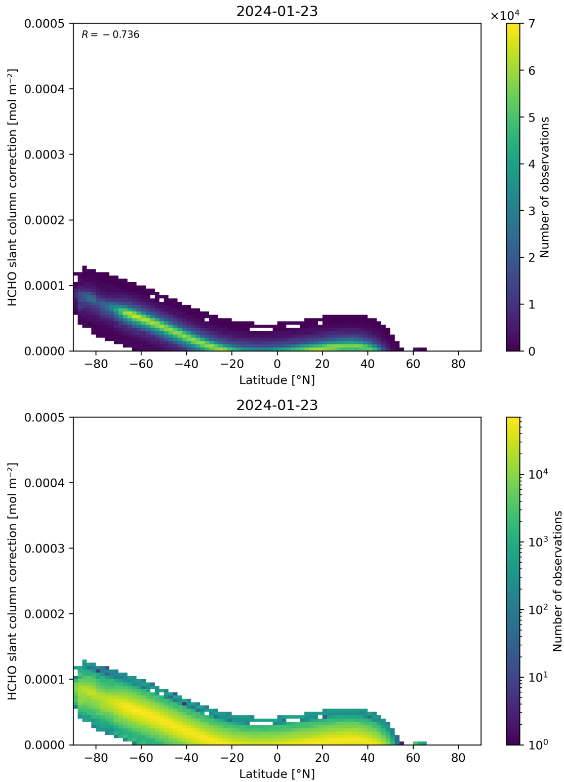
Figure 158: Scatter density plot of “Latitude” against “HCHO slant column correction” for 2024-01-22 to 2024-01-24.
