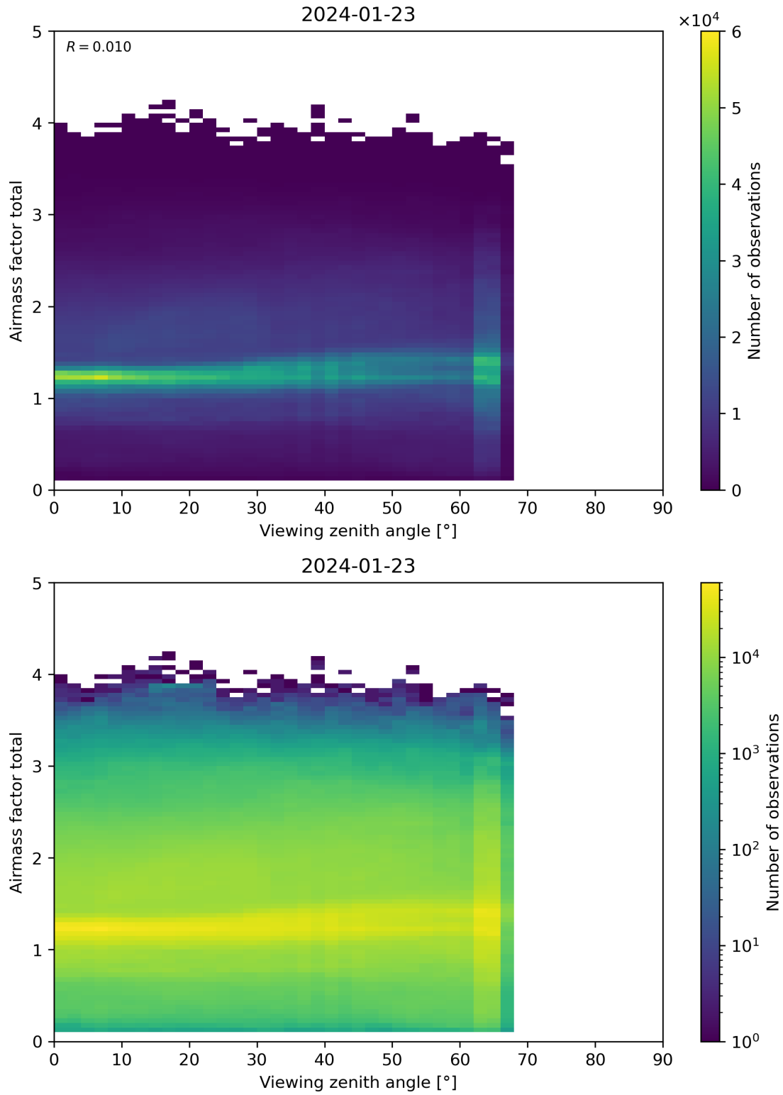
Figure 190: Scatter density plot of “Viewing zenith angle” against “Airmass factor total” for 2024-01-22 to 2024-01-24.
