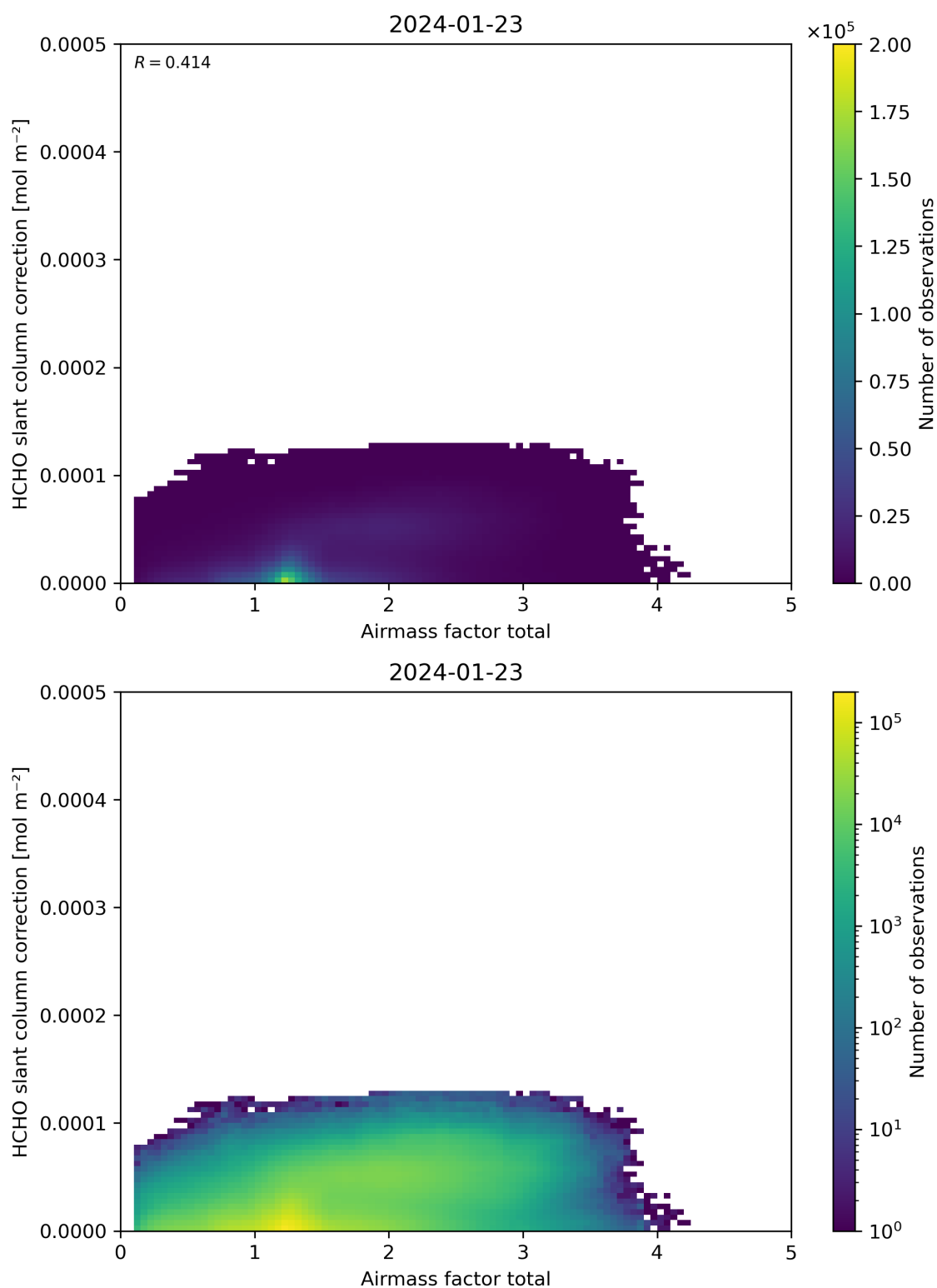
Figure 102: Scatter density plot of “Airmass factor total” against “HCHO slant column correction” for 2024-01-22 to 2024-01-24.
