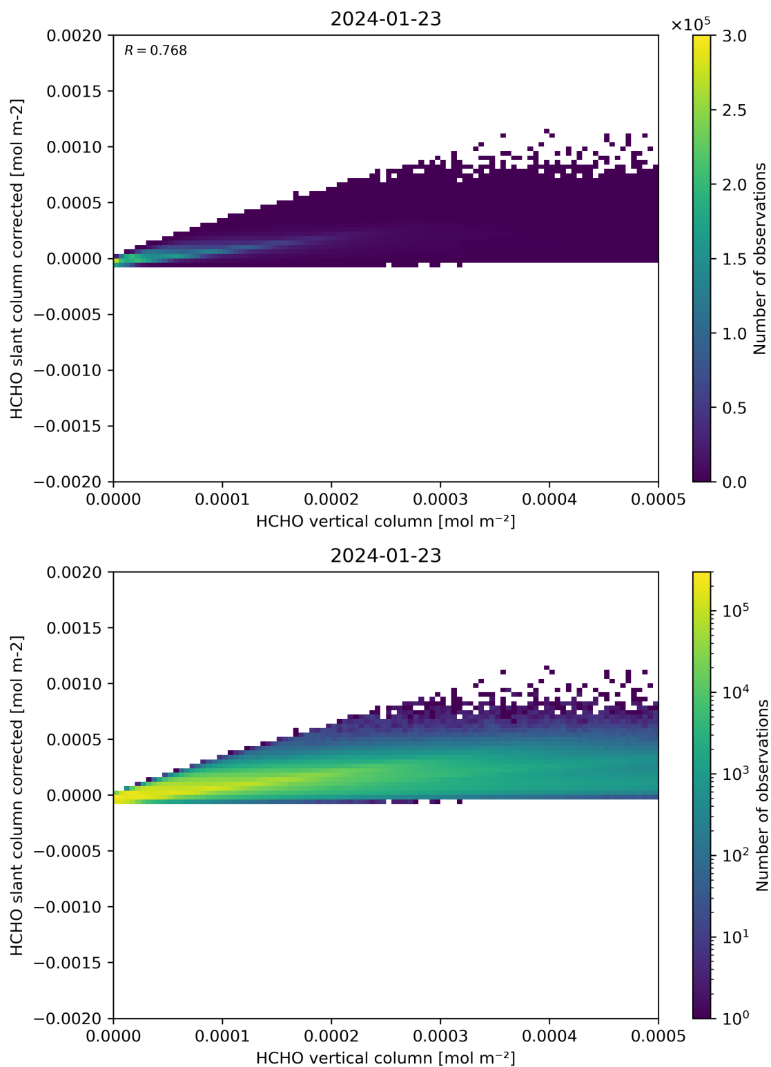
Figure 127: Scatter density plot of “HCHO vertical column” against “HCHO slant column corrected” for 2024-01-22 to 2024-01-24.
