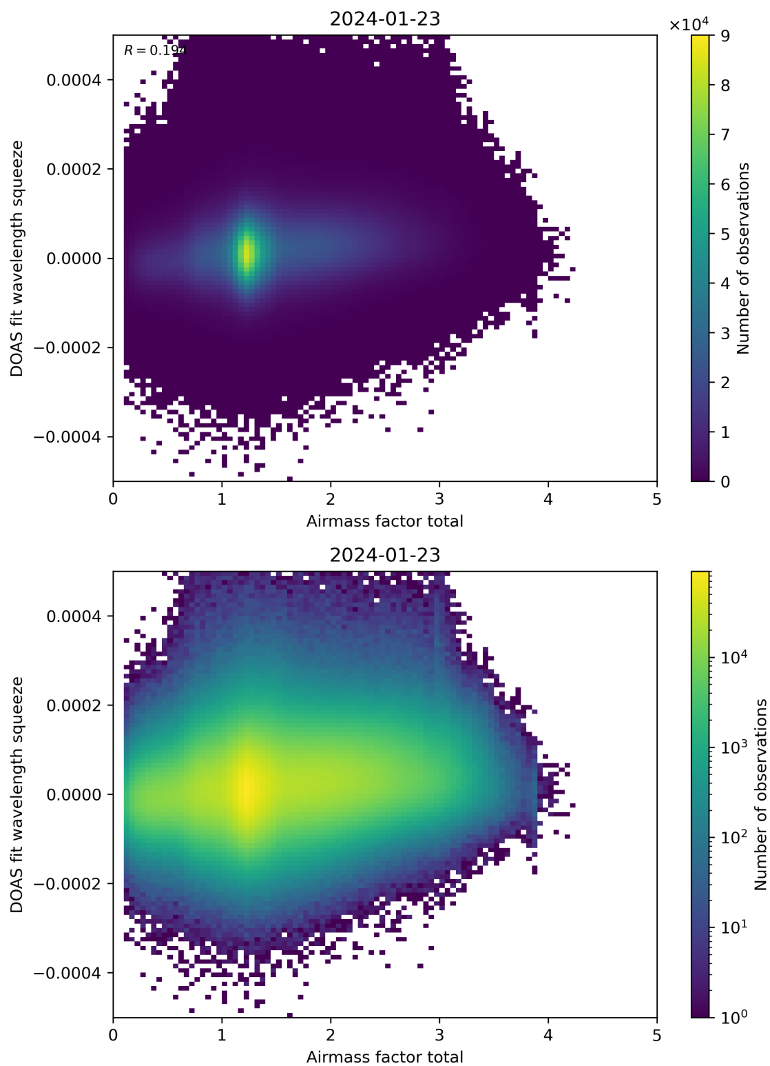
Figure 99: Scatter density plot of “Airmass factor total” against “DOAS fit wavelength squeeze” for 2024-01-22 to 2024-01-24.
