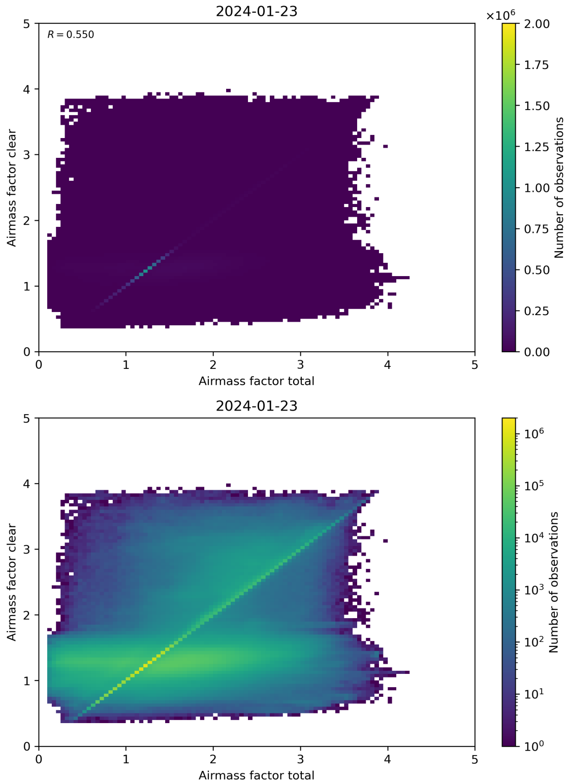
Figure 100: Scatter density plot of “Airmass factor total” against “Airmass factor clear” for 2024-01-22 to 2024-01-24.
