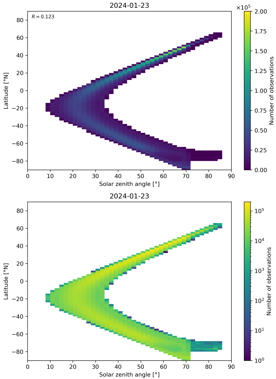
Figure 181: Scatter density plot of “Solar zenith angle” against “Latitude” for 2024-01-22 to 2024-01-24.
