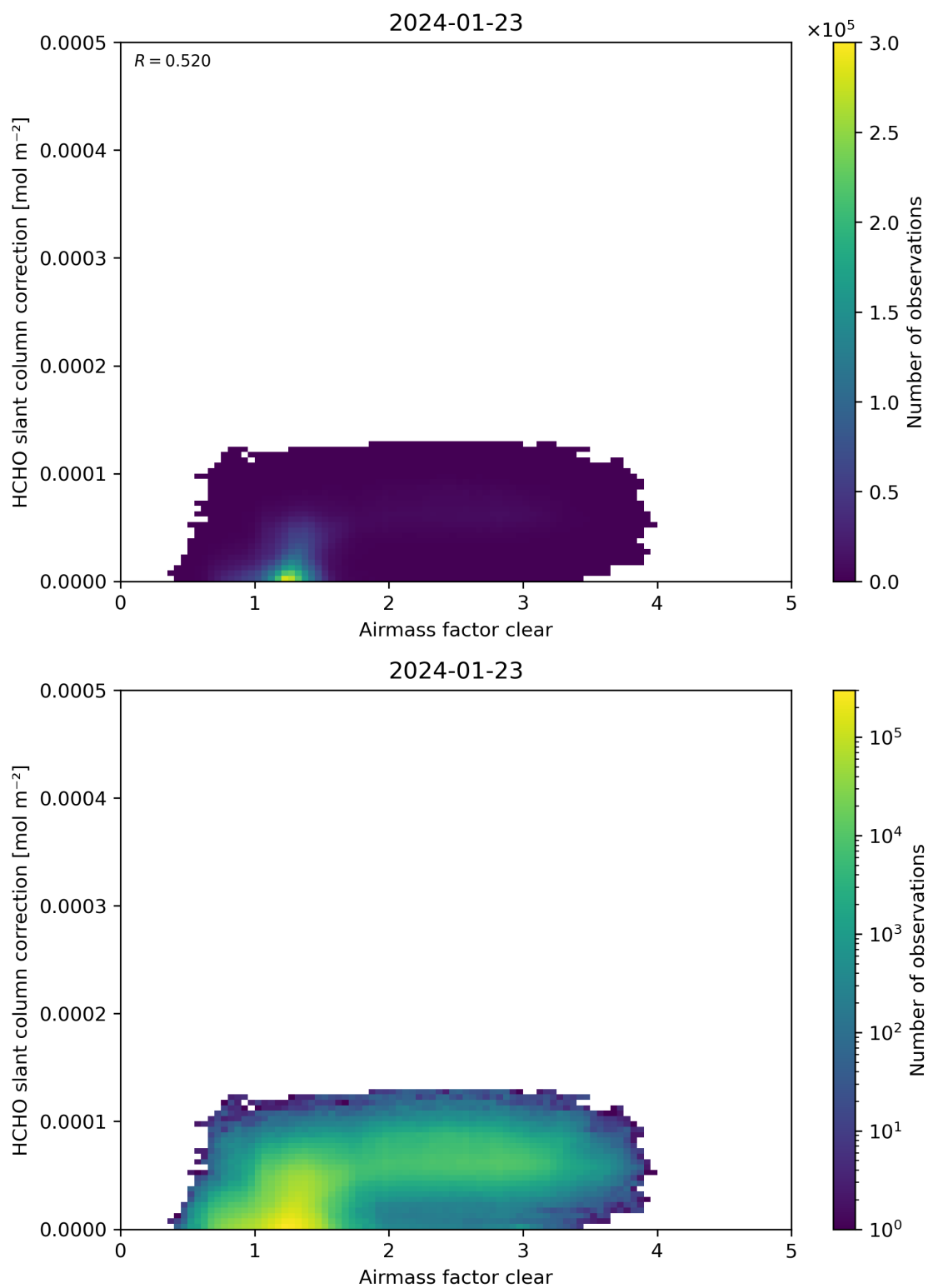
Figure 75: Scatter density plot of “Airmass factor clear” against “HCHO slant column correction” for 2024-01-22 to 2024-01-24.
