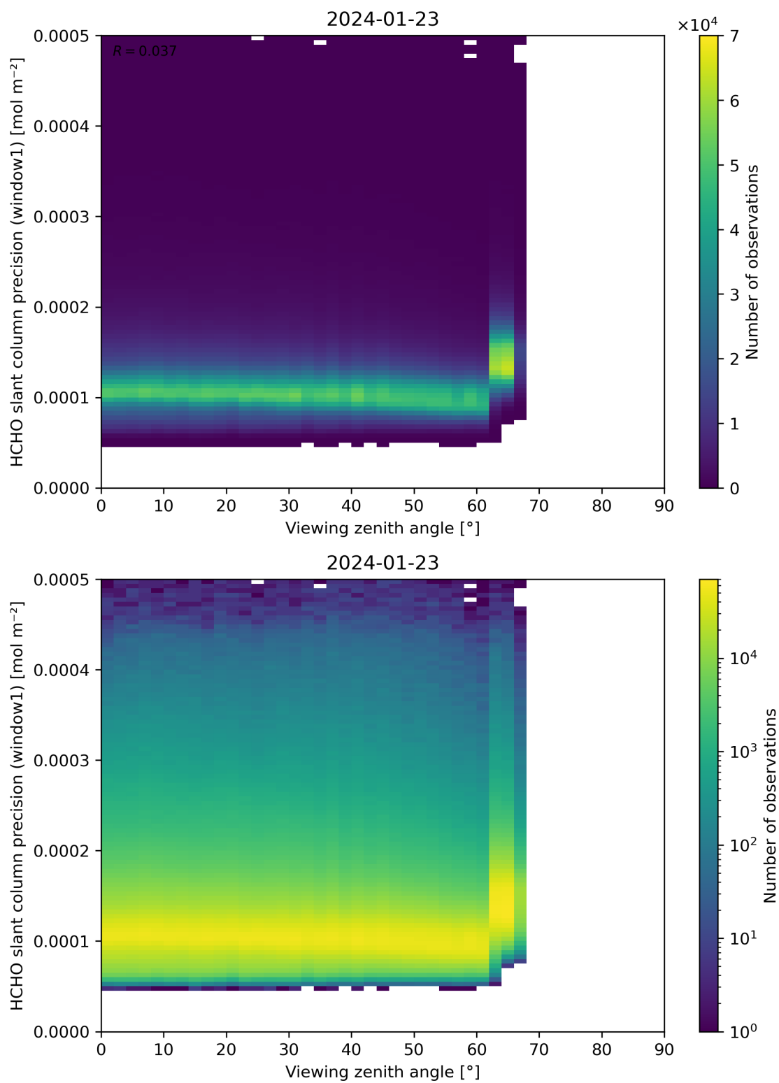
Figure 189: Scatter density plot of “Viewing zenith angle” against “HCHO slant column precision (window1)” for 2024-01-22 to 2024-01-24.
