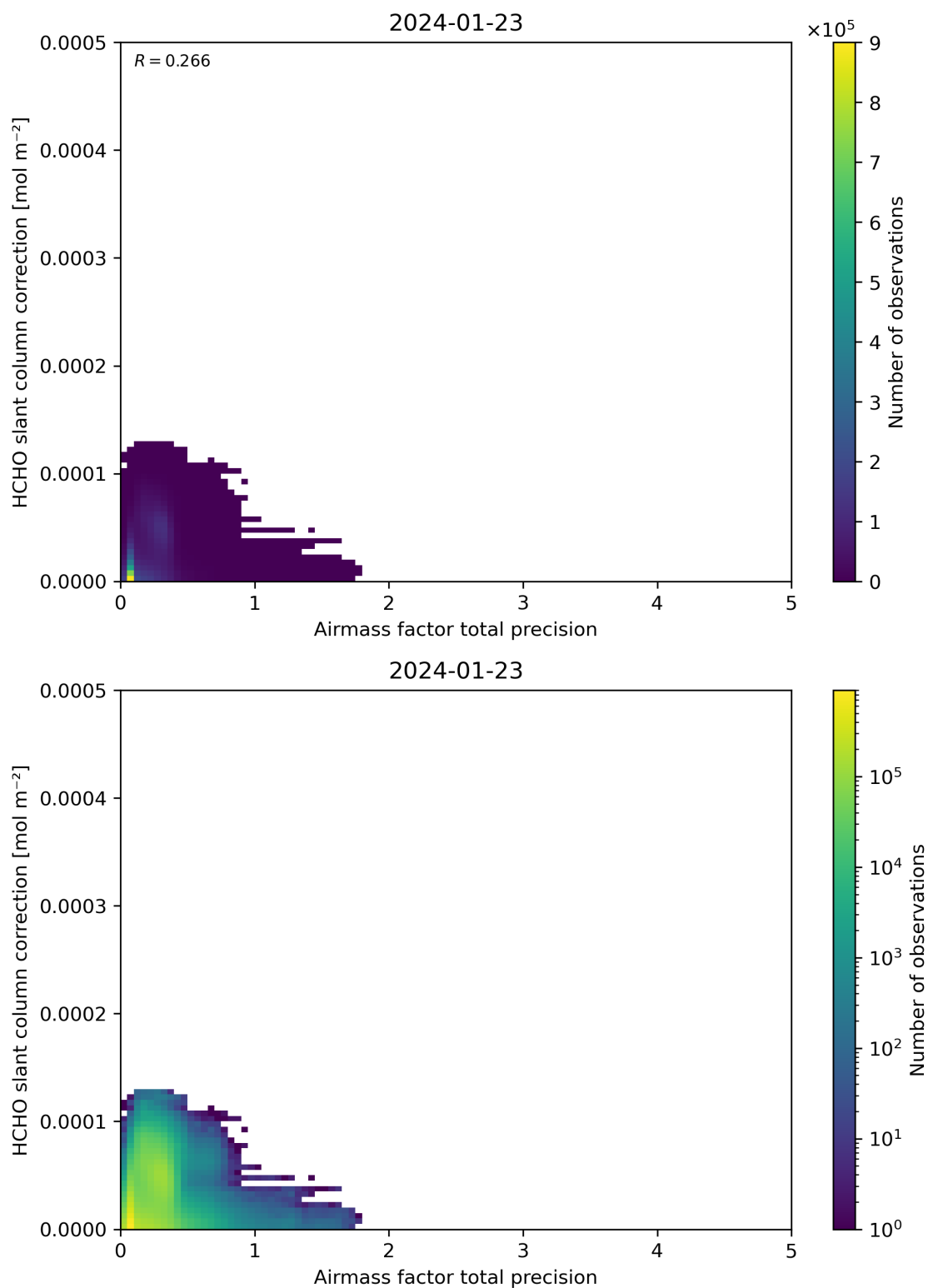
Figure 110: Scatter density plot of “Airmass factor total precision” against “HCHO slant column correction” for 2024-01-22 to 2024-01-24.
