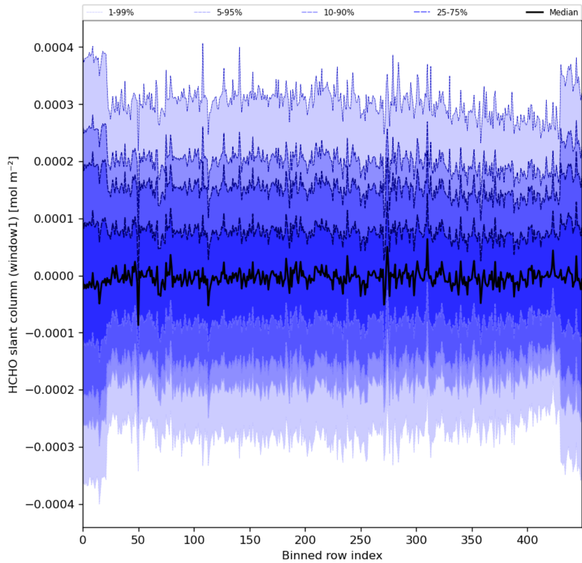
Figure 52: Along track statistics of “HCHO slant column (window1)” for 2024-01-22 to 2024-01-24
