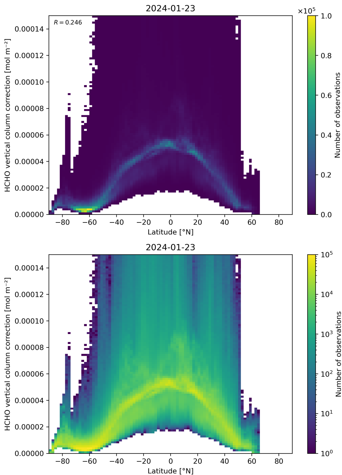
Figure 164: Scatter density plot of “Latitude” against “HCHO vertical column correction” for 2024-01-22 to 2024-01-24.
