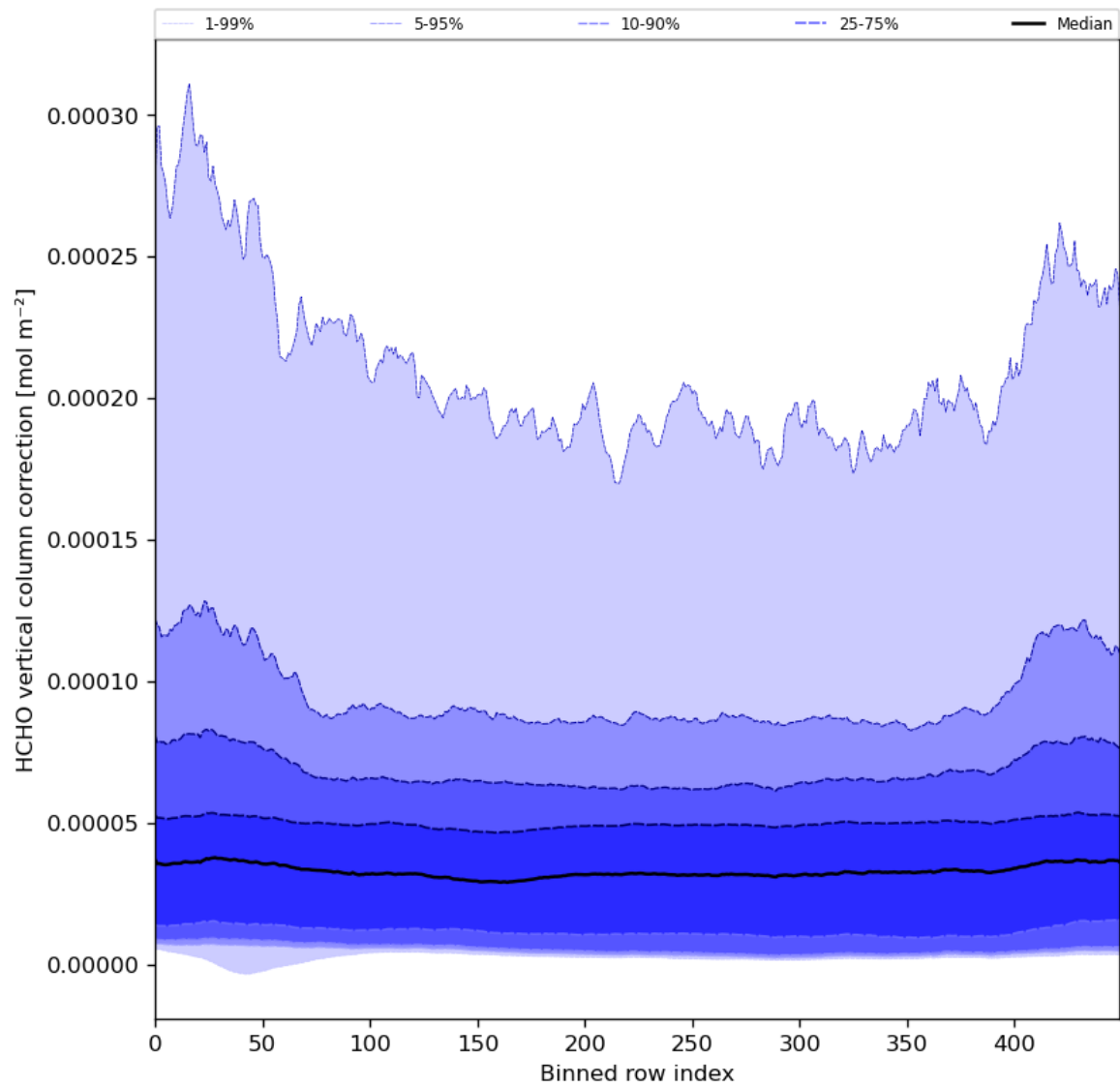
Figure 51: Along track statistics of “HCHO vertical column correction” for 2024-01-22 to 2024-01-24
