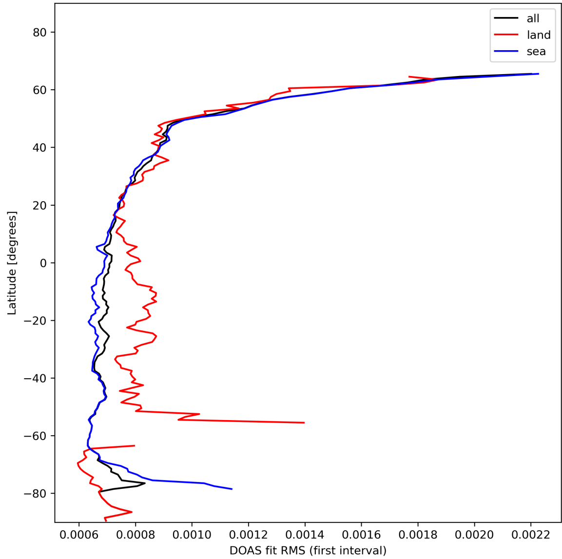
Figure 32: Zonal average of “DOAS fit RMS (first interval)” for 2024-01-22 to 2024-01-24.
