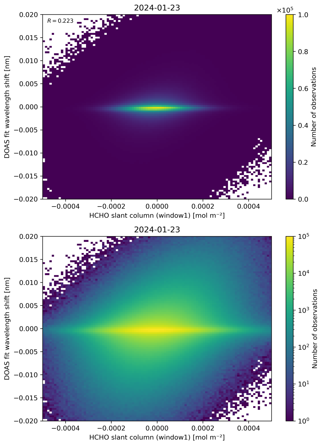
Figure 79: Scatter density plot of “HCHO slant column (window1)” against “DOAS fit wavelength shift” for 2024-01-22 to 2024-01-24.
