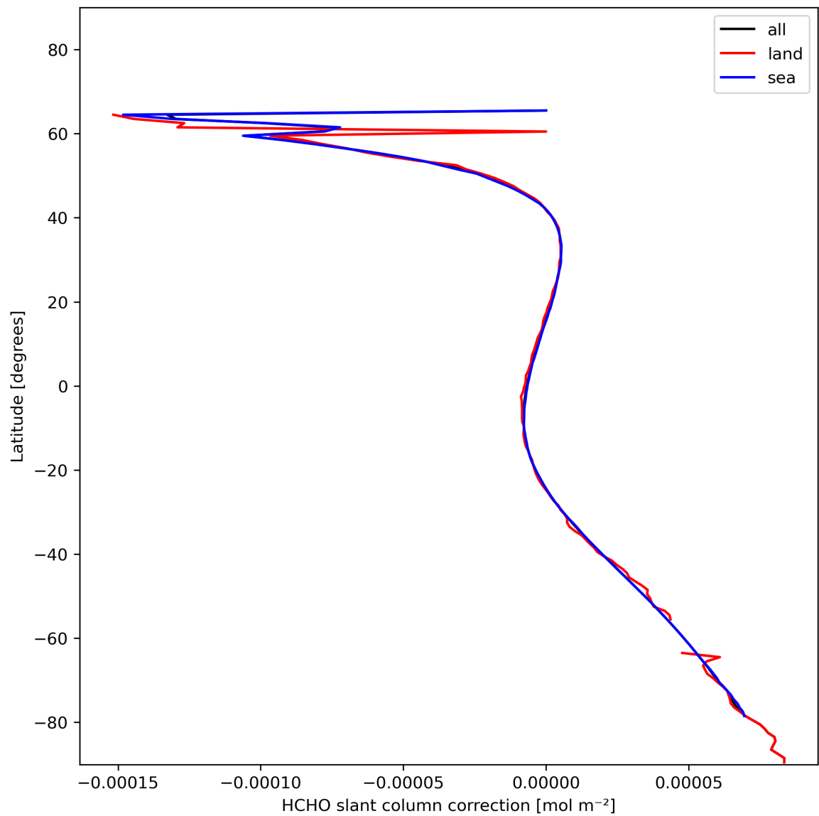
Figure 33: Zonal average of “HCHO slant column correction” for 2024-01-22 to 2024-01-24.
