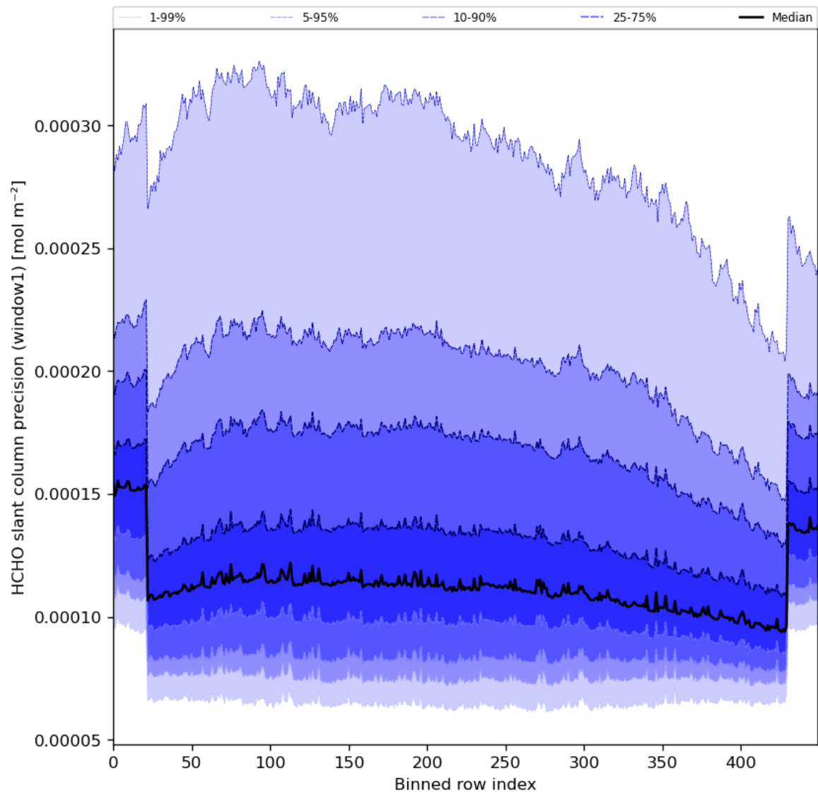
Figure 53: Along track statistics of “HCHO slant column precision (window1)” for 2024-01-22 to 2024-01-24
