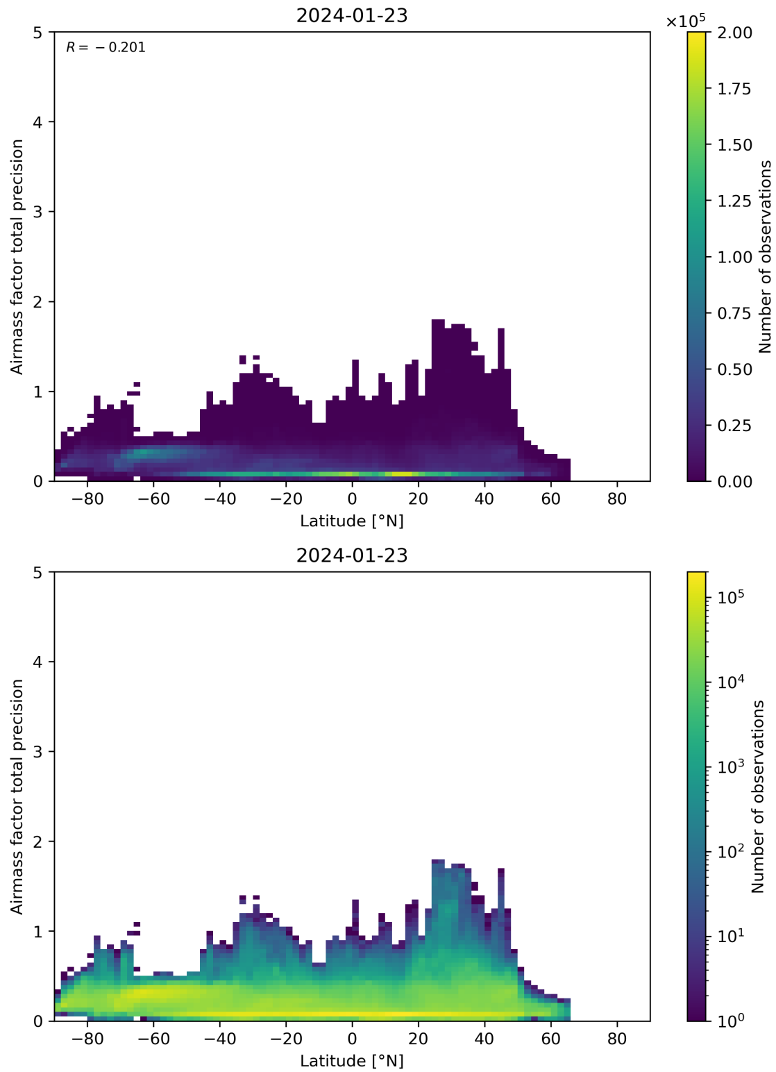
Figure 162: Scatter density plot of “Latitude” against “Airmass factor total precision” for 2024-01-22 to 2024-01-24.
