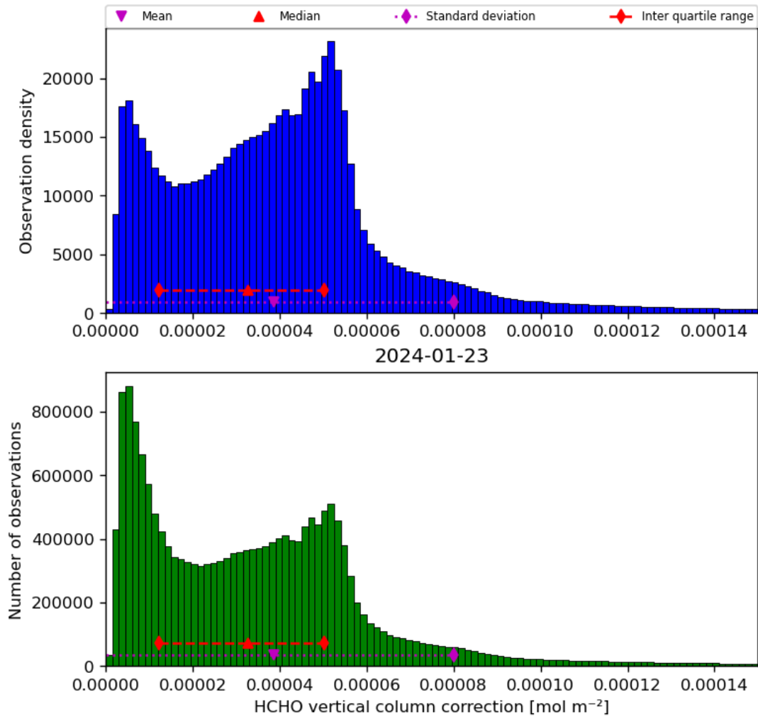
Figure 37: Histogram of “HCHO vertical column correction” for 2024-01-22 to 2024-01-24
