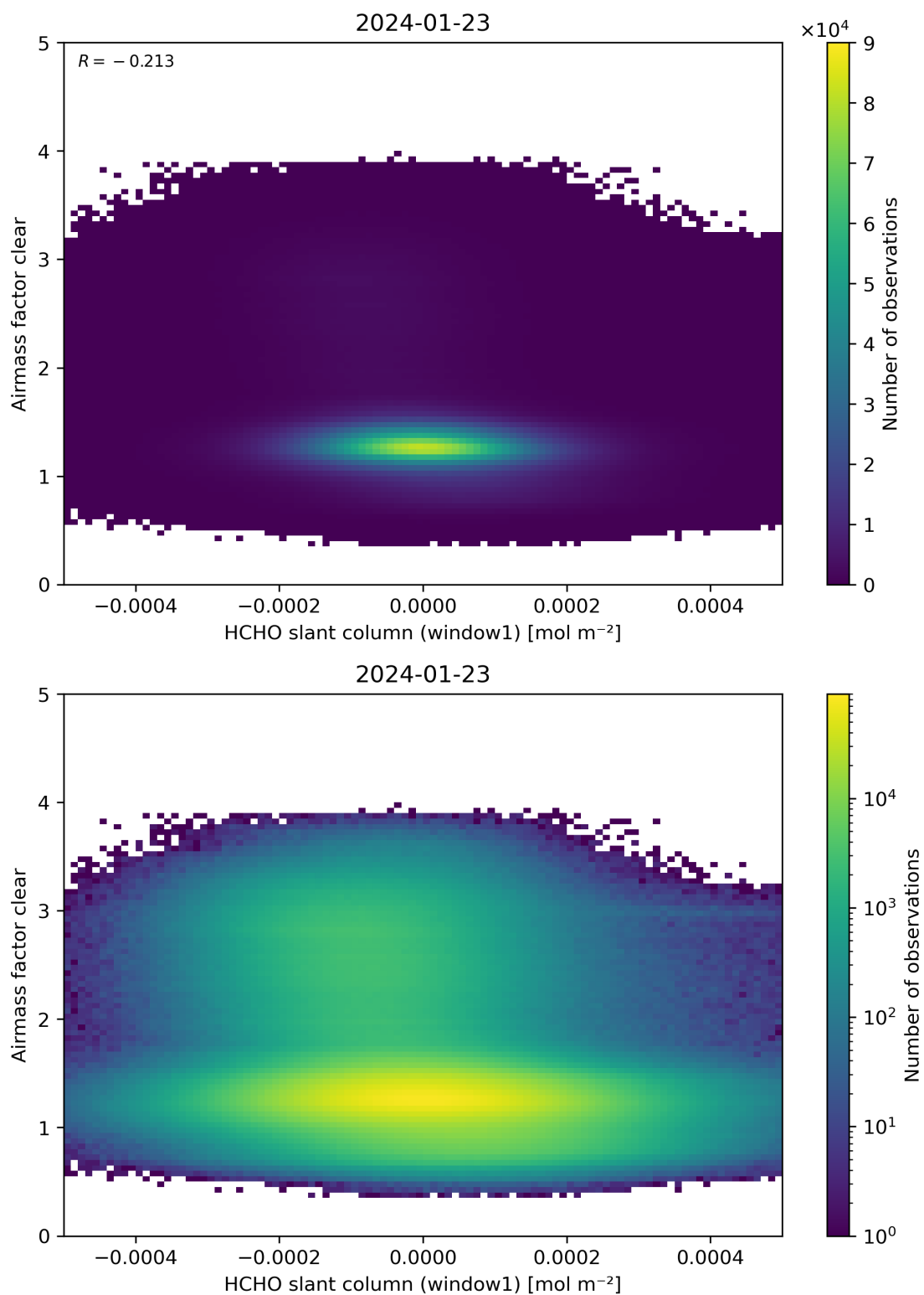
Figure 81: Scatter density plot of “HCHO slant column (window1)” against “Airmass factor clear” for 2024-01-22 to 2024-01-24.
