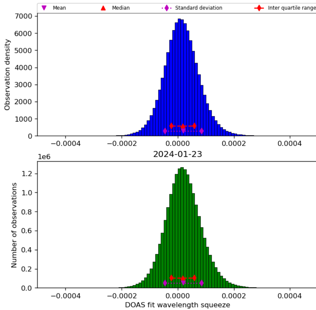
Figure 45: Histogram of “DOAS fit wavelength squeeze” for 2024-01-22 to 2024-01-24
