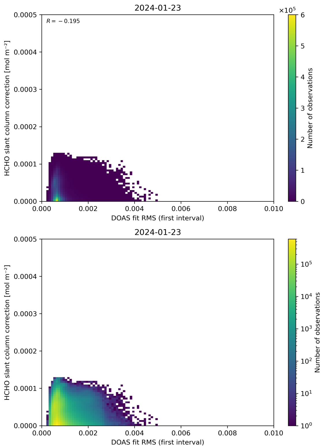
Figure 63: Scatter density plot of “DOAS fit RMS (first interval)” against “HCHO slant column correction” for 2024-01-22 to 2024-01-24.
