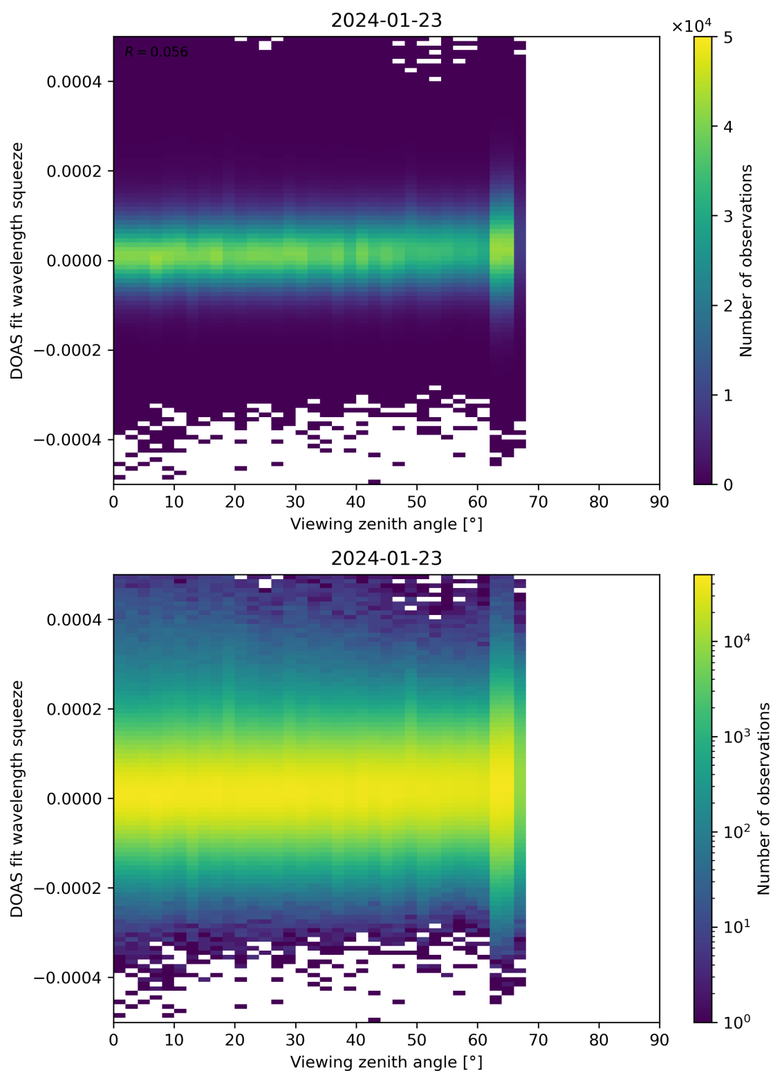
Figure 184: Scatter density plot of “Viewing zenith angle” against “DOAS fit wavelength squeeze” for 2024-01-22 to 2024-01-24.
