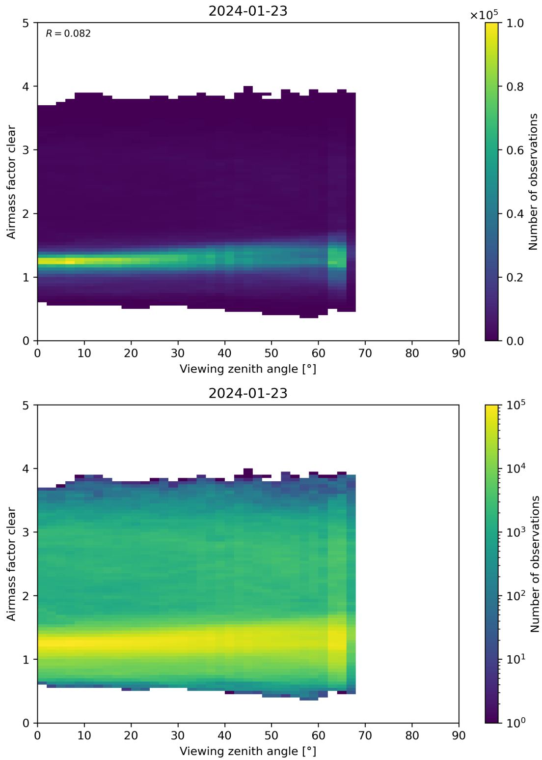
Figure 185: Scatter density plot of “Viewing zenith angle” against “Airmass factor clear” for 2024-01-22 to 2024-01-24.
