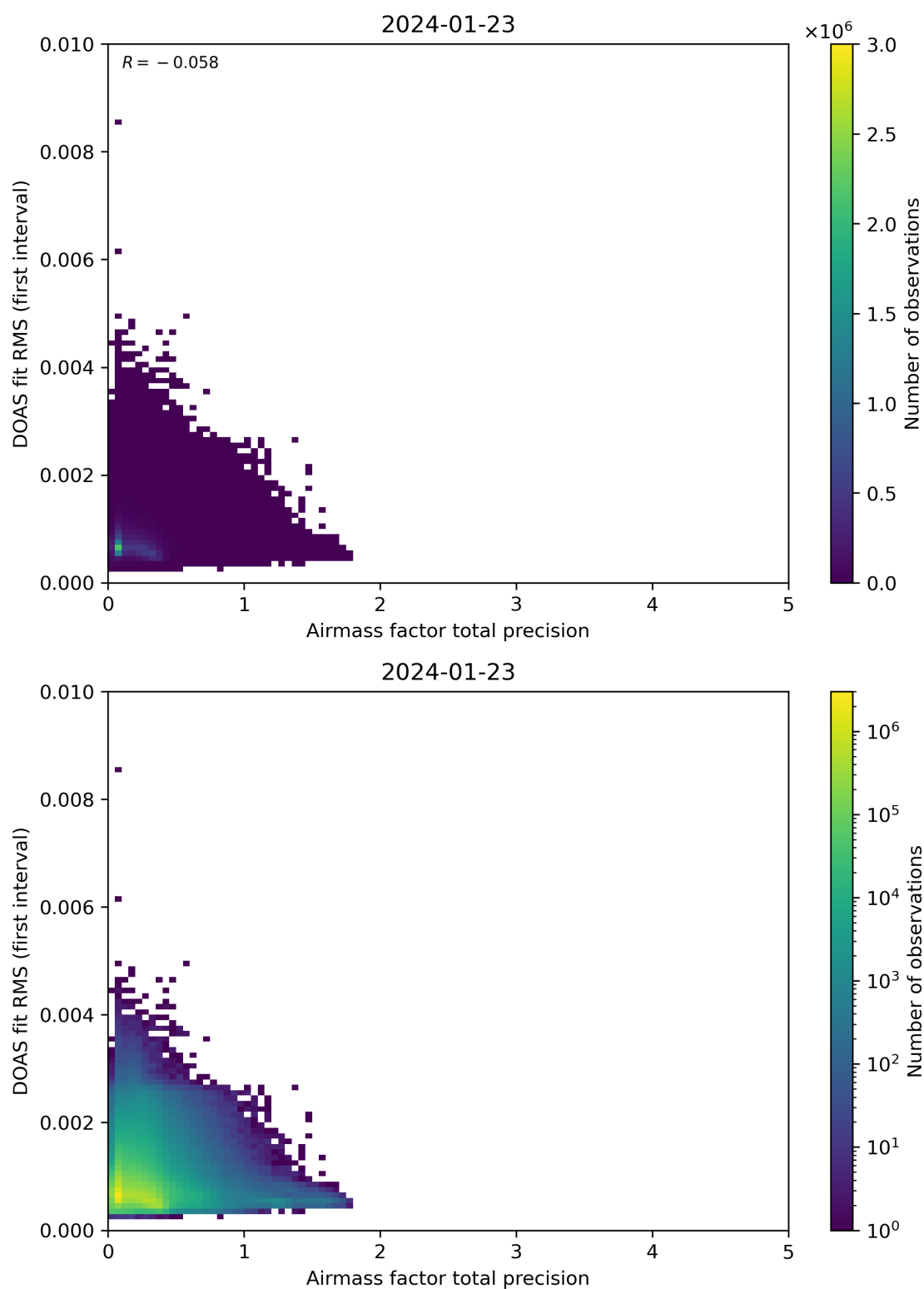
Figure 105: Scatter density plot of “Airmass factor total precision” against “DOAS fit RMS (first interval)” for 2024-01-22 to 2024-01-24.
