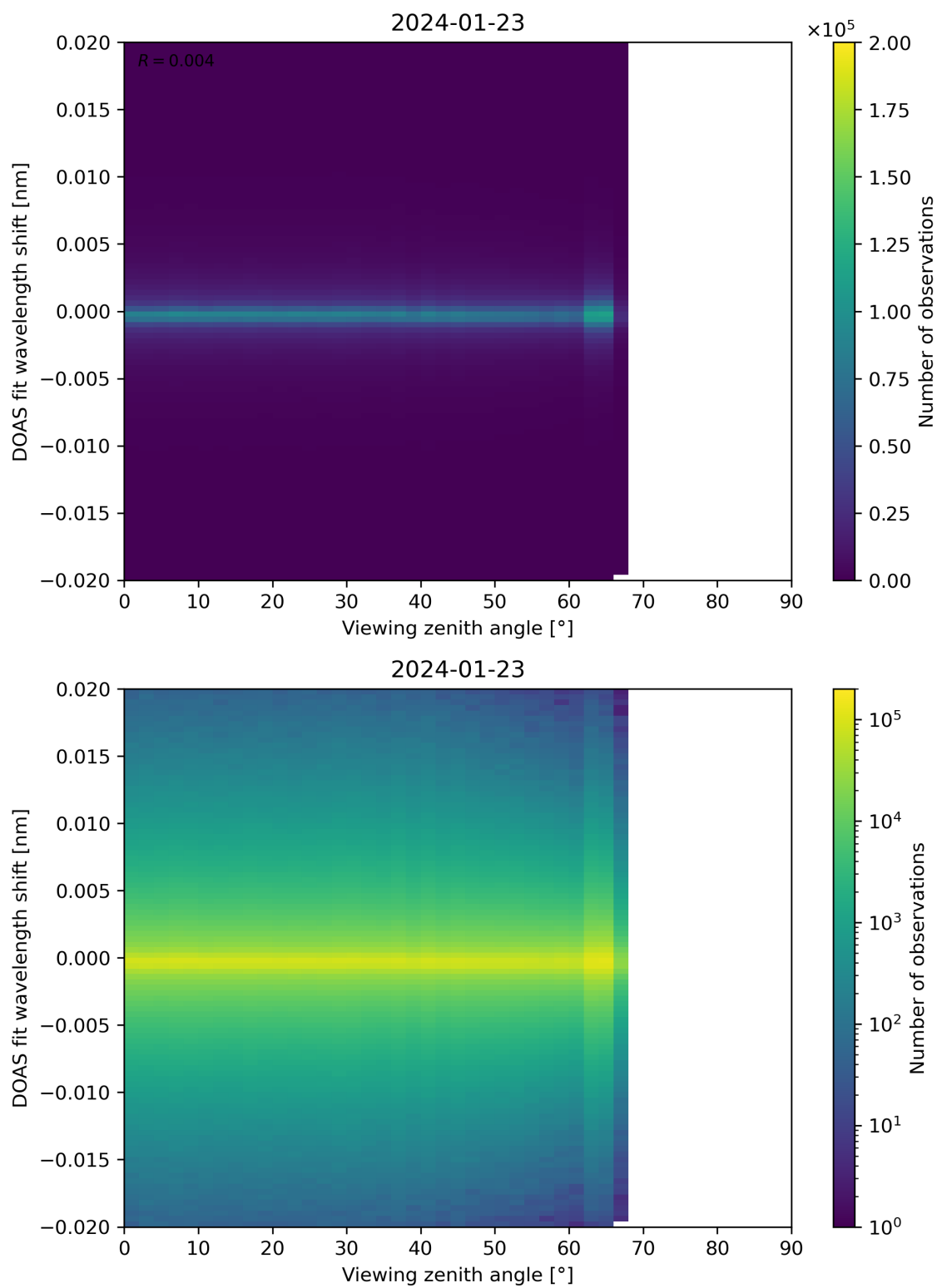
Figure 183: Scatter density plot of “Viewing zenith angle” against “DOAS fit wavelength shift” for 2024-01-22 to 2024-01-24.
