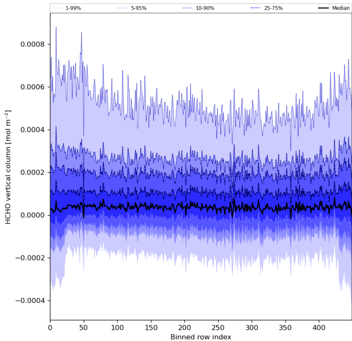
Figure 49: Along track statistics of “HCHO vertical column” for 2024-01-22 to 2024-01-24
