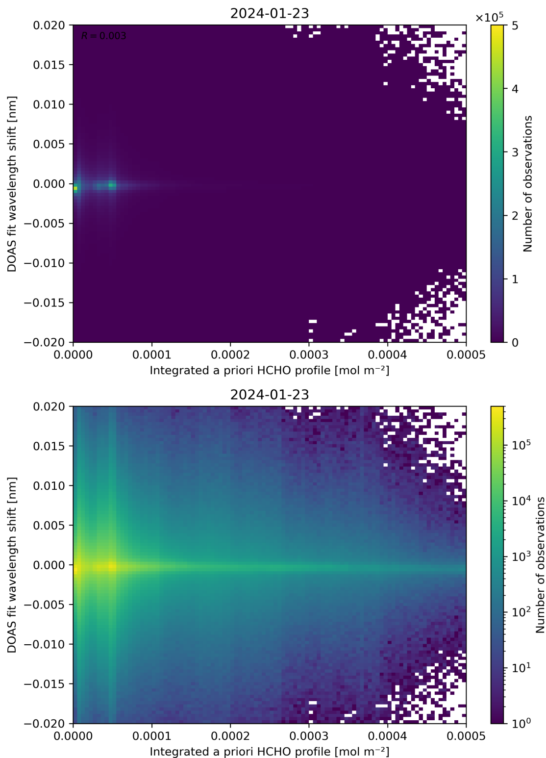
Figure 149: Scatter density plot of “Integrated a priori HCHO profile” against “DOAS fit wavelength shift” for 2024-01-22 to 2024-01-24.
