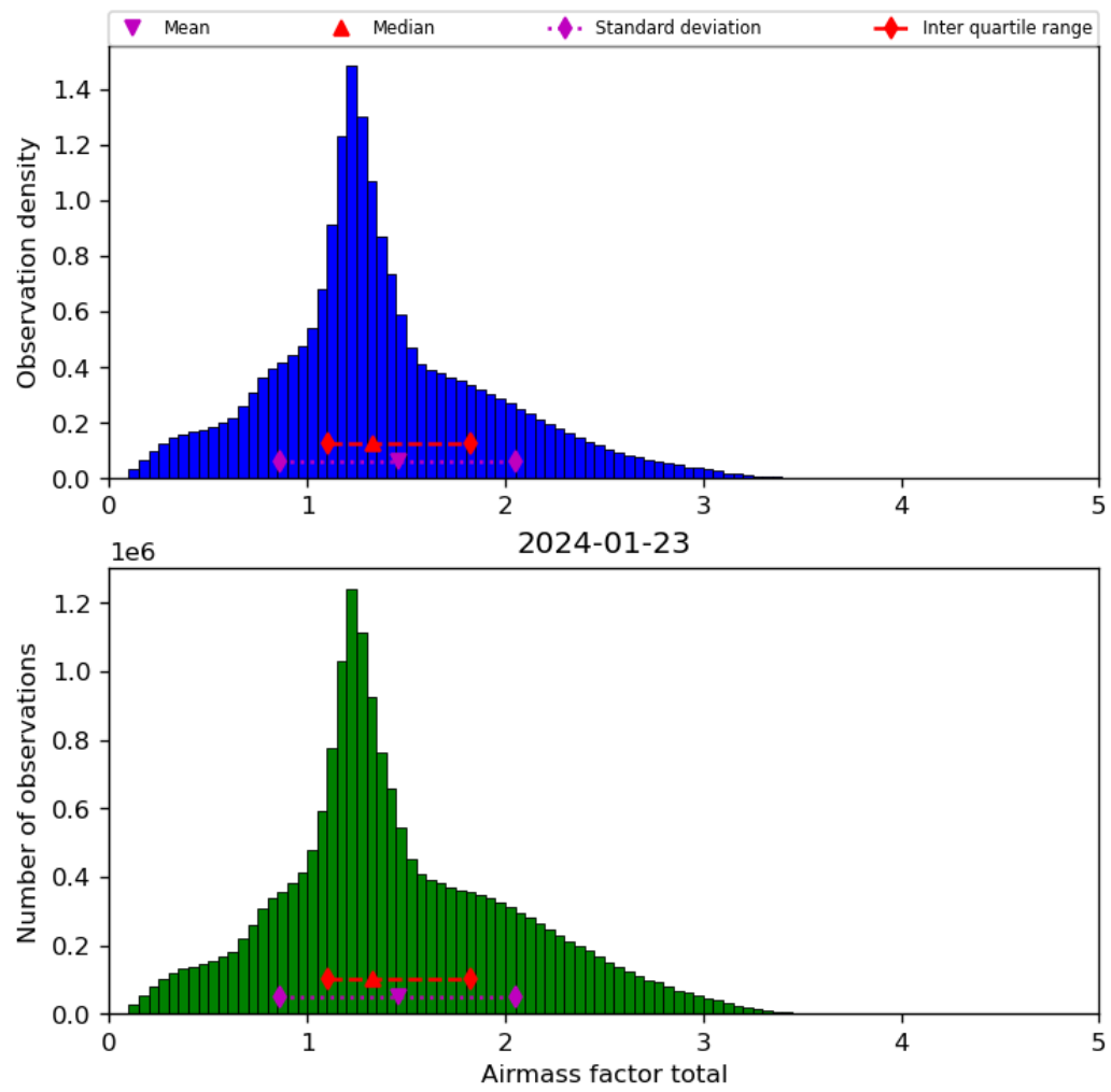
Figure 40: Histogram of “Airmass factor total” for 2024-01-22 to 2024-01-24
