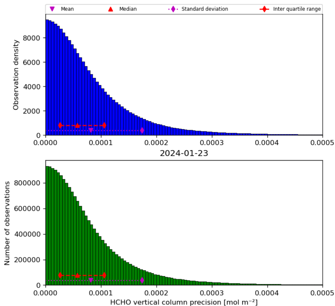
Figure 36: Histogram of “HCHO vertical column precision” for 2024-01-22 to 2024-01-24
