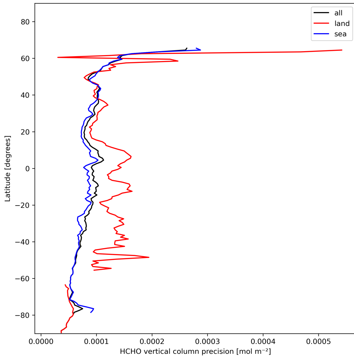
Figure 22: Zonal average of “HCHO vertical column precision” for 2024-01-22 to 2024-01-24.
