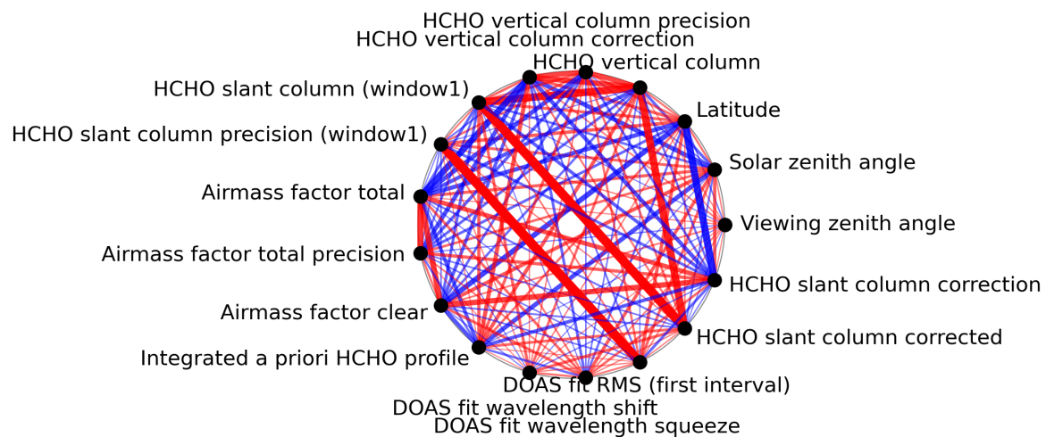
Figure 1: Map of correlation graph for 2024-01-22 to 2024-01-24.
