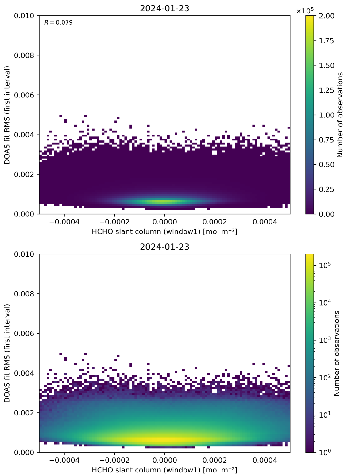
Figure 78: Scatter density plot of “HCHO slant column (window1)” against “DOAS fit RMS (first interval)” for 2024-01-22 to 2024-01-24.
