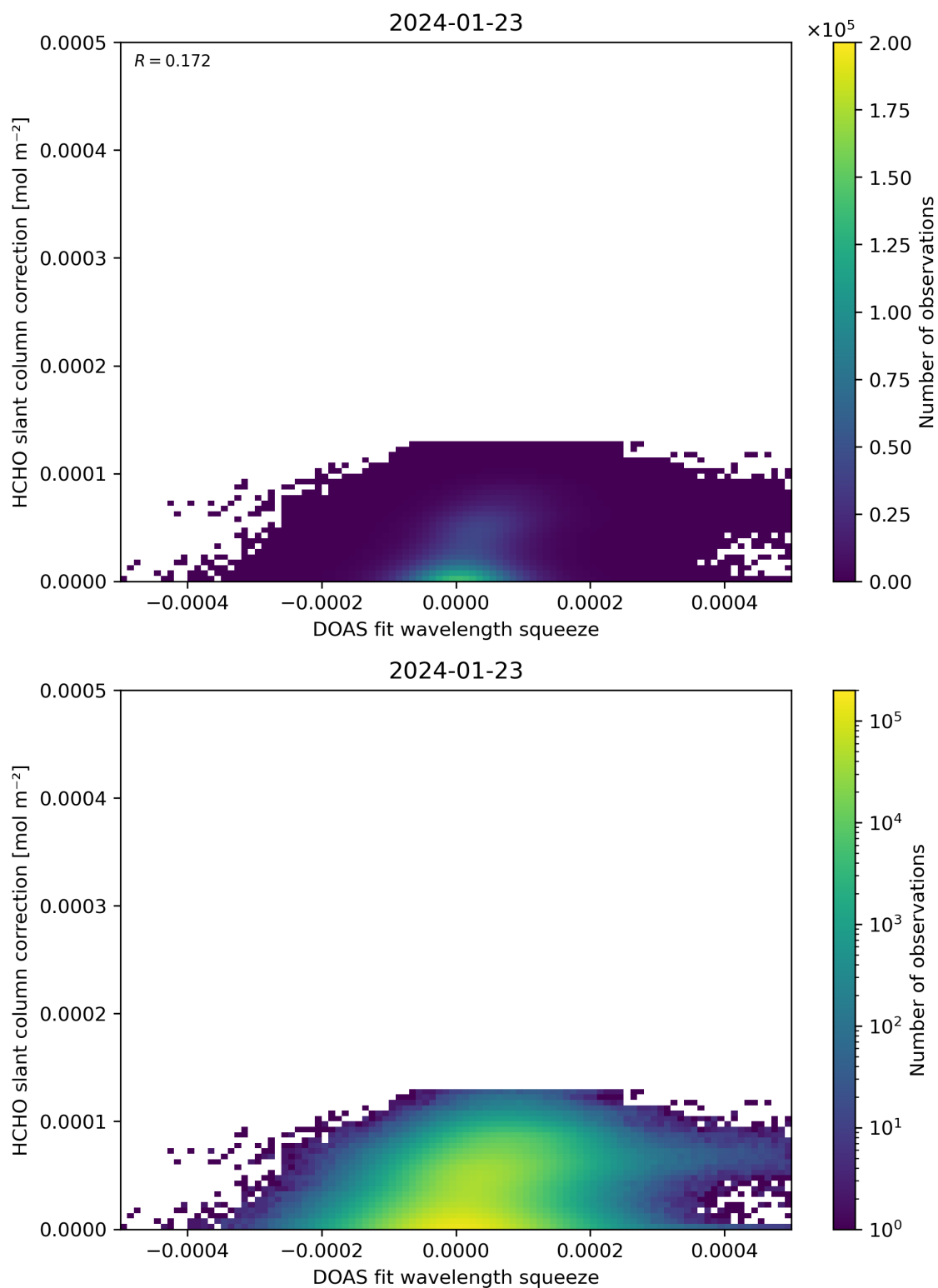
Figure 70: Scatter density plot of “DOAS fit wavelength squeeze” against “HCHO slant column correction” for 2024-01-22 to 2024-01-24.
