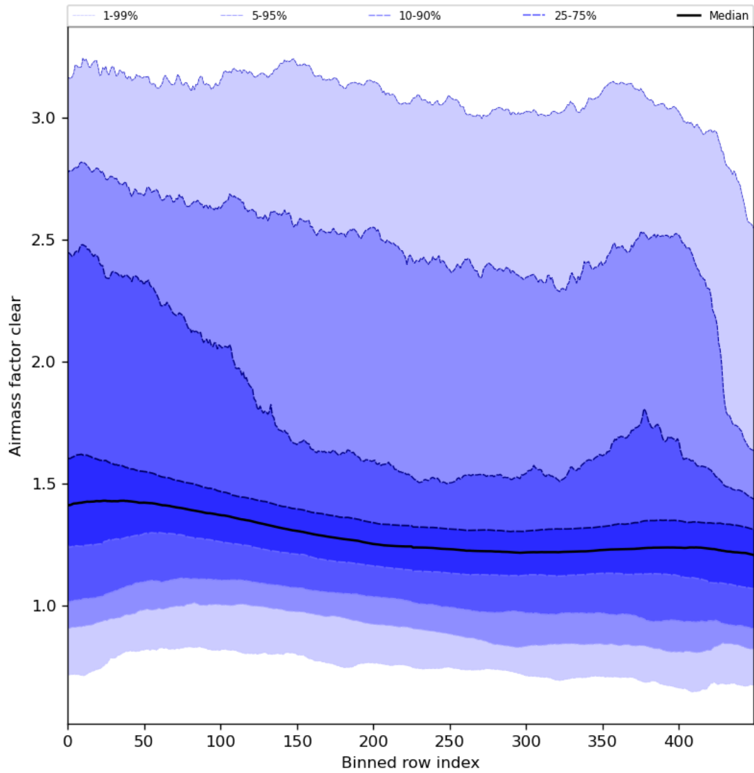
Figure 56: Along track statistics of “Airmass factor clear” for 2024-01-22 to 2024-01-24
