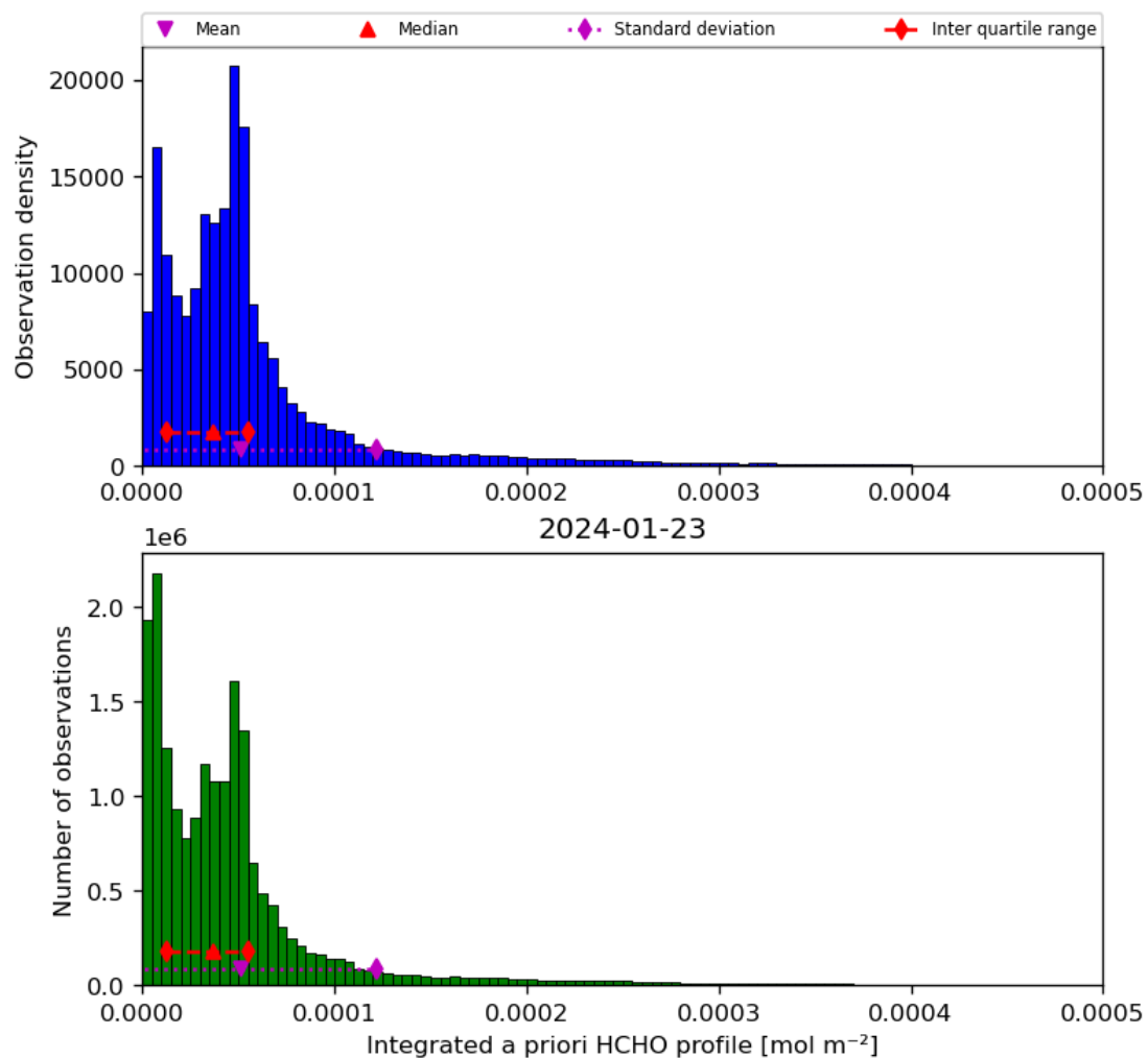
Figure 43: Histogram of “Integrated a priori HCHO profile” for 2024-01-22 to 2024-01-24
