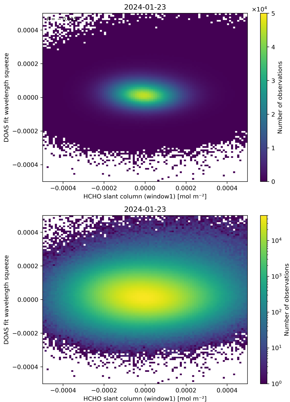
Figure 80: Scatter density plot of “HCHO slant column (window1)” against “DOAS fit wavelength squeeze” for 2024-01-22 to 2024-01-24.
