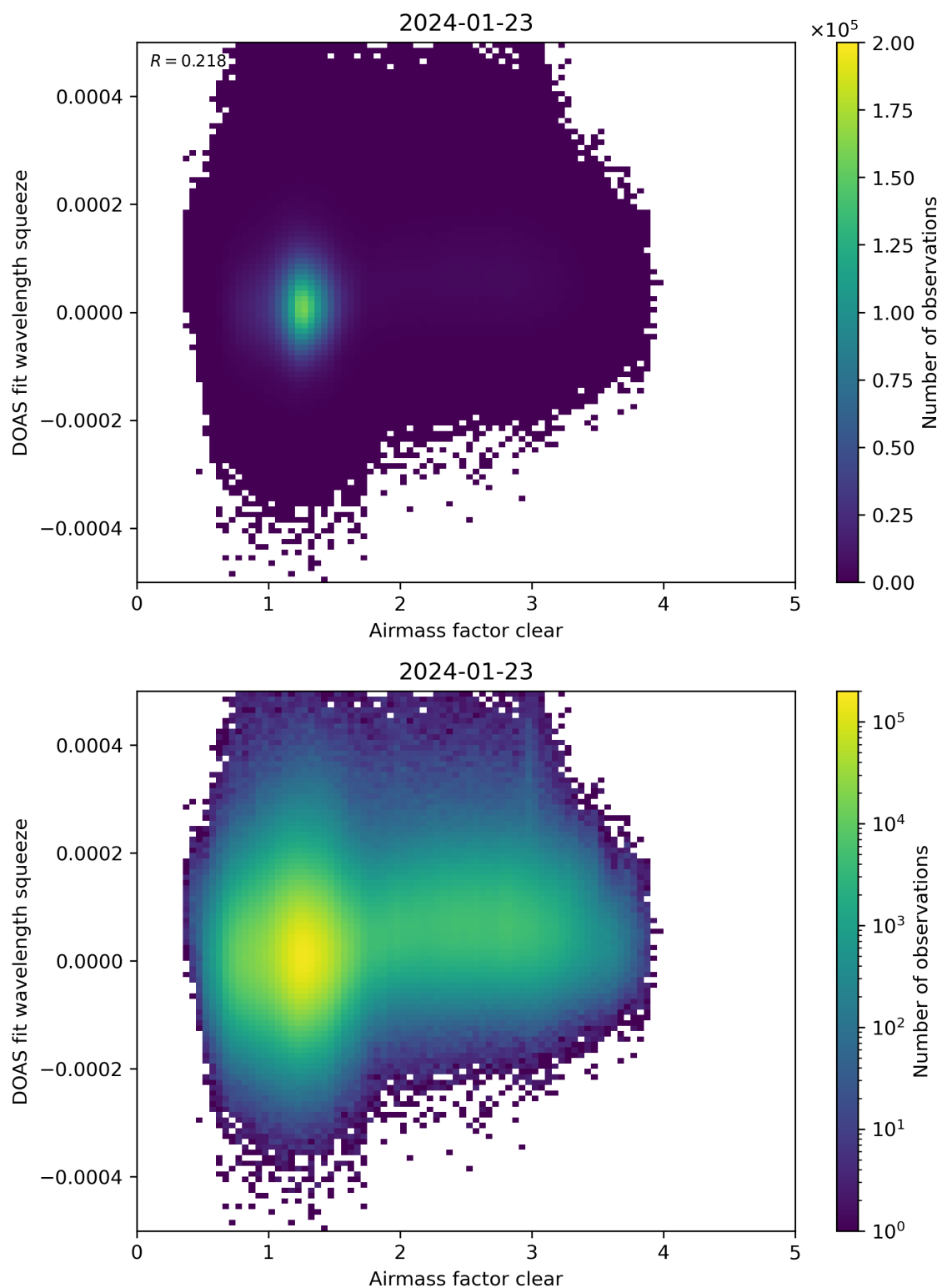
Figure 73: Scatter density plot of “Airmass factor clear” against “DOAS fit wavelength squeeze” for 2024-01-22 to 2024-01-24.
