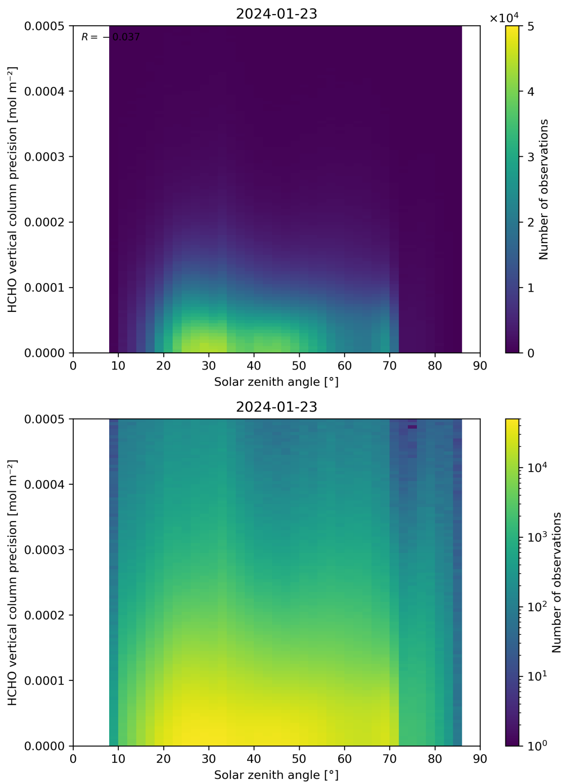
Figure 179: Scatter density plot of “Solar zenith angle” against “HCHO vertical column precision” for 2024-01-22 to 2024-01-24.
