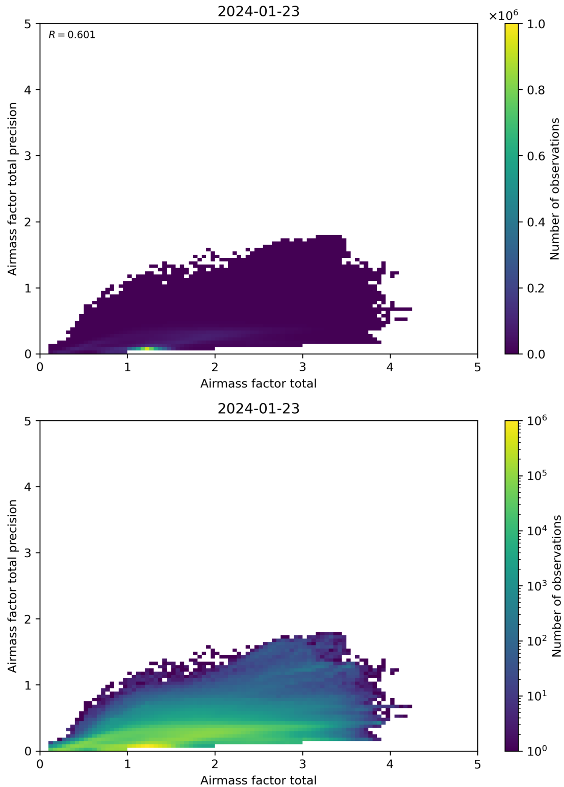
Figure 103: Scatter density plot of “Airmass factor total” against “Airmass factor total precision” for 2024-01-22 to 2024-01-24.
