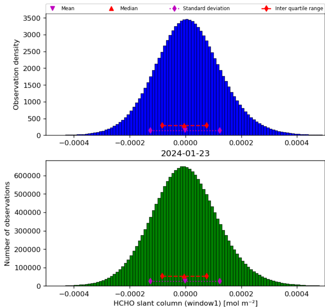
Figure 38: Histogram of “HCHO slant column (window1)” for 2024-01-22 to 2024-01-24
