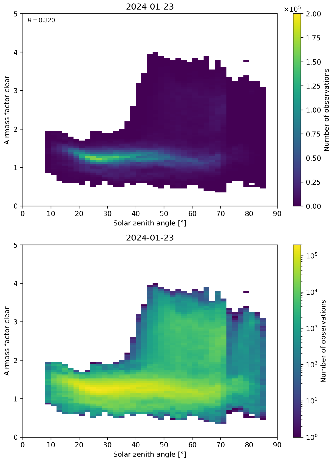
Figure 170: Scatter density plot of “Solar zenith angle” against “Airmass factor clear” for 2024-01-22 to 2024-01-24.
