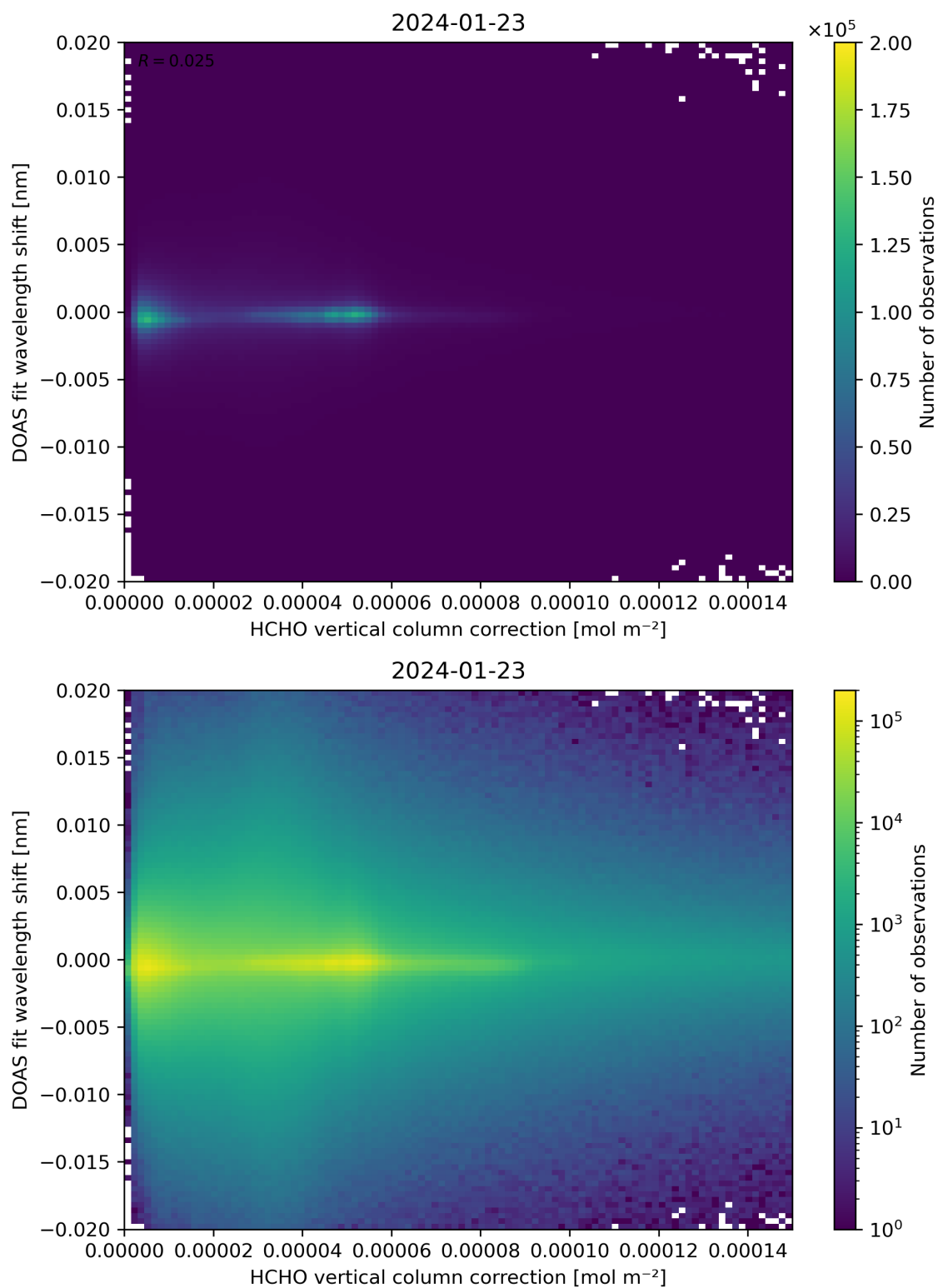
Figure 113: Scatter density plot of “HCHO vertical column correction” against “DOAS fit wavelength shift” for 2024-01-22 to 2024-01-24.
