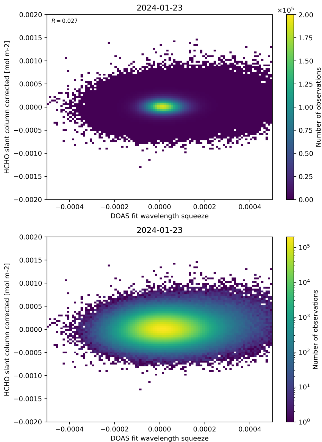
Figure 69: Scatter density plot of “DOAS fit wavelength squeeze” against “HCHO slant column corrected” for 2024-01-22 to 2024-01-24.
