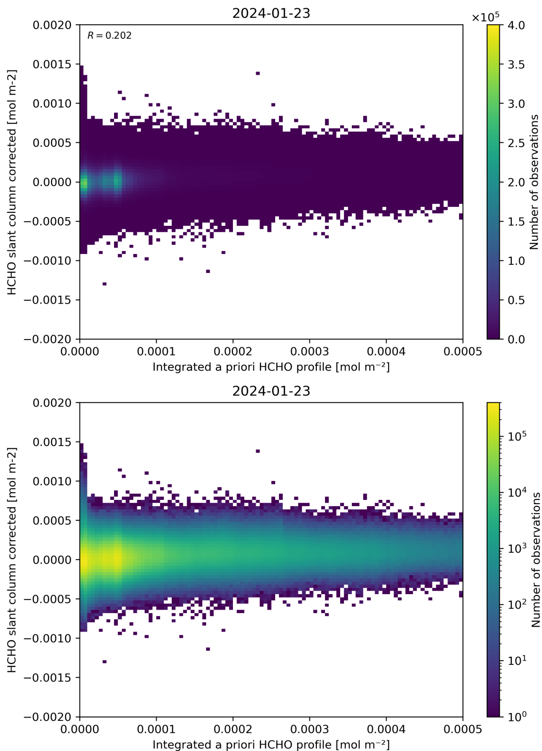
Figure 151: Scatter density plot of “Integrated a priori HCHO profile” against “HCHO slant column corrected” for 2024-01-22 to 2024-01-24.
