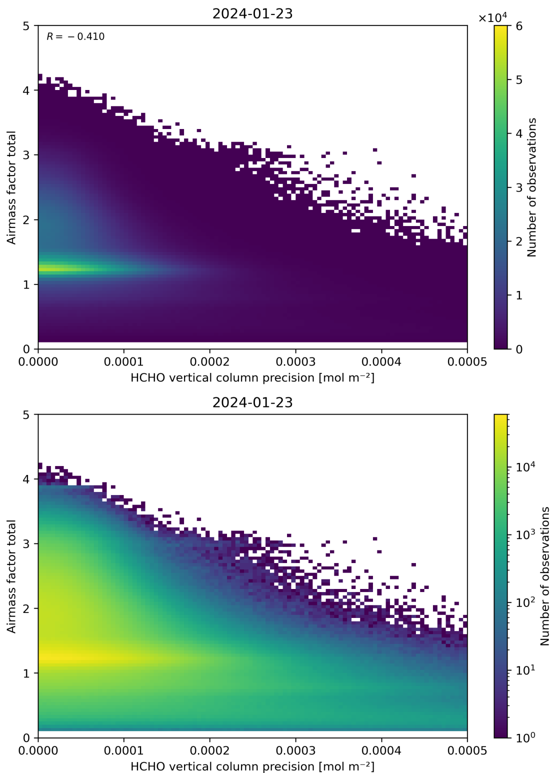
Figure 144: Scatter density plot of “HCHO vertical column precision” against “Airmass factor total” for 2024-01-22 to 2024-01-24.
