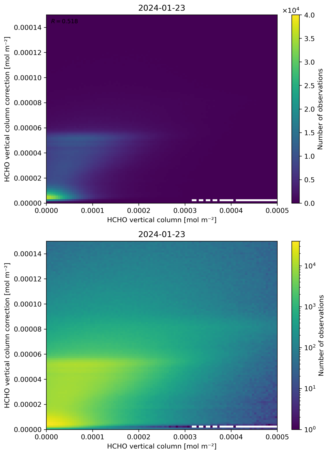
Figure 133: Scatter density plot of “HCHO vertical column” against “HCHO vertical column correction” for 2024-01-22 to 2024-01-24.
