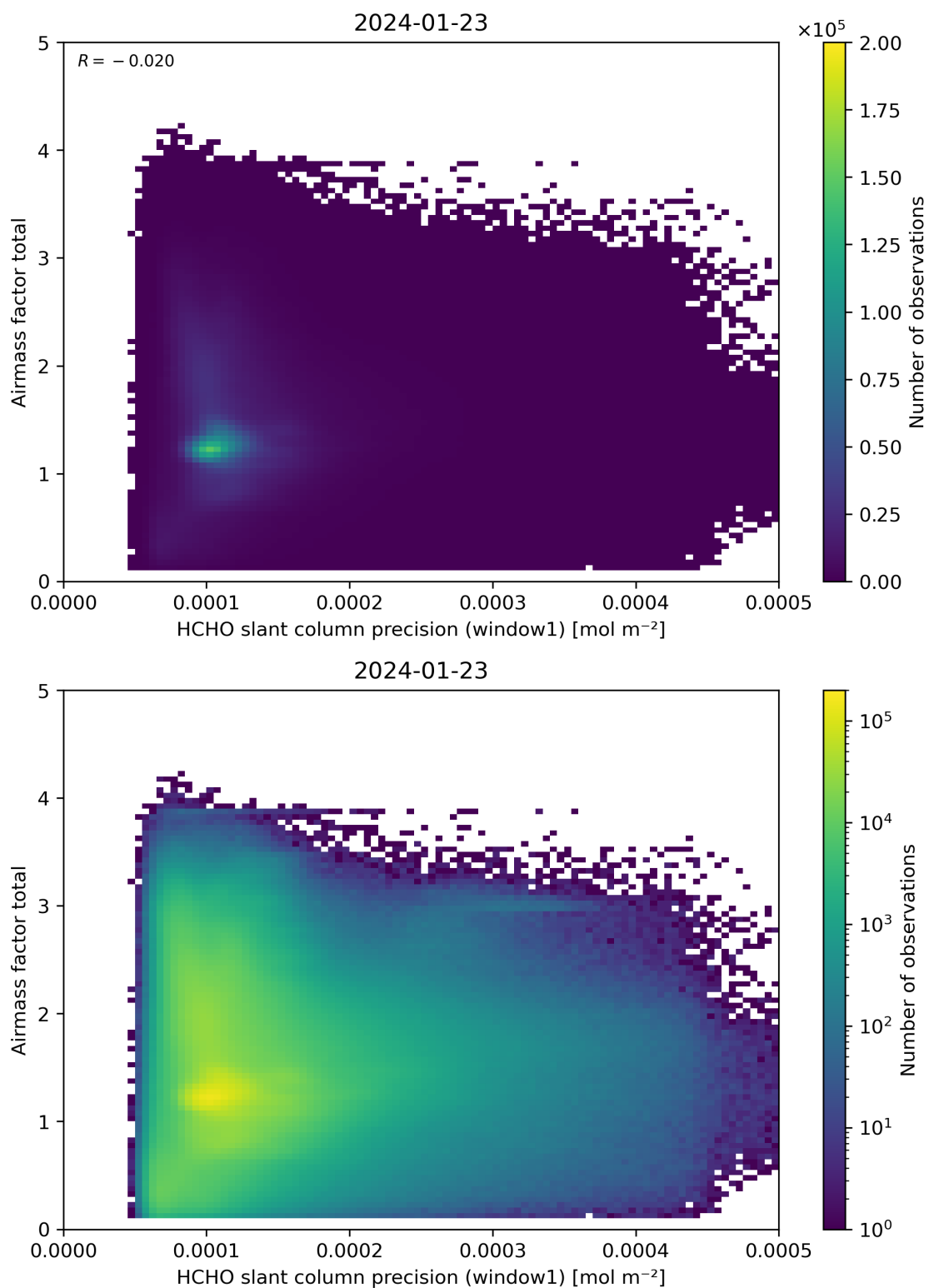
Figure 94: Scatter density plot of “HCHO slant column precision (window1)” against “Airmass factor total” for 2024-01-22 to 2024-01-24.
