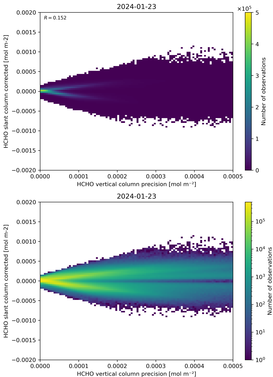
Figure 140: Scatter density plot of “HCHO vertical column precision” against “HCHO slant column corrected” for 2024-01-22 to 2024-01-24.
