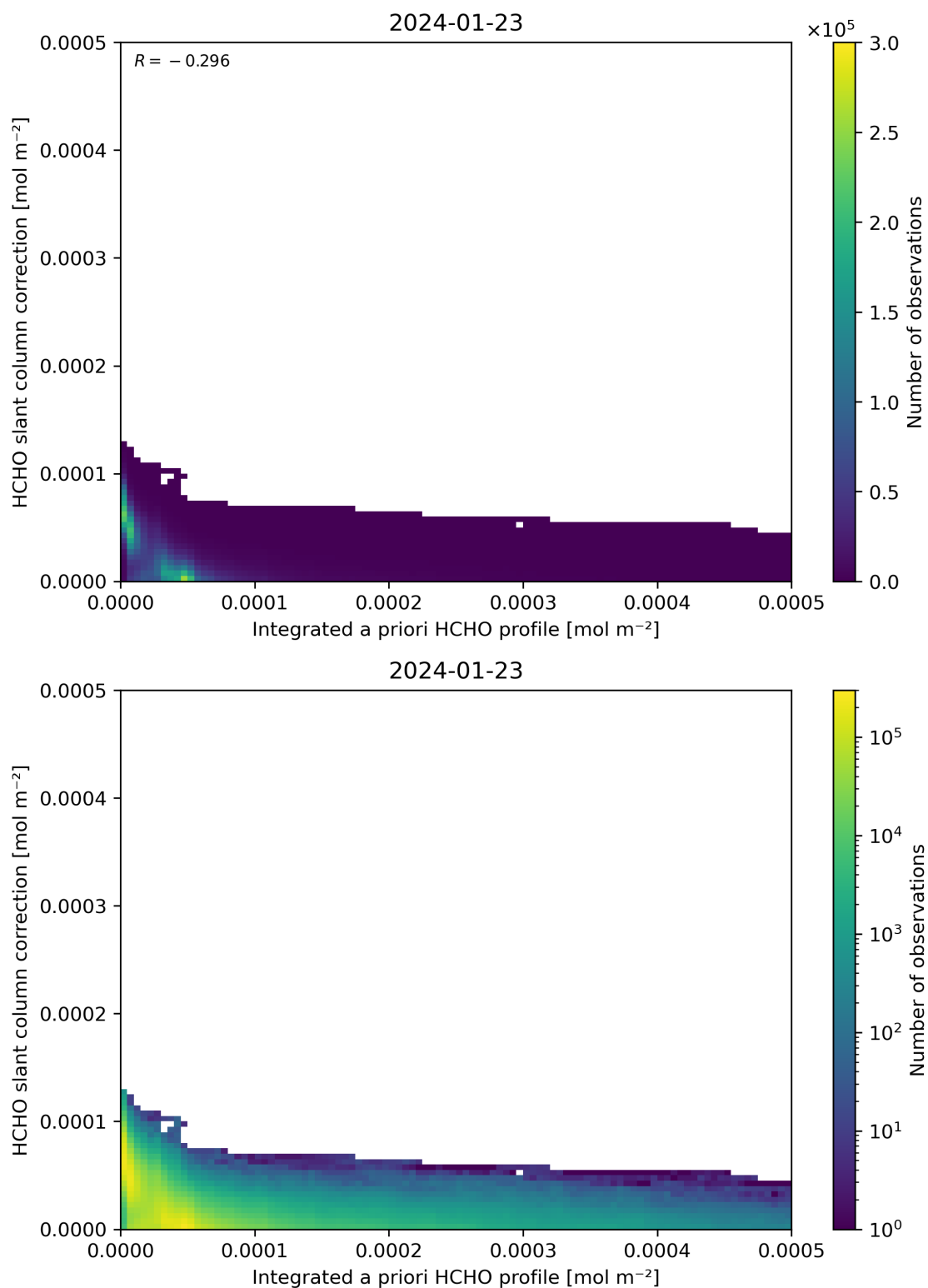
Figure 152: Scatter density plot of “Integrated a priori HCHO profile” against “HCHO slant column correction” for 2024-01-22 to 2024-01-24.
