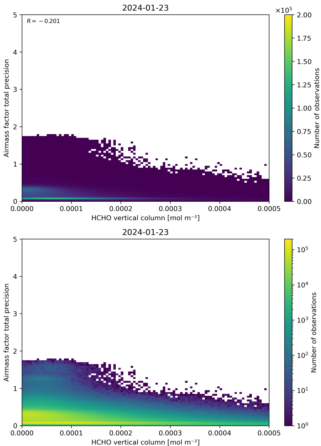
Figure 132: Scatter density plot of “HCHO vertical column” against “Airmass factor total precision” for 2024-01-22 to 2024-01-24.
