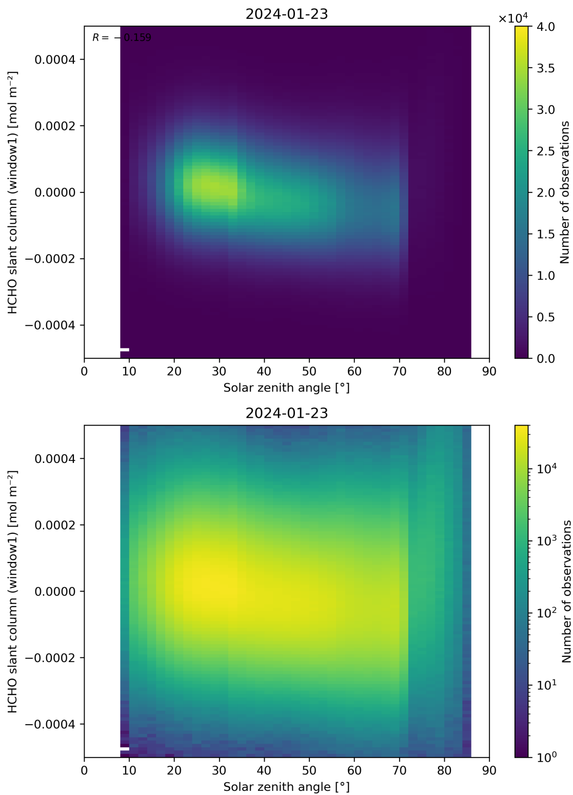
Figure 173: Scatter density plot of “Solar zenith angle” against “HCHO slant column (window1)” for 2024-01-22 to 2024-01-24.
