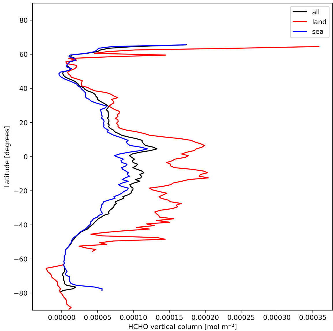
Figure 21: Zonal average of “HCHO vertical column” for 2024-01-22 to 2024-01-24.
