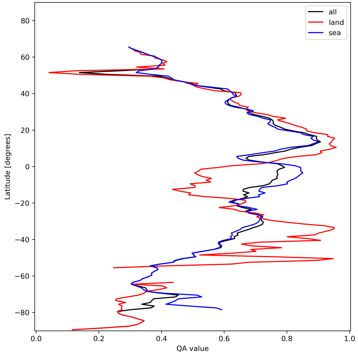
Figure 20: Zonal average of “QA value” for 2024-01-22 to 2024-01-24.
