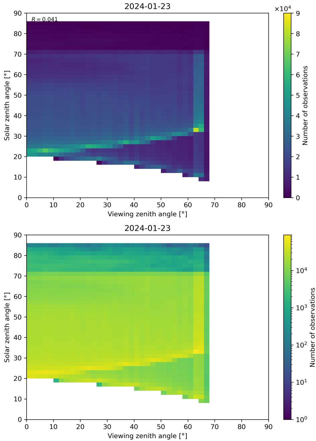
Figure 197: Scatter density plot of “Viewing zenith angle” against “Solar zenith angle” for 2024-01-22 to 2024-01-24.
