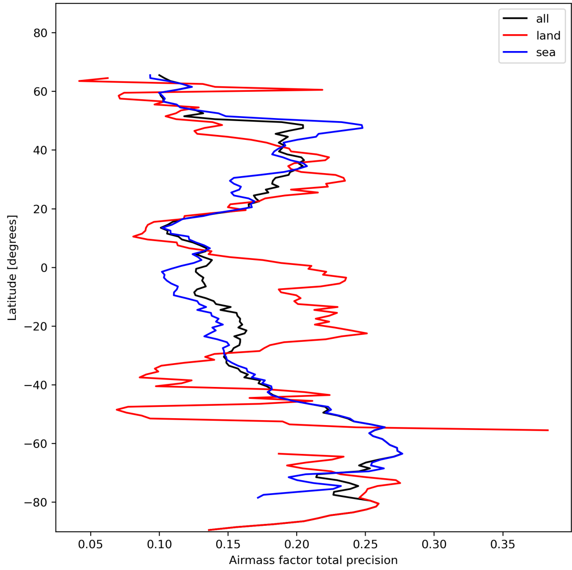
Figure 27: Zonal average of “Airmass factor total precision” for 2024-01-22 to 2024-01-24.
