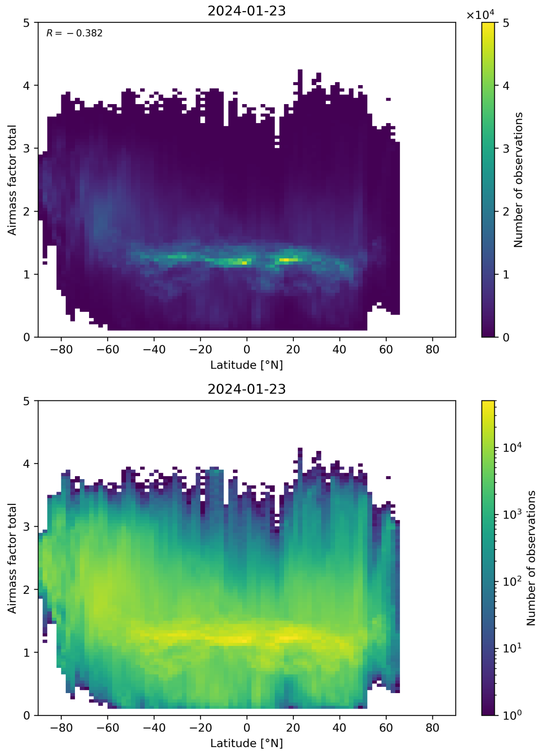
Figure 161: Scatter density plot of “Latitude” against “Airmass factor total” for 2024-01-22 to 2024-01-24.
