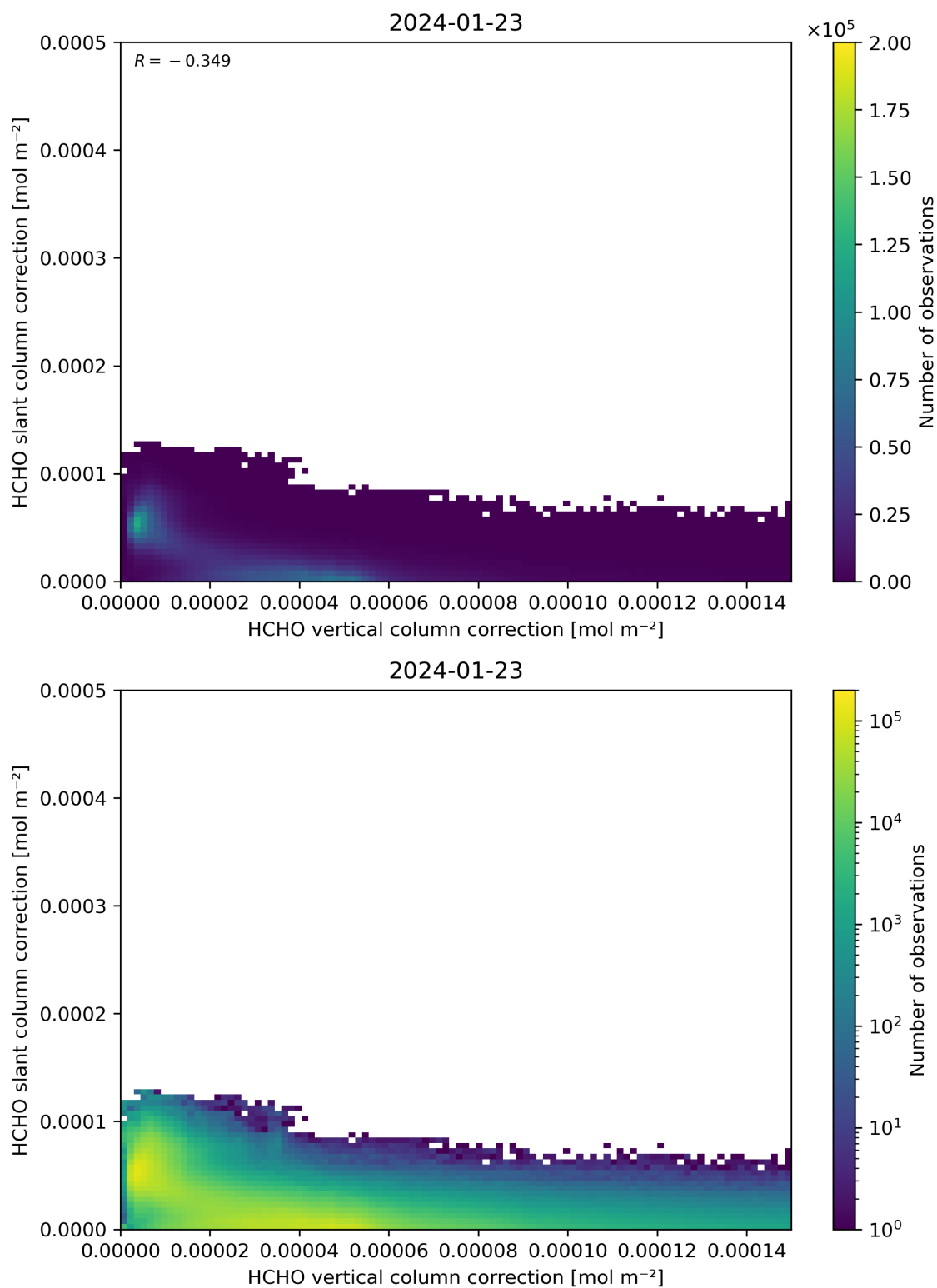
Figure 117: Scatter density plot of “HCHO vertical column correction” against “HCHO slant column correction” for 2024-01-22 to 2024-01-24.
