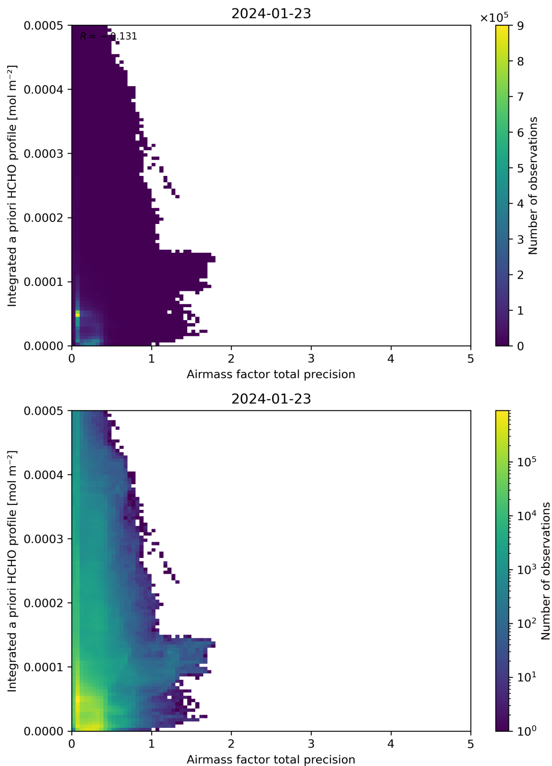
Figure 111: Scatter density plot of “Airmass factor total precision” against “Integrated a priori HCHO profile” for 2024-01-22 to 2024-01-24.
