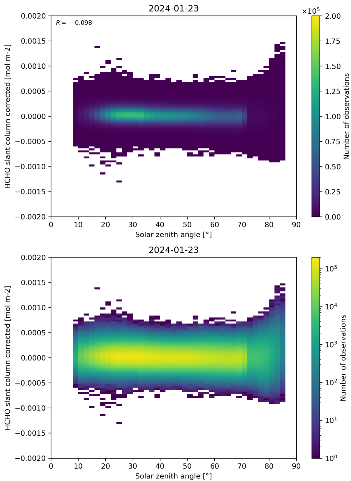
Figure 171: Scatter density plot of “Solar zenith angle” against “HCHO slant column corrected” for 2024-01-22 to 2024-01-24.
