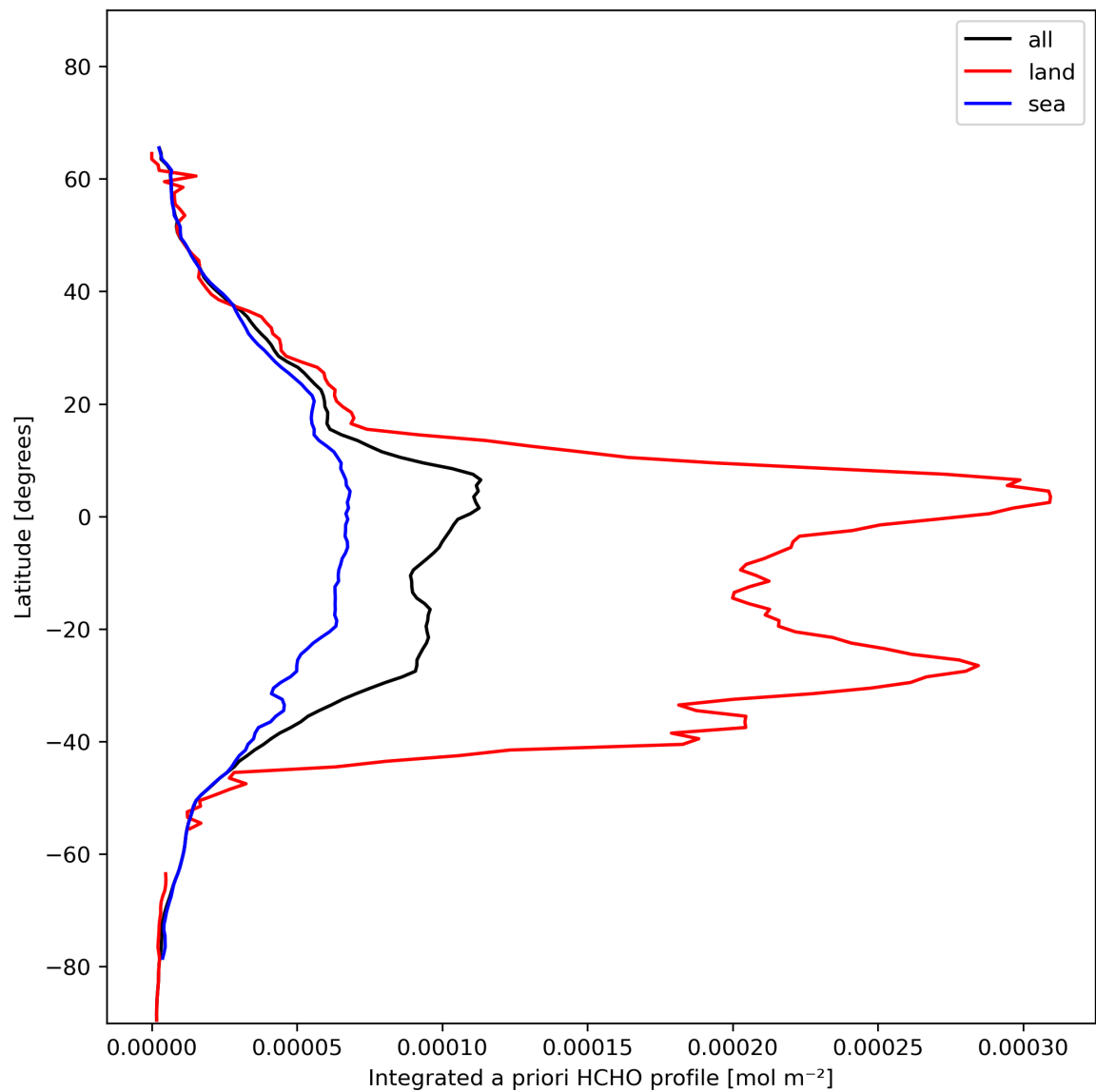
Figure 29: Zonal average of “Integrated a priori HCHO profile” for 2024-01-22 to 2024-01-24.
