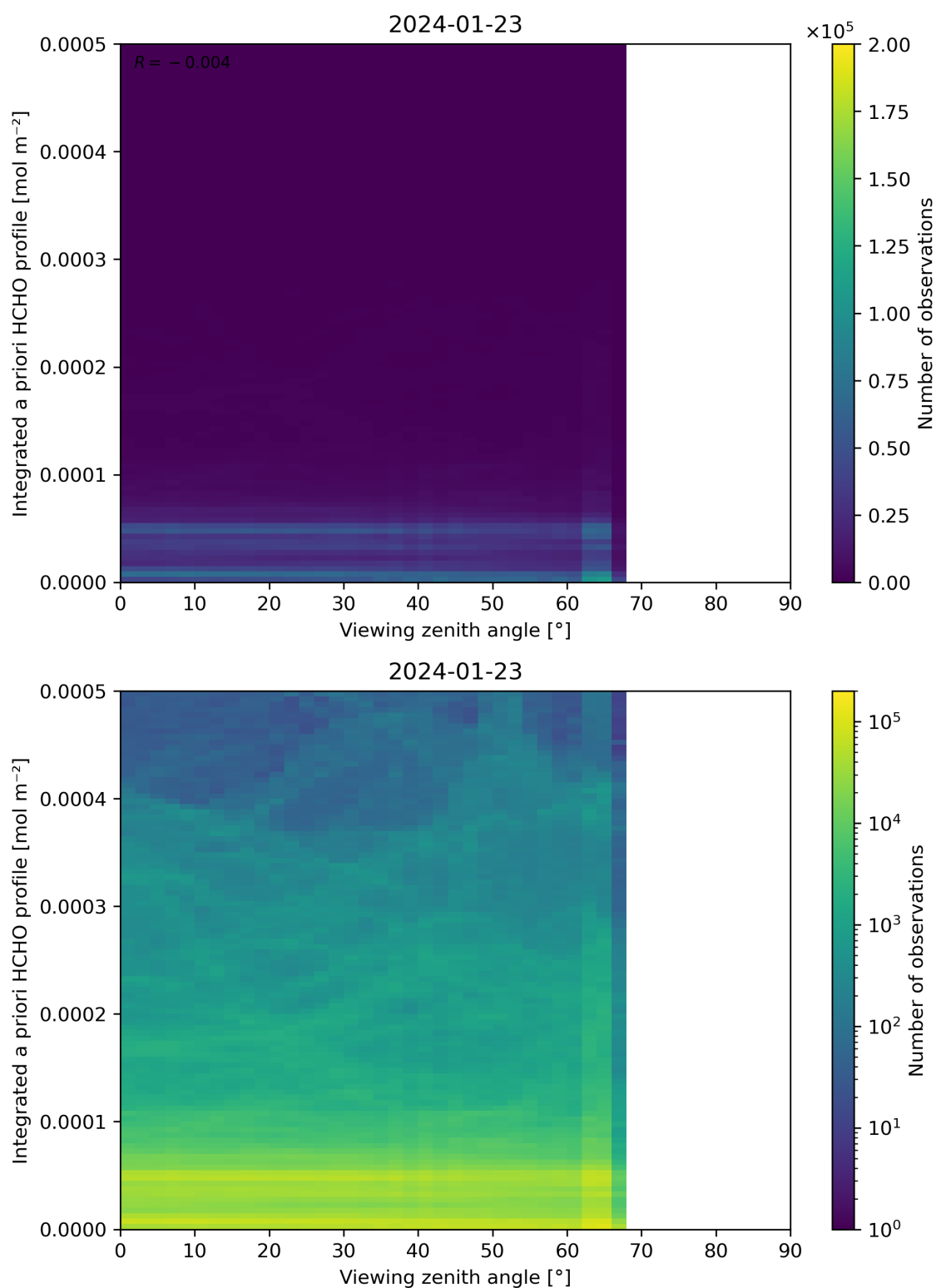
Figure 195: Scatter density plot of “Viewing zenith angle” against “Integrated a priori HCHO profile” for 2024-01-22 to 2024-01-24.
