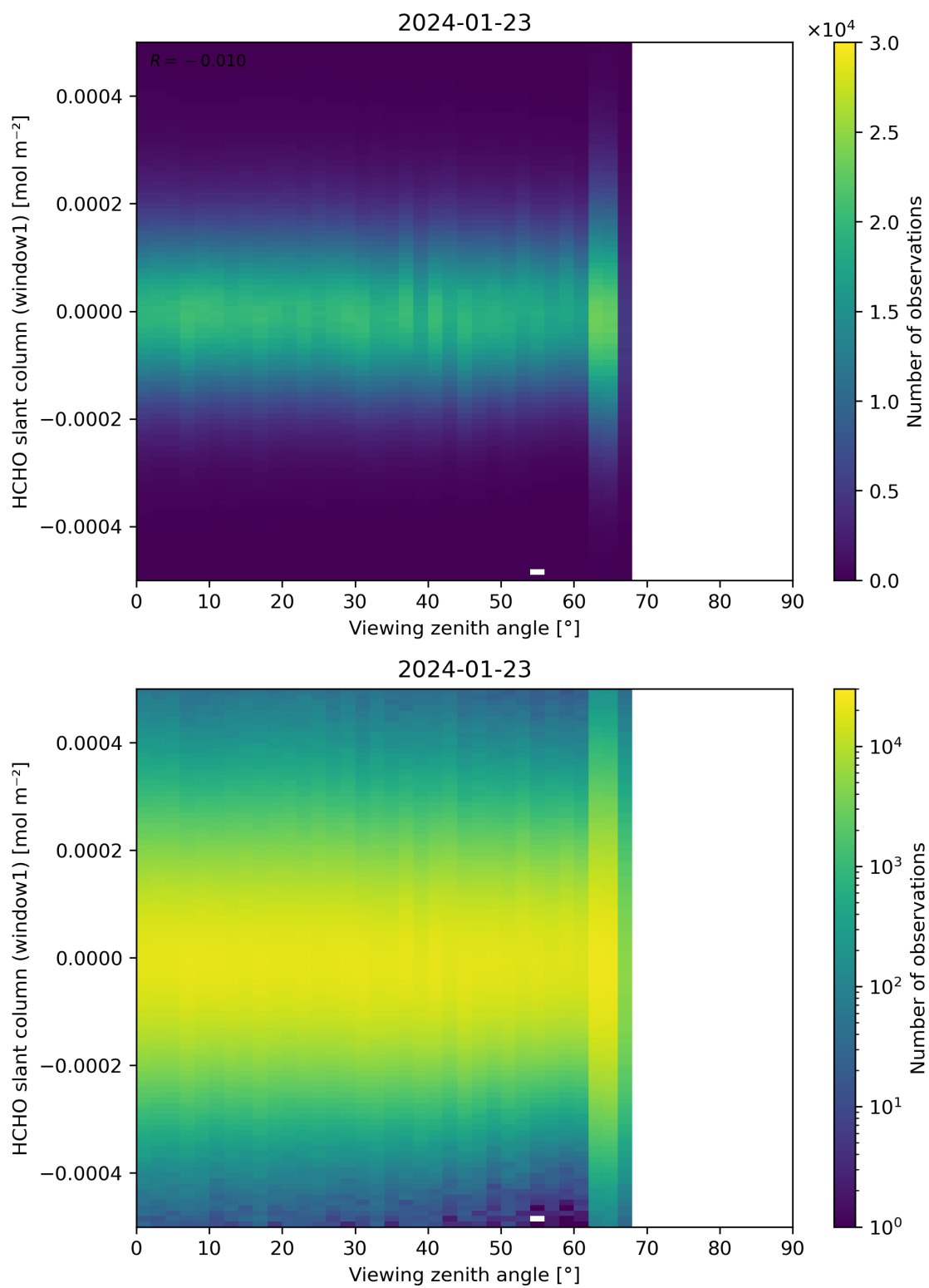
Figure 188: Scatter density plot of “Viewing zenith angle” against “HCHO slant column (window1)” for 2024-01-22 to 2024-01-24.
