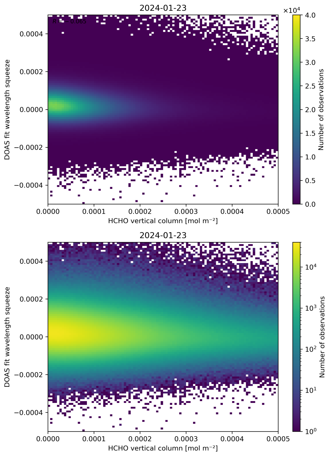
Figure 125: Scatter density plot of “HCHO vertical column” against “DOAS fit wavelength squeeze” for 2024-01-22 to 2024-01-24.
