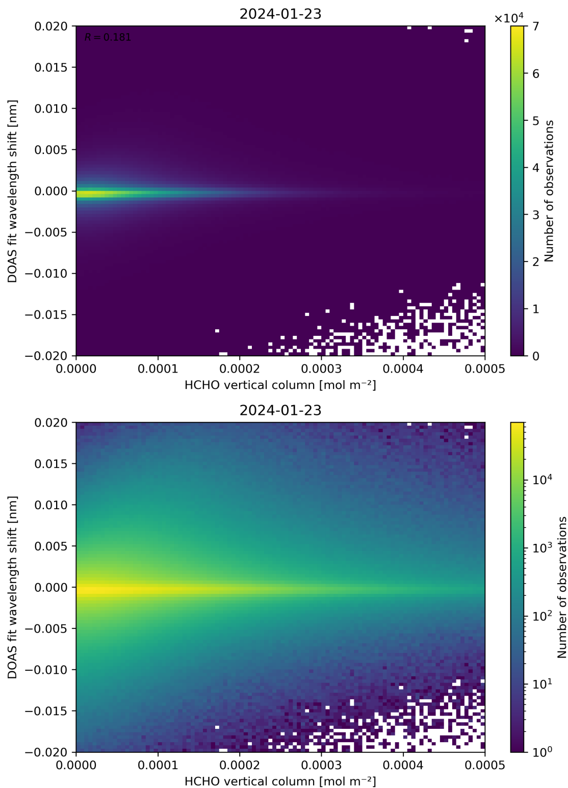
Figure 124: Scatter density plot of “HCHO vertical column” against “DOAS fit wavelength shift” for 2024-01-22 to 2024-01-24.
