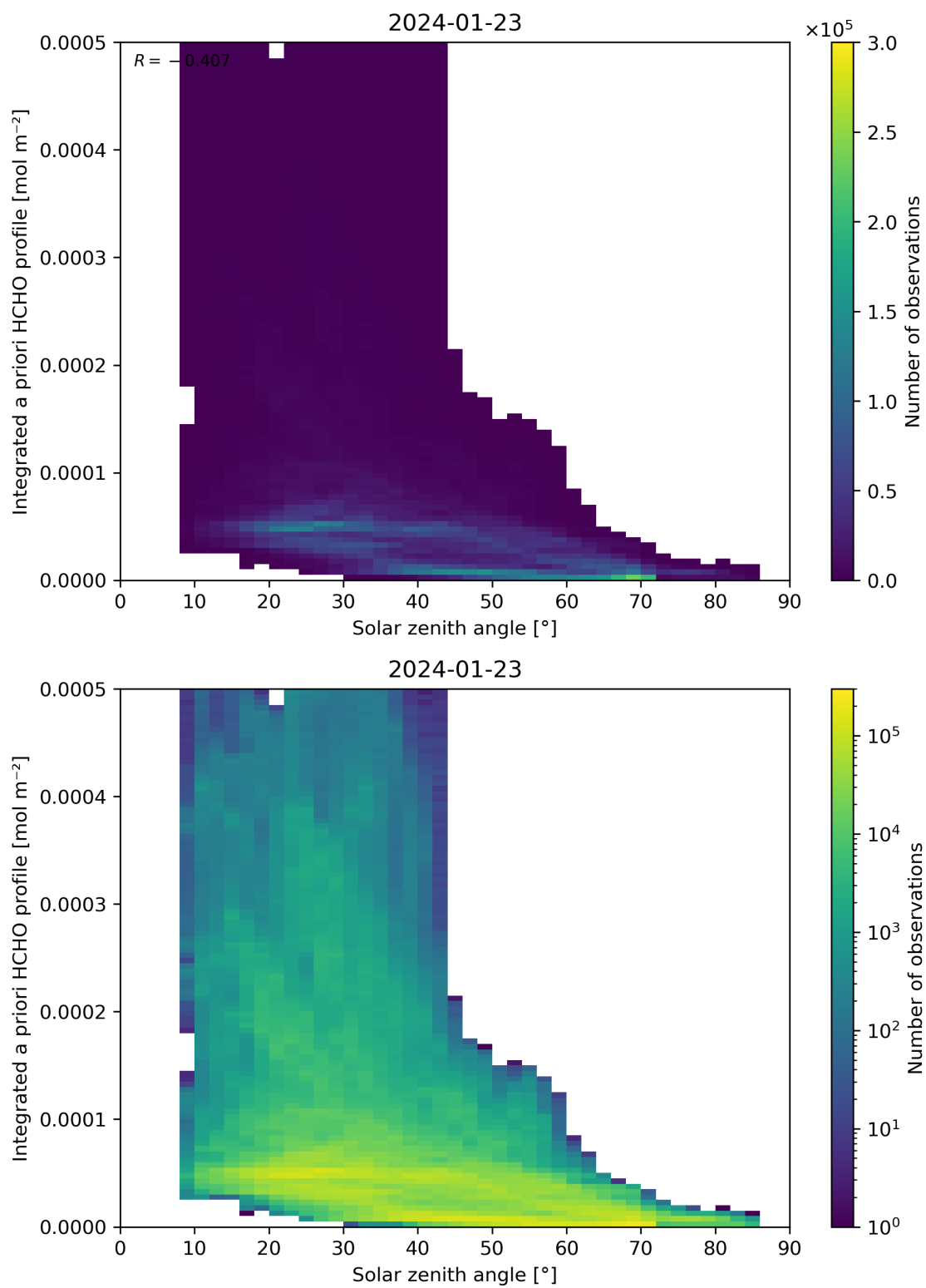
Figure 180: Scatter density plot of “Solar zenith angle” against “Integrated a priori HCHO profile” for 2024-01-22 to 2024-01-24.
