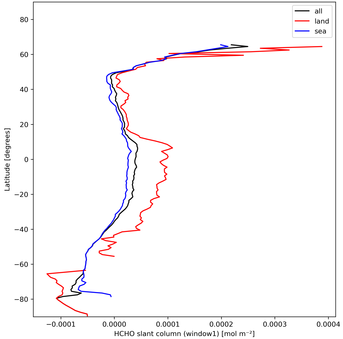
Figure 24: Zonal average of “HCHO slant column (window1)” for 2024-01-22 to 2024-01-24.
