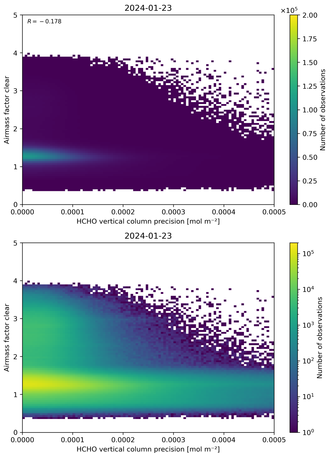
Figure 139: Scatter density plot of “HCHO vertical column precision” against “Airmass factor clear” for 2024-01-22 to 2024-01-24.
