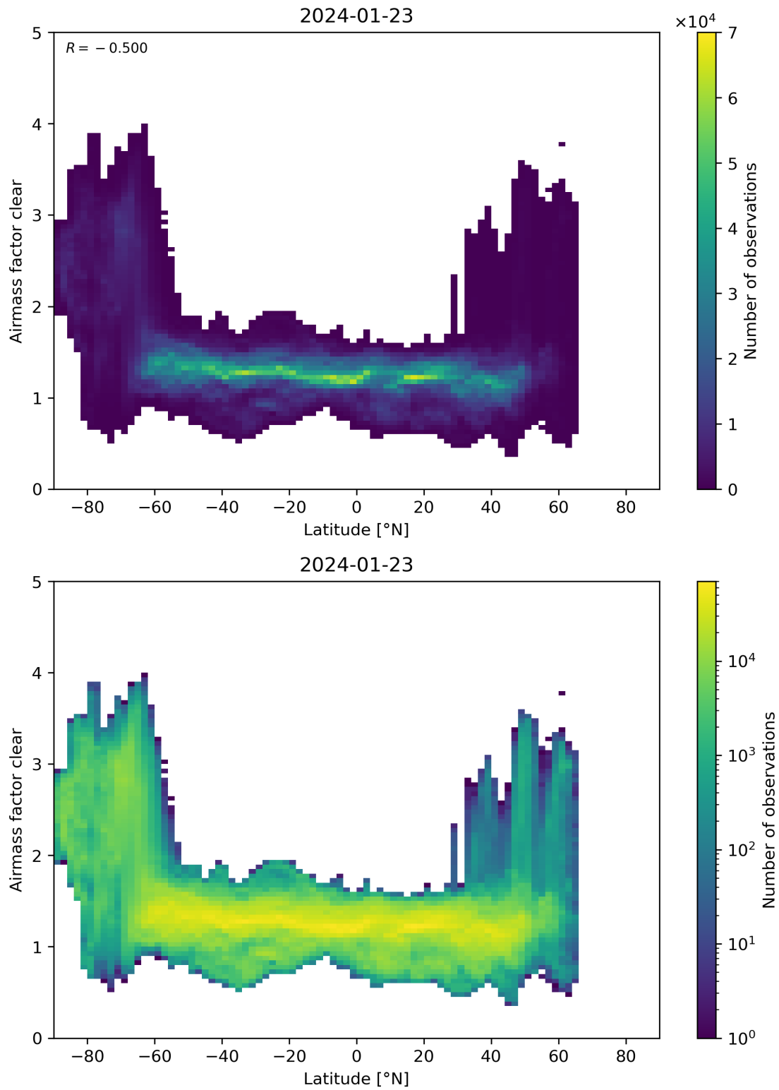
Figure 156: Scatter density plot of “Latitude” against “Airmass factor clear” for 2024-01-22 to 2024-01-24.
