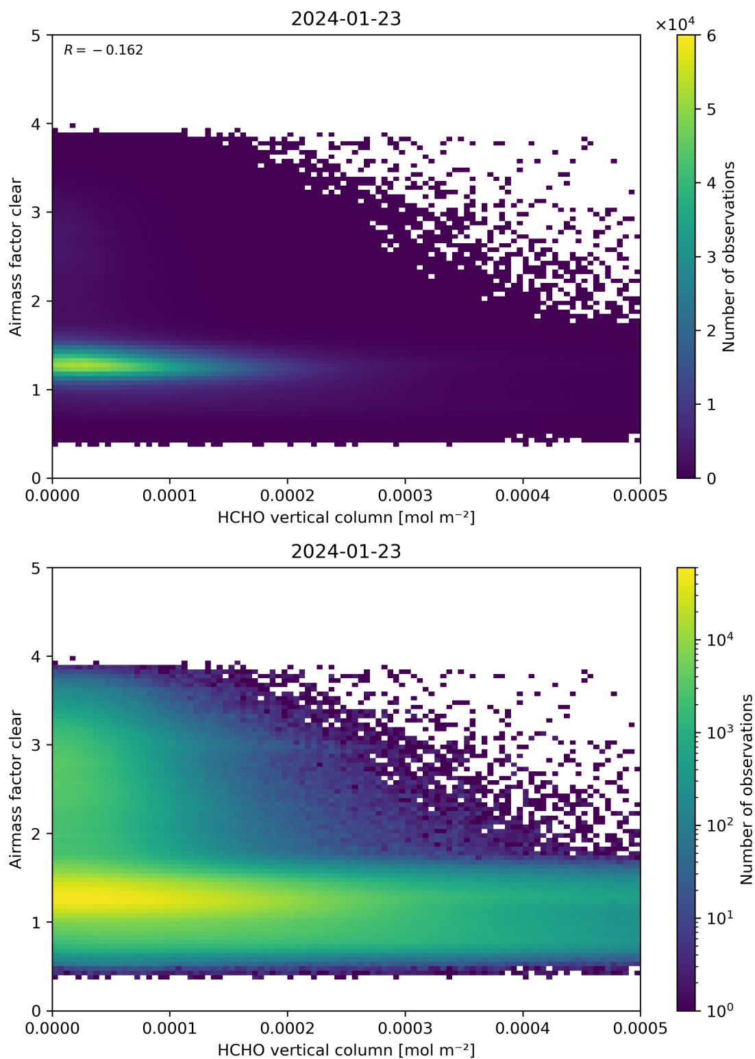
Figure 126: Scatter density plot of “HCHO vertical column” against “Airmass factor clear” for 2024-01-22 to 2024-01-24.
