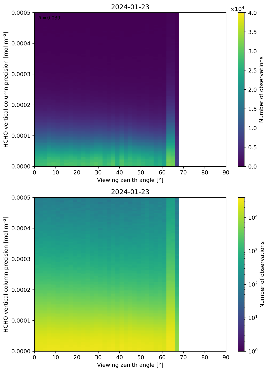
Figure 194: Scatter density plot of “Viewing zenith angle” against “HCHO vertical column precision” for 2024-01-22 to 2024-01-24.
