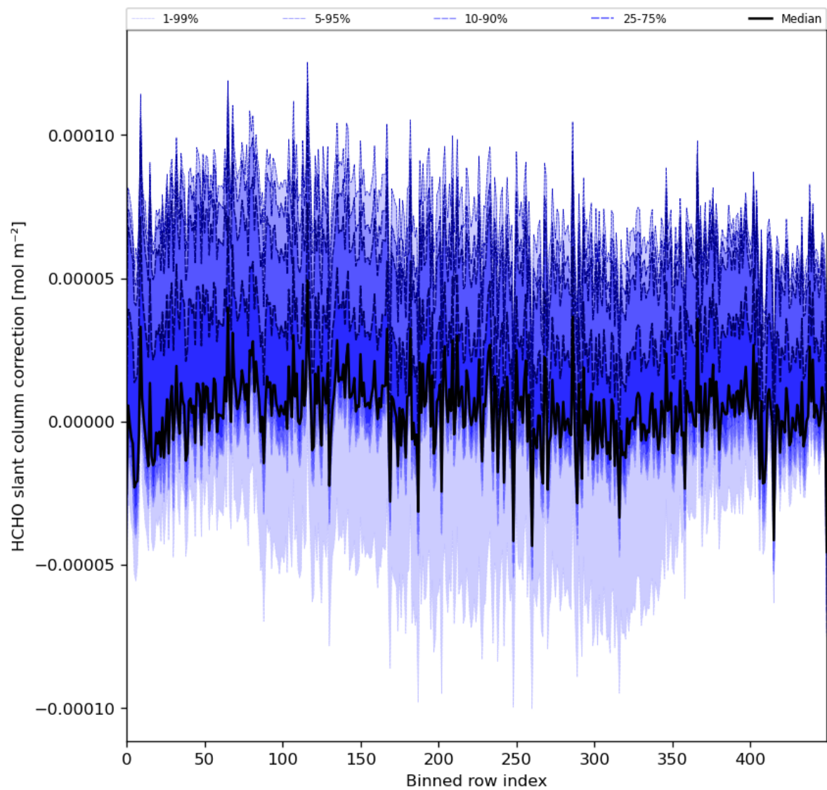
Figure 61: Along track statistics of “HCHO slant column correction” for 2024-01-22 to 2024-01-24
