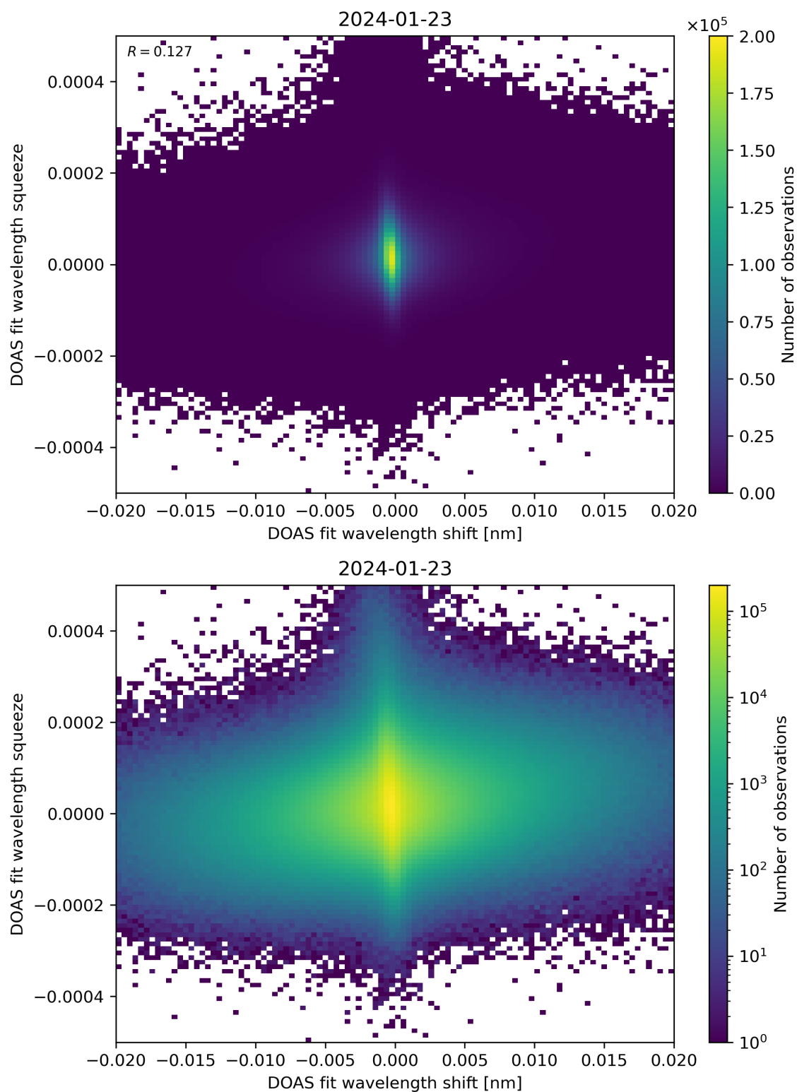
Figure 65: Scatter density plot of “DOAS fit wavelength shift” against “DOAS fit wavelength squeeze” for 2024-01-22 to 2024-01-24.
