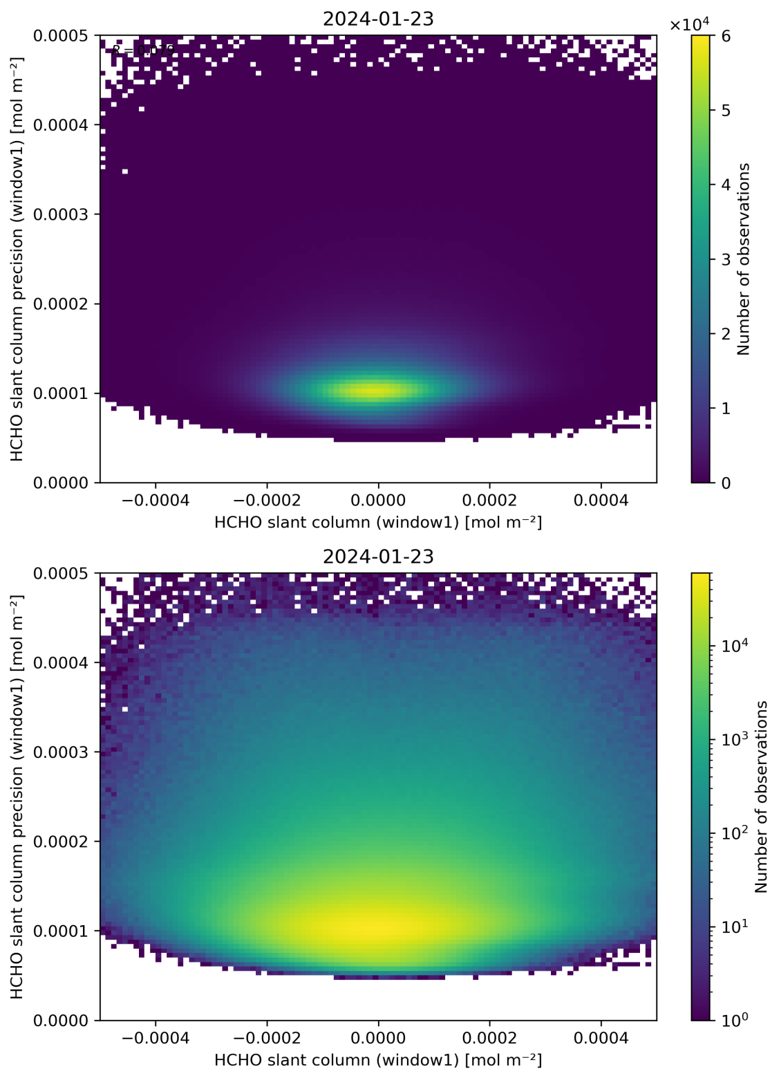
Figure 84: Scatter density plot of “HCHO slant column (window1)” against “HCHO slant column precision (window1)” for 2024-01-22 to 2024-01-24.
