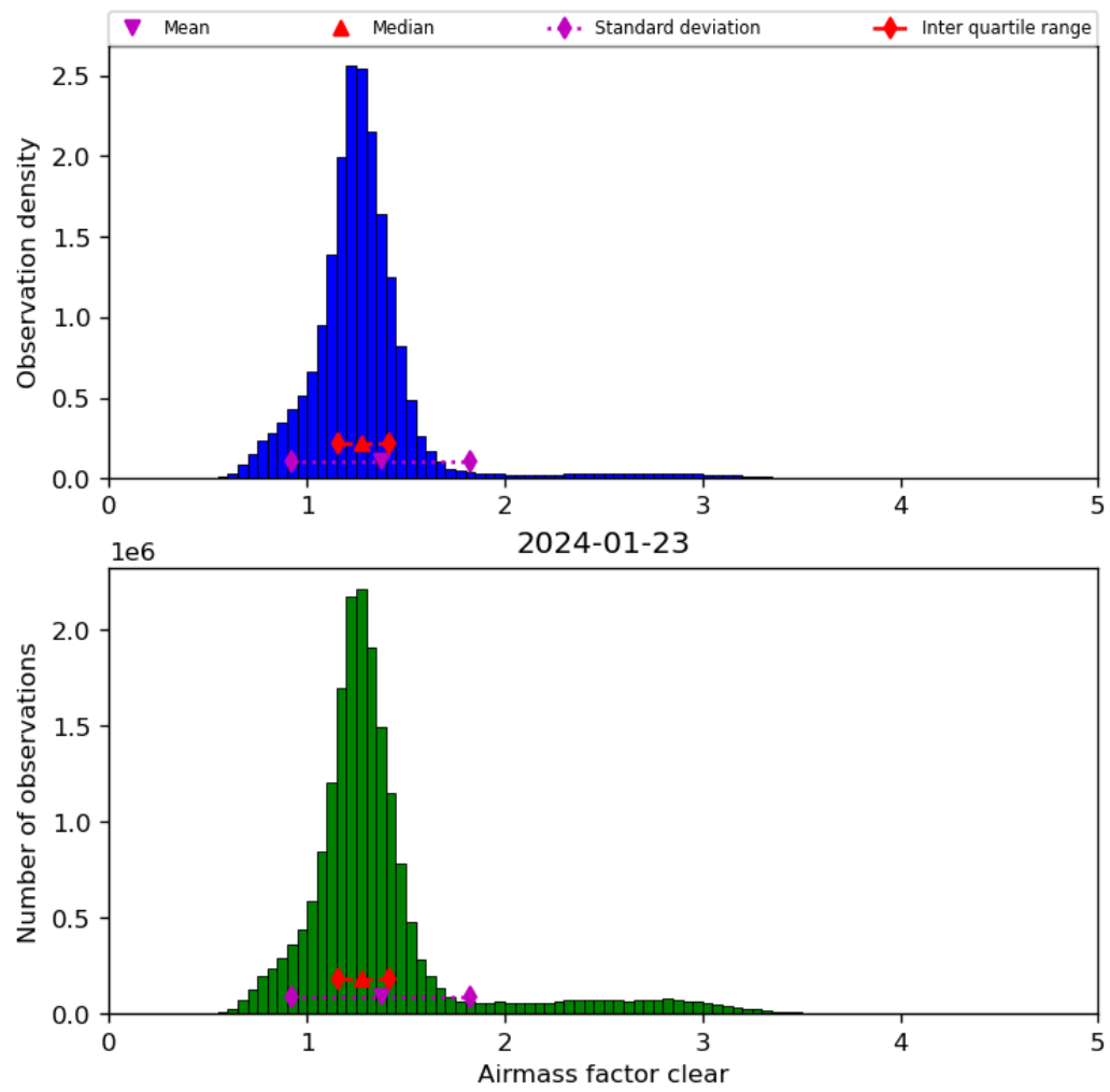
Figure 42: Histogram of “Airmass factor clear” for 2024-01-22 to 2024-01-24
