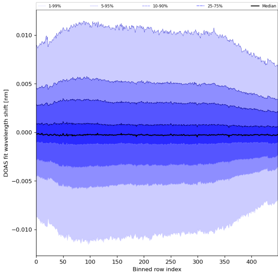
Figure 58: Along track statistics of “DOAS fit wavelength shift” for 2024-01-22 to 2024-01-24
