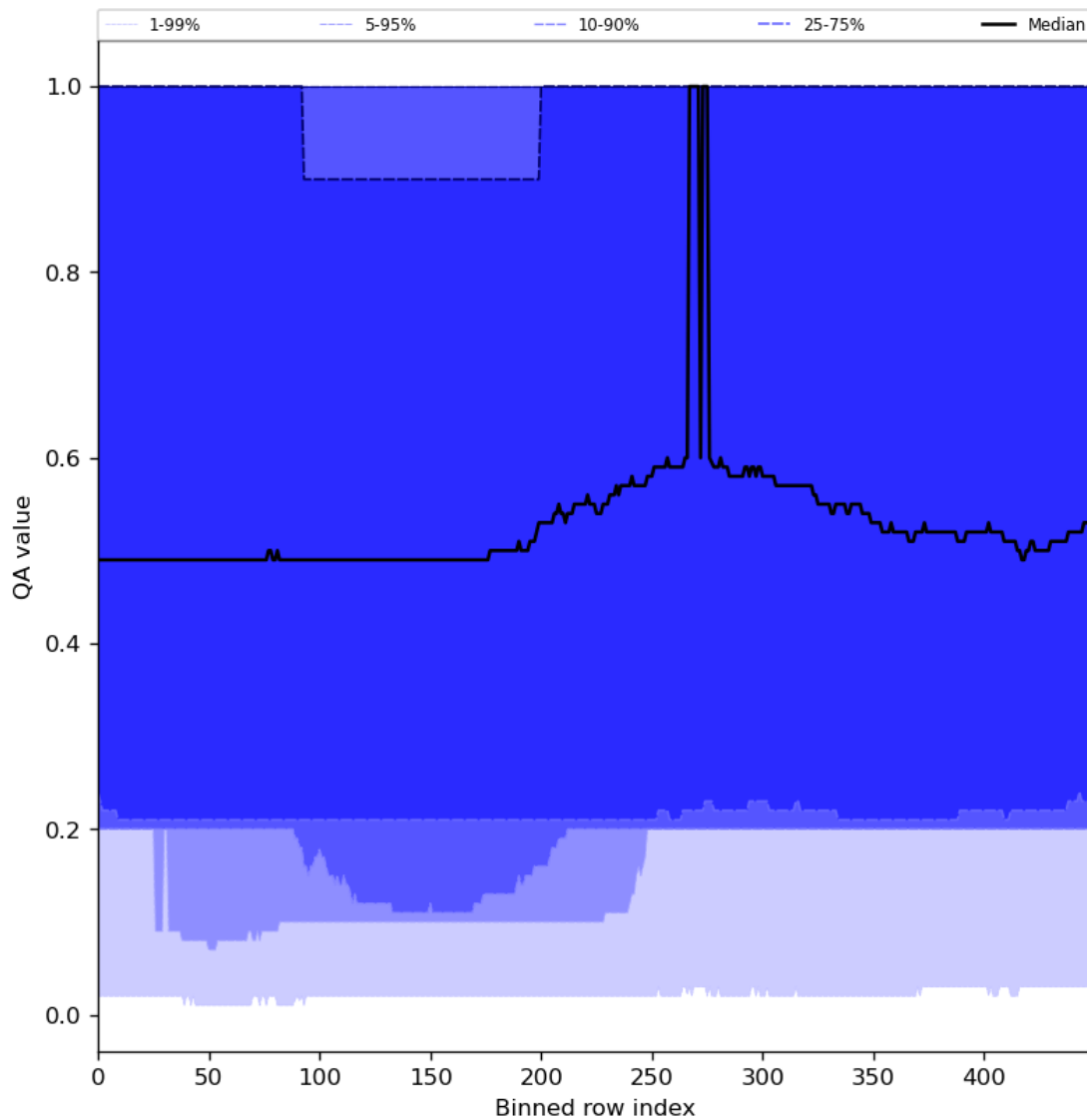
Figure 48: Along track statistics of “QA value” for 2024-01-22 to 2024-01-24
