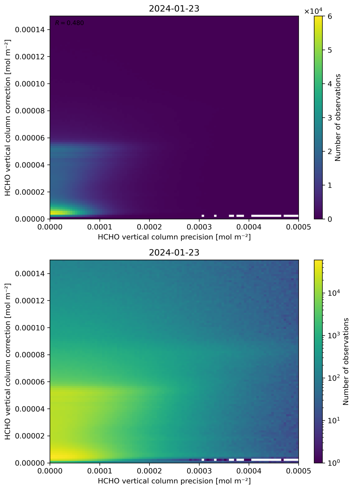
Figure 146: Scatter density plot of “HCHO vertical column precision” against “HCHO vertical column correction” for 2024-01-22 to 2024-01-24.
