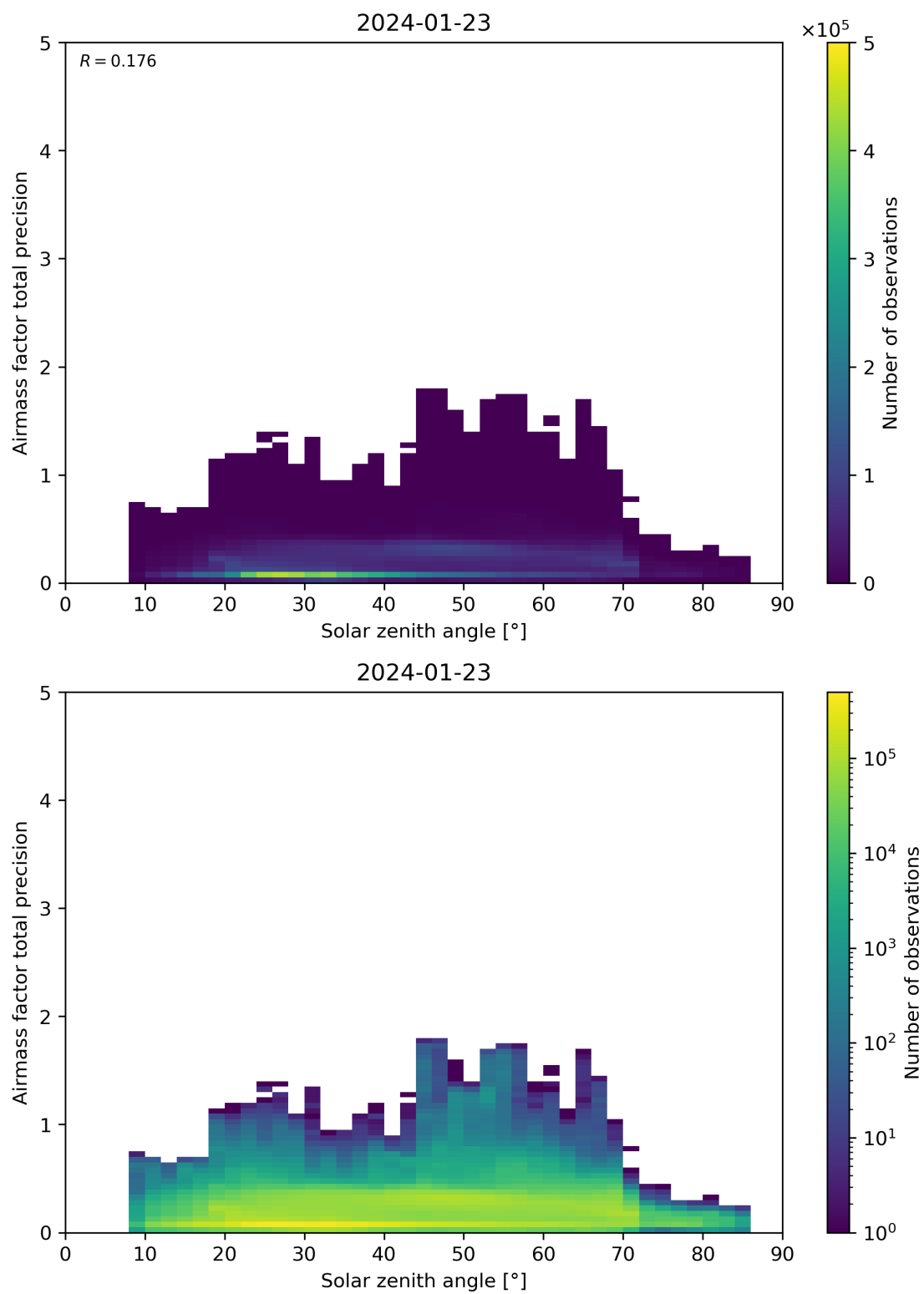
Figure 176: Scatter density plot of “Solar zenith angle” against “Airmass factor total precision” for 2024-01-22 to 2024-01-24.
