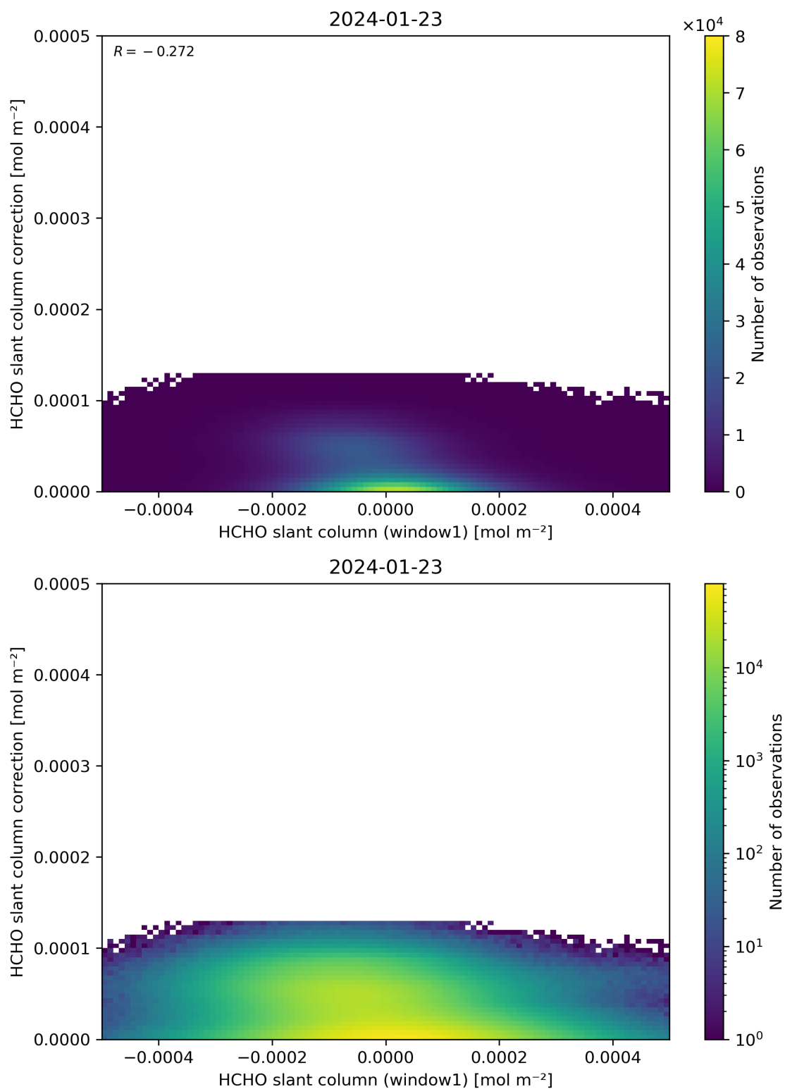
Figure 83: Scatter density plot of “HCHO slant column (window1)” against “HCHO slant column correction” for 2024-01-22 to 2024-01-24.
