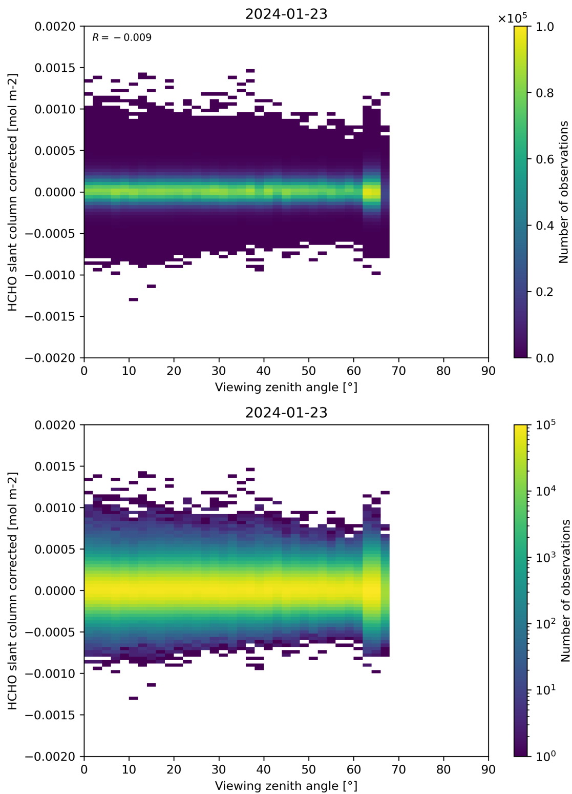
Figure 186: Scatter density plot of “Viewing zenith angle” against “HCHO slant column corrected” for 2024-01-22 to 2024-01-24.
