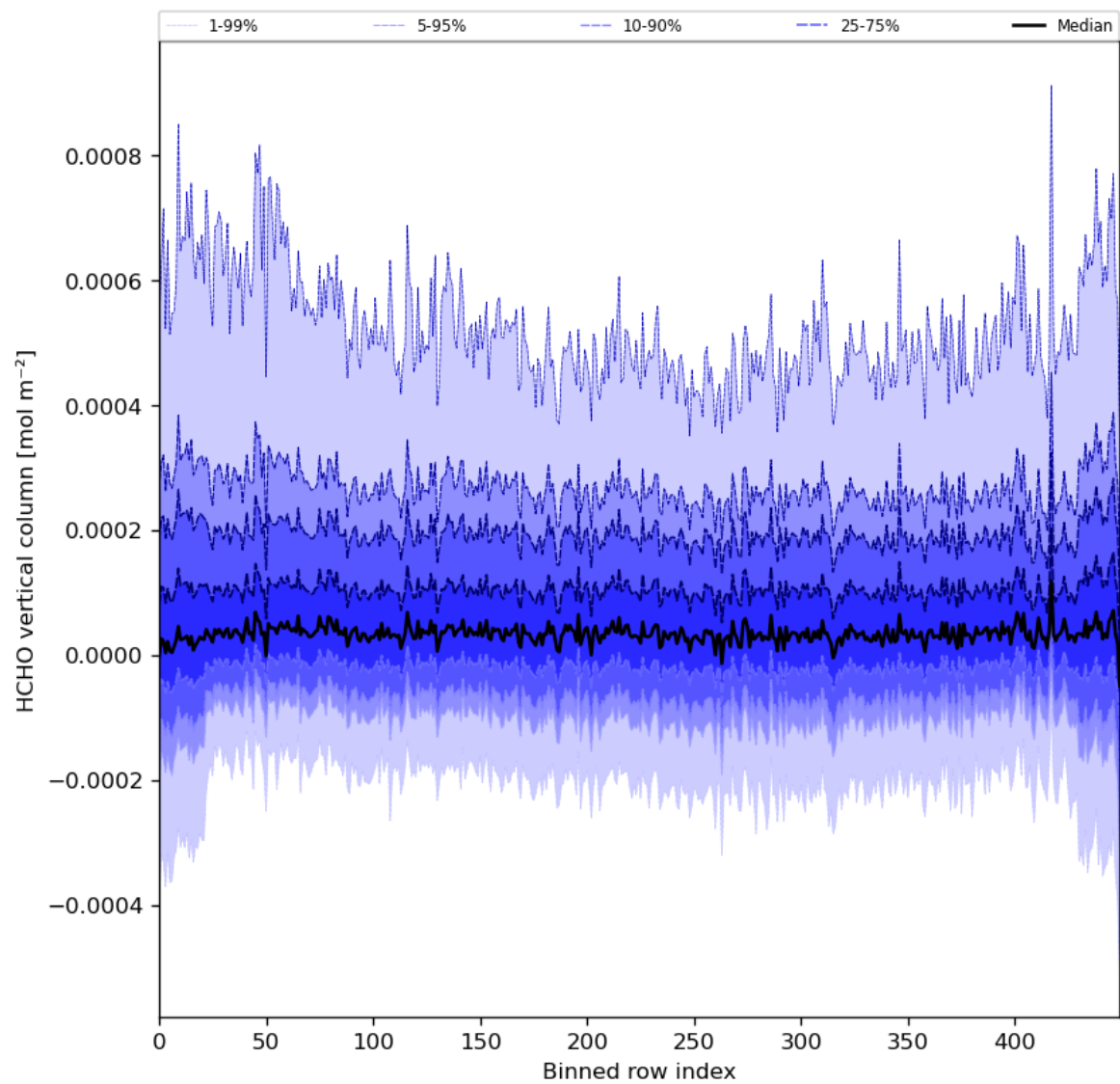
Figure 49: Along track statistics of “HCHO vertical column” for 2024-01-23 to 2024-01-25
