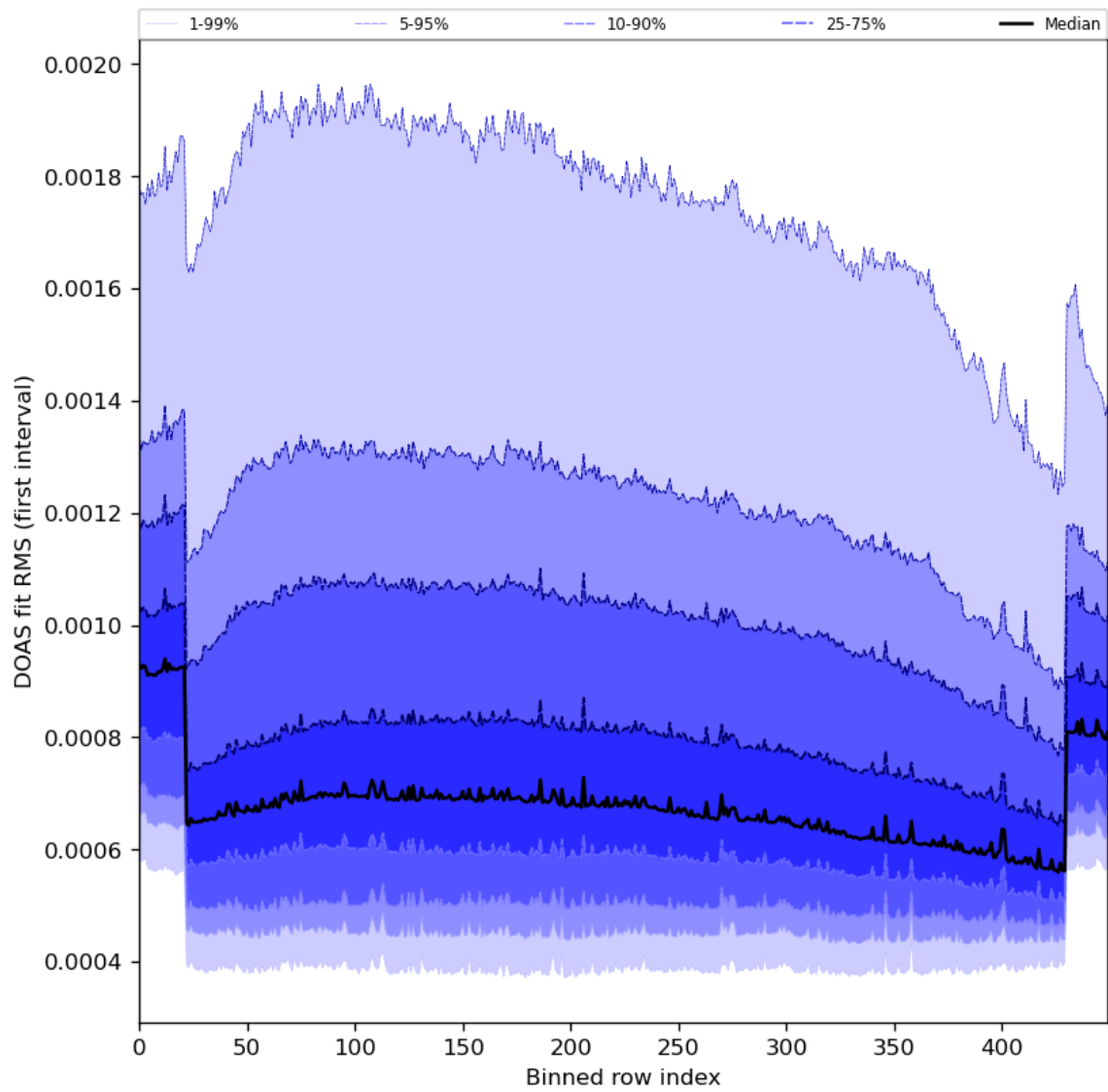
Figure 60: Along track statistics of “DOAS fit RMS (first interval)” for 2024-01-23 to 2024-01-25
