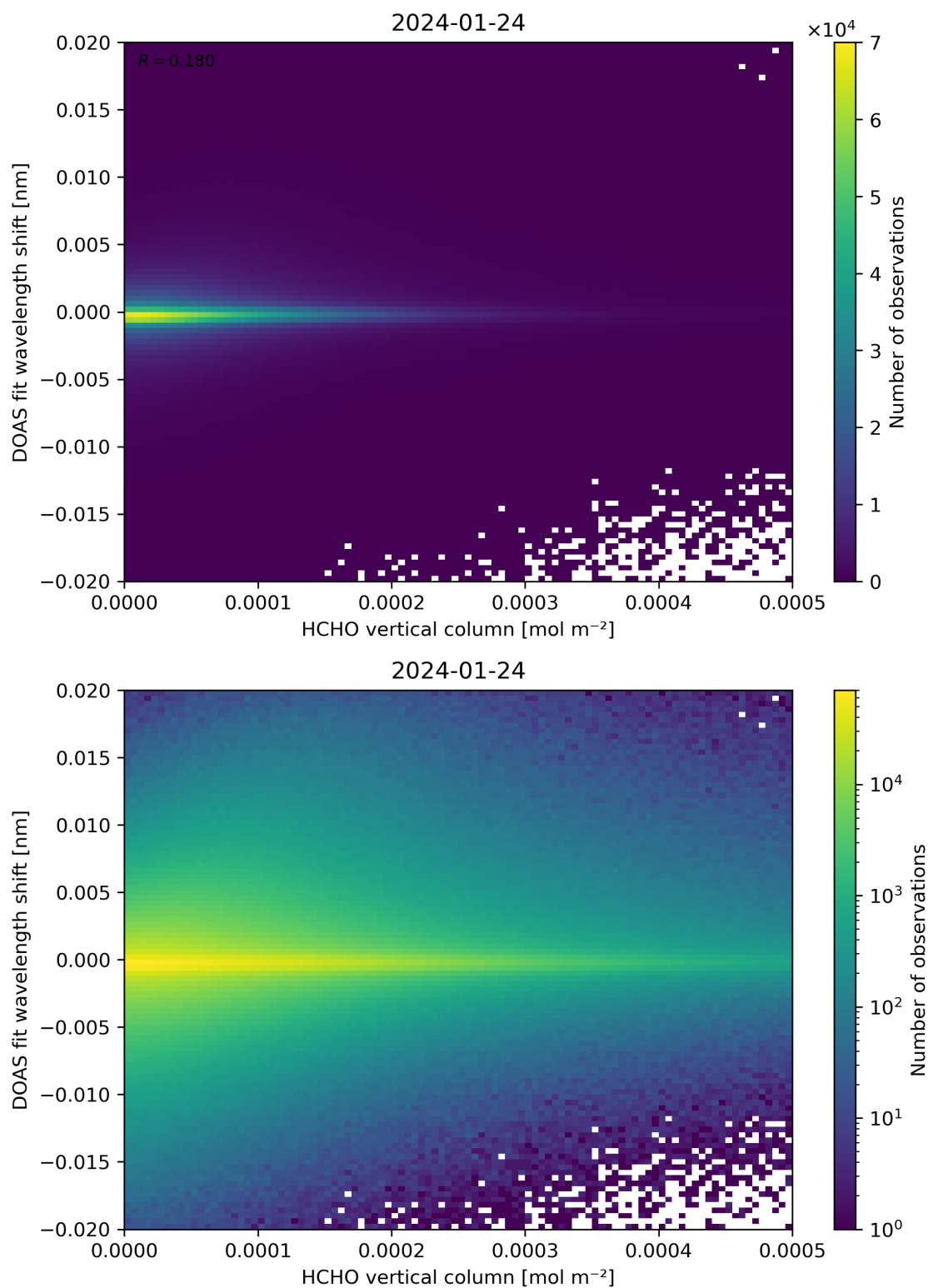
Figure 124: Scatter density plot of “HCHO vertical column” against “DOAS fit wavelength shift” for 2024-01-23 to 2024-01-25.
