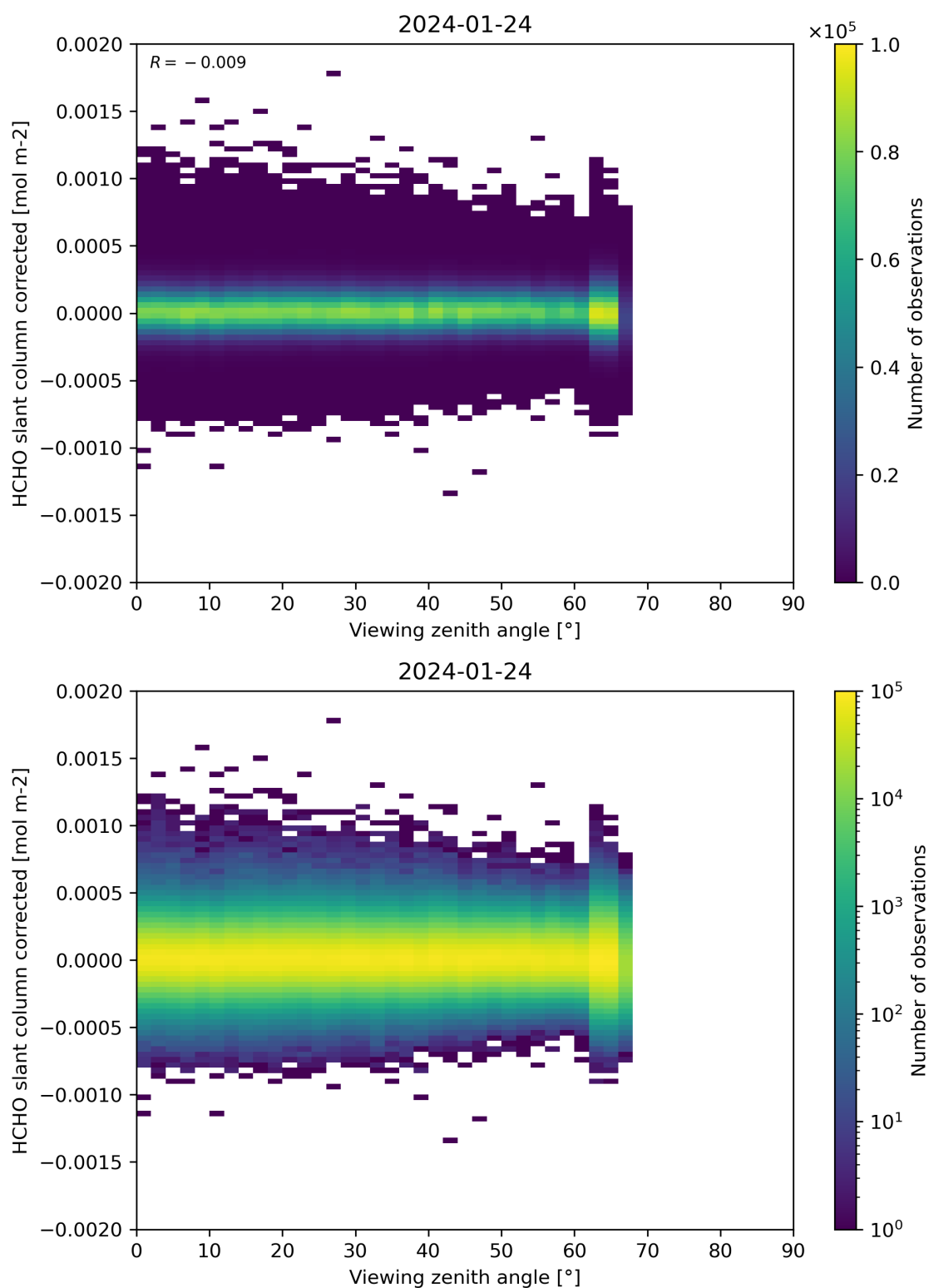
Figure 186: Scatter density plot of “Viewing zenith angle” against “HCHO slant column corrected” for 2024-01-23 to 2024-01-25.
