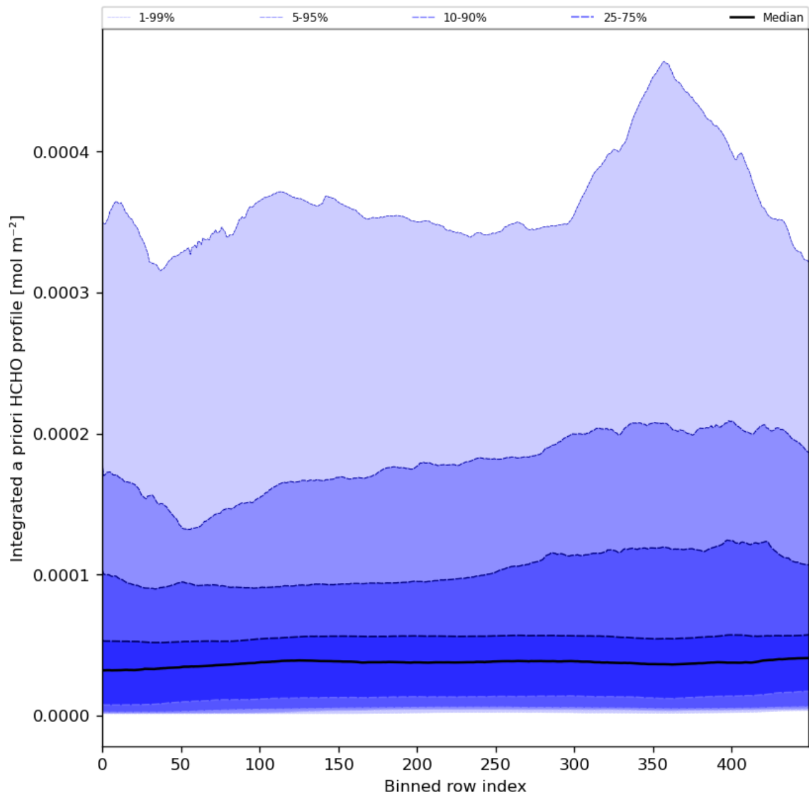
Figure 57: Along track statistics of “Integrated a priori HCHO profile” for 2024-01-23 to 2024-01-25
