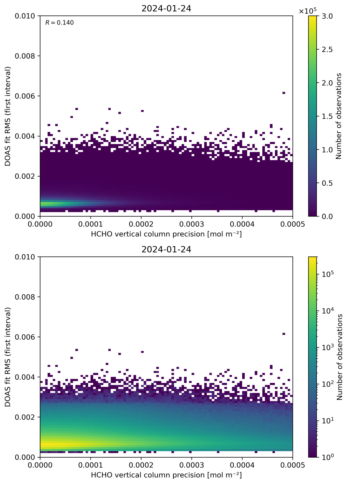
Figure 136: Scatter density plot of “HCHO vertical column precision” against “DOAS fit RMS (first interval)” for 2024-01-23 to 2024-01-25.
