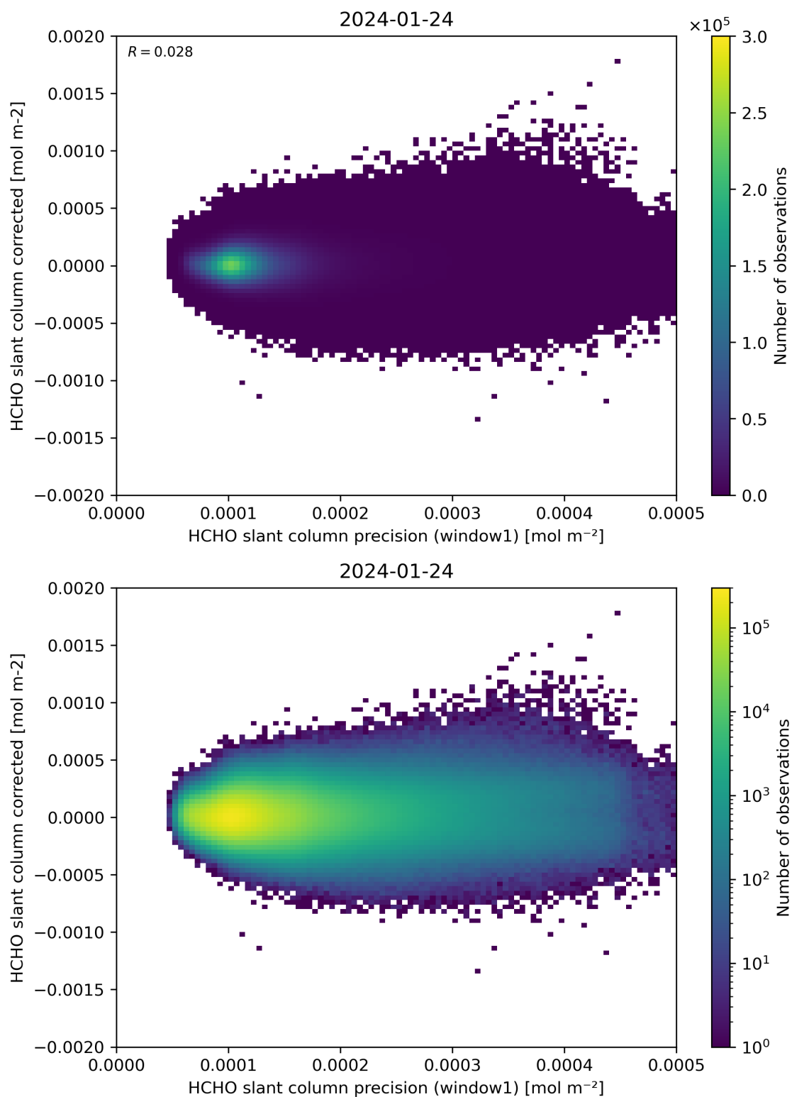
Figure 92: Scatter density plot of “HCHO slant column precision (window1)” against “HCHO slant column corrected” for 2024-01-23 to 2024-01-25.
