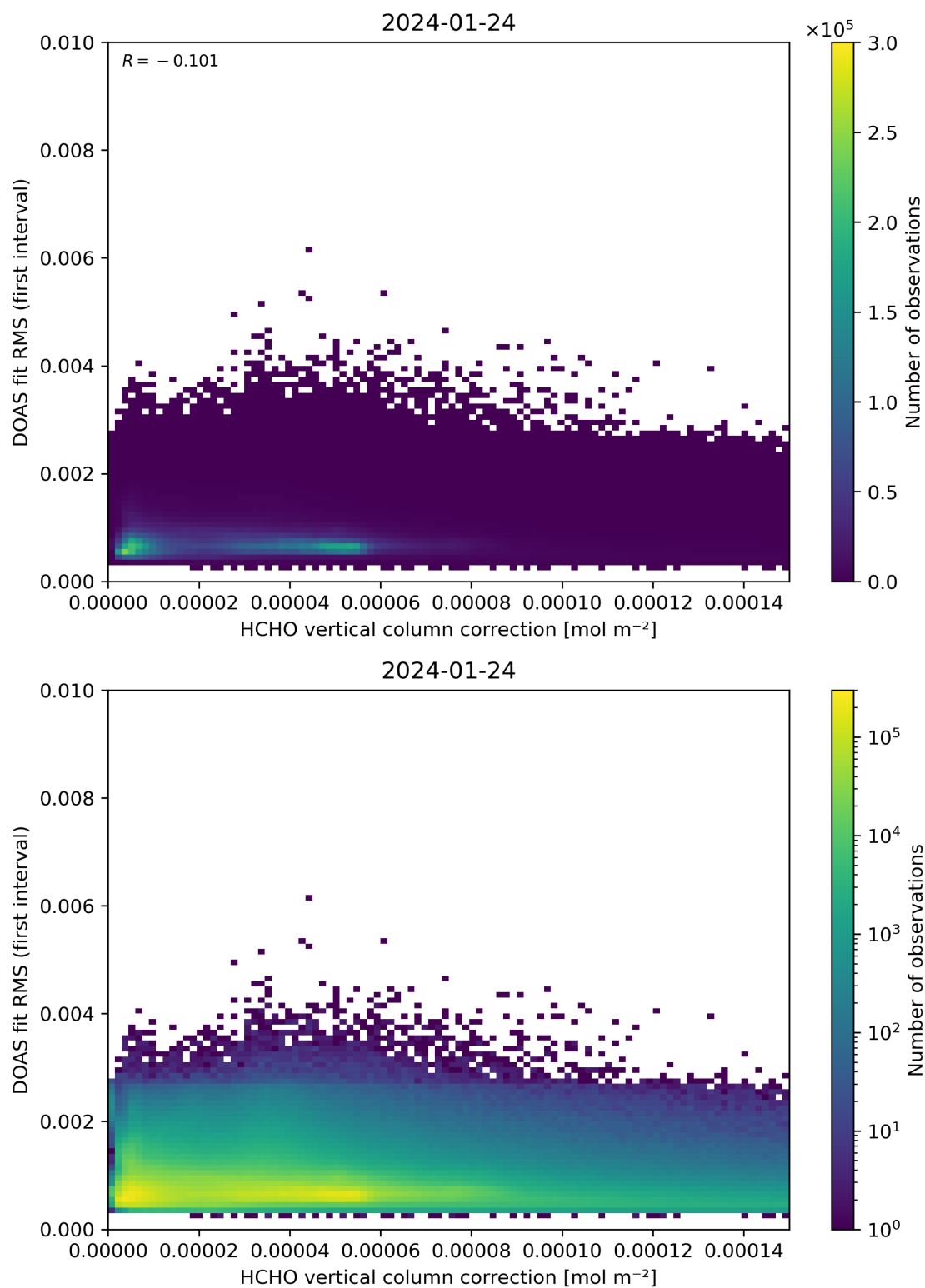
Figure 112: Scatter density plot of “HCHO vertical column correction” against “DOAS fit RMS (first interval)” for 2024-01-23 to 2024-01-25.
