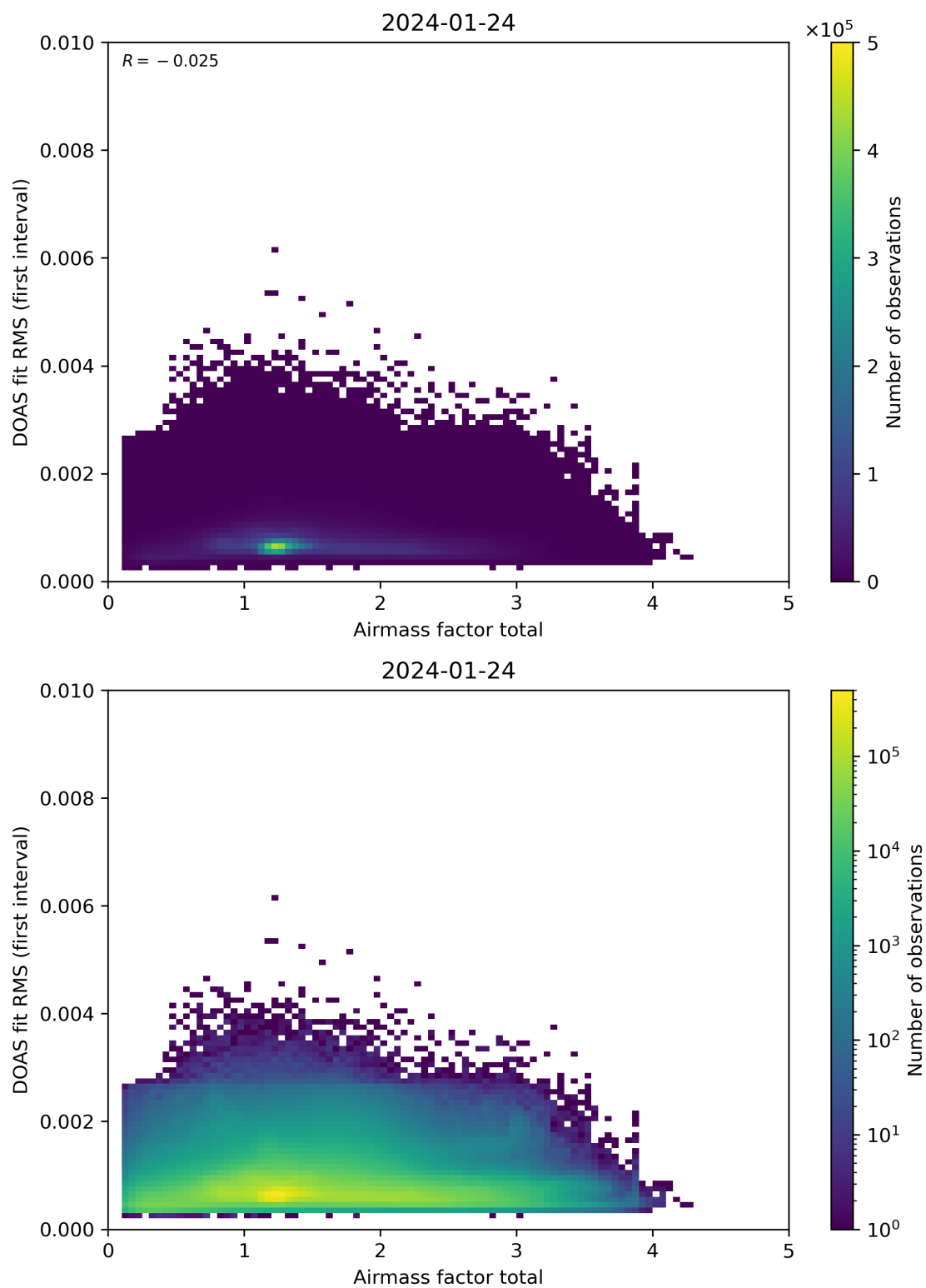
Figure 97: Scatter density plot of “Airmass factor total” against “DOAS fit RMS (first interval)” for 2024-01-23 to 2024-01-25.
