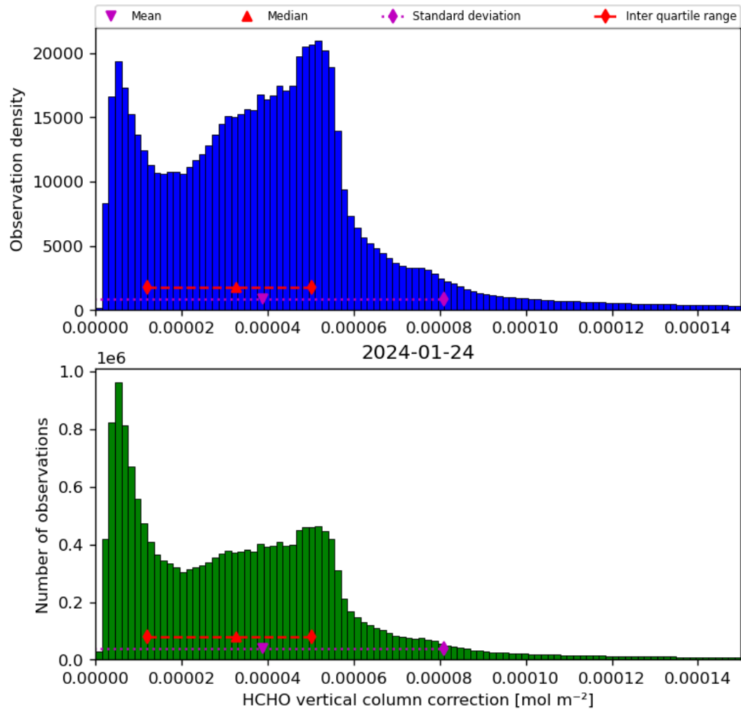
Figure 37: Histogram of “HCHO vertical column correction” for 2024-01-23 to 2024-01-25
