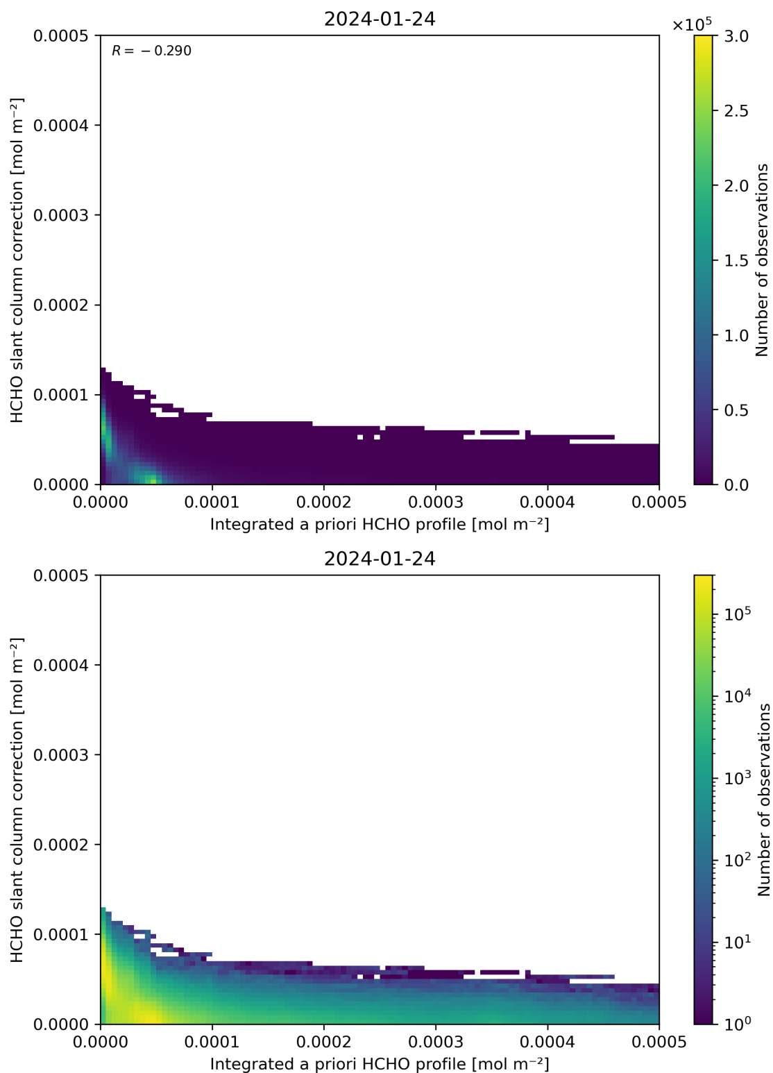
Figure 152: Scatter density plot of “Integrated a priori HCHO profile” against “HCHO slant column correction” for 2024-01-23 to 2024-01-25.
