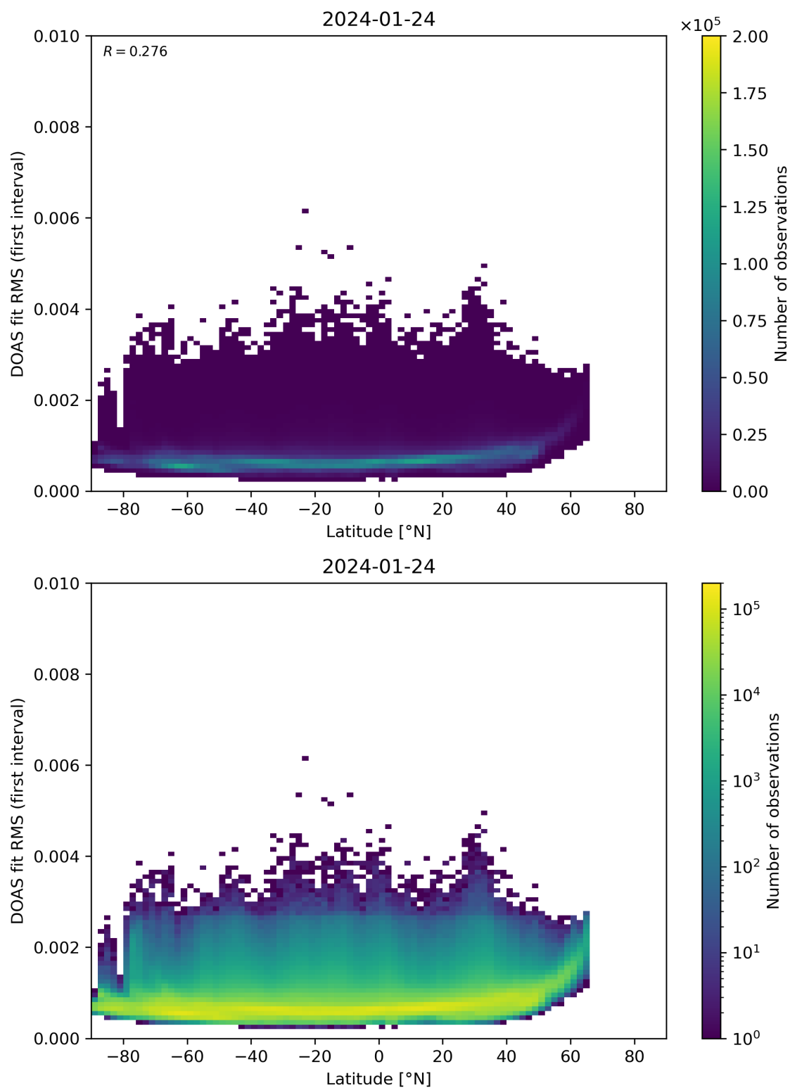
Figure 153: Scatter density plot of “Latitude” against “DOAS fit RMS (first interval)” for 2024-01-23 to 2024-01-25.
