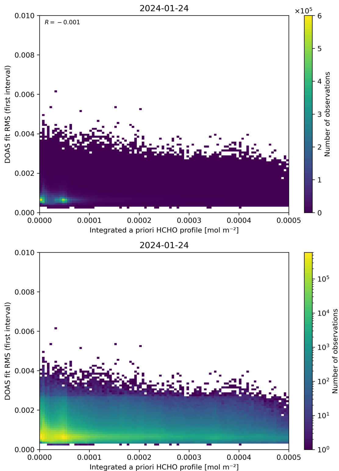
Figure 148: Scatter density plot of “Integrated a priori HCHO profile” against “DOAS fit RMS (first interval)” for 2024-01-23 to 2024-01-25.
