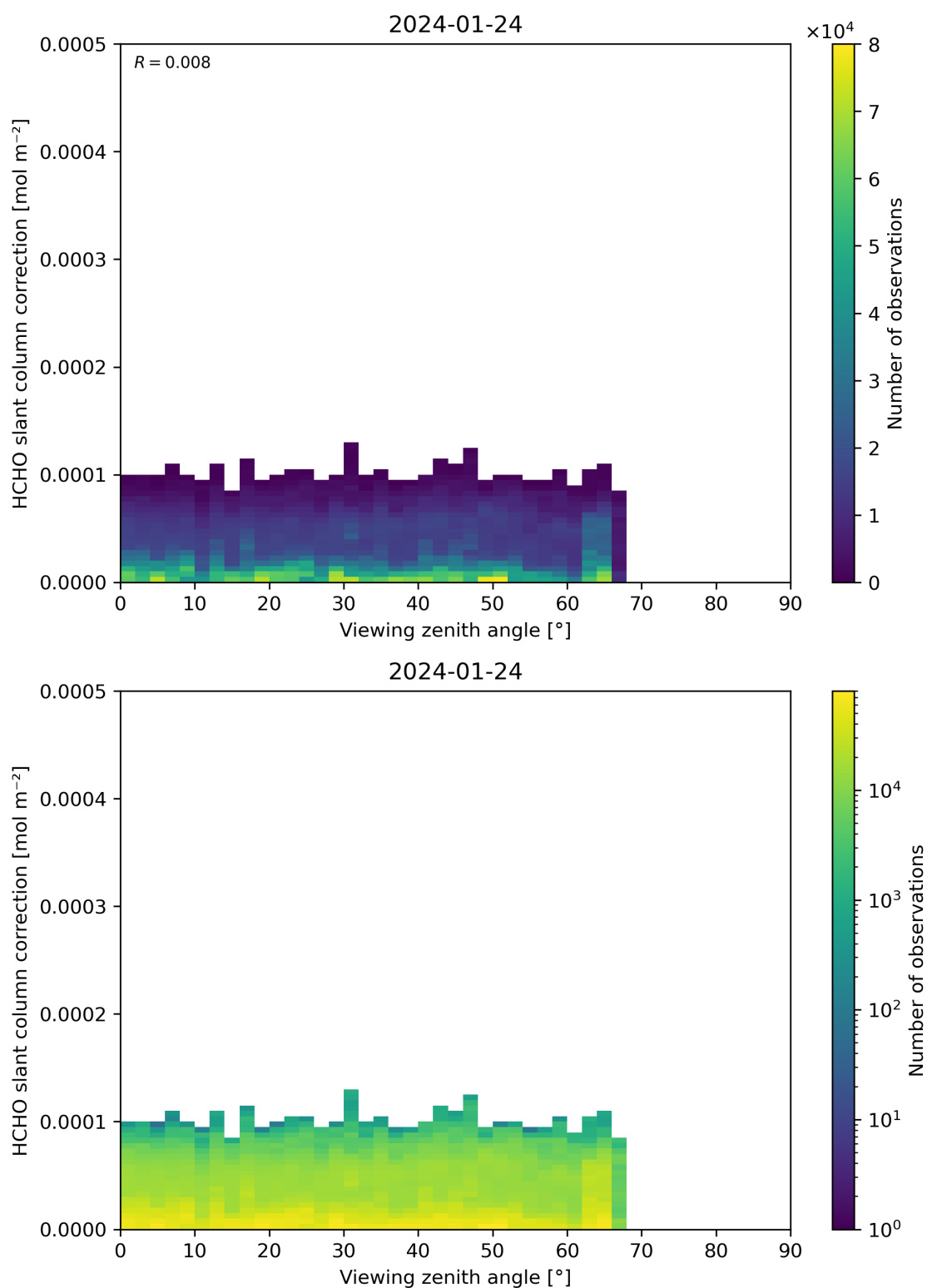
Figure 187: Scatter density plot of “Viewing zenith angle” against “HCHO slant column correction” for 2024-01-23 to 2024-01-25.
