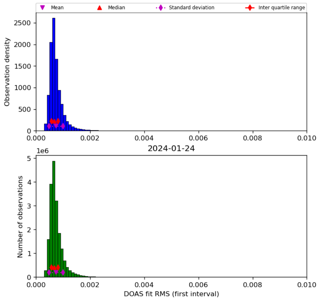
Figure 46: Histogram of “DOAS fit RMS (first interval)” for 2024-01-23 to 2024-01-25
