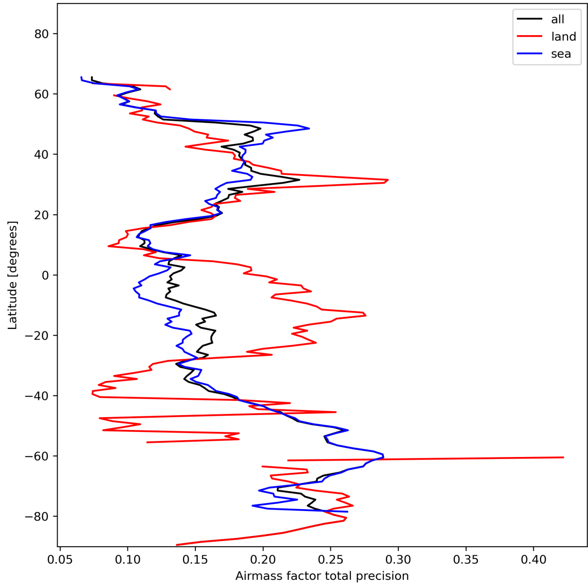
Figure 27: Zonal average of “Airmass factor total precision” for 2024-01-23 to 2024-01-25.
