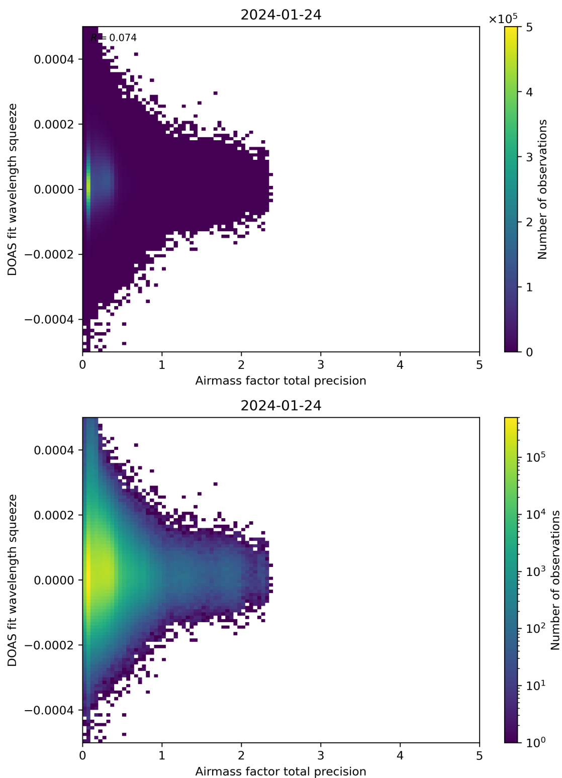
Figure 107: Scatter density plot of “Airmass factor total precision” against “DOAS fit wavelength squeeze” for 2024-01-23 to 2024-01-25.
