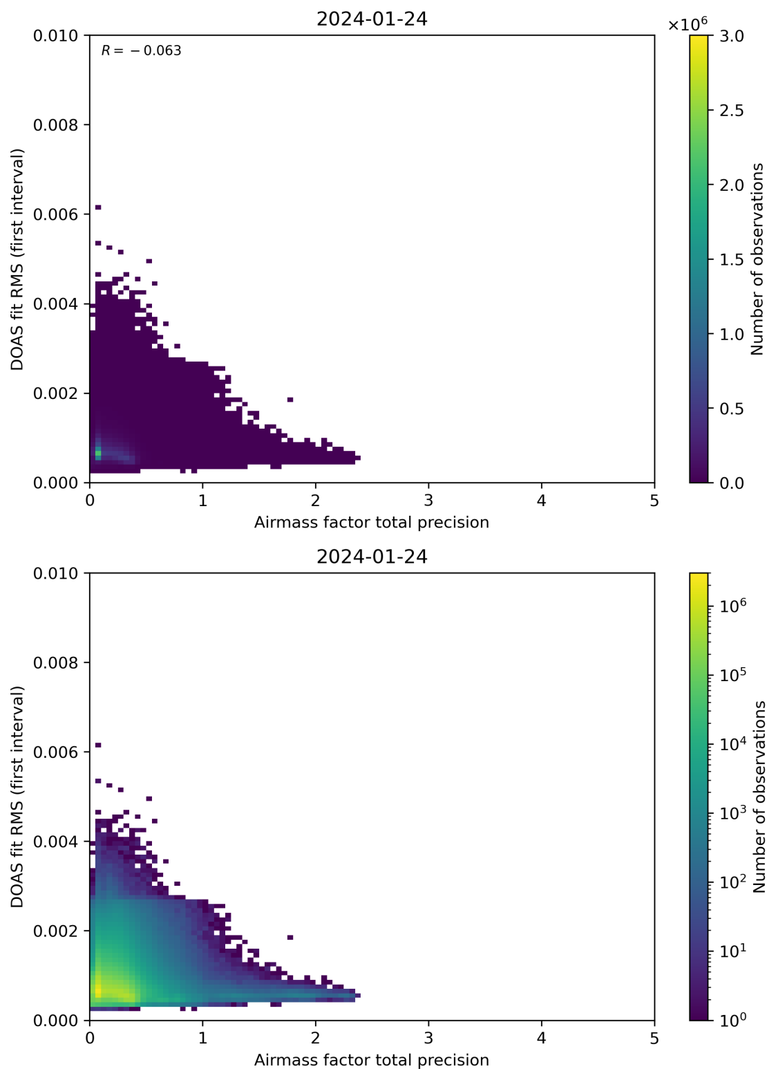
Figure 105: Scatter density plot of “Airmass factor total precision” against “DOAS fit RMS (first interval)” for 2024-01-23 to 2024-01-25.
