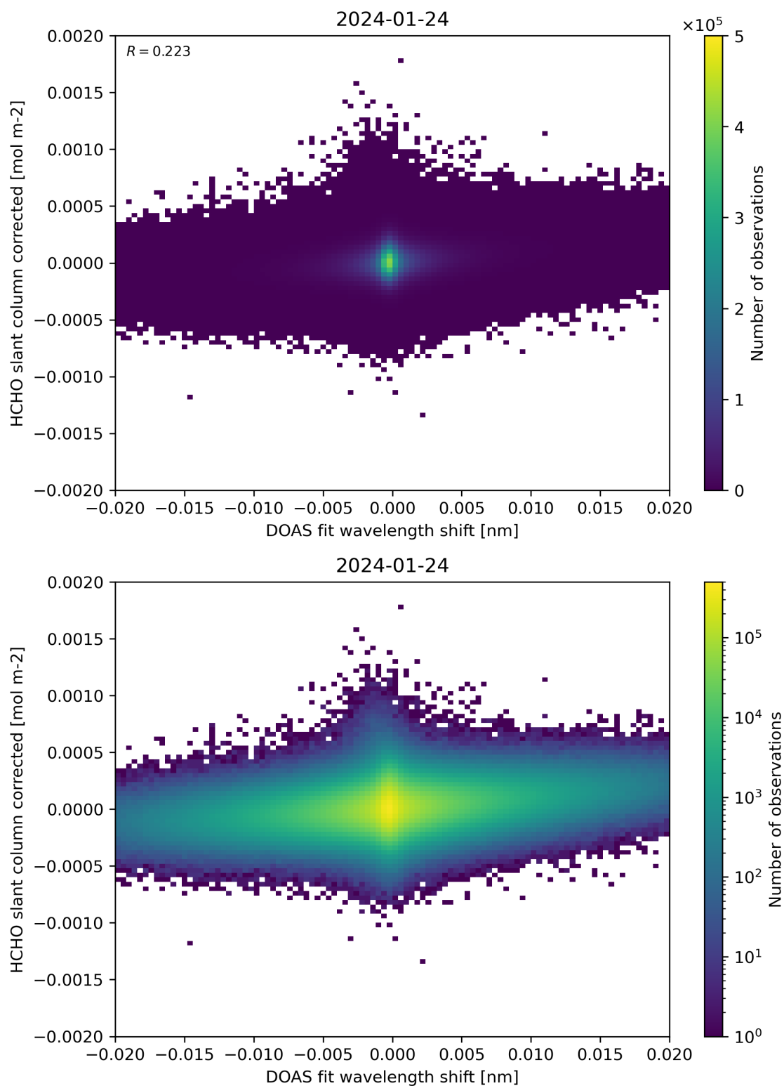
Figure 66: Scatter density plot of “DOAS fit wavelength shift” against “HCHO slant column corrected” for 2024-01-23 to 2024-01-25.
