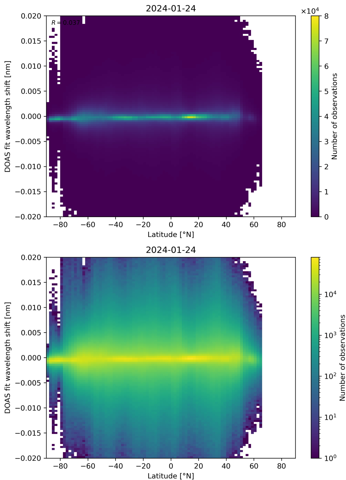
Figure 154: Scatter density plot of “Latitude” against “DOAS fit wavelength shift” for 2024-01-23 to 2024-01-25.
