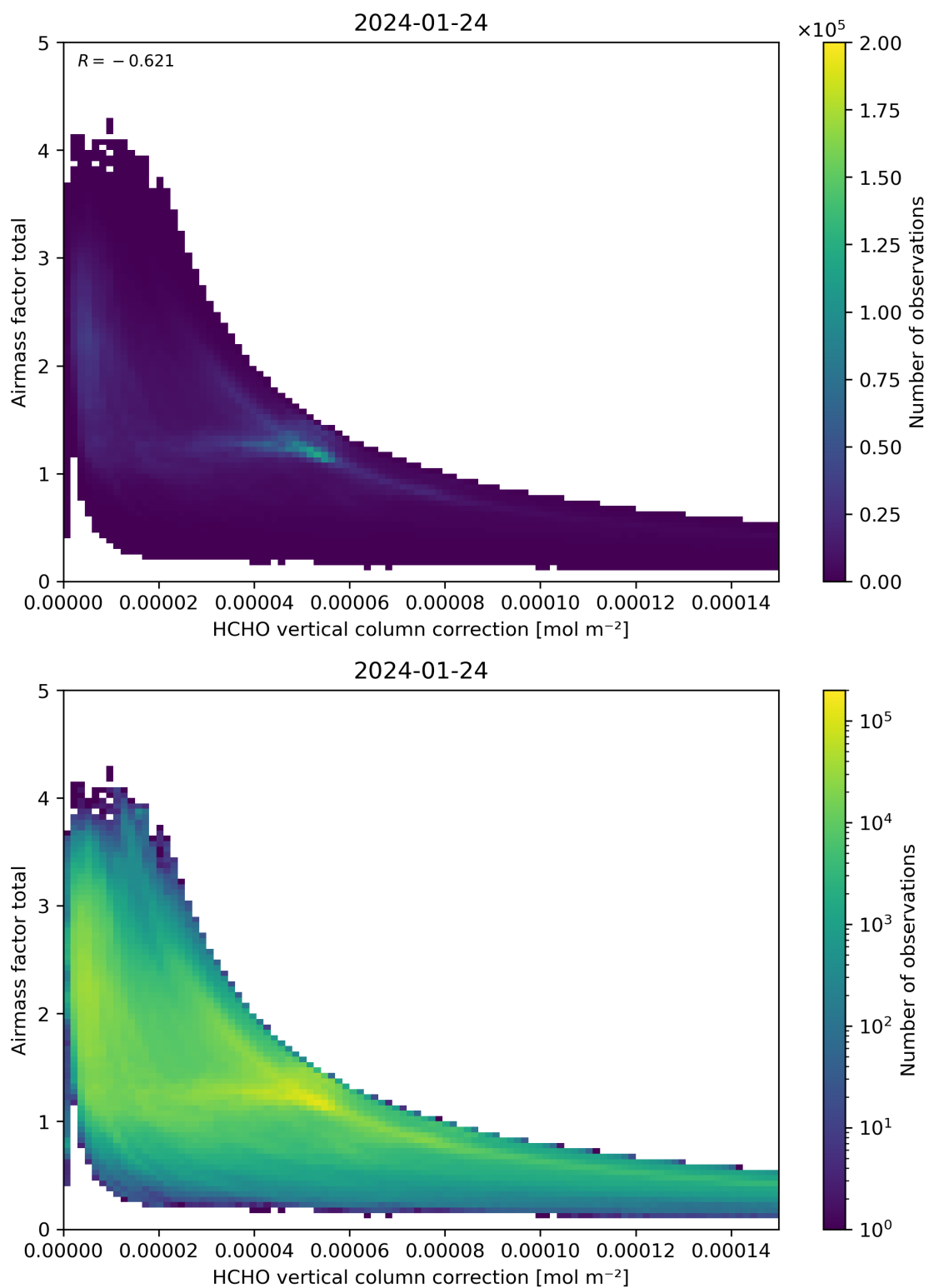
Figure 120: Scatter density plot of “HCHO vertical column correction” against “Airmass factor total” for 2024-01-23 to 2024-01-25.
