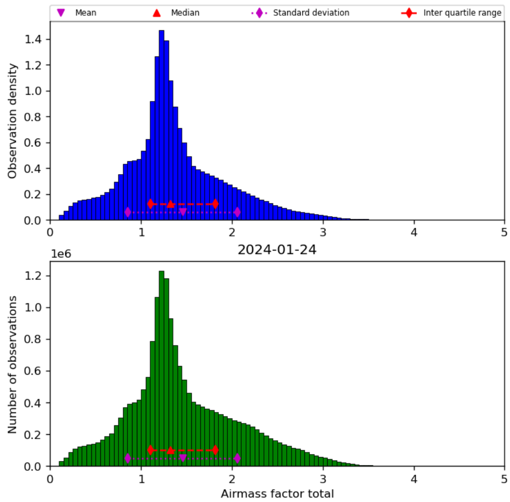
Figure 40: Histogram of “Airmass factor total” for 2024-01-23 to 2024-01-25
