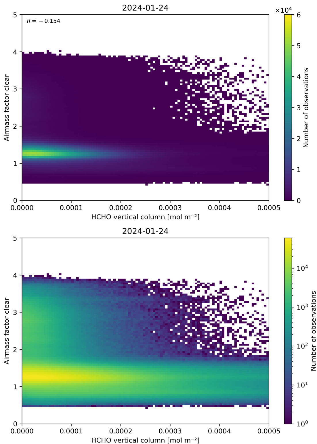
Figure 126: Scatter density plot of “HCHO vertical column” against “Airmass factor clear” for 2024-01-23 to 2024-01-25.
