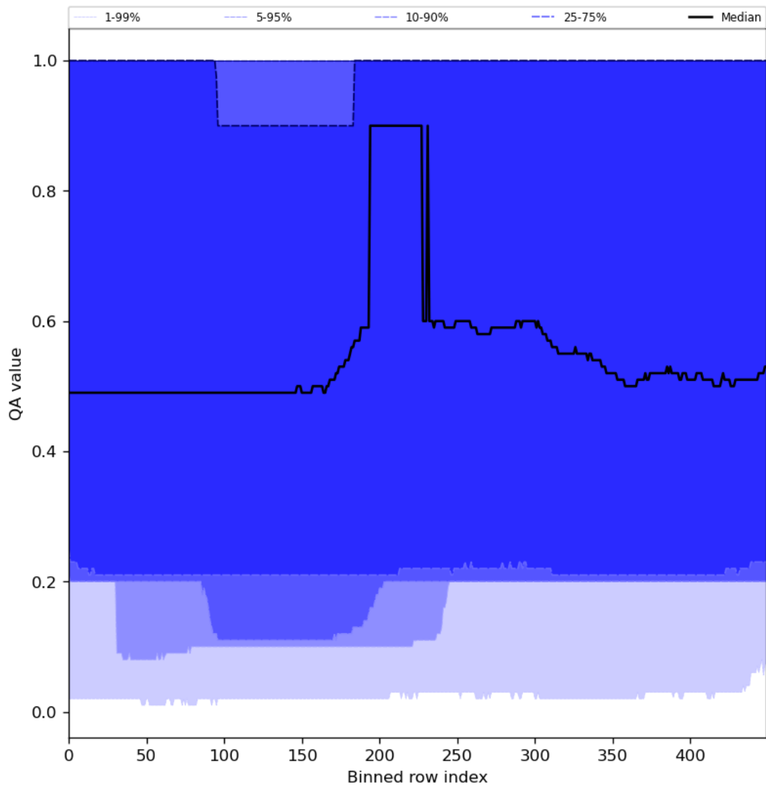
Figure 48: Along track statistics of “QA value” for 2024-01-23 to 2024-01-25
