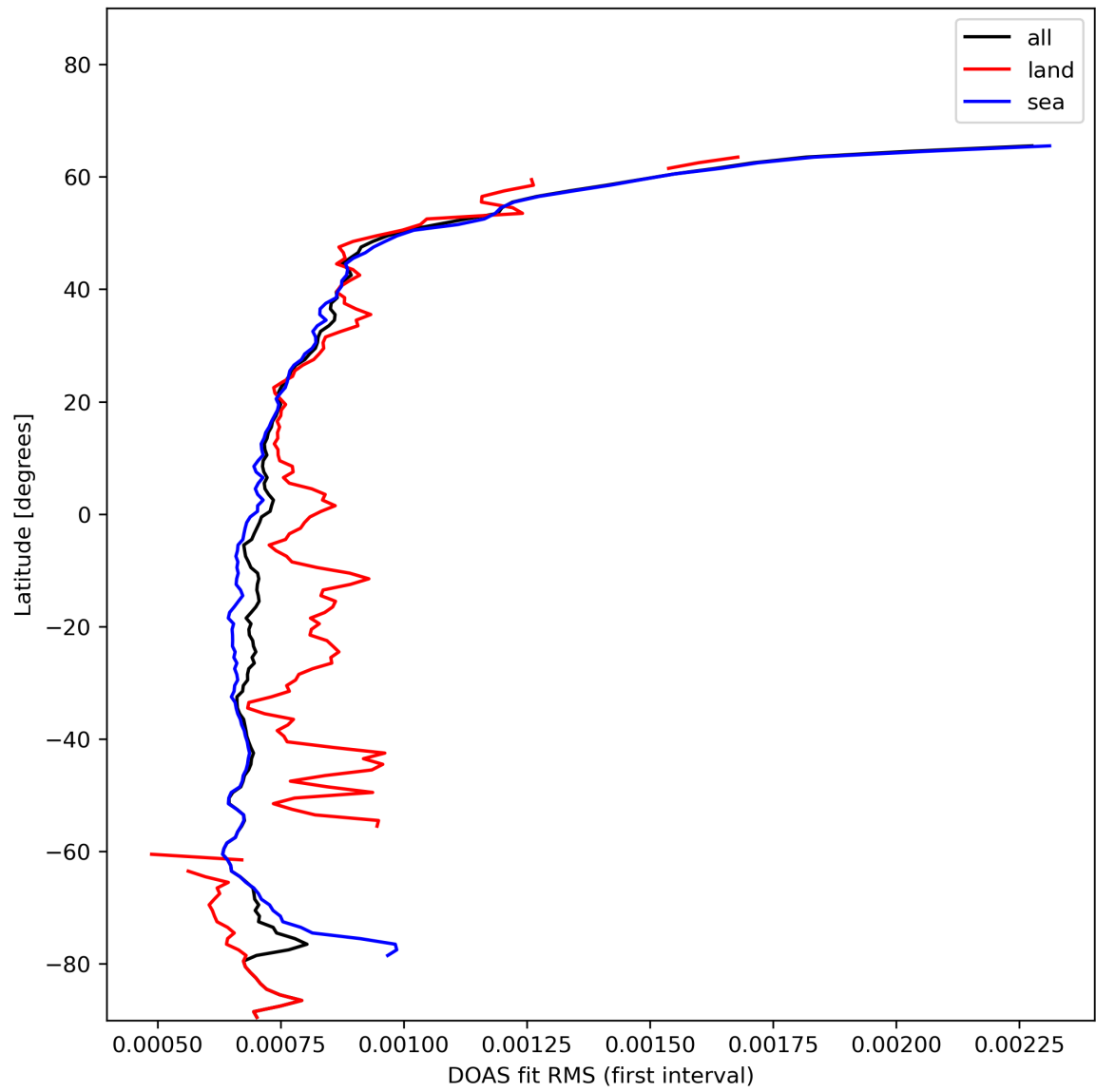
Figure 32: Zonal average of “DOAS fit RMS (first interval)” for 2024-01-23 to 2024-01-25.
