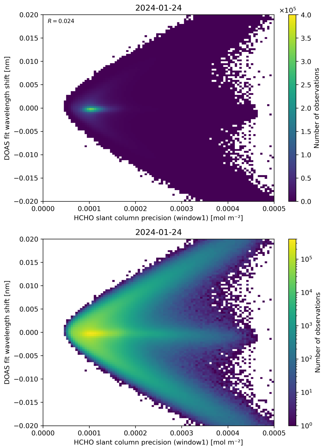
Figure 89: Scatter density plot of “HCHO slant column precision (window1)” against “DOAS fit wavelength shift” for 2024-01-23 to 2024-01-25.
