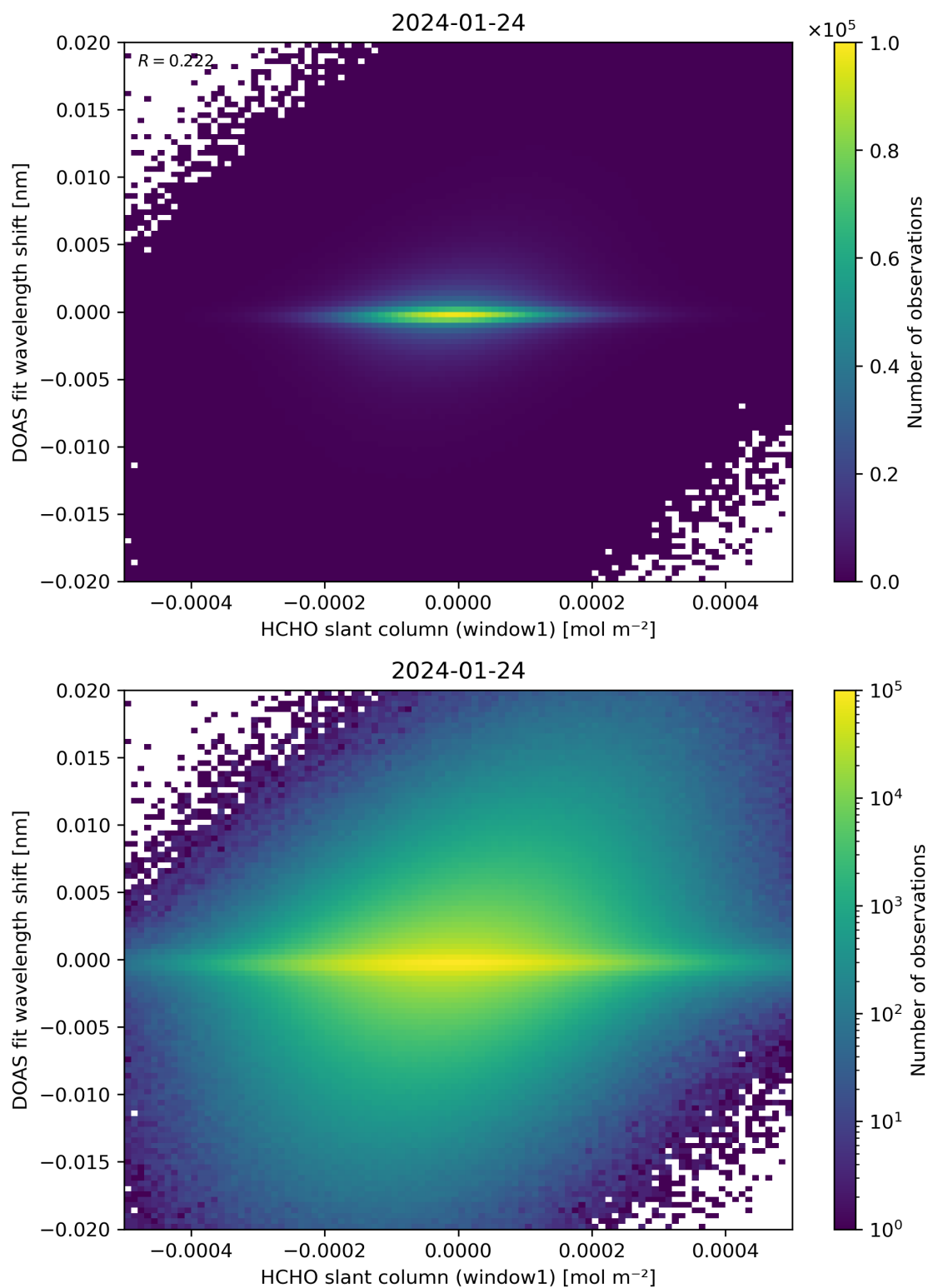
Figure 79: Scatter density plot of “HCHO slant column (window1)” against “DOAS fit wavelength shift” for 2024-01-23 to 2024-01-25.
