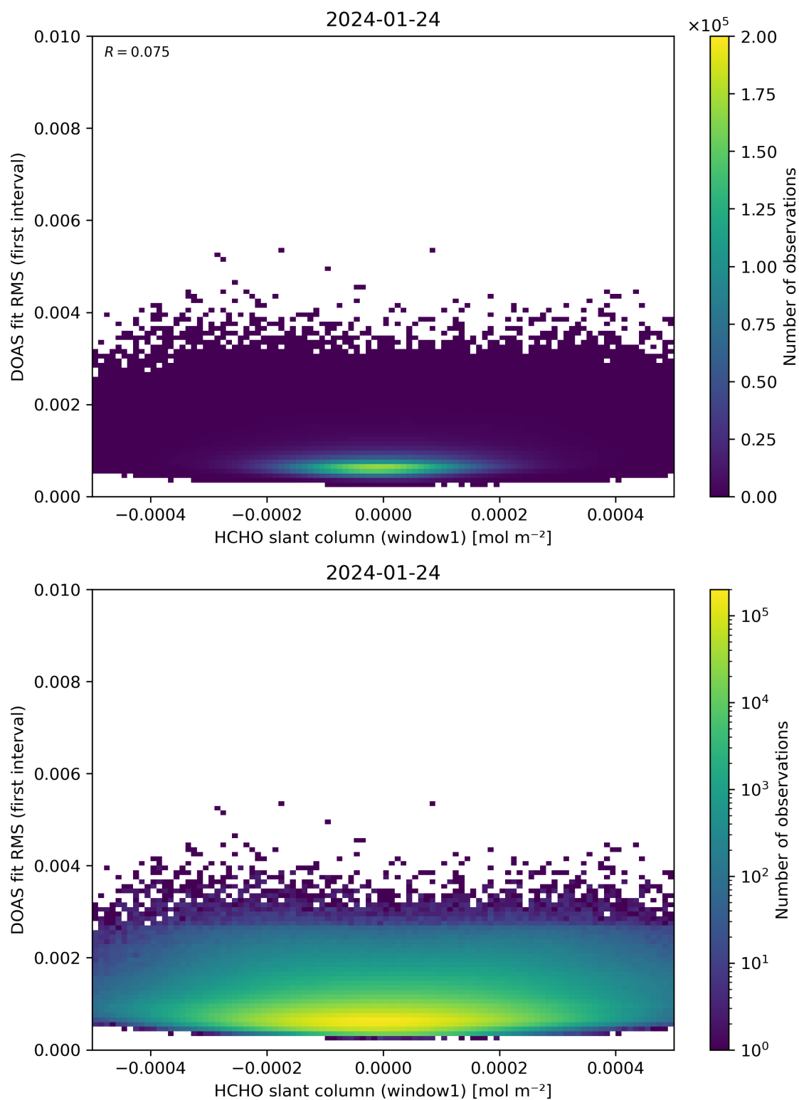
Figure 78: Scatter density plot of “HCHO slant column (window1)” against “DOAS fit RMS (first interval)” for 2024-01-23 to 2024-01-25.
