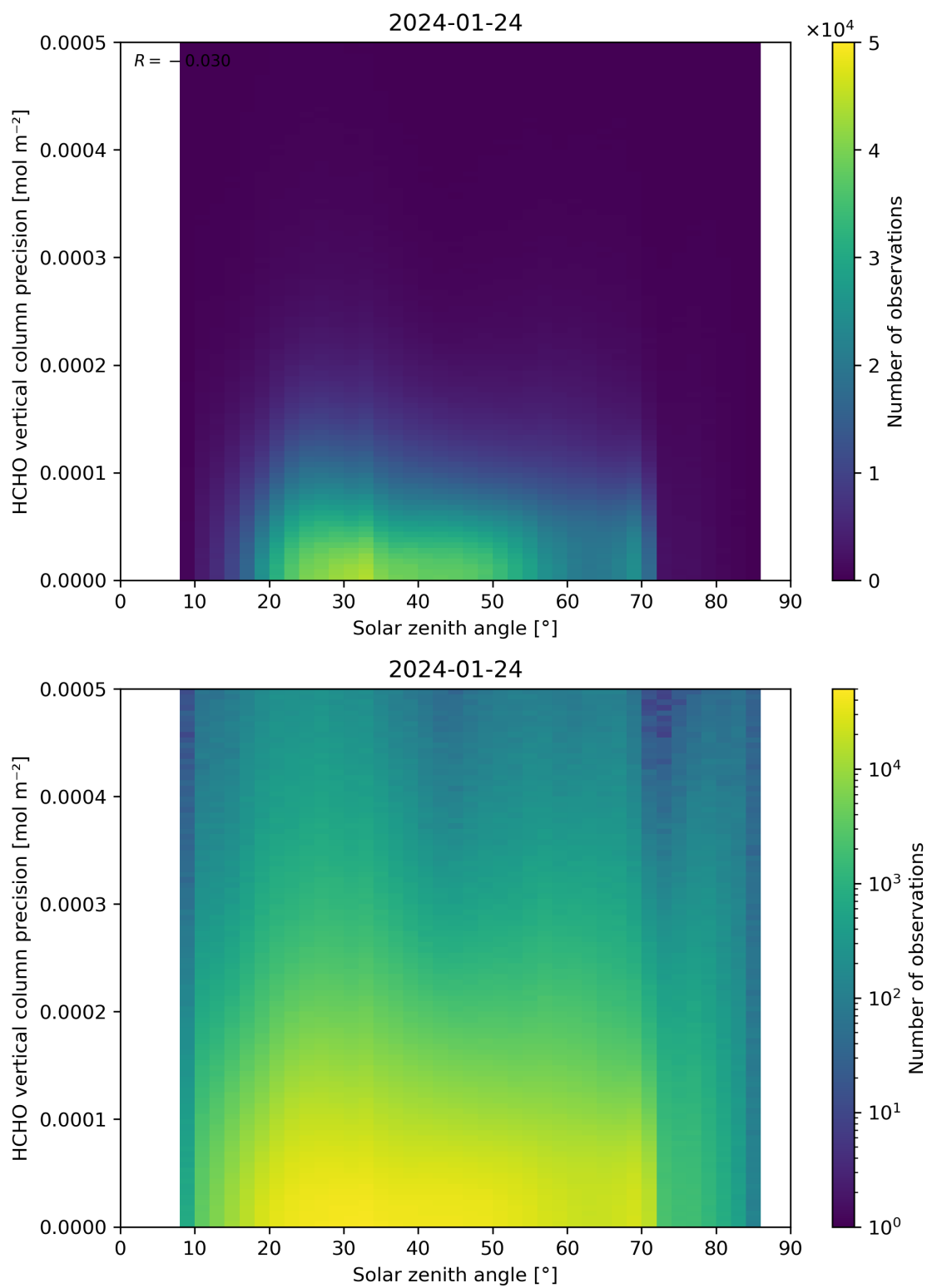
Figure 179: Scatter density plot of “Solar zenith angle” against “HCHO vertical column precision” for 2024-01-23 to 2024-01-25.
