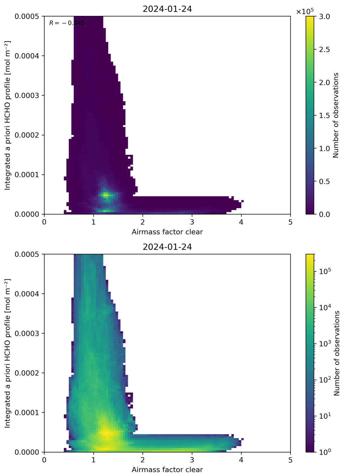
Figure 76: Scatter density plot of “Airmass factor clear” against “Integrated a priori HCHO profile” for 2024-01-23 to 2024-01-25.
