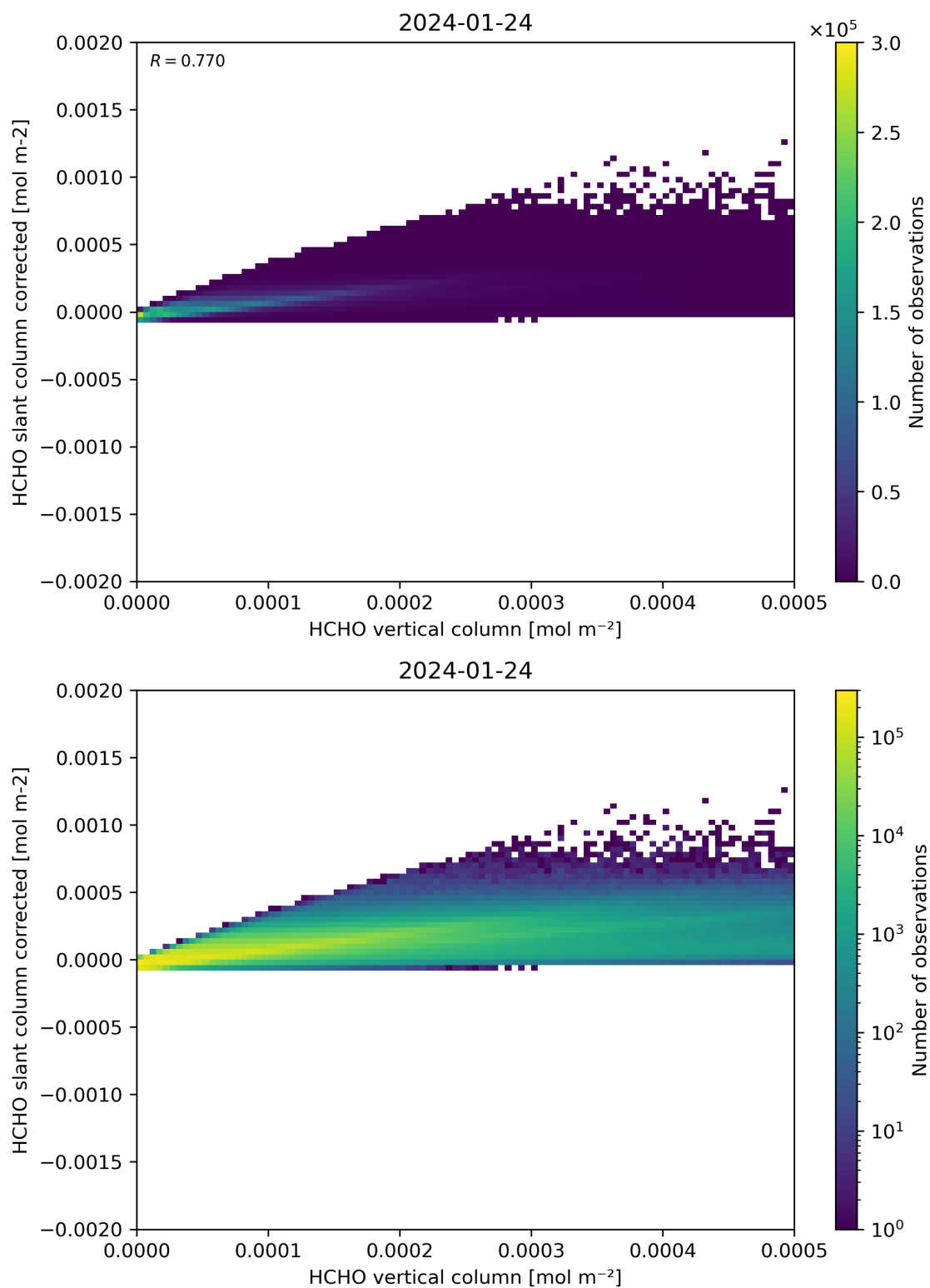
Figure 127: Scatter density plot of “HCHO vertical column” against “HCHO slant column corrected” for 2024-01-23 to 2024-01-25.
