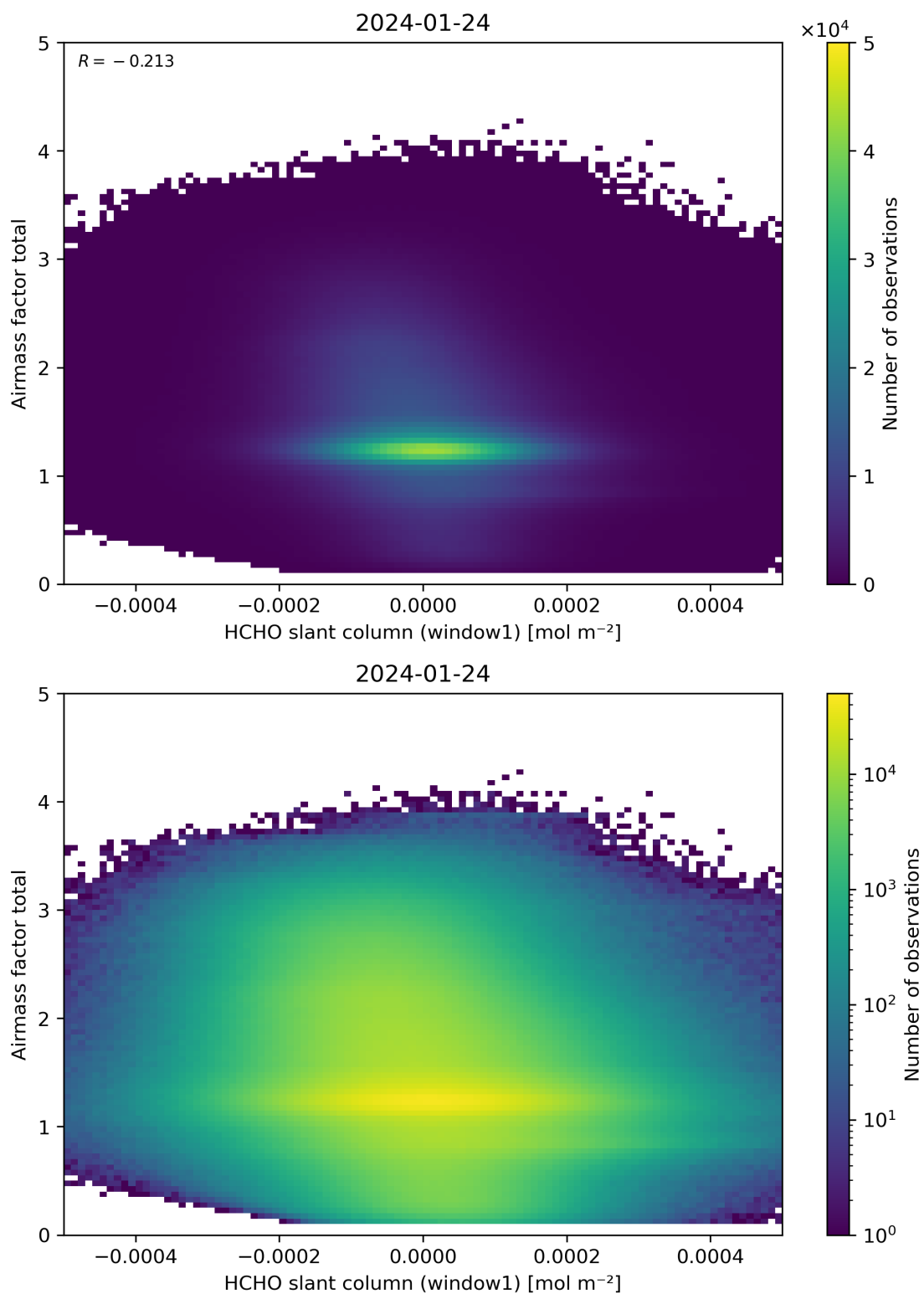
Figure 85: Scatter density plot of “HCHO slant column (window1)” against “Airmass factor total” for 2024-01-23 to 2024-01-25.
