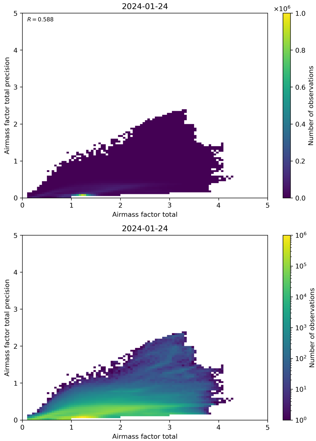
Figure 103: Scatter density plot of “Airmass factor total” against “Airmass factor total precision” for 2024-01-23 to 2024-01-25.
