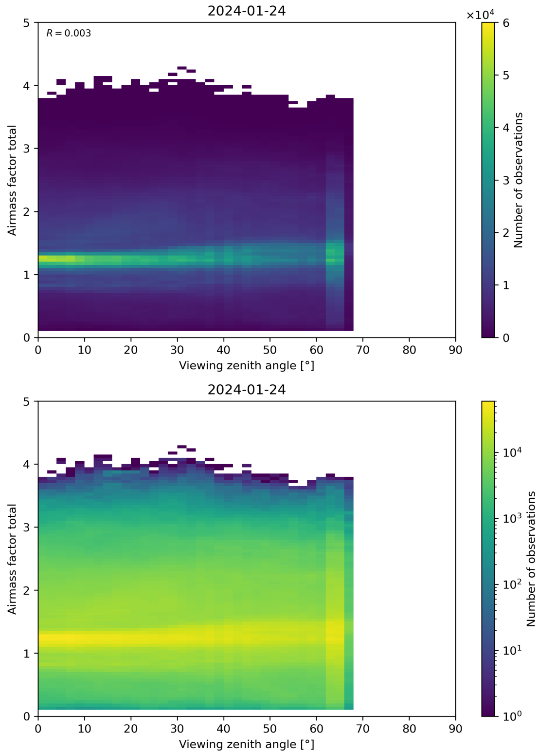
Figure 190: Scatter density plot of “Viewing zenith angle” against “Airmass factor total” for 2024-01-23 to 2024-01-25.
