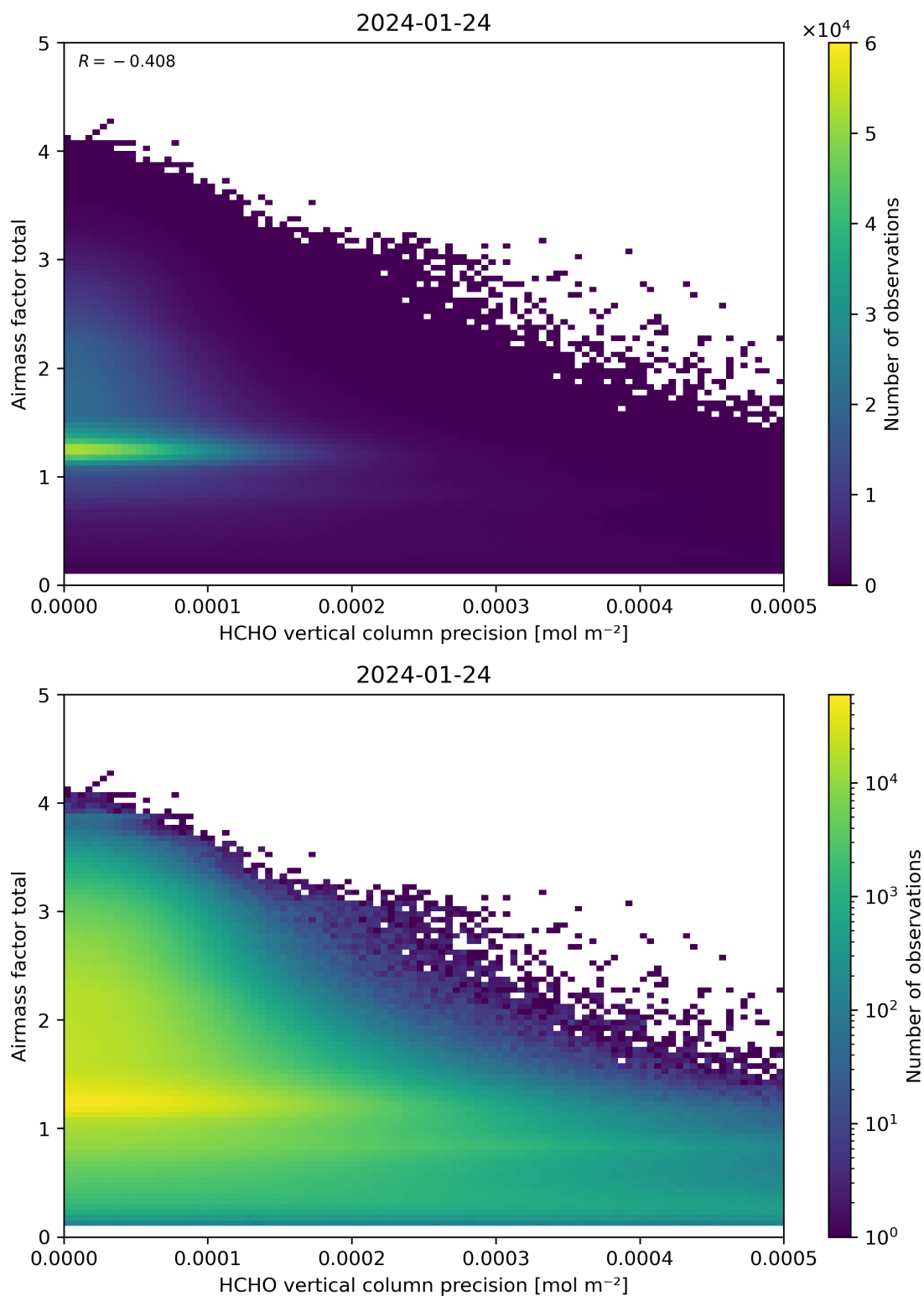
Figure 144: Scatter density plot of “HCHO vertical column precision” against “Airmass factor total” for 2024-01-23 to 2024-01-25.
