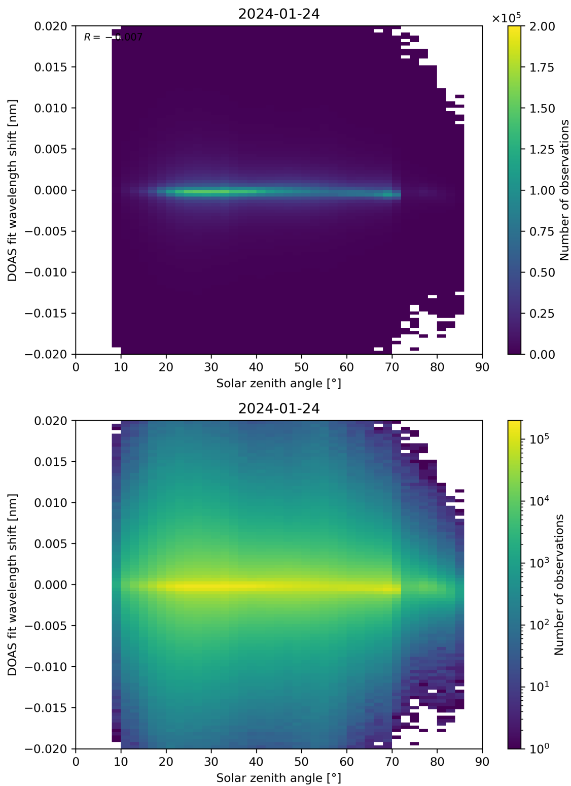
Figure 168: Scatter density plot of “Solar zenith angle” against “DOAS fit wavelength shift” for 2024-01-23 to 2024-01-25.
