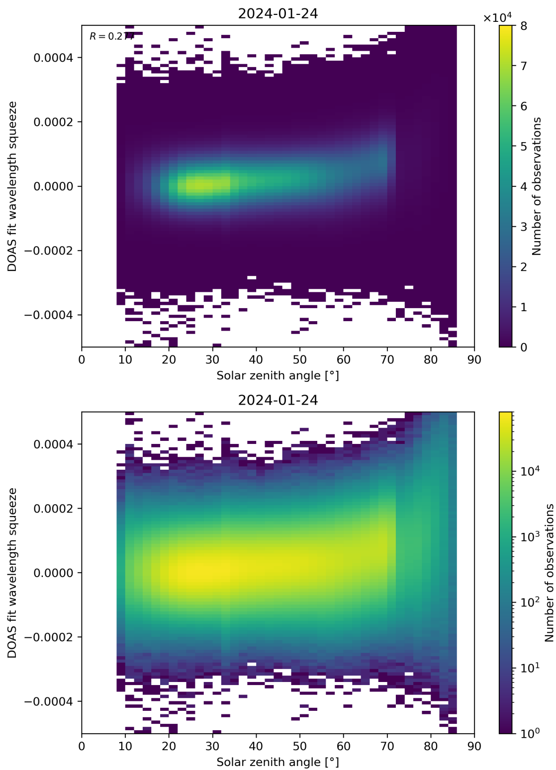
Figure 169: Scatter density plot of “Solar zenith angle” against “DOAS fit wavelength squeeze” for 2024-01-23 to 2024-01-25.
