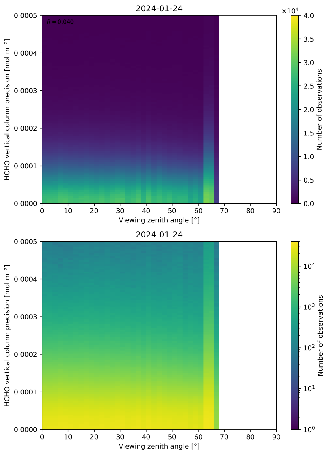
Figure 194: Scatter density plot of “Viewing zenith angle” against “HCHO vertical column precision” for 2024-01-23 to 2024-01-25.
