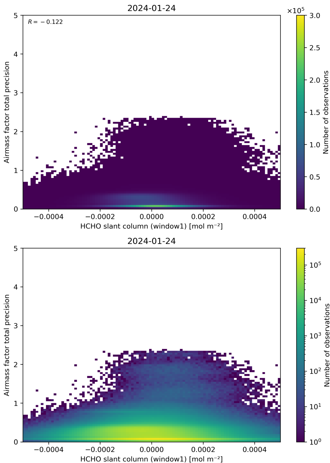
Figure 86: Scatter density plot of “HCHO slant column (window1)” against “Airmass factor total precision” for 2024-01-23 to 2024-01-25.
