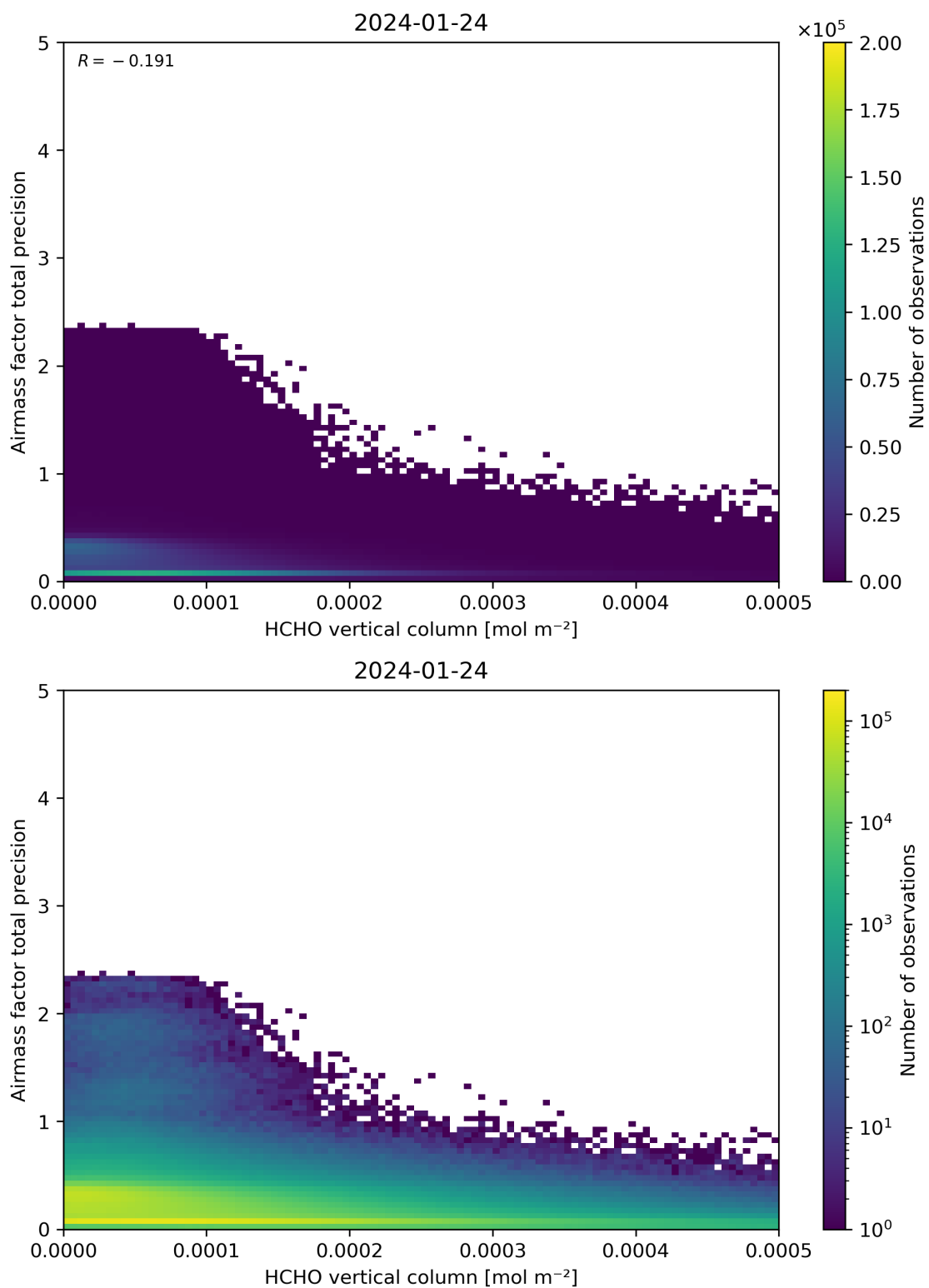
Figure 132: Scatter density plot of “HCHO vertical column” against “Airmass factor total precision” for 2024-01-23 to 2024-01-25.
