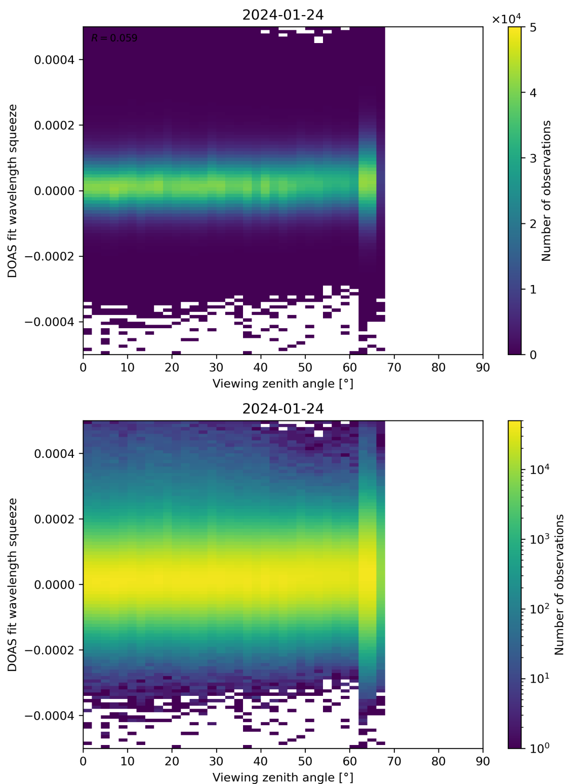
Figure 184: Scatter density plot of “Viewing zenith angle” against “DOAS fit wavelength squeeze” for 2024-01-23 to 2024-01-25.
