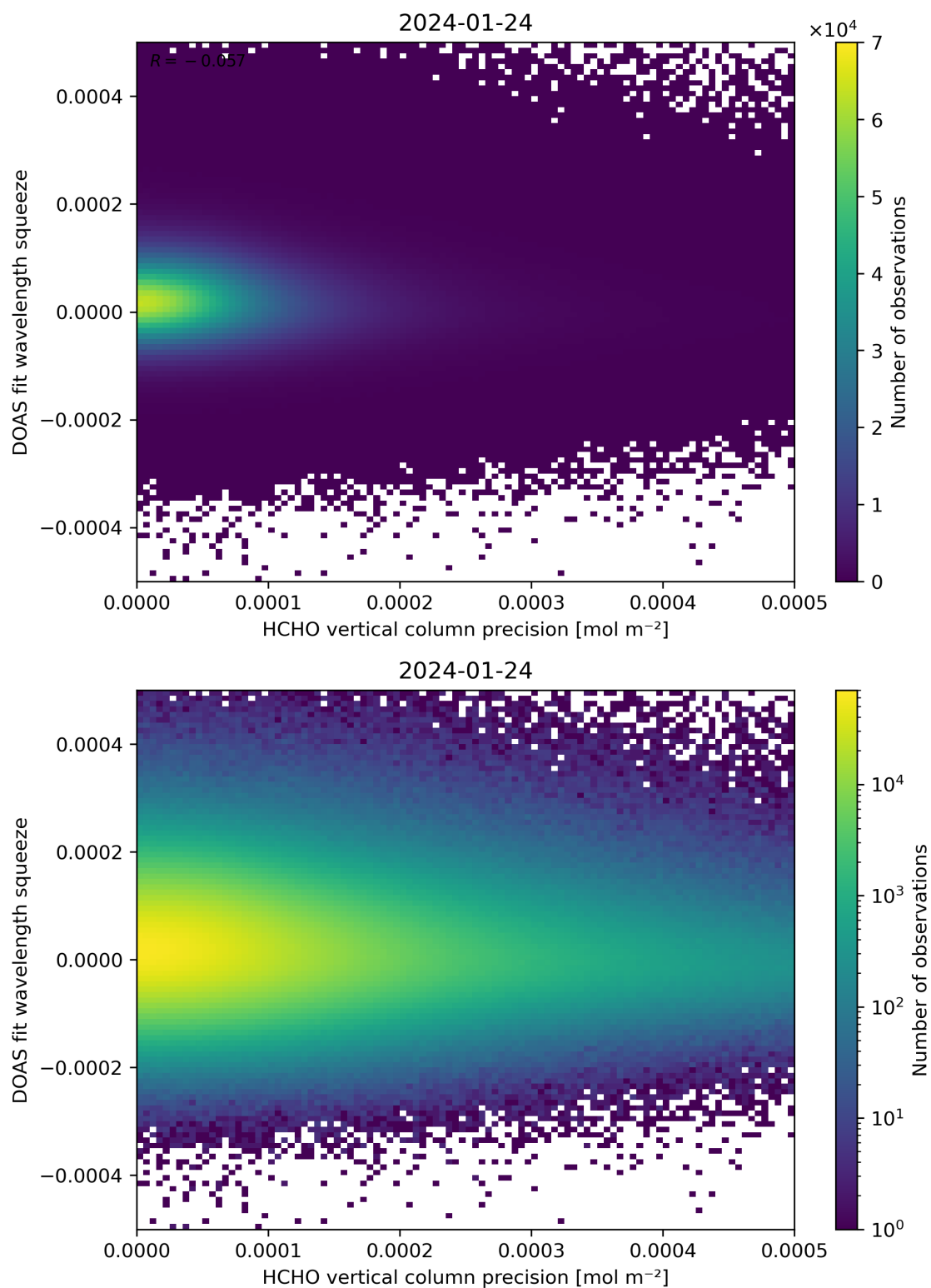
Figure 138: Scatter density plot of “HCHO vertical column precision” against “DOAS fit wavelength squeeze” for 2024-01-23 to 2024-01-25.
