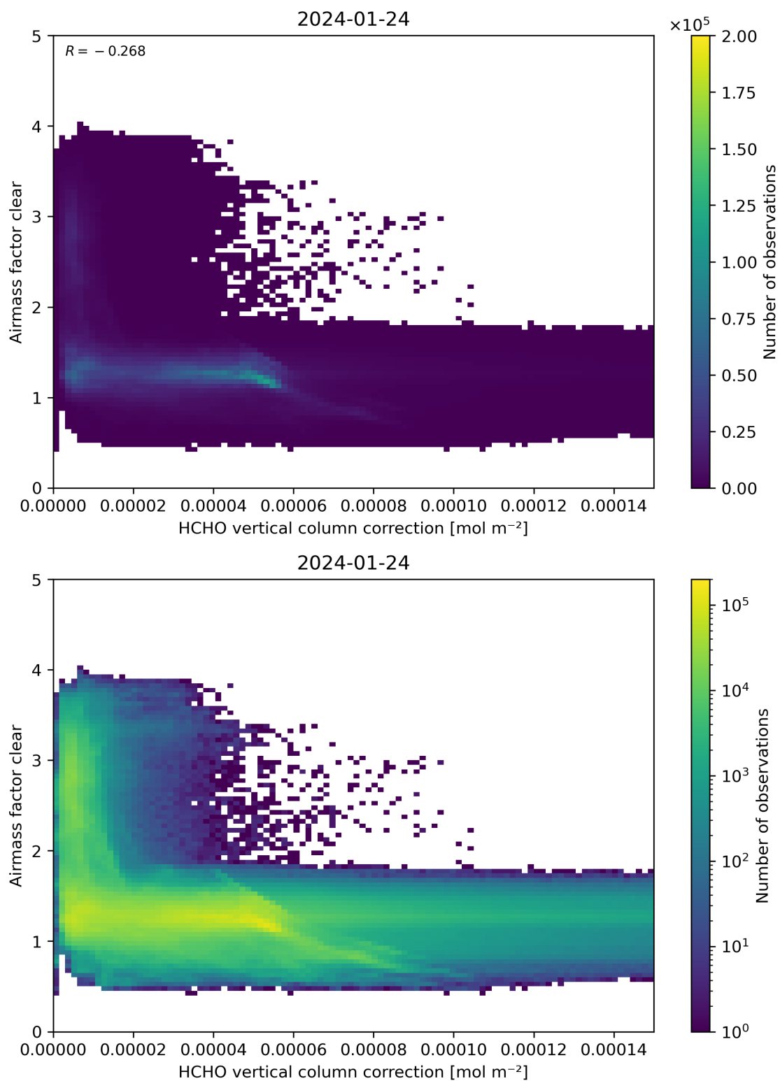
Figure 115: Scatter density plot of “HCHO vertical column correction” against “Airmass factor clear” for 2024-01-23 to 2024-01-25.
