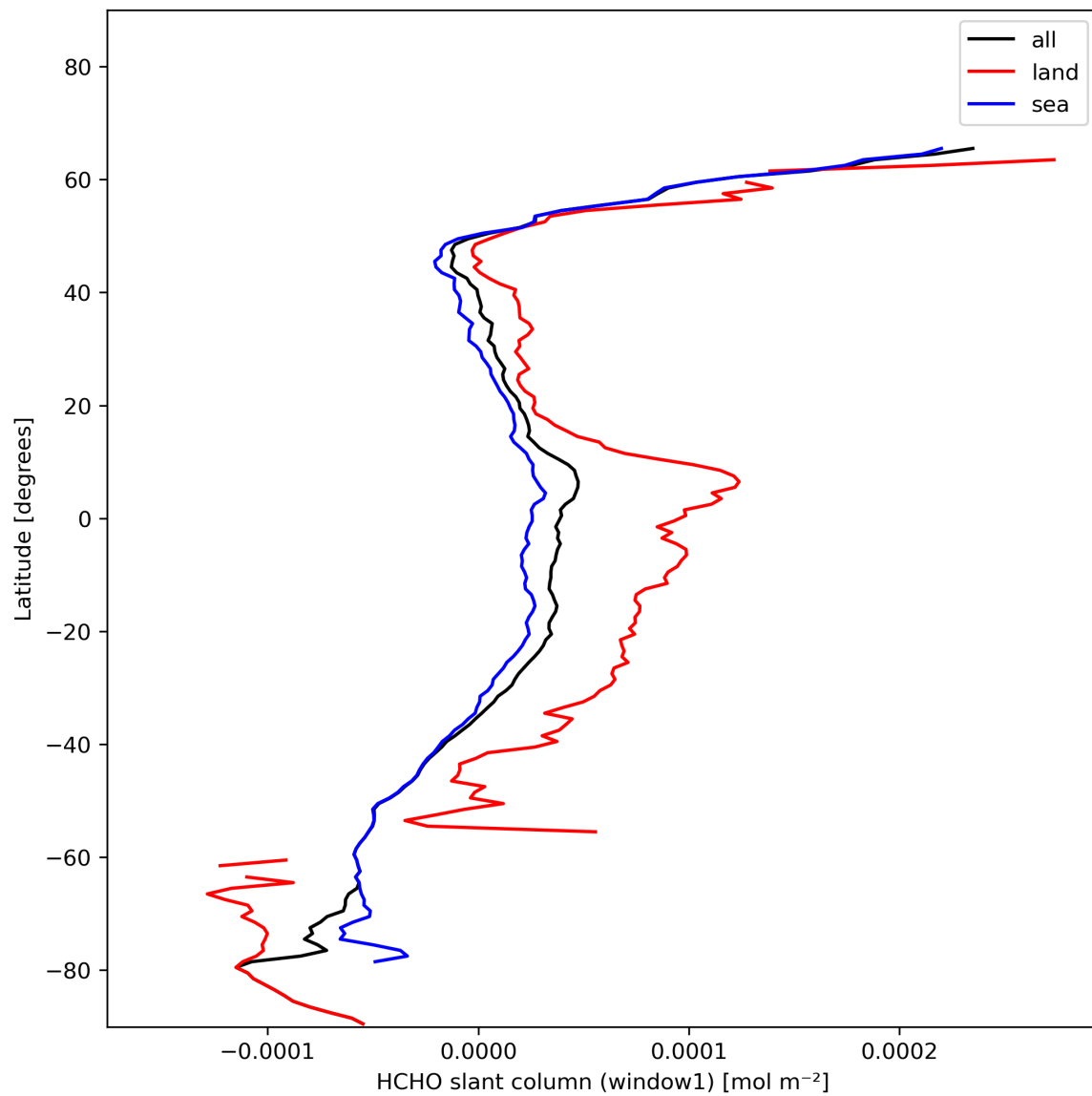
Figure 24: Zonal average of “HCHO slant column (window1)” for 2024-01-23 to 2024-01-25.
