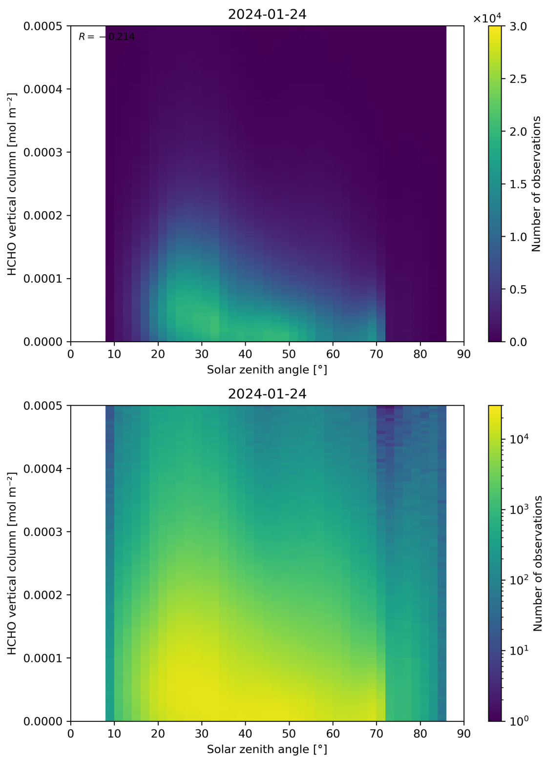
Figure 177: Scatter density plot of “Solar zenith angle” against “HCHO vertical column” for 2024-01-23 to 2024-01-25.
