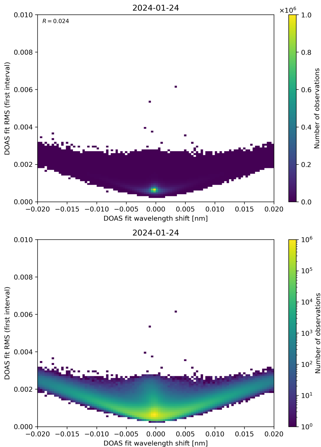
Figure 64: Scatter density plot of “DOAS fit wavelength shift” against “DOAS fit RMS (first interval)” for 2024-01-23 to 2024-01-25.
