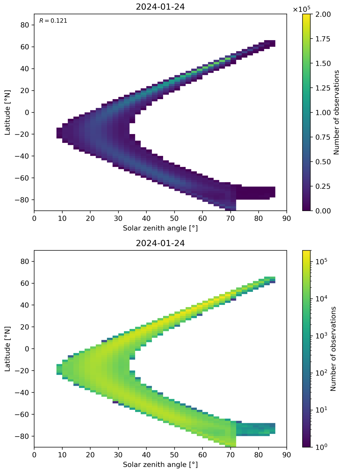
Figure 181: Scatter density plot of “Solar zenith angle” against “Latitude” for 2024-01-23 to 2024-01-25.
