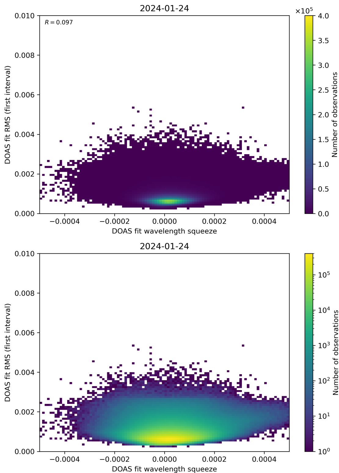
Figure 68: Scatter density plot of “DOAS fit wavelength squeeze” against “DOAS fit RMS (first interval)” for 2024-01-23 to 2024-01-25.
