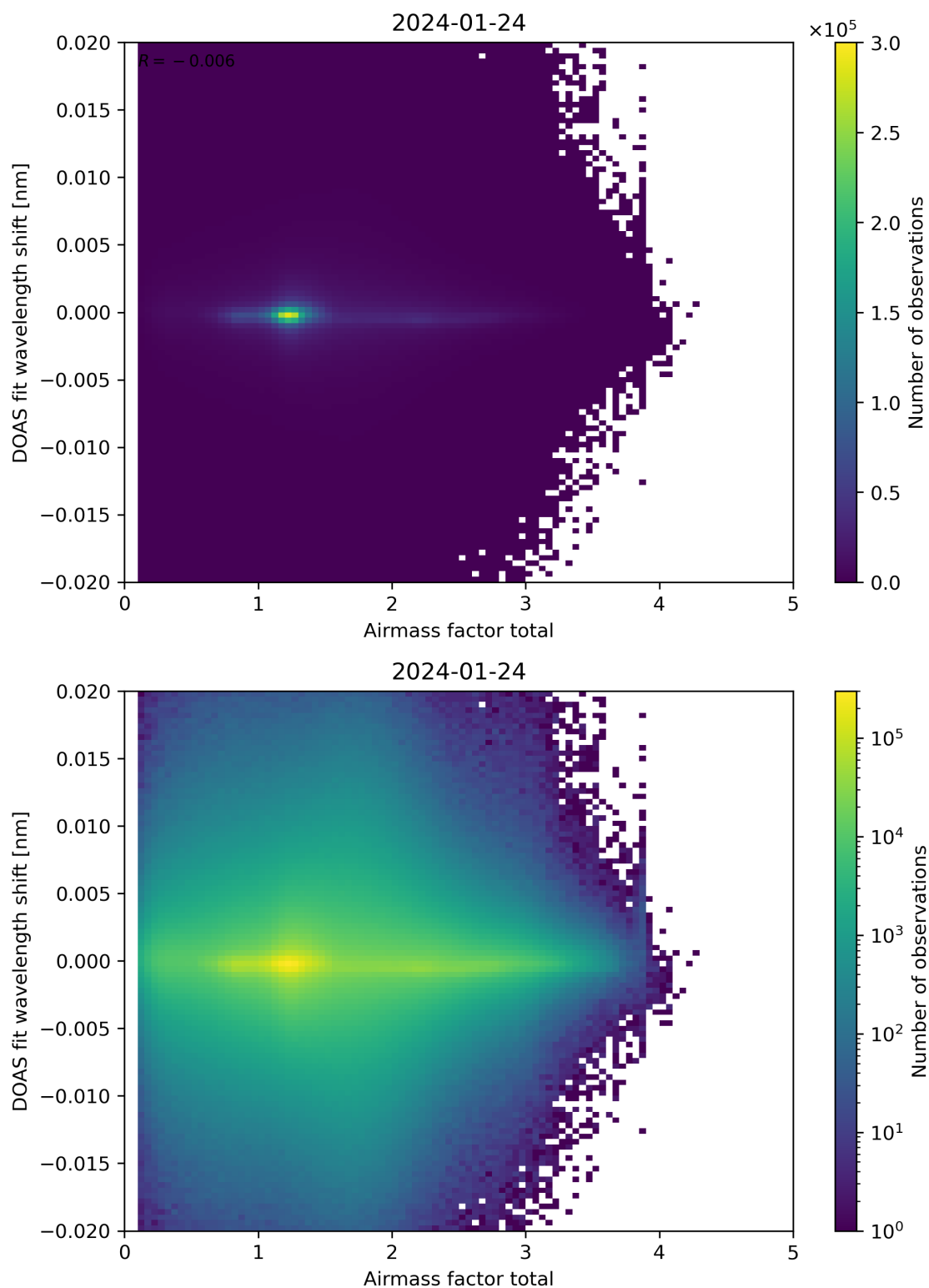
Figure 98: Scatter density plot of “Airmass factor total” against “DOAS fit wavelength shift” for 2024-01-23 to 2024-01-25.
