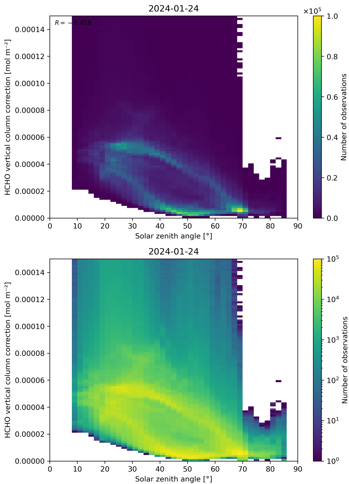
Figure 178: Scatter density plot of “Solar zenith angle” against “HCHO vertical column correction” for 2024-01-23 to 2024-01-25.
