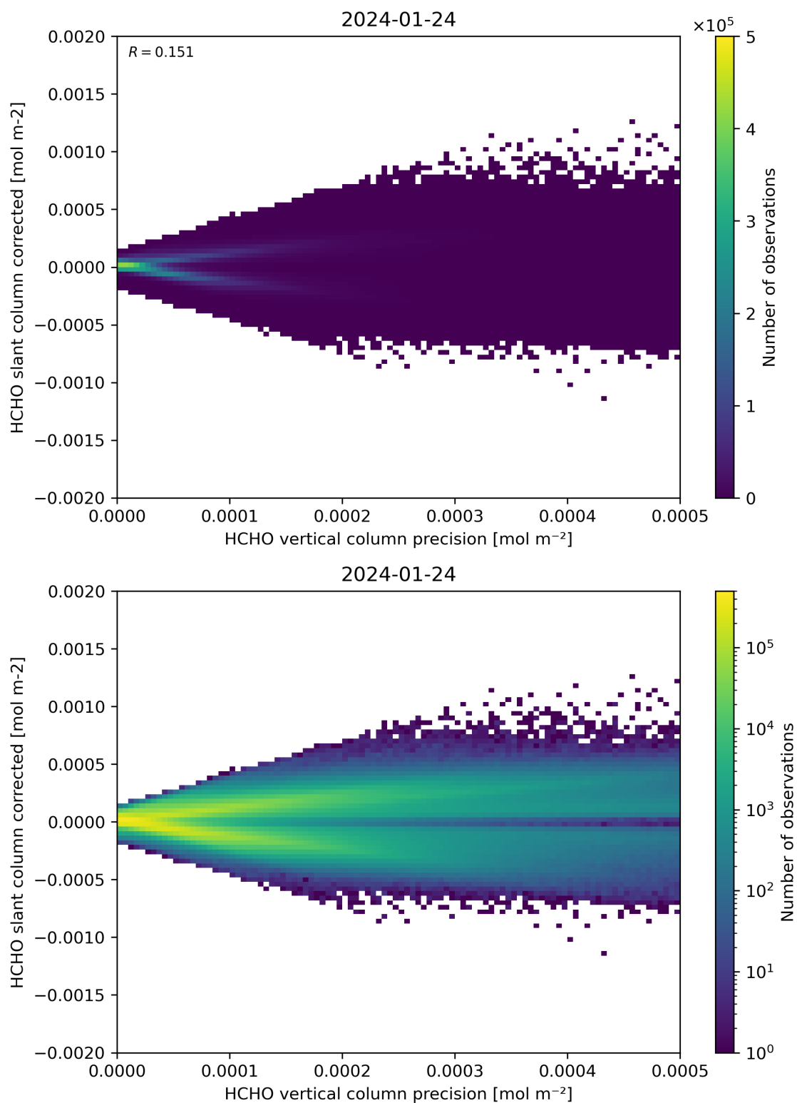
Figure 140: Scatter density plot of “HCHO vertical column precision” against “HCHO slant column corrected” for 2024-01-23 to 2024-01-25.
