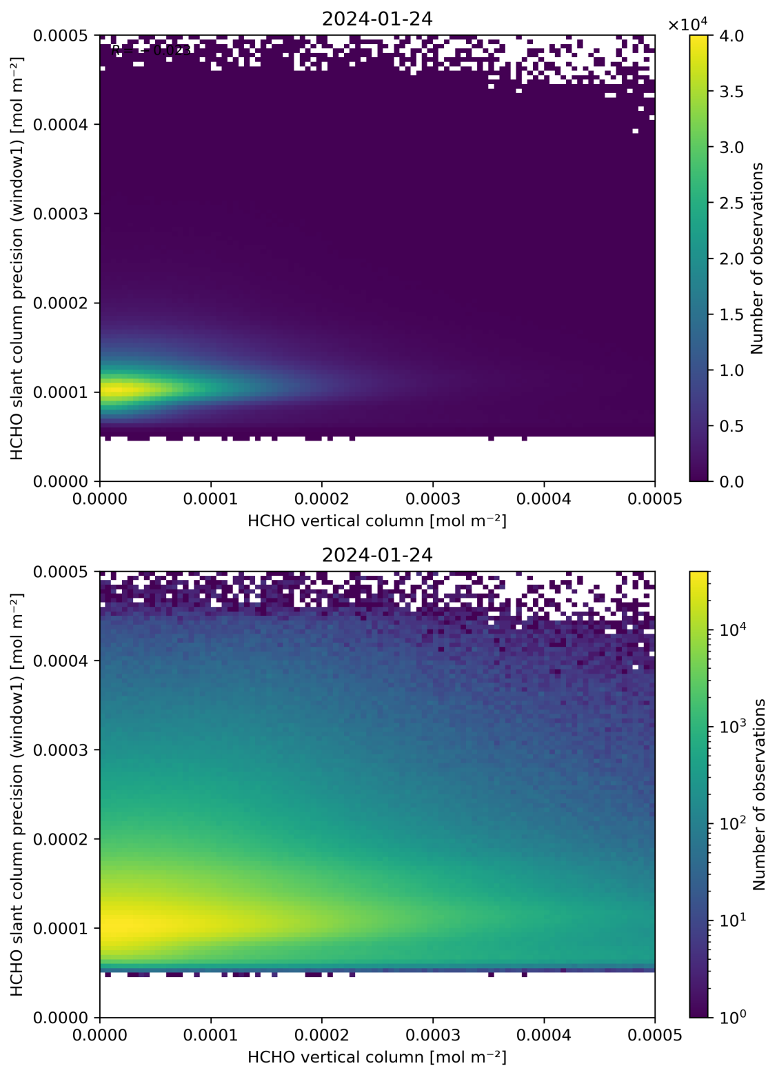
Figure 130: Scatter density plot of “HCHO vertical column” against “HCHO slant column precision (window1)” for 2024-01-23 to 2024-01-25.
