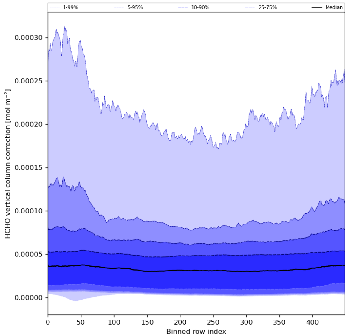
Figure 51: Along track statistics of “HCHO vertical column correction” for 2024-01-23 to 2024-01-25
