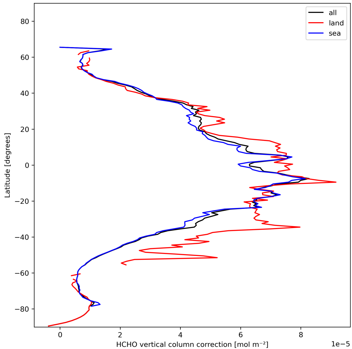
Figure 23: Zonal average of “HCHO vertical column correction” for 2024-01-23 to 2024-01-25.
