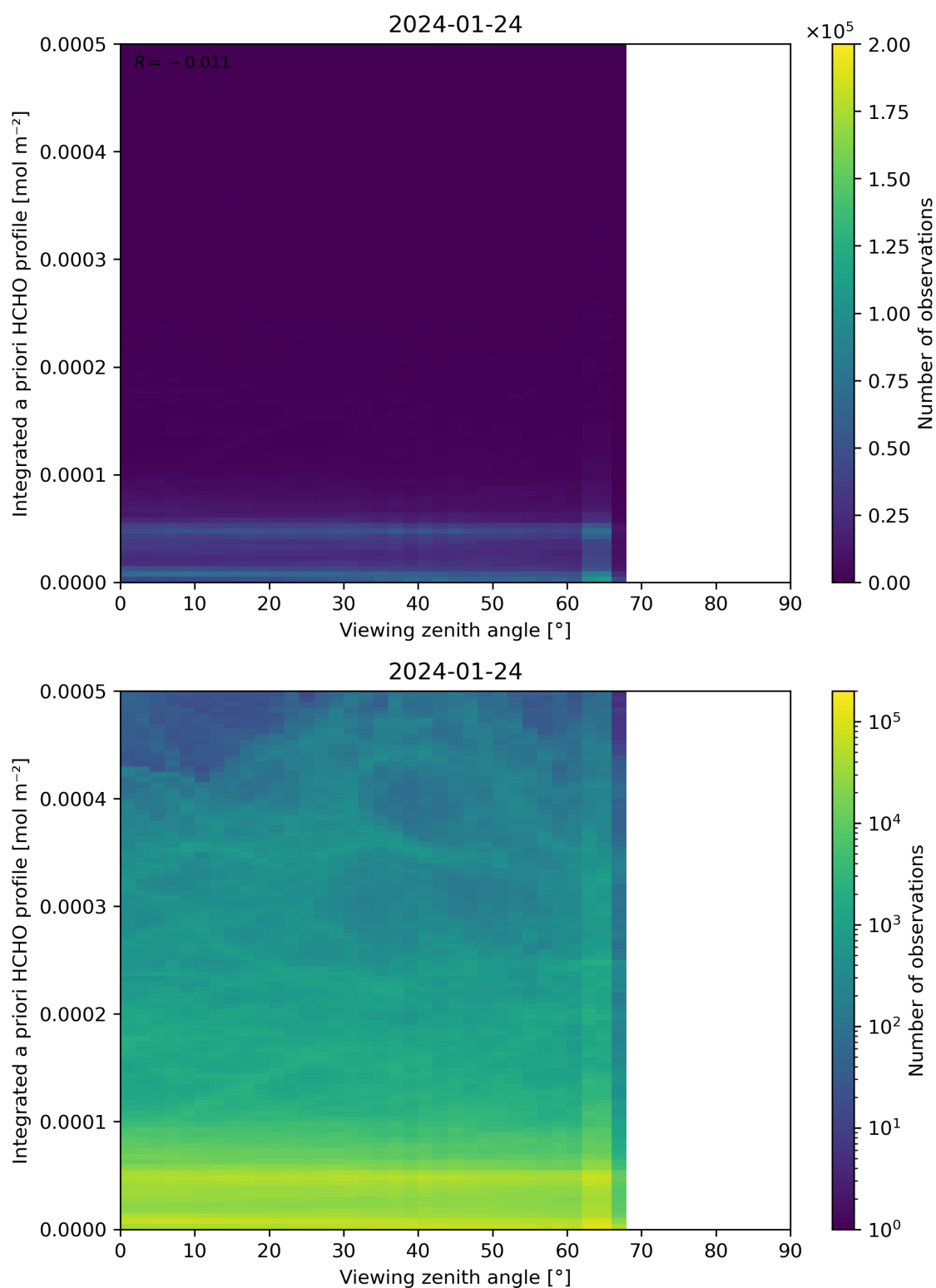
Figure 195: Scatter density plot of “Viewing zenith angle” against “Integrated a priori HCHO profile” for 2024-01-23 to 2024-01-25.
