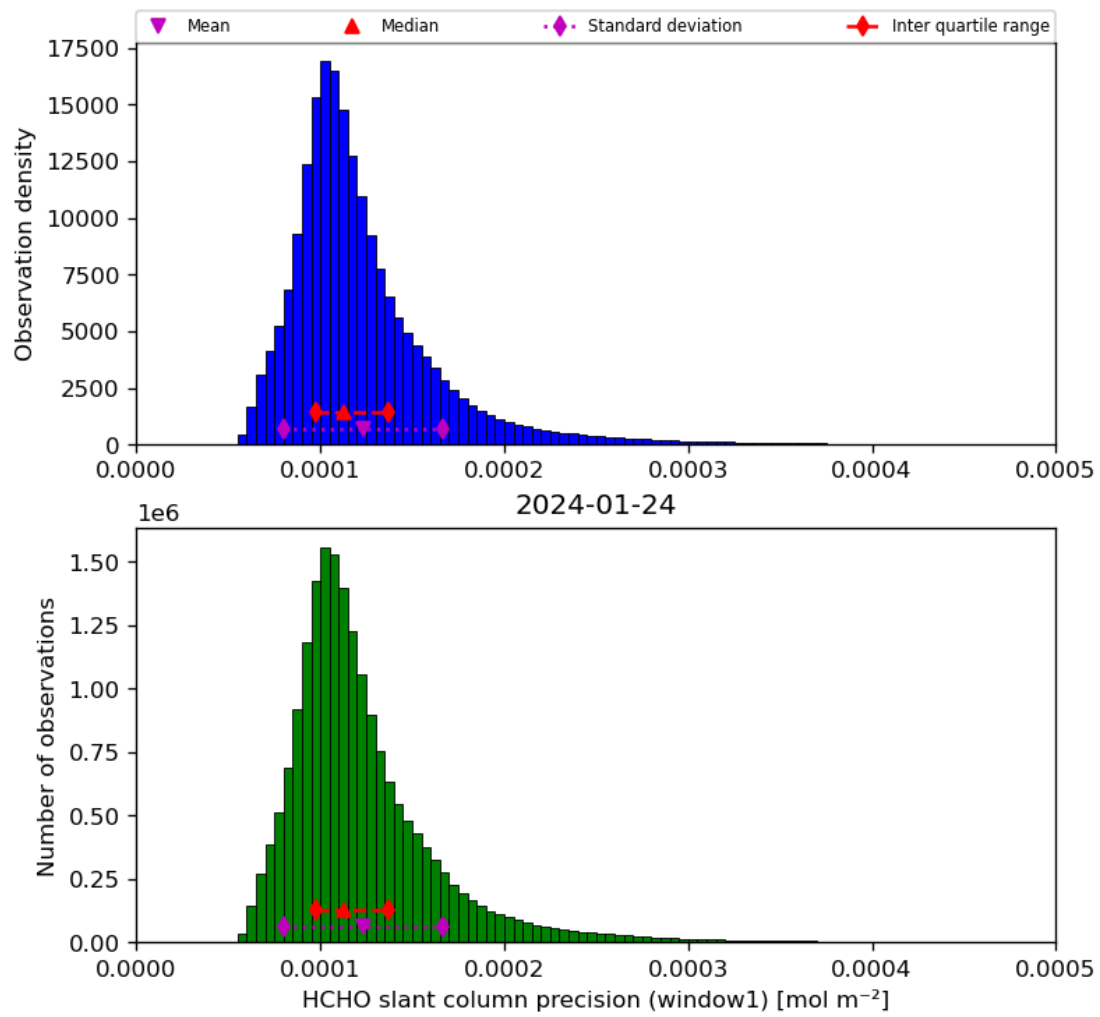
Figure 39: Histogram of “HCHO slant column precision (window1)” for 2024-01-23 to 2024-01-25
