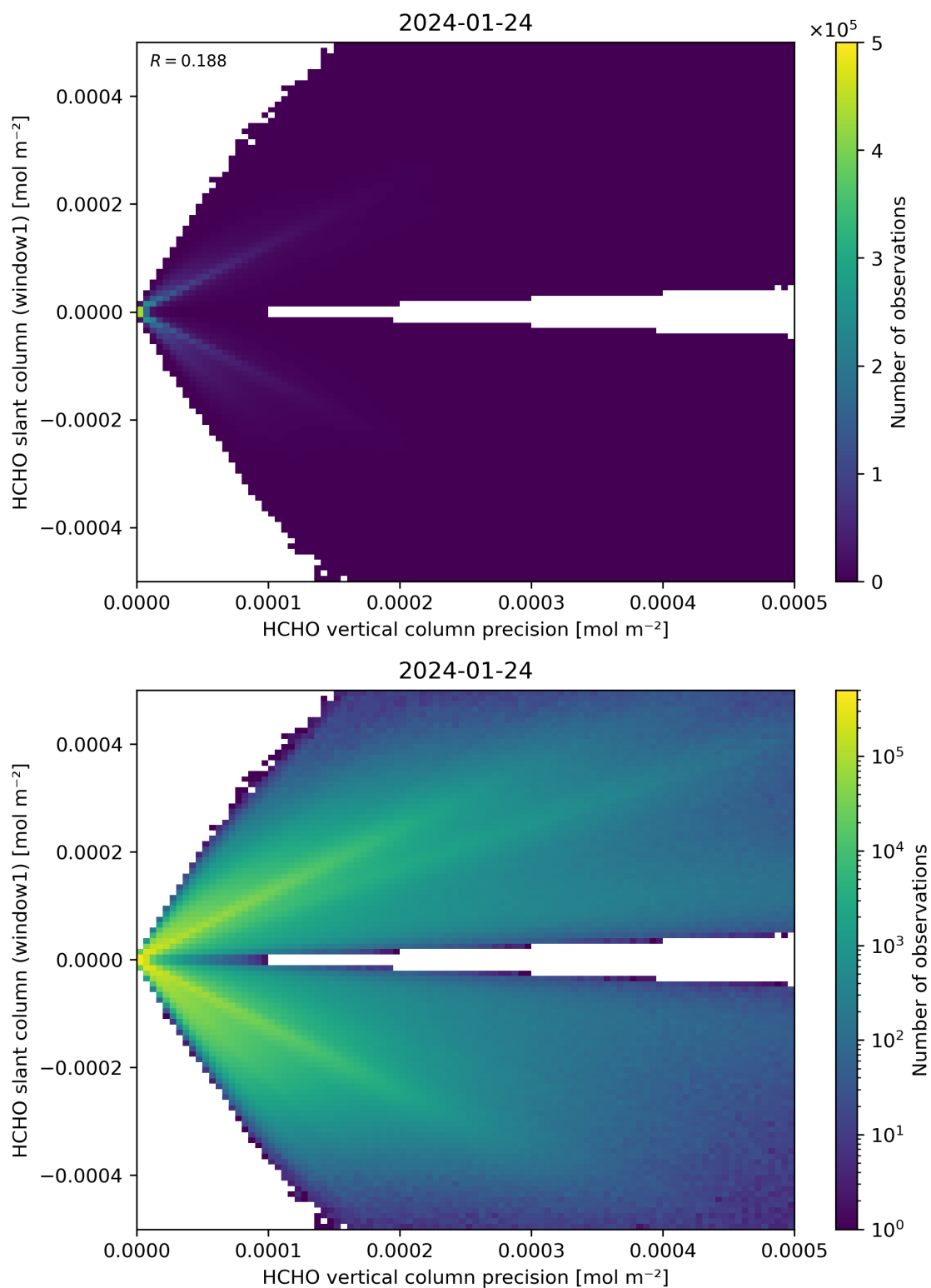
Figure 142: Scatter density plot of “HCHO vertical column precision” against “HCHO slant column (window1)” for 2024-01-23 to 2024-01-25.
