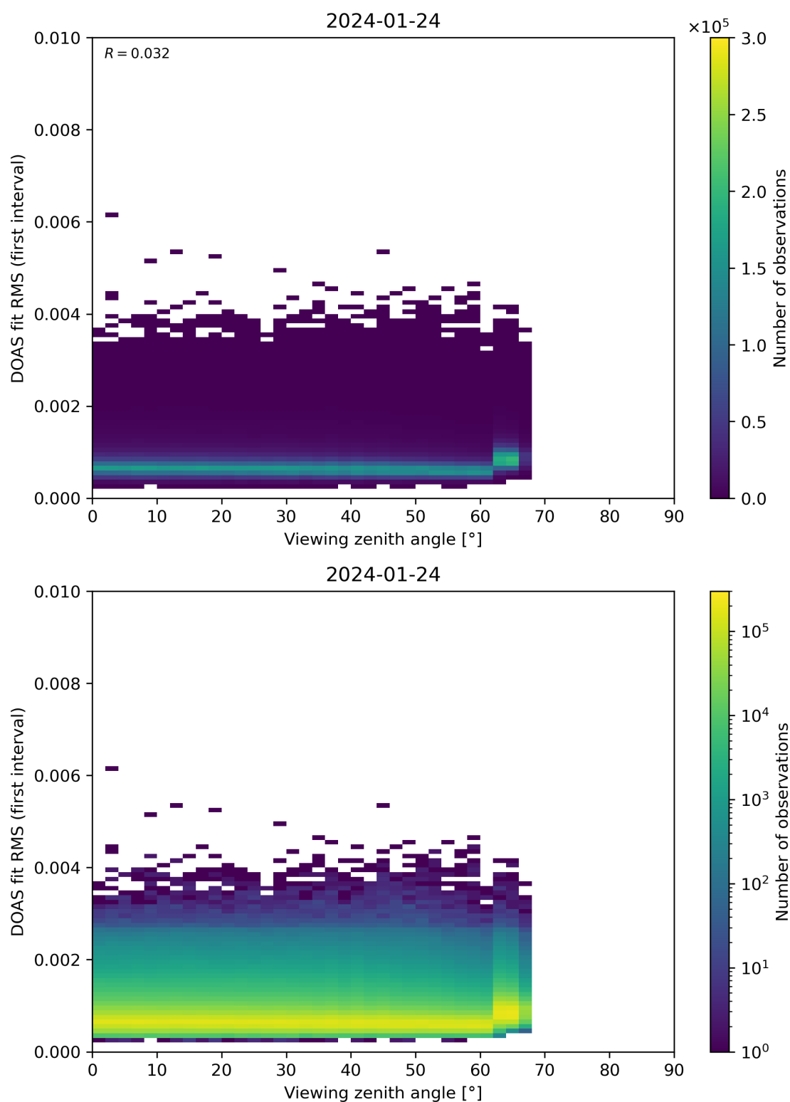
Figure 182: Scatter density plot of “Viewing zenith angle” against “DOAS fit RMS (first interval)” for 2024-01-23 to 2024-01-25.
