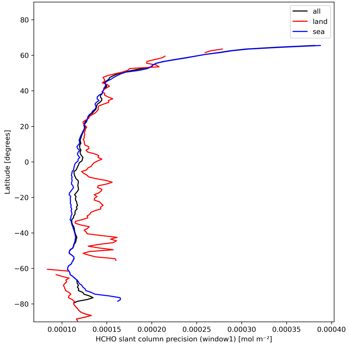
Figure 25: Zonal average of “HCHO slant column precision (window1)” for 2024-01-23 to 2024-01-25.
