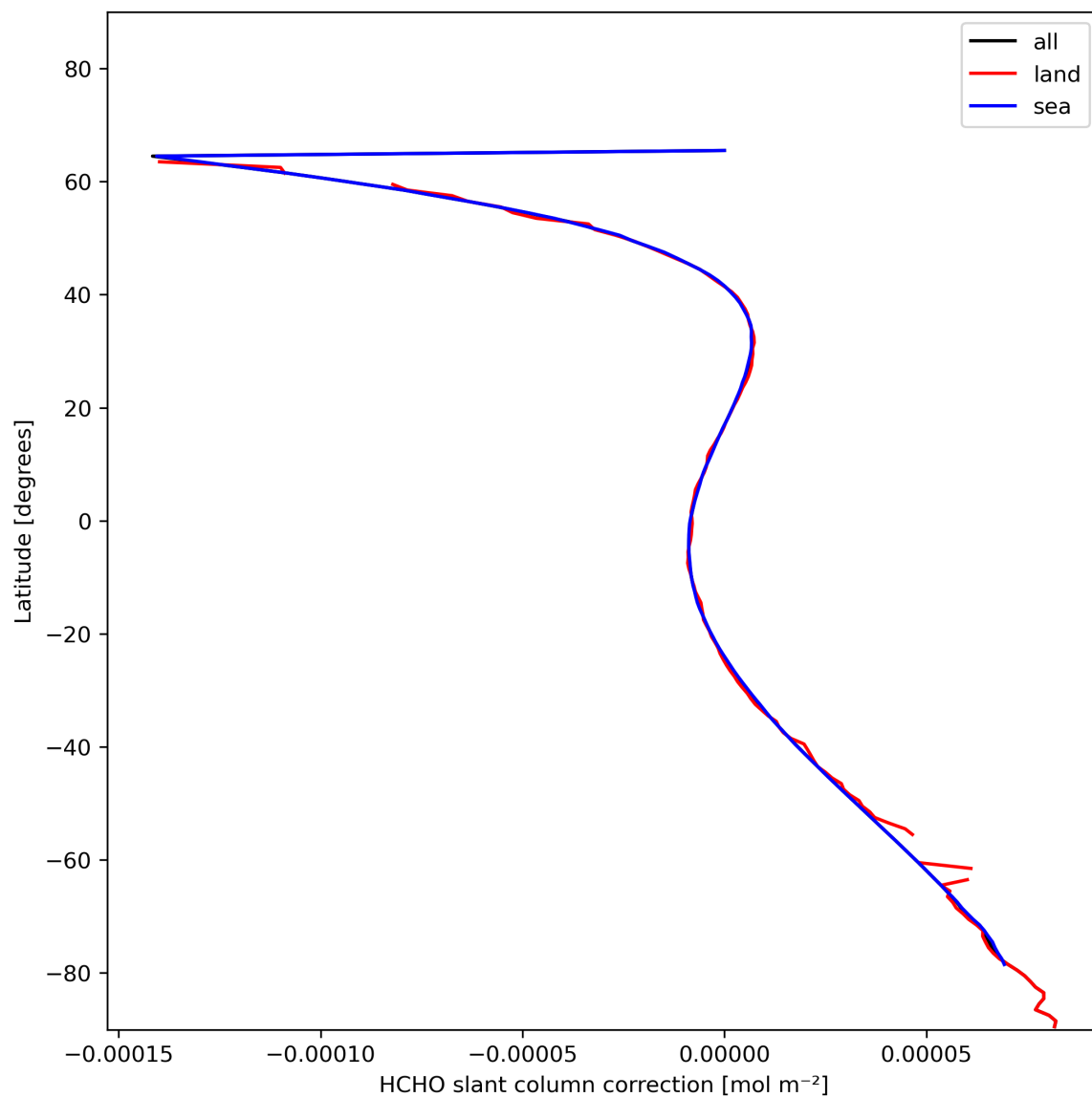
Figure 33: Zonal average of “HCHO slant column correction” for 2024-01-23 to 2024-01-25.
