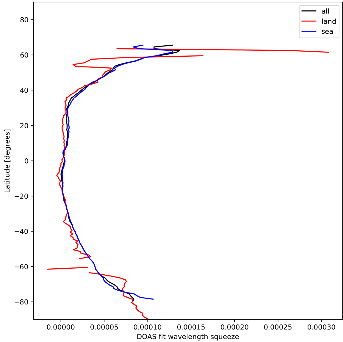
Figure 31: Zonal average of “DOAS fit wavelength squeeze” for 2024-01-23 to 2024-01-25.
