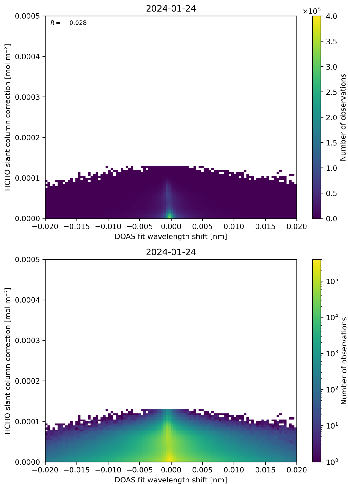
Figure 67: Scatter density plot of “DOAS fit wavelength shift” against “HCHO slant column correction” for 2024-01-23 to 2024-01-25.
