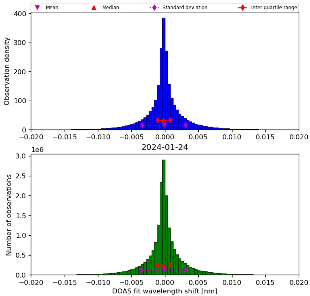
Figure 44: Histogram of “DOAS fit wavelength shift” for 2024-01-23 to 2024-01-25
