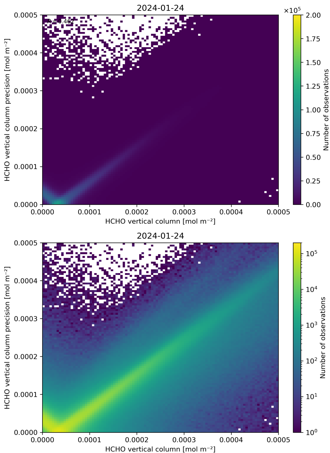
Figure 134: Scatter density plot of “HCHO vertical column” against “HCHO vertical column precision” for 2024-01-23 to 2024-01-25.
