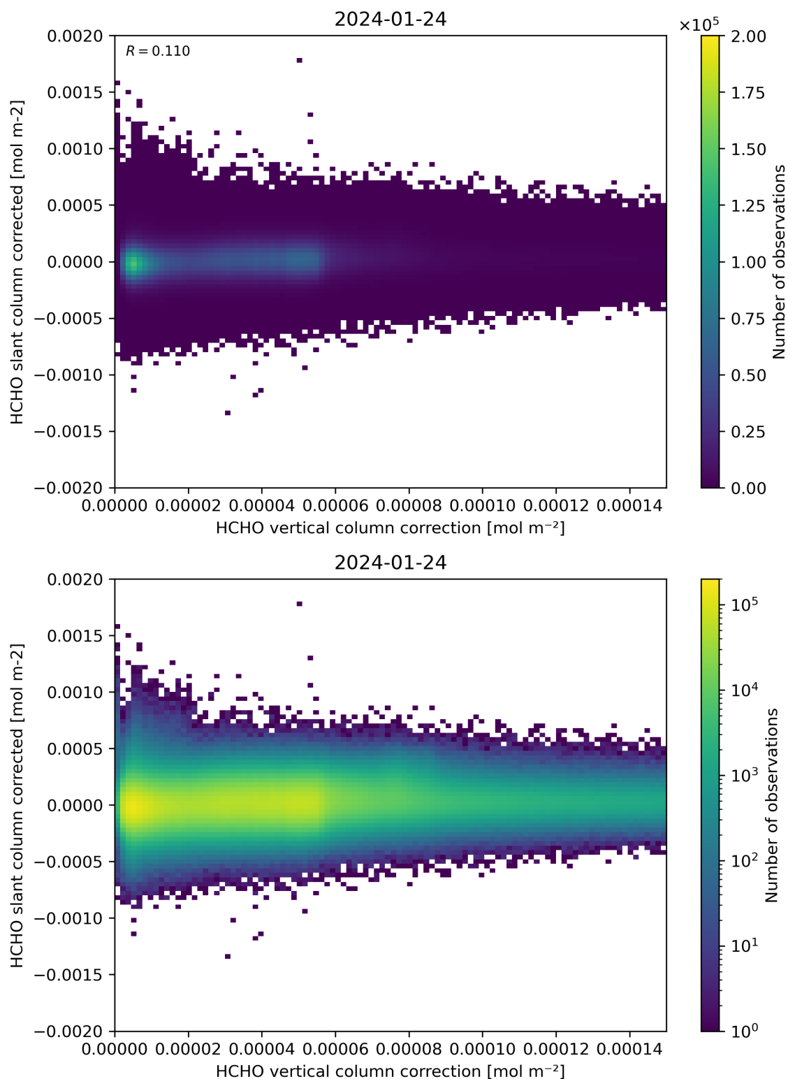
Figure 116: Scatter density plot of “HCHO vertical column correction” against “HCHO slant column corrected” for 2024-01-23 to 2024-01-25.
