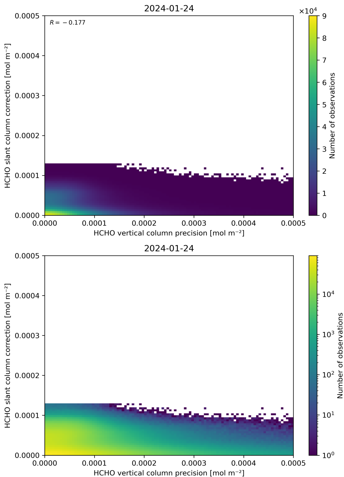
Figure 141: Scatter density plot of “HCHO vertical column precision” against “HCHO slant column correction” for 2024-01-23 to 2024-01-25.
