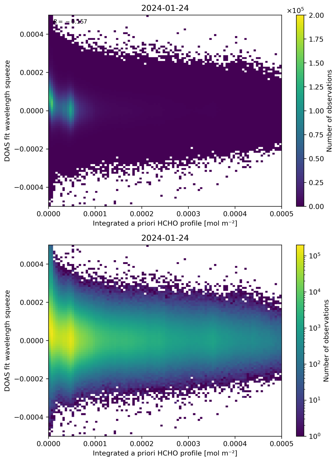
Figure 150: Scatter density plot of “Integrated a priori HCHO profile” against “DOAS fit wavelength squeeze” for 2024-01-23 to 2024-01-25.
