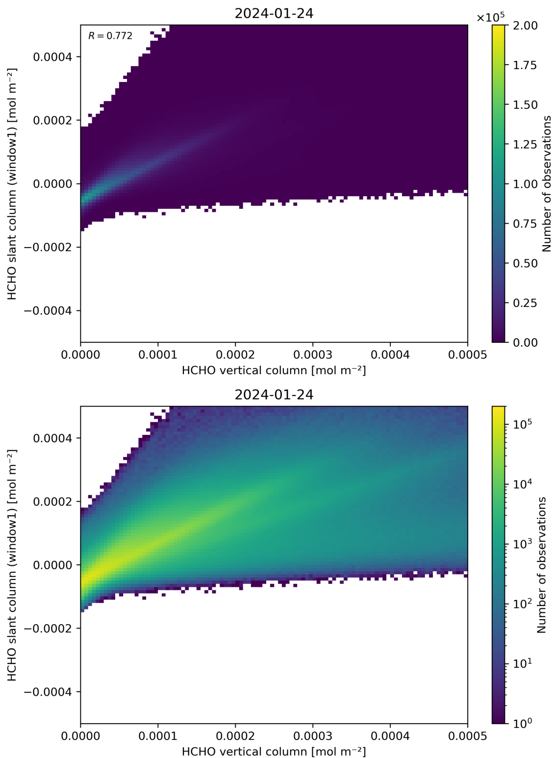
Figure 129: Scatter density plot of “HCHO vertical column” against “HCHO slant column (window1)” for 2024-01-23 to 2024-01-25.
