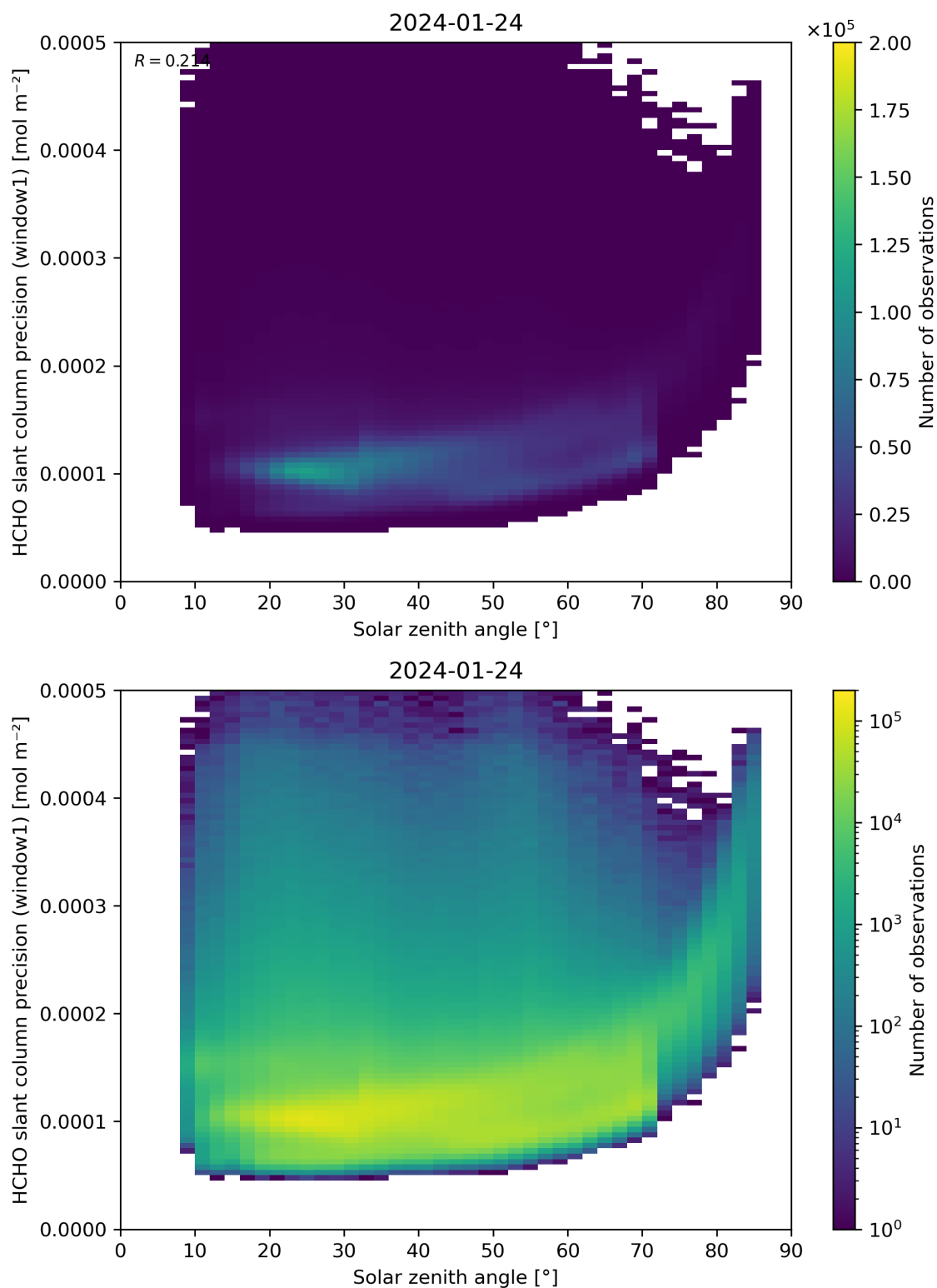
Figure 174: Scatter density plot of “Solar zenith angle” against “HCHO slant column precision (window1)” for 2024-01-23 to 2024-01-25.
