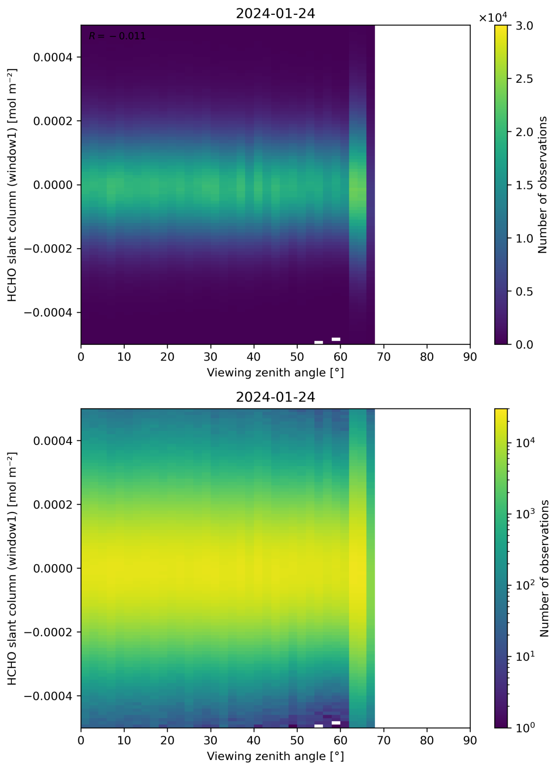
Figure 188: Scatter density plot of “Viewing zenith angle” against “HCHO slant column (window1)” for 2024-01-23 to 2024-01-25.
