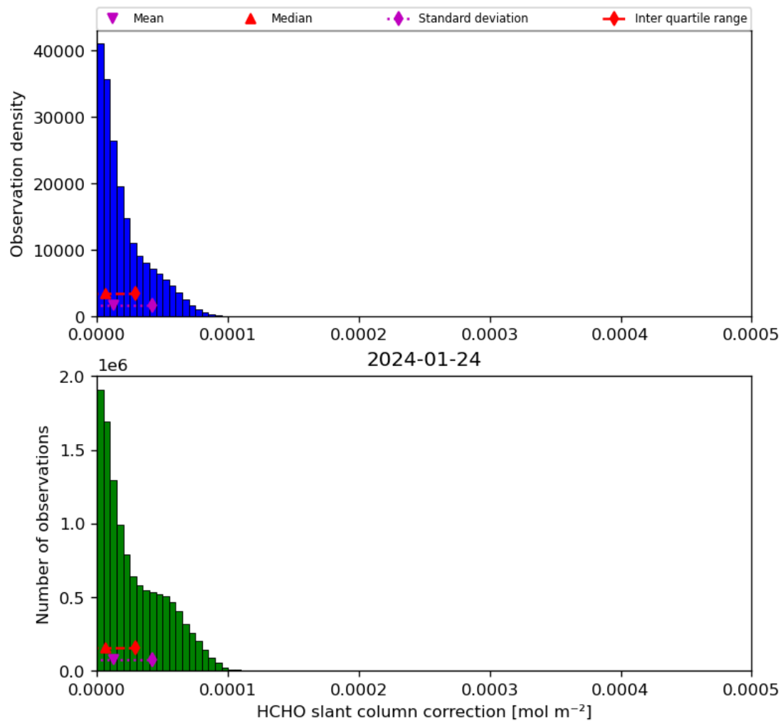
Figure 47: Histogram of “HCHO slant column correction” for 2024-01-23 to 2024-01-25
