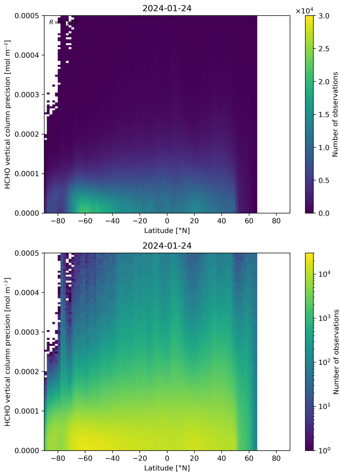
Figure 165: Scatter density plot of “Latitude” against “HCHO vertical column precision” for 2024-01-23 to 2024-01-25.
