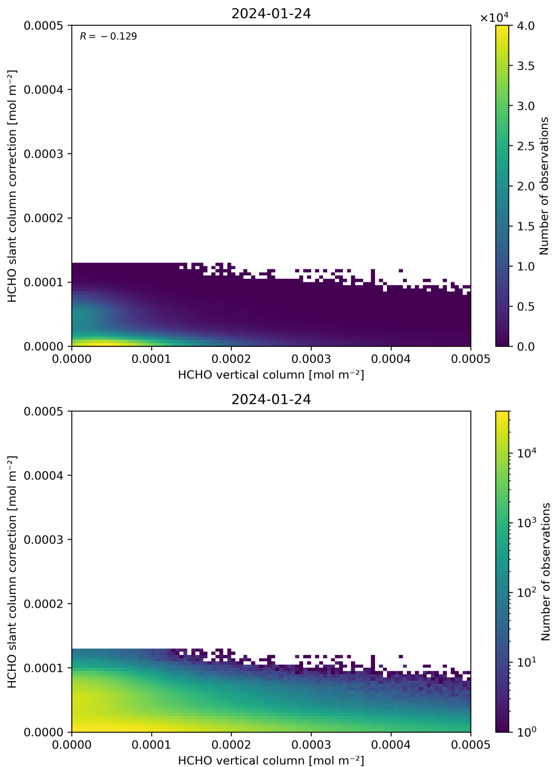
Figure 128: Scatter density plot of “HCHO vertical column” against “HCHO slant column correction” for 2024-01-23 to 2024-01-25.
