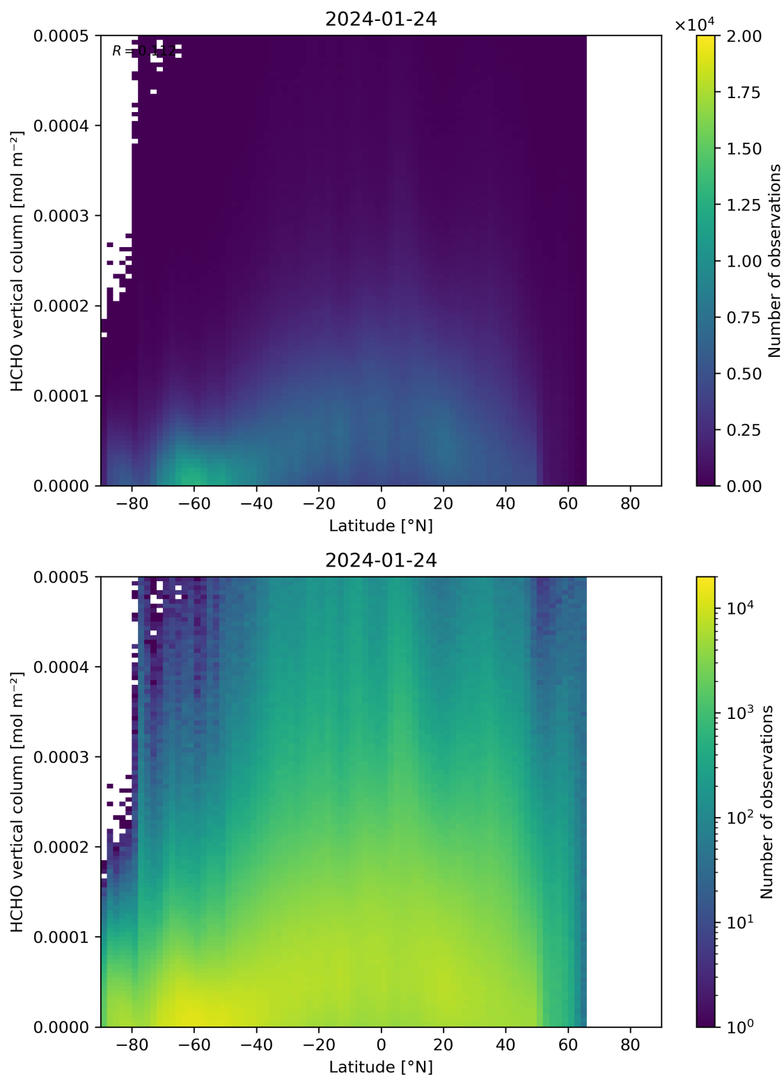
Figure 163: Scatter density plot of “Latitude” against “HCHO vertical column” for 2024-01-23 to 2024-01-25.
