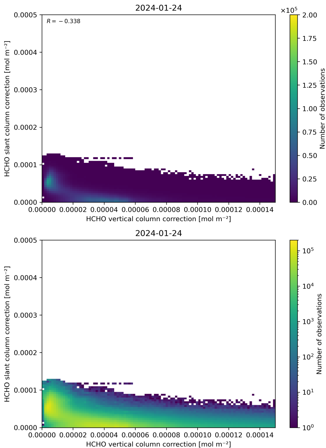
Figure 117: Scatter density plot of “HCHO vertical column correction” against “HCHO slant column correction” for 2024-01-23 to 2024-01-25.
