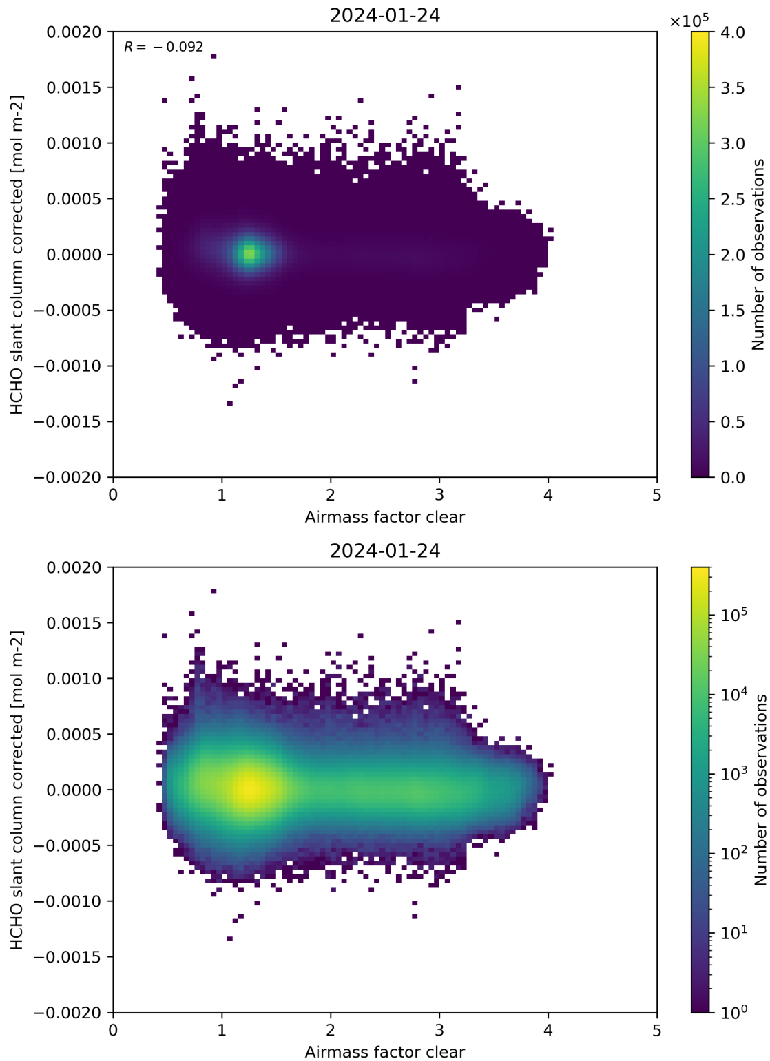
Figure 74: Scatter density plot of “Airmass factor clear” against “HCHO slant column corrected” for 2024-01-23 to 2024-01-25.
