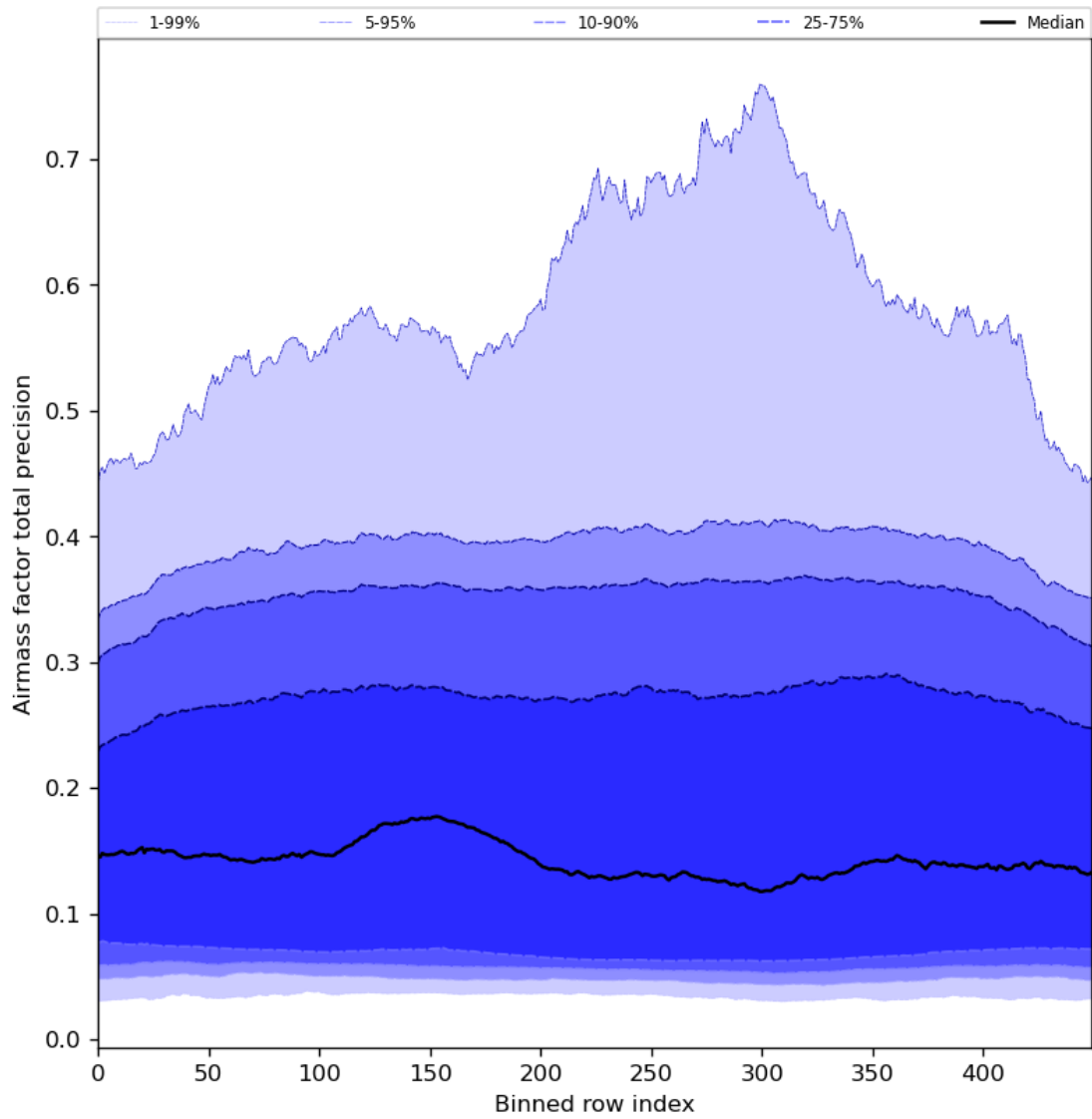
Figure 55: Along track statistics of “Airmass factor total precision” for 2024-01-23 to 2024-01-25
