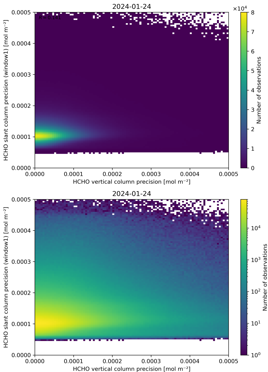
Figure 143: Scatter density plot of “HCHO vertical column precision” against “HCHO slant column precision (window1)” for 2024-01-23 to 2024-01-25.
