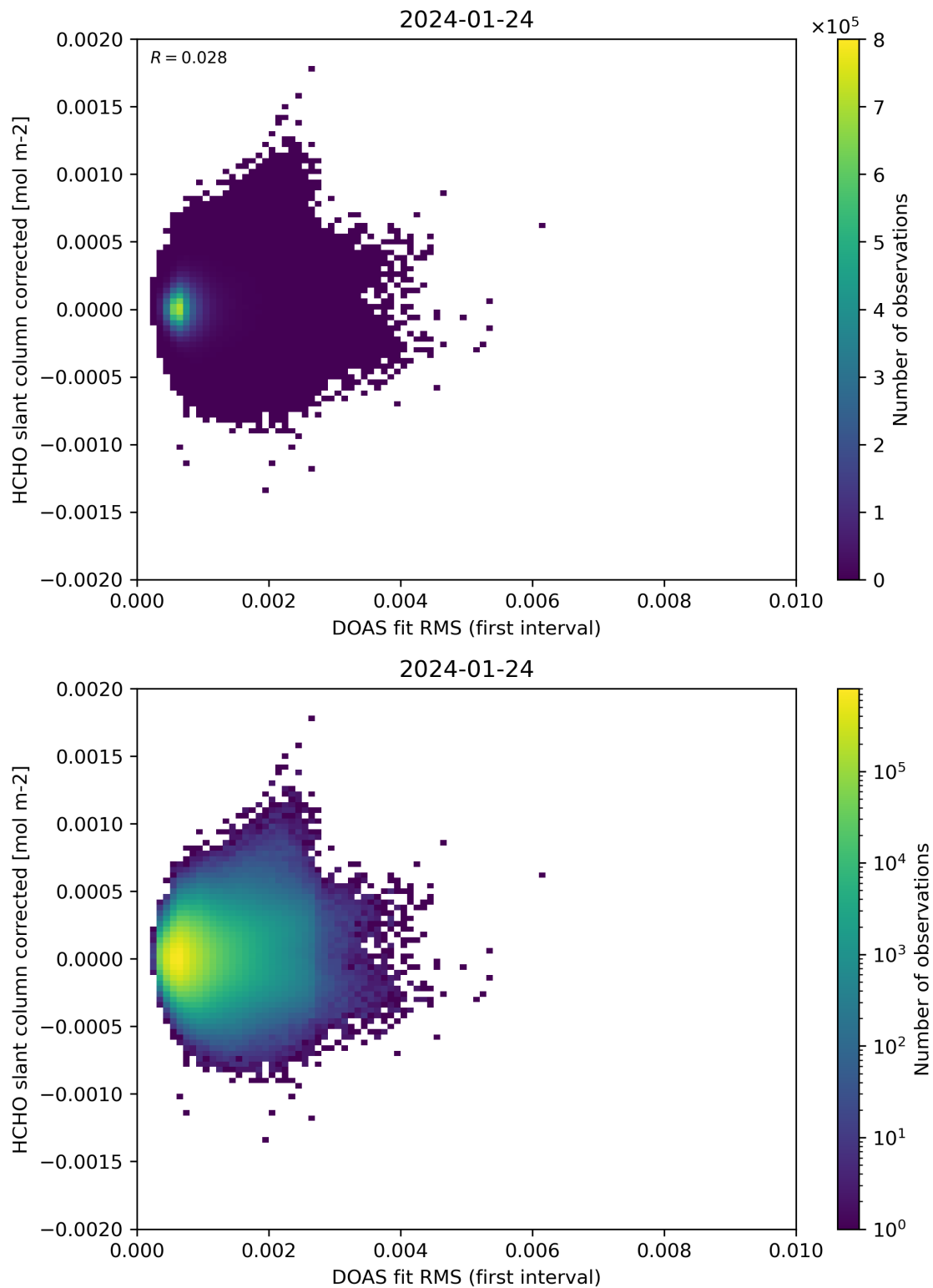
Figure 62: Scatter density plot of “DOAS fit RMS (first interval)” against “HCHO slant column corrected” for 2024-01-23 to 2024-01-25.
