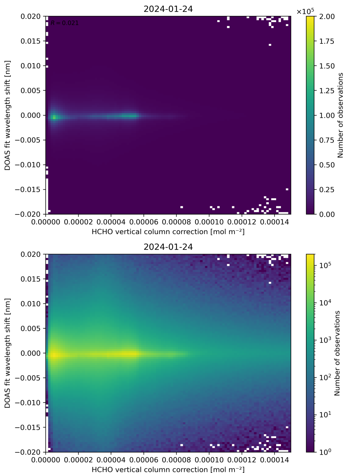
Figure 113: Scatter density plot of “HCHO vertical column correction” against “DOAS fit wavelength shift” for 2024-01-23 to 2024-01-25.
