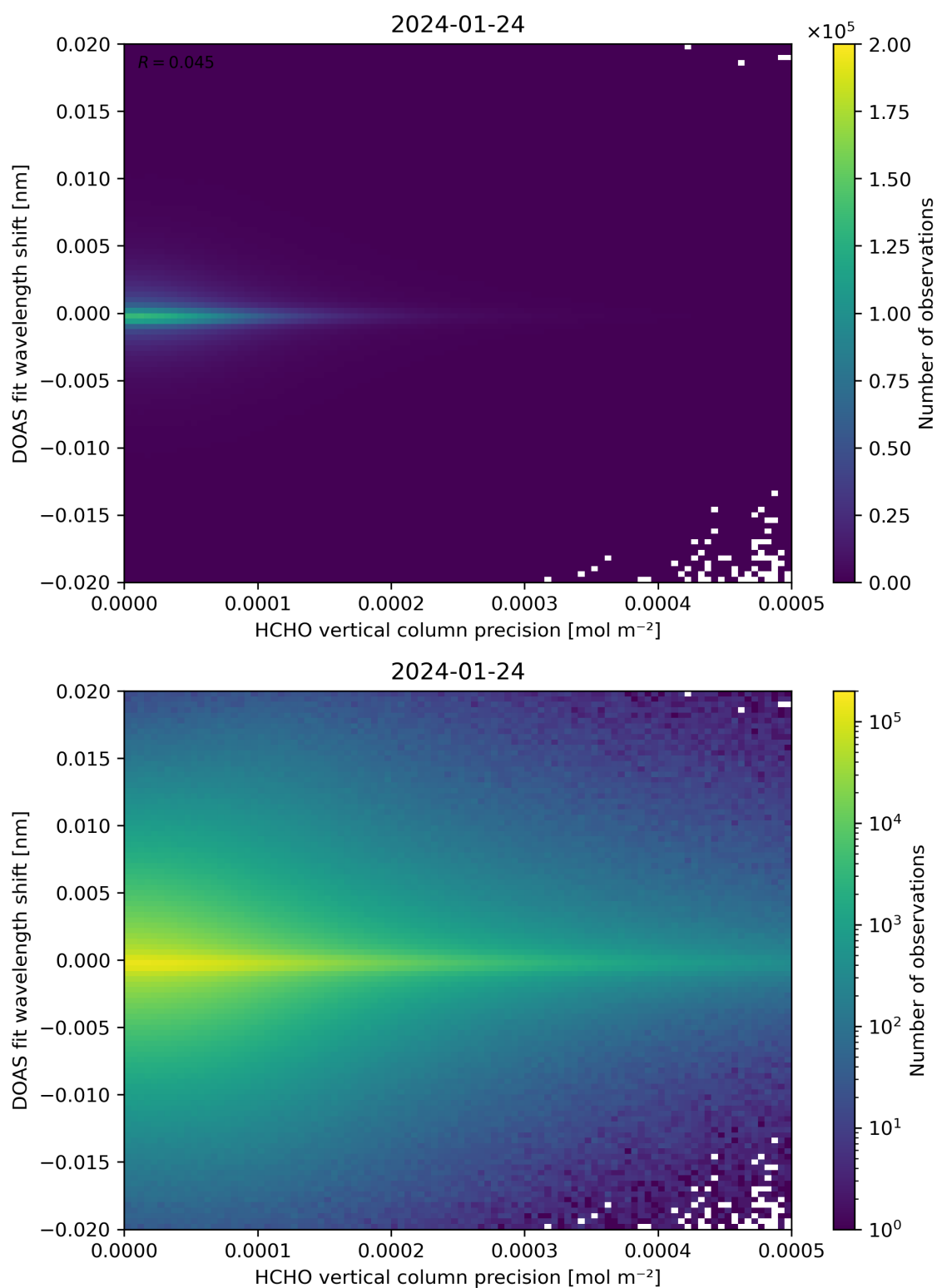
Figure 137: Scatter density plot of “HCHO vertical column precision” against “DOAS fit wavelength shift” for 2024-01-23 to 2024-01-25.
