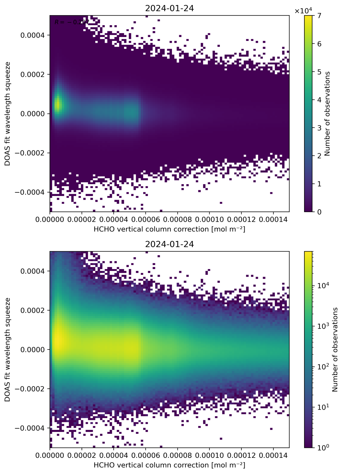
Figure 114: Scatter density plot of “HCHO vertical column correction” against “DOAS fit wavelength squeeze” for 2024-01-23 to 2024-01-25.
