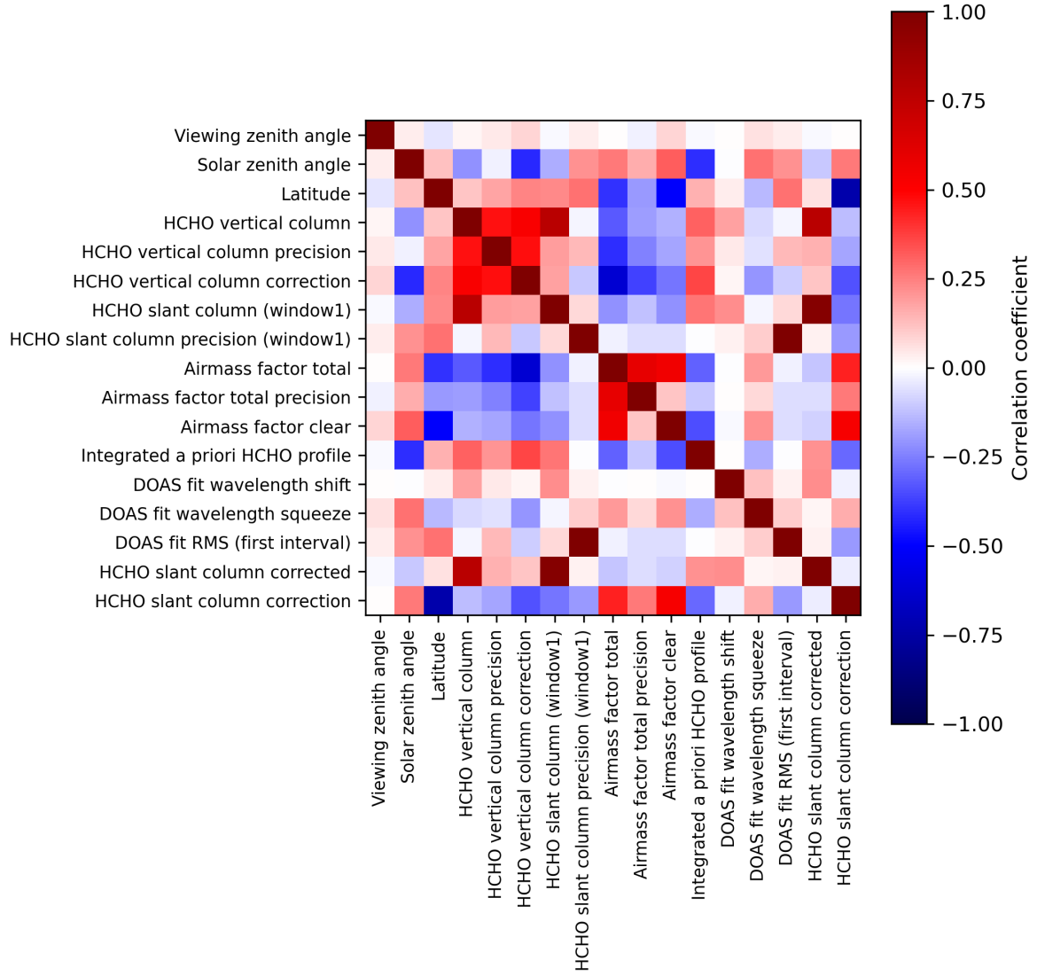
Figure 2: Map of correlation matrix for 2024-01-23 to 2024-01-25.
