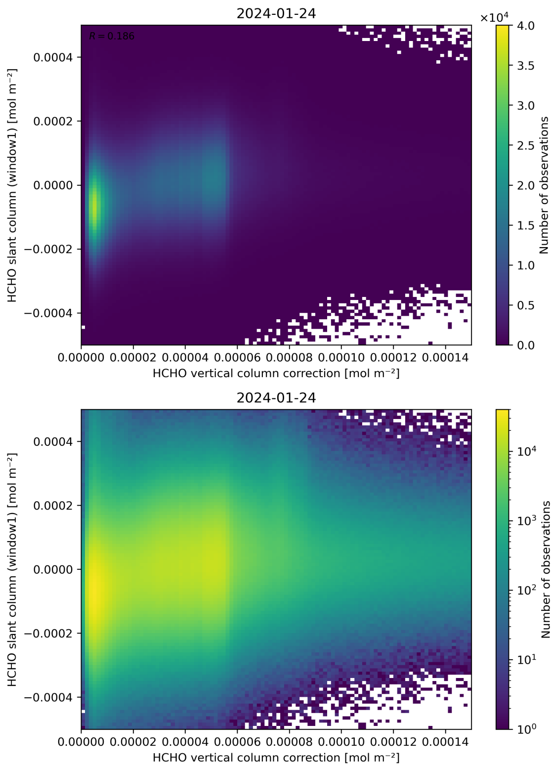
Figure 118: Scatter density plot of “HCHO vertical column correction” against “HCHO slant column (window1)” for 2024-01-23 to 2024-01-25.
