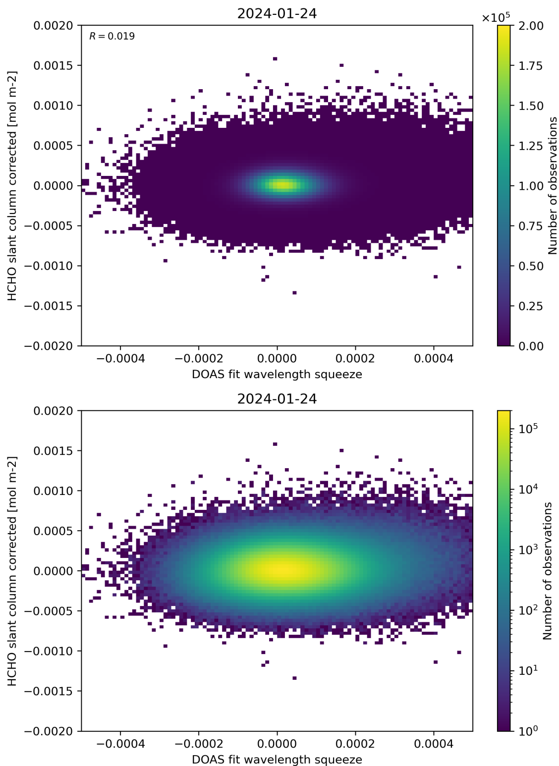
Figure 69: Scatter density plot of “DOAS fit wavelength squeeze” against “HCHO slant column corrected” for 2024-01-23 to 2024-01-25.
