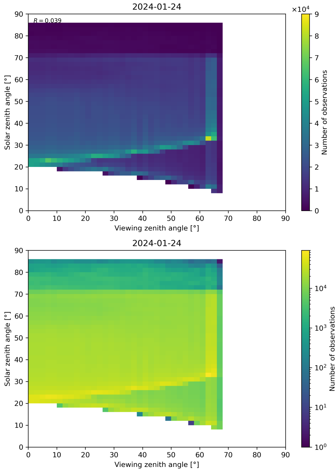
Figure 197: Scatter density plot of “Viewing zenith angle” against “Solar zenith angle” for 2024-01-23 to 2024-01-25.
