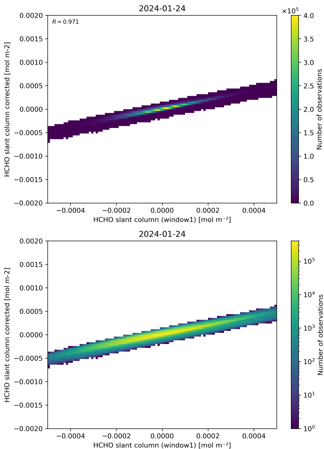
Figure 82: Scatter density plot of “HCHO slant column (window1)” against “HCHO slant column corrected” for 2024-01-23 to 2024-01-25.
