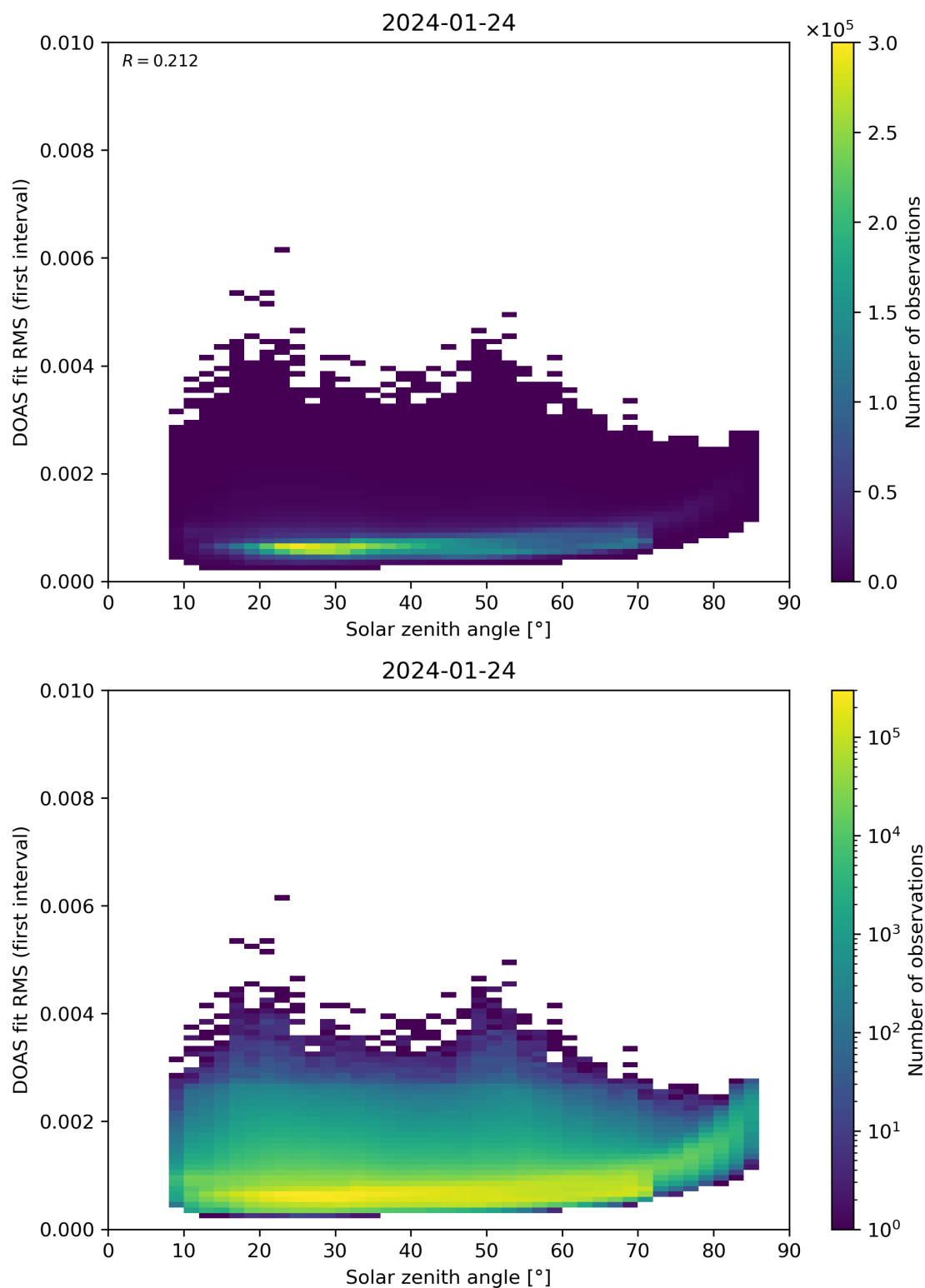
Figure 167: Scatter density plot of “Solar zenith angle” against “DOAS fit RMS (first interval)” for 2024-01-23 to 2024-01-25.
