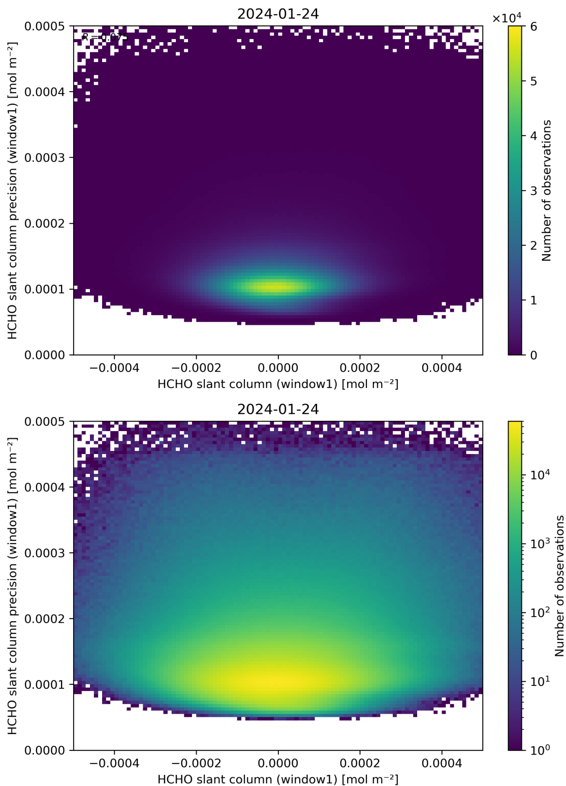
Figure 84: Scatter density plot of “HCHO slant column (window1)” against “HCHO slant column precision (window1)” for 2024-01-23 to 2024-01-25.
