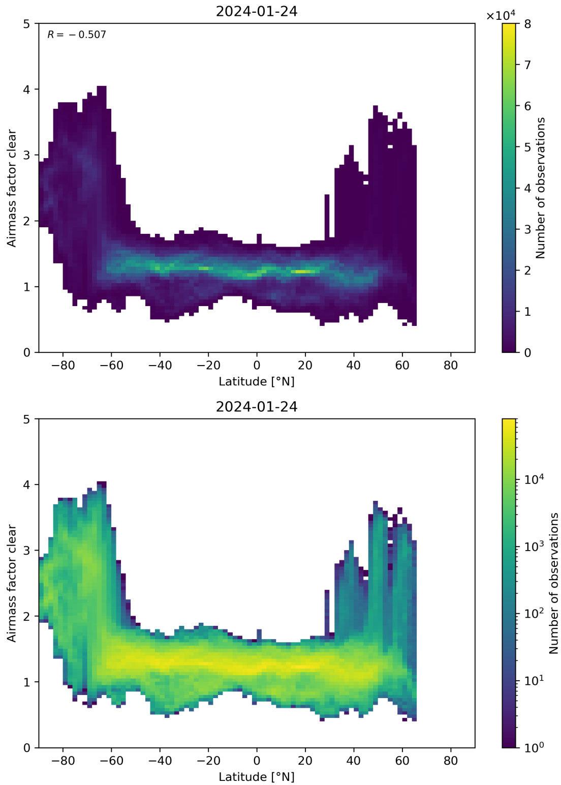
Figure 156: Scatter density plot of “Latitude” against “Airmass factor clear” for 2024-01-23 to 2024-01-25.
