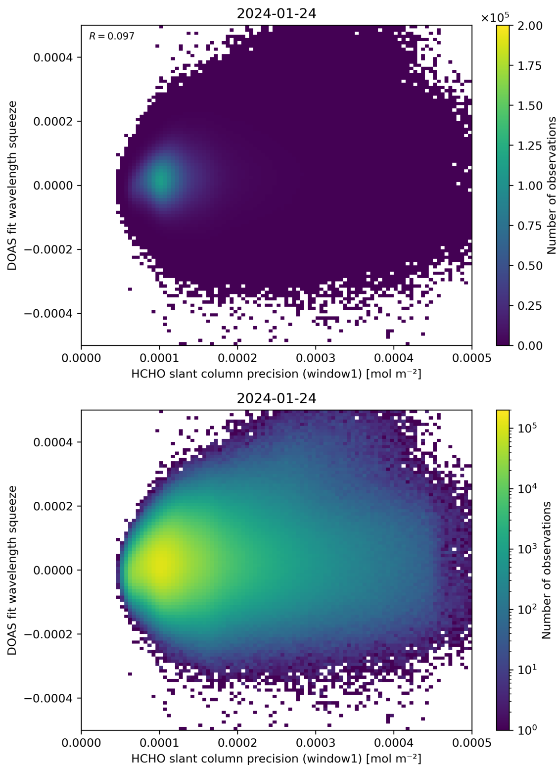
Figure 90: Scatter density plot of “HCHO slant column precision (window1)” against “DOAS fit wavelength squeeze” for 2024-01-23 to 2024-01-25.
