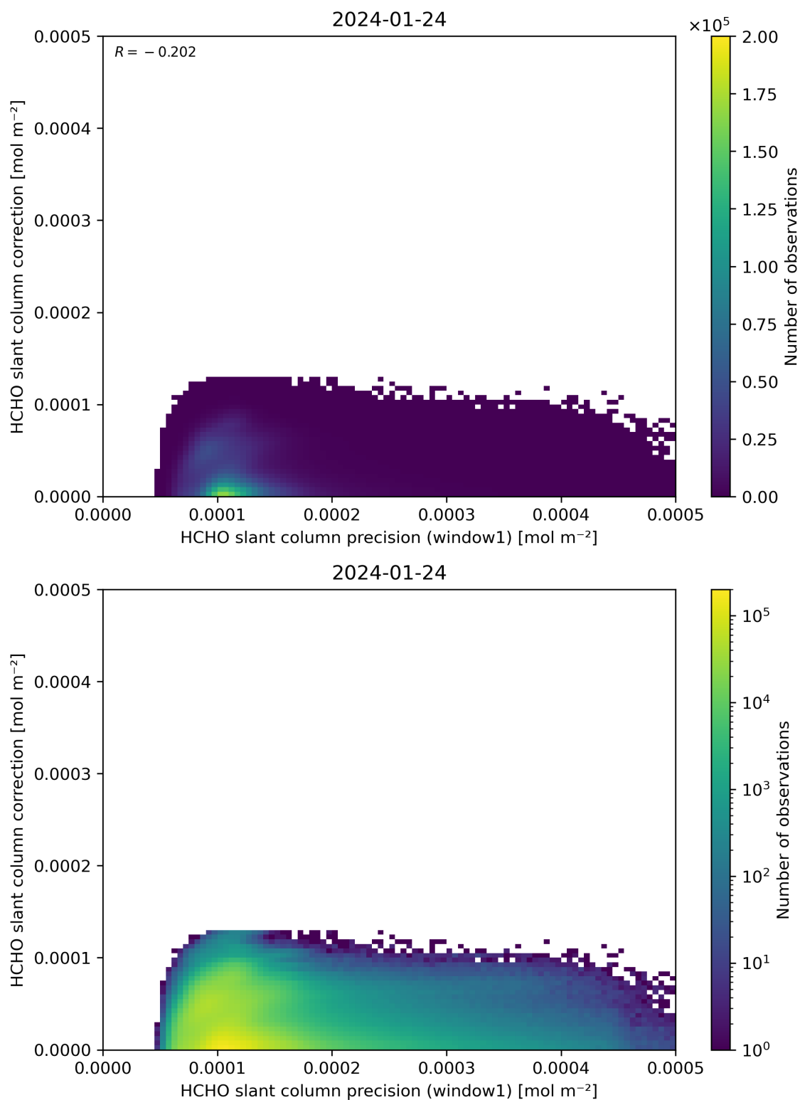
Figure 93: Scatter density plot of “HCHO slant column precision (window1)” against “HCHO slant column correction” for 2024-01-23 to 2024-01-25.
