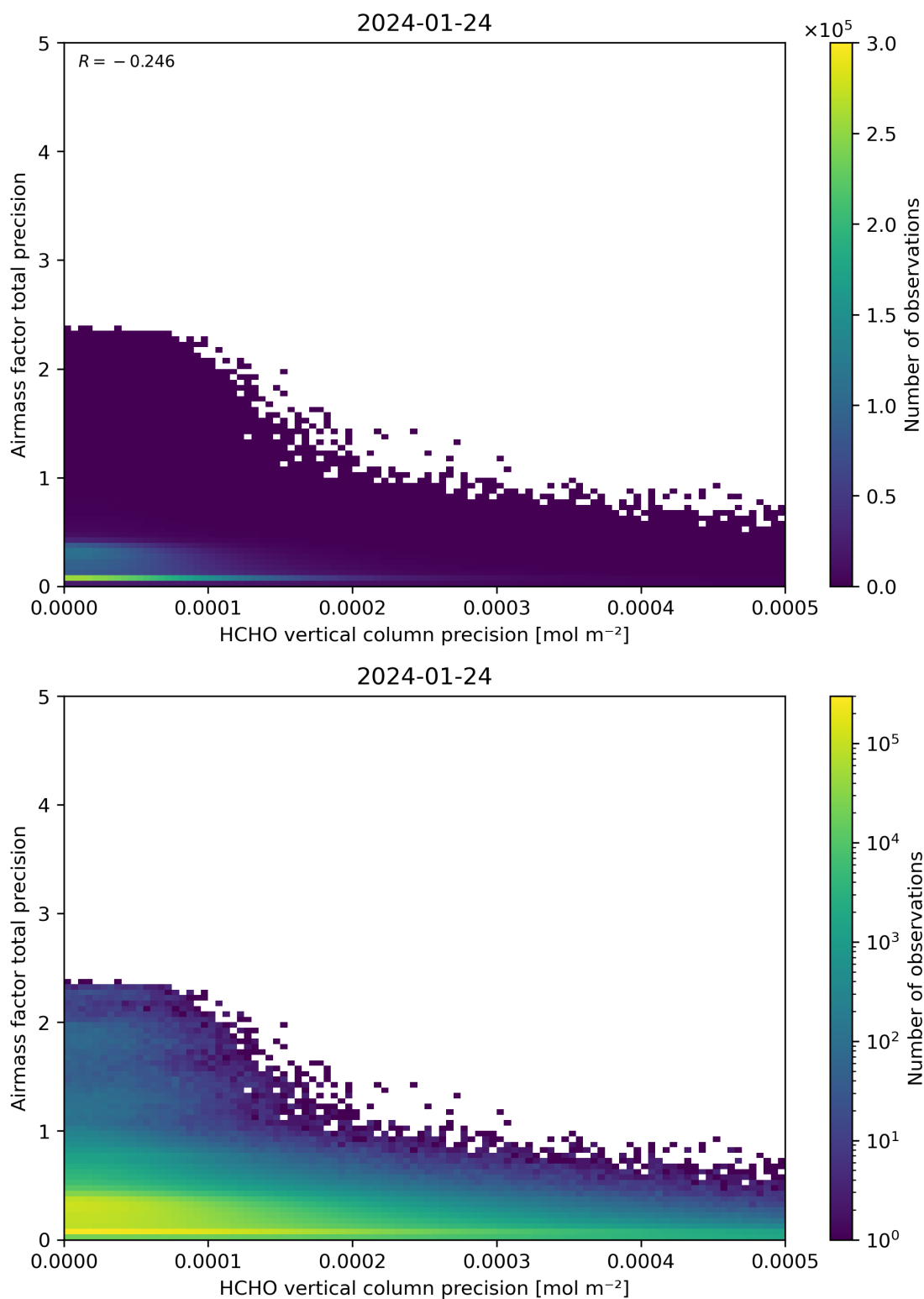
Figure 145: Scatter density plot of “HCHO vertical column precision” against “Airmass factor total precision” for 2024-01-23 to 2024-01-25.
