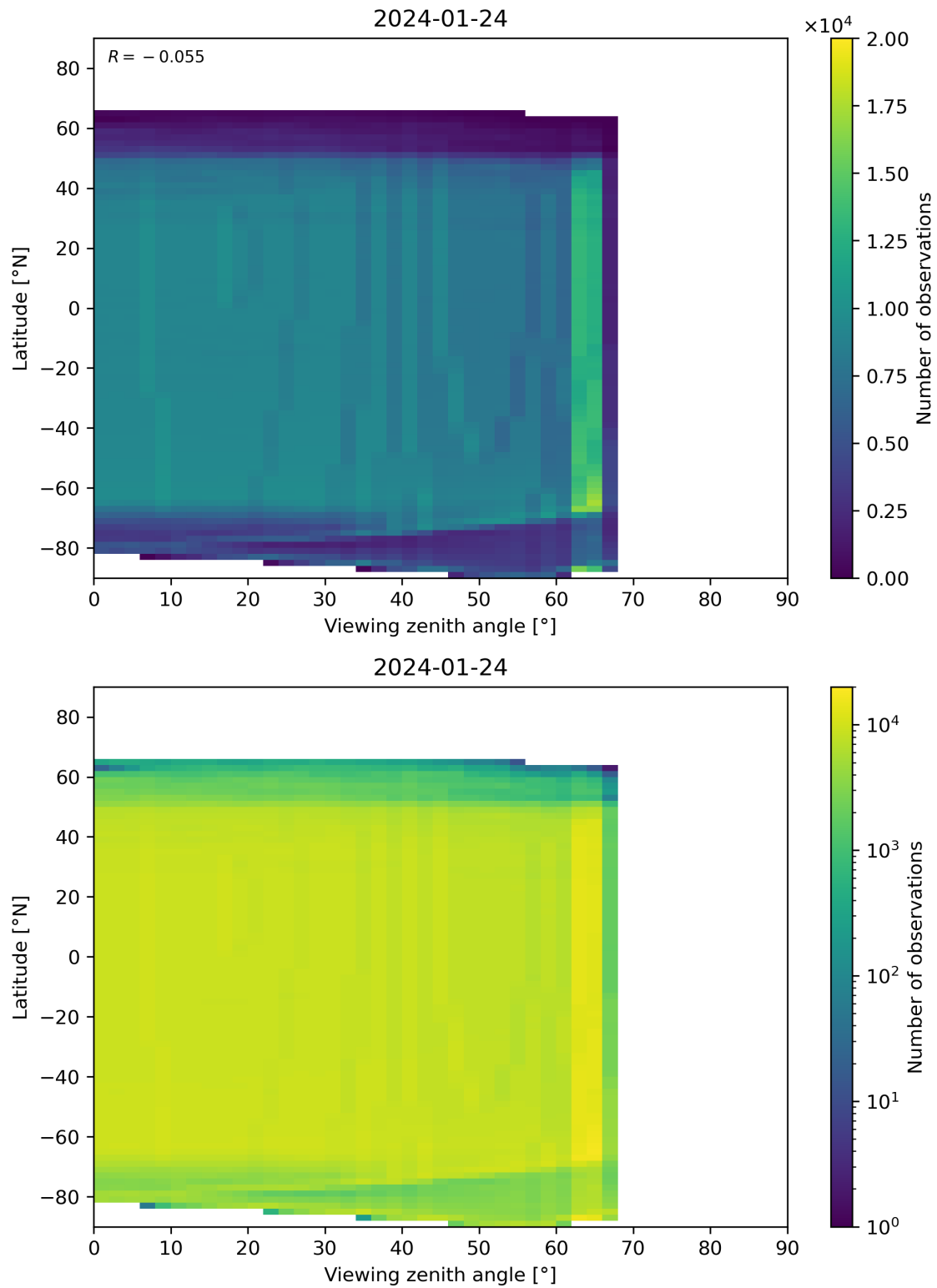
Figure 196: Scatter density plot of “Viewing zenith angle” against “Latitude” for 2024-01-23 to 2024-01-25.
