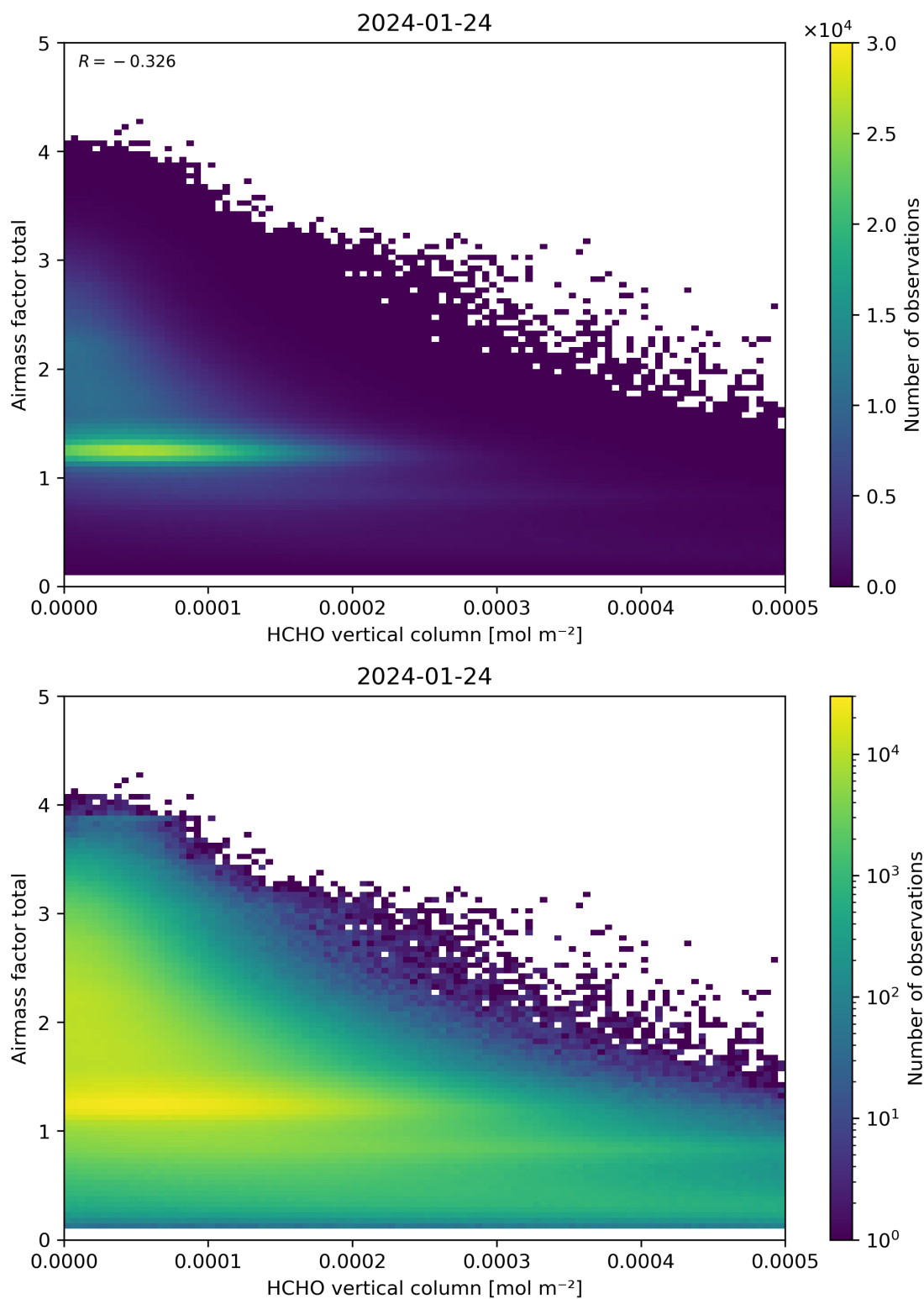
Figure 131: Scatter density plot of “HCHO vertical column” against “Airmass factor total” for 2024-01-23 to 2024-01-25.
