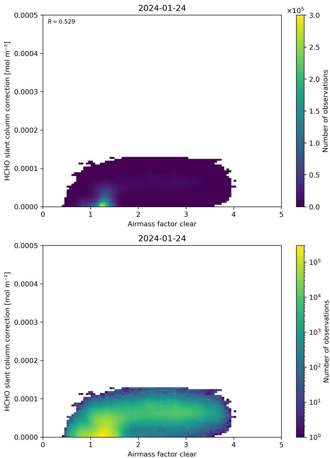
Figure 75: Scatter density plot of “Airmass factor clear” against “HCHO slant column correction” for 2024-01-23 to 2024-01-25.
