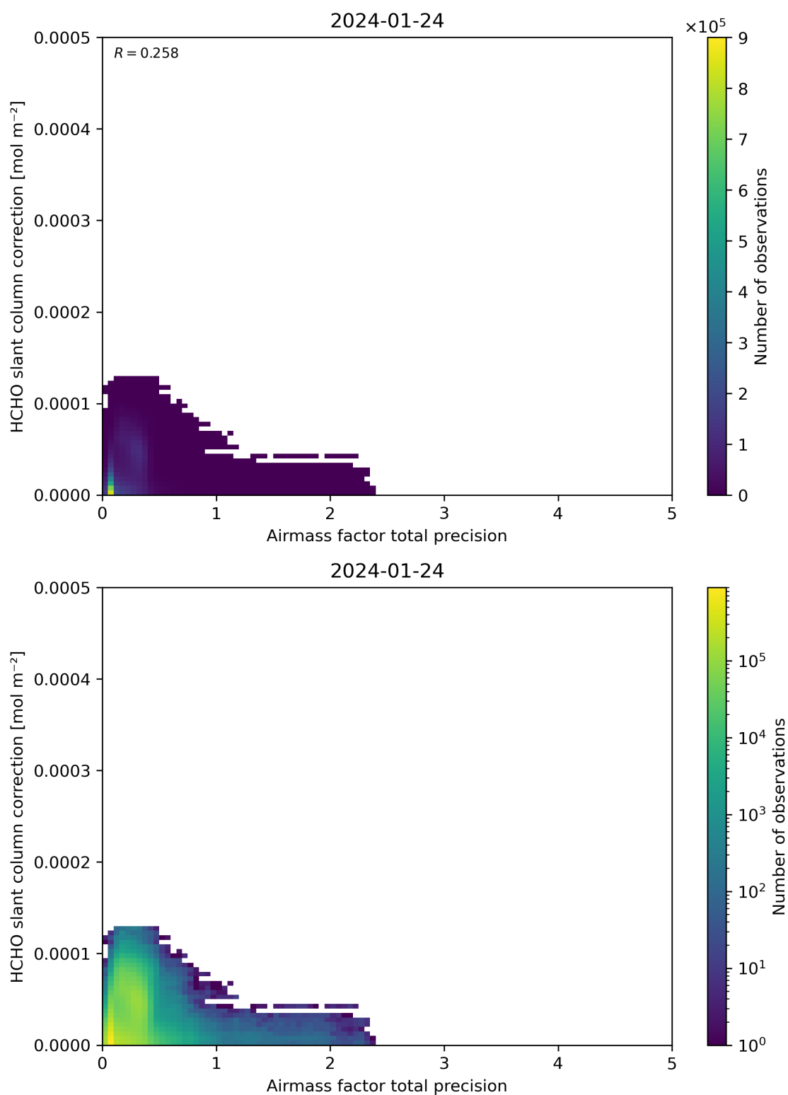
Figure 110: Scatter density plot of “Airmass factor total precision” against “HCHO slant column correction” for 2024-01-23 to 2024-01-25.
