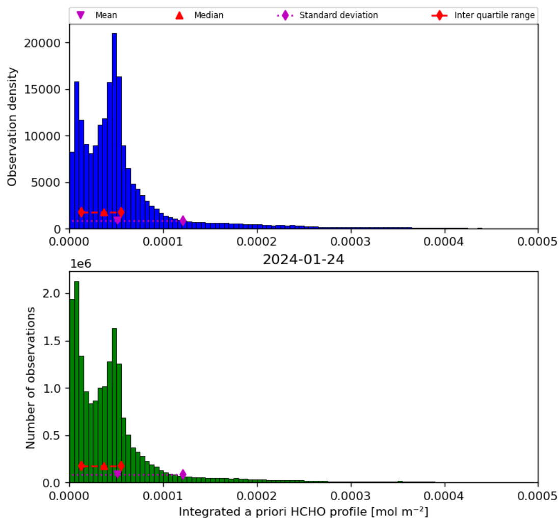
Figure 43: Histogram of “Integrated a priori HCHO profile” for 2024-01-23 to 2024-01-25
