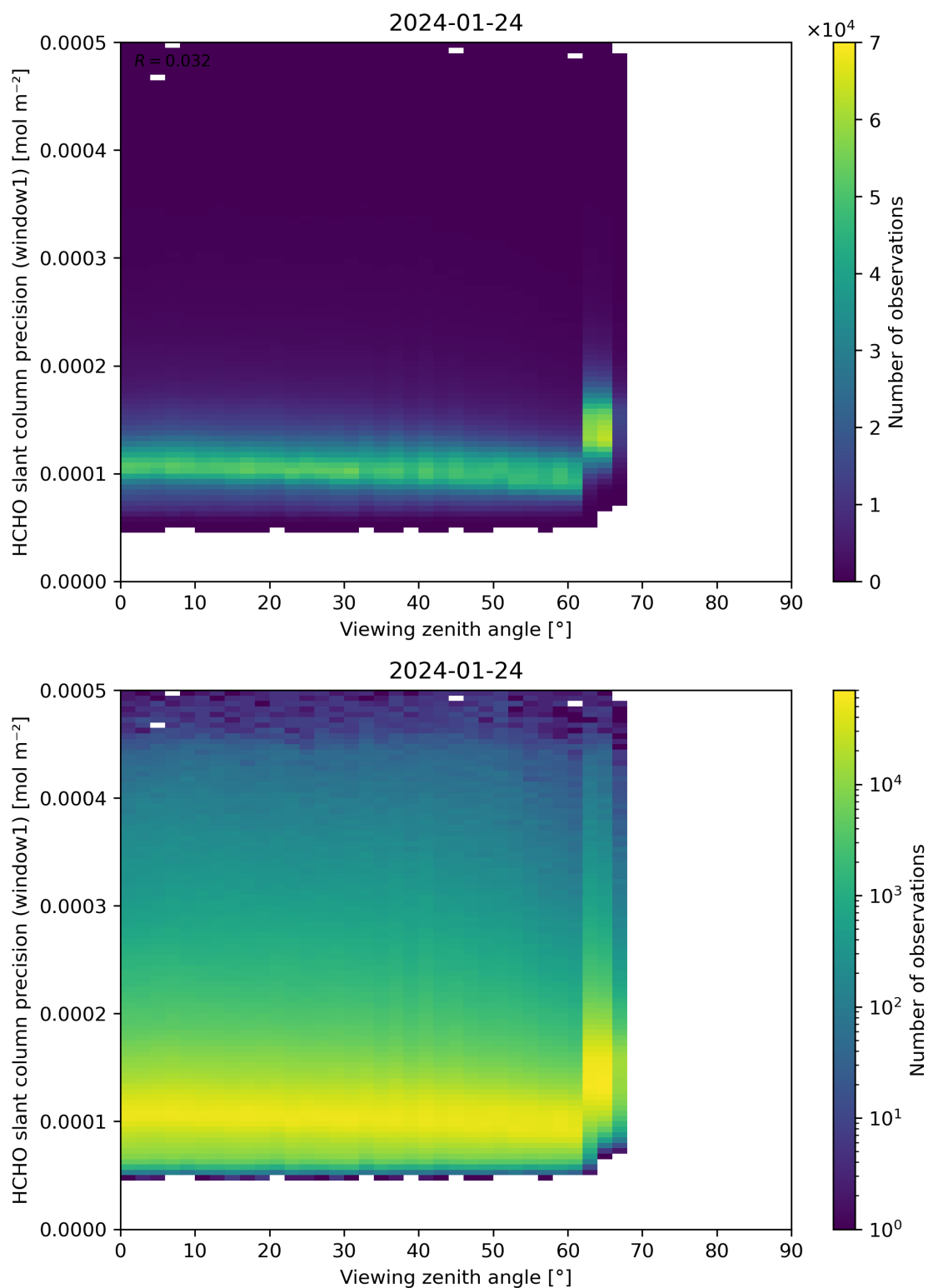
Figure 189: Scatter density plot of “Viewing zenith angle” against “HCHO slant column precision (window1)” for 2024-01-23 to 2024-01-25.
