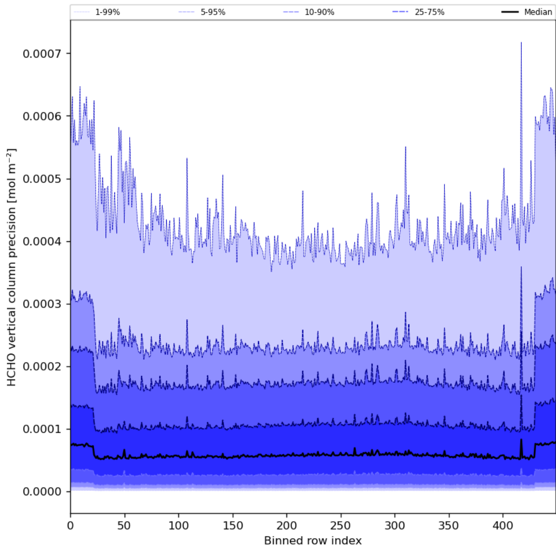
Figure 50: Along track statistics of “HCHO vertical column precision” for 2024-01-23 to 2024-01-25
