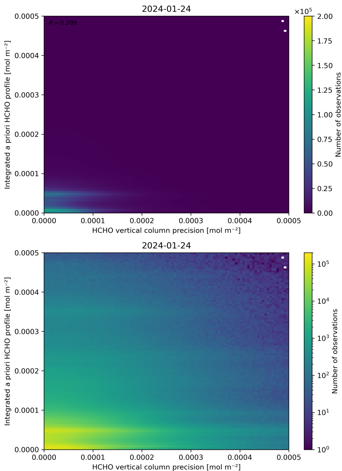
Figure 147: Scatter density plot of “HCHO vertical column precision” against “Integrated a priori HCHO profile” for 2024-01-23 to 2024-01-25.
