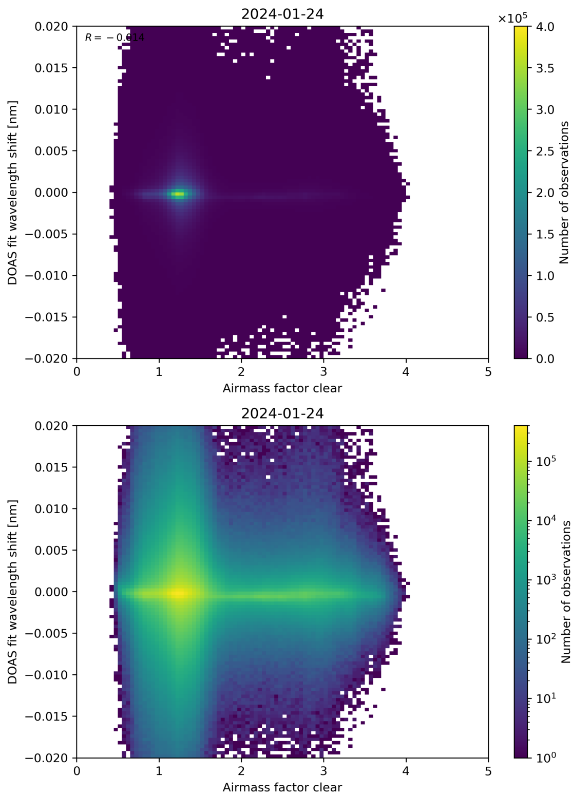
Figure 72: Scatter density plot of “Airmass factor clear” against “DOAS fit wavelength shift” for 2024-01-23 to 2024-01-25.
