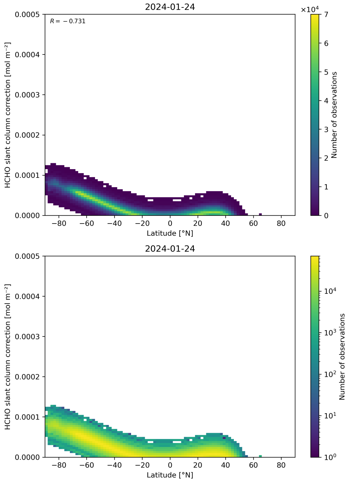
Figure 158: Scatter density plot of “Latitude” against “HCHO slant column correction” for 2024-01-23 to 2024-01-25.
