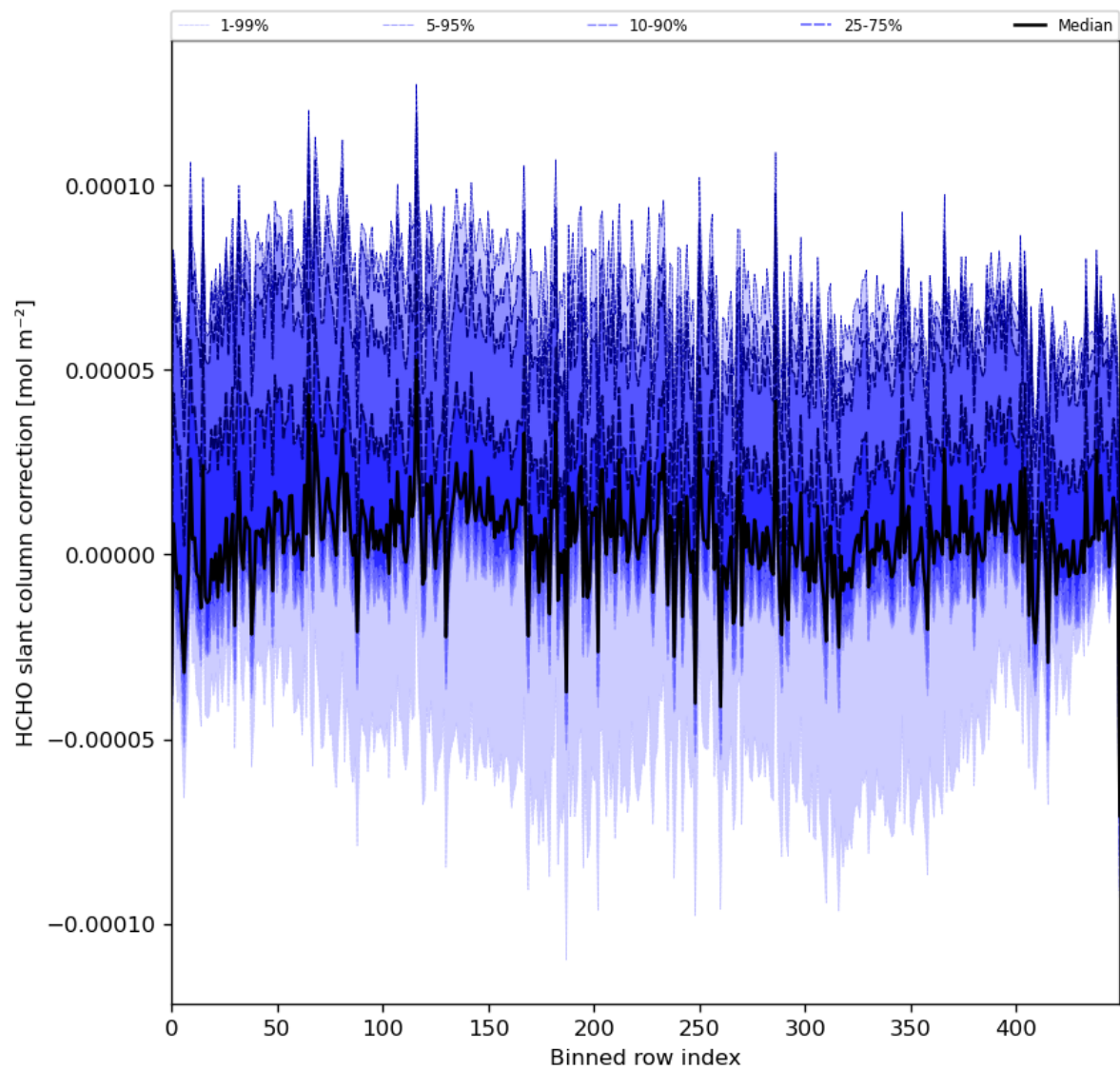
Figure 61: Along track statistics of “HCHO slant column correction” for 2024-01-23 to 2024-01-25
