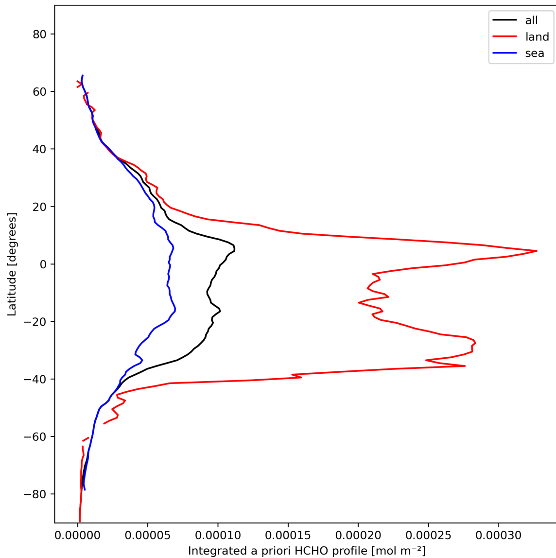
Figure 29: Zonal average of “Integrated a priori HCHO profile” for 2024-01-23 to 2024-01-25.
