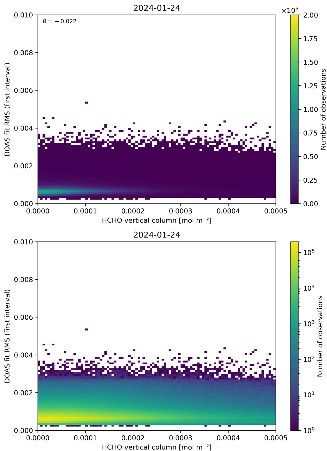
Figure 123: Scatter density plot of “HCHO vertical column” against “DOAS fit RMS (first interval)” for 2024-01-23 to 2024-01-25.
