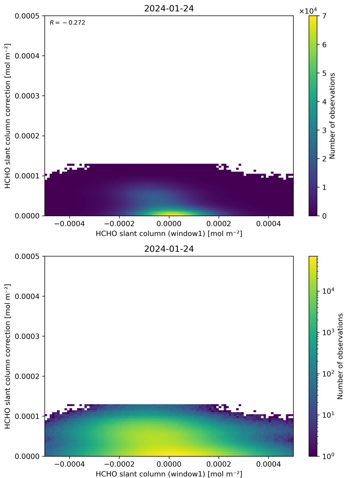
Figure 83: Scatter density plot of “HCHO slant column (window1)” against “HCHO slant column correction” for 2024-01-23 to 2024-01-25.
