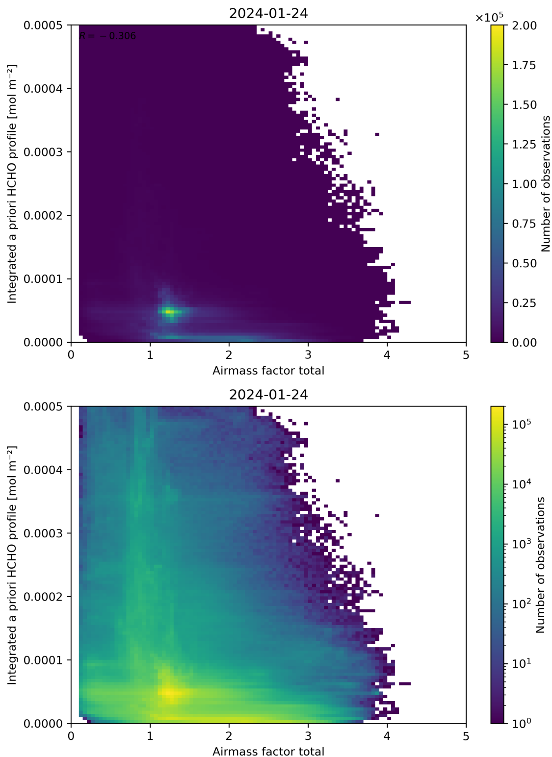
Figure 104: Scatter density plot of “Airmass factor total” against “Integrated a priori HCHO profile” for 2024-01-23 to 2024-01-25.
