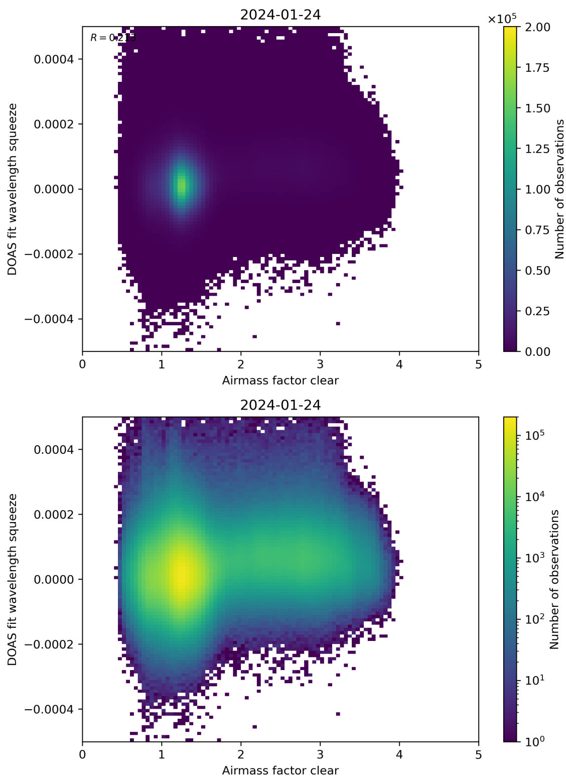
Figure 73: Scatter density plot of “Airmass factor clear” against “DOAS fit wavelength squeeze” for 2024-01-23 to 2024-01-25.
