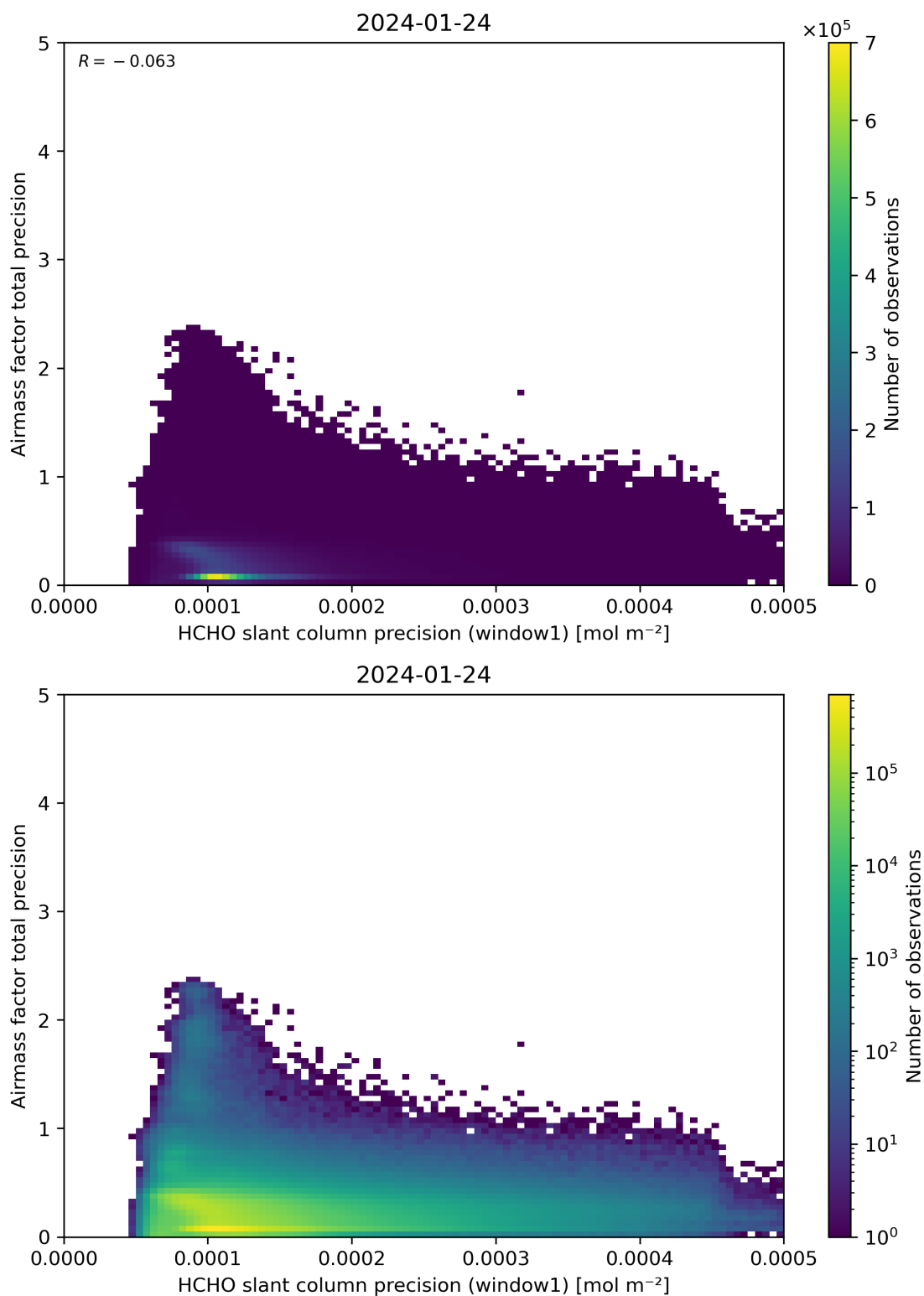
Figure 95: Scatter density plot of “HCHO slant column precision (window1)” against “Airmass factor total precision” for 2024-01-23 to 2024-01-25.
