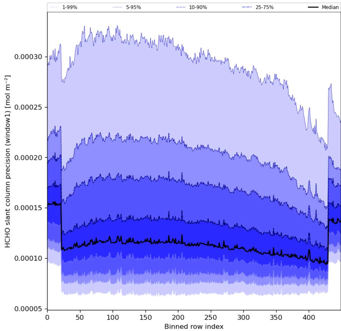
Figure 53: Along track statistics of “HCHO slant column precision (window1)” for 2024-01-23 to 2024-01-25
