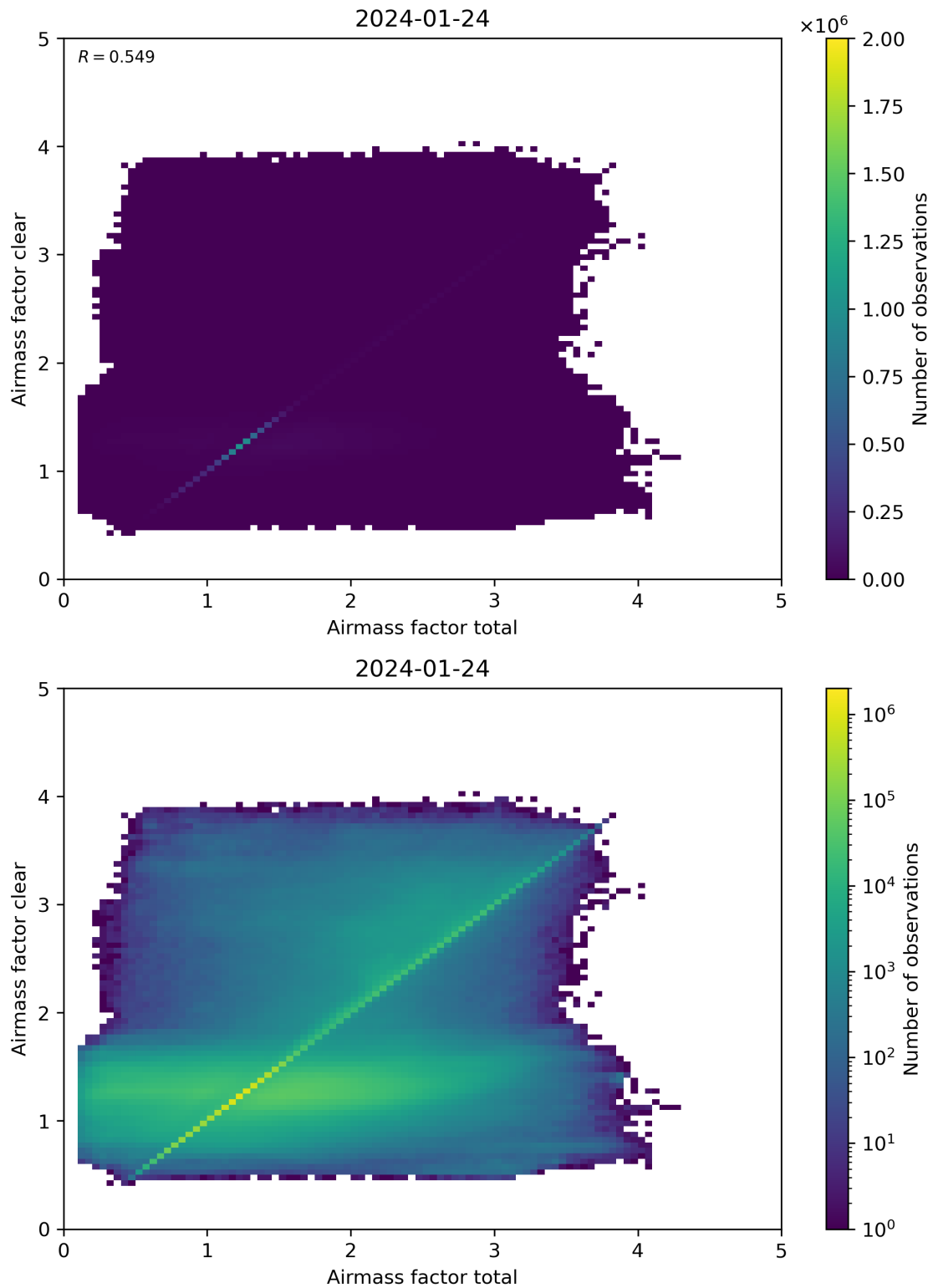
Figure 100: Scatter density plot of “Airmass factor total” against “Airmass factor clear” for 2024-01-23 to 2024-01-25.
