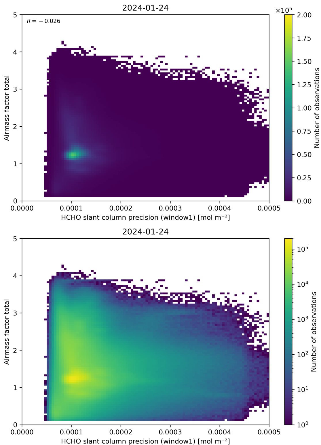
Figure 94: Scatter density plot of “HCHO slant column precision (window1)” against “Airmass factor total” for 2024-01-23 to 2024-01-25.
