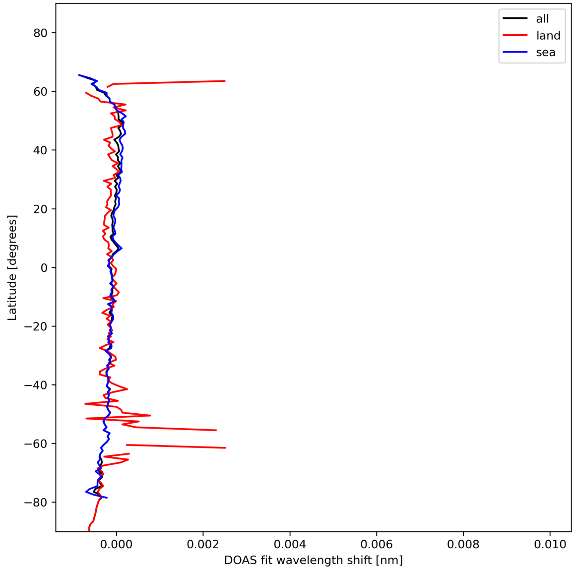
Figure 30: Zonal average of "DOAS fit wavelength shift" for 2024-01-23 to 2024-01-25.
