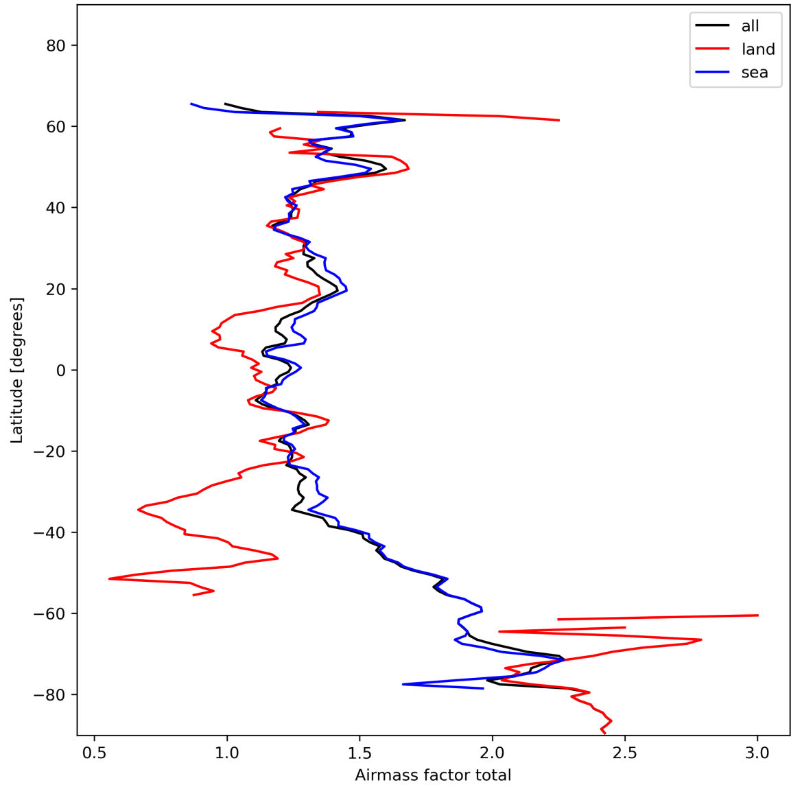
Figure 26: Zonal average of “Airmass factor total” for 2024-01-23 to 2024-01-25.
