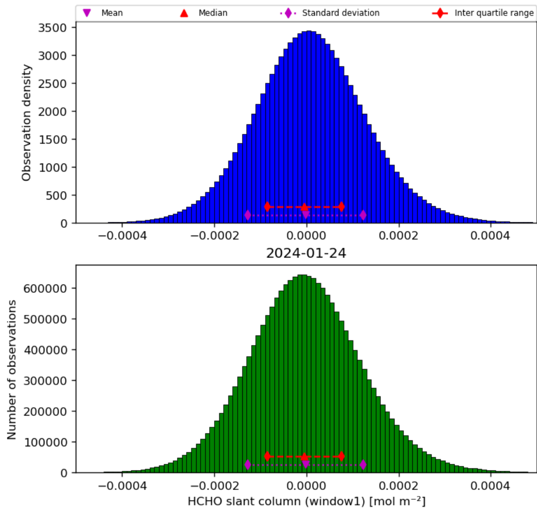
Figure 38: Histogram of “HCHO slant column (window1)” for 2024-01-23 to 2024-01-25
