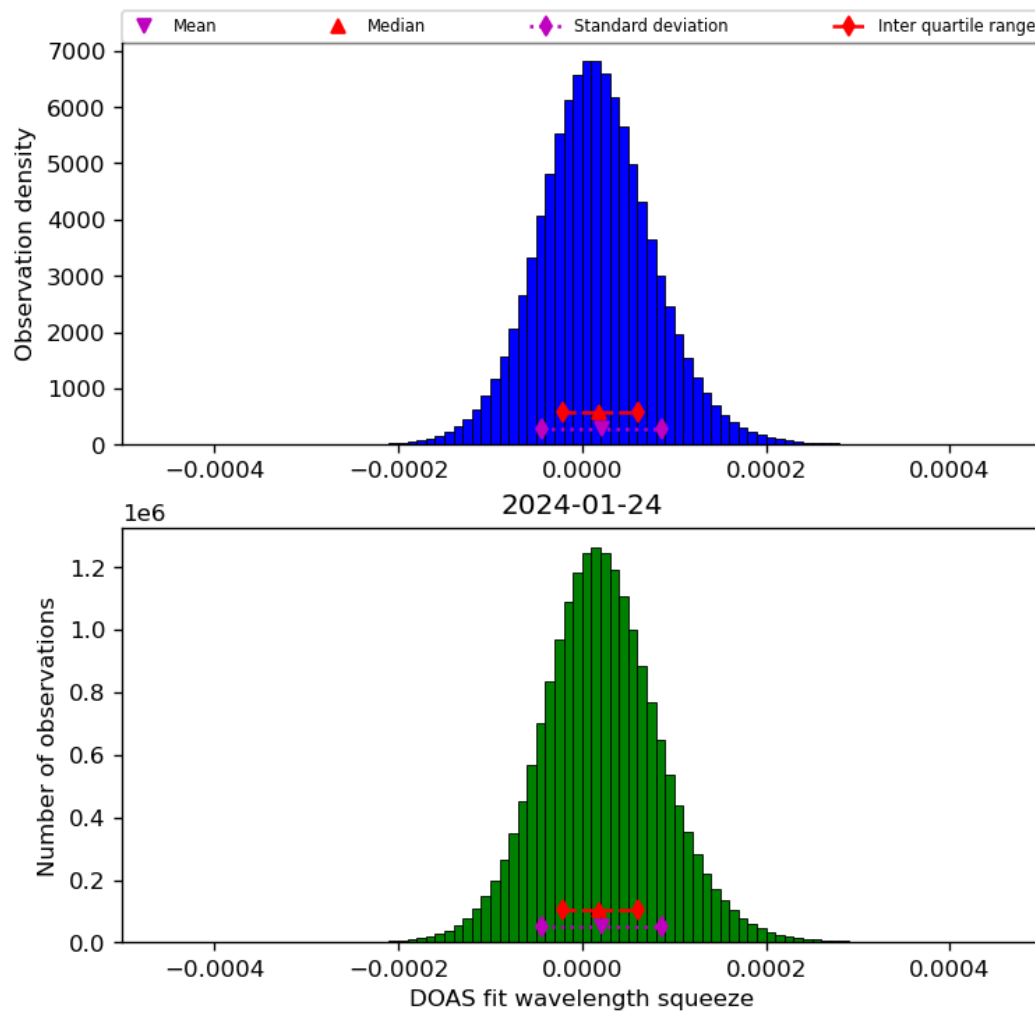
Figure 45: Histogram of “DOAS fit wavelength squeeze” for 2024-01-23 to 2024-01-25
