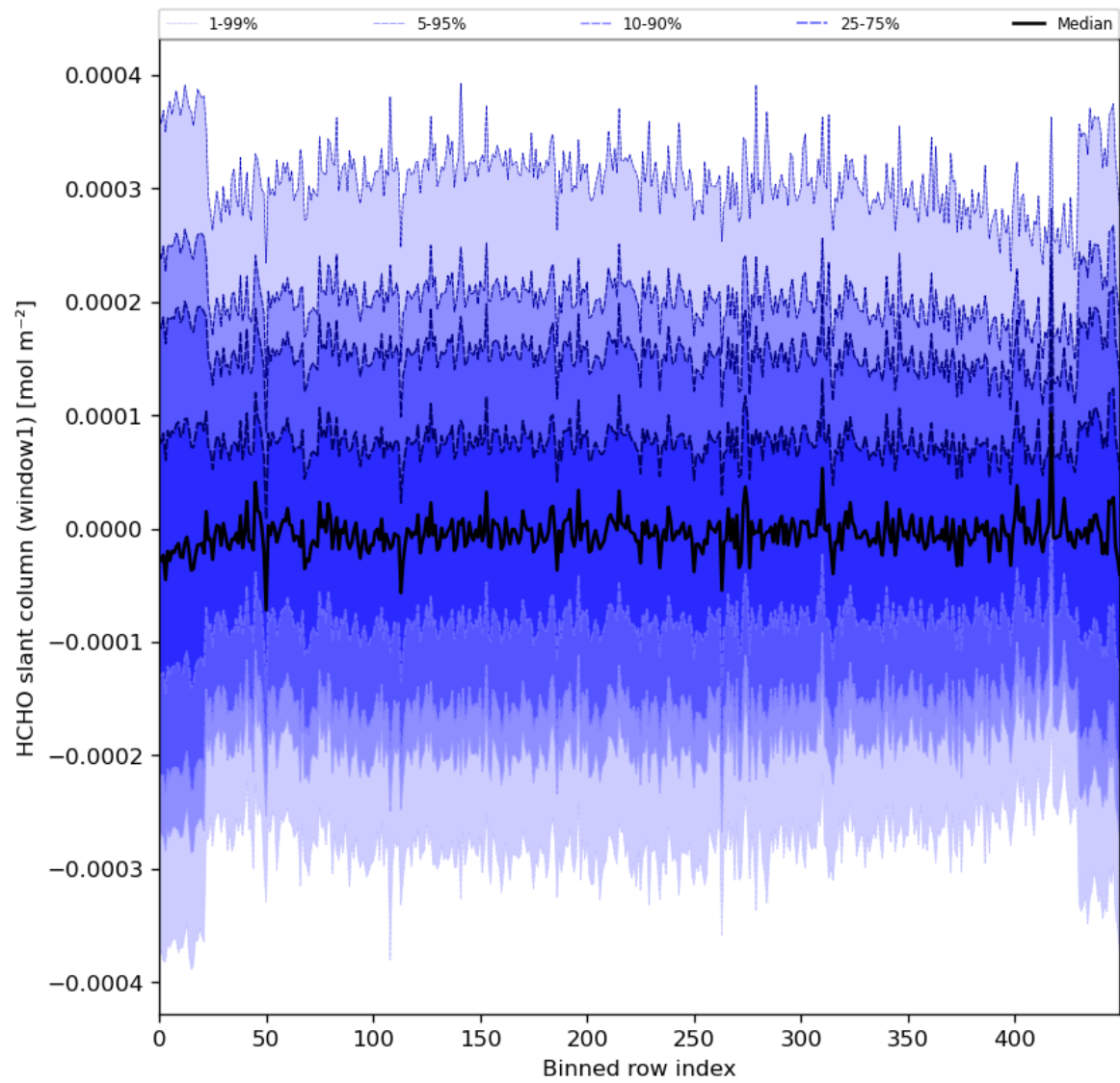
Figure 52: Along track statistics of “HCHO slant column (window1)” for 2024-01-23 to 2024-01-25
