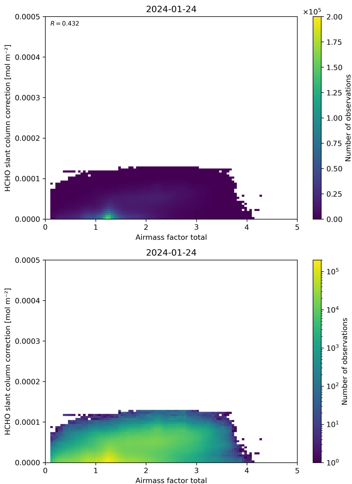
Figure 102: Scatter density plot of “Airmass factor total” against “HCHO slant column correction” for 2024-01-23 to 2024-01-25.
