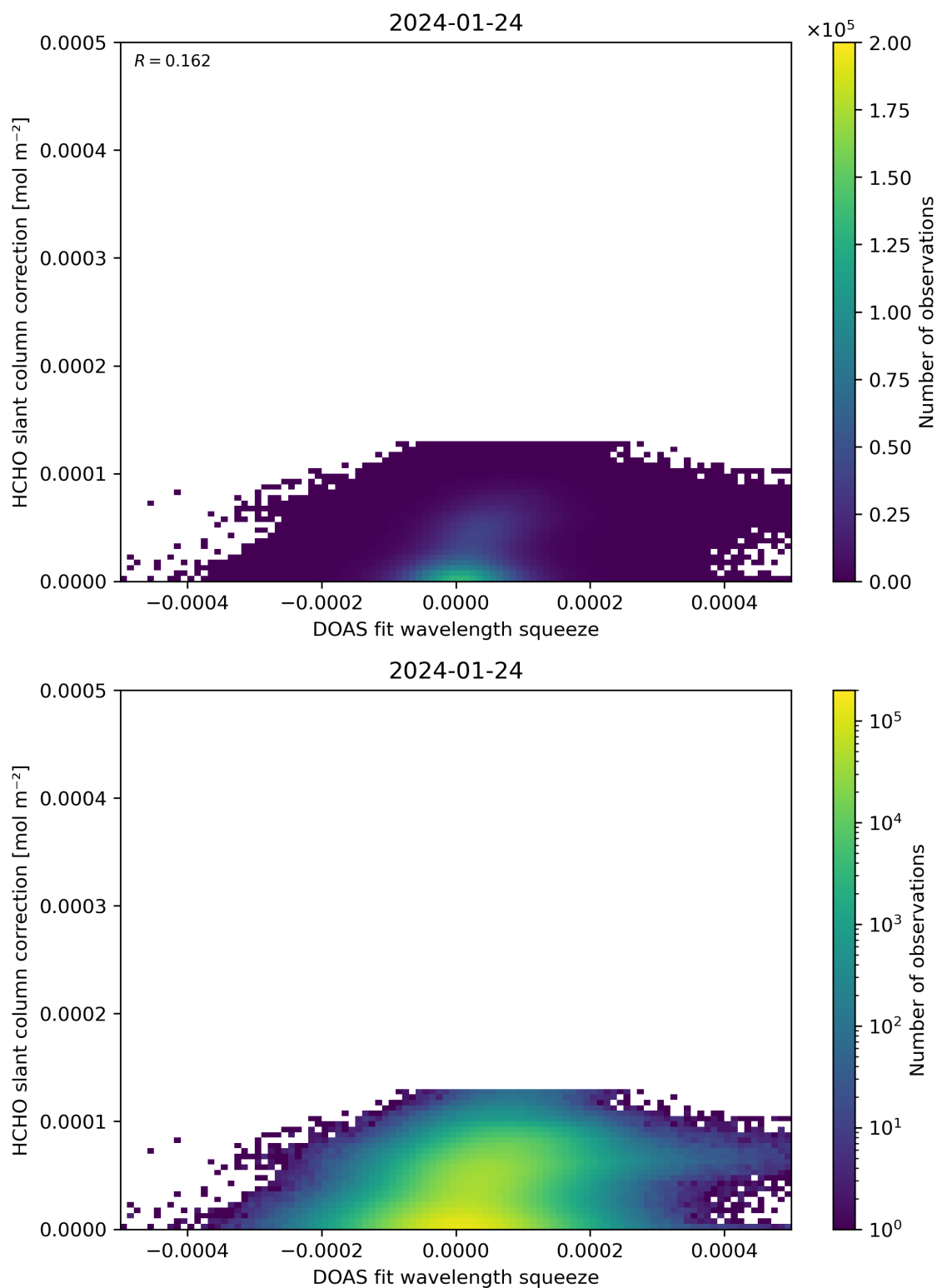
Figure 70: Scatter density plot of “DOAS fit wavelength squeeze” against “HCHO slant column correction” for 2024-01-23 to 2024-01-25.
