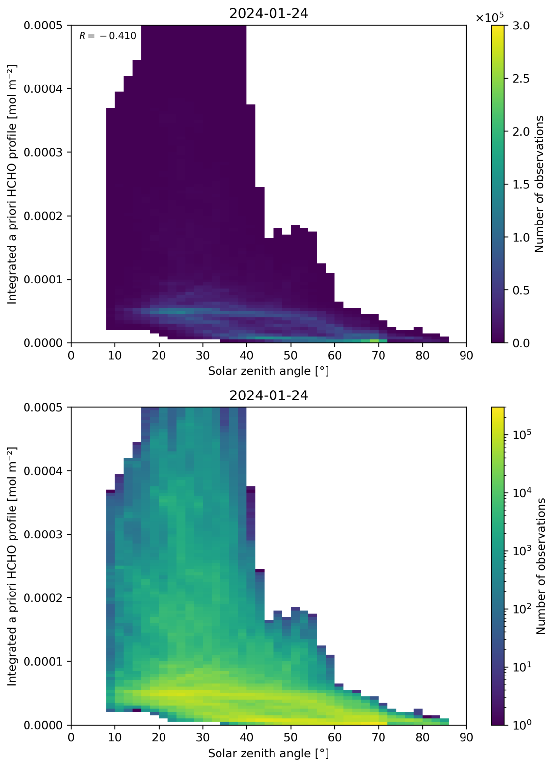
Figure 180: Scatter density plot of “Solar zenith angle” against “Integrated a priori HCHO profile” for 2024-01-23 to 2024-01-25.
