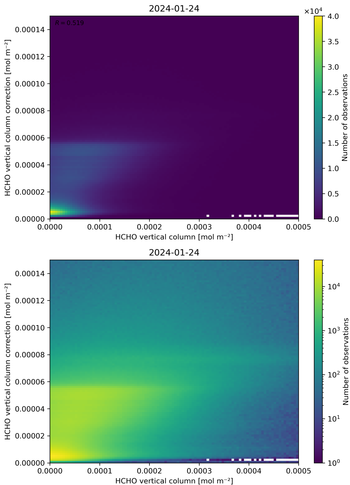
Figure 133: Scatter density plot of “HCHO vertical column” against “HCHO vertical column correction” for 2024-01-23 to 2024-01-25.
