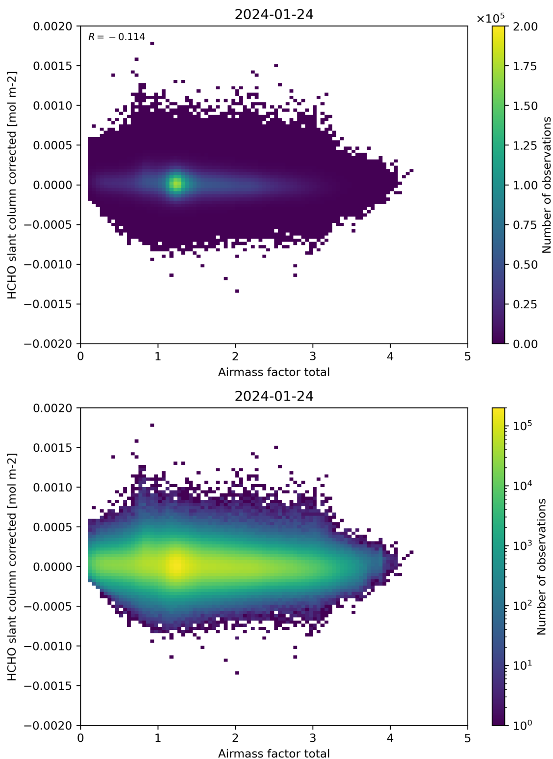
Figure 101: Scatter density plot of “Airmass factor total” against “HCHO slant column corrected” for 2024-01-23 to 2024-01-25.
