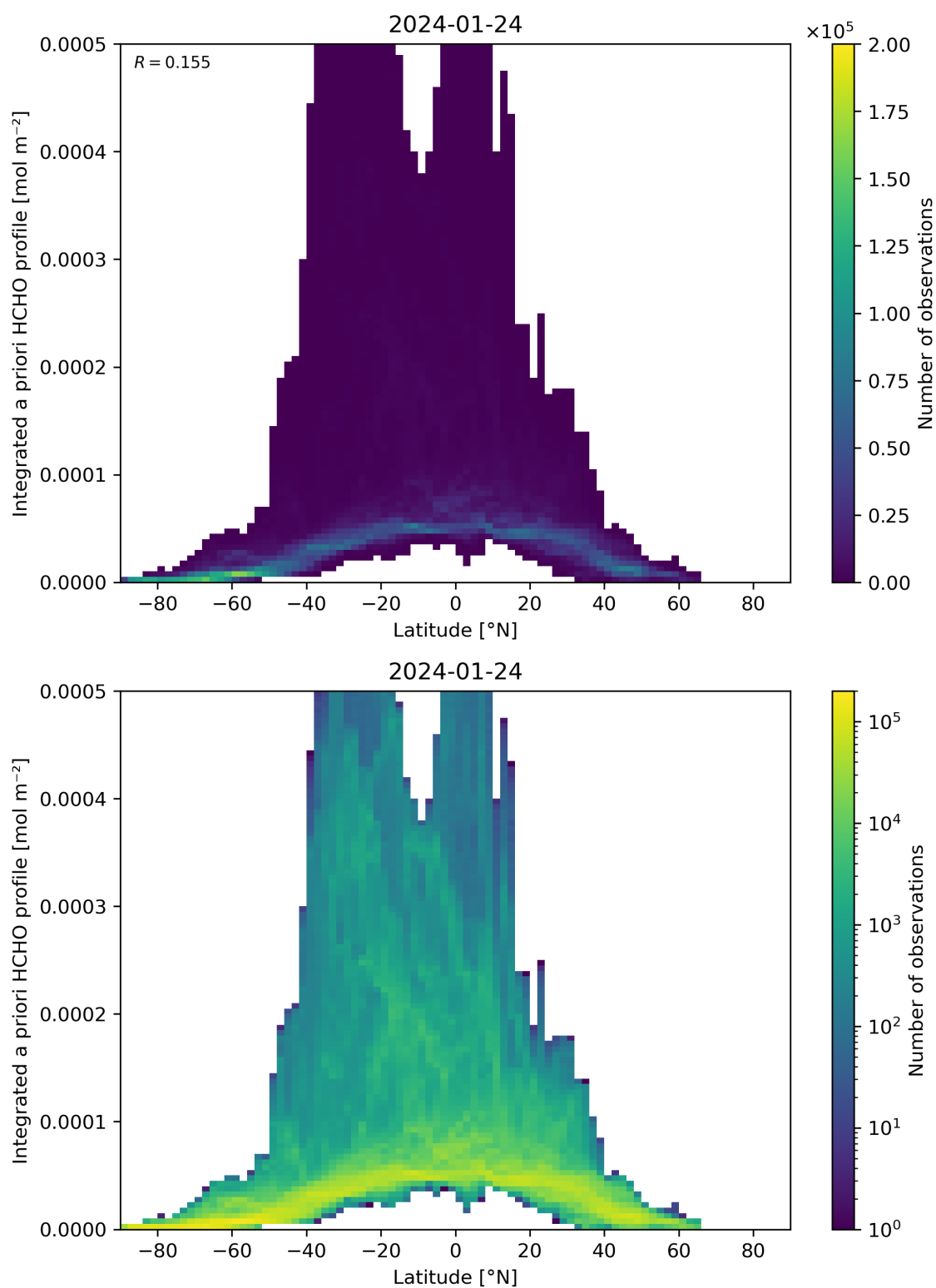
Figure 166: Scatter density plot of “Latitude” against “Integrated a priori HCHO profile” for 2024-01-23 to 2024-01-25.
