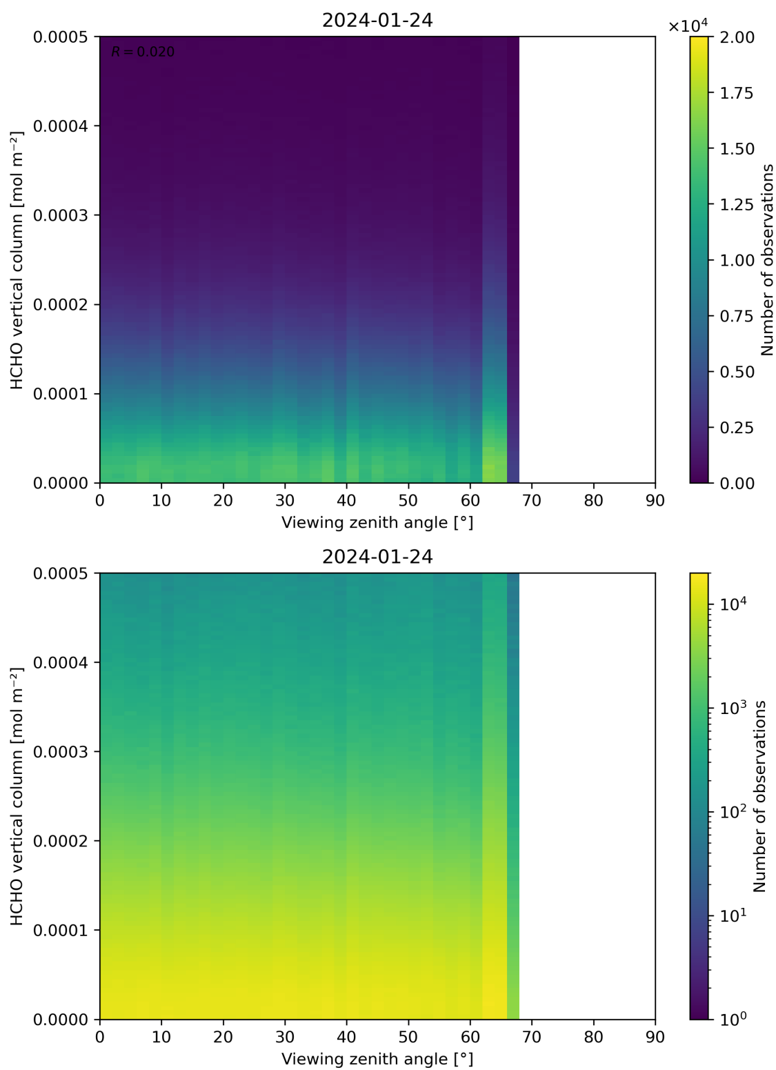
Figure 192: Scatter density plot of “Viewing zenith angle” against “HCHO vertical column” for 2024-01-23 to 2024-01-25.
