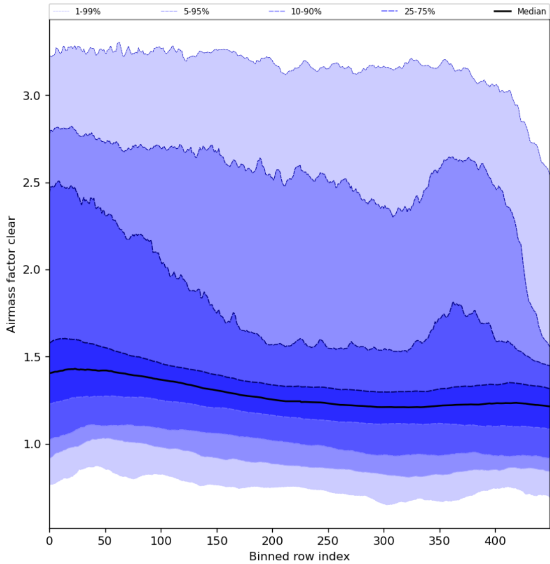
Figure 56: Along track statistics of “Airmass factor clear” for 2024-01-23 to 2024-01-25
