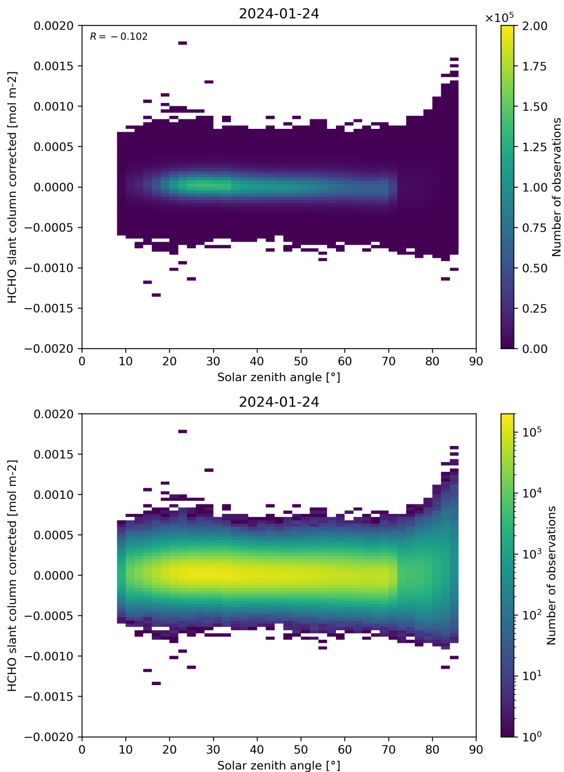
Figure 171: Scatter density plot of “Solar zenith angle” against “HCHO slant column corrected” for 2024-01-23 to 2024-01-25.
