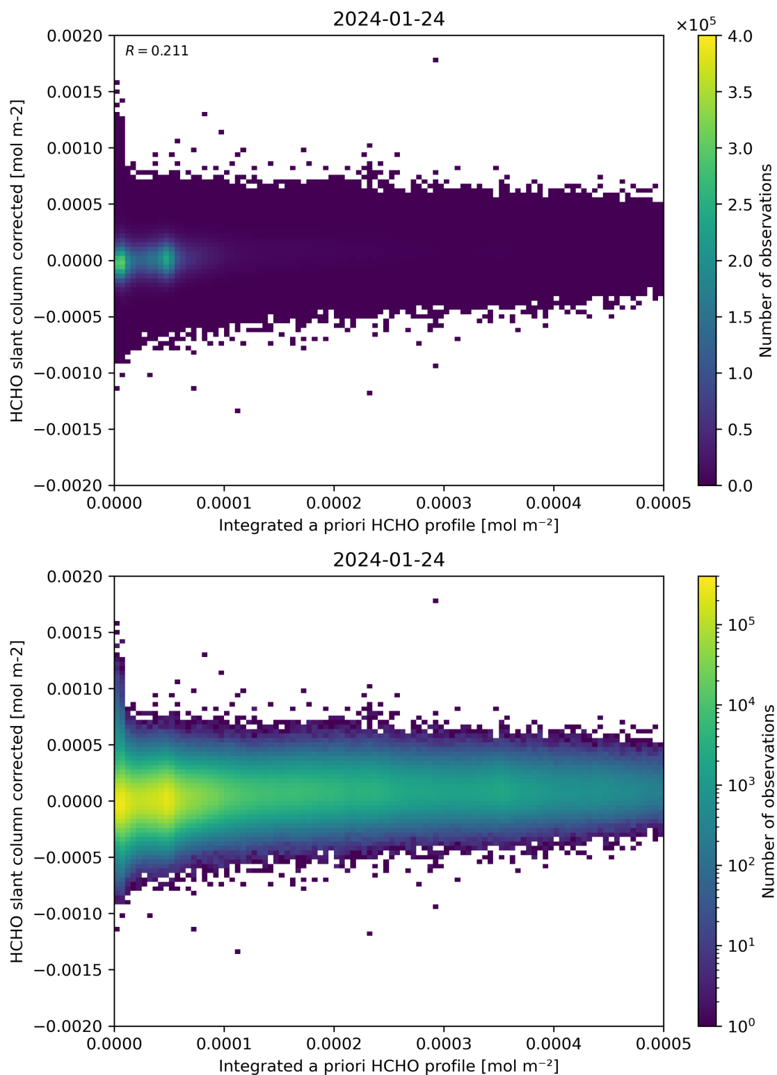
Figure 151: Scatter density plot of “Integrated a priori HCHO profile” against “HCHO slant column corrected” for 2024-01-23 to 2024-01-25.
