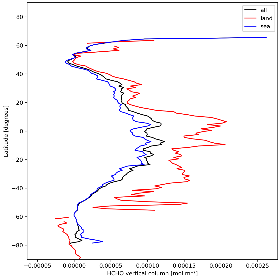
Figure 21: Zonal average of “HCHO vertical column” for 2024-01-23 to 2024-01-25.
