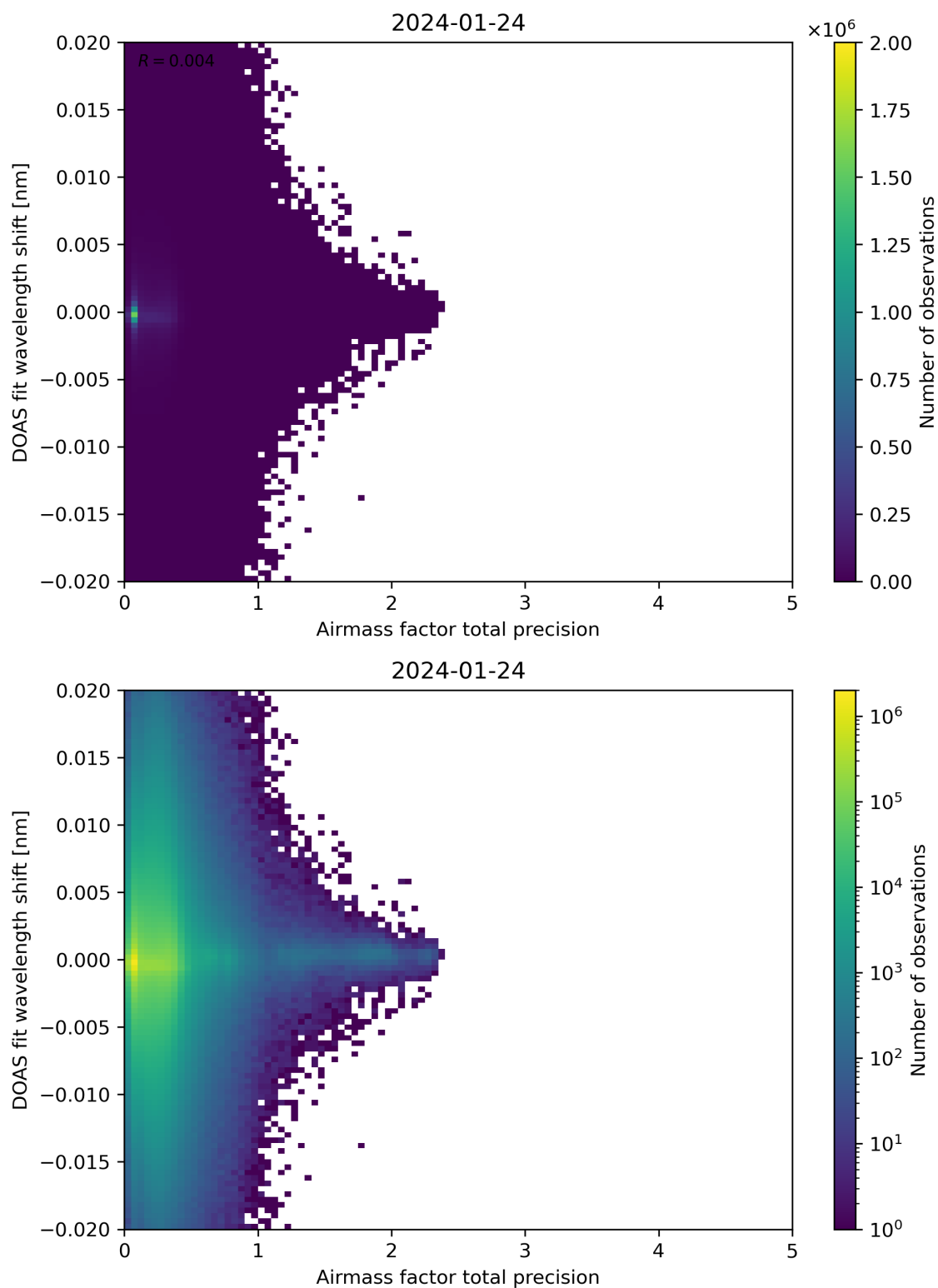
Figure 106: Scatter density plot of “Airmass factor total precision” against “DOAS fit wavelength shift” for 2024-01-23 to 2024-01-25.
