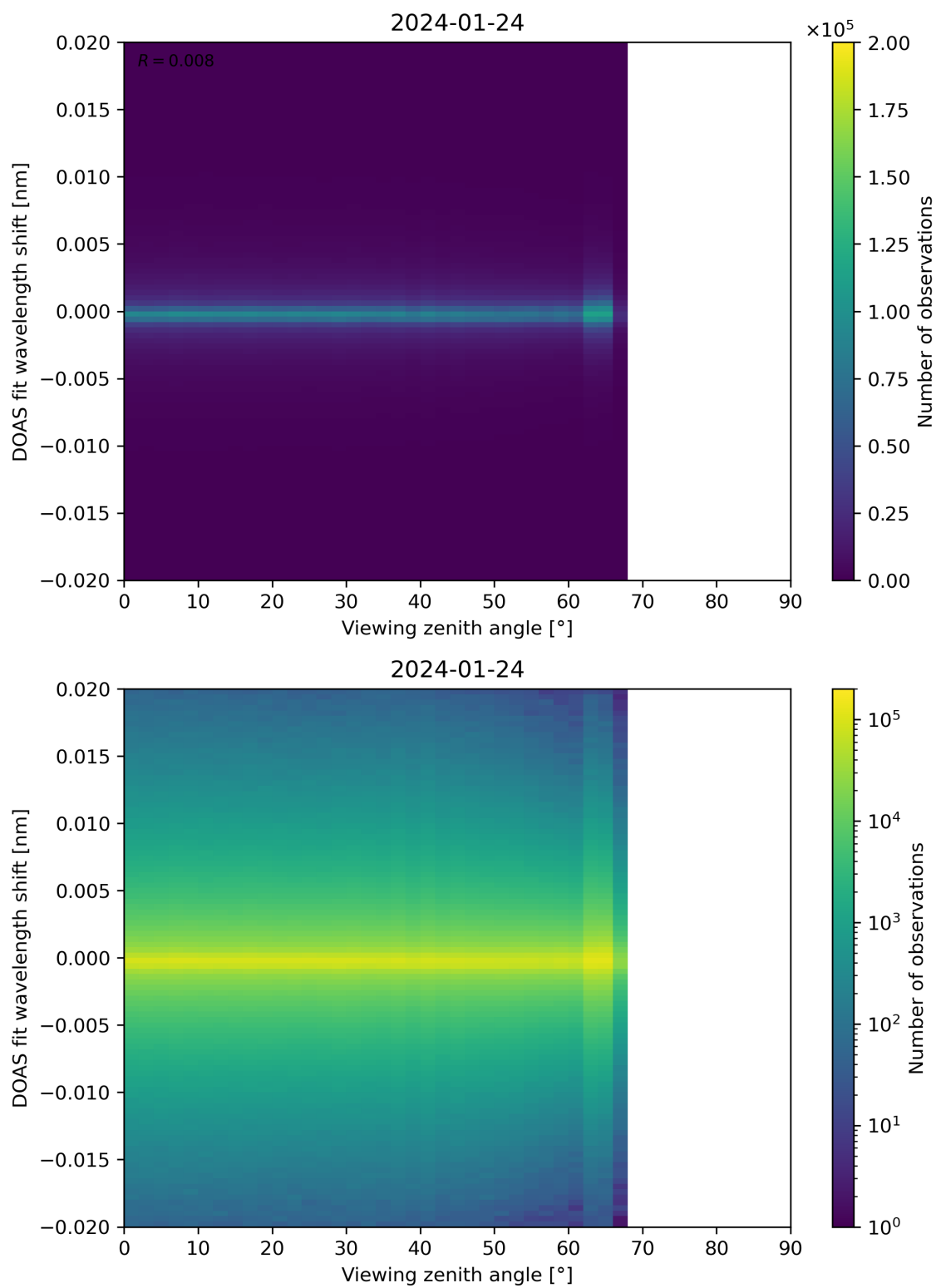
Figure 183: Scatter density plot of “Viewing zenith angle” against “DOAS fit wavelength shift” for 2024-01-23 to 2024-01-25.
