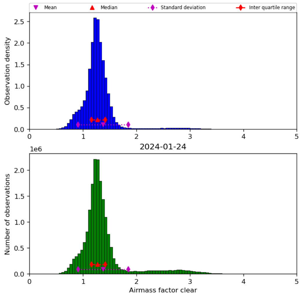
Figure 42: Histogram of “Airmass factor clear” for 2024-01-23 to 2024-01-25
