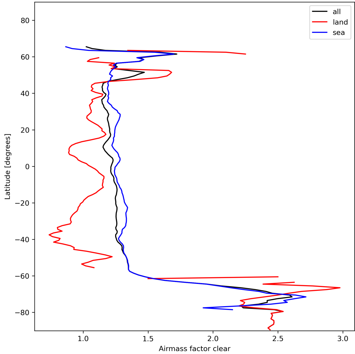
Figure 28: Zonal average of “Airmass factor clear” for 2024-01-23 to 2024-01-25.
