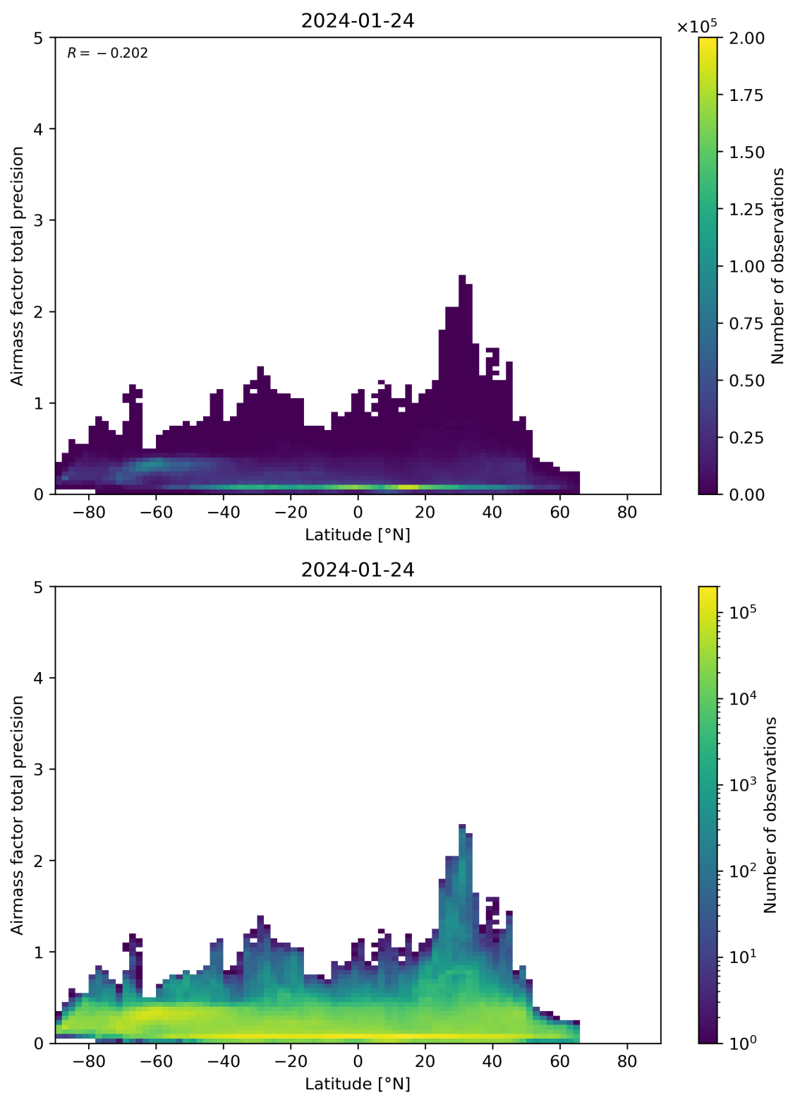
Figure 162: Scatter density plot of “Latitude” against “Airmass factor total precision” for 2024-01-23 to 2024-01-25.
