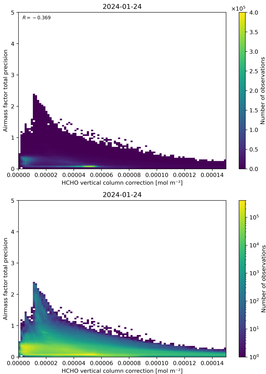
Figure 121: Scatter density plot of “HCHO vertical column correction” against “Airmass factor total precision” for 2024-01-23 to 2024-01-25.
