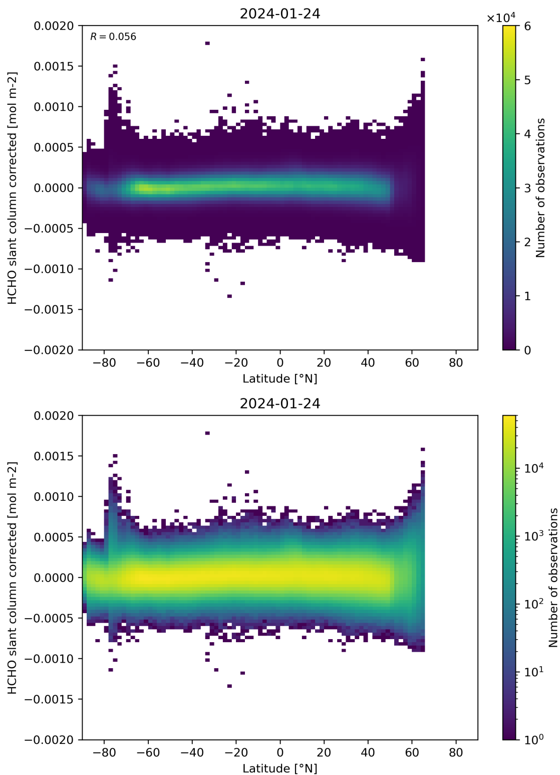
Figure 157: Scatter density plot of “Latitude” against “HCHO slant column corrected” for 2024-01-23 to 2024-01-25.
