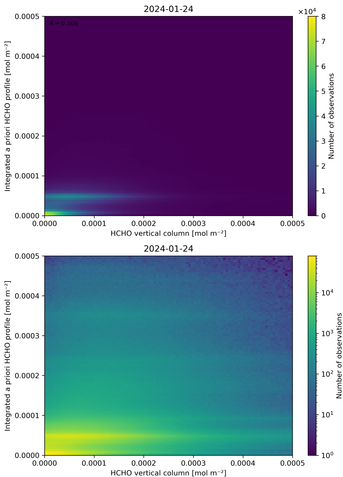
Figure 135: Scatter density plot of “HCHO vertical column” against “Integrated a priori HCHO profile” for 2024-01-23 to 2024-01-25.
