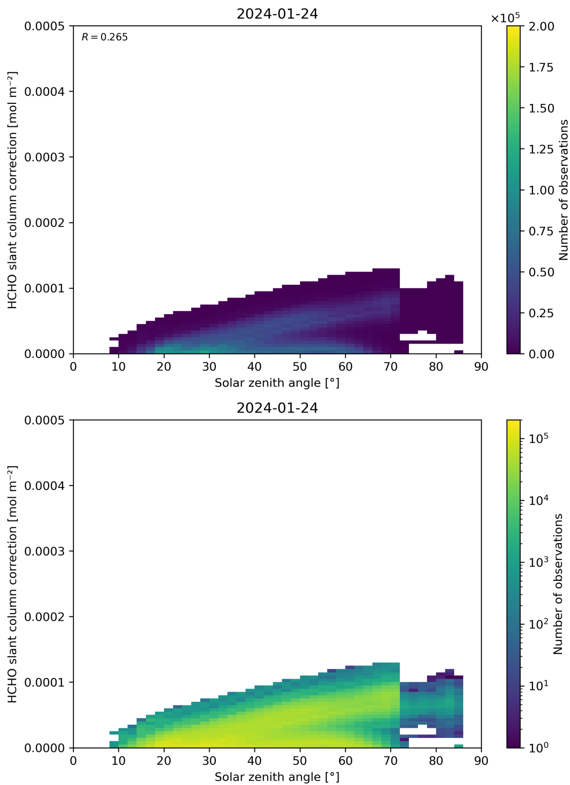
Figure 172: Scatter density plot of “Solar zenith angle” against “HCHO slant column correction” for 2024-01-23 to 2024-01-25.
