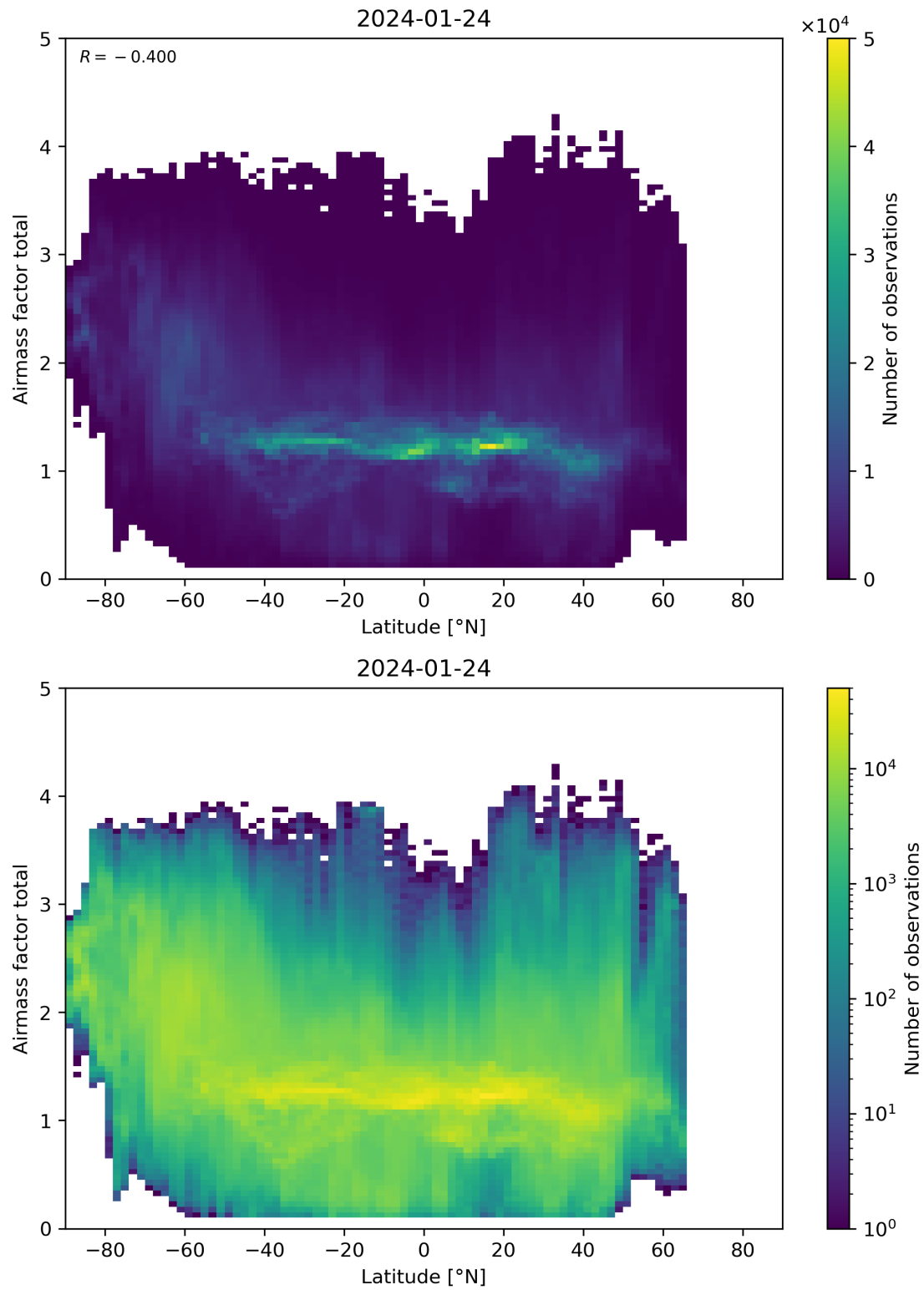
Figure 161: Scatter density plot of “Latitude” against “Airmass factor total” for 2024-01-23 to 2024-01-25.
