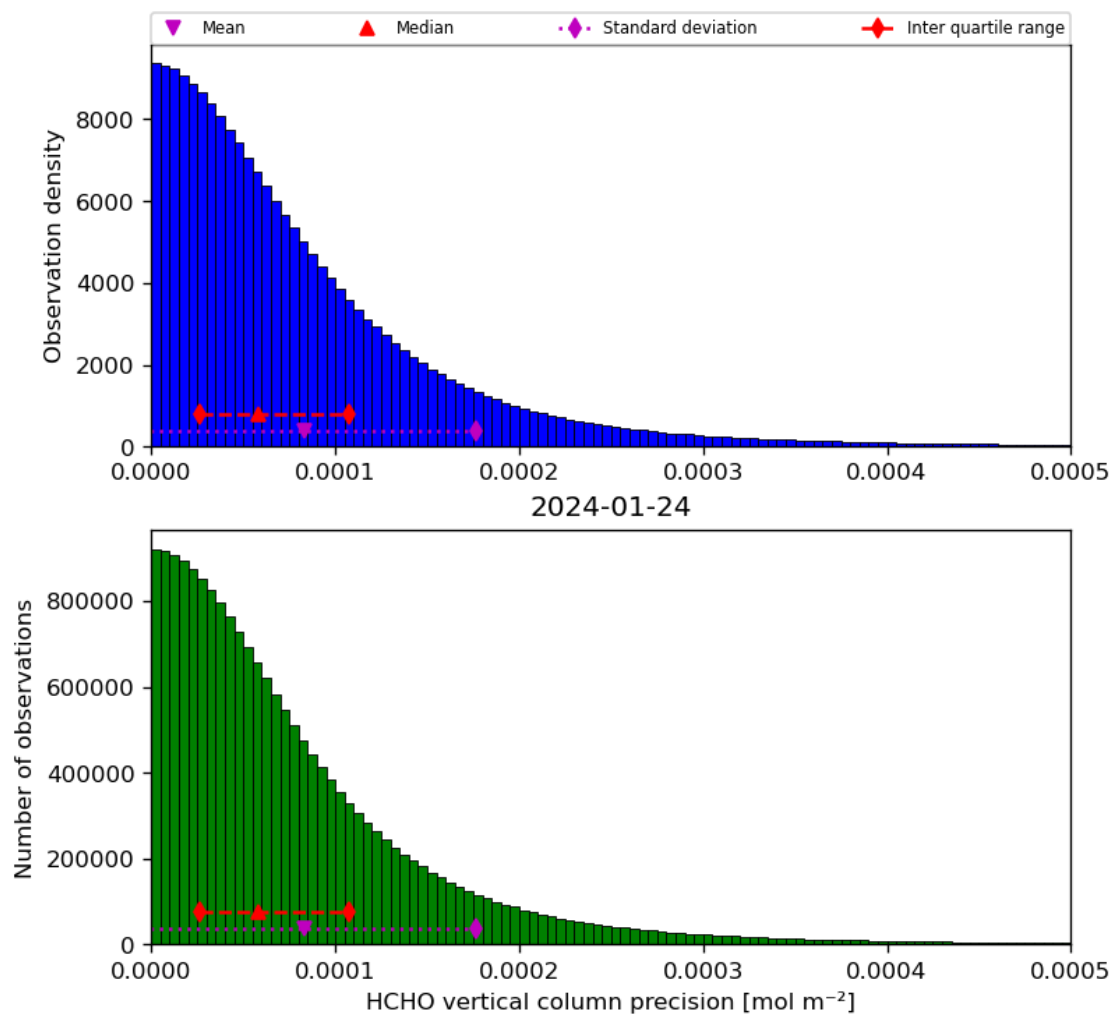
Figure 36: Histogram of “HCHO vertical column precision” for 2024-01-23 to 2024-01-25
