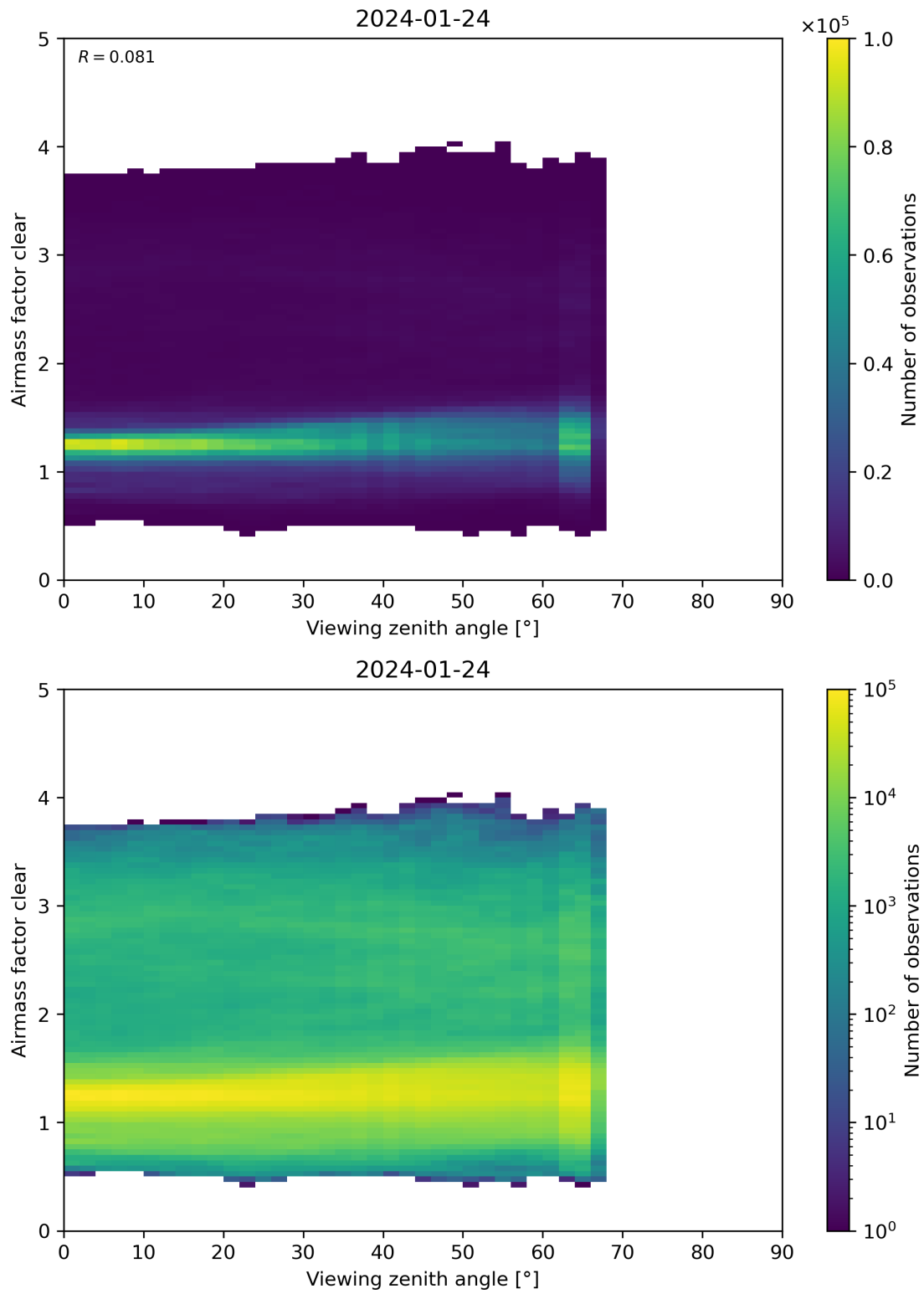
Figure 185: Scatter density plot of “Viewing zenith angle” against “Airmass factor clear” for 2024-01-23 to 2024-01-25.
