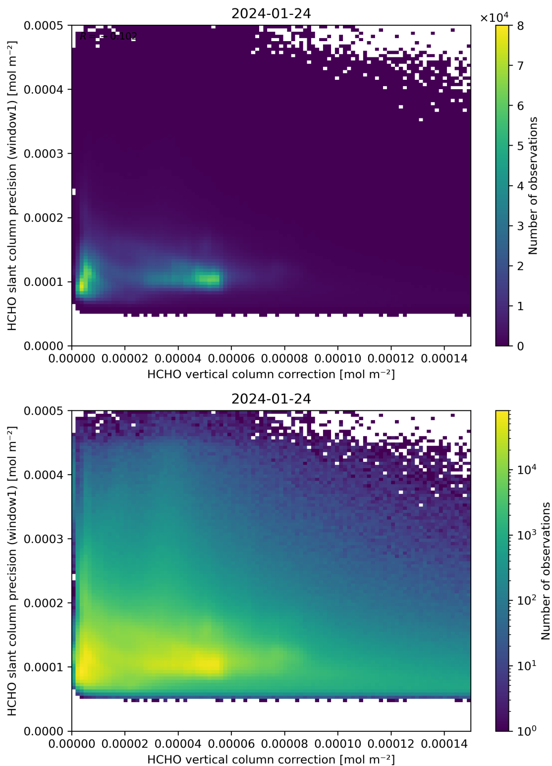
Figure 119: Scatter density plot of “HCHO vertical column correction” against “HCHO slant column precision (window1)” for 2024-01-23 to 2024-01-25.
