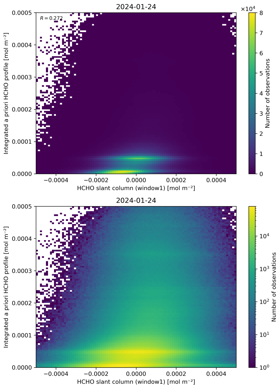
Figure 87: Scatter density plot of “HCHO slant column (window1)” against “Integrated a priori HCHO profile” for 2024-01-23 to 2024-01-25.
