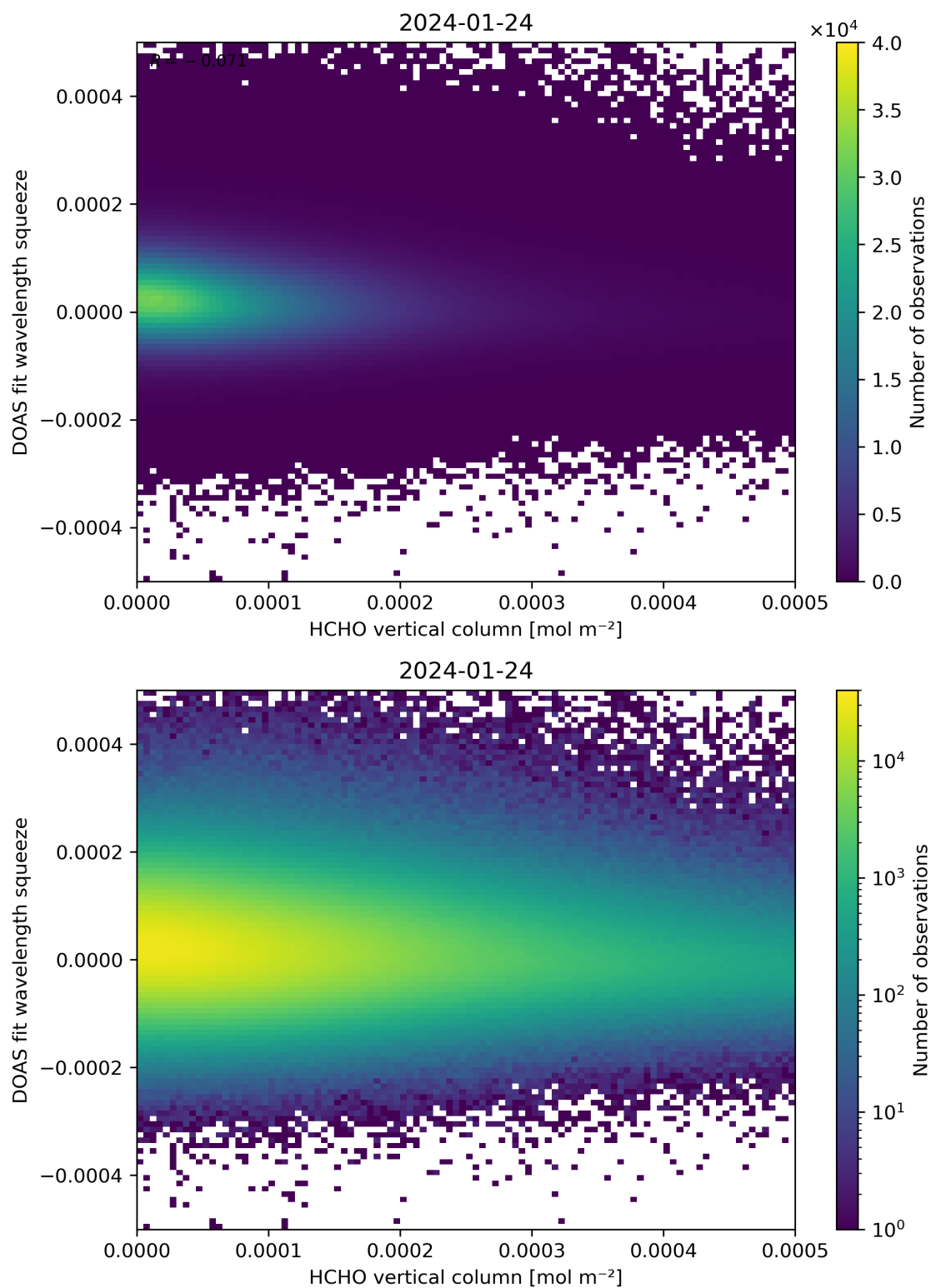
Figure 125: Scatter density plot of “HCHO vertical column” against “DOAS fit wavelength squeeze” for 2024-01-23 to 2024-01-25.
