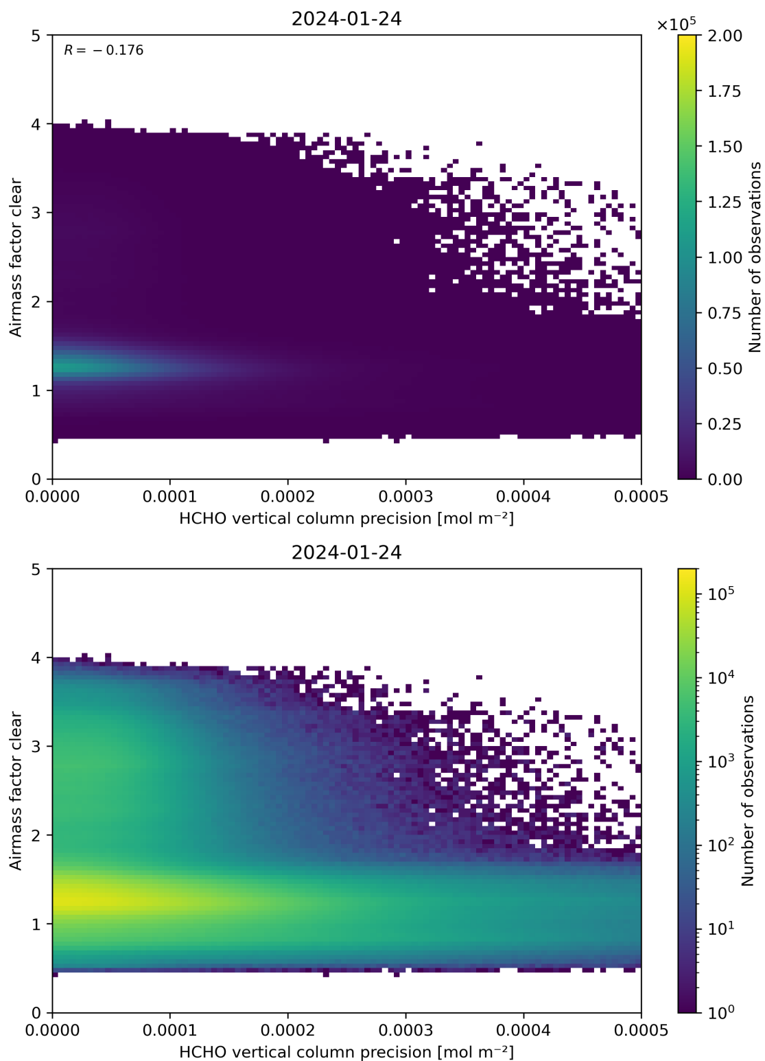
Figure 139: Scatter density plot of “HCHO vertical column precision” against “Airmass factor clear” for 2024-01-23 to 2024-01-25.
