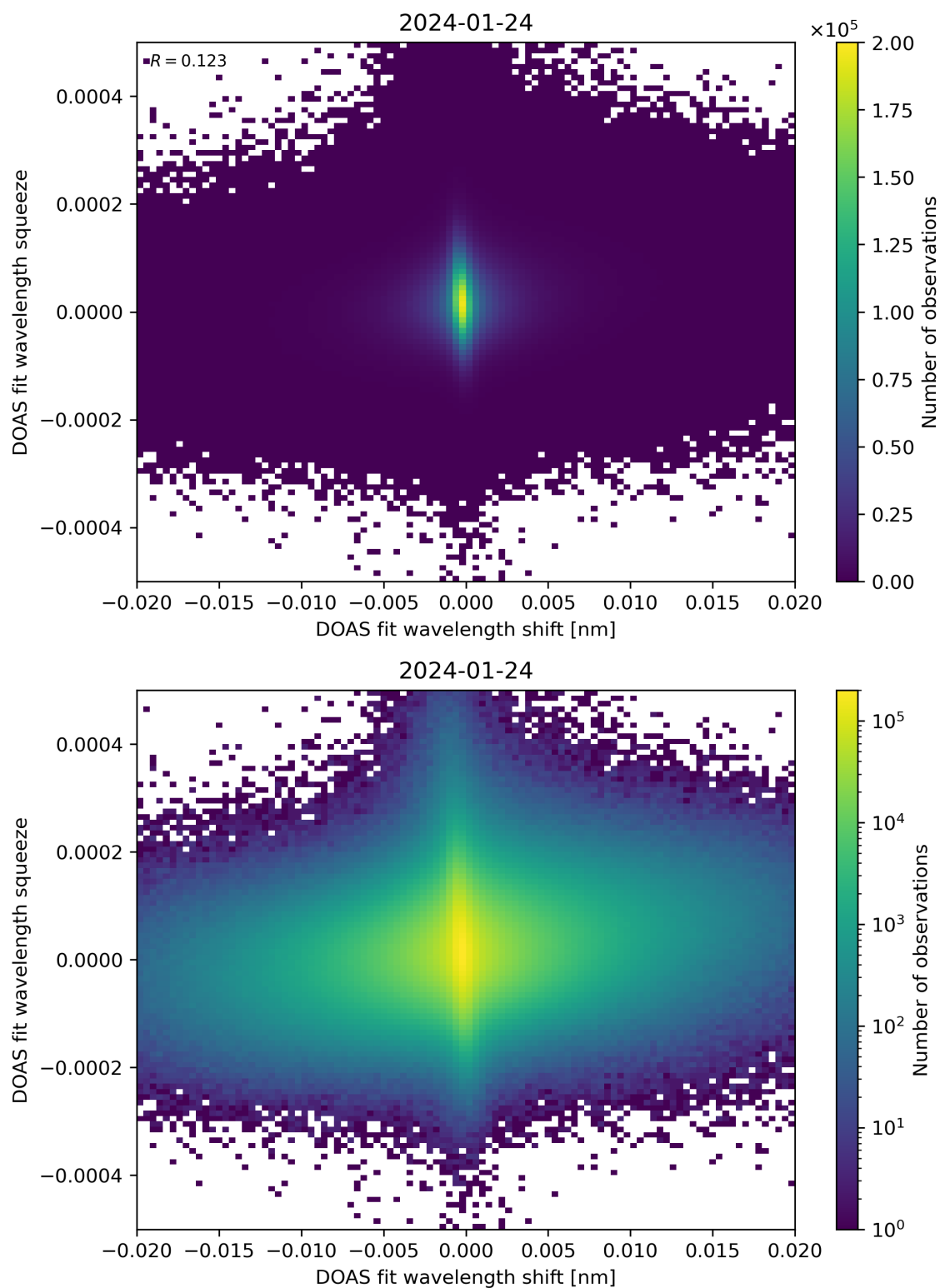
Figure 65: Scatter density plot of “DOAS fit wavelength shift” against “DOAS fit wavelength squeeze” for 2024-01-23 to 2024-01-25.
