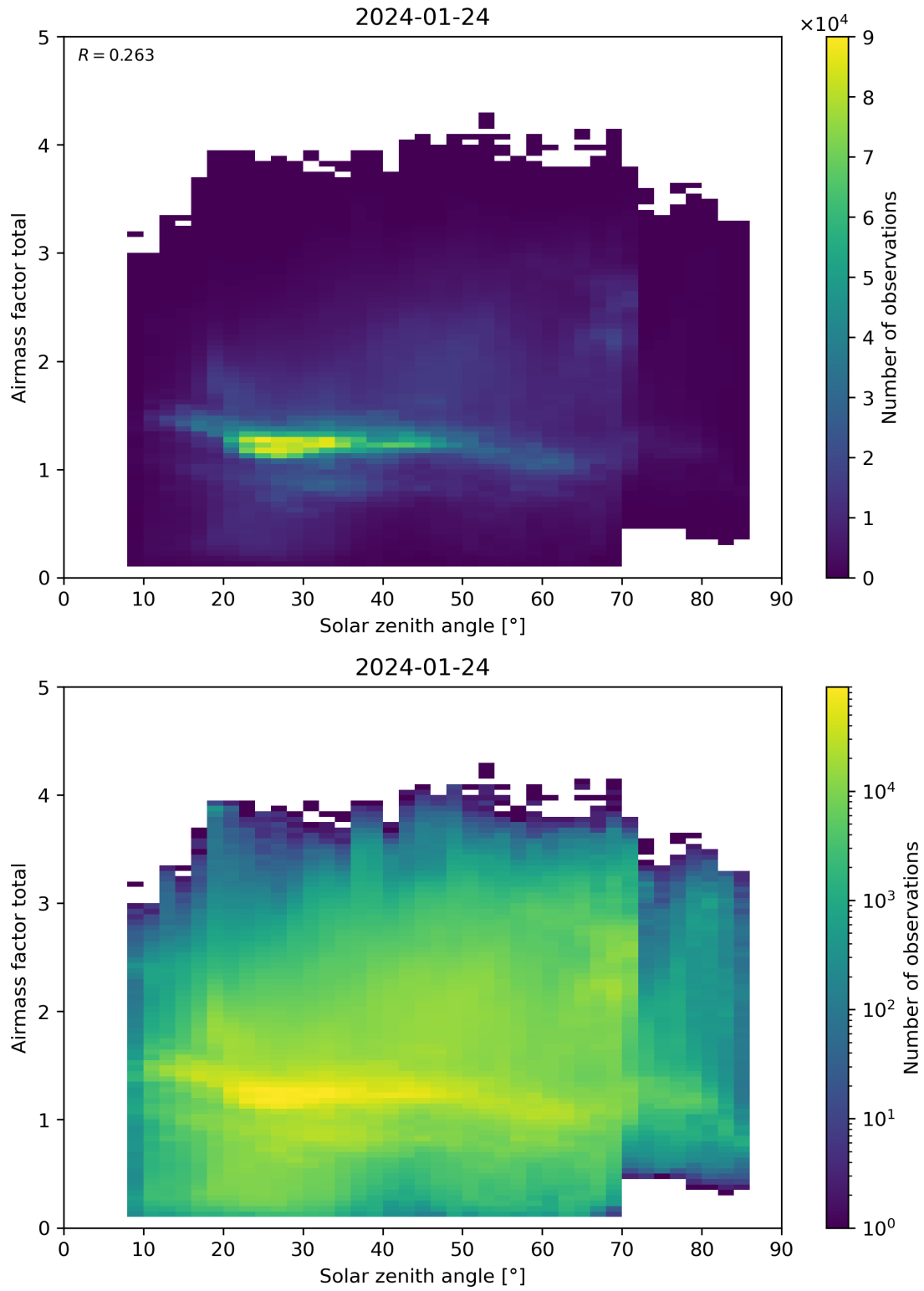
Figure 175: Scatter density plot of “Solar zenith angle” against “Airmass factor total” for 2024-01-23 to 2024-01-25.
