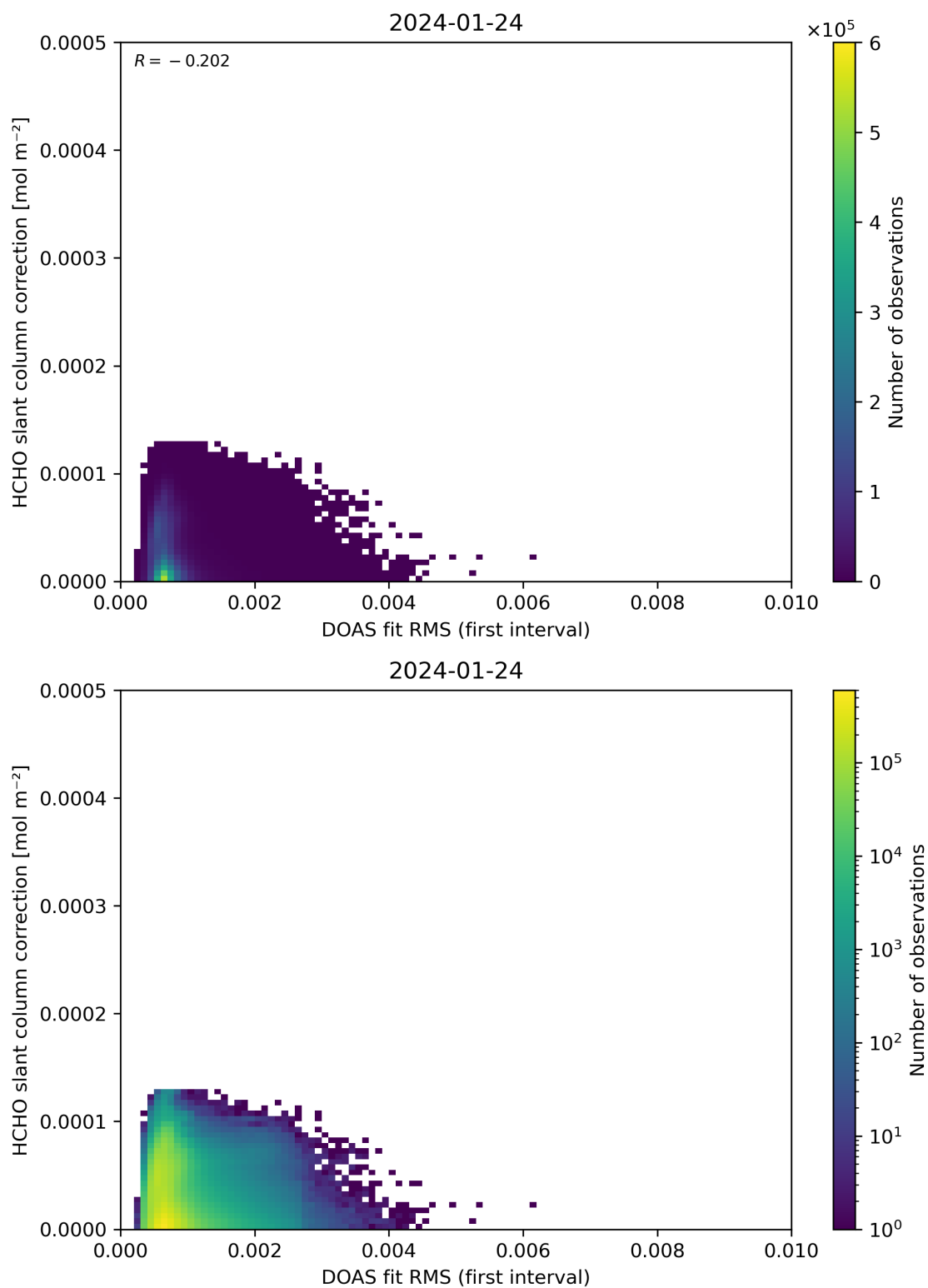
Figure 63: Scatter density plot of “DOAS fit RMS (first interval)” against “HCHO slant column correction” for 2024-01-23 to 2024-01-25.
