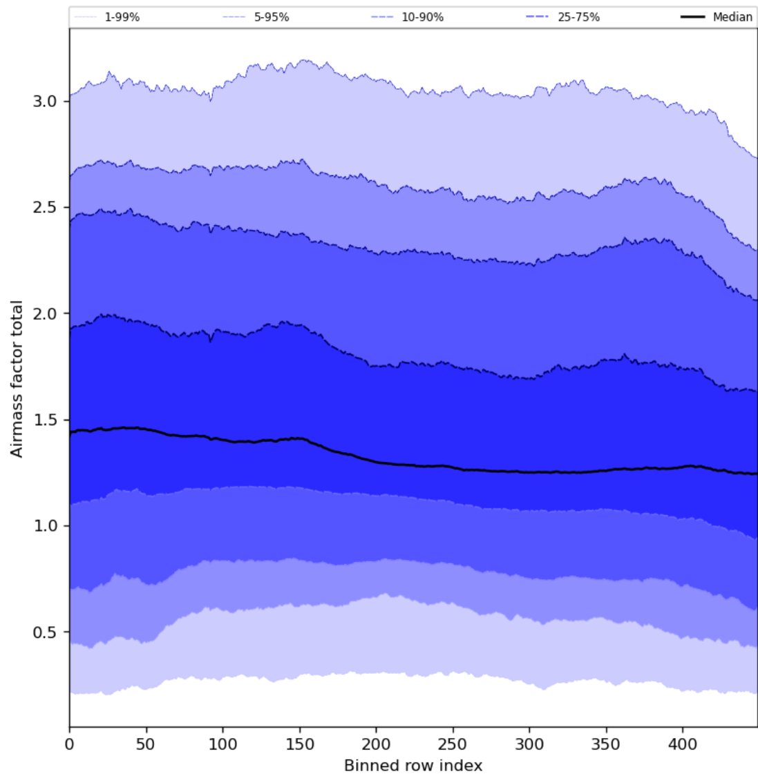
Figure 54: Along track statistics of “Airmass factor total” for 2024-01-23 to 2024-01-25
