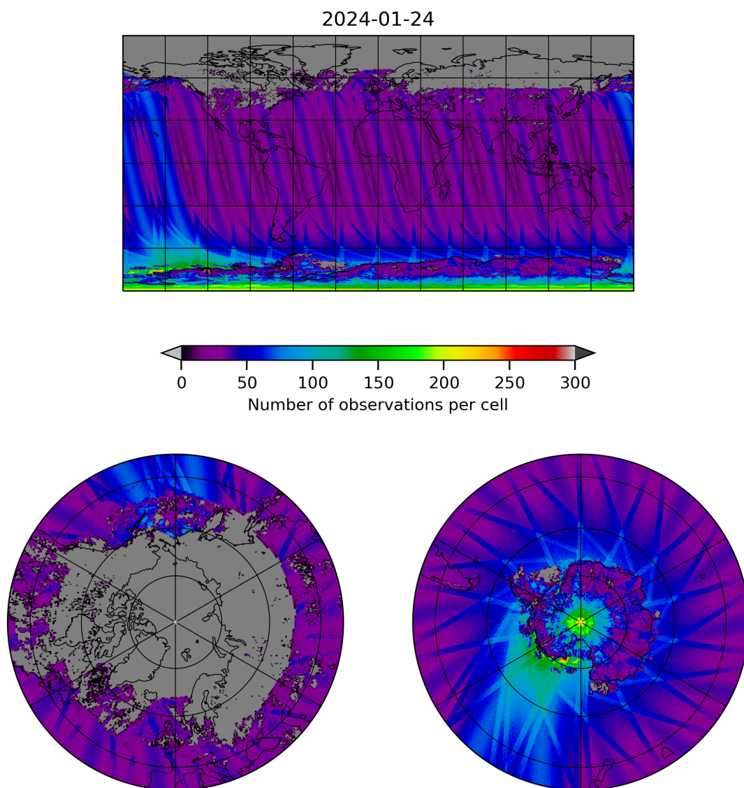
Figure 19: Map of the number of observations for 2024-01-23 to 2024-01-25
