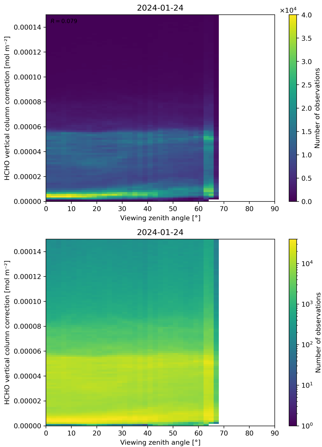
Figure 193: Scatter density plot of “Viewing zenith angle” against “HCHO vertical column correction” for 2024-01-23 to 2024-01-25.
