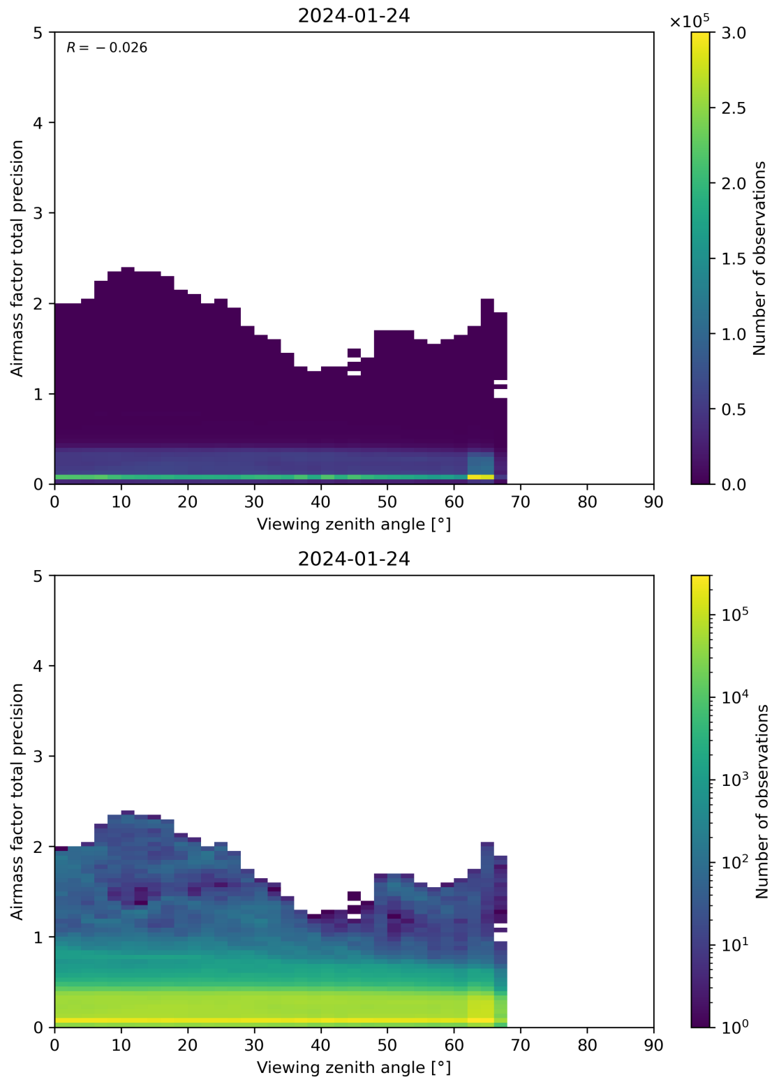
Figure 191: Scatter density plot of “Viewing zenith angle” against “Airmass factor total precision” for 2024-01-23 to 2024-01-25.
