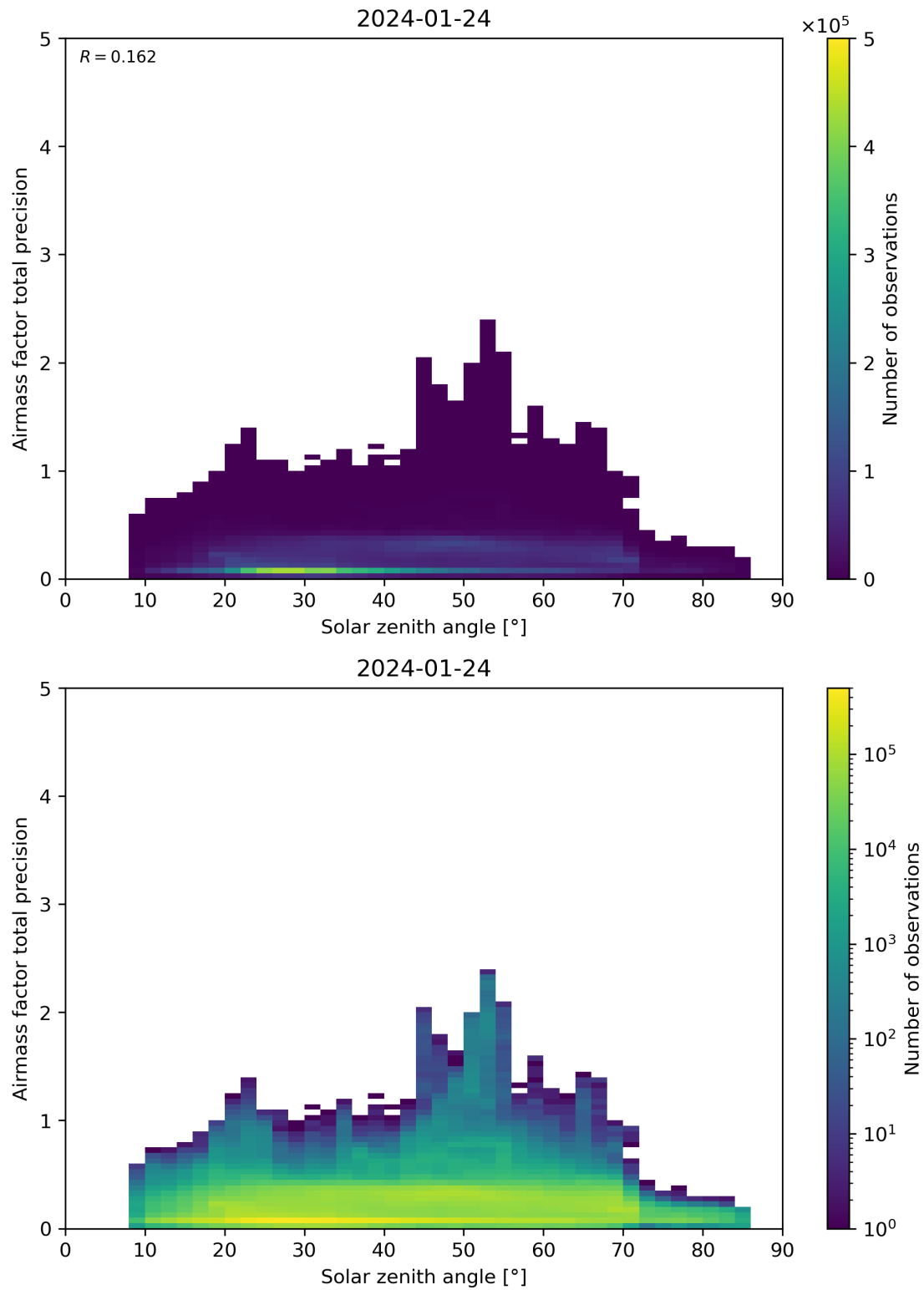
Figure 176: Scatter density plot of “Solar zenith angle” against “Airmass factor total precision” for 2024-01-23 to 2024-01-25.
