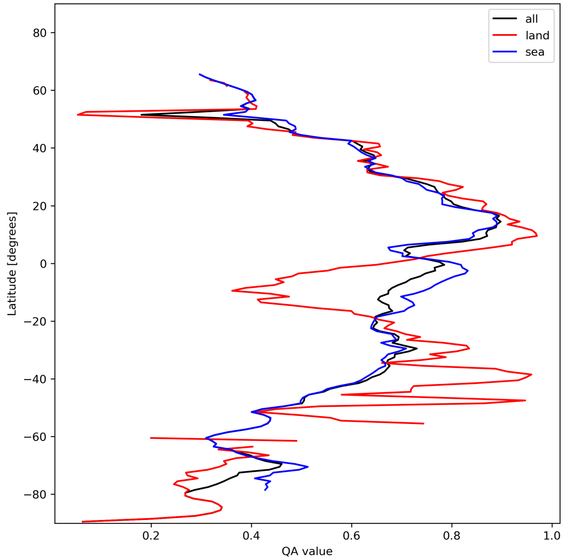
Figure 20: Zonal average of “QA value” for 2024-01-23 to 2024-01-25.
