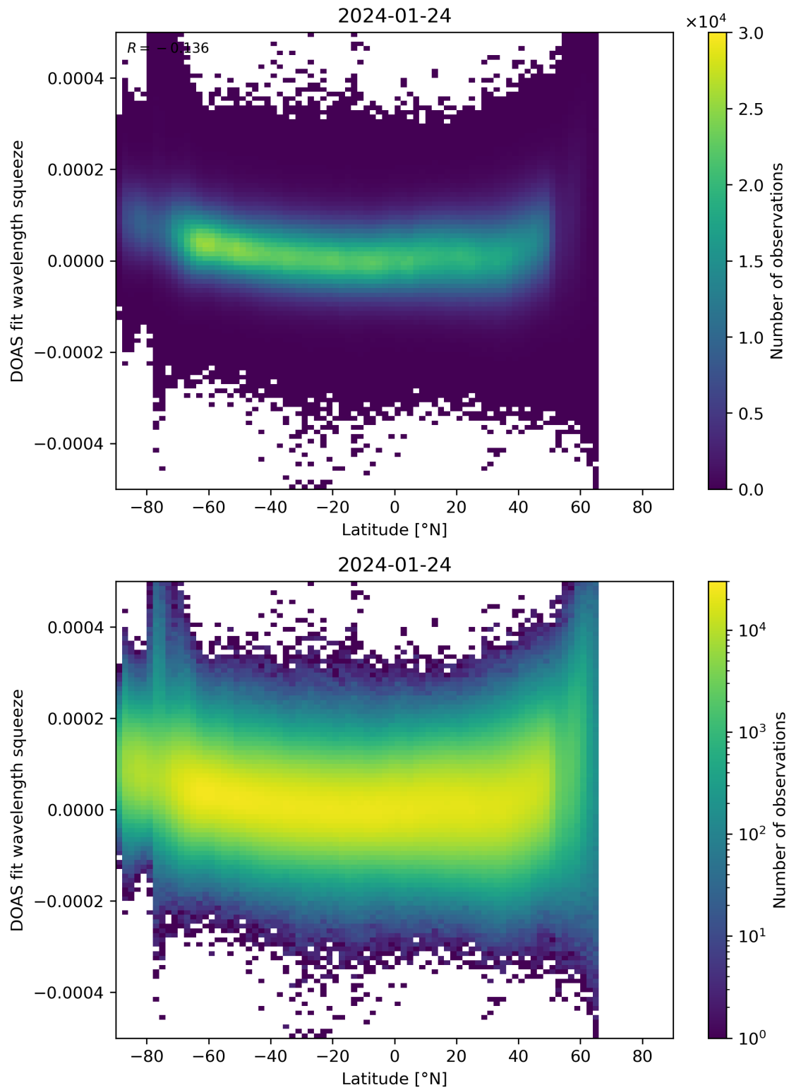
Figure 155: Scatter density plot of “Latitude” against “DOAS fit wavelength squeeze” for 2024-01-23 to 2024-01-25.
