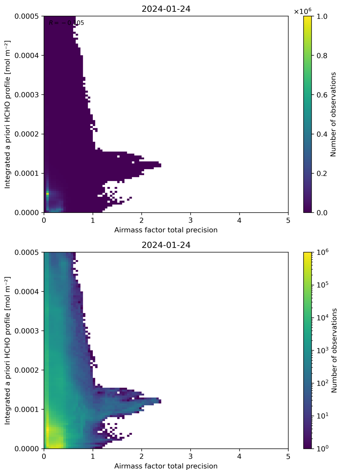
Figure 111: Scatter density plot of “Airmass factor total precision” against “Integrated a priori HCHO profile” for 2024-01-23 to 2024-01-25.
