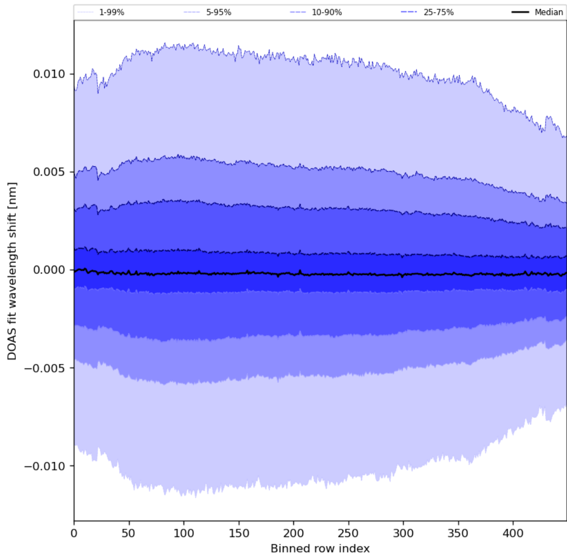
Figure 58: Along track statistics of “DOAS fit wavelength shift” for 2024-01-23 to 2024-01-25
