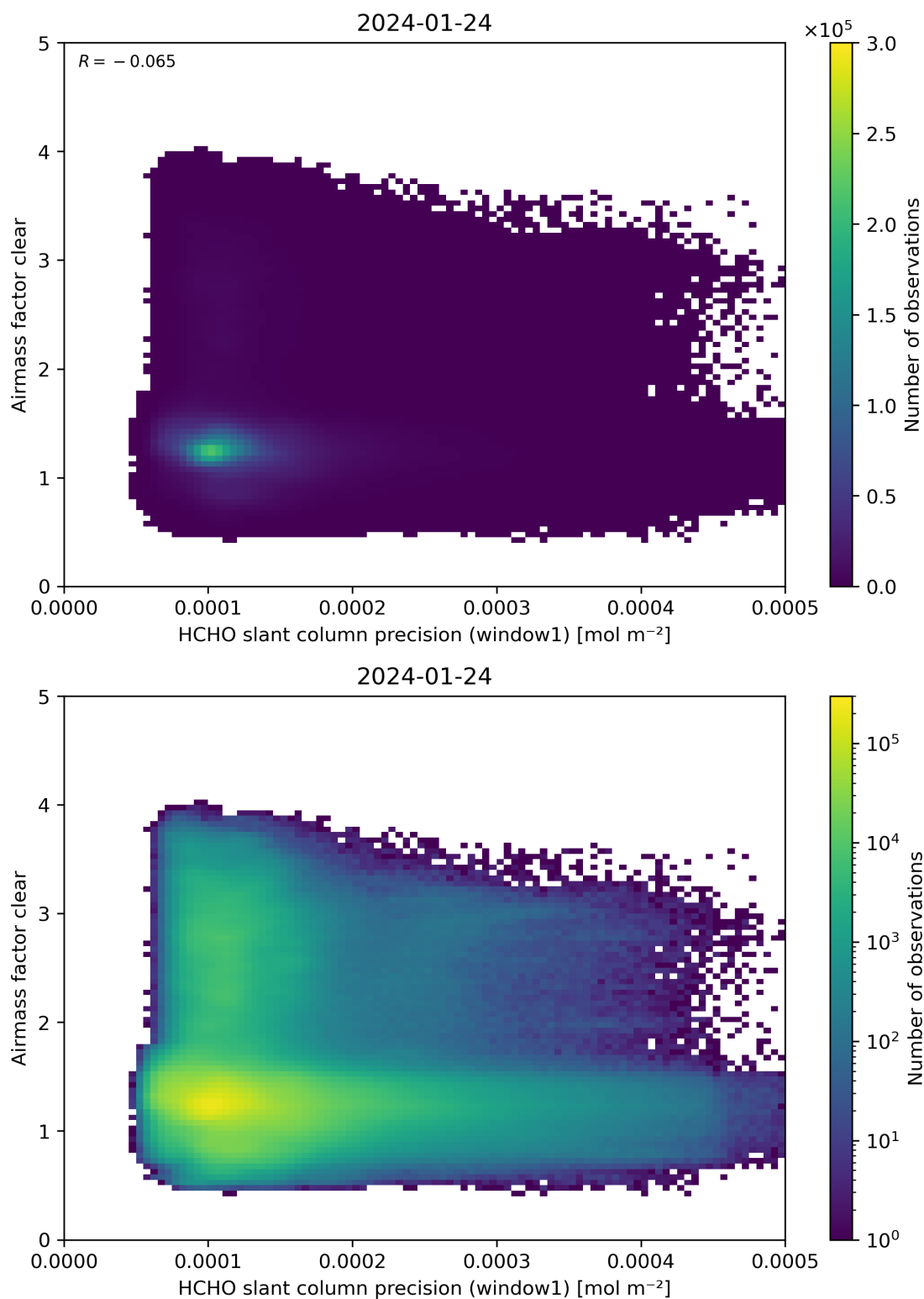
Figure 91: Scatter density plot of “HCHO slant column precision (window1)” against “Airmass factor clear” for 2024-01-23 to 2024-01-25.
