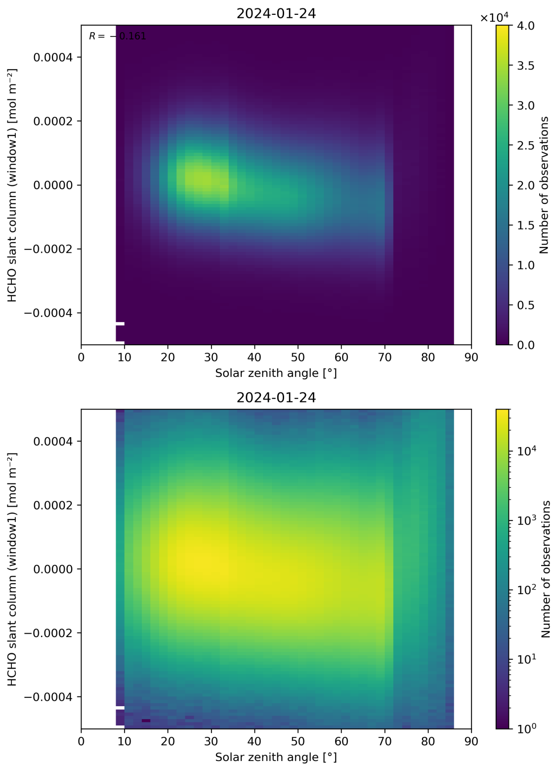
Figure 173: Scatter density plot of “Solar zenith angle” against “HCHO slant column (window1)” for 2024-01-23 to 2024-01-25.
