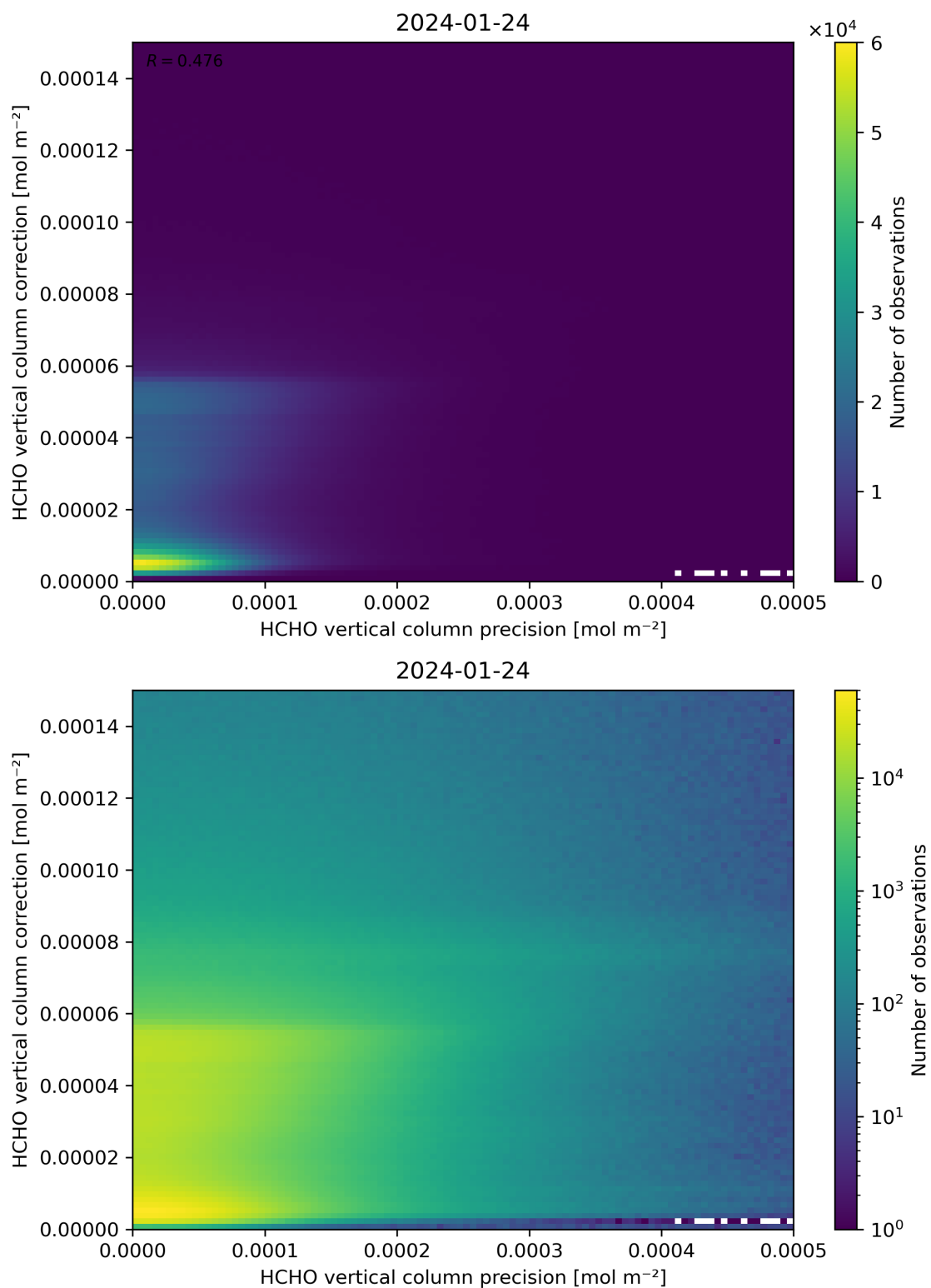
Figure 146: Scatter density plot of “HCHO vertical column precision” against “HCHO vertical column correction” for 2024-01-23 to 2024-01-25.
