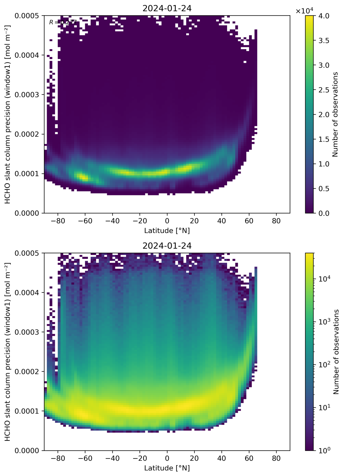
Figure 160: Scatter density plot of “Latitude” against “HCHO slant column precision (window1)” for 2024-01-23 to 2024-01-25.
