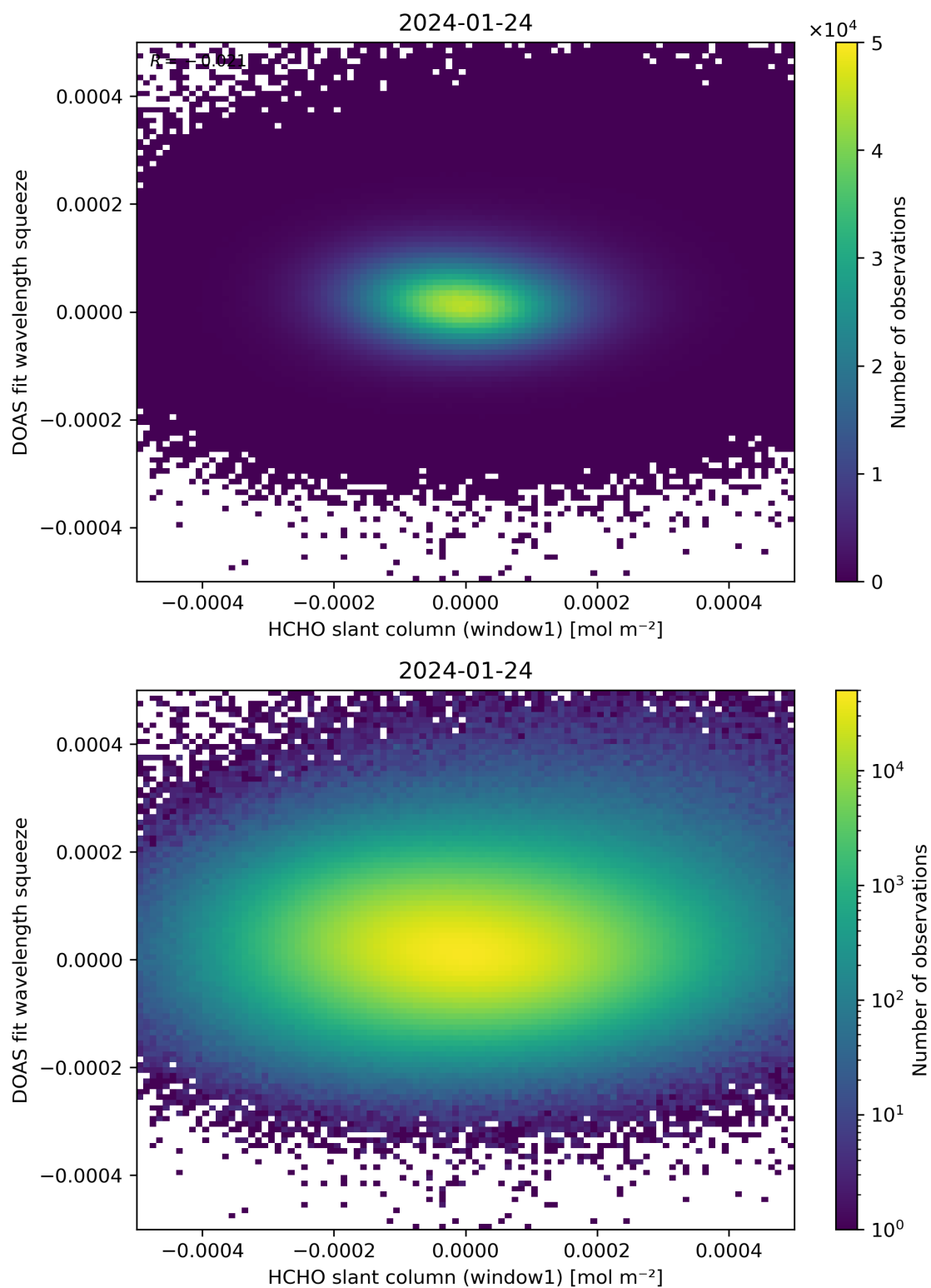
Figure 80: Scatter density plot of “HCHO slant column (window1)” against “DOAS fit wavelength squeeze” for 2024-01-23 to 2024-01-25.
