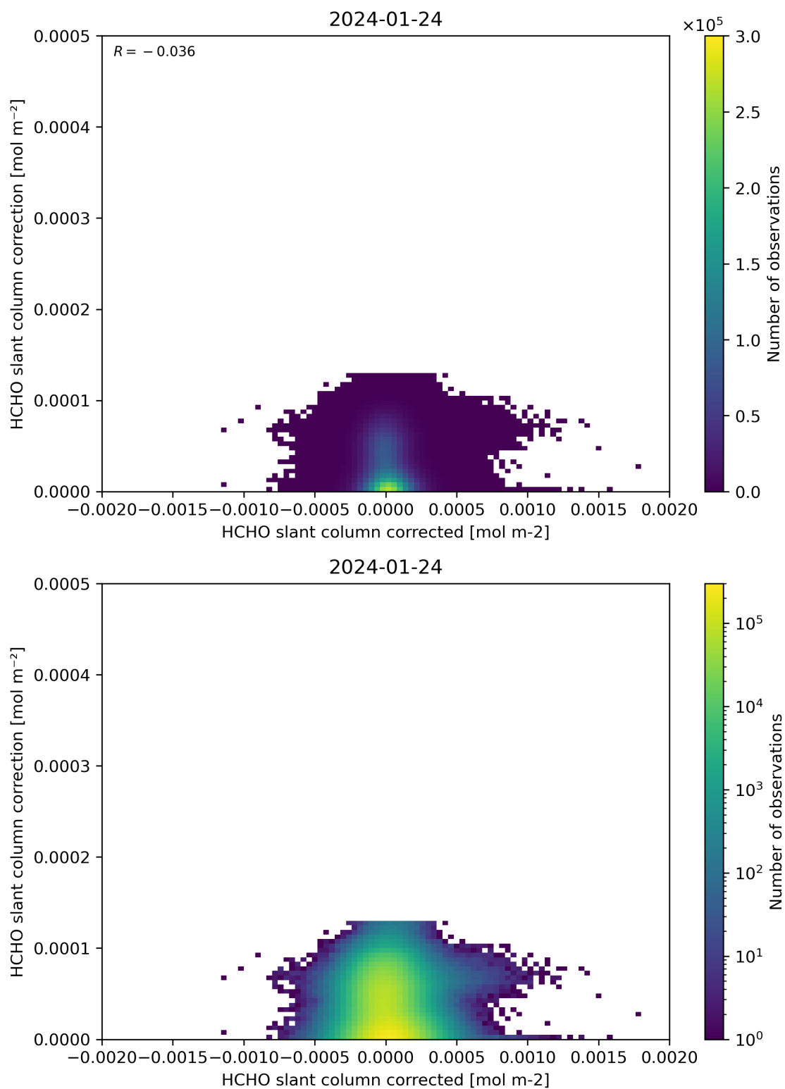
Figure 77: Scatter density plot of “HCHO slant column corrected” against “HCHO slant column correction” for 2024-01-23 to 2024-01-25.
