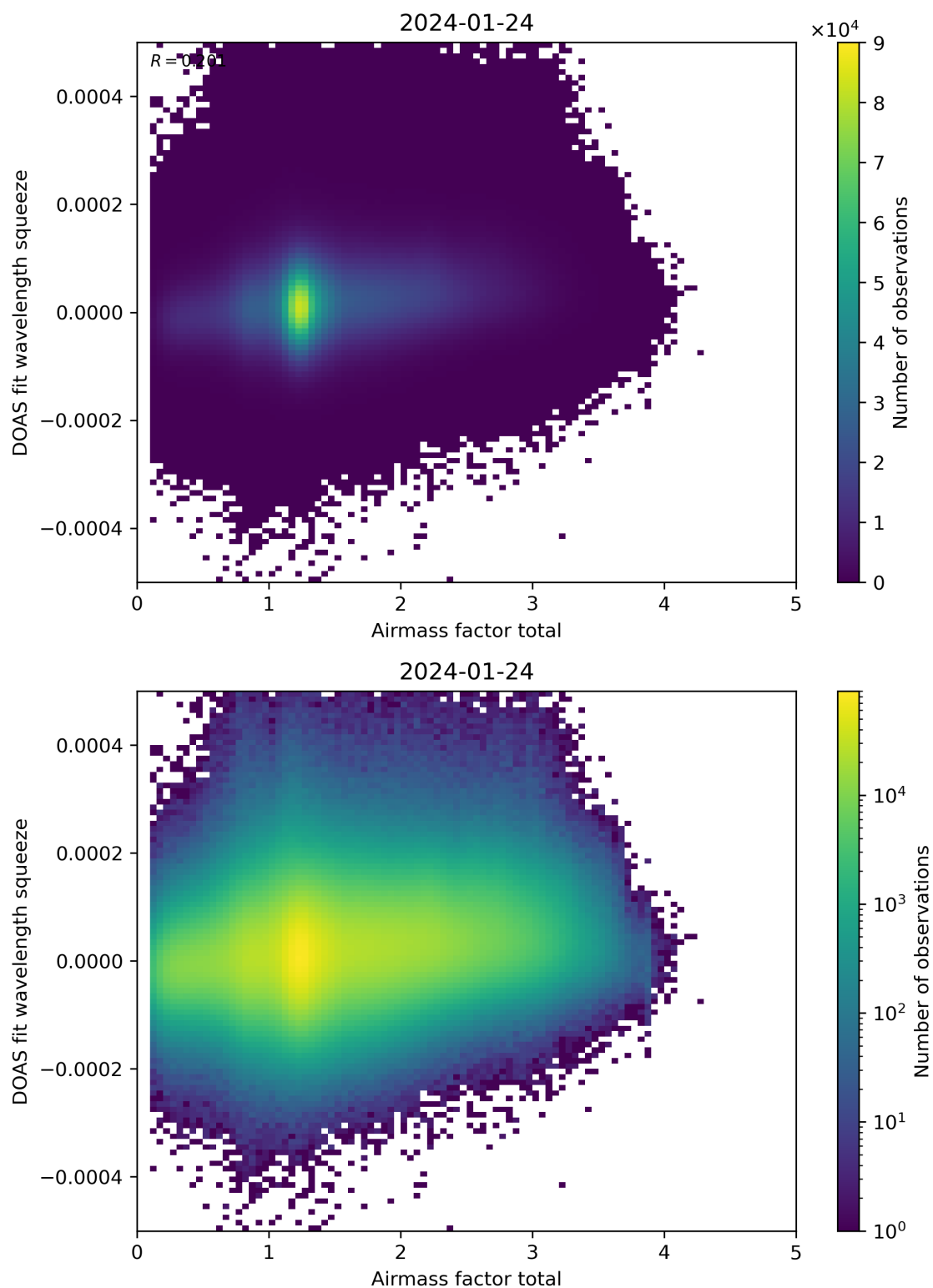
Figure 99: Scatter density plot of “Airmass factor total” against “DOAS fit wavelength squeeze” for 2024-01-23 to 2024-01-25.
