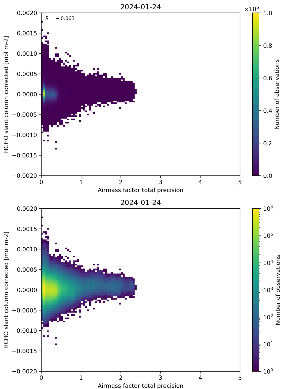
Figure 109: Scatter density plot of “Airmass factor total precision” against “HCHO slant column corrected” for 2024-01-23 to 2024-01-25.
