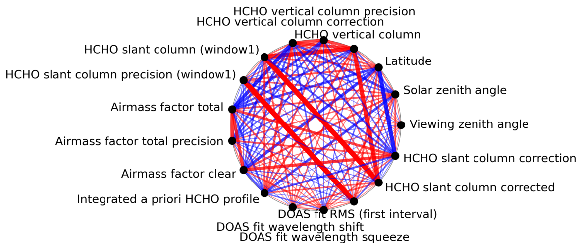
Figure 1: Map of correlation graph for 2024-01-23 to 2024-01-25.
