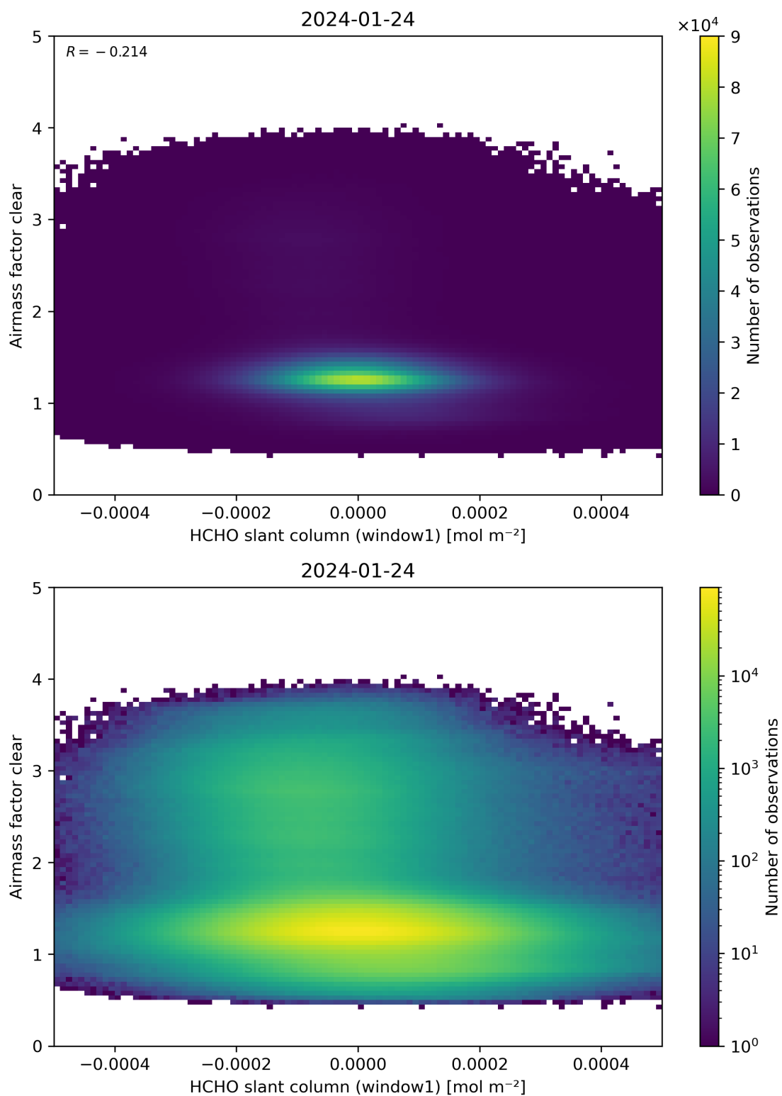
Figure 81: Scatter density plot of “HCHO slant column (window1)” against “Airmass factor clear” for 2024-01-23 to 2024-01-25.
