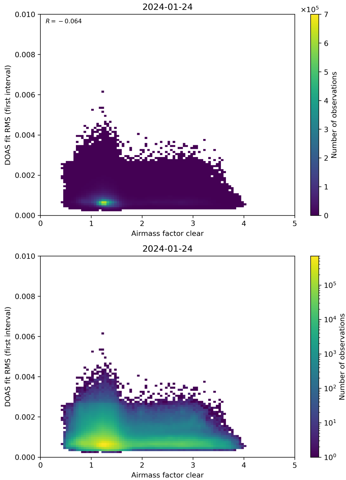
Figure 71: Scatter density plot of “Airmass factor clear” against “DOAS fit RMS (first interval)” for 2024-01-23 to 2024-01-25.
