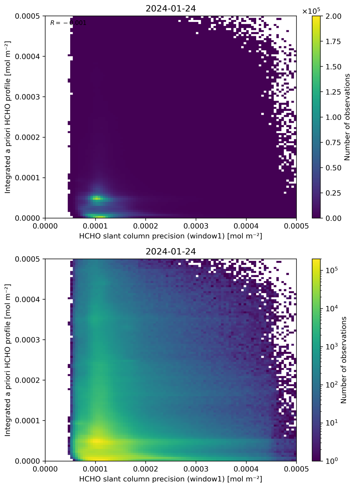
Figure 96: Scatter density plot of “HCHO slant column precision (window1)” against “Integrated a priori HCHO profile” for 2024-01-23 to 2024-01-25.
