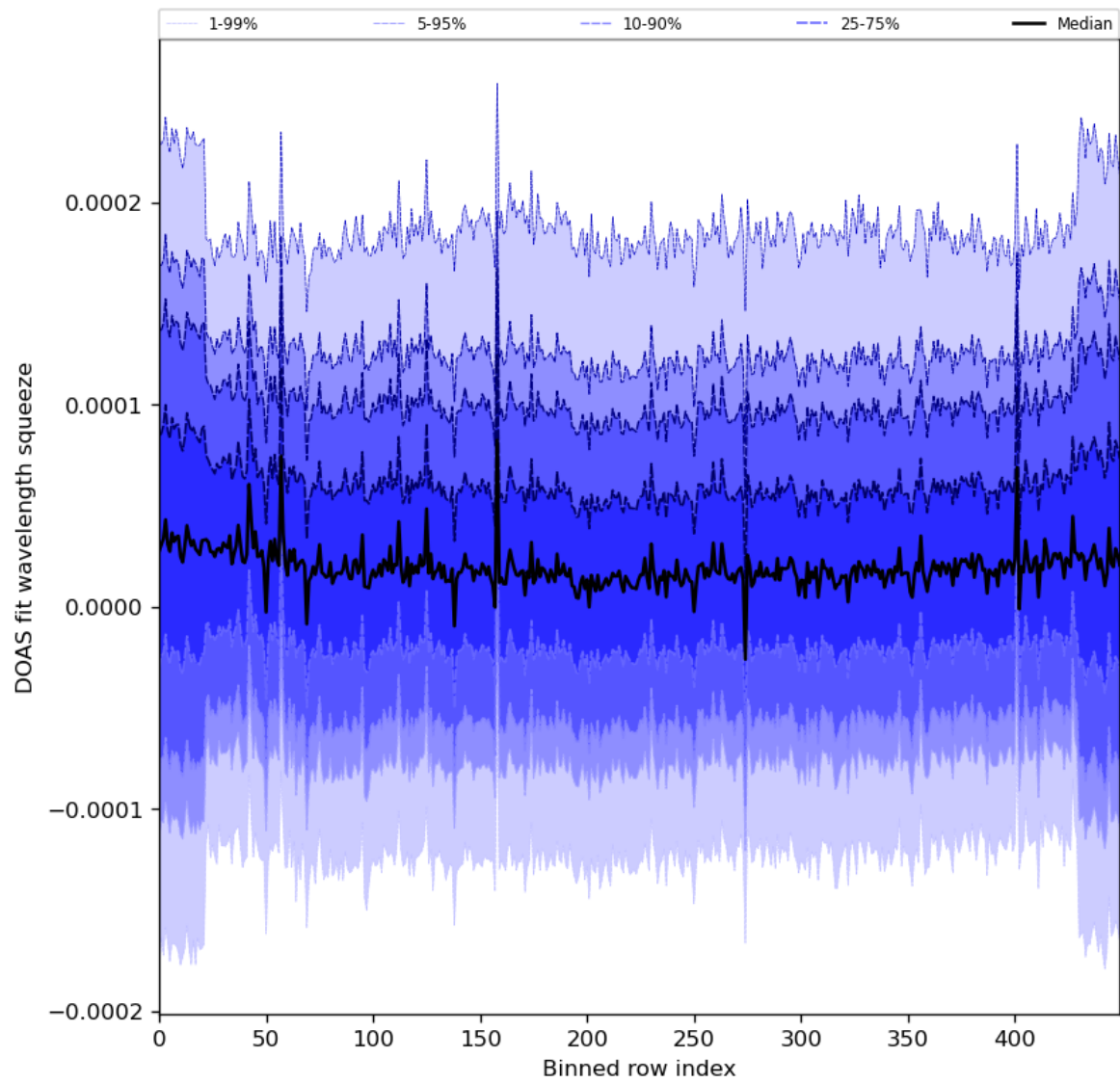
Figure 59: Along track statistics of “DOAS fit wavelength squeeze” for 2024-01-23 to 2024-01-25
