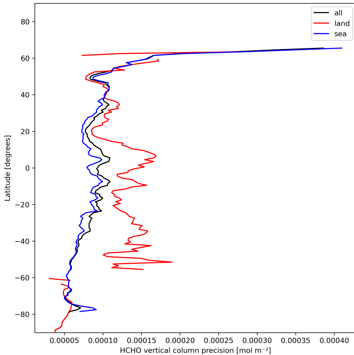
Figure 22: Zonal average of “HCHO vertical column precision” for 2024-01-23 to 2024-01-25.
