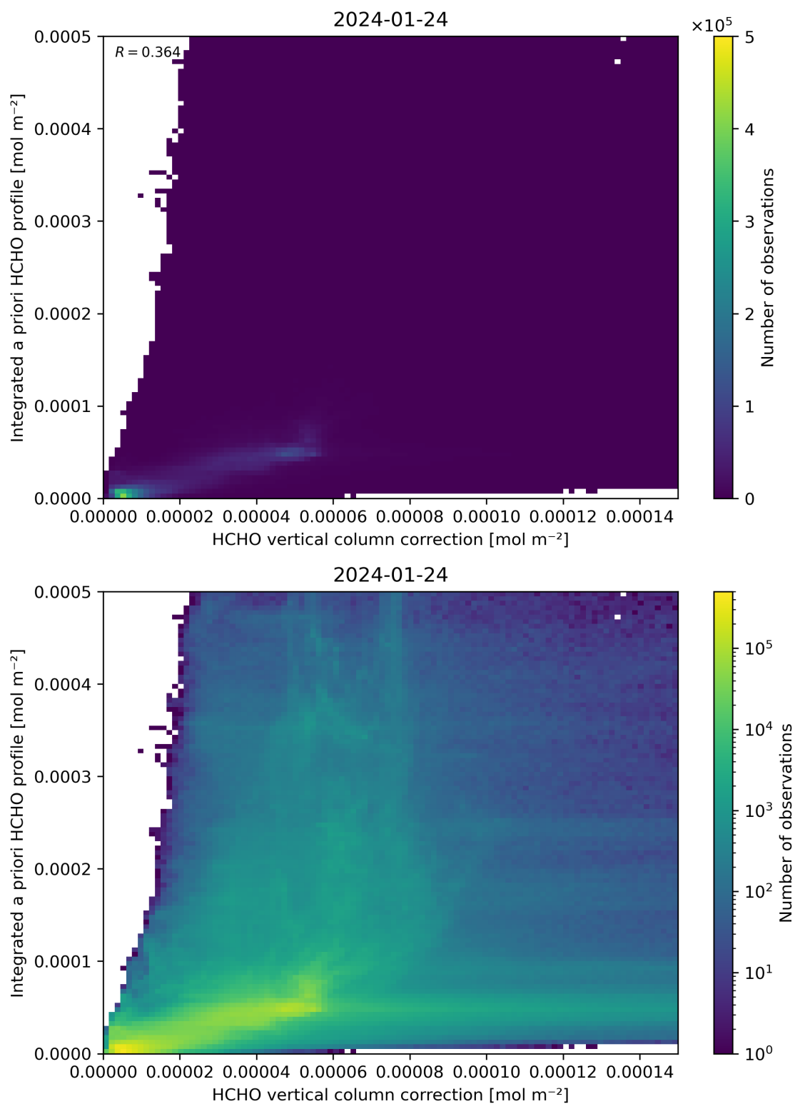
Figure 122: Scatter density plot of “HCHO vertical column correction” against “Integrated a priori HCHO profile” for 2024-01-23 to 2024-01-25.
