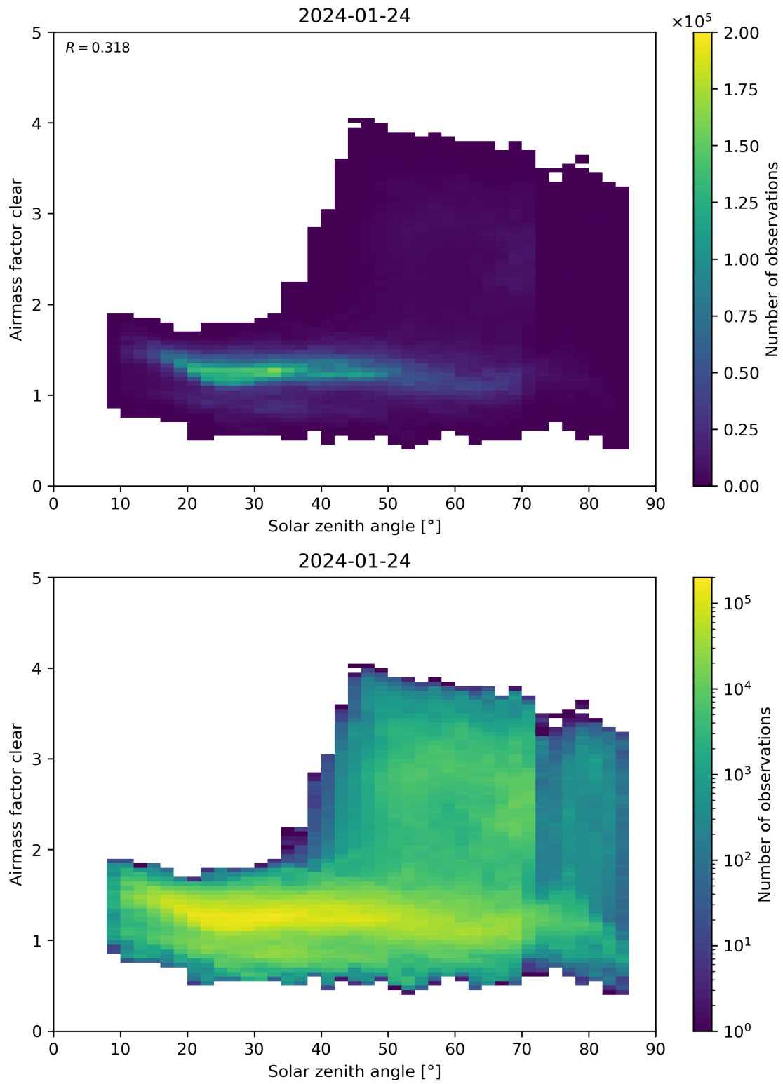
Figure 170: Scatter density plot of “Solar zenith angle” against “Airmass factor clear” for 2024-01-23 to 2024-01-25.
