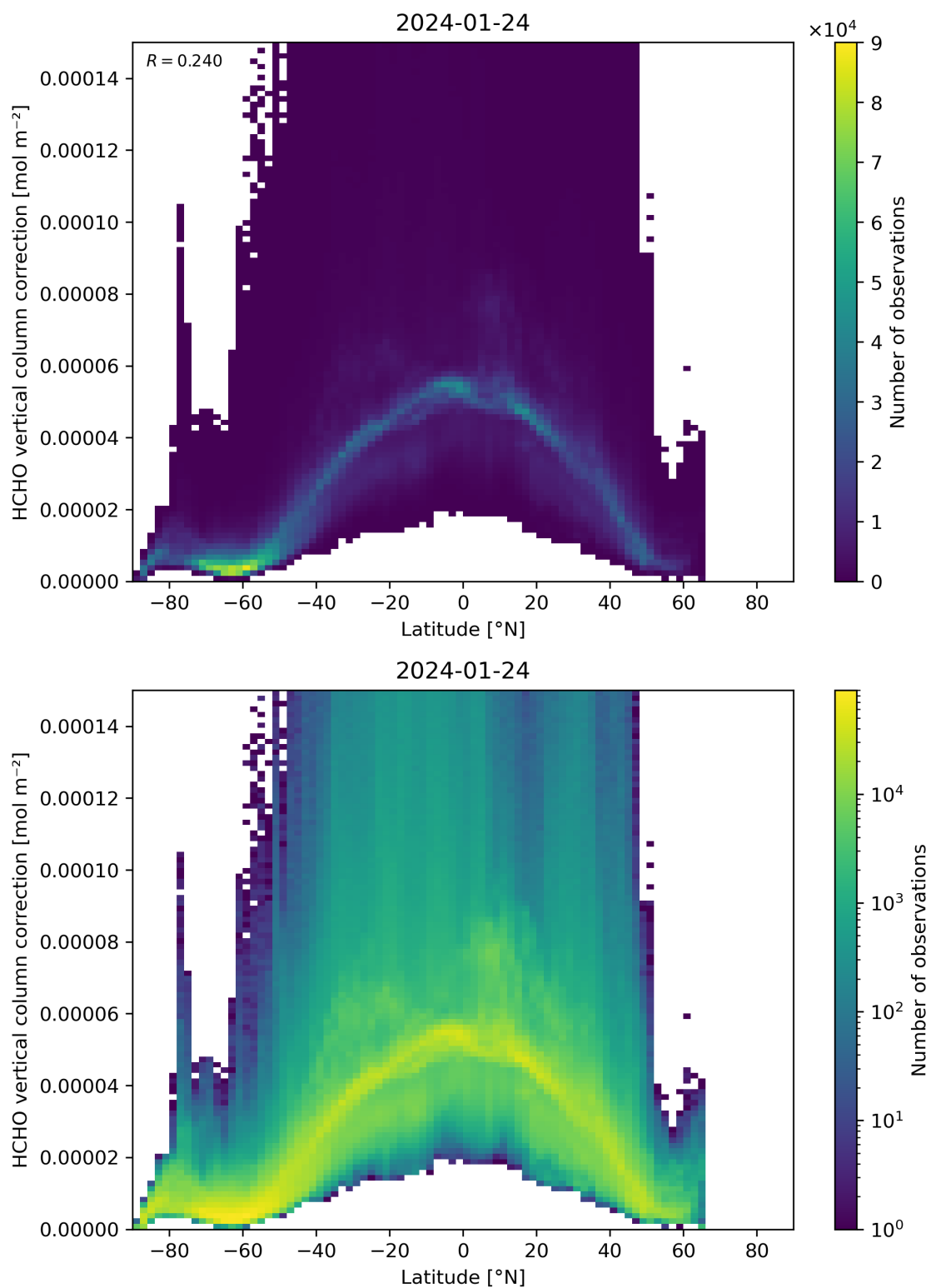
Figure 164: Scatter density plot of “Latitude” against “HCHO vertical column correction” for 2024-01-23 to 2024-01-25.
