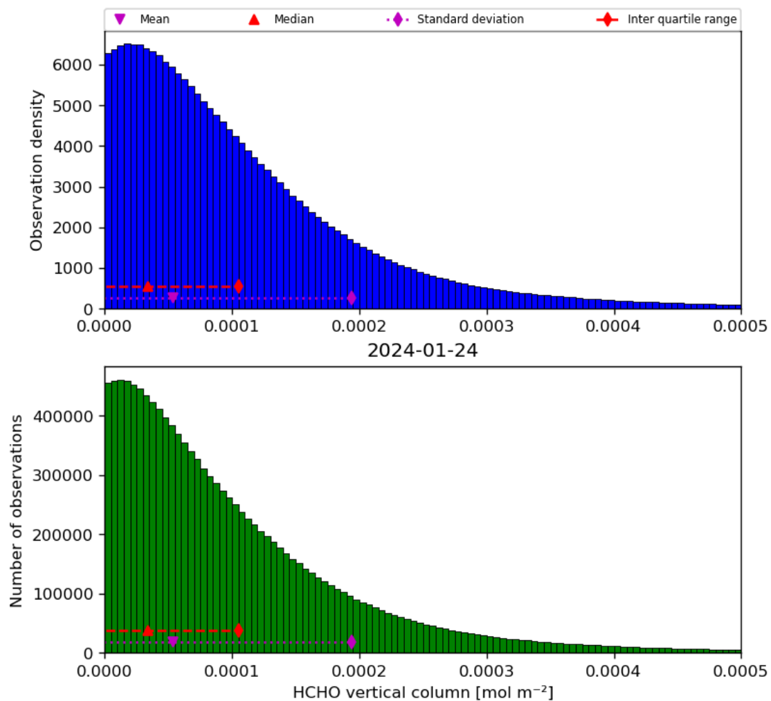
Figure 35: Histogram of “HCHO vertical column” for 2024-01-23 to 2024-01-25
