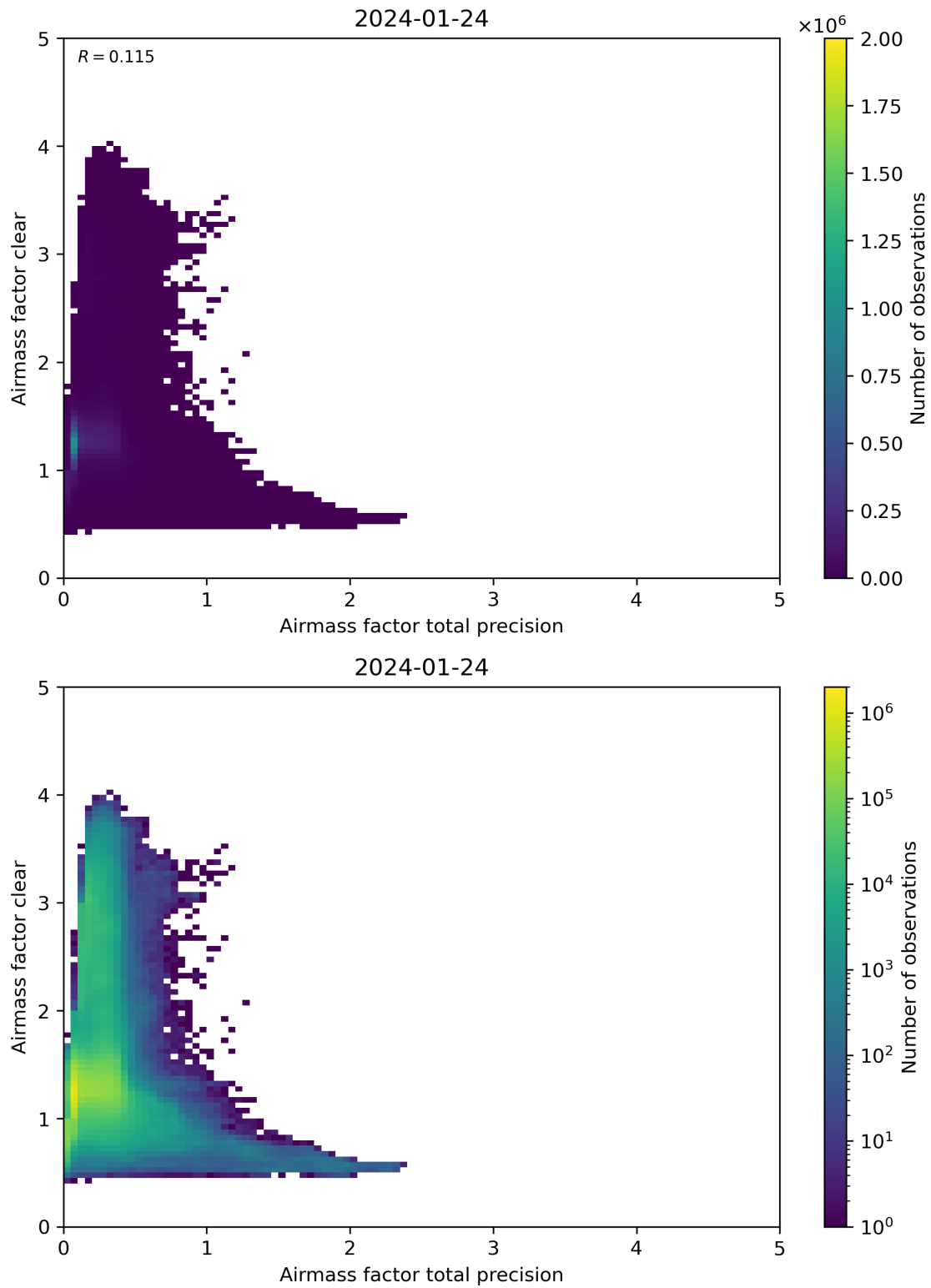
Figure 108: Scatter density plot of “Airmass factor total precision” against “Airmass factor clear” for 2024-01-23 to 2024-01-25.
