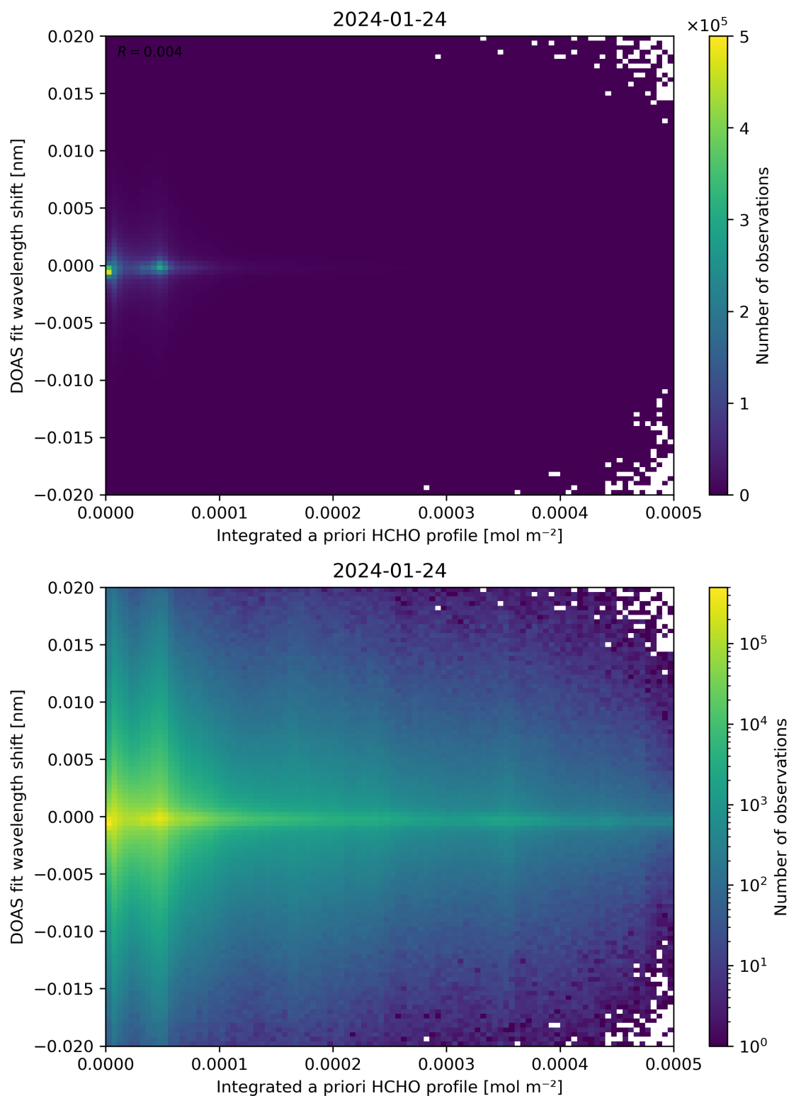
Figure 149: Scatter density plot of “Integrated a priori HCHO profile” against “DOAS fit wavelength shift” for 2024-01-23 to 2024-01-25.
