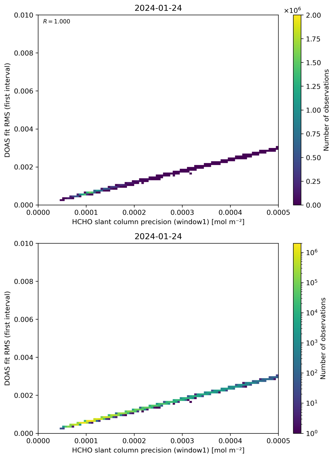
Figure 88: Scatter density plot of “HCHO slant column precision (window1)” against “DOAS fit RMS (first interval)” for 2024-01-23 to 2024-01-25.
