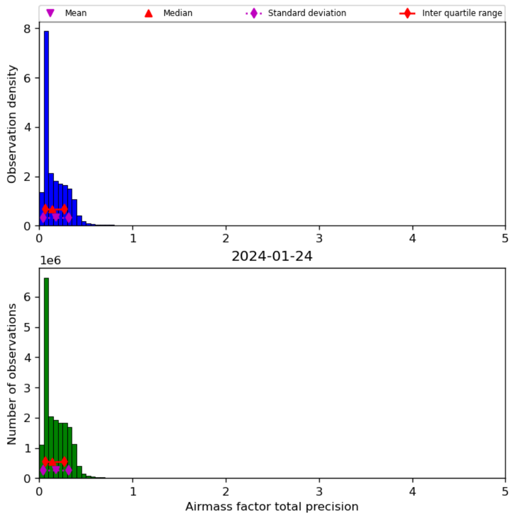
Figure 41: Histogram of “Airmass factor total precision” for 2024-01-23 to 2024-01-25
