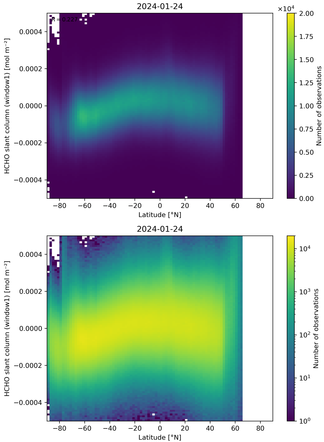
Figure 159: Scatter density plot of “Latitude” against “HCHO slant column (window1)” for 2024-01-23 to 2024-01-25.
