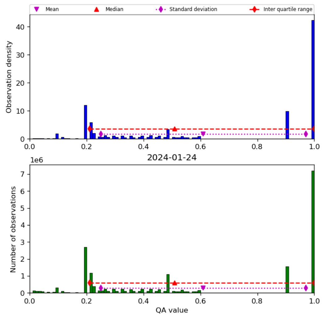
Figure 34: Histogram of “QA value” for 2024-01-23 to 2024-01-25
