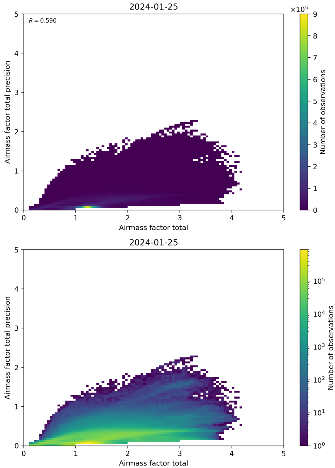
Figure 103: Scatter density plot of “Airmass factor total” against “Airmass factor total precision” for 2024-01-24 to 2024-01-26.
