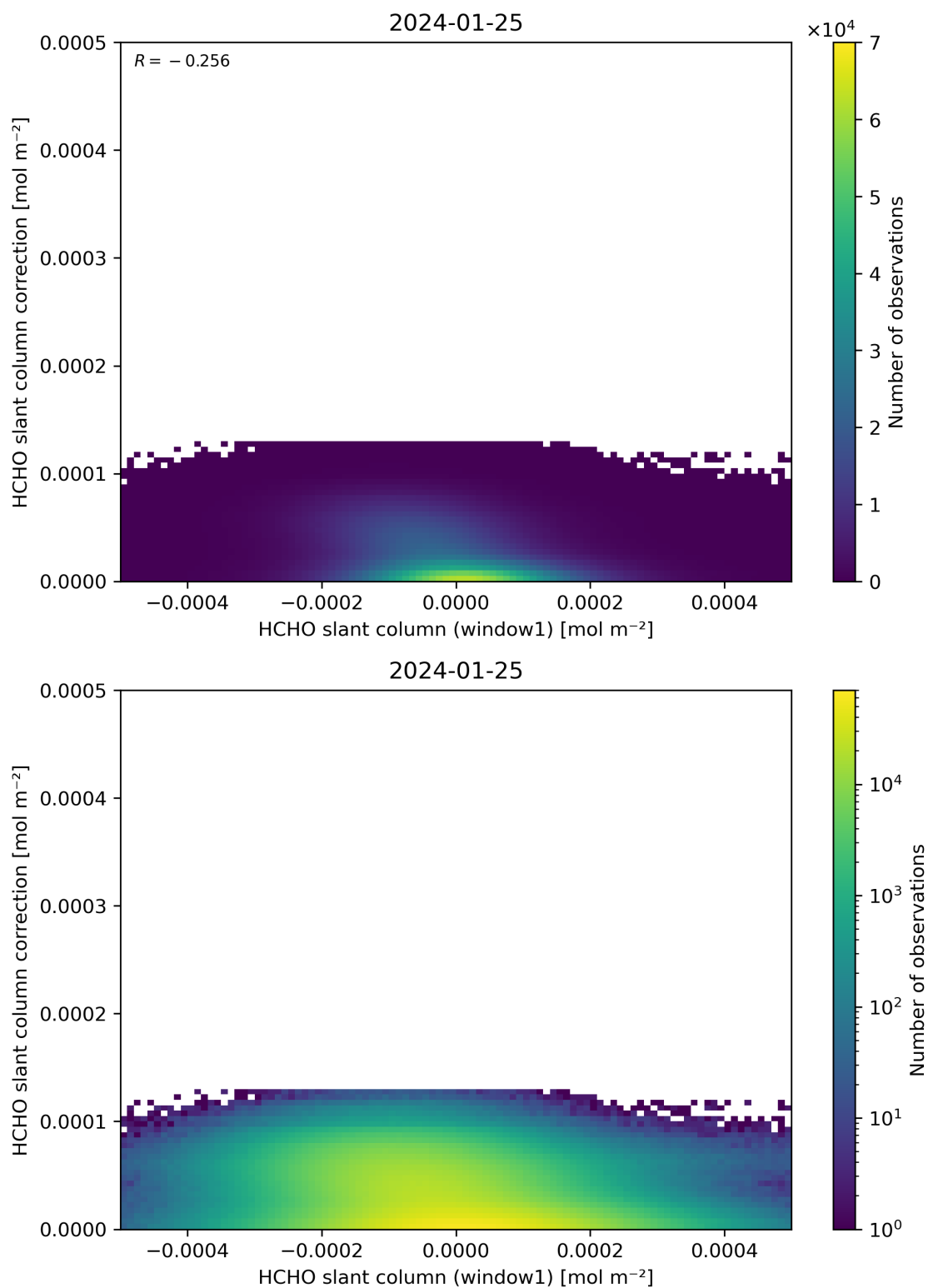
Figure 83: Scatter density plot of “HCHO slant column (window1)” against “HCHO slant column correction” for 2024-01-24 to 2024-01-26.
