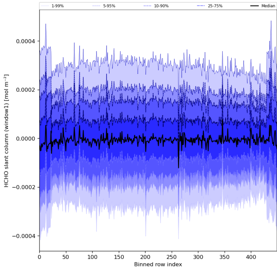
Figure 52: Along track statistics of “HCHO slant column (window1)” for 2024-01-24 to 2024-01-26
