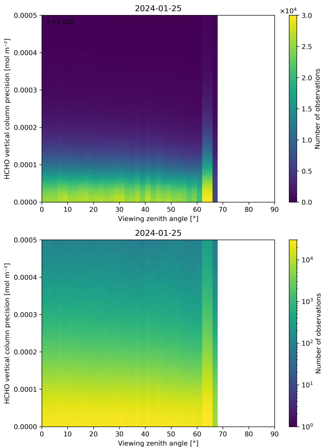
Figure 194: Scatter density plot of “Viewing zenith angle” against “HCHO vertical column precision” for 2024-01-24 to 2024-01-26.
