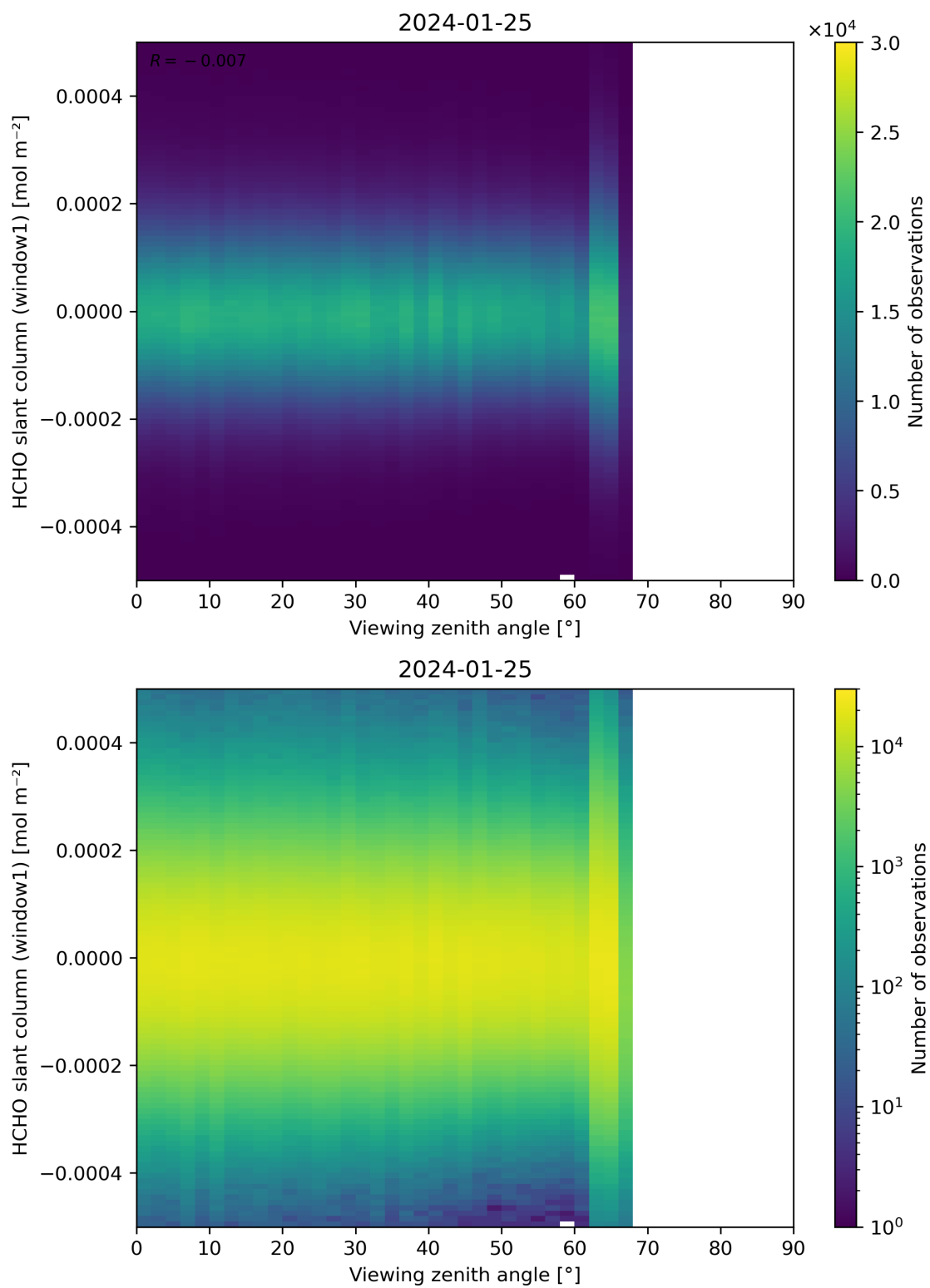
Figure 188: Scatter density plot of “Viewing zenith angle” against “HCHO slant column (window1)” for 2024-01-24 to 2024-01-26.
