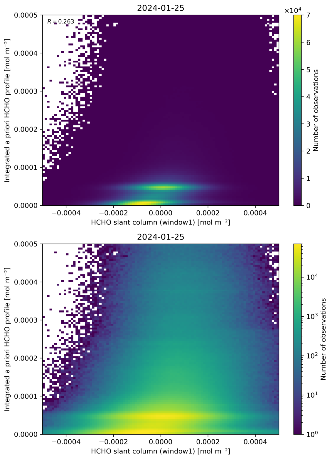
Figure 87: Scatter density plot of “HCHO slant column (window1)” against “Integrated a priori HCHO profile” for 2024-01-24 to 2024-01-26.
