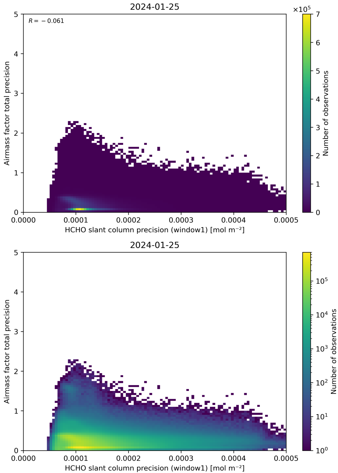
Figure 95: Scatter density plot of “HCHO slant column precision (window1)” against “Airmass factor total precision” for 2024-01-24 to 2024-01-26.
