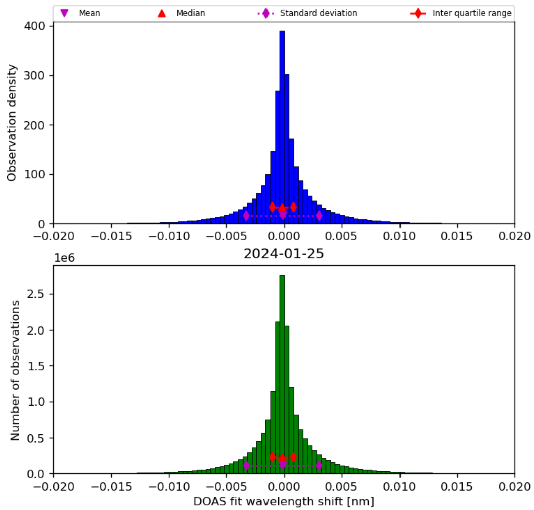
Figure 44: Histogram of “DOAS fit wavelength shift” for 2024-01-24 to 2024-01-26
