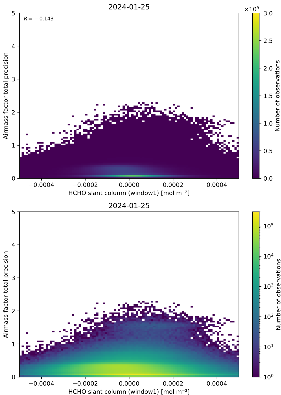
Figure 86: Scatter density plot of “HCHO slant column (window1)” against “Airmass factor total precision” for 2024-01-24 to 2024-01-26.
