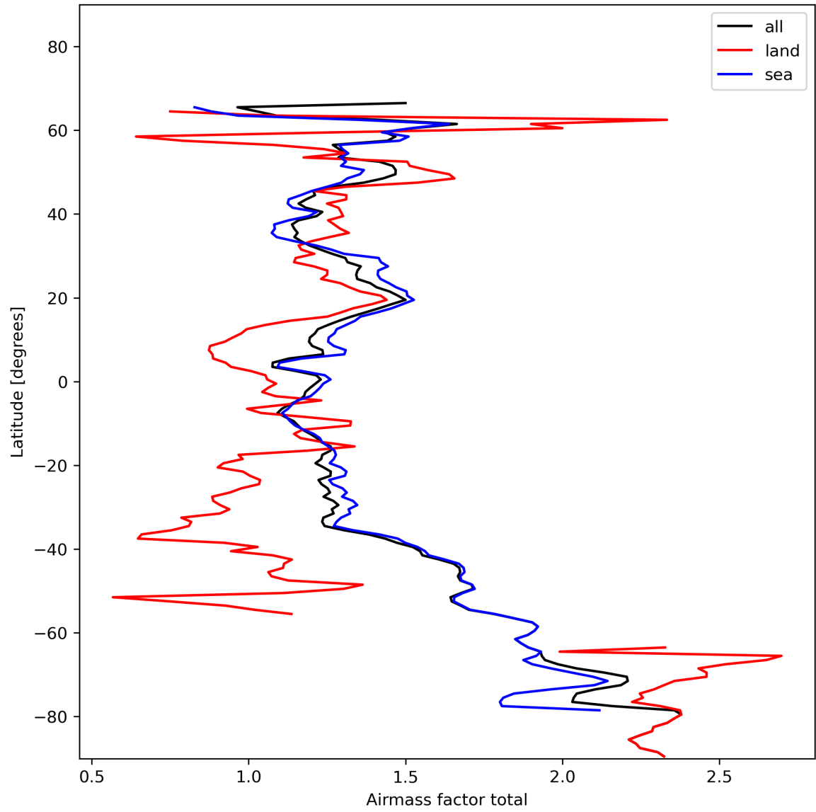
Figure 26: Zonal average of “Airmass factor total” for 2024-01-24 to 2024-01-26.
