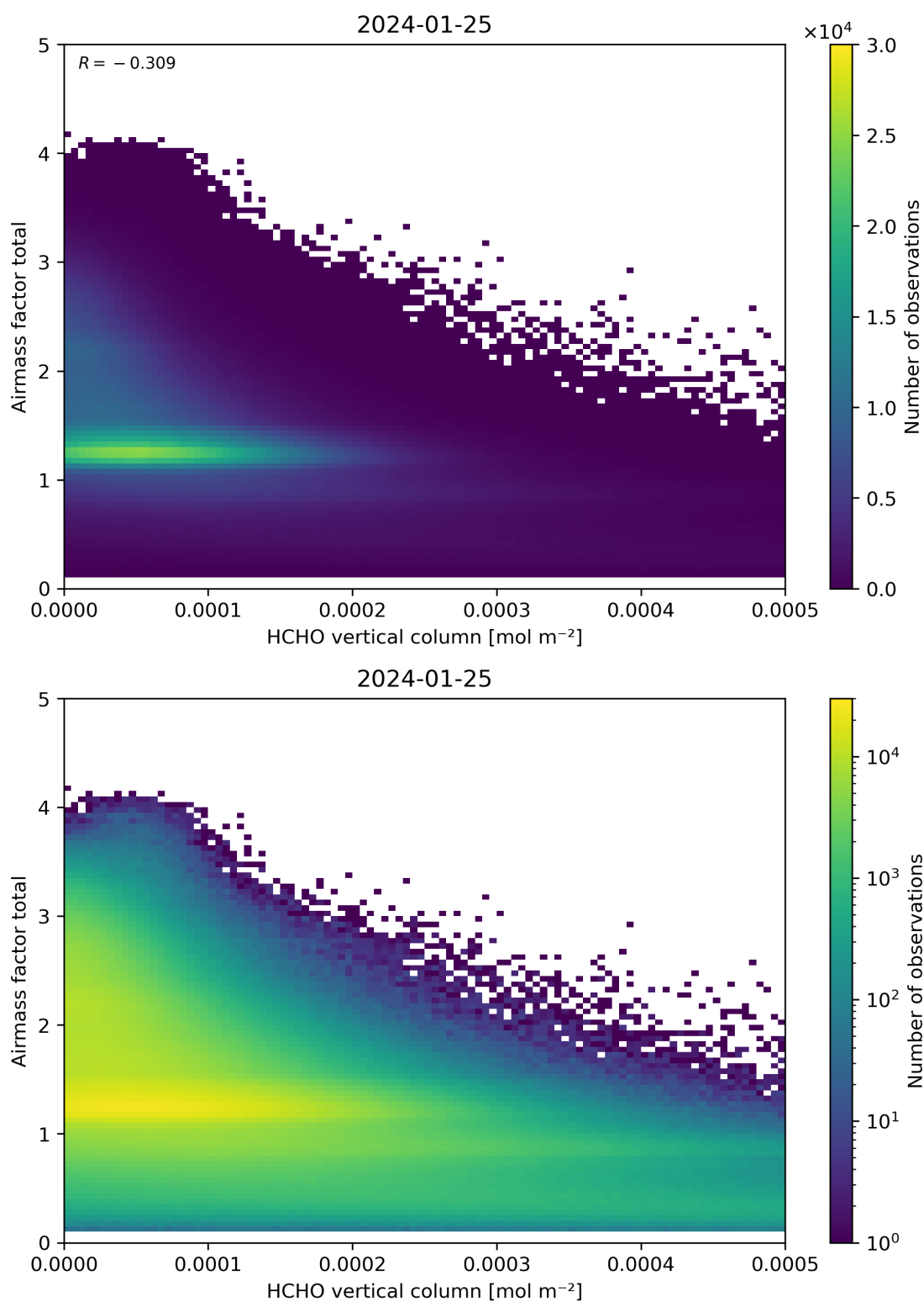
Figure 131: Scatter density plot of “HCHO vertical column” against “Airmass factor total” for 2024-01-24 to 2024-01-26.
