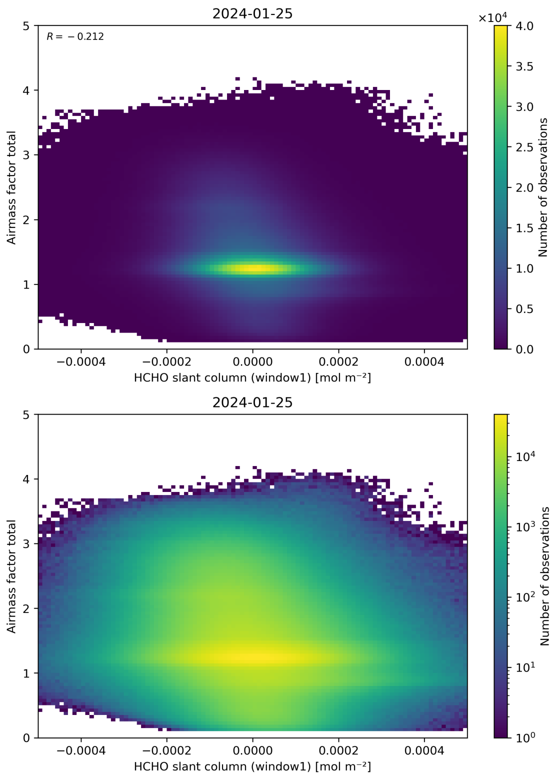
Figure 85: Scatter density plot of “HCHO slant column (window1)” against “Airmass factor total” for 2024-01-24 to 2024-01-26.
