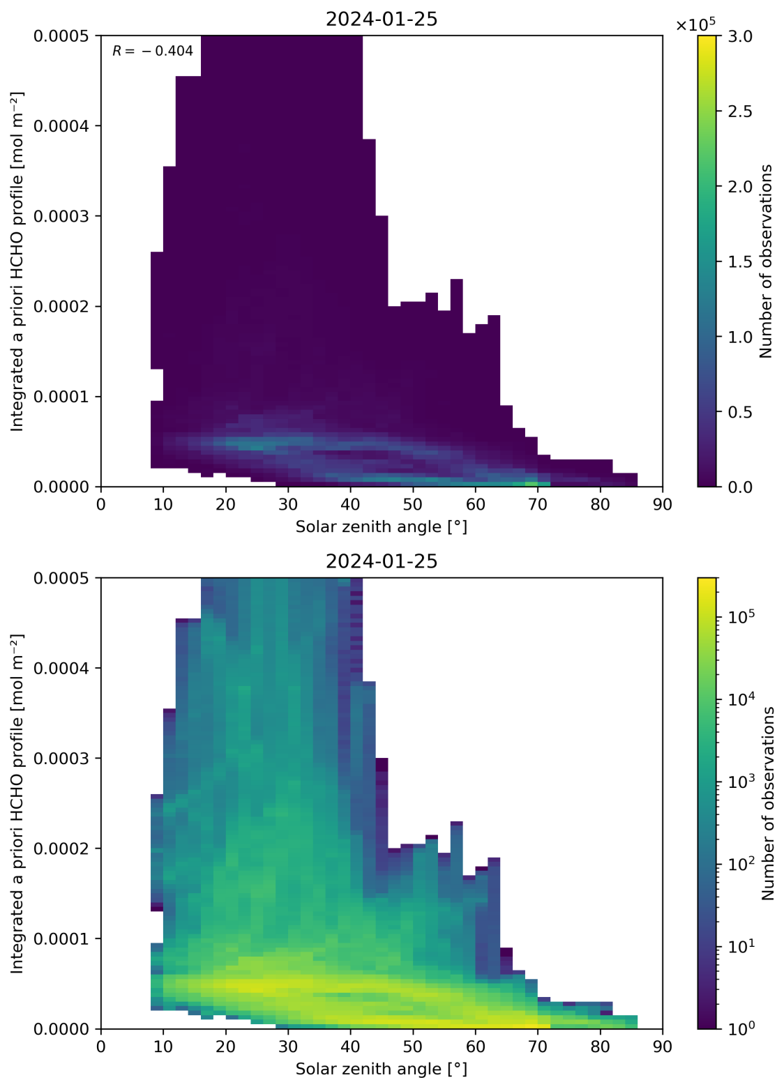
Figure 180: Scatter density plot of “Solar zenith angle” against “Integrated a priori HCHO profile” for 2024-01-24 to 2024-01-26.
