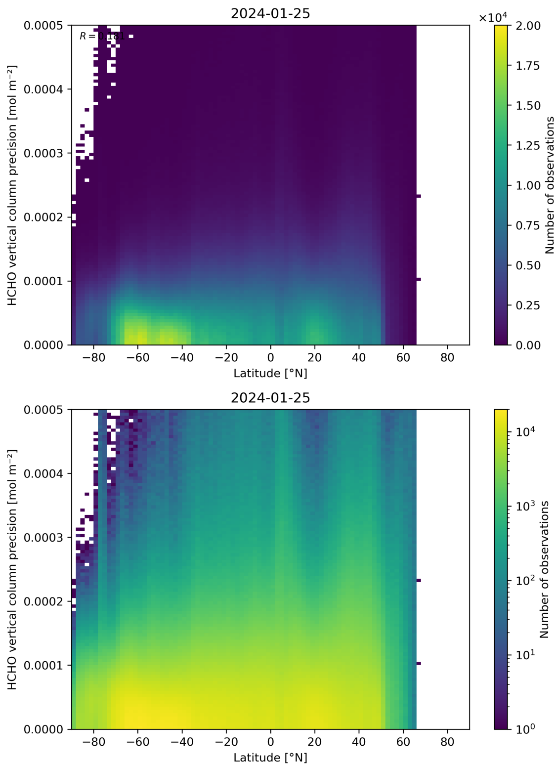
Figure 165: Scatter density plot of “Latitude” against “HCHO vertical column precision” for 2024-01-24 to 2024-01-26.
