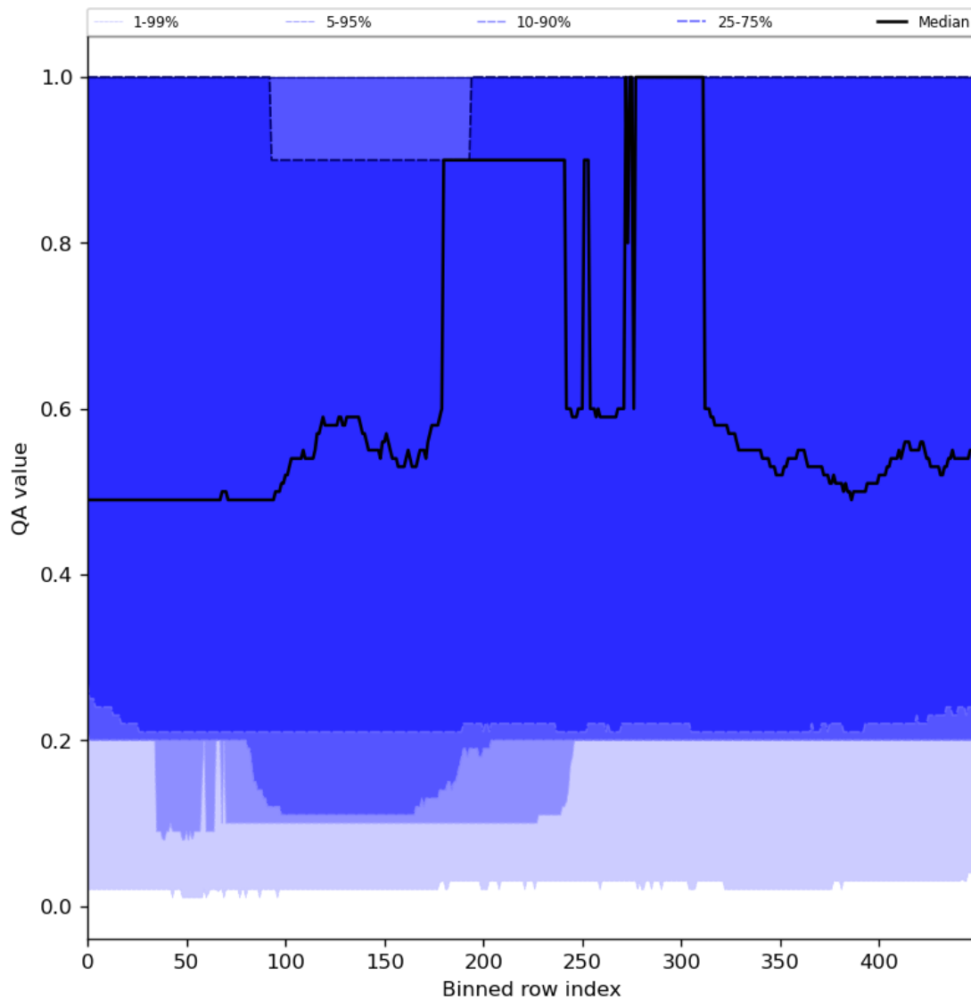
Figure 48: Along track statistics of “QA value” for 2024-01-24 to 2024-01-26
