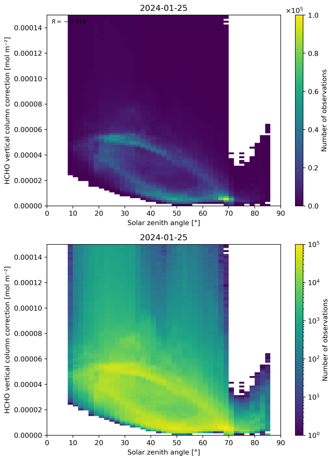
Figure 178: Scatter density plot of “Solar zenith angle” against “HCHO vertical column correction” for 2024-01-24 to 2024-01-26.
