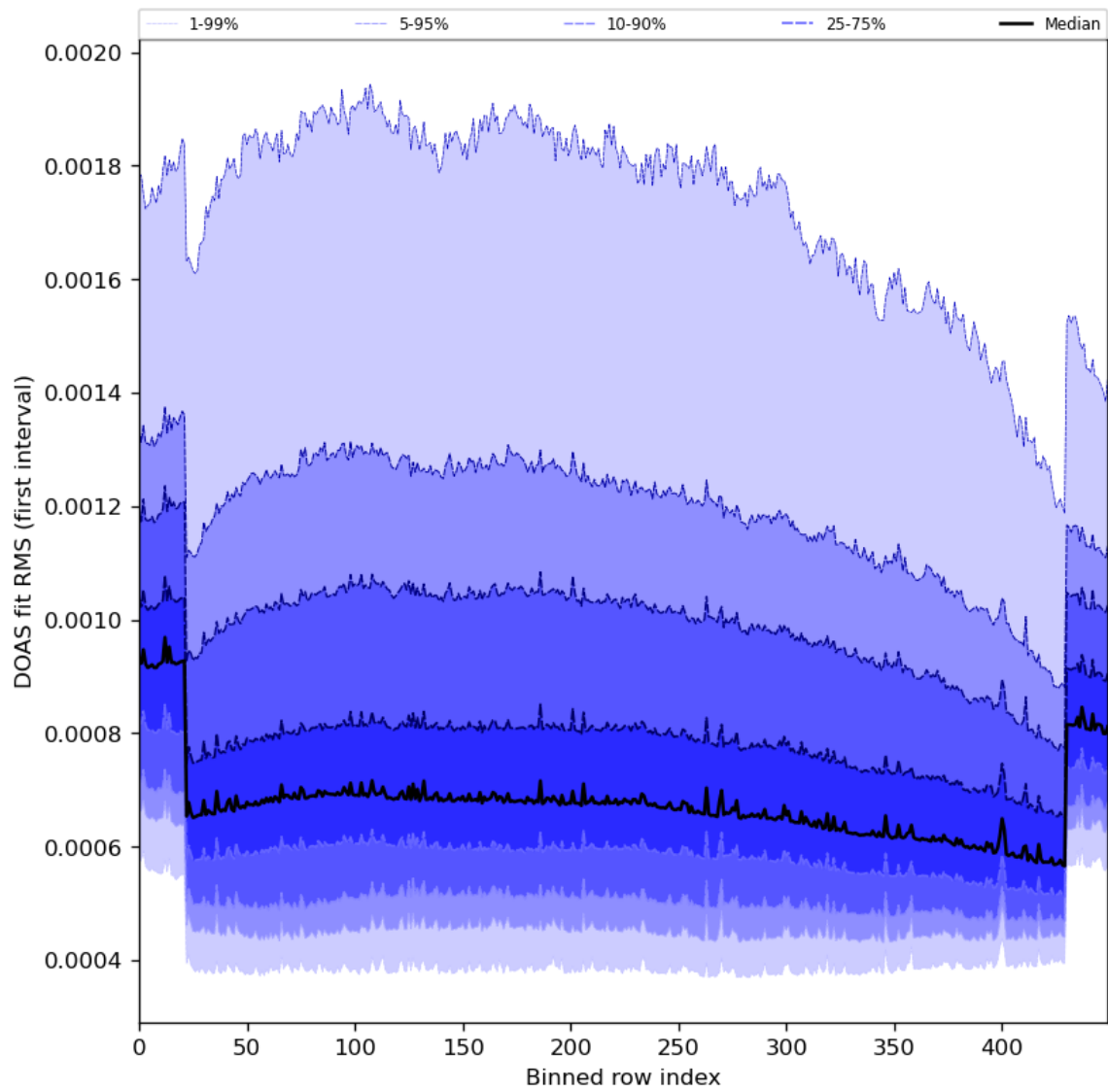
Figure 60: Along track statistics of “DOAS fit RMS (first interval)” for 2024-01-24 to 2024-01-26
