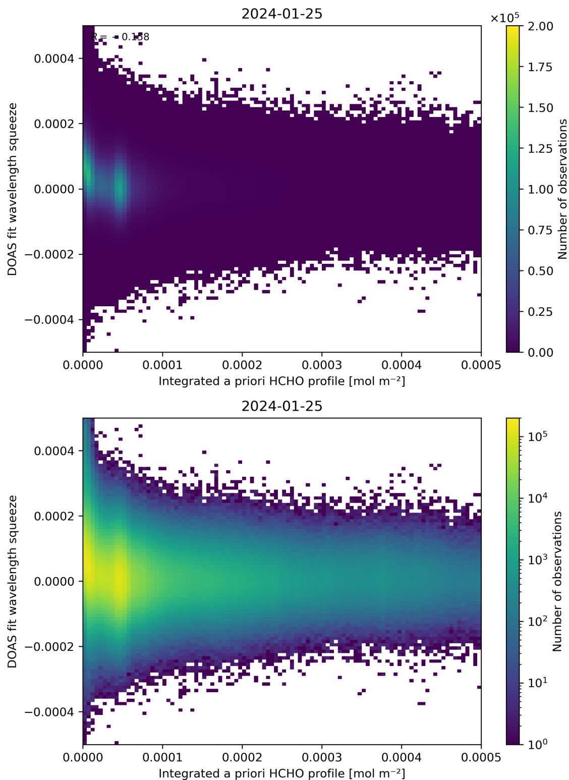
Figure 150: Scatter density plot of “Integrated a priori HCHO profile” against “DOAS fit wavelength squeeze” for 2024-01-24 to 2024-01-26.
