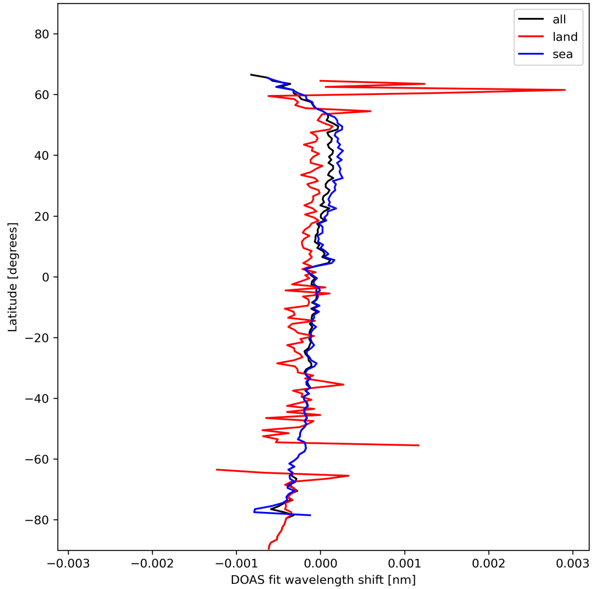
Figure 30: Zonal average of "DOAS fit wavelength shift" for 2024-01-24 to 2024-01-26.
