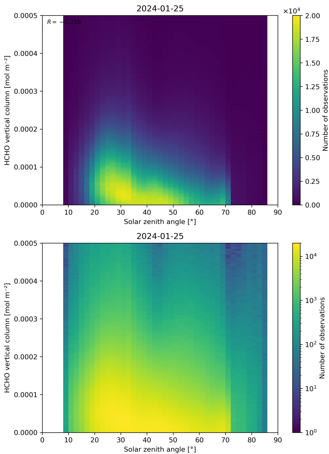
Figure 177: Scatter density plot of “Solar zenith angle” against “HCHO vertical column” for 2024-01-24 to 2024-01-26.
