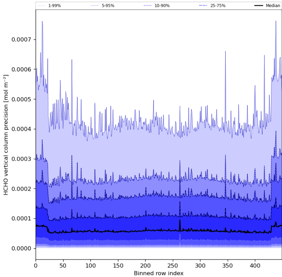
Figure 50: Along track statistics of "HCHO vertical column precision" for 2024-01-24 to 2024-01-26
