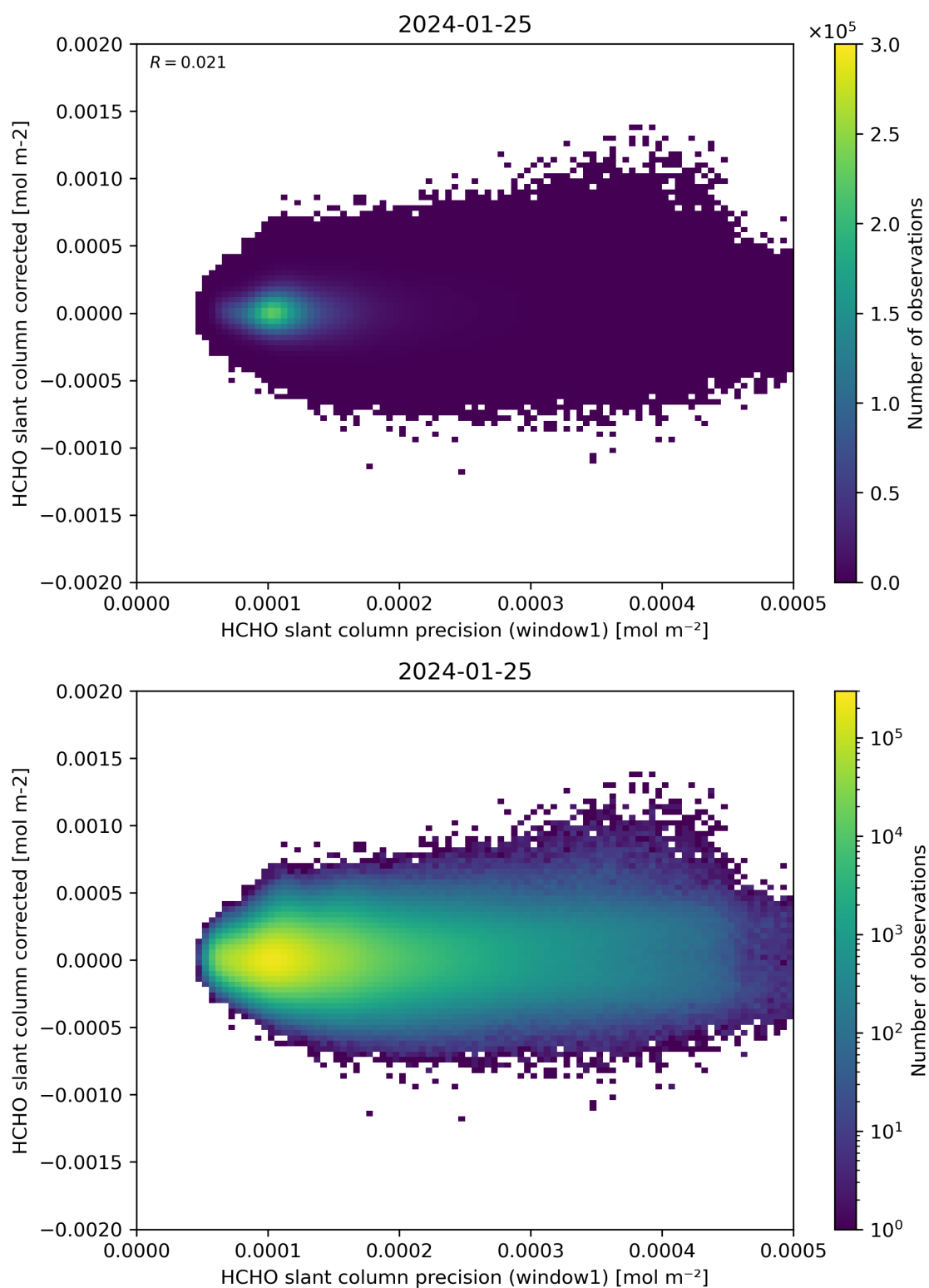
Figure 92: Scatter density plot of “HCHO slant column precision (window1)” against “HCHO slant column corrected” for 2024-01-24 to 2024-01-26.
