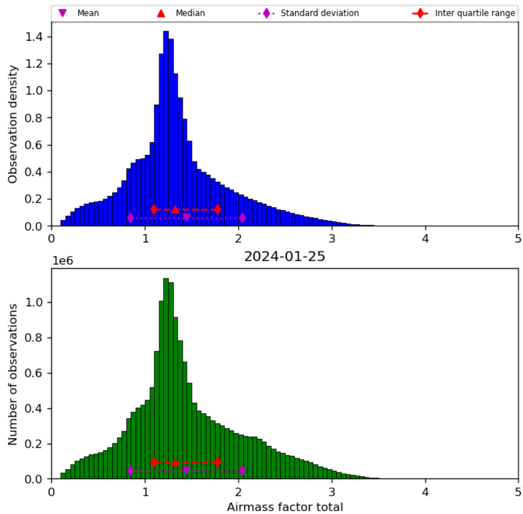
Figure 40: Histogram of “Airmass factor total” for 2024-01-24 to 2024-01-26
