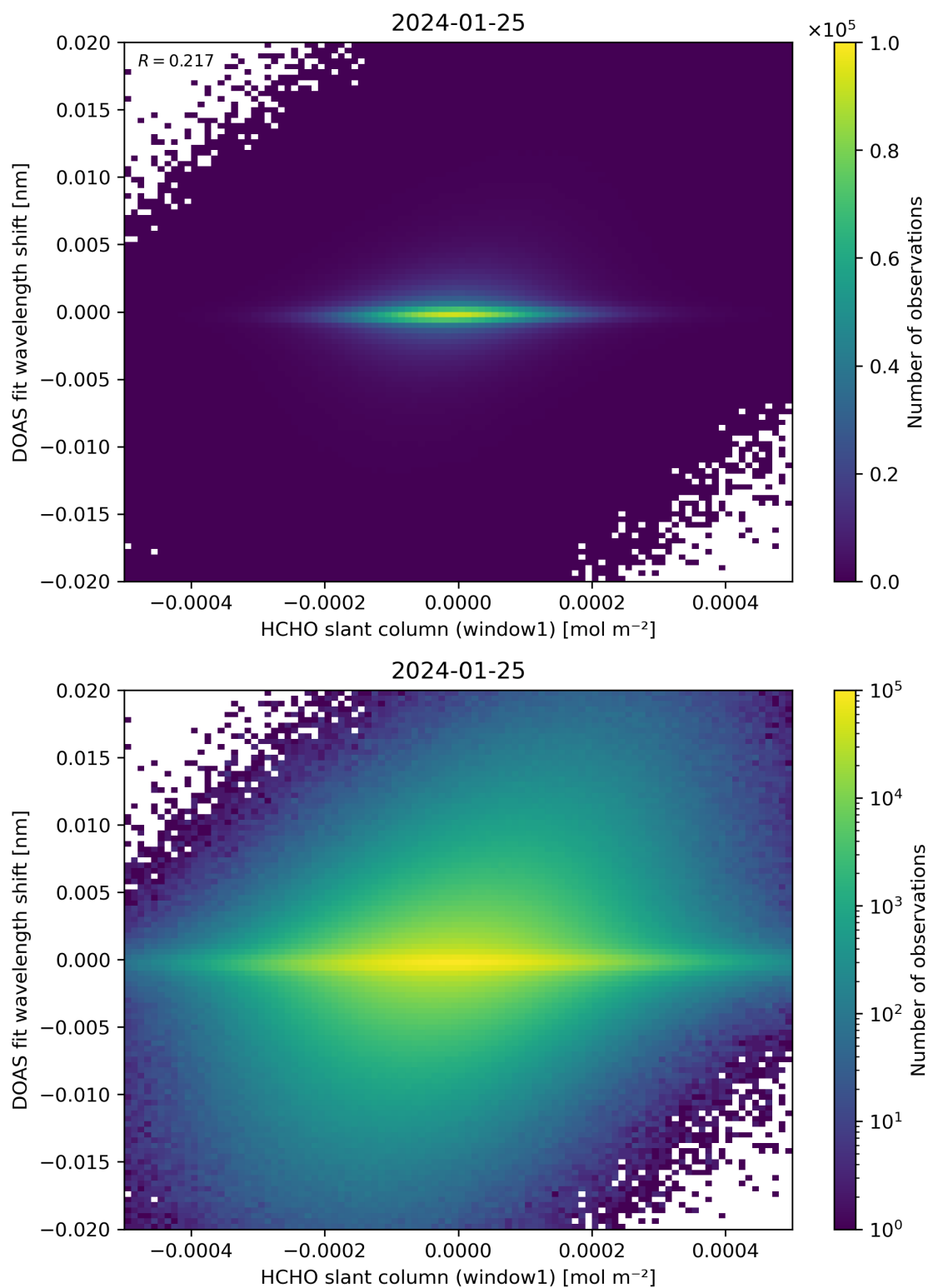
Figure 79: Scatter density plot of “HCHO slant column (window1)” against “DOAS fit wavelength shift” for 2024-01-24 to 2024-01-26.
