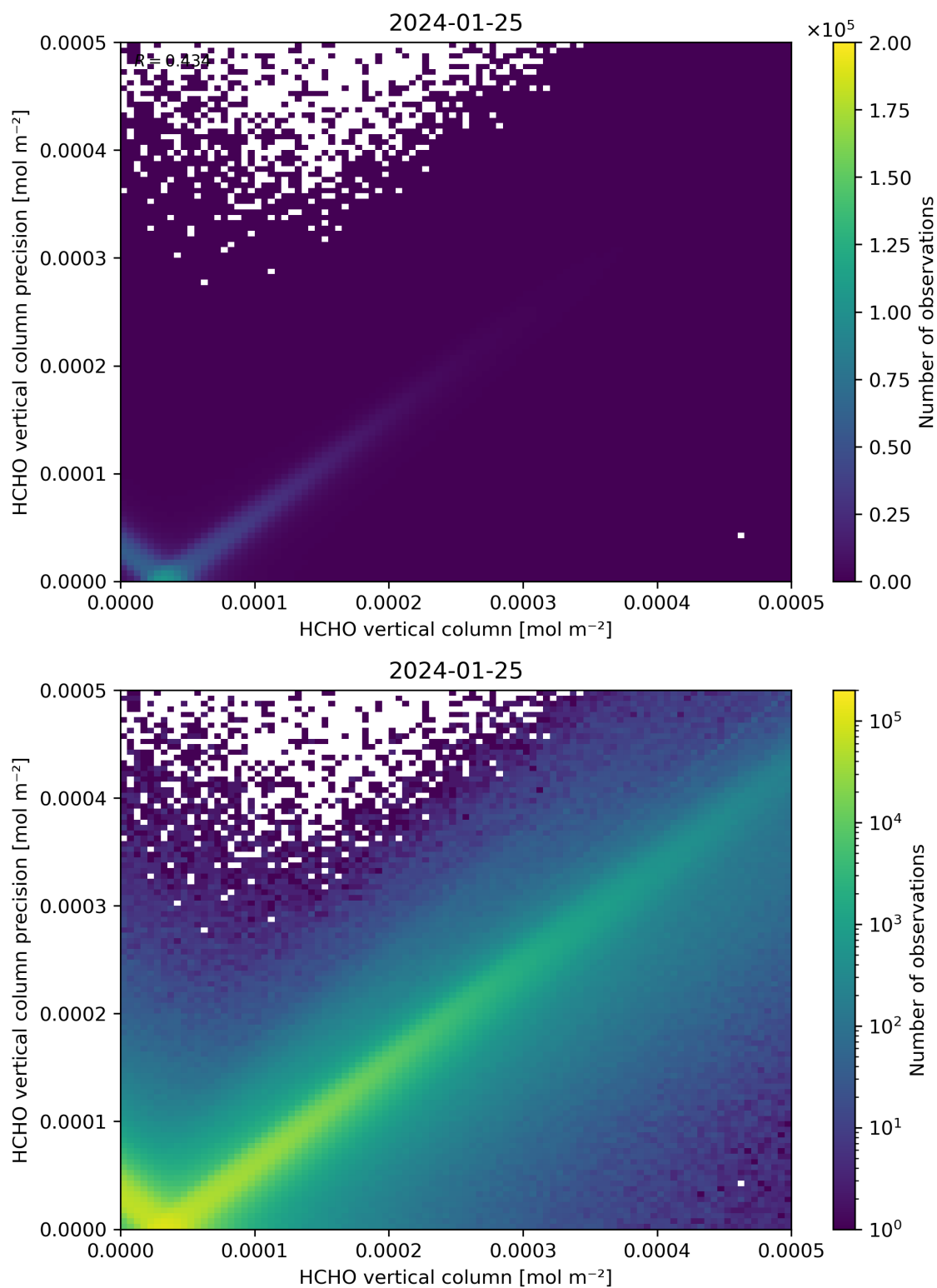
Figure 134: Scatter density plot of “HCHO vertical column” against “HCHO vertical column precision” for 2024-01-24 to 2024-01-26.
