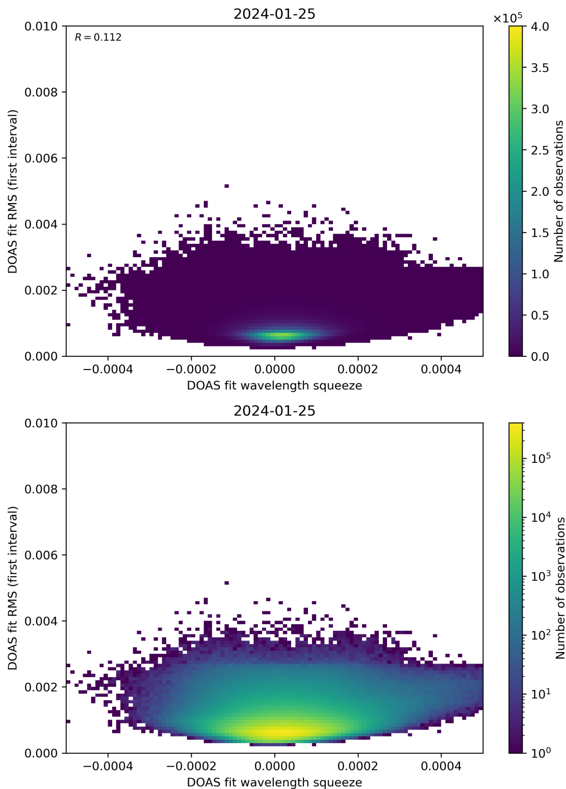
Figure 68: Scatter density plot of “DOAS fit wavelength squeeze” against “DOAS fit RMS (first interval)” for 2024-01-24 to 2024-01-26.
