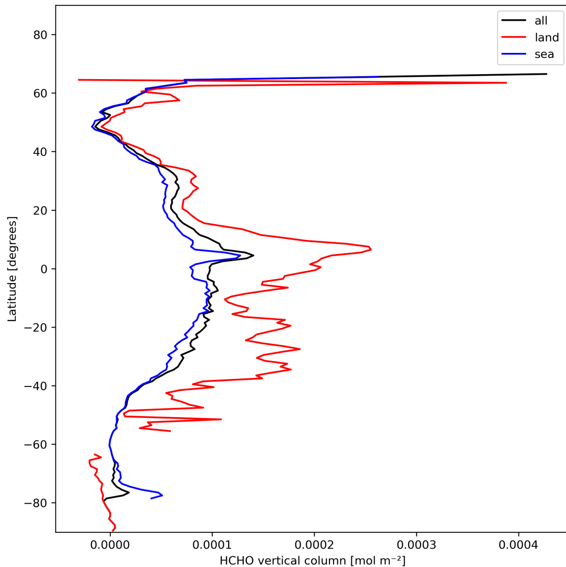
Figure 21: Zonal average of “HCHO vertical column” for 2024-01-24 to 2024-01-26.
