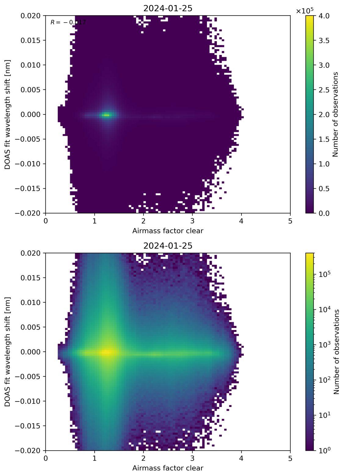
Figure 72: Scatter density plot of “Airmass factor clear” against “DOAS fit wavelength shift” for 2024-01-24 to 2024-01-26.
