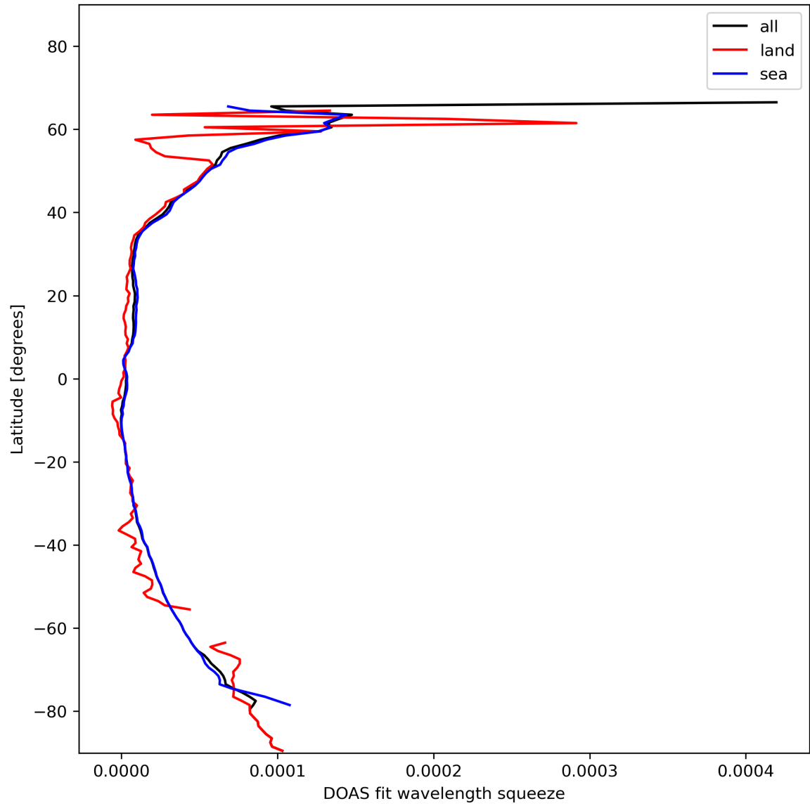
Figure 31: Zonal average of “DOAS fit wavelength squeeze” for 2024-01-24 to 2024-01-26.
