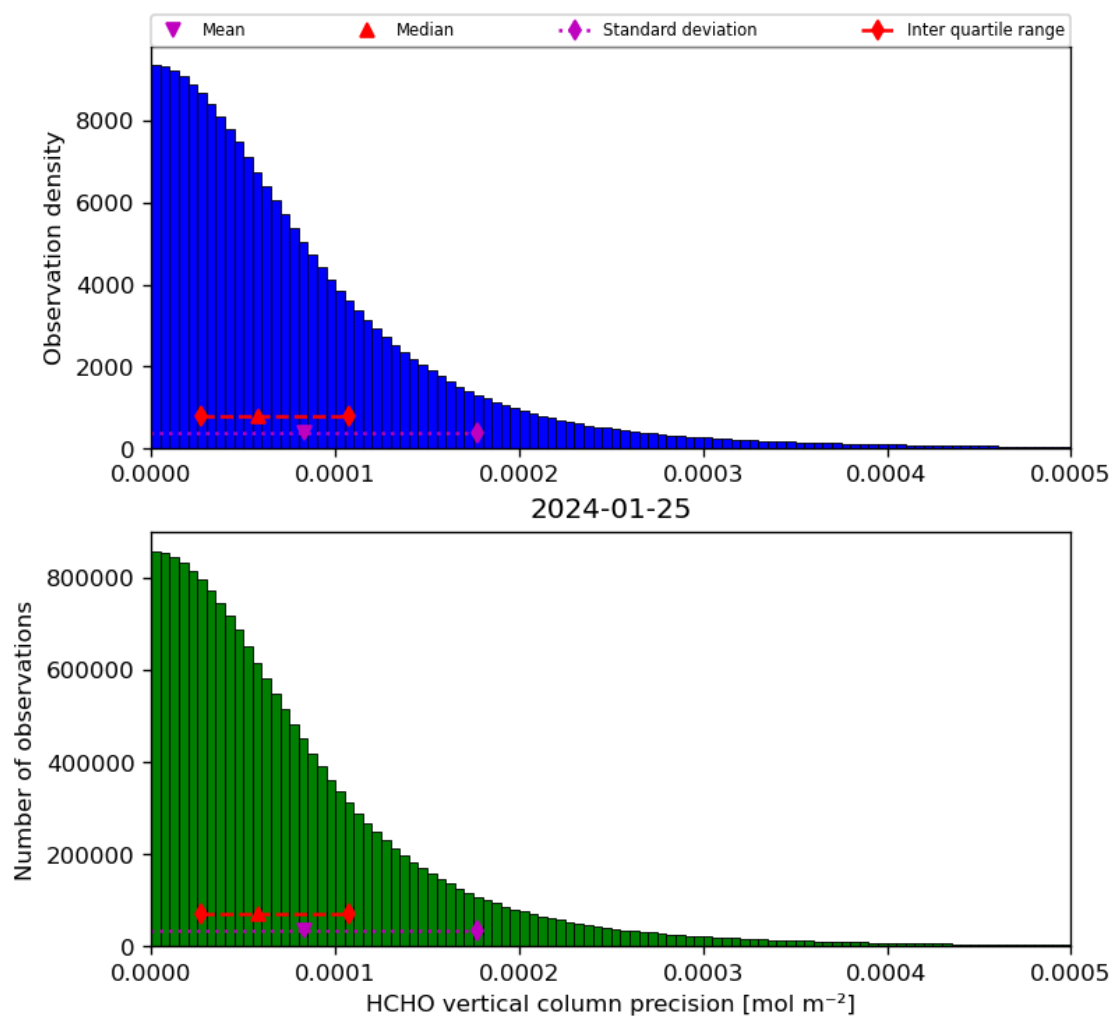
Figure 36: Histogram of “HCHO vertical column precision” for 2024-01-24 to 2024-01-26
