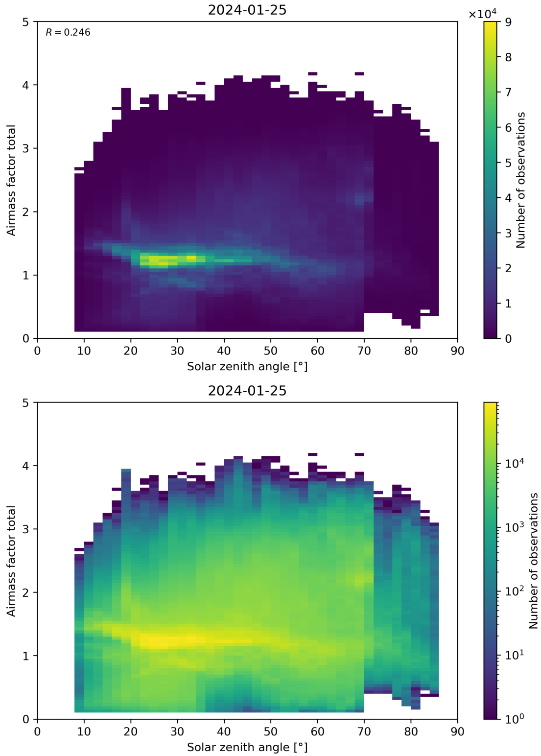
Figure 175: Scatter density plot of “Solar zenith angle” against “Airmass factor total” for 2024-01-24 to 2024-01-26.
