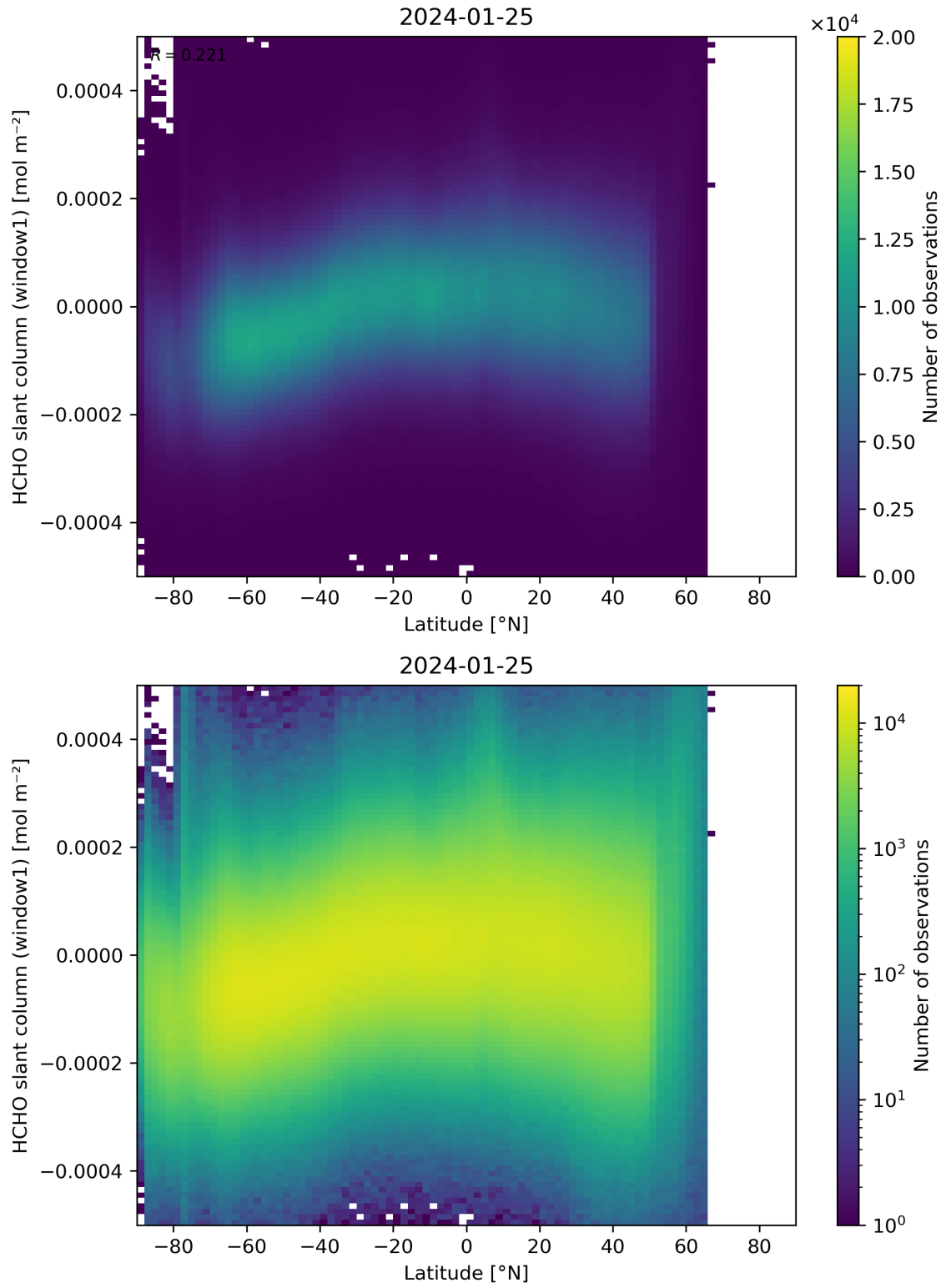
Figure 159: Scatter density plot of “Latitude” against “HCHO slant column (window1)” for 2024-01-24 to 2024-01-26.
