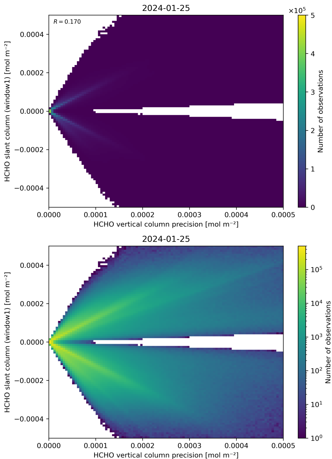
Figure 142: Scatter density plot of “HCHO vertical column precision” against “HCHO slant column (window1)” for 2024-01-24 to 2024-01-26.
