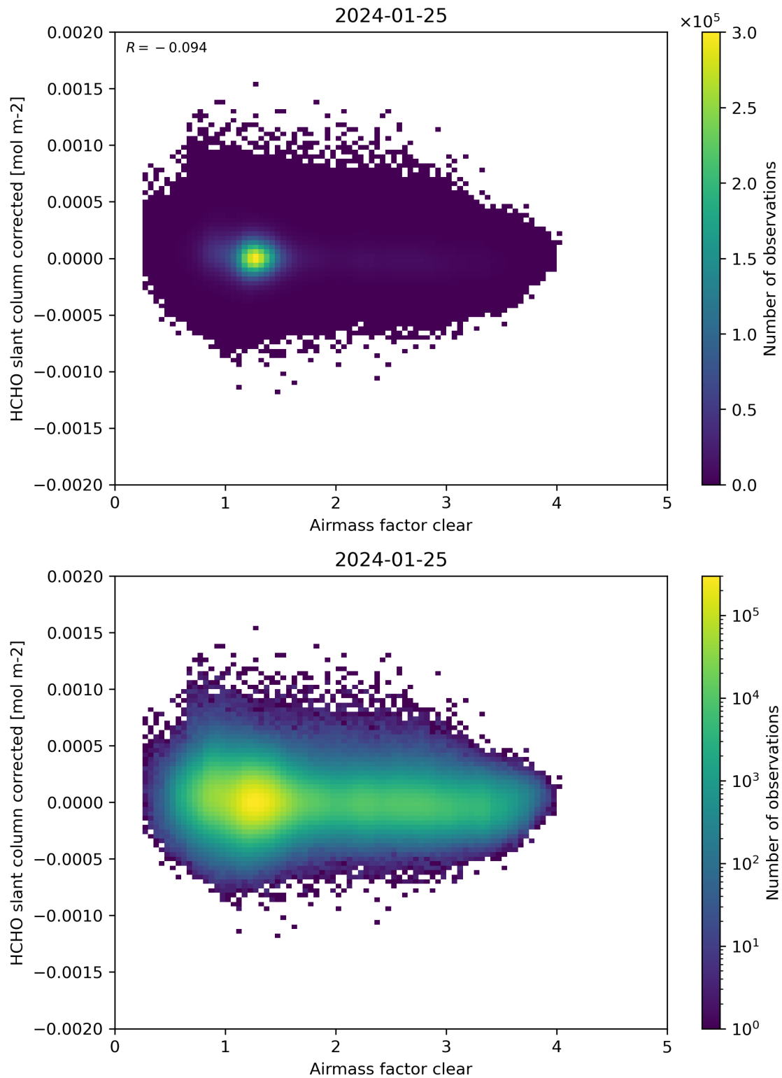
Figure 74: Scatter density plot of “Airmass factor clear” against “HCHO slant column corrected” for 2024-01-24 to 2024-01-26.
