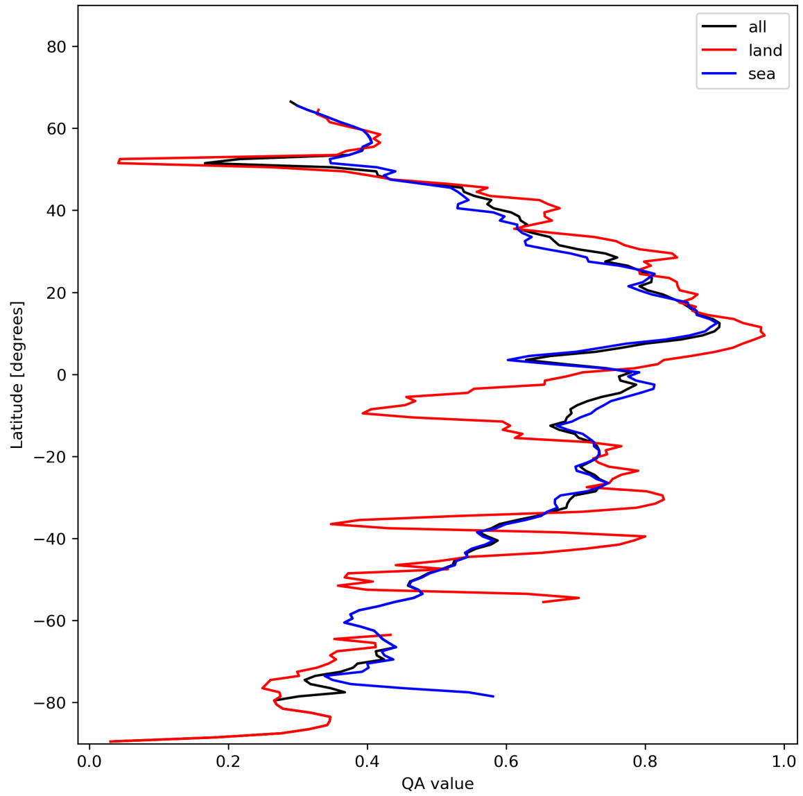
Figure 20: Zonal average of “QA value” for 2024-01-24 to 2024-01-26.
