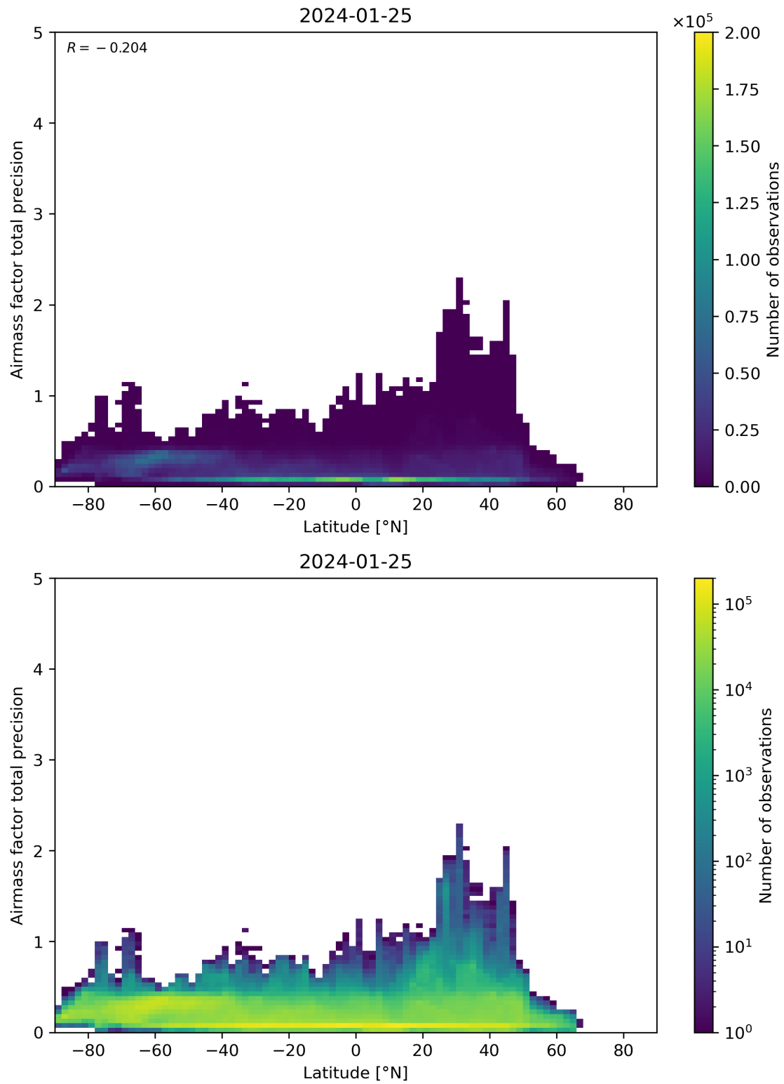
Figure 162: Scatter density plot of “Latitude” against “Airmass factor total precision” for 2024-01-24 to 2024-01-26.
