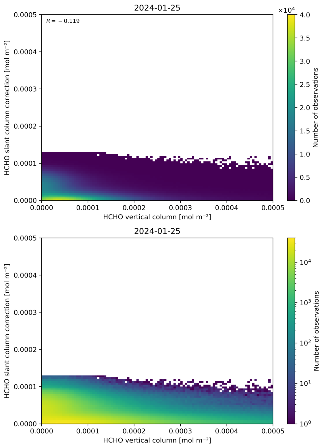
Figure 128: Scatter density plot of “HCHO vertical column” against “HCHO slant column correction” for 2024-01-24 to 2024-01-26.
