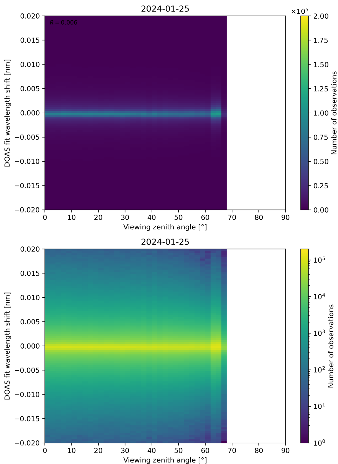
Figure 183: Scatter density plot of “Viewing zenith angle” against “DOAS fit wavelength shift” for 2024-01-24 to 2024-01-26.
