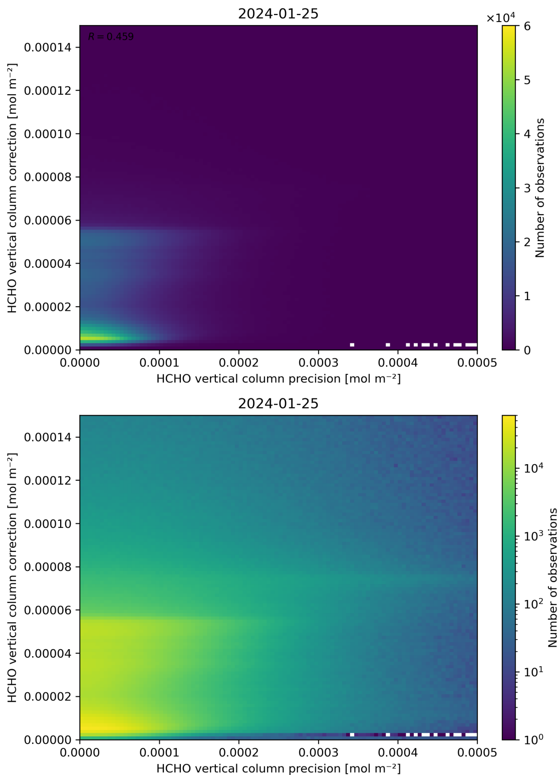
Figure 146: Scatter density plot of “HCHO vertical column precision” against “HCHO vertical column correction” for 2024-01-24 to 2024-01-26.
