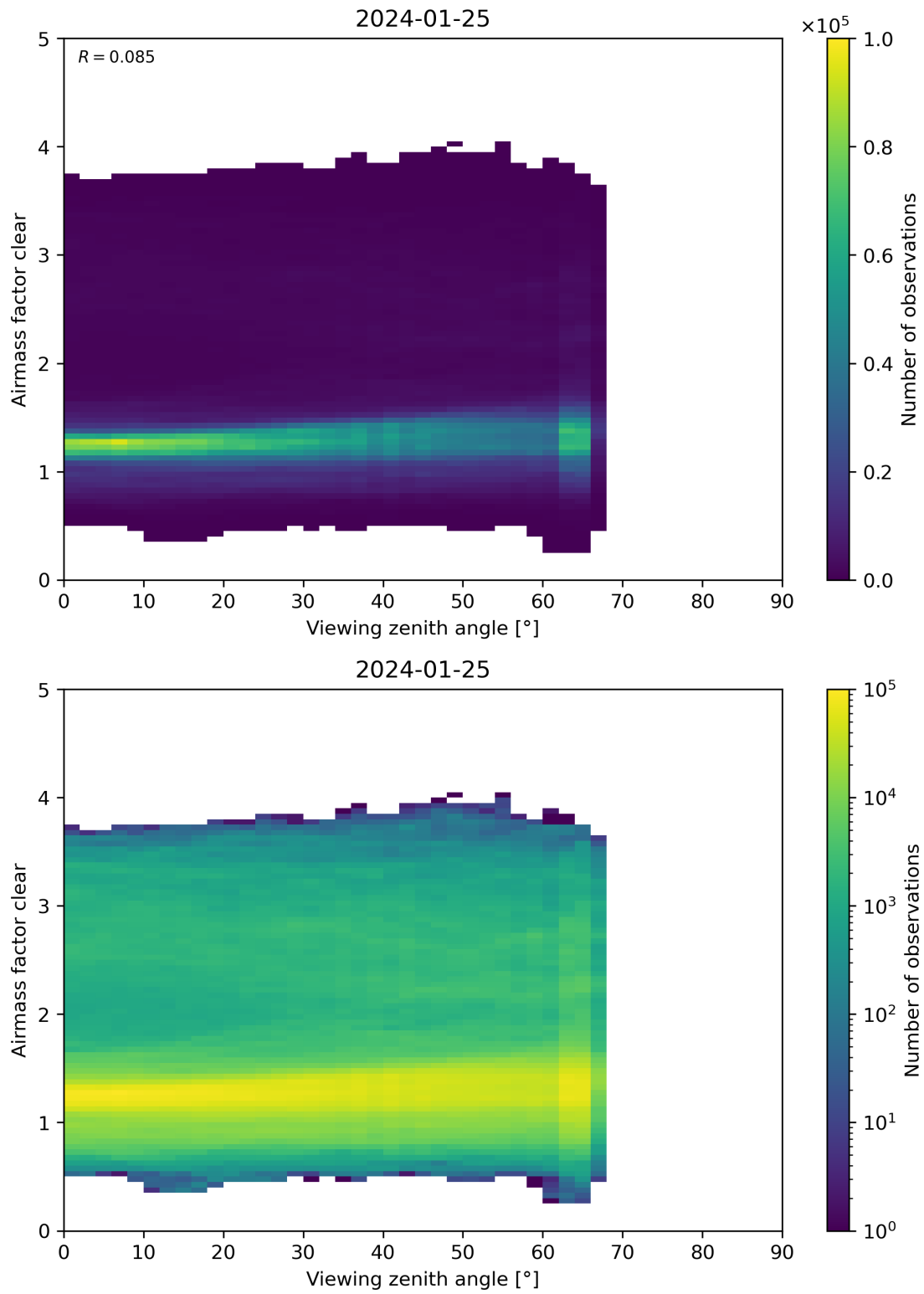
Figure 185: Scatter density plot of “Viewing zenith angle” against “Airmass factor clear” for 2024-01-24 to 2024-01-26.
