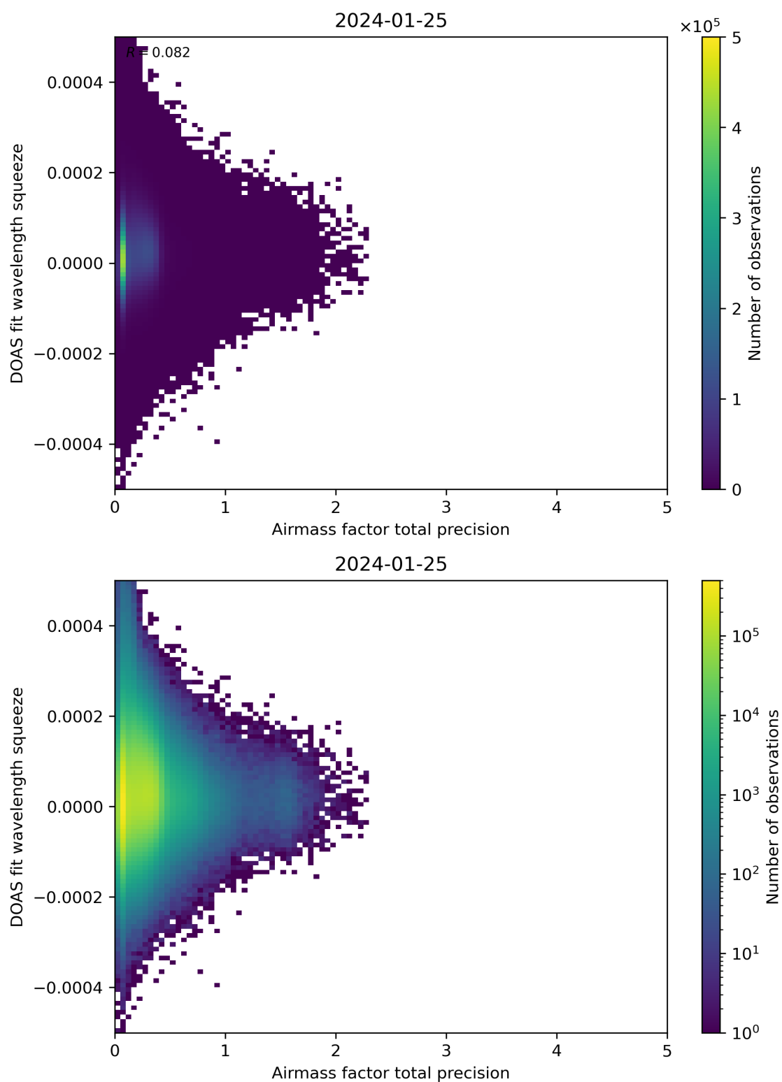
Figure 107: Scatter density plot of “Airmass factor total precision” against “DOAS fit wavelength squeeze” for 2024-01-24 to 2024-01-26.
