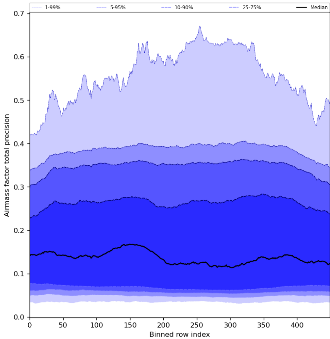
Figure 55: Along track statistics of “Airmass factor total precision” for 2024-01-24 to 2024-01-26
