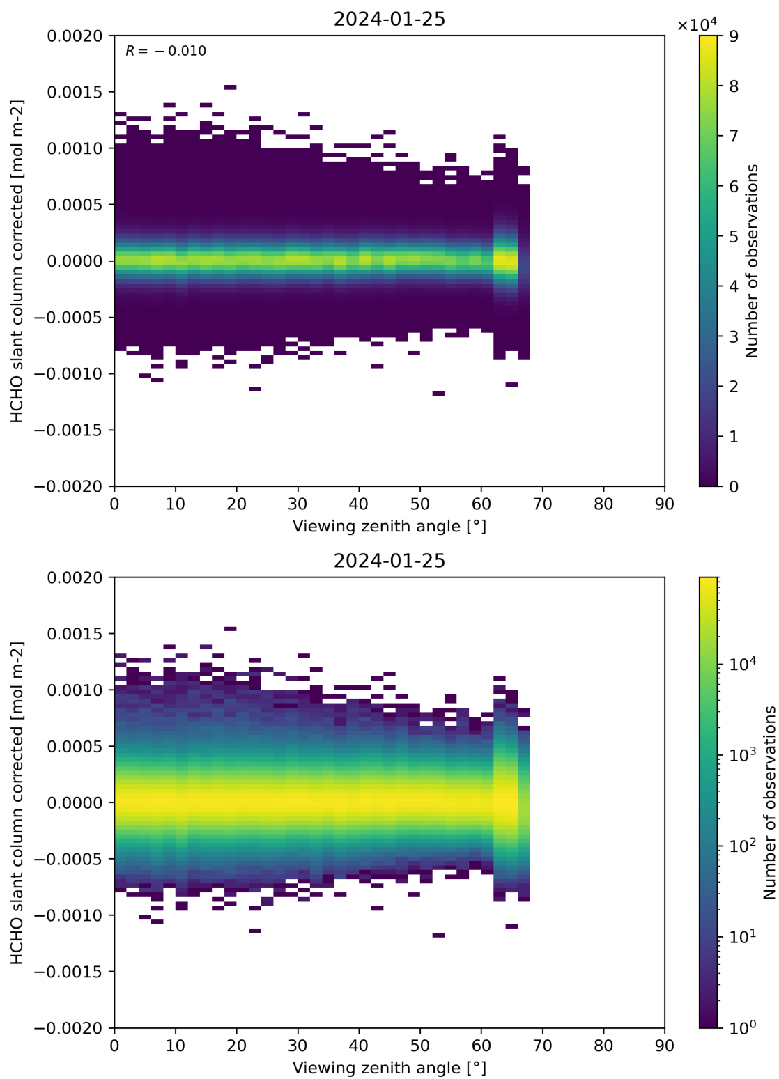
Figure 186: Scatter density plot of “Viewing zenith angle” against “HCHO slant column corrected” for 2024-01-24 to 2024-01-26.
