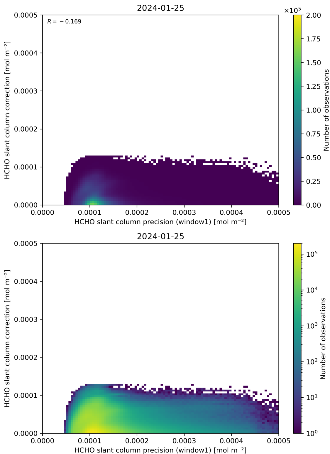
Figure 93: Scatter density plot of “HCHO slant column precision (window1)” against “HCHO slant column correction” for 2024-01-24 to 2024-01-26.
