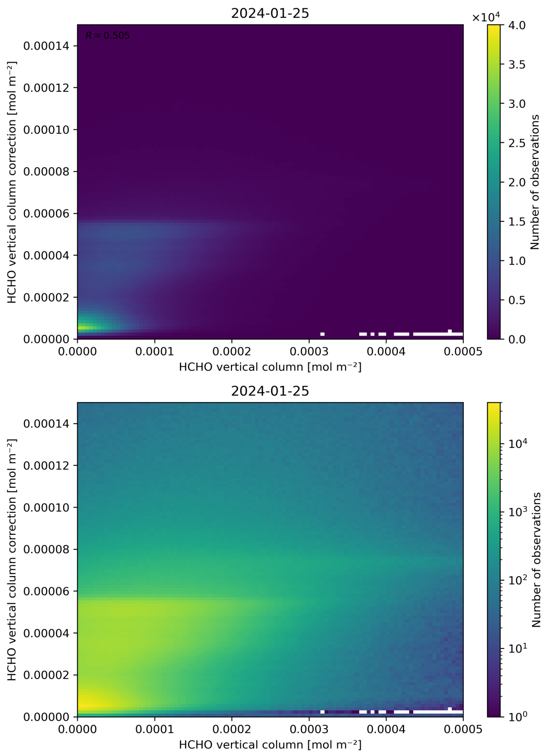
Figure 133: Scatter density plot of “HCHO vertical column” against “HCHO vertical column correction” for 2024-01-24 to 2024-01-26.
