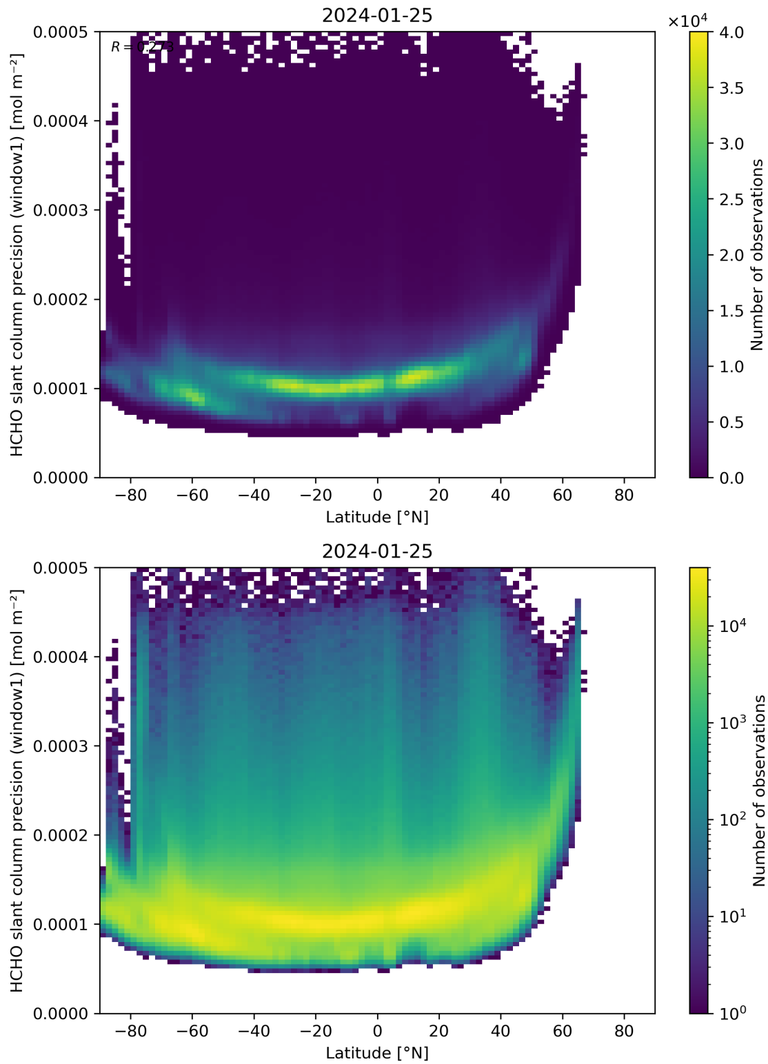
Figure 160: Scatter density plot of “Latitude” against “HCHO slant column precision (window1)” for 2024-01-24 to 2024-01-26.
