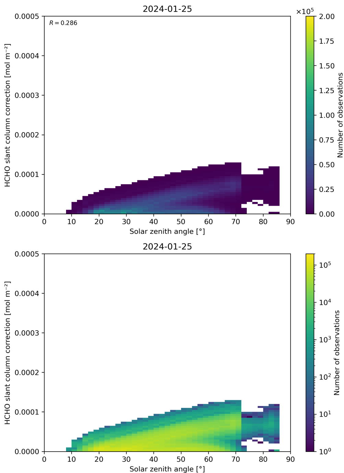
Figure 172: Scatter density plot of “Solar zenith angle” against “HCHO slant column correction” for 2024-01-24 to 2024-01-26.
