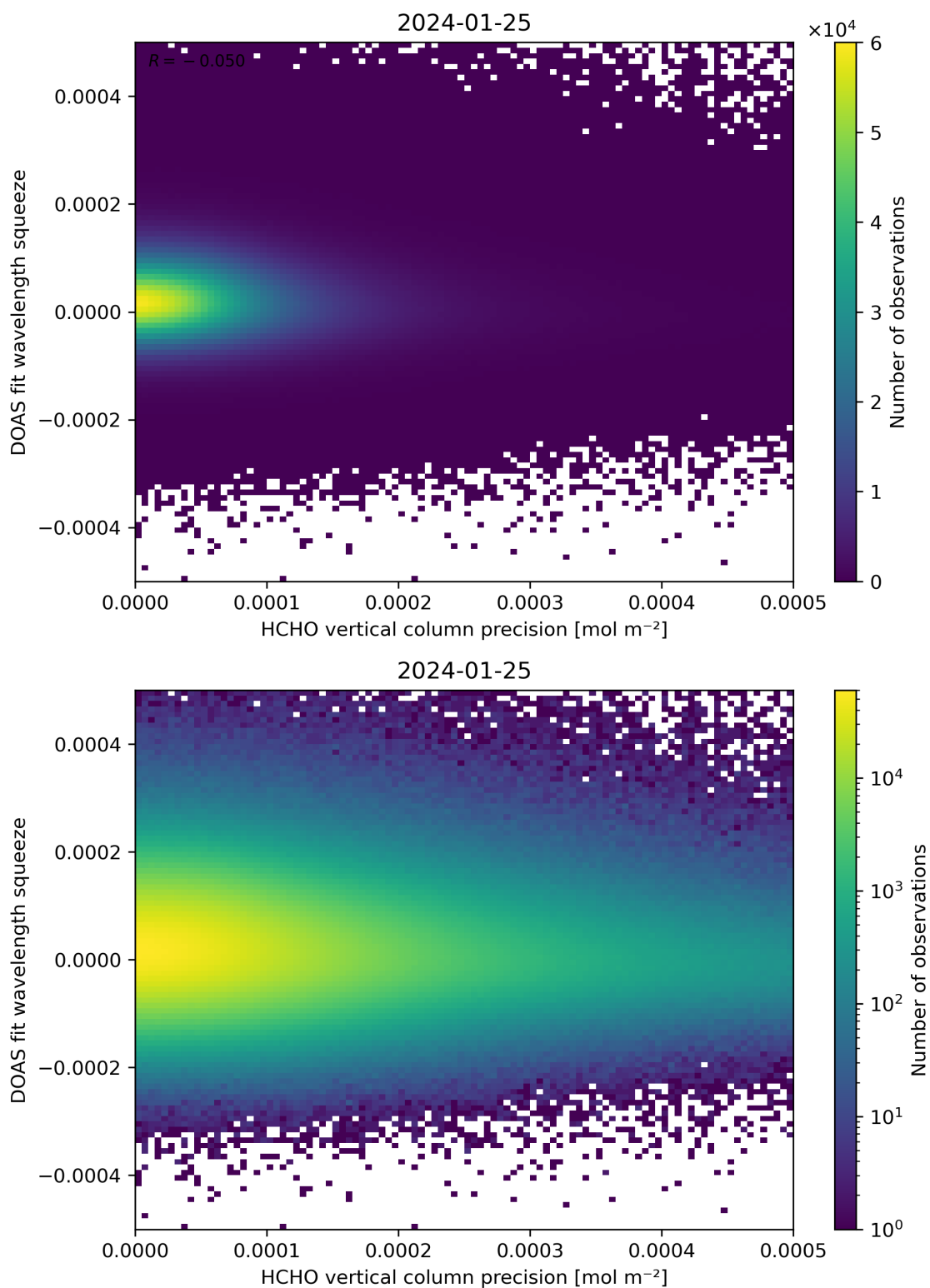
Figure 138: Scatter density plot of “HCHO vertical column precision” against “DOAS fit wavelength squeeze” for 2024-01-24 to 2024-01-26.
