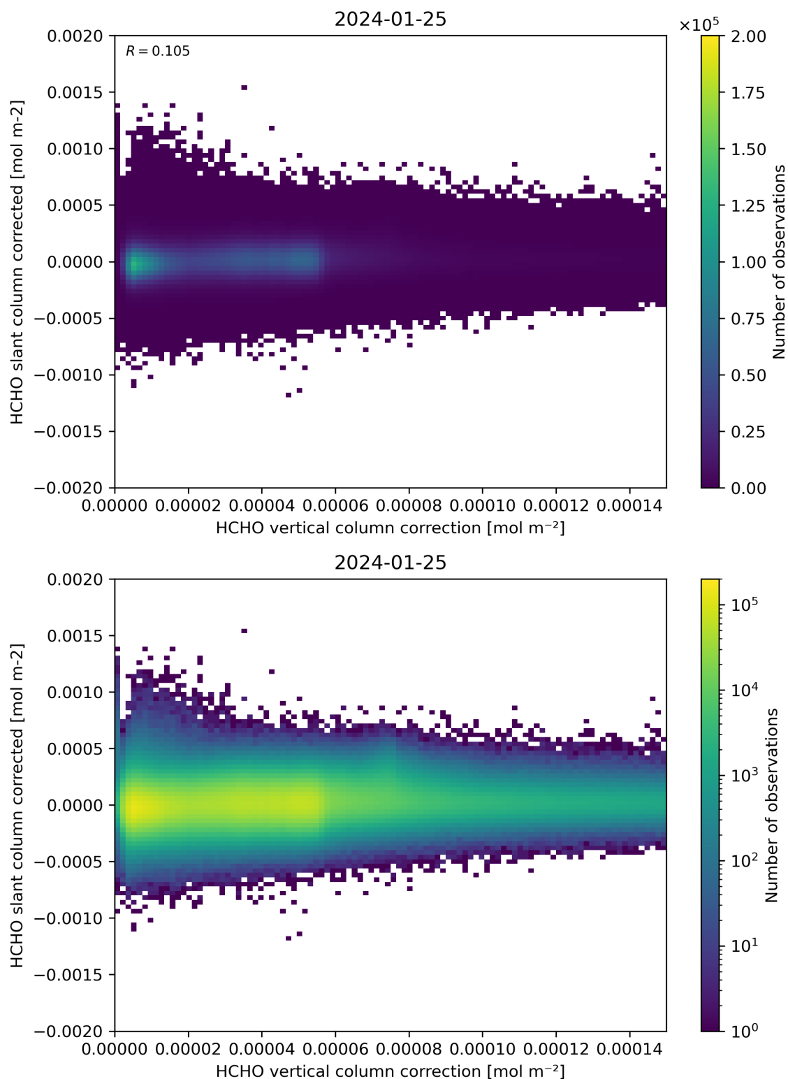
Figure 116: Scatter density plot of “HCHO vertical column correction” against “HCHO slant column corrected” for 2024-01-24 to 2024-01-26.
