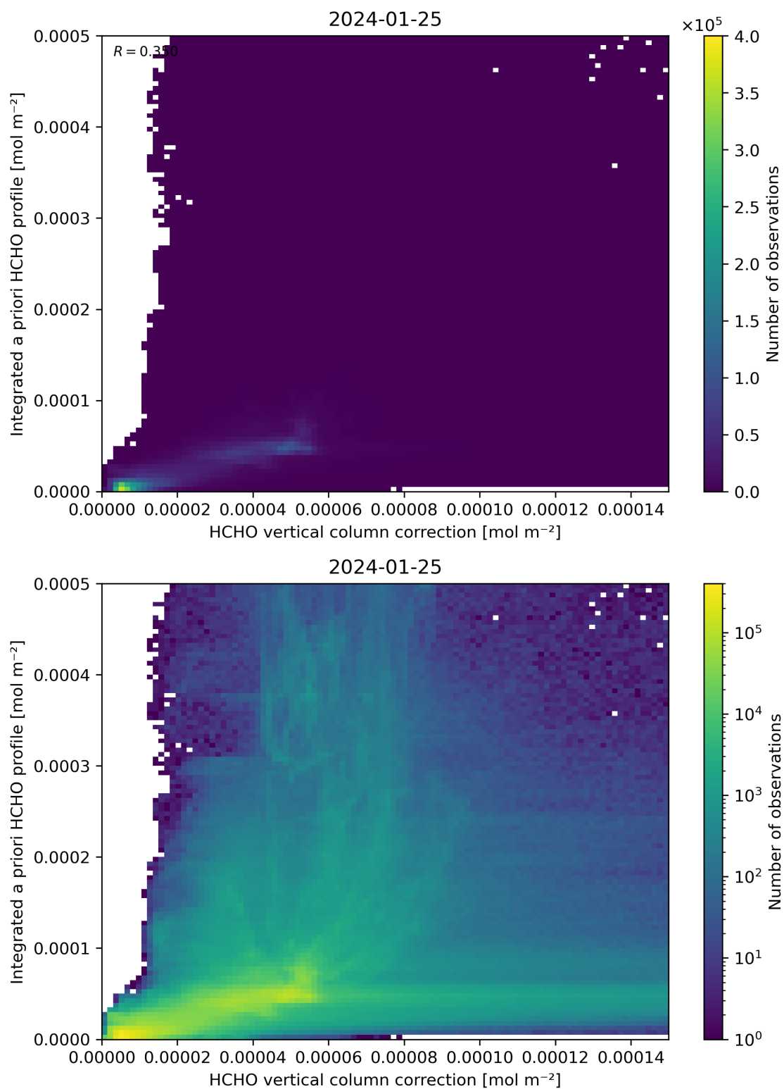
Figure 122: Scatter density plot of “HCHO vertical column correction” against “Integrated a priori HCHO profile” for 2024-01-24 to 2024-01-26.
