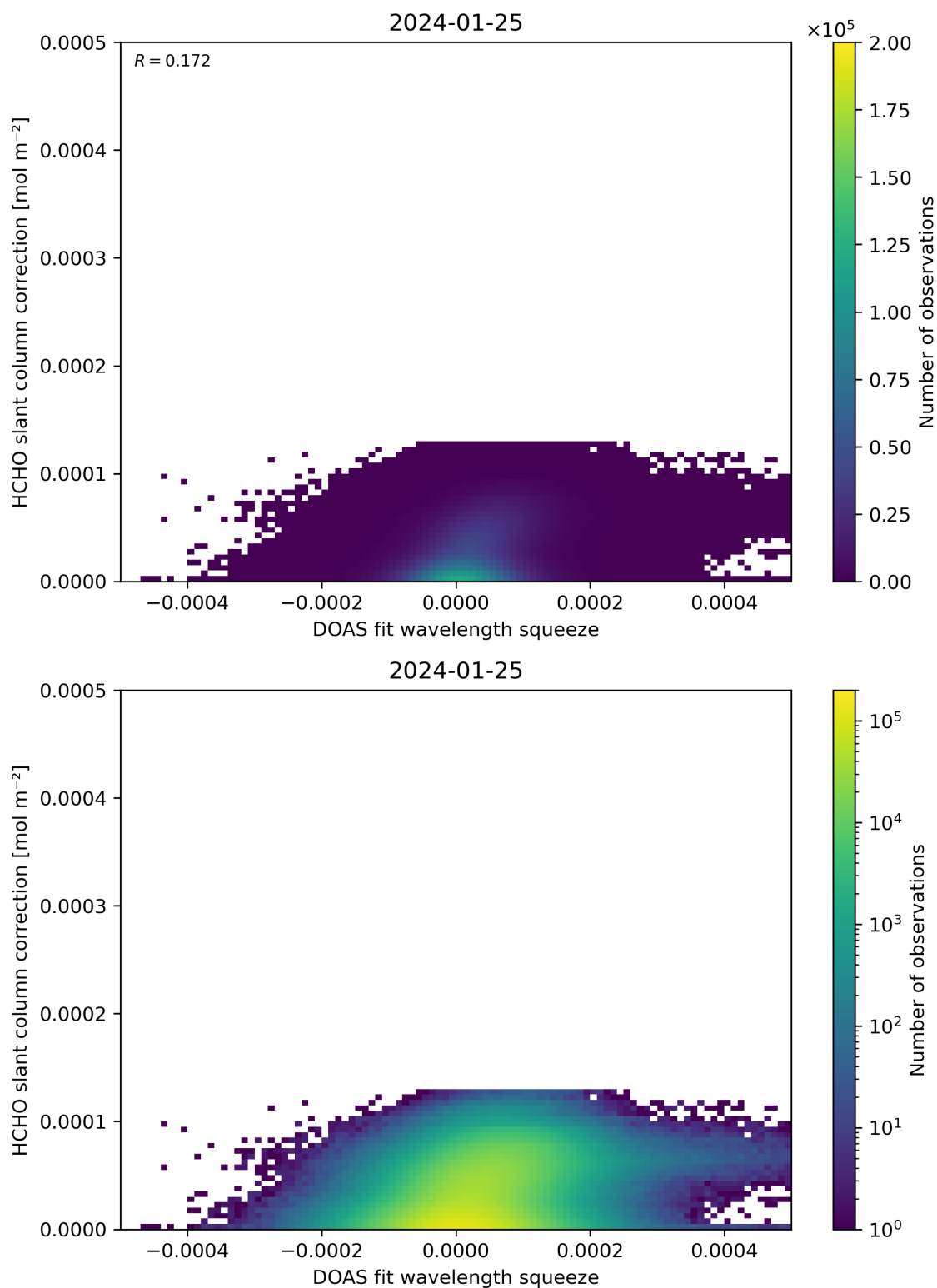
Figure 70: Scatter density plot of “DOAS fit wavelength squeeze” against “HCHO slant column correction” for 2024-01-24 to 2024-01-26.
