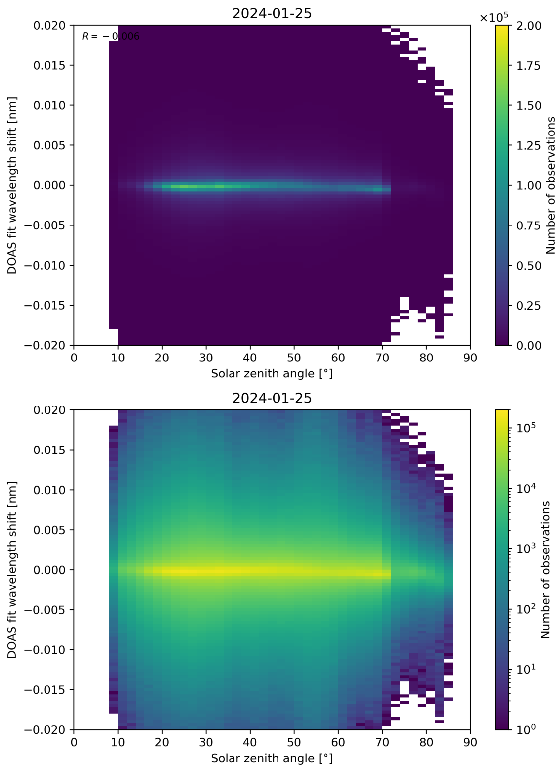
Figure 168: Scatter density plot of “Solar zenith angle” against “DOAS fit wavelength shift” for 2024-01-24 to 2024-01-26.
