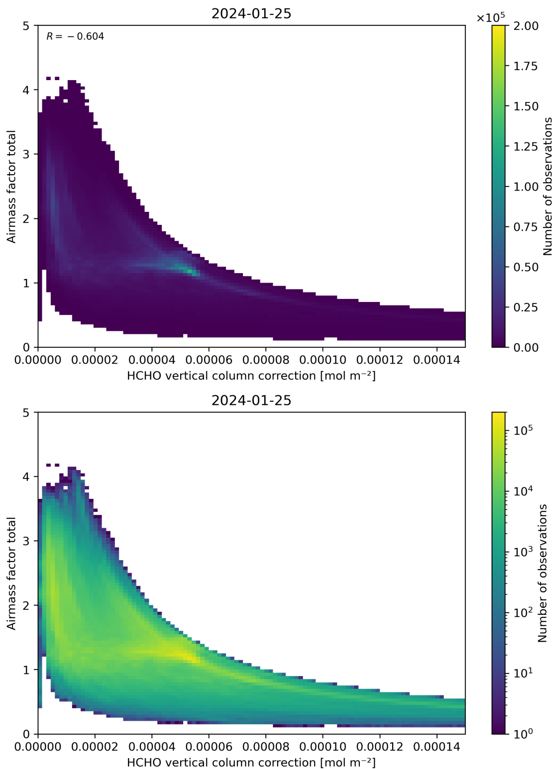
Figure 120: Scatter density plot of “HCHO vertical column correction” against “Airmass factor total” for 2024-01-24 to 2024-01-26.
