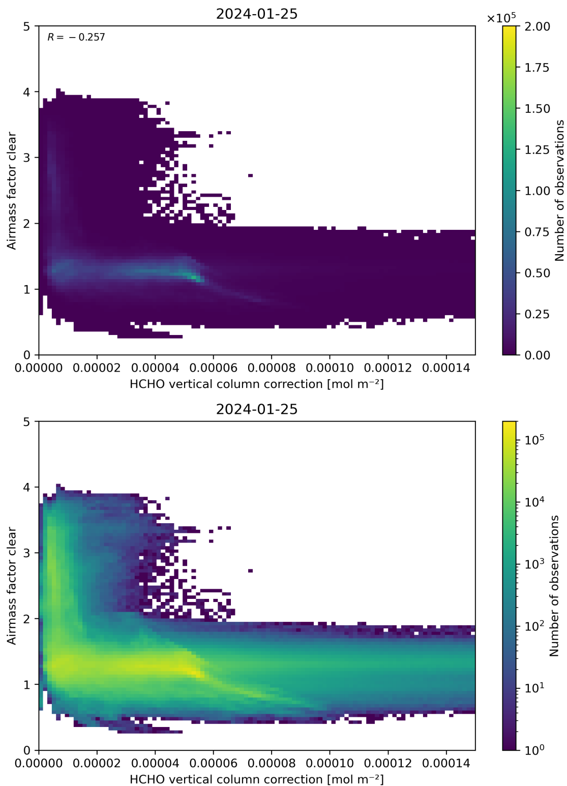
Figure 115: Scatter density plot of “HCHO vertical column correction” against “Airmass factor clear” for 2024-01-24 to 2024-01-26.
