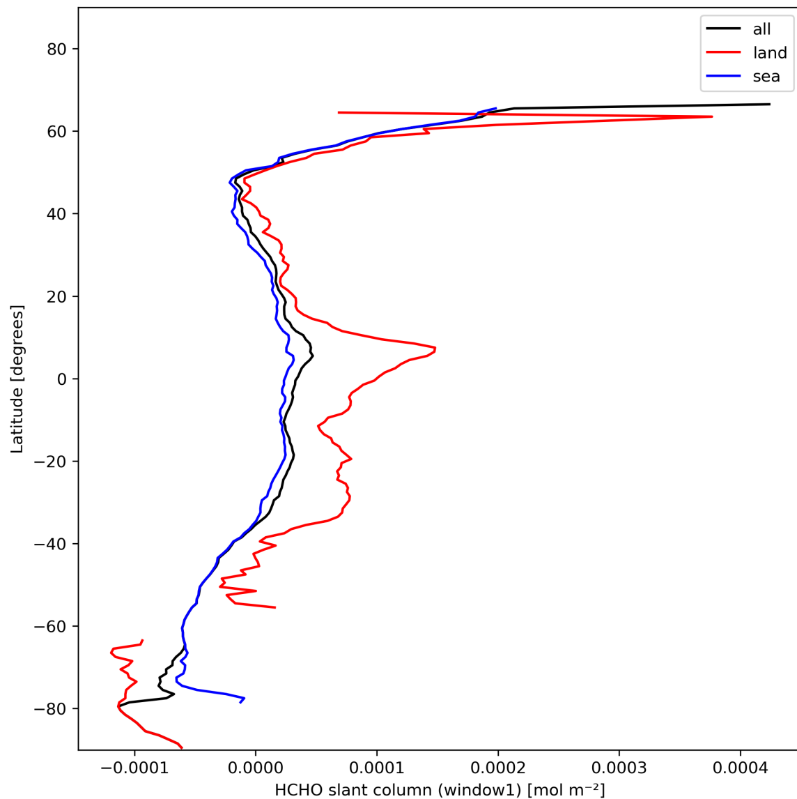
Figure 24: Zonal average of “HCHO slant column (window1)” for 2024-01-24 to 2024-01-26.
