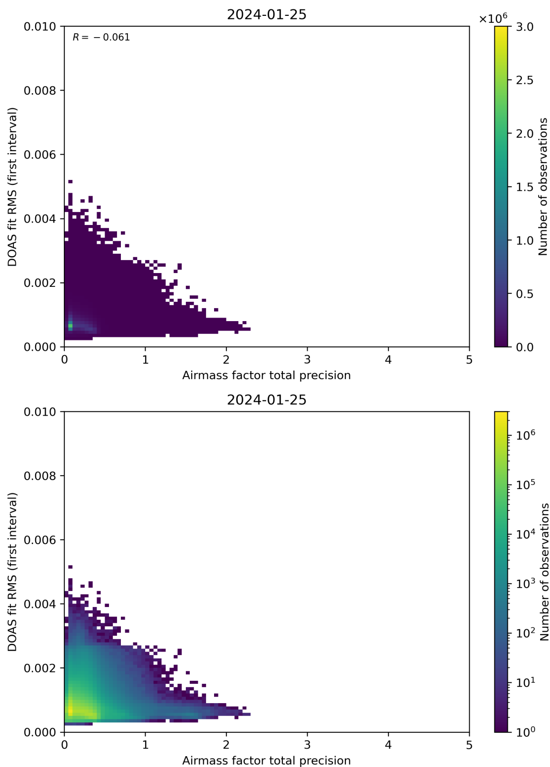
Figure 105: Scatter density plot of “Airmass factor total precision” against “DOAS fit RMS (first interval)” for 2024-01-24 to 2024-01-26.
