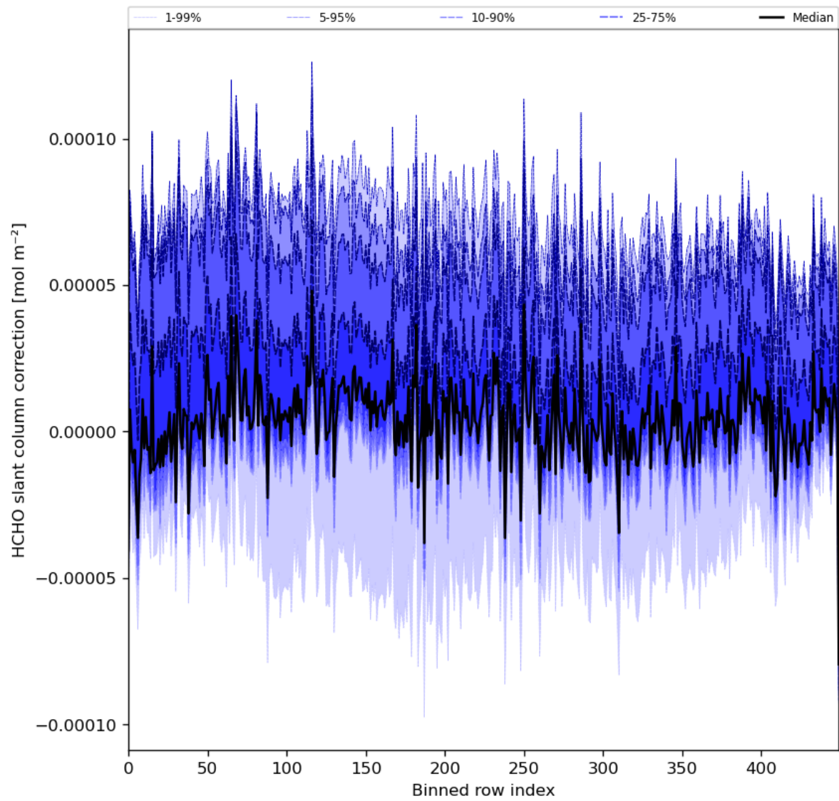
Figure 61: Along track statistics of “HCHO slant column correction” for 2024-01-24 to 2024-01-26
