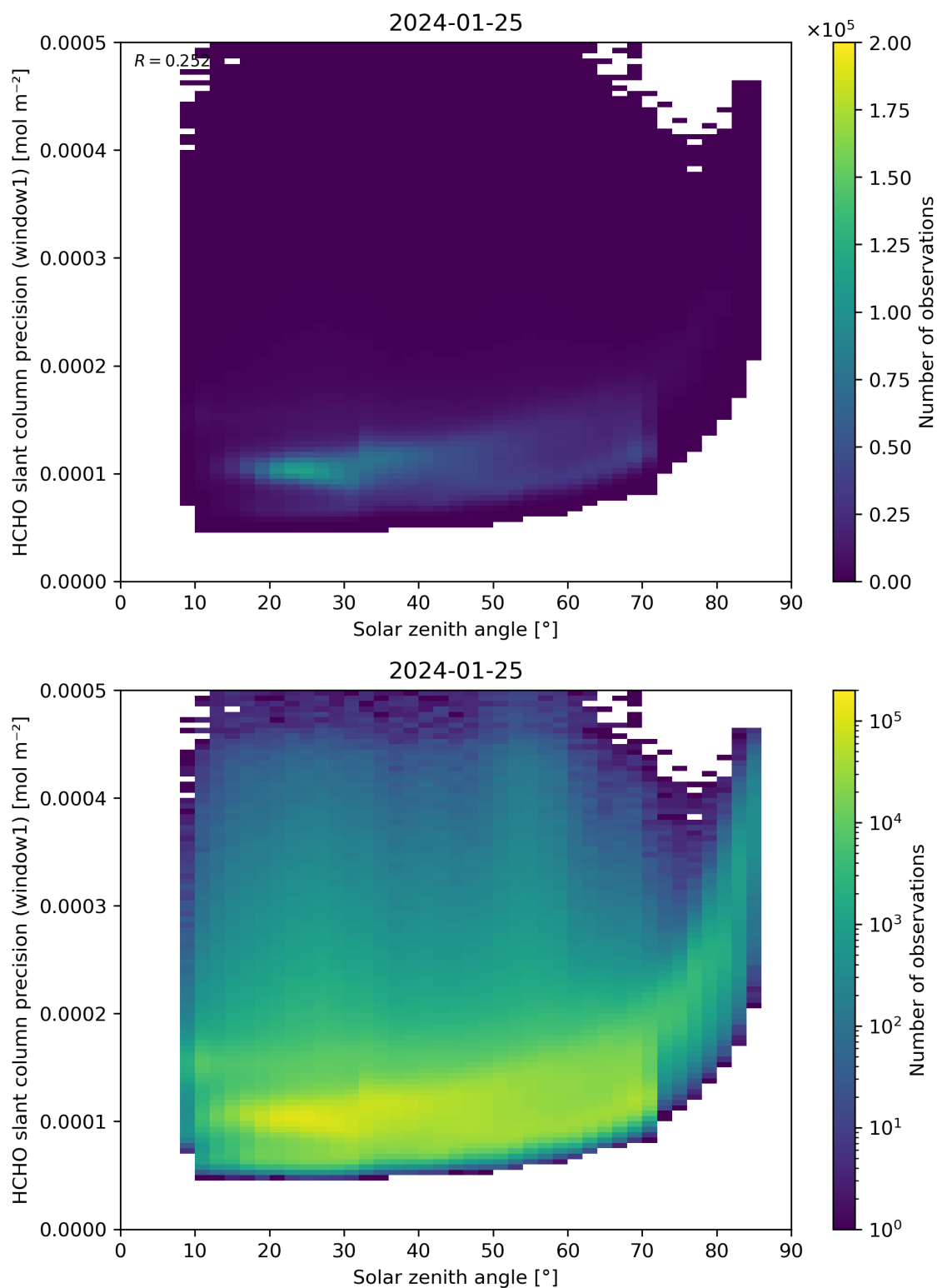
Figure 174: Scatter density plot of “Solar zenith angle” against “HCHO slant column precision (window1)” for 2024-01-24 to 2024-01-26.
