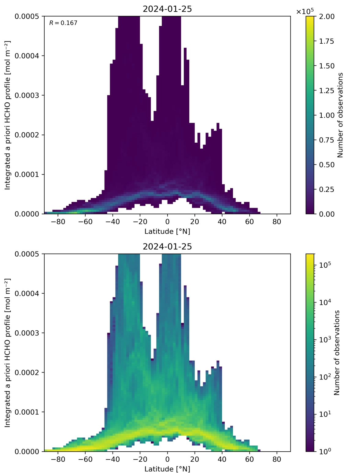
Figure 166: Scatter density plot of “Latitude” against “Integrated a priori HCHO profile” for 2024-01-24 to 2024-01-26.
