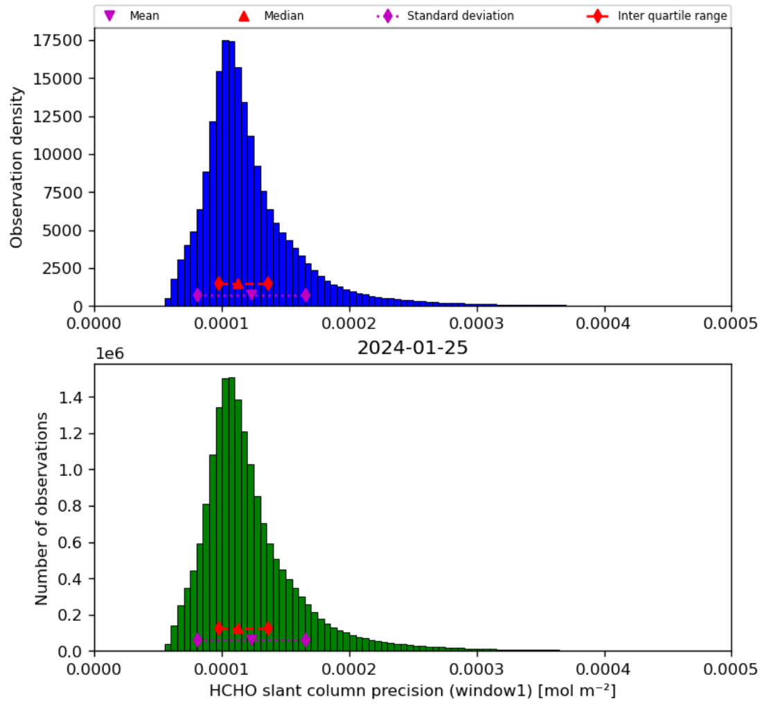
Figure 39: Histogram of “HCHO slant column precision (window1)” for 2024-01-24 to 2024-01-26
