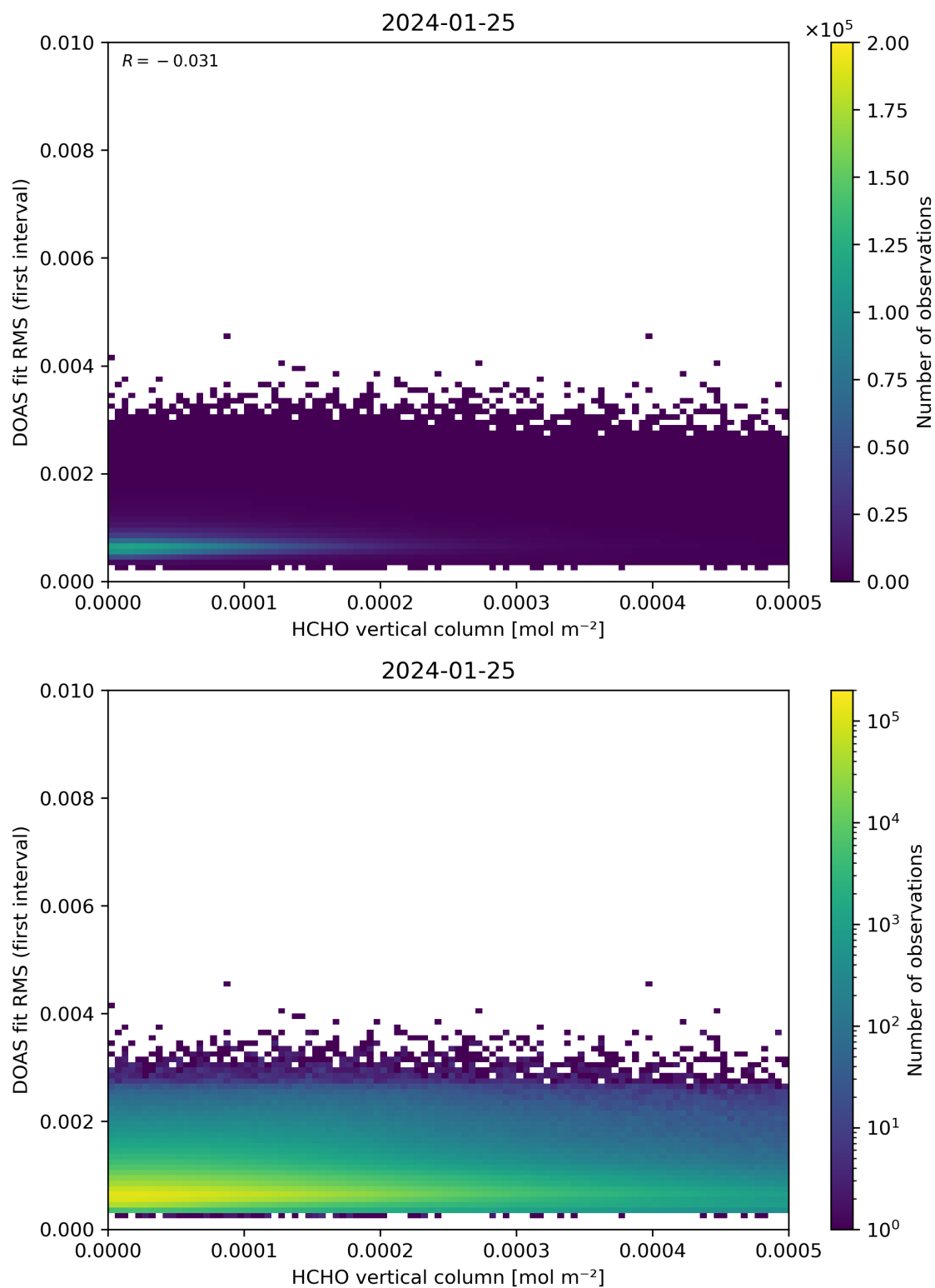
Figure 123: Scatter density plot of “HCHO vertical column” against “DOAS fit RMS (first interval)” for 2024-01-24 to 2024-01-26.
