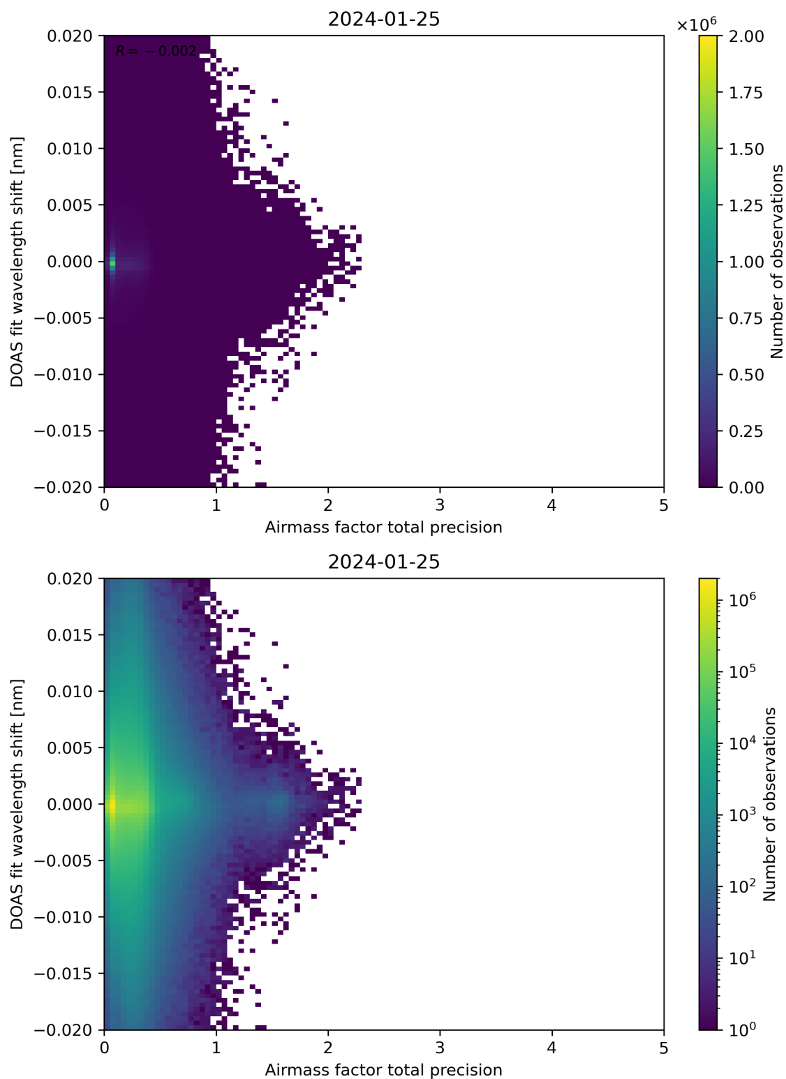
Figure 106: Scatter density plot of “Airmass factor total precision” against “DOAS fit wavelength shift” for 2024-01-24 to 2024-01-26.
