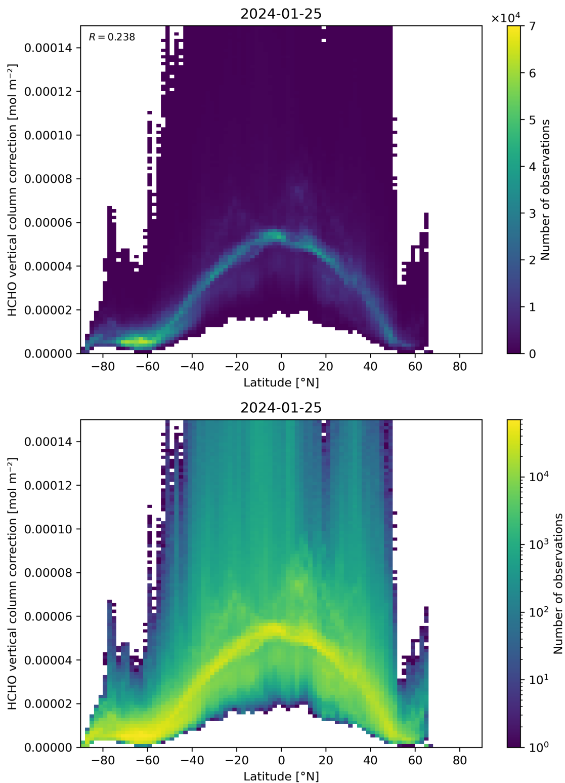
Figure 164: Scatter density plot of “Latitude” against “HCHO vertical column correction” for 2024-01-24 to 2024-01-26.
