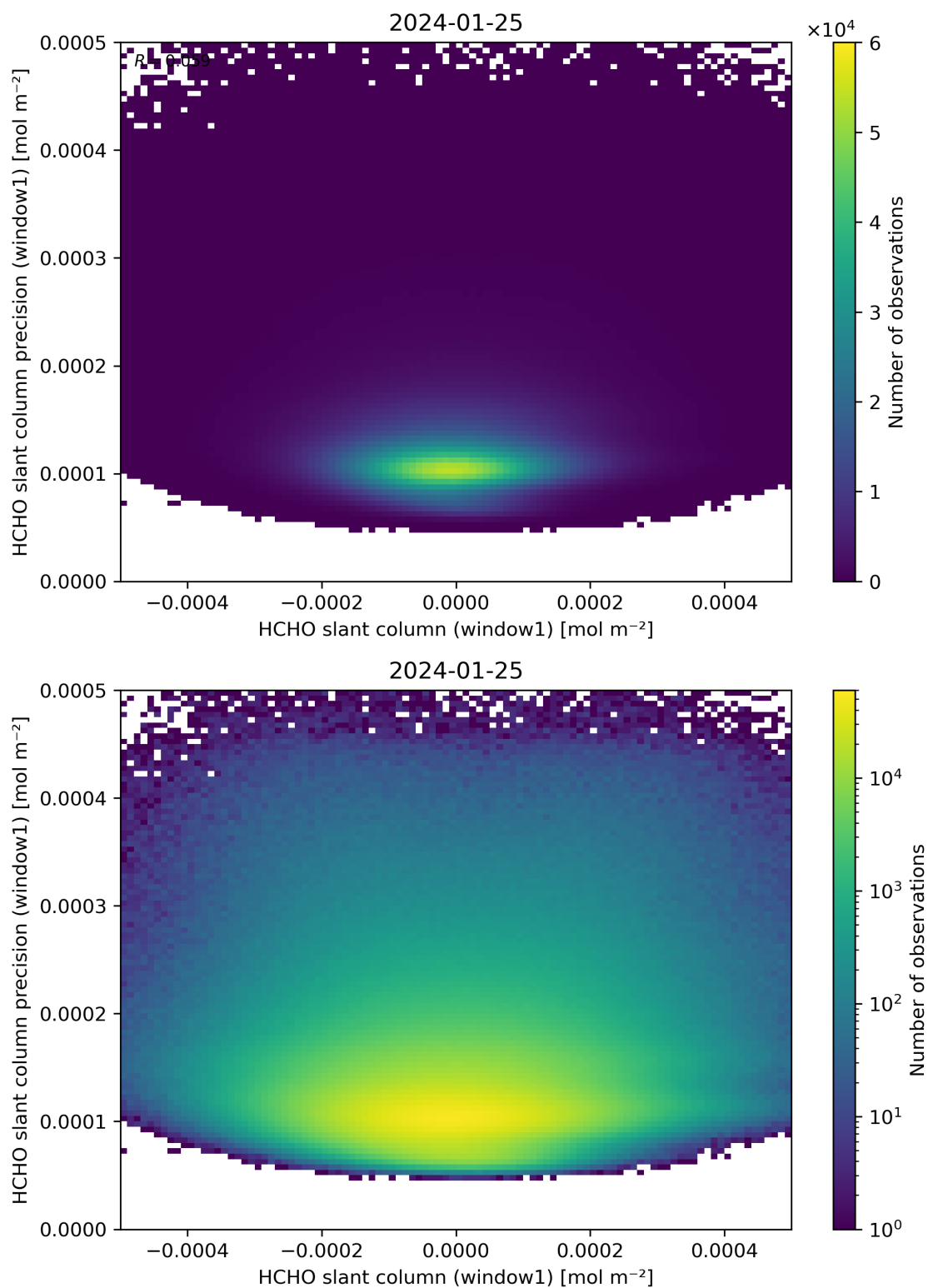
Figure 84: Scatter density plot of “HCHO slant column (window1)” against “HCHO slant column precision (window1)” for 2024-01-24 to 2024-01-26.
