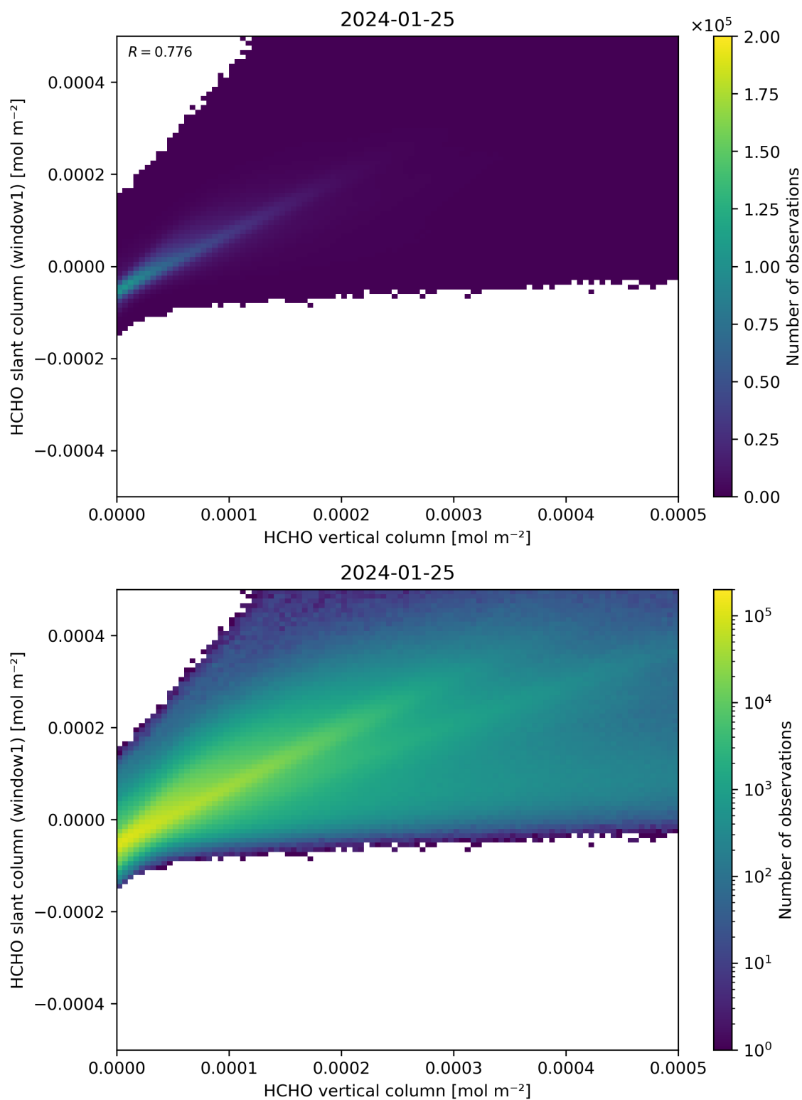
Figure 129: Scatter density plot of “HCHO vertical column” against “HCHO slant column (window1)” for 2024-01-24 to 2024-01-26.
