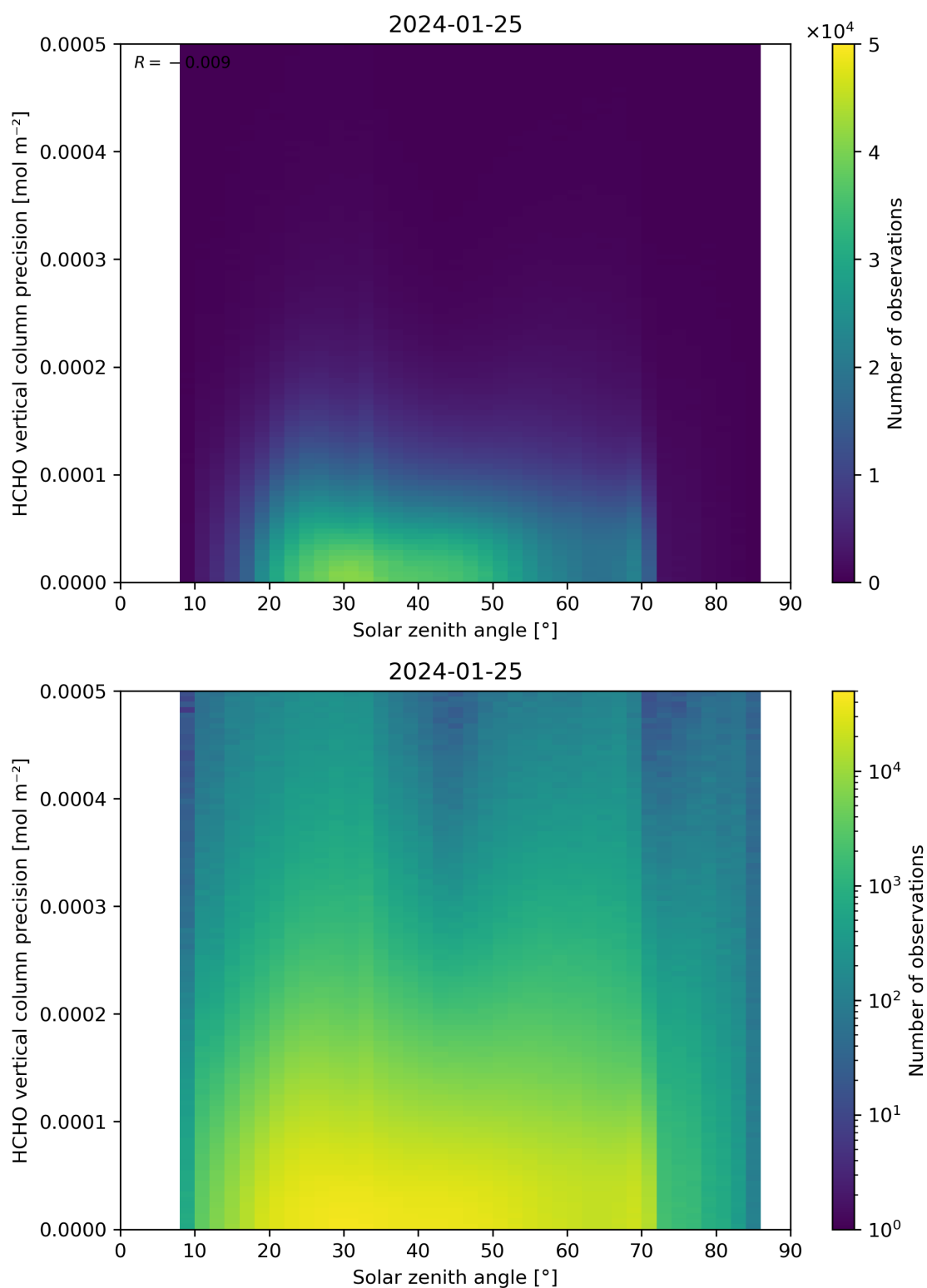
Figure 179: Scatter density plot of “Solar zenith angle” against “HCHO vertical column precision” for 2024-01-24 to 2024-01-26.
