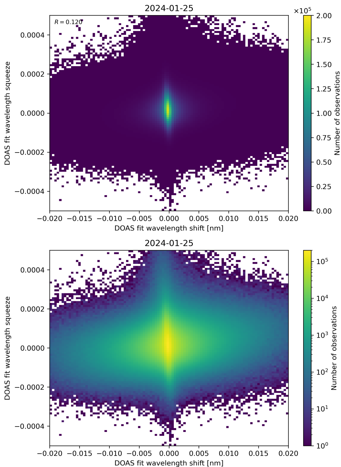
Figure 65: Scatter density plot of “DOAS fit wavelength shift” against “DOAS fit wavelength squeeze” for 2024-01-24 to 2024-01-26.
