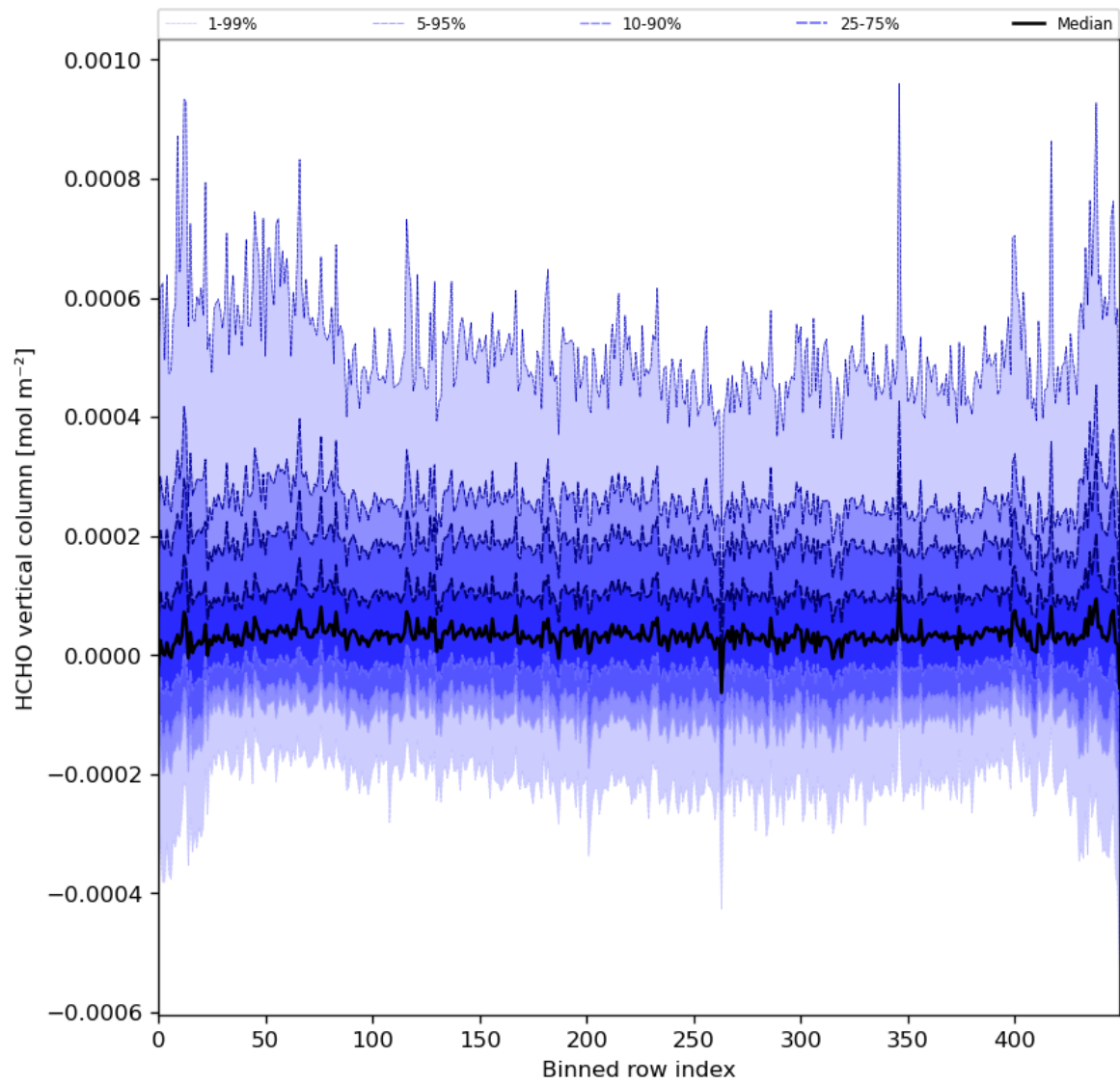
Figure 49: Along track statistics of “HCHO vertical column” for 2024-01-24 to 2024-01-26
