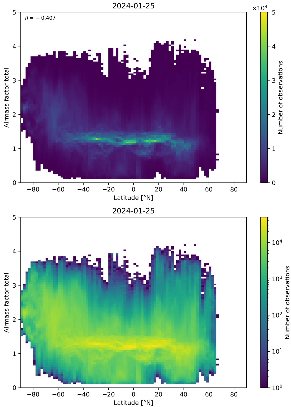
Figure 161: Scatter density plot of “Latitude” against “Airmass factor total” for 2024-01-24 to 2024-01-26.
