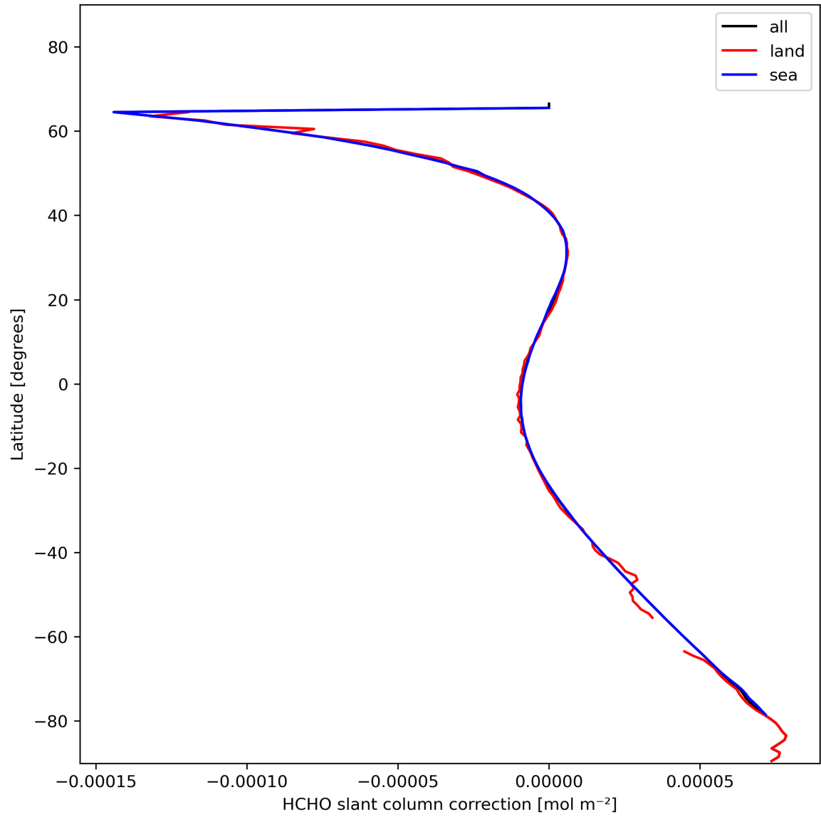
Figure 33: Zonal average of "HCHO slant column correction" for 2024-01-24 to 2024-01-26.
