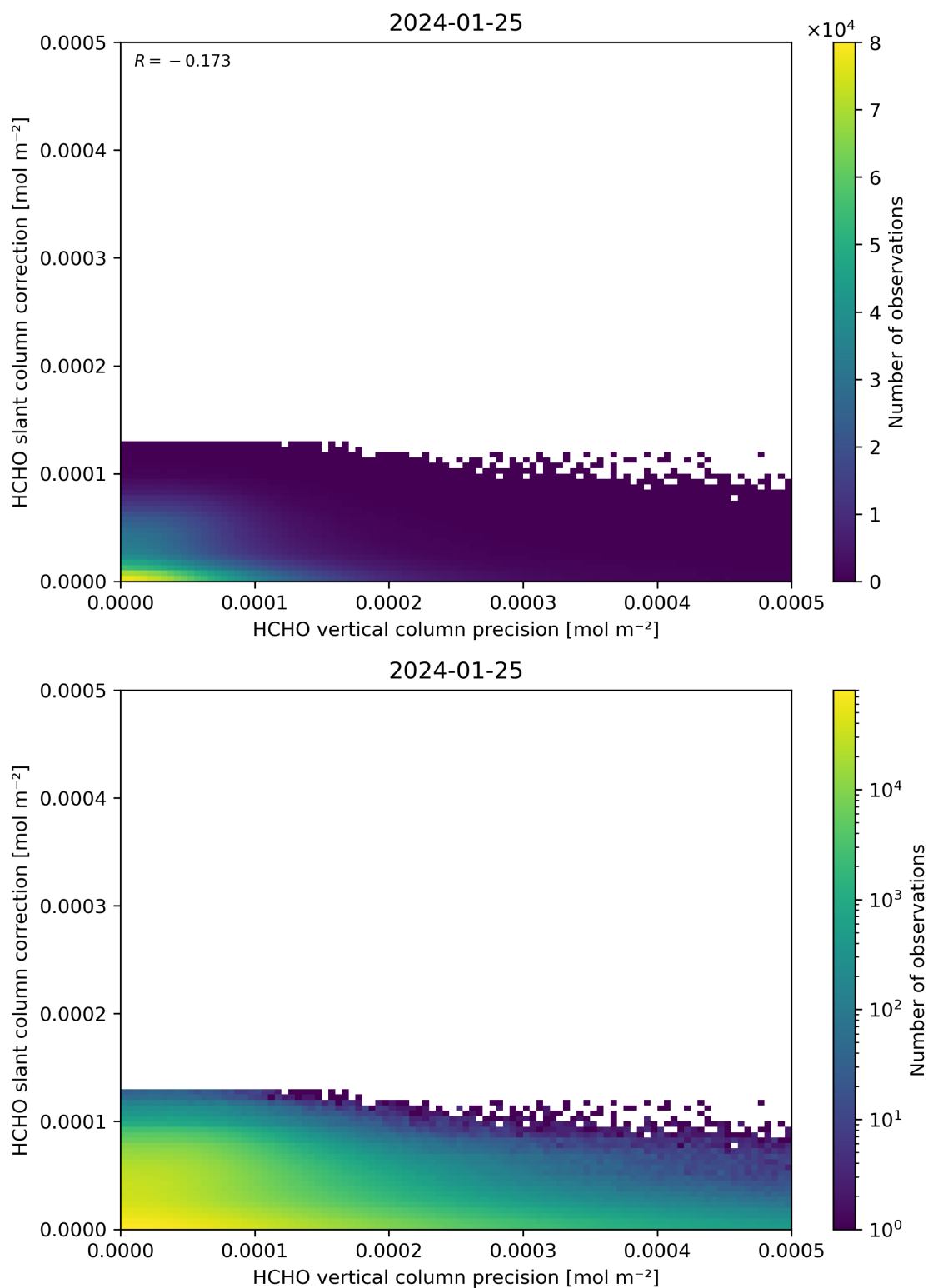
Figure 141: Scatter density plot of “HCHO vertical column precision” against “HCHO slant column correction” for 2024-01-24 to 2024-01-26.
