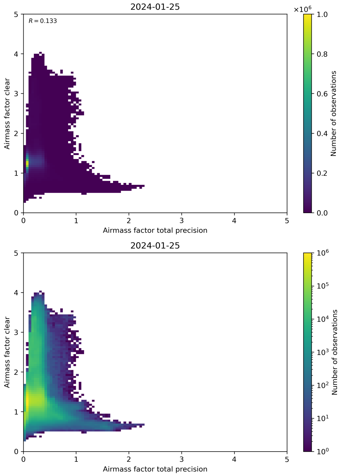
Figure 108: Scatter density plot of “Airmass factor total precision” against “Airmass factor clear” for 2024-01-24 to 2024-01-26.
