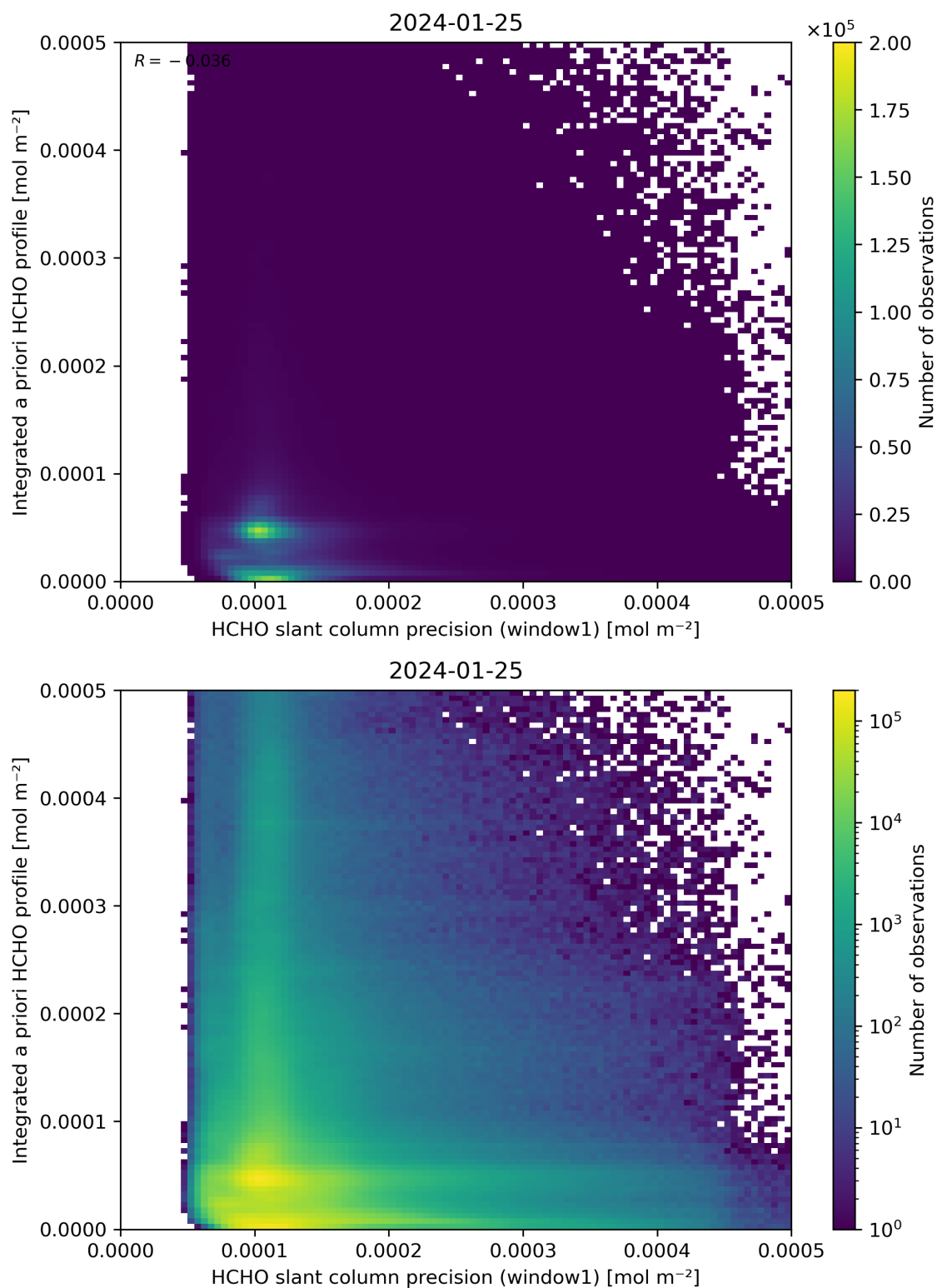
Figure 96: Scatter density plot of “HCHO slant column precision (window1)” against “Integrated a priori HCHO profile” for 2024-01-24 to 2024-01-26.
