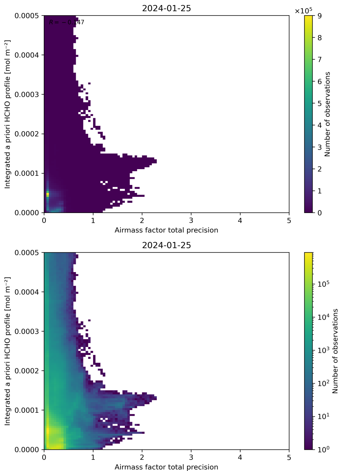
Figure 111: Scatter density plot of “Airmass factor total precision” against “Integrated a priori HCHO profile” for 2024-01-24 to 2024-01-26.
