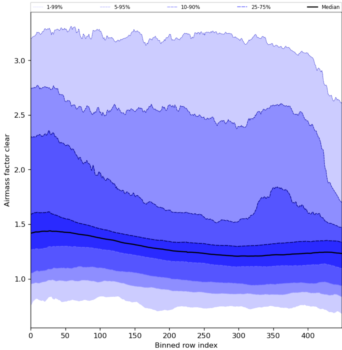
Figure 56: Along track statistics of “Airmass factor clear” for 2024-01-24 to 2024-01-26
