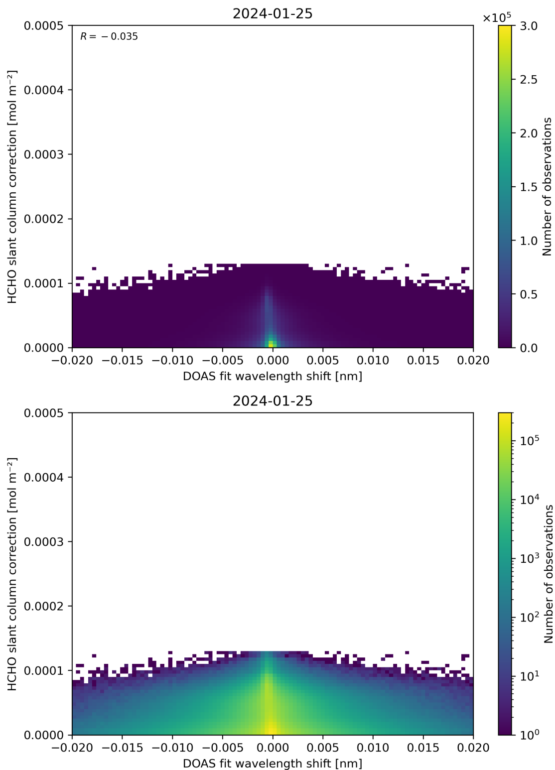
Figure 67: Scatter density plot of “DOAS fit wavelength shift” against “HCHO slant column correction” for 2024-01-24 to 2024-01-26.
