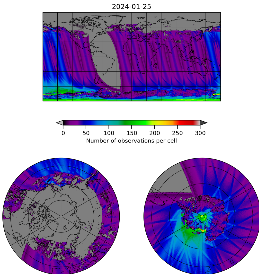
Figure 19: Map of the number of observations for 2024-01-24 to 2024-01-26
