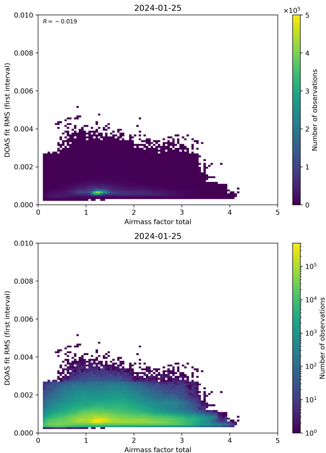
Figure 97: Scatter density plot of “Airmass factor total” against “DOAS fit RMS (first interval)” for 2024-01-24 to 2024-01-26.
