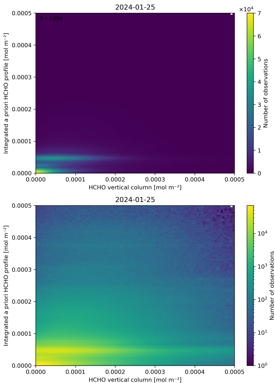
Figure 135: Scatter density plot of “HCHO vertical column” against “Integrated a priori HCHO profile” for 2024-01-24 to 2024-01-26.
