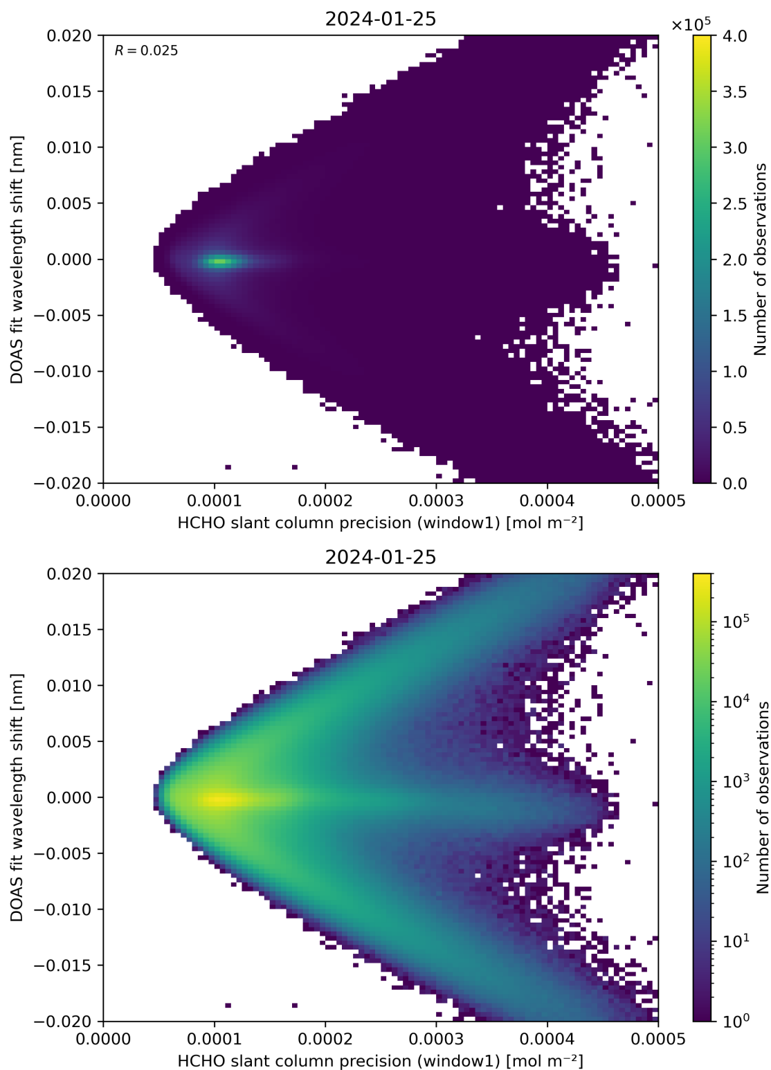
Figure 89: Scatter density plot of “HCHO slant column precision (window1)” against “DOAS fit wavelength shift” for 2024-01-24 to 2024-01-26.
