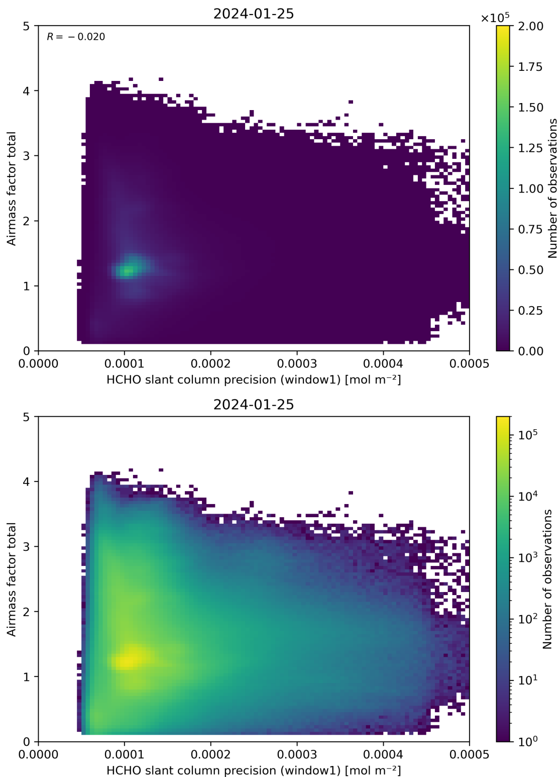
Figure 94: Scatter density plot of “HCHO slant column precision (window1)” against “Airmass factor total” for 2024-01-24 to 2024-01-26.
