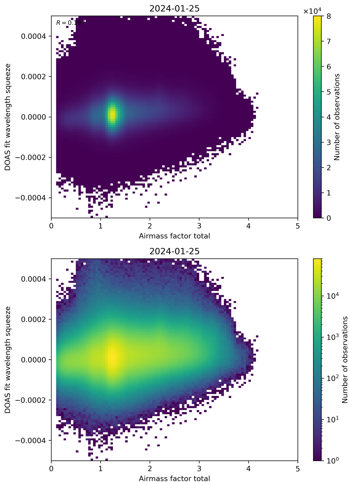
Figure 99: Scatter density plot of “Airmass factor total” against “DOAS fit wavelength squeeze” for 2024-01-24 to 2024-01-26.
