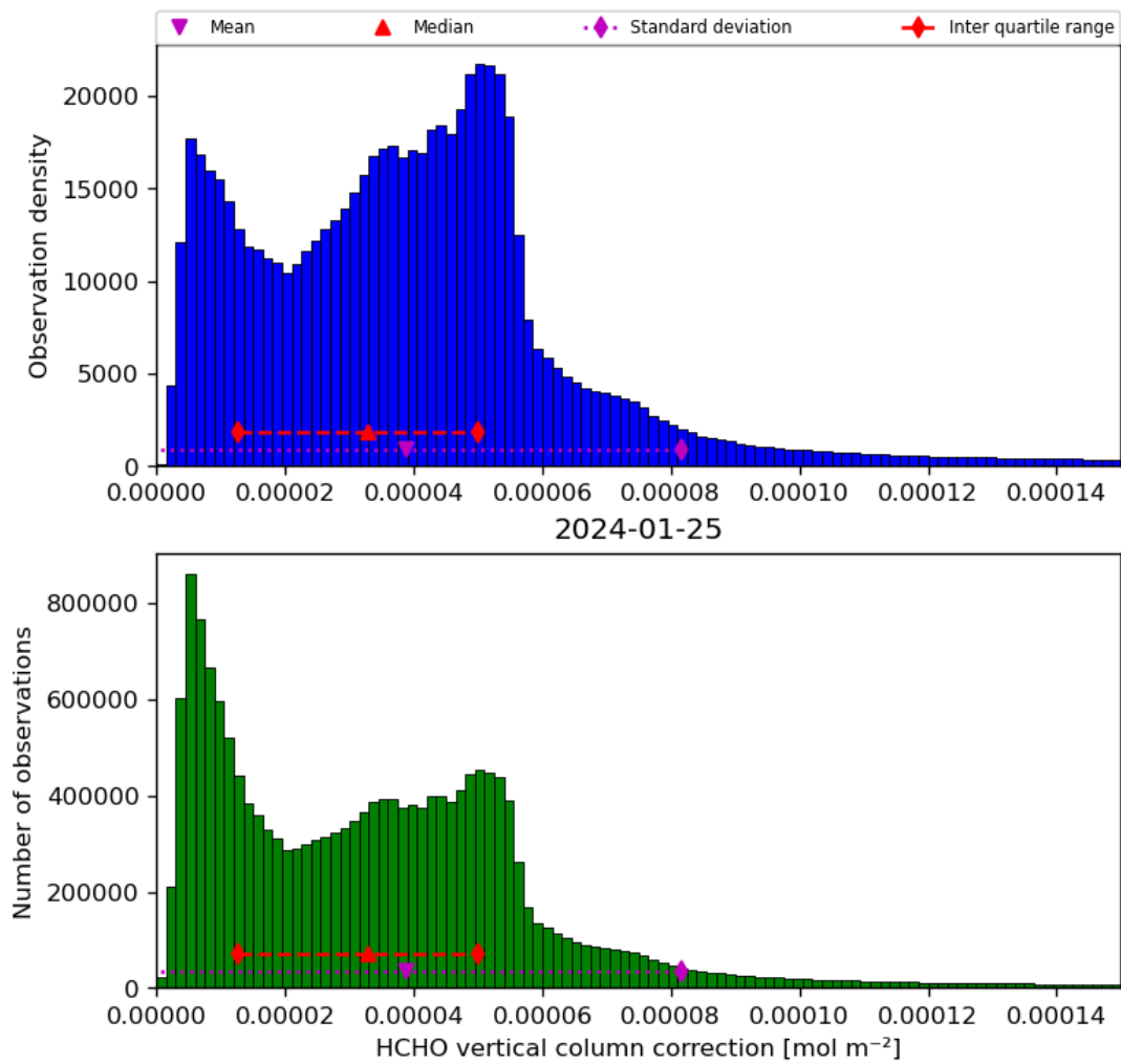
Figure 37: Histogram of “HCHO vertical column correction” for 2024-01-24 to 2024-01-26
