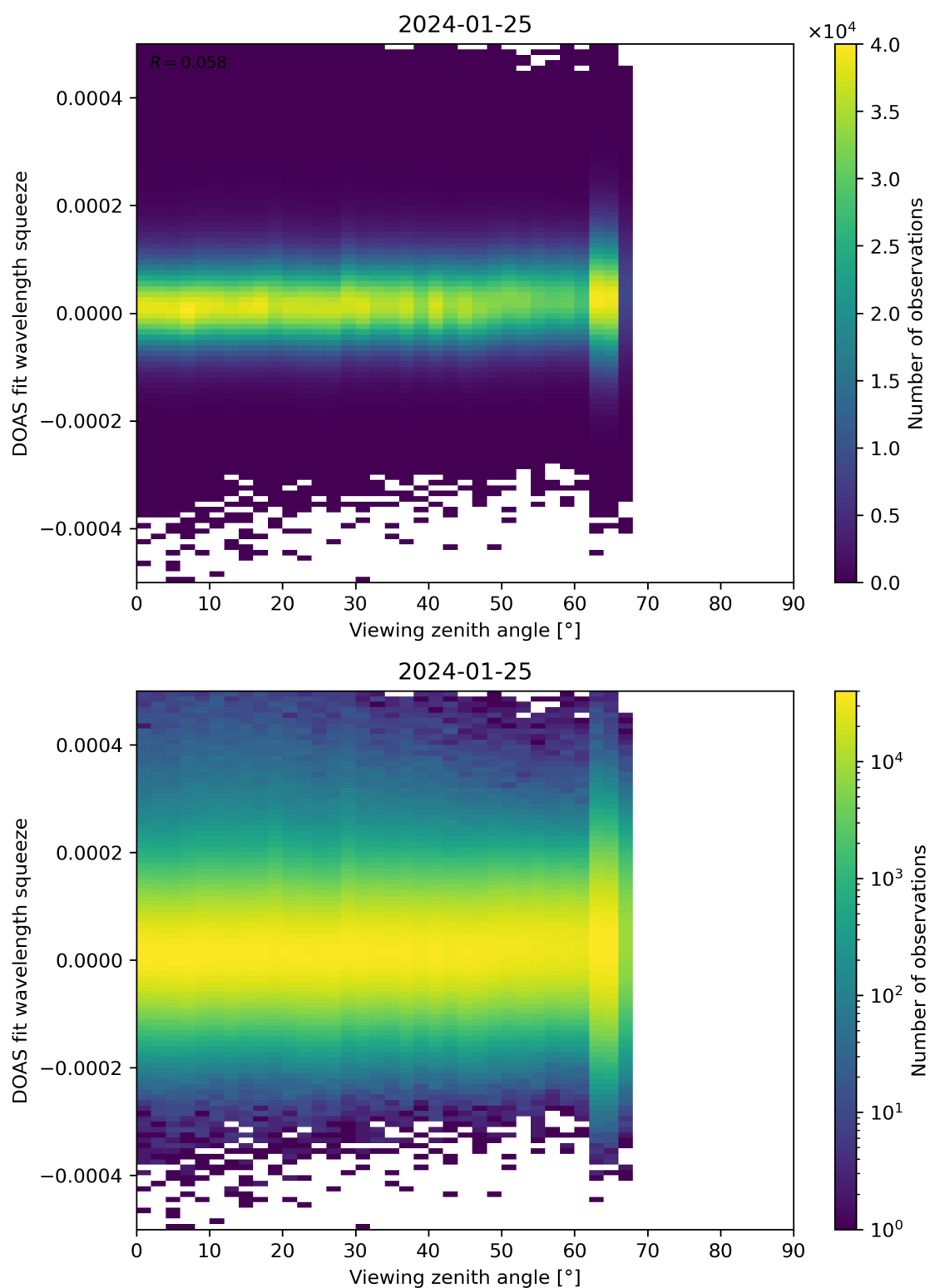
Figure 184: Scatter density plot of “Viewing zenith angle” against “DOAS fit wavelength squeeze” for 2024-01-24 to 2024-01-26.
