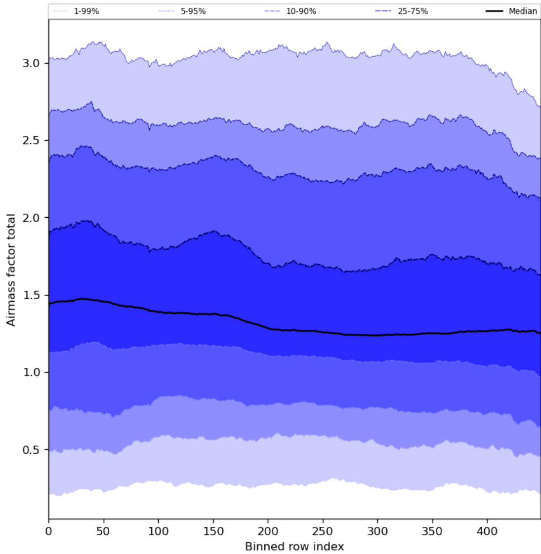
Figure 54: Along track statistics of “Airmass factor total” for 2024-01-24 to 2024-01-26
