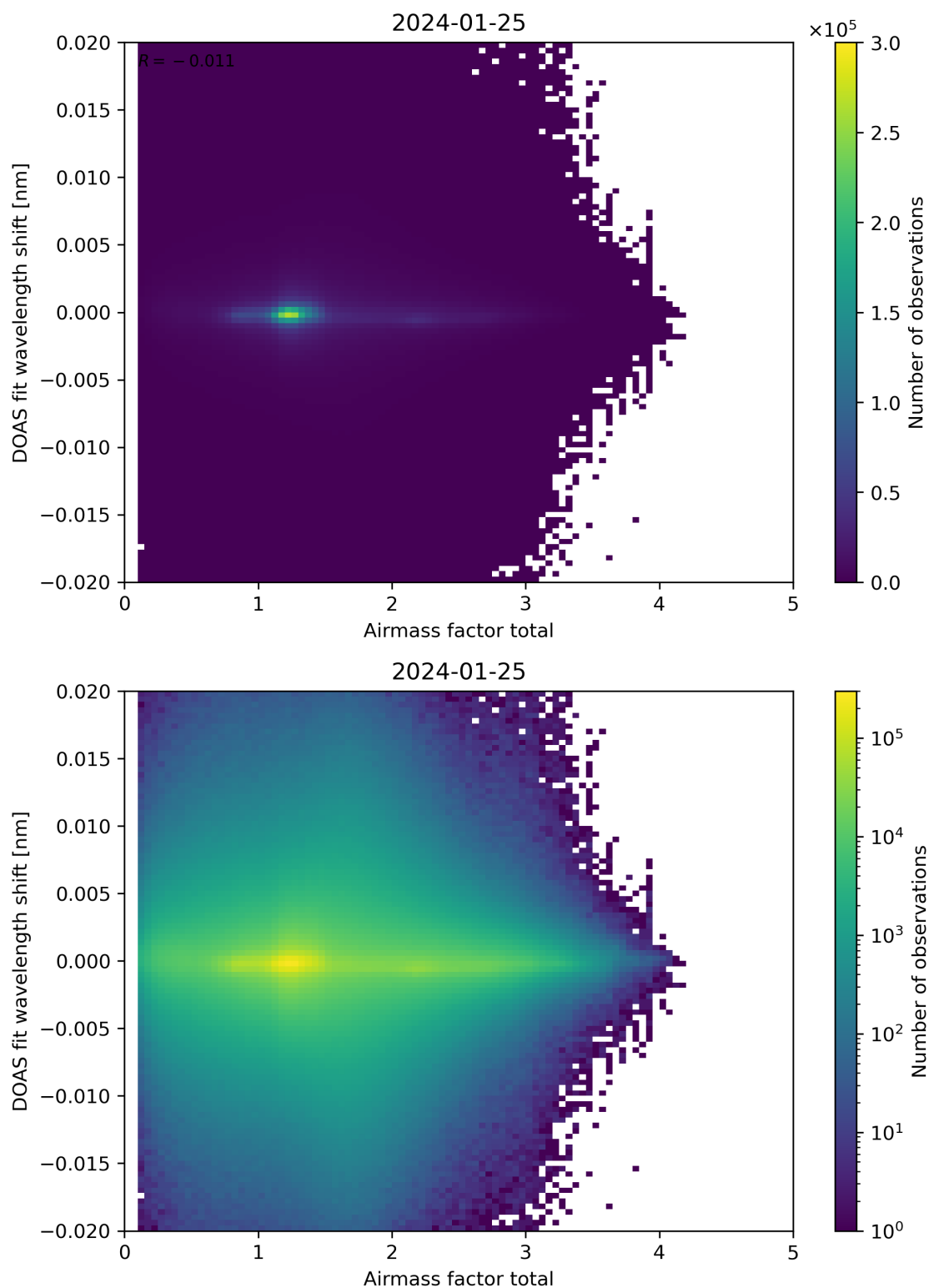
Figure 98: Scatter density plot of “Airmass factor total” against “DOAS fit wavelength shift” for 2024-01-24 to 2024-01-26.
