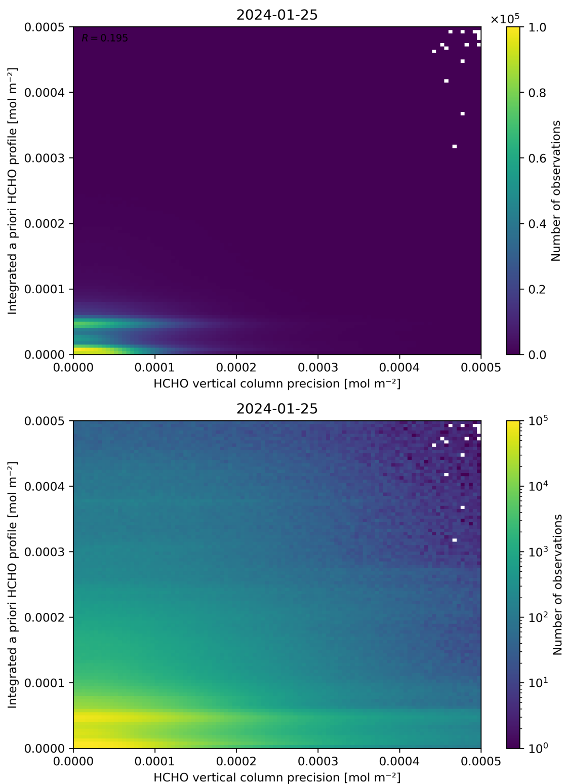
Figure 147: Scatter density plot of “HCHO vertical column precision” against “Integrated a priori HCHO profile” for 2024-01-24 to 2024-01-26.
