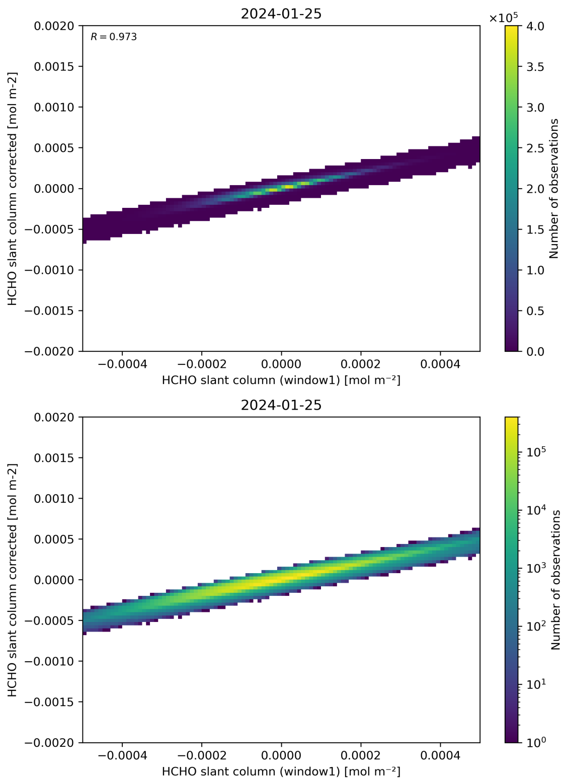
Figure 82: Scatter density plot of “HCHO slant column (window1)” against “HCHO slant column corrected” for 2024-01-24 to 2024-01-26.
