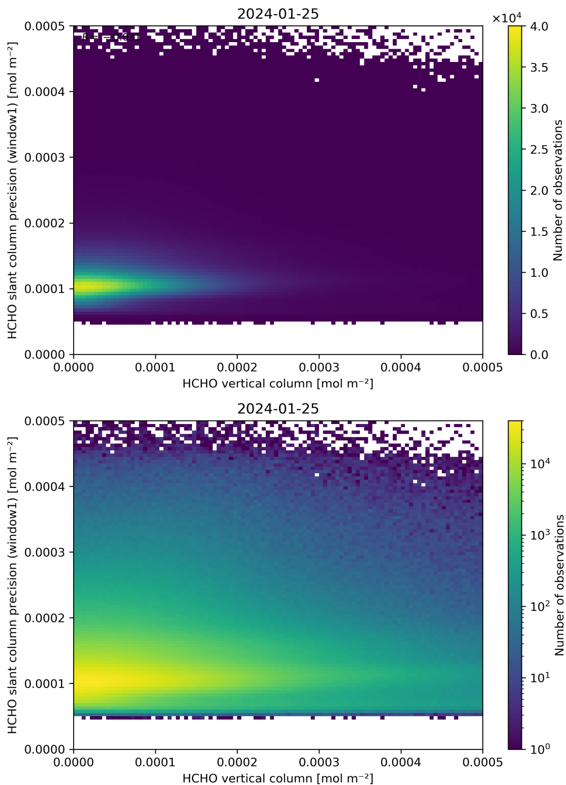
Figure 130: Scatter density plot of “HCHO vertical column” against “HCHO slant column precision (window1)” for 2024-01-24 to 2024-01-26.
