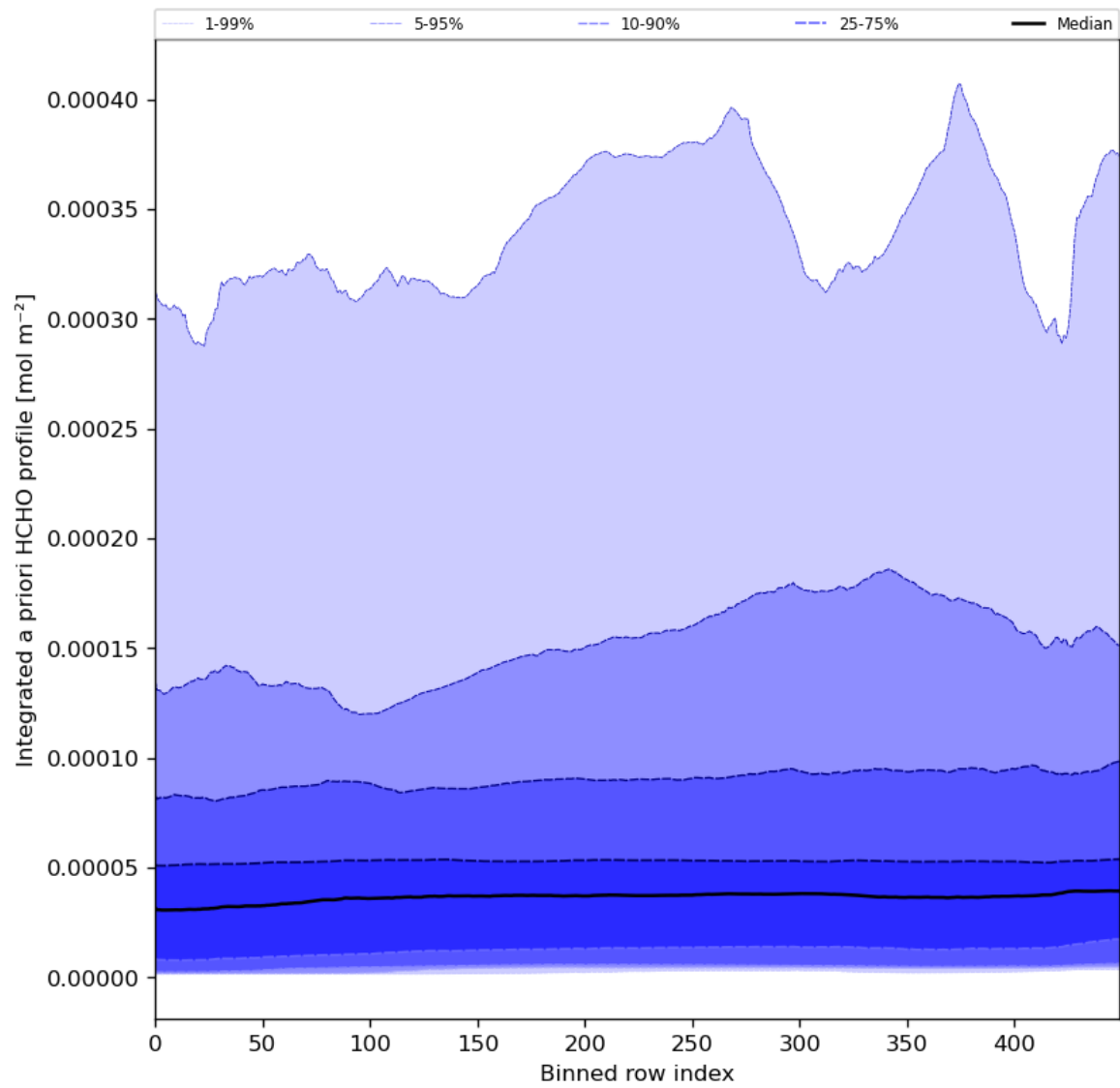
Figure 57: Along track statistics of “Integrated a priori HCHO profile” for 2024-01-24 to 2024-01-26
