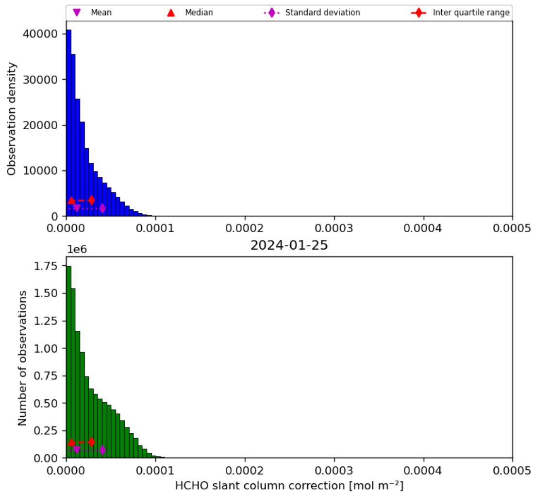
Figure 47: Histogram of “HCHO slant column correction” for 2024-01-24 to 2024-01-26
