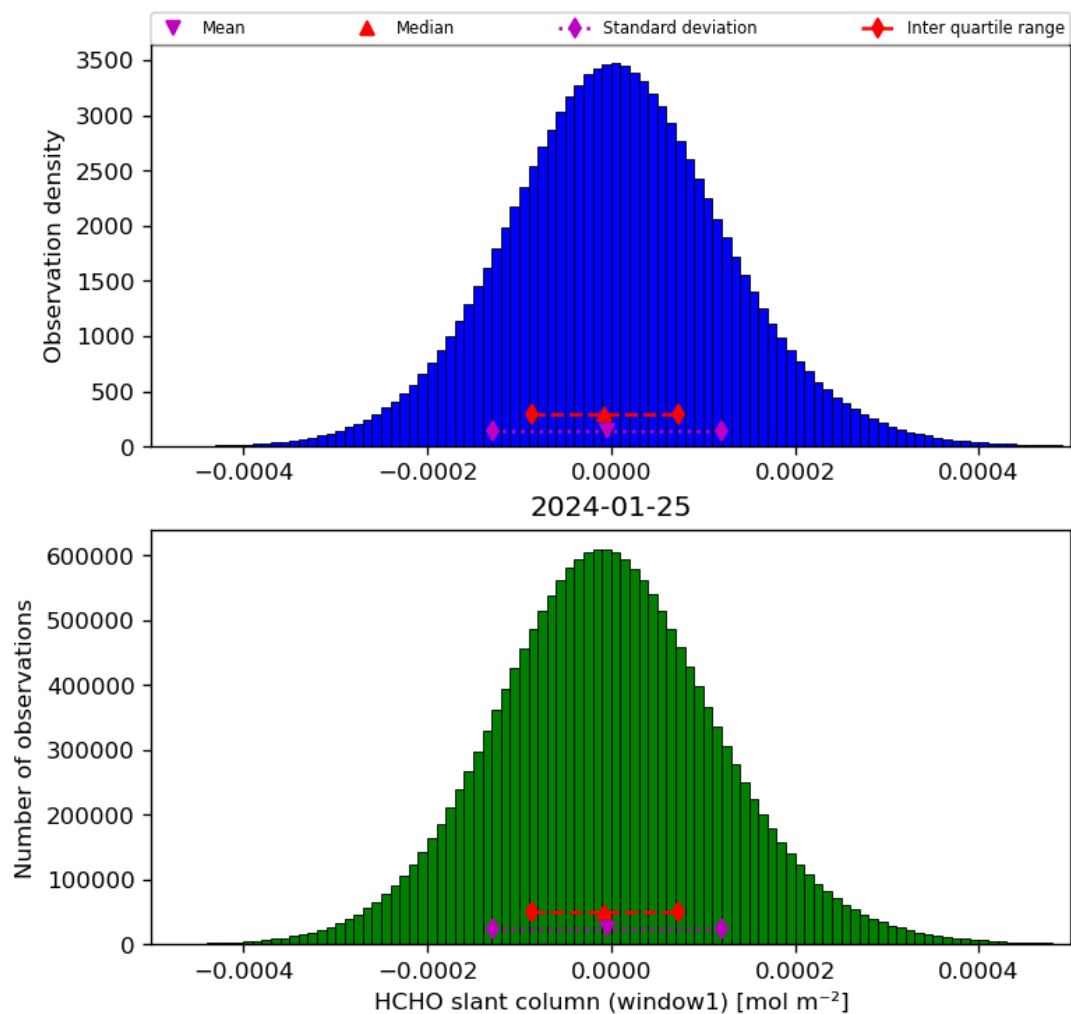
Figure 38: Histogram of “HCHO slant column (window1)” for 2024-01-24 to 2024-01-26
