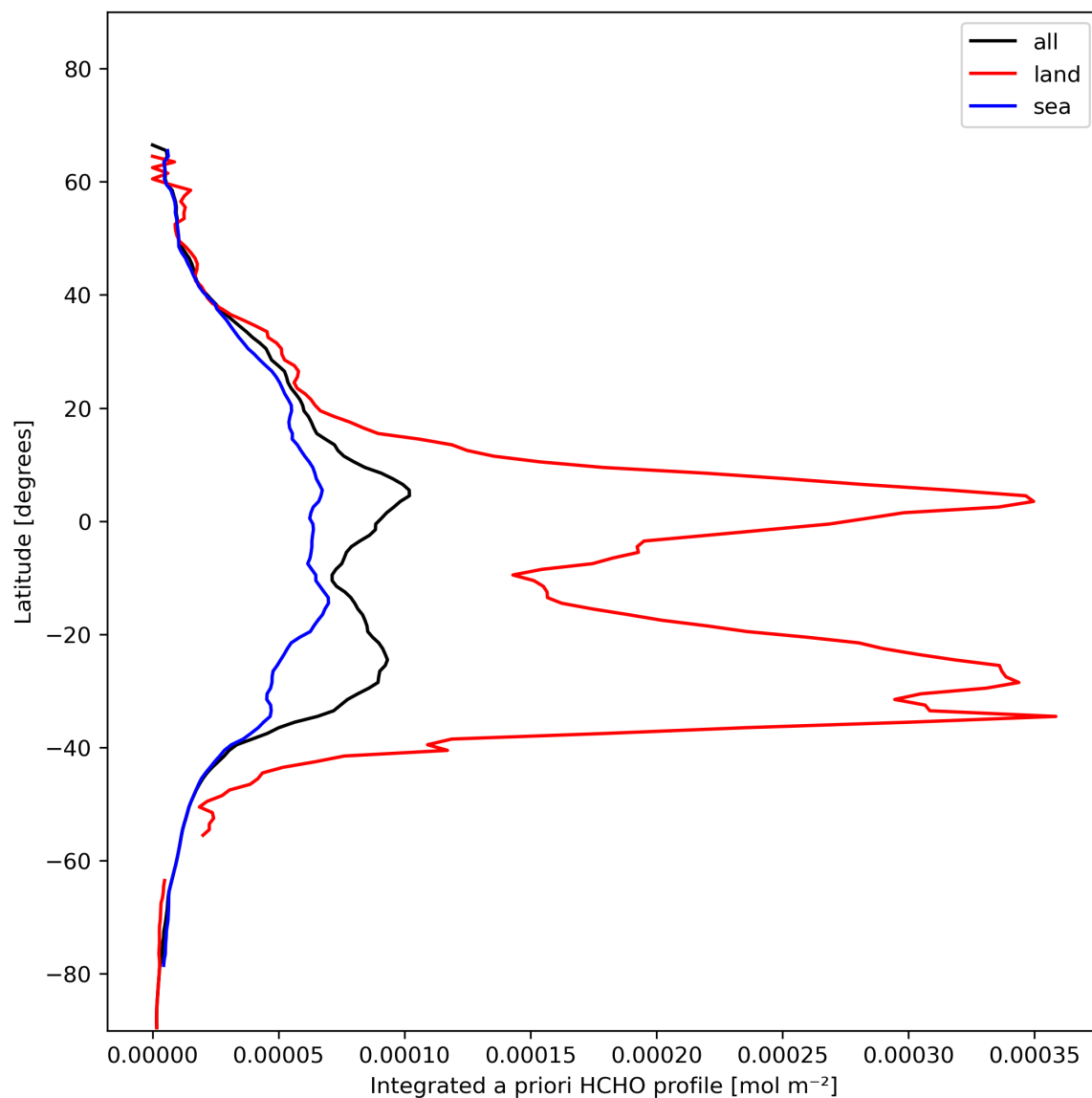
Figure 29: Zonal average of “Integrated a priori HCHO profile” for 2024-01-24 to 2024-01-26.
