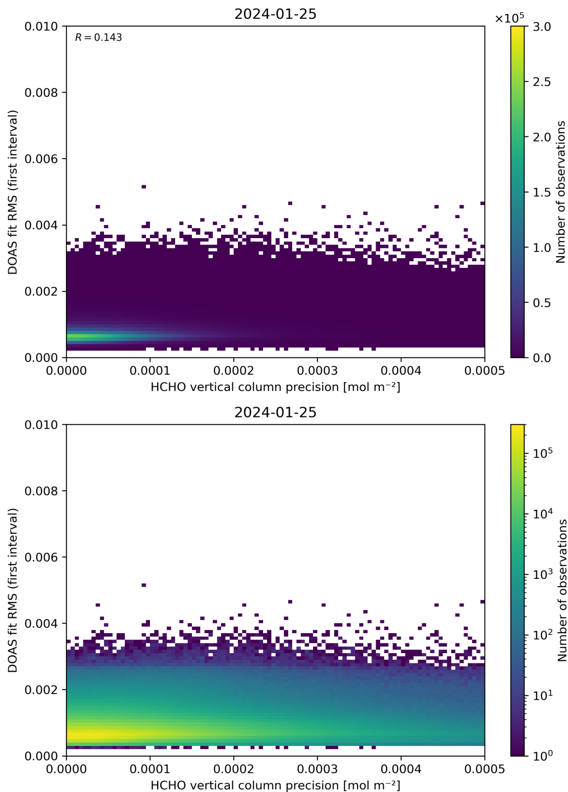
Figure 136: Scatter density plot of “HCHO vertical column precision” against “DOAS fit RMS (first interval)” for 2024-01-24 to 2024-01-26.
