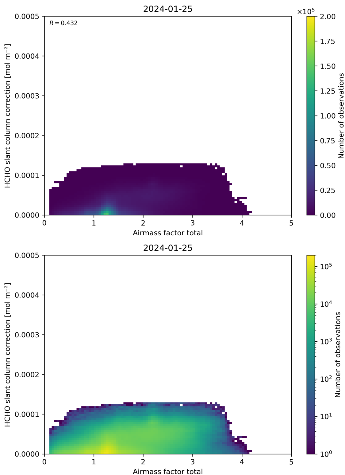
Figure 102: Scatter density plot of “Airmass factor total” against “HCHO slant column correction” for 2024-01-24 to 2024-01-26.
