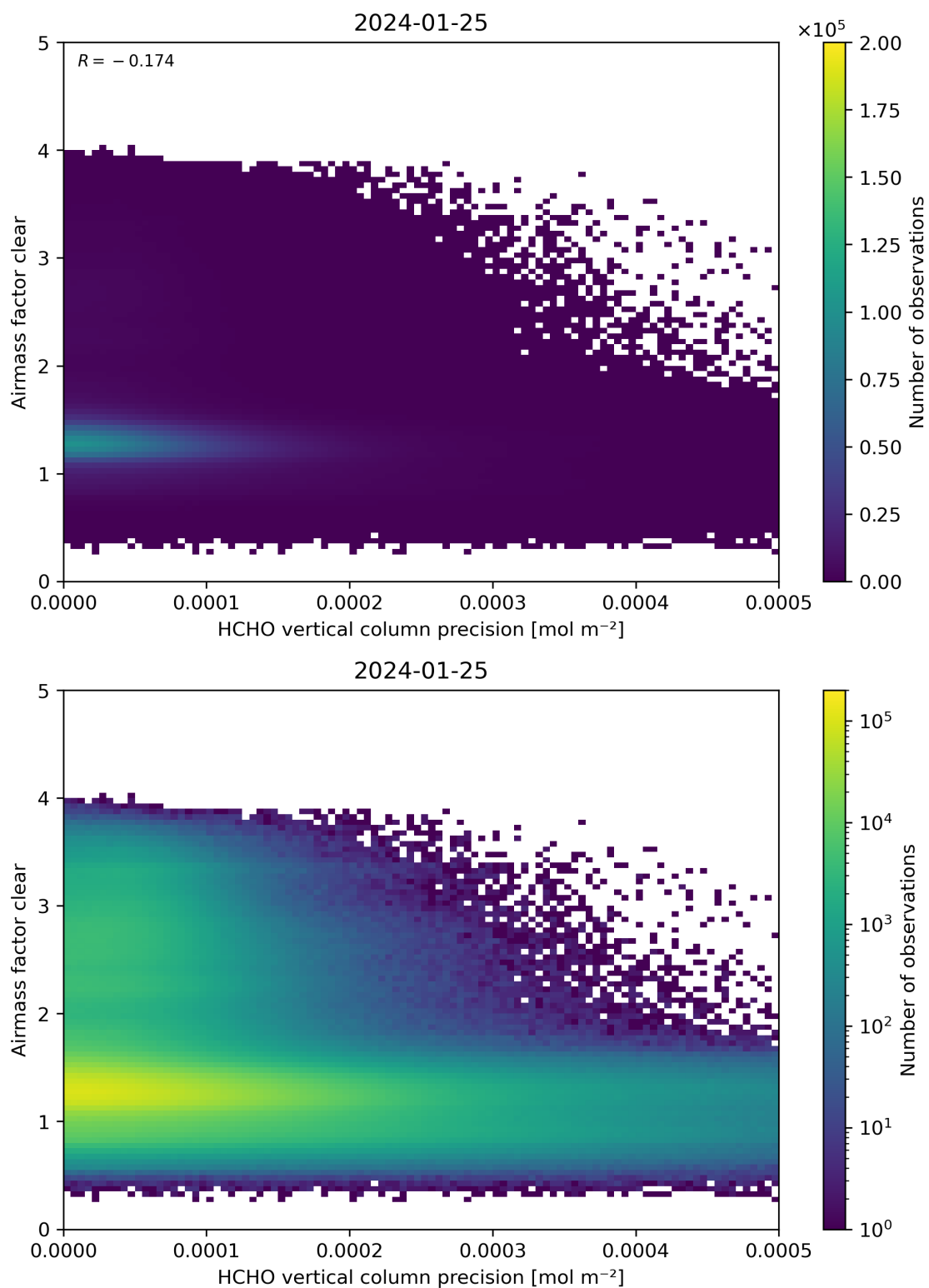
Figure 139: Scatter density plot of “HCHO vertical column precision” against “Airmass factor clear” for 2024-01-24 to 2024-01-26.
