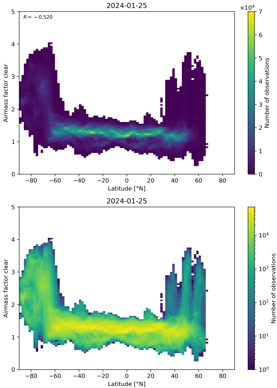
Figure 156: Scatter density plot of “Latitude” against “Airmass factor clear” for 2024-01-24 to 2024-01-26.
