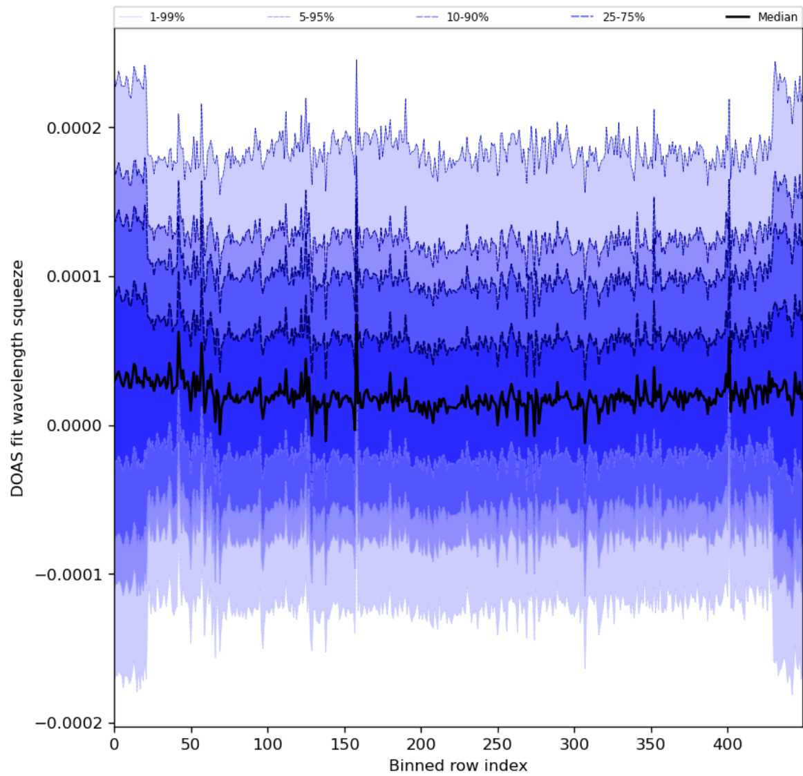
Figure 59: Along track statistics of “DOAS fit wavelength squeeze” for 2024-01-24 to 2024-01-26
