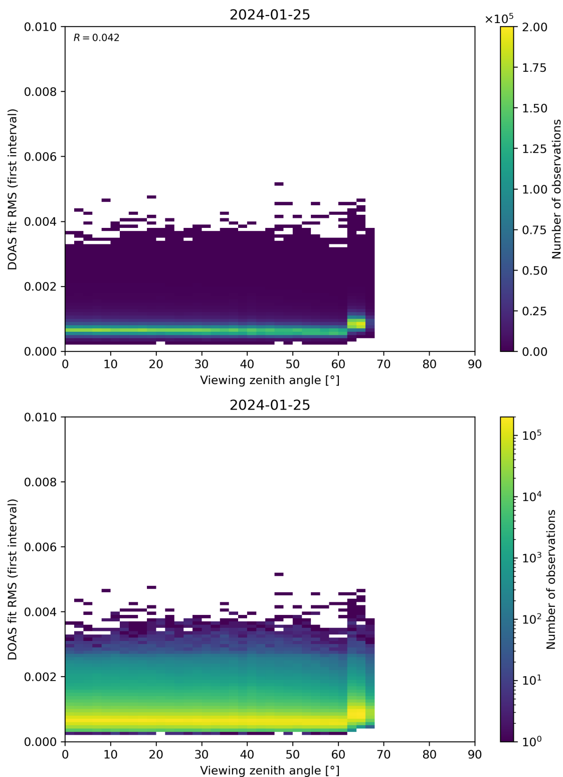
Figure 182: Scatter density plot of “Viewing zenith angle” against “DOAS fit RMS (first interval)” for 2024-01-24 to 2024-01-26.
