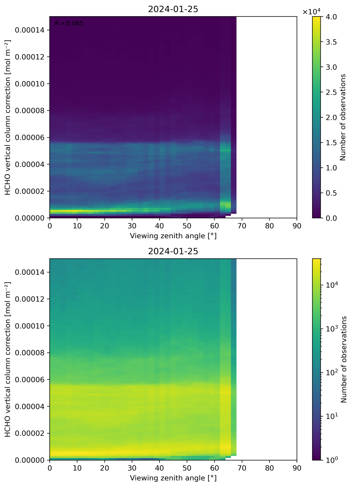
Figure 193: Scatter density plot of “Viewing zenith angle” against “HCHO vertical column correction” for 2024-01-24 to 2024-01-26.
