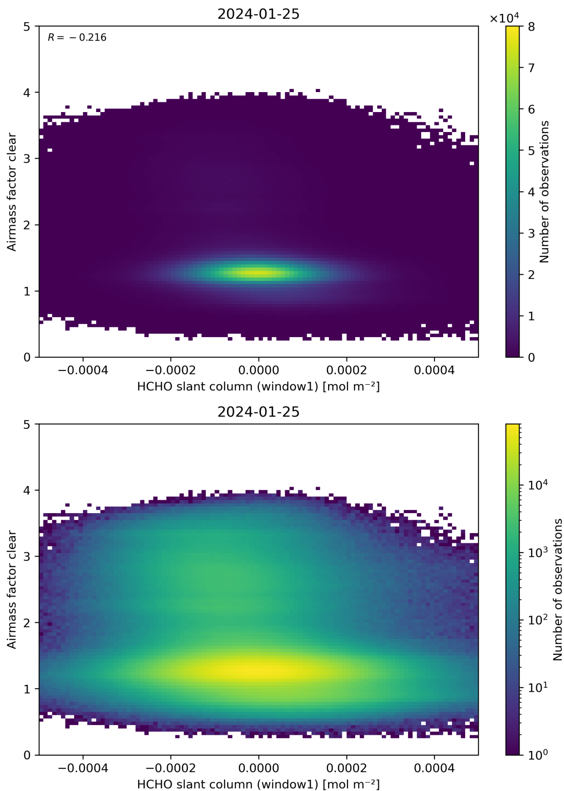
Figure 81: Scatter density plot of “HCHO slant column (window1)” against “Airmass factor clear” for 2024-01-24 to 2024-01-26.
