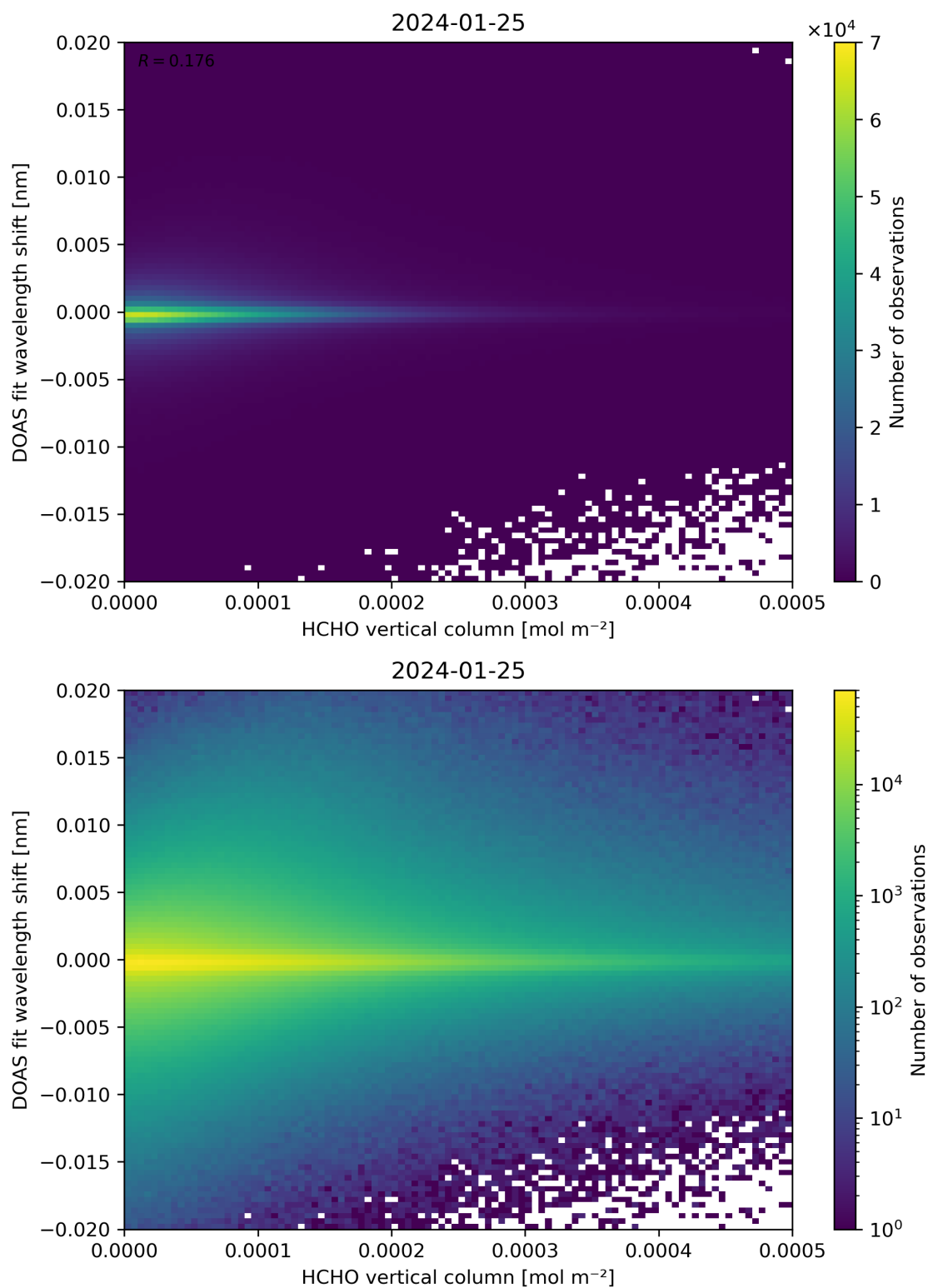
Figure 124: Scatter density plot of “HCHO vertical column” against “DOAS fit wavelength shift” for 2024-01-24 to 2024-01-26.
