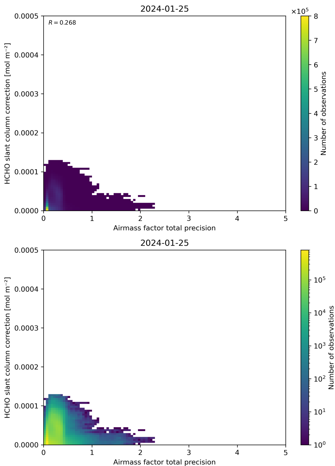
Figure 110: Scatter density plot of “Airmass factor total precision” against “HCHO slant column correction” for 2024-01-24 to 2024-01-26.
