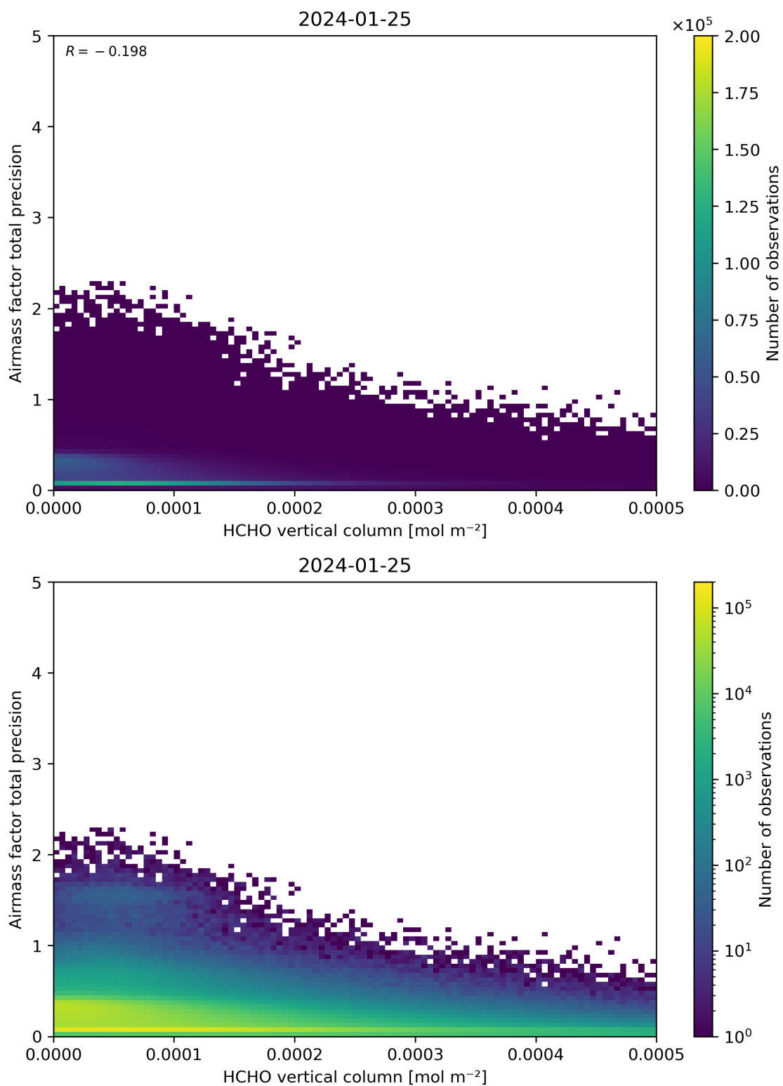
Figure 132: Scatter density plot of “HCHO vertical column” against “Airmass factor total precision” for 2024-01-24 to 2024-01-26.
