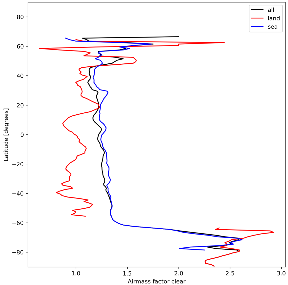
Figure 28: Zonal average of “Airmass factor clear” for 2024-01-24 to 2024-01-26.
