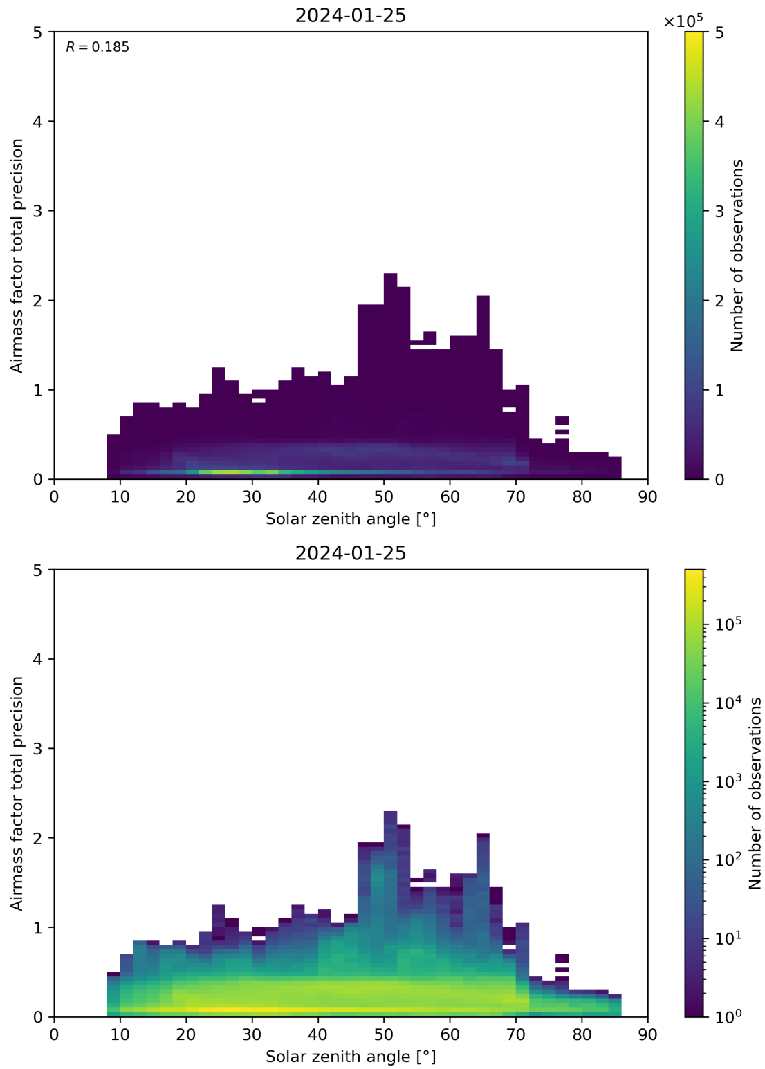
Figure 176: Scatter density plot of “Solar zenith angle” against “Airmass factor total precision” for 2024-01-24 to 2024-01-26.
