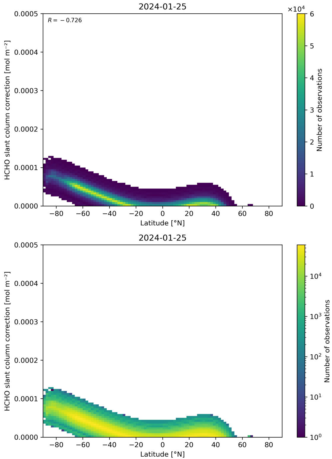
Figure 158: Scatter density plot of “Latitude” against “HCHO slant column correction” for 2024-01-24 to 2024-01-26.
