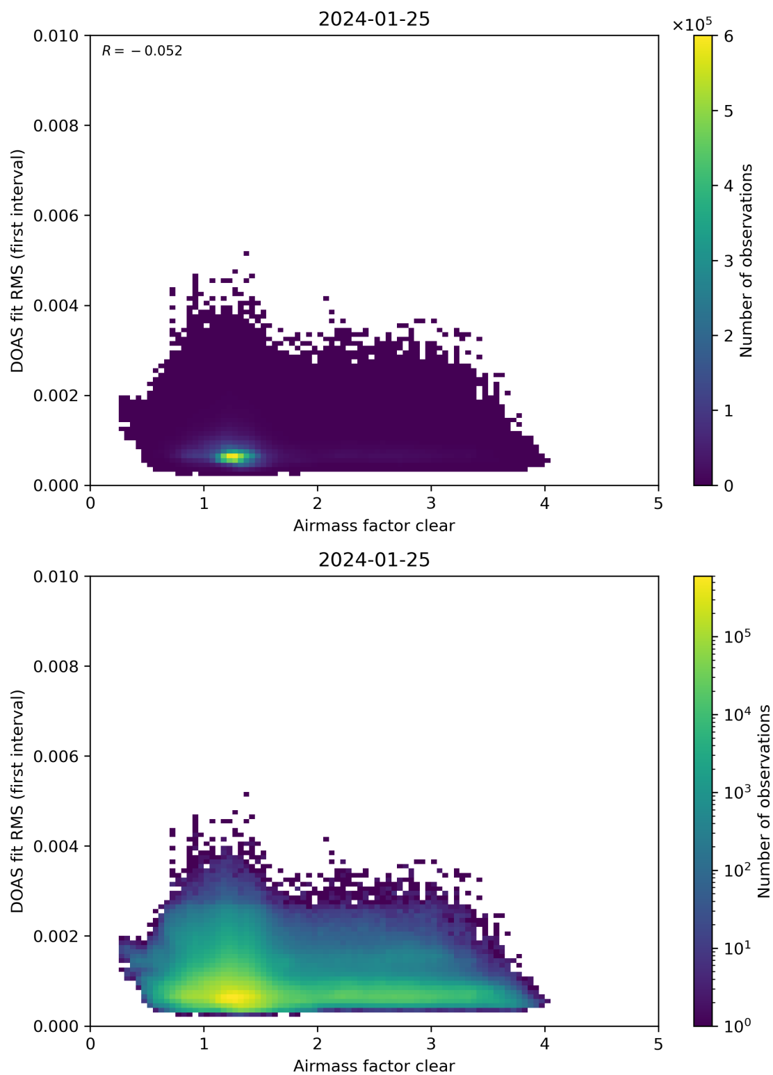
Figure 71: Scatter density plot of “Airmass factor clear” against “DOAS fit RMS (first interval)” for 2024-01-24 to 2024-01-26.
