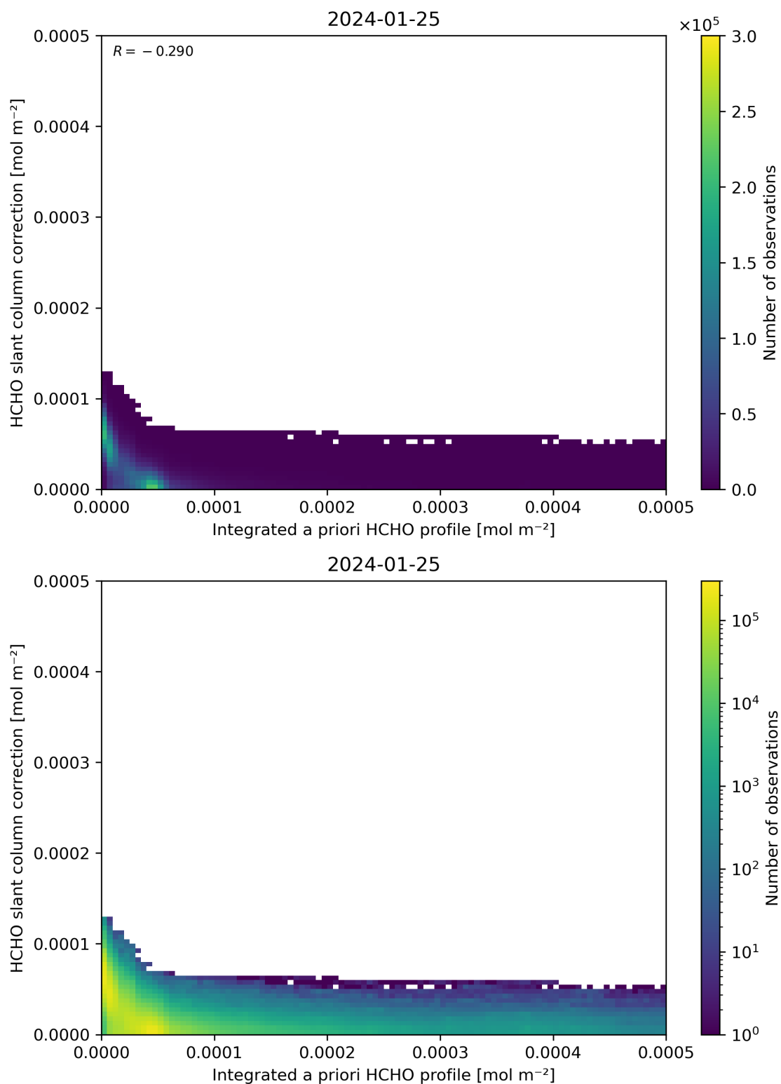
Figure 152: Scatter density plot of “Integrated a priori HCHO profile” against “HCHO slant column correction” for 2024-01-24 to 2024-01-26.
