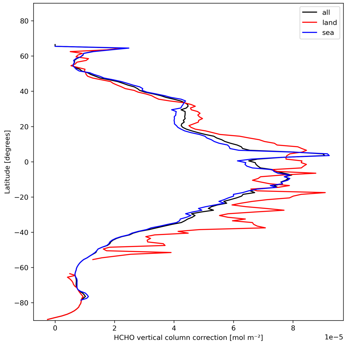
Figure 23: Zonal average of “HCHO vertical column correction” for 2024-01-24 to 2024-01-26.
