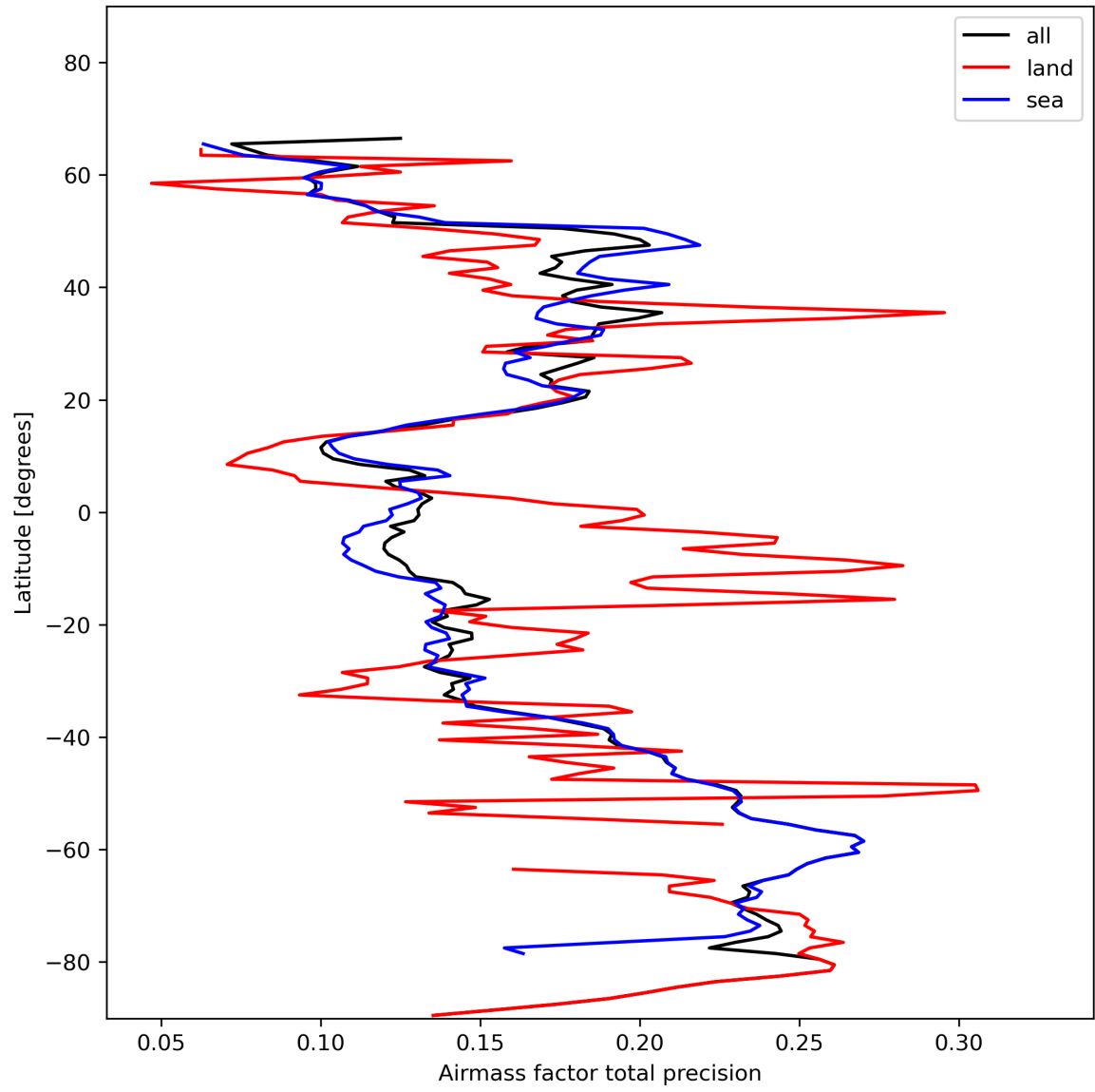
Figure 27: Zonal average of “Airmass factor total precision” for 2024-01-24 to 2024-01-26.
