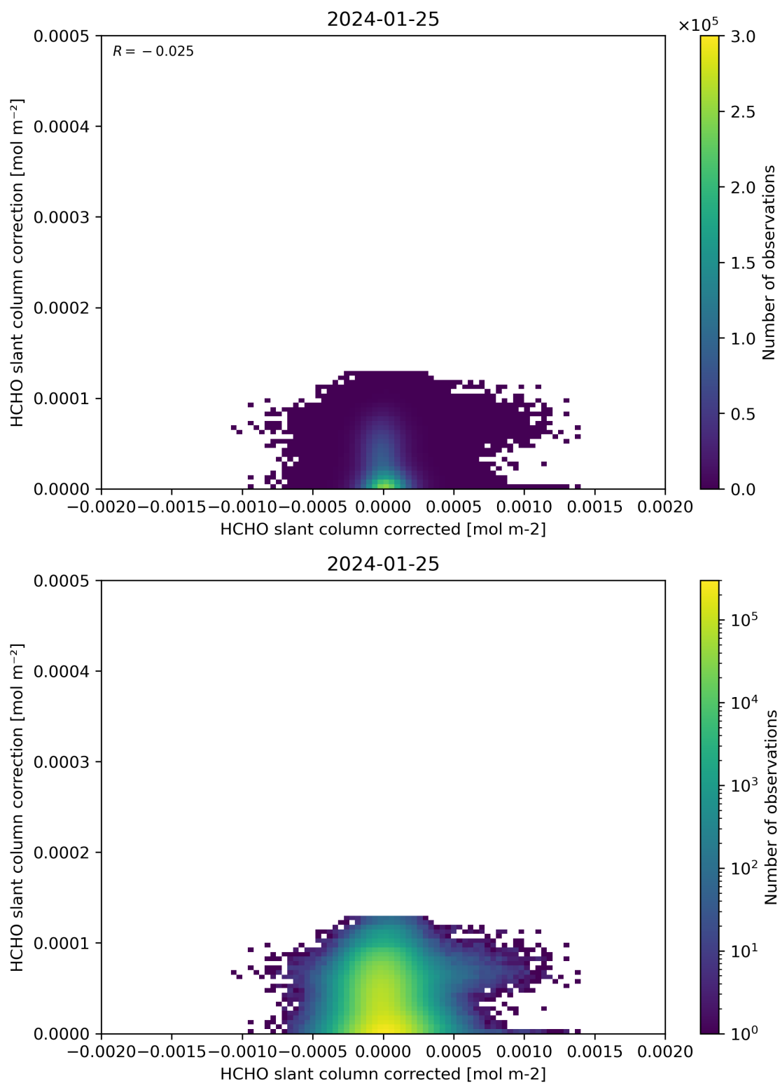
Figure 77: Scatter density plot of “HCHO slant column corrected” against “HCHO slant column correction” for 2024-01-24 to 2024-01-26.
