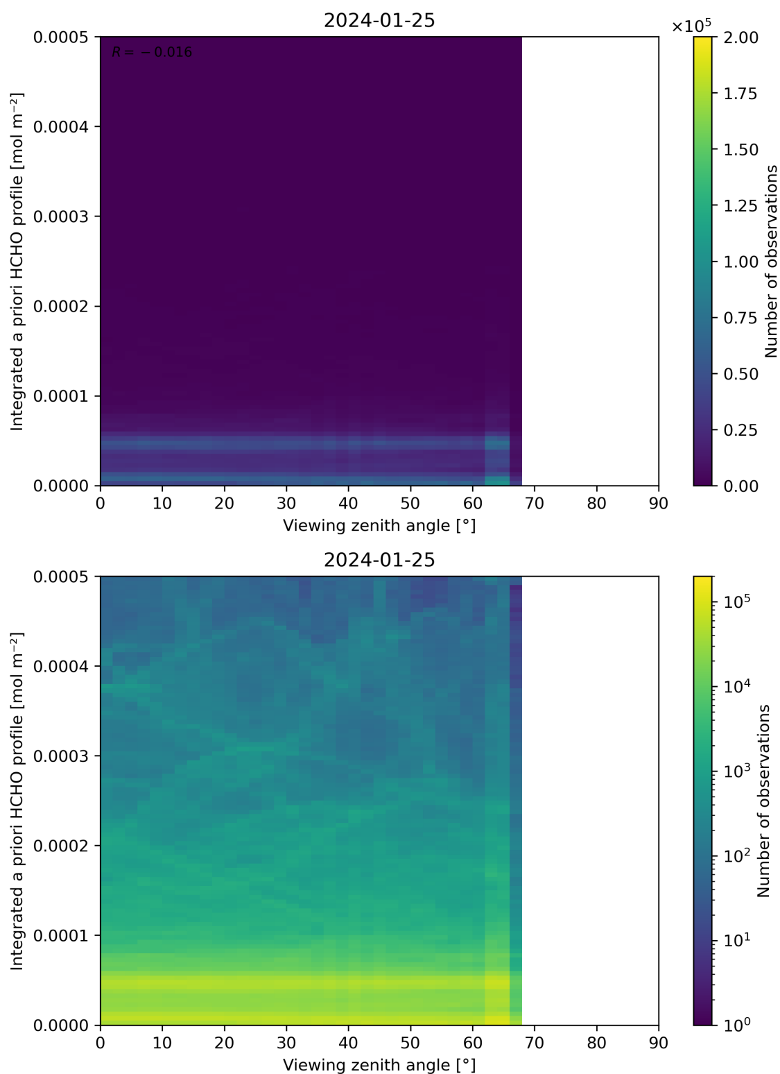
Figure 195: Scatter density plot of “Viewing zenith angle” against “Integrated a priori HCHO profile” for 2024-01-24 to 2024-01-26.
