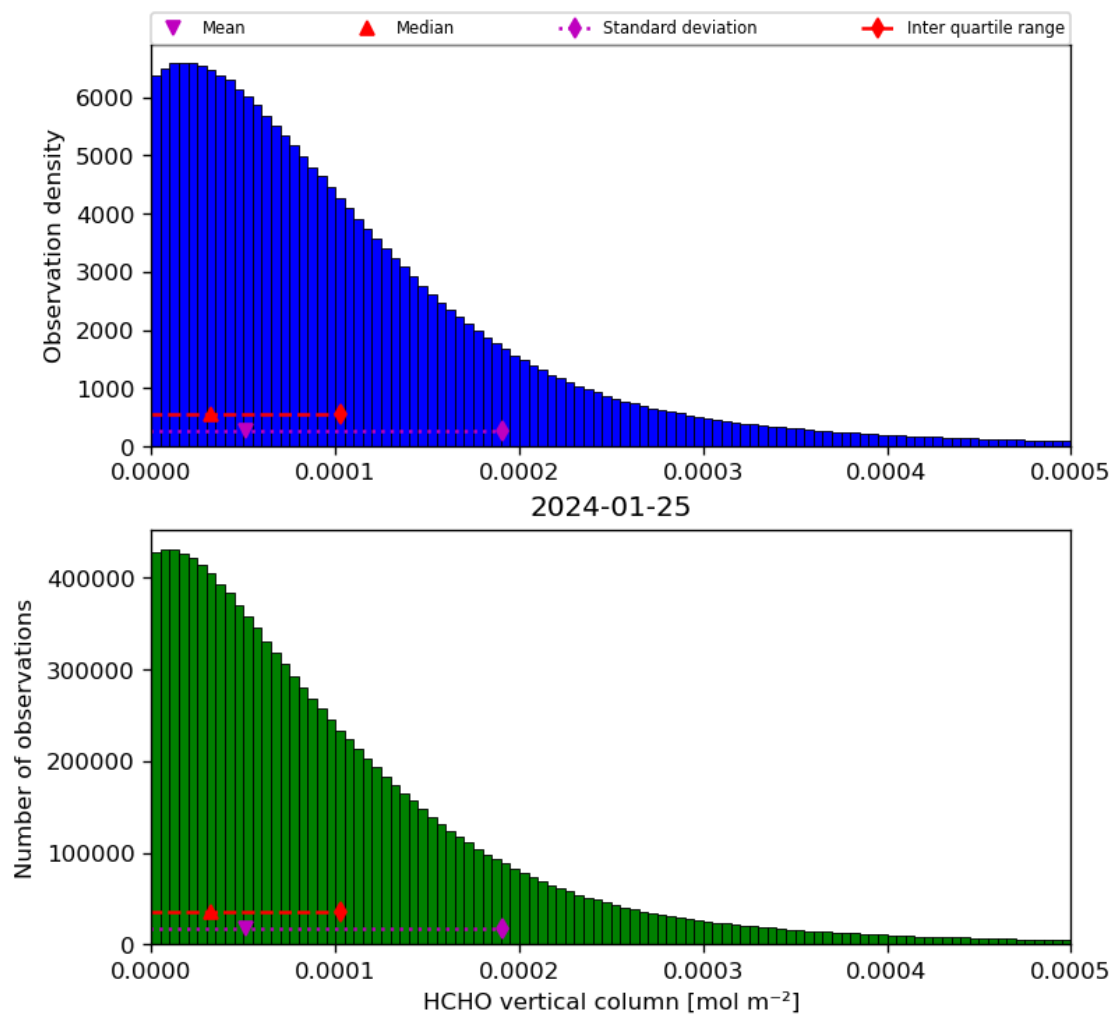
Figure 35: Histogram of “HCHO vertical column” for 2024-01-24 to 2024-01-26
