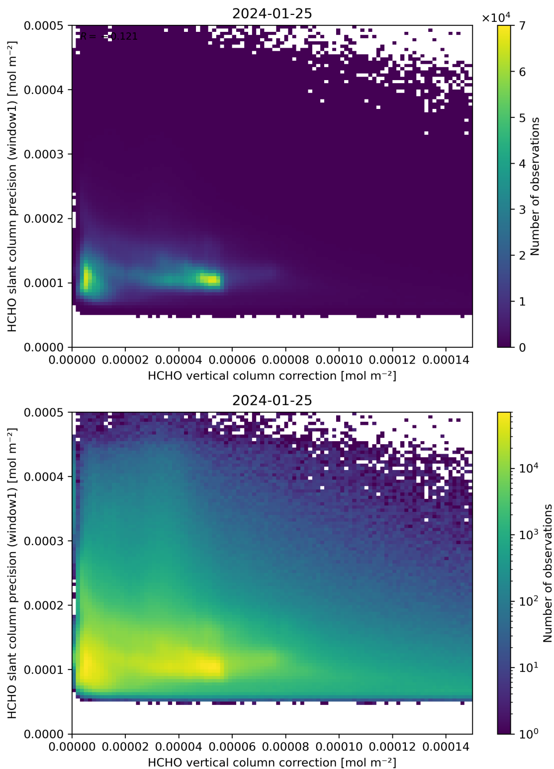
Figure 119: Scatter density plot of “HCHO vertical column correction” against “HCHO slant column precision (window1)” for 2024-01-24 to 2024-01-26.
