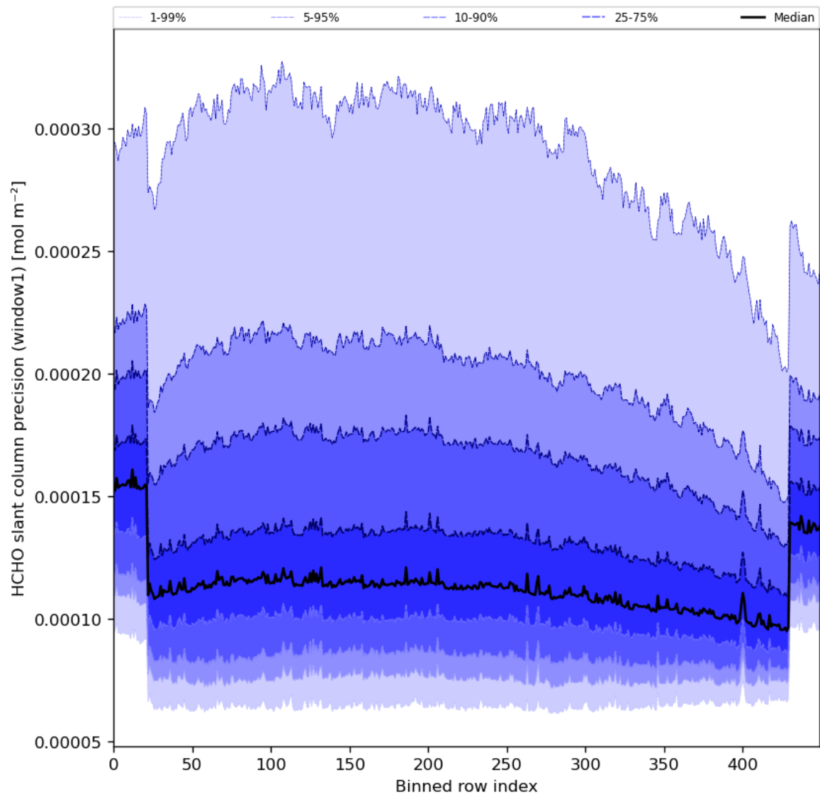
Figure 53: Along track statistics of “HCHO slant column precision (window1)” for 2024-01-24 to 2024-01-26
