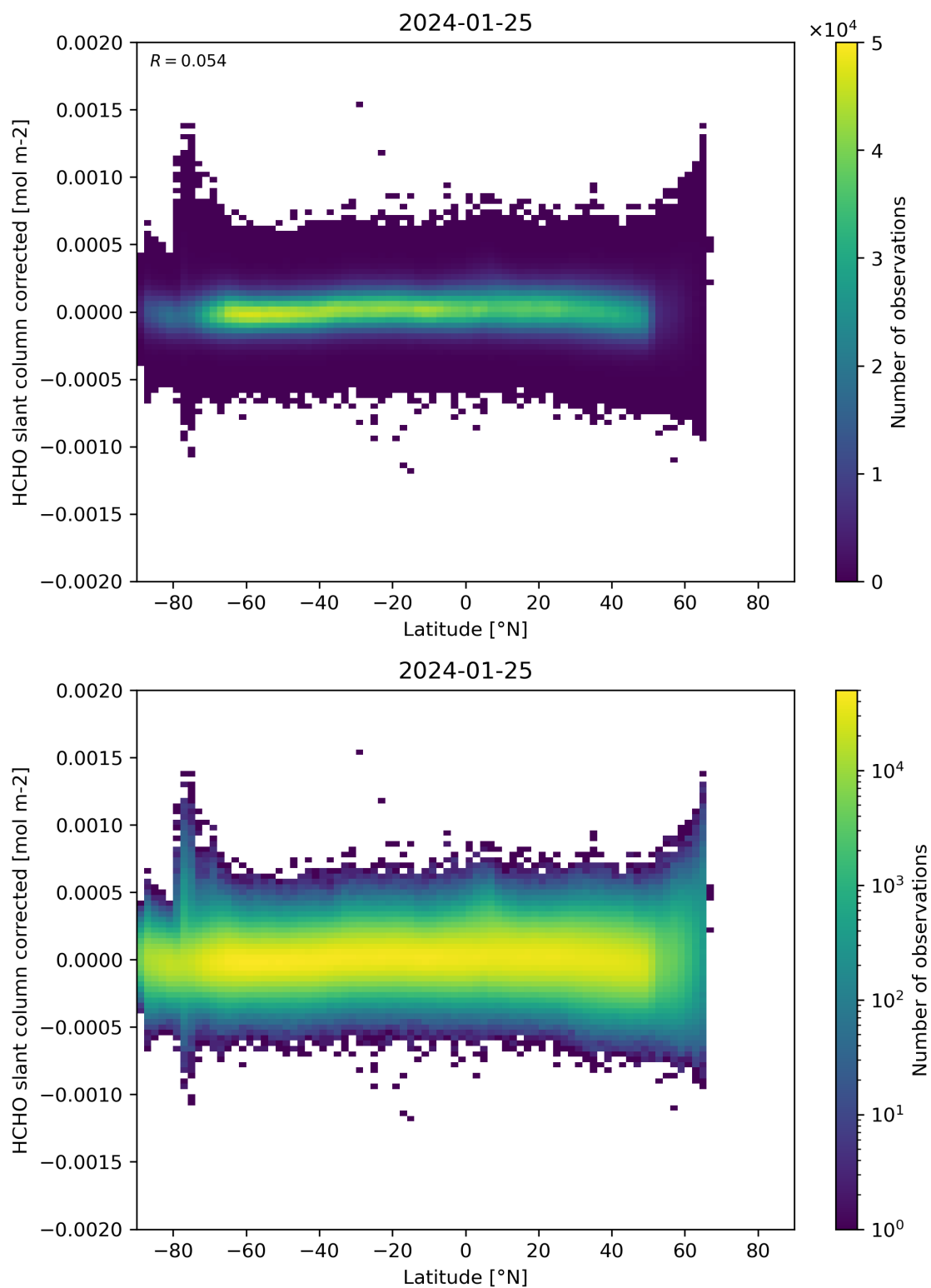
Figure 157: Scatter density plot of “Latitude” against “HCHO slant column corrected” for 2024-01-24 to 2024-01-26.
