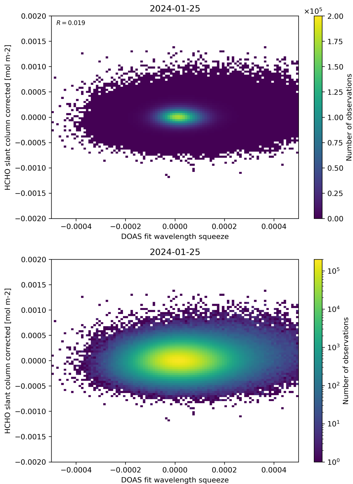
Figure 69: Scatter density plot of “DOAS fit wavelength squeeze” against “HCHO slant column corrected” for 2024-01-24 to 2024-01-26.
