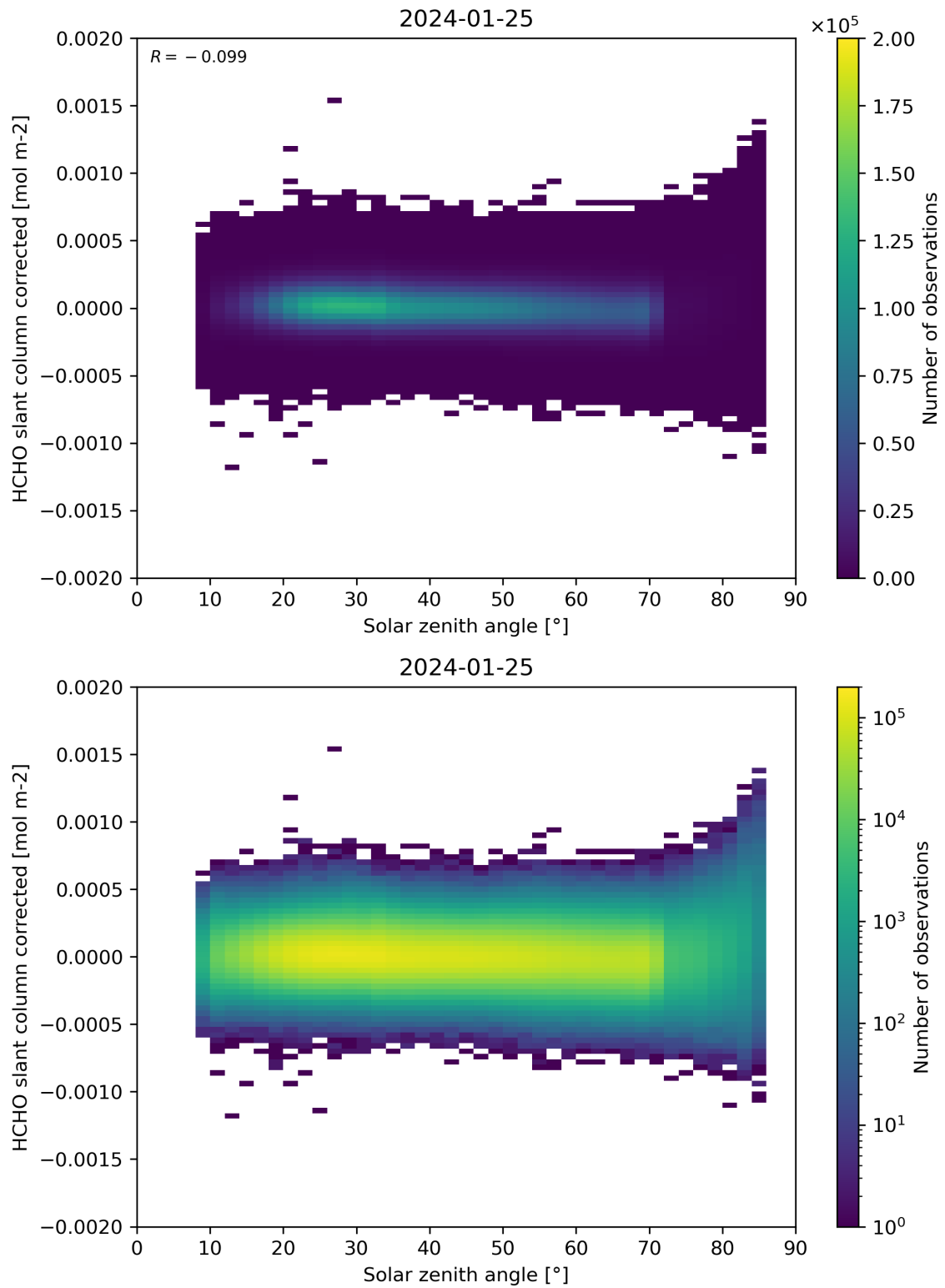
Figure 171: Scatter density plot of “Solar zenith angle” against “HCHO slant column corrected” for 2024-01-24 to 2024-01-26.
