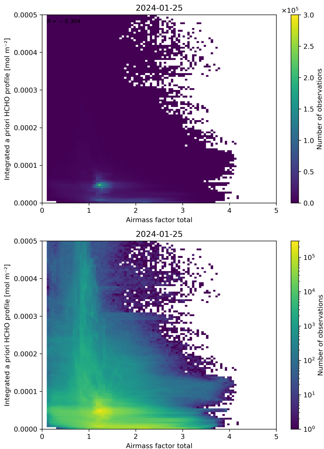
Figure 104: Scatter density plot of “Air mass factor total” against “Integrated a priori HCHO profile” for 2024-01-24 to 2024-01-26.
