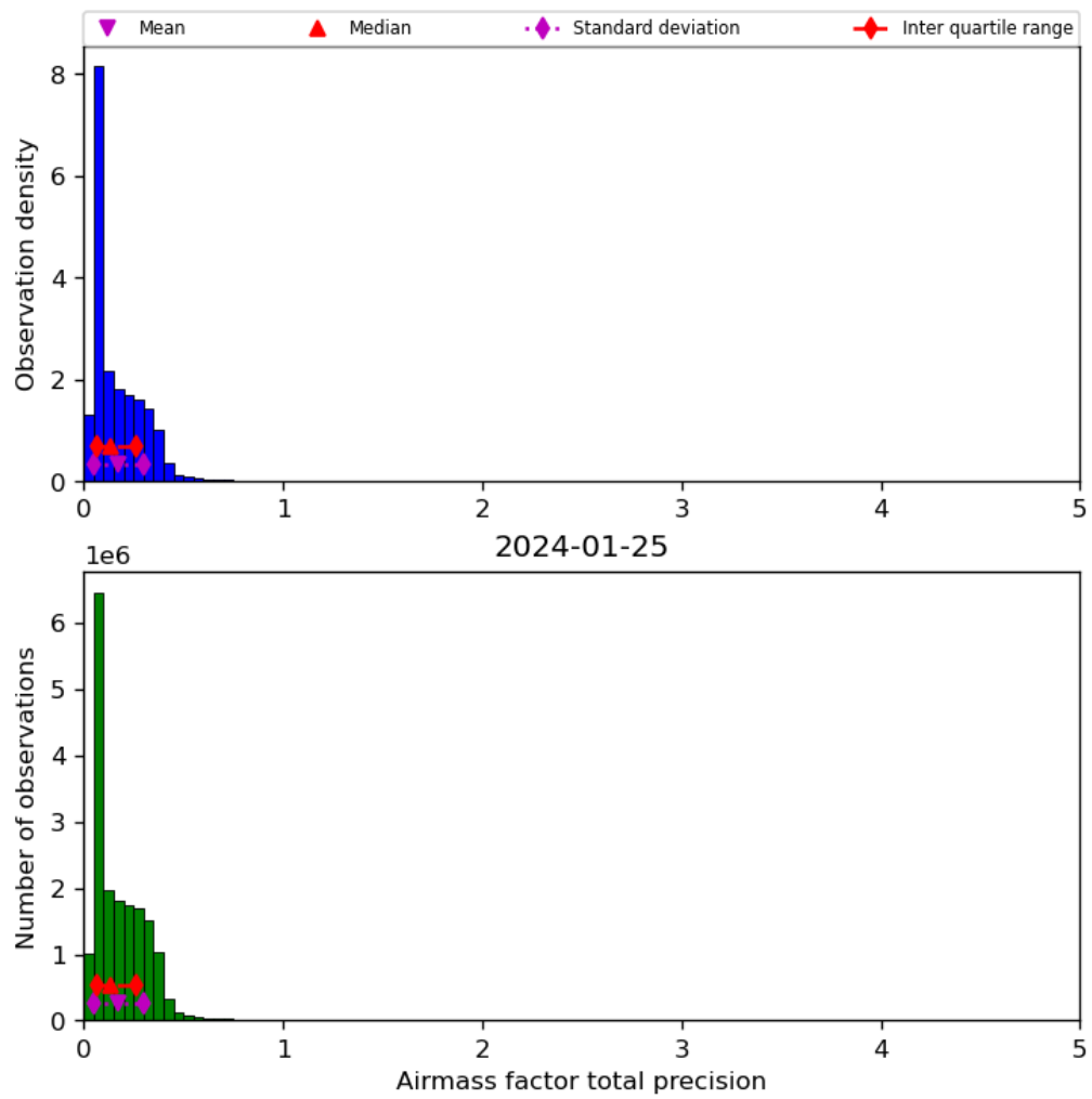
Figure 41: Histogram of “Airmass factor total precision” for 2024-01-24 to 2024-01-26
