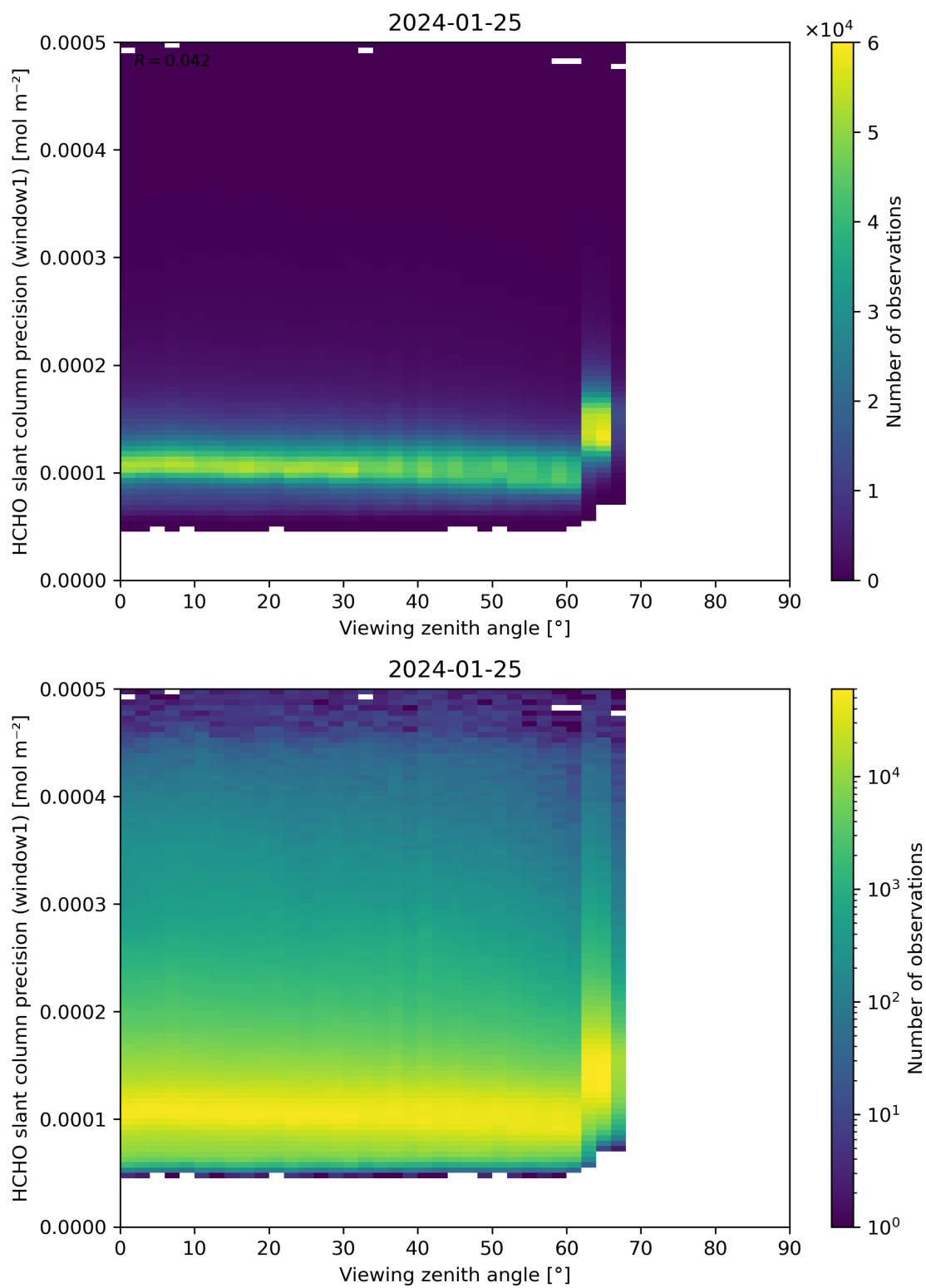
Figure 189: Scatter density plot of “Viewing zenith angle” against “HCHO slant column precision (window1)” for 2024-01-24 to 2024-01-26.
