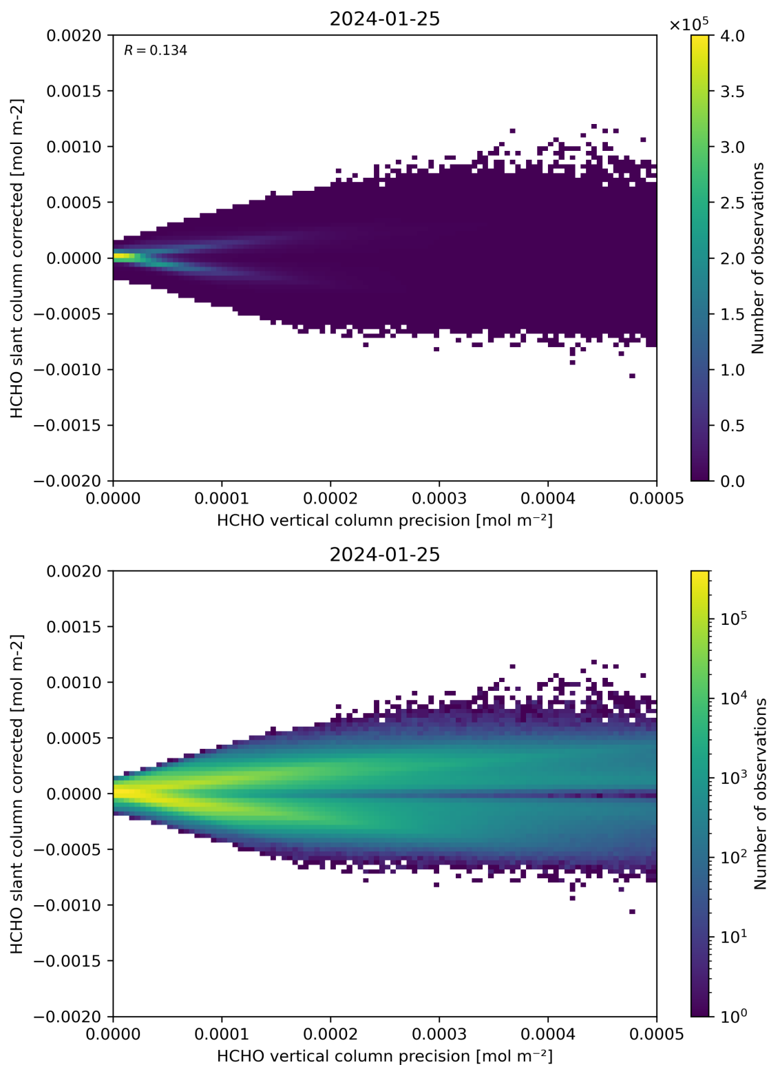
Figure 140: Scatter density plot of “HCHO vertical column precision” against “HCHO slant column corrected” for 2024-01-24 to 2024-01-26.
