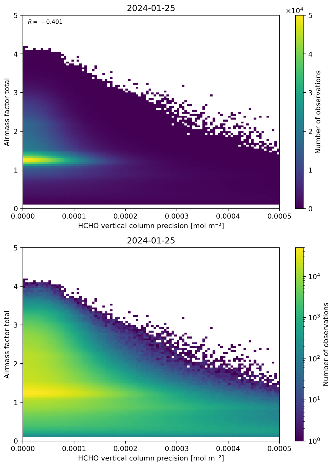
Figure 144: Scatter density plot of “HCHO vertical column precision” against “Airmass factor total” for 2024-01-24 to 2024-01-26.
