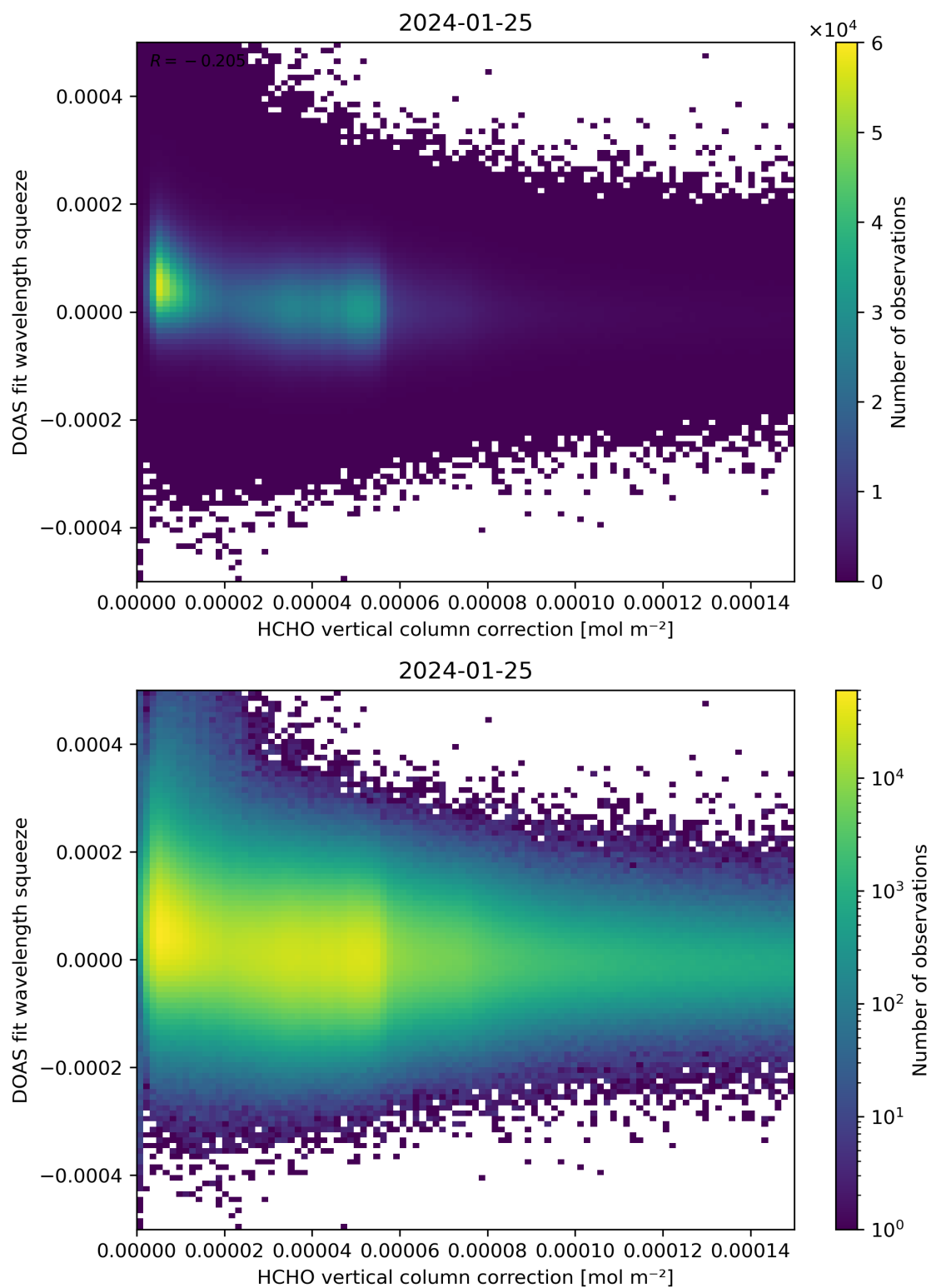
Figure 114: Scatter density plot of “HCHO vertical column correction” against “DOAS fit wavelength squeeze” for 2024-01-24 to 2024-01-26.
