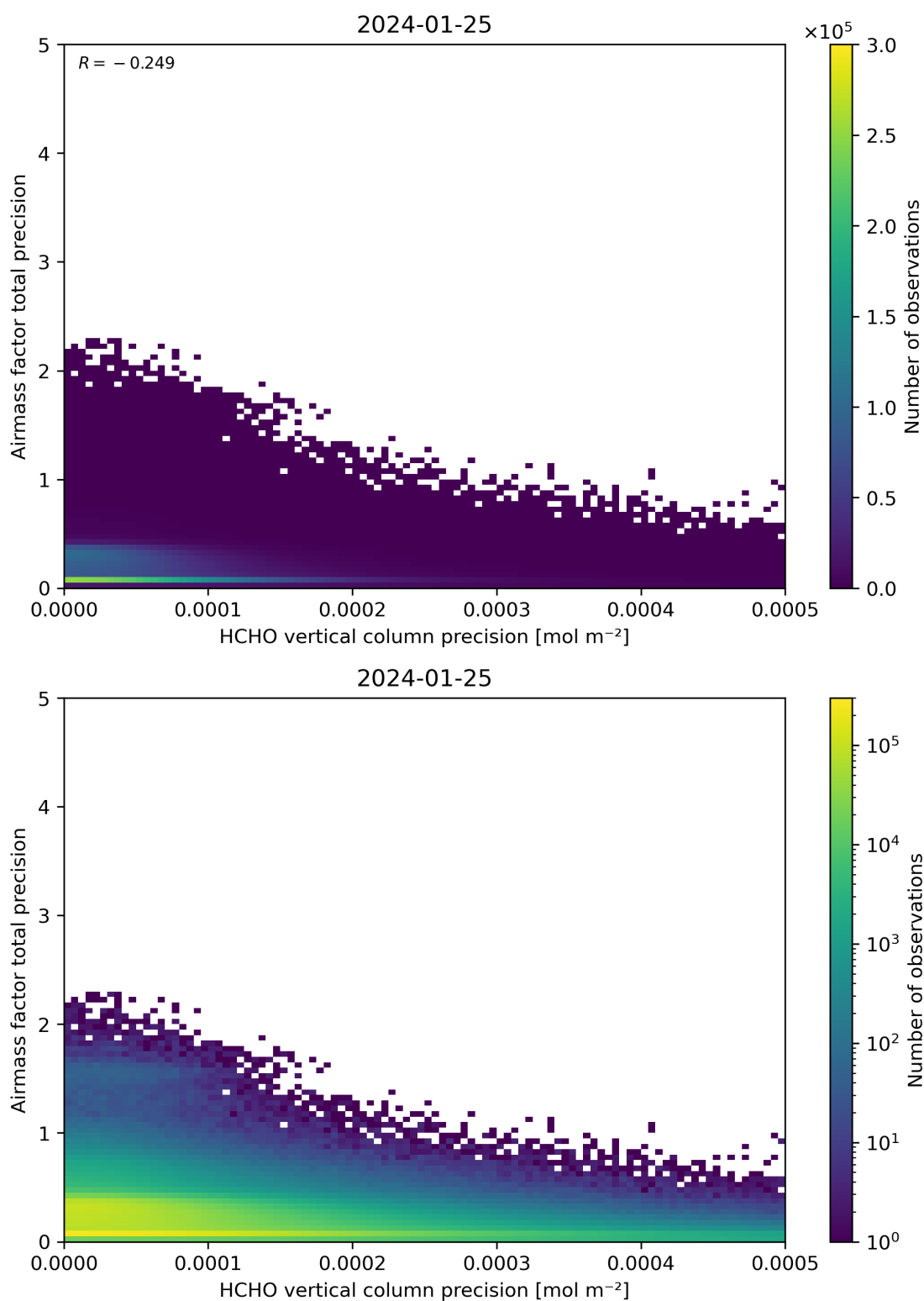
Figure 145: Scatter density plot of “HCHO vertical column precision” against “Airmass factor total precision” for 2024-01-24 to 2024-01-26.
