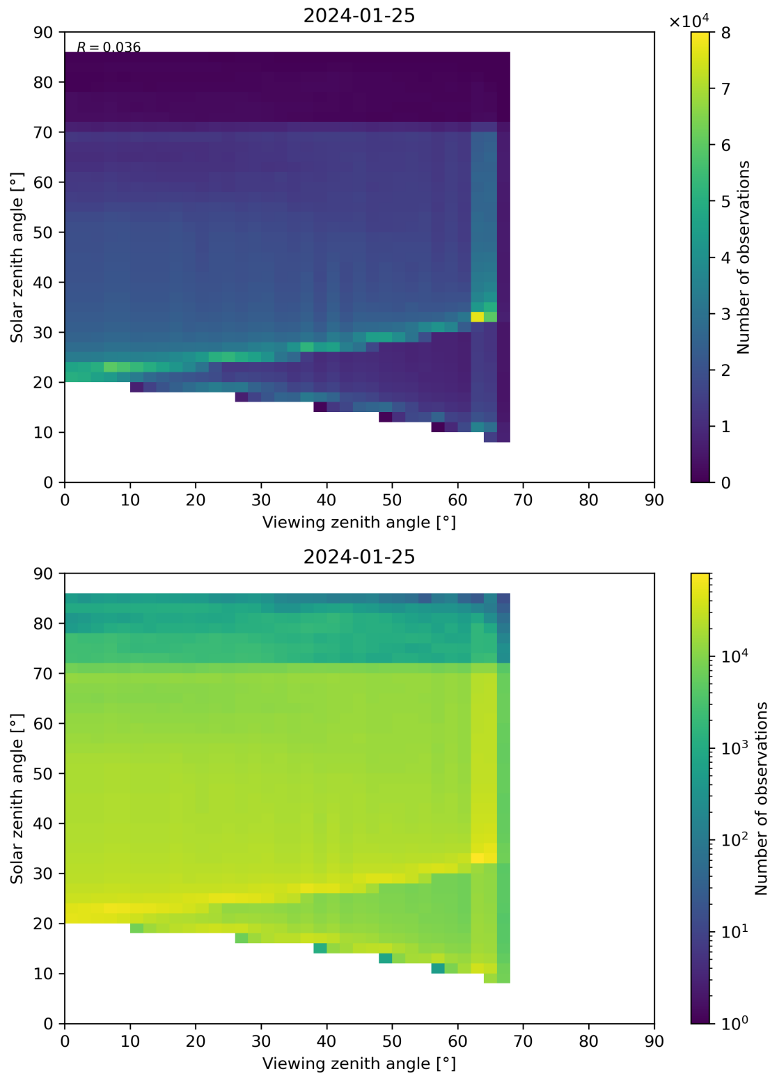
Figure 197: Scatter density plot of “Viewing zenith angle” against “Solar zenith angle” for 2024-01-24 to 2024-01-26.
