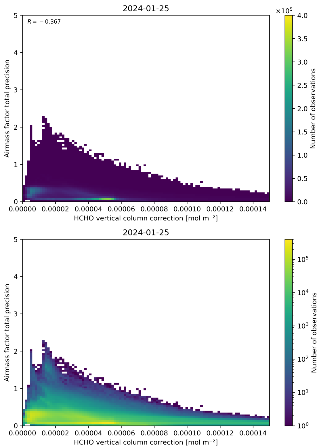
Figure 121: Scatter density plot of “HCHO vertical column correction” against “Airmass factor total precision” for 2024-01-24 to 2024-01-26.
