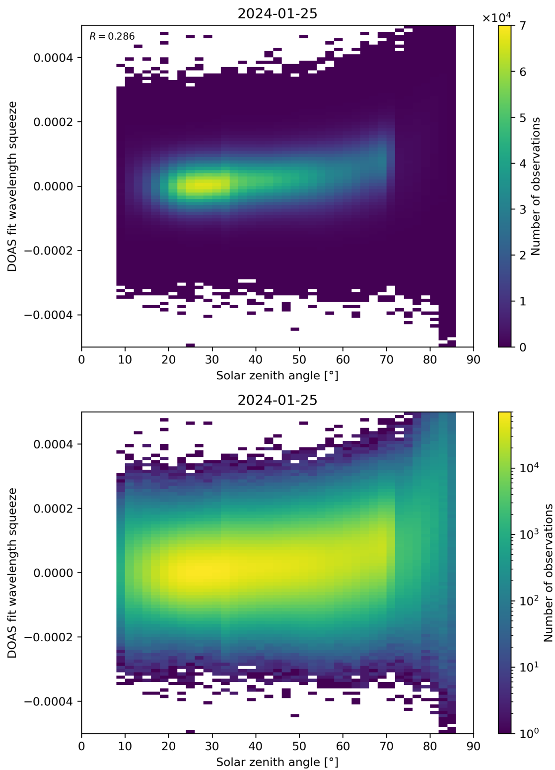
Figure 169: Scatter density plot of “Solar zenith angle” against “DOAS fit wavelength squeeze” for 2024-01-24 to 2024-01-26.
