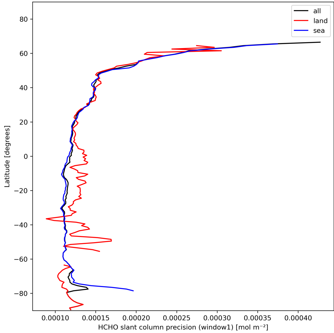
Figure 25: Zonal average of "HCHO slant column precision (window1)" for 2024-01-24 to 2024-01-26.
