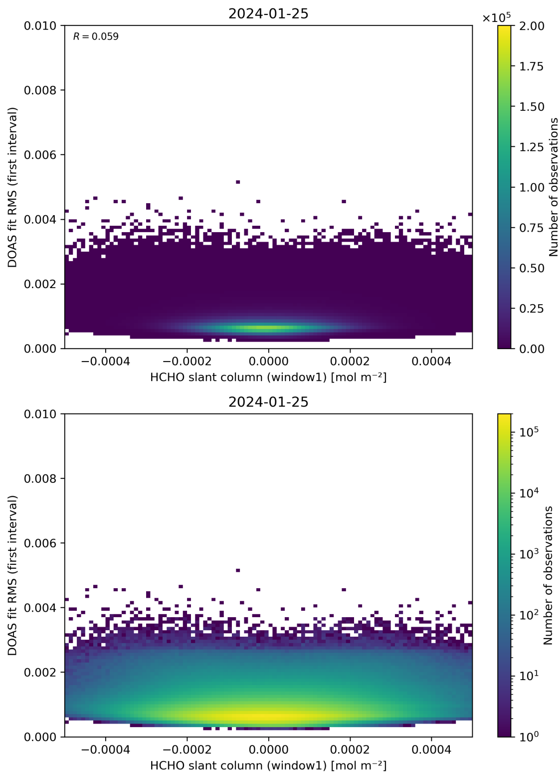
Figure 78: Scatter density plot of “HCHO slant column (window1)” against “DOAS fit RMS (first interval)” for 2024-01-24 to 2024-01-26.
