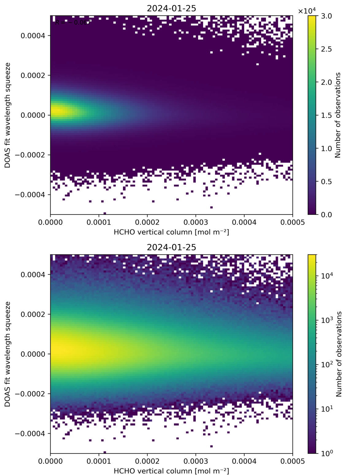
Figure 125: Scatter density plot of “HCHO vertical column” against “DOAS fit wavelength squeeze” for 2024-01-24 to 2024-01-26.
