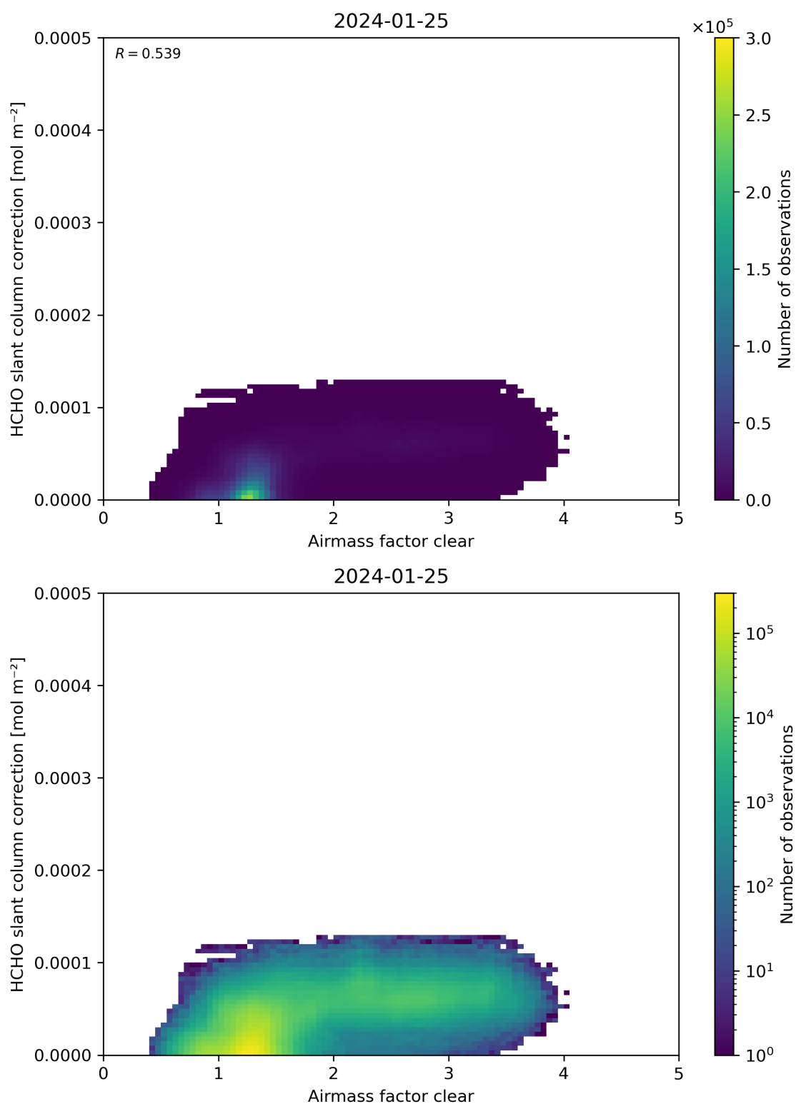
Figure 75: Scatter density plot of “Airmass factor clear” against “HCHO slant column correction” for 2024-01-24 to 2024-01-26.
