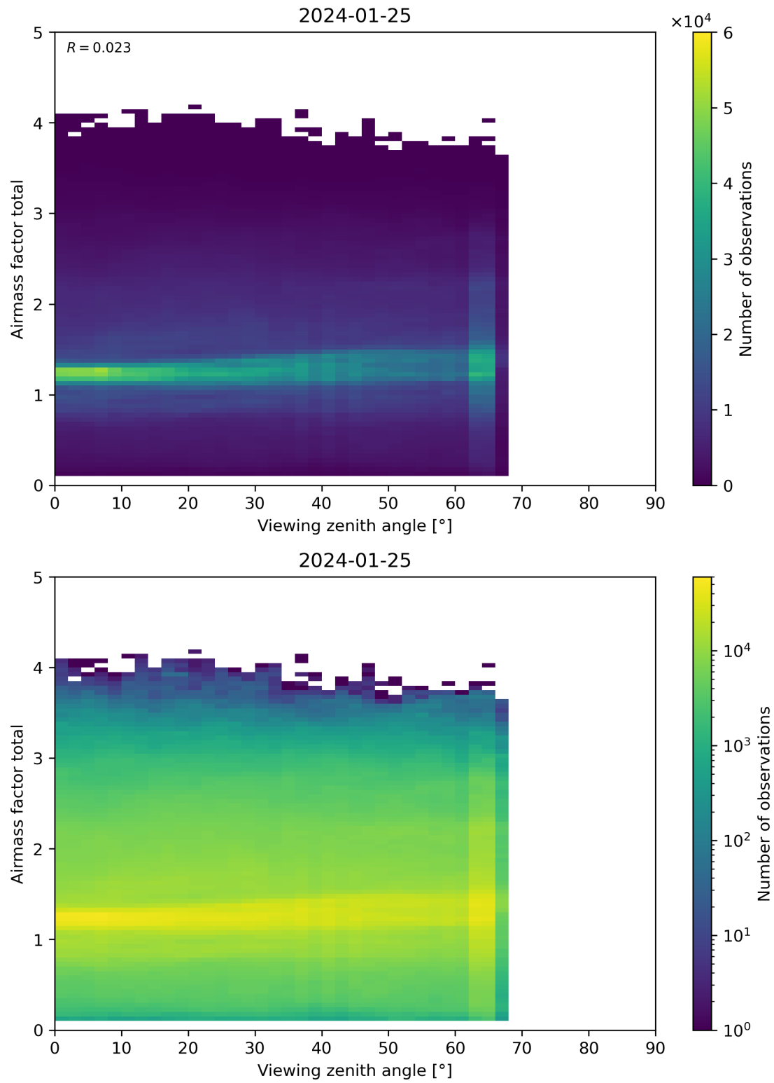
Figure 190: Scatter density plot of “Viewing zenith angle” against “Airmass factor total” for 2024-01-24 to 2024-01-26.
