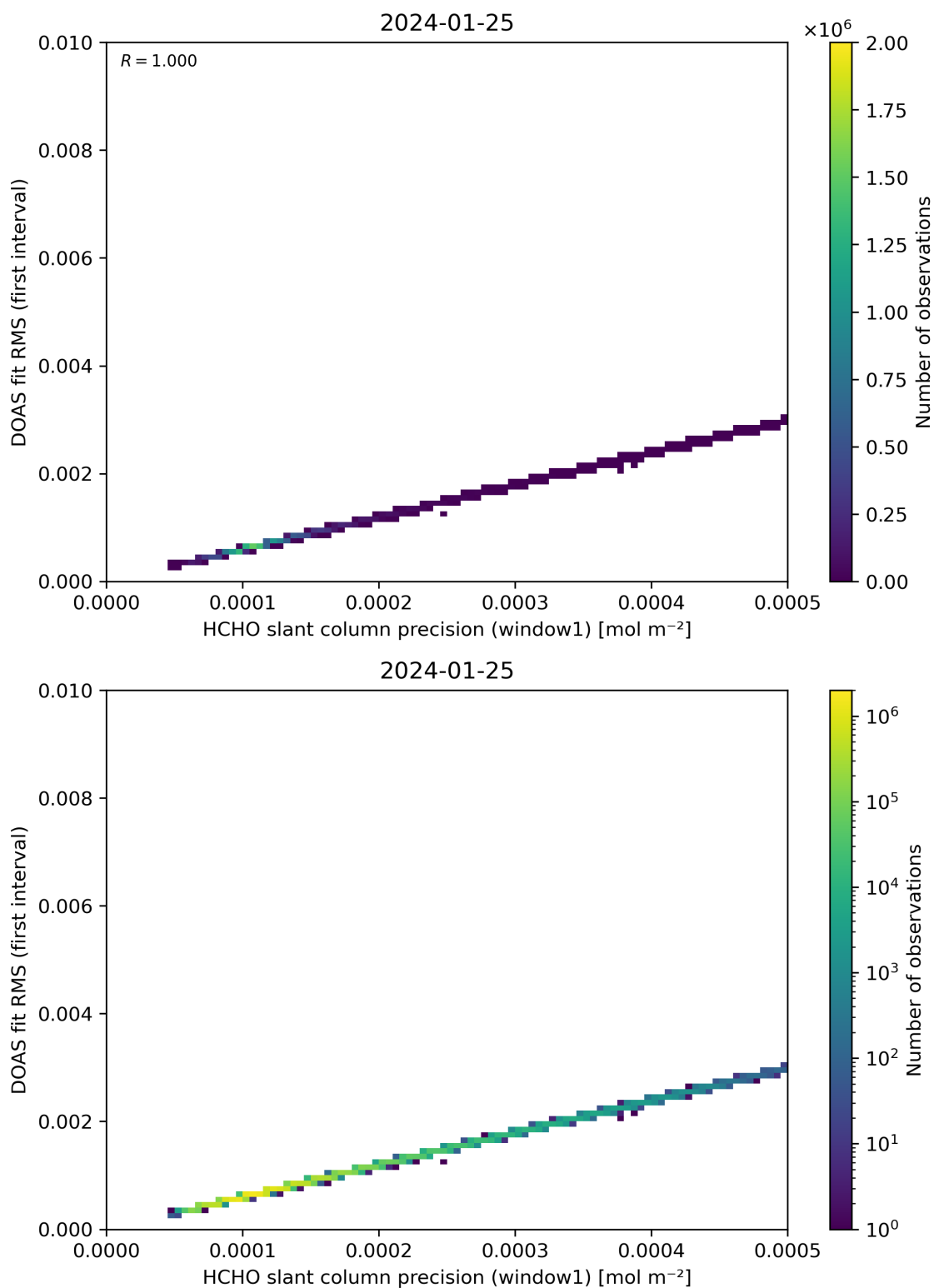
Figure 88: Scatter density plot of “HCHO slant column precision (window1)” against “DOAS fit RMS (first interval)” for 2024-01-24 to 2024-01-26.
