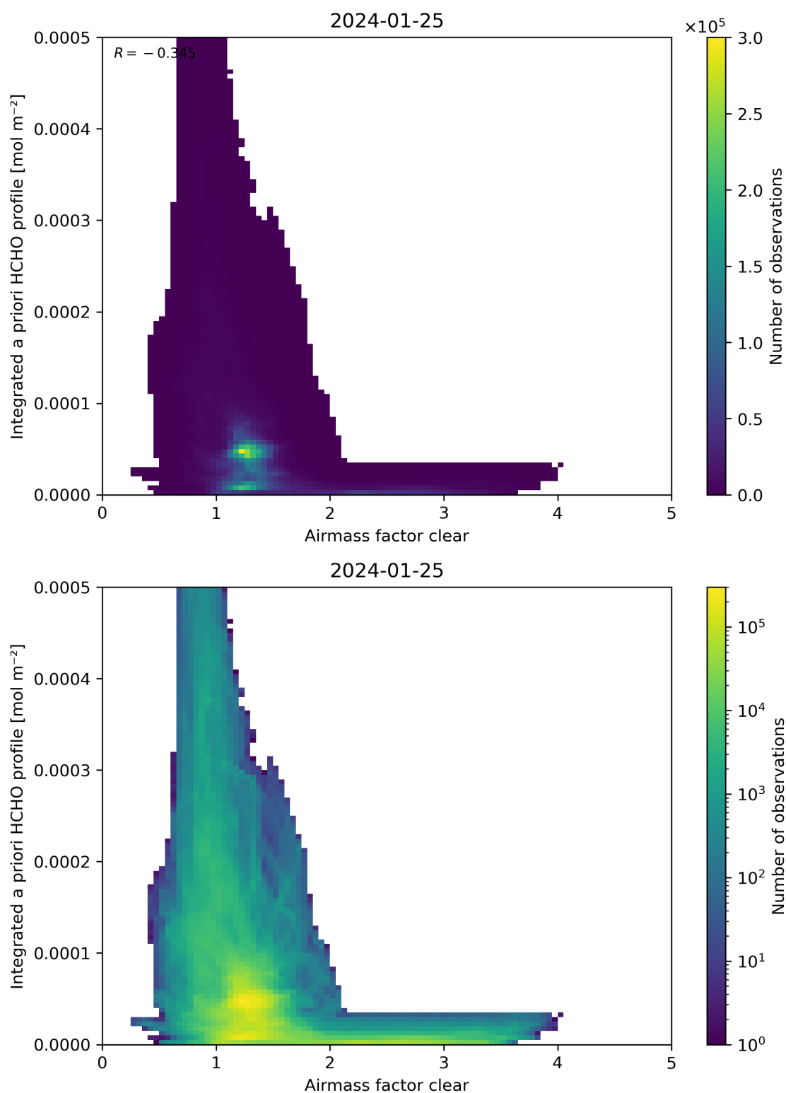
Figure 76: Scatter density plot of “Airmass factor clear” against “Integrated a priori HCHO profile” for 2024-01-24 to 2024-01-26.
