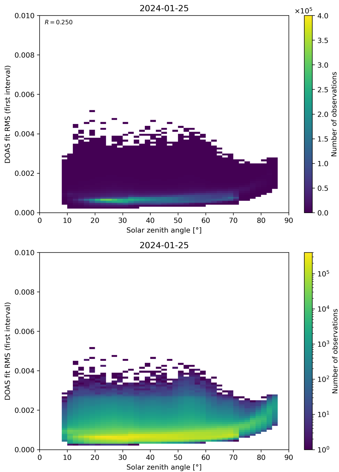
Figure 167: Scatter density plot of “Solar zenith angle” against “DOAS fit RMS (first interval)” for 2024-01-24 to 2024-01-26.
