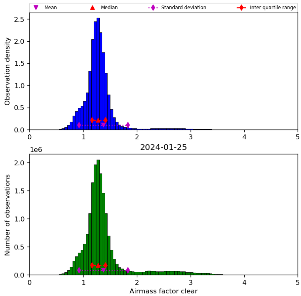
Figure 42: Histogram of “Airmass factor clear” for 2024-01-24 to 2024-01-26
