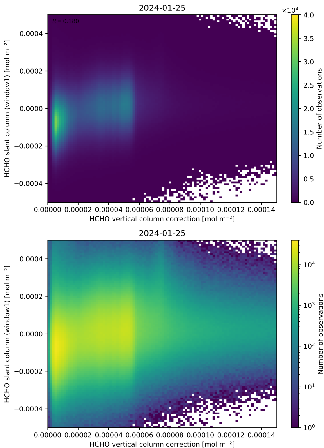
Figure 118: Scatter density plot of “HCHO vertical column correction” against “HCHO slant column (window1)” for 2024-01-24 to 2024-01-26.
