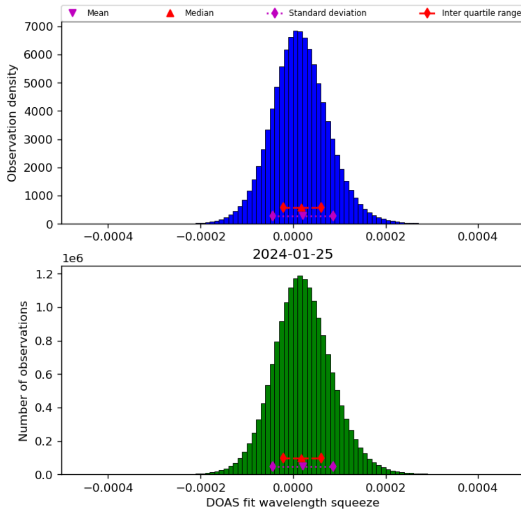
Figure 45: Histogram of “DOAS fit wavelength squeeze” for 2024-01-24 to 2024-01-26
