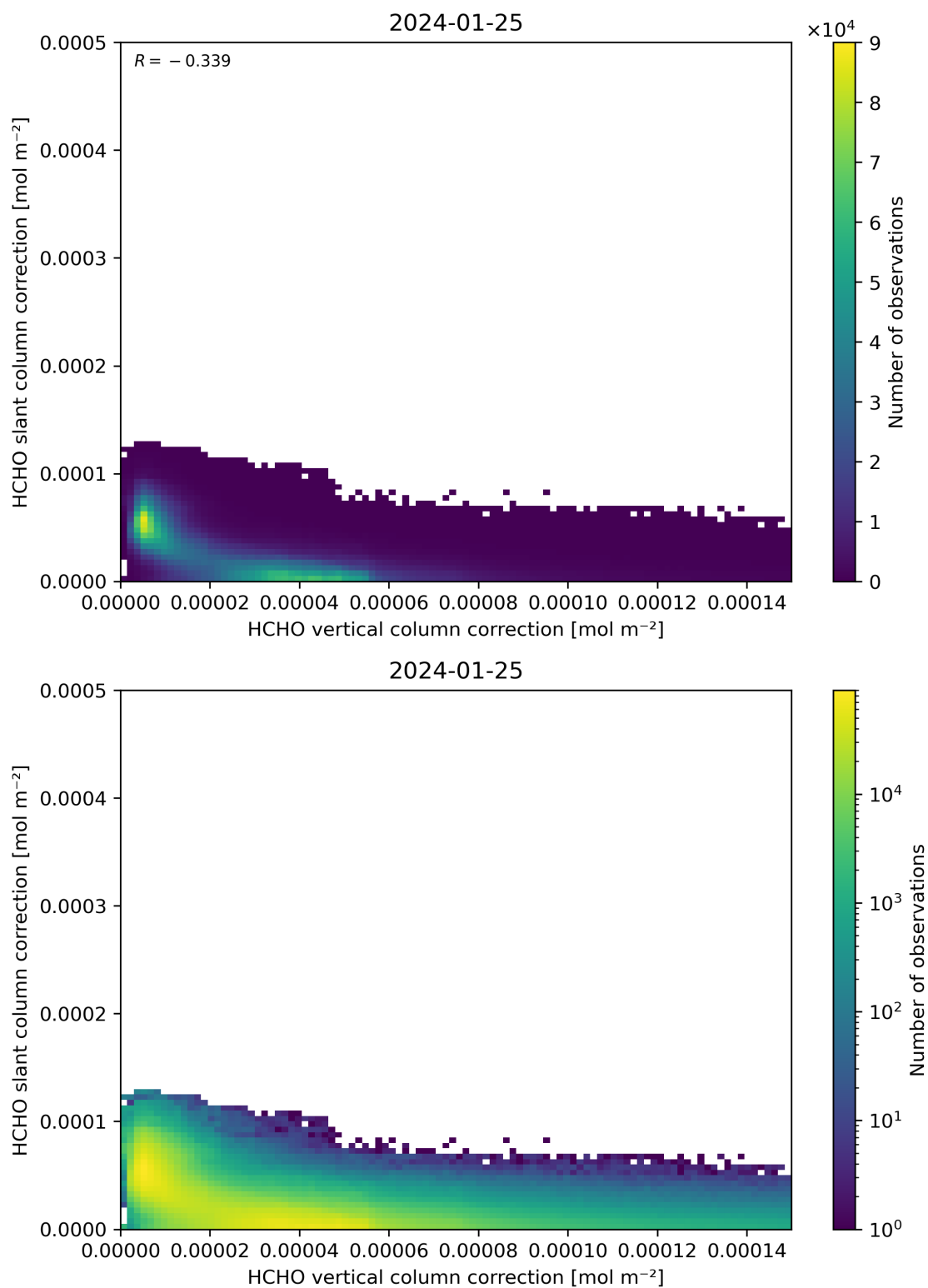
Figure 117: Scatter density plot of “HCHO vertical column correction” against “HCHO slant column correction” for 2024-01-24 to 2024-01-26.
