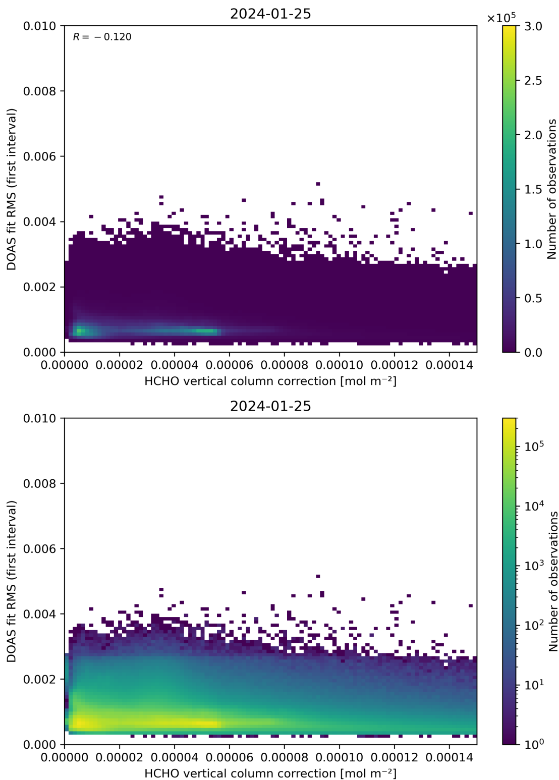
Figure 112: Scatter density plot of “HCHO vertical column correction” against “DOAS fit RMS (first interval)” for 2024-01-24 to 2024-01-26.
