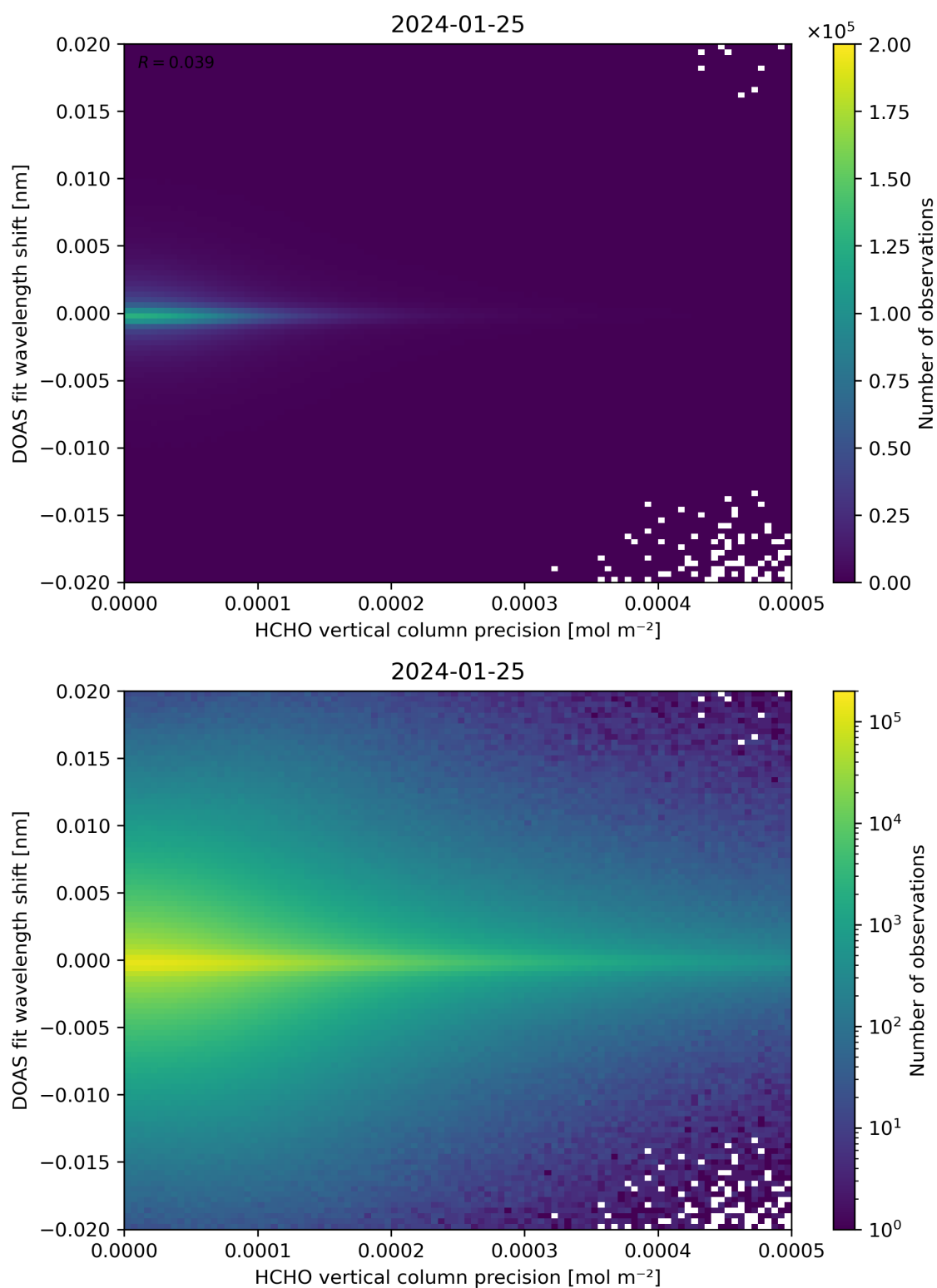
Figure 137: Scatter density plot of “HCHO vertical column precision” against “DOAS fit wavelength shift” for 2024-01-24 to 2024-01-26.
