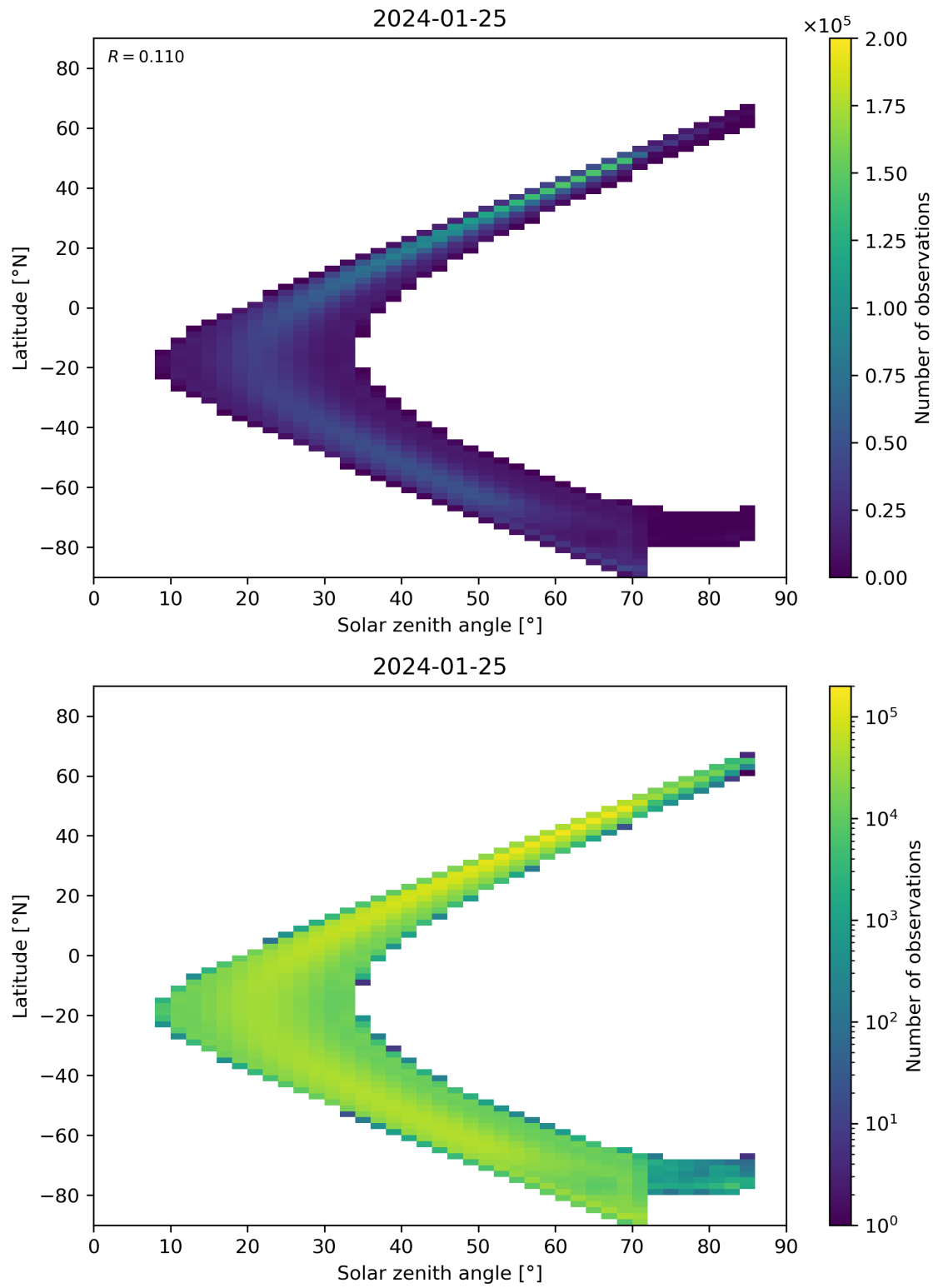
Figure 181: Scatter density plot of “Solar zenith angle” against “Latitude” for 2024-01-24 to 2024-01-26.
