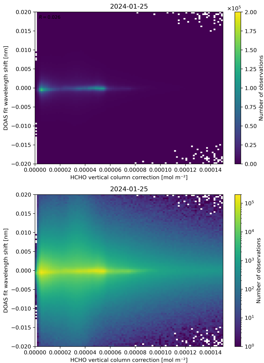
Figure 113: Scatter density plot of “HCHO vertical column correction” against “DOAS fit wavelength shift” for 2024-01-24 to 2024-01-26.
