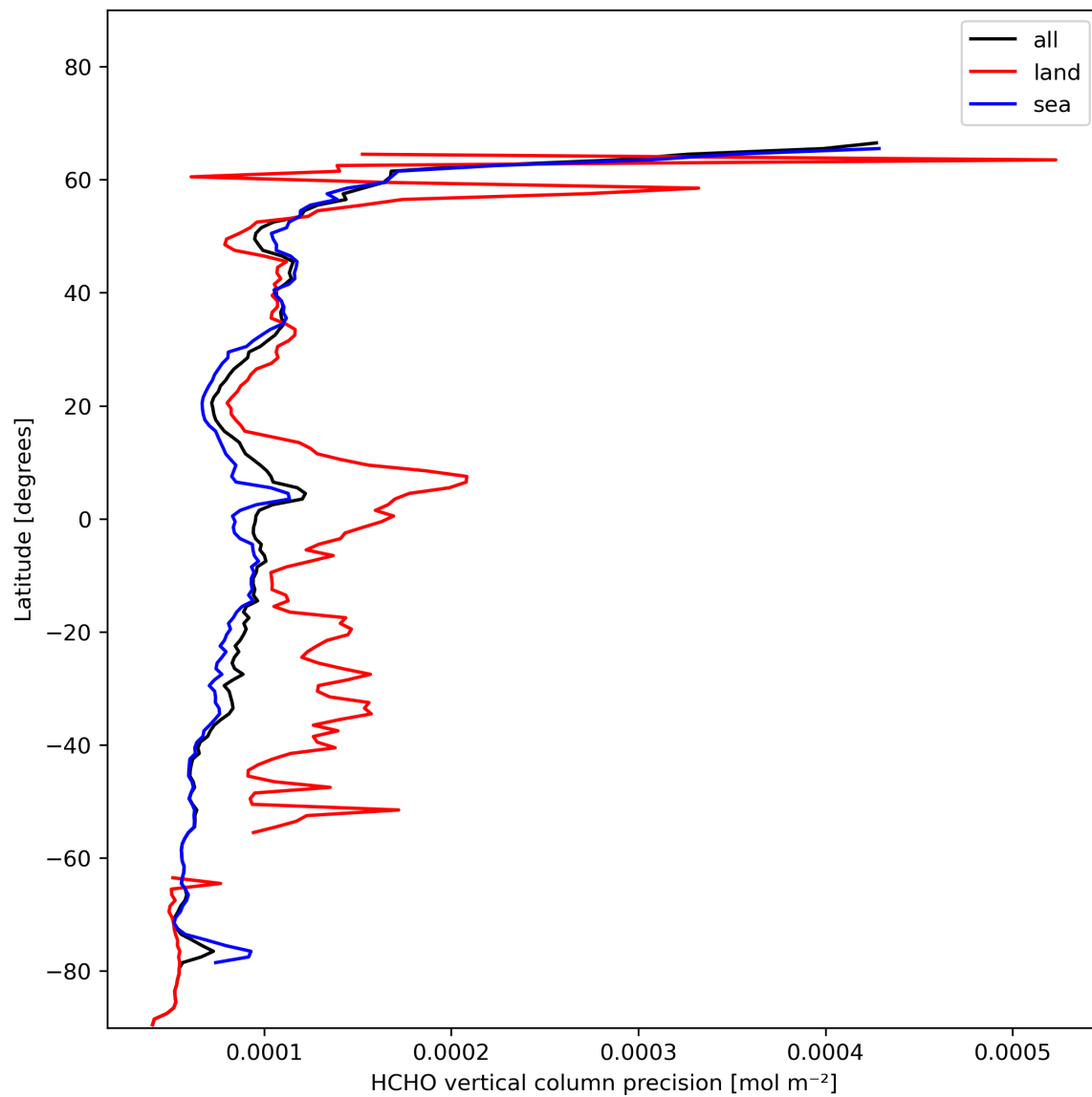
Figure 22: Zonal average of “HCHO vertical column precision” for 2024-01-24 to 2024-01-26.
