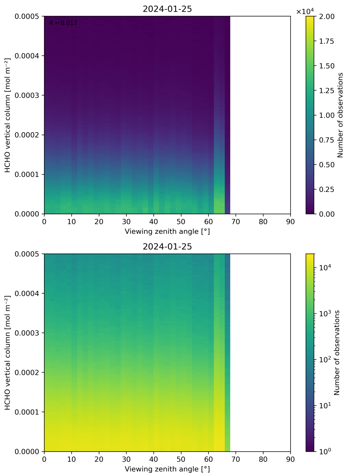
Figure 192: Scatter density plot of “Viewing zenith angle” against “HCHO vertical column” for 2024-01-24 to 2024-01-26.
