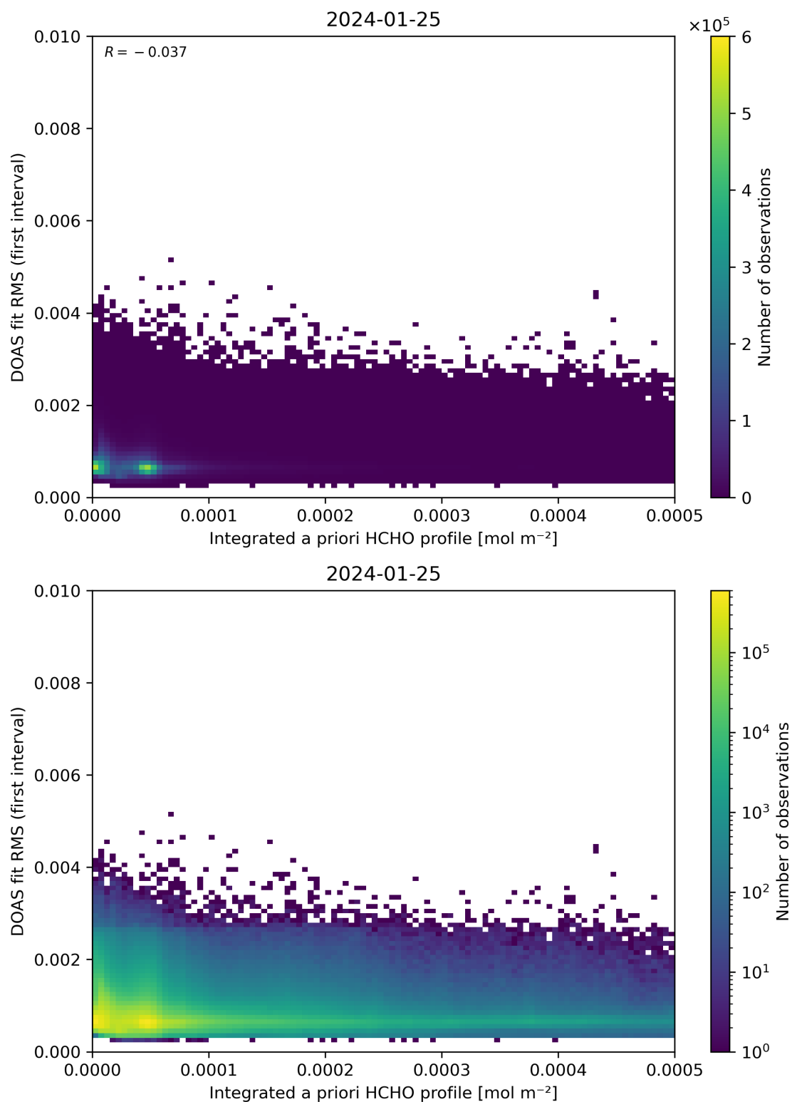
Figure 148: Scatter density plot of “Integrated a priori HCHO profile” against “DOAS fit RMS (first interval)” for 2024-01-24 to 2024-01-26.
