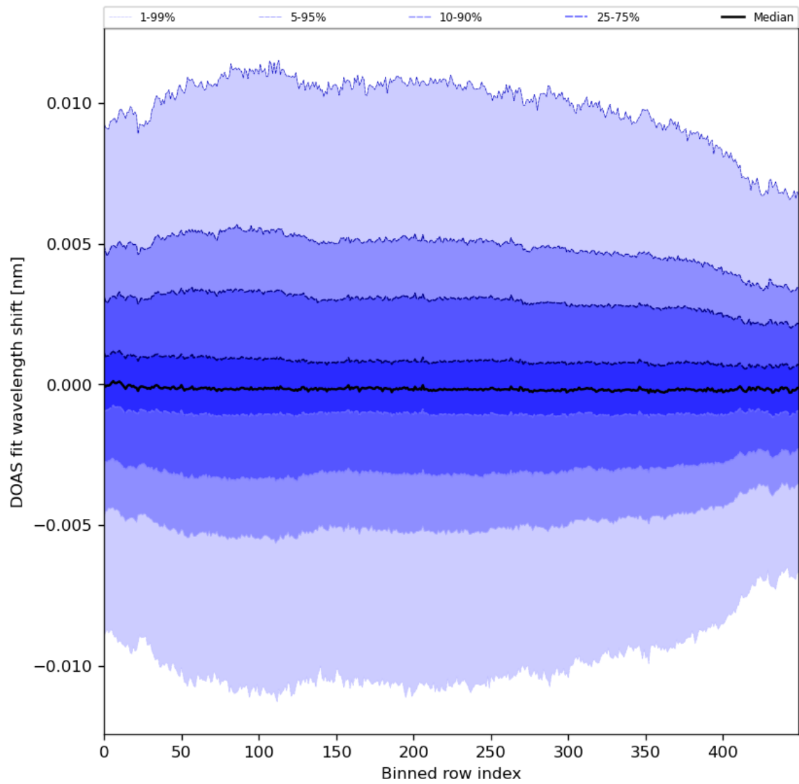
Figure 58: Along track statistics of “DOAS fit wavelength shift” for 2024-01-24 to 2024-01-26
