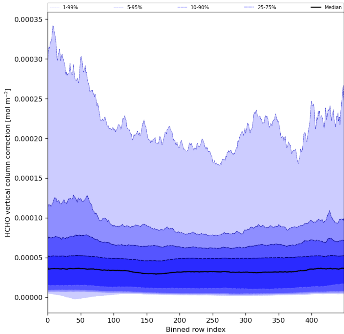
Figure 51: Along track statistics of “HCHO vertical column correction” for 2024-01-24 to 2024-01-26
