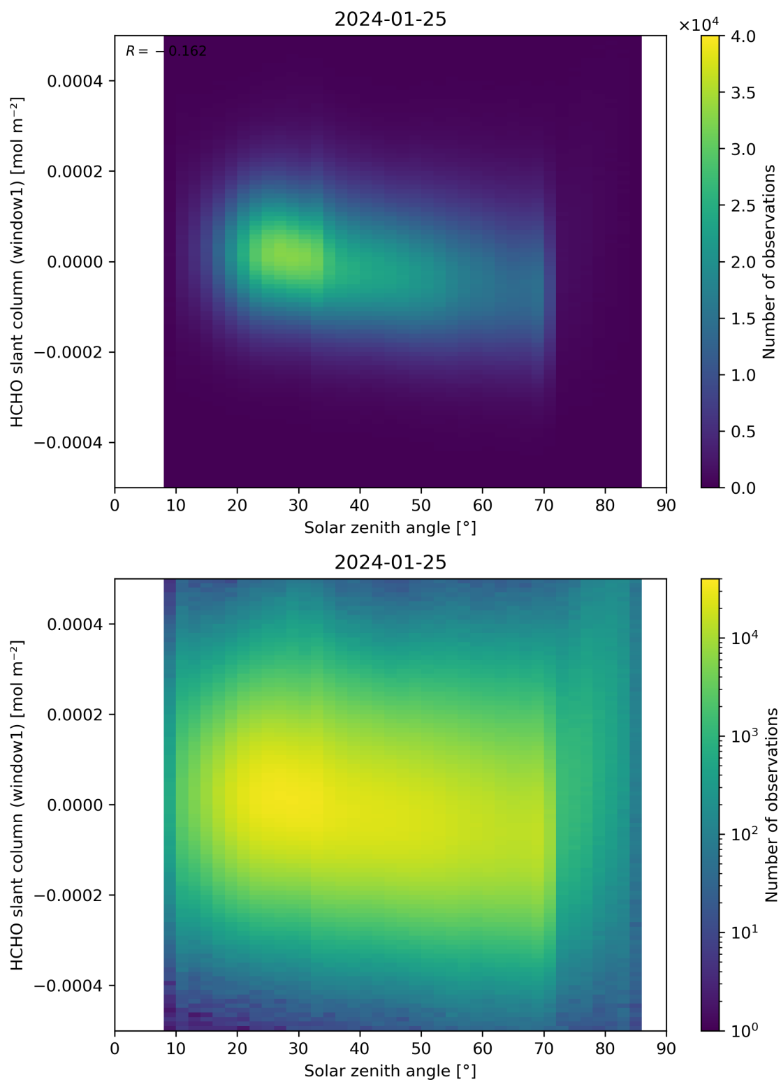
Figure 173: Scatter density plot of “Solar zenith angle” against “HCHO slant column (window1)” for 2024-01-24 to 2024-01-26.
