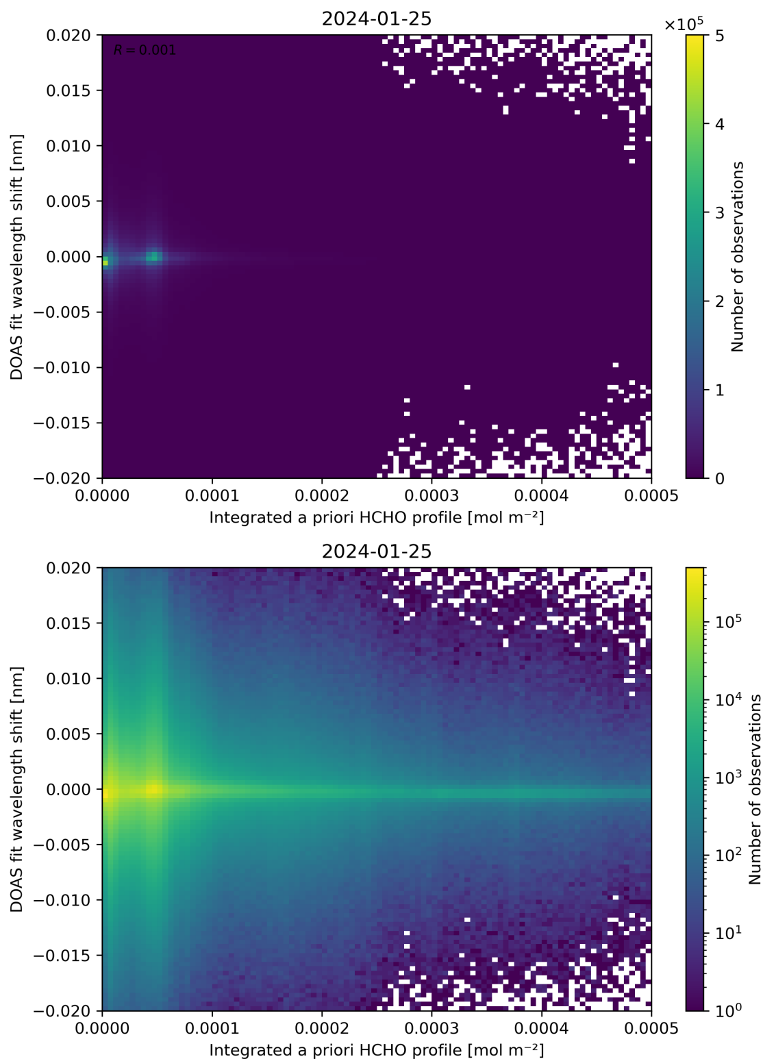
Figure 149: Scatter density plot of “Integrated a priori HCHO profile” against “DOAS fit wavelength shift” for 2024-01-24 to 2024-01-26.
