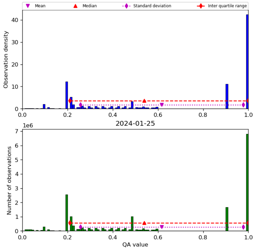
Figure 34: Histogram of “QA value” for 2024-01-24 to 2024-01-26
