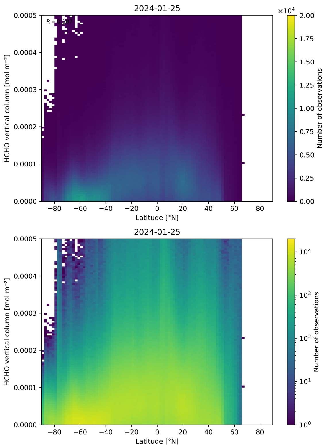
Figure 163: Scatter density plot of “Latitude” against “HCHO vertical column” for 2024-01-24 to 2024-01-26.
