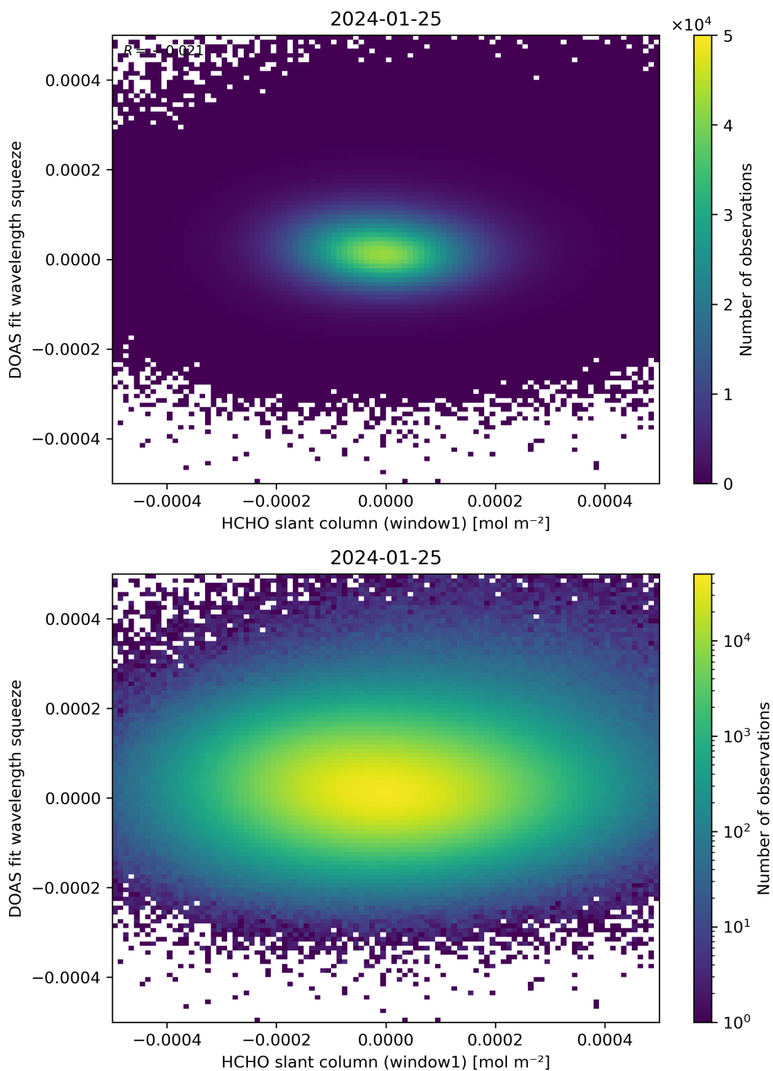
Figure 80: Scatter density plot of “HCHO slant column (window1)” against “DOAS fit wavelength squeeze” for 2024-01-24 to 2024-01-26.
