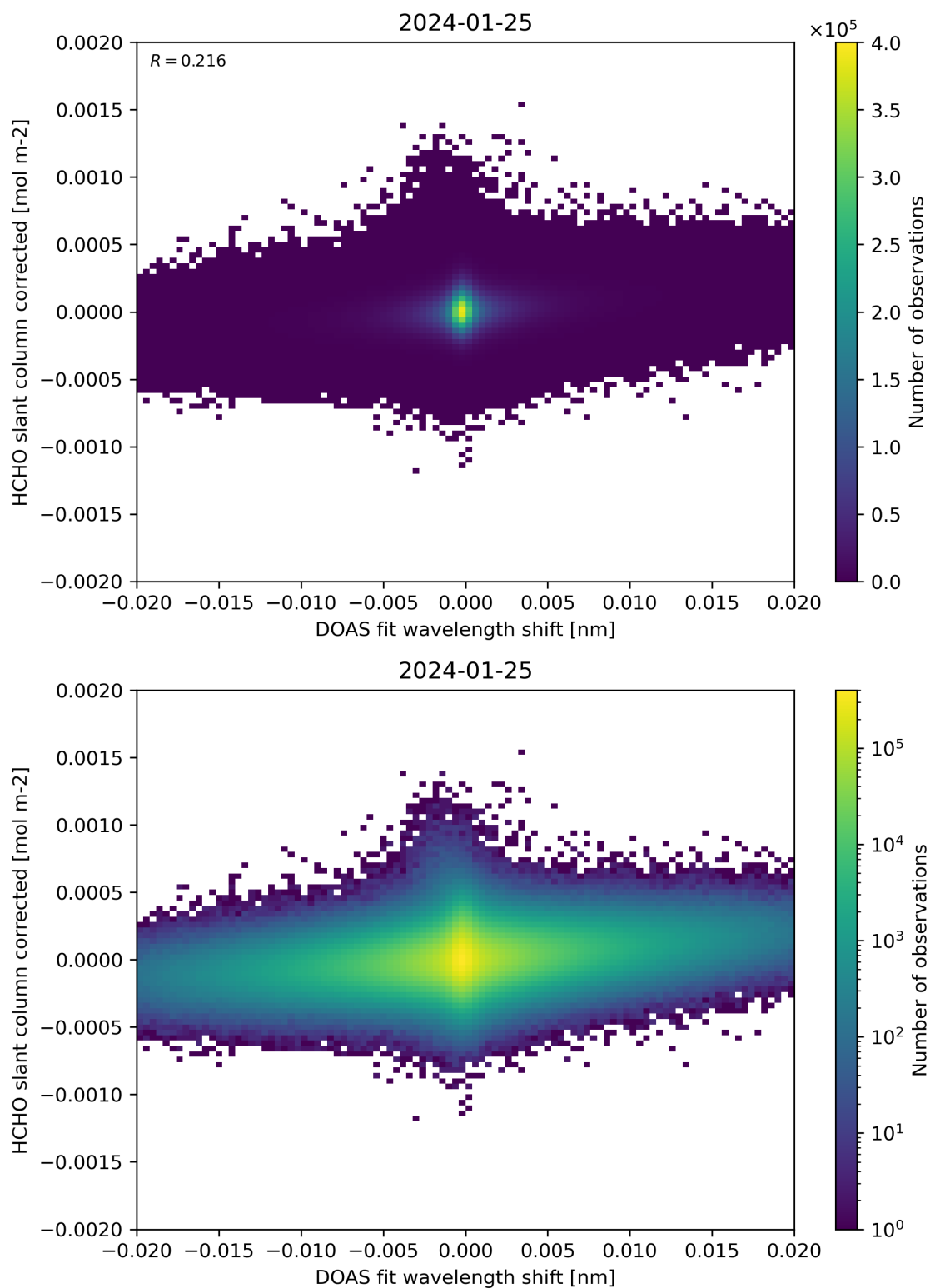
Figure 66: Scatter density plot of “DOAS fit wavelength shift” against “HCHO slant column corrected” for 2024-01-24 to 2024-01-26.
