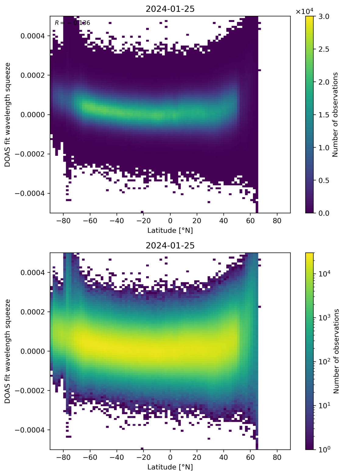
Figure 155: Scatter density plot of “Latitude” against “DOAS fit wavelength squeeze” for 2024-01-24 to 2024-01-26.
