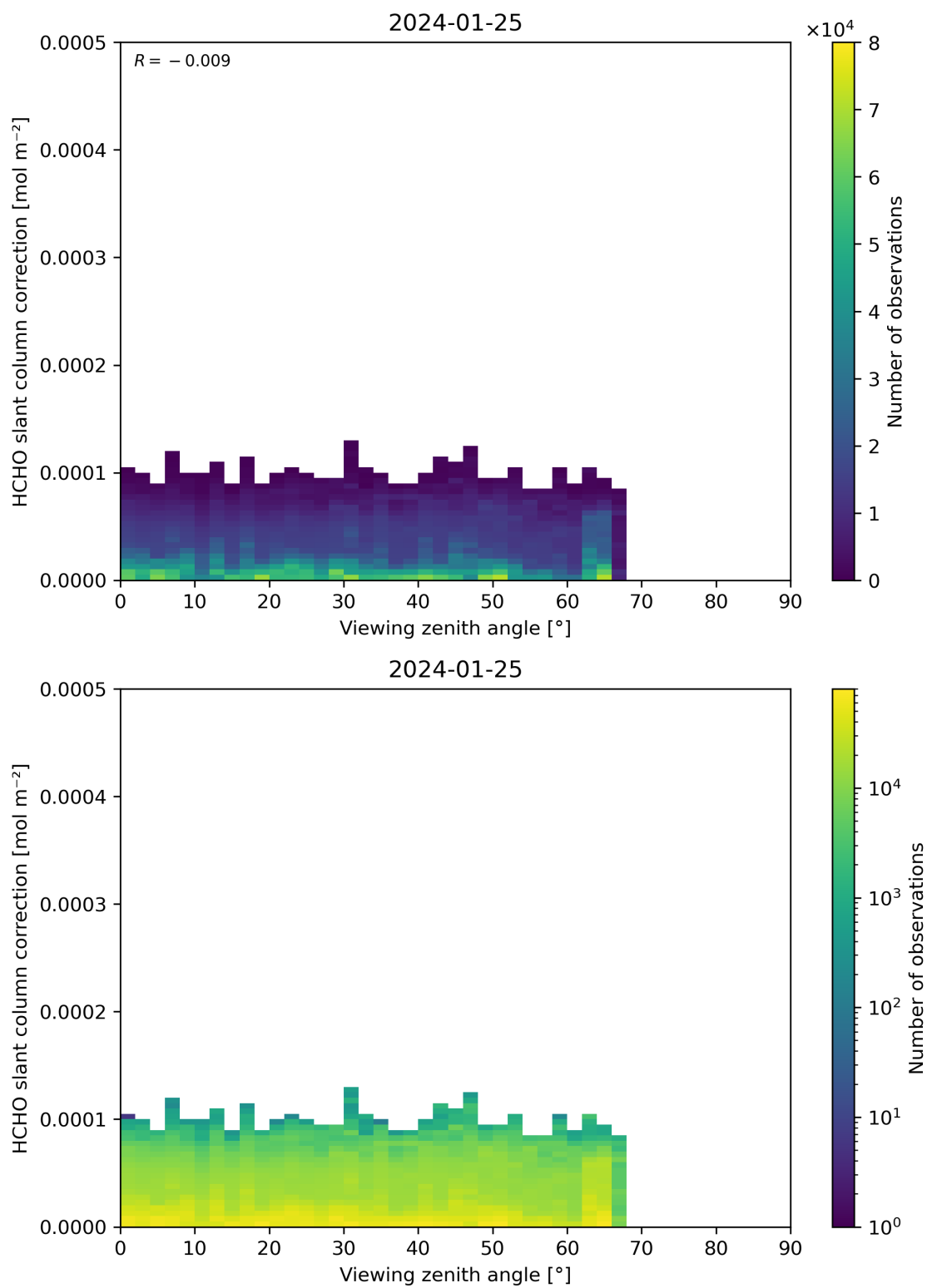
Figure 187: Scatter density plot of “Viewing zenith angle” against “HCHO slant column correction” for 2024-01-24 to 2024-01-26.
