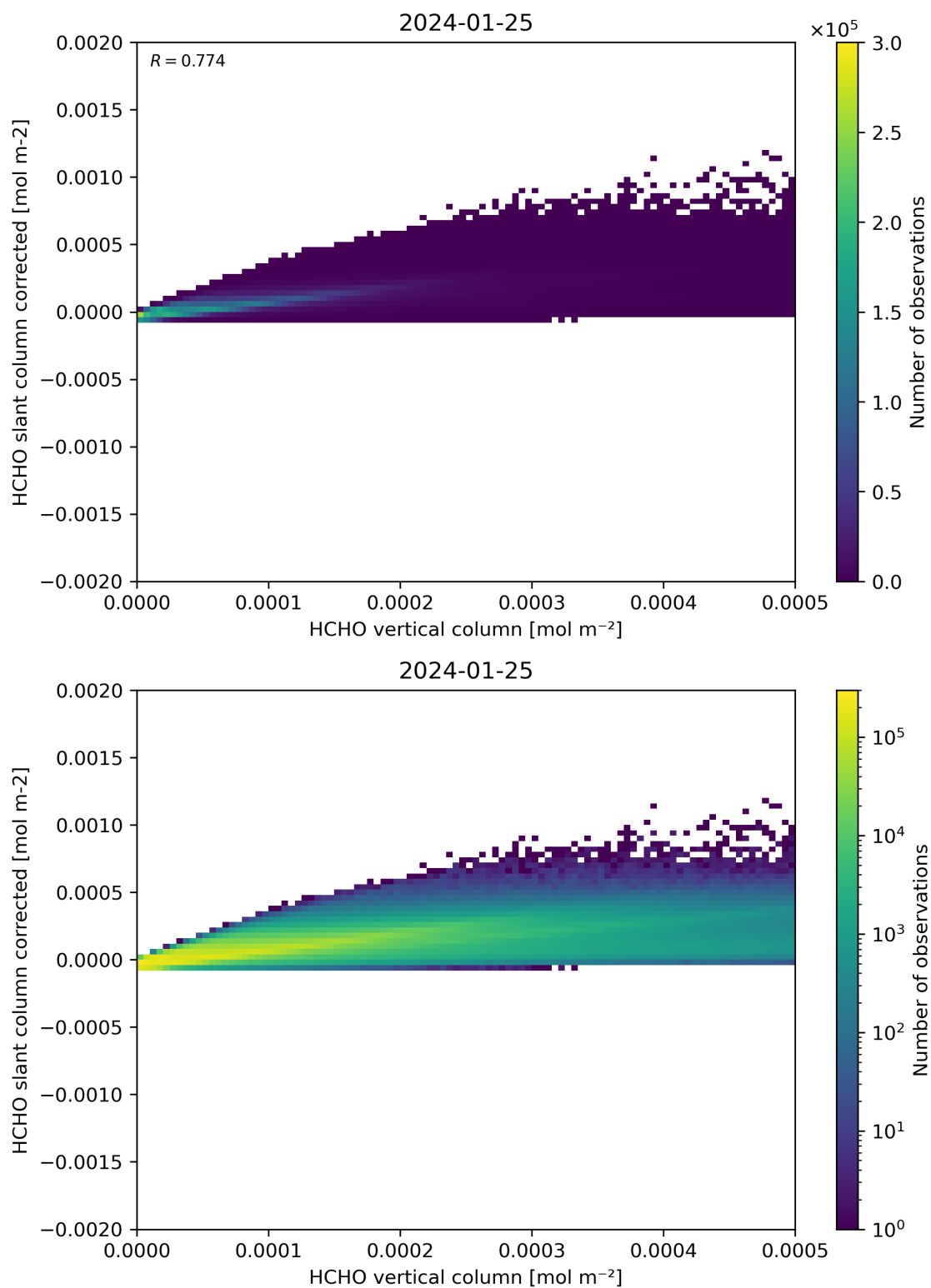
Figure 127: Scatter density plot of “HCHO vertical column” against “HCHO slant column corrected” for 2024-01-24 to 2024-01-26.
