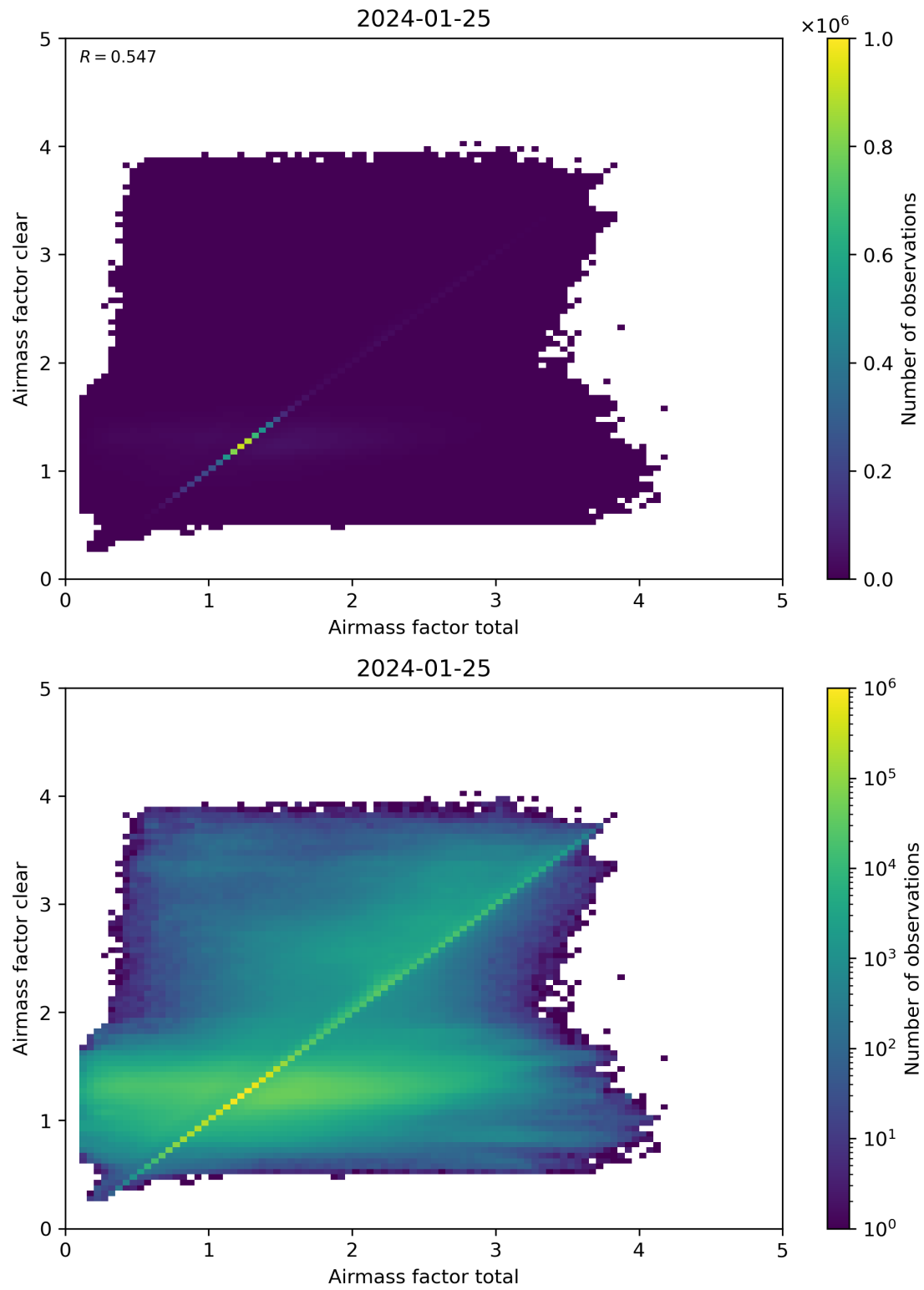
Figure 100: Scatter density plot of “Airmass factor total” against “Airmass factor clear” for 2024-01-24 to 2024-01-26.
