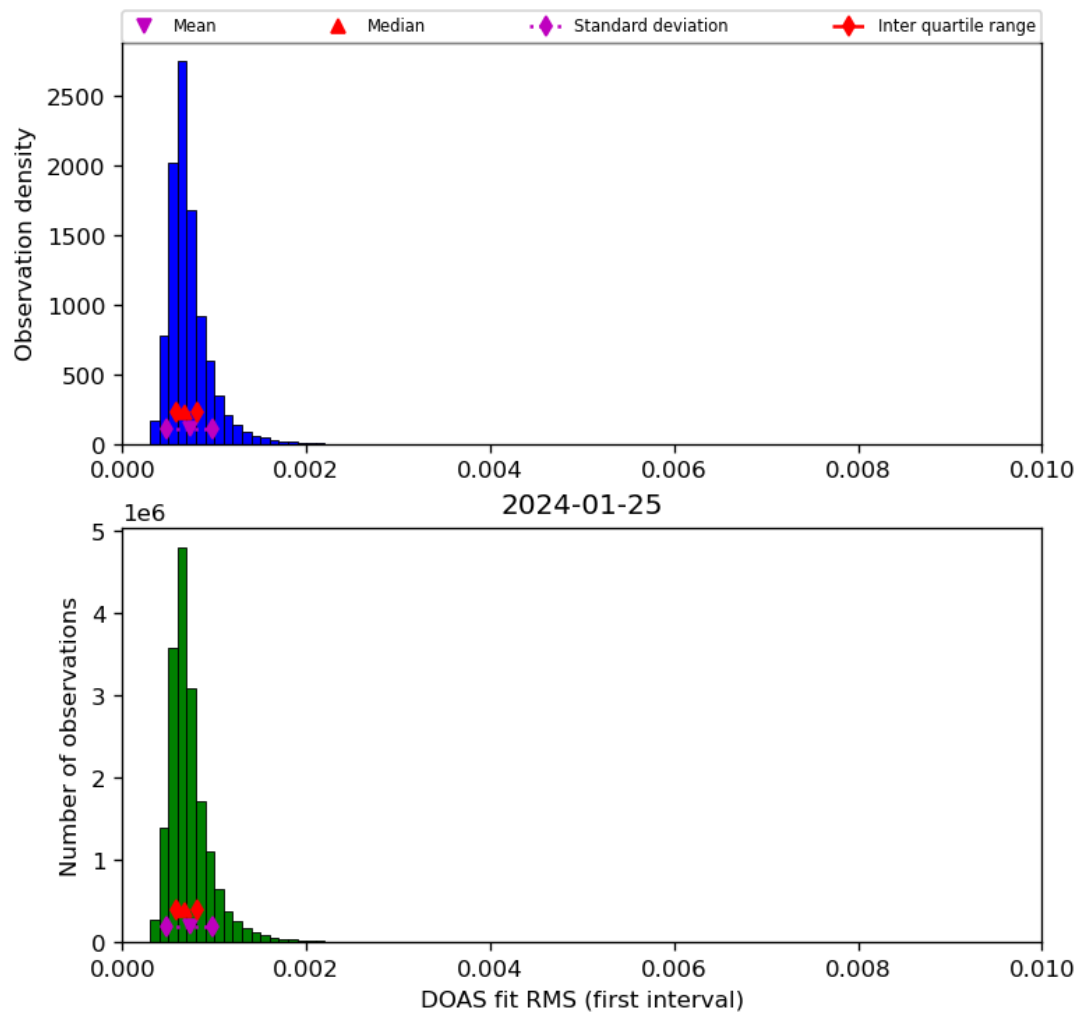
Figure 46: Histogram of “DOAS fit RMS (first interval)” for 2024-01-24 to 2024-01-26
