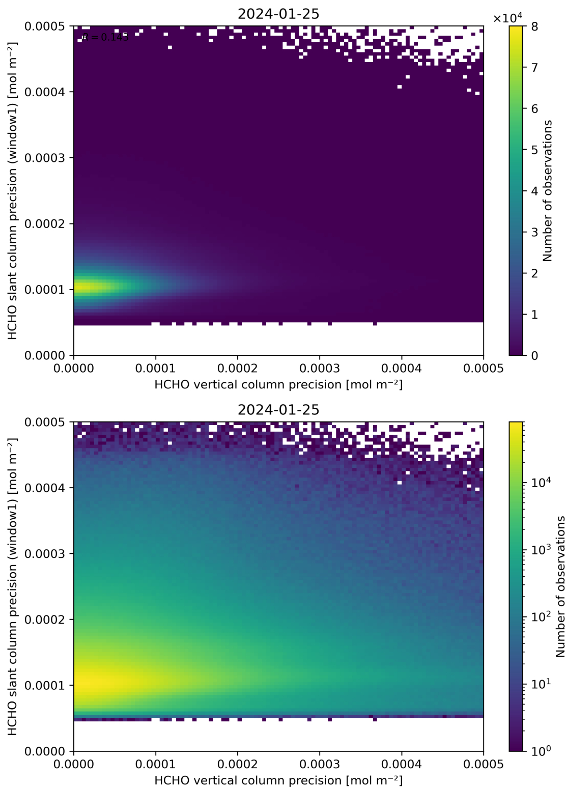
Figure 143: Scatter density plot of “HCHO vertical column precision” against “HCHO slant column precision (window1)” for 2024-01-24 to 2024-01-26.
