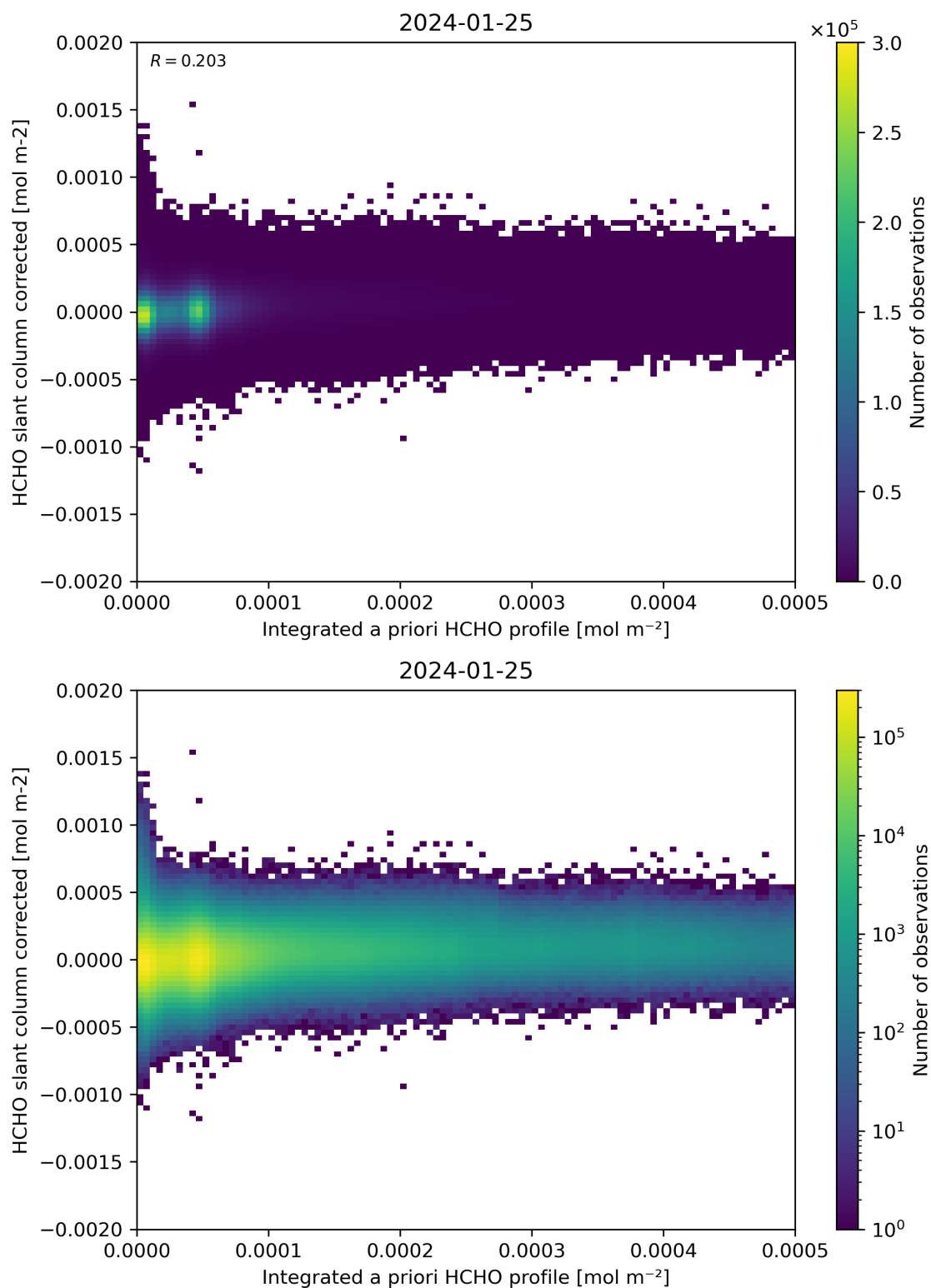
Figure 151: Scatter density plot of “Integrated a priori HCHO profile” against “HCHO slant column corrected” for 2024-01-24 to 2024-01-26.
