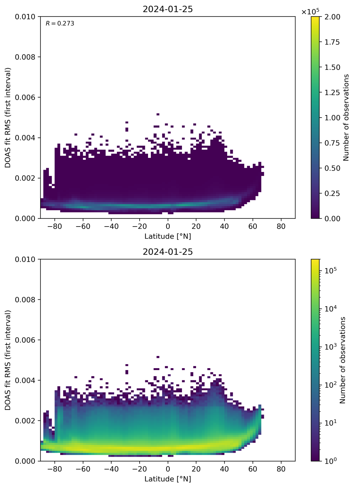
Figure 153: Scatter density plot of “Latitude” against “DOAS fit RMS (first interval)” for 2024-01-24 to 2024-01-26.
