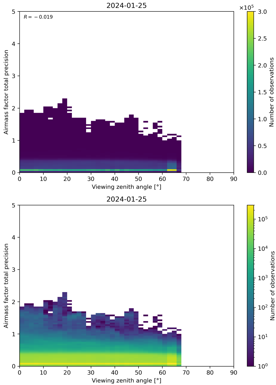
Figure 191: Scatter density plot of “Viewing zenith angle” against “Airmass factor total precision” for 2024-01-24 to 2024-01-26.
