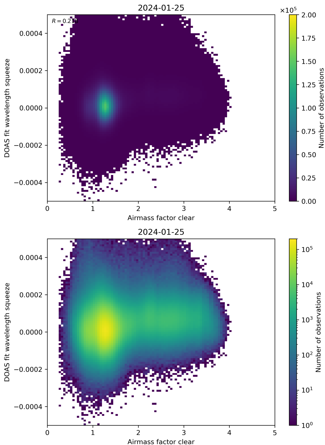
Figure 73: Scatter density plot of “Airmass factor clear” against “DOAS fit wavelength squeeze” for 2024-01-24 to 2024-01-26.
