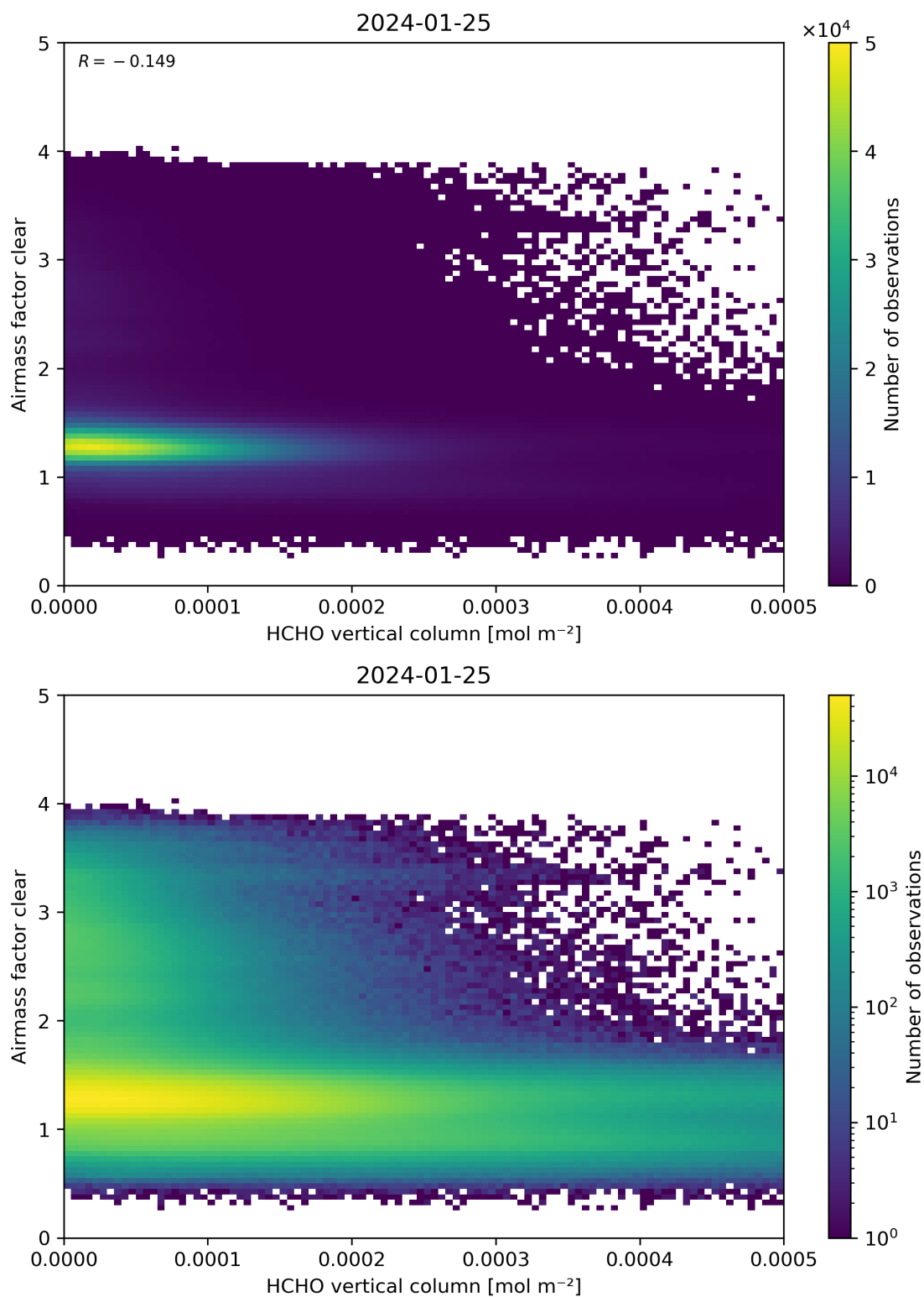
Figure 126: Scatter density plot of “HCHO vertical column” against “Airmass factor clear” for 2024-01-24 to 2024-01-26.
