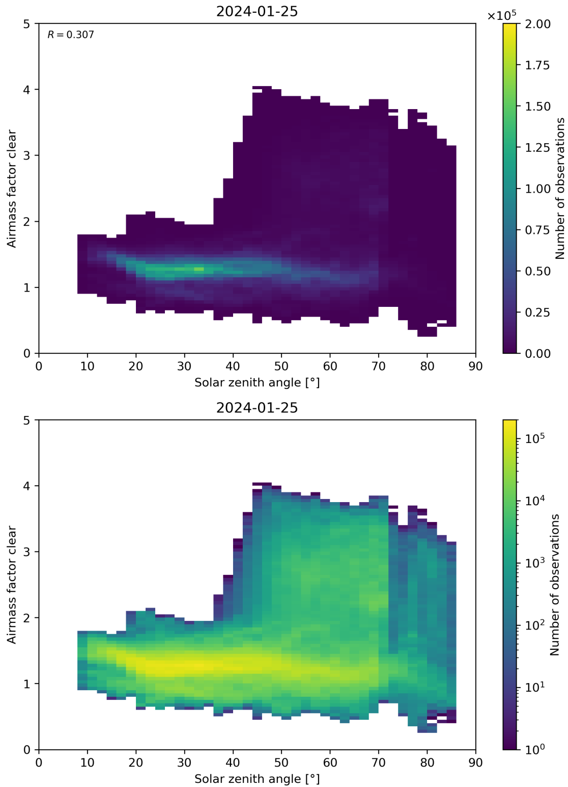
Figure 170: Scatter density plot of “Solar zenith angle” against “Airmass factor clear” for 2024-01-24 to 2024-01-26.
