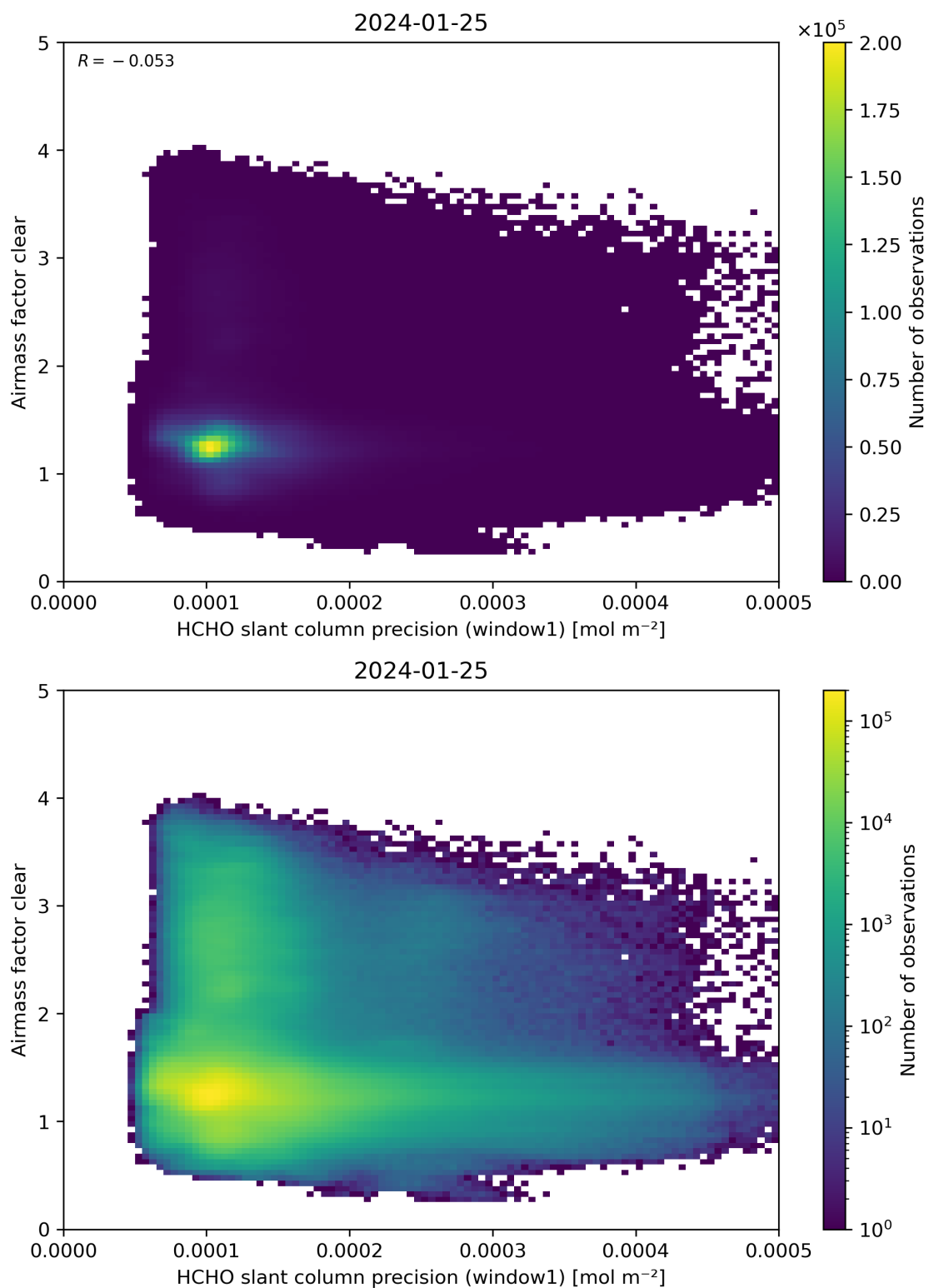
Figure 91: Scatter density plot of “HCHO slant column precision (window1)” against “Airmass factor clear” for 2024-01-24 to 2024-01-26.
