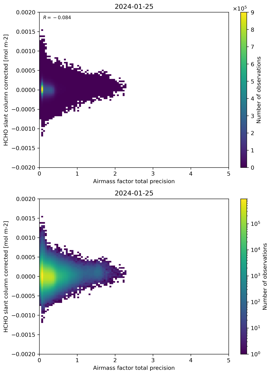
Figure 109: Scatter density plot of “Airmass factor total precision” against “HCHO slant column corrected” for 2024-01-24 to 2024-01-26.
