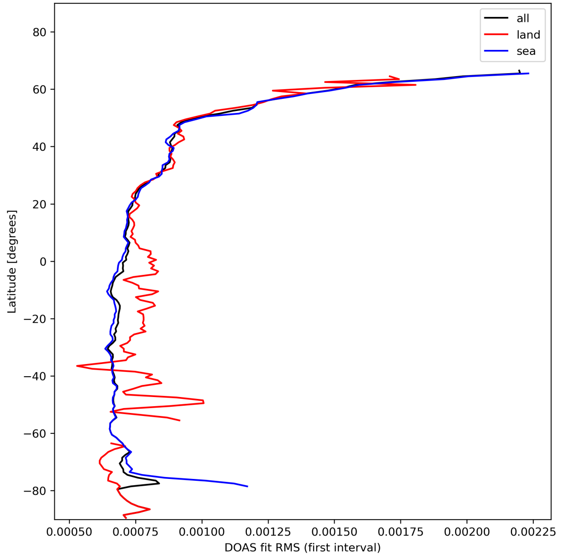
Figure 32: Zonal average of “DOAS fit RMS (first interval)” for 2024-01-24 to 2024-01-26.
