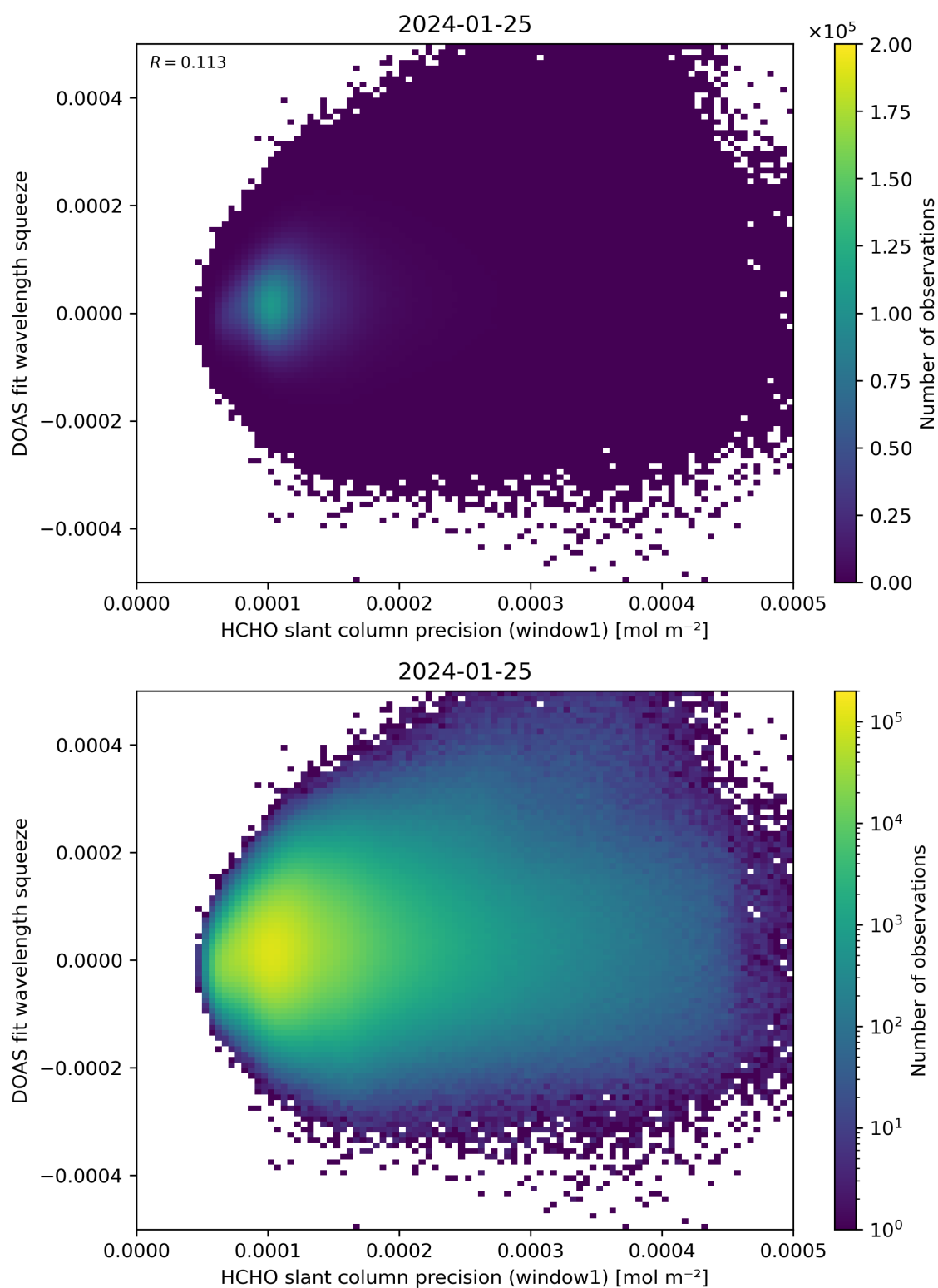
Figure 90: Scatter density plot of “HCHO slant column precision (window1)” against “DOAS fit wavelength squeeze” for 2024-01-24 to 2024-01-26.
