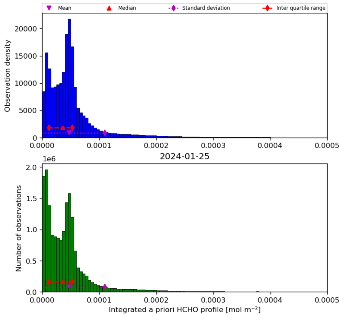
Figure 43: Histogram of “Integrated a priori HCHO profile” for 2024-01-24 to 2024-01-26
