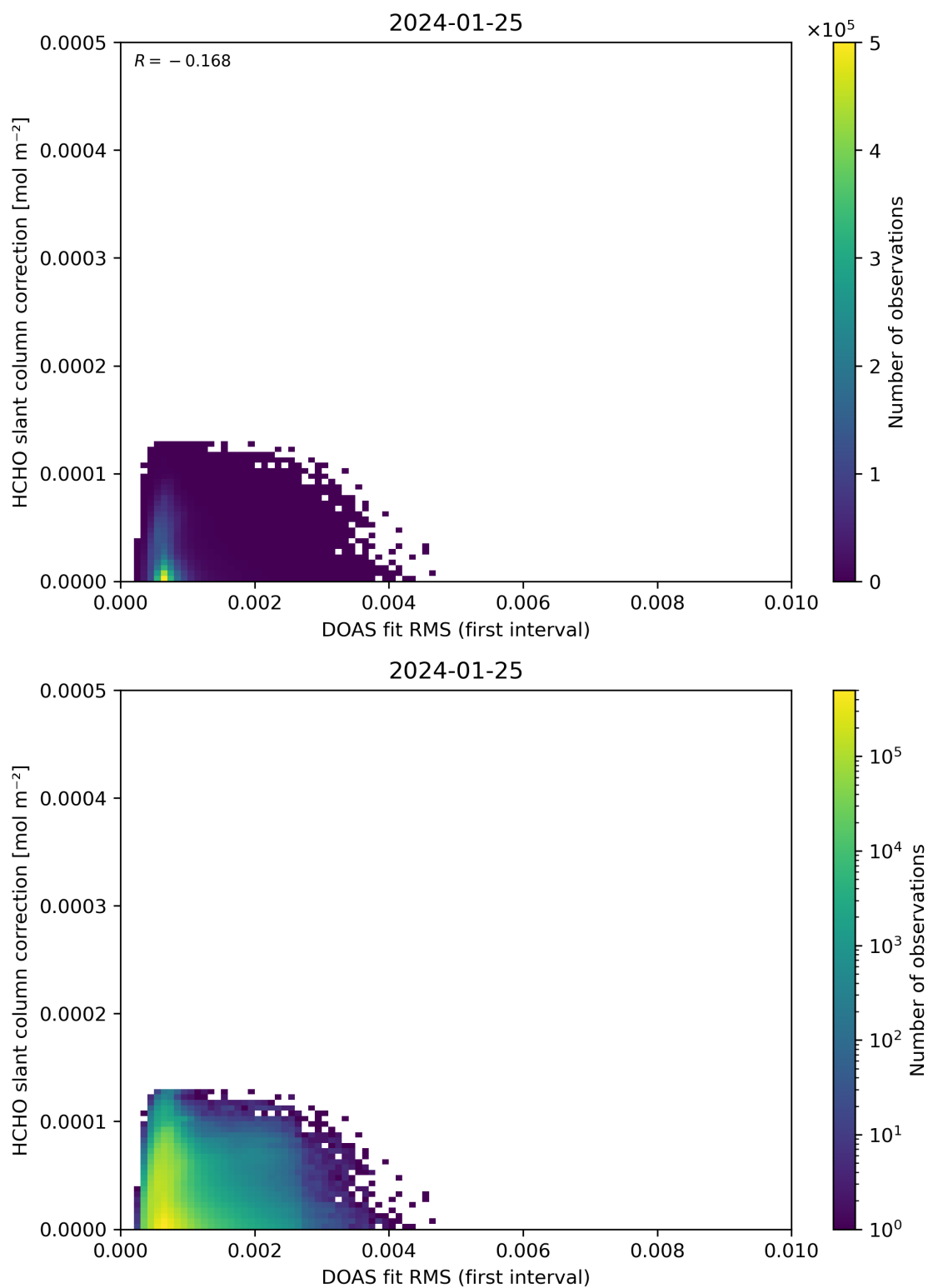
Figure 63: Scatter density plot of “DOAS fit RMS (first interval)” against “HCHO slant column correction” for 2024-01-24 to 2024-01-26.
