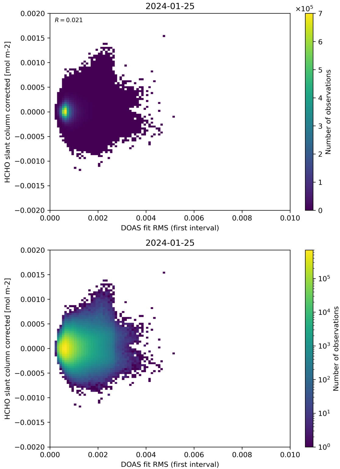
Figure 62: Scatter density plot of “DOAS fit RMS (first interval)” against “HCHO slant column corrected” for 2024-01-24 to 2024-01-26.
