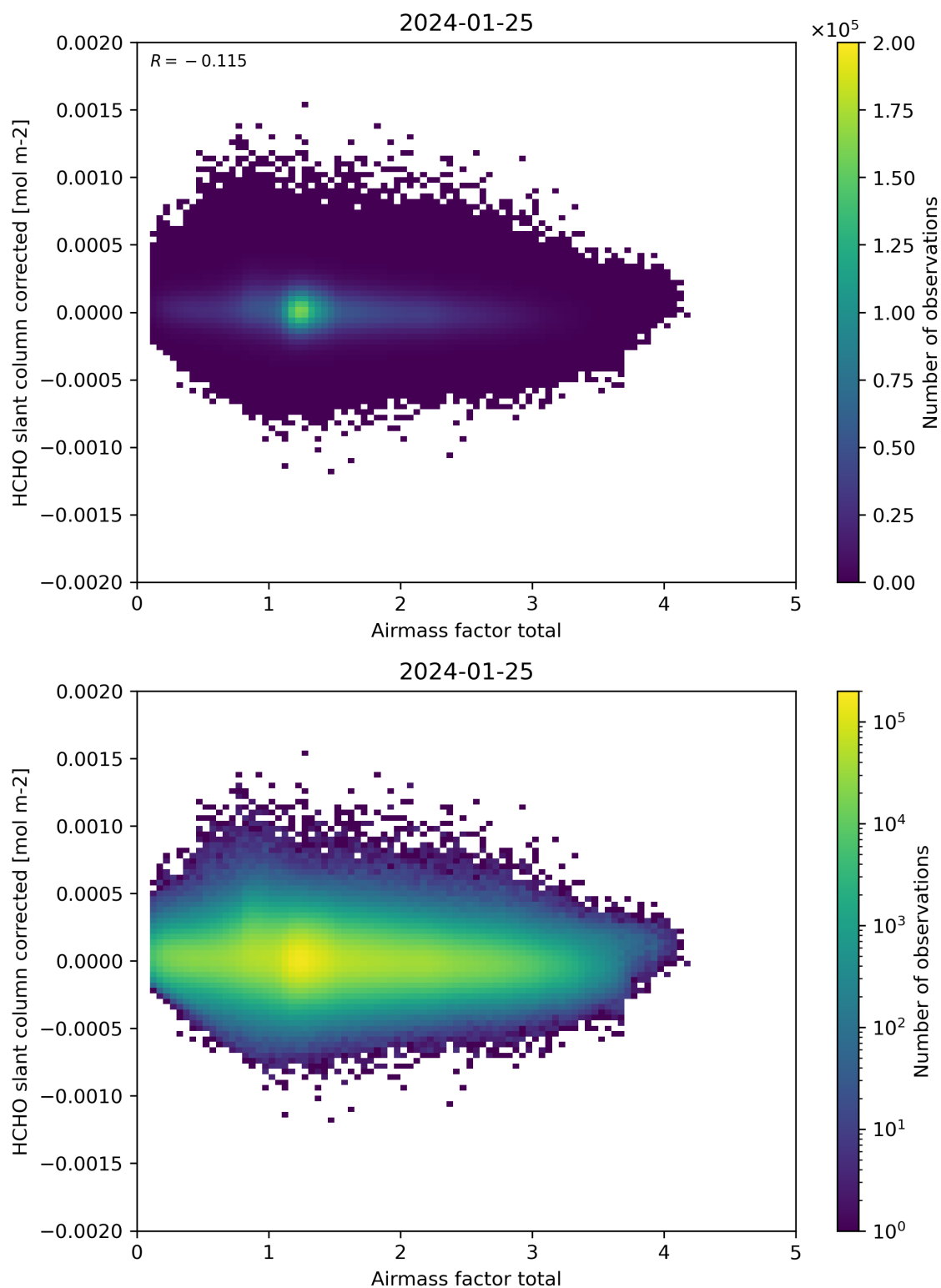
Figure 101: Scatter density plot of “Airmass factor total” against “HCHO slant column corrected” for 2024-01-24 to 2024-01-26.
