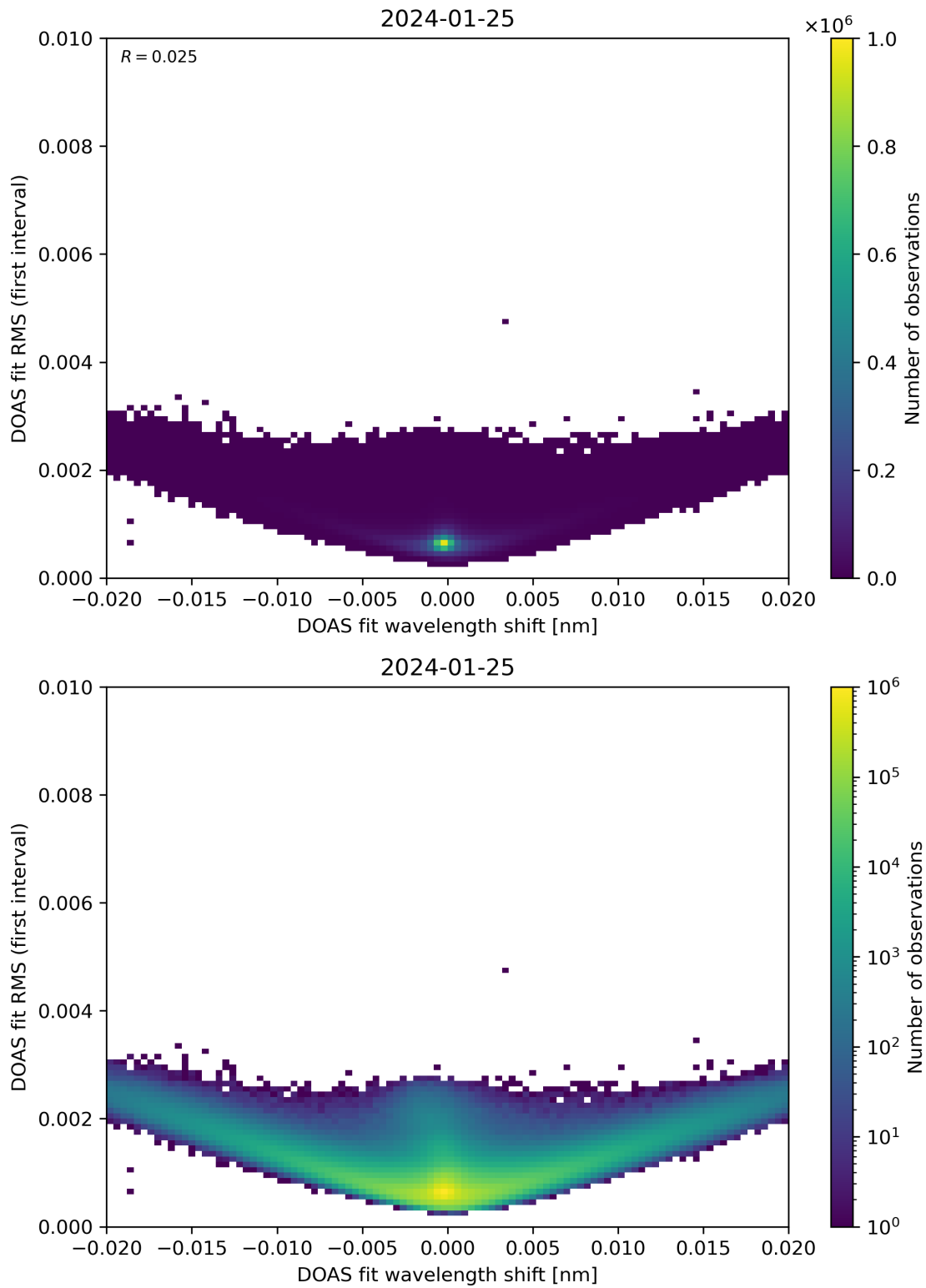
Figure 64: Scatter density plot of “DOAS fit wavelength shift” against “DOAS fit RMS (first interval)” for 2024-01-24 to 2024-01-26.
