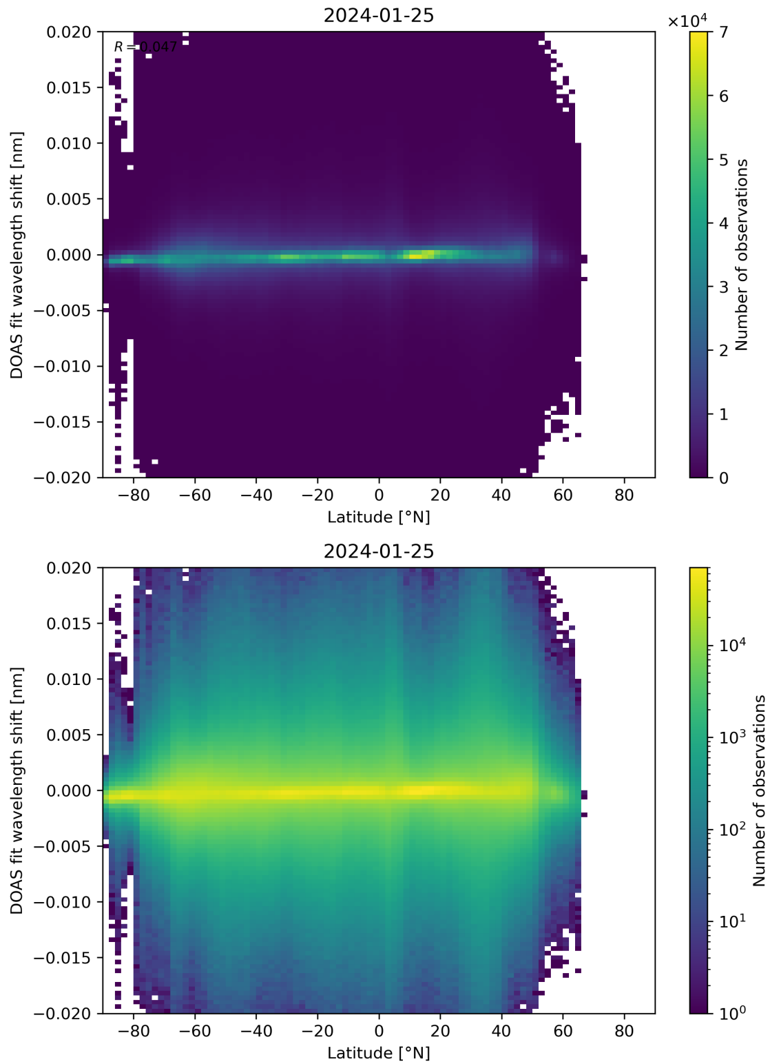
Figure 154: Scatter density plot of “Latitude” against “DOAS fit wavelength shift” for 2024-01-24 to 2024-01-26.
