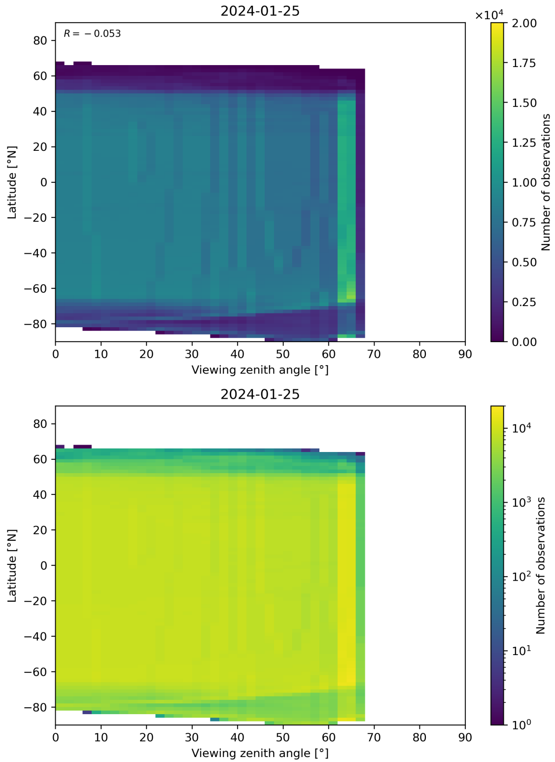
Figure 196: Scatter density plot of “Viewing zenith angle” against “Latitude” for 2024-01-24 to 2024-01-26.
