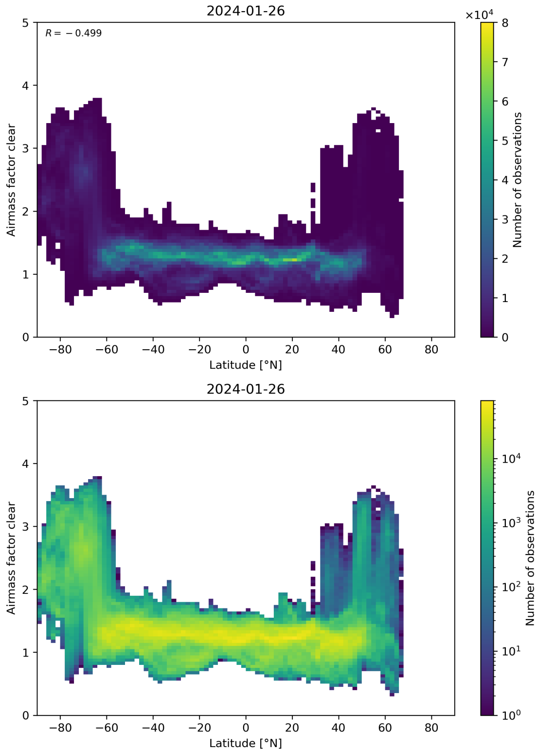
Figure 156: Scatter density plot of “Latitude” against “Airmass factor clear” for 2024-01-26 to 2024-01-27.
