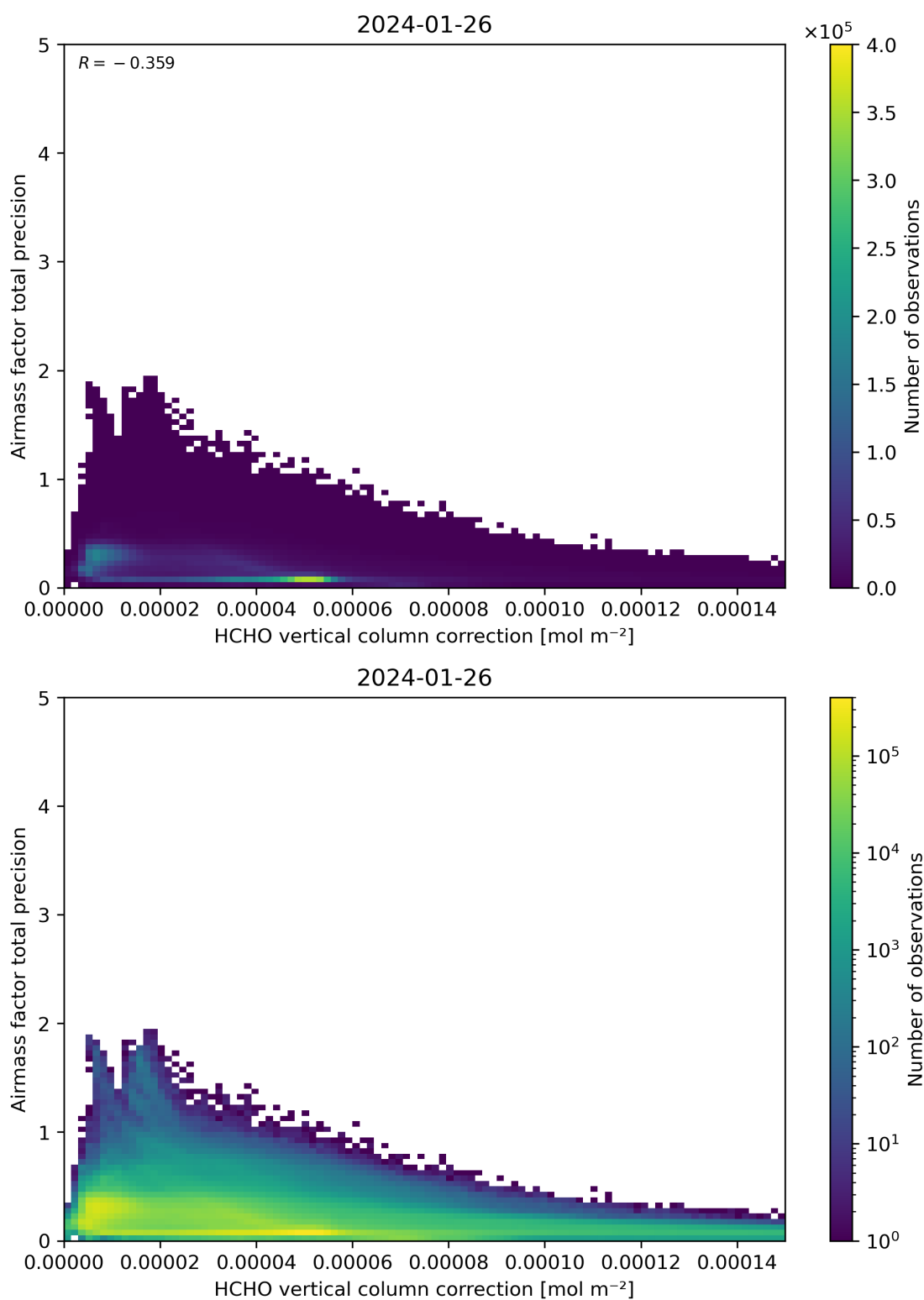
Figure 121: Scatter density plot of “HCHO vertical column correction” against “Airmass factor total precision” for 2024-01-26 to 2024-01-27.
