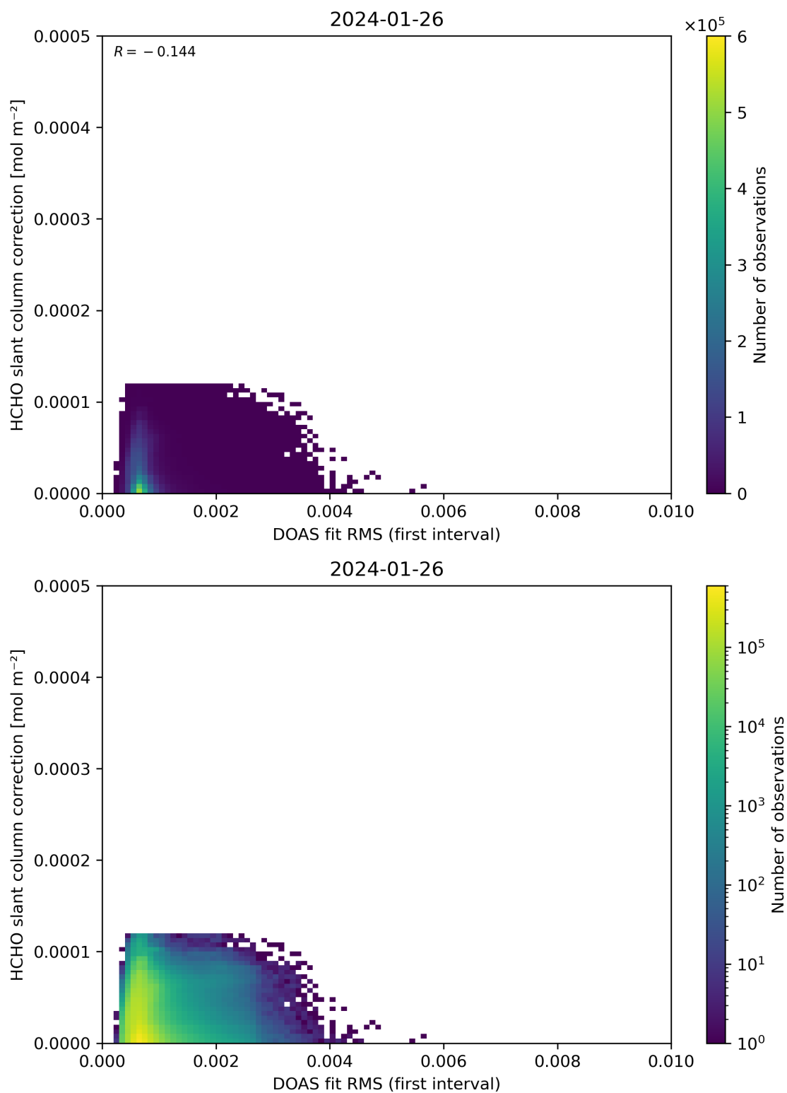
Figure 63: Scatter density plot of “DOAS fit RMS (first interval)” against “HCHO slant column correction” for 2024-01-26 to 2024-01-27.
