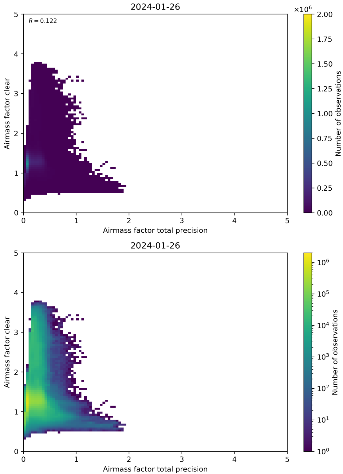
Figure 108: Scatter density plot of “Airmass factor total precision” against “Airmass factor clear” for 2024-01-26 to 2024-01-27.
