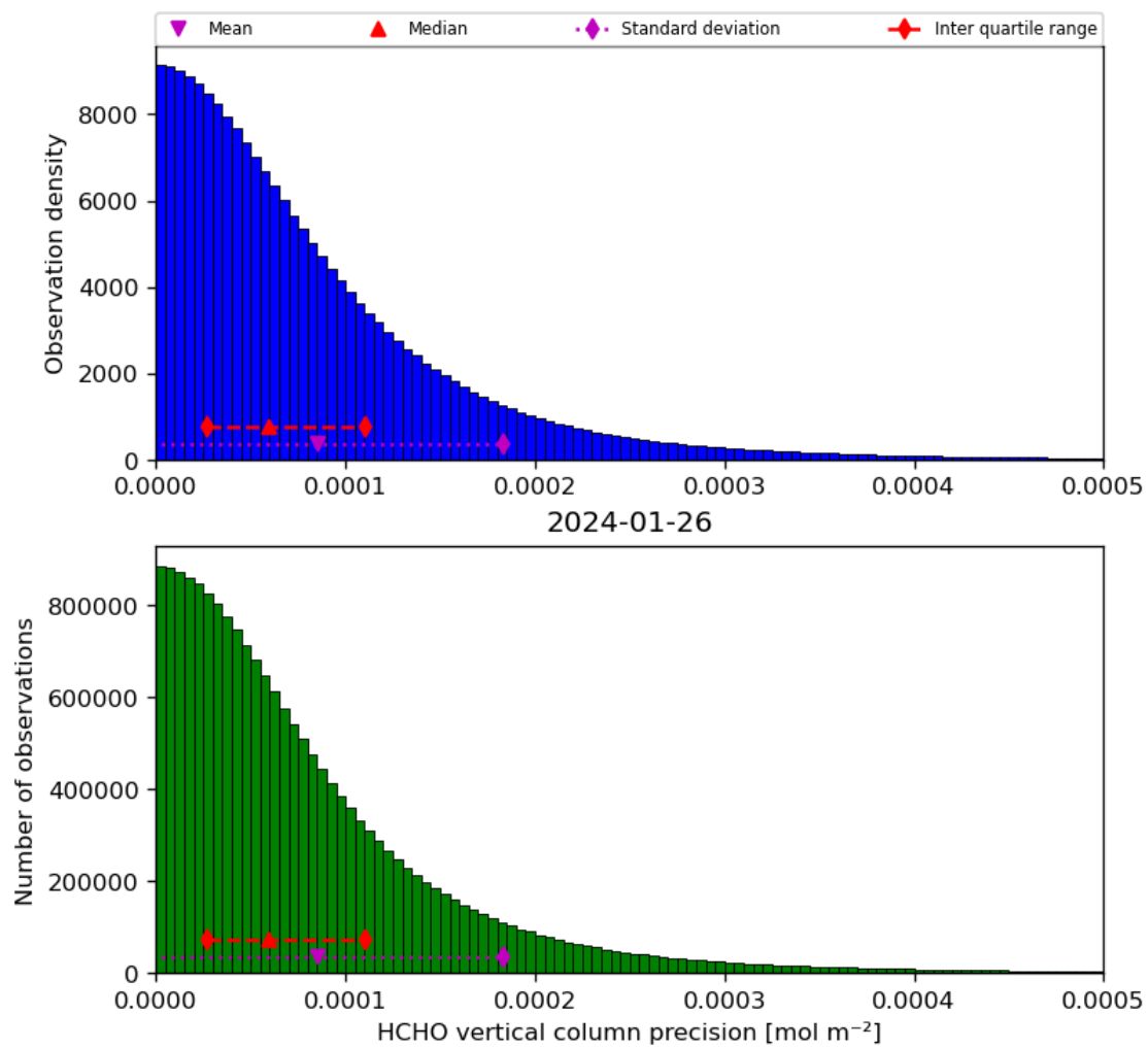
Figure 36: Histogram of “HCHO vertical column precision” for 2024-01-26 to 2024-01-27
