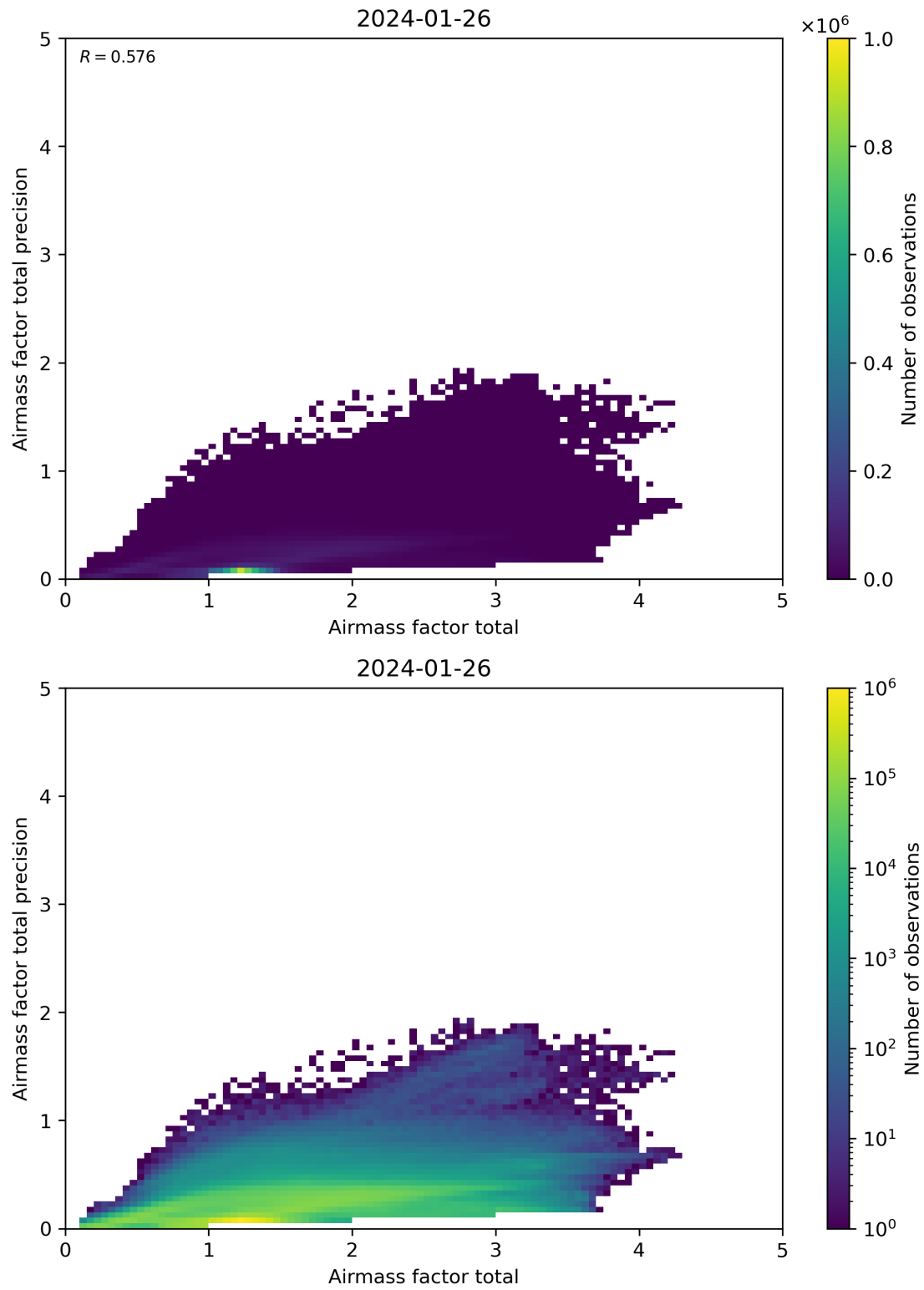
Figure 103: Scatter density plot of “Airmass factor total” against “Airmass factor total precision” for 2024-01-26 to 2024-01-27.
