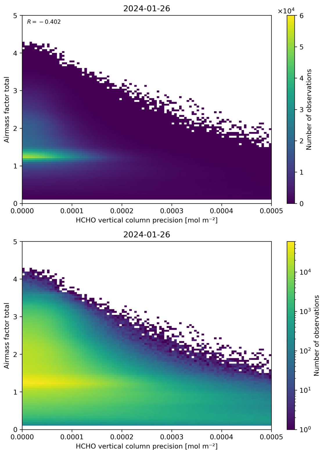
Figure 144: Scatter density plot of “HCHO vertical column precision” against “Airmass factor total” for 2024-01-26 to 2024-01-27.
