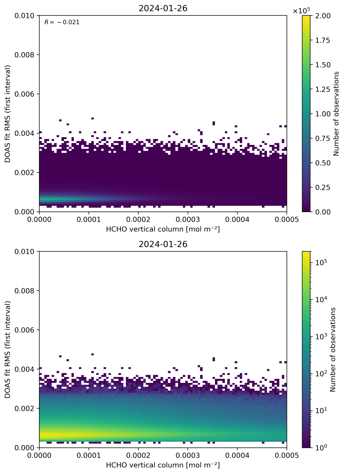
Figure 123: Scatter density plot of “HCHO vertical column” against “DOAS fit RMS (first interval)” for 2024-01-26 to 2024-01-27.
