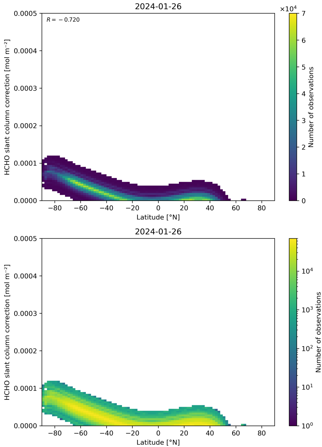
Figure 158: Scatter density plot of “Latitude” against “HCHO slant column correction” for 2024-01-26 to 2024-01-27.
