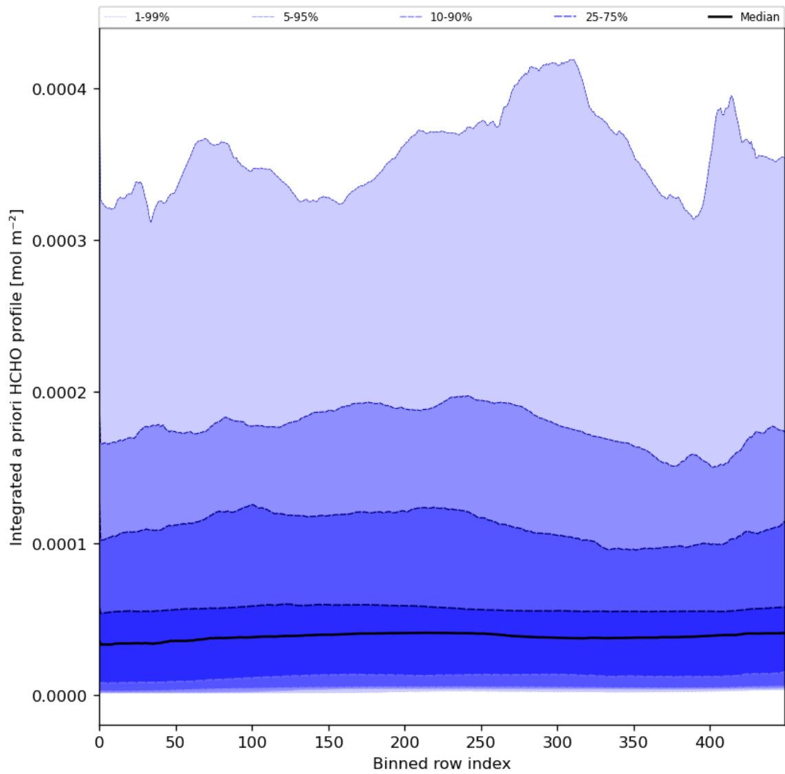
Figure 57: Along track statistics of “Integrated a priori HCHO profile” for 2024-01-26 to 2024-01-27
