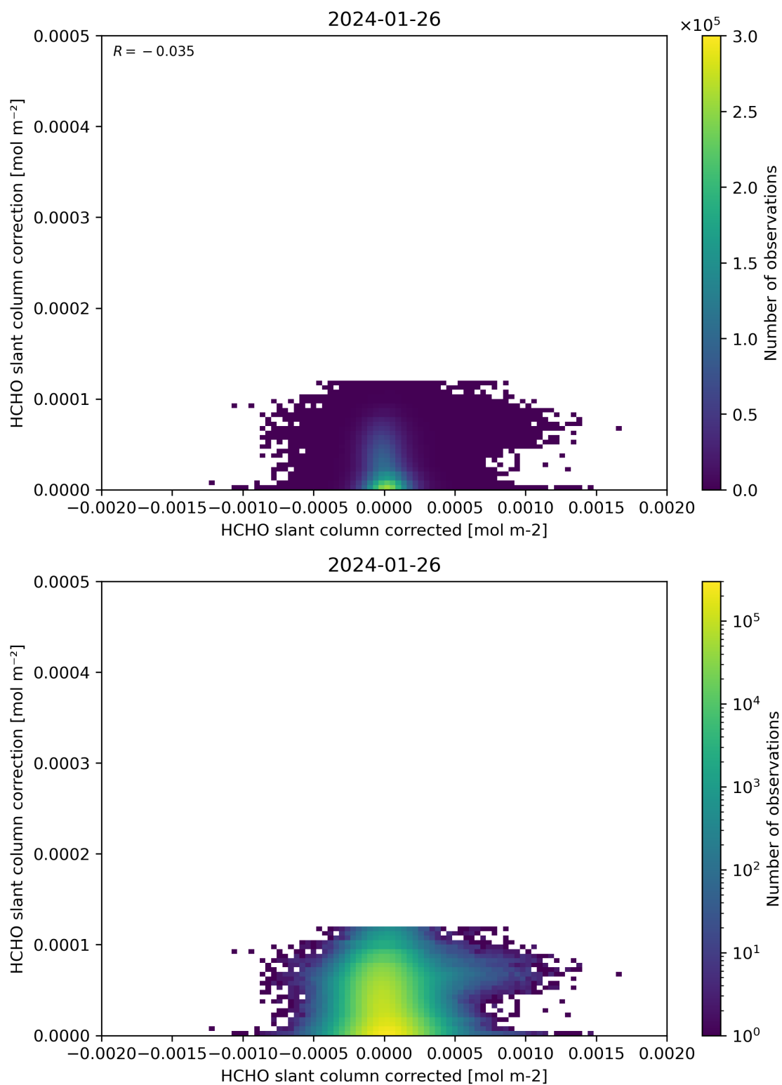
Figure 77: Scatter density plot of “HCHO slant column corrected” against “HCHO slant column correction” for 2024-01-26 to 2024-01-27.
