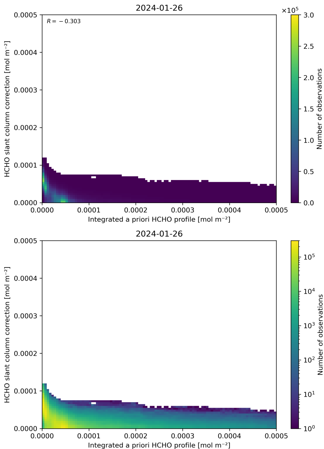
Figure 152: Scatter density plot of “Integrated a priori HCHO profile” against “HCHO slant column correction” for 2024-01-26 to 2024-01-27.
