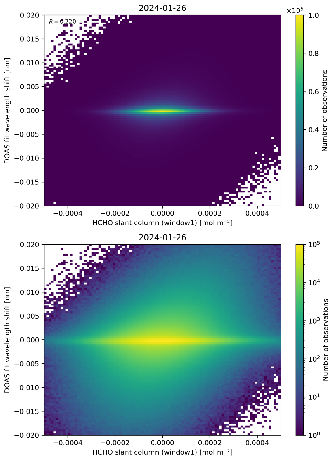
Figure 79: Scatter density plot of “HCHO slant column (window1)” against “DOAS fit wavelength shift” for 2024-01-26 to 2024-01-27.
