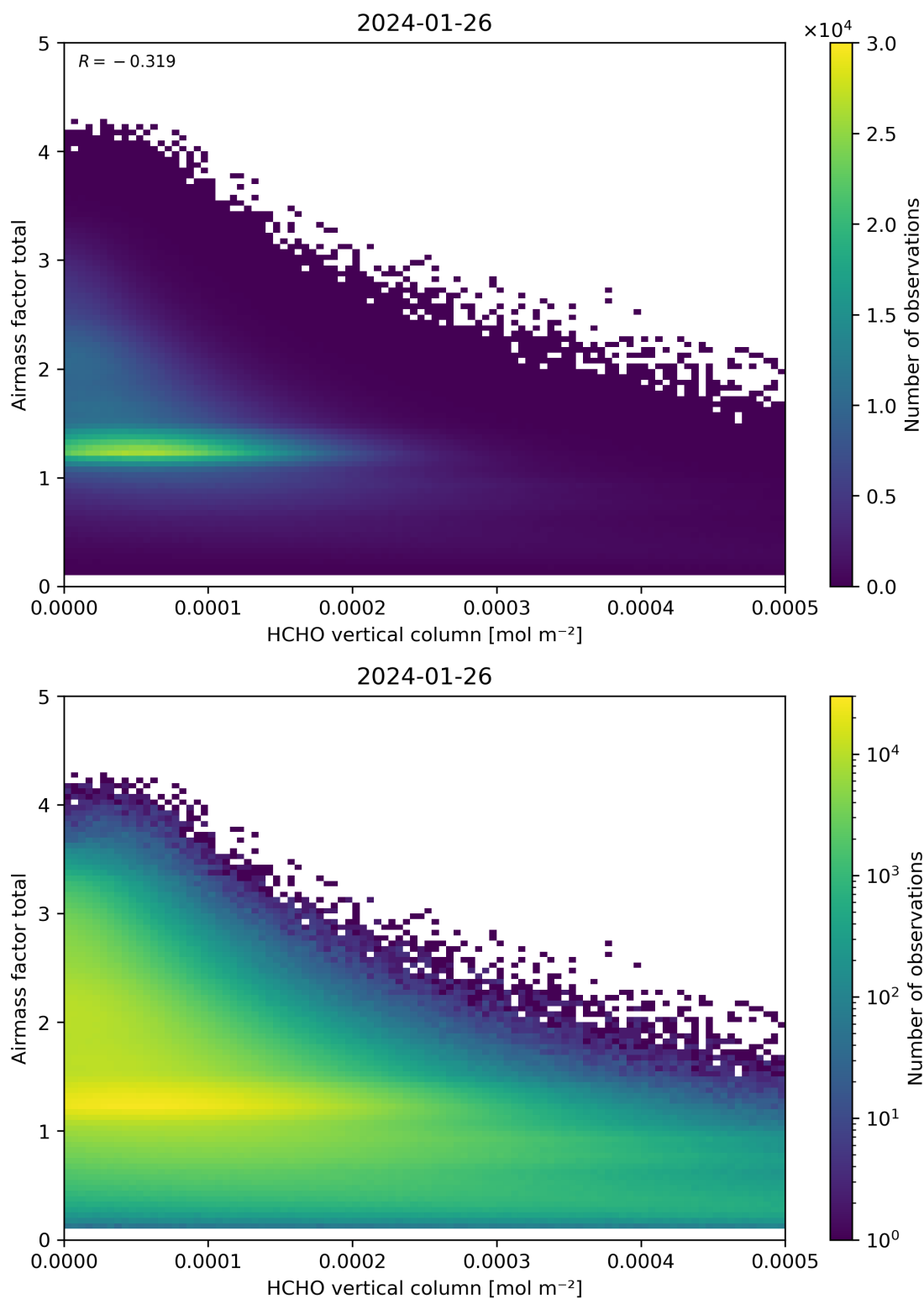
Figure 131: Scatter density plot of “HCHO vertical column” against “Airmass factor total” for 2024-01-26 to 2024-01-27.
