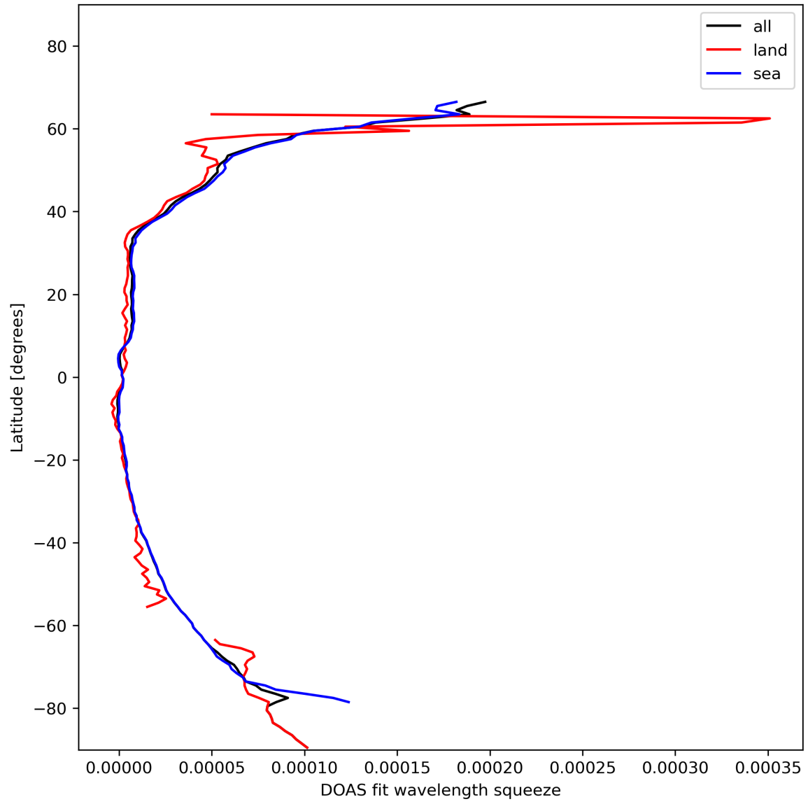
Figure 31: Zonal average of “DOAS fit wavelength squeeze” for 2024-01-26 to 2024-01-27.
