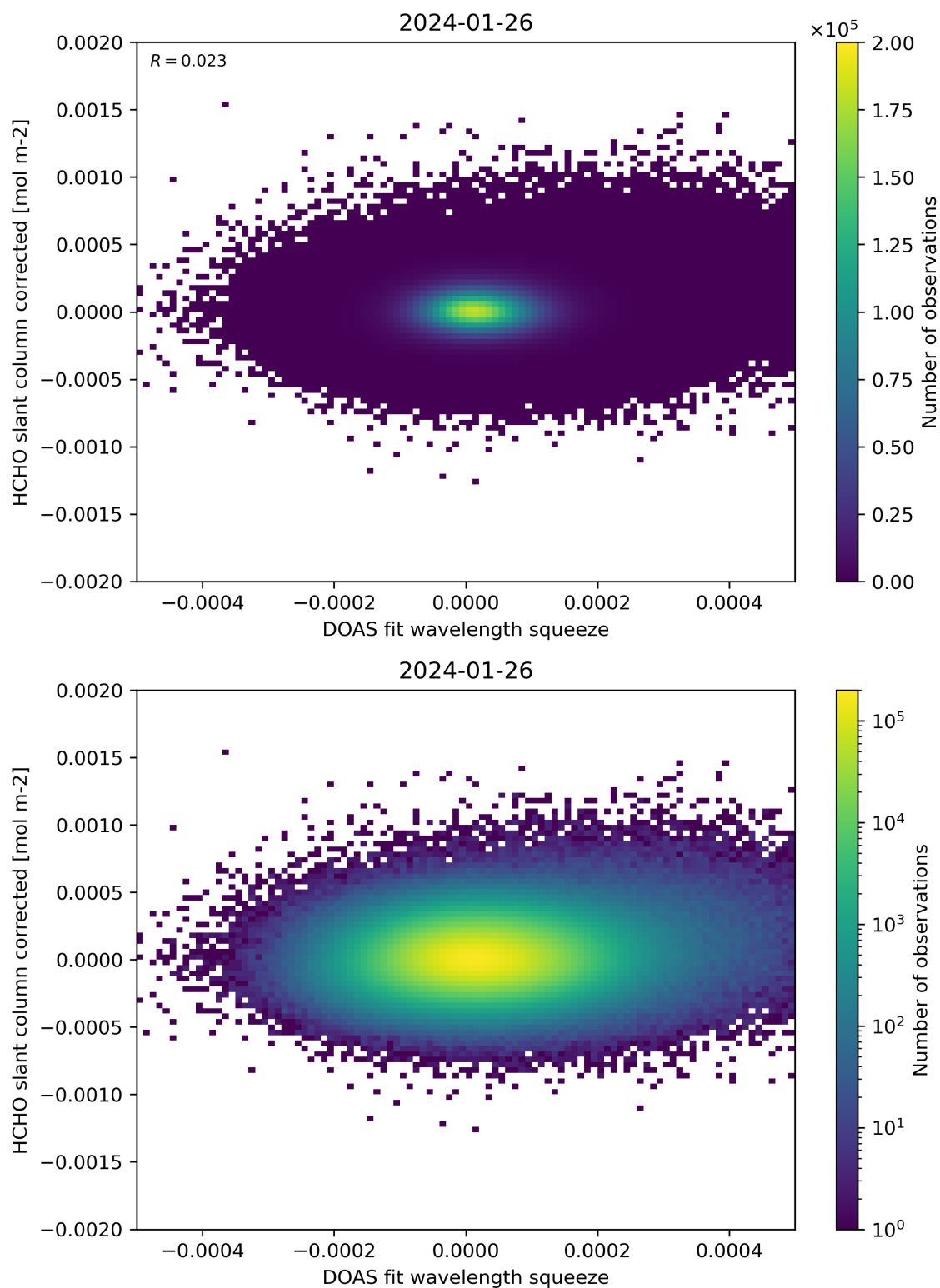
Figure 69: Scatter density plot of “DOAS fit wavelength squeeze” against “HCHO slant column corrected” for 2024-01-26 to 2024-01-27.
