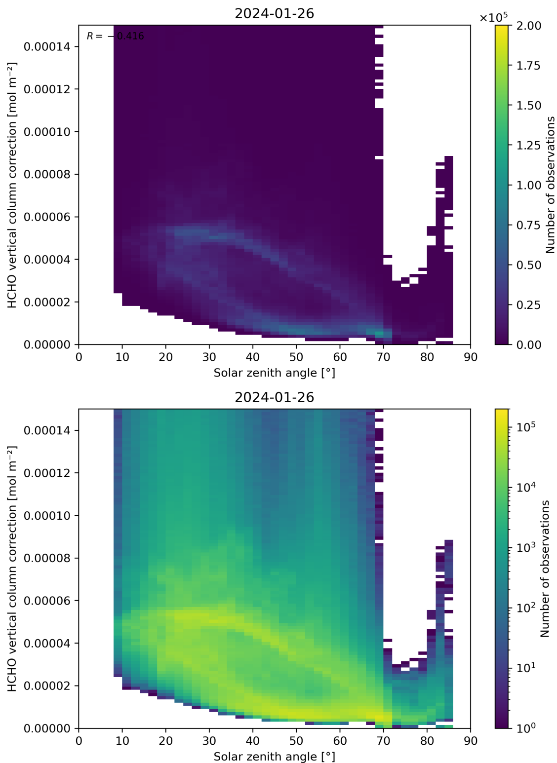
Figure 178: Scatter density plot of “Solar zenith angle” against “HCHO vertical column correction” for 2024-01-26 to 2024-01-27.
