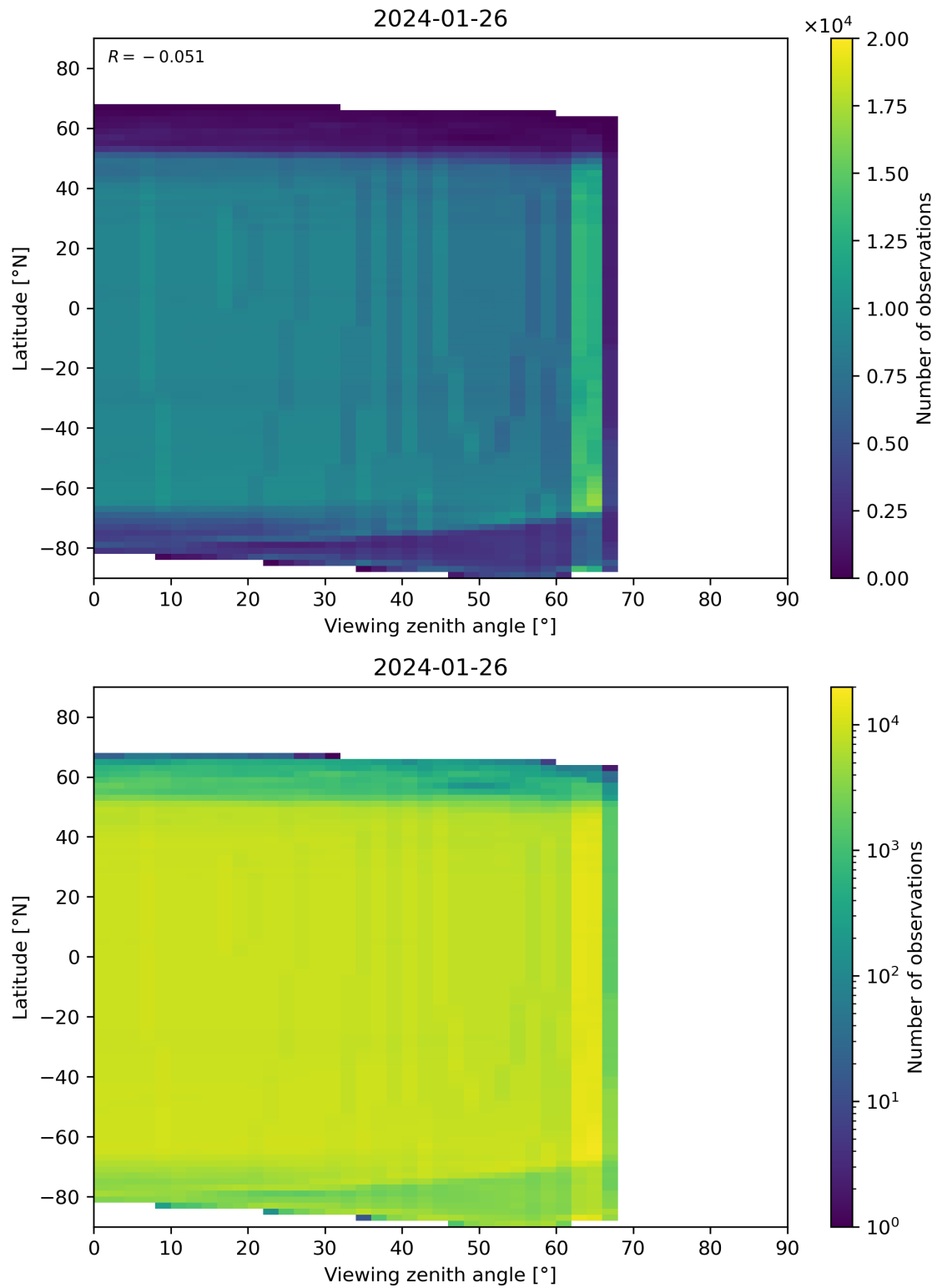
Figure 196: Scatter density plot of “Viewing zenith angle” against “Latitude” for 2024-01-26 to 2024-01-27.
