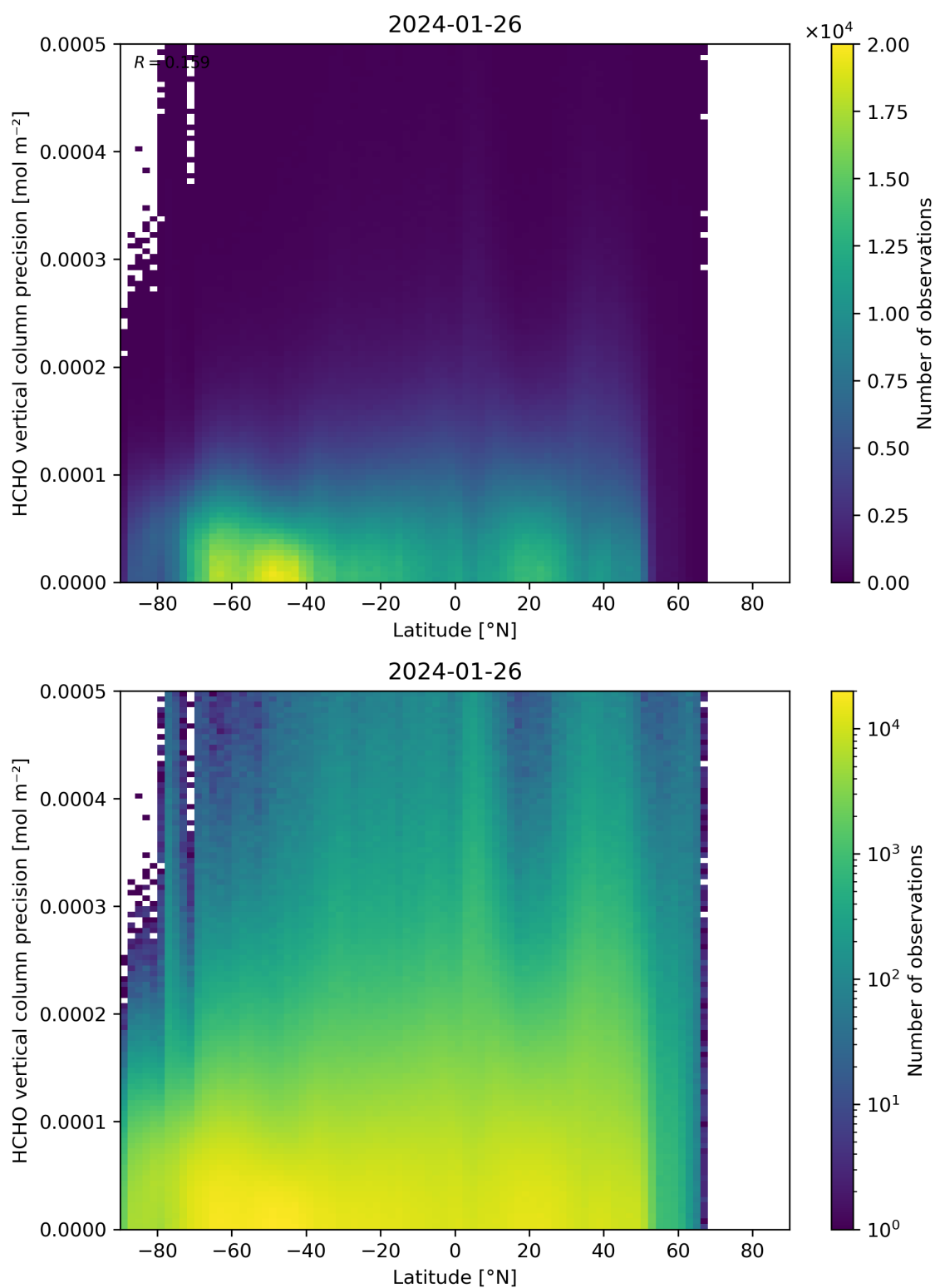
Figure 165: Scatter density plot of “Latitude” against “HCHO vertical column precision” for 2024-01-26 to 2024-01-27.
