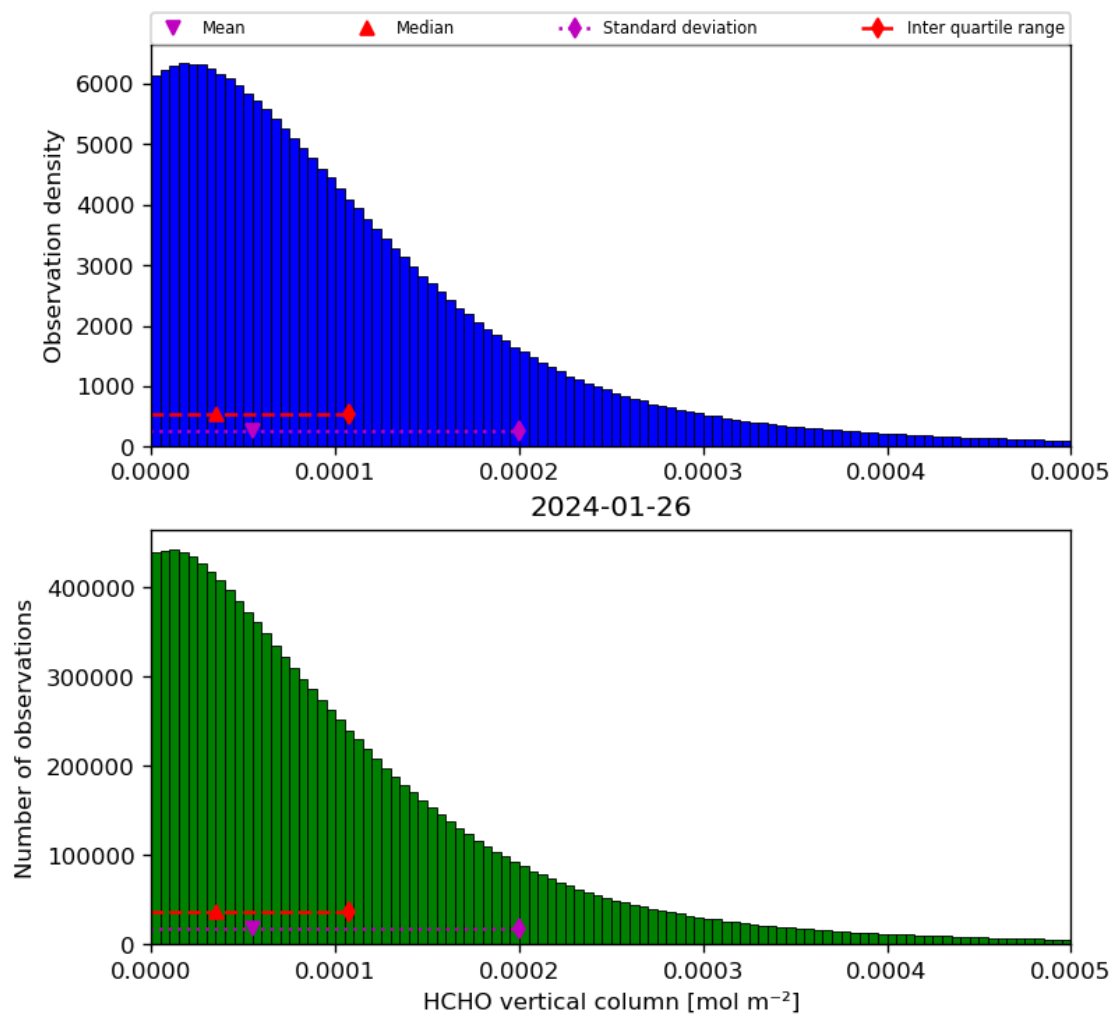
Figure 35: Histogram of “HCHO vertical column” for 2024-01-26 to 2024-01-27
