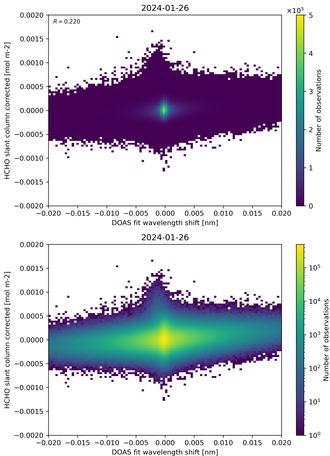
Figure 66: Scatter density plot of “DOAS fit wavelength shift” against “HCHO slant column corrected” for 2024-01-26 to 2024-01-27.
