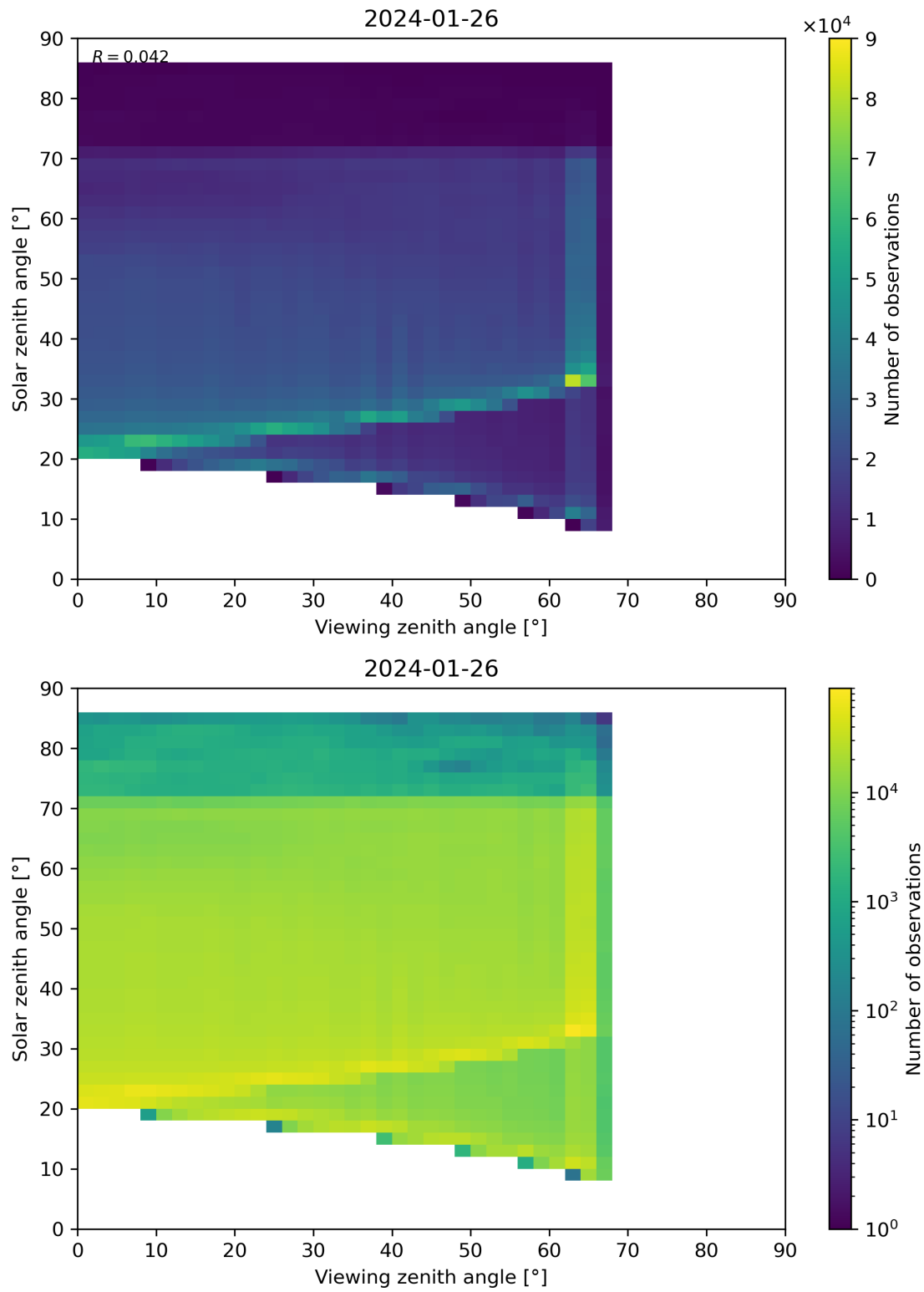
Figure 197: Scatter density plot of “Viewing zenith angle” against “Solar zenith angle” for 2024-01-26 to 2024-01-27.
