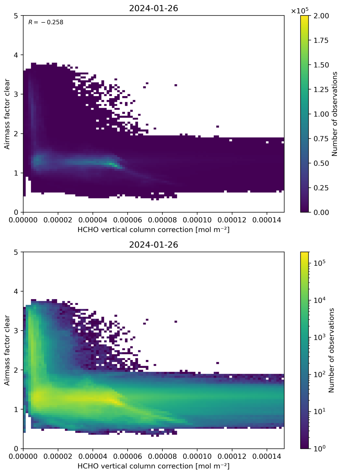
Figure 115: Scatter density plot of “HCHO vertical column correction” against “Airmass factor clear” for 2024-01-26 to 2024-01-27.
