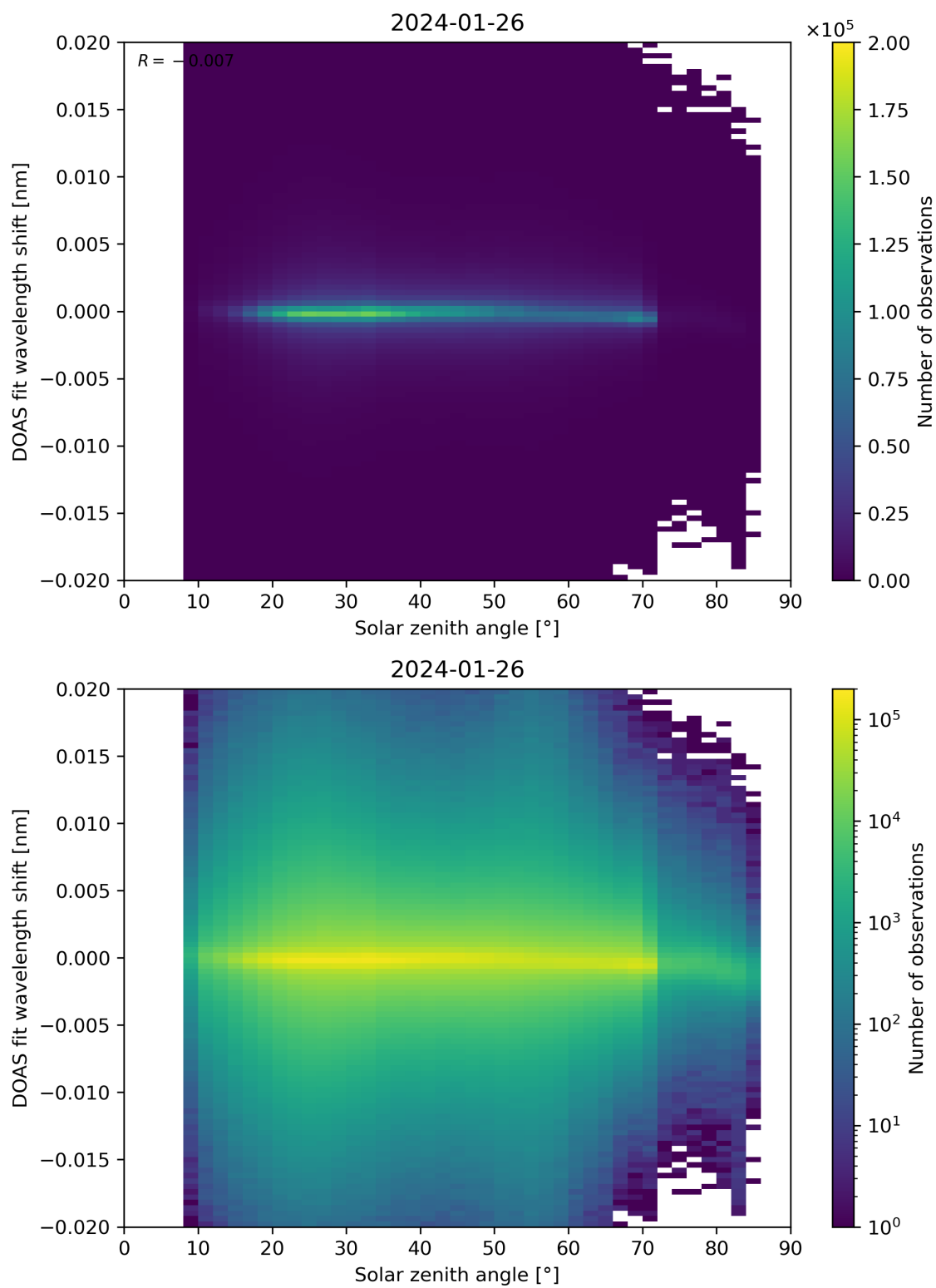
Figure 168: Scatter density plot of “Solar zenith angle” against “DOAS fit wavelength shift” for 2024-01-26 to 2024-01-27.
