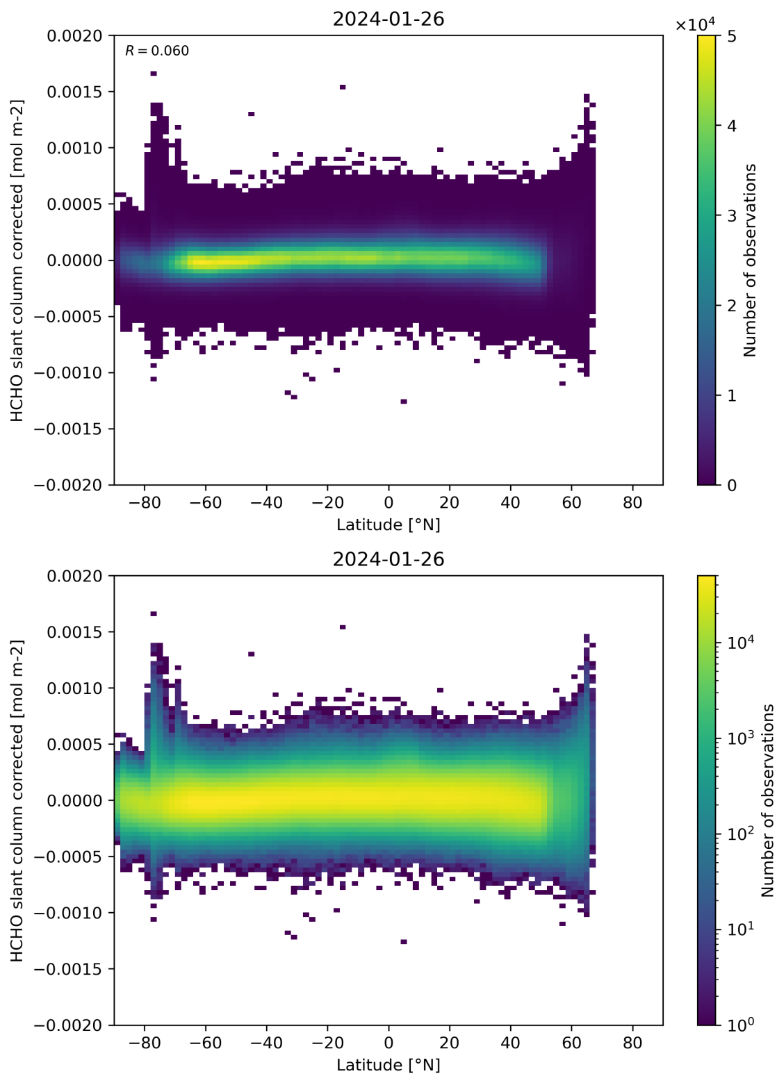
Figure 157: Scatter density plot of “Latitude” against “HCHO slant column corrected” for 2024-01-26 to 2024-01-27.
