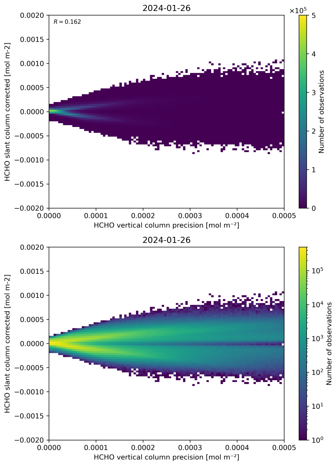
Figure 140: Scatter density plot of “HCHO vertical column precision” against “HCHO slant column corrected” for 2024-01-26 to 2024-01-27.
