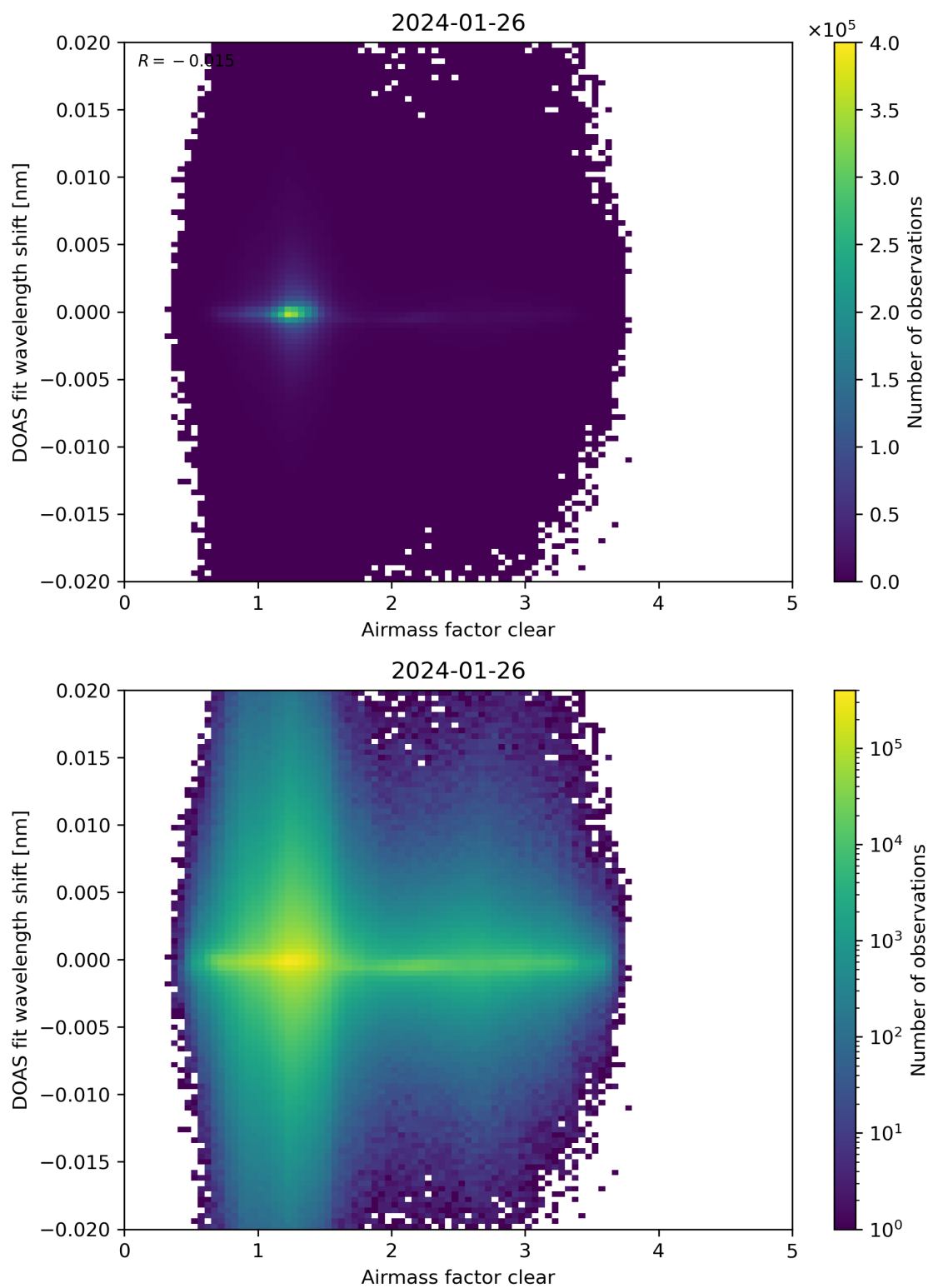
Figure 72: Scatter density plot of “Airmass factor clear” against “DOAS fit wavelength shift” for 2024-01-26 to 2024-01-27.
