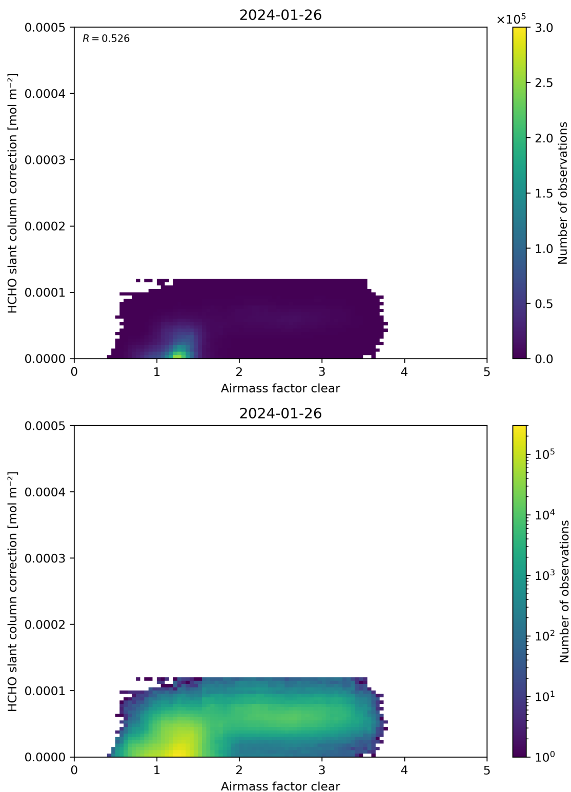
Figure 75: Scatter density plot of “Airmass factor clear” against “HCHO slant column correction” for 2024-01-26 to 2024-01-27.
