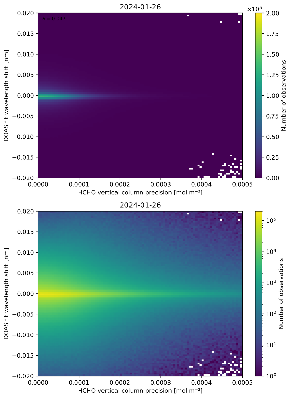
Figure 137: Scatter density plot of “HCHO vertical column precision” against “DOAS fit wavelength shift” for 2024-01-26 to 2024-01-27.
