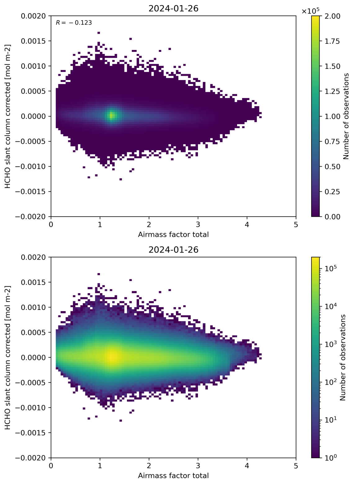
Figure 101: Scatter density plot of “Airmass factor total” against “HCHO slant column corrected” for 2024-01-26 to 2024-01-27.
