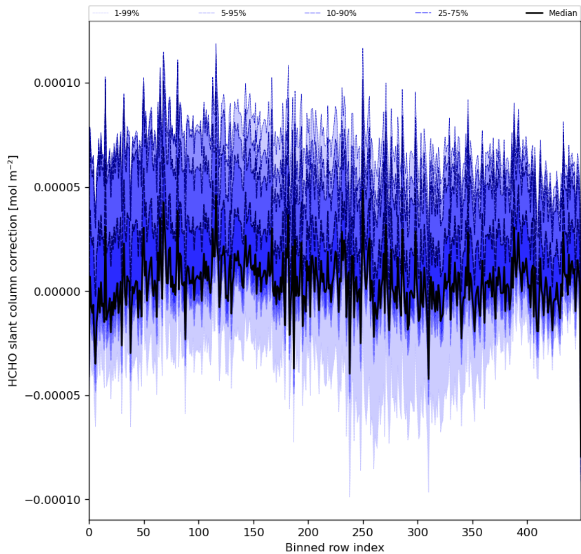
Figure 61: Along track statistics of “HCHO slant column correction” for 2024-01-26 to 2024-01-27
