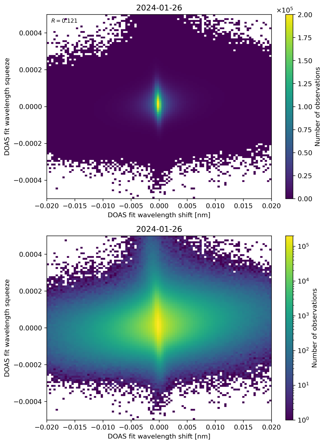
Figure 65: Scatter density plot of “DOAS fit wavelength shift” against “DOAS fit wavelength squeeze” for 2024-01-26 to 2024-01-27.
