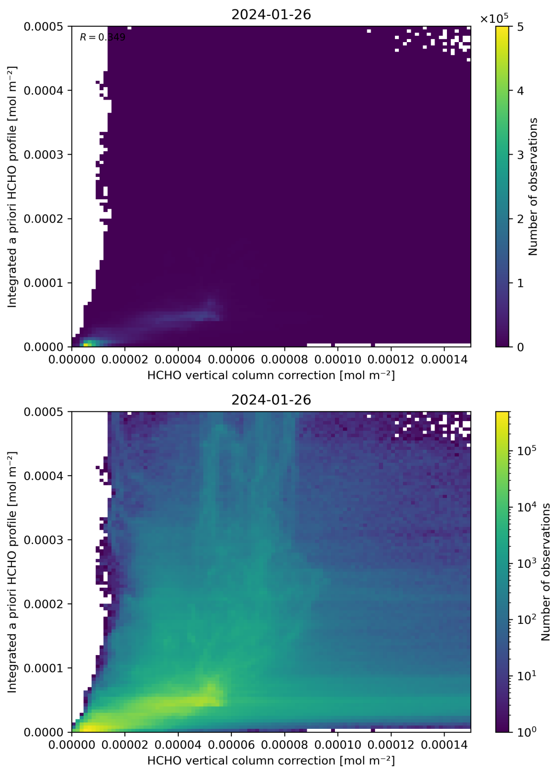
Figure 122: Scatter density plot of “HCHO vertical column correction” against “Integrated a priori HCHO profile” for 2024-01-26 to 2024-01-27.
