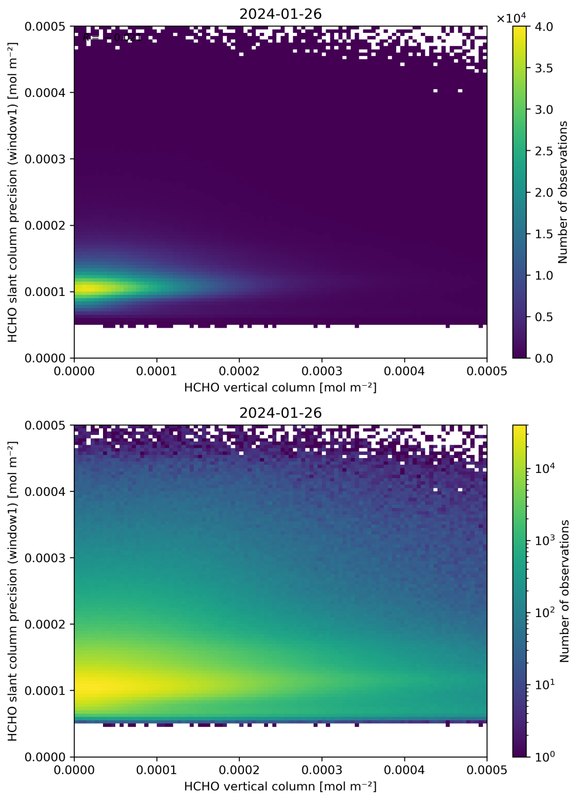
Figure 130: Scatter density plot of “HCHO vertical column” against “HCHO slant column precision (window1)” for 2024-01-26 to 2024-01-27.
