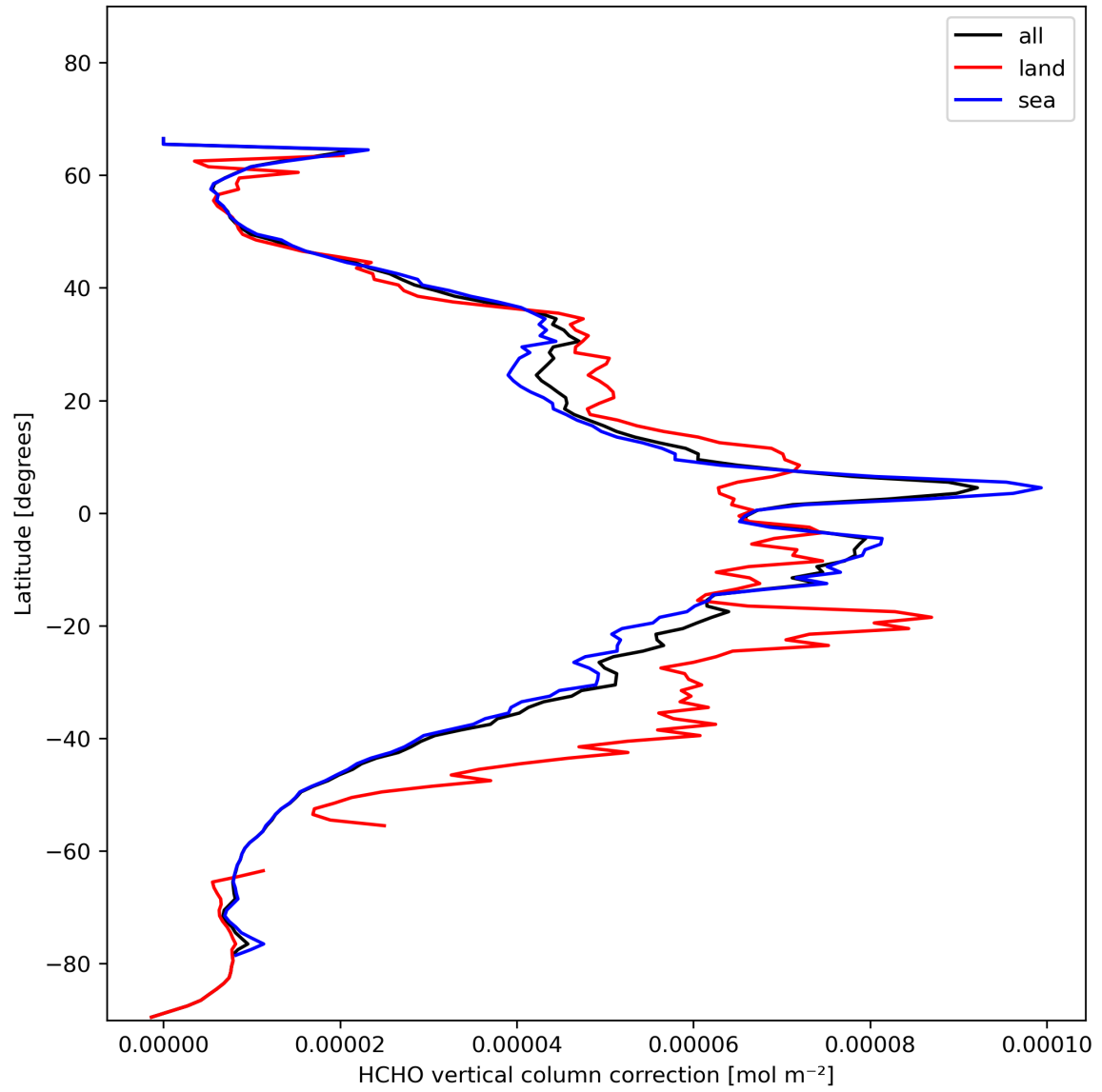
Figure 23: Zonal average of “HCHO vertical column correction” for 2024-01-26 to 2024-01-27.
