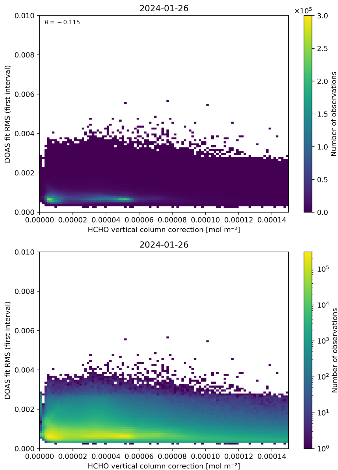
Figure 112: Scatter density plot of “HCHO vertical column correction” against “DOAS fit RMS (first interval)” for 2024-01-26 to 2024-01-27.
