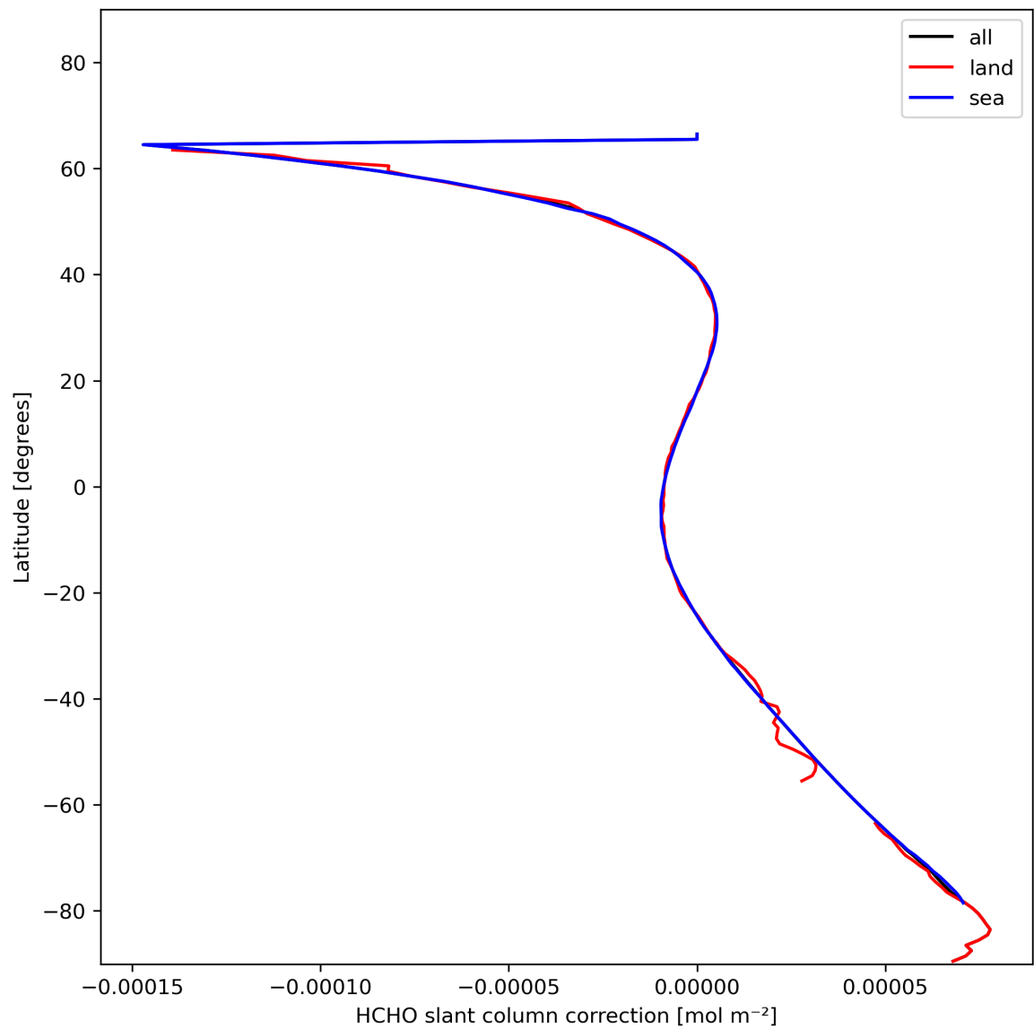
Figure 33: Zonal average of “HCHO slant column correction” for 2024-01-26 to 2024-01-27.
