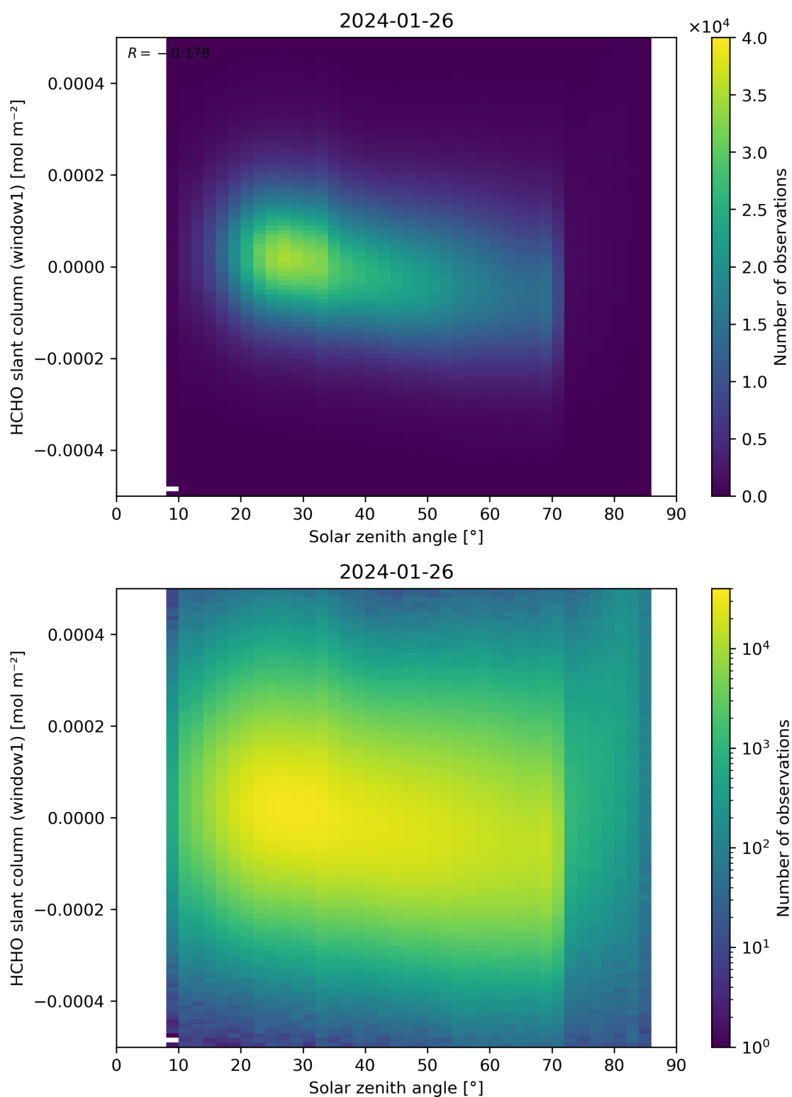
Figure 173: Scatter density plot of “Solar zenith angle” against “HCHO slant column (window1)” for 2024-01-26 to 2024-01-27.
