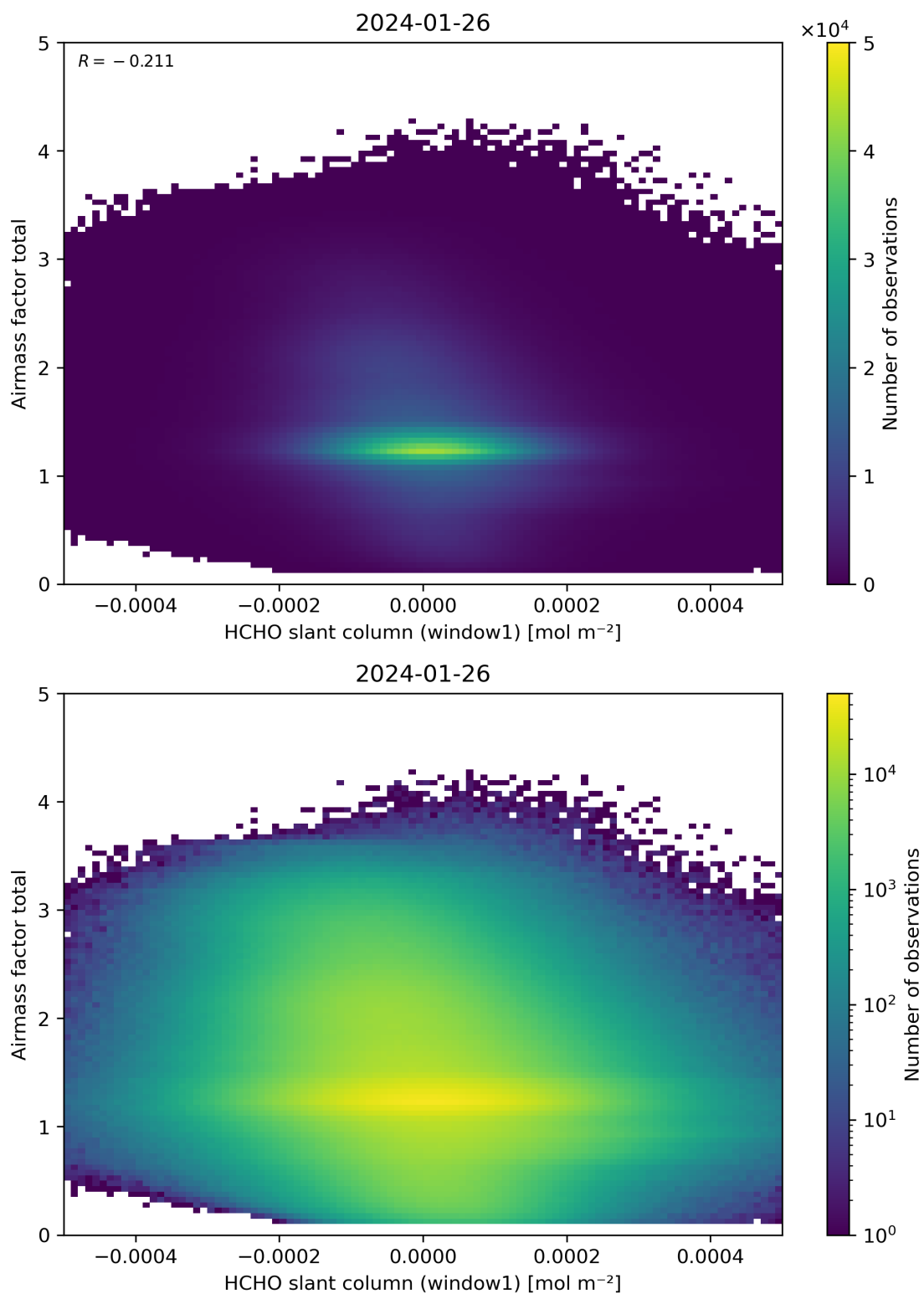
Figure 85: Scatter density plot of “HCHO slant column (window1)” against “Airmass factor total” for 2024-01-26 to 2024-01-27.
