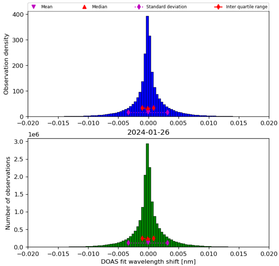
Figure 44: Histogram of “DOAS fit wavelength shift” for 2024-01-26 to 2024-01-27
