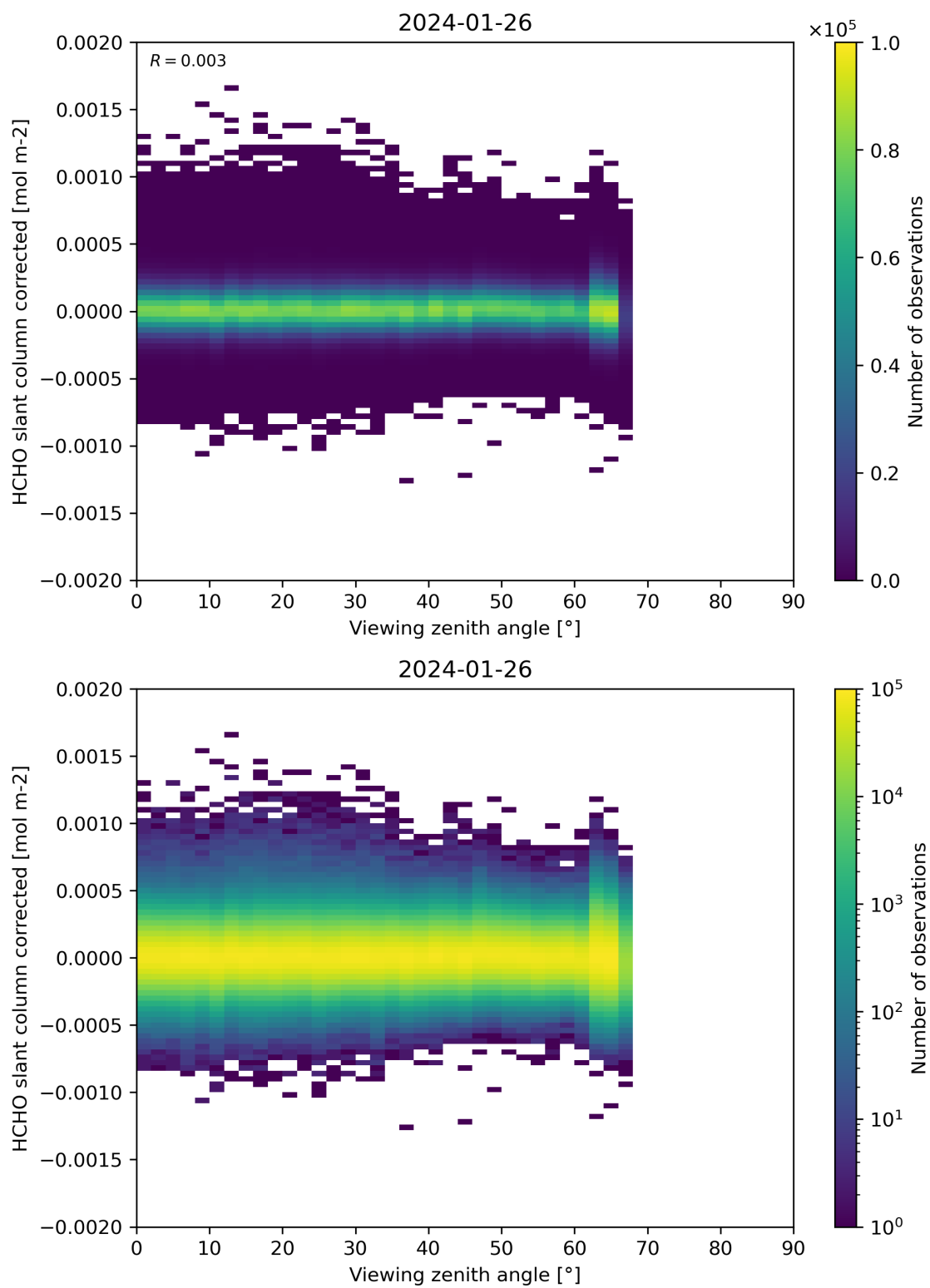
Figure 186: Scatter density plot of “Viewing zenith angle” against “HCHO slant column corrected” for 2024-01-26 to 2024-01-27.
