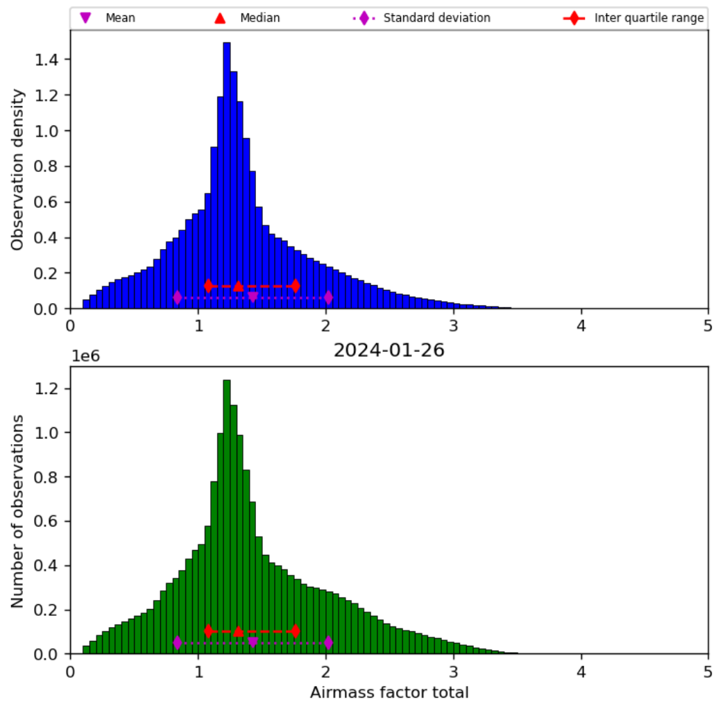
Figure 40: Histogram of “Airmass factor total” for 2024-01-26 to 2024-01-27
