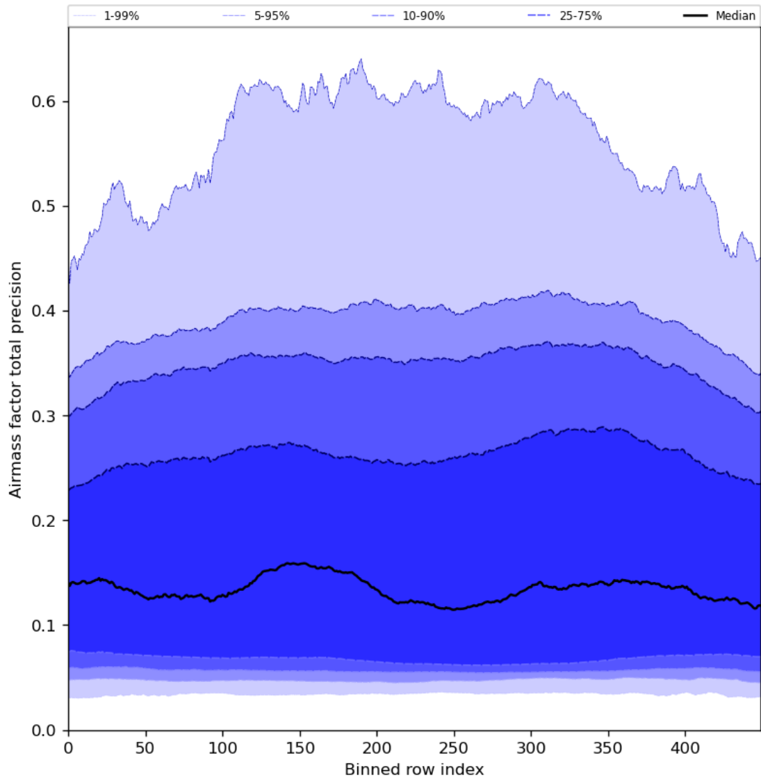
Figure 55: Along track statistics of “Airmass factor total precision” for 2024-01-26 to 2024-01-27
