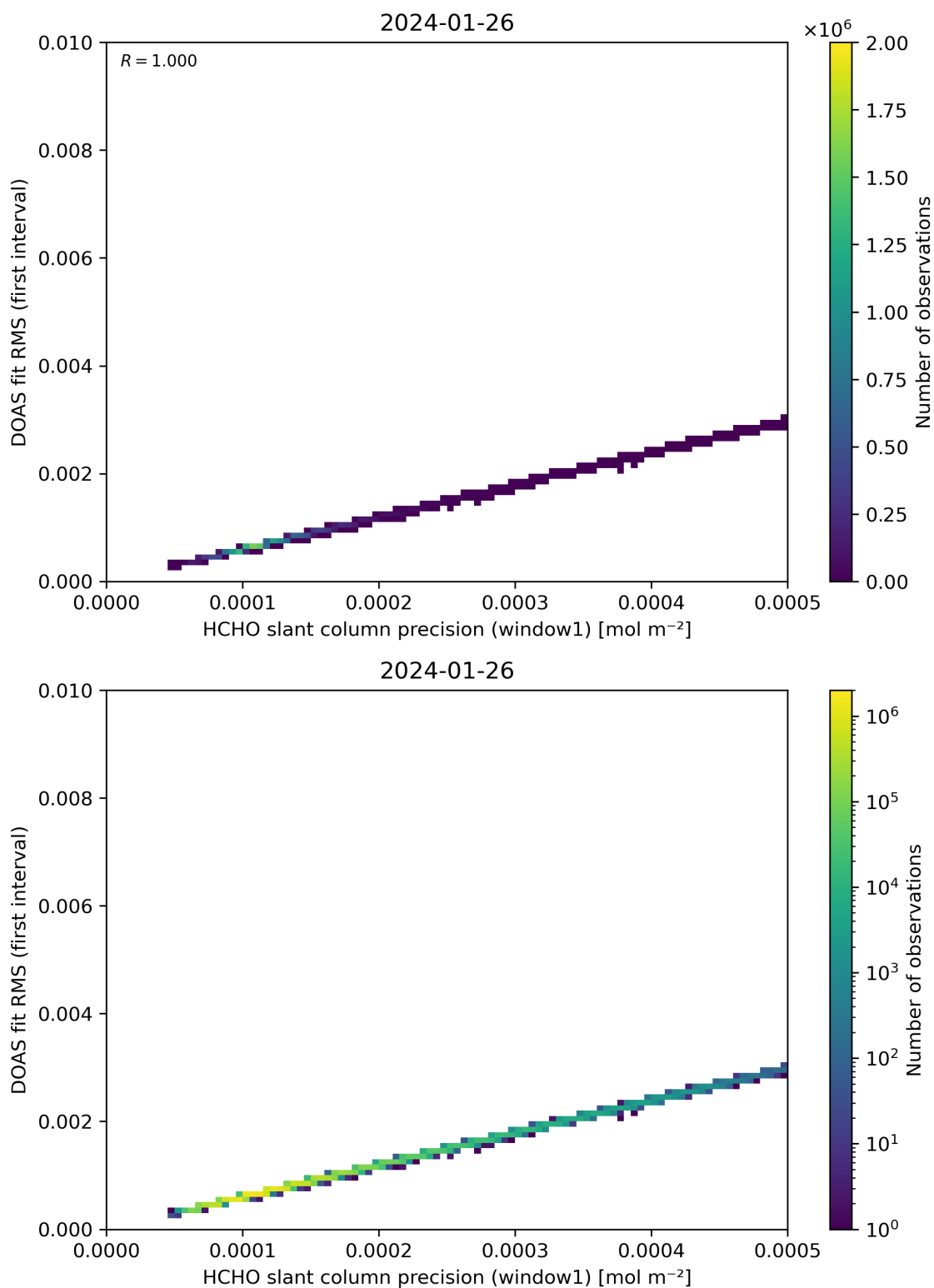
Figure 88: Scatter density plot of “HCHO slant column precision (window1)” against “DOAS fit RMS (first interval)” for 2024-01-26 to 2024-01-27.
