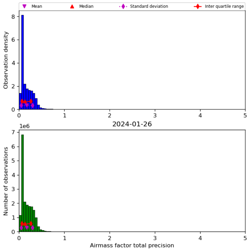
Figure 41: Histogram of “Airmass factor total precision” for 2024-01-26 to 2024-01-27
