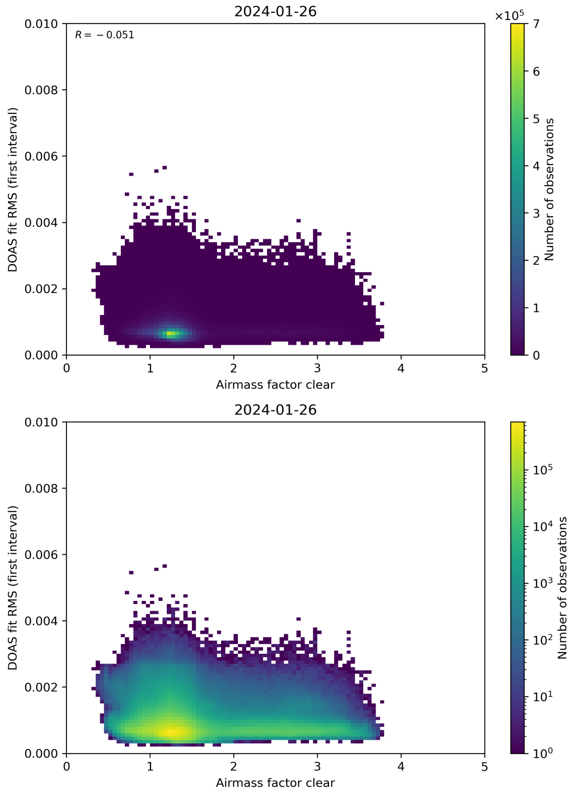
Figure 71: Scatter density plot of “Airmass factor clear” against “DOAS fit RMS (first interval)” for 2024-01-26 to 2024-01-27.
