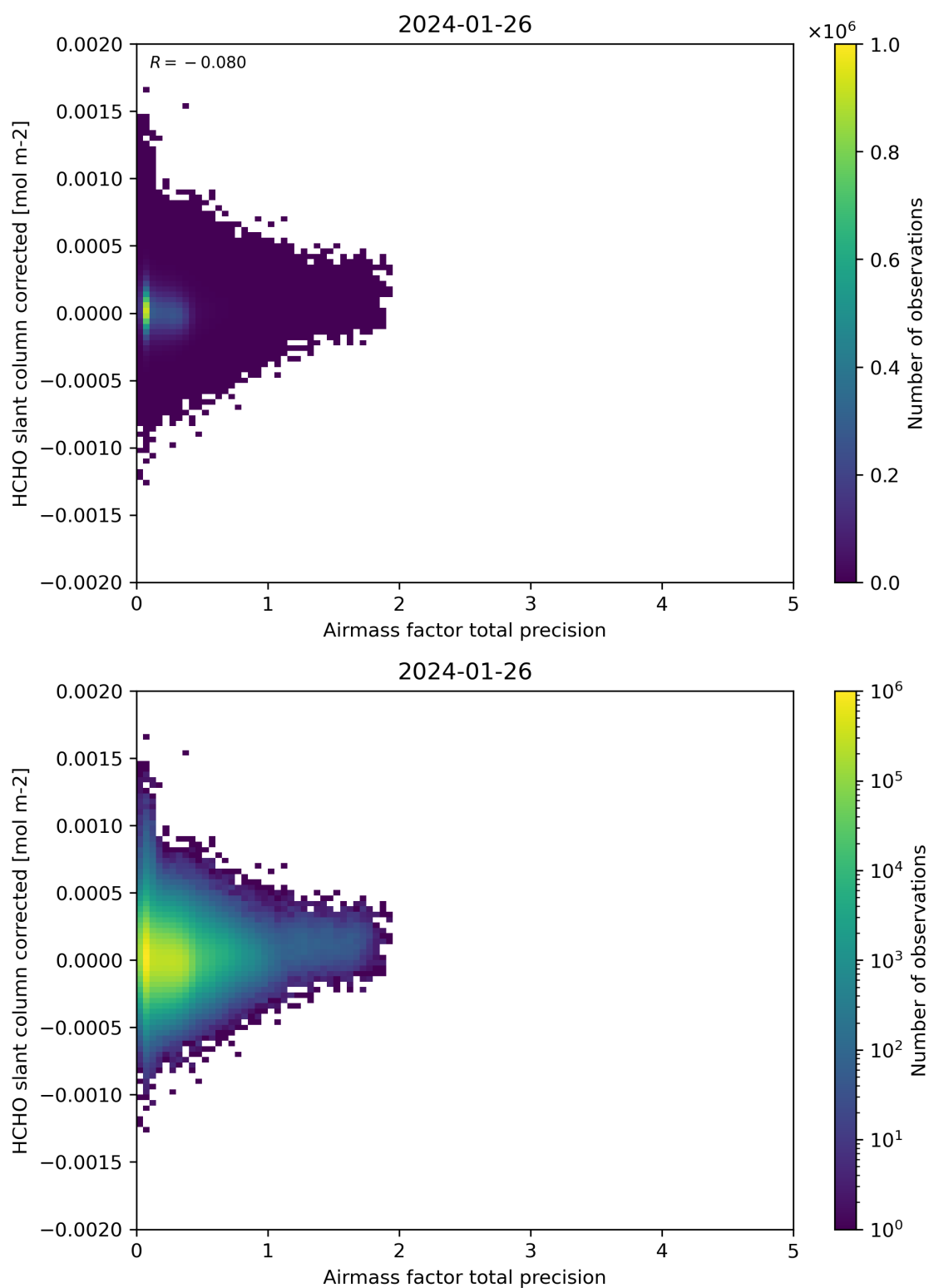
Figure 109: Scatter density plot of “Airmass factor total precision” against “HCHO slant column corrected” for 2024-01-26 to 2024-01-27.
