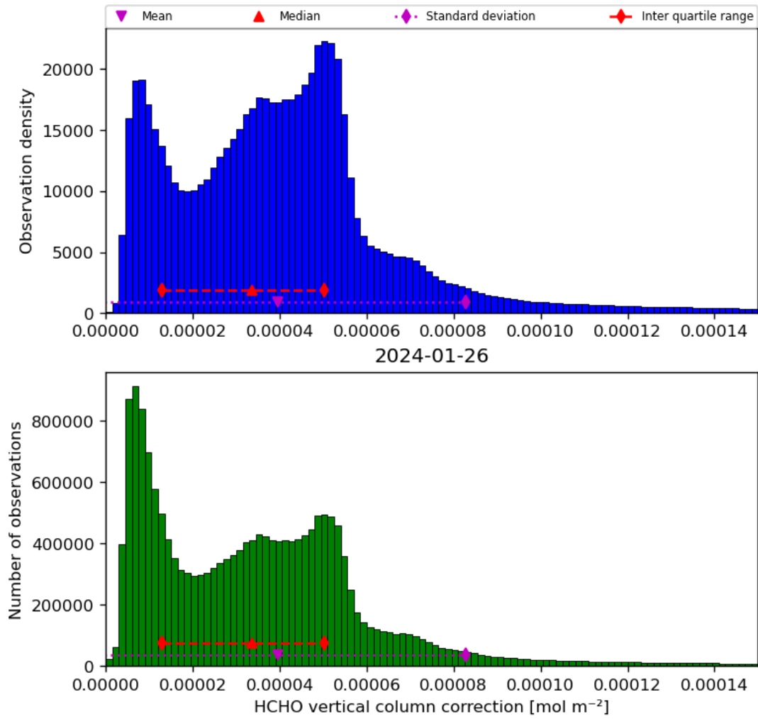
Figure 37: Histogram of “HCHO vertical column correction” for 2024-01-26 to 2024-01-27
