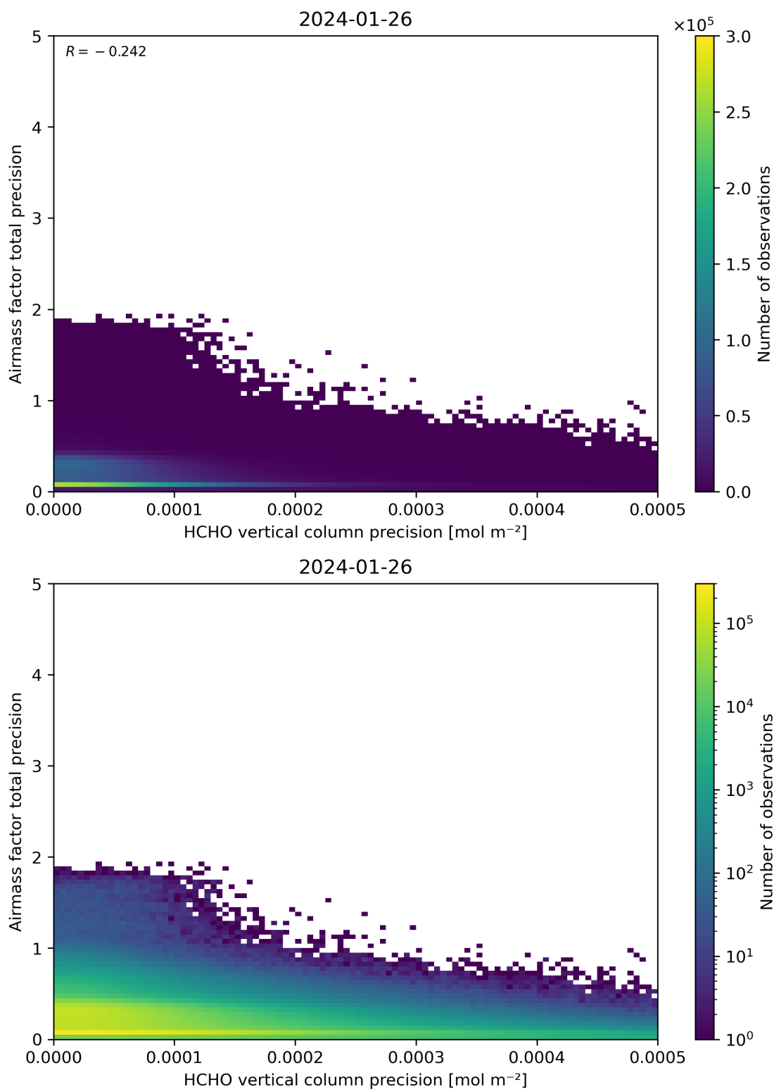
Figure 145: Scatter density plot of “HCHO vertical column precision” against “Airmass factor total precision” for 2024-01-26 to 2024-01-27.
