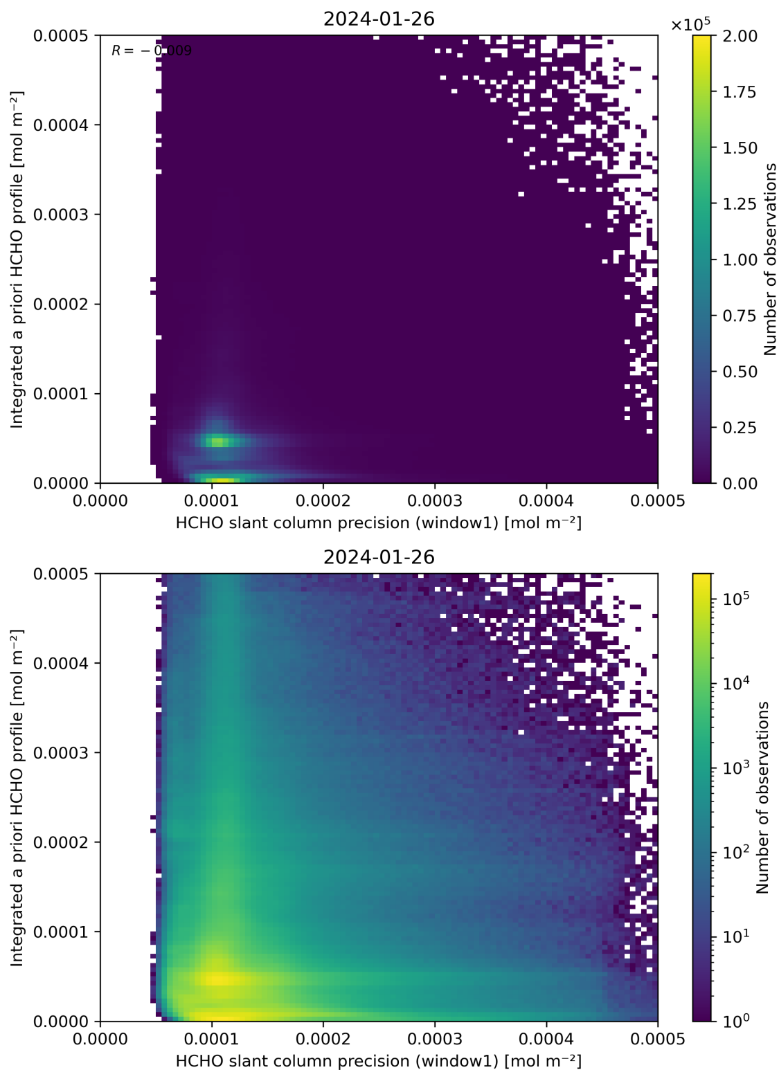
Figure 96: Scatter density plot of “HCHO slant column precision (window1)” against “Integrated a priori HCHO profile” for 2024-01-26 to 2024-01-27.
