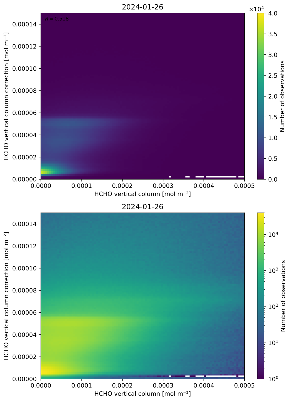
Figure 133: Scatter density plot of “HCHO vertical column” against “HCHO vertical column correction” for 2024-01-26 to 2024-01-27.
