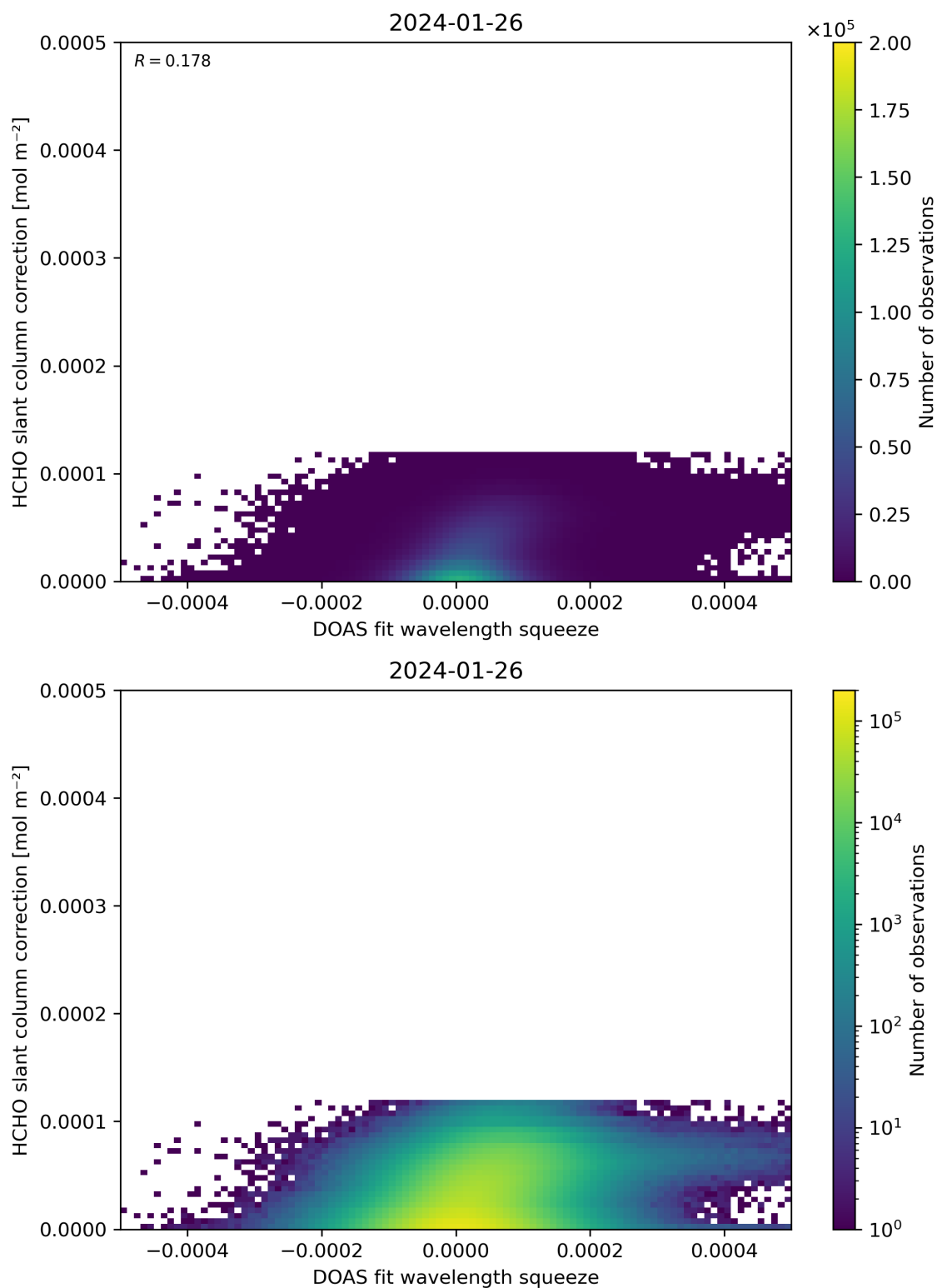
Figure 70: Scatter density plot of “DOAS fit wavelength squeeze” against “HCHO slant column correction” for 2024-01-26 to 2024-01-27.
