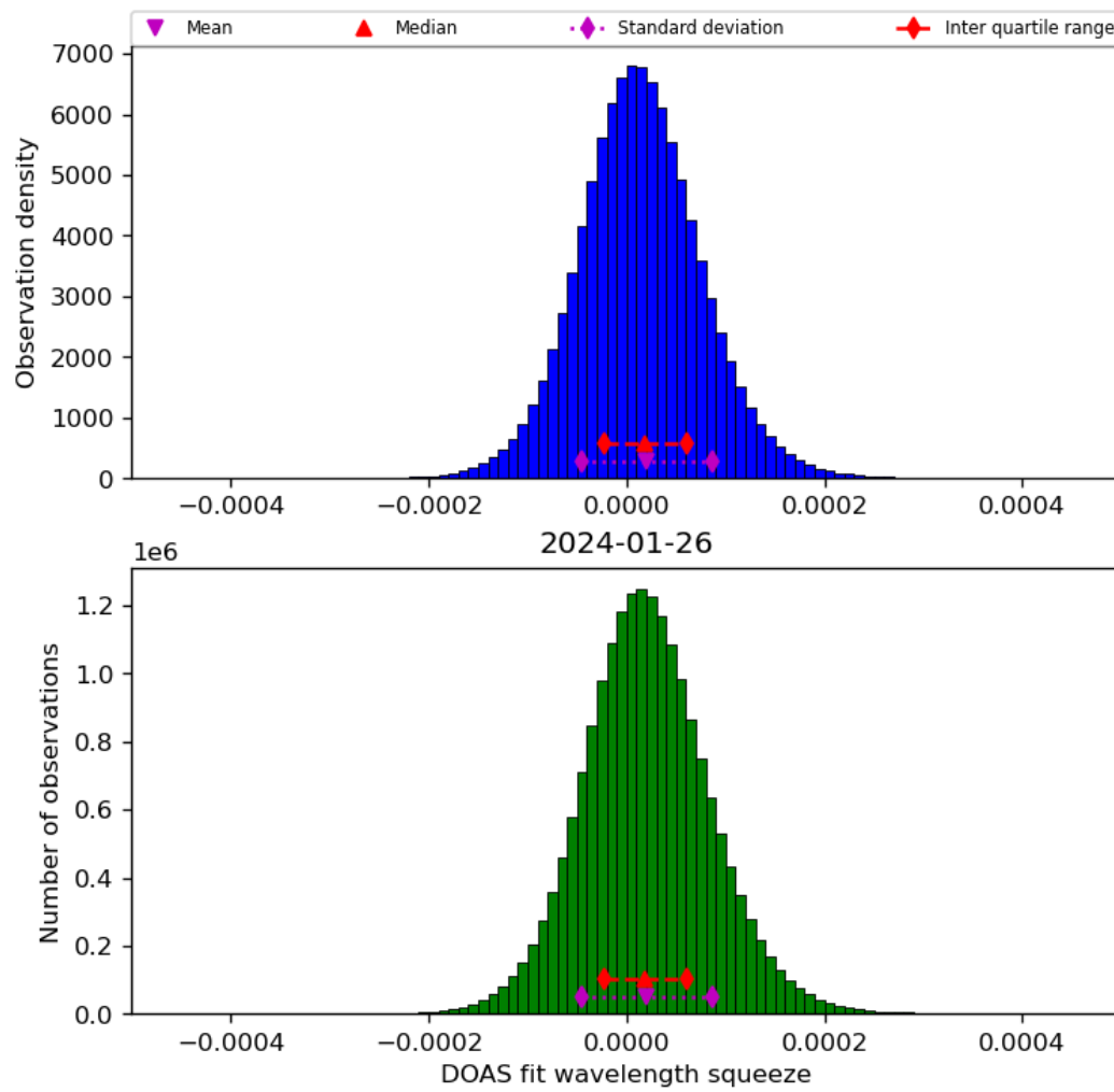
Figure 45: Histogram of “DOAS fit wavelength squeeze” for 2024-01-26 to 2024-01-27
