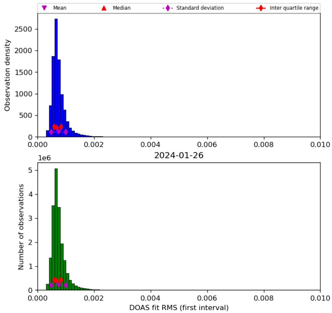
Figure 46: Histogram of “DOAS fit RMS (first interval)” for 2024-01-26 to 2024-01-27
