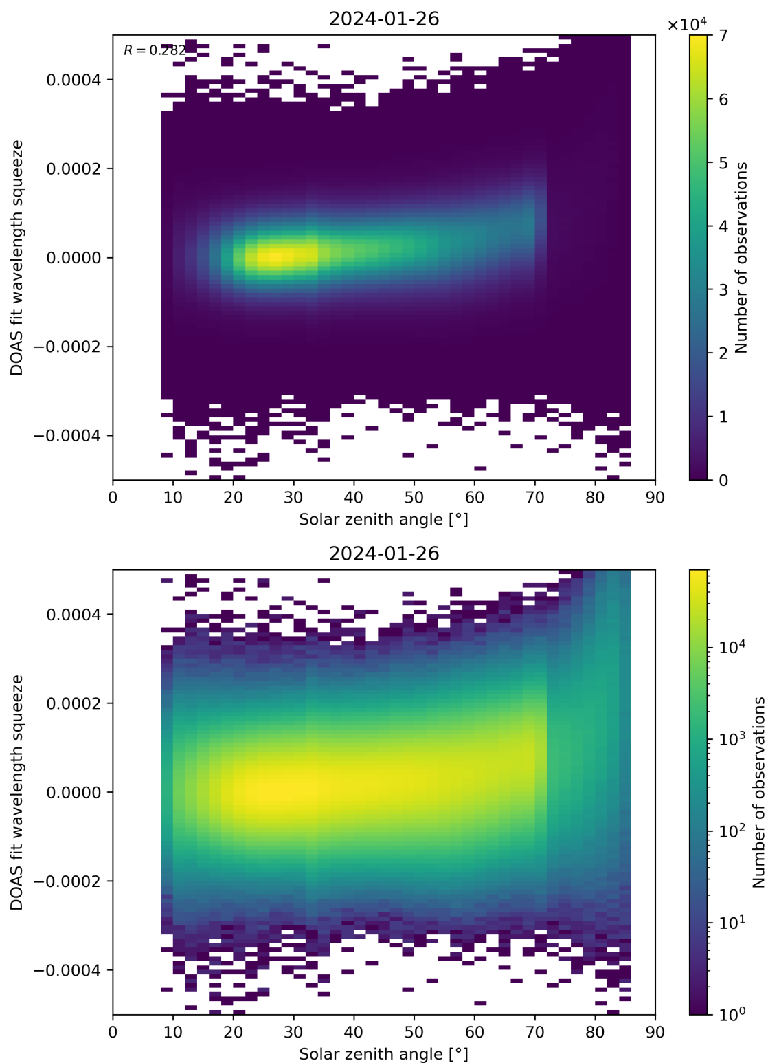
Figure 169: Scatter density plot of “Solar zenith angle” against “DOAS fit wavelength squeeze” for 2024-01-26 to 2024-01-27.
