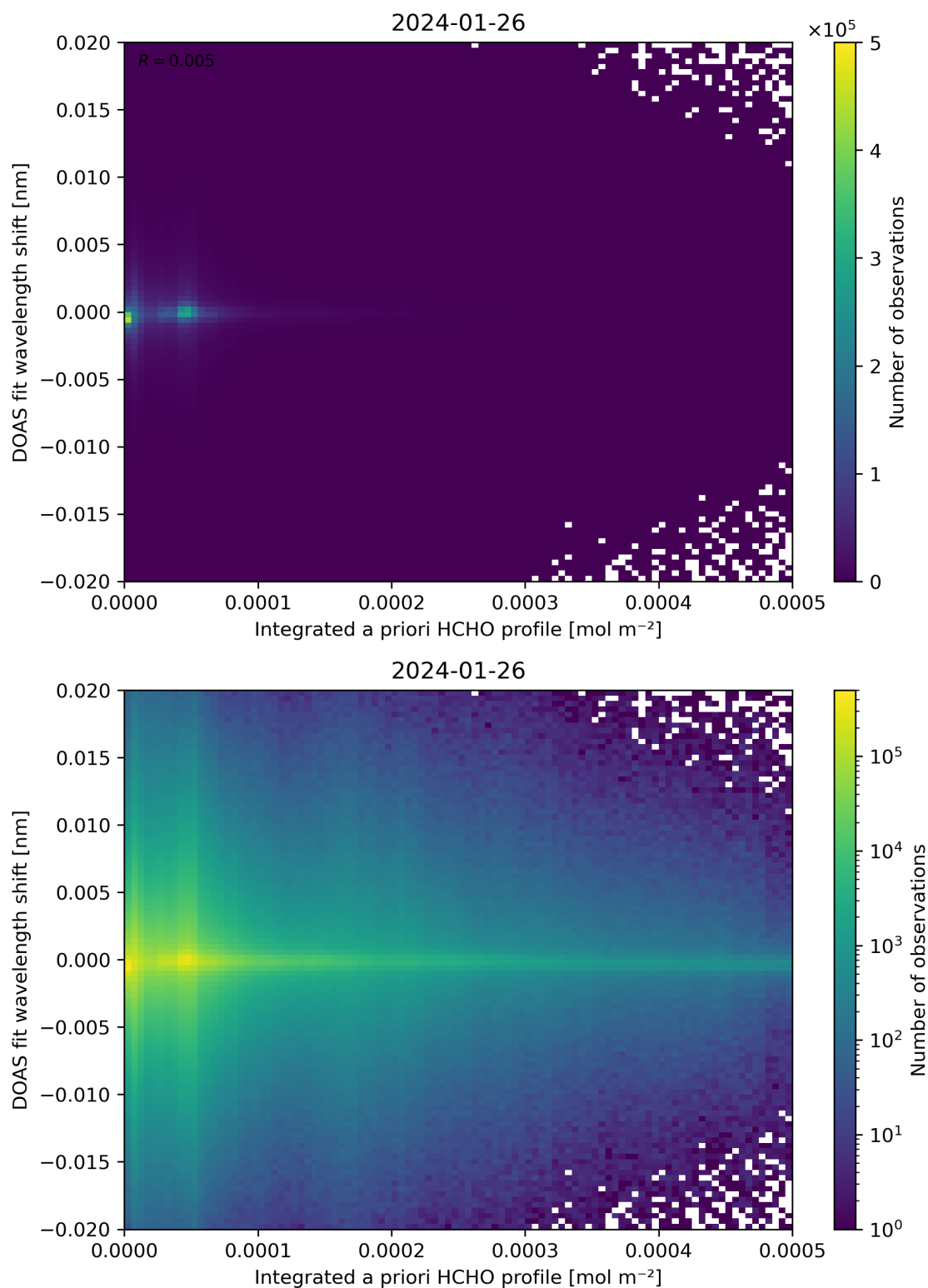
Figure 149: Scatter density plot of “Integrated a priori HCHO profile” against “DOAS fit wavelength shift” for 2024-01-26 to 2024-01-27.
