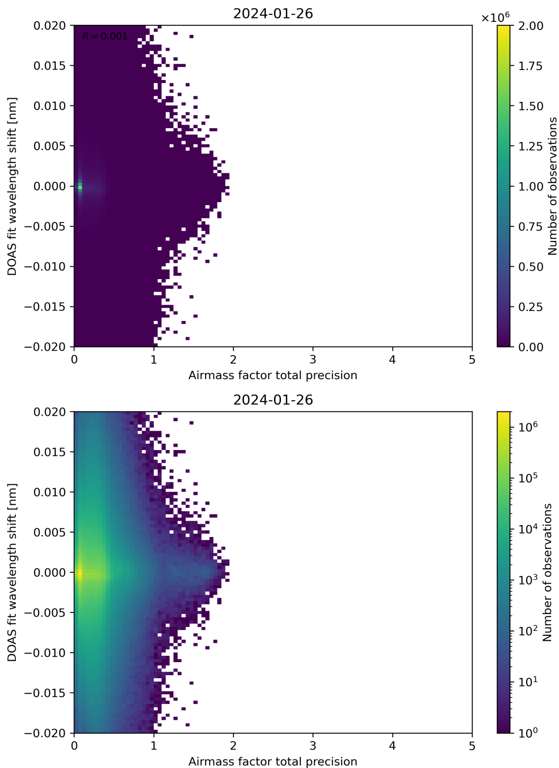
Figure 106: Scatter density plot of “Airmass factor total precision” against “DOAS fit wavelength shift” for 2024-01-26 to 2024-01-27.
