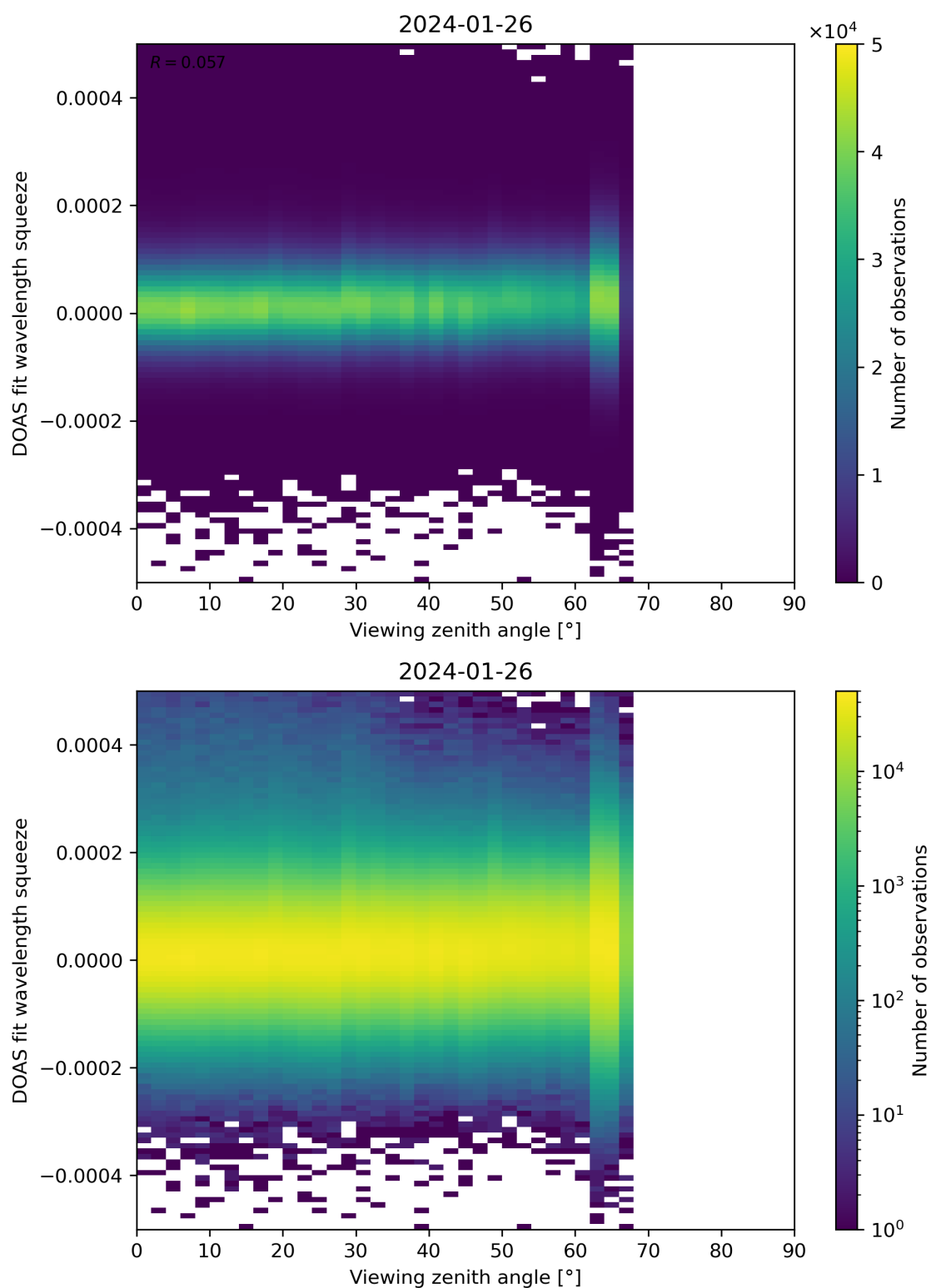
Figure 184: Scatter density plot of “Viewing zenith angle” against “DOAS fit wavelength squeeze” for 2024-01-26 to 2024-01-27.
