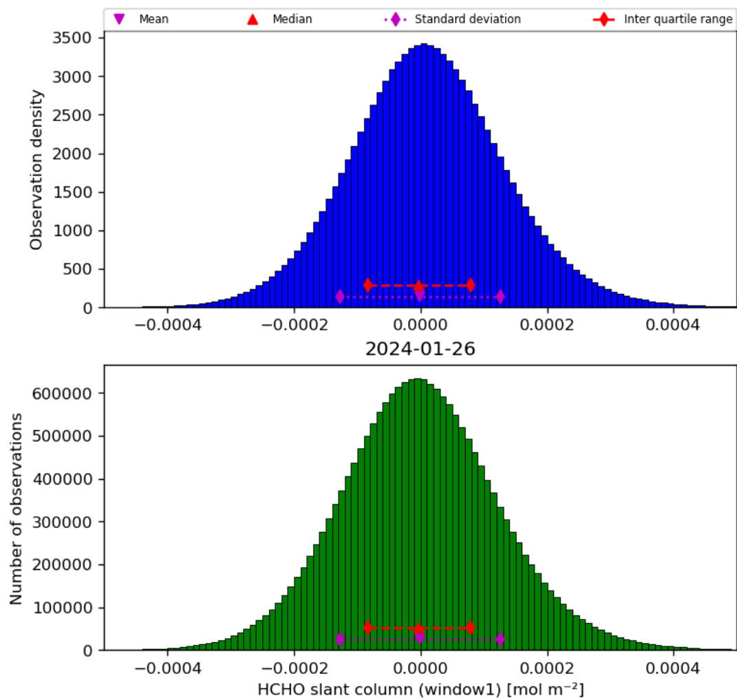
Figure 38: Histogram of “HCHO slant column (window1)” for 2024-01-26 to 2024-01-27
