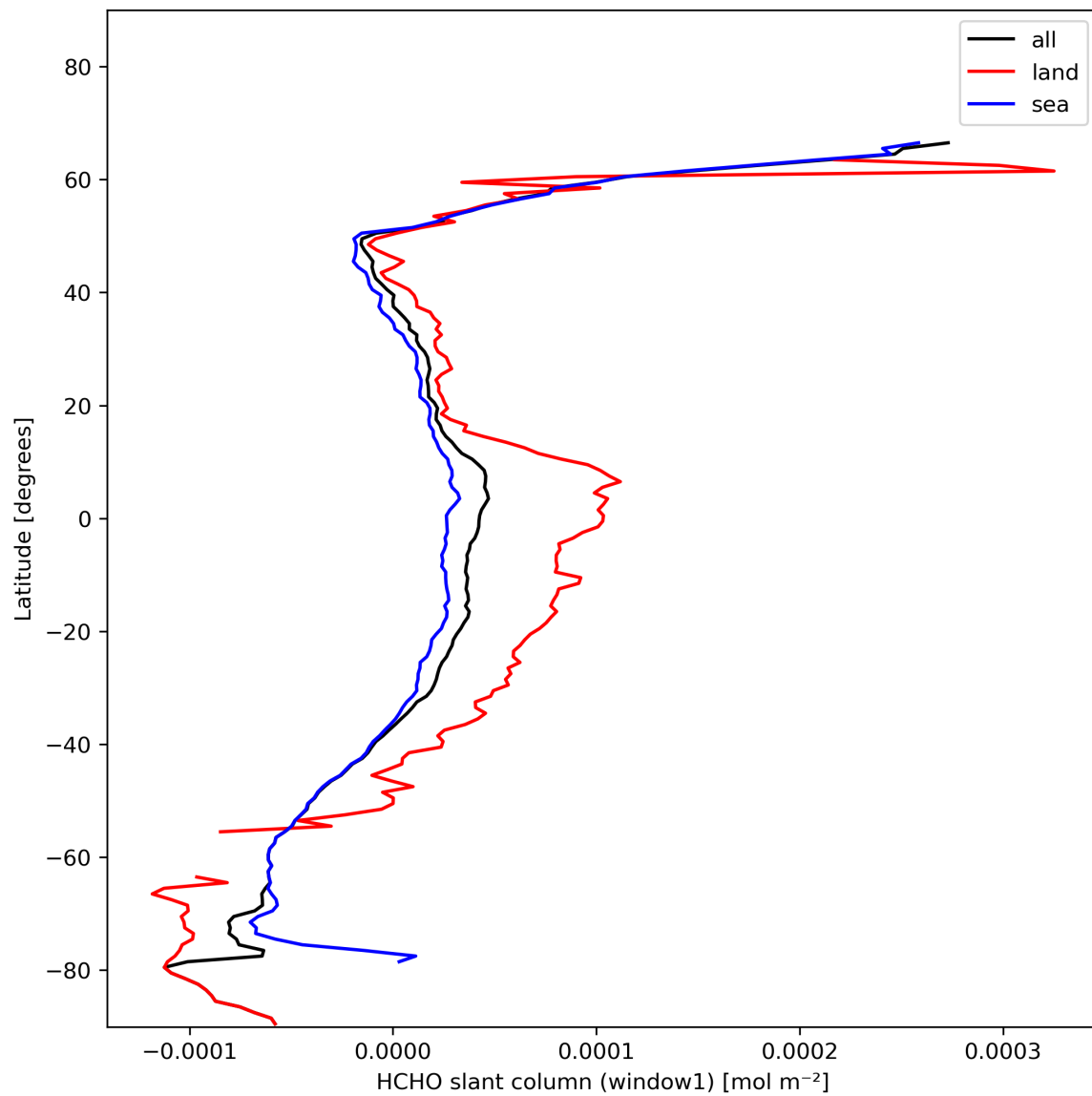
Figure 24: Zonal average of “HCHO slant column (window1)” for 2024-01-26 to 2024-01-27.
