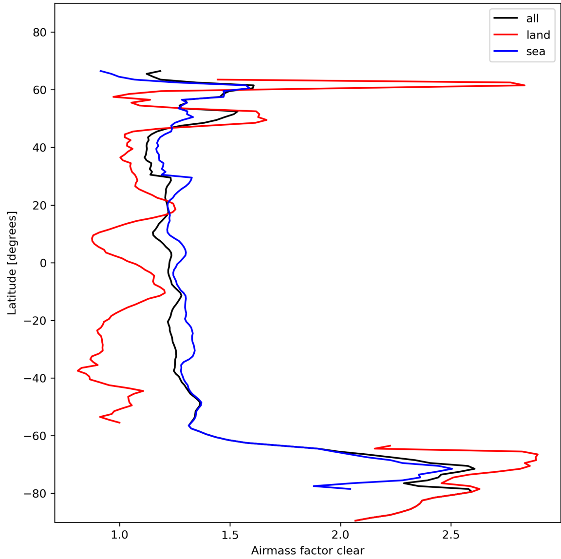
Figure 28: Zonal average of “Airmass factor clear” for 2024-01-26 to 2024-01-27.
