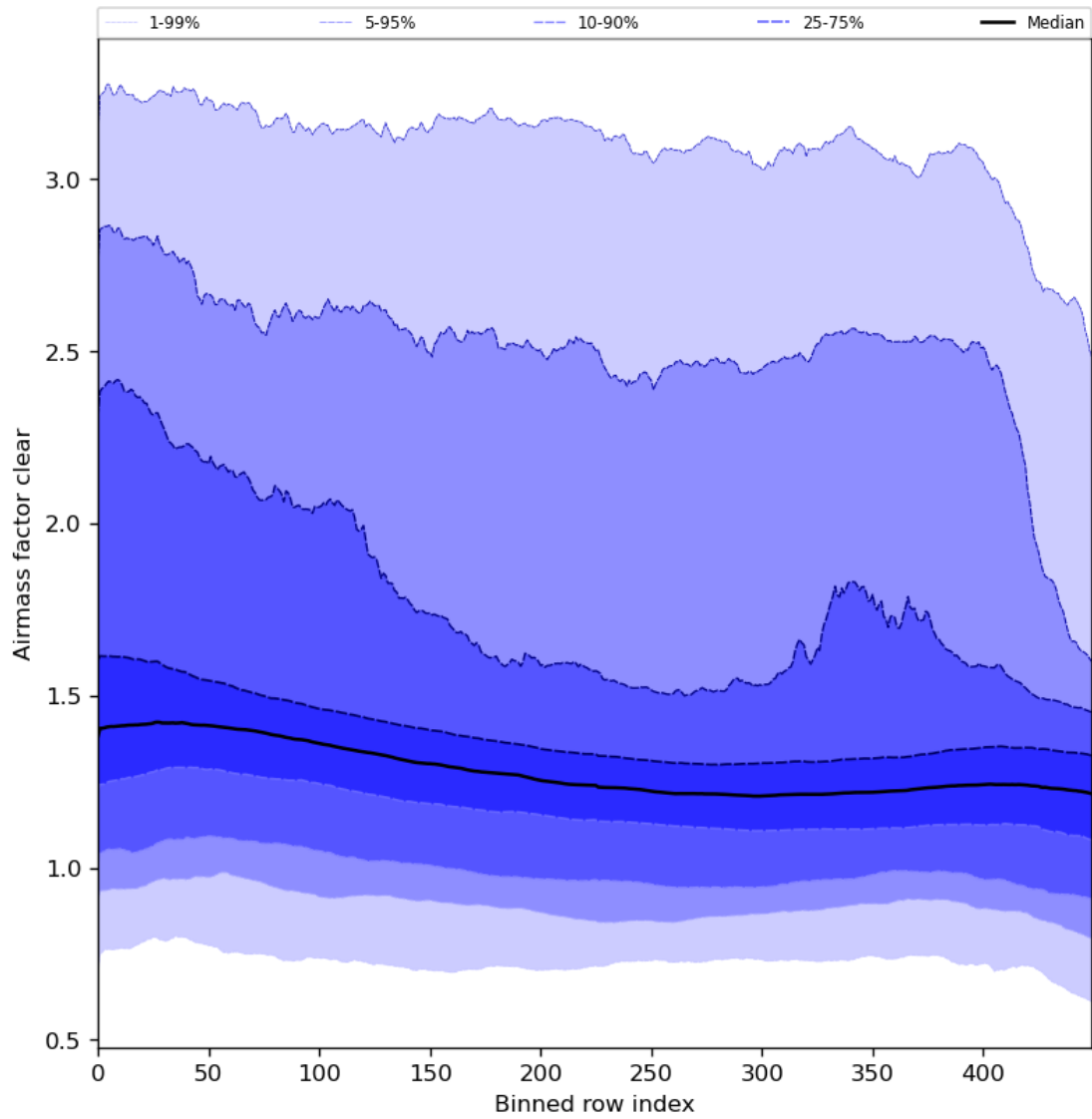
Figure 56: Along track statistics of “Airmass factor clear” for 2024-01-26 to 2024-01-27
