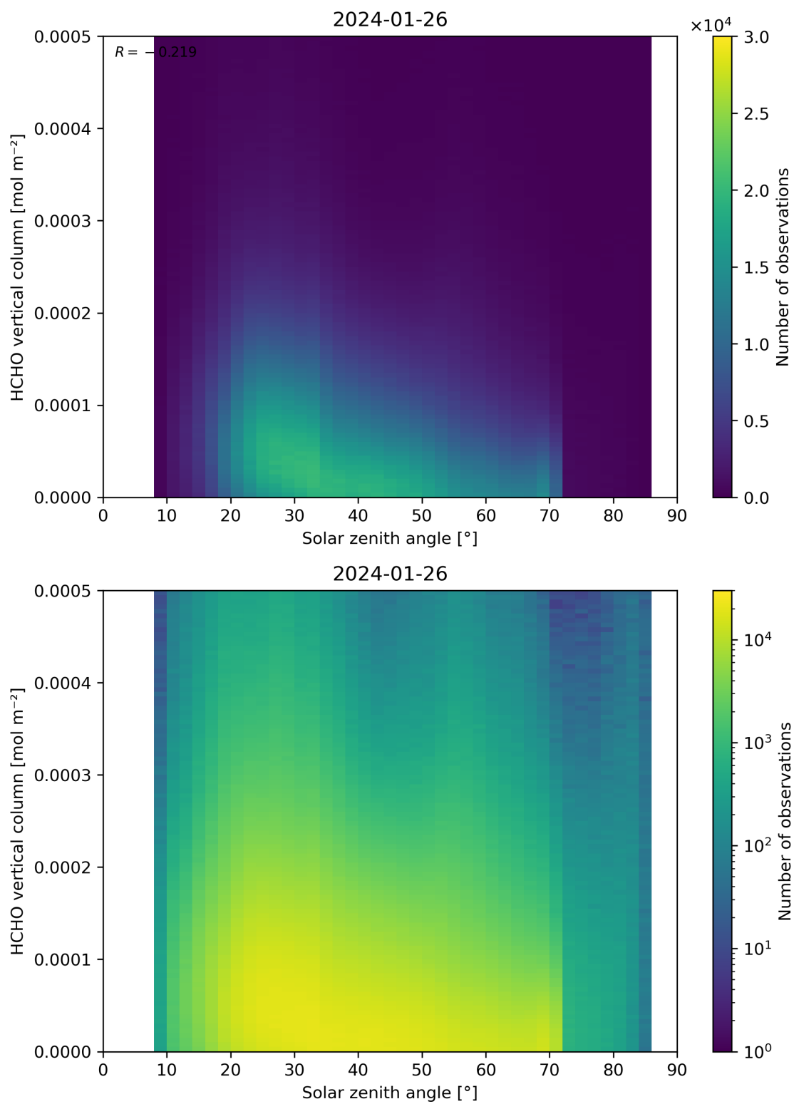
Figure 177: Scatter density plot of “Solar zenith angle” against “HCHO vertical column” for 2024-01-26 to 2024-01-27.
