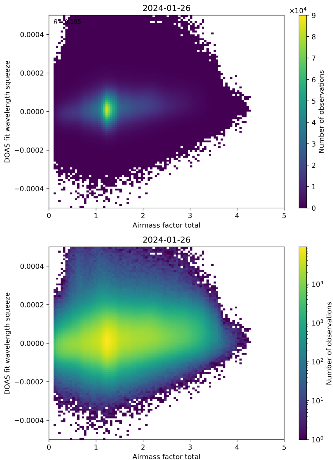
Figure 99: Scatter density plot of “Airmass factor total” against “DOAS fit wavelength squeeze” for 2024-01-26 to 2024-01-27.
