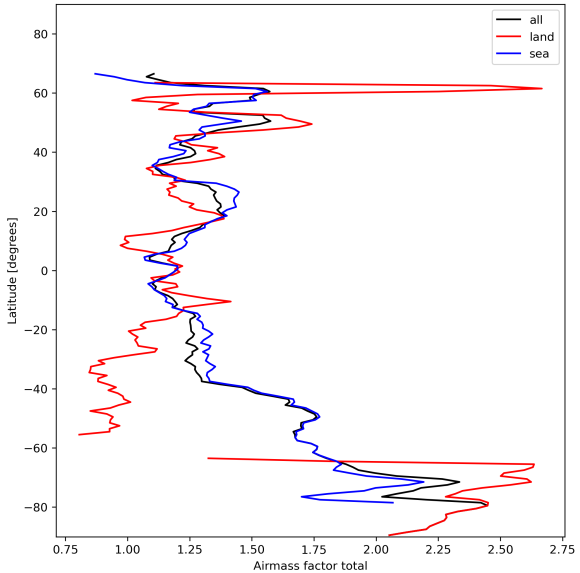
Figure 26: Zonal average of “Airmass factor total” for 2024-01-26 to 2024-01-27.
