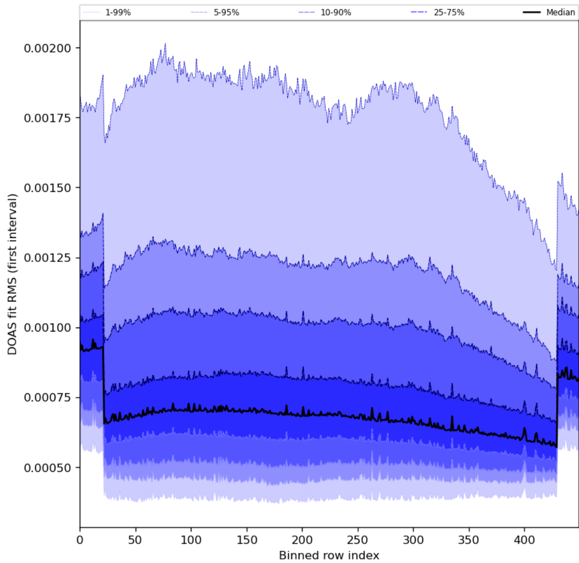
Figure 60: Along track statistics of “DOAS fit RMS (first interval)” for 2024-01-26 to 2024-01-27
