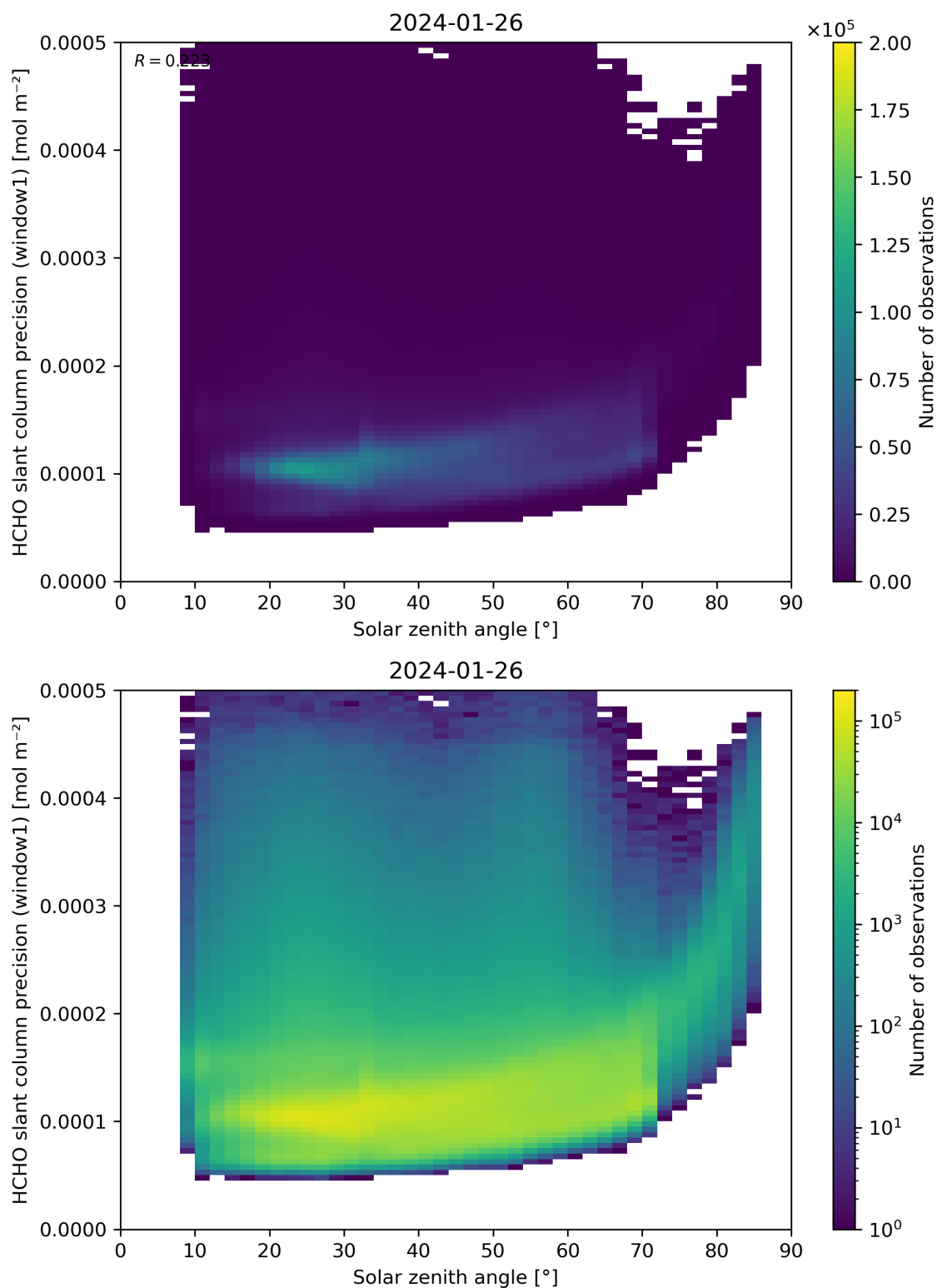
Figure 174: Scatter density plot of “Solar zenith angle” against “HCHO slant column precision (window1)” for 2024-01-26 to 2024-01-27.
