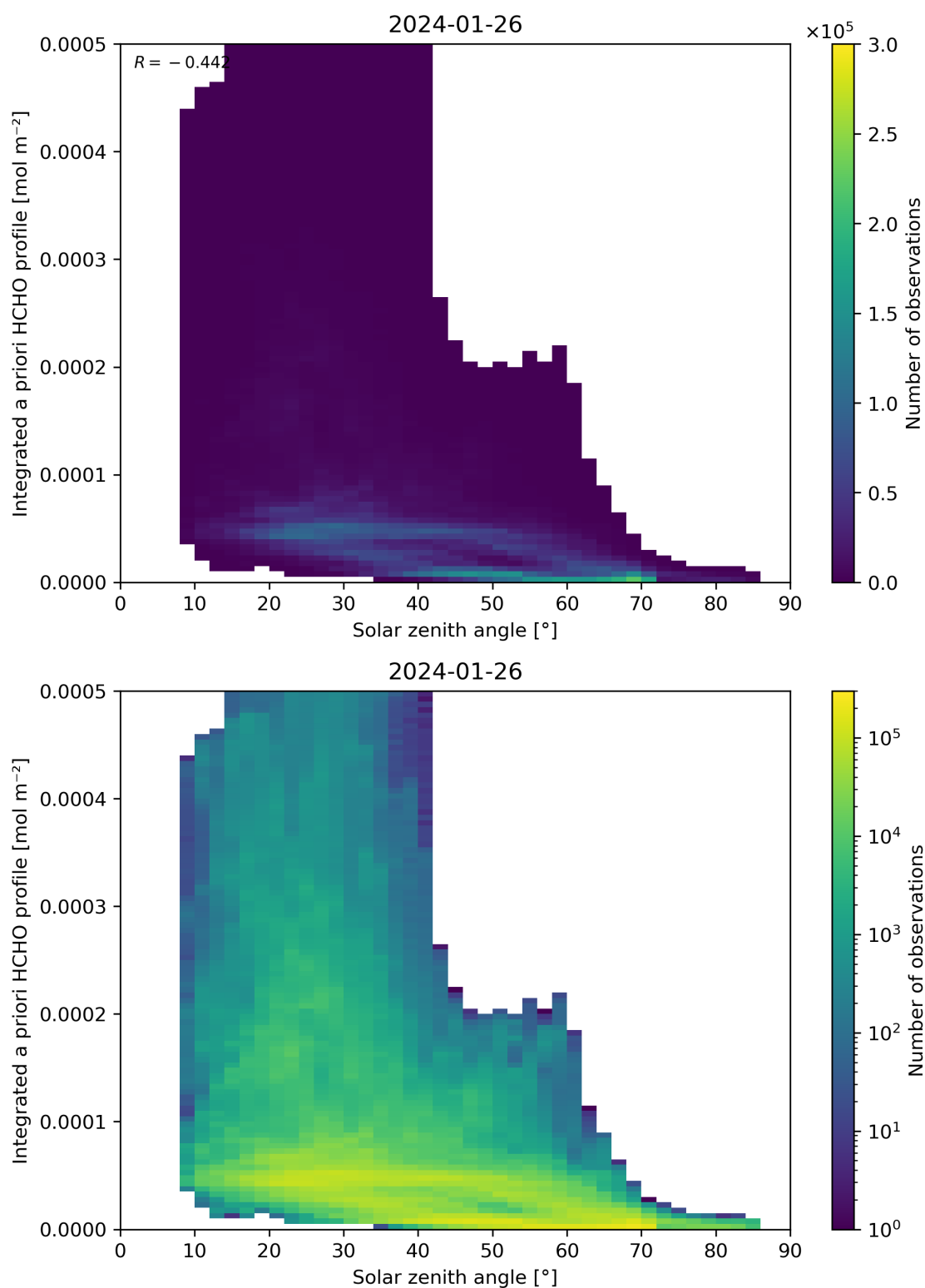
Figure 180: Scatter density plot of “Solar zenith angle” against “Integrated a priori HCHO profile” for 2024-01-26 to 2024-01-27.
