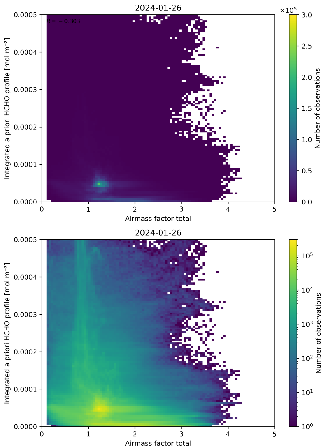
Figure 104: Scatter density plot of “Airmass factor total” against “Integrated a priori HCHO profile” for 2024-01-26 to 2024-01-27.
