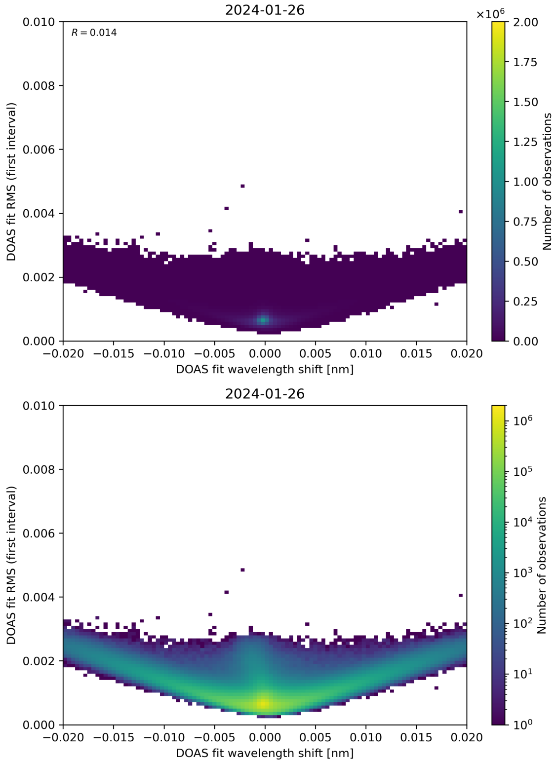
Figure 64: Scatter density plot of “DOAS fit wavelength shift” against “DOAS fit RMS (first interval)” for 2024-01-26 to 2024-01-27.
