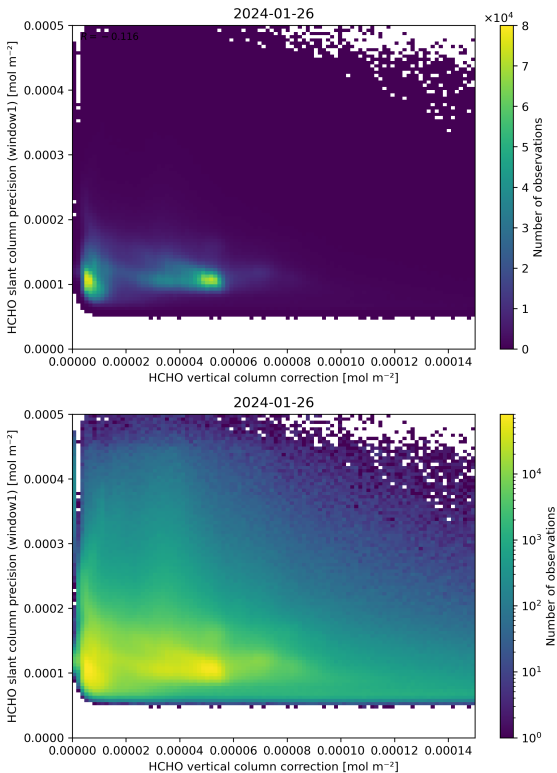
Figure 119: Scatter density plot of “HCHO vertical column correction” against “HCHO slant column precision (window1)” for 2024-01-26 to 2024-01-27.
