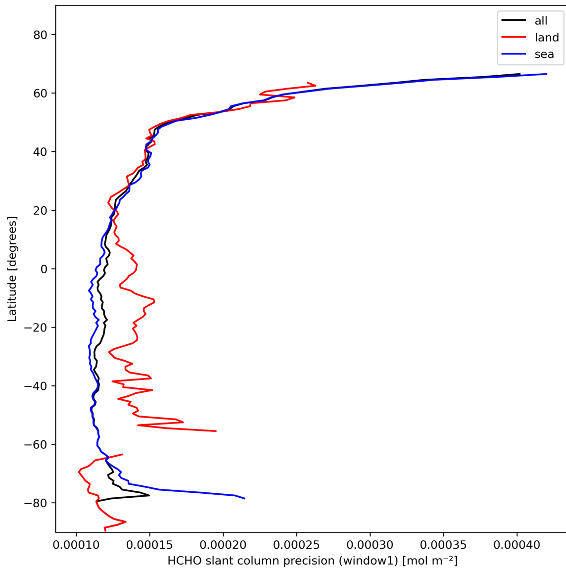
Figure 25: Zonal average of “HCHO slant column precision (window1)” for 2024-01-26 to 2024-01-27.
