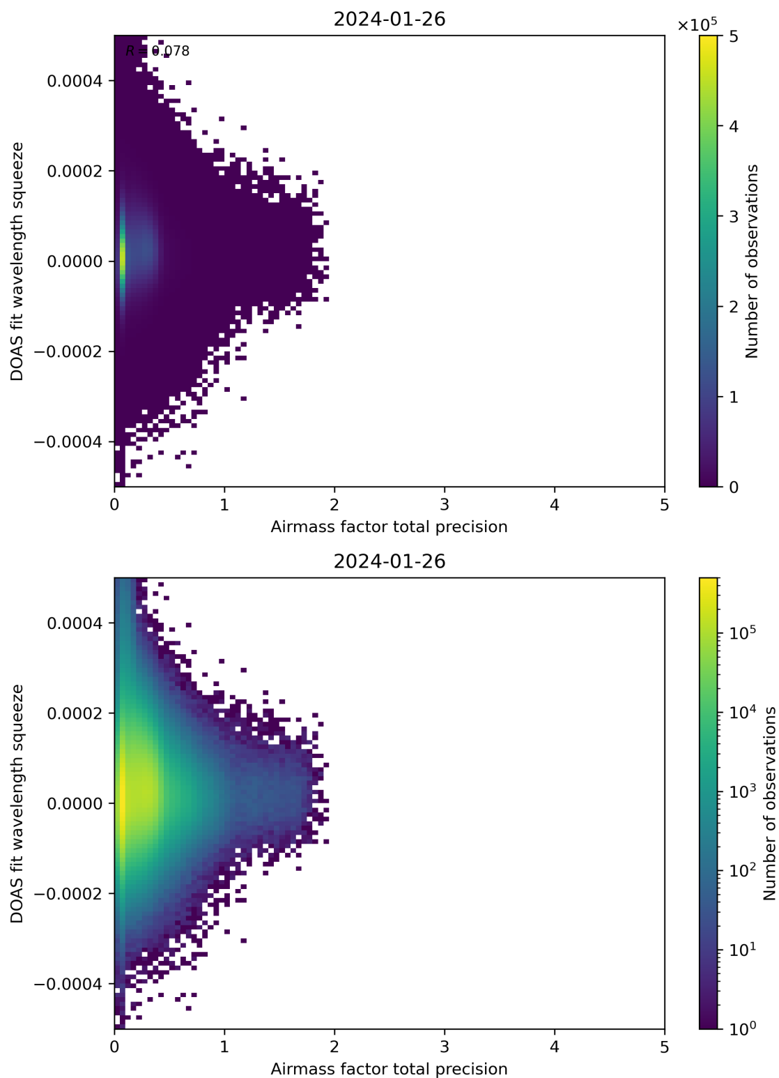
Figure 107: Scatter density plot of “Airmass factor total precision” against “DOAS fit wavelength squeeze” for 2024-01-26 to 2024-01-27.
