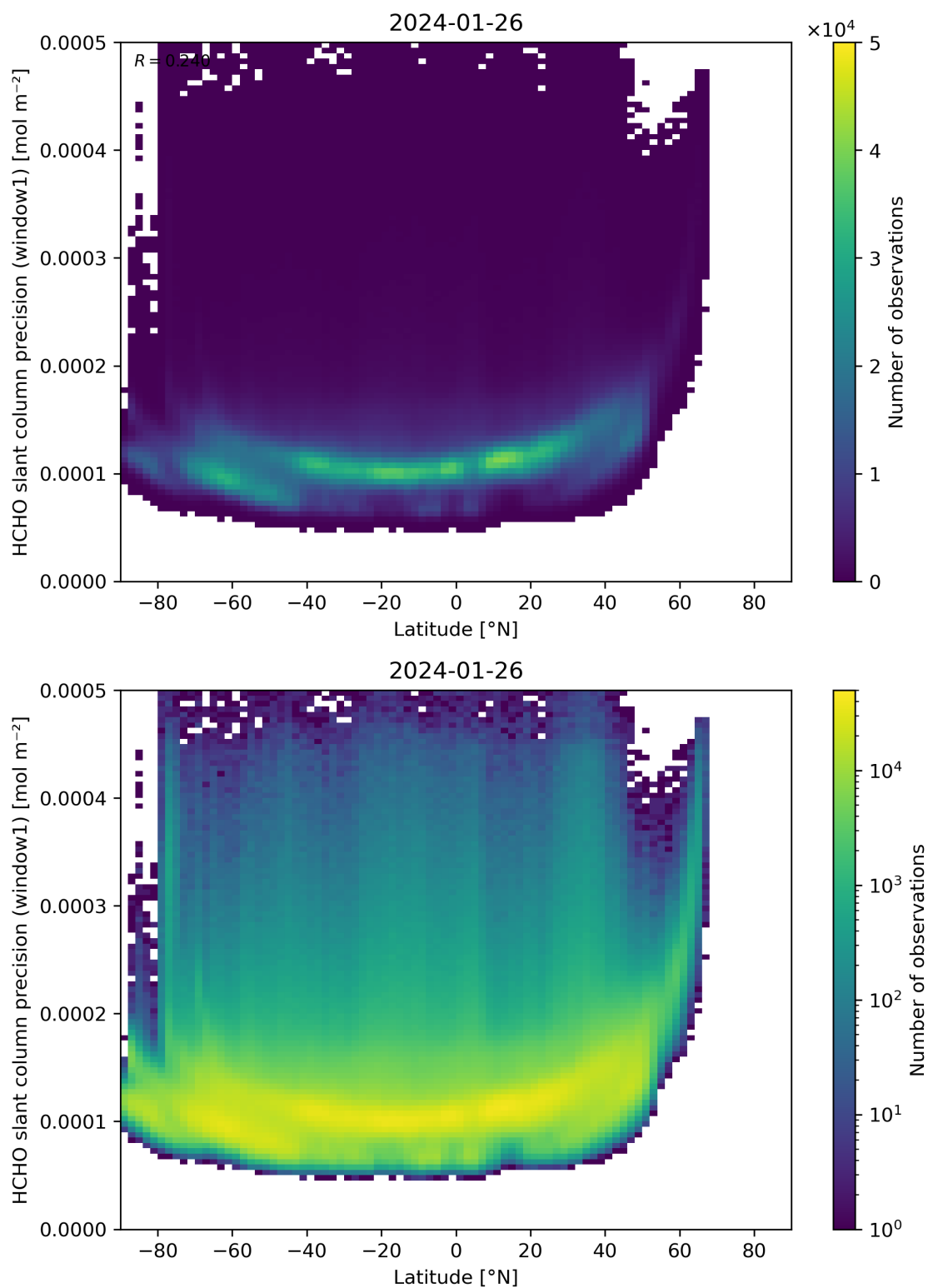
Figure 160: Scatter density plot of “Latitude” against “HCHO slant column precision (window1)” for 2024-01-26 to 2024-01-27.
