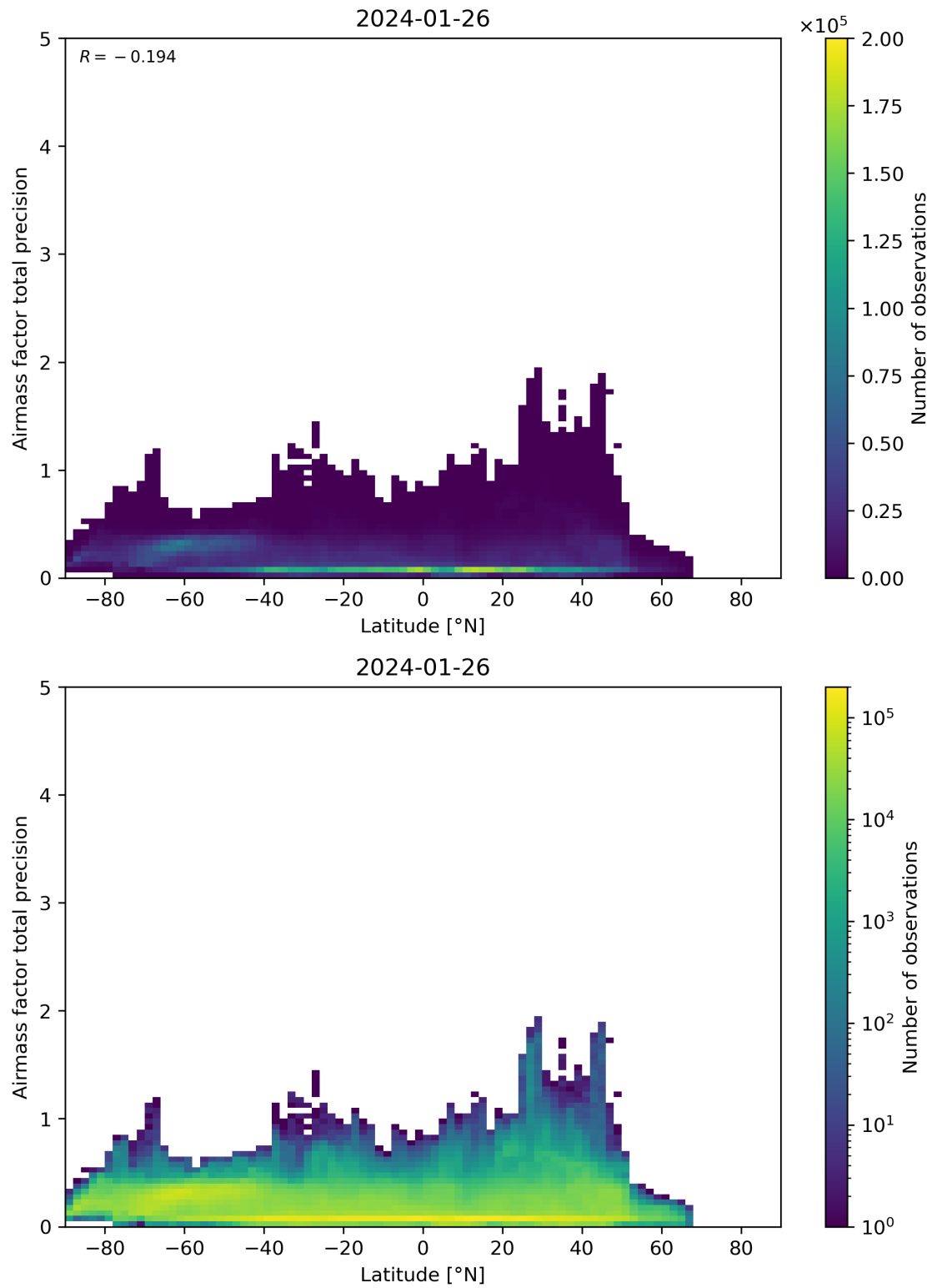
Figure 162: Scatter density plot of “Latitude” against “Airmass factor total precision” for 2024-01-26 to 2024-01-27.
