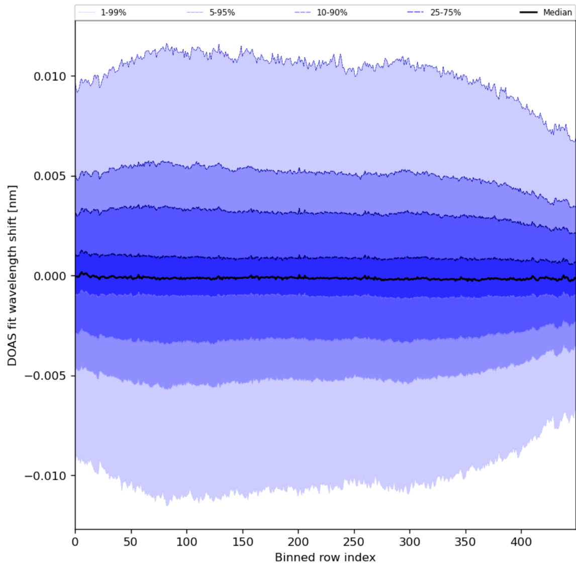
Figure 58: Along track statistics of “DOAS fit wavelength shift” for 2024-01-26 to 2024-01-27
