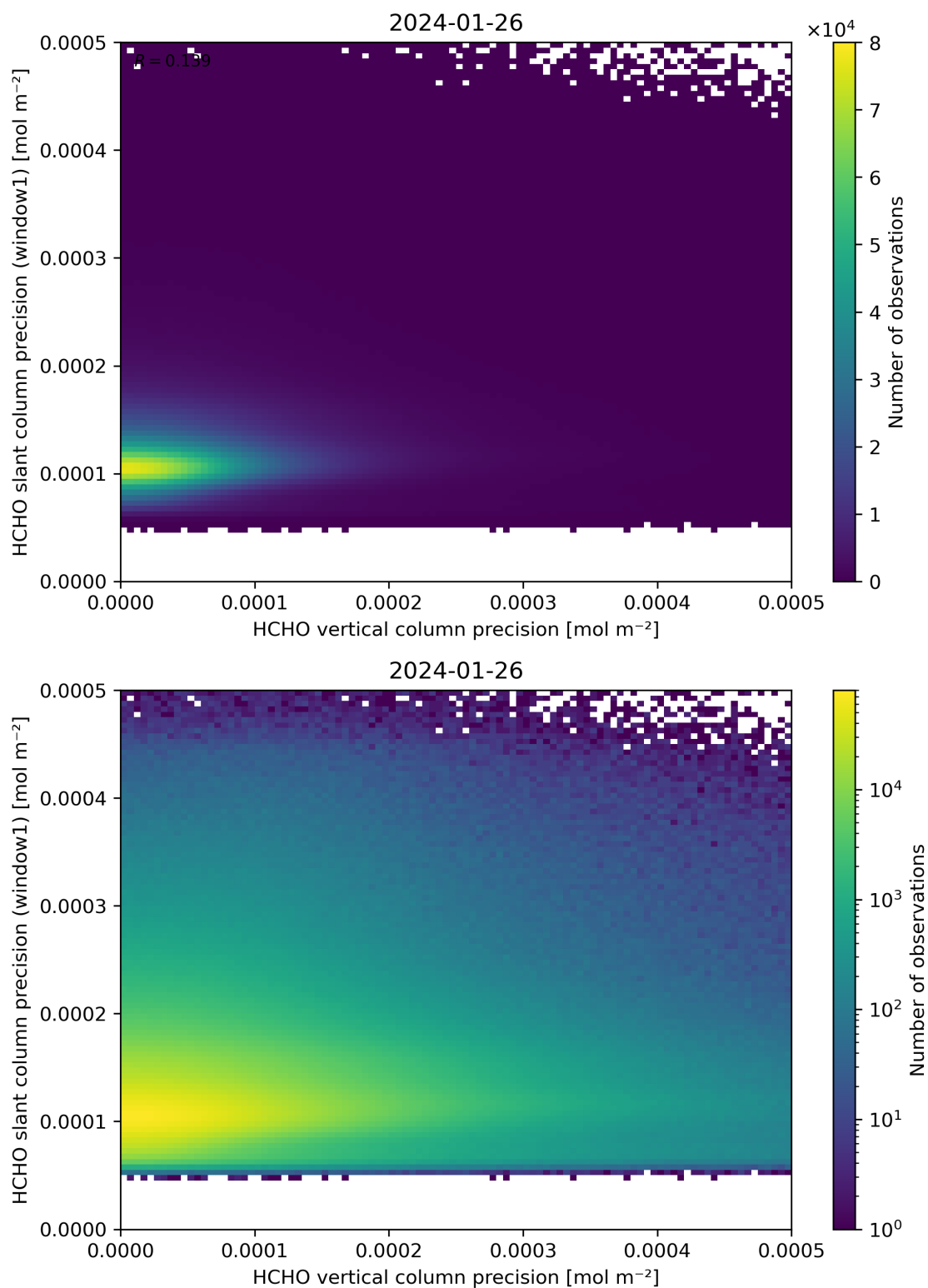
Figure 143: Scatter density plot of “HCHO vertical column precision” against “HCHO slant column precision (window1)” for 2024-01-26 to 2024-01-27.
