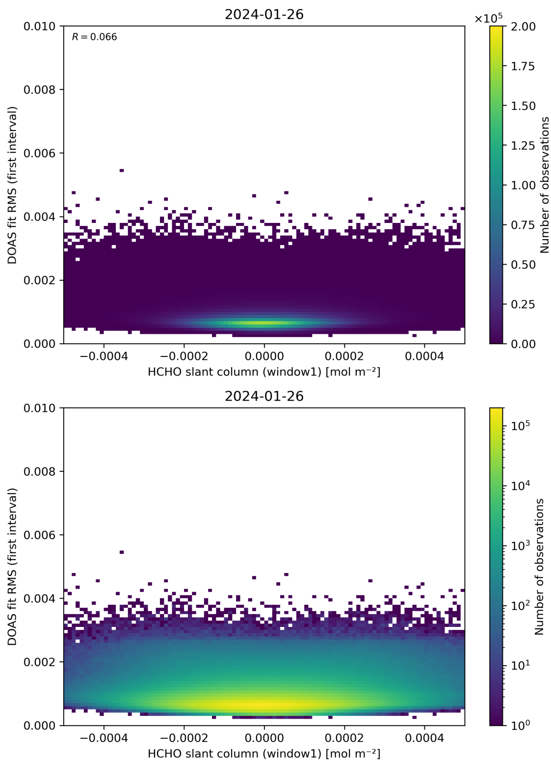
Figure 78: Scatter density plot of “HCHO slant column (window1)” against “DOAS fit RMS (first interval)” for 2024-01-26 to 2024-01-27.
