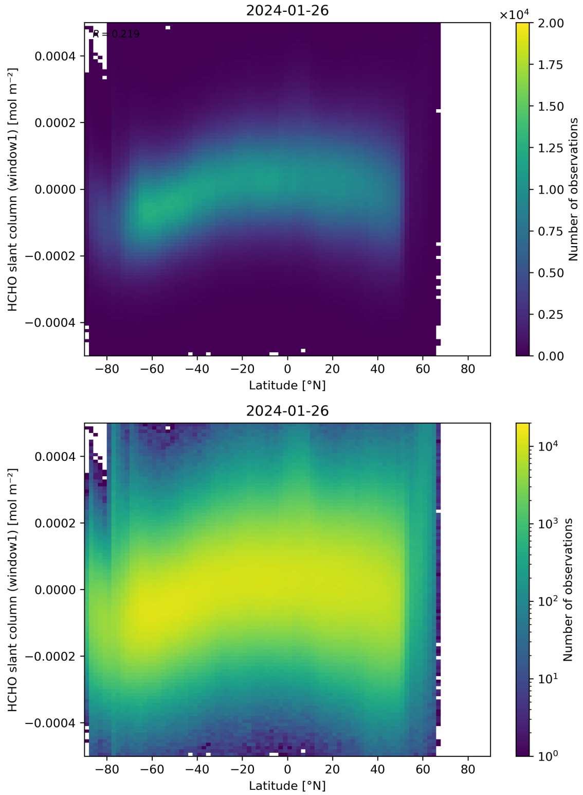
Figure 159: Scatter density plot of “Latitude” against “HCHO slant column (window1)” for 2024-01-26 to 2024-01-27.
