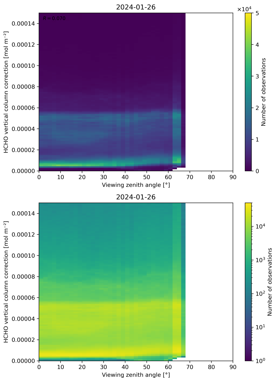
Figure 193: Scatter density plot of “Viewing zenith angle” against “HCHO vertical column correction” for 2024-01-26 to 2024-01-27.
