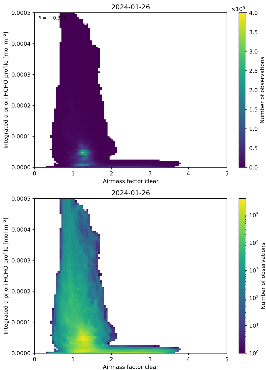
Figure 76: Scatter density plot of “Airmass factor clear” against “Integrated a priori HCHO profile” for 2024-01-26 to 2024-01-27.
