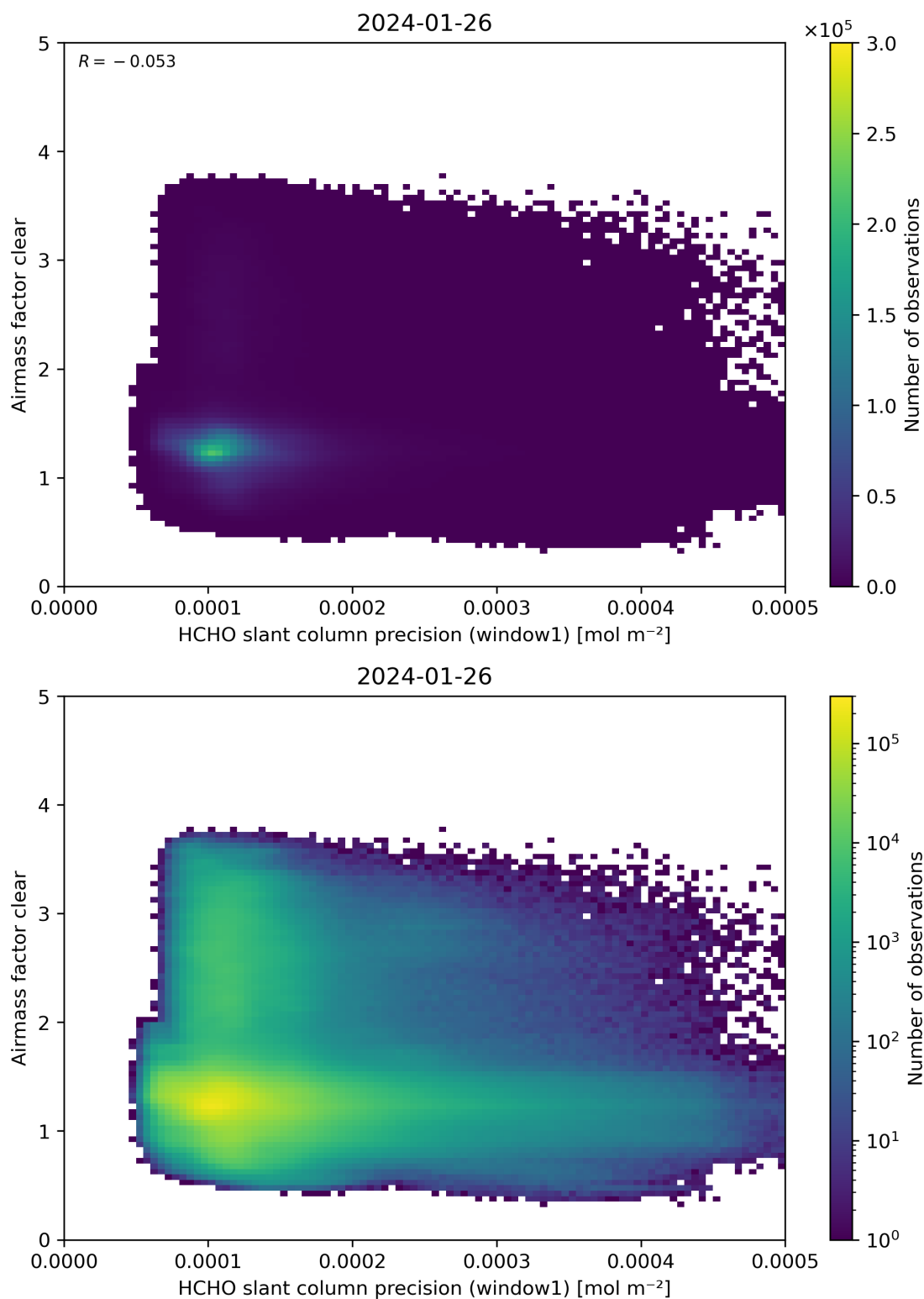
Figure 91: Scatter density plot of “HCHO slant column precision (window1)” against “Airmass factor clear” for 2024-01-26 to 2024-01-27.
