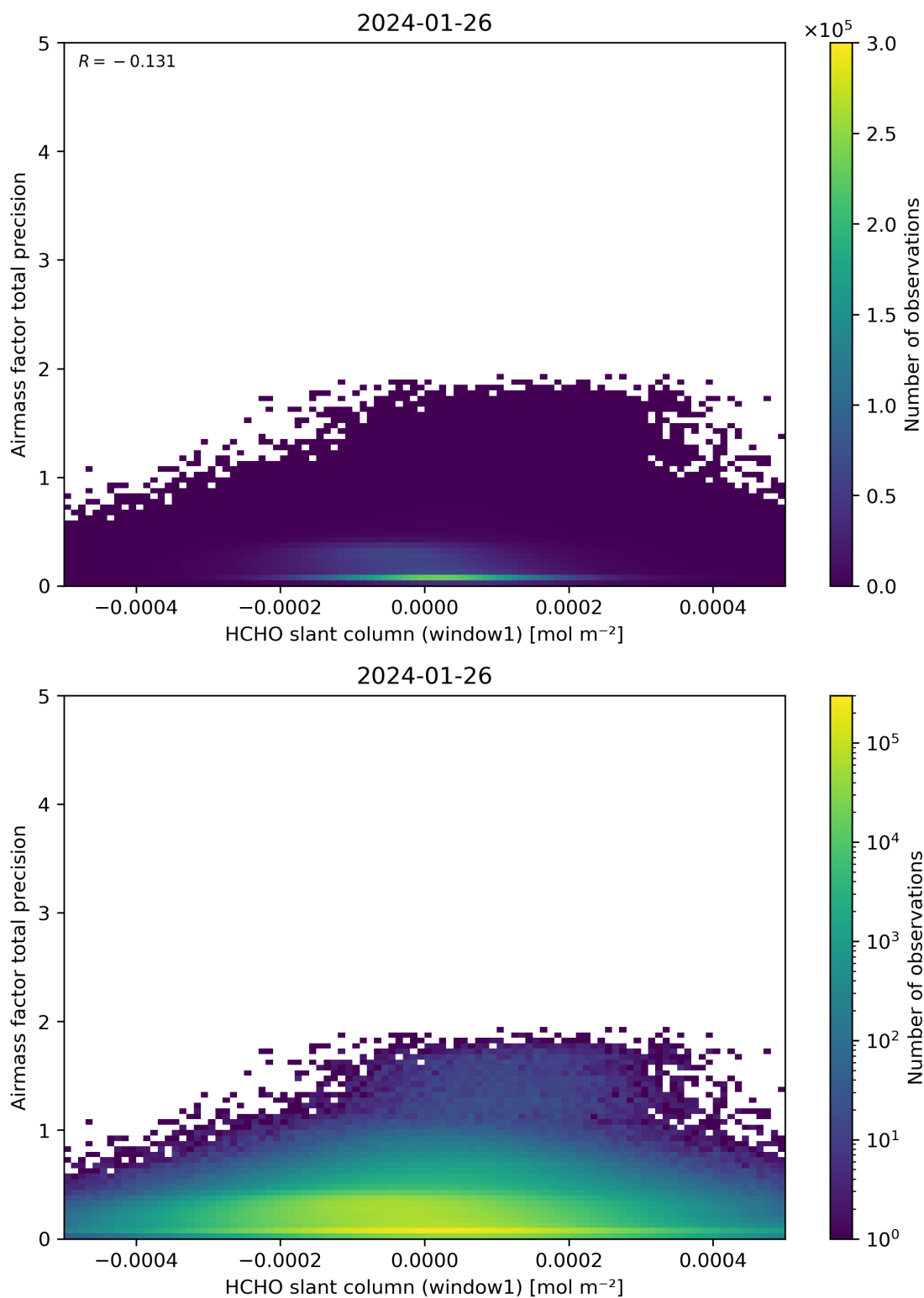
Figure 86: Scatter density plot of “HCHO slant column (window1)” against “Airmass factor total precision” for 2024-01-26 to 2024-01-27.
