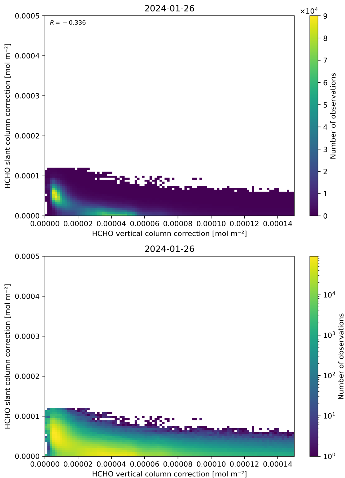
Figure 117: Scatter density plot of “HCHO vertical column correction” against “HCHO slant column correction” for 2024-01-26 to 2024-01-27.
