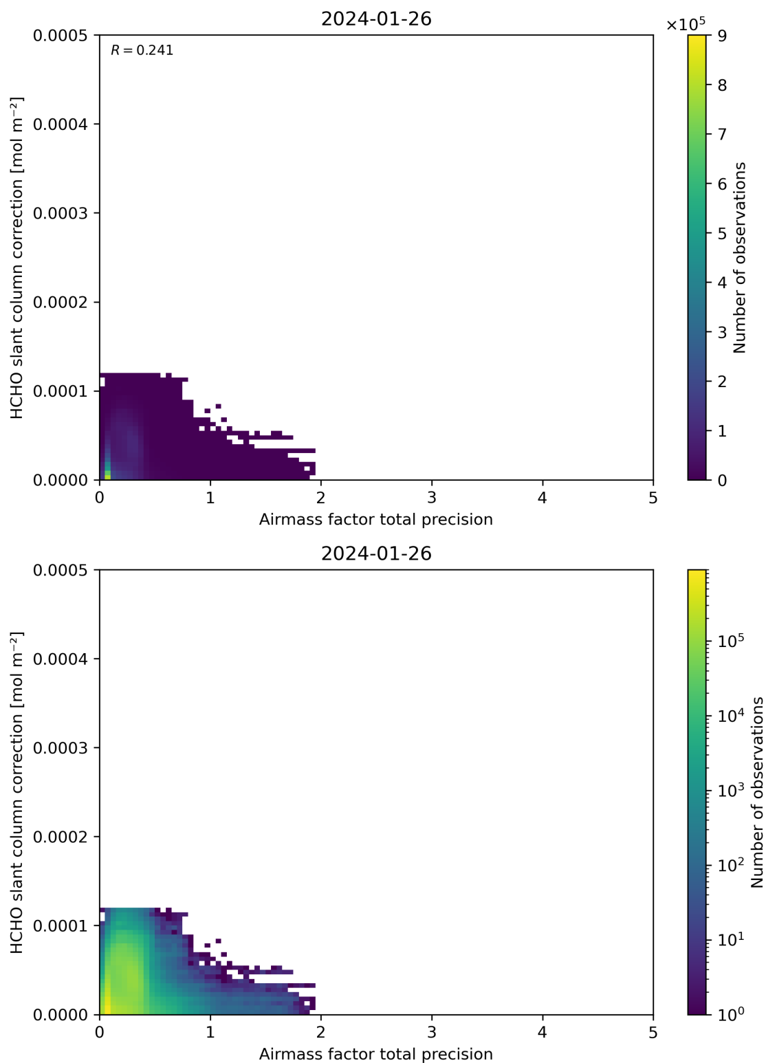
Figure 110: Scatter density plot of “Airmass factor total precision” against “HCHO slant column correction” for 2024-01-26 to 2024-01-27.
