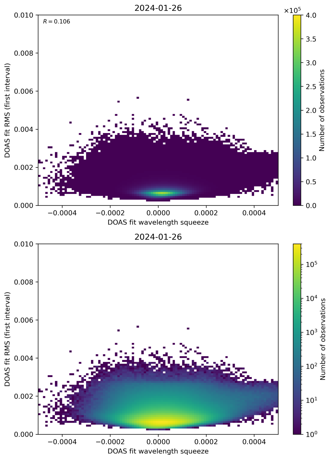
Figure 68: Scatter density plot of “DOAS fit wavelength squeeze” against “DOAS fit RMS (first interval)” for 2024-01-26 to 2024-01-27.
