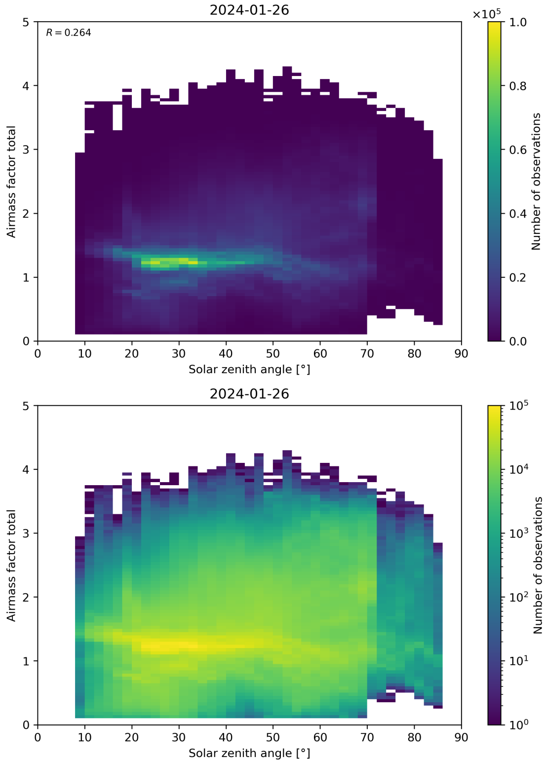
Figure 175: Scatter density plot of “Solar zenith angle” against “Airmass factor total” for 2024-01-26 to 2024-01-27.
