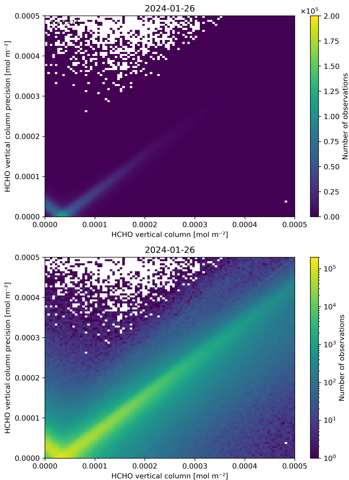
Figure 134: Scatter density plot of “HCHO vertical column” against “HCHO vertical column precision” for 2024-01-26 to 2024-01-27.
