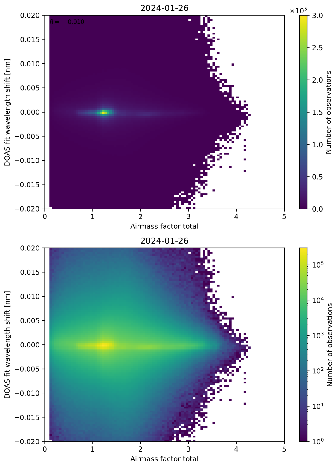
Figure 98: Scatter density plot of “Airmass factor total” against “DOAS fit wavelength shift” for 2024-01-26 to 2024-01-27.
