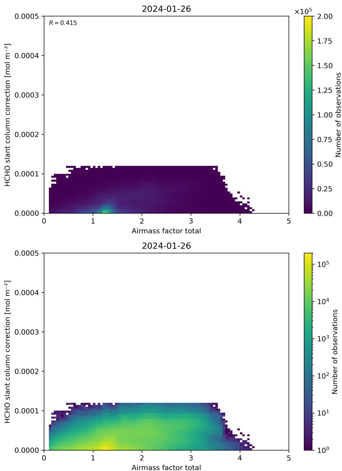
Figure 102: Scatter density plot of “Airmass factor total” against “HCHO slant column correction” for 2024-01-26 to 2024-01-27.
