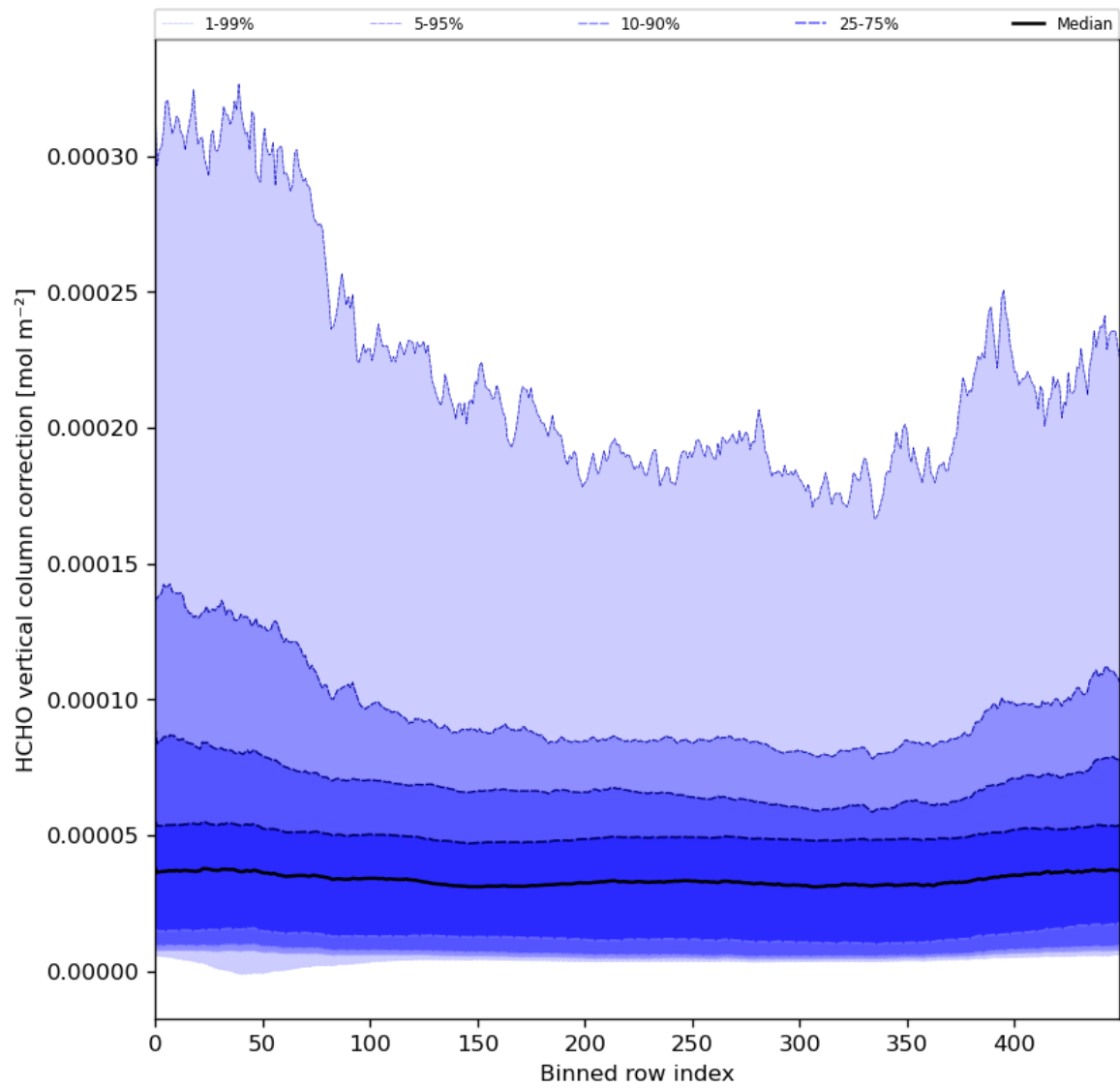
Figure 51: Along track statistics of “HCHO vertical column correction” for 2024-01-26 to 2024-01-27
