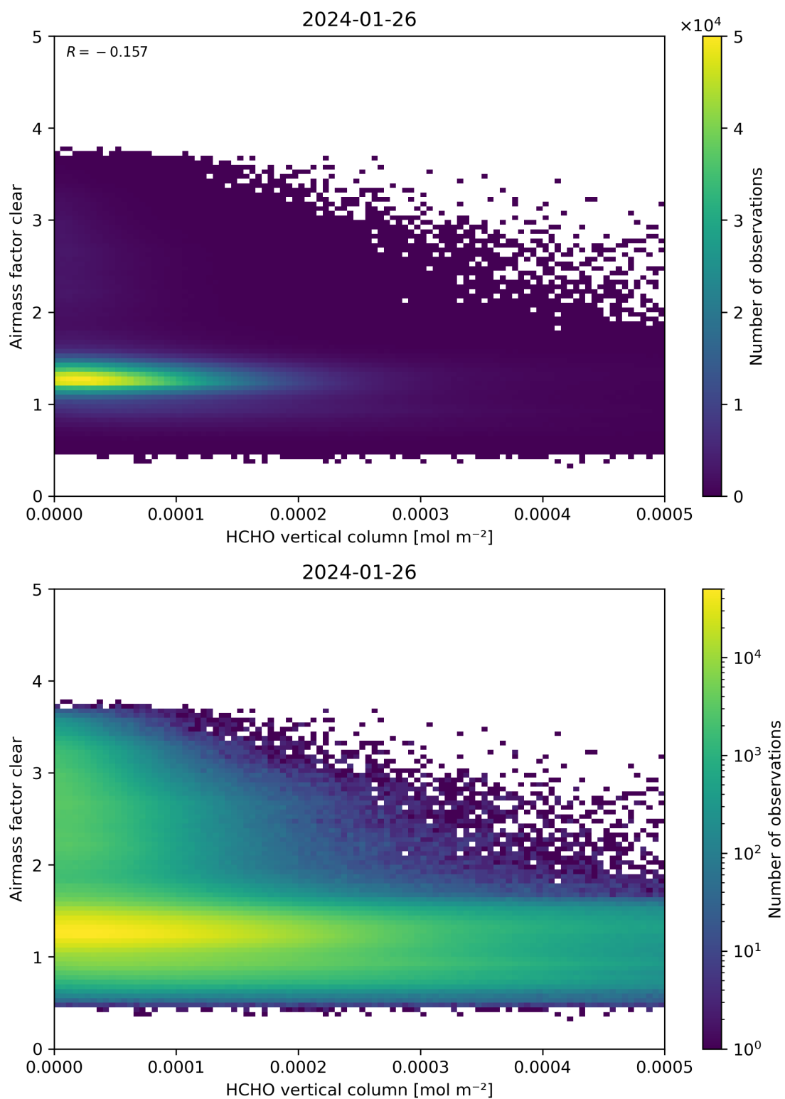
Figure 126: Scatter density plot of “HCHO vertical column” against “Airmass factor clear” for 2024-01-26 to 2024-01-27.
