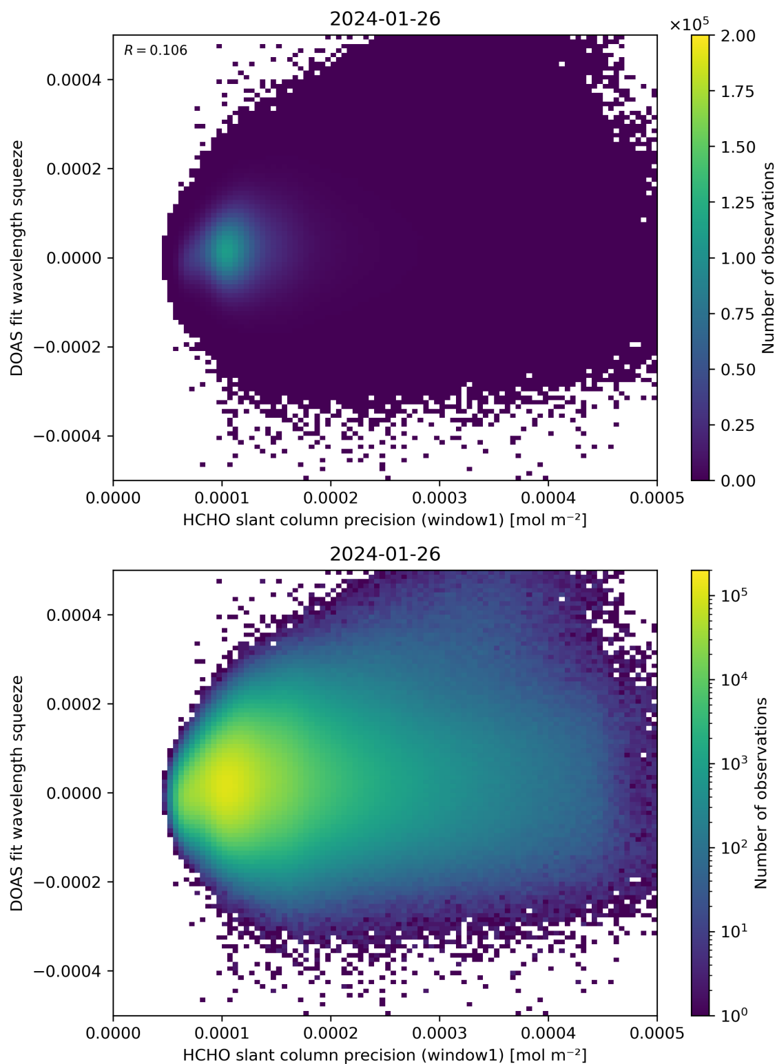
Figure 90: Scatter density plot of “HCHO slant column precision (window1)” against “DOAS fit wavelength squeeze” for 2024-01-26 to 2024-01-27.
