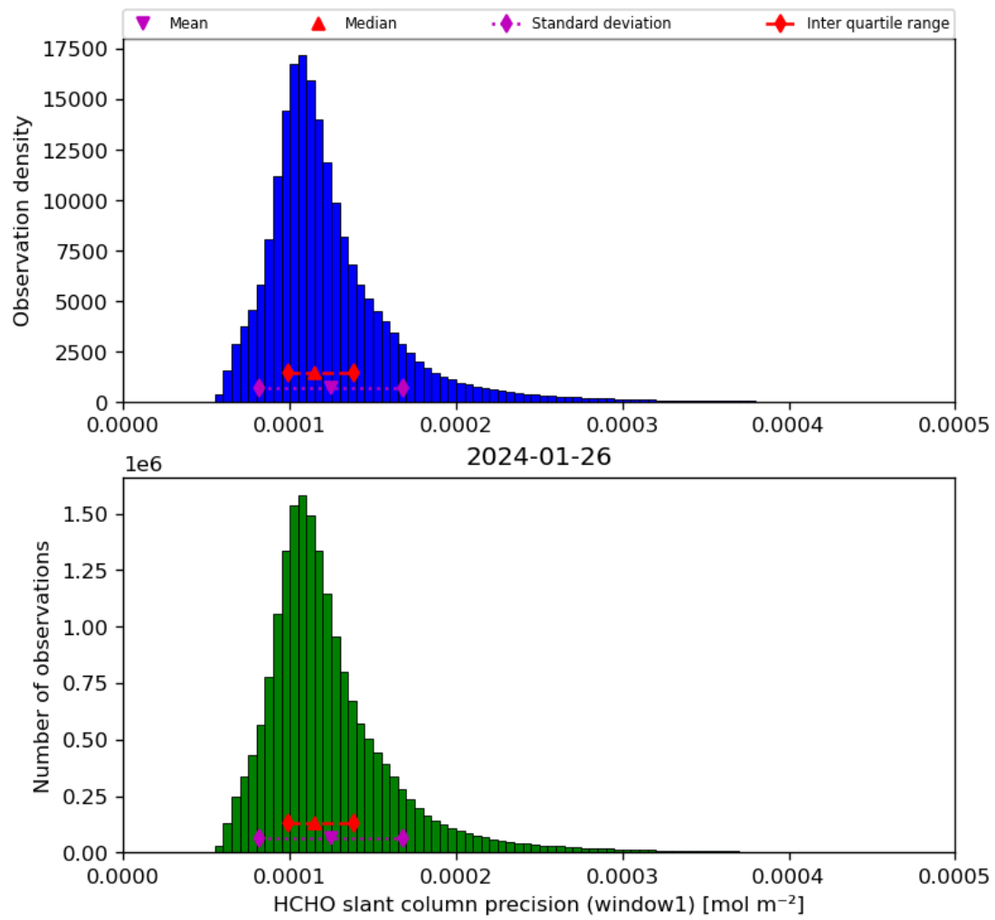
Figure 39: Histogram of “HCHO slant column precision (window1)” for 2024-01-26 to 2024-01-27
