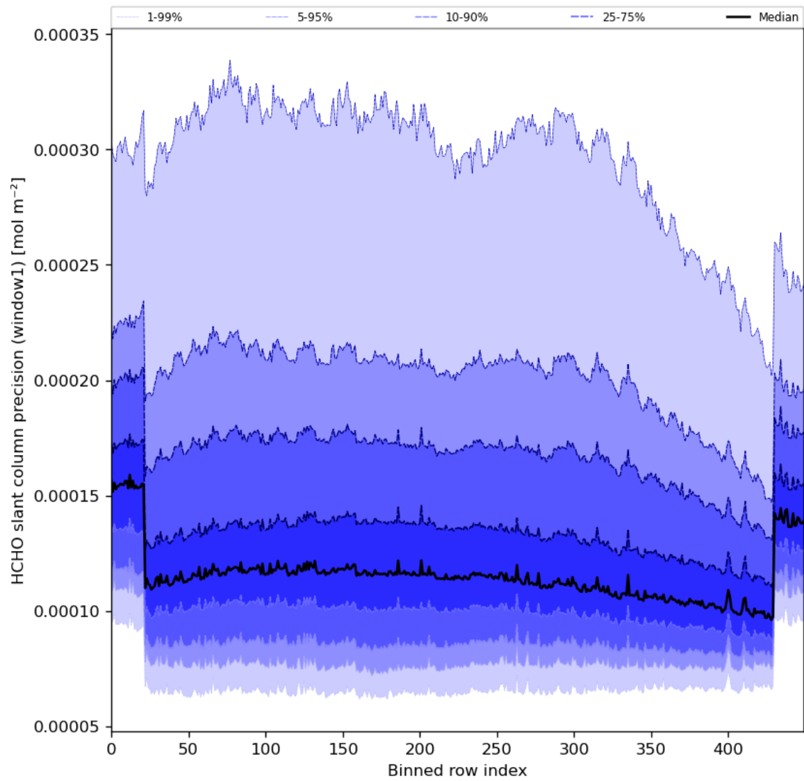
Figure 53: Along track statistics of "HCHO slant column precision (window1)" for 2024-01-26 to 2024-01-27
