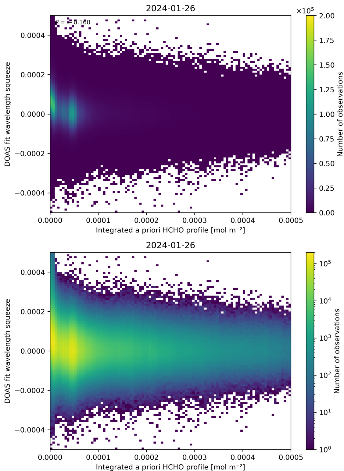
Figure 150: Scatter density plot of “Integrated a priori HCHO profile” against “DOAS fit wavelength squeeze” for 2024-01-26 to 2024-01-27.
