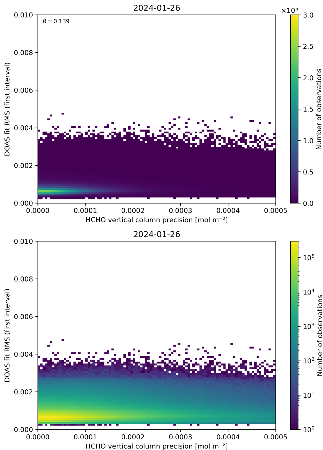
Figure 136: Scatter density plot of “HCHO vertical column precision” against “DOAS fit RMS (first interval)” for 2024-01-26 to 2024-01-27.
