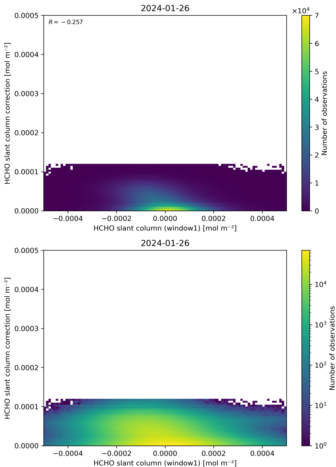
Figure 83: Scatter density plot of “HCHO slant column (window1)” against “HCHO slant column correction” for 2024-01-26 to 2024-01-27.
