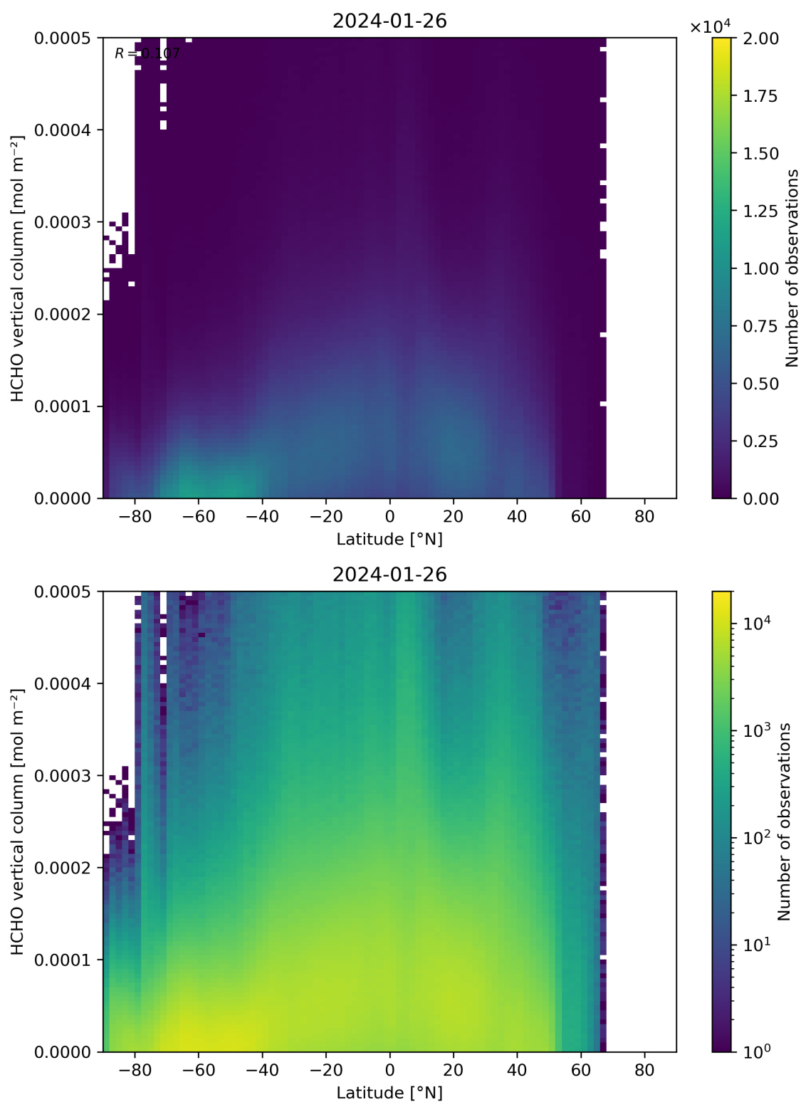
Figure 163: Scatter density plot of “Latitude” against “HCHO vertical column” for 2024-01-26 to 2024-01-27.
