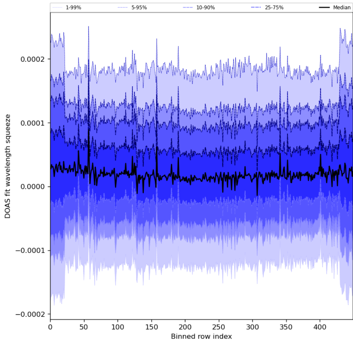
Figure 59: Along track statistics of “DOAS fit wavelength squeeze” for 2024-01-26 to 2024-01-27
