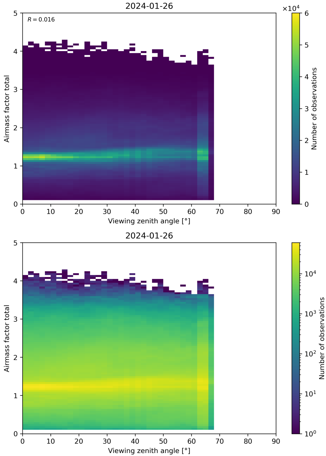
Figure 190: Scatter density plot of “Viewing zenith angle” against “Airmass factor total” for 2024-01-26 to 2024-01-27.
