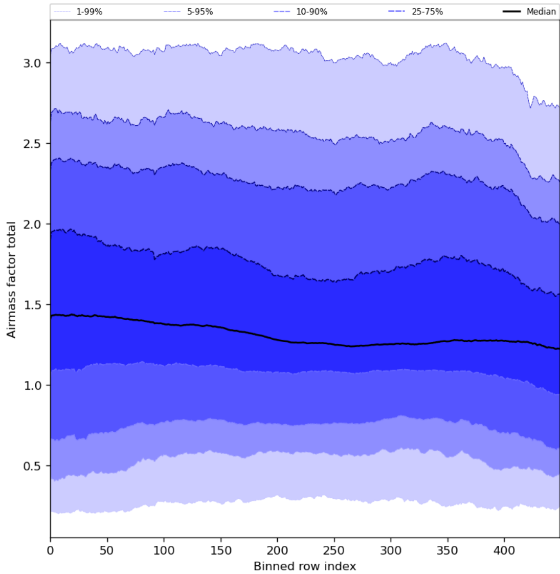
Figure 54: Along track statistics of “Airmass factor total” for 2024-01-26 to 2024-01-27
