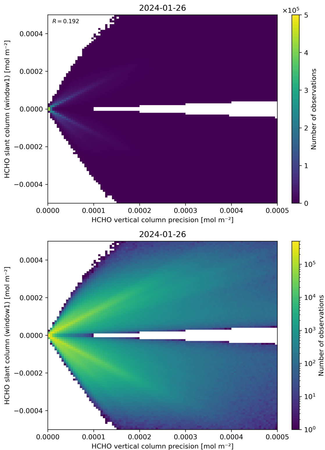
Figure 142: Scatter density plot of “HCHO vertical column precision” against “HCHO slant column (window1)” for 2024-01-26 to 2024-01-27.
