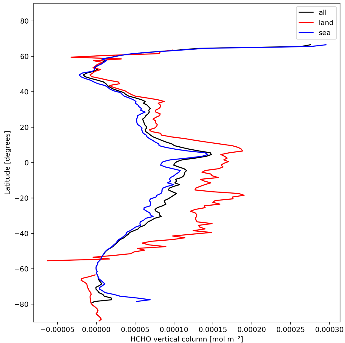
Figure 21: Zonal average of “HCHO vertical column” for 2024-01-26 to 2024-01-27.
