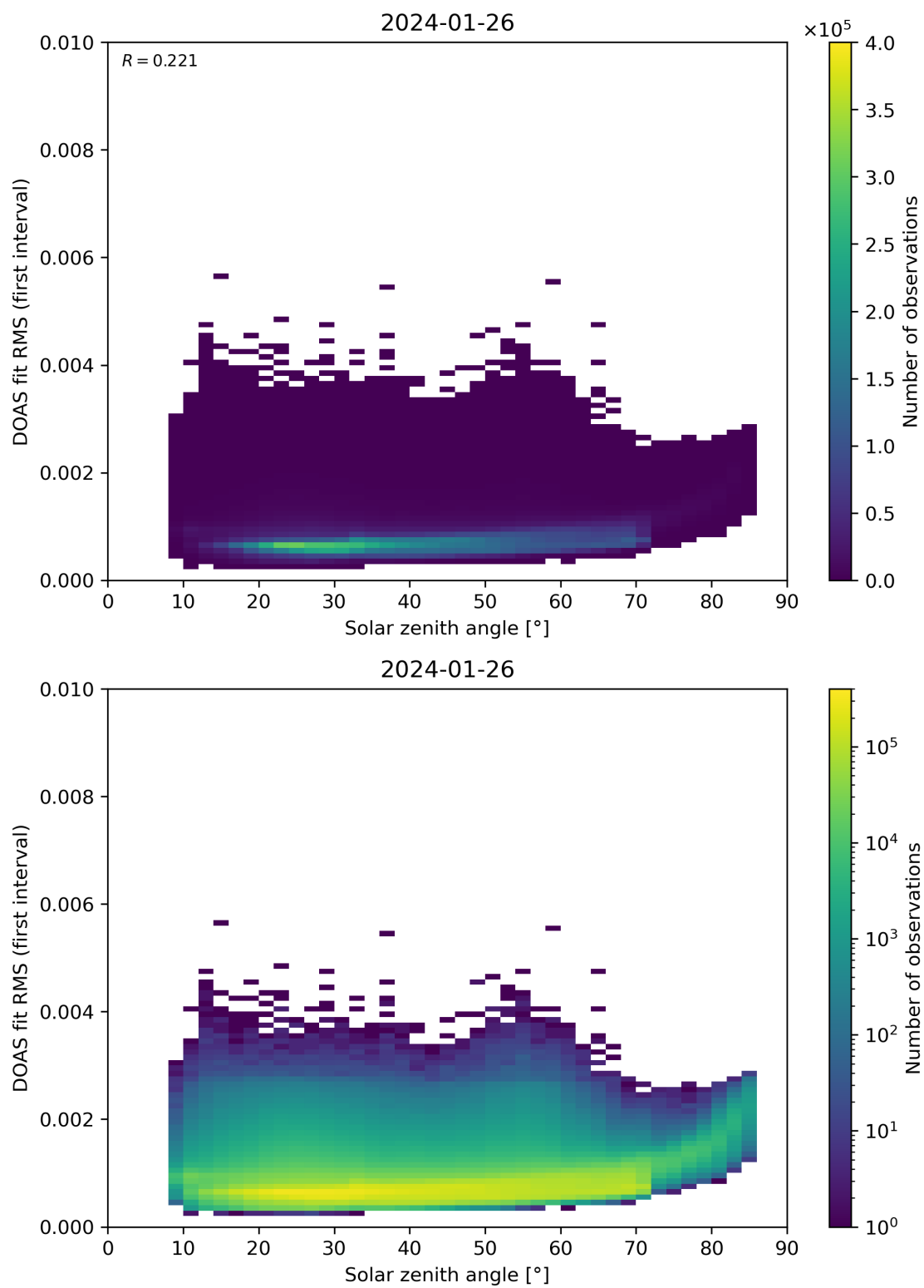
Figure 167: Scatter density plot of “Solar zenith angle” against “DOAS fit RMS (first interval)” for 2024-01-26 to 2024-01-27.
