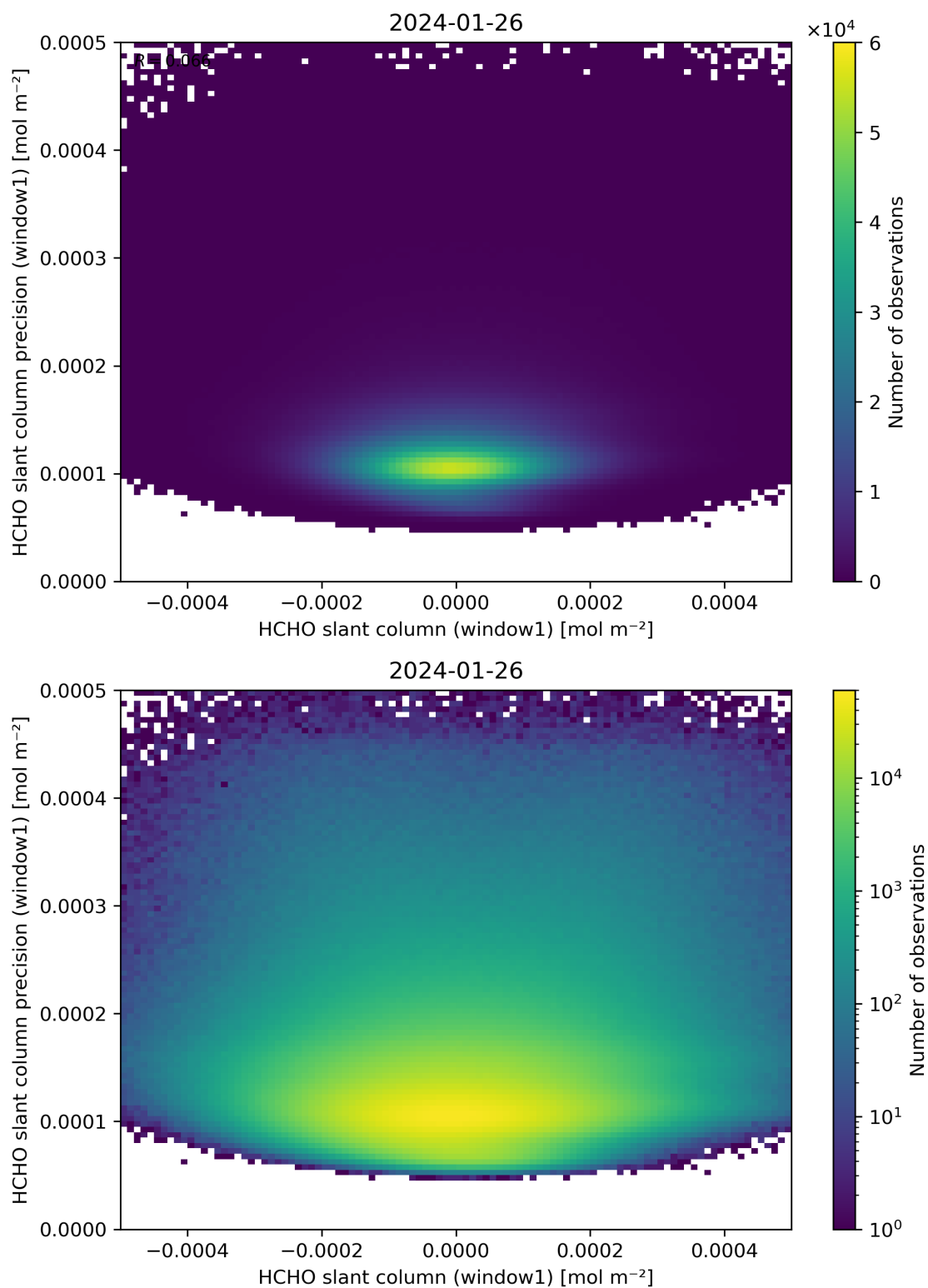
Figure 84: Scatter density plot of “HCHO slant column (window1)” against “HCHO slant column precision (window1)” for 2024-01-26 to 2024-01-27.
