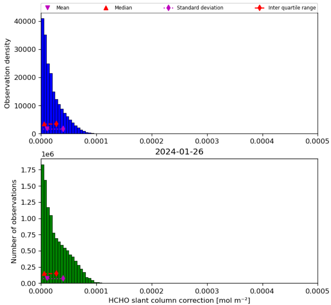
Figure 47: Histogram of “HCHO slant column correction” for 2024-01-26 to 2024-01-27
