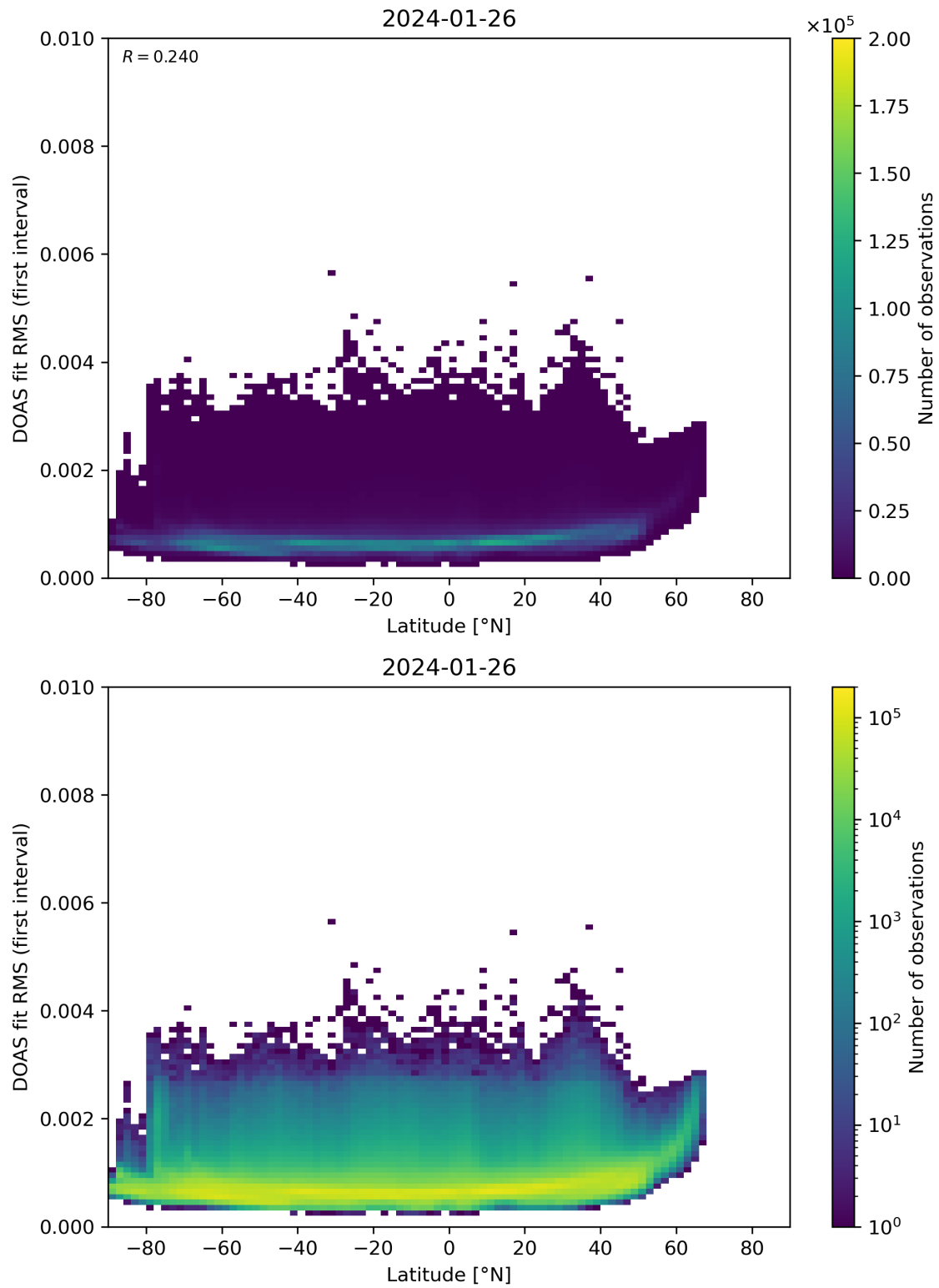
Figure 153: Scatter density plot of “Latitude” against “DOAS fit RMS (first interval)” for 2024-01-26 to 2024-01-27.
