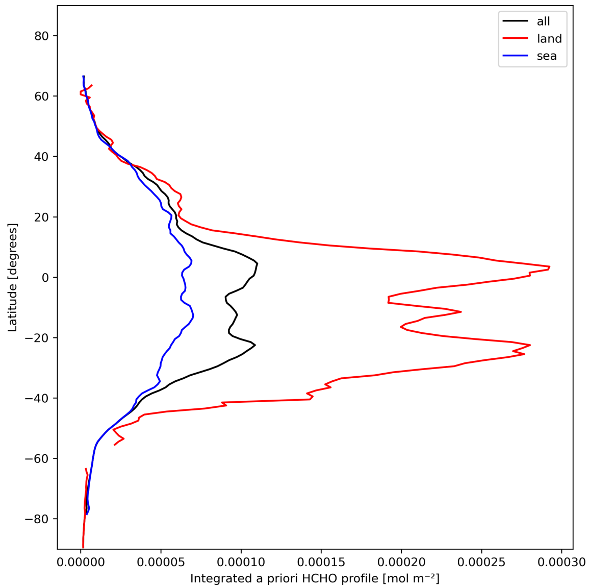
Figure 29: Zonal average of “Integrated a priori HCHO profile” for 2024-01-26 to 2024-01-27.
