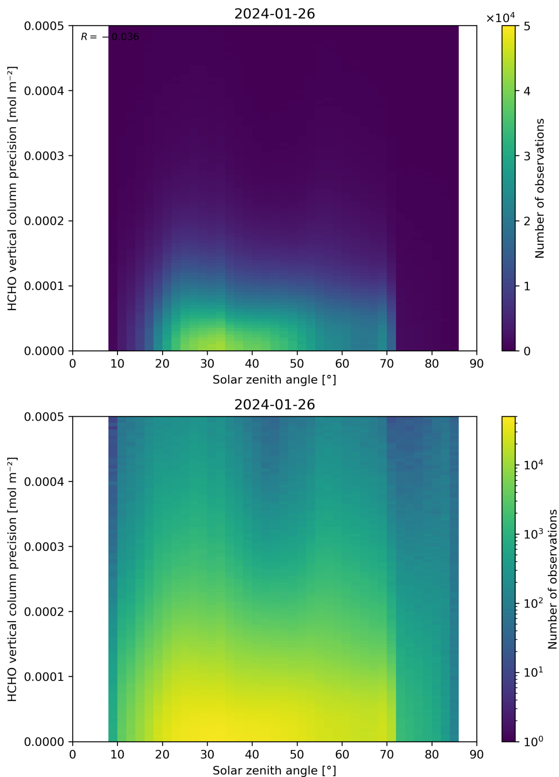
Figure 179: Scatter density plot of “Solar zenith angle” against “HCHO vertical column precision” for 2024-01-26 to 2024-01-27.
