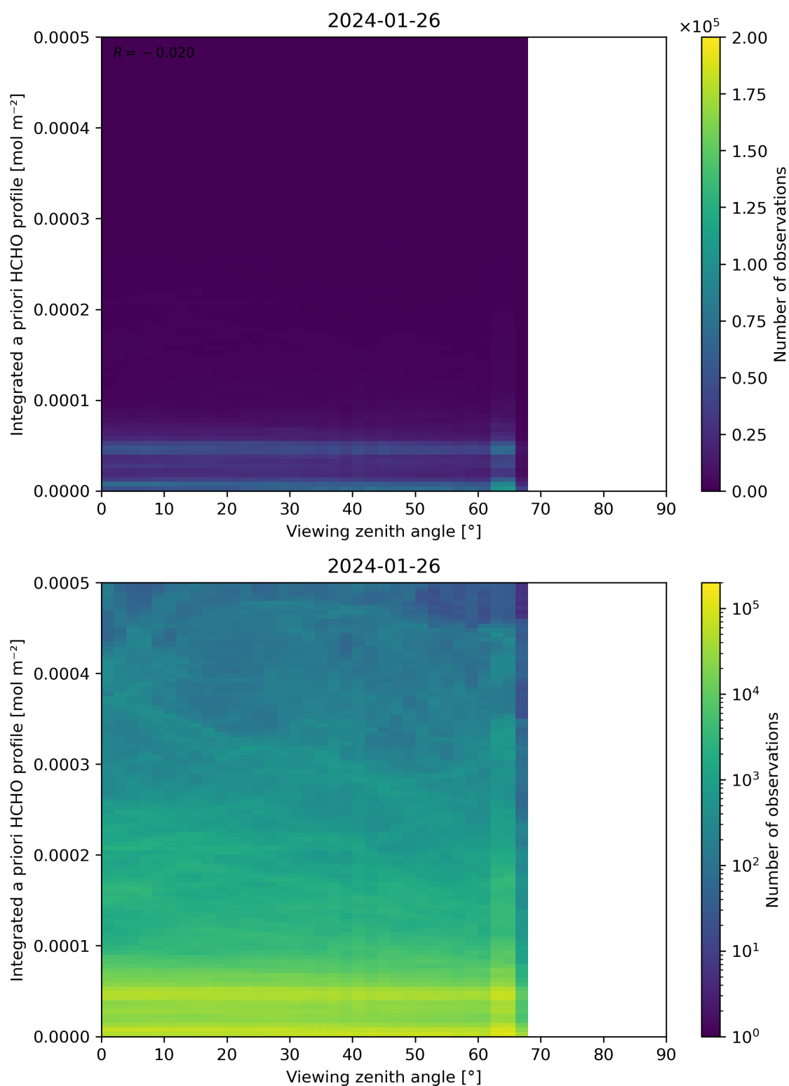
Figure 195: Scatter density plot of “Viewing zenith angle” against “Integrated a priori HCHO profile” for 2024-01-26 to 2024-01-27.
