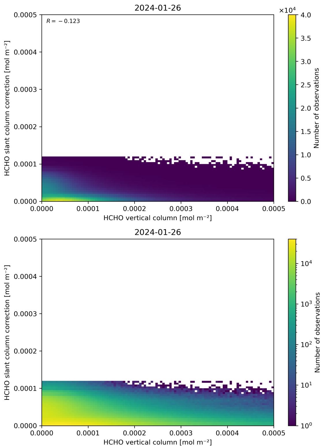
Figure 128: Scatter density plot of “HCHO vertical column” against “HCHO slant column correction” for 2024-01-26 to 2024-01-27.
