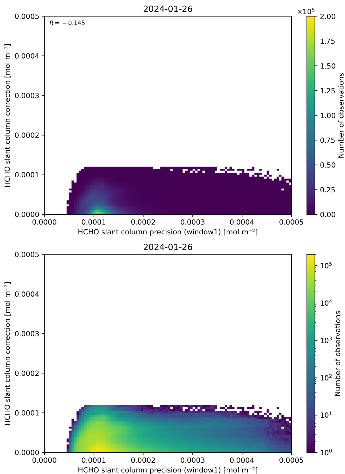
Figure 93: Scatter density plot of “HCHO slant column precision (window1)” against “HCHO slant column correction” for 2024-01-26 to 2024-01-27.
