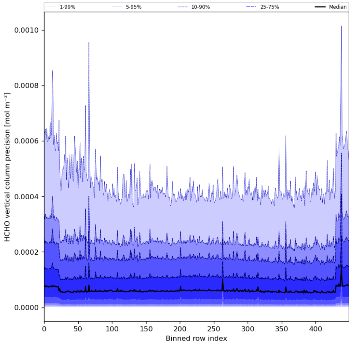
Figure 50: Along track statistics of "HCHO vertical column precision" for 2024-01-26 to 2024-01-27
