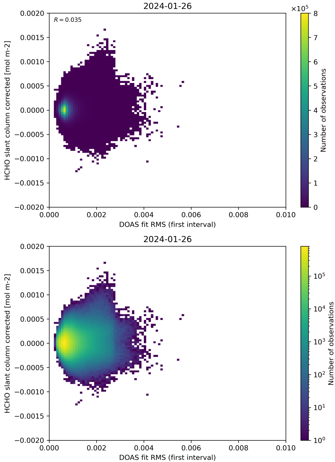
Figure 62: Scatter density plot of “DOAS fit RMS (first interval)” against “HCHO slant column corrected” for 2024-01-26 to 2024-01-27.
