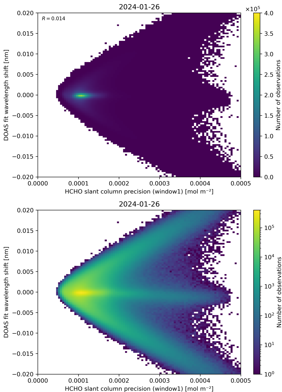
Figure 89: Scatter density plot of “HCHO slant column precision (window1)” against “DOAS fit wavelength shift” for 2024-01-26 to 2024-01-27.
