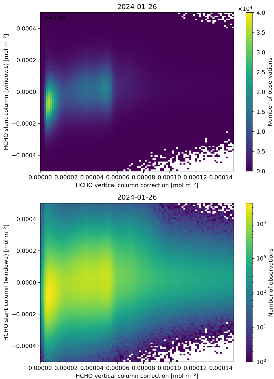
Figure 118: Scatter density plot of “HCHO vertical column correction” against “HCHO slant column (window1)” for 2024-01-26 to 2024-01-27.
