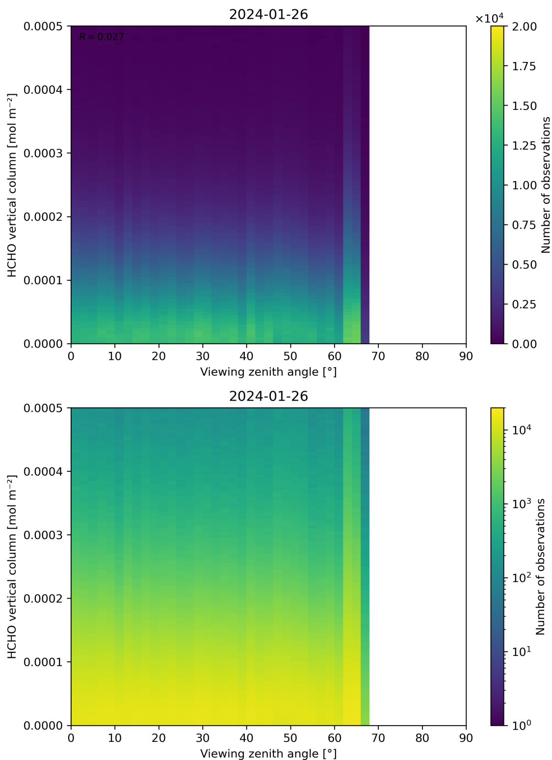
Figure 192: Scatter density plot of “Viewing zenith angle” against “HCHO vertical column” for 2024-01-26 to 2024-01-27.
