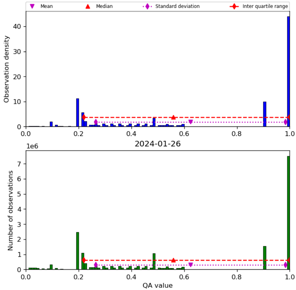
Figure 34: Histogram of “QA value” for 2024-01-26 to 2024-01-27
