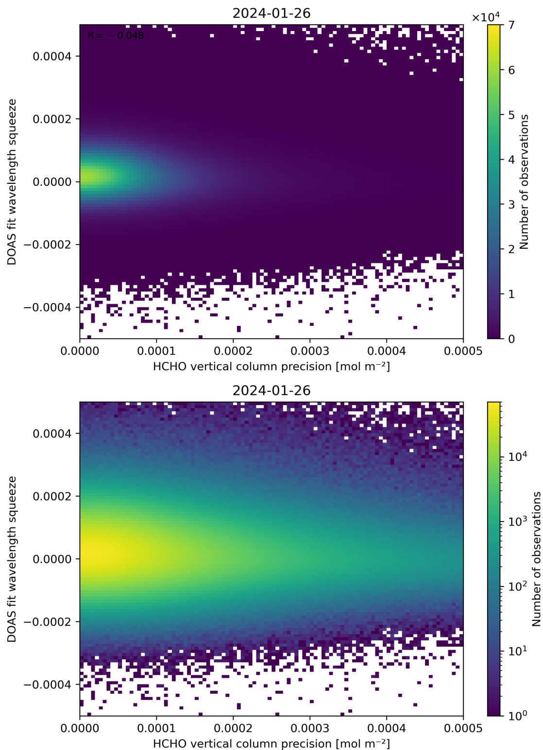
Figure 138: Scatter density plot of “HCHO vertical column precision” against “DOAS fit wavelength squeeze” for 2024-01-26 to 2024-01-27.
