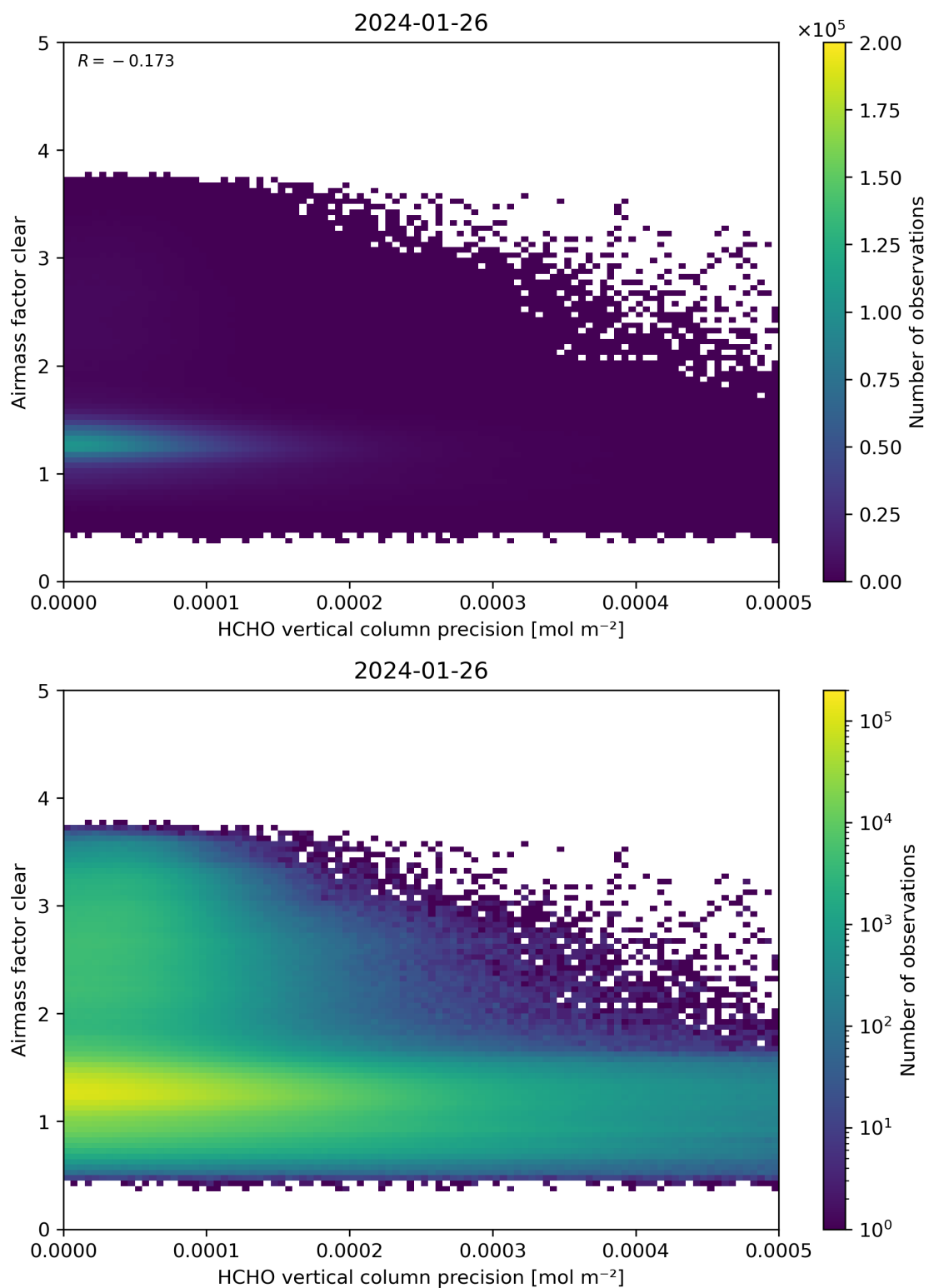
Figure 139: Scatter density plot of “HCHO vertical column precision” against “Airmass factor clear” for 2024-01-26 to 2024-01-27.
