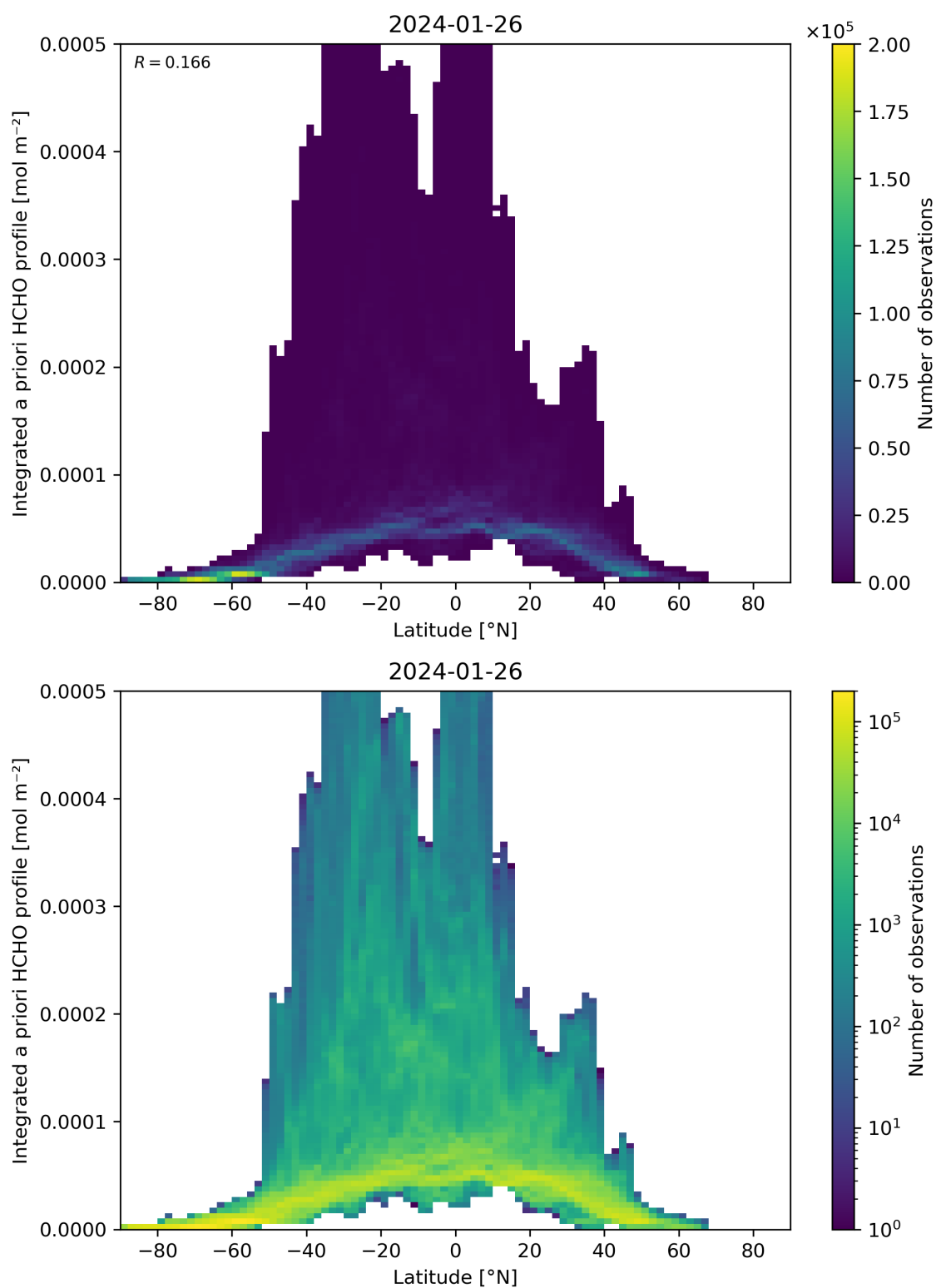
Figure 166: Scatter density plot of “Latitude” against “Integrated a priori HCHO profile” for 2024-01-26 to 2024-01-27.
