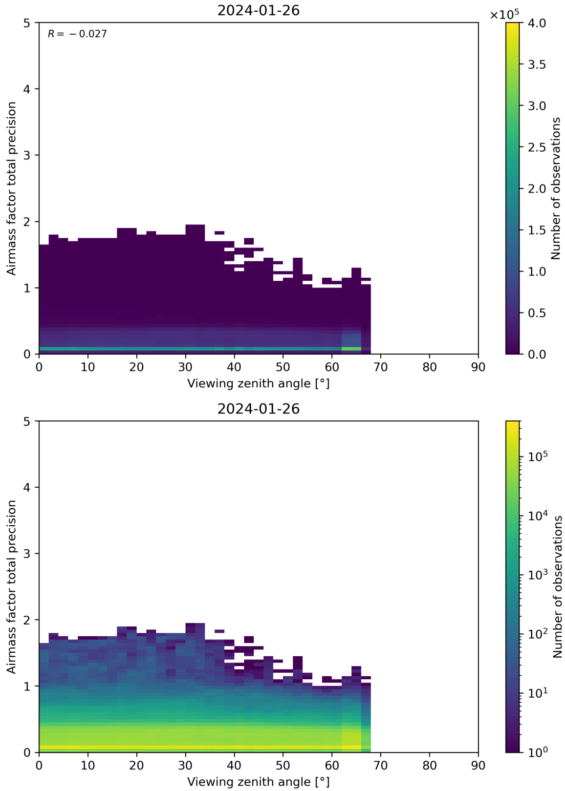
Figure 191: Scatter density plot of “Viewing zenith angle” against “Airmass factor total precision” for 2024-01-26 to 2024-01-27.
