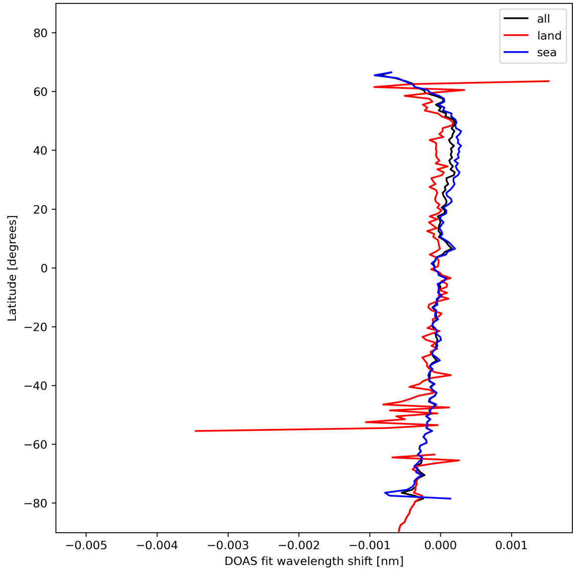
Figure 30: Zonal average of “DOAS fit wavelength shift” for 2024-01-26 to 2024-01-27.
