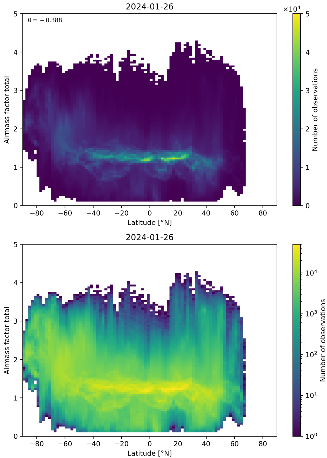
Figure 161: Scatter density plot of “Latitude” against “Airmass factor total” for 2024-01-26 to 2024-01-27.
