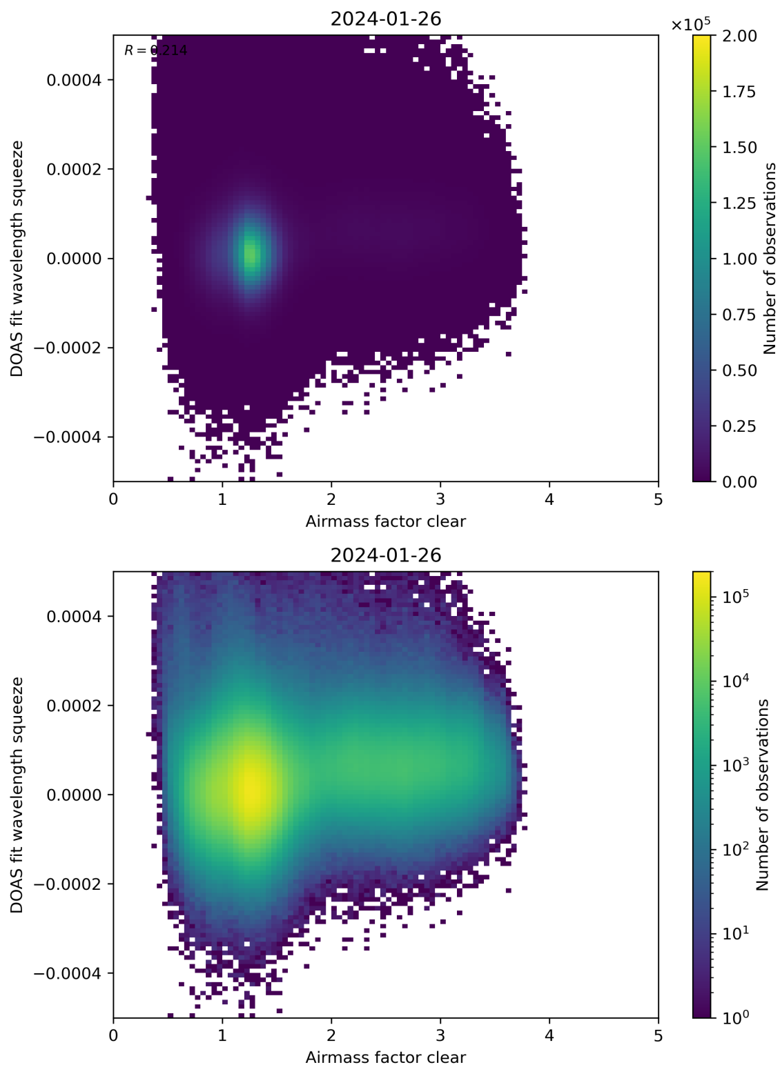
Figure 73: Scatter density plot of “Airmass factor clear” against “DOAS fit wavelength squeeze” for 2024-01-26 to 2024-01-27.
