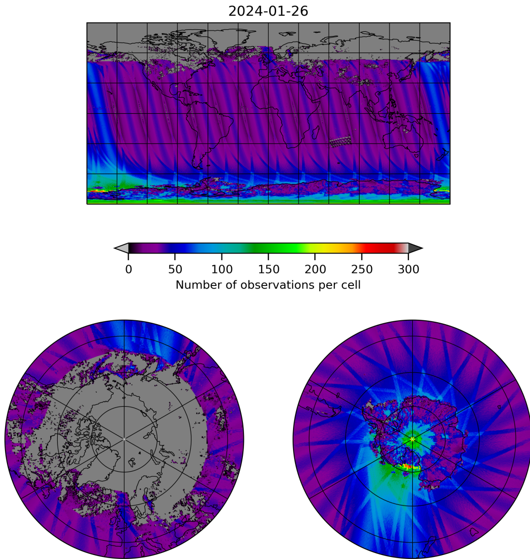
Figure 19: Map of the number of observations for 2024-01-26 to 2024-01-27
