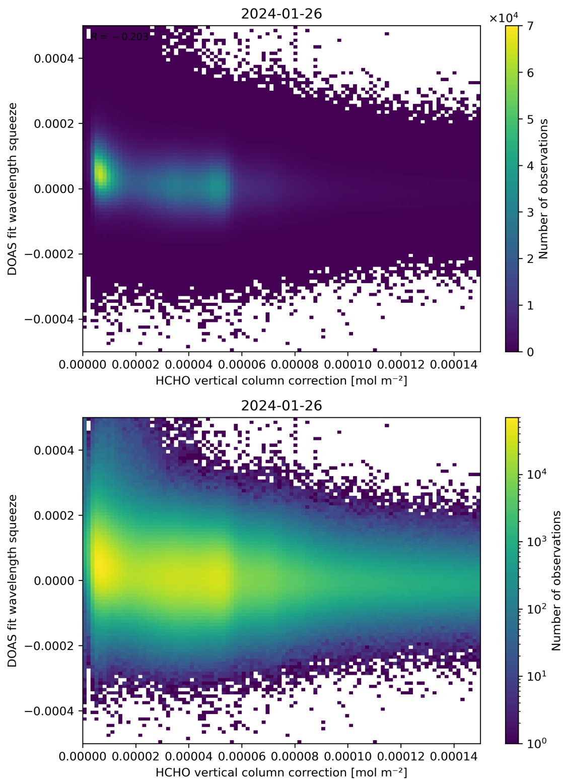
Figure 114: Scatter density plot of “HCHO vertical column correction” against “DOAS fit wavelength squeeze” for 2024-01-26 to 2024-01-27.
