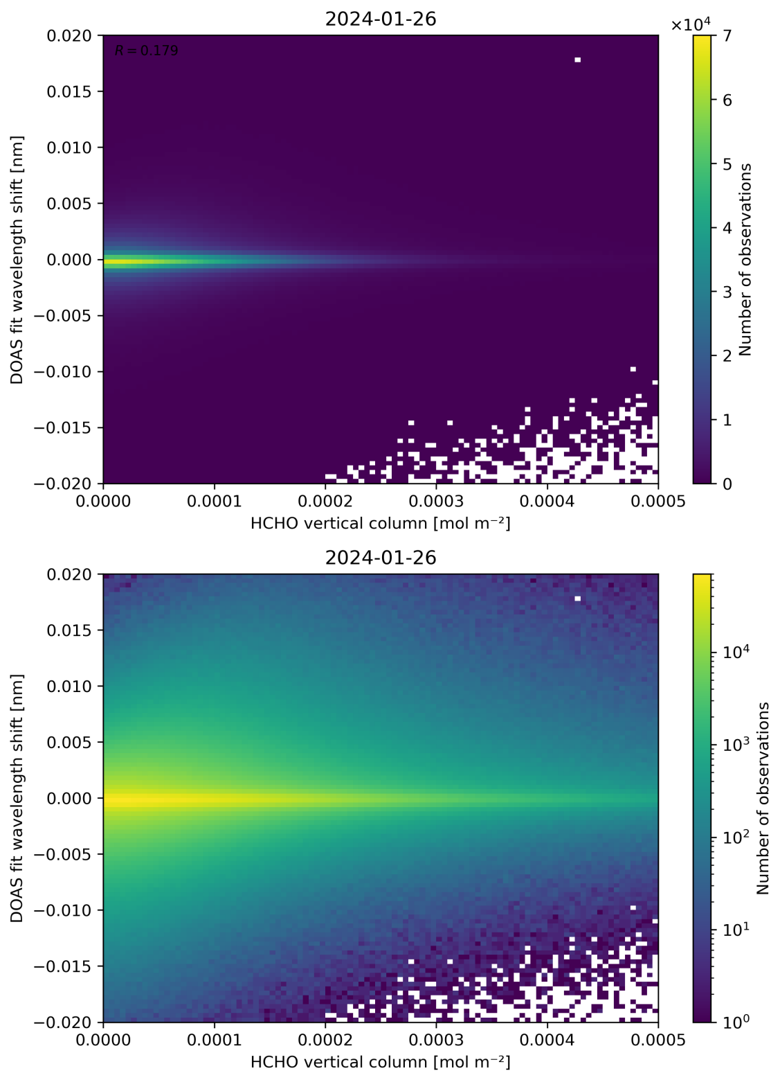
Figure 124: Scatter density plot of “HCHO vertical column” against “DOAS fit wavelength shift” for 2024-01-26 to 2024-01-27.
