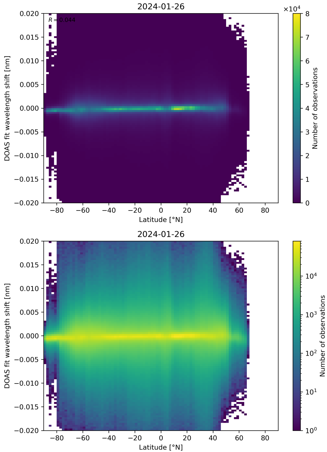
Figure 154: Scatter density plot of “Latitude” against “DOAS fit wavelength shift” for 2024-01-26 to 2024-01-27.
