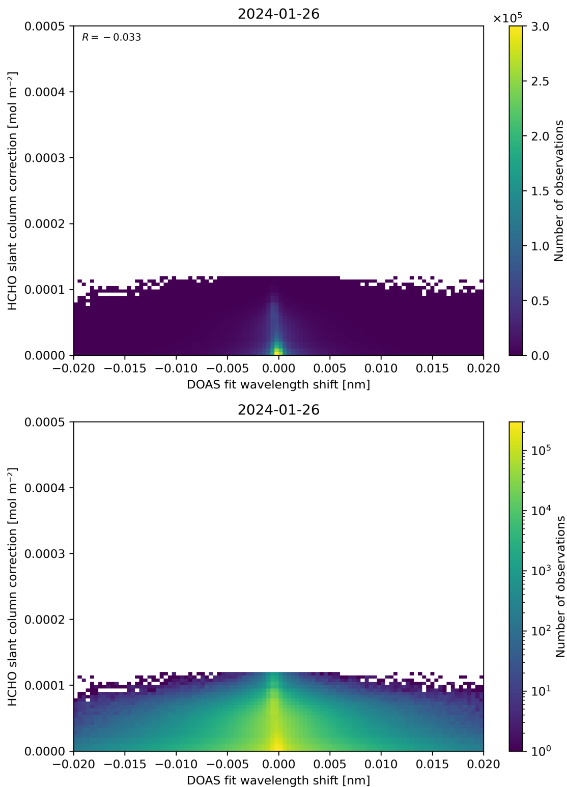
Figure 67: Scatter density plot of “DOAS fit wavelength shift” against “HCHO slant column correction” for 2024-01-26 to 2024-01-27.
