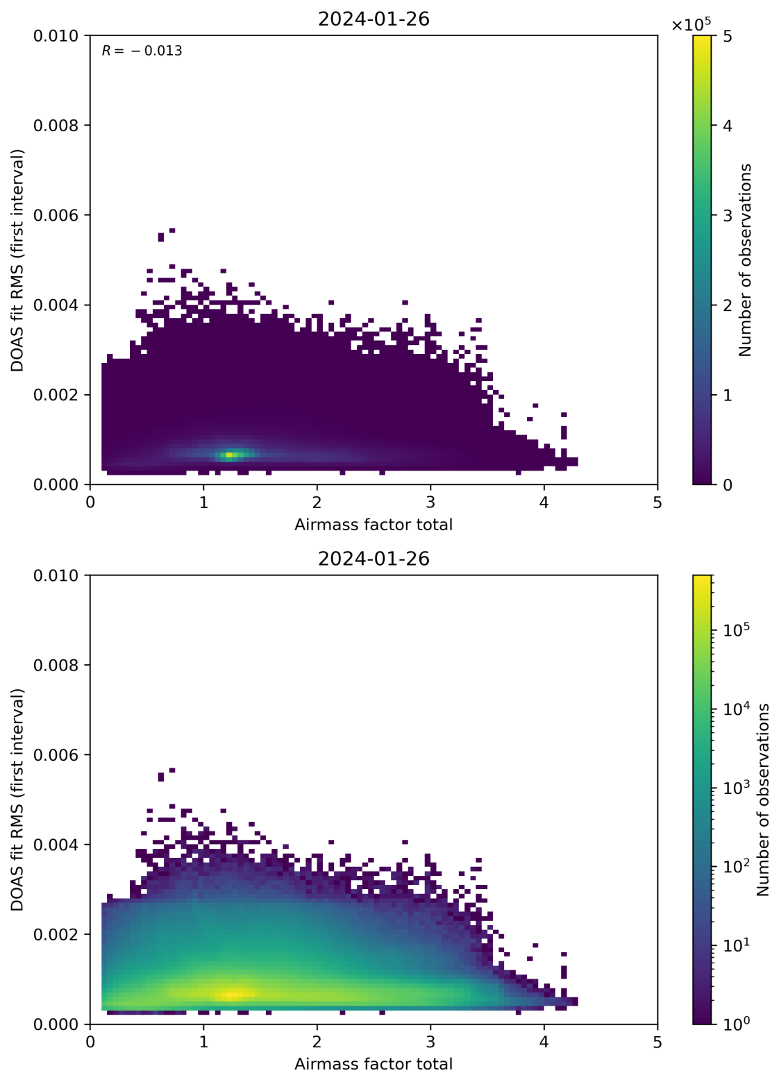
Figure 97: Scatter density plot of “Airmass factor total” against “DOAS fit RMS (first interval)” for 2024-01-26 to 2024-01-27.
