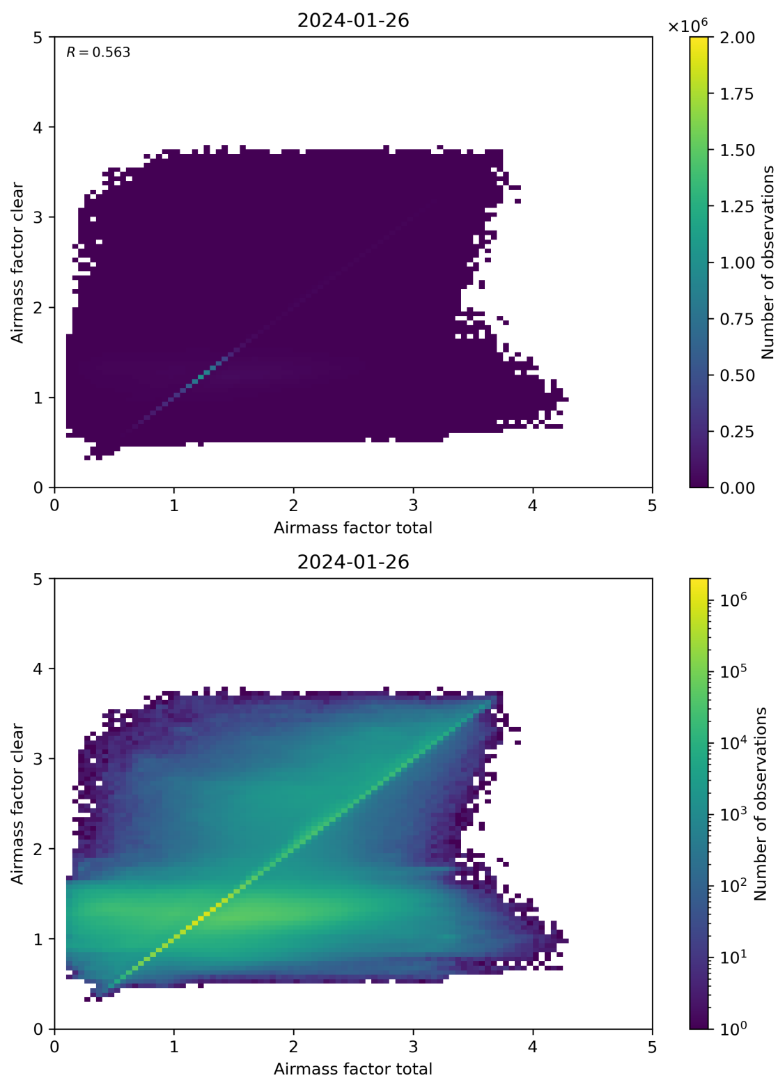
Figure 100: Scatter density plot of “Airmass factor total” against “Airmass factor clear” for 2024-01-26 to 2024-01-27.
