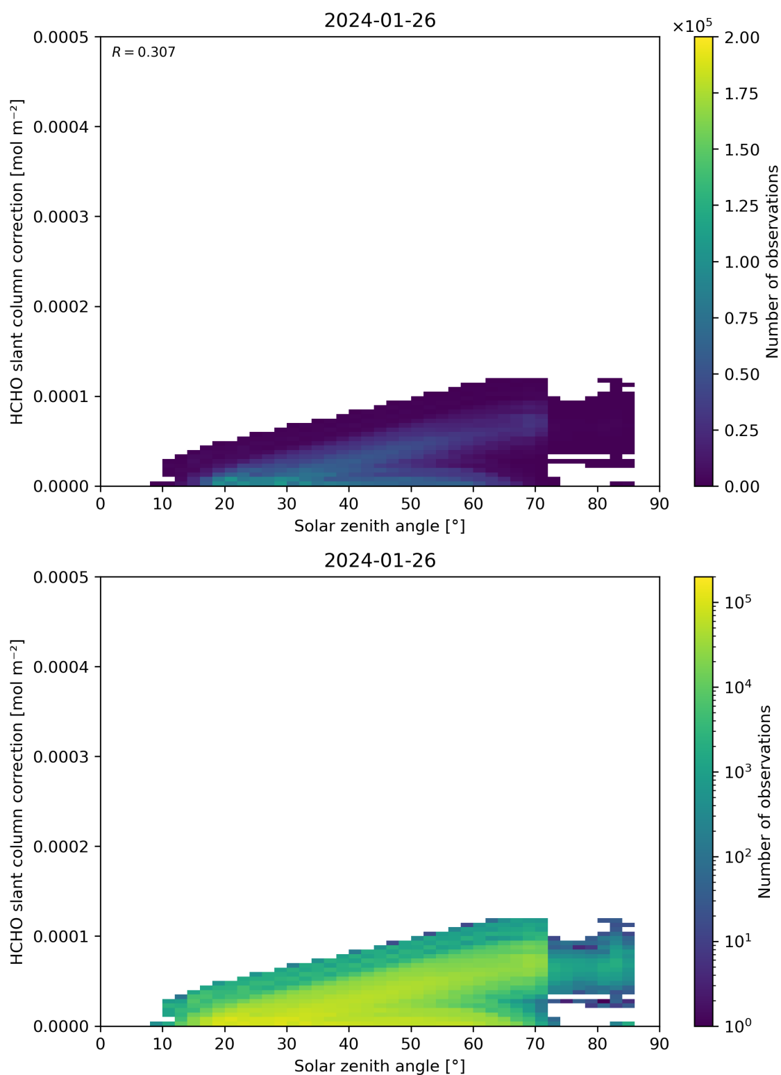
Figure 172: Scatter density plot of “Solar zenith angle” against “HCHO slant column correction” for 2024-01-26 to 2024-01-27.
