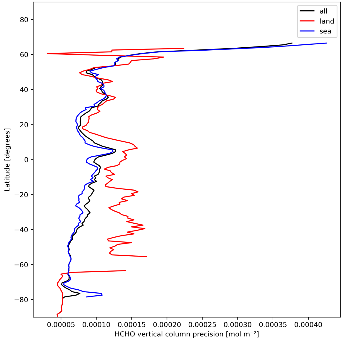
Figure 22: Zonal average of "HCHO vertical column precision" for 2024-01-26 to 2024-01-27.
