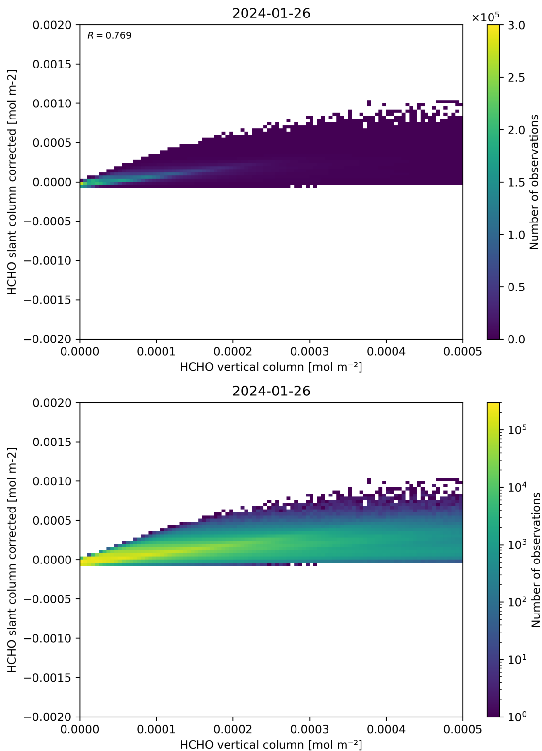
Figure 127: Scatter density plot of “HCHO vertical column” against “HCHO slant column corrected” for 2024-01-26 to 2024-01-27.
