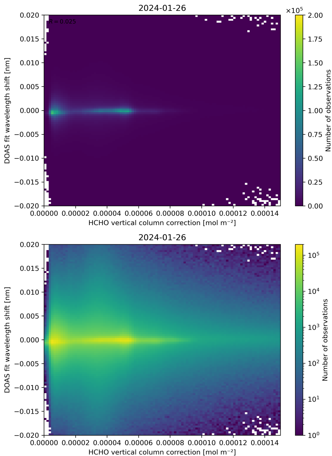
Figure 113: Scatter density plot of “HCHO vertical column correction” against “DOAS fit wavelength shift” for 2024-01-26 to 2024-01-27.
