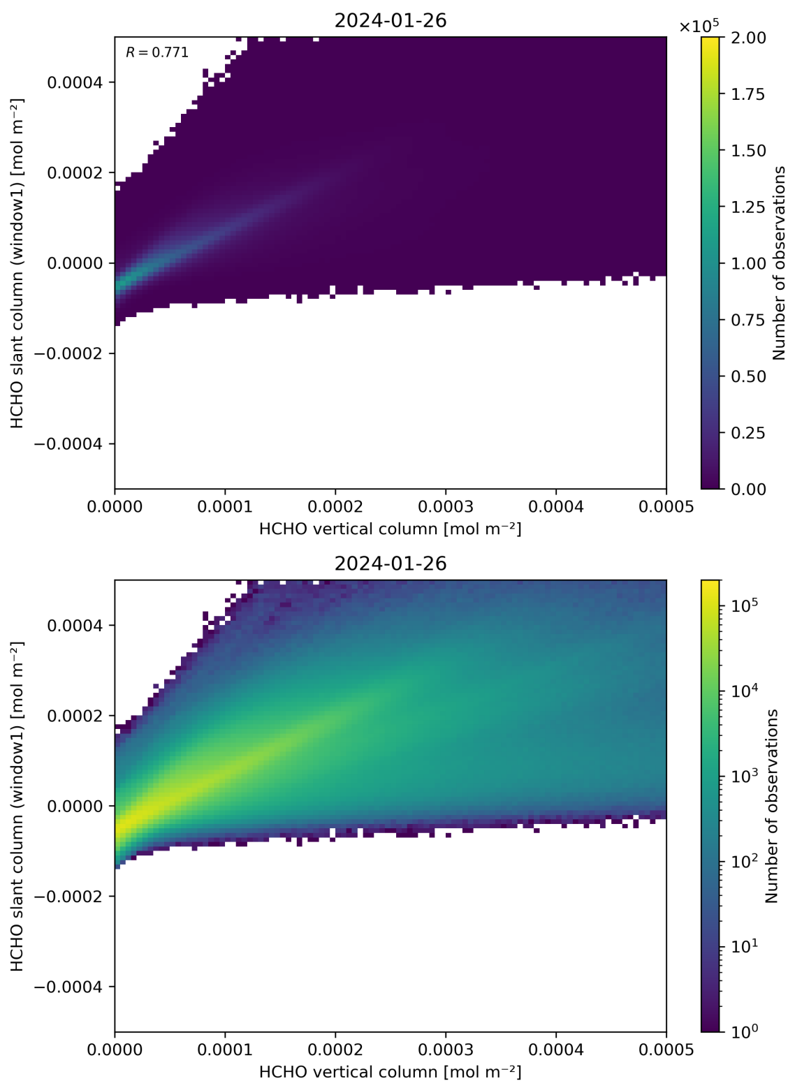
Figure 129: Scatter density plot of “HCHO vertical column” against “HCHO slant column (window1)” for 2024-01-26 to 2024-01-27.
