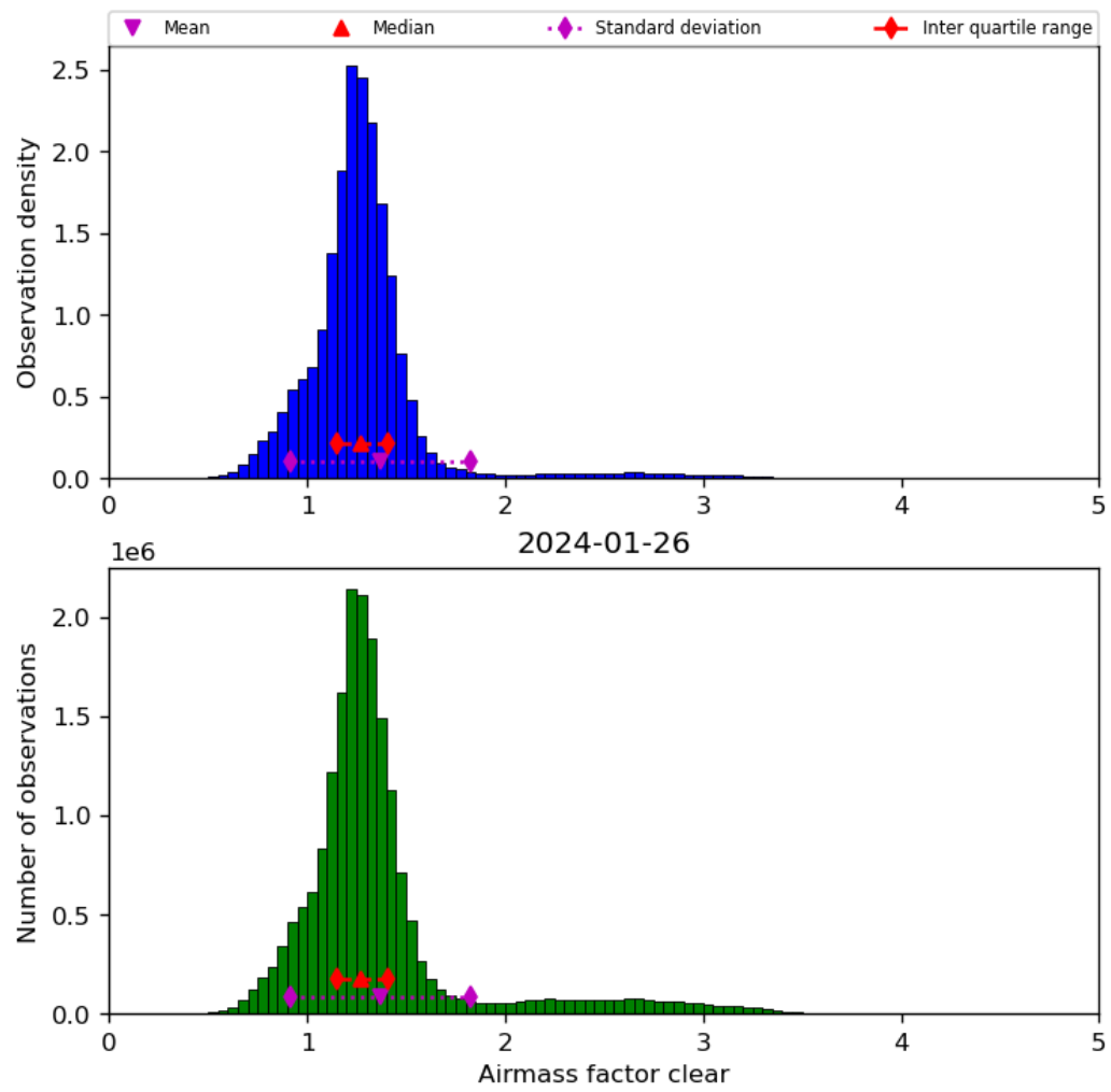
Figure 42: Histogram of “Airmass factor clear” for 2024-01-26 to 2024-01-27
