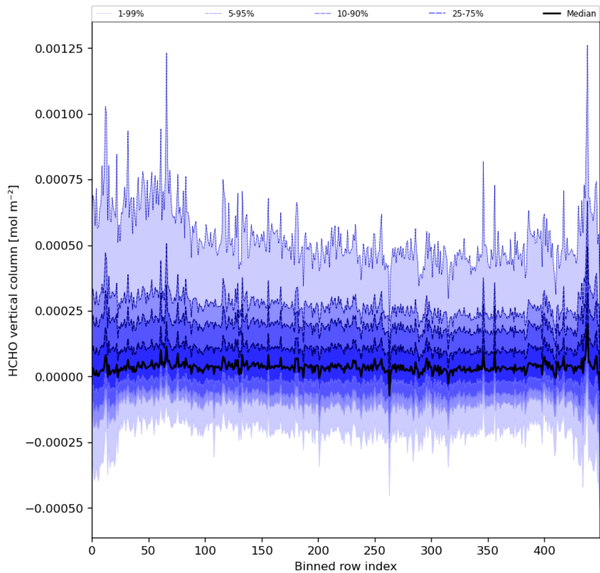
Figure 49: Along track statistics of “HCHO vertical column” for 2024-01-26 to 2024-01-27
