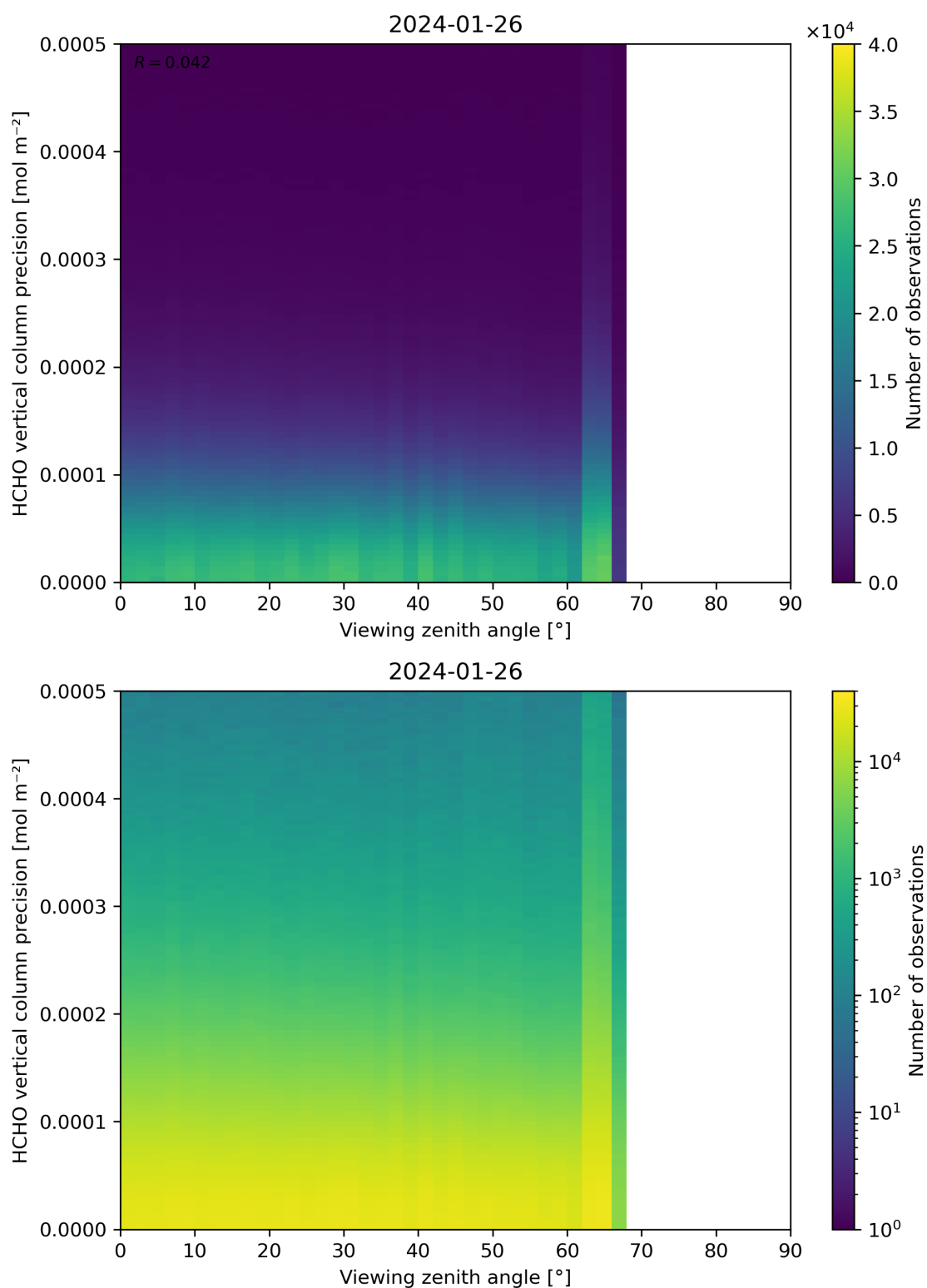
Figure 194: Scatter density plot of “Viewing zenith angle” against “HCHO vertical column precision” for 2024-01-26 to 2024-01-27.
