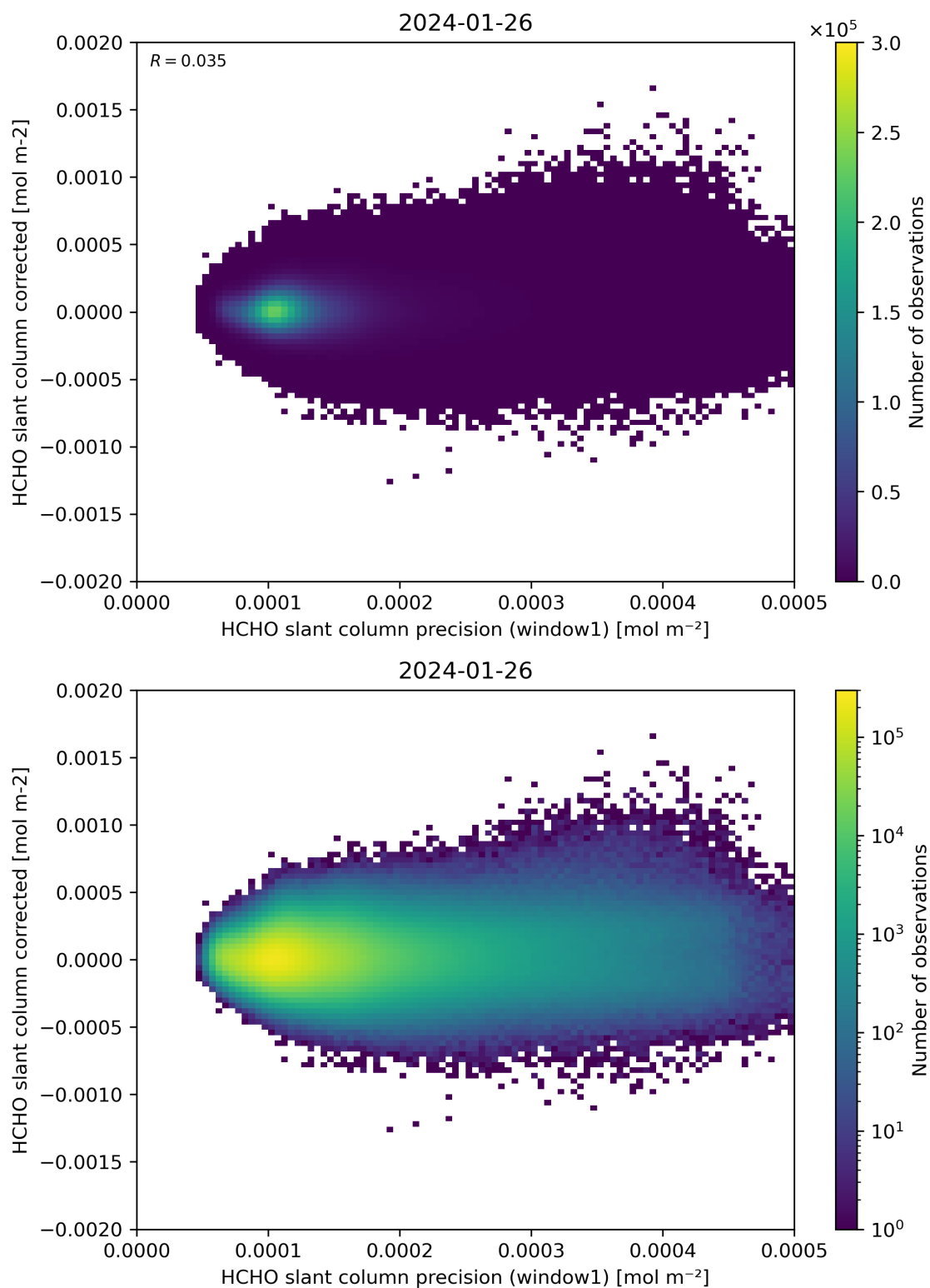
Figure 92: Scatter density plot of “HCHO slant column precision (window1)” against “HCHO slant column corrected” for 2024-01-26 to 2024-01-27.
