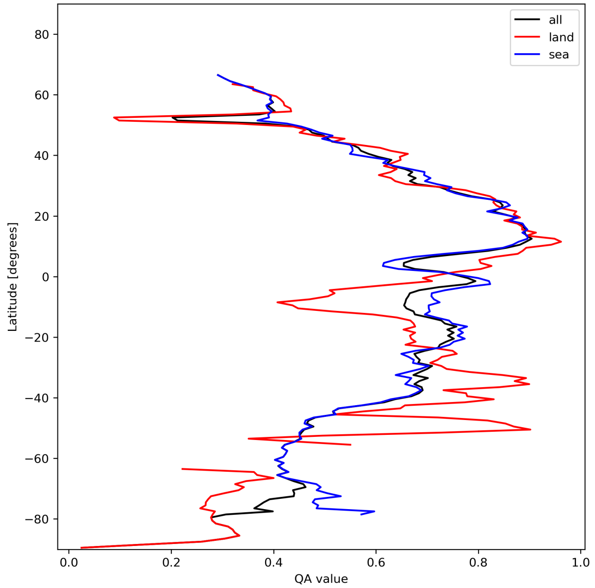
Figure 20: Zonal average of “QA value” for 2024-01-26 to 2024-01-27.
