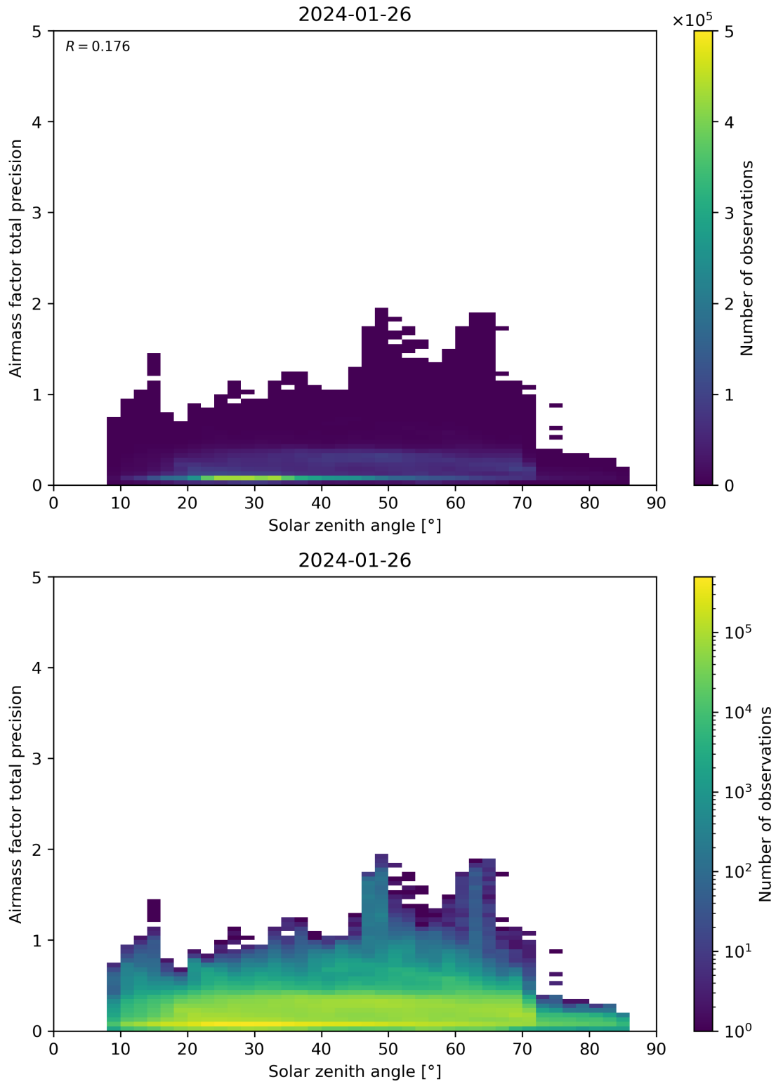
Figure 176: Scatter density plot of “Solar zenith angle” against “Airmass factor total precision” for 2024-01-26 to 2024-01-27.
