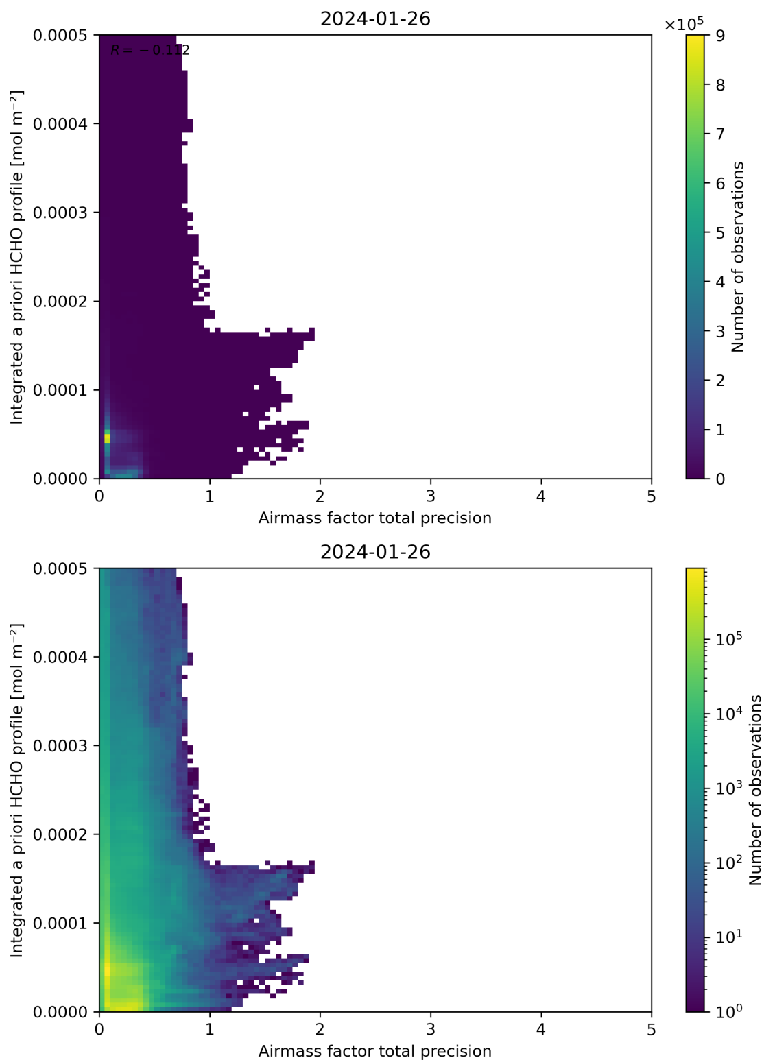
Figure 111: Scatter density plot of “Airmass factor total precision” against “Integrated a priori HCHO profile” for 2024-01-26 to 2024-01-27.
