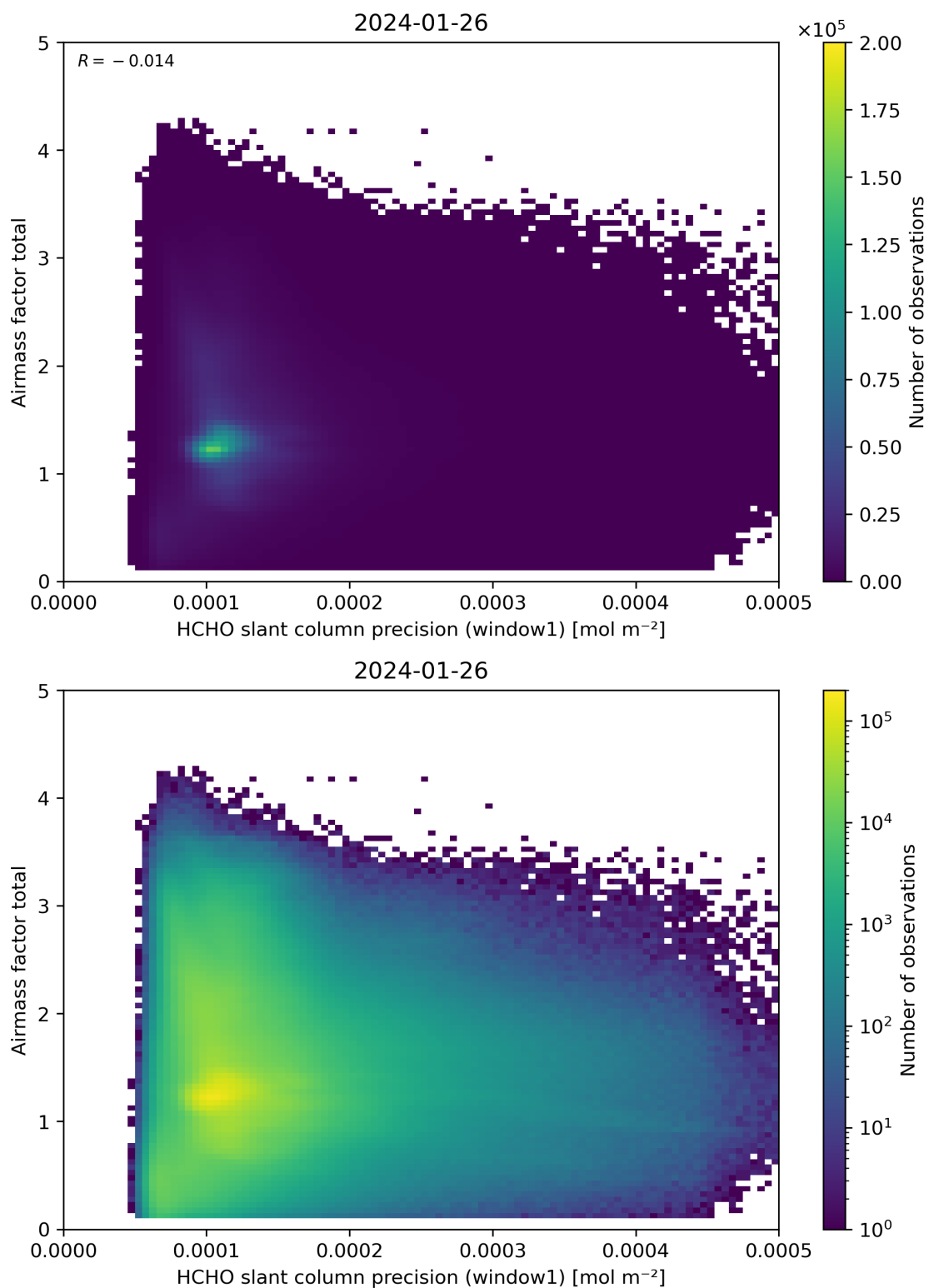
Figure 94: Scatter density plot of “HCHO slant column precision (window1)” against “Airmass factor total” for 2024-01-26 to 2024-01-27.
