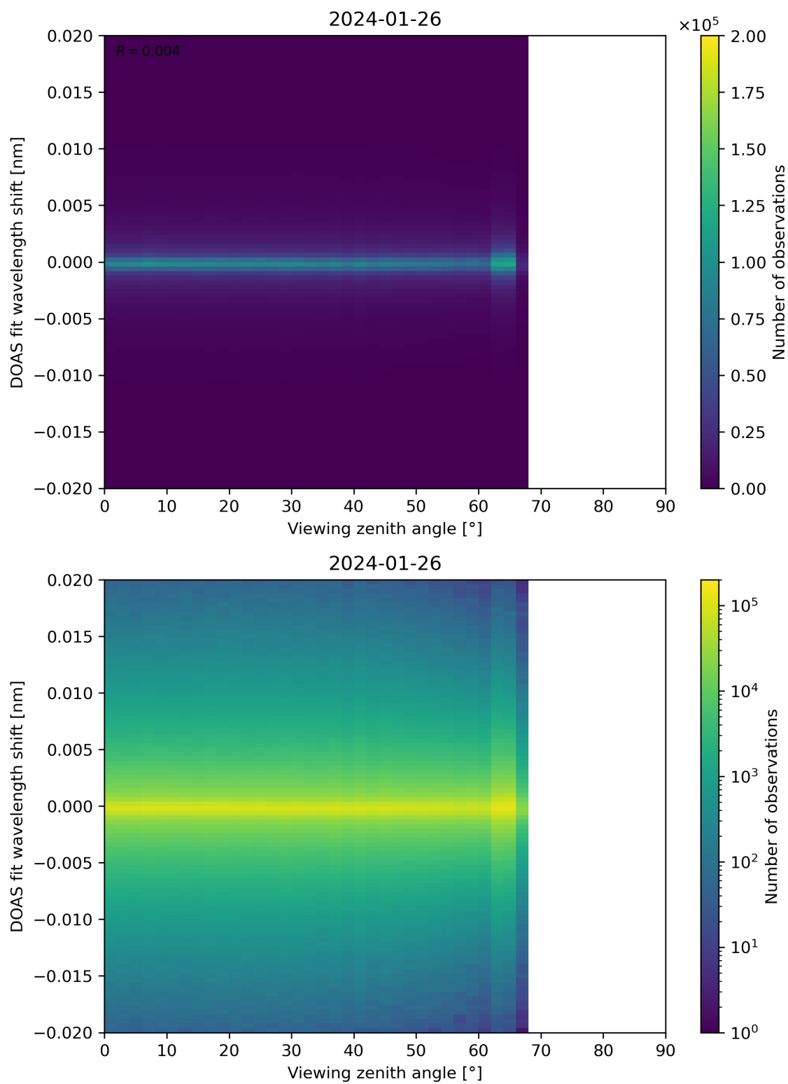
Figure 183: Scatter density plot of “Viewing zenith angle” against “DOAS fit wavelength shift” for 2024-01-26 to 2024-01-27.
