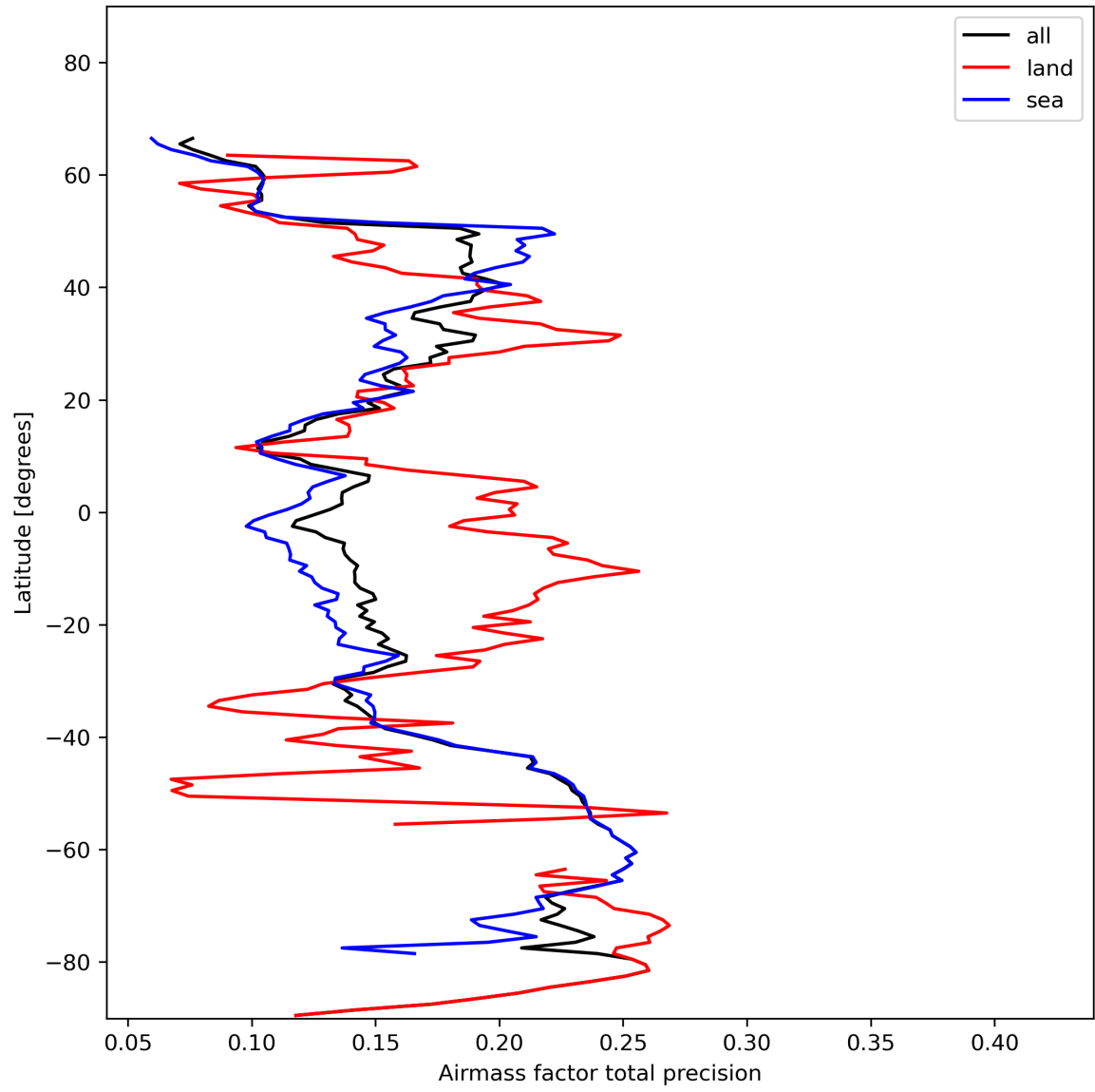
Figure 27: Zonal average of “Airmass factor total precision” for 2024-01-26 to 2024-01-27.
