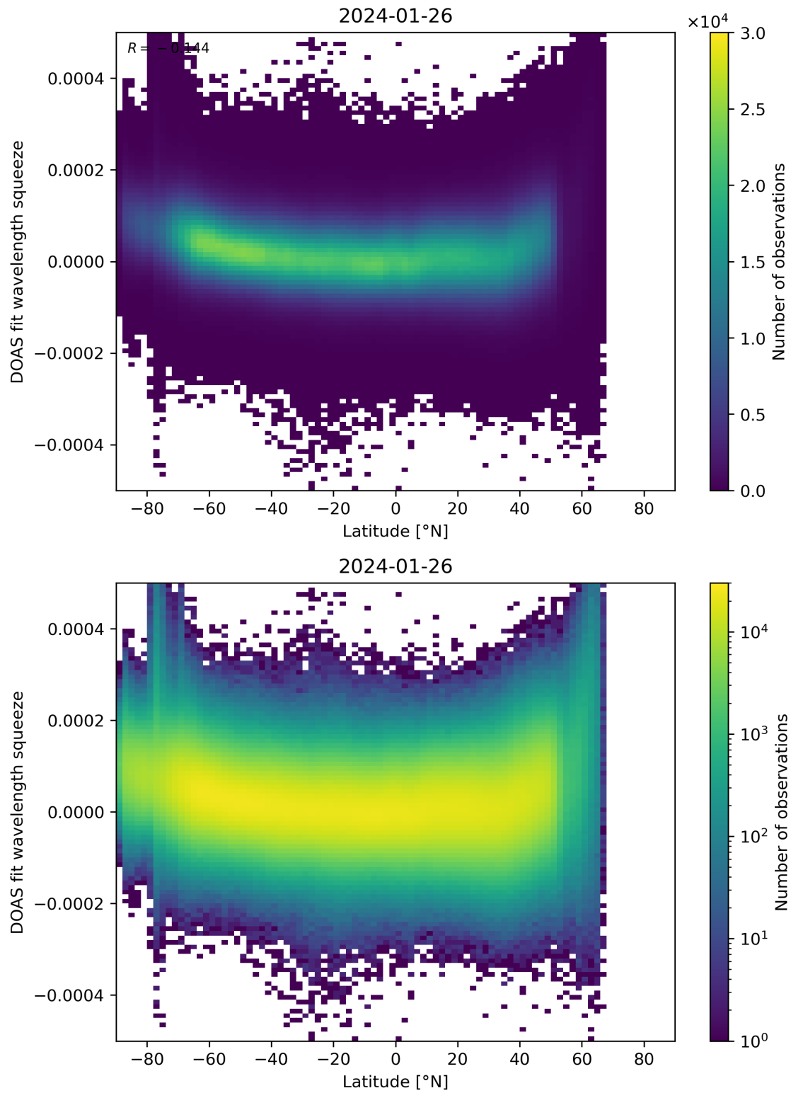
Figure 155: Scatter density plot of “Latitude” against “DOAS fit wavelength squeeze” for 2024-01-26 to 2024-01-27.
