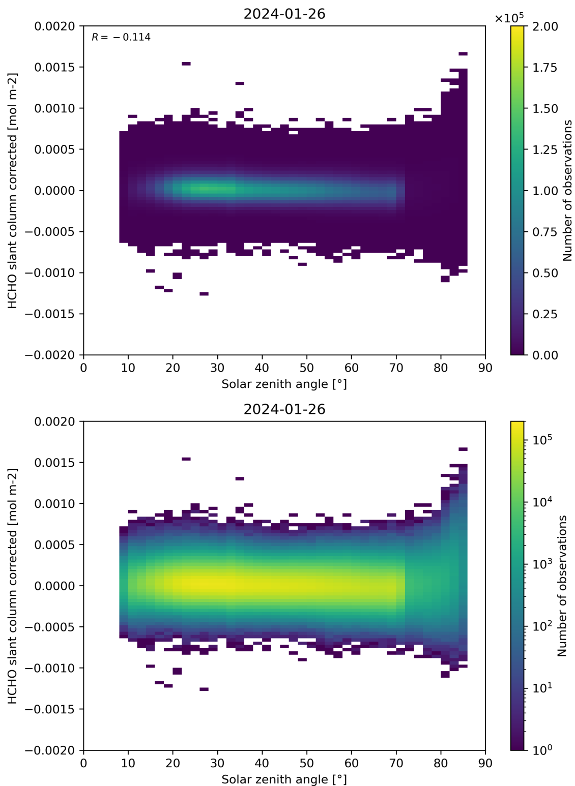
Figure 171: Scatter density plot of “Solar zenith angle” against “HCHO slant column corrected” for 2024-01-26 to 2024-01-27.
