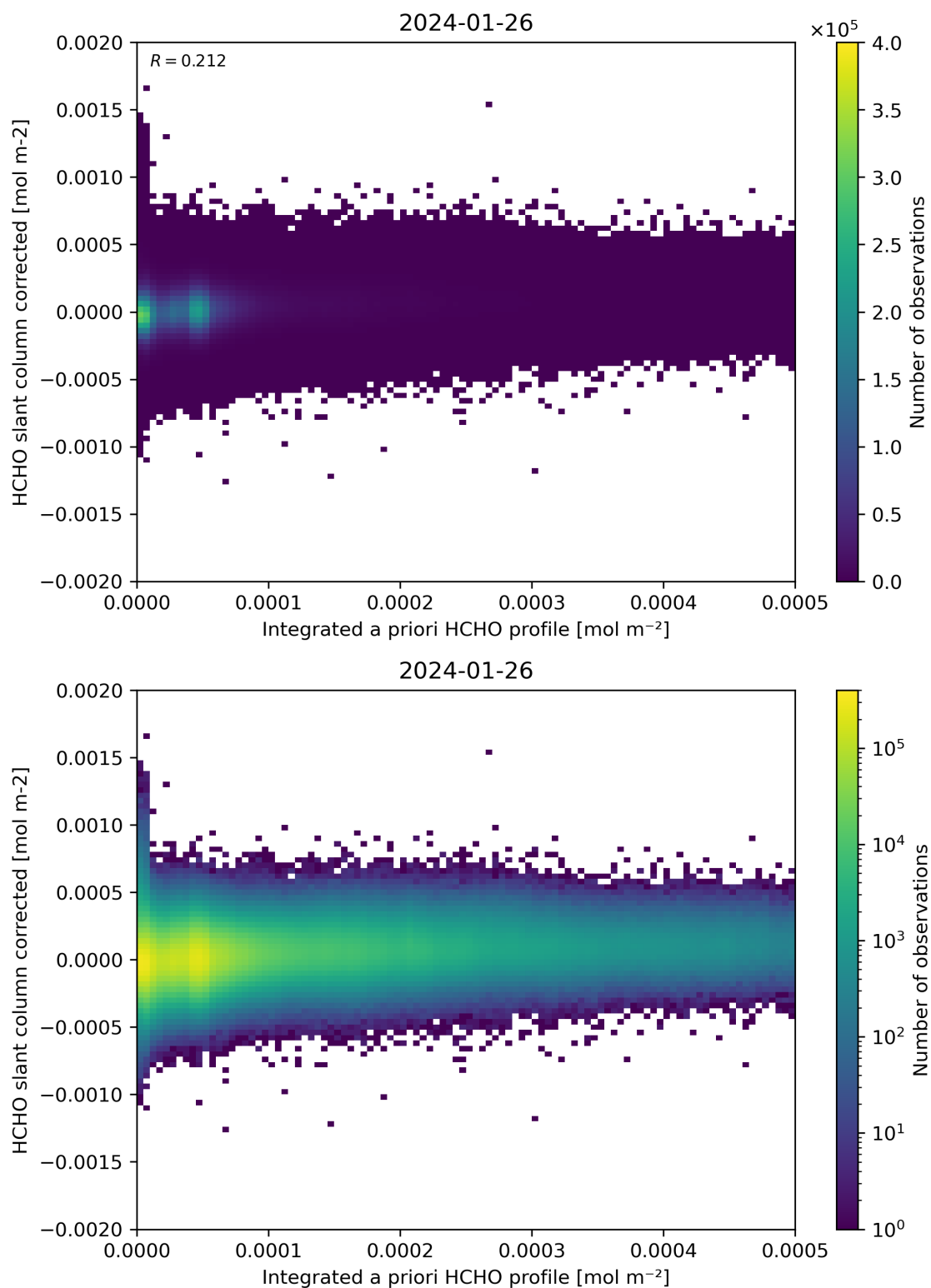
Figure 151: Scatter density plot of “Integrated a priori HCHO profile” against “HCHO slant column corrected” for 2024-01-26 to 2024-01-27.
