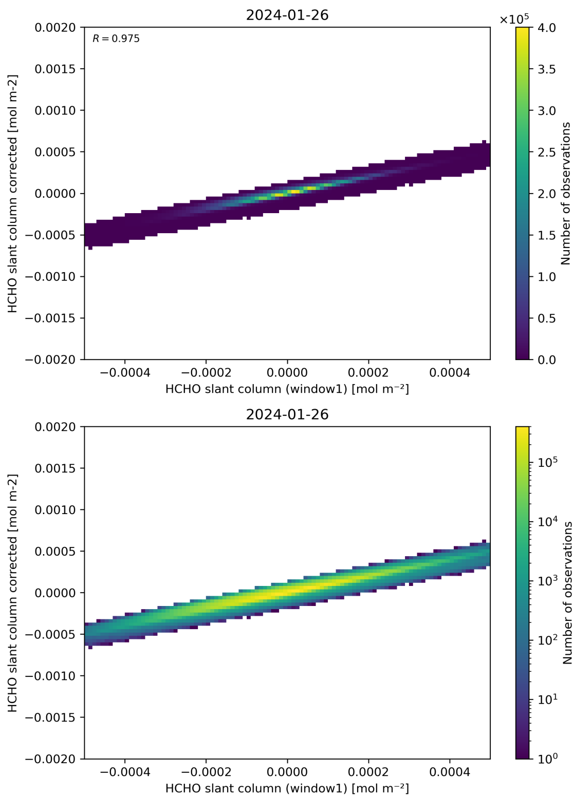
Figure 82: Scatter density plot of “HCHO slant column (window1)” against “HCHO slant column corrected” for 2024-01-26 to 2024-01-27.
