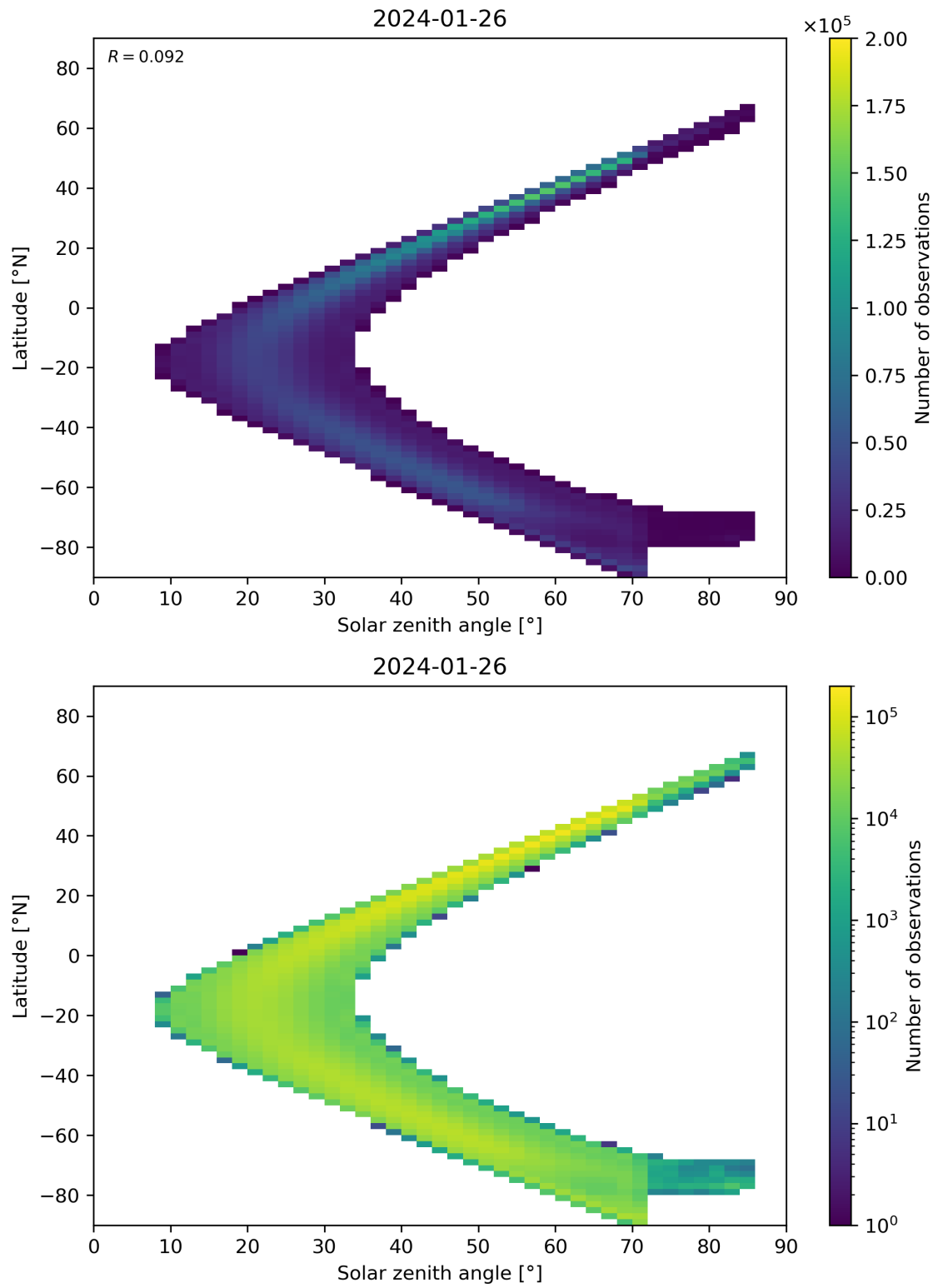
Figure 181: Scatter density plot of “Solar zenith angle” against “Latitude” for 2024-01-26 to 2024-01-27.
