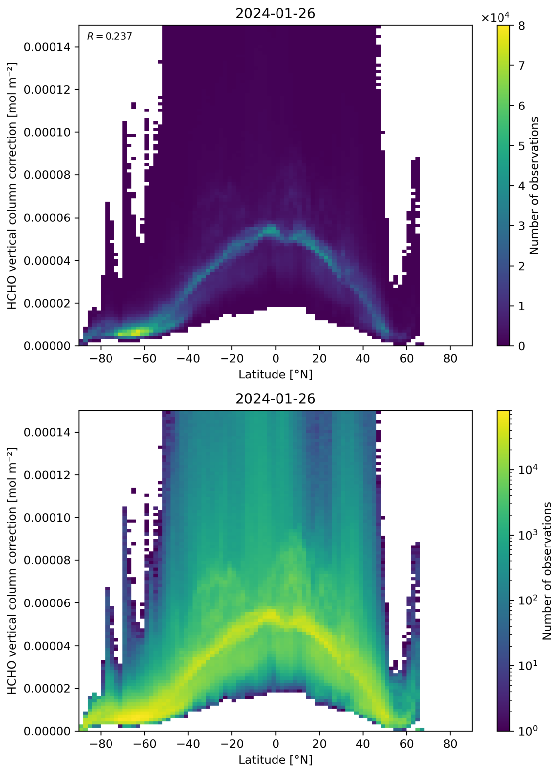
Figure 164: Scatter density plot of “Latitude” against “HCHO vertical column correction” for 2024-01-26 to 2024-01-27.
