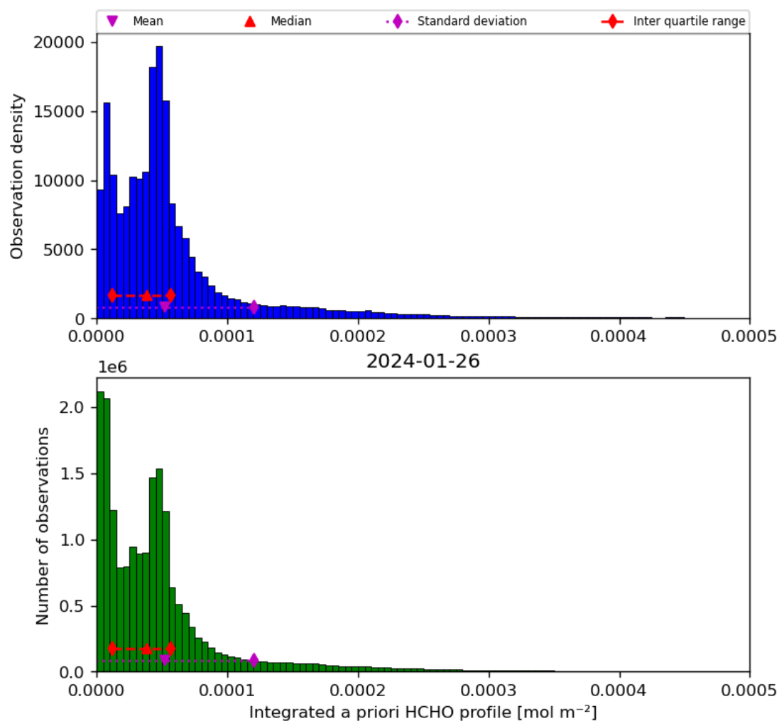
Figure 43: Histogram of “Integrated a priori HCHO profile” for 2024-01-26 to 2024-01-27
