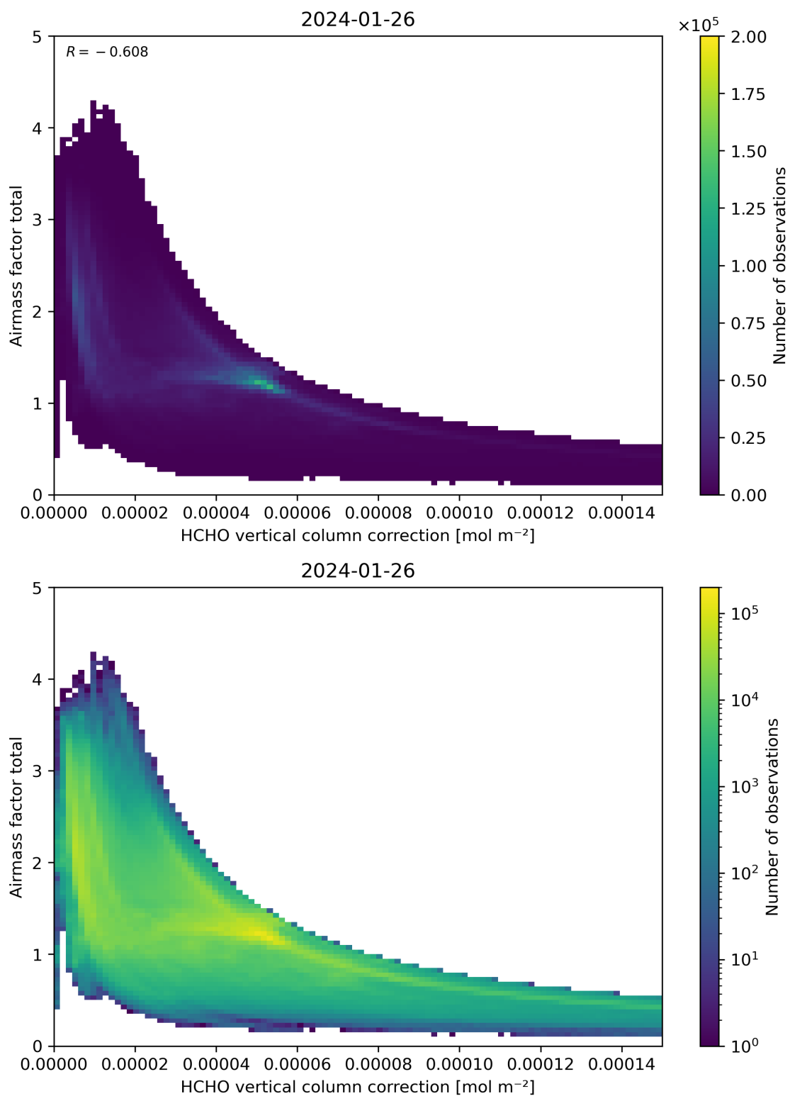
Figure 120: Scatter density plot of “HCHO vertical column correction” against “Airmass factor total” for 2024-01-26 to 2024-01-27.
