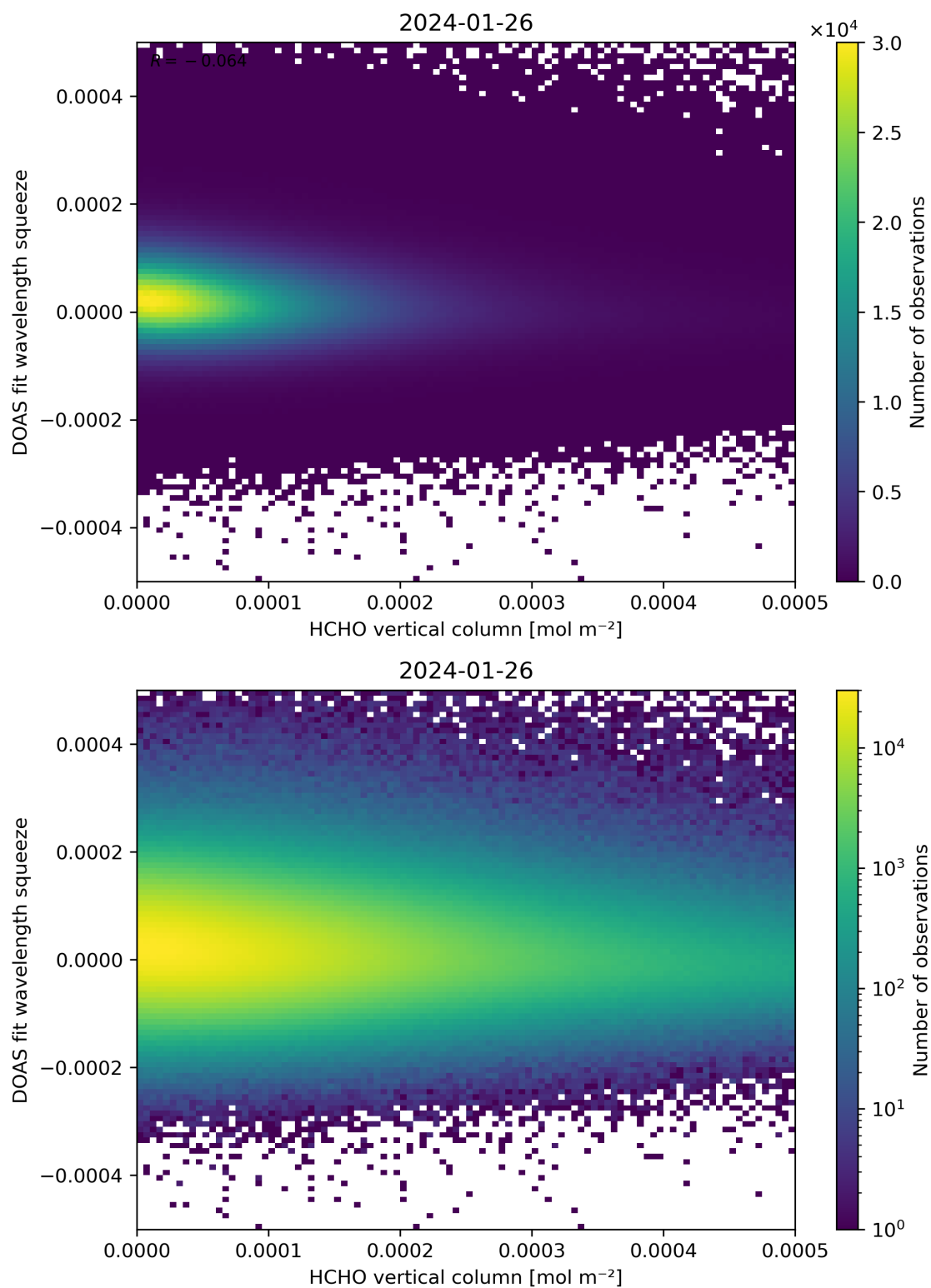
Figure 125: Scatter density plot of “HCHO vertical column” against “DOAS fit wavelength squeeze” for 2024-01-26 to 2024-01-27.
