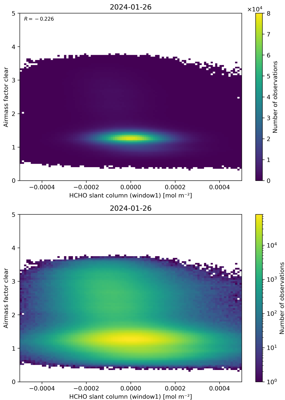
Figure 81: Scatter density plot of “HCHO slant column (window1)” against “Airmass factor clear” for 2024-01-26 to 2024-01-27.
