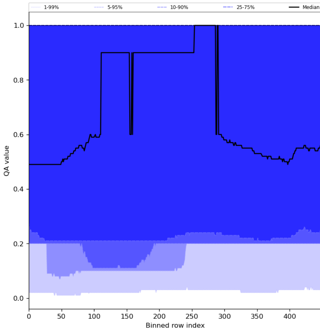
Figure 48: Along track statistics of “QA value” for 2024-01-26 to 2024-01-27
