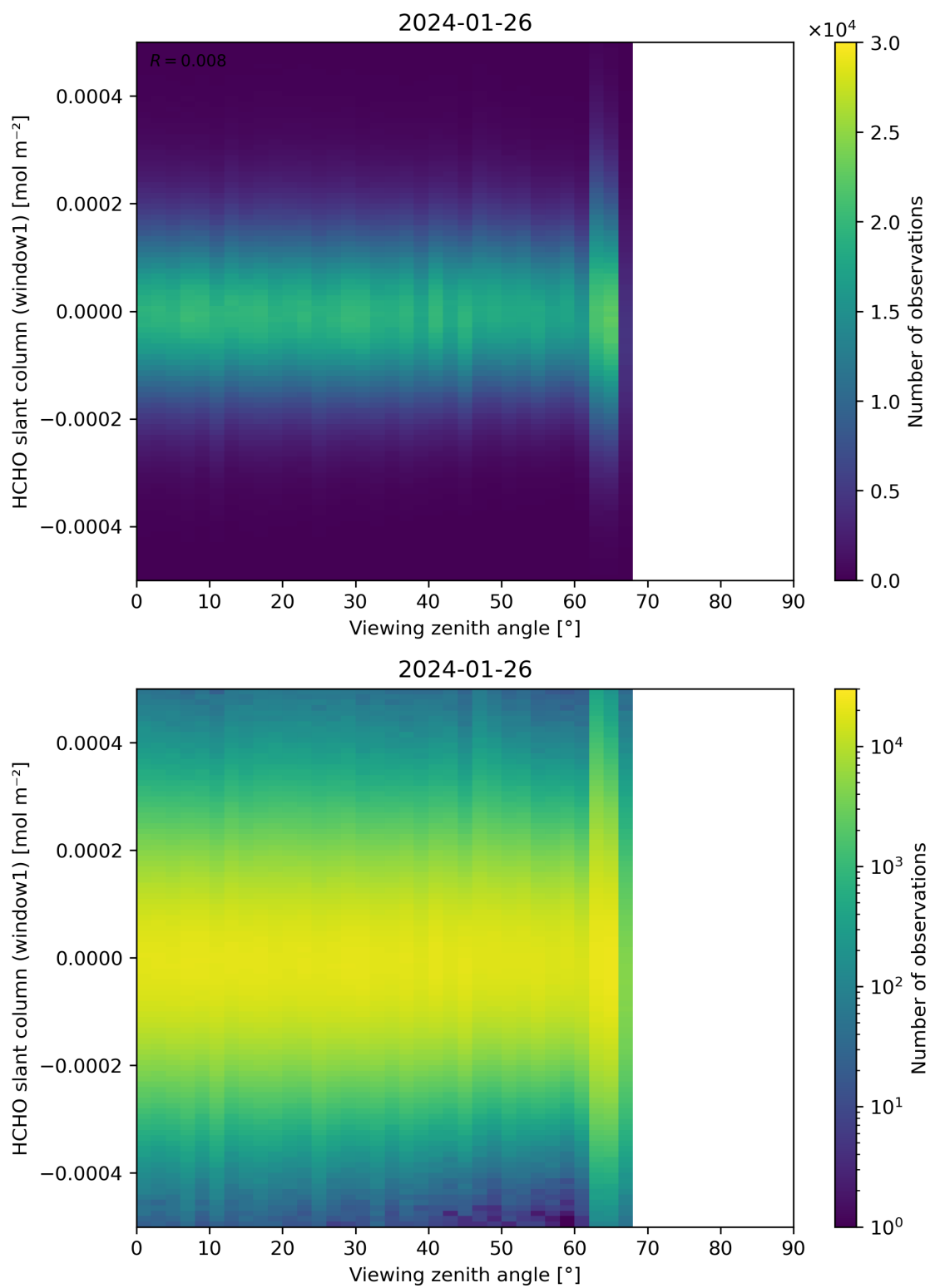
Figure 188: Scatter density plot of “Viewing zenith angle” against “HCHO slant column (window1)” for 2024-01-26 to 2024-01-27.
