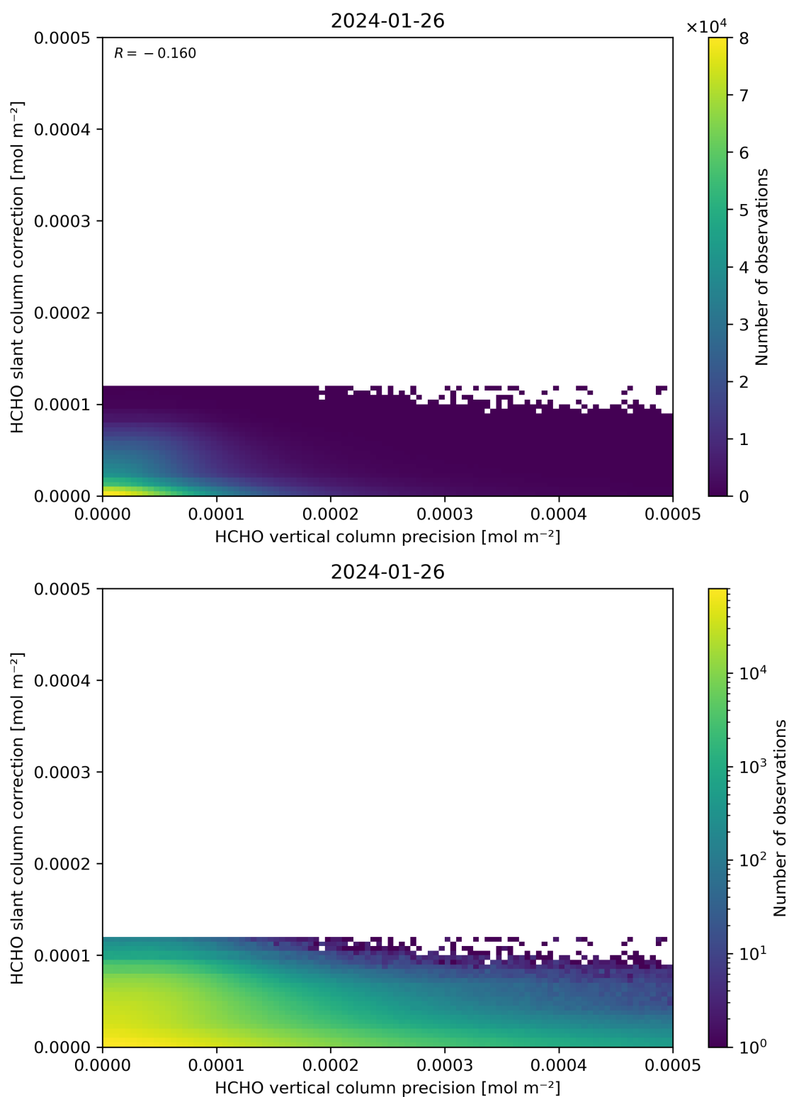
Figure 141: Scatter density plot of “HCHO vertical column precision” against “HCHO slant column correction” for 2024-01-26 to 2024-01-27.
