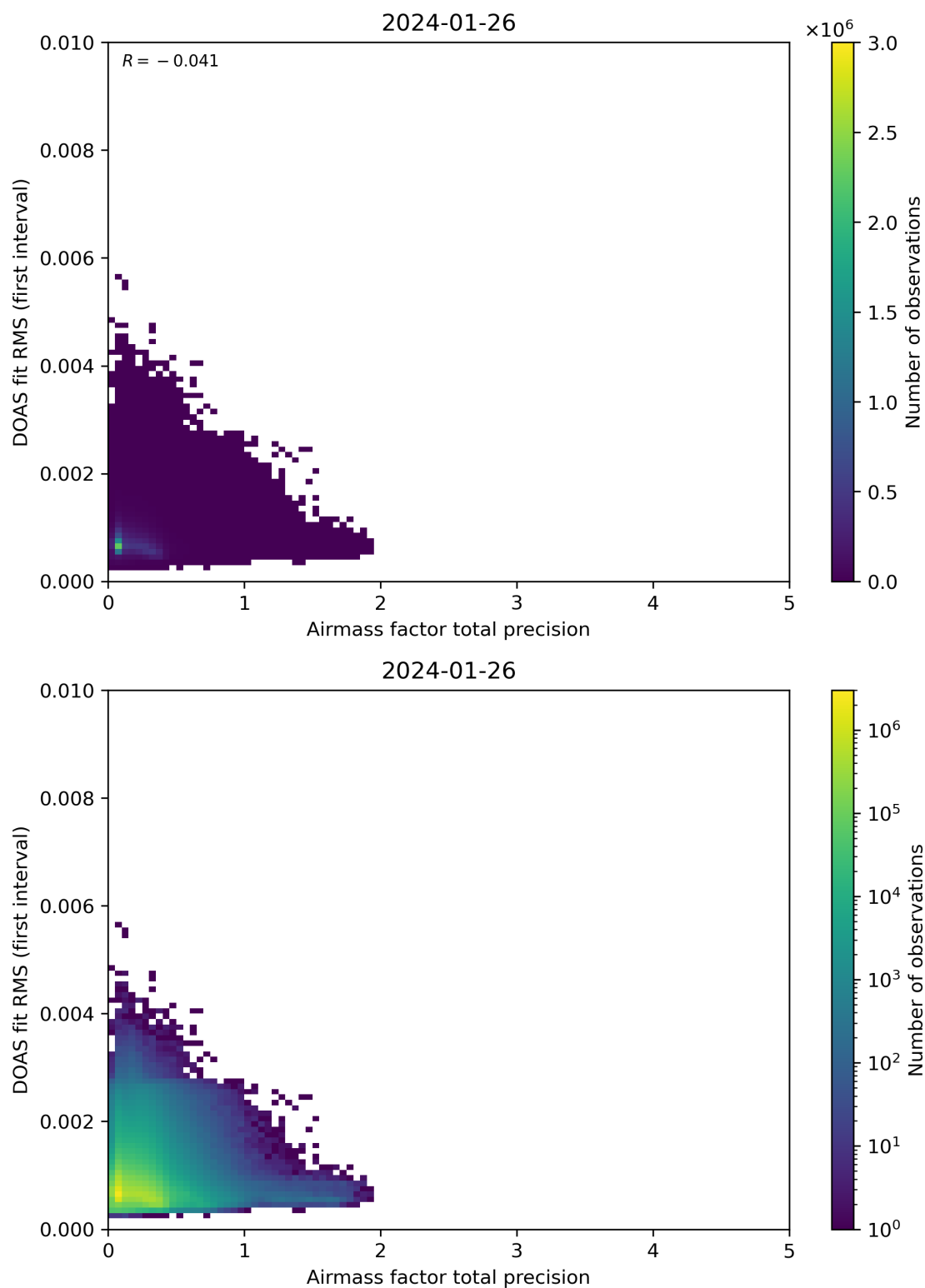
Figure 105: Scatter density plot of “Airmass factor total precision” against “DOAS fit RMS (first interval)” for 2024-01-26 to 2024-01-27.
