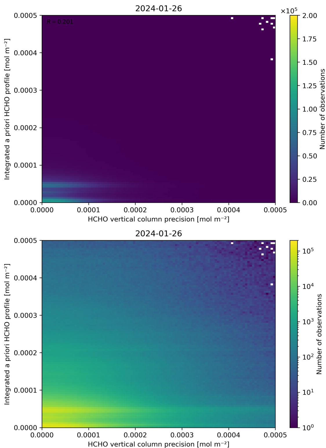
Figure 147: Scatter density plot of “HCHO vertical column precision” against “Integrated a priori HCHO profile” for 2024-01-26 to 2024-01-27.
