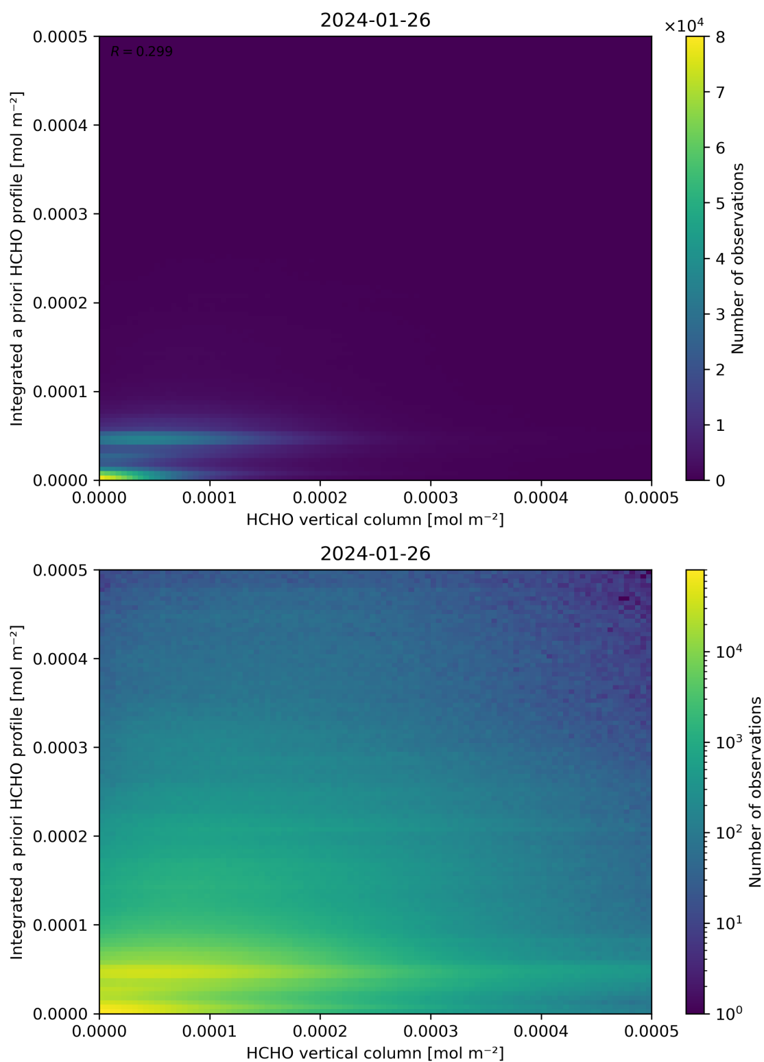
Figure 135: Scatter density plot of “HCHO vertical column” against “Integrated a priori HCHO profile” for 2024-01-26 to 2024-01-27.
