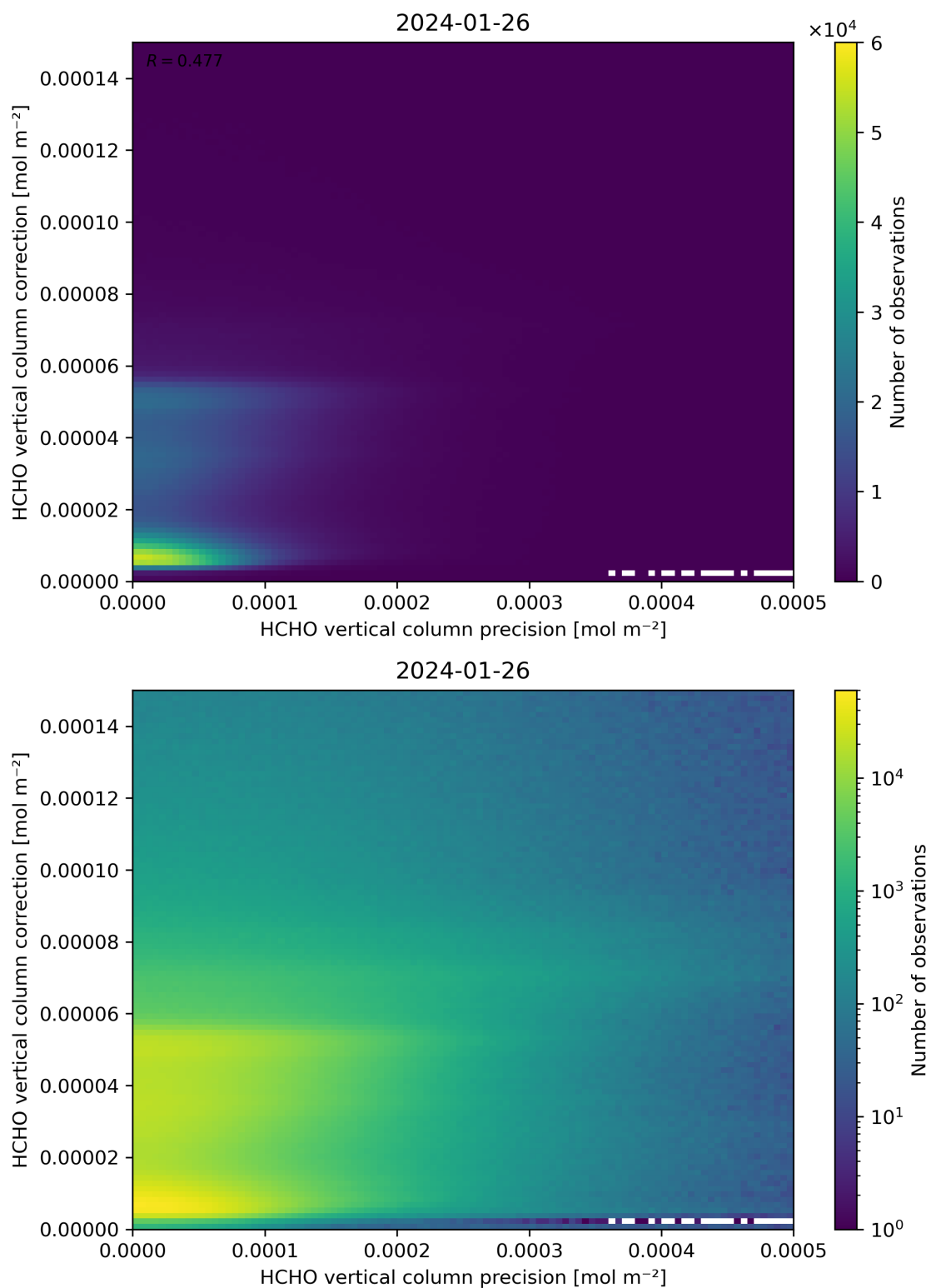
Figure 146: Scatter density plot of “HCHO vertical column precision” against “HCHO vertical column correction” for 2024-01-26 to 2024-01-27.
