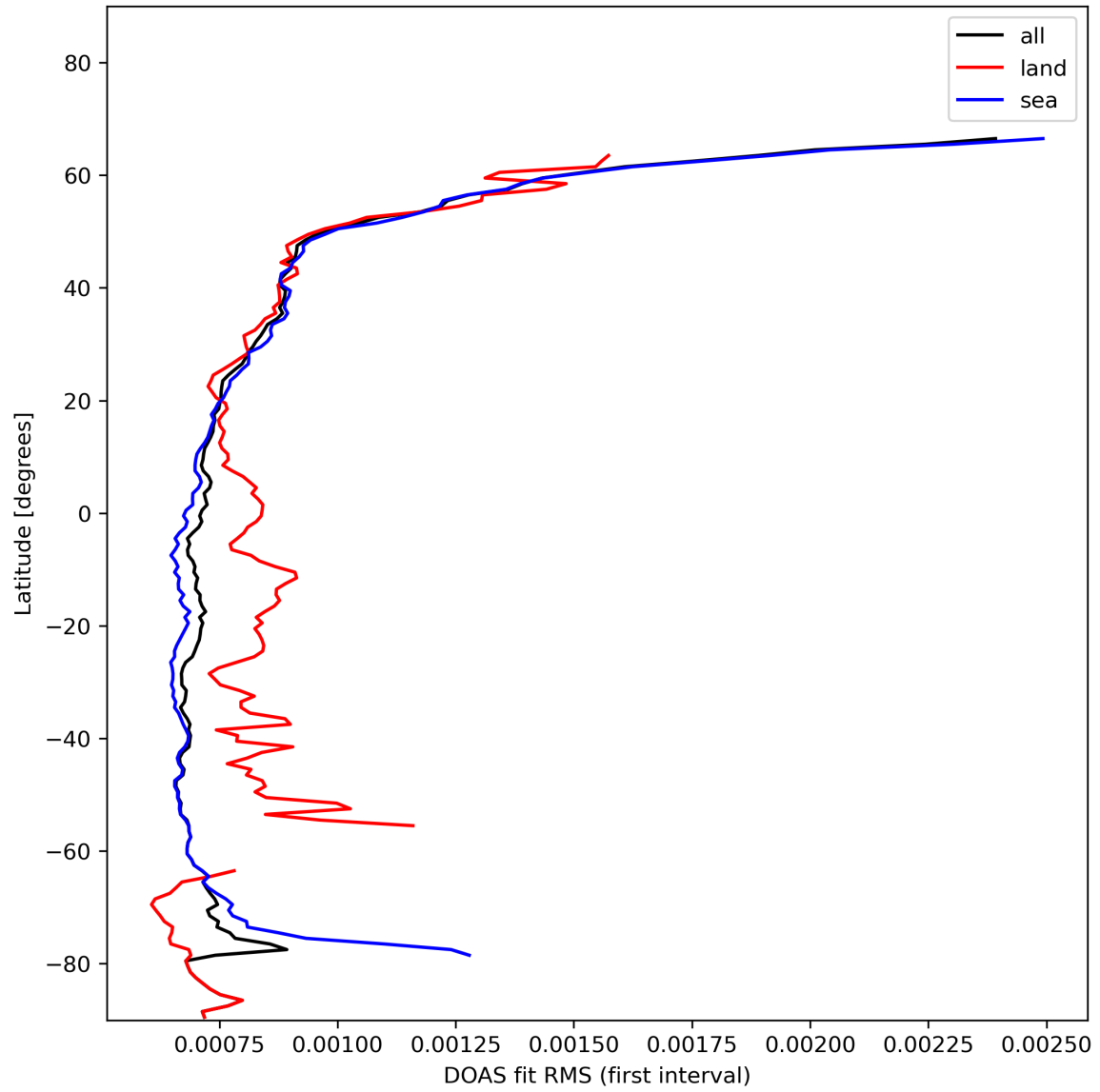
Figure 32: Zonal average of “DOAS fit RMS (first interval)” for 2024-01-26 to 2024-01-27.
