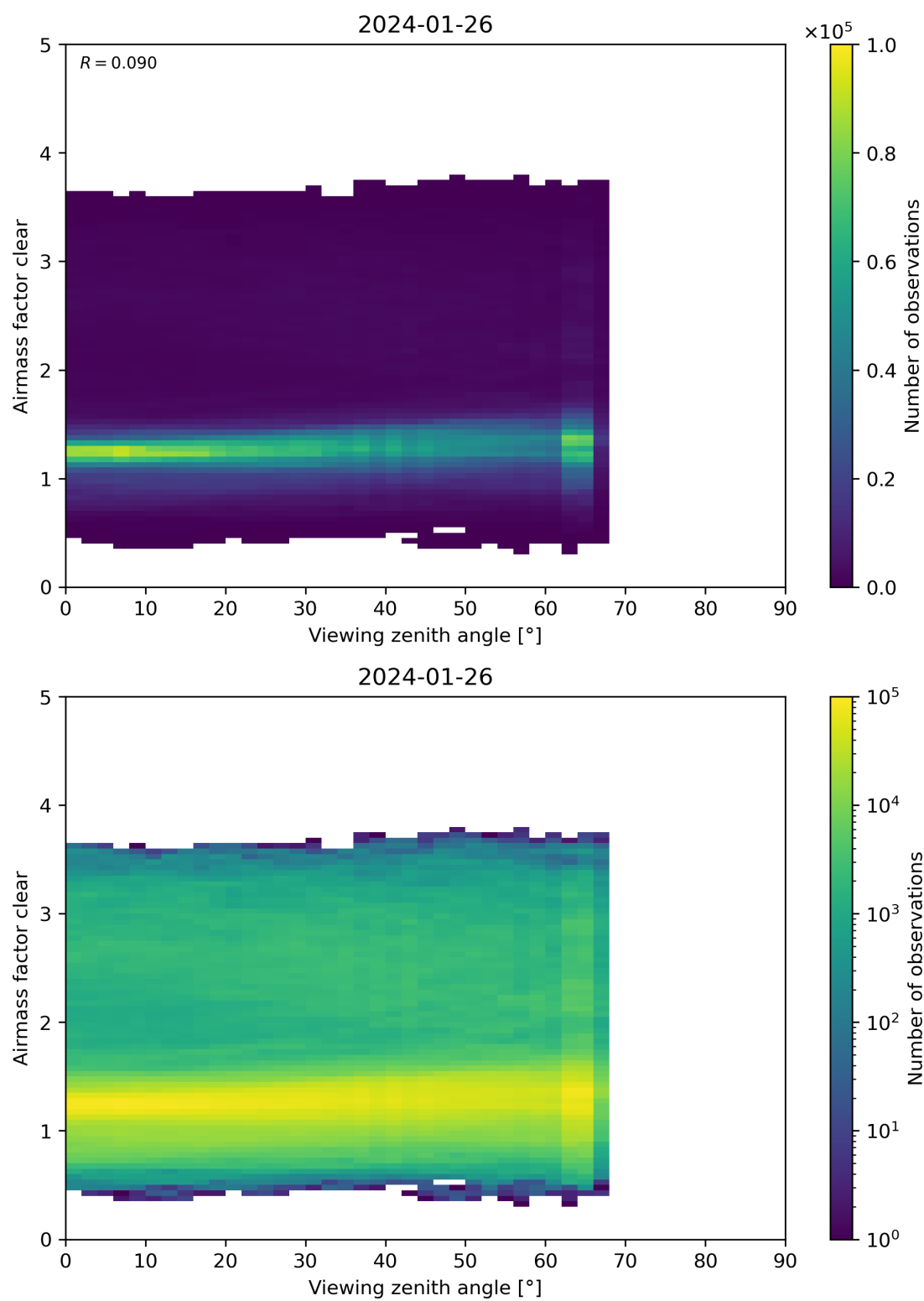
Figure 185: Scatter density plot of “Viewing zenith angle” against “Airmass factor clear” for 2024-01-26 to 2024-01-27.
