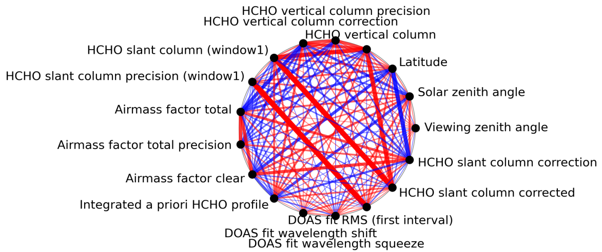
Figure 1: Map of correlation graph for 2024-01-26 to 2024-01-27.
