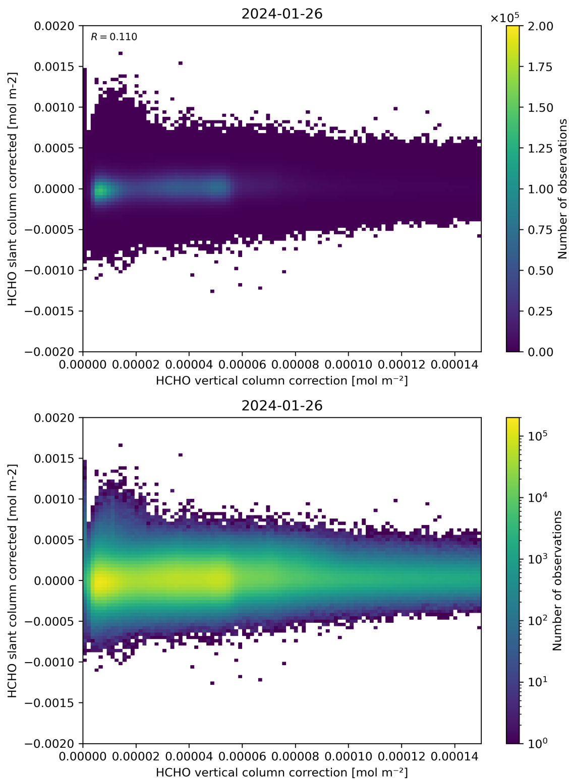
Figure 116: Scatter density plot of “HCHO vertical column correction” against “HCHO slant column corrected” for 2024-01-26 to 2024-01-27.
