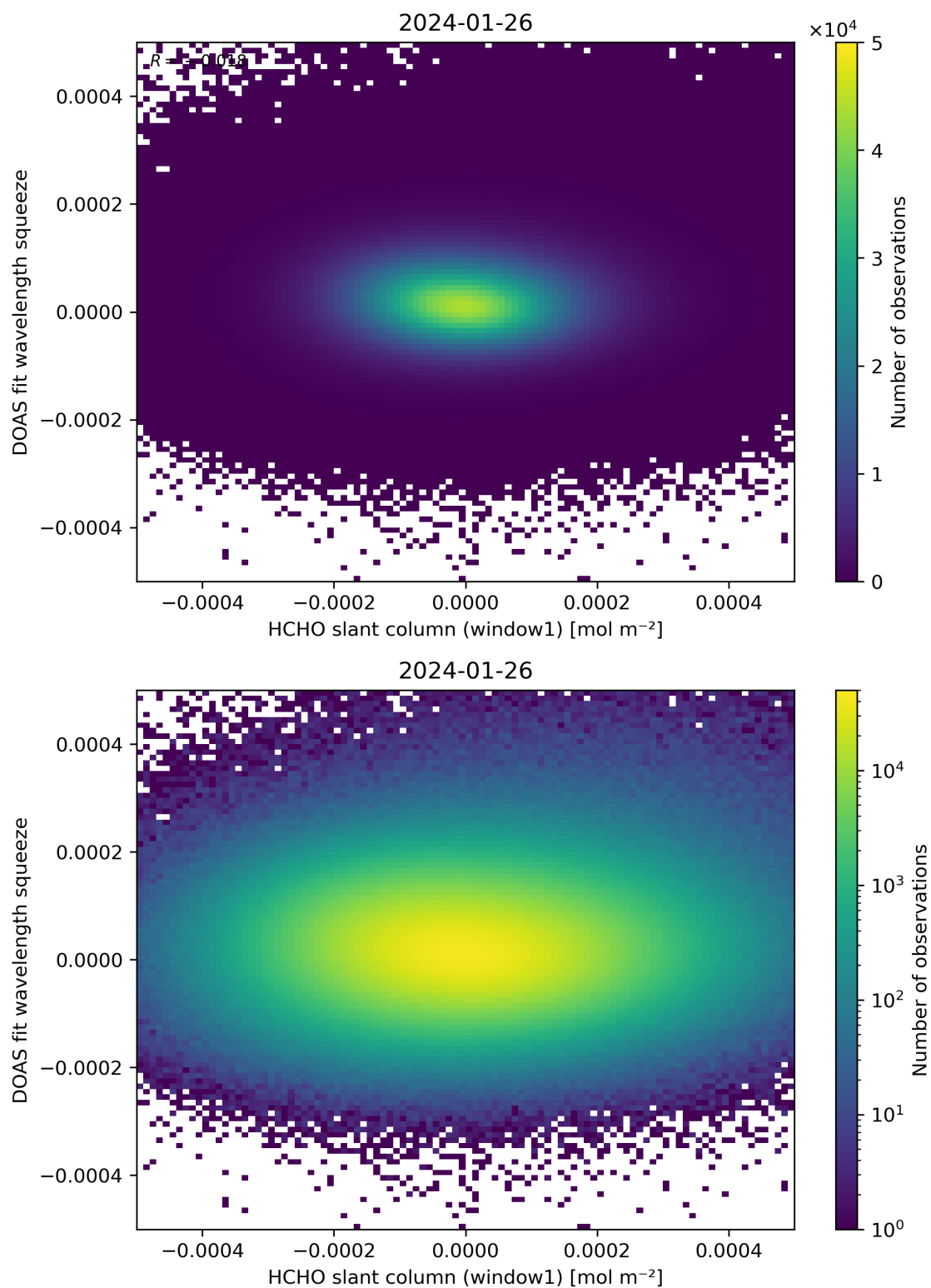
Figure 80: Scatter density plot of “HCHO slant column (window1)” against “DOAS fit wavelength squeeze” for 2024-01-26 to 2024-01-27.
