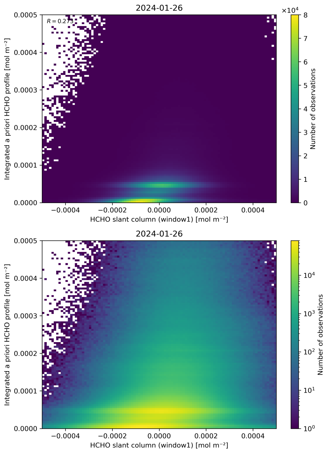
Figure 87: Scatter density plot of “HCHO slant column (window1)” against “Integrated a priori HCHO profile” for 2024-01-26 to 2024-01-27.
