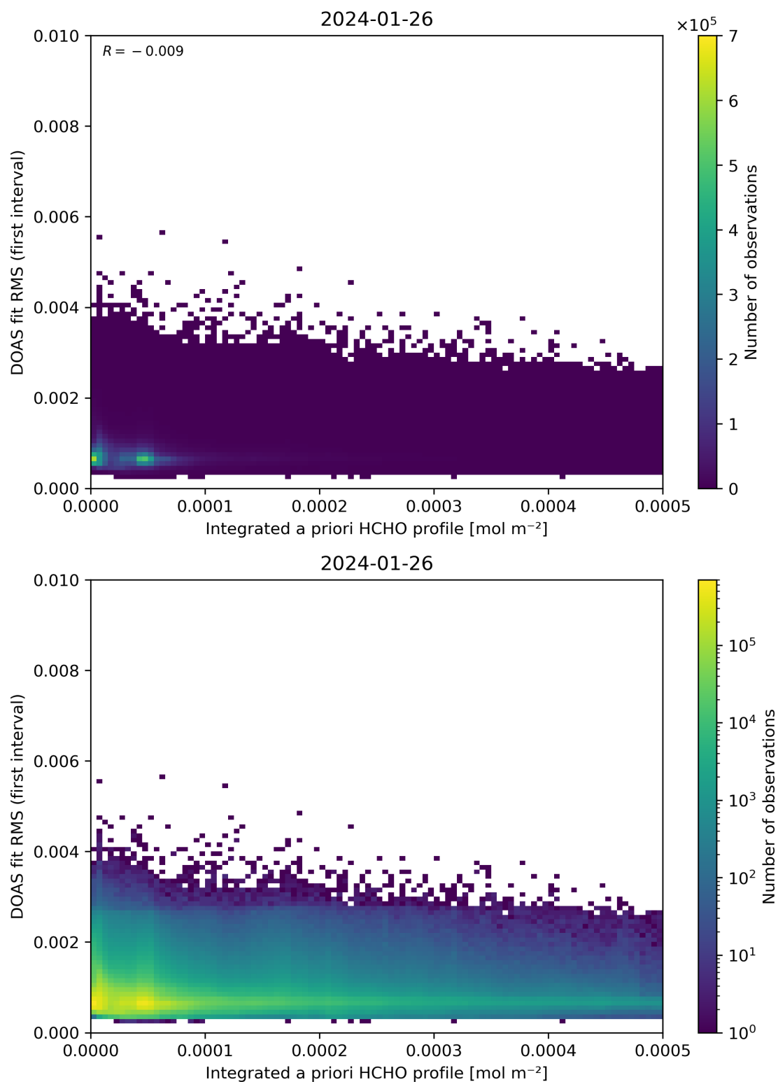
Figure 148: Scatter density plot of “Integrated a priori HCHO profile” against “DOAS fit RMS (first interval)” for 2024-01-26 to 2024-01-27.
