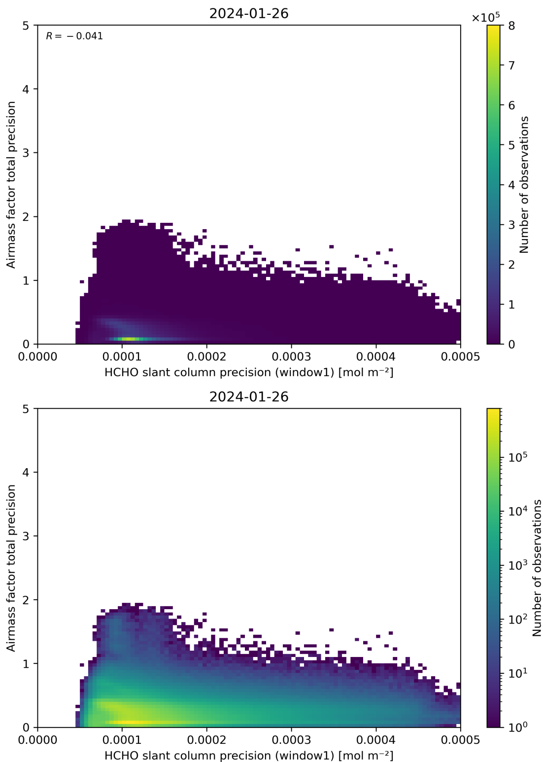
Figure 95: Scatter density plot of “HCHO slant column precision (window1)” against “Airmass factor total precision” for 2024-01-26 to 2024-01-27.
