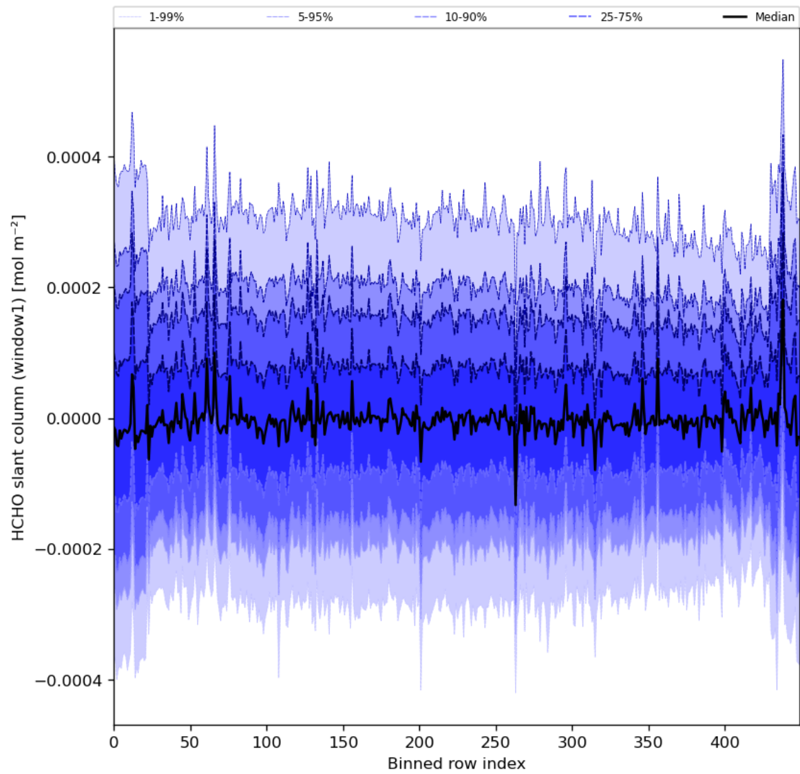
Figure 52: Along track statistics of “HCHO slant column (window1)” for 2024-01-26 to 2024-01-27
