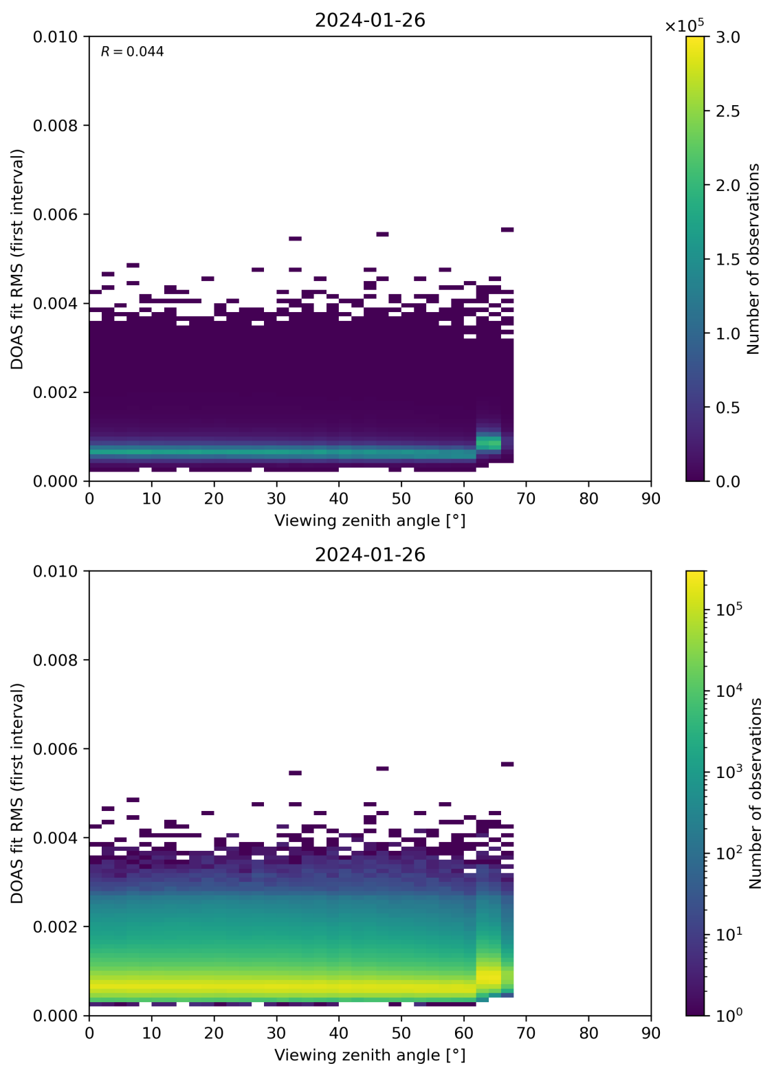
Figure 182: Scatter density plot of “Viewing zenith angle” against “DOAS fit RMS (first interval)” for 2024-01-26 to 2024-01-27.
