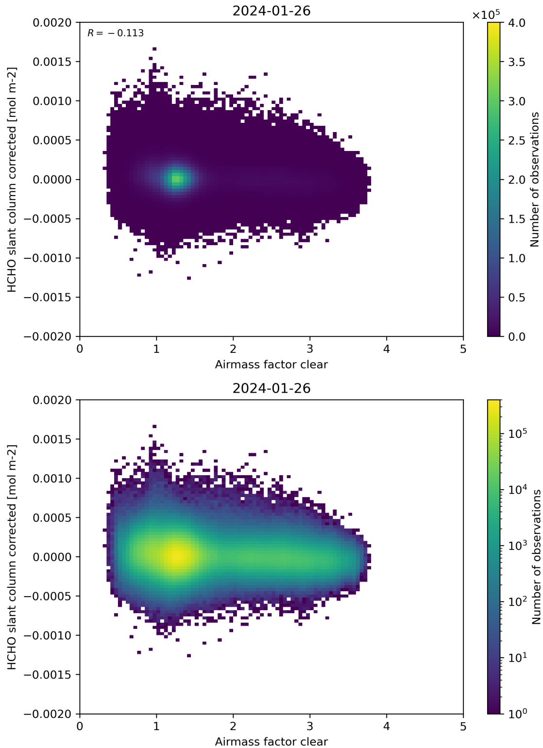
Figure 74: Scatter density plot of “Airmass factor clear” against “HCHO slant column corrected” for 2024-01-26 to 2024-01-27.
