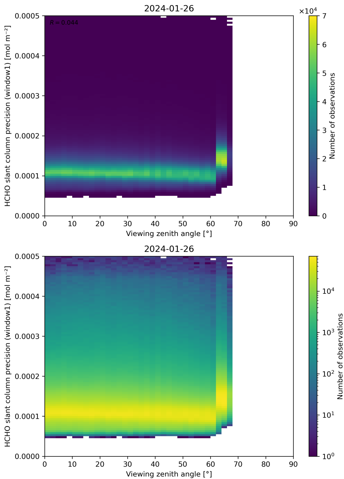
Figure 189: Scatter density plot of “Viewing zenith angle” against “HCHO slant column precision (window1)” for 2024-01-26 to 2024-01-27.
