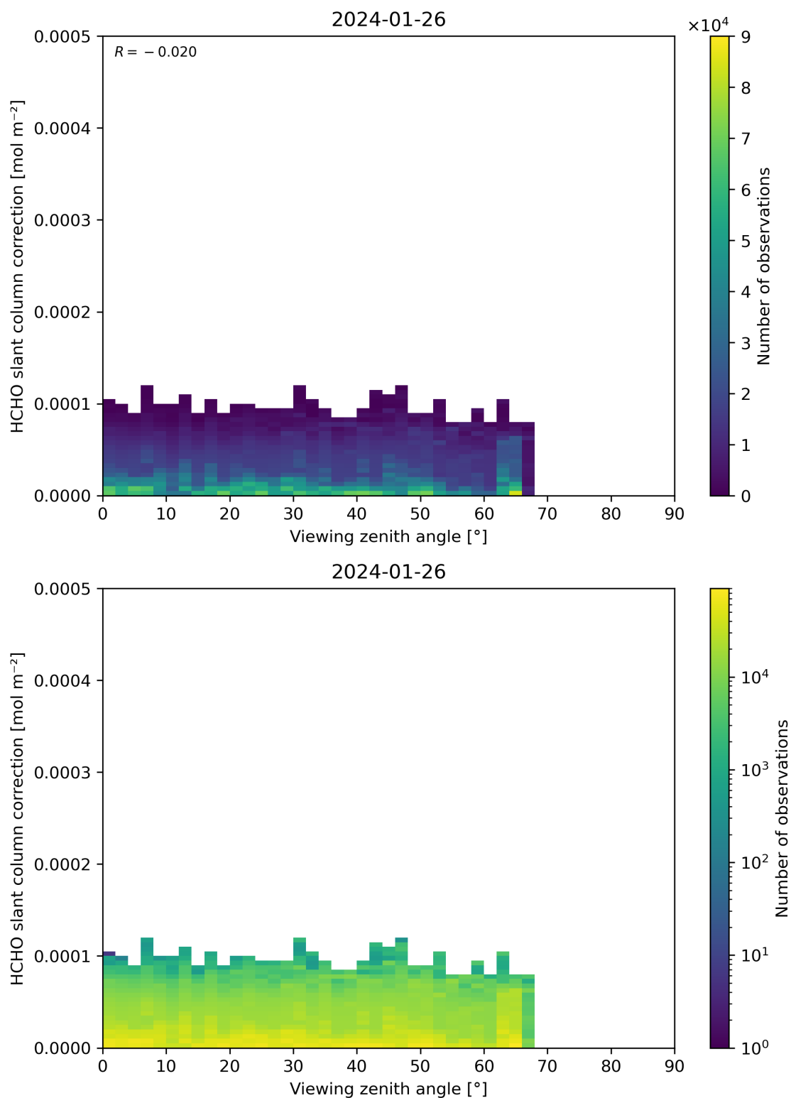
Figure 187: Scatter density plot of “Viewing zenith angle” against “HCHO slant column correction” for 2024-01-26 to 2024-01-27.
