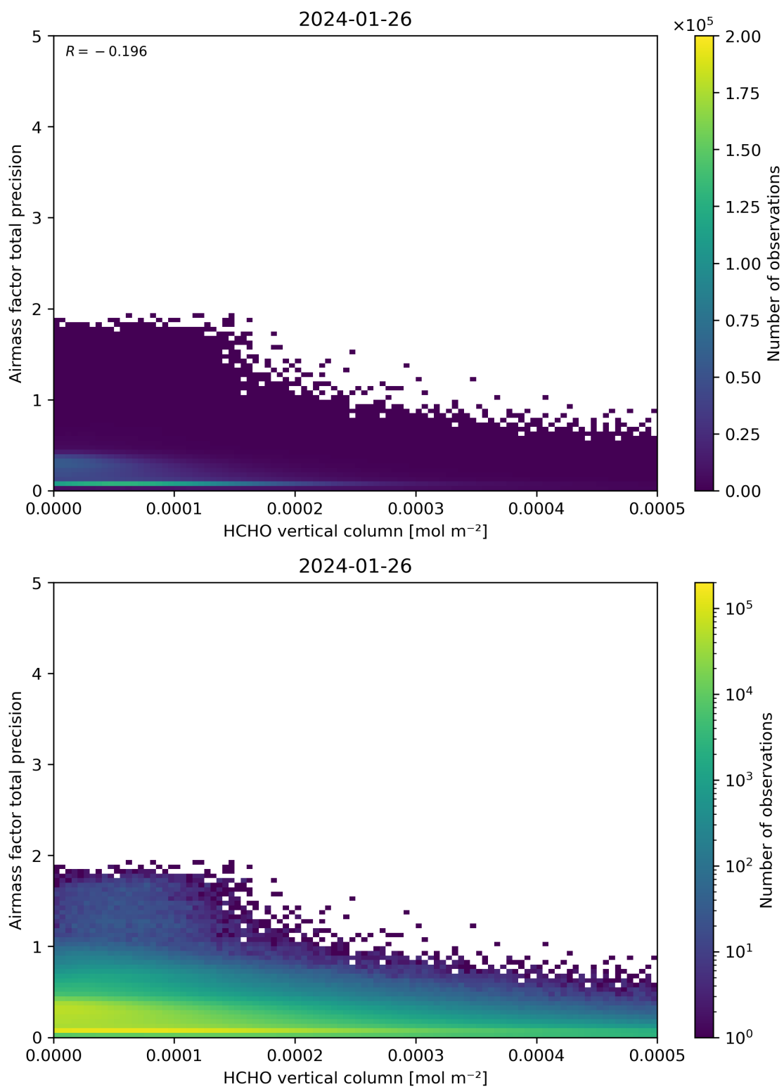
Figure 132: Scatter density plot of “HCHO vertical column” against “Airmass factor total precision” for 2024-01-26 to 2024-01-27.
