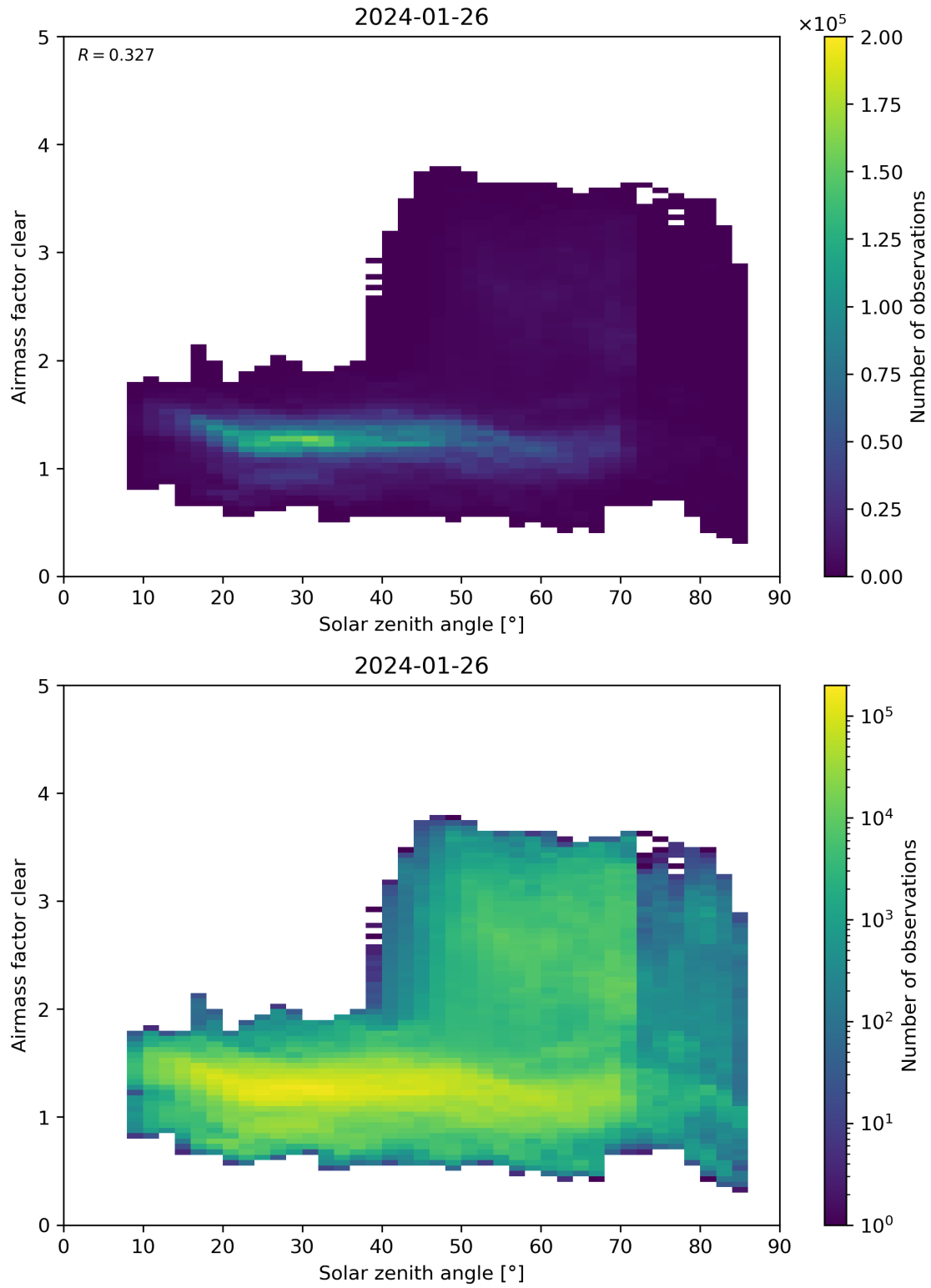
Figure 170: Scatter density plot of “Solar zenith angle” against “Airmass factor clear” for 2024-01-26 to 2024-01-27.
