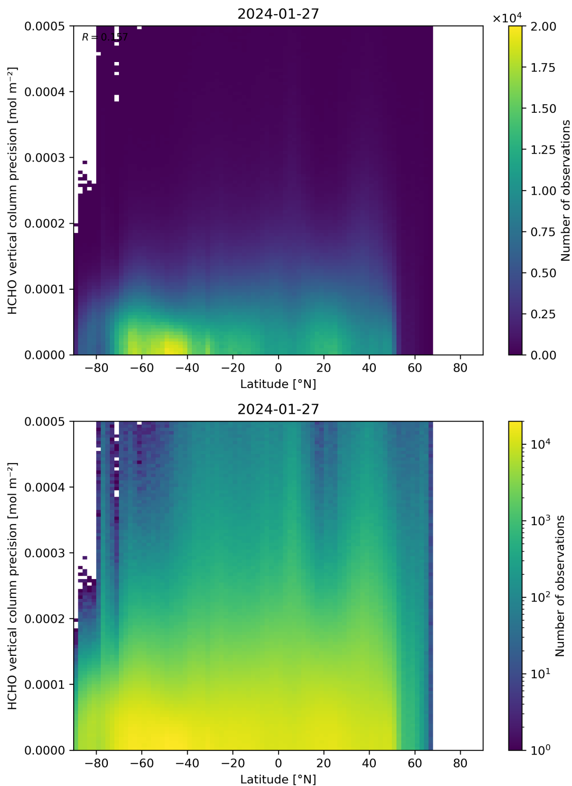
Figure 165: Scatter density plot of “Latitude” against “HCHO vertical column precision” for 2024-01-26 to 2024-01-28.
