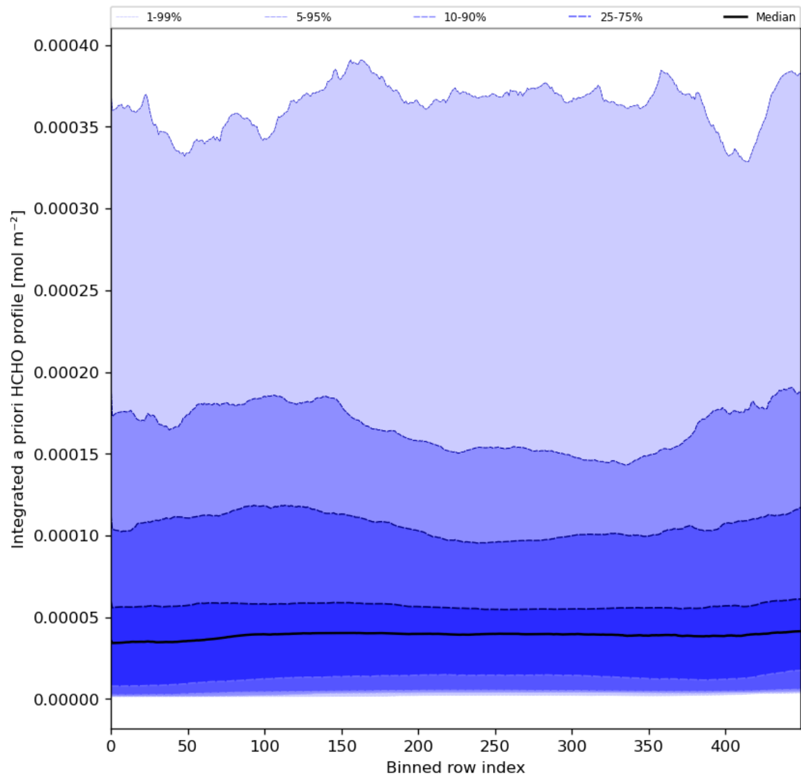
Figure 57: Along track statistics of “Integrated a priori HCHO profile” for 2024-01-26 to 2024-01-28
