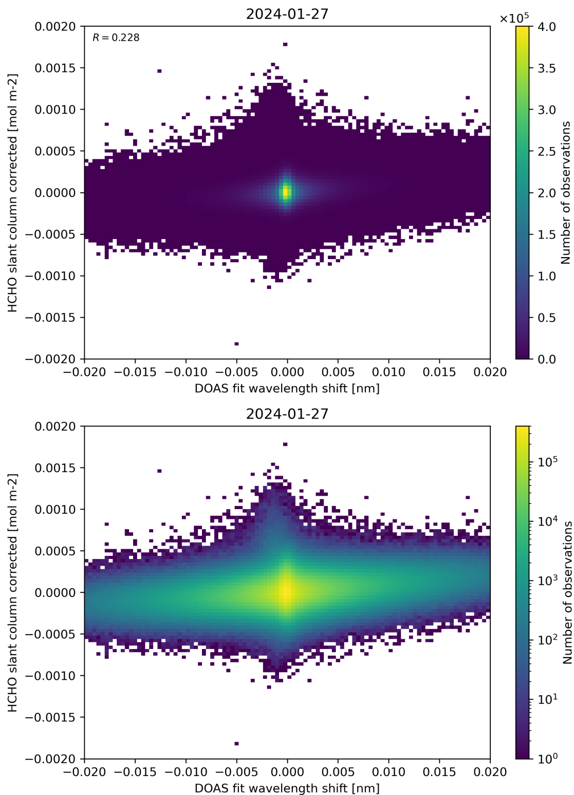
Figure 66: Scatter density plot of “DOAS fit wavelength shift” against “HCHO slant column corrected” for 2024-01-26 to 2024-01-28.
