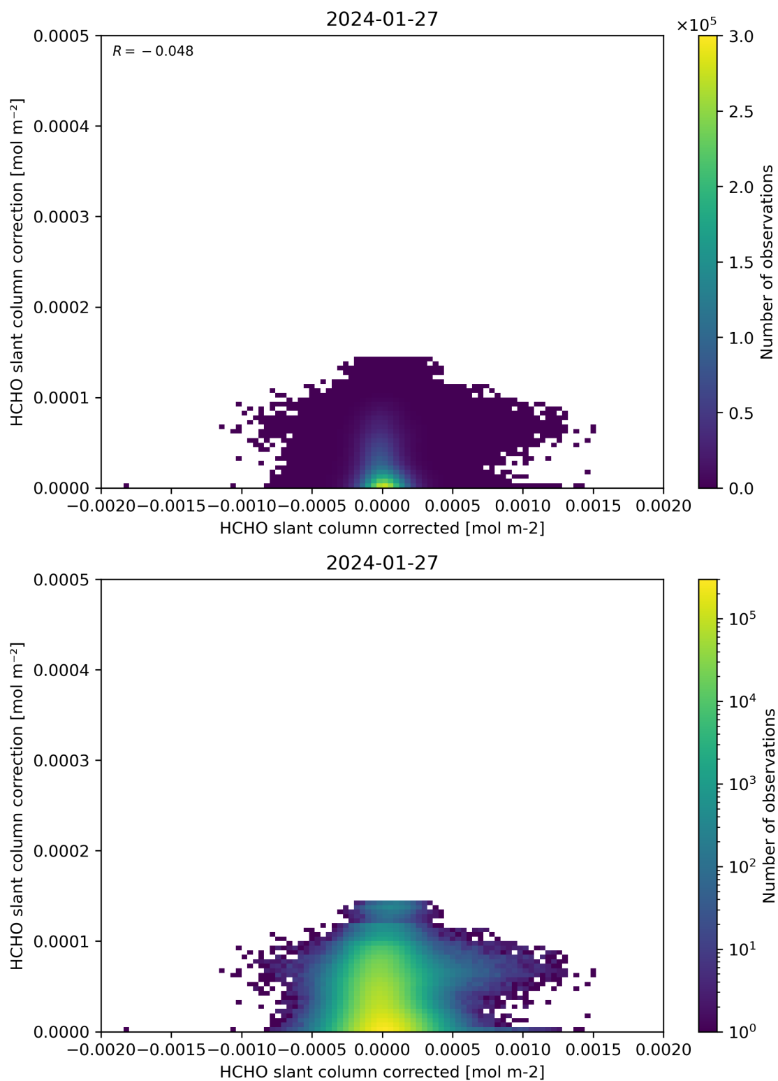
Figure 77: Scatter density plot of “HCHO slant column corrected” against “HCHO slant column correction” for 2024-01-26 to 2024-01-28.
