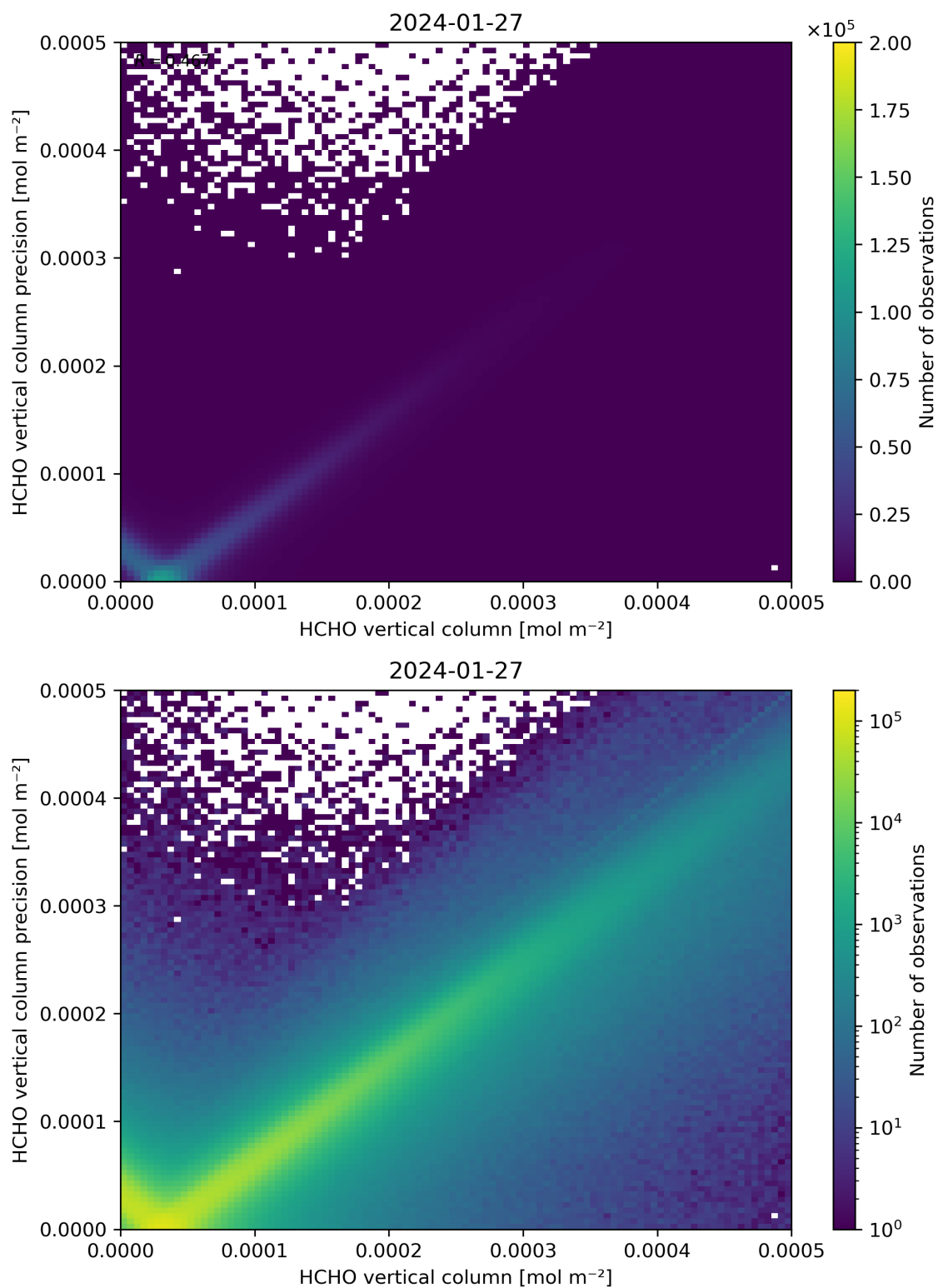
Figure 134: Scatter density plot of “HCHO vertical column” against “HCHO vertical column precision” for 2024-01-26 to 2024-01-28.
