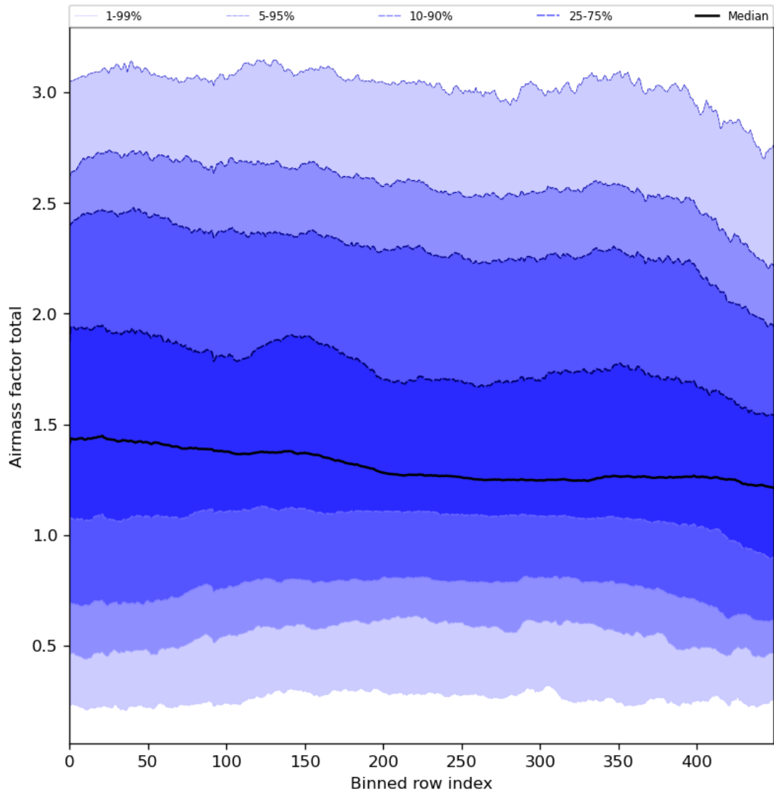
Figure 54: Along track statistics of “Airmass factor total” for 2024-01-26 to 2024-01-28
