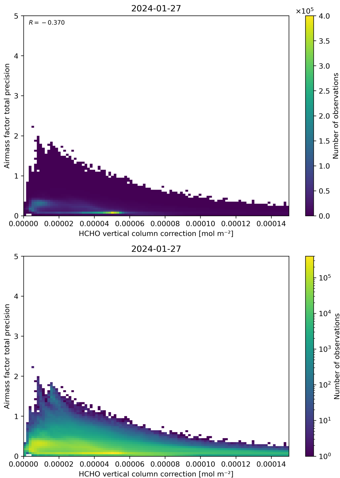
Figure 121: Scatter density plot of “HCHO vertical column correction” against “Airmass factor total precision” for 2024-01-26 to 2024-01-28.
