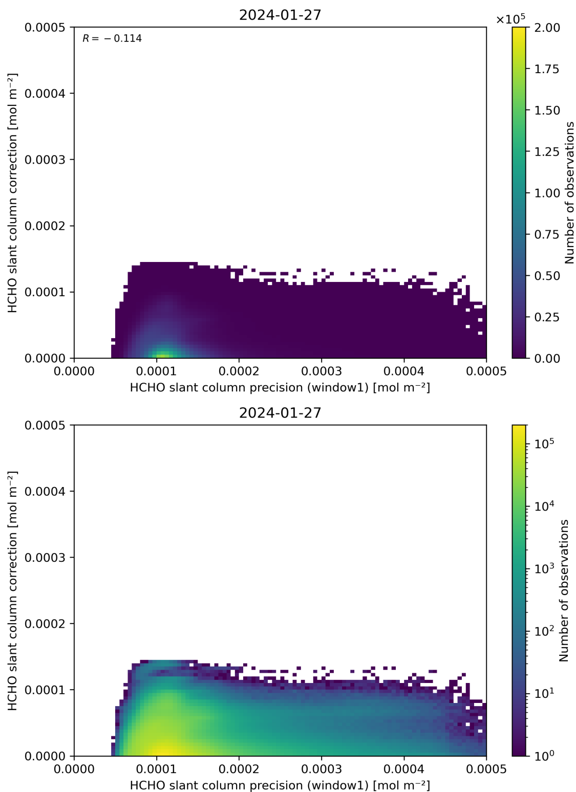
Figure 93: Scatter density plot of “HCHO slant column precision (window1)” against “HCHO slant column correction” for 2024-01-26 to 2024-01-28.
