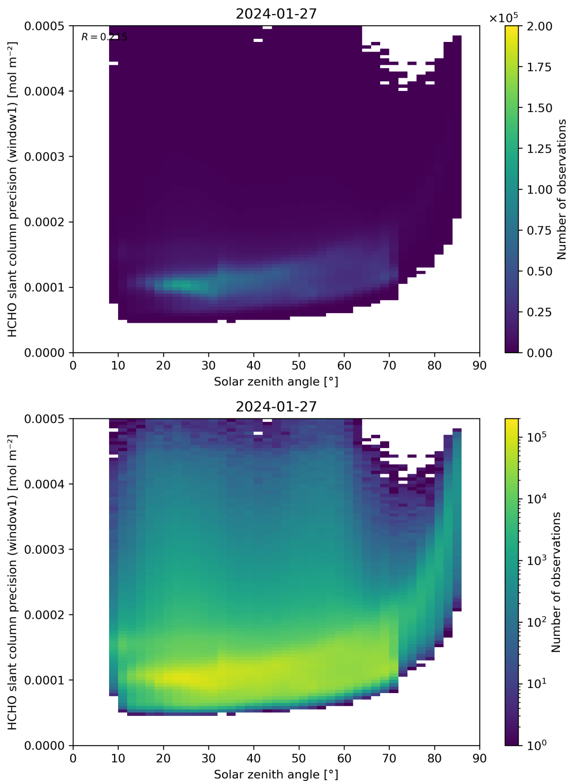
Figure 174: Scatter density plot of “Solar zenith angle” against “HCHO slant column precision (window1)” for 2024-01-26 to 2024-01-28.
