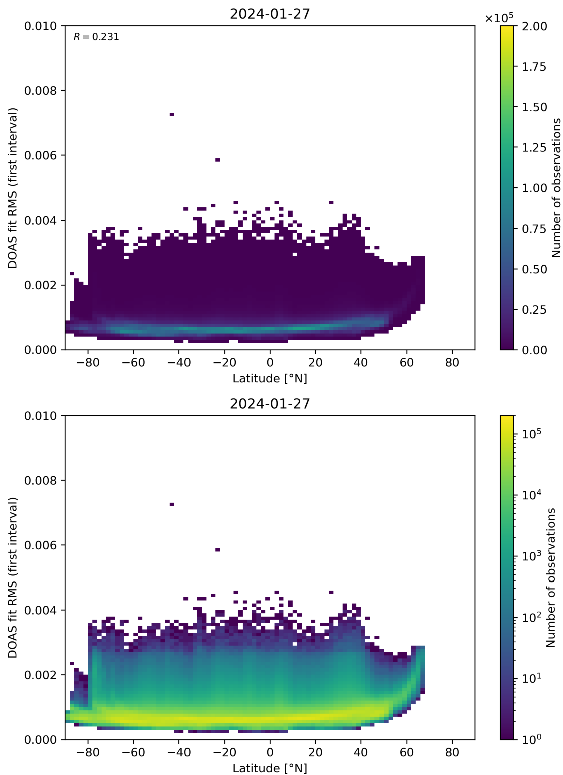
Figure 153: Scatter density plot of “Latitude” against “DOAS fit RMS (first interval)” for 2024-01-26 to 2024-01-28.
