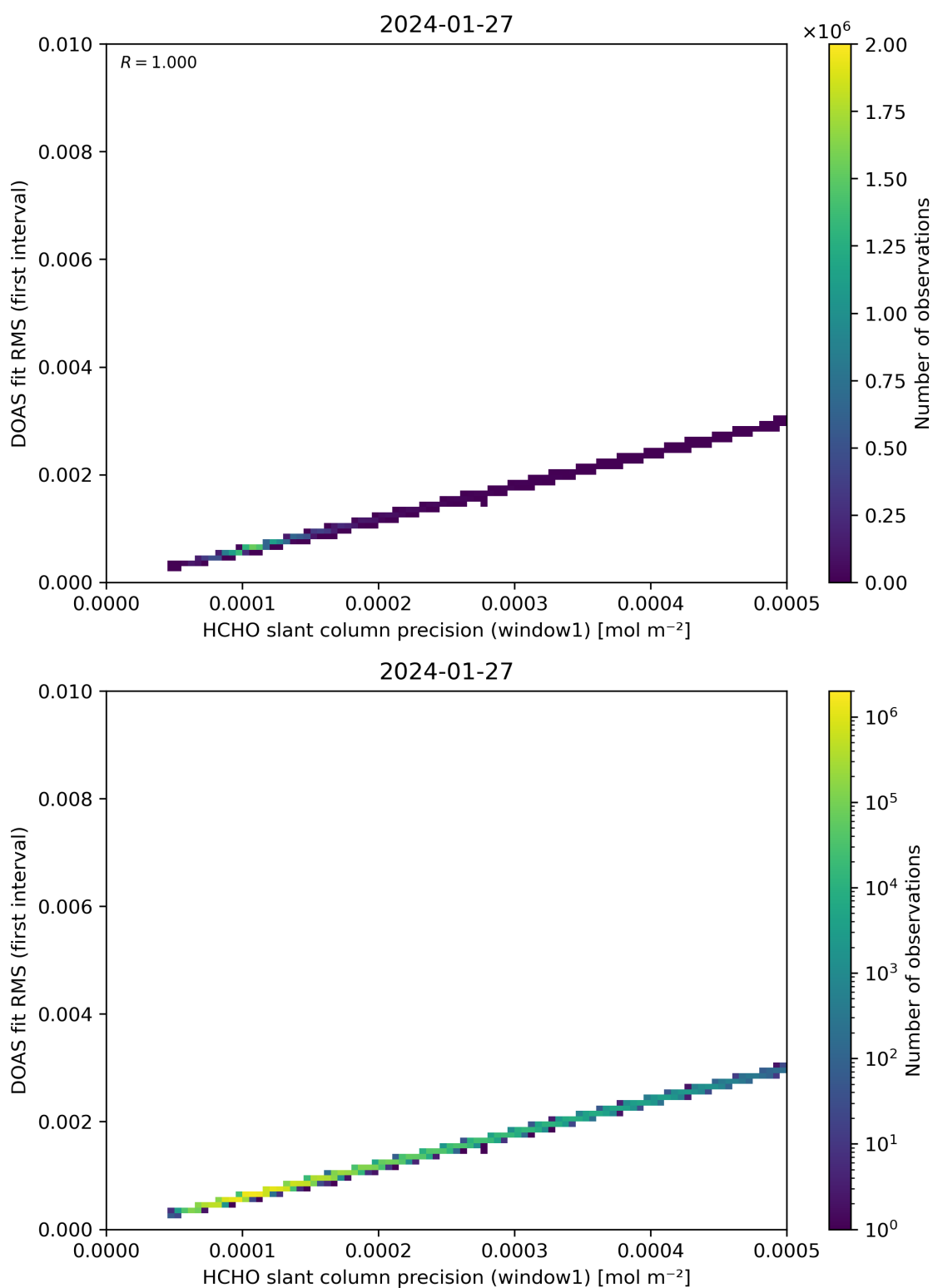
Figure 88: Scatter density plot of “HCHO slant column precision (window1)” against “DOAS fit RMS (first interval)” for 2024-01-26 to 2024-01-28.
