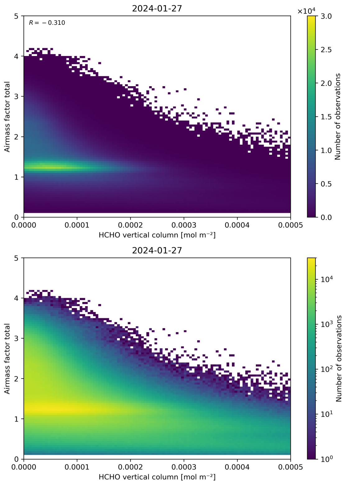
Figure 131: Scatter density plot of “HCHO vertical column” against “Airmass factor total” for 2024-01-26 to 2024-01-28.
