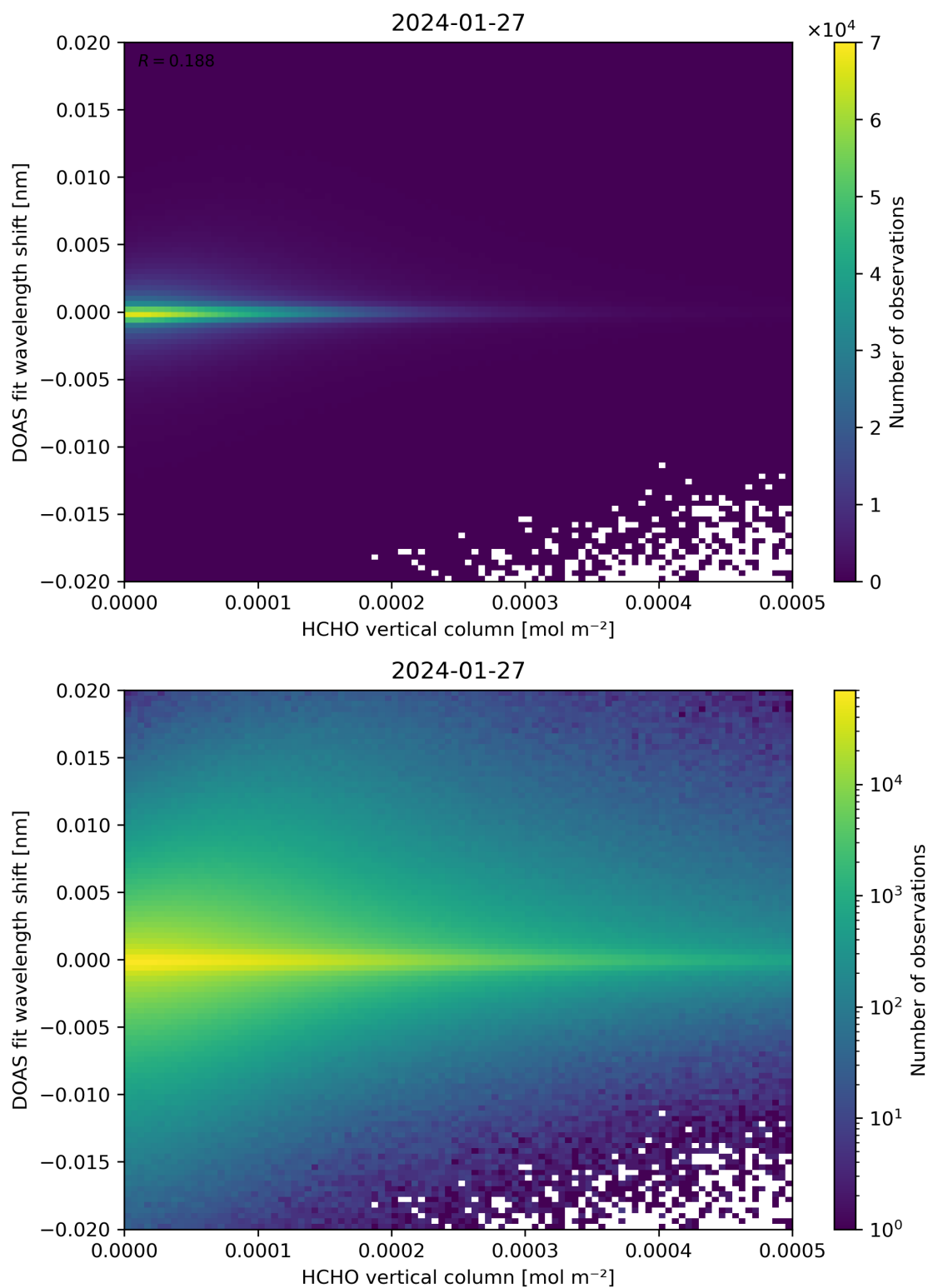
Figure 124: Scatter density plot of “HCHO vertical column” against “DOAS fit wavelength shift” for 2024-01-26 to 2024-01-28.
