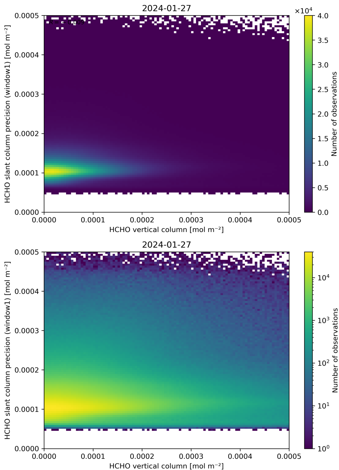
Figure 130: Scatter density plot of “HCHO vertical column” against “HCHO slant column precision (window1)” for 2024-01-26 to 2024-01-28.
