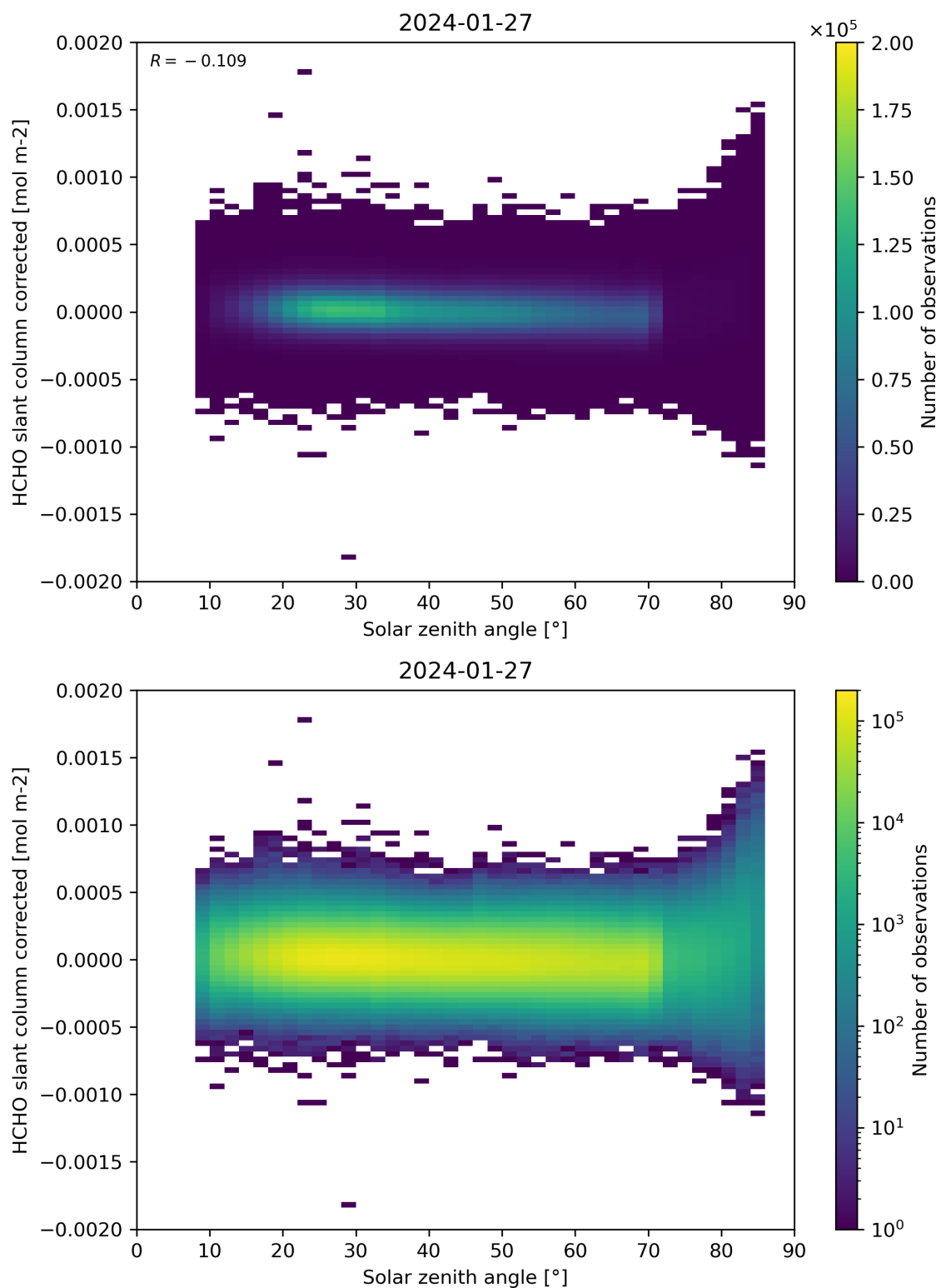
Figure 171: Scatter density plot of “Solar zenith angle” against “HCHO slant column corrected” for 2024-01-26 to 2024-01-28.
