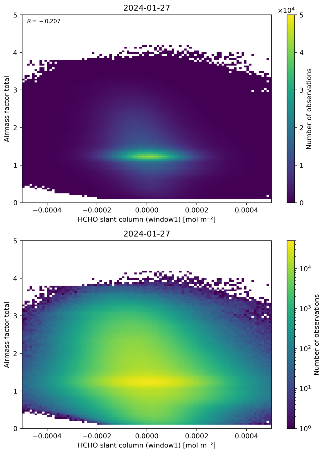
Figure 85: Scatter density plot of “HCHO slant column (window1)” against “Airmass factor total” for 2024-01-26 to 2024-01-28.
