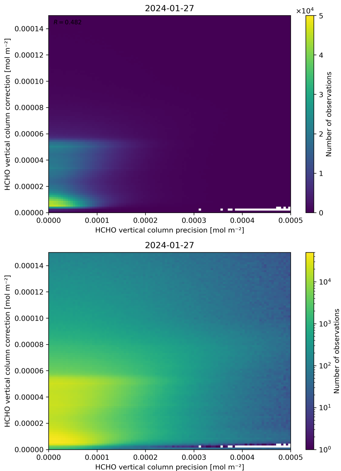
Figure 146: Scatter density plot of “HCHO vertical column precision” against “HCHO vertical column correction” for 2024-01-26 to 2024-01-28.
