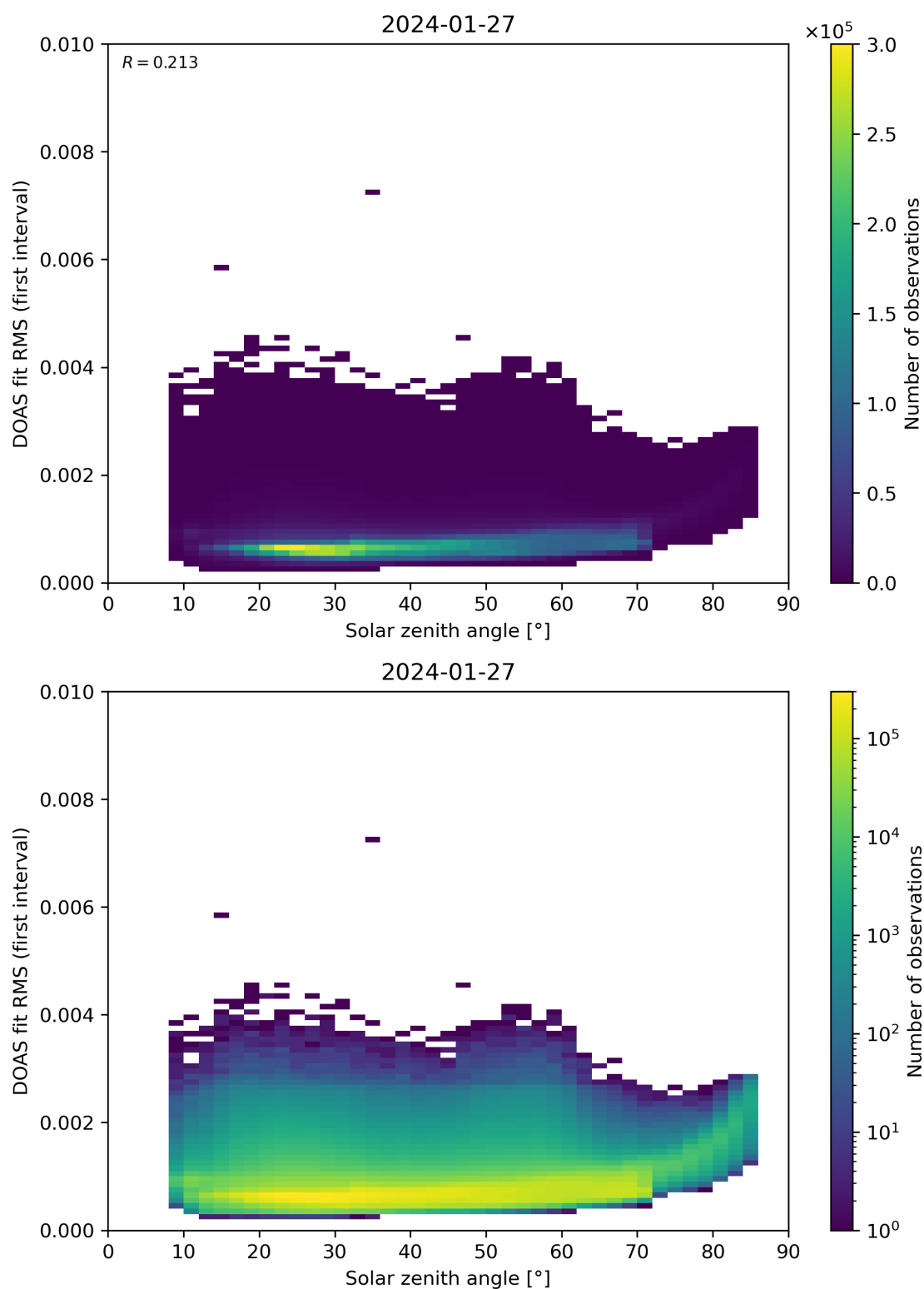
Figure 167: Scatter density plot of “Solar zenith angle” against “DOAS fit RMS (first interval)” for 2024-01-26 to 2024-01-28.
