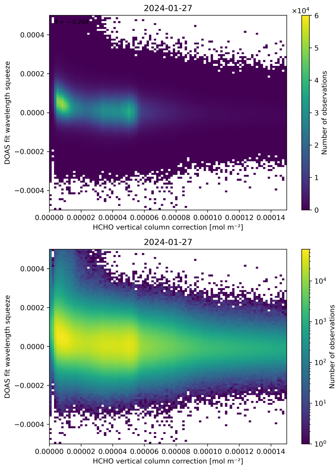
Figure 114: Scatter density plot of “HCHO vertical column correction” against “DOAS fit wavelength squeeze” for 2024-01-26 to 2024-01-28.
