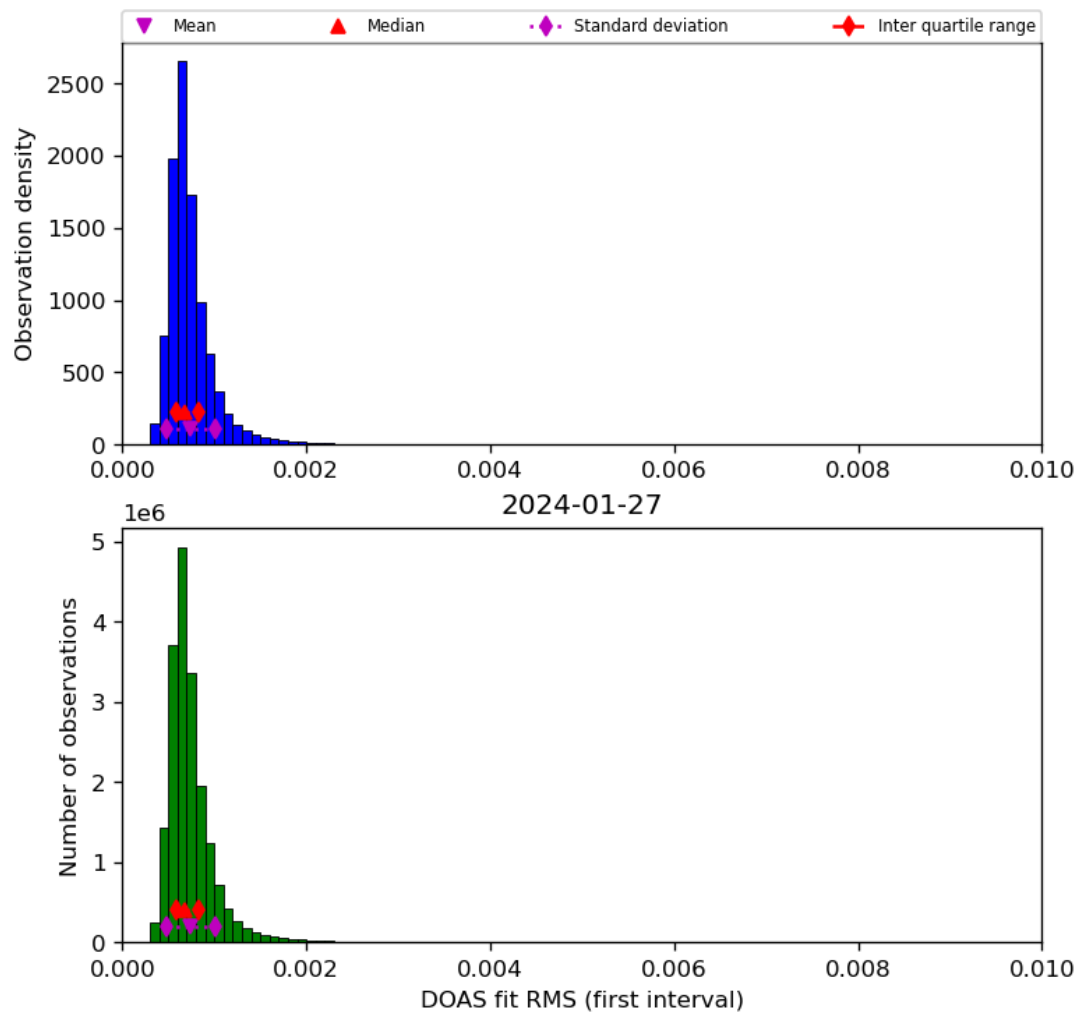
Figure 46: Histogram of “DOAS fit RMS (first interval)” for 2024-01-26 to 2024-01-28
