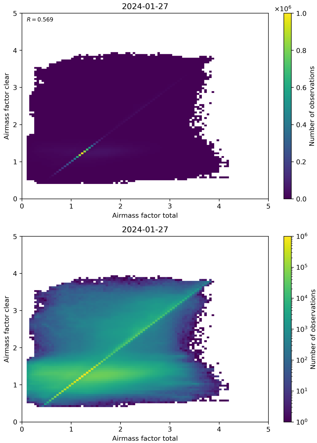
Figure 100: Scatter density plot of “Airmass factor total” against “Airmass factor clear” for 2024-01-26 to 2024-01-28.
