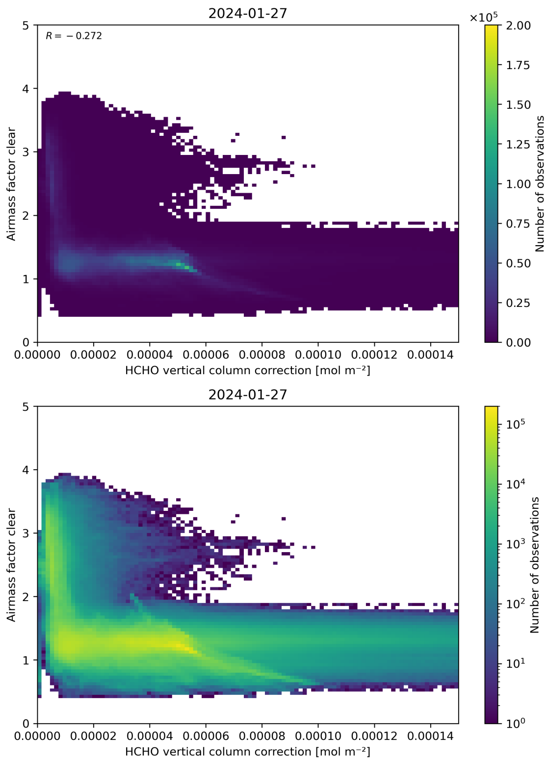
Figure 115: Scatter density plot of “HCHO vertical column correction” against “Airmass factor clear” for 2024-01-26 to 2024-01-28.
