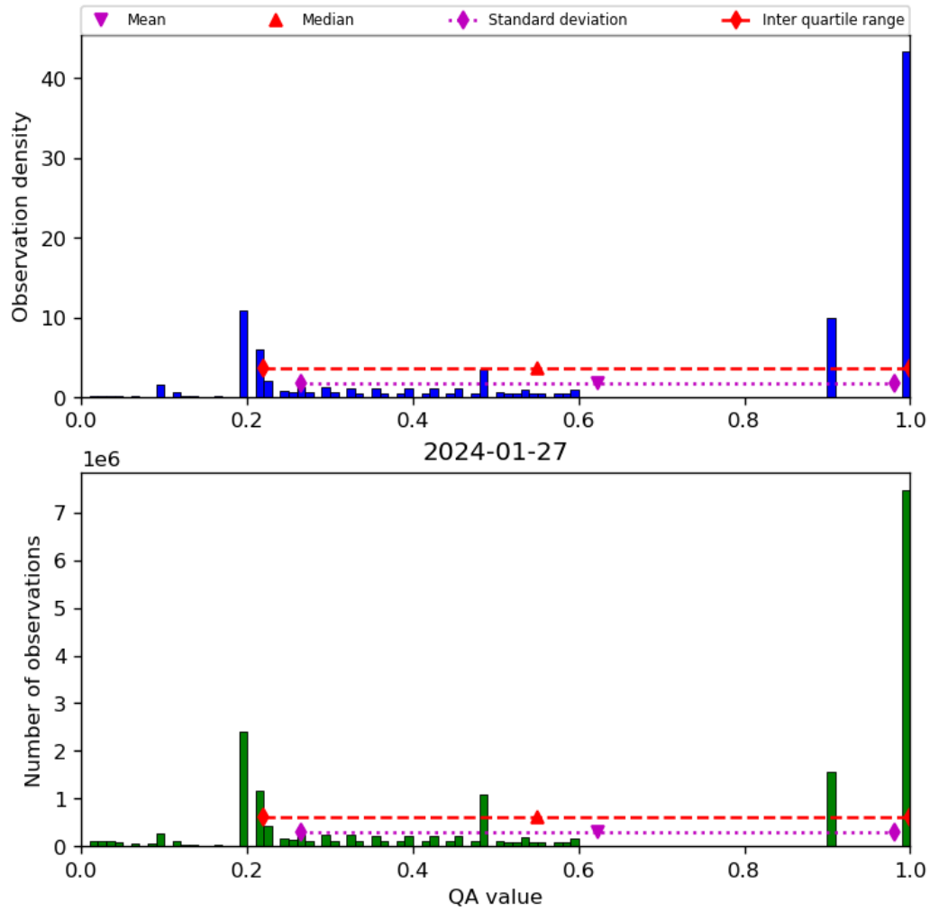
Figure 34: Histogram of “QA value” for 2024-01-26 to 2024-01-28
