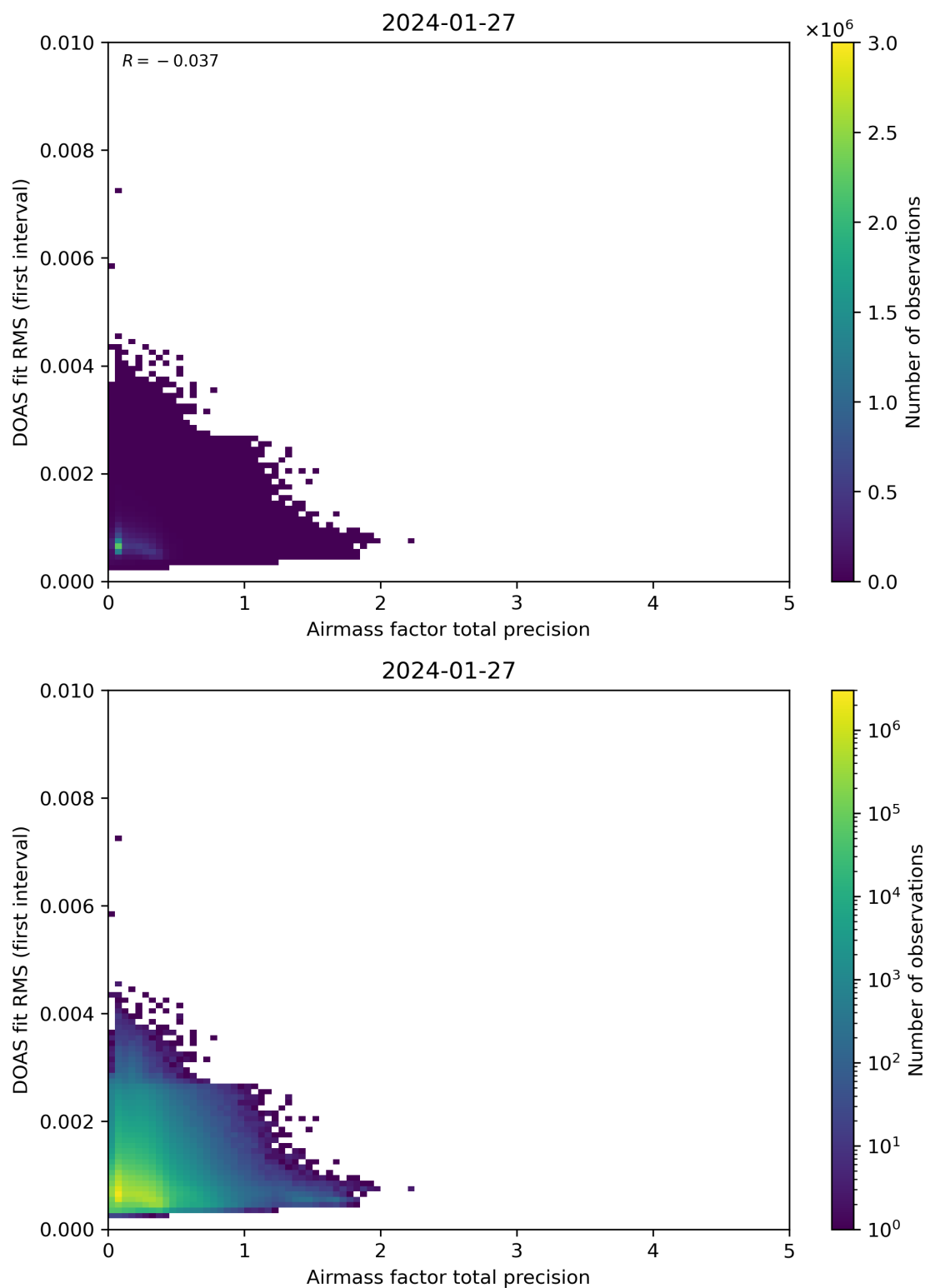
Figure 105: Scatter density plot of “Airmass factor total precision” against “DOAS fit RMS (first interval)” for 2024-01-26 to 2024-01-28.
