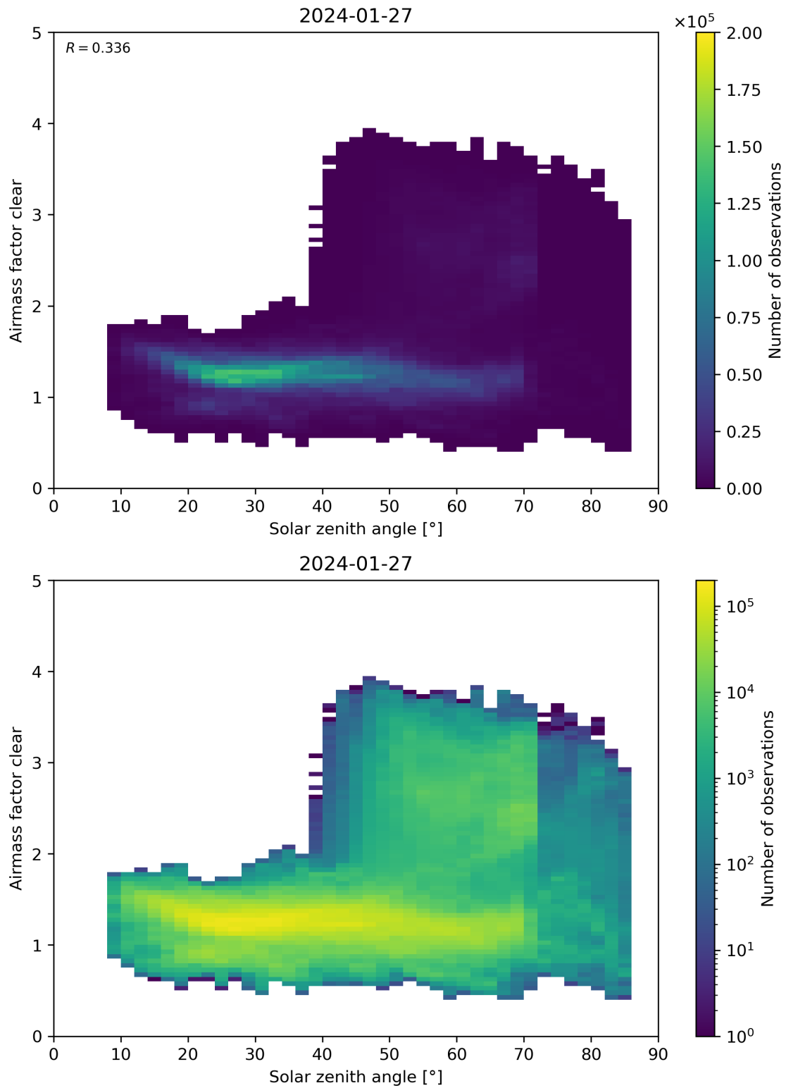
Figure 170: Scatter density plot of “Solar zenith angle” against “Airmass factor clear” for 2024-01-26 to 2024-01-28.
