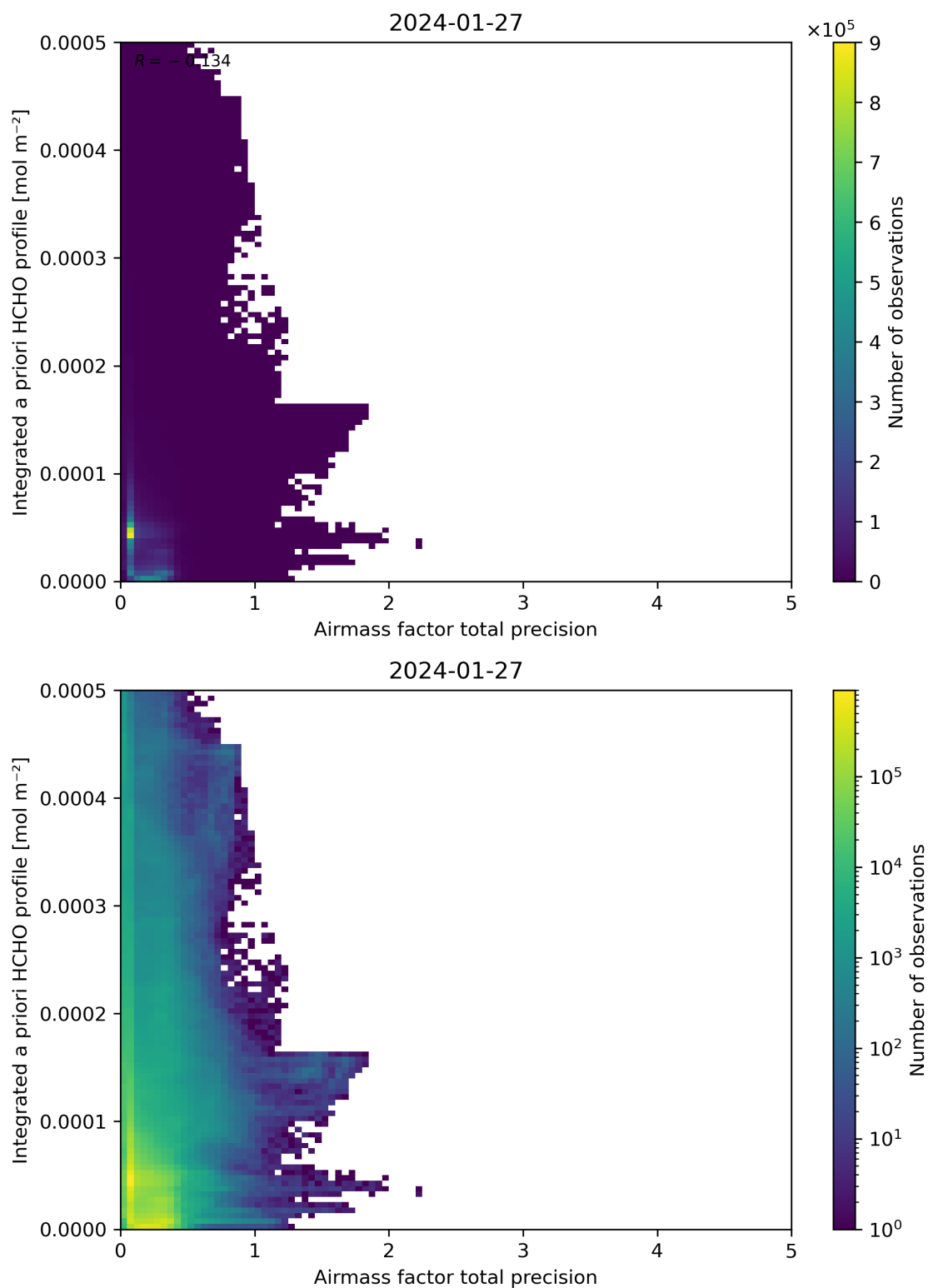
Figure 111: Scatter density plot of “Airmass factor total precision” against “Integrated a priori HCHO profile” for 2024-01-26 to 2024-01-28.
