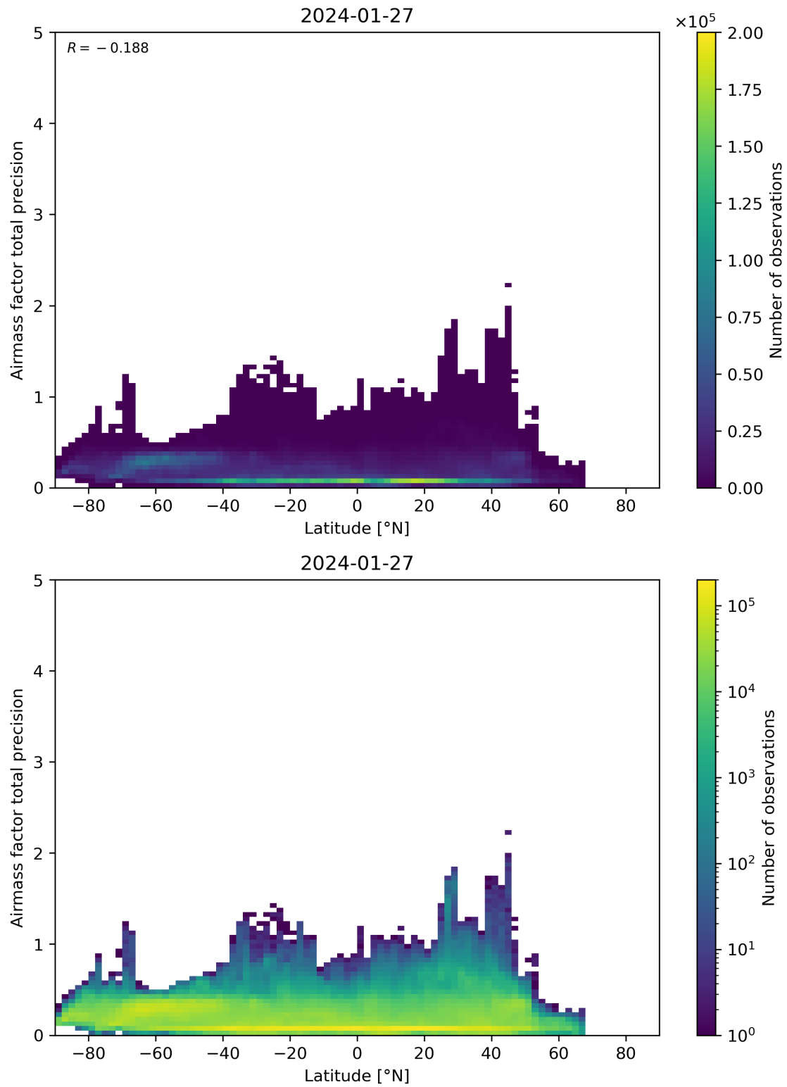
Figure 162: Scatter density plot of “Latitude” against “Airmass factor total precision” for 2024-01-26 to 2024-01-28.
