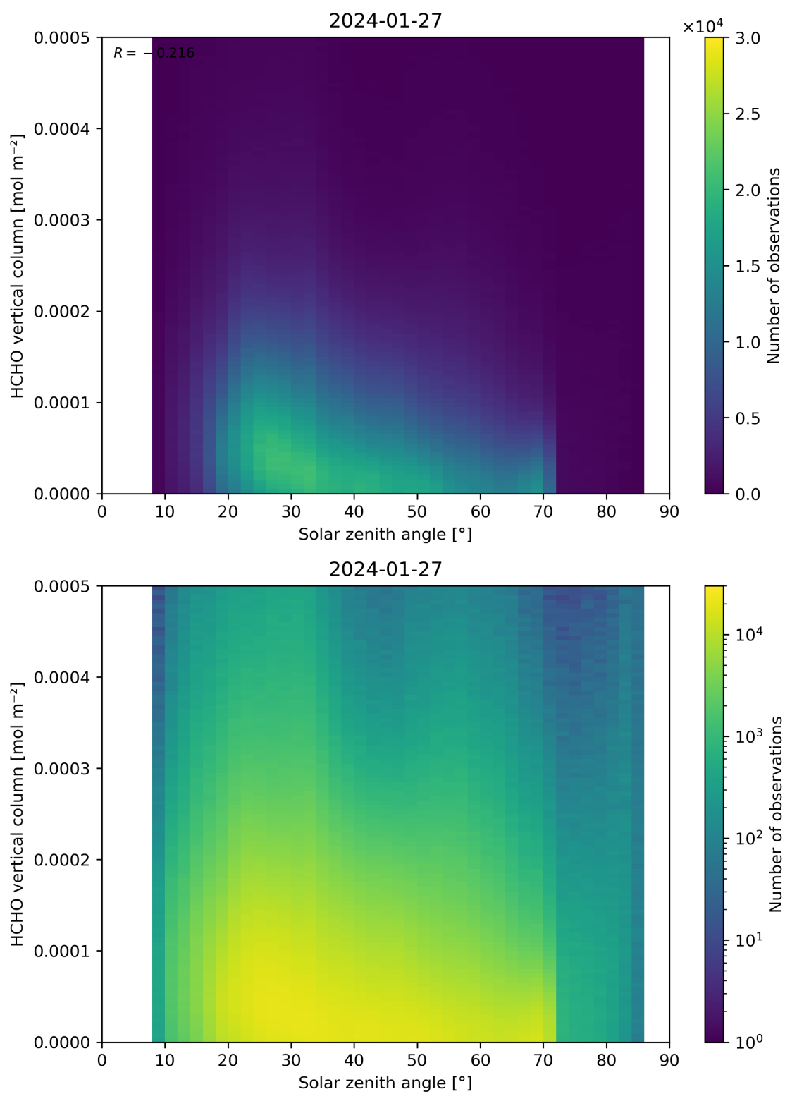
Figure 177: Scatter density plot of “Solar zenith angle” against “HCHO vertical column” for 2024-01-26 to 2024-01-28.
