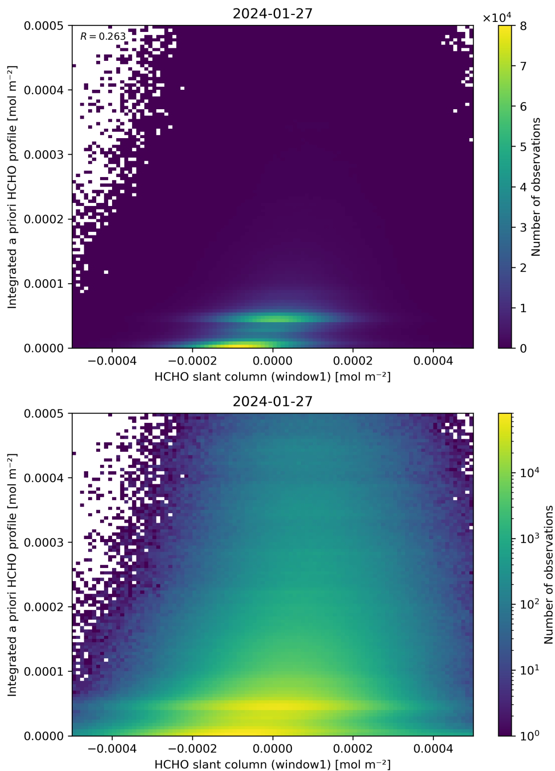
Figure 87: Scatter density plot of “HCHO slant column (window1)” against “Integrated a priori HCHO profile” for 2024-01-26 to 2024-01-28.
