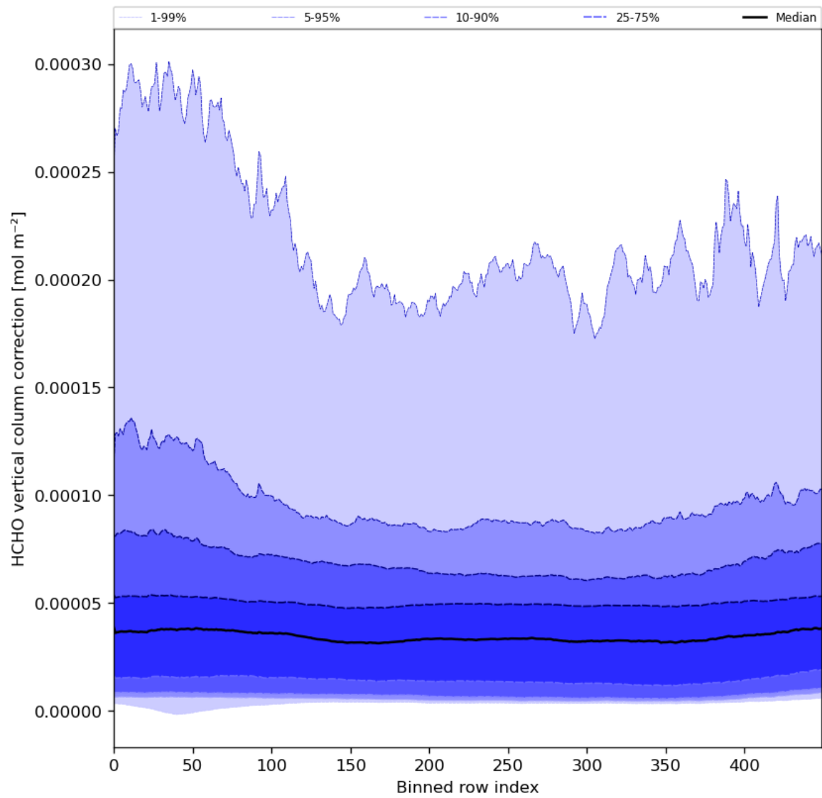
Figure 51: Along track statistics of “HCHO vertical column correction” for 2024-01-26 to 2024-01-28
