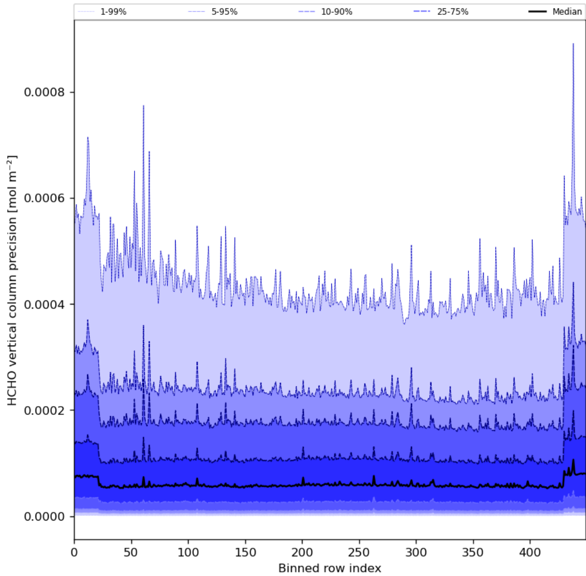
Figure 50: Along track statistics of “HCHO vertical column precision” for 2024-01-26 to 2024-01-28
