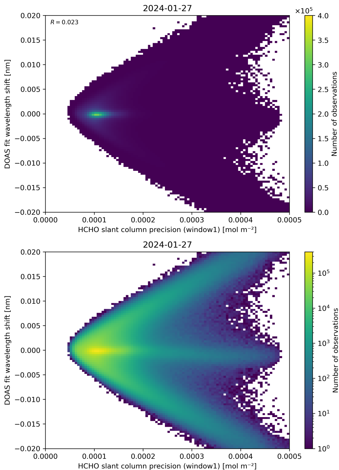
Figure 89: Scatter density plot of “HCHO slant column precision (window1)” against “DOAS fit wavelength shift” for 2024-01-26 to 2024-01-28.
