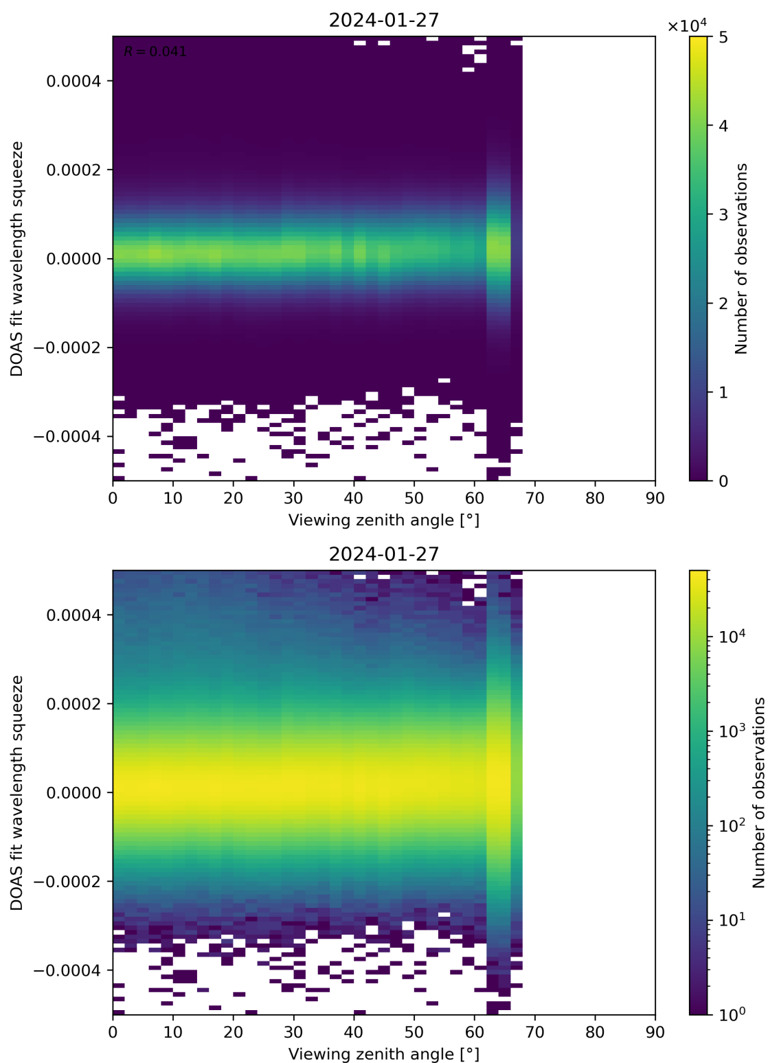
Figure 184: Scatter density plot of “Viewing zenith angle” against “DOAS fit wavelength squeeze” for 2024-01-26 to 2024-01-28.
