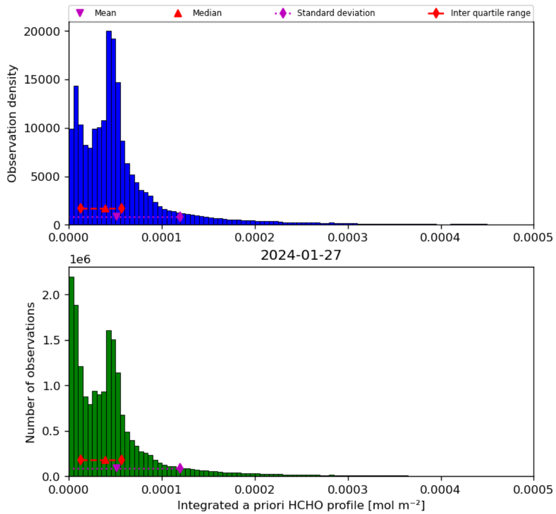
Figure 43: Histogram of “Integrated a priori HCHO profile” for 2024-01-26 to 2024-01-28
