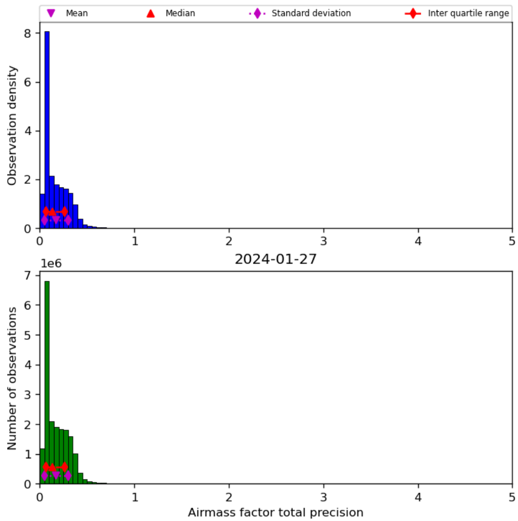
Figure 41: Histogram of “Airmass factor total precision” for 2024-01-26 to 2024-01-28
