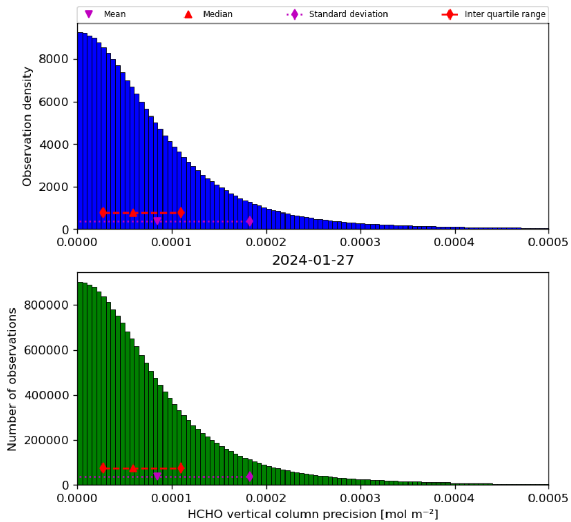
Figure 36: Histogram of “HCHO vertical column precision” for 2024-01-26 to 2024-01-28
