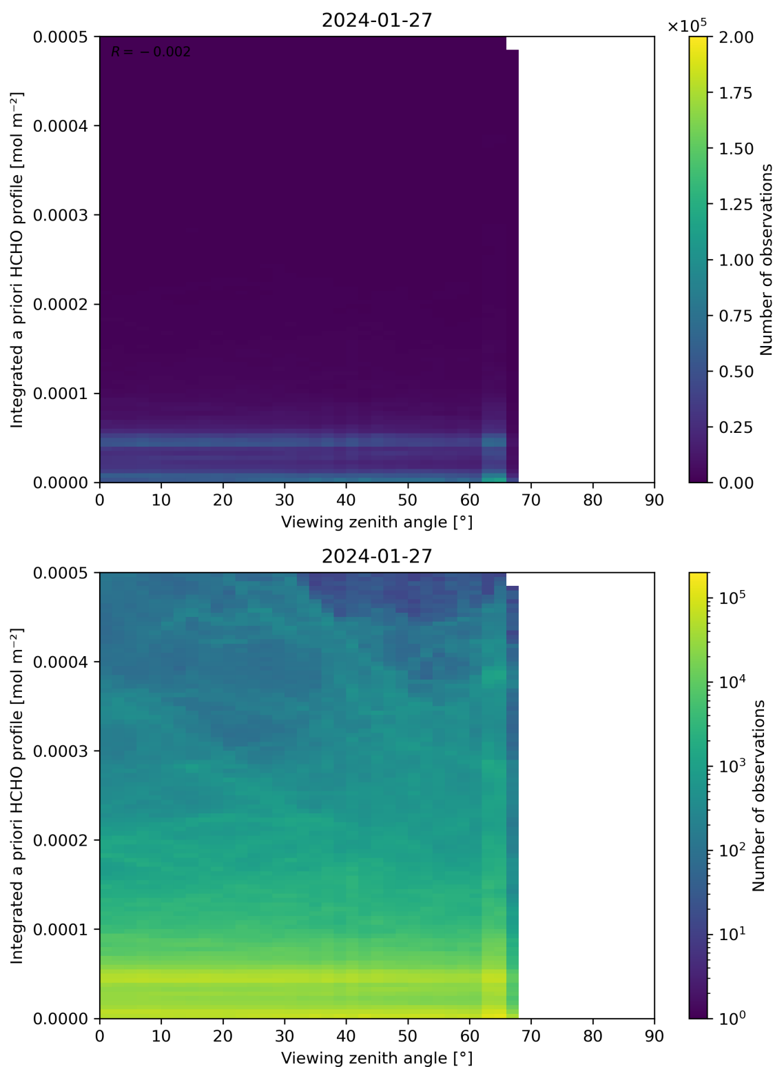
Figure 195: Scatter density plot of “Viewing zenith angle” against “Integrated a priori HCHO profile” for 2024-01-26 to 2024-01-28.
