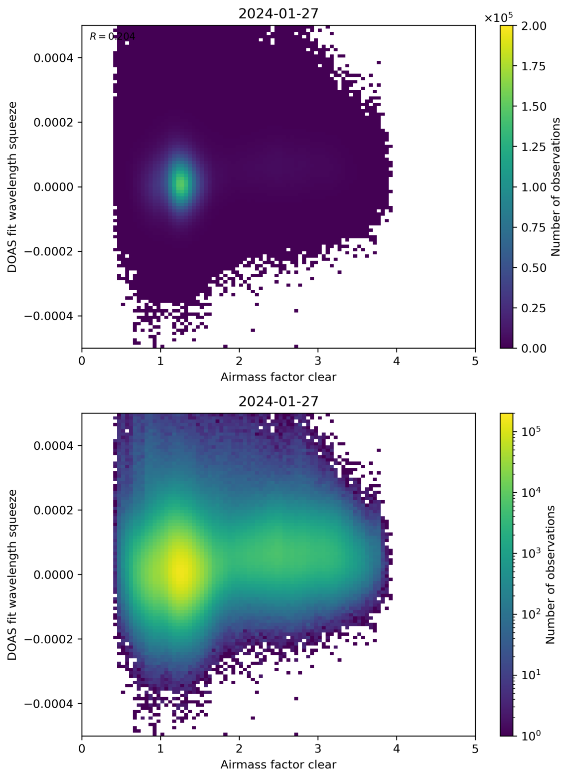
Figure 73: Scatter density plot of “Airmass factor clear” against “DOAS fit wavelength squeeze” for 2024-01-26 to 2024-01-28.
