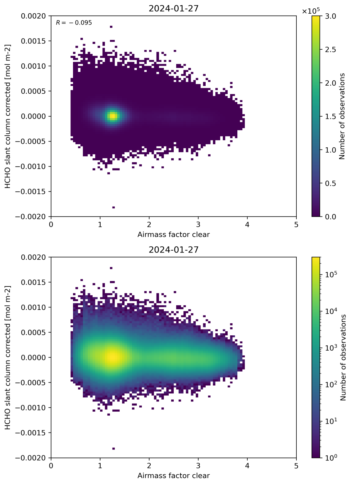
Figure 74: Scatter density plot of “Airmass factor clear” against “HCHO slant column corrected” for 2024-01-26 to 2024-01-28.
