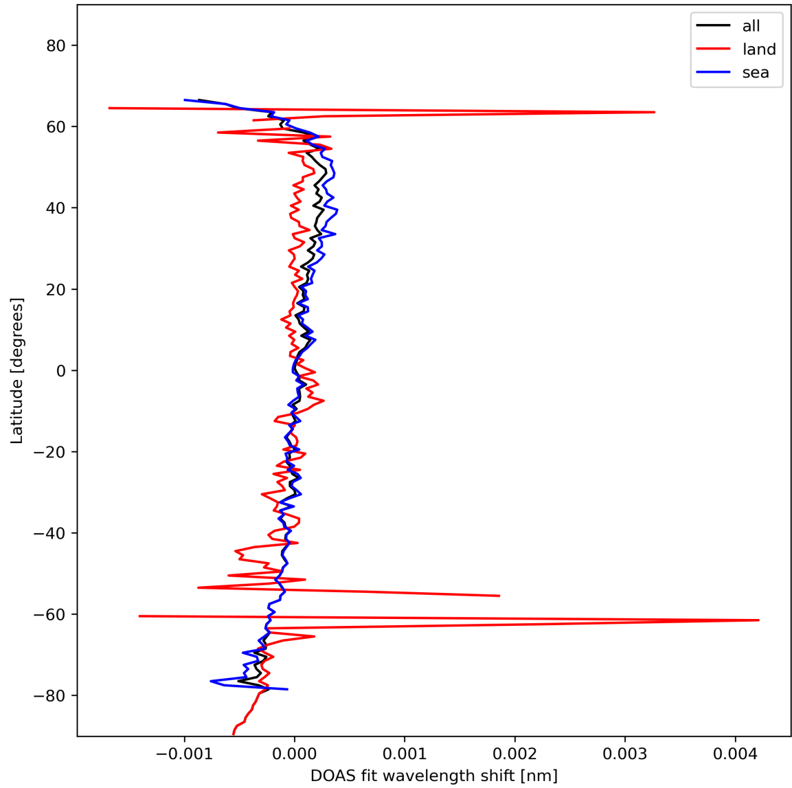
Figure 30: Zonal average of “DOAS fit wavelength shift” for 2024-01-26 to 2024-01-28.
