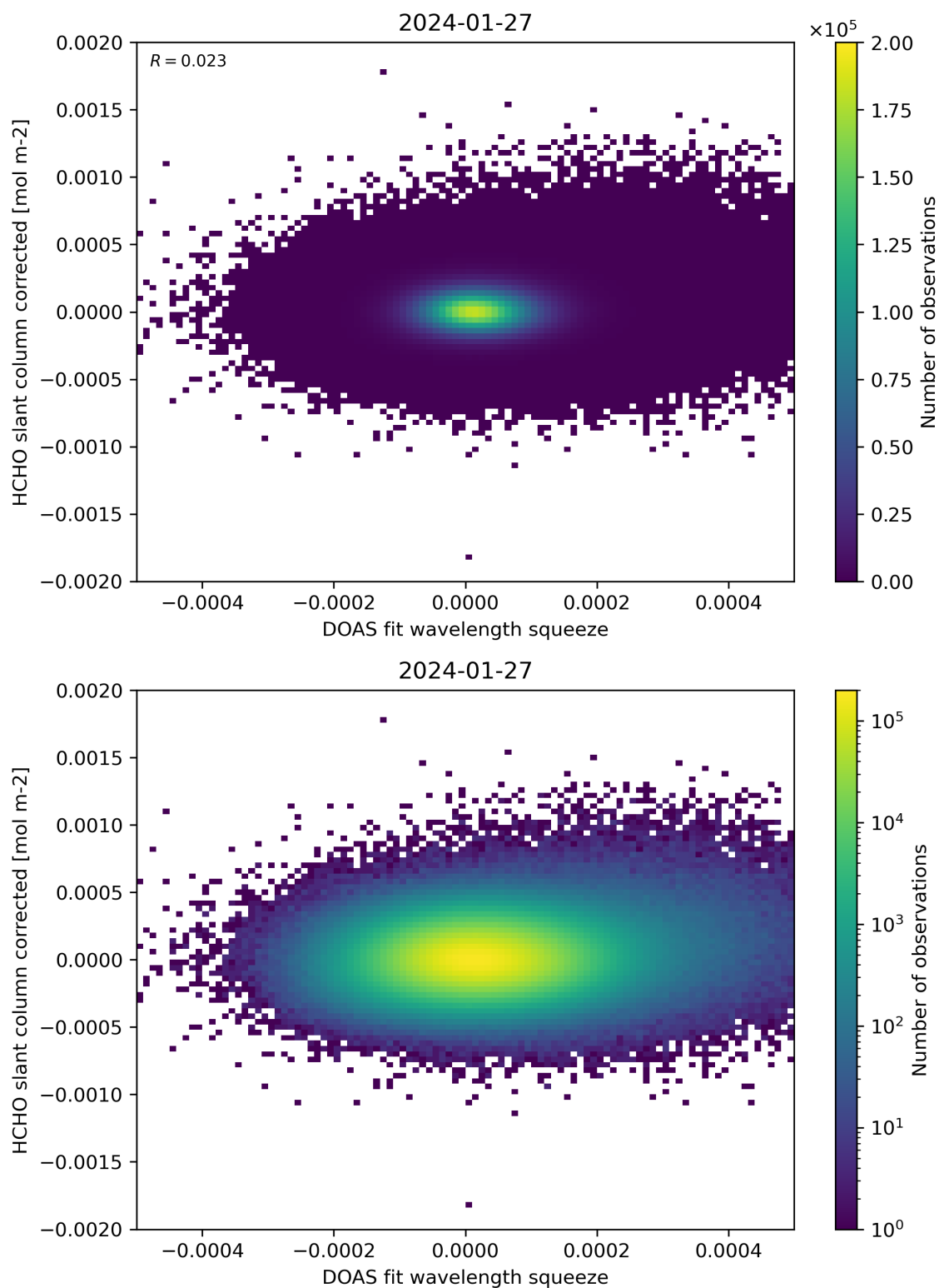
Figure 69: Scatter density plot of “DOAS fit wavelength squeeze” against “HCHO slant column corrected” for 2024-01-26 to 2024-01-28.
