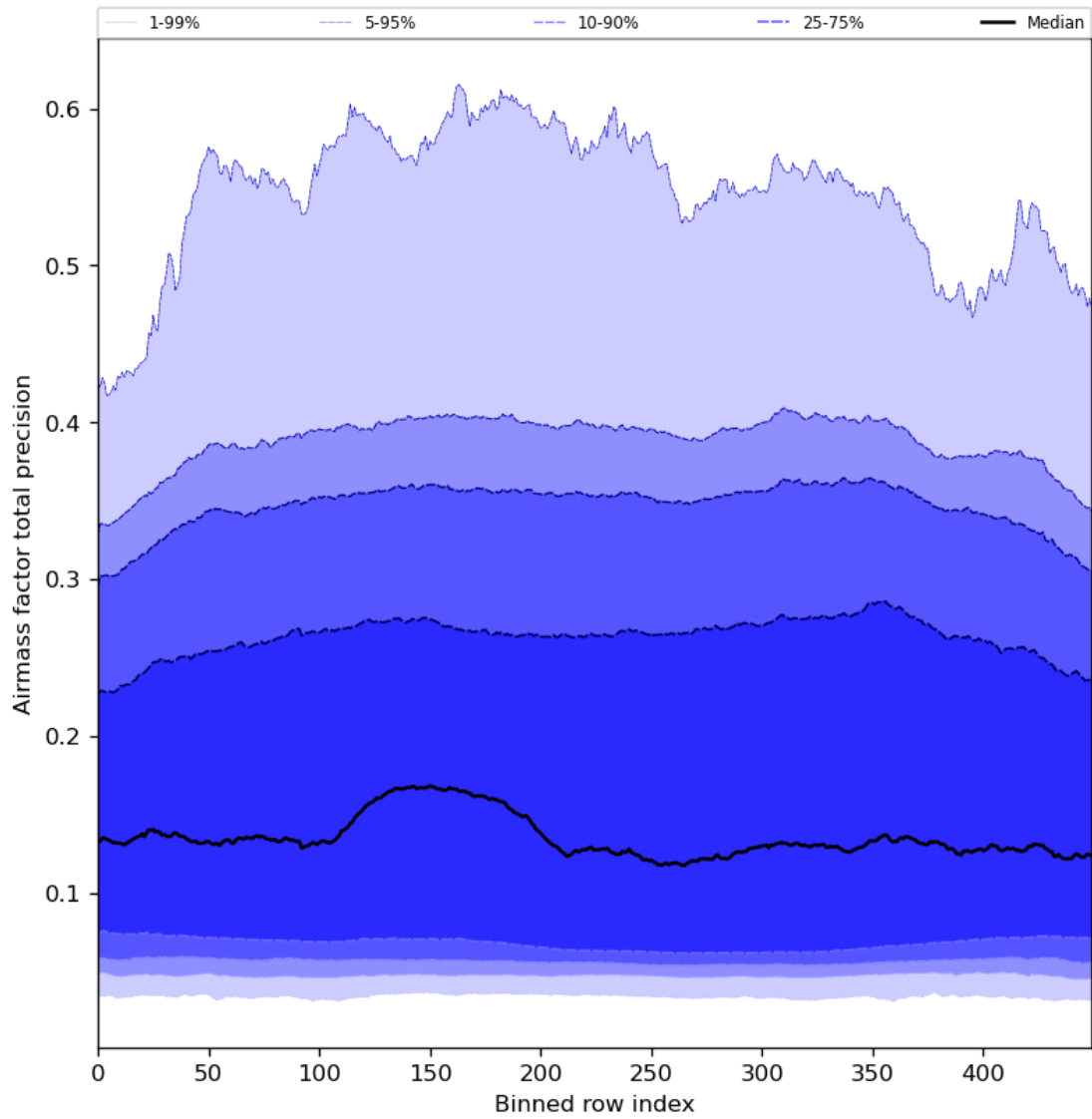
Figure 55: Along track statistics of “Airmass factor total precision” for 2024-01-26 to 2024-01-28
