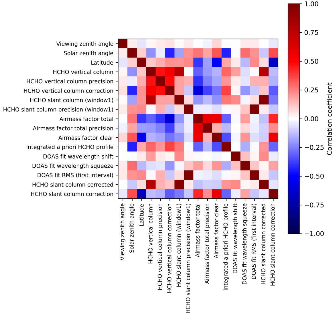
Figure 2: Map of correlation matrix for 2024-01-26 to 2024-01-28.
