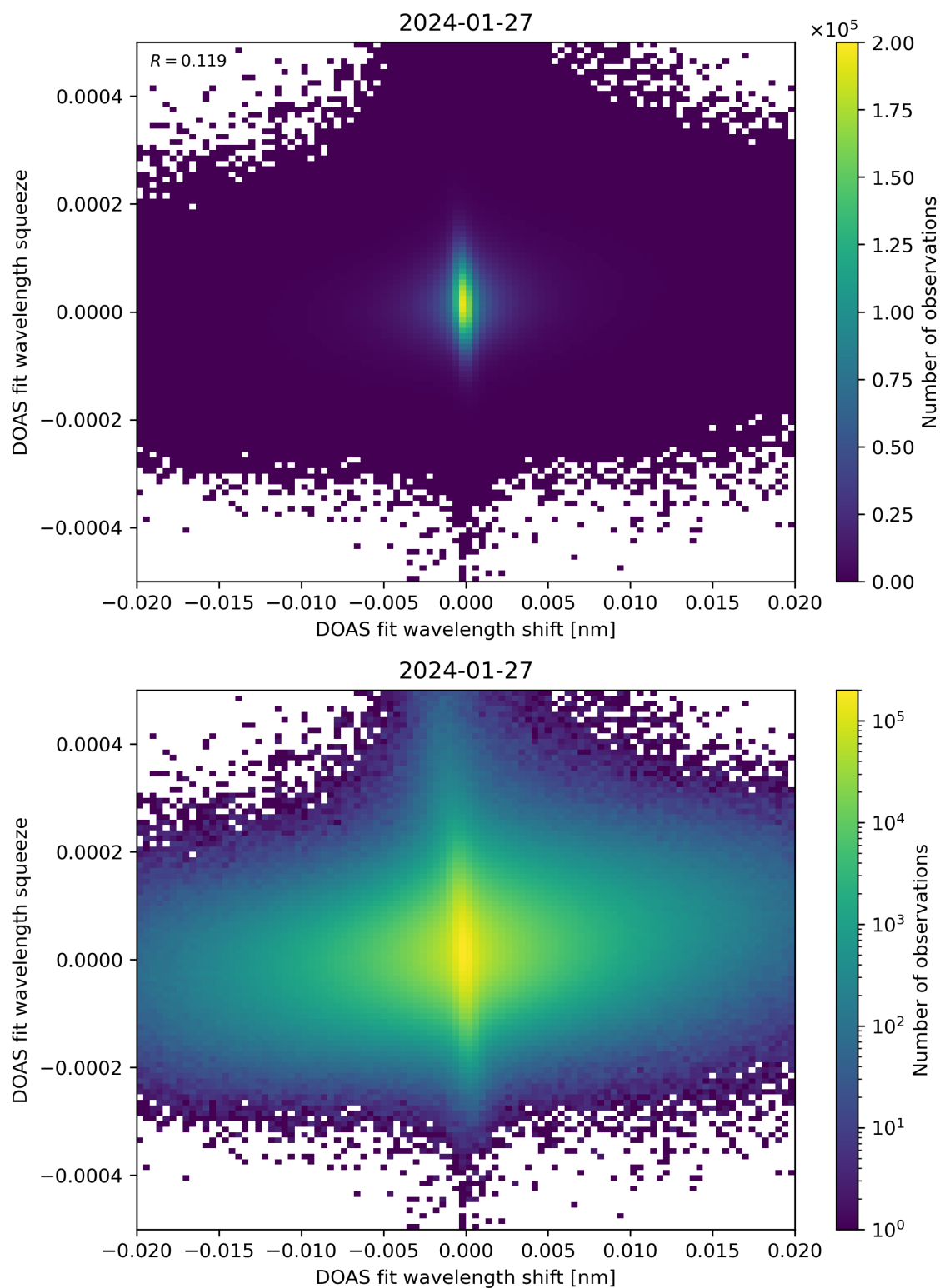
Figure 65: Scatter density plot of “DOAS fit wavelength shift” against “DOAS fit wavelength squeeze” for 2024-01-26 to 2024-01-28.
