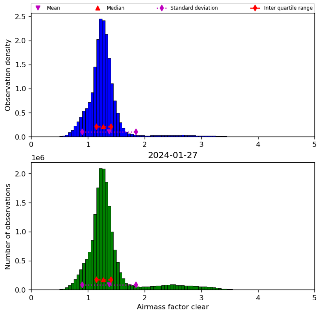
Figure 42: Histogram of “Airmass factor clear” for 2024-01-26 to 2024-01-28
