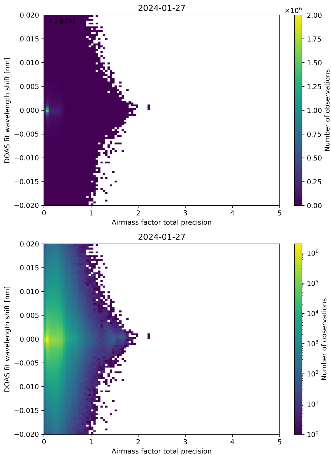
Figure 106: Scatter density plot of “Airmass factor total precision” against “DOAS fit wavelength shift” for 2024-01-26 to 2024-01-28.
