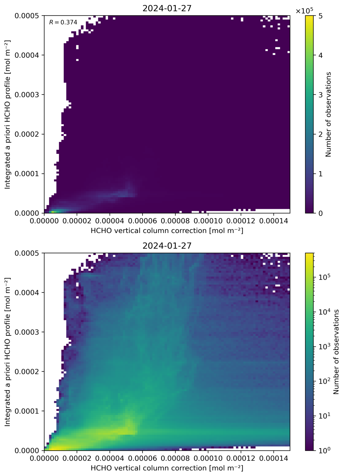
Figure 122: Scatter density plot of “HCHO vertical column correction” against “Integrated a priori HCHO profile” for 2024-01-26 to 2024-01-28.
