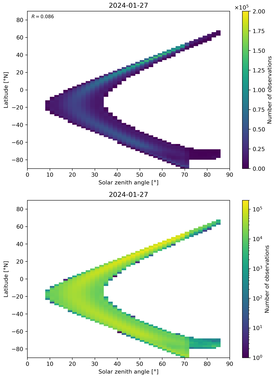
Figure 181: Scatter density plot of “Solar zenith angle” against “Latitude” for 2024-01-26 to 2024-01-28.
