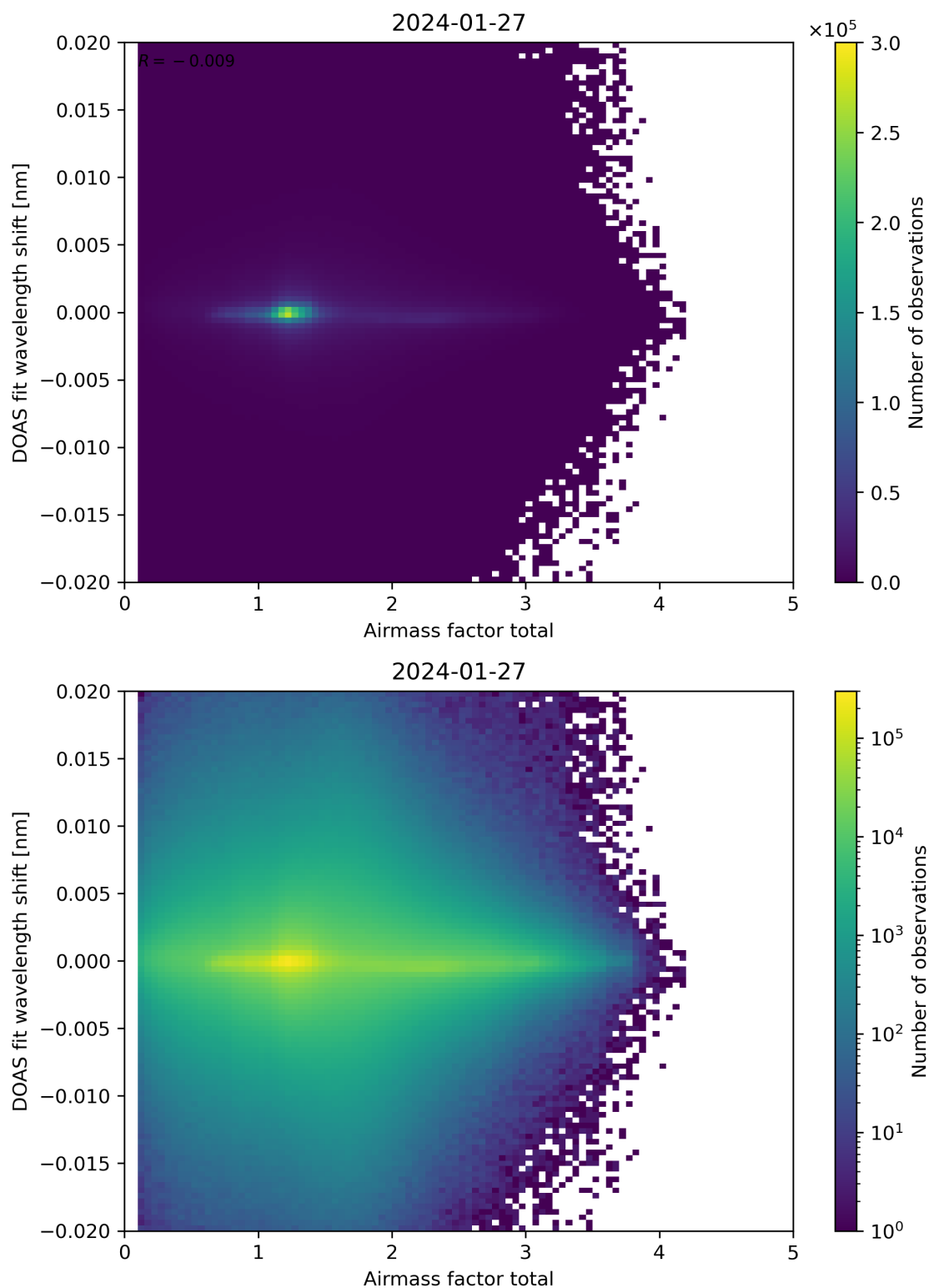
Figure 98: Scatter density plot of “Airmass factor total” against “DOAS fit wavelength shift” for 2024-01-26 to 2024-01-28.
