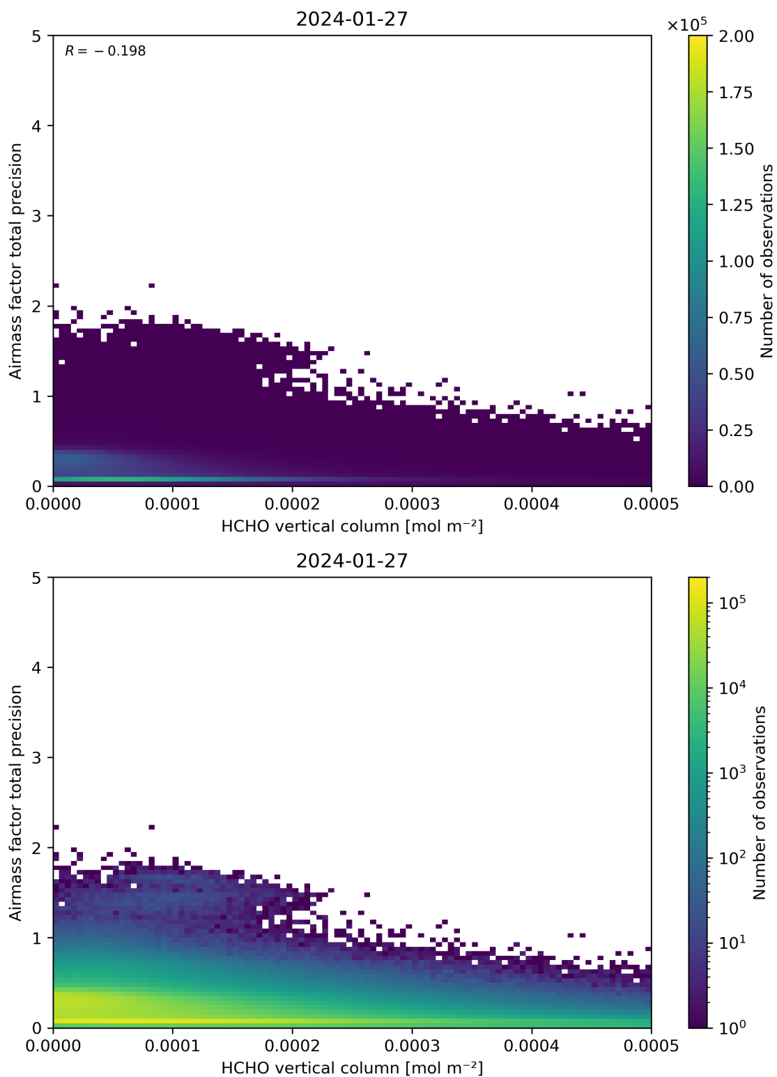
Figure 132: Scatter density plot of “HCHO vertical column” against “Airmass factor total precision” for 2024-01-26 to 2024-01-28.
