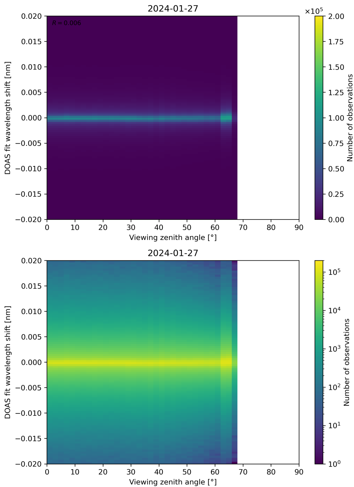
Figure 183: Scatter density plot of “Viewing zenith angle” against “DOAS fit wavelength shift” for 2024-01-26 to 2024-01-28.
