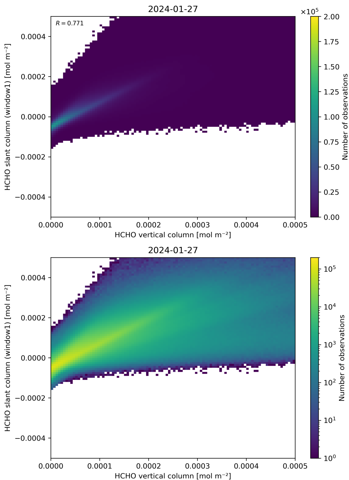
Figure 129: Scatter density plot of “HCHO vertical column” against “HCHO slant column (window1)” for 2024-01-26 to 2024-01-28.
