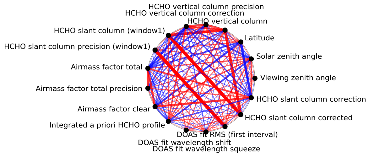
Figure 1: Map of correlation graph for 2024-01-26 to 2024-01-28.
