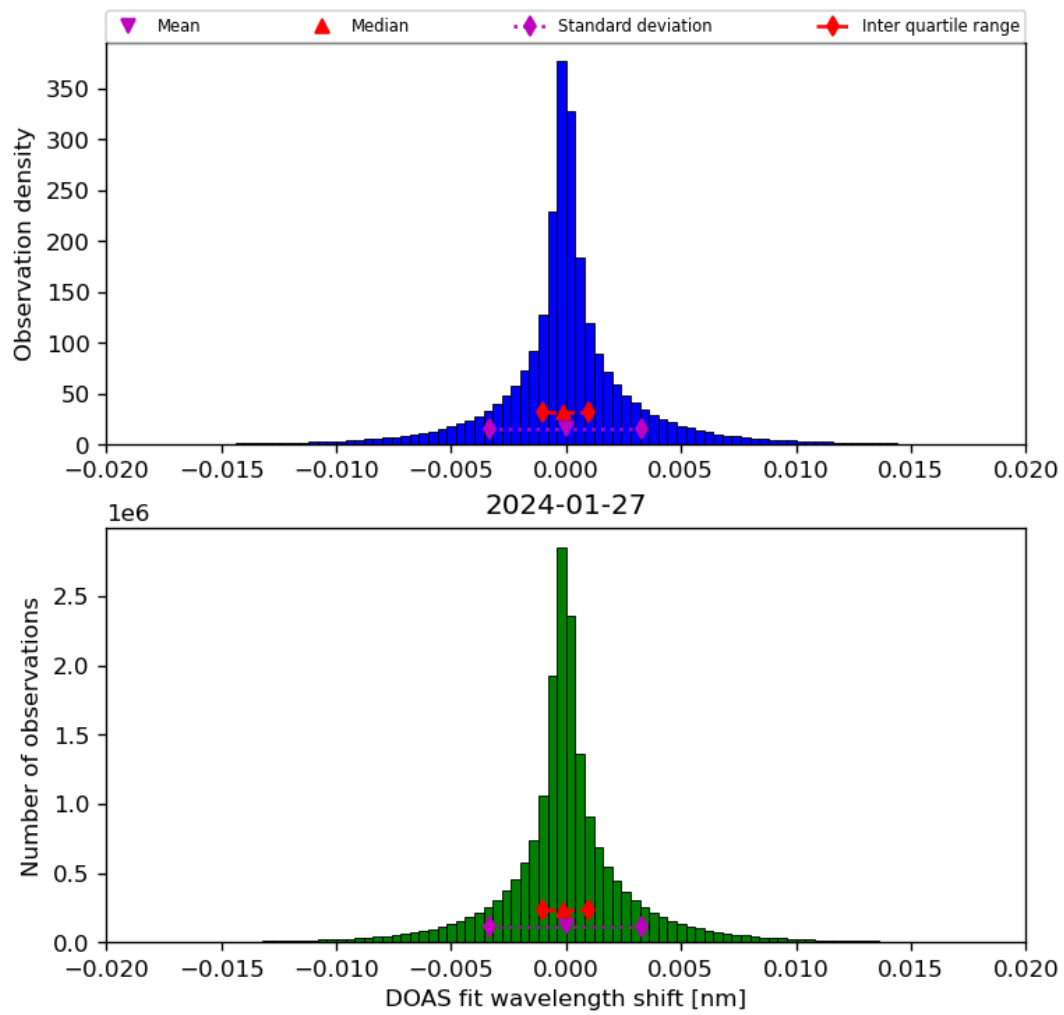
Figure 44: Histogram of “DOAS fit wavelength shift” for 2024-01-26 to 2024-01-28
