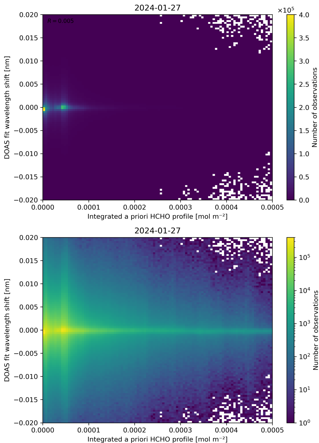
Figure 149: Scatter density plot of “Integrated a priori HCHO profile” against “DOAS fit wavelength shift” for 2024-01-26 to 2024-01-28.
