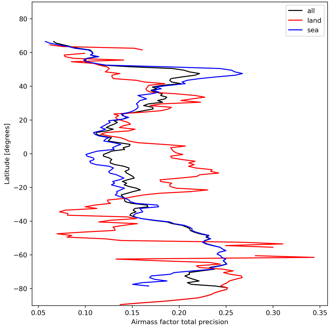
Figure 27: Zonal average of “Airmass factor total precision” for 2024-01-26 to 2024-01-28.
