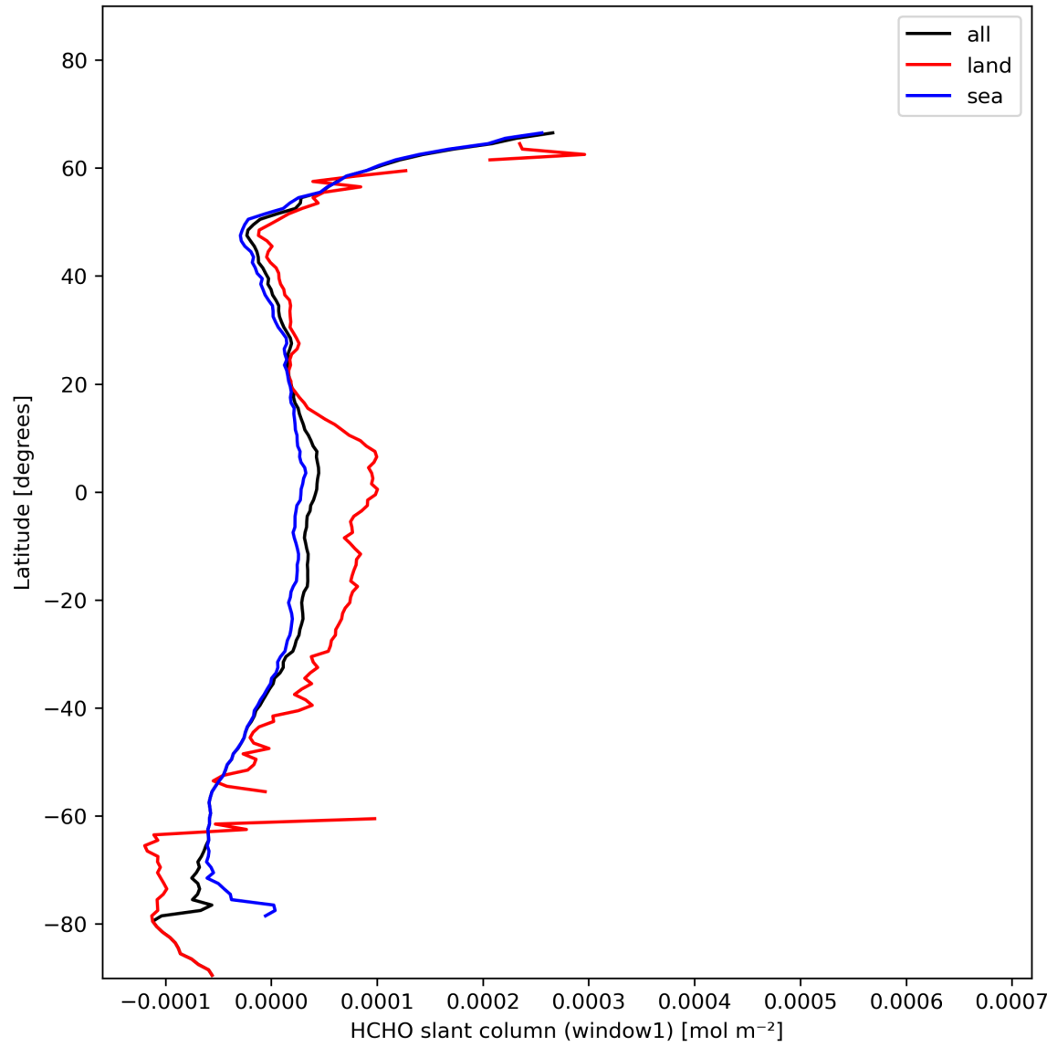
Figure 24: Zonal average of “HCHO slant column (window1)” for 2024-01-26 to 2024-01-28.
