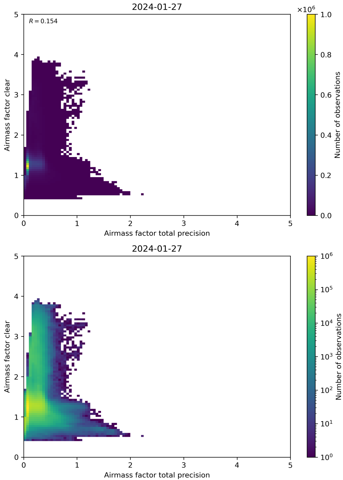
Figure 108: Scatter density plot of “Airmass factor total precision” against “Airmass factor clear” for 2024-01-26 to 2024-01-28.
