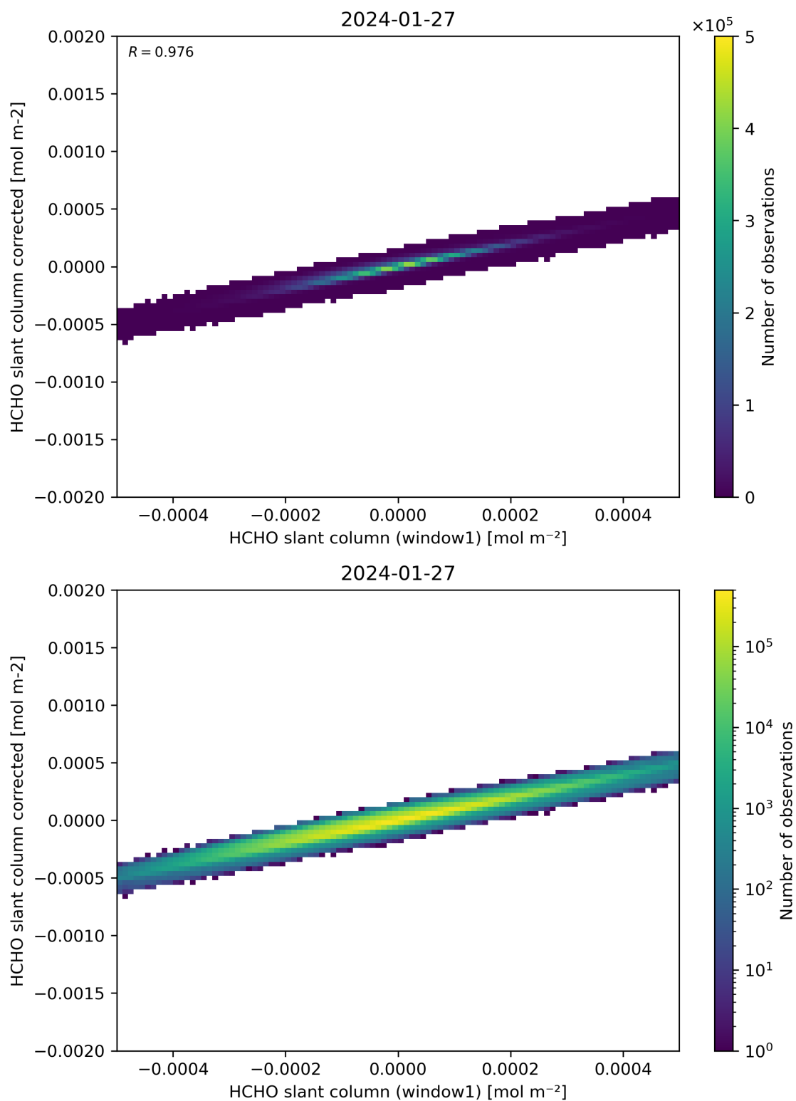
Figure 82: Scatter density plot of “HCHO slant column (window1)” against “HCHO slant column corrected” for 2024-01-26 to 2024-01-28.
