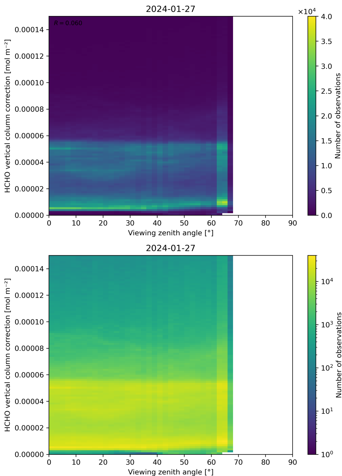
Figure 193: Scatter density plot of “Viewing zenith angle” against “HCHO vertical column correction” for 2024-01-26 to 2024-01-28.
