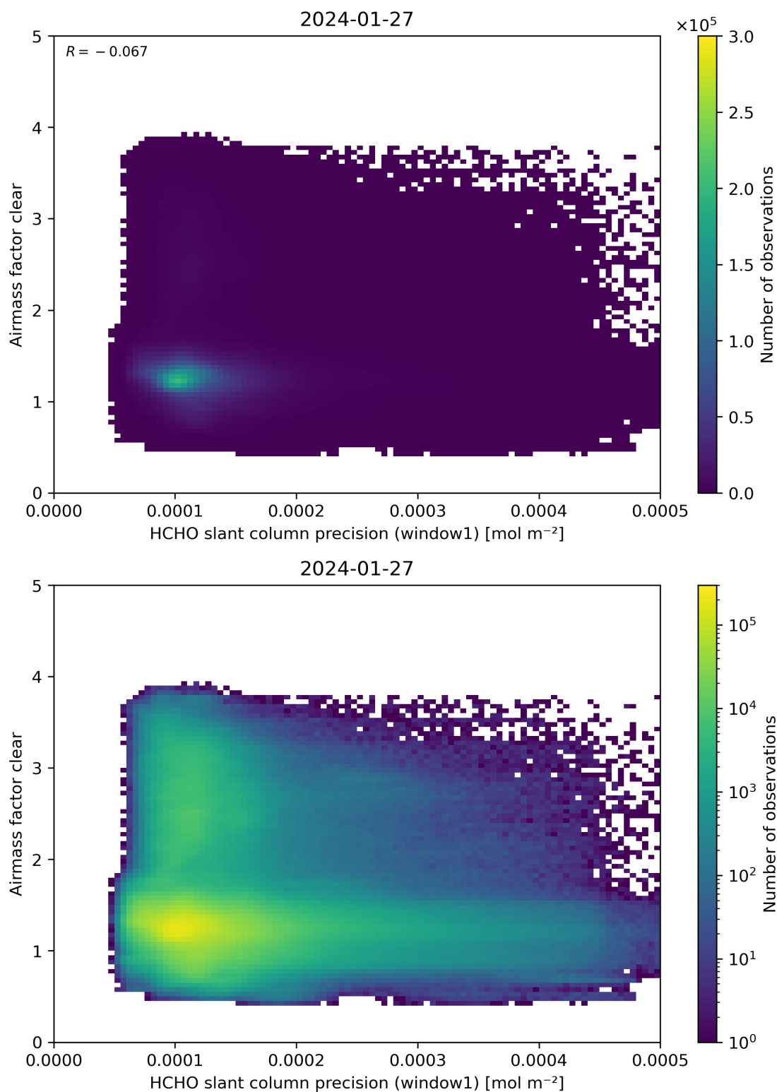
Figure 91: Scatter density plot of “HCHO slant column precision (window1)” against “Airmass factor clear” for 2024-01-26 to 2024-01-28.
