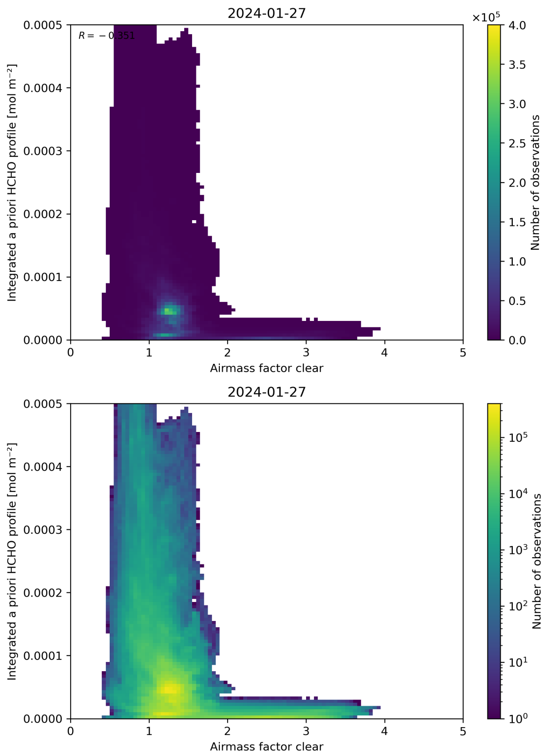
Figure 76: Scatter density plot of “Airmass factor clear” against “Integrated a priori HCHO profile” for 2024-01-26 to 2024-01-28.
