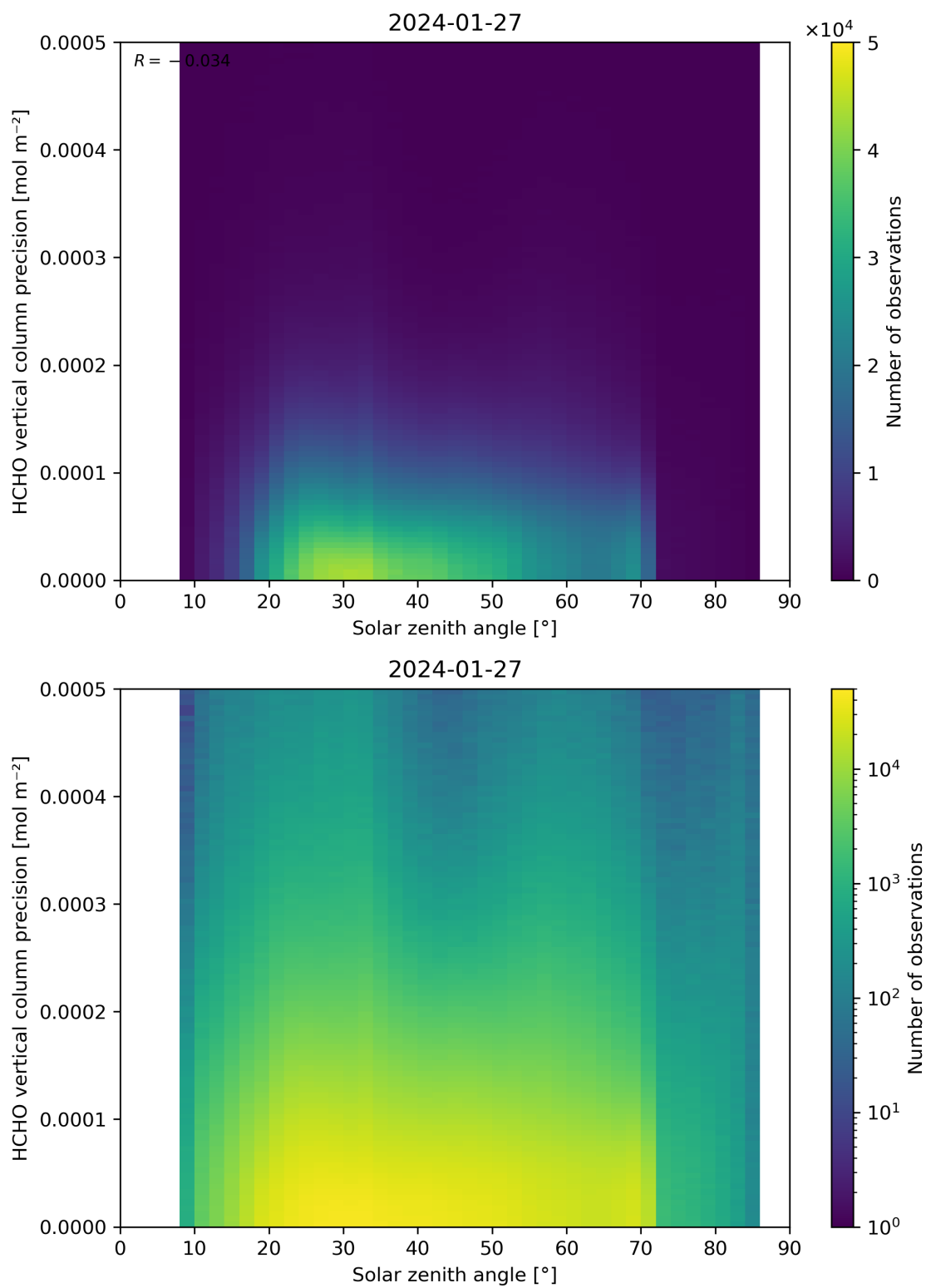
Figure 179: Scatter density plot of “Solar zenith angle” against “HCHO vertical column precision” for 2024-01-26 to 2024-01-28.
