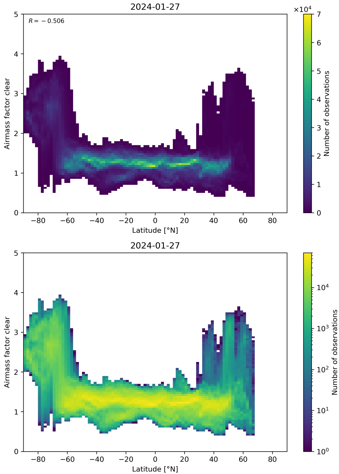
Figure 156: Scatter density plot of “Latitude” against “Airmass factor clear” for 2024-01-26 to 2024-01-28.
