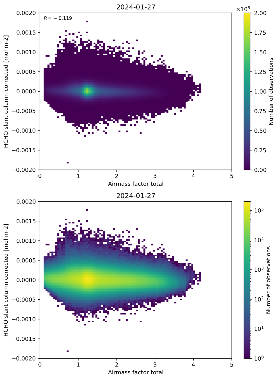
Figure 101: Scatter density plot of “Airmass factor total” against “HCHO slant column corrected” for 2024-01-26 to 2024-01-28.
