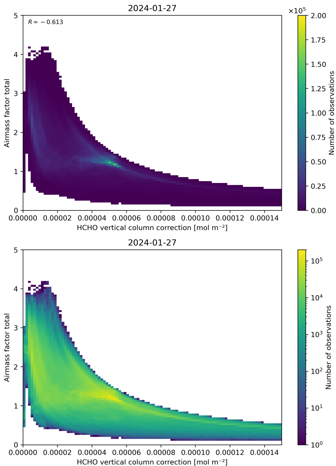
Figure 120: Scatter density plot of “HCHO vertical column correction” against “Airmass factor total” for 2024-01-26 to 2024-01-28.
