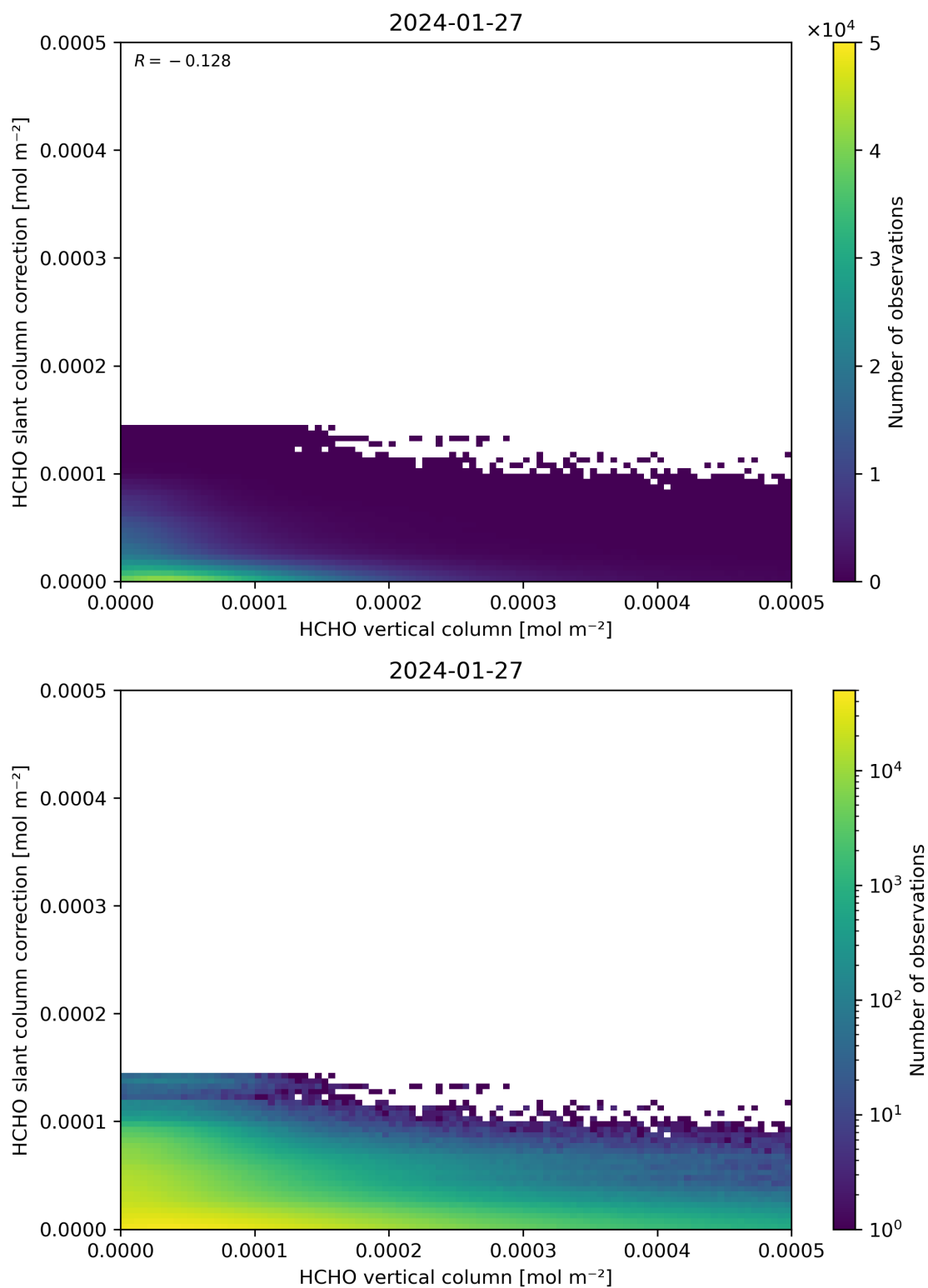
Figure 128: Scatter density plot of “HCHO vertical column” against “HCHO slant column correction” for 2024-01-26 to 2024-01-28.
