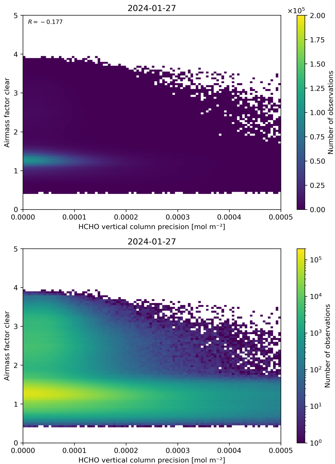
Figure 139: Scatter density plot of “HCHO vertical column precision” against “Airmass factor clear” for 2024-01-26 to 2024-01-28.
