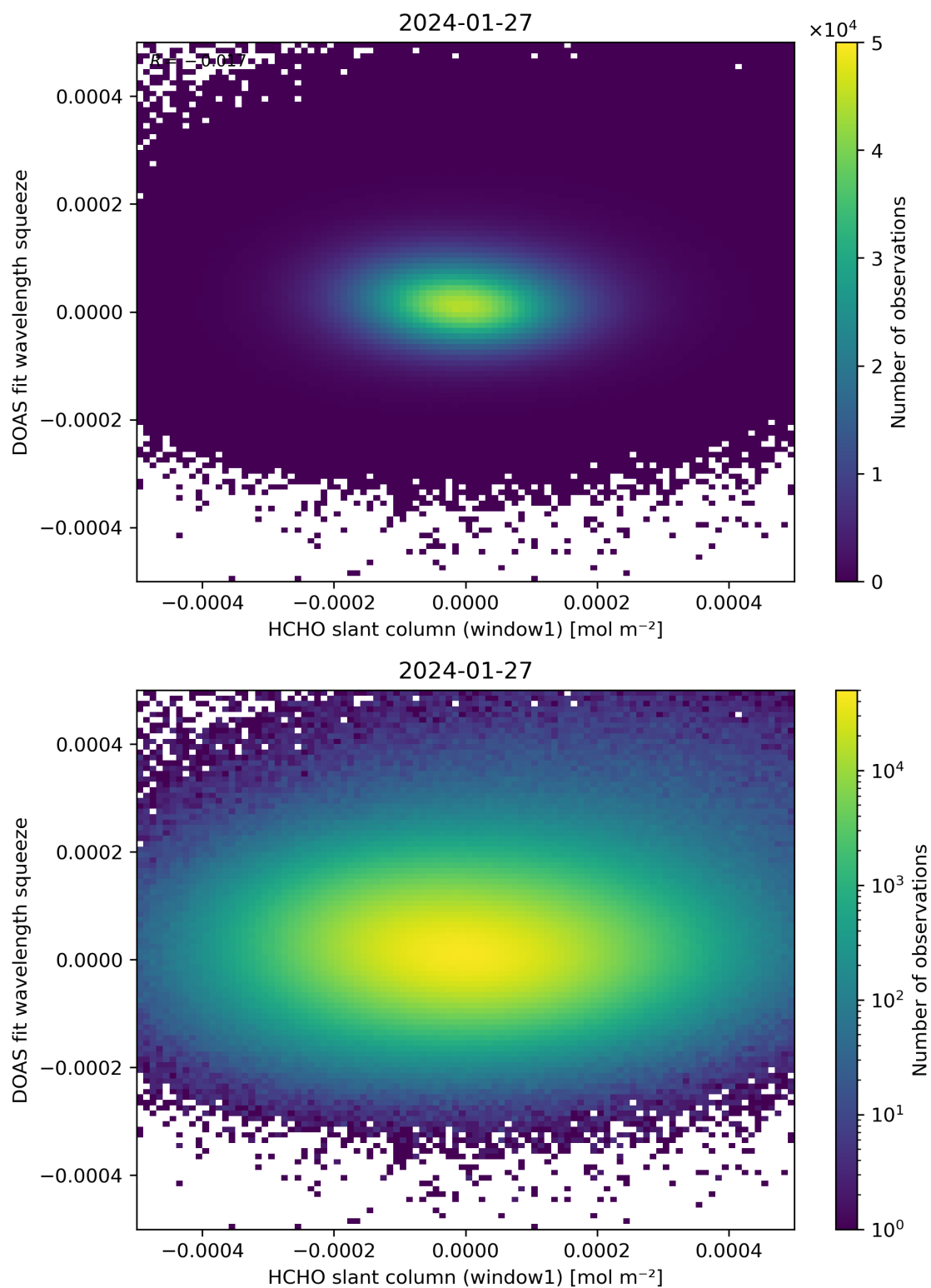
Figure 80: Scatter density plot of “HCHO slant column (window1)” against “DOAS fit wavelength squeeze” for 2024-01-26 to 2024-01-28.
