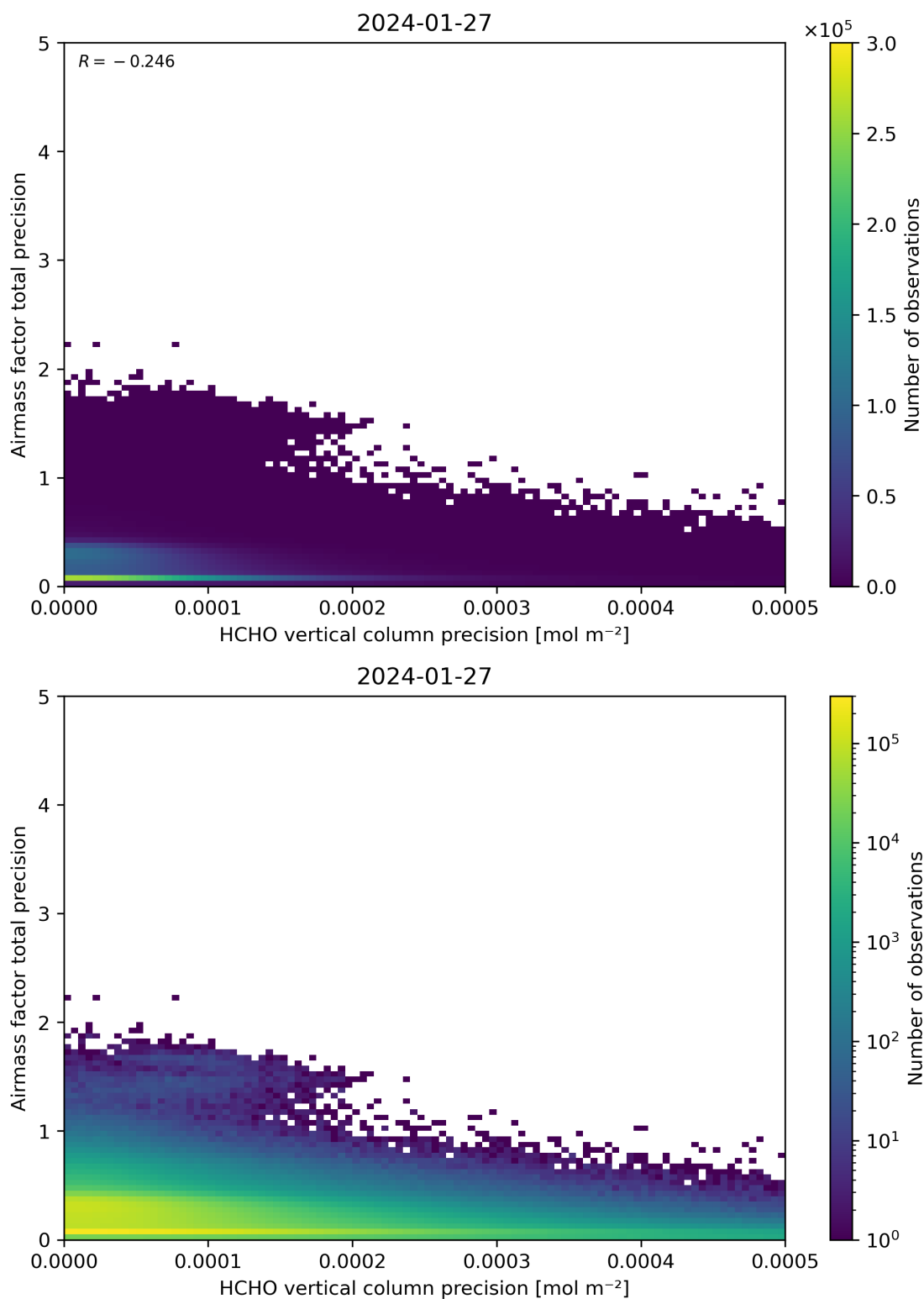
Figure 145: Scatter density plot of “HCHO vertical column precision” against “Airmass factor total precision” for 2024-01-26 to 2024-01-28.
