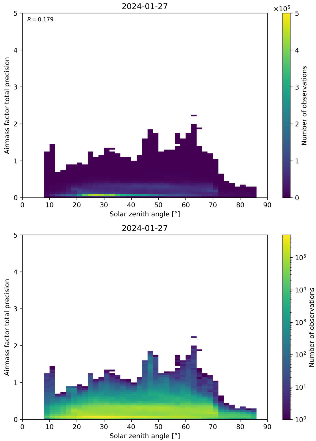
Figure 176: Scatter density plot of “Solar zenith angle” against “Airmass factor total precision” for 2024-01-26 to 2024-01-28.
