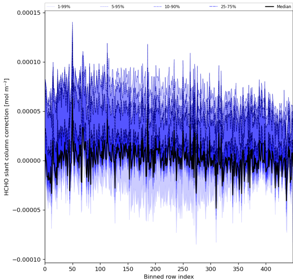
Figure 61: Along track statistics of “HCHO slant column correction” for 2024-01-26 to 2024-01-28
