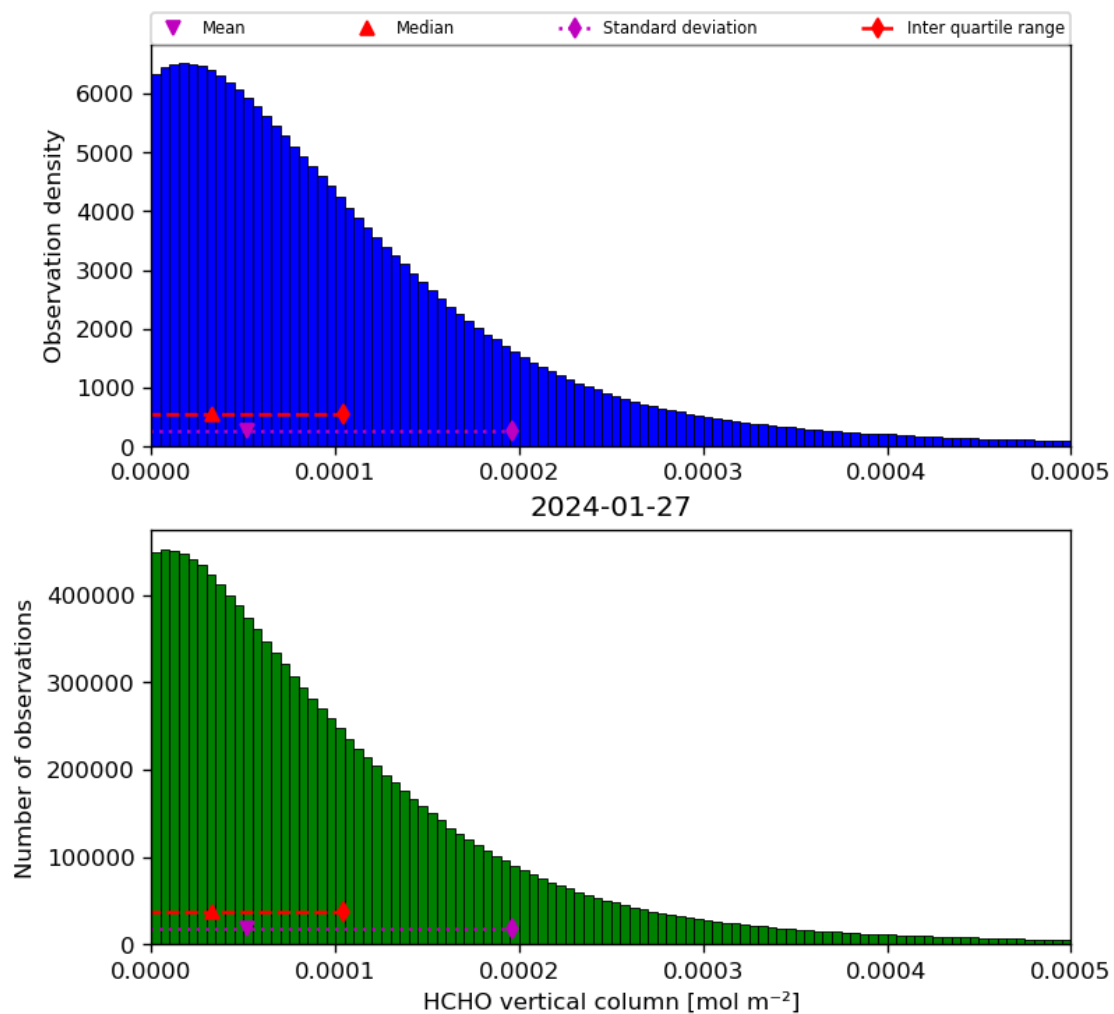
Figure 35: Histogram of “HCHO vertical column” for 2024-01-26 to 2024-01-28
