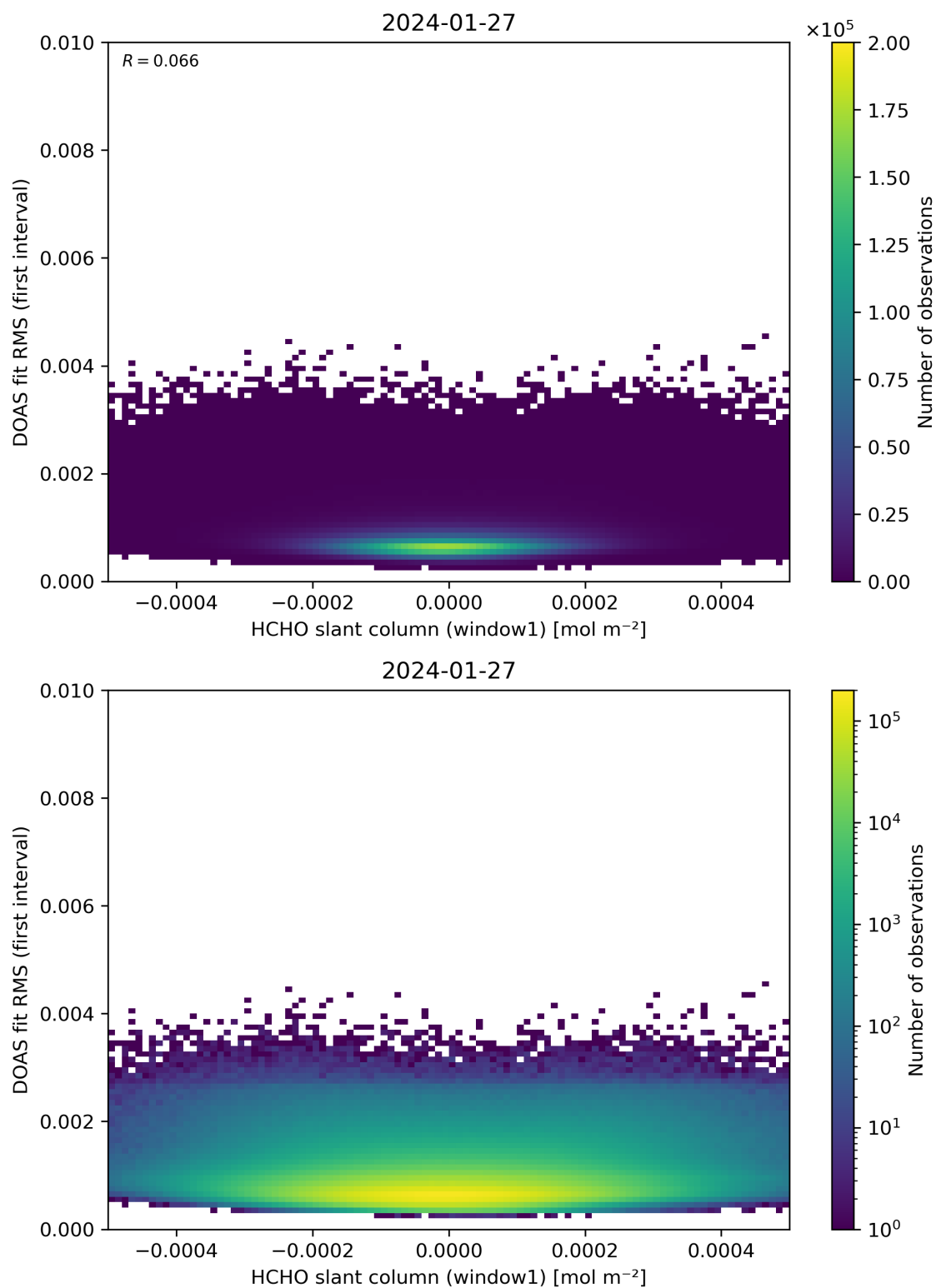
Figure 78: Scatter density plot of “HCHO slant column (window1)” against “DOAS fit RMS (first interval)” for 2024-01-26 to 2024-01-28.
