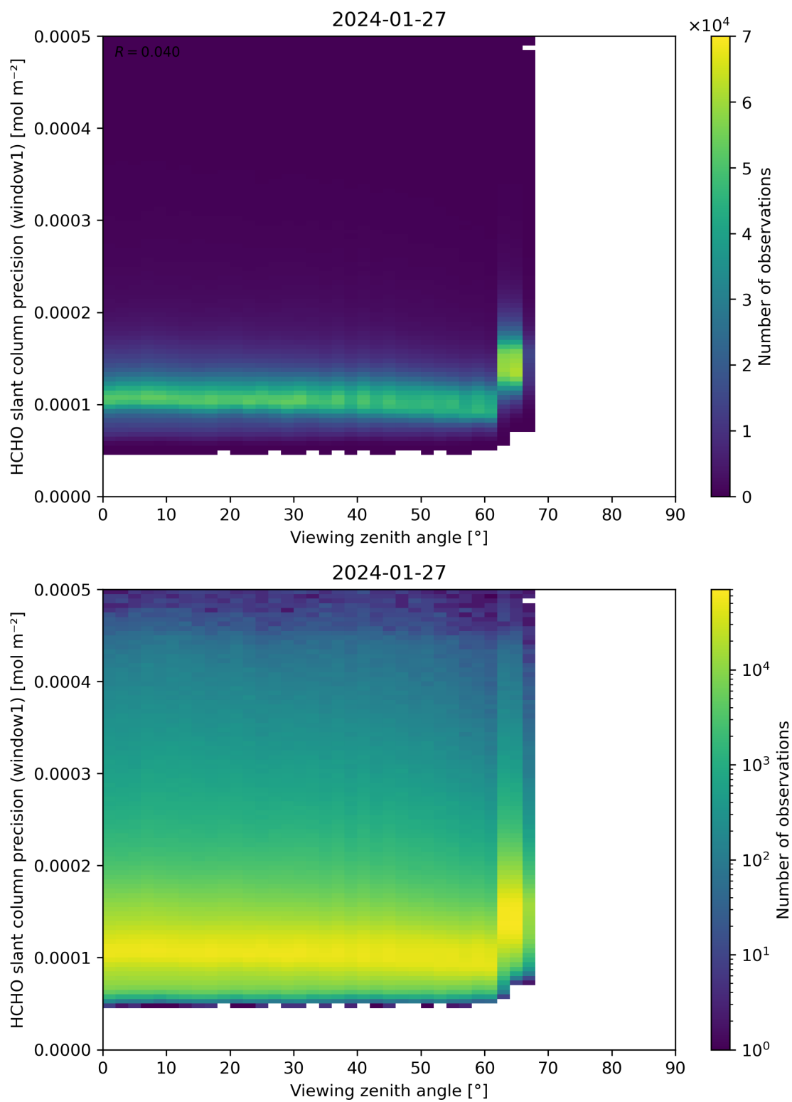
Figure 189: Scatter density plot of “Viewing zenith angle” against “HCHO slant column precision (window1)” for 2024-01-26 to 2024-01-28.
