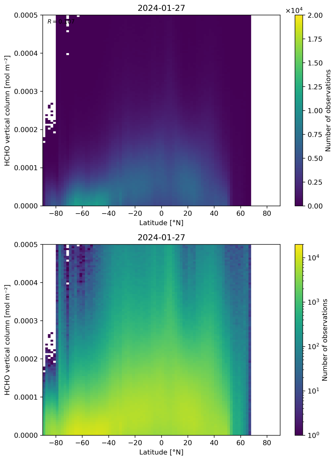
Figure 163: Scatter density plot of “Latitude” against “HCHO vertical column” for 2024-01-26 to 2024-01-28.
