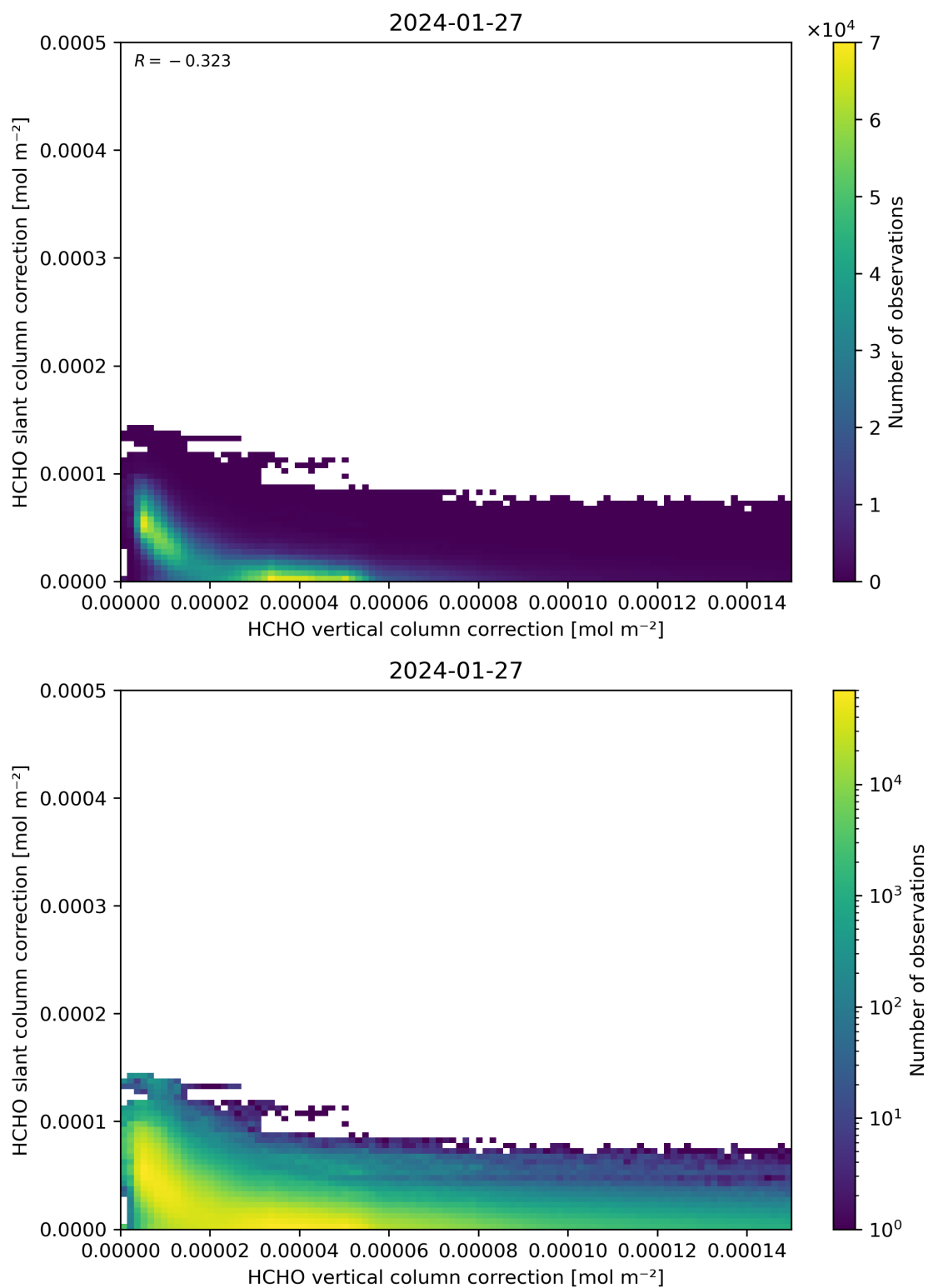
Figure 117: Scatter density plot of “HCHO vertical column correction” against “HCHO slant column correction” for 2024-01-26 to 2024-01-28.
