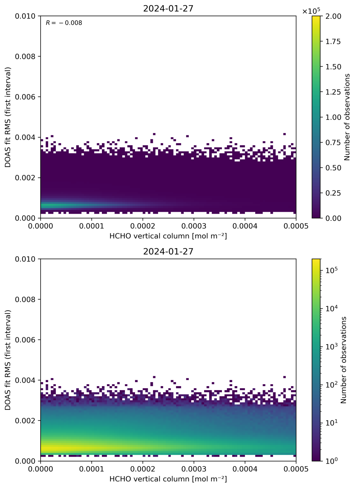
Figure 123: Scatter density plot of “HCHO vertical column” against “DOAS fit RMS (first interval)” for 2024-01-26 to 2024-01-28.
