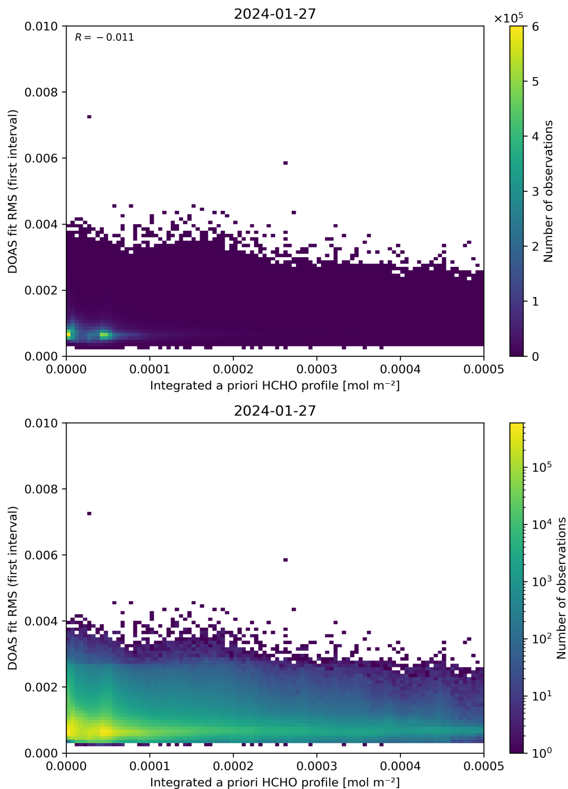
Figure 148: Scatter density plot of “Integrated a priori HCHO profile” against “DOAS fit RMS (first interval)” for 2024-01-26 to 2024-01-28.
