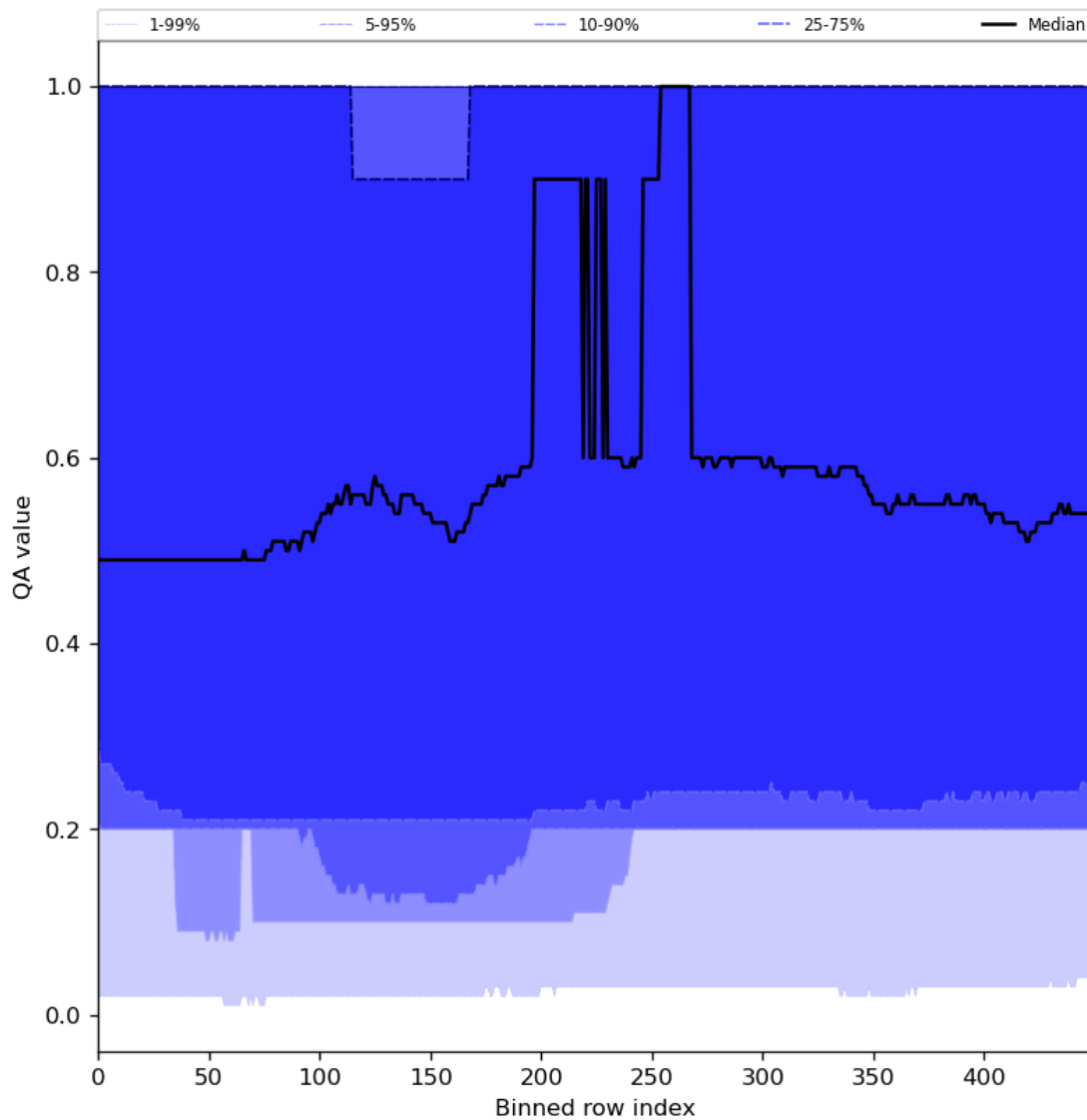
Figure 48: Along track statistics of “QA value” for 2024-01-26 to 2024-01-28
