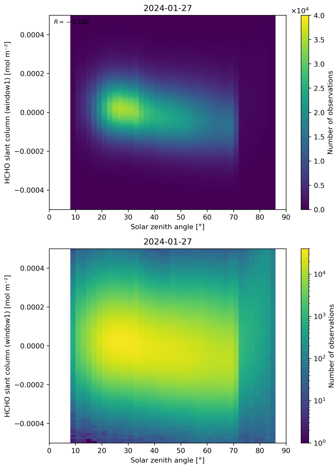
Figure 173: Scatter density plot of “Solar zenith angle” against “HCHO slant column (window1)” for 2024-01-26 to 2024-01-28.
