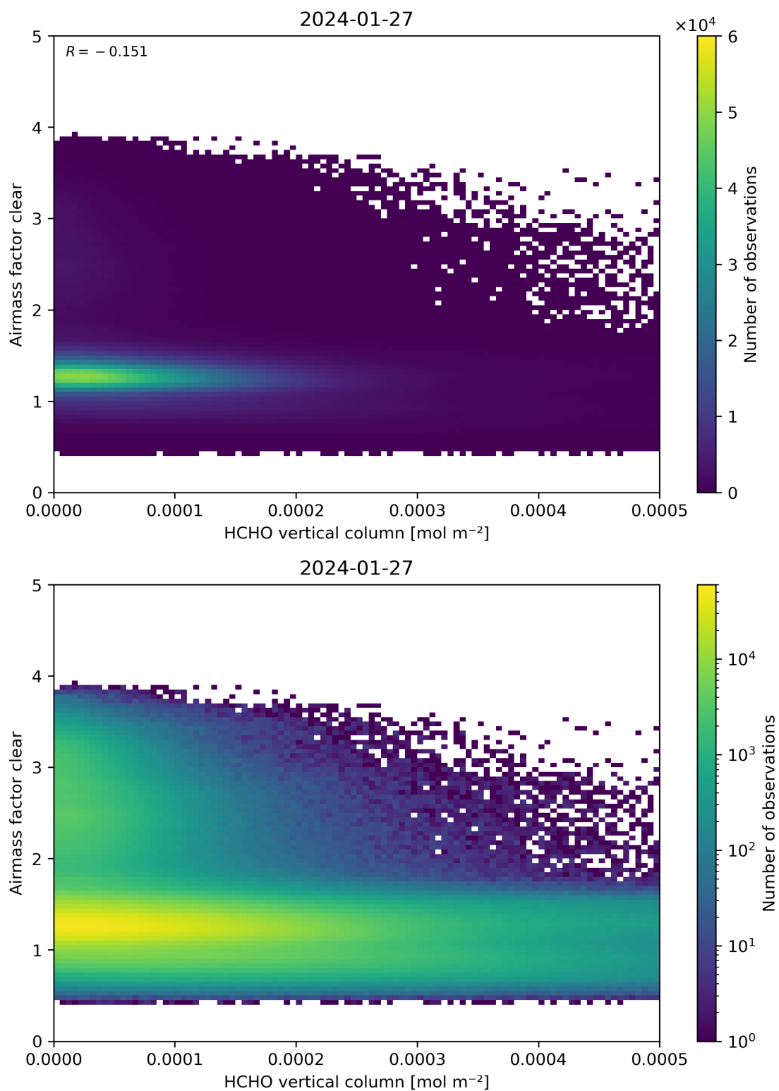
Figure 126: Scatter density plot of “HCHO vertical column” against “Airmass factor clear” for 2024-01-26 to 2024-01-28.
