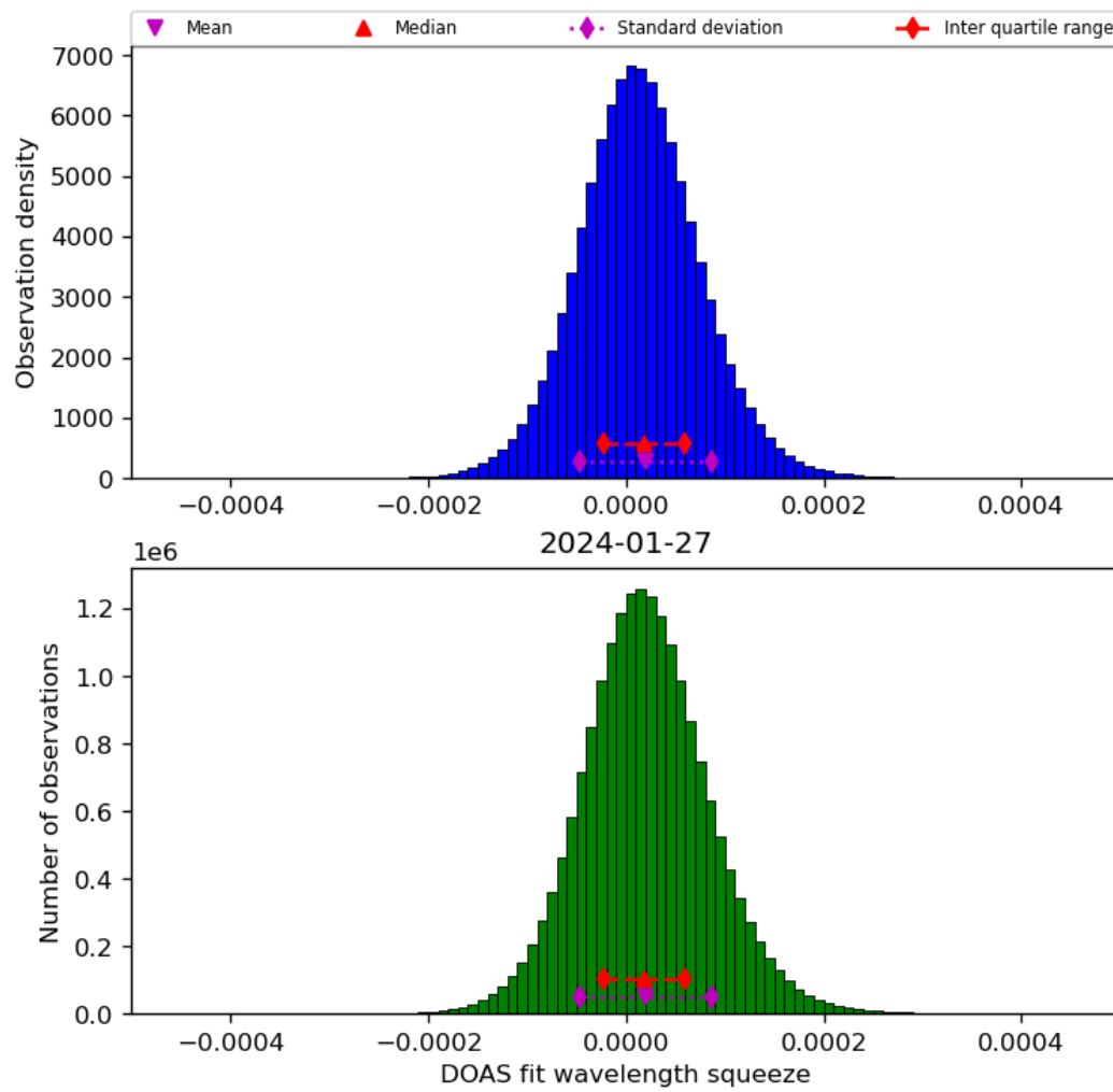
Figure 45: Histogram of “DOAS fit wavelength squeeze” for 2024-01-26 to 2024-01-28
