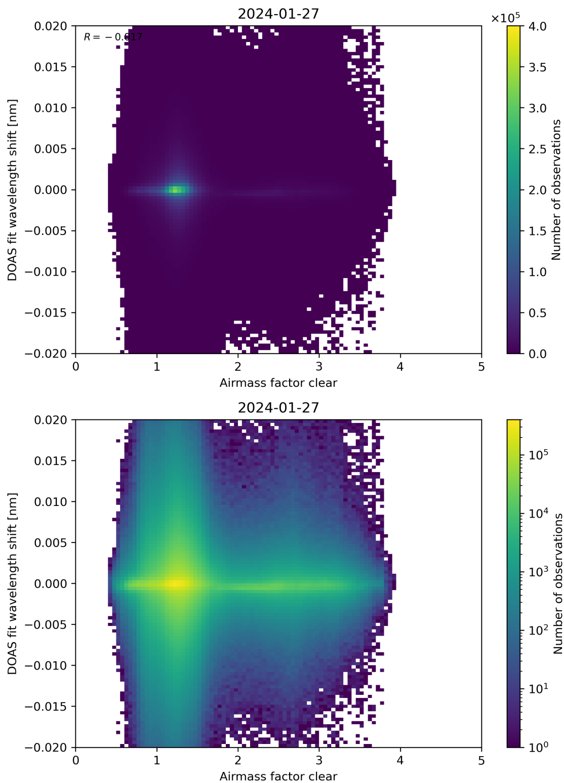
Figure 72: Scatter density plot of “Airmass factor clear” against “DOAS fit wavelength shift” for 2024-01-26 to 2024-01-28.
