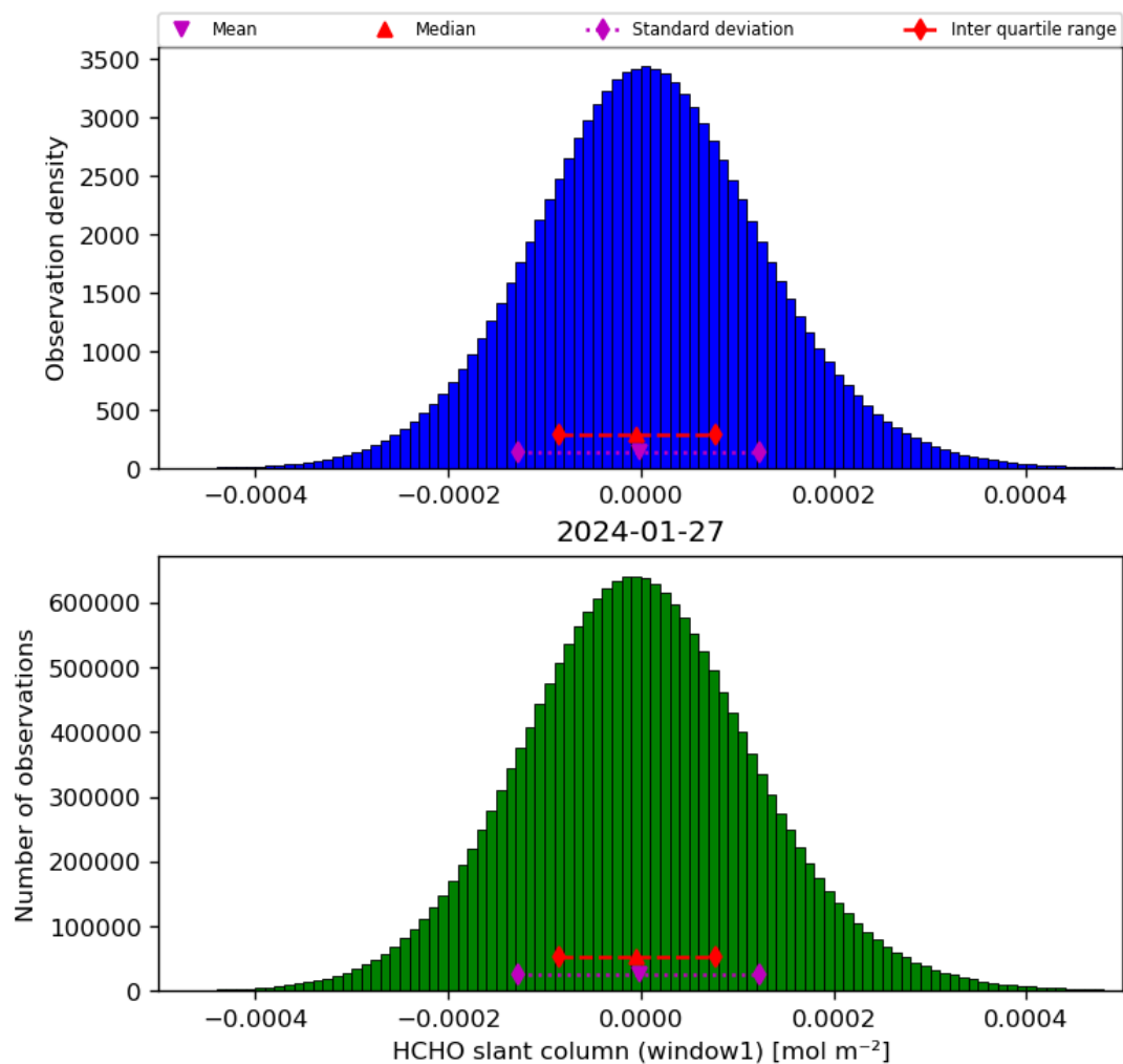
Figure 38: Histogram of “HCHO slant column (window1)” for 2024-01-26 to 2024-01-28
