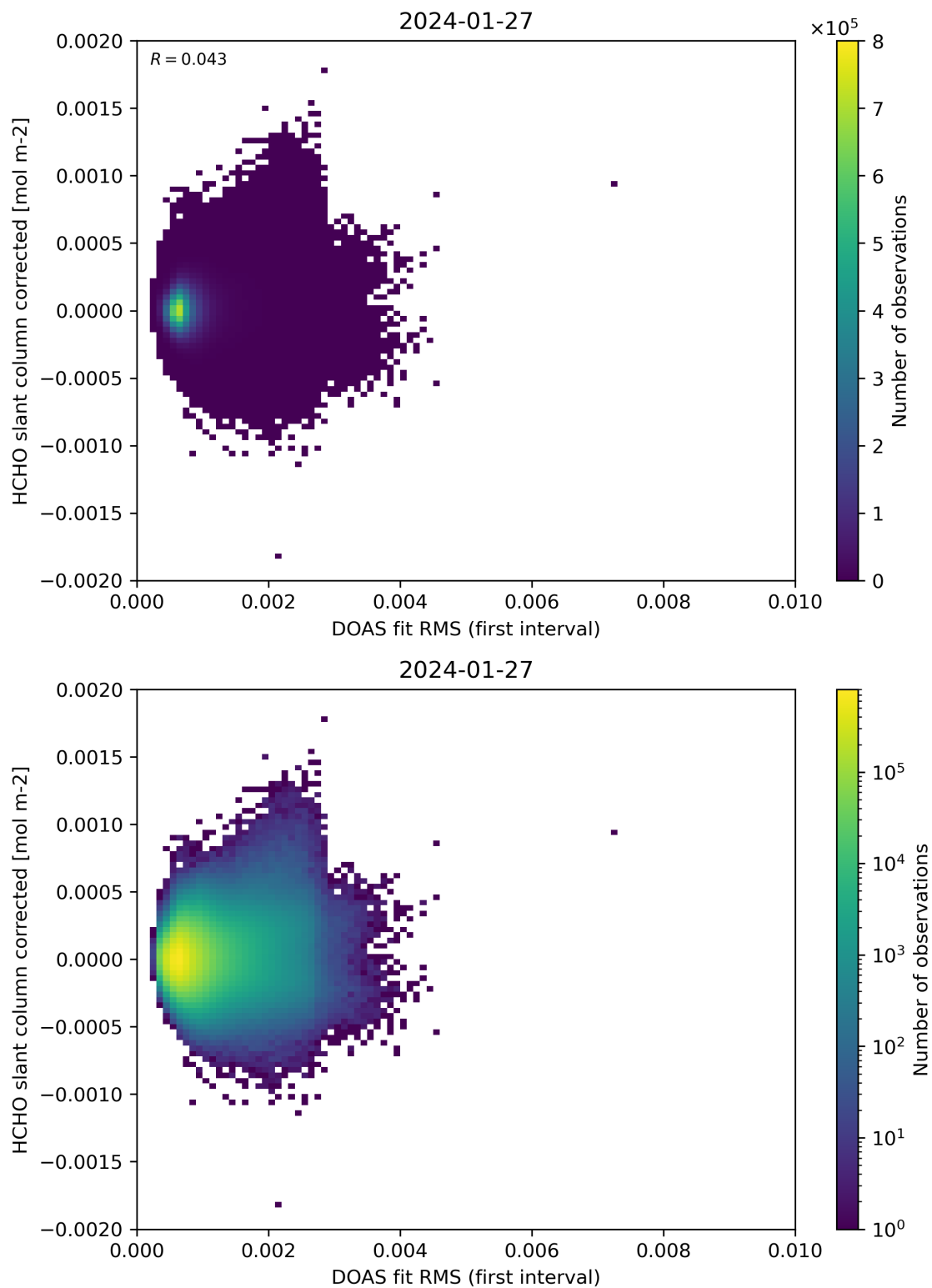
Figure 62: Scatter density plot of “DOAS fit RMS (first interval)” against “HCHO slant column corrected” for 2024-01-26 to 2024-01-28.
