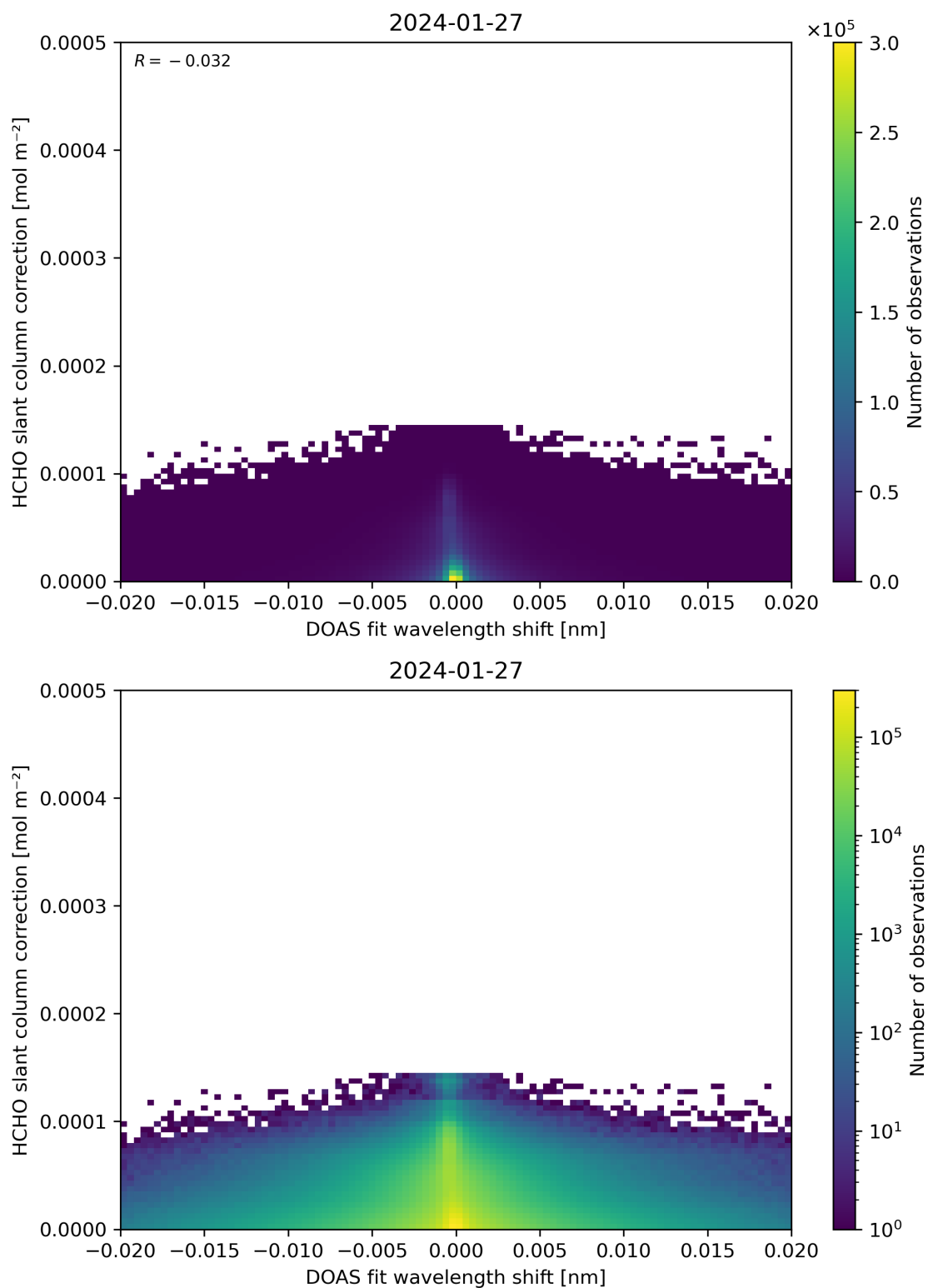
Figure 67: Scatter density plot of “DOAS fit wavelength shift” against “HCHO slant column correction” for 2024-01-26 to 2024-01-28.
