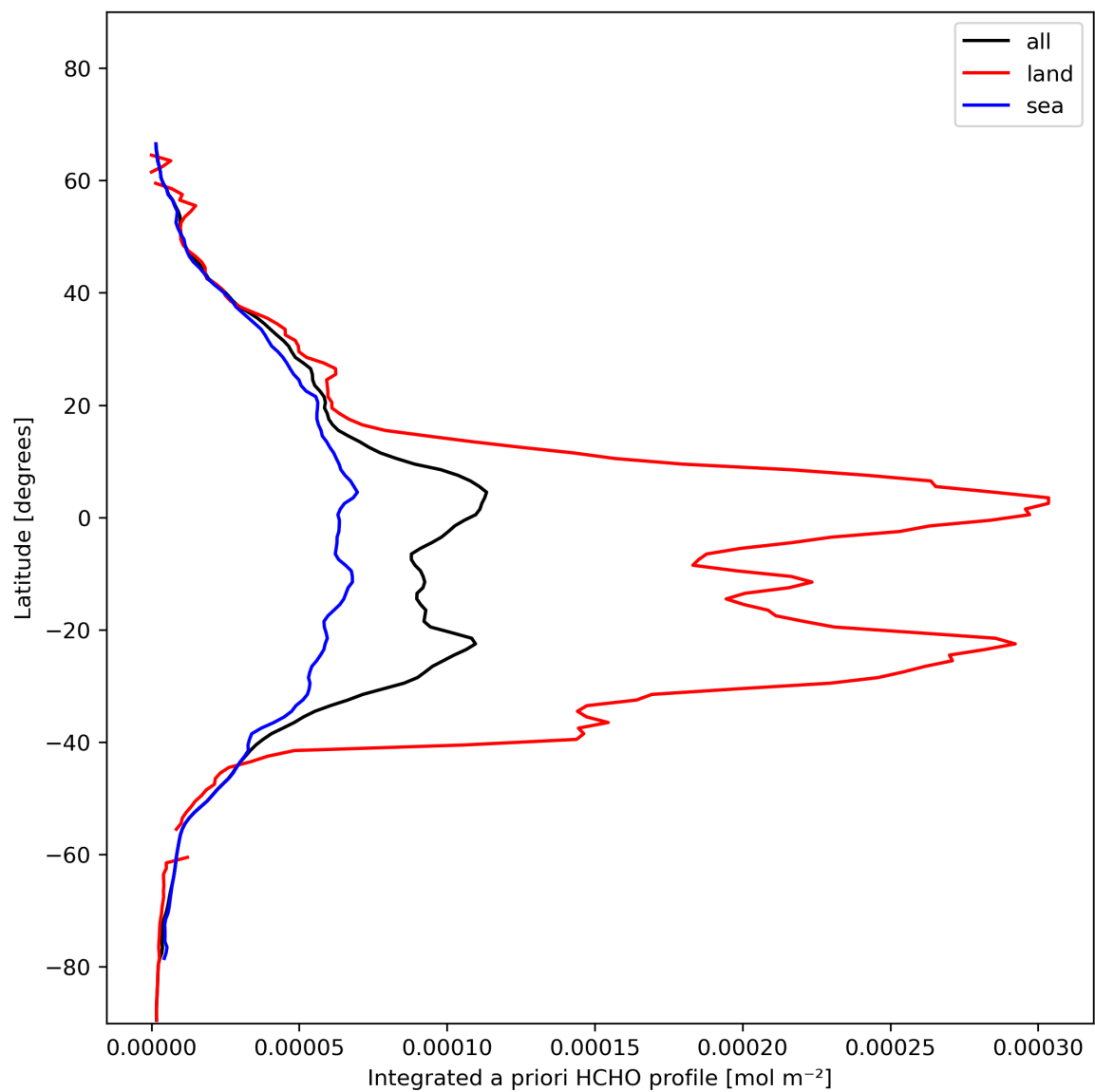
Figure 29: Zonal average of “Integrated a priori HCHO profile” for 2024-01-26 to 2024-01-28.
