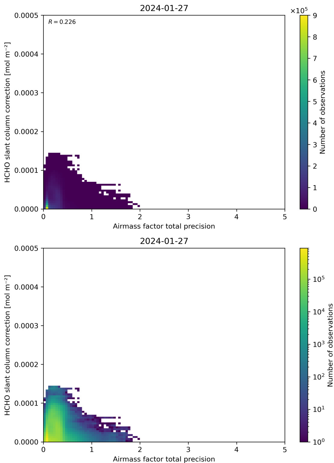
Figure 110: Scatter density plot of “Airmass factor total precision” against “HCHO slant column correction” for 2024-01-26 to 2024-01-28.
