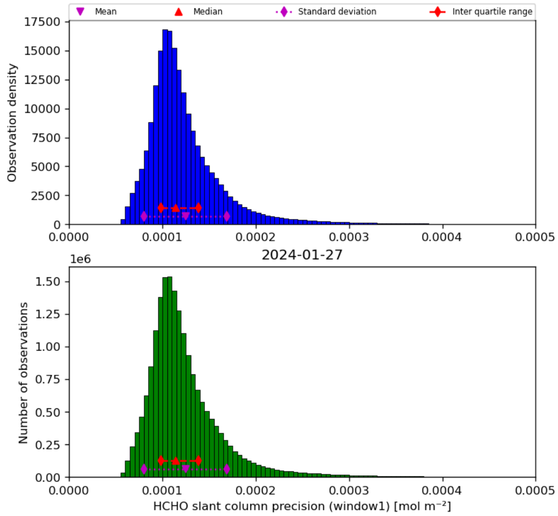
Figure 39: Histogram of “HCHO slant column precision (window1)” for 2024-01-26 to 2024-01-28
