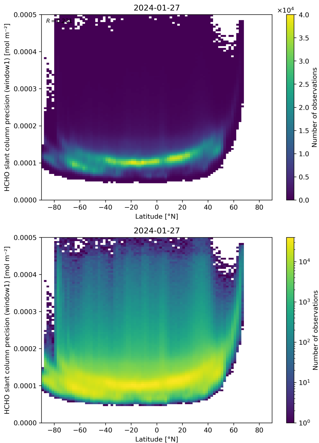
Figure 160: Scatter density plot of “Latitude” against “HCHO slant column precision (window1)” for 2024-01-26 to 2024-01-28.
