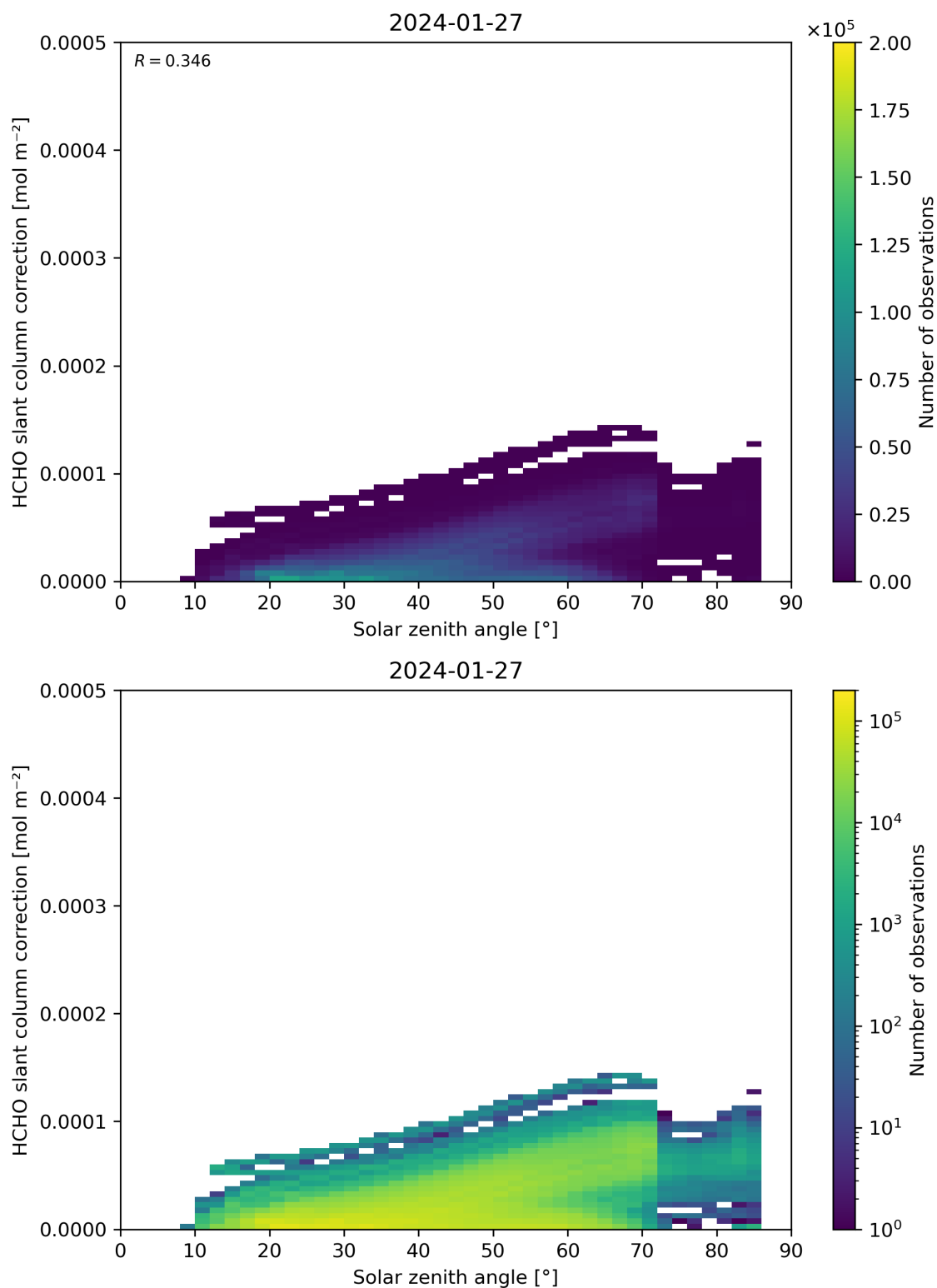
Figure 172: Scatter density plot of “Solar zenith angle” against “HCHO slant column correction” for 2024-01-26 to 2024-01-28.
