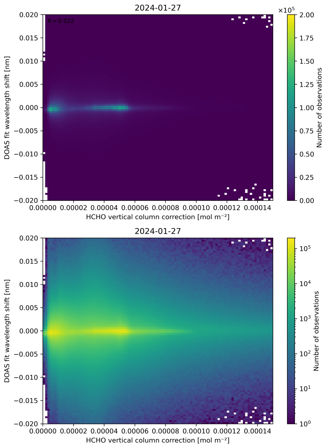
Figure 113: Scatter density plot of “HCHO vertical column correction” against “DOAS fit wavelength shift” for 2024-01-26 to 2024-01-28.
