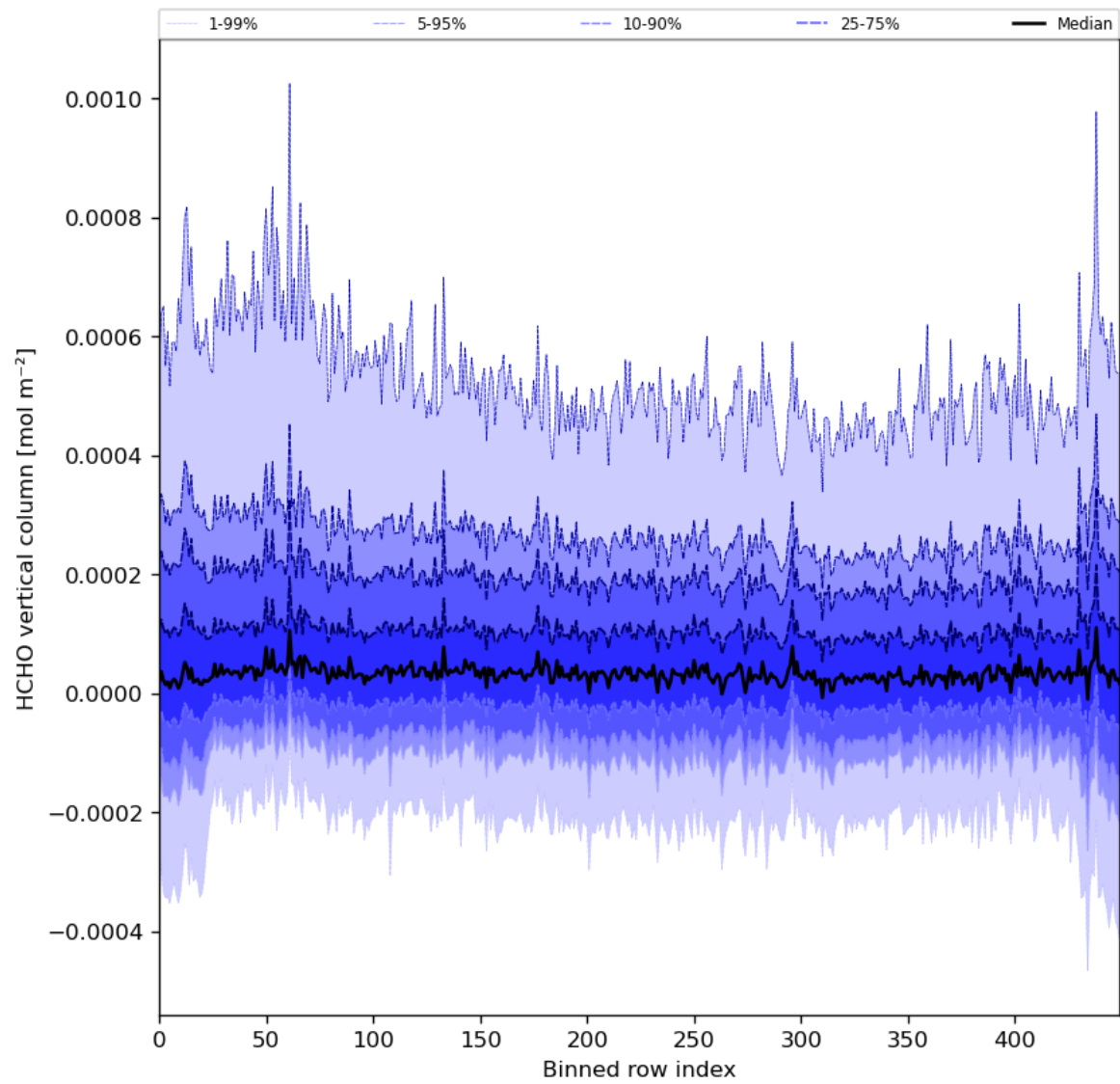
Figure 49: Along track statistics of “HCHO vertical column” for 2024-01-26 to 2024-01-28
