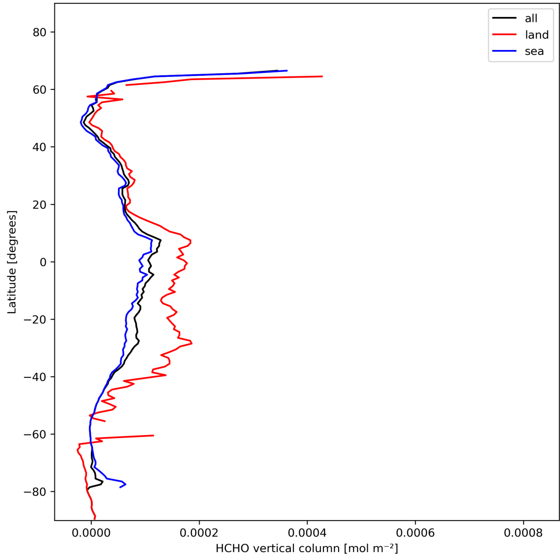
Figure 21: Zonal average of “HCHO vertical column” for 2024-01-26 to 2024-01-28.
