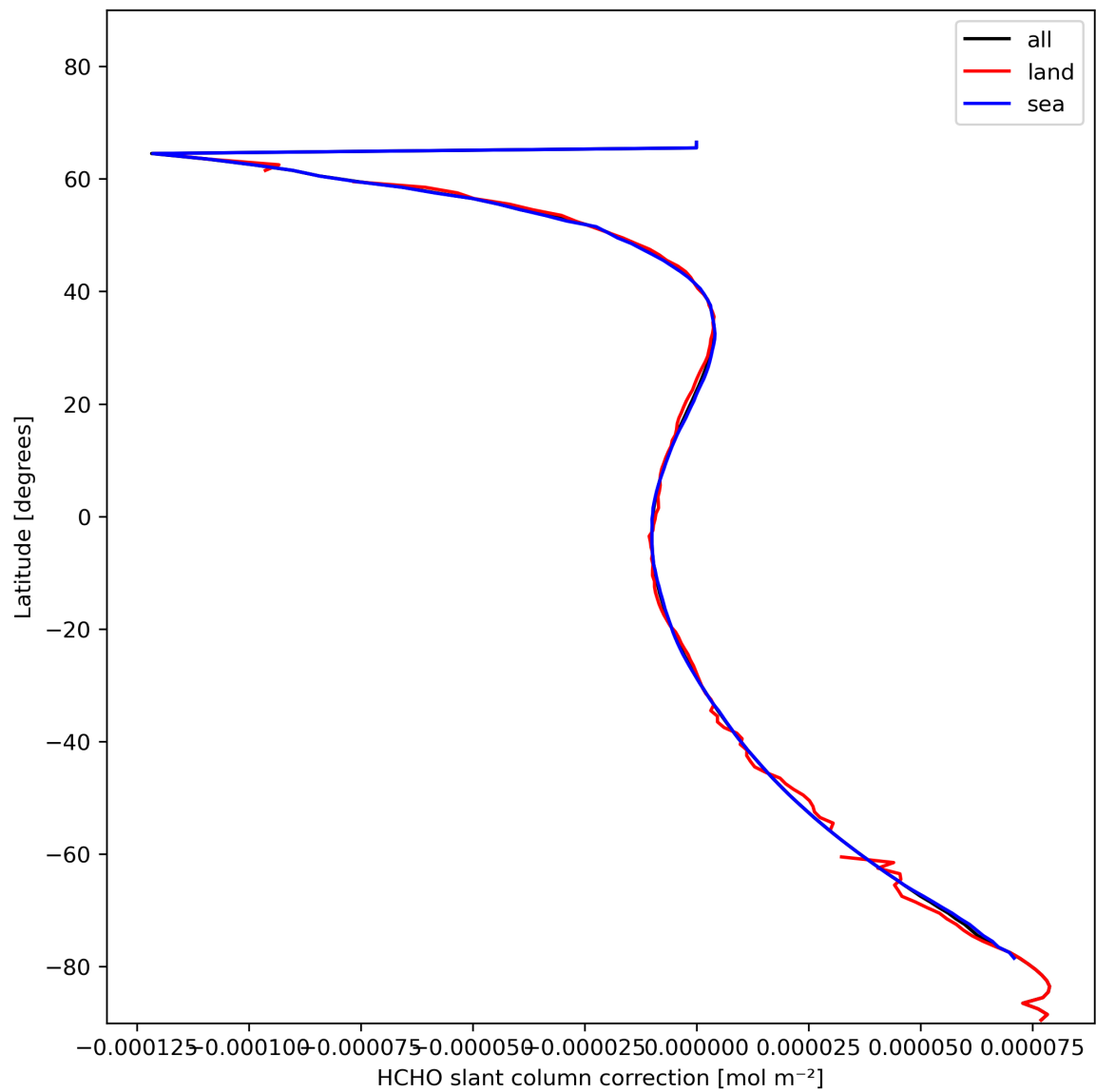
Figure 33: Zonal average of “HCHO slant column correction” for 2024-01-26 to 2024-01-28.
