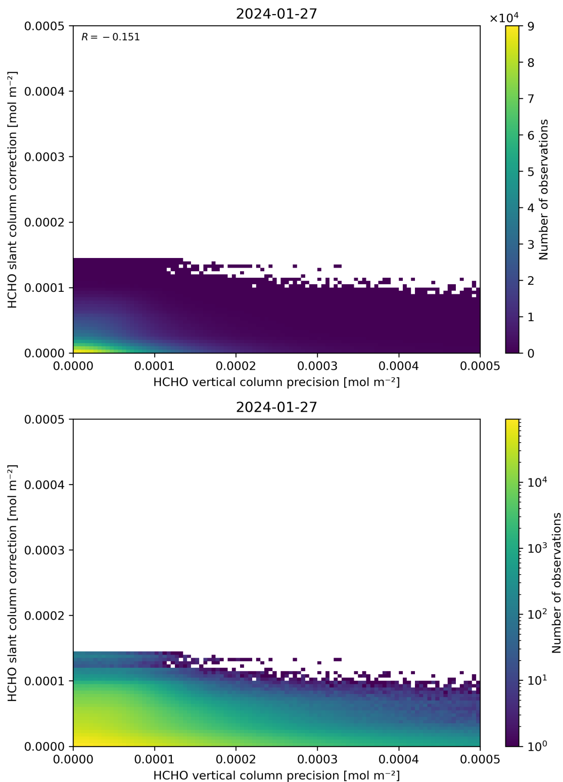
Figure 141: Scatter density plot of “HCHO vertical column precision” against “HCHO slant column correction” for 2024-01-26 to 2024-01-28.
