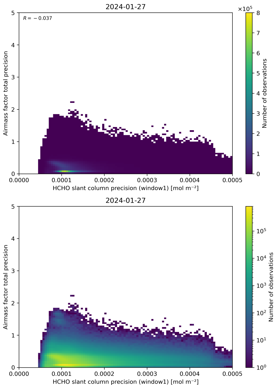
Figure 95: Scatter density plot of “HCHO slant column precision (window1)” against “Airmass factor total precision” for 2024-01-26 to 2024-01-28.
