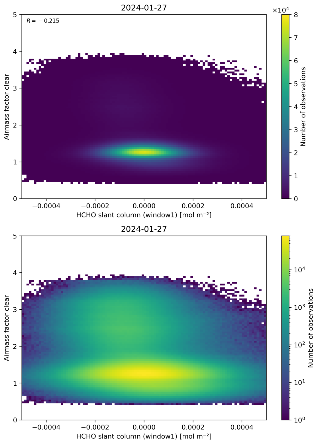
Figure 81: Scatter density plot of “HCHO slant column (window1)” against “Airmass factor clear” for 2024-01-26 to 2024-01-28.
