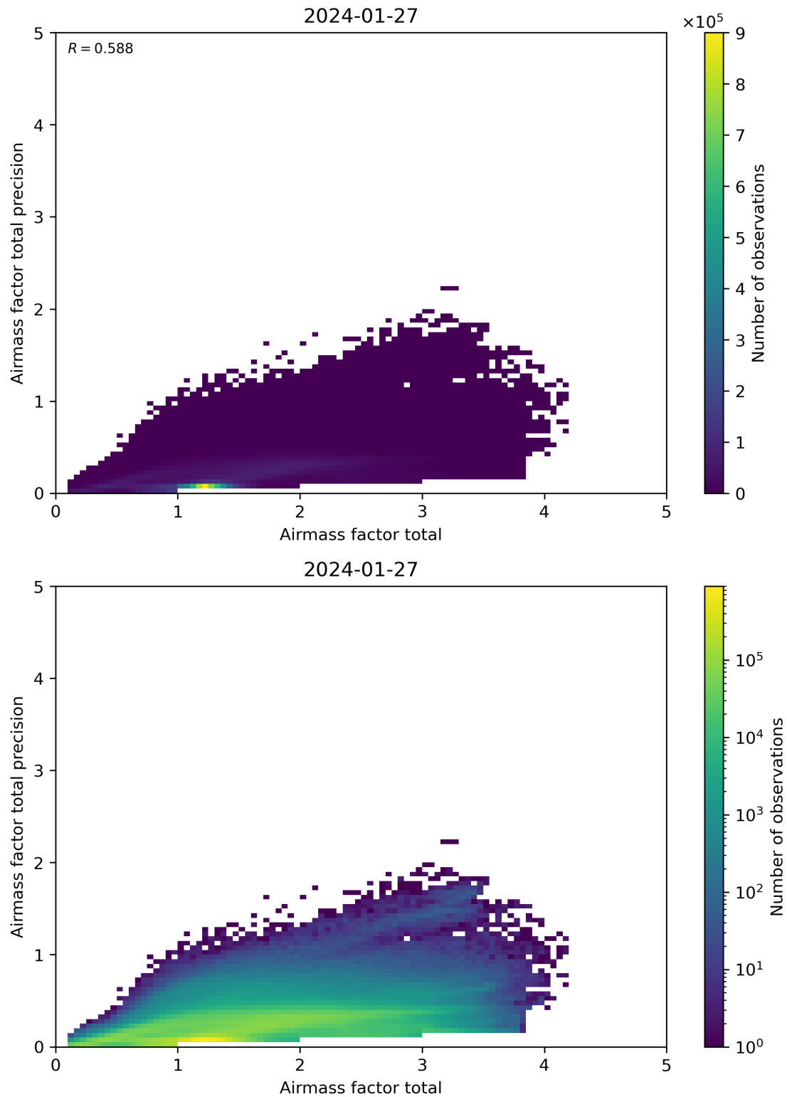
Figure 103: Scatter density plot of “Airmass factor total” against “Airmass factor total precision” for 2024-01-26 to 2024-01-28.
