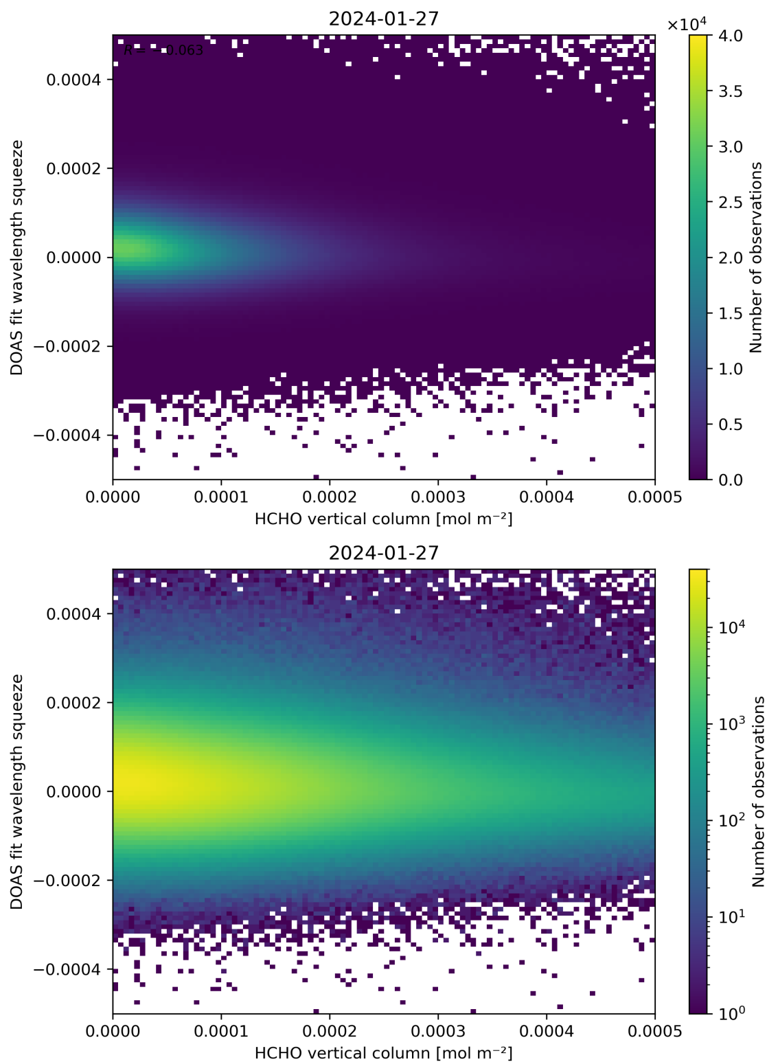
Figure 125: Scatter density plot of “HCHO vertical column” against “DOAS fit wavelength squeeze” for 2024-01-26 to 2024-01-28.
