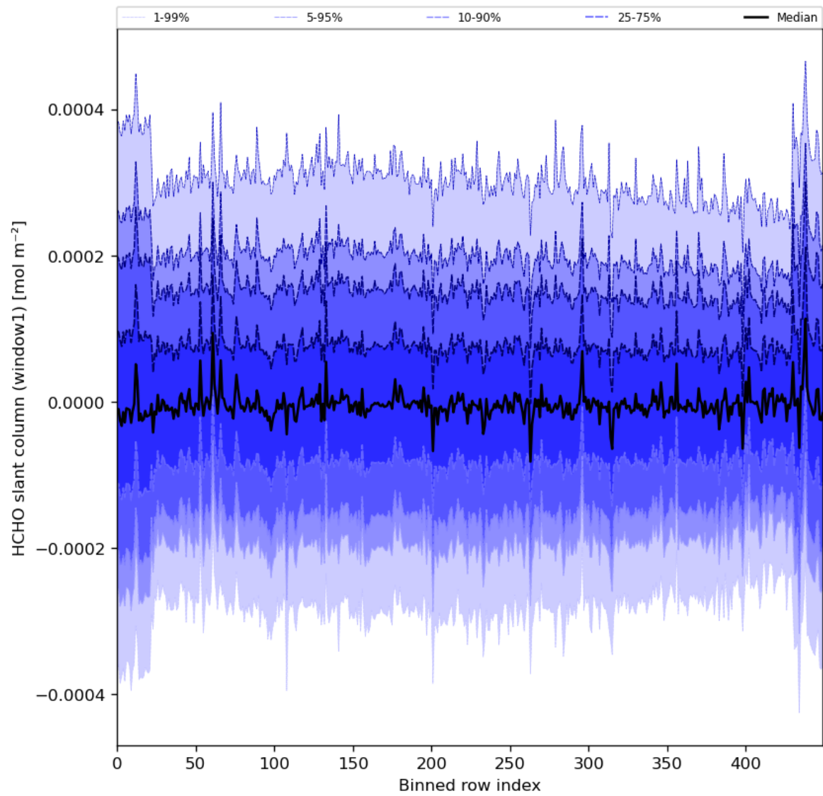
Figure 52: Along track statistics of “HCHO slant column (window1)” for 2024-01-26 to 2024-01-28
