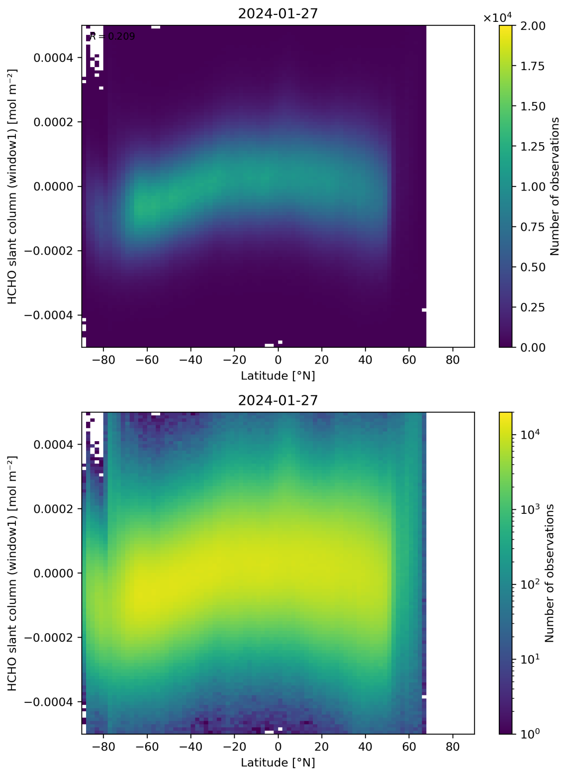
Figure 159: Scatter density plot of “Latitude” against “HCHO slant column (window1)” for 2024-01-26 to 2024-01-28.
