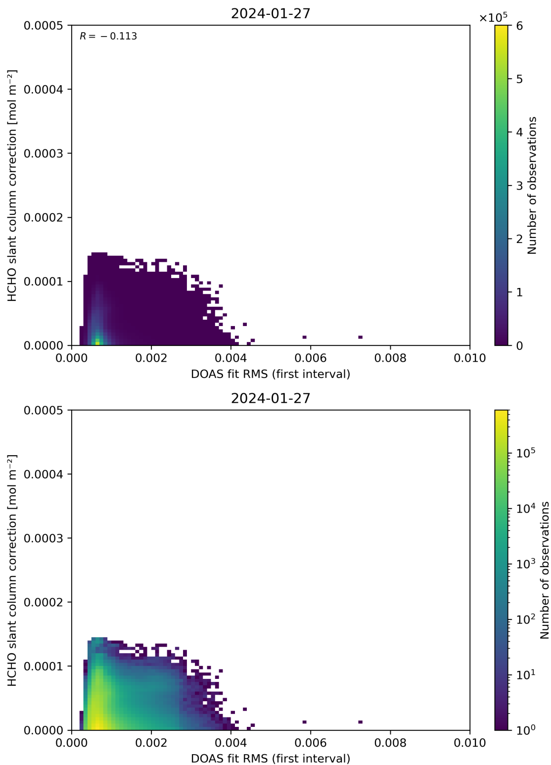
Figure 63: Scatter density plot of “DOAS fit RMS (first interval)” against “HCHO slant column correction” for 2024-01-26 to 2024-01-28.
