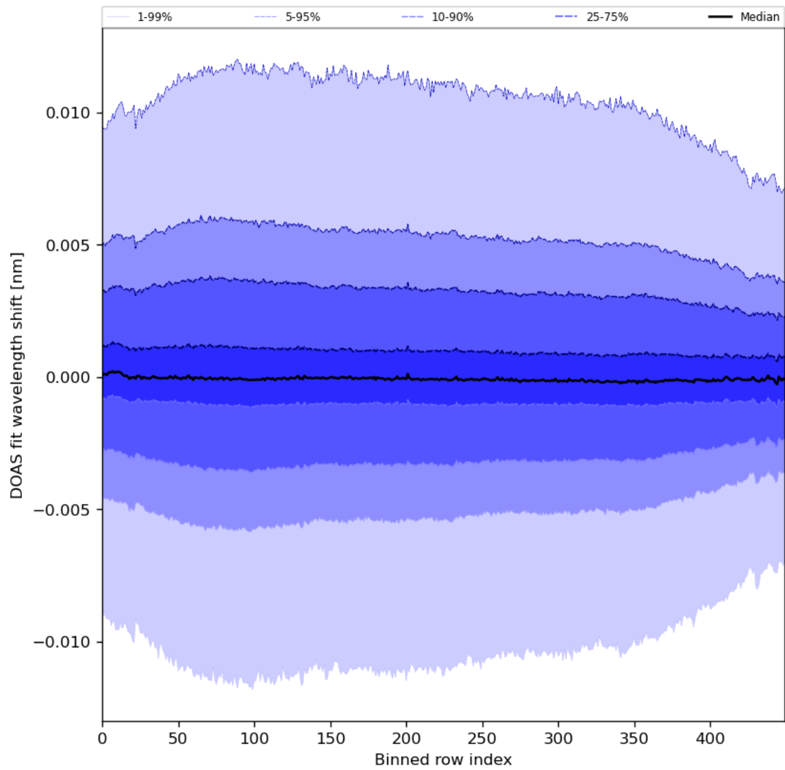
Figure 58: Along track statistics of “DOAS fit wavelength shift” for 2024-01-26 to 2024-01-28
