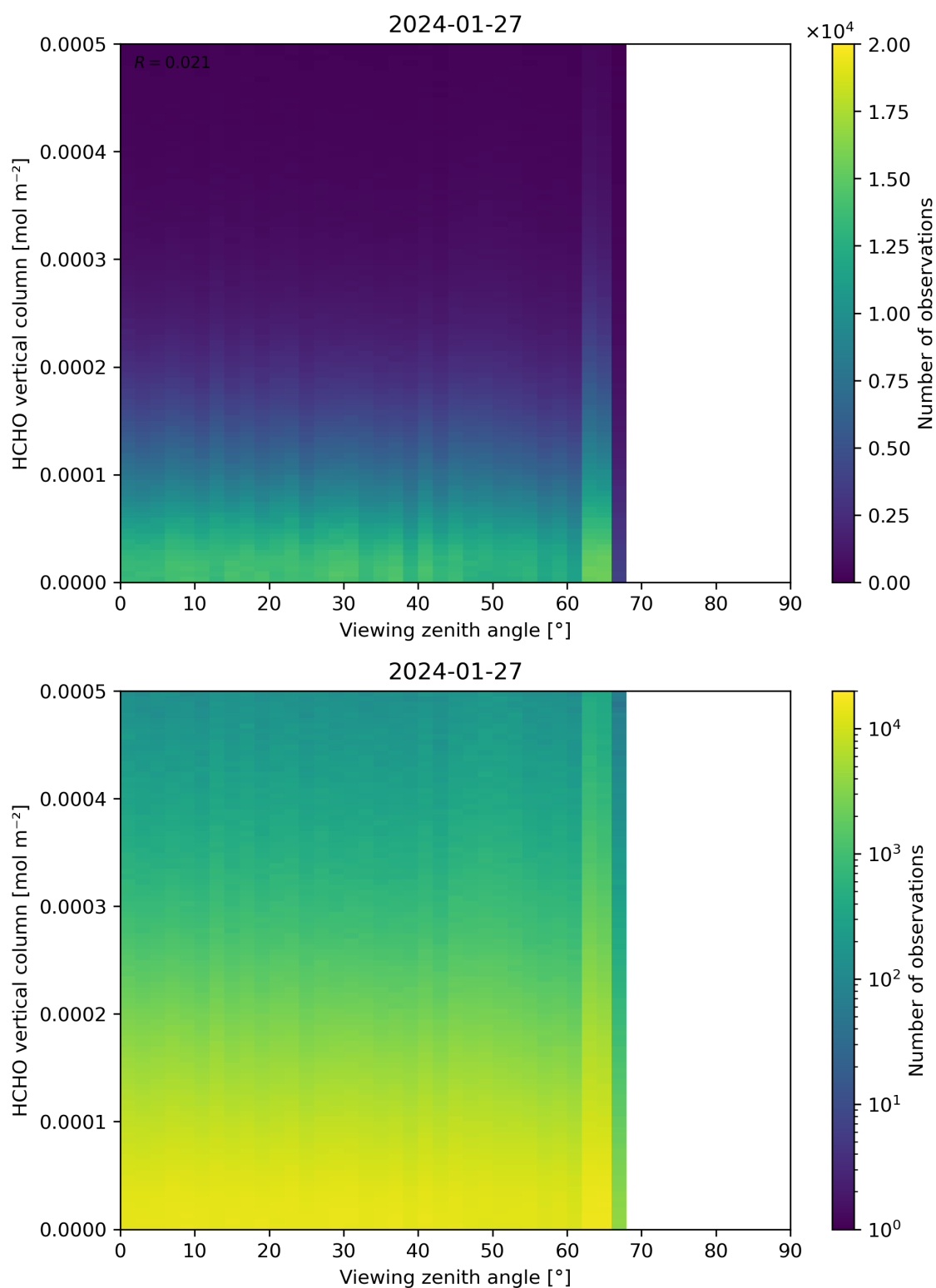
Figure 192: Scatter density plot of “Viewing zenith angle” against “HCHO vertical column” for 2024-01-26 to 2024-01-28.
