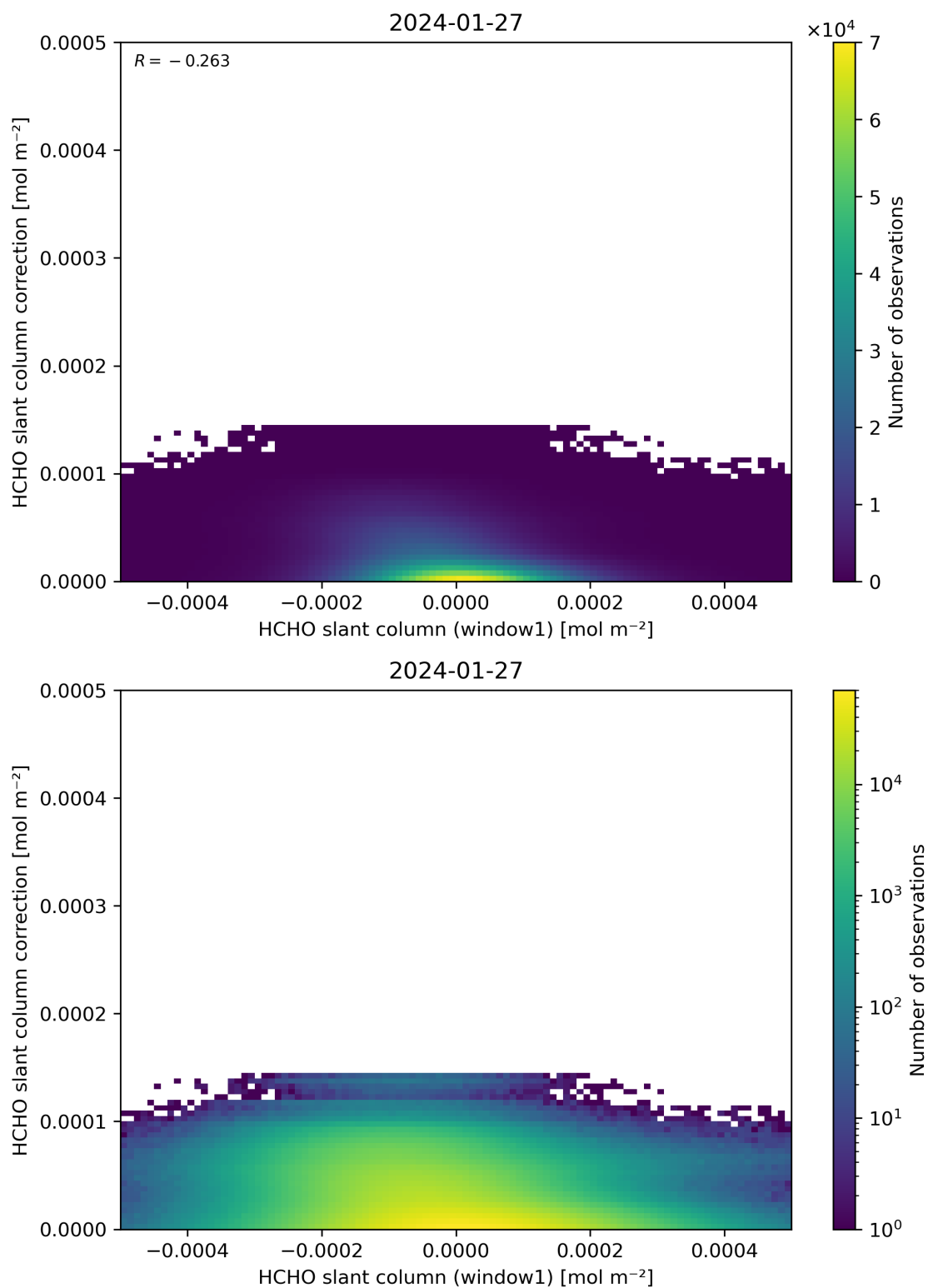
Figure 83: Scatter density plot of “HCHO slant column (window1)” against “HCHO slant column correction” for 2024-01-26 to 2024-01-28.
