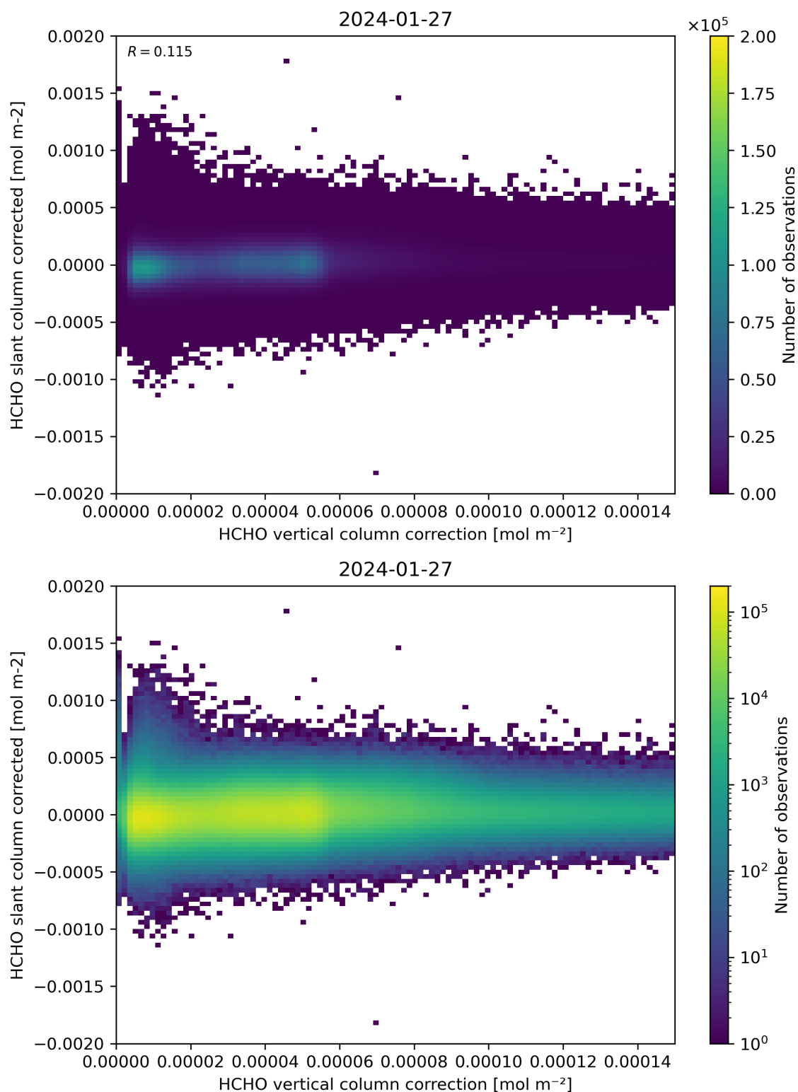
Figure 116: Scatter density plot of “HCHO vertical column correction” against “HCHO slant column corrected” for 2024-01-26 to 2024-01-28.
