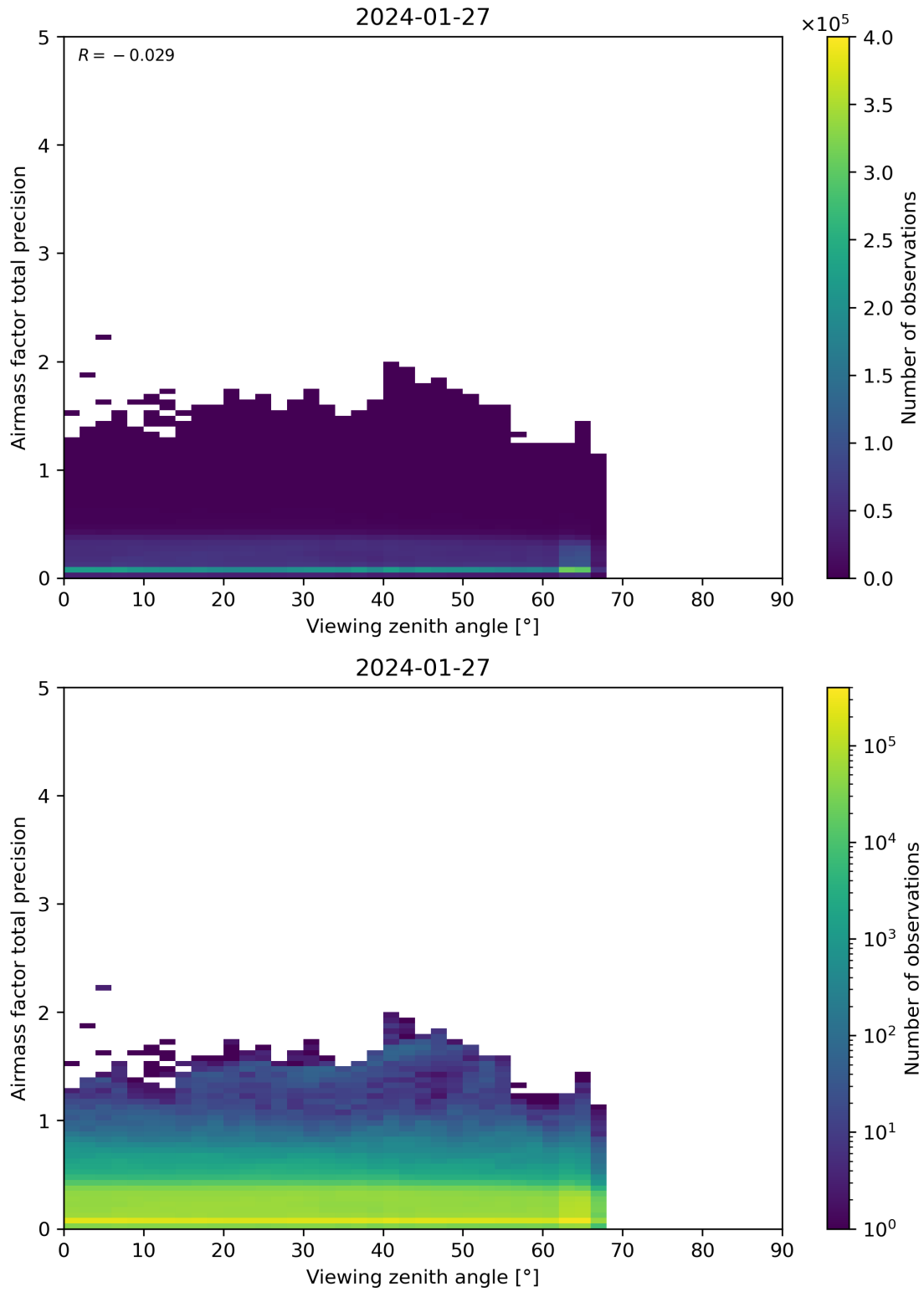
Figure 191: Scatter density plot of “Viewing zenith angle” against “Airmass factor total precision” for 2024-01-26 to 2024-01-28.
