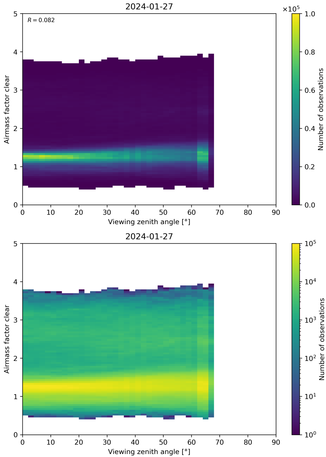
Figure 185: Scatter density plot of “Viewing zenith angle” against “Airmass factor clear” for 2024-01-26 to 2024-01-28.
