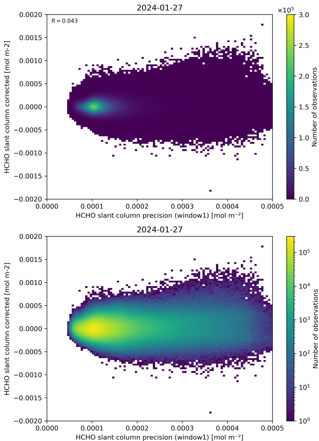
Figure 92: Scatter density plot of “HCHO slant column precision (window1)” against “HCHO slant column corrected” for 2024-01-26 to 2024-01-28.
