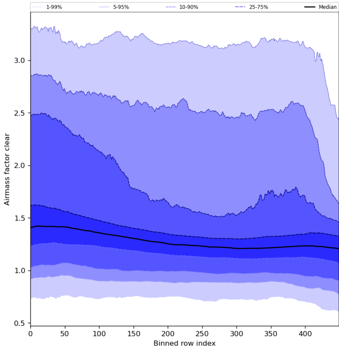
Figure 56: Along track statistics of “Airmass factor clear” for 2024-01-26 to 2024-01-28
