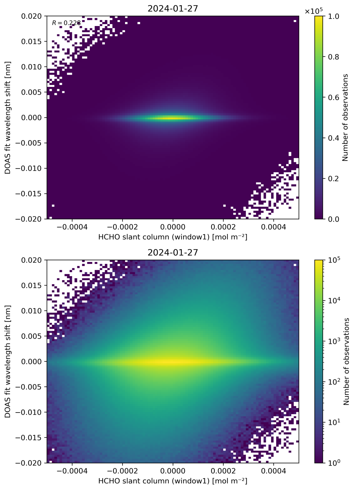
Figure 79: Scatter density plot of “HCHO slant column (window1)” against “DOAS fit wavelength shift” for 2024-01-26 to 2024-01-28.
