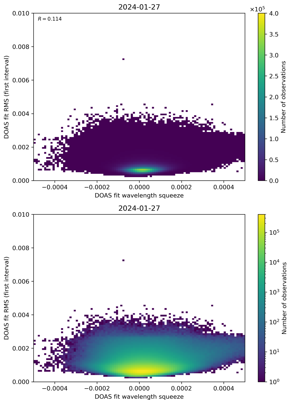
Figure 68: Scatter density plot of “DOAS fit wavelength squeeze” against “DOAS fit RMS (first interval)” for 2024-01-26 to 2024-01-28.
