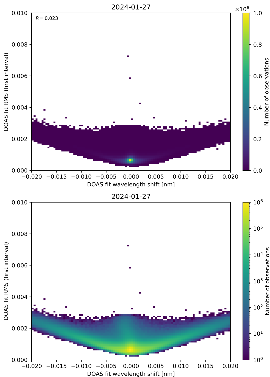
Figure 64: Scatter density plot of “DOAS fit wavelength shift” against “DOAS fit RMS (first interval)” for 2024-01-26 to 2024-01-28.
