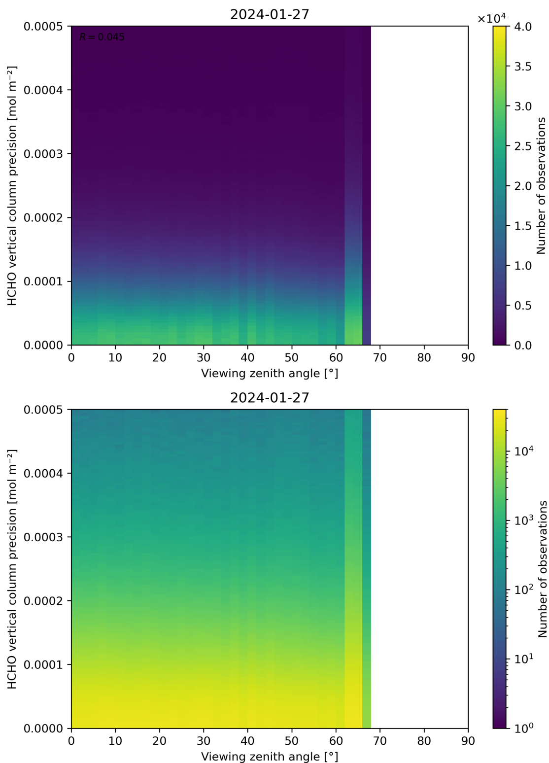
Figure 194: Scatter density plot of “Viewing zenith angle” against “HCHO vertical column precision” for 2024-01-26 to 2024-01-28.
