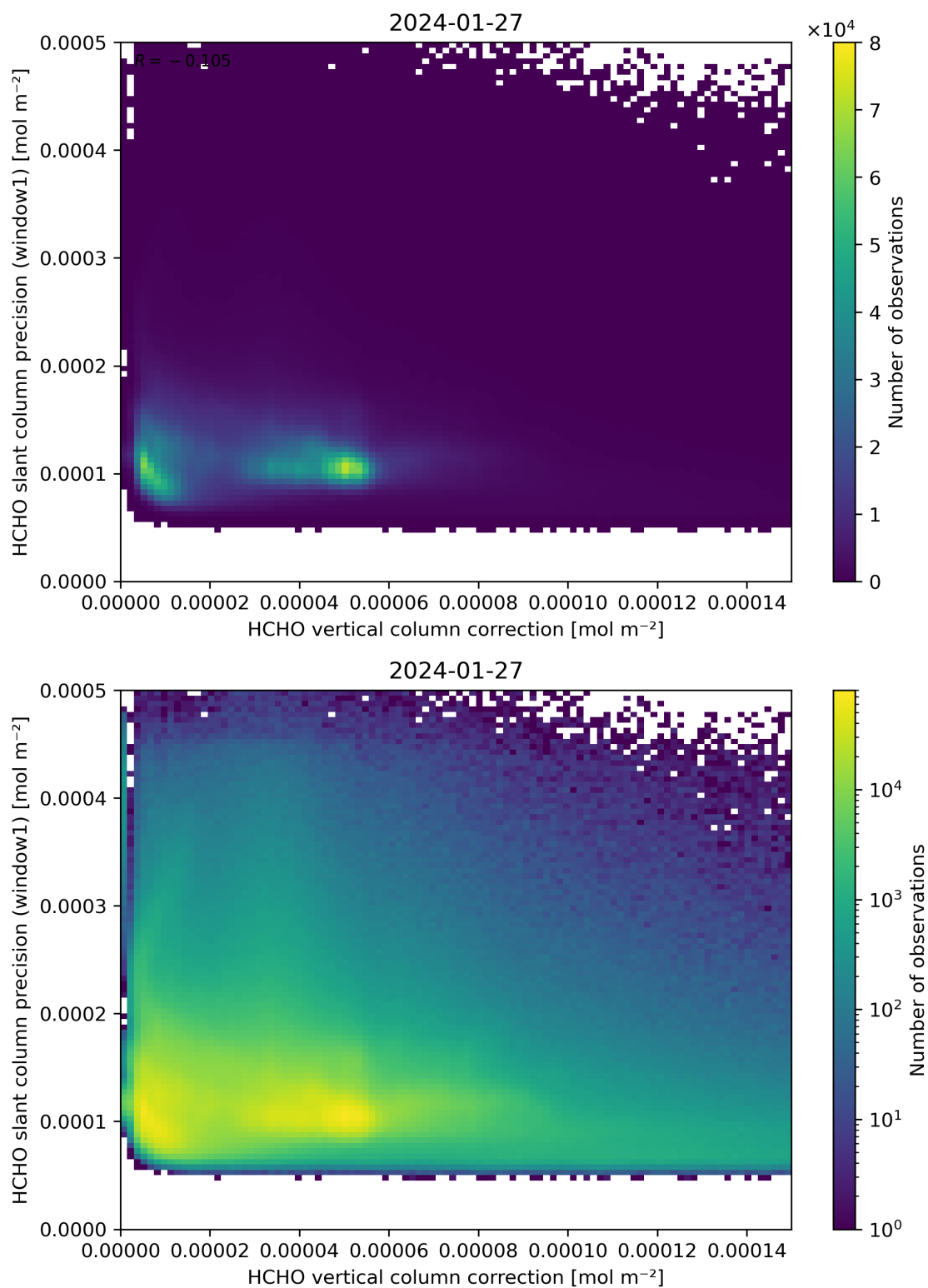
Figure 119: Scatter density plot of “HCHO vertical column correction” against “HCHO slant column precision (window1)” for 2024-01-26 to 2024-01-28.
