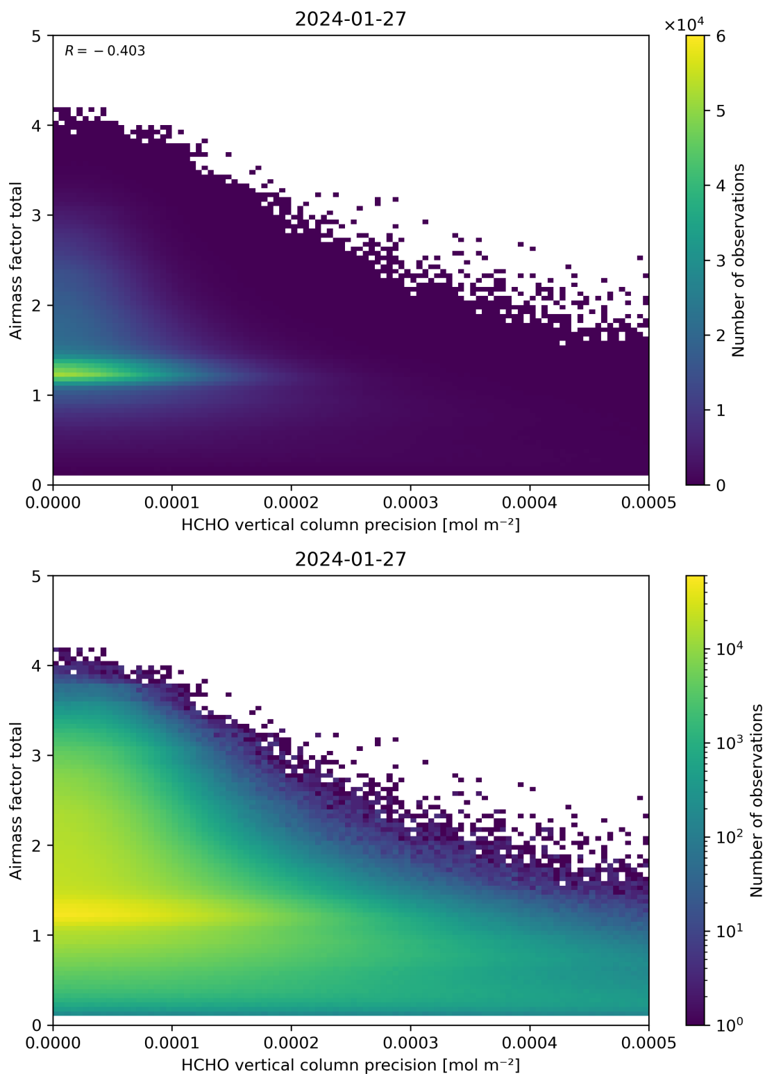
Figure 144: Scatter density plot of “HCHO vertical column precision” against “Airmass factor total” for 2024-01-26 to 2024-01-28.
