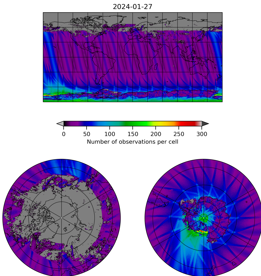
Figure 19: Map of the number of observations for 2024-01-26 to 2024-01-28
