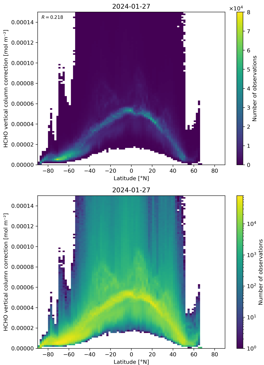
Figure 164: Scatter density plot of “Latitude” against “HCHO vertical column correction” for 2024-01-26 to 2024-01-28.
