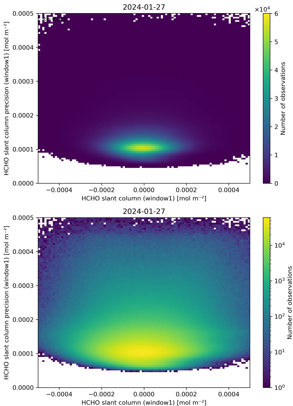
Figure 84: Scatter density plot of “HCHO slant column (window1)” against “HCHO slant column precision (window1)” for 2024-01-26 to 2024-01-28.
