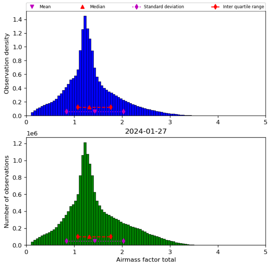
Figure 40: Histogram of “Airmass factor total” for 2024-01-26 to 2024-01-28
