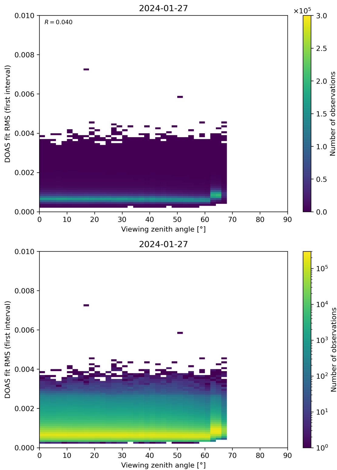
Figure 182: Scatter density plot of “Viewing zenith angle” against “DOAS fit RMS (first interval)” for 2024-01-26 to 2024-01-28.
