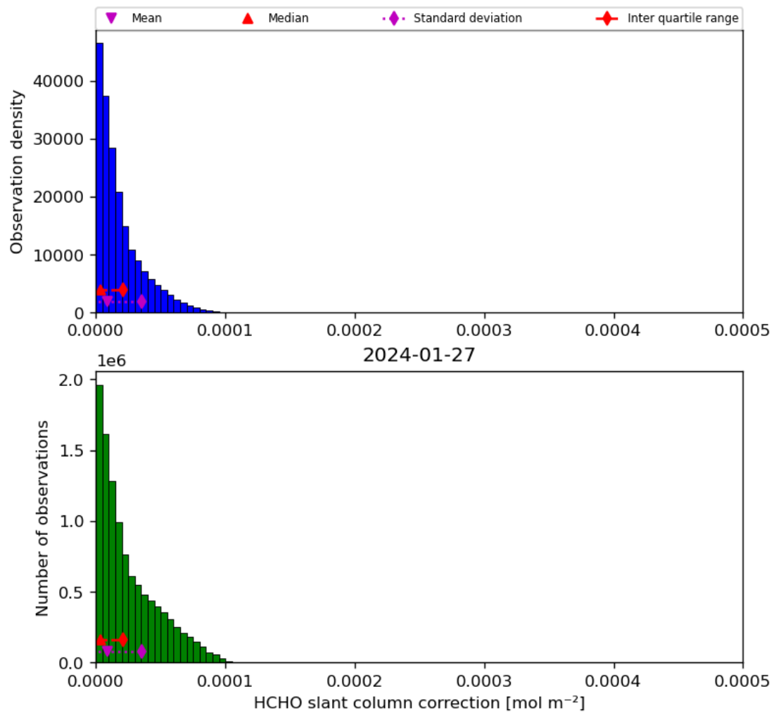
Figure 47: Histogram of “HCHO slant column correction” for 2024-01-26 to 2024-01-28
