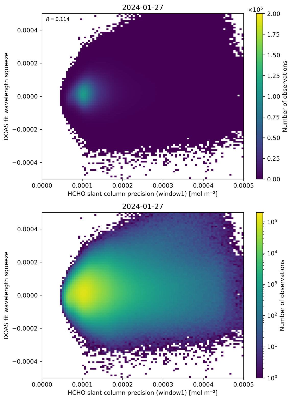
Figure 90: Scatter density plot of “HCHO slant column precision (window1)” against “DOAS fit wavelength squeeze” for 2024-01-26 to 2024-01-28.
