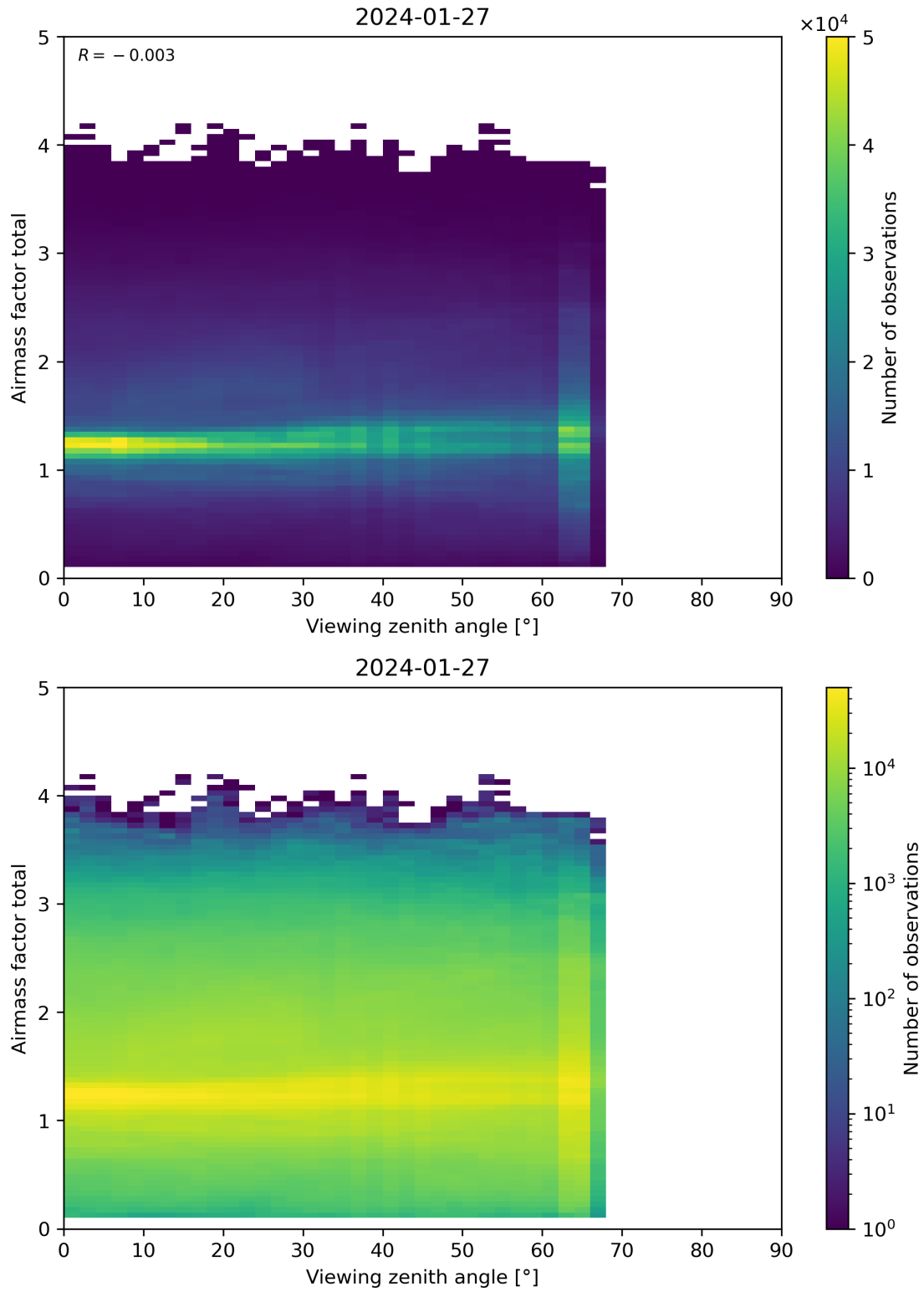
Figure 190: Scatter density plot of “Viewing zenith angle” against “Airmass factor total” for 2024-01-26 to 2024-01-28.
