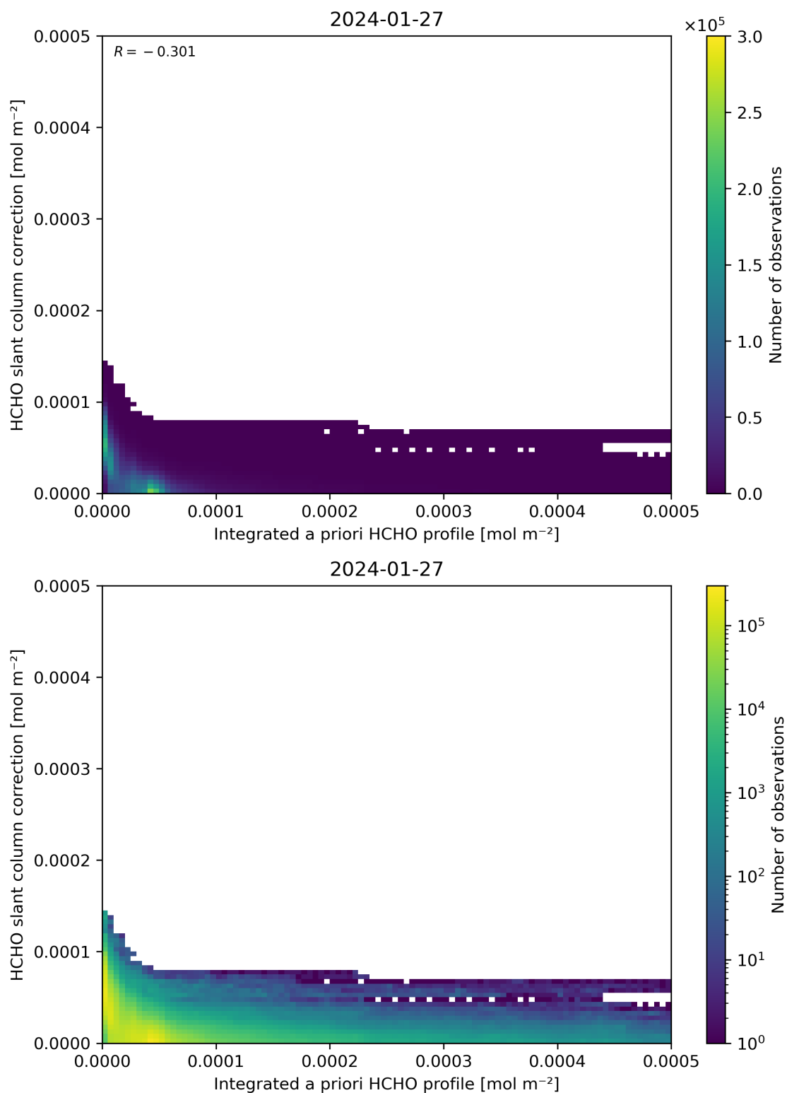
Figure 152: Scatter density plot of “Integrated a priori HCHO profile” against “HCHO slant column correction” for 2024-01-26 to 2024-01-28.
