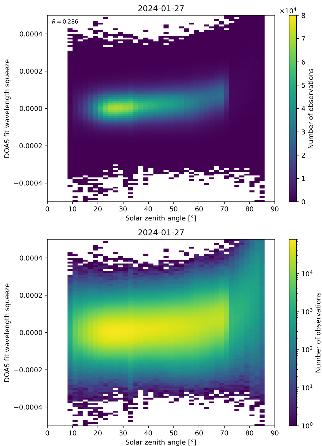
Figure 169: Scatter density plot of “Solar zenith angle” against “DOAS fit wavelength squeeze” for 2024-01-26 to 2024-01-28.
