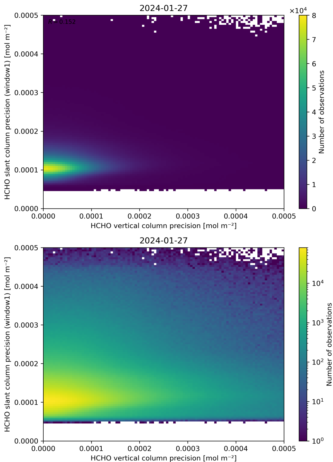
Figure 143: Scatter density plot of “HCHO vertical column precision” against “HCHO slant column precision (window1)” for 2024-01-26 to 2024-01-28.
