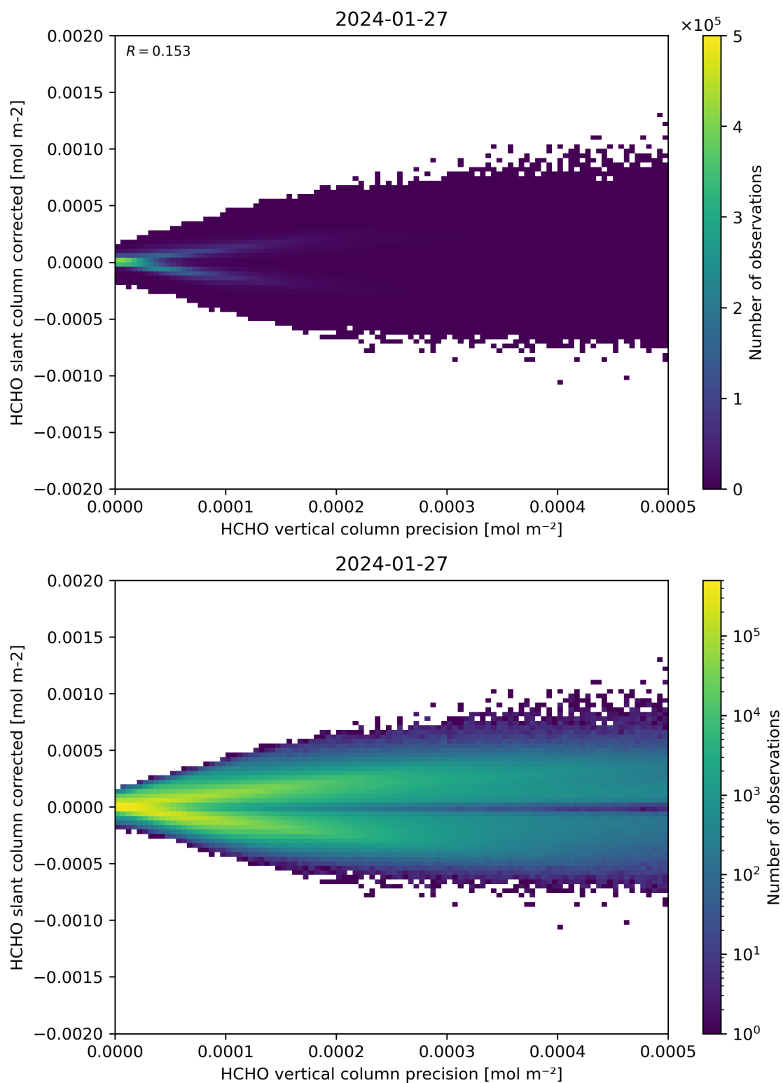
Figure 140: Scatter density plot of “HCHO vertical column precision” against “HCHO slant column corrected” for 2024-01-26 to 2024-01-28.
