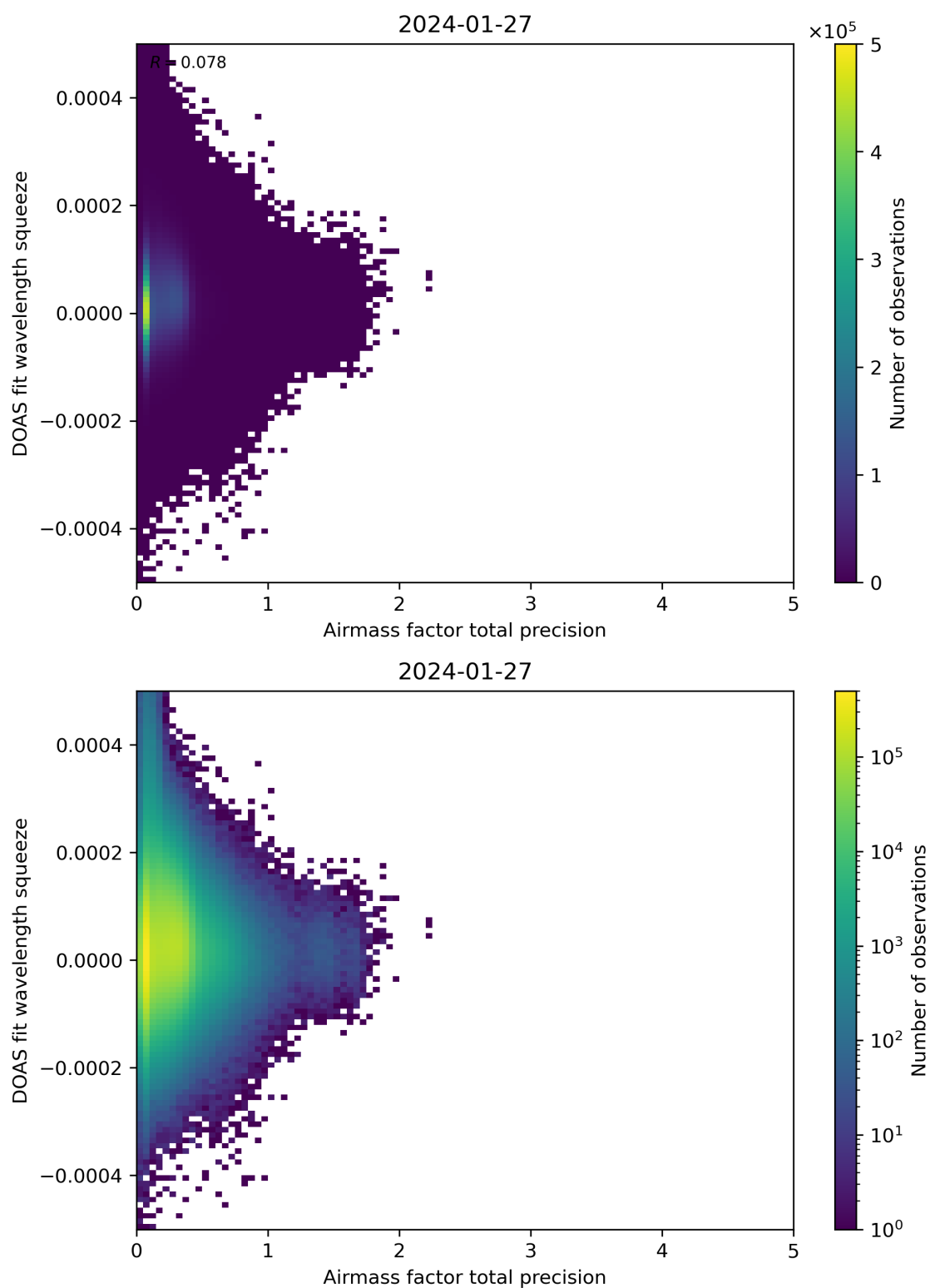
Figure 107: Scatter density plot of “Airmass factor total precision” against “DOAS fit wavelength squeeze” for 2024-01-26 to 2024-01-28.
