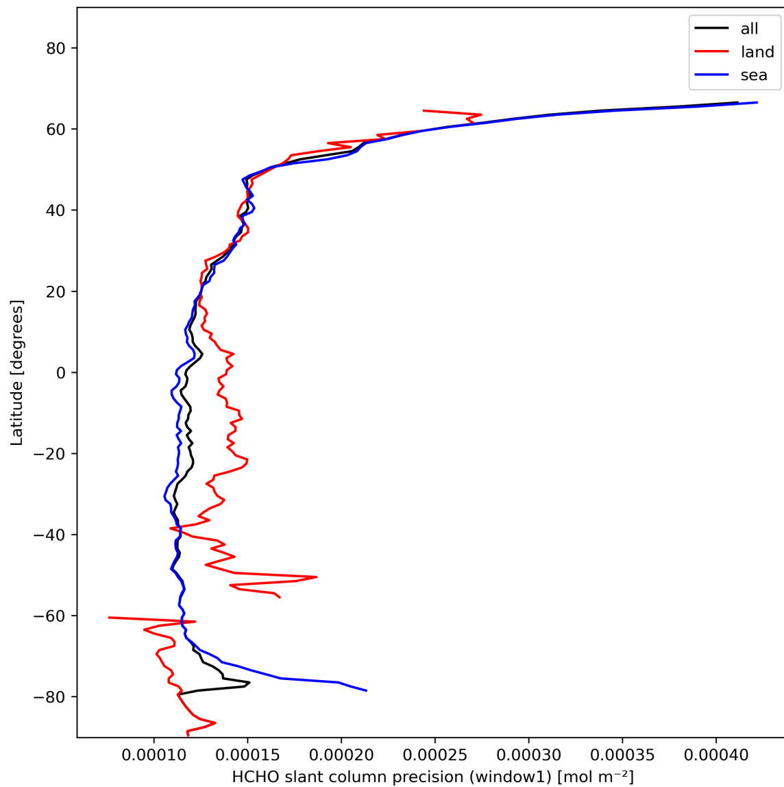
Figure 25: Zonal average of “HCHO slant column precision (window1)” for 2024-01-26 to 2024-01-28.
