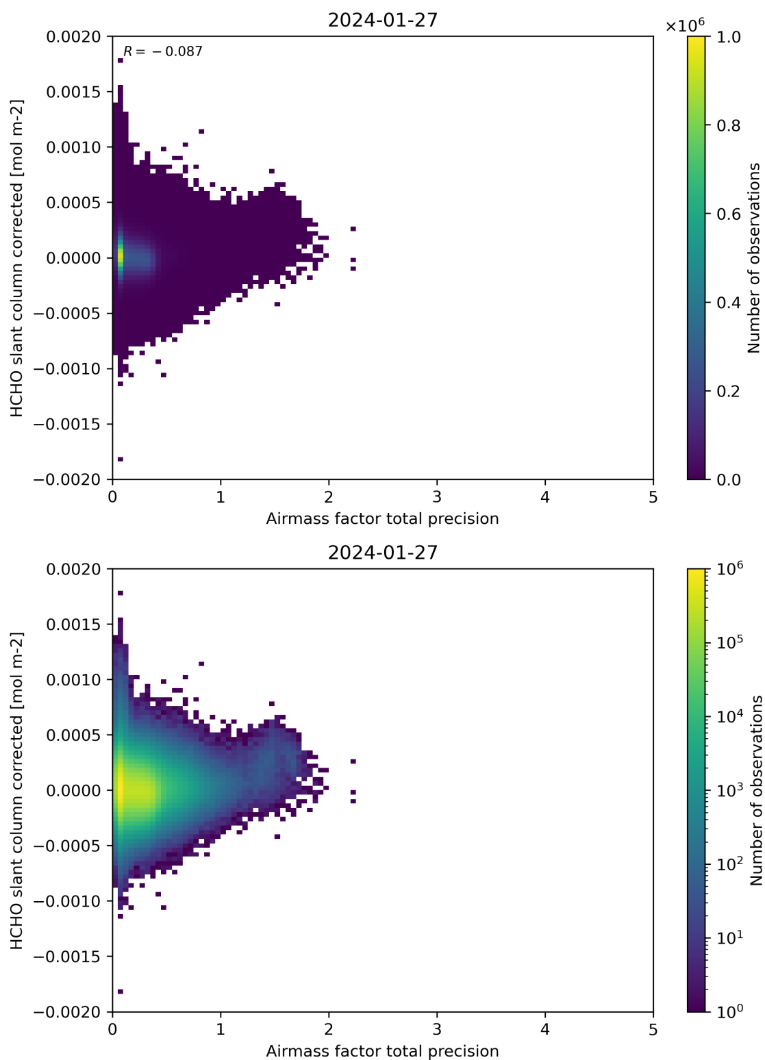
Figure 109: Scatter density plot of “Airmass factor total precision” against “HCHO slant column corrected” for 2024-01-26 to 2024-01-28.
