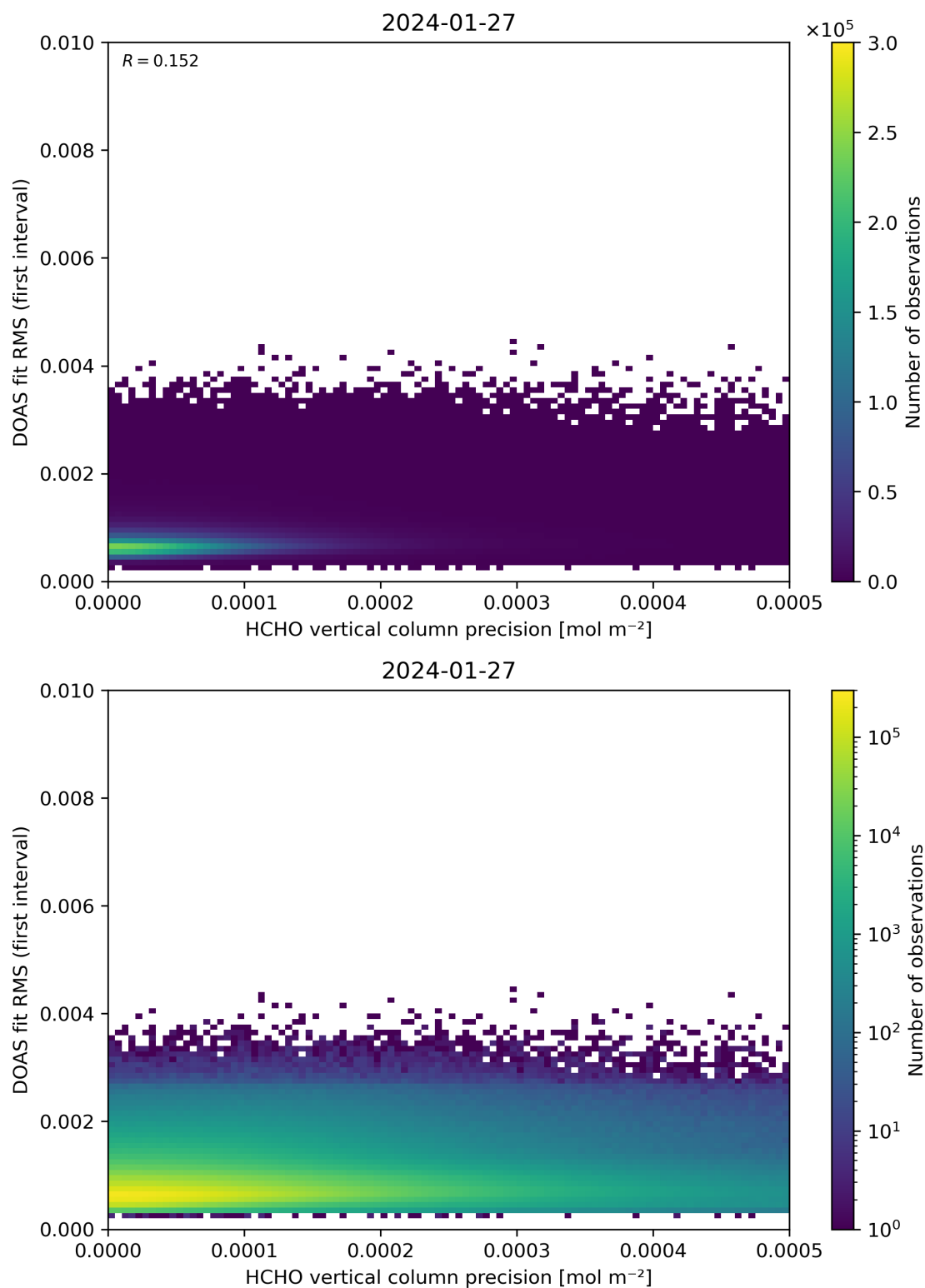
Figure 136: Scatter density plot of “HCHO vertical column precision” against “DOAS fit RMS (first interval)” for 2024-01-26 to 2024-01-28.
