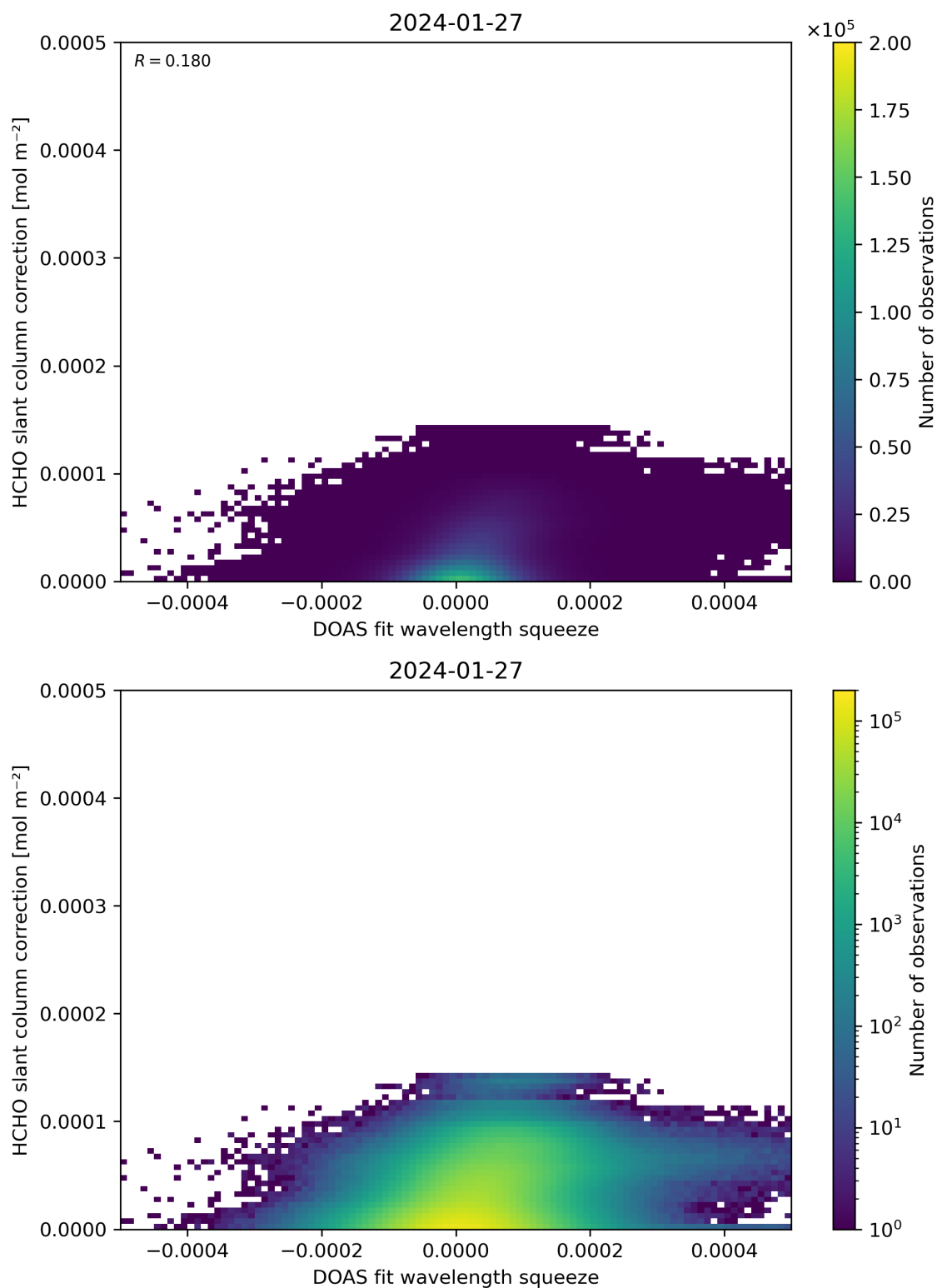
Figure 70: Scatter density plot of “DOAS fit wavelength squeeze” against “HCHO slant column correction” for 2024-01-26 to 2024-01-28.
