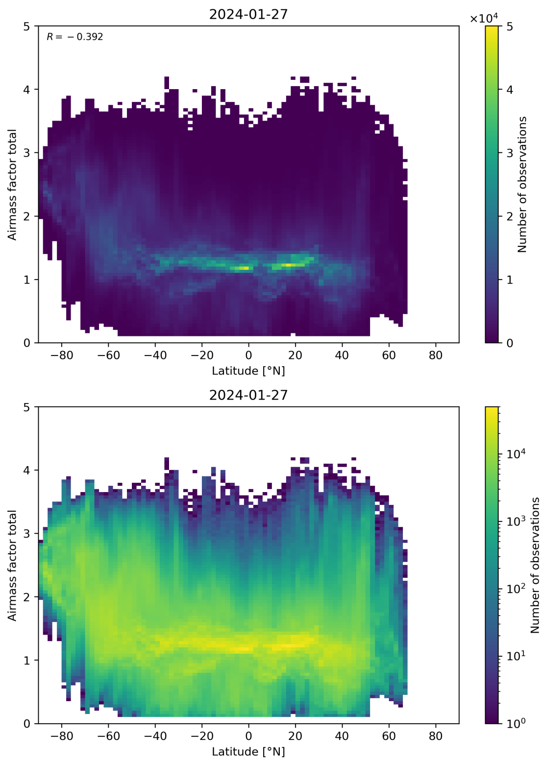
Figure 161: Scatter density plot of “Latitude” against “Airmass factor total” for 2024-01-26 to 2024-01-28.
