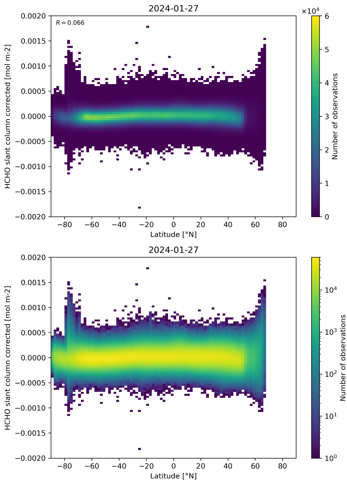
Figure 157: Scatter density plot of “Latitude” against “HCHO slant column corrected” for 2024-01-26 to 2024-01-28.
