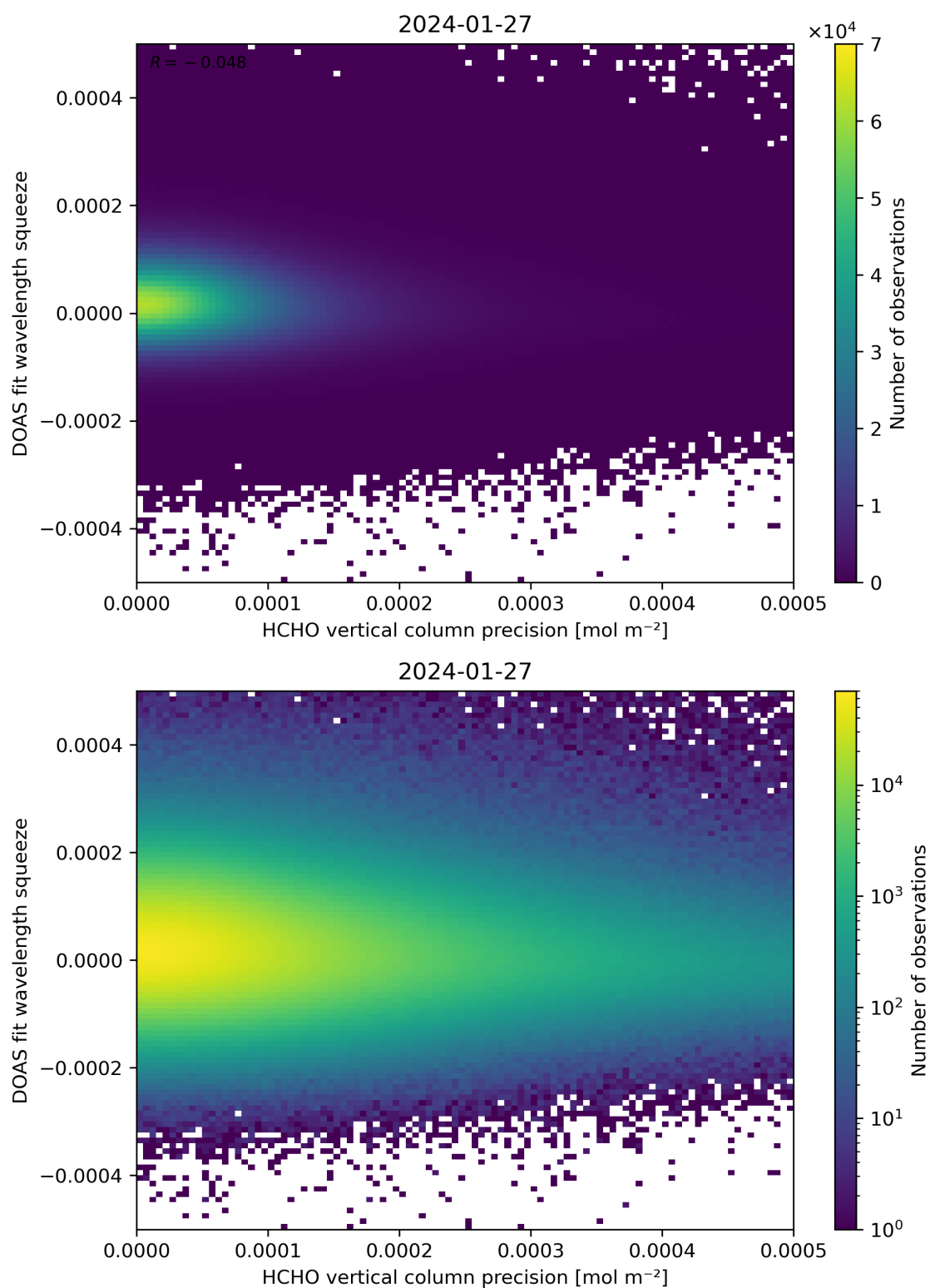
Figure 138: Scatter density plot of “HCHO vertical column precision” against “DOAS fit wavelength squeeze” for 2024-01-26 to 2024-01-28.
