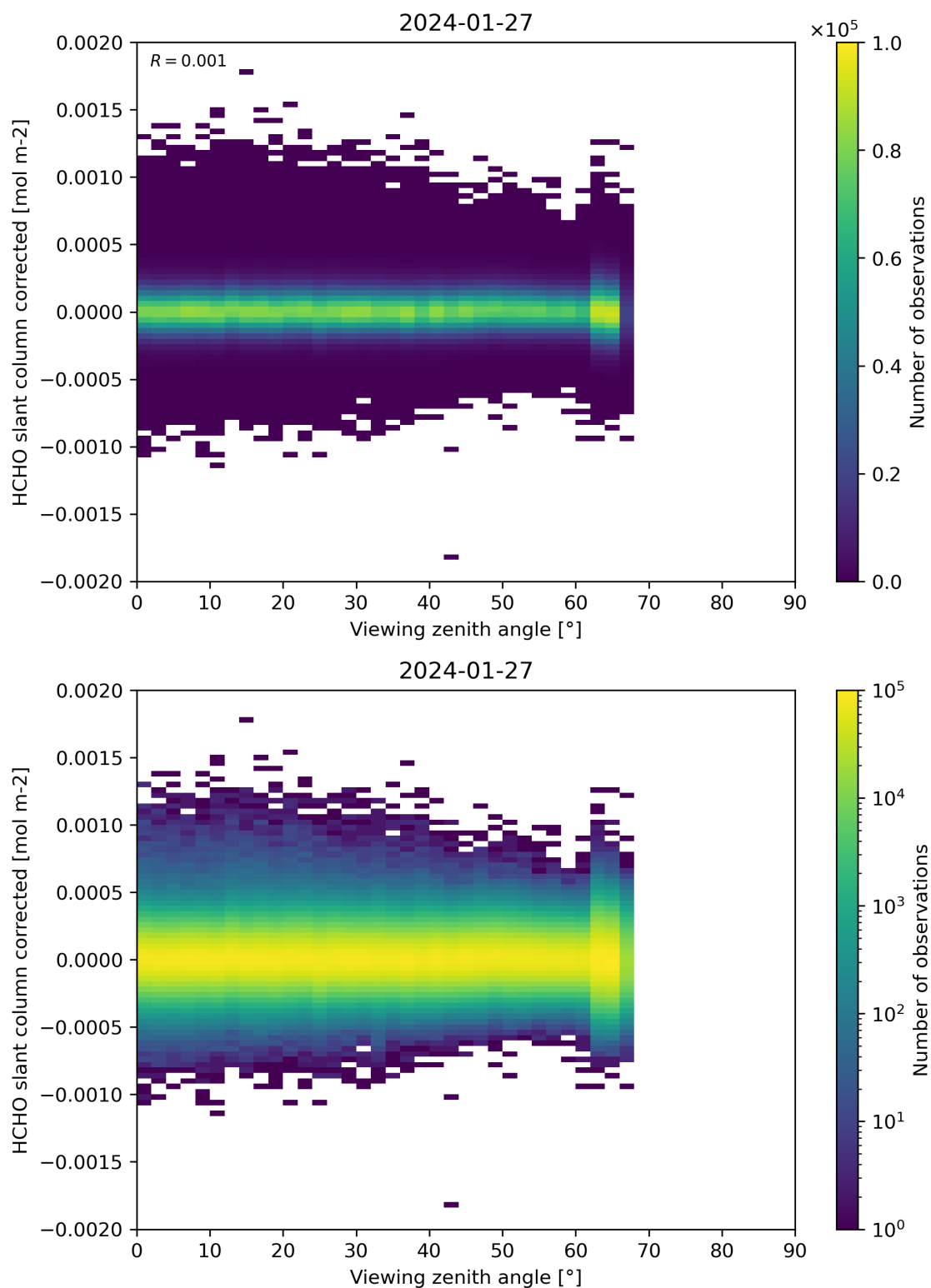
Figure 186: Scatter density plot of “Viewing zenith angle” against “HCHO slant column corrected” for 2024-01-26 to 2024-01-28.
