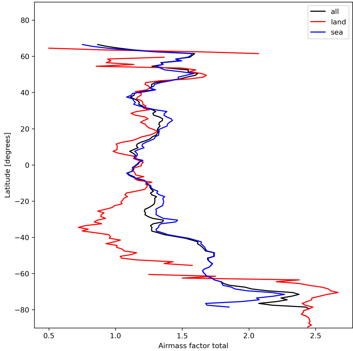
Figure 26: Zonal average of “Airmass factor total” for 2024-01-26 to 2024-01-28.
