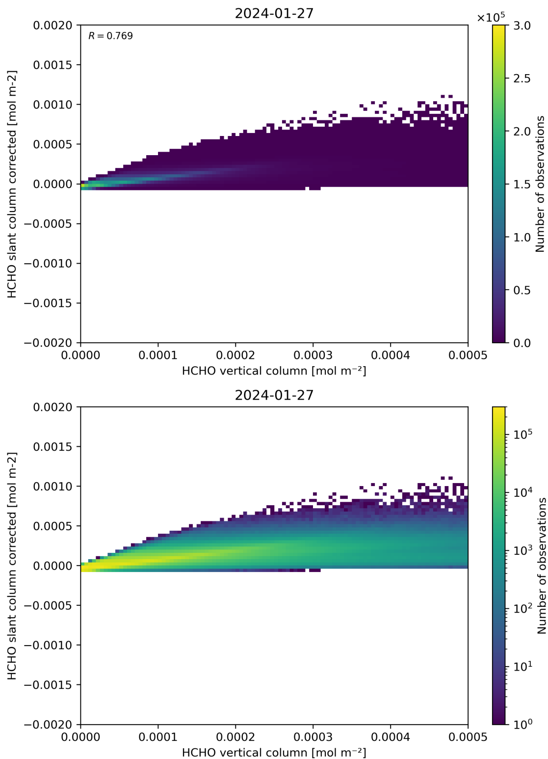
Figure 127: Scatter density plot of “HCHO vertical column” against “HCHO slant column corrected” for 2024-01-26 to 2024-01-28.
