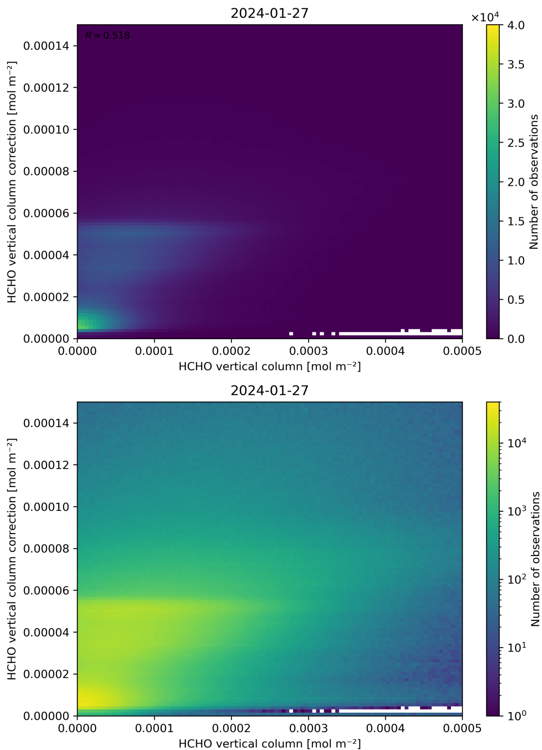
Figure 133: Scatter density plot of “HCHO vertical column” against “HCHO vertical column correction” for 2024-01-26 to 2024-01-28.
