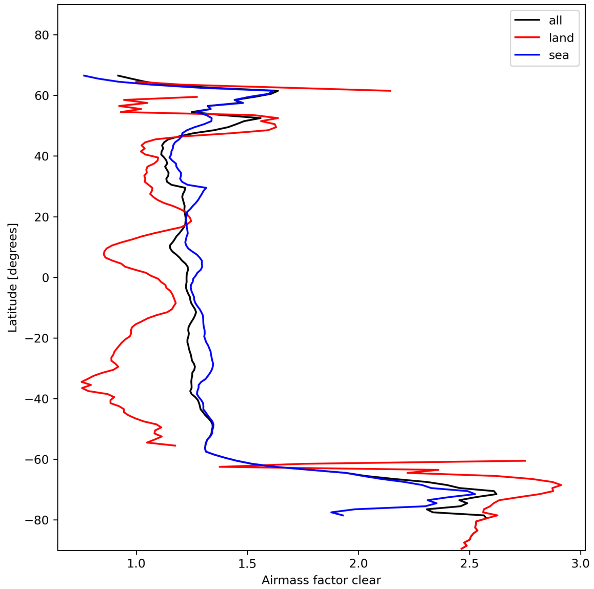
Figure 28: Zonal average of “Airmass factor clear” for 2024-01-26 to 2024-01-28.
