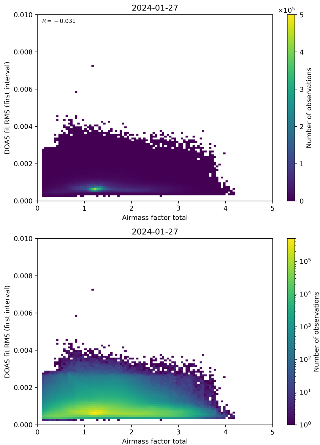
Figure 97: Scatter density plot of “Airmass factor total” against “DOAS fit RMS (first interval)” for 2024-01-26 to 2024-01-28.
