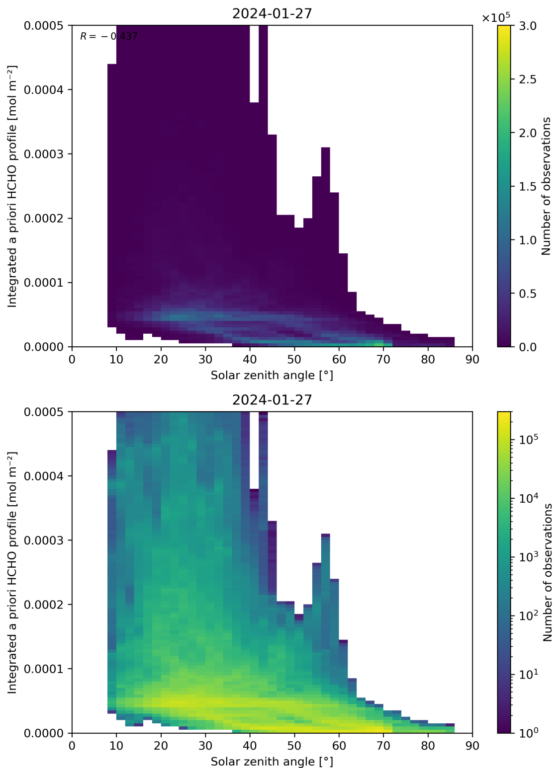
Figure 180: Scatter density plot of “Solar zenith angle” against “Integrated a priori HCHO profile” for 2024-01-26 to 2024-01-28.
