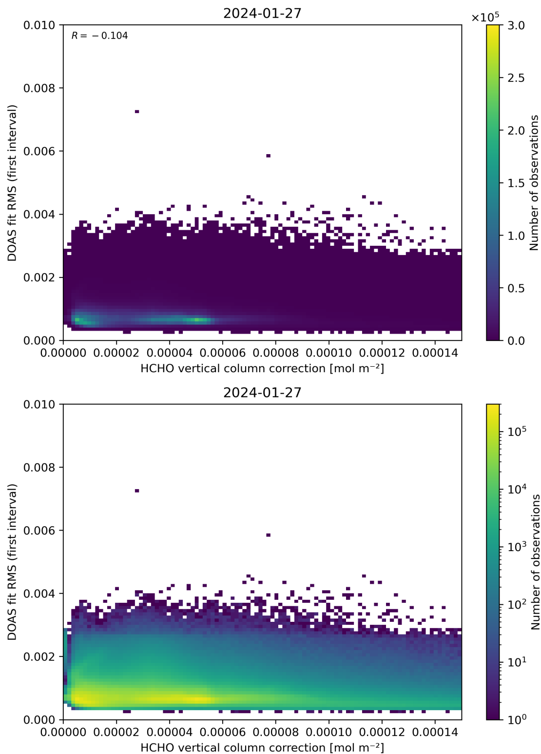
Figure 112: Scatter density plot of “HCHO vertical column correction” against “DOAS fit RMS (first interval)” for 2024-01-26 to 2024-01-28.
