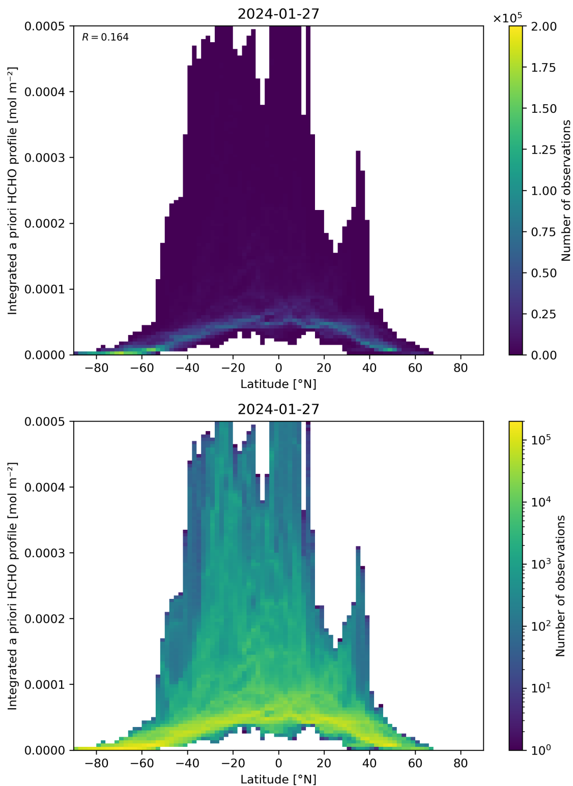
Figure 166: Scatter density plot of “Latitude” against “Integrated a priori HCHO profile” for 2024-01-26 to 2024-01-28.
