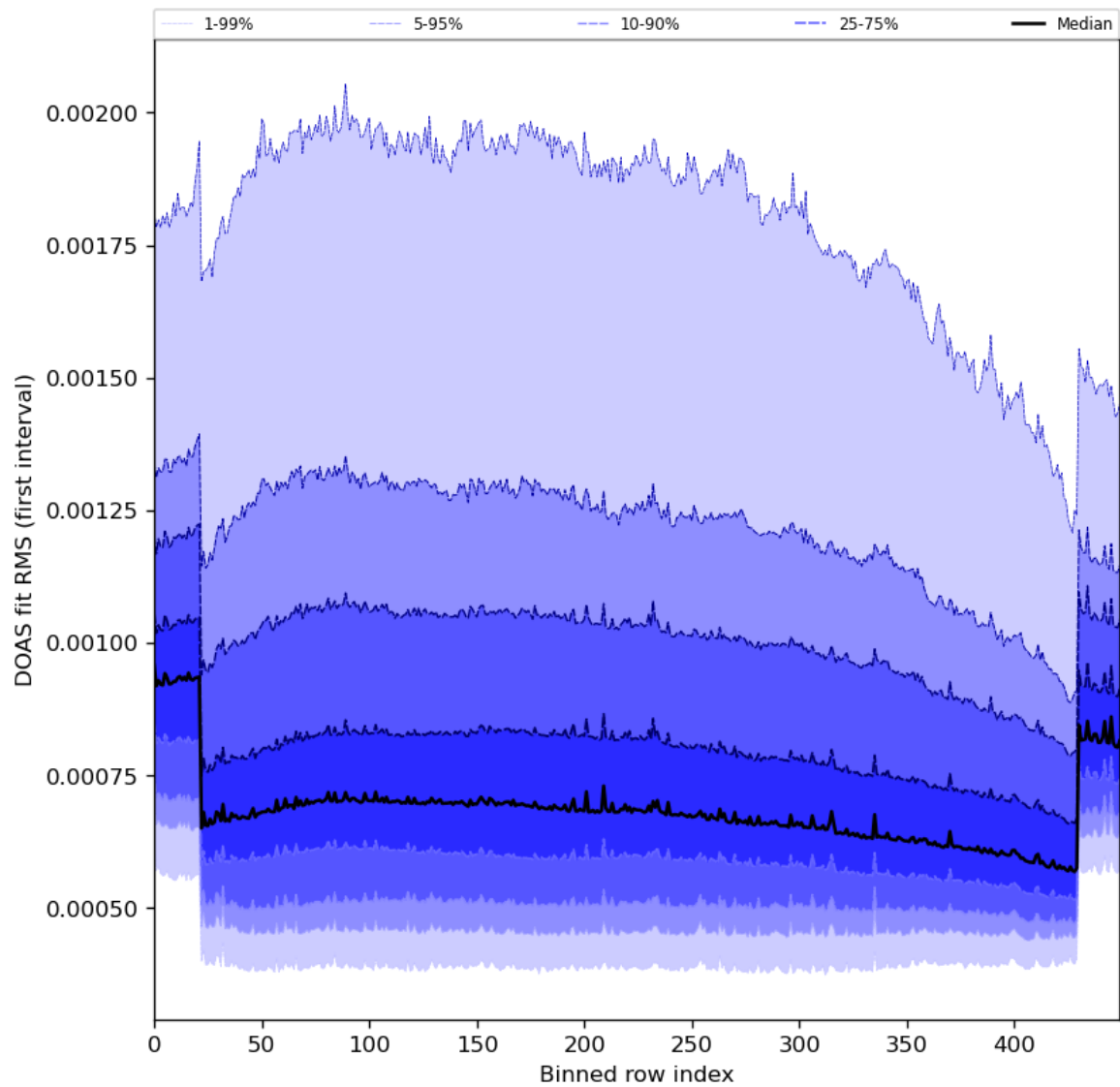
Figure 60: Along track statistics of “DOAS fit RMS (first interval)” for 2024-01-26 to 2024-01-28
