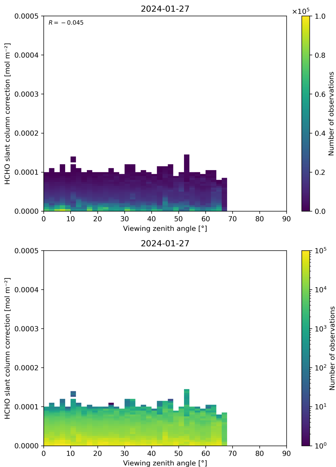
Figure 187: Scatter density plot of “Viewing zenith angle” against “HCHO slant column correction” for 2024-01-26 to 2024-01-28.
