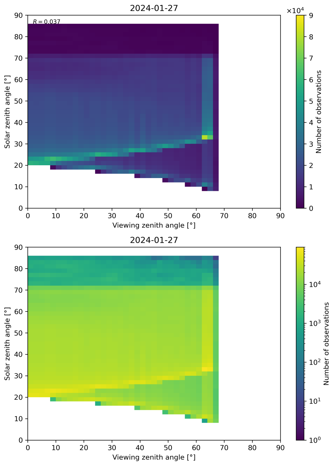
Figure 197: Scatter density plot of “Viewing zenith angle” against “Solar zenith angle” for 2024-01-26 to 2024-01-28.
