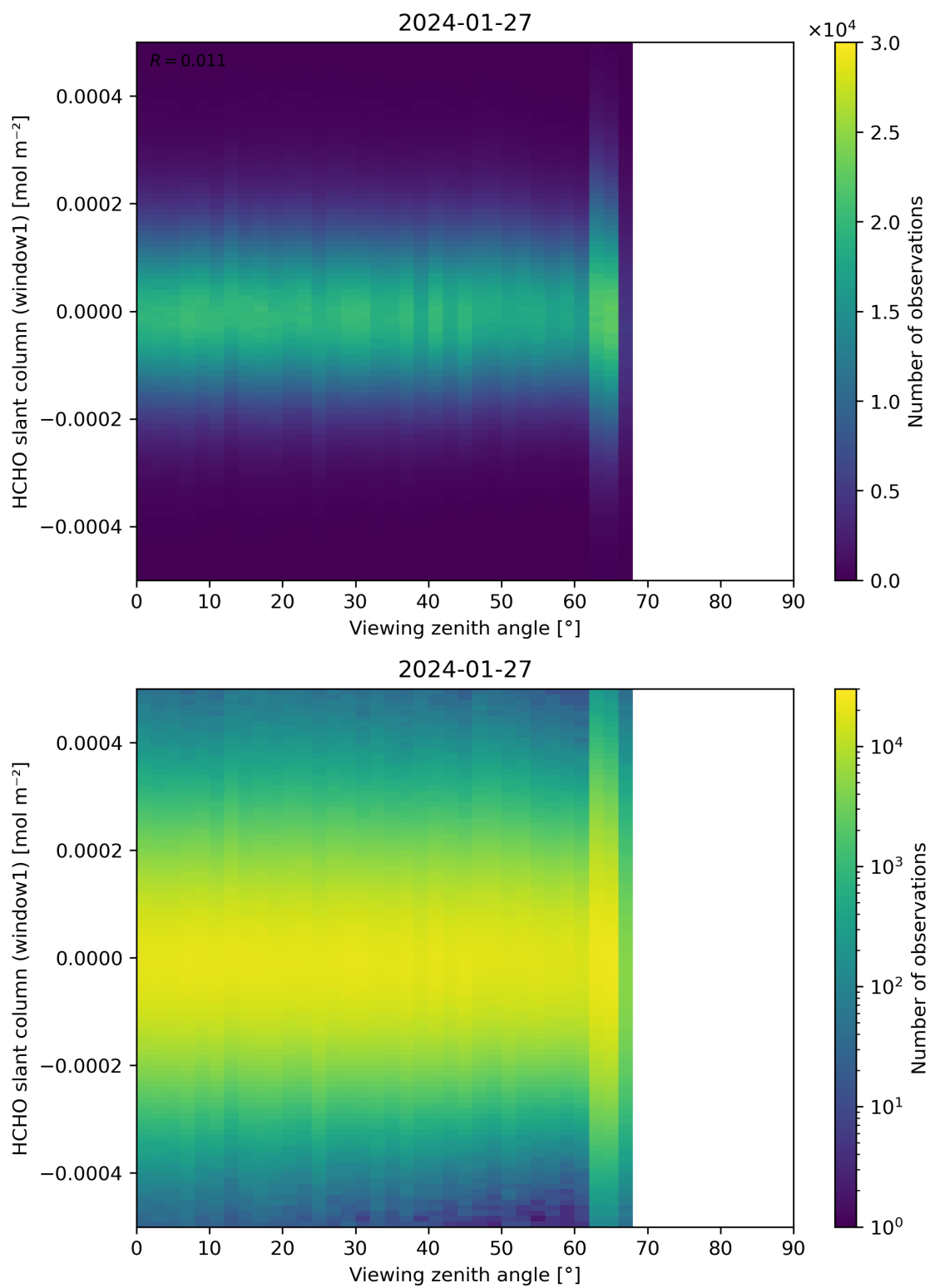
Figure 188: Scatter density plot of “Viewing zenith angle” against “HCHO slant column (window1)” for 2024-01-26 to 2024-01-28.
