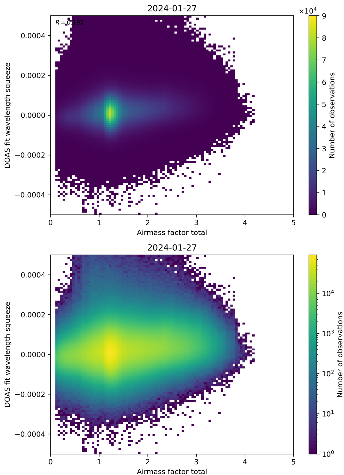
Figure 99: Scatter density plot of “Airmass factor total” against “DOAS fit wavelength squeeze” for 2024-01-26 to 2024-01-28.
