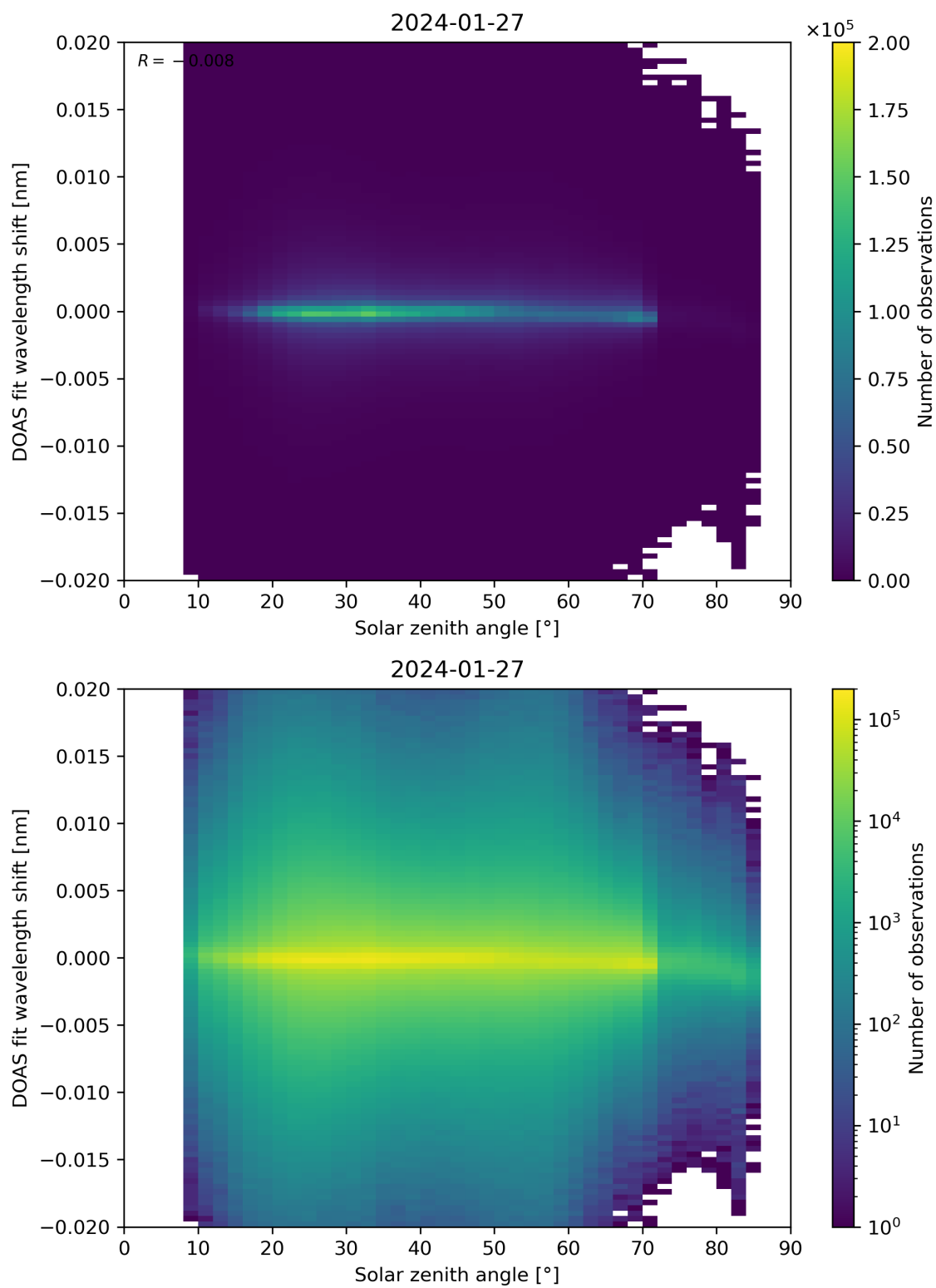
Figure 168: Scatter density plot of “Solar zenith angle” against “DOAS fit wavelength shift” for 2024-01-26 to 2024-01-28.
