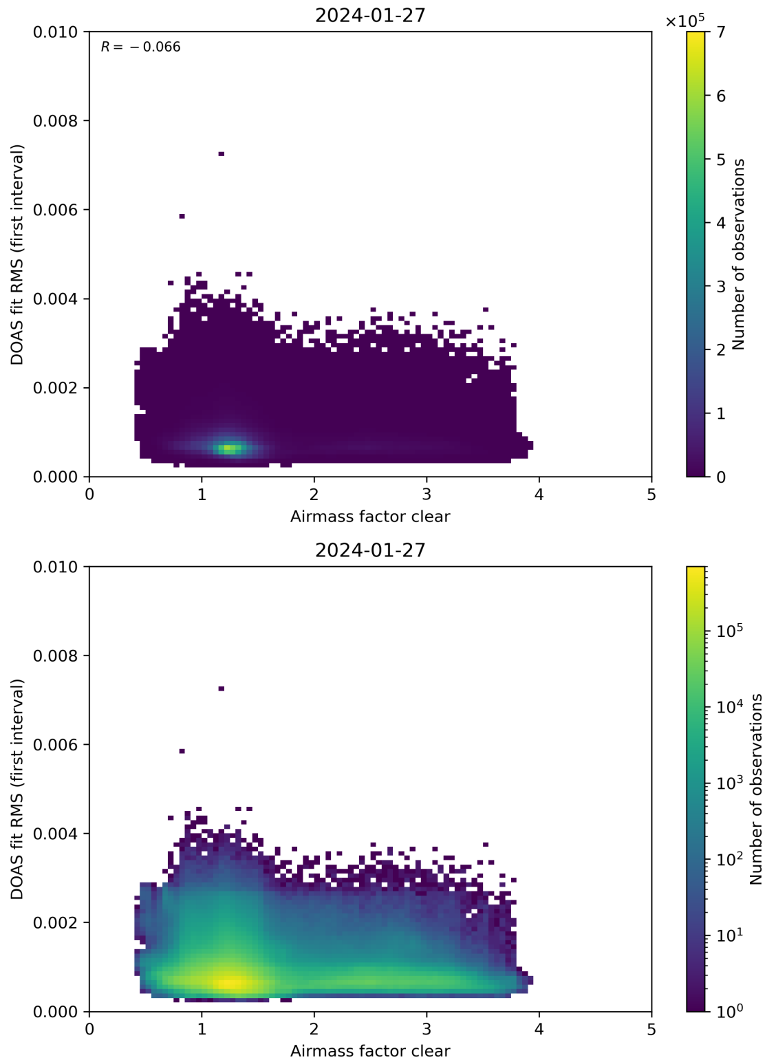
Figure 71: Scatter density plot of “Airmass factor clear” against “DOAS fit RMS (first interval)” for 2024-01-26 to 2024-01-28.
