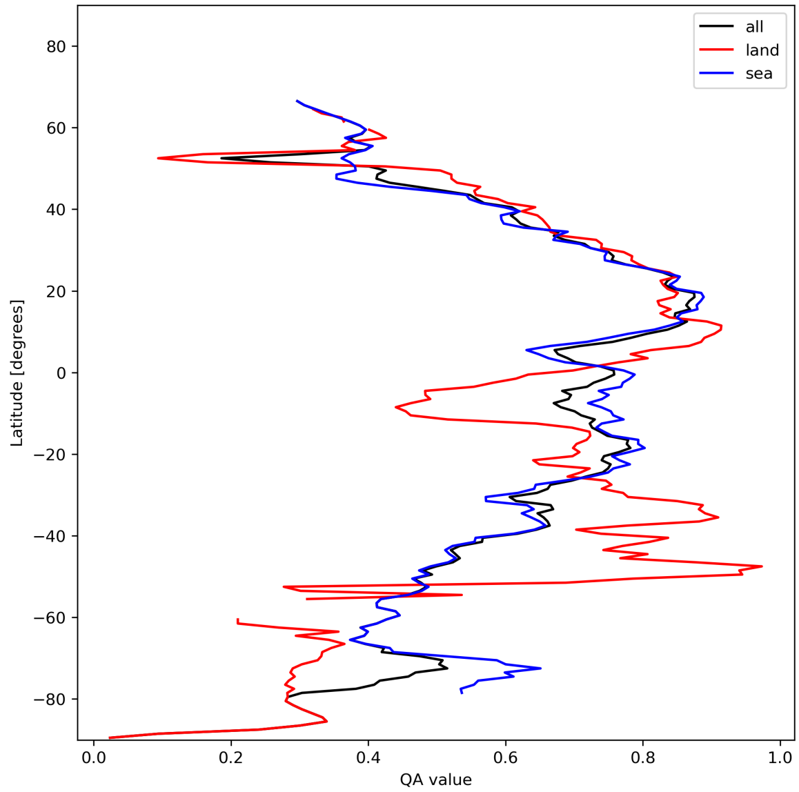
Figure 20: Zonal average of “QA value” for 2024-01-26 to 2024-01-28.
