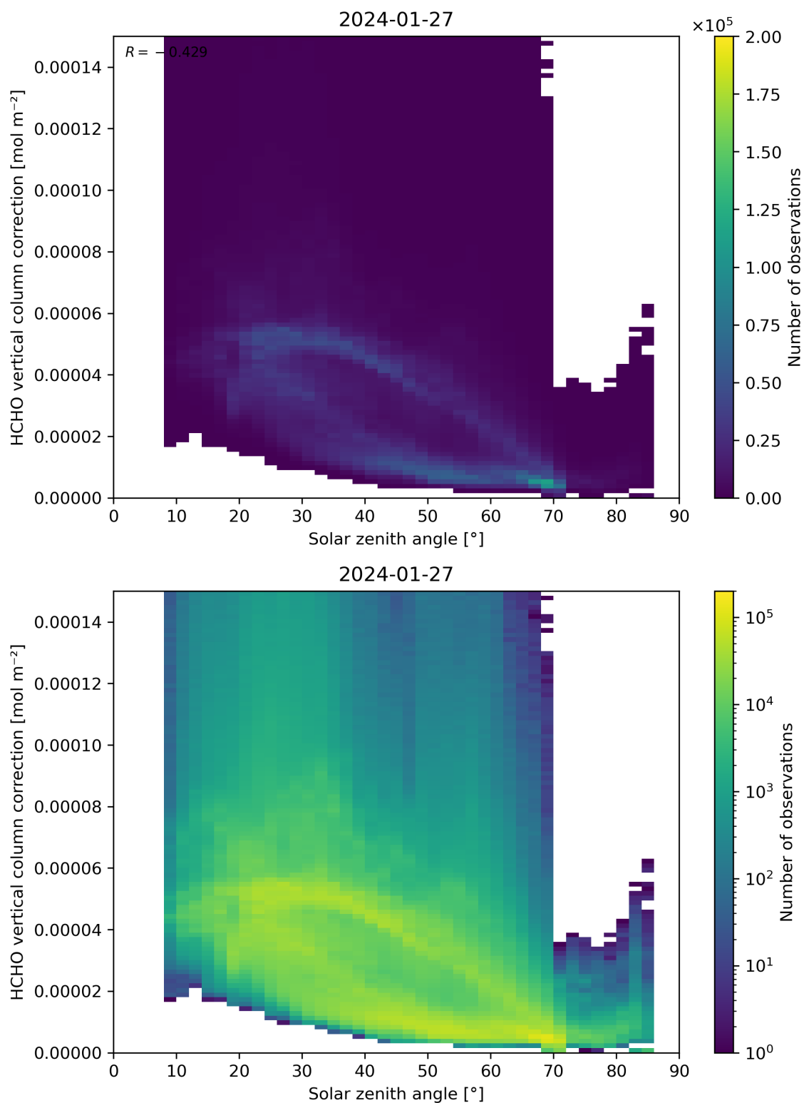
Figure 178: Scatter density plot of “Solar zenith angle” against “HCHO vertical column correction” for 2024-01-26 to 2024-01-28.
