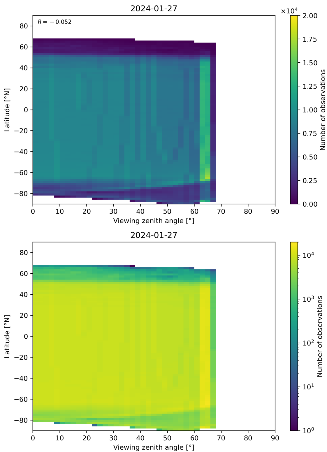
Figure 196: Scatter density plot of “Viewing zenith angle” against “Latitude” for 2024-01-26 to 2024-01-28.
