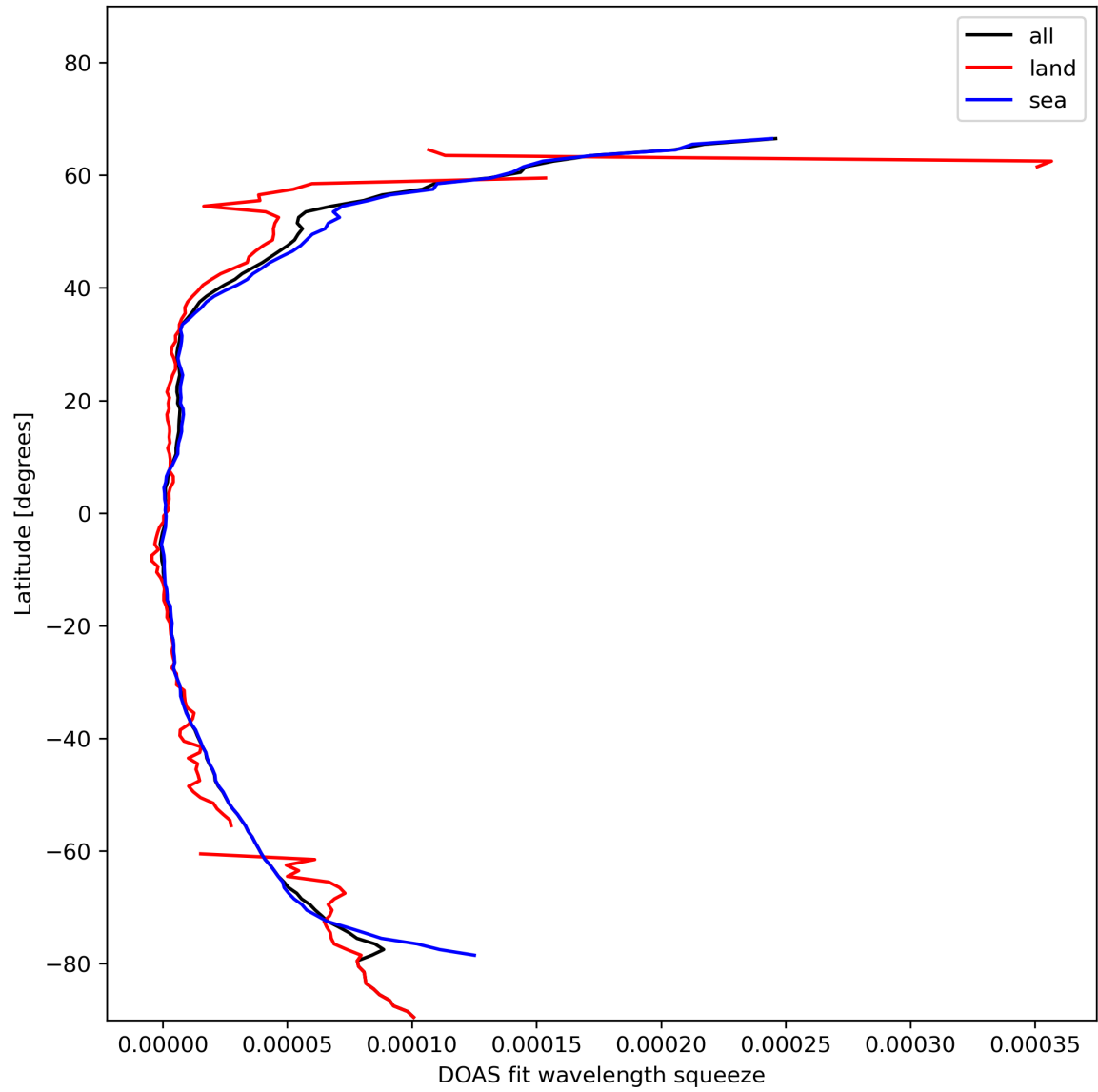
Figure 31: Zonal average of “DOAS fit wavelength squeeze” for 2024-01-26 to 2024-01-28.
