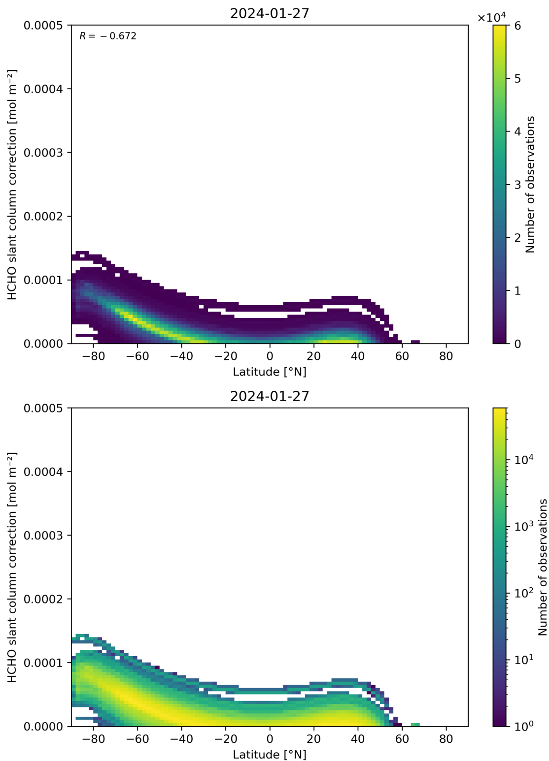
Figure 158: Scatter density plot of “Latitude” against “HCHO slant column correction” for 2024-01-26 to 2024-01-28.
