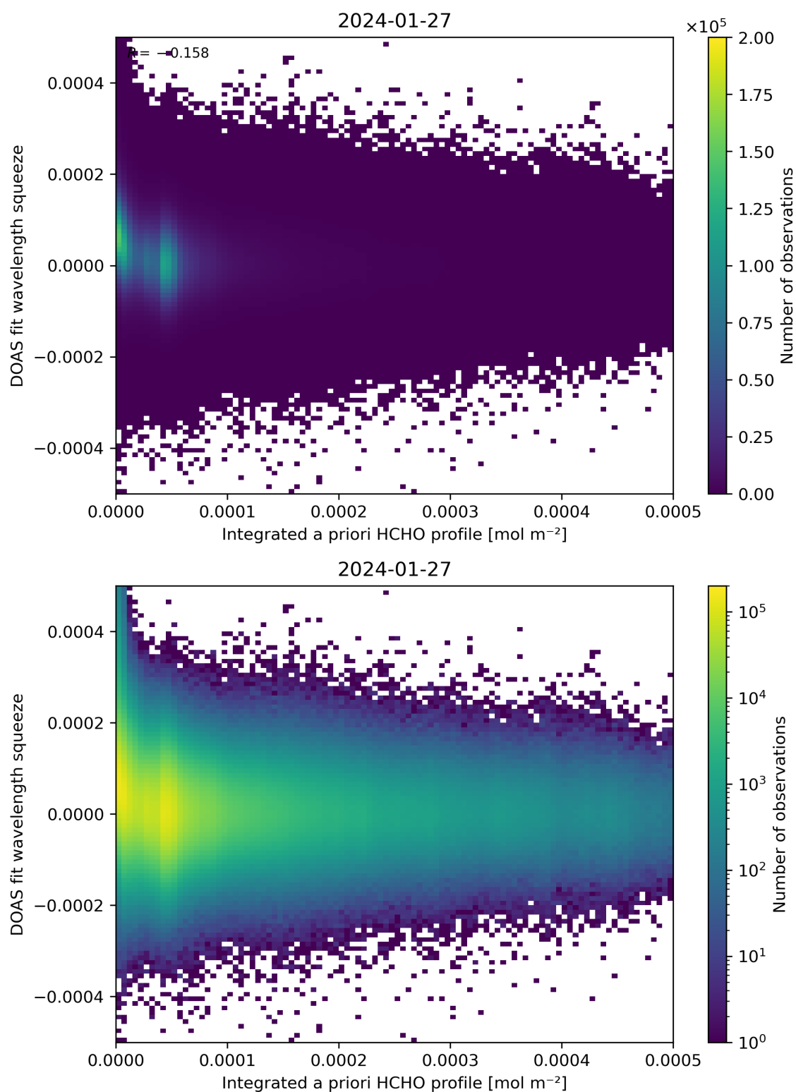
Figure 150: Scatter density plot of “Integrated a priori HCHO profile” against “DOAS fit wavelength squeeze” for 2024-01-26 to 2024-01-28.
