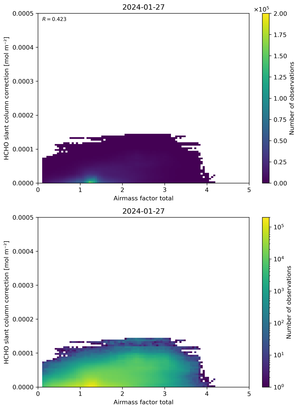
Figure 102: Scatter density plot of “Airmass factor total” against “HCHO slant column correction” for 2024-01-26 to 2024-01-28.
