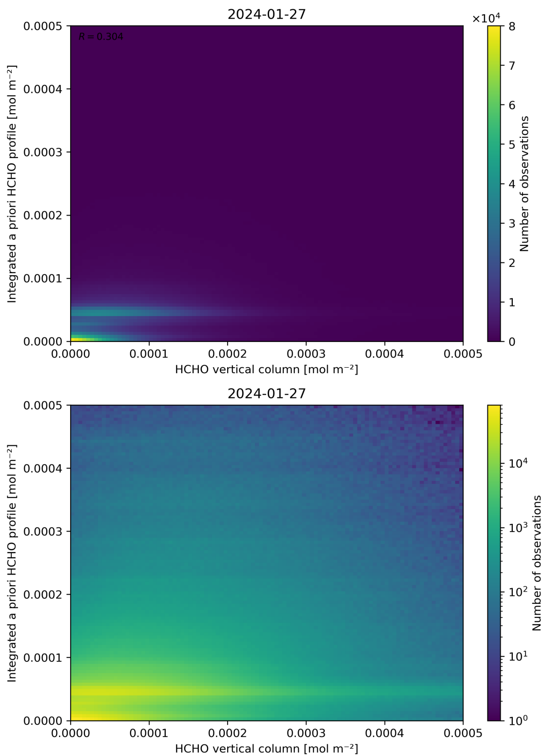
Figure 135: Scatter density plot of “HCHO vertical column” against “Integrated a priori HCHO profile” for 2024-01-26 to 2024-01-28.
