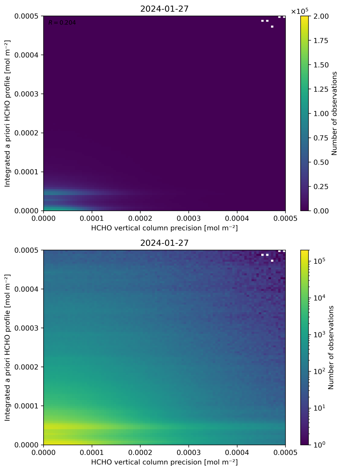
Figure 147: Scatter density plot of “HCHO vertical column precision” against “Integrated a priori HCHO profile” for 2024-01-26 to 2024-01-28.
