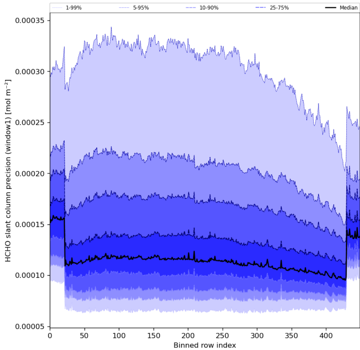
Figure 53: Along track statistics of “HCHO slant column precision (window1)” for 2024-01-26 to 2024-01-28
