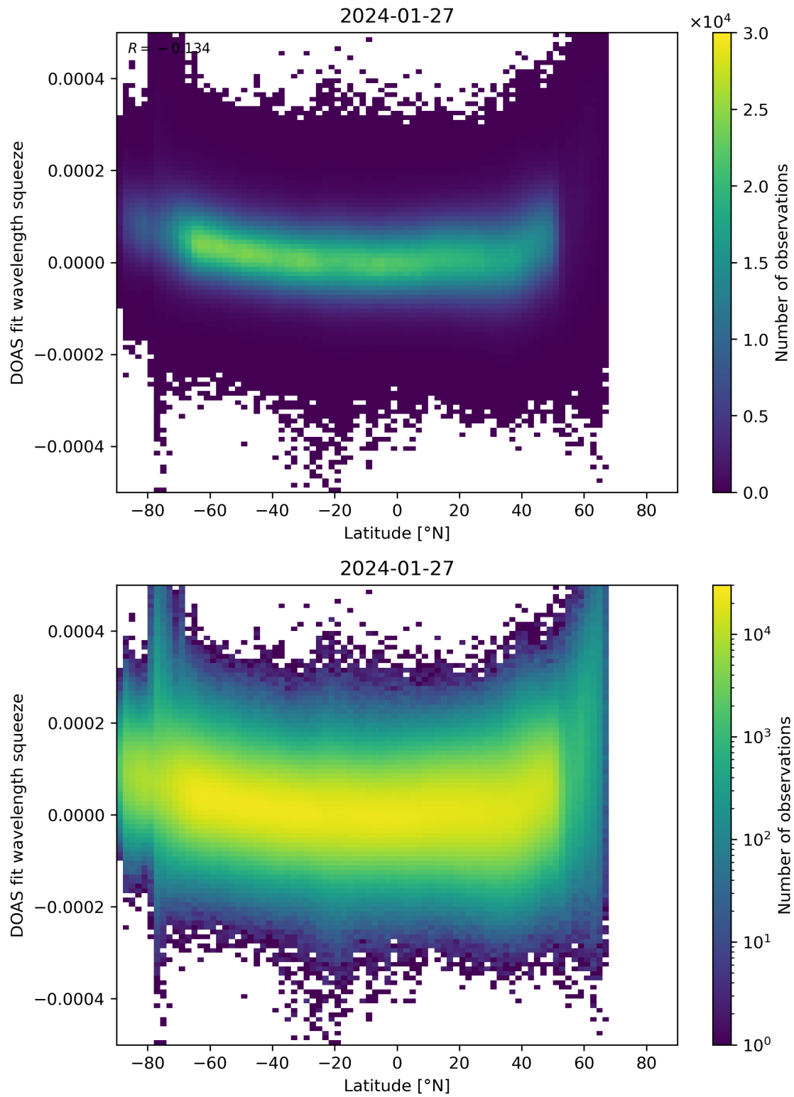
Figure 155: Scatter density plot of “Latitude” against “DOAS fit wavelength squeeze” for 2024-01-26 to 2024-01-28.
