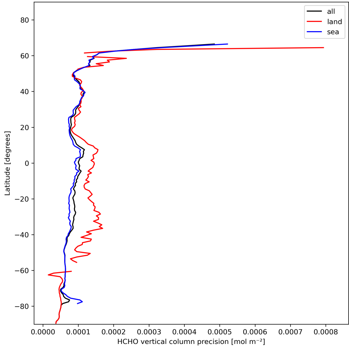
Figure 22: Zonal average of “HCHO vertical column precision” for 2024-01-26 to 2024-01-28.
