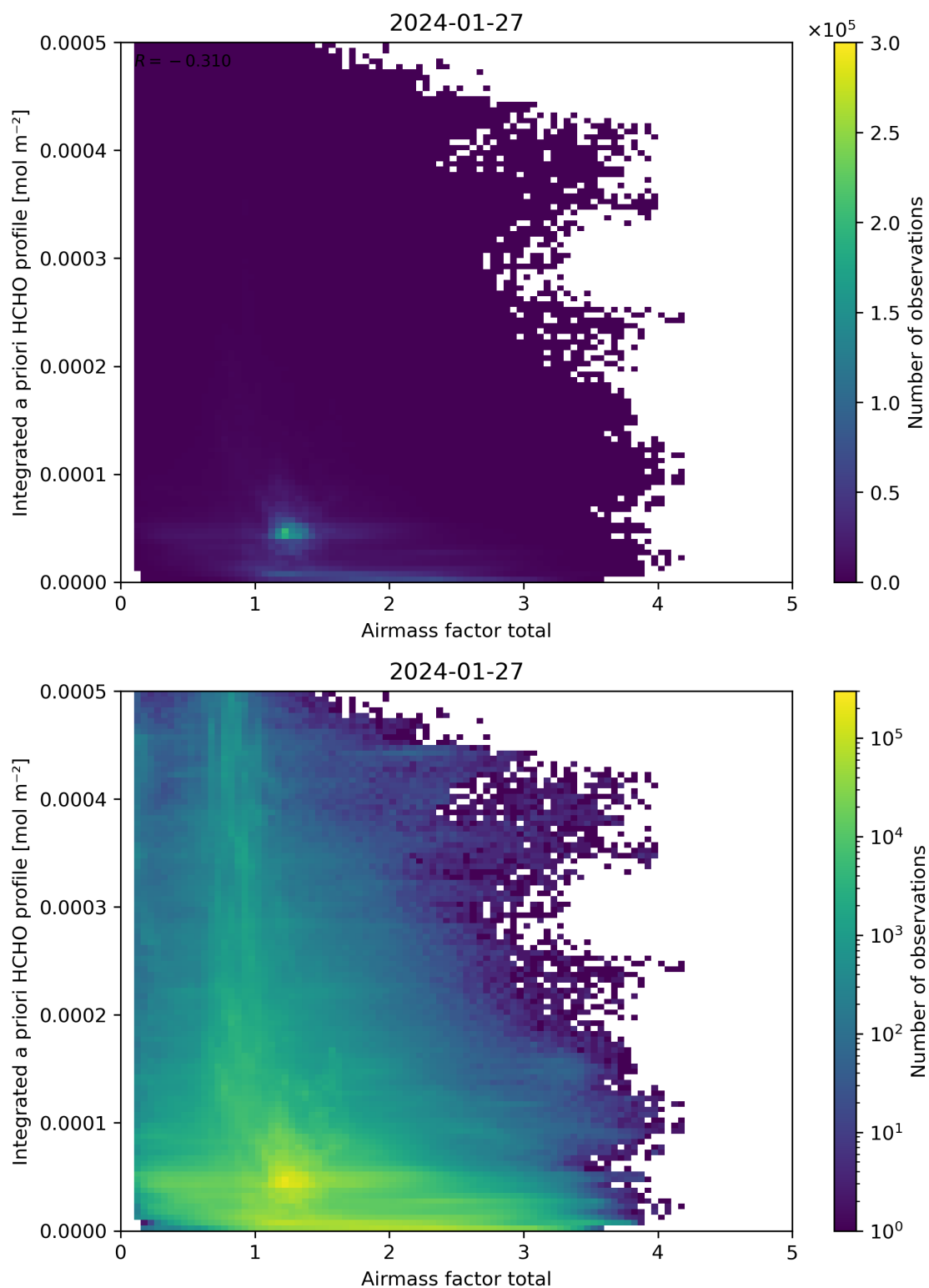
Figure 104: Scatter density plot of “Air mass factor total” against “Integrated a priori HCHO profile” for 2024-01-26 to 2024-01-28.
