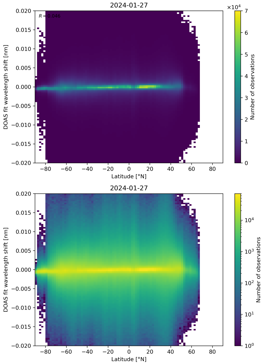
Figure 154: Scatter density plot of “Latitude” against “DOAS fit wavelength shift” for 2024-01-26 to 2024-01-28.
