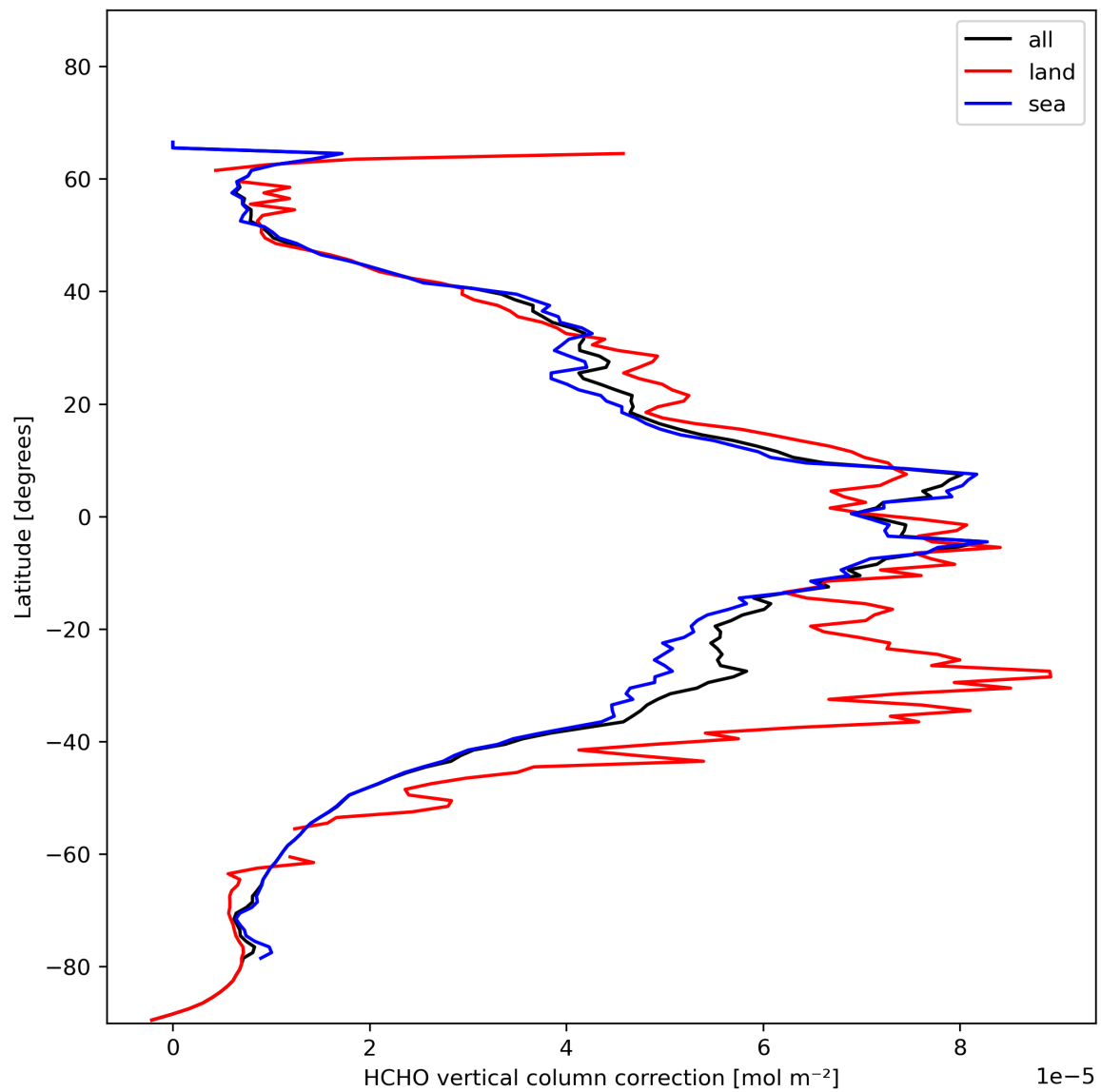
Figure 23: Zonal average of “HCHO vertical column correction” for 2024-01-26 to 2024-01-28.
