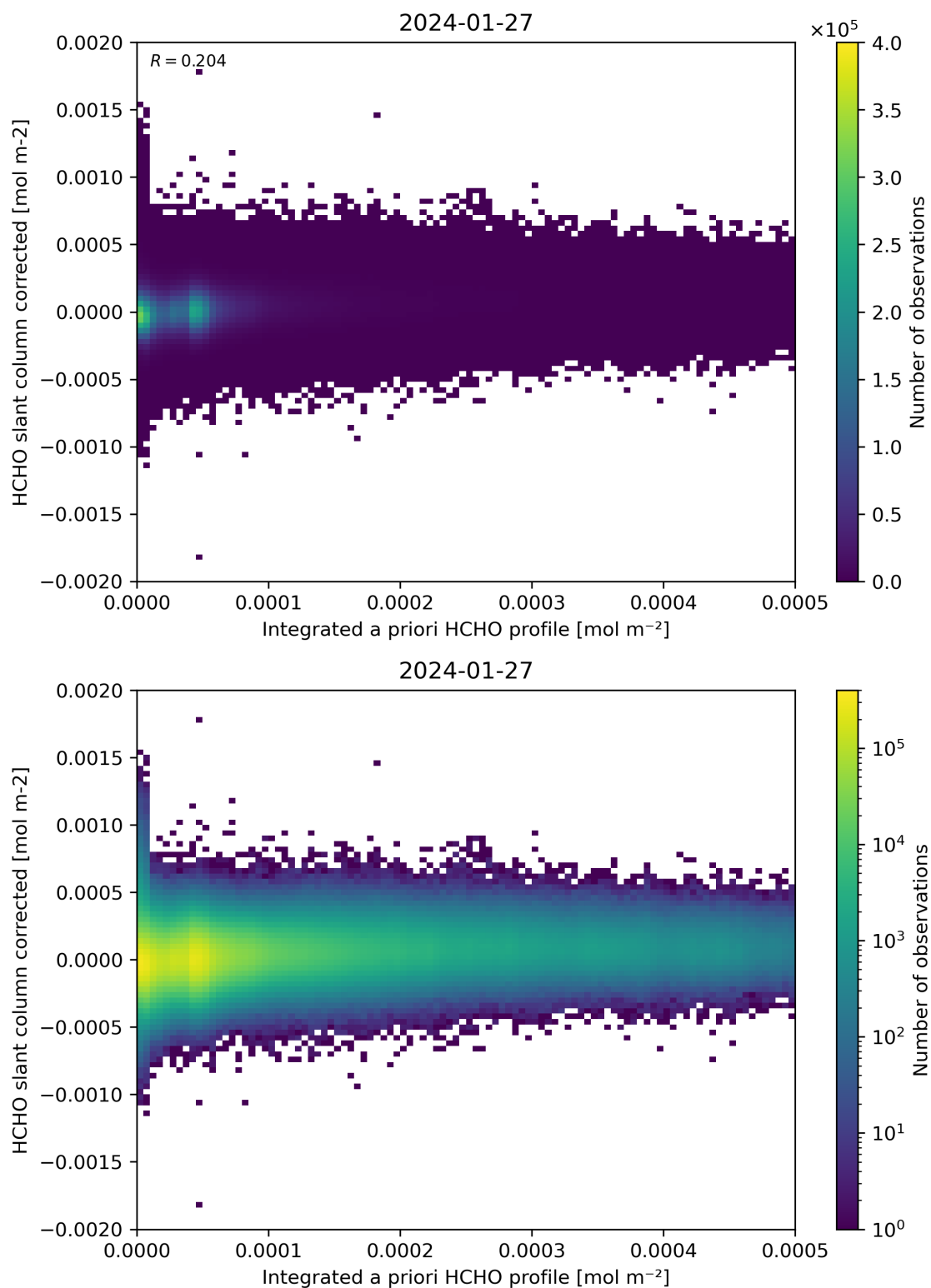
Figure 151: Scatter density plot of “Integrated a priori HCHO profile” against “HCHO slant column corrected” for 2024-01-26 to 2024-01-28.
