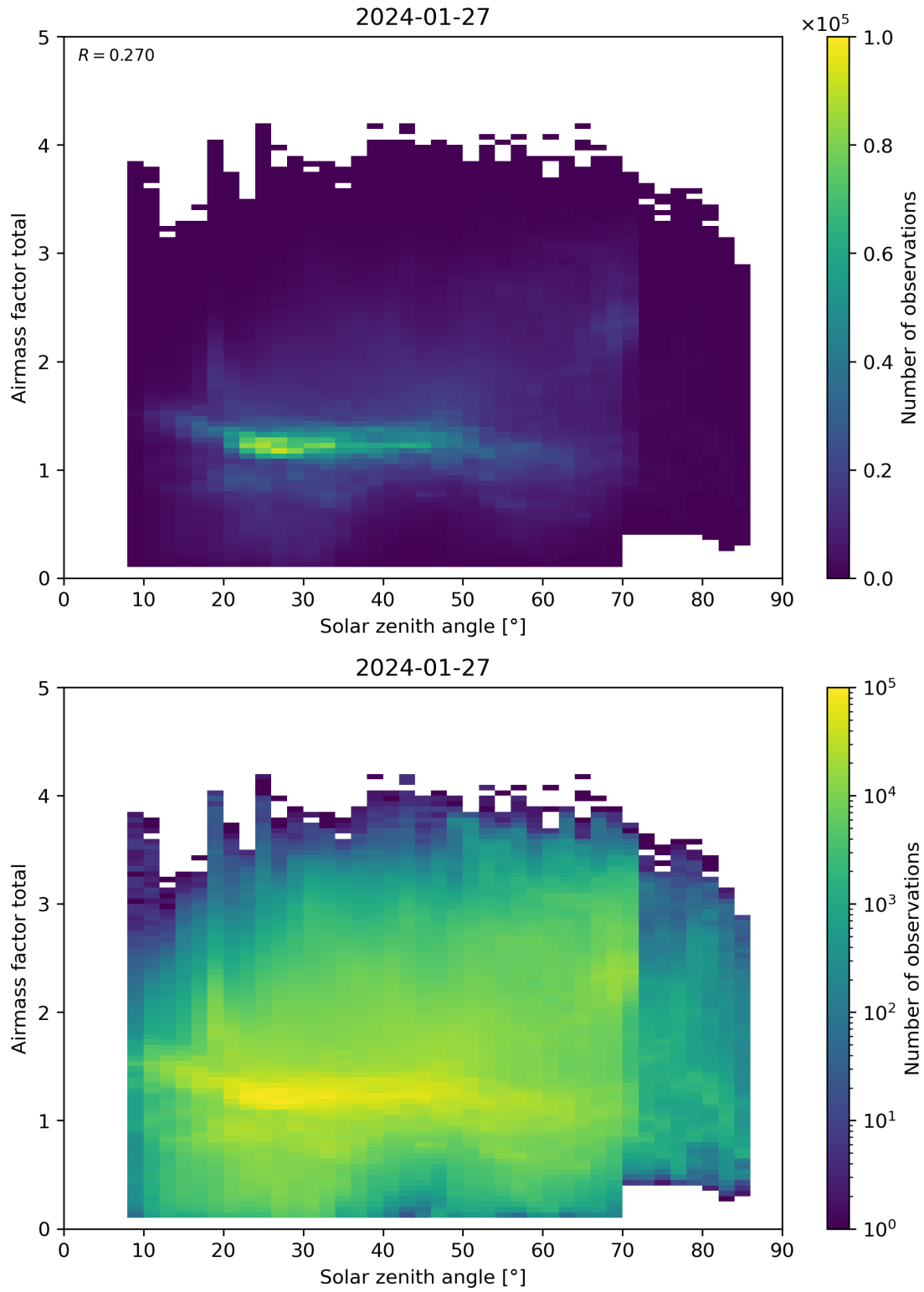
Figure 175: Scatter density plot of “Solar zenith angle” against “Airmass factor total” for 2024-01-26 to 2024-01-28.
