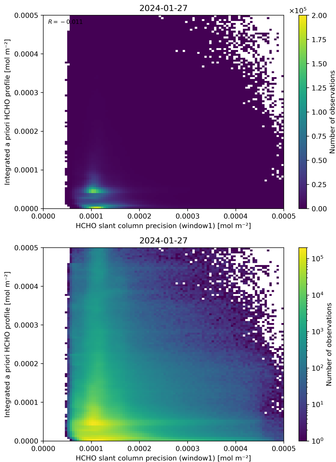
Figure 96: Scatter density plot of “HCHO slant column precision (window1)” against “Integrated a priori HCHO profile” for 2024-01-26 to 2024-01-28.
