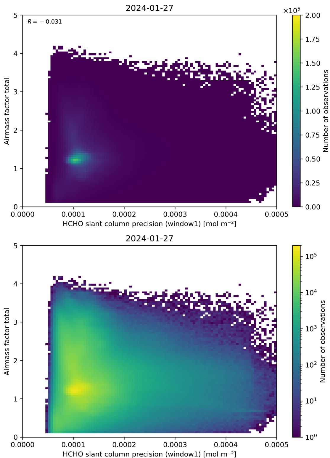
Figure 94: Scatter density plot of “HCHO slant column precision (window1)” against “Airmass factor total” for 2024-01-26 to 2024-01-28.
