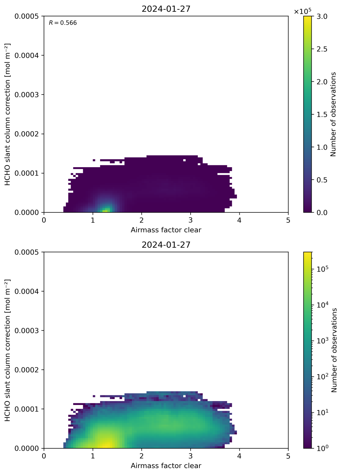
Figure 75: Scatter density plot of “Airmass factor clear” against “HCHO slant column correction” for 2024-01-26 to 2024-01-28.
