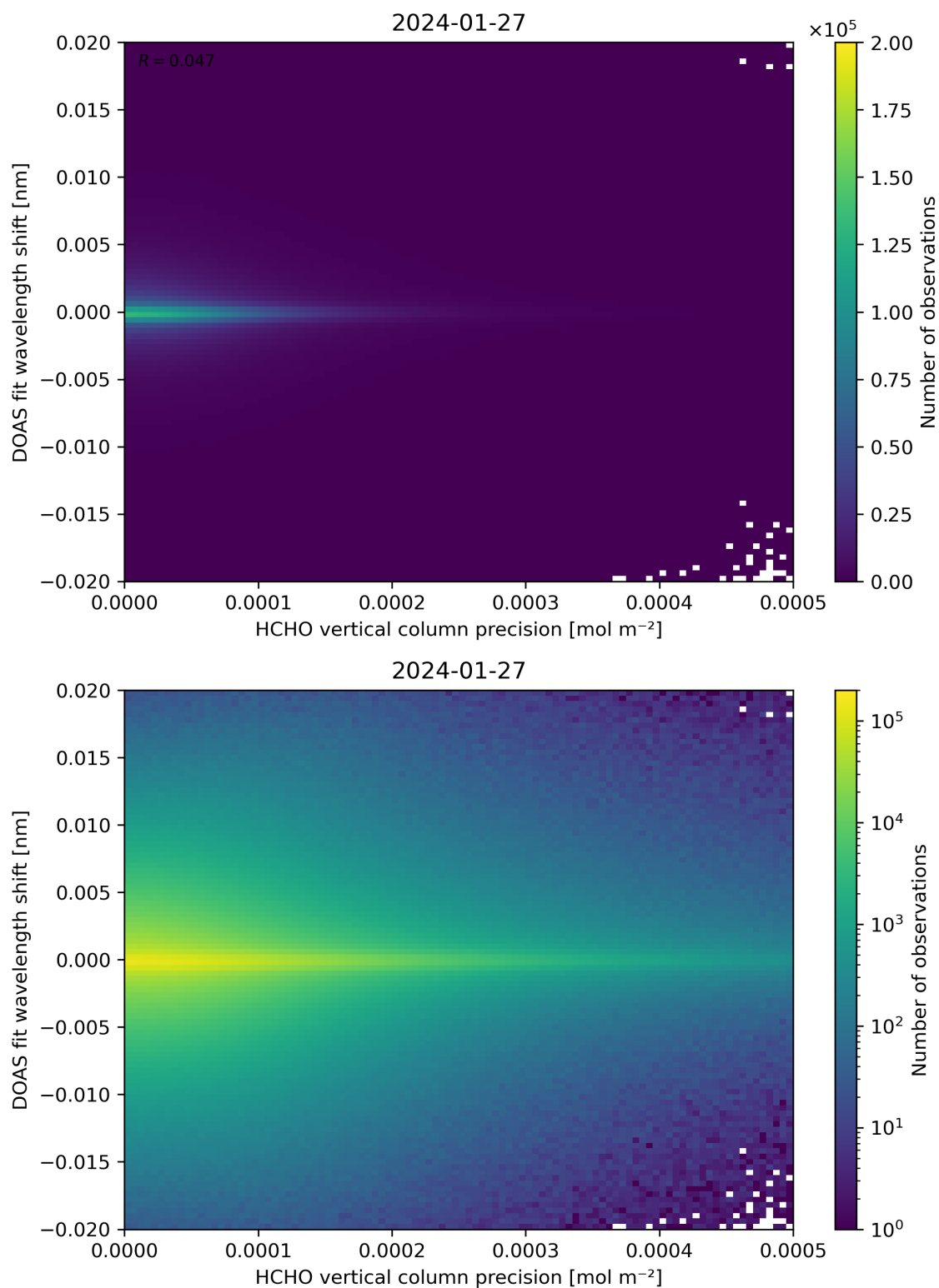
Figure 137: Scatter density plot of “HCHO vertical column precision” against “DOAS fit wavelength shift” for 2024-01-26 to 2024-01-28.
