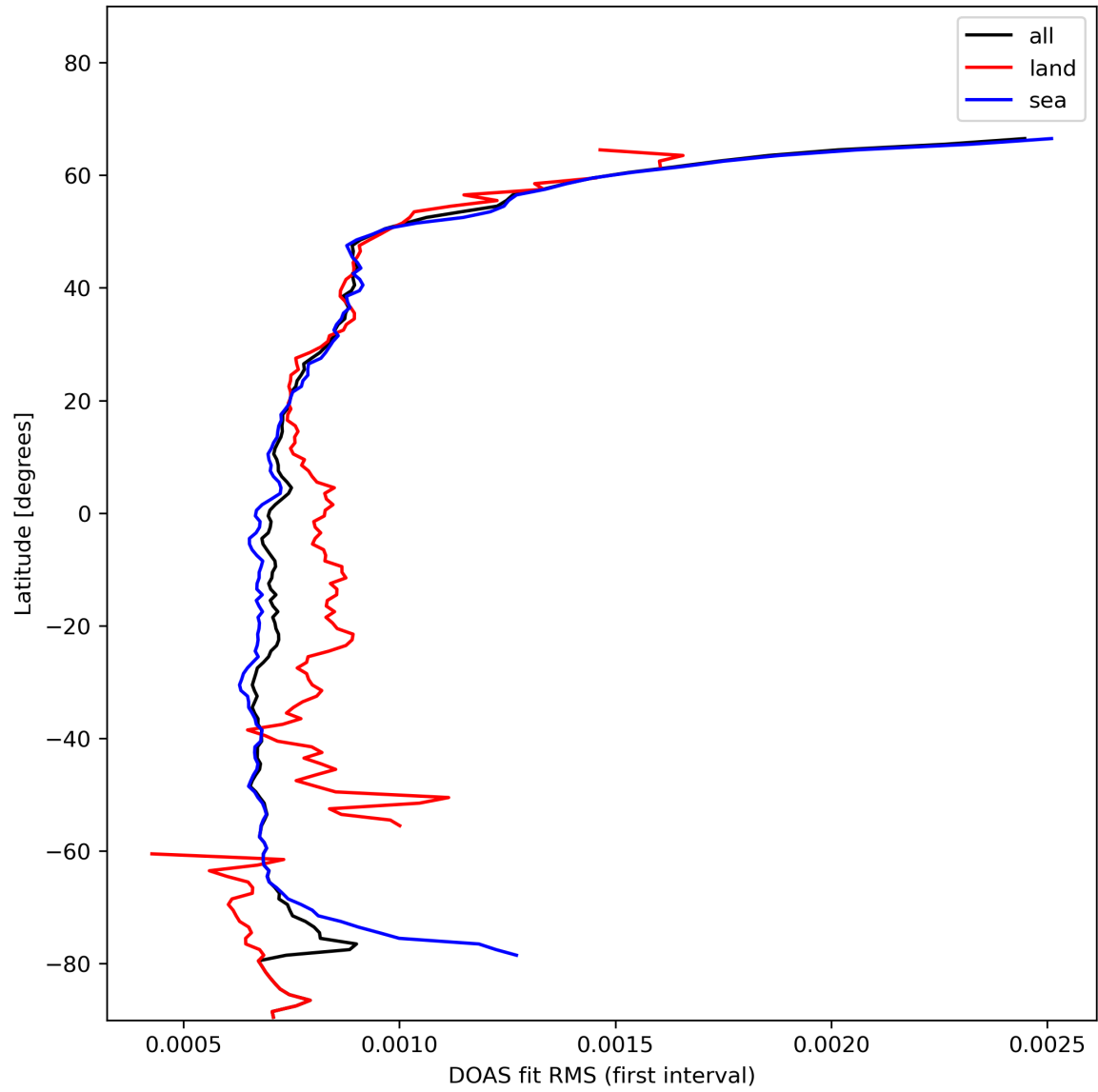
Figure 32: Zonal average of “DOAS fit RMS (first interval)” for 2024-01-26 to 2024-01-28.
