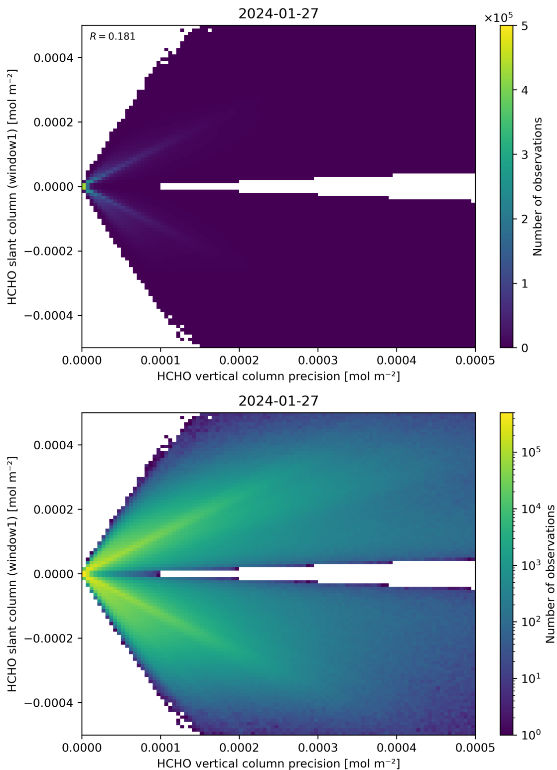
Figure 142: Scatter density plot of “HCHO vertical column precision” against “HCHO slant column (window1)” for 2024-01-26 to 2024-01-28.
