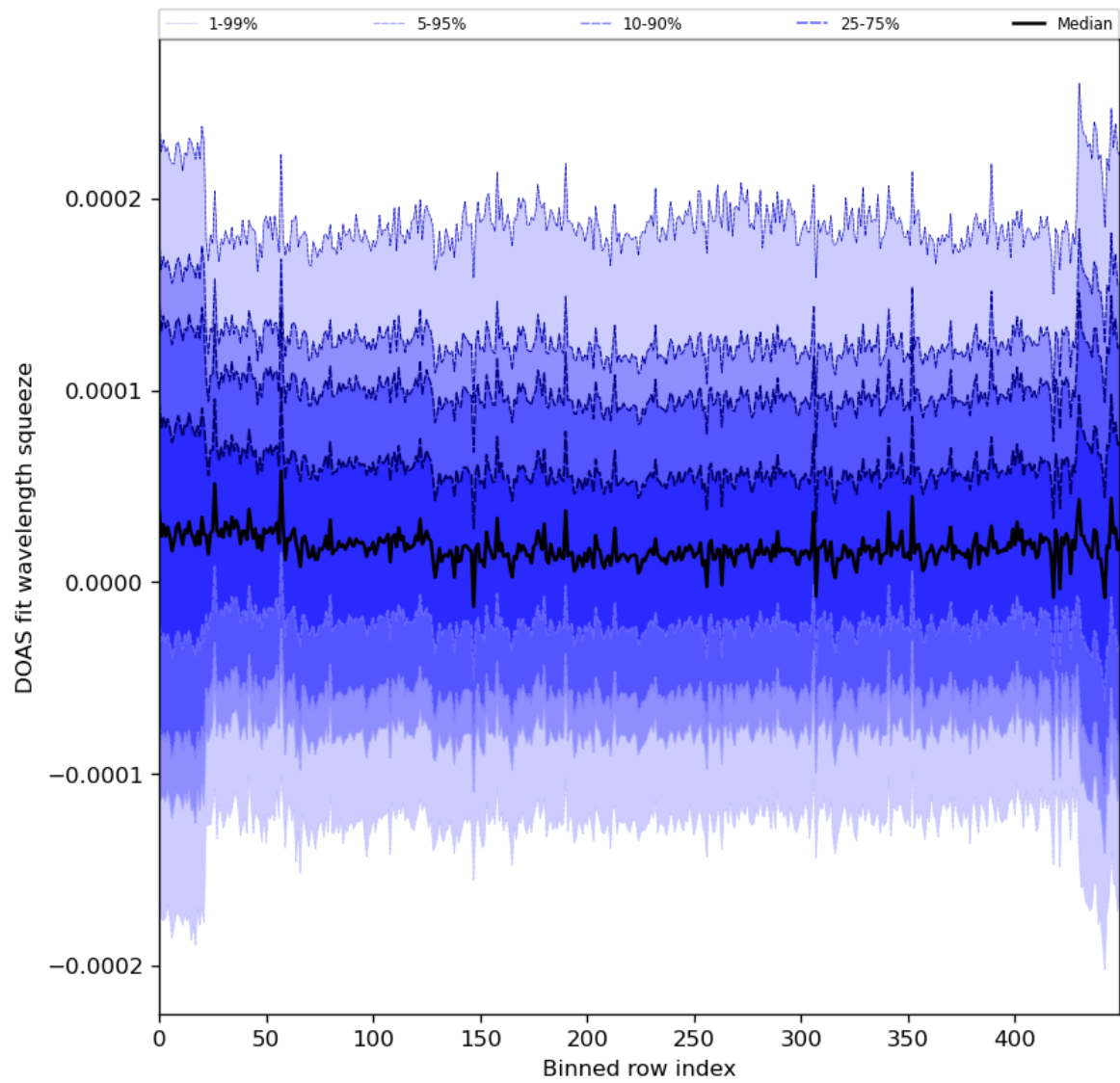
Figure 59: Along track statistics of “DOAS fit wavelength squeeze” for 2024-01-26 to 2024-01-28
