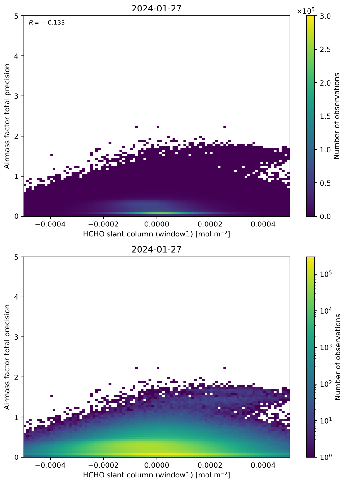
Figure 86: Scatter density plot of “HCHO slant column (window1)” against “Airmass factor total precision” for 2024-01-26 to 2024-01-28.
