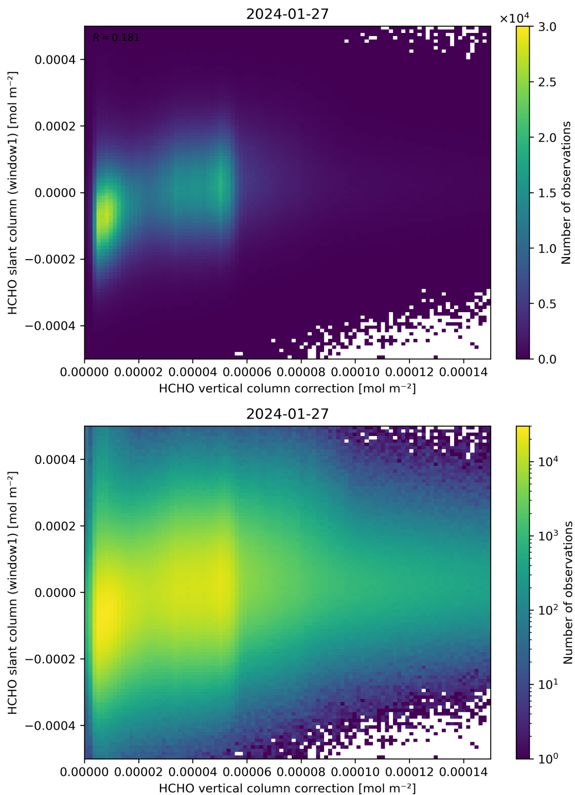
Figure 118: Scatter density plot of “HCHO vertical column correction” against “HCHO slant column (window1)” for 2024-01-26 to 2024-01-28.
