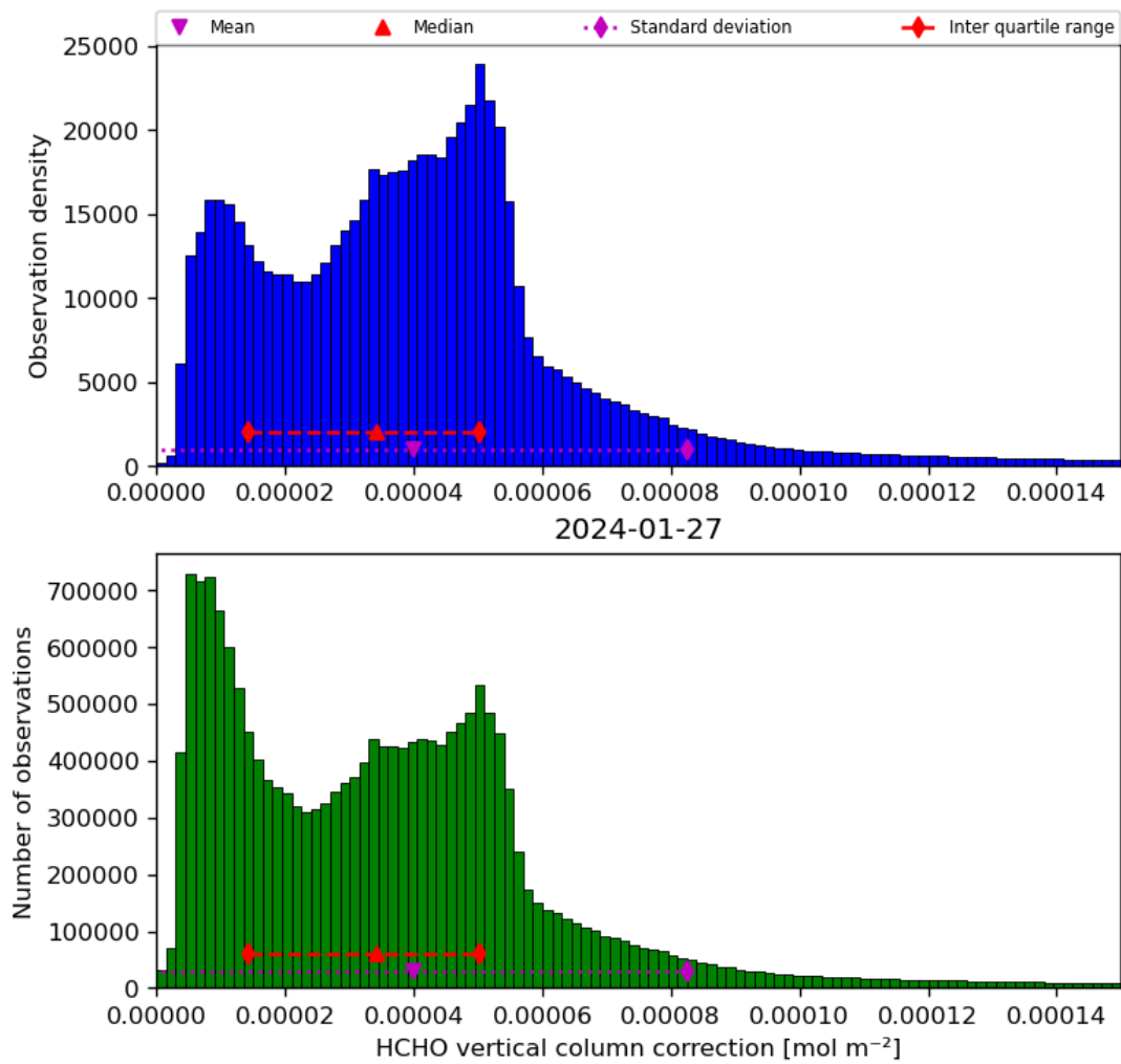
Figure 37: Histogram of “HCHO vertical column correction” for 2024-01-26 to 2024-01-28
