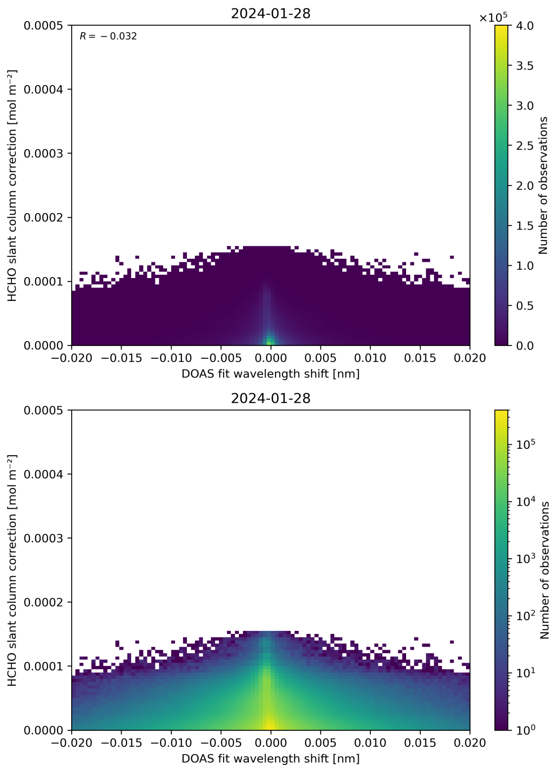
Figure 67: Scatter density plot of “DOAS fit wavelength shift” against “HCHO slant column correction” for 2024-01-27 to 2024-01-29.
