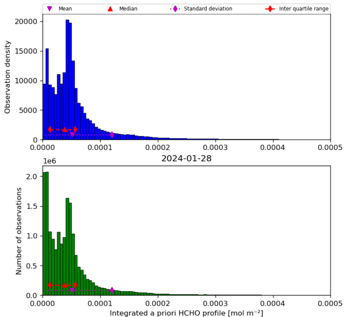
Figure 43: Histogram of “Integrated a priori HCHO profile” for 2024-01-27 to 2024-01-29
