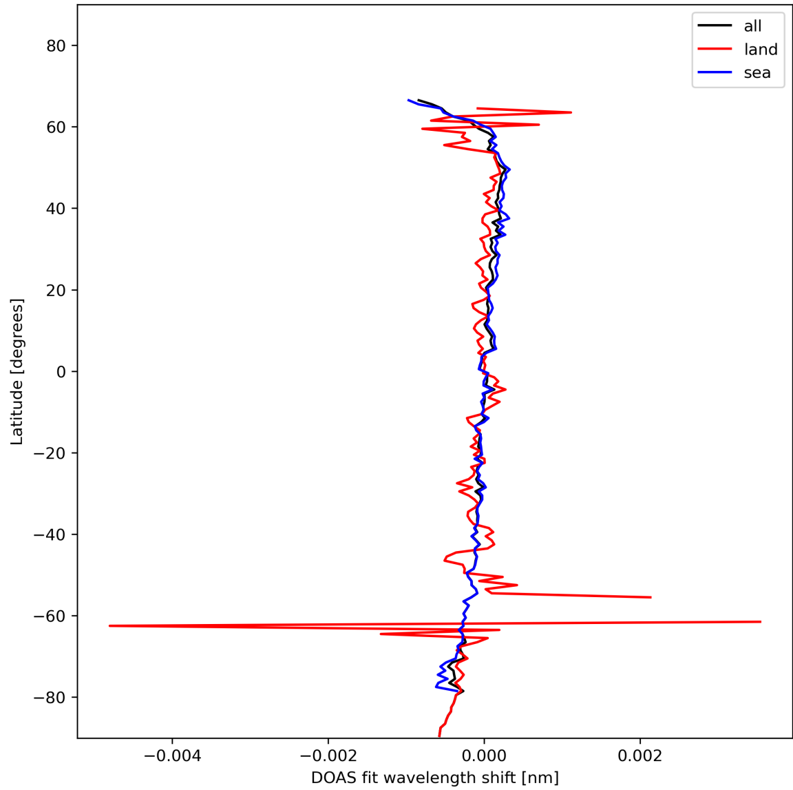
Figure 30: Zonal average of "DOAS fit wavelength shift" for 2024-01-27 to 2024-01-29.
