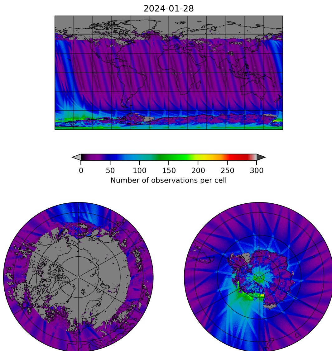
Figure 19: Map of the number of observations for 2024-01-27 to 2024-01-29
