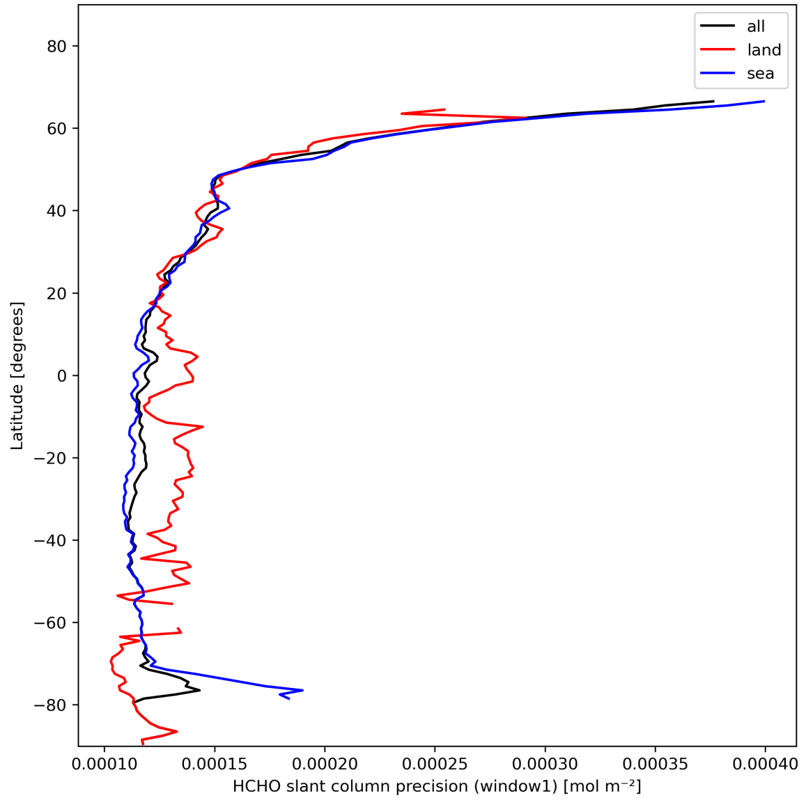
Figure 25: Zonal average of “HCHO slant column precision (window1)” for 2024-01-27 to 2024-01-29.
