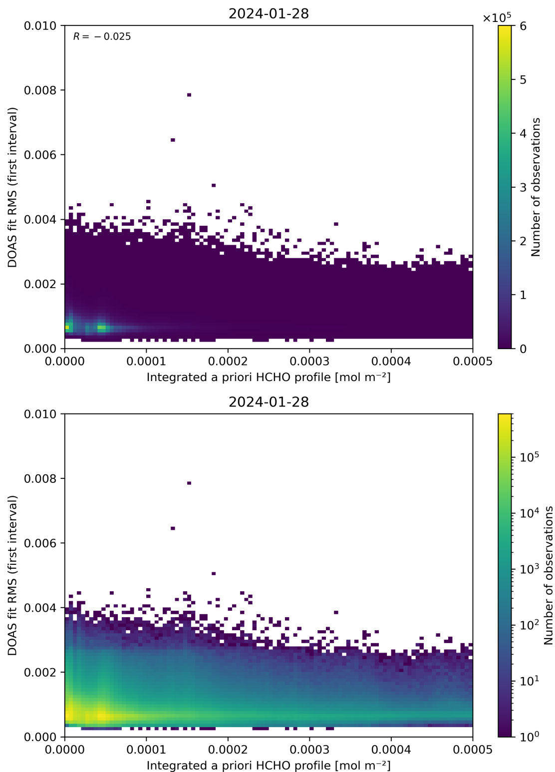
Figure 148: Scatter density plot of “Integrated a priori HCHO profile” against “DOAS fit RMS (first interval)” for 2024-01-27 to 2024-01-29.
