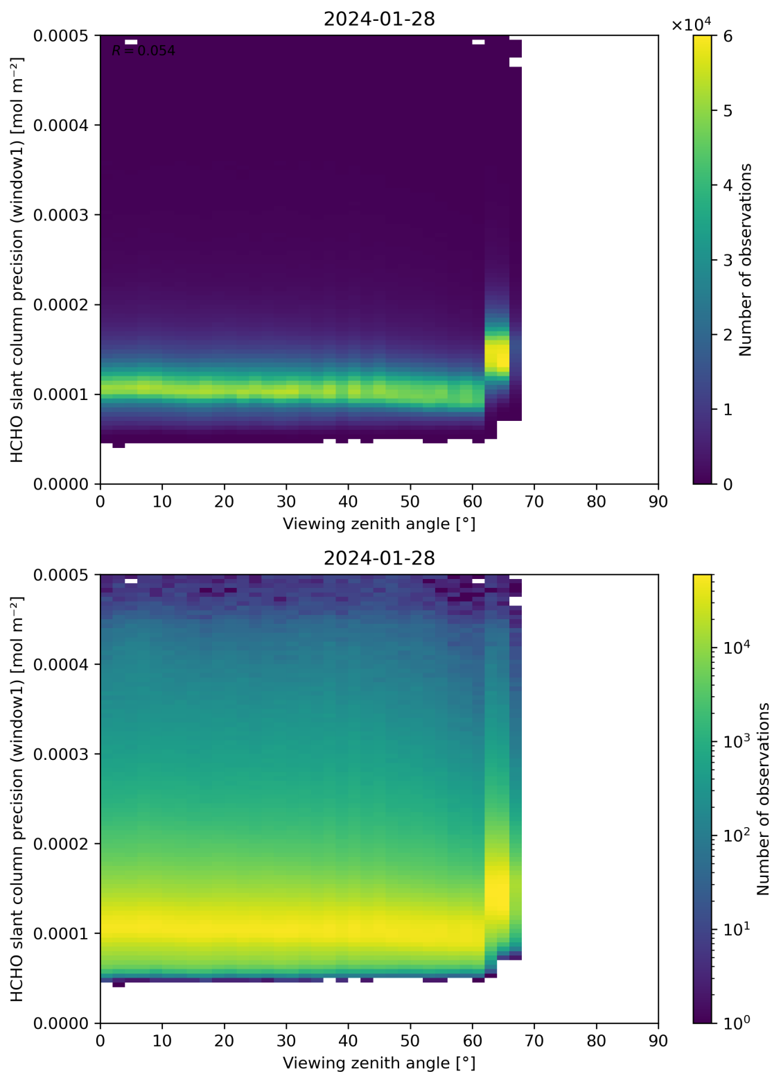
Figure 189: Scatter density plot of “Viewing zenith angle” against “HCHO slant column precision (window1)” for 2024-01-27 to 2024-01-29.
