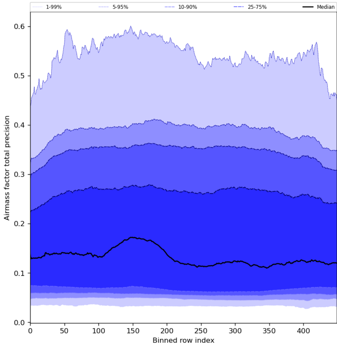
Figure 55: Along track statistics of “Airmass factor total precision” for 2024-01-27 to 2024-01-29
