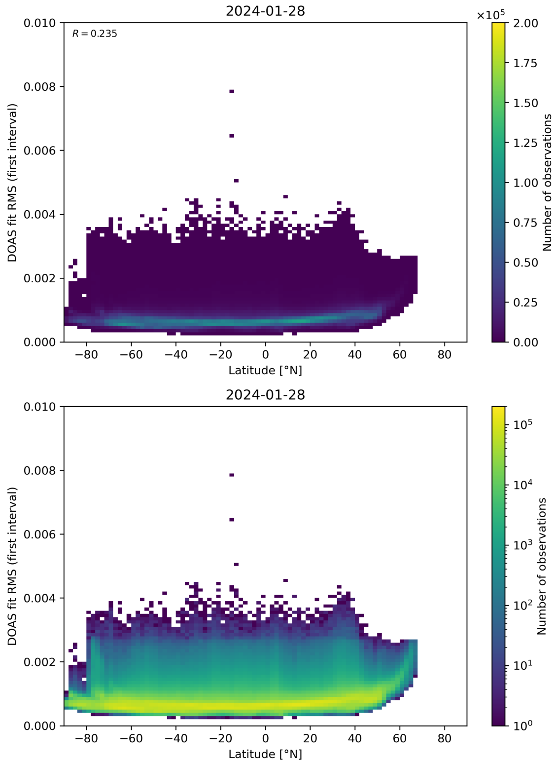
Figure 153: Scatter density plot of “Latitude” against “DOAS fit RMS (first interval)” for 2024-01-27 to 2024-01-29.
