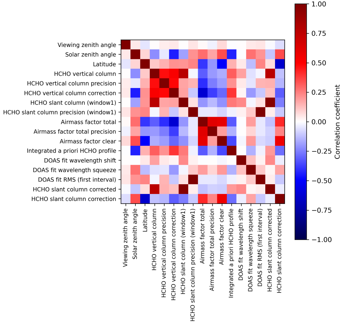
Figure 2: Map of correlation matrix for 2024-01-27 to 2024-01-29.
