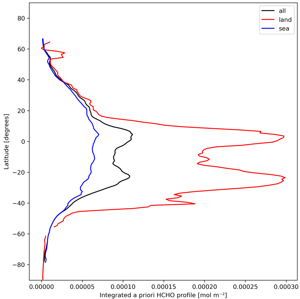
Figure 29: Zonal average of “Integrated a priori HCHO profile” for 2024-01-27 to 2024-01-29.
