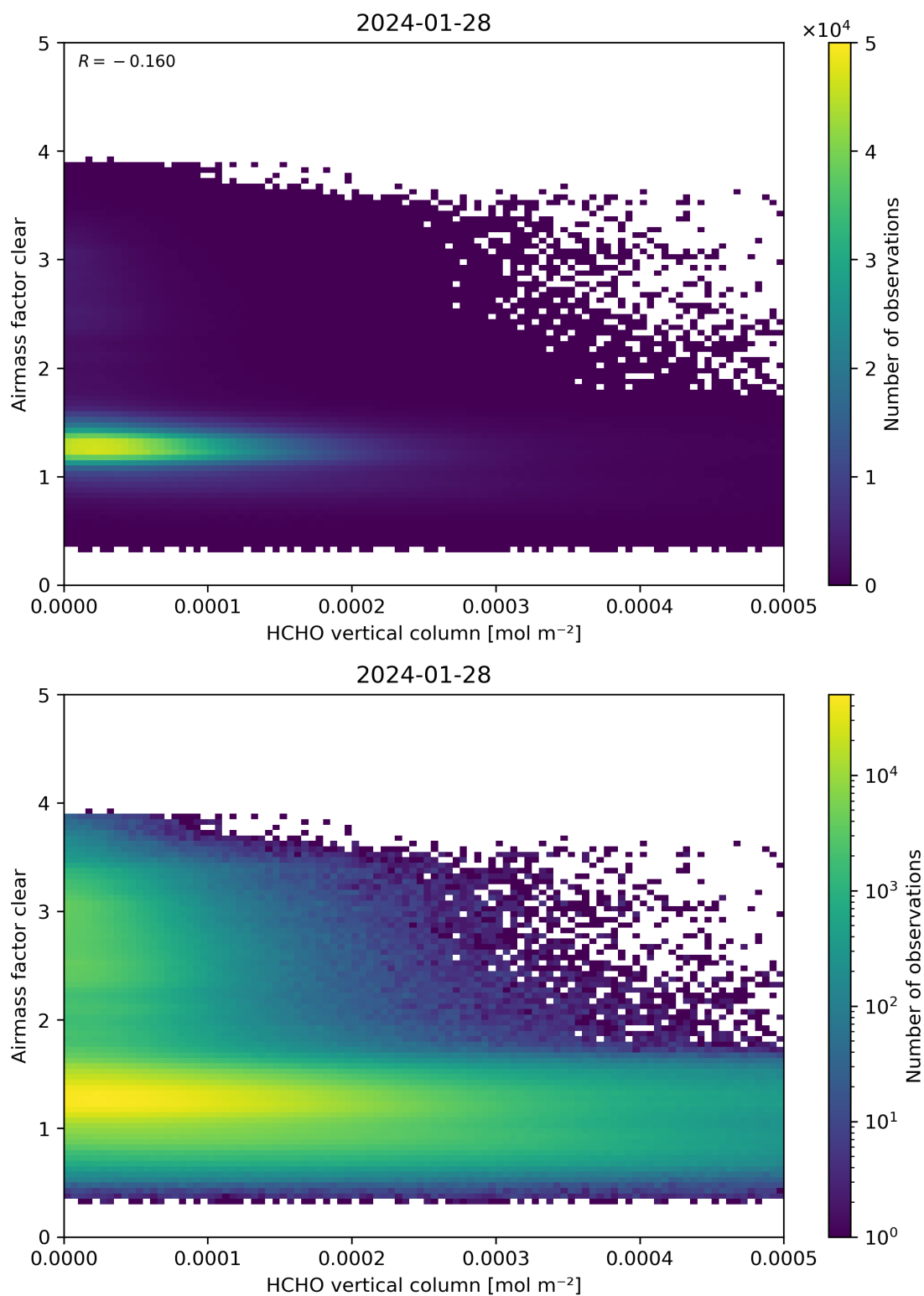
Figure 126: Scatter density plot of “HCHO vertical column” against “Airmass factor clear” for 2024-01-27 to 2024-01-29.
