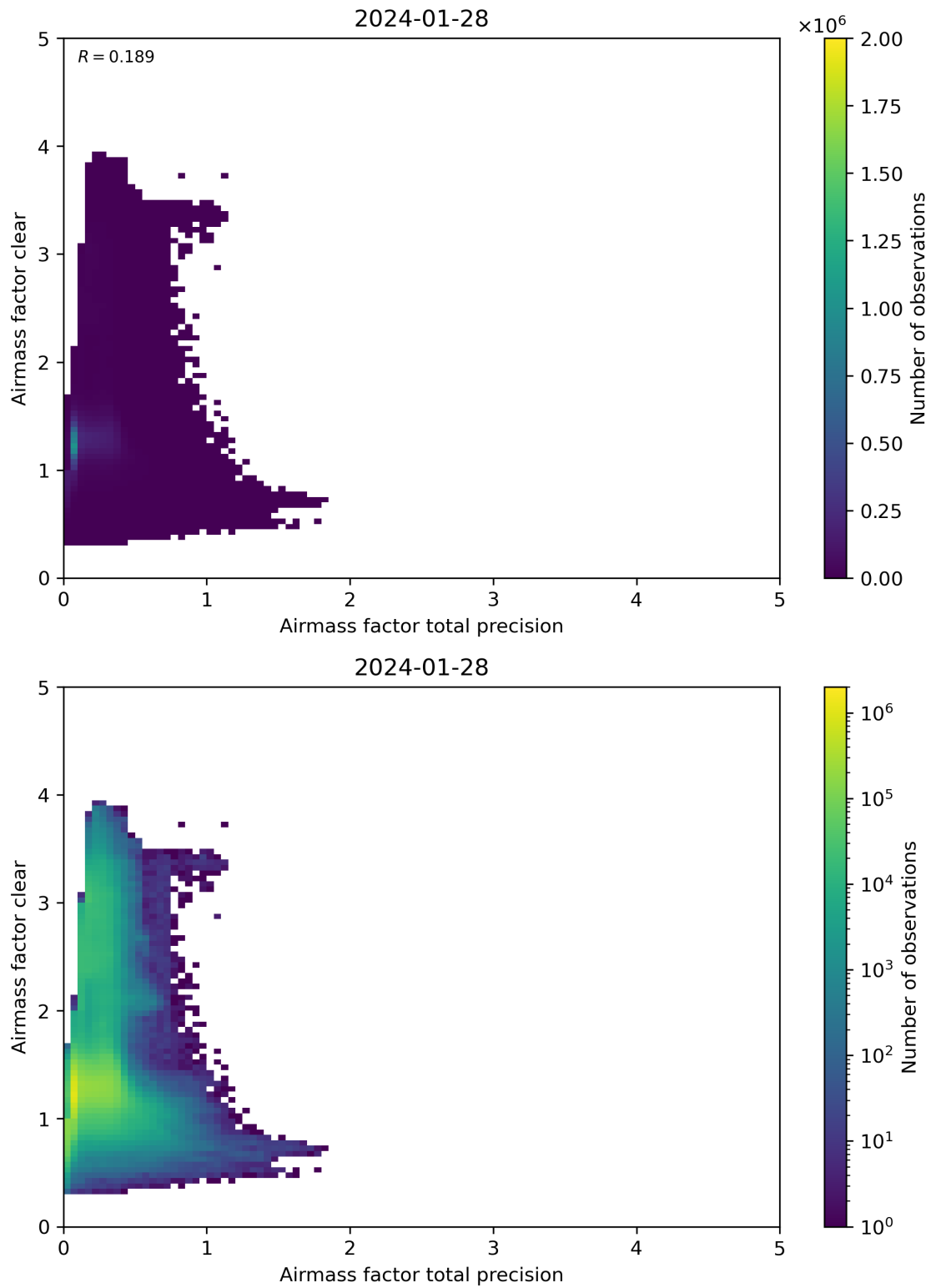
Figure 108: Scatter density plot of “Airmass factor total precision” against “Airmass factor clear” for 2024-01-27 to 2024-01-29.
