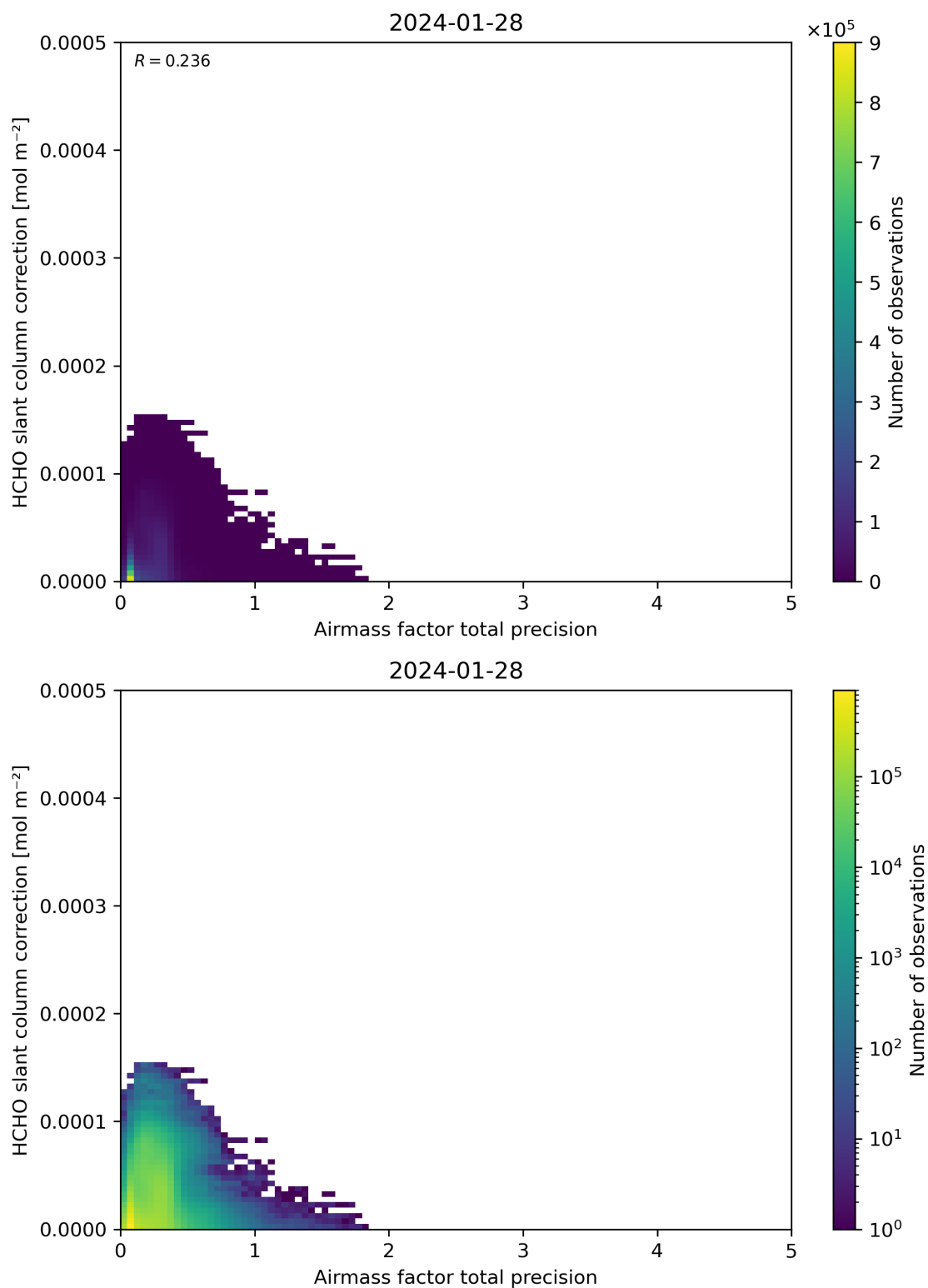
Figure 110: Scatter density plot of “Airmass factor total precision” against “HCHO slant column correction” for 2024-01-27 to 2024-01-29.
