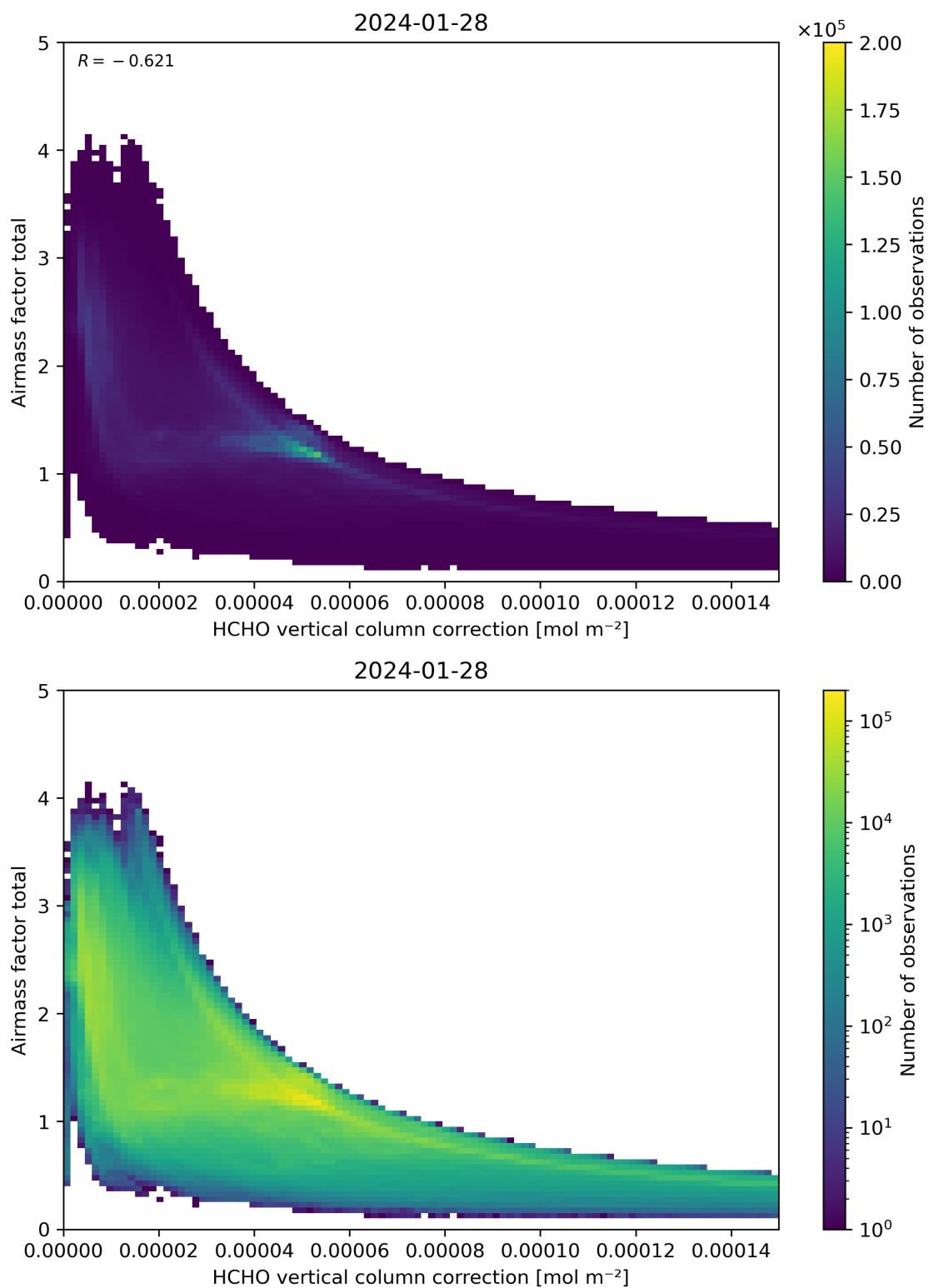
Figure 120: Scatter density plot of “HCHO vertical column correction” against “Airmass factor total” for 2024-01-27 to 2024-01-29.
