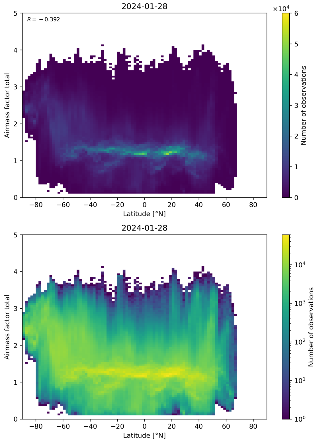
Figure 161: Scatter density plot of “Latitude” against “Airmass factor total” for 2024-01-27 to 2024-01-29.
