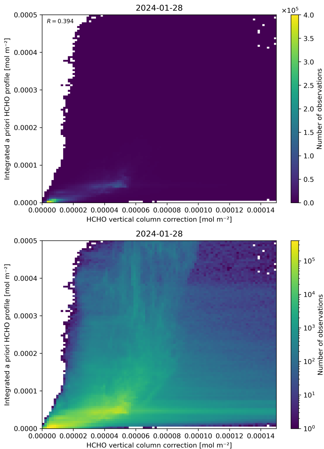
Figure 122: Scatter density plot of “HCHO vertical column correction” against “Integrated a priori HCHO profile” for 2024-01-27 to 2024-01-29.
