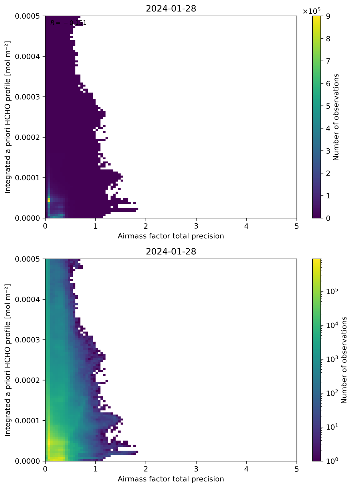
Figure 111: Scatter density plot of “Airmass factor total precision” against “Integrated a priori HCHO profile” for 2024-01-27 to 2024-01-29.
