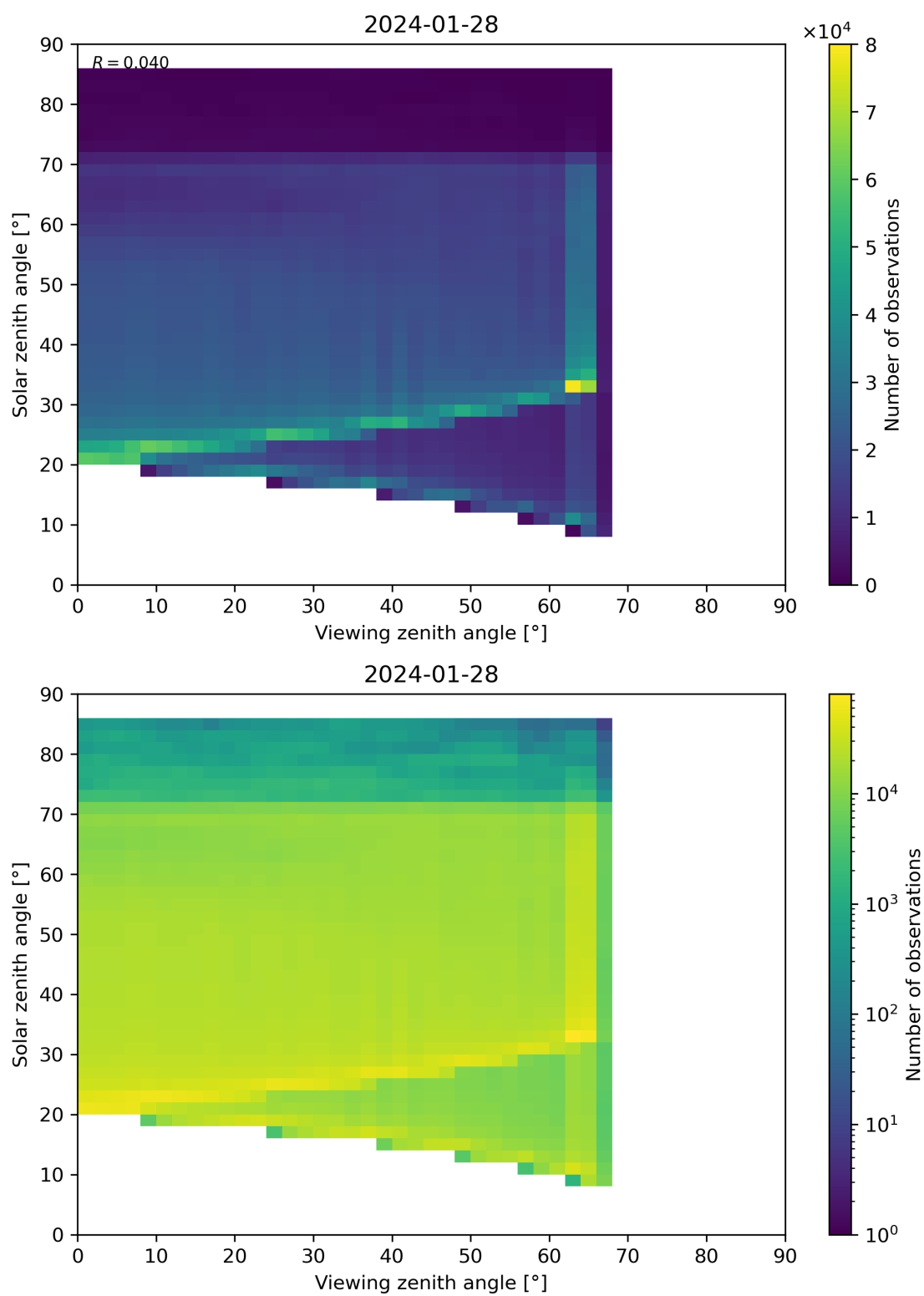
Figure 197: Scatter density plot of “Viewing zenith angle” against “Solar zenith angle” for 2024-01-27 to 2024-01-29.
