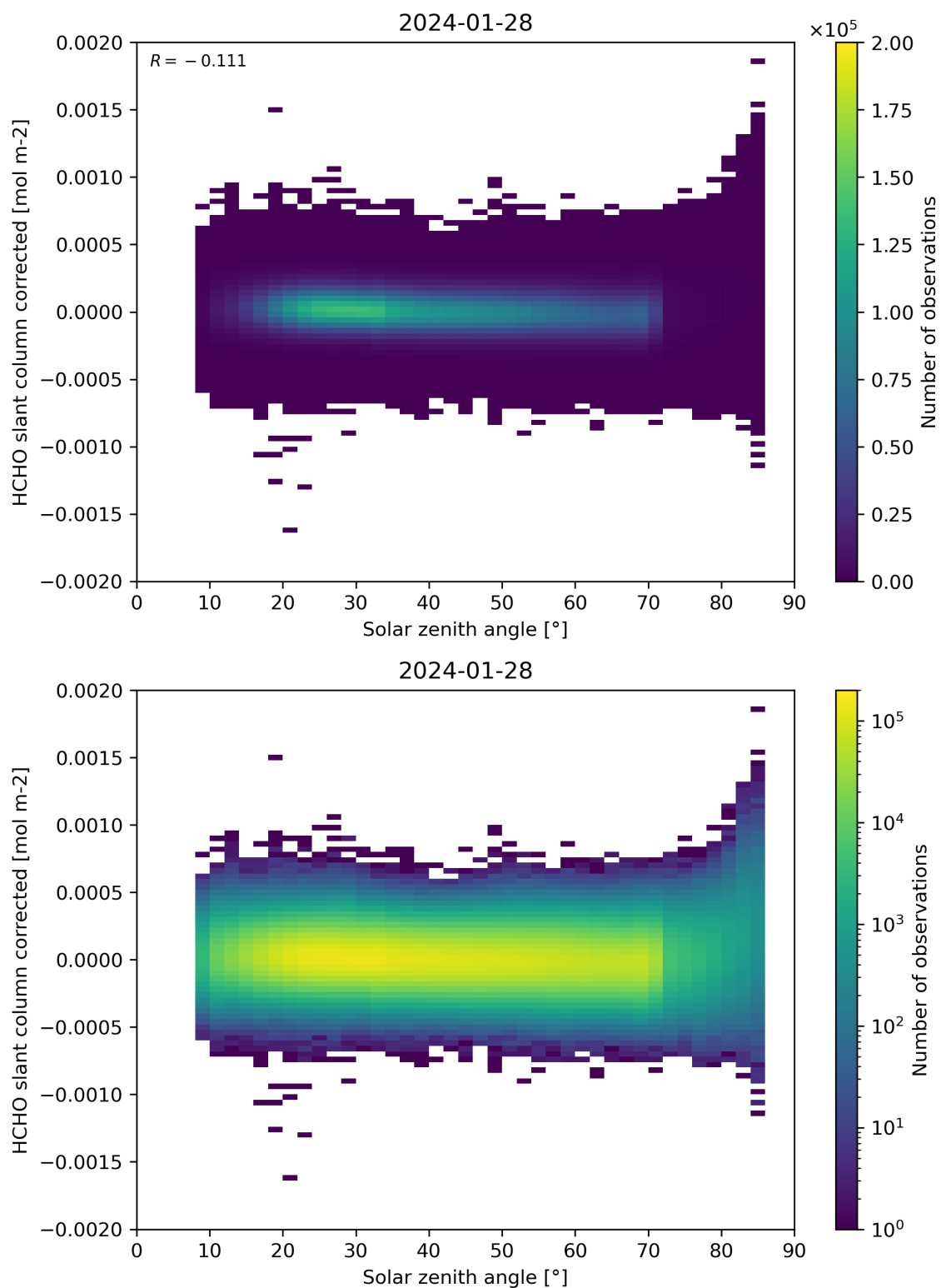
Figure 171: Scatter density plot of “Solar zenith angle” against “HCHO slant column corrected” for 2024-01-27 to 2024-01-29.
