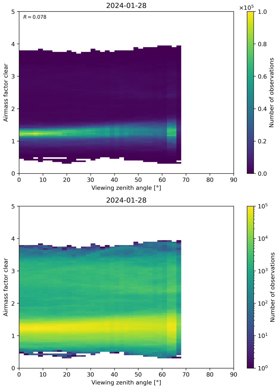
Figure 185: Scatter density plot of “Viewing zenith angle” against “Airmass factor clear” for 2024-01-27 to 2024-01-29.
