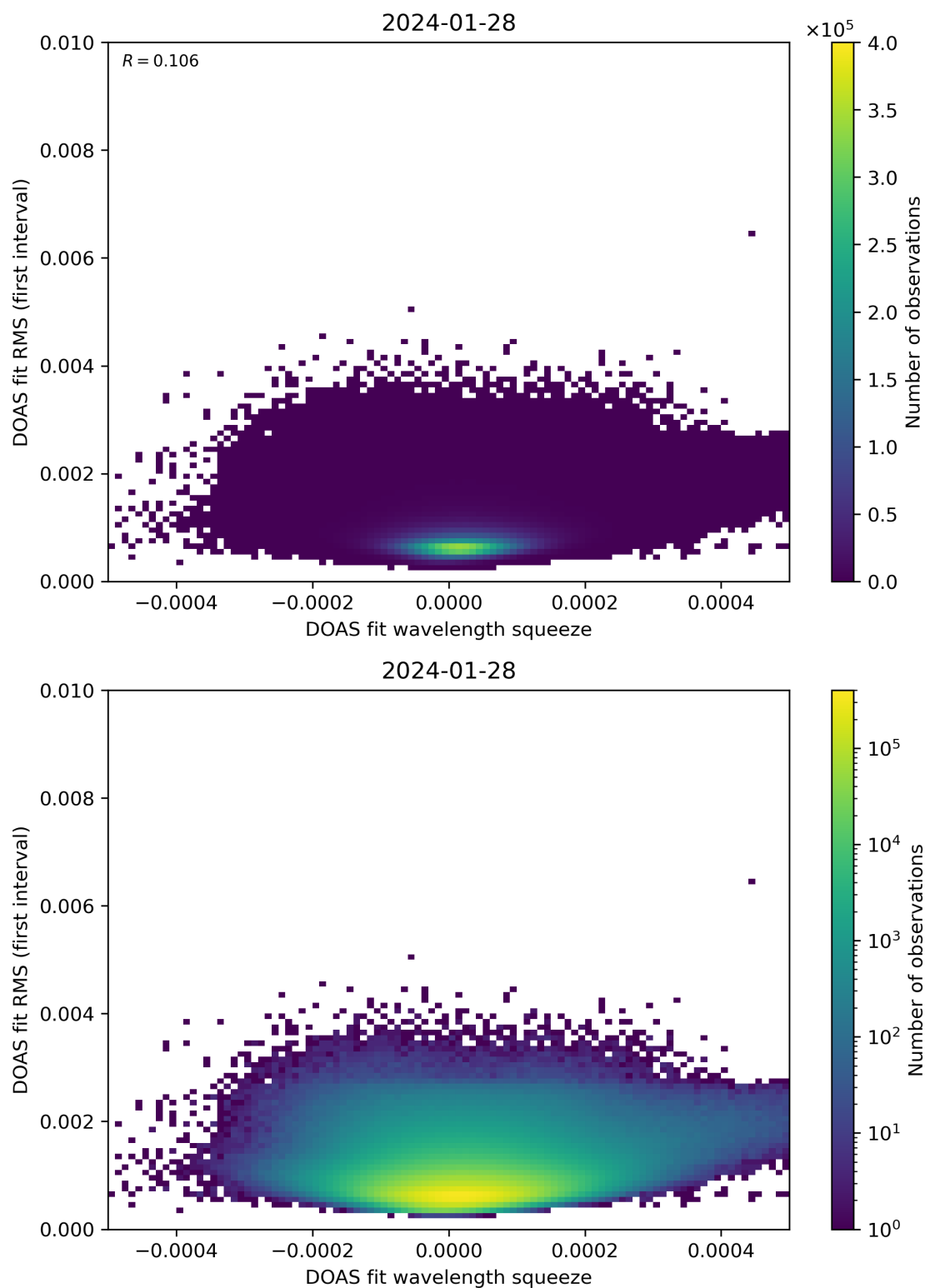
Figure 68: Scatter density plot of “DOAS fit wavelength squeeze” against “DOAS fit RMS (first interval)” for 2024-01-27 to 2024-01-29.
