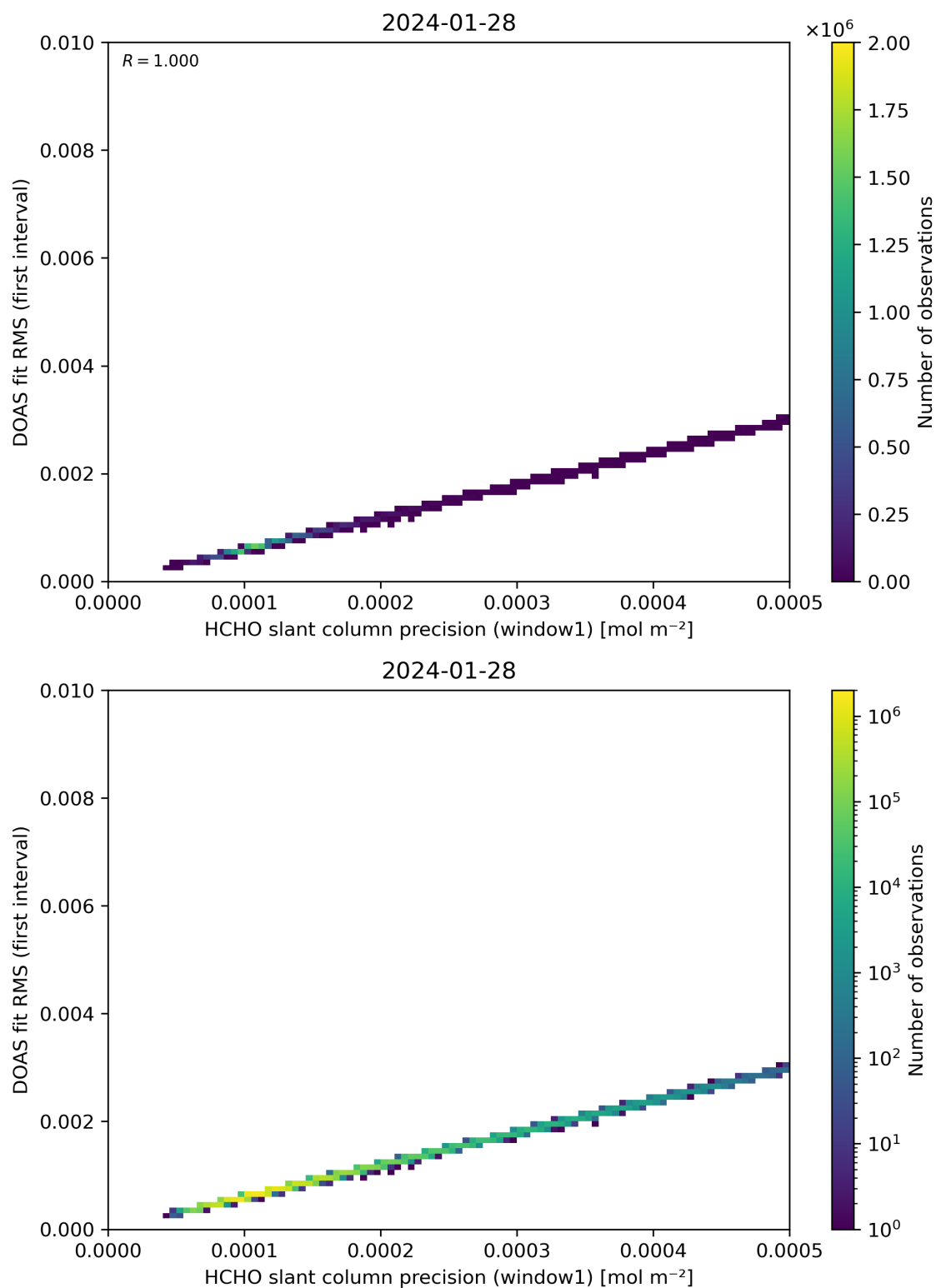
Figure 88: Scatter density plot of “HCHO slant column precision (window1)” against “DOAS fit RMS (first interval)” for 2024-01-27 to 2024-01-29.
