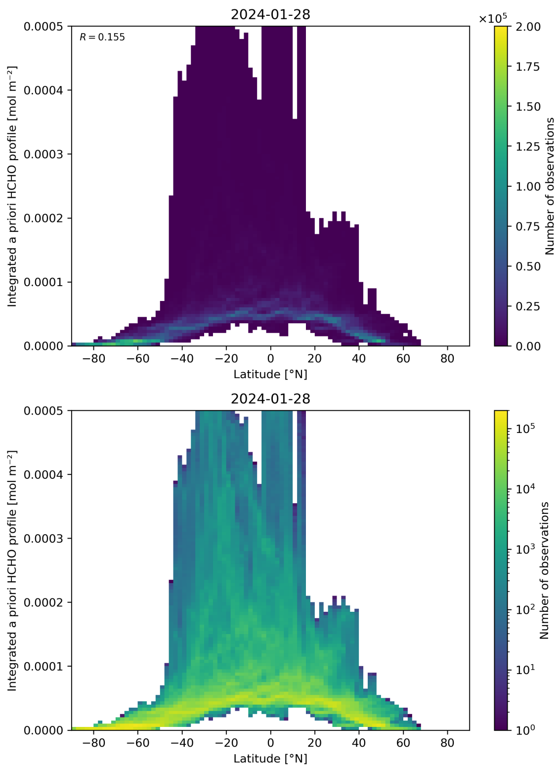
Figure 166: Scatter density plot of “Latitude” against “Integrated a priori HCHO profile” for 2024-01-27 to 2024-01-29.
