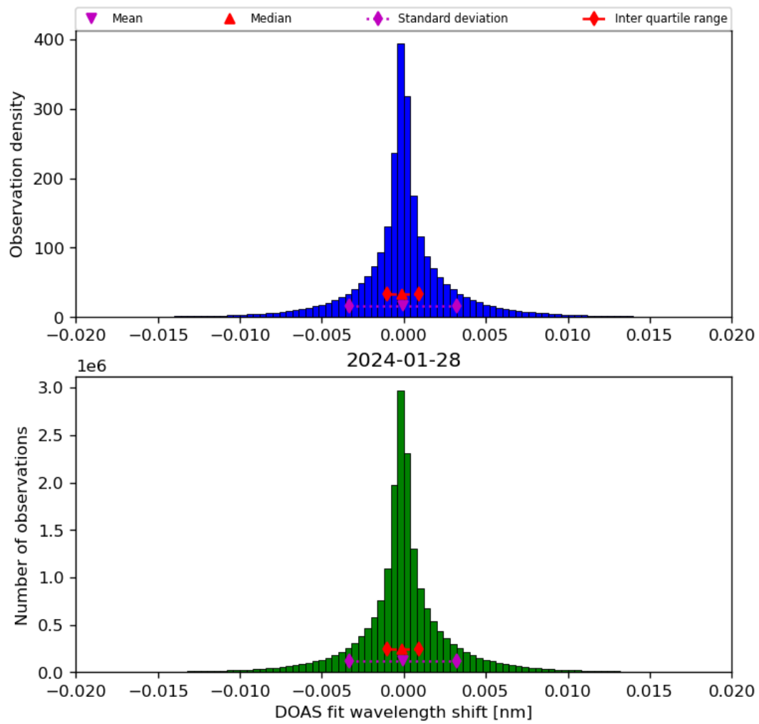
Figure 44: Histogram of “DOAS fit wavelength shift” for 2024-01-27 to 2024-01-29
