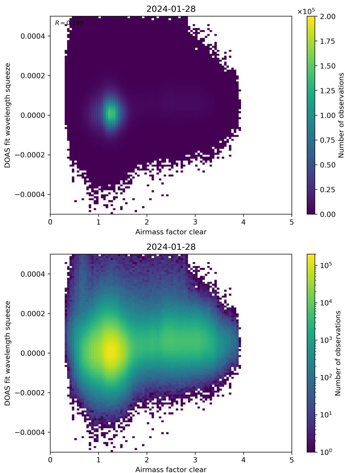
Figure 73: Scatter density plot of “Airmass factor clear” against “DOAS fit wavelength squeeze” for 2024-01-27 to 2024-01-29.
