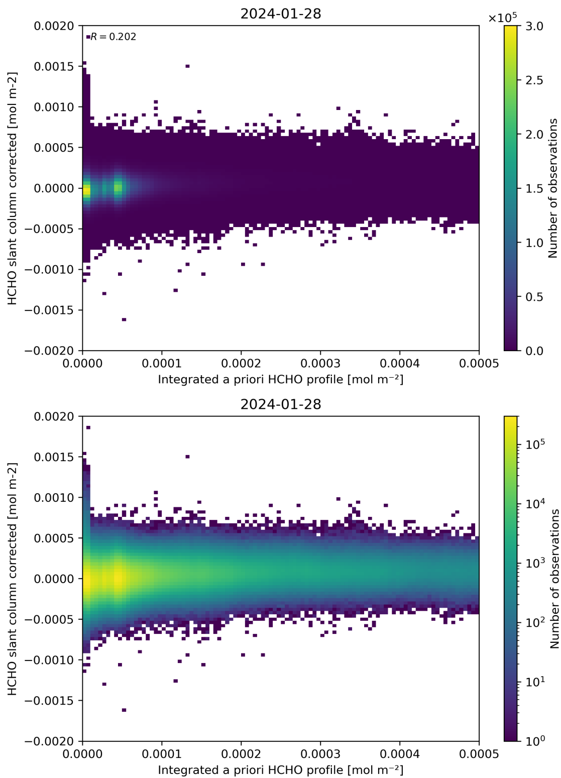
Figure 151: Scatter density plot of “Integrated a priori HCHO profile” against “HCHO slant column corrected” for 2024-01-27 to 2024-01-29.
