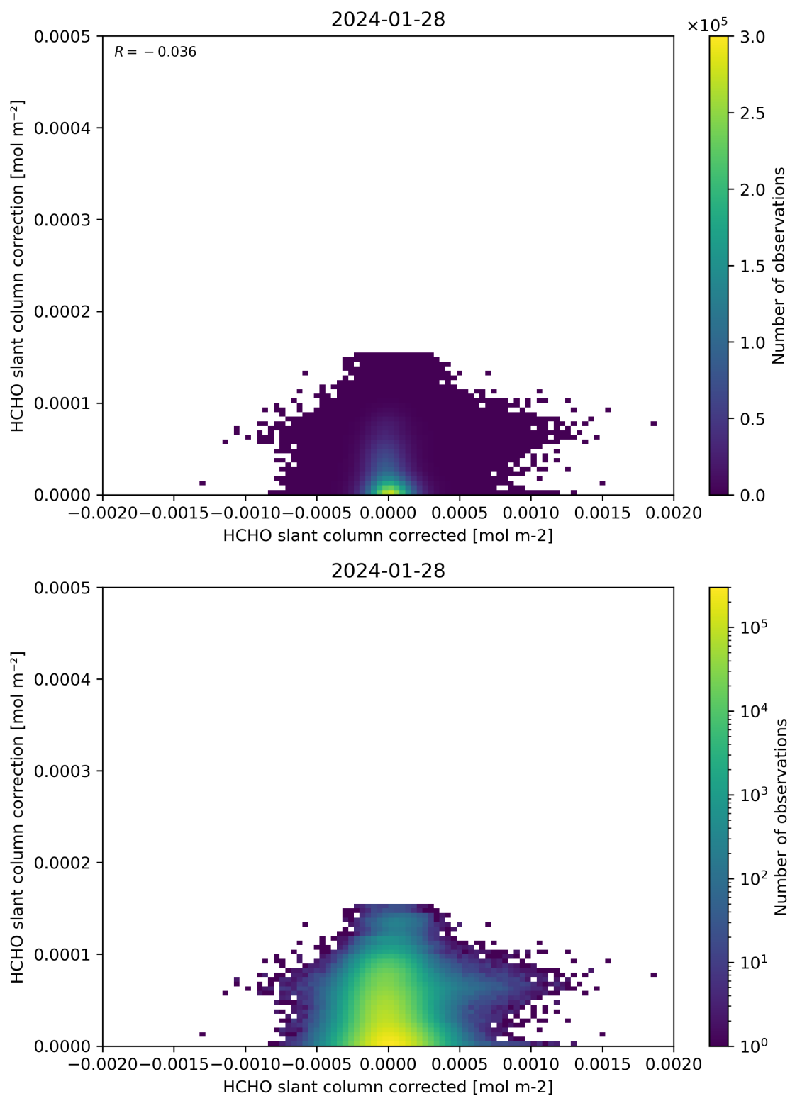
Figure 77: Scatter density plot of “HCHO slant column corrected” against “HCHO slant column correction” for 2024-01-27 to 2024-01-29.
