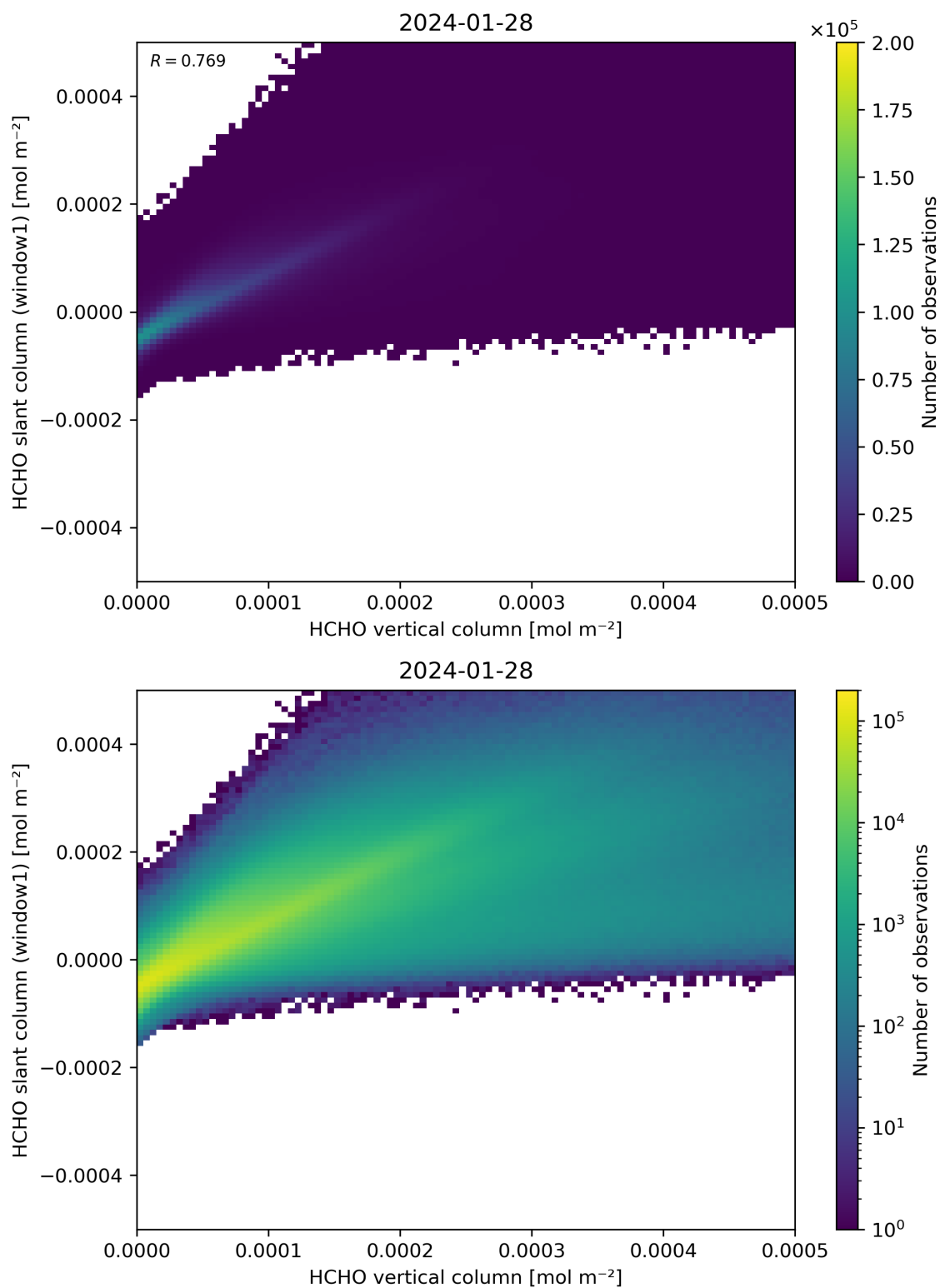
Figure 129: Scatter density plot of “HCHO vertical column” against “HCHO slant column (window1)” for 2024-01-27 to 2024-01-29.
