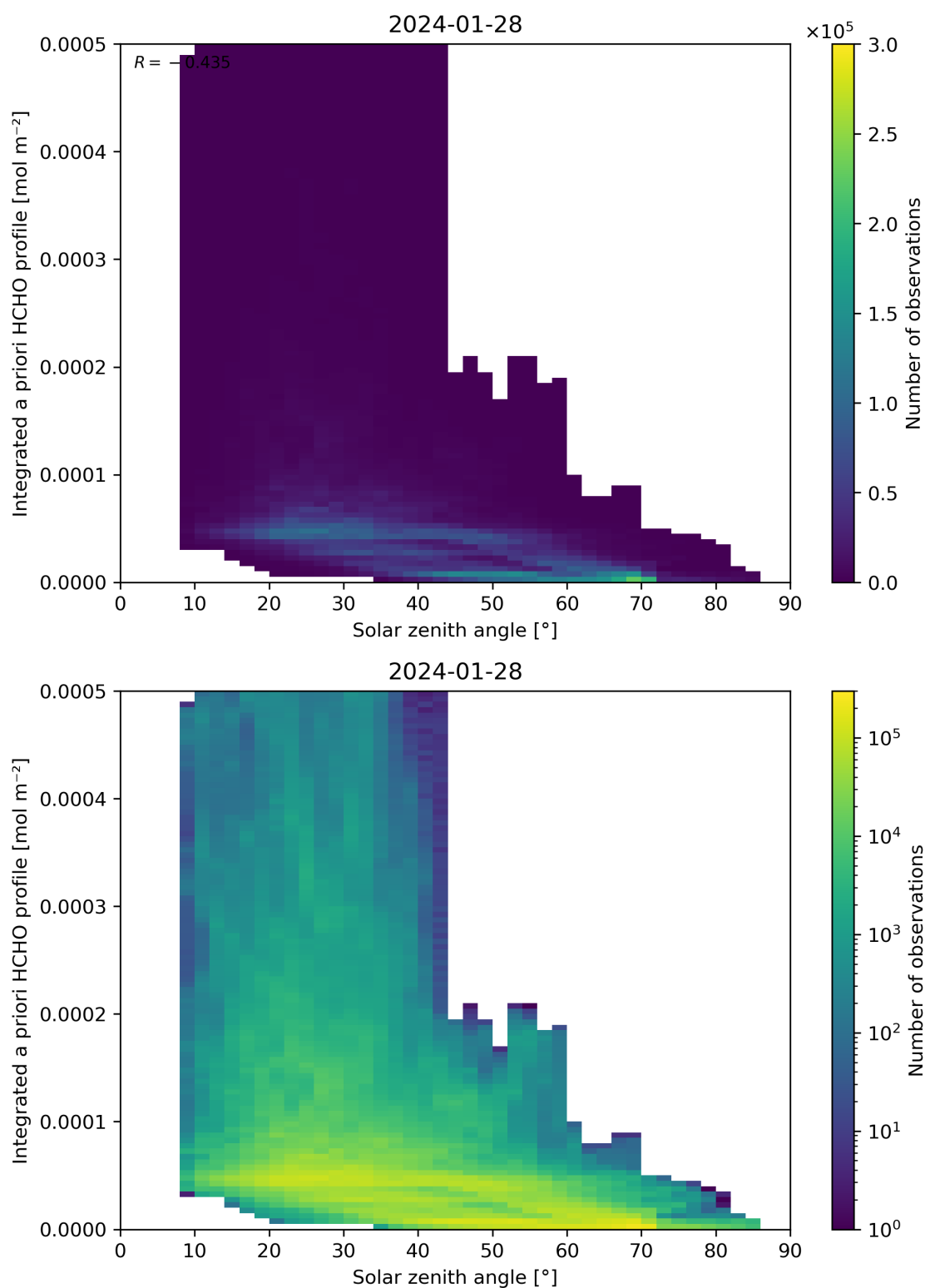
Figure 180: Scatter density plot of “Solar zenith angle” against “Integrated a priori HCHO profile” for 2024-01-27 to 2024-01-29.
