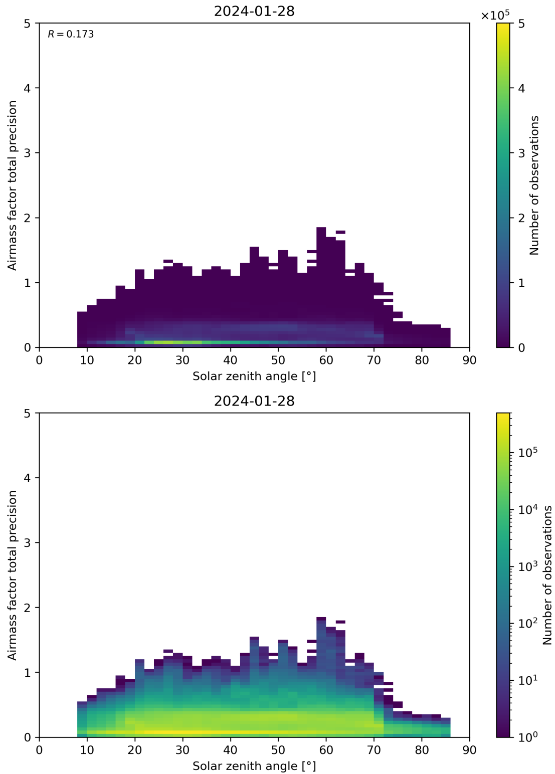
Figure 176: Scatter density plot of “Solar zenith angle” against “Airmass factor total precision” for 2024-01-27 to 2024-01-29.
