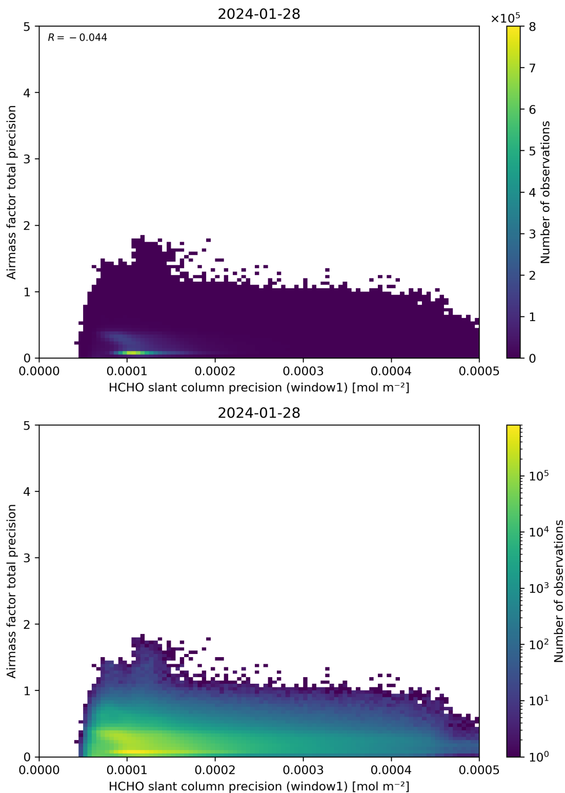
Figure 95: Scatter density plot of “HCHO slant column precision (window1)” against “Airmass factor total precision” for 2024-01-27 to 2024-01-29.
