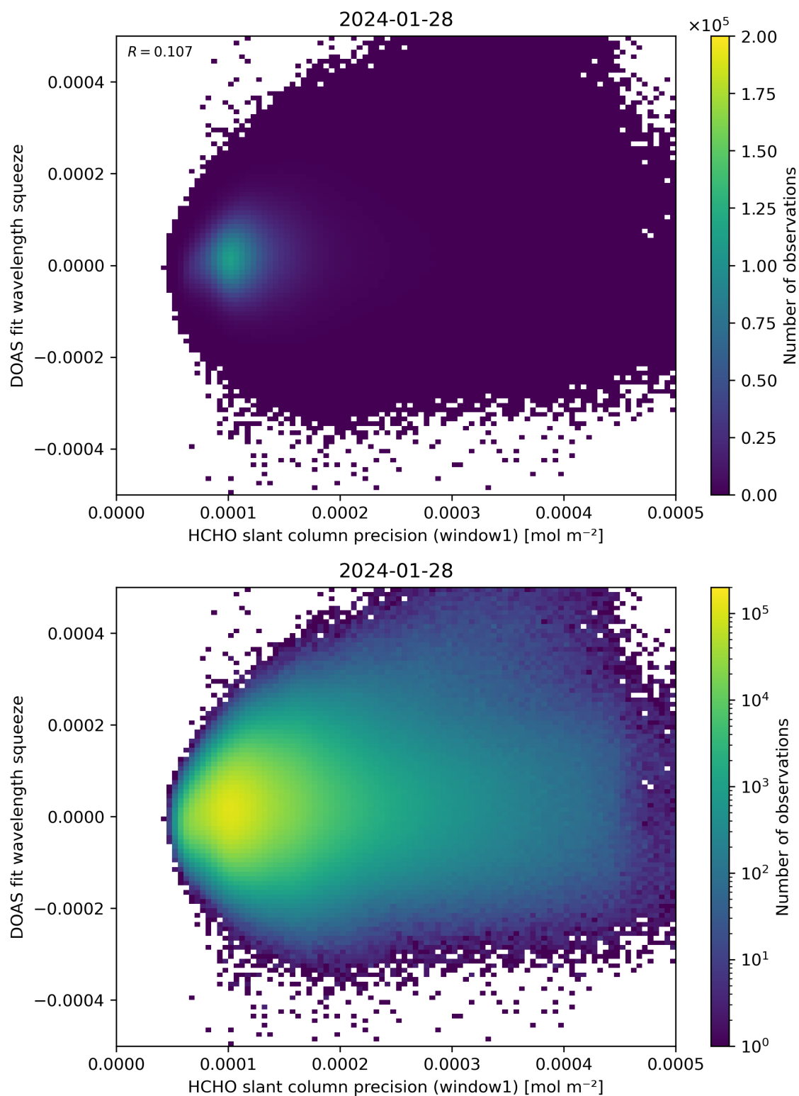
Figure 90: Scatter density plot of “HCHO slant column precision (window1)” against “DOAS fit wavelength squeeze” for 2024-01-27 to 2024-01-29.
