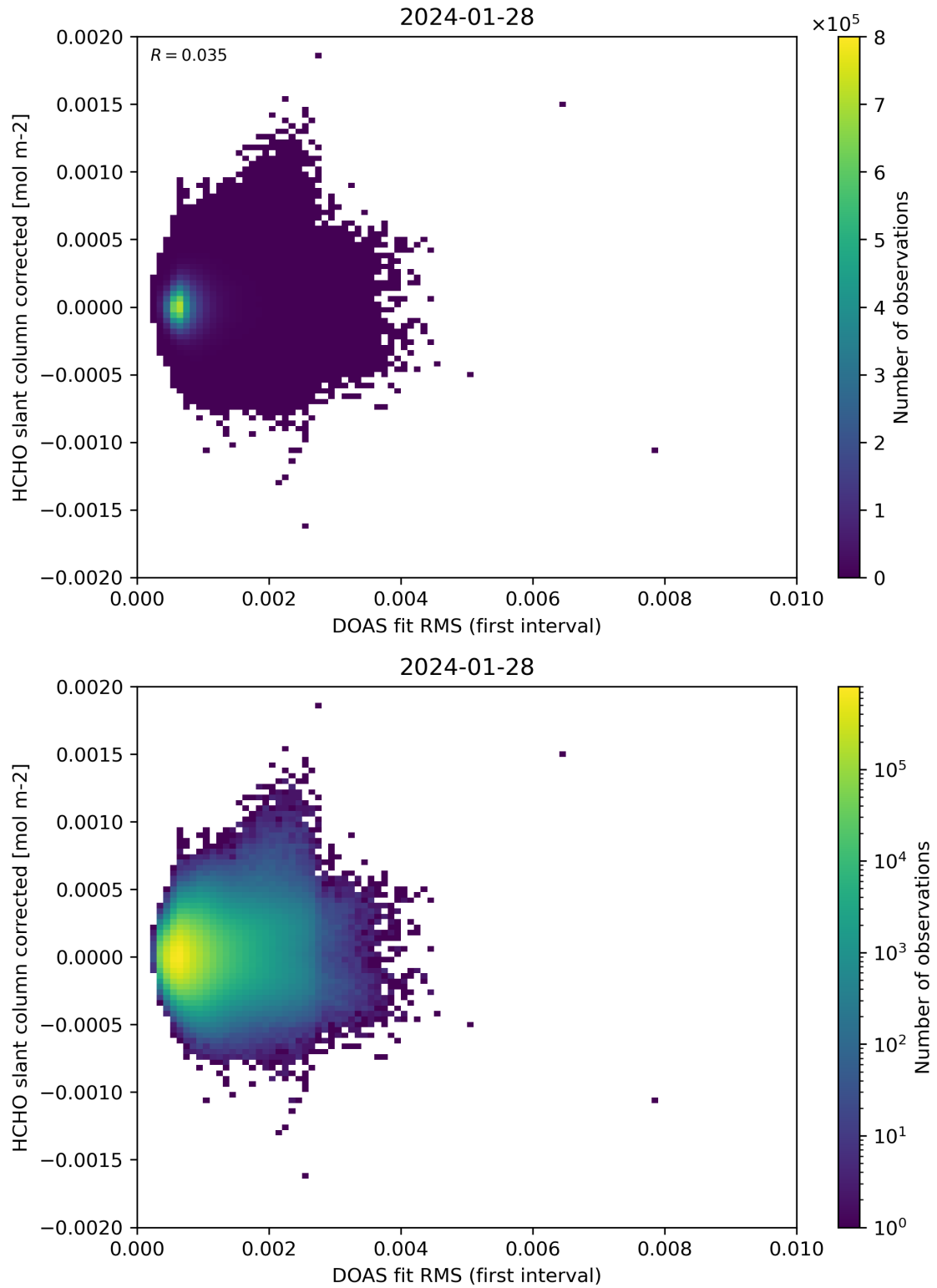
Figure 62: Scatter density plot of “DOAS fit RMS (first interval)” against “HCHO slant column corrected” for 2024-01-27 to 2024-01-29.
