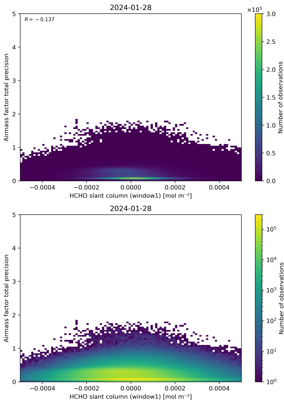
Figure 86: Scatter density plot of “HCHO slant column (window1)” against “Airmass factor total precision” for 2024-01-27 to 2024-01-29.
