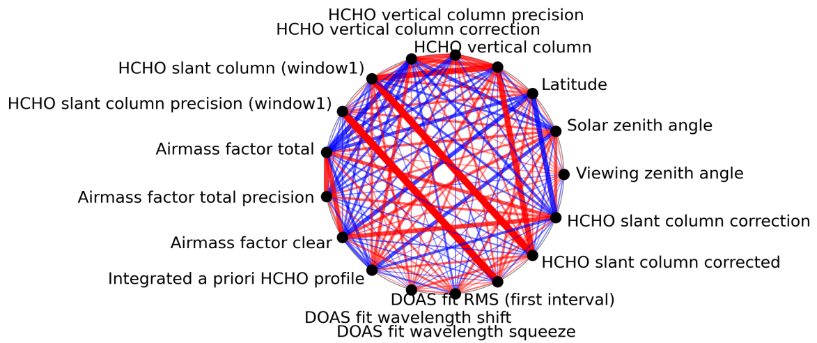
Figure 1: Map of correlation graph for 2024-01-27 to 2024-01-29.
