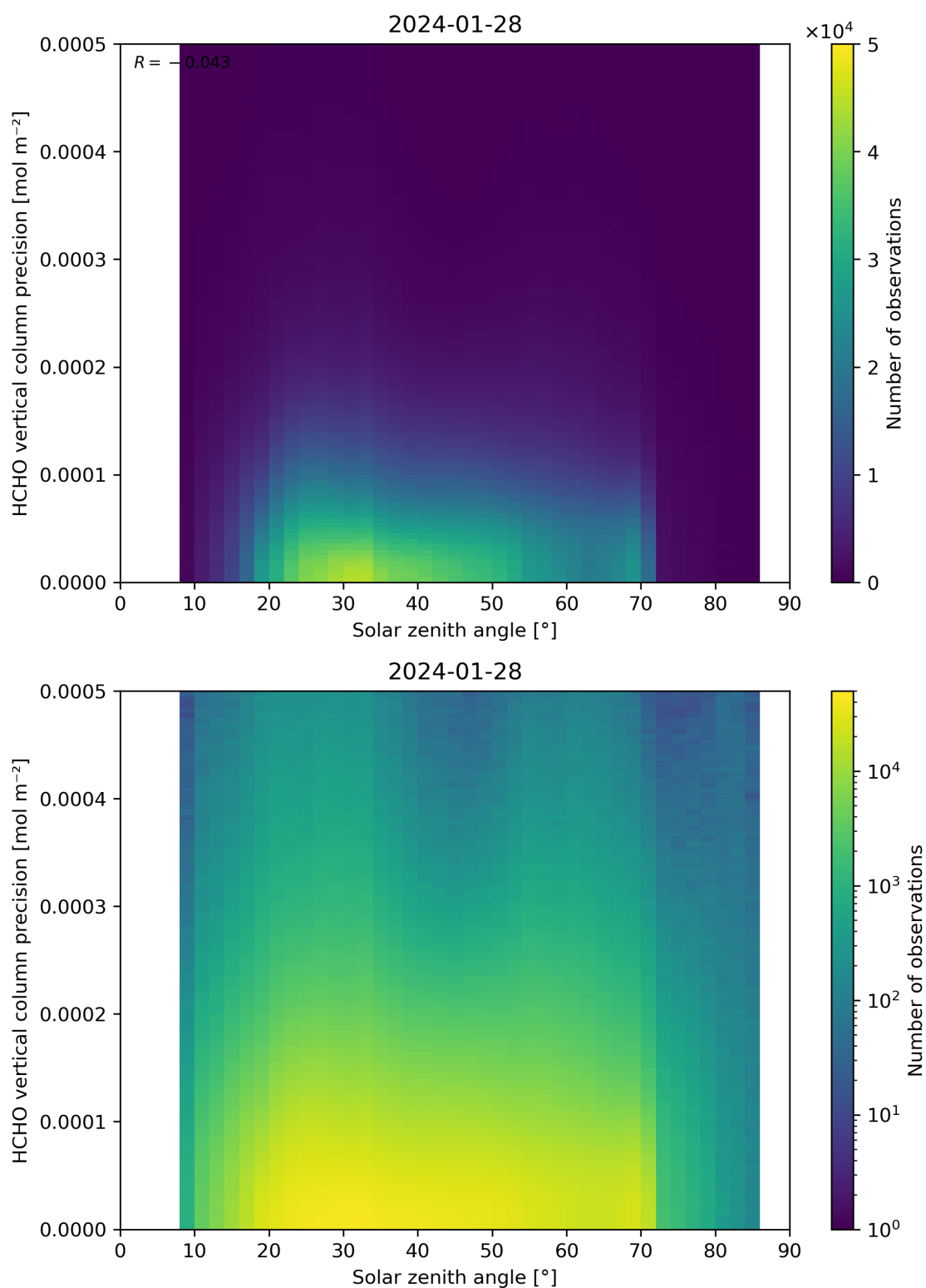
Figure 179: Scatter density plot of “Solar zenith angle” against “HCHO vertical column precision” for 2024-01-27 to 2024-01-29.
