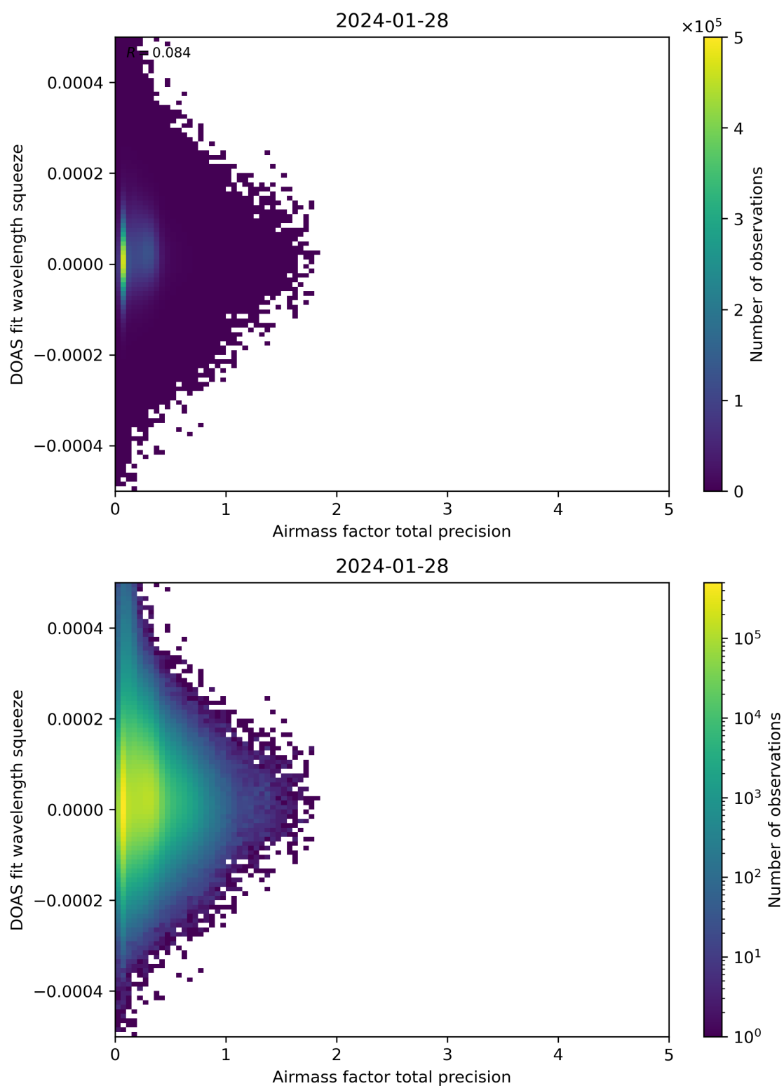
Figure 107: Scatter density plot of “Airmass factor total precision” against “DOAS fit wavelength squeeze” for 2024-01-27 to 2024-01-29.
