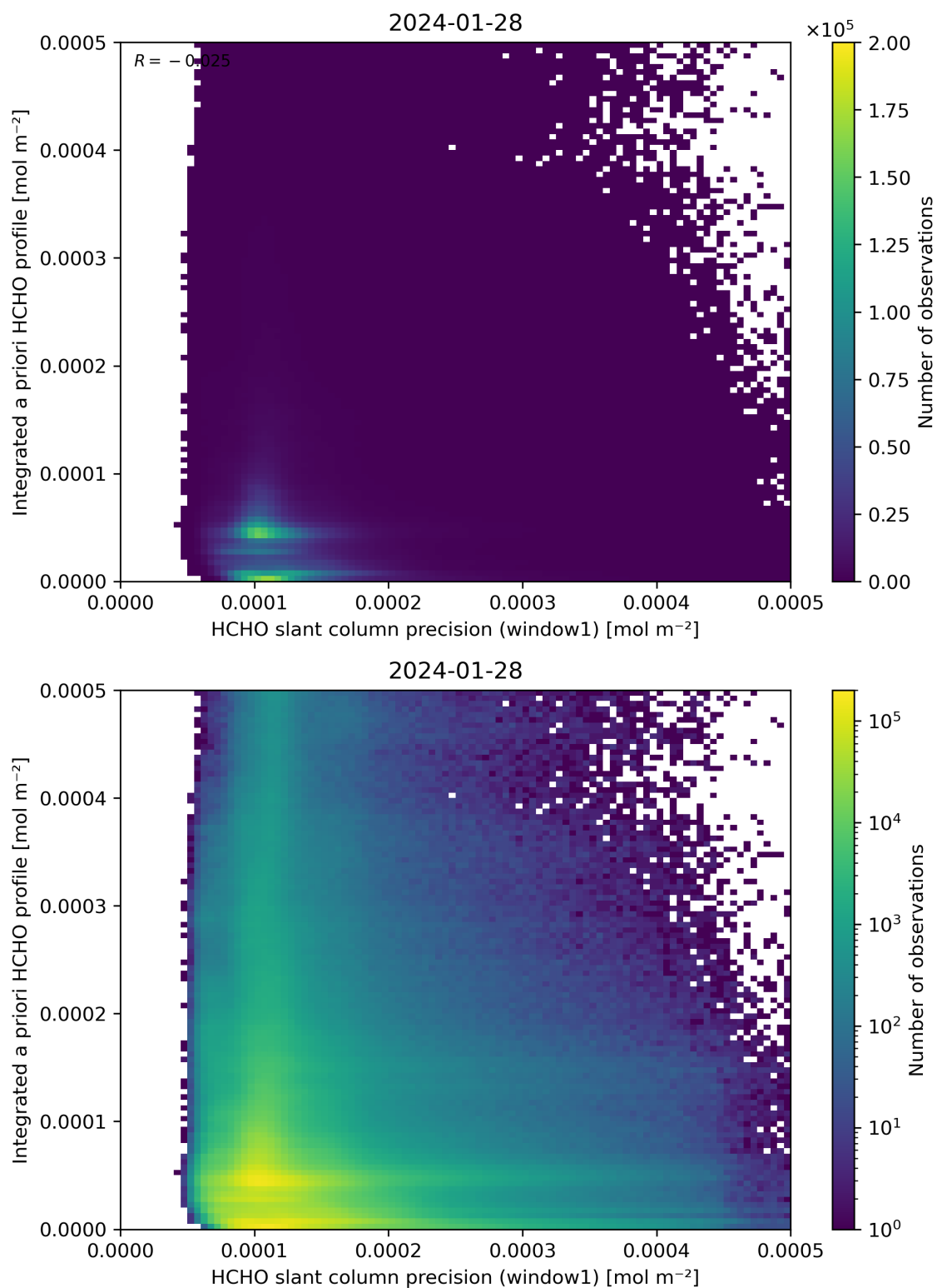
Figure 96: Scatter density plot of “HCHO slant column precision (window1)” against “Integrated a priori HCHO profile” for 2024-01-27 to 2024-01-29.
