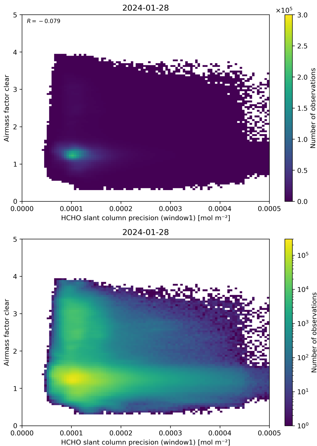
Figure 91: Scatter density plot of “HCHO slant column precision (window1)” against “Airmass factor clear” for 2024-01-27 to 2024-01-29.
