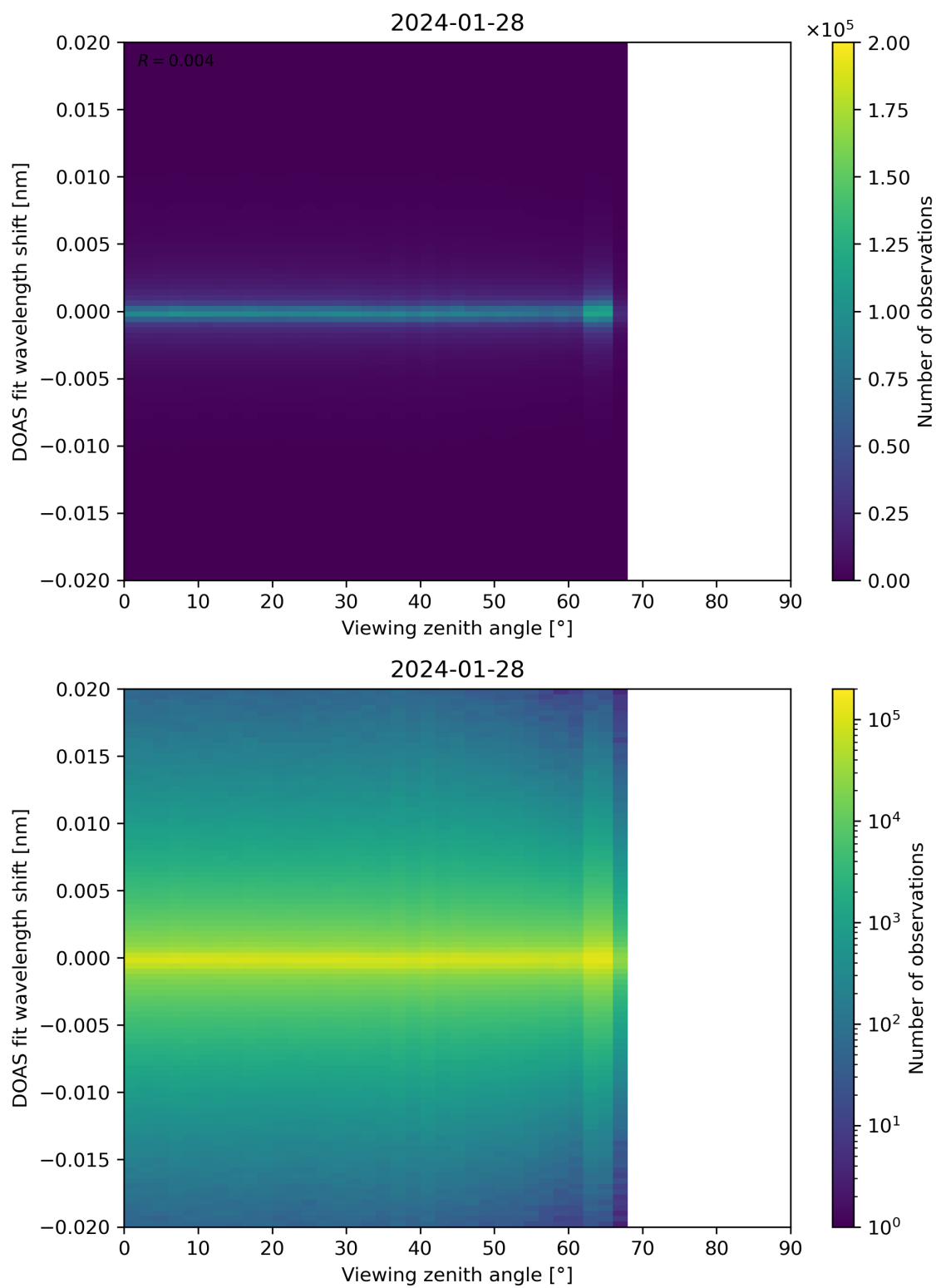
Figure 183: Scatter density plot of “Viewing zenith angle” against “DOAS fit wavelength shift” for 2024-01-27 to 2024-01-29.
