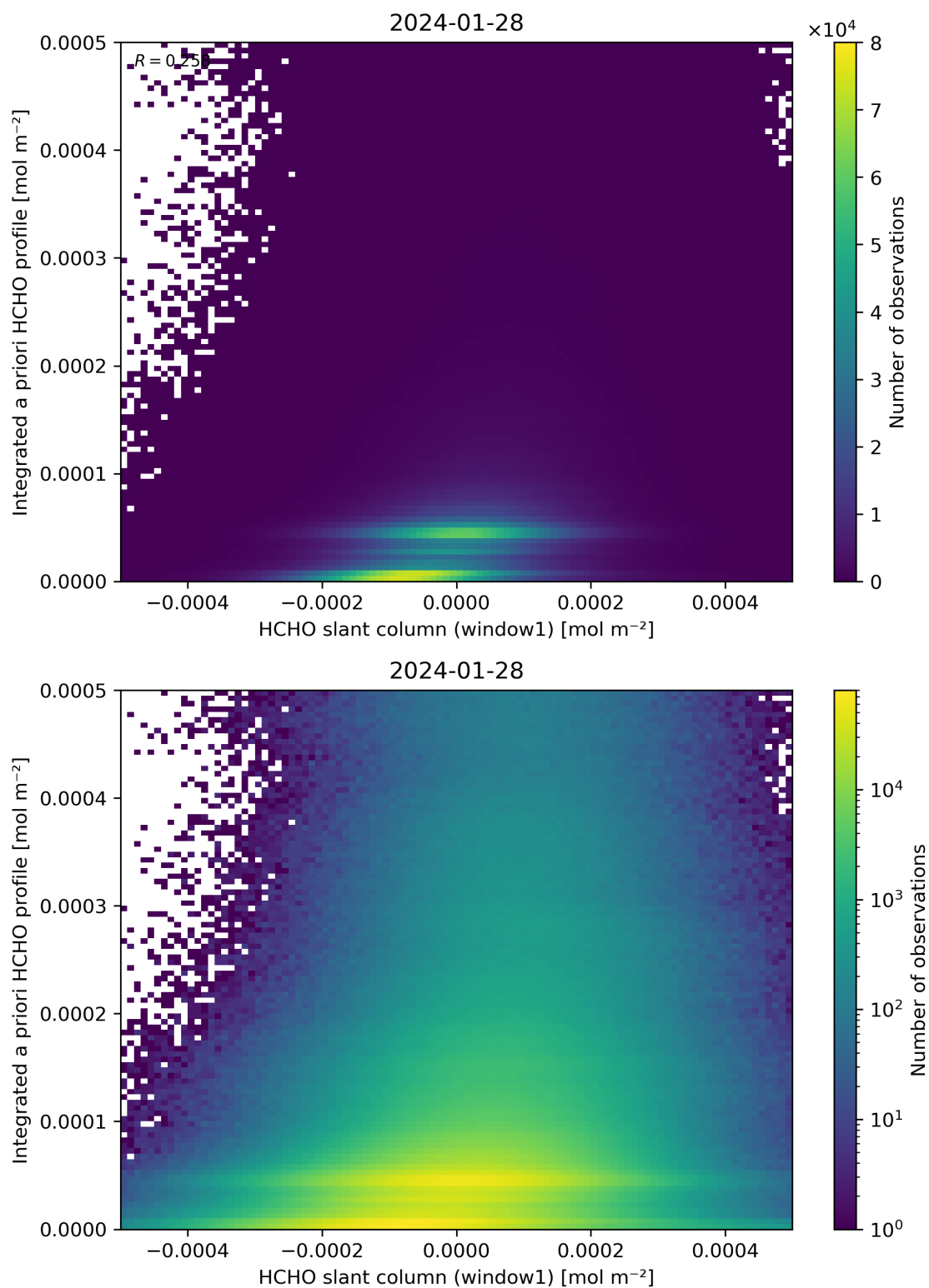
Figure 87: Scatter density plot of “HCHO slant column (window1)” against “Integrated a priori HCHO profile” for 2024-01-27 to 2024-01-29.
