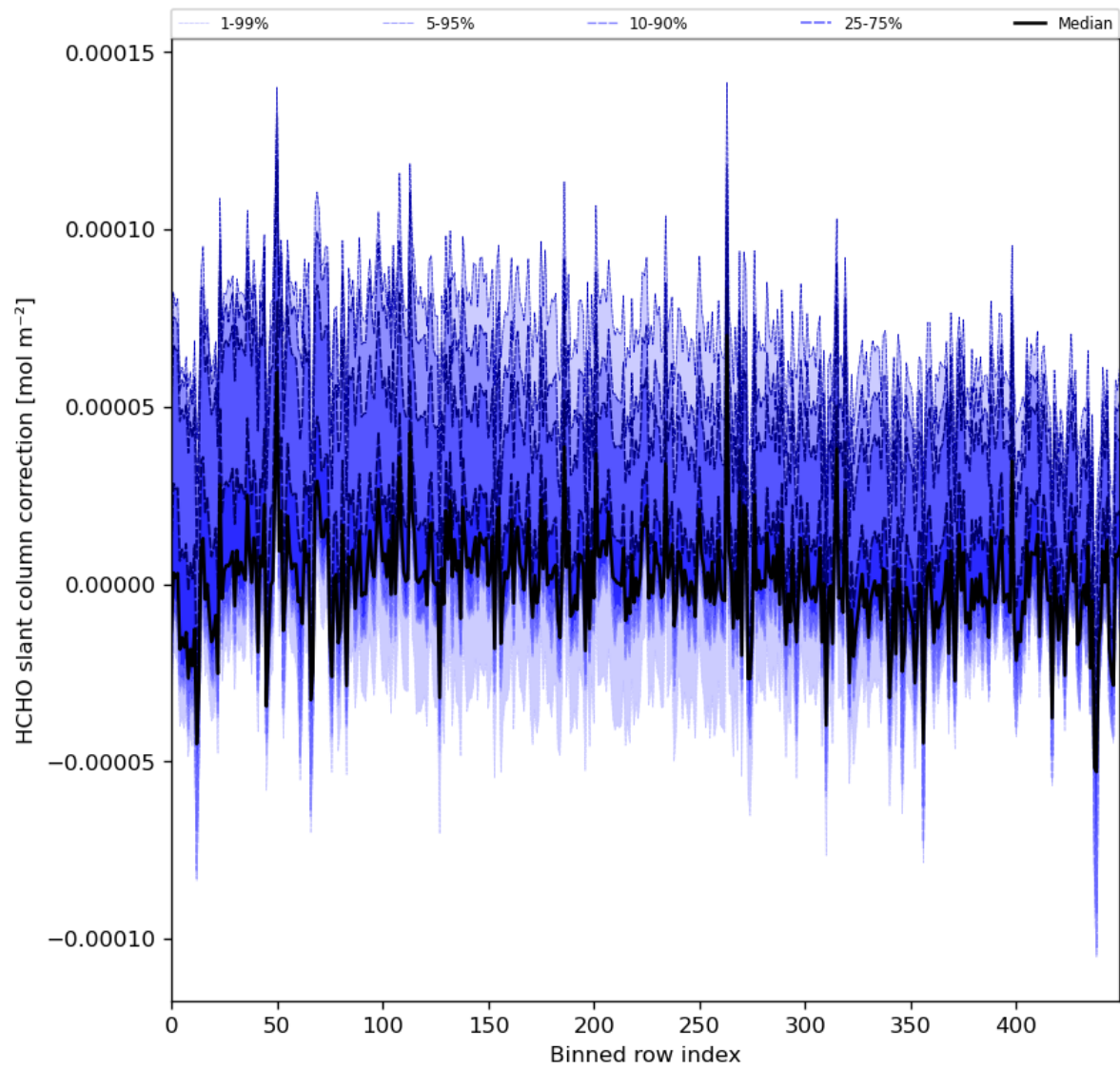
Figure 61: Along track statistics of “HCHO slant column correction” for 2024-01-27 to 2024-01-29
