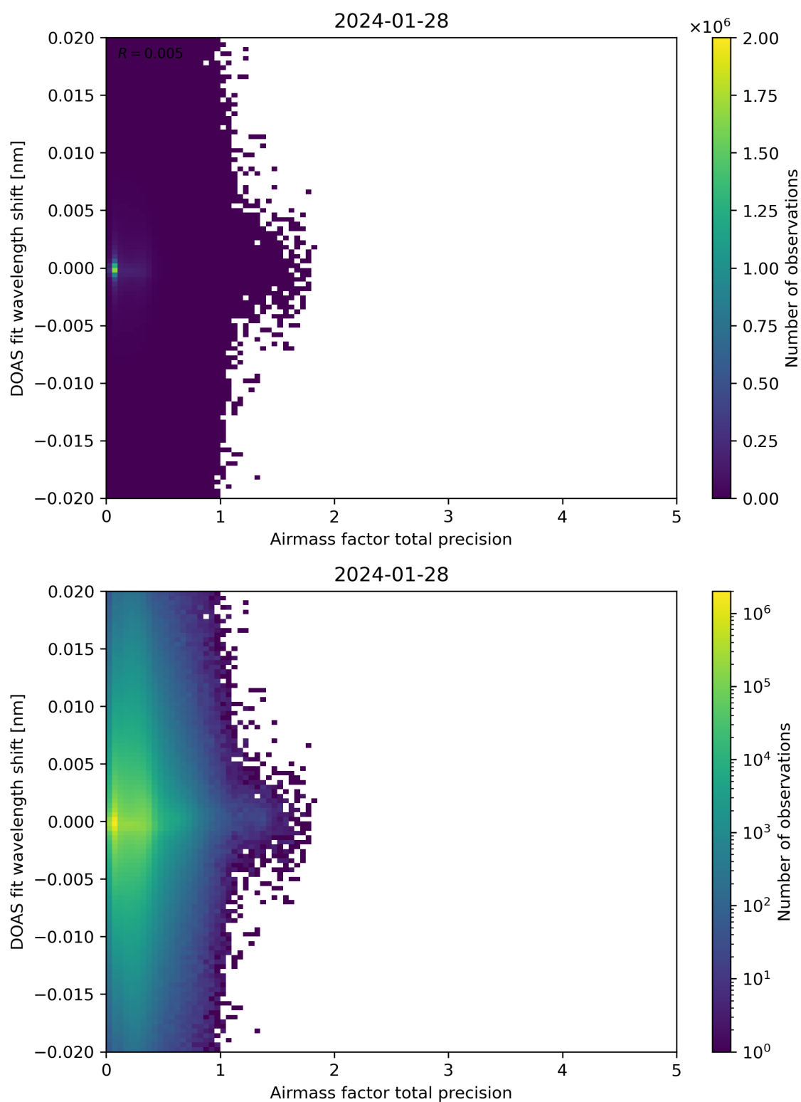
Figure 106: Scatter density plot of “Airmass factor total precision” against “DOAS fit wavelength shift” for 2024-01-27 to 2024-01-29.
