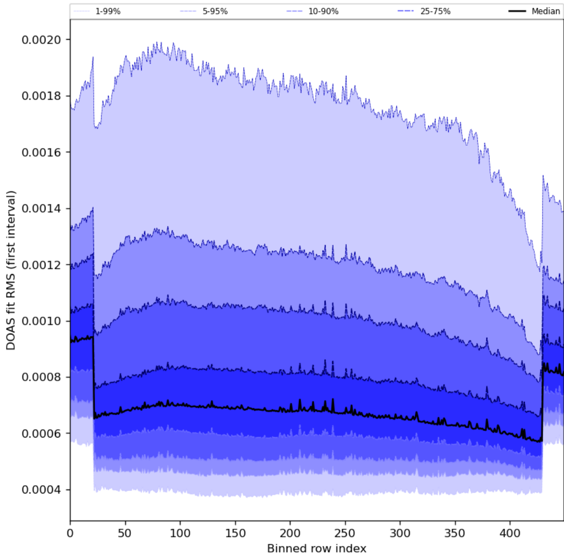
Figure 60: Along track statistics of “DOAS fit RMS (first interval)” for 2024-01-27 to 2024-01-29
