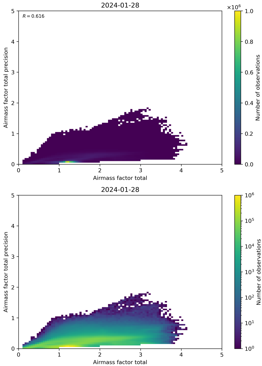
Figure 103: Scatter density plot of “Airmass factor total” against “Airmass factor total precision” for 2024-01-27 to 2024-01-29.
