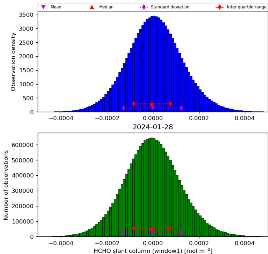
Figure 38: Histogram of “HCHO slant column (window1)” for 2024-01-27 to 2024-01-29
