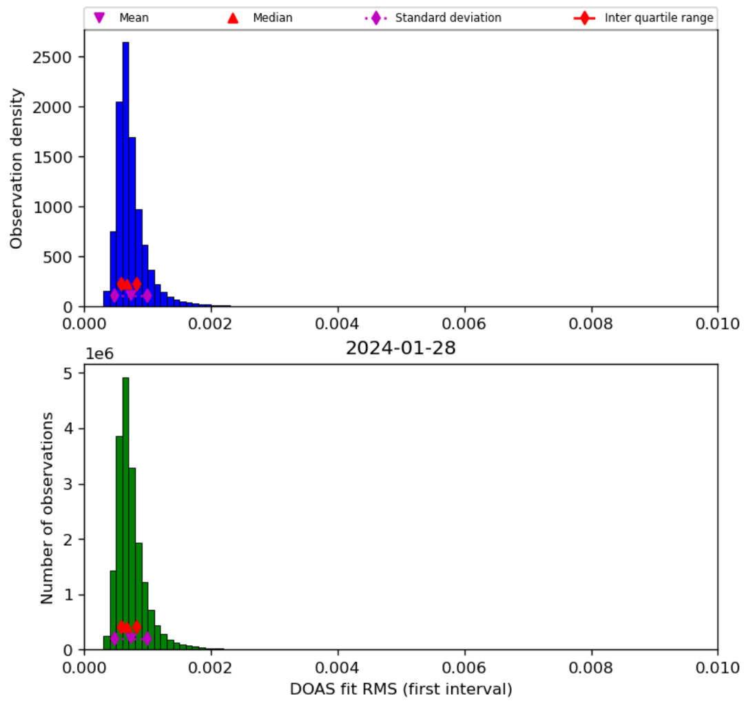
Figure 46: Histogram of “DOAS fit RMS (first interval)” for 2024-01-27 to 2024-01-29
