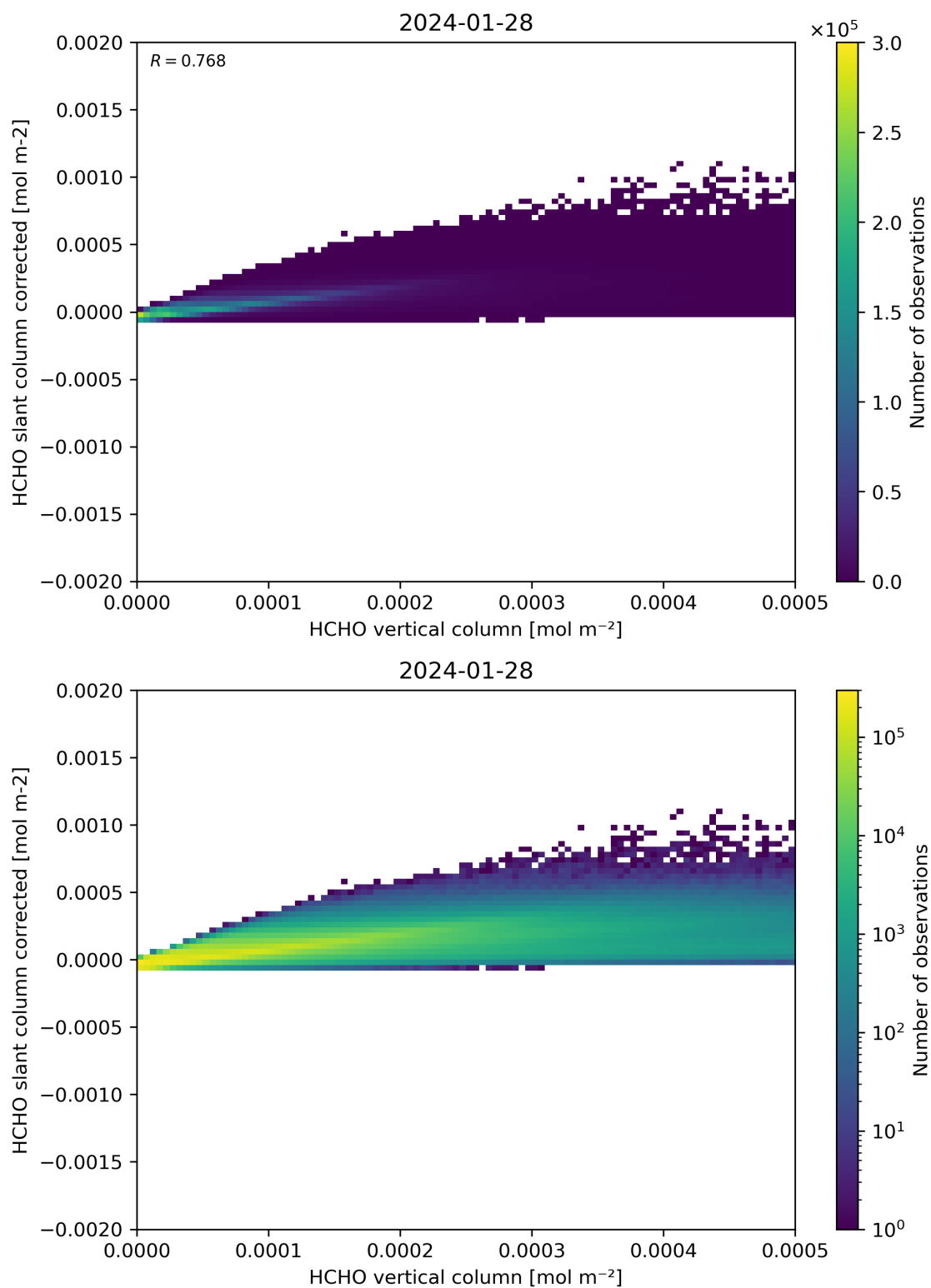
Figure 127: Scatter density plot of “HCHO vertical column” against “HCHO slant column corrected” for 2024-01-27 to 2024-01-29.
