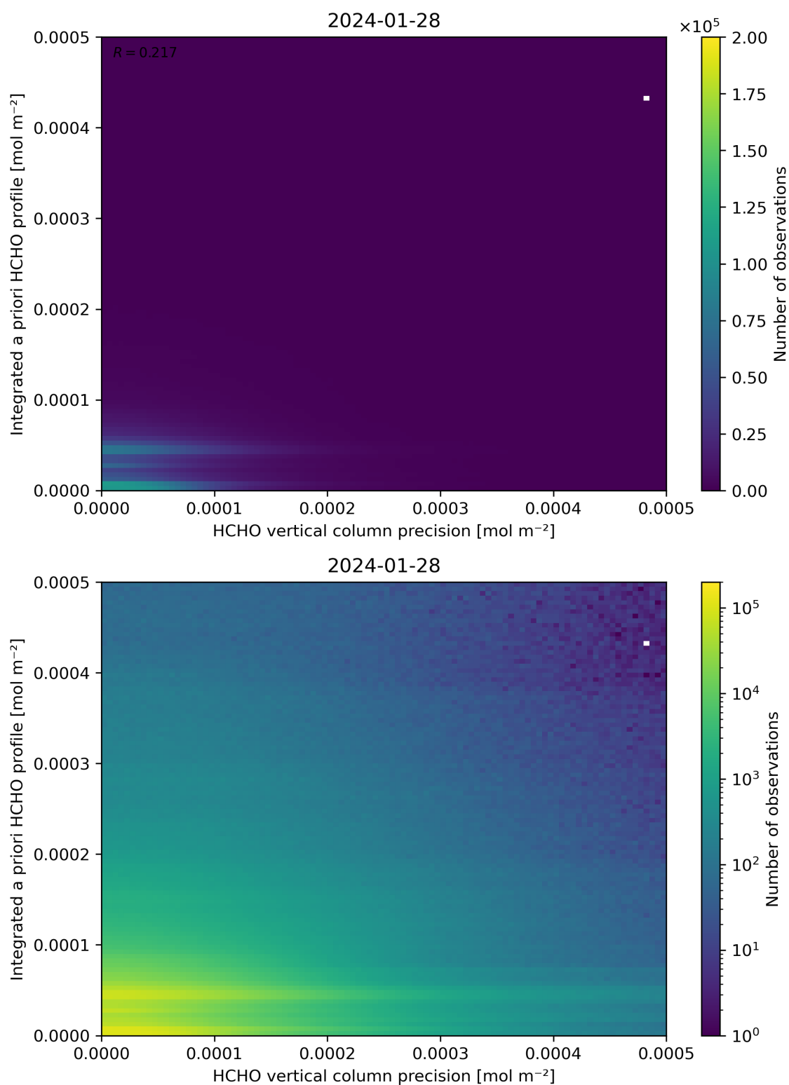
Figure 147: Scatter density plot of “HCHO vertical column precision” against “Integrated a priori HCHO profile” for 2024-01-27 to 2024-01-29.
