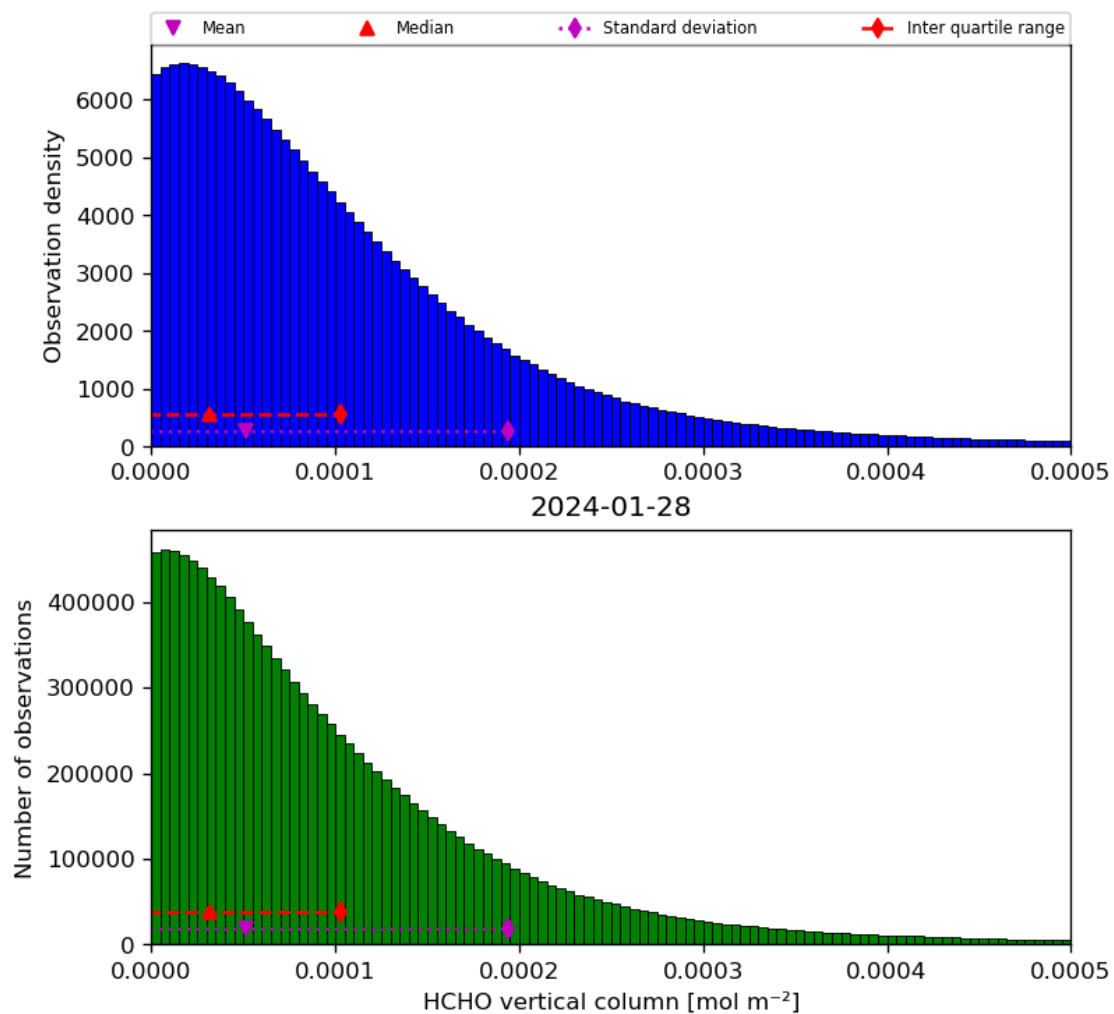
Figure 35: Histogram of “HCHO vertical column” for 2024-01-27 to 2024-01-29
