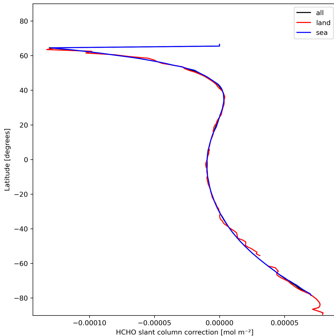
Figure 33: Zonal average of “HCHO slant column correction” for 2024-01-27 to 2024-01-29.
