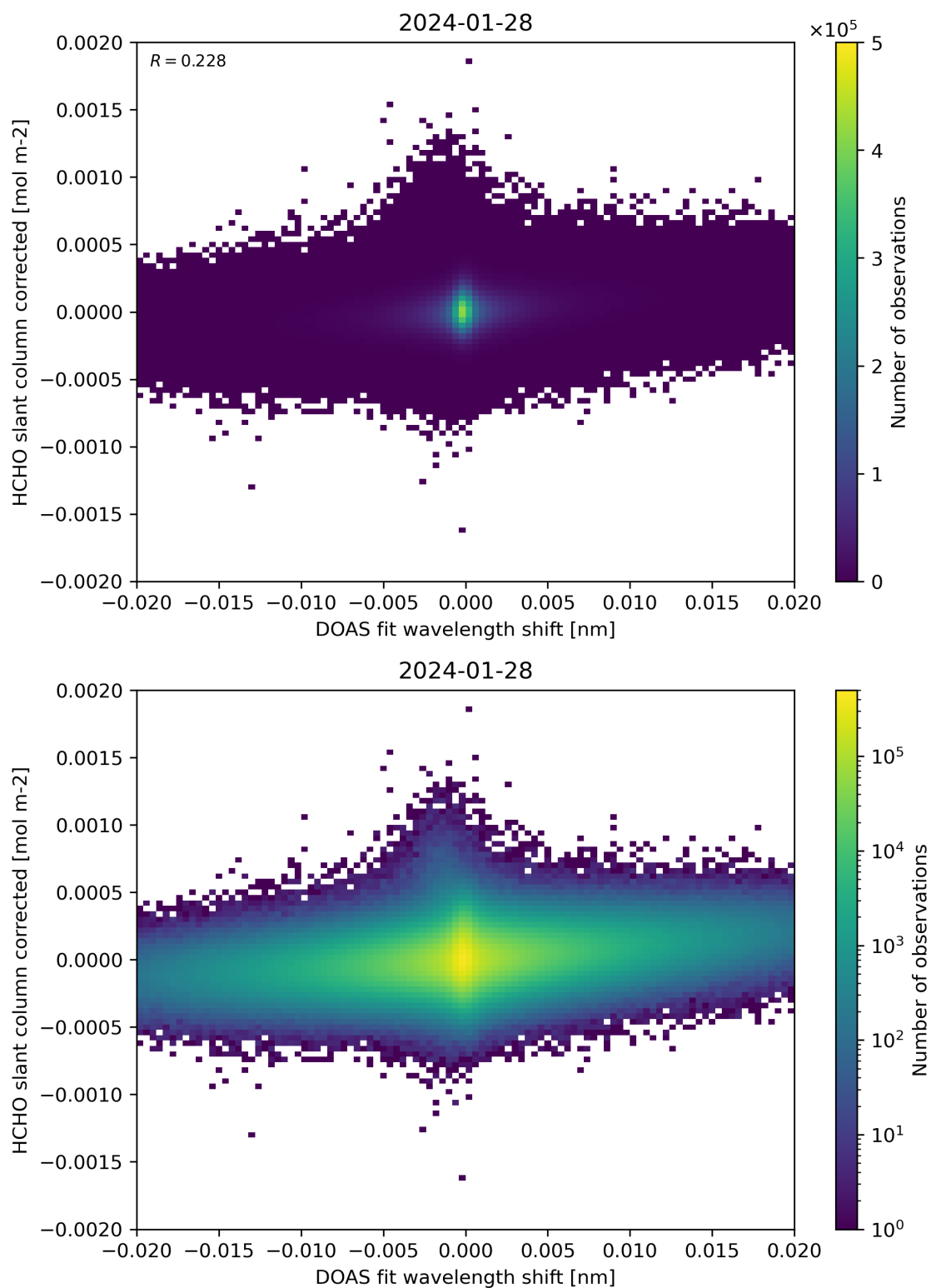
Figure 66: Scatter density plot of “DOAS fit wavelength shift” against “HCHO slant column corrected” for 2024-01-27 to 2024-01-29.
