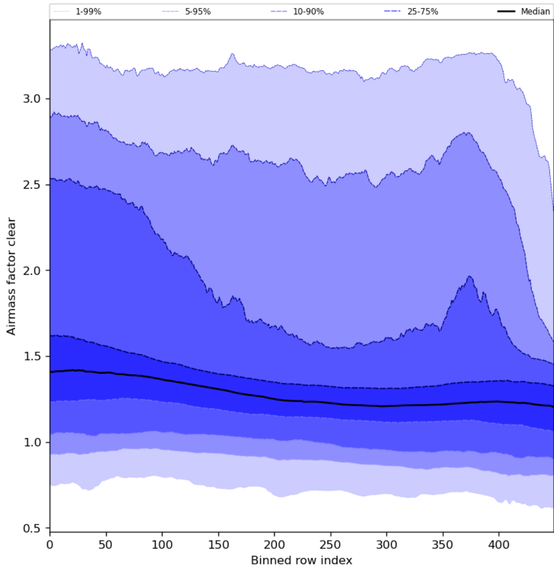
Figure 56: Along track statistics of “Airmass factor clear” for 2024-01-27 to 2024-01-29
