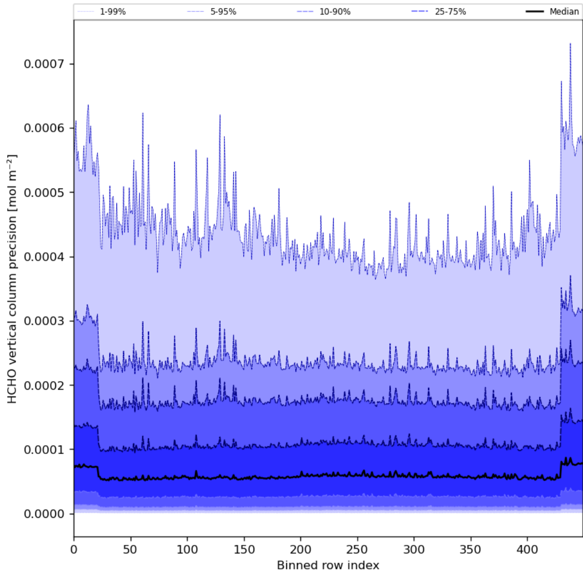
Figure 50: Along track statistics of “HCHO vertical column precision” for 2024-01-27 to 2024-01-29
