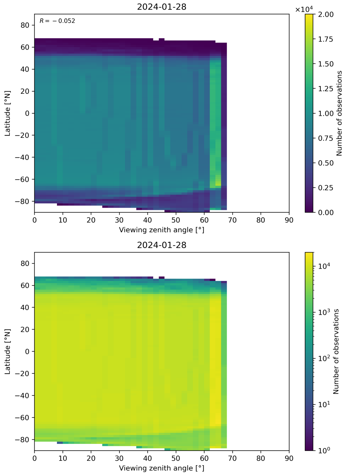
Figure 196: Scatter density plot of “Viewing zenith angle” against “Latitude” for 2024-01-27 to 2024-01-29.
