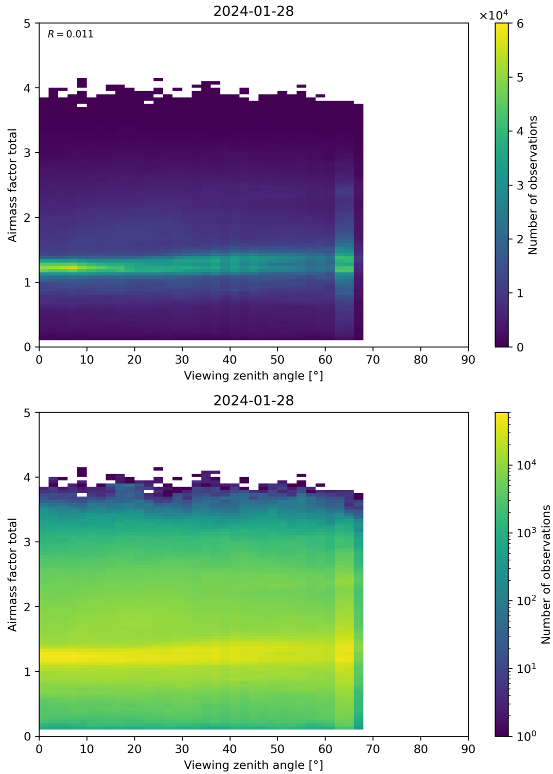
Figure 190: Scatter density plot of “Viewing zenith angle” against “Airmass factor total” for 2024-01-27 to 2024-01-29.
