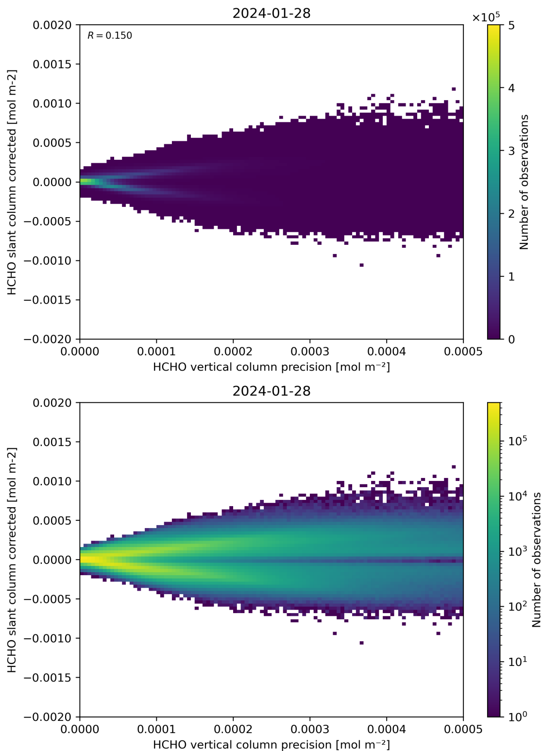
Figure 140: Scatter density plot of “HCHO vertical column precision” against “HCHO slant column corrected” for 2024-01-27 to 2024-01-29.
