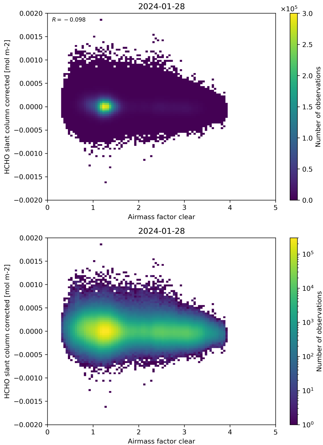
Figure 74: Scatter density plot of “Airmass factor clear” against “HCHO slant column corrected” for 2024-01-27 to 2024-01-29.
