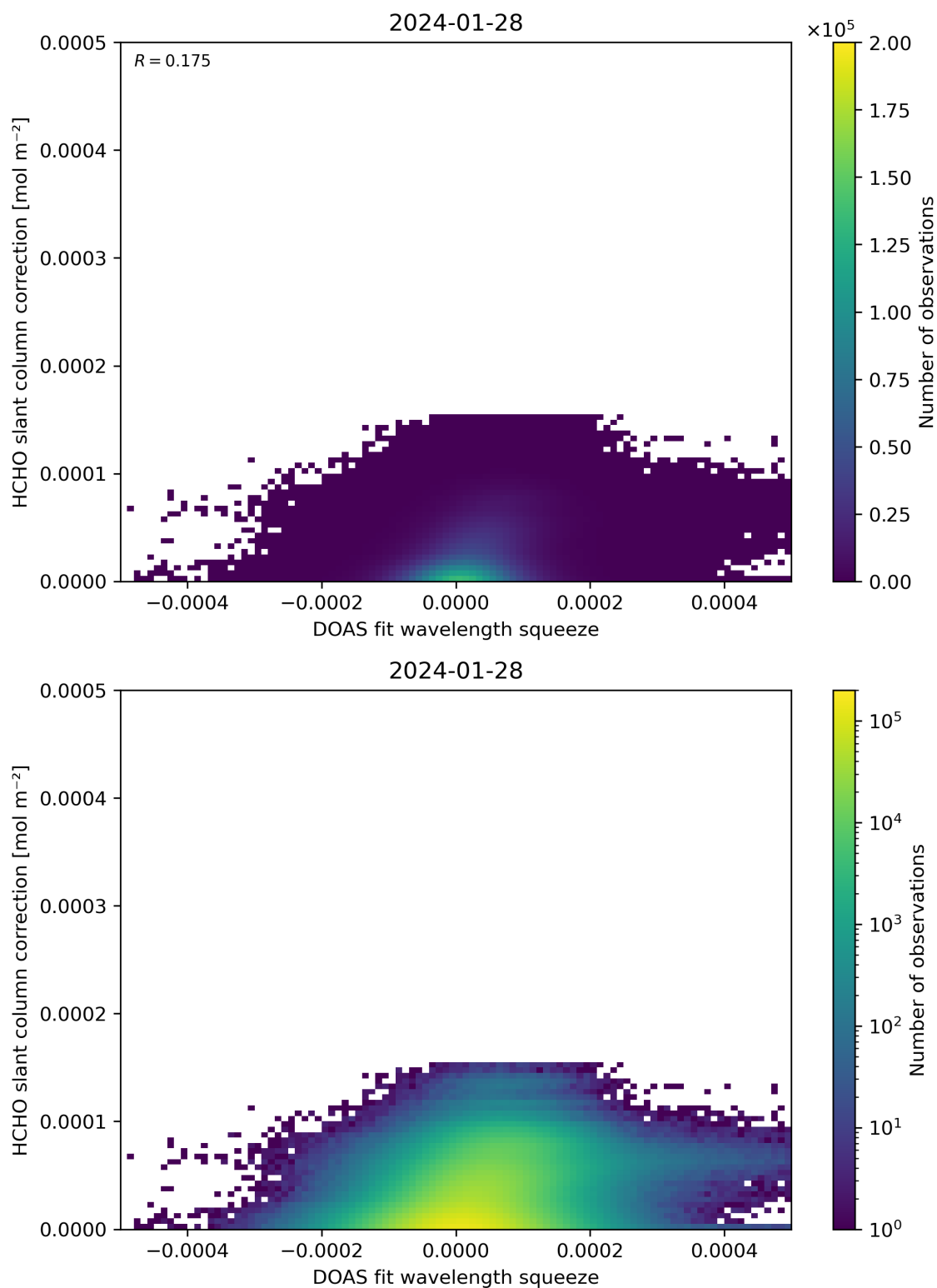
Figure 70: Scatter density plot of “DOAS fit wavelength squeeze” against “HCHO slant column correction” for 2024-01-27 to 2024-01-29.
