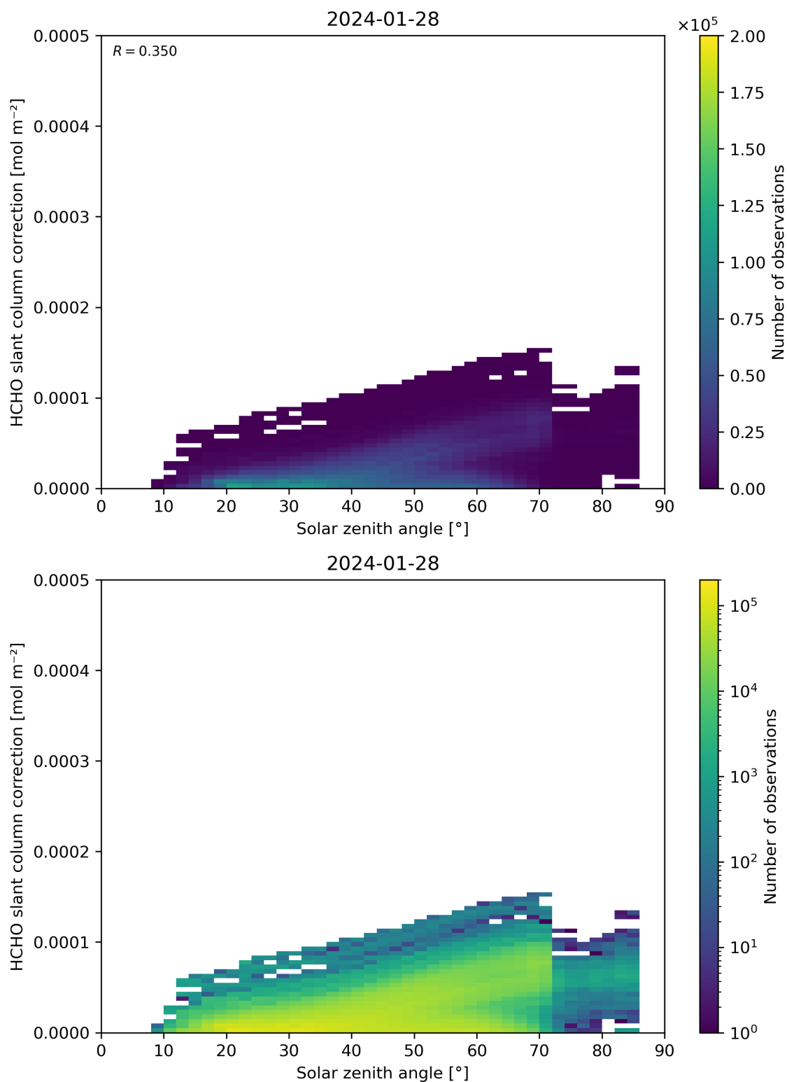
Figure 172: Scatter density plot of “Solar zenith angle” against “HCHO slant column correction” for 2024-01-27 to 2024-01-29.
