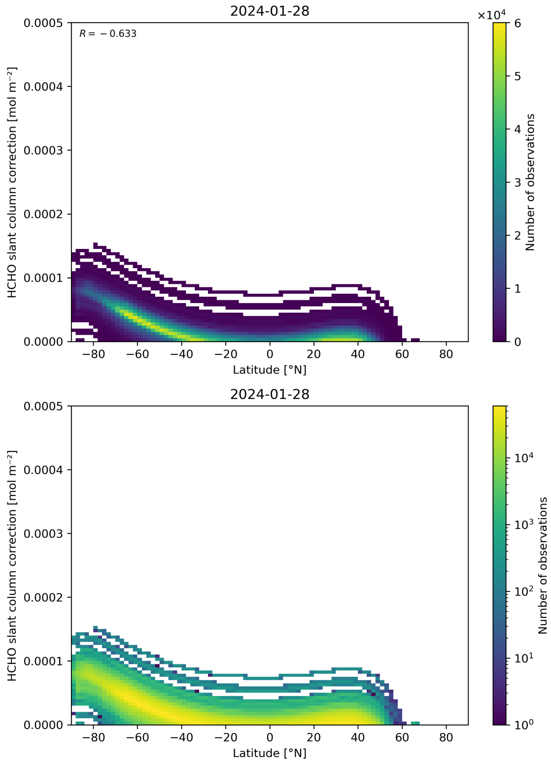
Figure 158: Scatter density plot of “Latitude” against “HCHO slant column correction” for 2024-01-27 to 2024-01-29.
