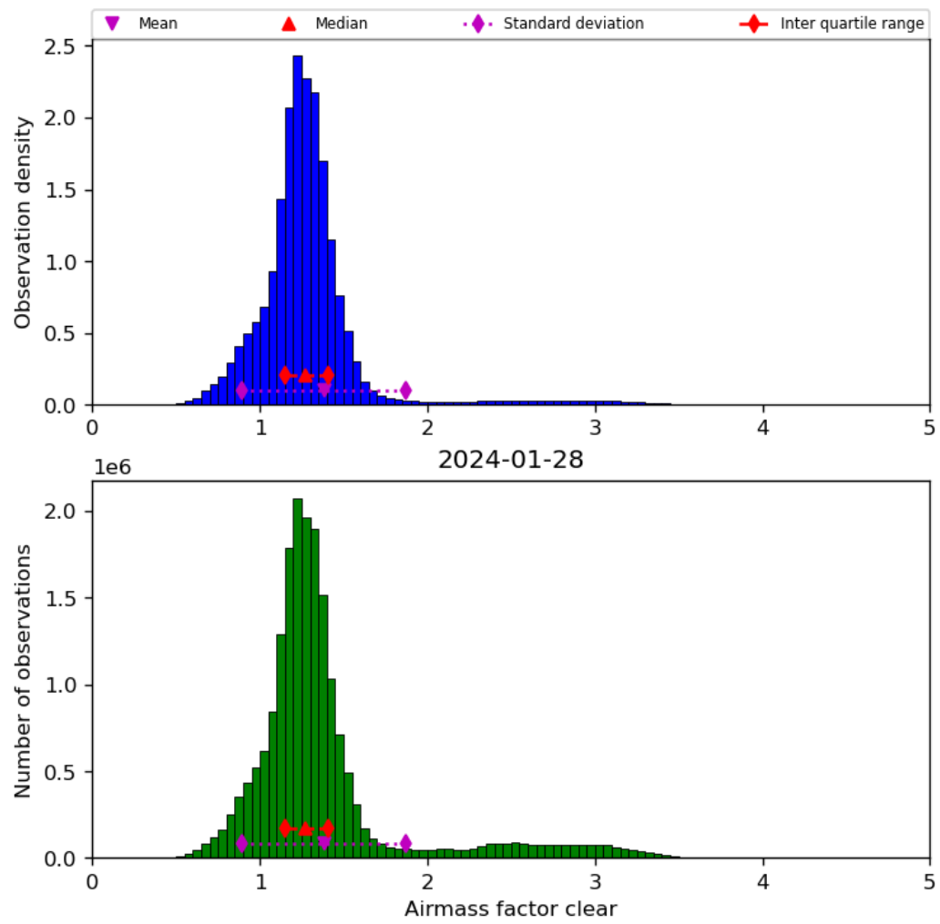
Figure 42: Histogram of “Airmass factor clear” for 2024-01-27 to 2024-01-29
