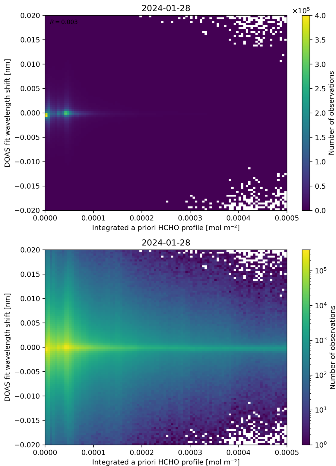
Figure 149: Scatter density plot of “Integrated a priori HCHO profile” against “DOAS fit wavelength shift” for 2024-01-27 to 2024-01-29.
