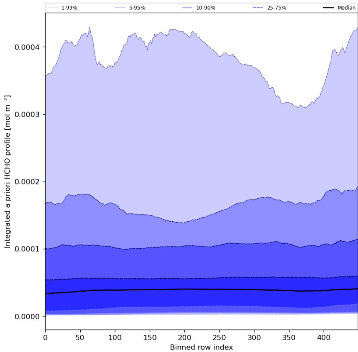
Figure 57: Along track statistics of “Integrated a priori HCHO profile” for 2024-01-27 to 2024-01-29
