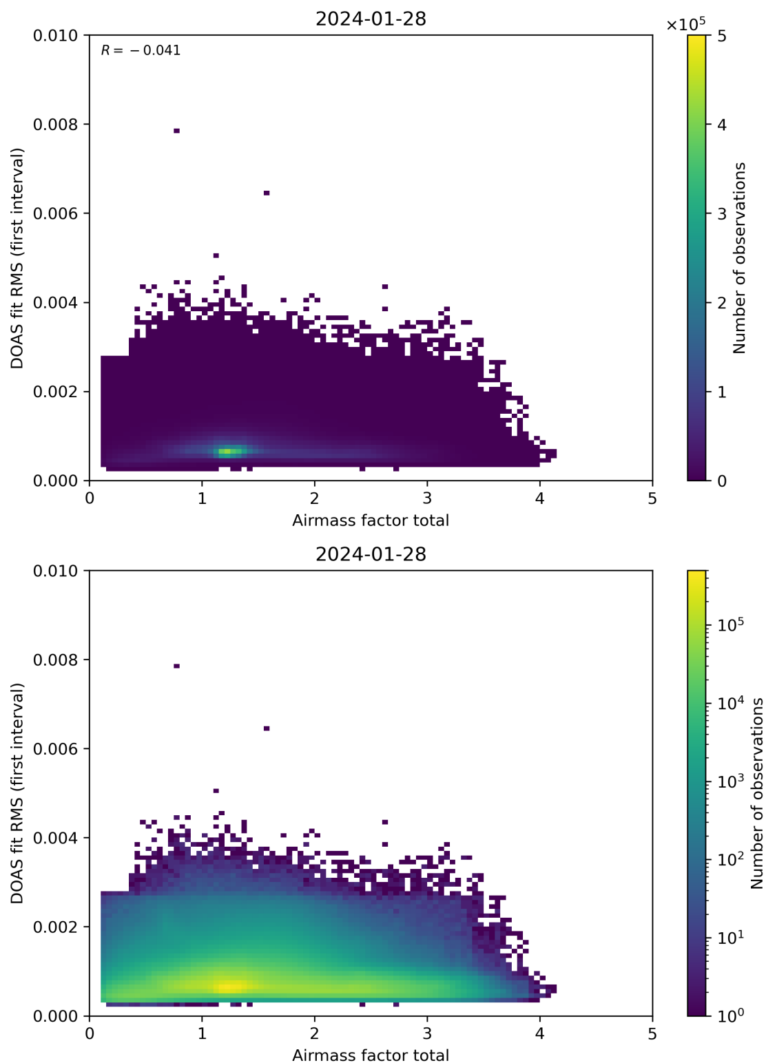
Figure 97: Scatter density plot of “Airmass factor total” against “DOAS fit RMS (first interval)” for 2024-01-27 to 2024-01-29.
