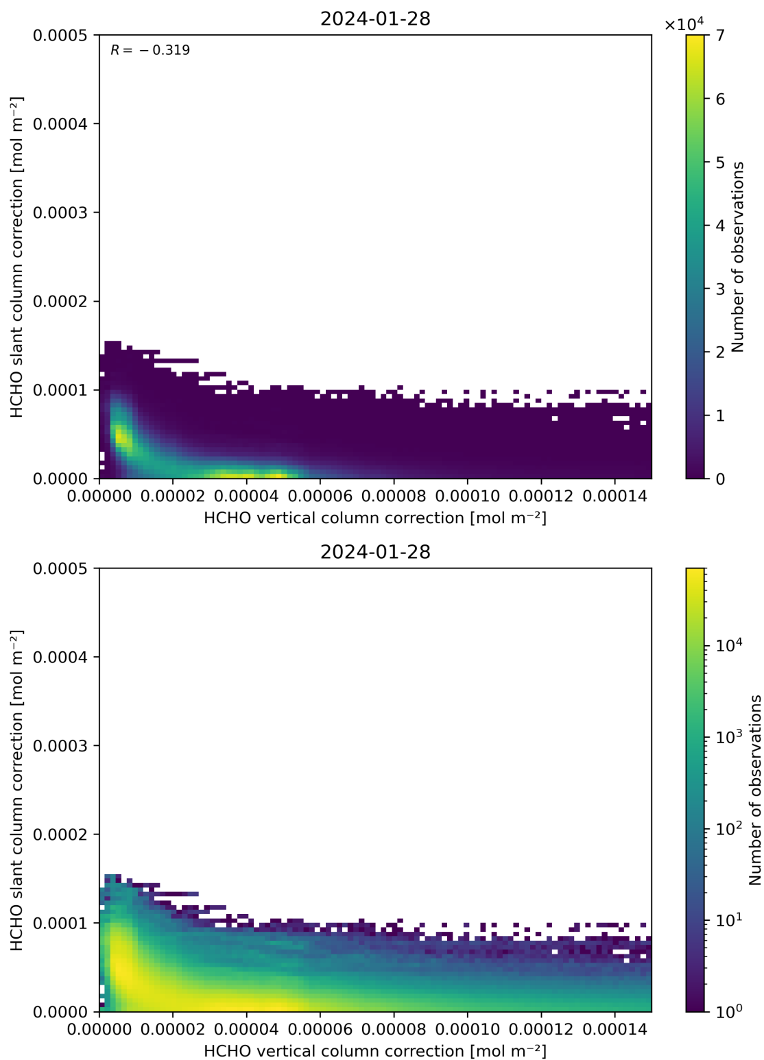
Figure 117: Scatter density plot of “HCHO vertical column correction” against “HCHO slant column correction” for 2024-01-27 to 2024-01-29.
