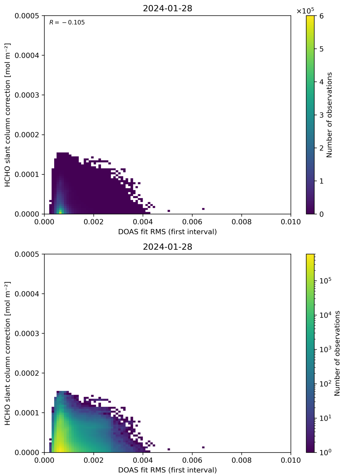
Figure 63: Scatter density plot of “DOAS fit RMS (first interval)” against “HCHO slant column correction” for 2024-01-27 to 2024-01-29.
