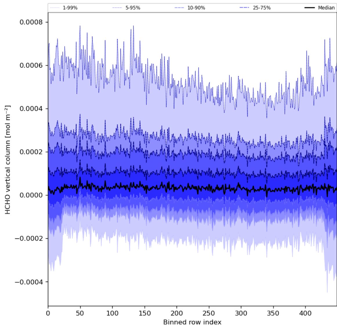
Figure 49: Along track statistics of “HCHO vertical column” for 2024-01-27 to 2024-01-29
