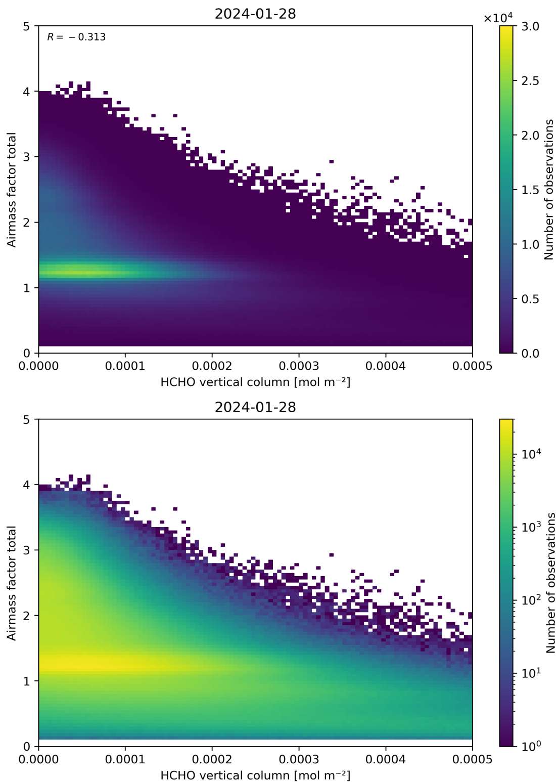
Figure 131: Scatter density plot of “HCHO vertical column” against “Airmass factor total” for 2024-01-27 to 2024-01-29.
