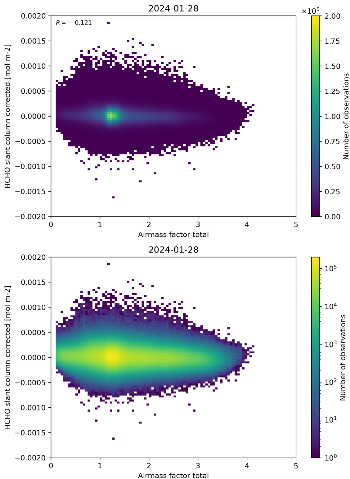
Figure 101: Scatter density plot of “Airmass factor total” against “HCHO slant column corrected” for 2024-01-27 to 2024-01-29.
