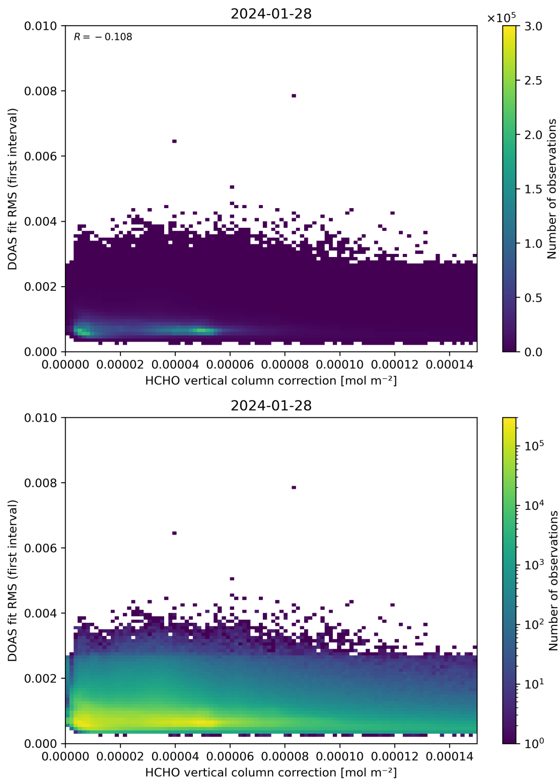
Figure 112: Scatter density plot of “HCHO vertical column correction” against “DOAS fit RMS (first interval)” for 2024-01-27 to 2024-01-29.
