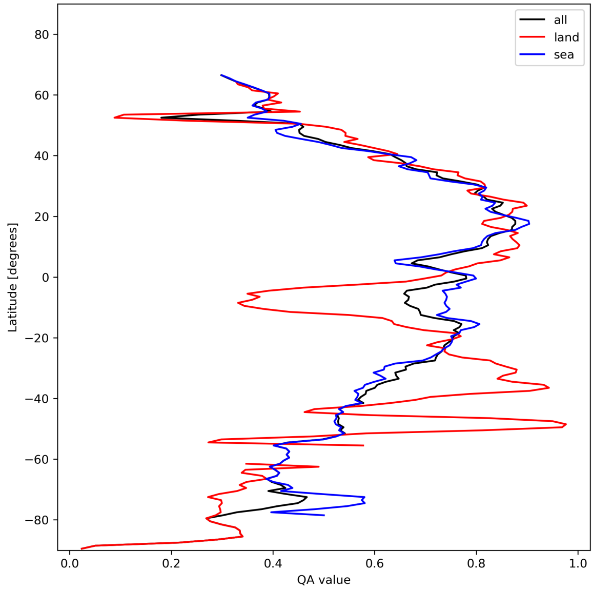
Figure 20: Zonal average of “QA value” for 2024-01-27 to 2024-01-29.
