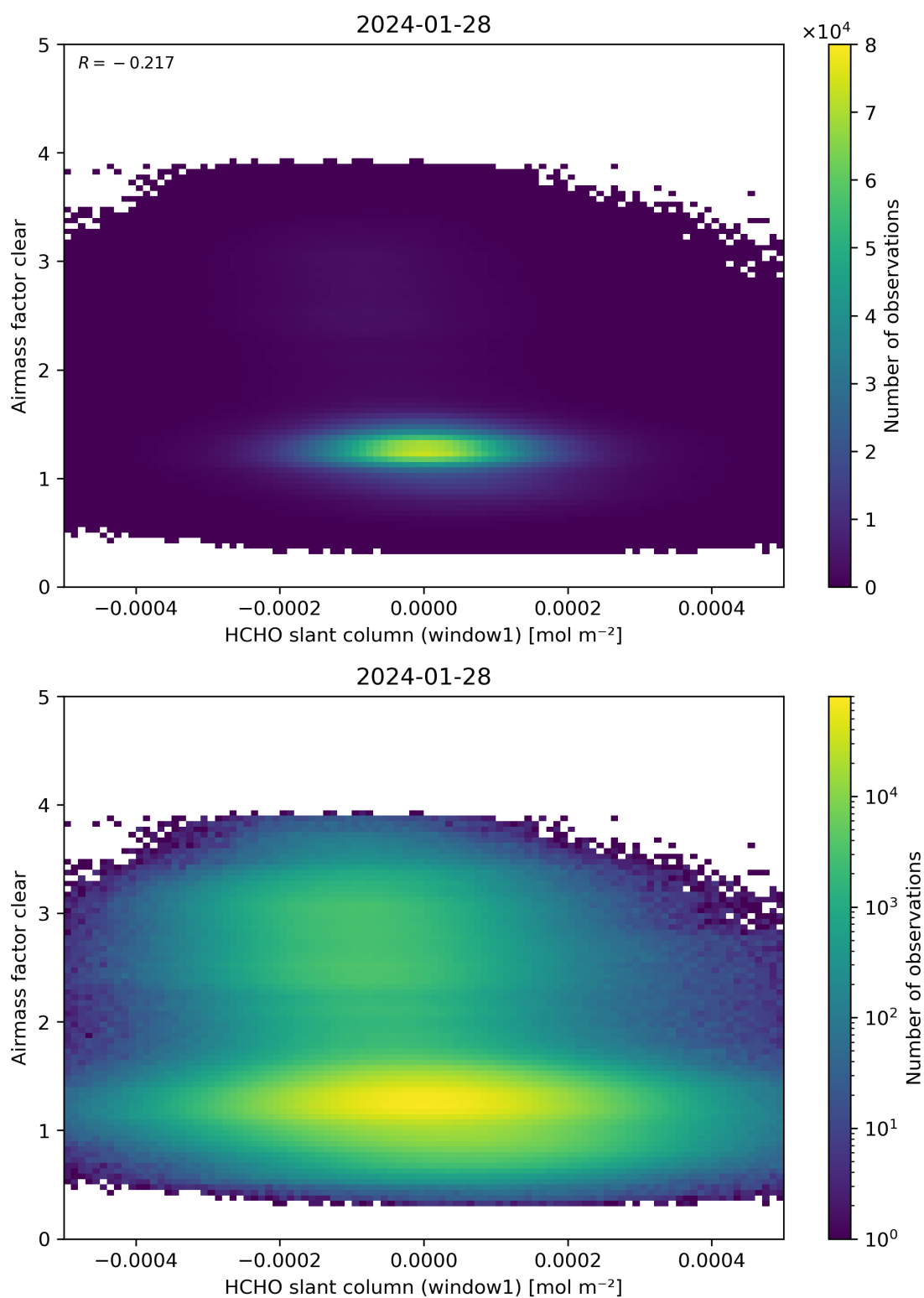
Figure 81: Scatter density plot of “HCHO slant column (window1)” against “Airmass factor clear” for 2024-01-27 to 2024-01-29.
