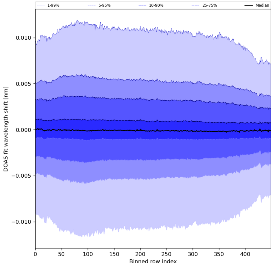
Figure 58: Along track statistics of “DOAS fit wavelength shift” for 2024-01-27 to 2024-01-29
