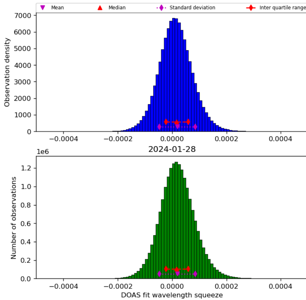
Figure 45: Histogram of “DOAS fit wavelength squeeze” for 2024-01-27 to 2024-01-29
