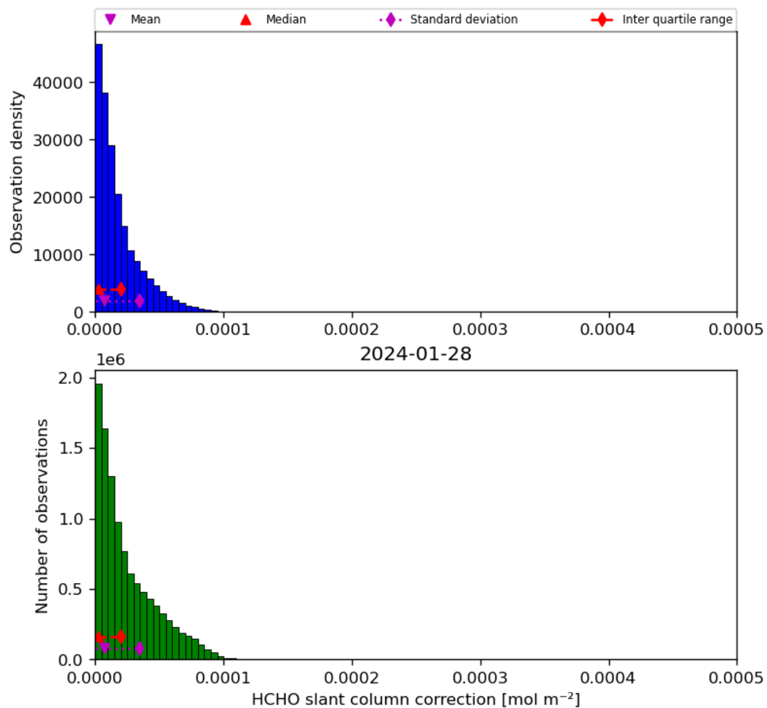
Figure 47: Histogram of “HCHO slant column correction” for 2024-01-27 to 2024-01-29
