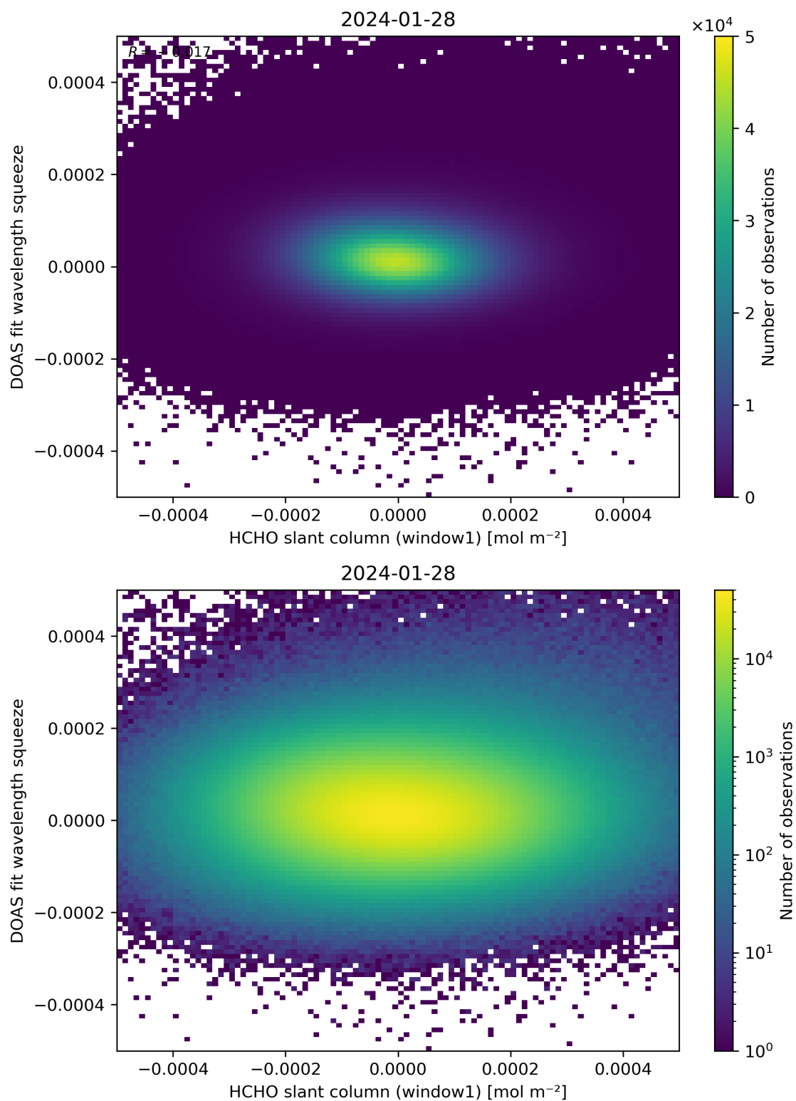
Figure 80: Scatter density plot of “HCHO slant column (window1)” against “DOAS fit wavelength squeeze” for 2024-01-27 to 2024-01-29.
