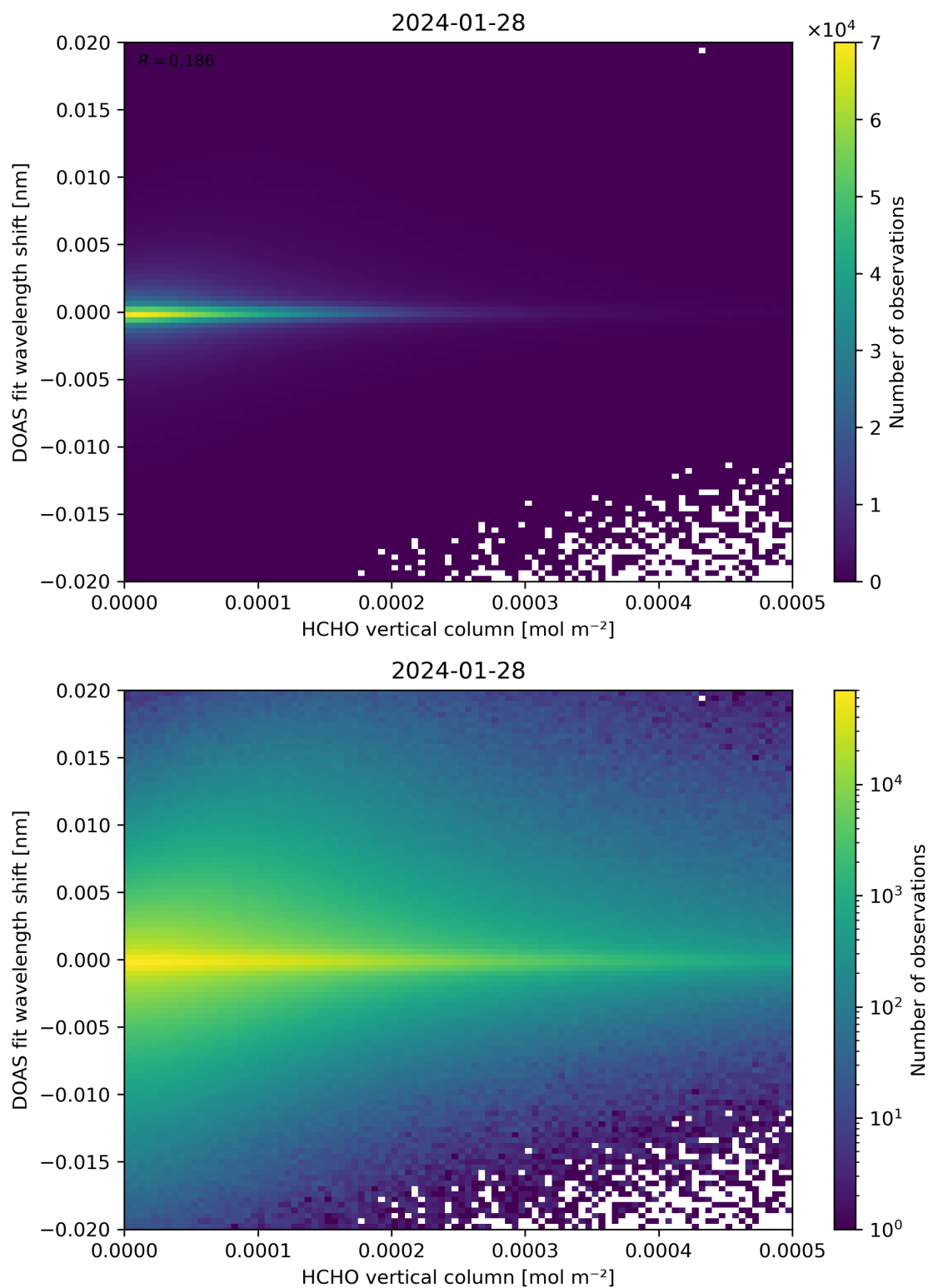
Figure 124: Scatter density plot of “HCHO vertical column” against “DOAS fit wavelength shift” for 2024-01-27 to 2024-01-29.
