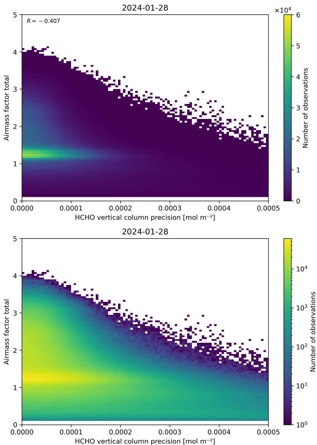
Figure 144: Scatter density plot of “HCHO vertical column precision” against “Airmass factor total” for 2024-01-27 to 2024-01-29.
