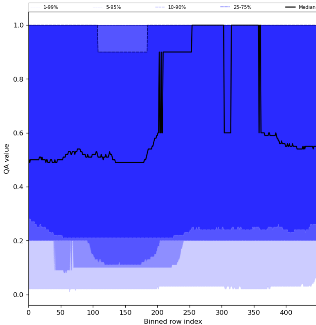
Figure 48: Along track statistics of “QA value” for 2024-01-27 to 2024-01-29
