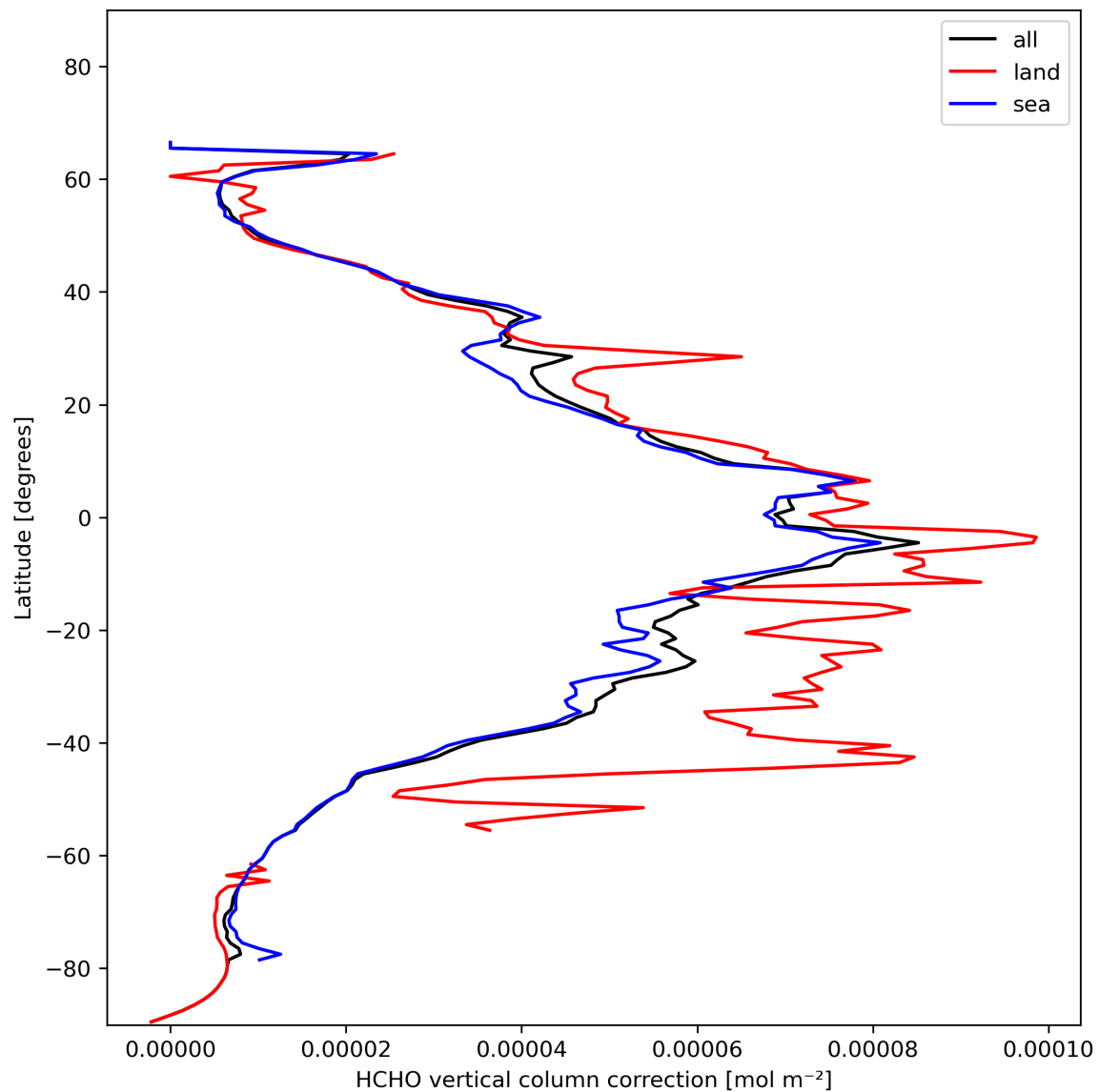
Figure 23: Zonal average of “HCHO vertical column correction” for 2024-01-27 to 2024-01-29.
