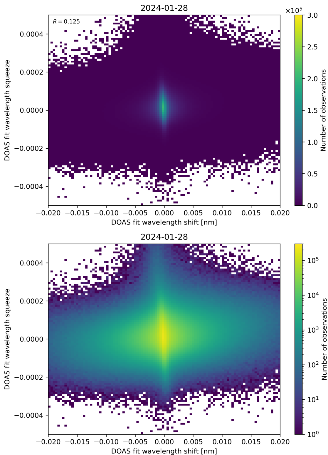
Figure 65: Scatter density plot of “DOAS fit wavelength shift” against “DOAS fit wavelength squeeze” for 2024-01-27 to 2024-01-29.
