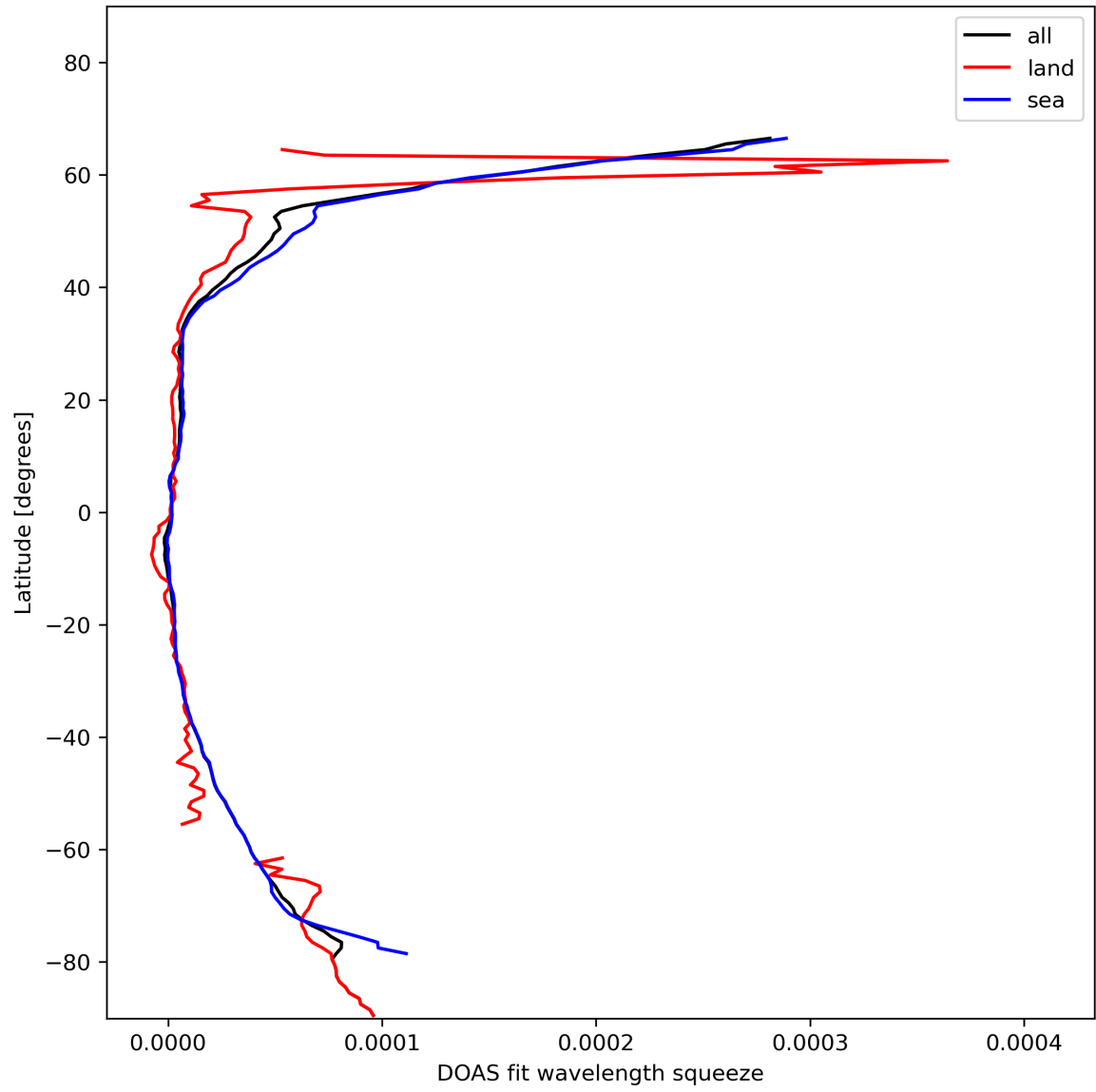
Figure 31: Zonal average of “DOAS fit wavelength squeeze” for 2024-01-27 to 2024-01-29.
