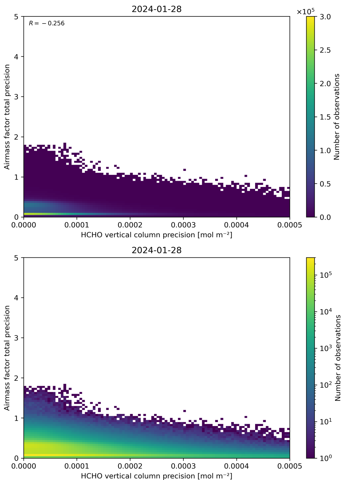
Figure 145: Scatter density plot of “HCHO vertical column precision” against “Airmass factor total precision” for 2024-01-27 to 2024-01-29.
