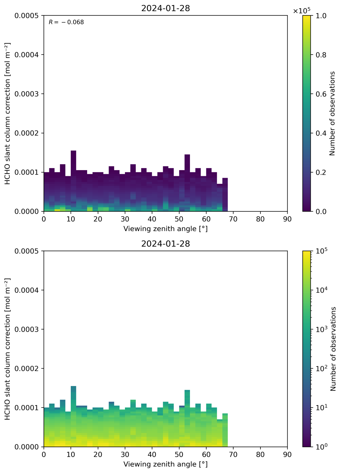
Figure 187: Scatter density plot of “Viewing zenith angle” against “HCHO slant column correction” for 2024-01-27 to 2024-01-29.
