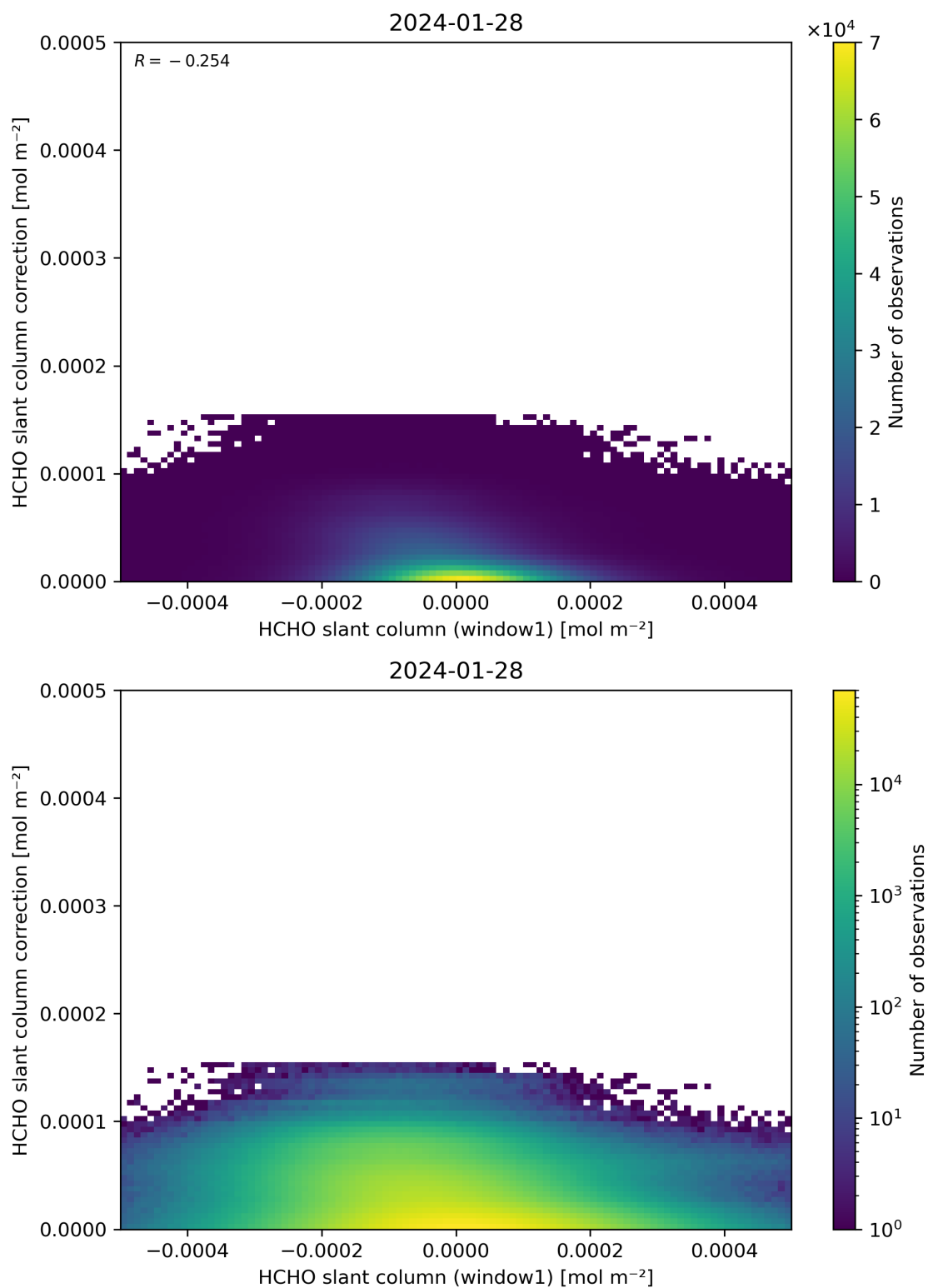
Figure 83: Scatter density plot of “HCHO slant column (window1)” against “HCHO slant column correction” for 2024-01-27 to 2024-01-29.
