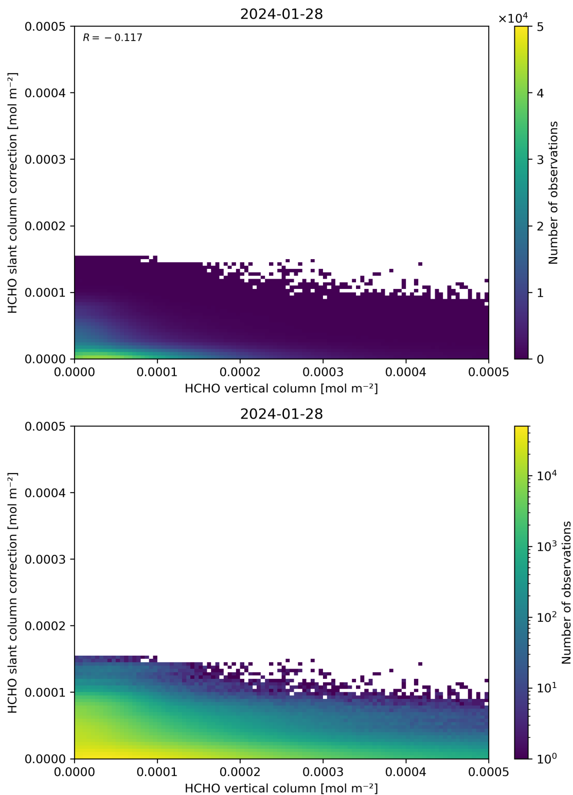
Figure 128: Scatter density plot of “HCHO vertical column” against “HCHO slant column correction” for 2024-01-27 to 2024-01-29.
