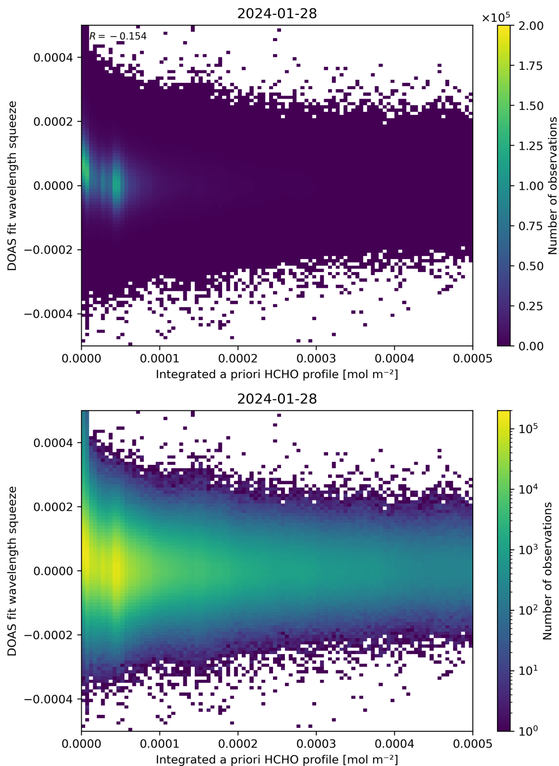
Figure 150: Scatter density plot of “Integrated a priori HCHO profile” against “DOAS fit wavelength squeeze” for 2024-01-27 to 2024-01-29.
