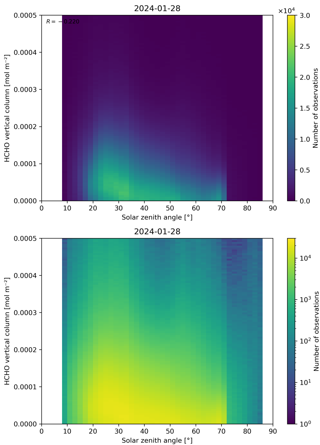
Figure 177: Scatter density plot of “Solar zenith angle” against “HCHO vertical column” for 2024-01-27 to 2024-01-29.
