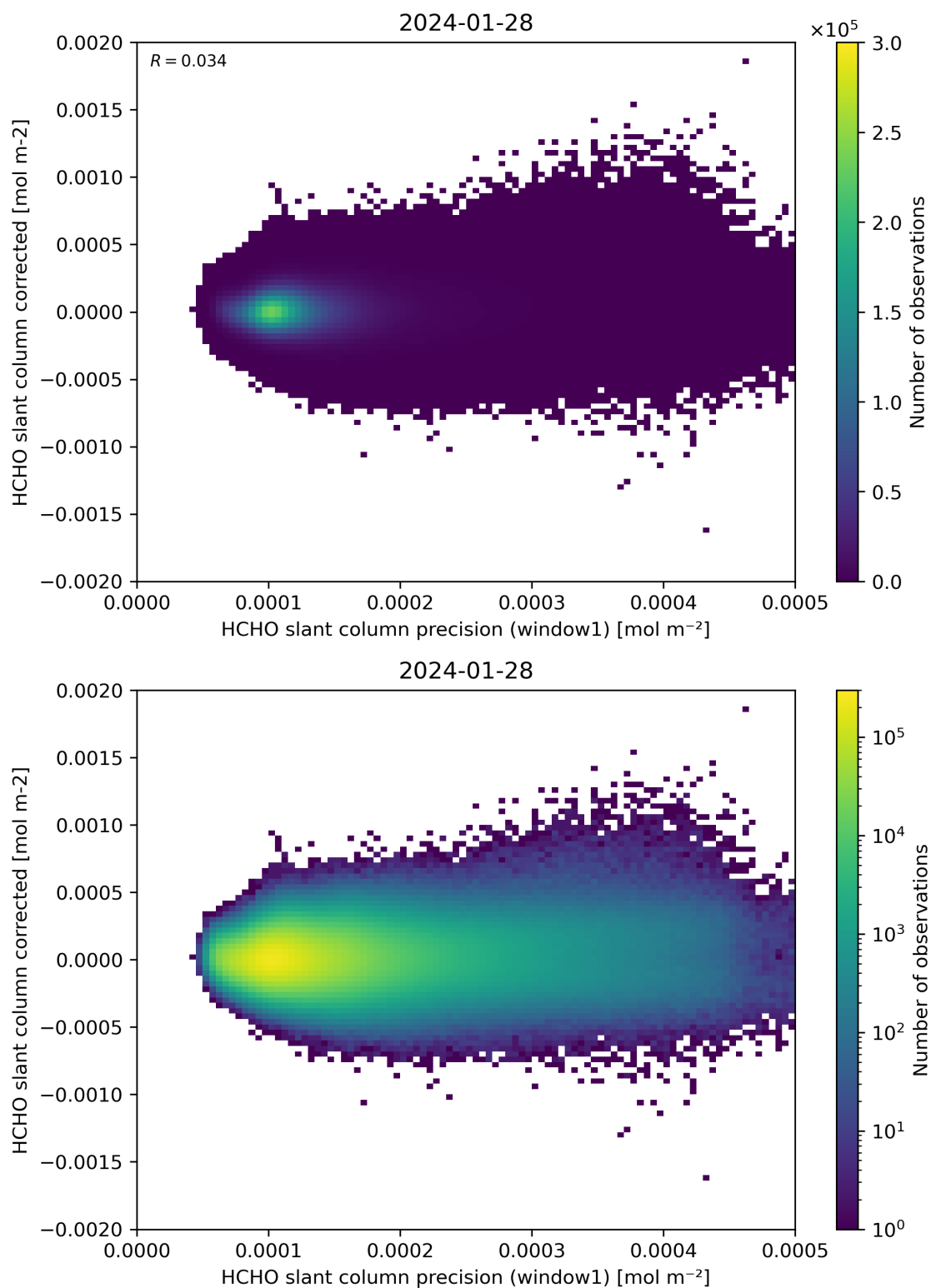
Figure 92: Scatter density plot of “HCHO slant column precision (window1)” against “HCHO slant column corrected” for 2024-01-27 to 2024-01-29.
