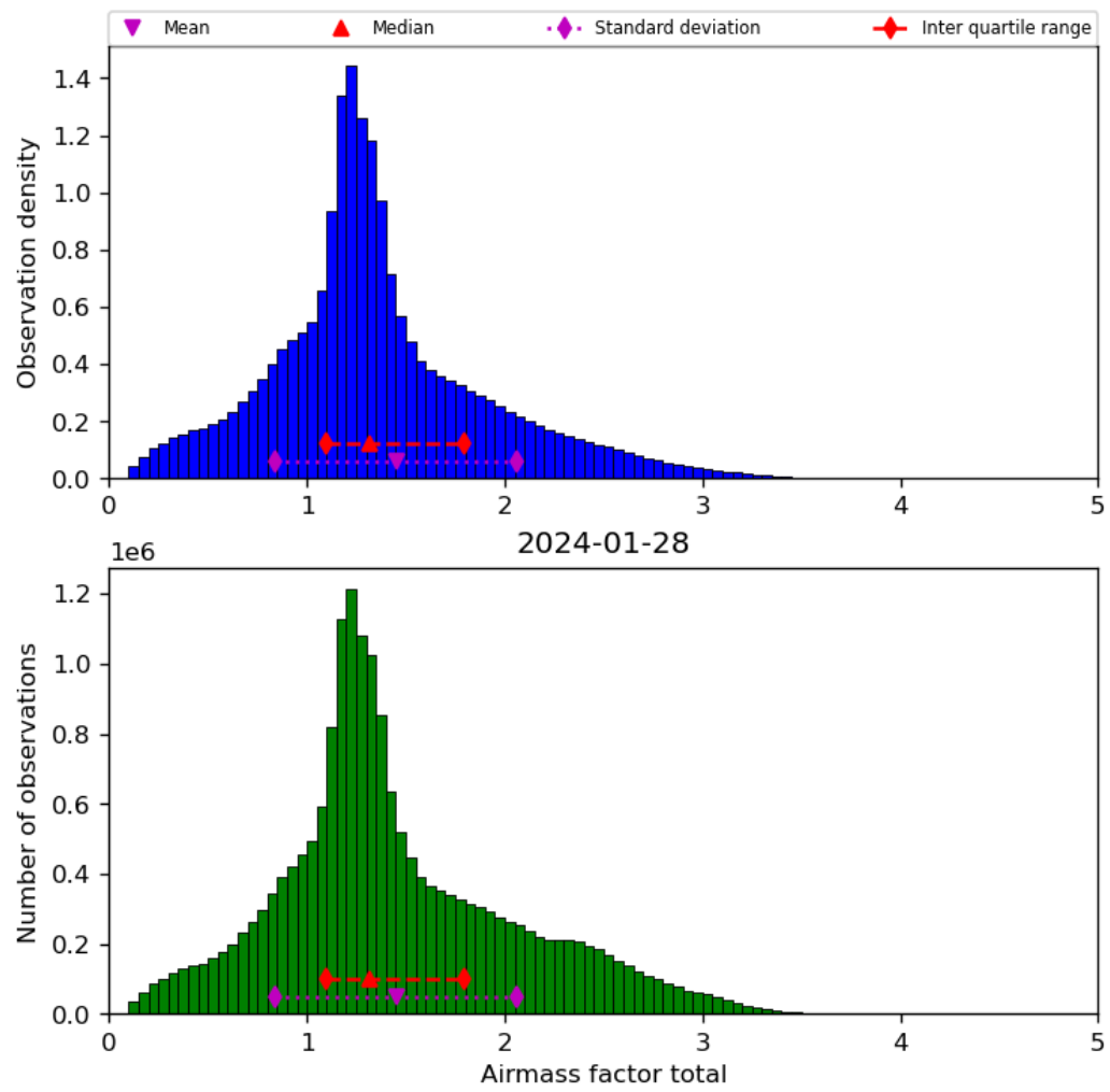
Figure 40: Histogram of “Airmass factor total” for 2024-01-27 to 2024-01-29
