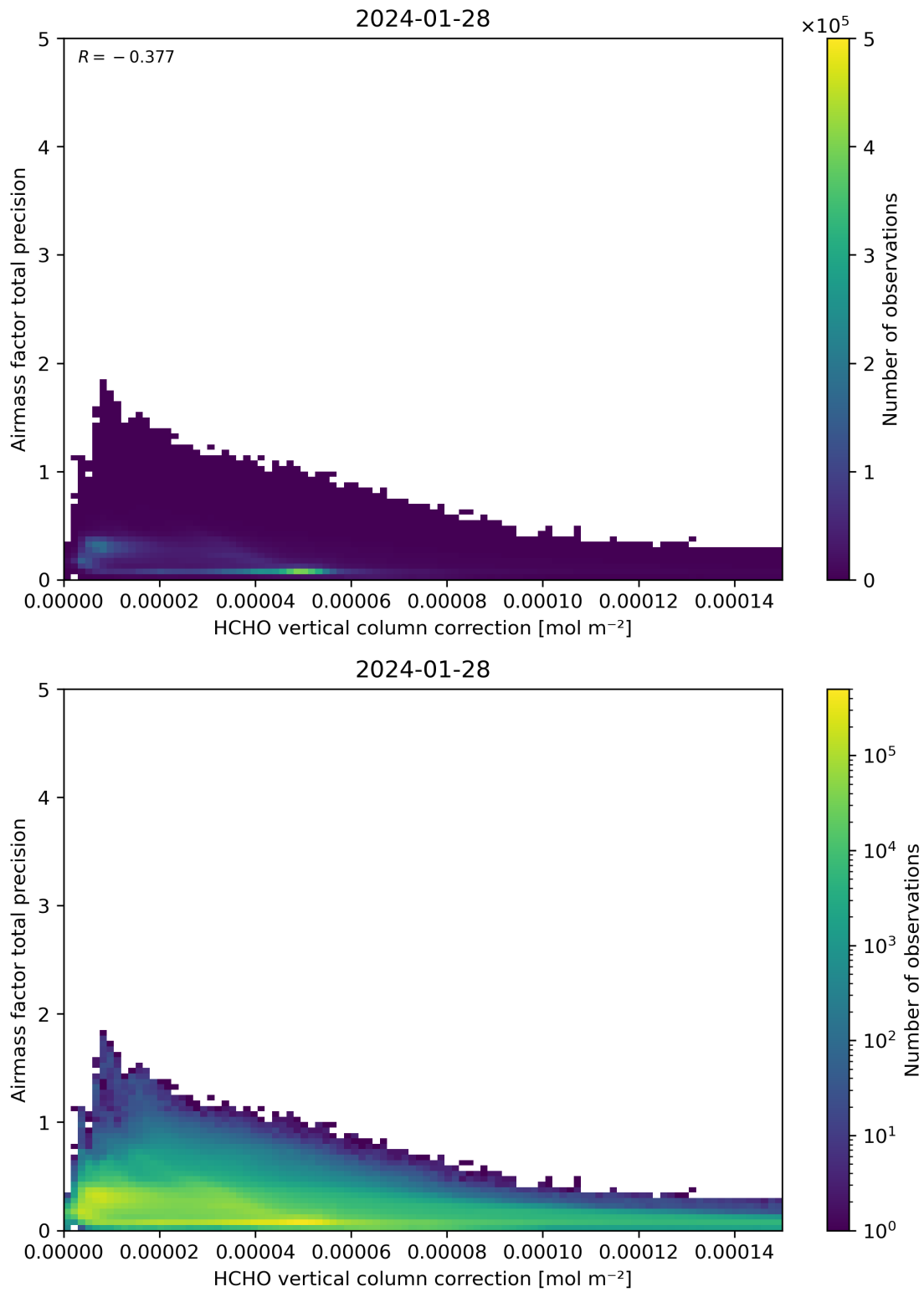
Figure 121: Scatter density plot of “HCHO vertical column correction” against “Airmass factor total precision” for 2024-01-27 to 2024-01-29.
