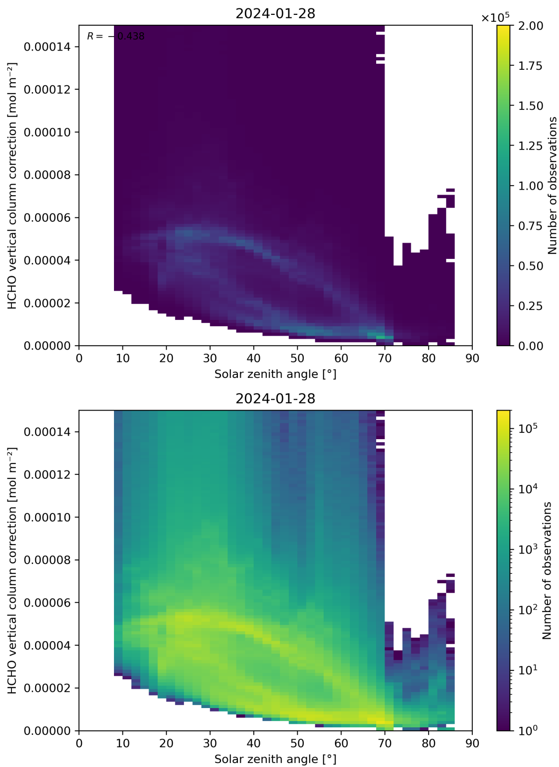
Figure 178: Scatter density plot of “Solar zenith angle” against “HCHO vertical column correction” for 2024-01-27 to 2024-01-29.
