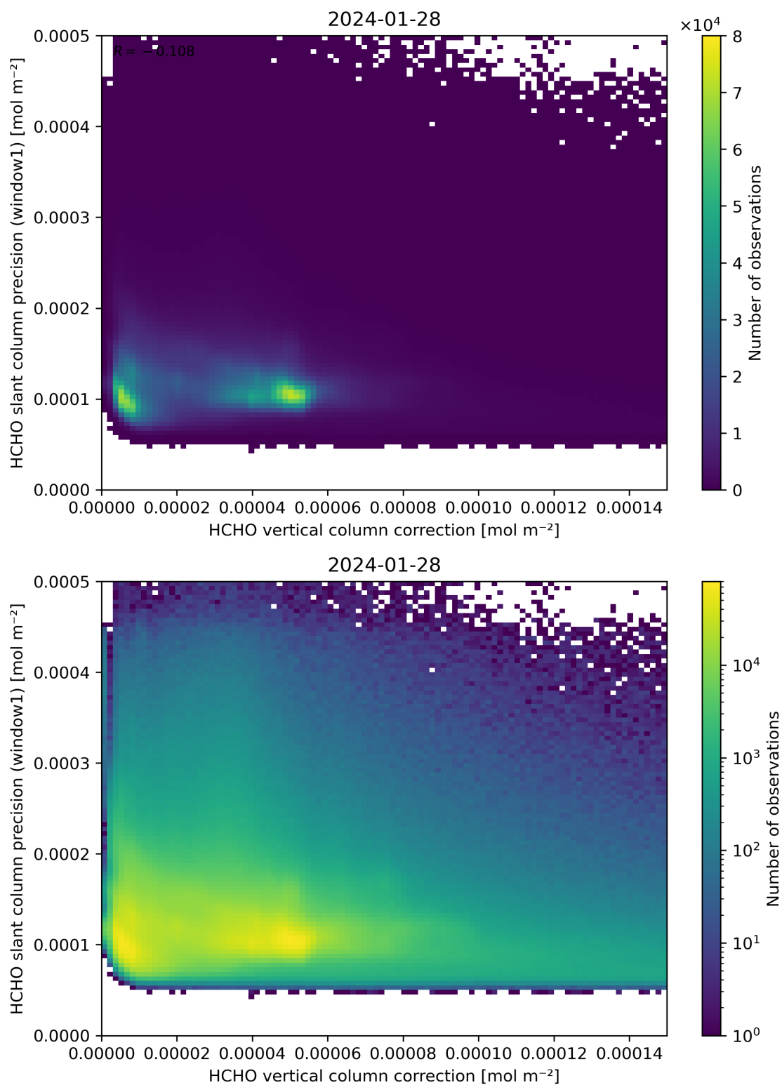
Figure 119: Scatter density plot of “HCHO vertical column correction” against “HCHO slant column precision (window1)” for 2024-01-27 to 2024-01-29.
