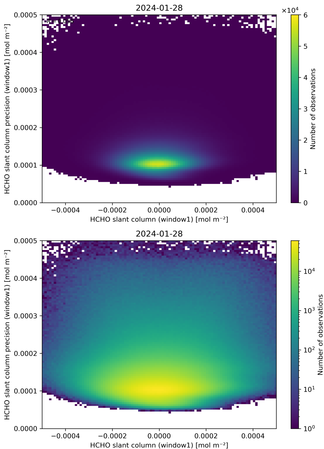
Figure 84: Scatter density plot of “HCHO slant column (window1)” against “HCHO slant column precision (window1)” for 2024-01-27 to 2024-01-29.
