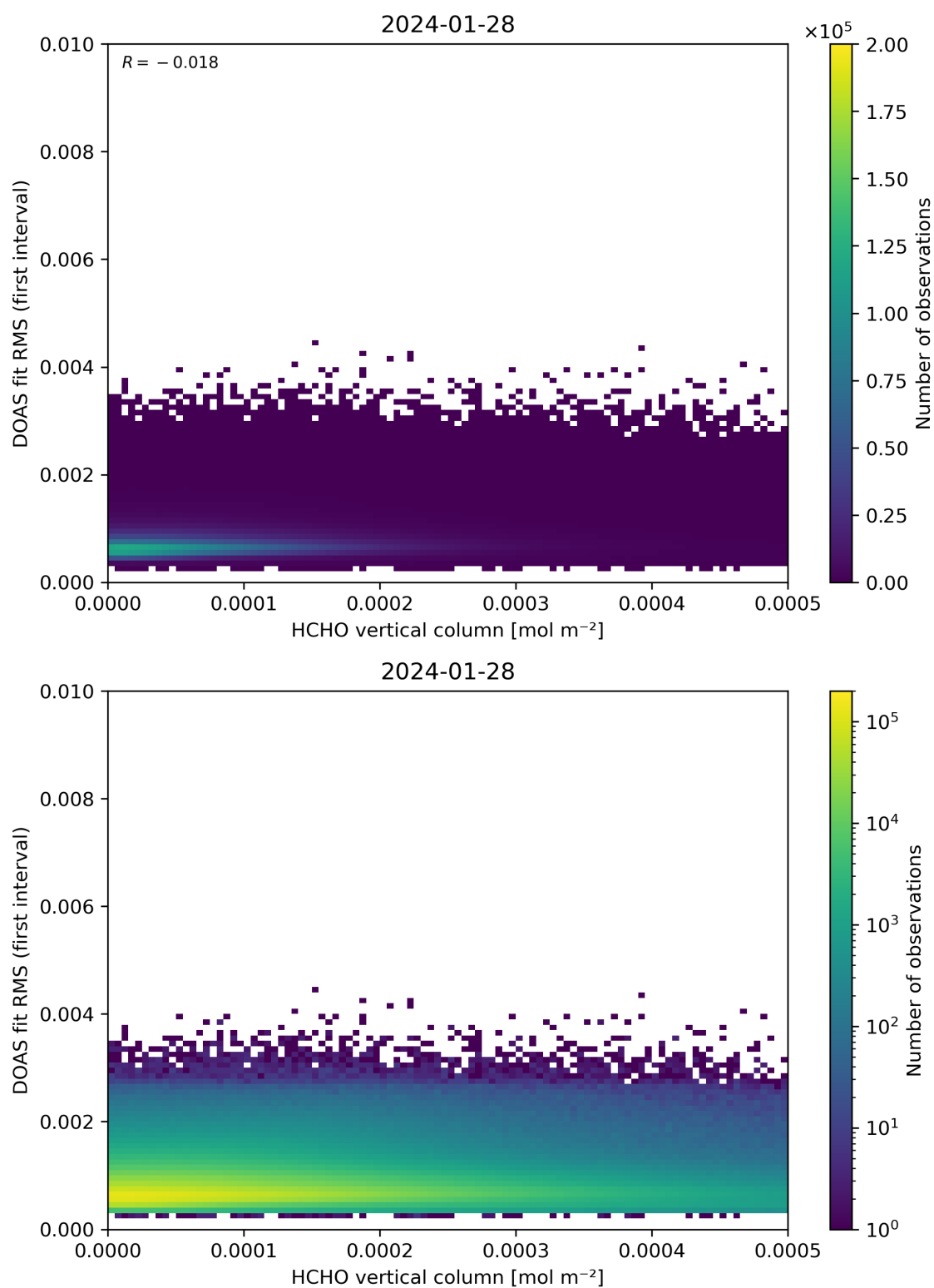
Figure 123: Scatter density plot of “HCHO vertical column” against “DOAS fit RMS (first interval)” for 2024-01-27 to 2024-01-29.
