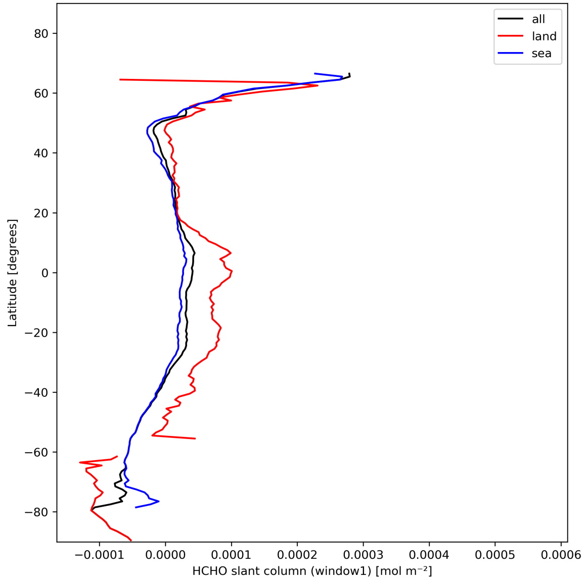
Figure 24: Zonal average of “HCHO slant column (window1)” for 2024-01-27 to 2024-01-29.
