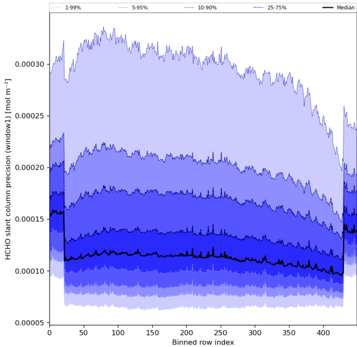
Figure 53: Along track statistics of “HCHO slant column precision (window1)” for 2024-01-27 to 2024-01-29
