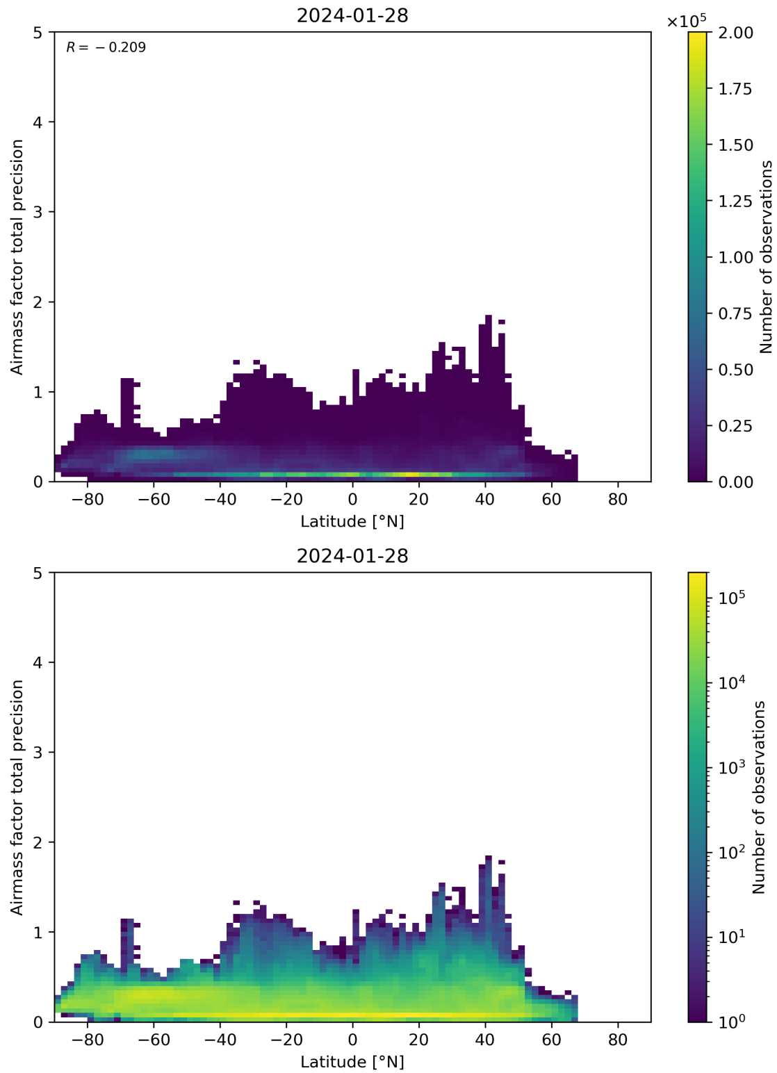
Figure 162: Scatter density plot of “Latitude” against “Airmass factor total precision” for 2024-01-27 to 2024-01-29.
