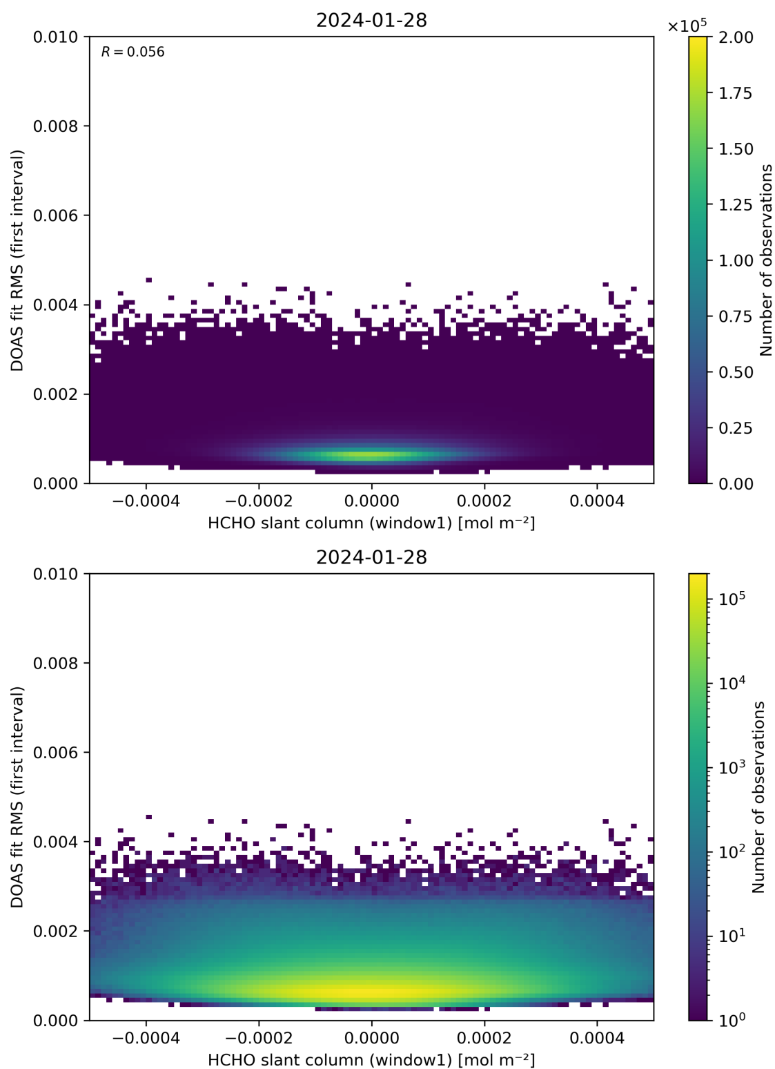
Figure 78: Scatter density plot of “HCHO slant column (window1)” against “DOAS fit RMS (first interval)” for 2024-01-27 to 2024-01-29.
