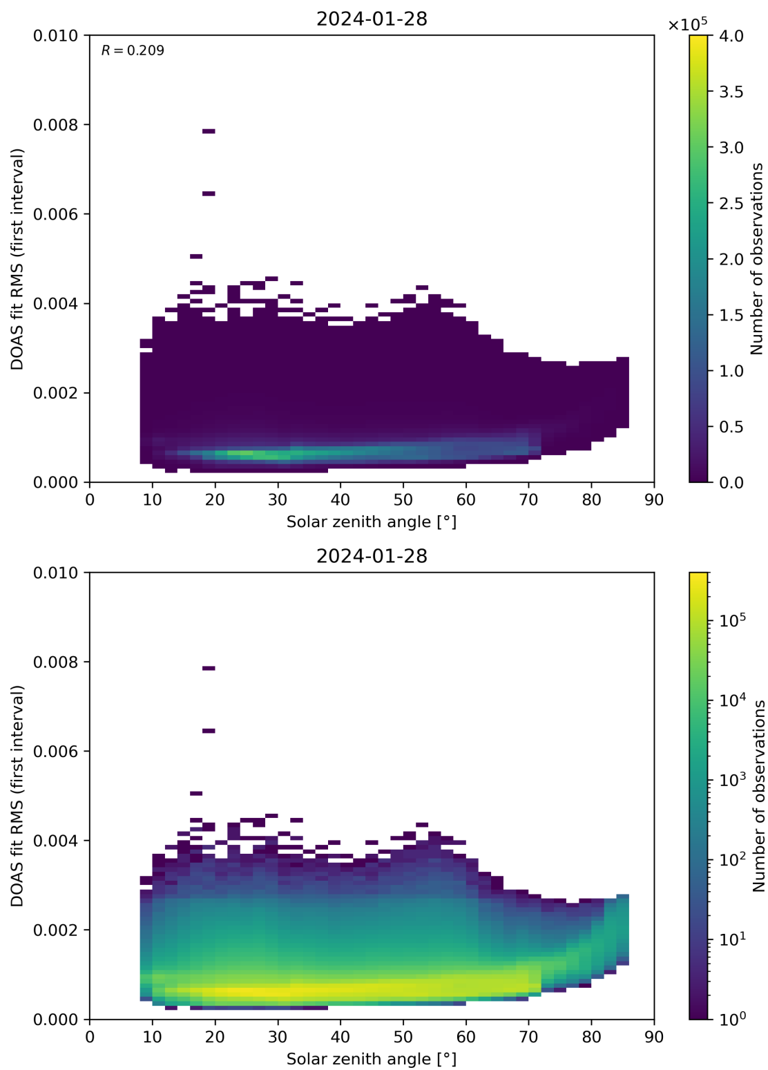
Figure 167: Scatter density plot of “Solar zenith angle” against “DOAS fit RMS (first interval)” for 2024-01-27 to 2024-01-29.
