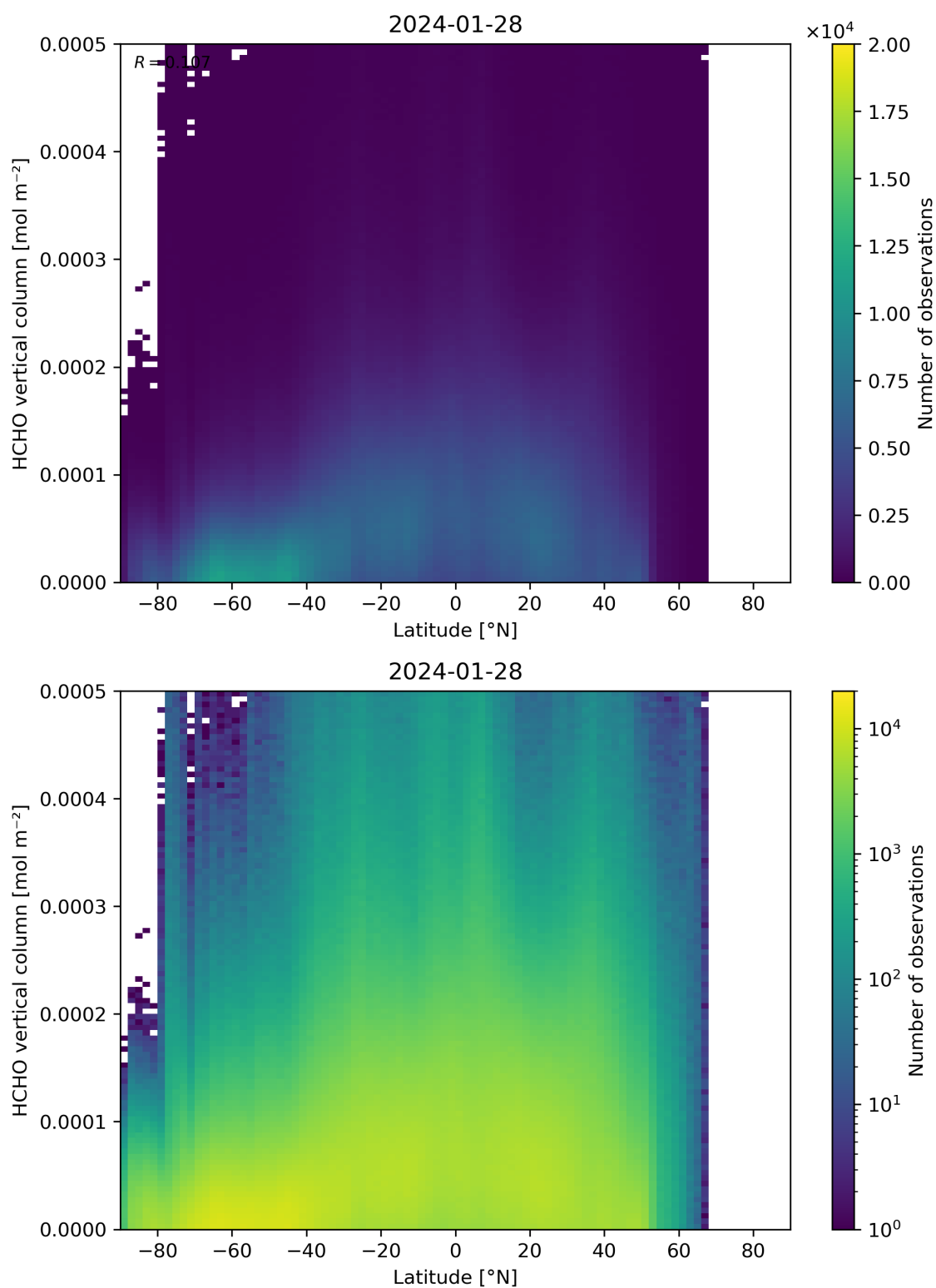
Figure 163: Scatter density plot of “Latitude” against “HCHO vertical column” for 2024-01-27 to 2024-01-29.
