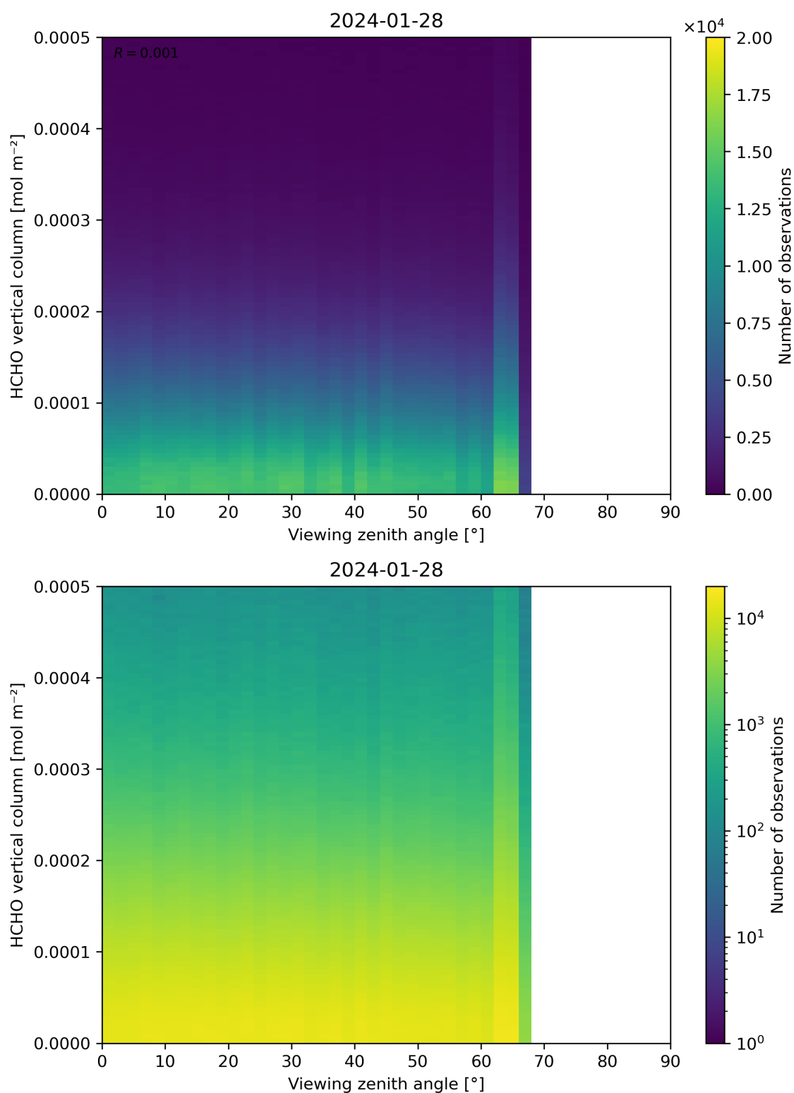
Figure 192: Scatter density plot of “Viewing zenith angle” against “HCHO vertical column” for 2024-01-27 to 2024-01-29.
