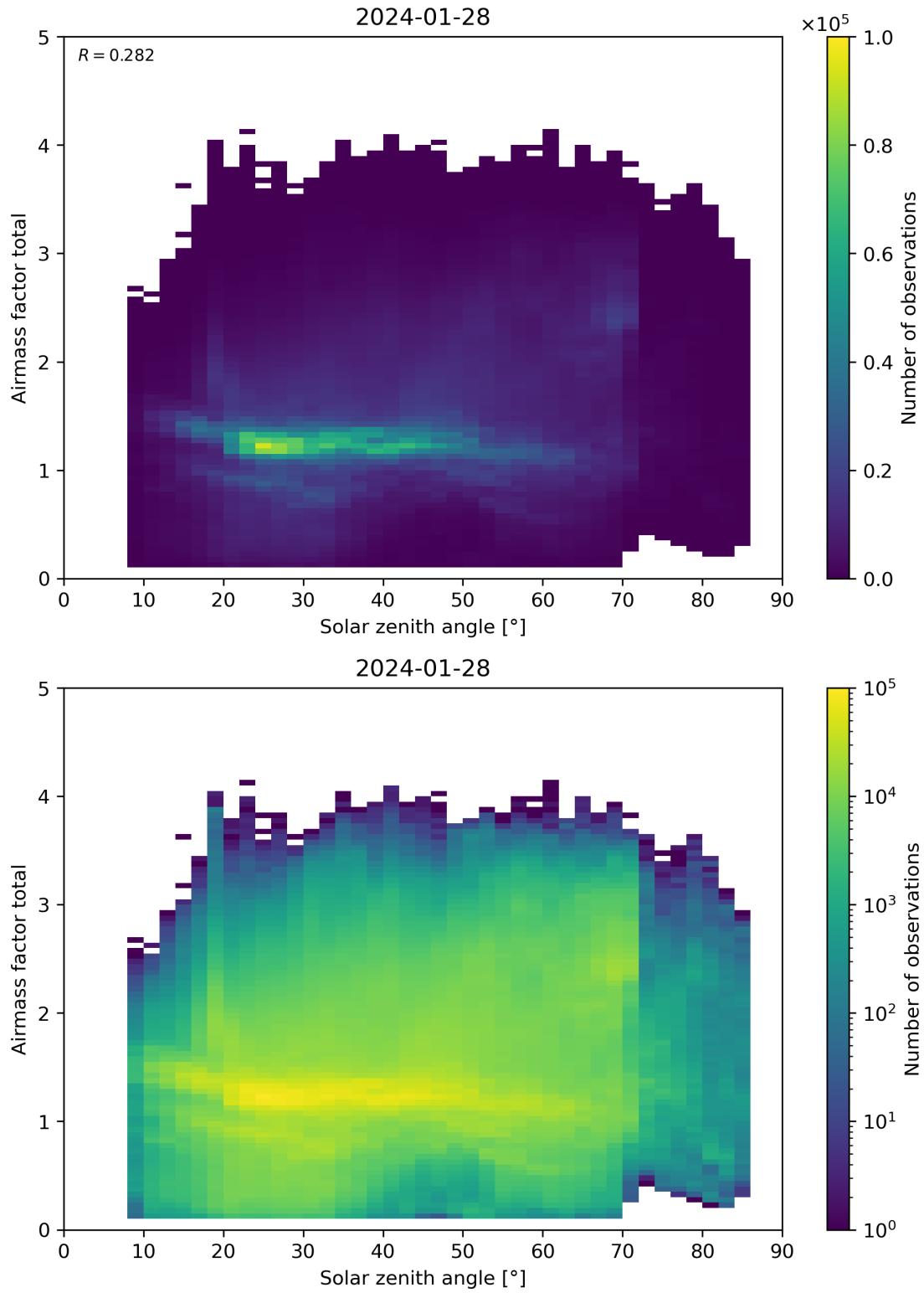
Figure 175: Scatter density plot of “Solar zenith angle” against “Airmass factor total” for 2024-01-27 to 2024-01-29.
