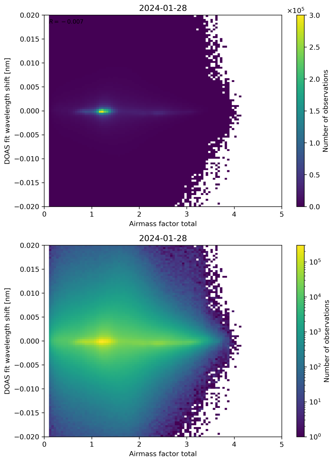
Figure 98: Scatter density plot of “Airmass factor total” against “DOAS fit wavelength shift” for 2024-01-27 to 2024-01-29.
