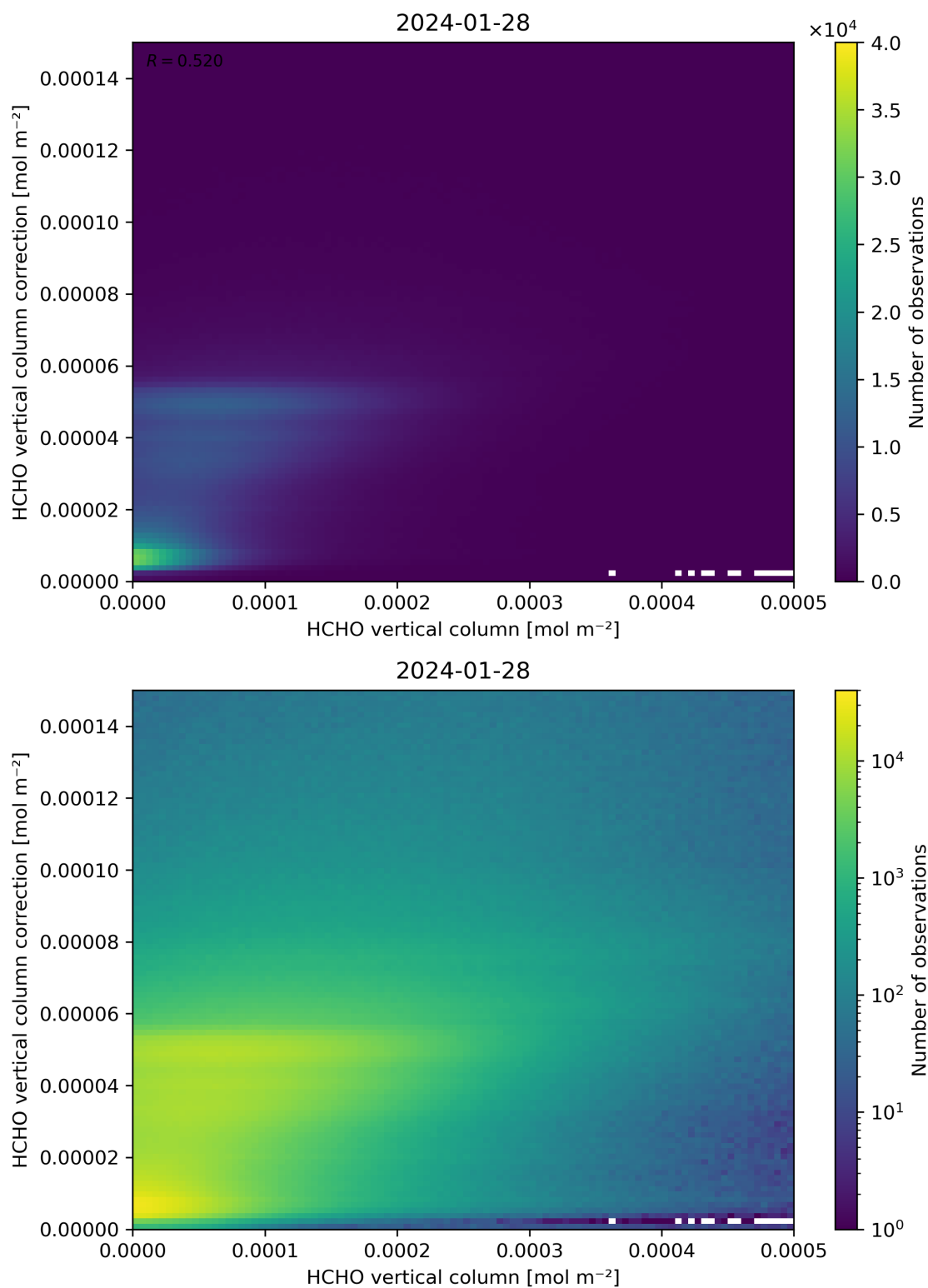
Figure 133: Scatter density plot of “HCHO vertical column” against “HCHO vertical column correction” for 2024-01-27 to 2024-01-29.
