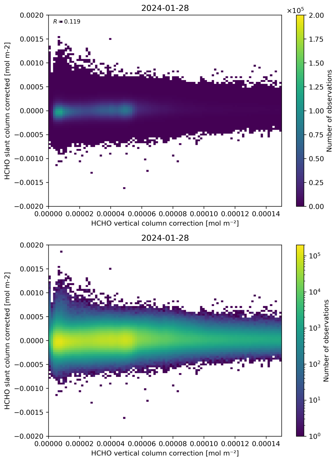
Figure 116: Scatter density plot of “HCHO vertical column correction” against “HCHO slant column corrected” for 2024-01-27 to 2024-01-29.
