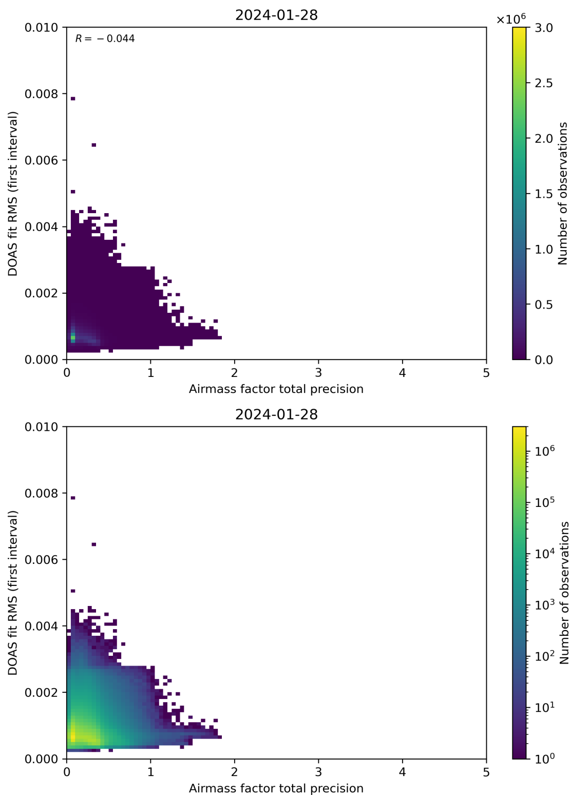
Figure 105: Scatter density plot of “Airmass factor total precision” against “DOAS fit RMS (first interval)” for 2024-01-27 to 2024-01-29.
