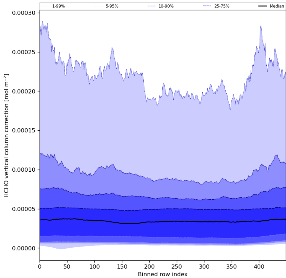
Figure 51: Along track statistics of “HCHO vertical column correction” for 2024-01-27 to 2024-01-29
