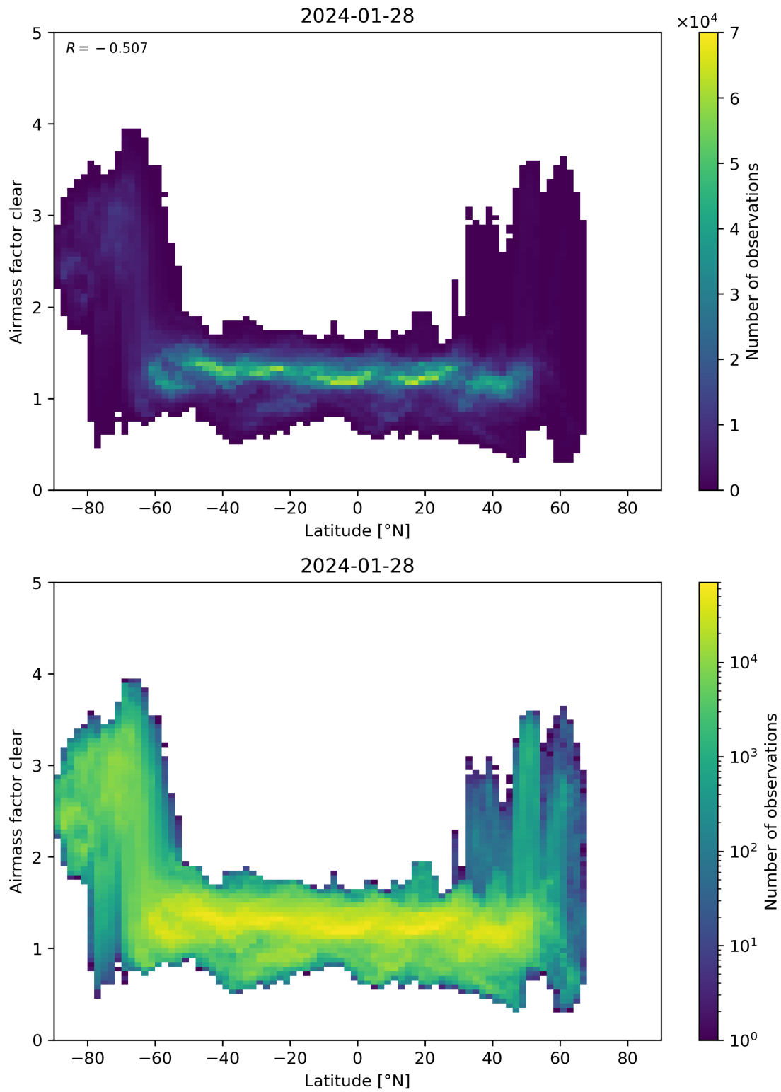
Figure 156: Scatter density plot of “Latitude” against “Airmass factor clear” for 2024-01-27 to 2024-01-29.
