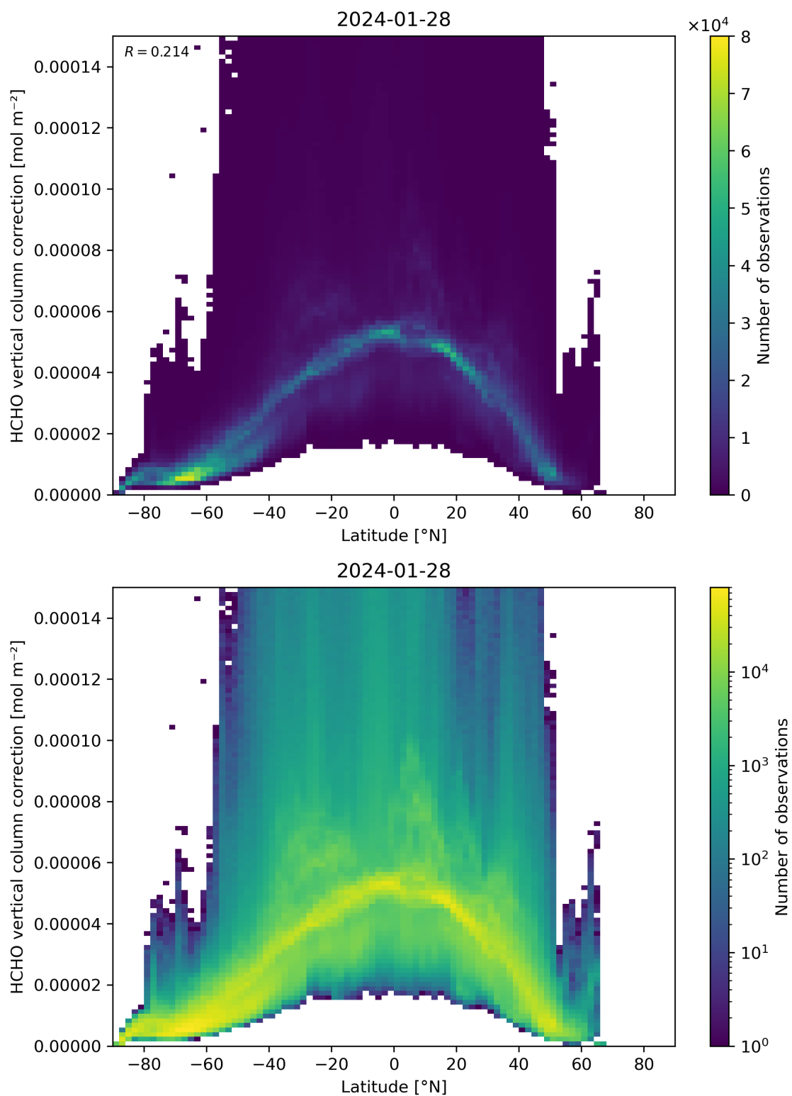
Figure 164: Scatter density plot of “Latitude” against “HCHO vertical column correction” for 2024-01-27 to 2024-01-29.
