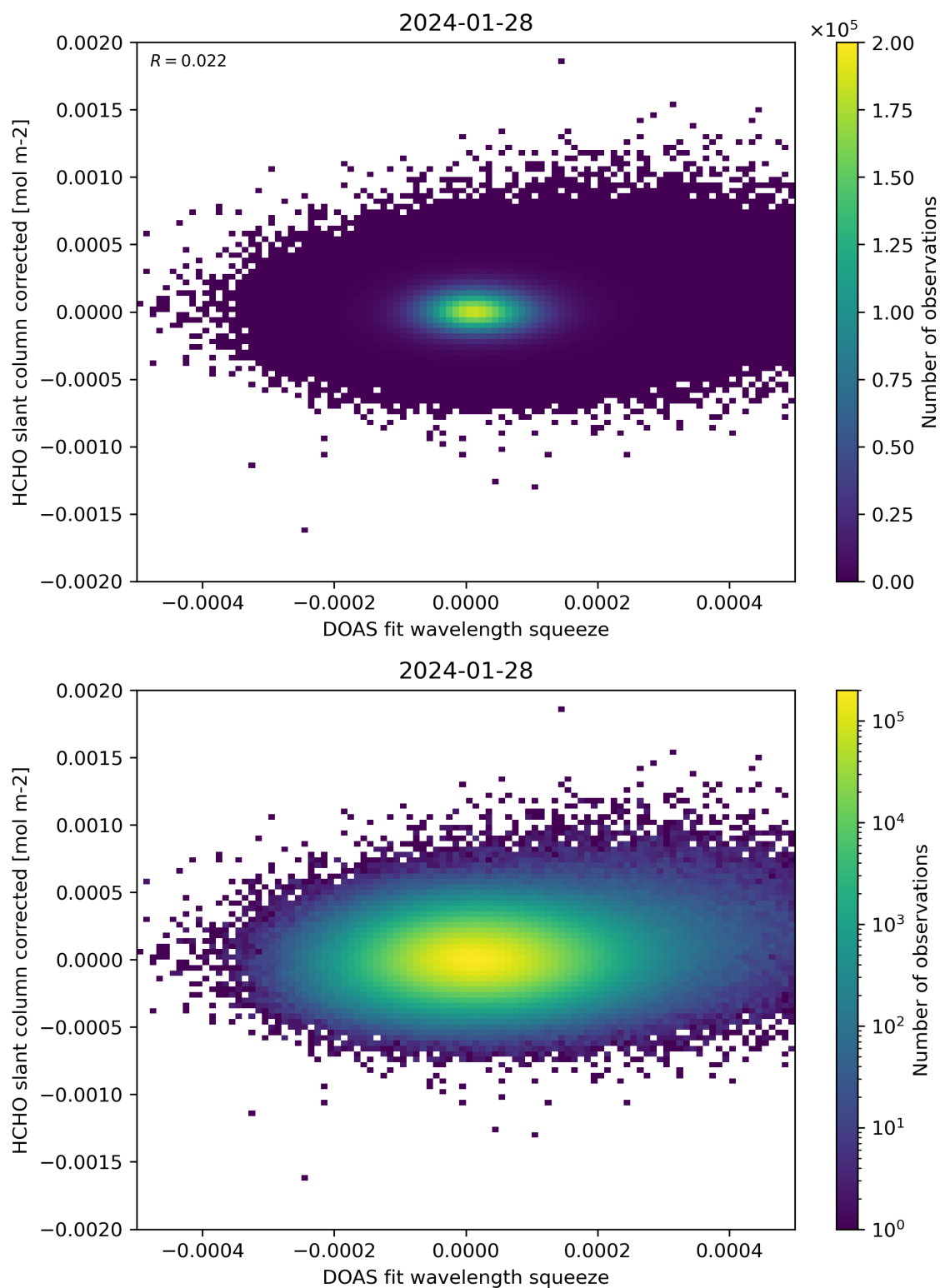
Figure 69: Scatter density plot of “DOAS fit wavelength squeeze” against “HCHO slant column corrected” for 2024-01-27 to 2024-01-29.
