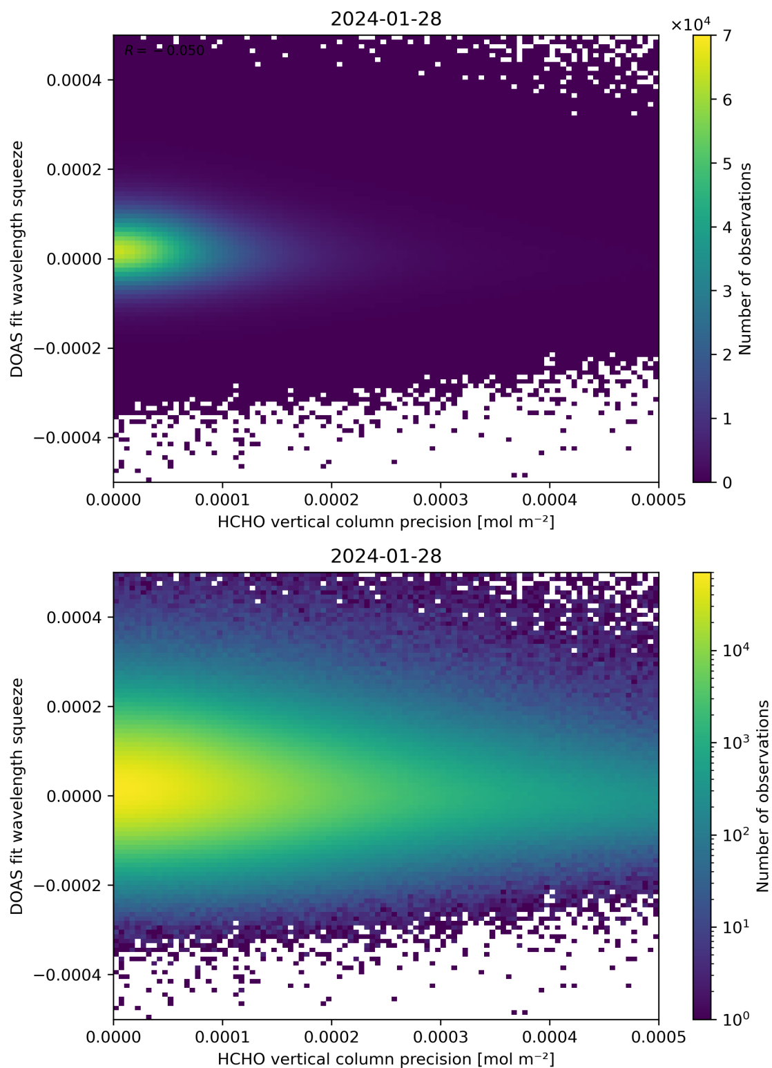
Figure 138: Scatter density plot of “HCHO vertical column precision” against “DOAS fit wavelength squeeze” for 2024-01-27 to 2024-01-29.
