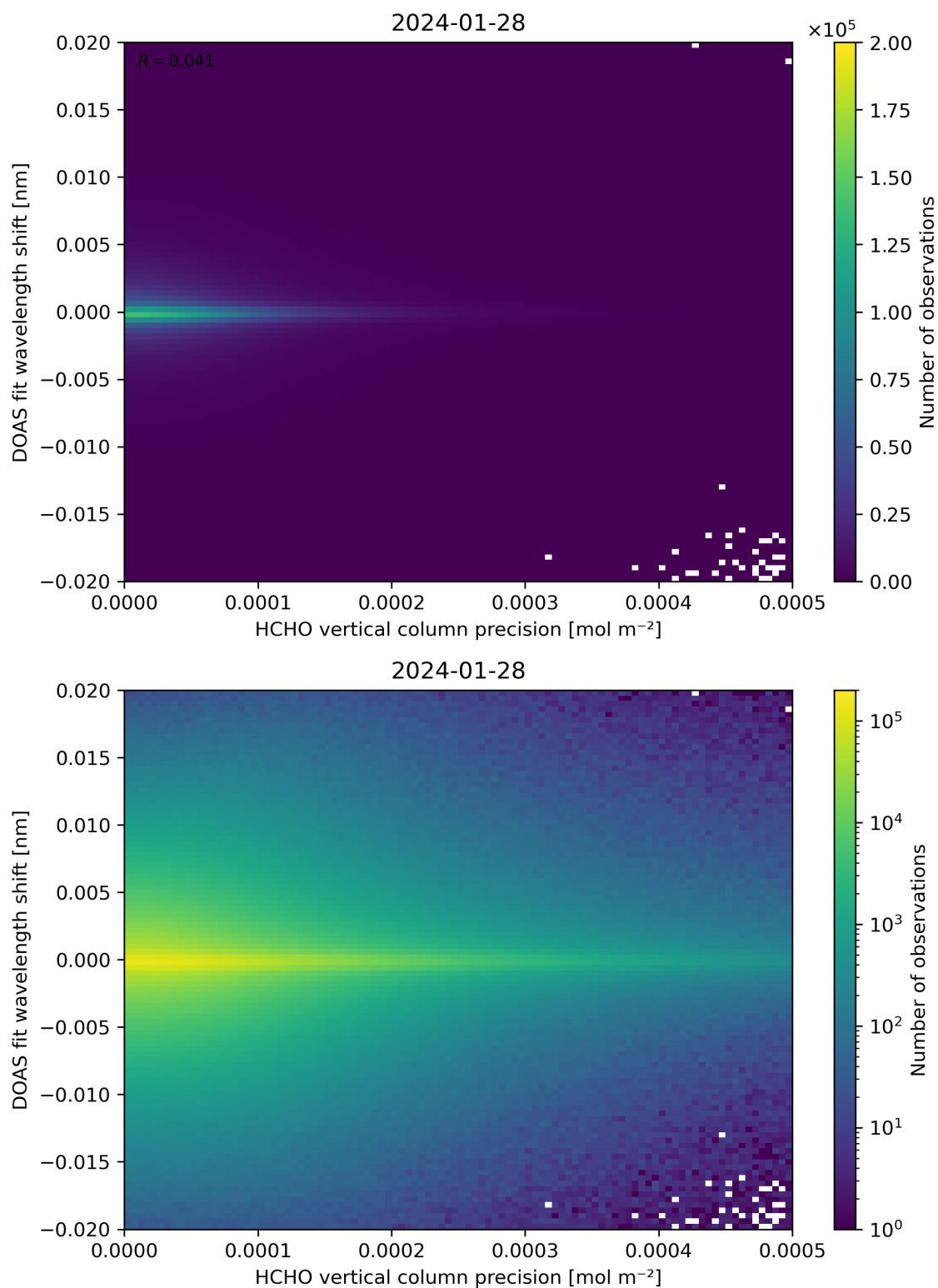
Figure 137: Scatter density plot of “HCHO vertical column precision” against “DOAS fit wavelength shift” for 2024-01-27 to 2024-01-29.
