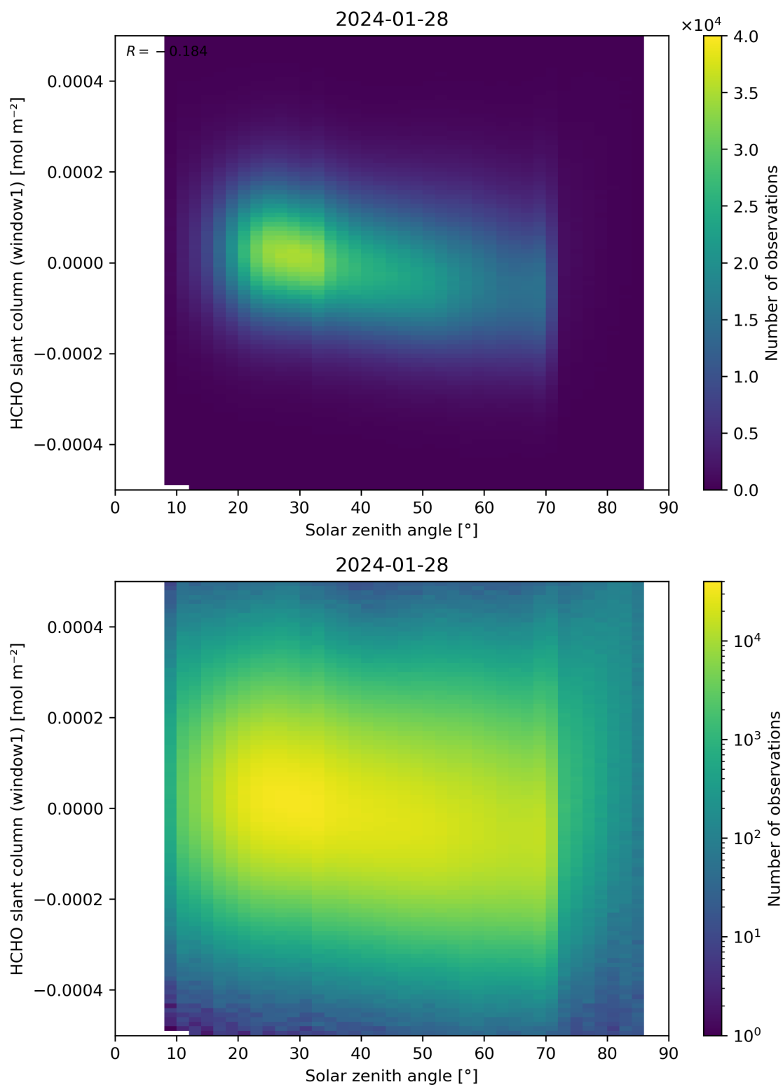
Figure 173: Scatter density plot of “Solar zenith angle” against “HCHO slant column (window1)” for 2024-01-27 to 2024-01-29.
