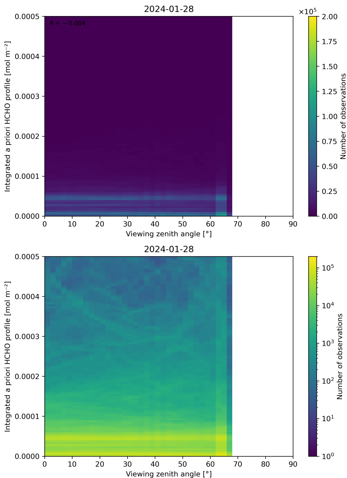
Figure 195: Scatter density plot of “Viewing zenith angle” against “Integrated a priori HCHO profile” for 2024-01-27 to 2024-01-29.
