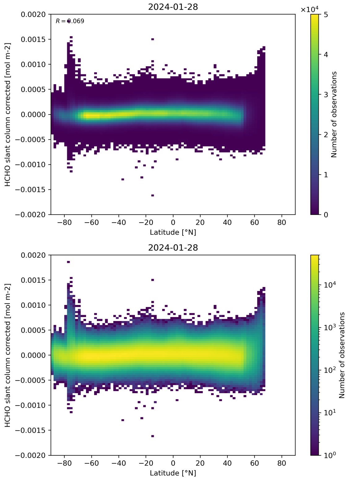
Figure 157: Scatter density plot of “Latitude” against “HCHO slant column corrected” for 2024-01-27 to 2024-01-29.
