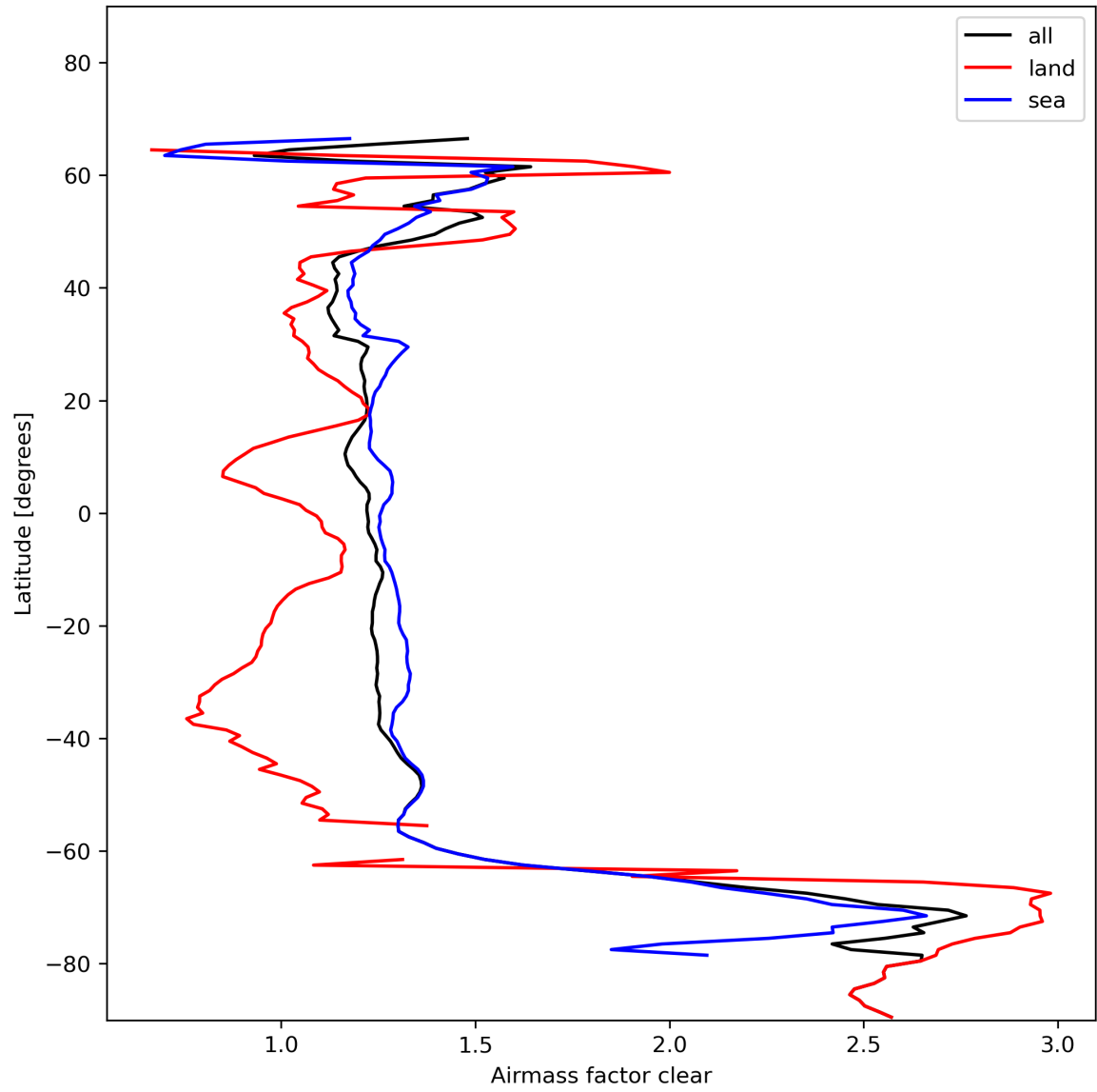
Figure 28: Zonal average of “Airmass factor clear” for 2024-01-27 to 2024-01-29.
