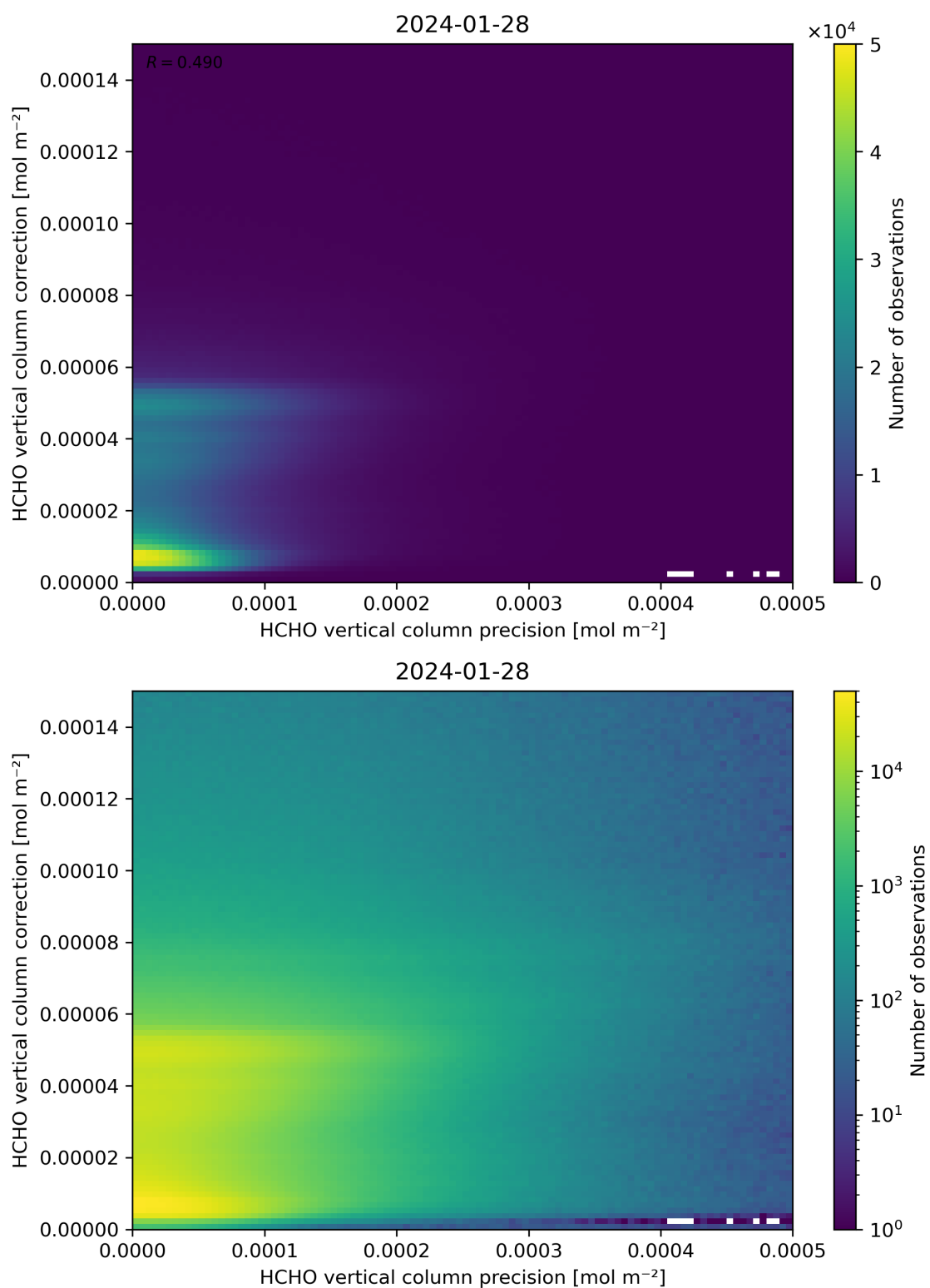
Figure 146: Scatter density plot of “HCHO vertical column precision” against “HCHO vertical column correction” for 2024-01-27 to 2024-01-29.
