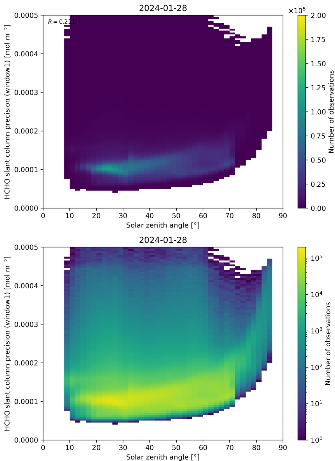
Figure 174: Scatter density plot of “Solar zenith angle” against “HCHO slant column precision (window1)” for 2024-01-27 to 2024-01-29.
