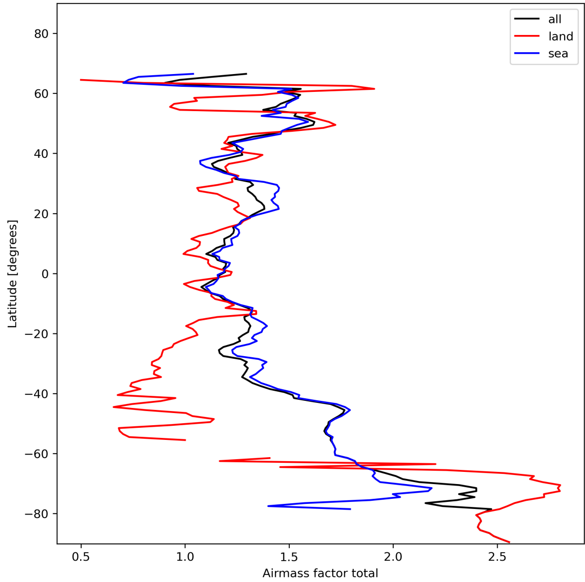
Figure 26: Zonal average of “Airmass factor total” for 2024-01-27 to 2024-01-29.
