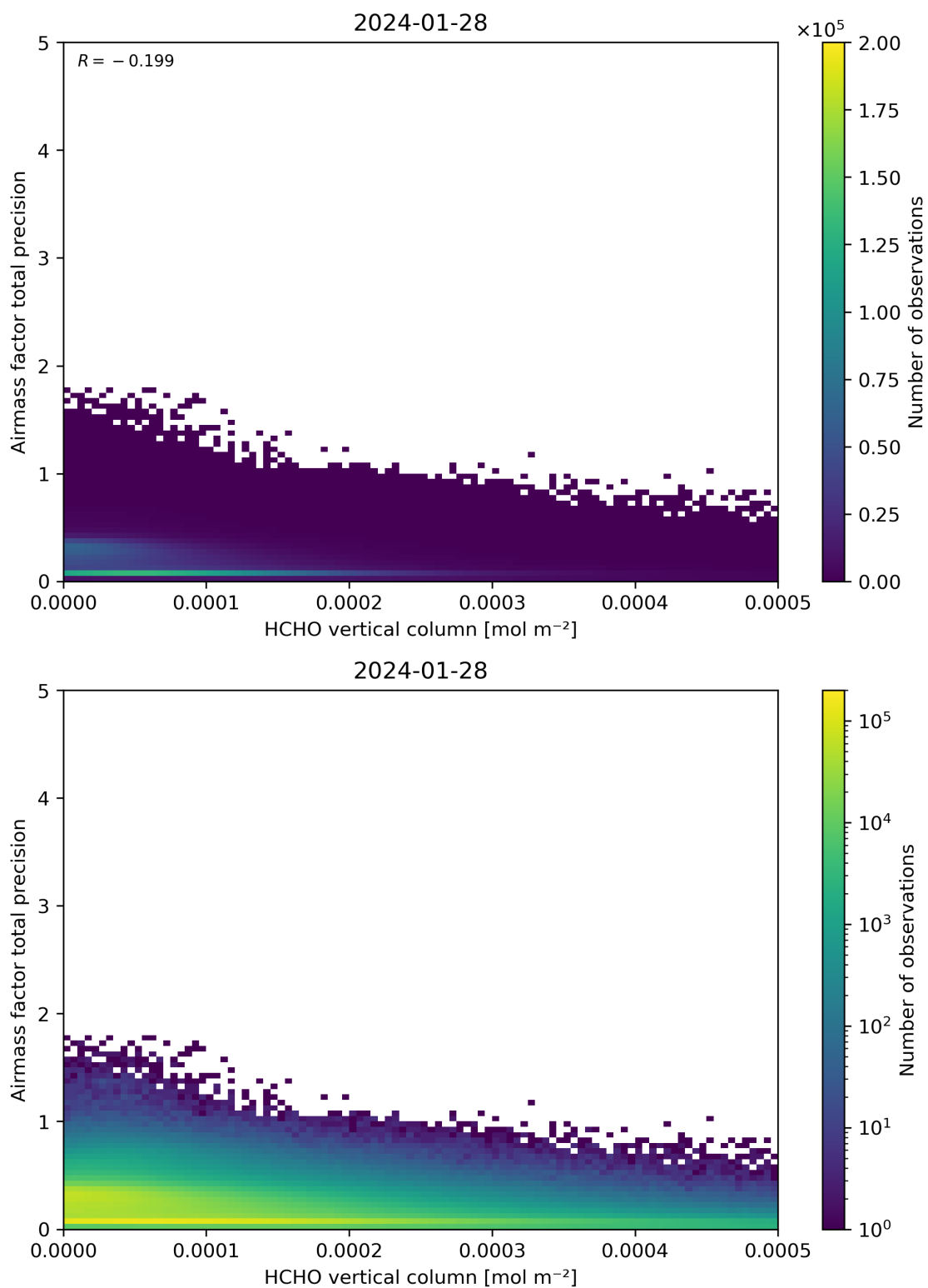
Figure 132: Scatter density plot of “HCHO vertical column” against “Airmass factor total precision” for 2024-01-27 to 2024-01-29.
