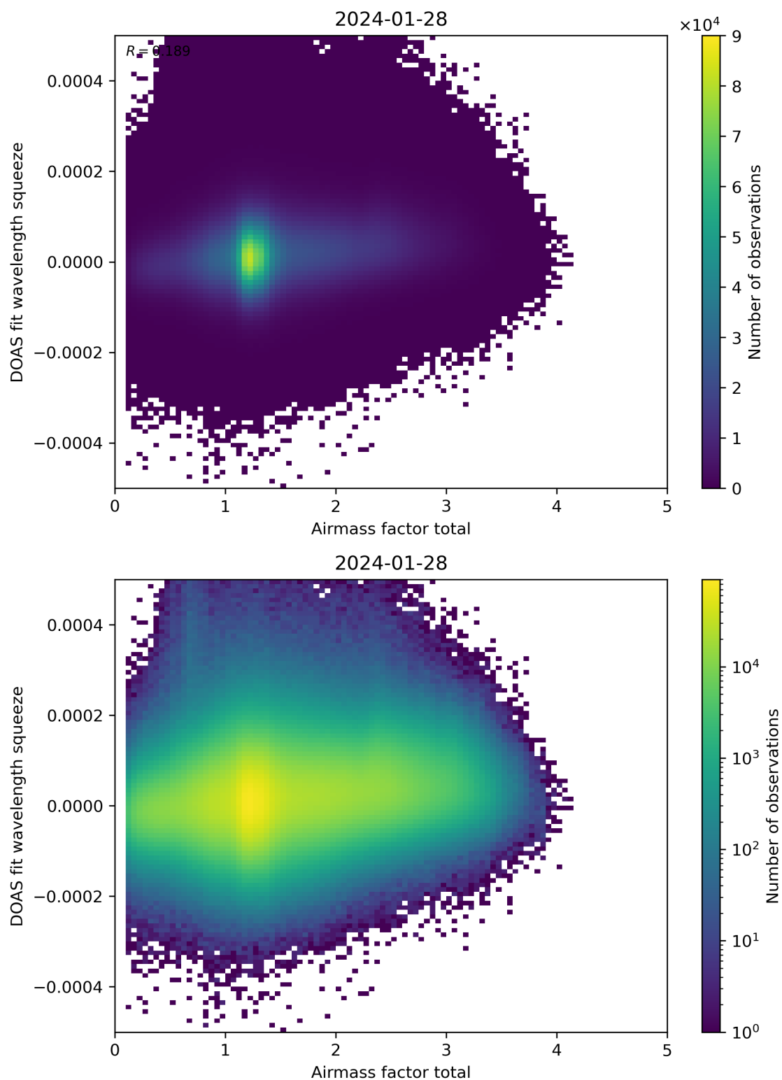
Figure 99: Scatter density plot of “Airmass factor total” against “DOAS fit wavelength squeeze” for 2024-01-27 to 2024-01-29.
