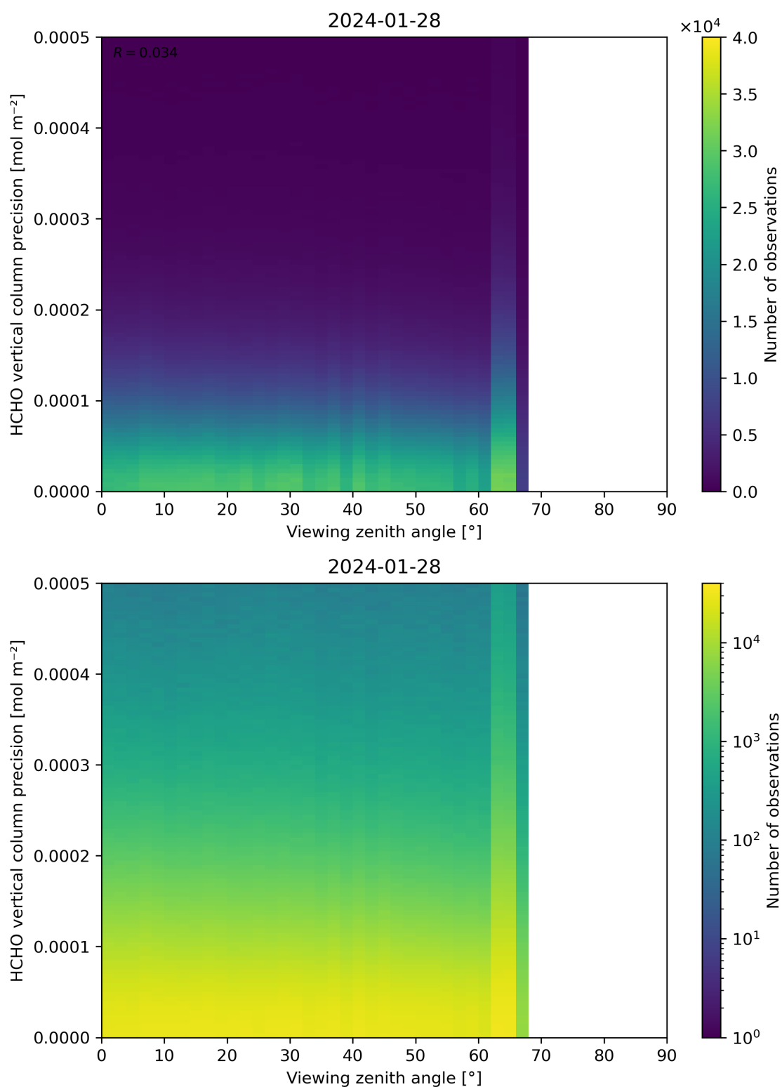
Figure 194: Scatter density plot of “Viewing zenith angle” against “HCHO vertical column precision” for 2024-01-27 to 2024-01-29.
