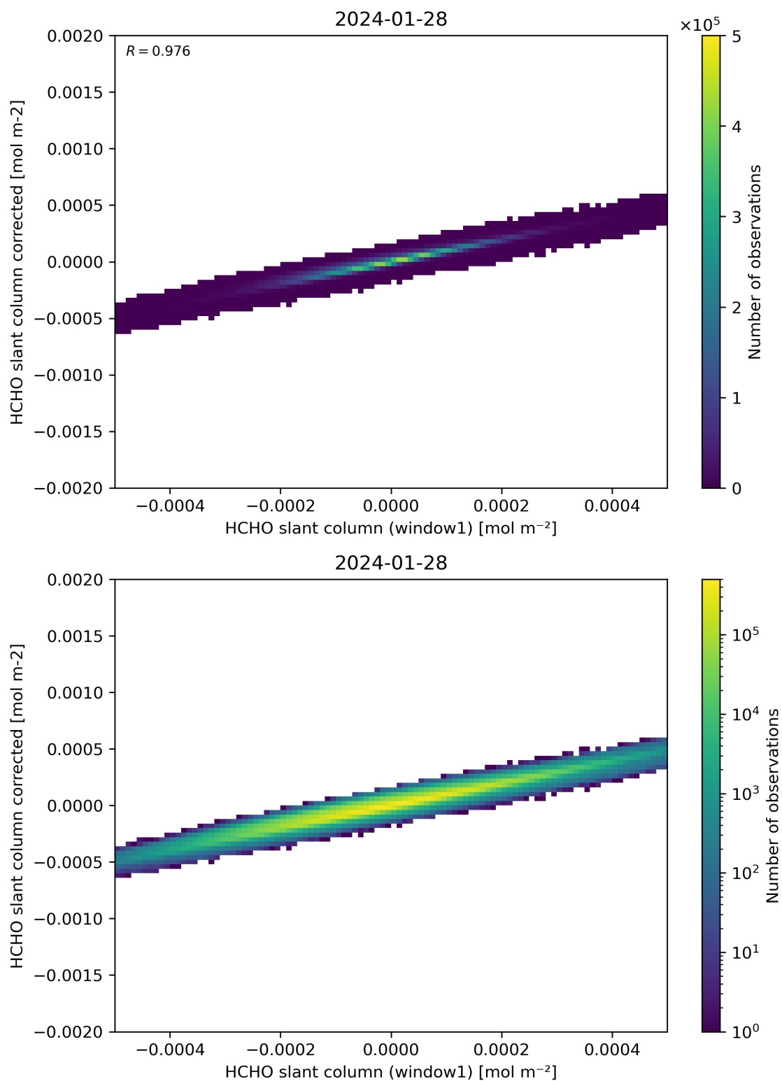
Figure 82: Scatter density plot of “HCHO slant column (window1)” against “HCHO slant column corrected” for 2024-01-27 to 2024-01-29.
