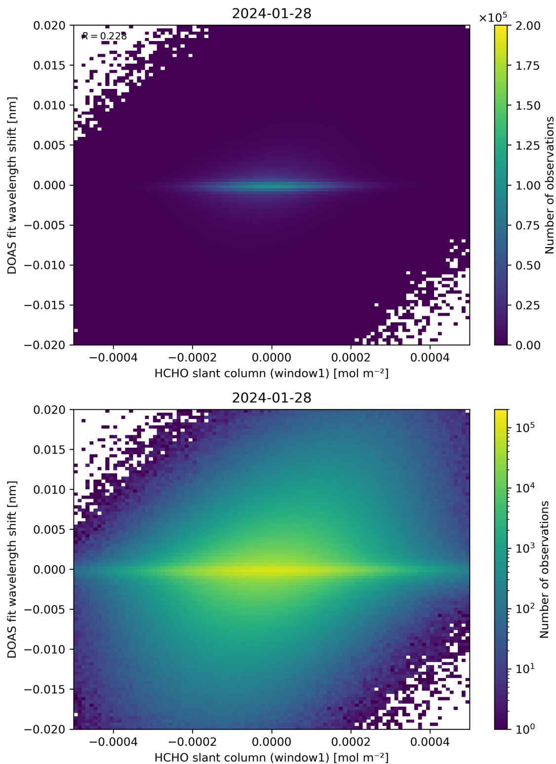
Figure 79: Scatter density plot of “HCHO slant column (window1)” against “DOAS fit wavelength shift” for 2024-01-27 to 2024-01-29.
