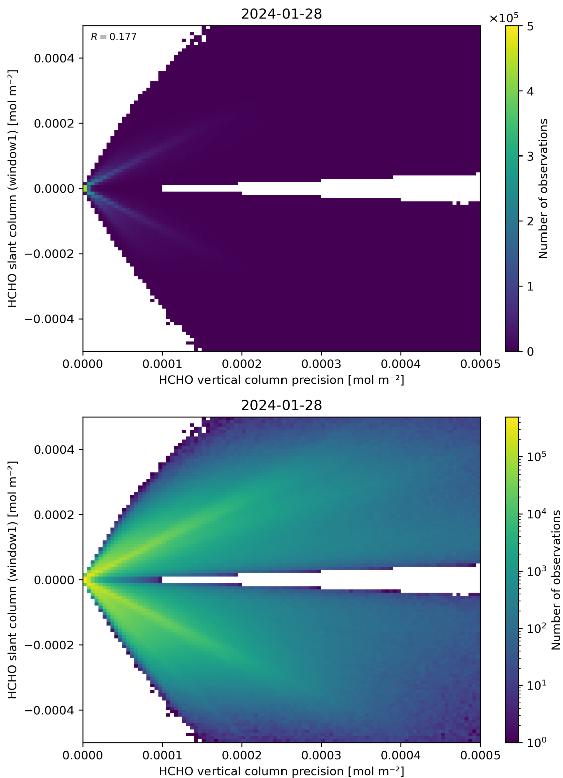
Figure 142: Scatter density plot of “HCHO vertical column precision” against “HCHO slant column (window1)” for 2024-01-27 to 2024-01-29.
