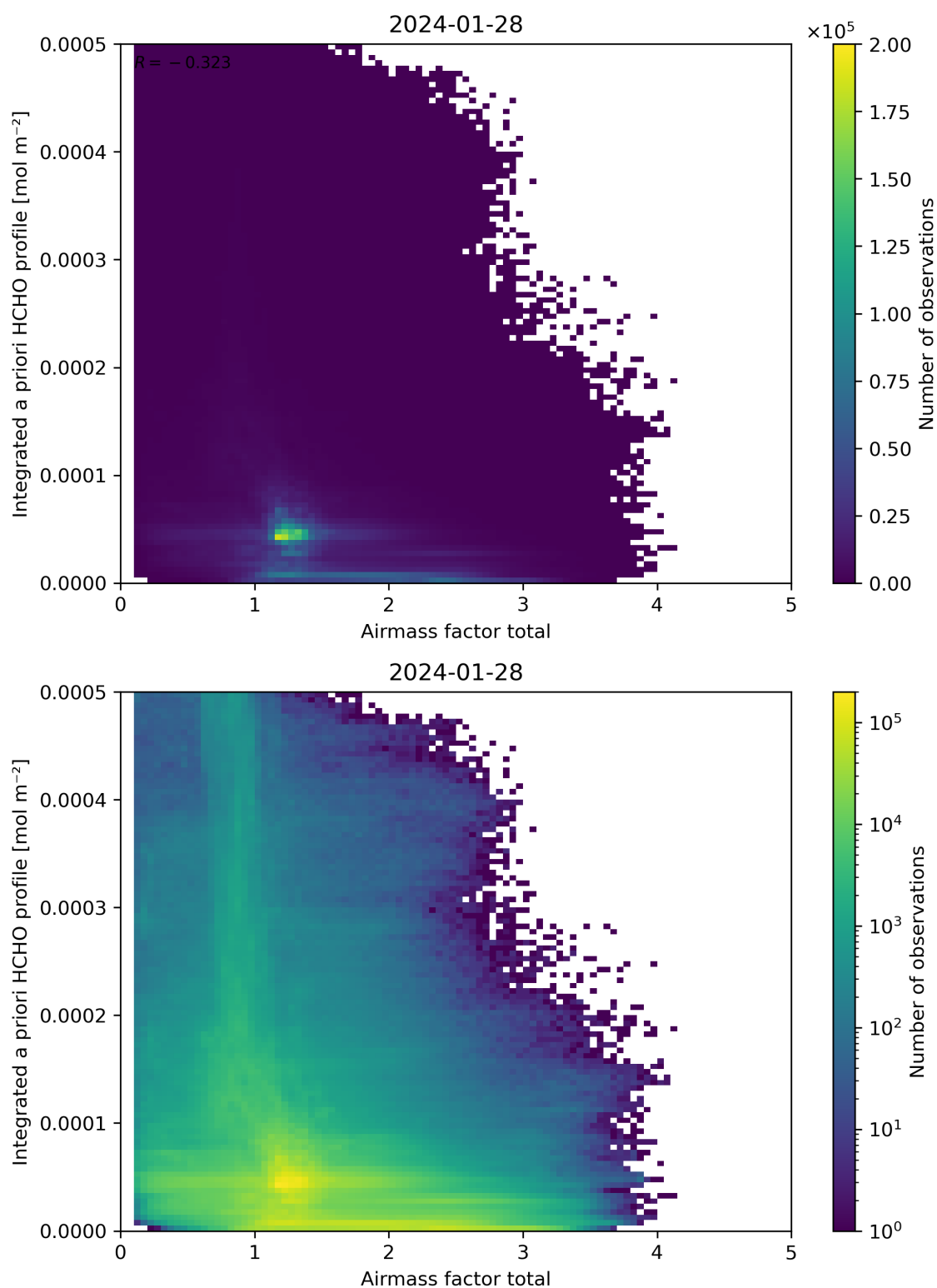
Figure 104: Scatter density plot of “Airmass factor total” against “Integrated a priori HCHO profile” for 2024-01-27 to 2024-01-29.
