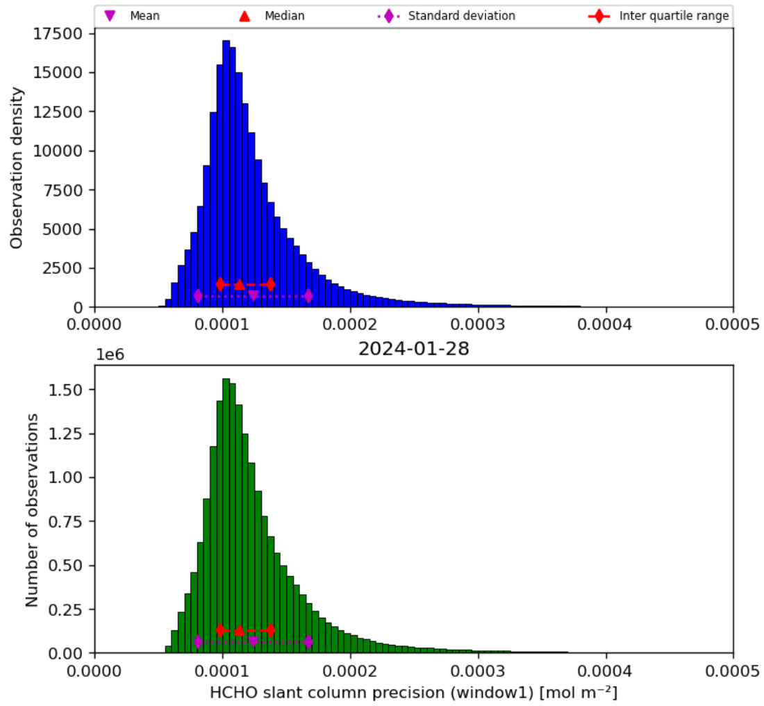
Figure 39: Histogram of “HCHO slant column precision (window1)” for 2024-01-27 to 2024-01-29
