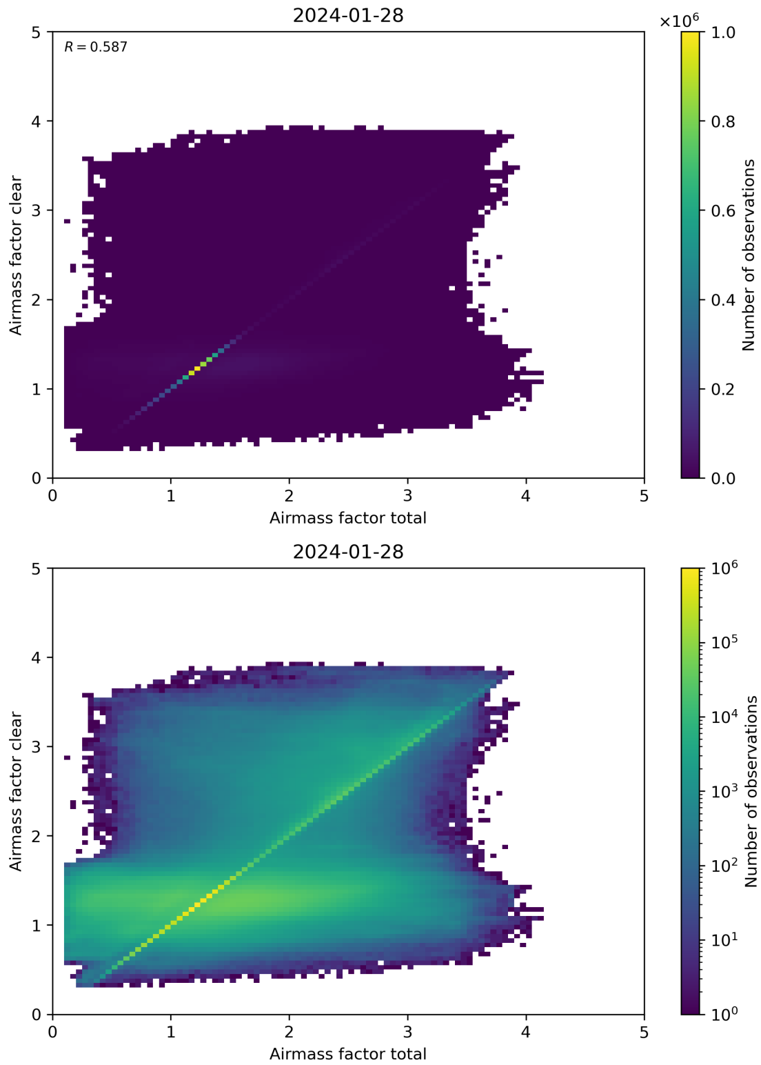
Figure 100: Scatter density plot of “Airmass factor total” against “Airmass factor clear” for 2024-01-27 to 2024-01-29.
