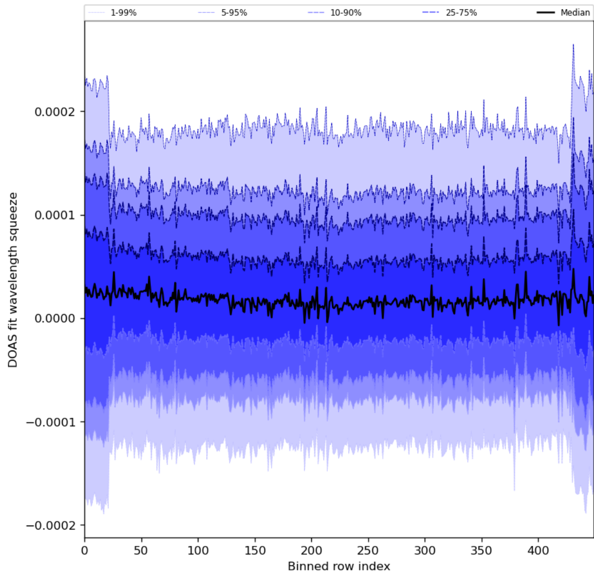
Figure 59: Along track statistics of “DOAS fit wavelength squeeze” for 2024-01-27 to 2024-01-29
