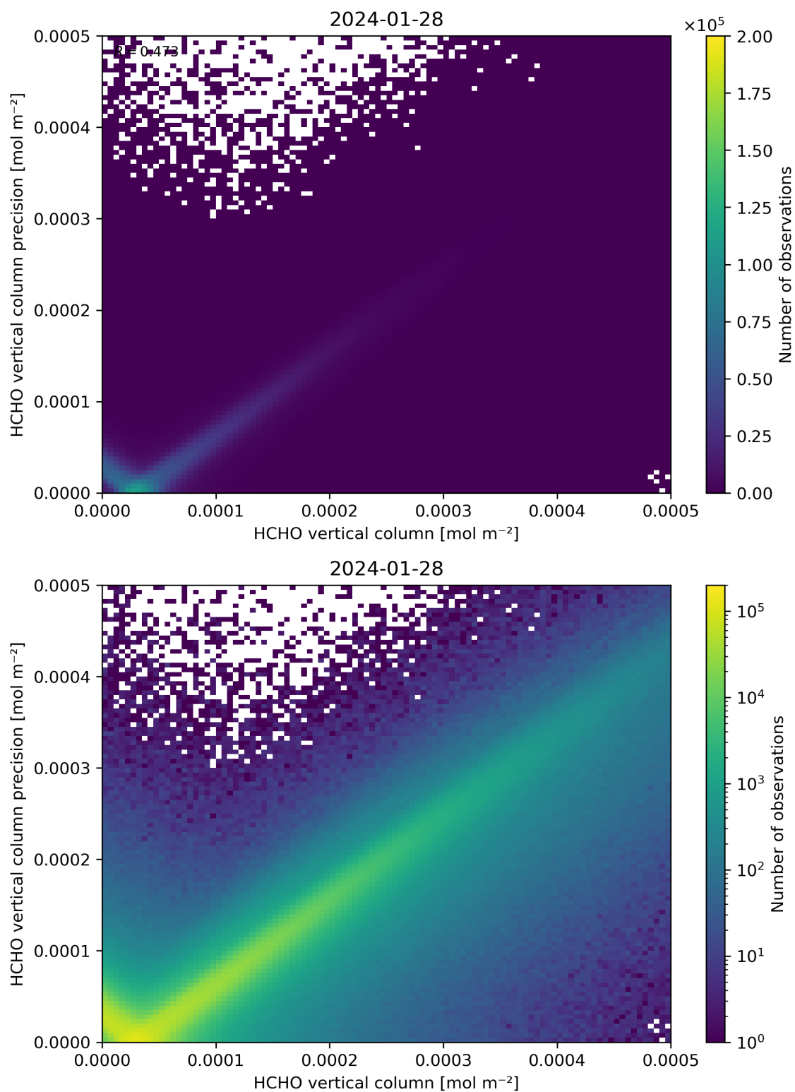
Figure 134: Scatter density plot of “HCHO vertical column” against “HCHO vertical column precision” for 2024-01-27 to 2024-01-29.
