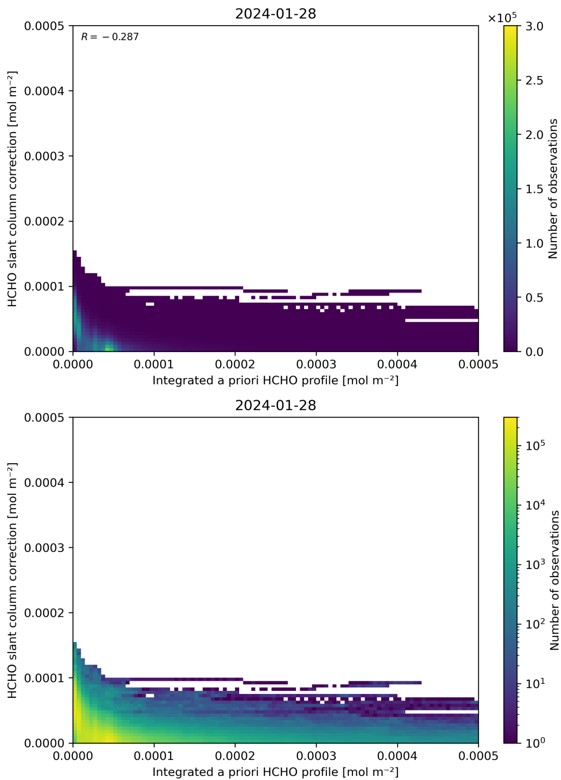
Figure 152: Scatter density plot of “Integrated a priori HCHO profile” against “HCHO slant column correction” for 2024-01-27 to 2024-01-29.
