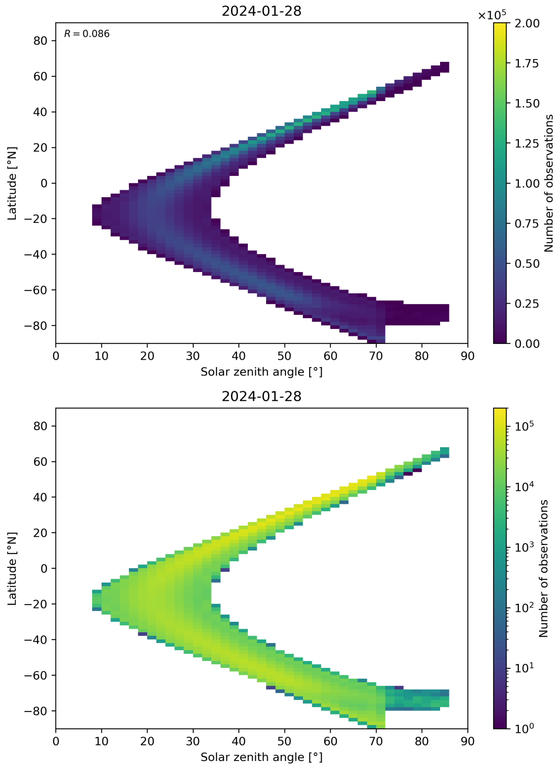
Figure 181: Scatter density plot of “Solar zenith angle” against “Latitude” for 2024-01-27 to 2024-01-29.
