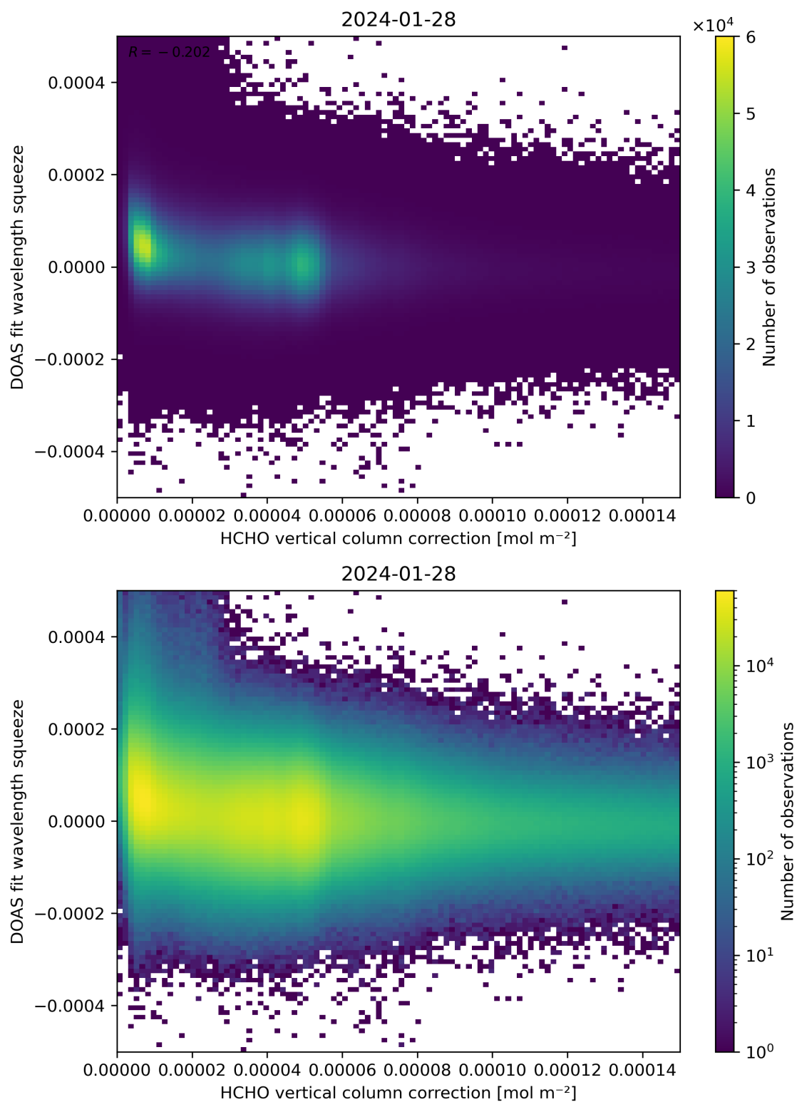
Figure 114: Scatter density plot of “HCHO vertical column correction” against “DOAS fit wavelength squeeze” for 2024-01-27 to 2024-01-29.
