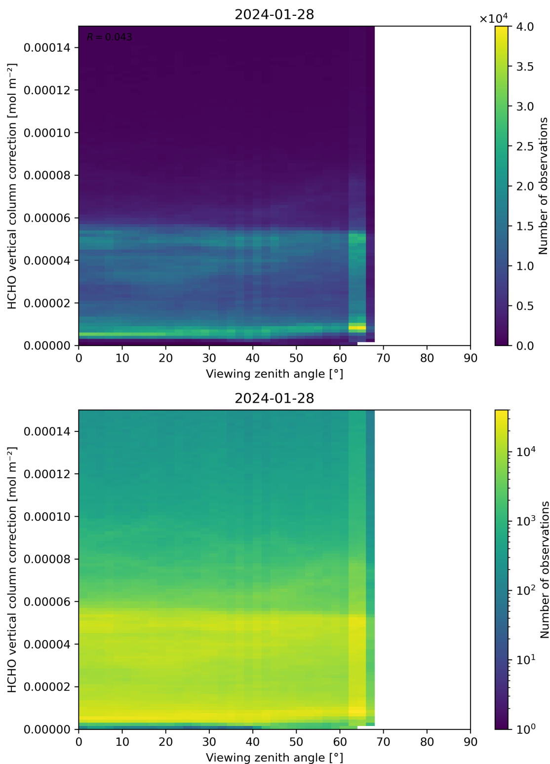
Figure 193: Scatter density plot of “Viewing zenith angle” against “HCHO vertical column correction” for 2024-01-27 to 2024-01-29.
