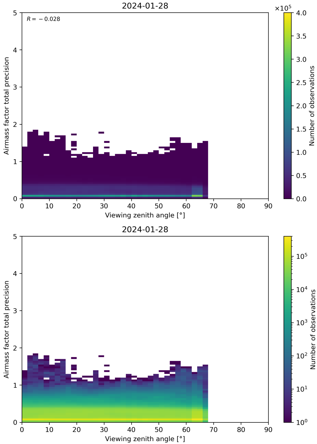
Figure 191: Scatter density plot of “Viewing zenith angle” against “Airmass factor total precision” for 2024-01-27 to 2024-01-29.
