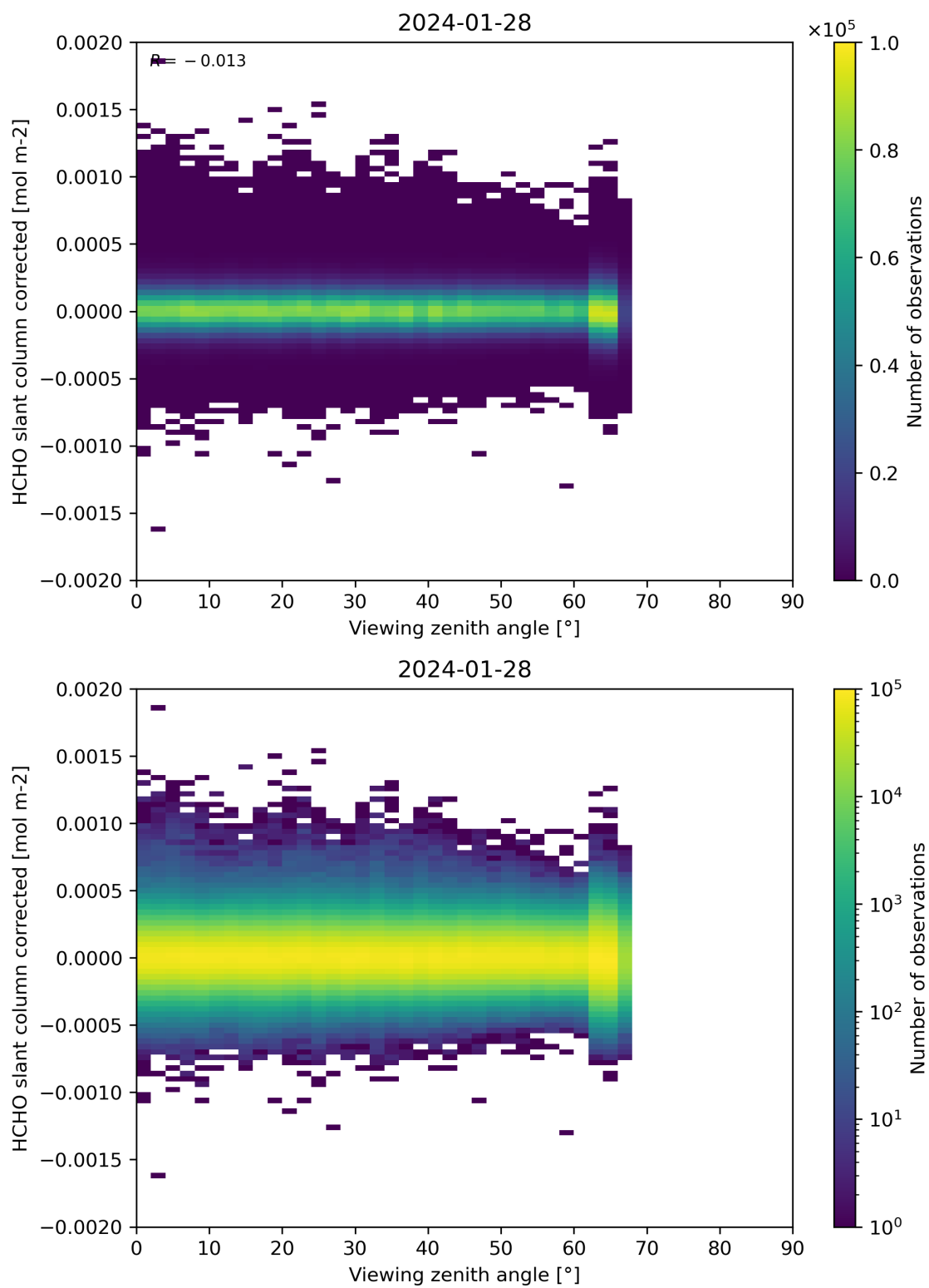
Figure 186: Scatter density plot of “Viewing zenith angle” against “HCHO slant column corrected” for 2024-01-27 to 2024-01-29.
