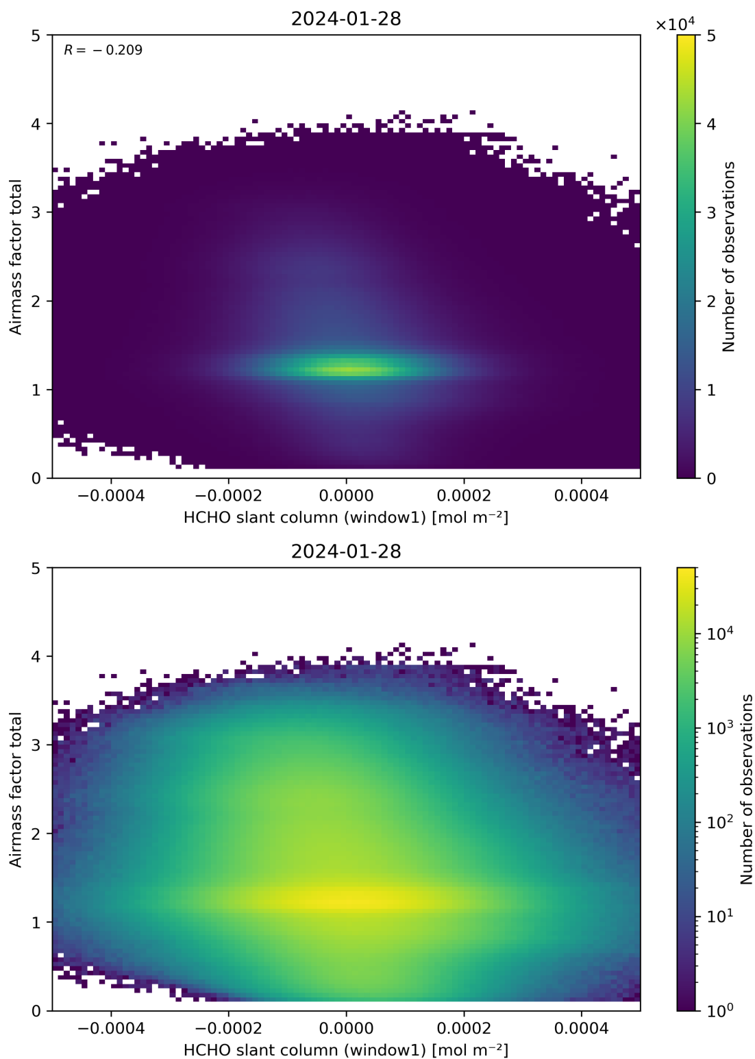
Figure 85: Scatter density plot of “HCHO slant column (window1)” against “Airmass factor total” for 2024-01-27 to 2024-01-29.
