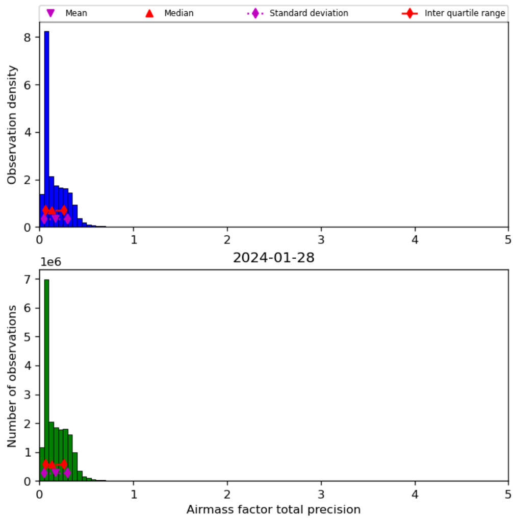
Figure 41: Histogram of “Airmass factor total precision” for 2024-01-27 to 2024-01-29
