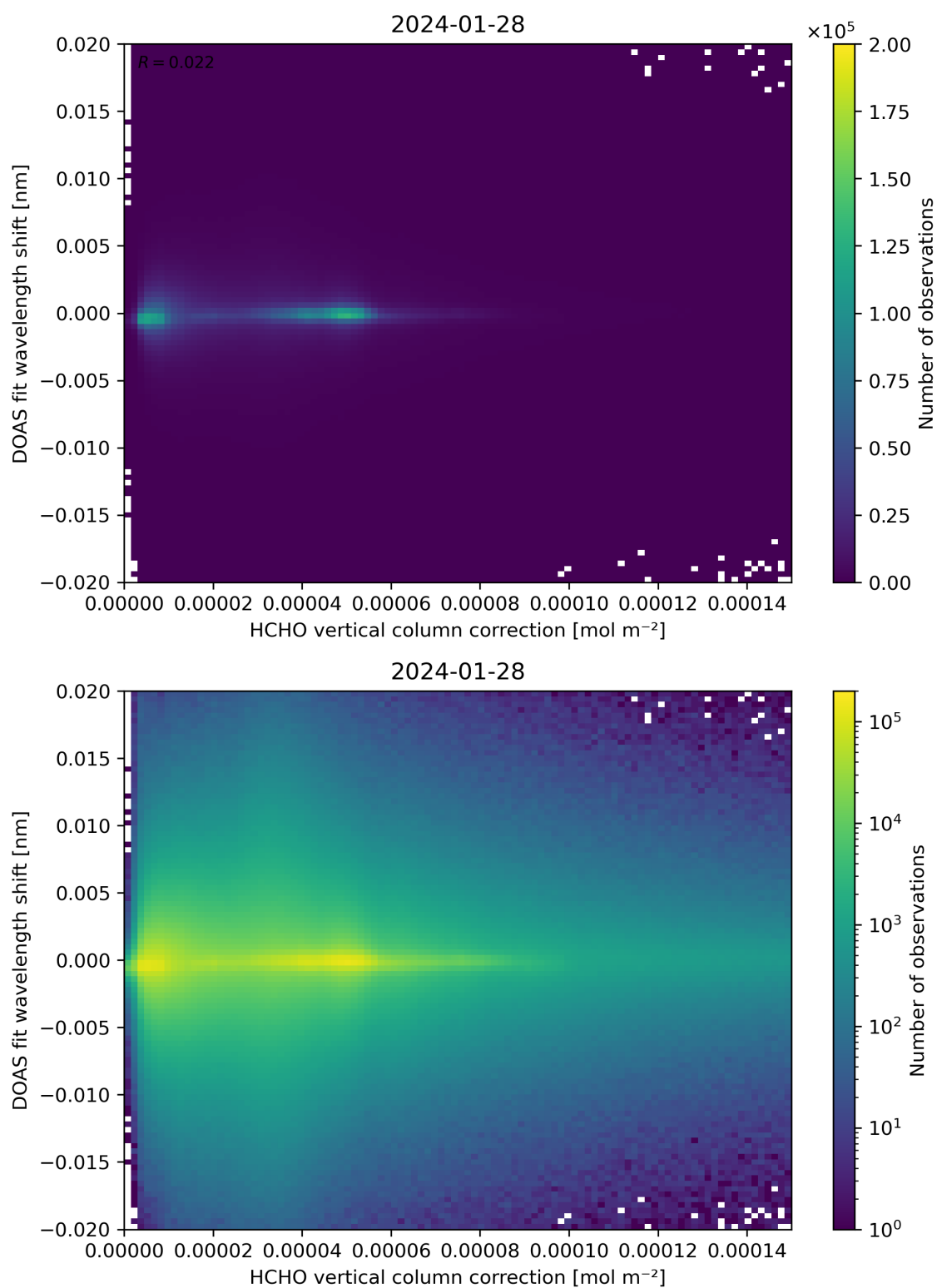
Figure 113: Scatter density plot of “HCHO vertical column correction” against “DOAS fit wavelength shift” for 2024-01-27 to 2024-01-29.
