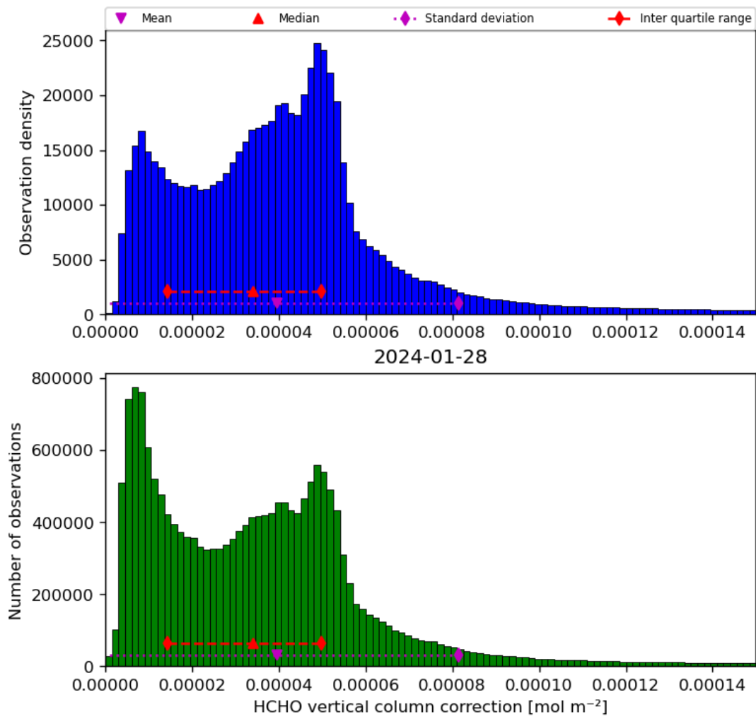
Figure 37: Histogram of “HCHO vertical column correction” for 2024-01-27 to 2024-01-29
