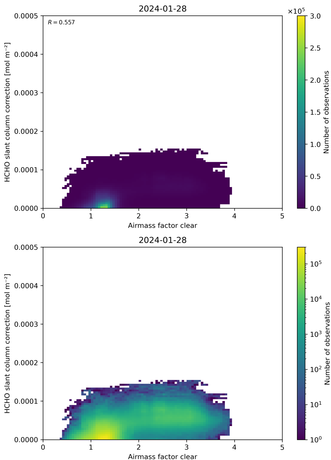
Figure 75: Scatter density plot of “Airmass factor clear” against “HCHO slant column correction” for 2024-01-27 to 2024-01-29.
