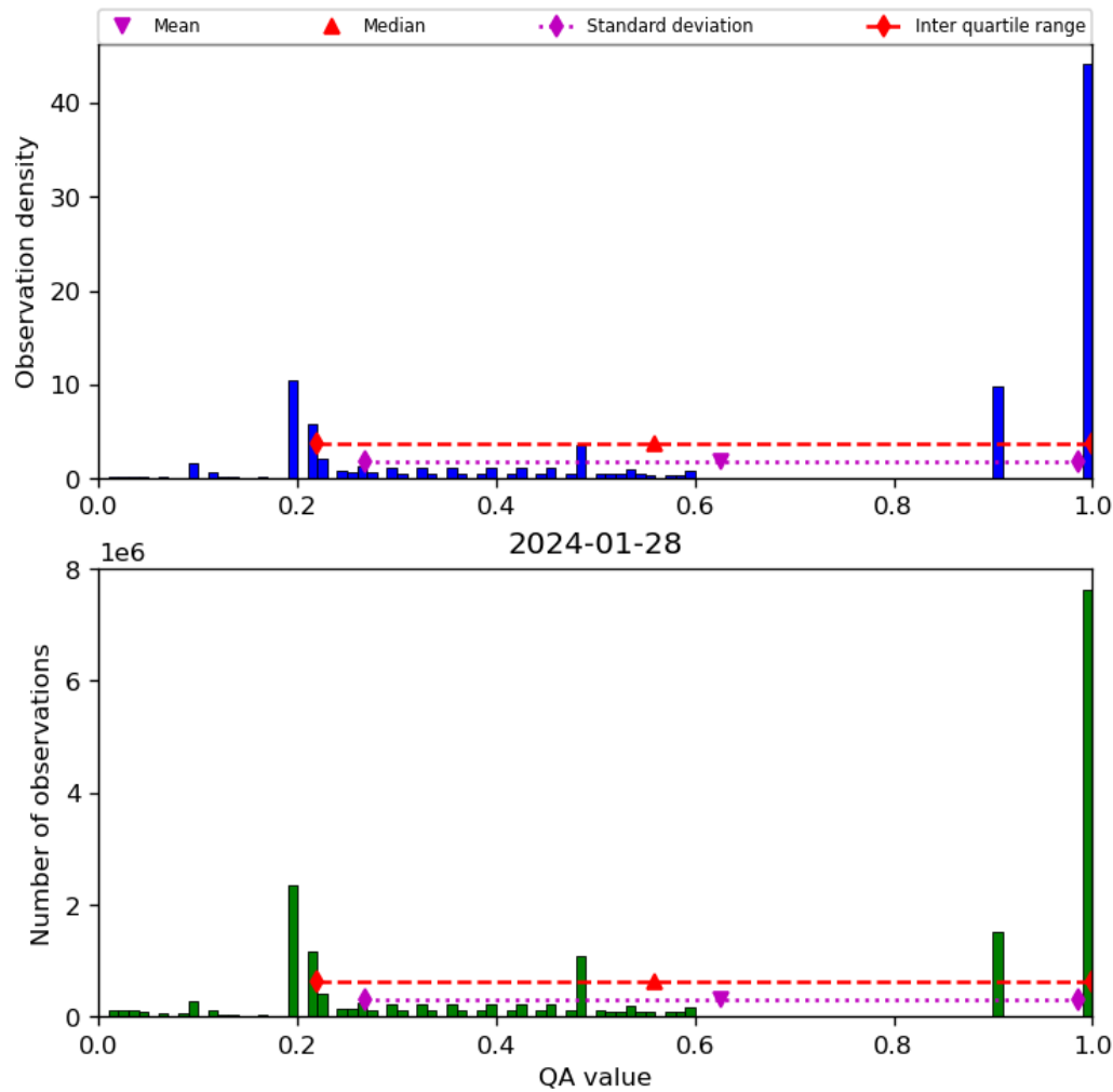
Figure 34: Histogram of “QA value” for 2024-01-27 to 2024-01-29
