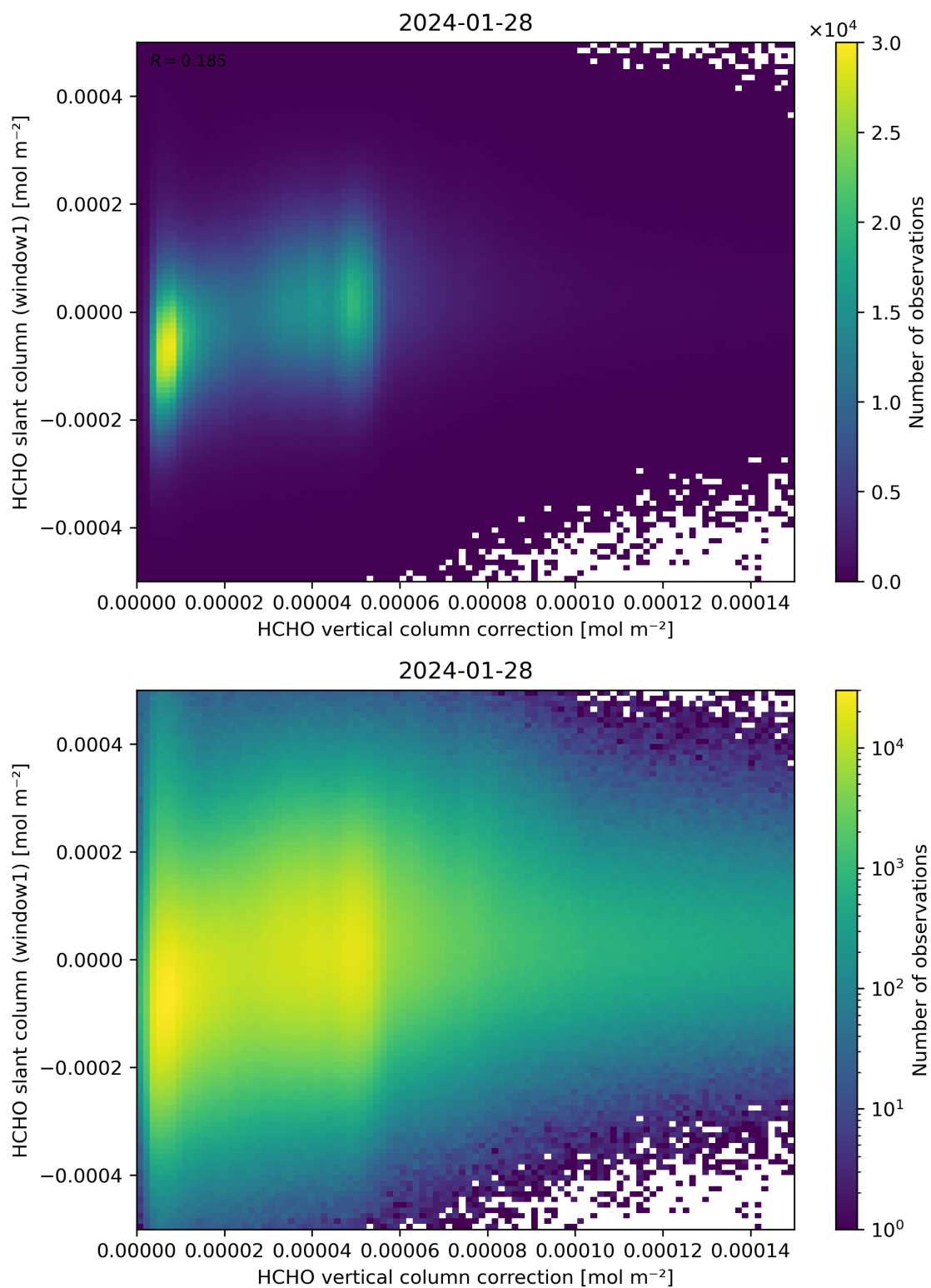
Figure 118: Scatter density plot of “HCHO vertical column correction” against “HCHO slant column (window1)” for 2024-01-27 to 2024-01-29.
