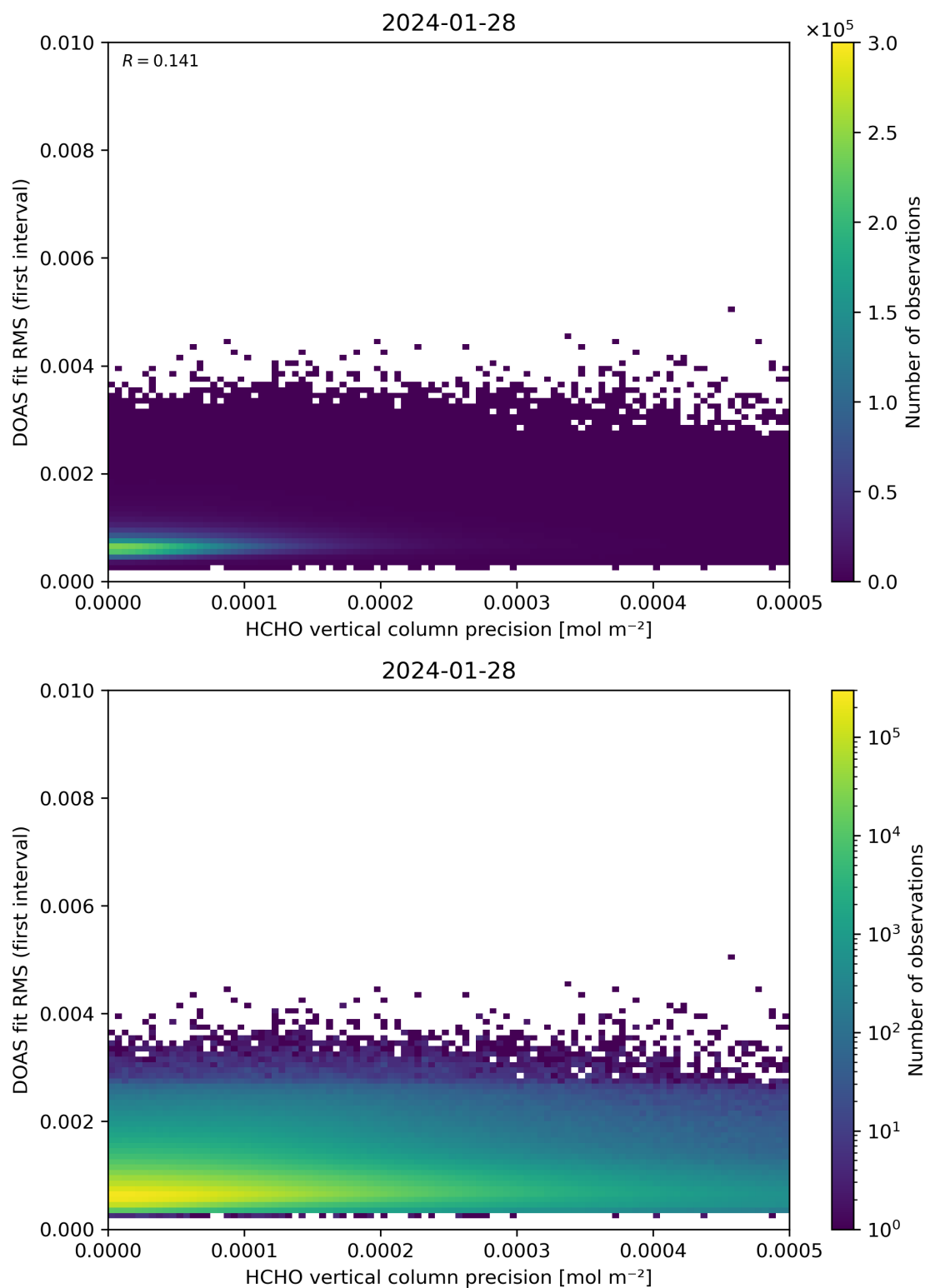
Figure 136: Scatter density plot of “HCHO vertical column precision” against “DOAS fit RMS (first interval)” for 2024-01-27 to 2024-01-29.
