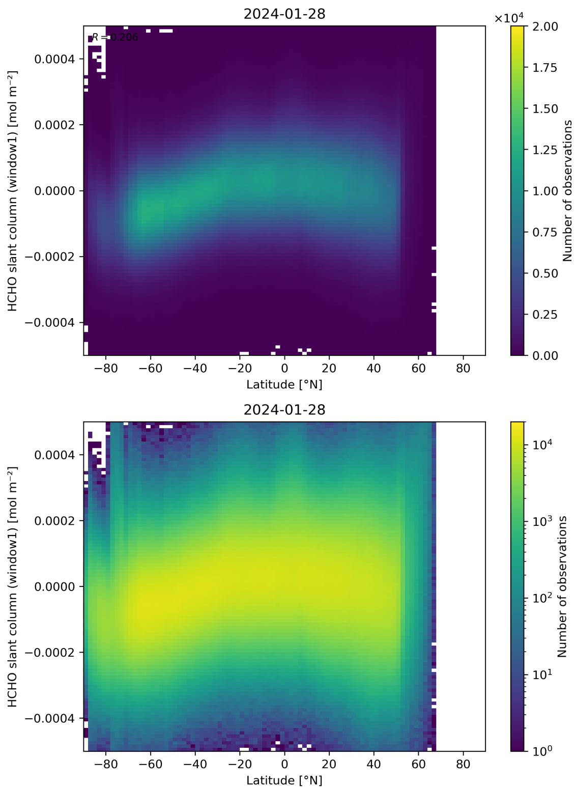
Figure 159: Scatter density plot of “Latitude” against “HCHO slant column (window1)” for 2024-01-27 to 2024-01-29.
