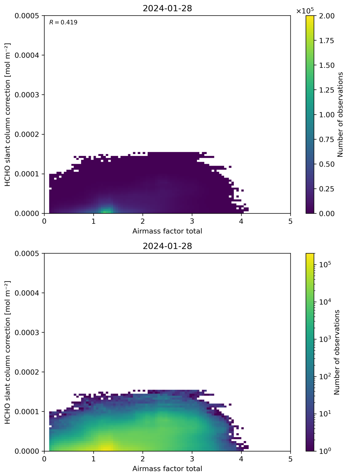
Figure 102: Scatter density plot of “Airmass factor total” against “HCHO slant column correction” for 2024-01-27 to 2024-01-29.
