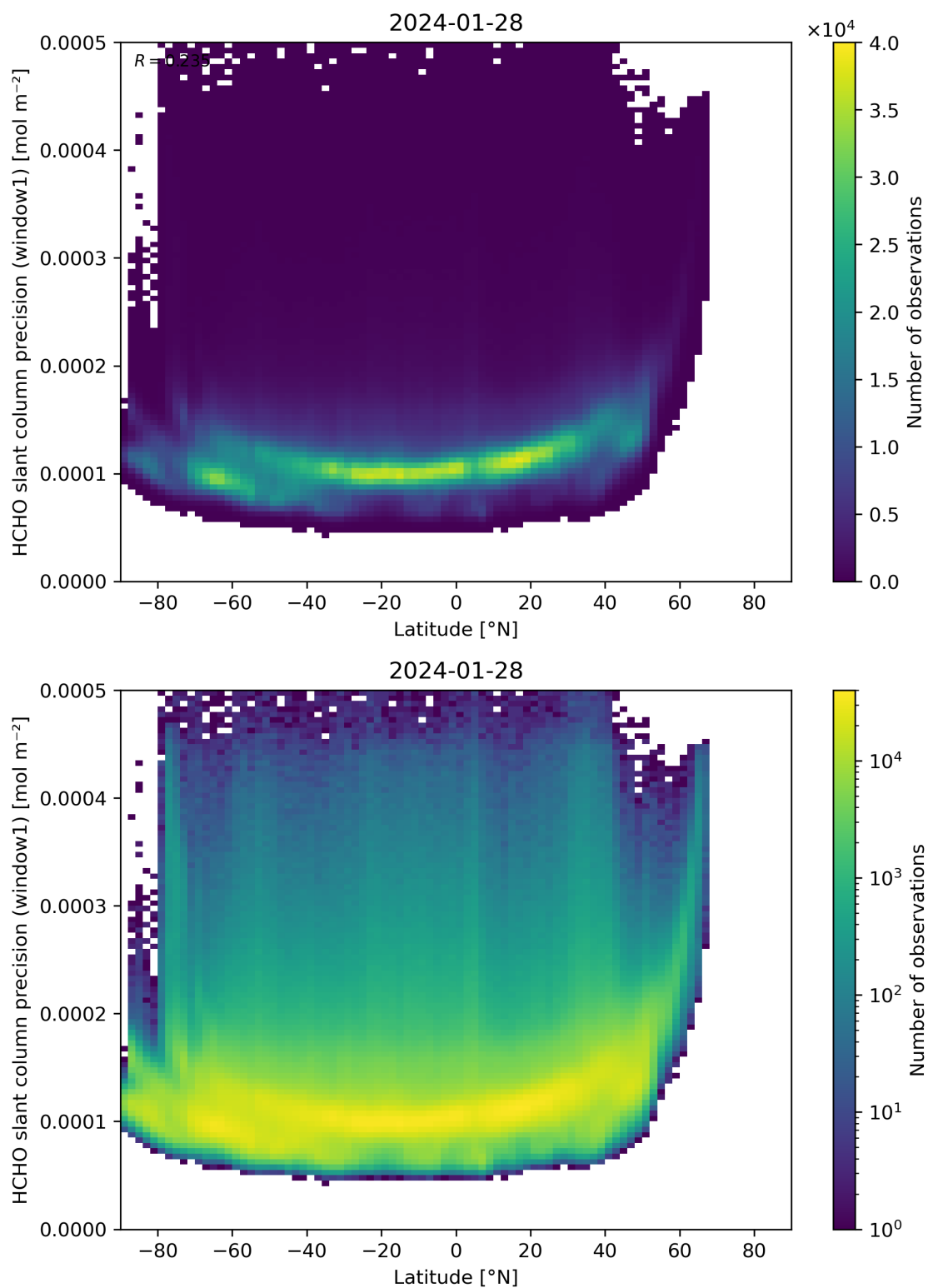
Figure 160: Scatter density plot of “Latitude” against “HCHO slant column precision (window1)” for 2024-01-27 to 2024-01-29.
