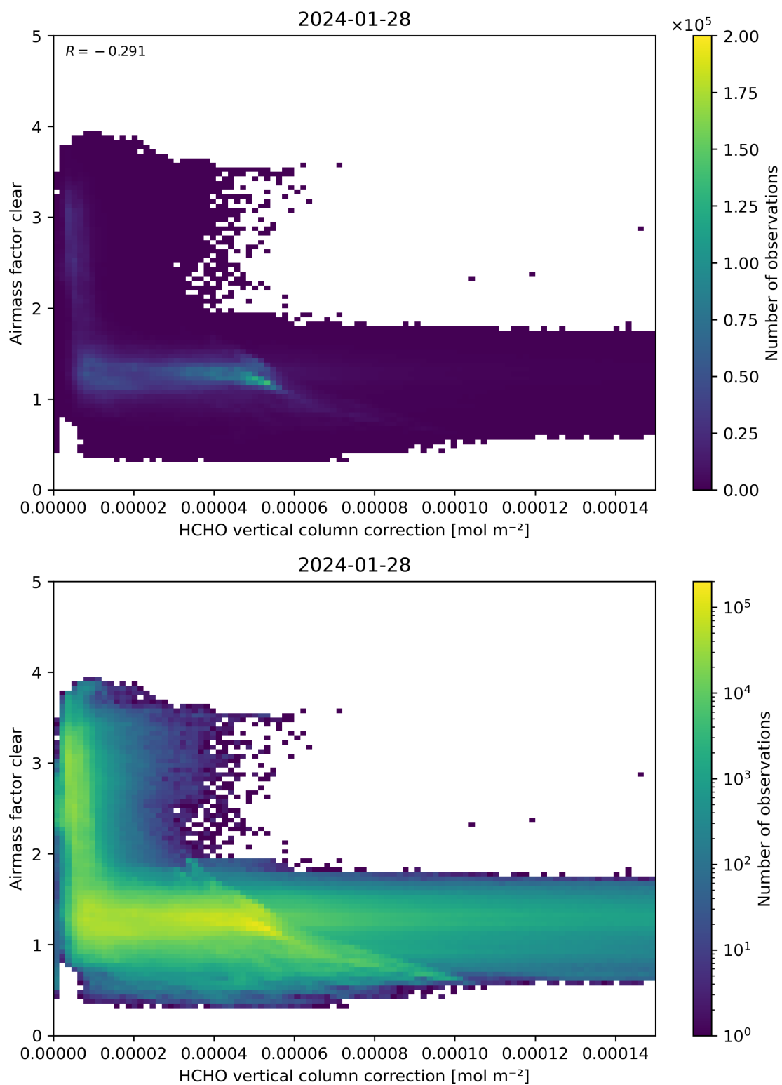
Figure 115: Scatter density plot of “HCHO vertical column correction” against “Airmass factor clear” for 2024-01-27 to 2024-01-29.
