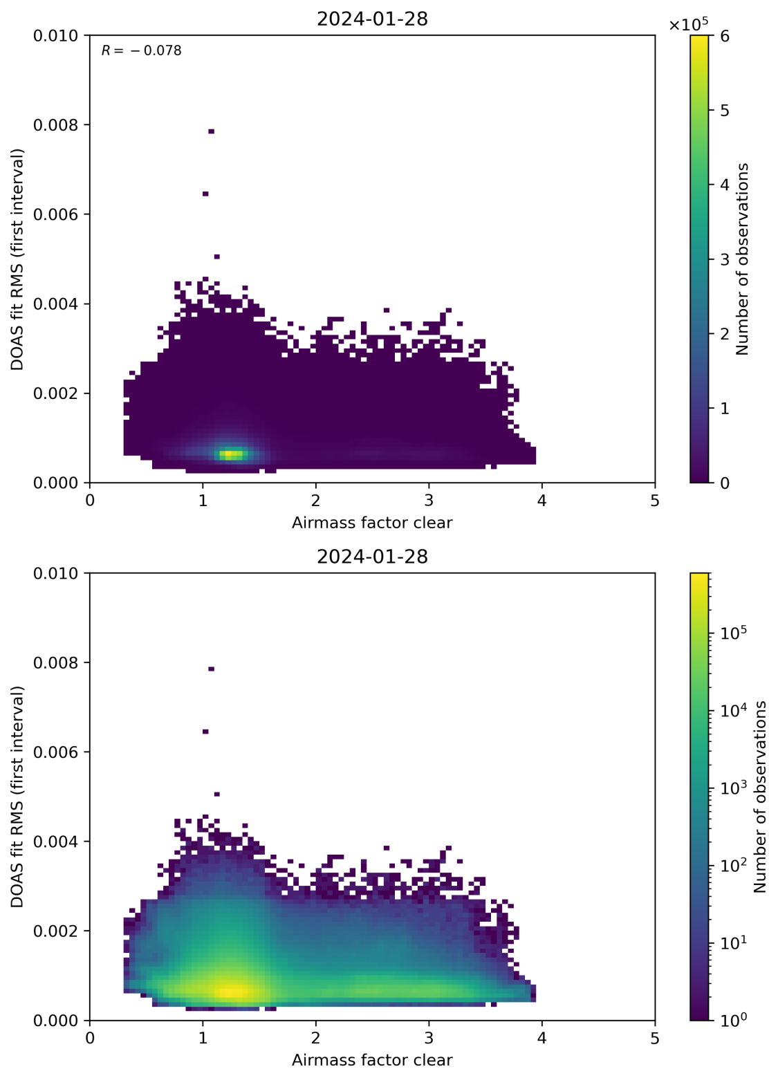
Figure 71: Scatter density plot of “Airmass factor clear” against “DOAS fit RMS (first interval)” for 2024-01-27 to 2024-01-29.
