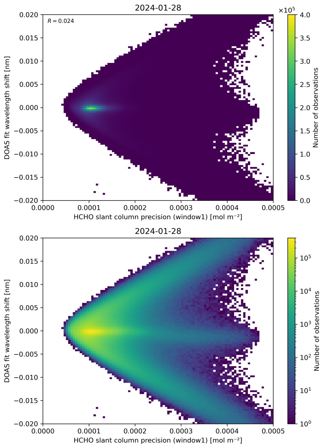
Figure 89: Scatter density plot of “HCHO slant column precision (window1)” against “DOAS fit wavelength shift” for 2024-01-27 to 2024-01-29.
