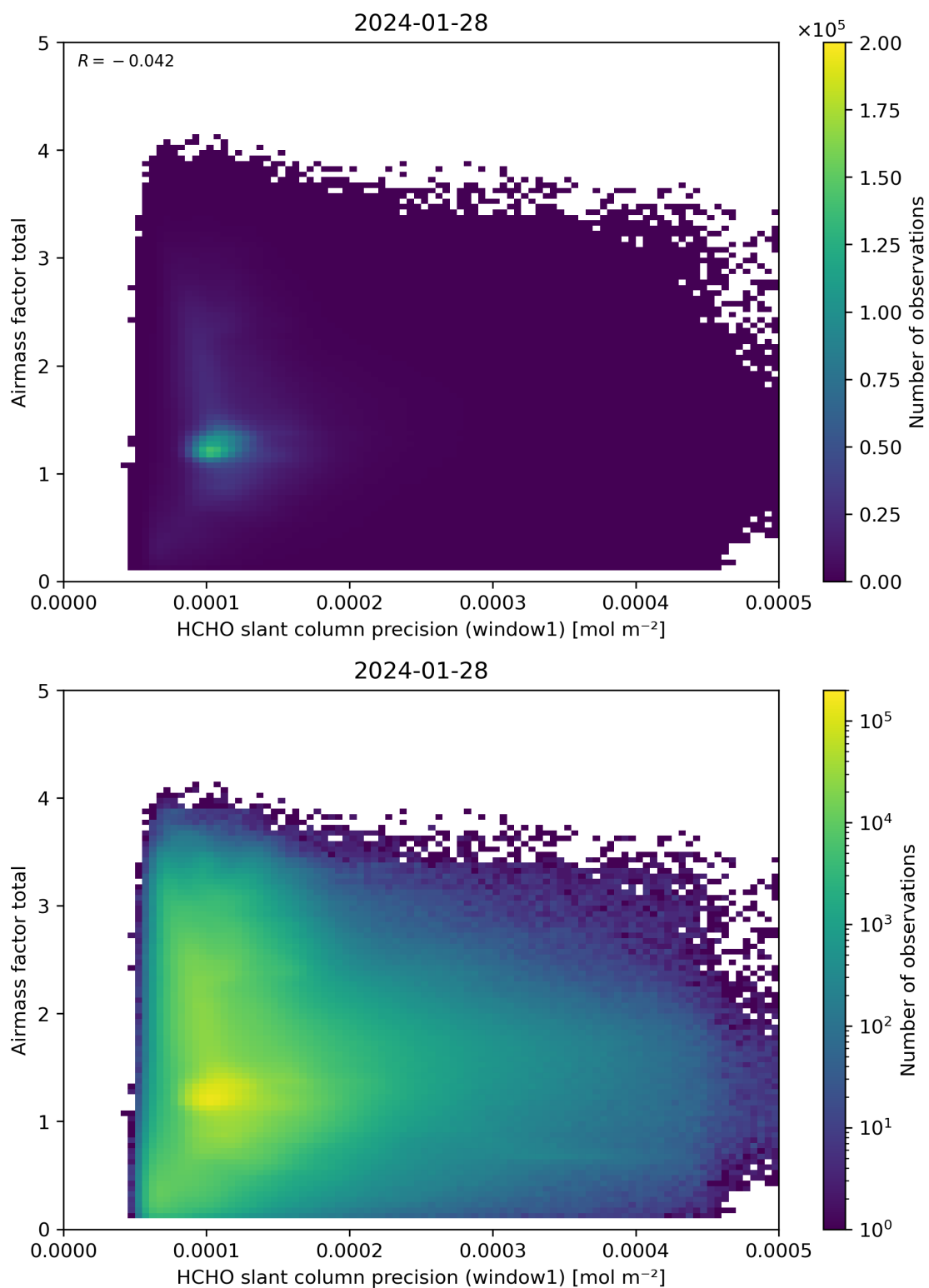
Figure 94: Scatter density plot of “HCHO slant column precision (window1)” against “Airmass factor total” for 2024-01-27 to 2024-01-29.
