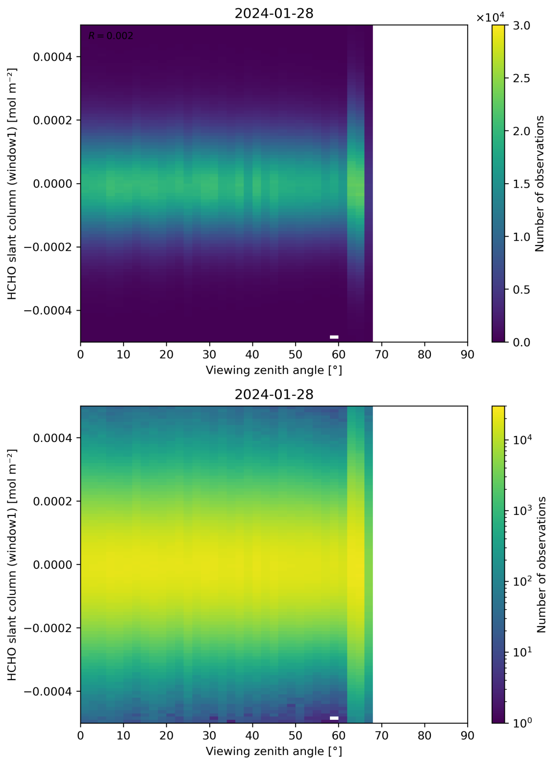
Figure 188: Scatter density plot of “Viewing zenith angle” against “HCHO slant column (window1)” for 2024-01-27 to 2024-01-29.
