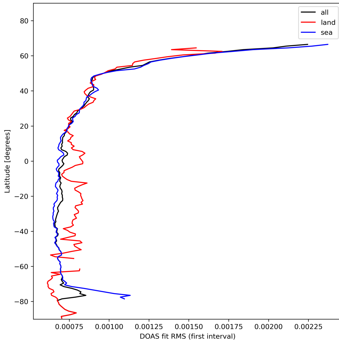
Figure 32: Zonal average of “DOAS fit RMS (first interval)” for 2024-01-27 to 2024-01-29.
