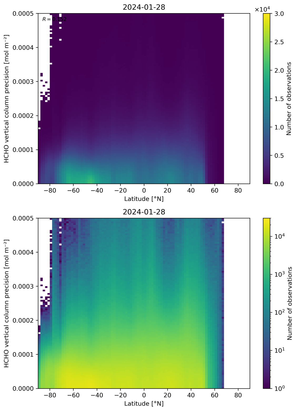
Figure 165: Scatter density plot of “Latitude” against “HCHO vertical column precision” for 2024-01-27 to 2024-01-29.
