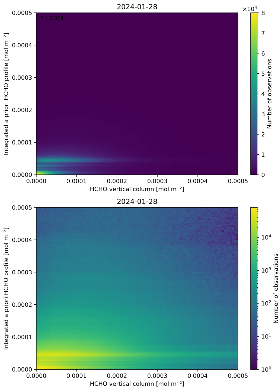
Figure 135: Scatter density plot of “HCHO vertical column” against “Integrated a priori HCHO profile” for 2024-01-27 to 2024-01-29.
