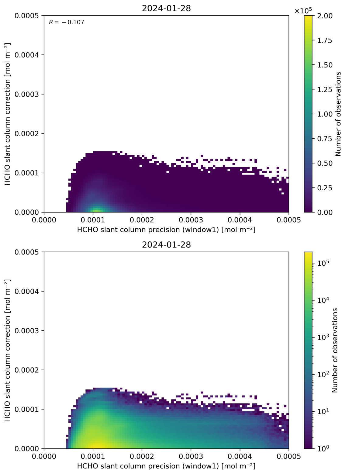
Figure 93: Scatter density plot of “HCHO slant column precision (window1)” against “HCHO slant column correction” for 2024-01-27 to 2024-01-29.
