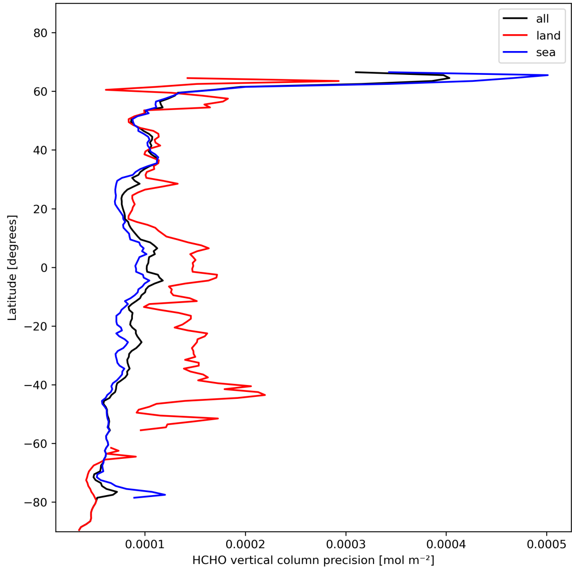
Figure 22: Zonal average of “HCHO vertical column precision” for 2024-01-27 to 2024-01-29.
