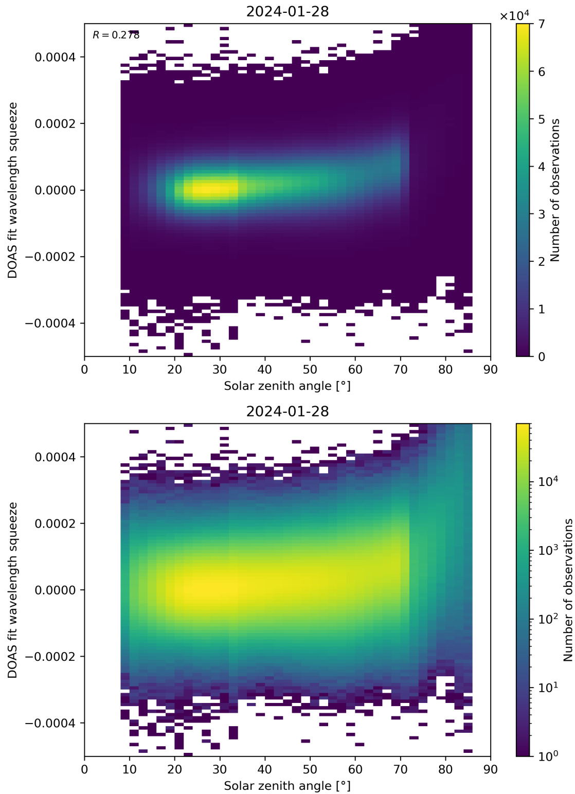
Figure 169: Scatter density plot of “Solar zenith angle” against “DOAS fit wavelength squeeze” for 2024-01-27 to 2024-01-29.
