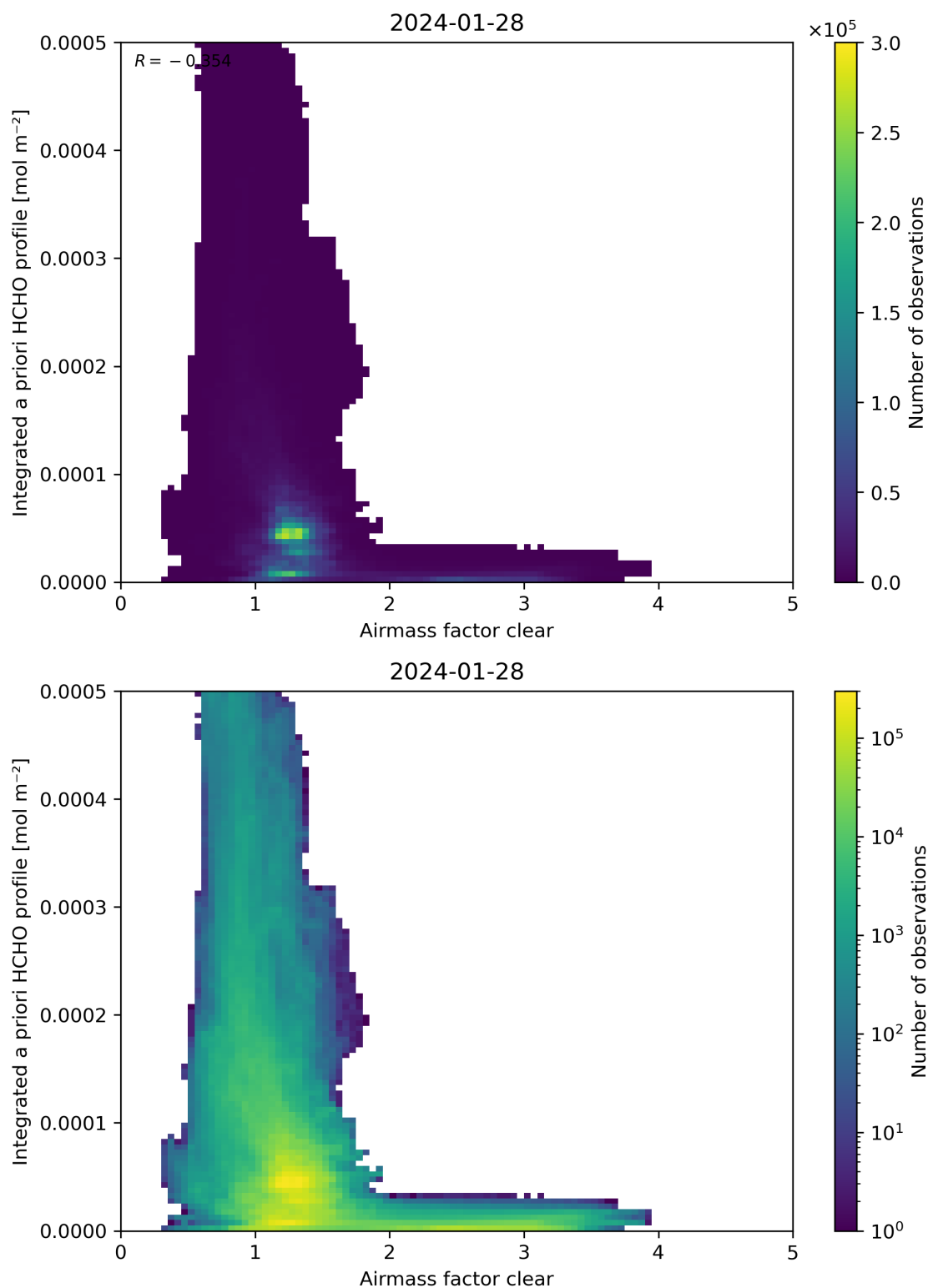
Figure 76: Scatter density plot of “Airmass factor clear” against “Integrated a priori HCHO profile” for 2024-01-27 to 2024-01-29.
