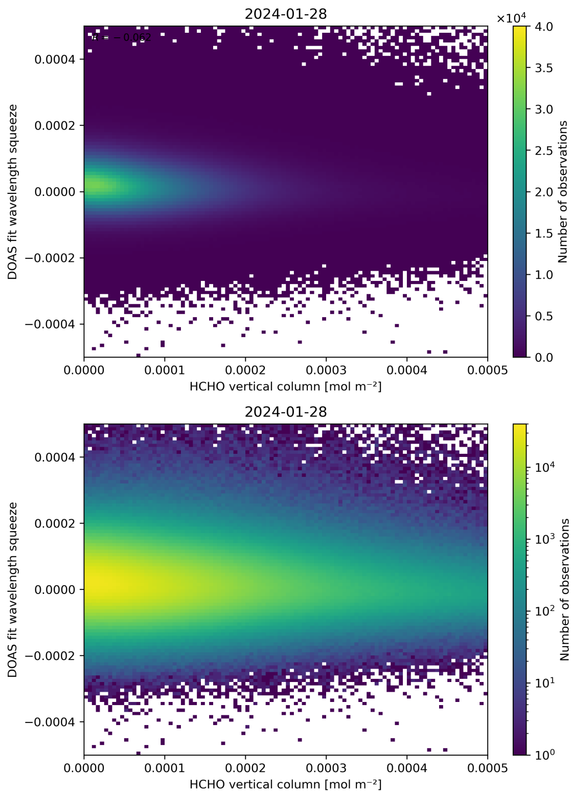
Figure 125: Scatter density plot of “HCHO vertical column” against “DOAS fit wavelength squeeze” for 2024-01-27 to 2024-01-29.
