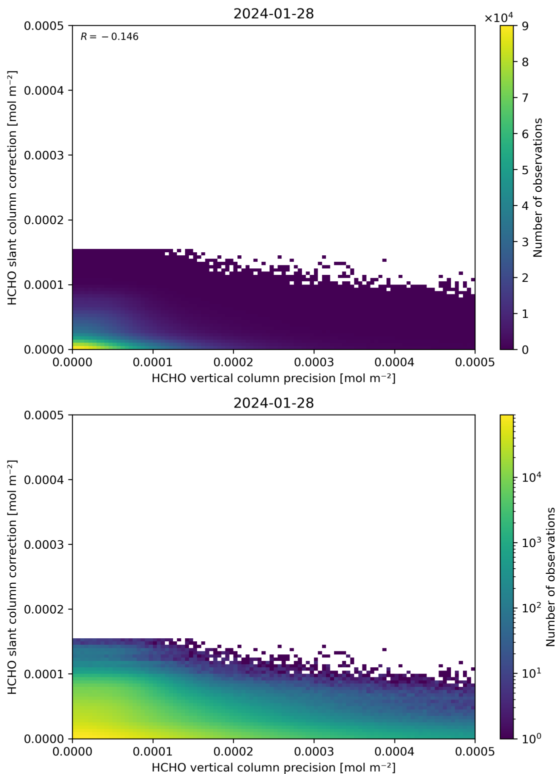
Figure 141: Scatter density plot of “HCHO vertical column precision” against “HCHO slant column correction” for 2024-01-27 to 2024-01-29.
