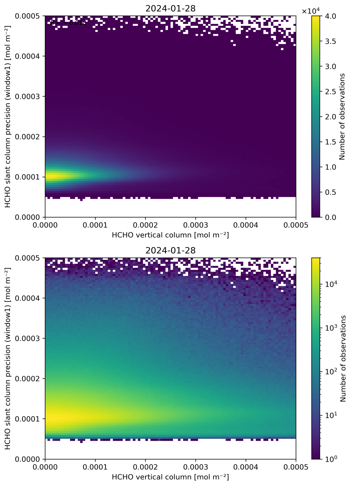
Figure 130: Scatter density plot of “HCHO vertical column” against “HCHO slant column precision (window1)” for 2024-01-27 to 2024-01-29.
