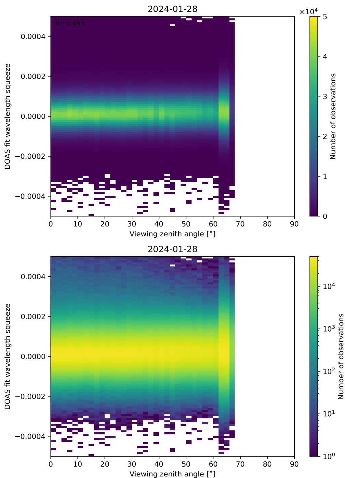
Figure 184: Scatter density plot of “Viewing zenith angle” against “DOAS fit wavelength squeeze” for 2024-01-27 to 2024-01-29.
