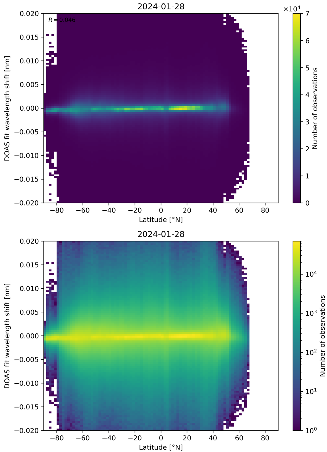
Figure 154: Scatter density plot of “Latitude” against “DOAS fit wavelength shift” for 2024-01-27 to 2024-01-29.
