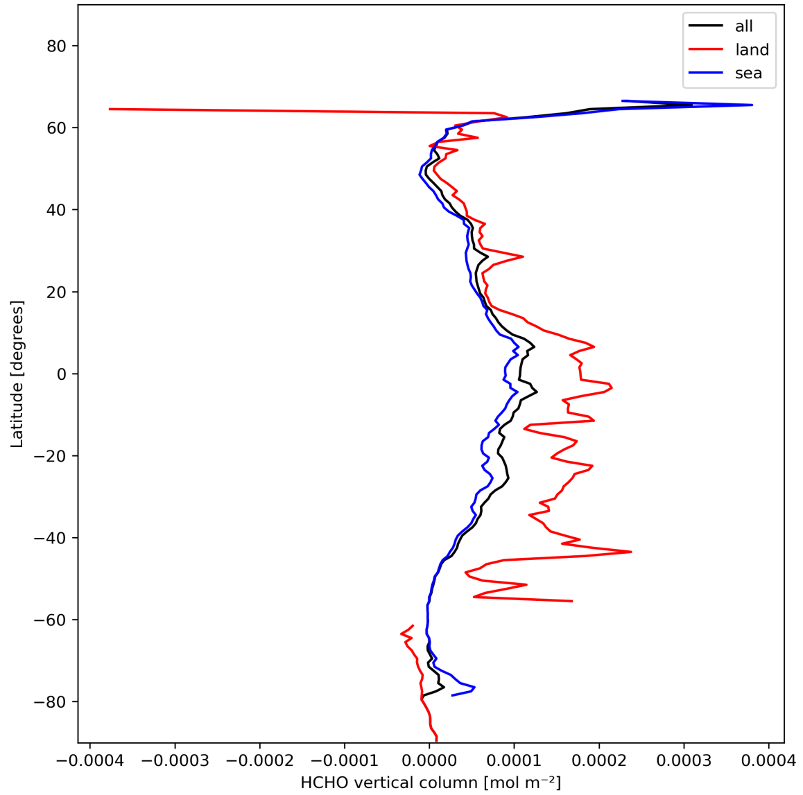
Figure 21: Zonal average of “HCHO vertical column” for 2024-01-27 to 2024-01-29.
