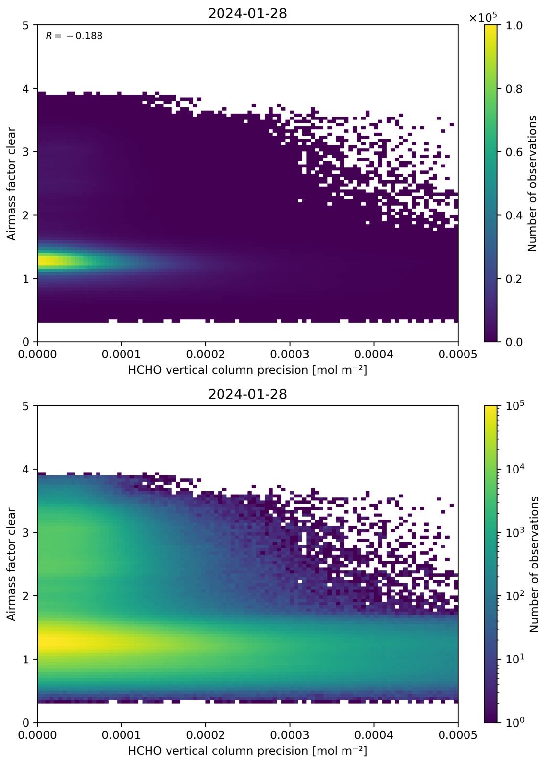
Figure 139: Scatter density plot of “HCHO vertical column precision” against “Airmass factor clear” for 2024-01-27 to 2024-01-29.
