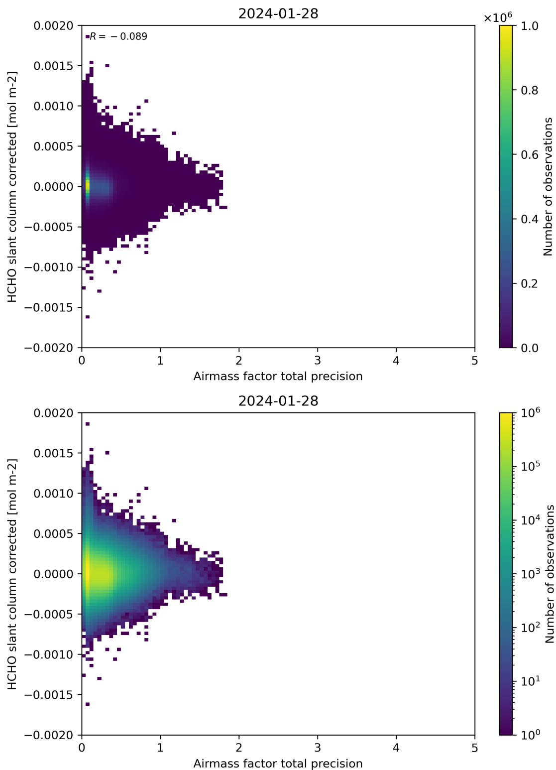
Figure 109: Scatter density plot of “Airmass factor total precision” against “HCHO slant column corrected” for 2024-01-27 to 2024-01-29.
