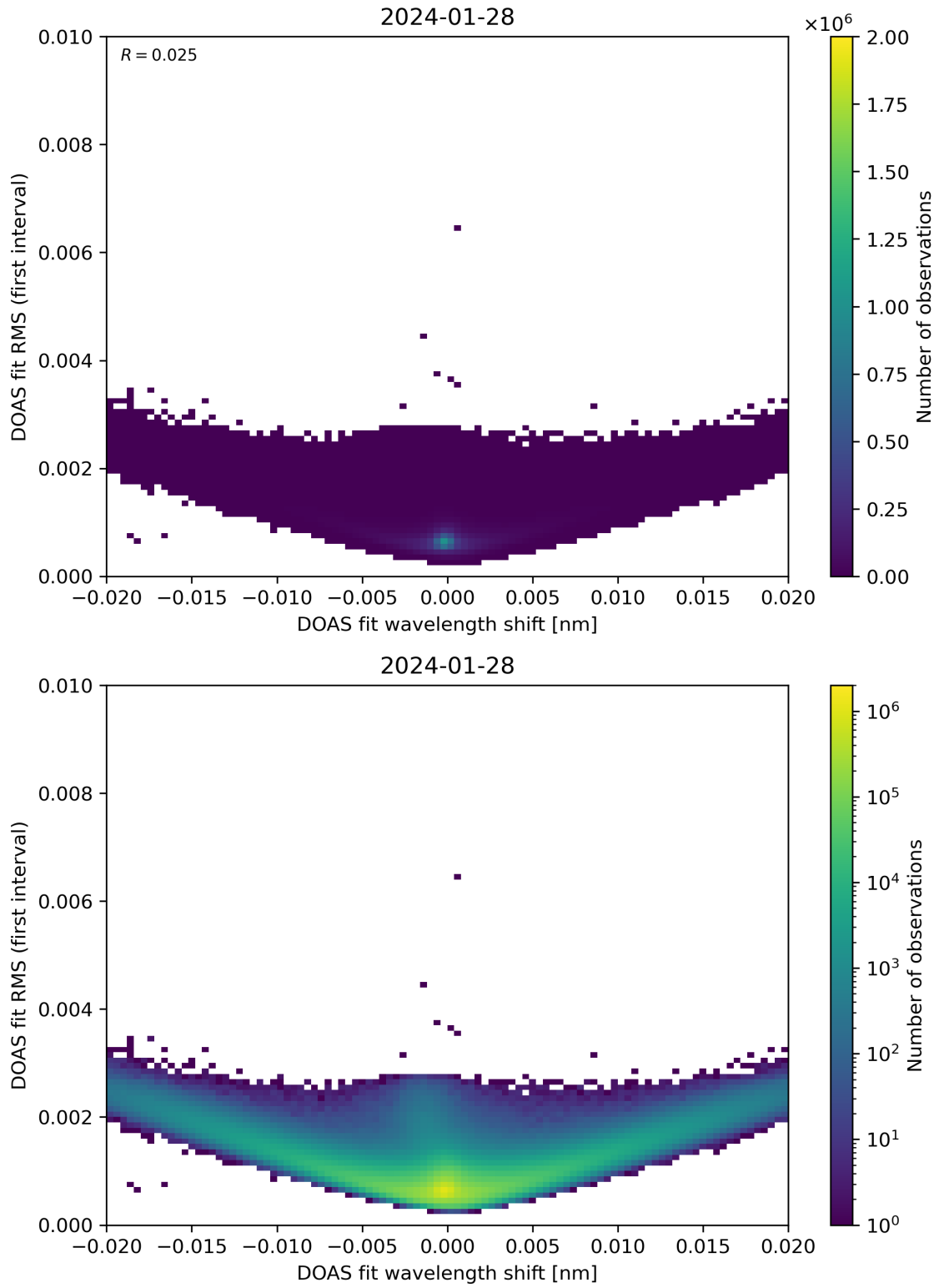
Figure 64: Scatter density plot of “DOAS fit wavelength shift” against “DOAS fit RMS (first interval)” for 2024-01-27 to 2024-01-29.
