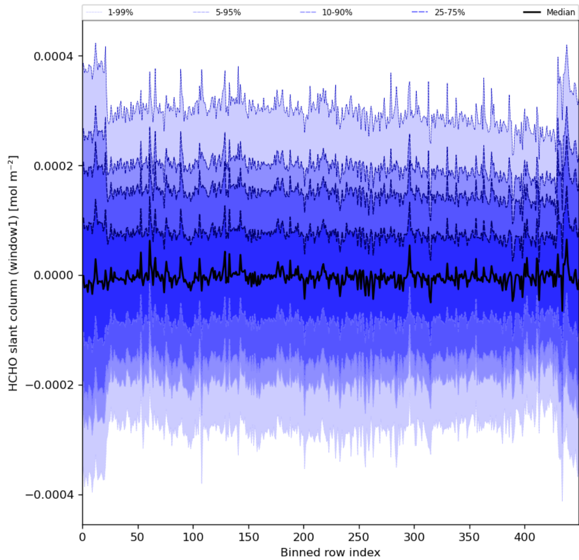
Figure 52: Along track statistics of “HCHO slant column (window1)” for 2024-01-27 to 2024-01-29
