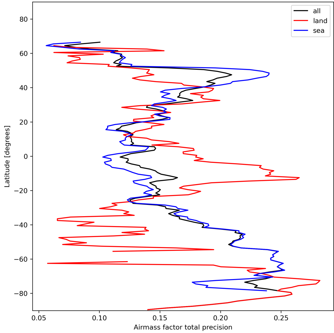
Figure 27: Zonal average of “Airmass factor total precision” for 2024-01-27 to 2024-01-29.
