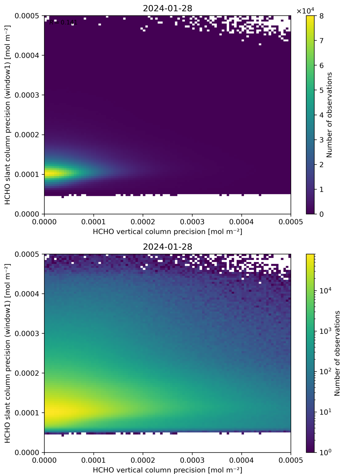
Figure 143: Scatter density plot of “HCHO vertical column precision” against “HCHO slant column precision (window1)” for 2024-01-27 to 2024-01-29.
