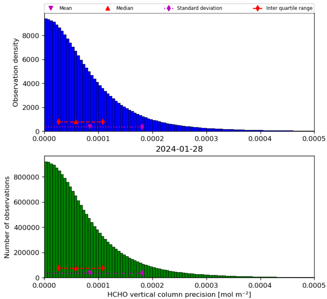
Figure 36: Histogram of “HCHO vertical column precision” for 2024-01-27 to 2024-01-29
