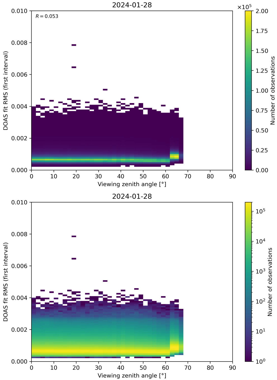
Figure 182: Scatter density plot of “Viewing zenith angle” against “DOAS fit RMS (first interval)” for 2024-01-27 to 2024-01-29.
