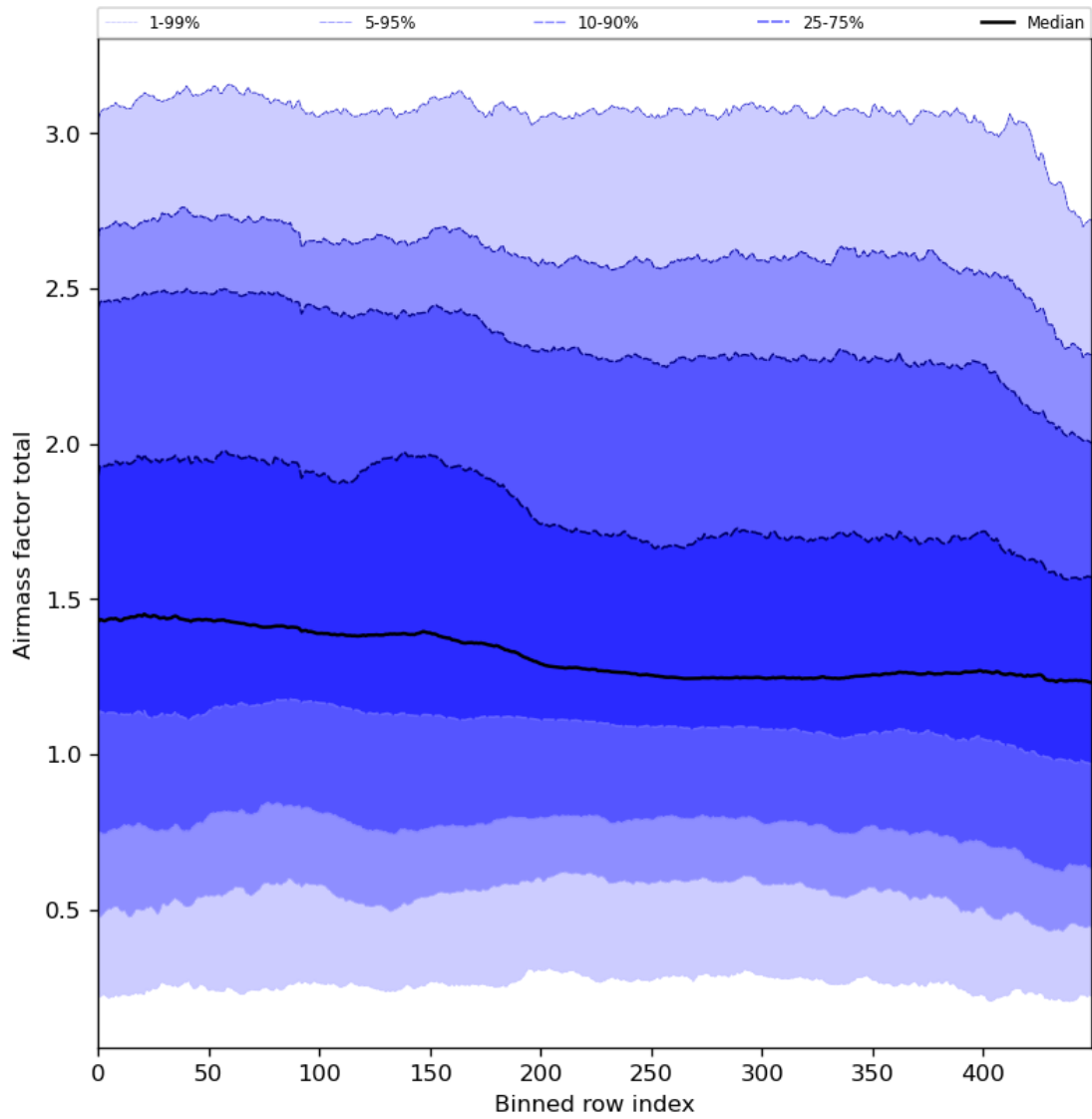
Figure 54: Along track statistics of “Airmass factor total” for 2024-01-27 to 2024-01-29
