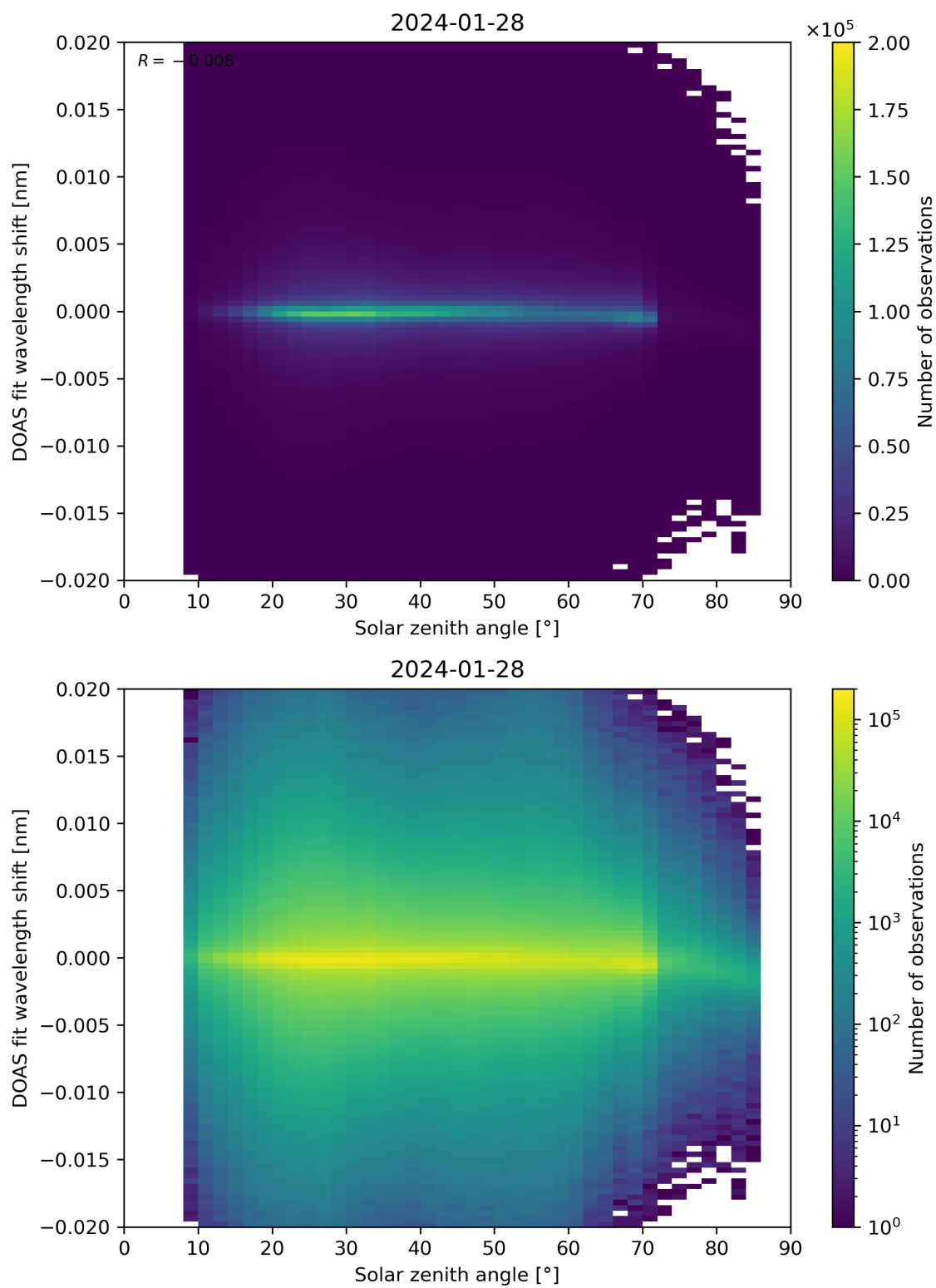
Figure 168: Scatter density plot of “Solar zenith angle” against “DOAS fit wavelength shift” for 2024-01-27 to 2024-01-29.
