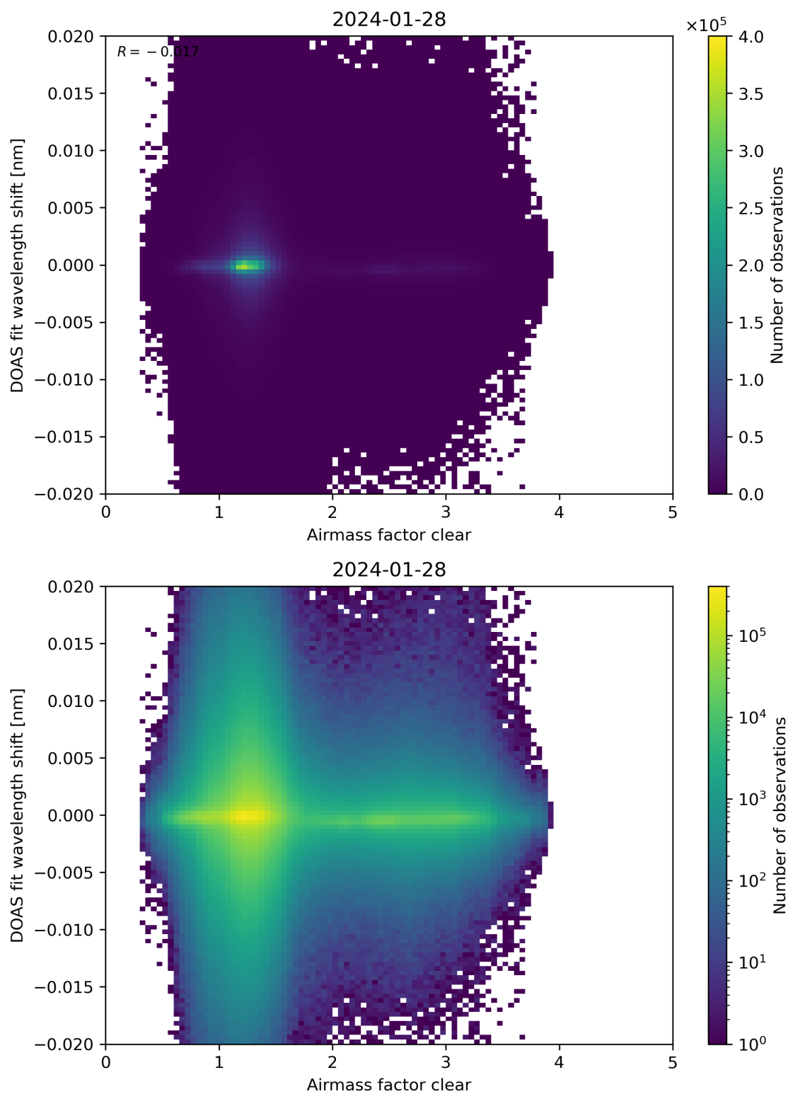
Figure 72: Scatter density plot of “Airmass factor clear” against “DOAS fit wavelength shift” for 2024-01-27 to 2024-01-29.
