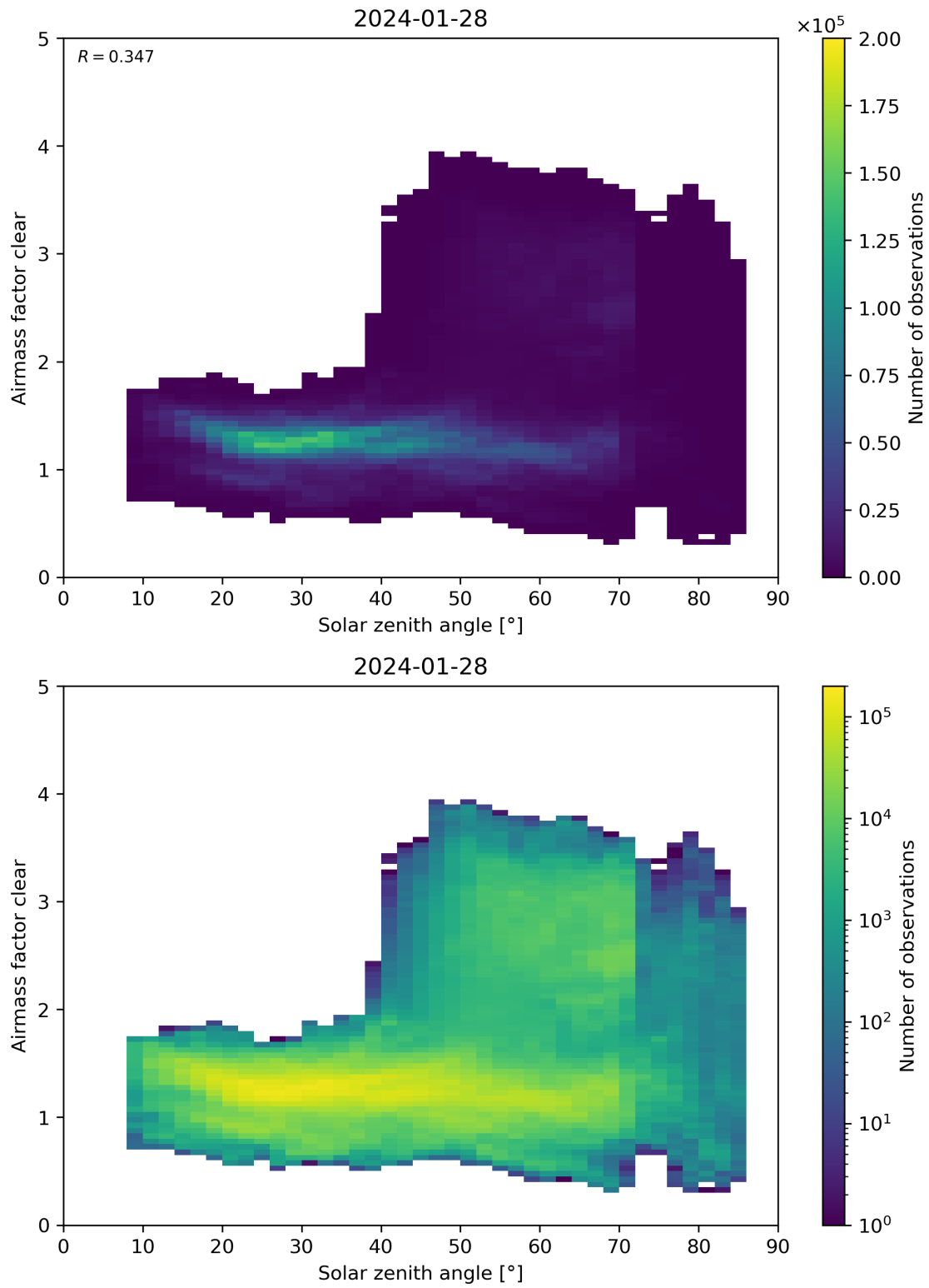
Figure 170: Scatter density plot of “Solar zenith angle” against “Airmass factor clear” for 2024-01-27 to 2024-01-29.
