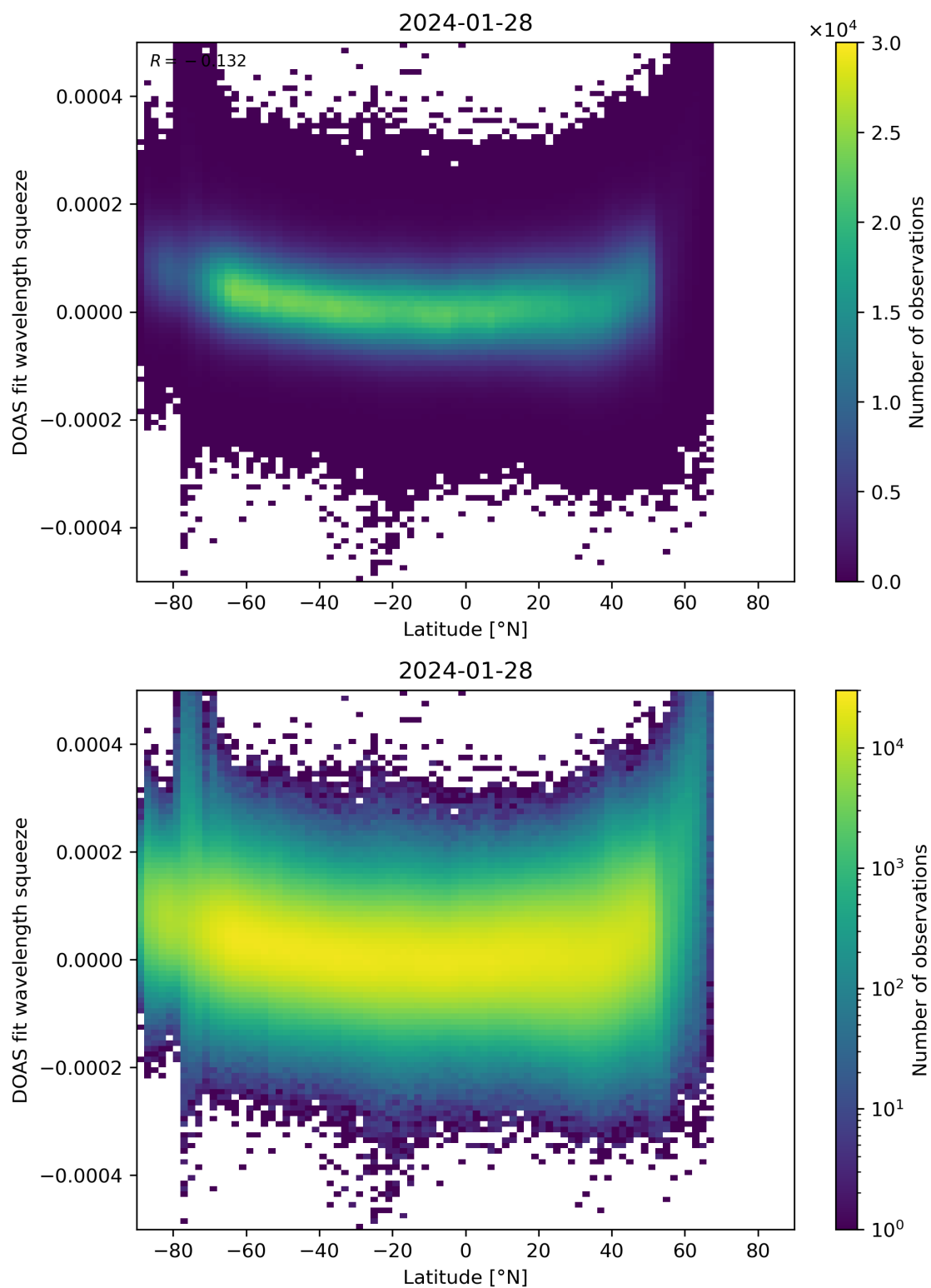
Figure 155: Scatter density plot of “Latitude” against “DOAS fit wavelength squeeze” for 2024-01-27 to 2024-01-29.
