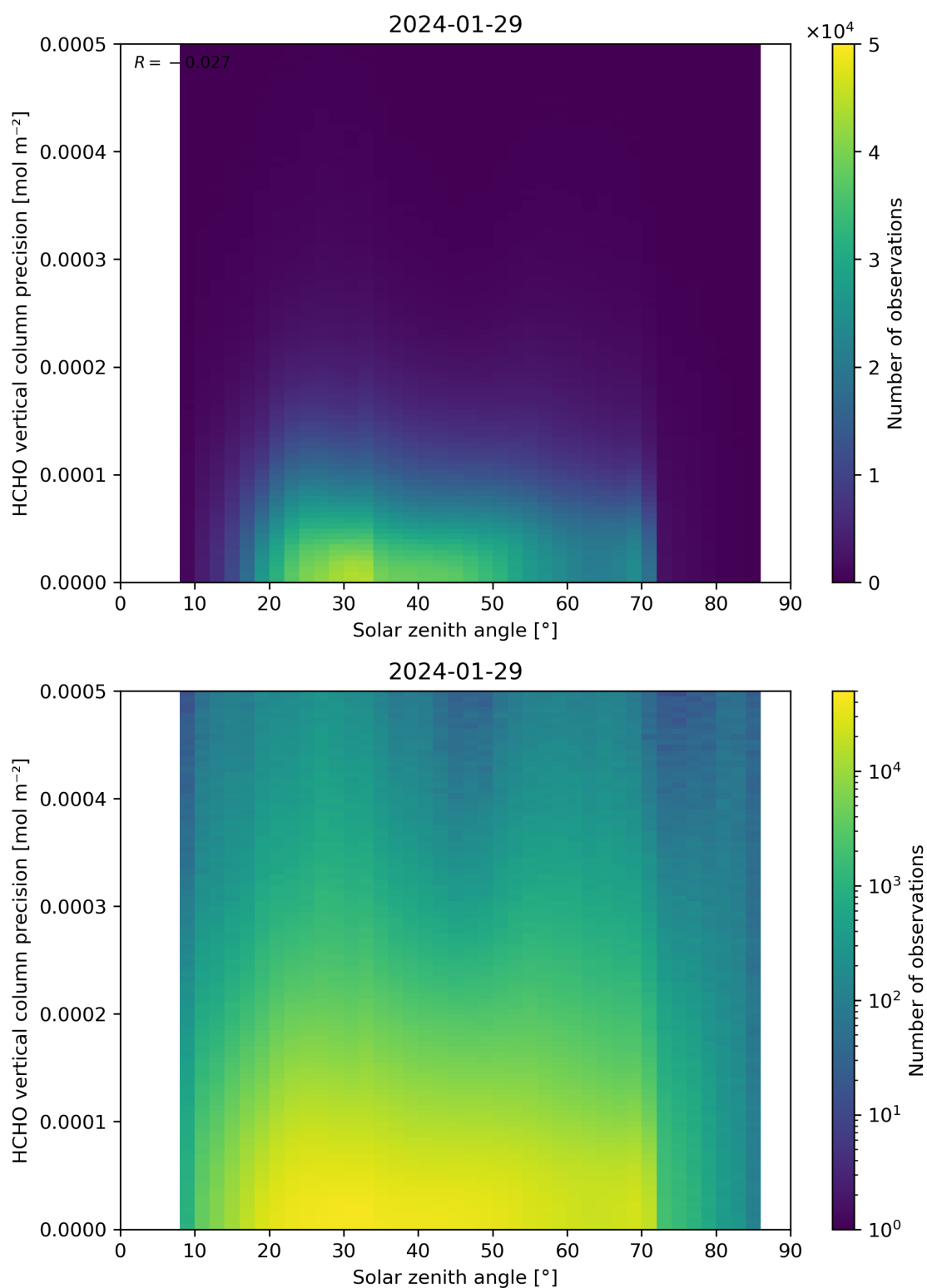
Figure 179: Scatter density plot of “Solar zenith angle” against “HCHO vertical column precision” for 2024-01-28 to 2024-01-30.
