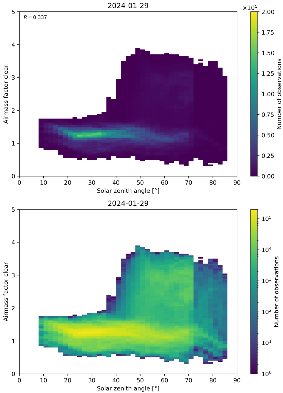
Figure 170: Scatter density plot of “Solar zenith angle” against “Airmass factor clear” for 2024-01-28 to 2024-01-30.
