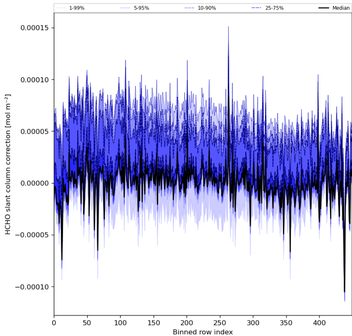
Figure 61: Along track statistics of “HCHO slant column correction” for 2024-01-28 to 2024-01-30
