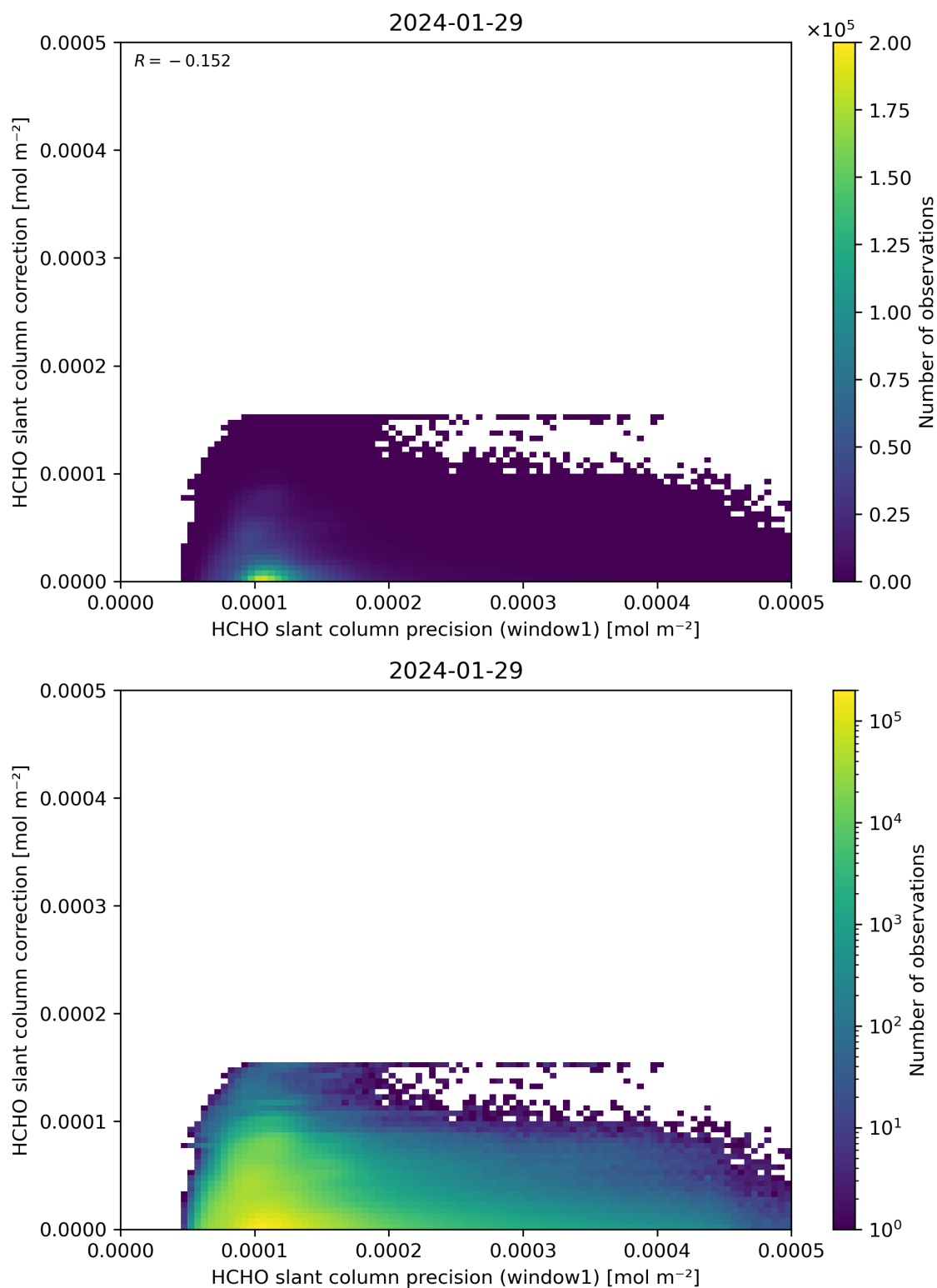
Figure 93: Scatter density plot of “HCHO slant column precision (window1)” against “HCHO slant column correction” for 2024-01-28 to 2024-01-30.
