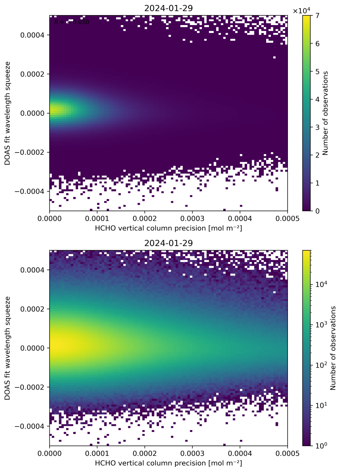
Figure 138: Scatter density plot of “HCHO vertical column precision” against “DOAS fit wavelength squeeze” for 2024-01-28 to 2024-01-30.
