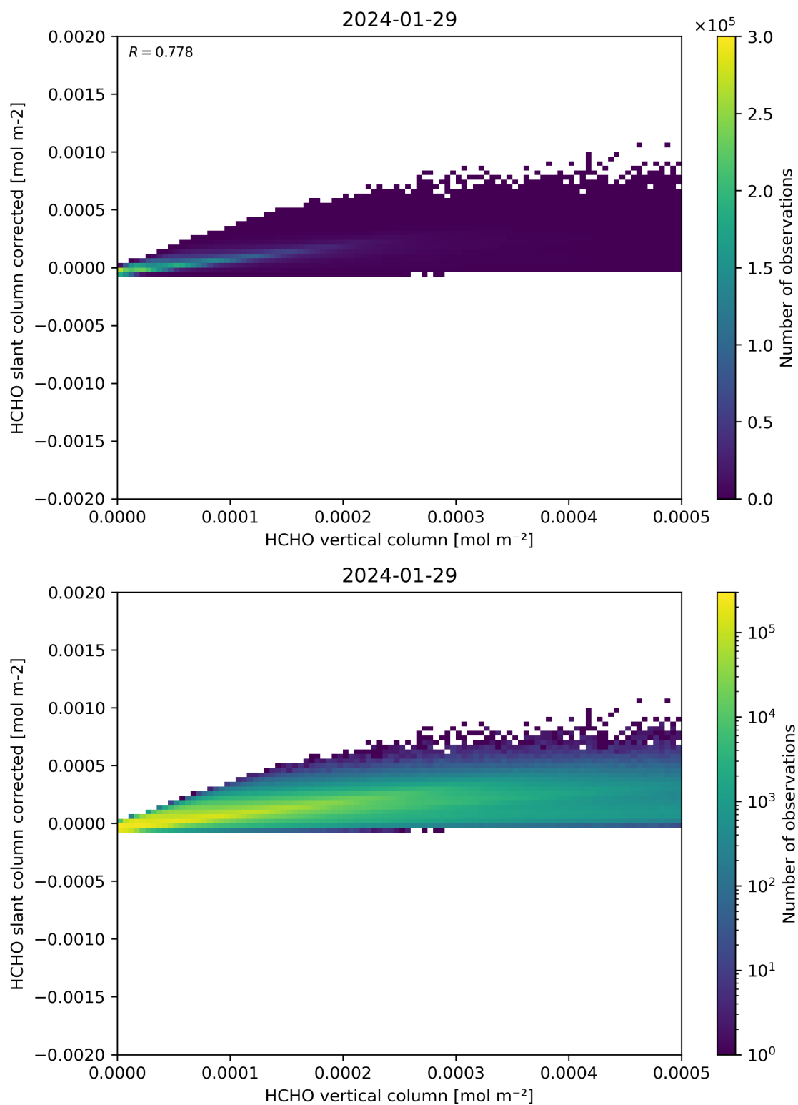
Figure 127: Scatter density plot of “HCHO vertical column” against “HCHO slant column corrected” for 2024-01-28 to 2024-01-30.
