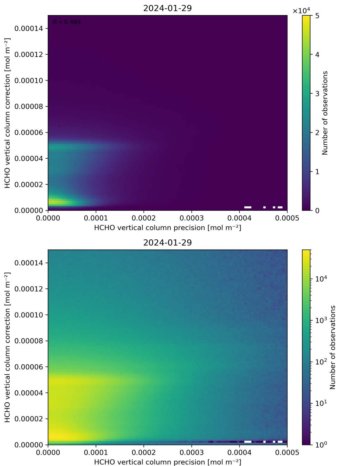
Figure 146: Scatter density plot of “HCHO vertical column precision” against “HCHO vertical column correction” for 2024-01-28 to 2024-01-30.
