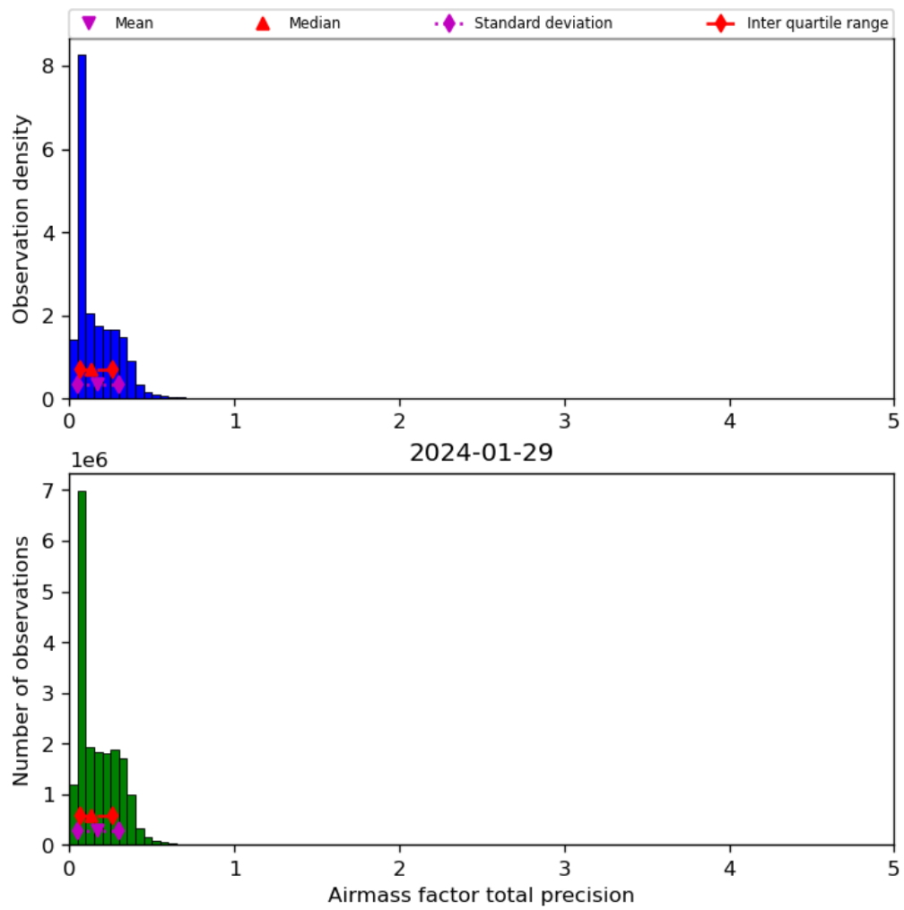
Figure 41: Histogram of “Airmass factor total precision” for 2024-01-28 to 2024-01-30
