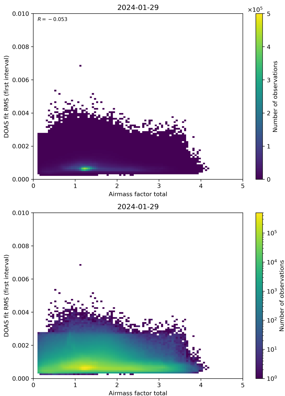
Figure 97: Scatter density plot of “Airmass factor total” against “DOAS fit RMS (first interval)” for 2024-01-28 to 2024-01-30.
