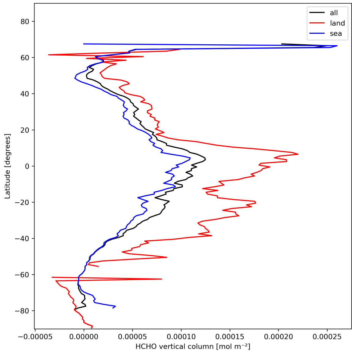
Figure 21: Zonal average of “HCHO vertical column” for 2024-01-28 to 2024-01-30.
