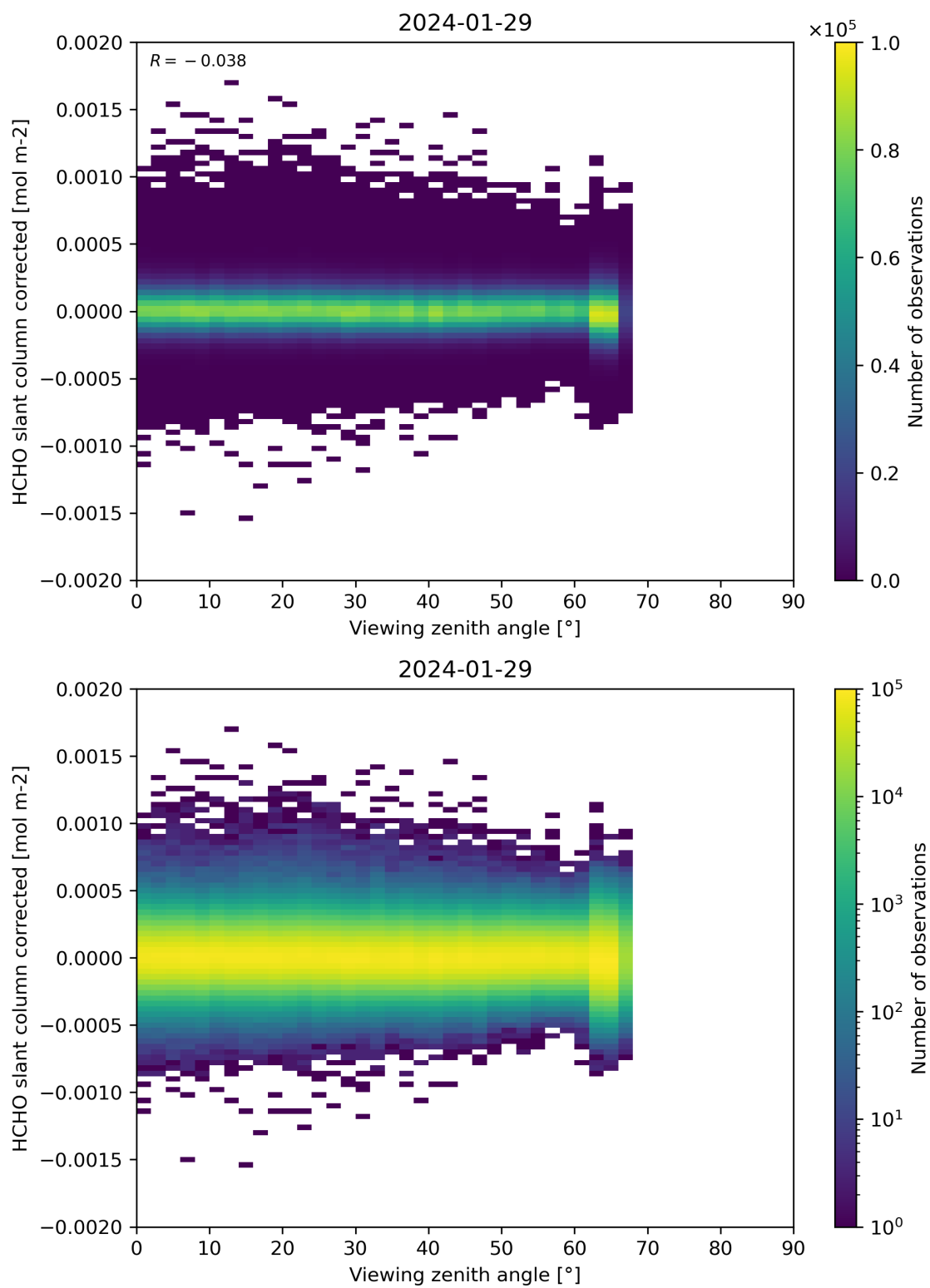
Figure 186: Scatter density plot of “Viewing zenith angle” against “HCHO slant column corrected” for 2024-01-28 to 2024-01-30.
