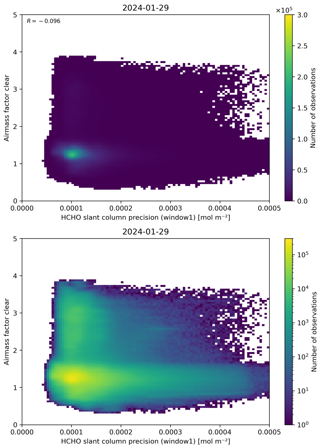
Figure 91: Scatter density plot of “HCHO slant column precision (window1)” against “Airmass factor clear” for 2024-01-28 to 2024-01-30.
