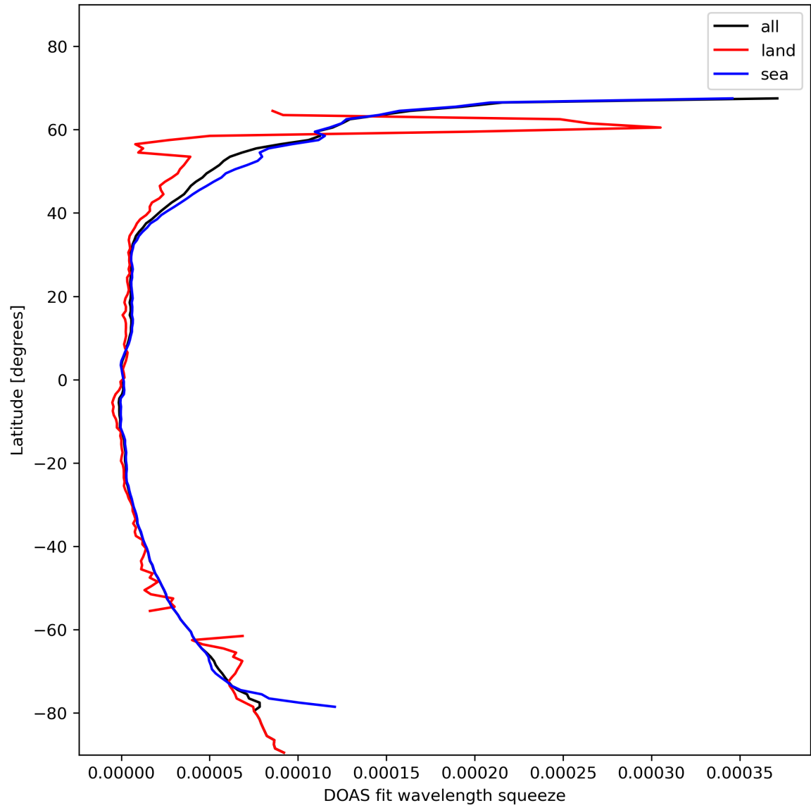
Figure 31: Zonal average of “DOAS fit wavelength squeeze” for 2024-01-28 to 2024-01-30.
