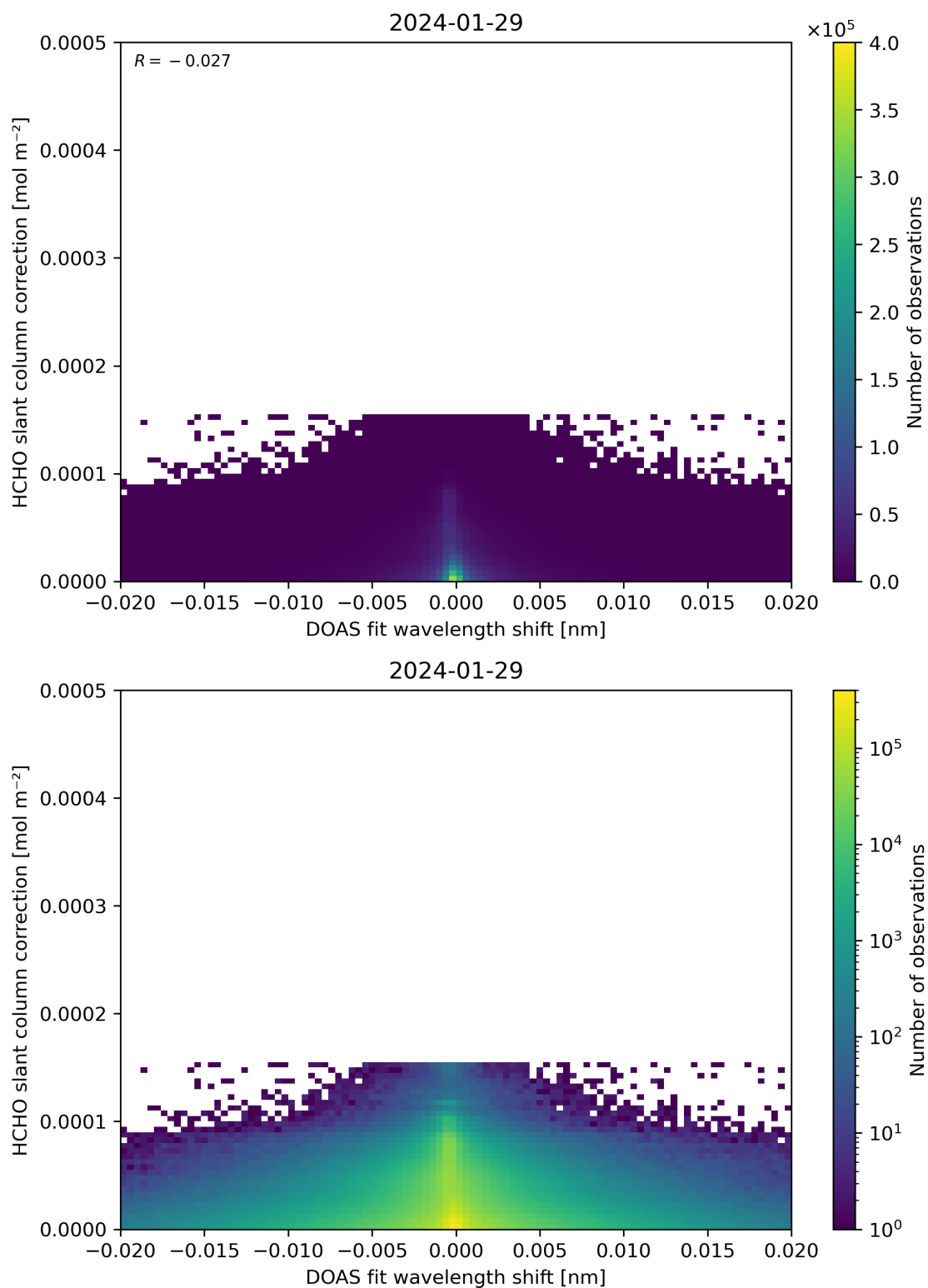
Figure 67: Scatter density plot of “DOAS fit wavelength shift” against “HCHO slant column correction” for 2024-01-28 to 2024-01-30.
