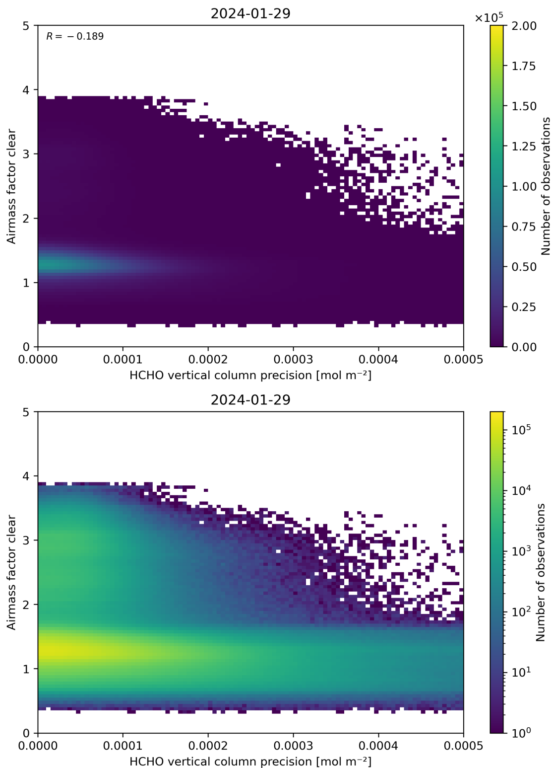
Figure 139: Scatter density plot of “HCHO vertical column precision” against “Airmass factor clear” for 2024-01-28 to 2024-01-30.
