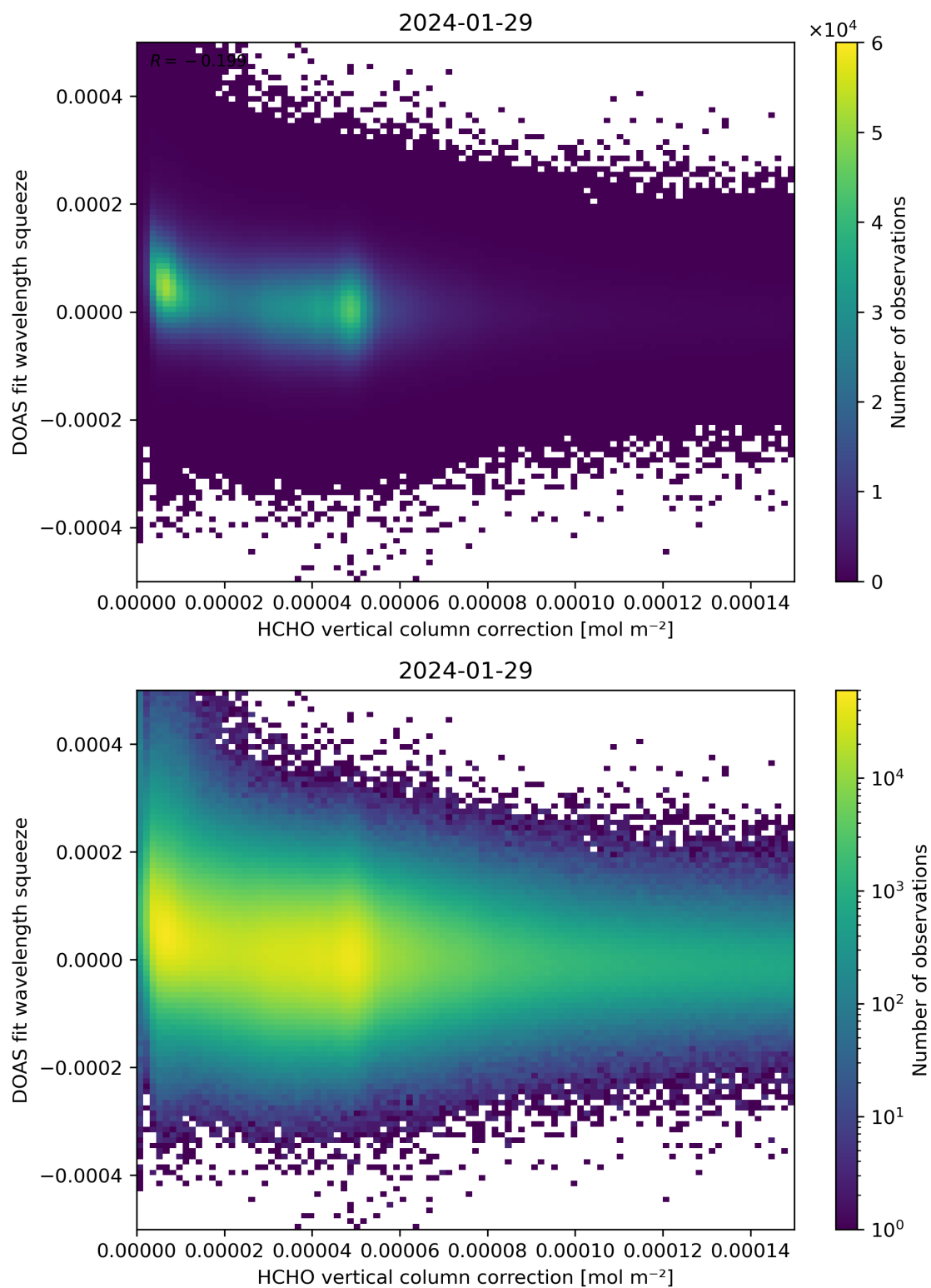
Figure 114: Scatter density plot of “HCHO vertical column correction” against “DOAS fit wavelength squeeze” for 2024-01-28 to 2024-01-30.
