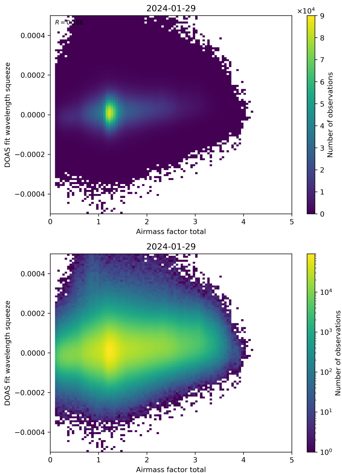
Figure 99: Scatter density plot of “Airmass factor total” against “DOAS fit wavelength squeeze” for 2024-01-28 to 2024-01-30.
