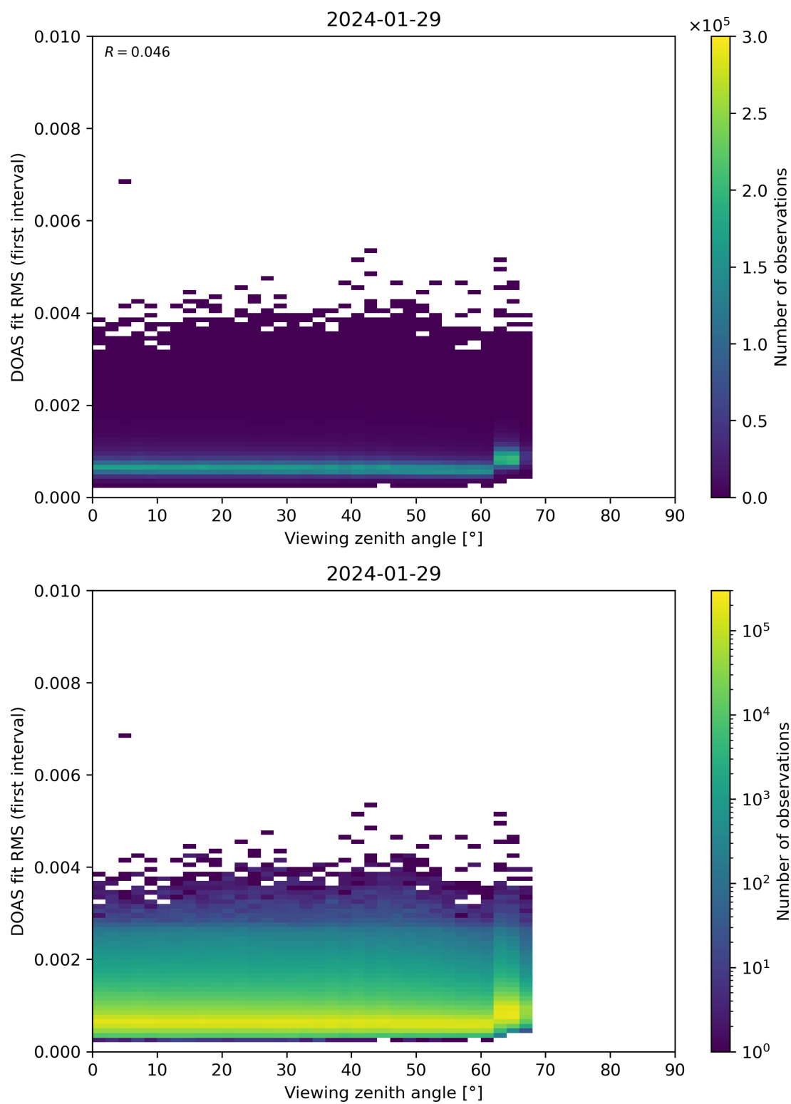
Figure 182: Scatter density plot of “Viewing zenith angle” against “DOAS fit RMS (first interval)” for 2024-01-28 to 2024-01-30.
