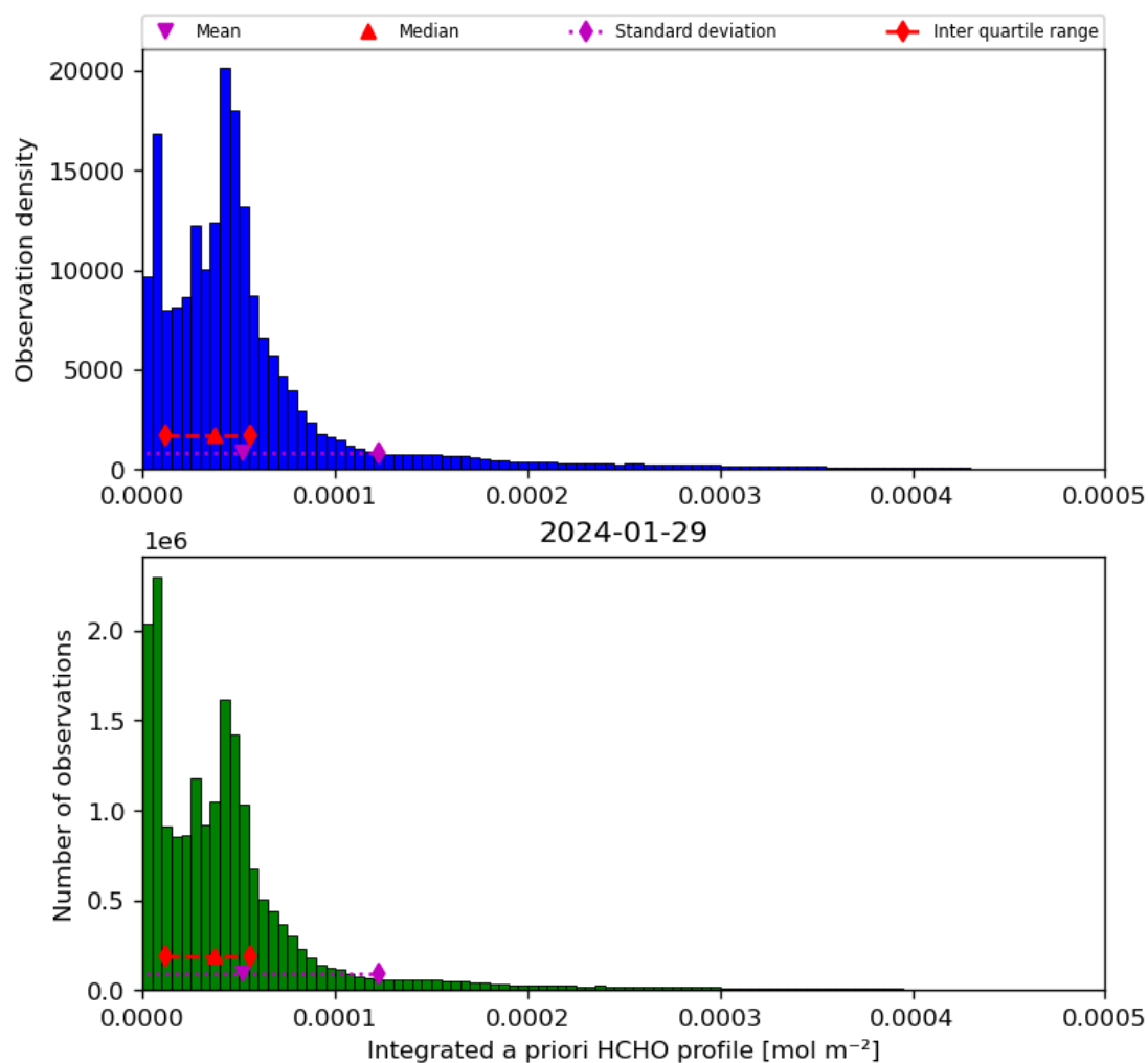
Figure 43: Histogram of “Integrated a priori HCHO profile” for 2024-01-28 to 2024-01-30
