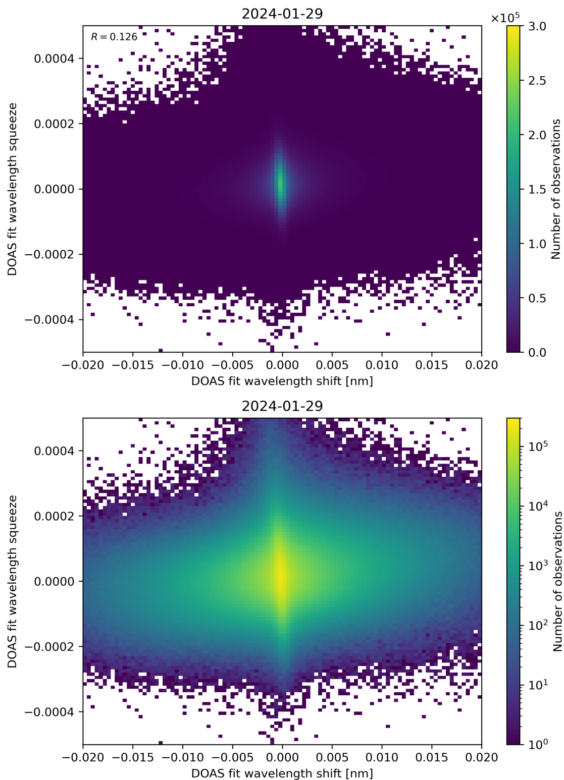
Figure 65: Scatter density plot of “DOAS fit wavelength shift” against “DOAS fit wavelength squeeze” for 2024-01-28 to 2024-01-30.
