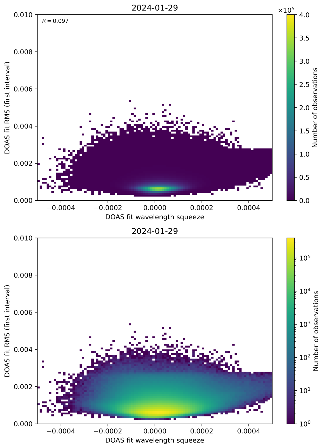
Figure 68: Scatter density plot of “DOAS fit wavelength squeeze” against “DOAS fit RMS (first interval)” for 2024-01-28 to 2024-01-30.
