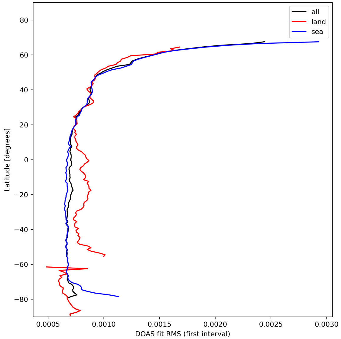
Figure 32: Zonal average of “DOAS fit RMS (first interval)” for 2024-01-28 to 2024-01-30.
