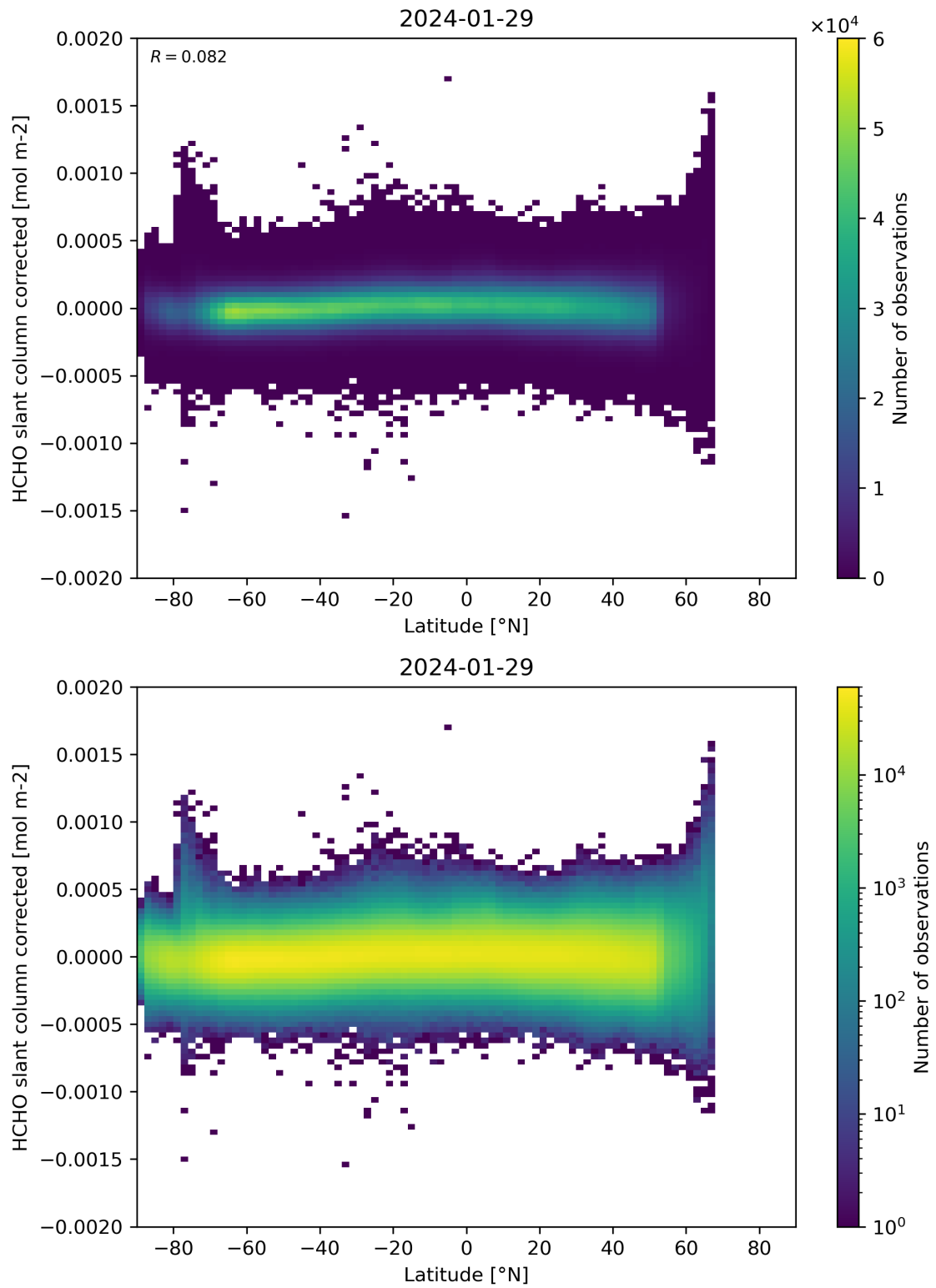
Figure 157: Scatter density plot of “Latitude” against “HCHO slant column corrected” for 2024-01-28 to 2024-01-30.
