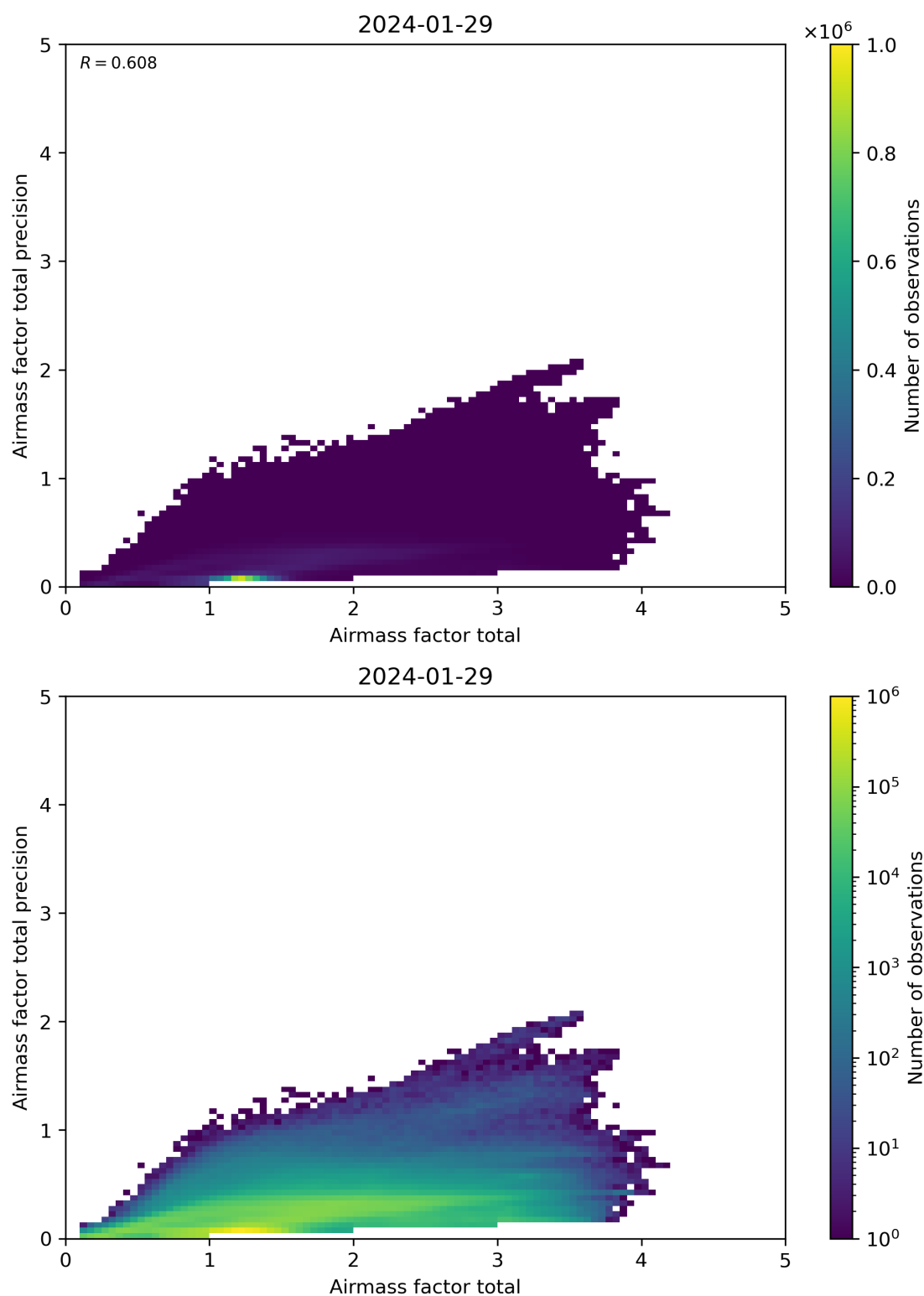
Figure 103: Scatter density plot of “Airmass factor total” against “Airmass factor total precision” for 2024-01-28 to 2024-01-30.
