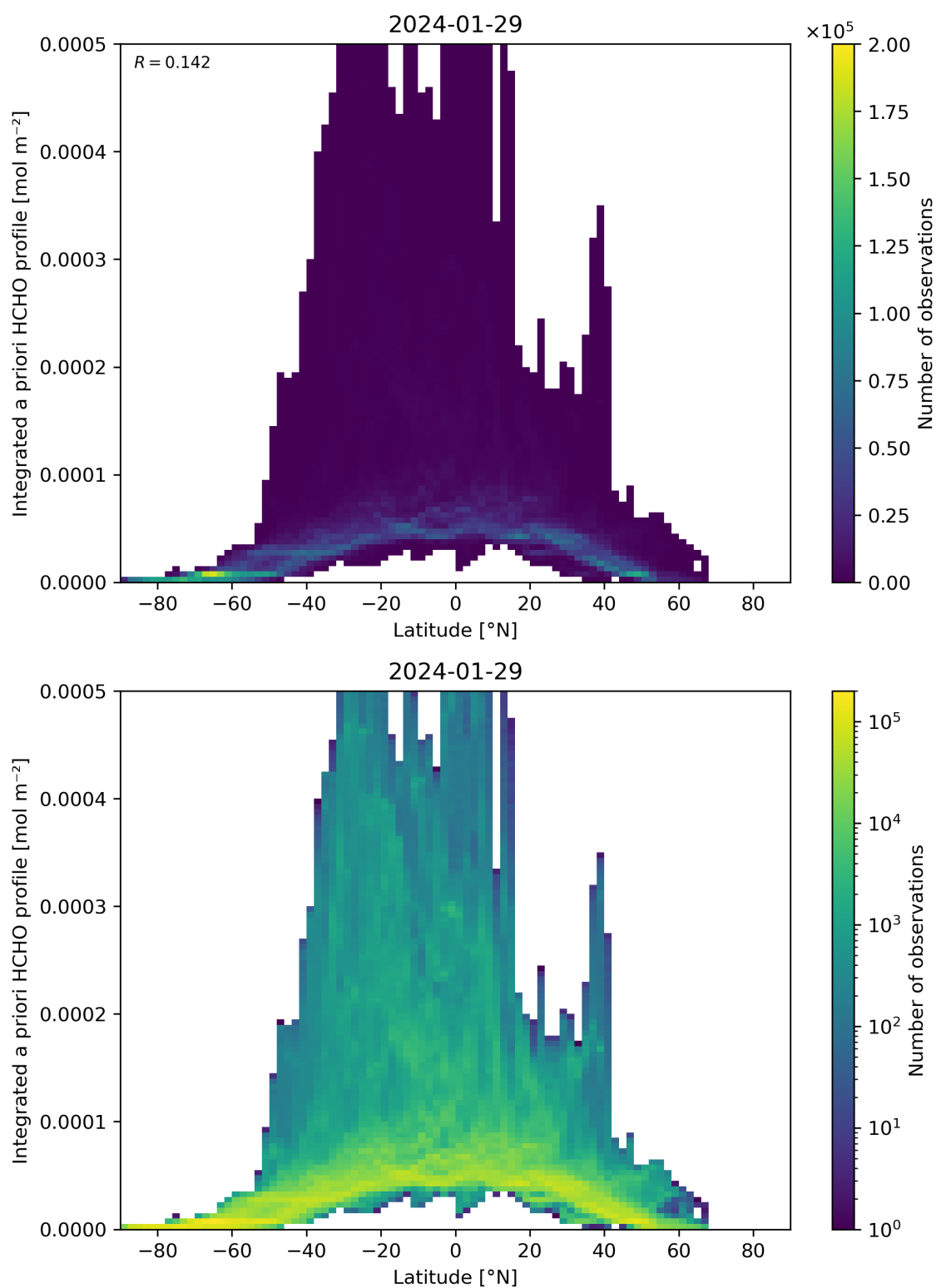
Figure 166: Scatter density plot of “Latitude” against “Integrated a priori HCHO profile” for 2024-01-28 to 2024-01-30.
