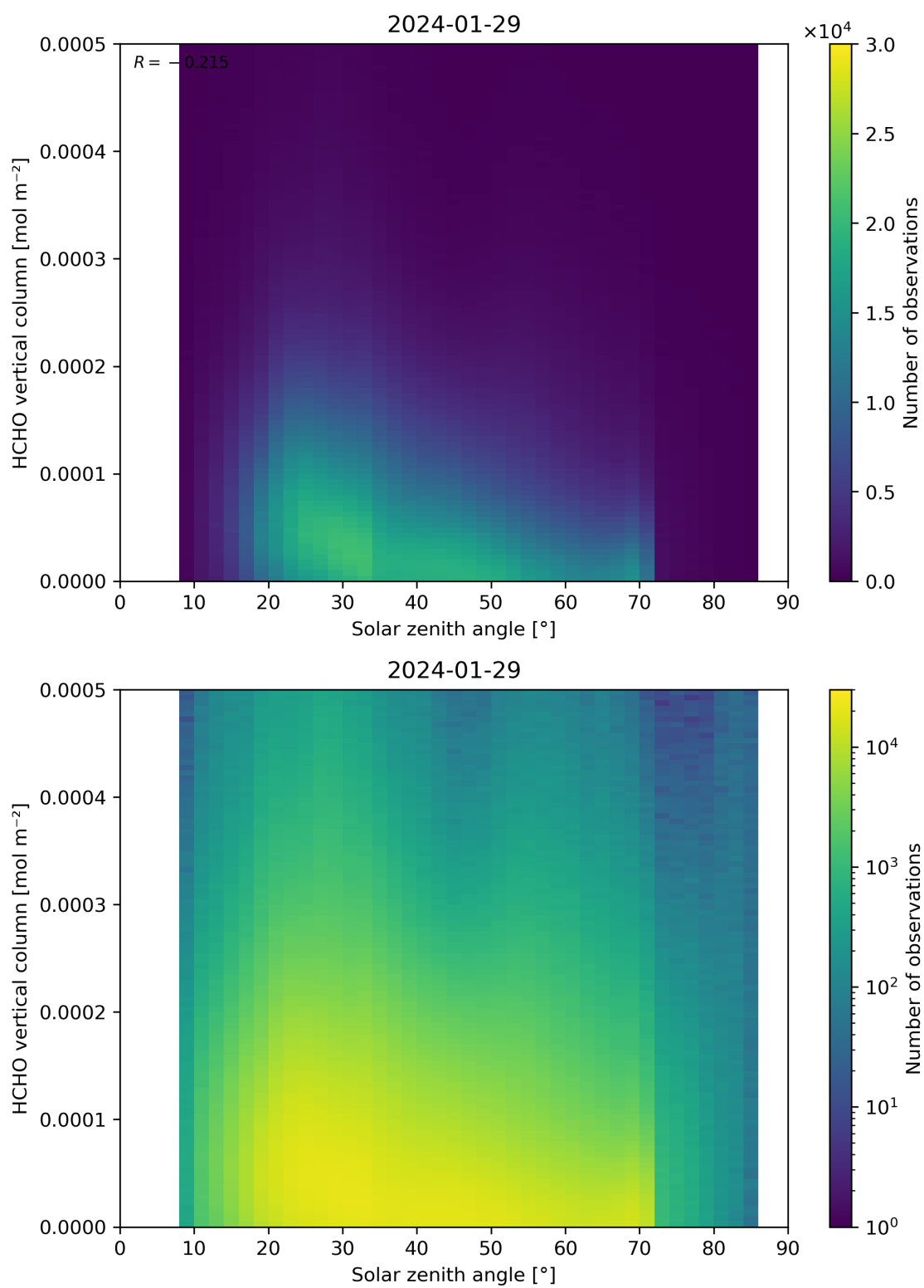
Figure 177: Scatter density plot of “Solar zenith angle” against “HCHO vertical column” for 2024-01-28 to 2024-01-30.
