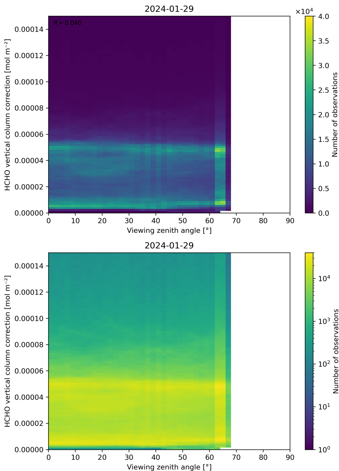
Figure 193: Scatter density plot of “Viewing zenith angle” against “HCHO vertical column correction” for 2024-01-28 to 2024-01-30.
