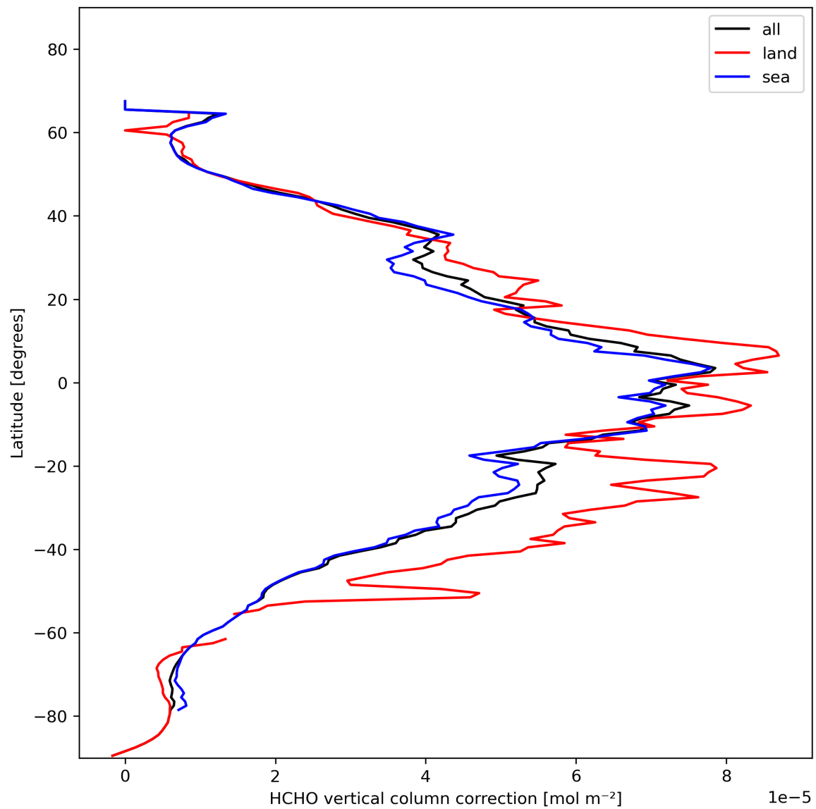
Figure 23: Zonal average of “HCHO vertical column correction” for 2024-01-28 to 2024-01-30.
