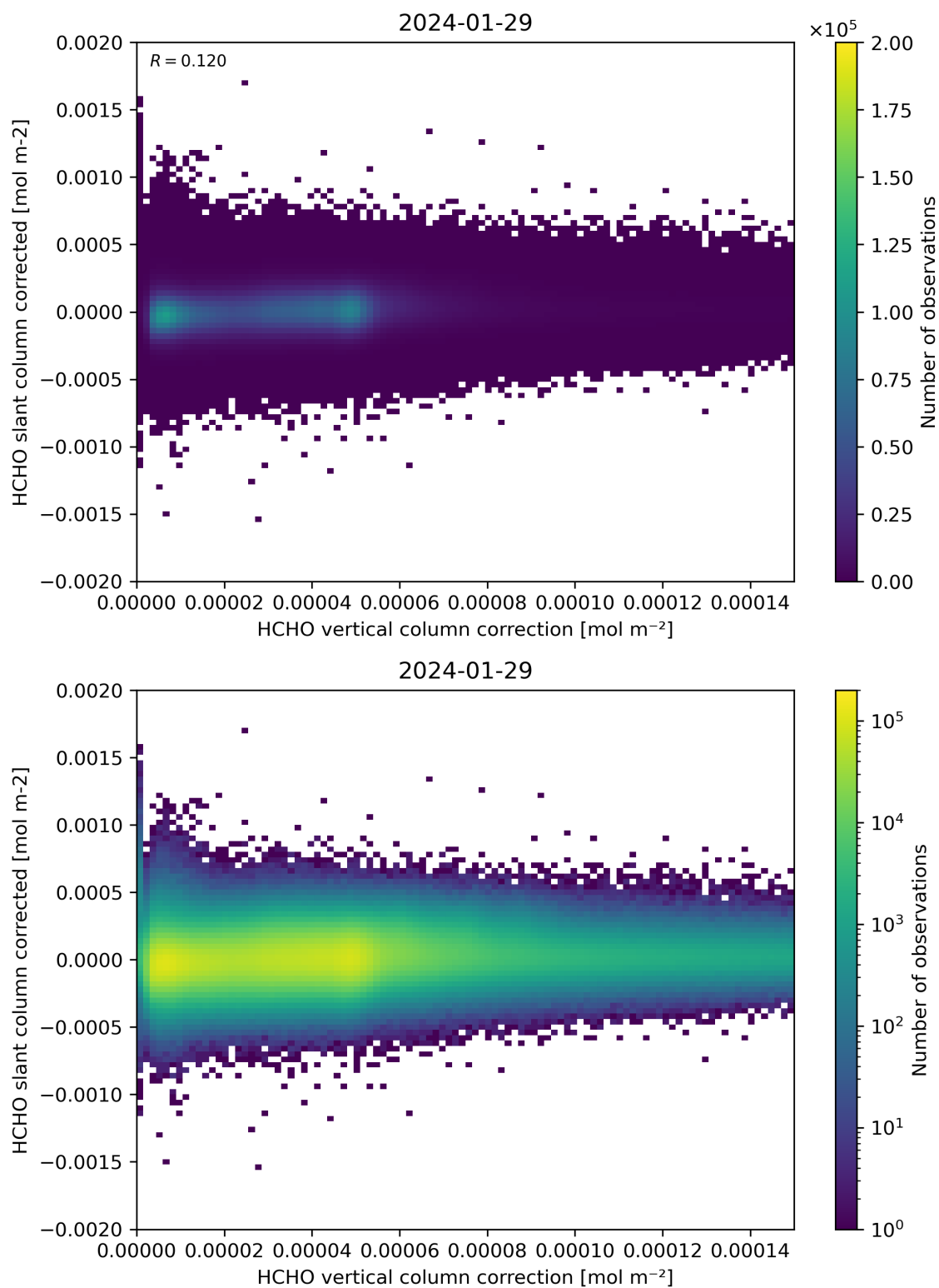
Figure 116: Scatter density plot of “HCHO vertical column correction” against “HCHO slant column corrected” for 2024-01-28 to 2024-01-30.
