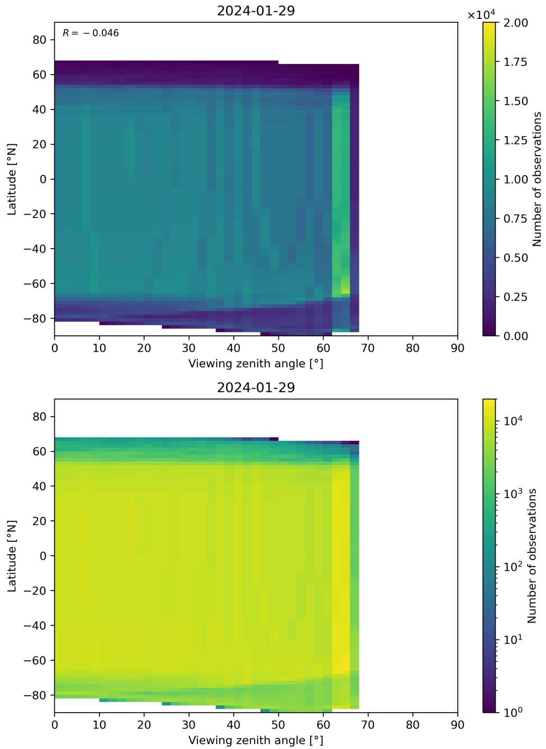
Figure 196: Scatter density plot of “Viewing zenith angle” against “Latitude” for 2024-01-28 to 2024-01-30.
