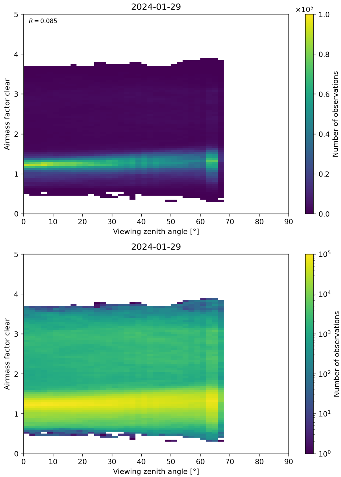
Figure 185: Scatter density plot of “Viewing zenith angle” against “Airmass factor clear” for 2024-01-28 to 2024-01-30.
