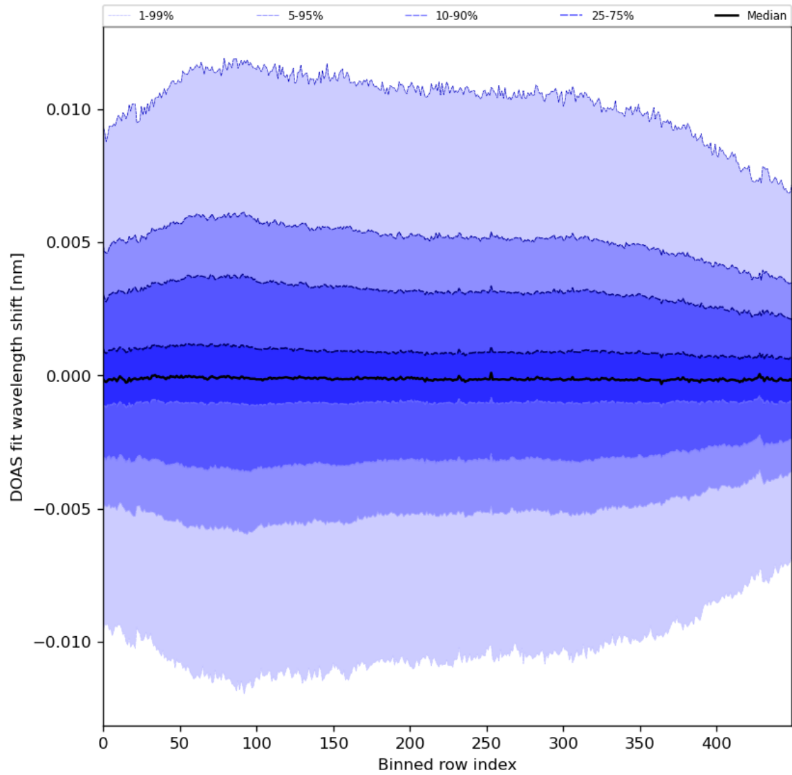
Figure 58: Along track statistics of “DOAS fit wavelength shift” for 2024-01-28 to 2024-01-30
