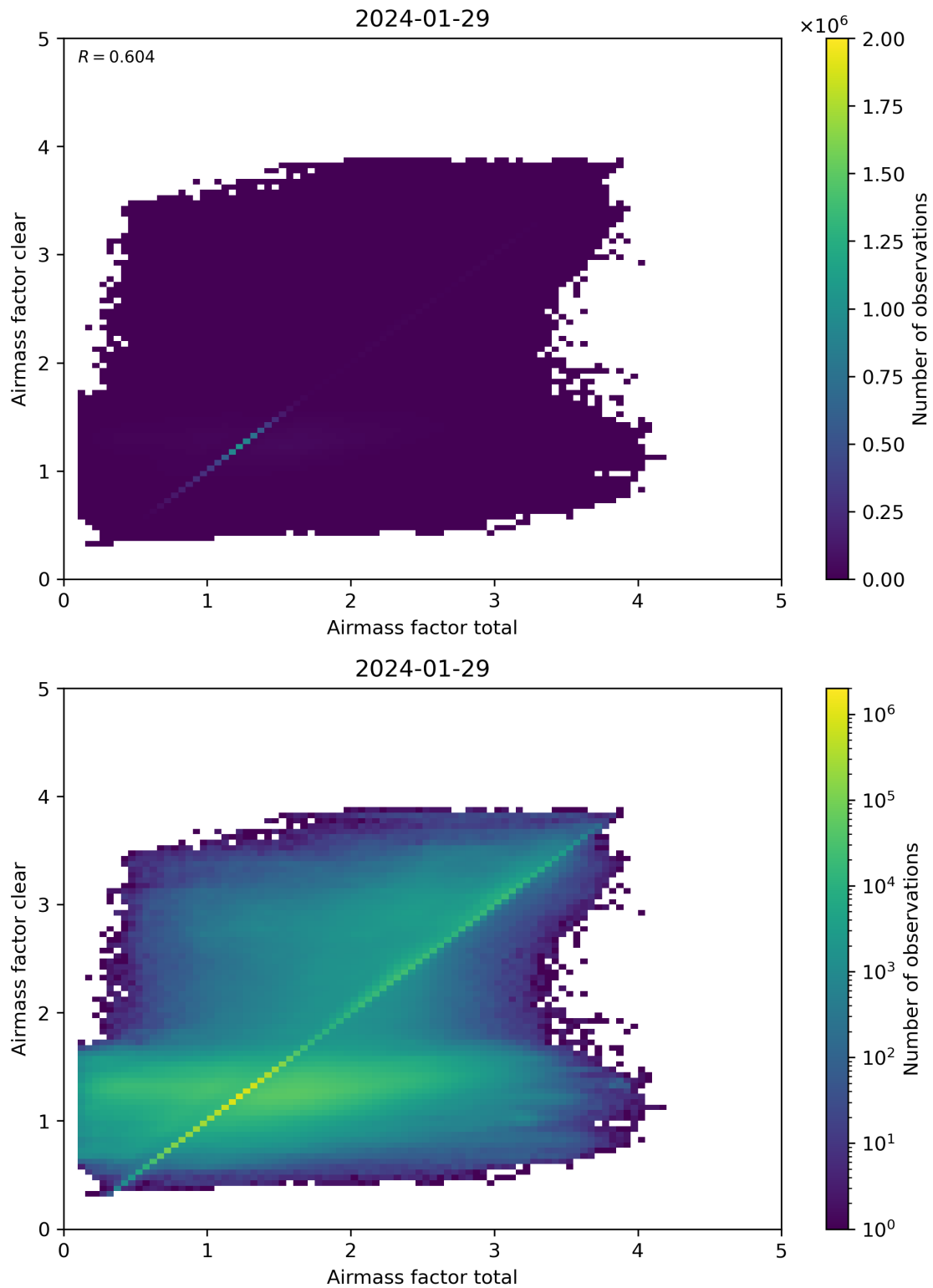
Figure 100: Scatter density plot of “Airmass factor total” against “Airmass factor clear” for 2024-01-28 to 2024-01-30.
