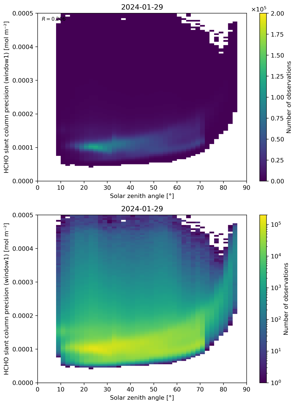
Figure 174: Scatter density plot of “Solar zenith angle” against “HCHO slant column precision (window1)” for 2024-01-28 to 2024-01-30.
