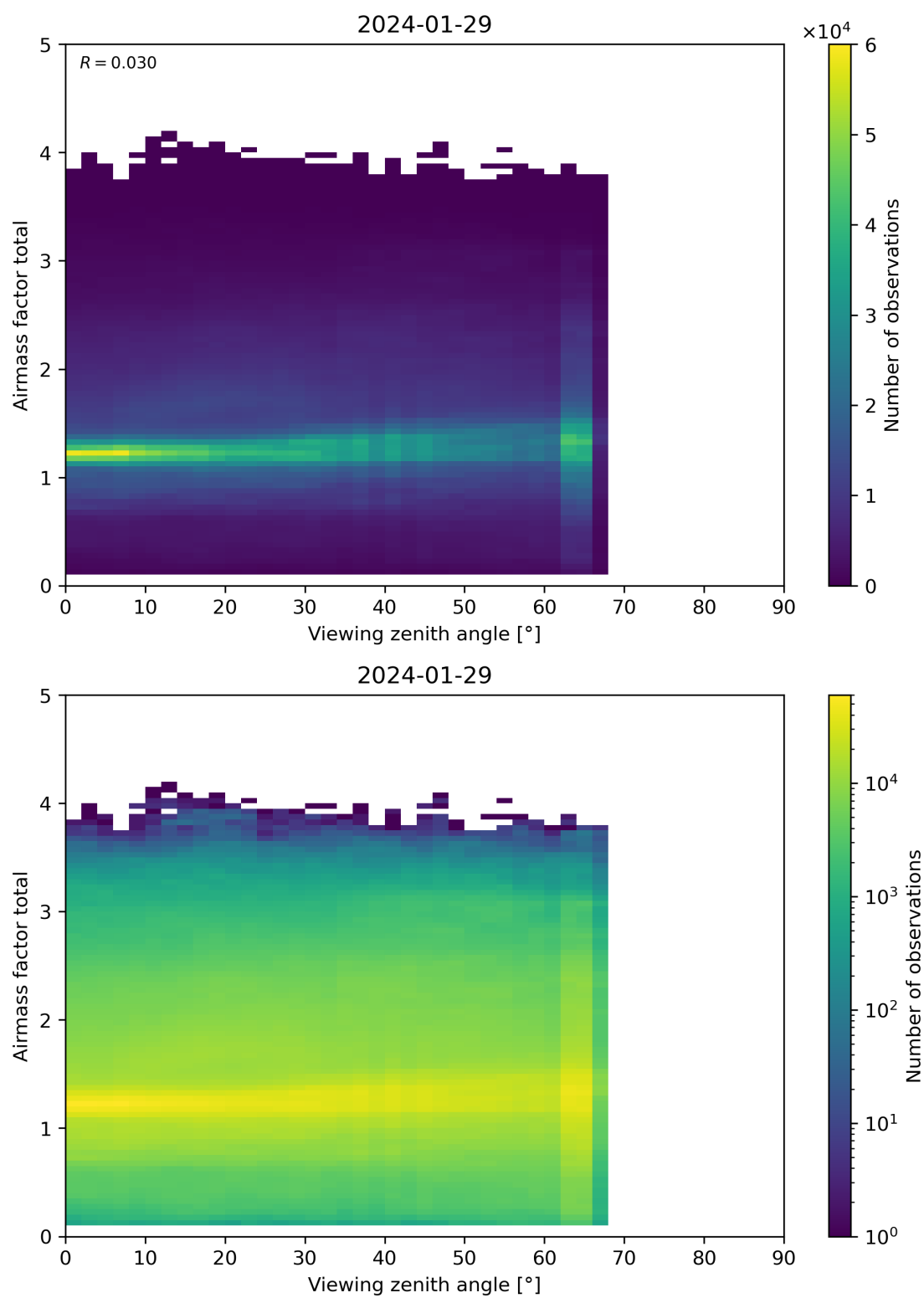
Figure 190: Scatter density plot of “Viewing zenith angle” against “Airmass factor total” for 2024-01-28 to 2024-01-30.
