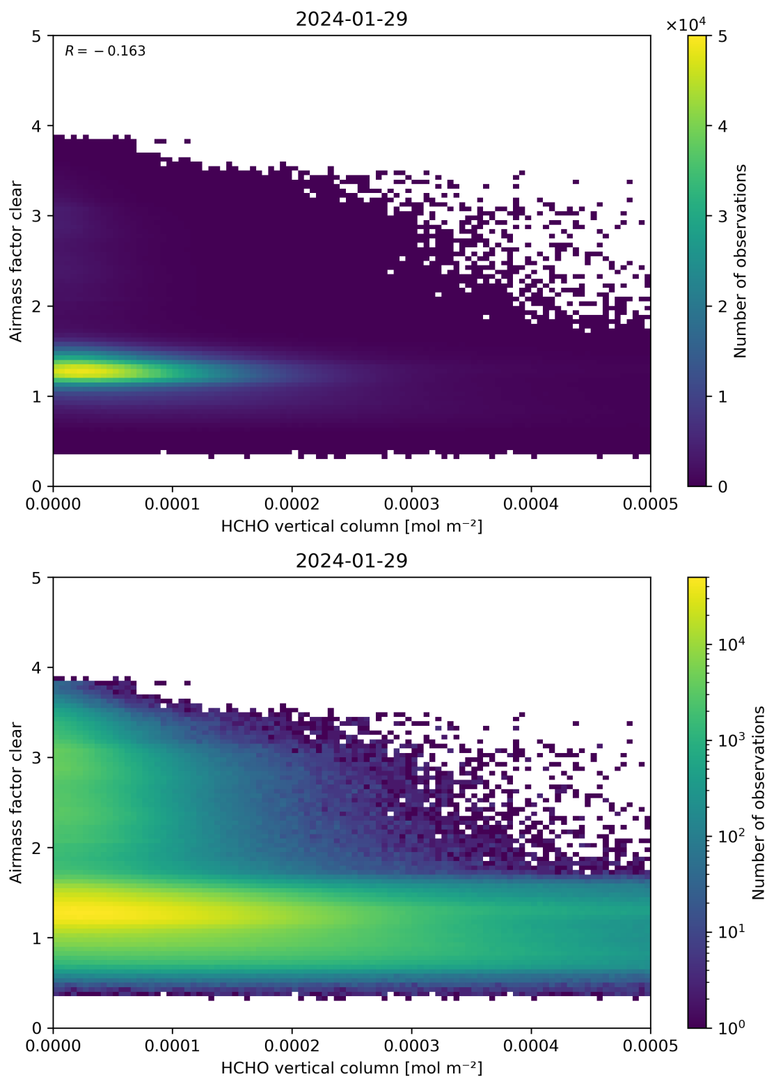
Figure 126: Scatter density plot of “HCHO vertical column” against “Airmass factor clear” for 2024-01-28 to 2024-01-30.
