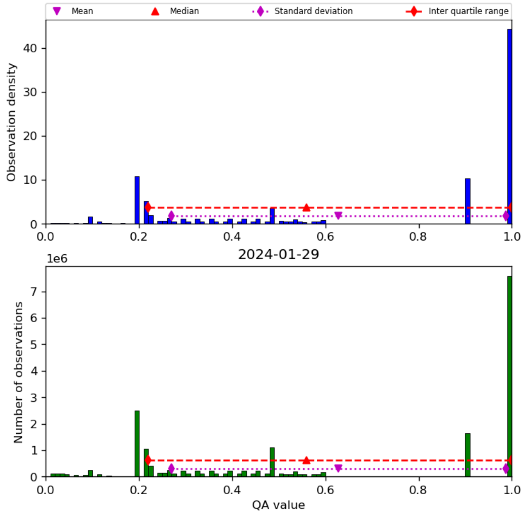
Figure 34: Histogram of “QA value” for 2024-01-28 to 2024-01-30
