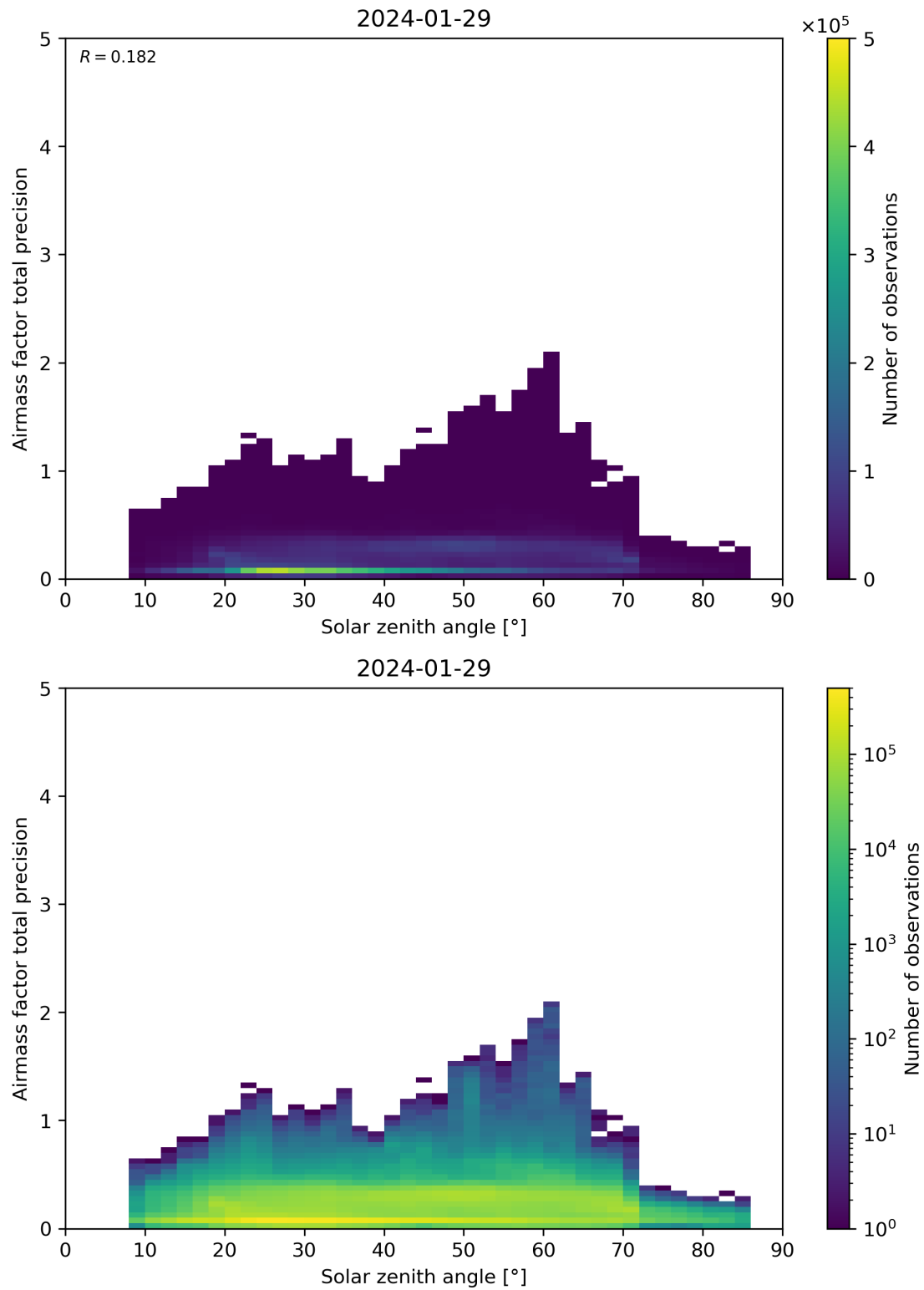
Figure 176: Scatter density plot of “Solar zenith angle” against “Airmass factor total precision” for 2024-01-28 to 2024-01-30.
