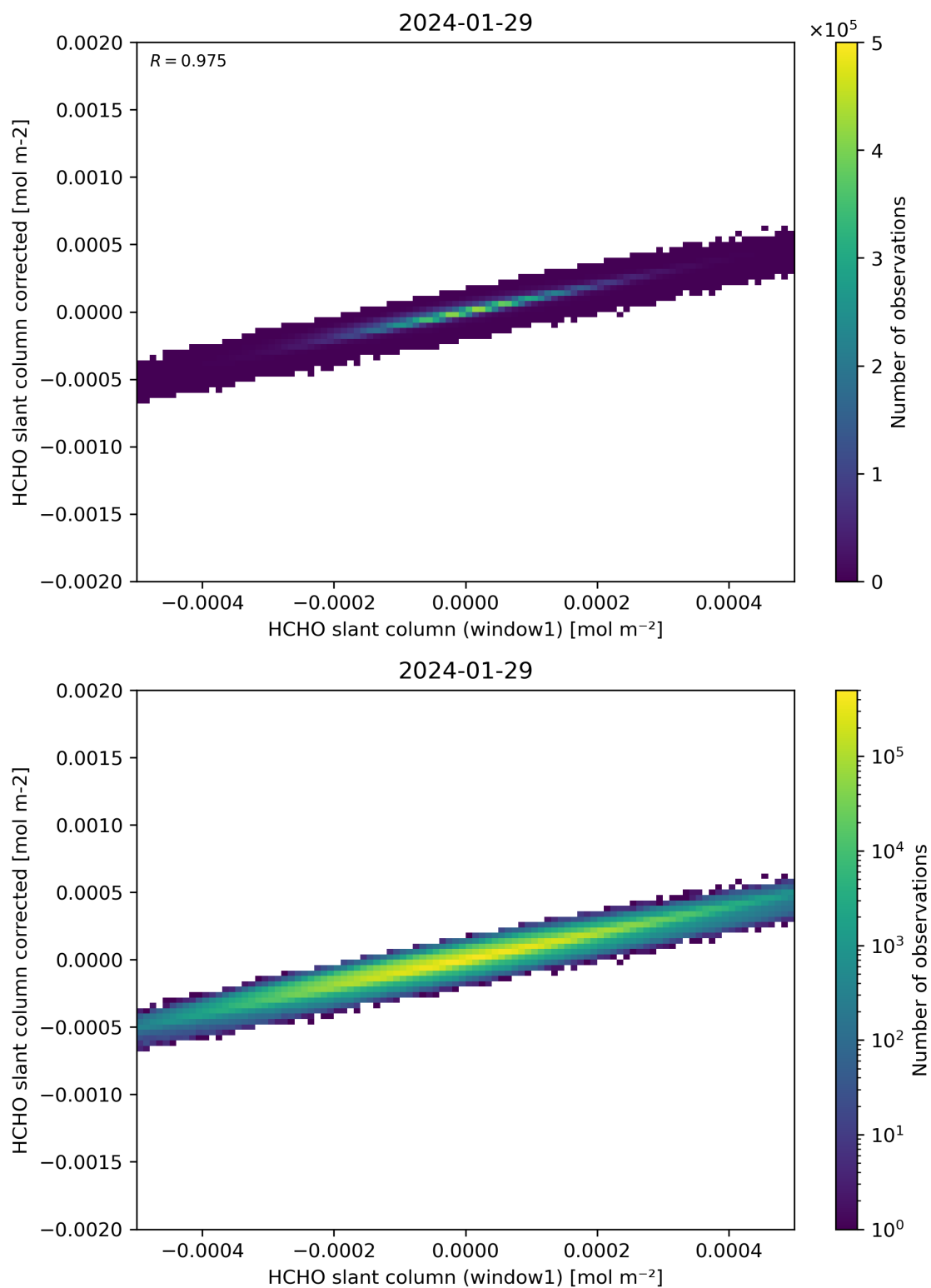
Figure 82: Scatter density plot of “HCHO slant column (window1)” against “HCHO slant column corrected” for 2024-01-28 to 2024-01-30.
