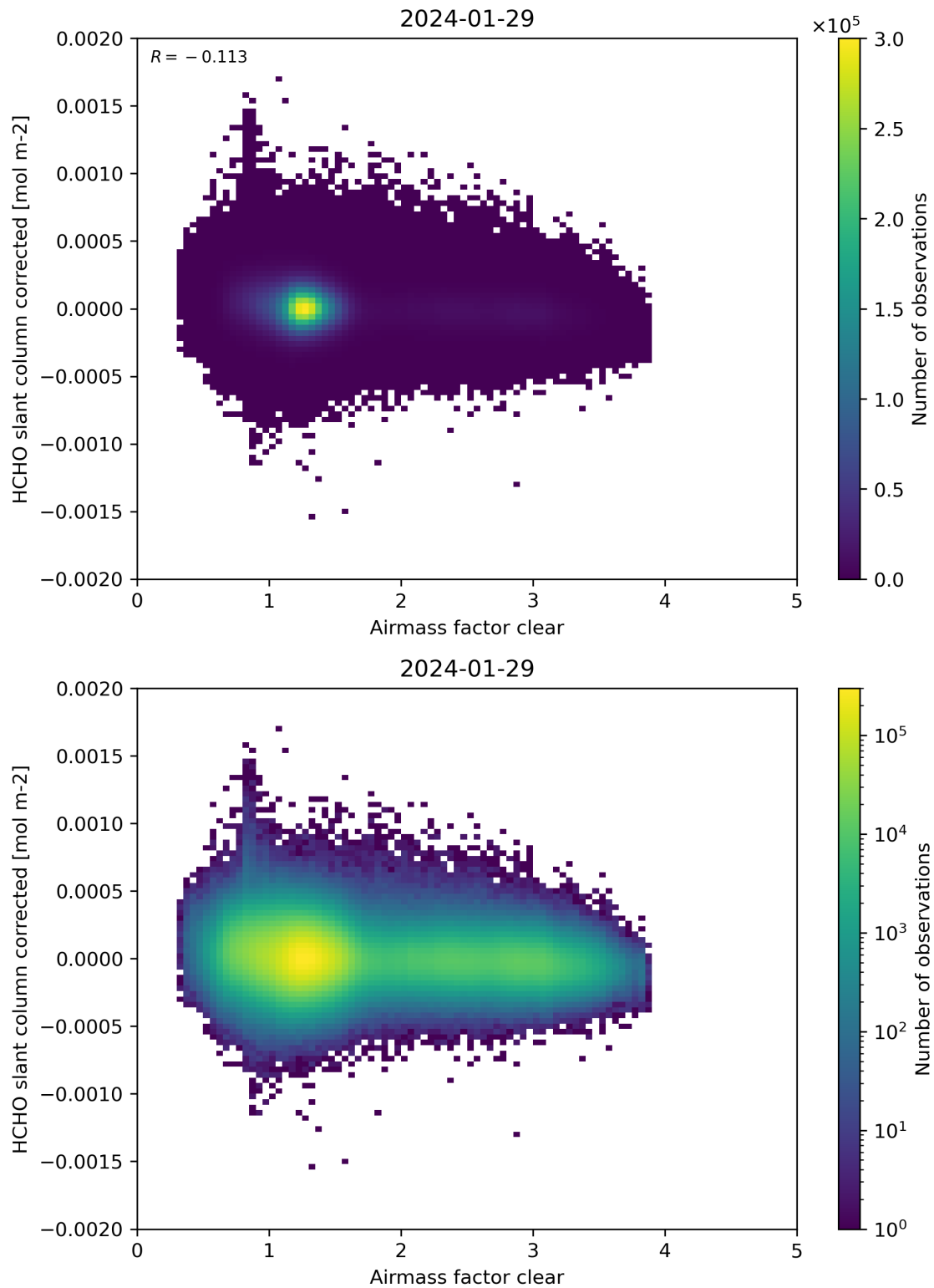
Figure 74: Scatter density plot of “Airmass factor clear” against “HCHO slant column corrected” for 2024-01-28 to 2024-01-30.
