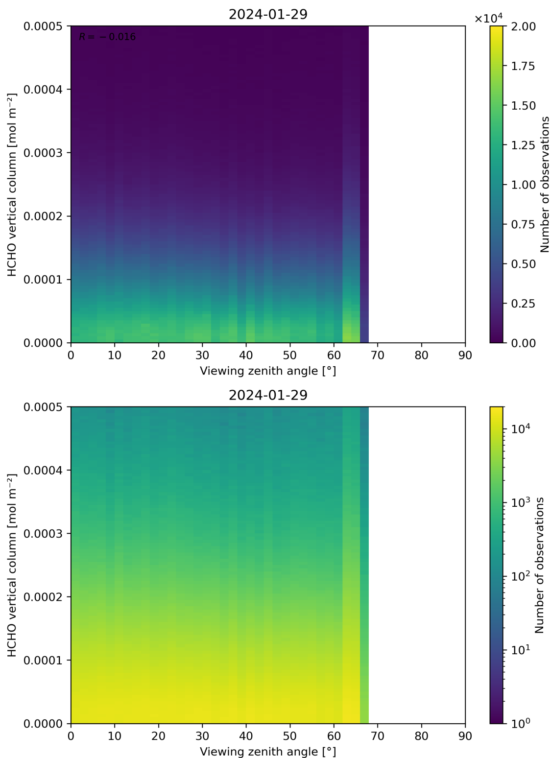
Figure 192: Scatter density plot of “Viewing zenith angle” against “HCHO vertical column” for 2024-01-28 to 2024-01-30.
