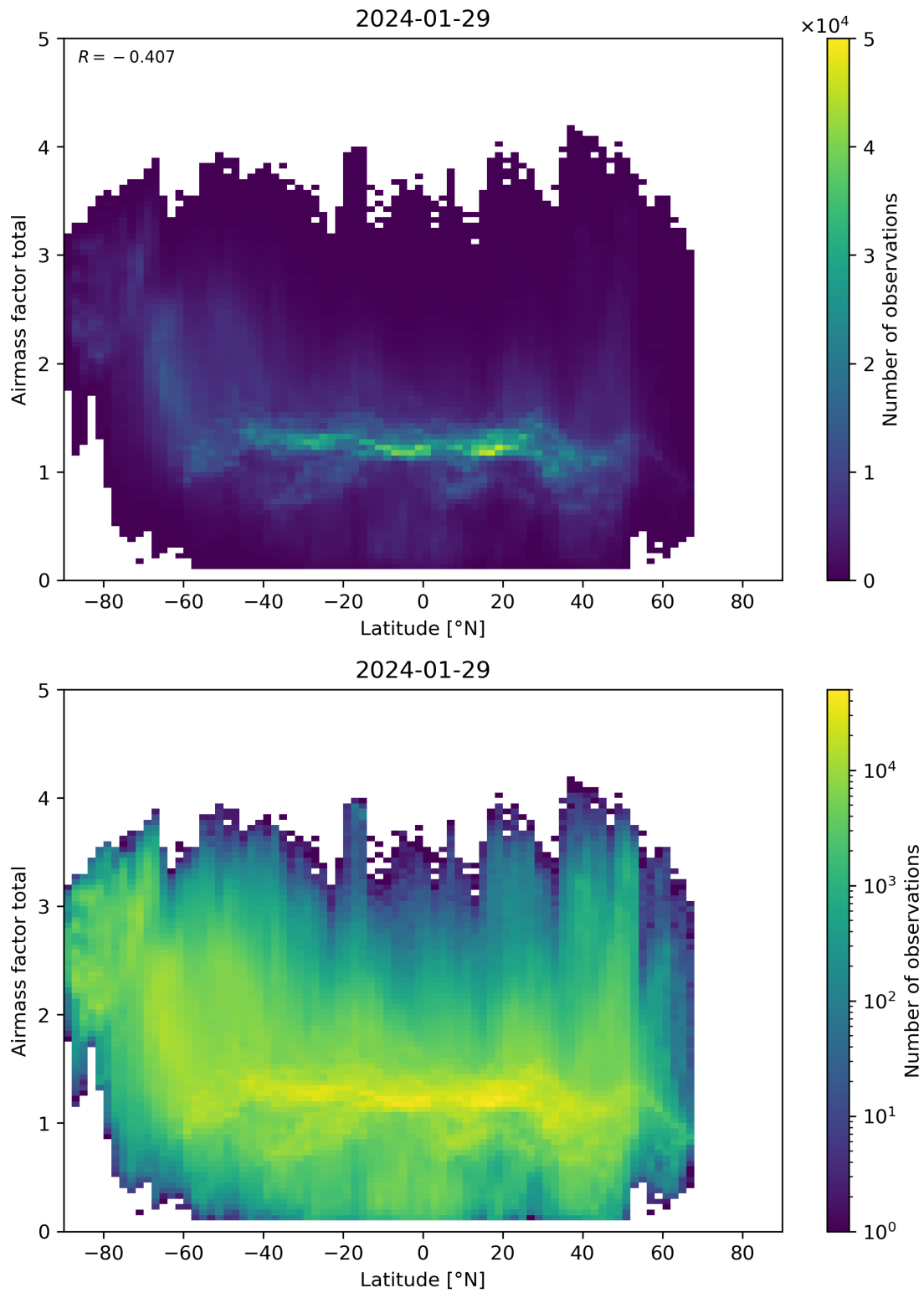
Figure 161: Scatter density plot of “Latitude” against “Airmass factor total” for 2024-01-28 to 2024-01-30.
