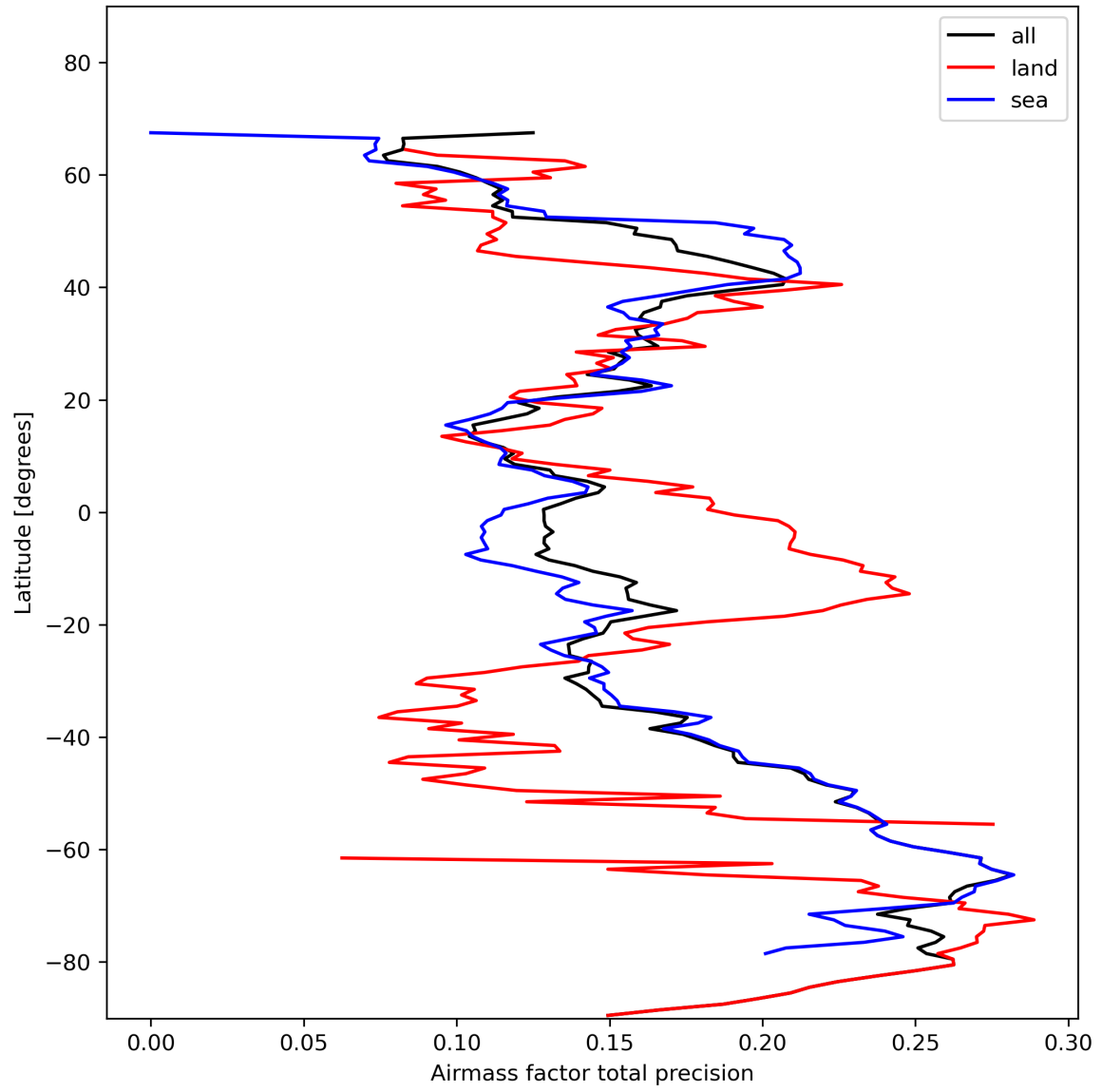
Figure 27: Zonal average of “Airmass factor total precision” for 2024-01-28 to 2024-01-30.
