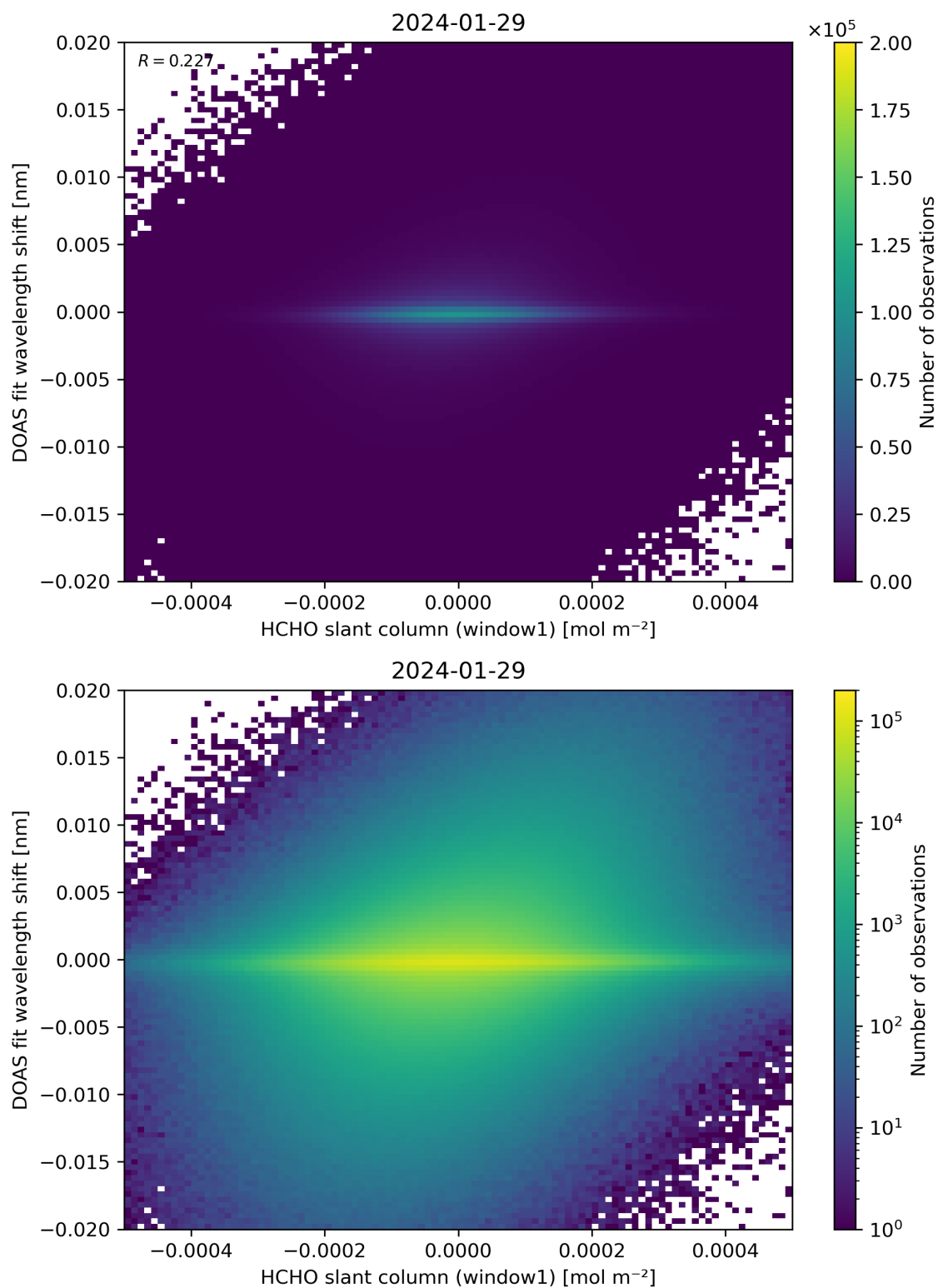
Figure 79: Scatter density plot of “HCHO slant column (window1)” against “DOAS fit wavelength shift” for 2024-01-28 to 2024-01-30.
