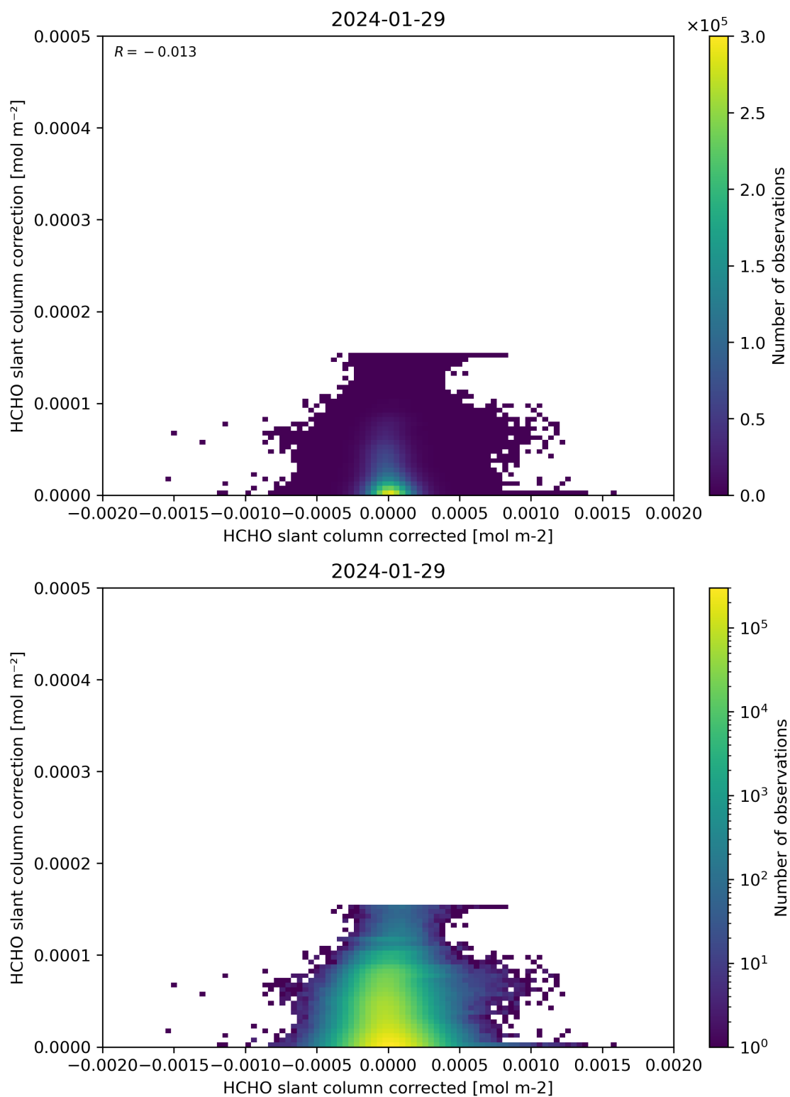
Figure 77: Scatter density plot of “HCHO slant column corrected” against “HCHO slant column correction” for 2024-01-28 to 2024-01-30.
