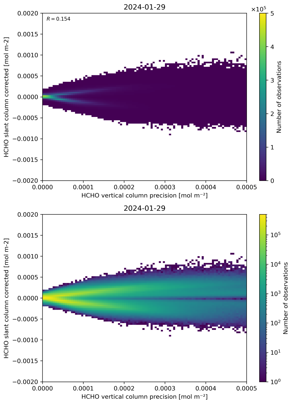
Figure 140: Scatter density plot of “HCHO vertical column precision” against “HCHO slant column corrected” for 2024-01-28 to 2024-01-30.
