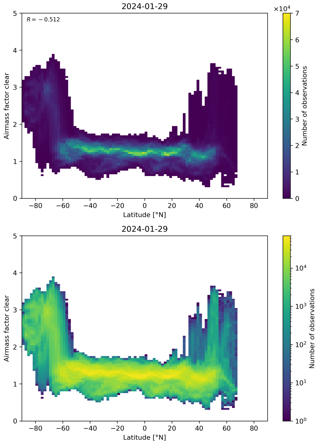
Figure 156: Scatter density plot of “Latitude” against “Airmass factor clear” for 2024-01-28 to 2024-01-30.
