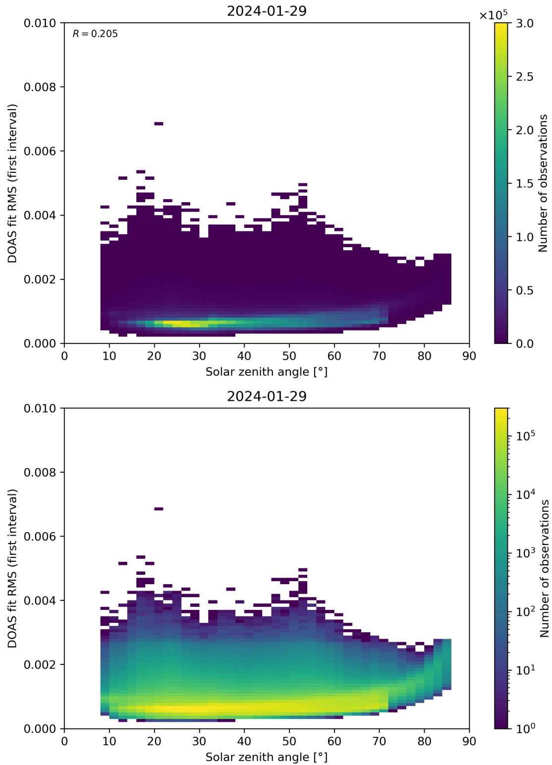
Figure 167: Scatter density plot of “Solar zenith angle” against “DOAS fit RMS (first interval)” for 2024-01-28 to 2024-01-30.
