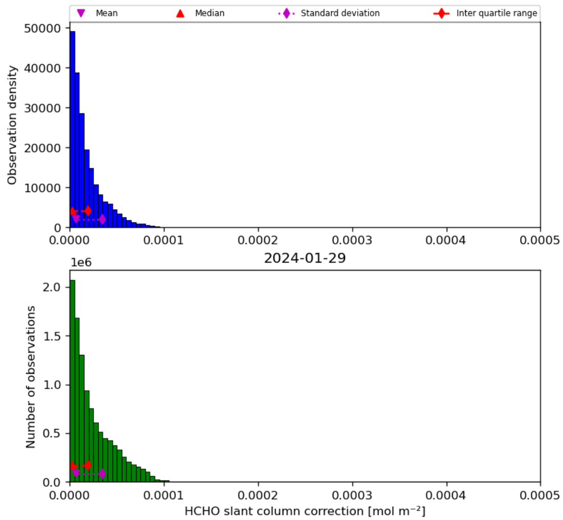
Figure 47: Histogram of “HCHO slant column correction” for 2024-01-28 to 2024-01-30
