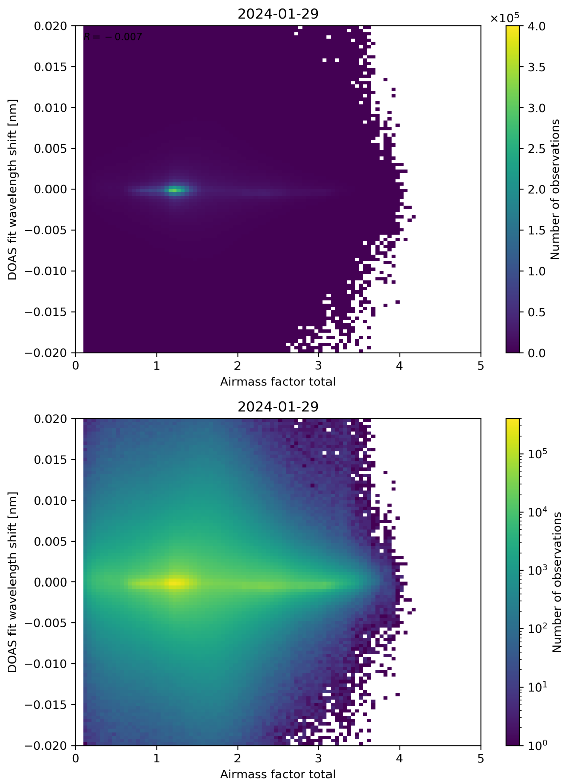
Figure 98: Scatter density plot of “Airmass factor total” against “DOAS fit wavelength shift” for 2024-01-28 to 2024-01-30.
