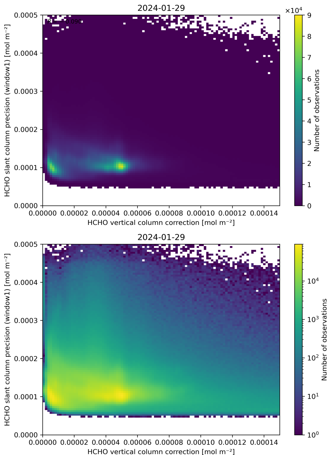
Figure 119: Scatter density plot of “HCHO vertical column correction” against “HCHO slant column precision (window1)” for 2024-01-28 to 2024-01-30.
