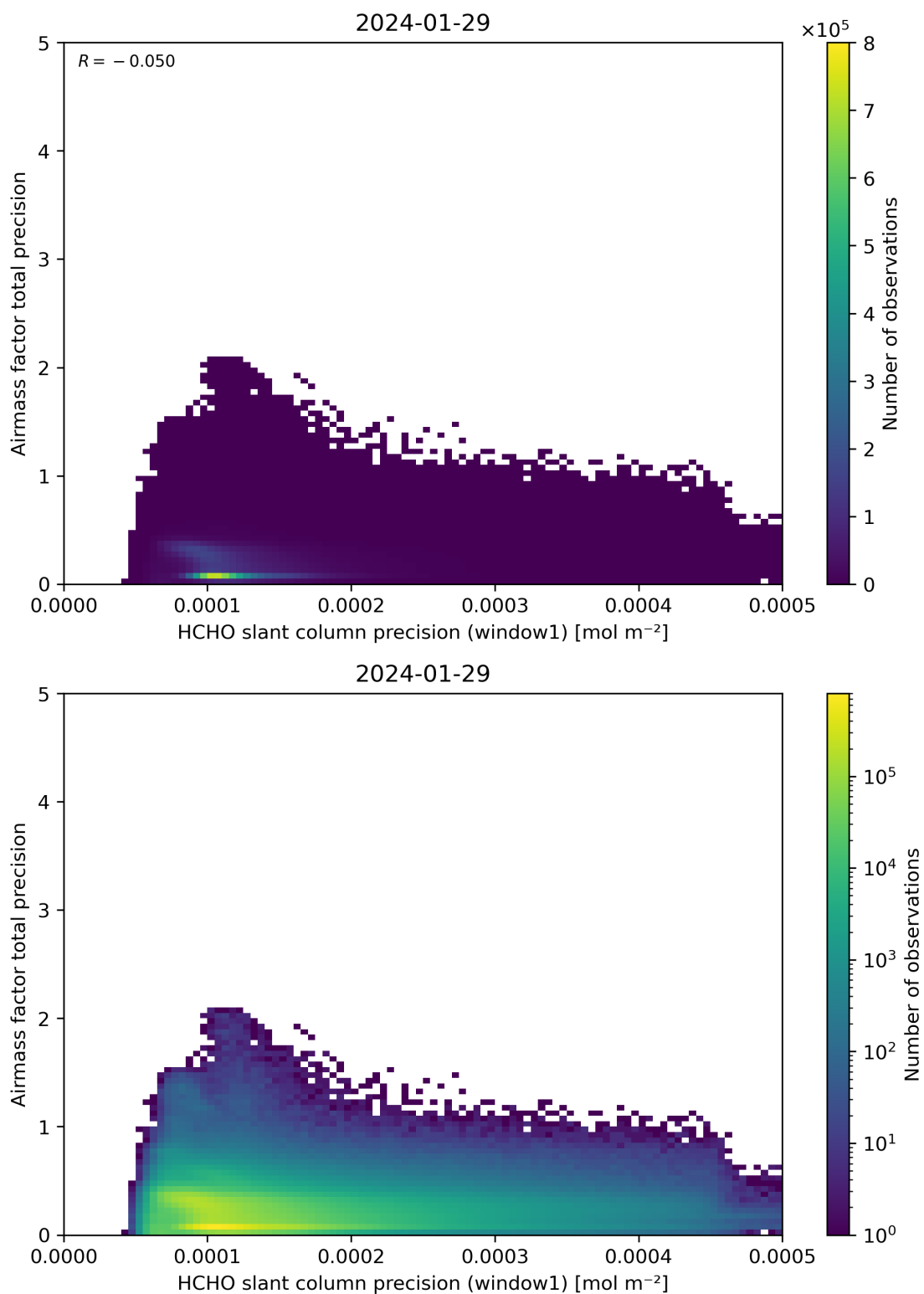
Figure 95: Scatter density plot of “HCHO slant column precision (window1)” against “Airmass factor total precision” for 2024-01-28 to 2024-01-30.
