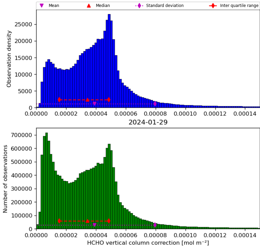
Figure 37: Histogram of “HCHO vertical column correction” for 2024-01-28 to 2024-01-30
