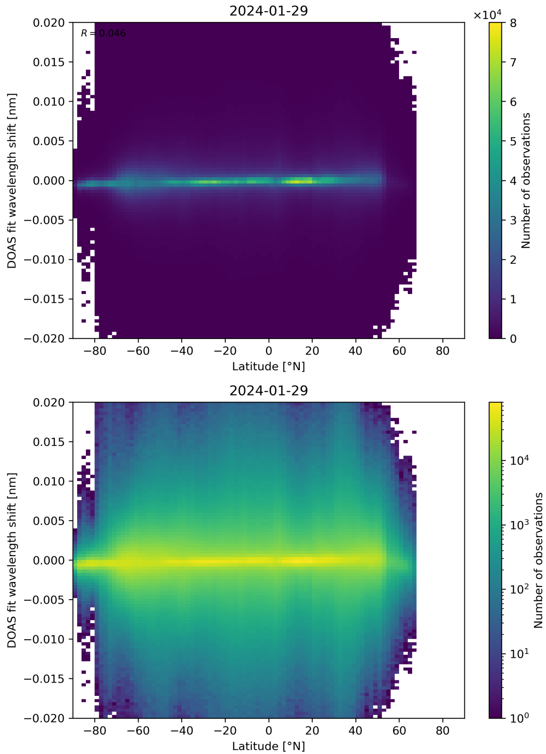
Figure 154: Scatter density plot of “Latitude” against “DOAS fit wavelength shift” for 2024-01-28 to 2024-01-30.
