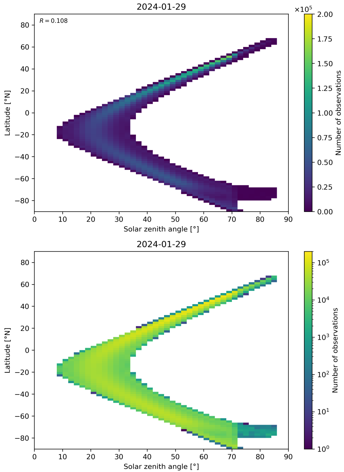
Figure 181: Scatter density plot of “Solar zenith angle” against “Latitude” for 2024-01-28 to 2024-01-30.
