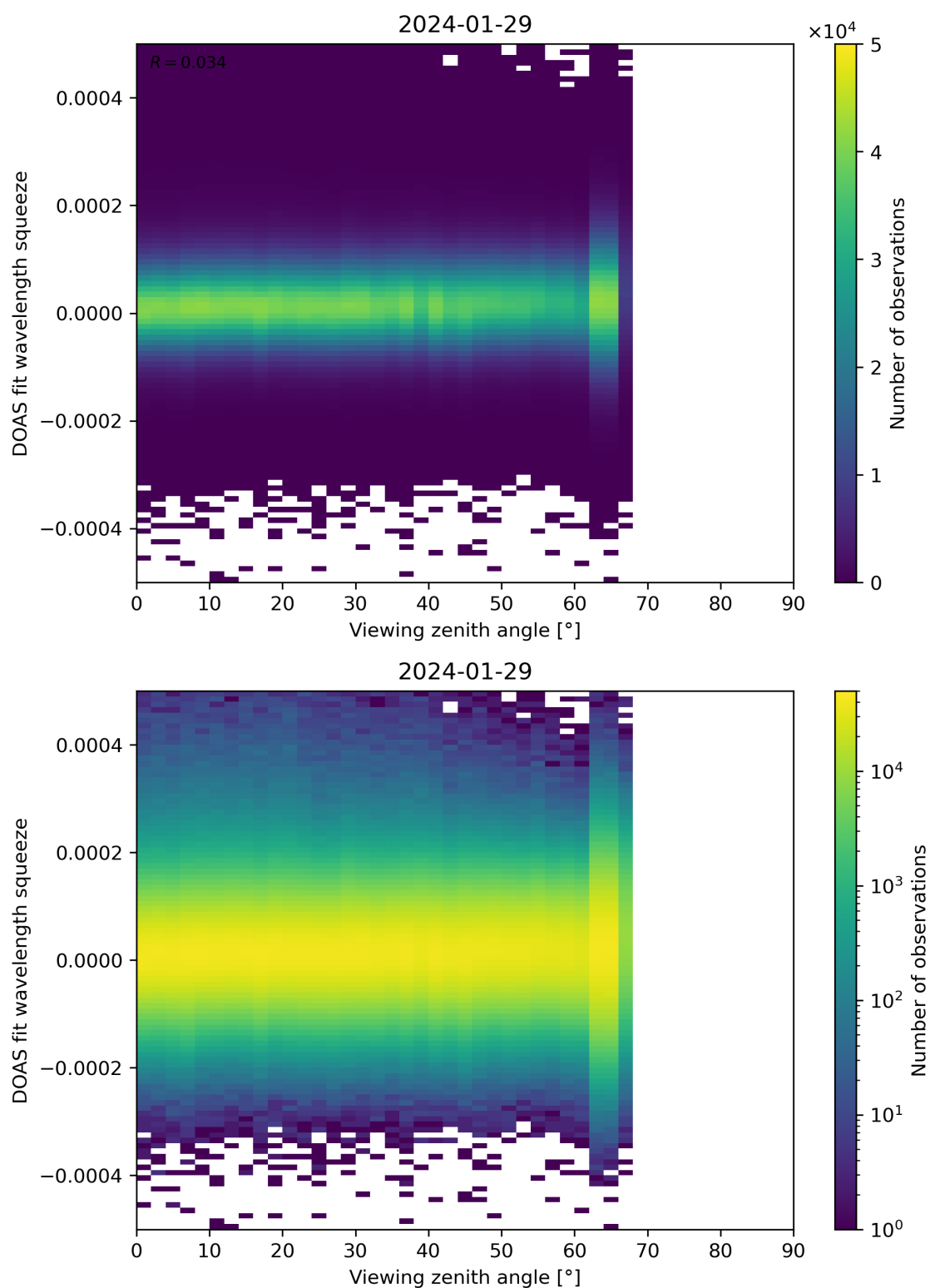
Figure 184: Scatter density plot of “Viewing zenith angle” against “DOAS fit wavelength squeeze” for 2024-01-28 to 2024-01-30.
