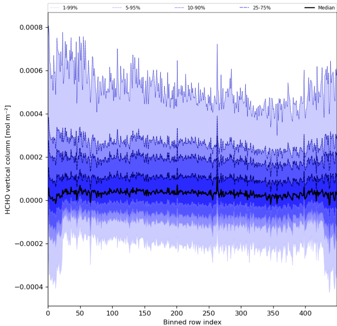
Figure 49: Along track statistics of “HCHO vertical column” for 2024-01-28 to 2024-01-30
