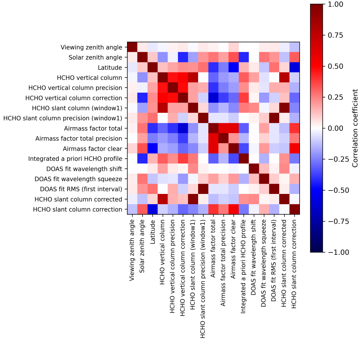
Figure 2: Map of correlation matrix for 2024-01-28 to 2024-01-30.
