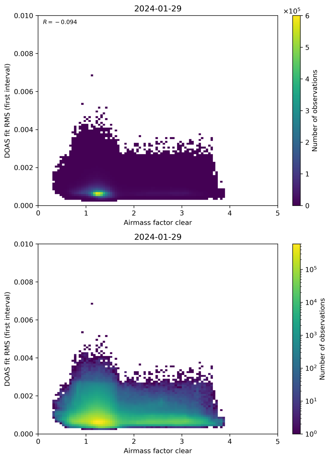
Figure 71: Scatter density plot of “Airmass factor clear” against “DOAS fit RMS (first interval)” for 2024-01-28 to 2024-01-30.
