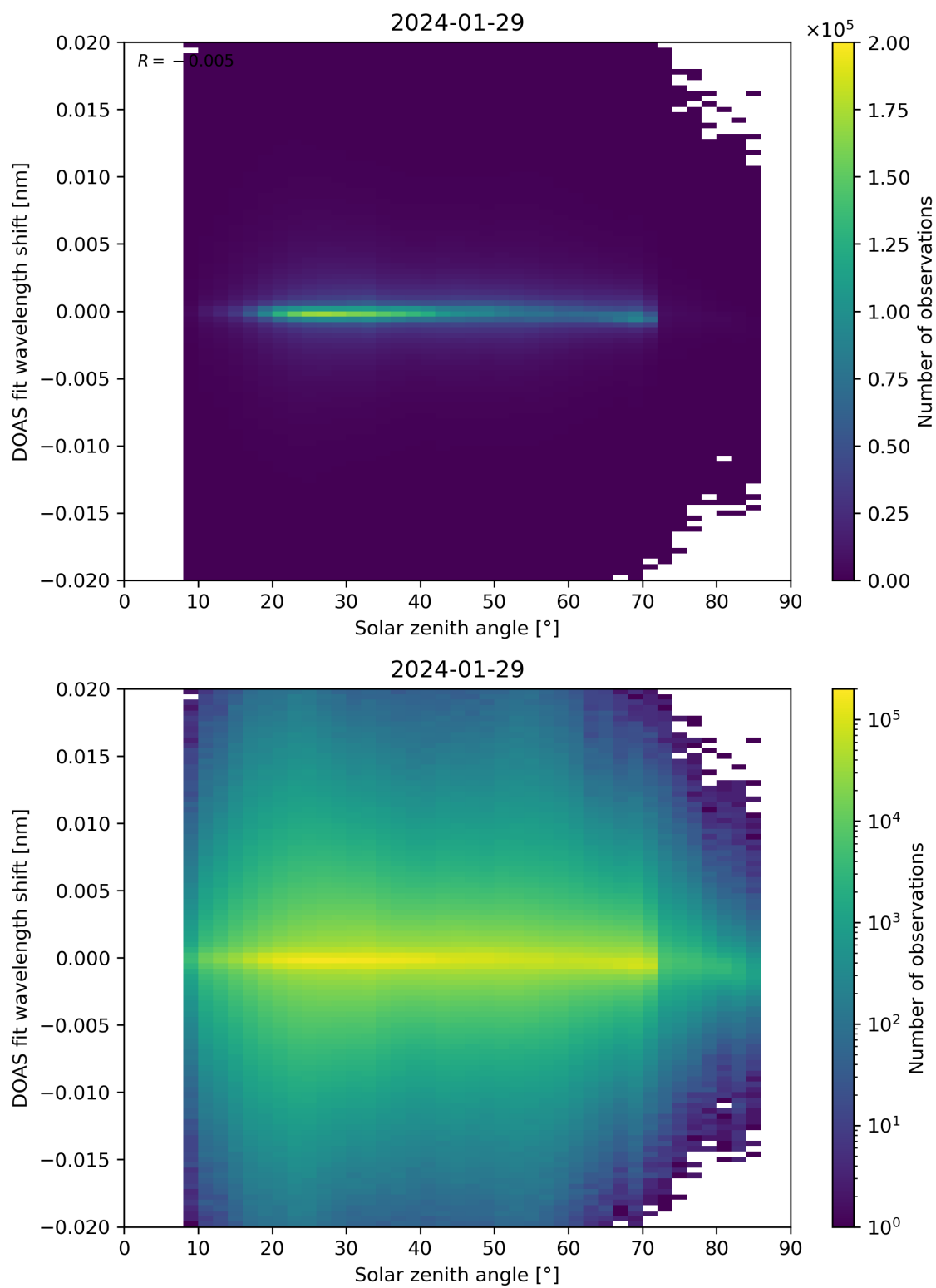
Figure 168: Scatter density plot of “Solar zenith angle” against “DOAS fit wavelength shift” for 2024-01-28 to 2024-01-30.
