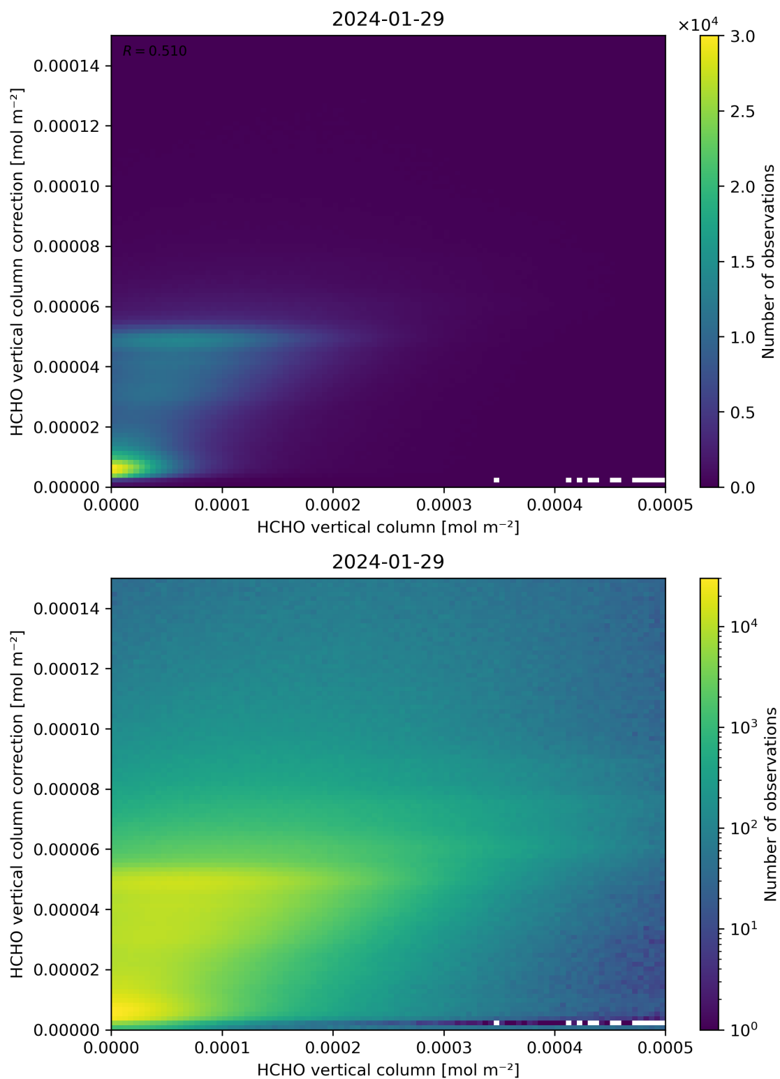
Figure 133: Scatter density plot of “HCHO vertical column” against “HCHO vertical column correction” for 2024-01-28 to 2024-01-30.
