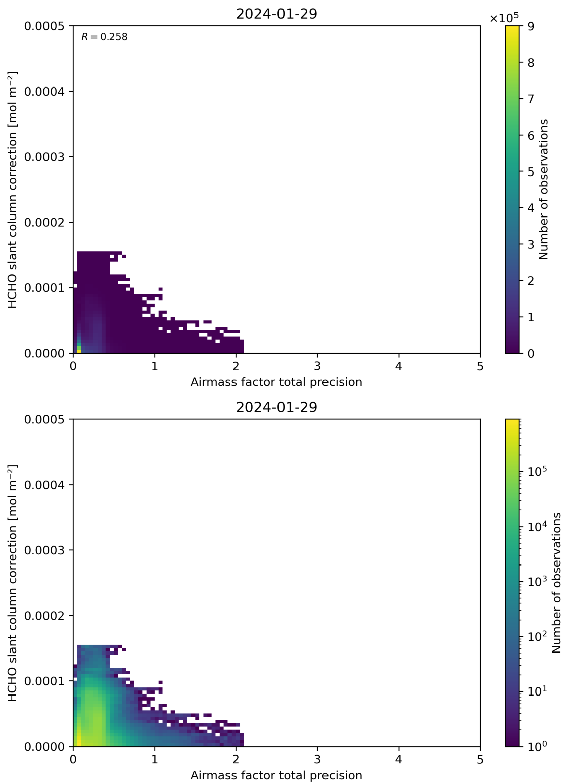
Figure 110: Scatter density plot of “Airmass factor total precision” against “HCHO slant column correction” for 2024-01-28 to 2024-01-30.
