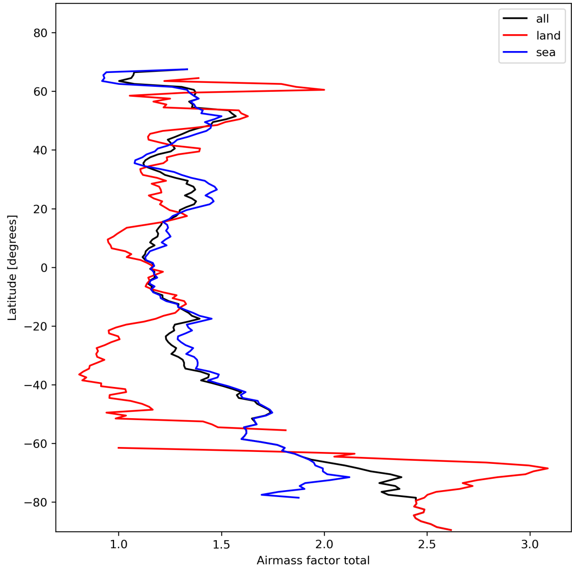
Figure 26: Zonal average of “Airmass factor total” for 2024-01-28 to 2024-01-30.
