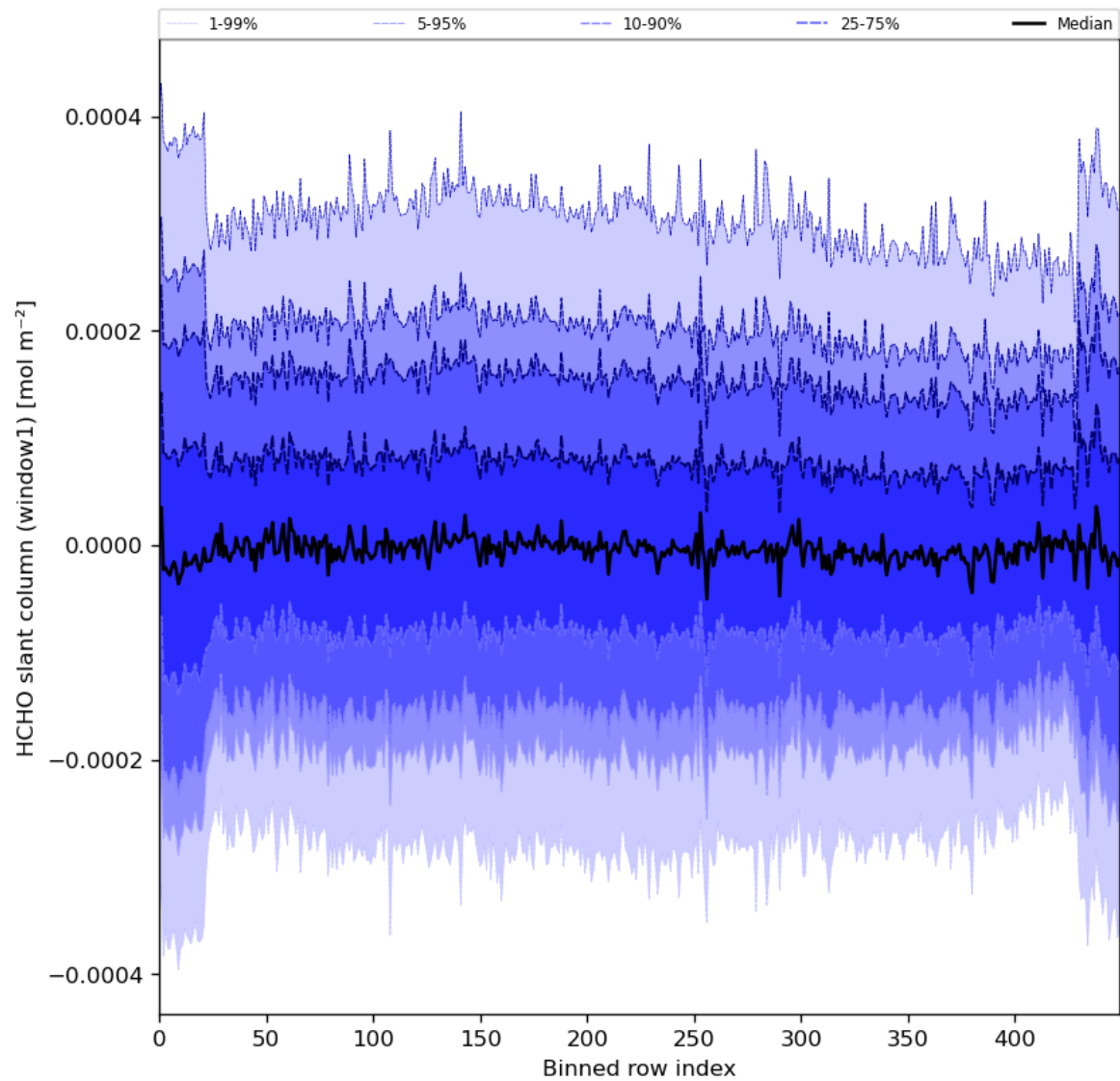
Figure 52: Along track statistics of “HCHO slant column (window1)” for 2024-01-28 to 2024-01-30
