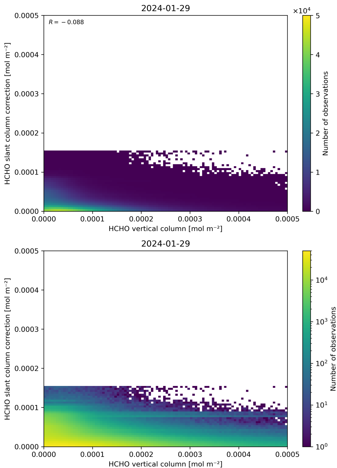
Figure 128: Scatter density plot of “HCHO vertical column” against “HCHO slant column correction” for 2024-01-28 to 2024-01-30.
