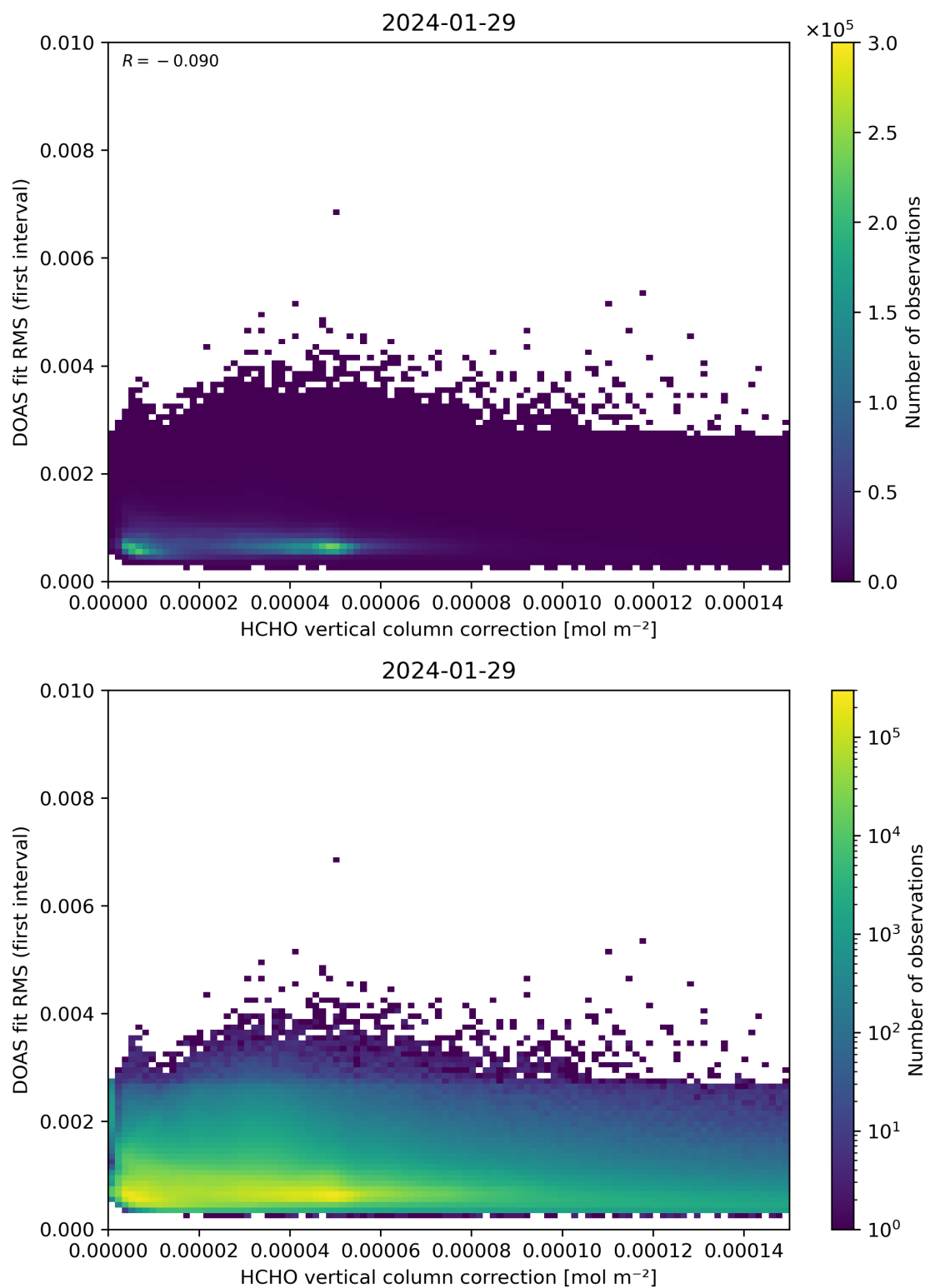
Figure 112: Scatter density plot of “HCHO vertical column correction” against “DOAS fit RMS (first interval)” for 2024-01-28 to 2024-01-30.
