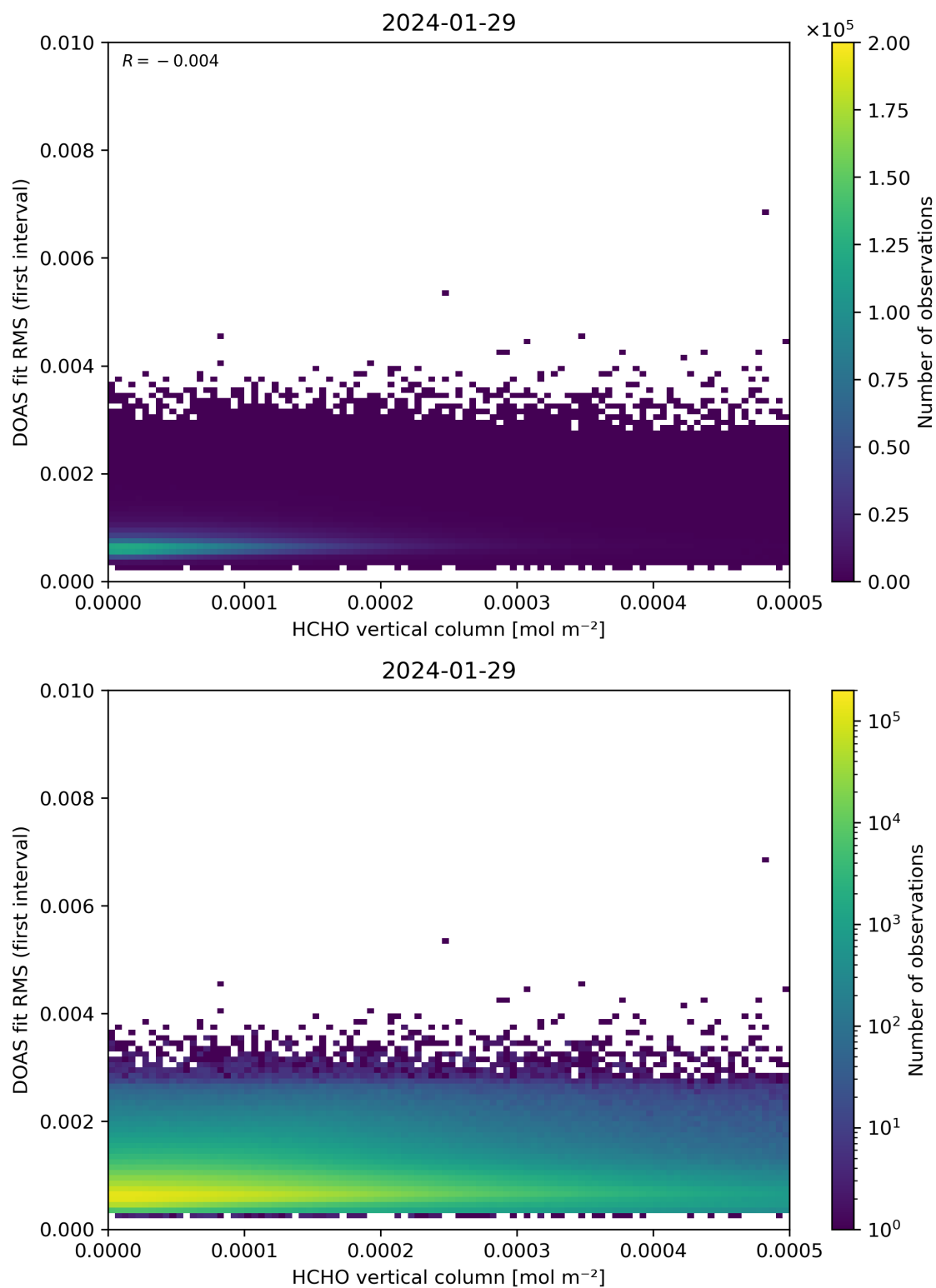
Figure 123: Scatter density plot of “HCHO vertical column” against “DOAS fit RMS (first interval)” for 2024-01-28 to 2024-01-30.
