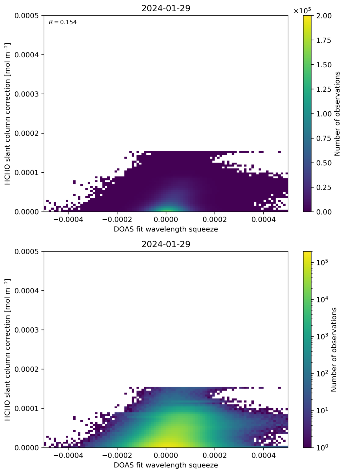
Figure 70: Scatter density plot of “DOAS fit wavelength squeeze” against “HCHO slant column correction” for 2024-01-28 to 2024-01-30.
