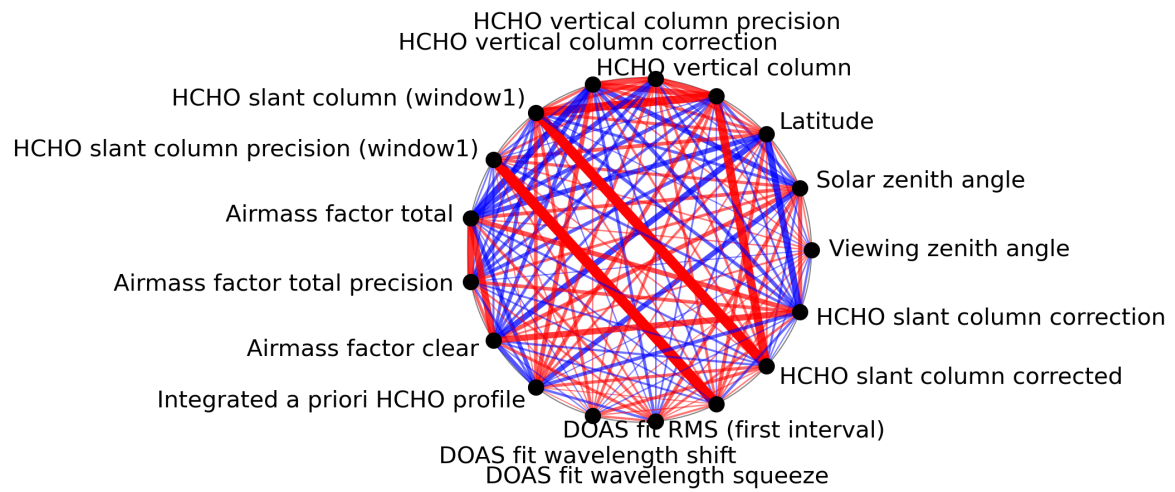
Figure 1: Map of correlation graph for 2024-01-28 to 2024-01-30.
