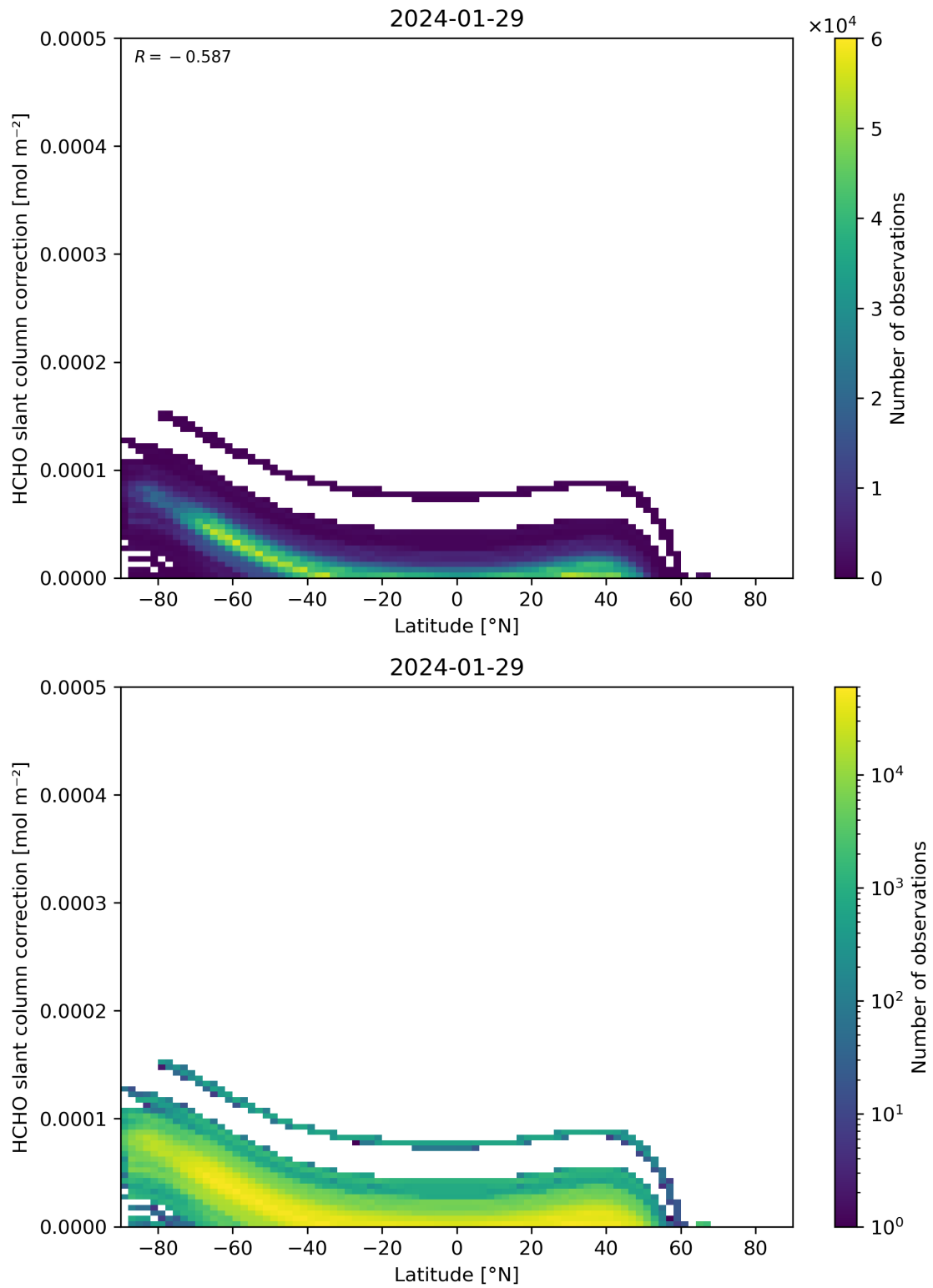
Figure 158: Scatter density plot of “Latitude” against “HCHO slant column correction” for 2024-01-28 to 2024-01-30.
