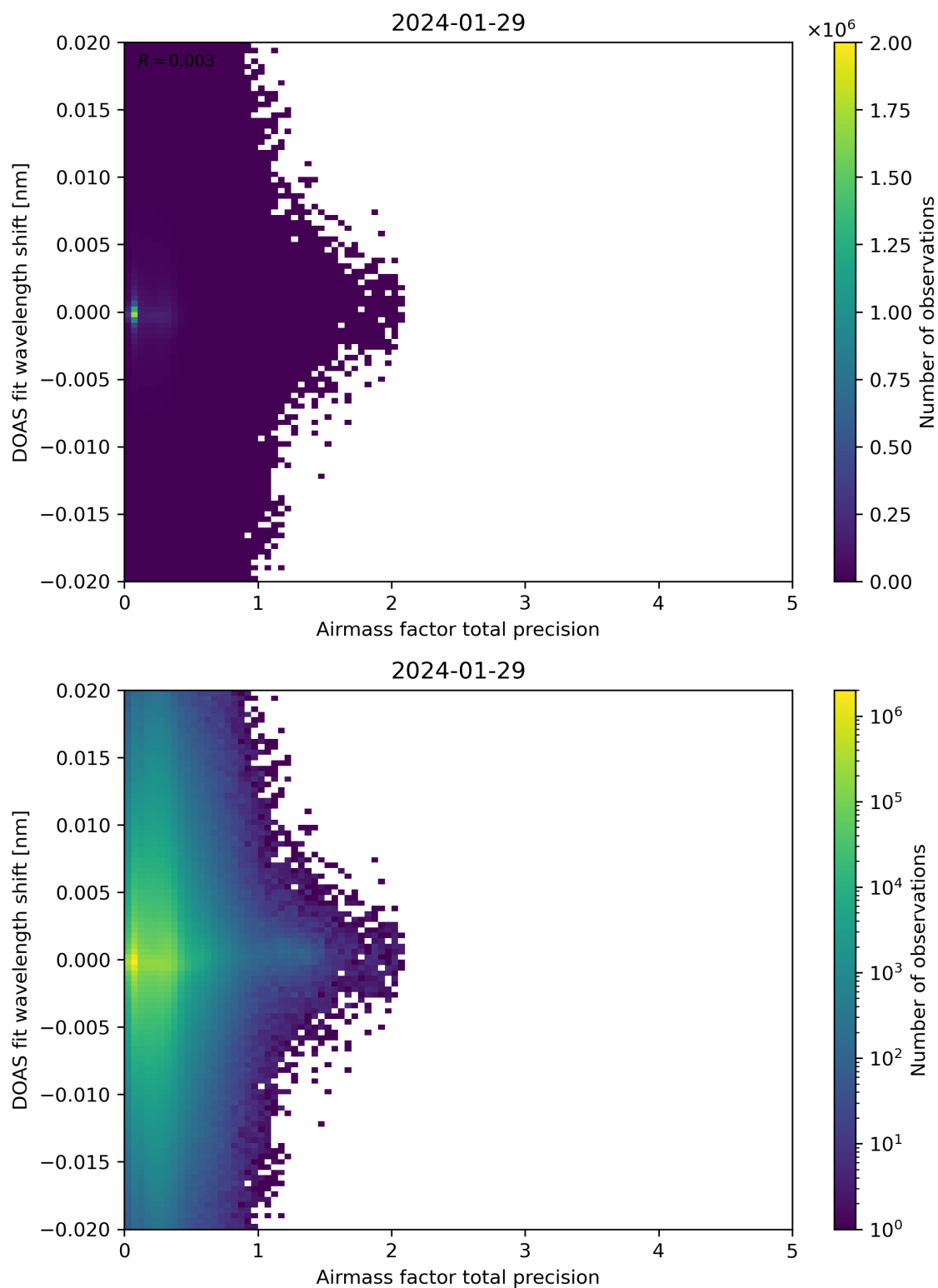
Figure 106: Scatter density plot of “Airmass factor total precision” against “DOAS fit wavelength shift” for 2024-01-28 to 2024-01-30.
