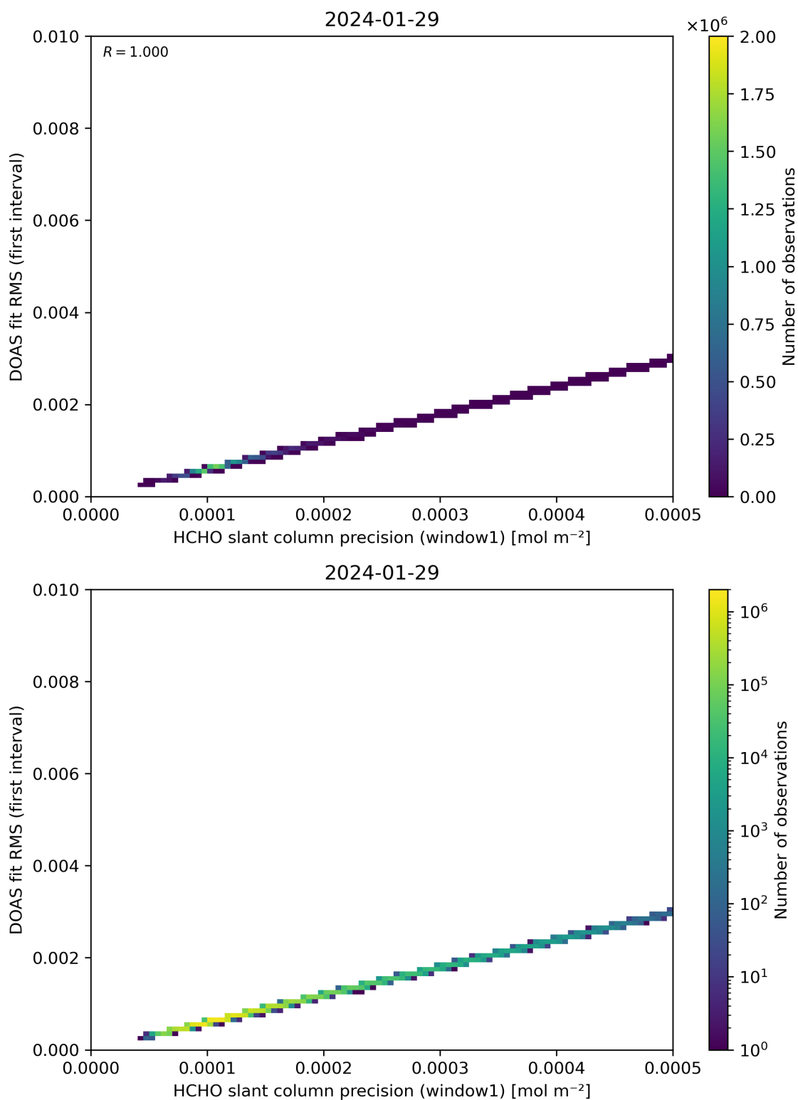
Figure 88: Scatter density plot of “HCHO slant column precision (window1)” against “DOAS fit RMS (first interval)” for 2024-01-28 to 2024-01-30.
