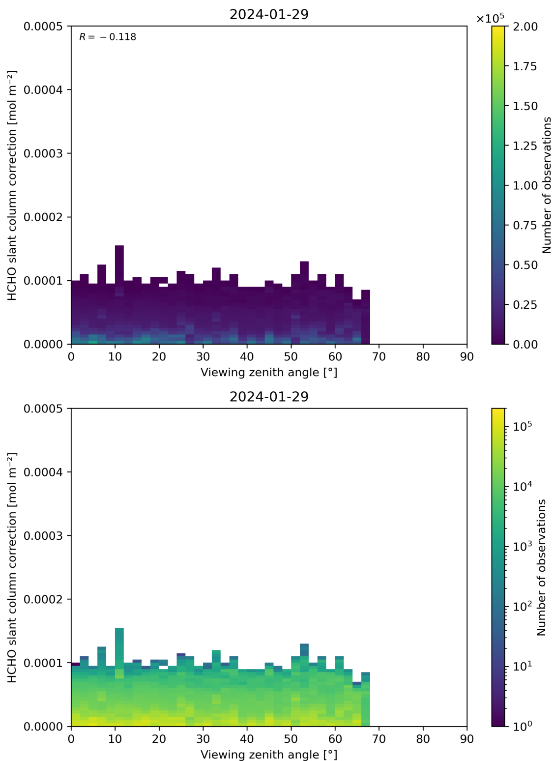
Figure 187: Scatter density plot of “Viewing zenith angle” against “HCHO slant column correction” for 2024-01-28 to 2024-01-30.
