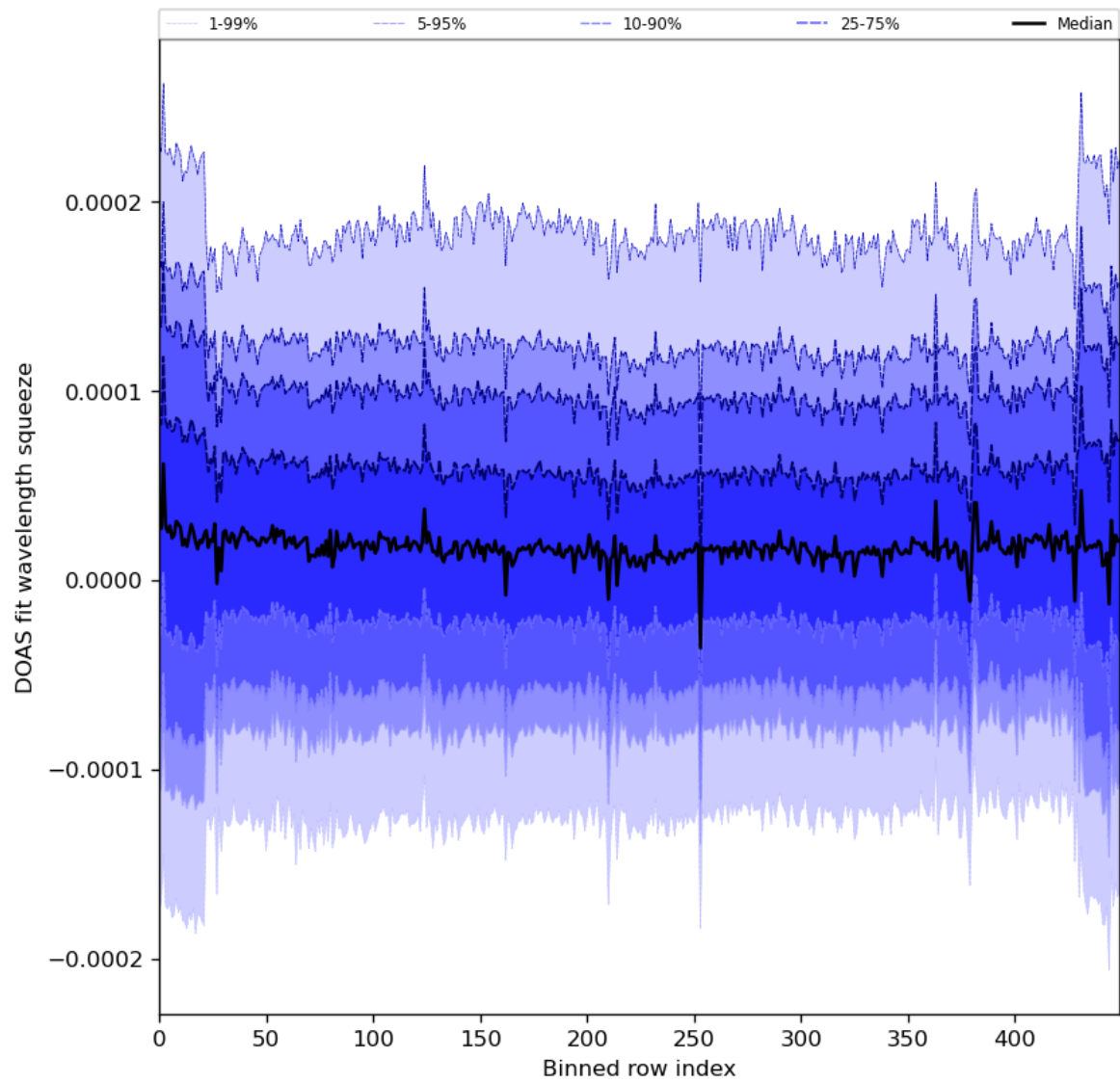
Figure 59: Along track statistics of “DOAS fit wavelength squeeze” for 2024-01-28 to 2024-01-30
