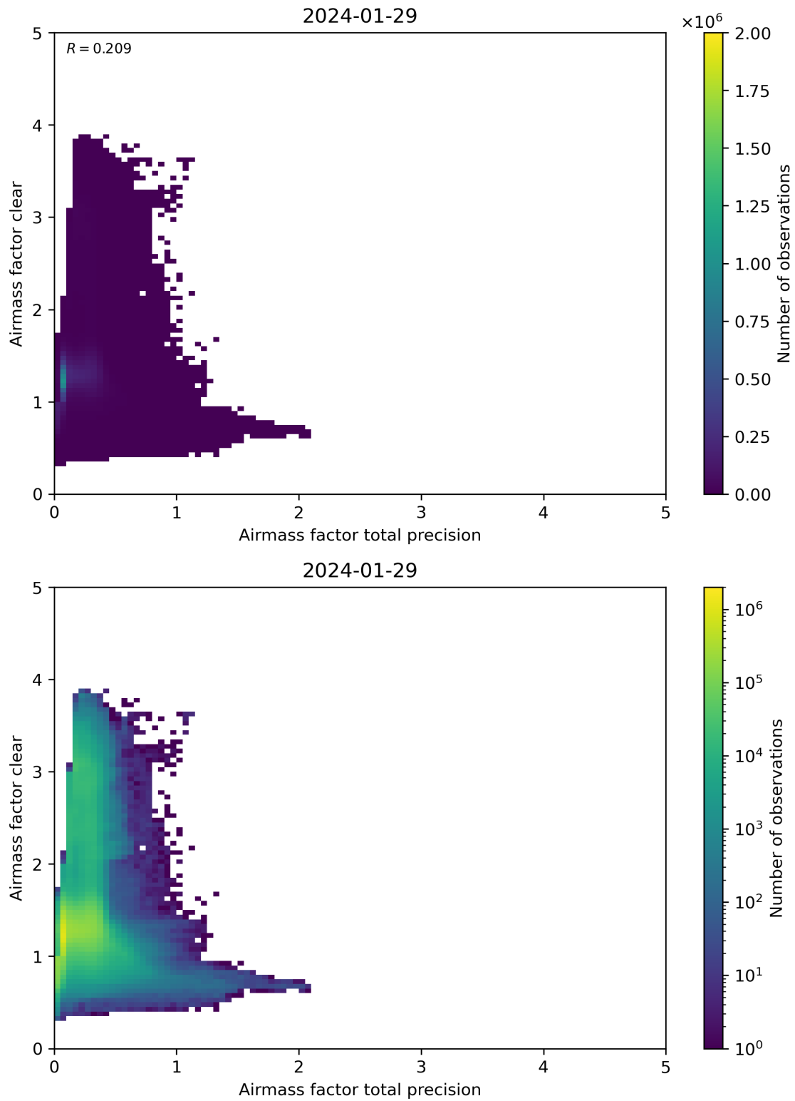
Figure 108: Scatter density plot of “Airmass factor total precision” against “Airmass factor clear” for 2024-01-28 to 2024-01-30.
