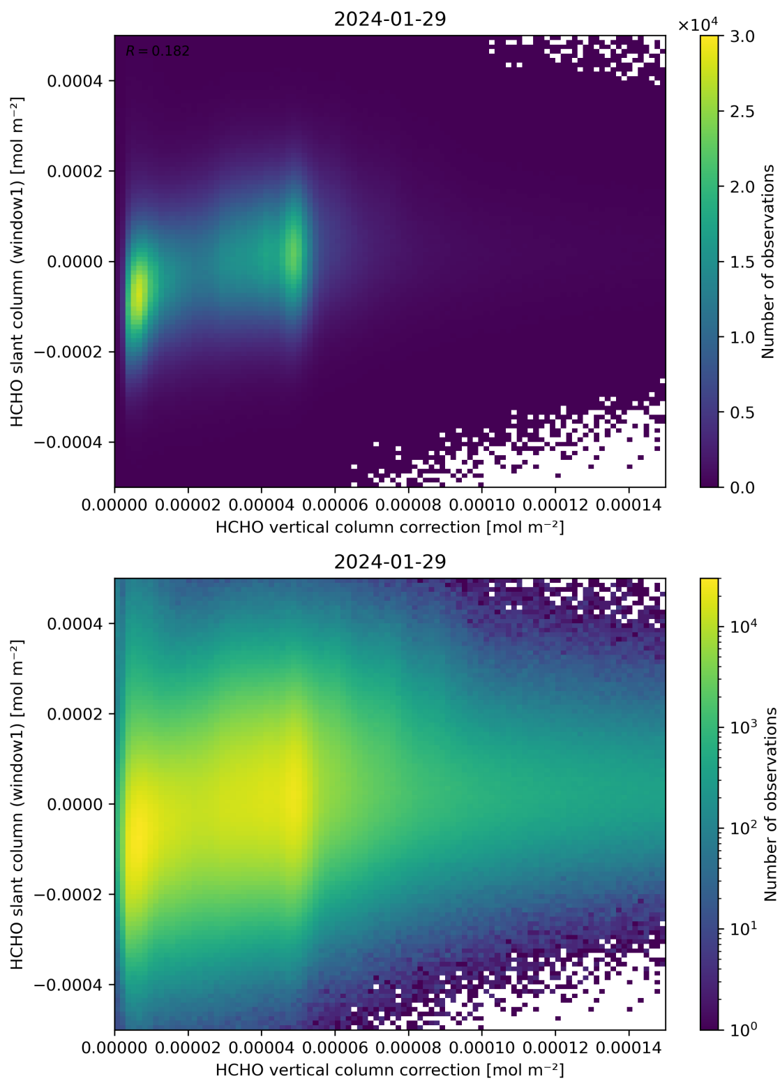
Figure 118: Scatter density plot of “HCHO vertical column correction” against “HCHO slant column (window1)” for 2024-01-28 to 2024-01-30.
