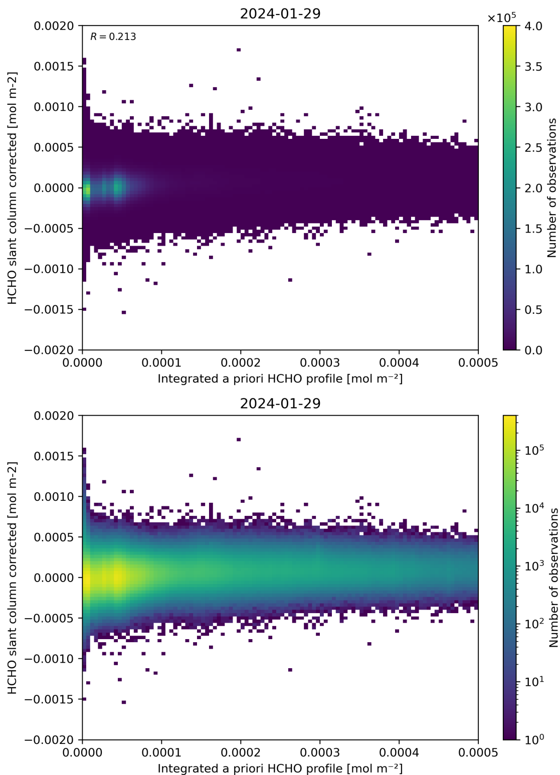
Figure 151: Scatter density plot of “Integrated a priori HCHO profile” against “HCHO slant column corrected” for 2024-01-28 to 2024-01-30.
