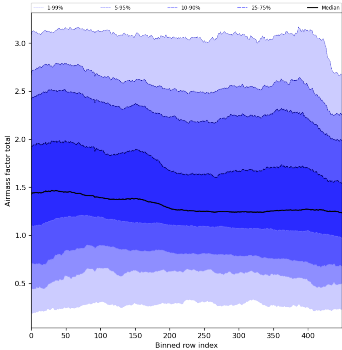
Figure 54: Along track statistics of “Airmass factor total” for 2024-01-28 to 2024-01-30
