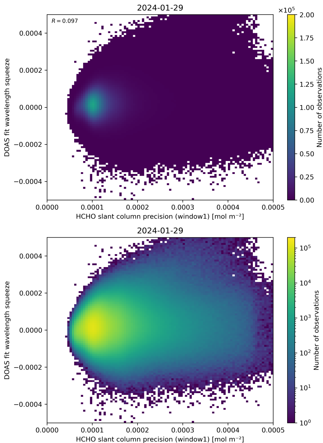
Figure 90: Scatter density plot of “HCHO slant column precision (window1)” against “DOAS fit wavelength squeeze” for 2024-01-28 to 2024-01-30.
