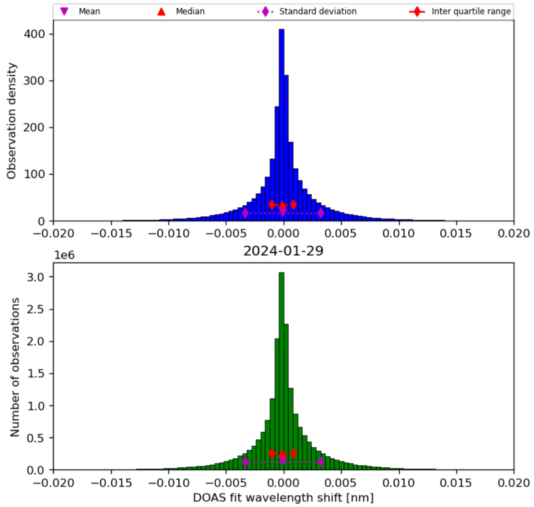
Figure 44: Histogram of “DOAS fit wavelength shift” for 2024-01-28 to 2024-01-30
