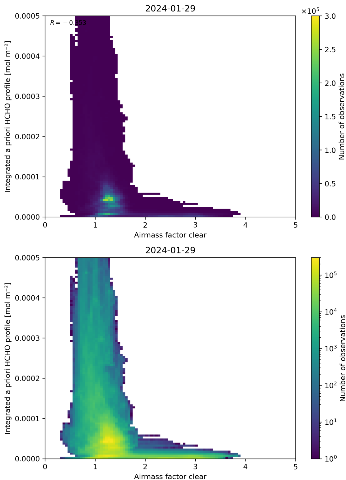
Figure 76: Scatter density plot of “Airmass factor clear” against “Integrated a priori HCHO profile” for 2024-01-28 to 2024-01-30.
