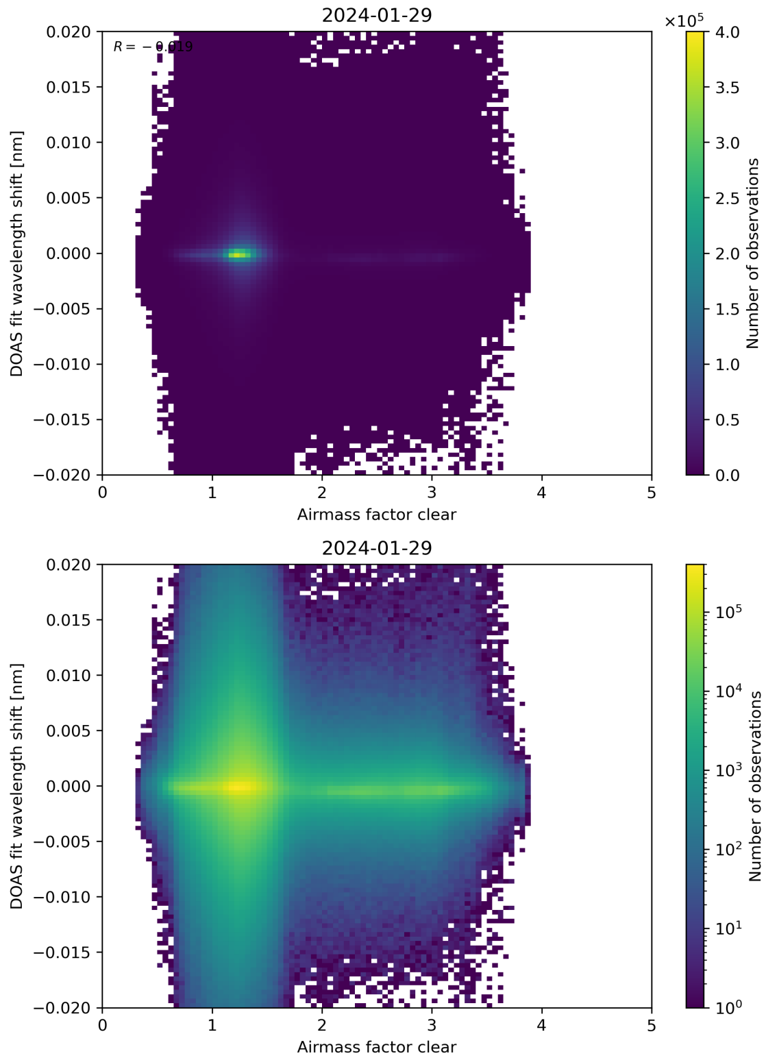
Figure 72: Scatter density plot of “Airmass factor clear” against “DOAS fit wavelength shift” for 2024-01-28 to 2024-01-30.
