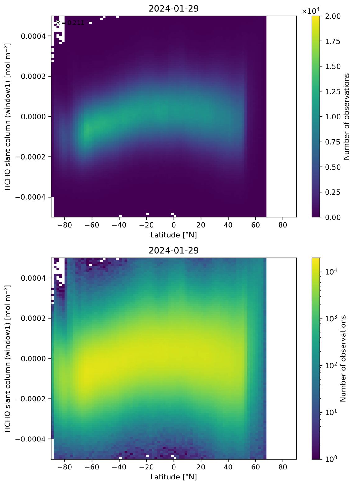
Figure 159: Scatter density plot of “Latitude” against “HCHO slant column (window1)” for 2024-01-28 to 2024-01-30.
