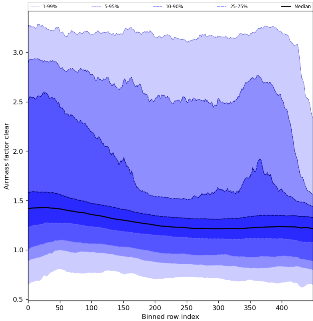
Figure 56: Along track statistics of “Airmass factor clear” for 2024-01-28 to 2024-01-30
