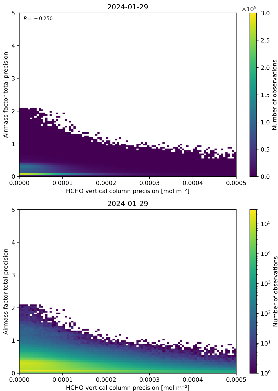
Figure 145: Scatter density plot of “HCHO vertical column precision” against “Airmass factor total precision” for 2024-01-28 to 2024-01-30.
