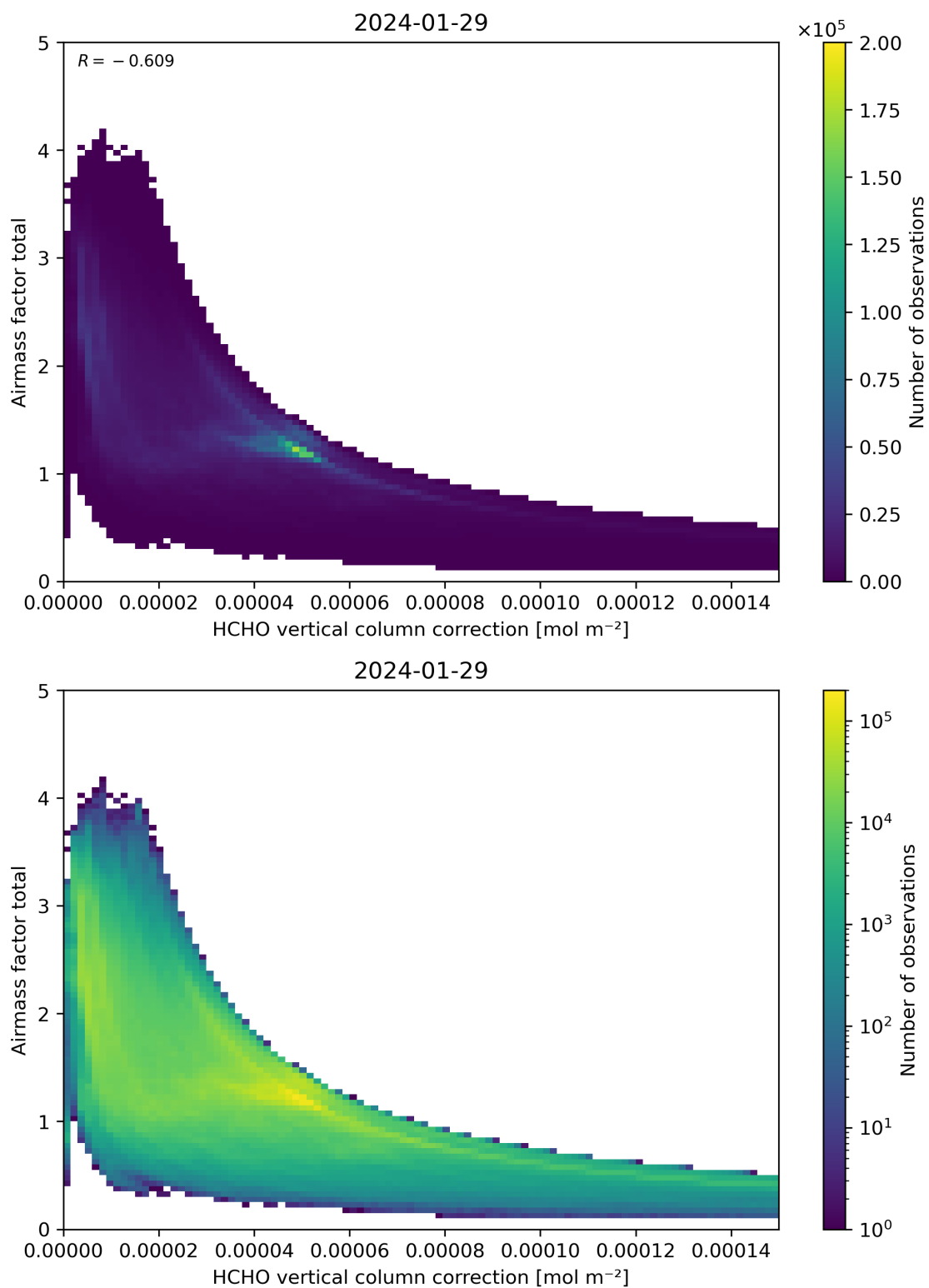
Figure 120: Scatter density plot of “HCHO vertical column correction” against “Airmass factor total” for 2024-01-28 to 2024-01-30.
