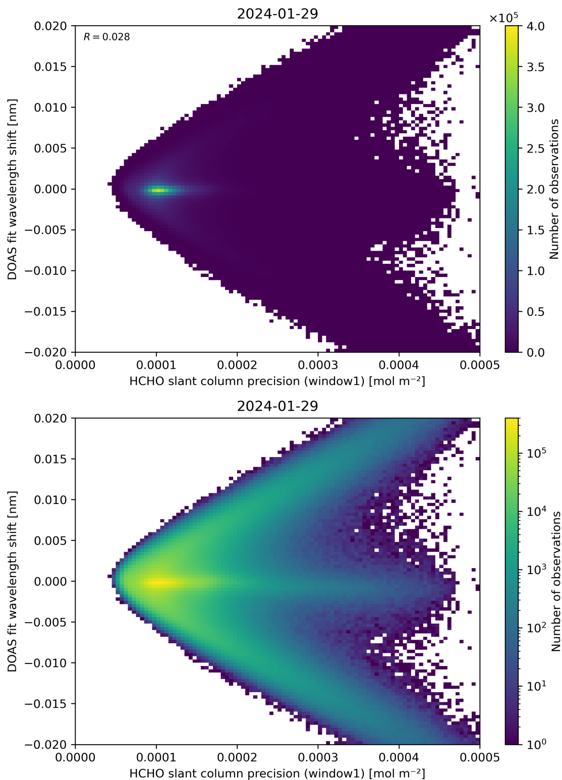
Figure 89: Scatter density plot of “HCHO slant column precision (window1)” against “DOAS fit wavelength shift” for 2024-01-28 to 2024-01-30.
