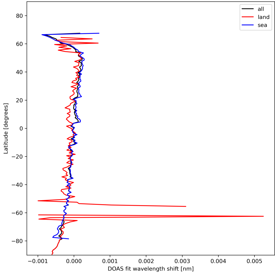
Figure 30: Zonal average of “DOAS fit wavelength shift” for 2024-01-28 to 2024-01-30.
