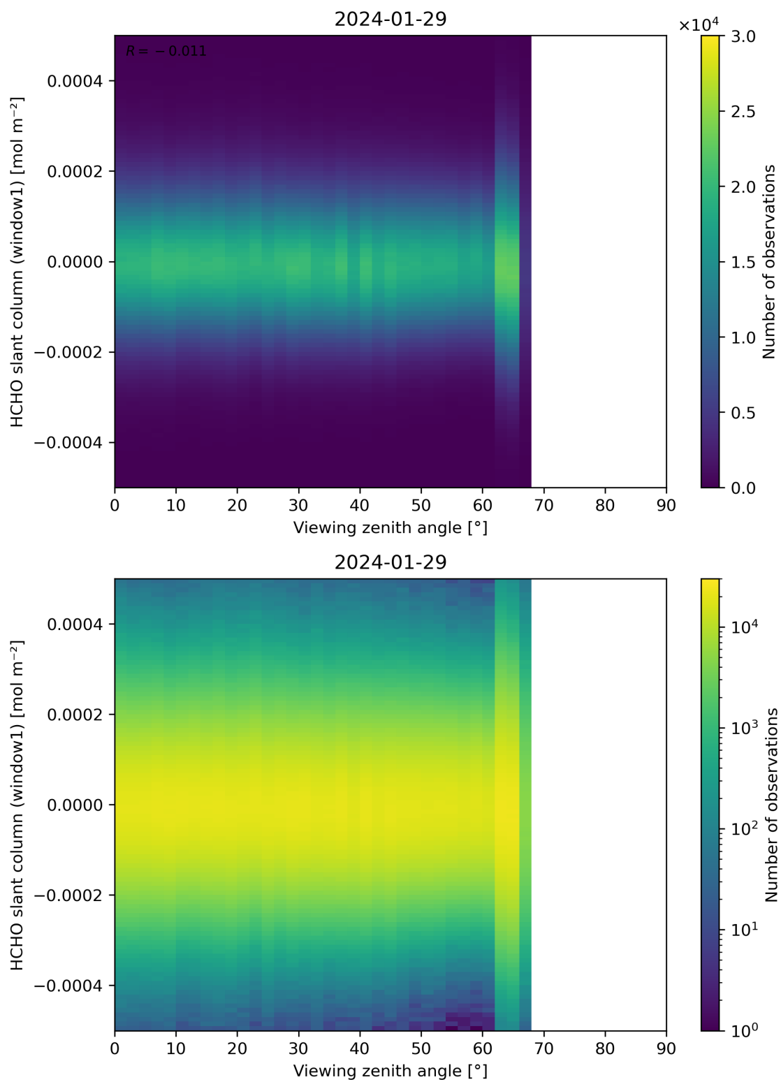
Figure 188: Scatter density plot of “Viewing zenith angle” against “HCHO slant column (window1)” for 2024-01-28 to 2024-01-30.
