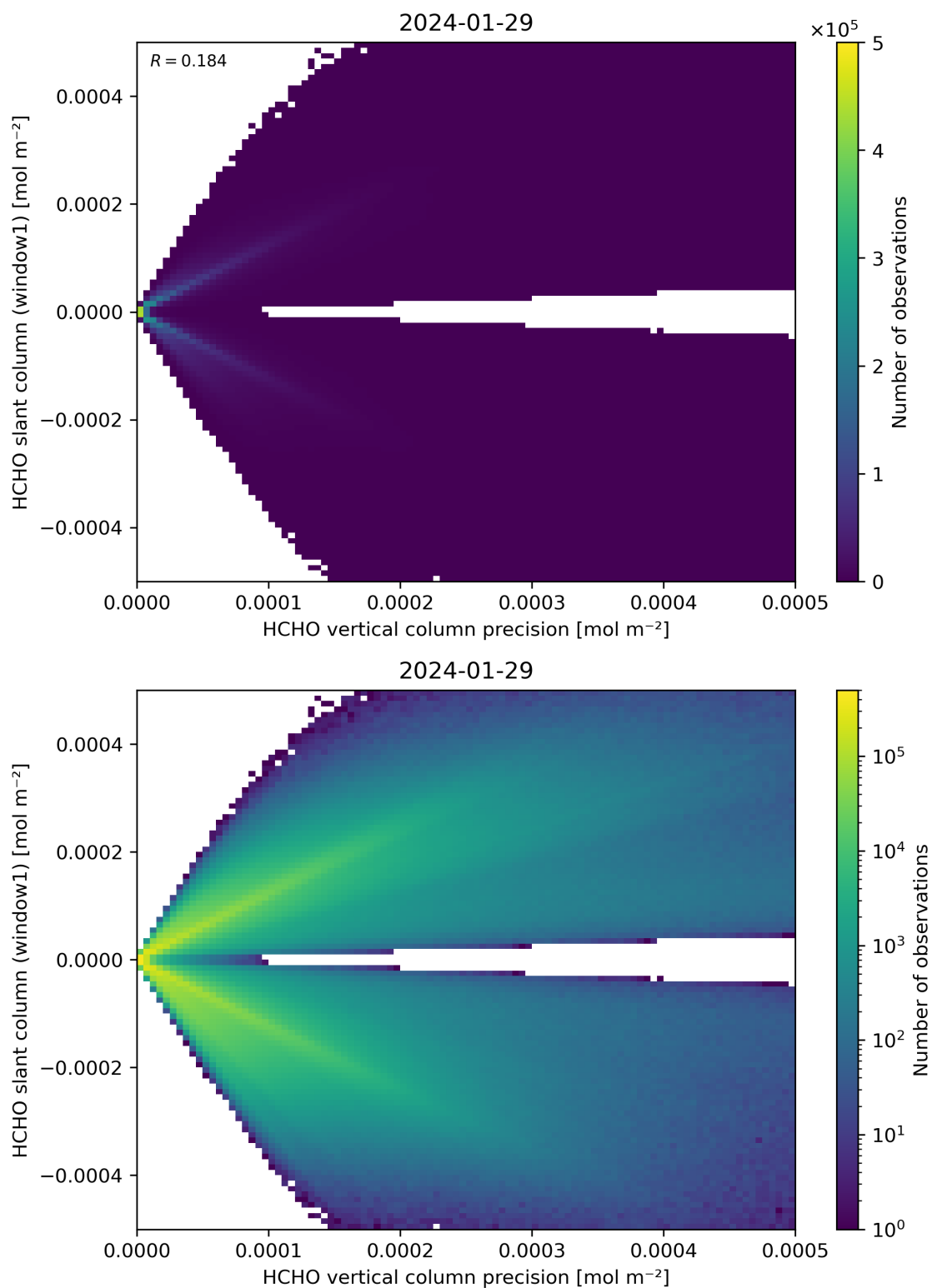
Figure 142: Scatter density plot of “HCHO vertical column precision” against “HCHO slant column (window1)” for 2024-01-28 to 2024-01-30.
