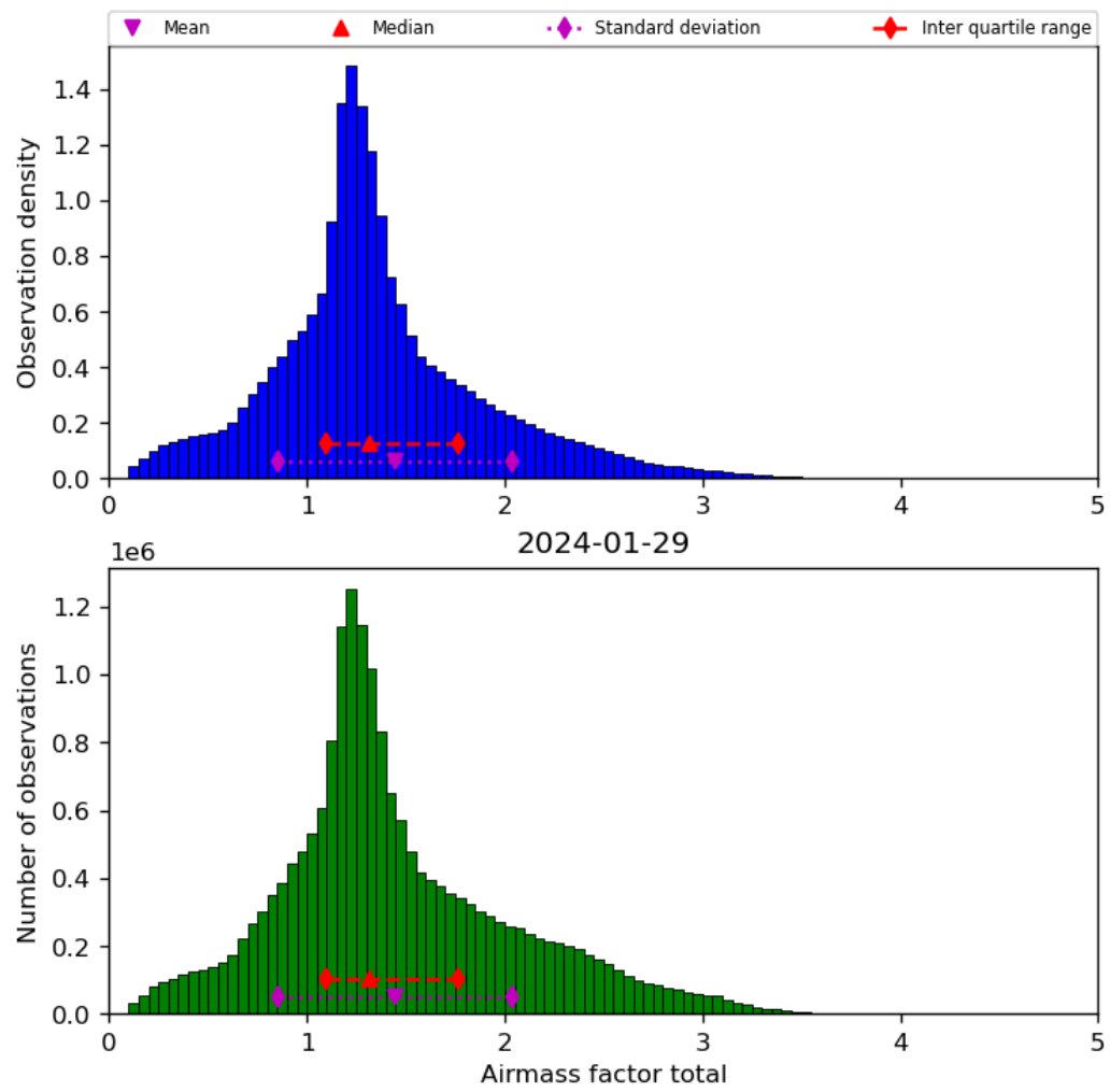
Figure 40: Histogram of “Airmass factor total” for 2024-01-28 to 2024-01-30
