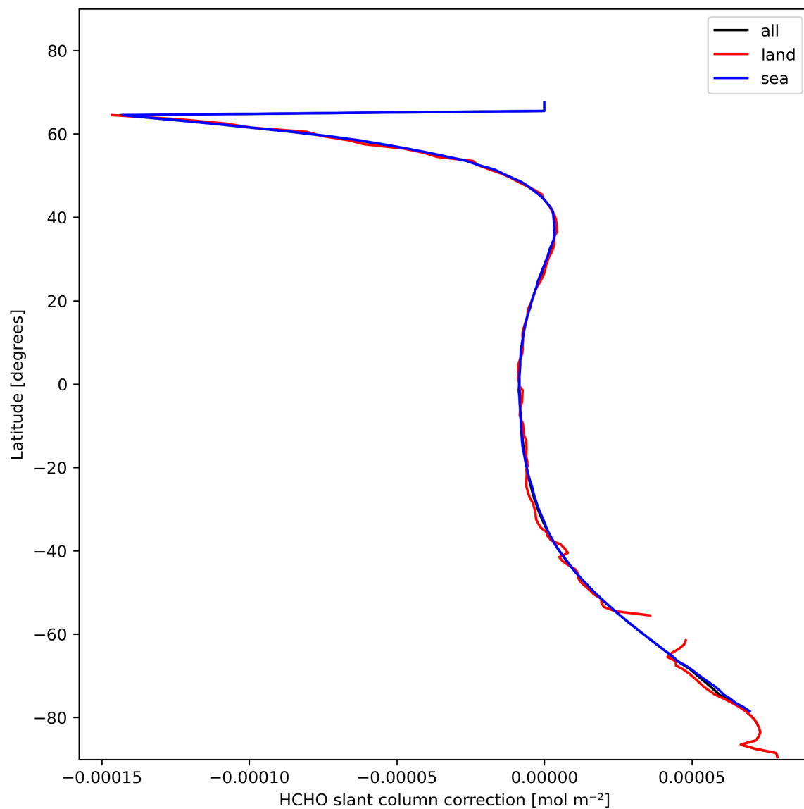
Figure 33: Zonal average of “HCHO slant column correction” for 2024-01-28 to 2024-01-30.
