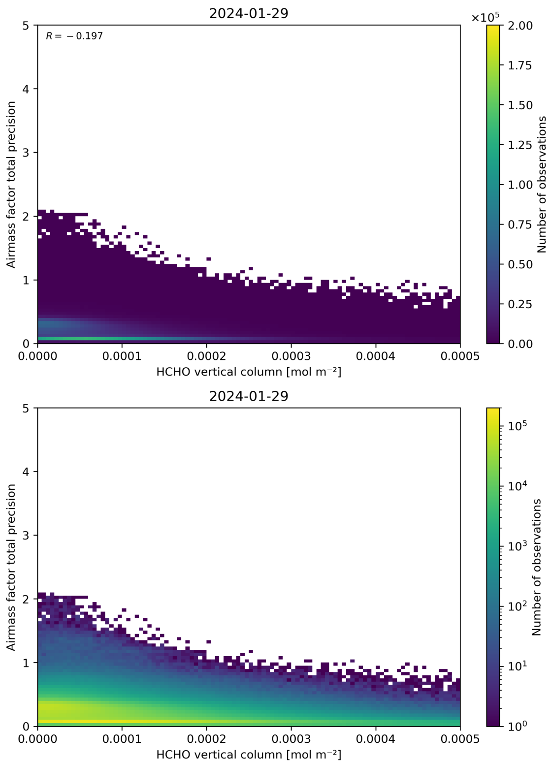
Figure 132: Scatter density plot of “HCHO vertical column” against “Airmass factor total precision” for 2024-01-28 to 2024-01-30.
