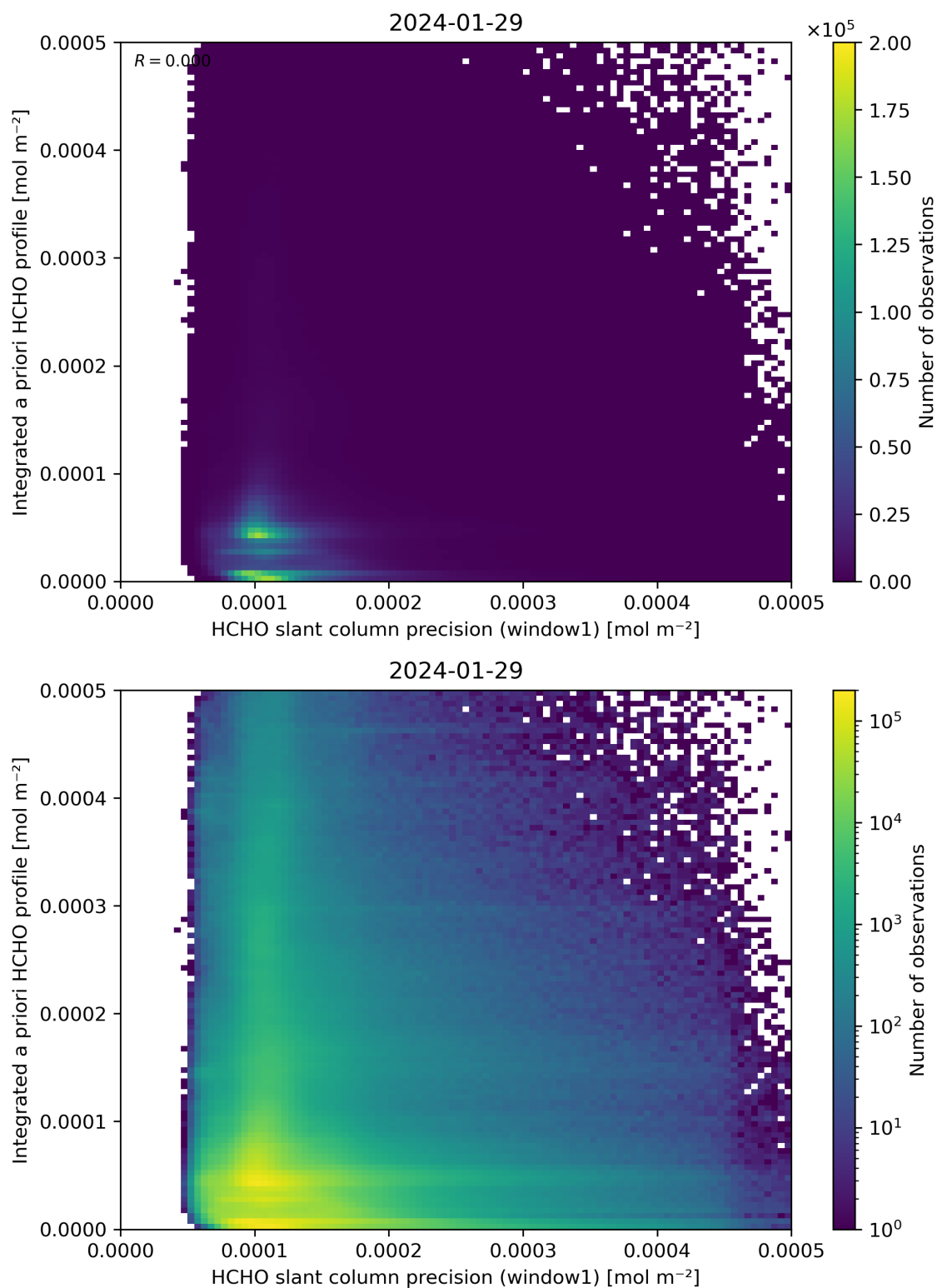
Figure 96: Scatter density plot of “HCHO slant column precision (window1)” against “Integrated a priori HCHO profile” for 2024-01-28 to 2024-01-30.
