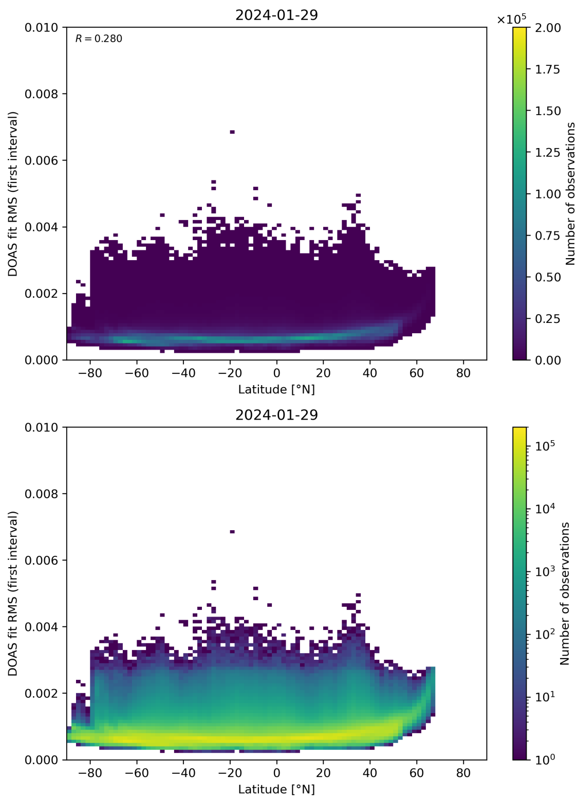
Figure 153: Scatter density plot of “Latitude” against “DOAS fit RMS (first interval)” for 2024-01-28 to 2024-01-30.
