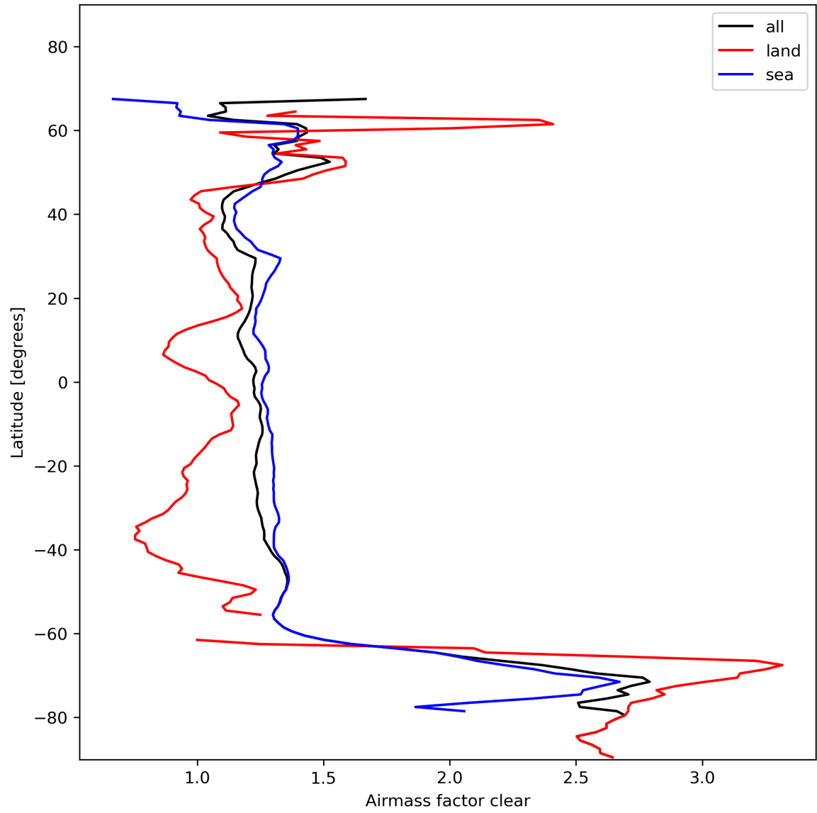
Figure 28: Zonal average of “Airmass factor clear” for 2024-01-28 to 2024-01-30.
