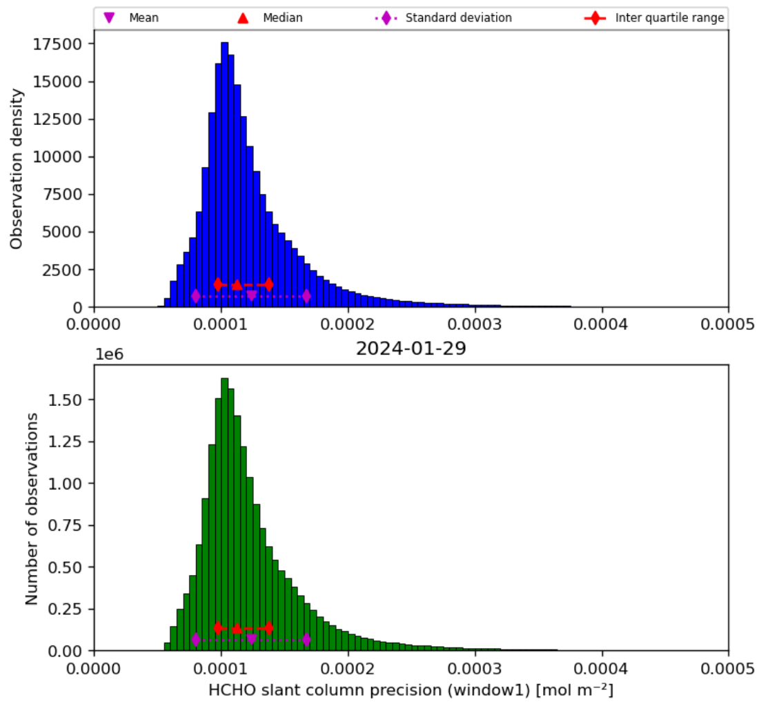
Figure 39: Histogram of “HCHO slant column precision (window1)” for 2024-01-28 to 2024-01-30
