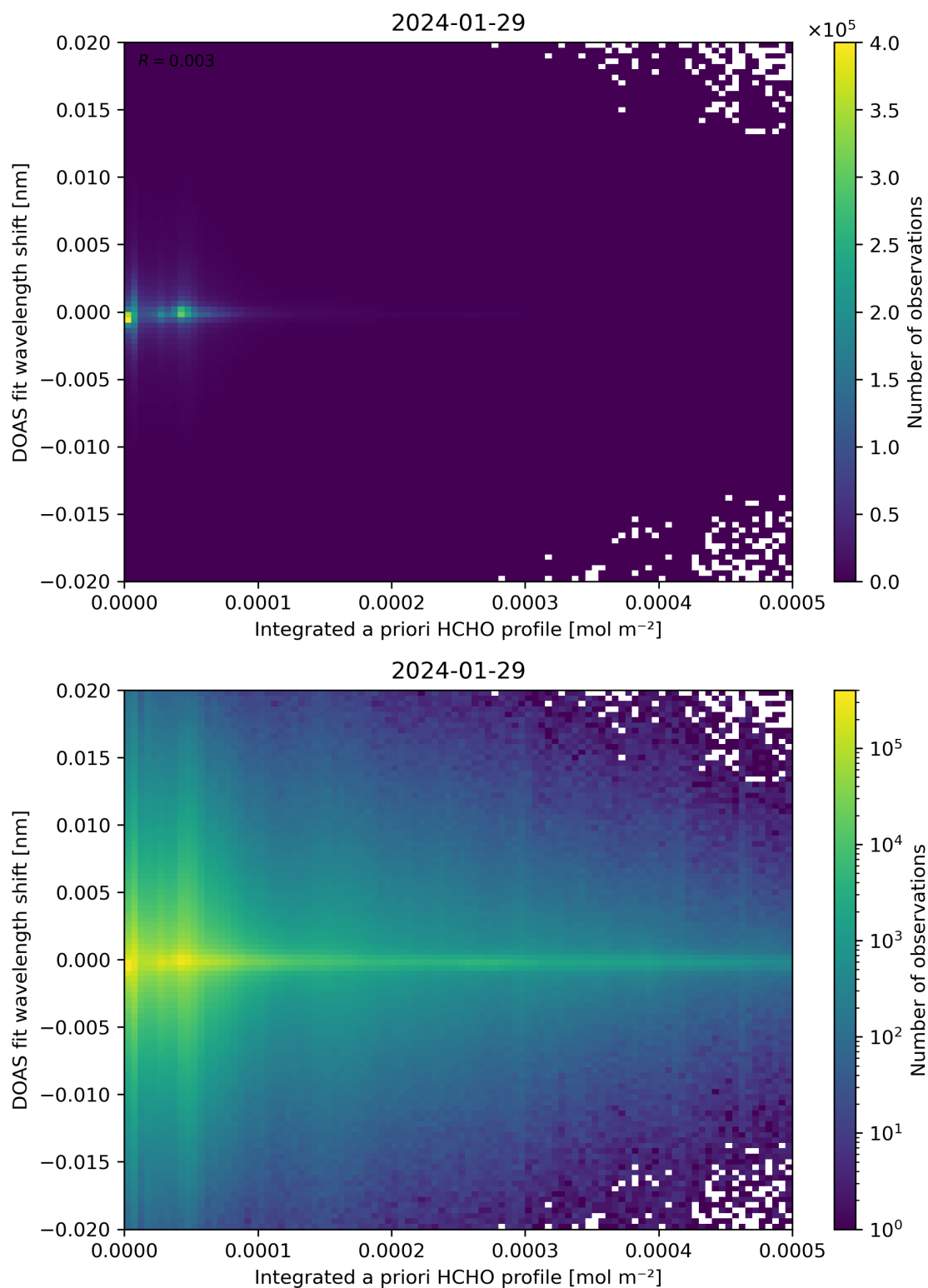
Figure 149: Scatter density plot of “Integrated a priori HCHO profile” against “DOAS fit wavelength shift” for 2024-01-28 to 2024-01-30.
