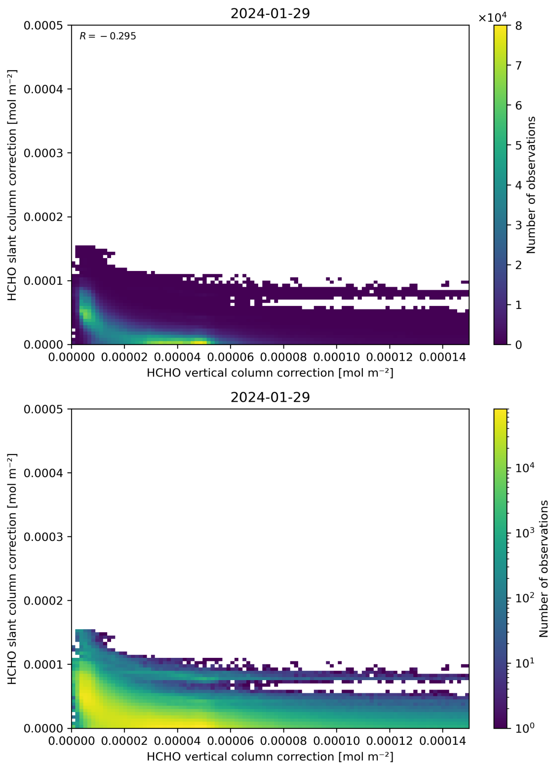
Figure 117: Scatter density plot of “HCHO vertical column correction” against “HCHO slant column correction” for 2024-01-28 to 2024-01-30.
