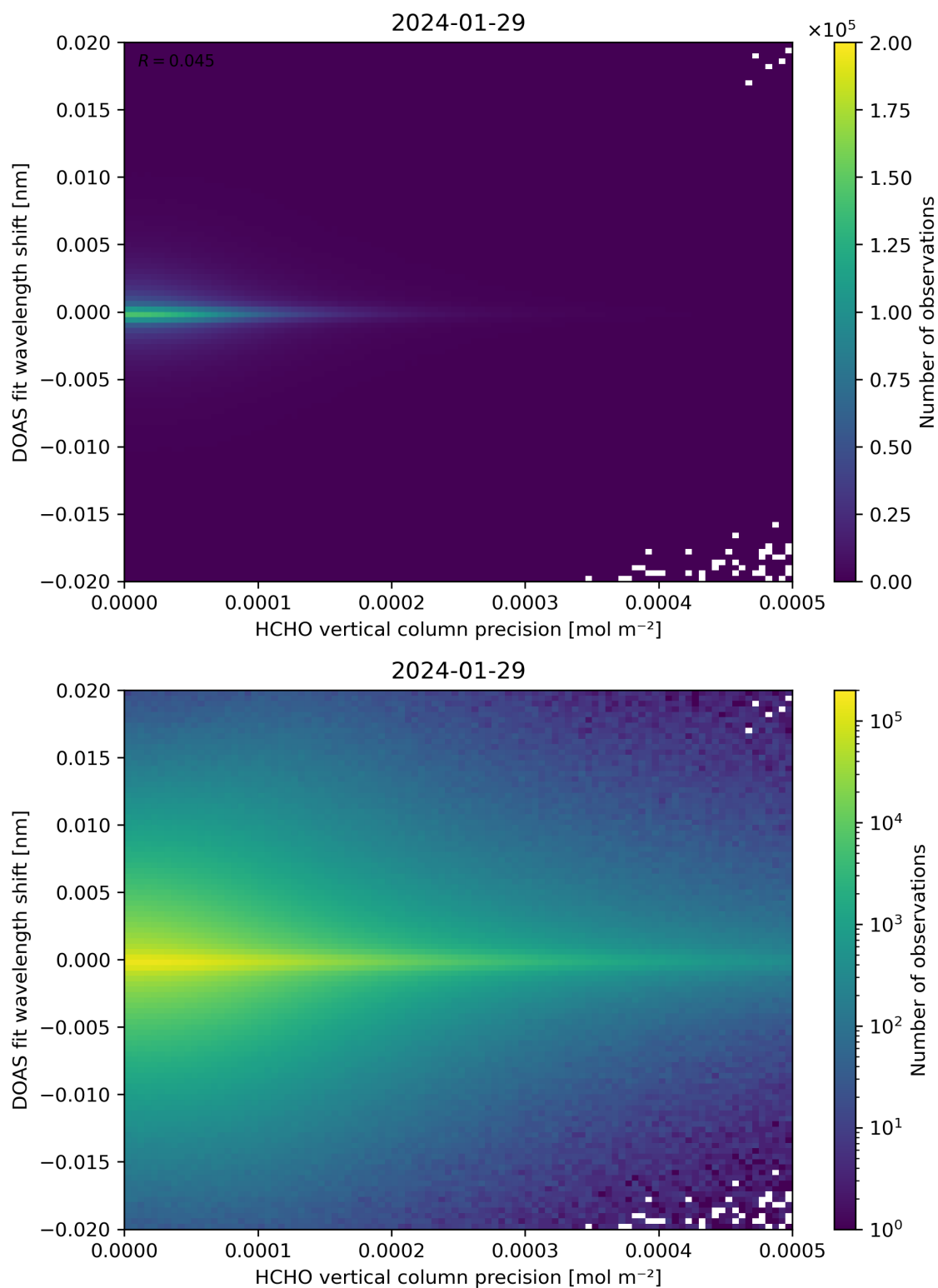
Figure 137: Scatter density plot of “HCHO vertical column precision” against “DOAS fit wavelength shift” for 2024-01-28 to 2024-01-30.
