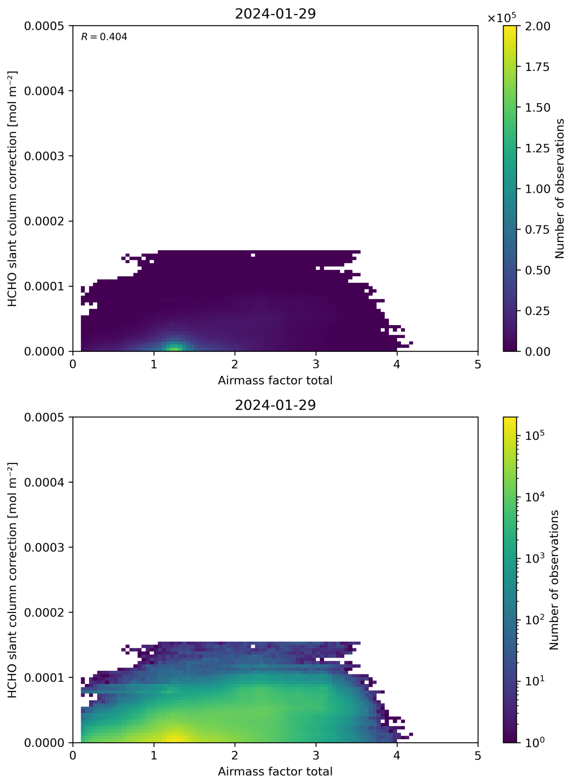
Figure 102: Scatter density plot of “Airmass factor total” against “HCHO slant column correction” for 2024-01-28 to 2024-01-30.
