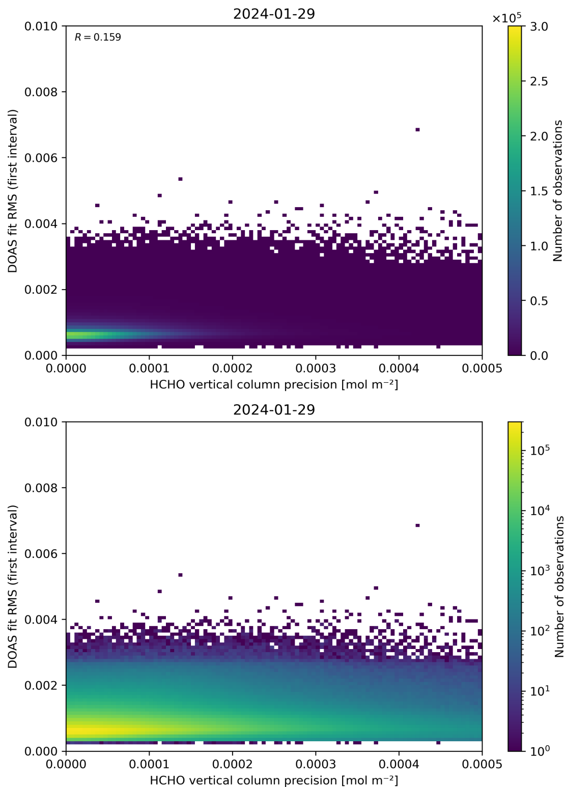
Figure 136: Scatter density plot of “HCHO vertical column precision” against “DOAS fit RMS (first interval)” for 2024-01-28 to 2024-01-30.
