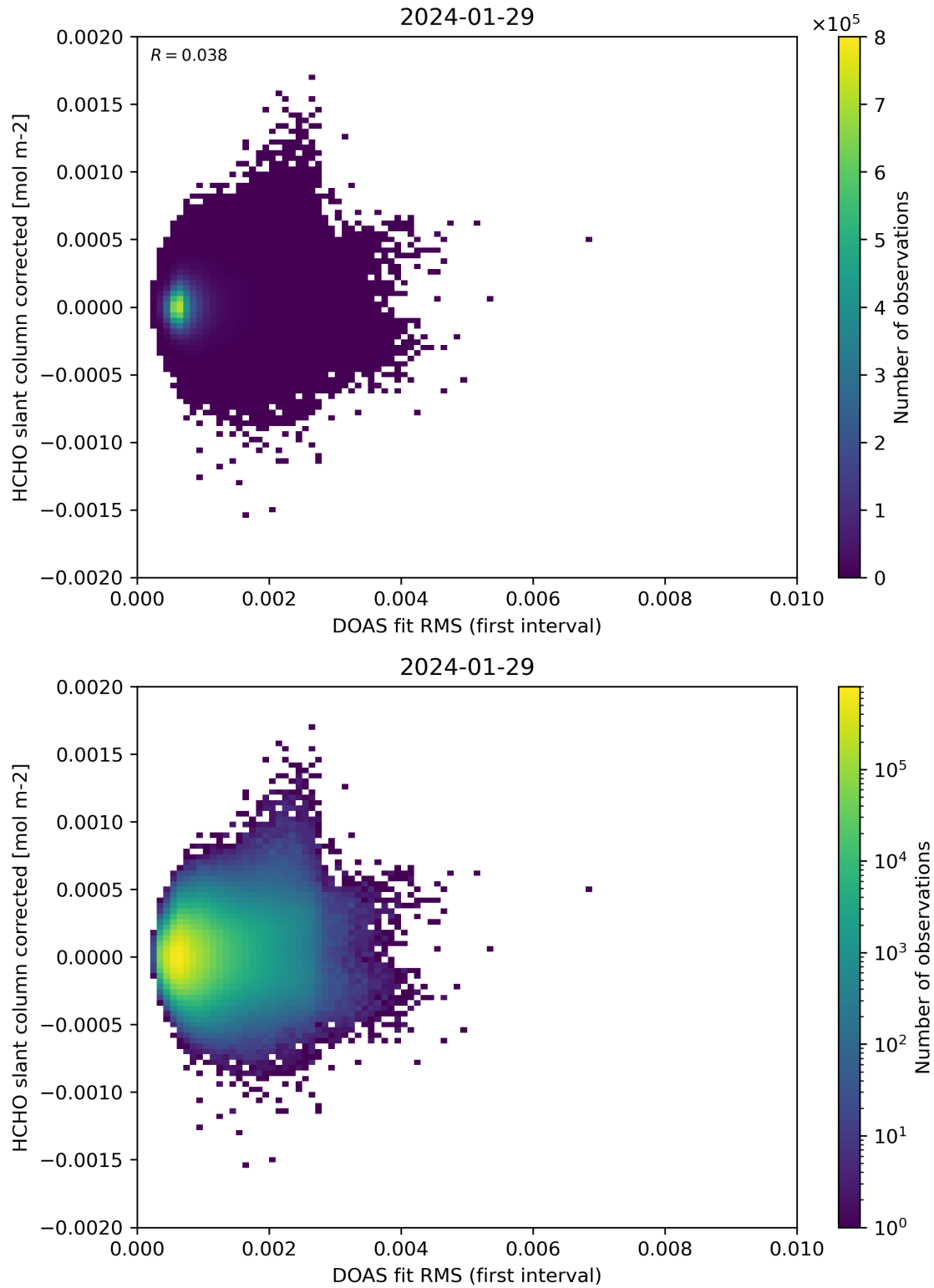
Figure 62: Scatter density plot of “DOAS fit RMS (first interval)” against “HCHO slant column corrected” for 2024-01-28 to 2024-01-30.
