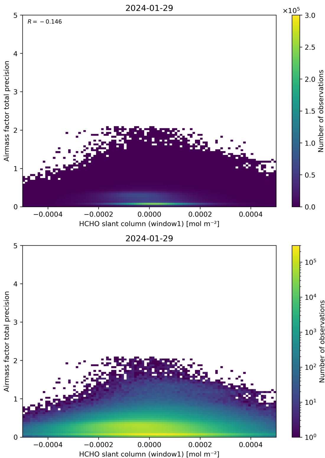
Figure 86: Scatter density plot of “HCHO slant column (window1)” against “Airmass factor total precision” for 2024-01-28 to 2024-01-30.
