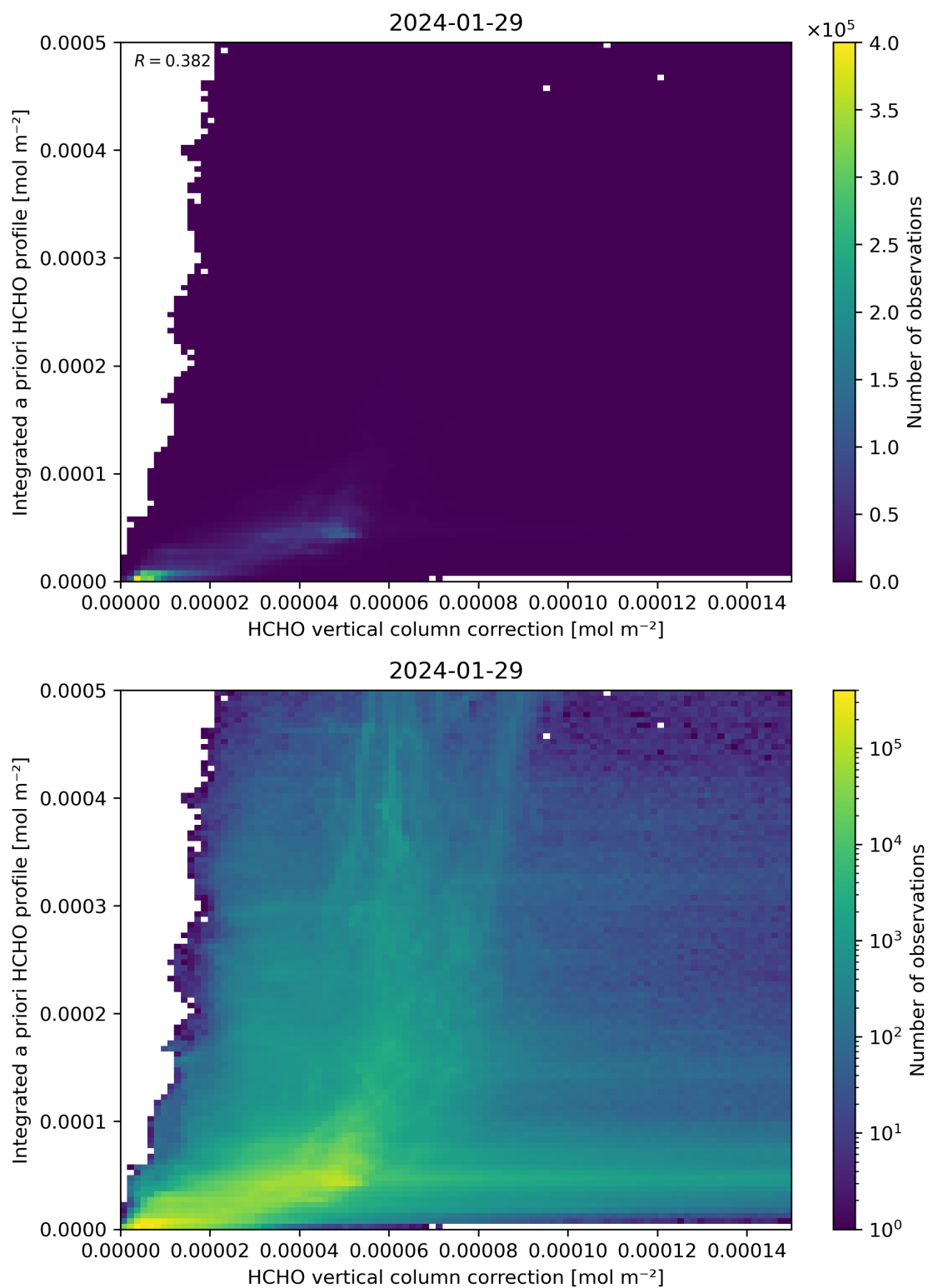
Figure 122: Scatter density plot of “HCHO vertical column correction” against “Integrated a priori HCHO profile” for 2024-01-28 to 2024-01-30.
