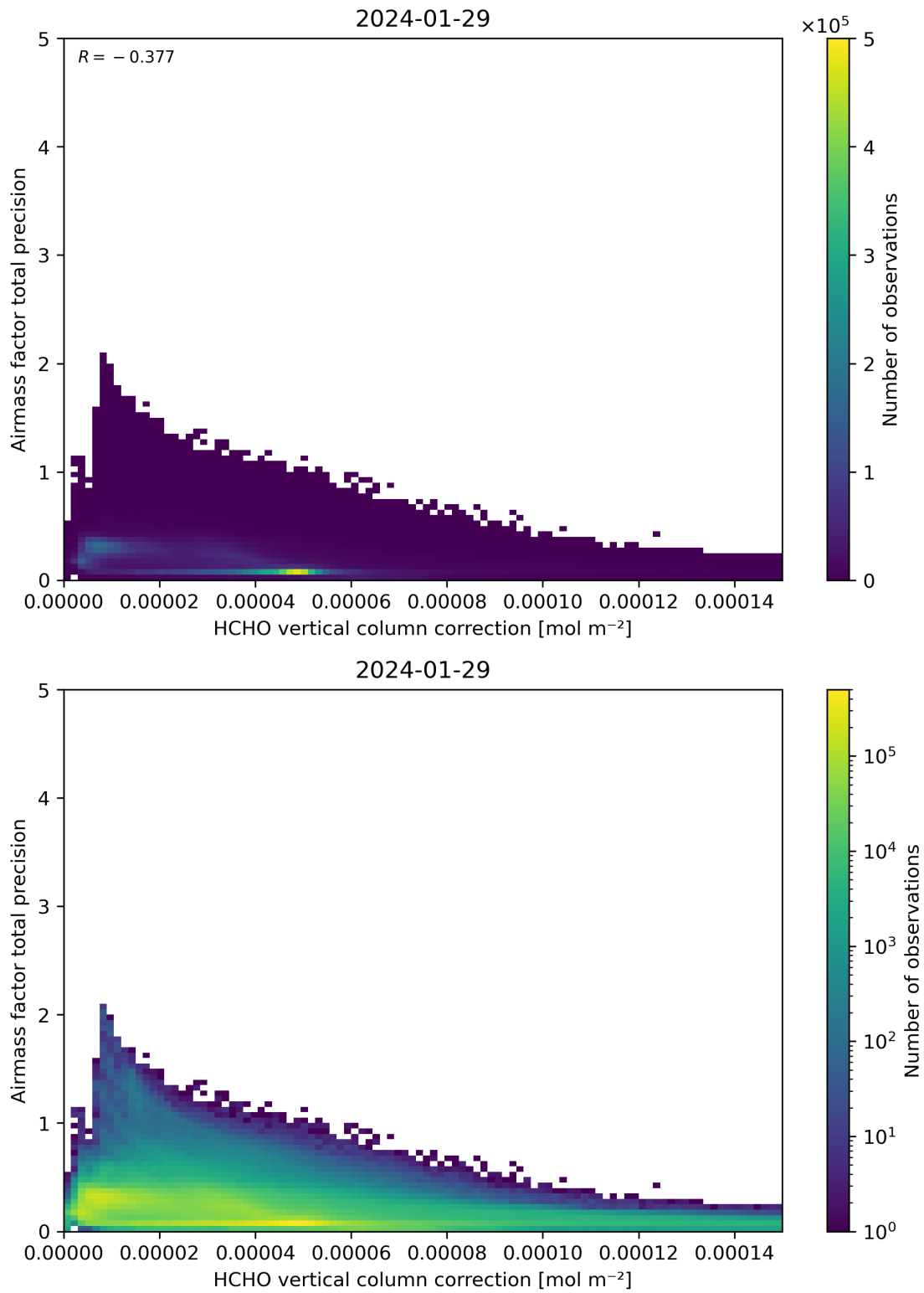
Figure 121: Scatter density plot of “HCHO vertical column correction” against “Airmass factor total precision” for 2024-01-28 to 2024-01-30.
