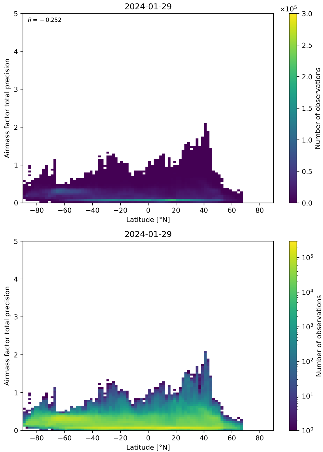
Figure 162: Scatter density plot of “Latitude” against “Airmass factor total precision” for 2024-01-28 to 2024-01-30.
