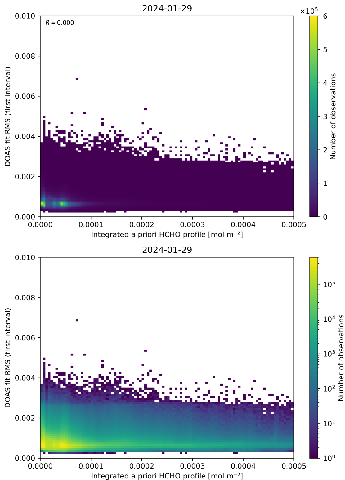
Figure 148: Scatter density plot of “Integrated a priori HCHO profile” against “DOAS fit RMS (first interval)” for 2024-01-28 to 2024-01-30.
