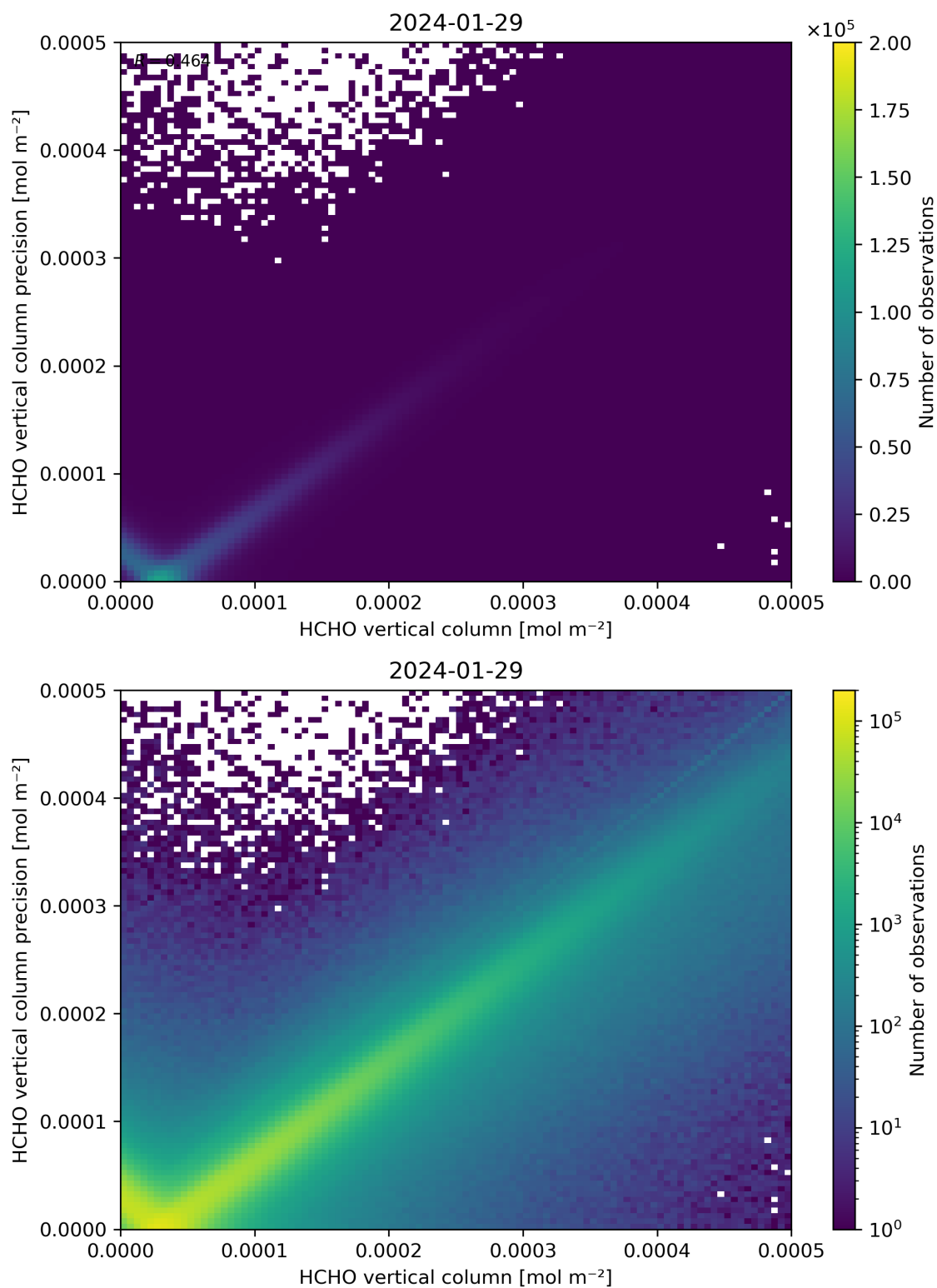
Figure 134: Scatter density plot of “HCHO vertical column” against “HCHO vertical column precision” for 2024-01-28 to 2024-01-30.
