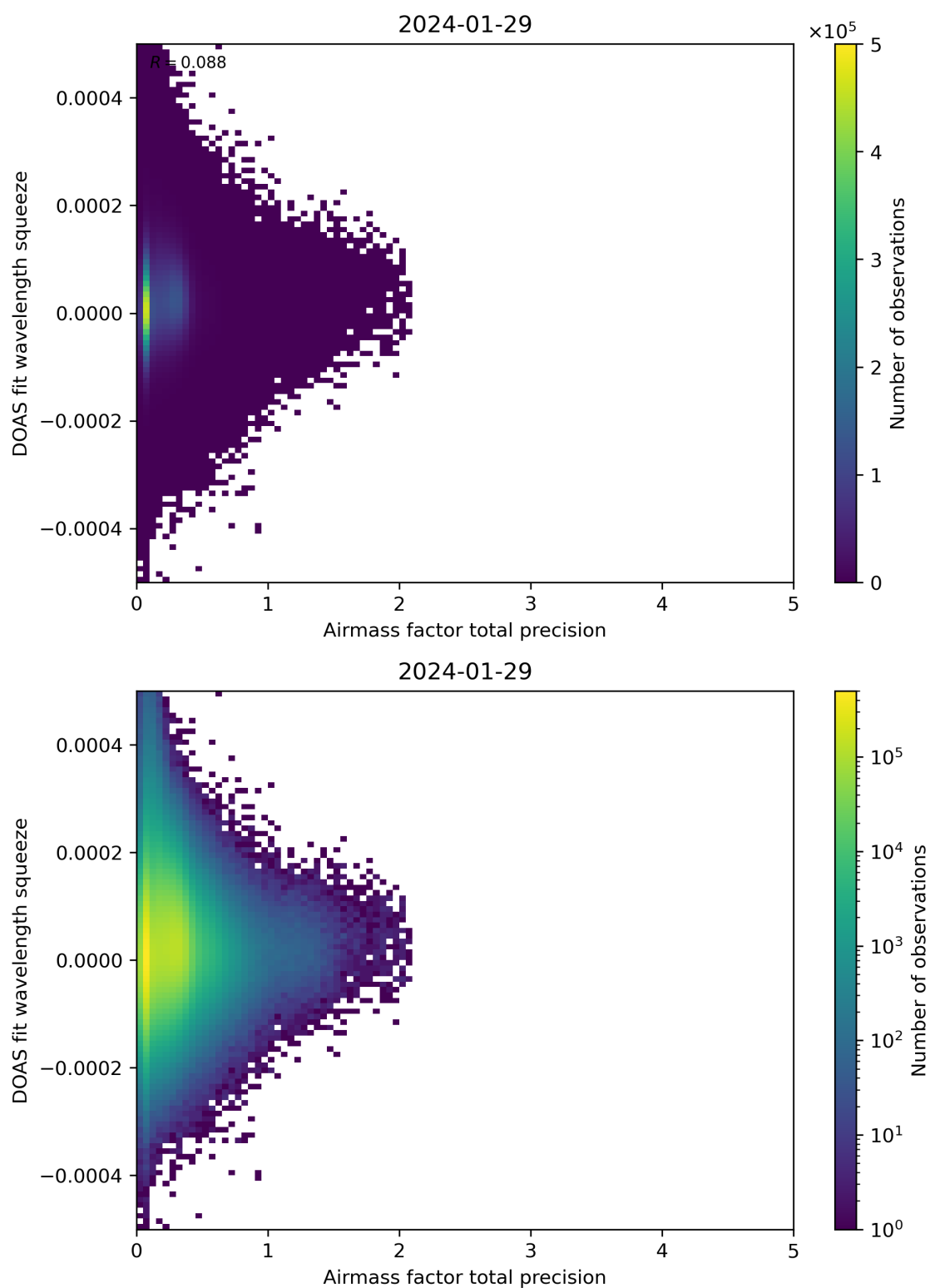
Figure 107: Scatter density plot of “Airmass factor total precision” against “DOAS fit wavelength squeeze” for 2024-01-28 to 2024-01-30.
