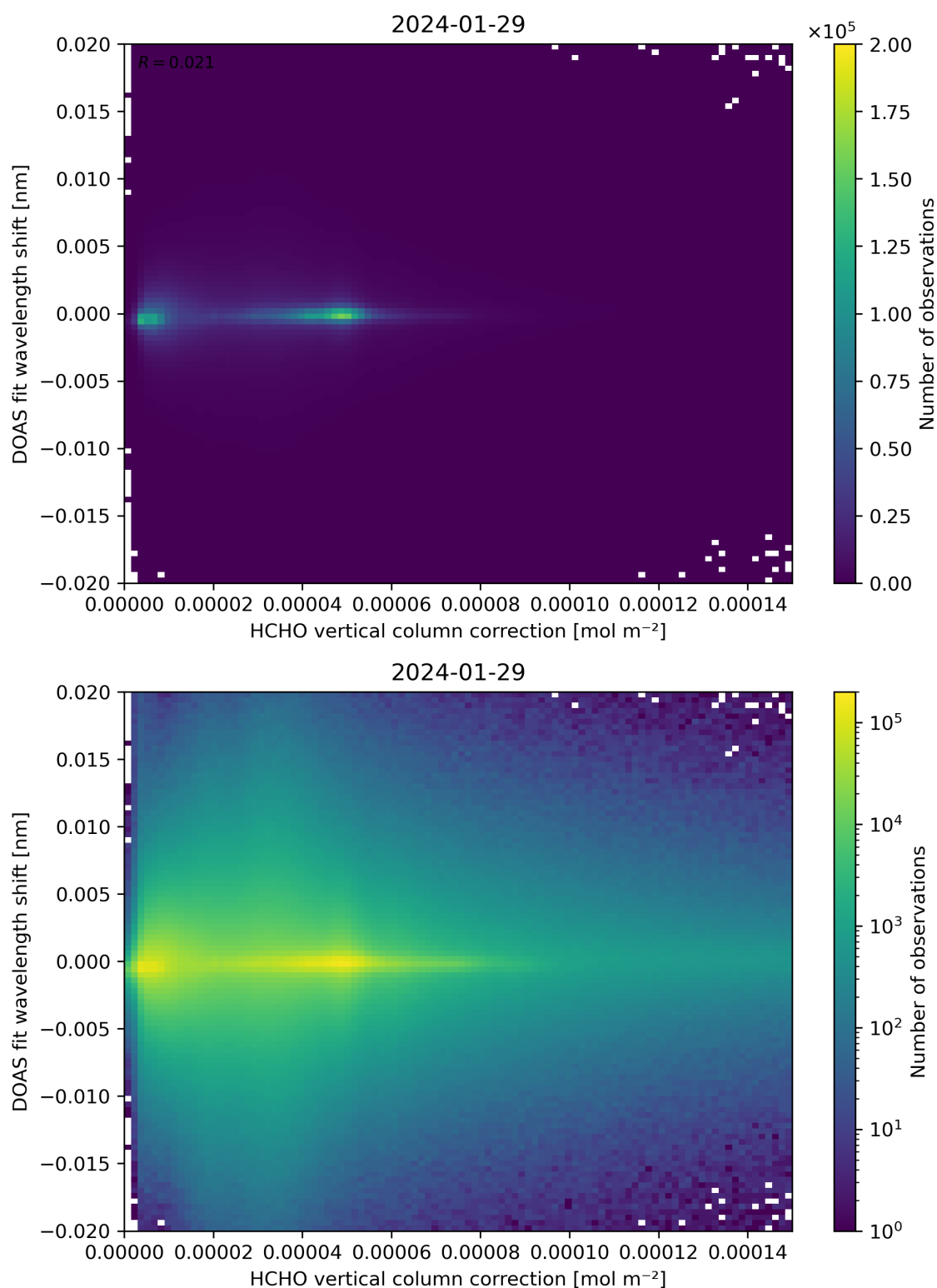
Figure 113: Scatter density plot of “HCHO vertical column correction” against “DOAS fit wavelength shift” for 2024-01-28 to 2024-01-30.
