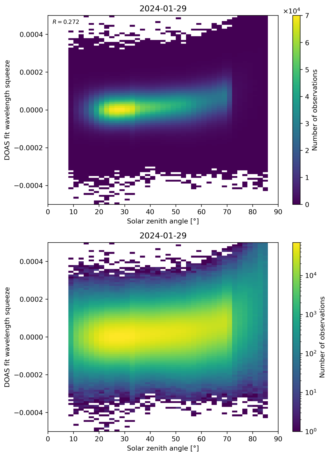
Figure 169: Scatter density plot of “Solar zenith angle” against “DOAS fit wavelength squeeze” for 2024-01-28 to 2024-01-30.
