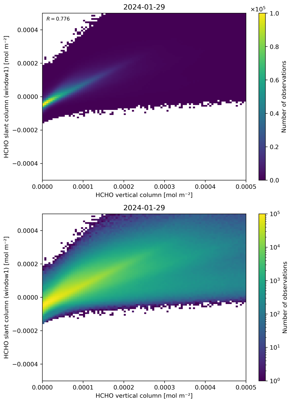
Figure 129: Scatter density plot of “HCHO vertical column” against “HCHO slant column (window1)” for 2024-01-28 to 2024-01-30.
