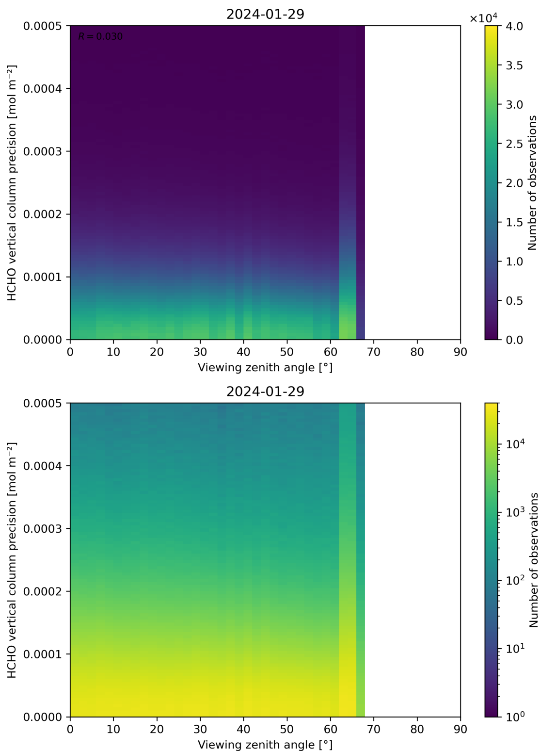
Figure 194: Scatter density plot of “Viewing zenith angle” against “HCHO vertical column precision” for 2024-01-28 to 2024-01-30.
