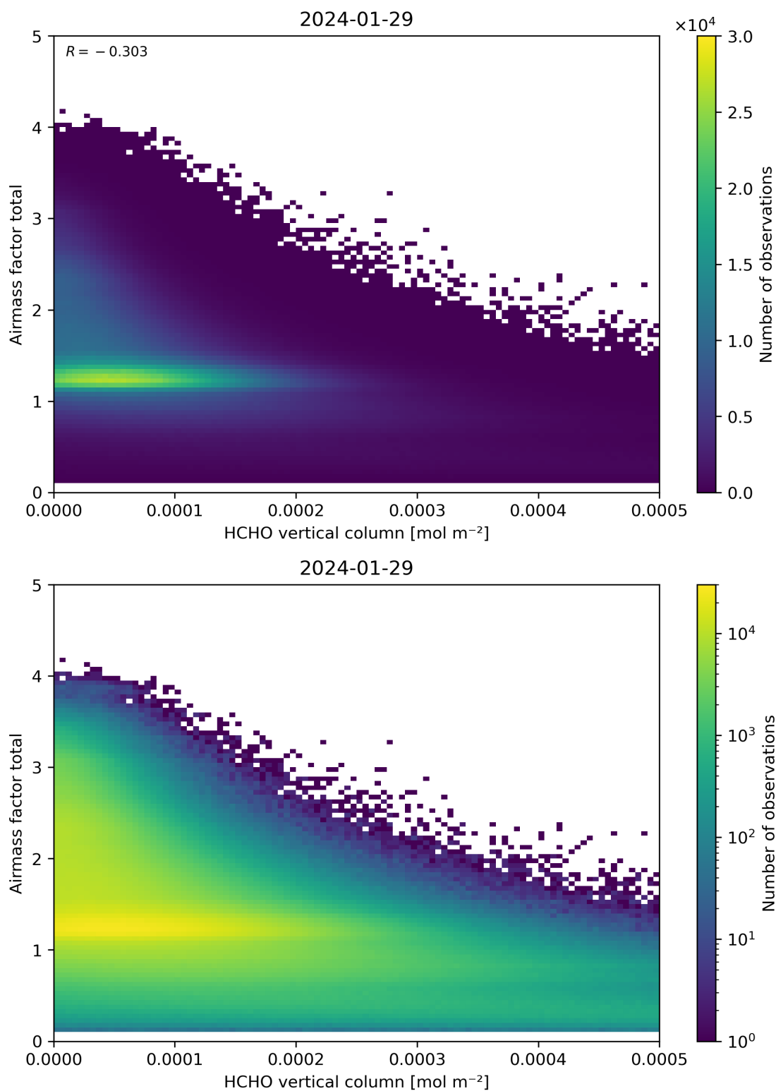
Figure 131: Scatter density plot of “HCHO vertical column” against “Airmass factor total” for 2024-01-28 to 2024-01-30.
