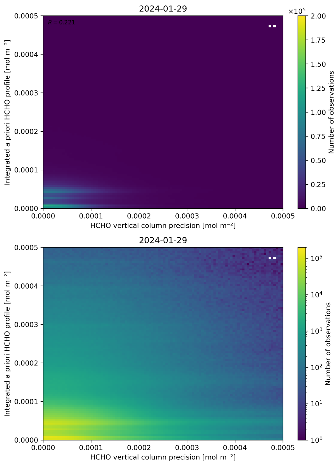
Figure 147: Scatter density plot of “HCHO vertical column precision” against “Integrated a priori HCHO profile” for 2024-01-28 to 2024-01-30.
