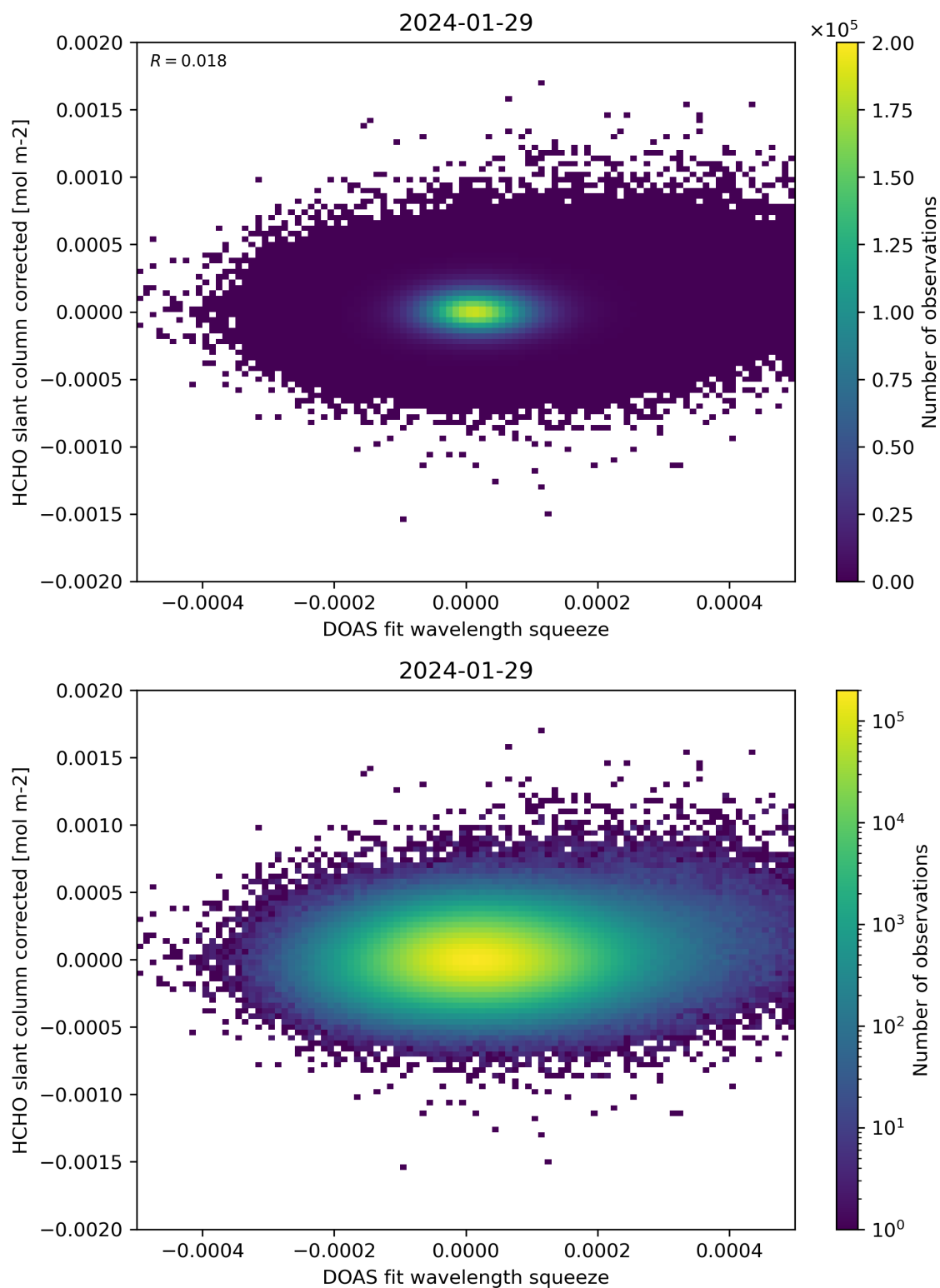
Figure 69: Scatter density plot of “DOAS fit wavelength squeeze” against “HCHO slant column corrected” for 2024-01-28 to 2024-01-30.
