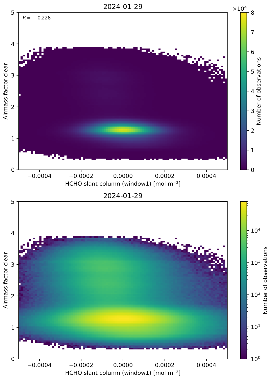
Figure 81: Scatter density plot of “HCHO slant column (window1)” against “Airmass factor clear” for 2024-01-28 to 2024-01-30.
