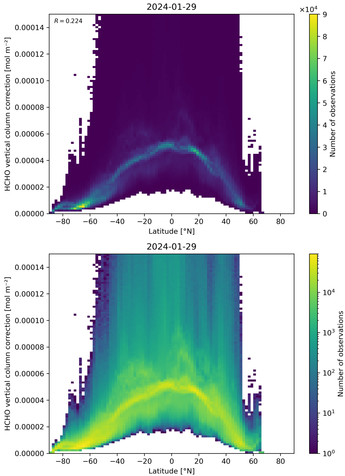
Figure 164: Scatter density plot of “Latitude” against “HCHO vertical column correction” for 2024-01-28 to 2024-01-30.
