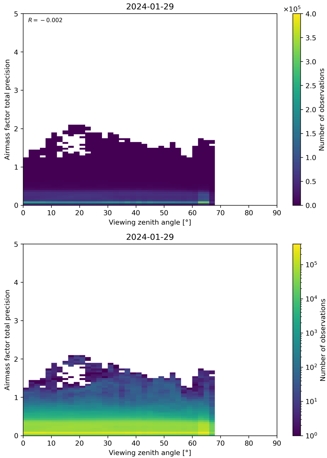
Figure 191: Scatter density plot of “Viewing zenith angle” against “Airmass factor total precision” for 2024-01-28 to 2024-01-30.
