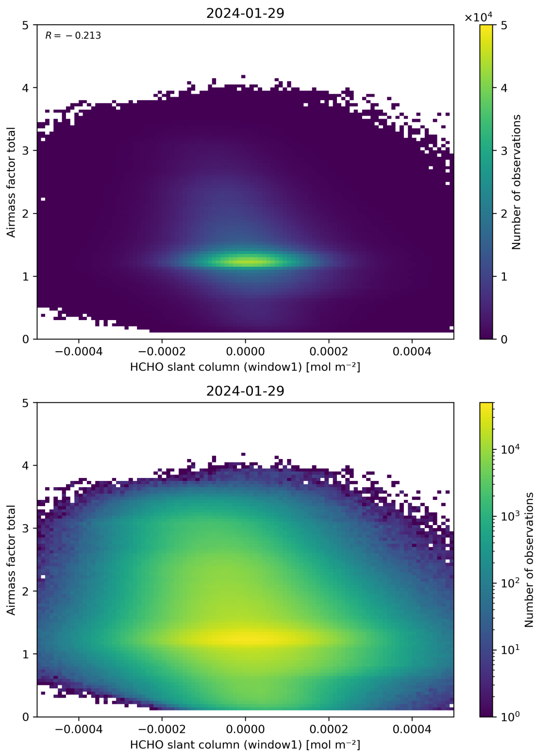
Figure 85: Scatter density plot of “HCHO slant column (window1)” against “Airmass factor total” for 2024-01-28 to 2024-01-30.
