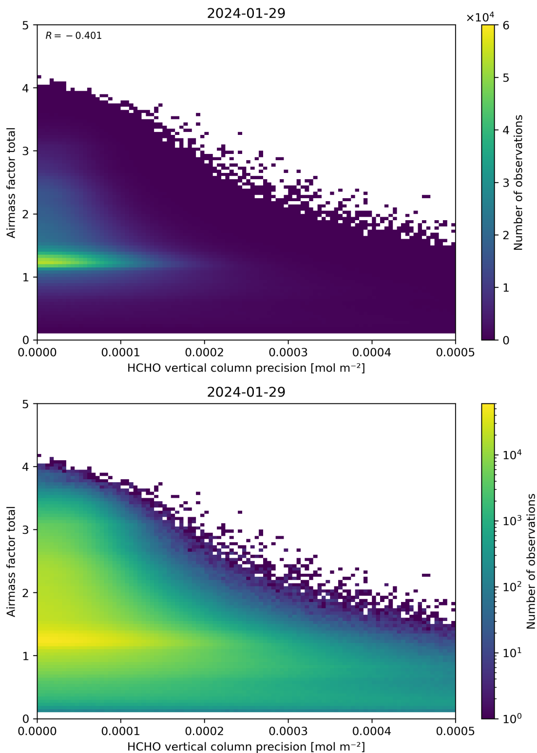
Figure 144: Scatter density plot of “HCHO vertical column precision” against “Airmass factor total” for 2024-01-28 to 2024-01-30.
