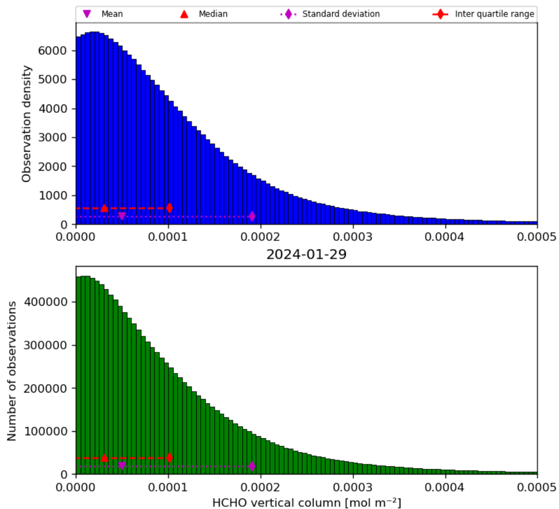
Figure 35: Histogram of “HCHO vertical column” for 2024-01-28 to 2024-01-30
