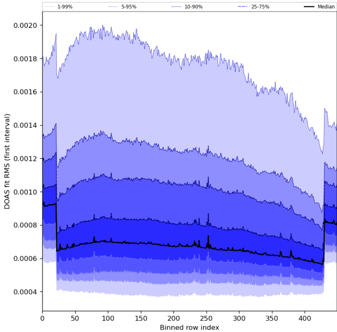
Figure 60: Along track statistics of “DOAS fit RMS (first interval)” for 2024-01-28 to 2024-01-30
