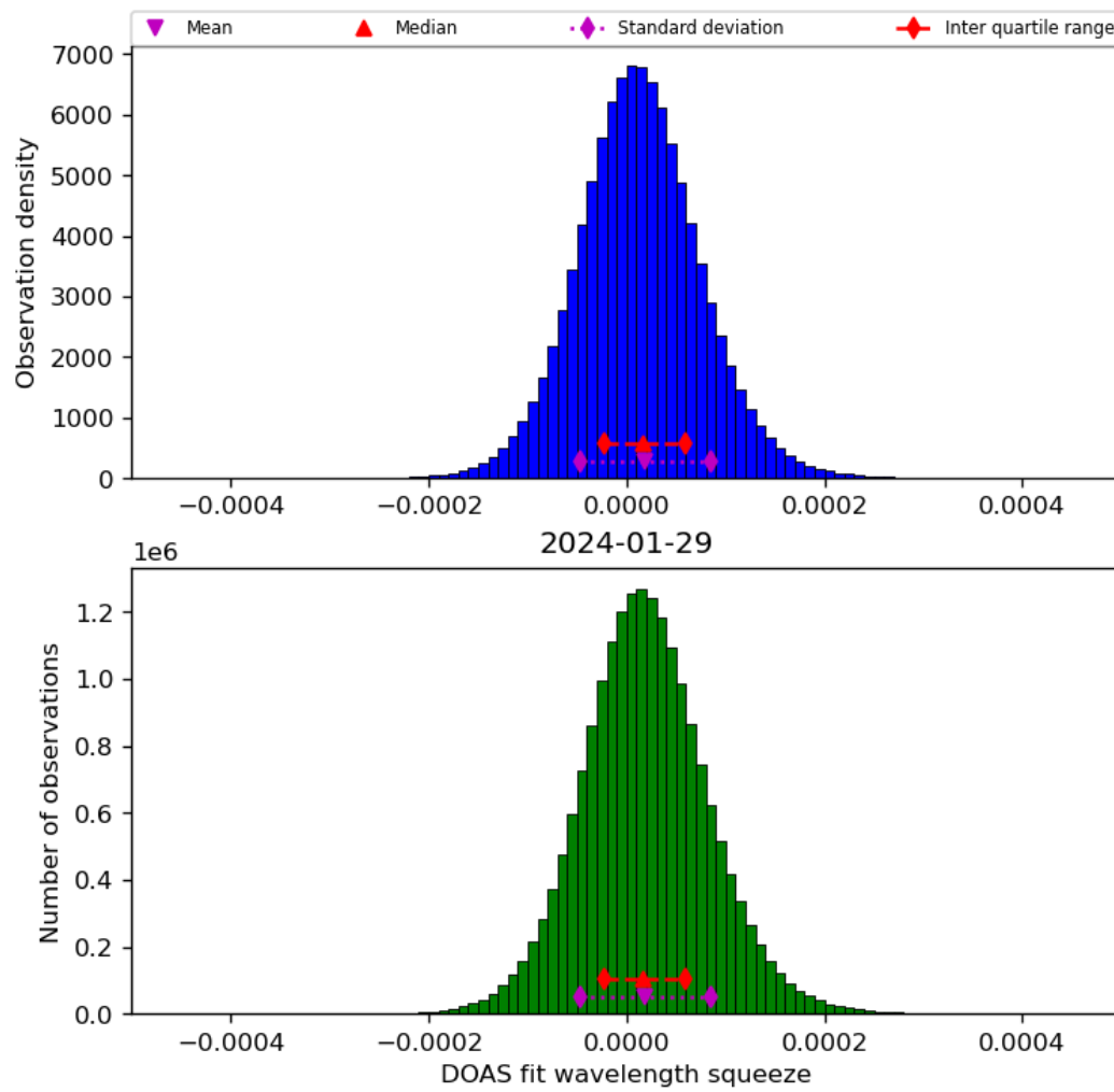
Figure 45: Histogram of “DOAS fit wavelength squeeze” for 2024-01-28 to 2024-01-30
