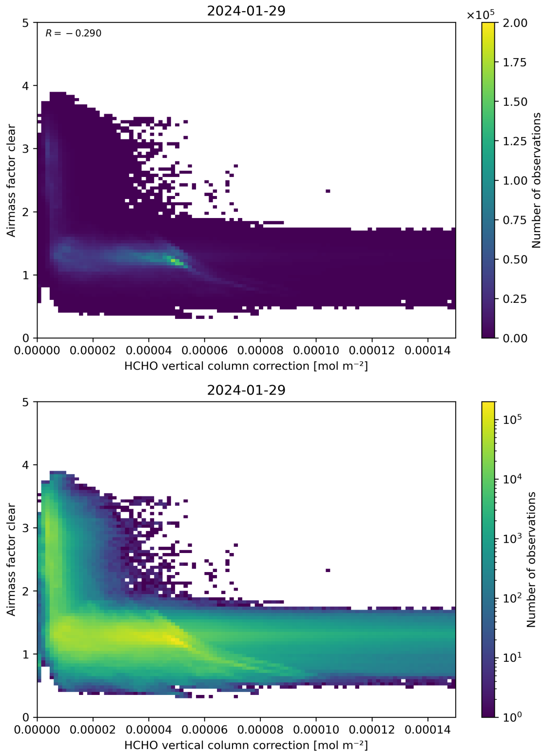
Figure 115: Scatter density plot of “HCHO vertical column correction” against “Airmass factor clear” for 2024-01-28 to 2024-01-30.
