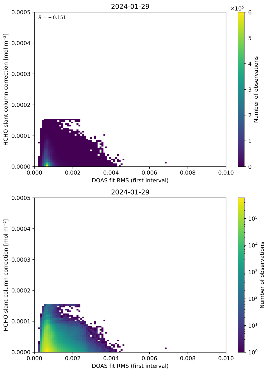
Figure 63: Scatter density plot of “DOAS fit RMS (first interval)” against “HCHO slant column correction” for 2024-01-28 to 2024-01-30.
