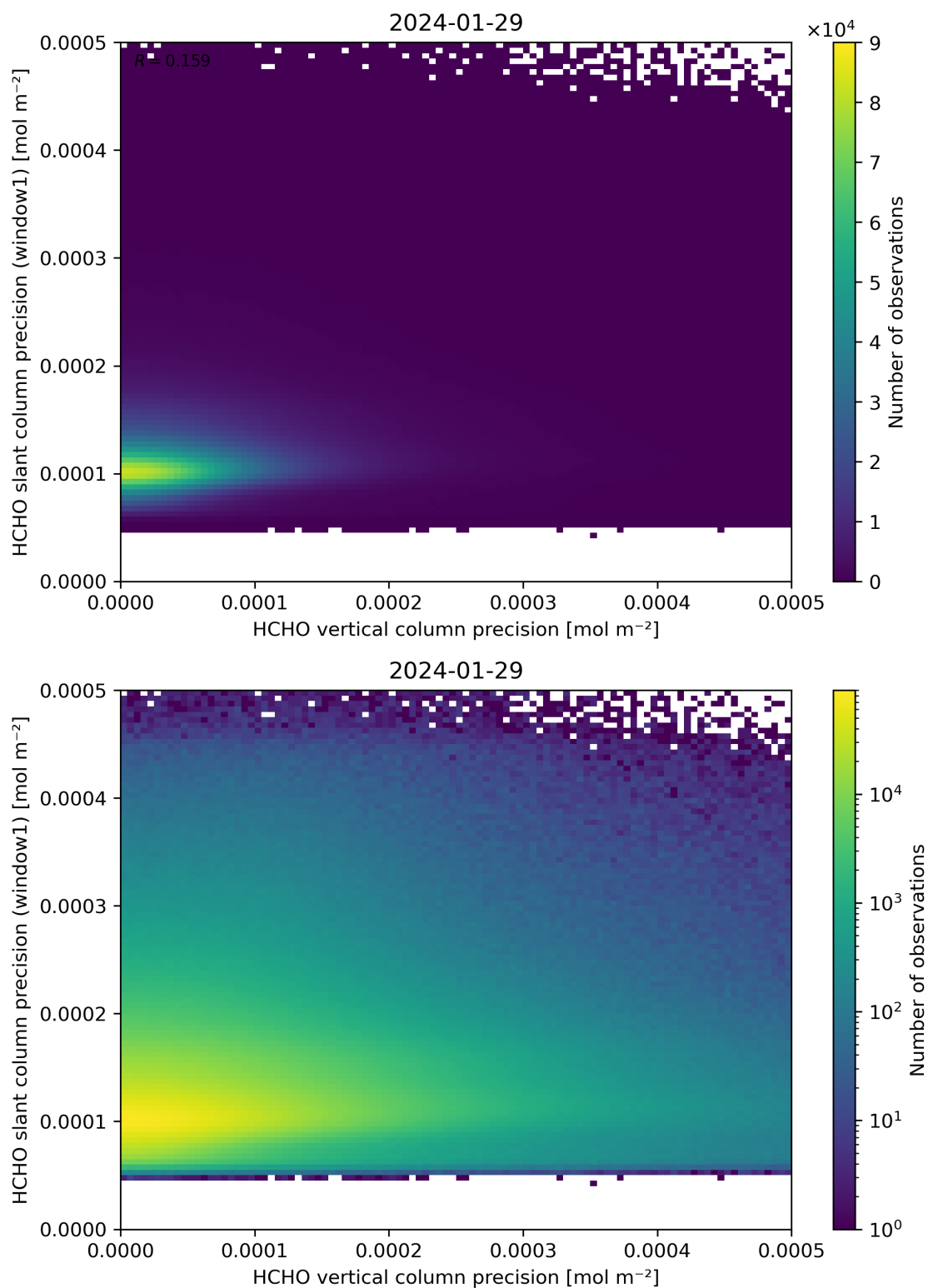
Figure 143: Scatter density plot of “HCHO vertical column precision” against “HCHO slant column precision (window1)” for 2024-01-28 to 2024-01-30.
