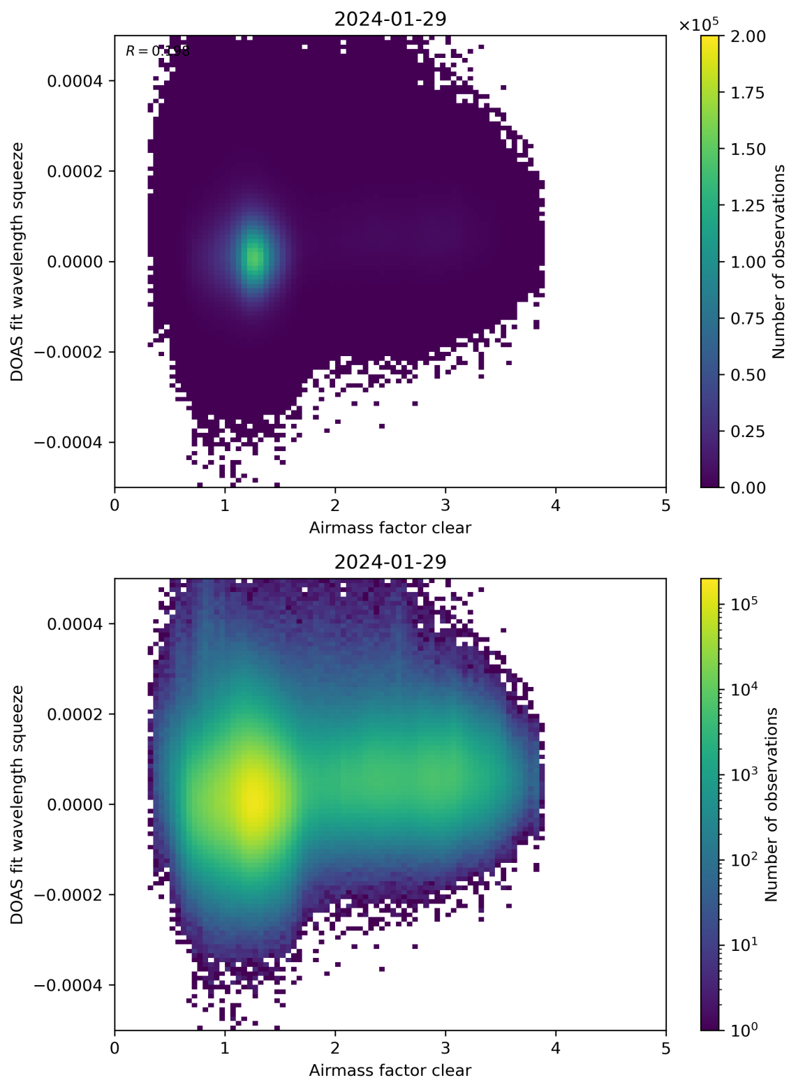
Figure 73: Scatter density plot of “Airmass factor clear” against “DOAS fit wavelength squeeze” for 2024-01-28 to 2024-01-30.
