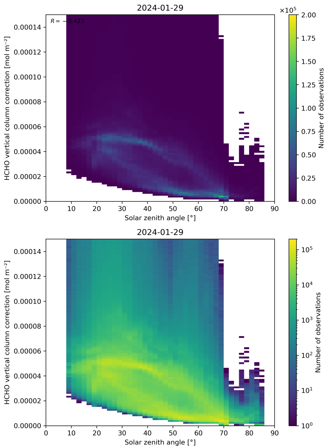
Figure 178: Scatter density plot of “Solar zenith angle” against “HCHO vertical column correction” for 2024-01-28 to 2024-01-30.
