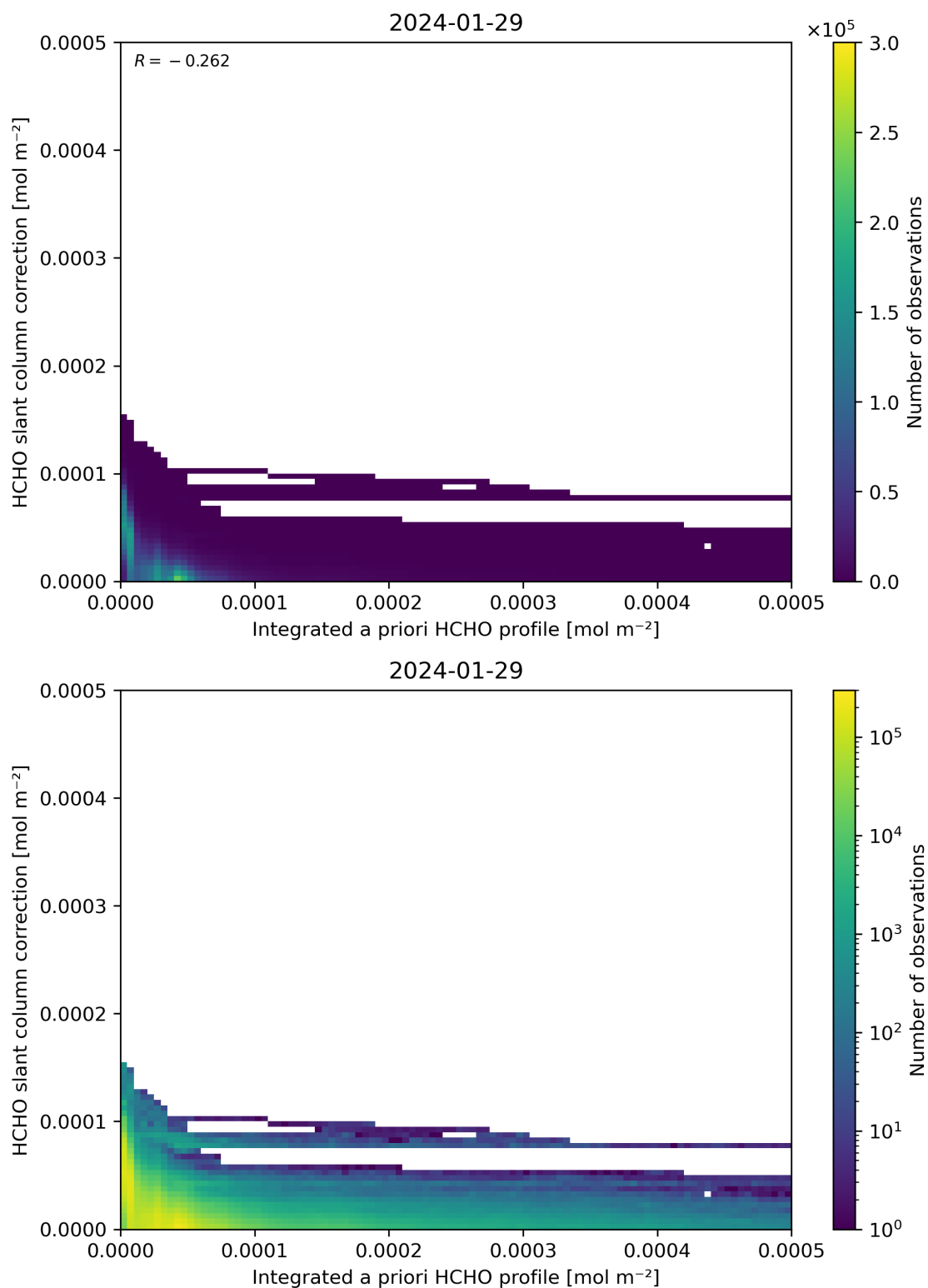
Figure 152: Scatter density plot of “Integrated a priori HCHO profile” against “HCHO slant column correction” for 2024-01-28 to 2024-01-30.
