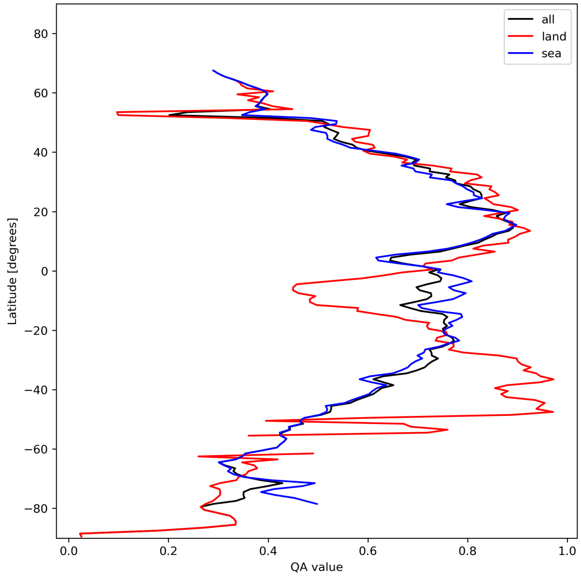
Figure 20: Zonal average of “QA value” for 2024-01-28 to 2024-01-30.
