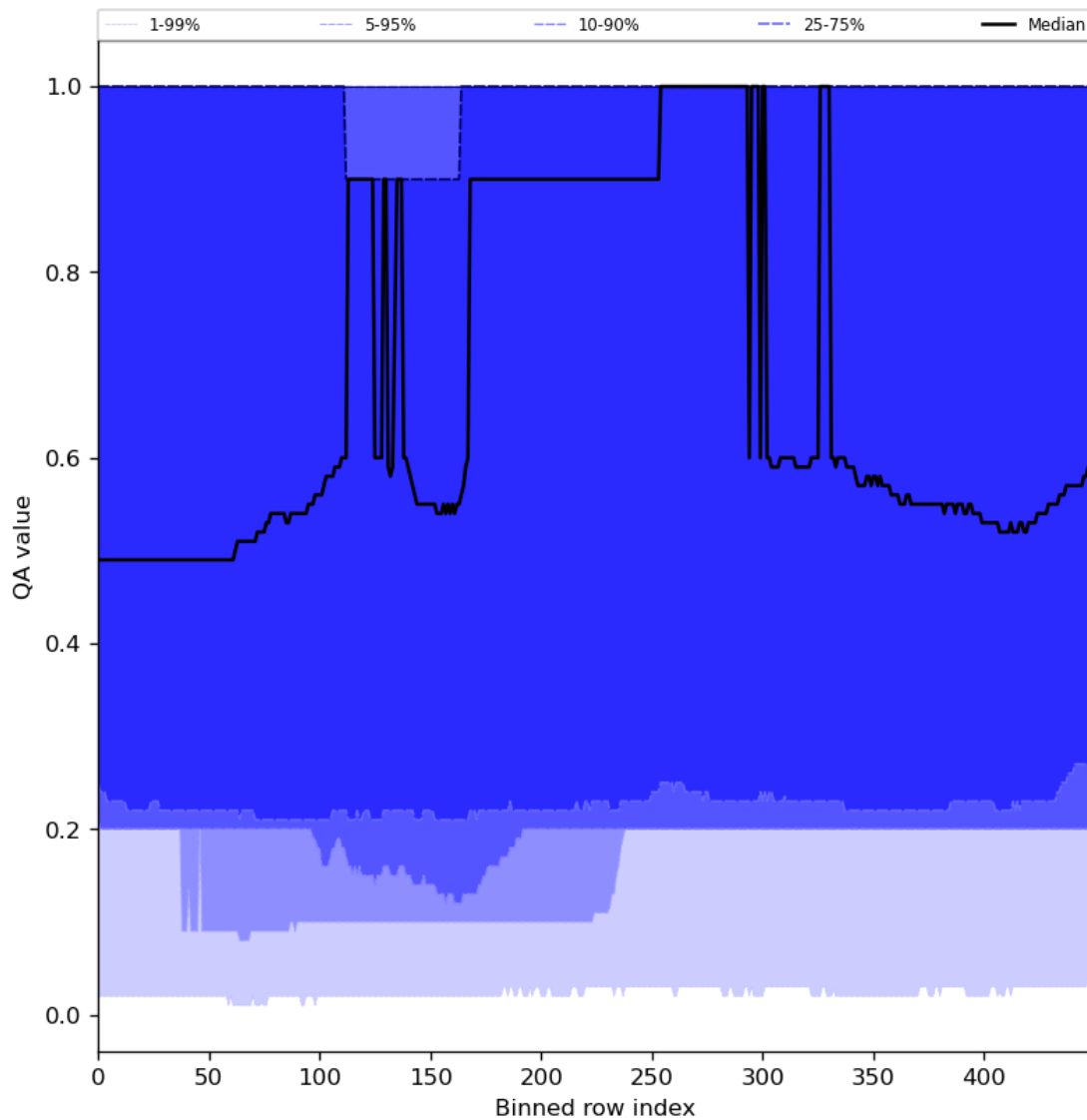
Figure 48: Along track statistics of “QA value” for 2024-01-28 to 2024-01-30
