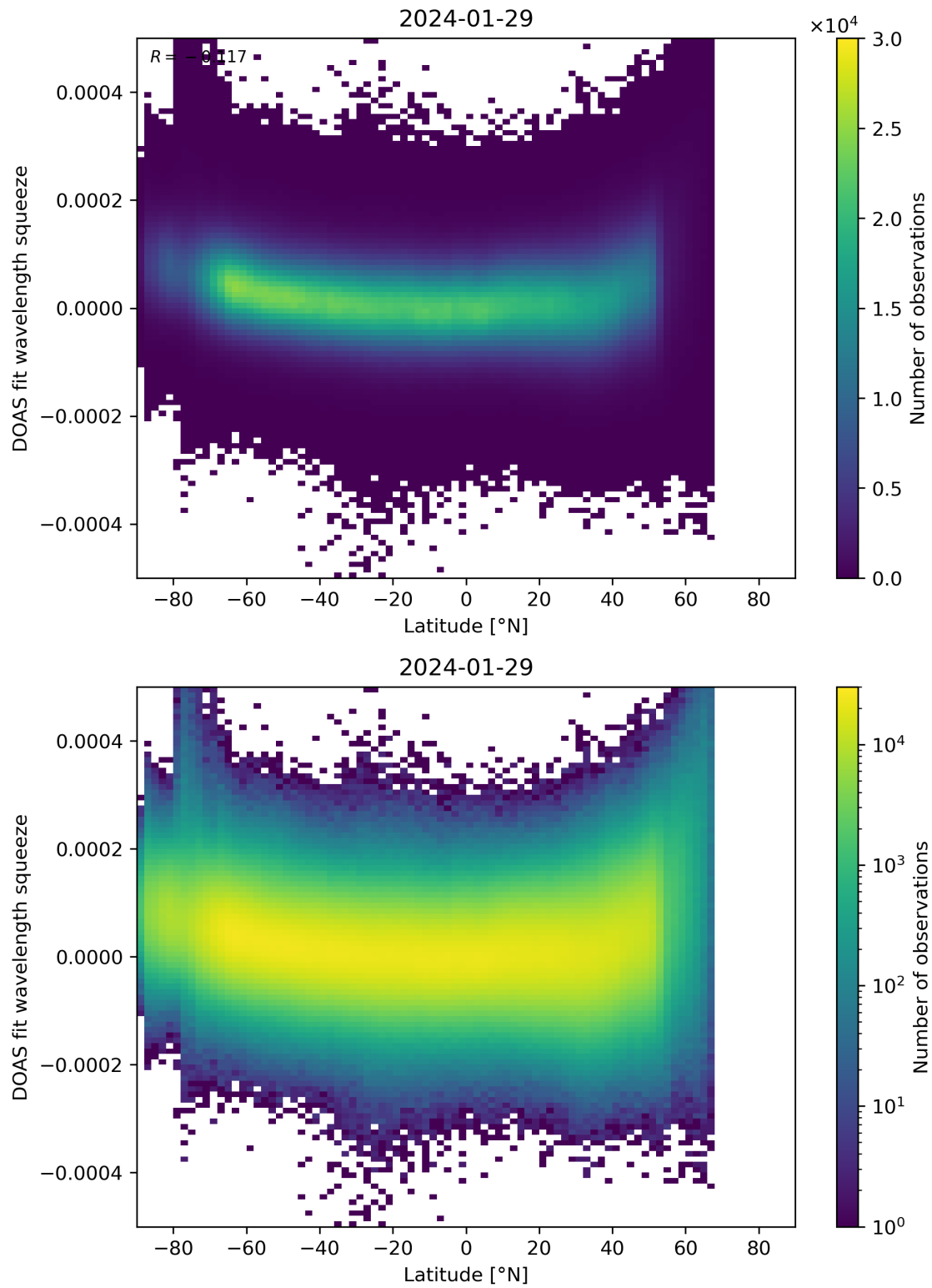
Figure 155: Scatter density plot of “Latitude” against “DOAS fit wavelength squeeze” for 2024-01-28 to 2024-01-30.
