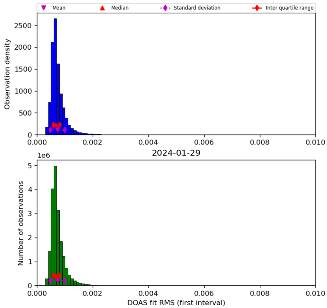
Figure 46: Histogram of “DOAS fit RMS (first interval)” for 2024-01-28 to 2024-01-30
