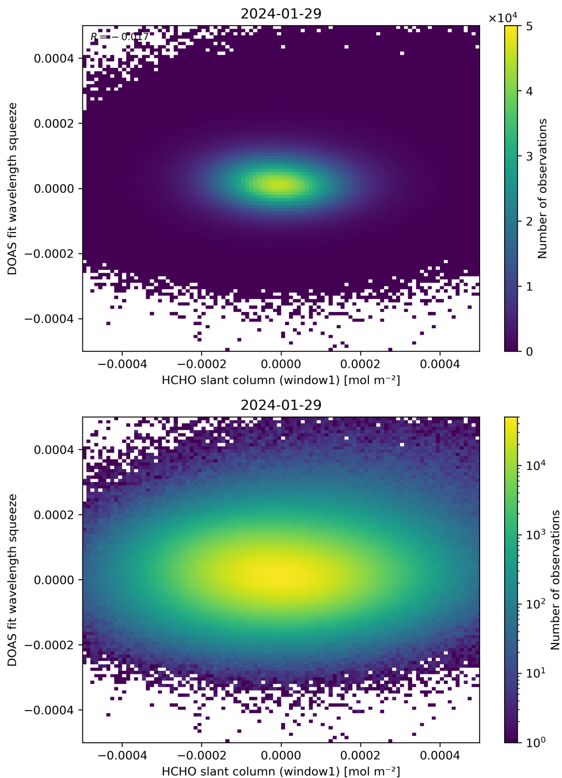
Figure 80: Scatter density plot of “HCHO slant column (window1)” against “DOAS fit wavelength squeeze” for 2024-01-28 to 2024-01-30.
