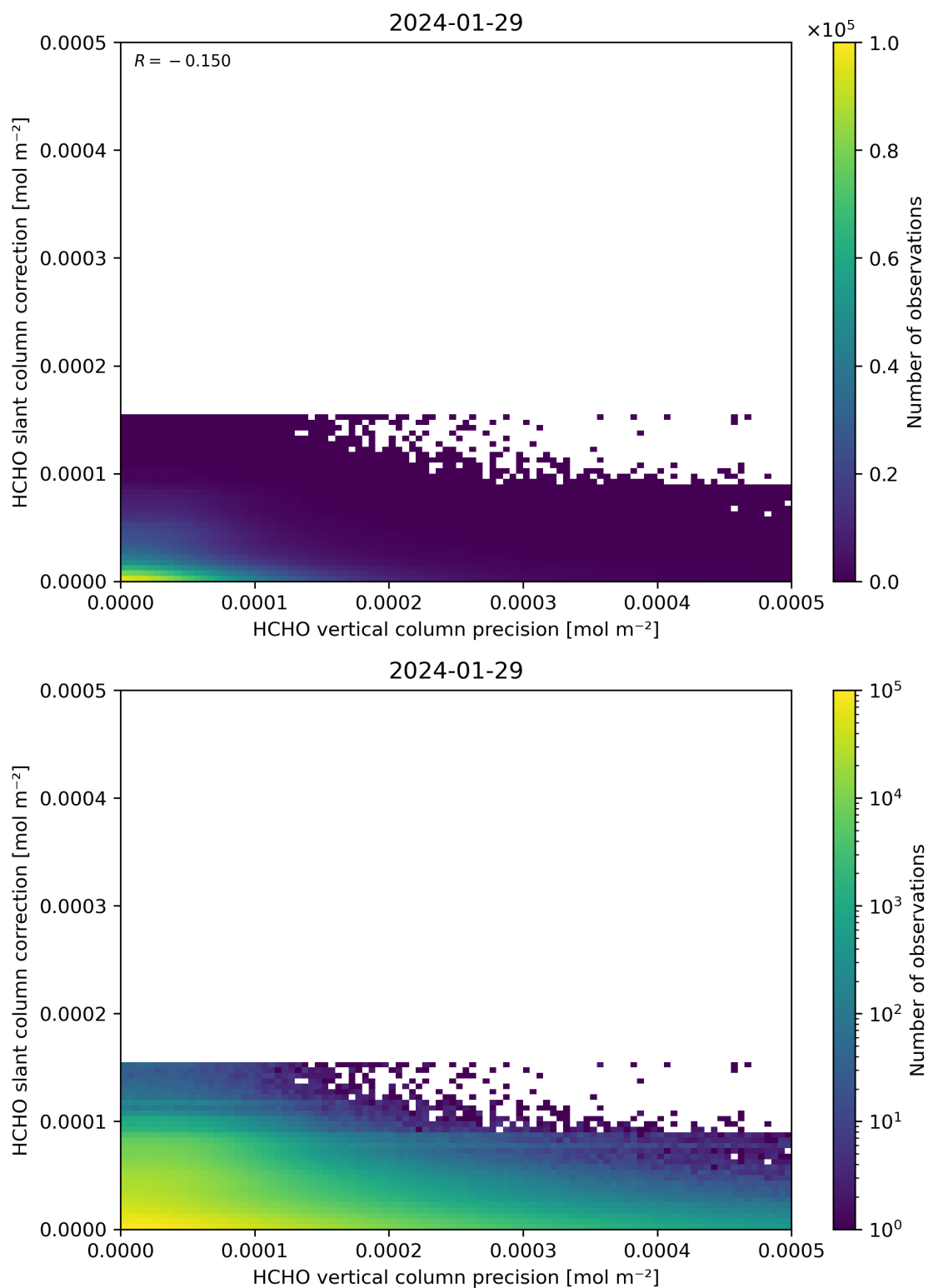
Figure 141: Scatter density plot of “HCHO vertical column precision” against “HCHO slant column correction” for 2024-01-28 to 2024-01-30.
