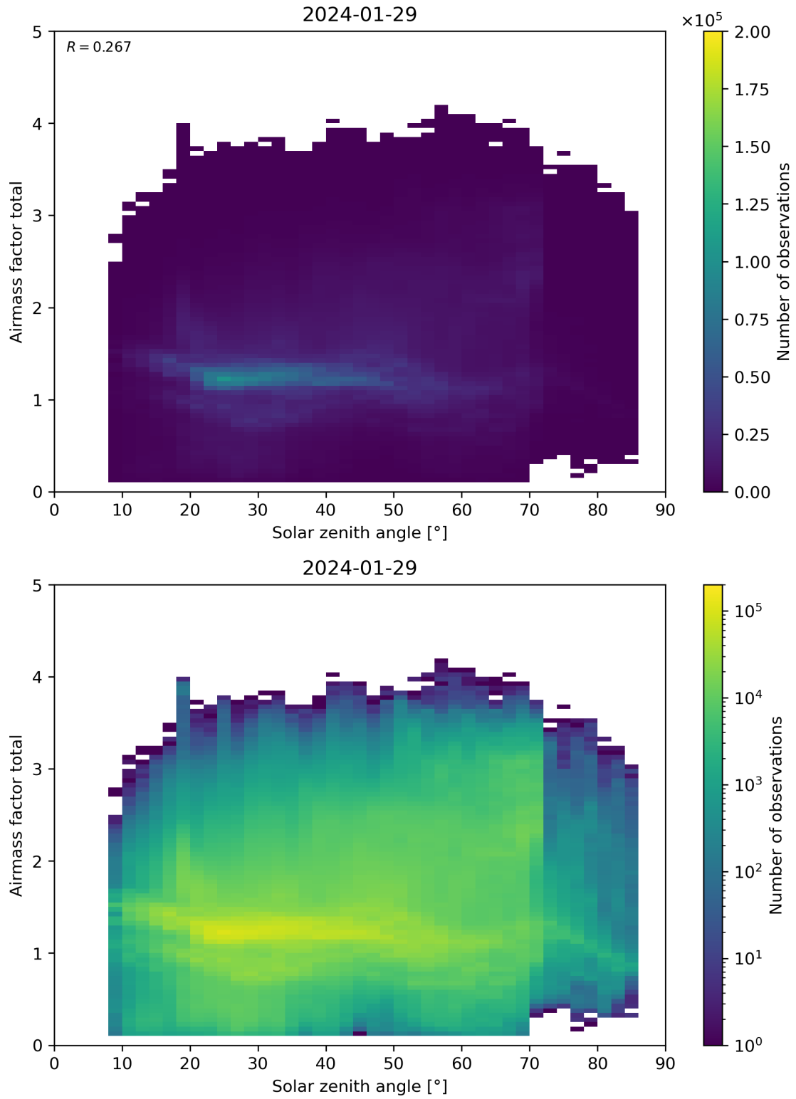
Figure 175: Scatter density plot of “Solar zenith angle” against “Airmass factor total” for 2024-01-28 to 2024-01-30.
