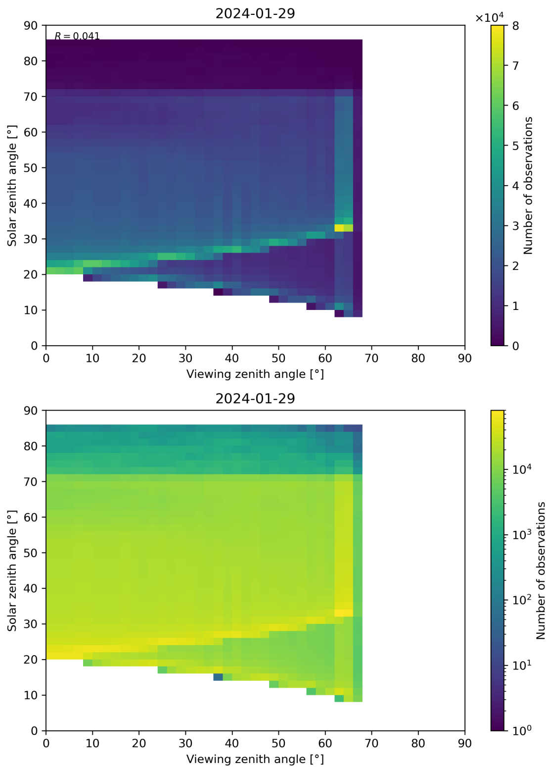
Figure 197: Scatter density plot of “Viewing zenith angle” against “Solar zenith angle” for 2024-01-28 to 2024-01-30.
