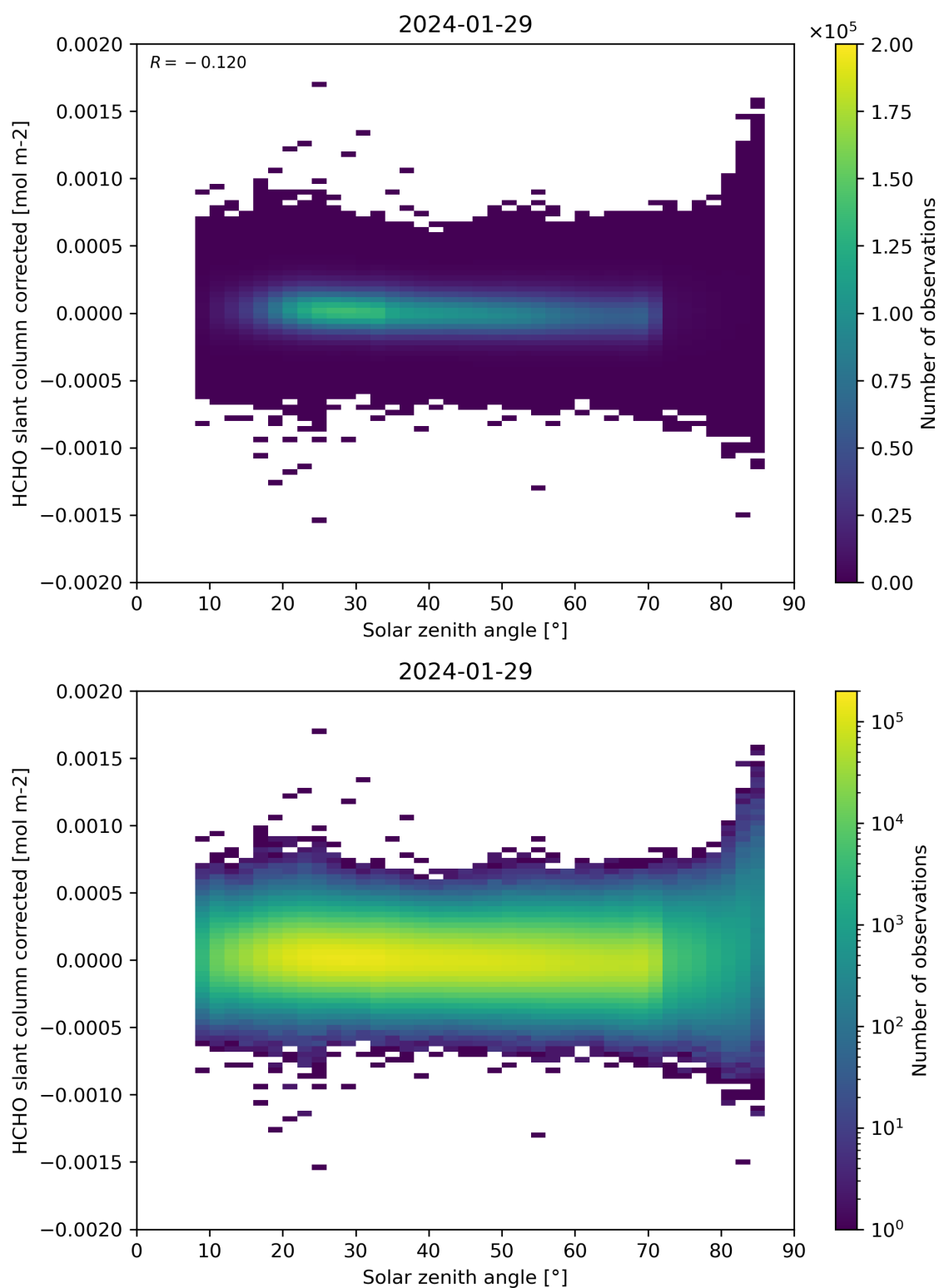
Figure 171: Scatter density plot of “Solar zenith angle” against “HCHO slant column corrected” for 2024-01-28 to 2024-01-30.
