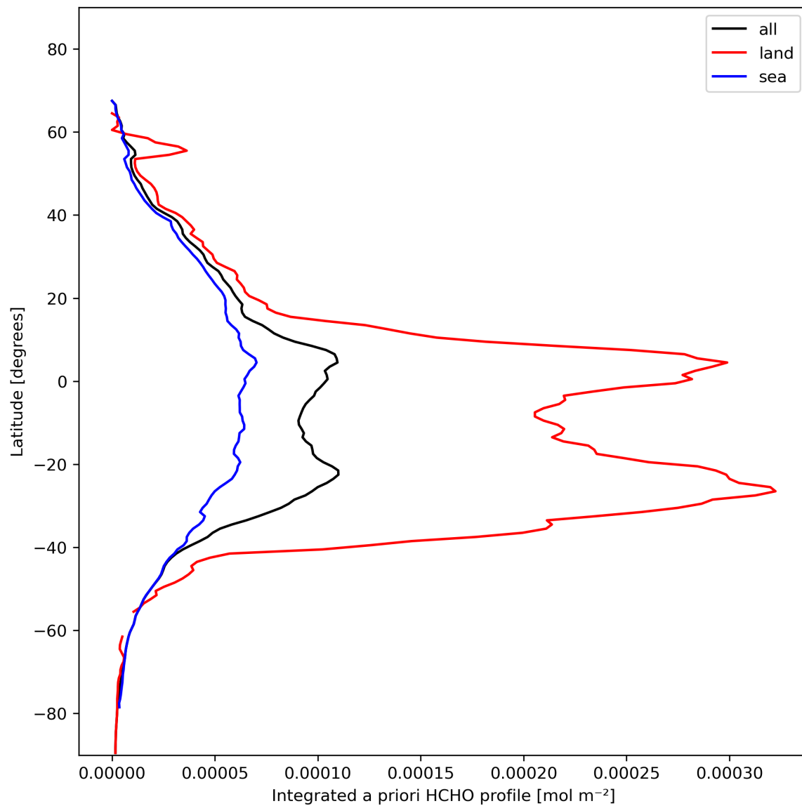
Figure 29: Zonal average of “Integrated a priori HCHO profile” for 2024-01-28 to 2024-01-30.
