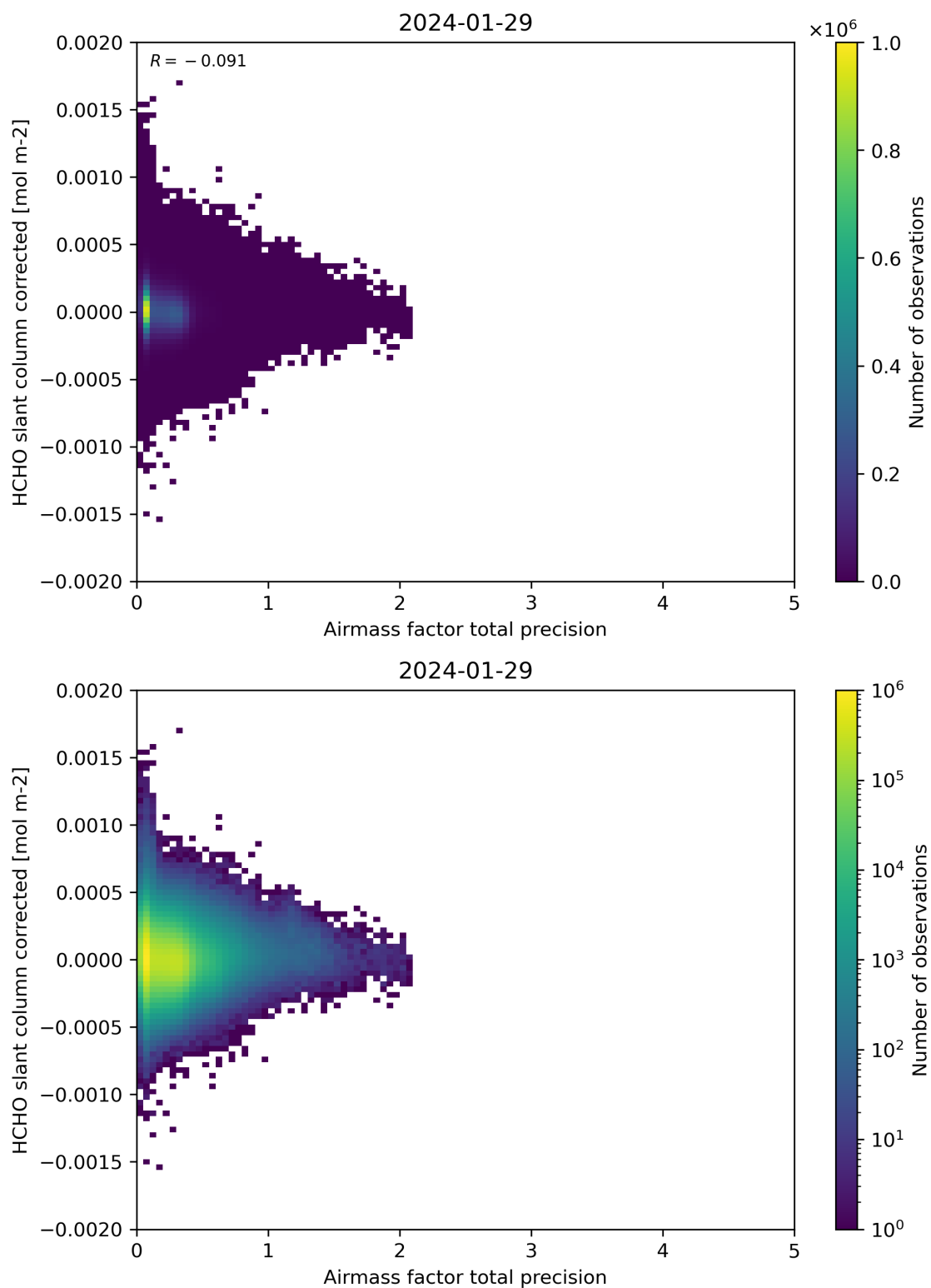
Figure 109: Scatter density plot of “Airmass factor total precision” against “HCHO slant column corrected” for 2024-01-28 to 2024-01-30.
