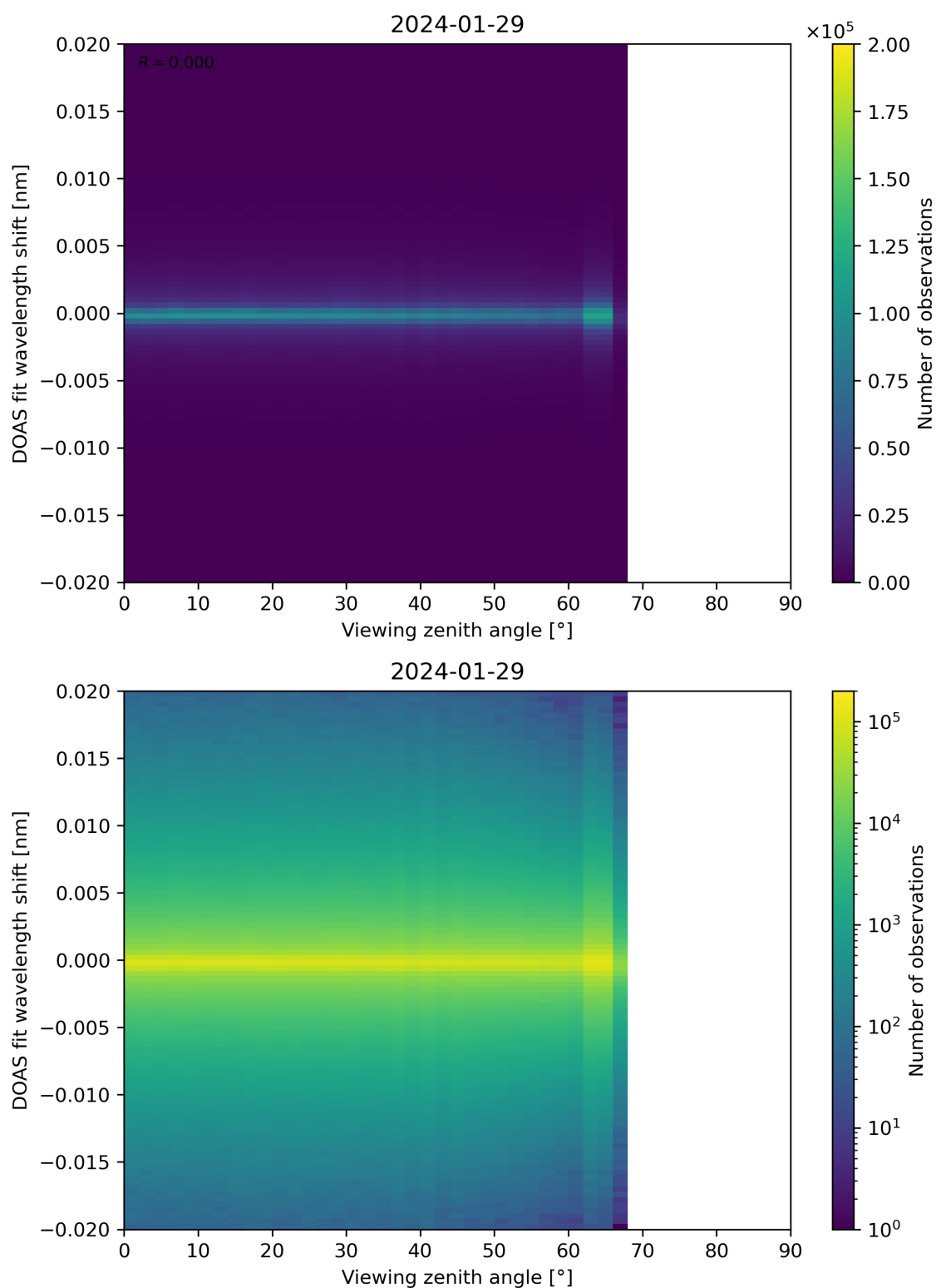
Figure 183: Scatter density plot of “Viewing zenith angle” against “DOAS fit wavelength shift” for 2024-01-28 to 2024-01-30.
