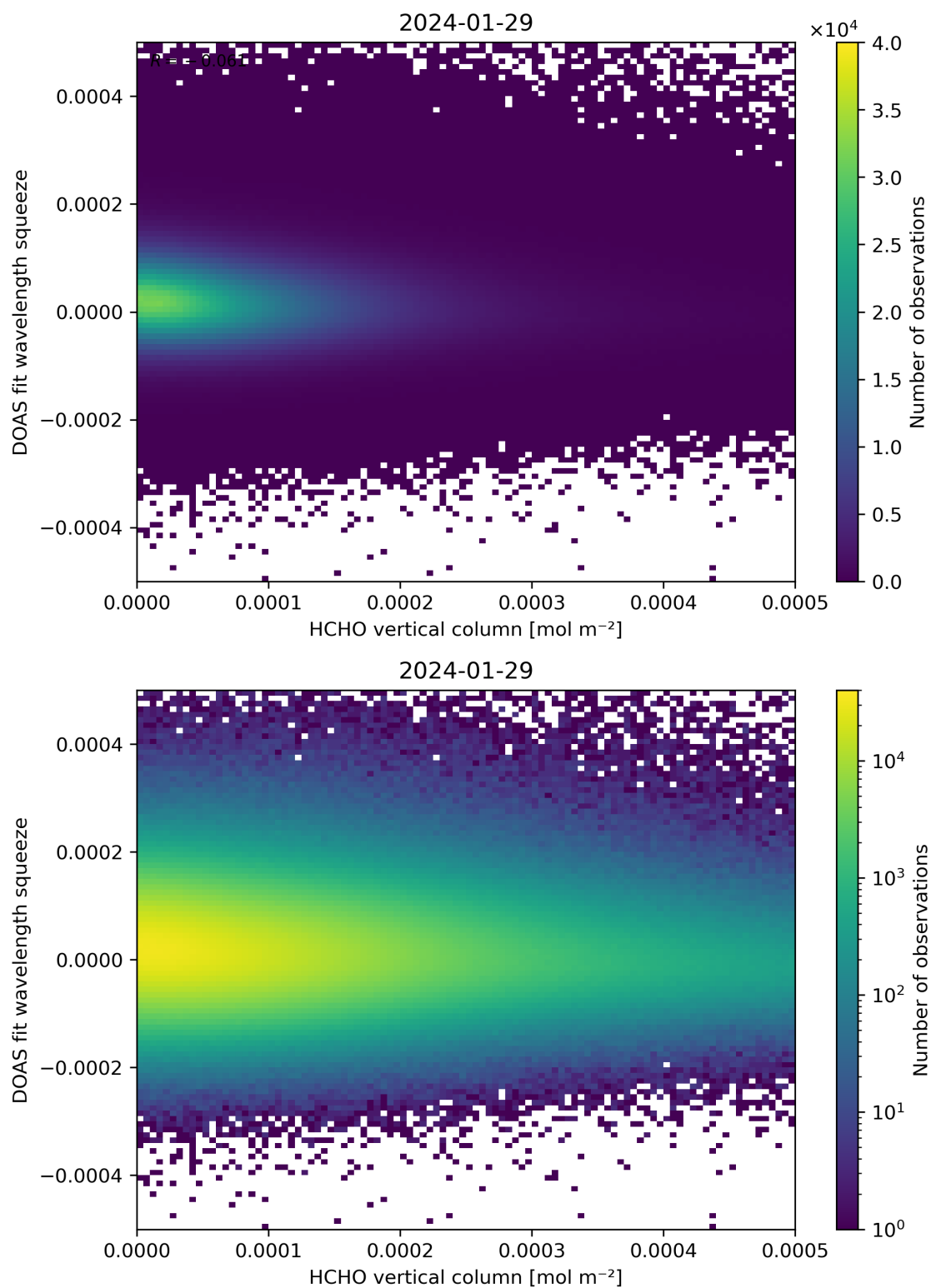
Figure 125: Scatter density plot of “HCHO vertical column” against “DOAS fit wavelength squeeze” for 2024-01-28 to 2024-01-30.
