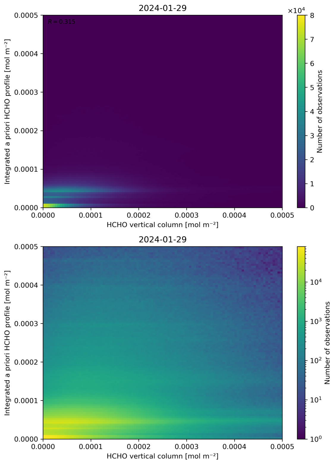
Figure 135: Scatter density plot of “HCHO vertical column” against “Integrated a priori HCHO profile” for 2024-01-28 to 2024-01-30.
