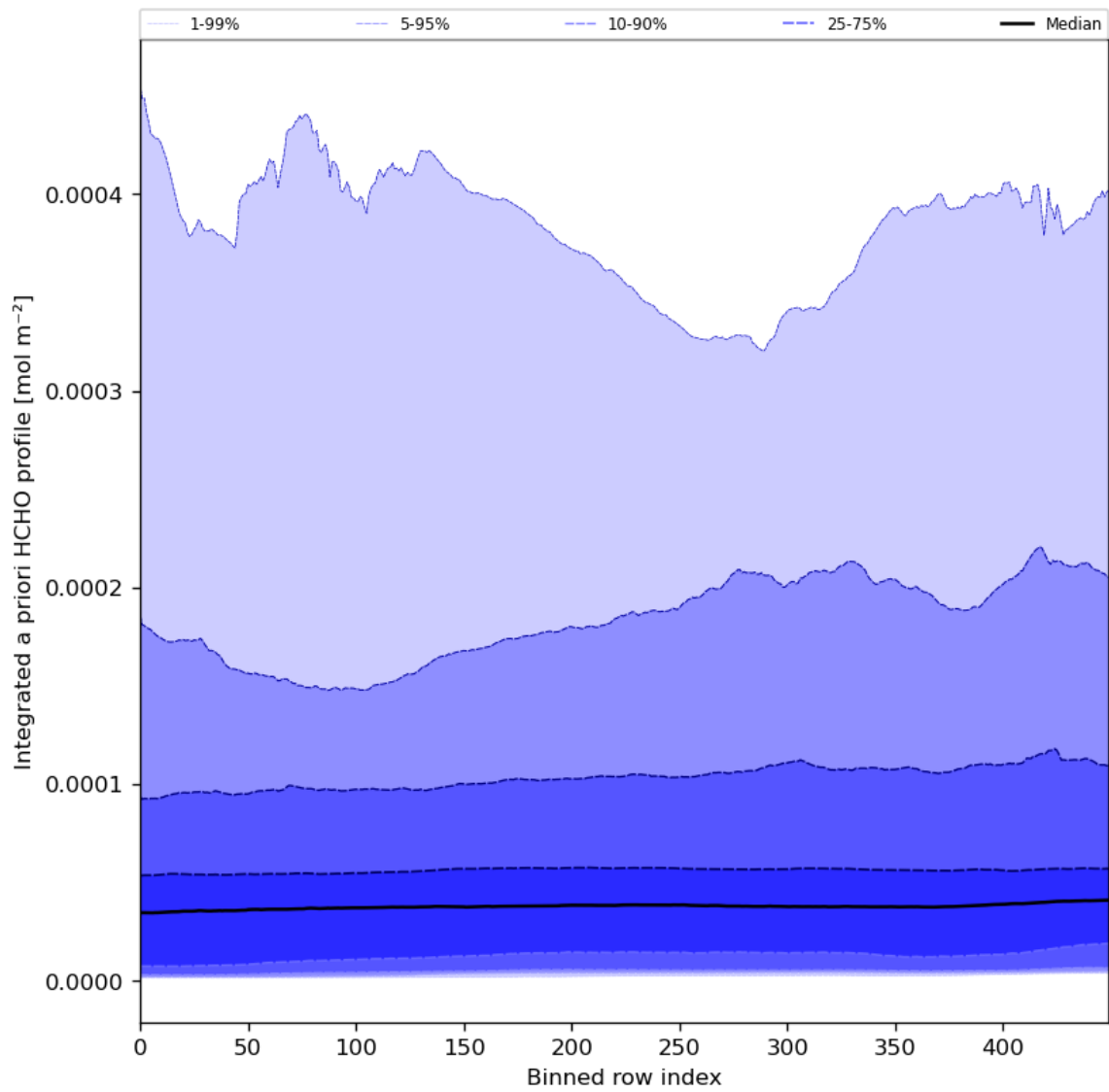
Figure 57: Along track statistics of "Integrated a priori HCHO profile" for 2024-01-28 to 2024-01-30
