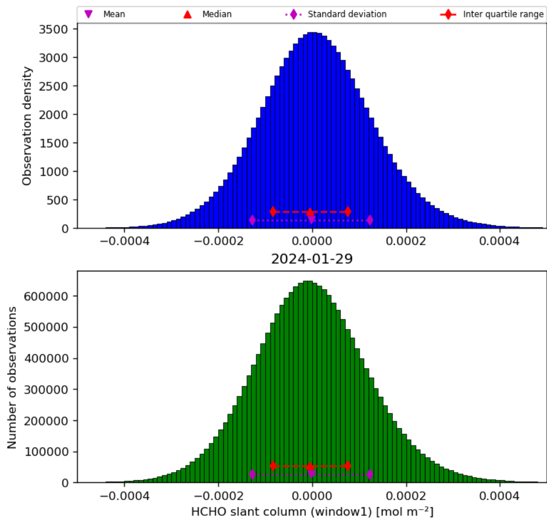
Figure 38: Histogram of “HCHO slant column (window1)” for 2024-01-28 to 2024-01-30
