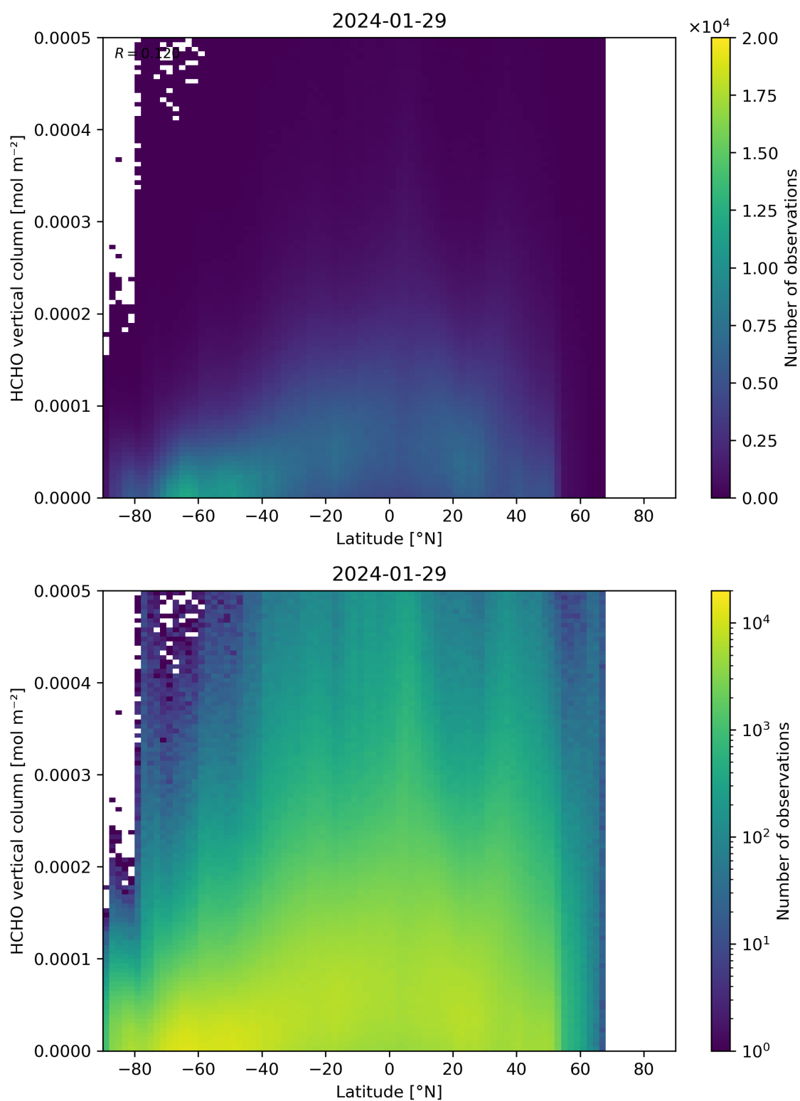
Figure 163: Scatter density plot of “Latitude” against “HCHO vertical column” for 2024-01-28 to 2024-01-30.
