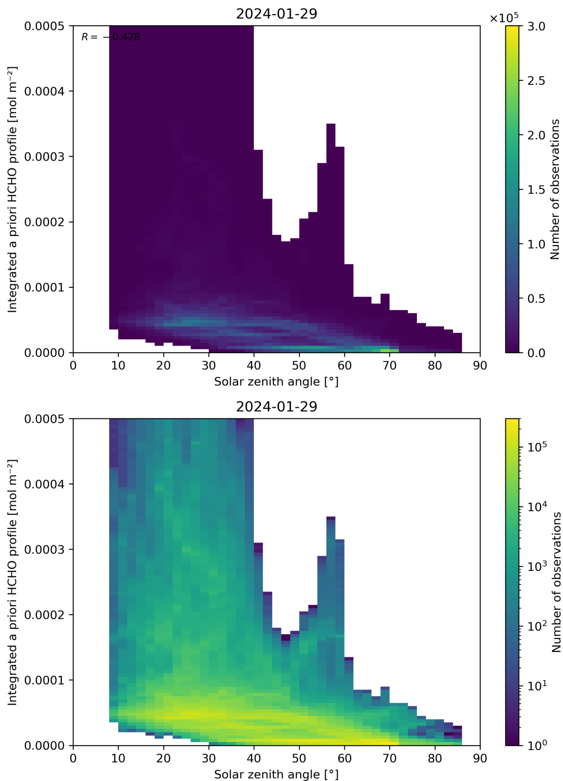
Figure 180: Scatter density plot of “Solar zenith angle” against “Integrated a priori HCHO profile” for 2024-01-28 to 2024-01-30.
