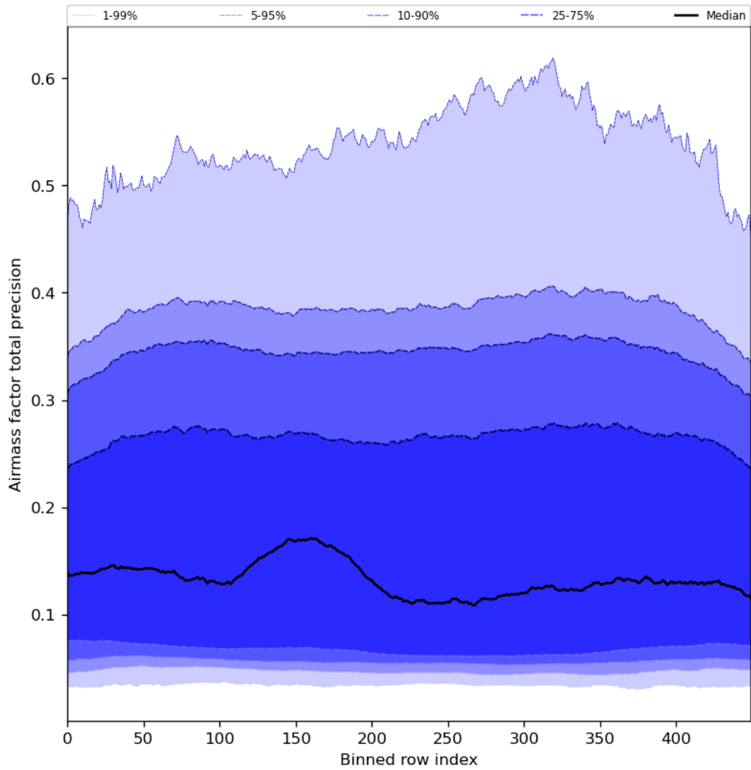
Figure 55: Along track statistics of “Airmass factor total precision” for 2024-01-28 to 2024-01-30
