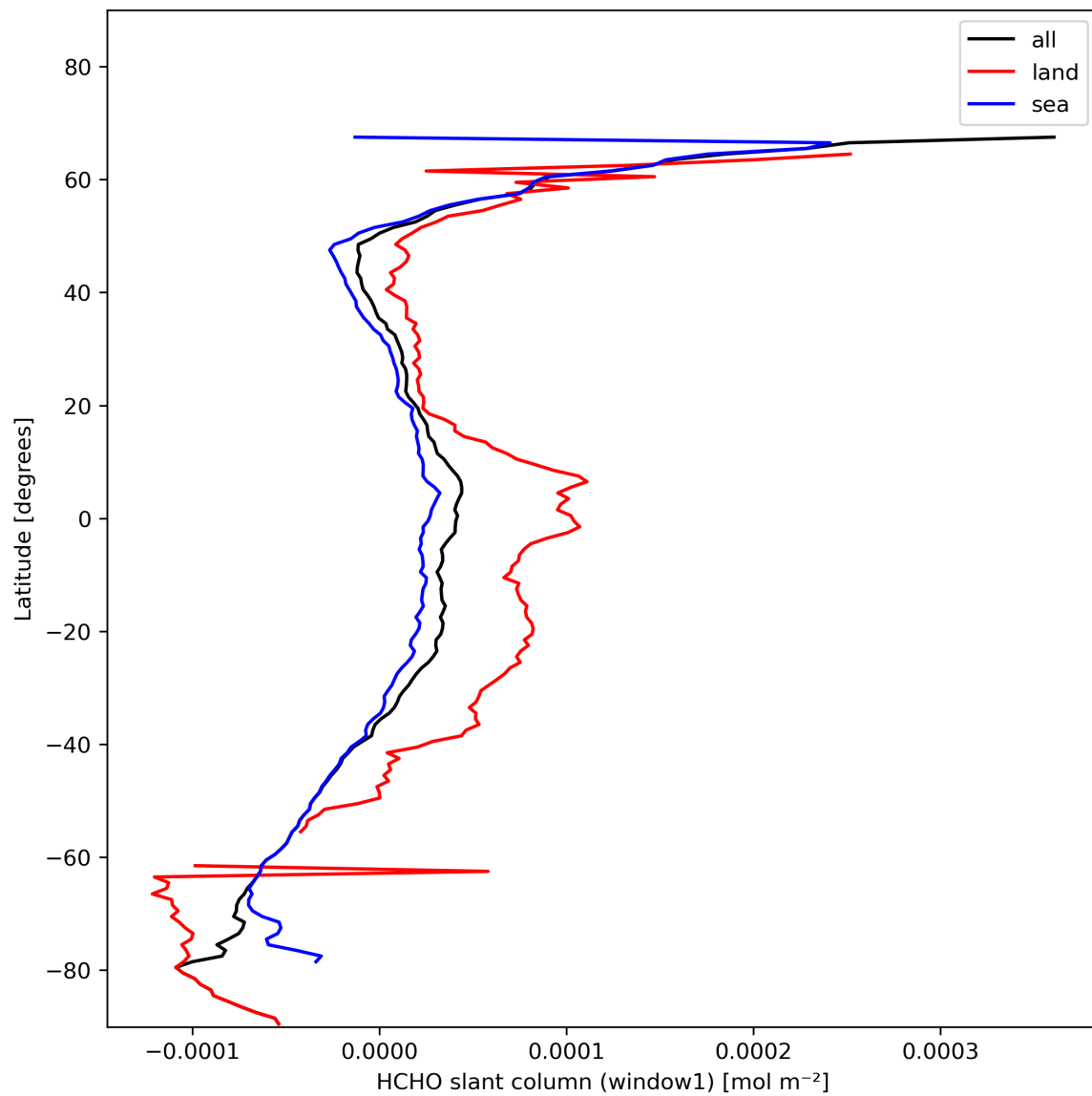
Figure 24: Zonal average of “HCHO slant column (window1)” for 2024-01-28 to 2024-01-30.
