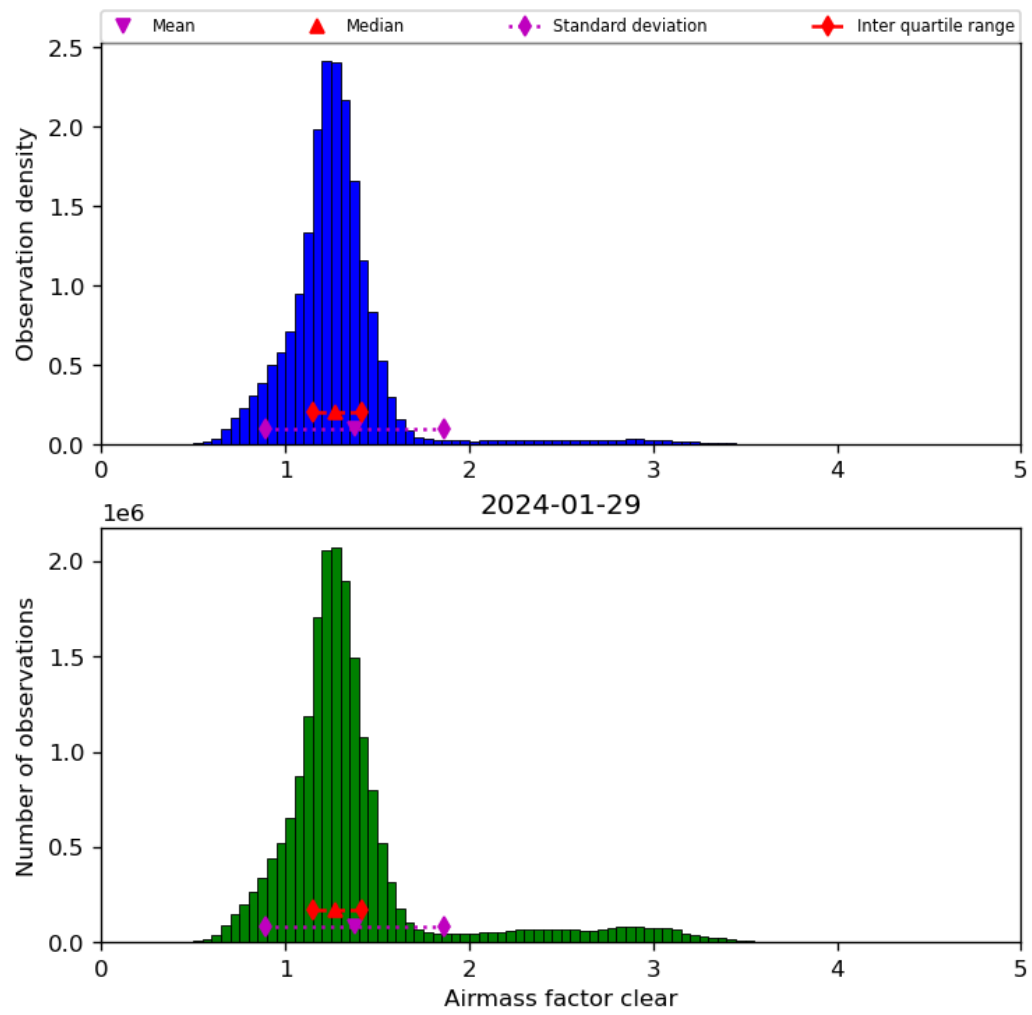
Figure 42: Histogram of “Airmass factor clear” for 2024-01-28 to 2024-01-30
