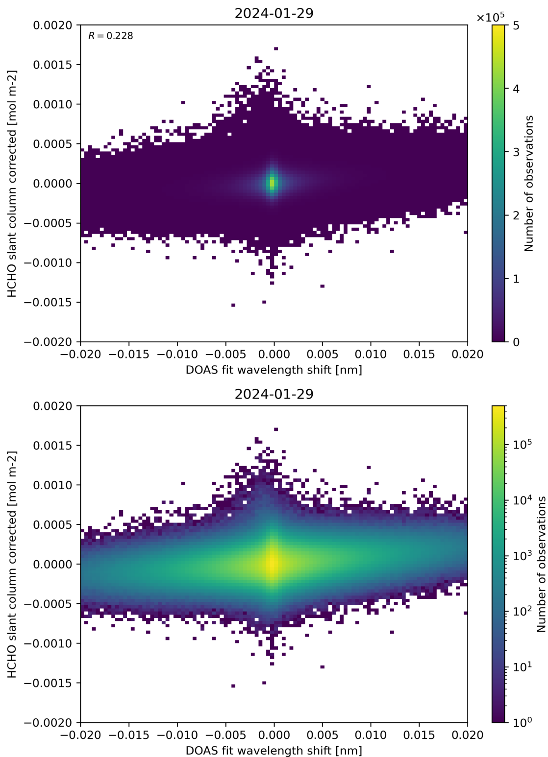
Figure 66: Scatter density plot of “DOAS fit wavelength shift” against “HCHO slant column corrected” for 2024-01-28 to 2024-01-30.
