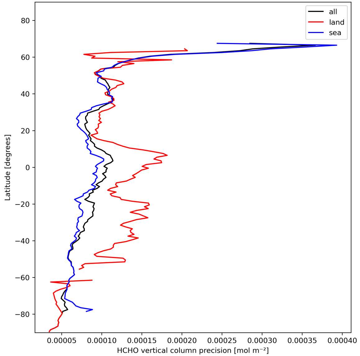
Figure 22: Zonal average of “HCHO vertical column precision” for 2024-01-28 to 2024-01-30.
