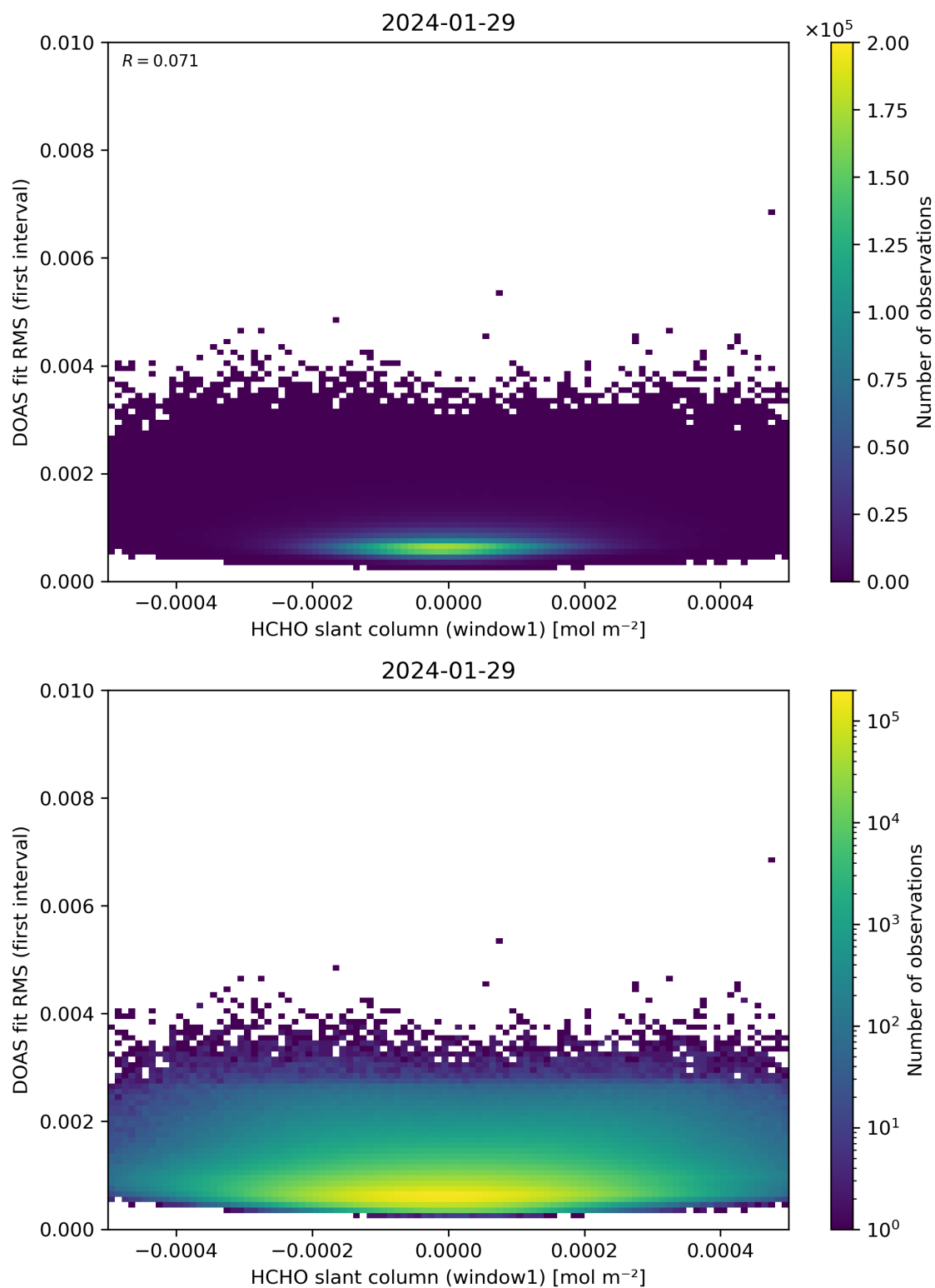
Figure 78: Scatter density plot of “HCHO slant column (window1)” against “DOAS fit RMS (first interval)” for 2024-01-28 to 2024-01-30.
