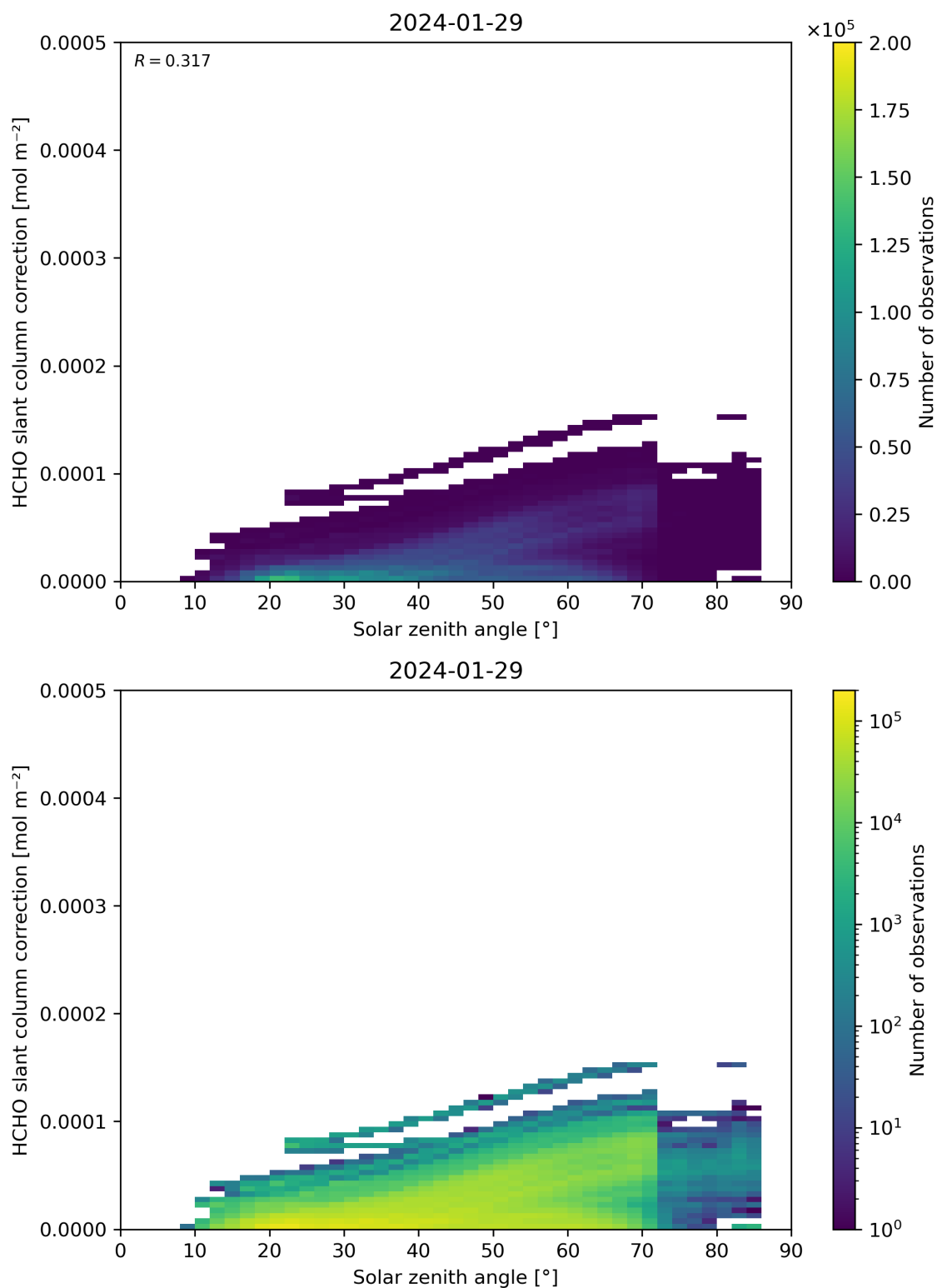
Figure 172: Scatter density plot of “Solar zenith angle” against “HCHO slant column correction” for 2024-01-28 to 2024-01-30.
