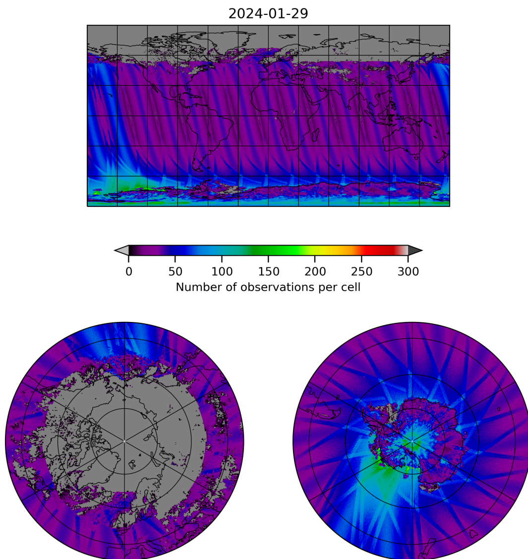
Figure 19: Map of the number of observations for 2024-01-28 to 2024-01-30
