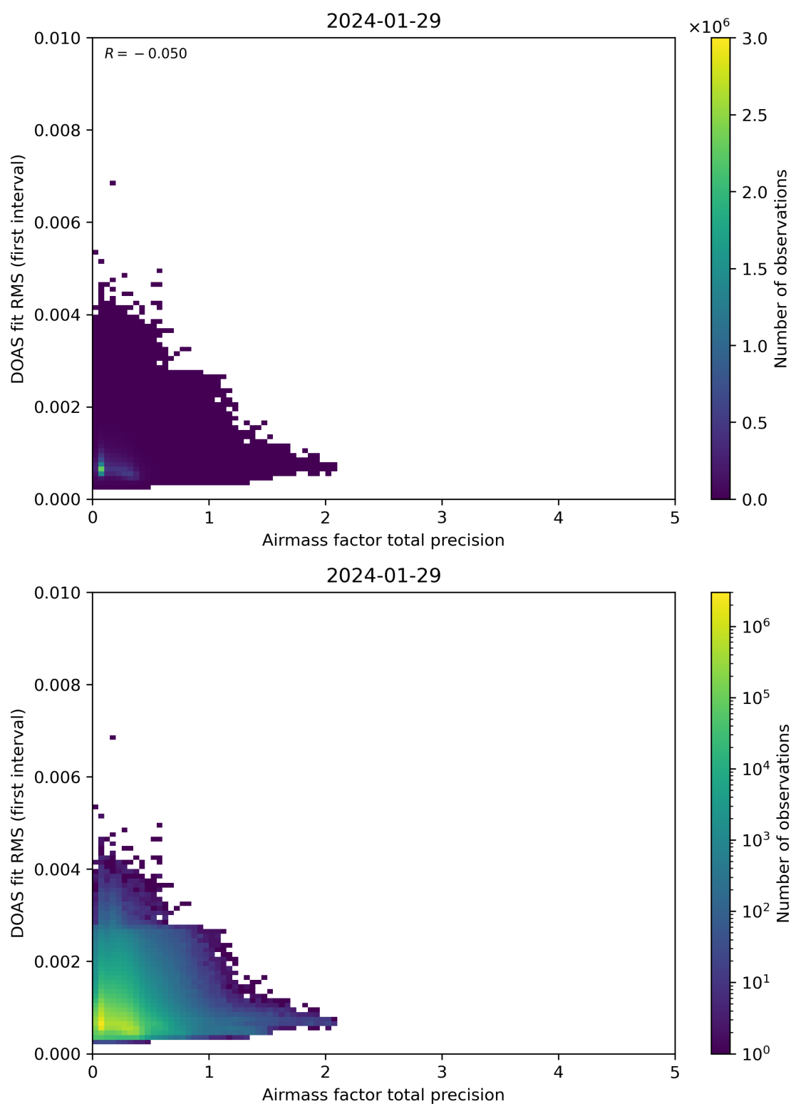
Figure 105: Scatter density plot of “Airmass factor total precision” against “DOAS fit RMS (first interval)” for 2024-01-28 to 2024-01-30.
