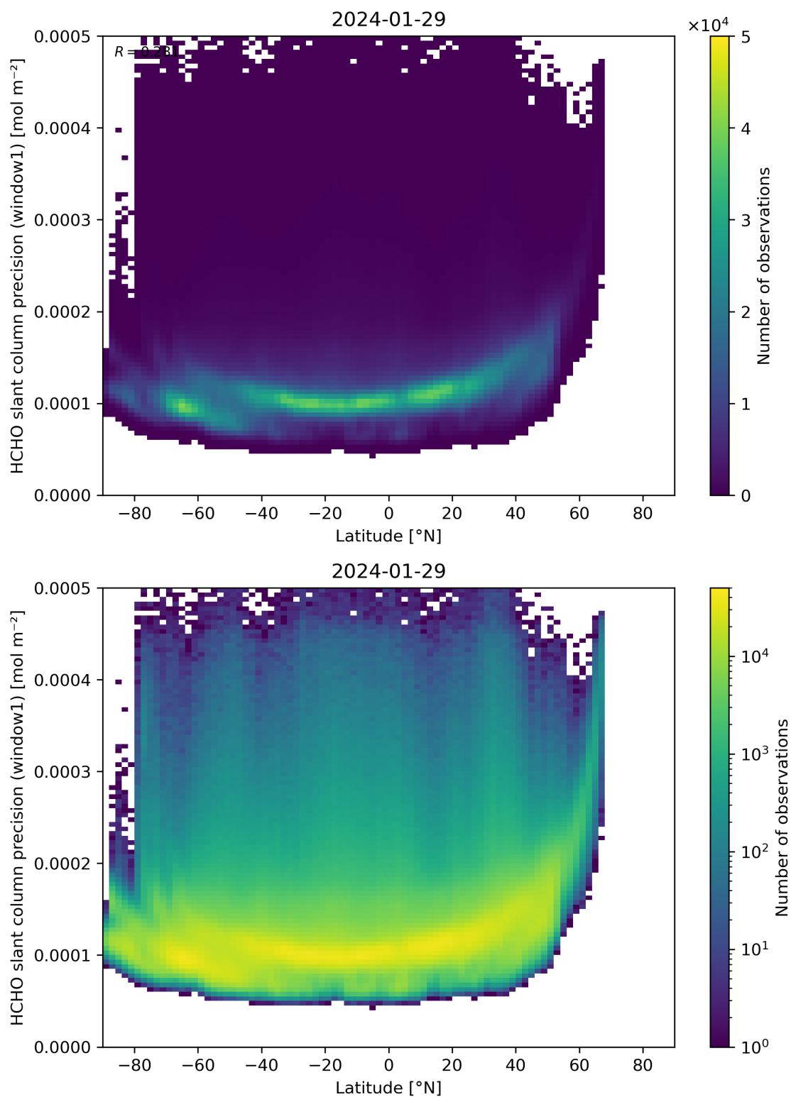
Figure 160: Scatter density plot of “Latitude” against “HCHO slant column precision (window1)” for 2024-01-28 to 2024-01-30.
