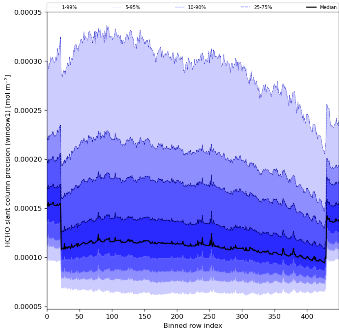
Figure 53: Along track statistics of “HCHO slant column precision (window1)” for 2024-01-28 to 2024-01-30
