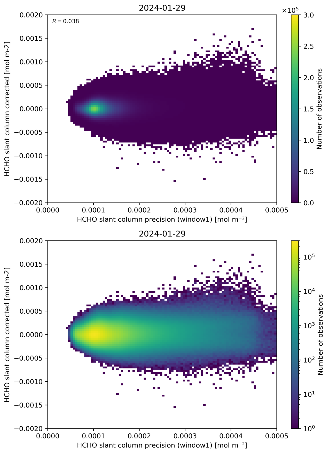
Figure 92: Scatter density plot of “HCHO slant column precision (window1)” against “HCHO slant column corrected” for 2024-01-28 to 2024-01-30.
