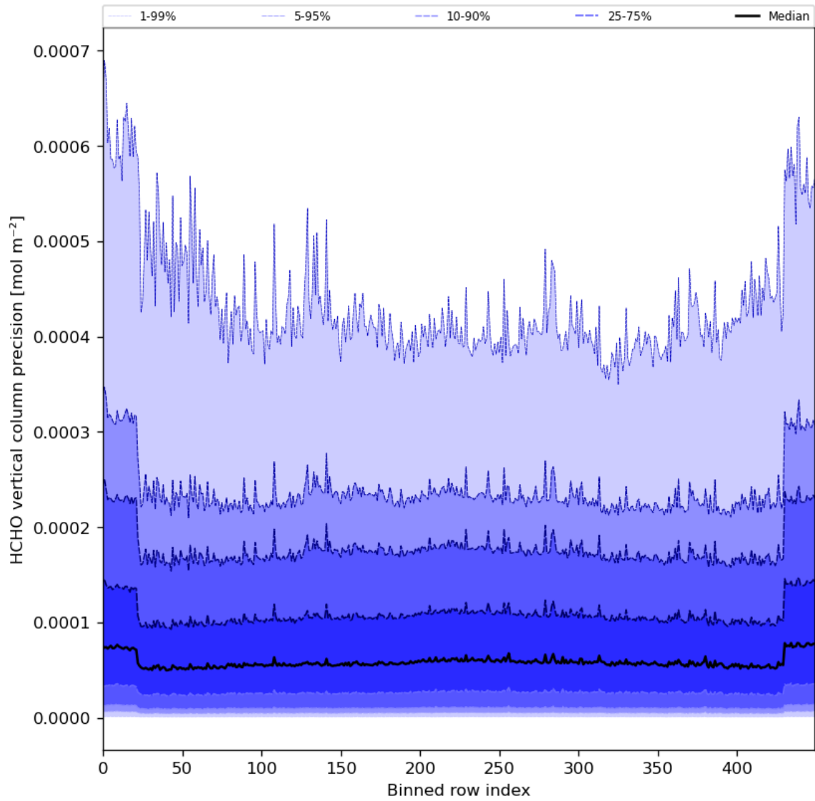
Figure 50: Along track statistics of “HCHO vertical column precision” for 2024-01-28 to 2024-01-30
