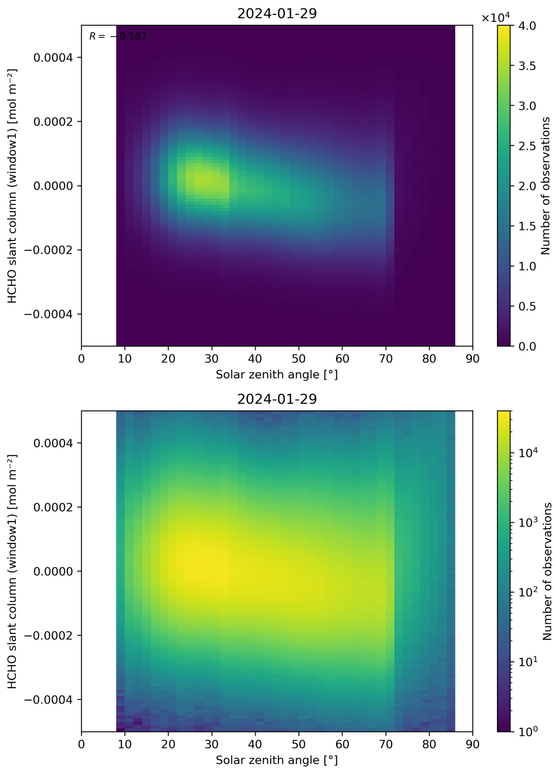
Figure 173: Scatter density plot of “Solar zenith angle” against “HCHO slant column (window1)” for 2024-01-28 to 2024-01-30.
