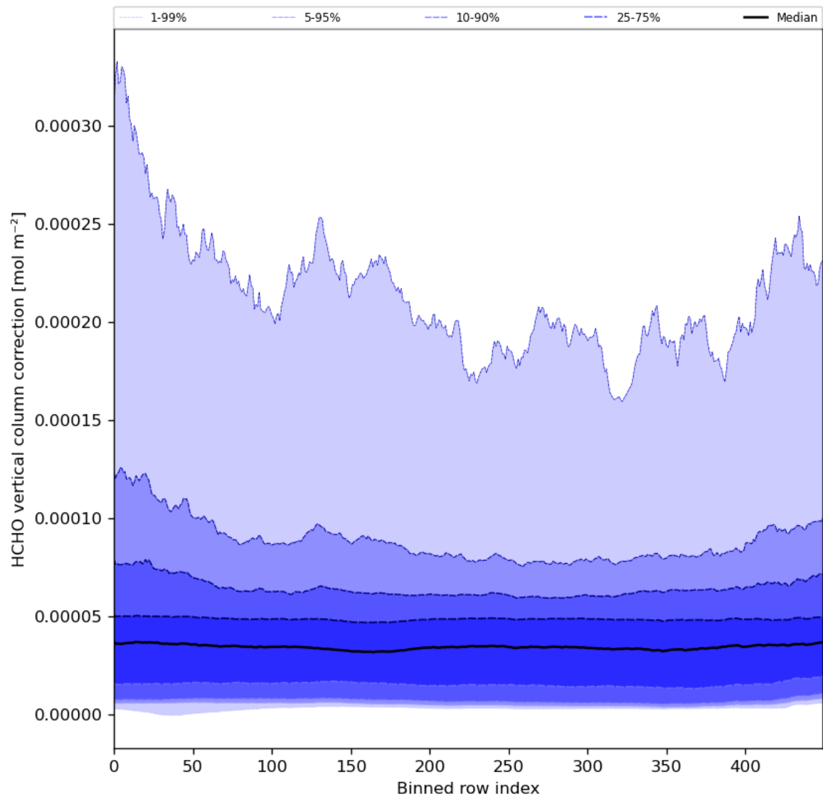
Figure 51: Along track statistics of “HCHO vertical column correction” for 2024-01-28 to 2024-01-30
