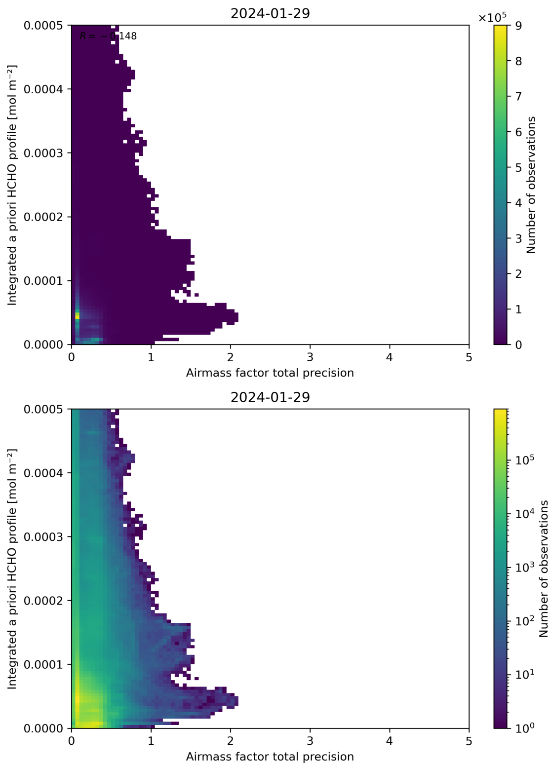
Figure 111: Scatter density plot of “Airmass factor total precision” against “Integrated a priori HCHO profile” for 2024-01-28 to 2024-01-30.
