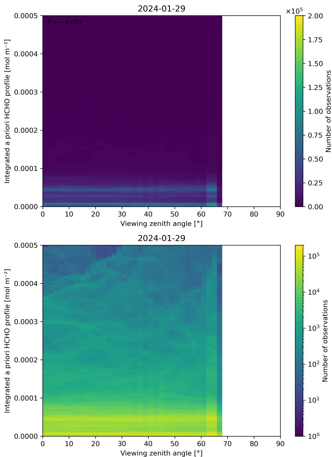
Figure 195: Scatter density plot of “Viewing zenith angle” against “Integrated a priori HCHO profile” for 2024-01-28 to 2024-01-30.
