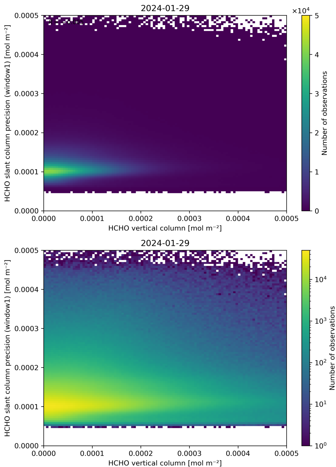
Figure 130: Scatter density plot of “HCHO vertical column” against “HCHO slant column precision (window1)” for 2024-01-28 to 2024-01-30.
