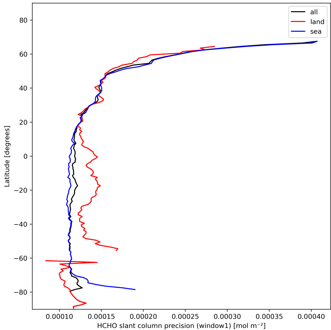
Figure 25: Zonal average of “HCHO slant column precision (window1)” for 2024-01-28 to 2024-01-30.
