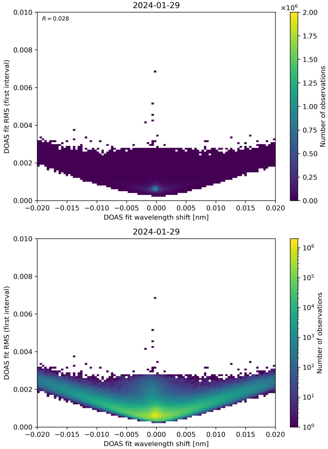
Figure 64: Scatter density plot of “DOAS fit wavelength shift” against “DOAS fit RMS (first interval)” for 2024-01-28 to 2024-01-30.
