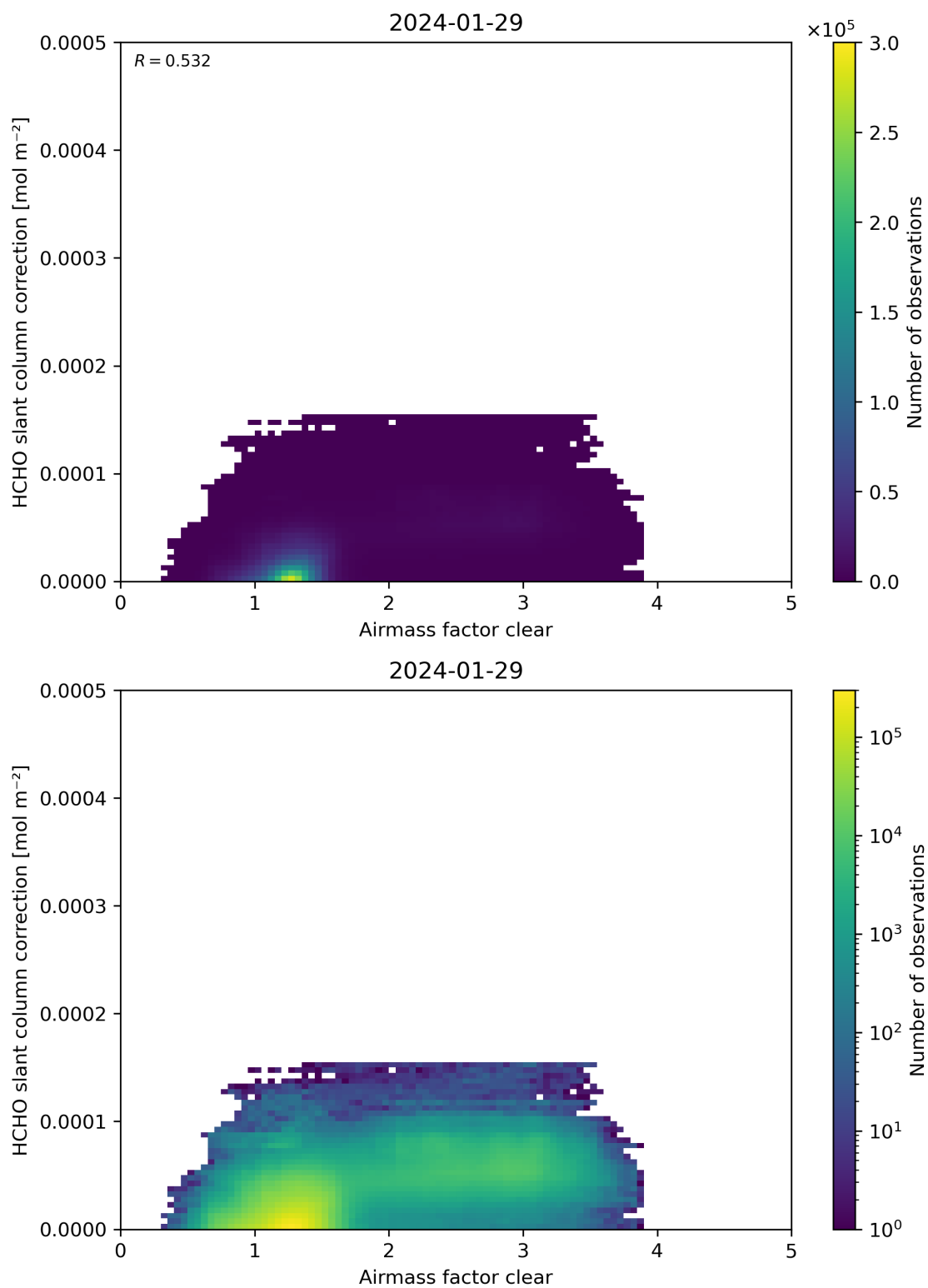
Figure 75: Scatter density plot of “Airmass factor clear” against “HCHO slant column correction” for 2024-01-28 to 2024-01-30.
