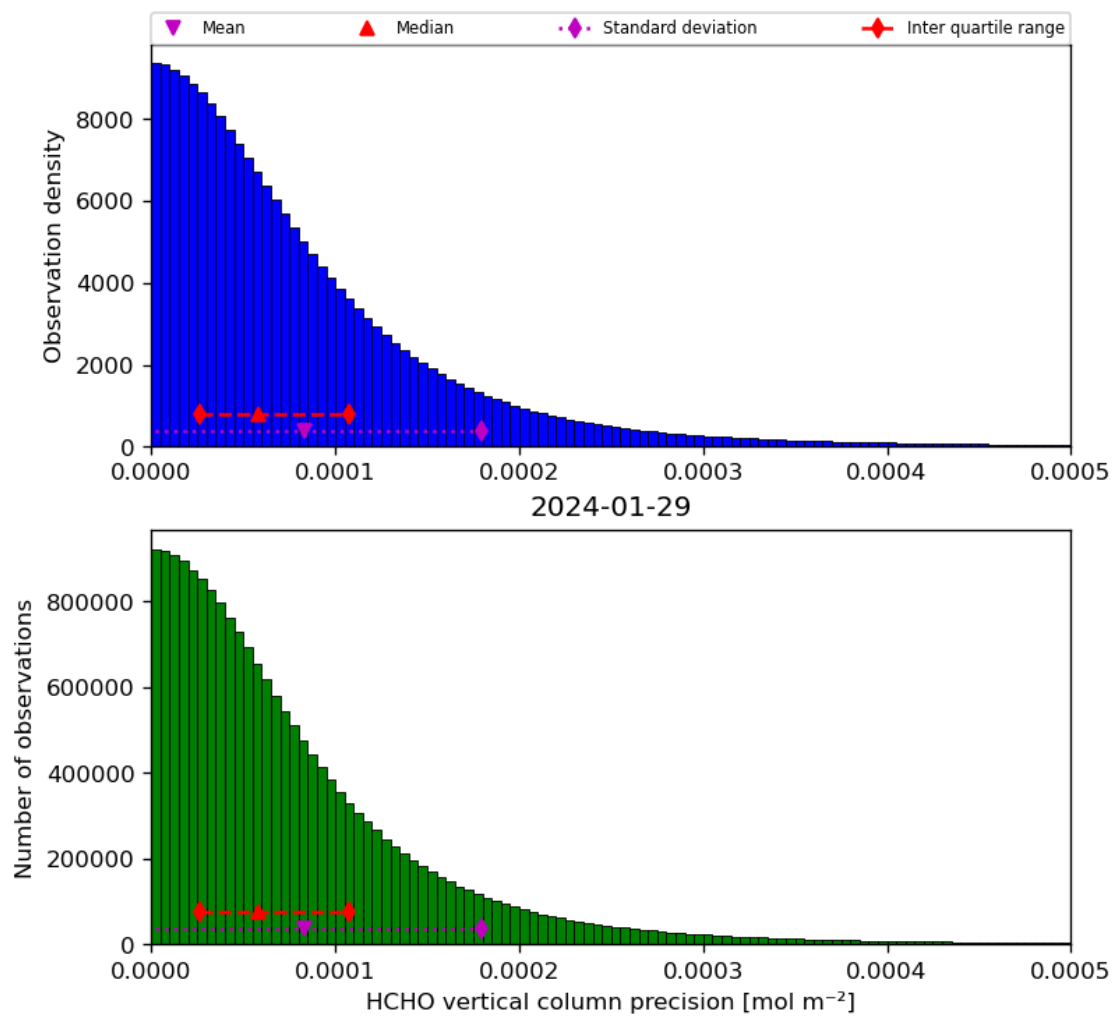
Figure 36: Histogram of “HCHO vertical column precision” for 2024-01-28 to 2024-01-30
