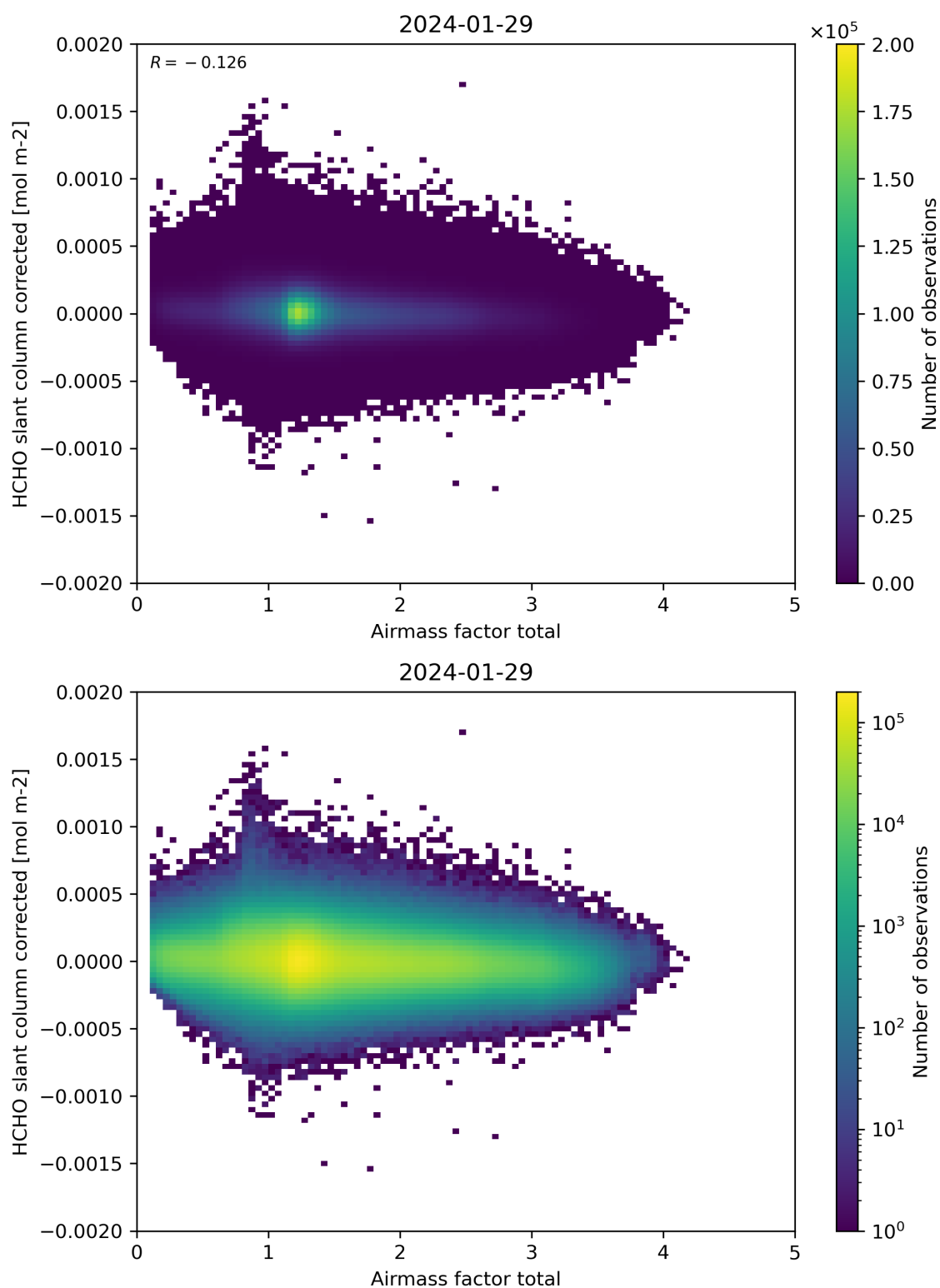
Figure 101: Scatter density plot of “Airmass factor total” against “HCHO slant column corrected” for 2024-01-28 to 2024-01-30.
