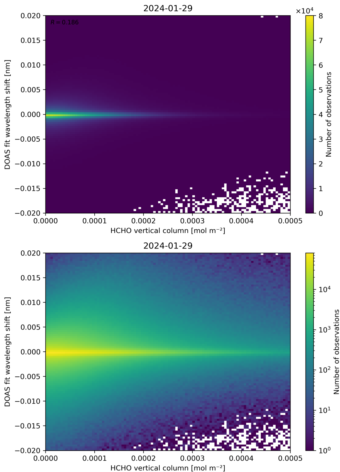
Figure 124: Scatter density plot of “HCHO vertical column” against “DOAS fit wavelength shift” for 2024-01-28 to 2024-01-30.
