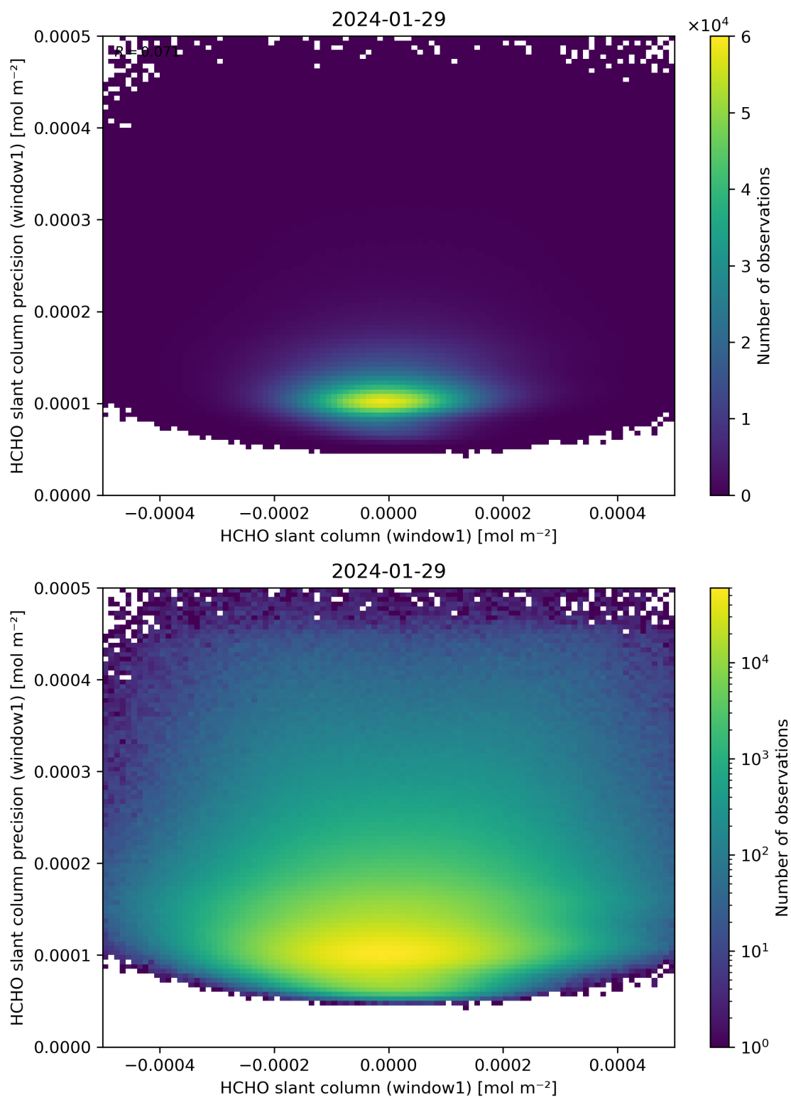
Figure 84: Scatter density plot of “HCHO slant column (window1)” against “HCHO slant column precision (window1)” for 2024-01-28 to 2024-01-30.
