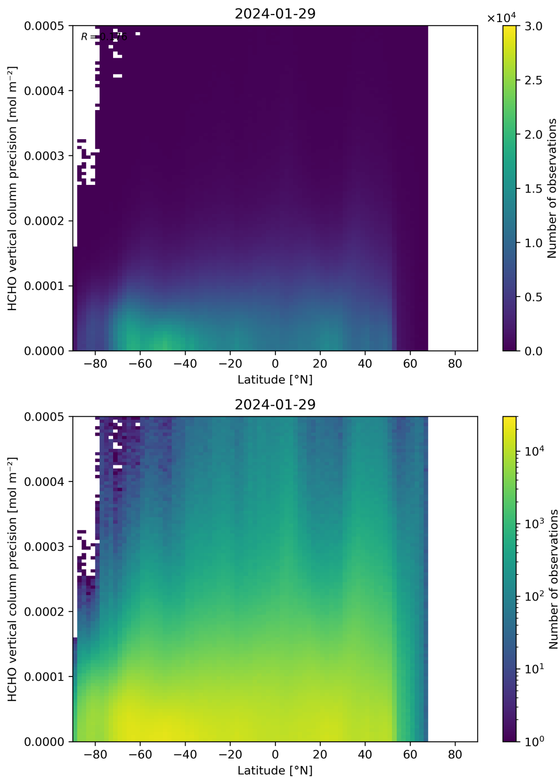
Figure 165: Scatter density plot of “Latitude” against “HCHO vertical column precision” for 2024-01-28 to 2024-01-30.
