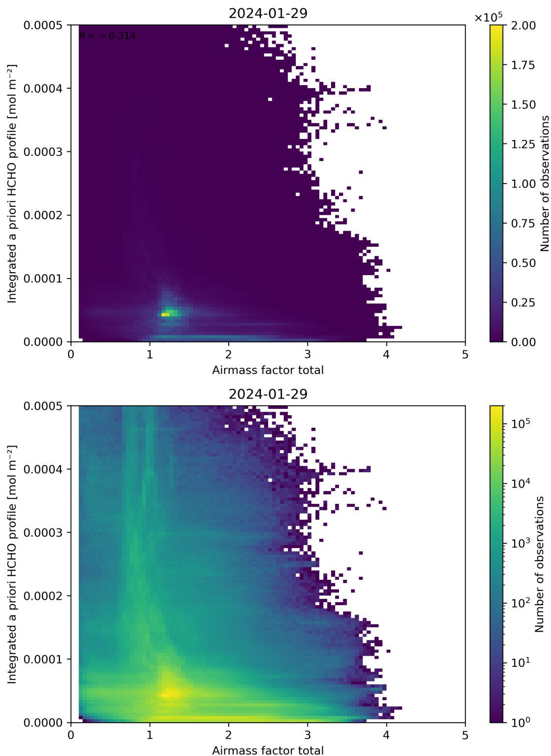
Figure 104: Scatter density plot of “Airmass factor total” against “Integrated a priori HCHO profile” for 2024-01-28 to 2024-01-30.
