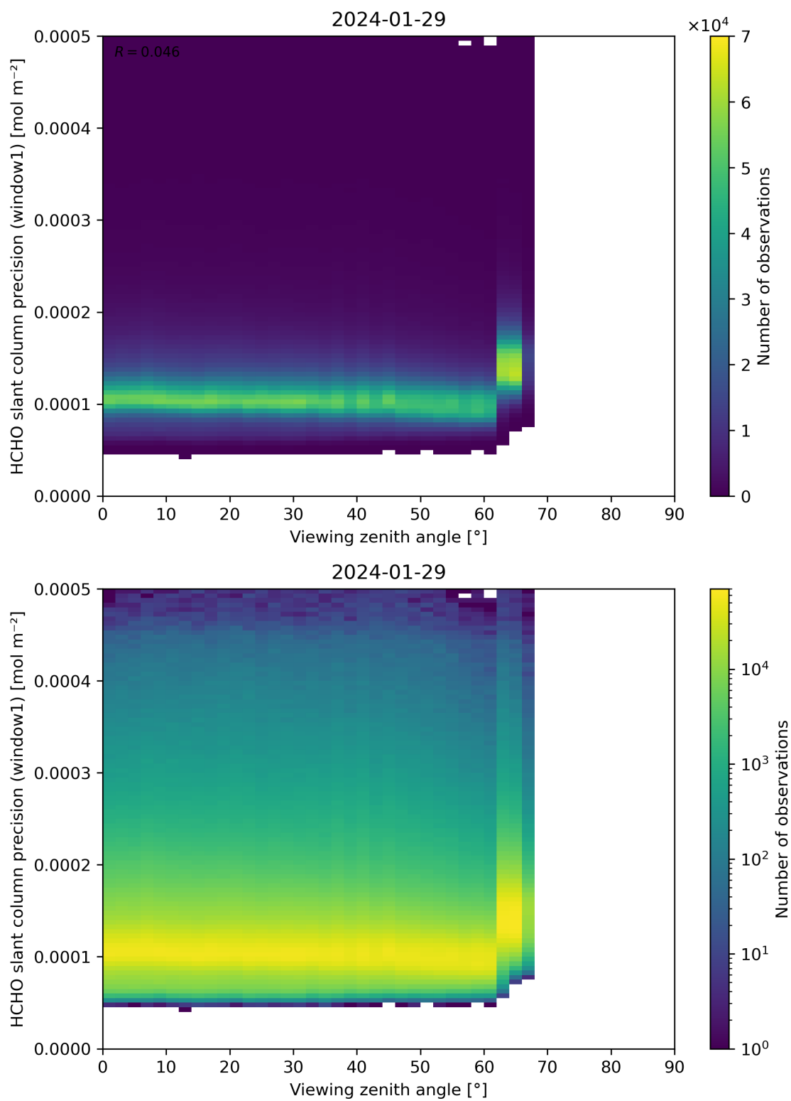
Figure 189: Scatter density plot of “Viewing zenith angle” against “HCHO slant column precision (window1)” for 2024-01-28 to 2024-01-30.
