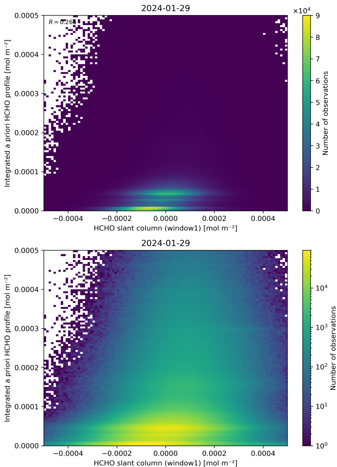
Figure 87: Scatter density plot of “HCHO slant column (window1)” against “Integrated a priori HCHO profile” for 2024-01-28 to 2024-01-30.
