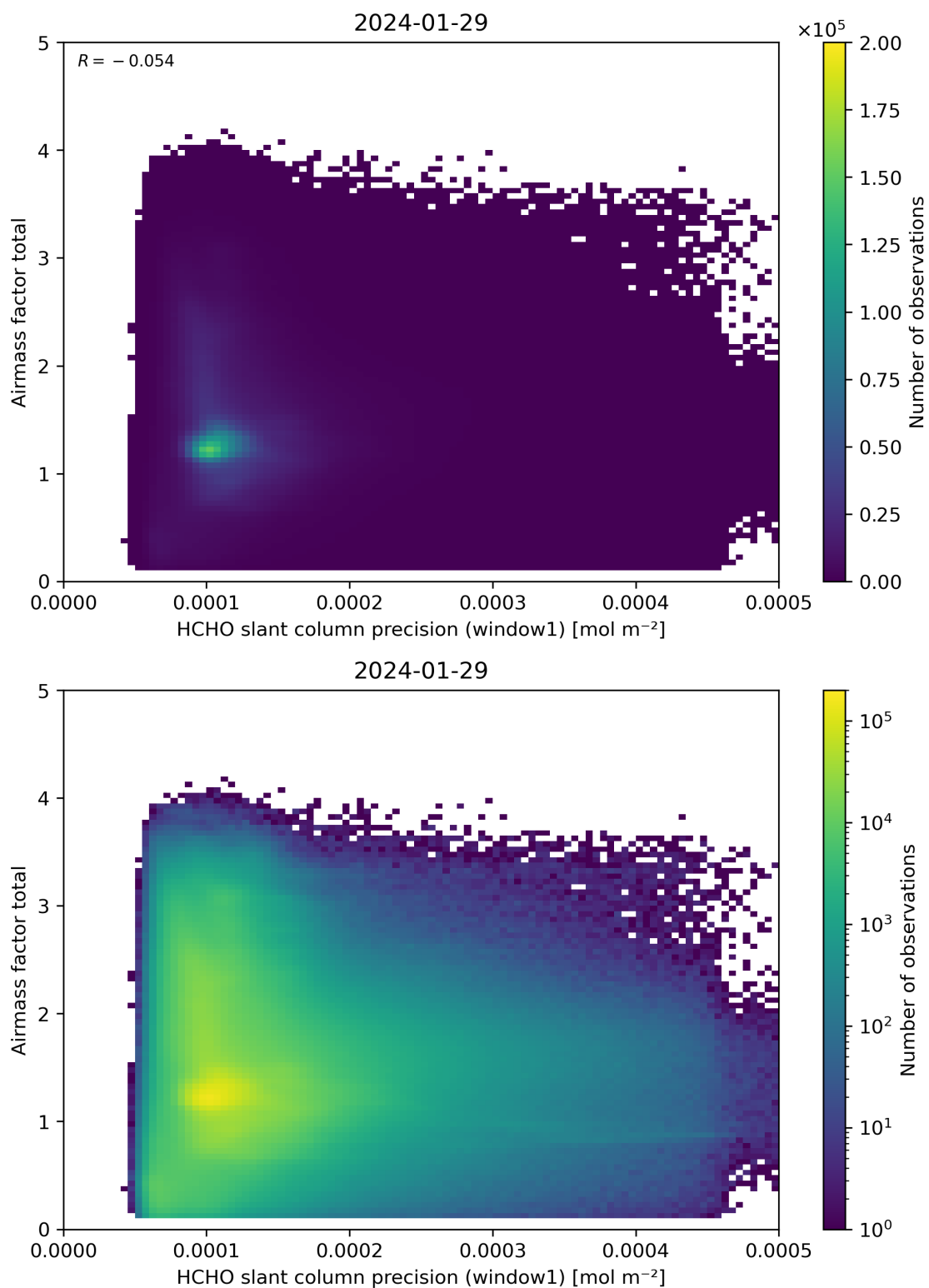
Figure 94: Scatter density plot of “HCHO slant column precision (window1)” against “Airmass factor total” for 2024-01-28 to 2024-01-30.
