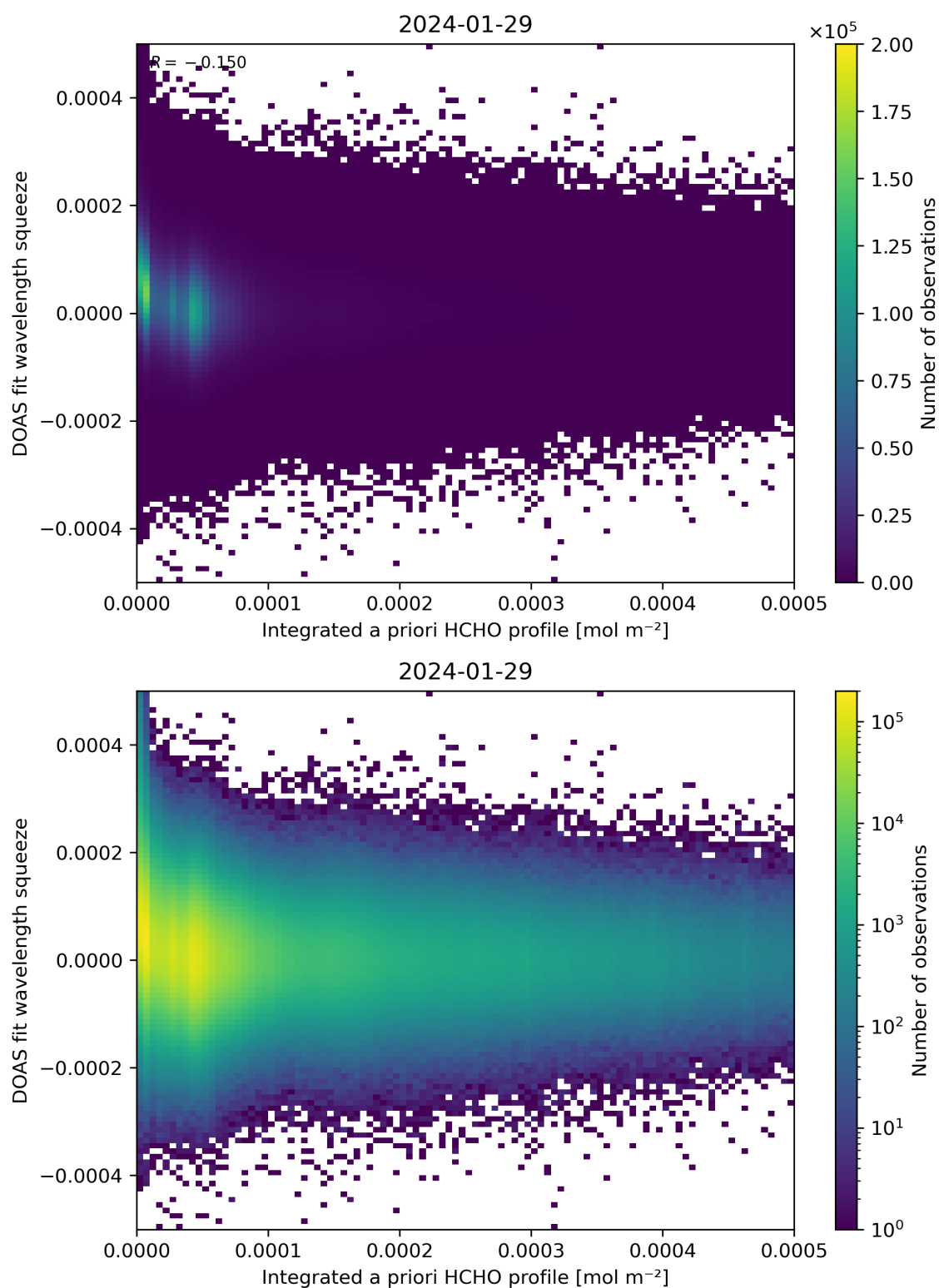
Figure 150: Scatter density plot of “Integrated a priori HCHO profile” against “DOAS fit wavelength squeeze” for 2024-01-28 to 2024-01-30.
