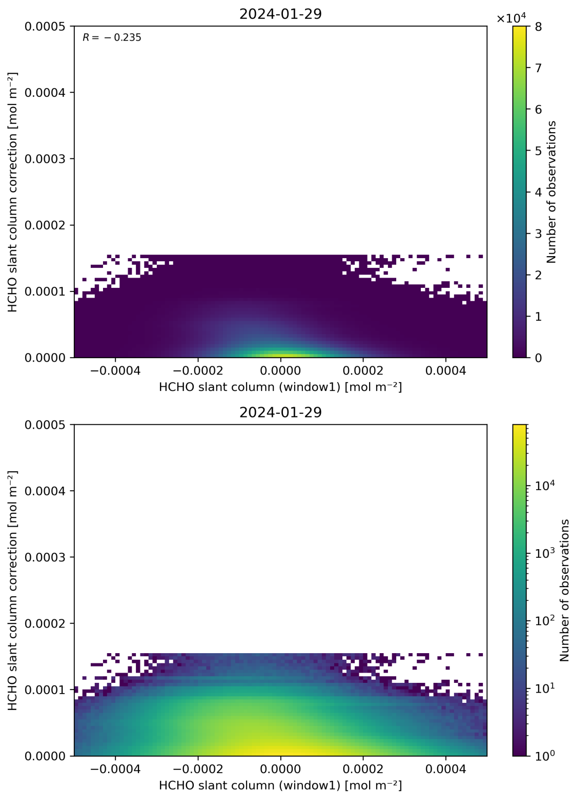
Figure 83: Scatter density plot of “HCHO slant column (window1)” against “HCHO slant column correction” for 2024-01-28 to 2024-01-30.
