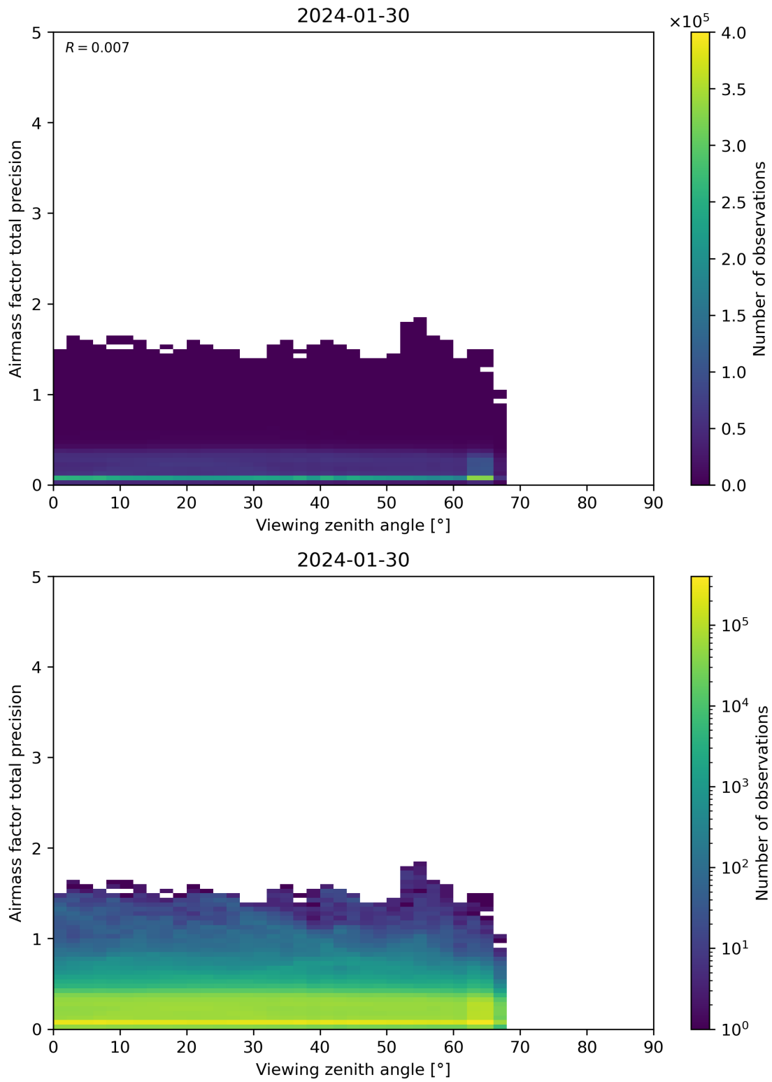
Figure 191: Scatter density plot of “Viewing zenith angle” against “Airmass factor total precision” for 2024-01-29 to 2024-01-31.
