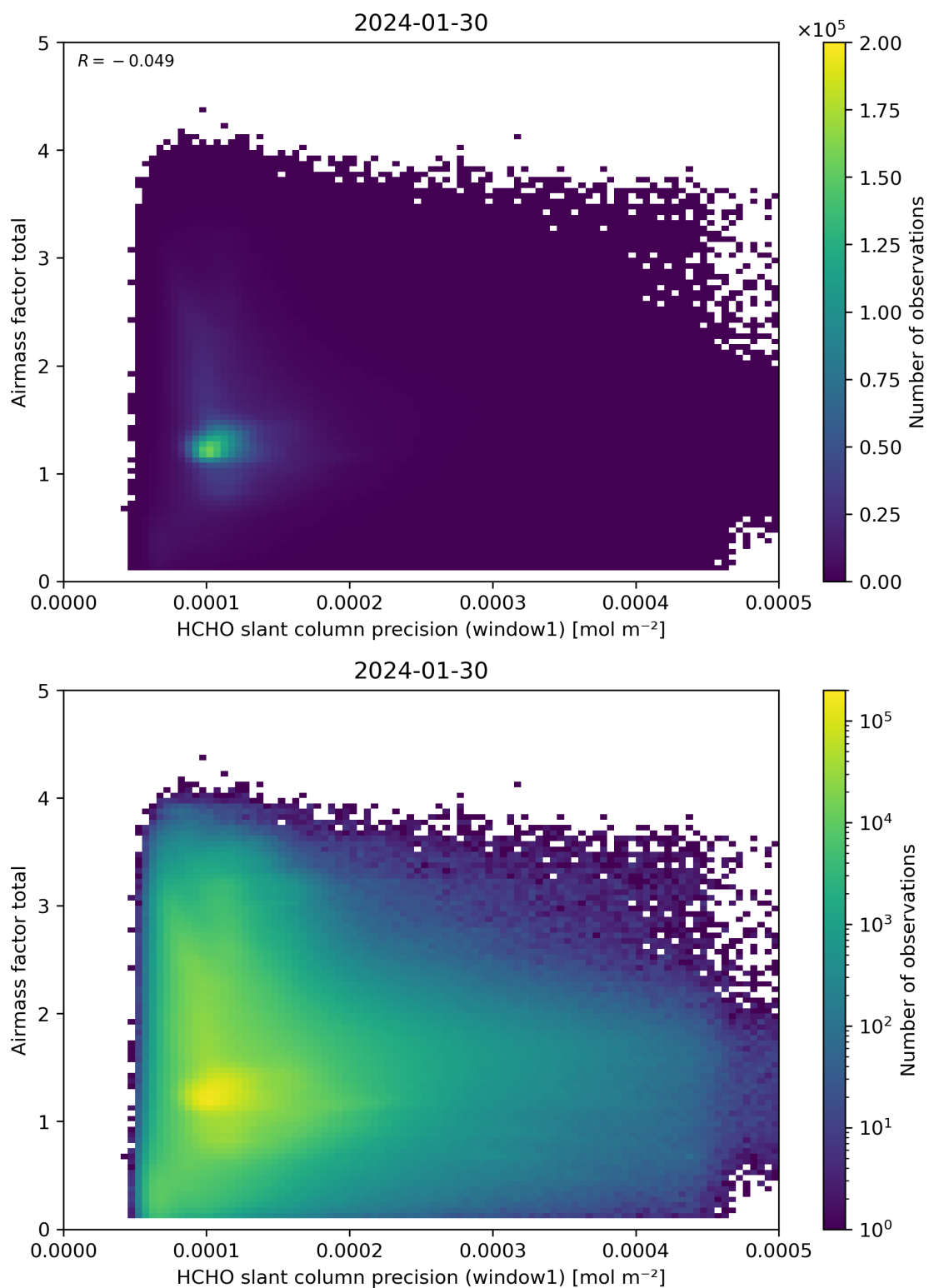
Figure 94: Scatter density plot of “HCHO slant column precision (window1)” against “Airmass factor total” for 2024-01-29 to 2024-01-31.
