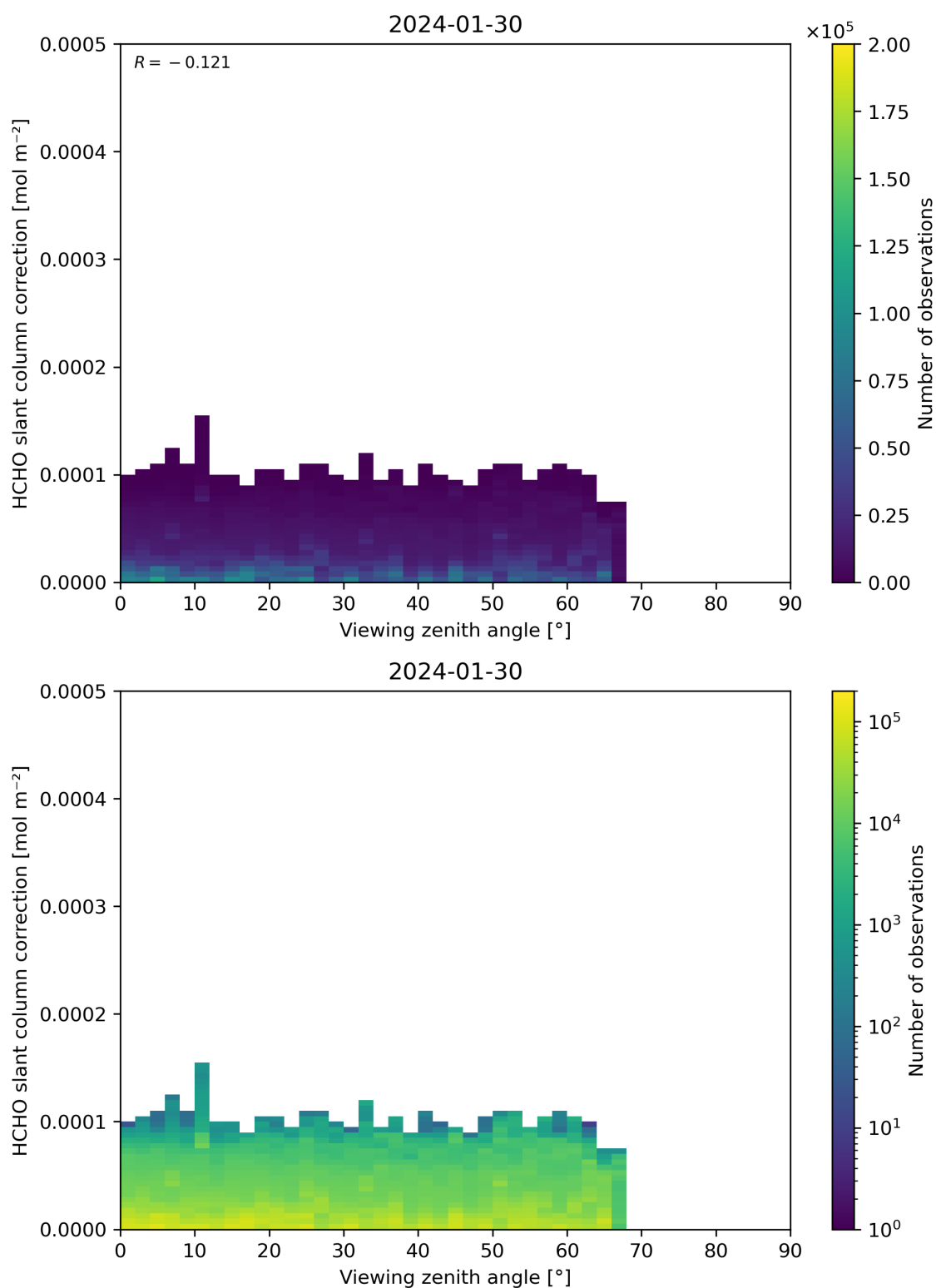
Figure 187: Scatter density plot of “Viewing zenith angle” against “HCHO slant column correction” for 2024-01-29 to 2024-01-31.
