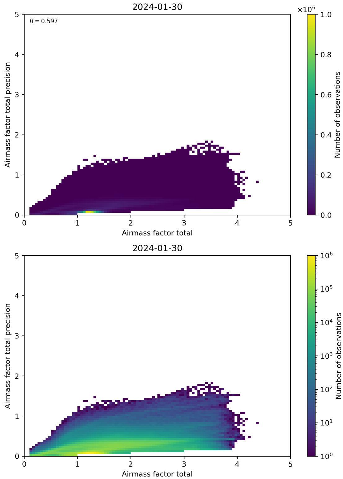
Figure 103: Scatter density plot of “Airmass factor total” against “Airmass factor total precision” for 2024-01-29 to 2024-01-31.
