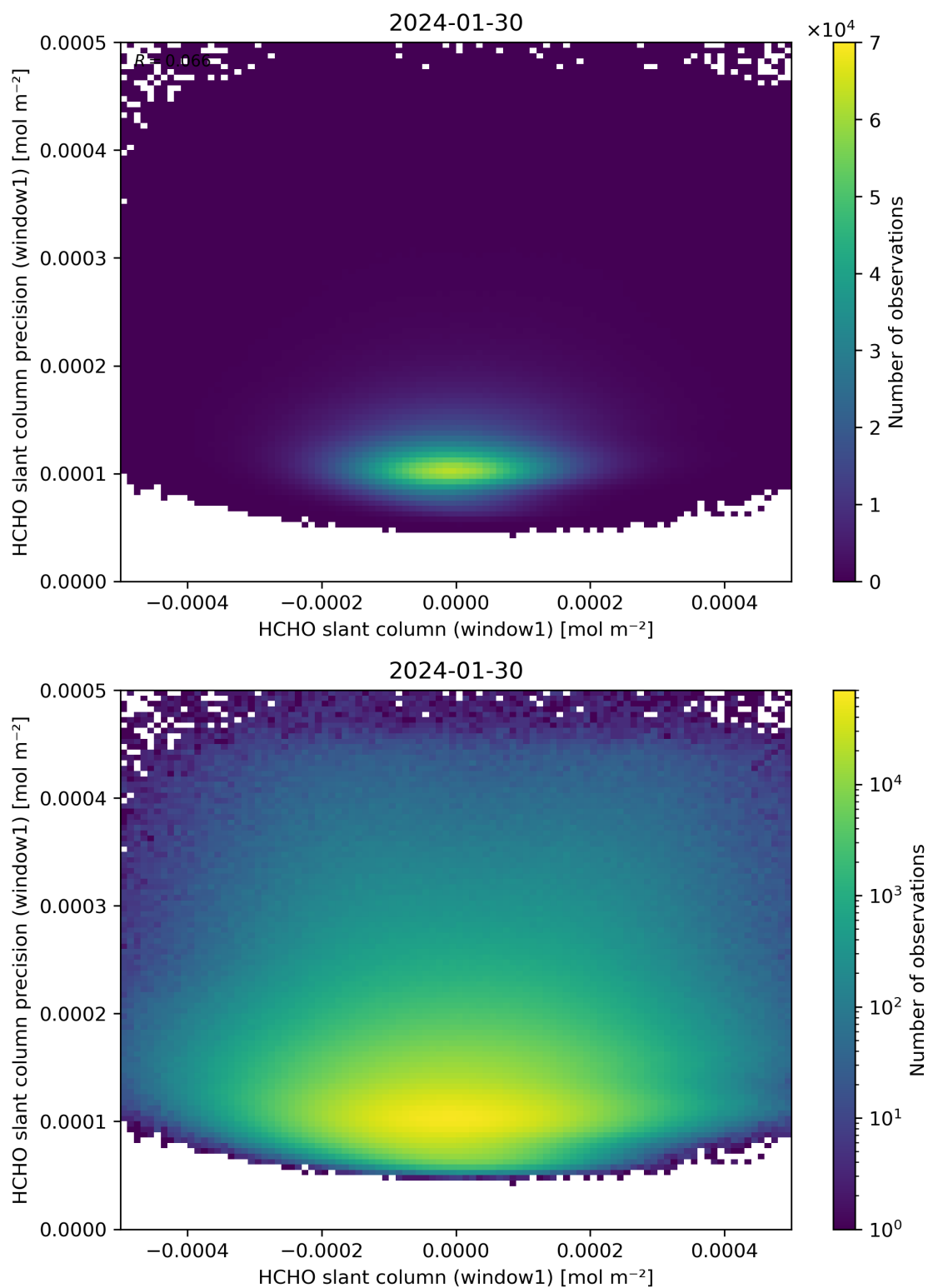
Figure 84: Scatter density plot of “HCHO slant column (window1)” against “HCHO slant column precision (window1)” for 2024-01-29 to 2024-01-31.
