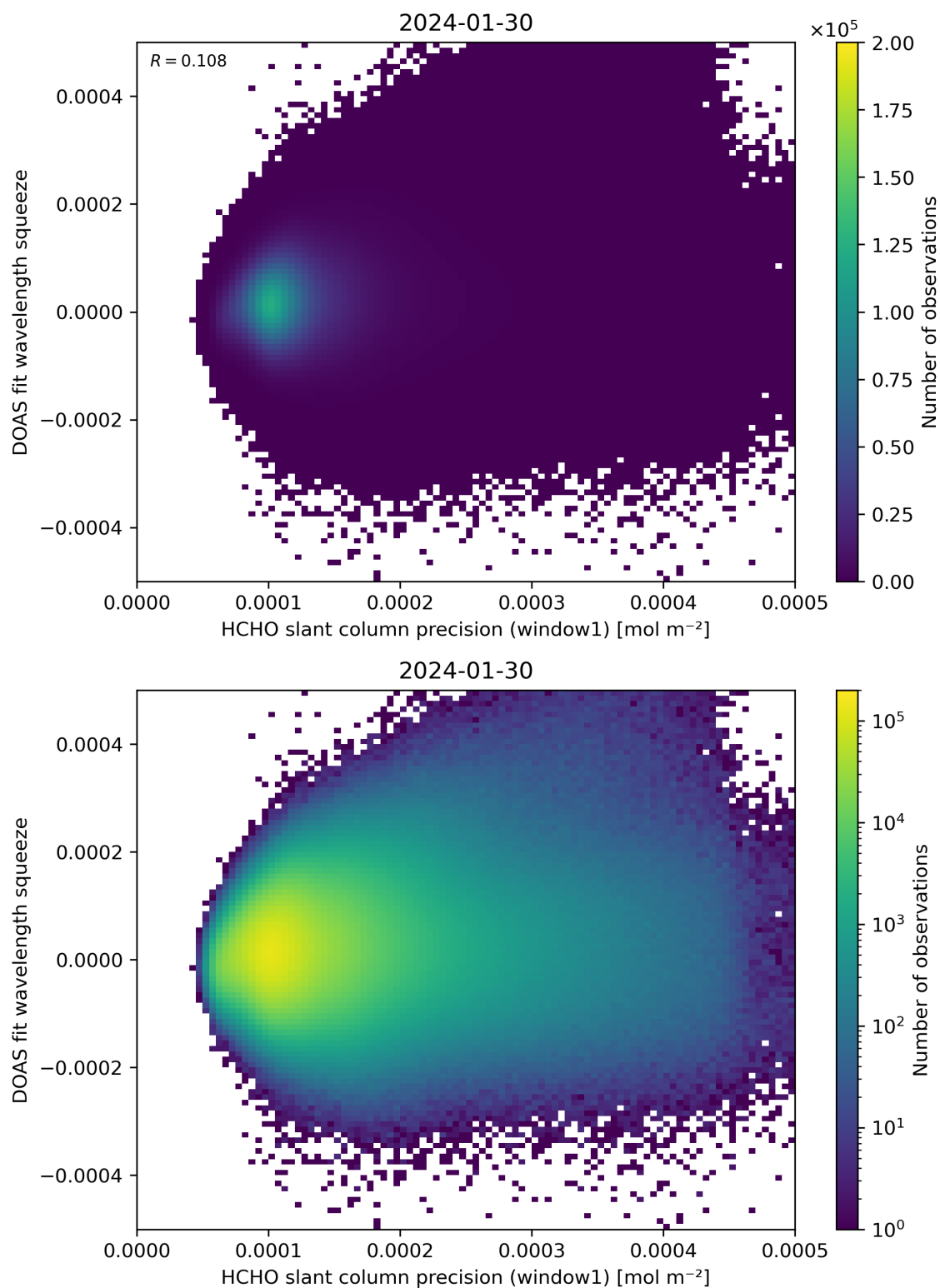
Figure 90: Scatter density plot of “HCHO slant column precision (window1)” against “DOAS fit wavelength squeeze” for 2024-01-29 to 2024-01-31.
