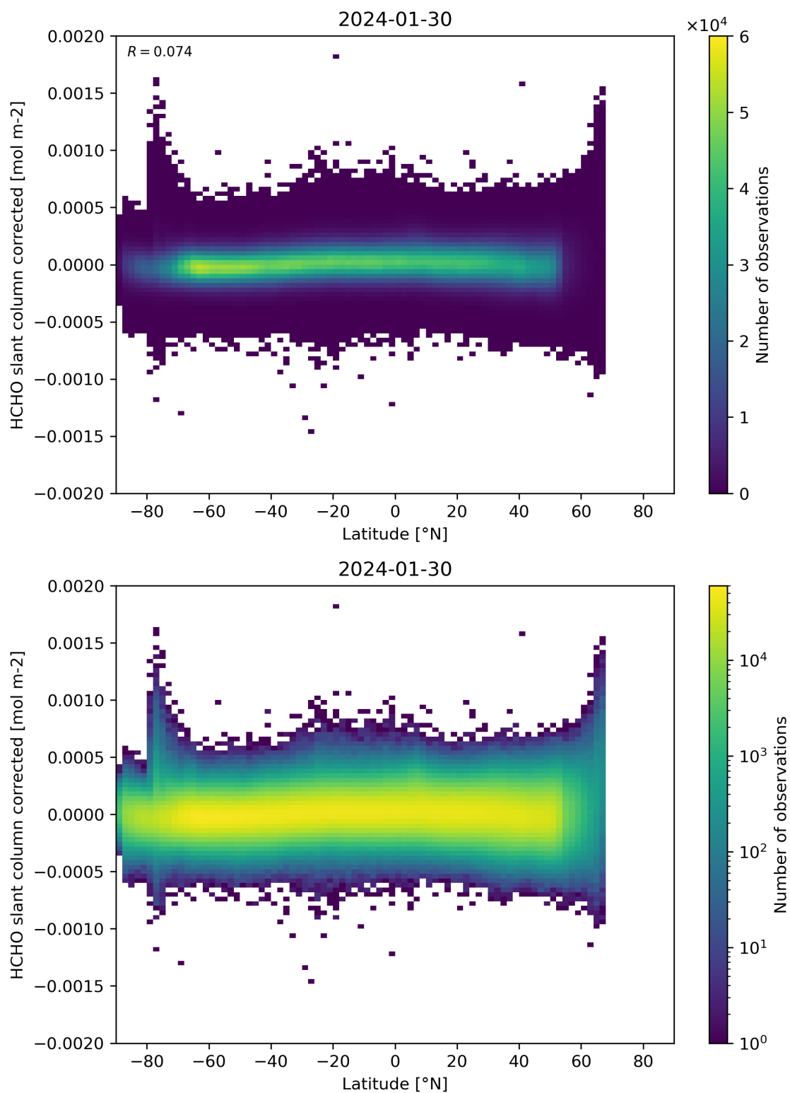
Figure 157: Scatter density plot of “Latitude” against “HCHO slant column corrected” for 2024-01-29 to 2024-01-31.
