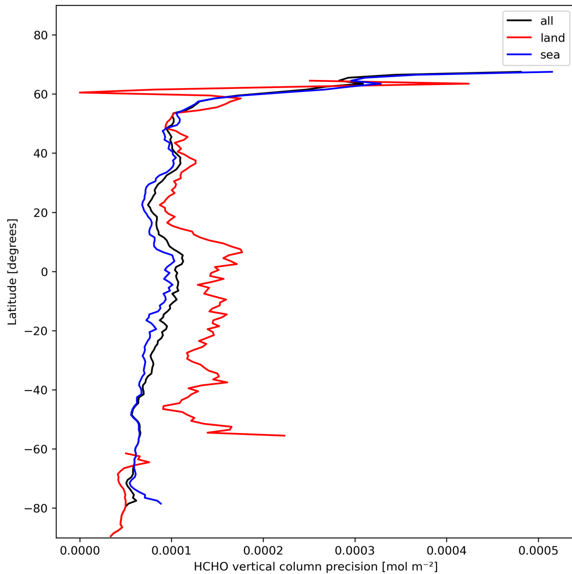
Figure 22: Zonal average of “HCHO vertical column precision” for 2024-01-29 to 2024-01-31.
