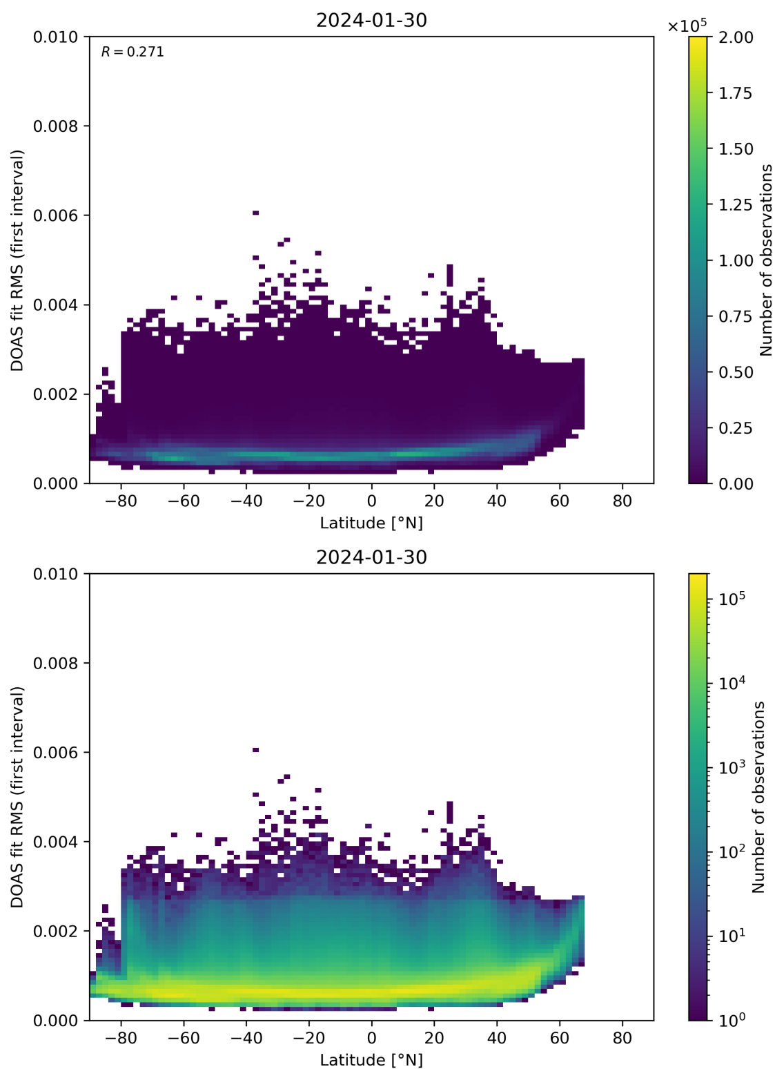
Figure 153: Scatter density plot of “Latitude” against “DOAS fit RMS (first interval)” for 2024-01-29 to 2024-01-31.
