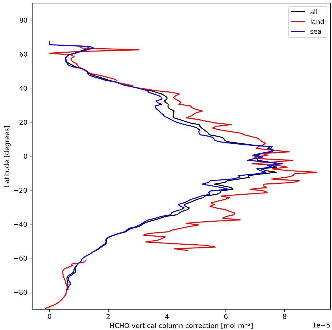
Figure 23: Zonal average of “HCHO vertical column correction” for 2024-01-29 to 2024-01-31.
