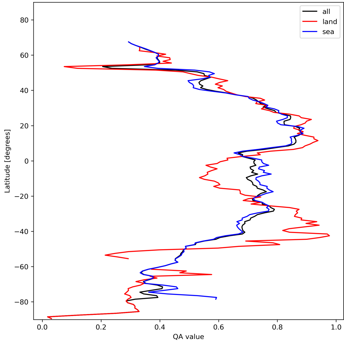
Figure 20: Zonal average of “QA value” for 2024-01-29 to 2024-01-31.
