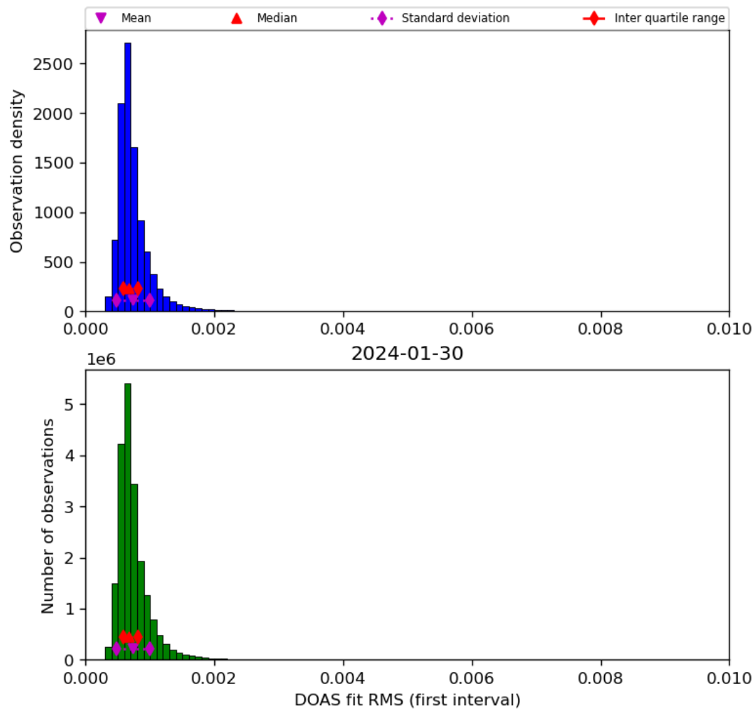
Figure 46: Histogram of “DOAS fit RMS (first interval)” for 2024-01-29 to 2024-01-31
