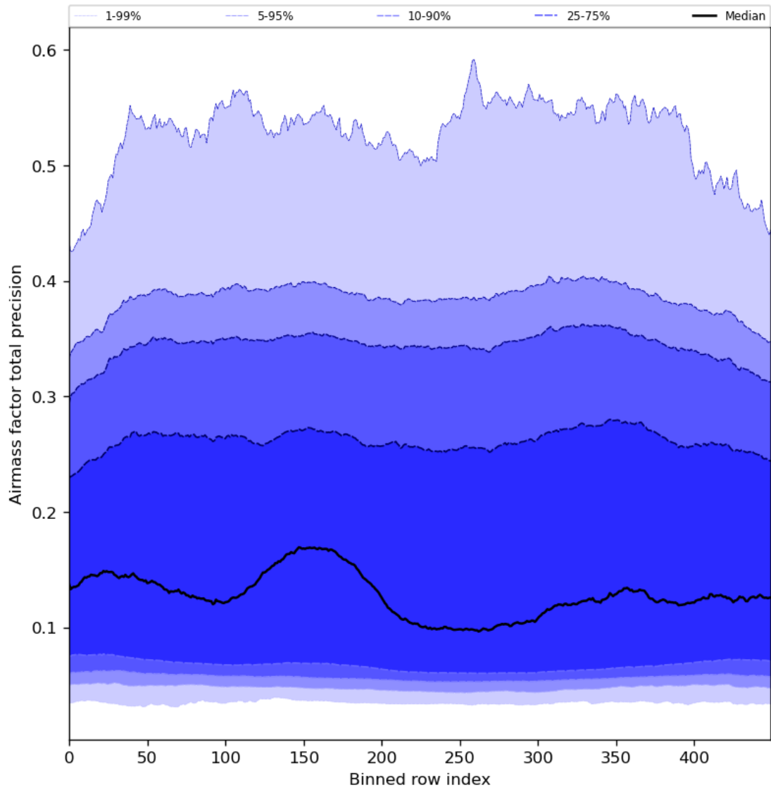
Figure 55: Along track statistics of “Airmass factor total precision” for 2024-01-29 to 2024-01-31
