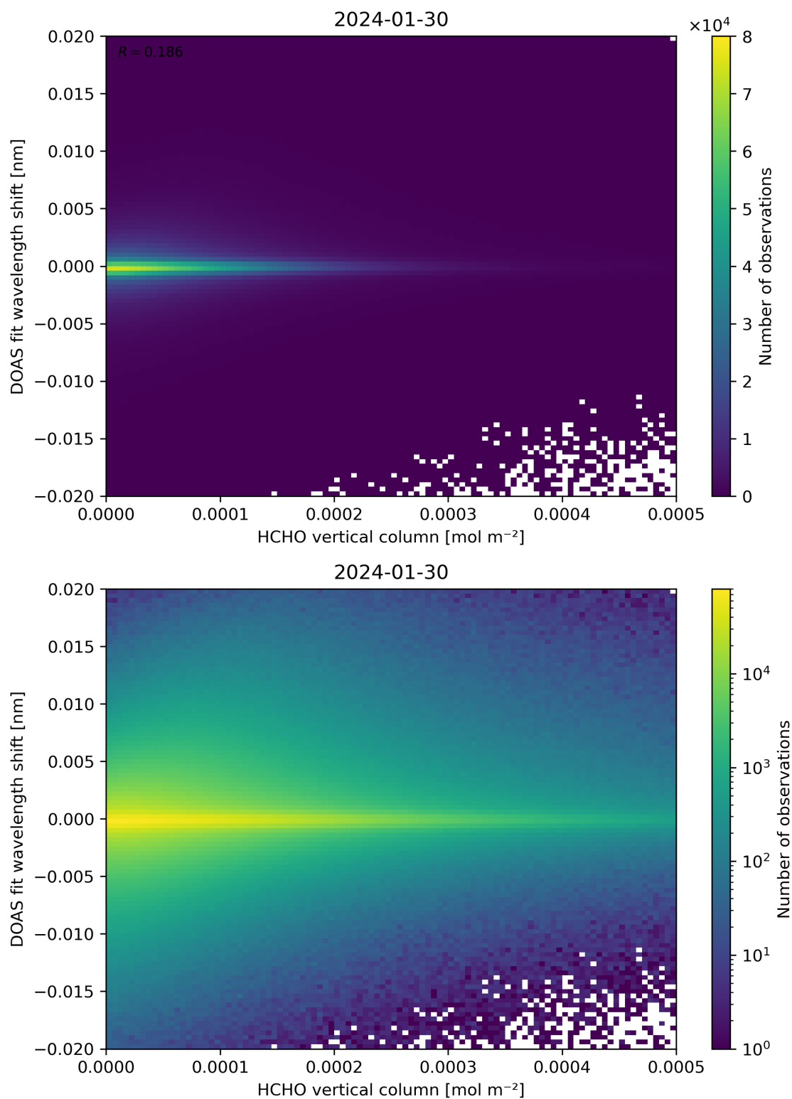
Figure 124: Scatter density plot of “HCHO vertical column” against “DOAS fit wavelength shift” for 2024-01-29 to 2024-01-31.
