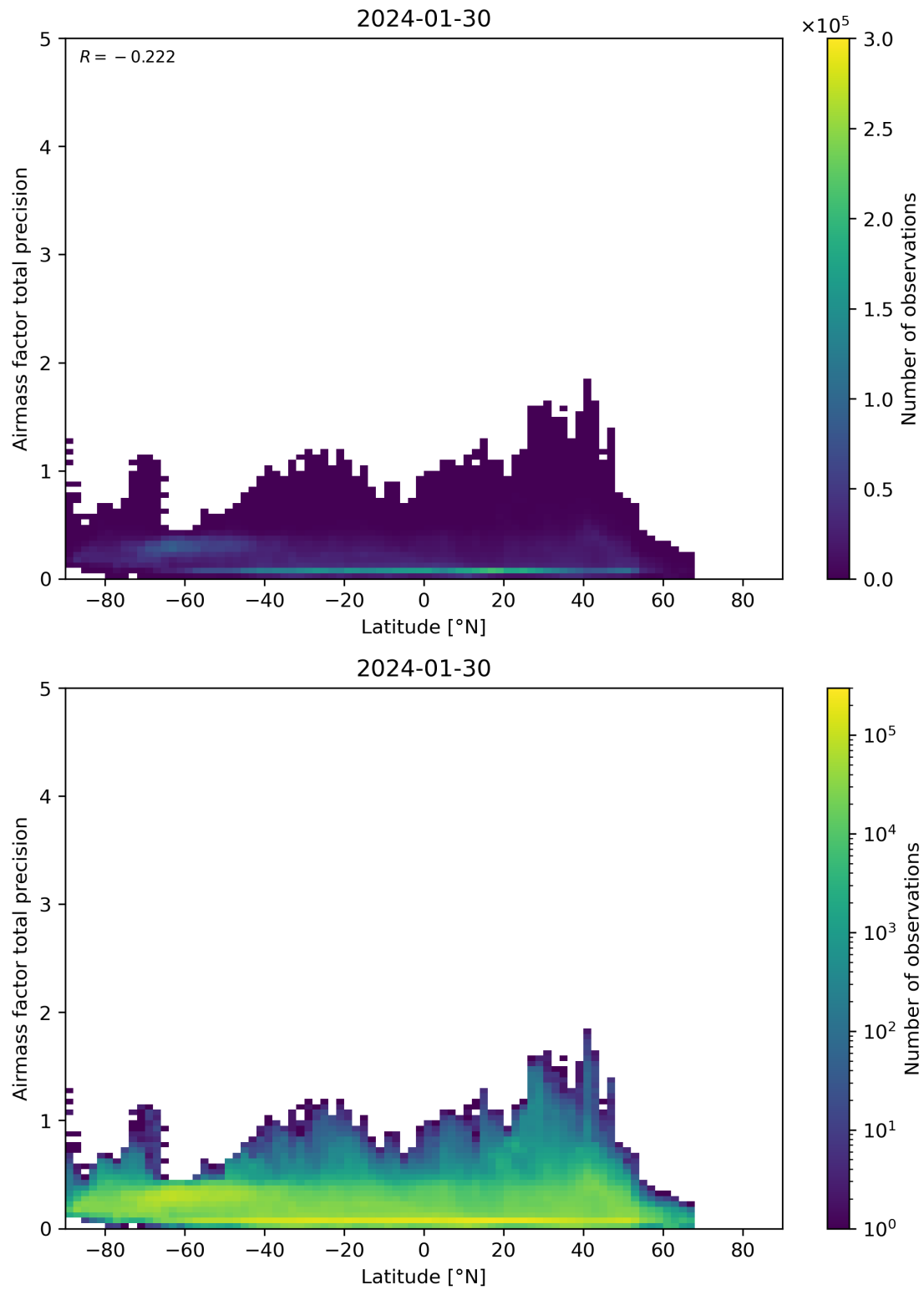
Figure 162: Scatter density plot of “Latitude” against “Airmass factor total precision” for 2024-01-29 to 2024-01-31.
