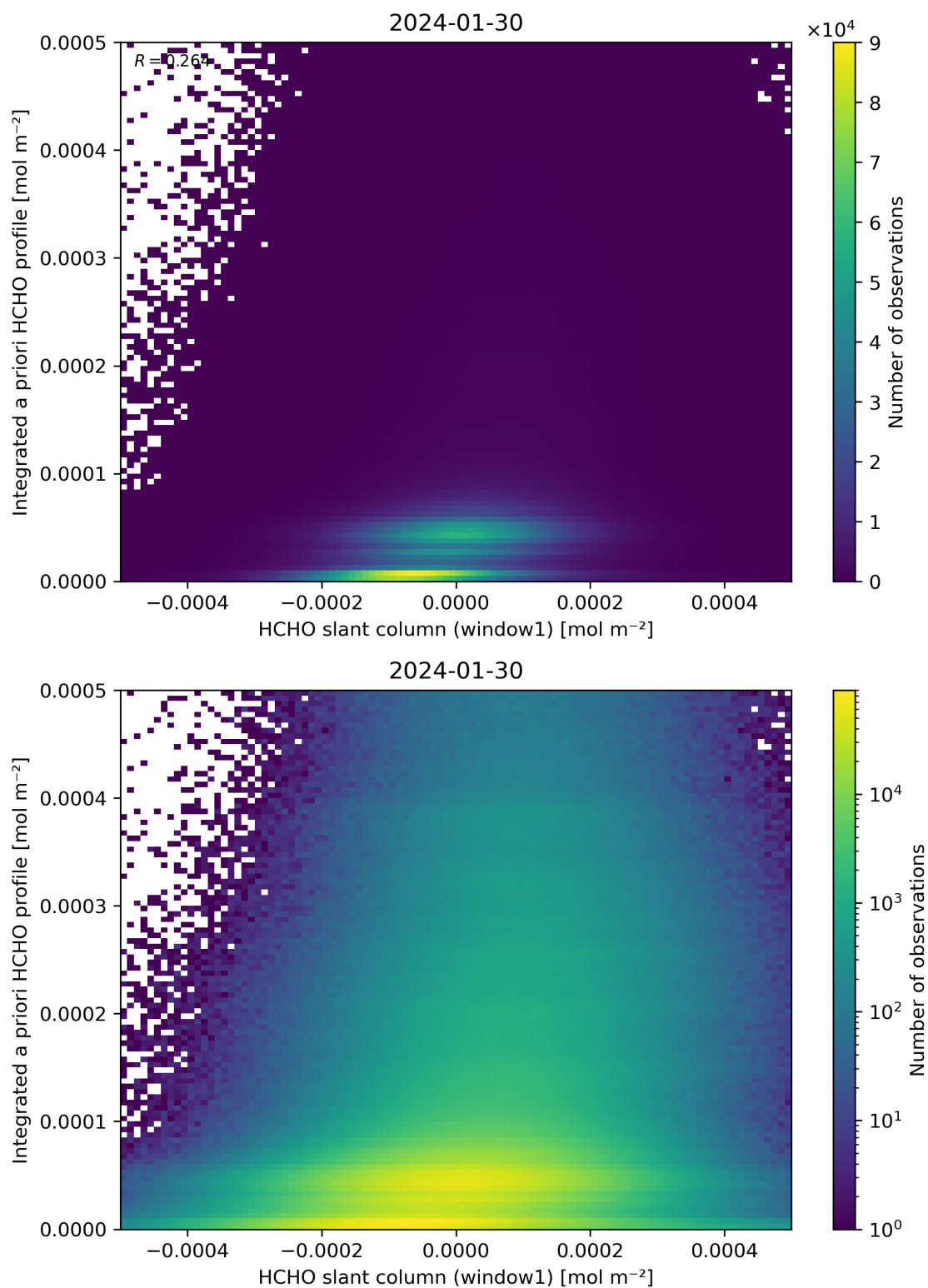
Figure 87: Scatter density plot of “HCHO slant column (window1)” against “Integrated a priori HCHO profile” for 2024-01-29 to 2024-01-31.
