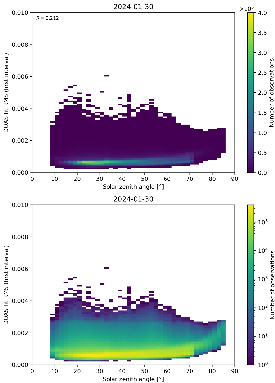
Figure 167: Scatter density plot of “Solar zenith angle” against “DOAS fit RMS (first interval)” for 2024-01-29 to 2024-01-31.
