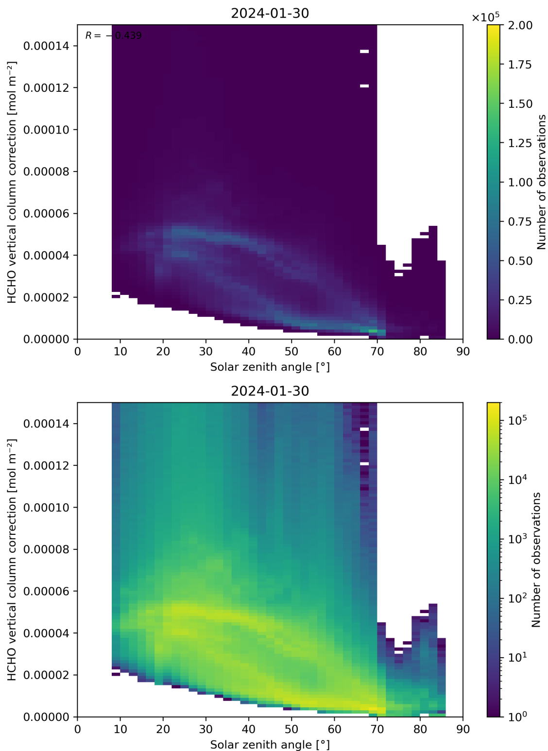
Figure 178: Scatter density plot of “Solar zenith angle” against “HCHO vertical column correction” for 2024-01-29 to 2024-01-31.
