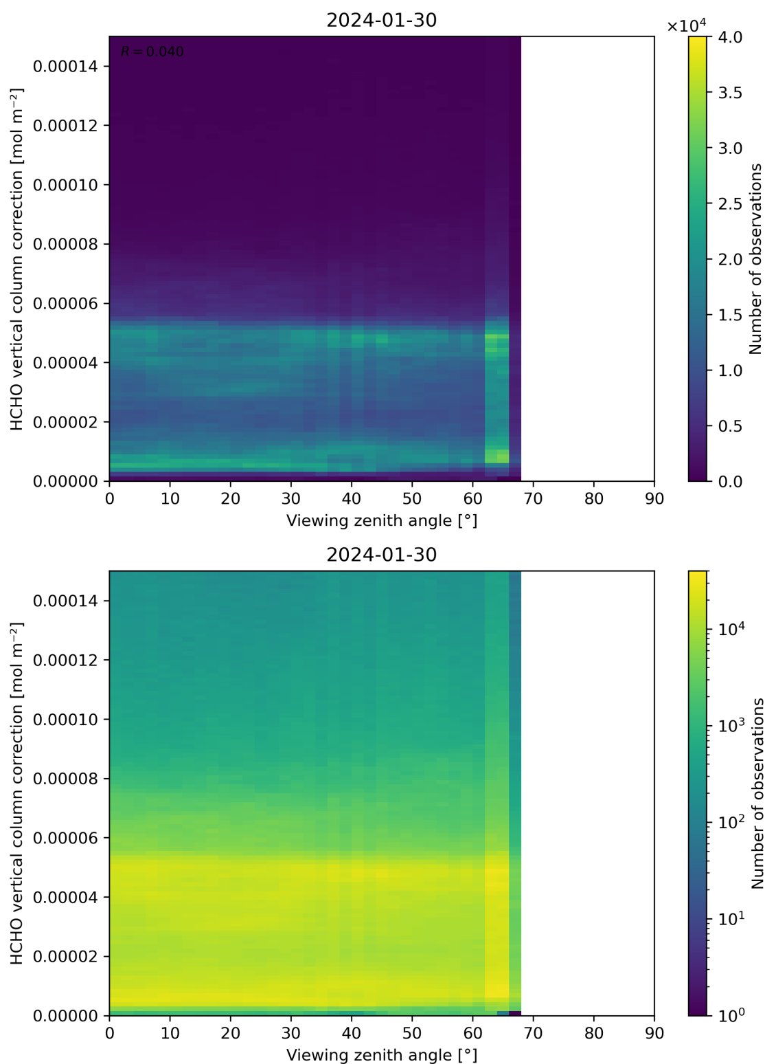
Figure 193: Scatter density plot of “Viewing zenith angle” against “HCHO vertical column correction” for 2024-01-29 to 2024-01-31.
