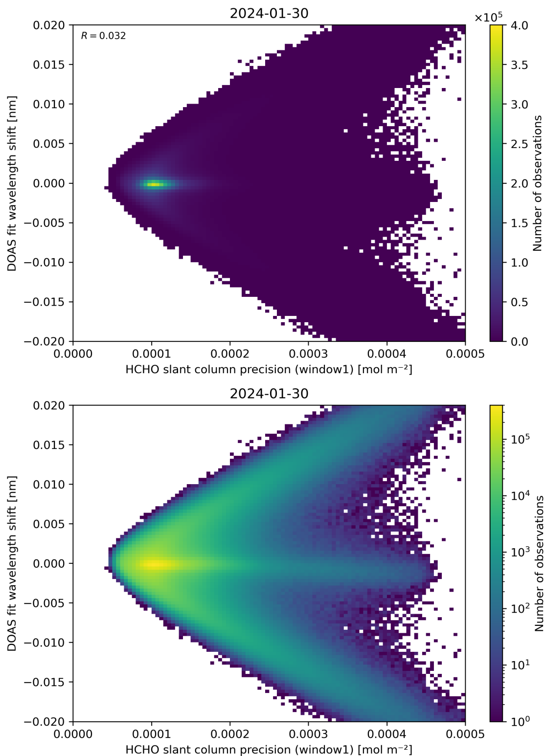
Figure 89: Scatter density plot of “HCHO slant column precision (window1)” against “DOAS fit wavelength shift” for 2024-01-29 to 2024-01-31.
