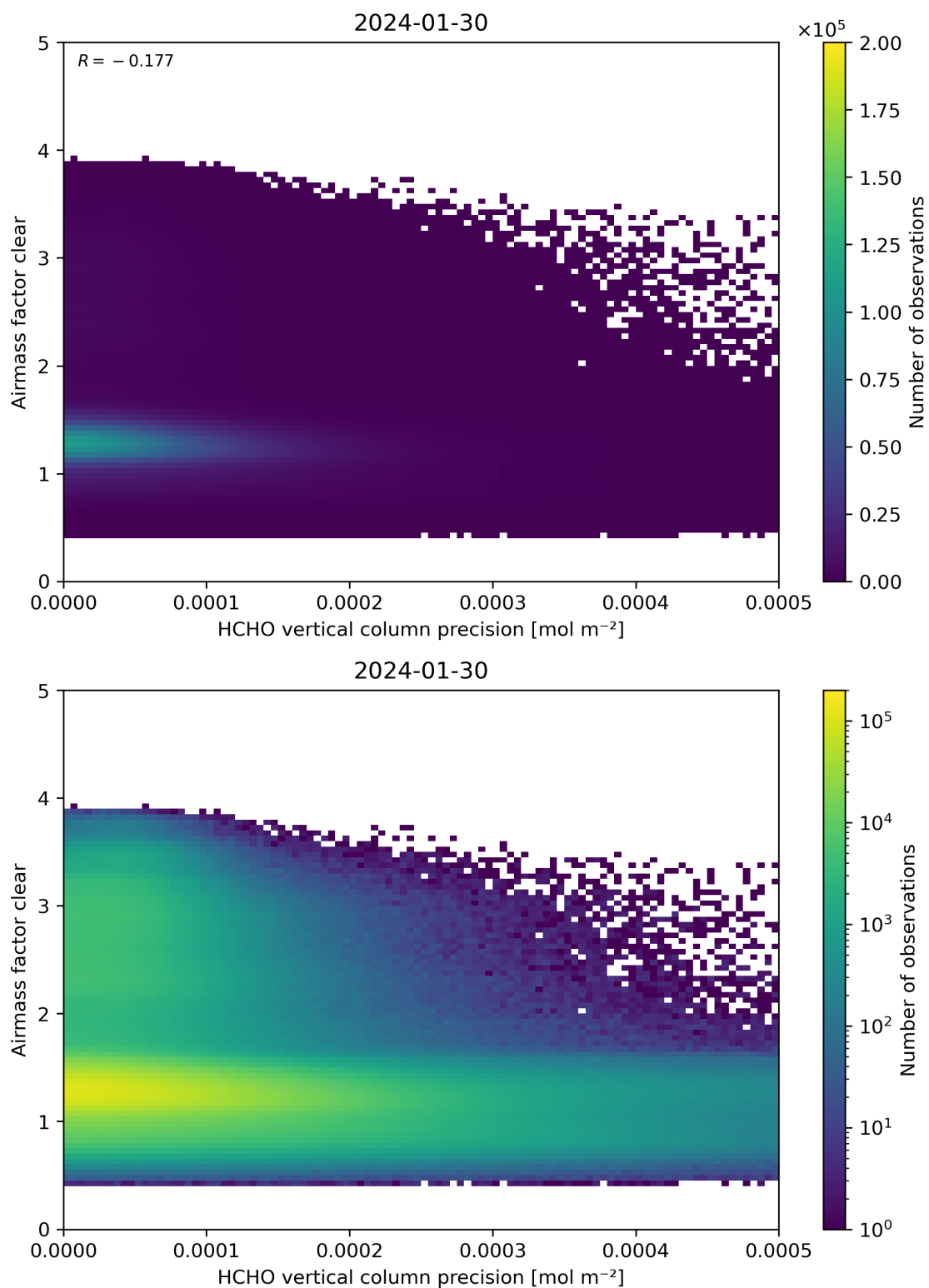
Figure 139: Scatter density plot of “HCHO vertical column precision” against “Airmass factor clear” for 2024-01-29 to 2024-01-31.
