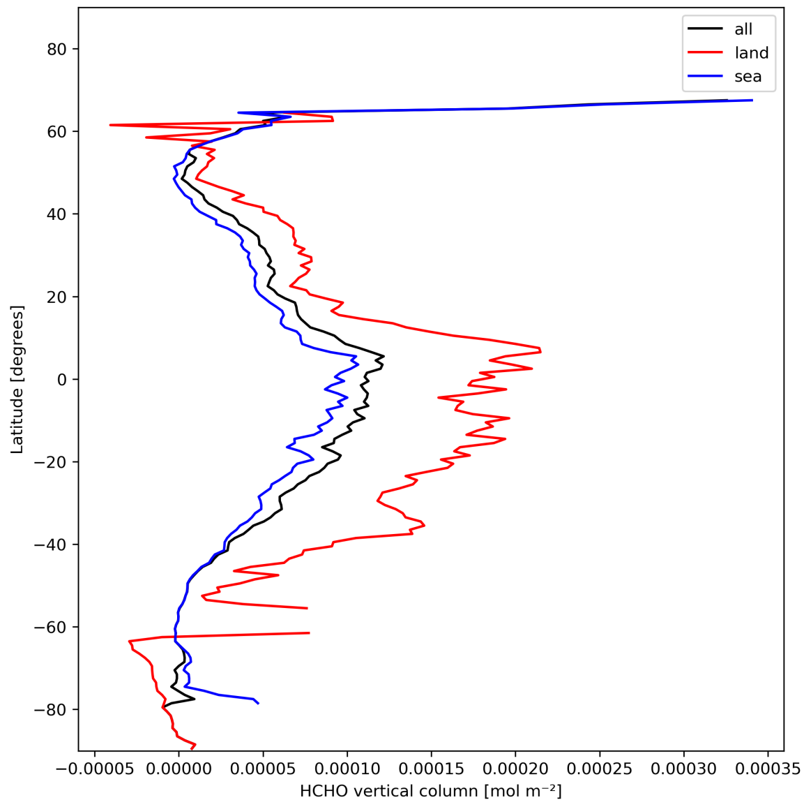
Figure 21: Zonal average of “HCHO vertical column” for 2024-01-29 to 2024-01-31.
