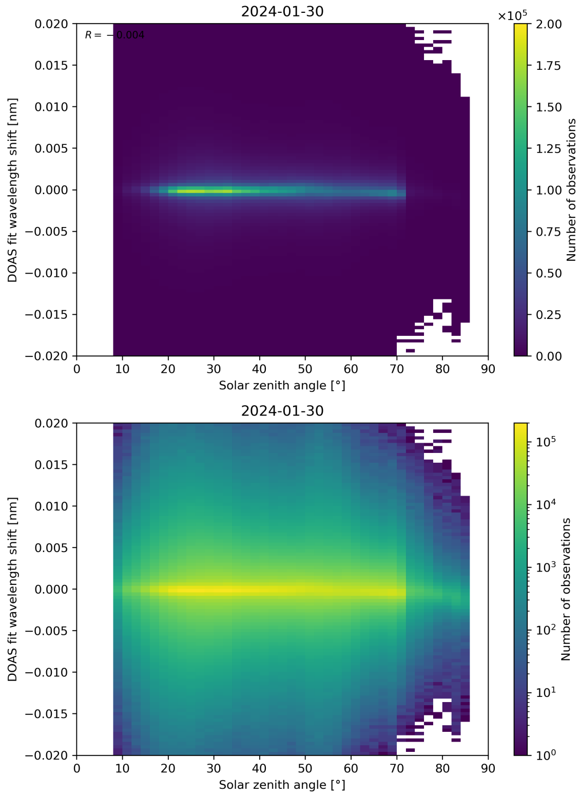
Figure 168: Scatter density plot of “Solar zenith angle” against “DOAS fit wavelength shift” for 2024-01-29 to 2024-01-31.
