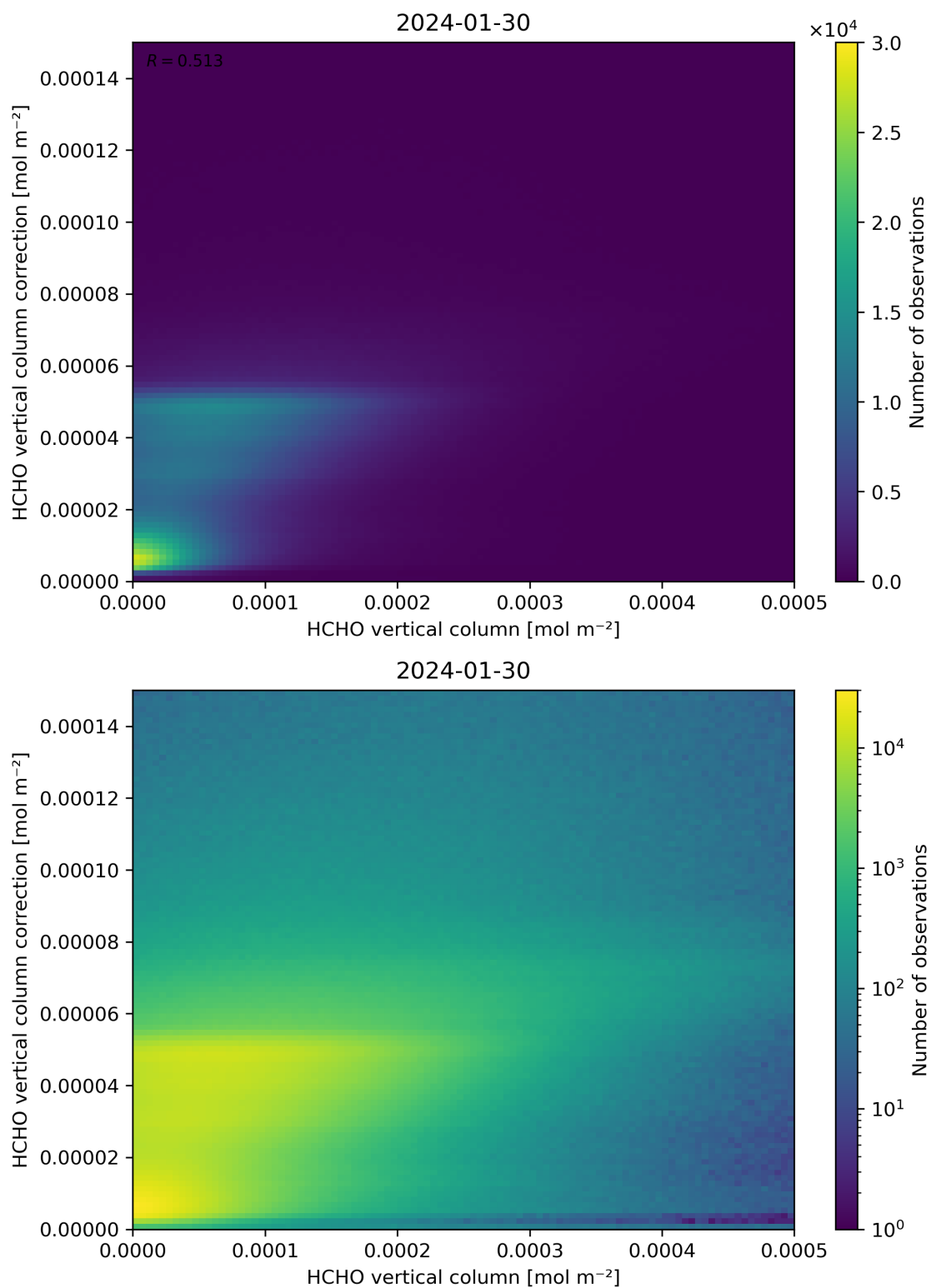
Figure 133: Scatter density plot of “HCHO vertical column” against “HCHO vertical column correction” for 2024-01-29 to 2024-01-31.
