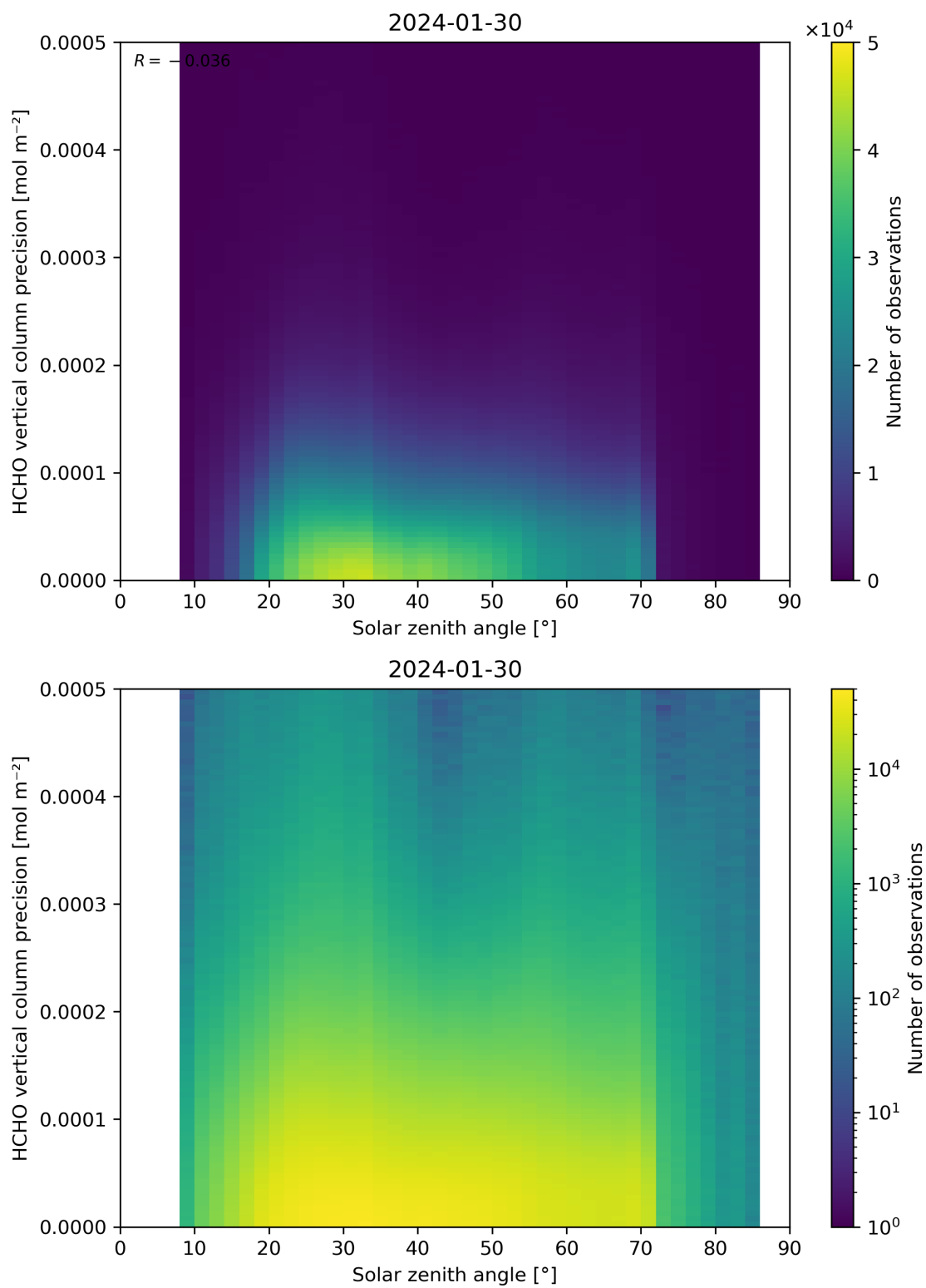
Figure 179: Scatter density plot of “Solar zenith angle” against “HCHO vertical column precision” for 2024-01-29 to 2024-01-31.
