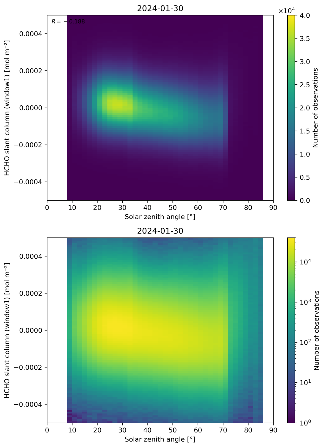
Figure 173: Scatter density plot of “Solar zenith angle” against “HCHO slant column (window1)” for 2024-01-29 to 2024-01-31.
