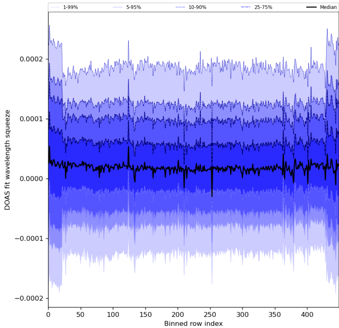
Figure 59: Along track statistics of “DOAS fit wavelength squeeze” for 2024-01-29 to 2024-01-31
