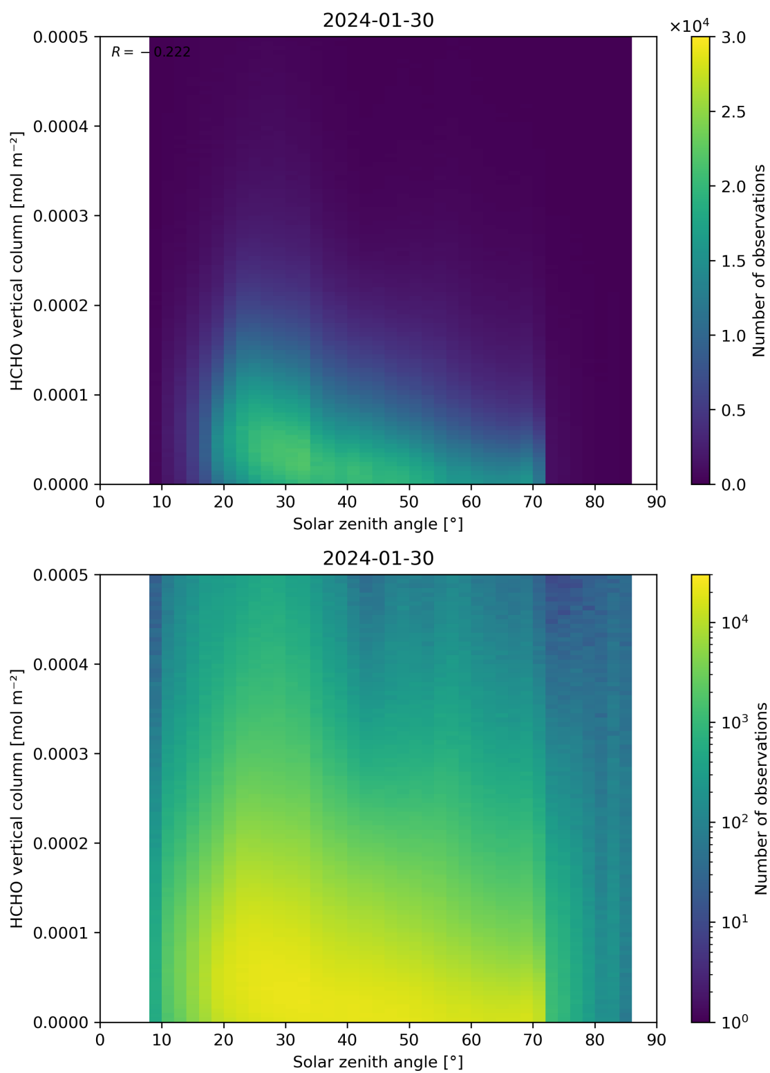
Figure 177: Scatter density plot of “Solar zenith angle” against “HCHO vertical column” for 2024-01-29 to 2024-01-31.
