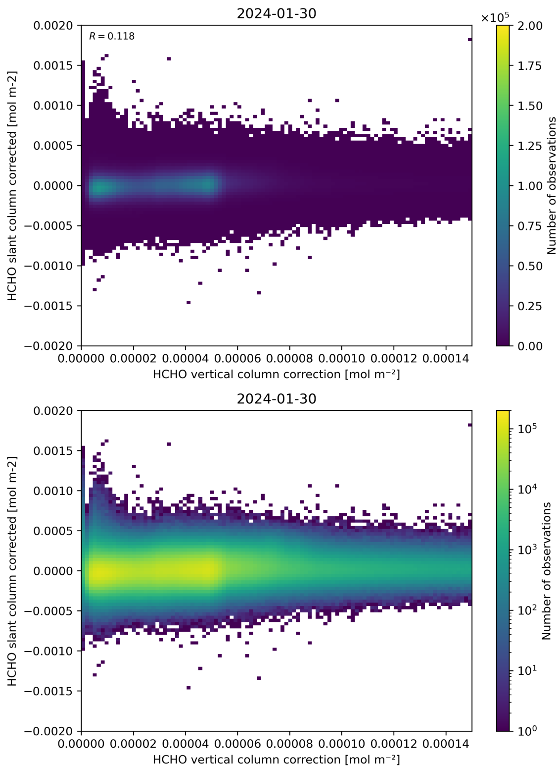
Figure 116: Scatter density plot of “HCHO vertical column correction” against “HCHO slant column corrected” for 2024-01-29 to 2024-01-31.
