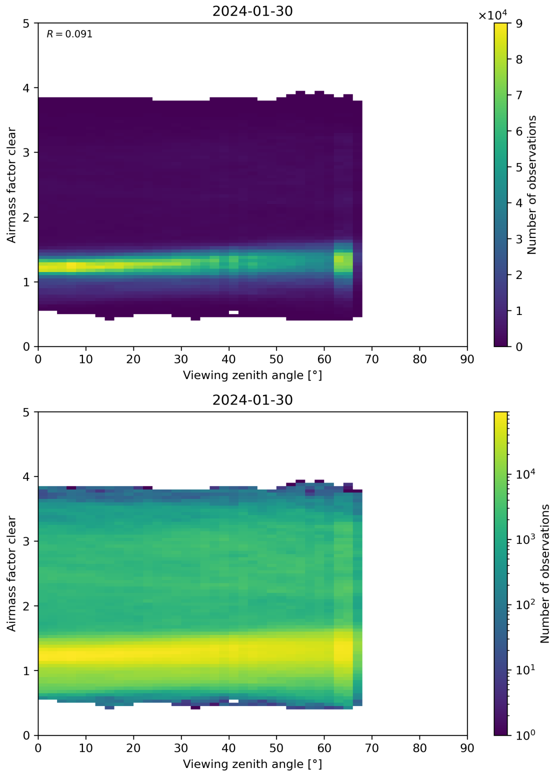
Figure 185: Scatter density plot of “Viewing zenith angle” against “Airmass factor clear” for 2024-01-29 to 2024-01-31.
