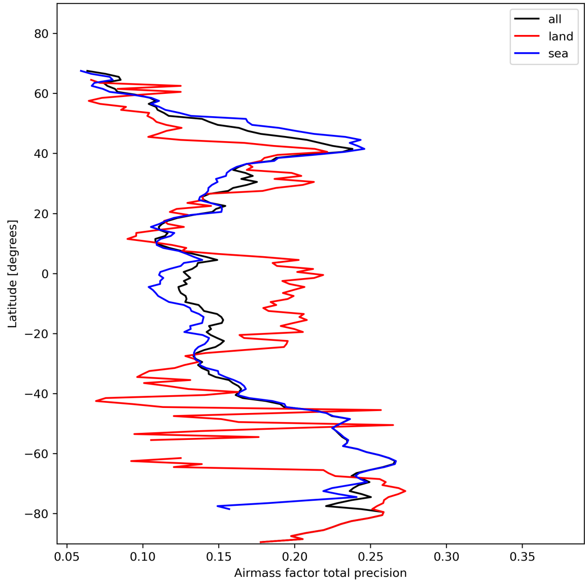
Figure 27: Zonal average of “Airmass factor total precision” for 2024-01-29 to 2024-01-31.
