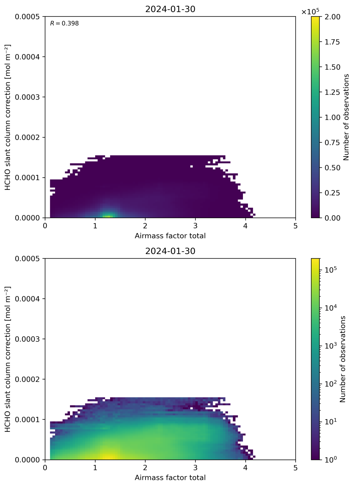
Figure 102: Scatter density plot of “Airmass factor total” against “HCHO slant column correction” for 2024-01-29 to 2024-01-31.
