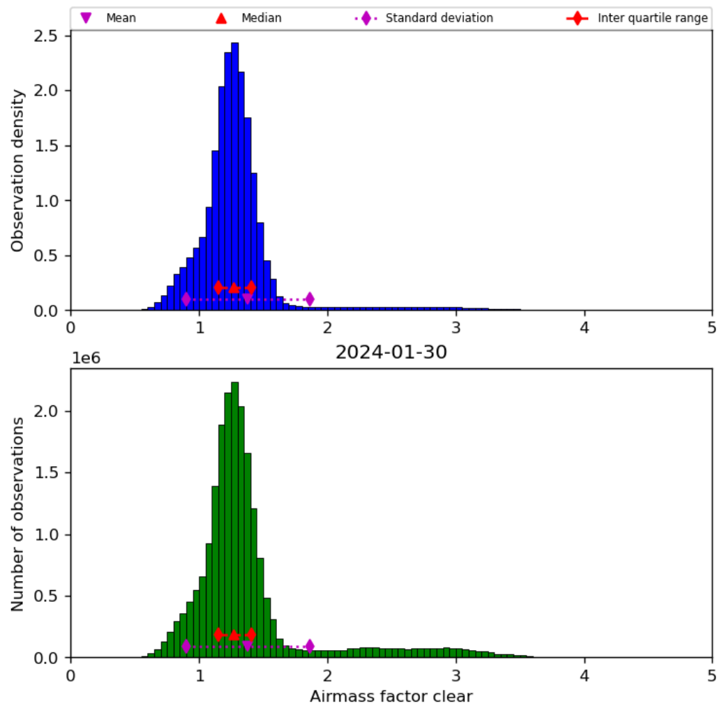
Figure 42: Histogram of “Airmass factor clear” for 2024-01-29 to 2024-01-31
