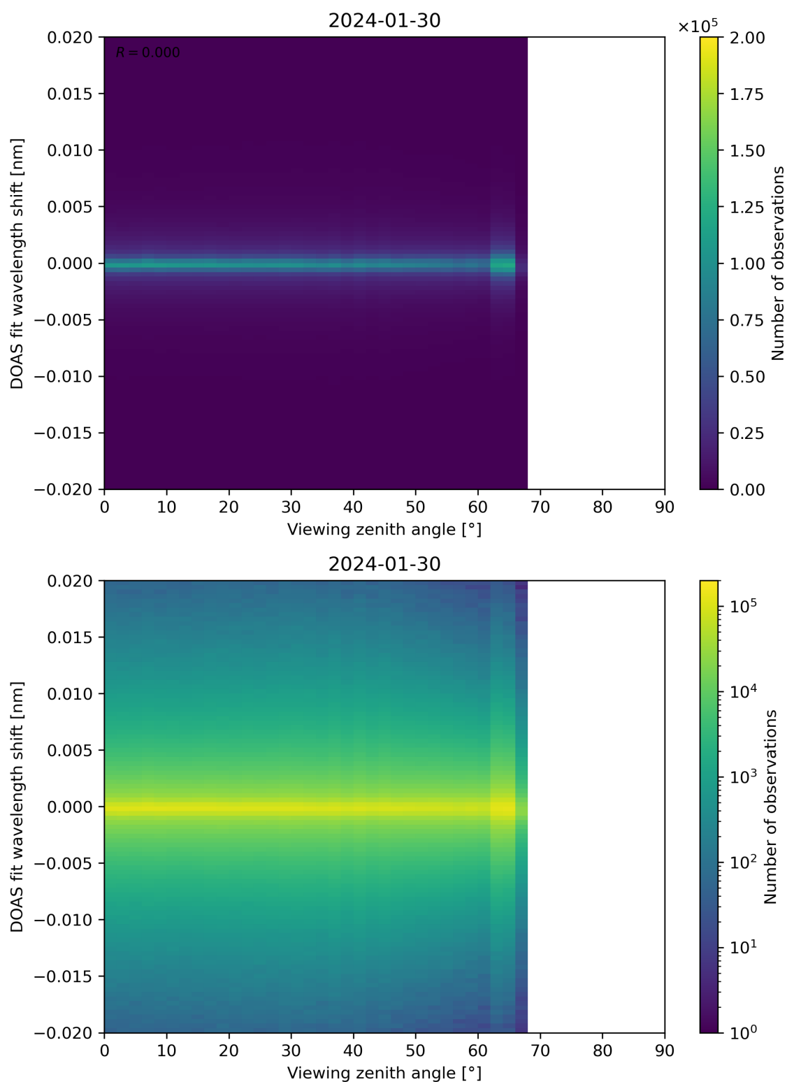
Figure 183: Scatter density plot of “Viewing zenith angle” against “DOAS fit wavelength shift” for 2024-01-29 to 2024-01-31.
