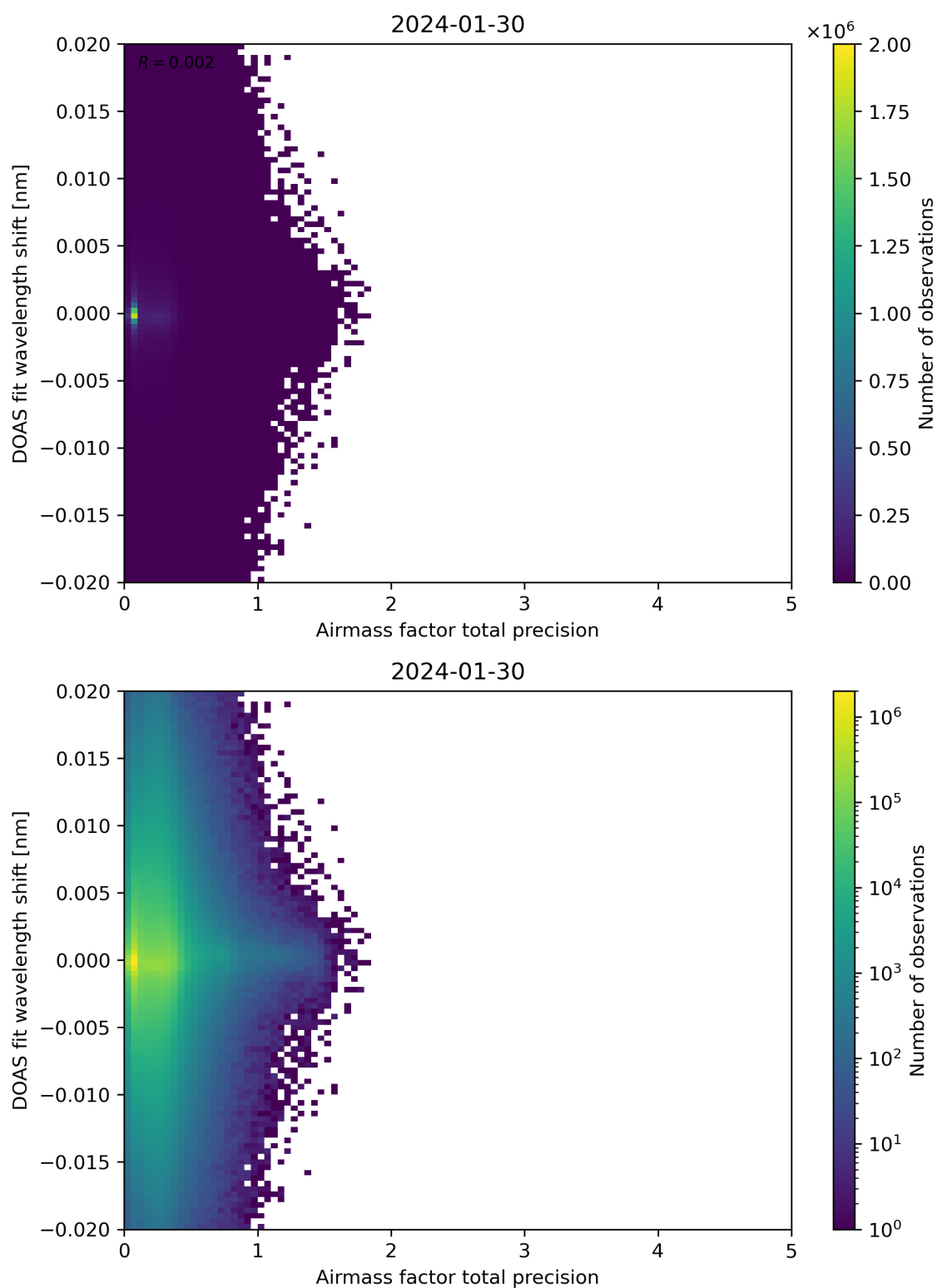
Figure 106: Scatter density plot of “Airmass factor total precision” against “DOAS fit wavelength shift” for 2024-01-29 to 2024-01-31.
