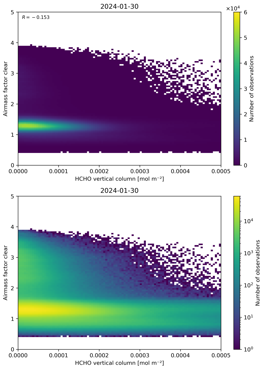
Figure 126: Scatter density plot of “HCHO vertical column” against “Airmass factor clear” for 2024-01-29 to 2024-01-31.
