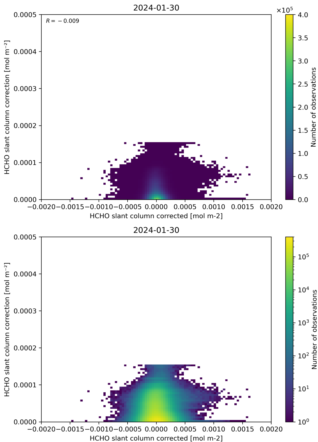
Figure 77: Scatter density plot of “HCHO slant column corrected” against “HCHO slant column correction” for 2024-01-29 to 2024-01-31.
