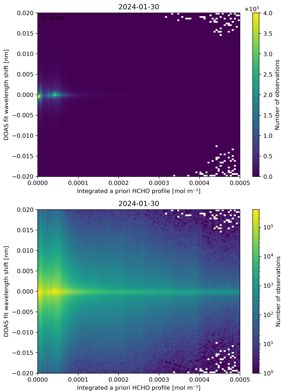
Figure 149: Scatter density plot of “Integrated a priori HCHO profile” against “DOAS fit wavelength shift” for 2024-01-29 to 2024-01-31.
