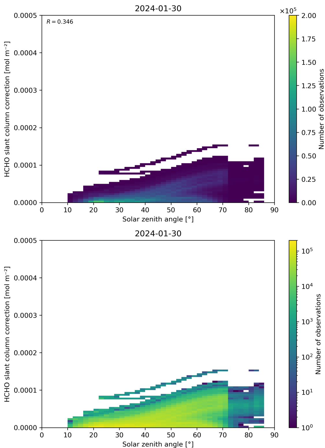
Figure 172: Scatter density plot of “Solar zenith angle” against “HCHO slant column correction” for 2024-01-29 to 2024-01-31.
