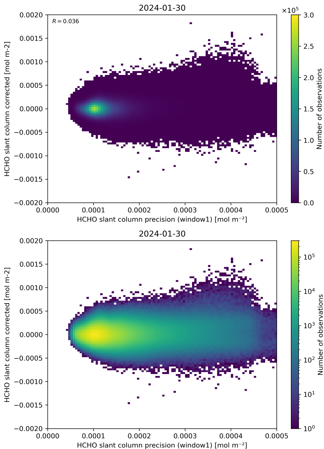
Figure 92: Scatter density plot of “HCHO slant column precision (window1)” against “HCHO slant column corrected” for 2024-01-29 to 2024-01-31.
