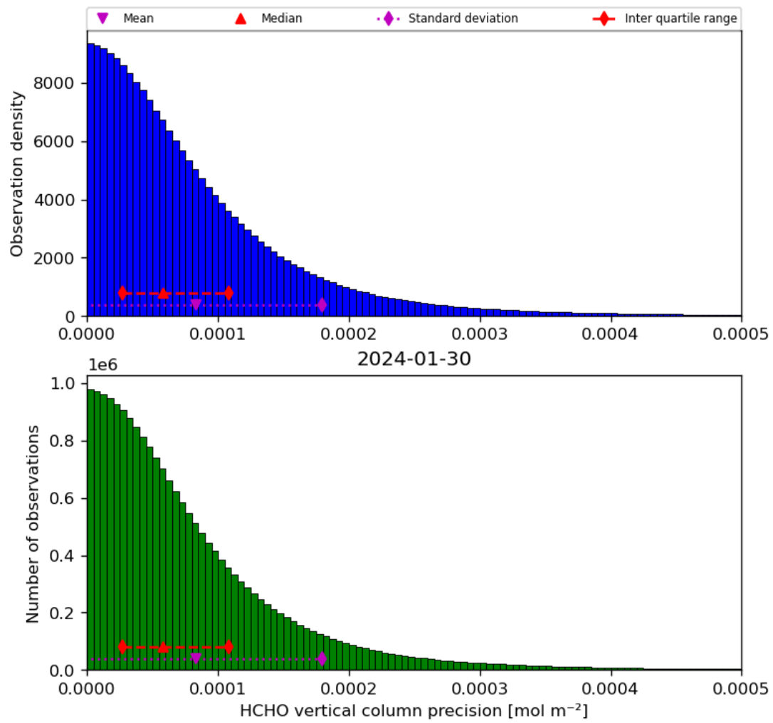
Figure 36: Histogram of “HCHO vertical column precision” for 2024-01-29 to 2024-01-31
