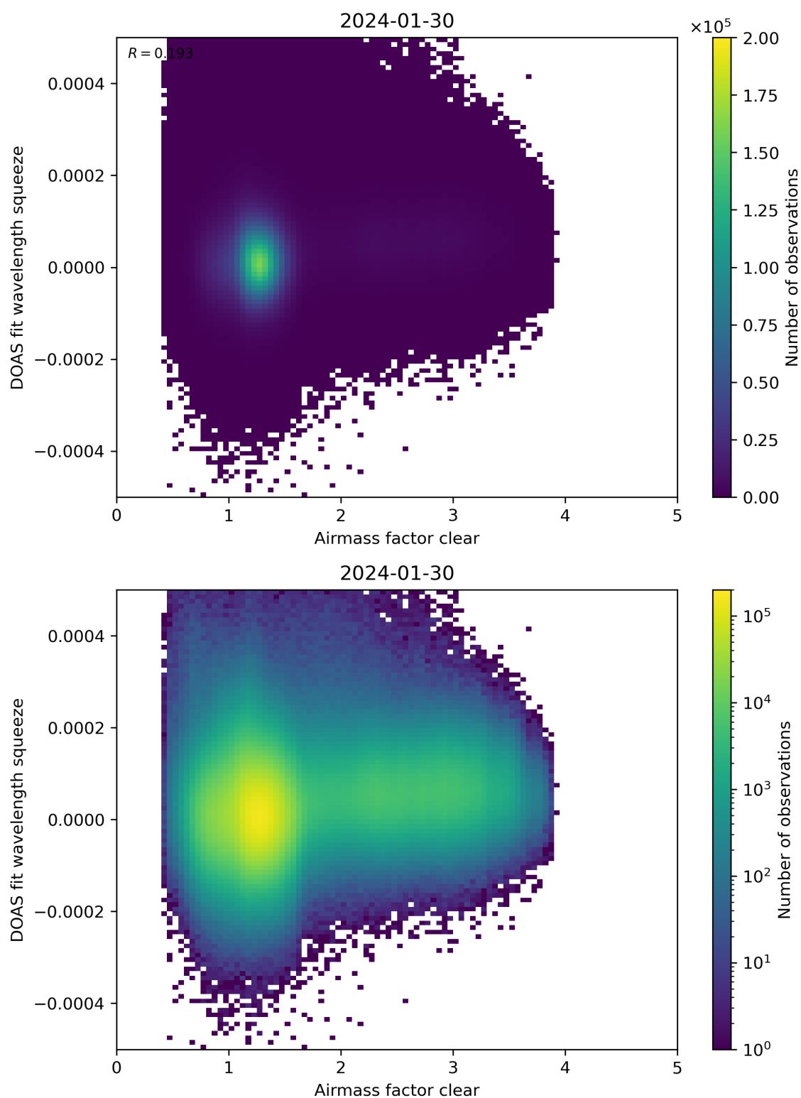
Figure 73: Scatter density plot of “Airmass factor clear” against “DOAS fit wavelength squeeze” for 2024-01-29 to 2024-01-31.
