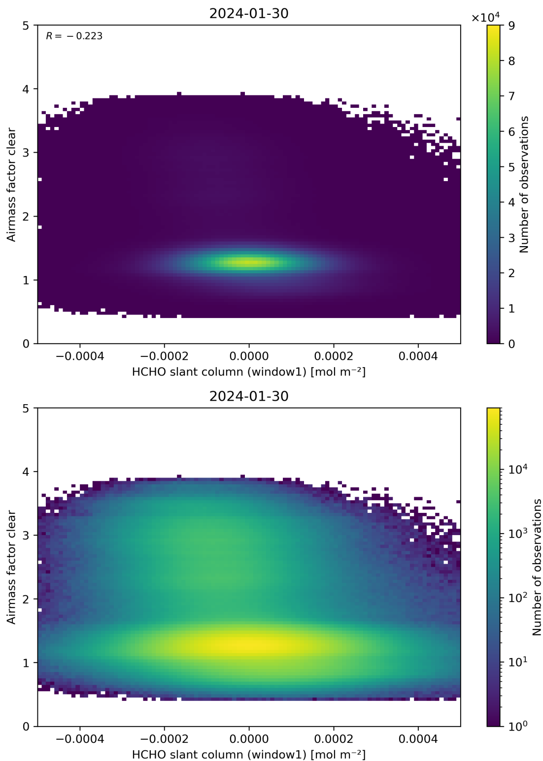
Figure 81: Scatter density plot of “HCHO slant column (window1)” against “Airmass factor clear” for 2024-01-29 to 2024-01-31.
