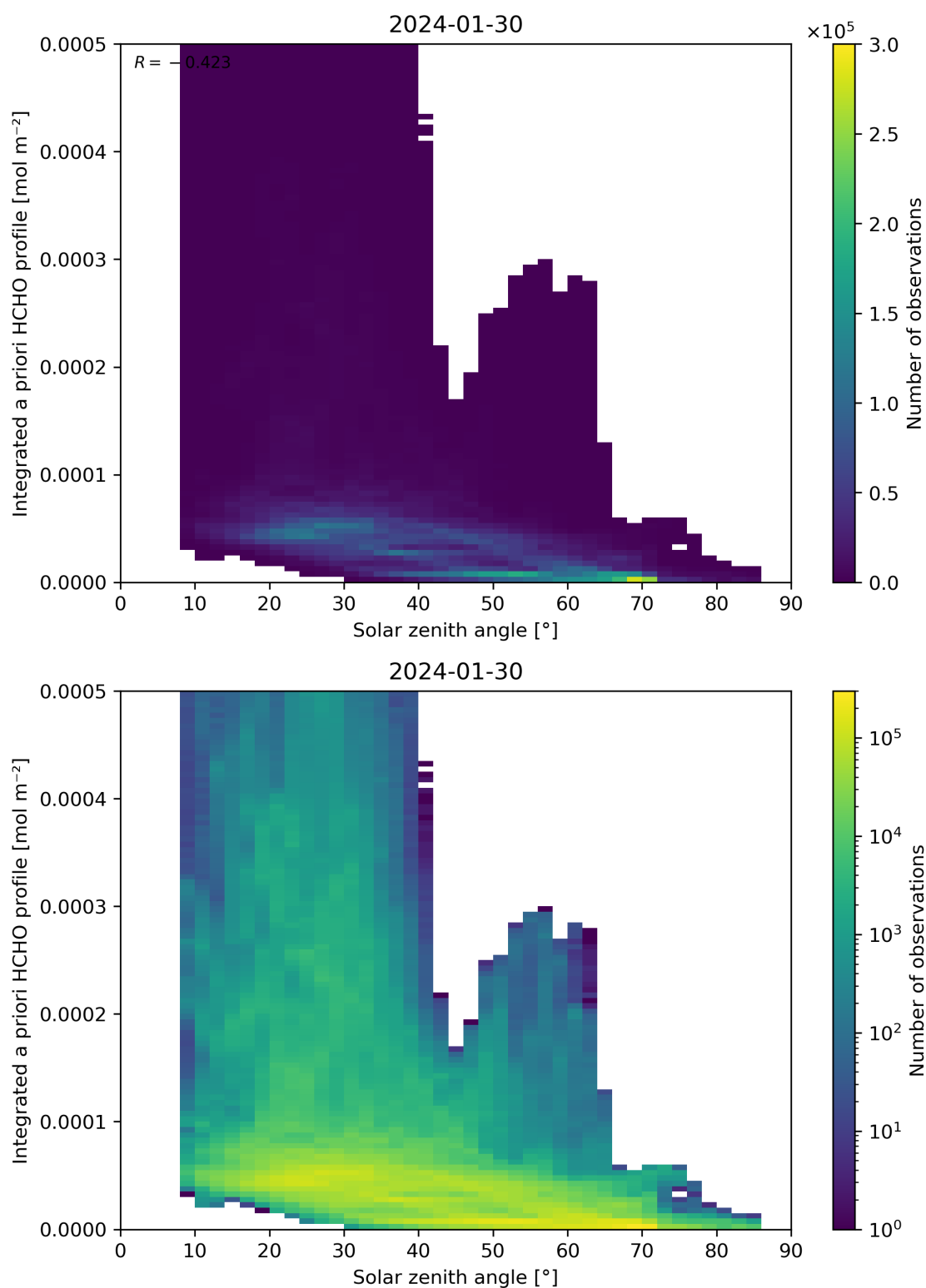
Figure 180: Scatter density plot of “Solar zenith angle” against “Integrated a priori HCHO profile” for 2024-01-29 to 2024-01-31.
