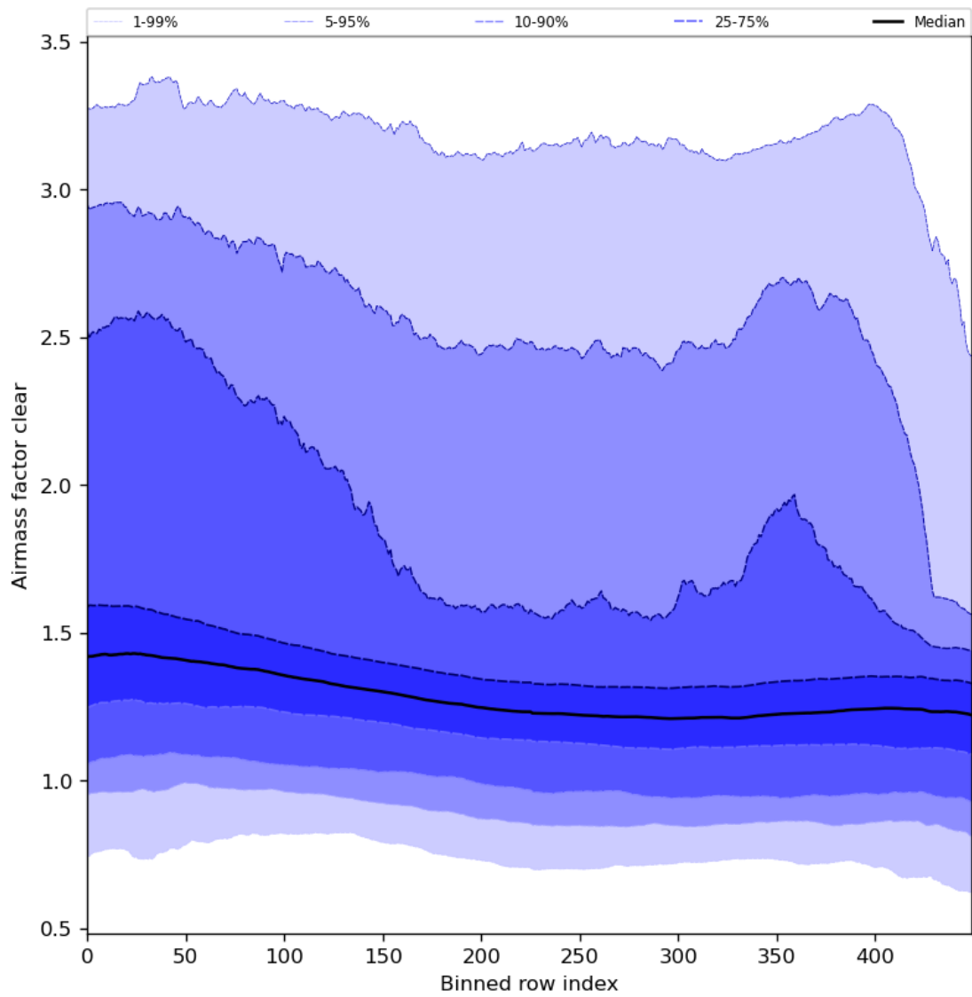
Figure 56: Along track statistics of “Air mass factor clear” for 2024-01-29 to 2024-01-31
