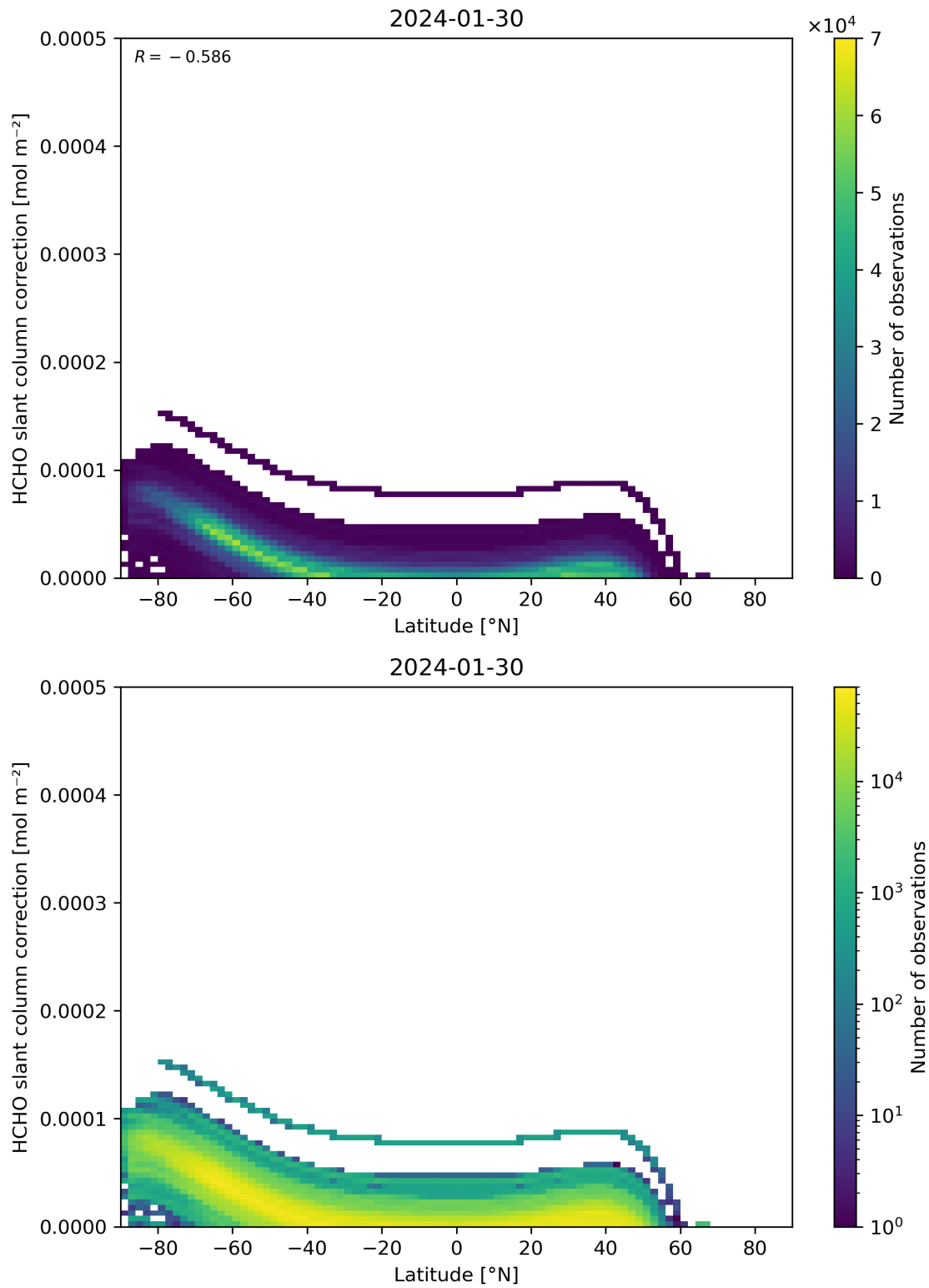
Figure 158: Scatter density plot of “Latitude” against “HCHO slant column correction” for 2024-01-29 to 2024-01-31.
