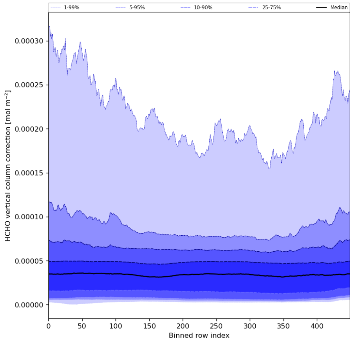
Figure 51: Along track statistics of “HCHO vertical column correction” for 2024-01-29 to 2024-01-31
