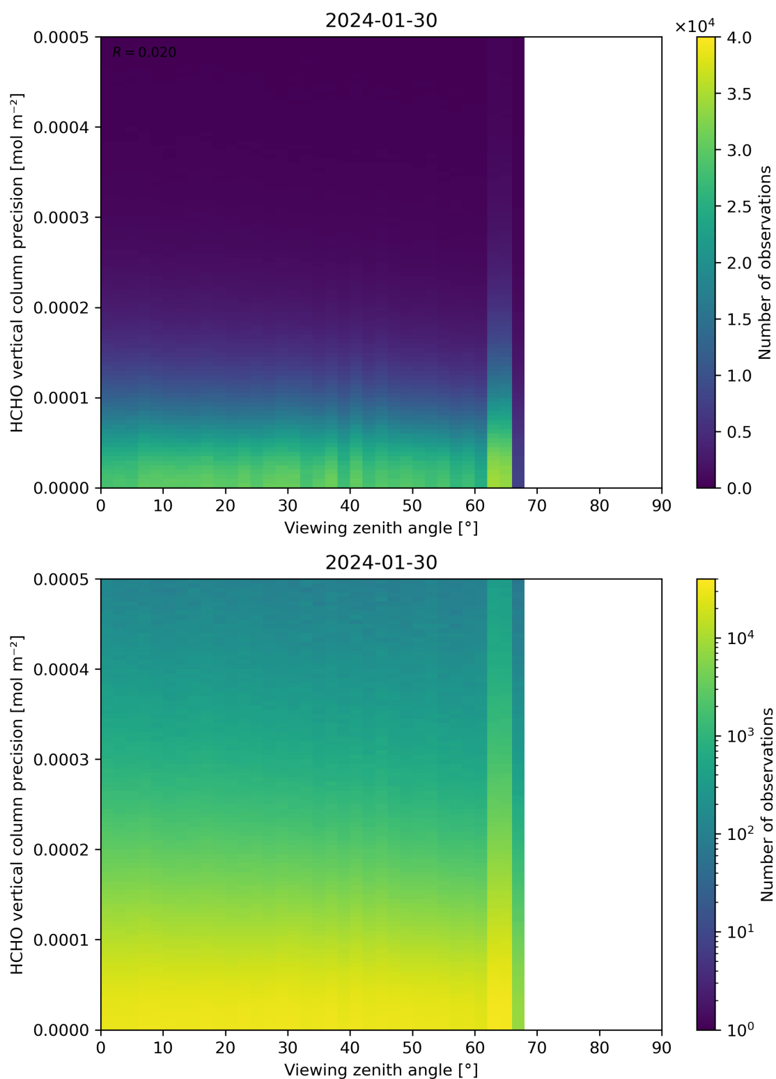
Figure 194: Scatter density plot of “Viewing zenith angle” against “HCHO vertical column precision” for 2024-01-29 to 2024-01-31.
