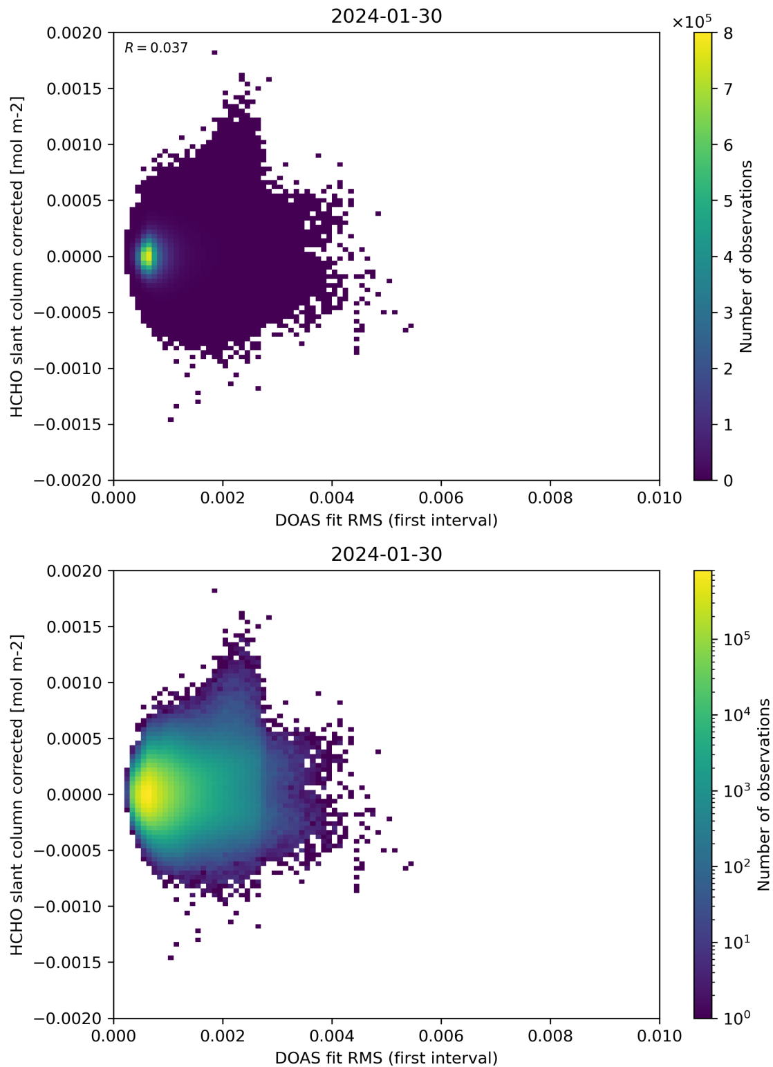
Figure 62: Scatter density plot of “DOAS fit RMS (first interval)” against “HCHO slant column corrected” for 2024-01-29 to 2024-01-31.
