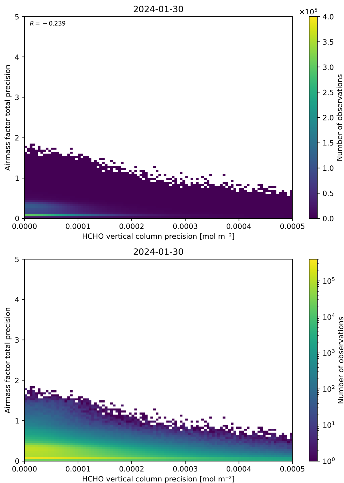
Figure 145: Scatter density plot of “HCHO vertical column precision” against “Airmass factor total precision” for 2024-01-29 to 2024-01-31.
