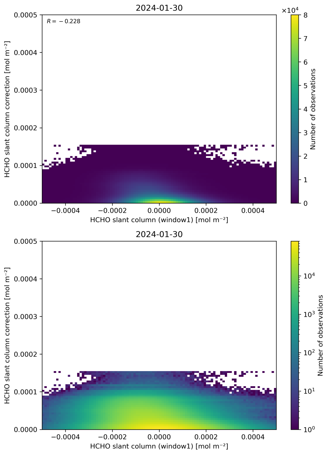
Figure 83: Scatter density plot of “HCHO slant column (window1)” against “HCHO slant column correction” for 2024-01-29 to 2024-01-31.
