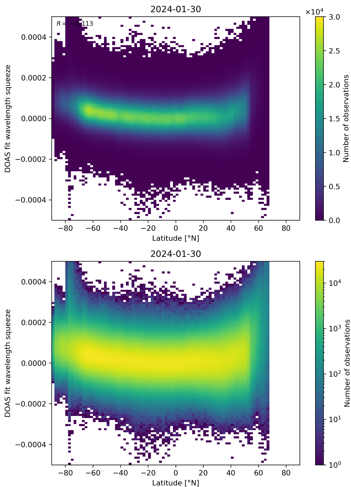
Figure 155: Scatter density plot of “Latitude” against “DOAS fit wavelength squeeze” for 2024-01-29 to 2024-01-31.
