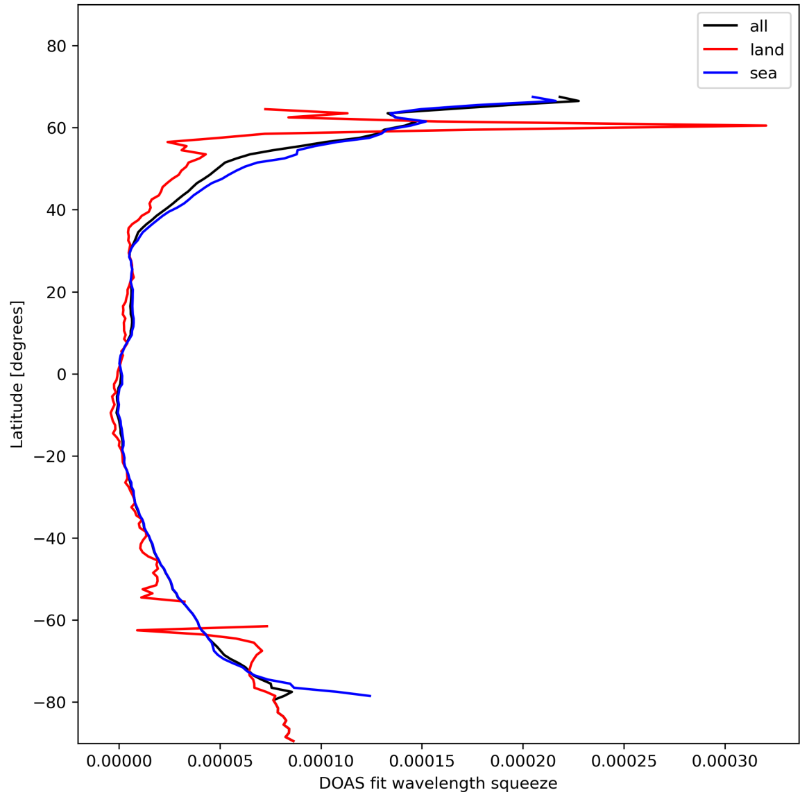
Figure 31: Zonal average of “DOAS fit wavelength squeeze” for 2024-01-29 to 2024-01-31.
