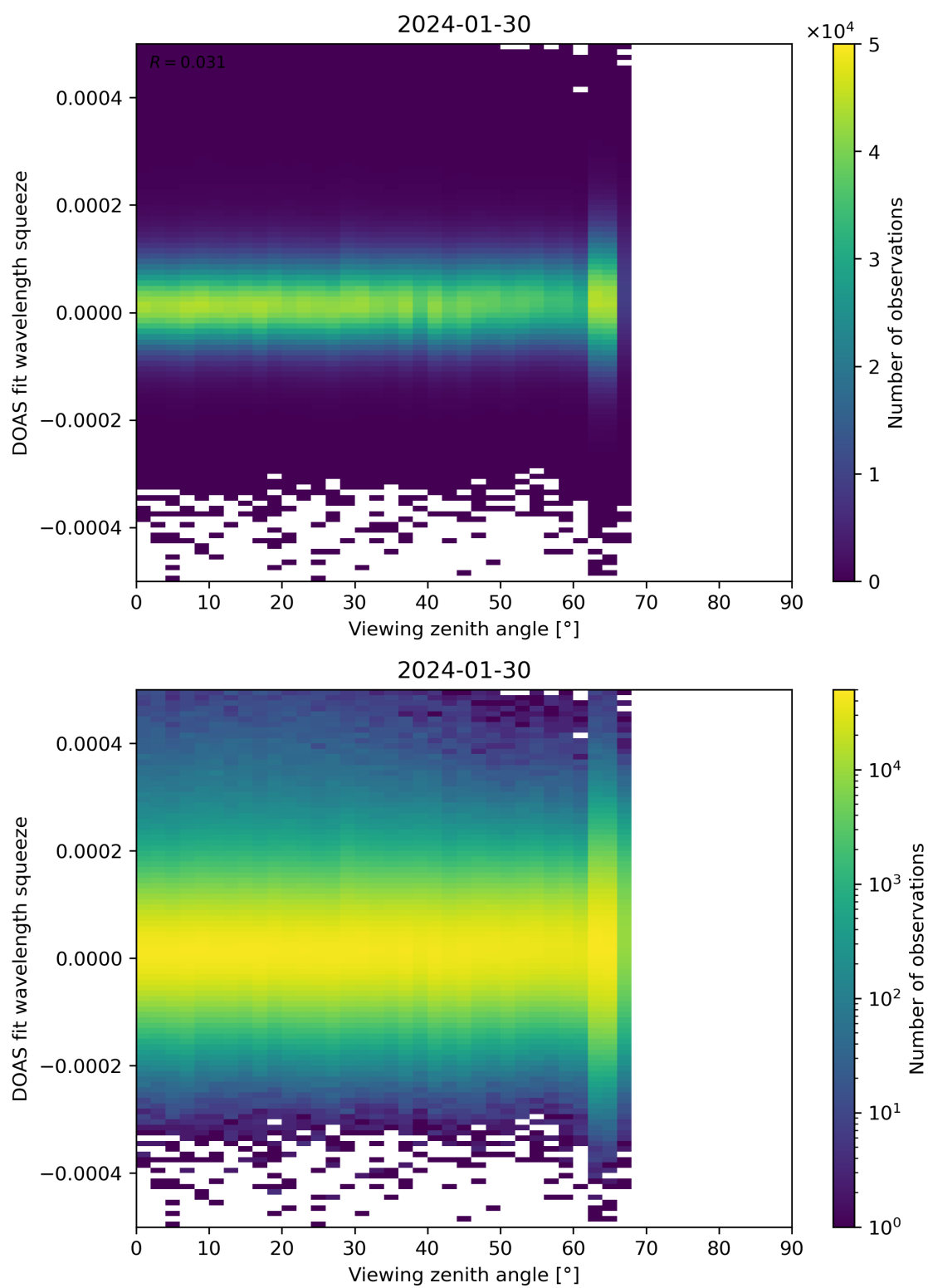
Figure 184: Scatter density plot of “Viewing zenith angle” against “DOAS fit wavelength squeeze” for 2024-01-29 to 2024-01-31.
