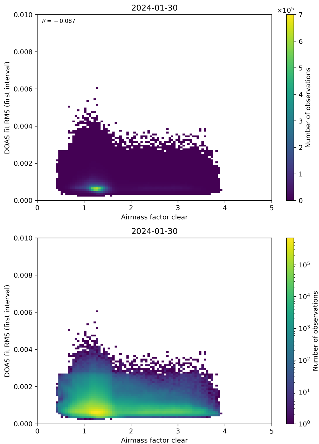
Figure 71: Scatter density plot of “Airmass factor clear” against “DOAS fit RMS (first interval)” for 2024-01-29 to 2024-01-31.
