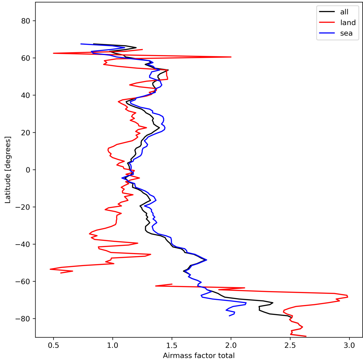
Figure 26: Zonal average of “Airmass factor total” for 2024-01-29 to 2024-01-31.
