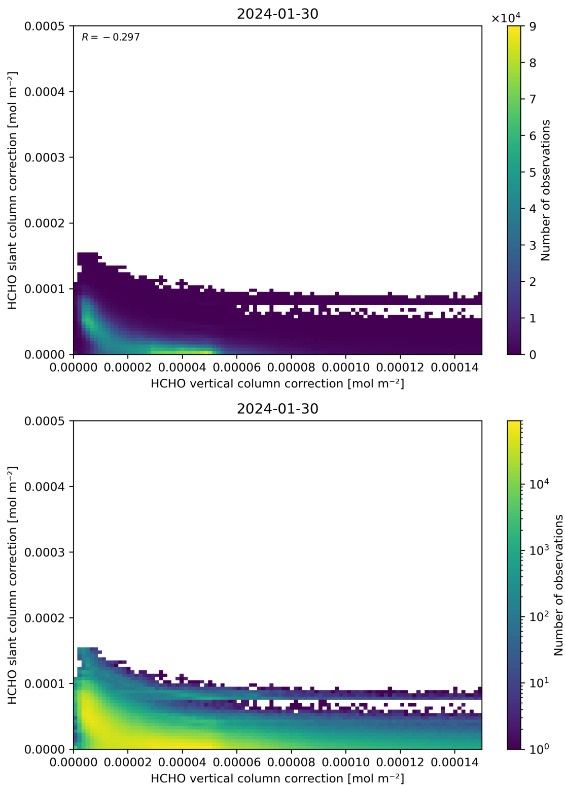
Figure 117: Scatter density plot of “HCHO vertical column correction” against “HCHO slant column correction” for 2024-01-29 to 2024-01-31.
