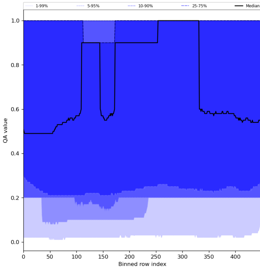
Figure 48: Along track statistics of “QA value” for 2024-01-29 to 2024-01-31
