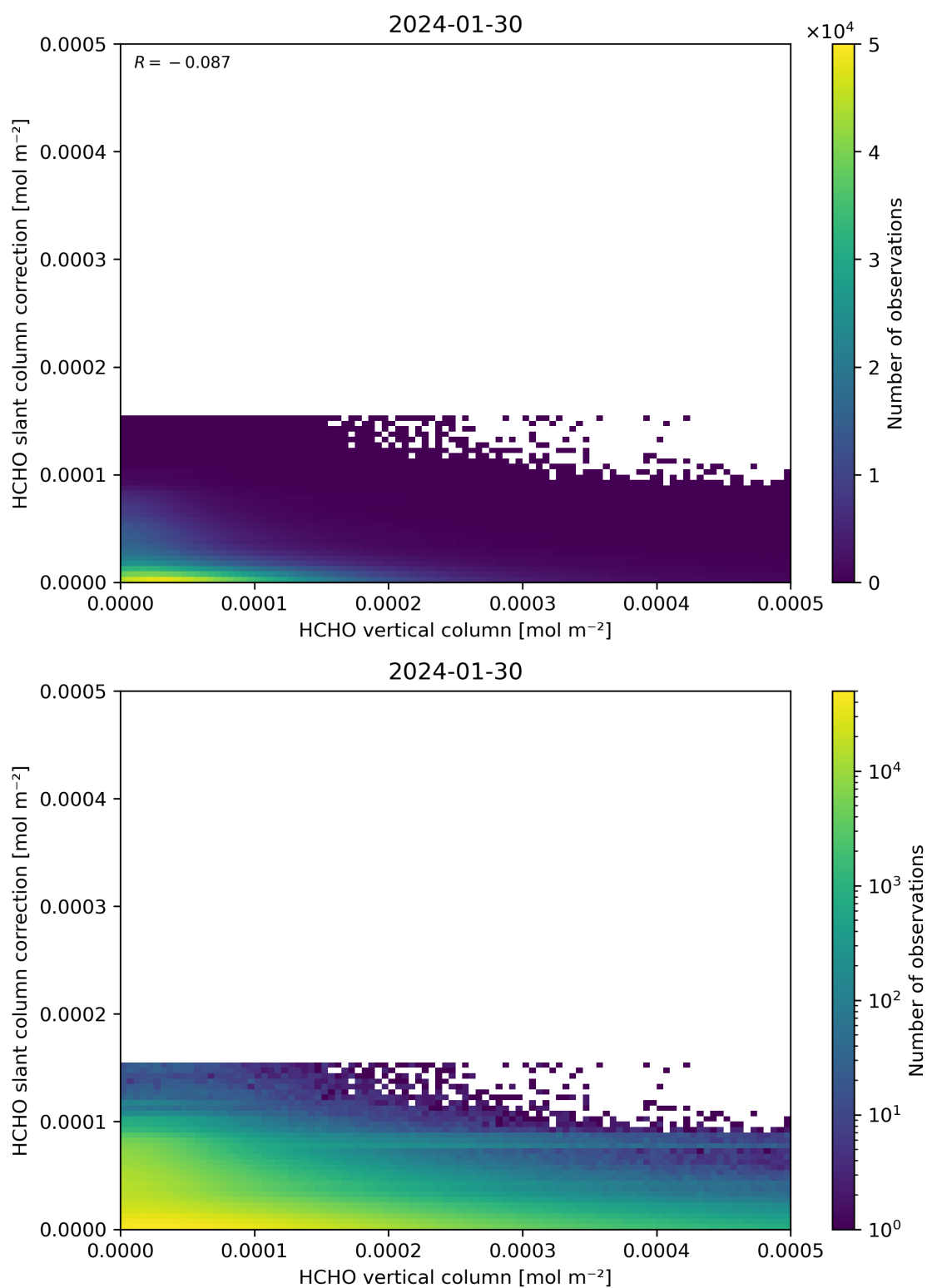
Figure 128: Scatter density plot of “HCHO vertical column” against “HCHO slant column correction” for 2024-01-29 to 2024-01-31.
