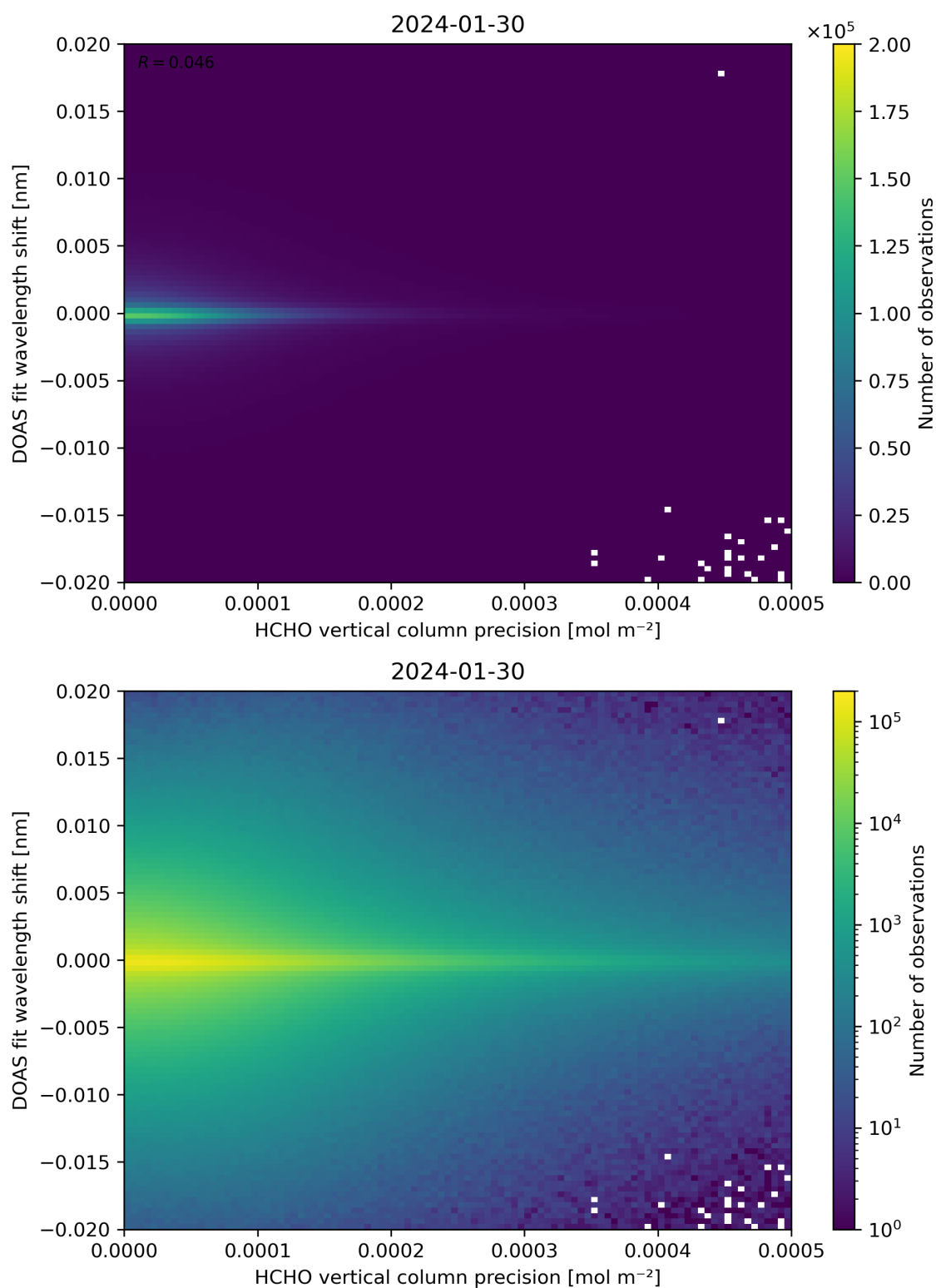
Figure 137: Scatter density plot of “HCHO vertical column precision” against “DOAS fit wavelength shift” for 2024-01-29 to 2024-01-31.
