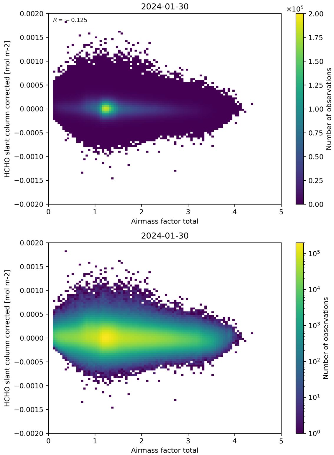
Figure 101: Scatter density plot of “Airmass factor total” against “HCHO slant column corrected” for 2024-01-29 to 2024-01-31.
