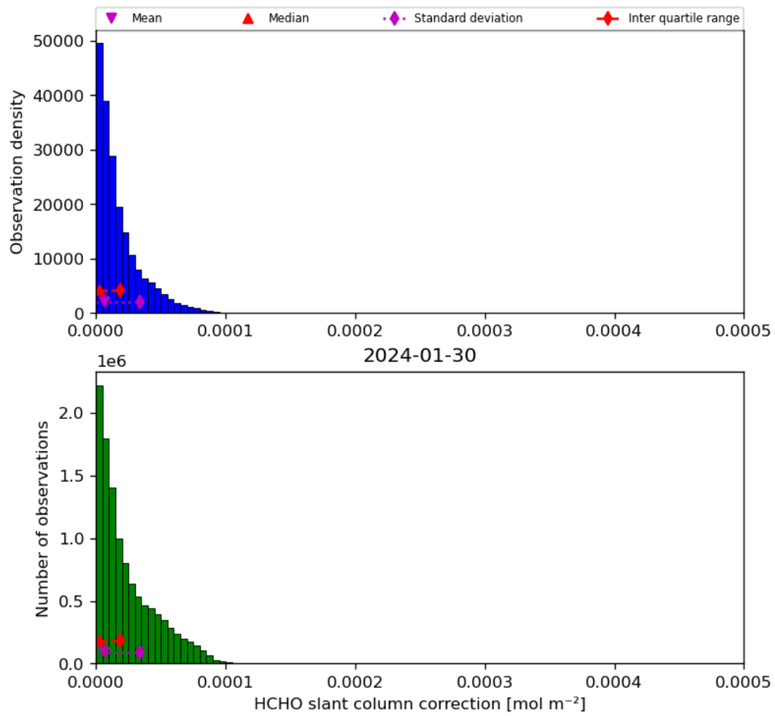
Figure 47: Histogram of “HCHO slant column correction” for 2024-01-29 to 2024-01-31
