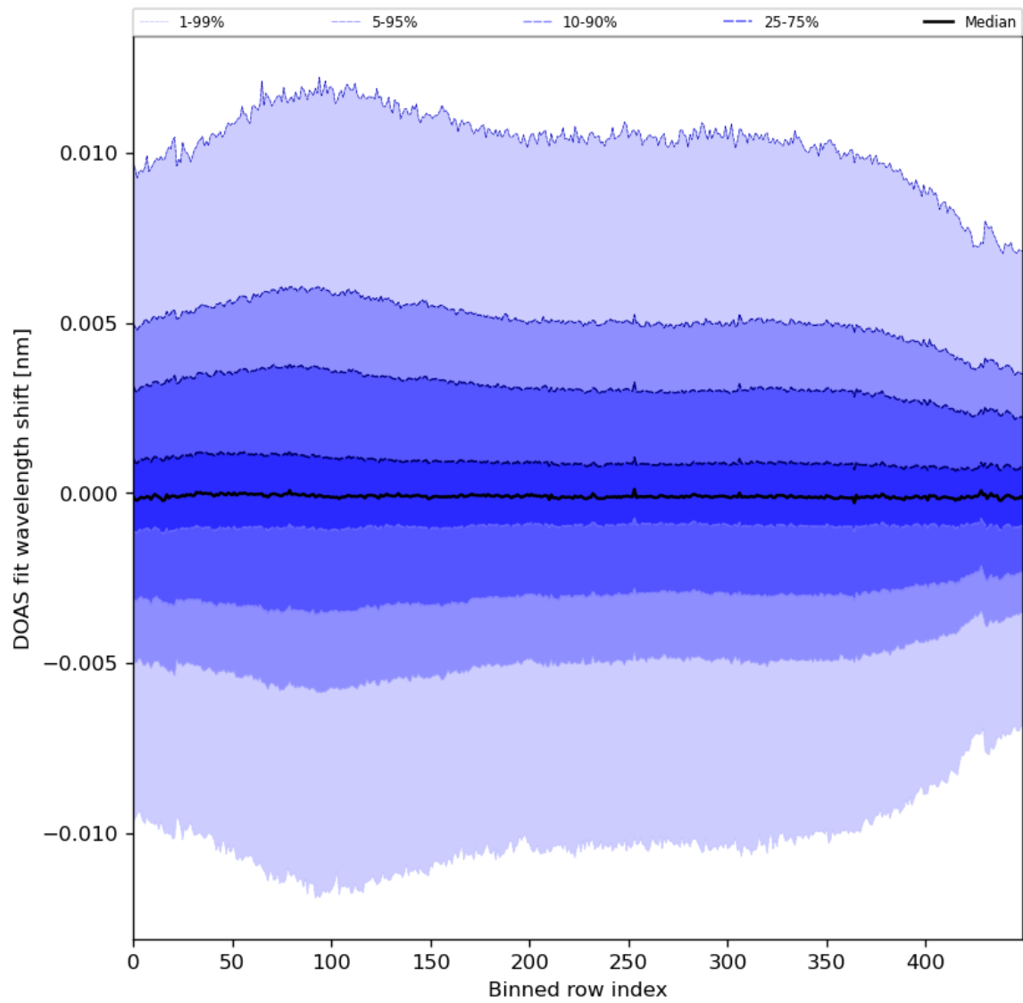
Figure 58: Along track statistics of “DOAS fit wavelength shift” for 2024-01-29 to 2024-01-31
