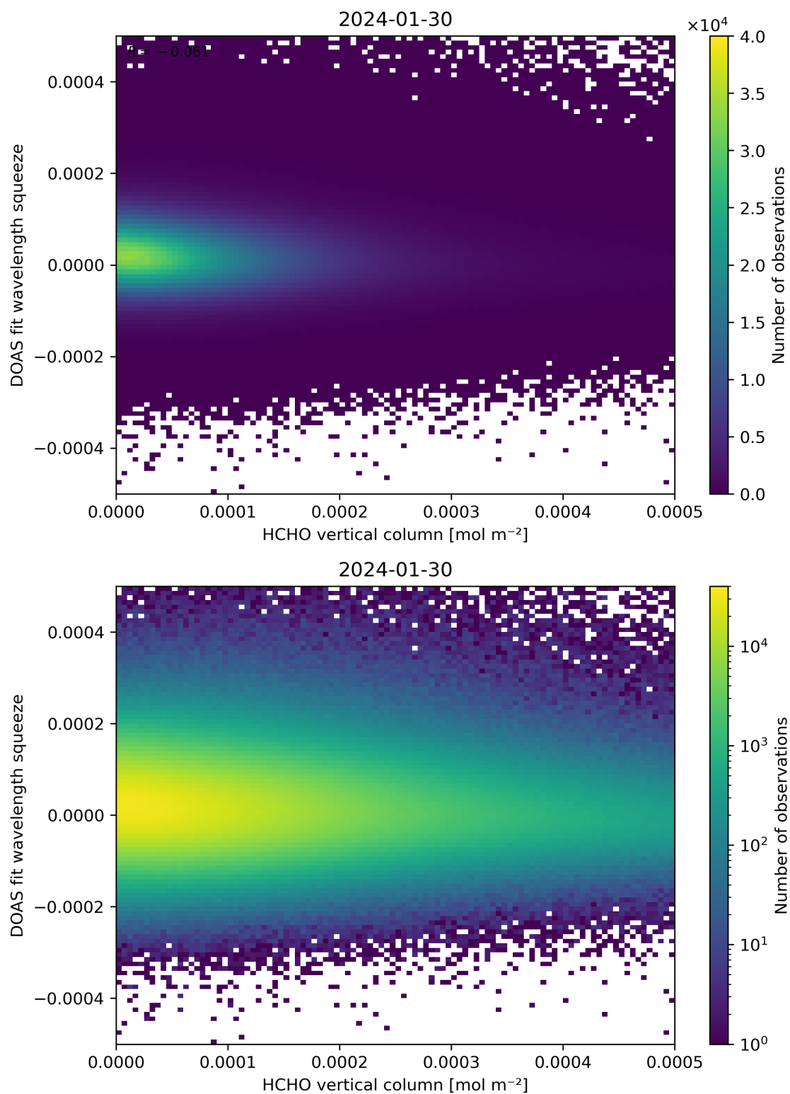
Figure 125: Scatter density plot of “HCHO vertical column” against “DOAS fit wavelength squeeze” for 2024-01-29 to 2024-01-31.
