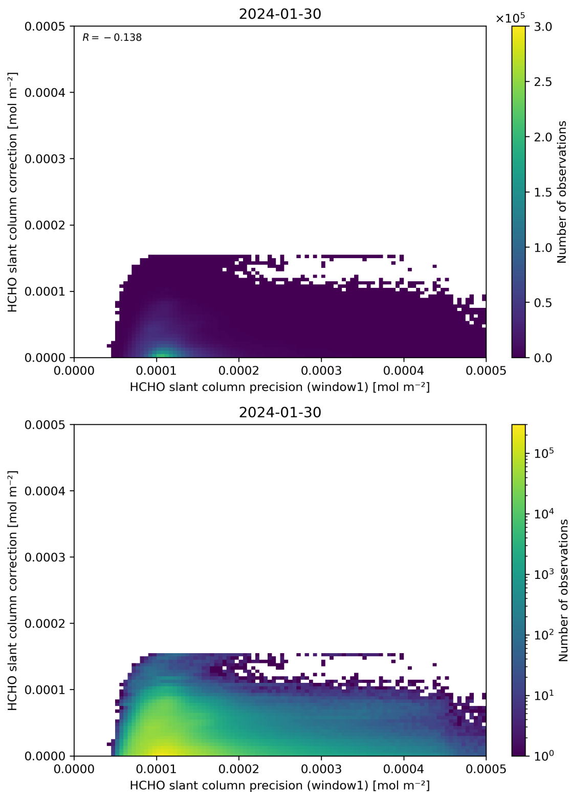
Figure 93: Scatter density plot of “HCHO slant column precision (window1)” against “HCHO slant column correction” for 2024-01-29 to 2024-01-31.
