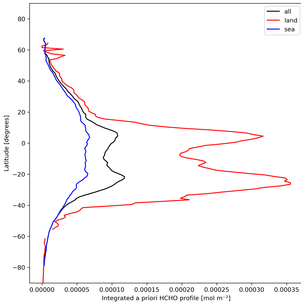
Figure 29: Zonal average of “Integrated a priori HCHO profile” for 2024-01-29 to 2024-01-31.
