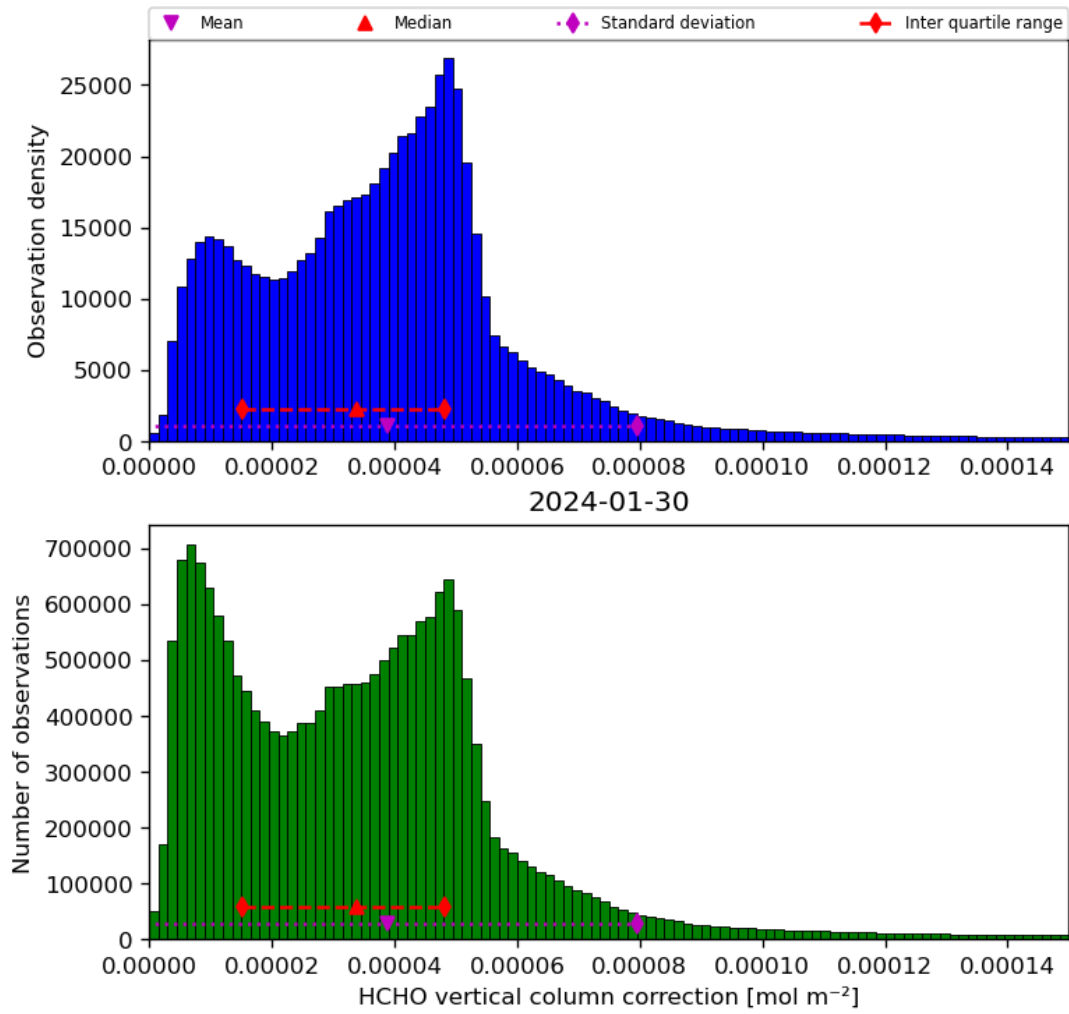
Figure 37: Histogram of “HCHO vertical column correction” for 2024-01-29 to 2024-01-31
