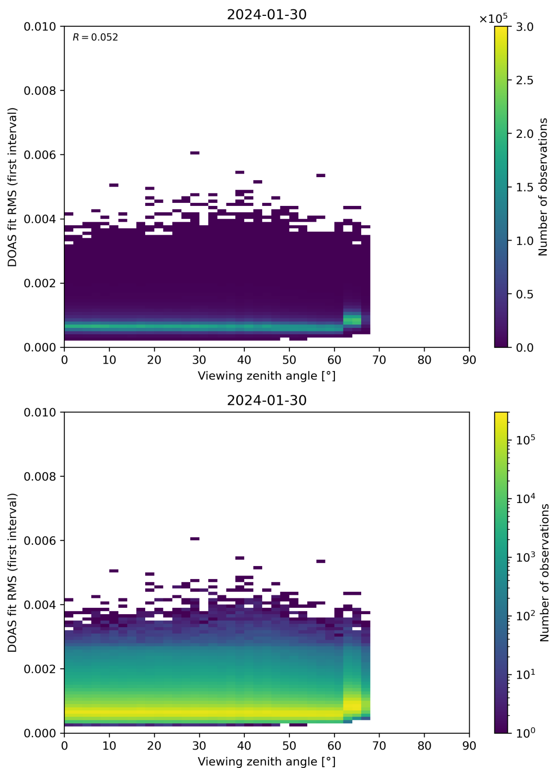
Figure 182: Scatter density plot of “Viewing zenith angle” against “DOAS fit RMS (first interval)” for 2024-01-29 to 2024-01-31.
