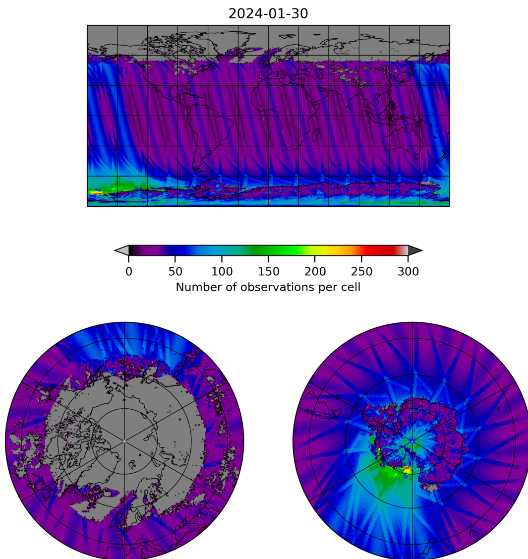
Figure 19: Map of the number of observations for 2024-01-29 to 2024-01-31
