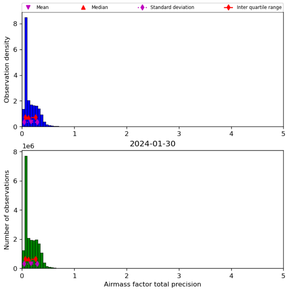
Figure 41: Histogram of "Airmass factor total precision" for 2024-01-29 to 2024-01-31
