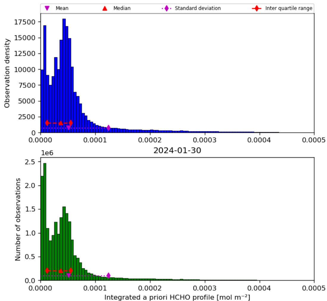
Figure 43: Histogram of “Integrated a priori HCHO profile” for 2024-01-29 to 2024-01-31
