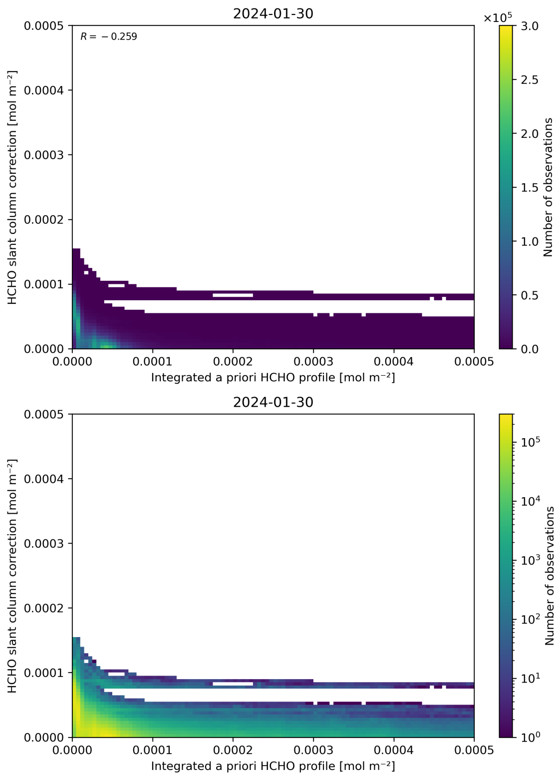
Figure 152: Scatter density plot of “Integrated a priori HCHO profile” against “HCHO slant column correction” for 2024-01-29 to 2024-01-31.
