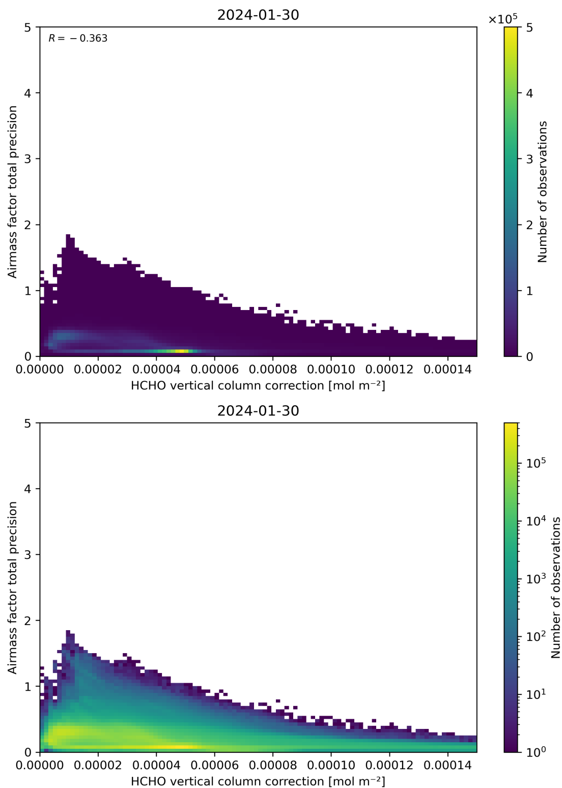
Figure 121: Scatter density plot of “HCHO vertical column correction” against “Airmass factor total precision” for 2024-01-29 to 2024-01-31.
