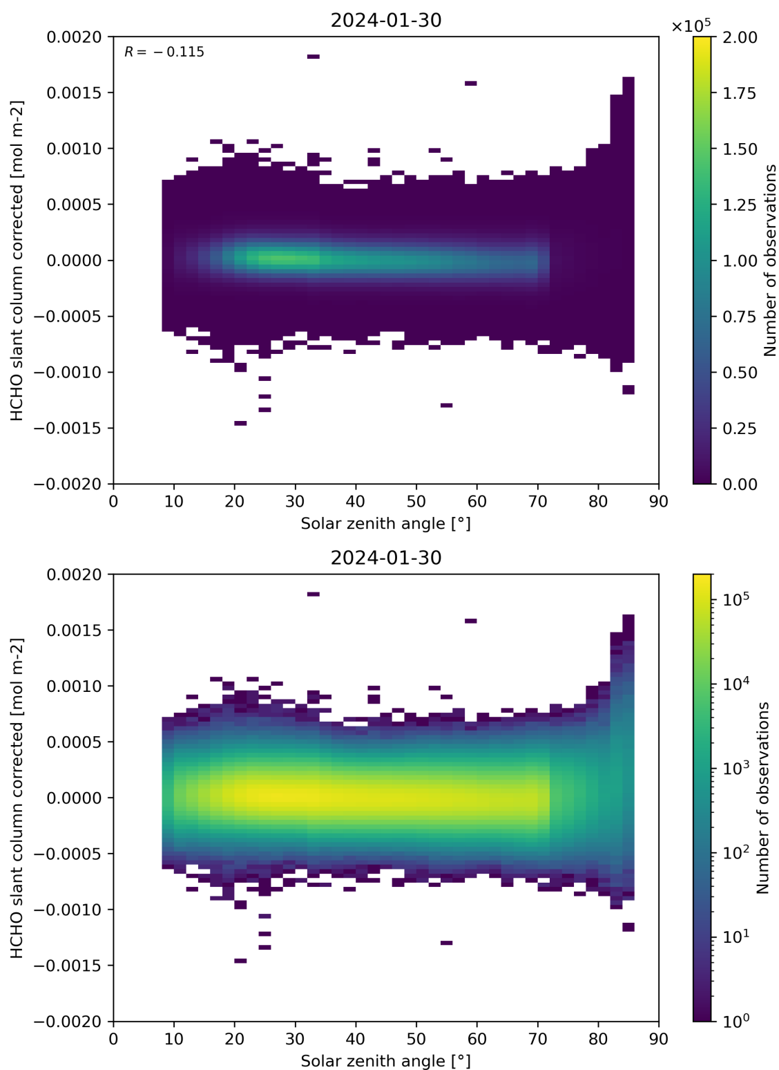
Figure 171: Scatter density plot of “Solar zenith angle” against “HCHO slant column corrected” for 2024-01-29 to 2024-01-31.
