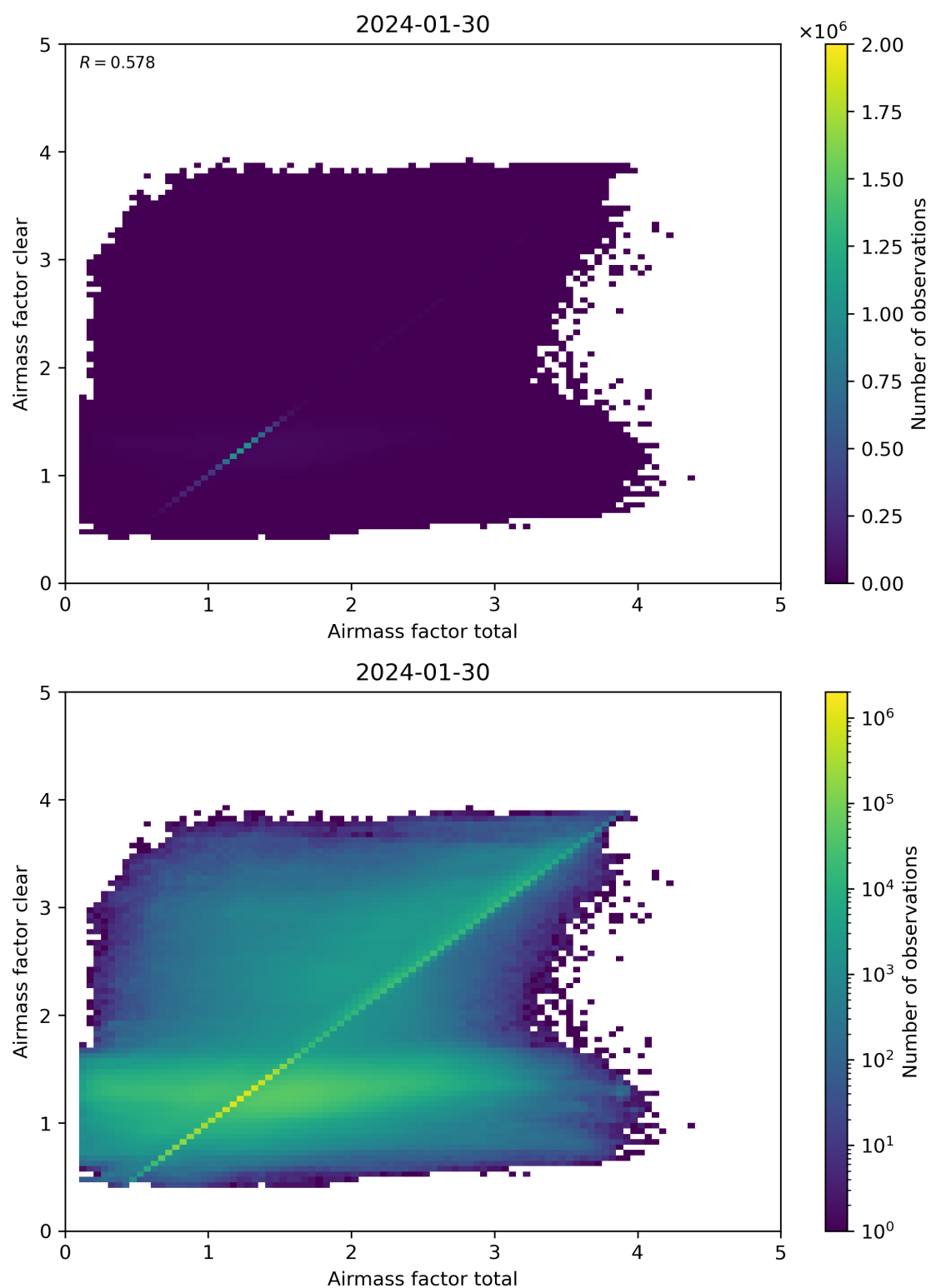
Figure 100: Scatter density plot of “Airmass factor total” against “Airmass factor clear” for 2024-01-29 to 2024-01-31.
