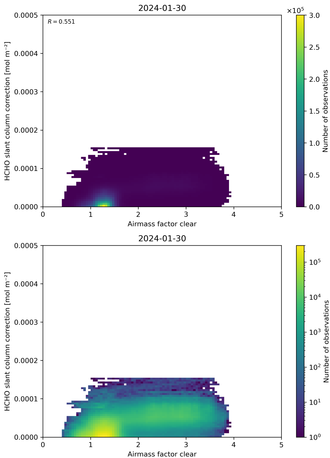
Figure 75: Scatter density plot of “Airmass factor clear” against “HCHO slant column correction” for 2024-01-29 to 2024-01-31.
