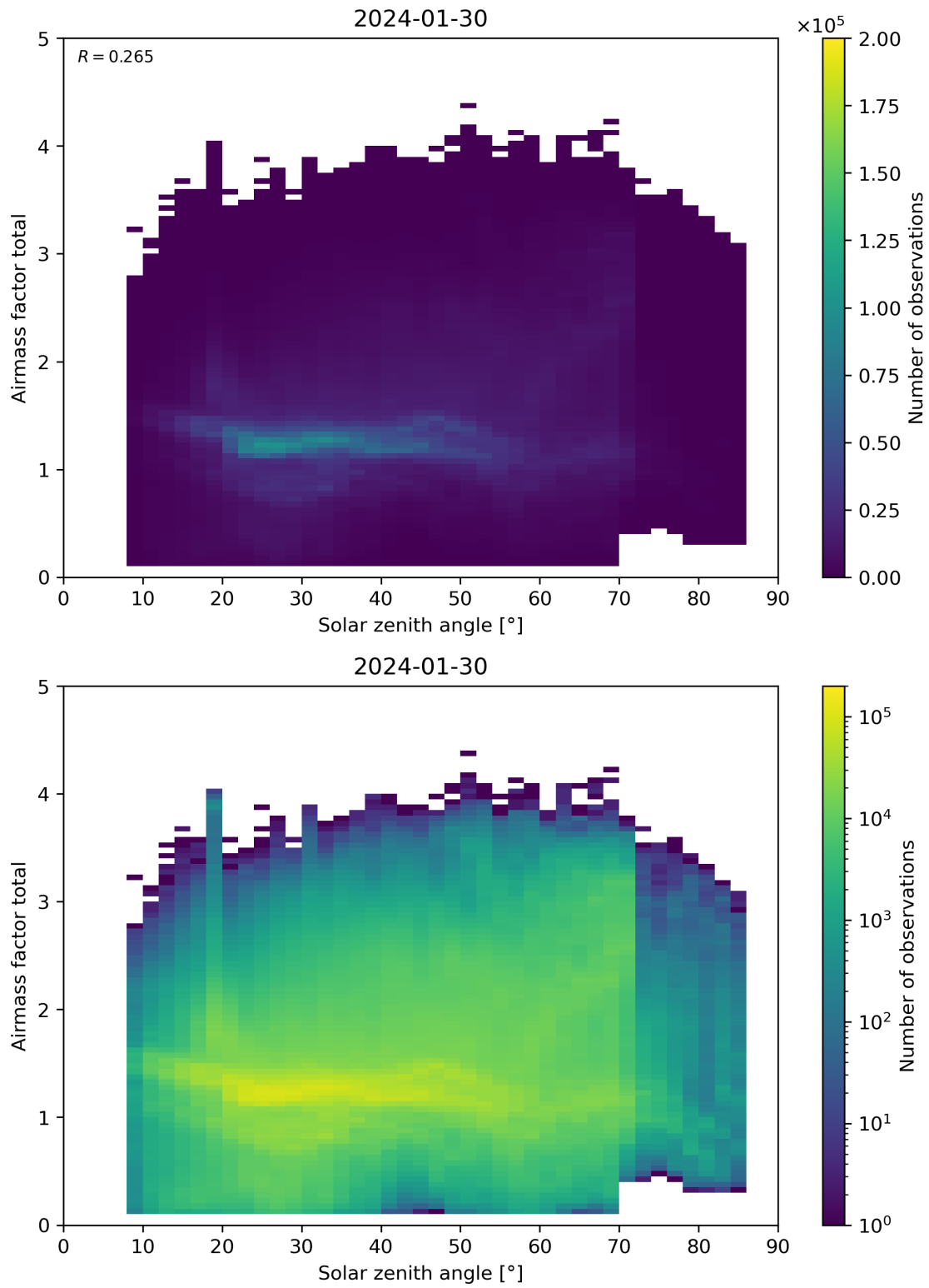
Figure 175: Scatter density plot of “Solar zenith angle” against “Airmass factor total” for 2024-01-29 to 2024-01-31.
