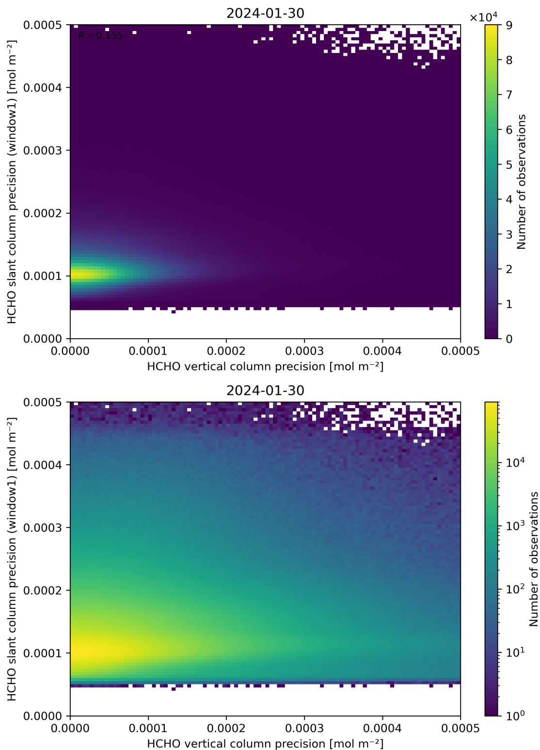
Figure 143: Scatter density plot of “HCHO vertical column precision” against “HCHO slant column precision (window1)” for 2024-01-29 to 2024-01-31.
