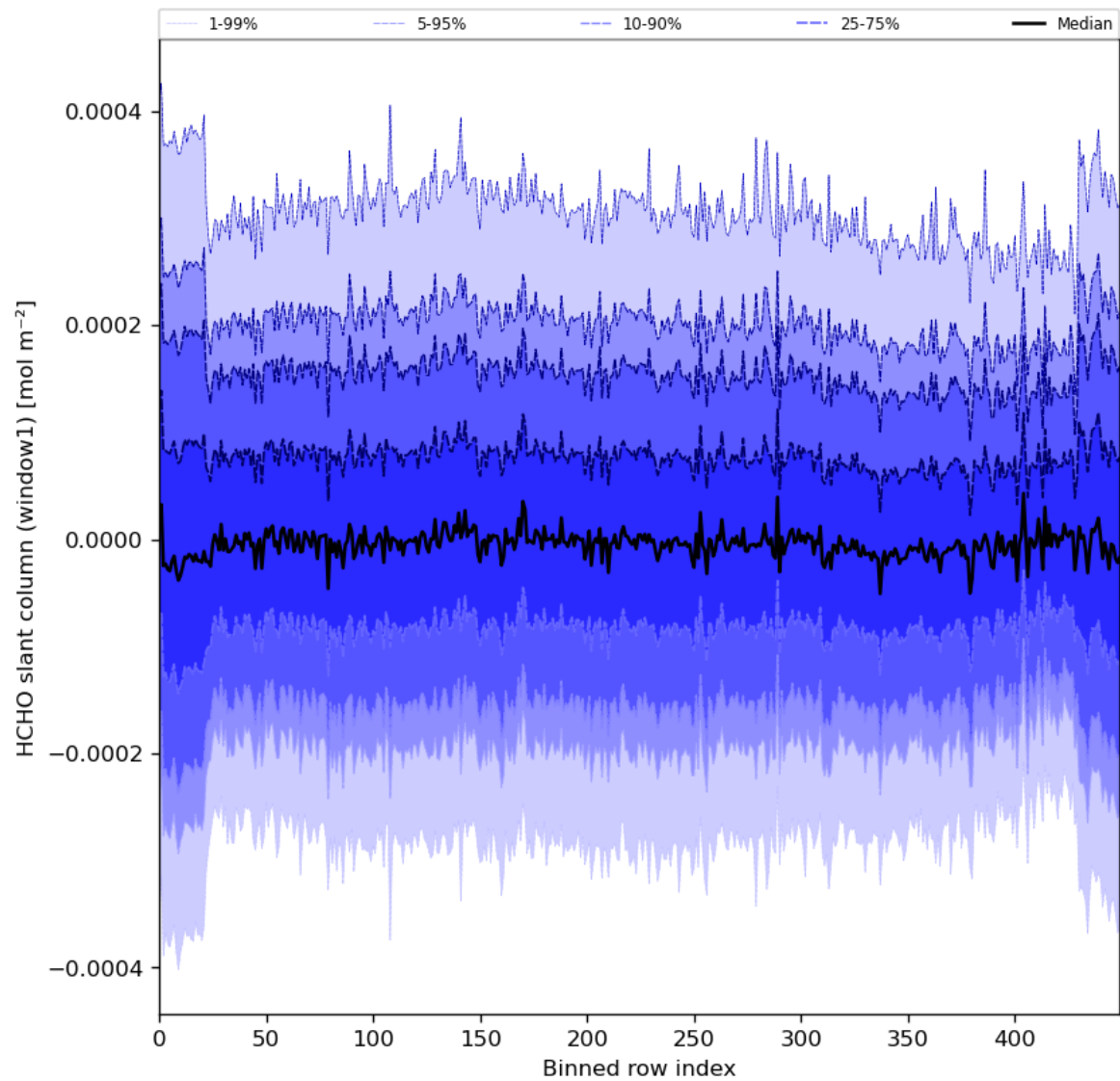
Figure 52: Along track statistics of “HCHO slant column (window1)” for 2024-01-29 to 2024-01-31
