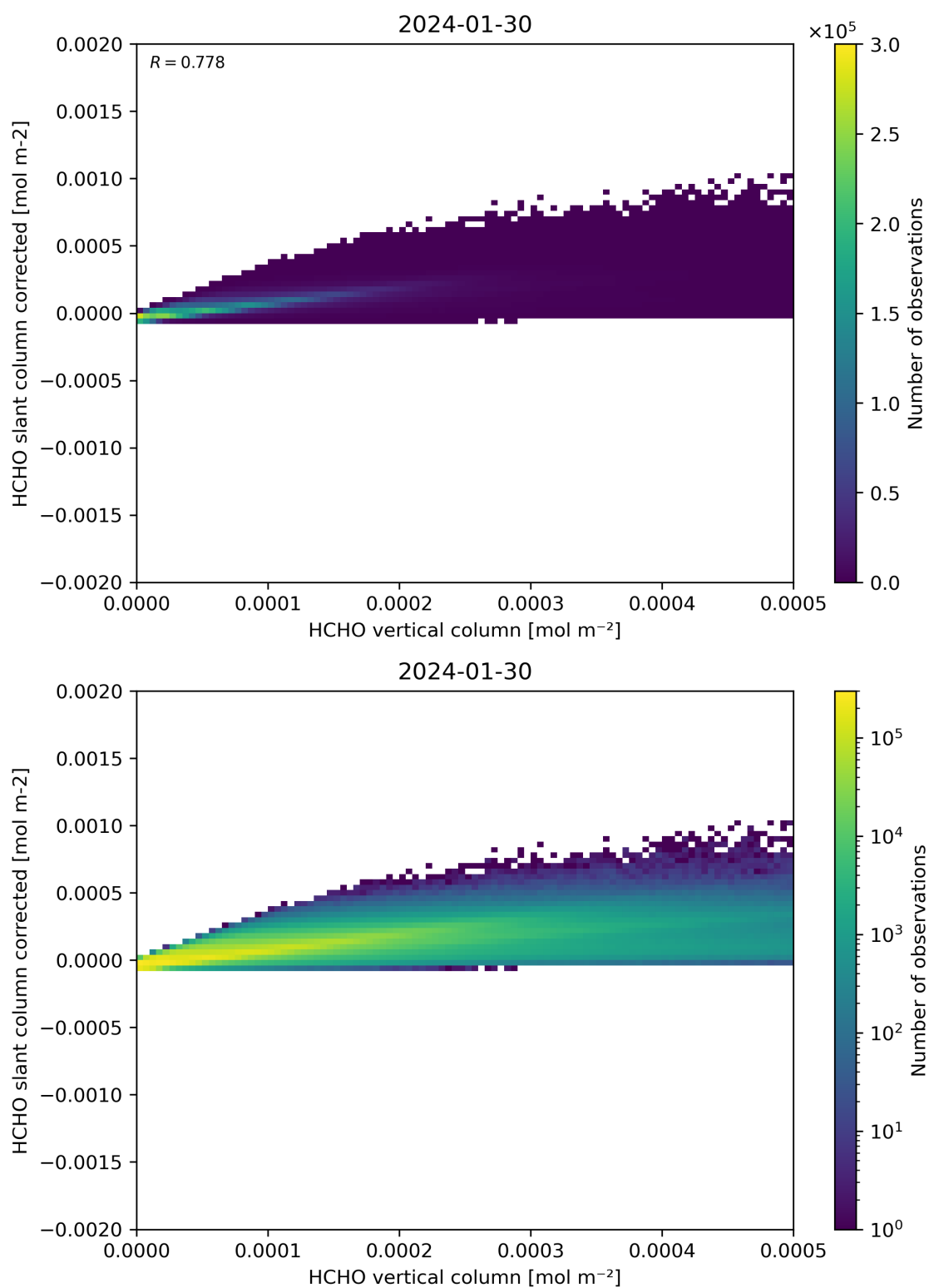
Figure 127: Scatter density plot of “HCHO vertical column” against “HCHO slant column corrected” for 2024-01-29 to 2024-01-31.
