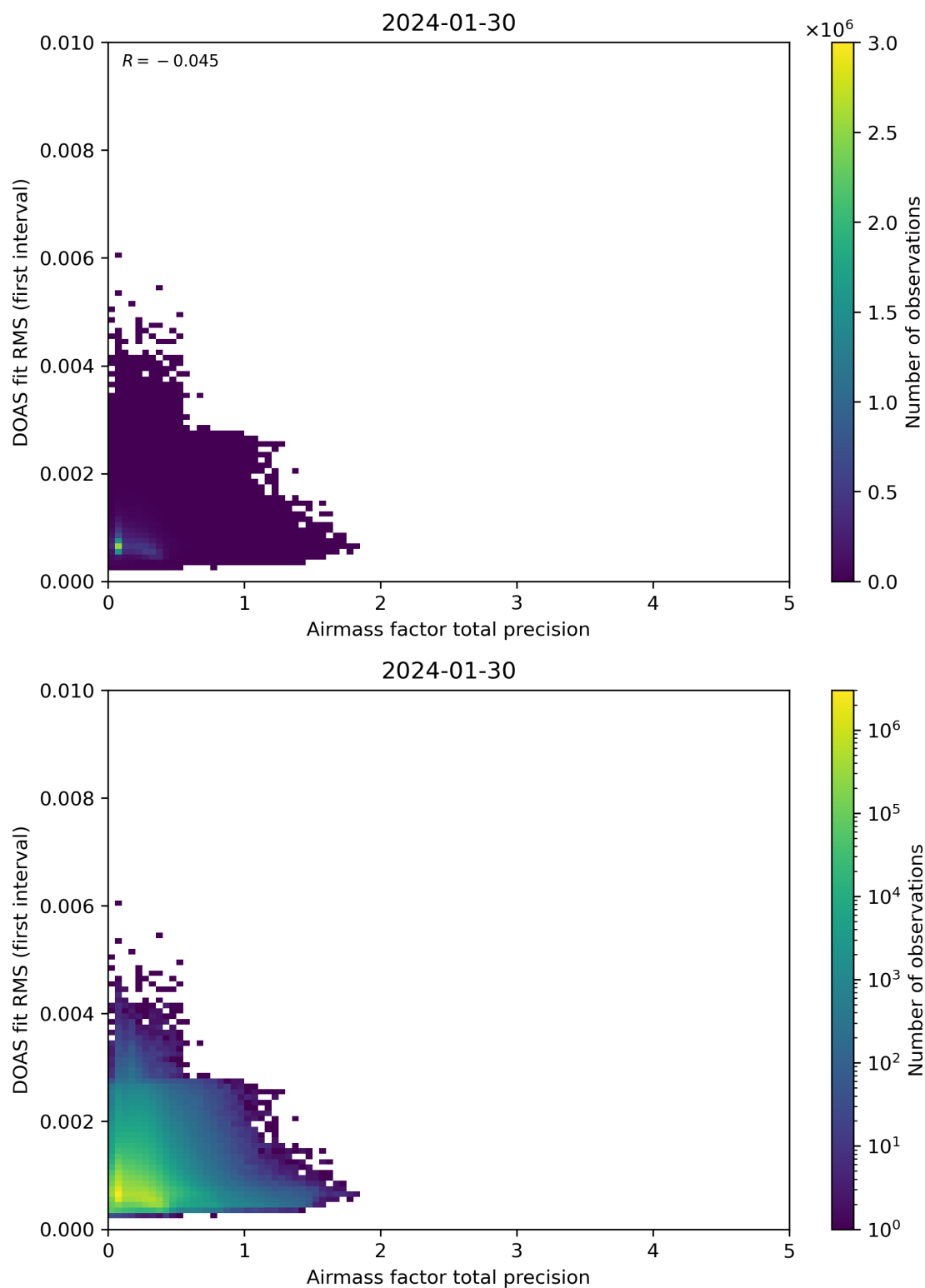
Figure 105: Scatter density plot of “Airmass factor total precision” against “DOAS fit RMS (first interval)” for 2024-01-29 to 2024-01-31.
