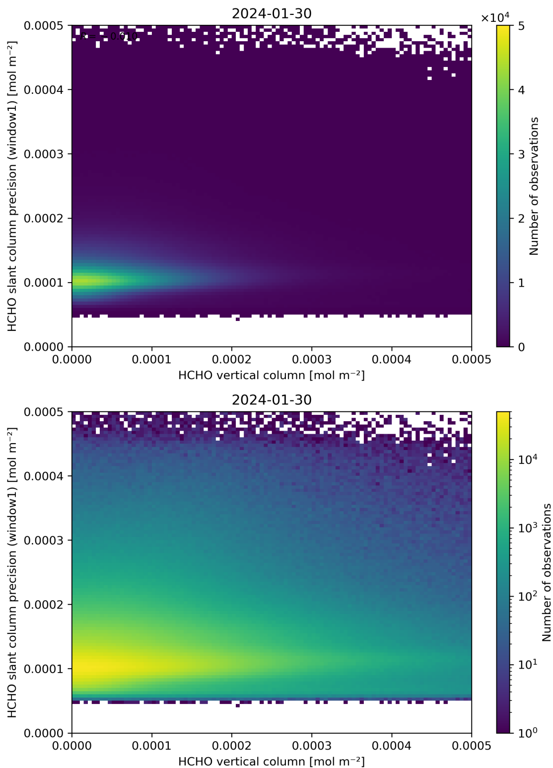
Figure 130: Scatter density plot of “HCHO vertical column” against “HCHO slant column precision (window1)” for 2024-01-29 to 2024-01-31.
