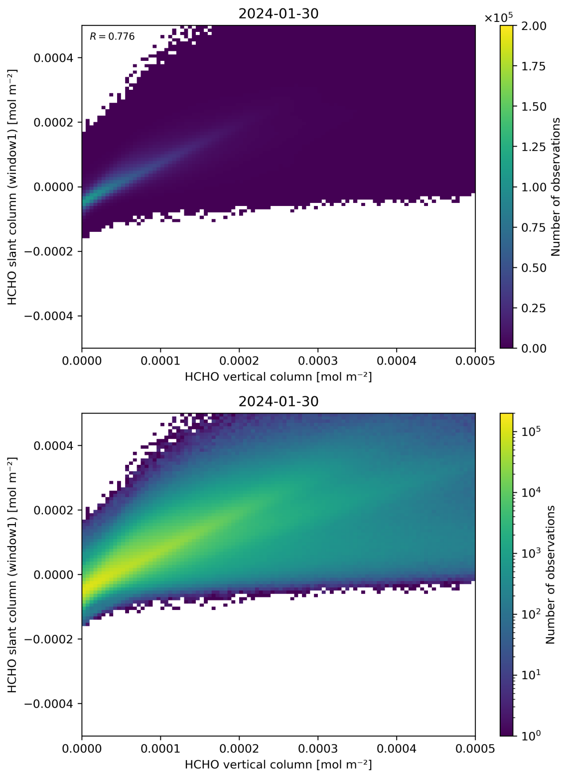
Figure 129: Scatter density plot of “HCHO vertical column” against “HCHO slant column (window1)” for 2024-01-29 to 2024-01-31.
