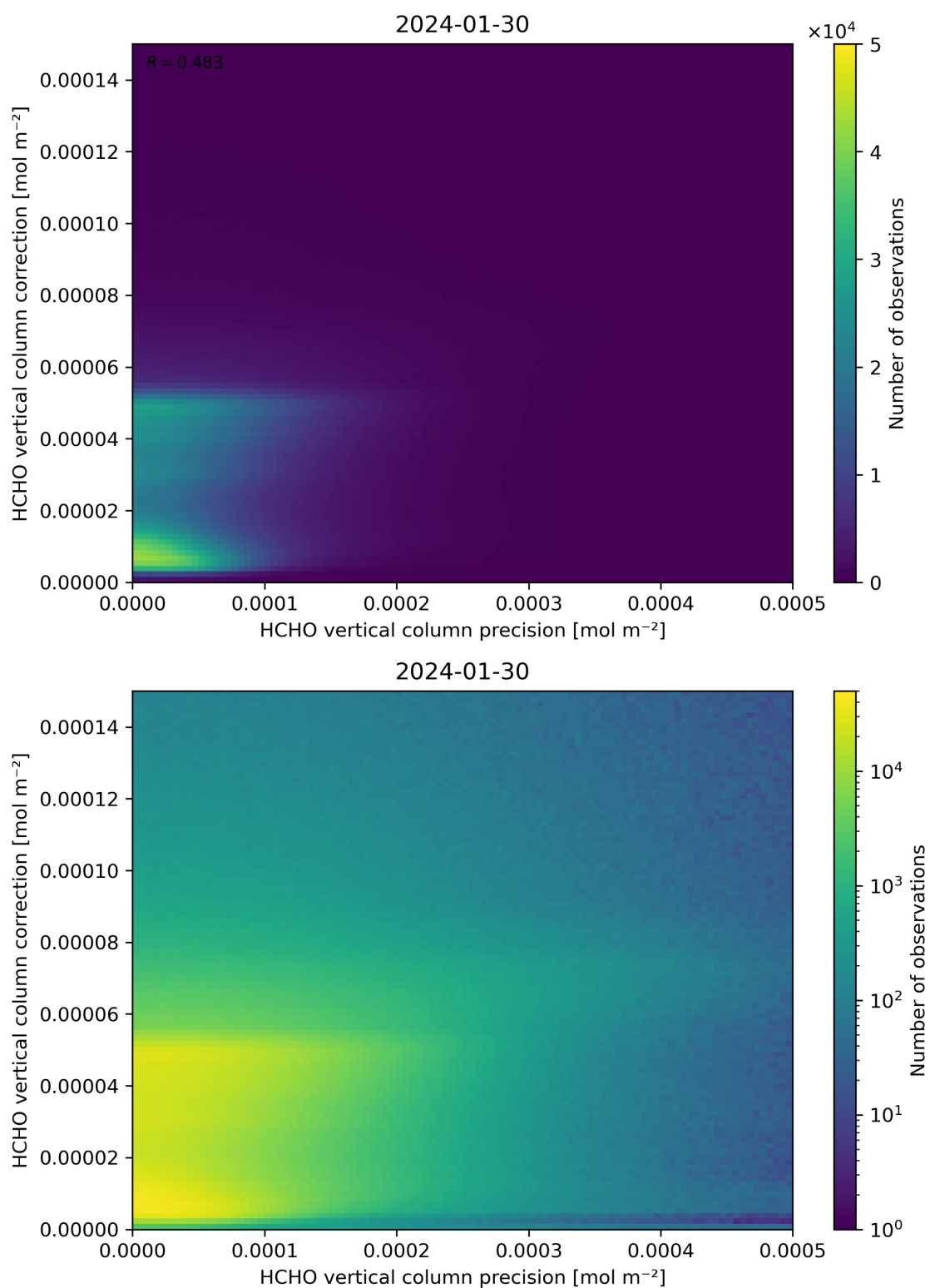
Figure 146: Scatter density plot of “HCHO vertical column precision” against “HCHO vertical column correction” for 2024-01-29 to 2024-01-31.
