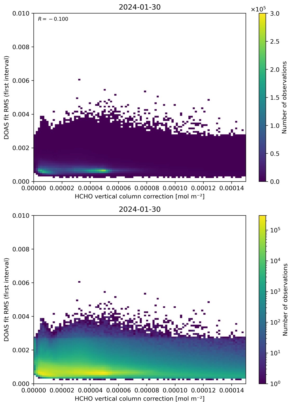
Figure 112: Scatter density plot of “HCHO vertical column correction” against “DOAS fit RMS (first interval)” for 2024-01-29 to 2024-01-31.
