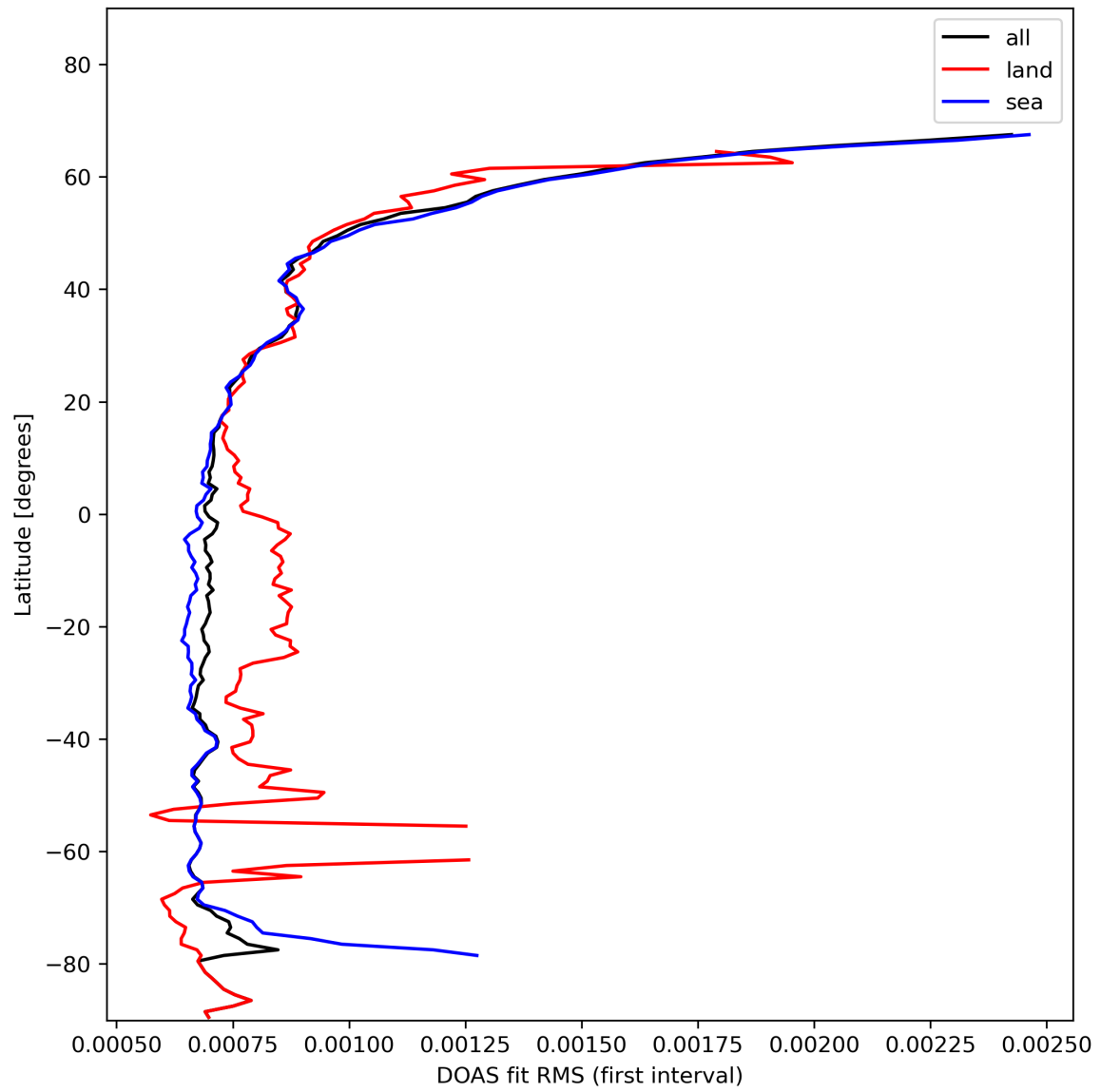
Figure 32: Zonal average of “DOAS fit RMS (first interval)” for 2024-01-29 to 2024-01-31.
