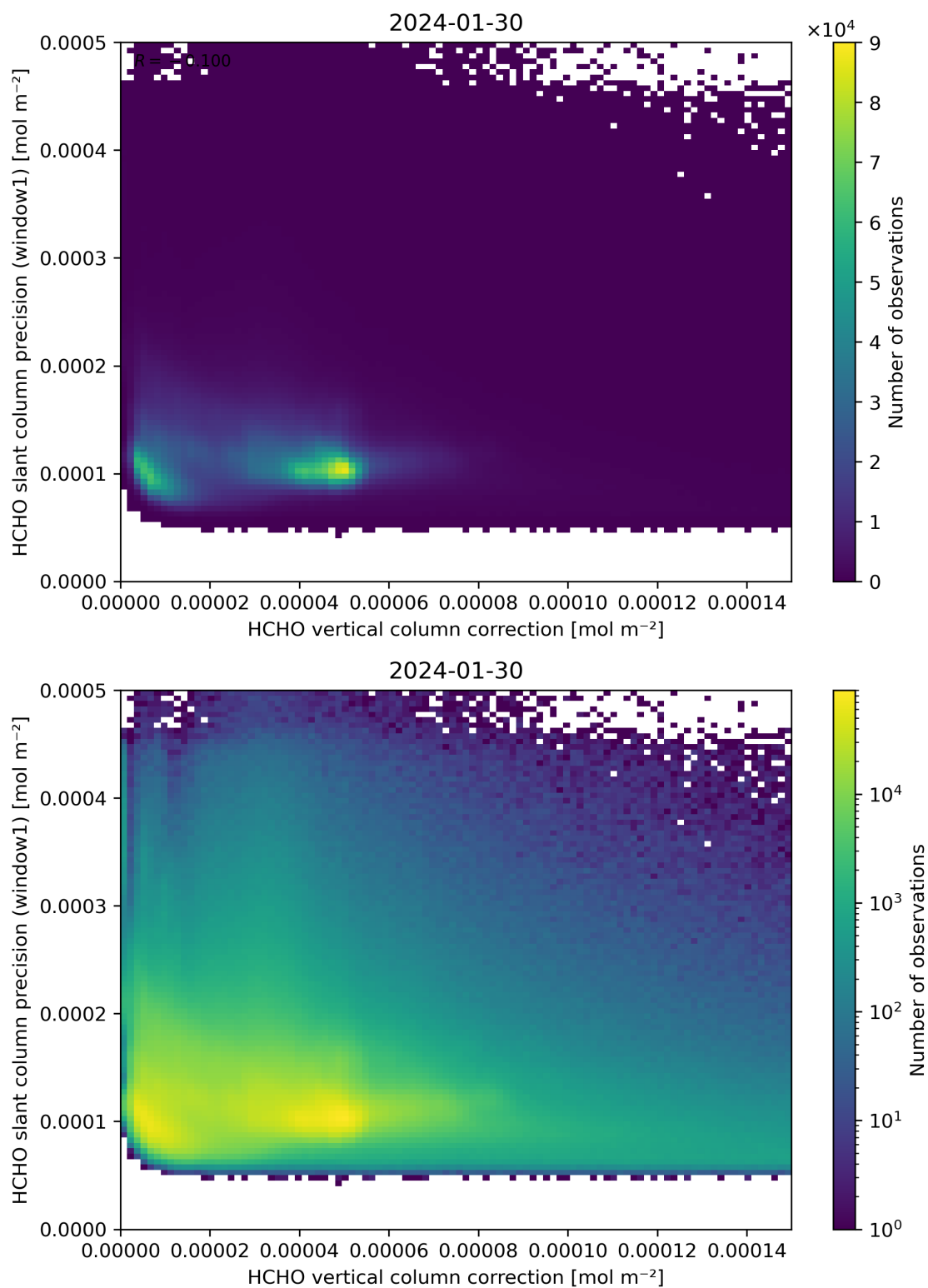
Figure 119: Scatter density plot of “HCHO vertical column correction” against “HCHO slant column precision (window1)” for 2024-01-29 to 2024-01-31.
