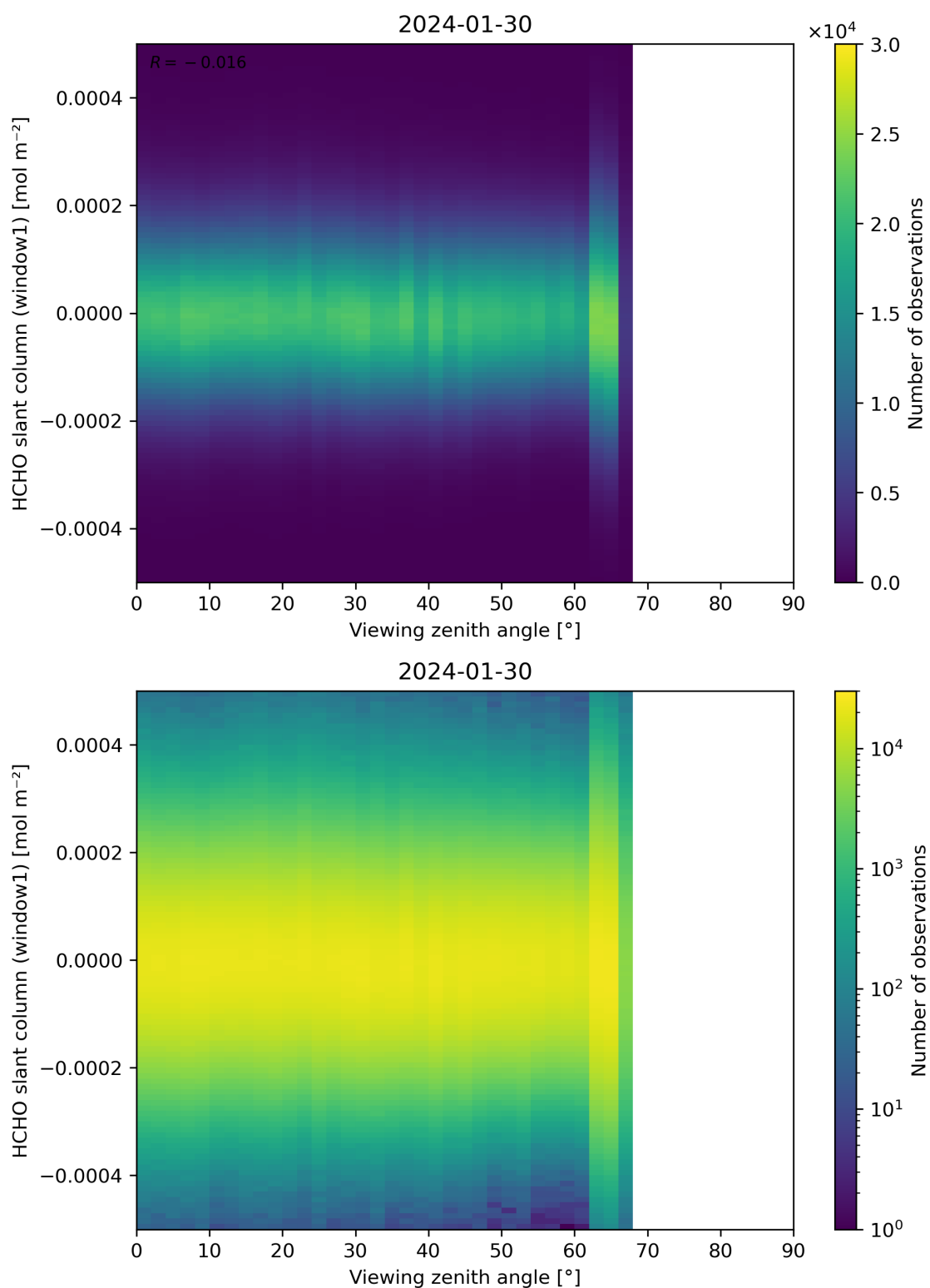
Figure 188: Scatter density plot of “Viewing zenith angle” against “HCHO slant column (window1)” for 2024-01-29 to 2024-01-31.
