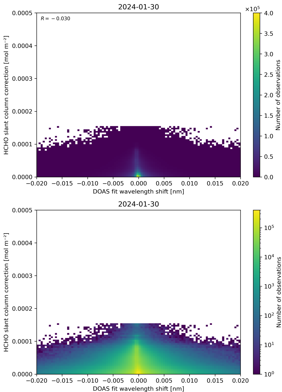
Figure 67: Scatter density plot of “DOAS fit wavelength shift” against “HCHO slant column correction” for 2024-01-29 to 2024-01-31.
