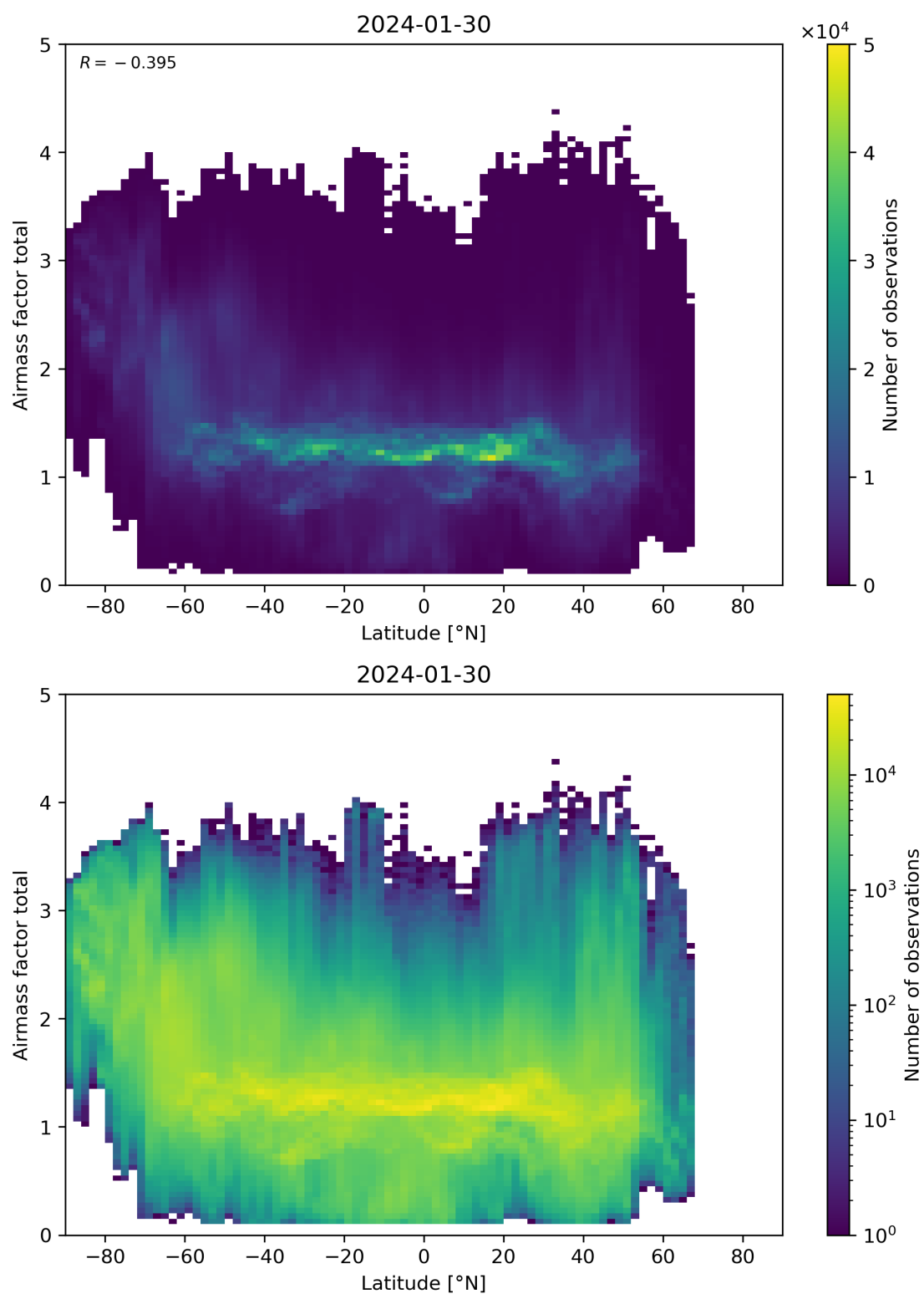
Figure 161: Scatter density plot of “Latitude” against “Airmass factor total” for 2024-01-29 to 2024-01-31.
