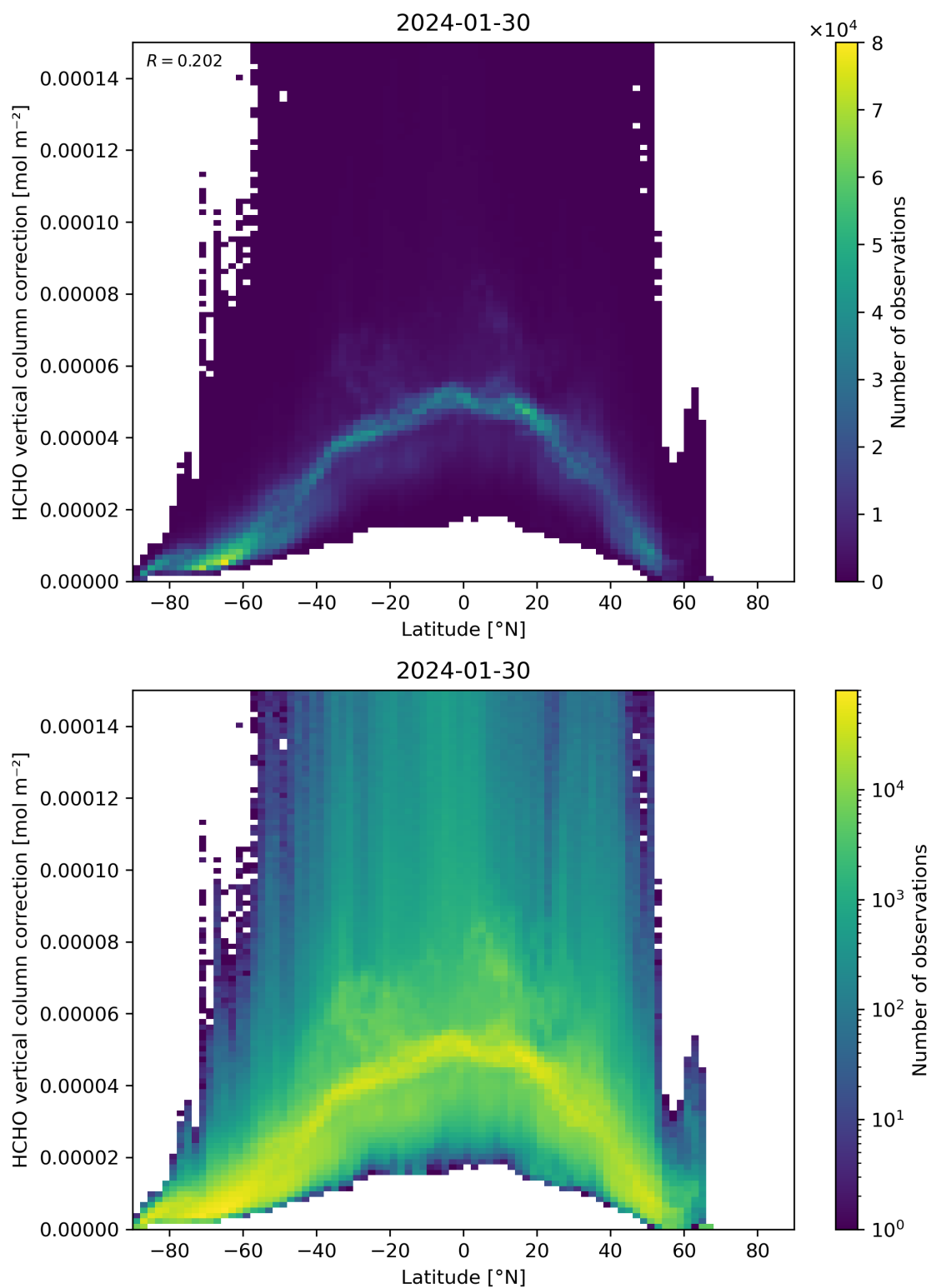
Figure 164: Scatter density plot of “Latitude” against “HCHO vertical column correction” for 2024-01-29 to 2024-01-31.
