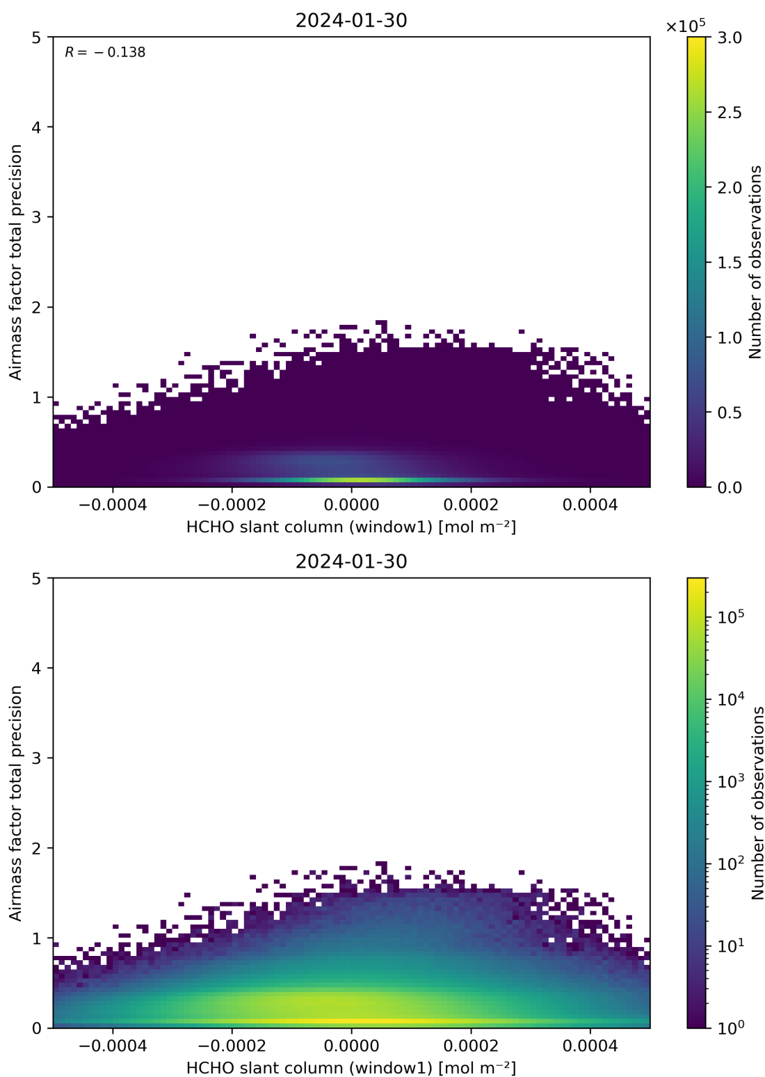
Figure 86: Scatter density plot of “HCHO slant column (window1)” against “Airmass factor total precision” for 2024-01-29 to 2024-01-31.
