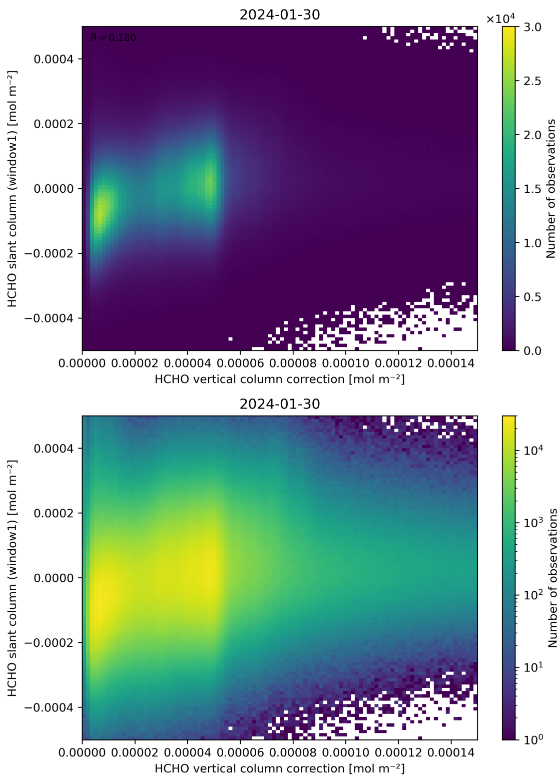
Figure 118: Scatter density plot of “HCHO vertical column correction” against “HCHO slant column (window1)” for 2024-01-29 to 2024-01-31.
