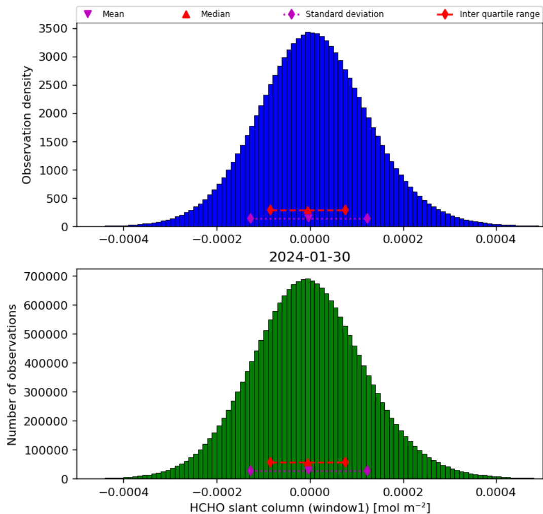
Figure 38: Histogram of “HCHO slant column (window1)” for 2024-01-29 to 2024-01-31
