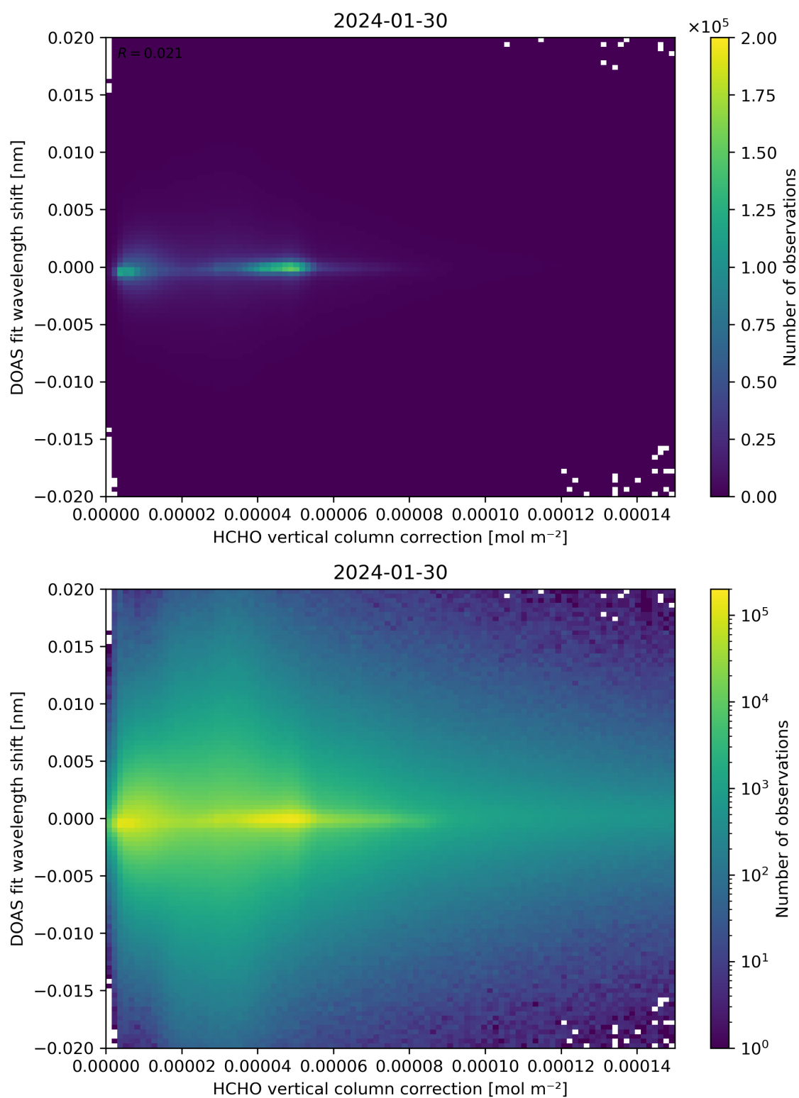
Figure 113: Scatter density plot of “HCHO vertical column correction” against “DOAS fit wavelength shift” for 2024-01-29 to 2024-01-31.
