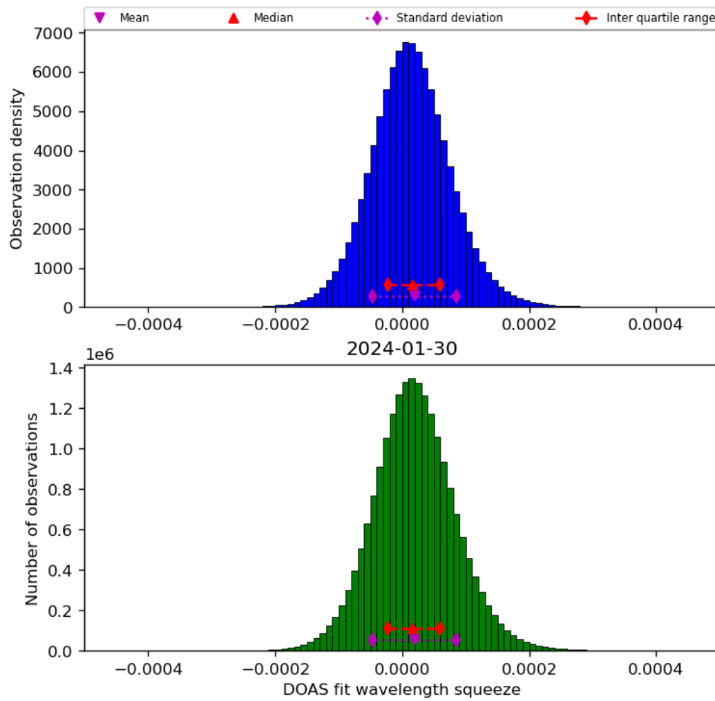
Figure 45: Histogram of “DOAS fit wavelength squeeze” for 2024-01-29 to 2024-01-31
