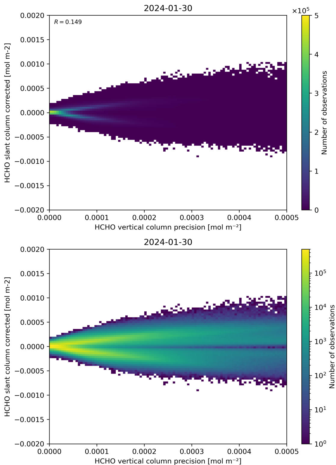
Figure 140: Scatter density plot of “HCHO vertical column precision” against “HCHO slant column corrected” for 2024-01-29 to 2024-01-31.
