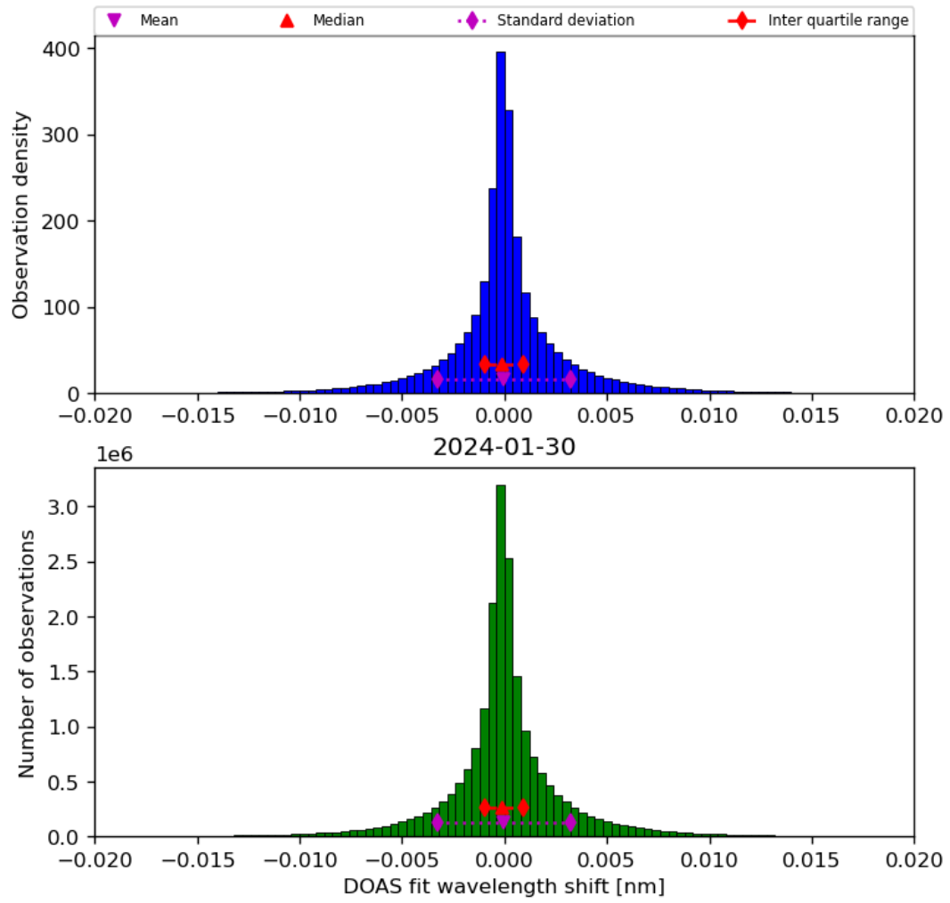
Figure 44: Histogram of “DOAS fit wavelength shift” for 2024-01-29 to 2024-01-31
