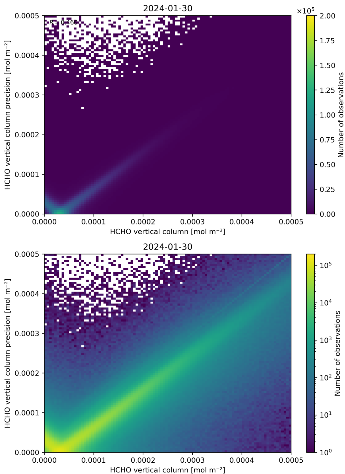
Figure 134: Scatter density plot of “HCHO vertical column” against “HCHO vertical column precision” for 2024-01-29 to 2024-01-31.
