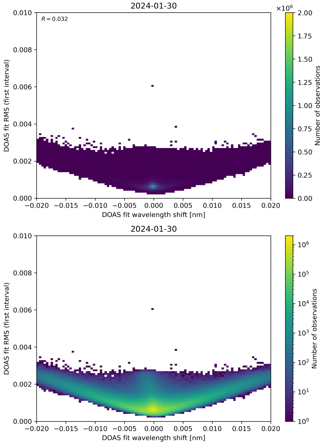
Figure 64: Scatter density plot of “DOAS fit wavelength shift” against “DOAS fit RMS (first interval)” for 2024-01-29 to 2024-01-31.
