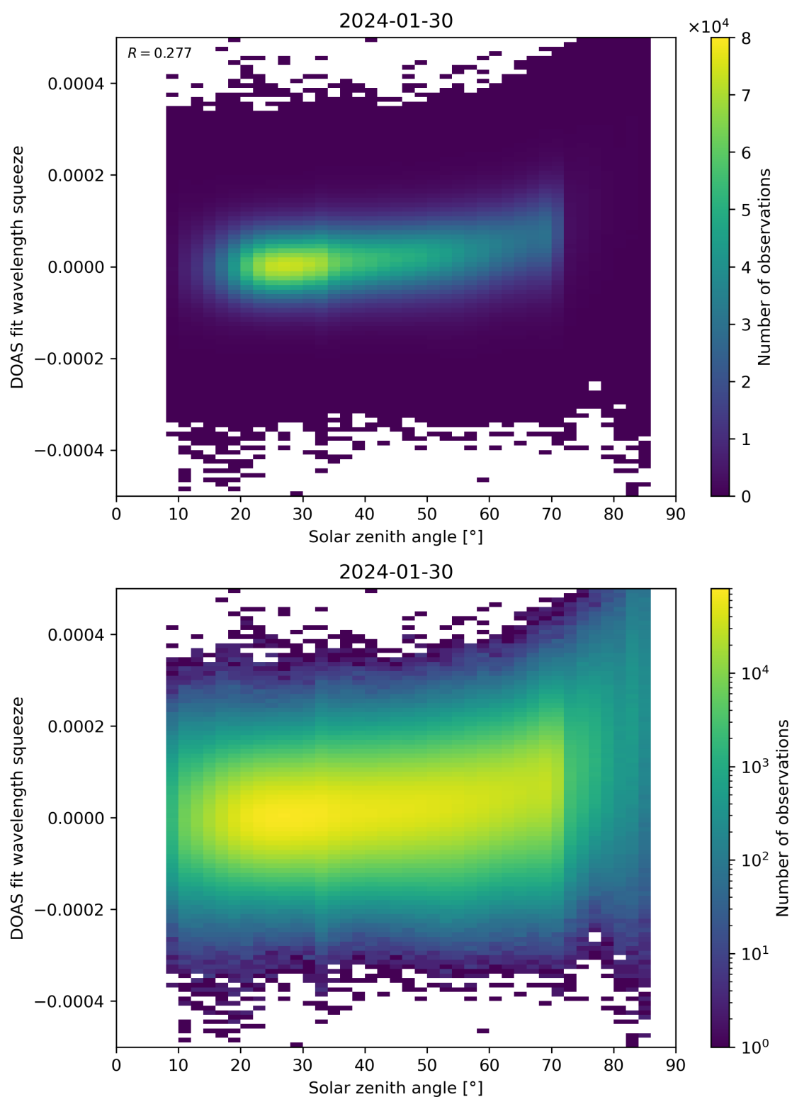
Figure 169: Scatter density plot of “Solar zenith angle” against “DOAS fit wavelength squeeze” for 2024-01-29 to 2024-01-31.
