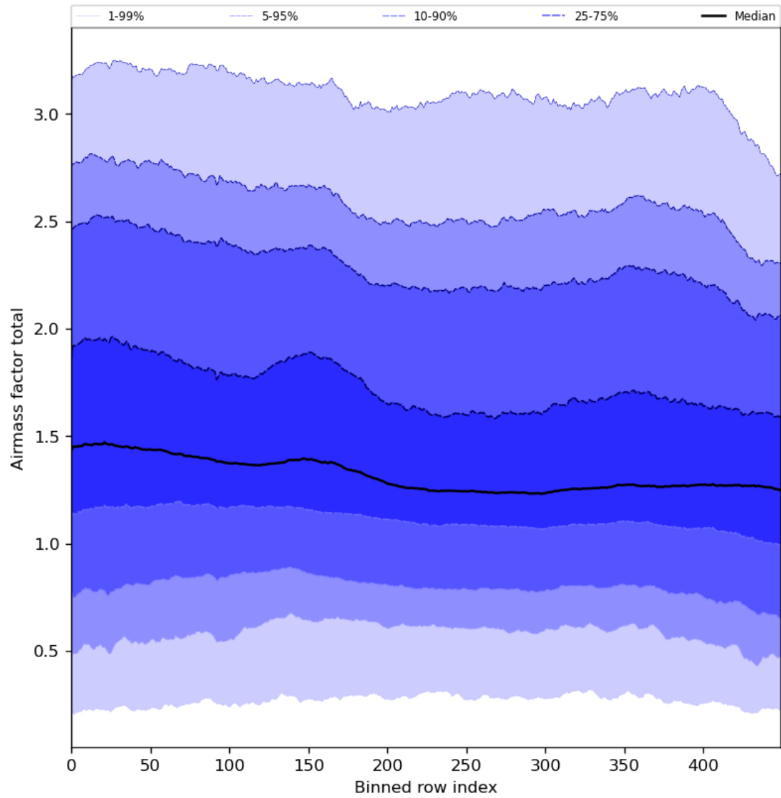
Figure 54: Along track statistics of “Airmass factor total” for 2024-01-29 to 2024-01-31
