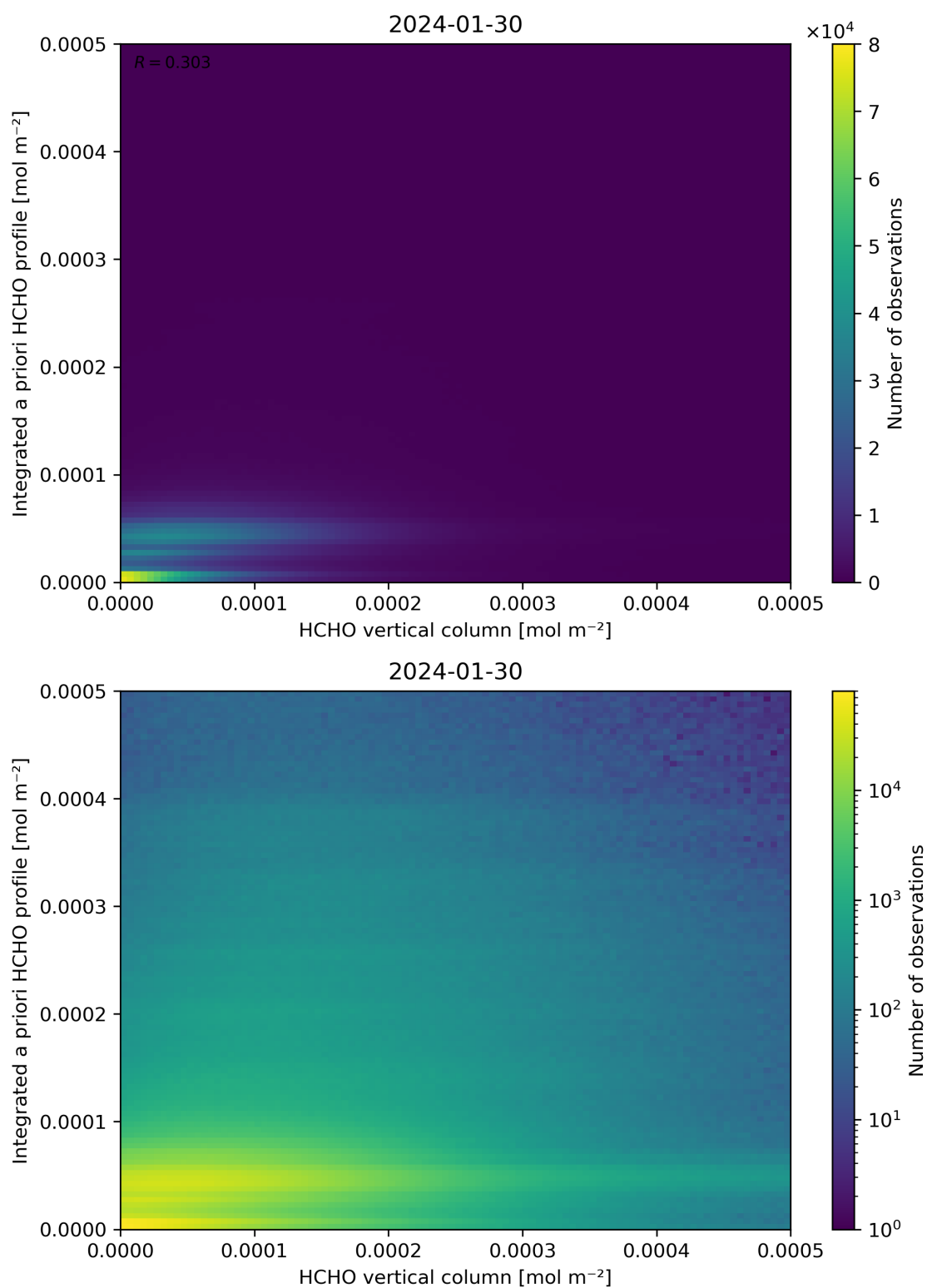
Figure 135: Scatter density plot of “HCHO vertical column” against “Integrated a priori HCHO profile” for 2024-01-29 to 2024-01-31.
