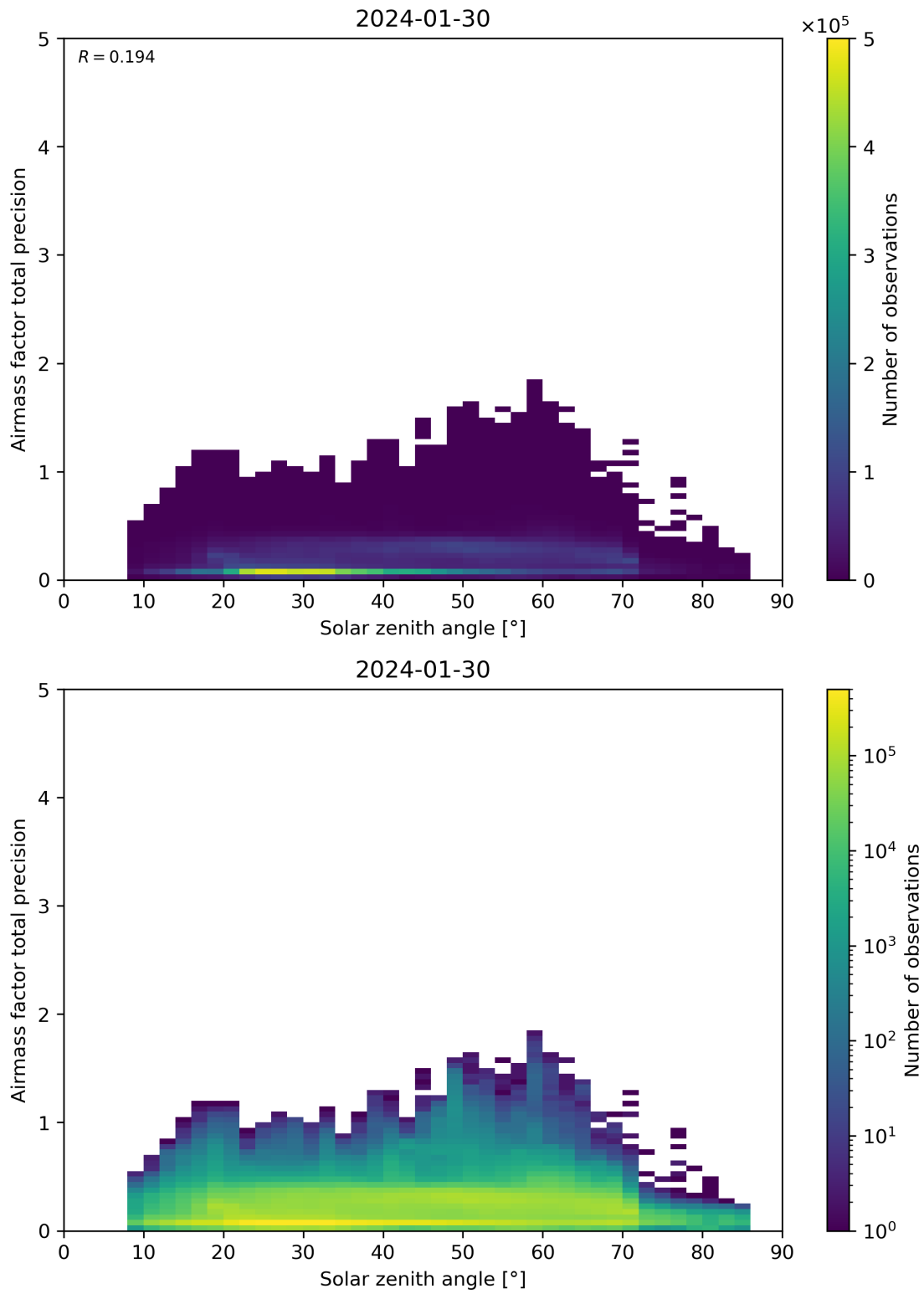
Figure 176: Scatter density plot of “Solar zenith angle” against “Airmass factor total precision” for 2024-01-29 to 2024-01-31.
