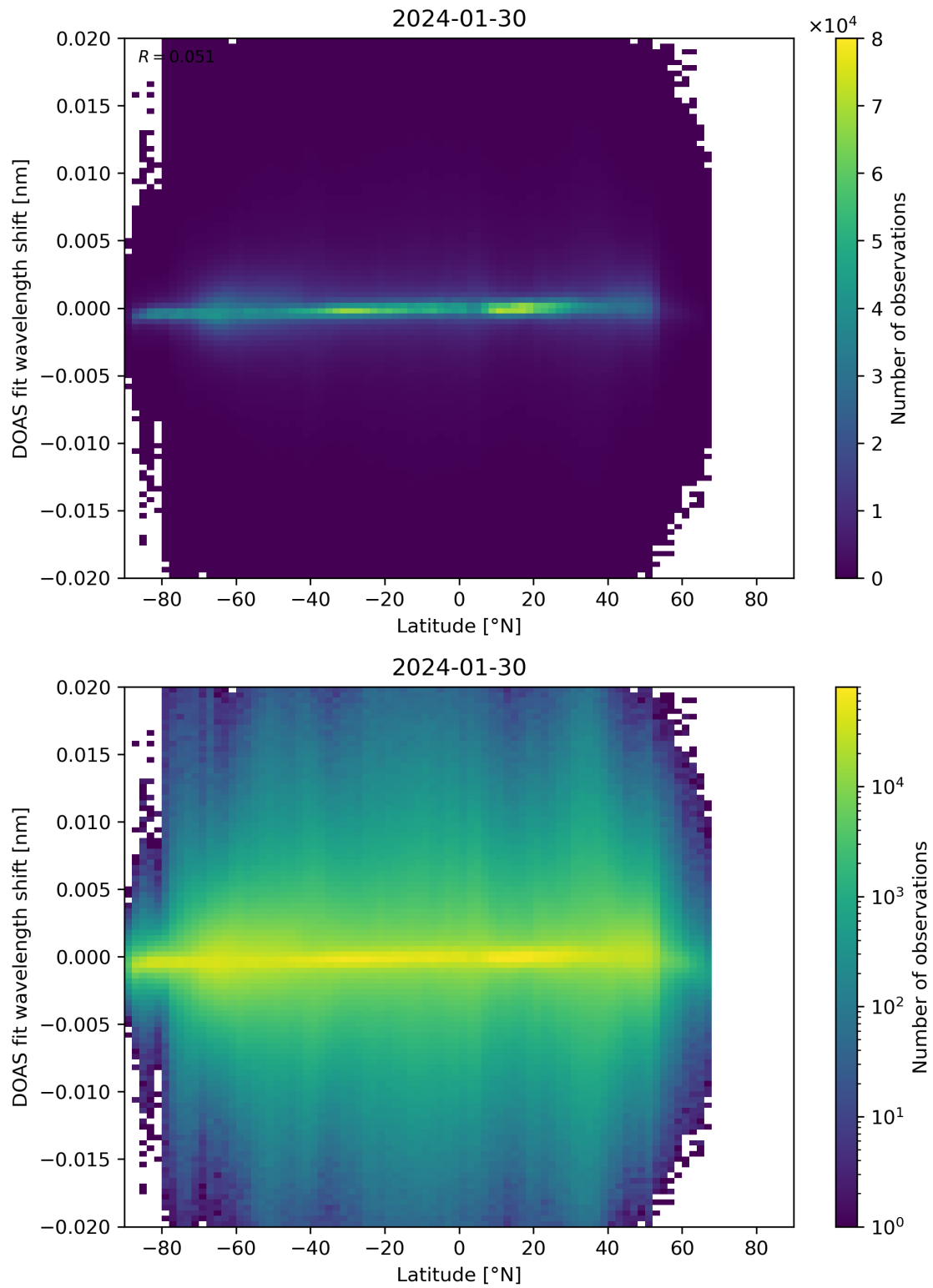
Figure 154: Scatter density plot of “Latitude” against “DOAS fit wavelength shift” for 2024-01-29 to 2024-01-31.
