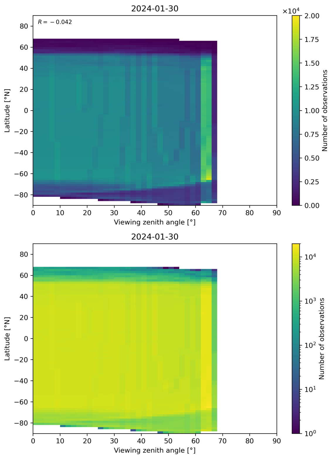
Figure 196: Scatter density plot of “Viewing zenith angle” against “Latitude” for 2024-01-29 to 2024-01-31.
