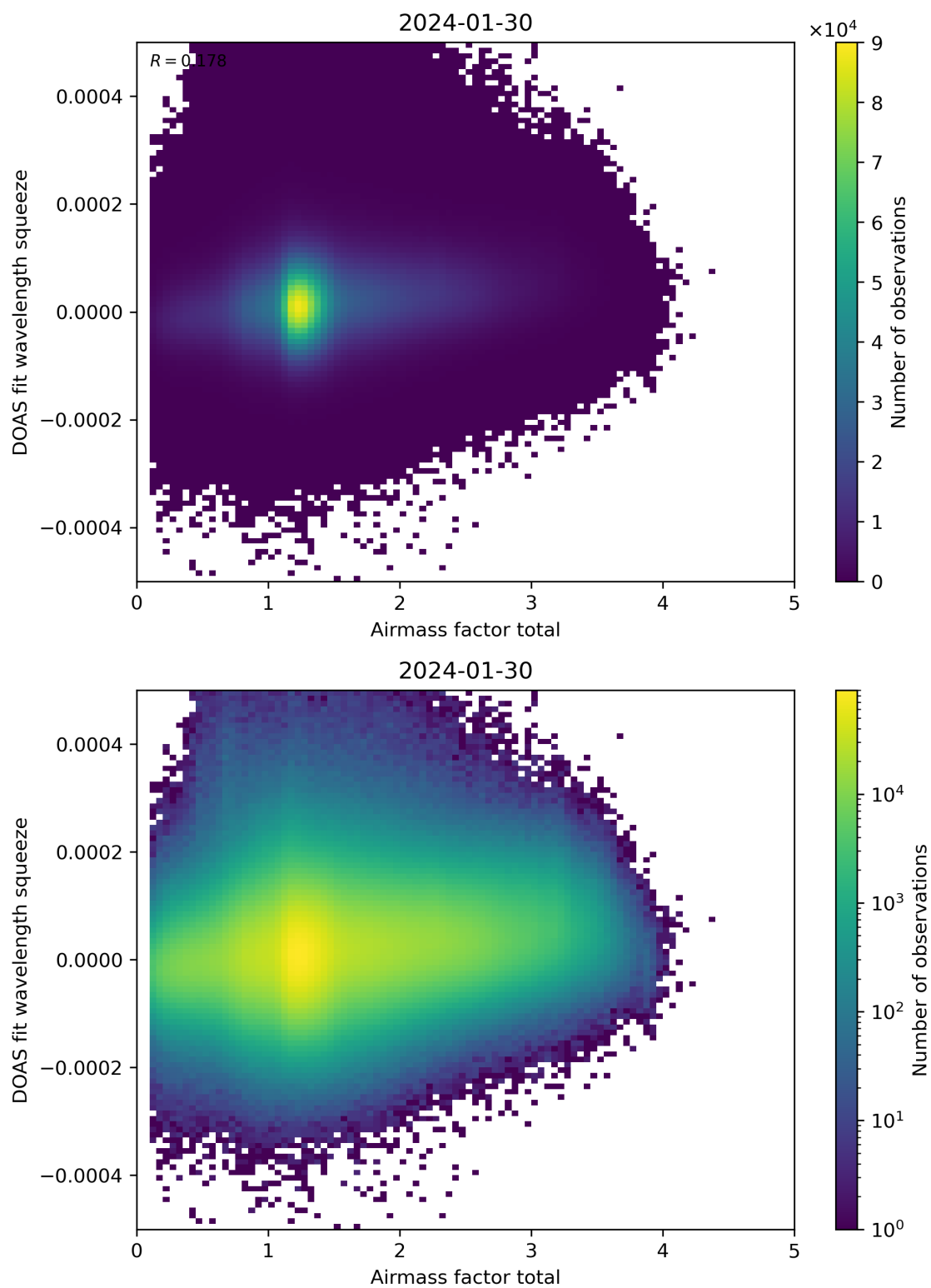
Figure 99: Scatter density plot of “Airmass factor total” against “DOAS fit wavelength squeeze” for 2024-01-29 to 2024-01-31.
