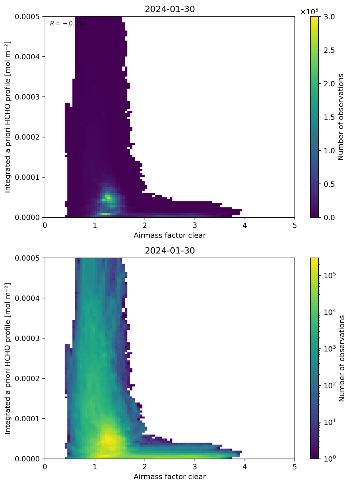
Figure 76: Scatter density plot of “Airmass factor clear” against “Integrated a priori HCHO profile” for 2024-01-29 to 2024-01-31.
