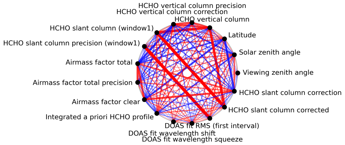
Figure 1: Map of correlation graph for 2024-01-29 to 2024-01-31.
