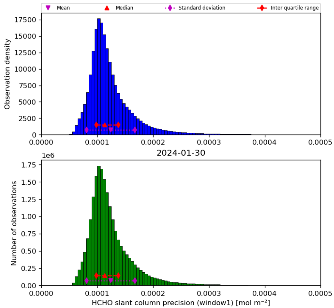
Figure 39: Histogram of “HCHO slant column precision (window1)” for 2024-01-29 to 2024-01-31
