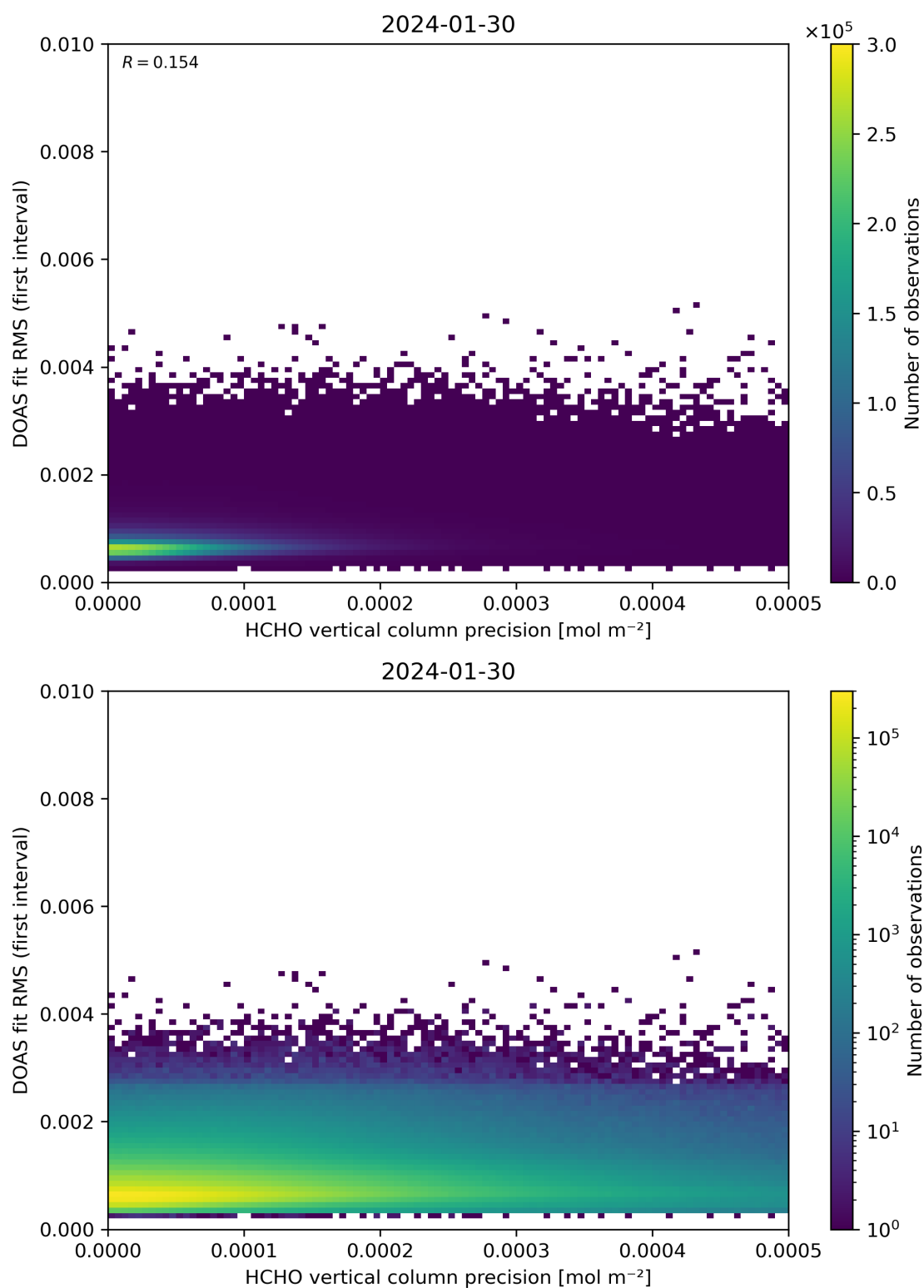
Figure 136: Scatter density plot of “HCHO vertical column precision” against “DOAS fit RMS (first interval)” for 2024-01-29 to 2024-01-31.
