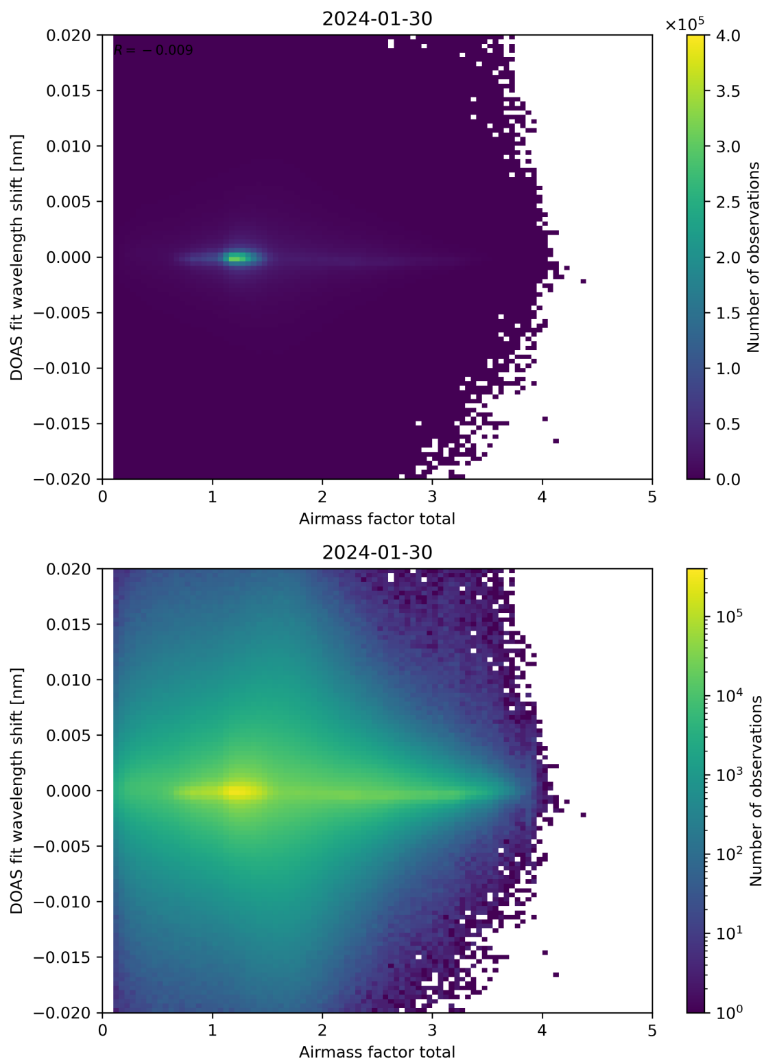
Figure 98: Scatter density plot of “Airmass factor total” against “DOAS fit wavelength shift” for 2024-01-29 to 2024-01-31.
