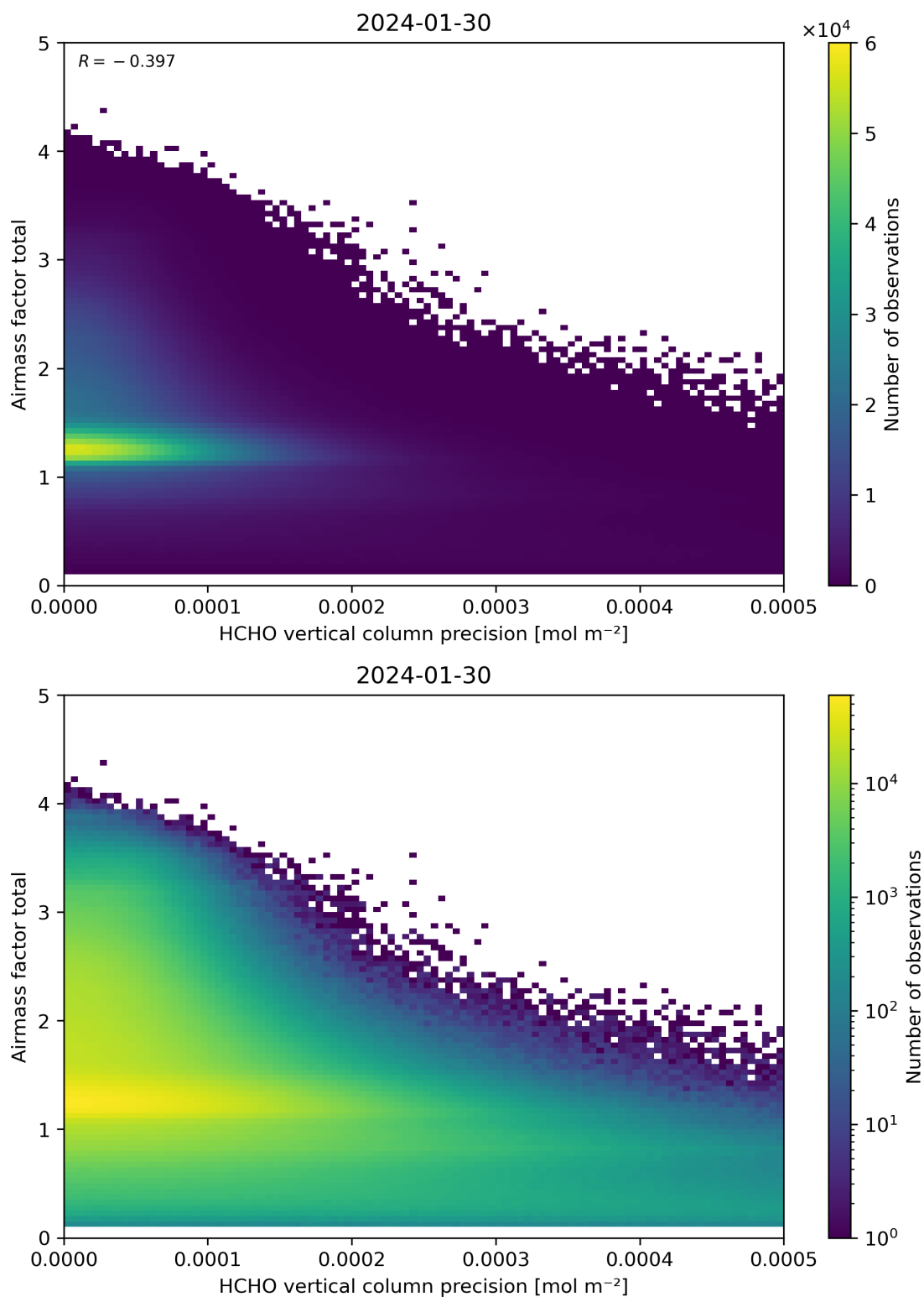
Figure 144: Scatter density plot of “HCHO vertical column precision” against “Airmass factor total” for 2024-01-29 to 2024-01-31.
