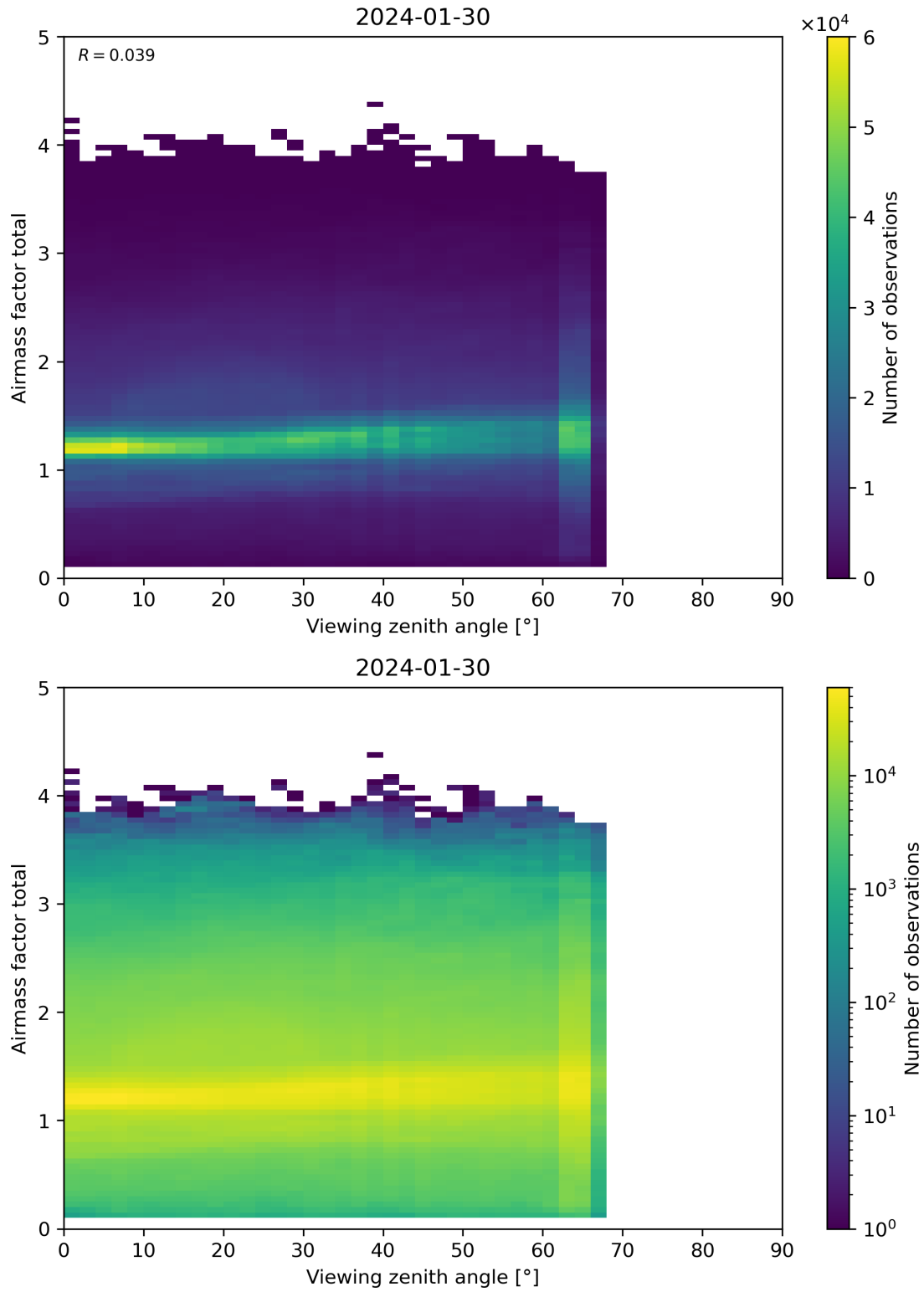
Figure 190: Scatter density plot of “Viewing zenith angle” against “Airmass factor total” for 2024-01-29 to 2024-01-31.
