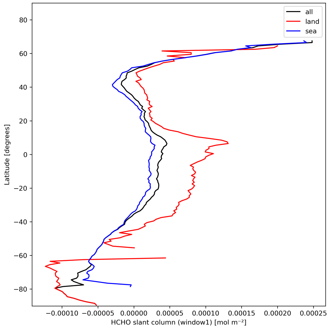
Figure 24: Zonal average of “HCHO slant column (window1)” for 2024-01-29 to 2024-01-31.
