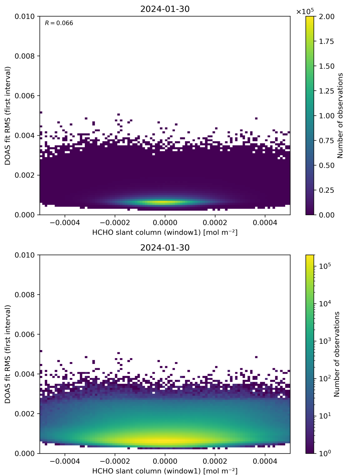
Figure 78: Scatter density plot of “HCHO slant column (window1)” against “DOAS fit RMS (first interval)” for 2024-01-29 to 2024-01-31.
