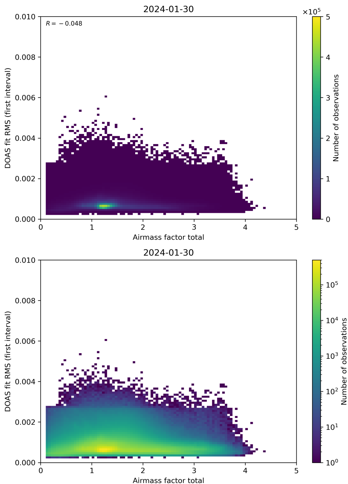
Figure 97: Scatter density plot of “Airmass factor total” against “DOAS fit RMS (first interval)” for 2024-01-29 to 2024-01-31.
