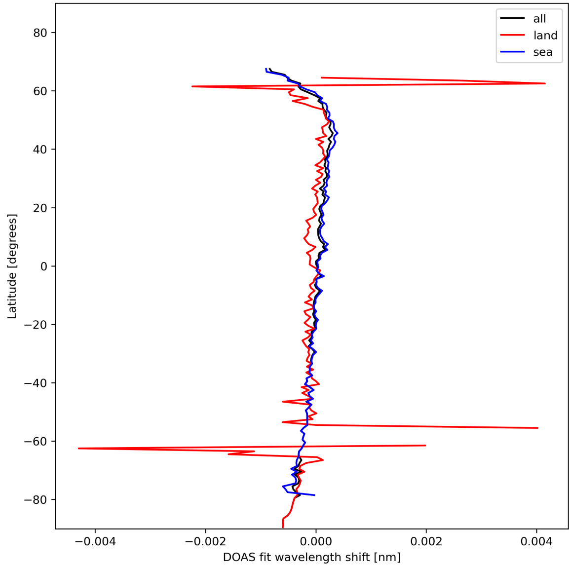
Figure 30: Zonal average of "DOAS fit wavelength shift" for 2024-01-29 to 2024-01-31.
