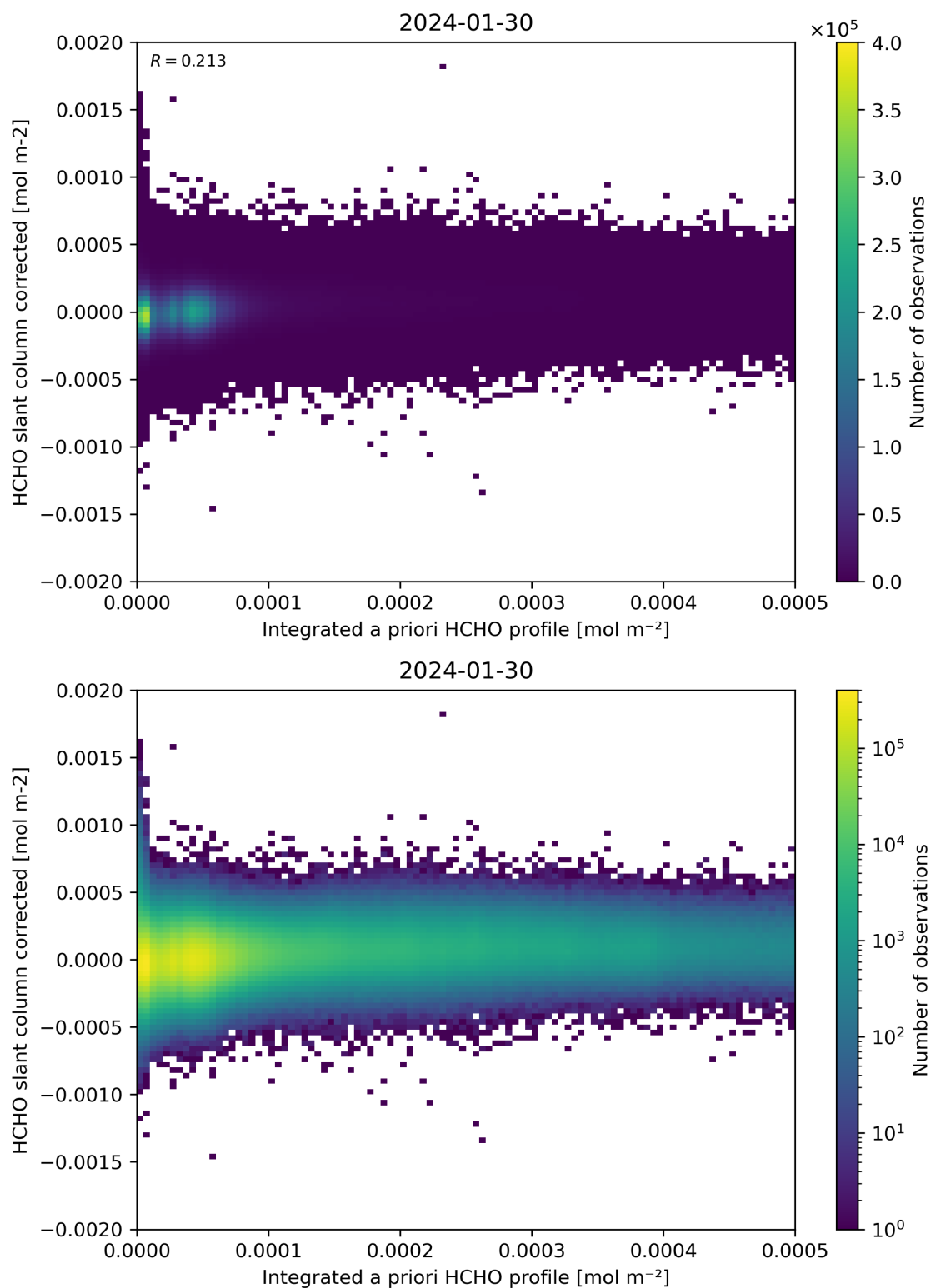
Figure 151: Scatter density plot of “Integrated a priori HCHO profile” against “HCHO slant column corrected” for 2024-01-29 to 2024-01-31.
