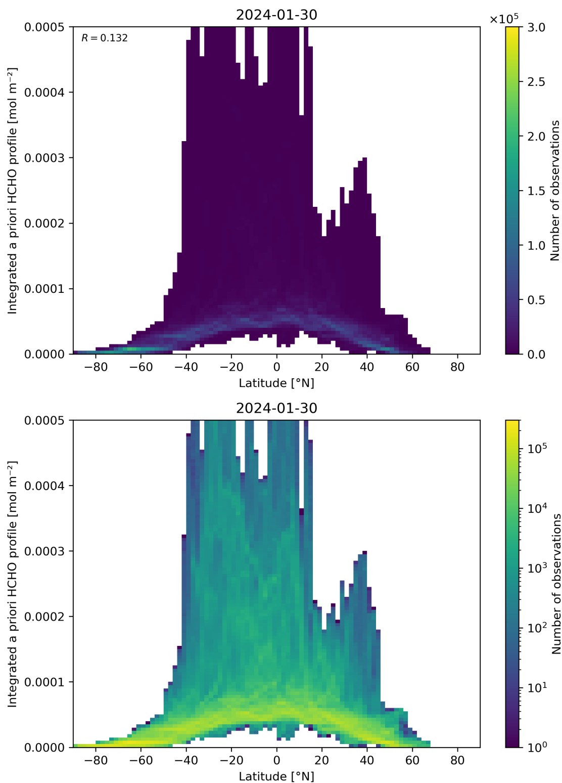
Figure 166: Scatter density plot of “Latitude” against “Integrated a priori HCHO profile” for 2024-01-29 to 2024-01-31.
