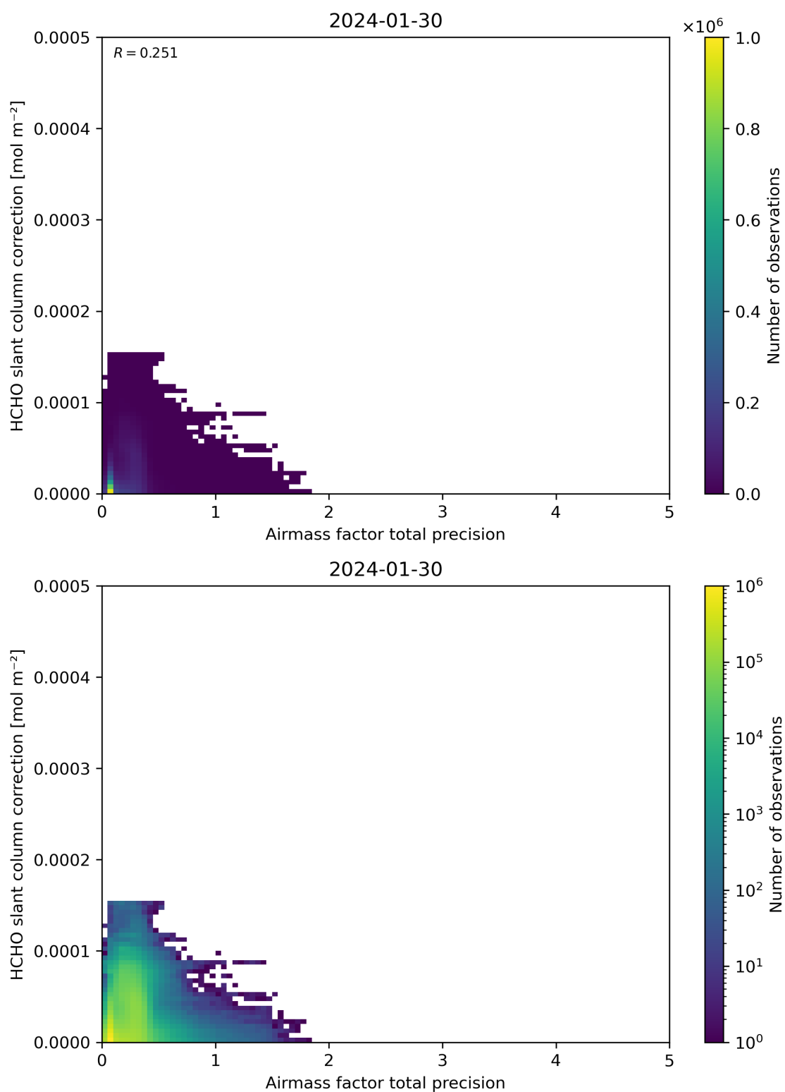
Figure 110: Scatter density plot of “Airmass factor total precision” against “HCHO slant column correction” for 2024-01-29 to 2024-01-31.
