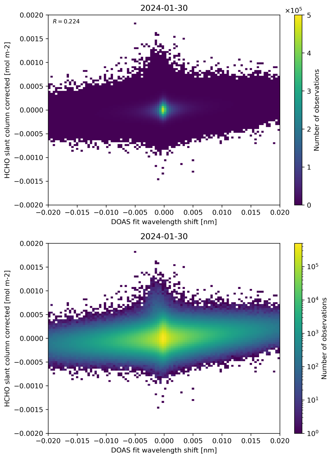
Figure 66: Scatter density plot of “DOAS fit wavelength shift” against “HCHO slant column corrected” for 2024-01-29 to 2024-01-31.
