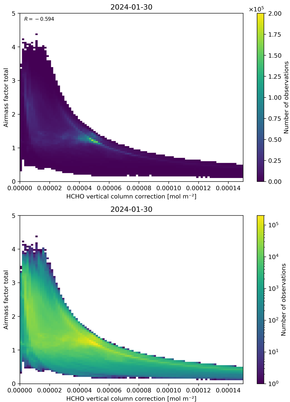
Figure 120: Scatter density plot of “HCHO vertical column correction” against “Airmass factor total” for 2024-01-29 to 2024-01-31.
