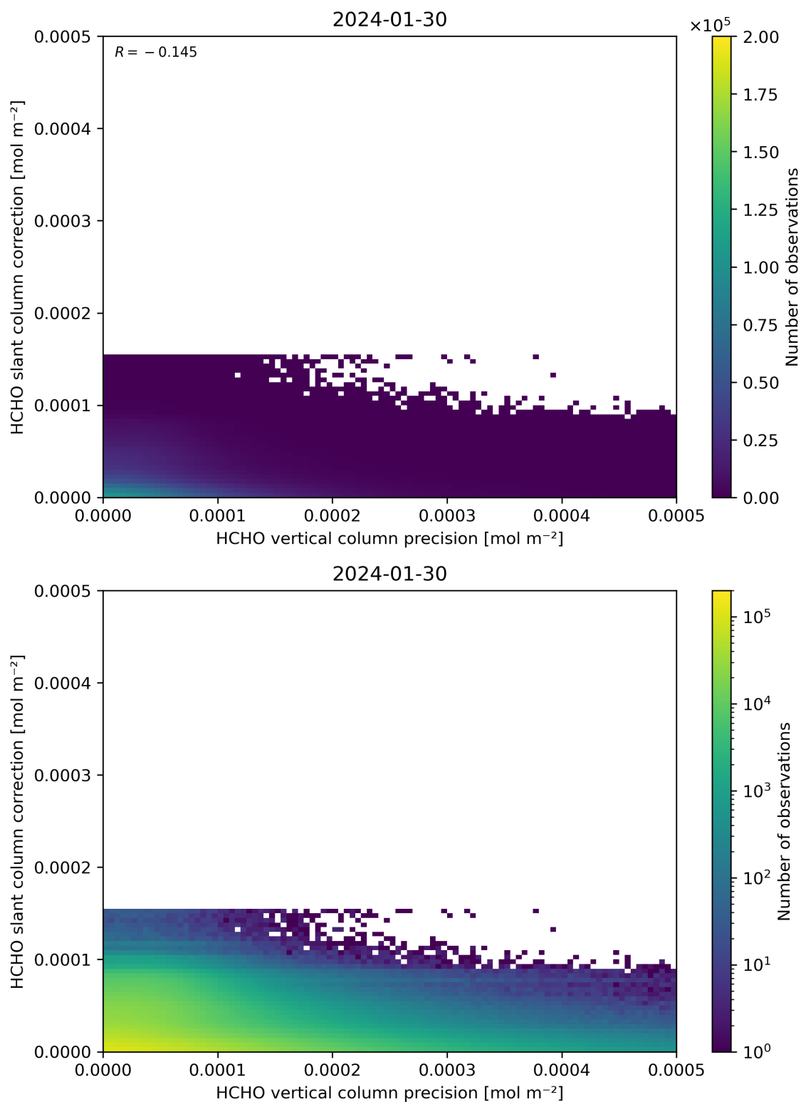
Figure 141: Scatter density plot of “HCHO vertical column precision” against “HCHO slant column correction” for 2024-01-29 to 2024-01-31.
