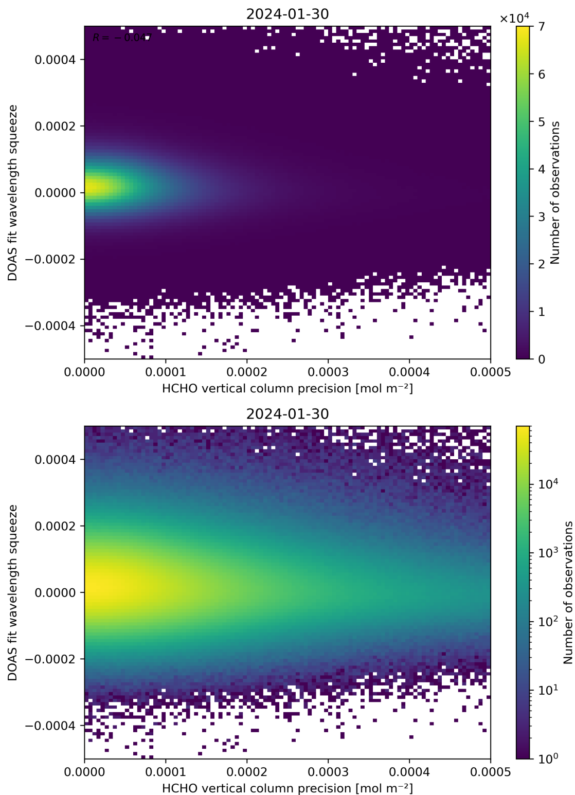
Figure 138: Scatter density plot of “HCHO vertical column precision” against “DOAS fit wavelength squeeze” for 2024-01-29 to 2024-01-31.
