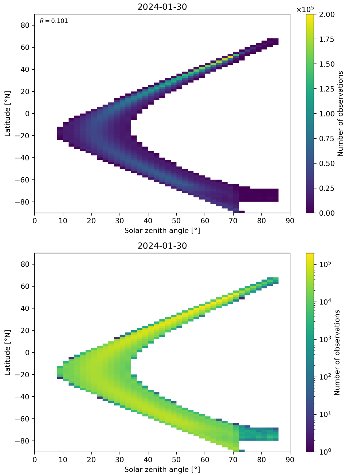
Figure 181: Scatter density plot of “Solar zenith angle” against “Latitude” for 2024-01-29 to 2024-01-31.
