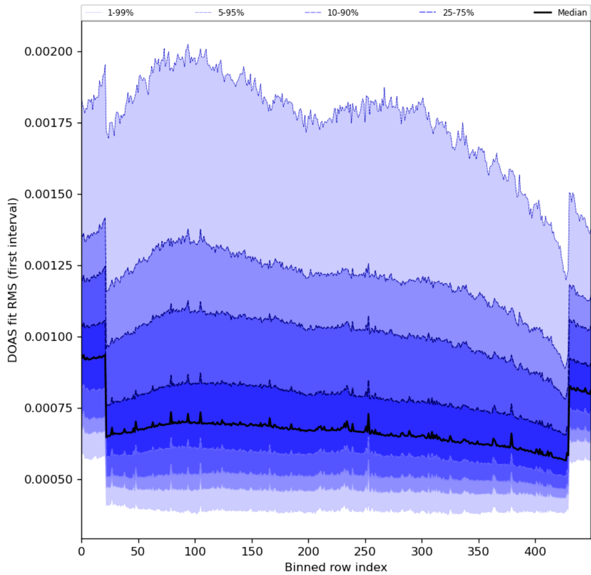
Figure 60: Along track statistics of “DOAS fit RMS (first interval)” for 2024-01-29 to 2024-01-31
