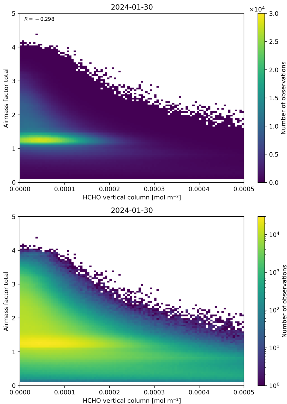
Figure 131: Scatter density plot of “HCHO vertical column” against “Airmass factor total” for 2024-01-29 to 2024-01-31.
