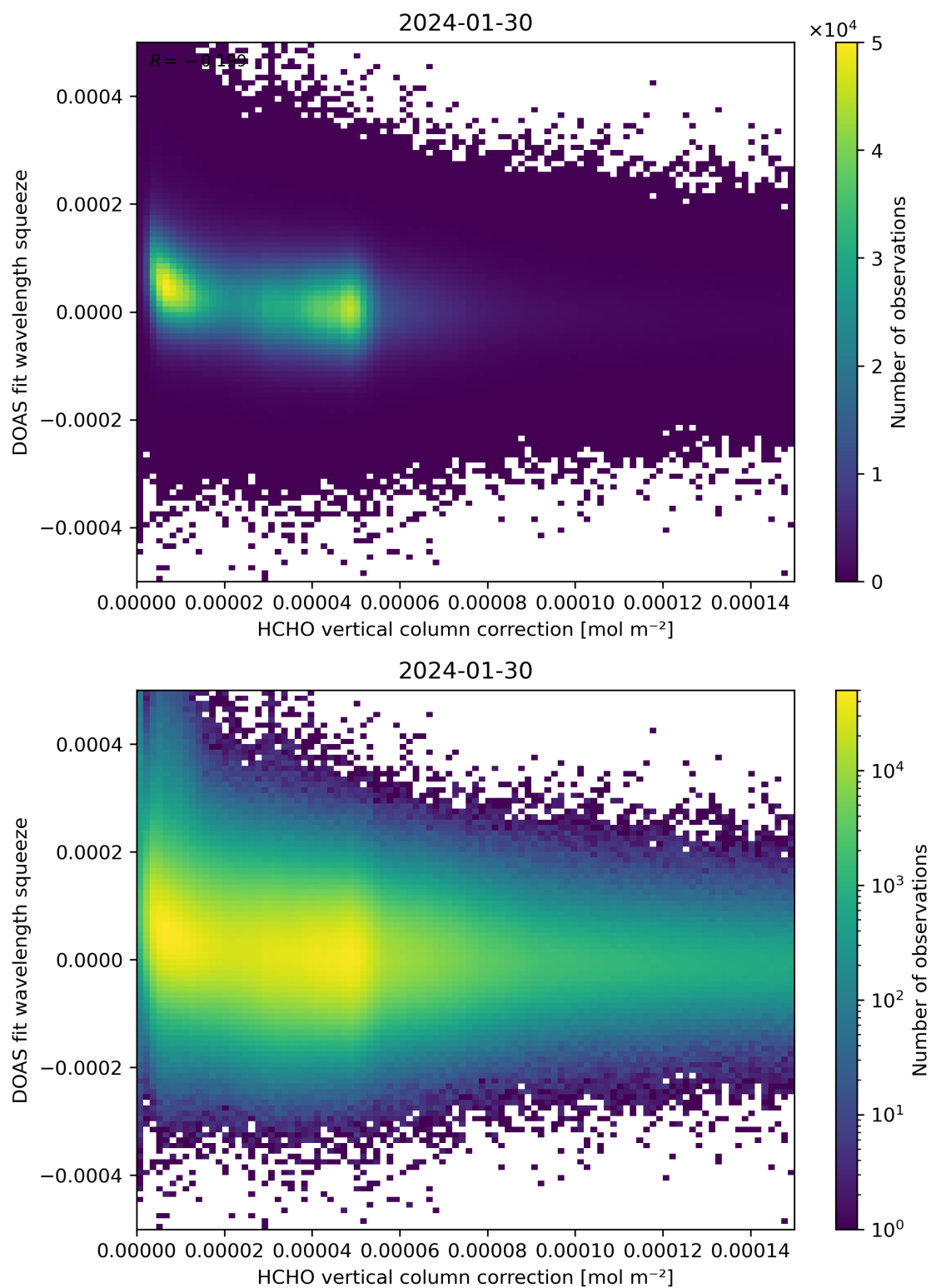
Figure 114: Scatter density plot of “HCHO vertical column correction” against “DOAS fit wavelength squeeze” for 2024-01-29 to 2024-01-31.
