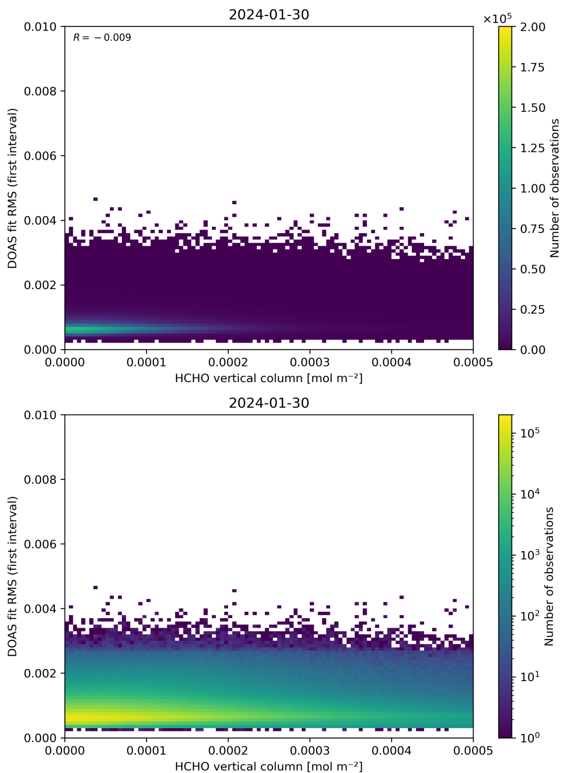
Figure 123: Scatter density plot of “HCHO vertical column” against “DOAS fit RMS (first interval)” for 2024-01-29 to 2024-01-31.
