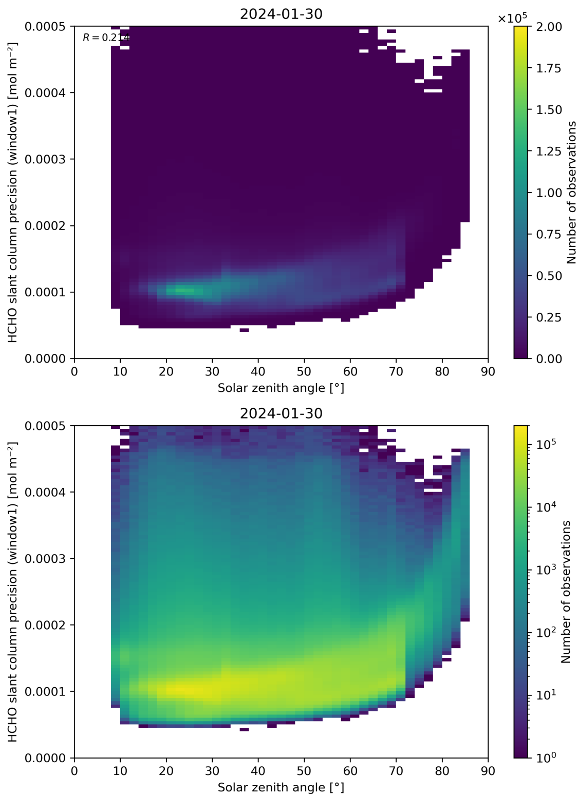
Figure 174: Scatter density plot of “Solar zenith angle” against “HCHO slant column precision (window1)” for 2024-01-29 to 2024-01-31.
