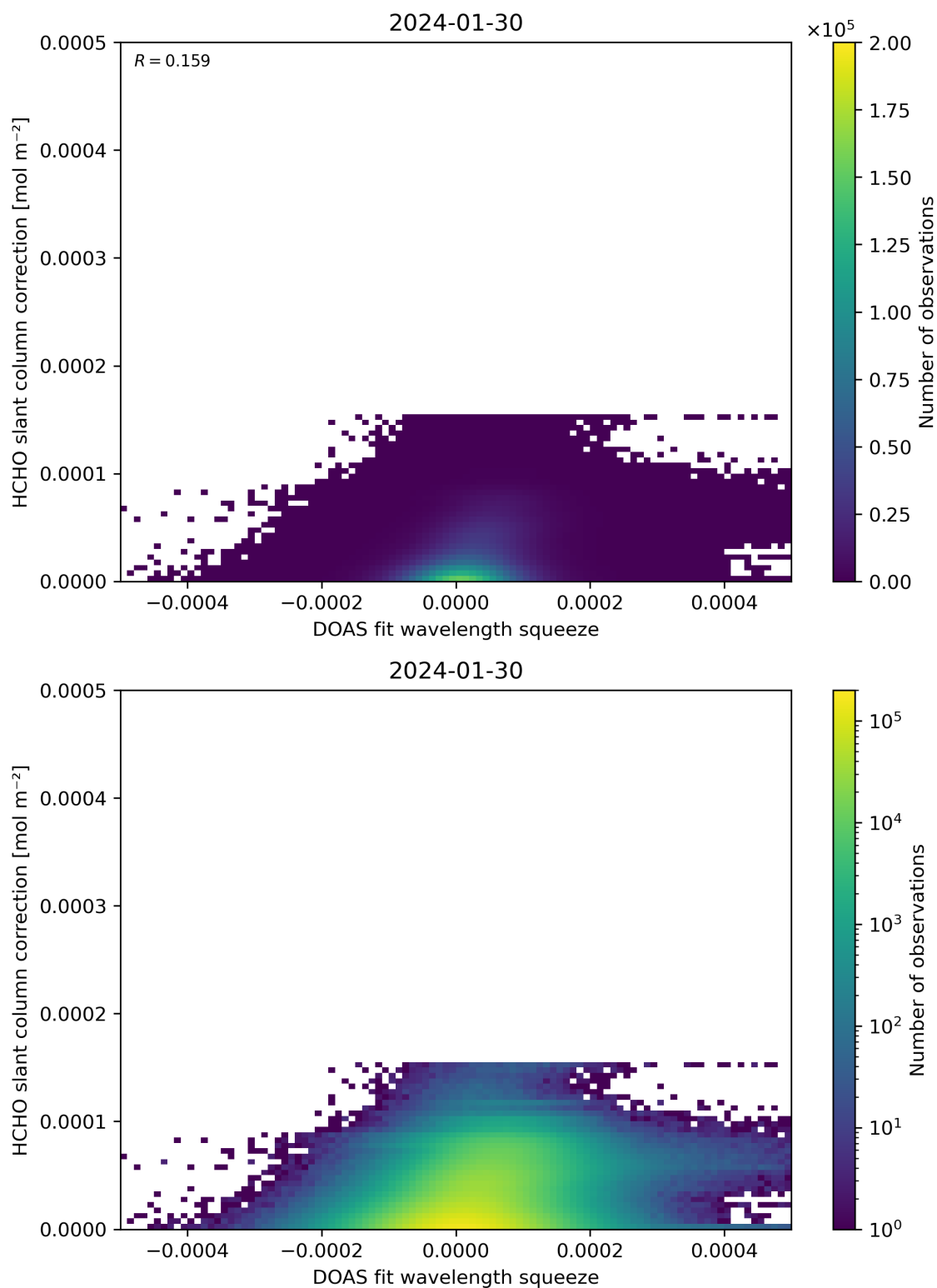
Figure 70: Scatter density plot of “DOAS fit wavelength squeeze” against “HCHO slant column correction” for 2024-01-29 to 2024-01-31.
