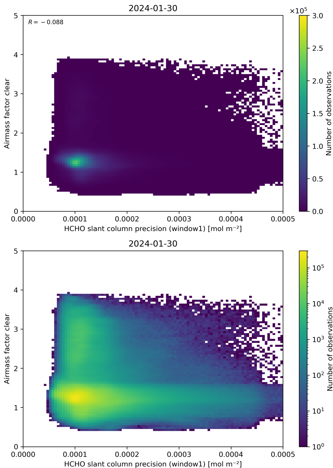
Figure 91: Scatter density plot of “HCHO slant column precision (window1)” against “Airmass factor clear” for 2024-01-29 to 2024-01-31.
