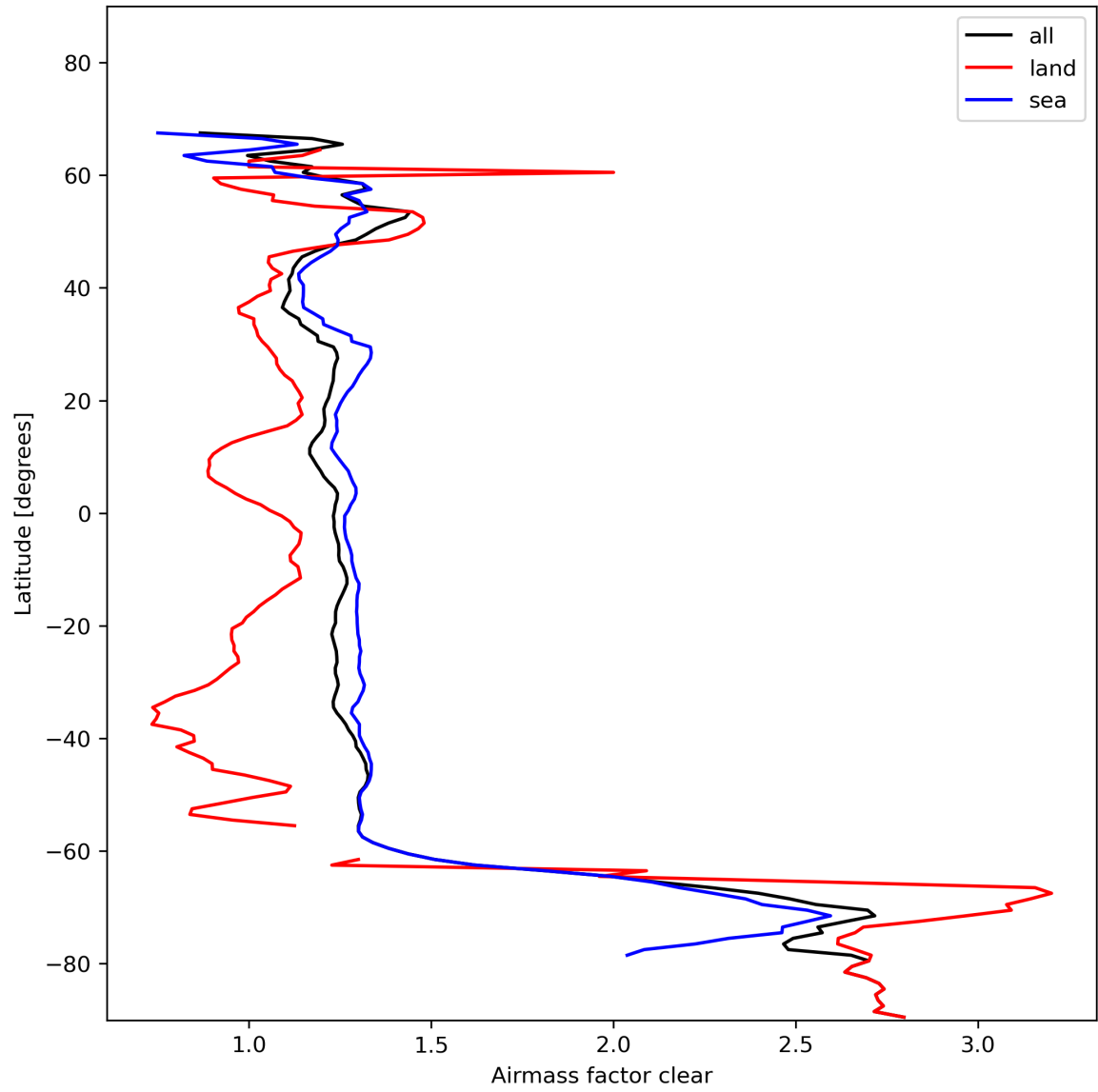
Figure 28: Zonal average of “Airmass factor clear” for 2024-01-29 to 2024-01-31.
