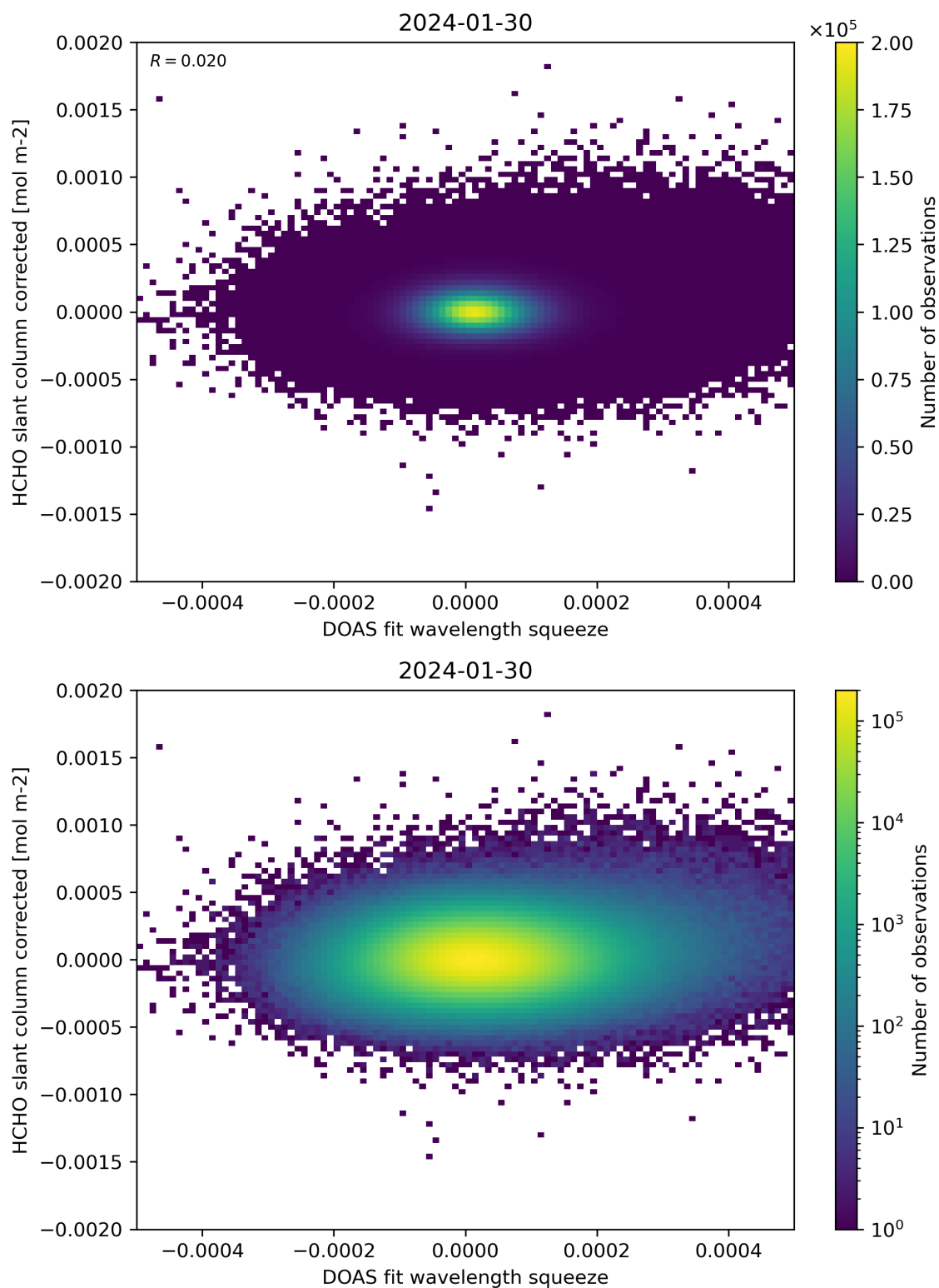
Figure 69: Scatter density plot of “DOAS fit wavelength squeeze” against “HCHO slant column corrected” for 2024-01-29 to 2024-01-31.
