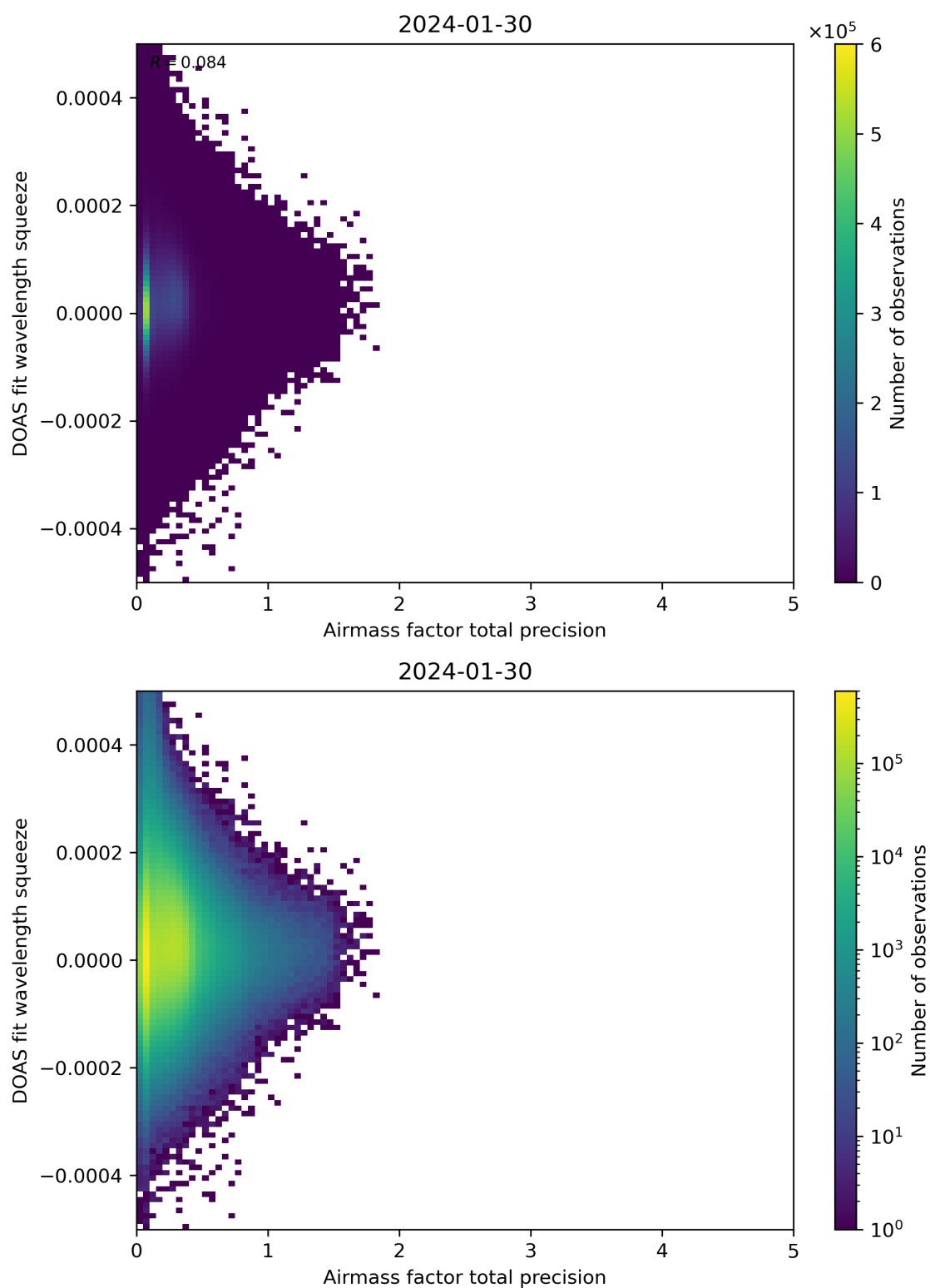
Figure 107: Scatter density plot of “Airmass factor total precision” against “DOAS fit wavelength squeeze” for 2024-01-29 to 2024-01-31.
