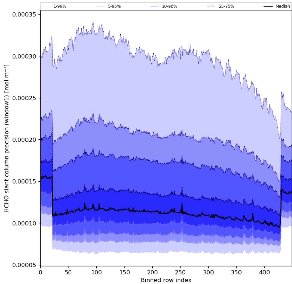
Figure 53: Along track statistics of “HCHO slant column precision (window1)” for 2024-01-29 to 2024-01-31
