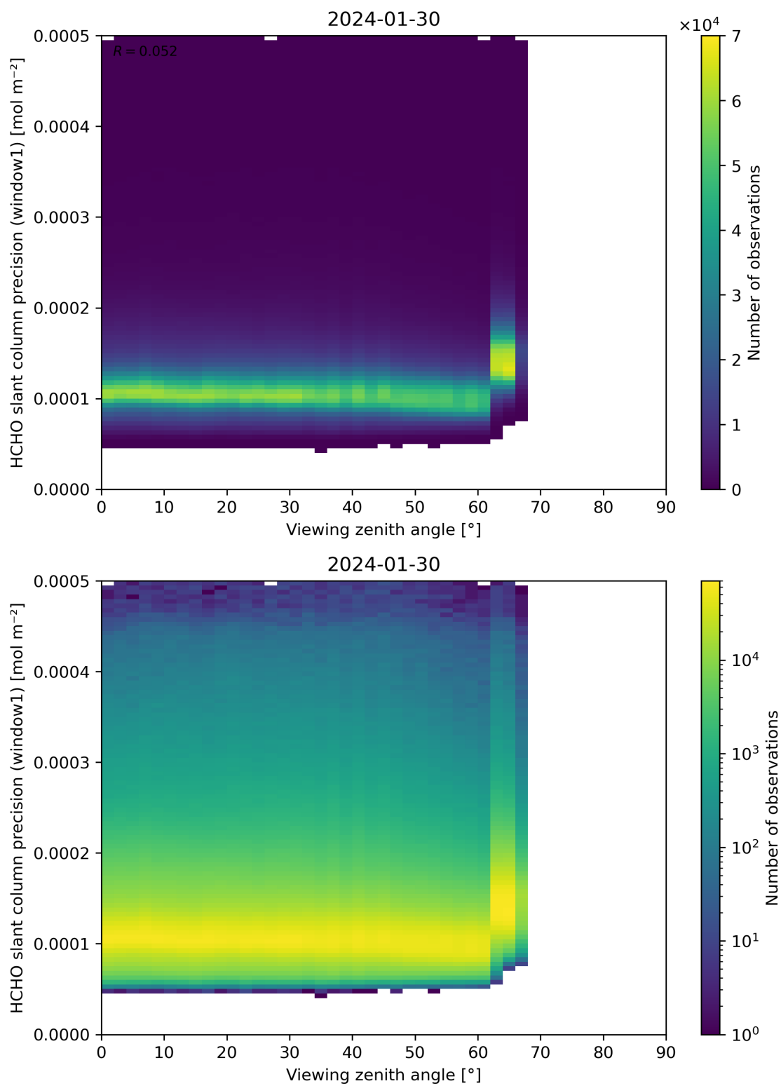
Figure 189: Scatter density plot of “Viewing zenith angle” against “HCHO slant column precision (window1)” for 2024-01-29 to 2024-01-31.
