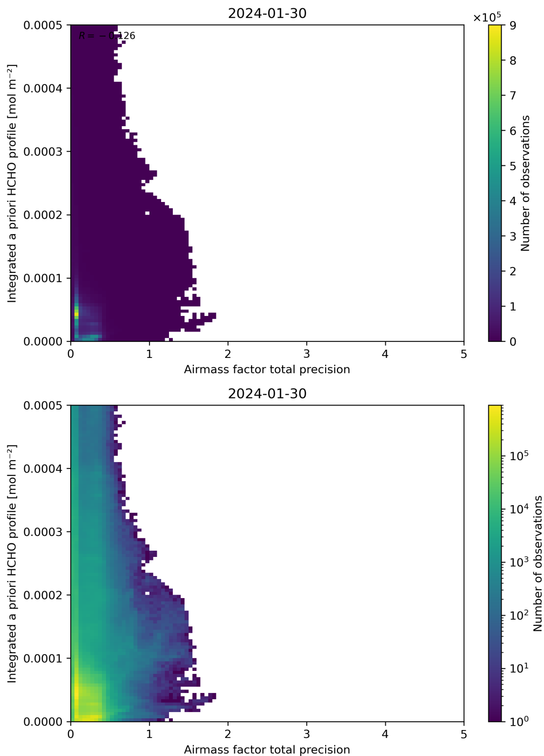
Figure 111: Scatter density plot of “Airmass factor total precision” against “Integrated a priori HCHO profile” for 2024-01-29 to 2024-01-31.
