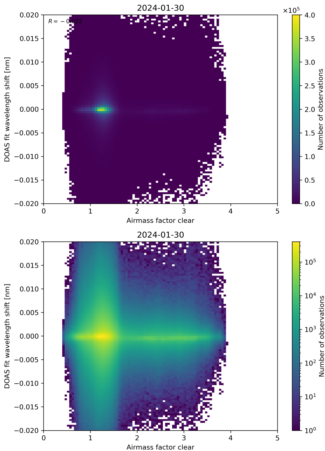
Figure 72: Scatter density plot of “Airmass factor clear” against “DOAS fit wavelength shift” for 2024-01-29 to 2024-01-31.
