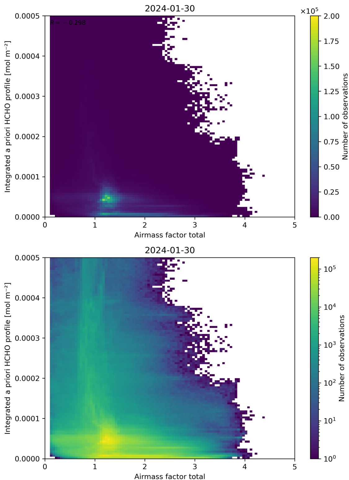
Figure 104: Scatter density plot of “Airmass factor total” against “Integrated a priori HCHO profile” for 2024-01-29 to 2024-01-31.
