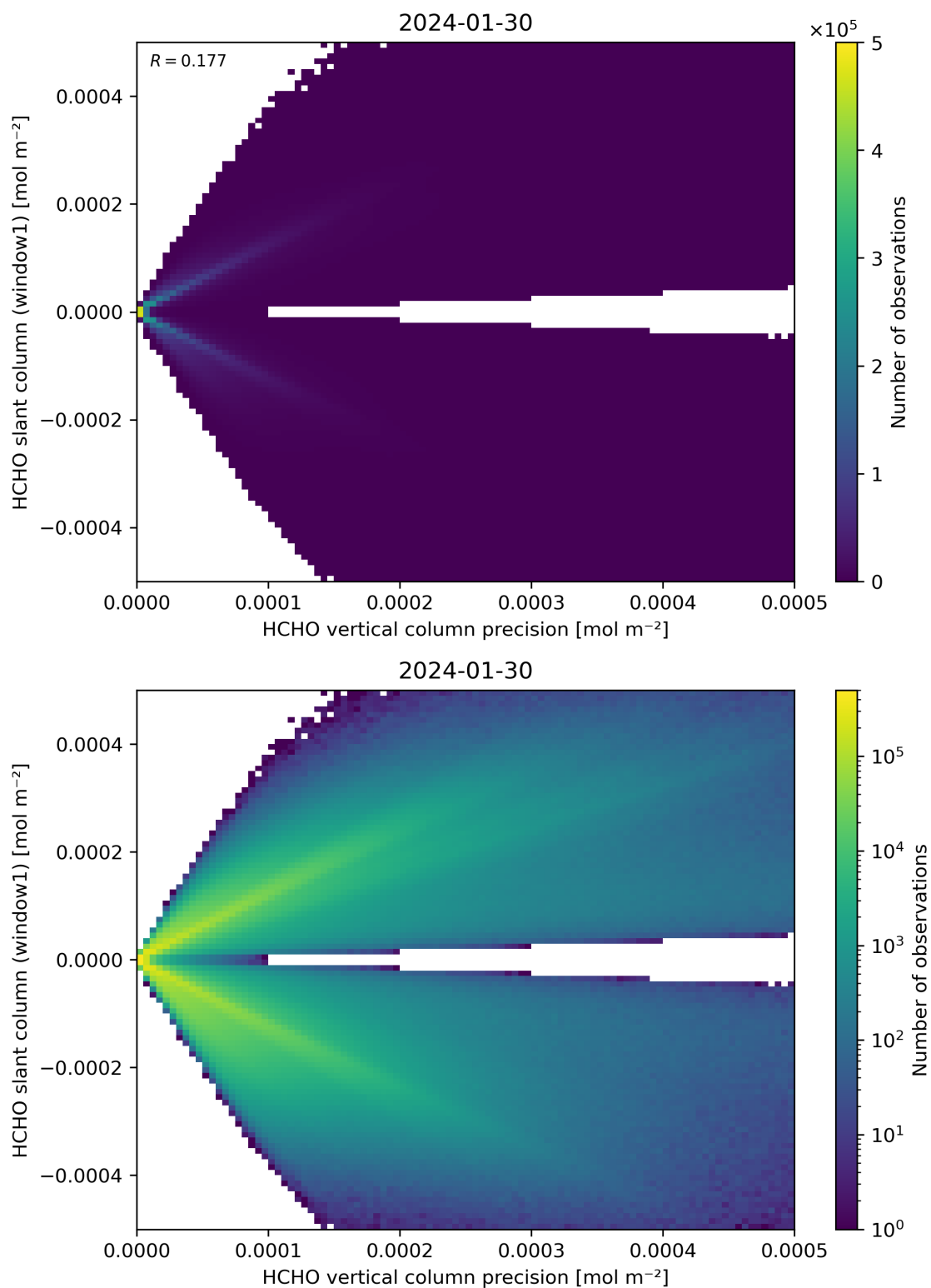
Figure 142: Scatter density plot of “HCHO vertical column precision” against “HCHO slant column (window1)” for 2024-01-29 to 2024-01-31.
