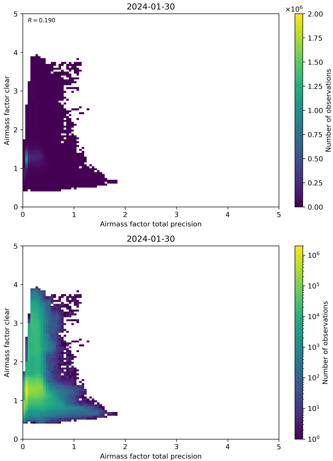
Figure 108: Scatter density plot of “Airmass factor total precision” against “Airmass factor clear” for 2024-01-29 to 2024-01-31.
