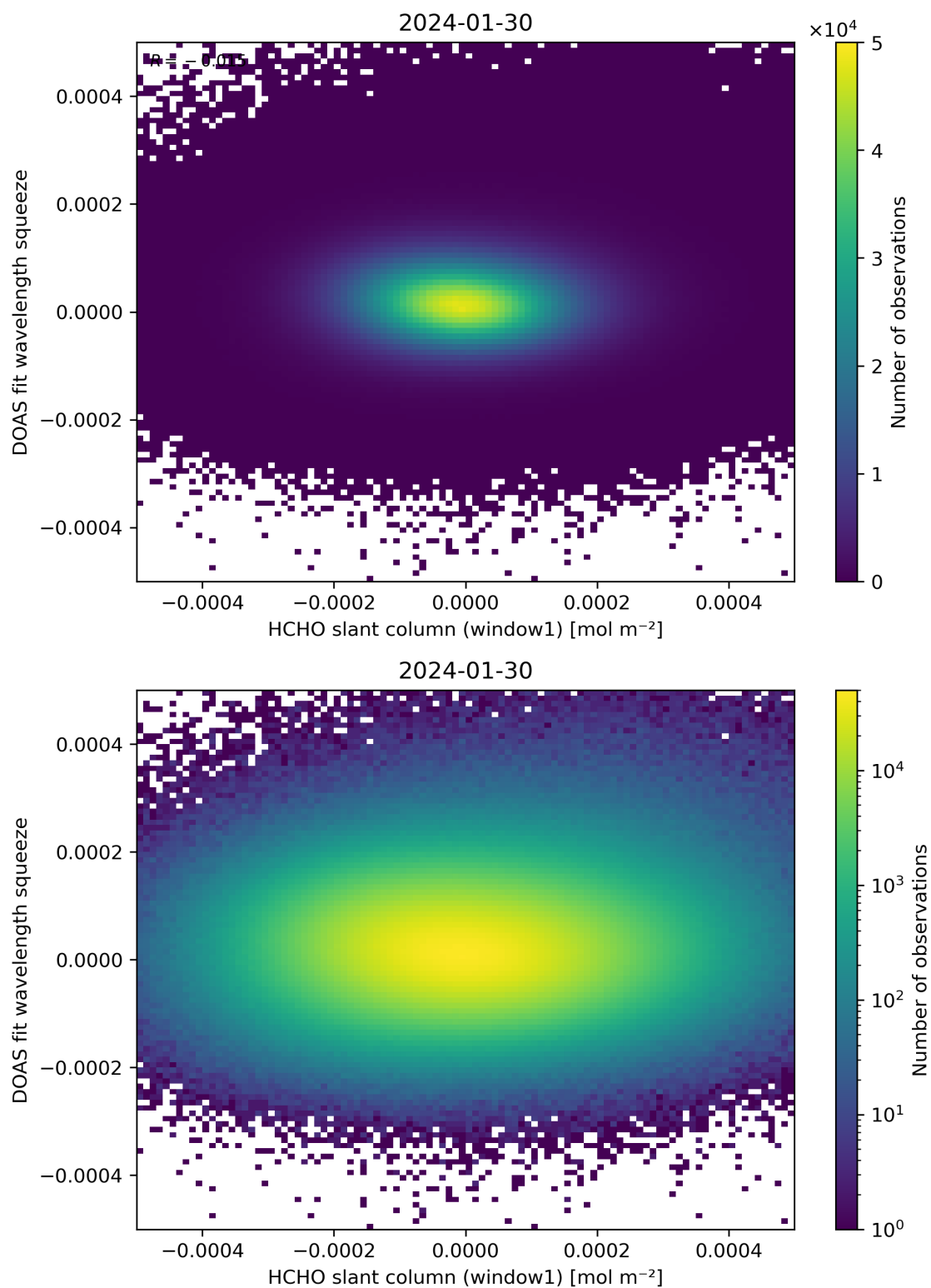
Figure 80: Scatter density plot of “HCHO slant column (window1)” against “DOAS fit wavelength squeeze” for 2024-01-29 to 2024-01-31.
