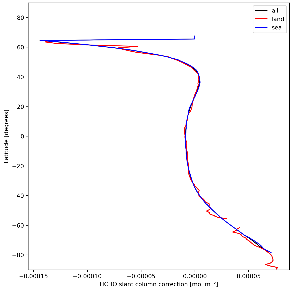
Figure 33: Zonal average of “HCHO slant column correction” for 2024-01-29 to 2024-01-31.
