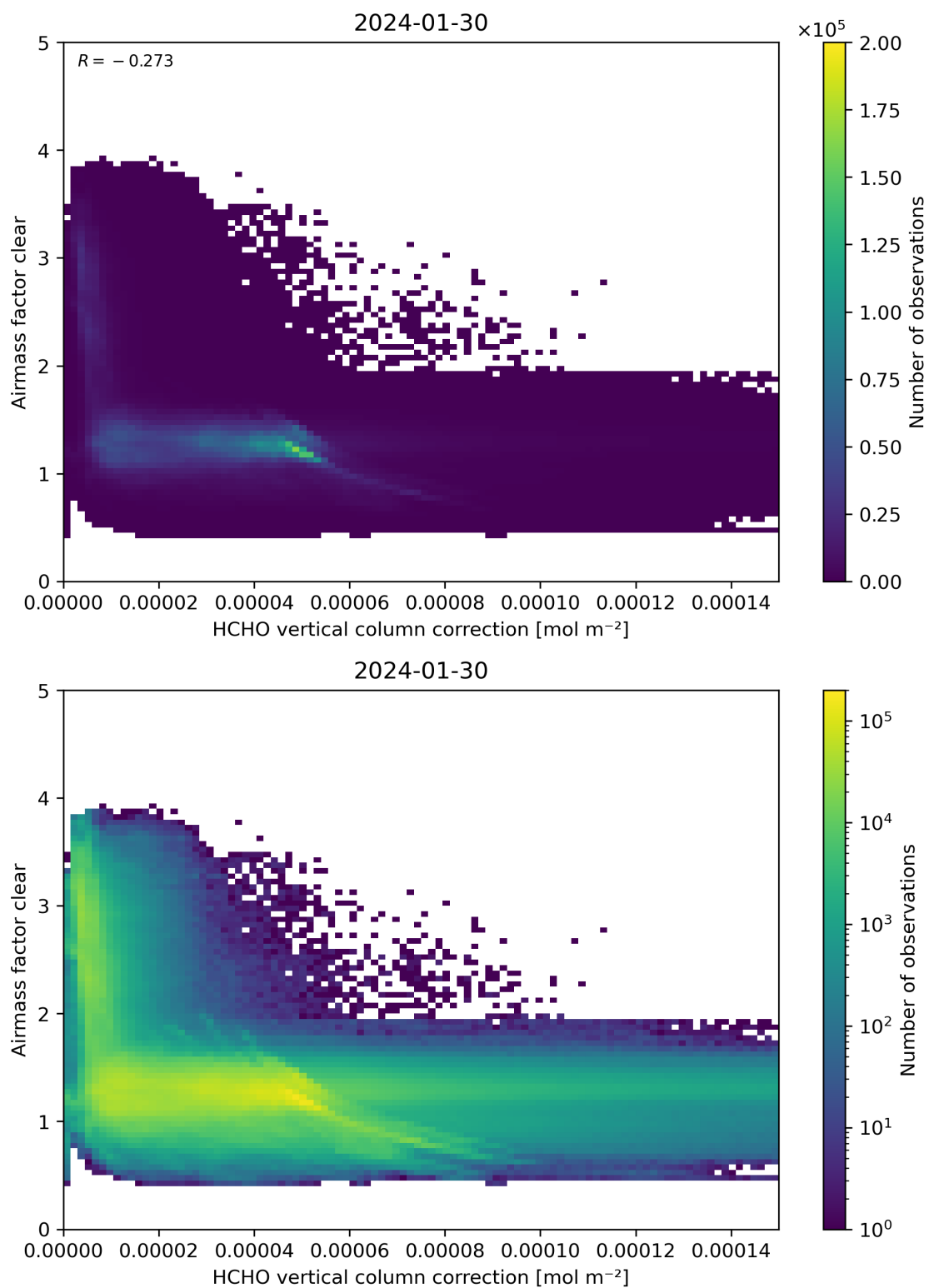
Figure 115: Scatter density plot of “HCHO vertical column correction” against “Airmass factor clear” for 2024-01-29 to 2024-01-31.
