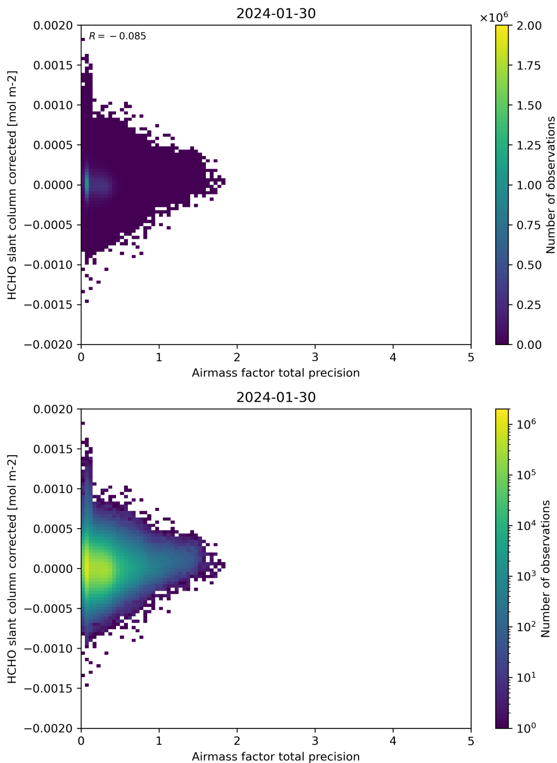
Figure 109: Scatter density plot of “Airmass factor total precision” against “HCHO slant column corrected” for 2024-01-29 to 2024-01-31.
