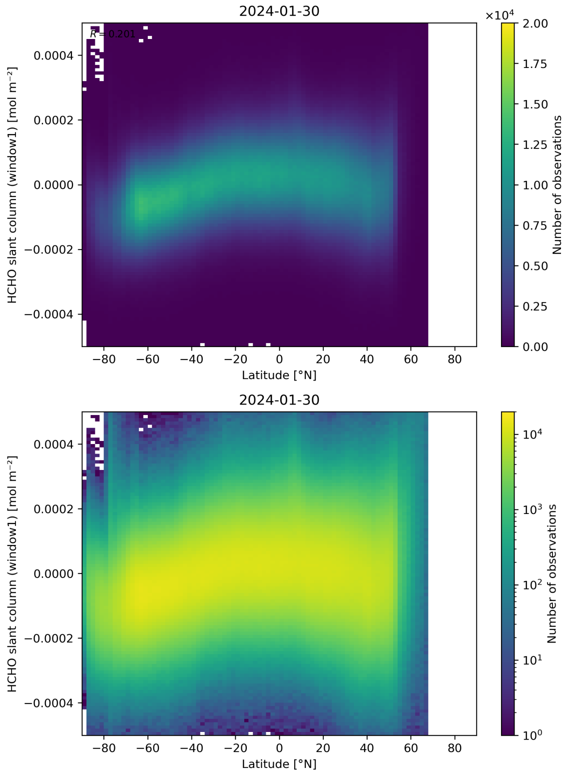
Figure 159: Scatter density plot of “Latitude” against “HCHO slant column (window1)” for 2024-01-29 to 2024-01-31.
