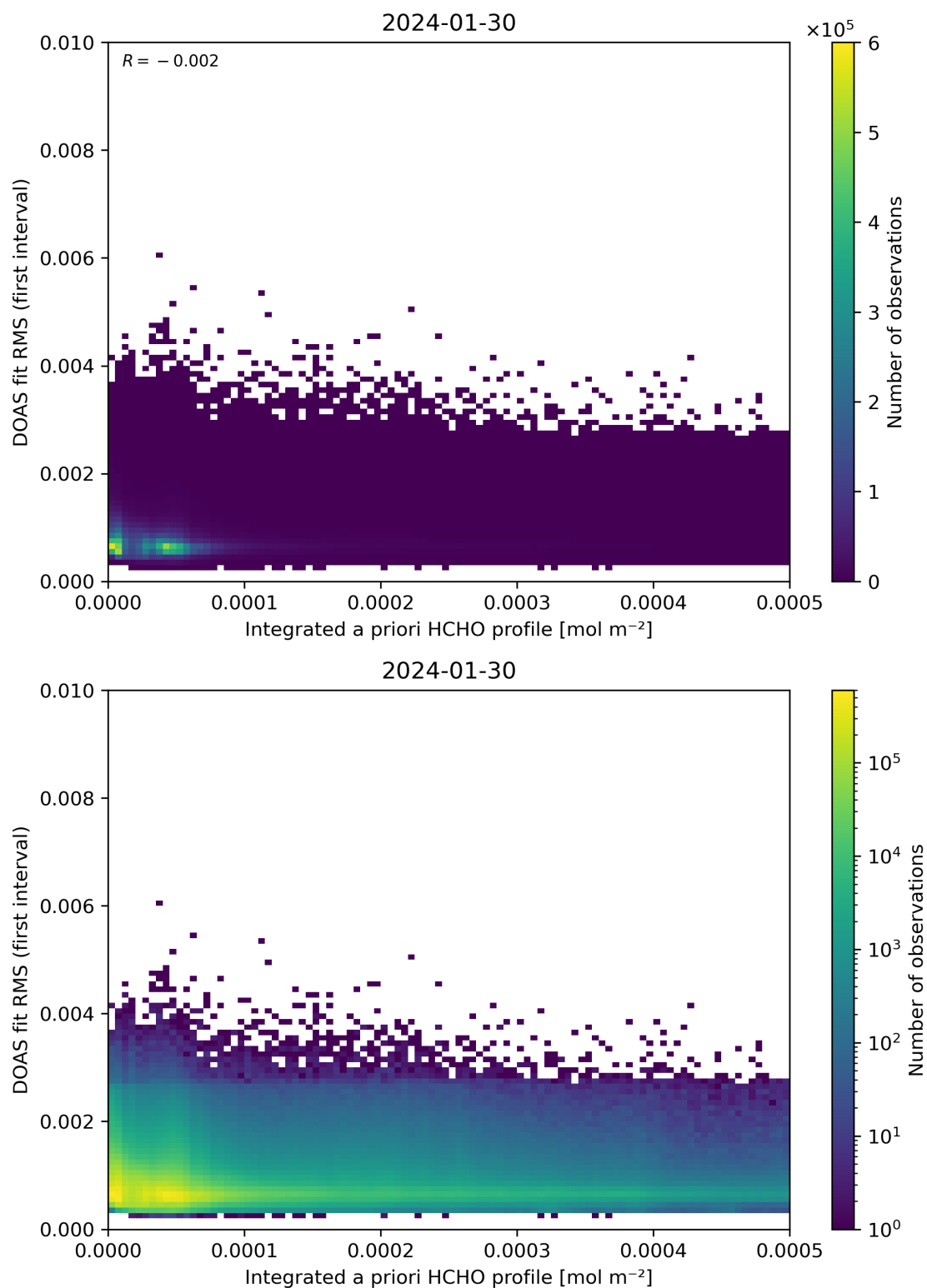
Figure 148: Scatter density plot of “Integrated a priori HCHO profile” against “DOAS fit RMS (first interval)” for 2024-01-29 to 2024-01-31.
