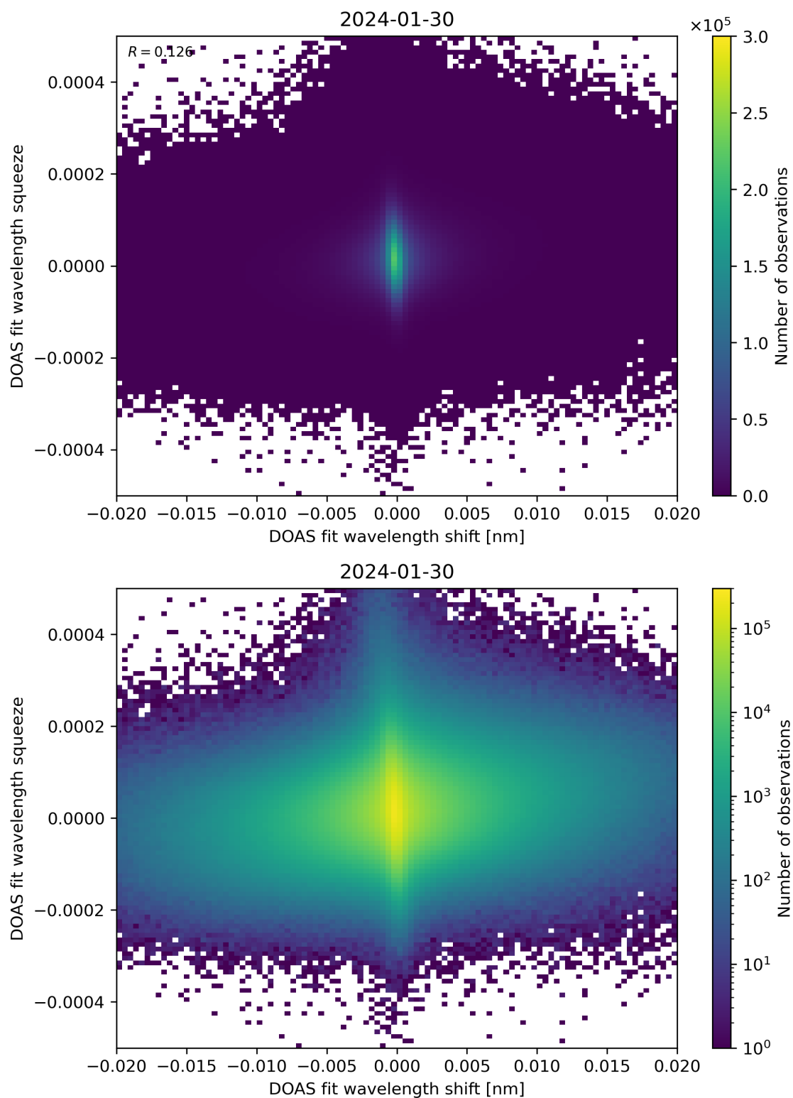
Figure 65: Scatter density plot of “DOAS fit wavelength shift” against “DOAS fit wavelength squeeze” for 2024-01-29 to 2024-01-31.
