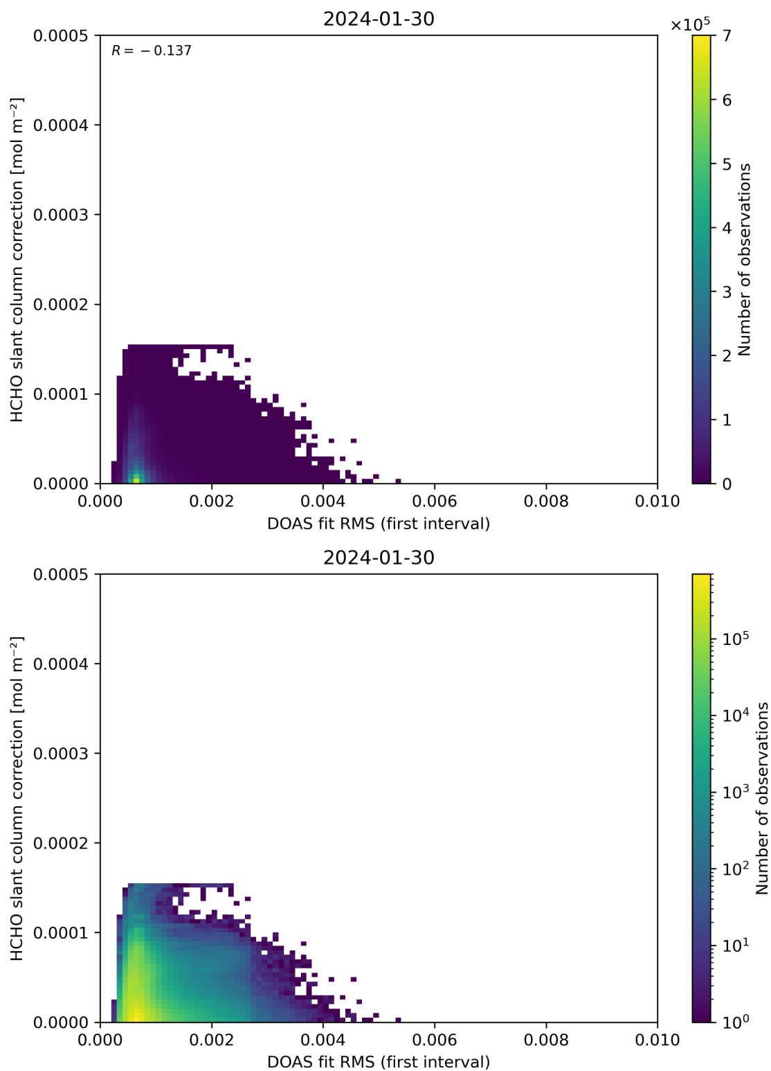
Figure 63: Scatter density plot of “DOAS fit RMS (first interval)” against “HCHO slant column correction” for 2024-01-29 to 2024-01-31.
