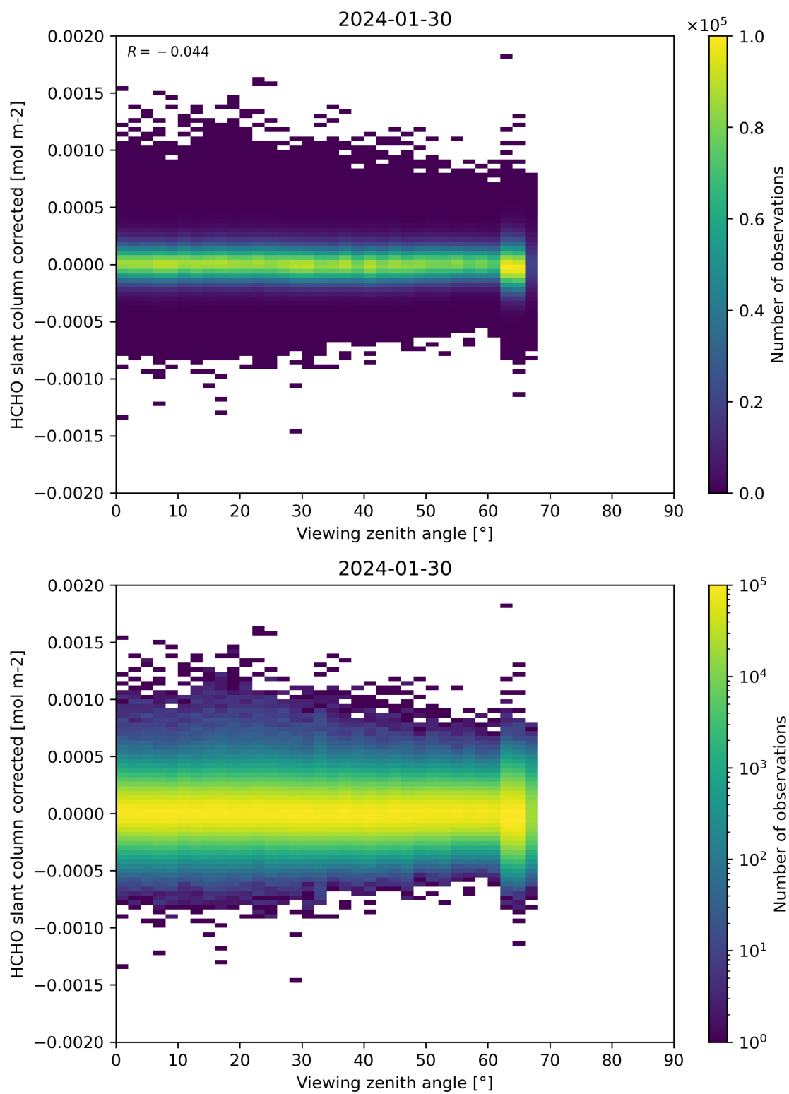
Figure 186: Scatter density plot of “Viewing zenith angle” against “HCHO slant column corrected” for 2024-01-29 to 2024-01-31.
