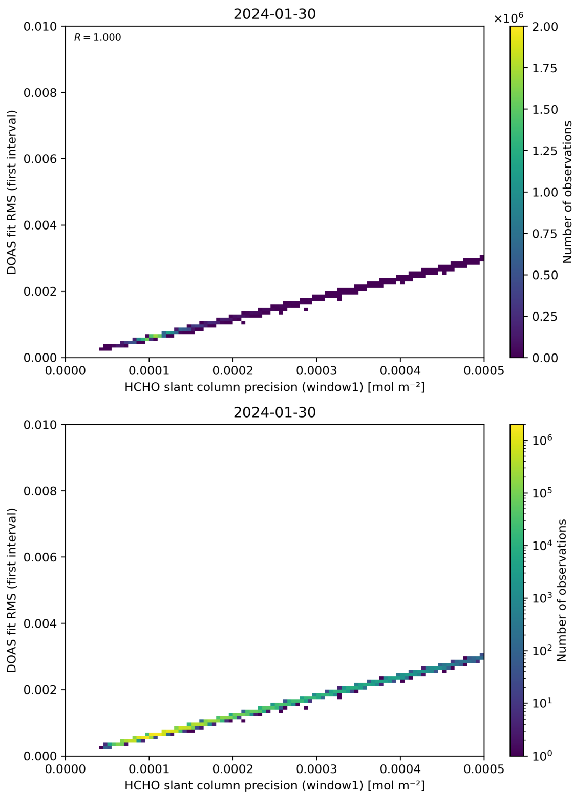
Figure 88: Scatter density plot of “HCHO slant column precision (window1)” against “DOAS fit RMS (first interval)” for 2024-01-29 to 2024-01-31.
