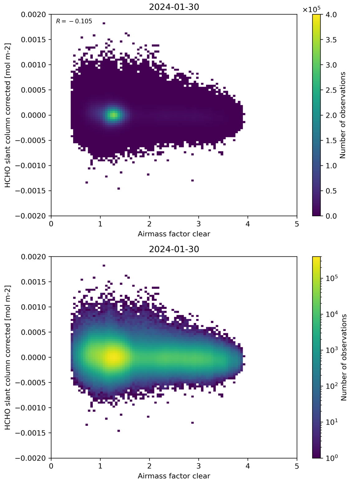
Figure 74: Scatter density plot of “Airmass factor clear” against “HCHO slant column corrected” for 2024-01-29 to 2024-01-31.
