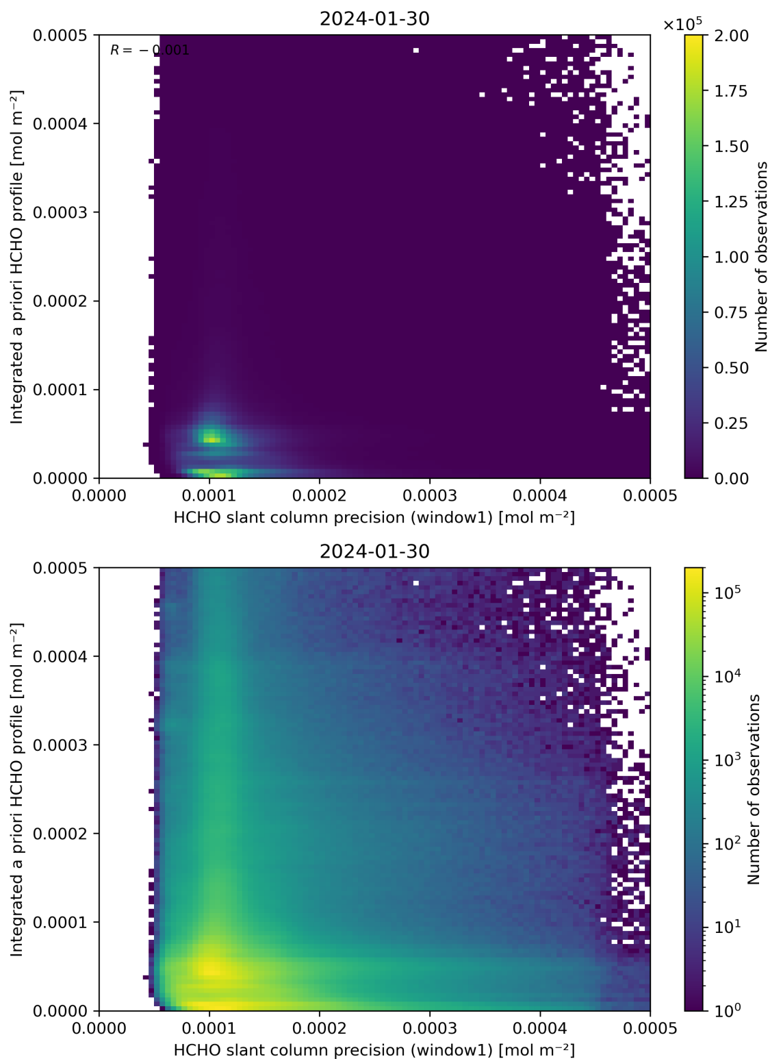
Figure 96: Scatter density plot of “HCHO slant column precision (window1)” against “Integrated a priori HCHO profile” for 2024-01-29 to 2024-01-31.
