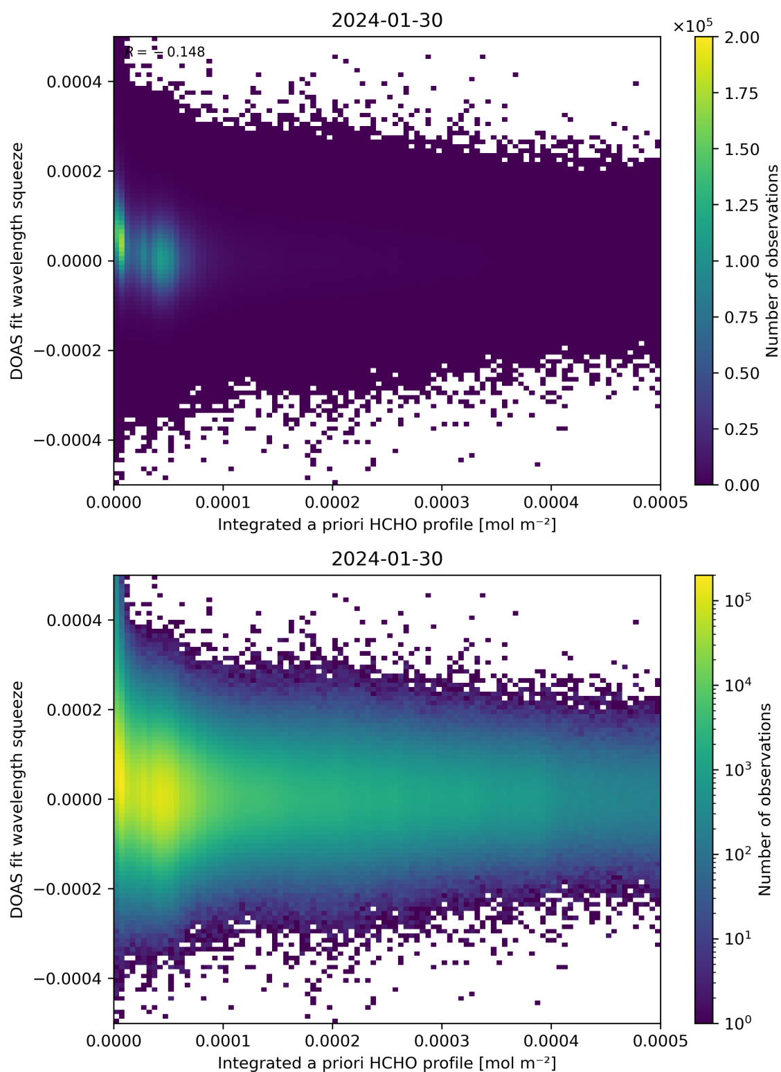
Figure 150: Scatter density plot of “Integrated a priori HCHO profile” against “DOAS fit wavelength squeeze” for 2024-01-29 to 2024-01-31.
