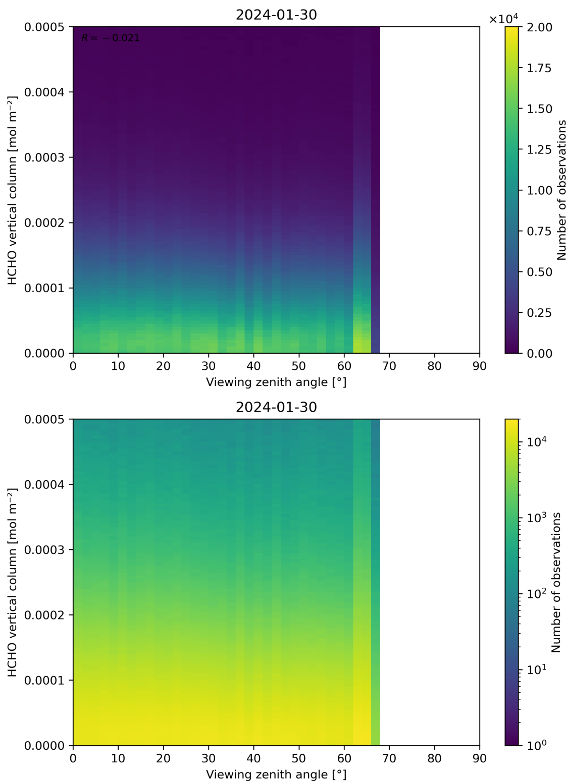
Figure 192: Scatter density plot of “Viewing zenith angle” against “HCHO vertical column” for 2024-01-29 to 2024-01-31.
