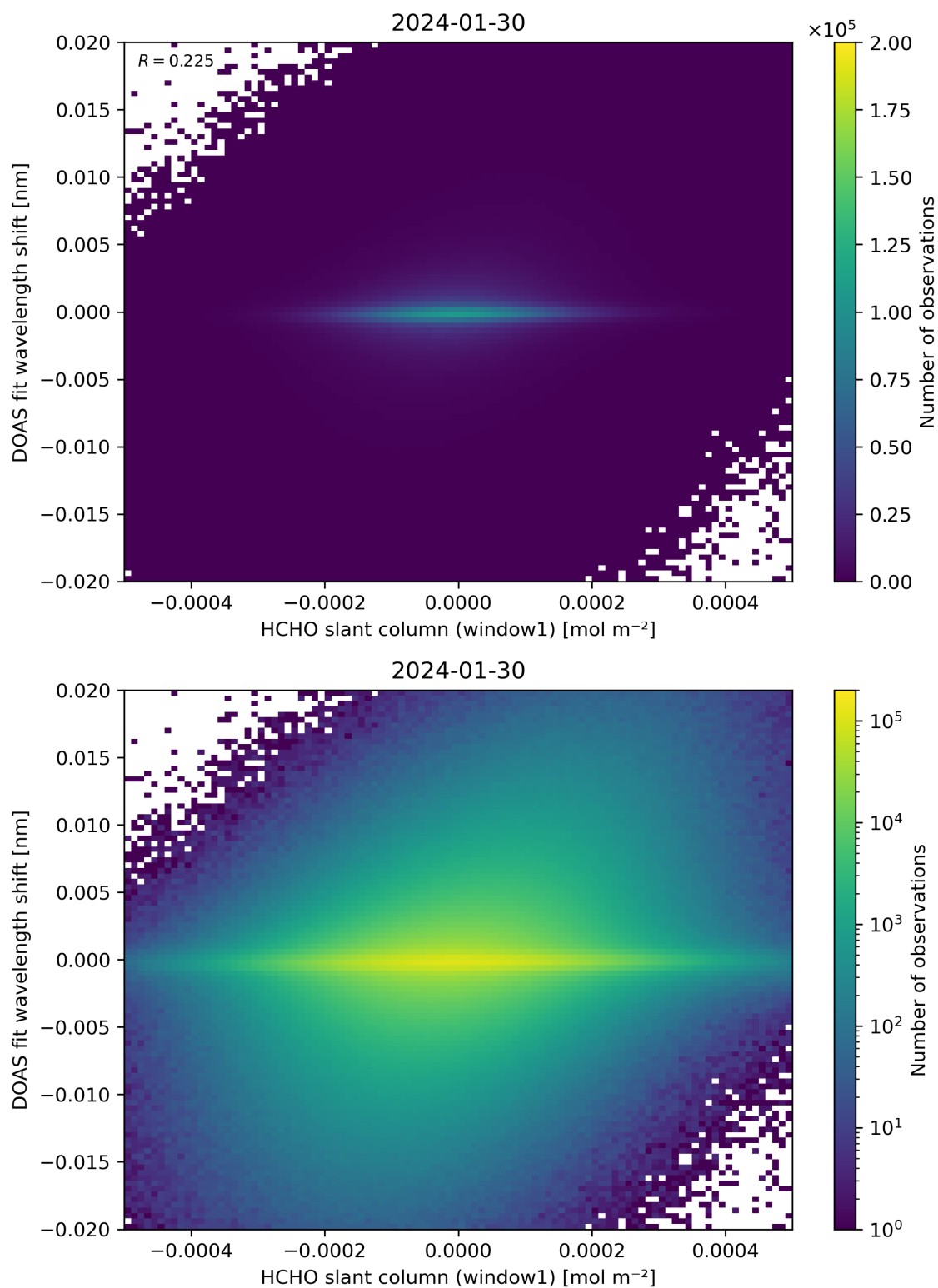
Figure 79: Scatter density plot of “HCHO slant column (window1)” against “DOAS fit wavelength shift” for 2024-01-29 to 2024-01-31.
