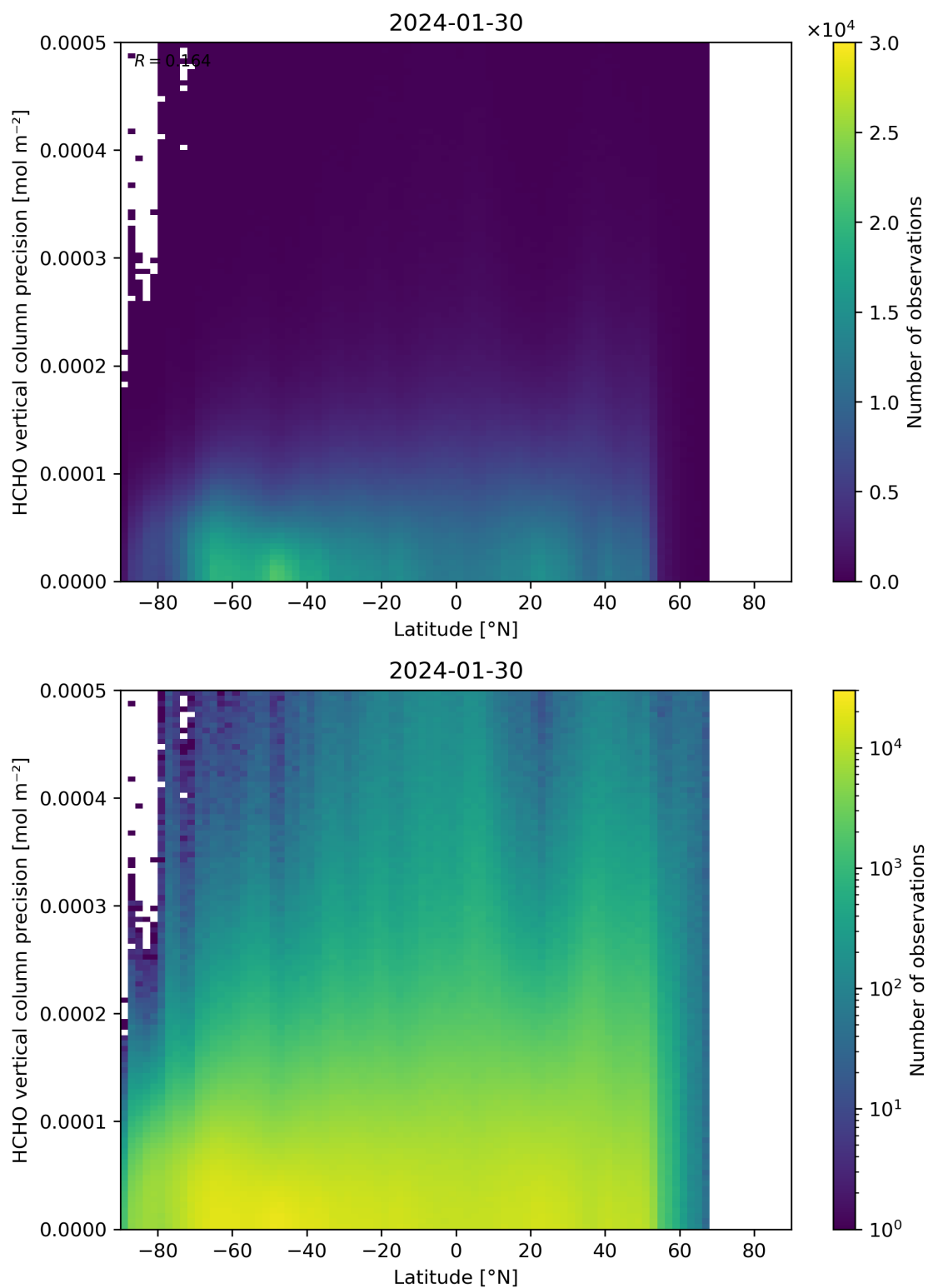
Figure 165: Scatter density plot of “Latitude” against “HCHO vertical column precision” for 2024-01-29 to 2024-01-31.
