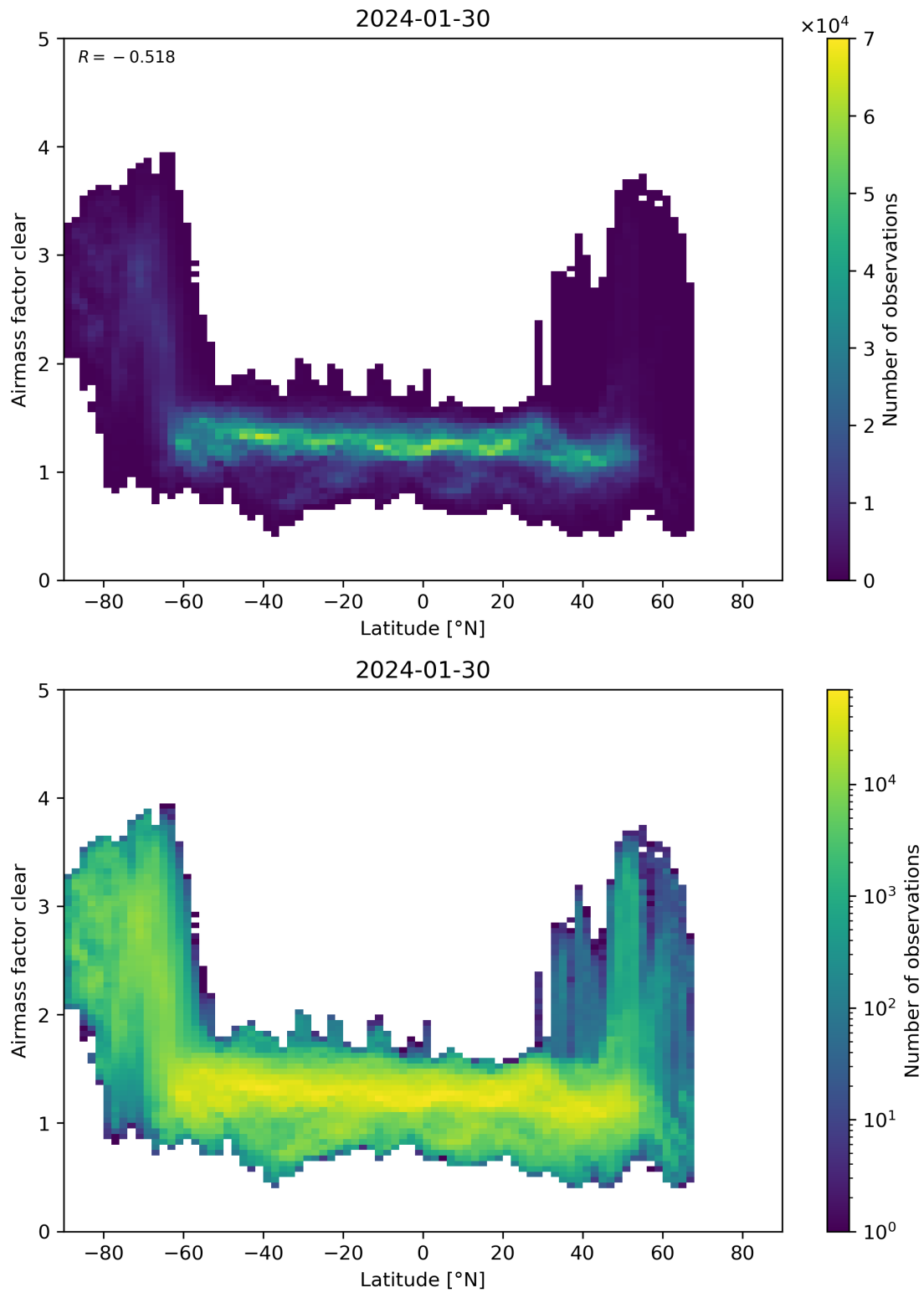
Figure 156: Scatter density plot of “Latitude” against “Airmass factor clear” for 2024-01-29 to 2024-01-31.
