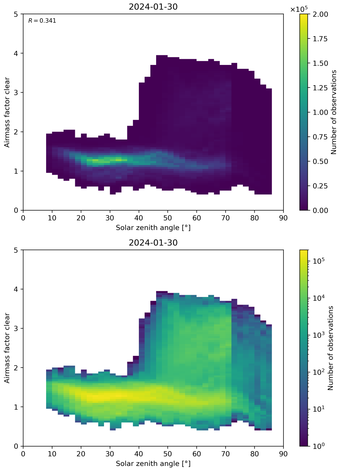
Figure 170: Scatter density plot of “Solar zenith angle” against “Airmass factor clear” for 2024-01-29 to 2024-01-31.
