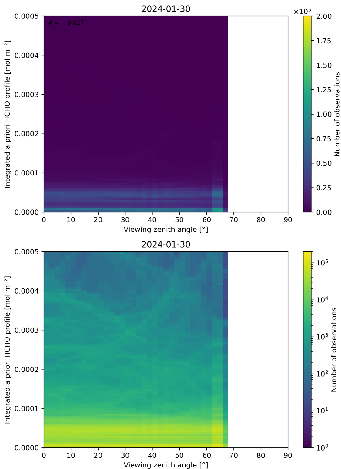
Figure 195: Scatter density plot of “Viewing zenith angle” against “Integrated a priori HCHO profile” for 2024-01-29 to 2024-01-31.
