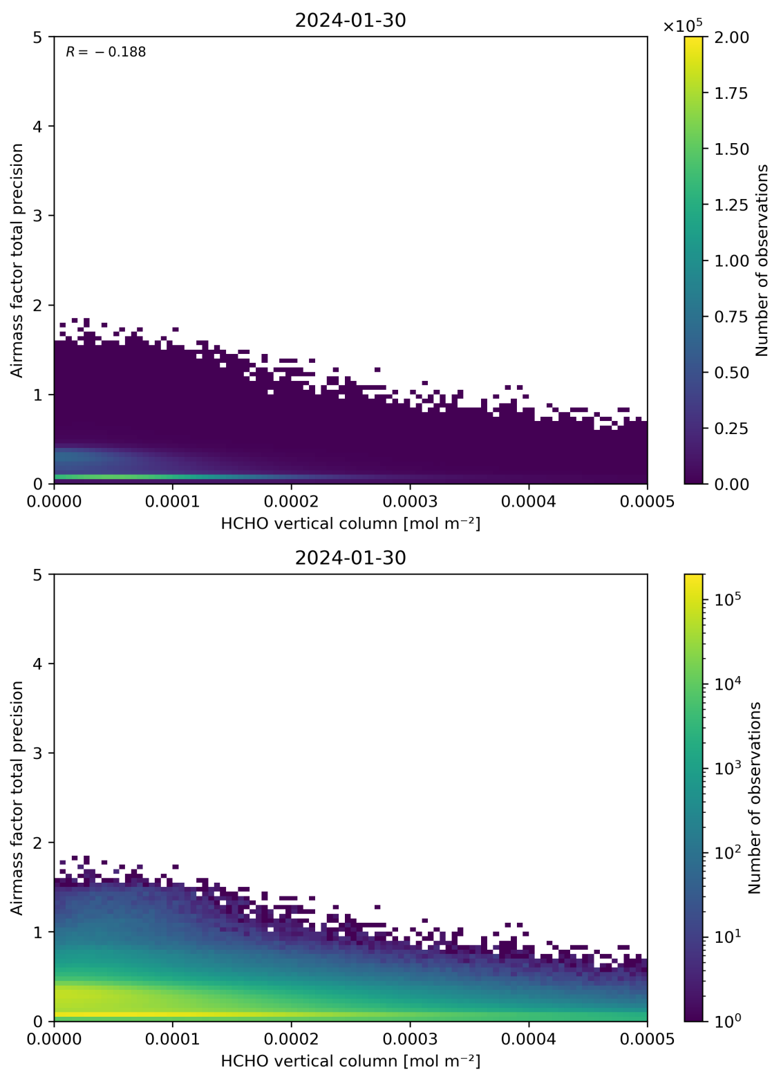
Figure 132: Scatter density plot of “HCHO vertical column” against “Airmass factor total precision” for 2024-01-29 to 2024-01-31.
