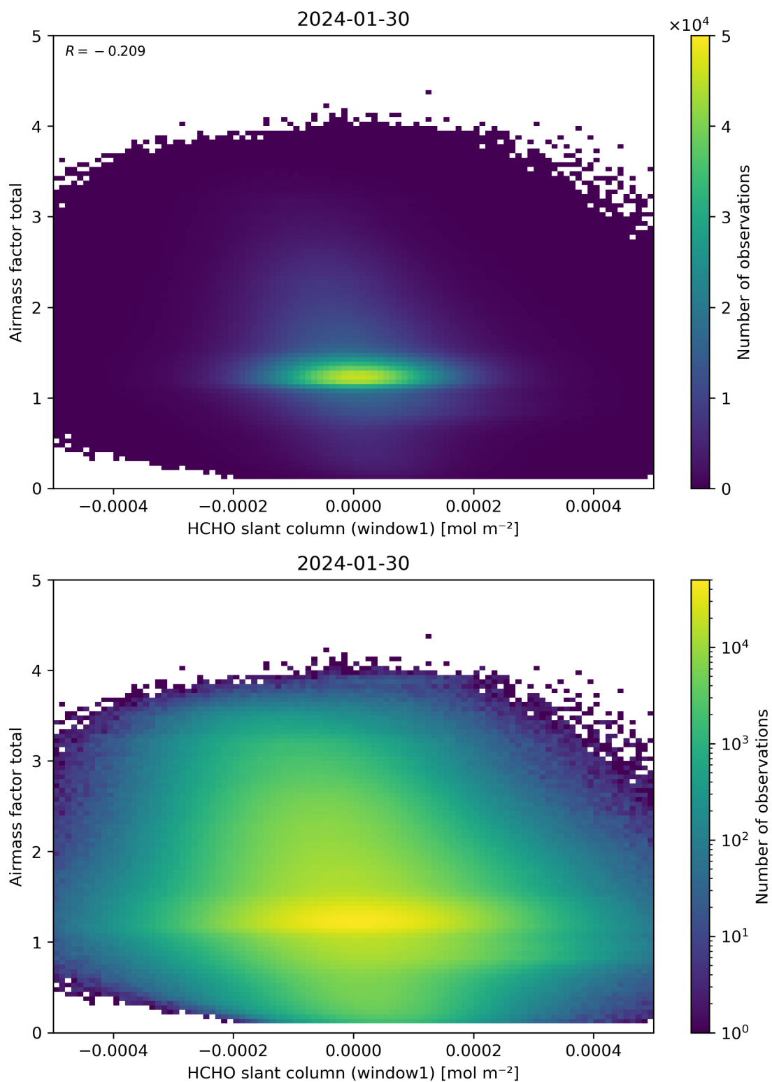
Figure 85: Scatter density plot of “HCHO slant column (window1)” against “Airmass factor total” for 2024-01-29 to 2024-01-31.
