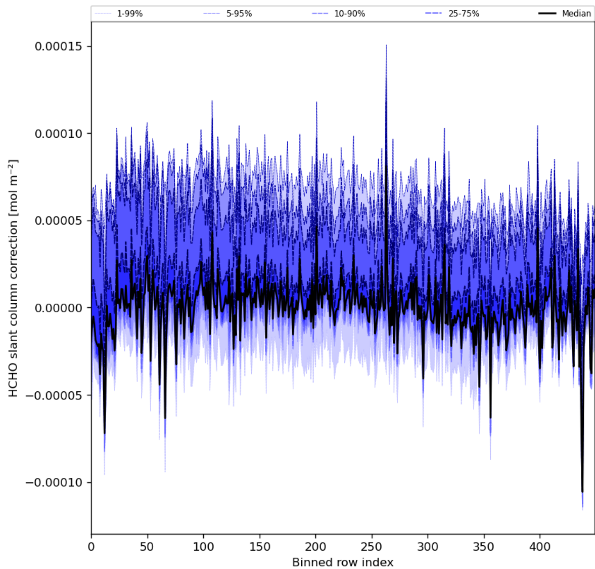
Figure 61: Along track statistics of “HCHO slant column correction” for 2024-01-29 to 2024-01-31
