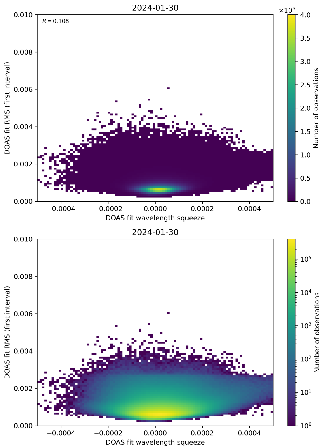
Figure 68: Scatter density plot of “DOAS fit wavelength squeeze” against “DOAS fit RMS (first interval)” for 2024-01-29 to 2024-01-31.
