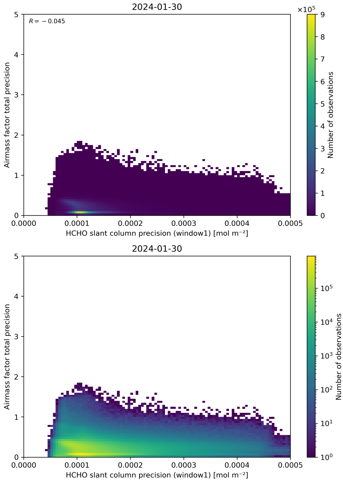
Figure 95: Scatter density plot of “HCHO slant column precision (window1)” against “Airmass factor total precision” for 2024-01-29 to 2024-01-31.
