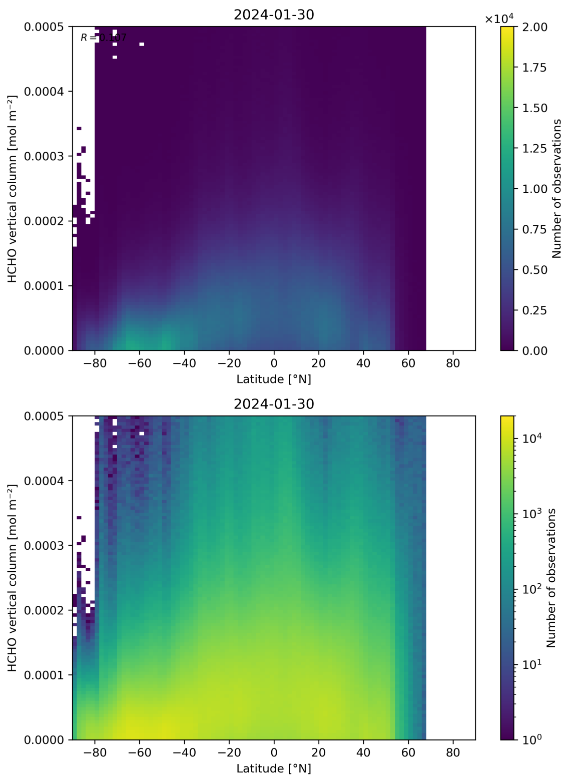
Figure 163: Scatter density plot of “Latitude” against “HCHO vertical column” for 2024-01-29 to 2024-01-31.
