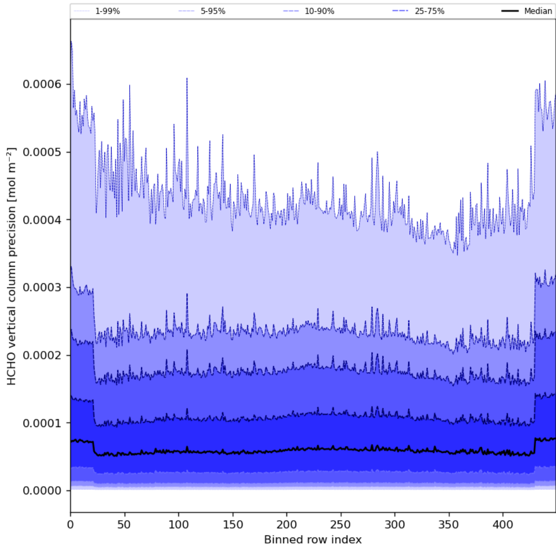
Figure 50: Along track statistics of “HCHO vertical column precision” for 2024-01-29 to 2024-01-31
