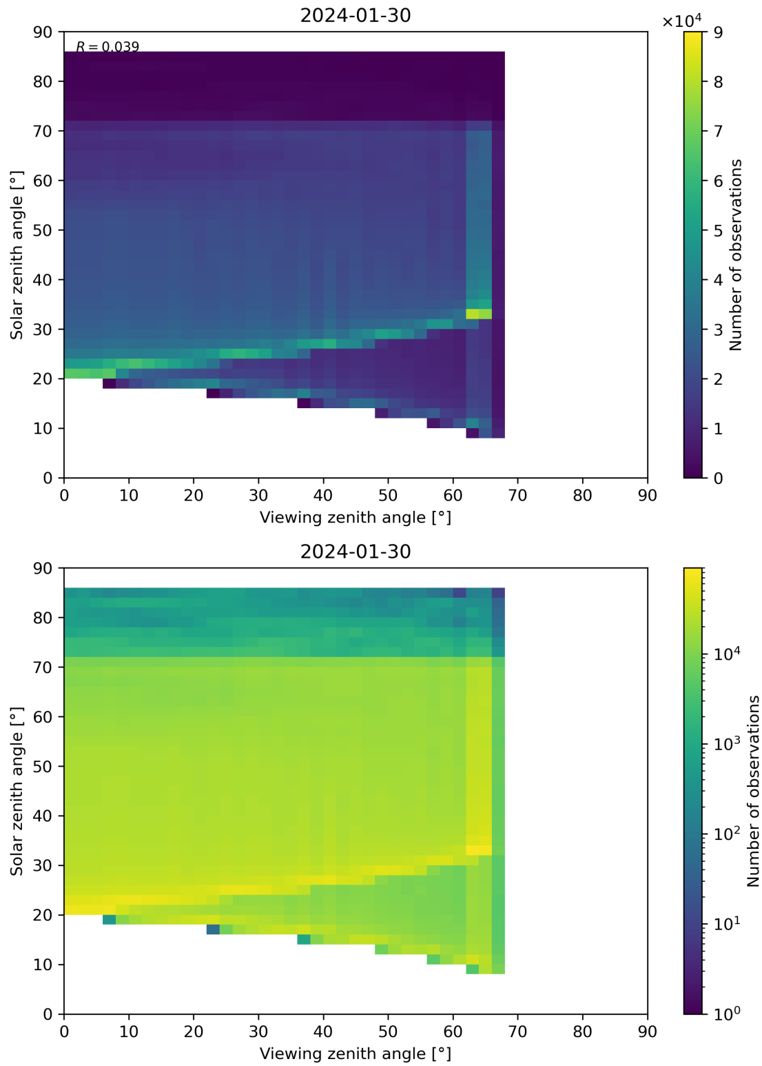
Figure 197: Scatter density plot of “Viewing zenith angle” against “Solar zenith angle” for 2024-01-29 to 2024-01-31.
