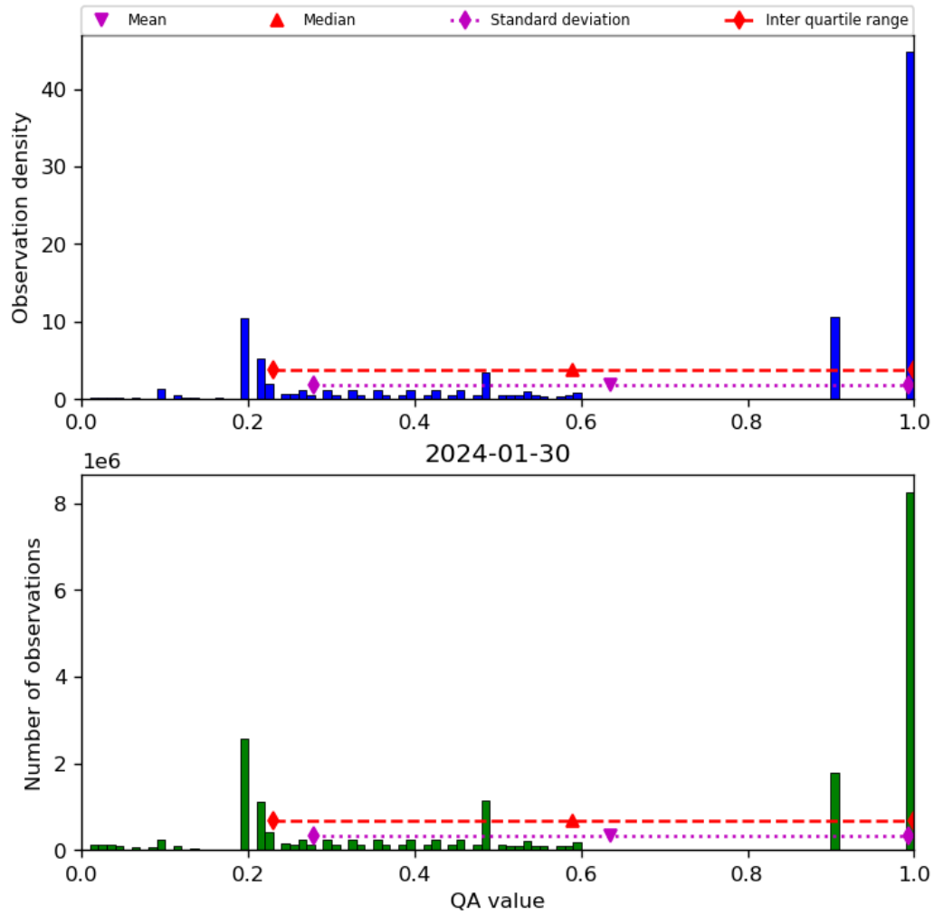
Figure 34: Histogram of “QA value” for 2024-01-29 to 2024-01-31
