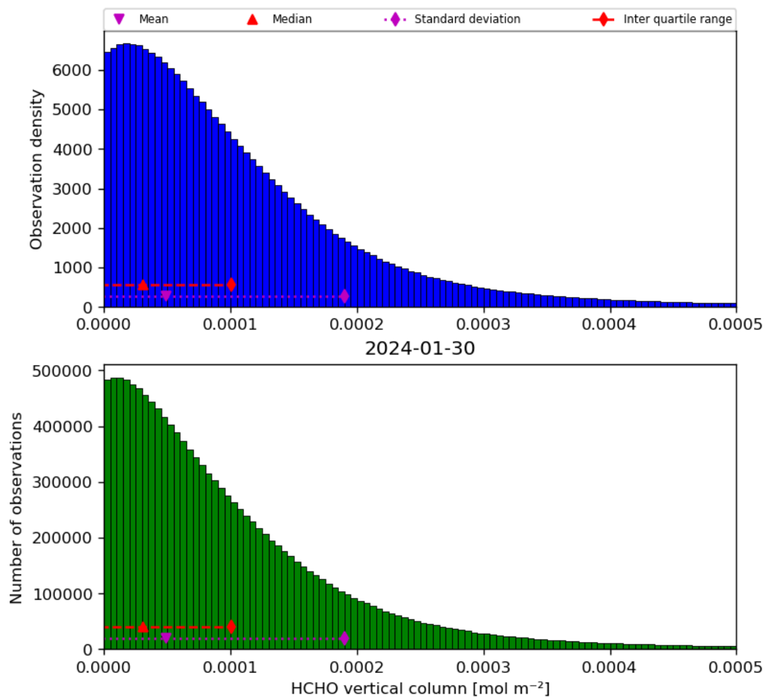
Figure 35: Histogram of “HCHO vertical column” for 2024-01-29 to 2024-01-31
