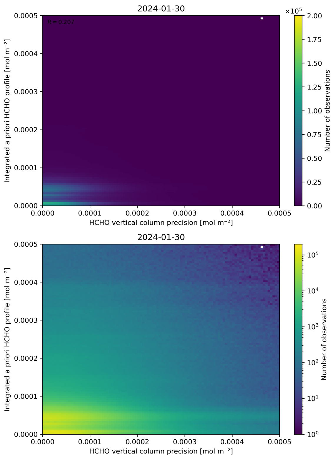
Figure 147: Scatter density plot of “HCHO vertical column precision” against “Integrated a priori HCHO profile” for 2024-01-29 to 2024-01-31.
