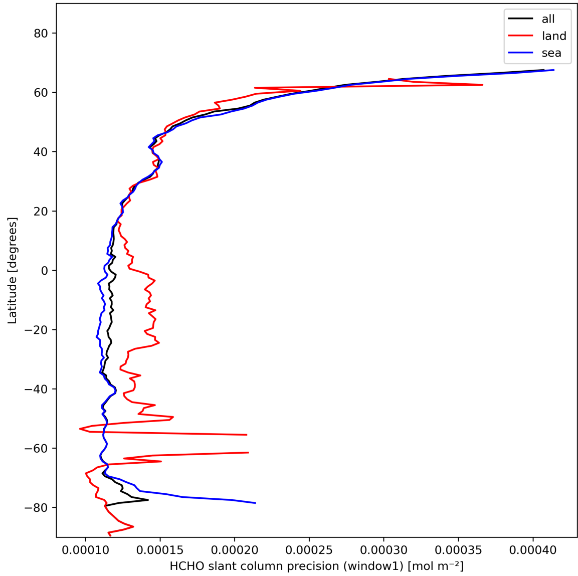
Figure 25: Zonal average of “HCHO slant column precision (window1)” for 2024-01-29 to 2024-01-31.
