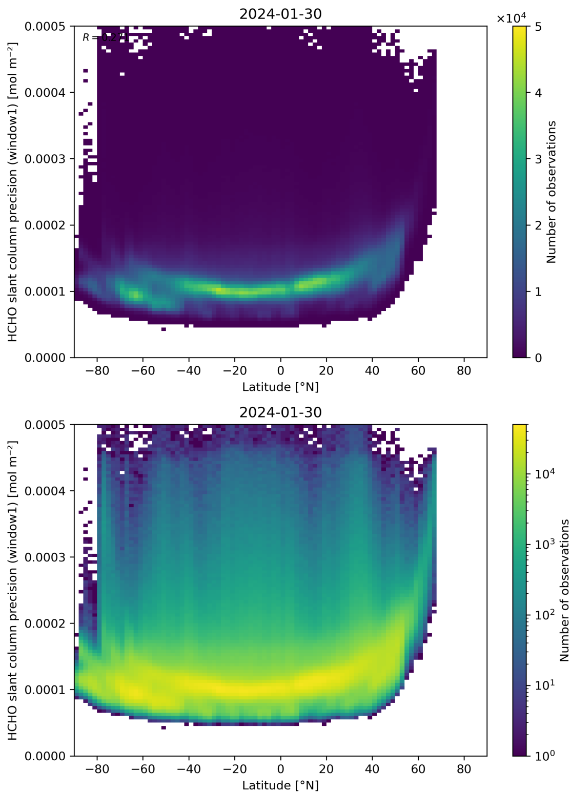
Figure 160: Scatter density plot of “Latitude” against “HCHO slant column precision (window1)” for 2024-01-29 to 2024-01-31.
