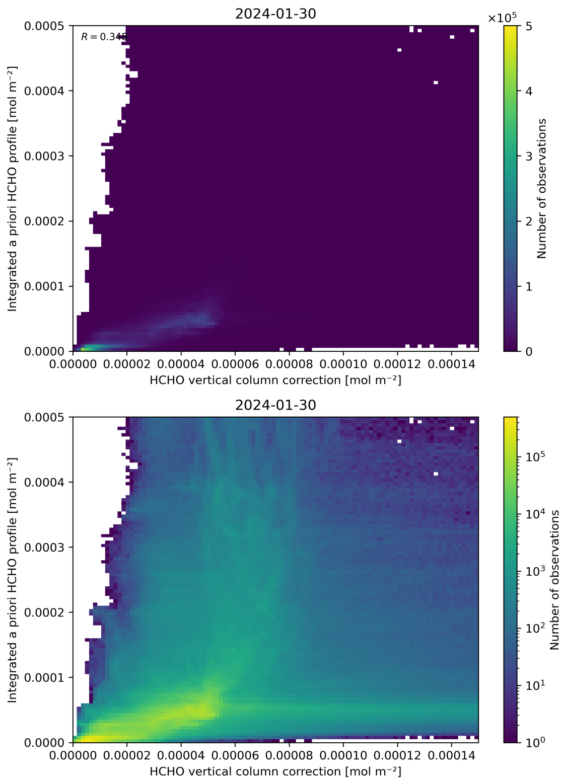
Figure 122: Scatter density plot of “HCHO vertical column correction” against “Integrated a priori HCHO profile” for 2024-01-29 to 2024-01-31.
