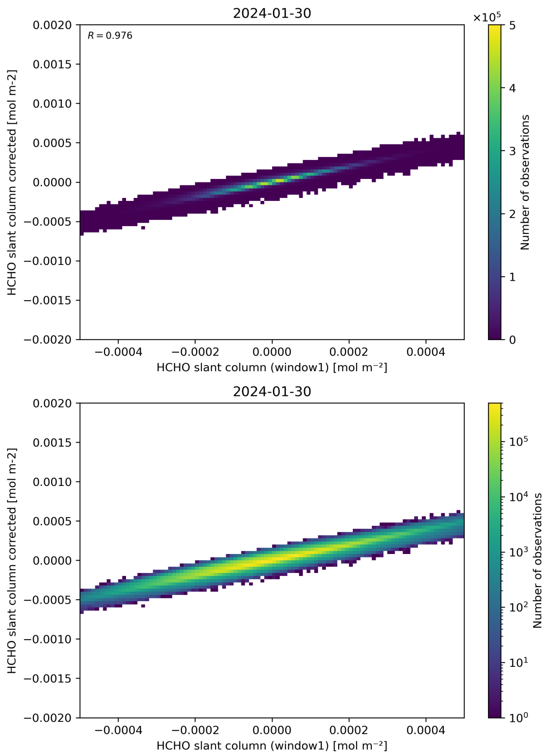
Figure 82: Scatter density plot of “HCHO slant column (window1)” against “HCHO slant column corrected” for 2024-01-29 to 2024-01-31.
