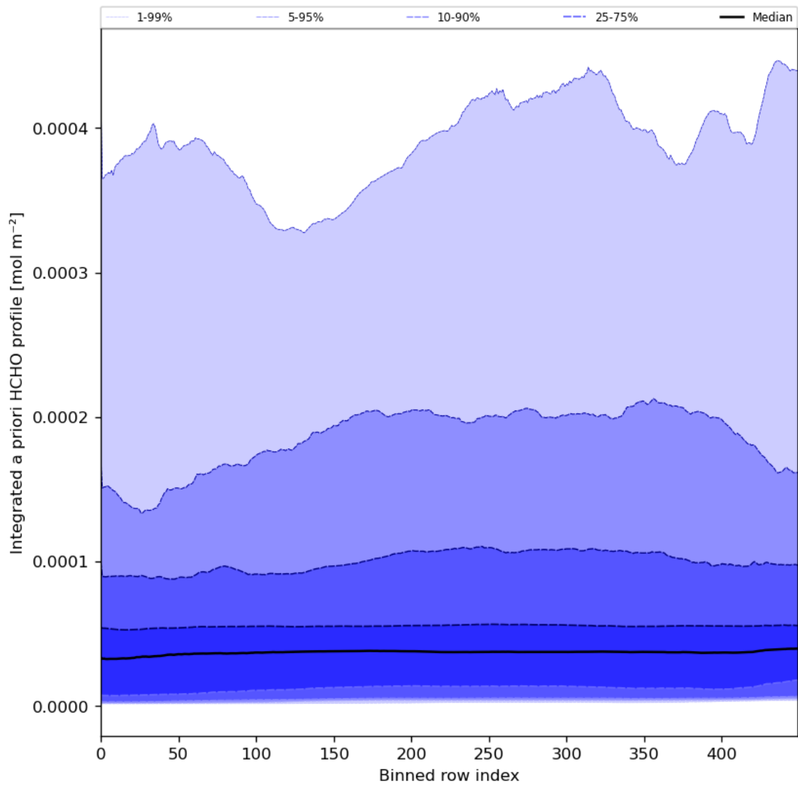
Figure 57: Along track statistics of “Integrated a priori HCHO profile” for 2024-01-29 to 2024-01-31
