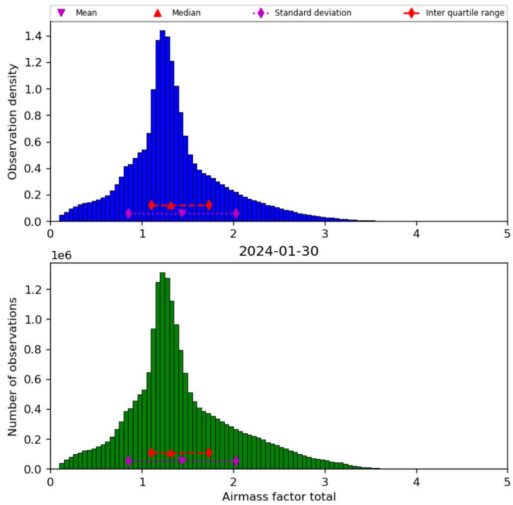
Figure 40: Histogram of “Airmass factor total” for 2024-01-29 to 2024-01-31
