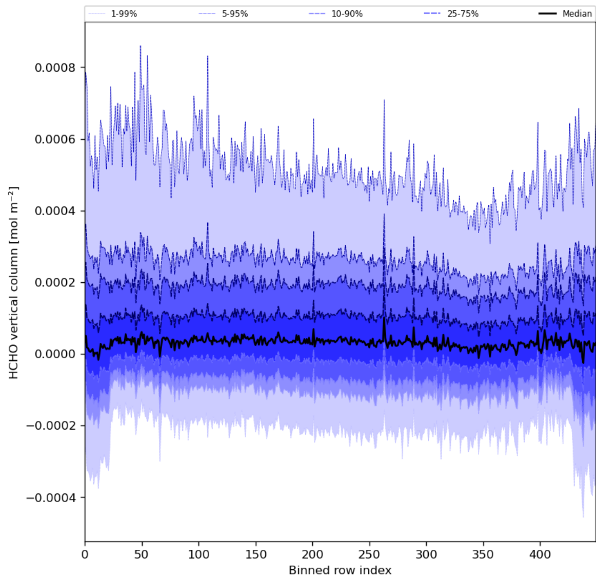
Figure 49: Along track statistics of “HCHO vertical column” for 2024-01-29 to 2024-01-31
