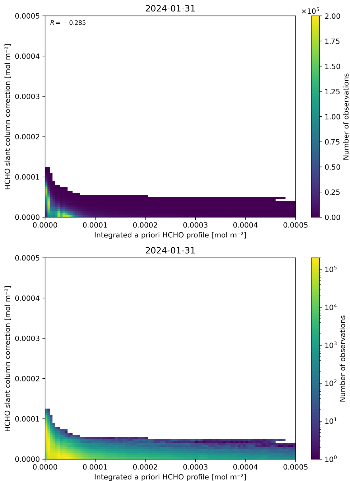
Figure 152: Scatter density plot of “Integrated a priori HCHO profile” against “HCHO slant column correction” for 2024-01-31 to 2024-02-01.
