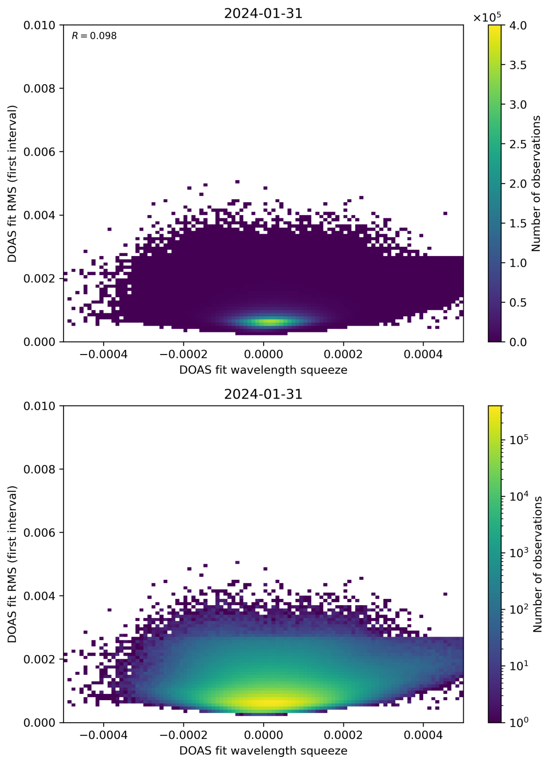
Figure 68: Scatter density plot of “DOAS fit wavelength squeeze” against “DOAS fit RMS (first interval)” for 2024-01-31 to 2024-02-01.
