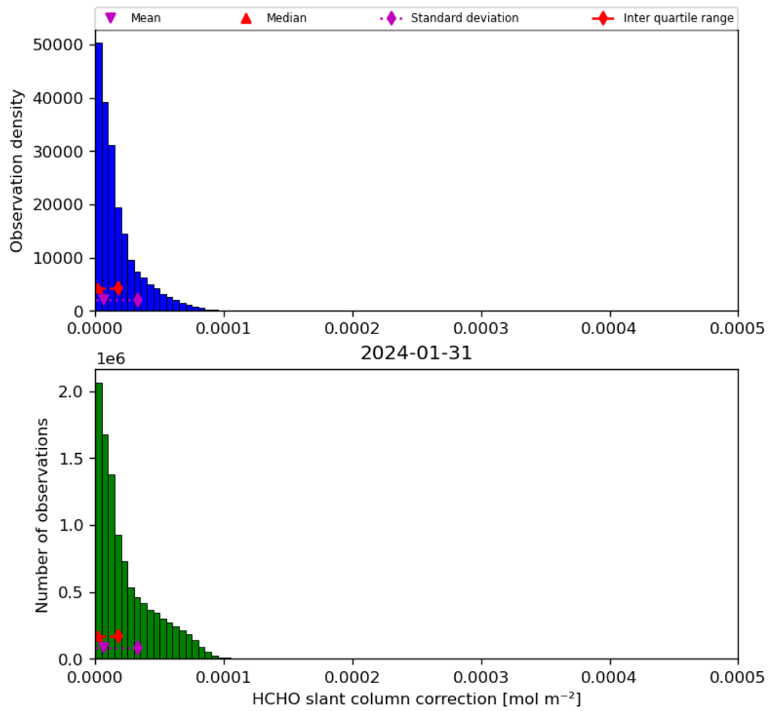
Figure 47: Histogram of “HCHO slant column correction” for 2024-01-31 to 2024-02-01
