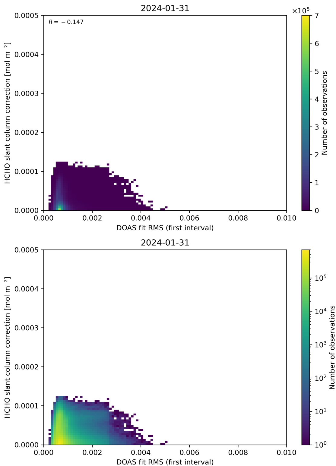
Figure 63: Scatter density plot of “DOAS fit RMS (first interval)” against “HCHO slant column correction” for 2024-01-31 to 2024-02-01.
