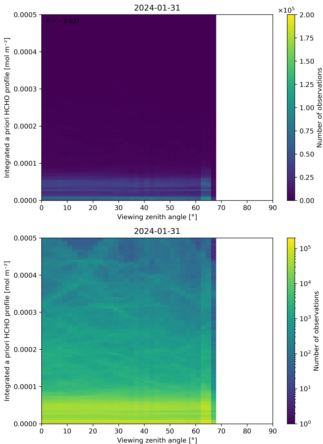
Figure 195: Scatter density plot of “Viewing zenith angle” against “Integrated a priori HCHO profile” for 2024-01-31 to 2024-02-01.
