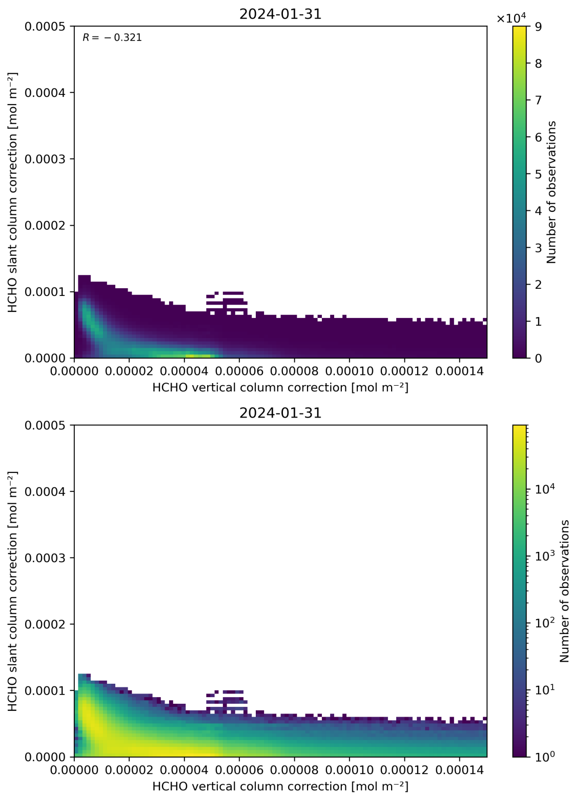
Figure 117: Scatter density plot of “HCHO vertical column correction” against “HCHO slant column correction” for 2024-01-31 to 2024-02-01.
