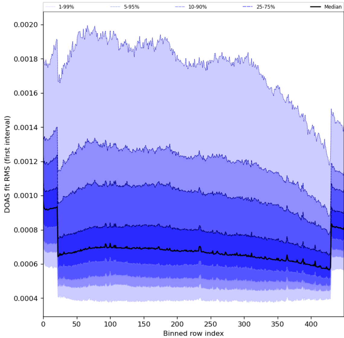
Figure 60: Along track statistics of “DOAS fit RMS (first interval)” for 2024-01-31 to 2024-02-01
