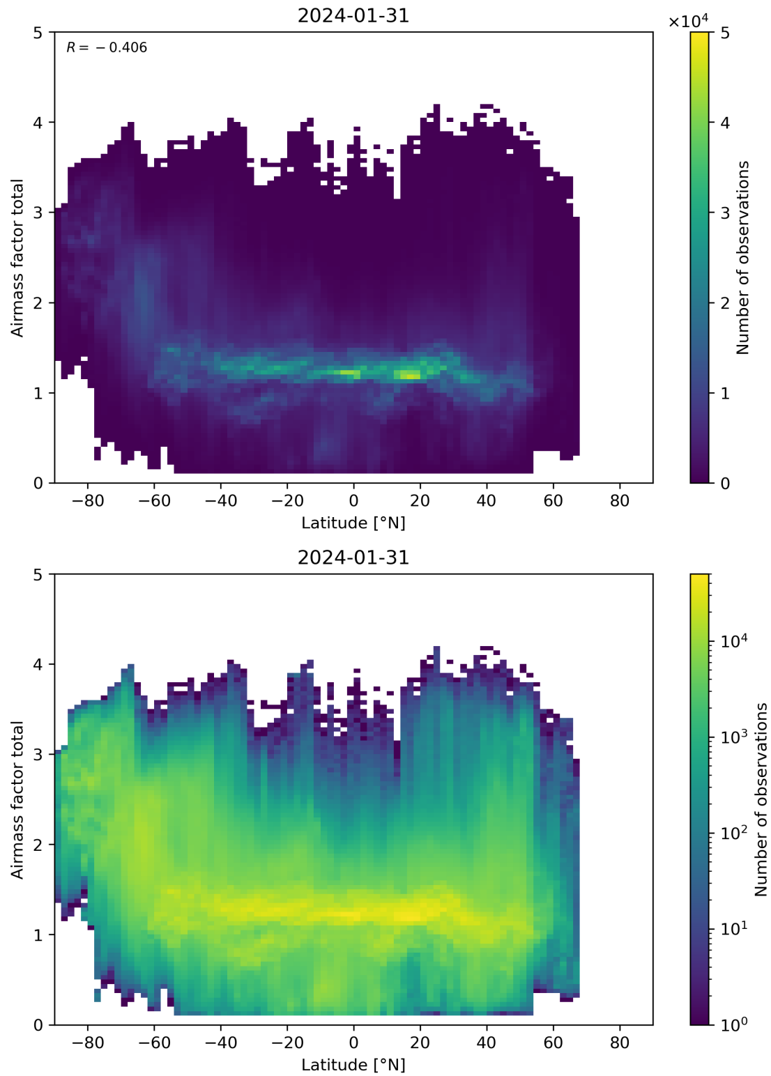
Figure 161: Scatter density plot of “Latitude” against “Airmass factor total” for 2024-01-31 to 2024-02-01.
