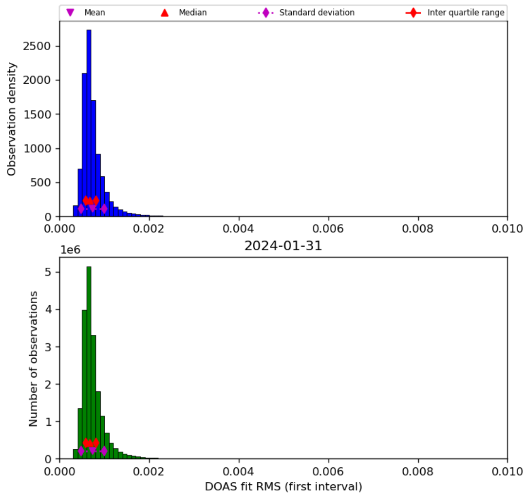
Figure 46: Histogram of “DOAS fit RMS (first interval)” for 2024-01-31 to 2024-02-01
