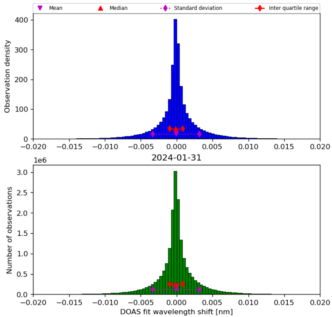
Figure 44: Histogram of “DOAS fit wavelength shift” for 2024-01-31 to 2024-02-01
