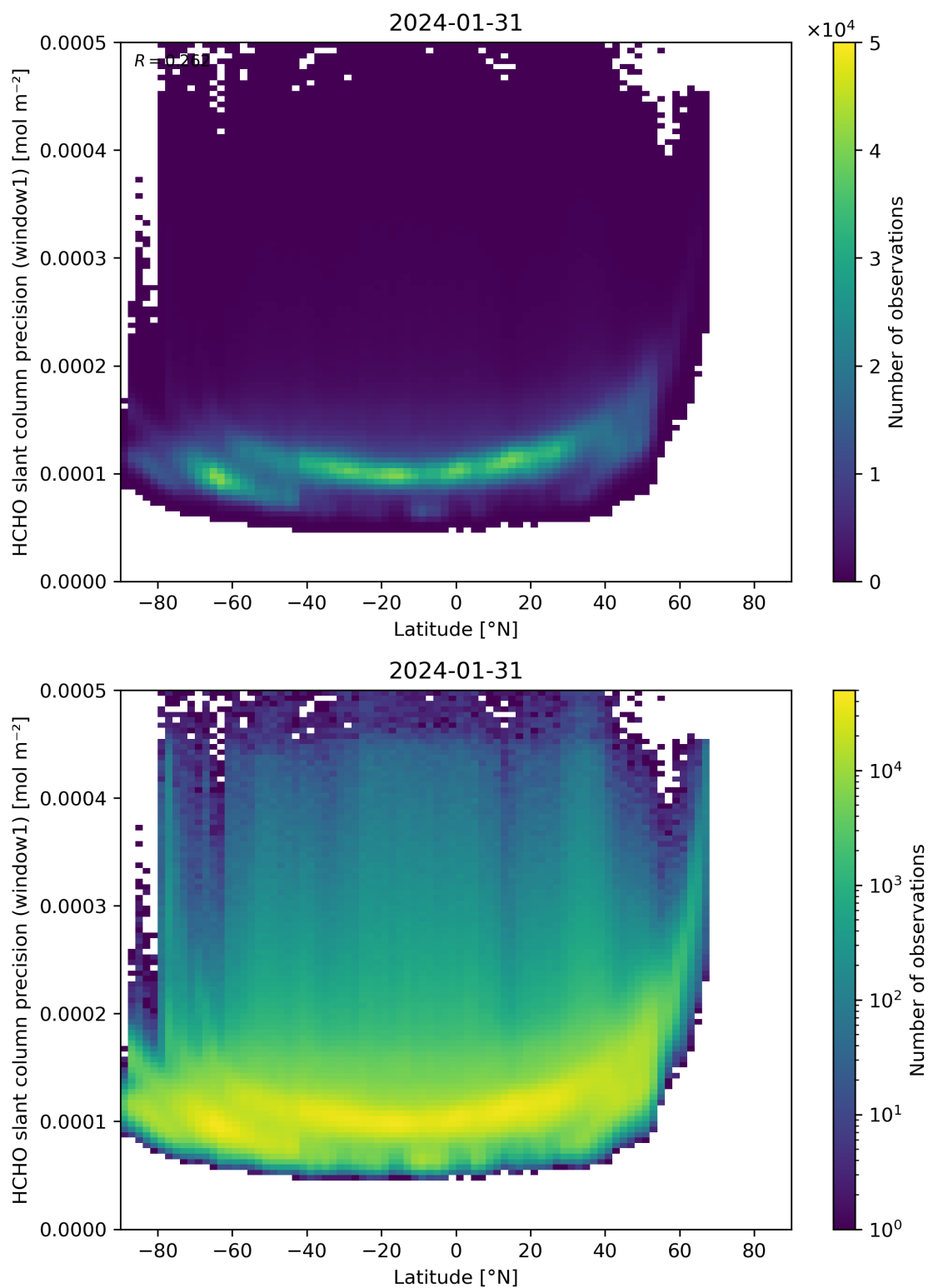
Figure 160: Scatter density plot of “Latitude” against “HCHO slant column precision (window1)” for 2024-01-31 to 2024-02-01.
