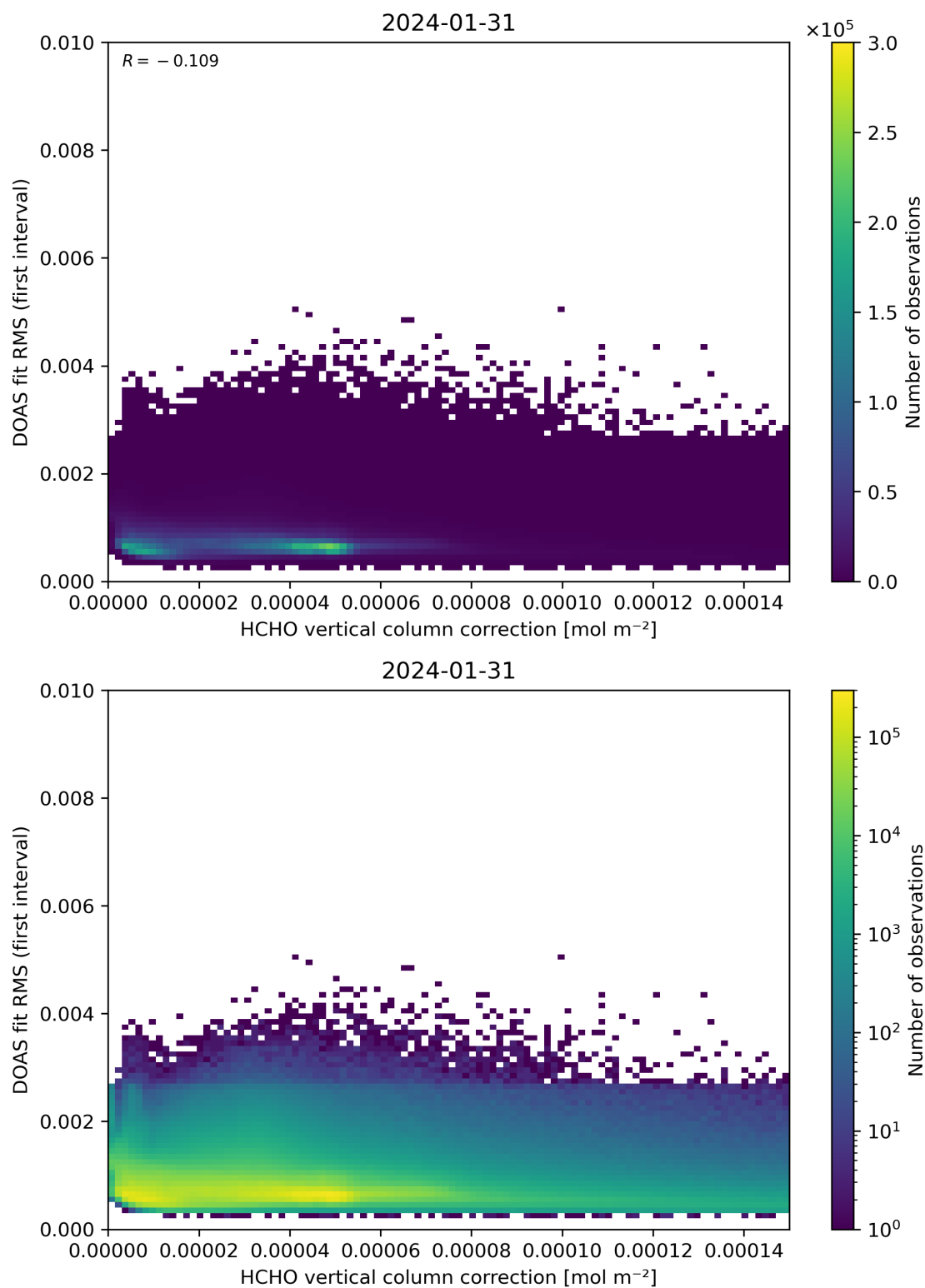
Figure 112: Scatter density plot of “HCHO vertical column correction” against “DOAS fit RMS (first interval)” for 2024-01-31 to 2024-02-01.
