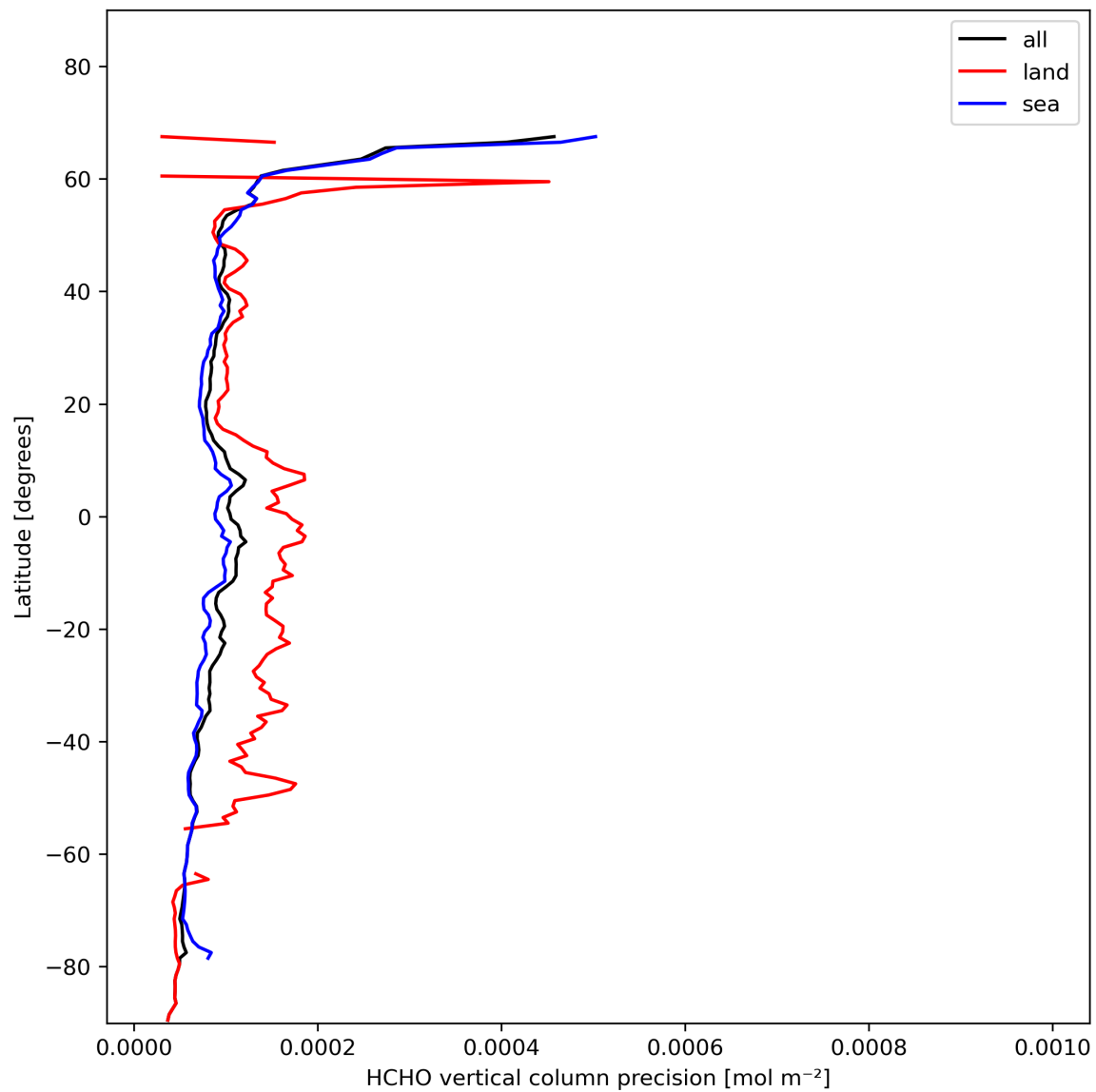
Figure 22: Zonal average of “HCHO vertical column precision” for 2024-01-31 to 2024-02-01.
