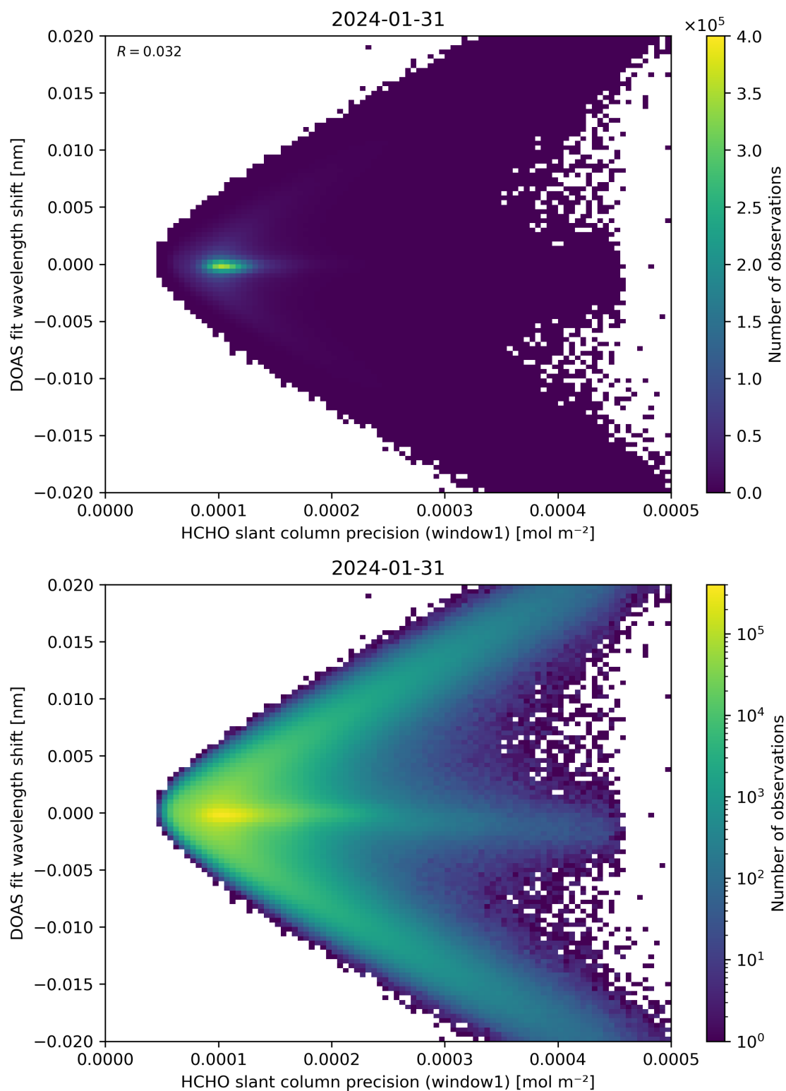
Figure 89: Scatter density plot of “HCHO slant column precision (window1)” against “DOAS fit wavelength shift” for 2024-01-31 to 2024-02-01.
