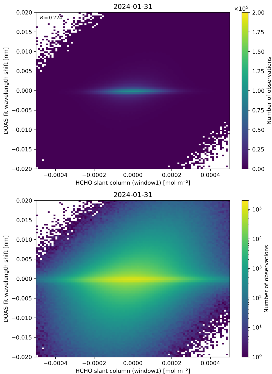
Figure 79: Scatter density plot of “HCHO slant column (window1)” against “DOAS fit wavelength shift” for 2024-01-31 to 2024-02-01.
