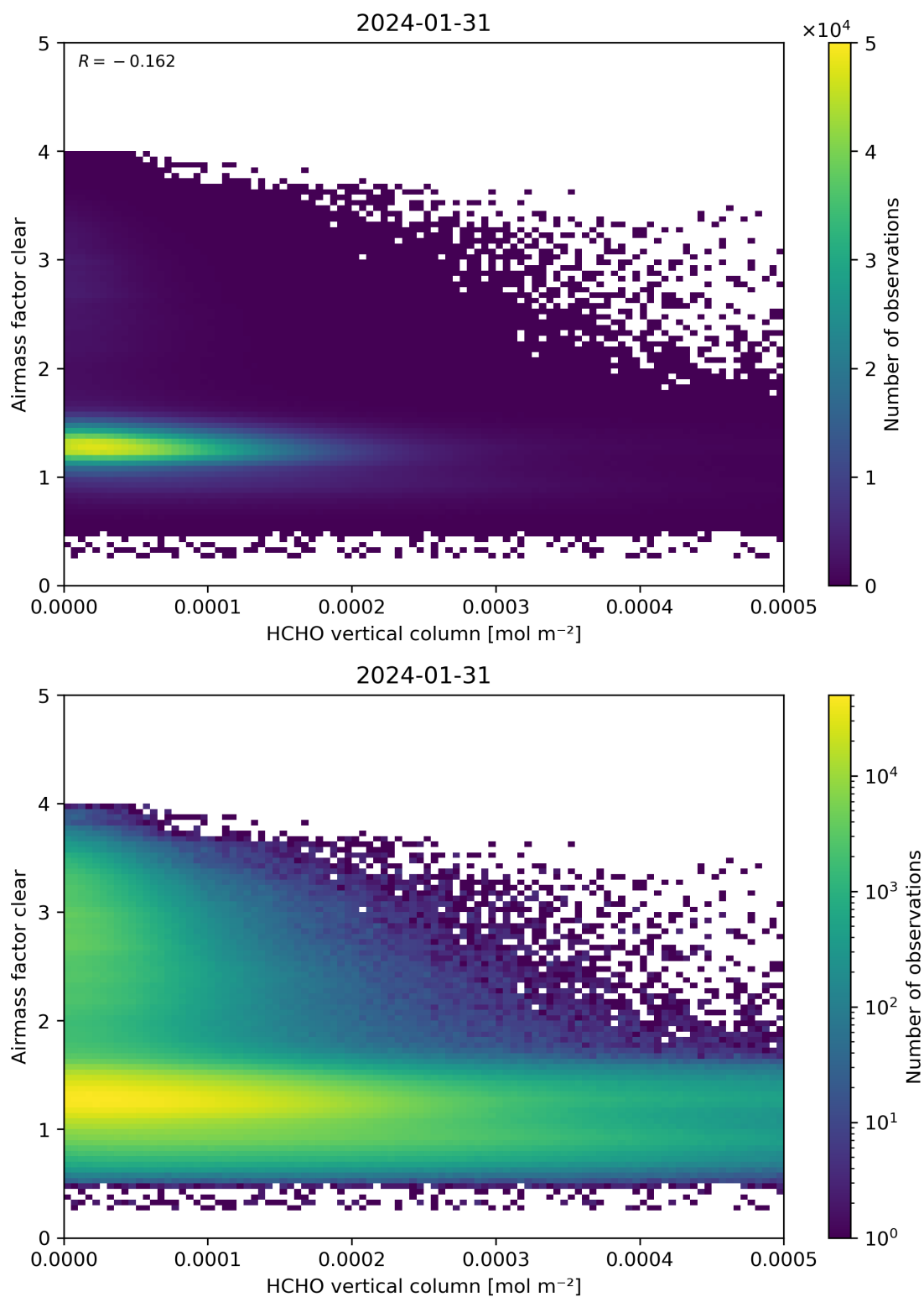
Figure 126: Scatter density plot of “HCHO vertical column” against “Airmass factor clear” for 2024-01-31 to 2024-02-01.
