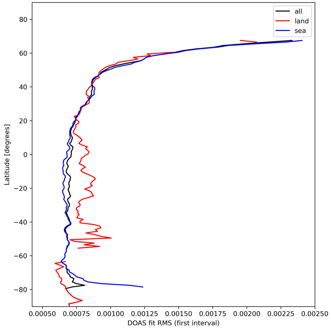
Figure 32: Zonal average of “DOAS fit RMS (first interval)” for 2024-01-31 to 2024-02-01.
