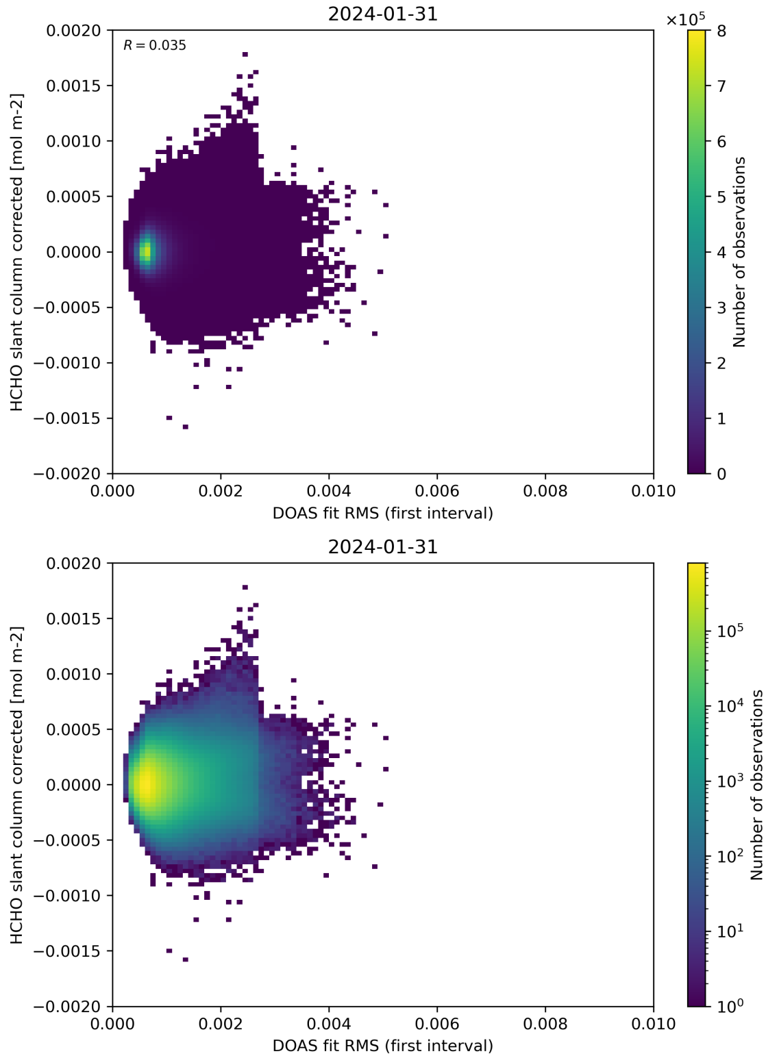
Figure 62: Scatter density plot of “DOAS fit RMS (first interval)” against “HCHO slant column corrected” for 2024-01-31 to 2024-02-01.
