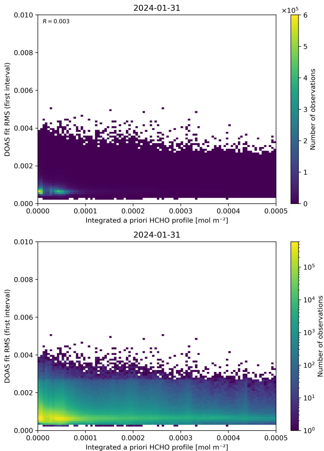
Figure 148: Scatter density plot of “Integrated a priori HCHO profile” against “DOAS fit RMS (first interval)” for 2024-01-31 to 2024-02-01.
