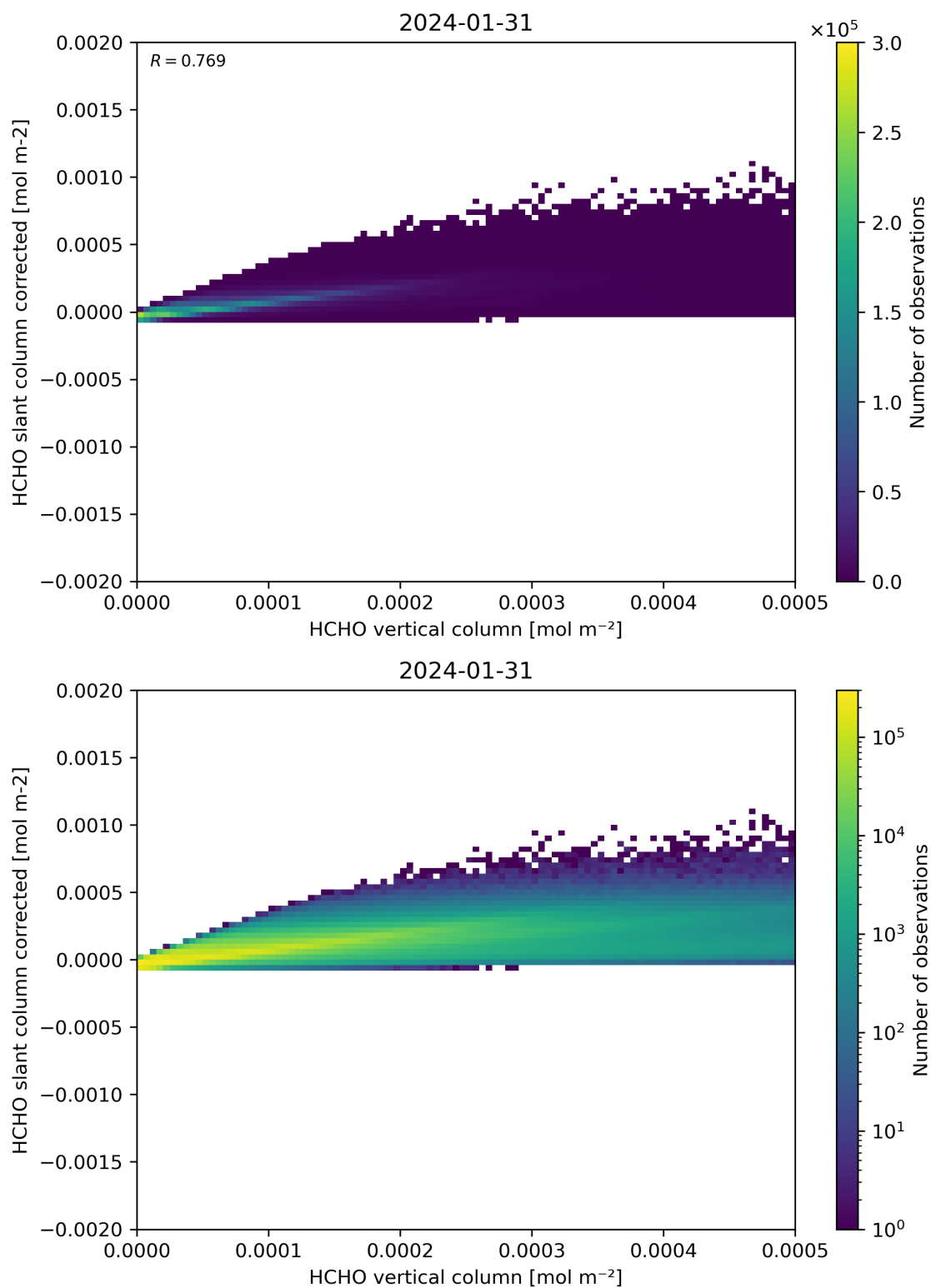
Figure 127: Scatter density plot of “HCHO vertical column” against “HCHO slant column corrected” for 2024-01-31 to 2024-02-01.
