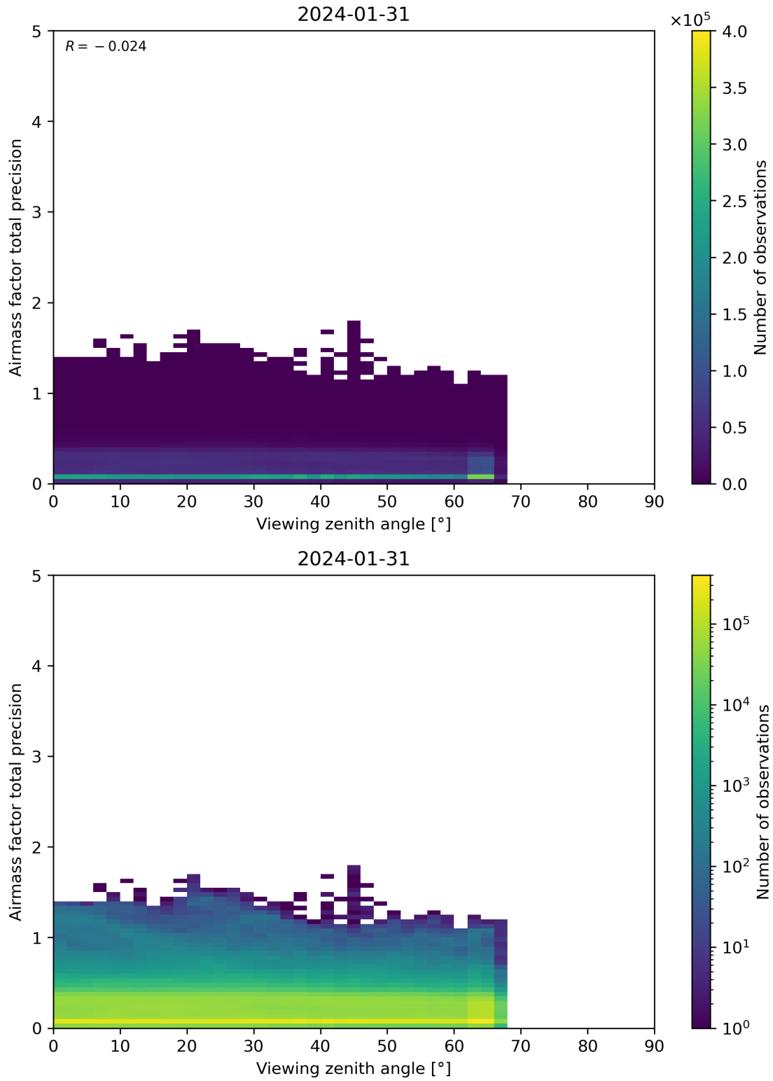
Figure 191: Scatter density plot of “Viewing zenith angle” against “Airmass factor total precision” for 2024-01-31 to 2024-02-01.
