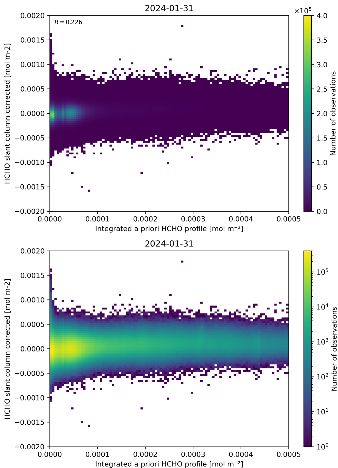
Figure 151: Scatter density plot of “Integrated a priori HCHO profile” against “HCHO slant column corrected” for 2024-01-31 to 2024-02-01.
