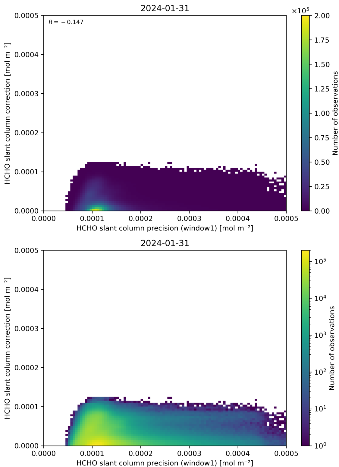
Figure 93: Scatter density plot of “HCHO slant column precision (window1)” against “HCHO slant column correction” for 2024-01-31 to 2024-02-01.
