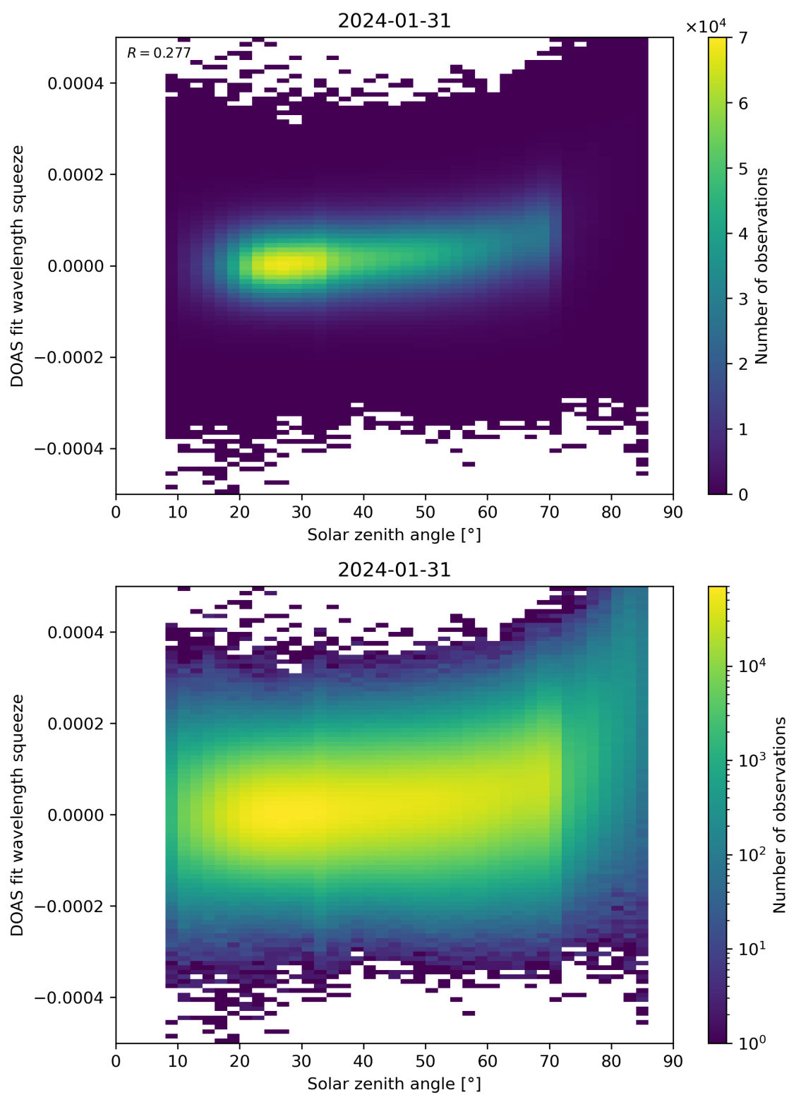
Figure 169: Scatter density plot of “Solar zenith angle” against “DOAS fit wavelength squeeze” for 2024-01-31 to 2024-02-01.
