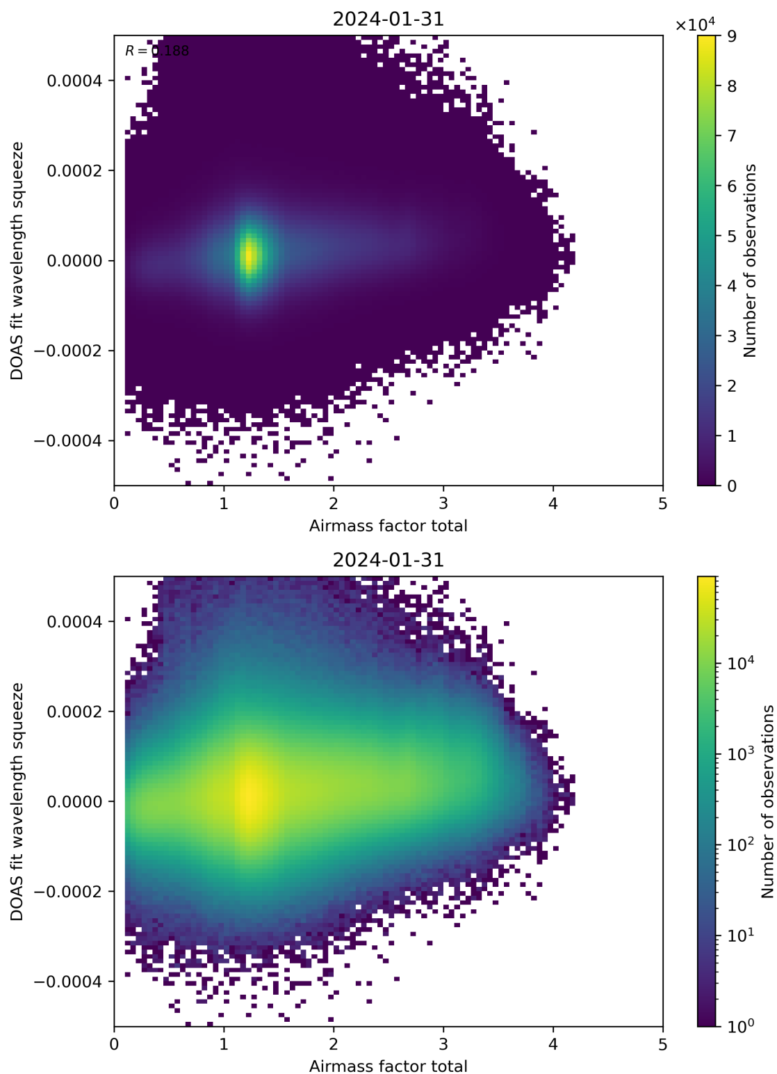
Figure 99: Scatter density plot of “Airmass factor total” against “DOAS fit wavelength squeeze” for 2024-01-31 to 2024-02-01.
