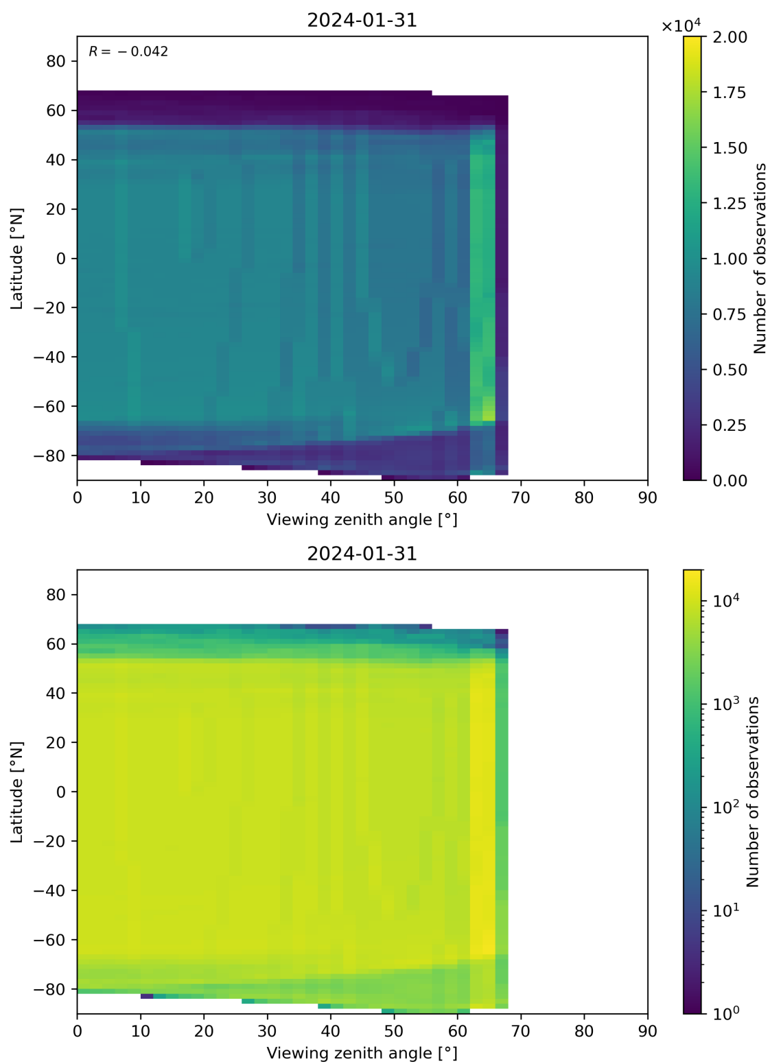
Figure 196: Scatter density plot of “Viewing zenith angle” against “Latitude” for 2024-01-31 to 2024-02-01.
