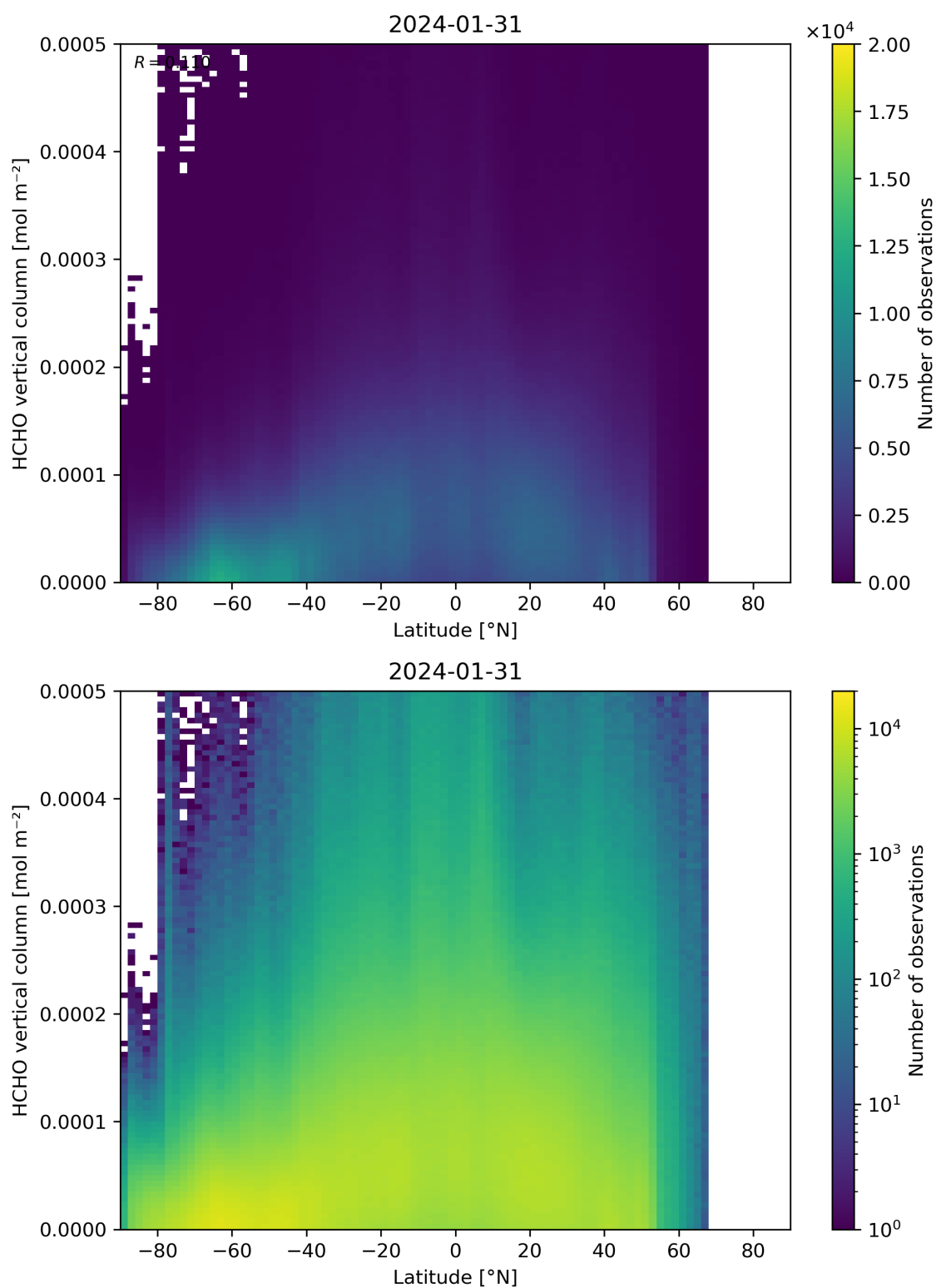
Figure 163: Scatter density plot of “Latitude” against “HCHO vertical column” for 2024-01-31 to 2024-02-01.
