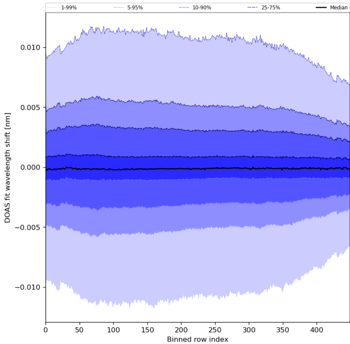
Figure 58: Along track statistics of “DOAS fit wavelength shift” for 2024-01-31 to 2024-02-01
