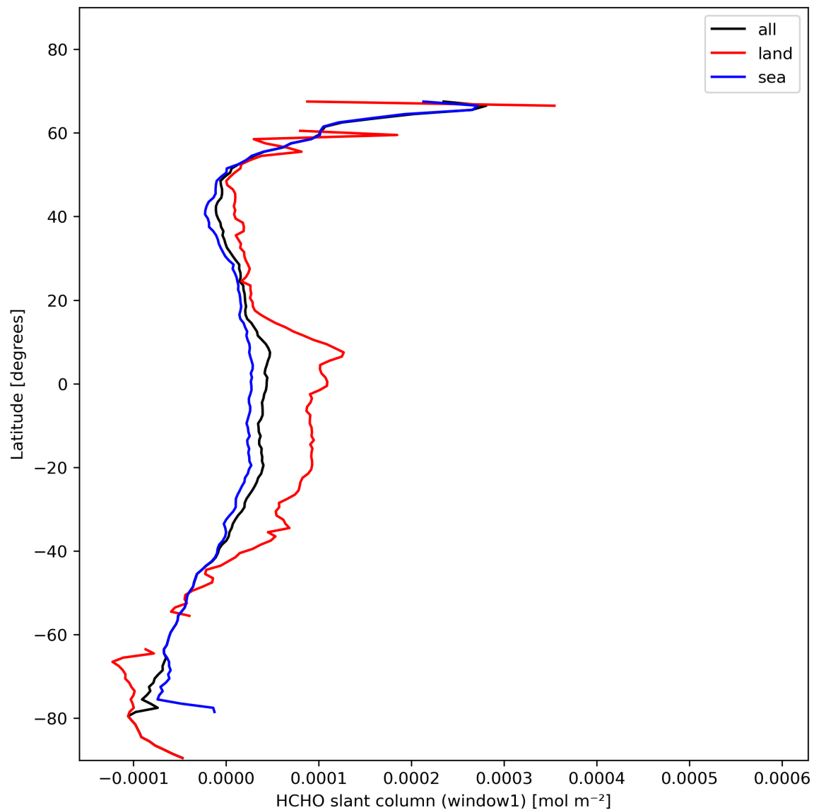
Figure 24: Zonal average of “HCHO slant column (window1)” for 2024-01-31 to 2024-02-01.
