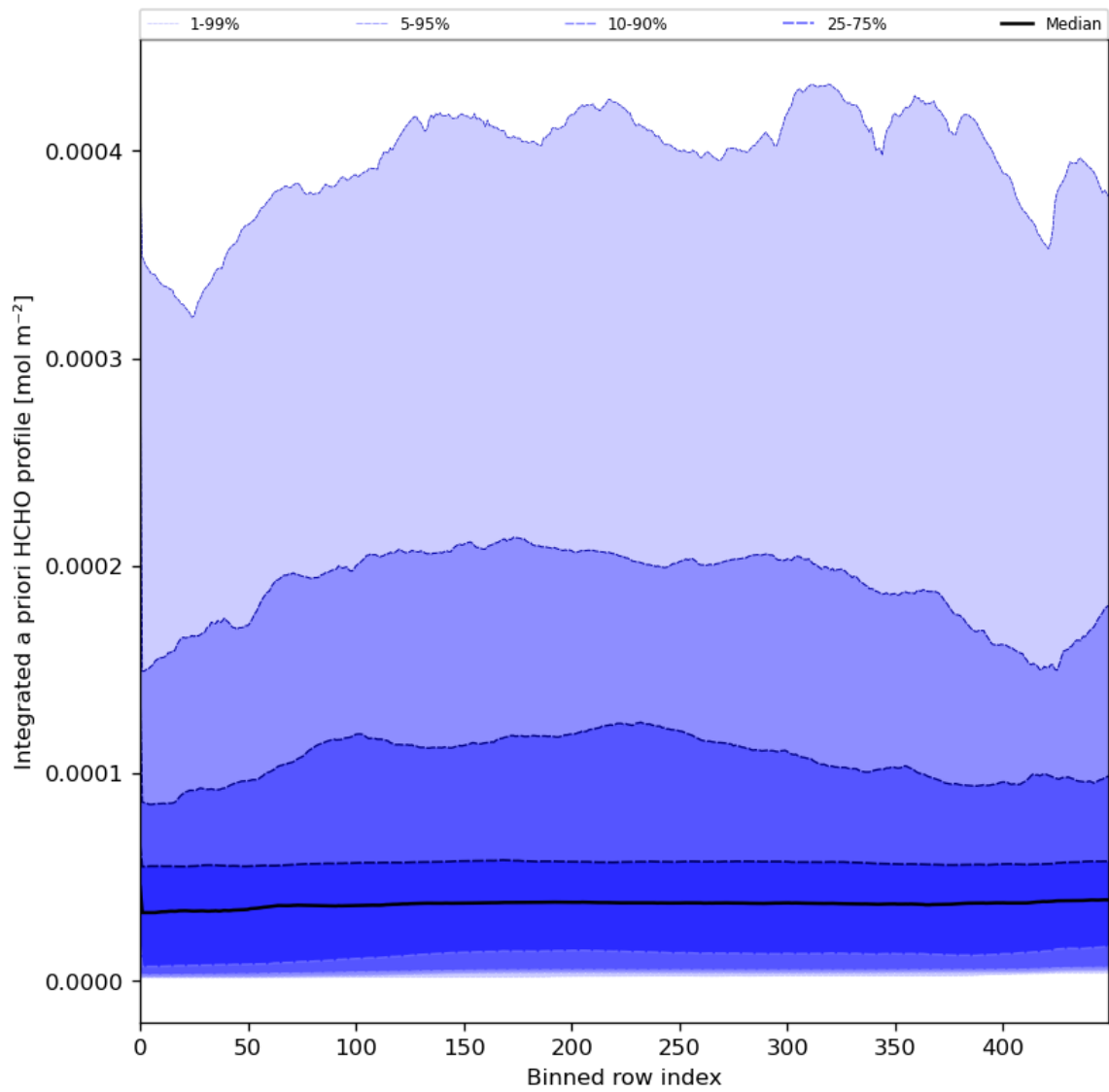
Figure 57: Along track statistics of "Integrated a priori HCHO profile" for 2024-01-31 to 2024-02-01
