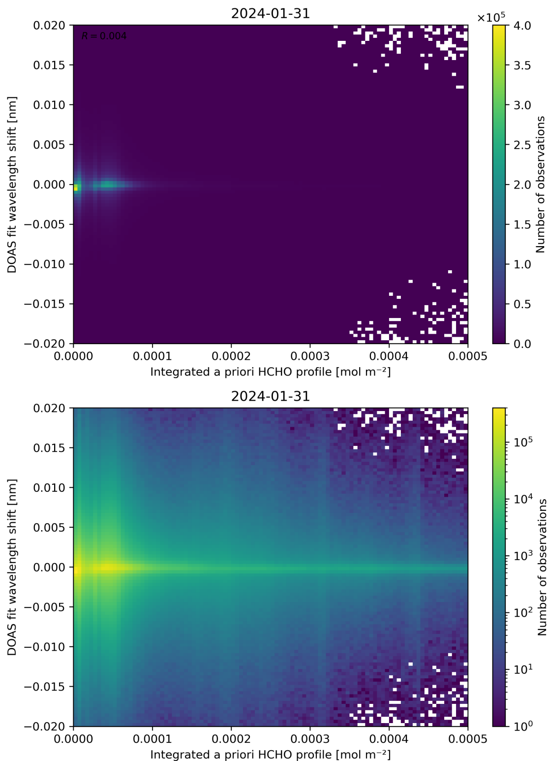
Figure 149: Scatter density plot of “Integrated a priori HCHO profile” against “DOAS fit wavelength shift” for 2024-01-31 to 2024-02-01.
