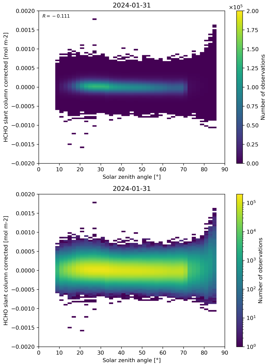
Figure 171: Scatter density plot of “Solar zenith angle” against “HCHO slant column corrected” for 2024-01-31 to 2024-02-01.
