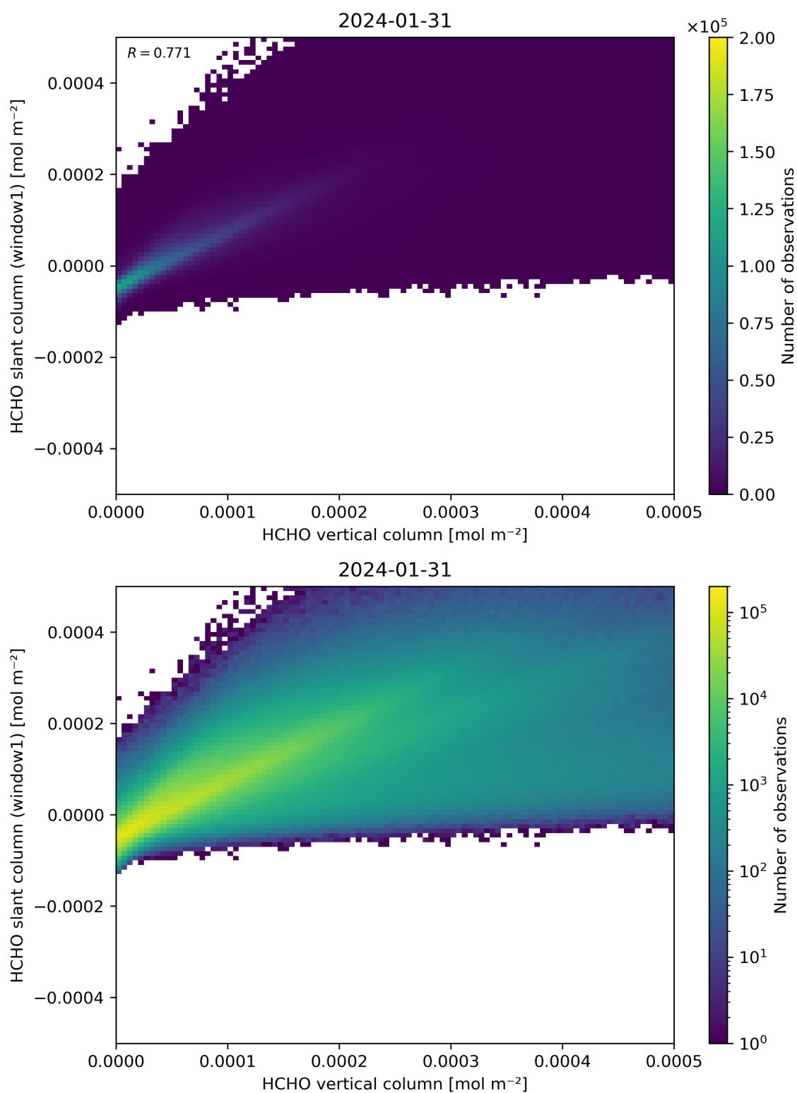
Figure 129: Scatter density plot of “HCHO vertical column” against “HCHO slant column (window1)” for 2024-01-31 to 2024-02-01.
