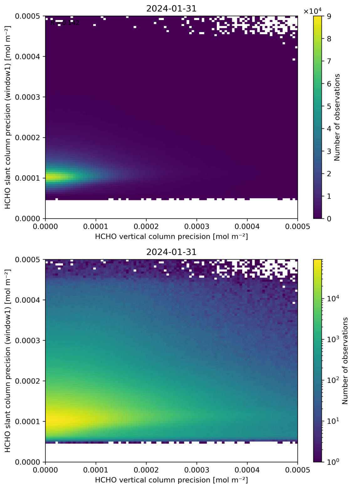
Figure 143: Scatter density plot of “HCHO vertical column precision” against “HCHO slant column precision (window1)” for 2024-01-31 to 2024-02-01.
