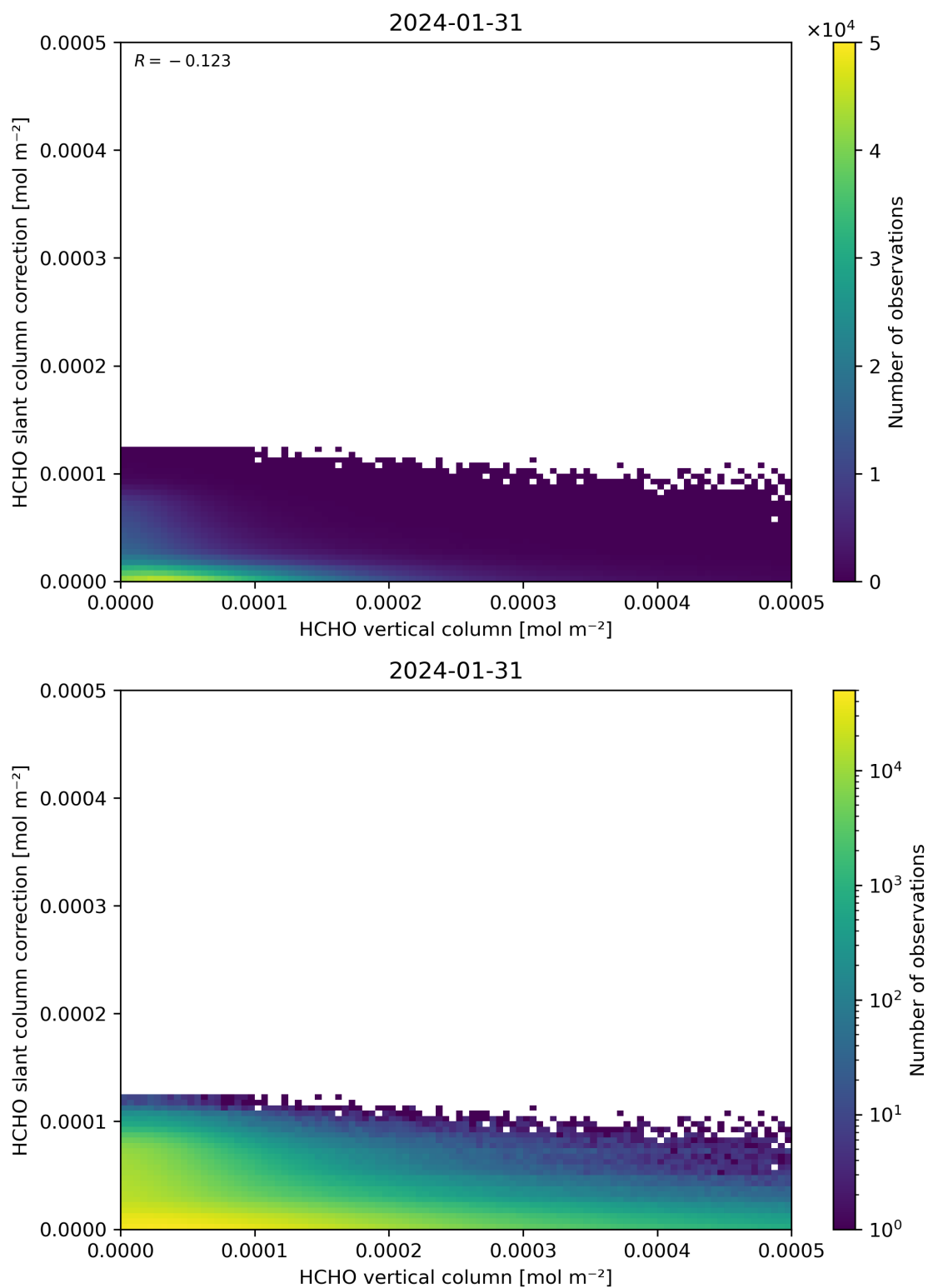
Figure 128: Scatter density plot of “HCHO vertical column” against “HCHO slant column correction” for 2024-01-31 to 2024-02-01.
