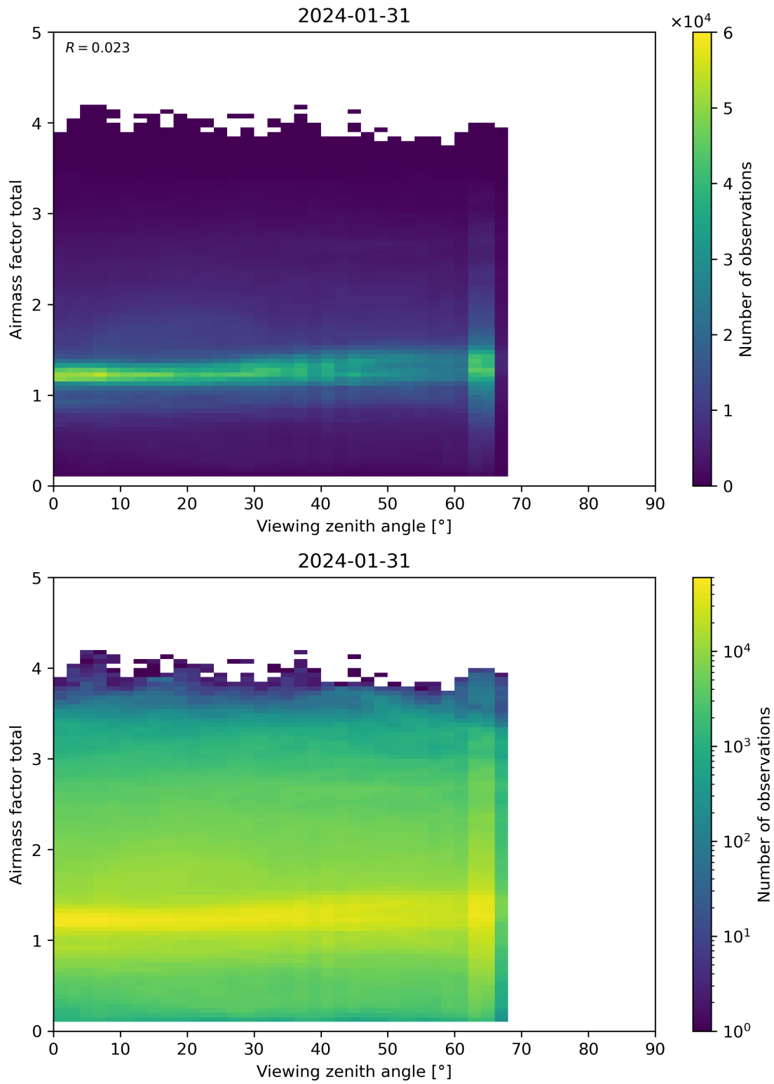
Figure 190: Scatter density plot of “Viewing zenith angle” against “Airmass factor total” for 2024-01-31 to 2024-02-01.
