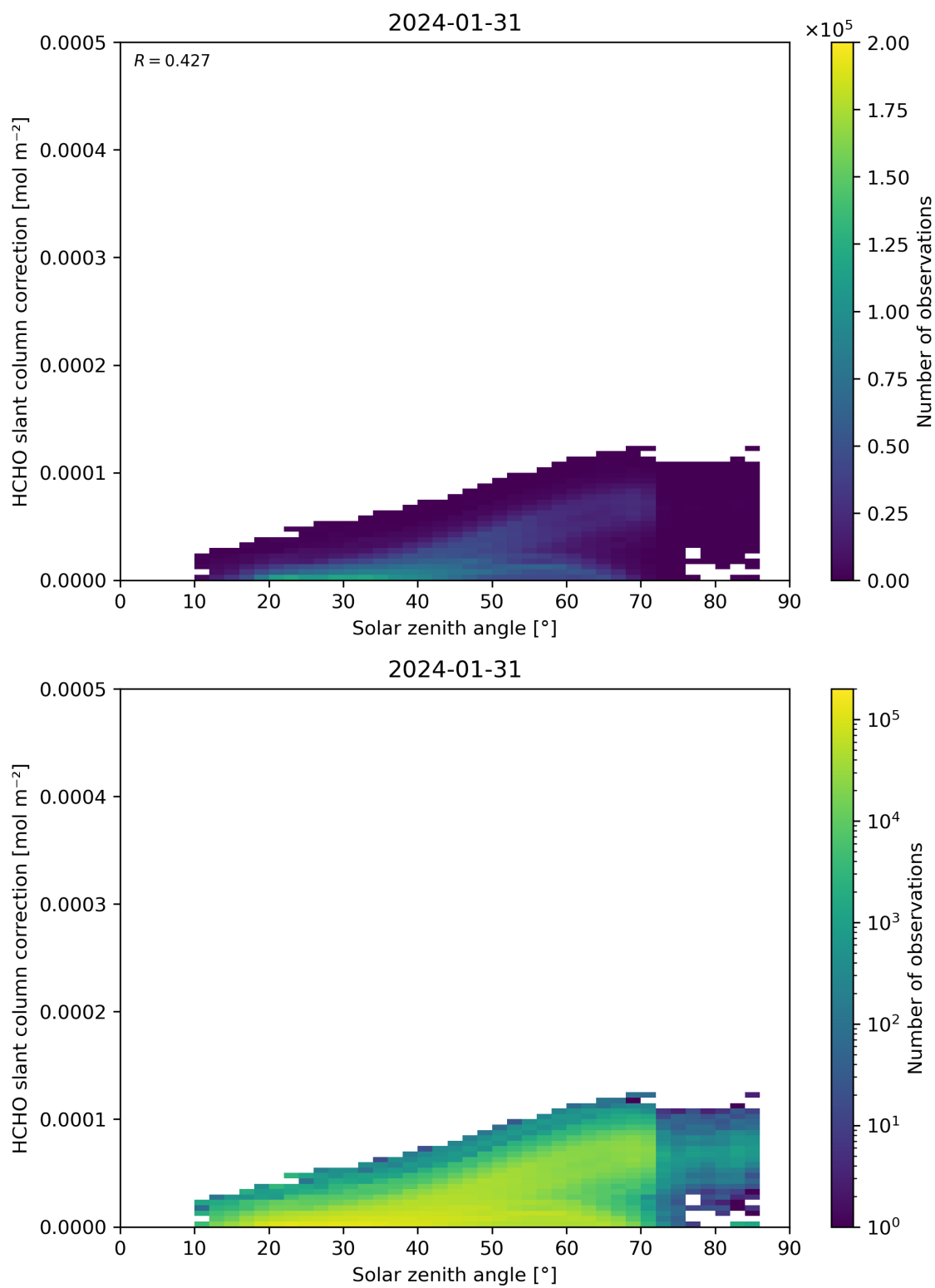
Figure 172: Scatter density plot of “Solar zenith angle” against “HCHO slant column correction” for 2024-01-31 to 2024-02-01.
