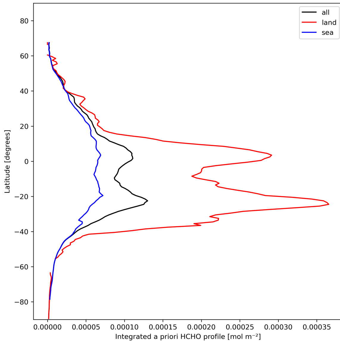
Figure 29: Zonal average of “Integrated a priori HCHO profile” for 2024-01-31 to 2024-02-01.
