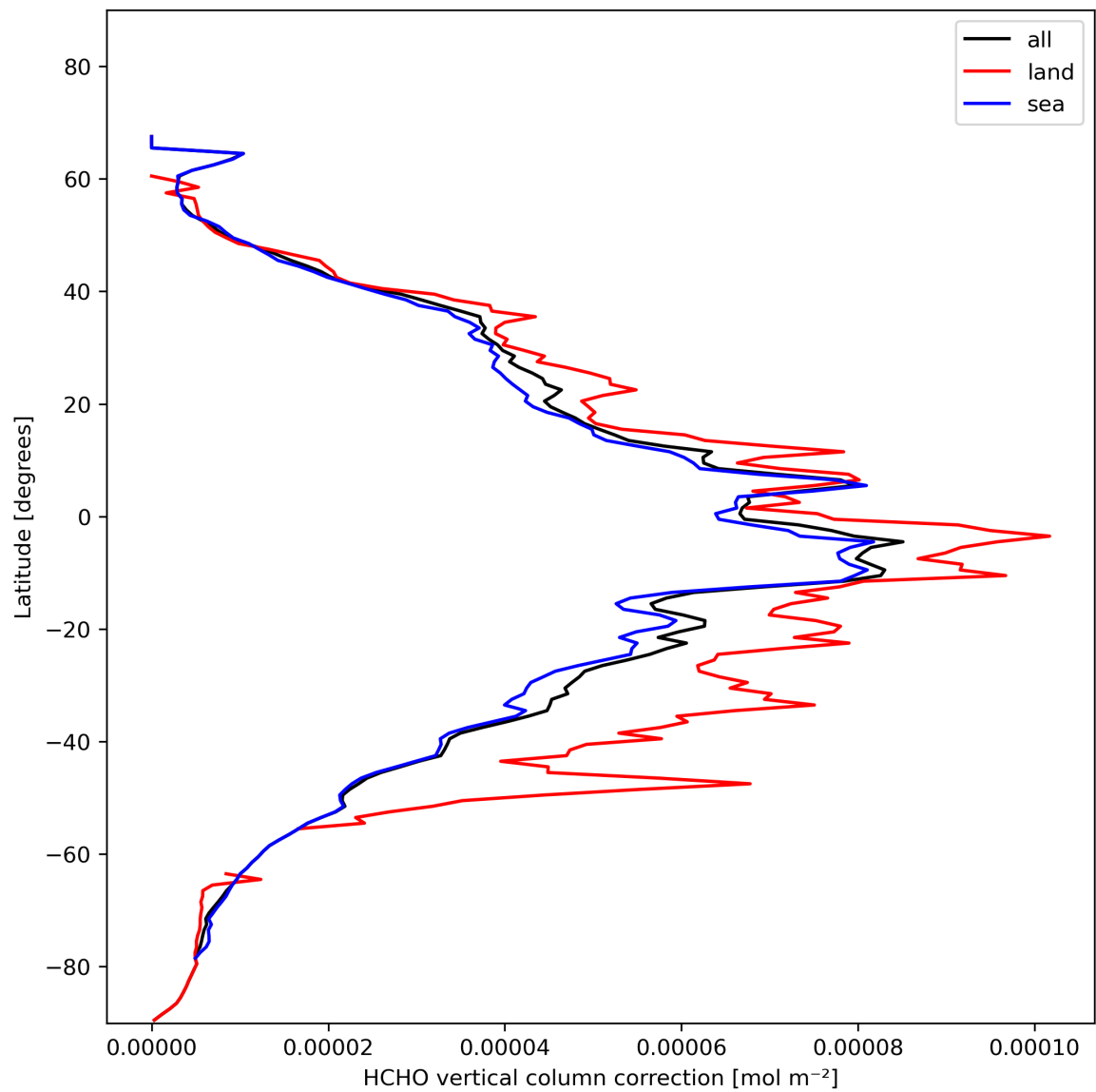
Figure 23: Zonal average of “HCHO vertical column correction” for 2024-01-31 to 2024-02-01.
