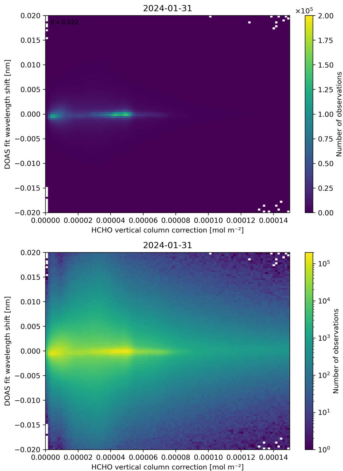
Figure 113: Scatter density plot of “HCHO vertical column correction” against “DOAS fit wavelength shift” for 2024-01-31 to 2024-02-01.
