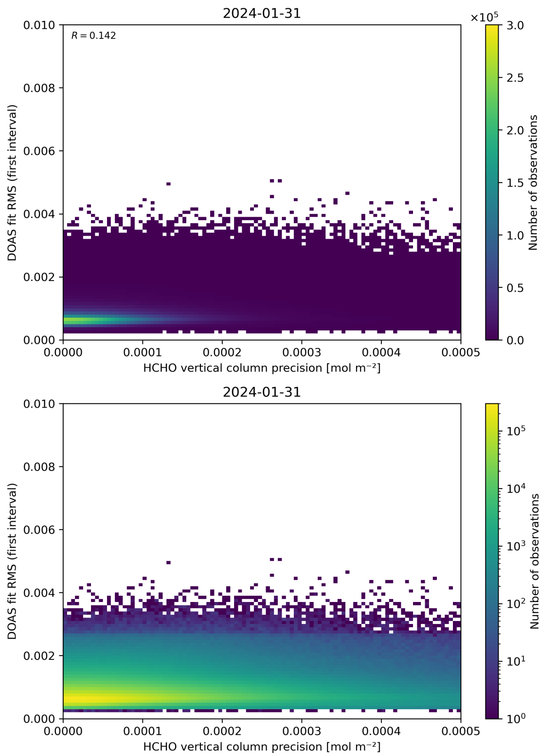
Figure 136: Scatter density plot of “HCHO vertical column precision” against “DOAS fit RMS (first interval)” for 2024-01-31 to 2024-02-01.
