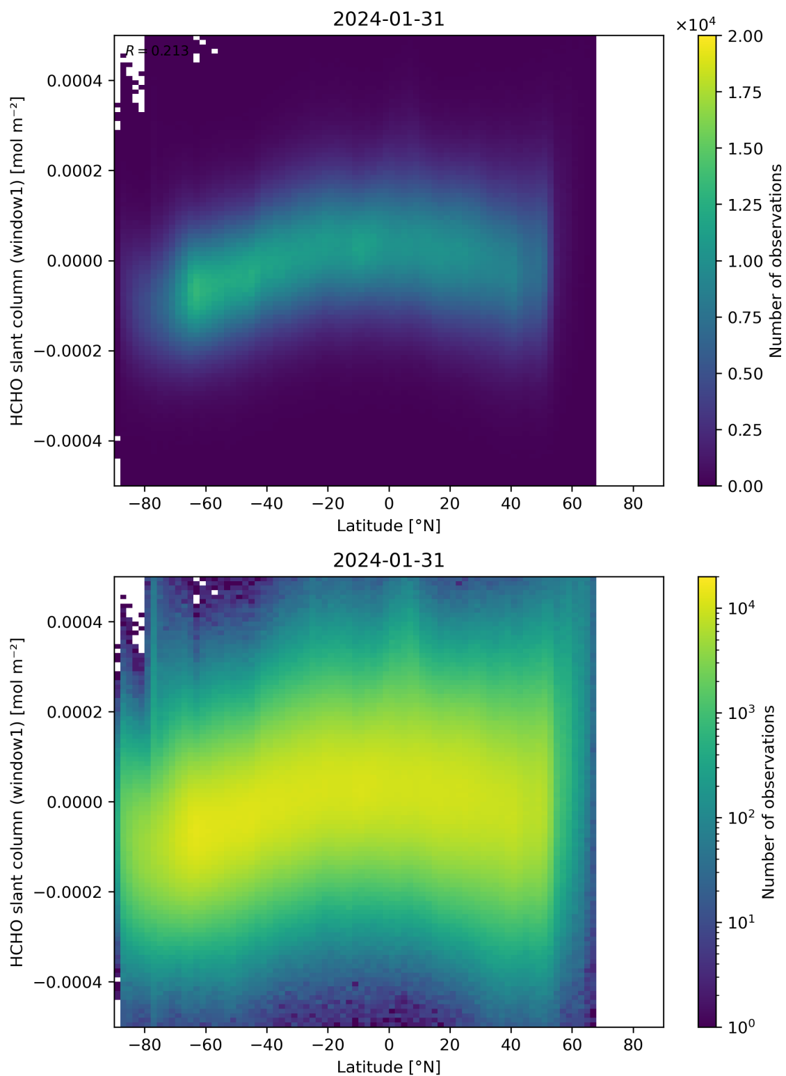
Figure 159: Scatter density plot of “Latitude” against “HCHO slant column (window1)” for 2024-01-31 to 2024-02-01.
