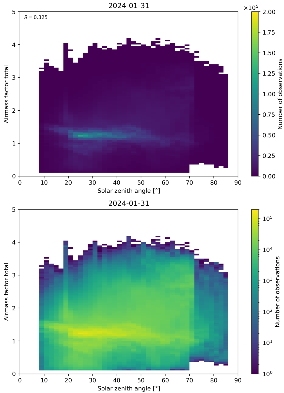
Figure 175: Scatter density plot of “Solar zenith angle” against “Airmass factor total” for 2024-01-31 to 2024-02-01.
