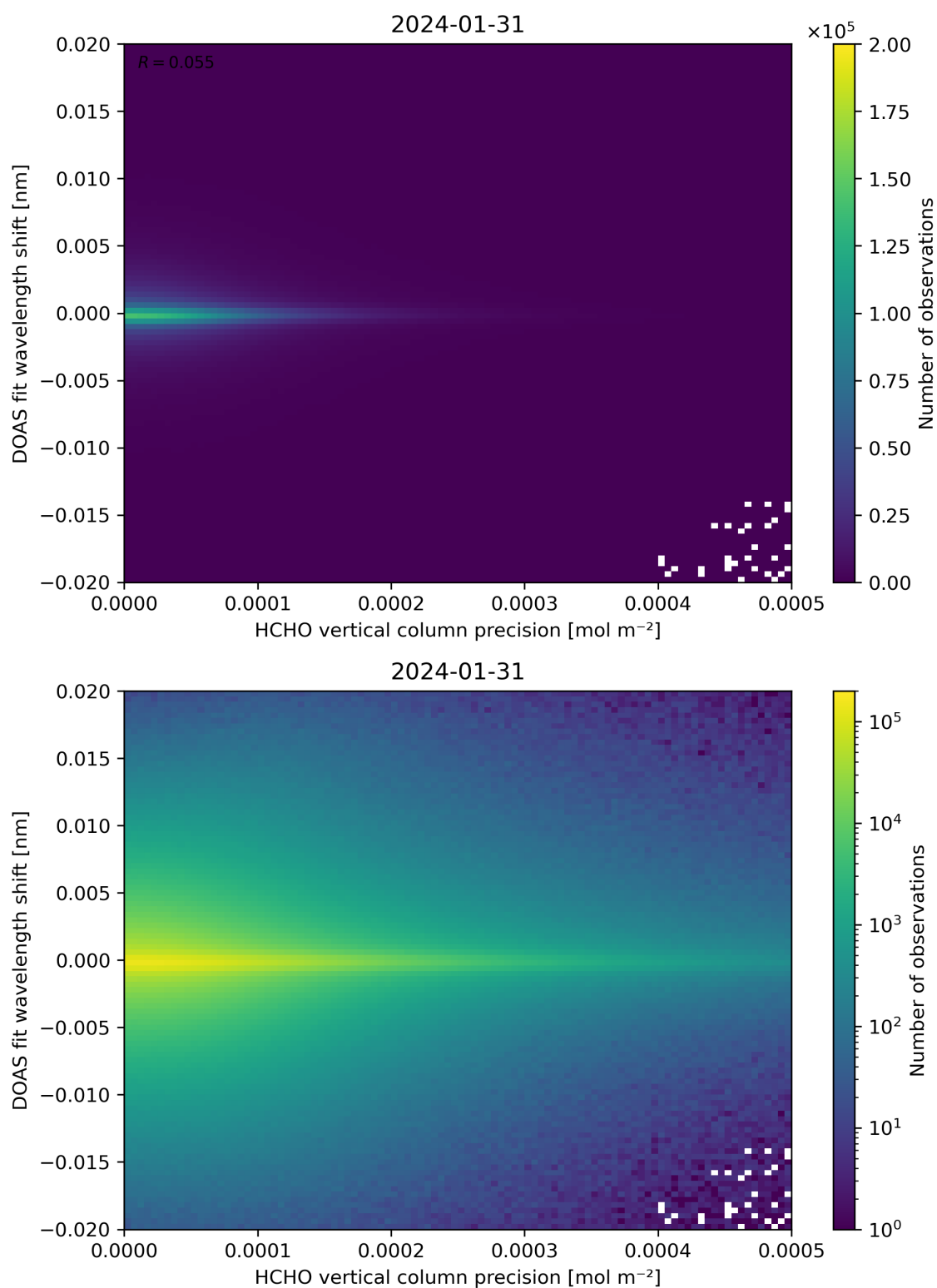
Figure 137: Scatter density plot of “HCHO vertical column precision” against “DOAS fit wavelength shift” for 2024-01-31 to 2024-02-01.
