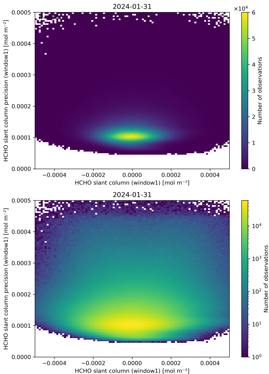
Figure 84: Scatter density plot of “HCHO slant column (window1)” against “HCHO slant column precision (window1)” for 2024-01-31 to 2024-02-01.
