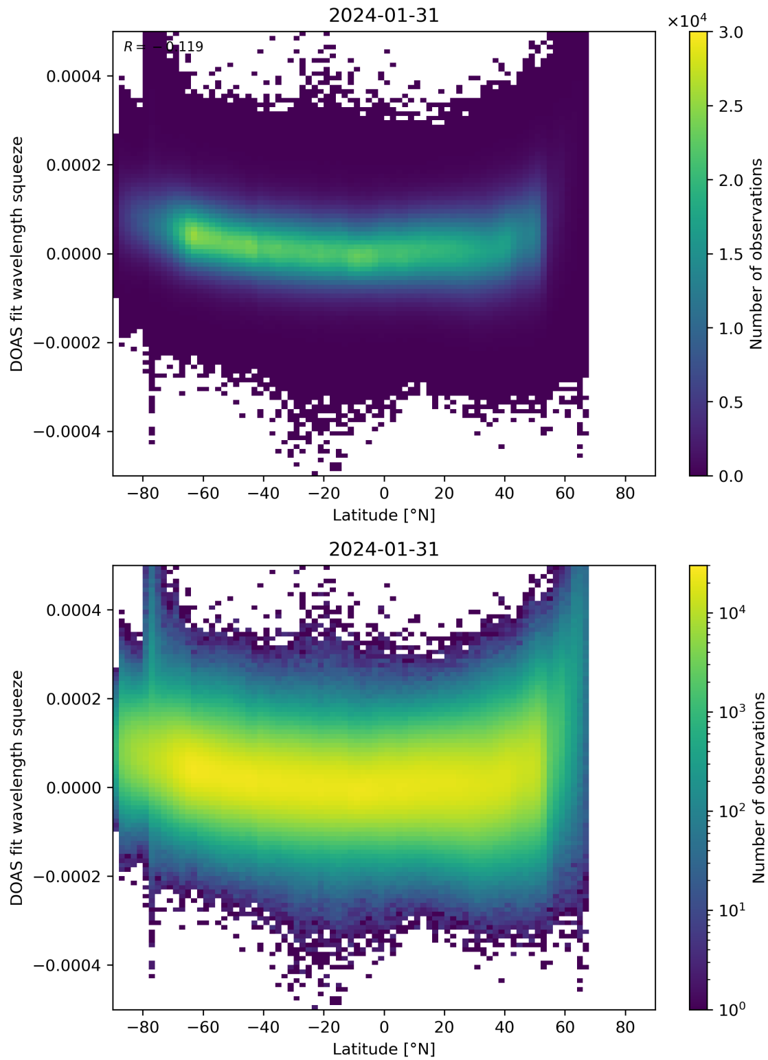
Figure 155: Scatter density plot of “Latitude” against “DOAS fit wavelength squeeze” for 2024-01-31 to 2024-02-01.
