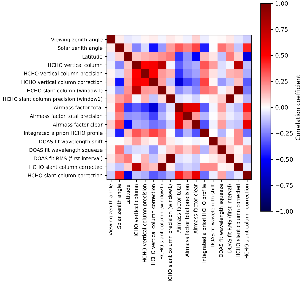
Figure 2: Map of correlation matrix for 2024-01-31 to 2024-02-01.
