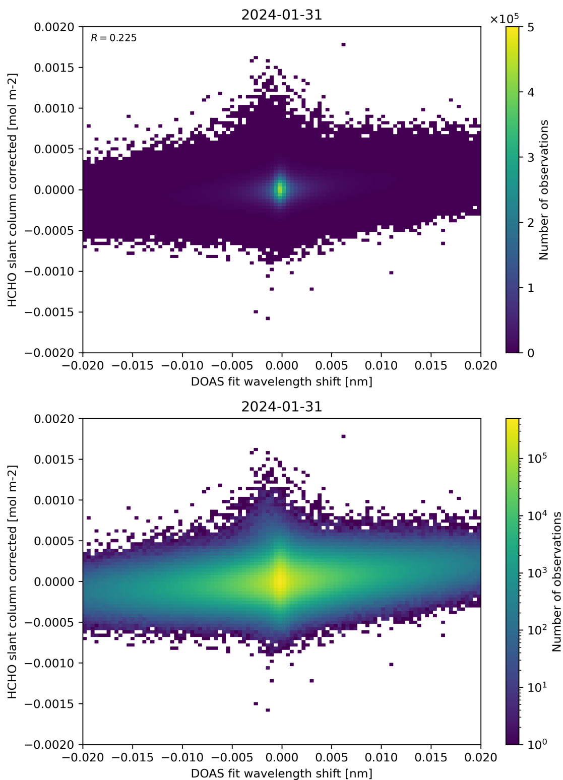
Figure 66: Scatter density plot of “DOAS fit wavelength shift” against “HCHO slant column corrected” for 2024-01-31 to 2024-02-01.
