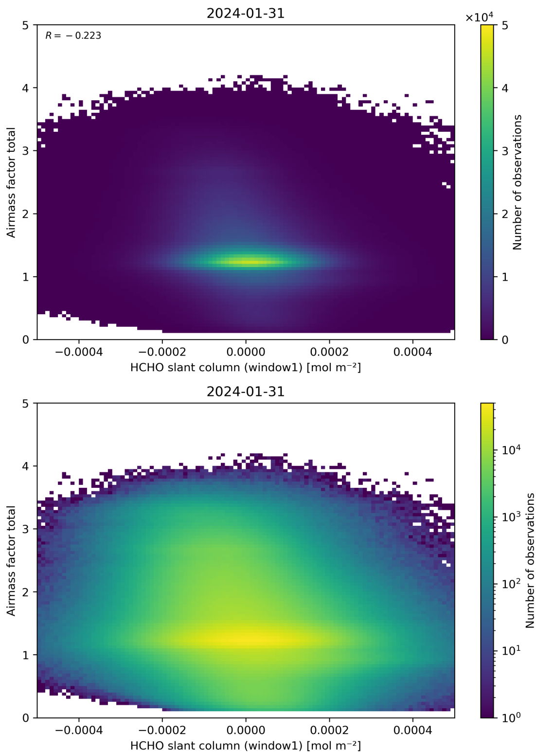
Figure 85: Scatter density plot of “HCHO slant column (window1)” against “Airmass factor total” for 2024-01-31 to 2024-02-01.
