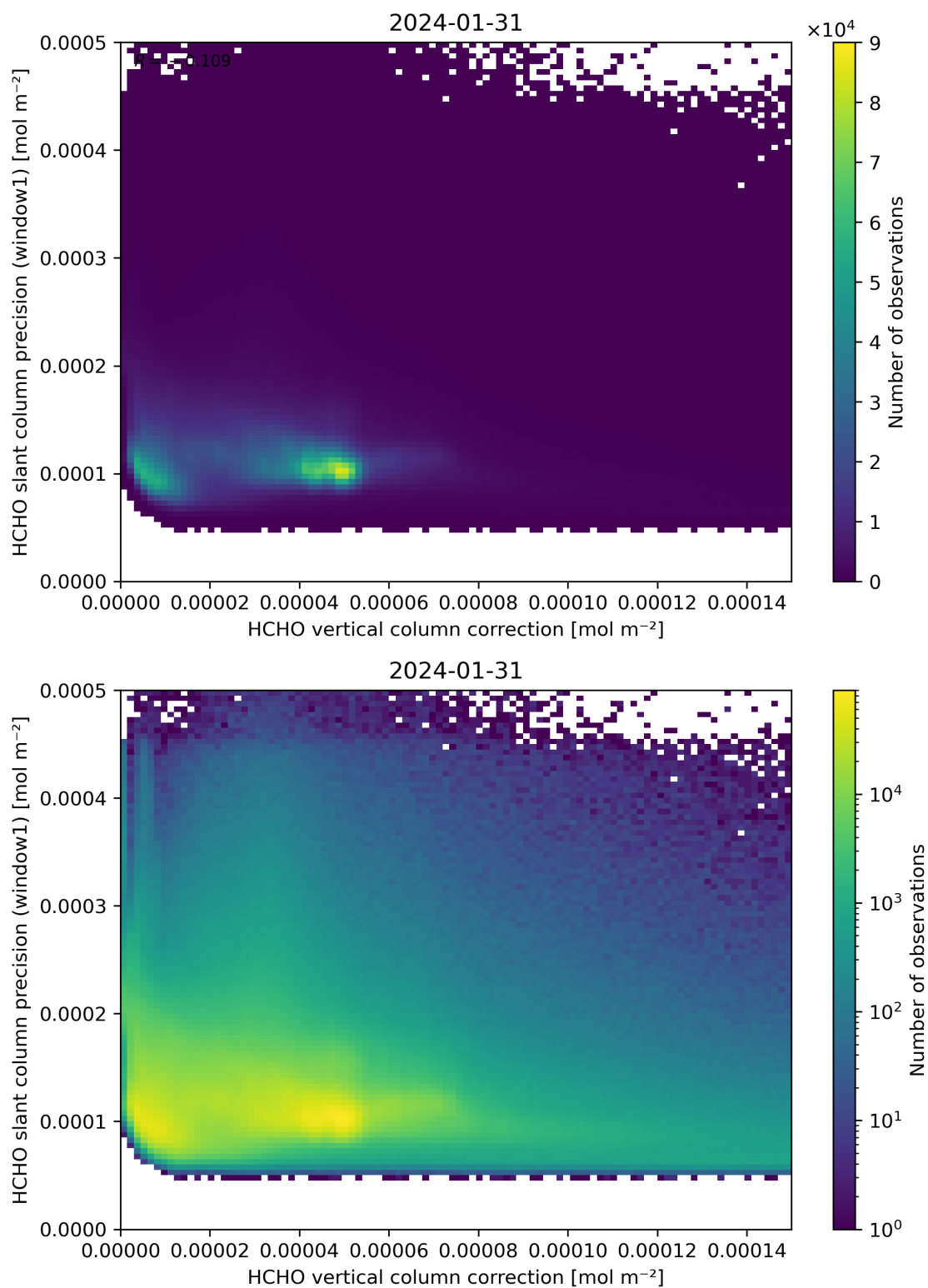
Figure 119: Scatter density plot of “HCHO vertical column correction” against “HCHO slant column precision (window1)” for 2024-01-31 to 2024-02-01.
