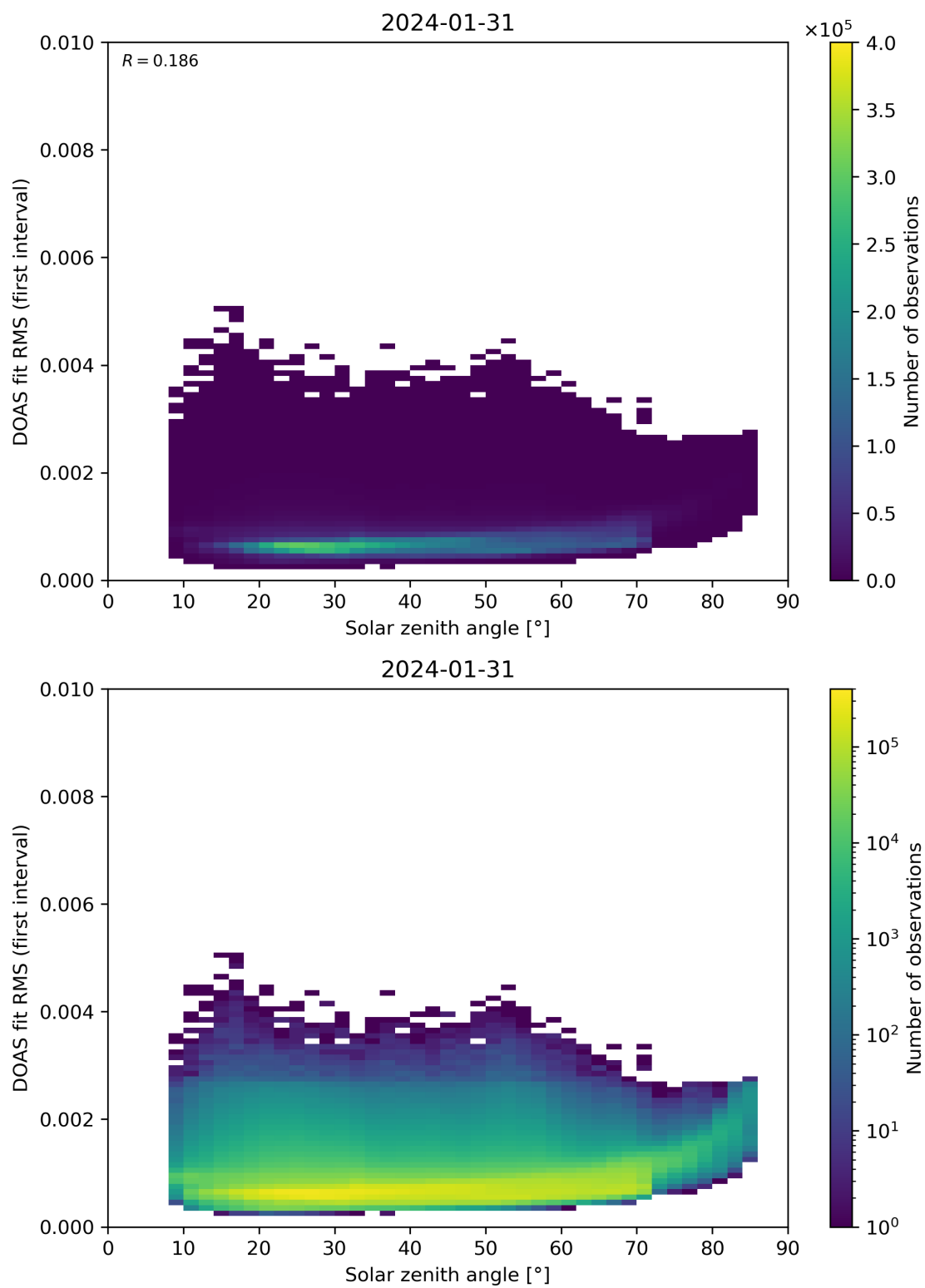
Figure 167: Scatter density plot of “Solar zenith angle” against “DOAS fit RMS (first interval)” for 2024-01-31 to 2024-02-01.
