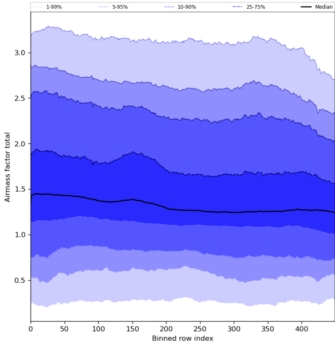
Figure 54: Along track statistics of “Airmass factor total” for 2024-01-31 to 2024-02-01
