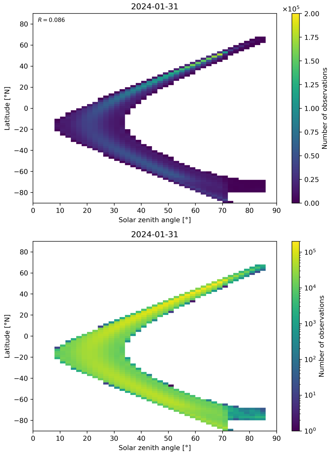
Figure 181: Scatter density plot of “Solar zenith angle” against “Latitude” for 2024-01-31 to 2024-02-01.
