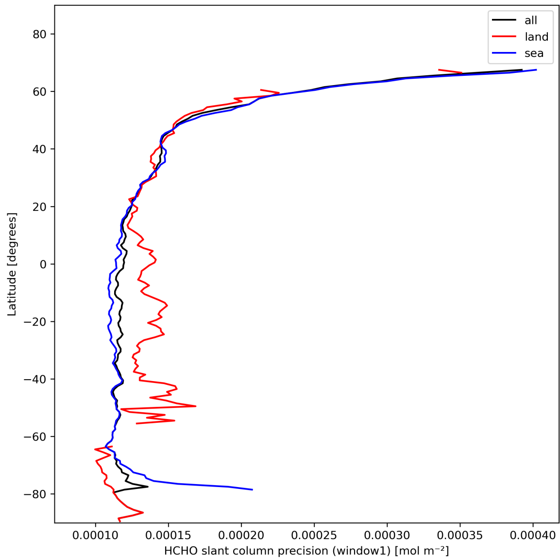
Figure 25: Zonal average of “HCHO slant column precision (window1)” for 2024-01-31 to 2024-02-01.
