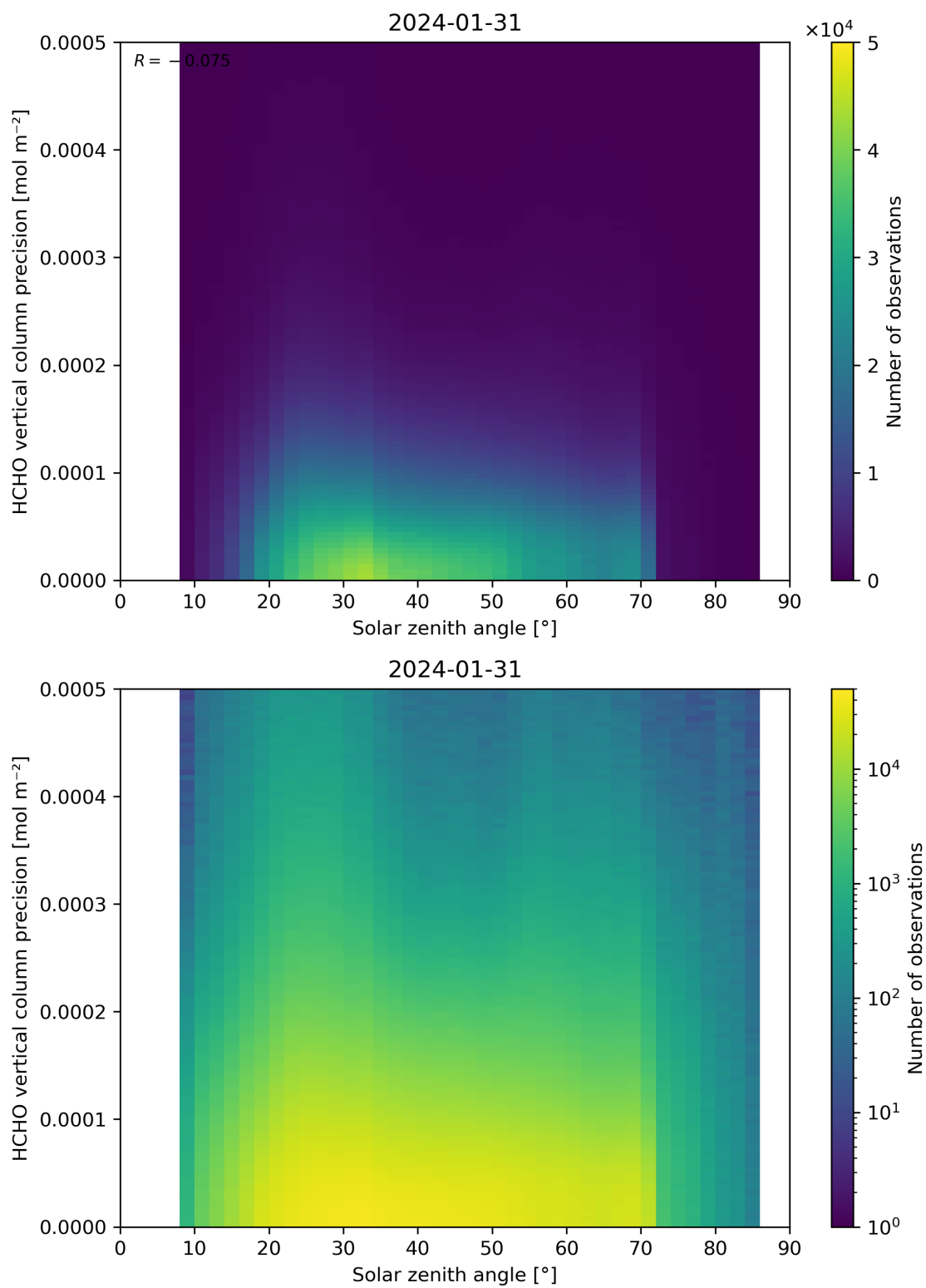
Figure 179: Scatter density plot of “Solar zenith angle” against “HCHO vertical column precision” for 2024-01-31 to 2024-02-01.
