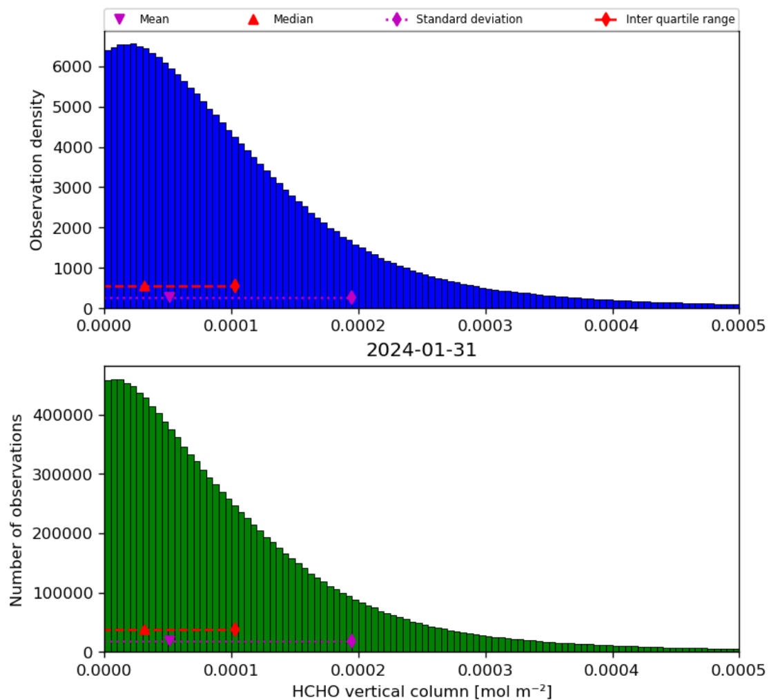
Figure 35: Histogram of “HCHO vertical column” for 2024-01-31 to 2024-02-01
