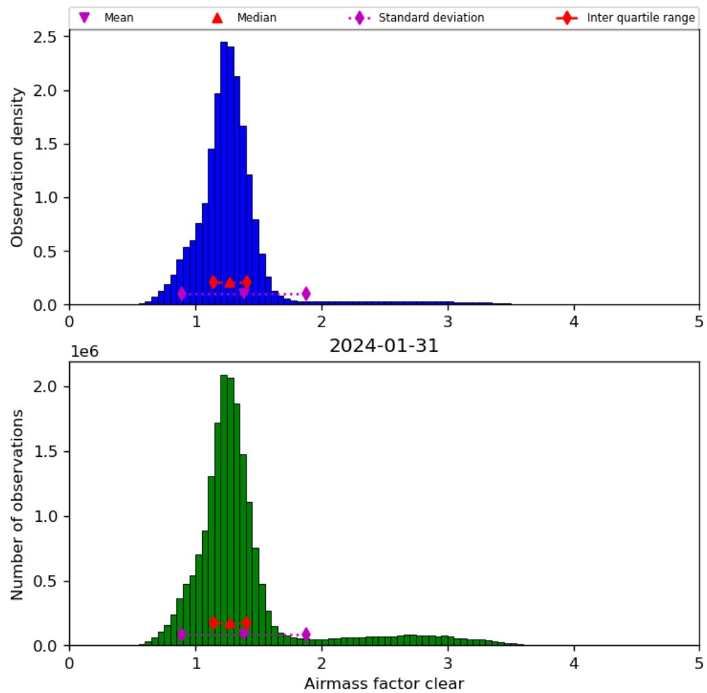
Figure 42: Histogram of “Airmass factor clear” for 2024-01-31 to 2024-02-01
