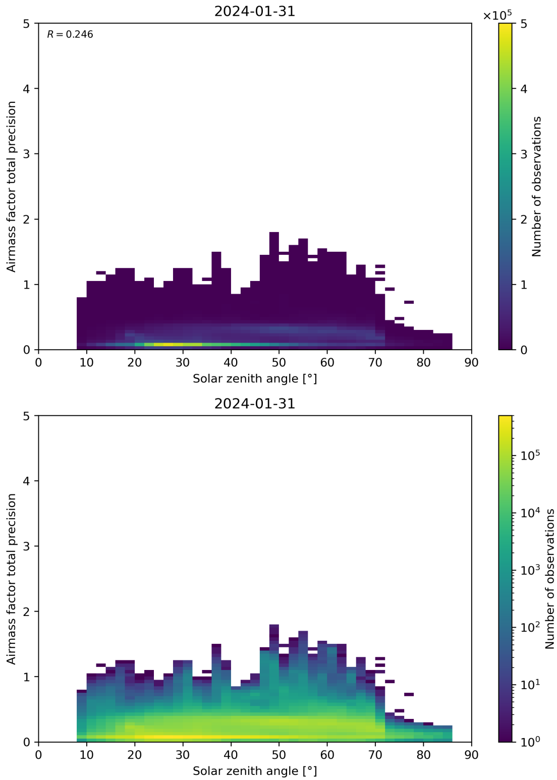
Figure 176: Scatter density plot of “Solar zenith angle” against “Airmass factor total precision” for 2024-01-31 to 2024-02-01.
