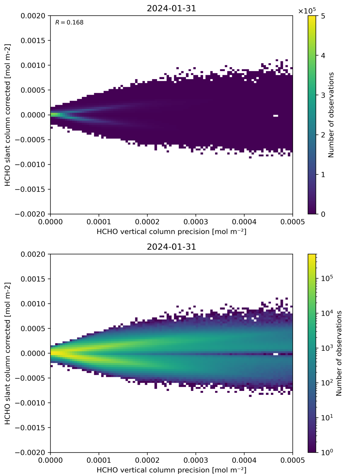
Figure 140: Scatter density plot of “HCHO vertical column precision” against “HCHO slant column corrected” for 2024-01-31 to 2024-02-01.
