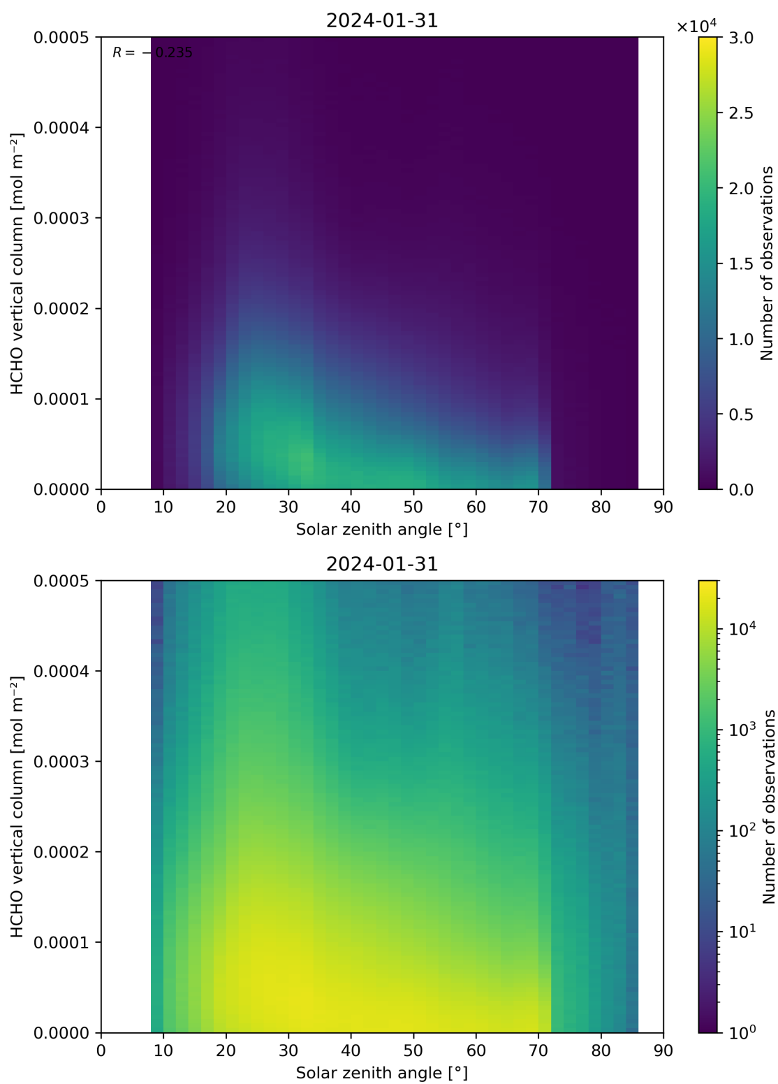
Figure 177: Scatter density plot of “Solar zenith angle” against “HCHO vertical column” for 2024-01-31 to 2024-02-01.
