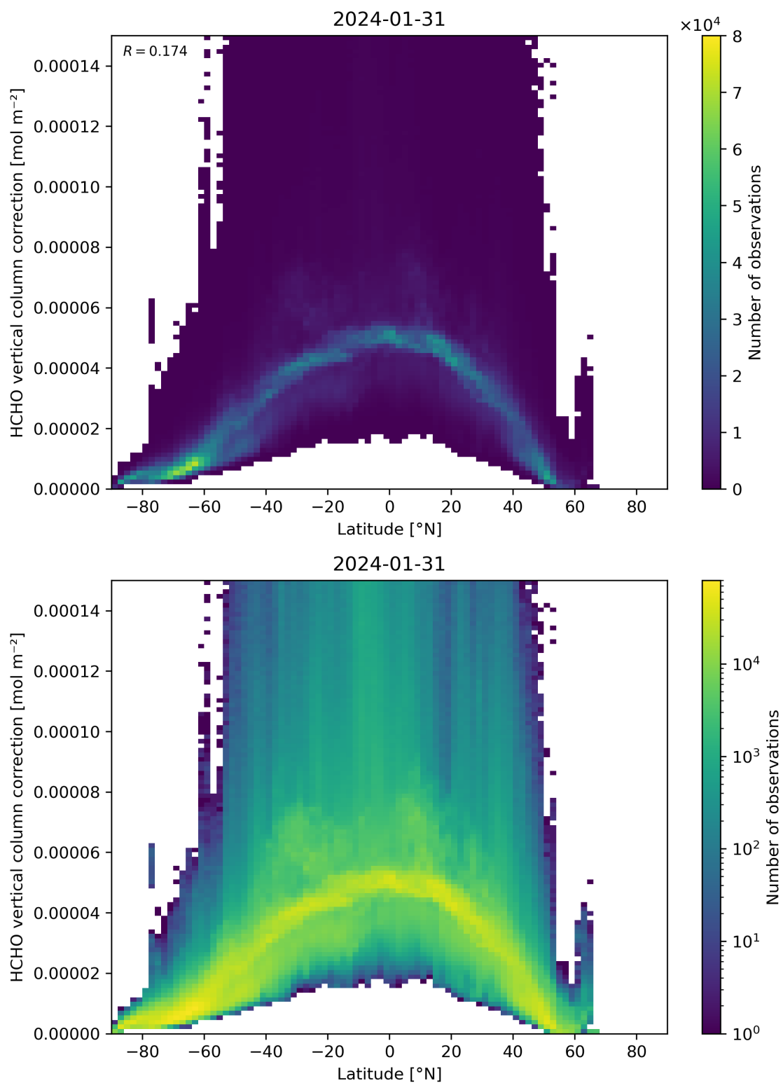
Figure 164: Scatter density plot of “Latitude” against “HCHO vertical column correction” for 2024-01-31 to 2024-02-01.
