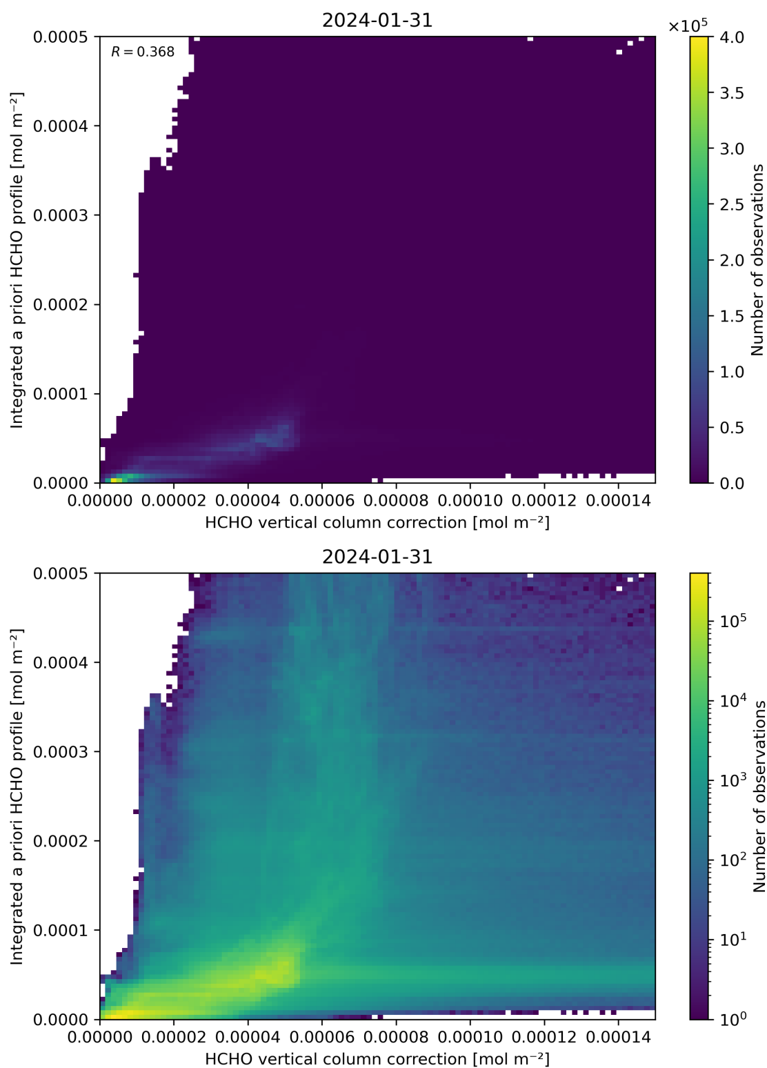
Figure 122: Scatter density plot of “HCHO vertical column correction” against “Integrated a priori HCHO profile” for 2024-01-31 to 2024-02-01.
