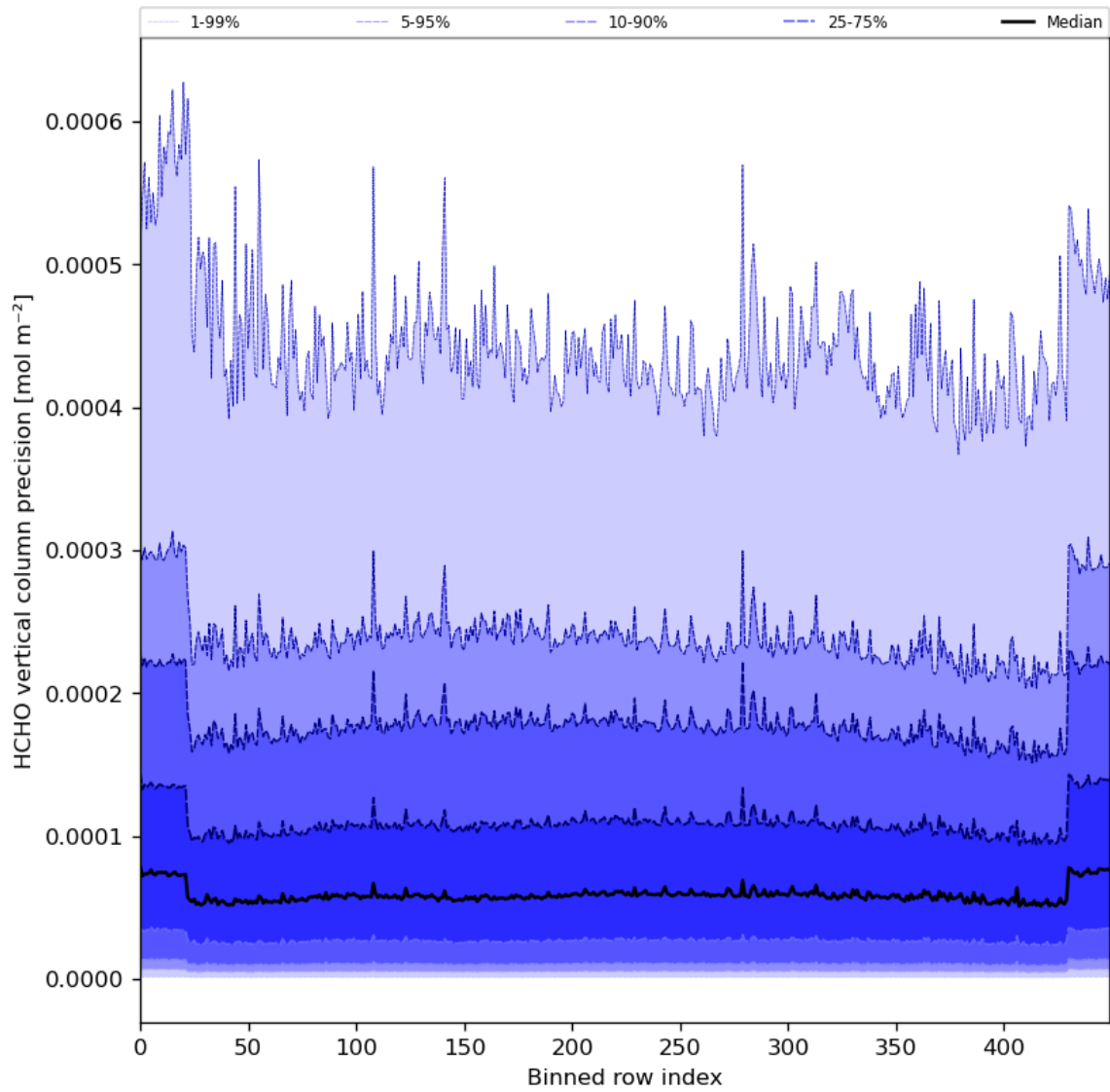
Figure 50: Along track statistics of “HCHO vertical column precision” for 2024-01-31 to 2024-02-01
