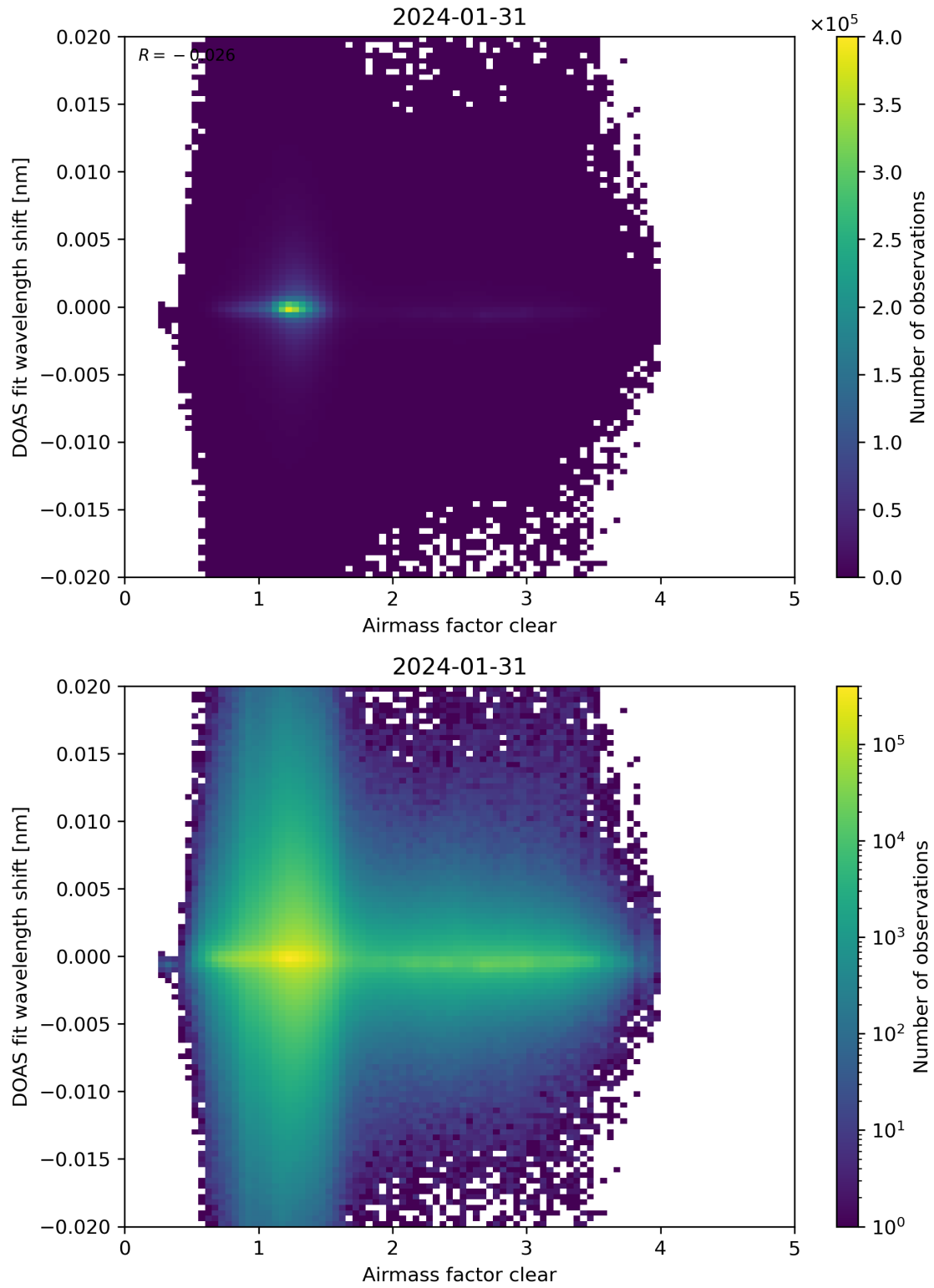
Figure 72: Scatter density plot of “Airmass factor clear” against “DOAS fit wavelength shift” for 2024-01-31 to 2024-02-01.
