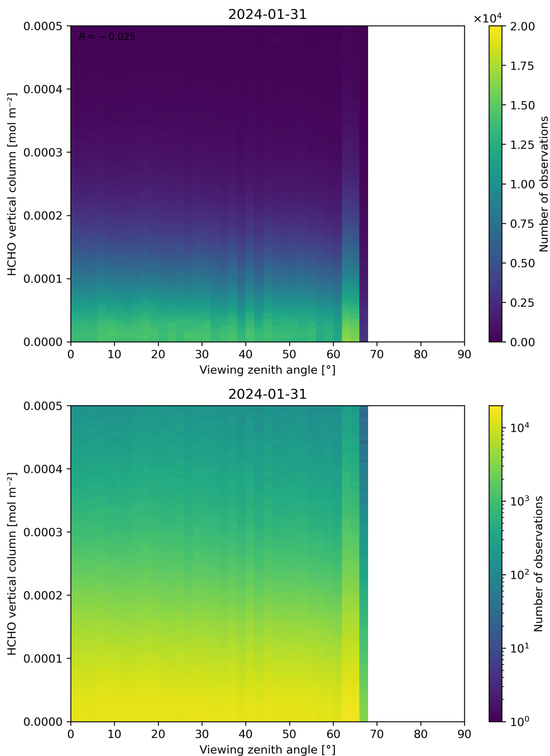
Figure 192: Scatter density plot of “Viewing zenith angle” against “HCHO vertical column” for 2024-01-31 to 2024-02-01.
