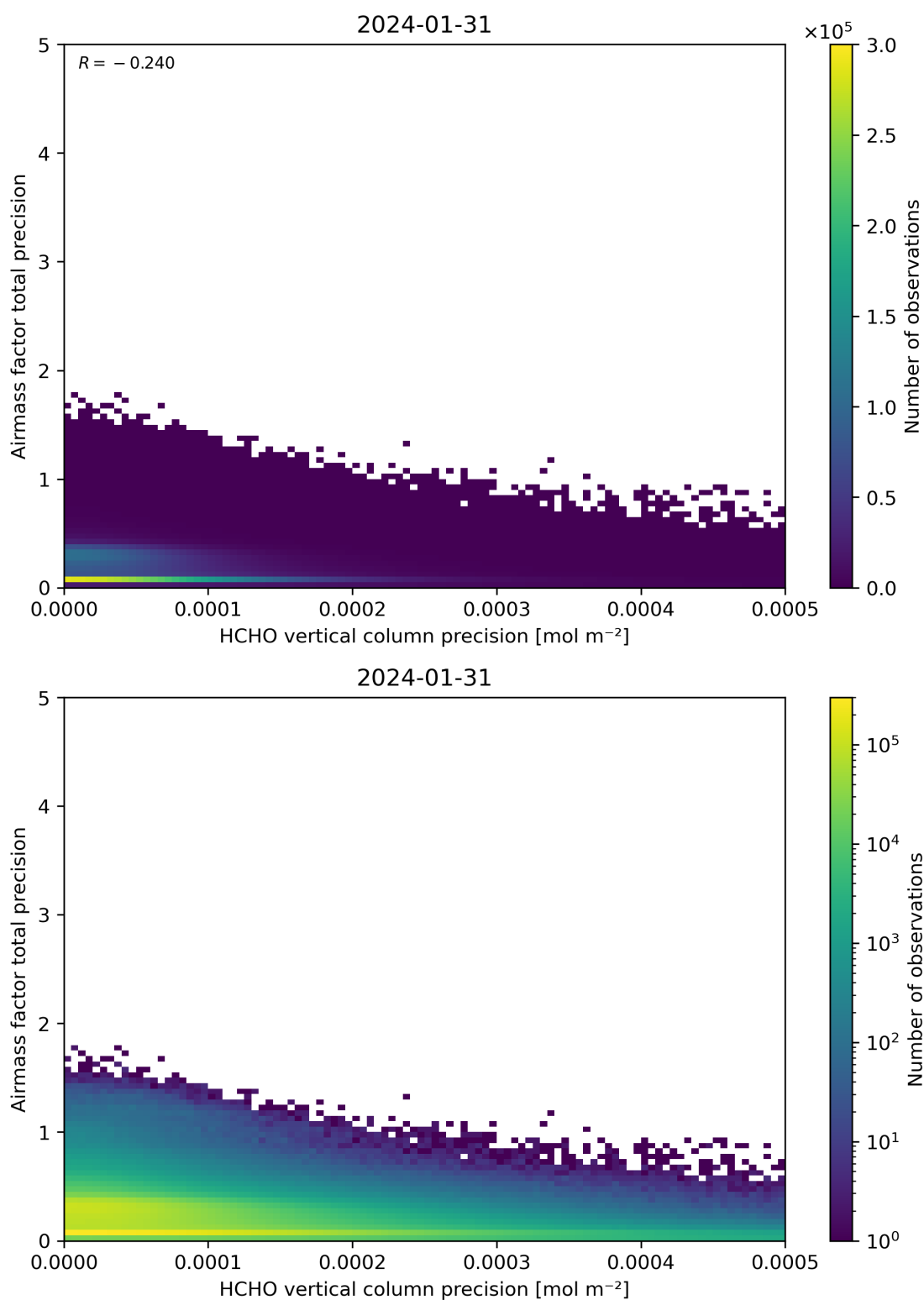
Figure 145: Scatter density plot of “HCHO vertical column precision” against “Airmass factor total precision” for 2024-01-31 to 2024-02-01.
