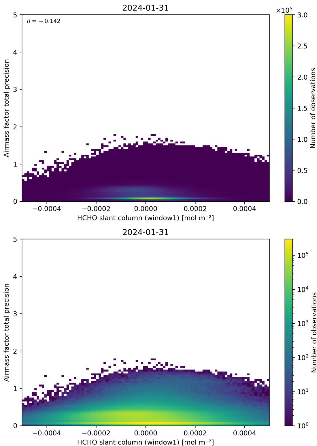
Figure 86: Scatter density plot of “HCHO slant column (window1)” against “Airmass factor total precision” for 2024-01-31 to 2024-02-01.
