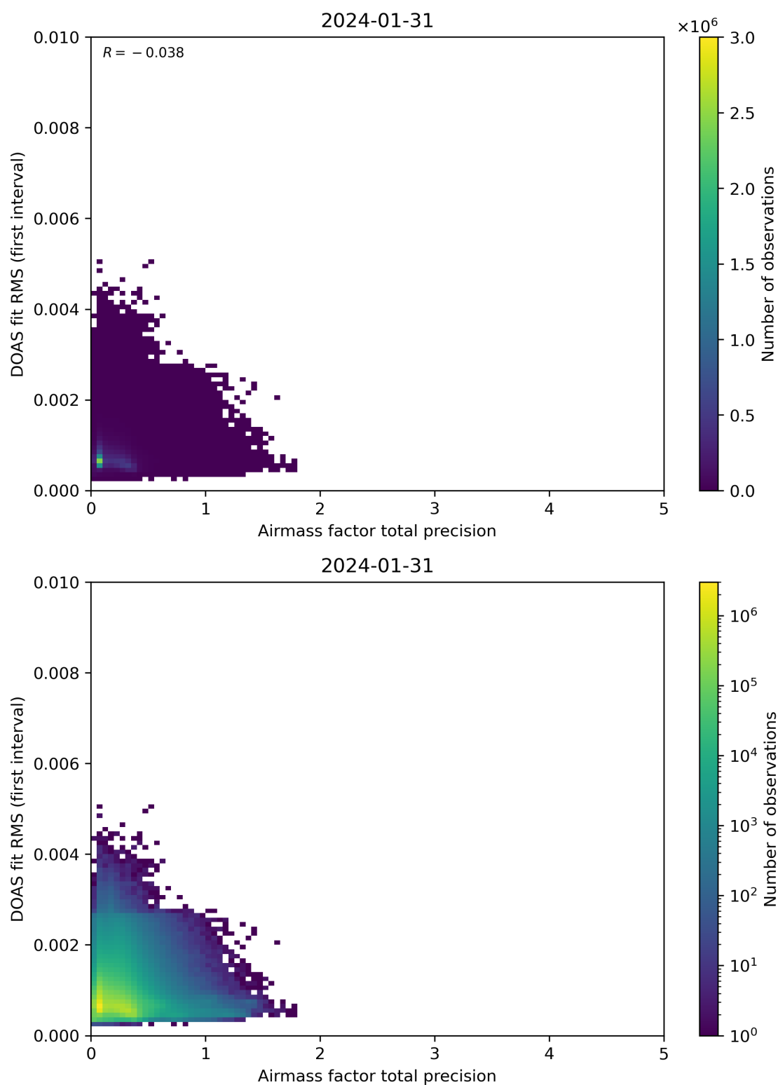
Figure 105: Scatter density plot of “Airmass factor total precision” against “DOAS fit RMS (first interval)” for 2024-01-31 to 2024-02-01.
