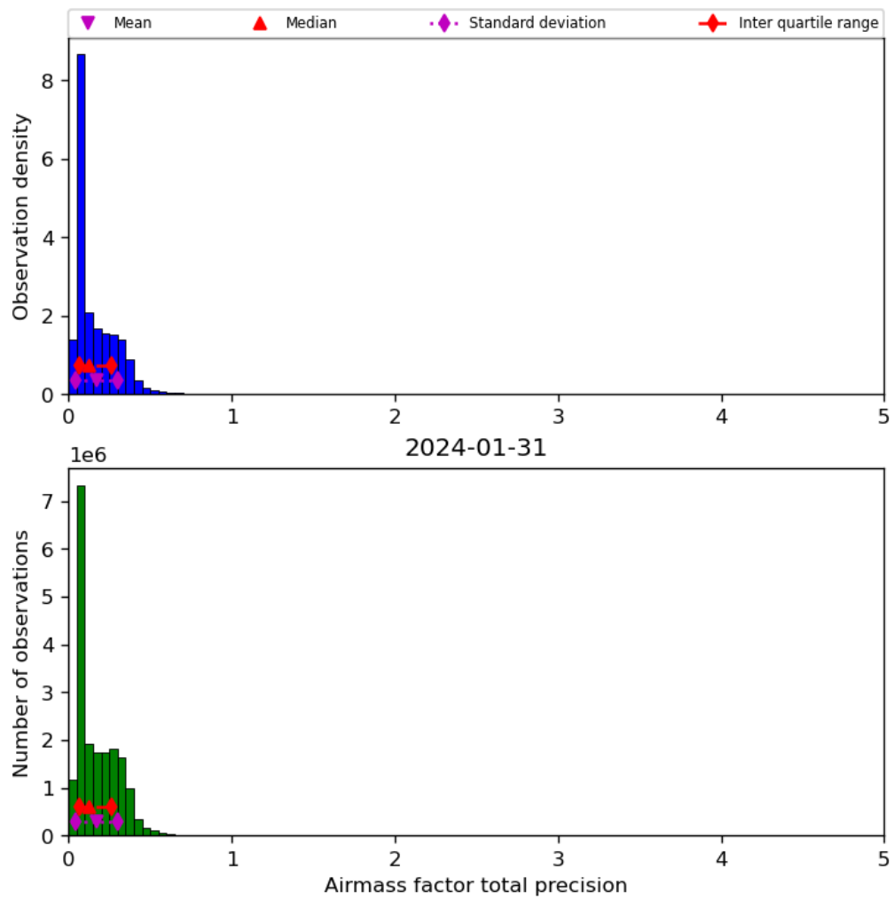
Figure 41: Histogram of “Airmass factor total precision” for 2024-01-31 to 2024-02-01
