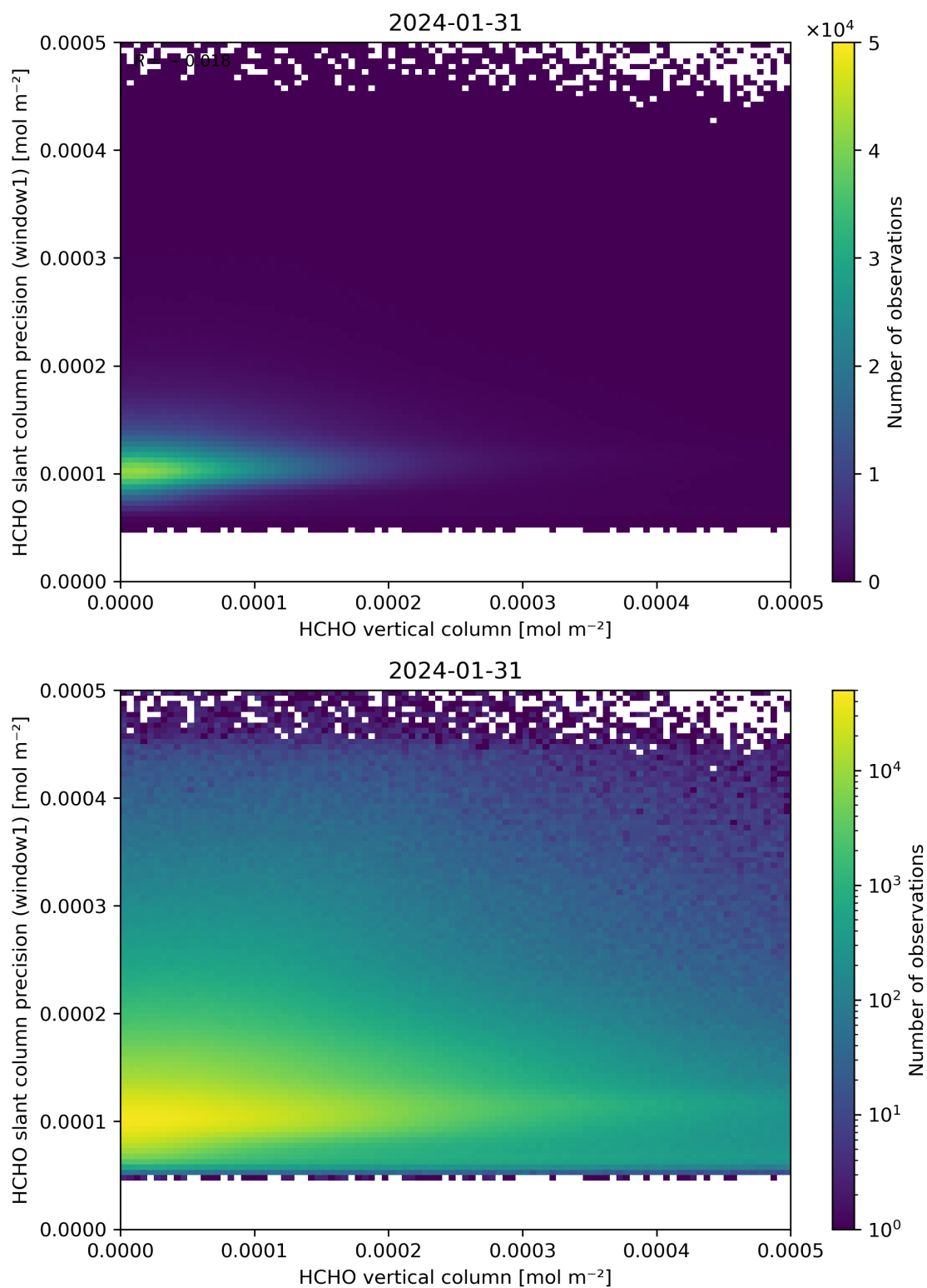
Figure 130: Scatter density plot of “HCHO vertical column” against “HCHO slant column precision (window1)” for 2024-01-31 to 2024-02-01.
