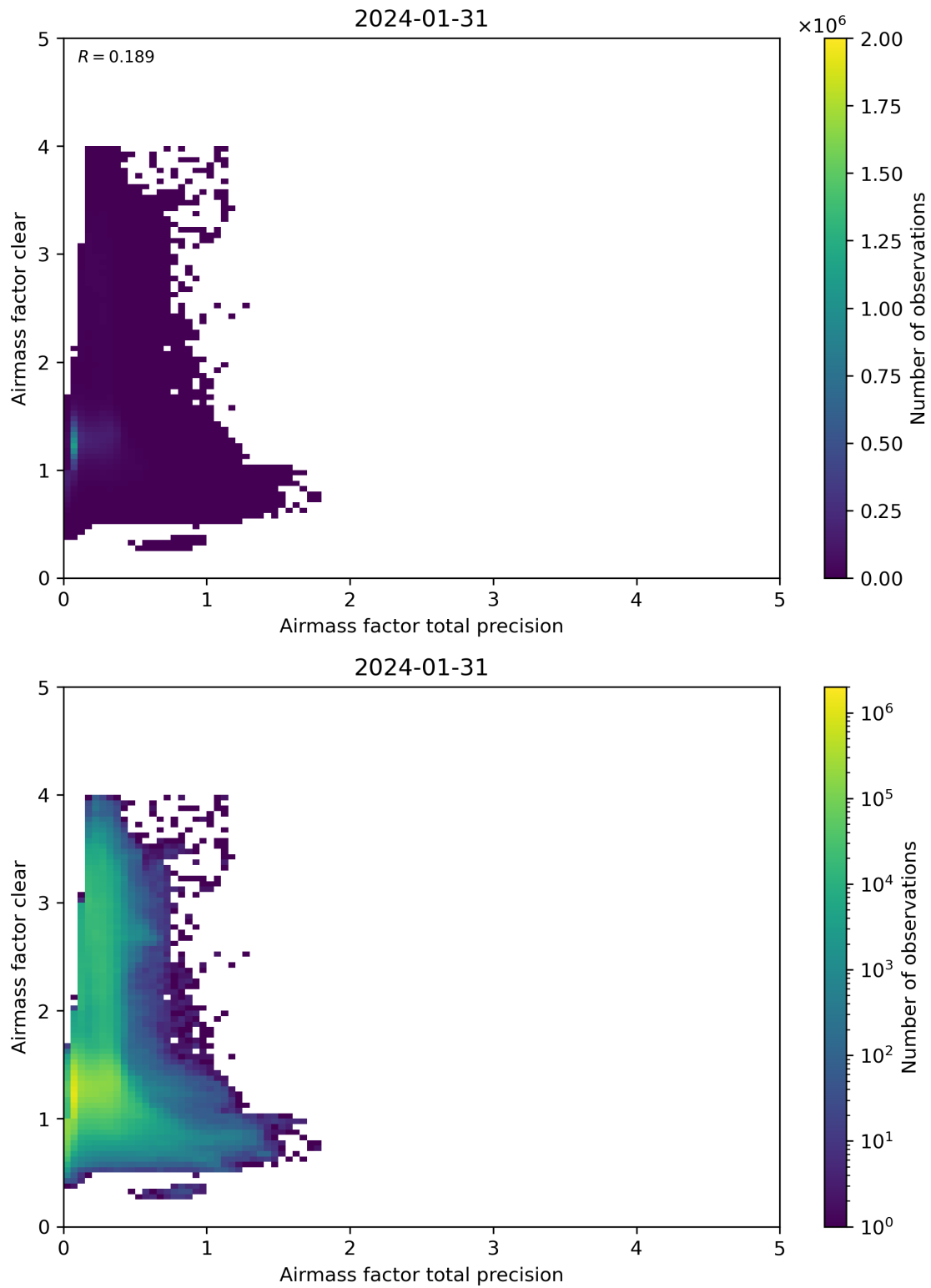
Figure 108: Scatter density plot of “Airmass factor total precision” against “Airmass factor clear” for 2024-01-31 to 2024-02-01.
