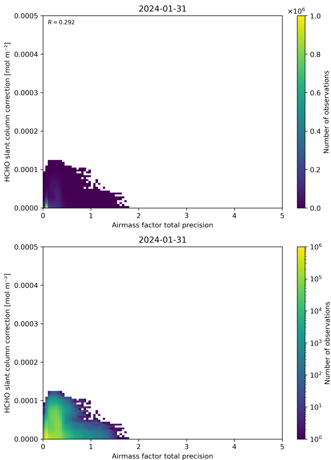
Figure 110: Scatter density plot of “Airmass factor total precision” against “HCHO slant column correction” for 2024-01-31 to 2024-02-01.
