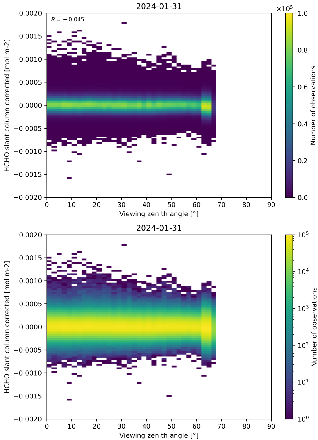
Figure 186: Scatter density plot of “Viewing zenith angle” against “HCHO slant column corrected” for 2024-01-31 to 2024-02-01.
