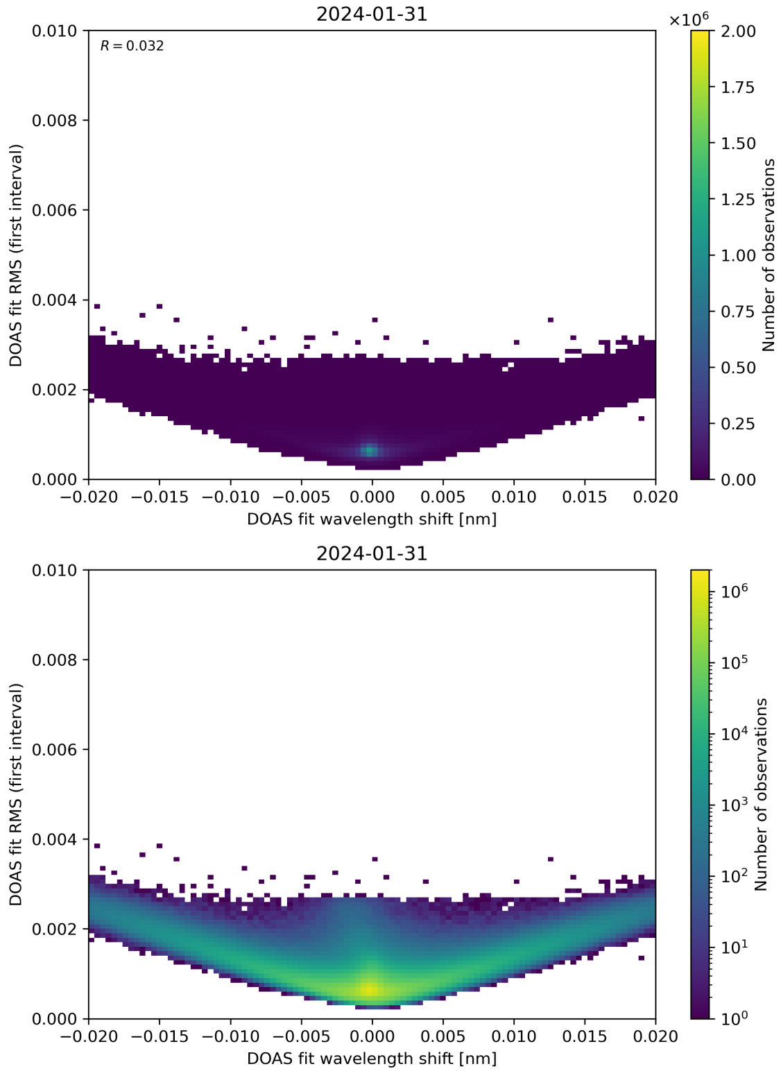
Figure 64: Scatter density plot of “DOAS fit wavelength shift” against “DOAS fit RMS (first interval)” for 2024-01-31 to 2024-02-01.
