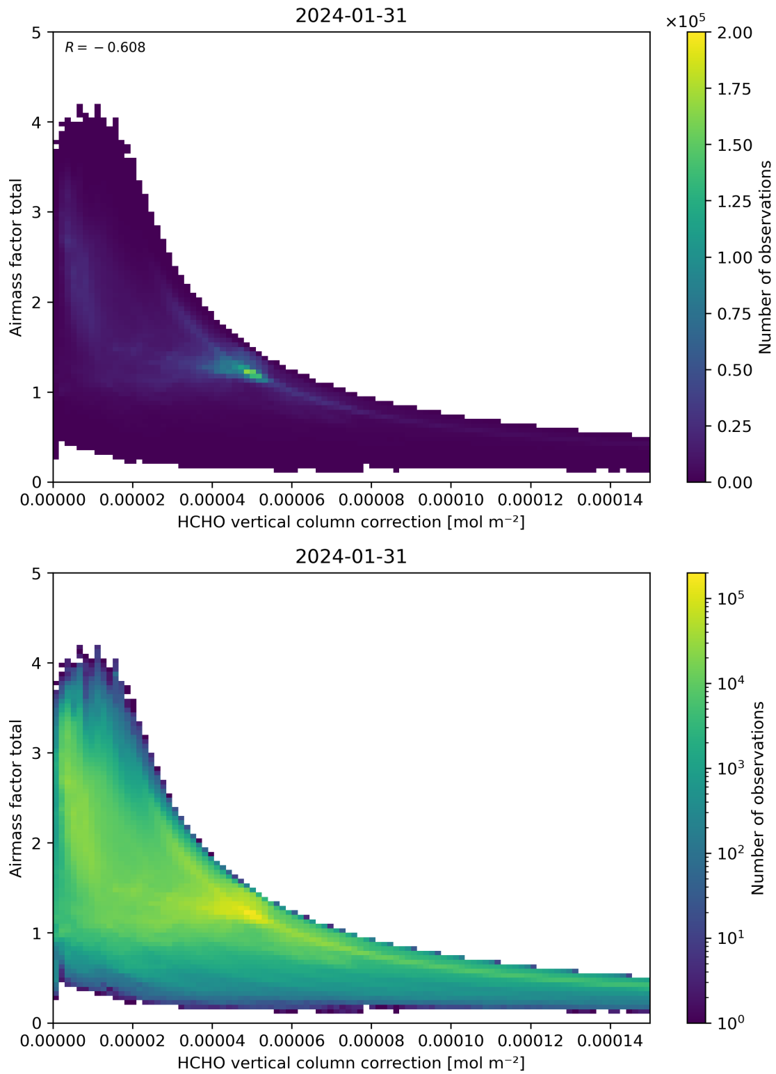
Figure 120: Scatter density plot of “HCHO vertical column correction” against “Airmass factor total” for 2024-01-31 to 2024-02-01.
