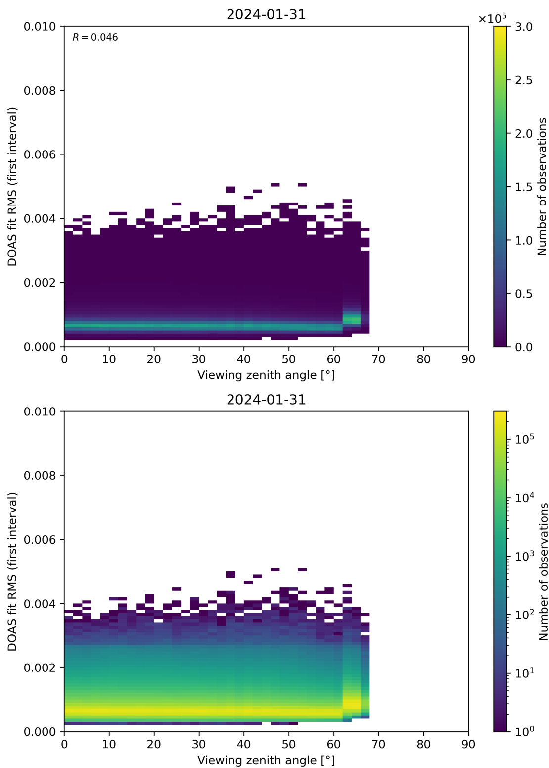
Figure 182: Scatter density plot of “Viewing zenith angle” against “DOAS fit RMS (first interval)” for 2024-01-31 to 2024-02-01.
