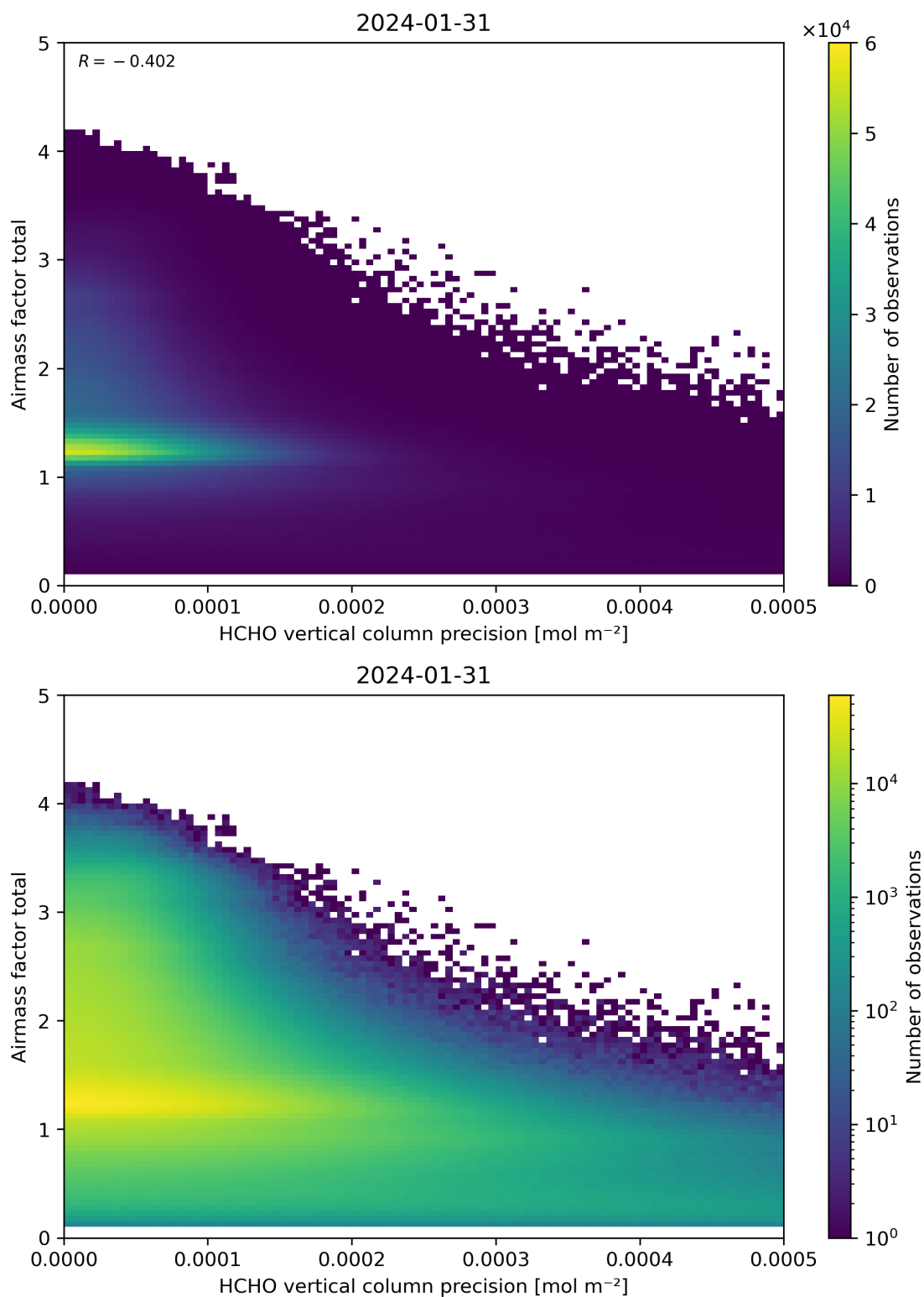
Figure 144: Scatter density plot of “HCHO vertical column precision” against “Airmass factor total” for 2024-01-31 to 2024-02-01.
