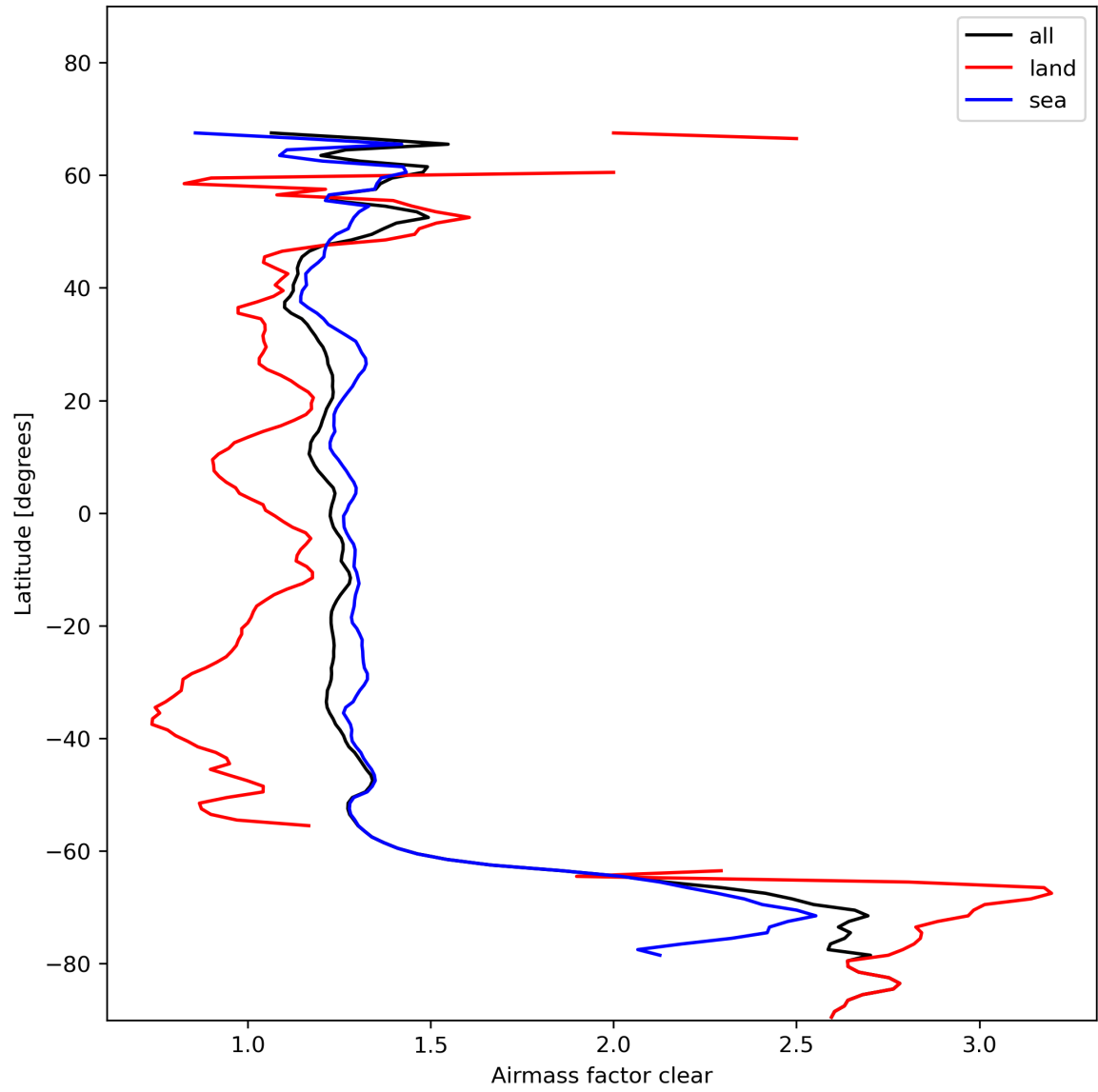
Figure 28: Zonal average of “Airmass factor clear” for 2024-01-31 to 2024-02-01.
