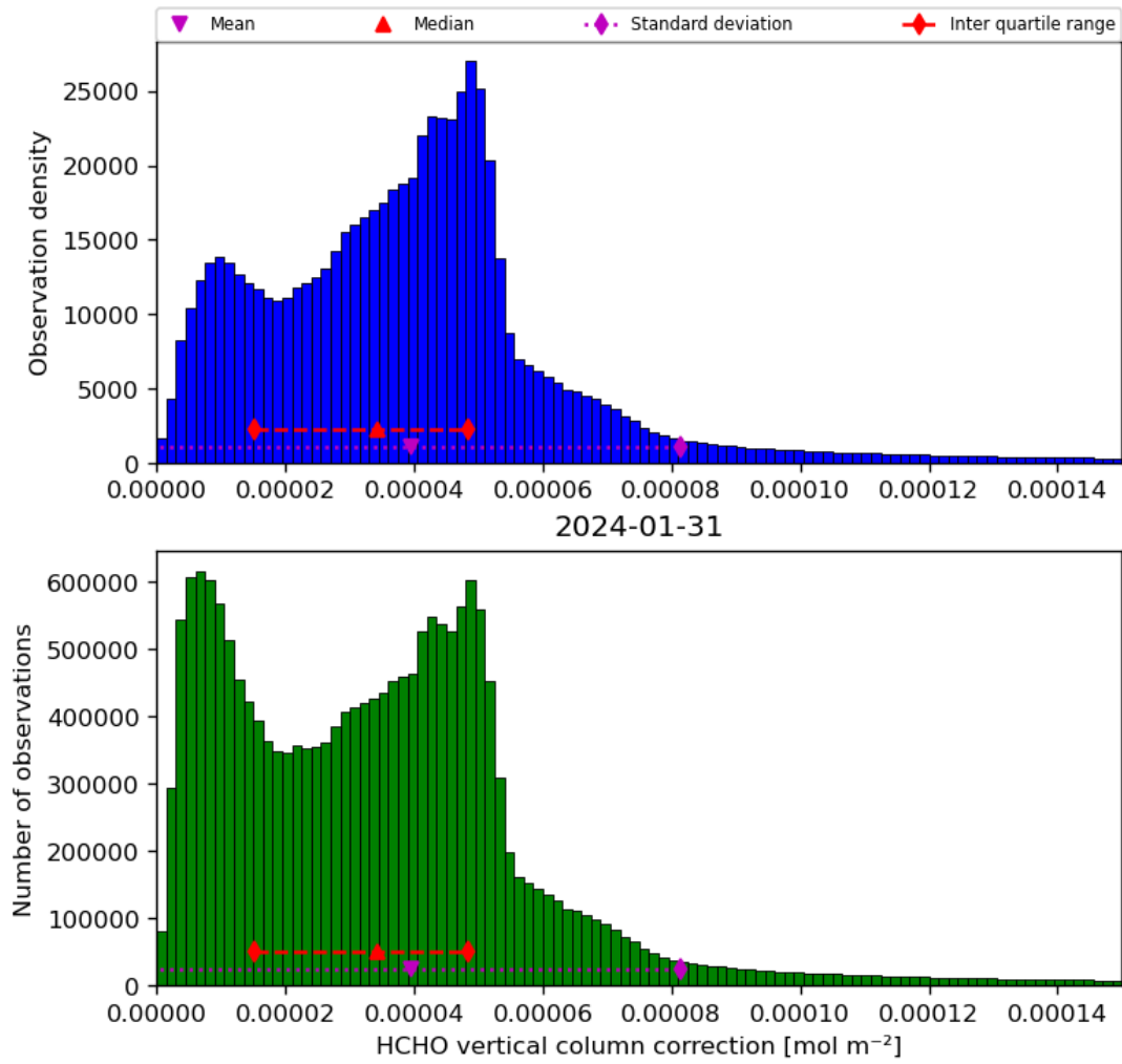
Figure 37: Histogram of “HCHO vertical column correction” for 2024-01-31 to 2024-02-01
