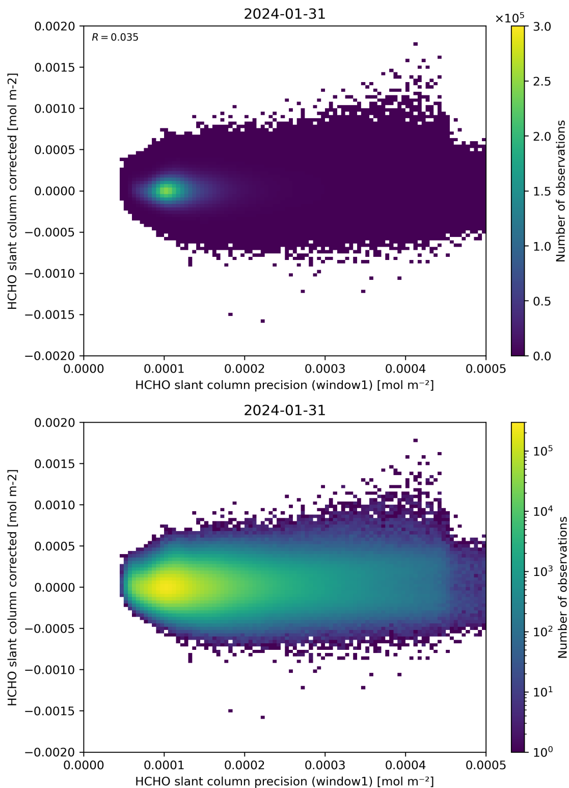
Figure 92: Scatter density plot of “HCHO slant column precision (window1)” against “HCHO slant column corrected” for 2024-01-31 to 2024-02-01.
