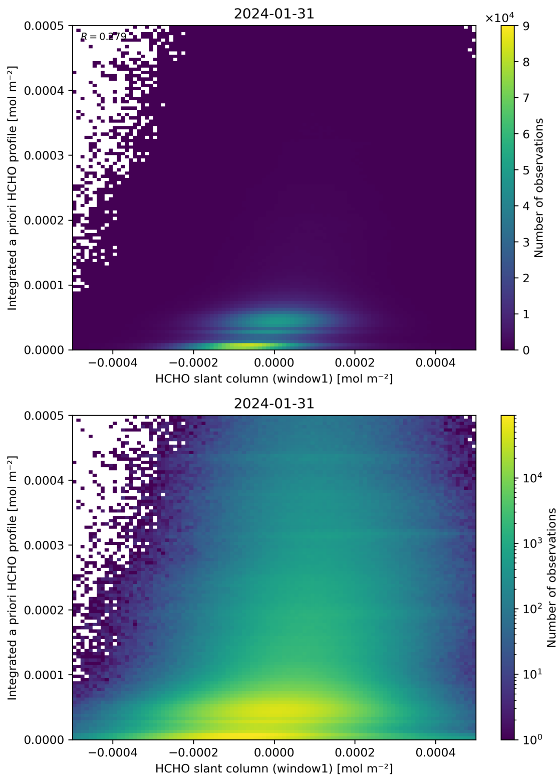
Figure 87: Scatter density plot of “HCHO slant column (window1)” against “Integrated a priori HCHO profile” for 2024-01-31 to 2024-02-01.
