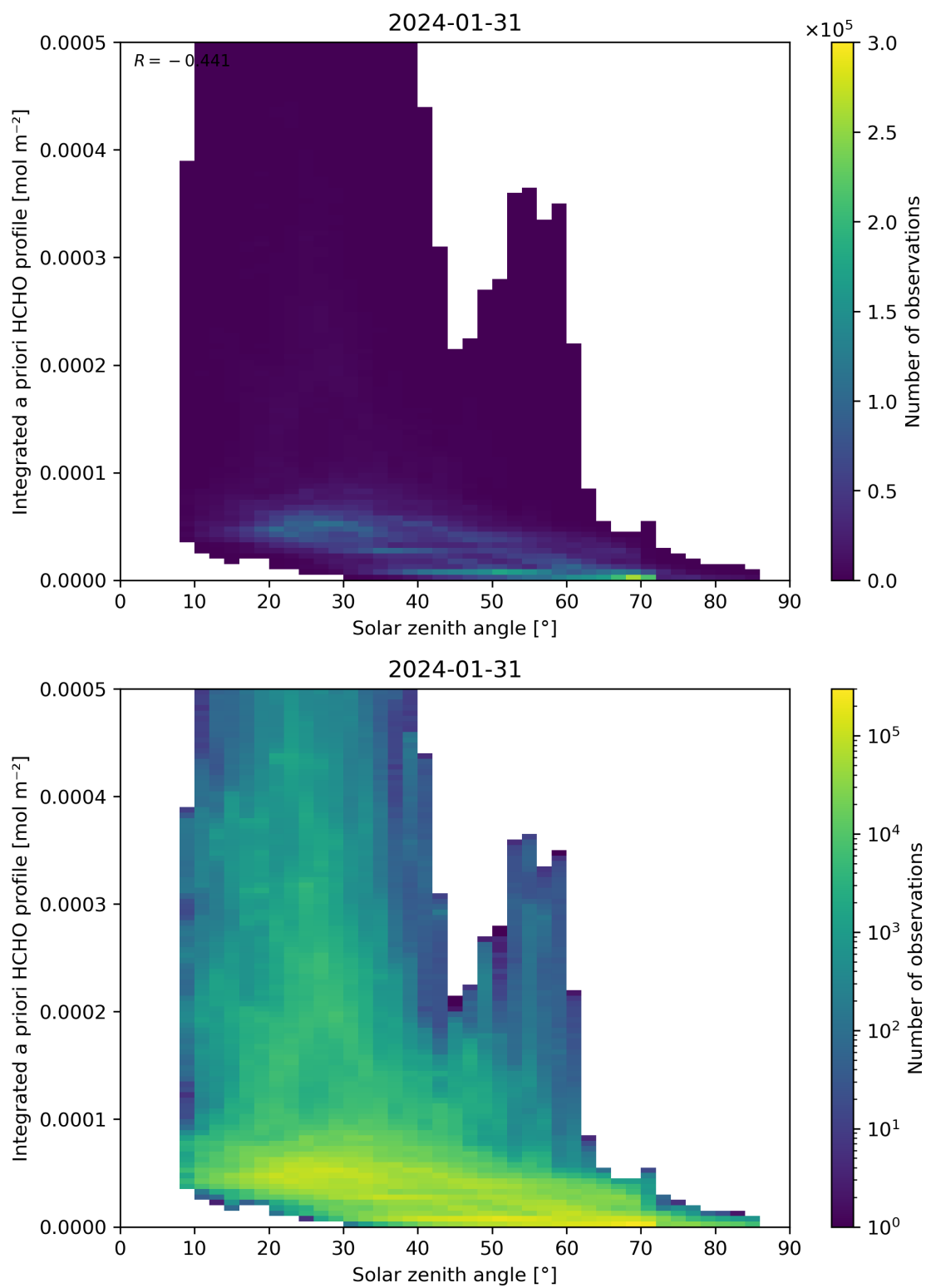
Figure 180: Scatter density plot of “Solar zenith angle” against “Integrated a priori HCHO profile” for 2024-01-31 to 2024-02-01.
