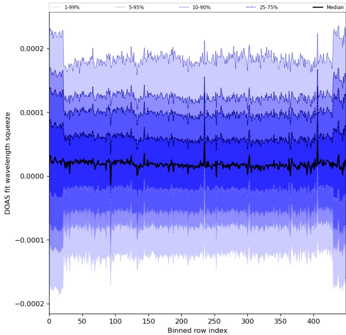
Figure 59: Along track statistics of “DOAS fit wavelength squeeze” for 2024-01-31 to 2024-02-01
