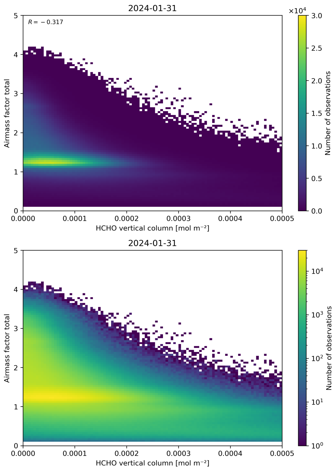
Figure 131: Scatter density plot of “HCHO vertical column” against “Airmass factor total” for 2024-01-31 to 2024-02-01.
