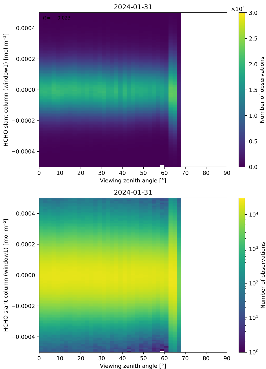
Figure 188: Scatter density plot of “Viewing zenith angle” against “HCHO slant column (window1)” for 2024-01-31 to 2024-02-01.
