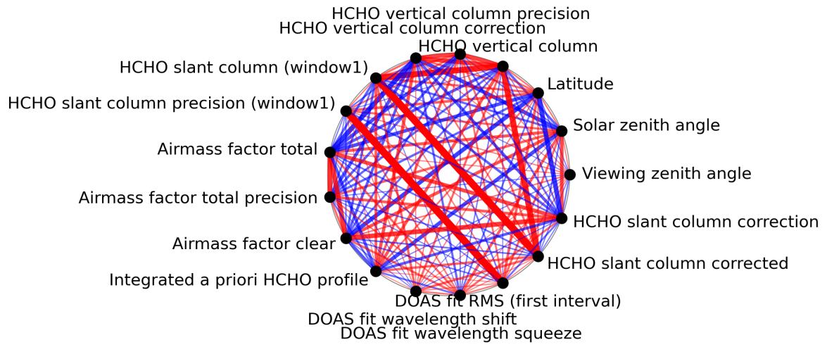
Figure 1: Map of correlation graph for 2024-01-31 to 2024-02-01.
