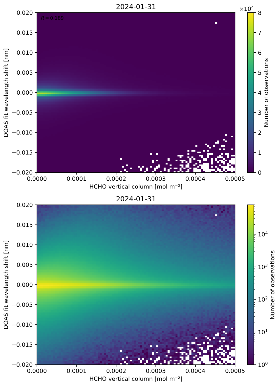
Figure 124: Scatter density plot of “HCHO vertical column” against “DOAS fit wavelength shift” for 2024-01-31 to 2024-02-01.
