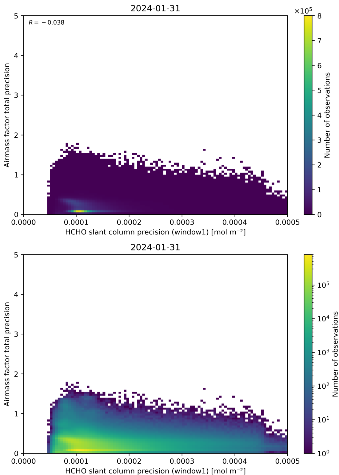
Figure 95: Scatter density plot of “HCHO slant column precision (window1)” against “Airmass factor total precision” for 2024-01-31 to 2024-02-01.
