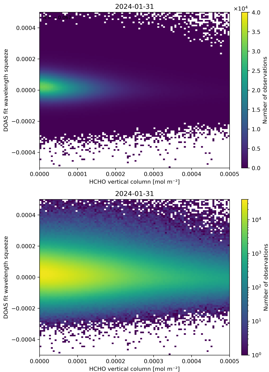
Figure 125: Scatter density plot of “HCHO vertical column” against “DOAS fit wavelength squeeze” for 2024-01-31 to 2024-02-01.
