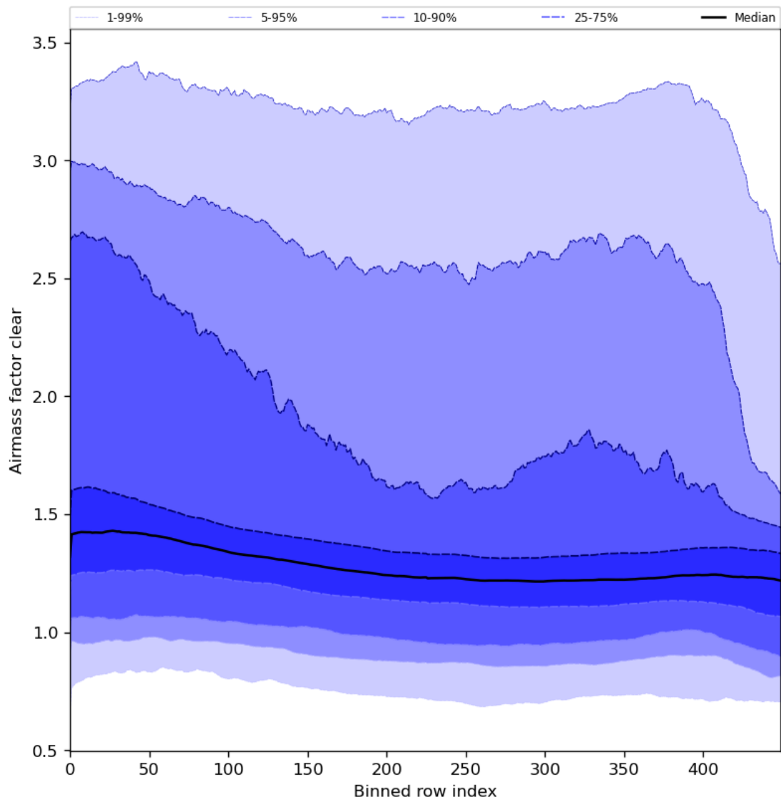
Figure 56: Along track statistics of “Airmass factor clear” for 2024-01-31 to 2024-02-01
