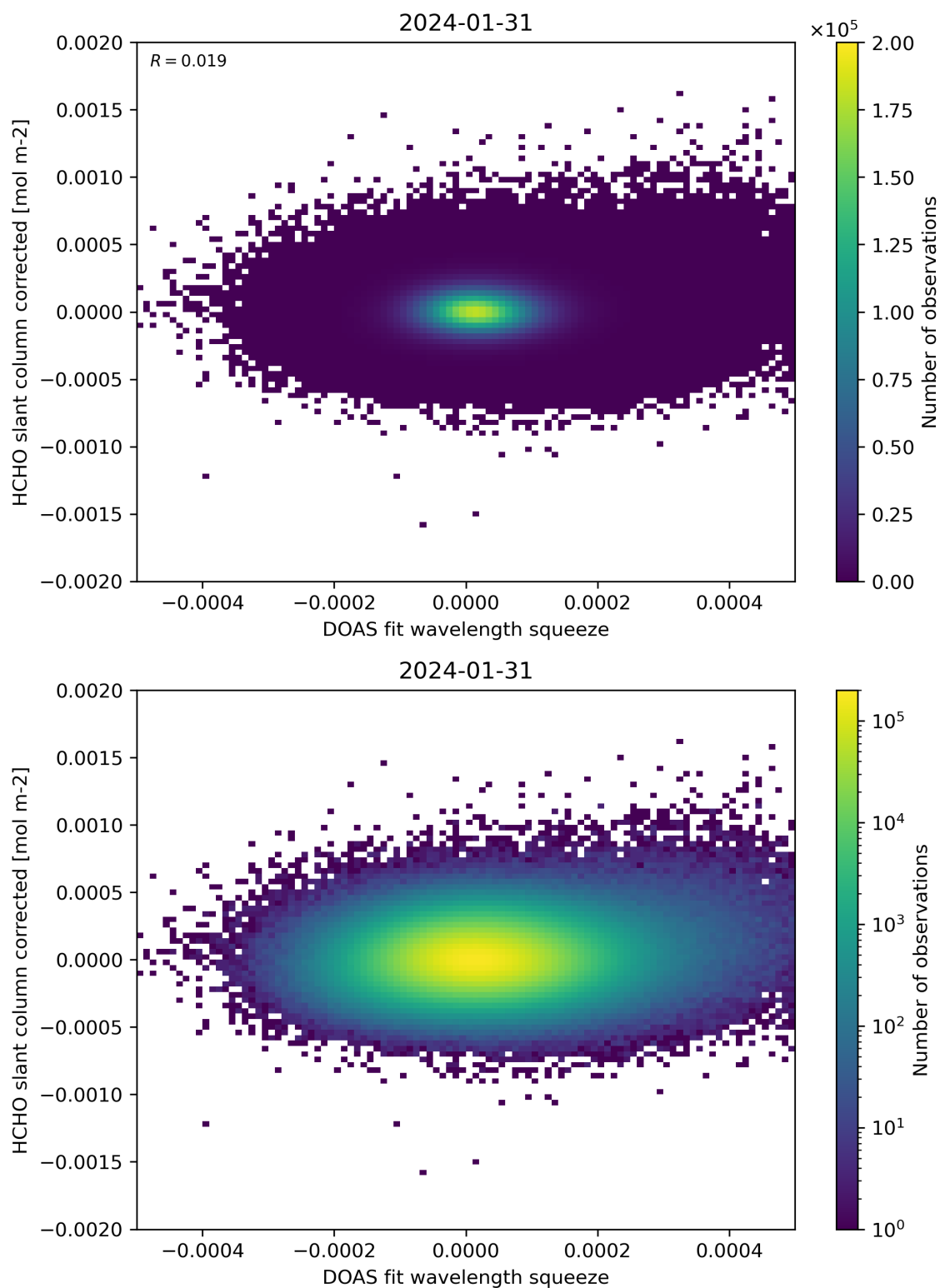
Figure 69: Scatter density plot of “DOAS fit wavelength squeeze” against “HCHO slant column corrected” for 2024-01-31 to 2024-02-01.
