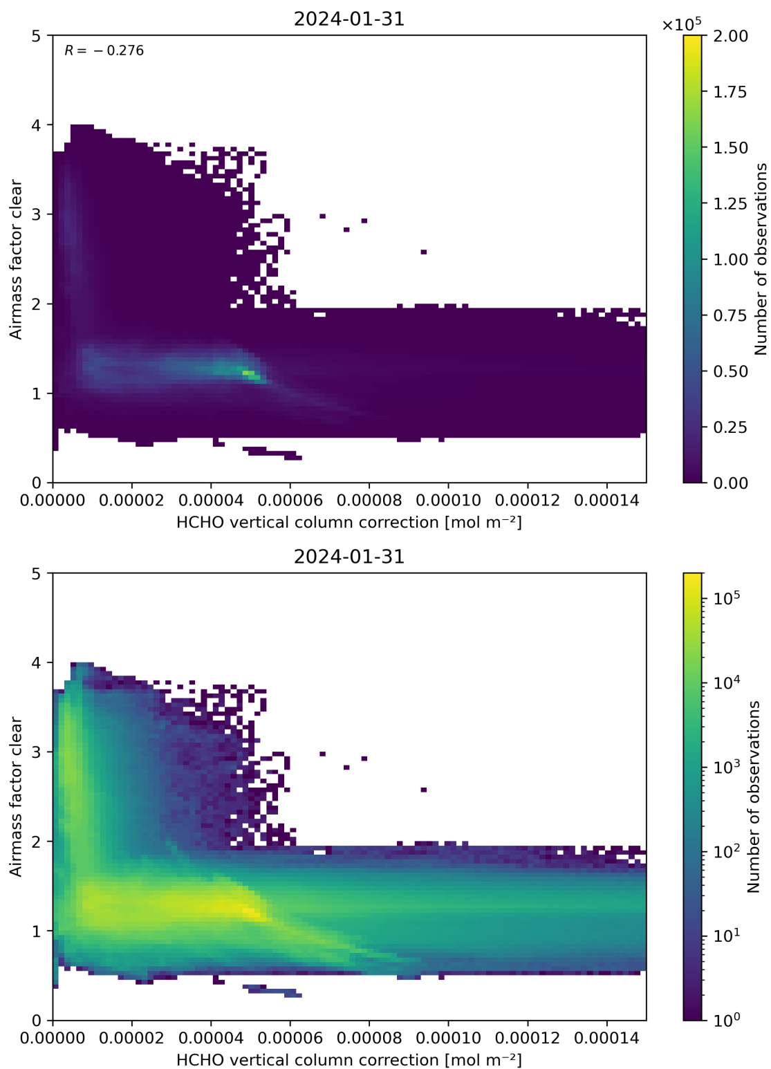
Figure 115: Scatter density plot of “HCHO vertical column correction” against “Airmass factor clear” for 2024-01-31 to 2024-02-01.
