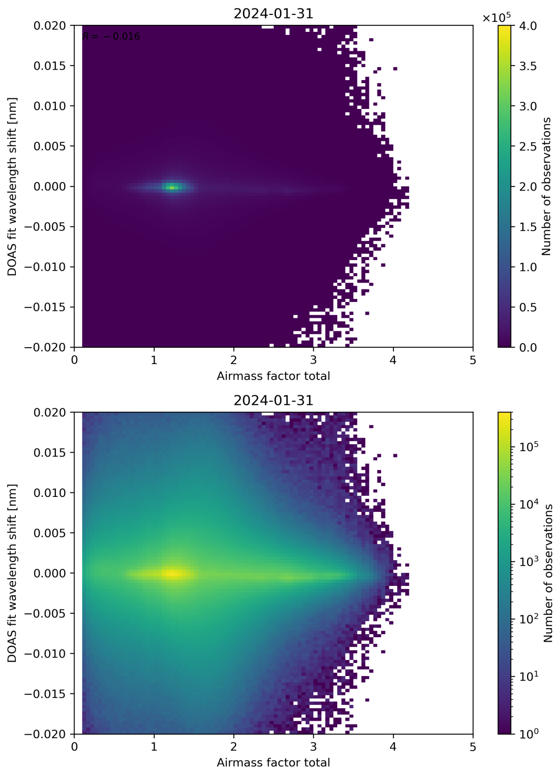
Figure 98: Scatter density plot of “Airmass factor total” against “DOAS fit wavelength shift” for 2024-01-31 to 2024-02-01.
