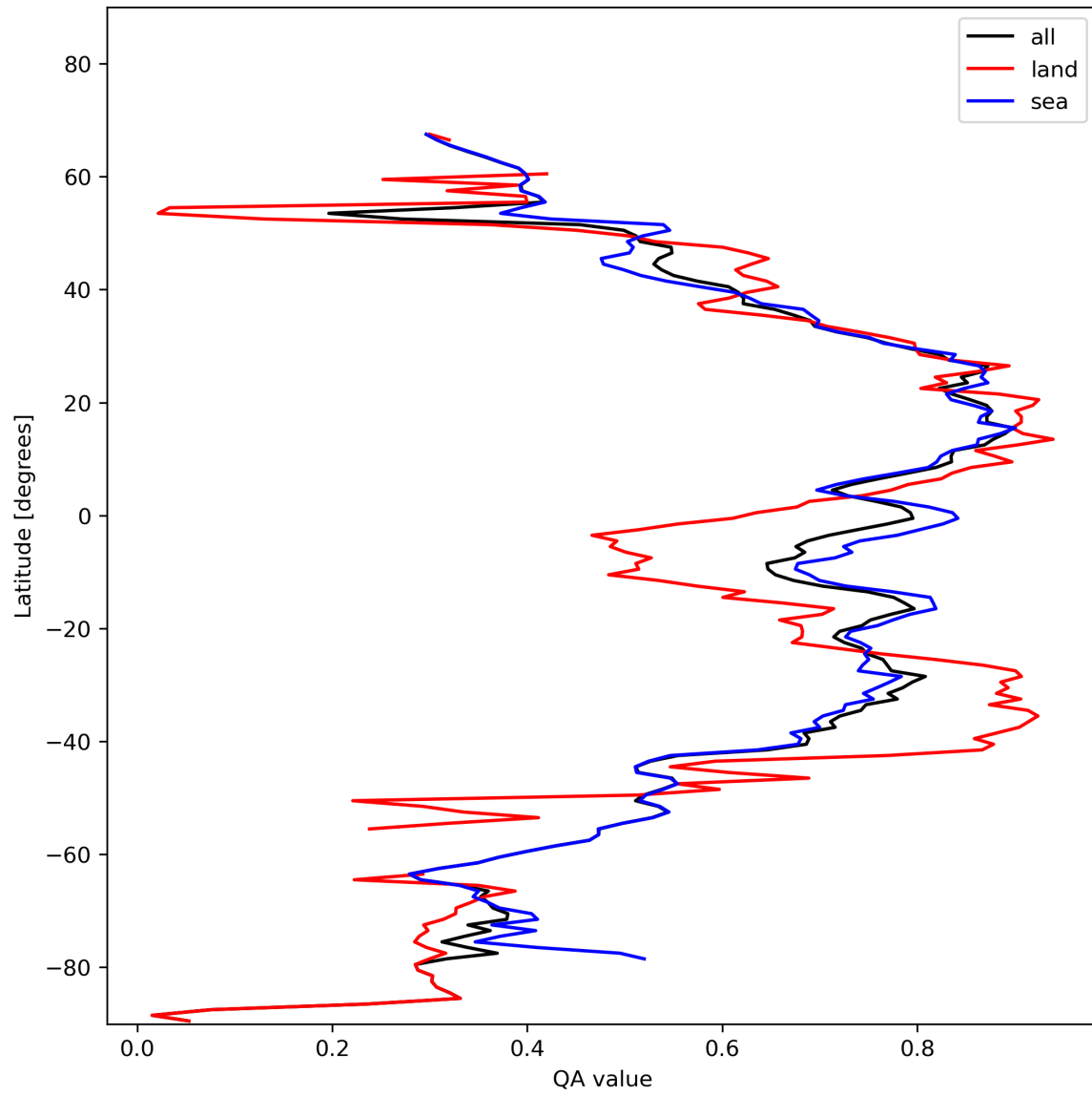
Figure 20: Zonal average of “QA value” for 2024-01-31 to 2024-02-01.
