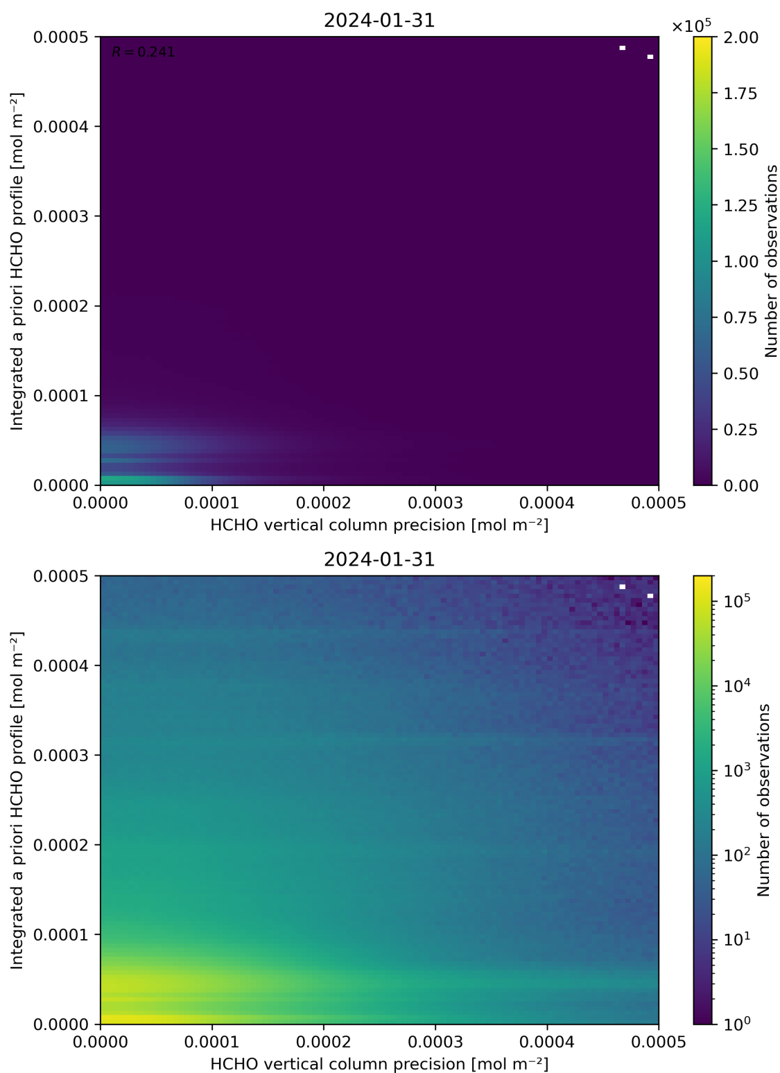
Figure 147: Scatter density plot of “HCHO vertical column precision” against “Integrated a priori HCHO profile” for 2024-01-31 to 2024-02-01.
