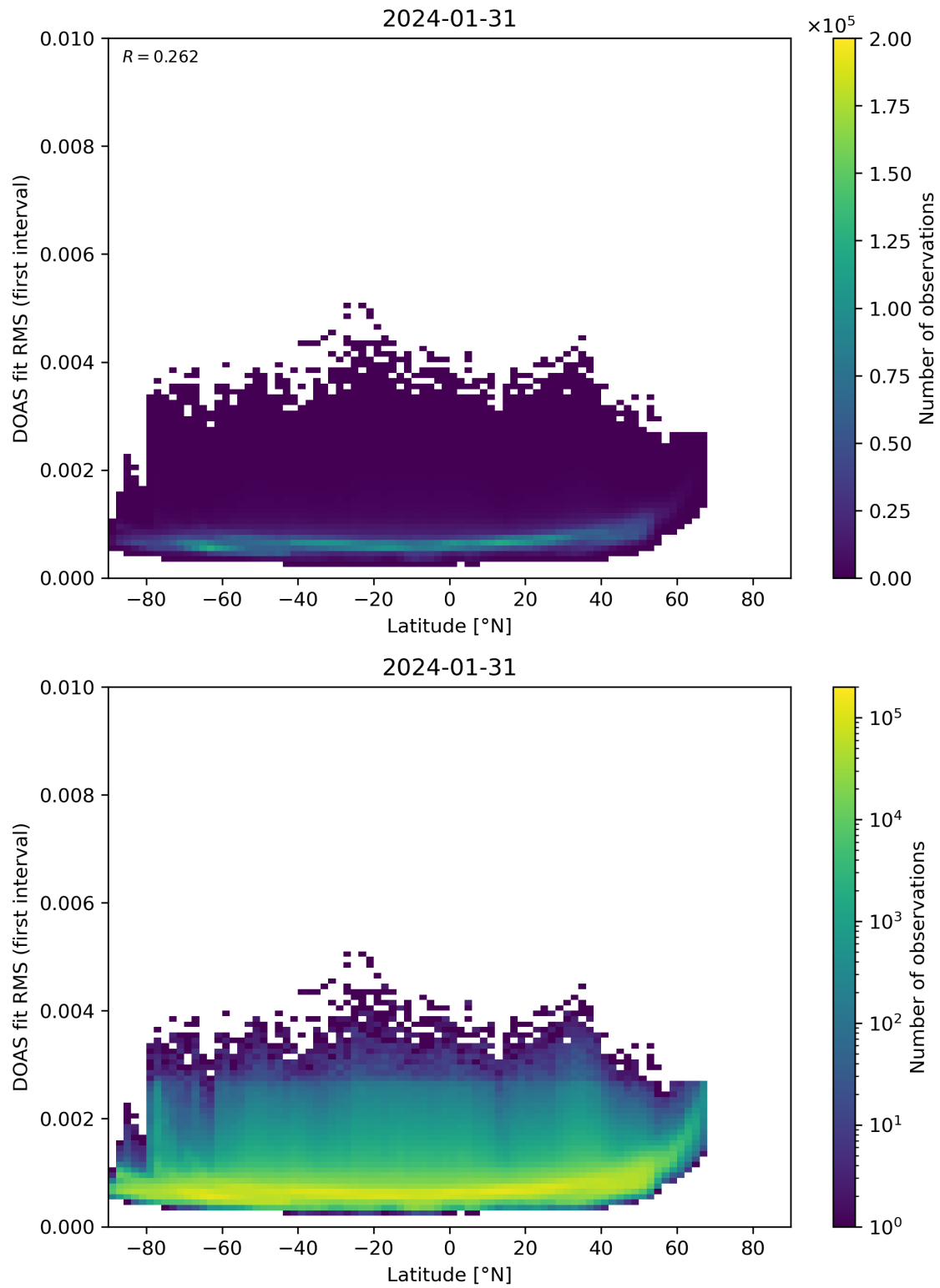
Figure 153: Scatter density plot of “Latitude” against “DOAS fit RMS (first interval)” for 2024-01-31 to 2024-02-01.
