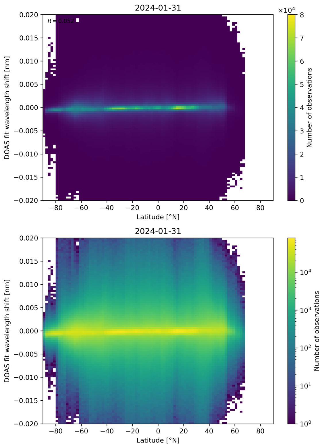
Figure 154: Scatter density plot of “Latitude” against “DOAS fit wavelength shift” for 2024-01-31 to 2024-02-01.
