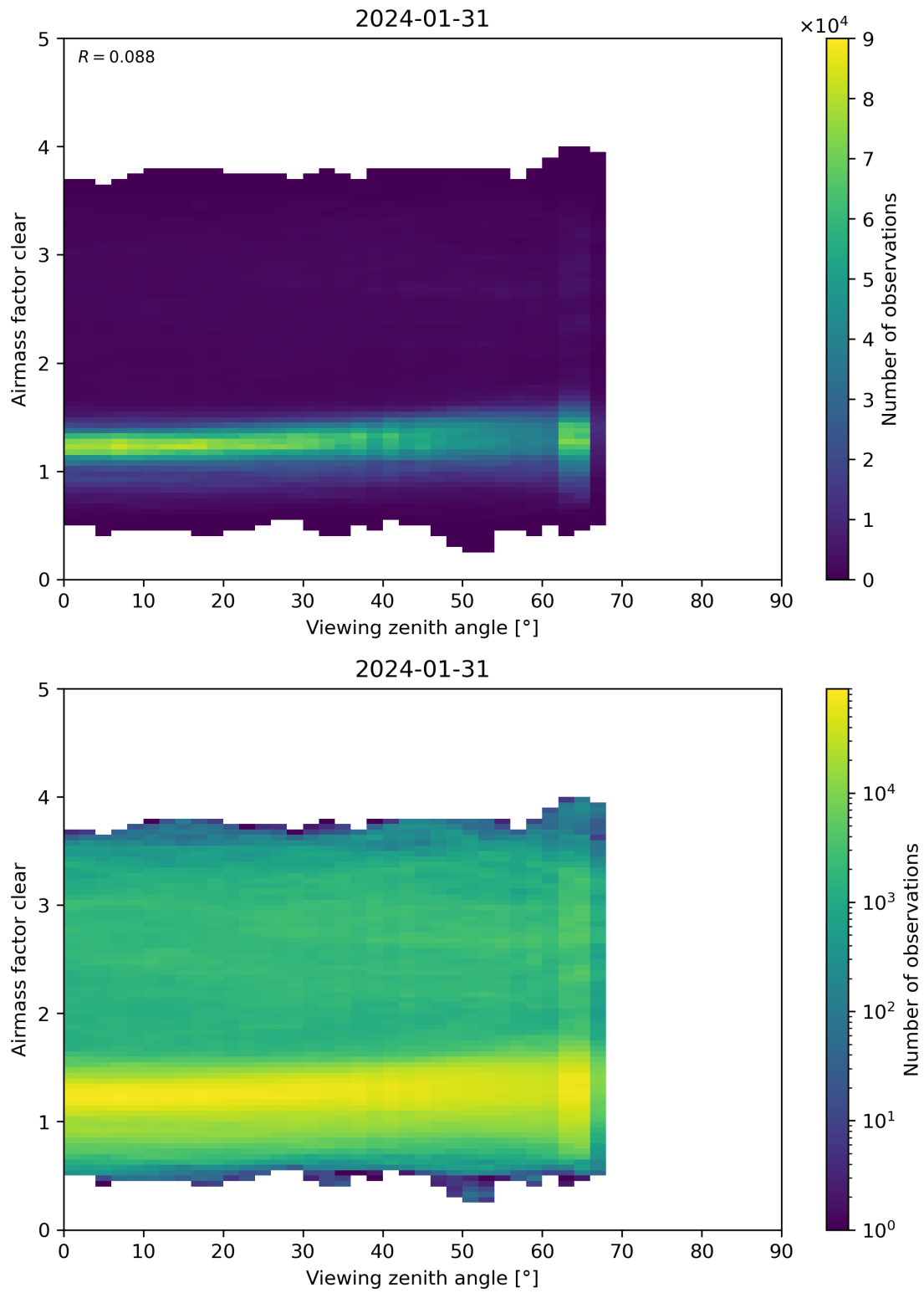
Figure 185: Scatter density plot of “Viewing zenith angle” against “Airmass factor clear” for 2024-01-31 to 2024-02-01.
