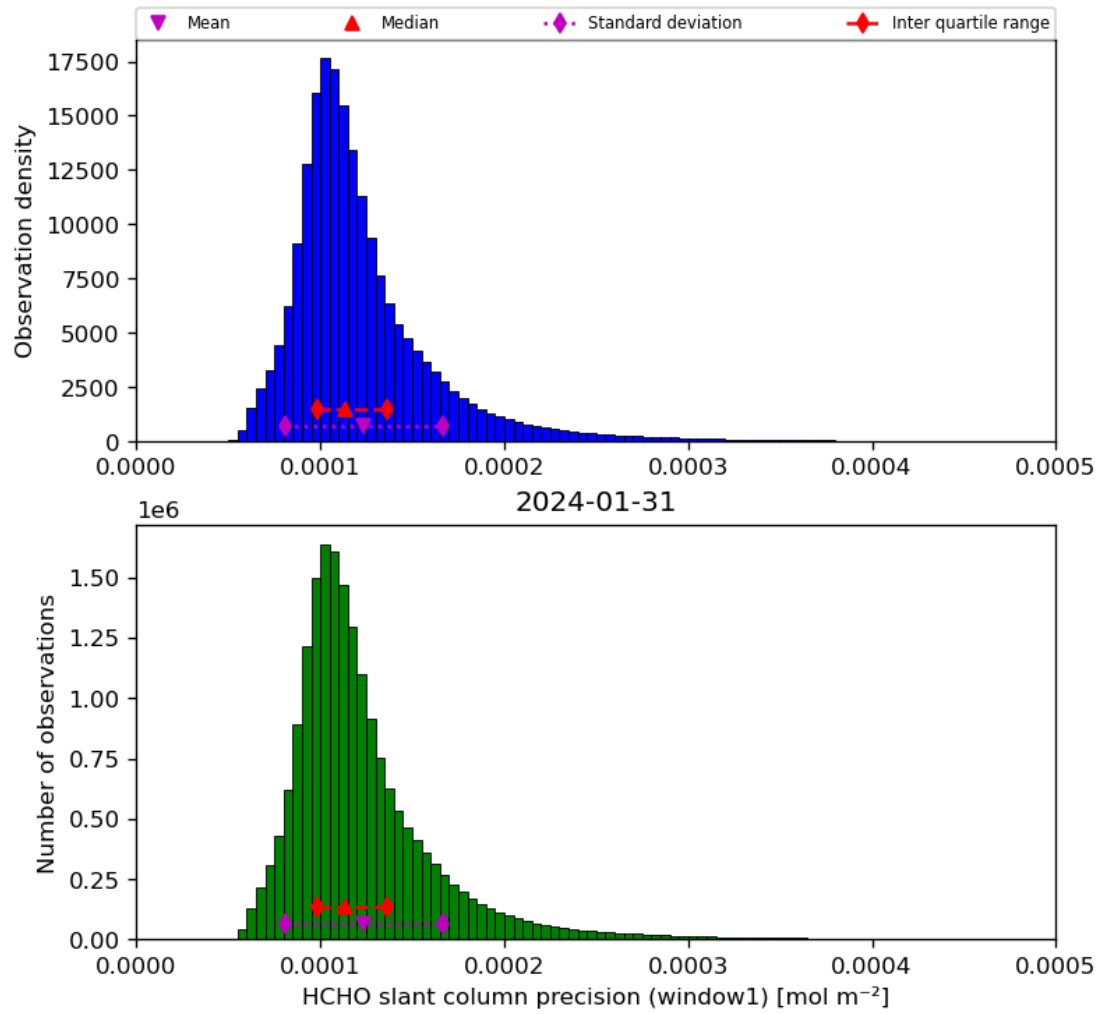
Figure 39: Histogram of “HCHO slant column precision (window1)” for 2024-01-31 to 2024-02-01
