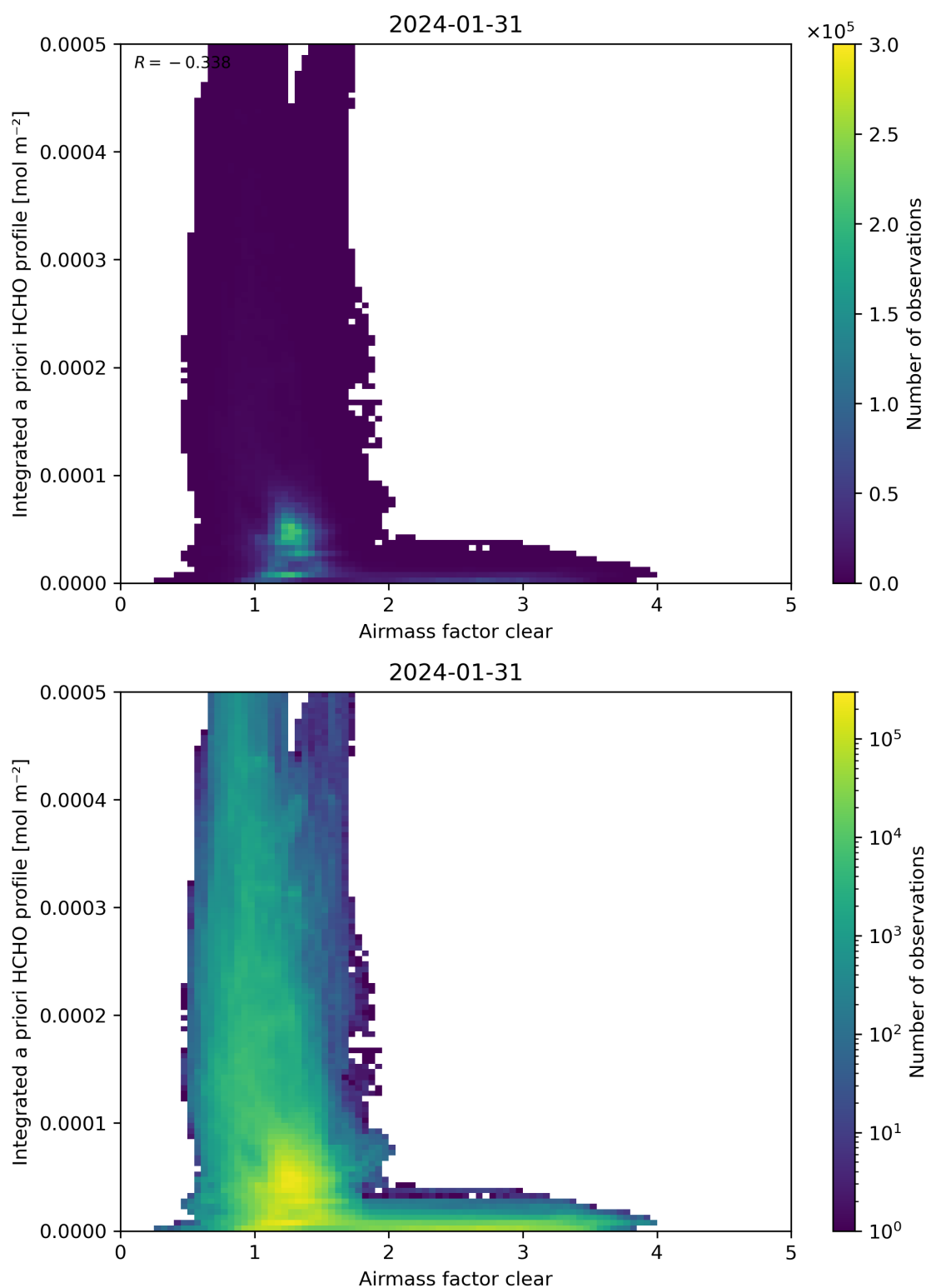
Figure 76: Scatter density plot of “Airmass factor clear” against “Integrated a priori HCHO profile” for 2024-01-31 to 2024-02-01.
