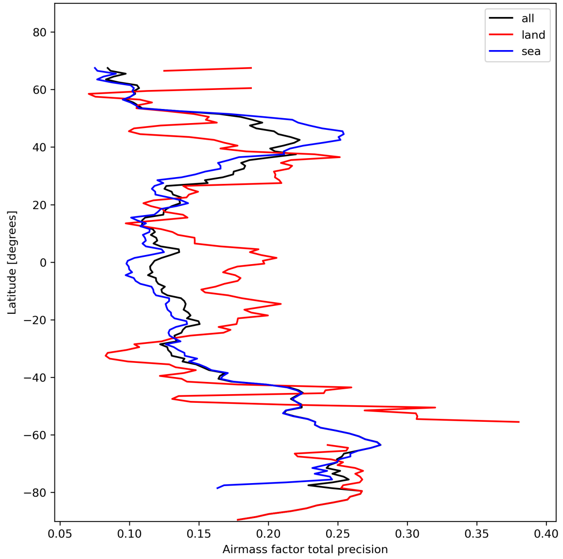
Figure 27: Zonal average of “Airmass factor total precision” for 2024-01-31 to 2024-02-01.
