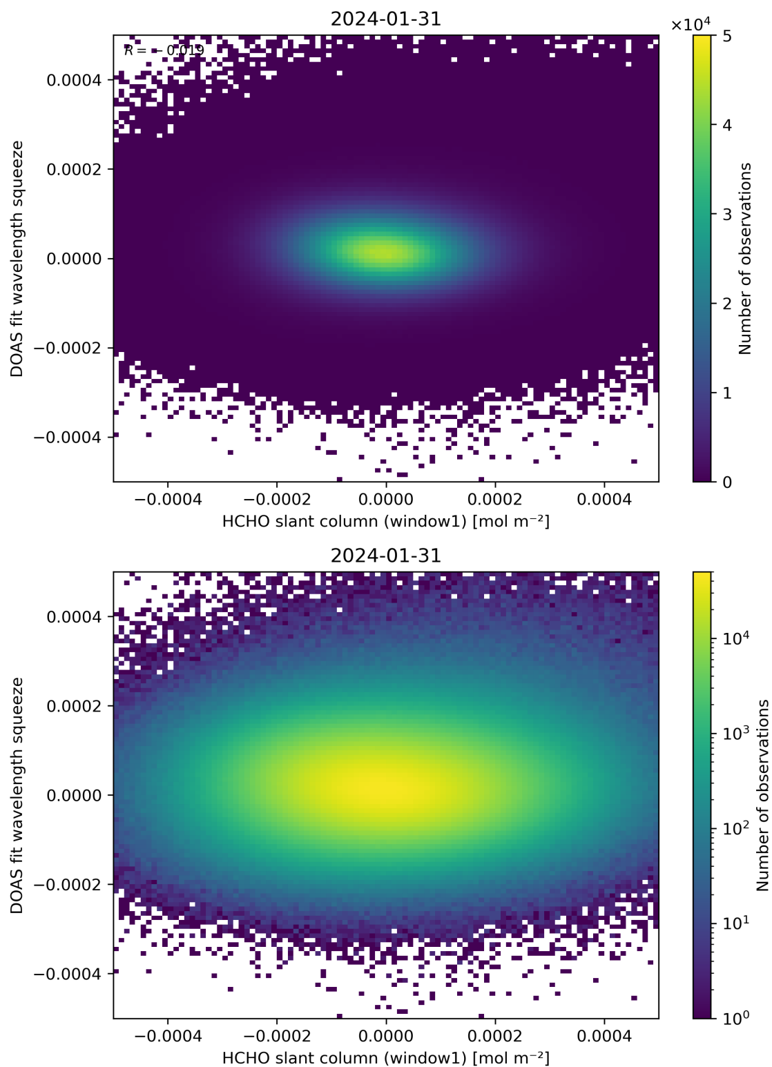
Figure 80: Scatter density plot of “HCHO slant column (window1)” against “DOAS fit wavelength squeeze” for 2024-01-31 to 2024-02-01.
