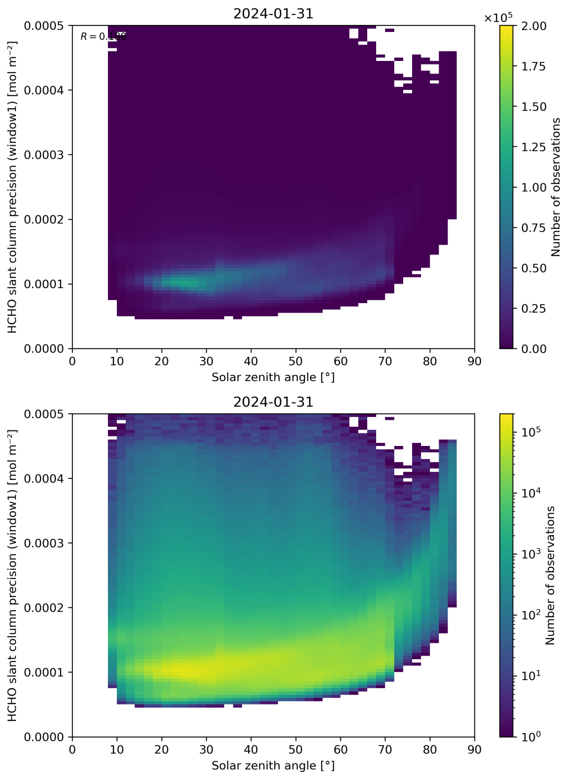
Figure 174: Scatter density plot of “Solar zenith angle” against “HCHO slant column precision (window1)” for 2024-01-31 to 2024-02-01.
