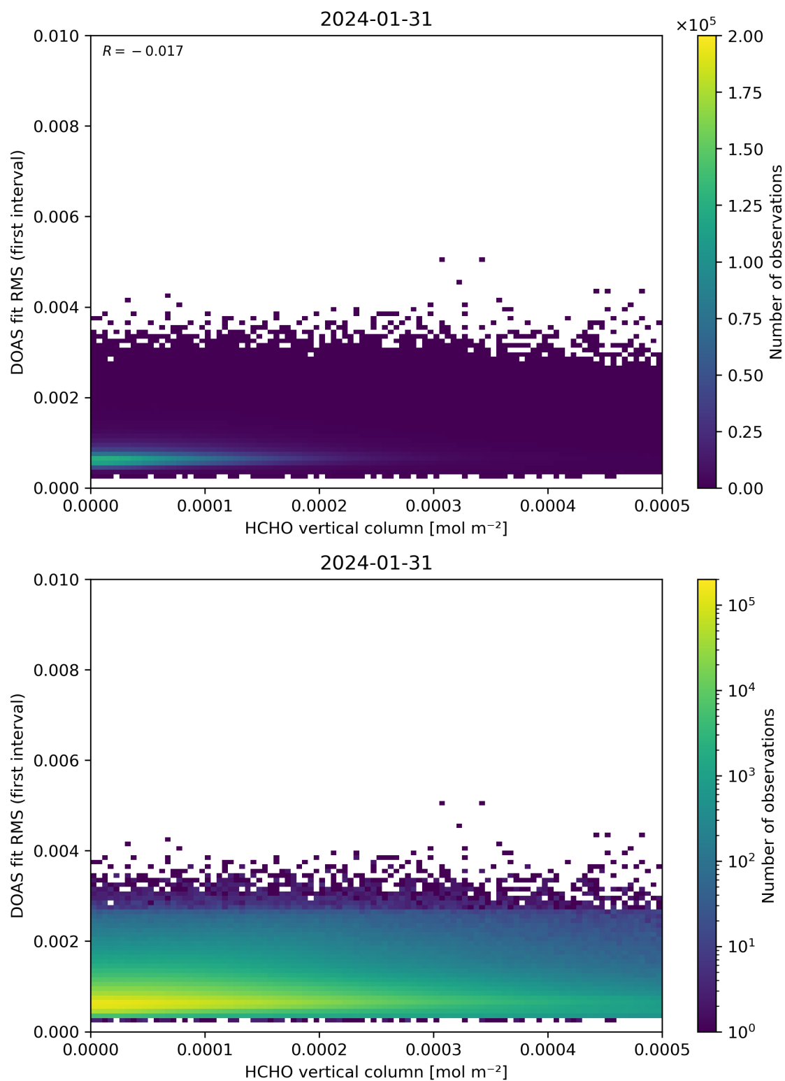
Figure 123: Scatter density plot of “HCHO vertical column” against “DOAS fit RMS (first interval)” for 2024-01-31 to 2024-02-01.
