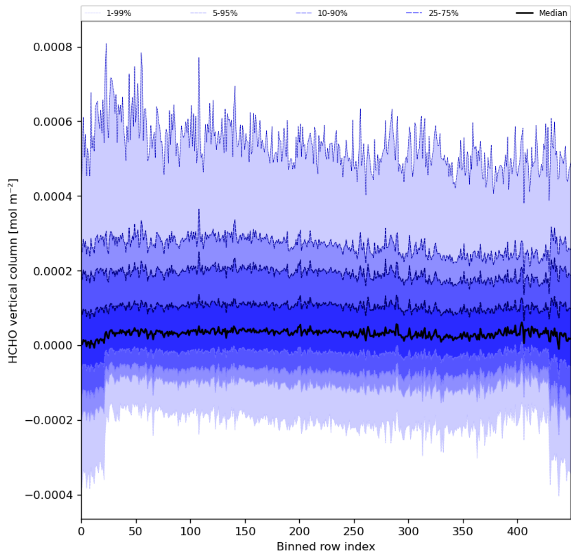
Figure 49: Along track statistics of “HCHO vertical column” for 2024-01-31 to 2024-02-01
