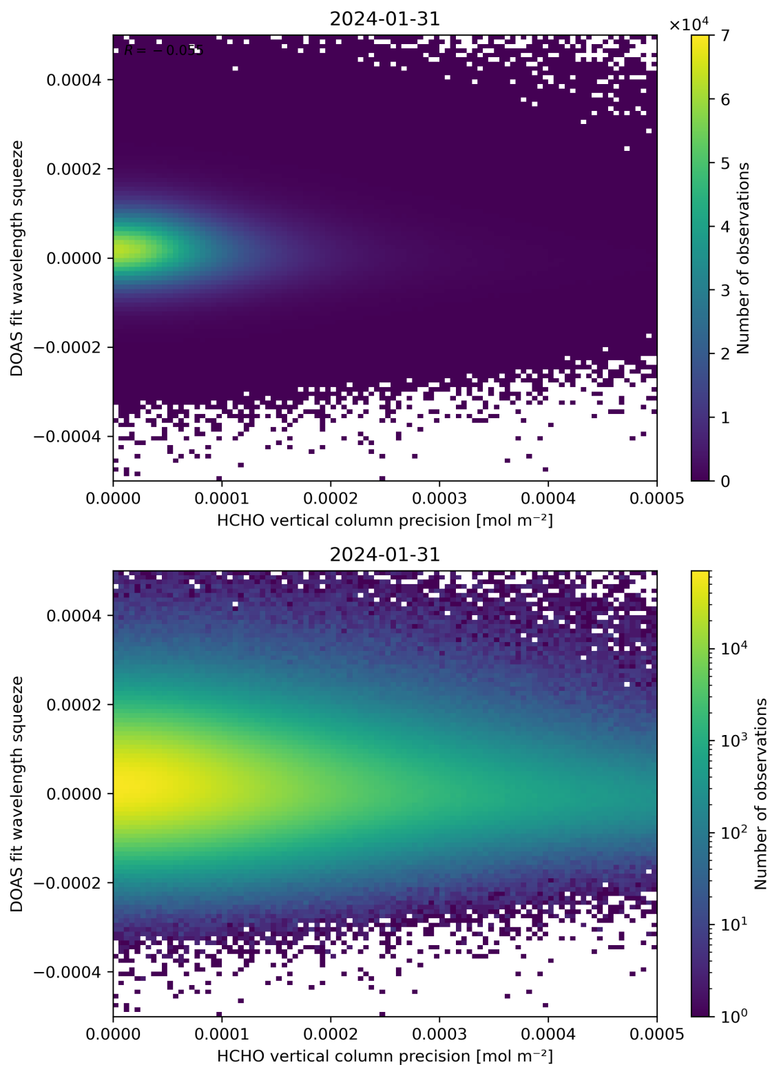
Figure 138: Scatter density plot of “HCHO vertical column precision” against “DOAS fit wavelength squeeze” for 2024-01-31 to 2024-02-01.
