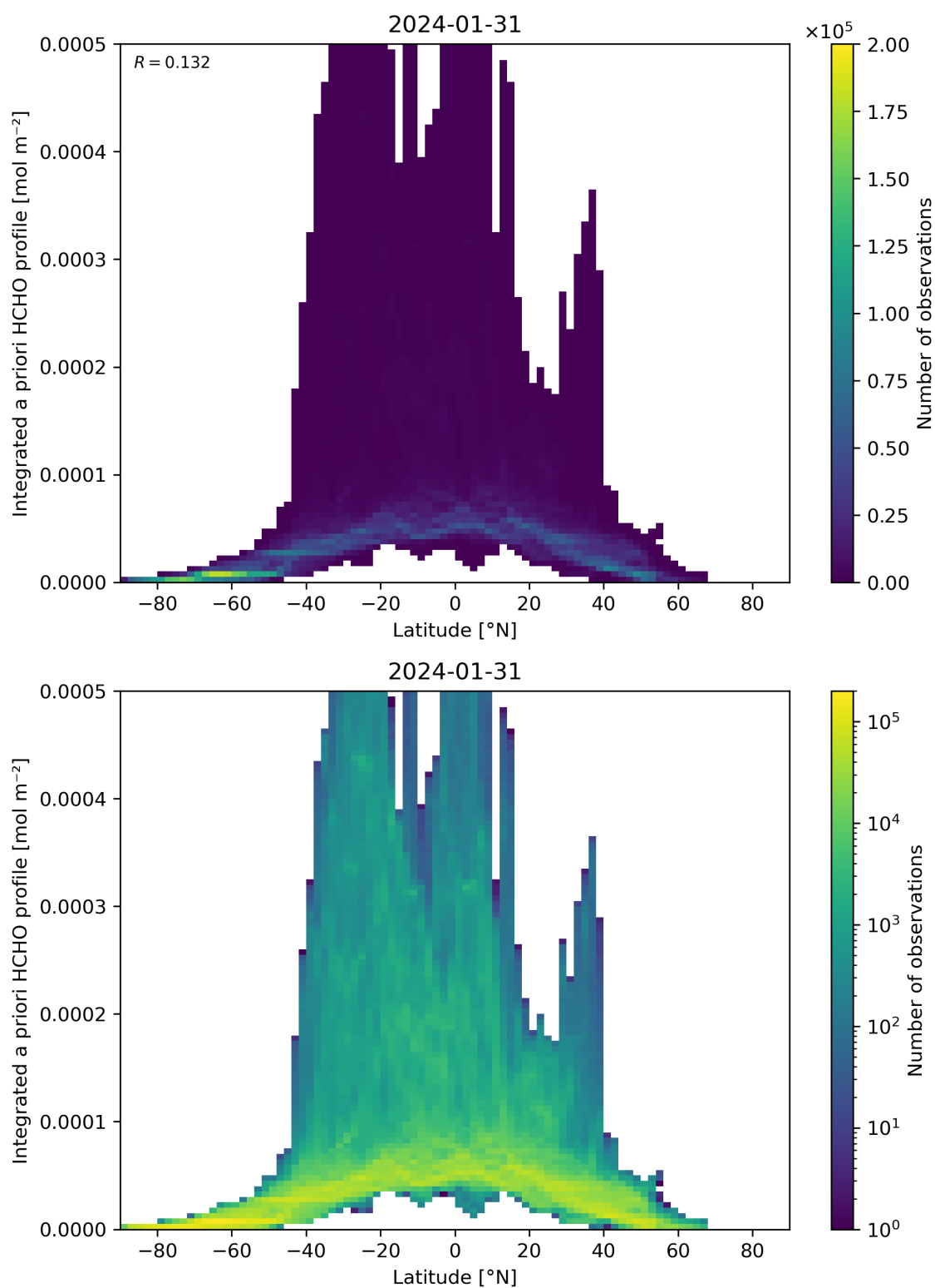
Figure 166: Scatter density plot of “Latitude” against “Integrated a priori HCHO profile” for 2024-01-31 to 2024-02-01.
