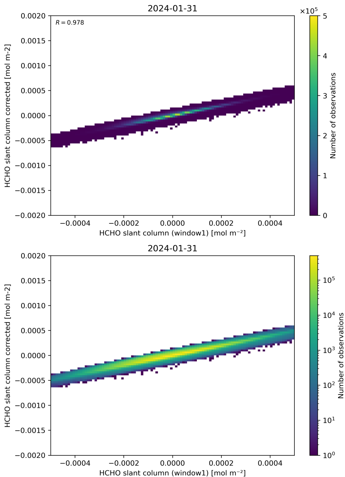
Figure 82: Scatter density plot of “HCHO slant column (window1)” against “HCHO slant column corrected” for 2024-01-31 to 2024-02-01.
