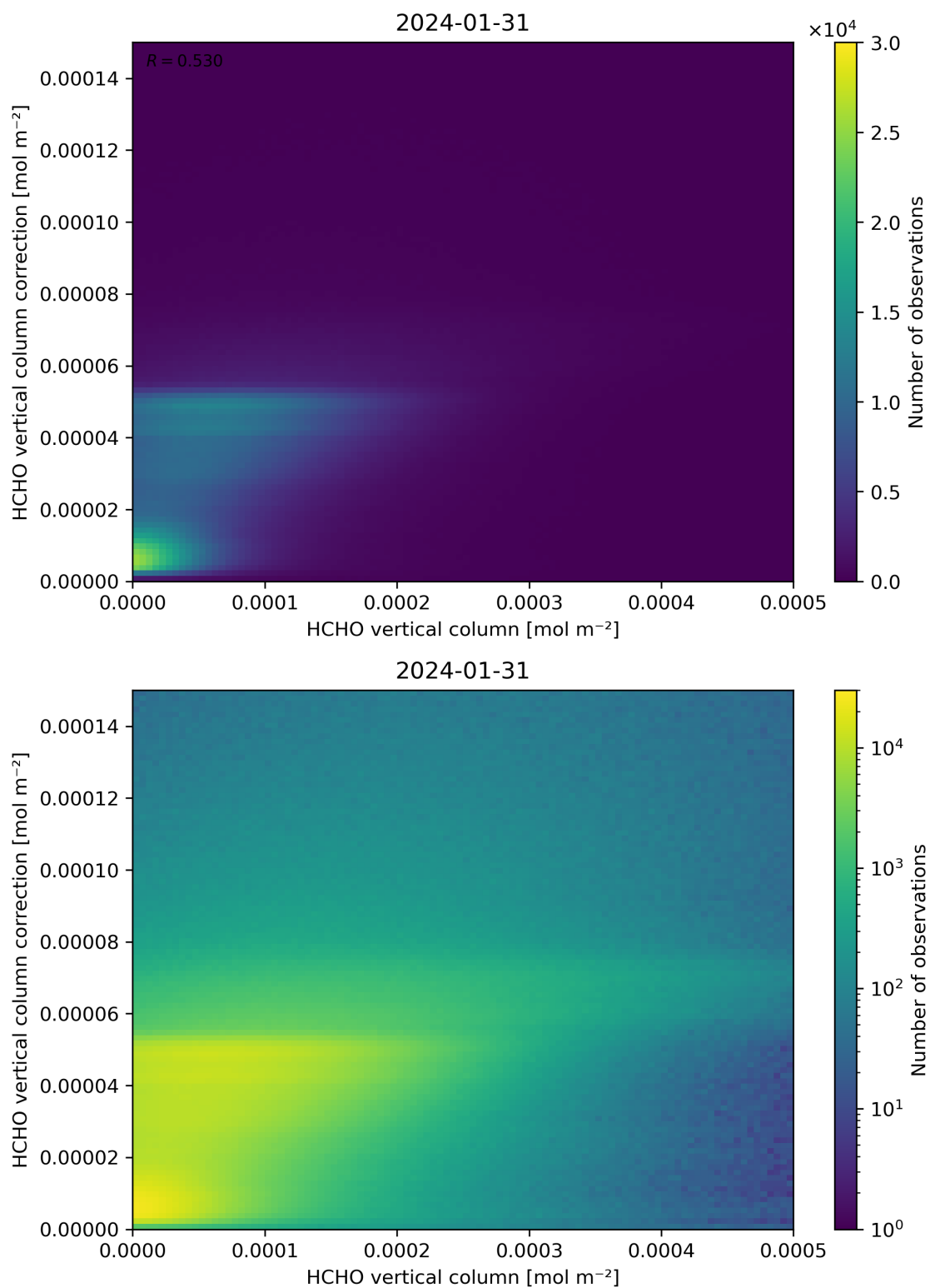
Figure 133: Scatter density plot of “HCHO vertical column” against “HCHO vertical column correction” for 2024-01-31 to 2024-02-01.
