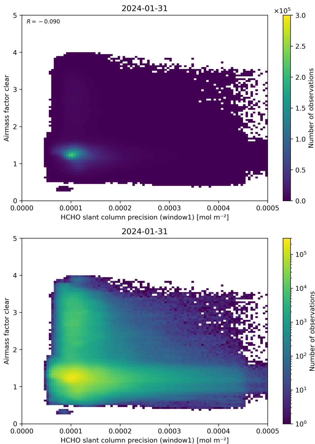
Figure 91: Scatter density plot of “HCHO slant column precision (window1)” against “Airmass factor clear” for 2024-01-31 to 2024-02-01.
