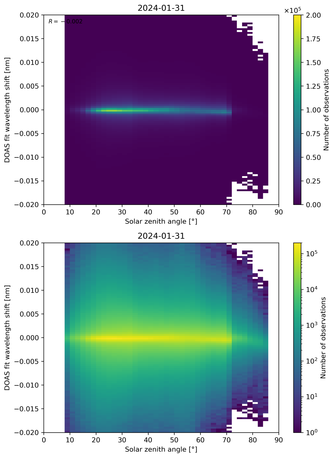
Figure 168: Scatter density plot of “Solar zenith angle” against “DOAS fit wavelength shift” for 2024-01-31 to 2024-02-01.
