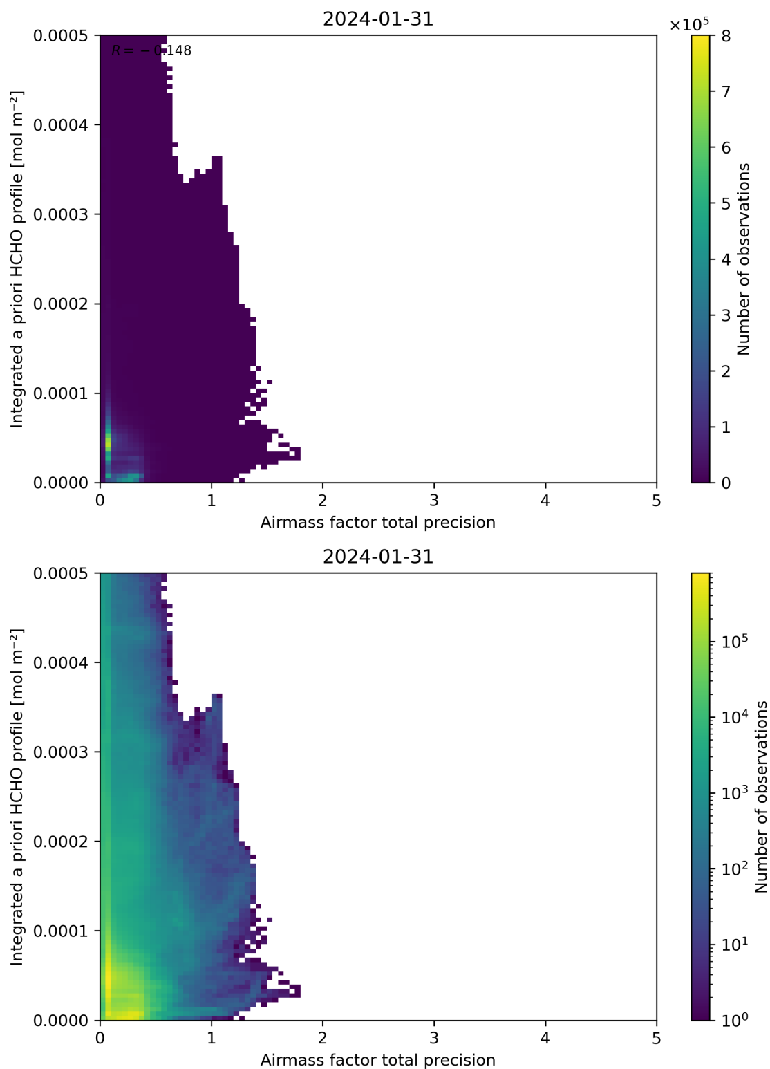
Figure 111: Scatter density plot of “Airmass factor total precision” against “Integrated a priori HCHO profile” for 2024-01-31 to 2024-02-01.
