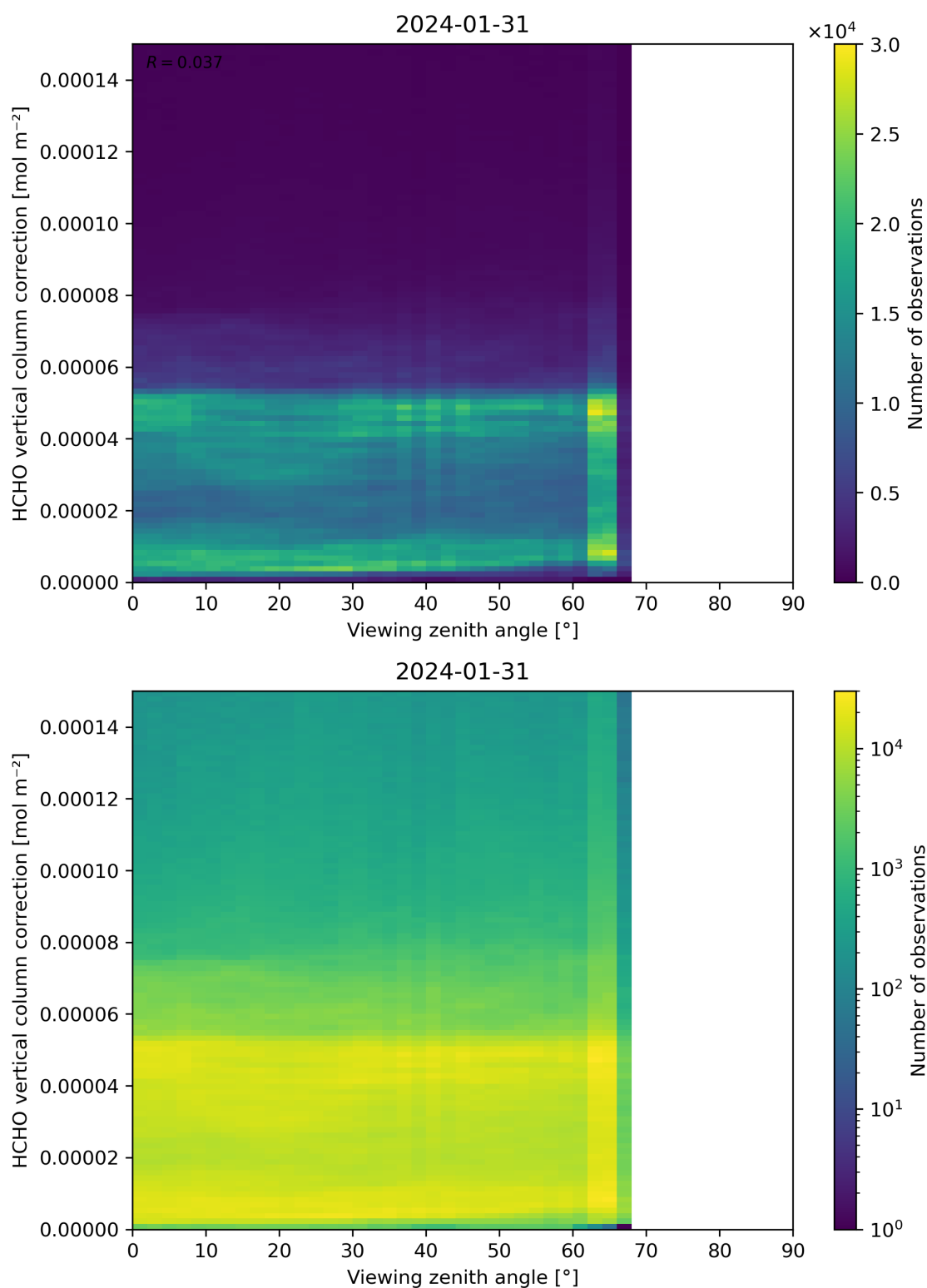
Figure 193: Scatter density plot of “Viewing zenith angle” against “HCHO vertical column correction” for 2024-01-31 to 2024-02-01.
