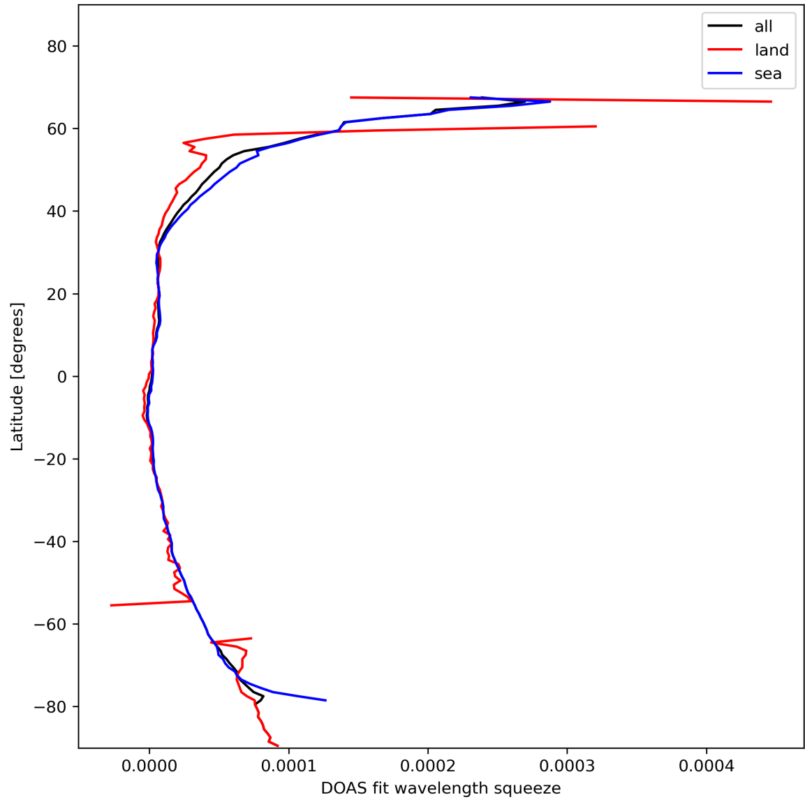
Figure 31: Zonal average of “DOAS fit wavelength squeeze” for 2024-01-31 to 2024-02-01.
