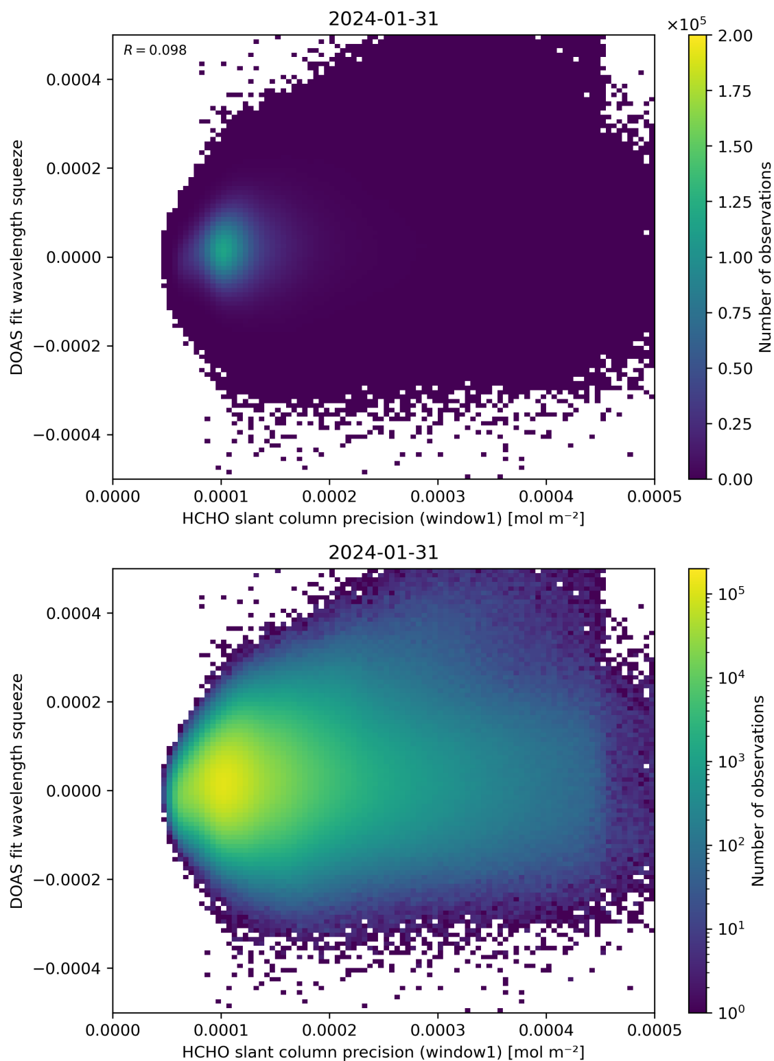
Figure 90: Scatter density plot of “HCHO slant column precision (window1)” against “DOAS fit wavelength squeeze” for 2024-01-31 to 2024-02-01.
