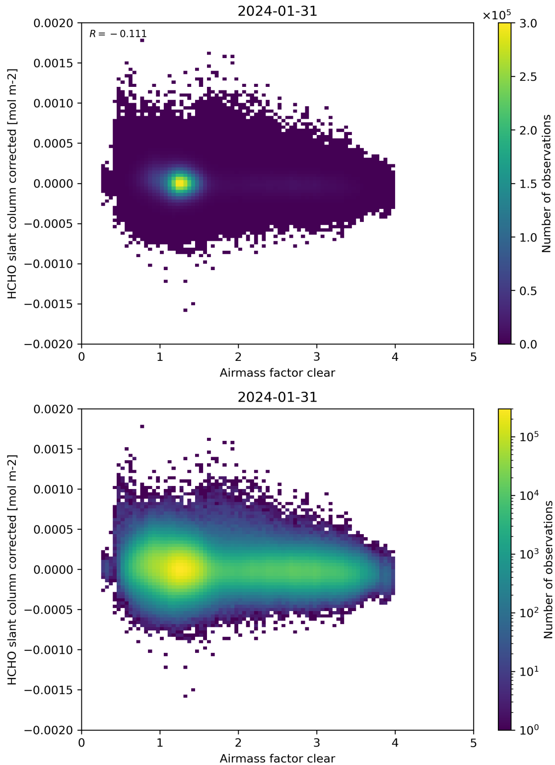
Figure 74: Scatter density plot of “Airmass factor clear” against “HCHO slant column corrected” for 2024-01-31 to 2024-02-01.
