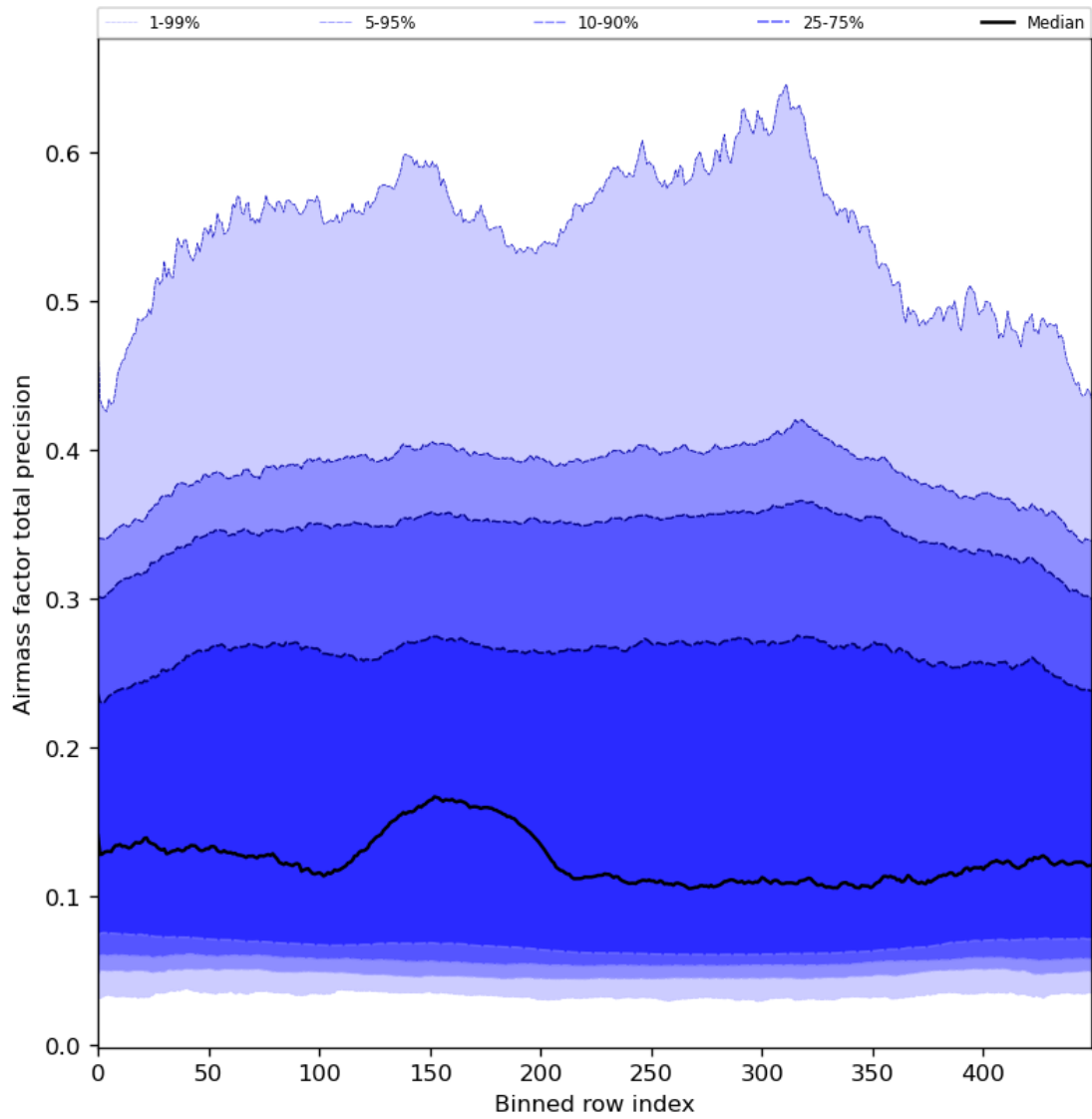
Figure 55: Along track statistics of “Airmass factor total precision” for 2024-01-31 to 2024-02-01
