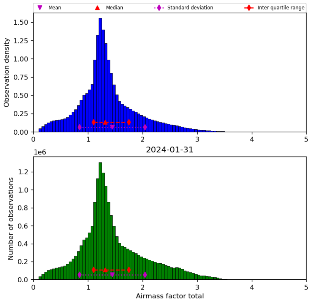
Figure 40: Histogram of “Airmass factor total” for 2024-01-31 to 2024-02-01
