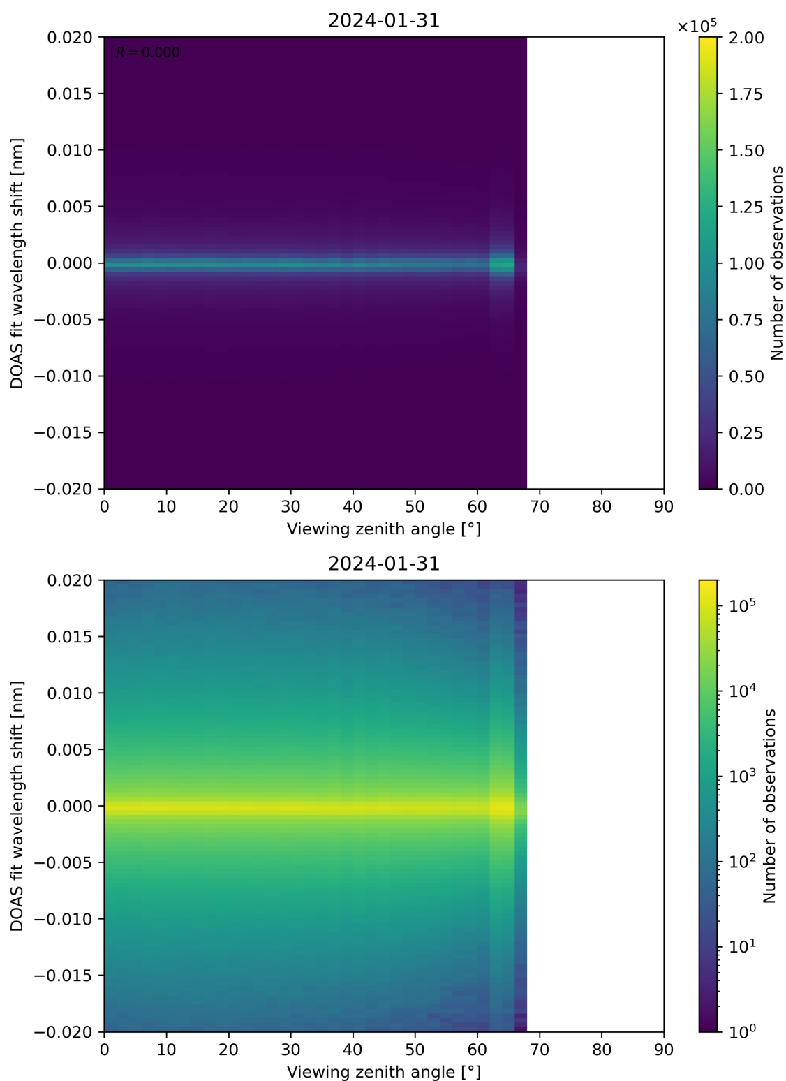
Figure 183: Scatter density plot of “Viewing zenith angle” against “DOAS fit wavelength shift” for 2024-01-31 to 2024-02-01.
