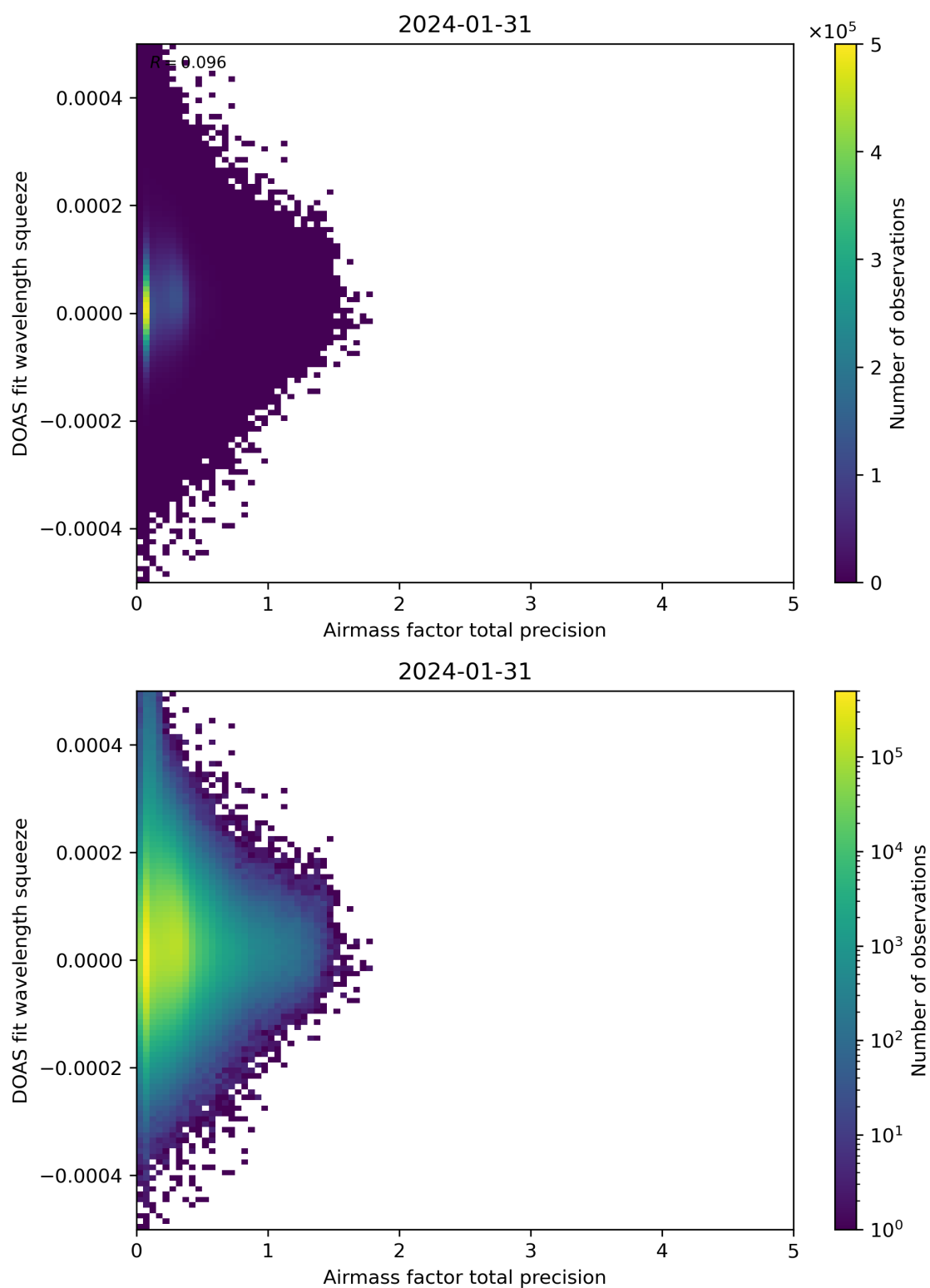
Figure 107: Scatter density plot of “Airmass factor total precision” against “DOAS fit wavelength squeeze” for 2024-01-31 to 2024-02-01.
