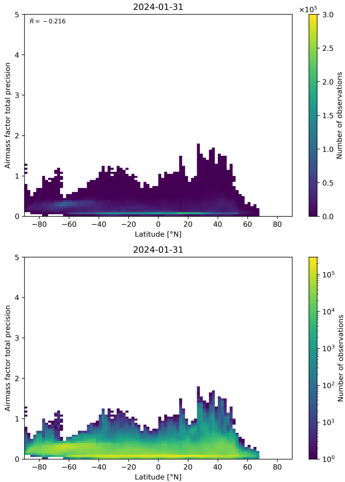
Figure 162: Scatter density plot of “Latitude” against “Airmass factor total precision” for 2024-01-31 to 2024-02-01.
