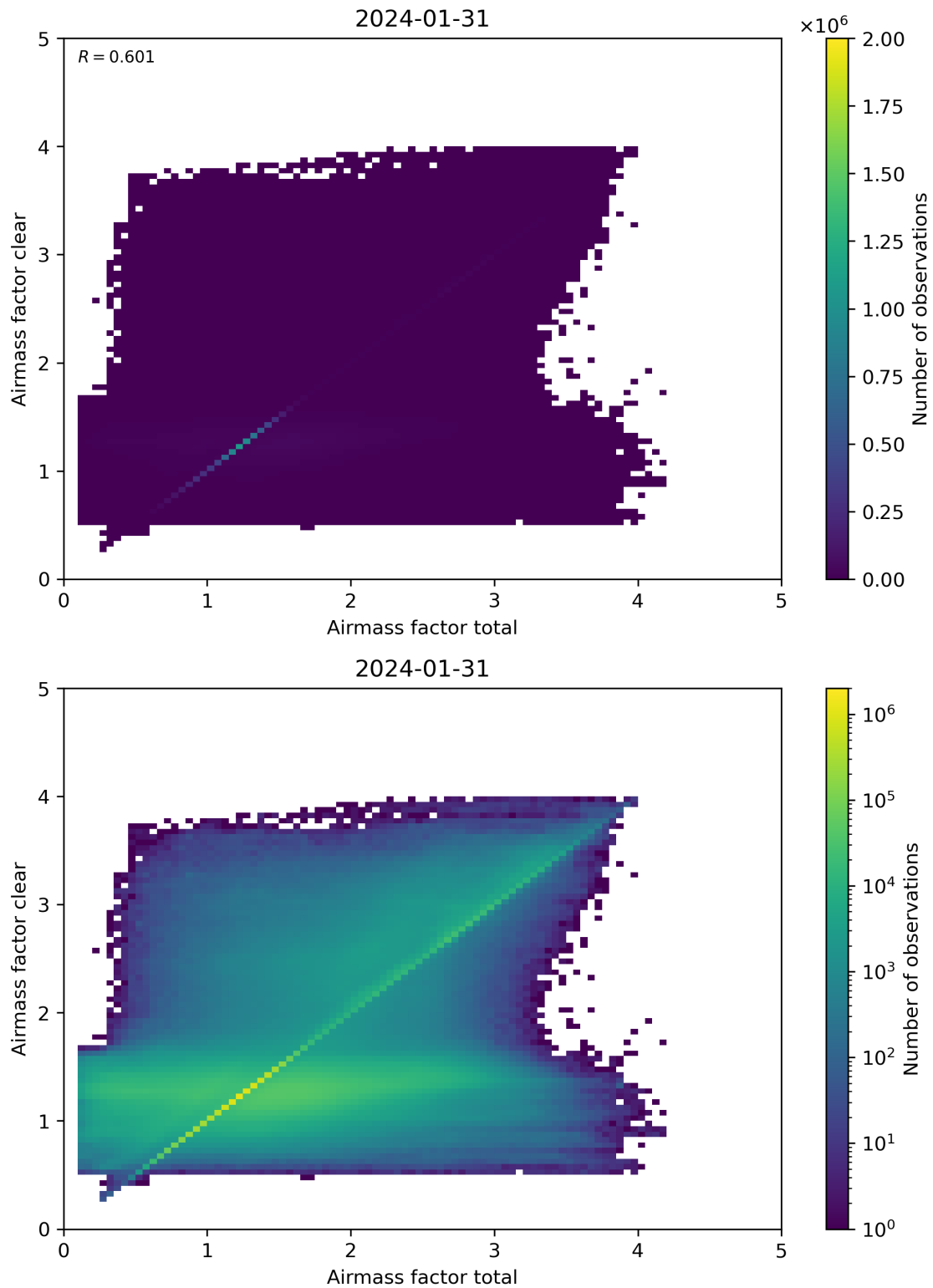
Figure 100: Scatter density plot of “Airmass factor total” against “Airmass factor clear” for 2024-01-31 to 2024-02-01.
