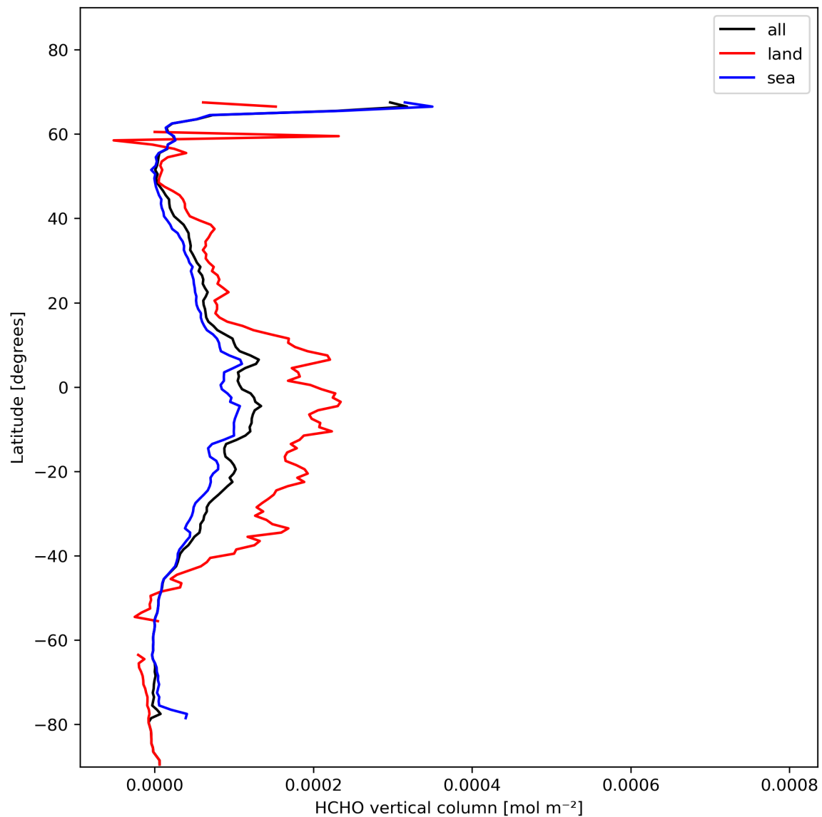
Figure 21: Zonal average of “HCHO vertical column” for 2024-01-31 to 2024-02-01.
