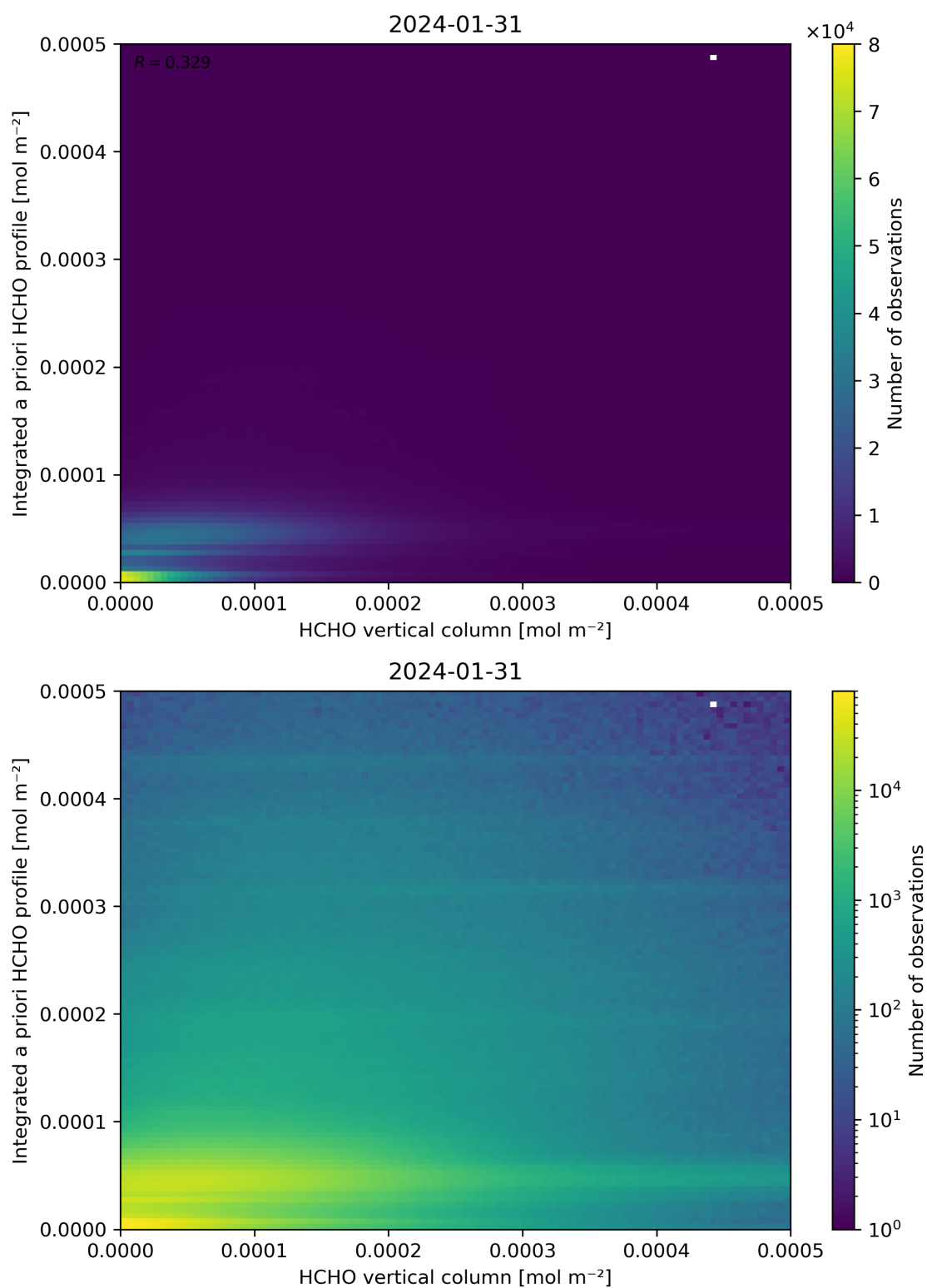
Figure 135: Scatter density plot of “HCHO vertical column” against “Integrated a priori HCHO profile” for 2024-01-31 to 2024-02-01.
