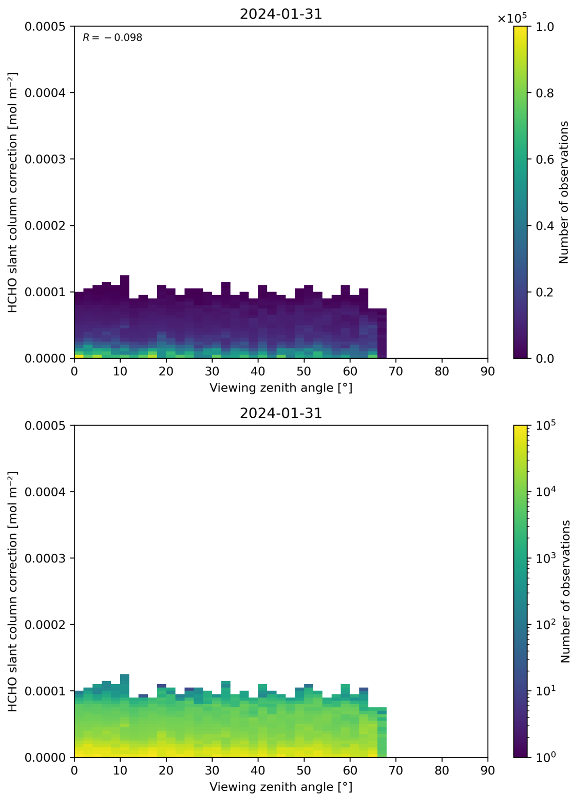
Figure 187: Scatter density plot of “Viewing zenith angle” against “HCHO slant column correction” for 2024-01-31 to 2024-02-01.
