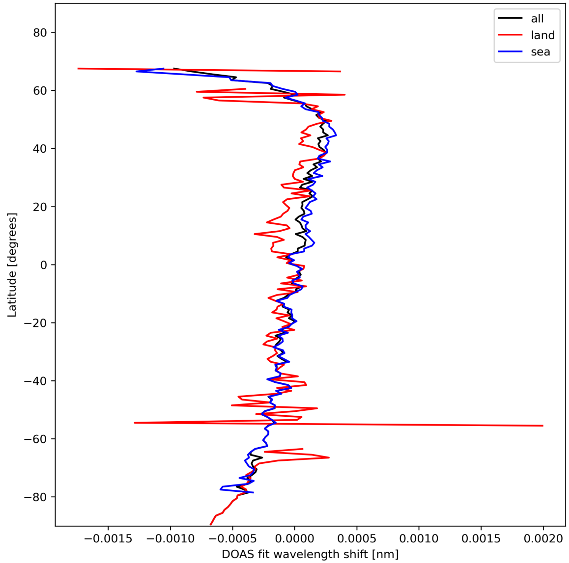
Figure 30: Zonal average of "DOAS fit wavelength shift" for 2024-01-31 to 2024-02-01.
