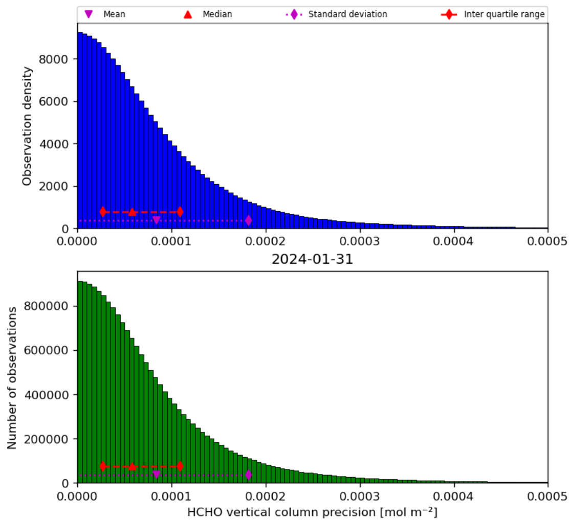
Figure 36: Histogram of “HCHO vertical column precision” for 2024-01-31 to 2024-02-01
