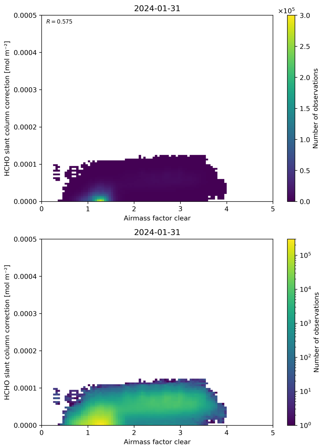
Figure 75: Scatter density plot of “Air mass factor clear” against “HCHO slant column correction” for 2024-01-31 to 2024-02-01.
