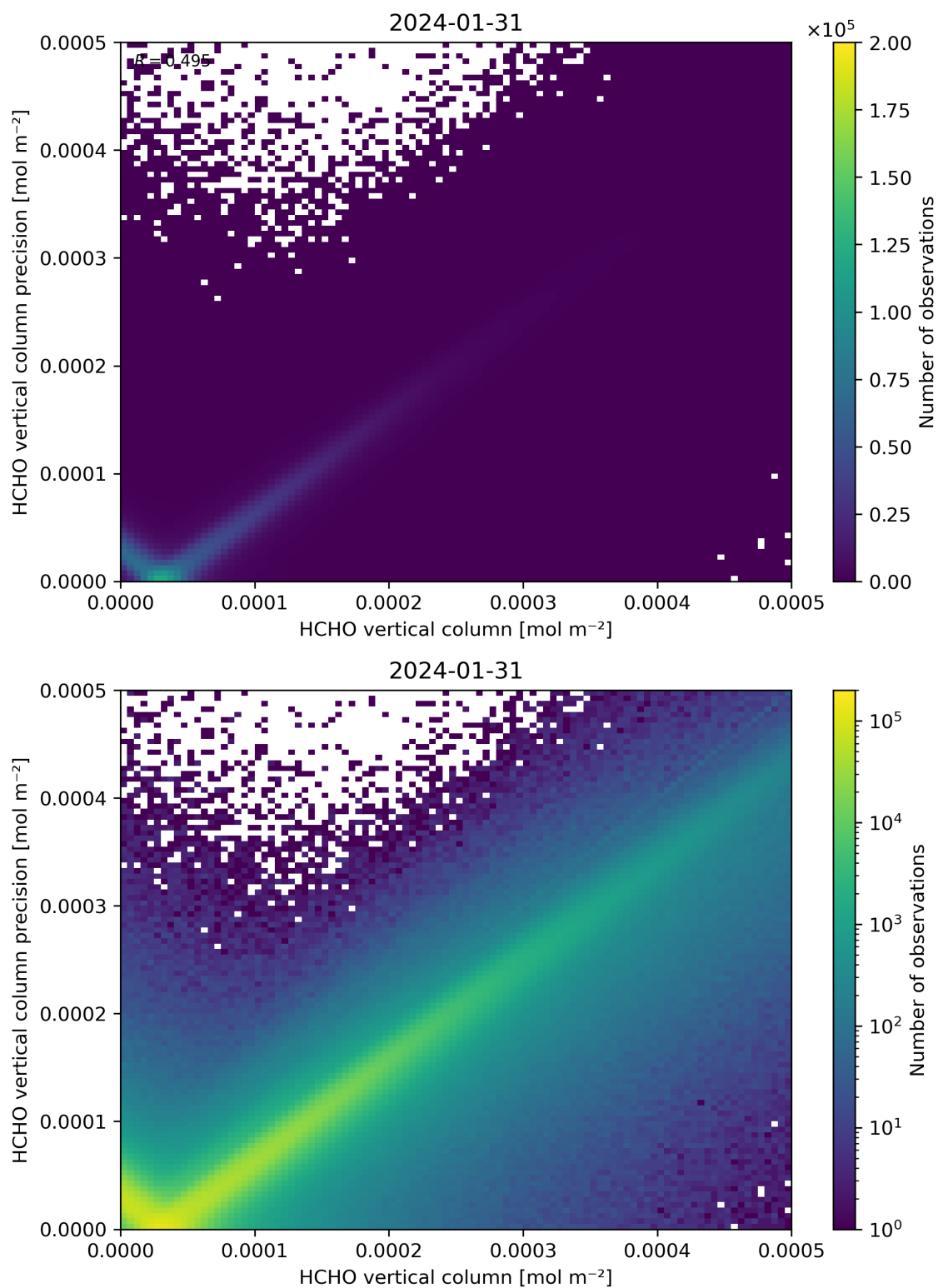
Figure 134: Scatter density plot of “HCHO vertical column” against “HCHO vertical column precision” for 2024-01-31 to 2024-02-01.
