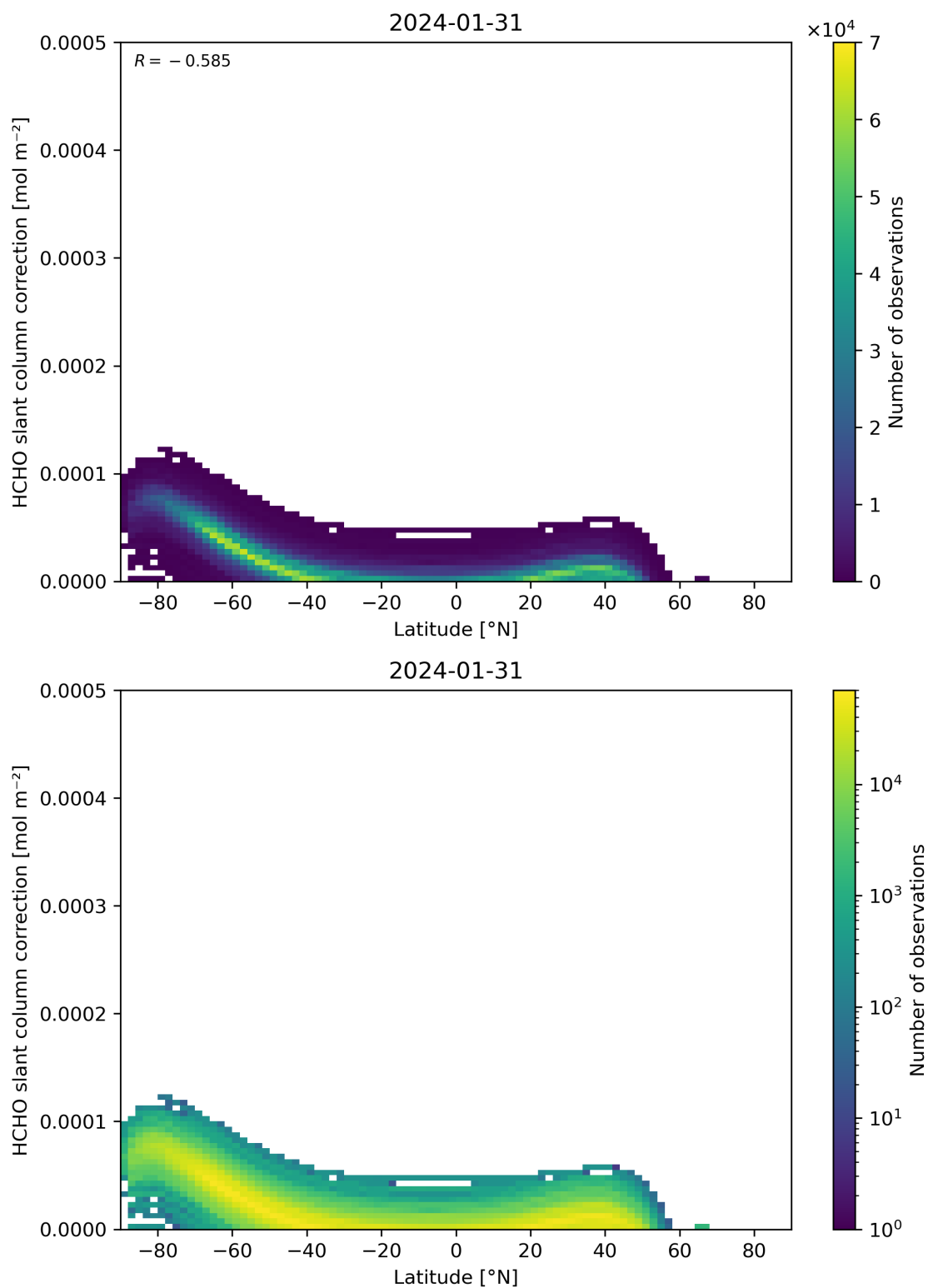
Figure 158: Scatter density plot of “Latitude” against “HCHO slant column correction” for 2024-01-31 to 2024-02-01.
