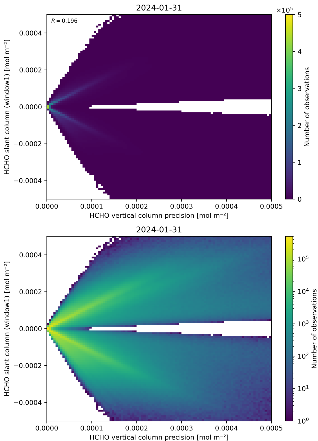
Figure 142: Scatter density plot of “HCHO vertical column precision” against “HCHO slant column (window1)” for 2024-01-31 to 2024-02-01.
