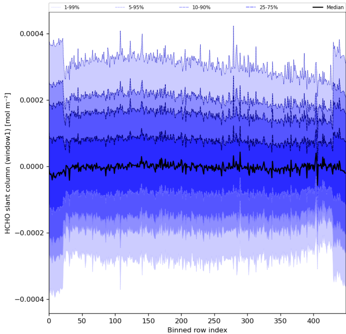
Figure 52: Along track statistics of “HCHO slant column (window1)” for 2024-01-31 to 2024-02-01
