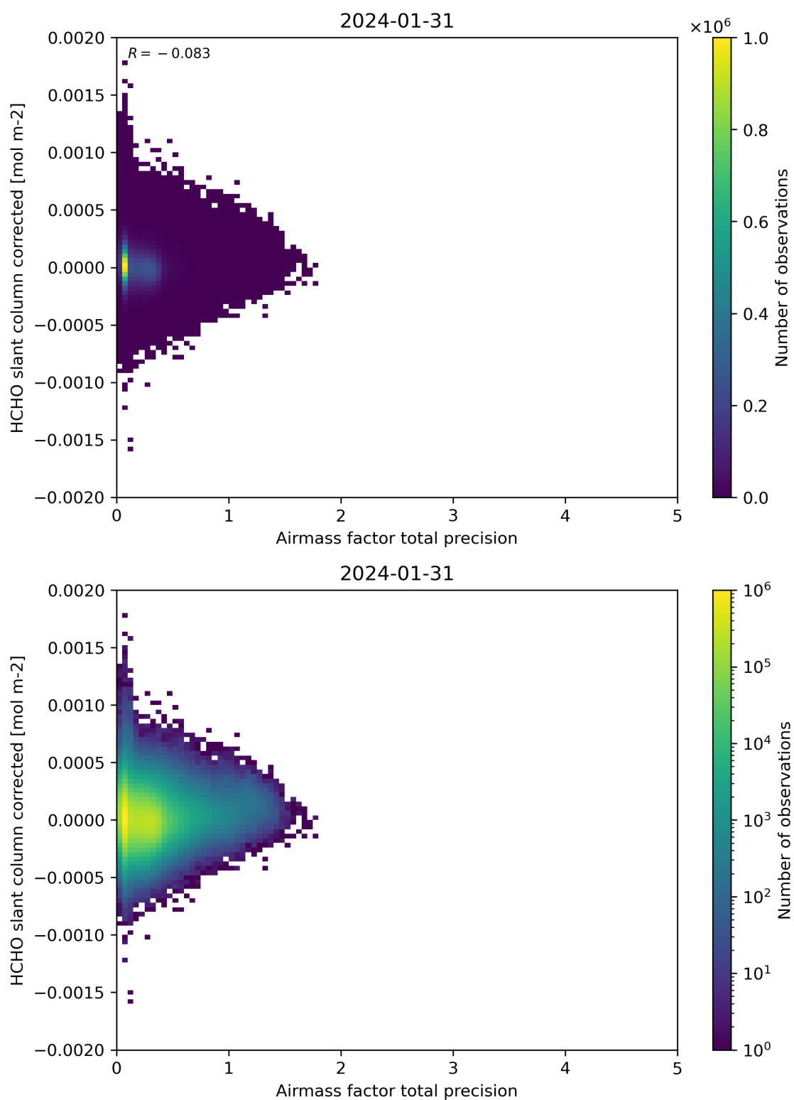
Figure 109: Scatter density plot of “Airmass factor total precision” against “HCHO slant column corrected” for 2024-01-31 to 2024-02-01.
