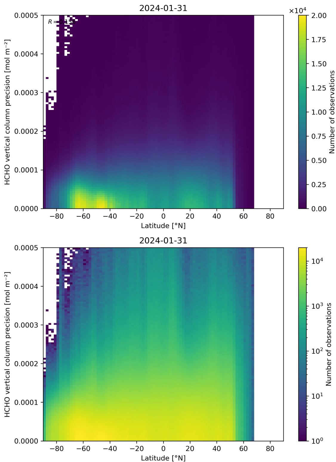
Figure 165: Scatter density plot of “Latitude” against “HCHO vertical column precision” for 2024-01-31 to 2024-02-01.
