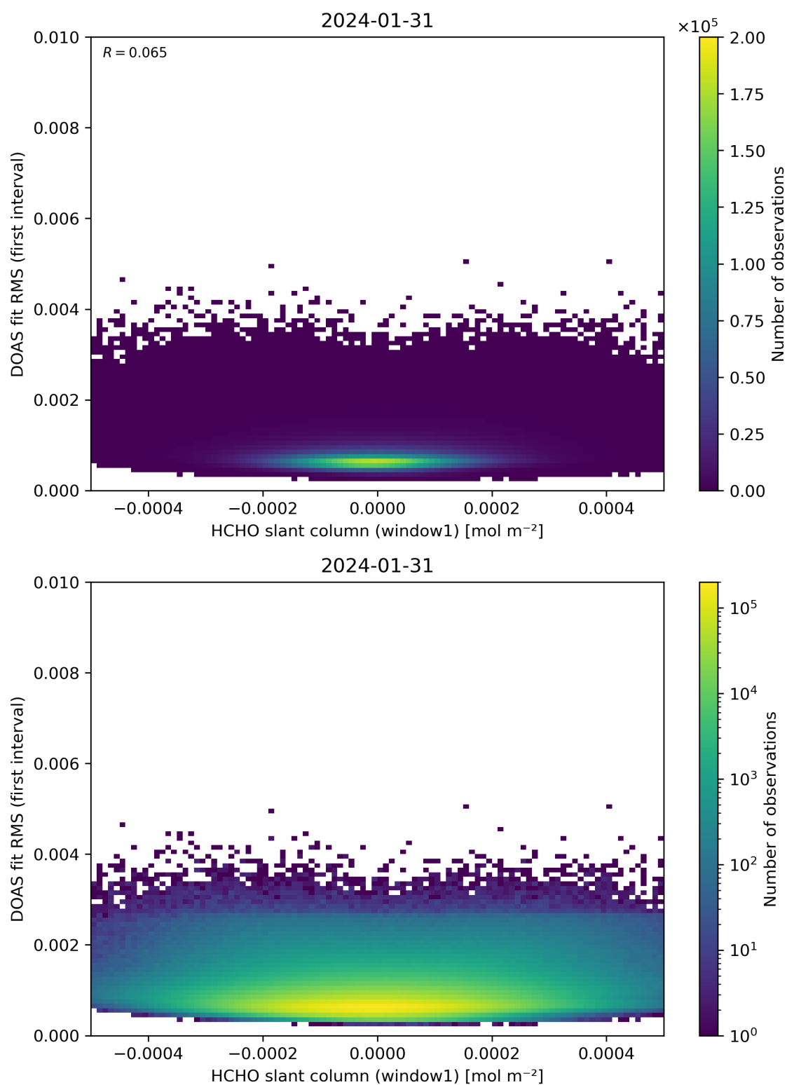
Figure 78: Scatter density plot of “HCHO slant column (window1)” against “DOAS fit RMS (first interval)” for 2024-01-31 to 2024-02-01.
