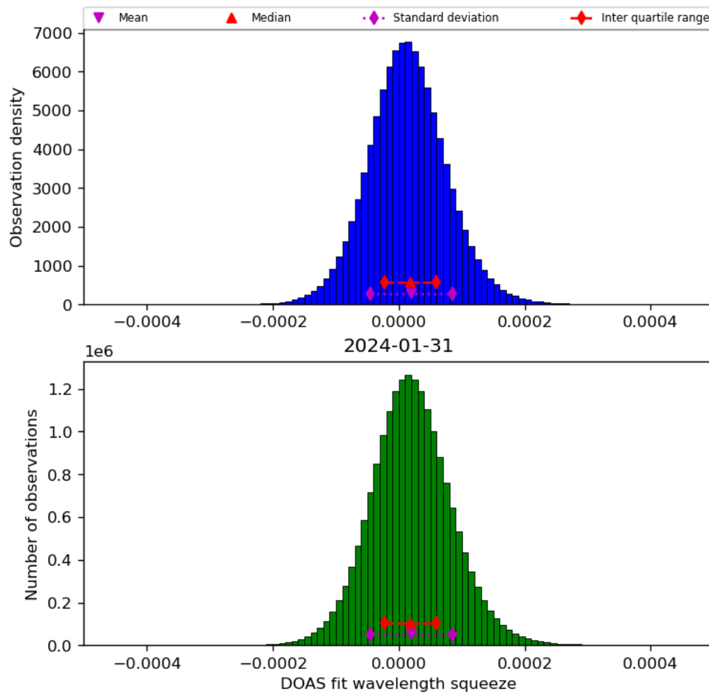
Figure 45: Histogram of “DOAS fit wavelength squeeze” for 2024-01-31 to 2024-02-01
