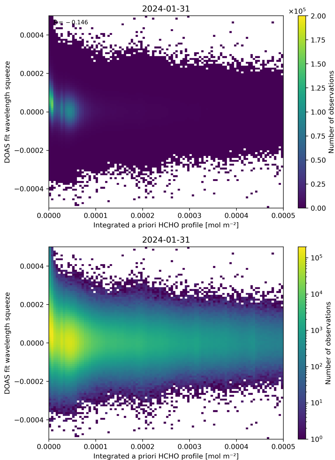
Figure 150: Scatter density plot of “Integrated a priori HCHO profile” against “DOAS fit wavelength squeeze” for 2024-01-31 to 2024-02-01.
