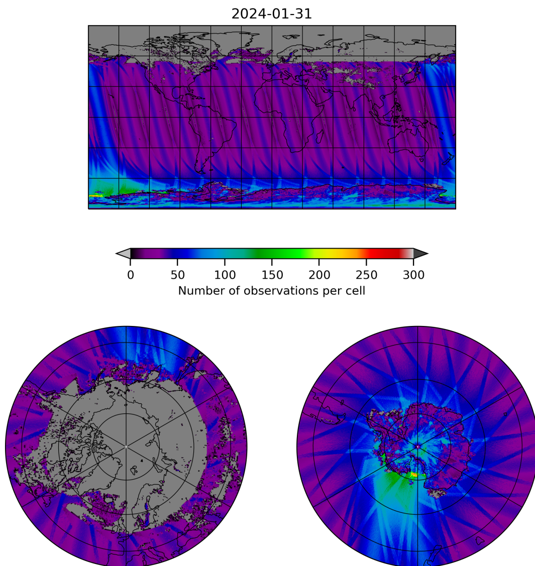
Figure 19: Map of the number of observations for 2024-01-31 to 2024-02-01
