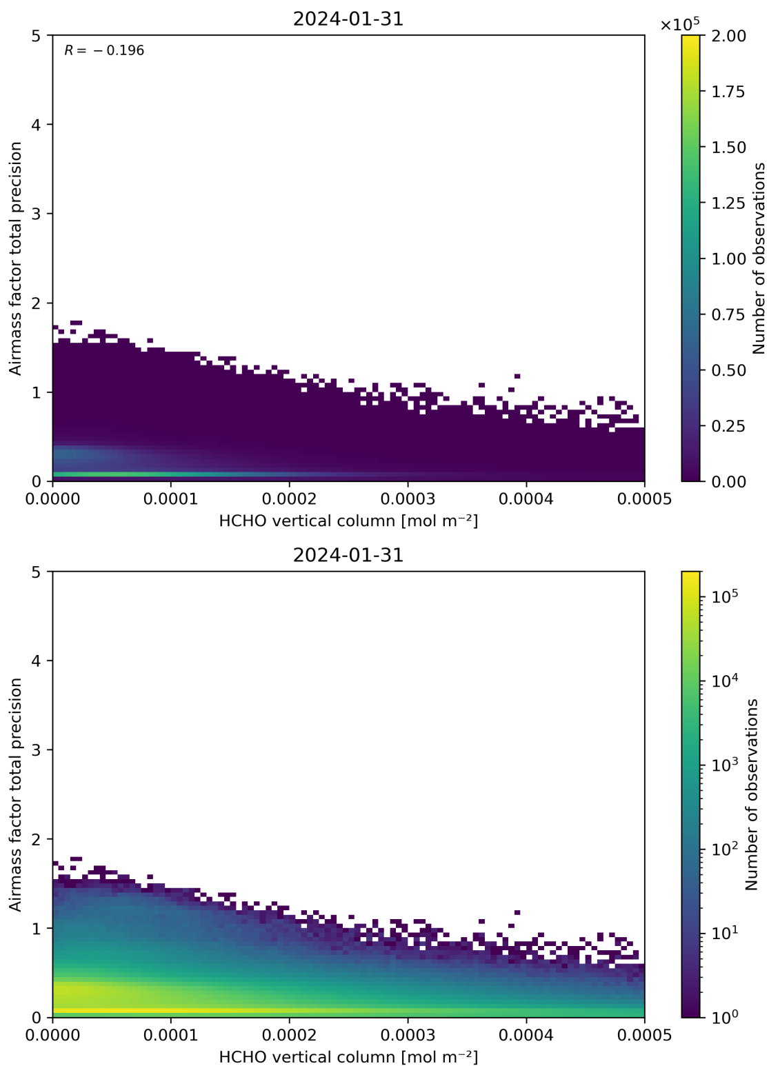
Figure 132: Scatter density plot of “HCHO vertical column” against “Airmass factor total precision” for 2024-01-31 to 2024-02-01.
