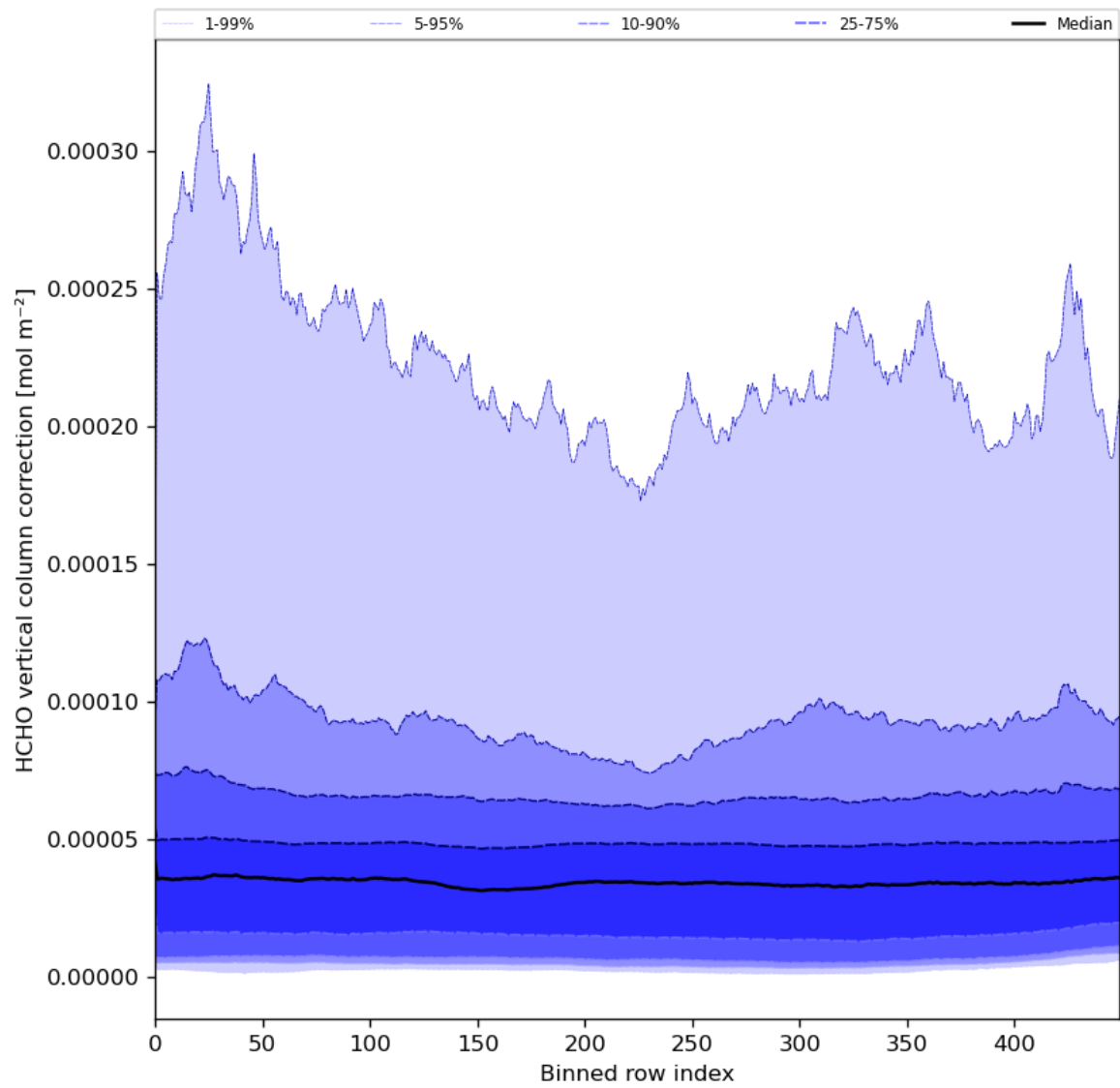
Figure 51: Along track statistics of “HCHO vertical column correction” for 2024-01-31 to 2024-02-01
