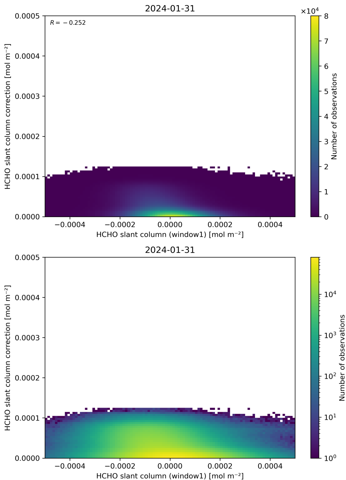
Figure 83: Scatter density plot of “HCHO slant column (window1)” against “HCHO slant column correction” for 2024-01-31 to 2024-02-01.
