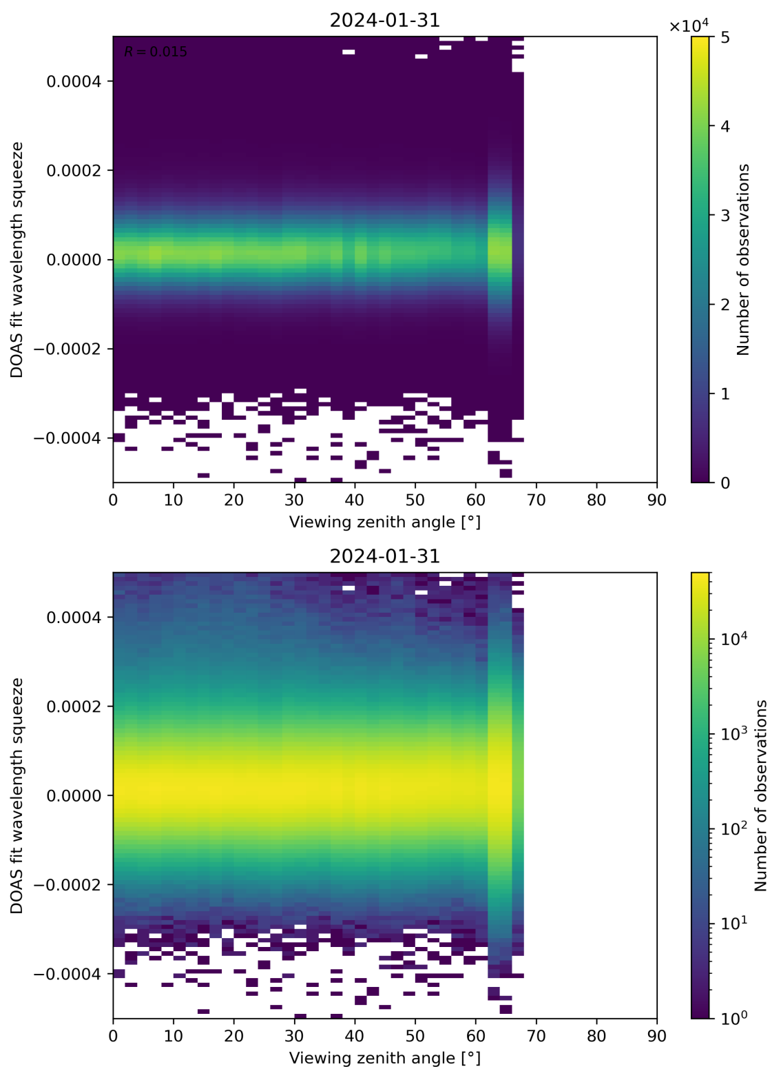
Figure 184: Scatter density plot of “Viewing zenith angle” against “DOAS fit wavelength squeeze” for 2024-01-31 to 2024-02-01.
