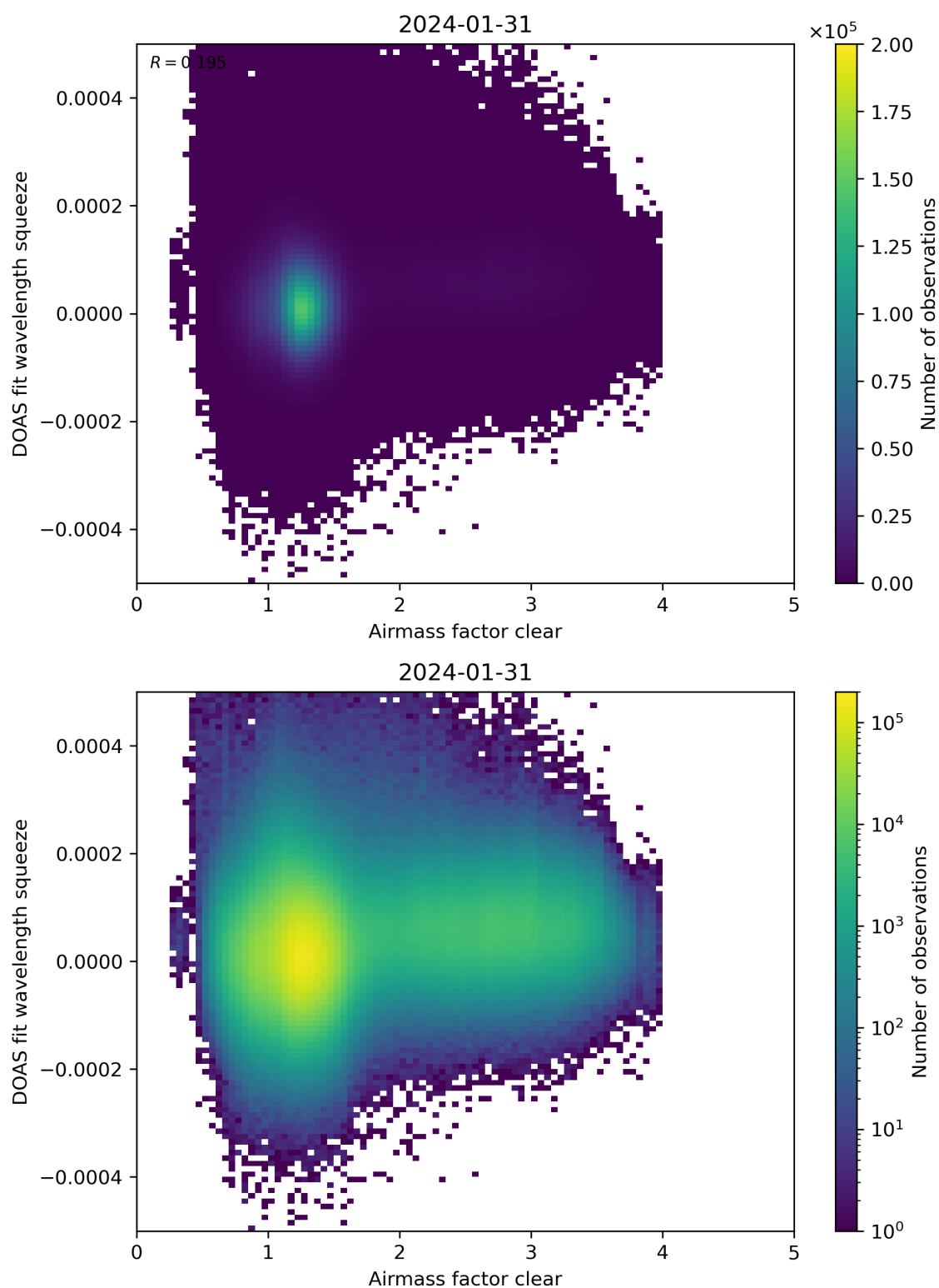
Figure 73: Scatter density plot of “Airmass factor clear” against “DOAS fit wavelength squeeze” for 2024-01-31 to 2024-02-01.
