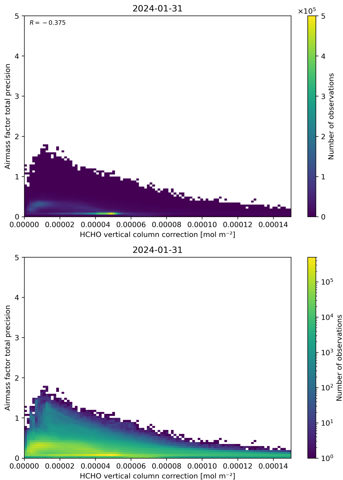
Figure 121: Scatter density plot of “HCHO vertical column correction” against “Airmass factor total precision” for 2024-01-31 to 2024-02-01.
