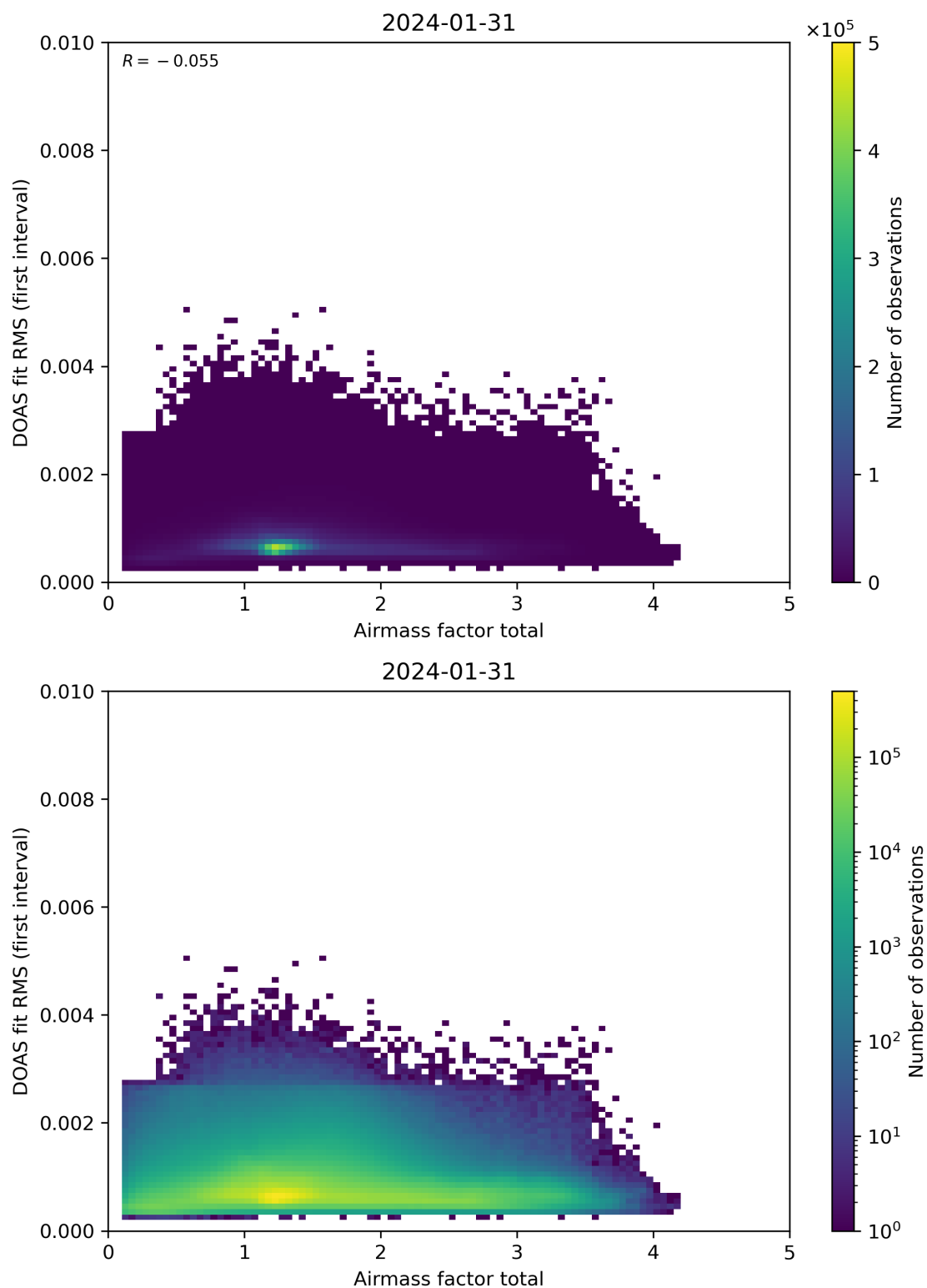
Figure 97: Scatter density plot of “Airmass factor total” against “DOAS fit RMS (first interval)” for 2024-01-31 to 2024-02-01.
