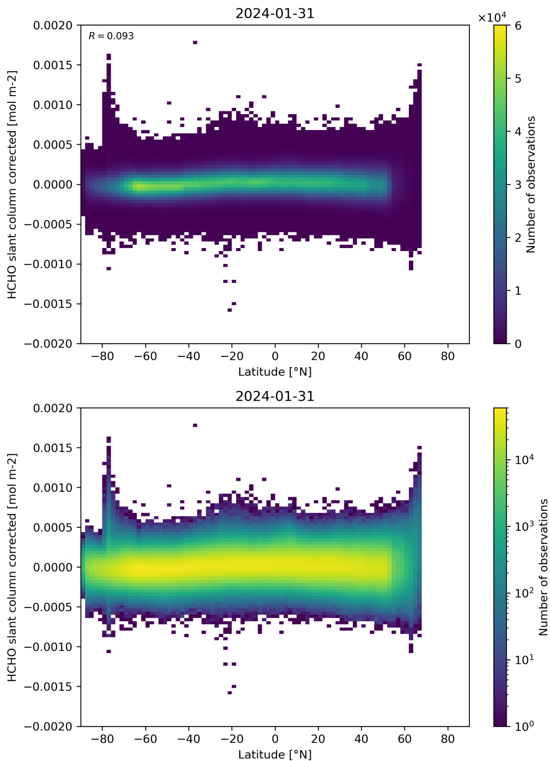
Figure 157: Scatter density plot of “Latitude” against “HCHO slant column corrected” for 2024-01-31 to 2024-02-01.
