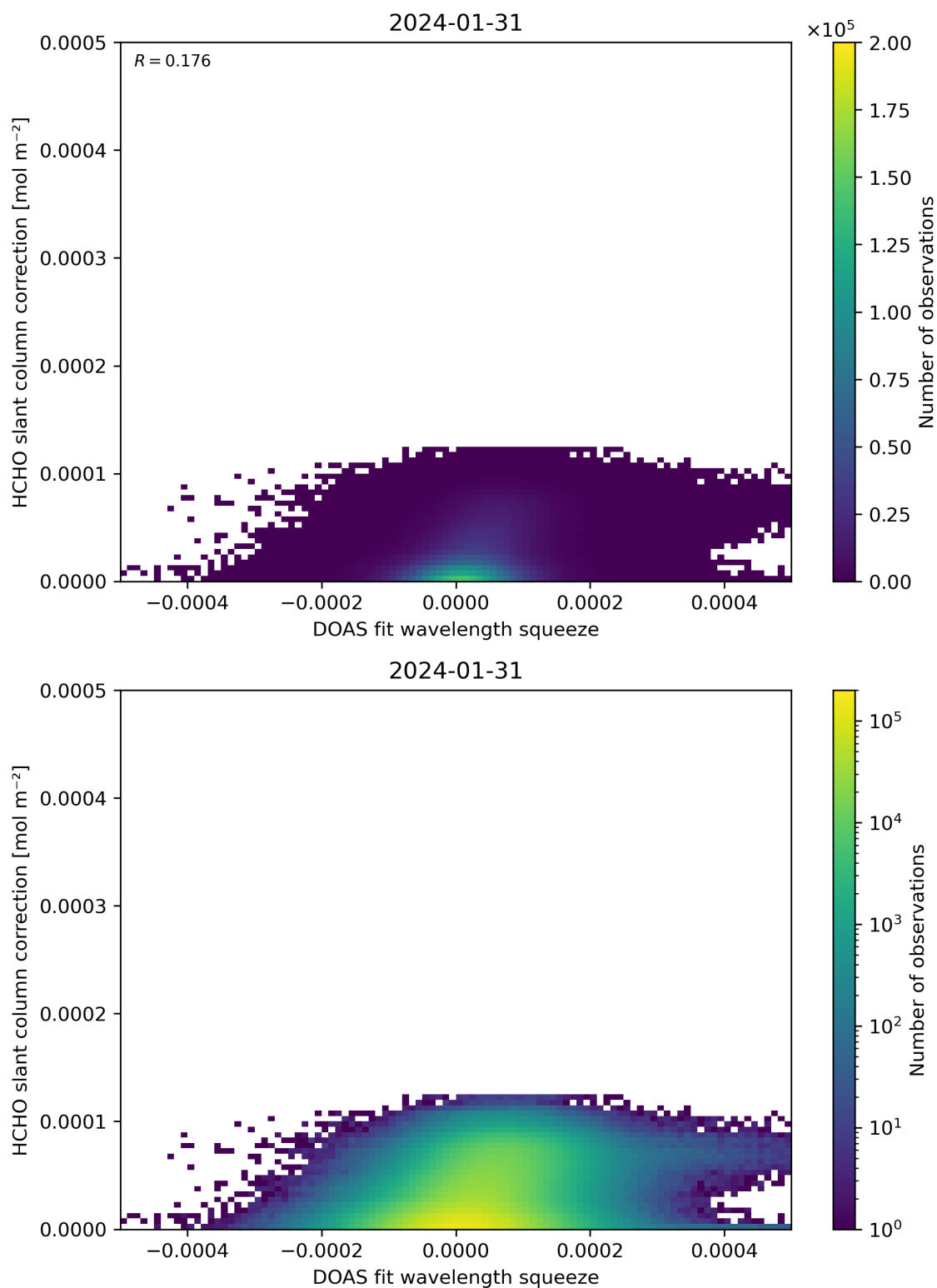
Figure 70: Scatter density plot of “DOAS fit wavelength squeeze” against “HCHO slant column correction” for 2024-01-31 to 2024-02-01.
