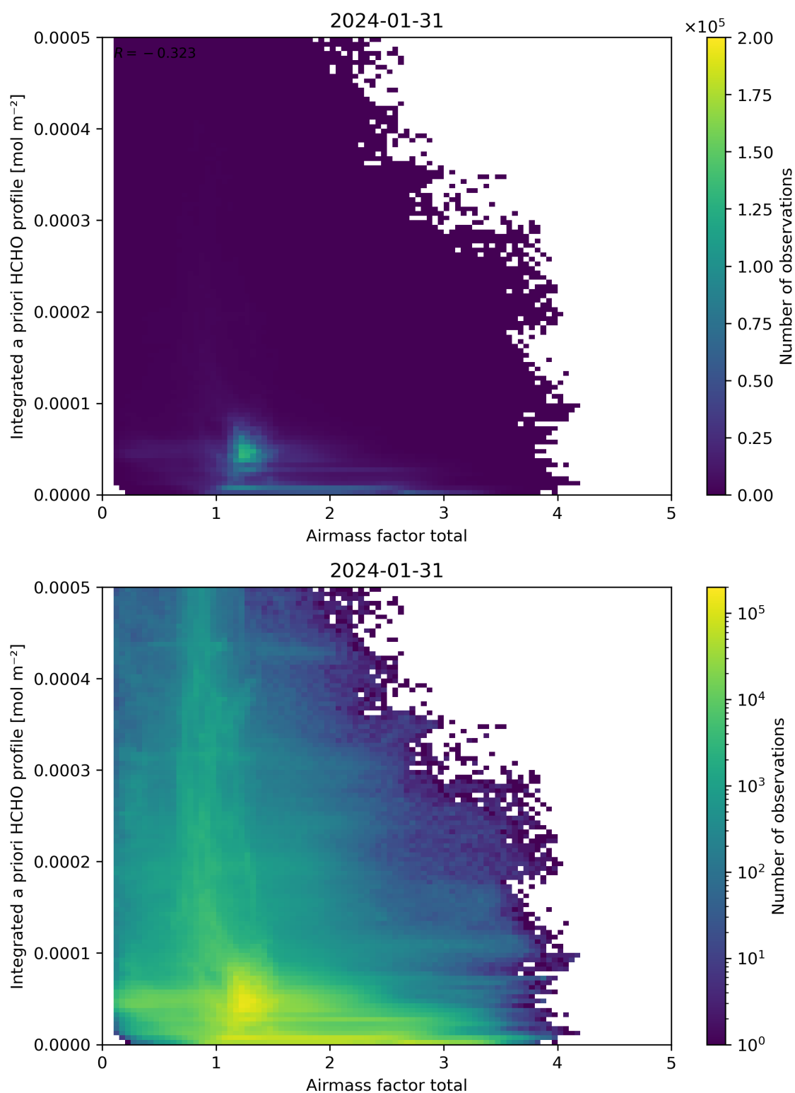
Figure 104: Scatter density plot of “Airmass factor total” against “Integrated a priori HCHO profile” for 2024-01-31 to 2024-02-01.
