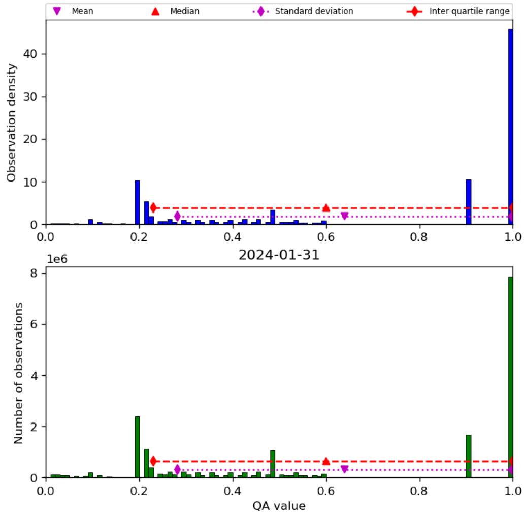
Figure 34: Histogram of “QA value” for 2024-01-31 to 2024-02-01
