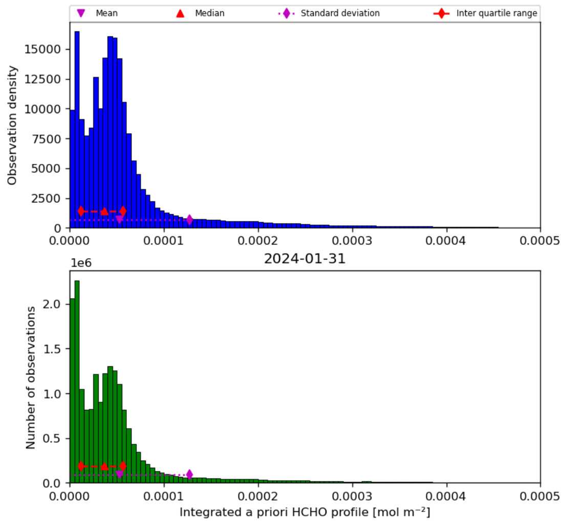
Figure 43: Histogram of “Integrated a priori HCHO profile” for 2024-01-31 to 2024-02-01
