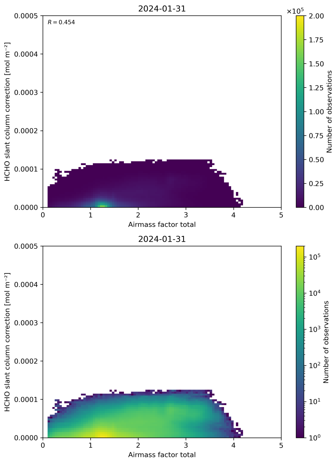
Figure 102: Scatter density plot of “Airmass factor total” against “HCHO slant column correction” for 2024-01-31 to 2024-02-01.
