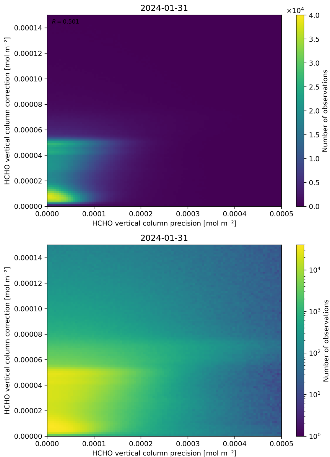
Figure 146: Scatter density plot of “HCHO vertical column precision” against “HCHO vertical column correction” for 2024-01-31 to 2024-02-01.
