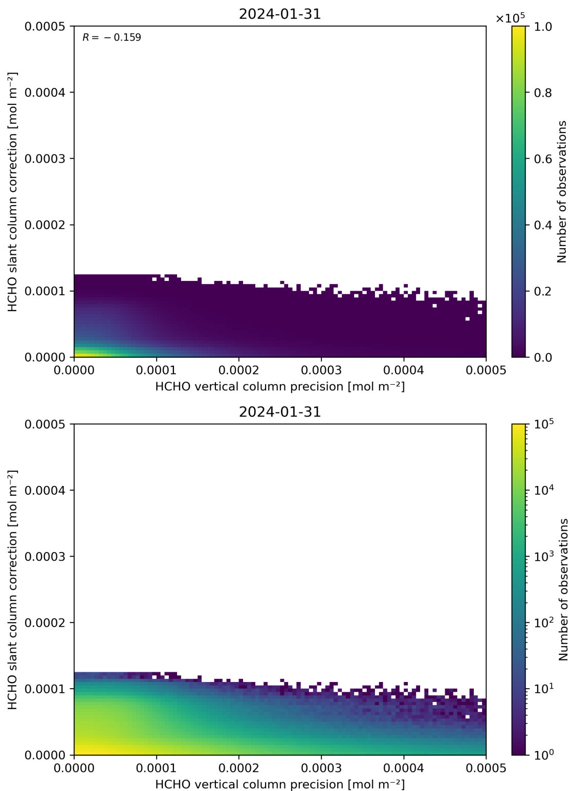
Figure 141: Scatter density plot of “HCHO vertical column precision” against “HCHO slant column correction” for 2024-01-31 to 2024-02-01.
