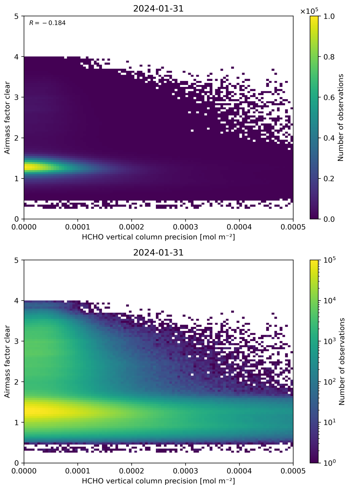
Figure 139: Scatter density plot of “HCHO vertical column precision” against “Airmass factor clear” for 2024-01-31 to 2024-02-01.
