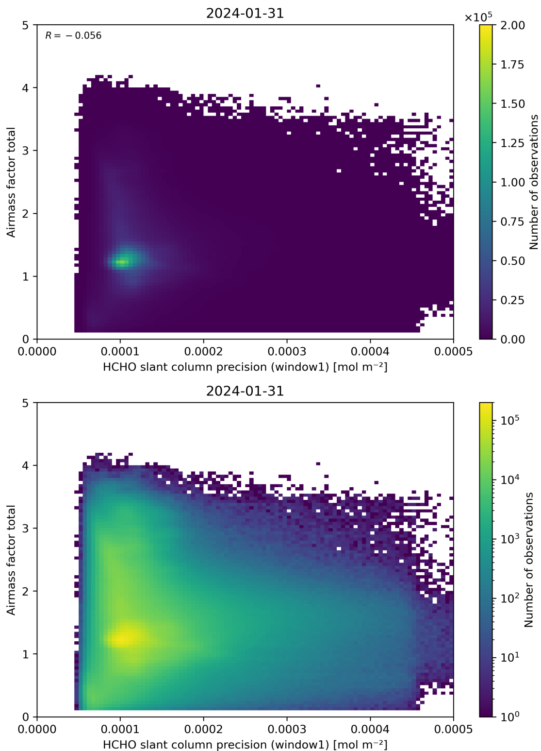
Figure 94: Scatter density plot of “HCHO slant column precision (window1)” against “Airmass factor total” for 2024-01-31 to 2024-02-01.
