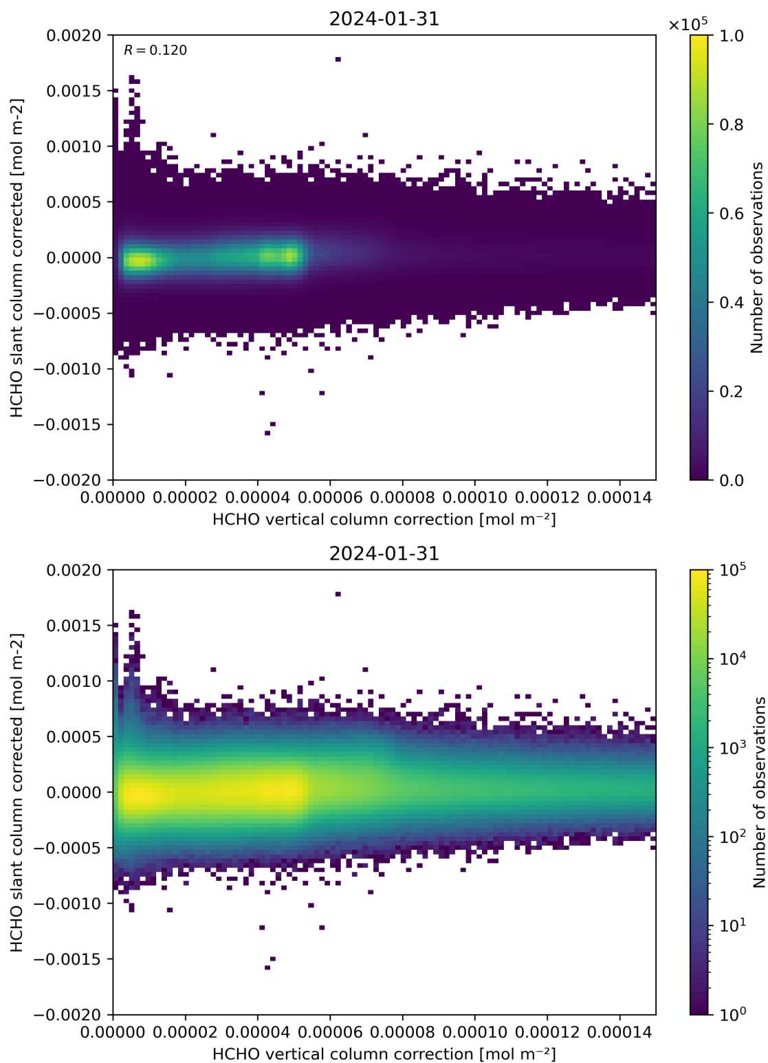
Figure 116: Scatter density plot of “HCHO vertical column correction” against “HCHO slant column corrected” for 2024-01-31 to 2024-02-01.
