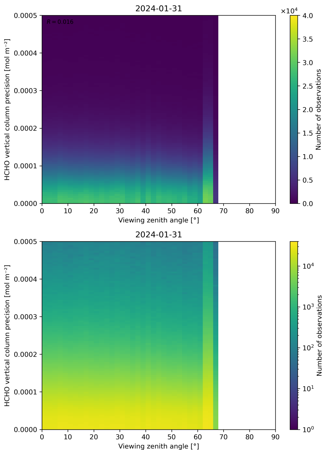
Figure 194: Scatter density plot of “Viewing zenith angle” against “HCHO vertical column precision” for 2024-01-31 to 2024-02-01.
