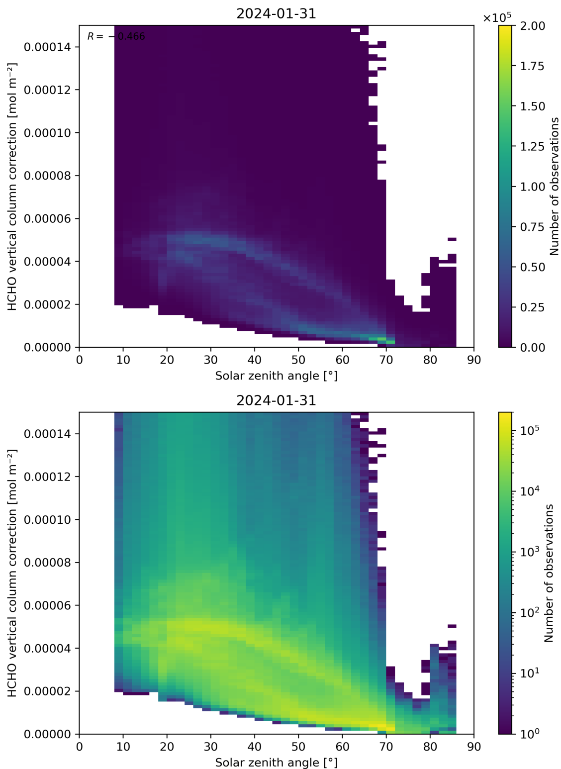
Figure 178: Scatter density plot of “Solar zenith angle” against “HCHO vertical column correction” for 2024-01-31 to 2024-02-01.
