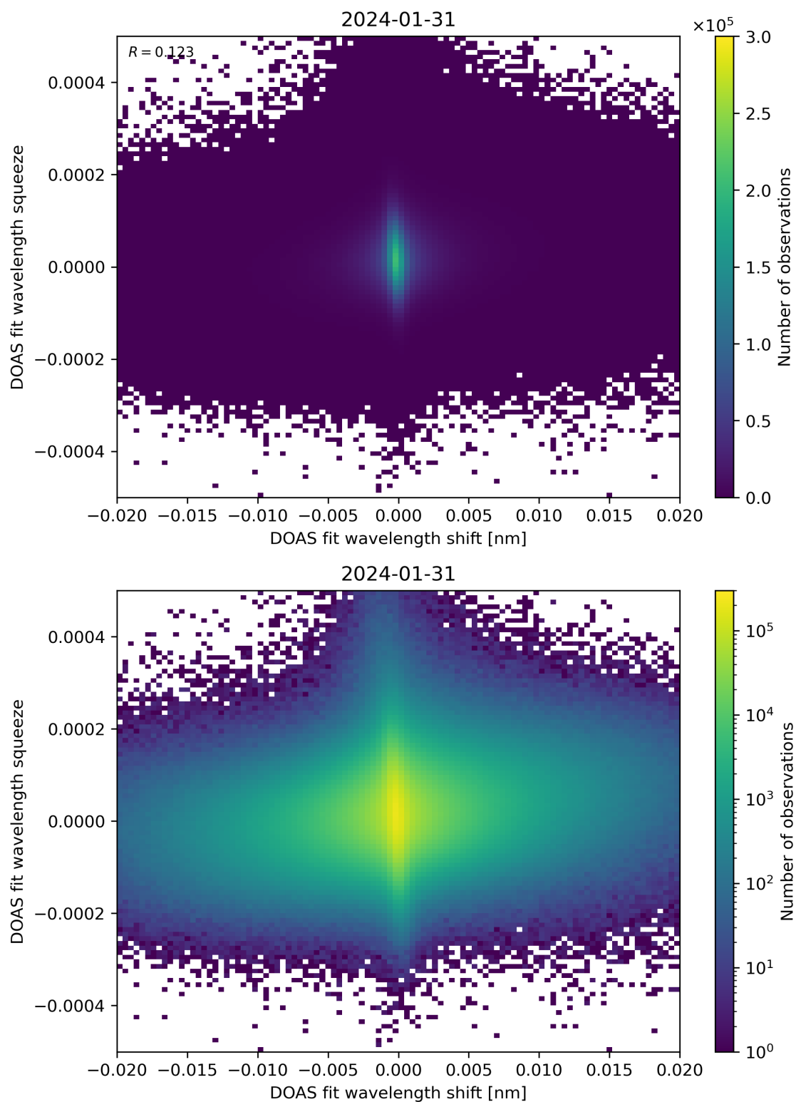
Figure 65: Scatter density plot of “DOAS fit wavelength shift” against “DOAS fit wavelength squeeze” for 2024-01-31 to 2024-02-01.
