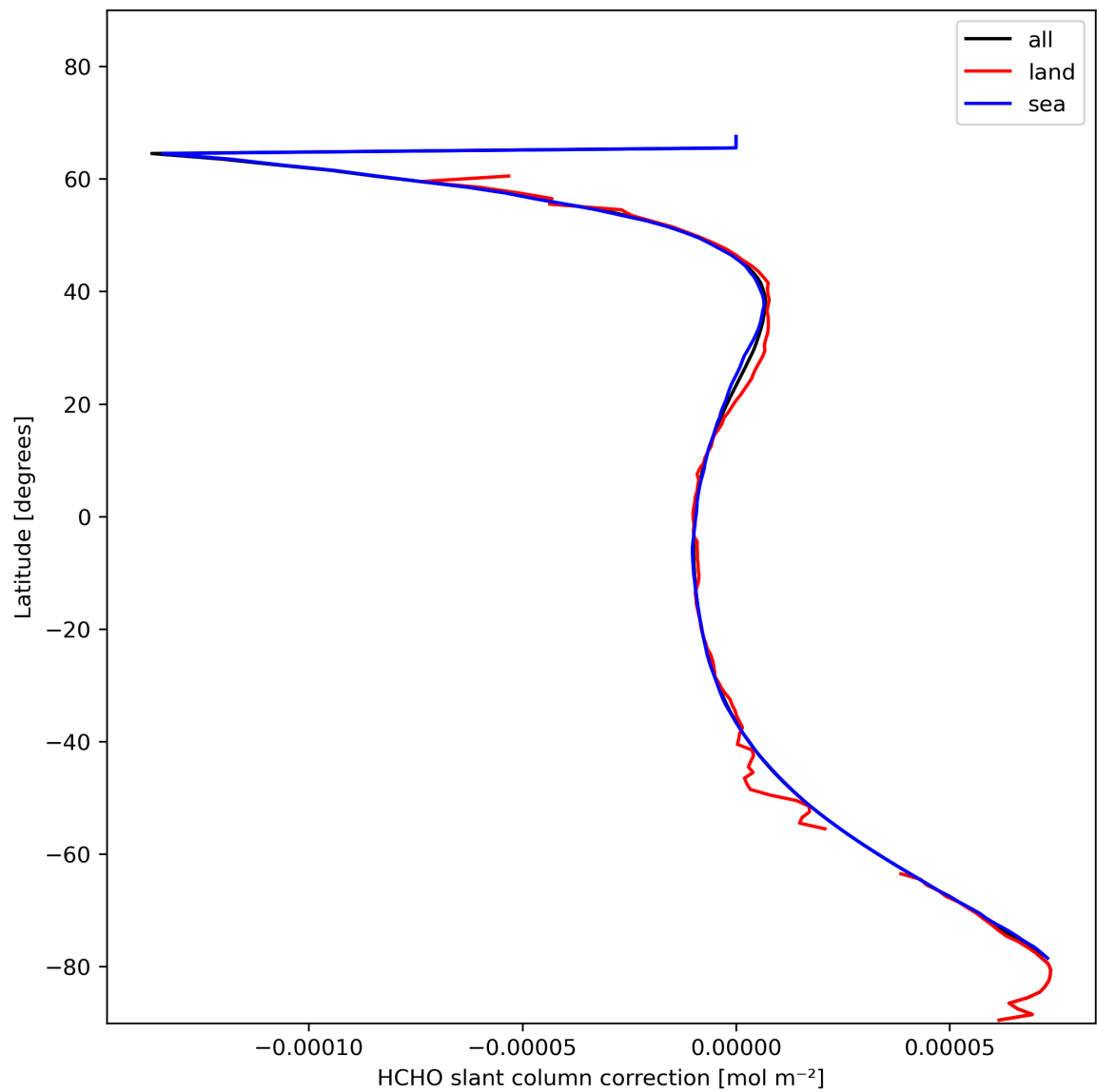
Figure 33: Zonal average of “HCHO slant column correction” for 2024-01-31 to 2024-02-01.
