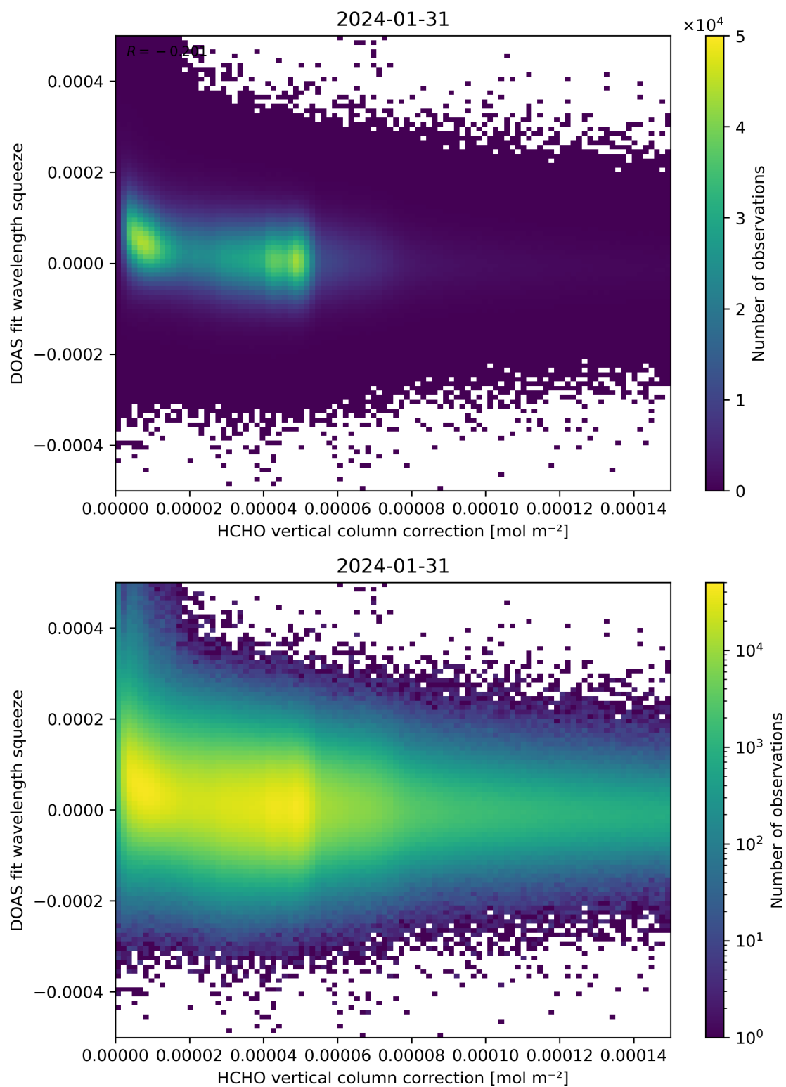
Figure 114: Scatter density plot of “HCHO vertical column correction” against “DOAS fit wavelength squeeze” for 2024-01-31 to 2024-02-01.
