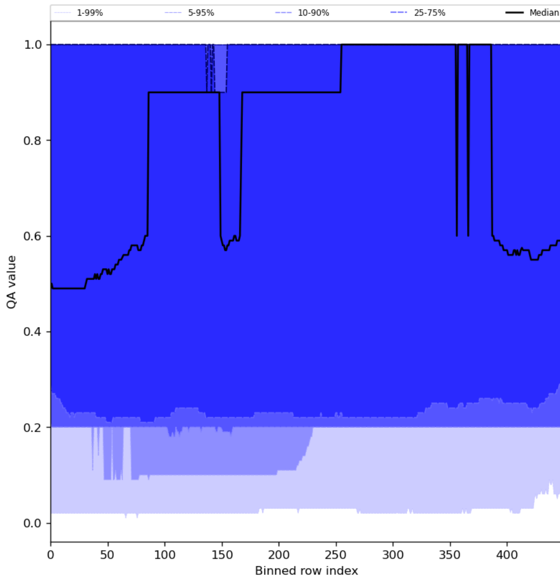
Figure 48: Along track statistics of “QA value” for 2024-01-31 to 2024-02-01
