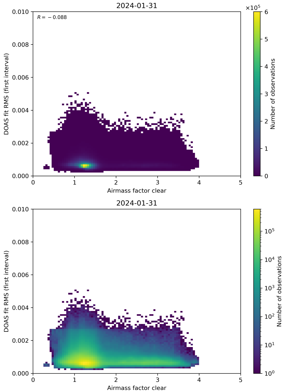
Figure 71: Scatter density plot of “Airmass factor clear” against “DOAS fit RMS (first interval)” for 2024-01-31 to 2024-02-01.
