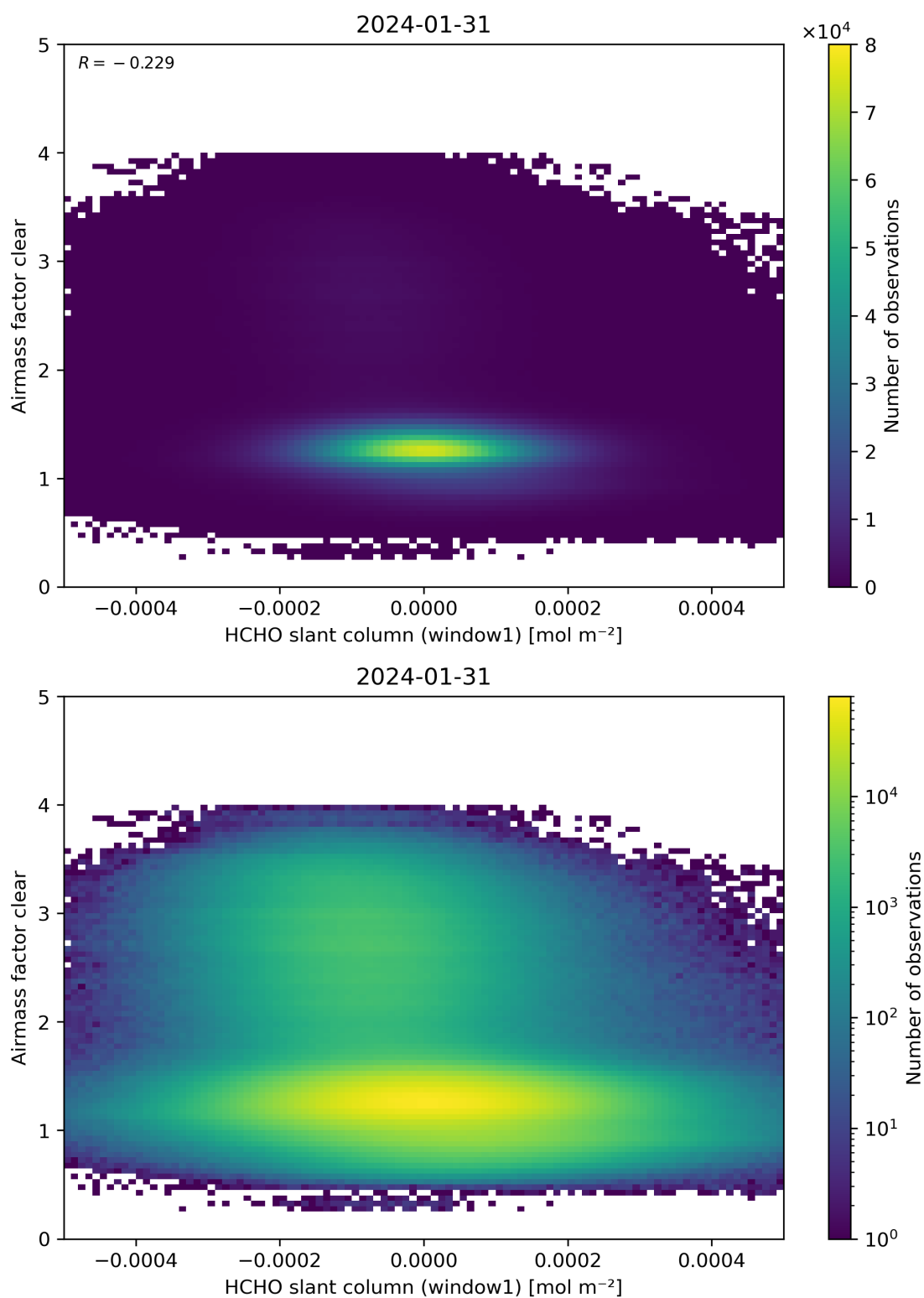
Figure 81: Scatter density plot of “HCHO slant column (window1)” against “Airmass factor clear” for 2024-01-31 to 2024-02-01.
