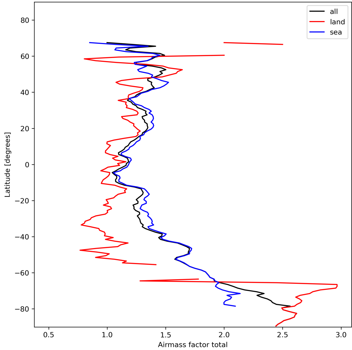
Figure 26: Zonal average of “Airmass factor total” for 2024-01-31 to 2024-02-01.
