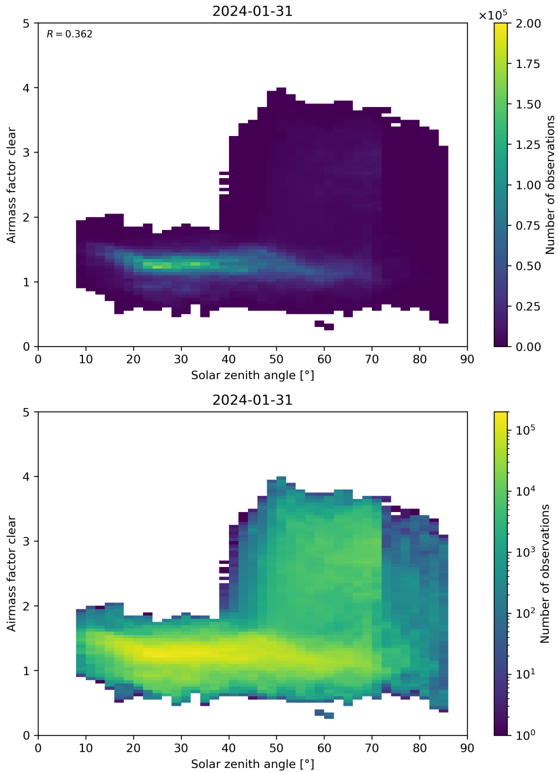
Figure 170: Scatter density plot of “Solar zenith angle” against “Airmass factor clear” for 2024-01-31 to 2024-02-01.
