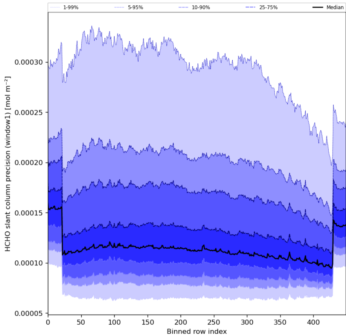
Figure 53: Along track statistics of “HCHO slant column precision (window1)” for 2024-01-31 to 2024-02-01
