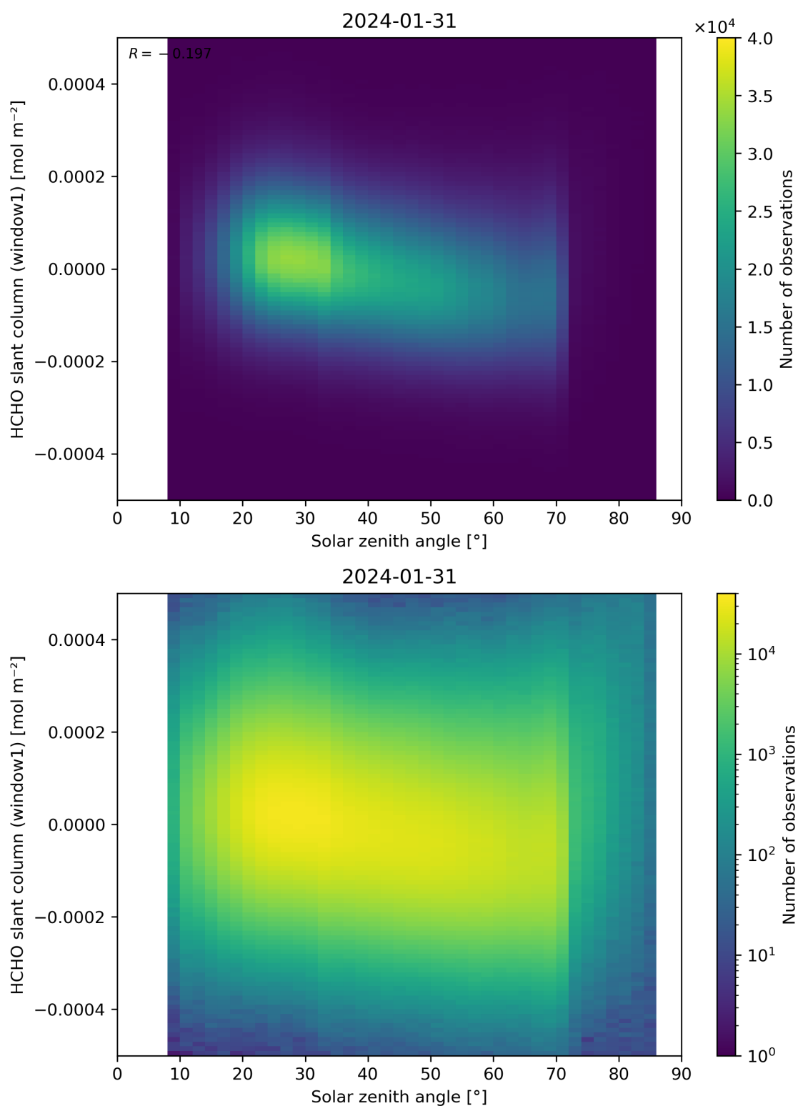
Figure 173: Scatter density plot of “Solar zenith angle” against “HCHO slant column (window1)” for 2024-01-31 to 2024-02-01.
