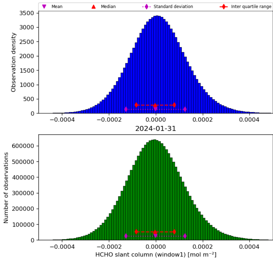
Figure 38: Histogram of “HCHO slant column (window1)” for 2024-01-31 to 2024-02-01
