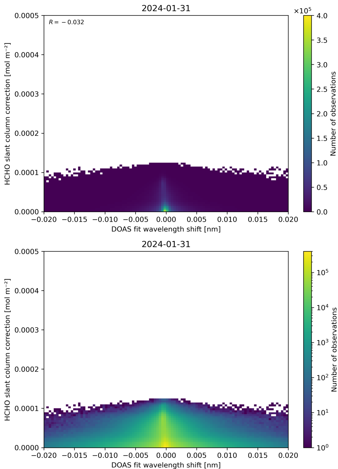
Figure 67: Scatter density plot of “DOAS fit wavelength shift” against “HCHO slant column correction” for 2024-01-31 to 2024-02-01.
