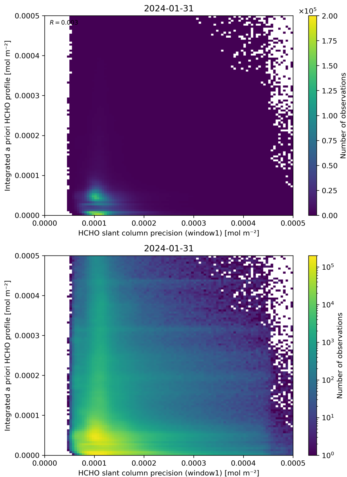
Figure 96: Scatter density plot of “HCHO slant column precision (window1)” against “Integrated a priori HCHO profile” for 2024-01-31 to 2024-02-01.
