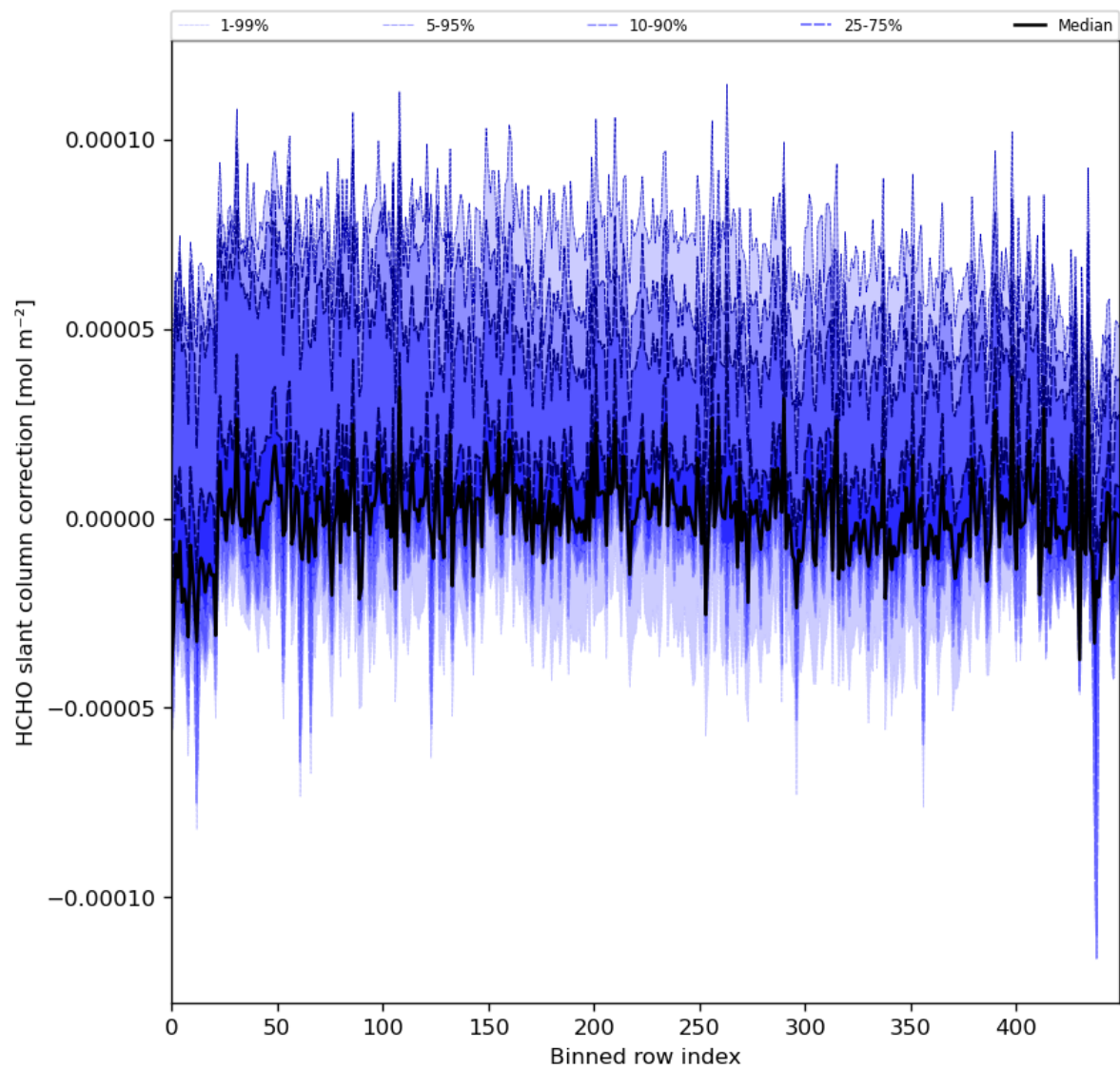
Figure 61: Along track statistics of “HCHO slant column correction” for 2024-01-31 to 2024-02-01
