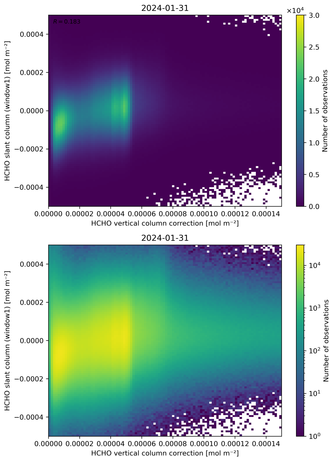
Figure 118: Scatter density plot of “HCHO vertical column correction” against “HCHO slant column (window1)” for 2024-01-31 to 2024-02-01.
