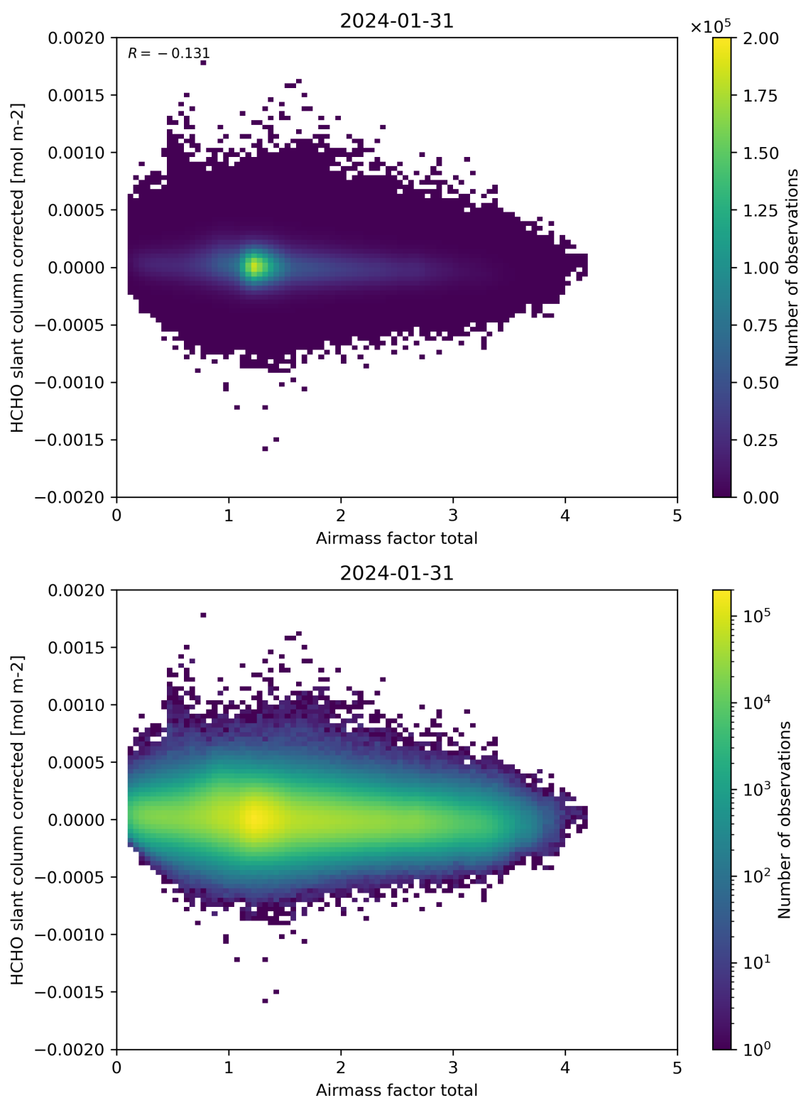
Figure 101: Scatter density plot of “Airmass factor total” against “HCHO slant column corrected” for 2024-01-31 to 2024-02-01.
