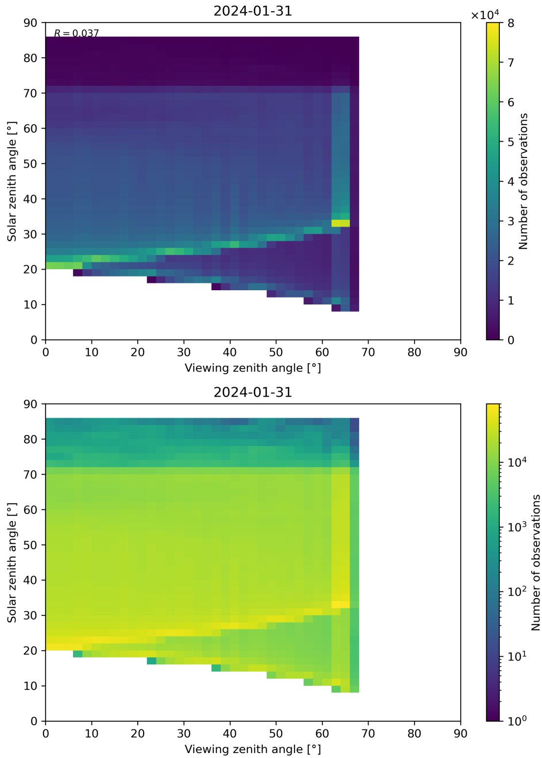
Figure 197: Scatter density plot of “Viewing zenith angle” against “Solar zenith angle” for 2024-01-31 to 2024-02-01.
