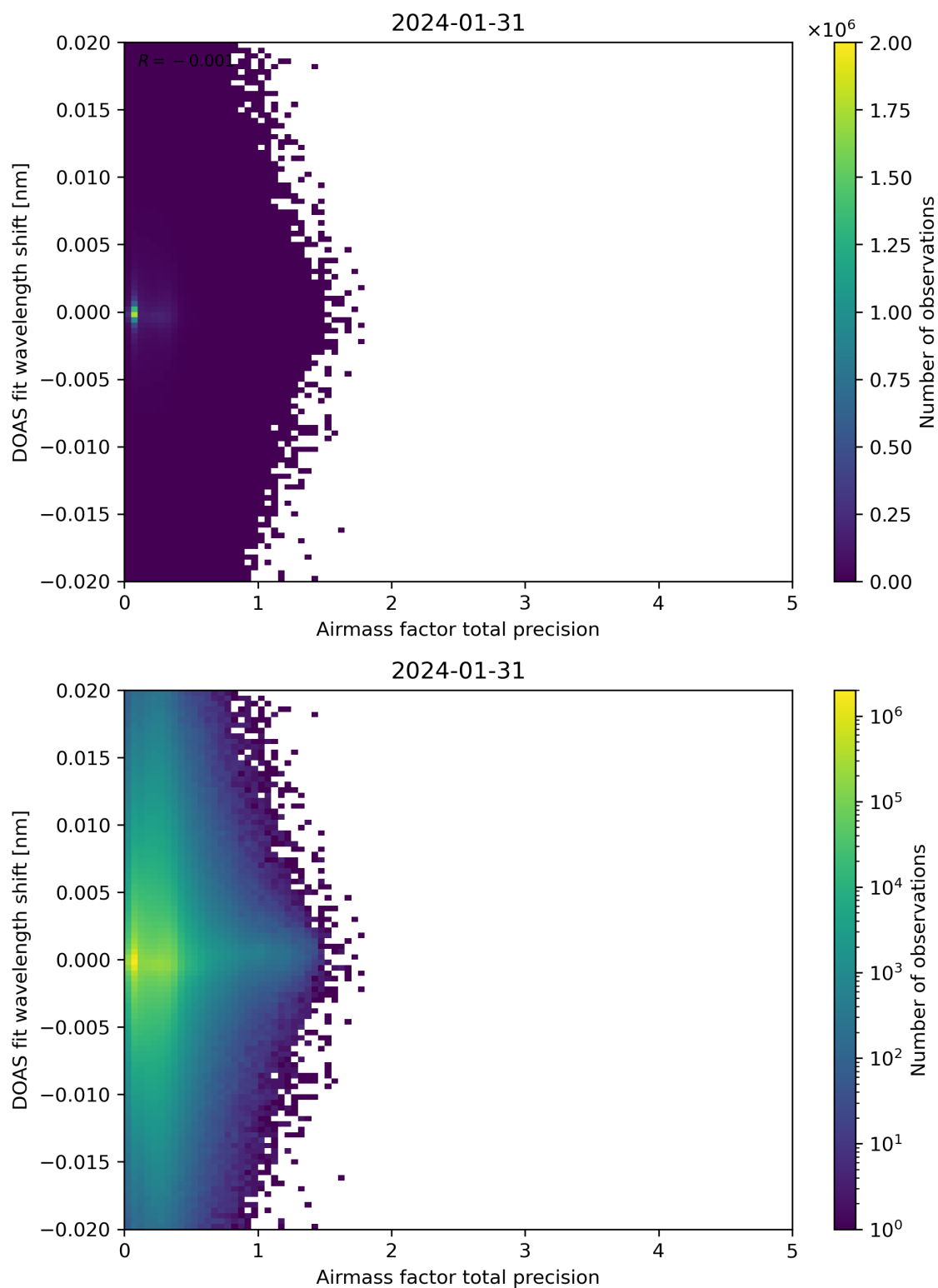
Figure 106: Scatter density plot of “Airmass factor total precision” against “DOAS fit wavelength shift” for 2024-01-31 to 2024-02-01.
