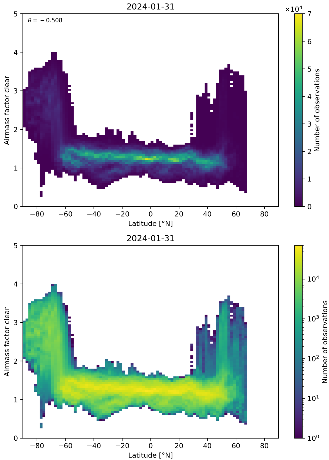
Figure 156: Scatter density plot of “Latitude” against “Airmass factor clear” for 2024-01-31 to 2024-02-01.
