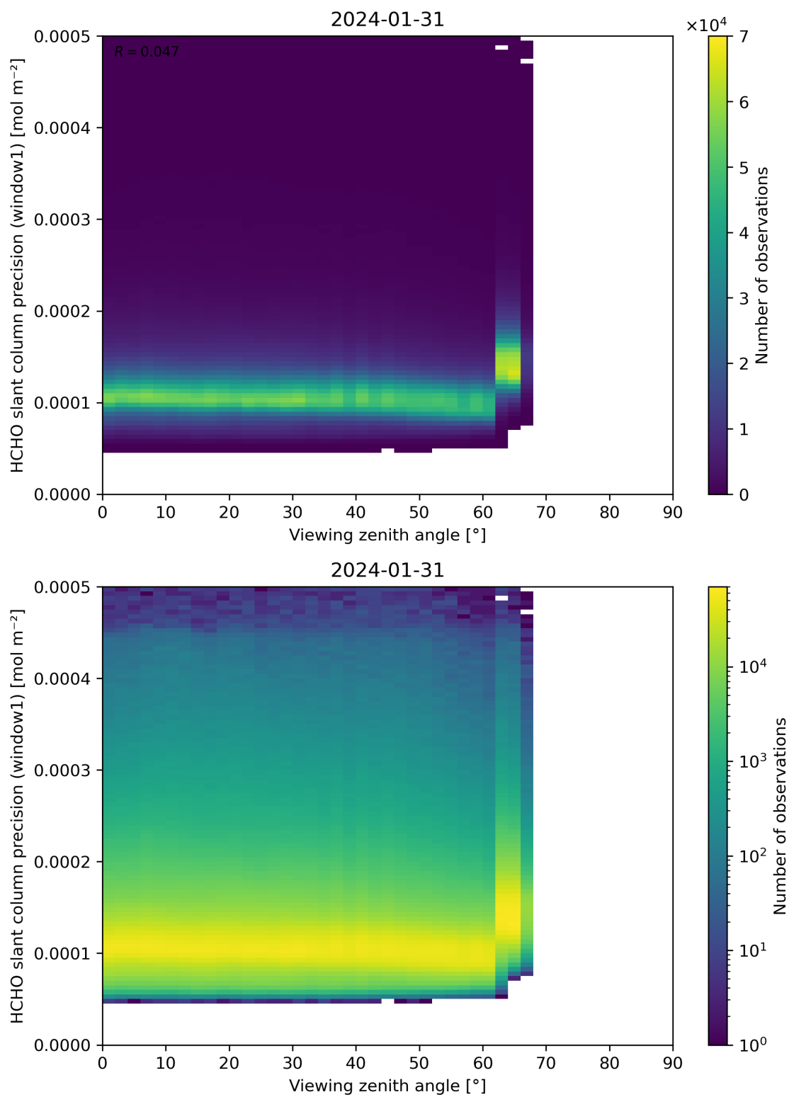
Figure 189: Scatter density plot of “Viewing zenith angle” against “HCHO slant column precision (window1)” for 2024-01-31 to 2024-02-01.
