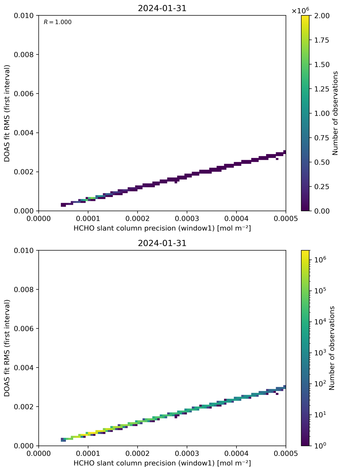
Figure 88: Scatter density plot of “HCHO slant column precision (window1)” against “DOAS fit RMS (first interval)” for 2024-01-31 to 2024-02-01.
