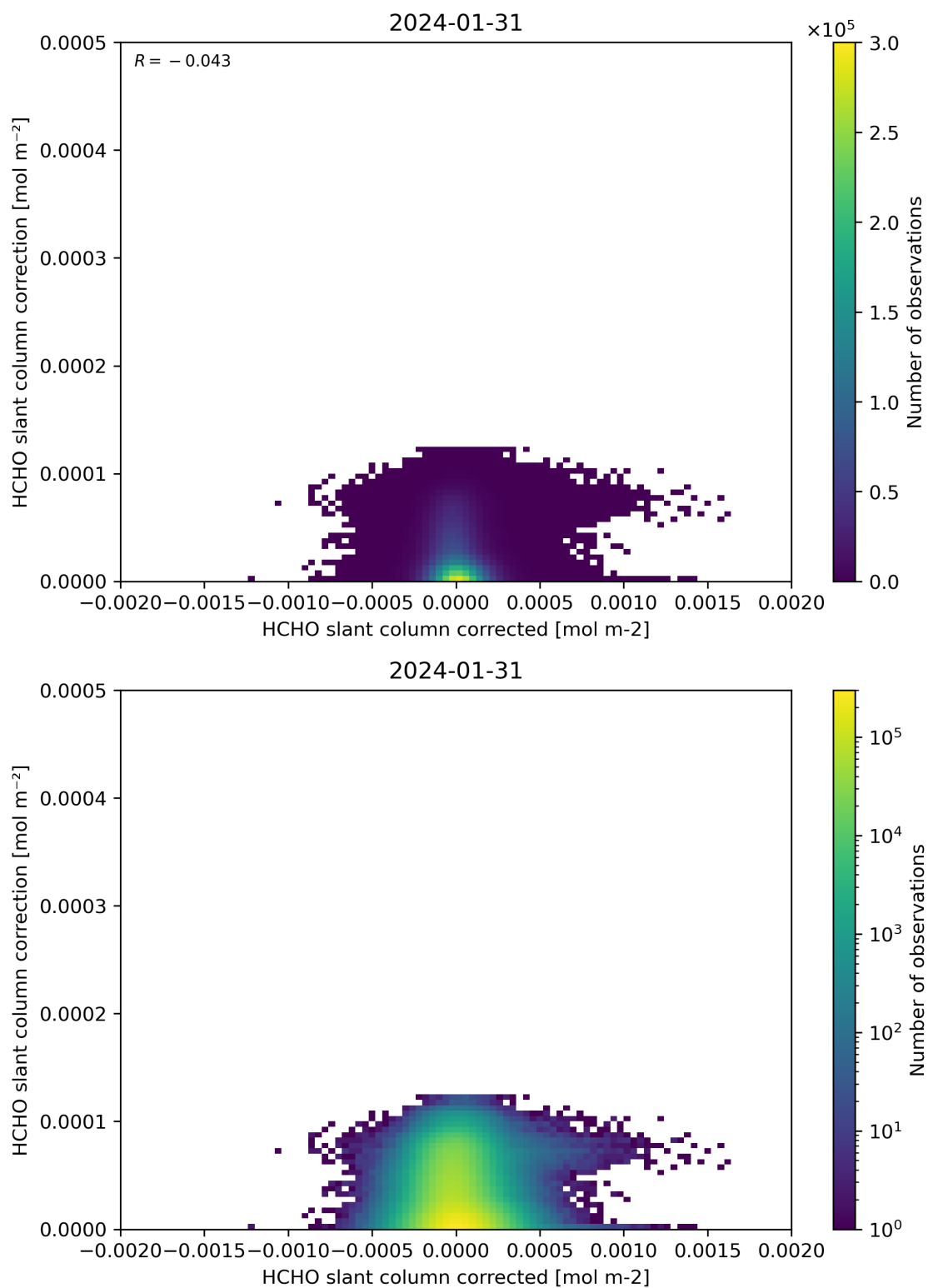
Figure 77: Scatter density plot of “HCHO slant column corrected” against “HCHO slant column correction” for 2024-01-31 to 2024-02-01.
