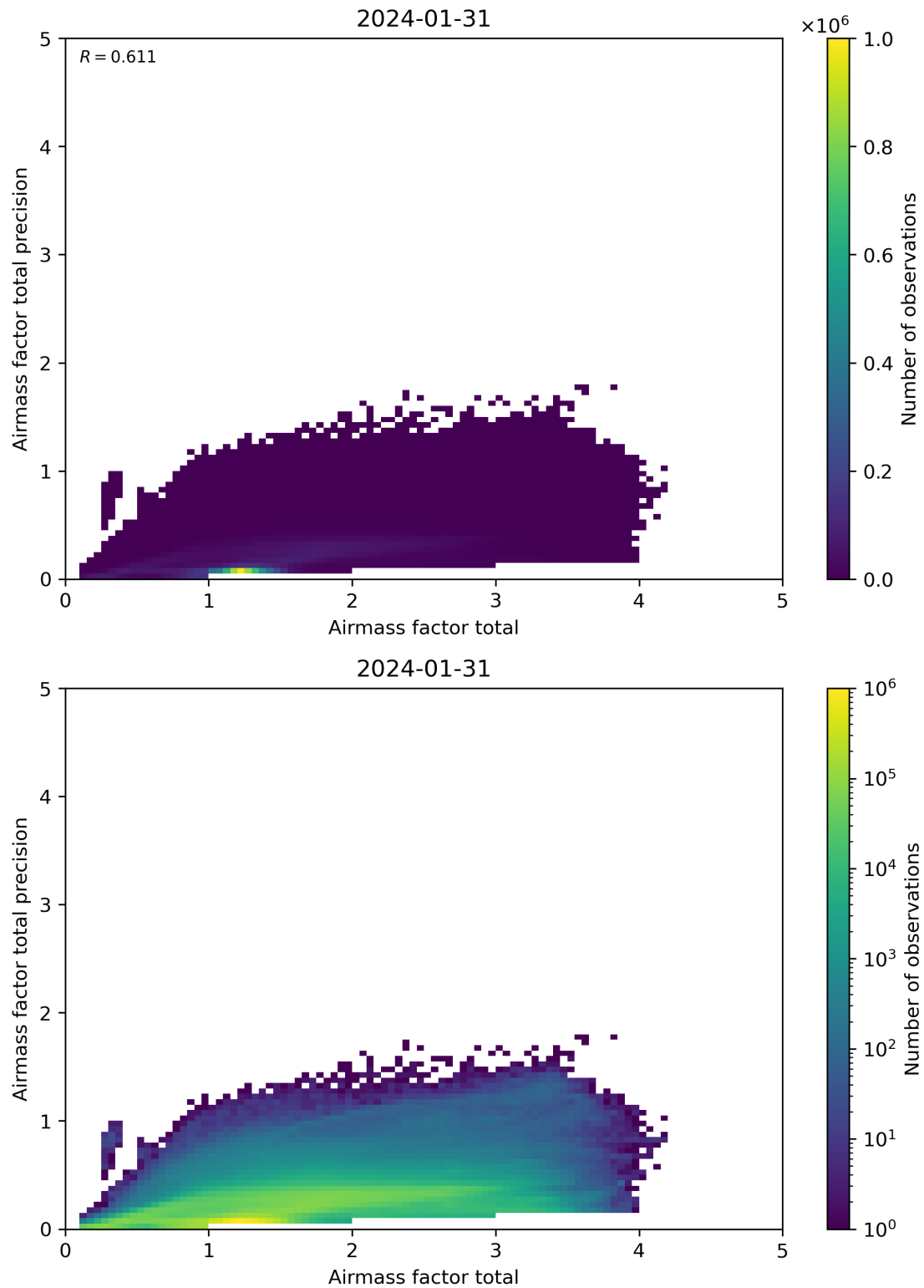
Figure 103: Scatter density plot of “Airmass factor total” against “Airmass factor total precision” for 2024-01-31 to 2024-02-01.
