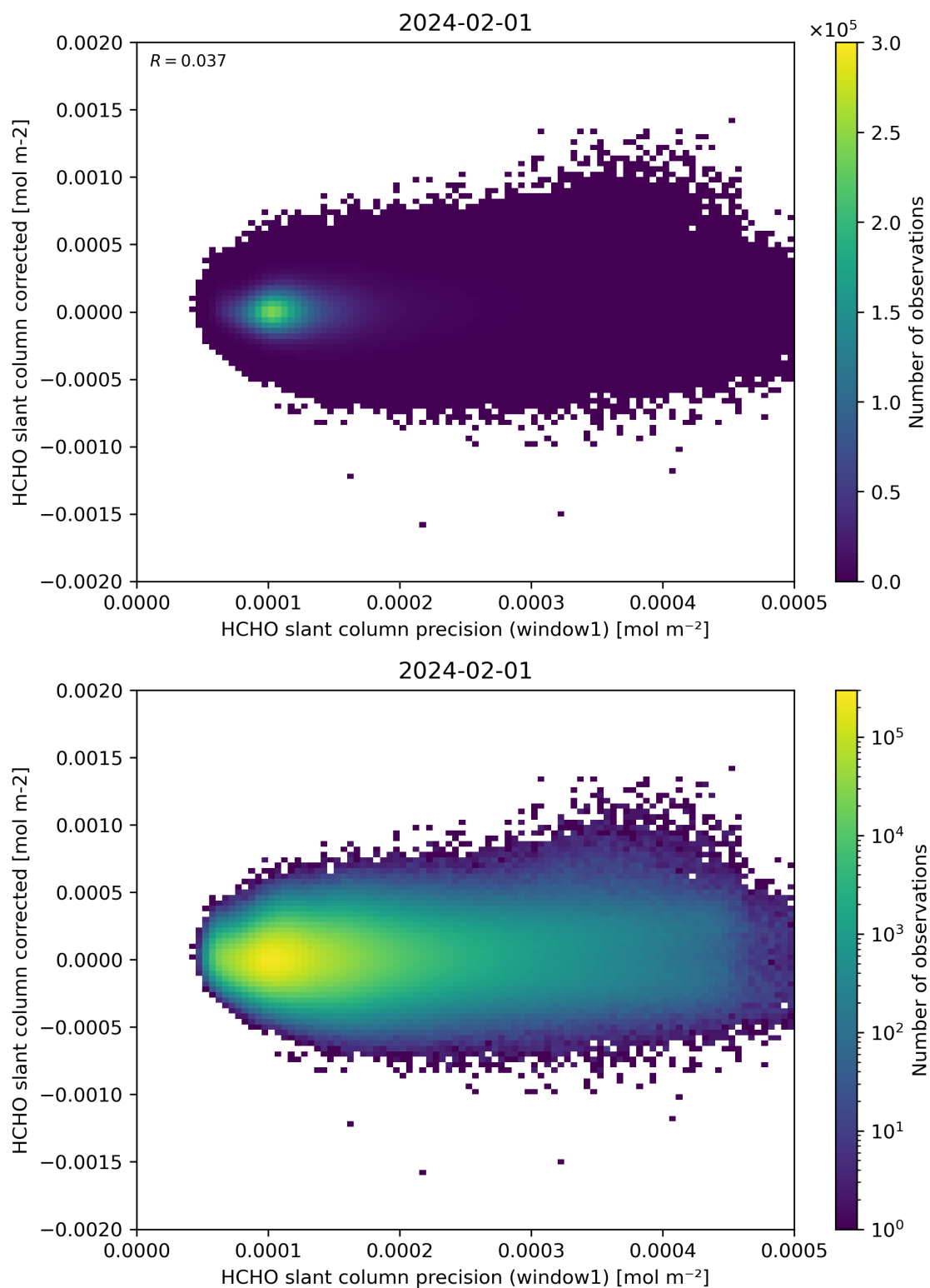
Figure 92: Scatter density plot of “HCHO slant column precision (window1)” against “HCHO slant column corrected” for 2024-01-31 to 2024-02-02.
