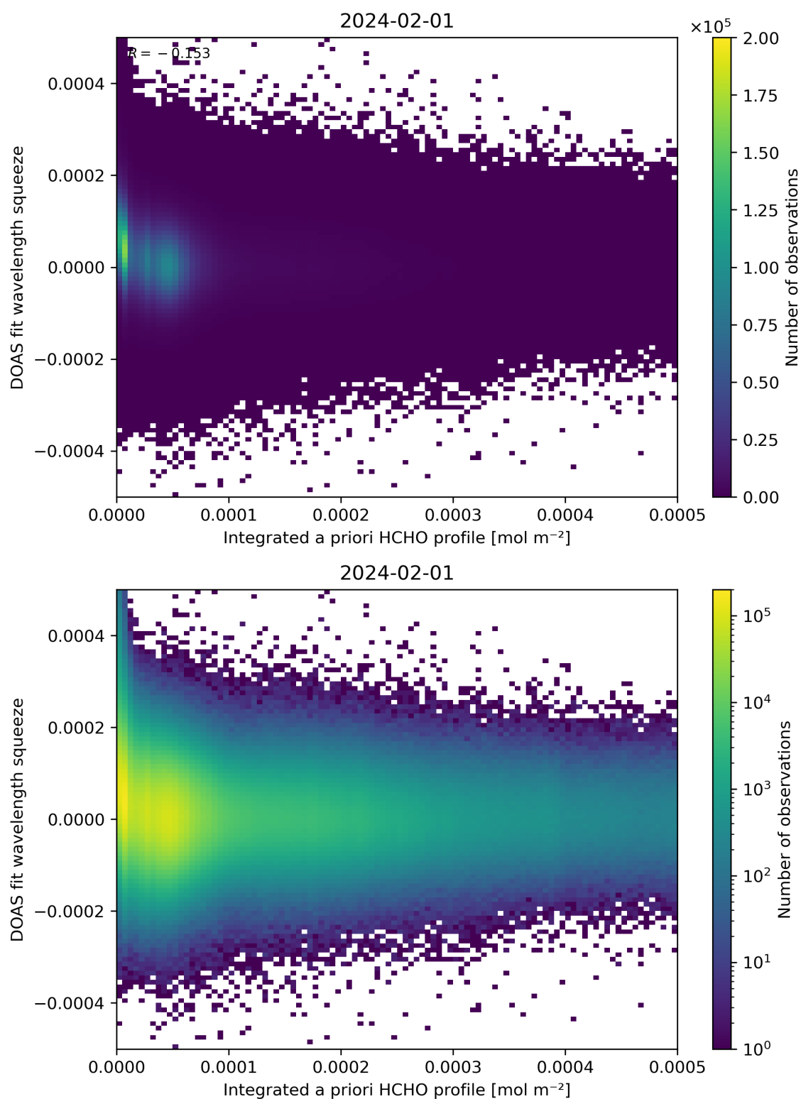
Figure 150: Scatter density plot of “Integrated a priori HCHO profile” against “DOAS fit wavelength squeeze” for 2024-01-31 to 2024-02-02.
