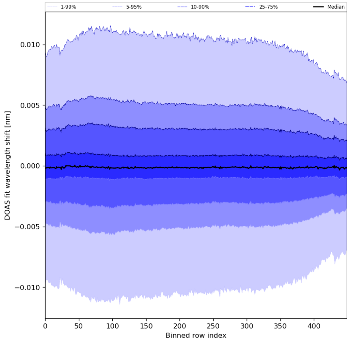
Figure 58: Along track statistics of “DOAS fit wavelength shift” for 2024-01-31 to 2024-02-02
