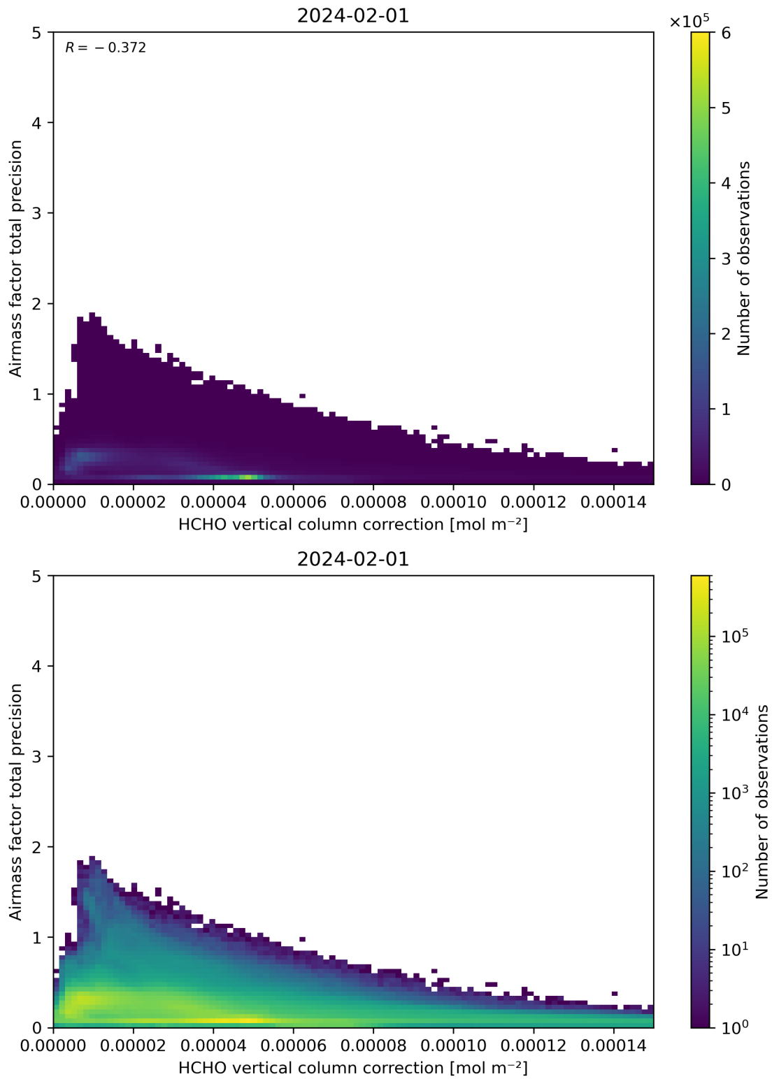
Figure 121: Scatter density plot of “HCHO vertical column correction” against “Airmass factor total precision” for 2024-01-31 to 2024-02-02.
