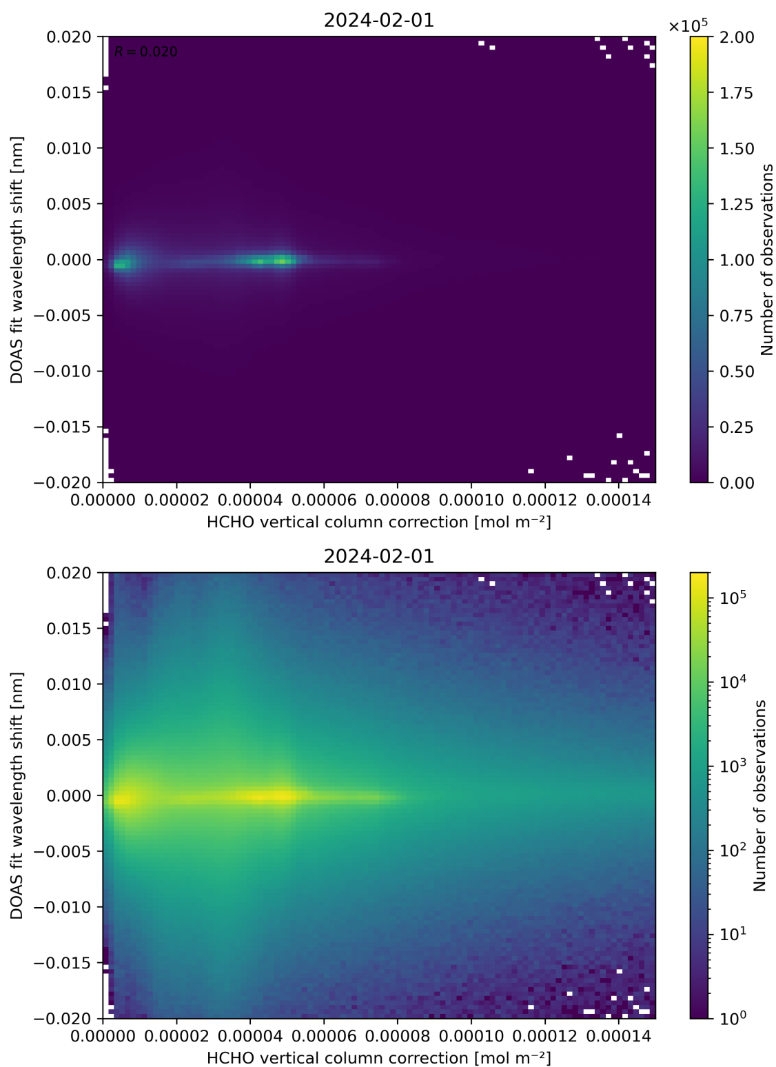
Figure 113: Scatter density plot of “HCHO vertical column correction” against “DOAS fit wavelength shift” for 2024-01-31 to 2024-02-02.
