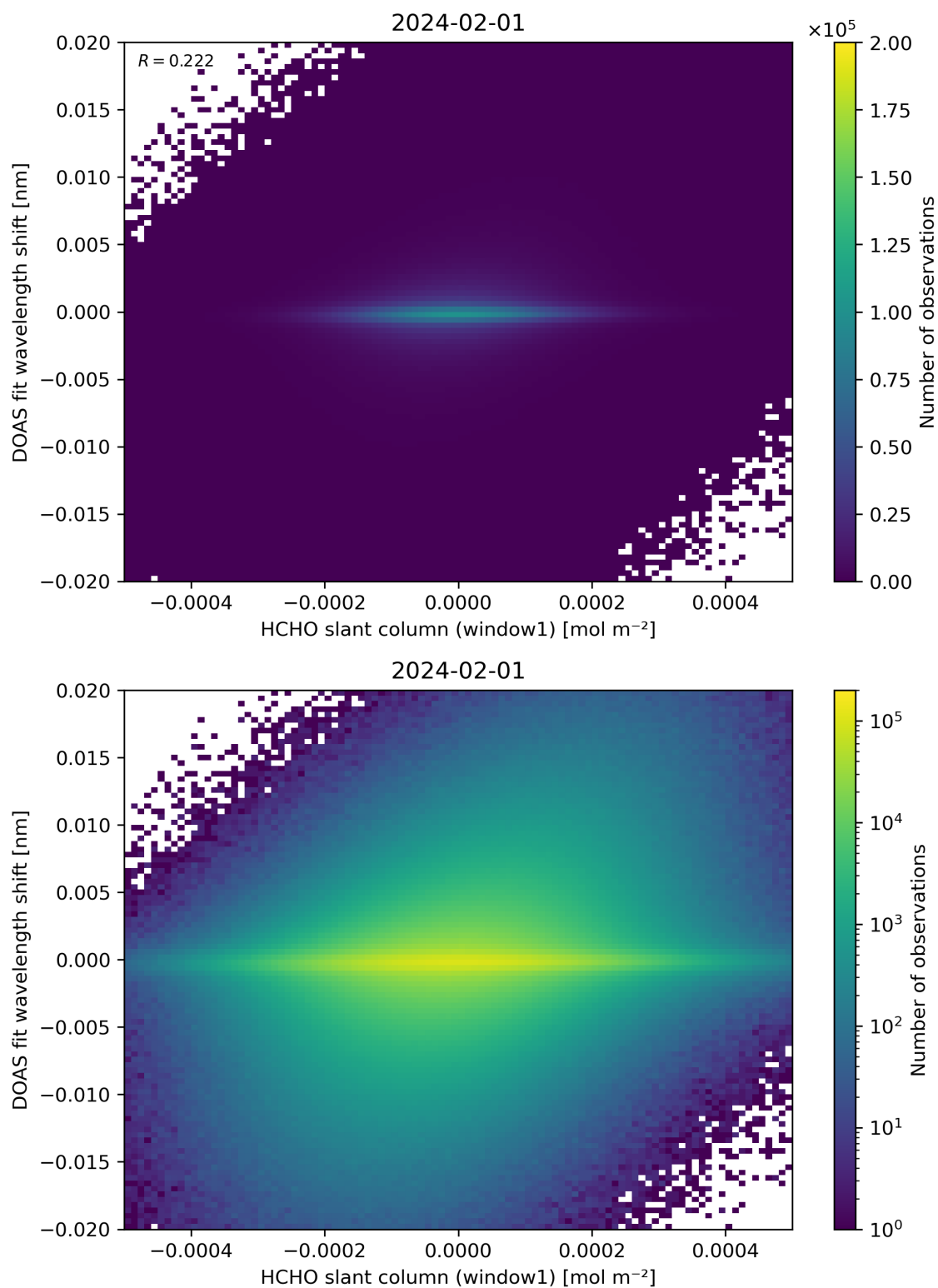
Figure 79: Scatter density plot of “HCHO slant column (window1)” against “DOAS fit wavelength shift” for 2024-01-31 to 2024-02-02.
