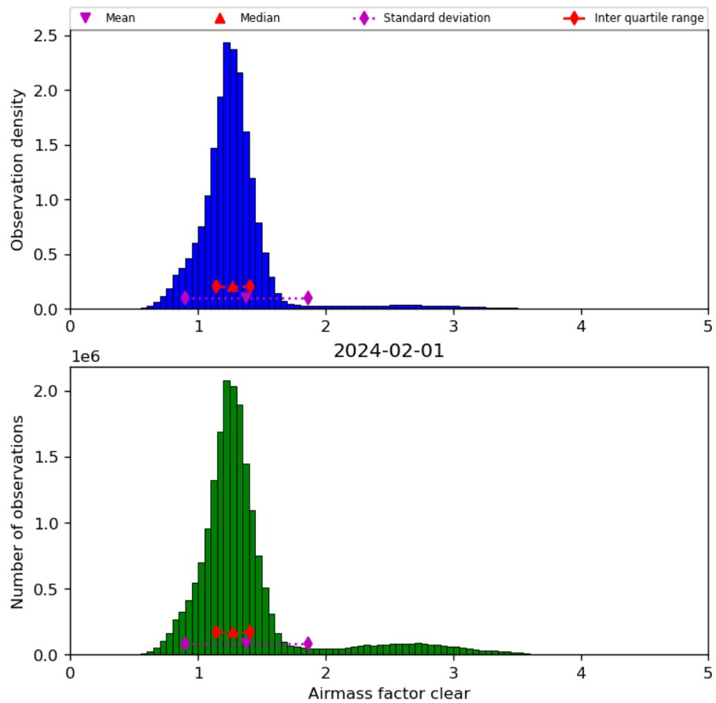
Figure 42: Histogram of “Airmass factor clear” for 2024-01-31 to 2024-02-02
