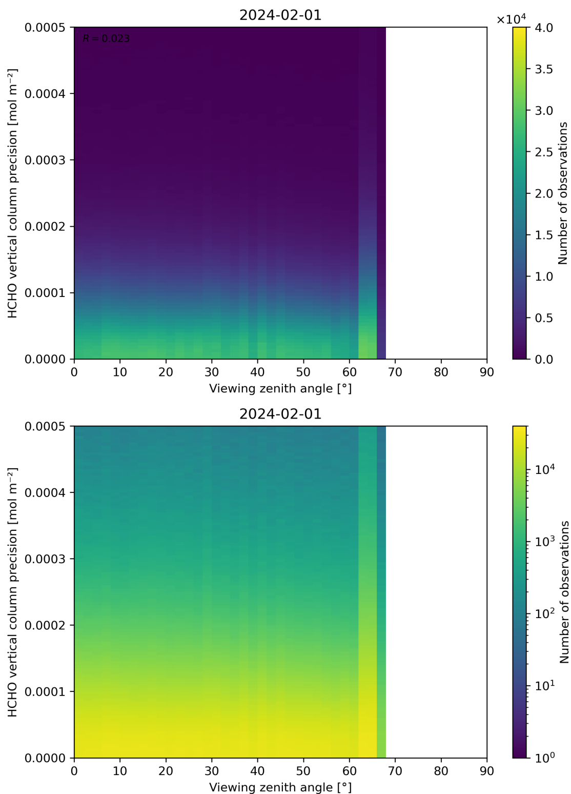
Figure 194: Scatter density plot of “Viewing zenith angle” against “HCHO vertical column precision” for 2024-01-31 to 2024-02-02.
