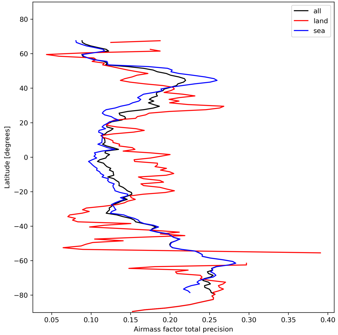
Figure 27: Zonal average of “Airmass factor total precision” for 2024-01-31 to 2024-02-02.
