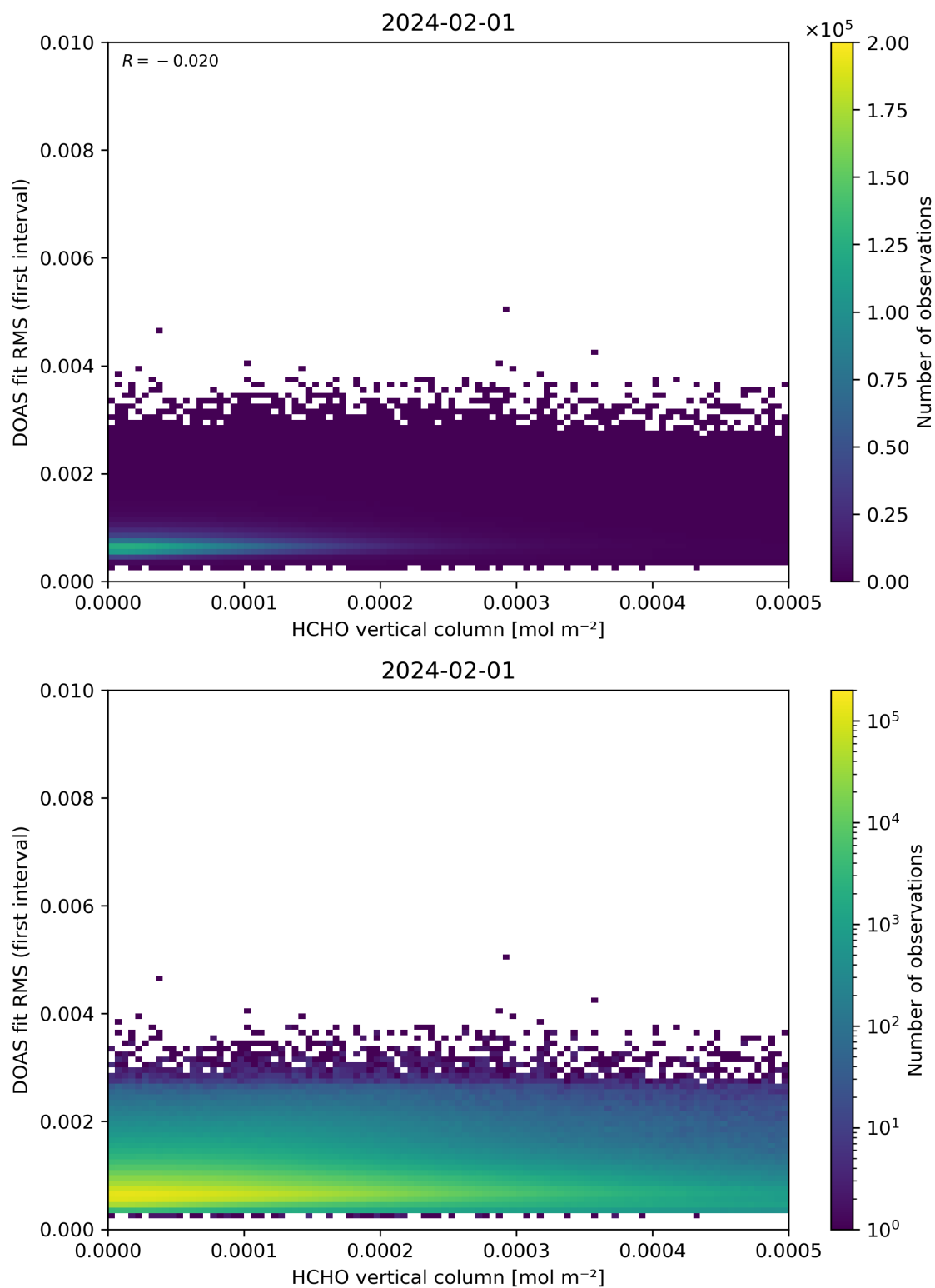
Figure 123: Scatter density plot of “HCHO vertical column” against “DOAS fit RMS (first interval)” for 2024-01-31 to 2024-02-02.
