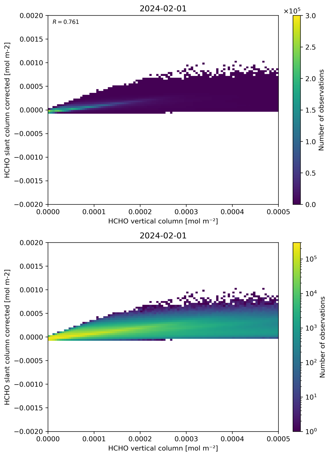
Figure 127: Scatter density plot of “HCHO vertical column” against “HCHO slant column corrected” for 2024-01-31 to 2024-02-02.
