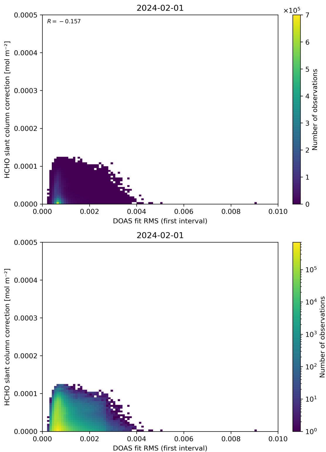
Figure 63: Scatter density plot of “DOAS fit RMS (first interval)” against “HCHO slant column correction” for 2024-01-31 to 2024-02-02.
