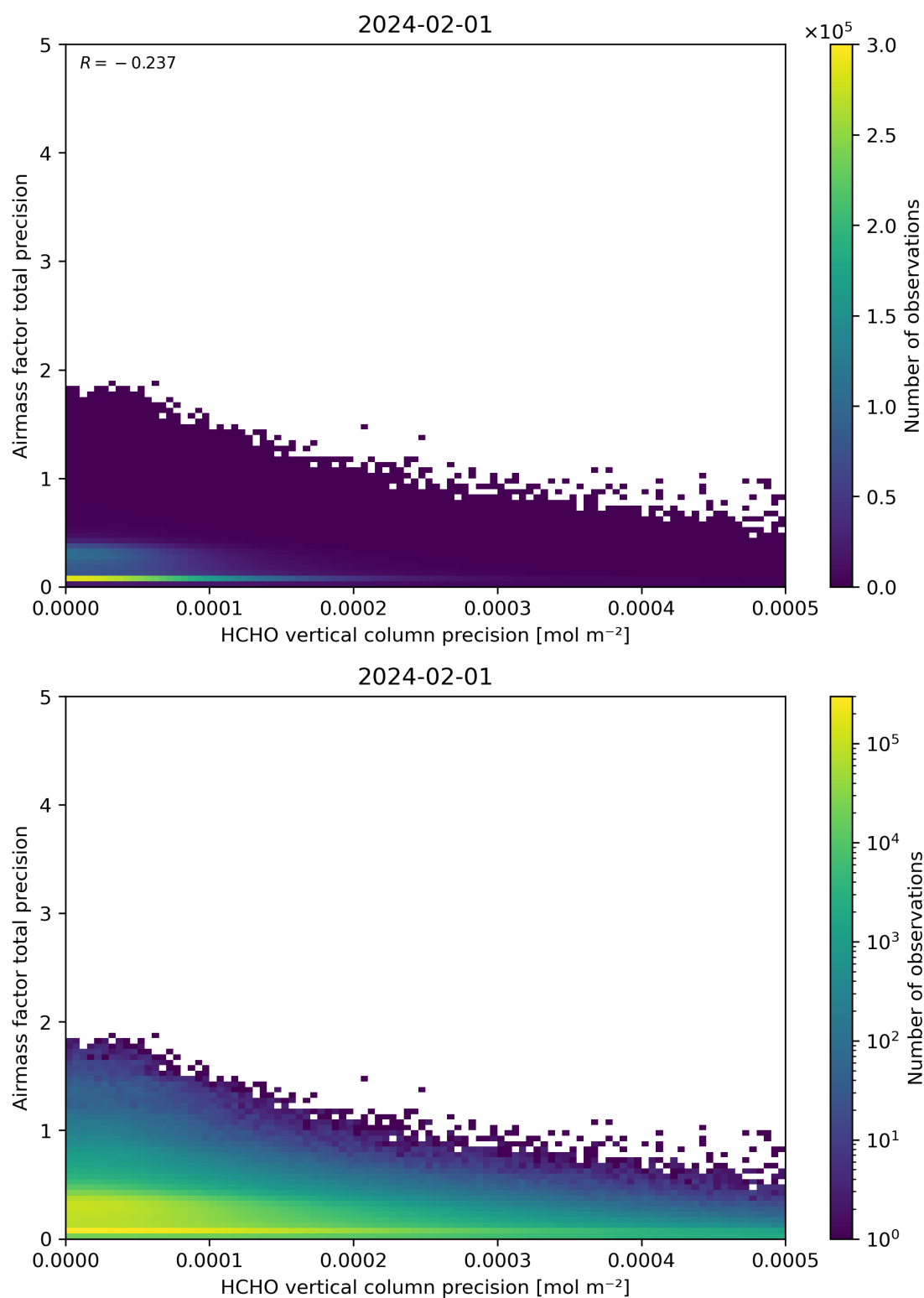
Figure 145: Scatter density plot of “HCHO vertical column precision” against “Airmass factor total precision” for 2024-01-31 to 2024-02-02.
