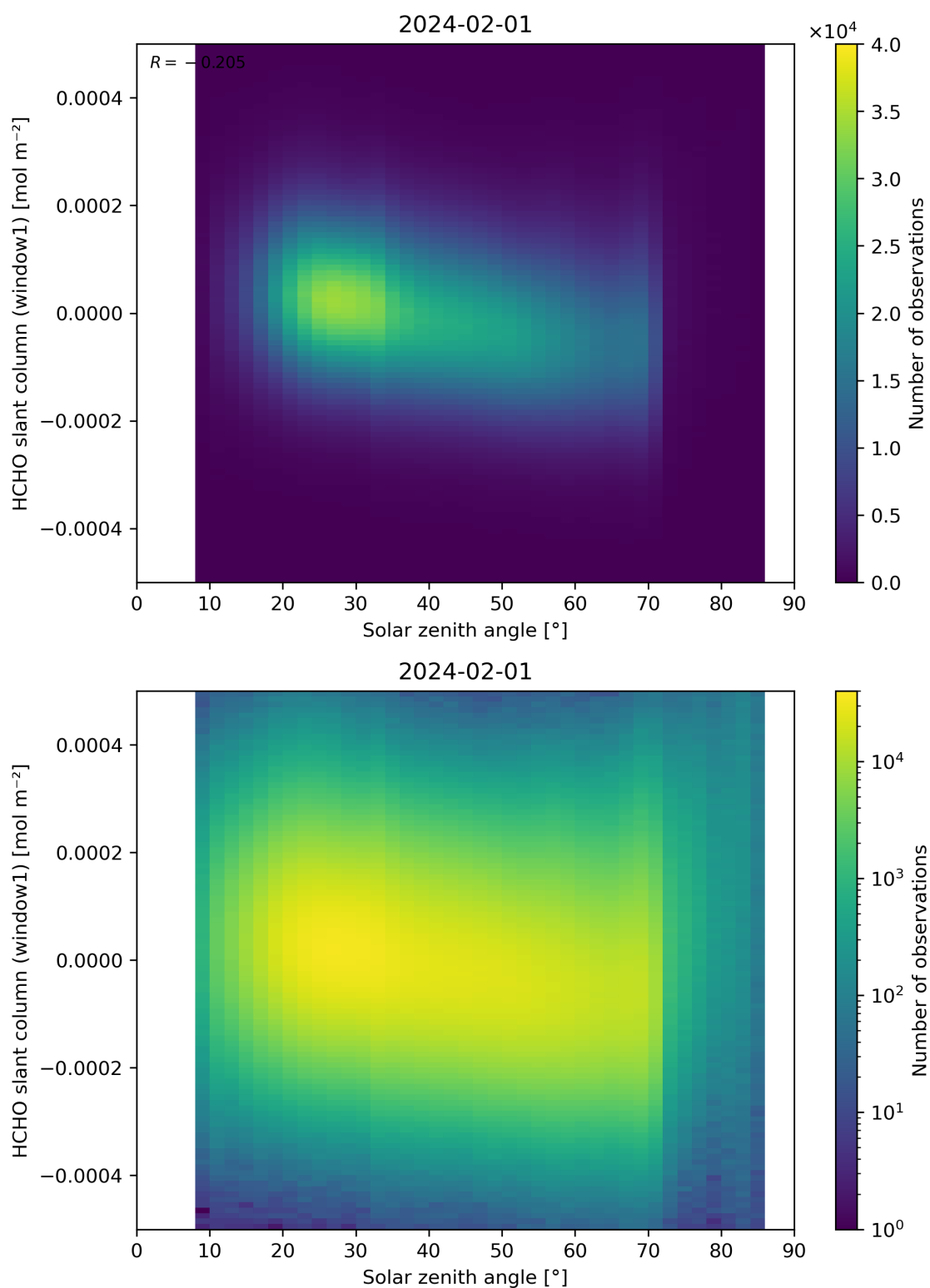
Figure 173: Scatter density plot of “Solar zenith angle” against “HCHO slant column (window1)” for 2024-01-31 to 2024-02-02.
