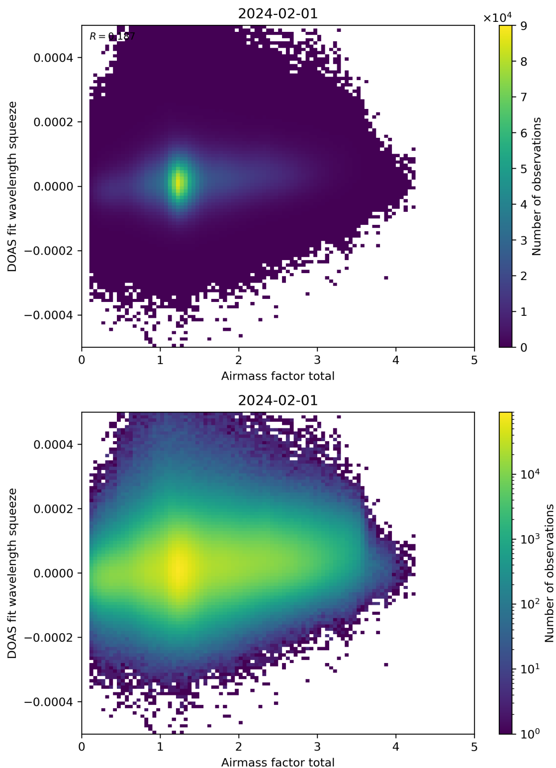
Figure 99: Scatter density plot of “Airmass factor total” against “DOAS fit wavelength squeeze” for 2024-01-31 to 2024-02-02.
