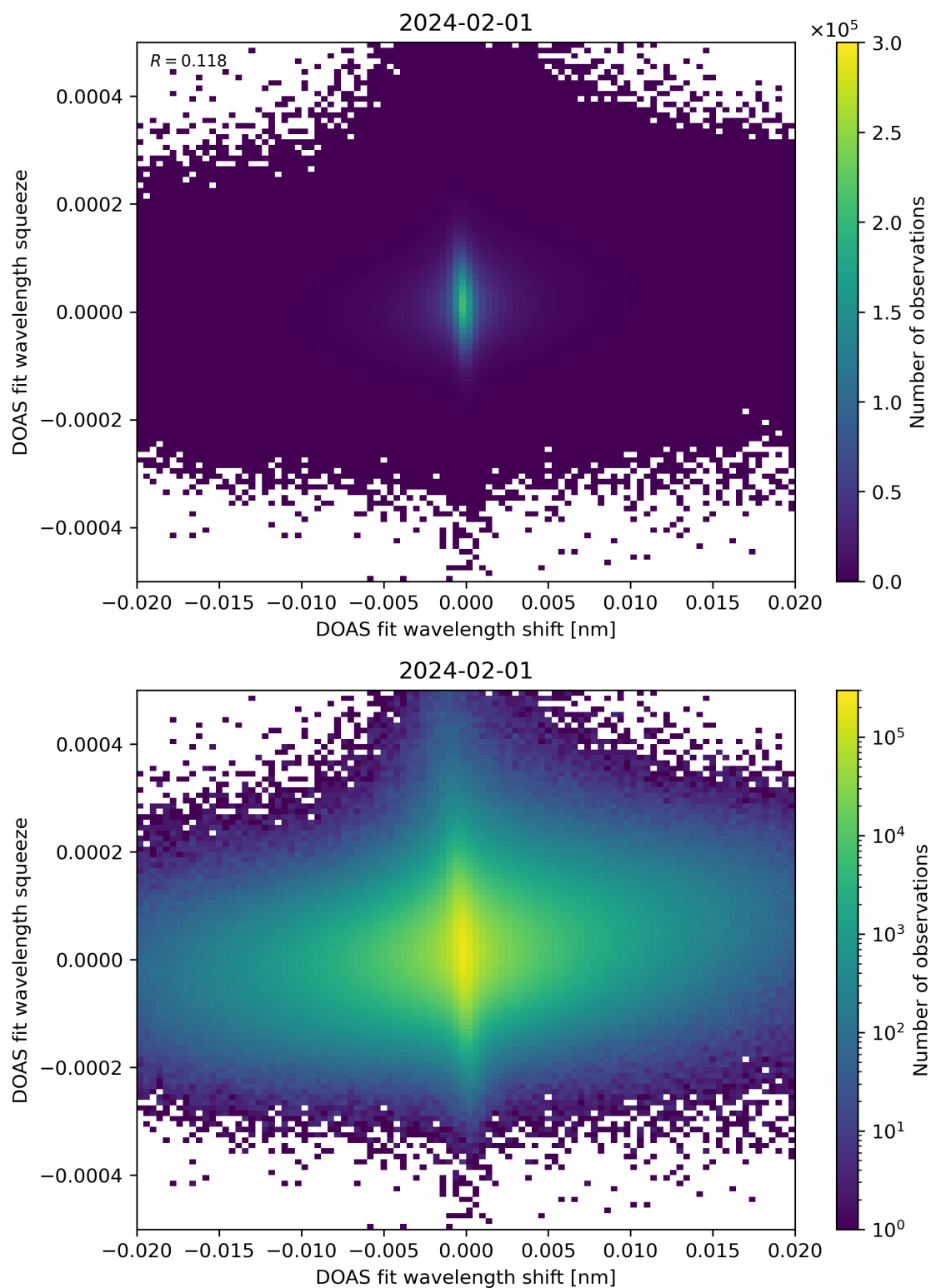
Figure 65: Scatter density plot of “DOAS fit wavelength shift” against “DOAS fit wavelength squeeze” for 2024-01-31 to 2024-02-02.
