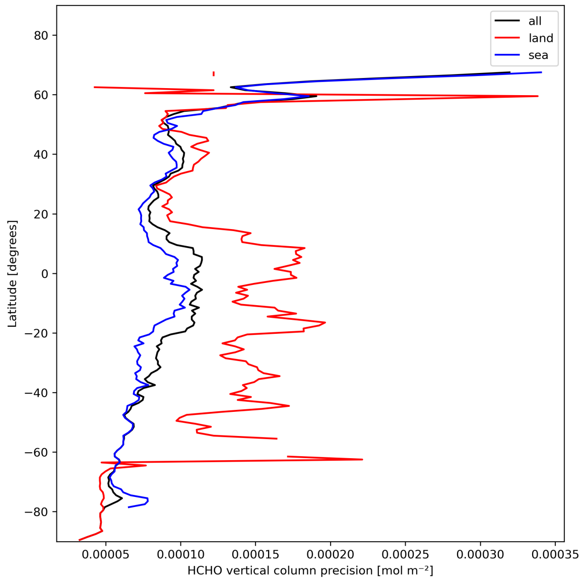
Figure 22: Zonal average of “HCHO vertical column precision” for 2024-01-31 to 2024-02-02.
