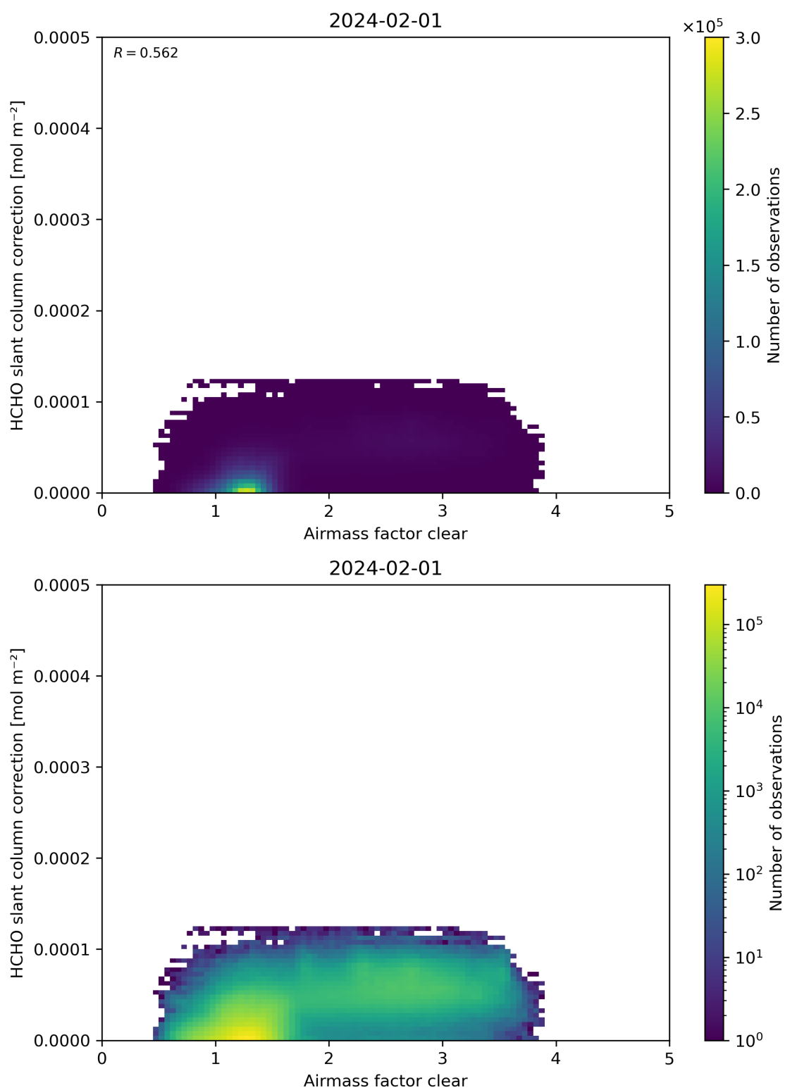
Figure 75: Scatter density plot of “Airmass factor clear” against “HCHO slant column correction” for 2024-01-31 to 2024-02-02.
