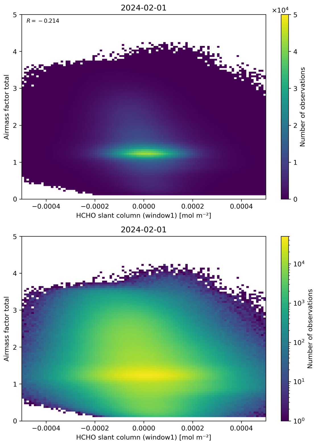
Figure 85: Scatter density plot of “HCHO slant column (window1)” against “Airmass factor total” for 2024-01-31 to 2024-02-02.
