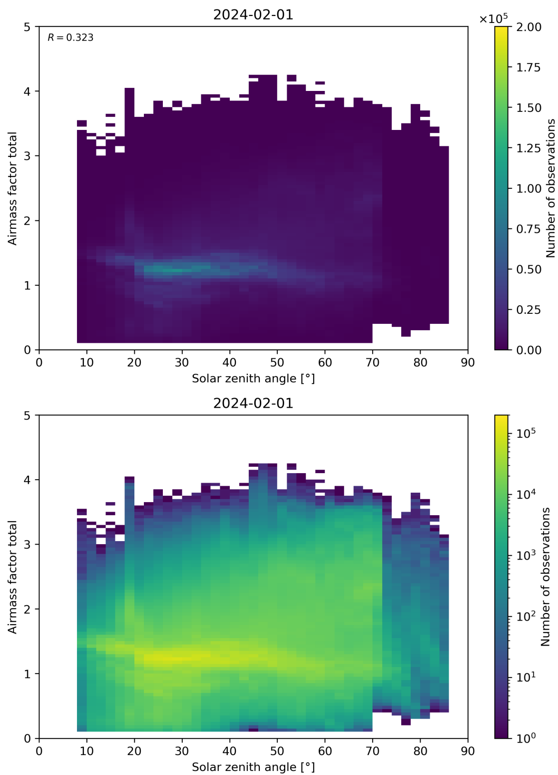
Figure 175: Scatter density plot of “Solar zenith angle” against “Airmass factor total” for 2024-01-31 to 2024-02-02.
