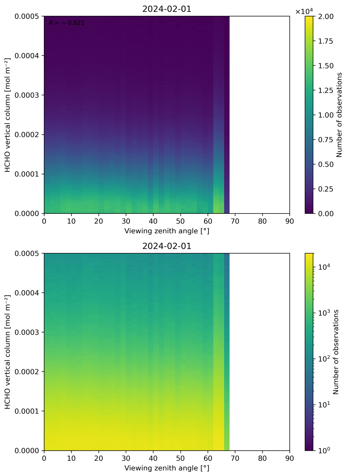
Figure 192: Scatter density plot of “Viewing zenith angle” against “HCHO vertical column” for 2024-01-31 to 2024-02-02.
