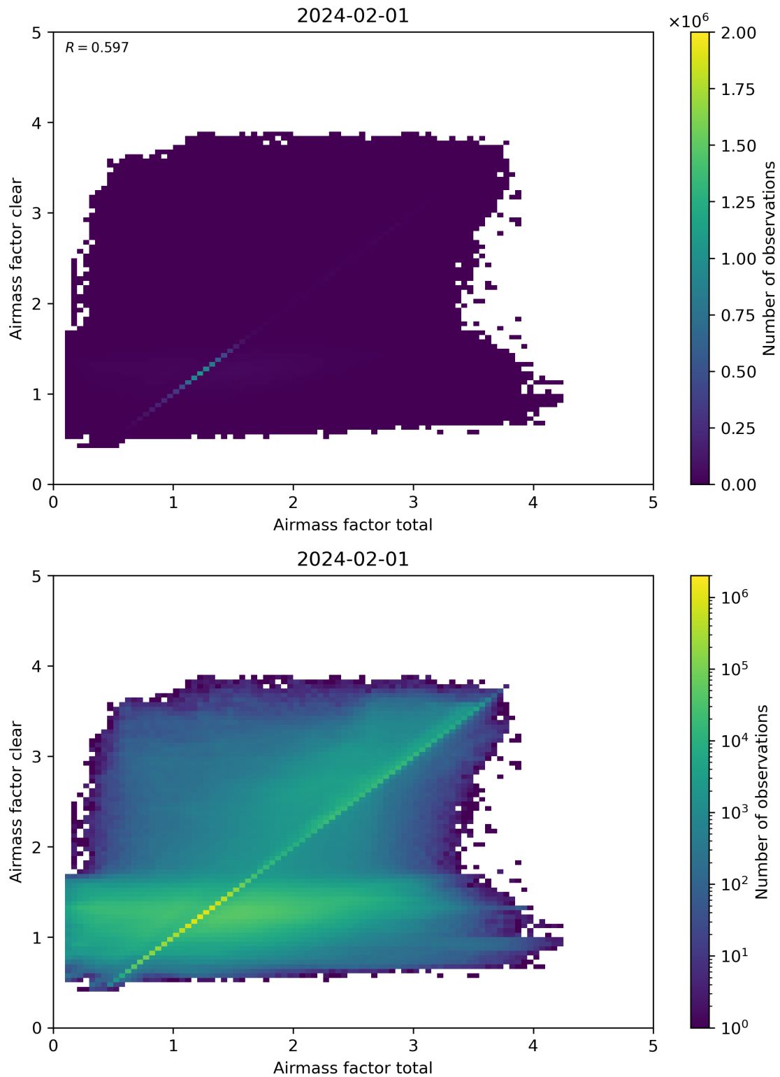
Figure 100: Scatter density plot of “Airmass factor total” against “Airmass factor clear” for 2024-01-31 to 2024-02-02.
