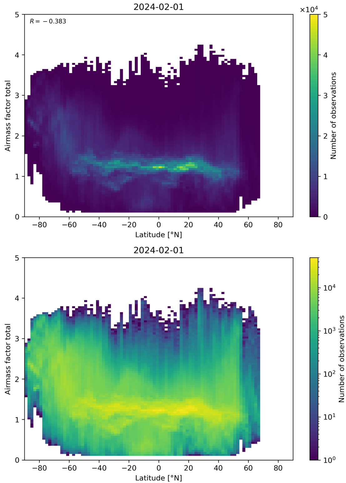
Figure 161: Scatter density plot of “Latitude” against “Airmass factor total” for 2024-01-31 to 2024-02-02.
