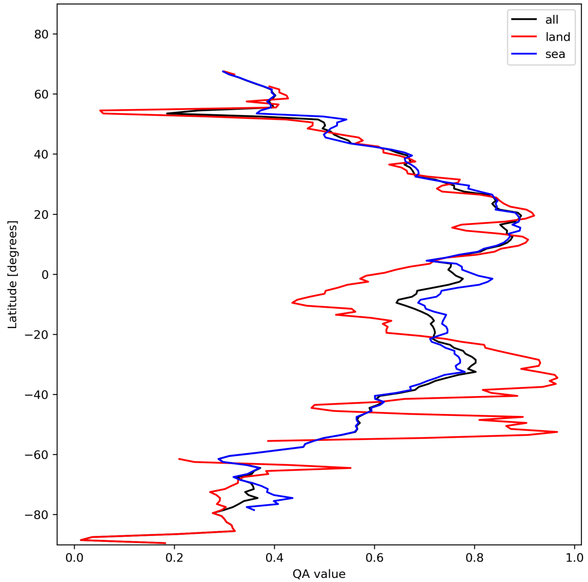
Figure 20: Zonal average of “QA value” for 2024-01-31 to 2024-02-02.
