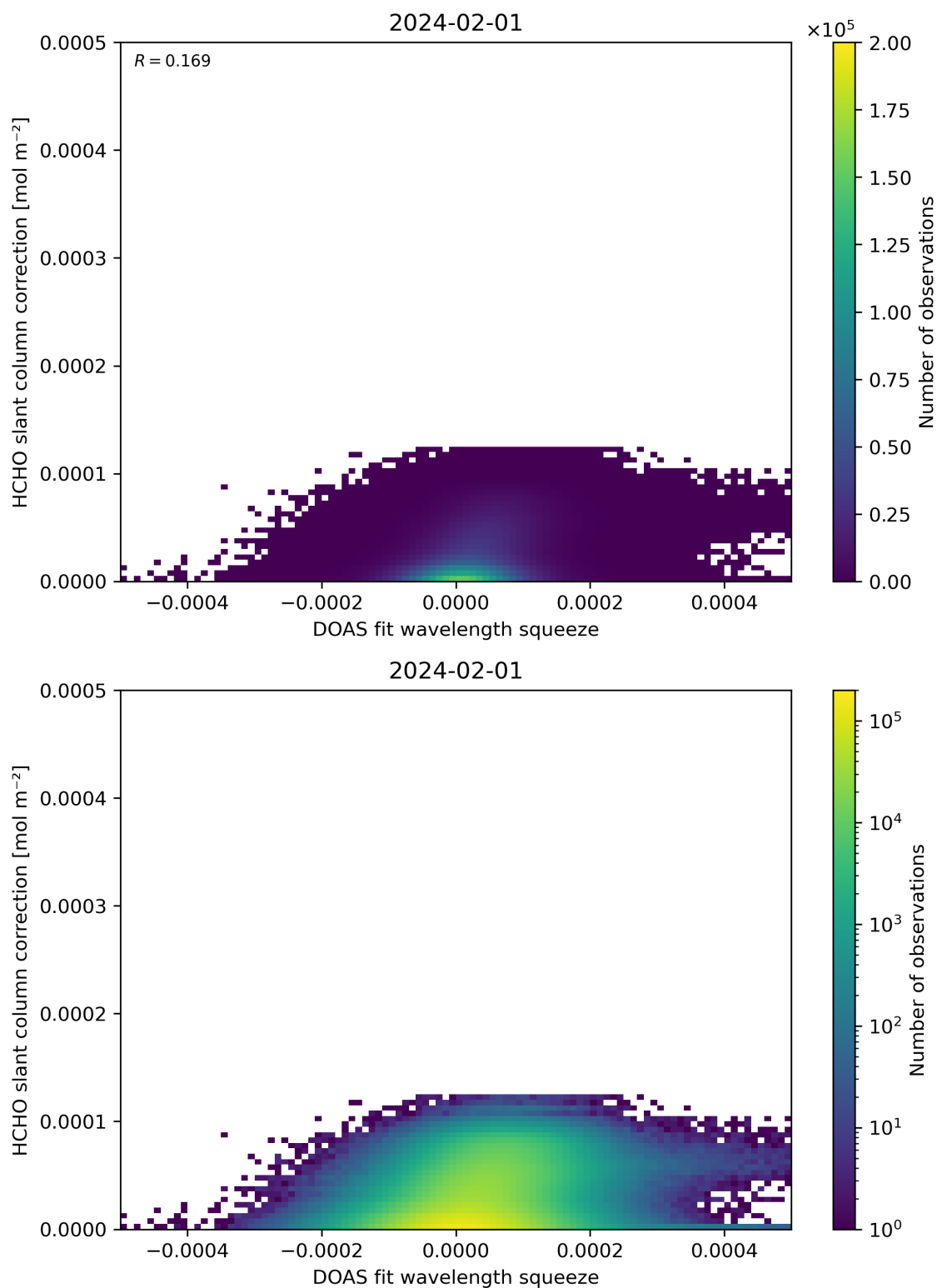
Figure 70: Scatter density plot of “DOAS fit wavelength squeeze” against “HCHO slant column correction” for 2024-01-31 to 2024-02-02.
