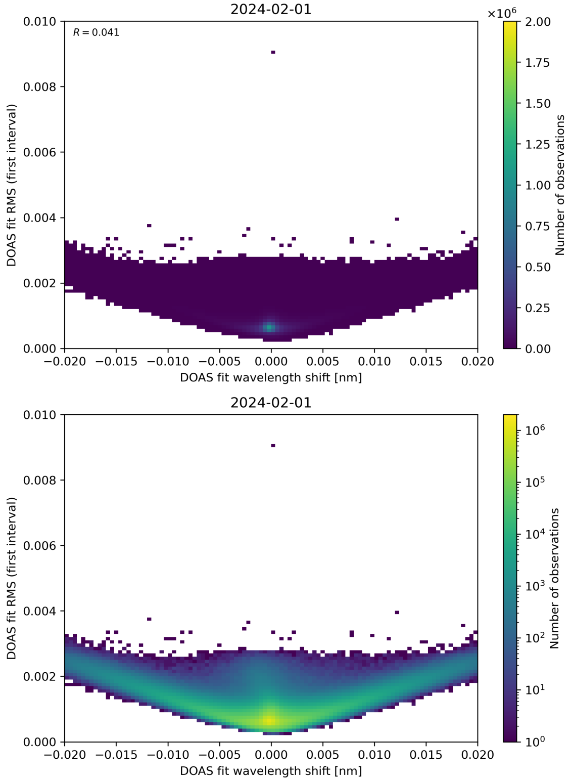
Figure 64: Scatter density plot of “DOAS fit wavelength shift” against “DOAS fit RMS (first interval)” for 2024-01-31 to 2024-02-02.
