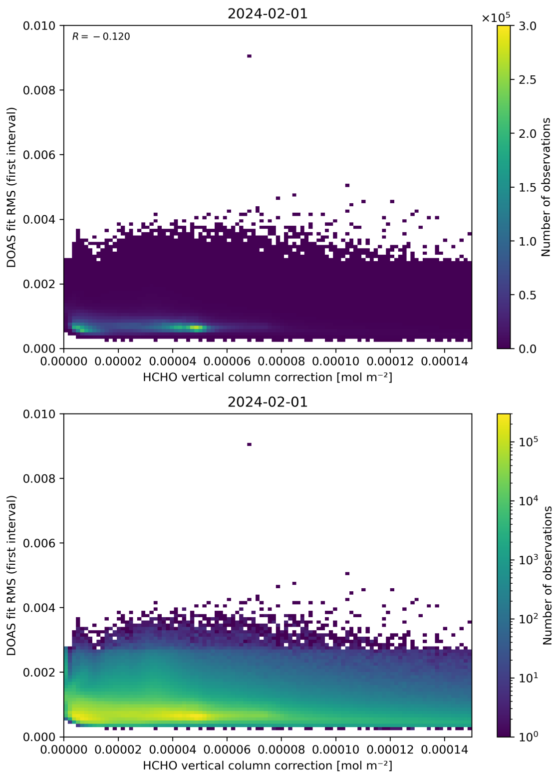
Figure 112: Scatter density plot of “HCHO vertical column correction” against “DOAS fit RMS (first interval)” for 2024-01-31 to 2024-02-02.
