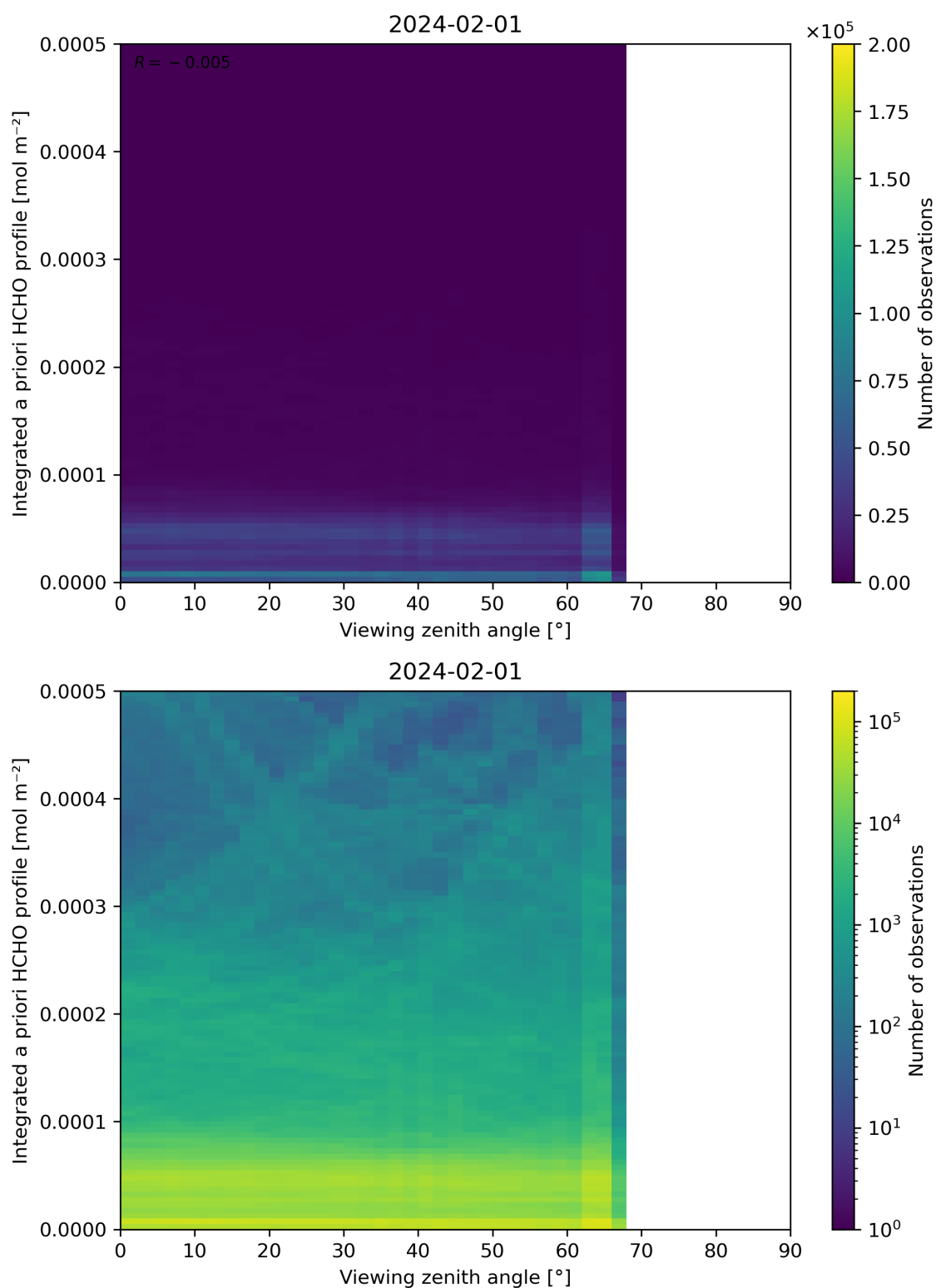
Figure 195: Scatter density plot of “Viewing zenith angle” against “Integrated a priori HCHO profile” for 2024-01-31 to 2024-02-02.
