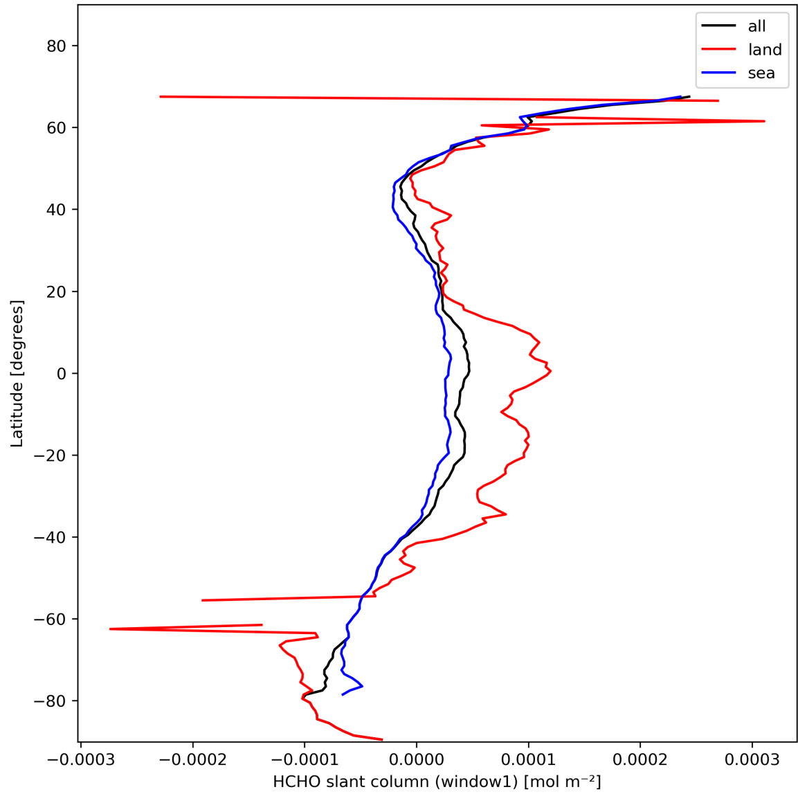
Figure 24: Zonal average of “HCHO slant column (window1)” for 2024-01-31 to 2024-02-02.
