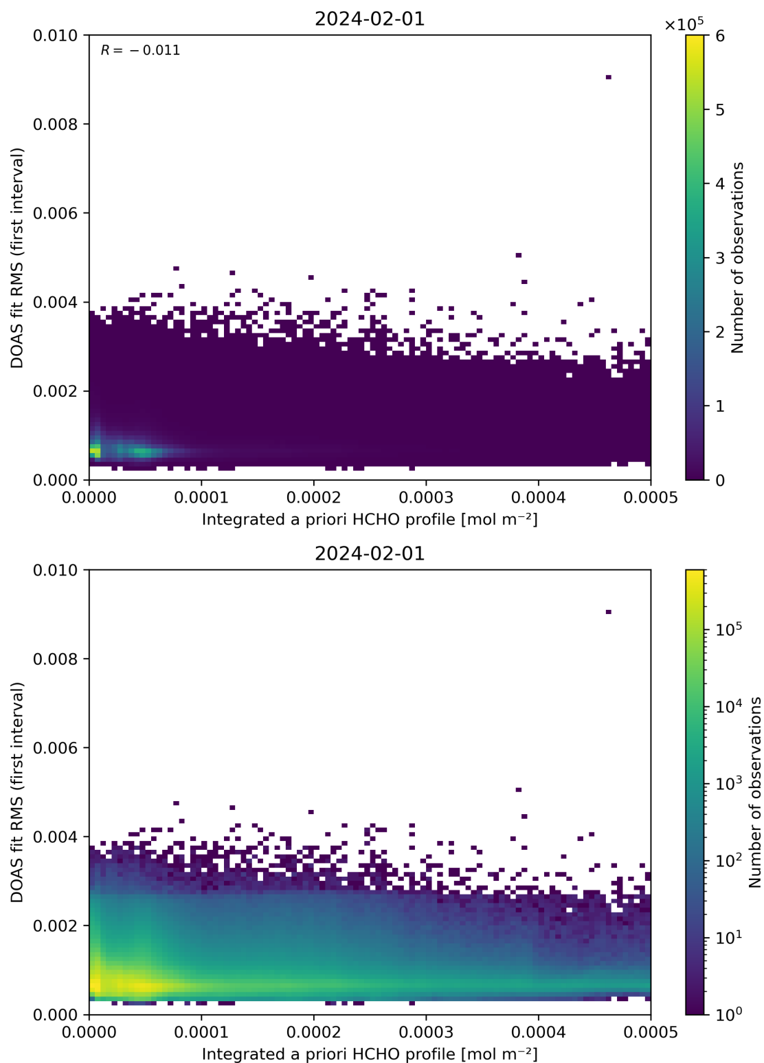
Figure 148: Scatter density plot of “Integrated a priori HCHO profile” against “DOAS fit RMS (first interval)” for 2024-01-31 to 2024-02-02.
