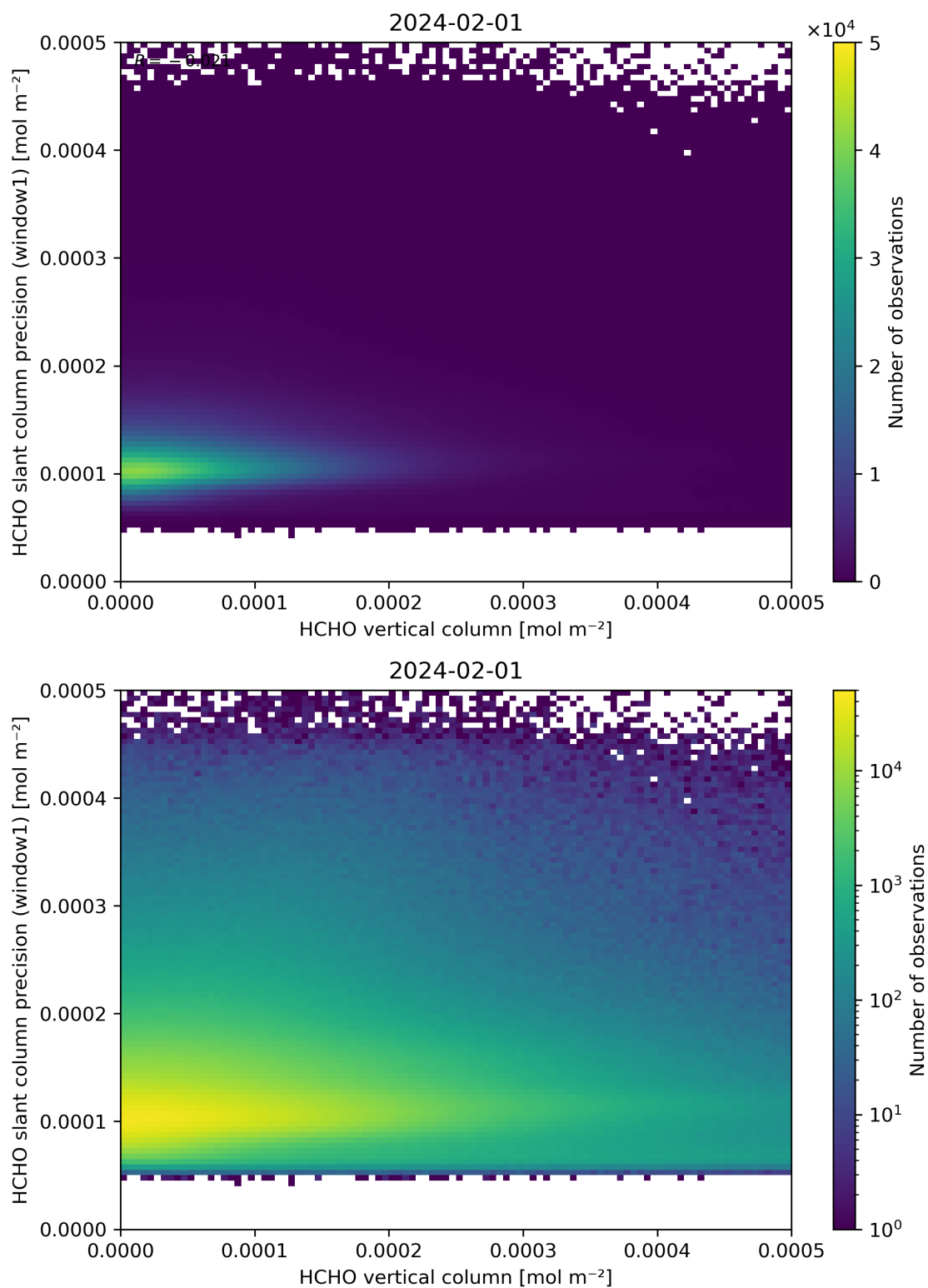
Figure 130: Scatter density plot of “HCHO vertical column” against “HCHO slant column precision (window1)” for 2024-01-31 to 2024-02-02.
