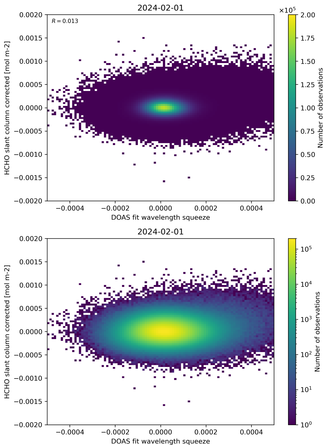
Figure 69: Scatter density plot of “DOAS fit wavelength squeeze” against “HCHO slant column corrected” for 2024-01-31 to 2024-02-02.
