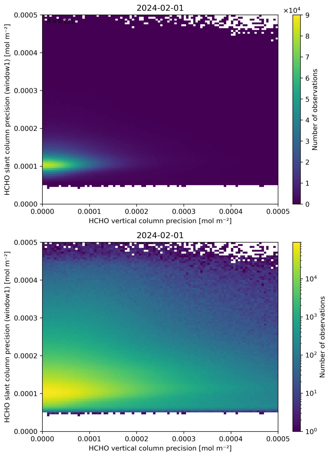
Figure 143: Scatter density plot of “HCHO vertical column precision” against “HCHO slant column precision (window1)” for 2024-01-31 to 2024-02-02.
