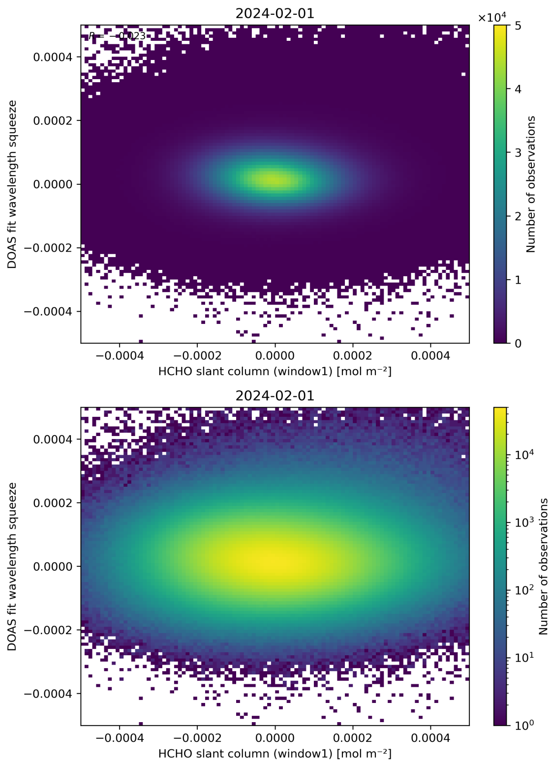
Figure 80: Scatter density plot of “HCHO slant column (window1)” against “DOAS fit wavelength squeeze” for 2024-01-31 to 2024-02-02.
