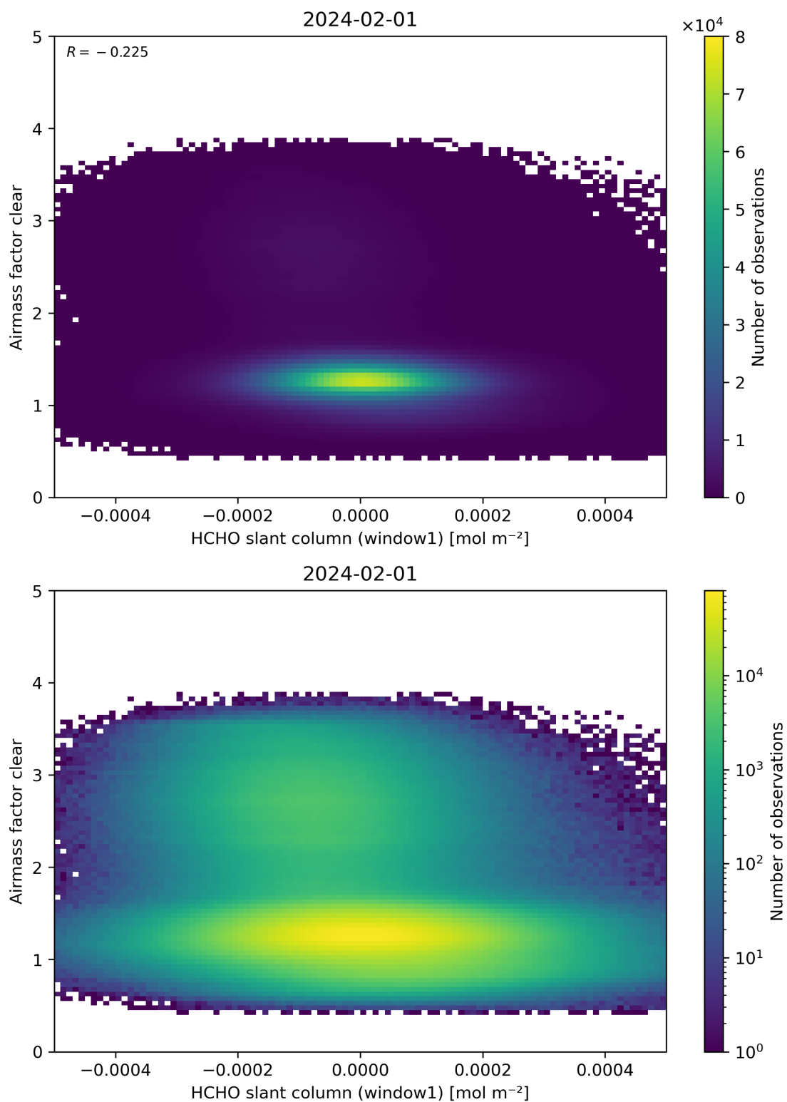
Figure 81: Scatter density plot of “HCHO slant column (window1)” against “Airmass factor clear” for 2024-01-31 to 2024-02-02.
