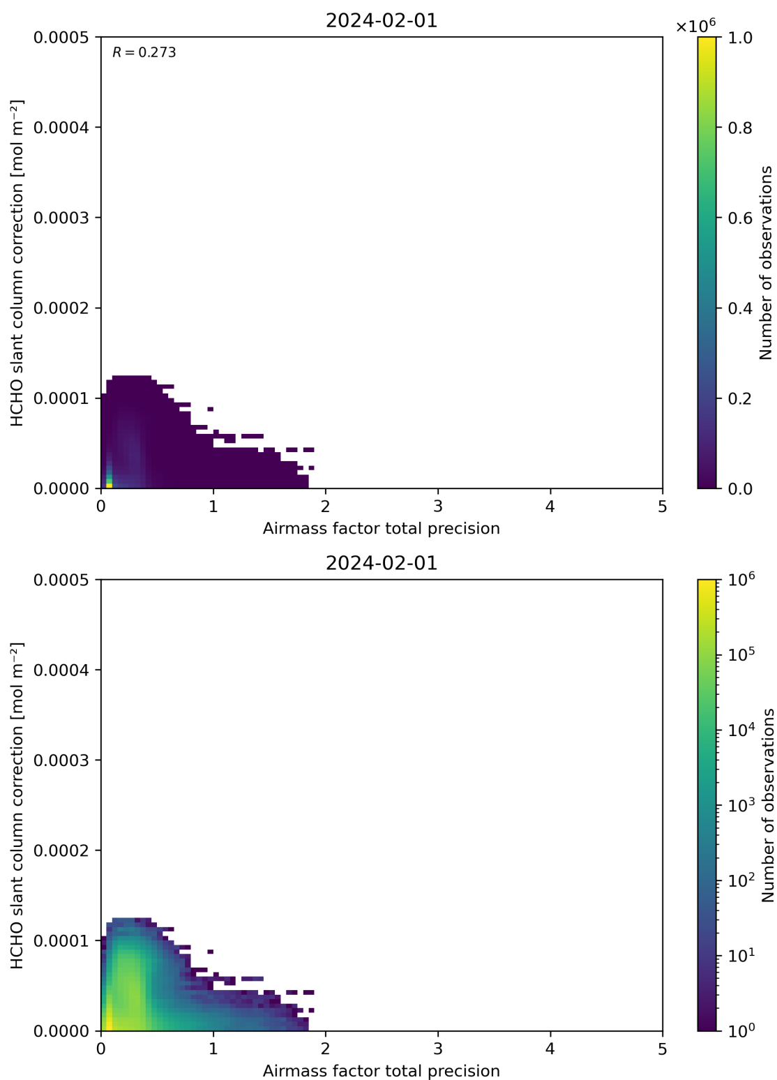
Figure 110: Scatter density plot of “Airmass factor total precision” against “HCHO slant column correction” for 2024-01-31 to 2024-02-02.
