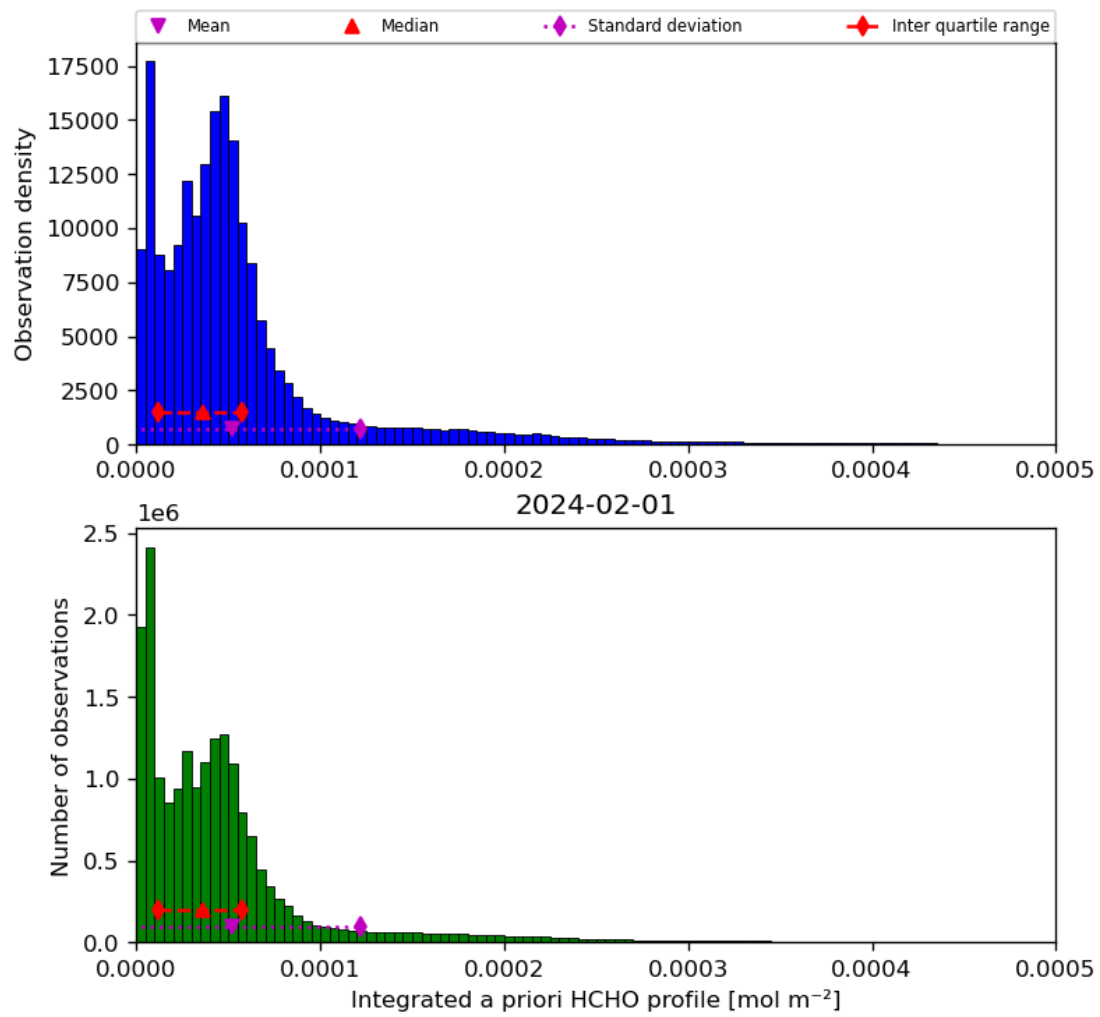
Figure 43: Histogram of “Integrated a priori HCHO profile” for 2024-01-31 to 2024-02-02
