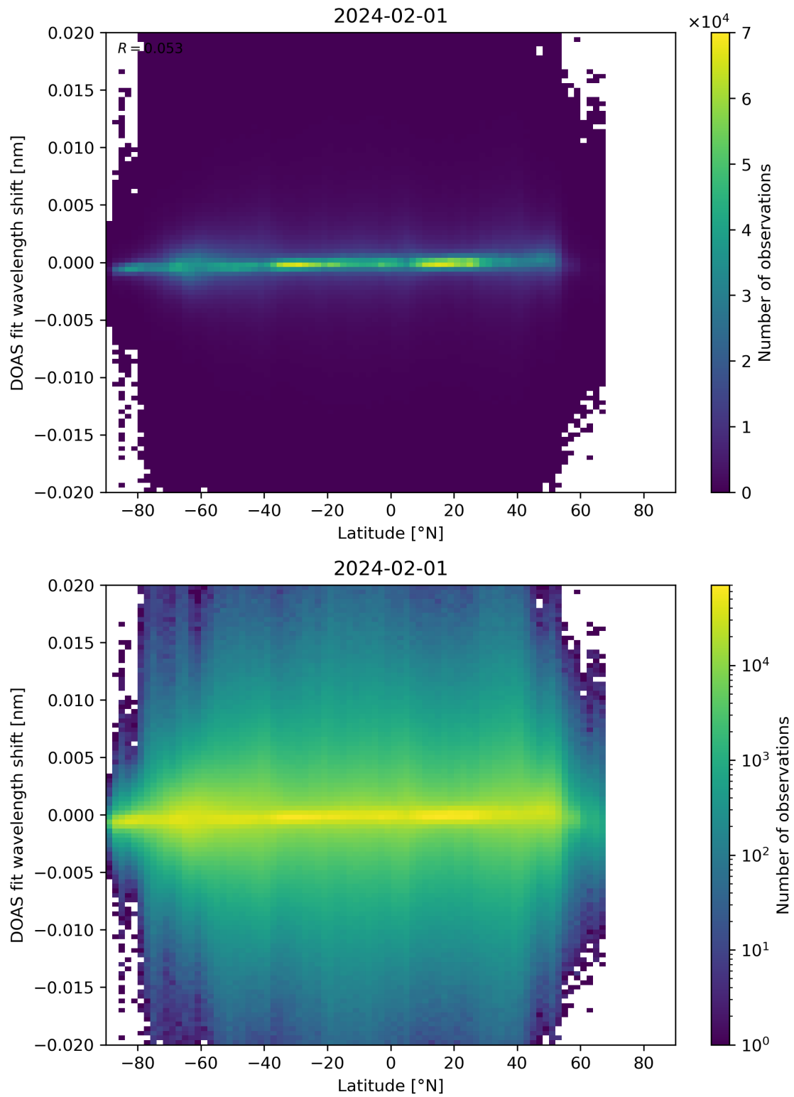
Figure 154: Scatter density plot of “Latitude” against “DOAS fit wavelength shift” for 2024-01-31 to 2024-02-02.
