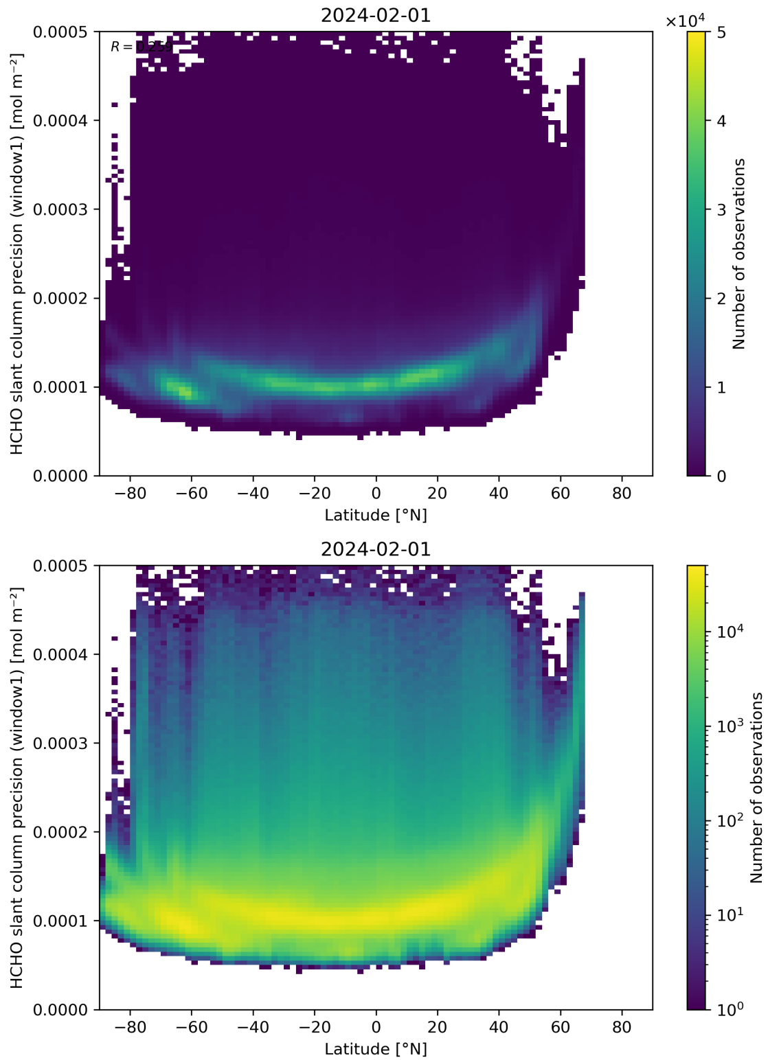
Figure 160: Scatter density plot of “Latitude” against “HCHO slant column precision (window1)” for 2024-01-31 to 2024-02-02.
