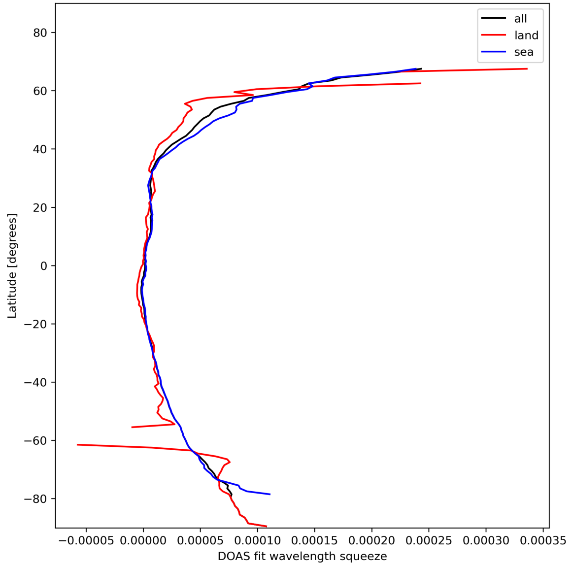
Figure 31: Zonal average of “DOAS fit wavelength squeeze” for 2024-01-31 to 2024-02-02.
