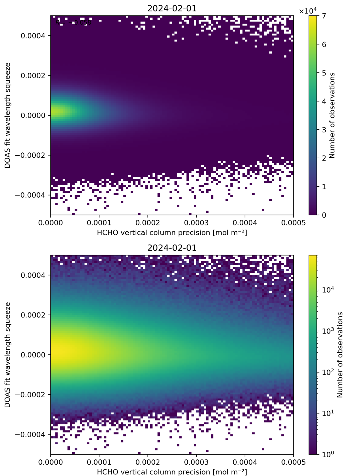
Figure 138: Scatter density plot of “HCHO vertical column precision” against “DOAS fit wavelength squeeze” for 2024-01-31 to 2024-02-02.
