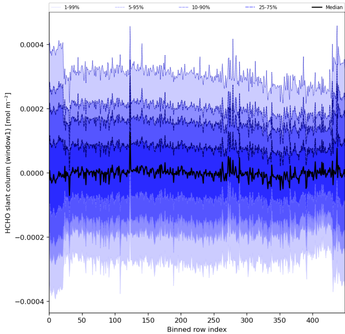
Figure 52: Along track statistics of “HCHO slant column (window1)” for 2024-01-31 to 2024-02-02
