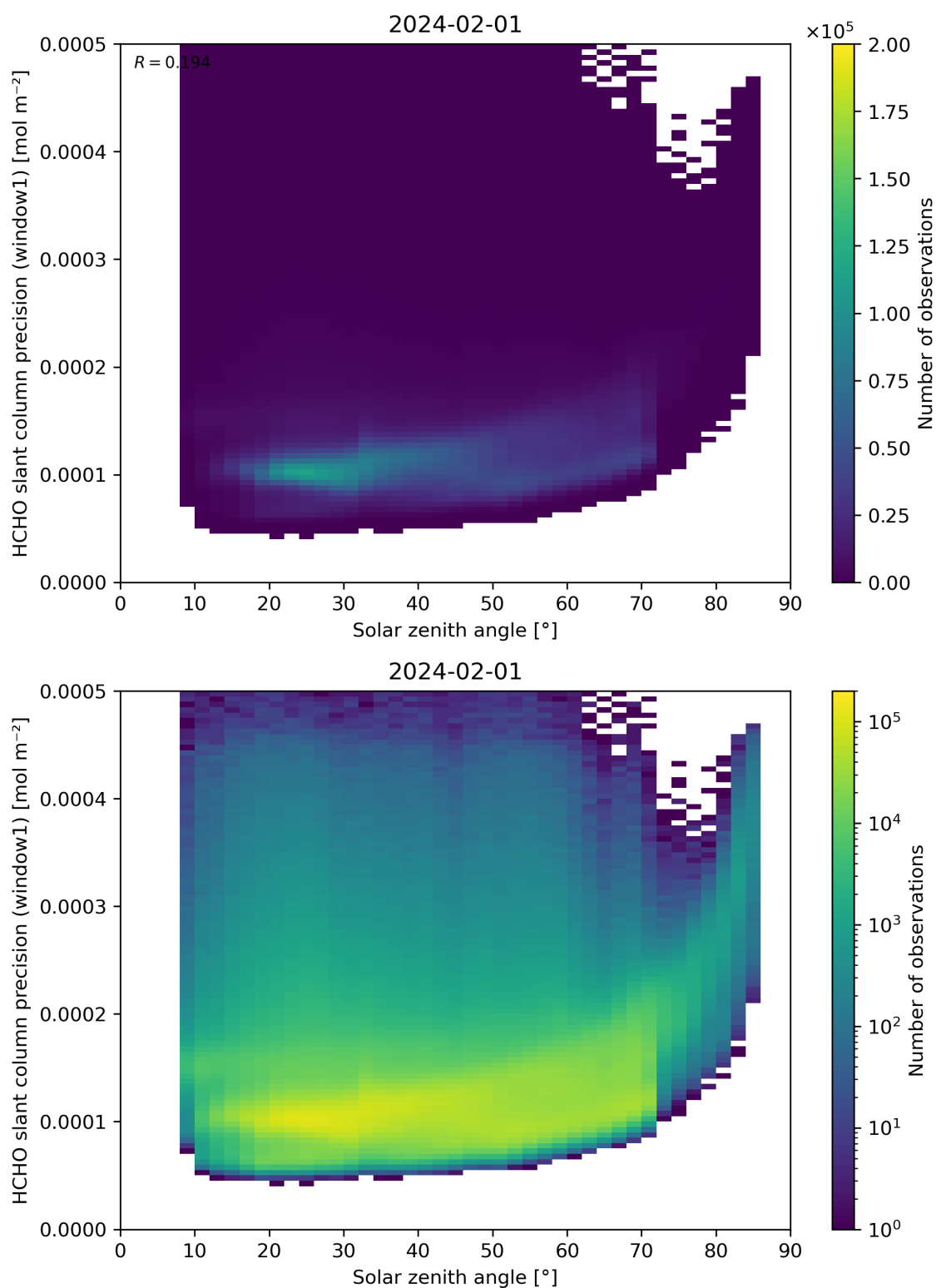
Figure 174: Scatter density plot of “Solar zenith angle” against “HCHO slant column precision (window1)” for 2024-01-31 to 2024-02-02.
