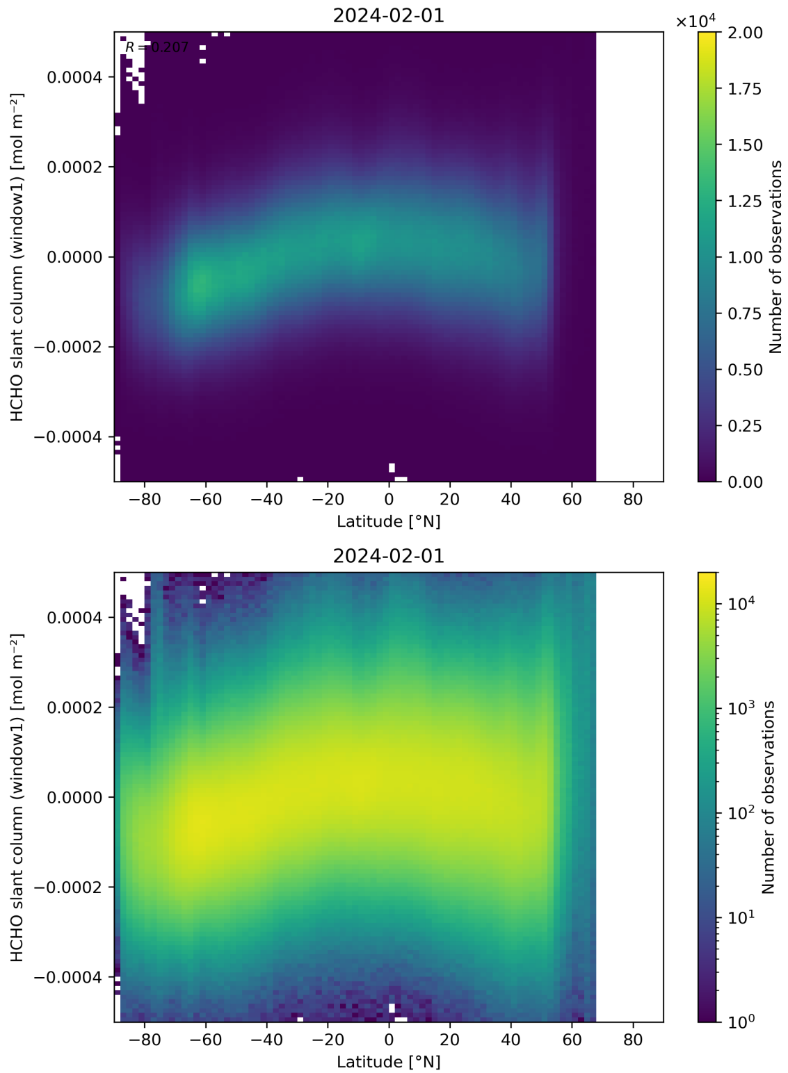
Figure 159: Scatter density plot of “Latitude” against “HCHO slant column (window1)” for 2024-01-31 to 2024-02-02.
