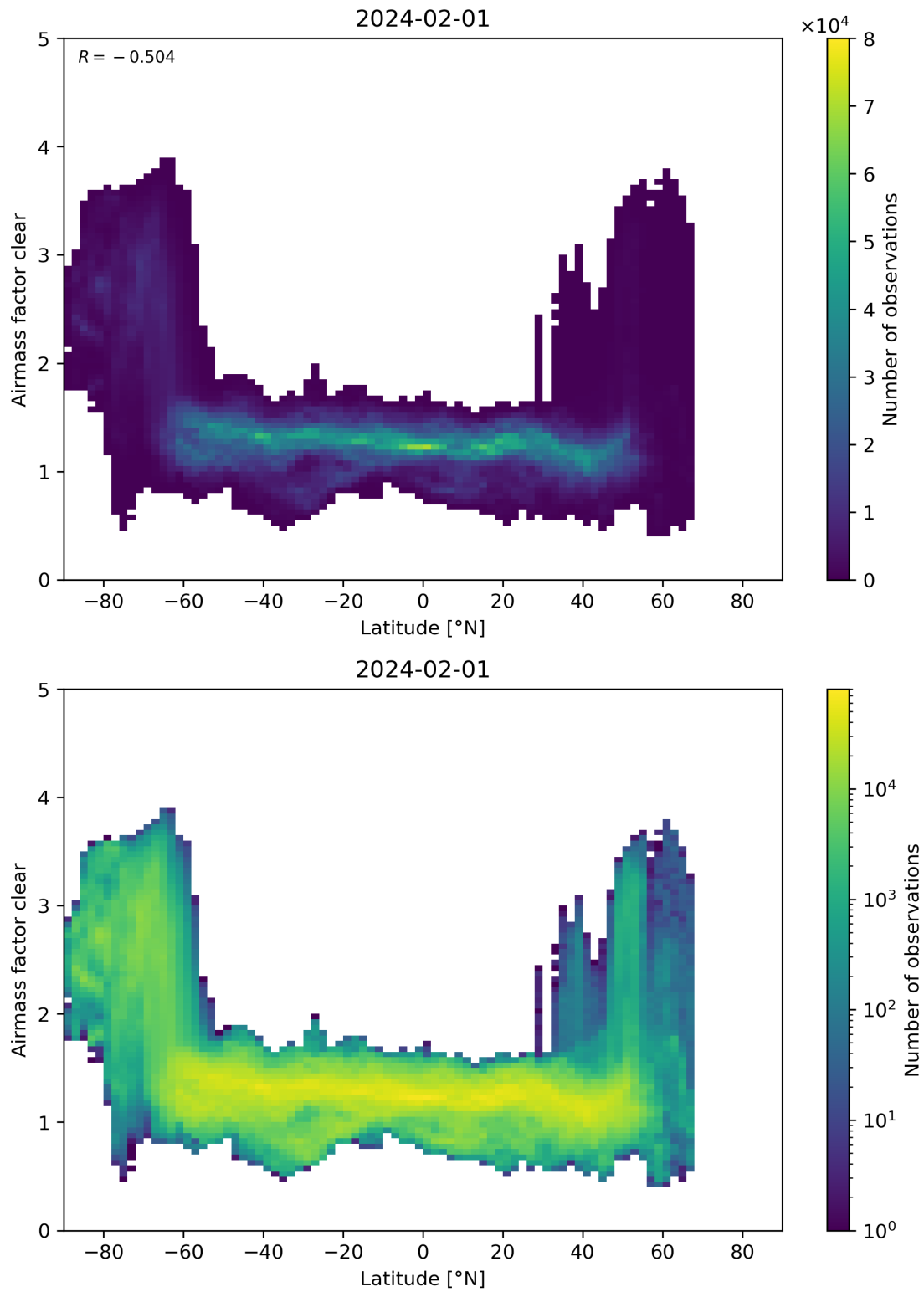
Figure 156: Scatter density plot of “Latitude” against “Airmass factor clear” for 2024-01-31 to 2024-02-02.
