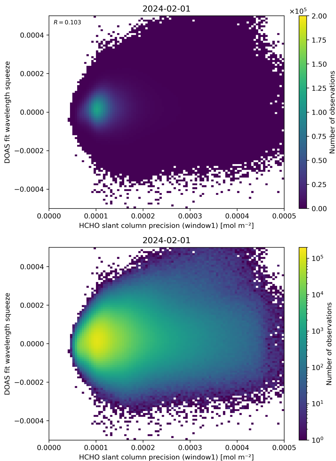
Figure 90: Scatter density plot of “HCHO slant column precision (window1)” against “DOAS fit wavelength squeeze” for 2024-01-31 to 2024-02-02.
