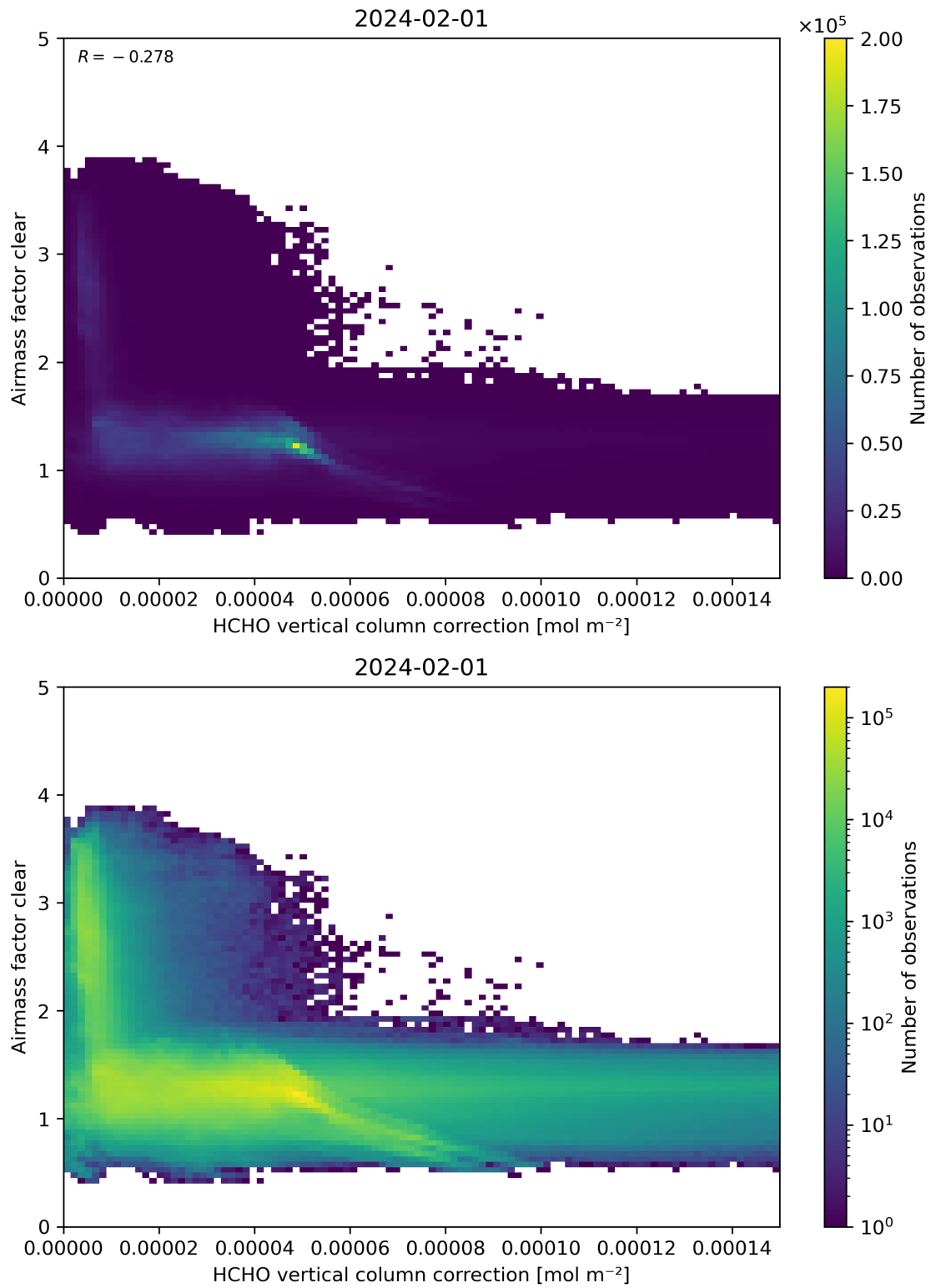
Figure 115: Scatter density plot of “HCHO vertical column correction” against “Airmass factor clear” for 2024-01-31 to 2024-02-02.
