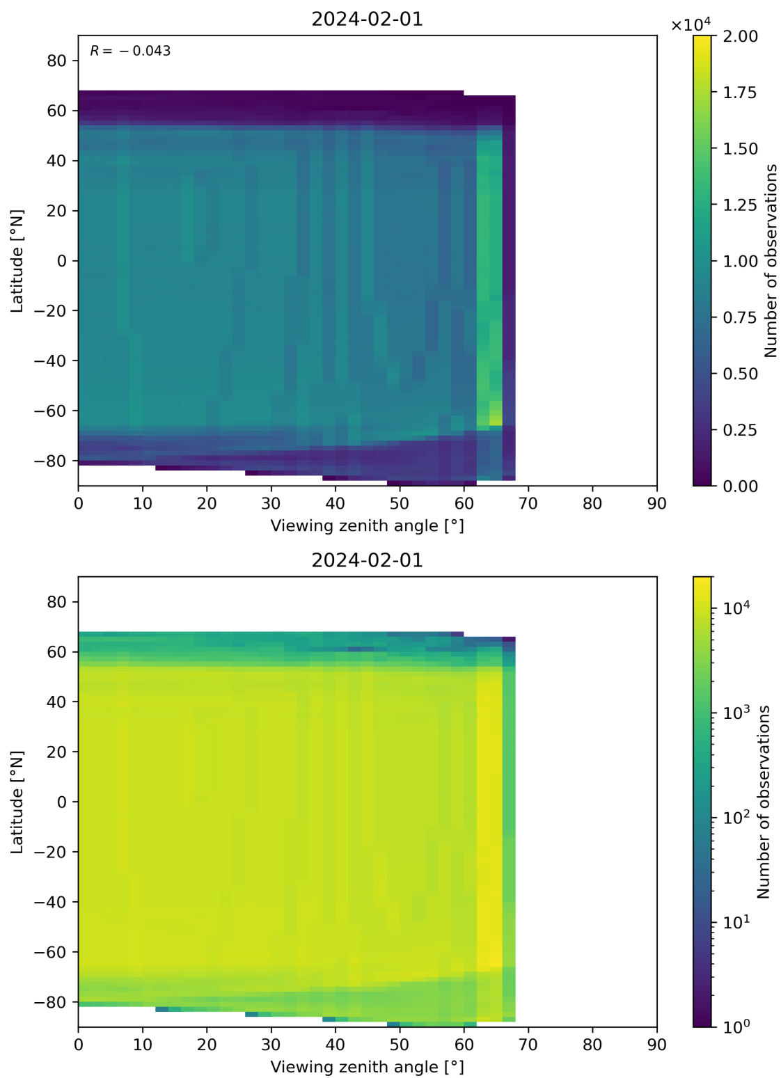
Figure 196: Scatter density plot of “Viewing zenith angle” against “Latitude” for 2024-01-31 to 2024-02-02.
