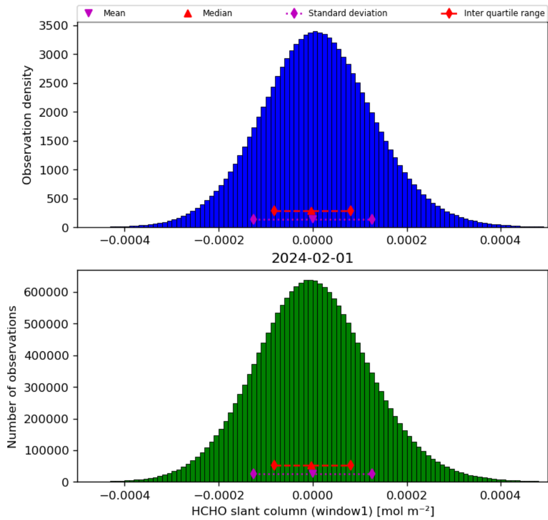
Figure 38: Histogram of “HCHO slant column (window1)” for 2024-01-31 to 2024-02-02
