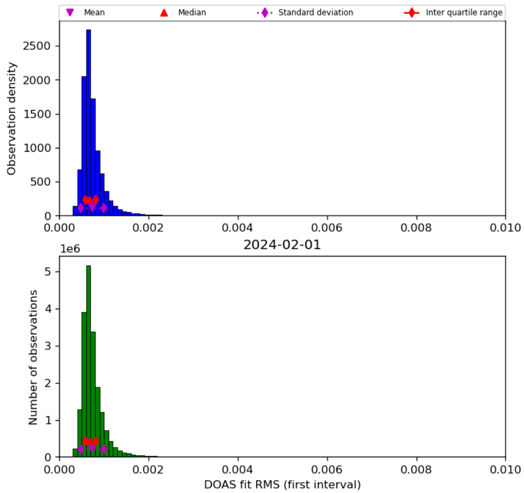
Figure 46: Histogram of “DOAS fit RMS (first interval)” for 2024-01-31 to 2024-02-02
