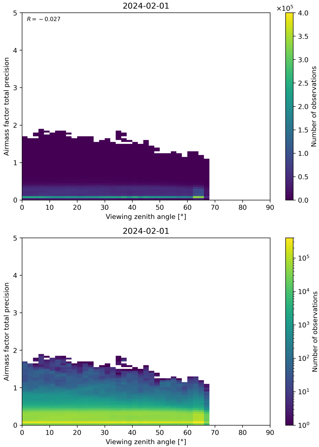
Figure 191: Scatter density plot of “Viewing zenith angle” against “Airmass factor total precision” for 2024-01-31 to 2024-02-02.
