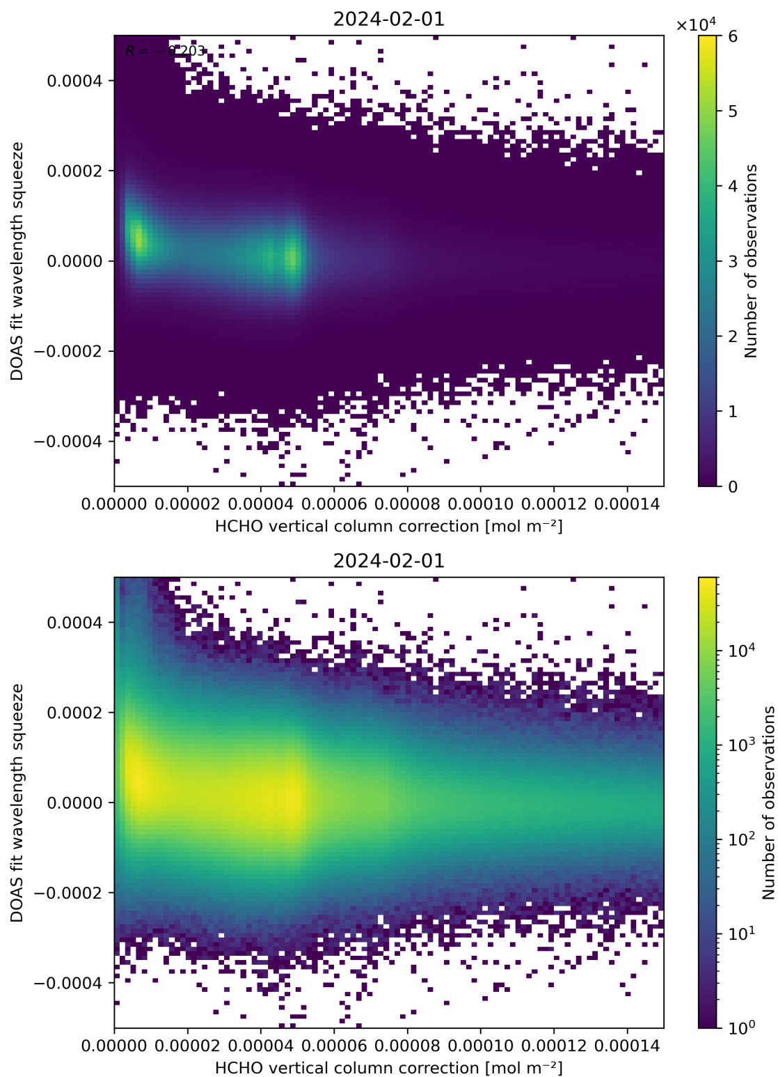
Figure 114: Scatter density plot of “HCHO vertical column correction” against “DOAS fit wavelength squeeze” for 2024-01-31 to 2024-02-02.
