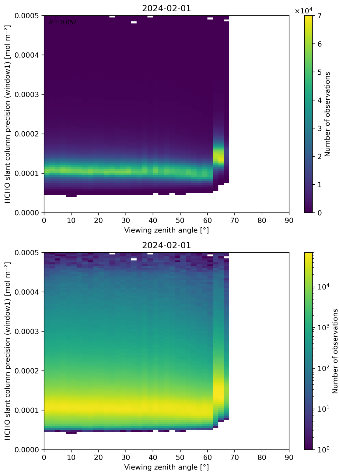
Figure 189: Scatter density plot of “Viewing zenith angle” against “HCHO slant column precision (window1)” for 2024-01-31 to 2024-02-02.
