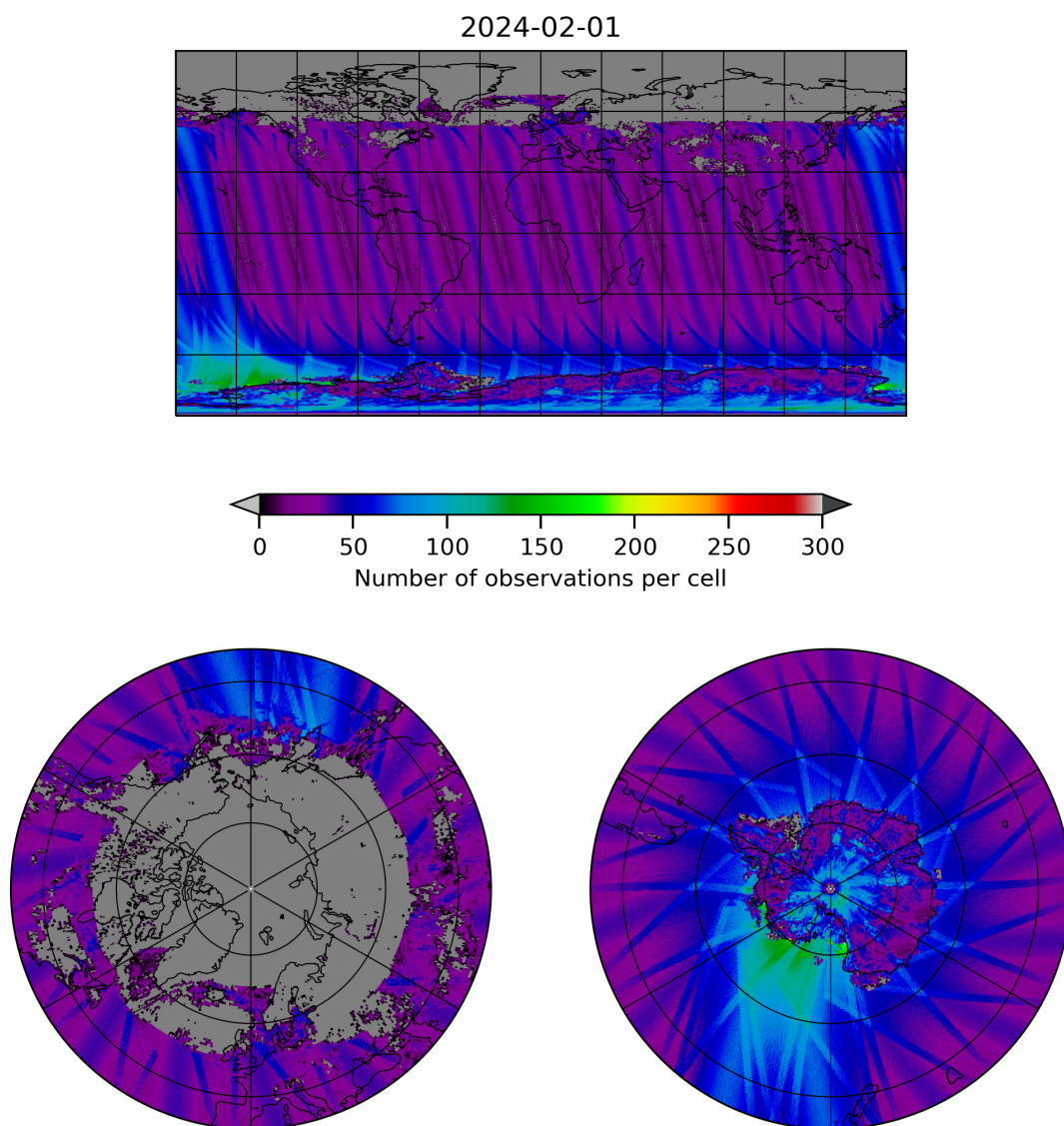
Figure 19: Map of the number of observations for 2024-01-31 to 2024-02-02
