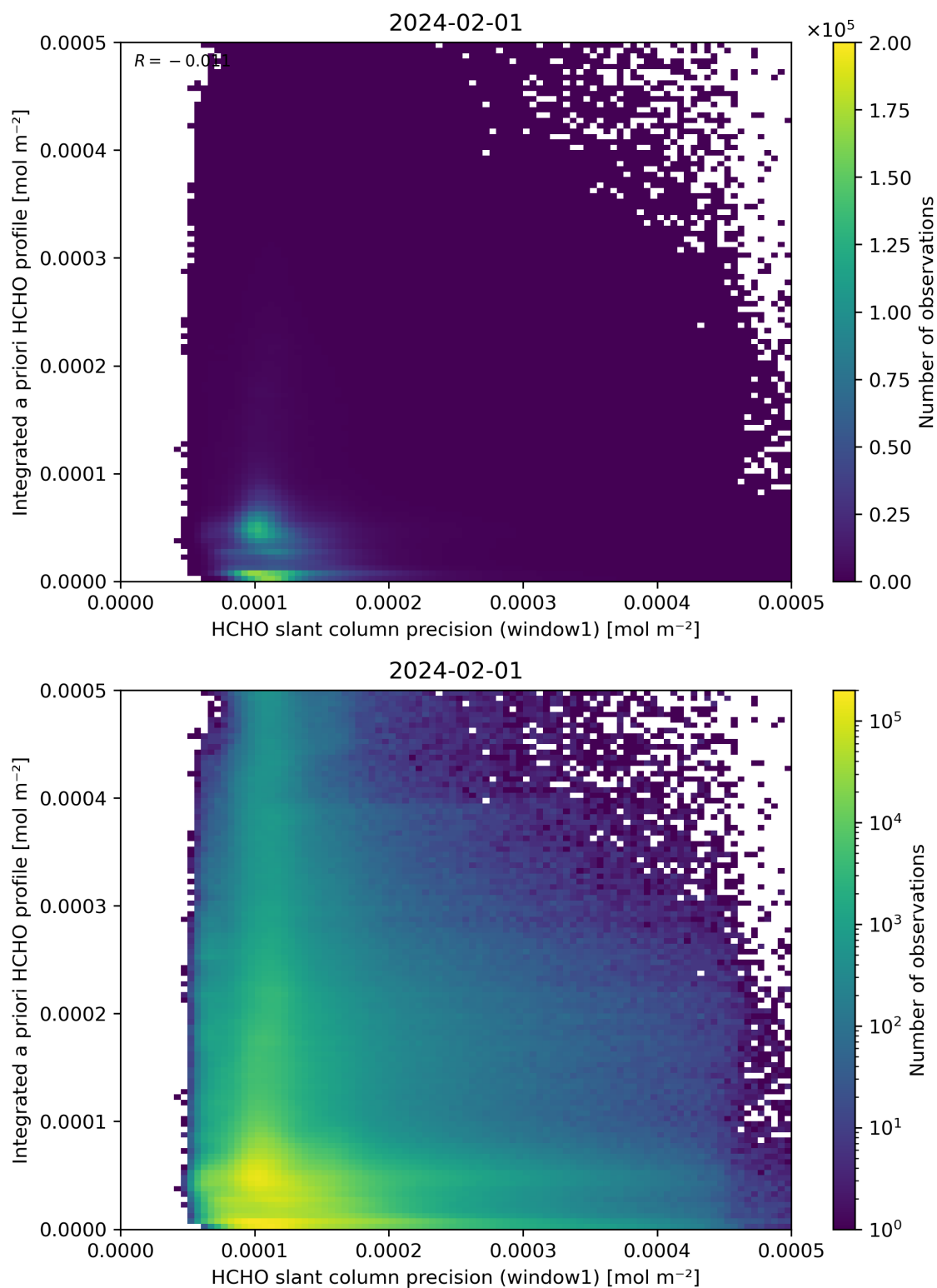
Figure 96: Scatter density plot of “HCHO slant column precision (window1)” against “Integrated a priori HCHO profile” for 2024-01-31 to 2024-02-02.
