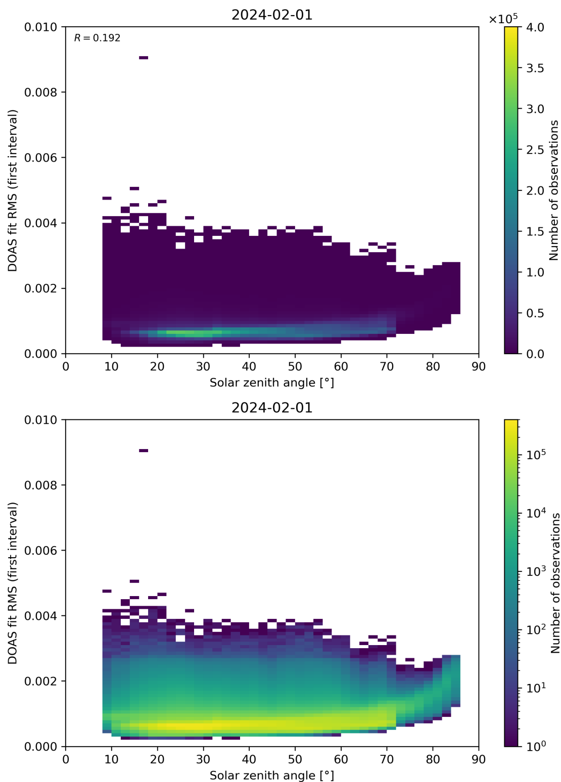
Figure 167: Scatter density plot of “Solar zenith angle” against “DOAS fit RMS (first interval)” for 2024-01-31 to 2024-02-02.
