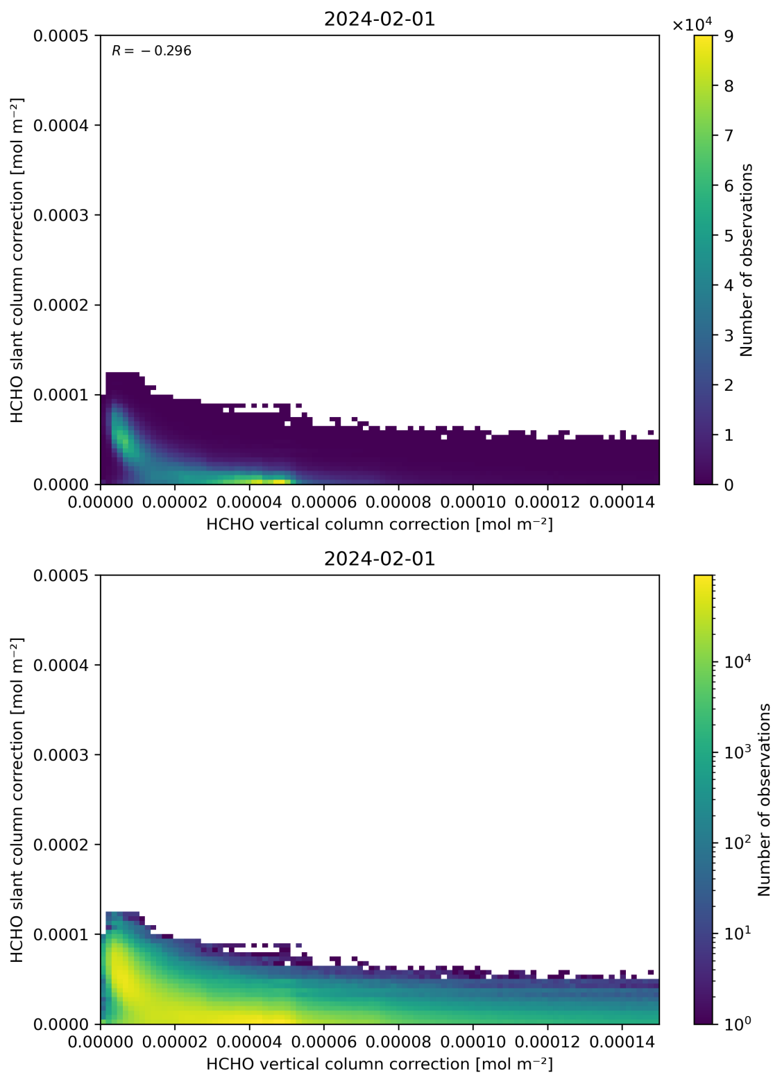
Figure 117: Scatter density plot of “HCHO vertical column correction” against “HCHO slant column correction” for 2024-01-31 to 2024-02-02.
