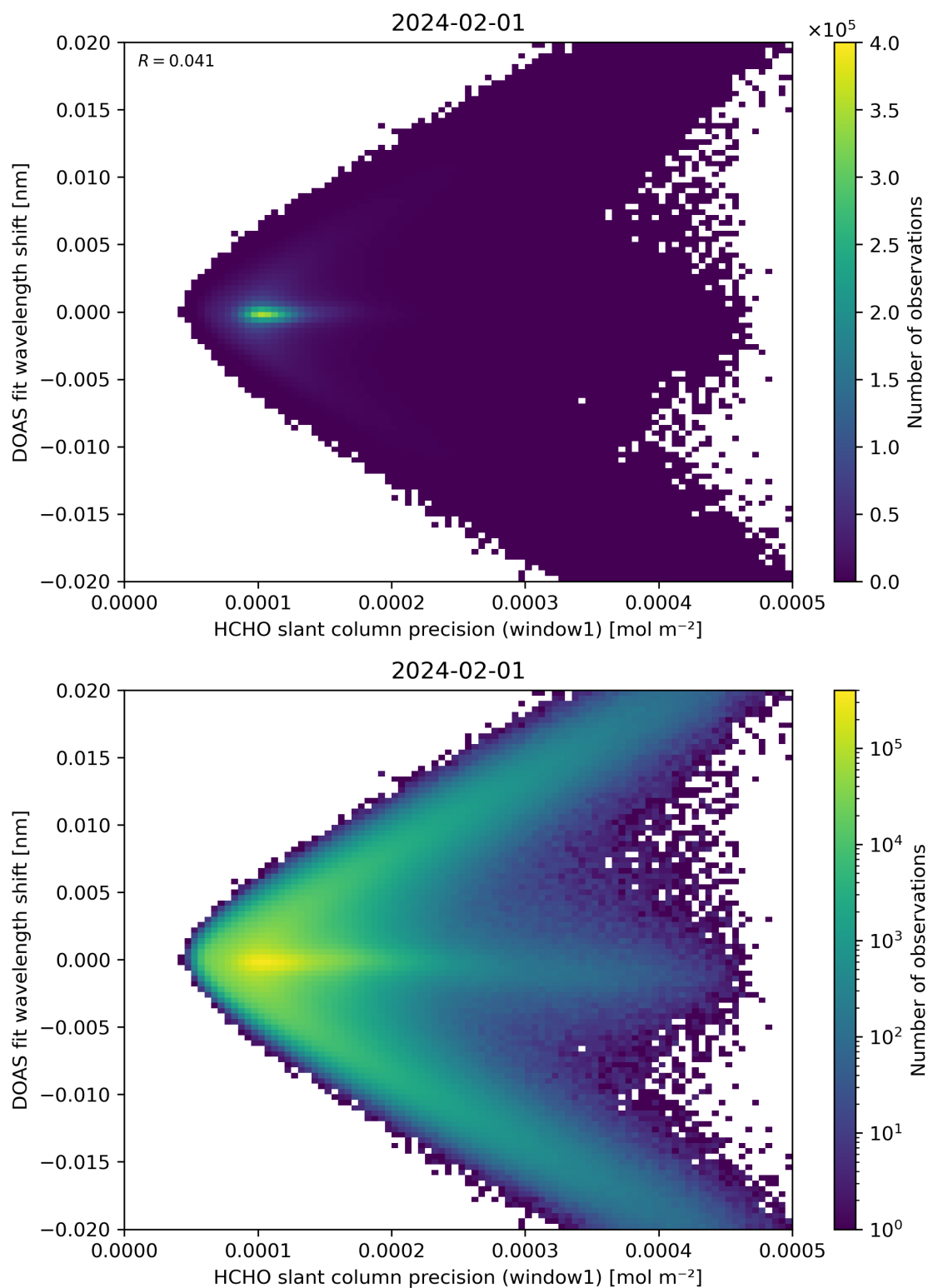
Figure 89: Scatter density plot of “HCHO slant column precision (window1)” against “DOAS fit wavelength shift” for 2024-01-31 to 2024-02-02.
