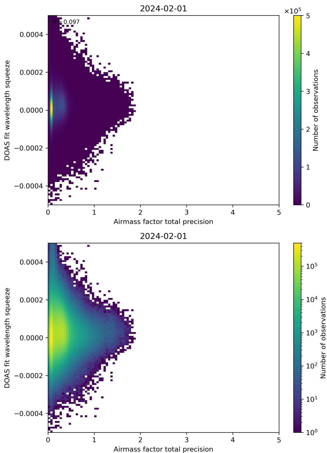
Figure 107: Scatter density plot of “Airmass factor total precision” against “DOAS fit wavelength squeeze” for 2024-01-31 to 2024-02-02.
