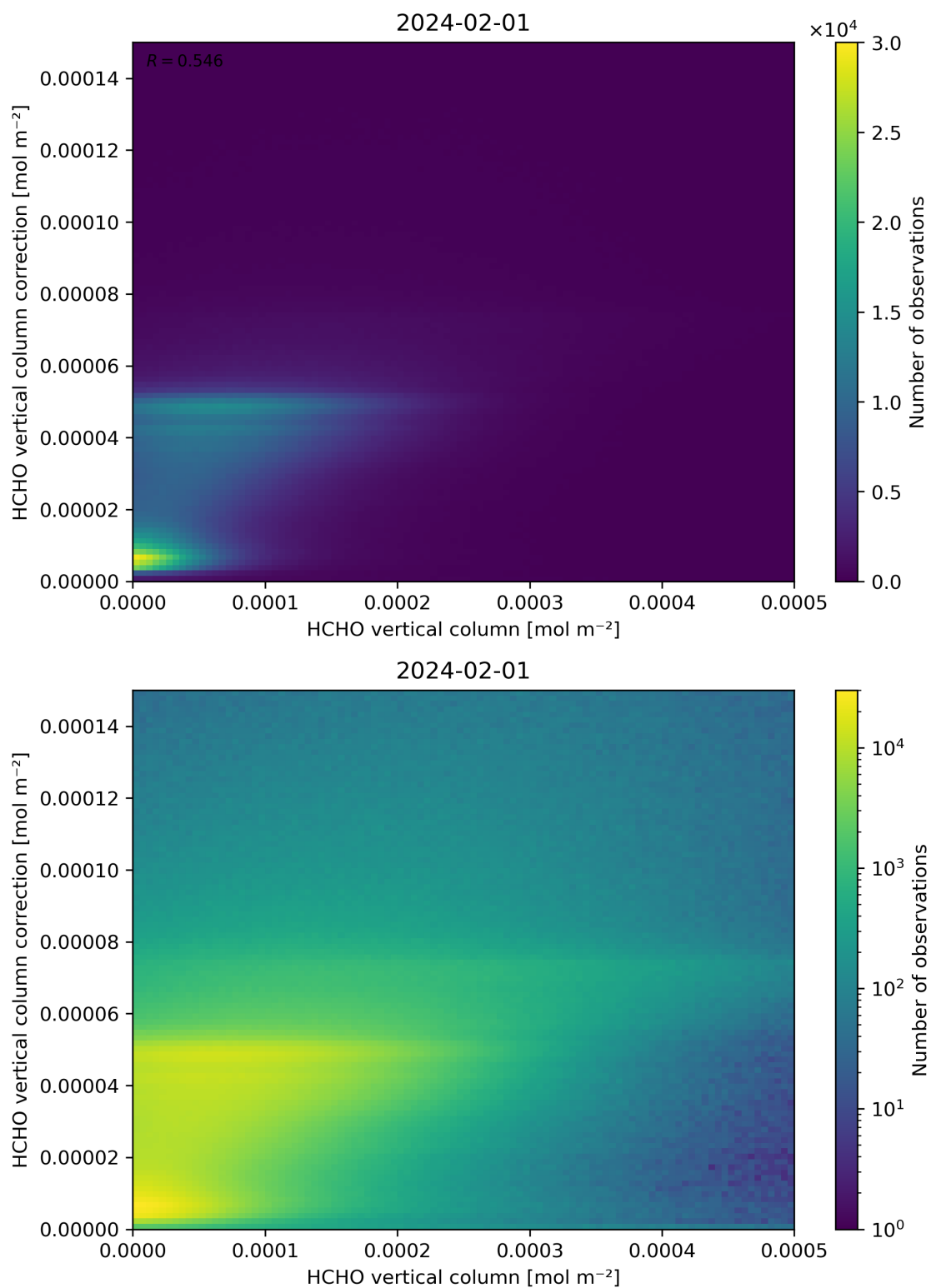
Figure 133: Scatter density plot of “HCHO vertical column” against “HCHO vertical column correction” for 2024-01-31 to 2024-02-02.
