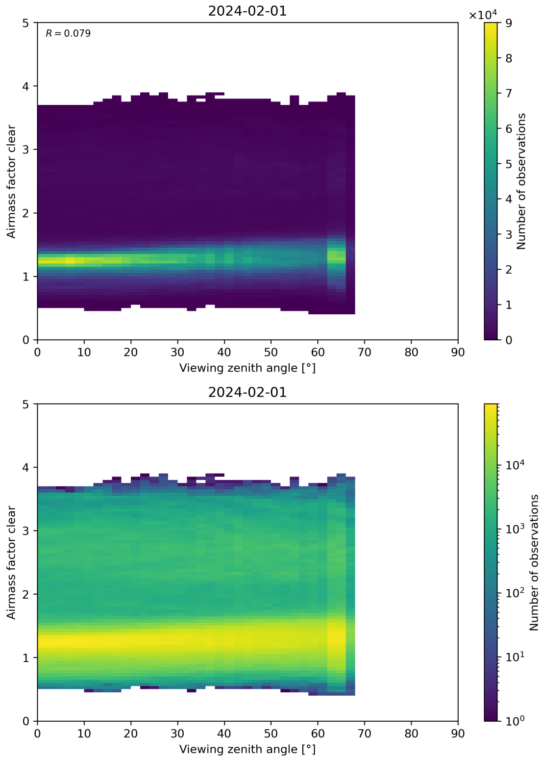
Figure 185: Scatter density plot of “Viewing zenith angle” against “Airmass factor clear” for 2024-01-31 to 2024-02-02.
