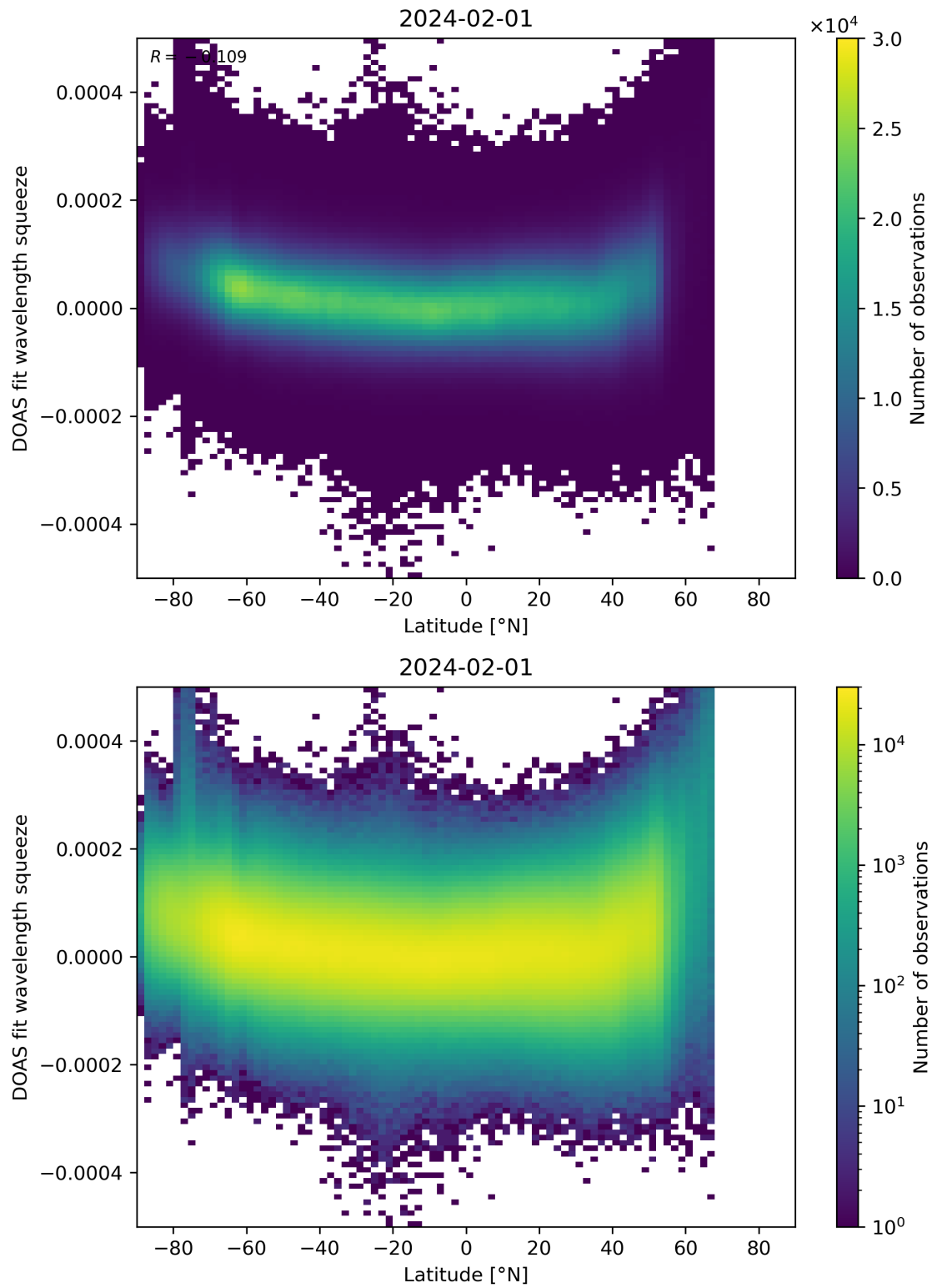
Figure 155: Scatter density plot of “Latitude” against “DOAS fit wavelength squeeze” for 2024-01-31 to 2024-02-02.
