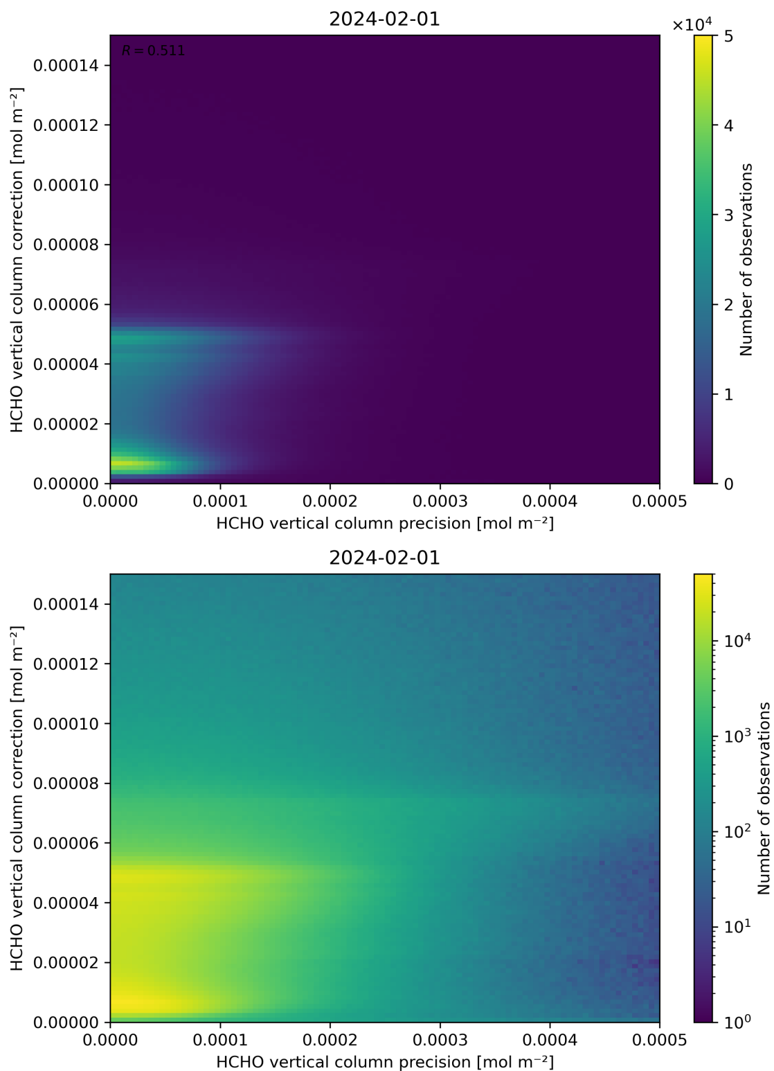
Figure 146: Scatter density plot of “HCHO vertical column precision” against “HCHO vertical column correction” for 2024-01-31 to 2024-02-02.
