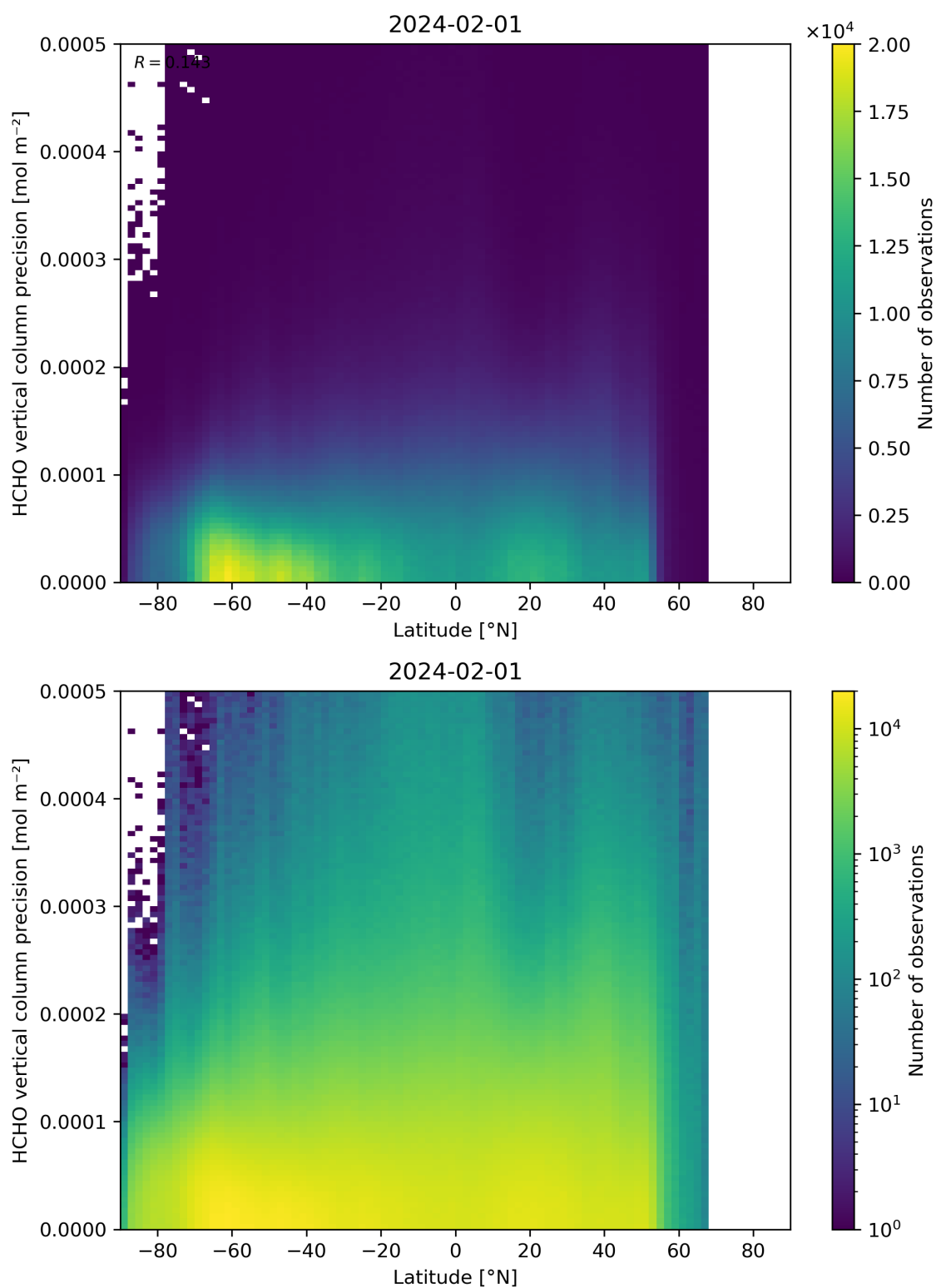
Figure 165: Scatter density plot of “Latitude” against “HCHO vertical column precision” for 2024-01-31 to 2024-02-02.
