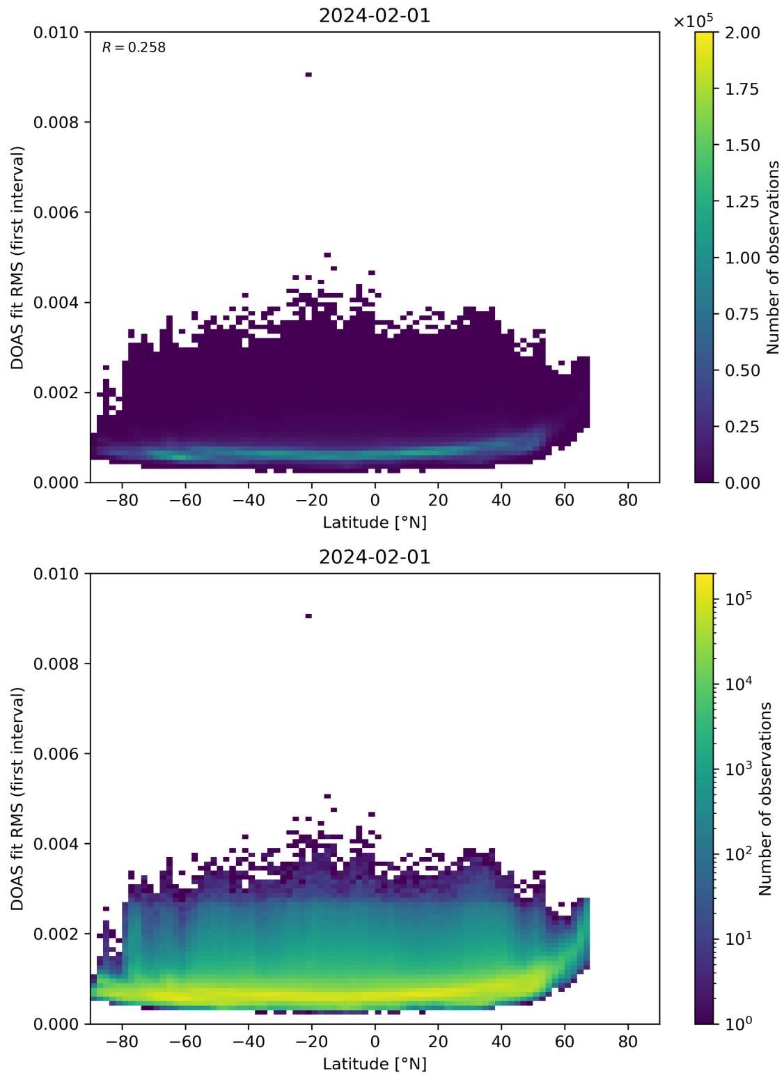
Figure 153: Scatter density plot of “Latitude” against “DOAS fit RMS (first interval)” for 2024-01-31 to 2024-02-02.
