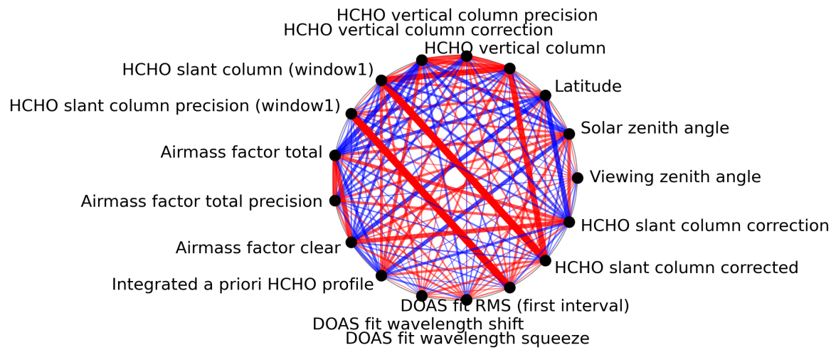
Figure 1: Map of correlation graph for 2024-01-31 to 2024-02-02.
