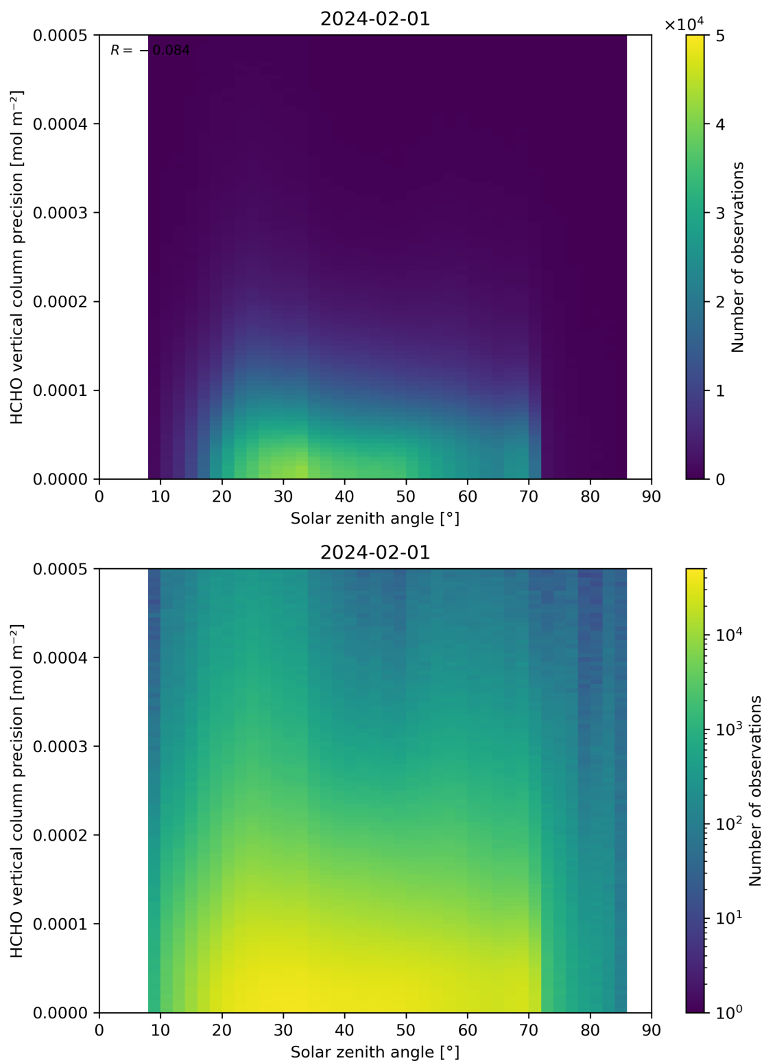
Figure 179: Scatter density plot of “Solar zenith angle” against “HCHO vertical column precision” for 2024-01-31 to 2024-02-02.
