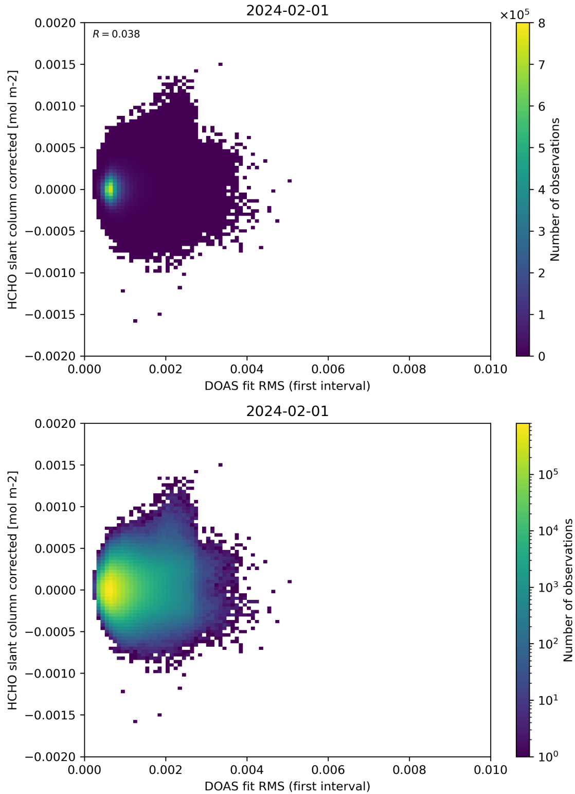
Figure 62: Scatter density plot of “DOAS fit RMS (first interval)” against “HCHO slant column corrected” for 2024-01-31 to 2024-02-02.
