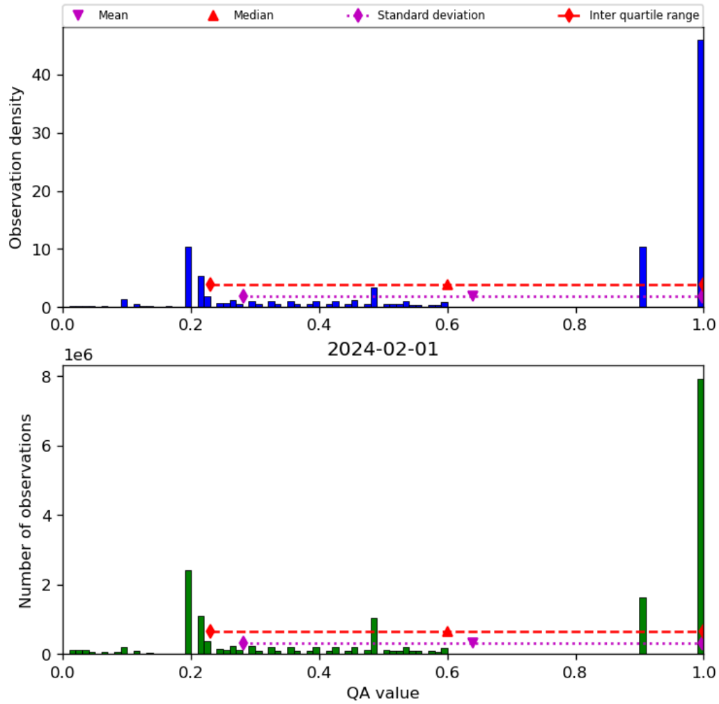
Figure 34: Histogram of “QA value” for 2024-01-31 to 2024-02-02
