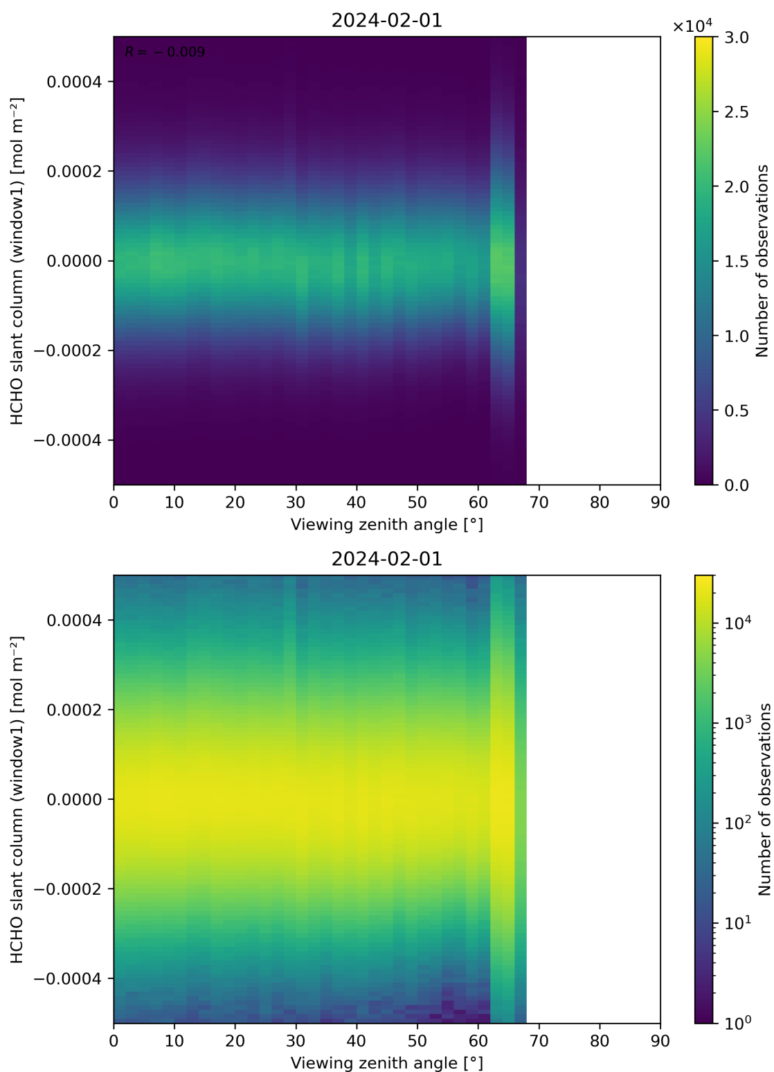
Figure 188: Scatter density plot of “Viewing zenith angle” against “HCHO slant column (window1)” for 2024-01-31 to 2024-02-02.
