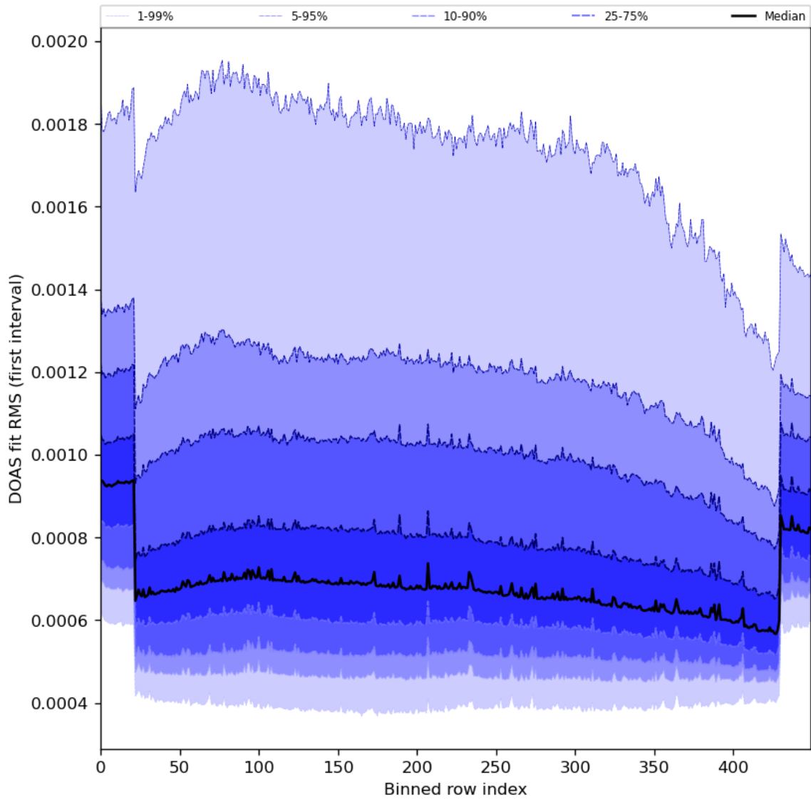
Figure 60: Along track statistics of “DOAS fit RMS (first interval)” for 2024-01-31 to 2024-02-02
