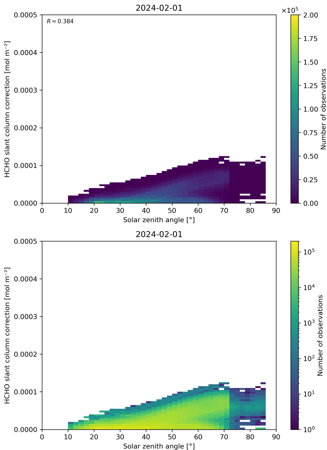
Figure 172: Scatter density plot of “Solar zenith angle” against “HCHO slant column correction” for 2024-01-31 to 2024-02-02.
