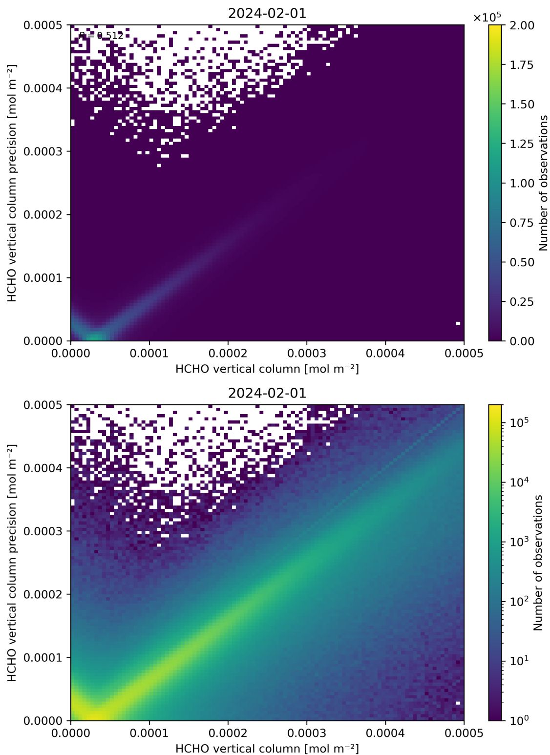
Figure 134: Scatter density plot of “HCHO vertical column” against “HCHO vertical column precision” for 2024-01-31 to 2024-02-02.
