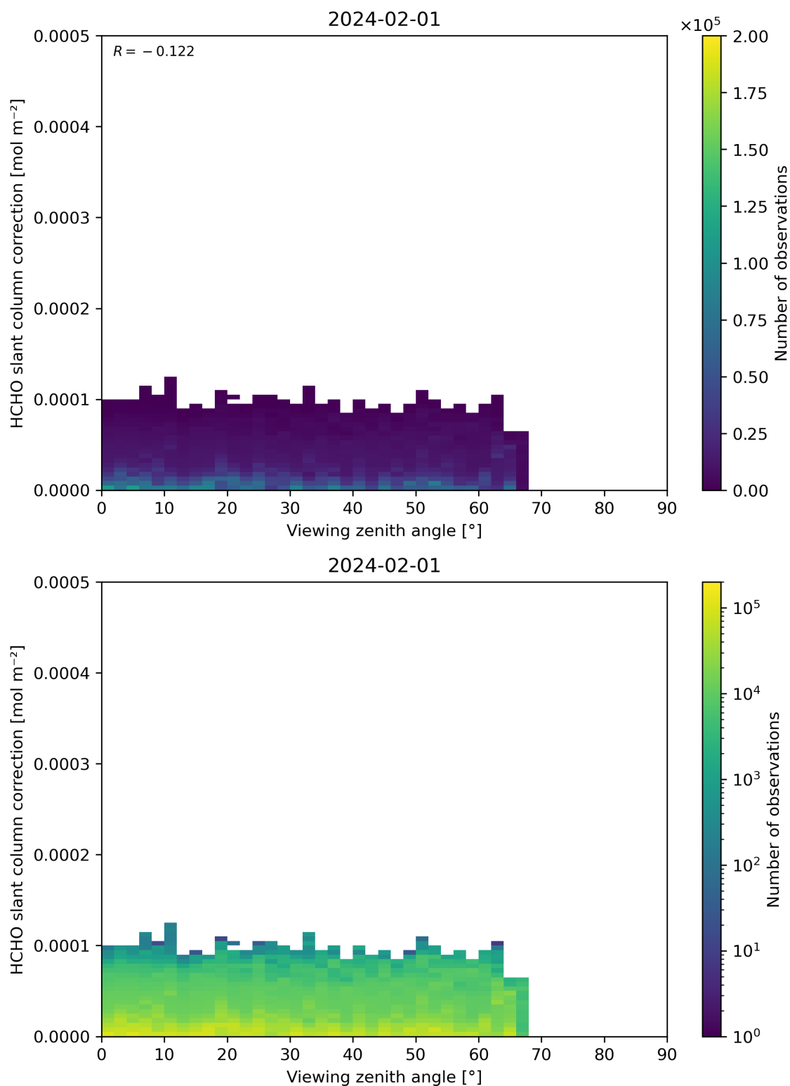
Figure 187: Scatter density plot of “Viewing zenith angle” against “HCHO slant column correction” for 2024-01-31 to 2024-02-02.
