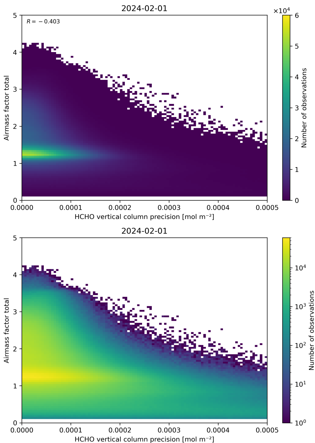
Figure 144: Scatter density plot of “HCHO vertical column precision” against “Airmass factor total” for 2024-01-31 to 2024-02-02.
