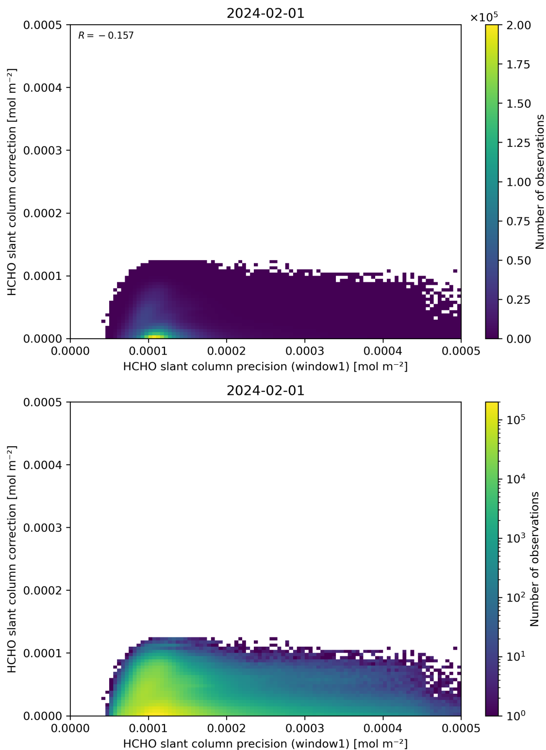
Figure 93: Scatter density plot of “HCHO slant column precision (window1)” against “HCHO slant column correction” for 2024-01-31 to 2024-02-02.
