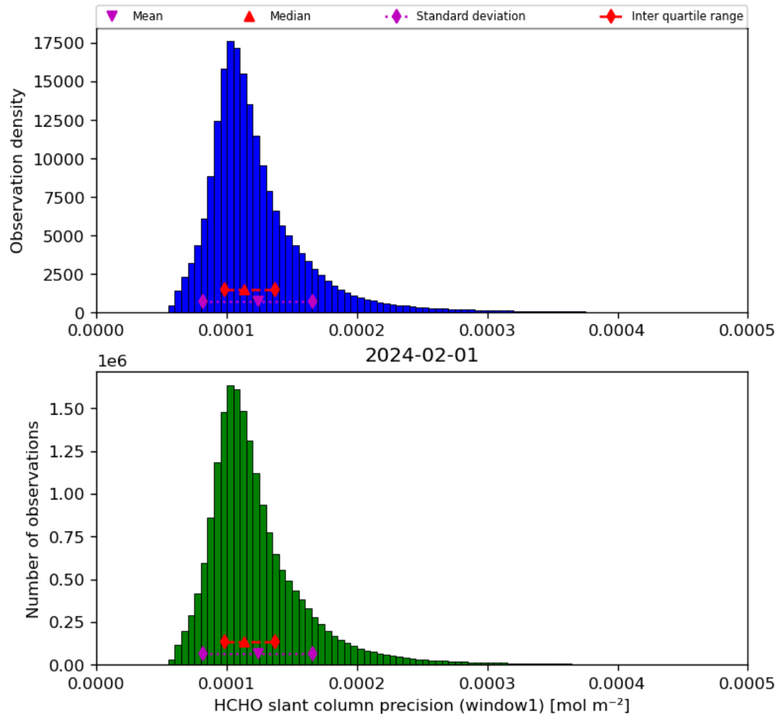
Figure 39: Histogram of “HCHO slant column precision (window1)” for 2024-01-31 to 2024-02-02
