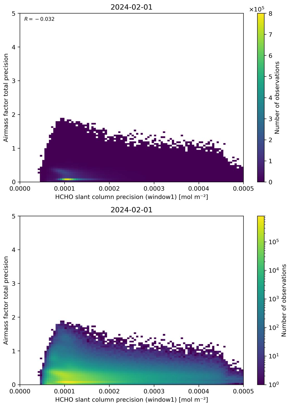
Figure 95: Scatter density plot of “HCHO slant column precision (window1)” against “Airmass factor total precision” for 2024-01-31 to 2024-02-02.
