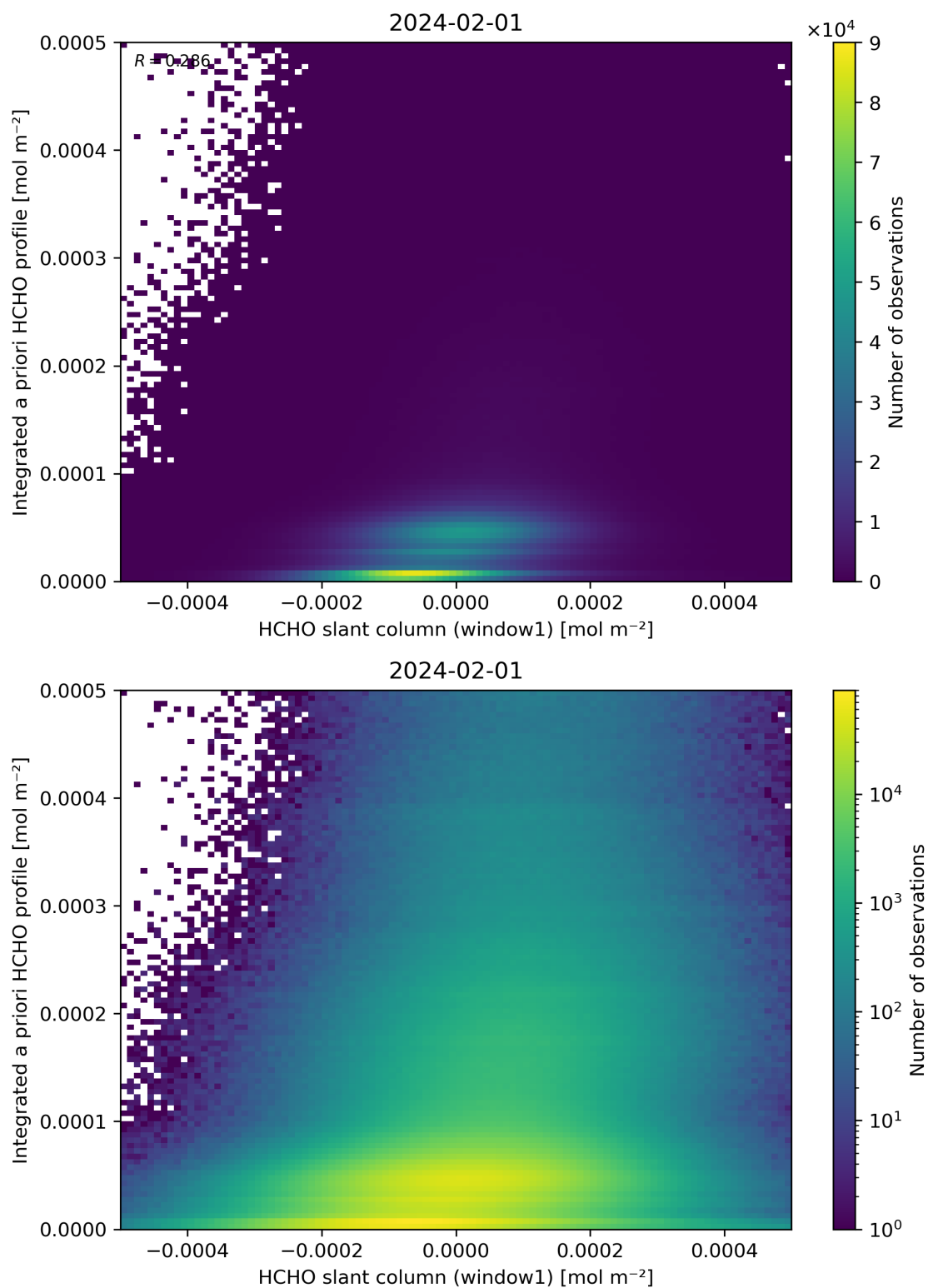
Figure 87: Scatter density plot of “HCHO slant column (window1)” against “Integrated a priori HCHO profile” for 2024-01-31 to 2024-02-02.
