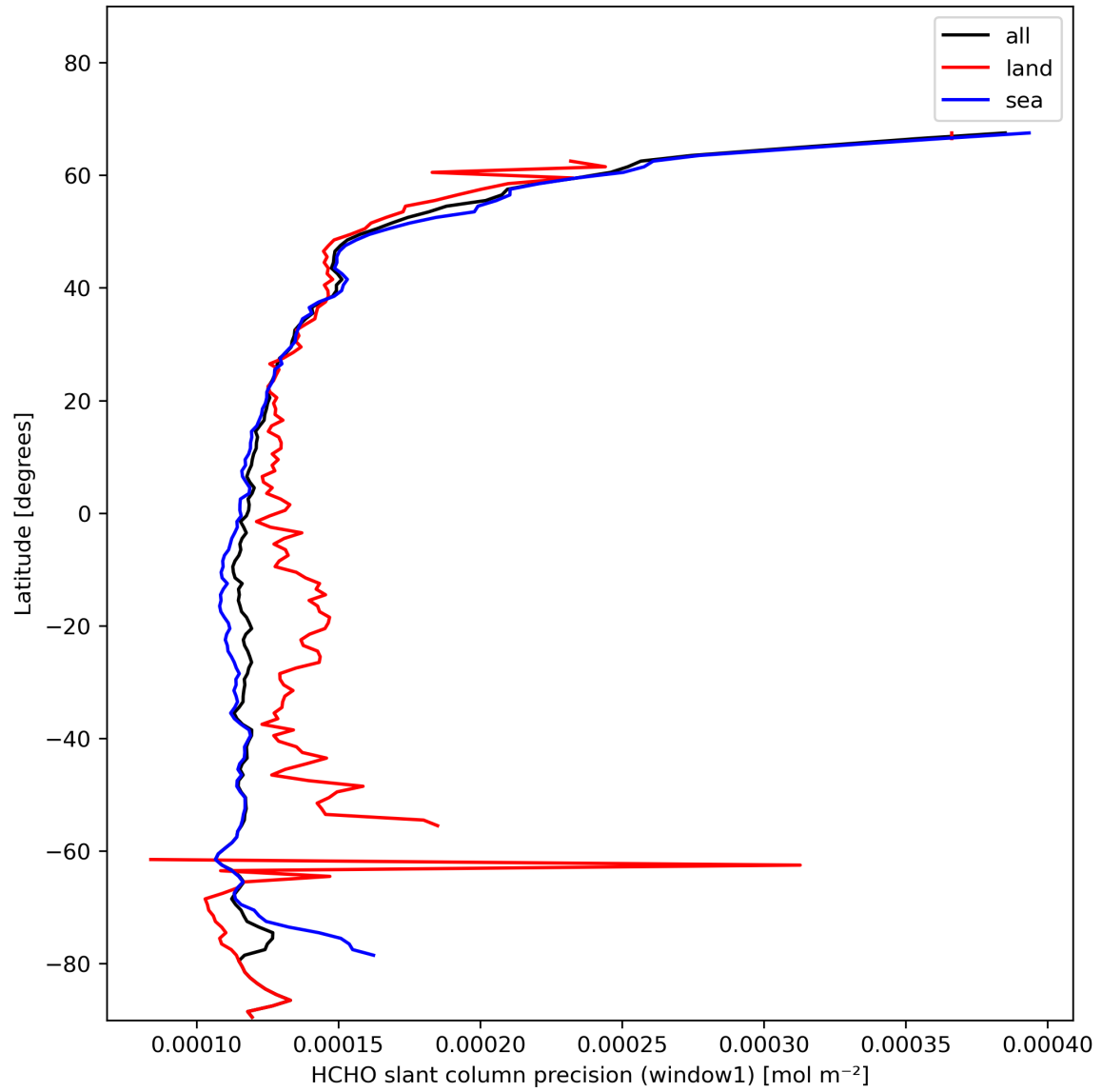
Figure 25: Zonal average of “HCHO slant column precision (window1)” for 2024-01-31 to 2024-02-02.
