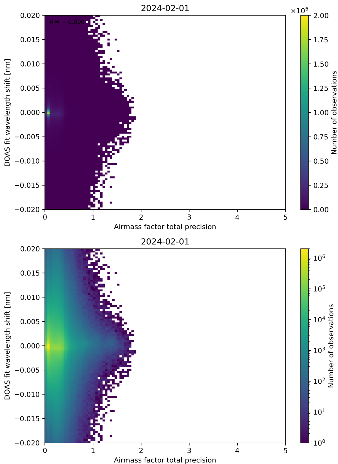
Figure 106: Scatter density plot of “Airmass factor total precision” against “DOAS fit wavelength shift” for 2024-01-31 to 2024-02-02.
