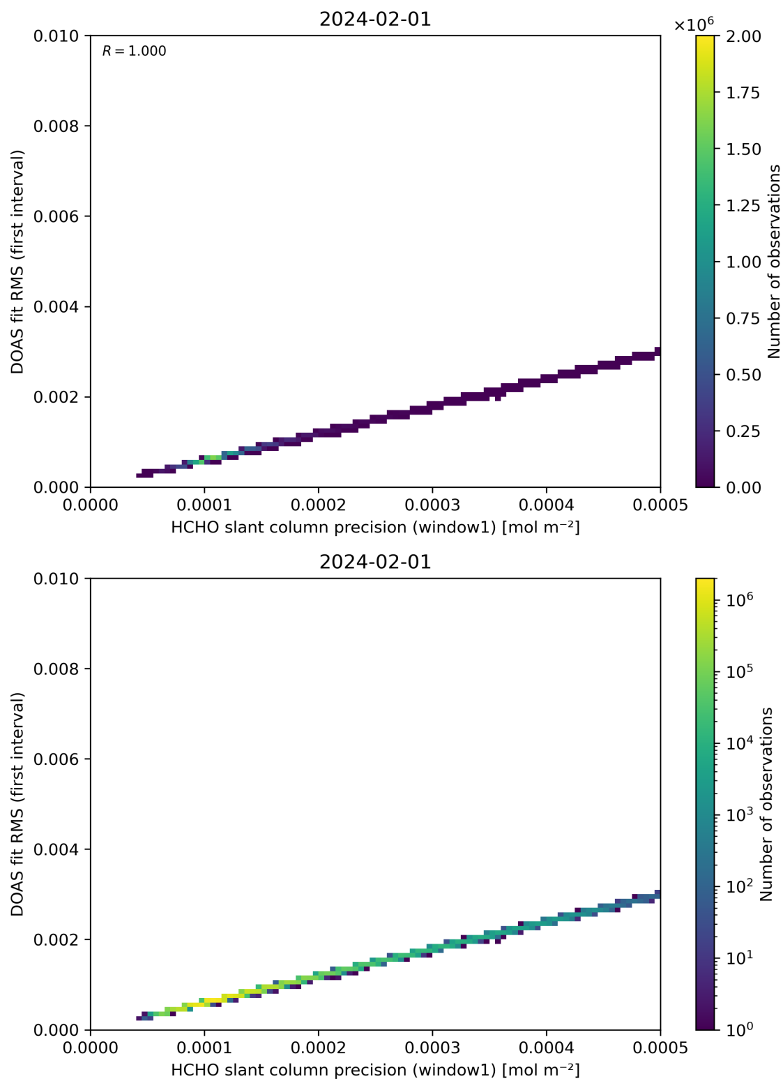
Figure 88: Scatter density plot of “HCHO slant column precision (window1)” against “DOAS fit RMS (first interval)” for 2024-01-31 to 2024-02-02.
