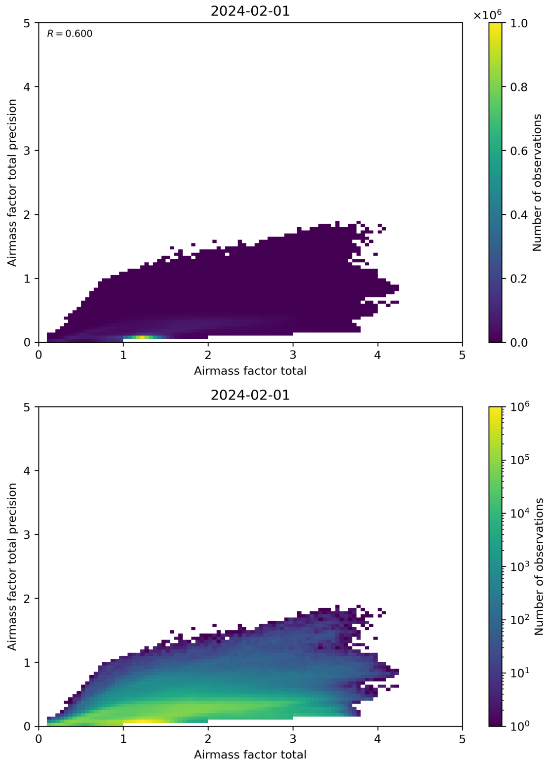
Figure 103: Scatter density plot of “Airmass factor total” against “Airmass factor total precision” for 2024-01-31 to 2024-02-02.
