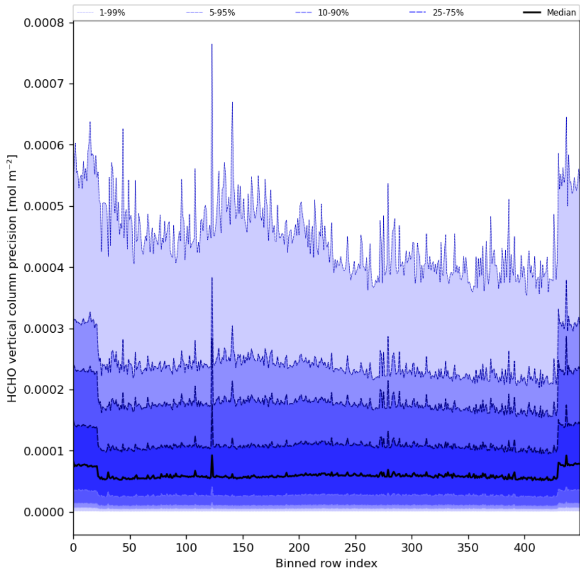
Figure 50: Along track statistics of “HCHO vertical column precision” for 2024-01-31 to 2024-02-02
