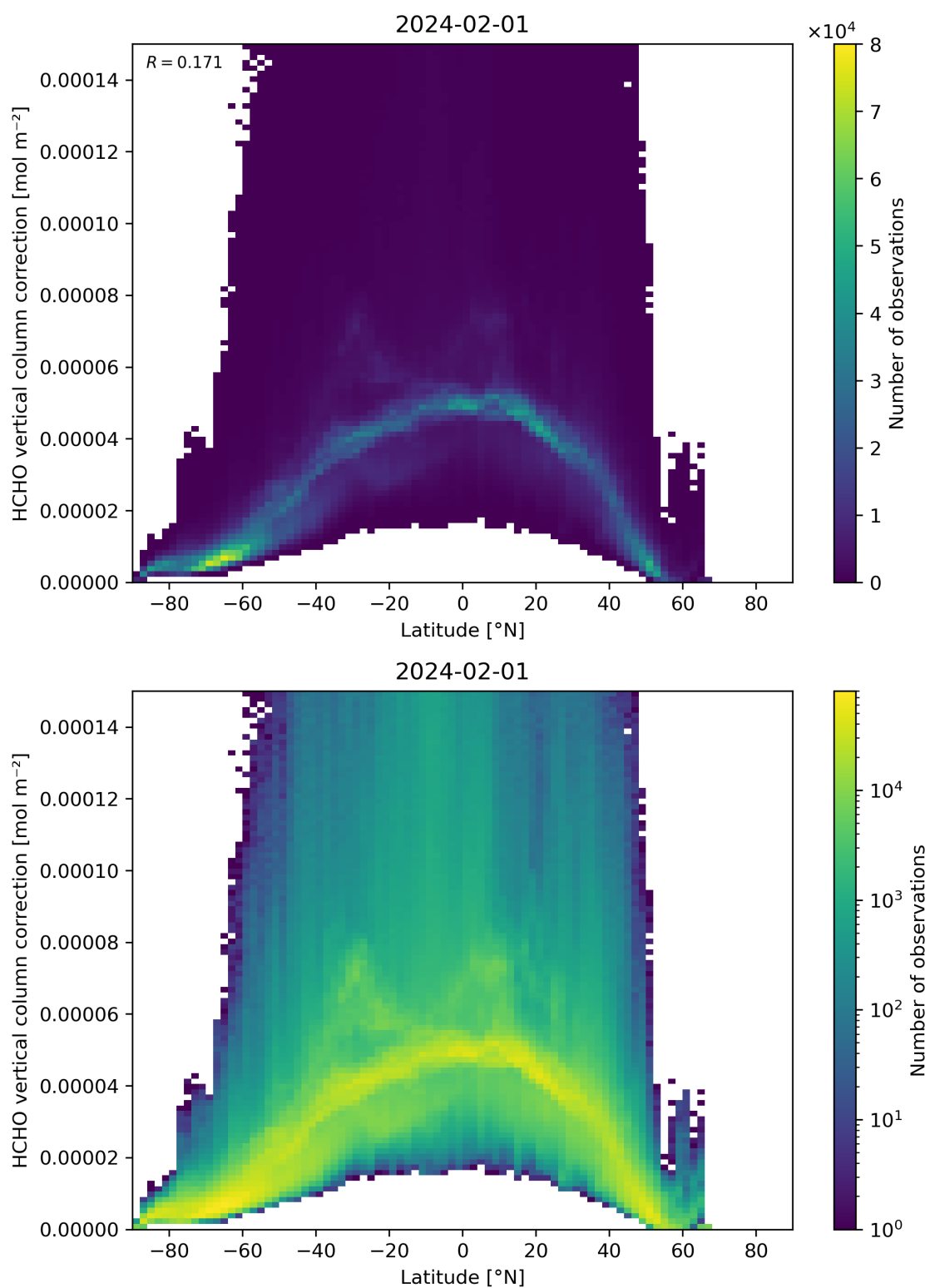
Figure 164: Scatter density plot of “Latitude” against “HCHO vertical column correction” for 2024-01-31 to 2024-02-02.
