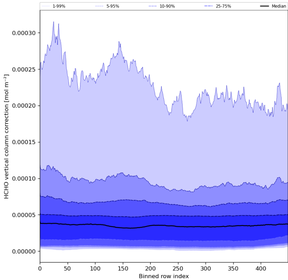
Figure 51: Along track statistics of “HCHO vertical column correction” for 2024-01-31 to 2024-02-02
