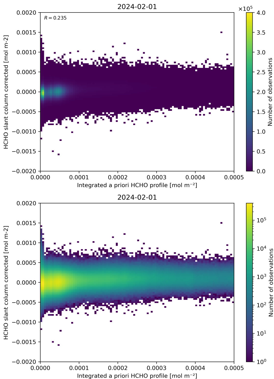
Figure 151: Scatter density plot of “Integrated a priori HCHO profile” against “HCHO slant column corrected” for 2024-01-31 to 2024-02-02.
