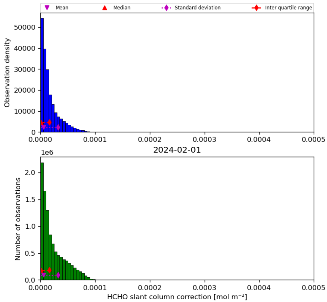
Figure 47: Histogram of “HCHO slant column correction” for 2024-01-31 to 2024-02-02
