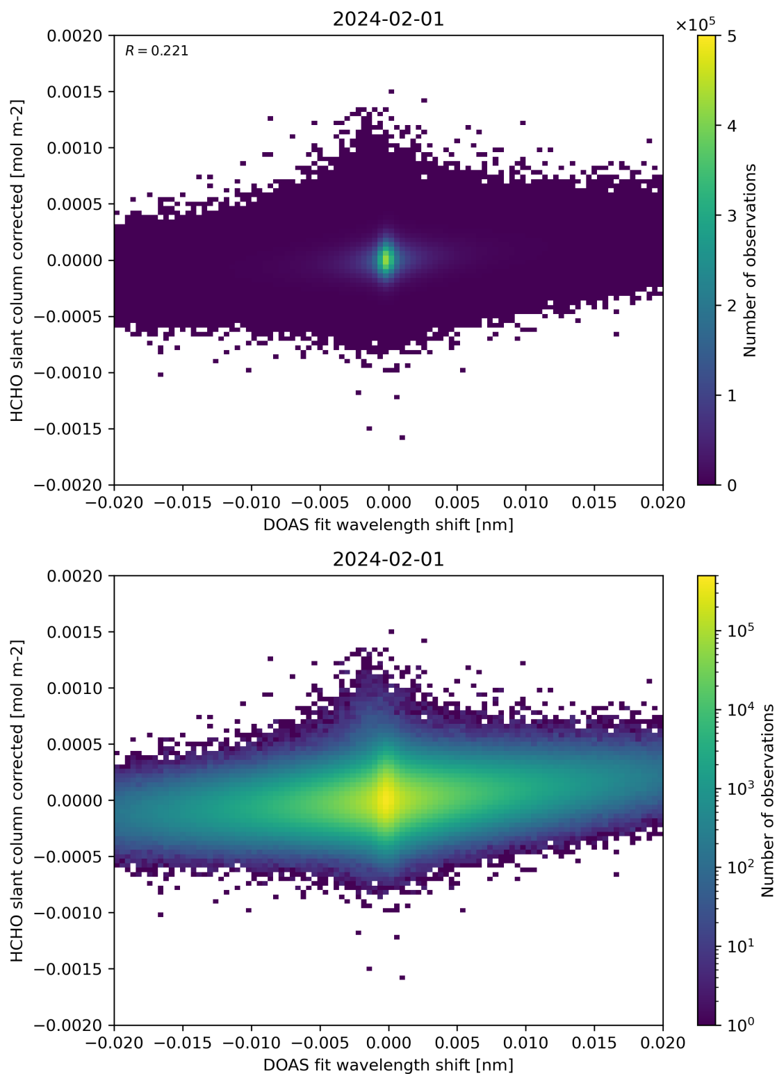
Figure 66: Scatter density plot of “DOAS fit wavelength shift” against “HCHO slant column corrected” for 2024-01-31 to 2024-02-02.
