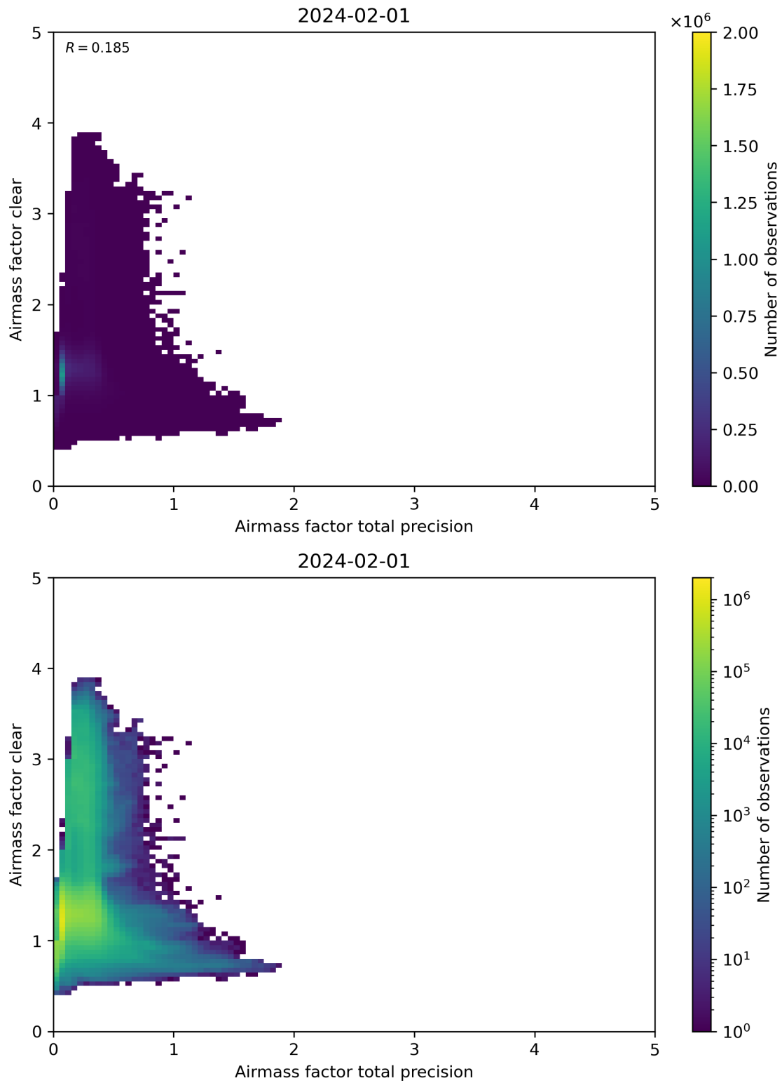
Figure 108: Scatter density plot of “Airmass factor total precision” against “Airmass factor clear” for 2024-01-31 to 2024-02-02.
