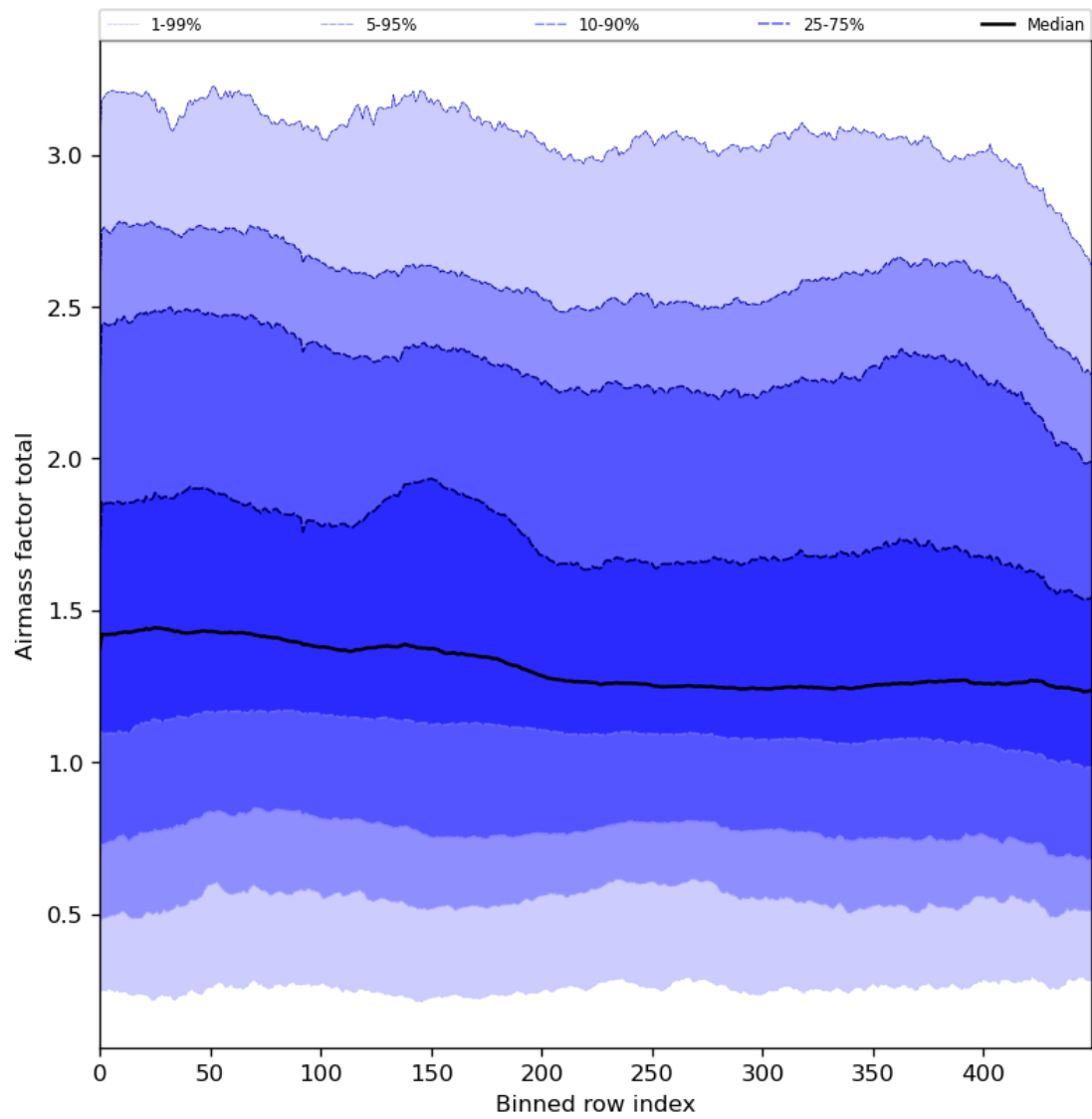
Figure 54: Along track statistics of “Airmass factor total” for 2024-01-31 to 2024-02-02
