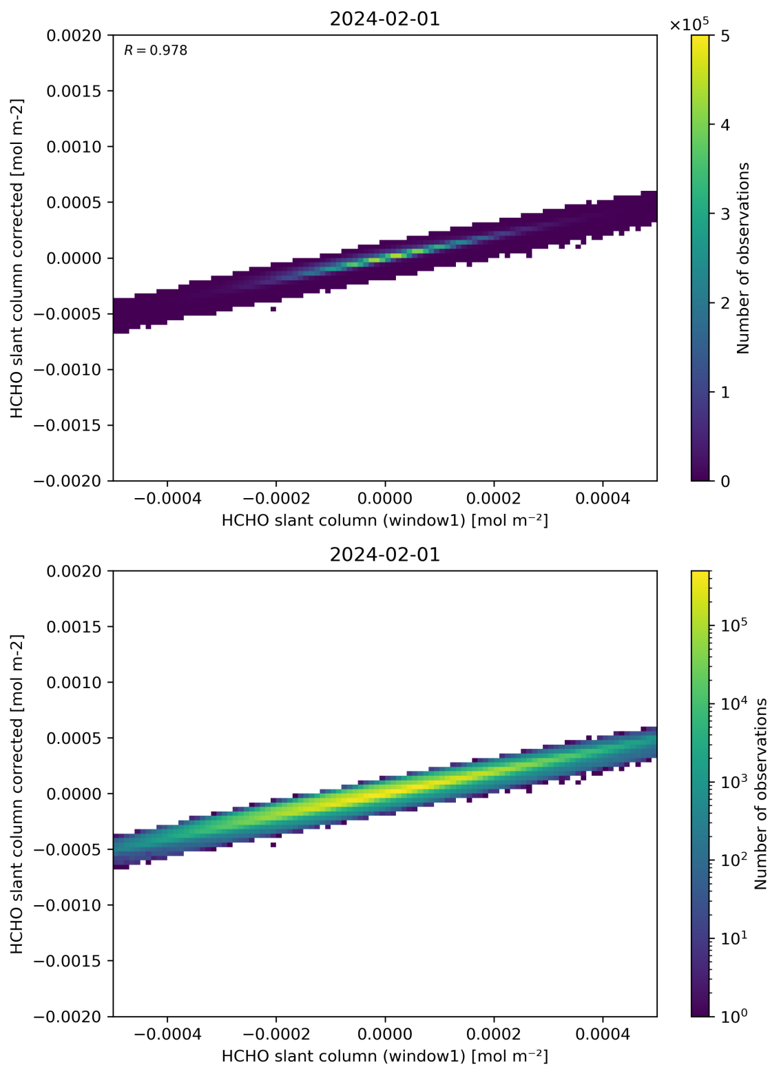
Figure 82: Scatter density plot of “HCHO slant column (window1)” against “HCHO slant column corrected” for 2024-01-31 to 2024-02-02.
