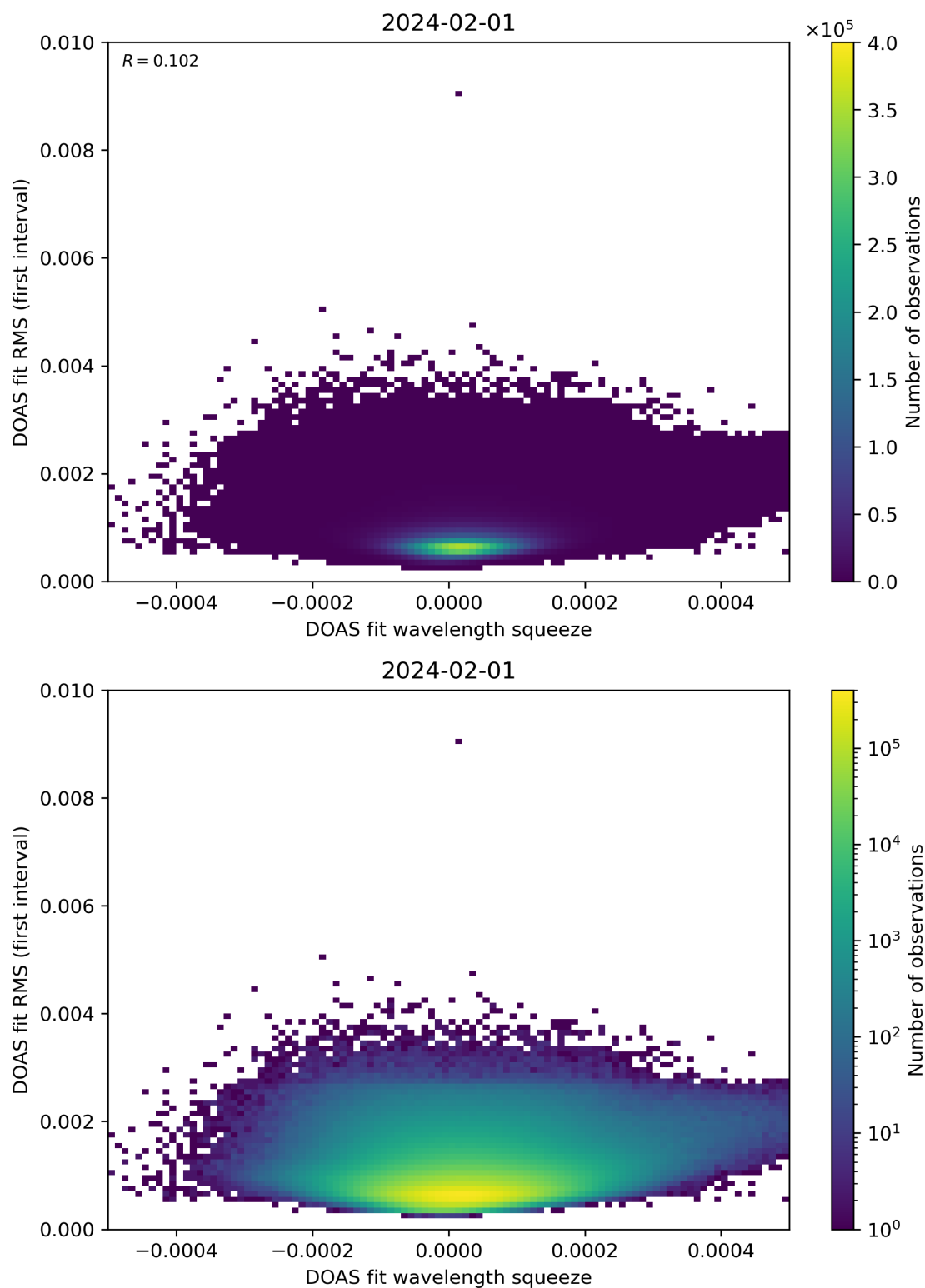
Figure 68: Scatter density plot of “DOAS fit wavelength squeeze” against “DOAS fit RMS (first interval)” for 2024-01-31 to 2024-02-02.
