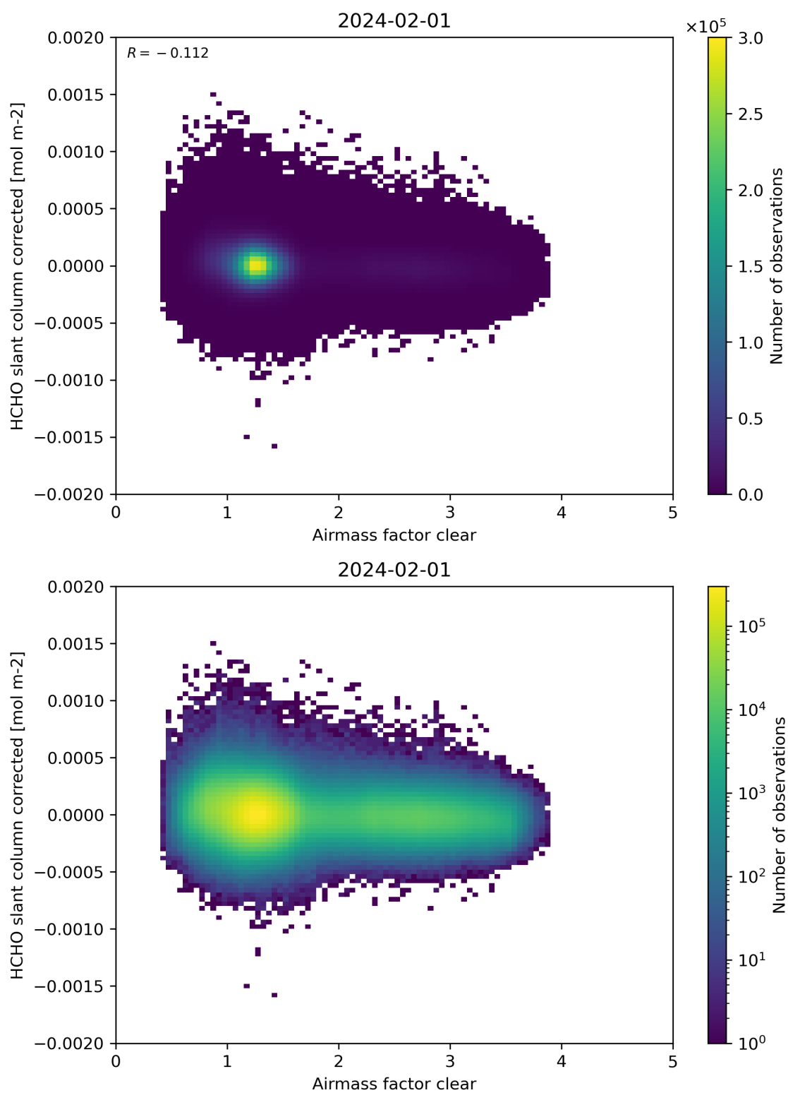
Figure 74: Scatter density plot of “Airmass factor clear” against “HCHO slant column corrected” for 2024-01-31 to 2024-02-02.
