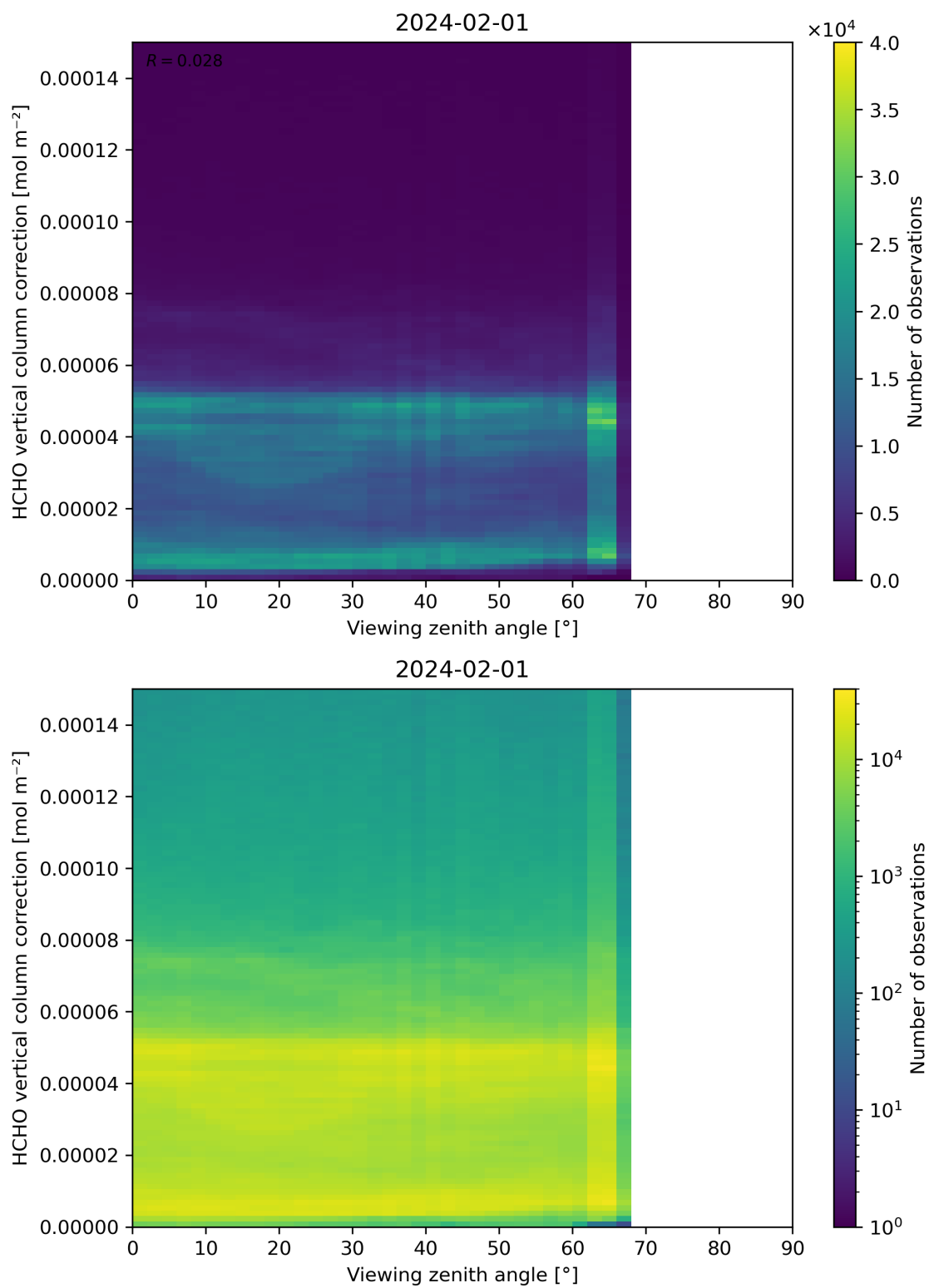
Figure 193: Scatter density plot of “Viewing zenith angle” against “HCHO vertical column correction” for 2024-01-31 to 2024-02-02.
