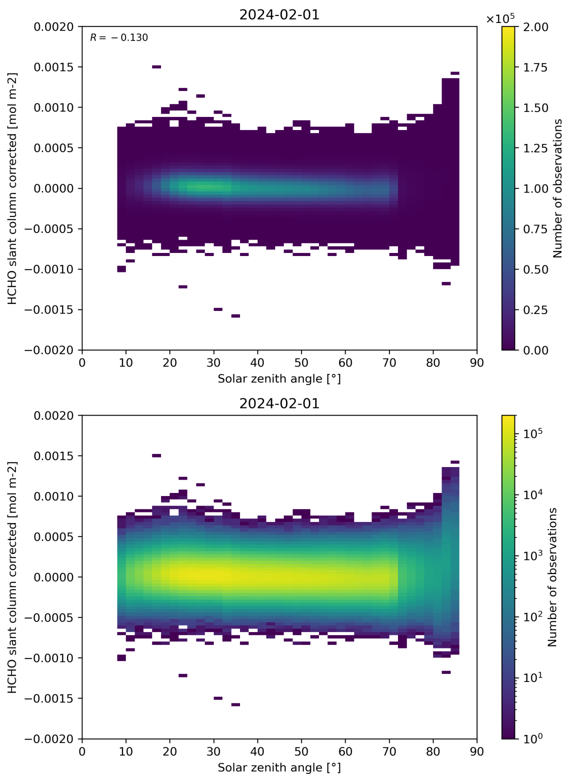
Figure 171: Scatter density plot of “Solar zenith angle” against “HCHO slant column corrected” for 2024-01-31 to 2024-02-02.
