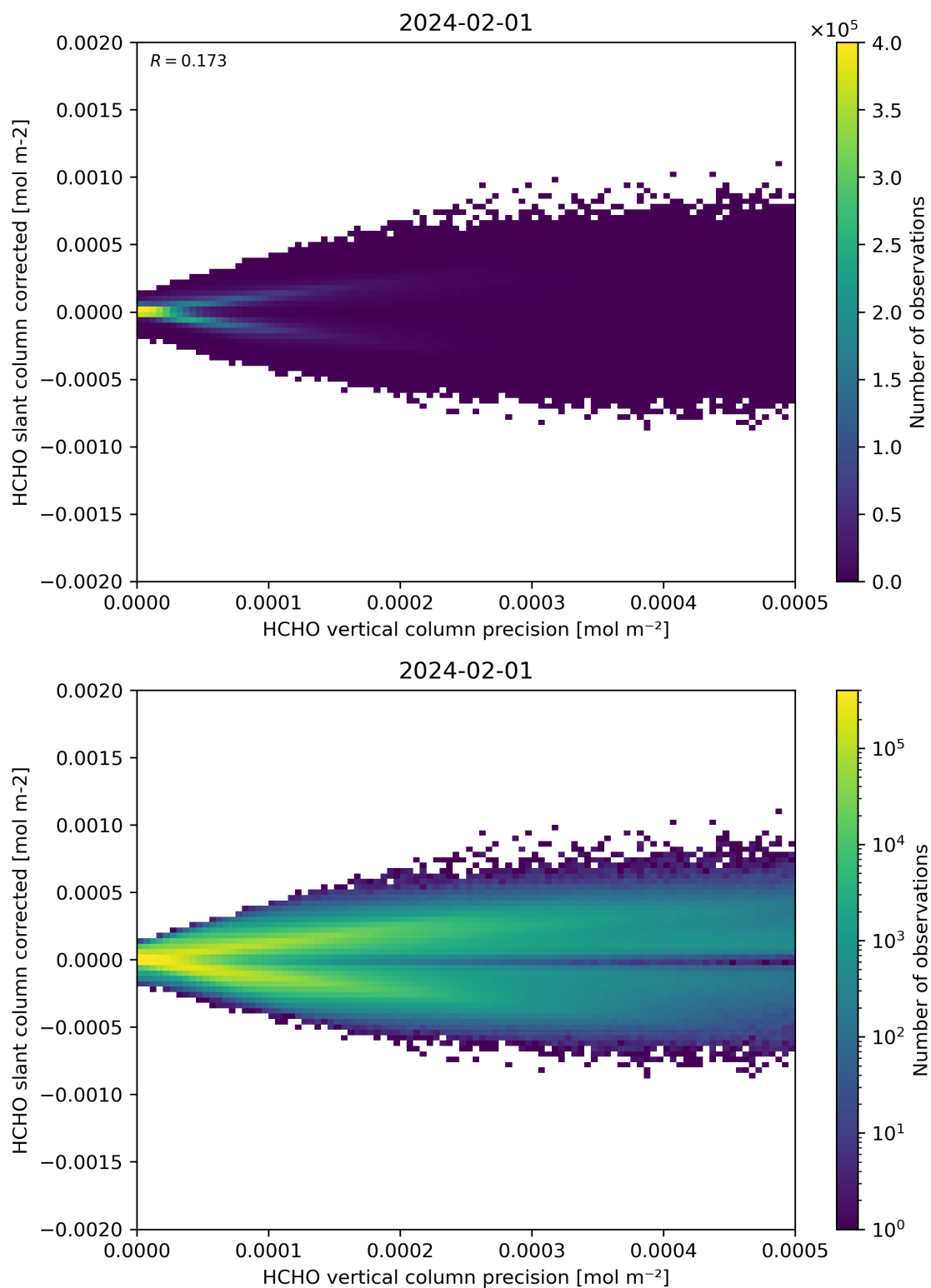
Figure 140: Scatter density plot of “HCHO vertical column precision” against “HCHO slant column corrected” for 2024-01-31 to 2024-02-02.
