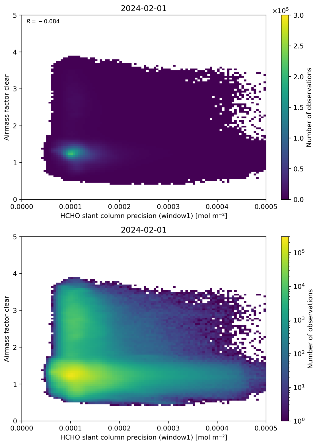
Figure 91: Scatter density plot of “HCHO slant column precision (window1)” against “Airmass factor clear” for 2024-01-31 to 2024-02-02.
