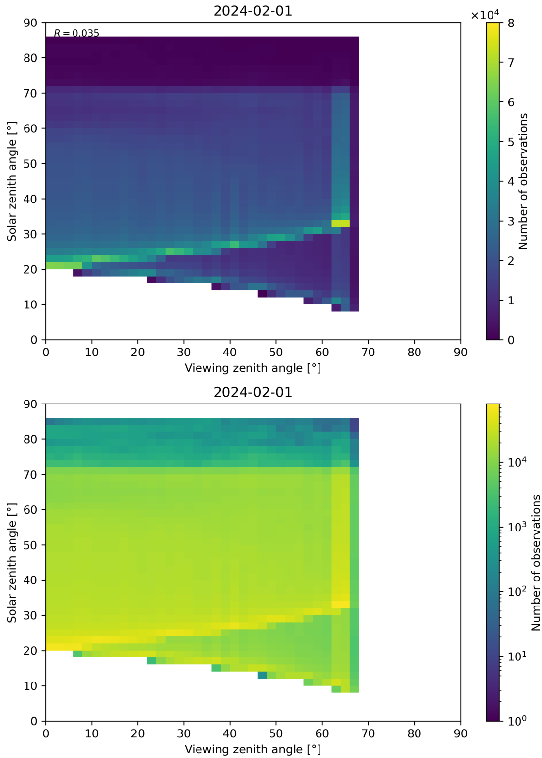
Figure 197: Scatter density plot of “Viewing zenith angle” against “Solar zenith angle” for 2024-01-31 to 2024-02-02.
