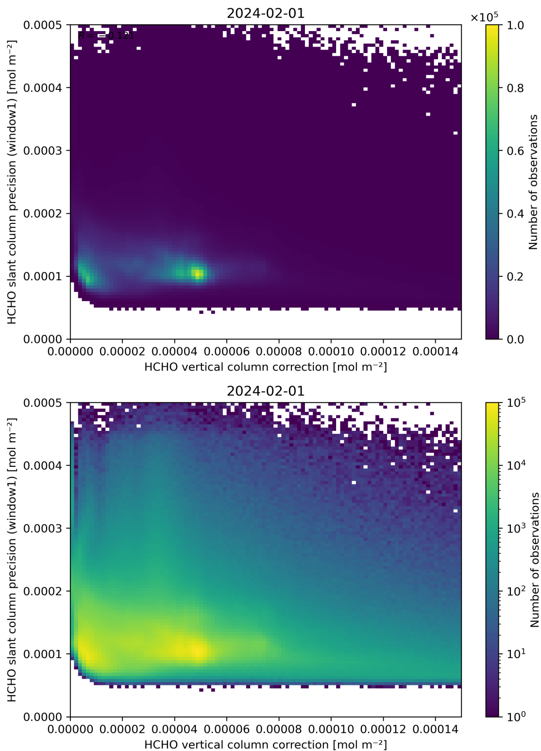
Figure 119: Scatter density plot of “HCHO vertical column correction” against “HCHO slant column precision (window1)” for 2024-01-31 to 2024-02-02.
