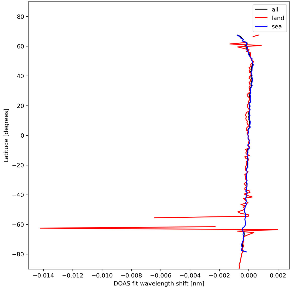
Figure 30: Zonal average of “DOAS fit wavelength shift” for 2024-01-31 to 2024-02-02.
