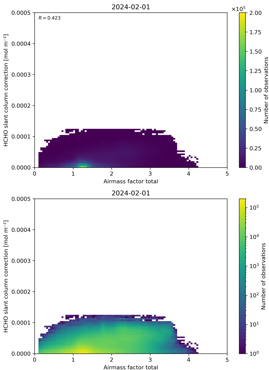
Figure 102: Scatter density plot of “Airmass factor total” against “HCHO slant column correction” for 2024-01-31 to 2024-02-02.
