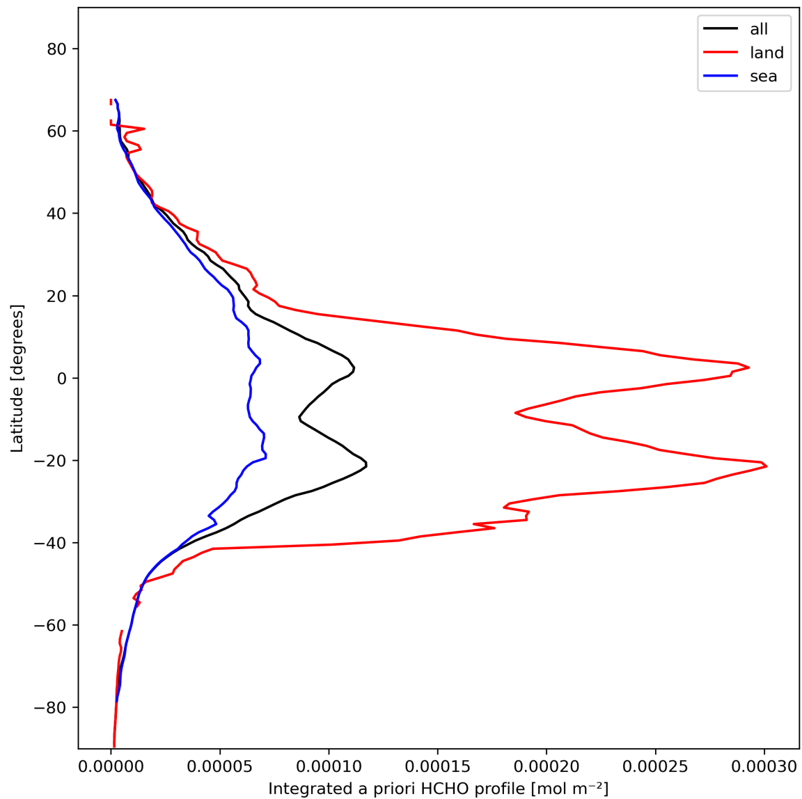
Figure 29: Zonal average of “Integrated a priori HCHO profile” for 2024-01-31 to 2024-02-02.
