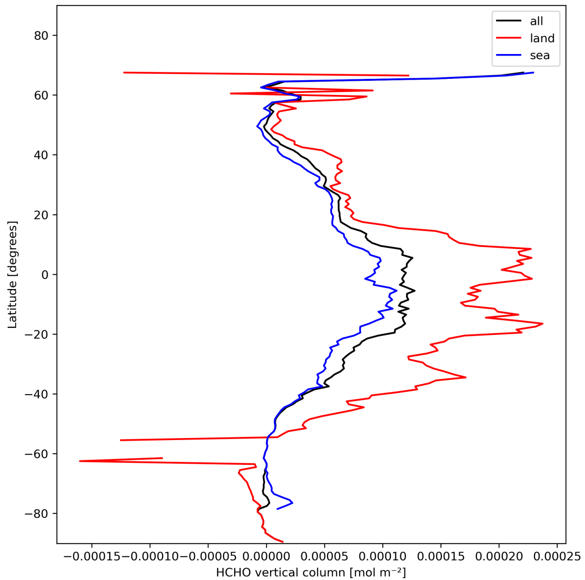
Figure 21: Zonal average of “HCHO vertical column” for 2024-01-31 to 2024-02-02.
