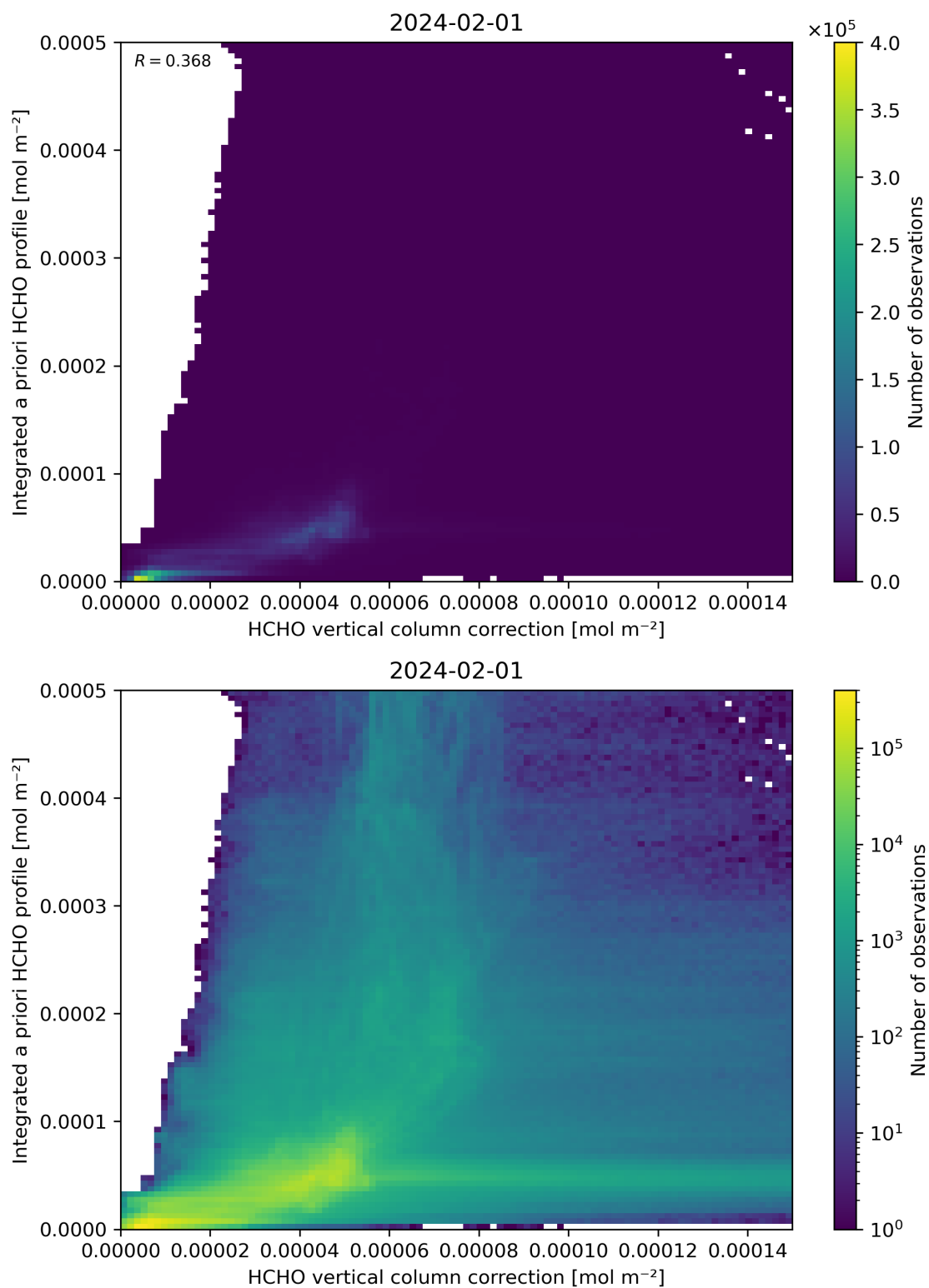
Figure 122: Scatter density plot of “HCHO vertical column correction” against “Integrated a priori HCHO profile” for 2024-01-31 to 2024-02-02.
