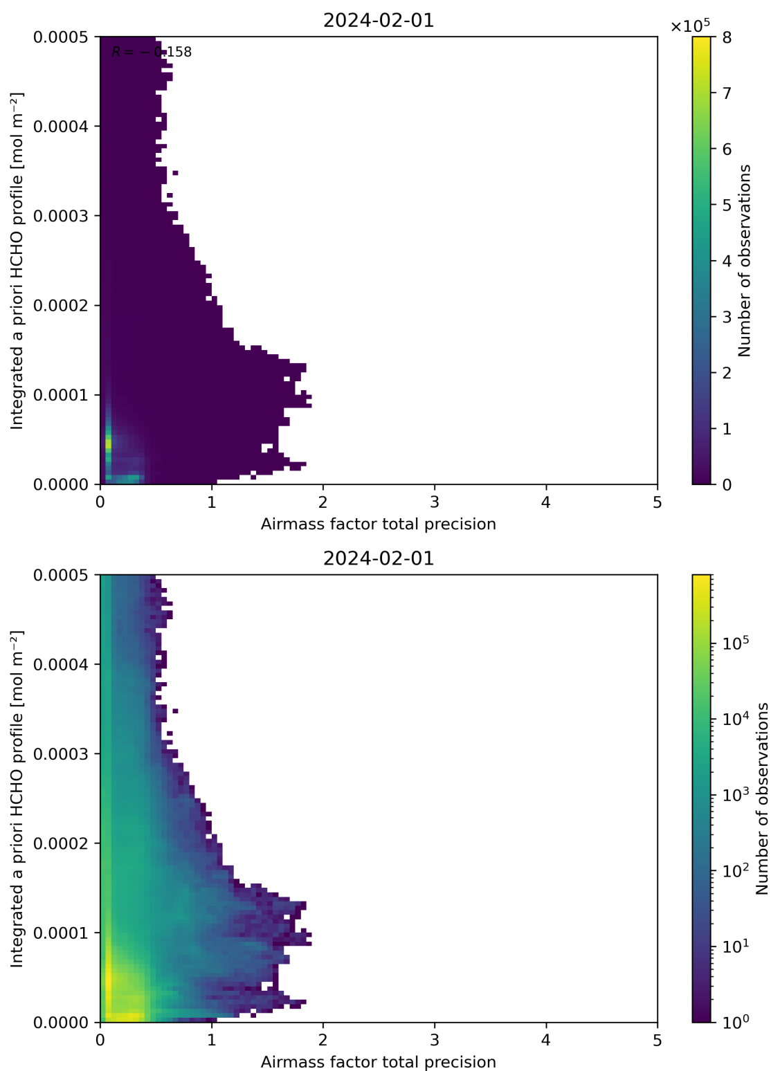
Figure 111: Scatter density plot of “Airmass factor total precision” against “Integrated a priori HCHO profile” for 2024-01-31 to 2024-02-02.
