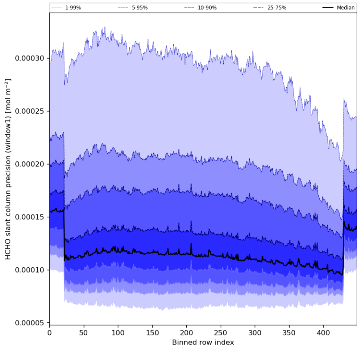
Figure 53: Along track statistics of “HCHO slant column precision (window1)” for 2024-01-31 to 2024-02-02
