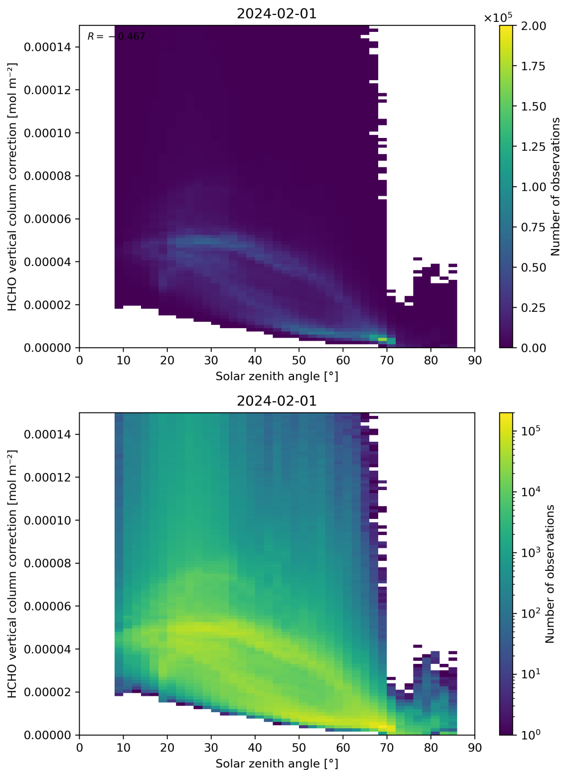
Figure 178: Scatter density plot of “Solar zenith angle” against “HCHO vertical column correction” for 2024-01-31 to 2024-02-02.
