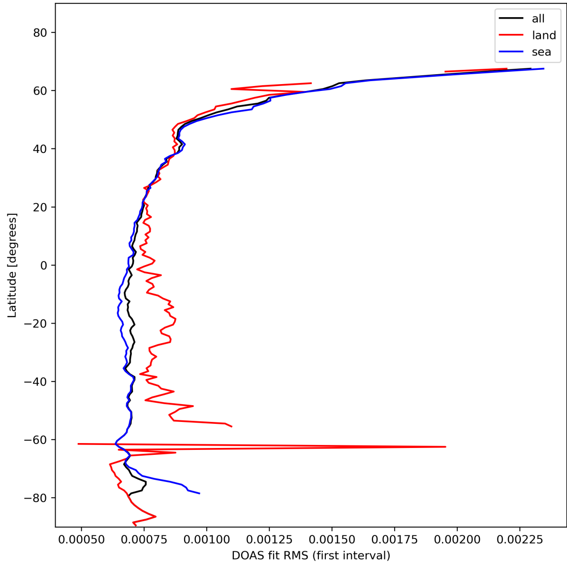
Figure 32: Zonal average of “DOAS fit RMS (first interval)” for 2024-01-31 to 2024-02-02.
