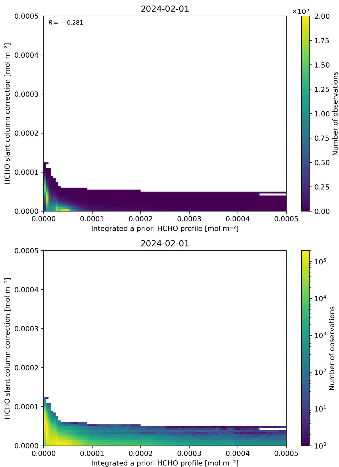
Figure 152: Scatter density plot of “Integrated a priori HCHO profile” against “HCHO slant column correction” for 2024-01-31 to 2024-02-02.
