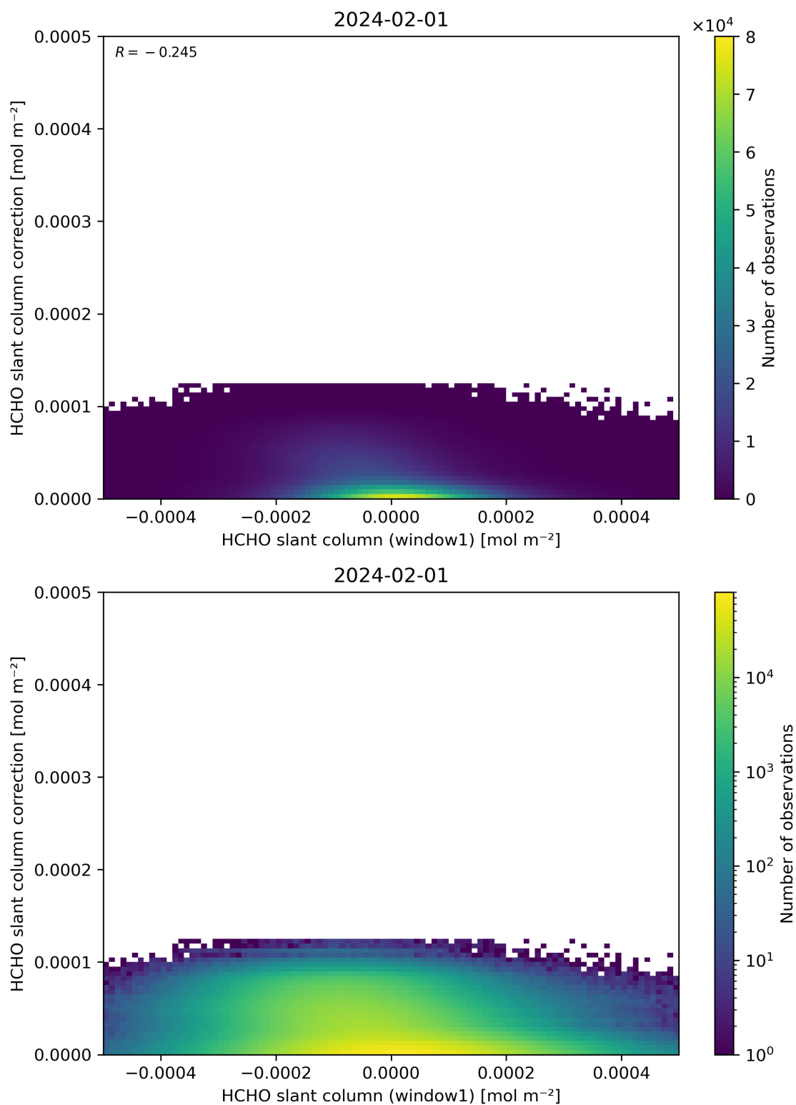
Figure 83: Scatter density plot of “HCHO slant column (window1)” against “HCHO slant column correction” for 2024-01-31 to 2024-02-02.
