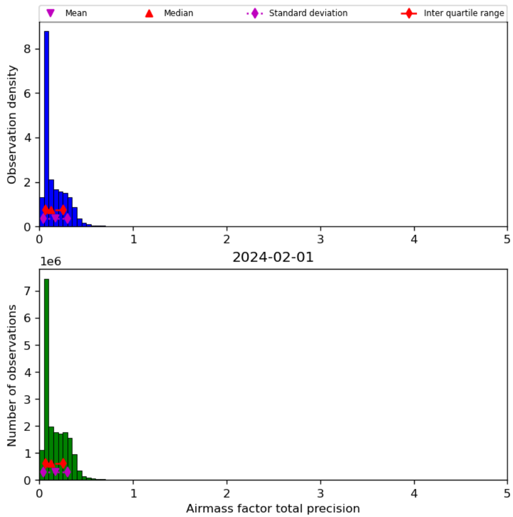
Figure 41: Histogram of “Airmass factor total precision” for 2024-01-31 to 2024-02-02
