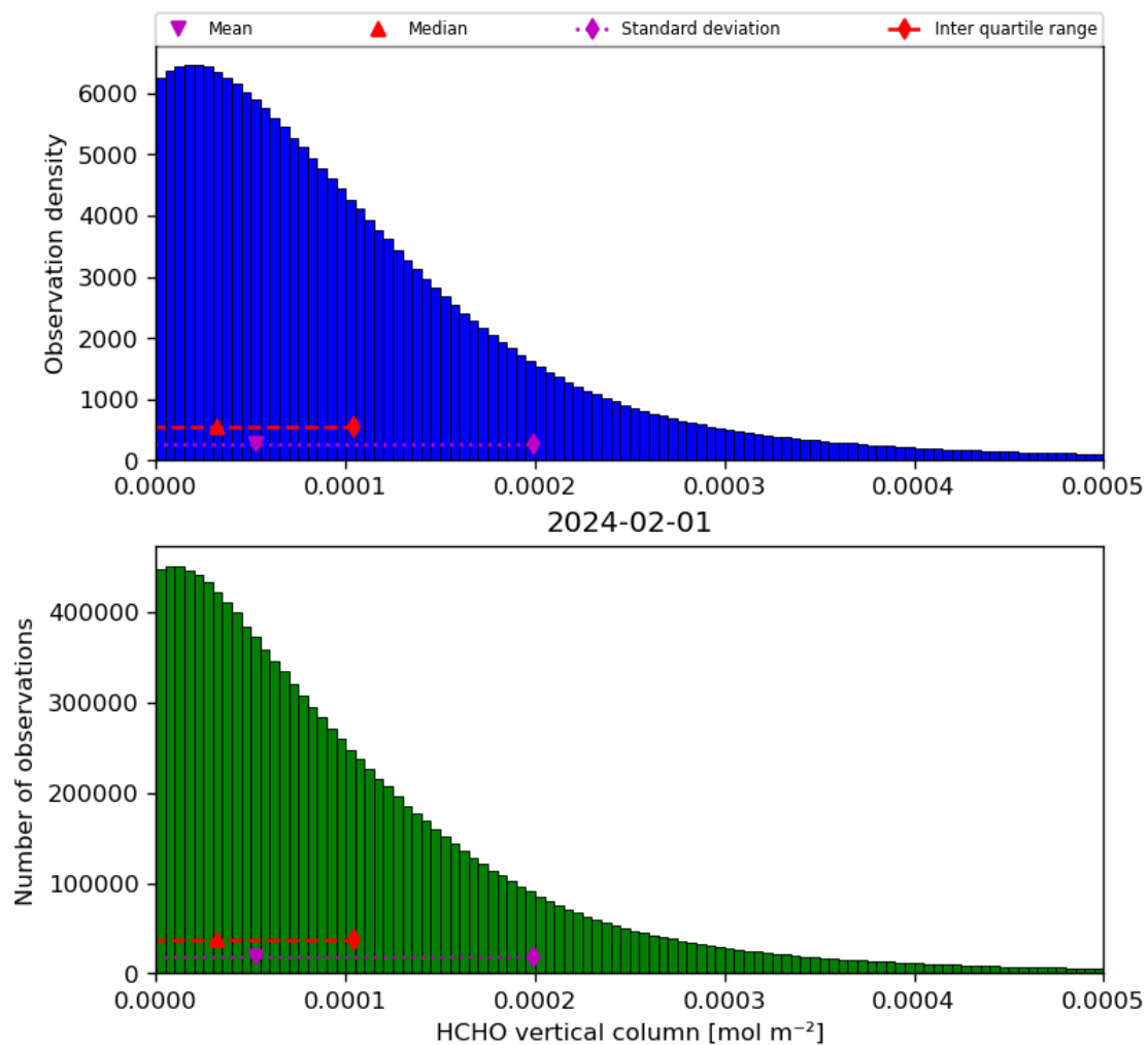
Figure 35: Histogram of “HCHO vertical column” for 2024-01-31 to 2024-02-02
