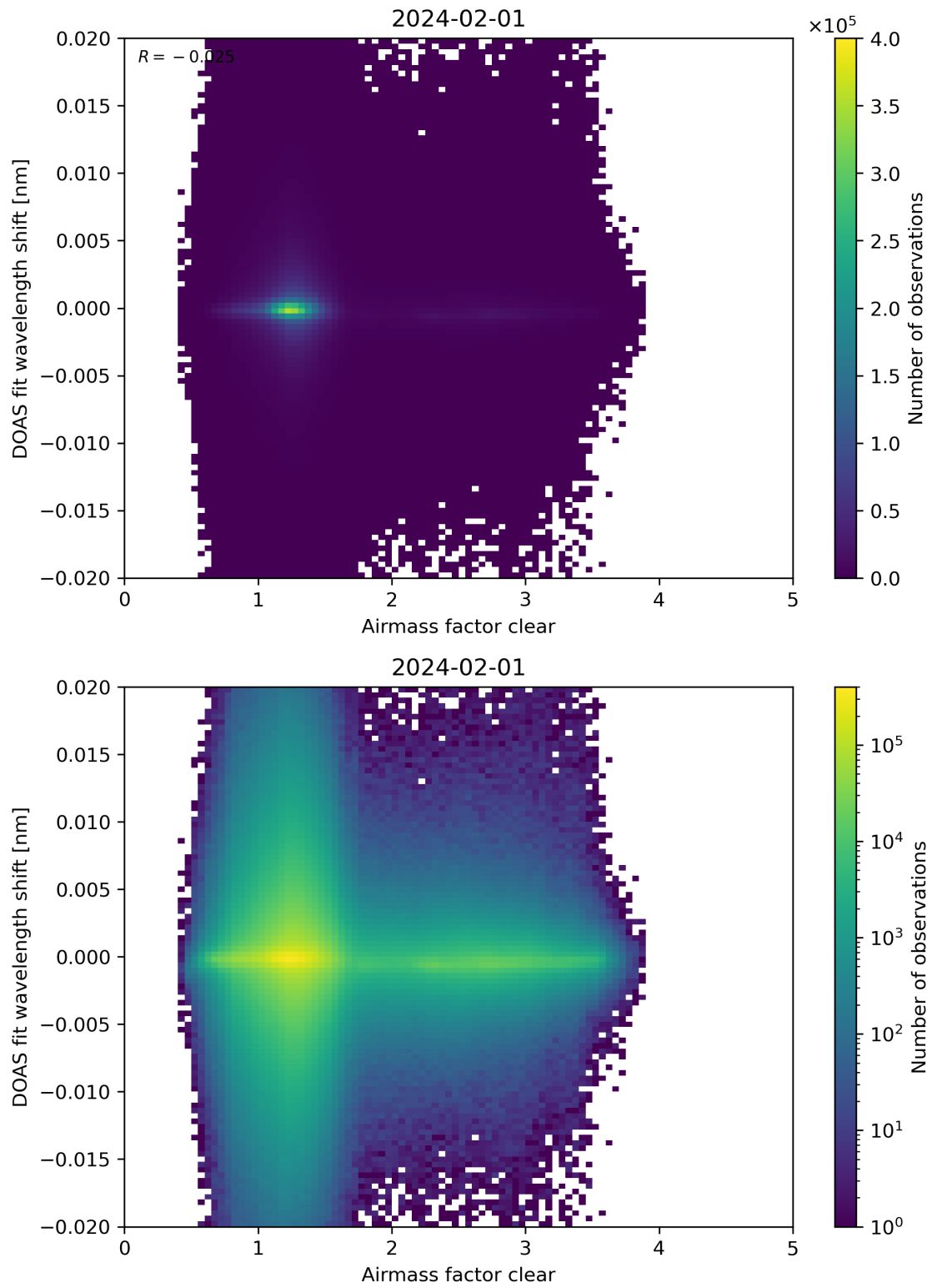
Figure 72: Scatter density plot of “Airmass factor clear” against “DOAS fit wavelength shift” for 2024-01-31 to 2024-02-02.
