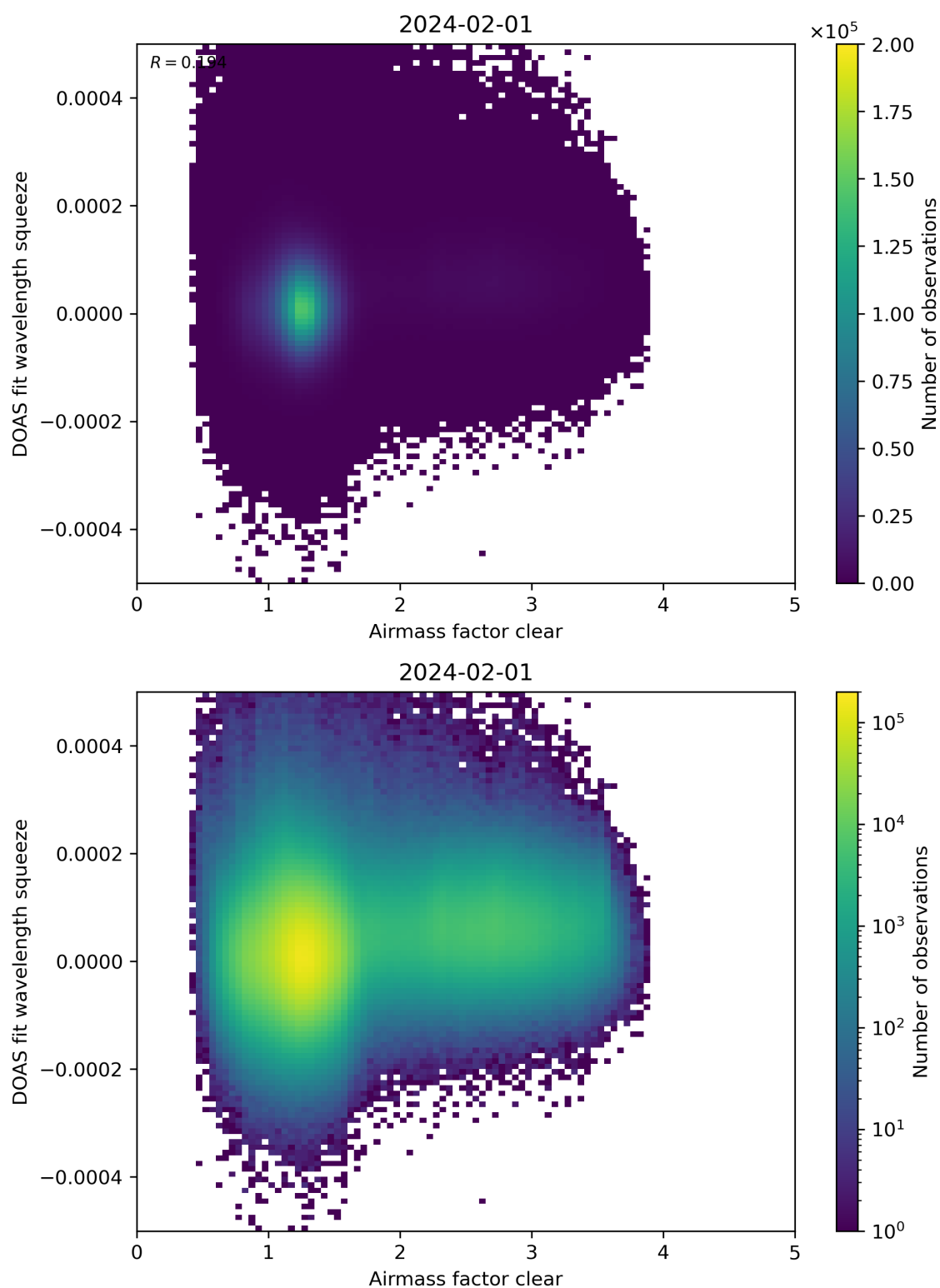
Figure 73: Scatter density plot of “Airmass factor clear” against “DOAS fit wavelength squeeze” for 2024-01-31 to 2024-02-02.
