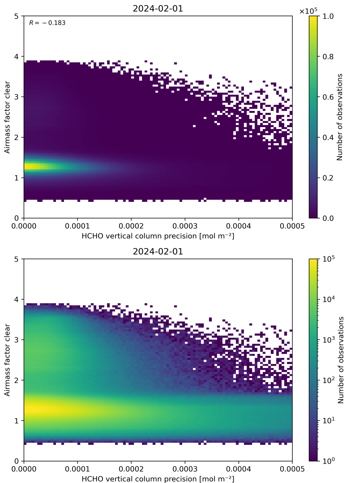
Figure 139: Scatter density plot of “HCHO vertical column precision” against “Airmass factor clear” for 2024-01-31 to 2024-02-02.
