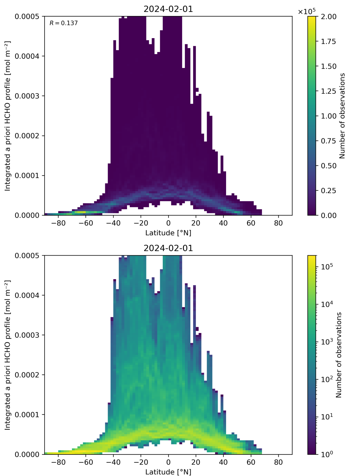
Figure 166: Scatter density plot of “Latitude” against “Integrated a priori HCHO profile” for 2024-01-31 to 2024-02-02.
