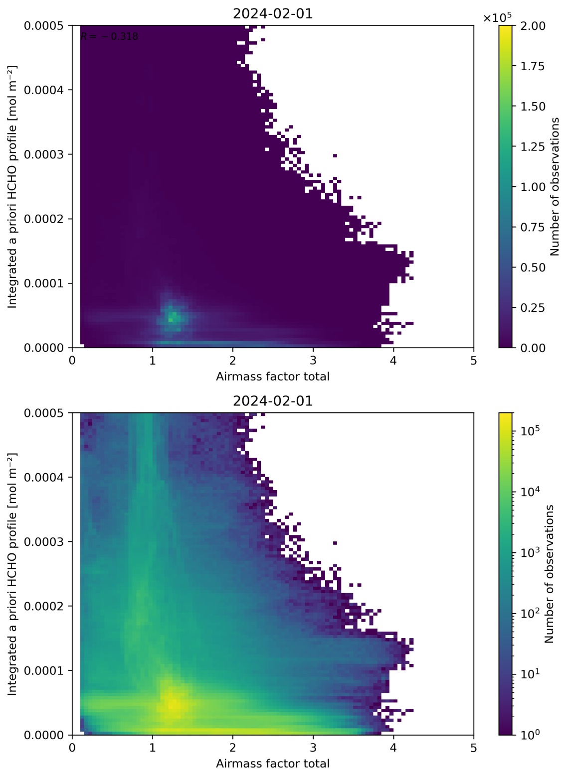
Figure 104: Scatter density plot of “Airmass factor total” against “Integrated a priori HCHO profile” for 2024-01-31 to 2024-02-02.
