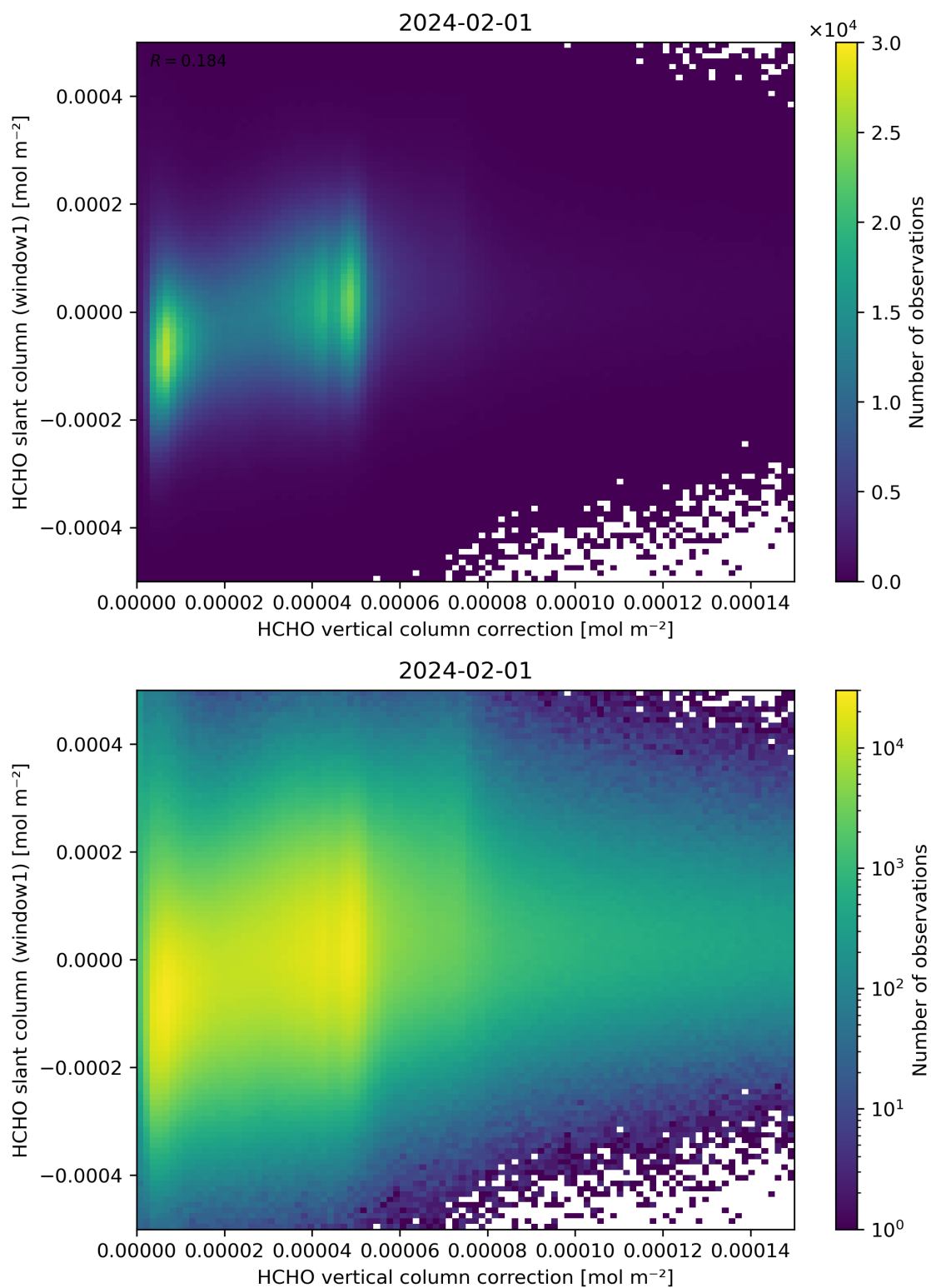
Figure 118: Scatter density plot of “HCHO vertical column correction” against “HCHO slant column (window1)” for 2024-01-31 to 2024-02-02.
