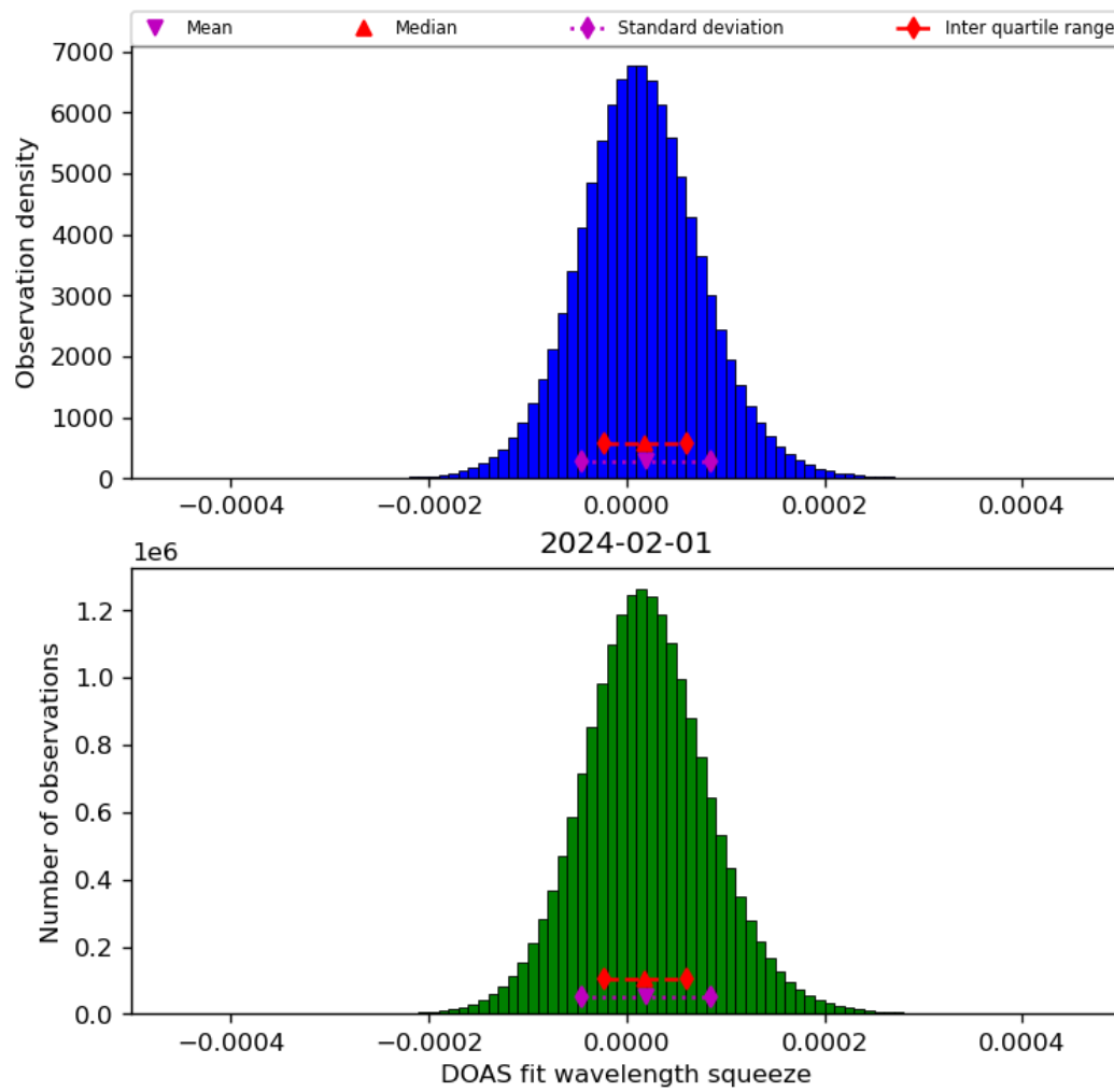
Figure 45: Histogram of “DOAS fit wavelength squeeze” for 2024-01-31 to 2024-02-02
