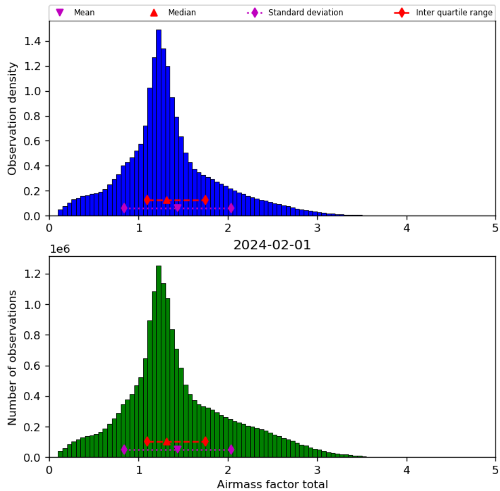
Figure 40: Histogram of “Airmass factor total” for 2024-01-31 to 2024-02-02
