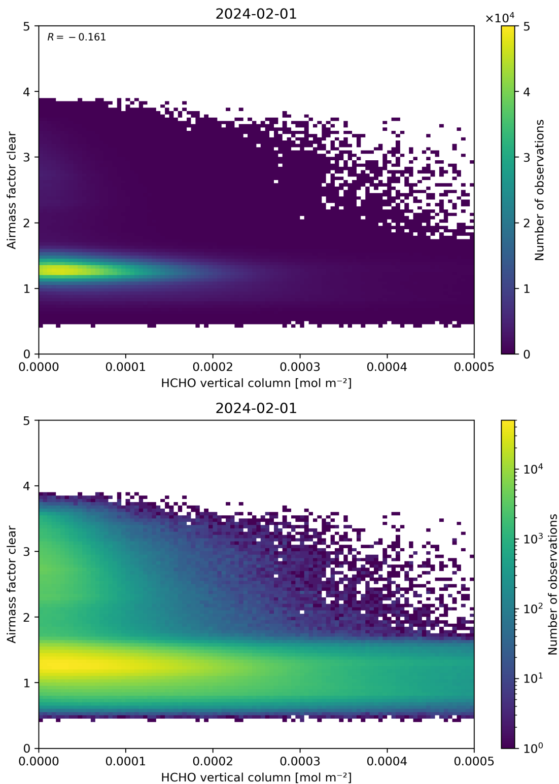
Figure 126: Scatter density plot of “HCHO vertical column” against “Airmass factor clear” for 2024-01-31 to 2024-02-02.
