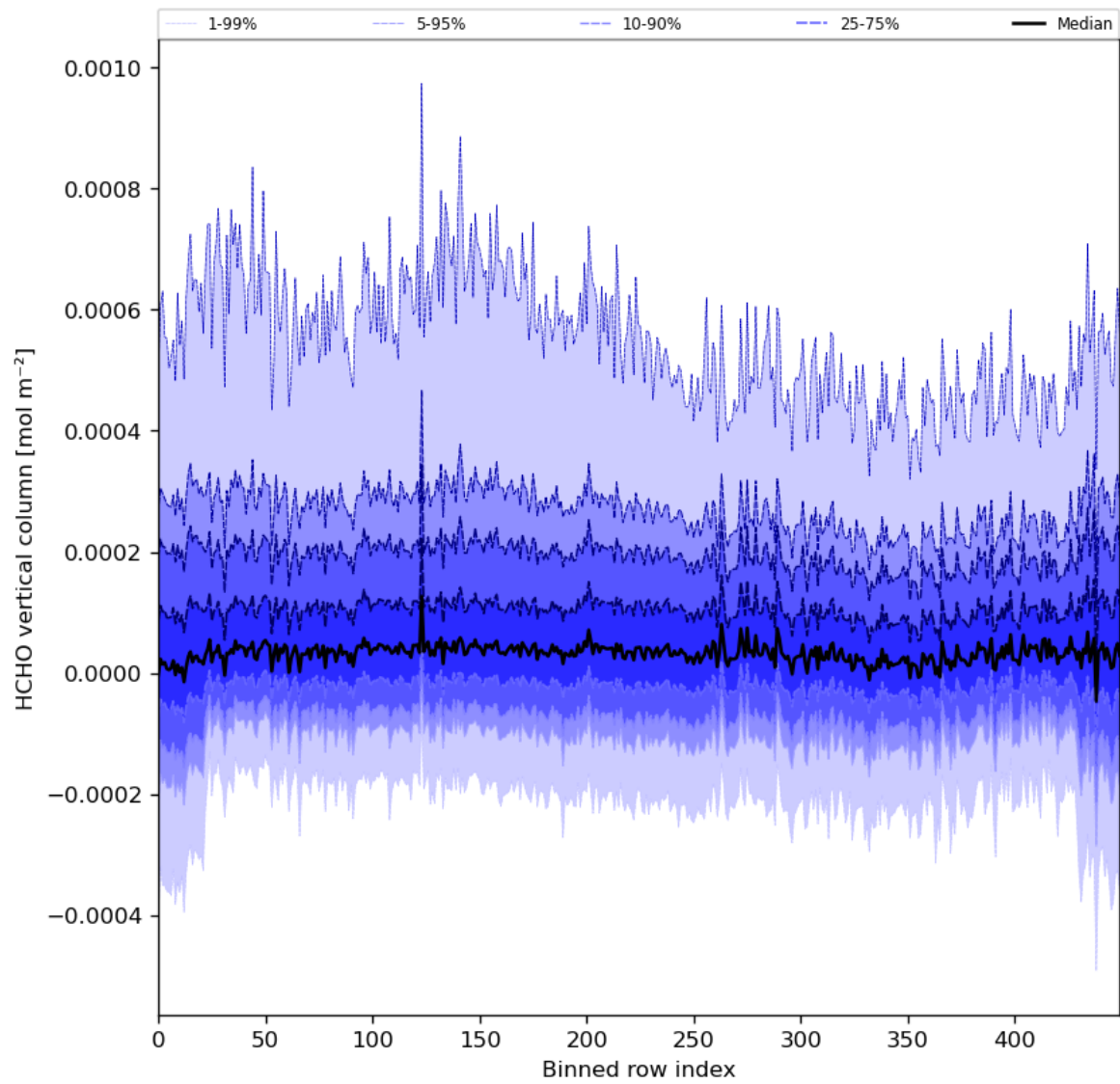
Figure 49: Along track statistics of “HCHO vertical column” for 2024-01-31 to 2024-02-02
