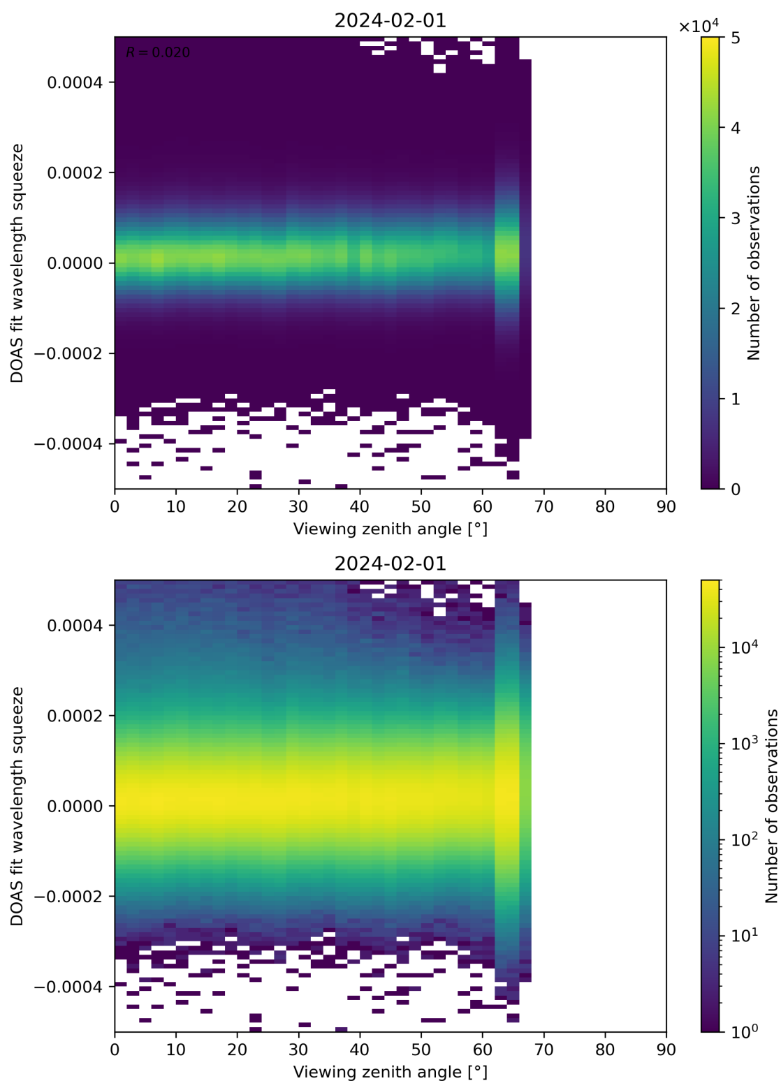
Figure 184: Scatter density plot of “Viewing zenith angle” against “DOAS fit wavelength squeeze” for 2024-01-31 to 2024-02-02.
