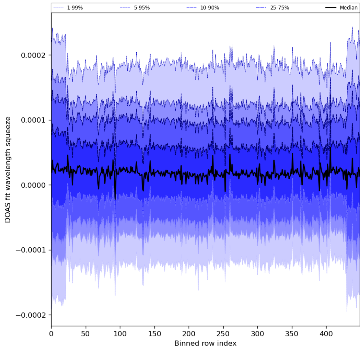
Figure 59: Along track statistics of “DOAS fit wavelength squeeze” for 2024-01-31 to 2024-02-02
