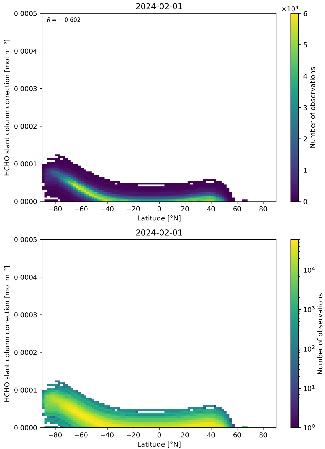
Figure 158: Scatter density plot of “Latitude” against “HCHO slant column correction” for 2024-01-31 to 2024-02-02.
