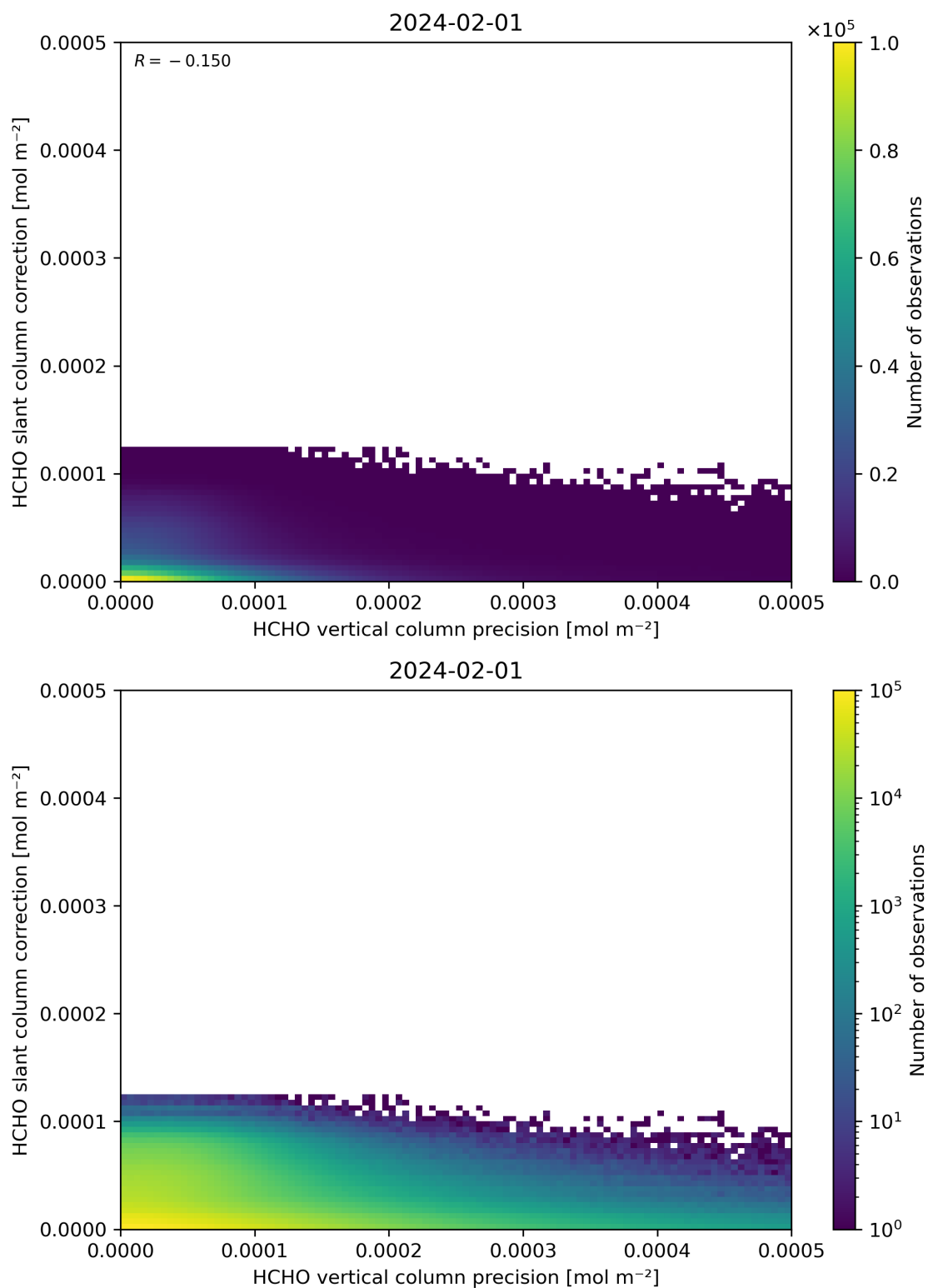
Figure 141: Scatter density plot of “HCHO vertical column precision” against “HCHO slant column correction” for 2024-01-31 to 2024-02-02.
