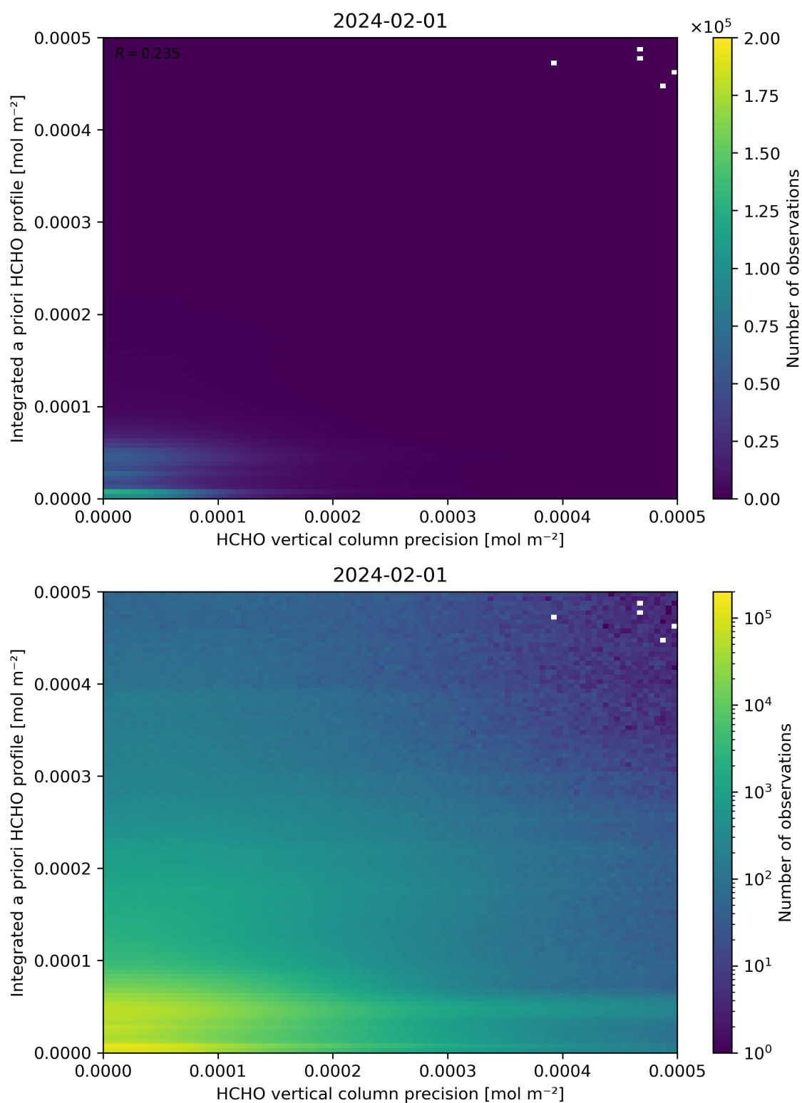
Figure 147: Scatter density plot of “HCHO vertical column precision” against “Integrated a priori HCHO profile” for 2024-01-31 to 2024-02-02.
