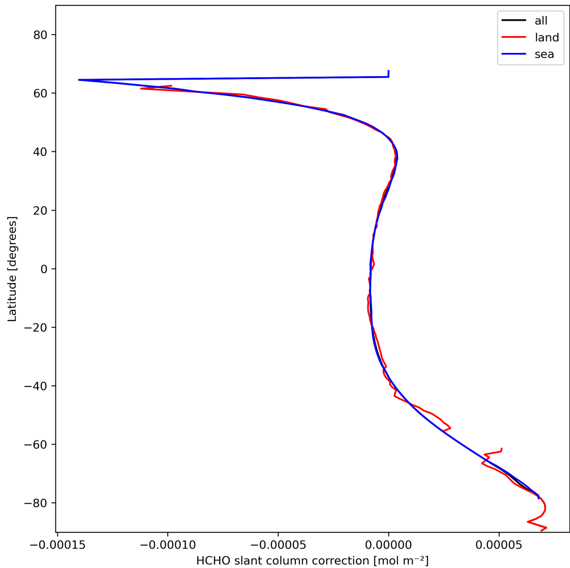
Figure 33: Zonal average of “HCHO slant column correction” for 2024-01-31 to 2024-02-02.
