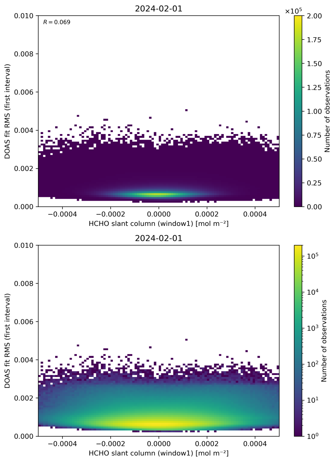
Figure 78: Scatter density plot of “HCHO slant column (window1)” against “DOAS fit RMS (first interval)” for 2024-01-31 to 2024-02-02.
