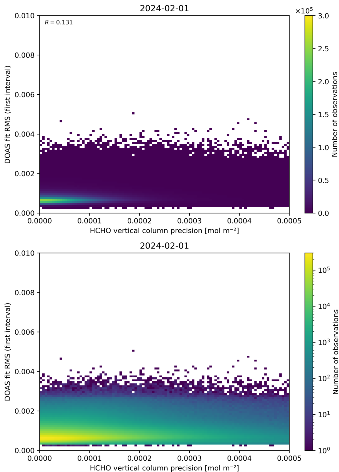
Figure 136: Scatter density plot of “HCHO vertical column precision” against “DOAS fit RMS (first interval)” for 2024-01-31 to 2024-02-02.
