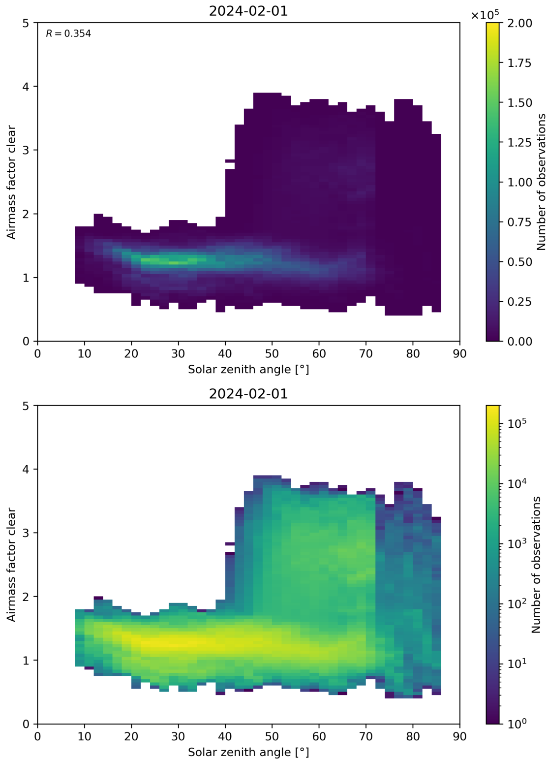
Figure 170: Scatter density plot of “Solar zenith angle” against “Airmass factor clear” for 2024-01-31 to 2024-02-02.
