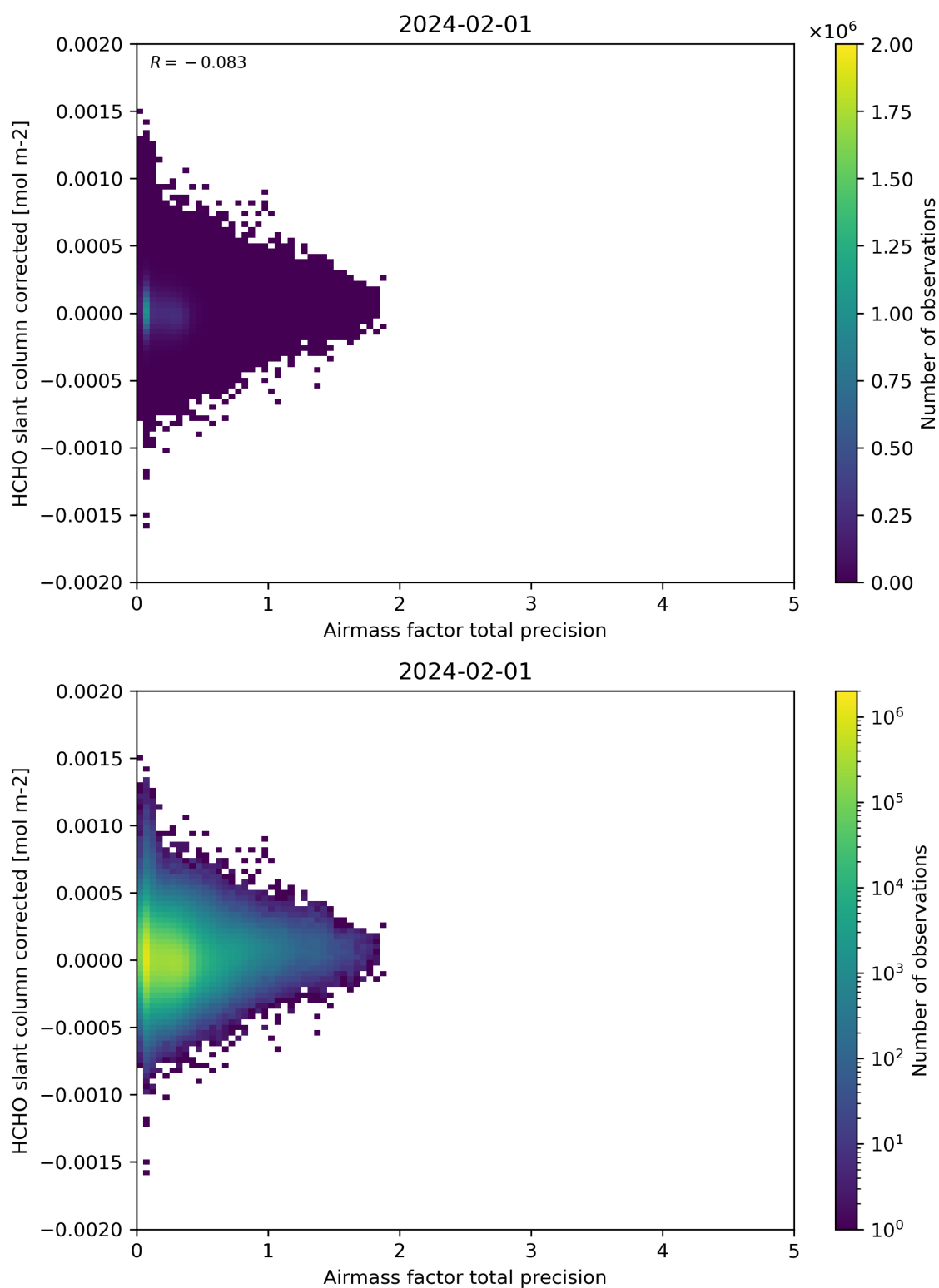
Figure 109: Scatter density plot of “Airmass factor total precision” against “HCHO slant column corrected” for 2024-01-31 to 2024-02-02.
