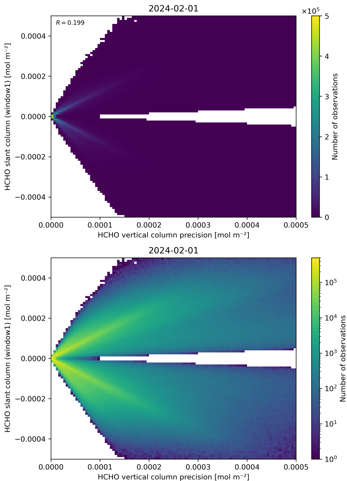
Figure 142: Scatter density plot of “HCHO vertical column precision” against “HCHO slant column (window1)” for 2024-01-31 to 2024-02-02.
