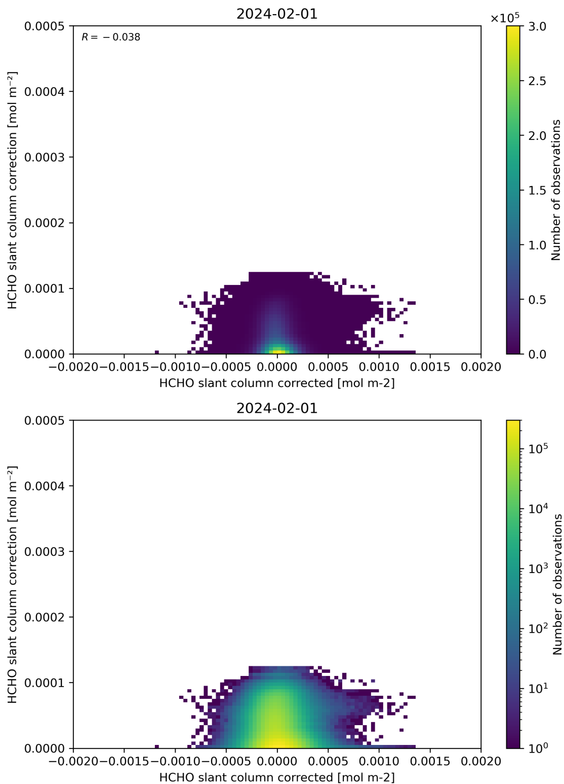
Figure 77: Scatter density plot of “HCHO slant column corrected” against “HCHO slant column correction” for 2024-01-31 to 2024-02-02.
