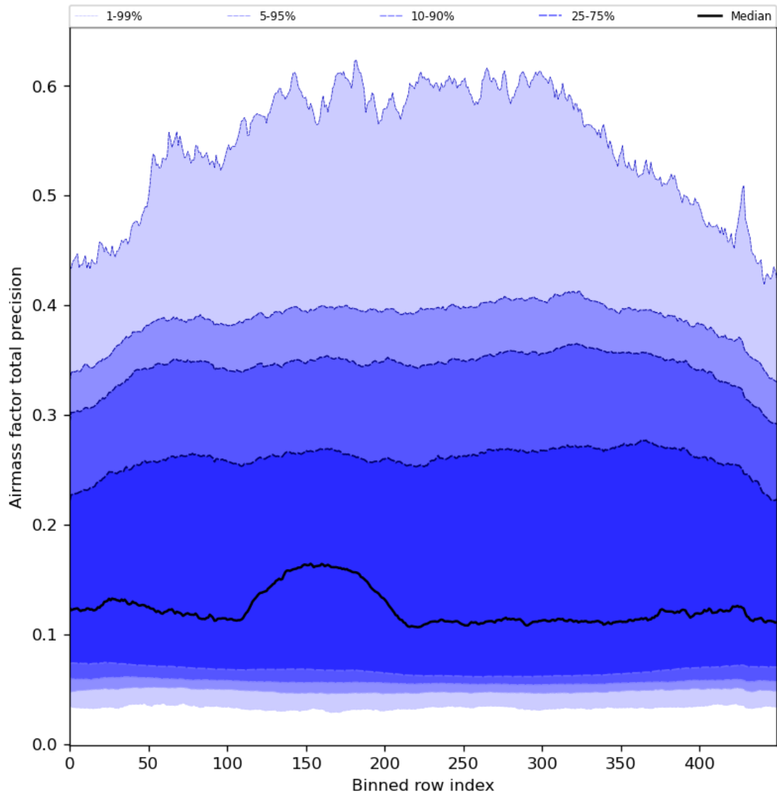
Figure 55: Along track statistics of “Airmass factor total precision” for 2024-01-31 to 2024-02-02
