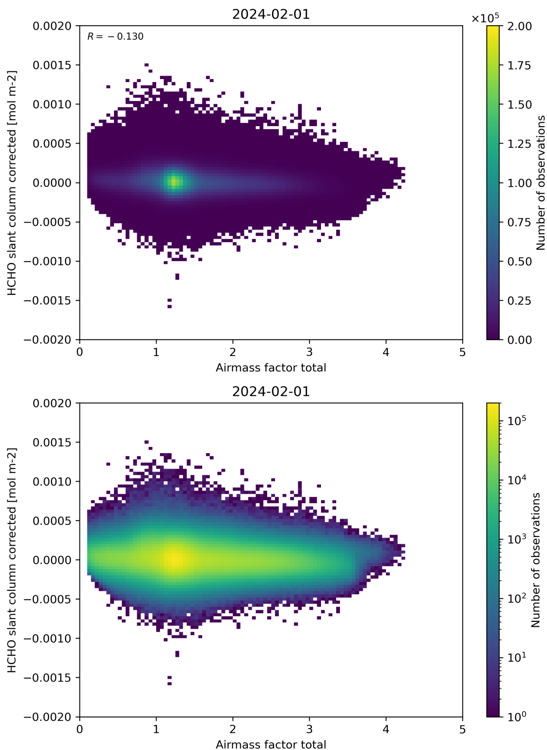
Figure 101: Scatter density plot of “Airmass factor total” against “HCHO slant column corrected” for 2024-01-31 to 2024-02-02.
