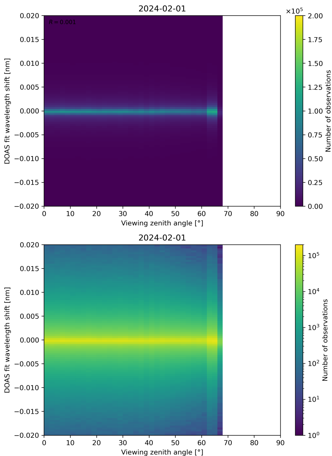
Figure 183: Scatter density plot of “Viewing zenith angle” against “DOAS fit wavelength shift” for 2024-01-31 to 2024-02-02.
