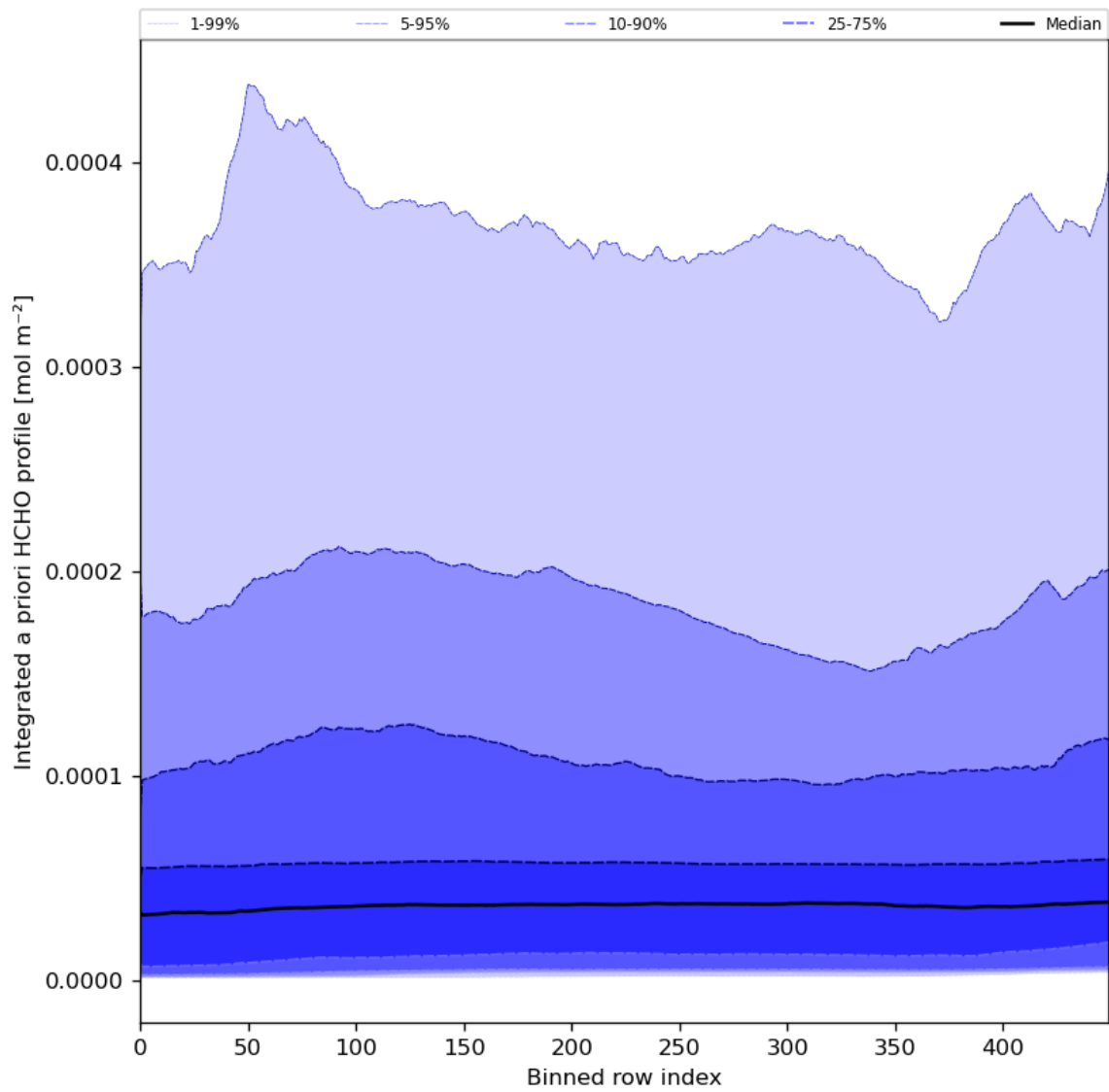
Figure 57: Along track statistics of “Integrated a priori HCHO profile” for 2024-01-31 to 2024-02-02
