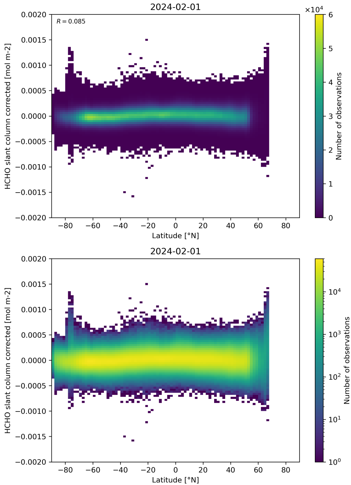
Figure 157: Scatter density plot of “Latitude” against “HCHO slant column corrected” for 2024-01-31 to 2024-02-02.
