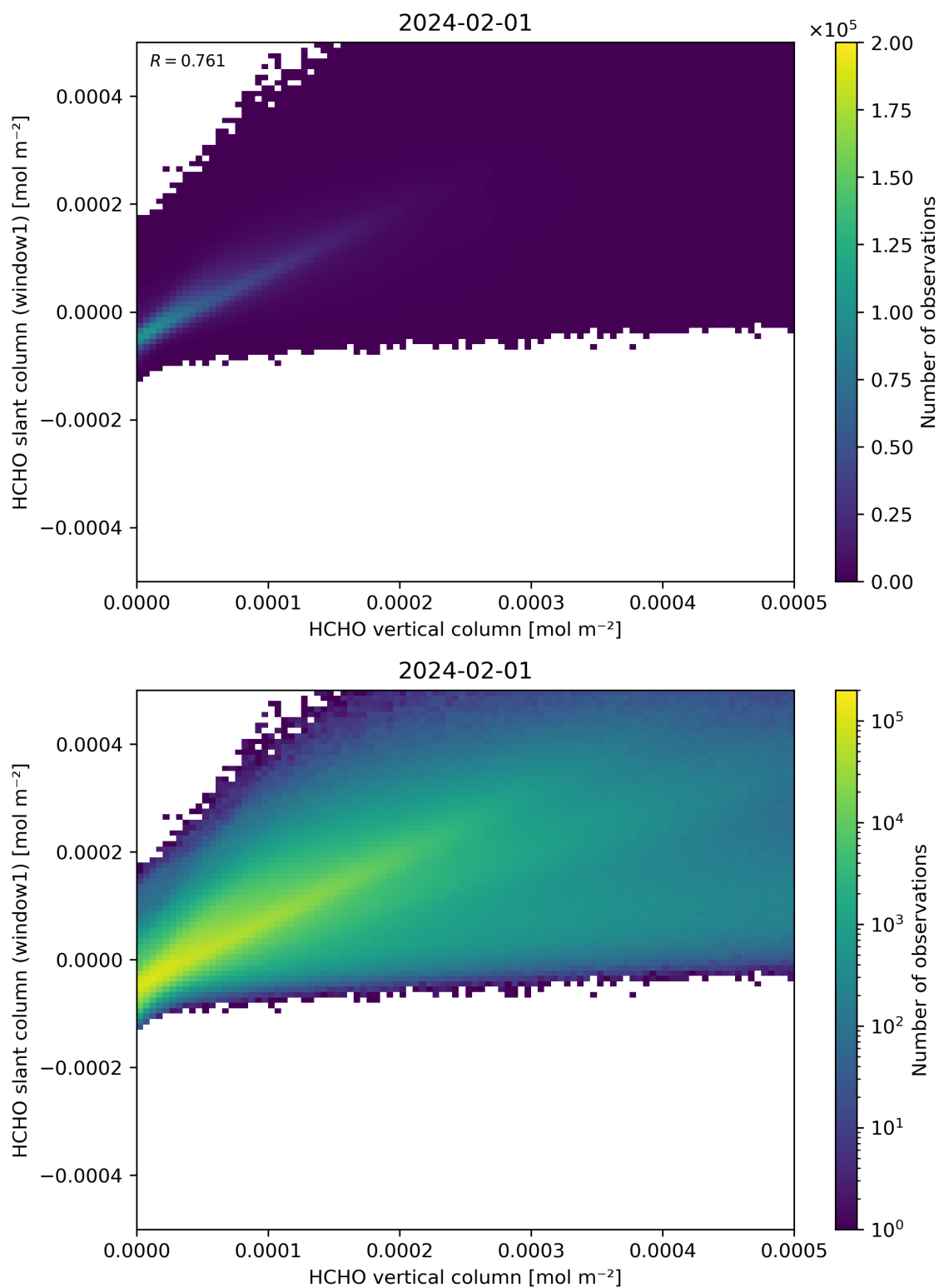
Figure 129: Scatter density plot of “HCHO vertical column” against “HCHO slant column (window1)” for 2024-01-31 to 2024-02-02.
