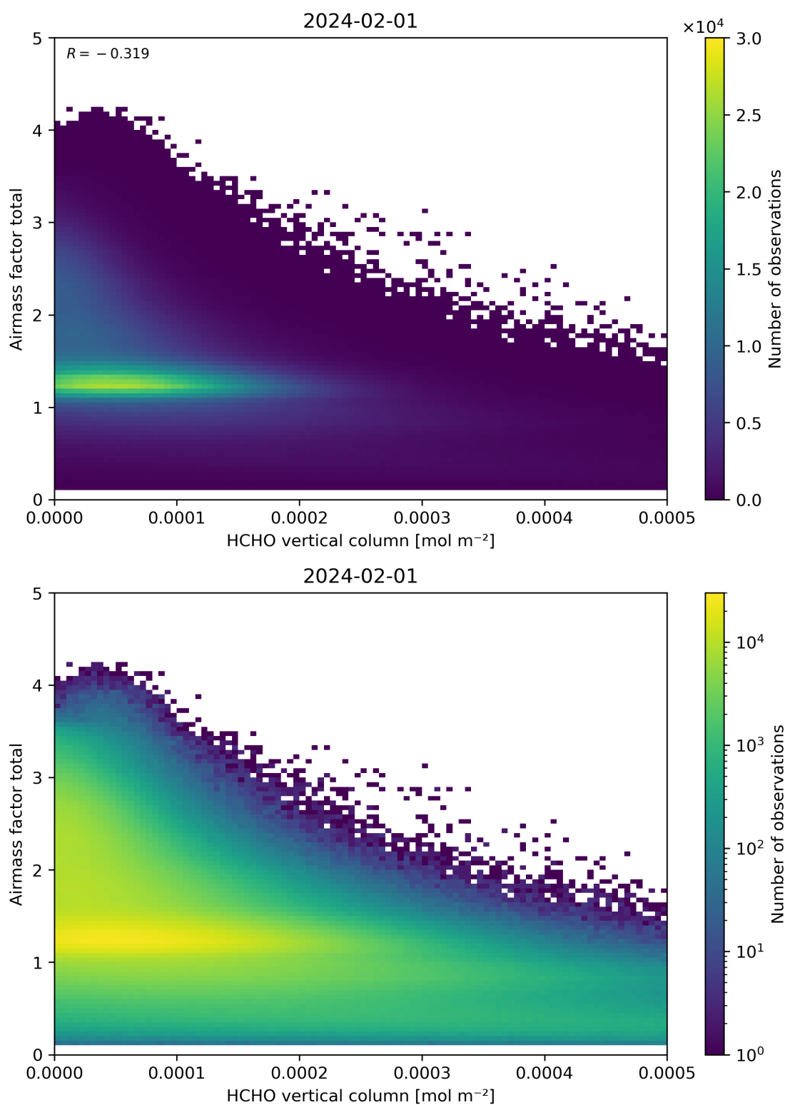
Figure 131: Scatter density plot of “HCHO vertical column” against “Airmass factor total” for 2024-01-31 to 2024-02-02.
