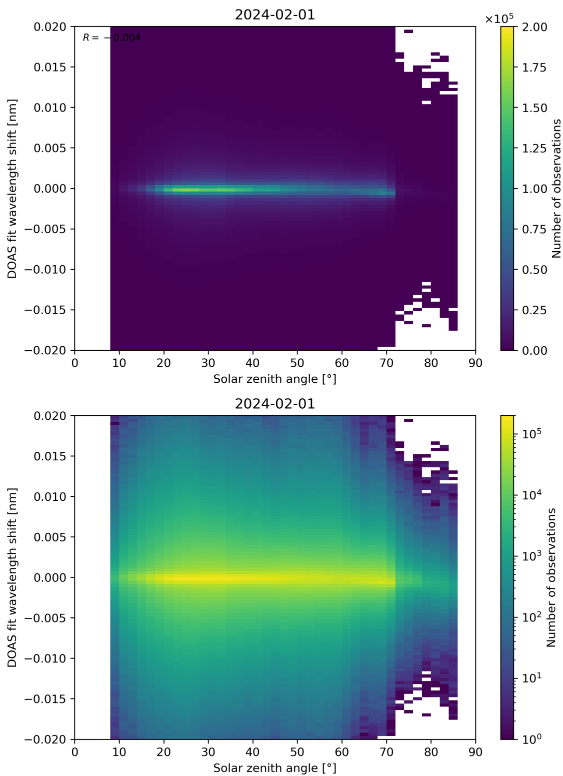
Figure 168: Scatter density plot of “Solar zenith angle” against “DOAS fit wavelength shift” for 2024-01-31 to 2024-02-02.
