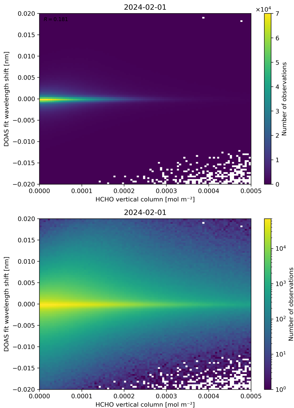
Figure 124: Scatter density plot of “HCHO vertical column” against “DOAS fit wavelength shift” for 2024-01-31 to 2024-02-02.
