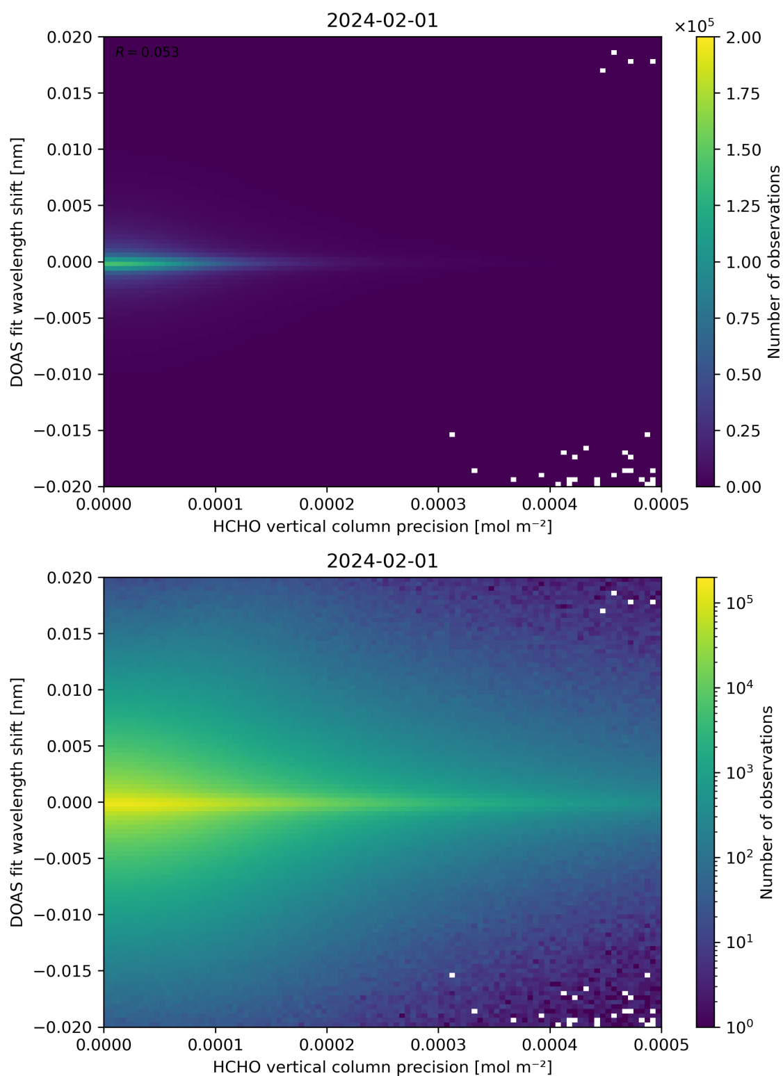
Figure 137: Scatter density plot of “HCHO vertical column precision” against “DOAS fit wavelength shift” for 2024-01-31 to 2024-02-02.
