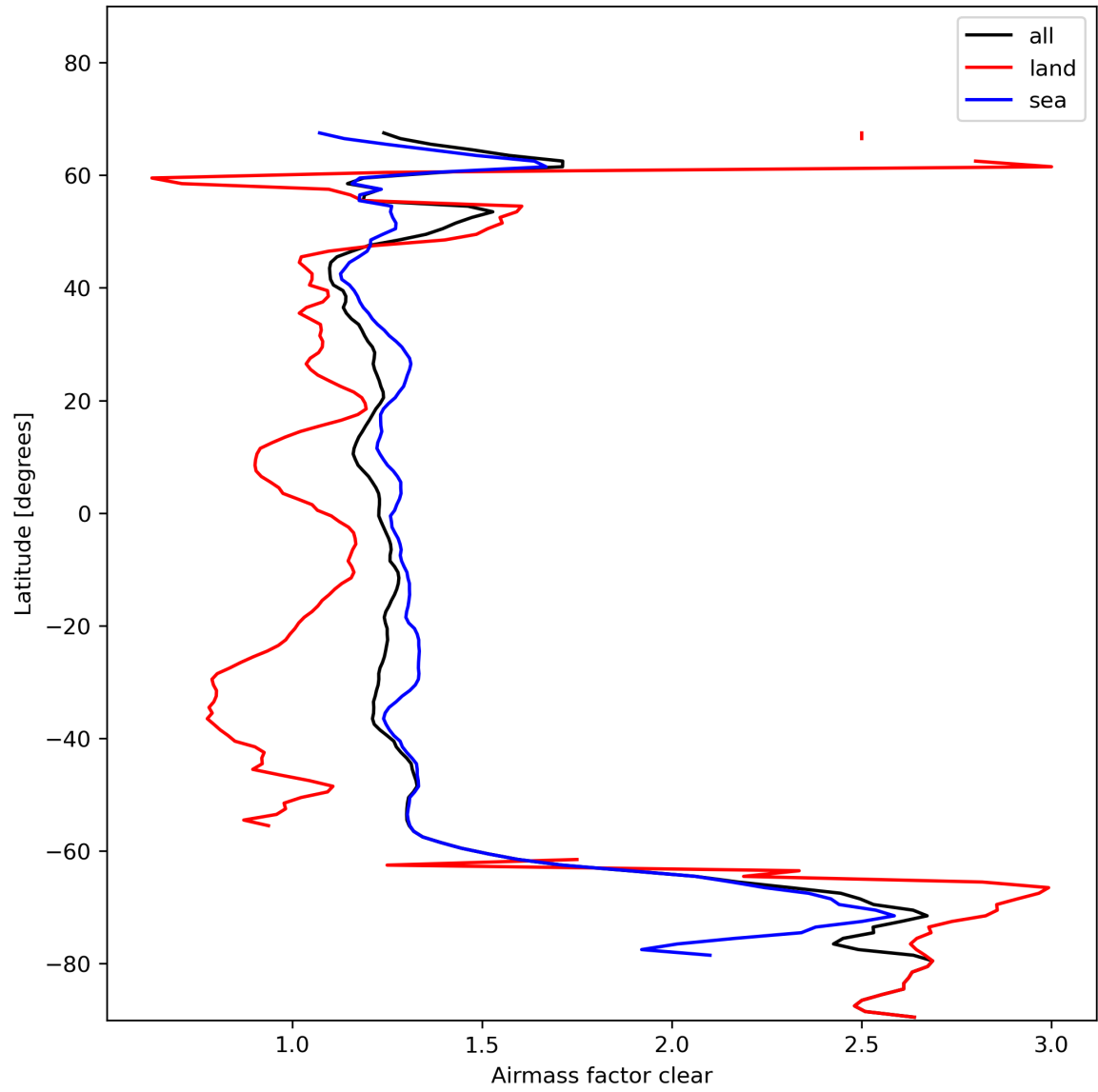
Figure 28: Zonal average of “Airmass factor clear” for 2024-01-31 to 2024-02-02.
