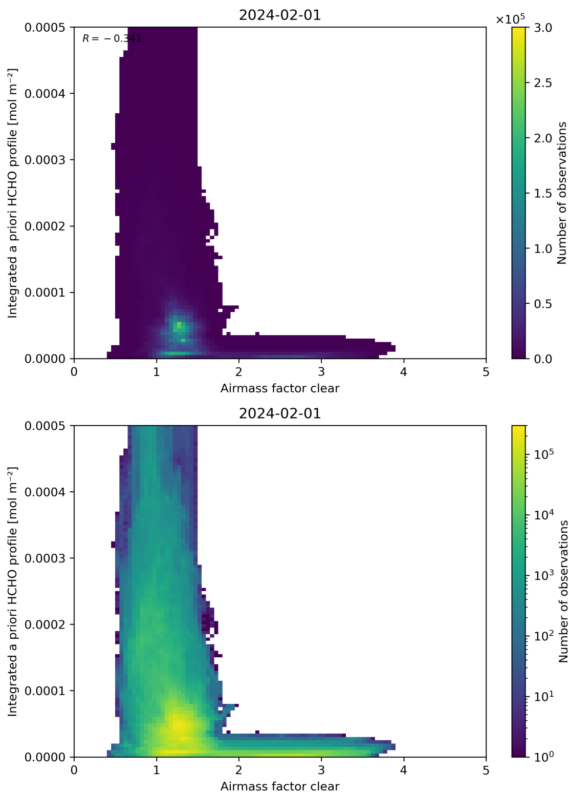
Figure 76: Scatter density plot of “Airmass factor clear” against “Integrated a priori HCHO profile” for 2024-01-31 to 2024-02-02.
