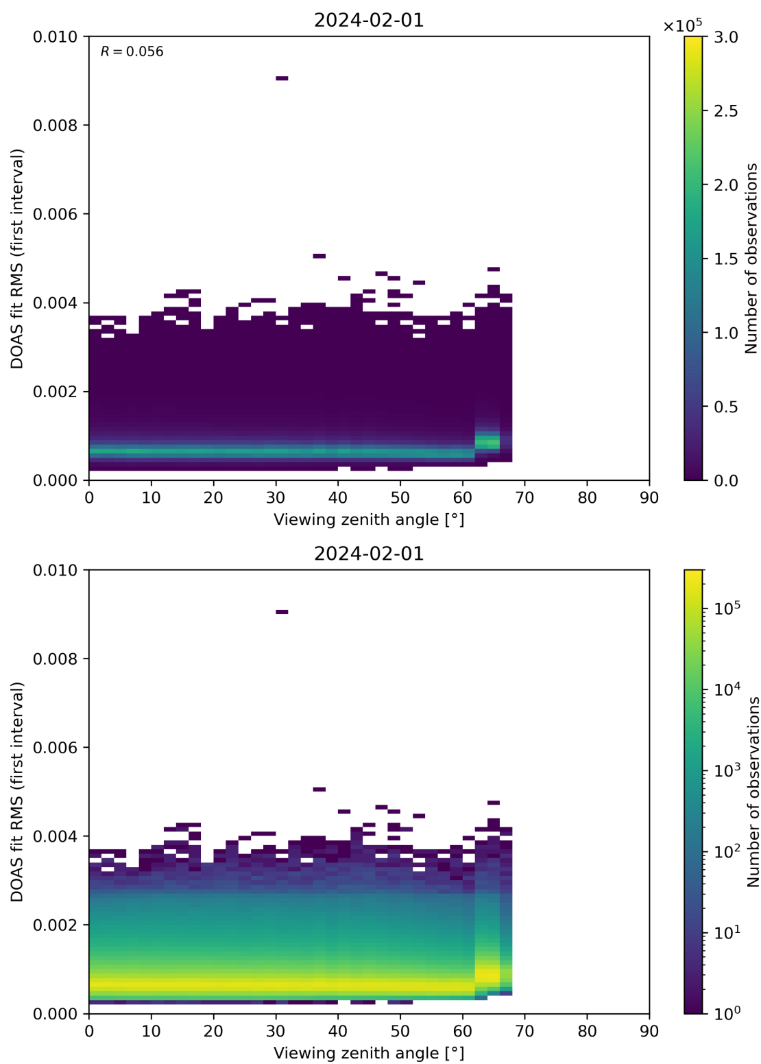
Figure 182: Scatter density plot of “Viewing zenith angle” against “DOAS fit RMS (first interval)” for 2024-01-31 to 2024-02-02.
