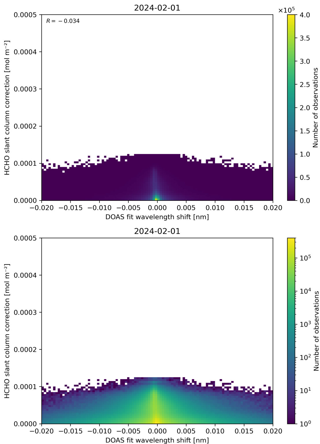
Figure 67: Scatter density plot of “DOAS fit wavelength shift” against “HCHO slant column correction” for 2024-01-31 to 2024-02-02.
