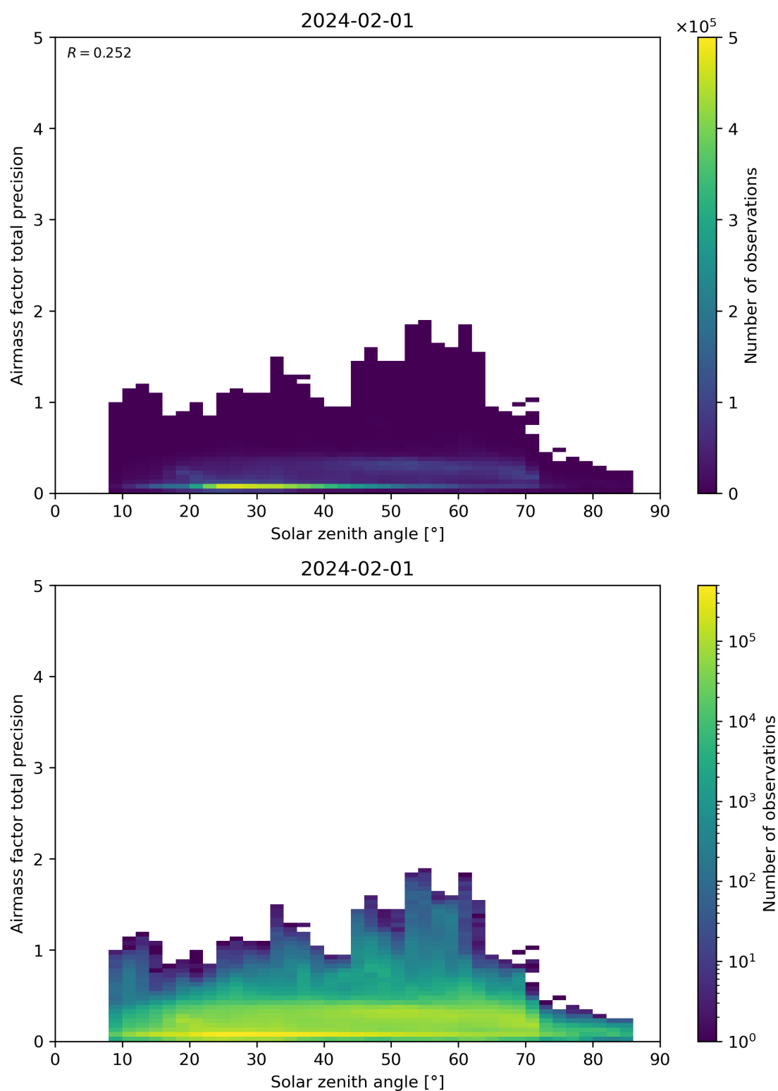
Figure 176: Scatter density plot of “Solar zenith angle” against “Airmass factor total precision” for 2024-01-31 to 2024-02-02.
