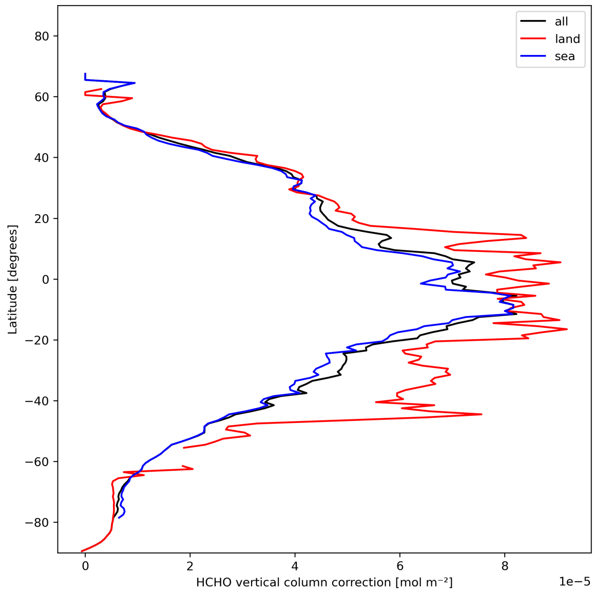
Figure 23: Zonal average of “HCHO vertical column correction” for 2024-01-31 to 2024-02-02.
