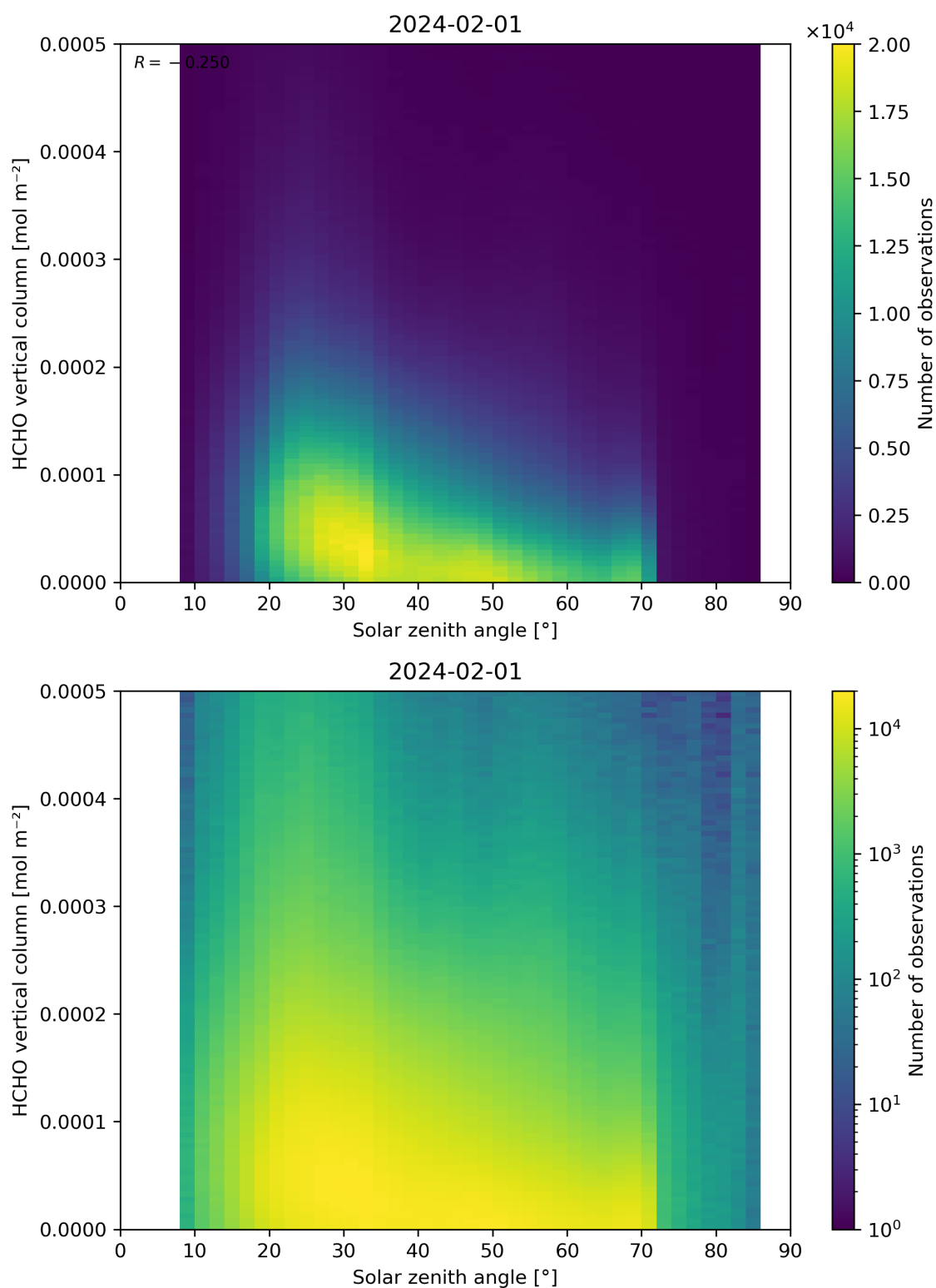
Figure 177: Scatter density plot of “Solar zenith angle” against “HCHO vertical column” for 2024-01-31 to 2024-02-02.
