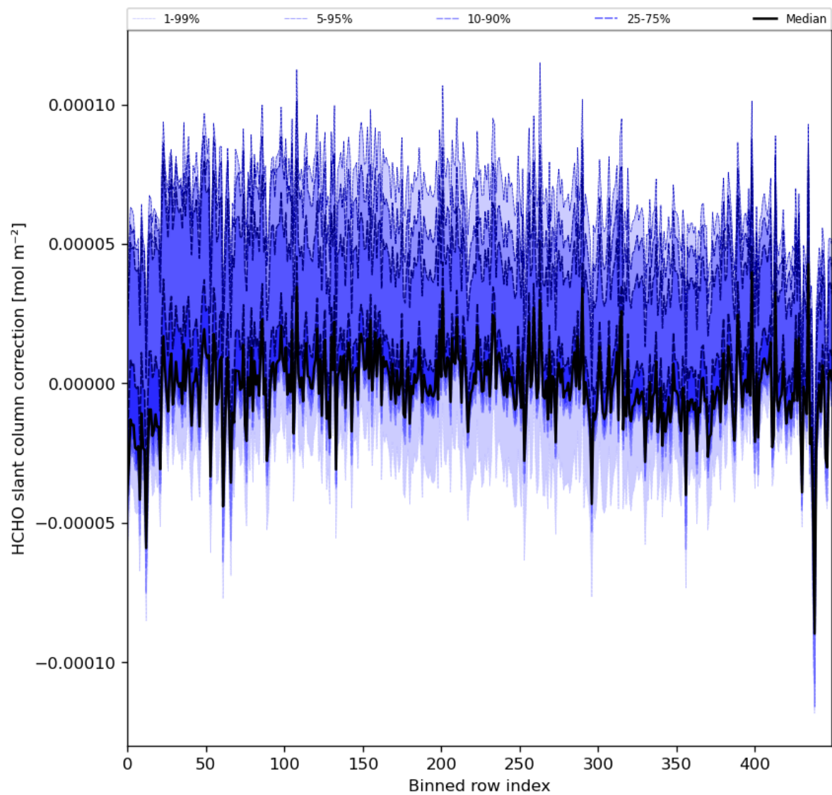
Figure 61: Along track statistics of “HCHO slant column correction” for 2024-01-31 to 2024-02-02
