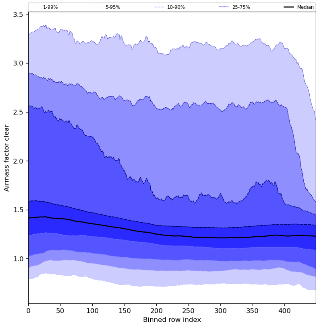
Figure 56: Along track statistics of “Airmass factor clear” for 2024-01-31 to 2024-02-02
