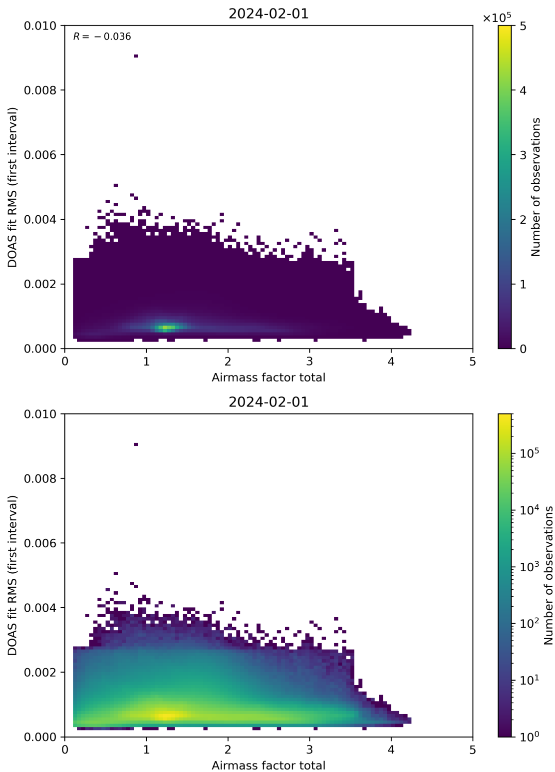
Figure 97: Scatter density plot of “Airmass factor total” against “DOAS fit RMS (first interval)” for 2024-01-31 to 2024-02-02.
