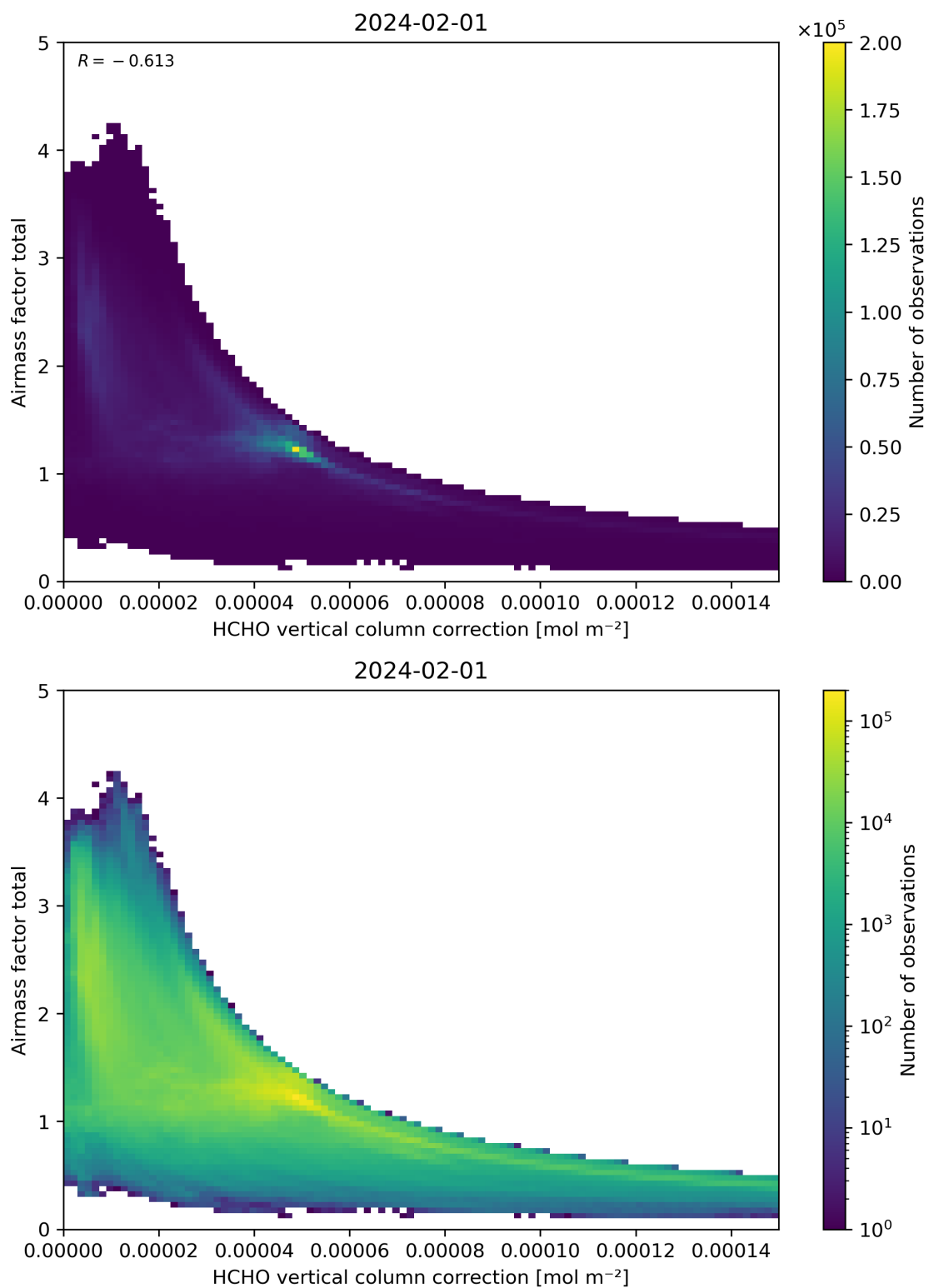
Figure 120: Scatter density plot of “HCHO vertical column correction” against “Airmass factor total” for 2024-01-31 to 2024-02-02.
