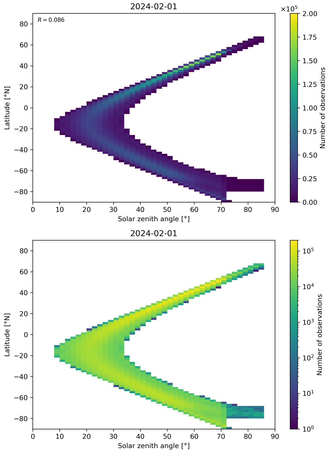
Figure 181: Scatter density plot of “Solar zenith angle” against “Latitude” for 2024-01-31 to 2024-02-02.
