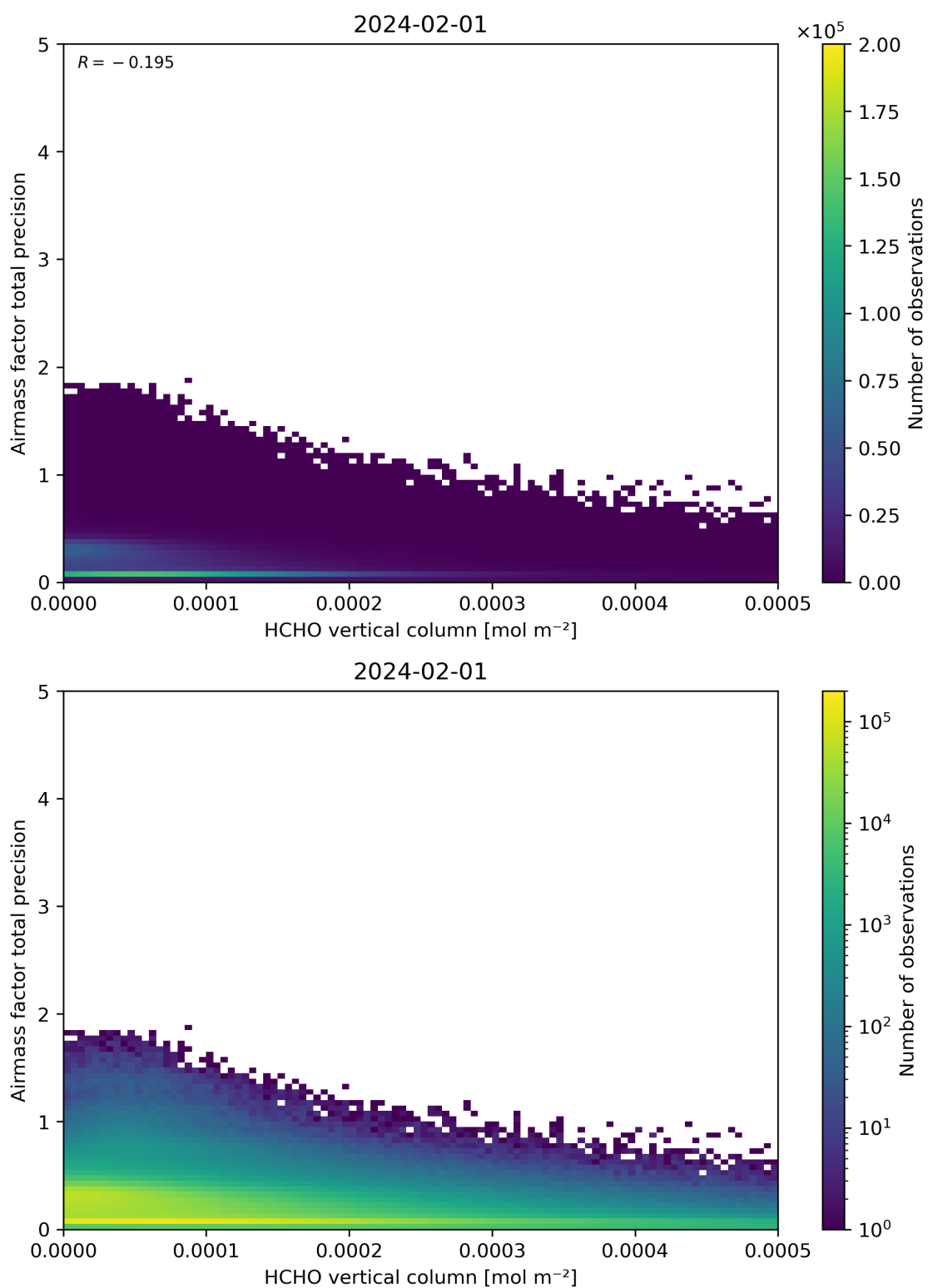
Figure 132: Scatter density plot of “HCHO vertical column” against “Airmass factor total precision” for 2024-01-31 to 2024-02-02.
