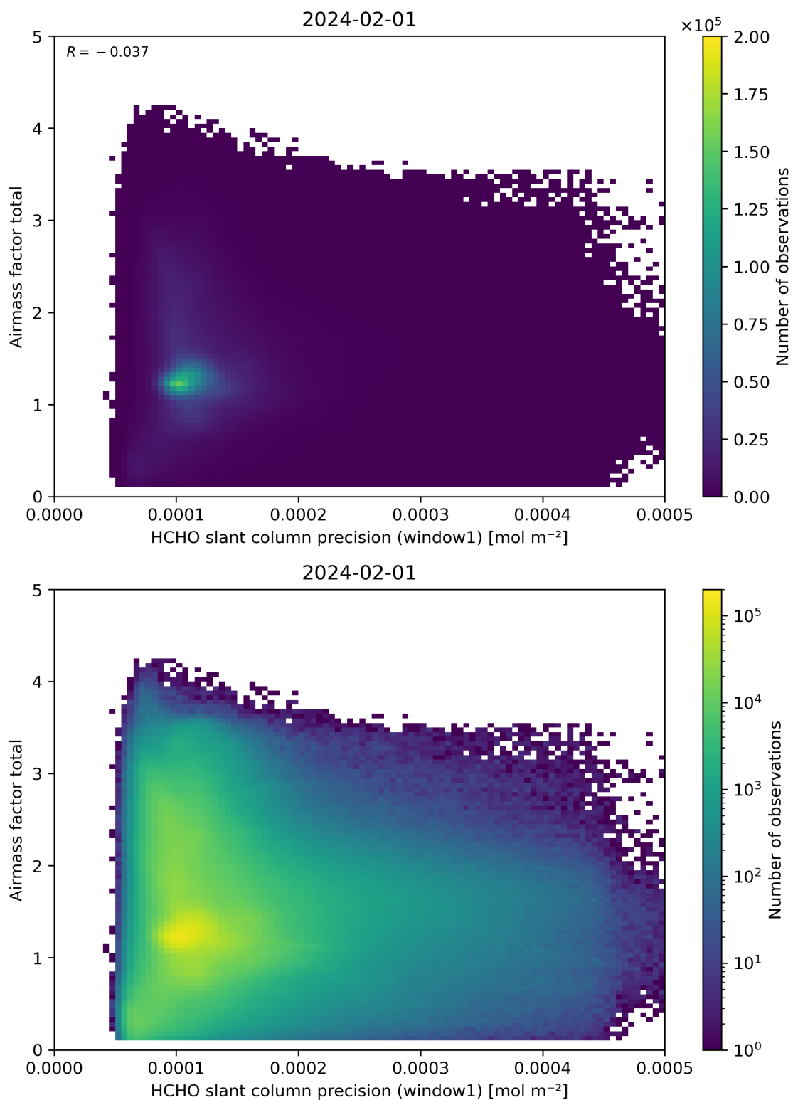
Figure 94: Scatter density plot of “HCHO slant column precision (window1)” against “Airmass factor total” for 2024-01-31 to 2024-02-02.
