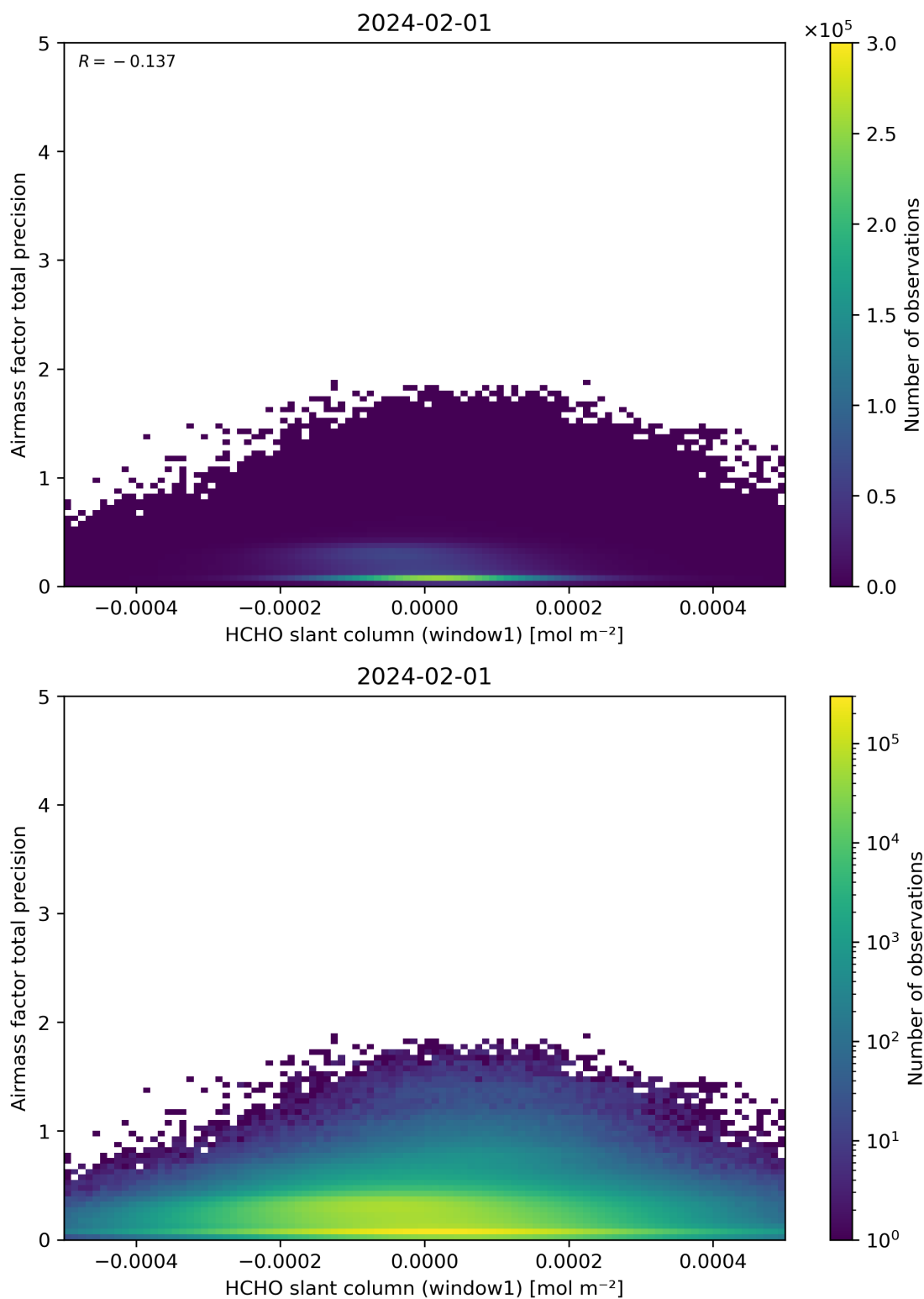
Figure 86: Scatter density plot of “HCHO slant column (window1)” against “Airmass factor total precision” for 2024-01-31 to 2024-02-02.
