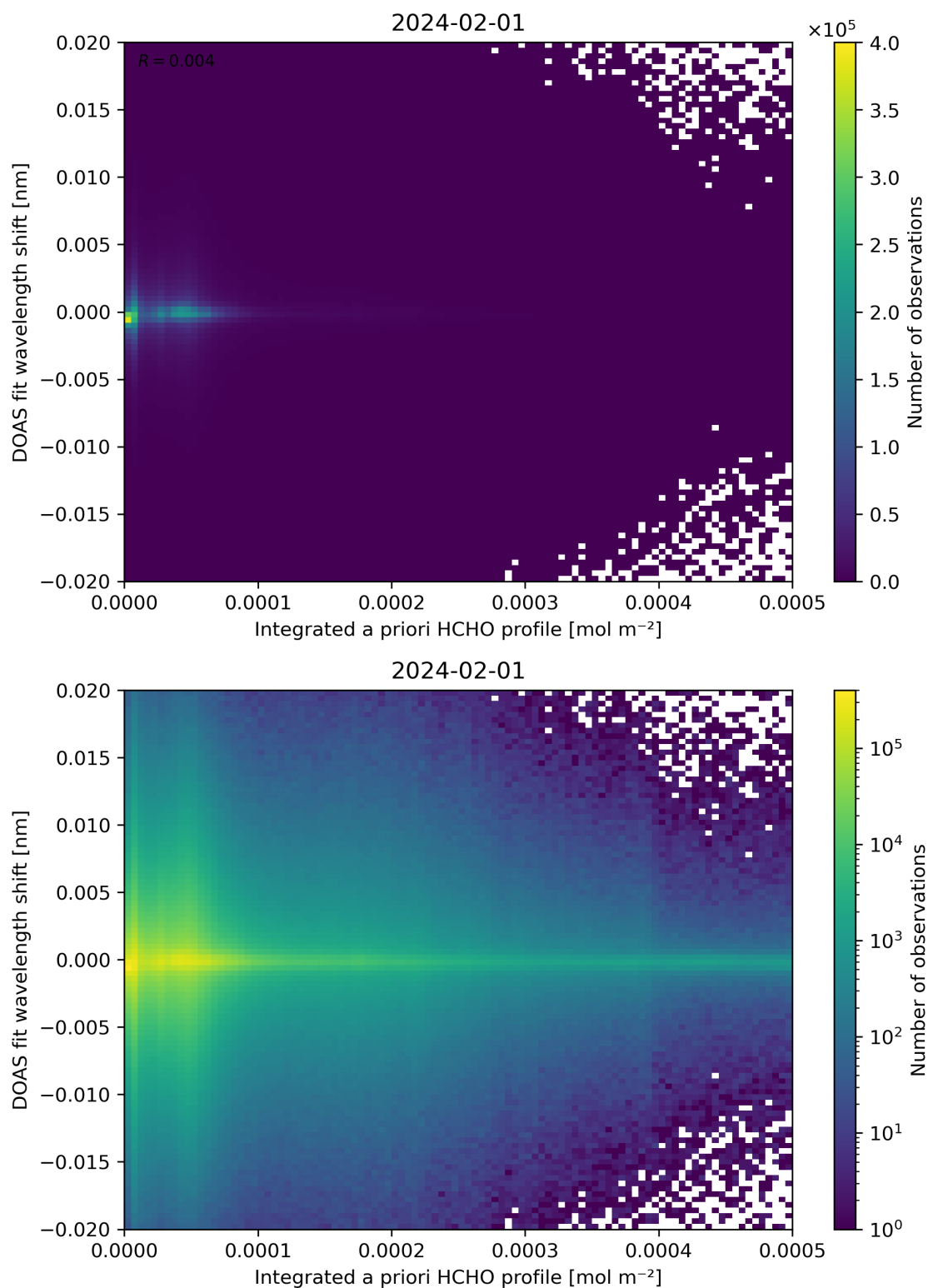
Figure 149: Scatter density plot of “Integrated a priori HCHO profile” against “DOAS fit wavelength shift” for 2024-01-31 to 2024-02-02.
