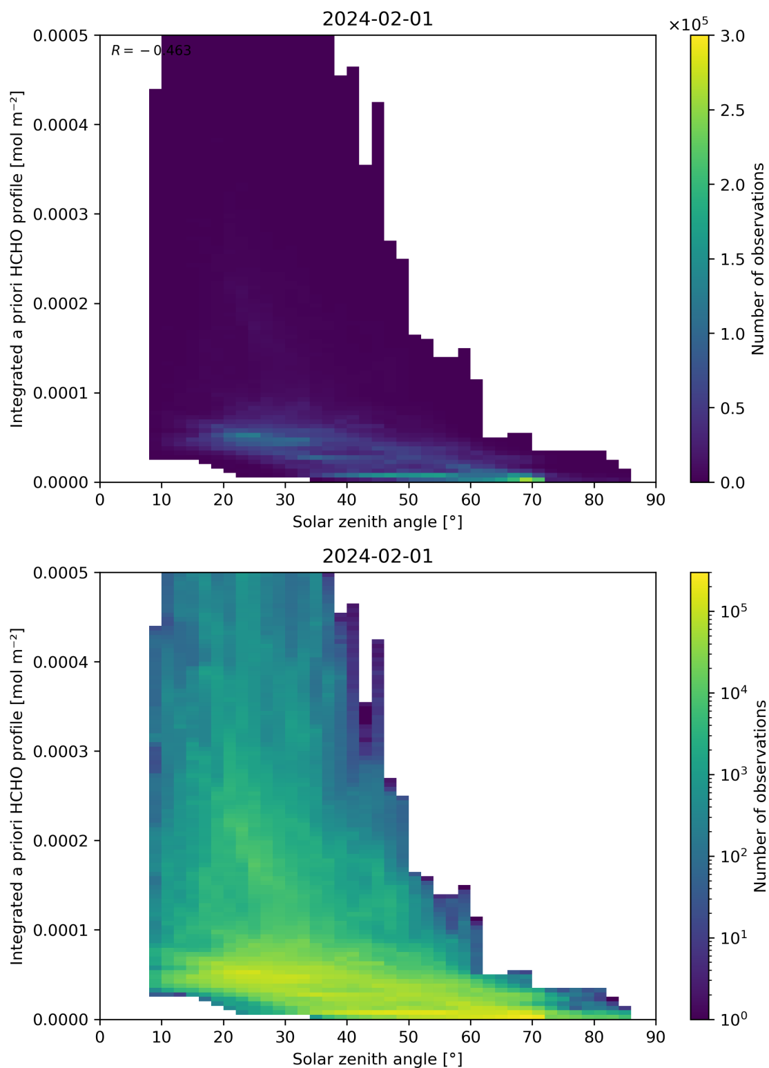
Figure 180: Scatter density plot of “Solar zenith angle” against “Integrated a priori HCHO profile” for 2024-01-31 to 2024-02-02.
