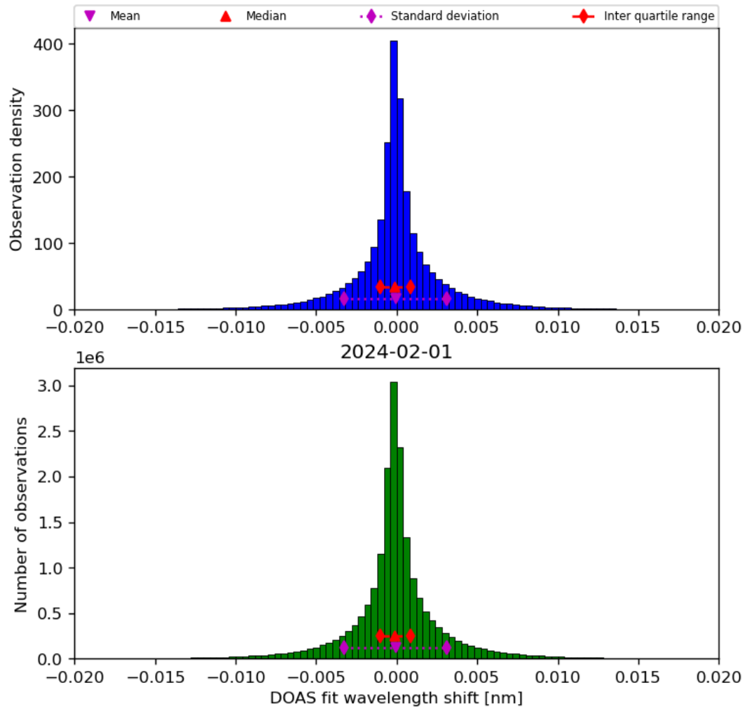
Figure 44: Histogram of “DOAS fit wavelength shift” for 2024-01-31 to 2024-02-02
