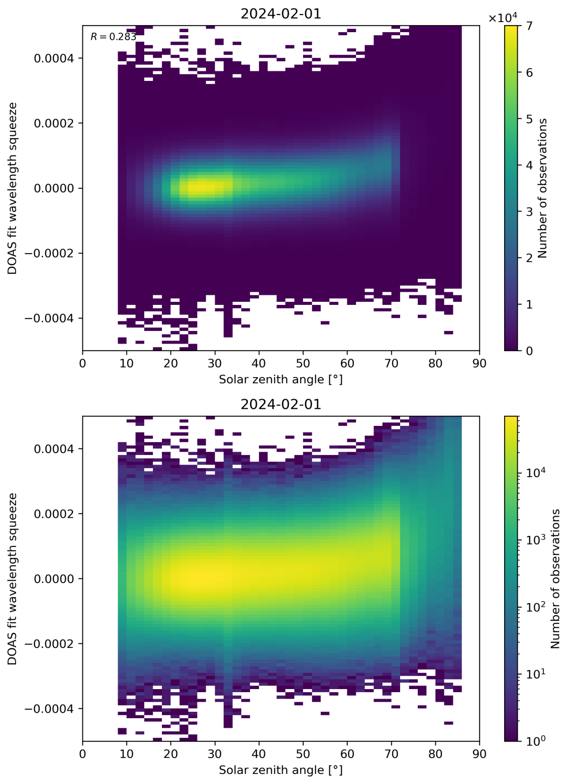
Figure 169: Scatter density plot of “Solar zenith angle” against “DOAS fit wavelength squeeze” for 2024-01-31 to 2024-02-02.
