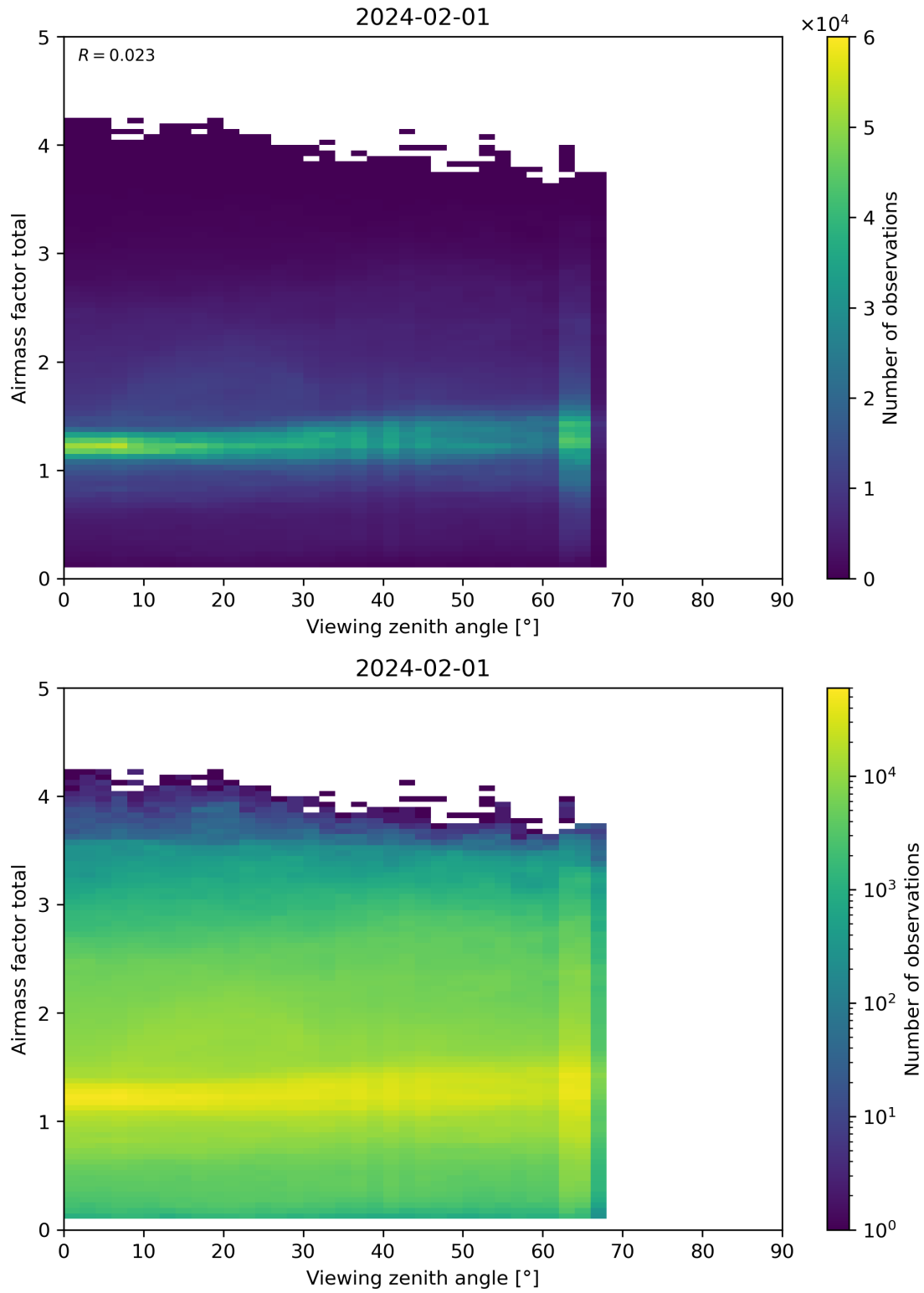
Figure 190: Scatter density plot of “Viewing zenith angle” against “Airmass factor total” for 2024-01-31 to 2024-02-02.
