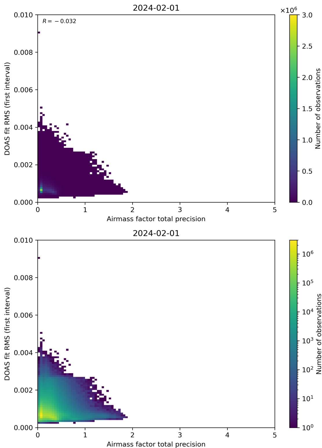
Figure 105: Scatter density plot of “Airmass factor total precision” against “DOAS fit RMS (first interval)” for 2024-01-31 to 2024-02-02.
