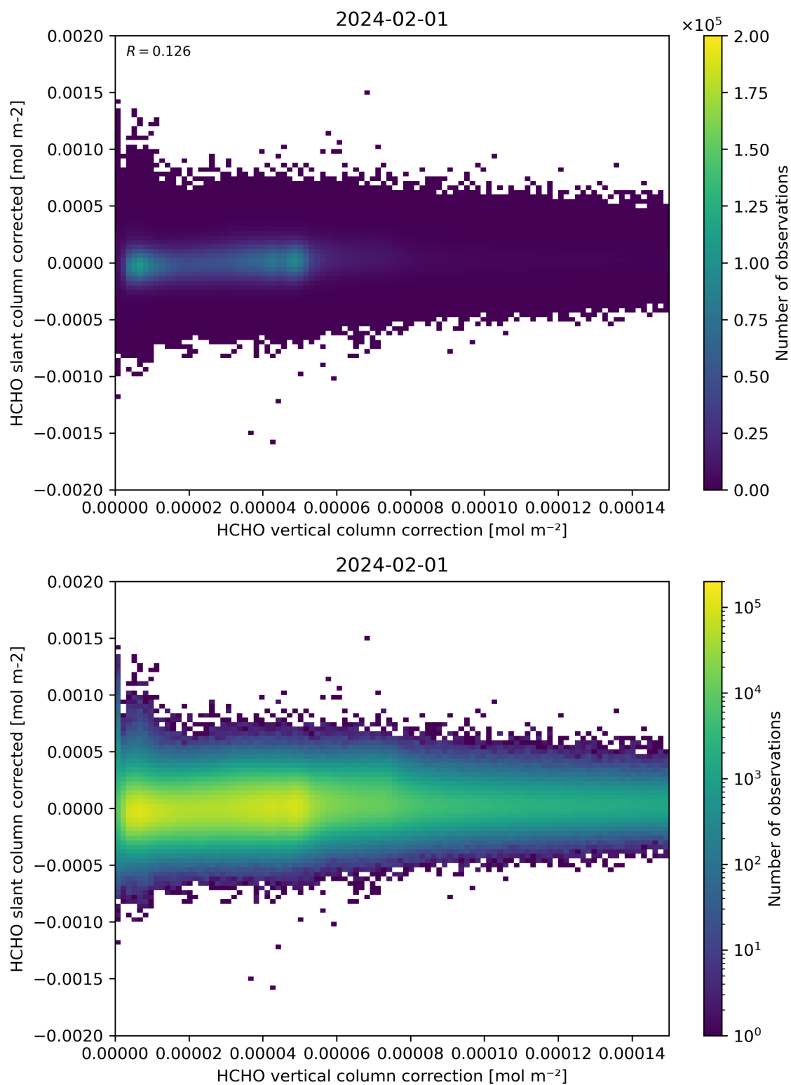
Figure 116: Scatter density plot of “HCHO vertical column correction” against “HCHO slant column corrected” for 2024-01-31 to 2024-02-02.
