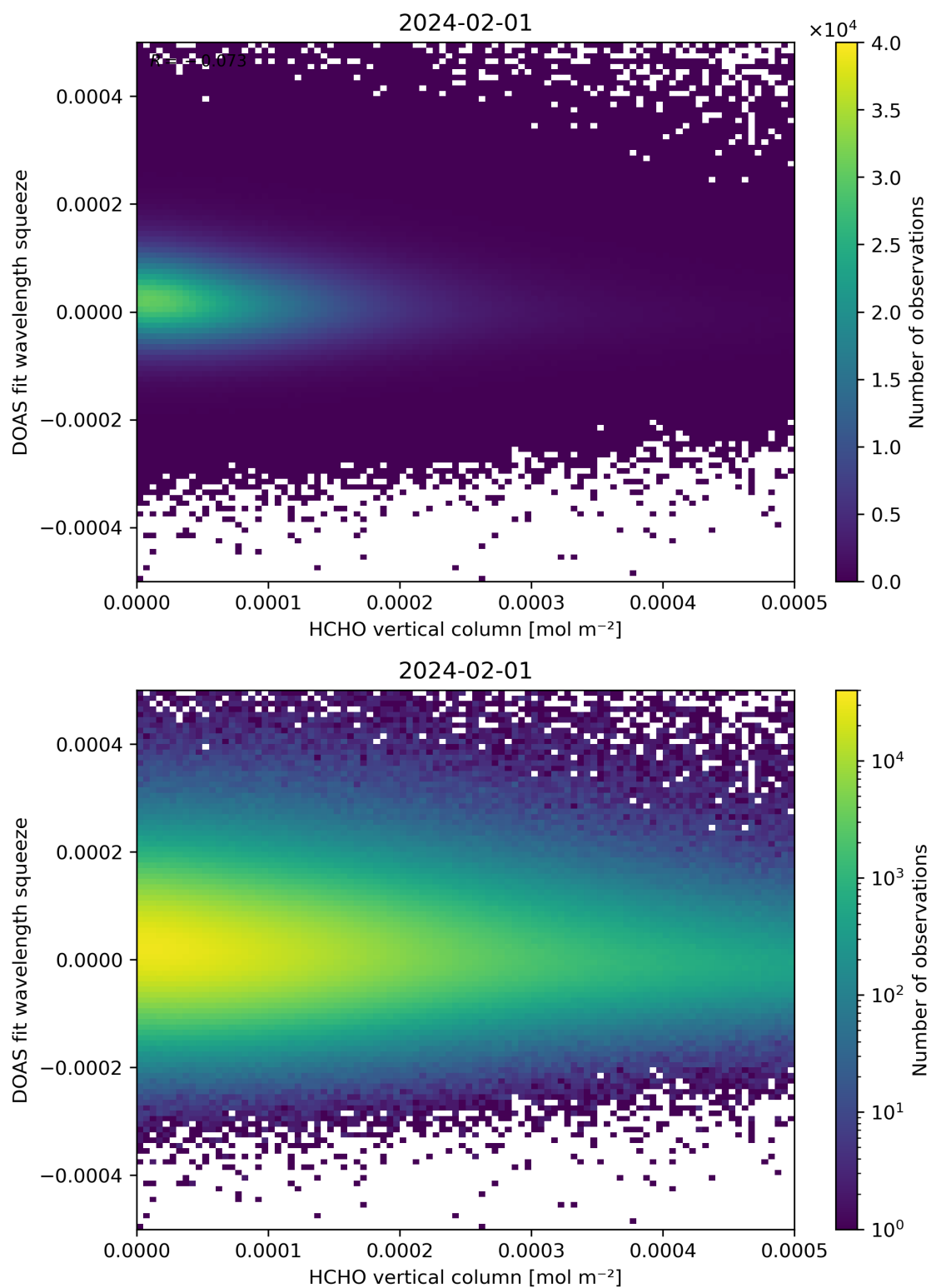
Figure 125: Scatter density plot of “HCHO vertical column” against “DOAS fit wavelength squeeze” for 2024-01-31 to 2024-02-02.
