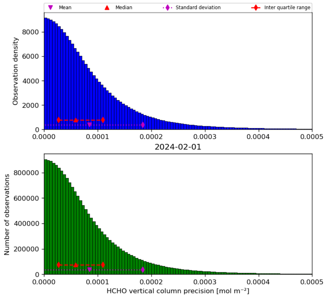
Figure 36: Histogram of “HCHO vertical column precision” for 2024-01-31 to 2024-02-02
