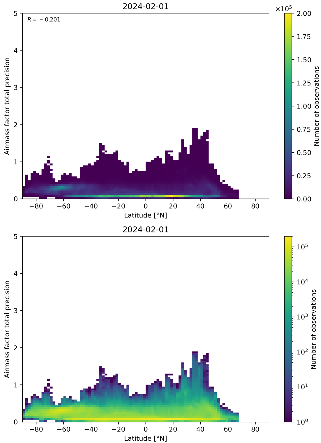
Figure 162: Scatter density plot of “Latitude” against “Airmass factor total precision” for 2024-01-31 to 2024-02-02.
