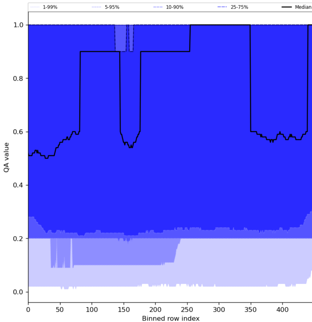
Figure 48: Along track statistics of “QA value” for 2024-01-31 to 2024-02-02
