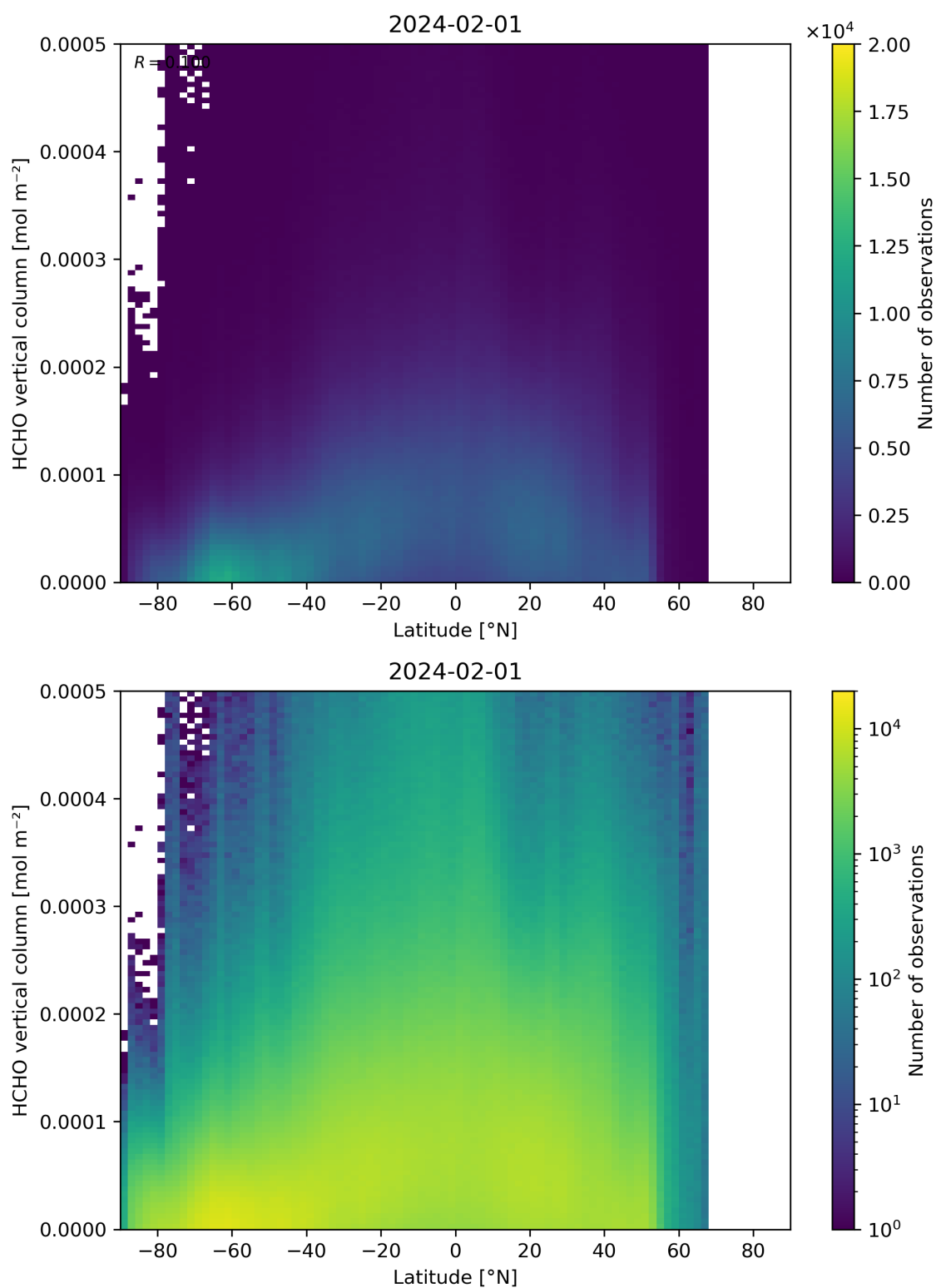
Figure 163: Scatter density plot of “Latitude” against “HCHO vertical column” for 2024-01-31 to 2024-02-02.
