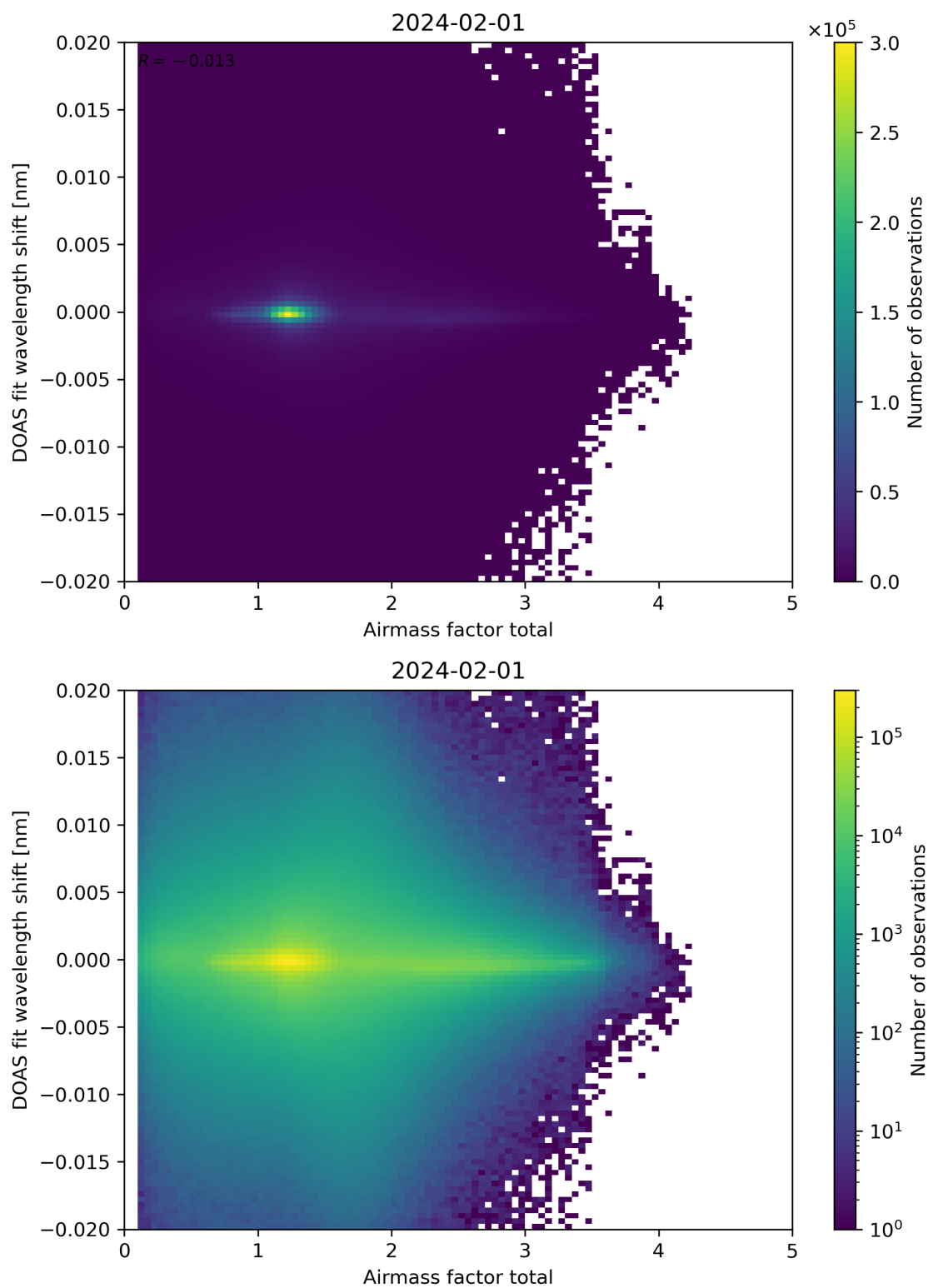
Figure 98: Scatter density plot of “Airmass factor total” against “DOAS fit wavelength shift” for 2024-01-31 to 2024-02-02.
