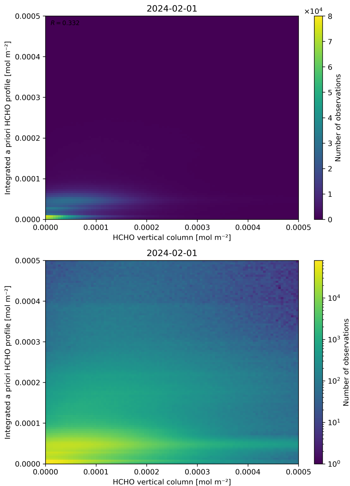
Figure 135: Scatter density plot of “HCHO vertical column” against “Integrated a priori HCHO profile” for 2024-01-31 to 2024-02-02.
