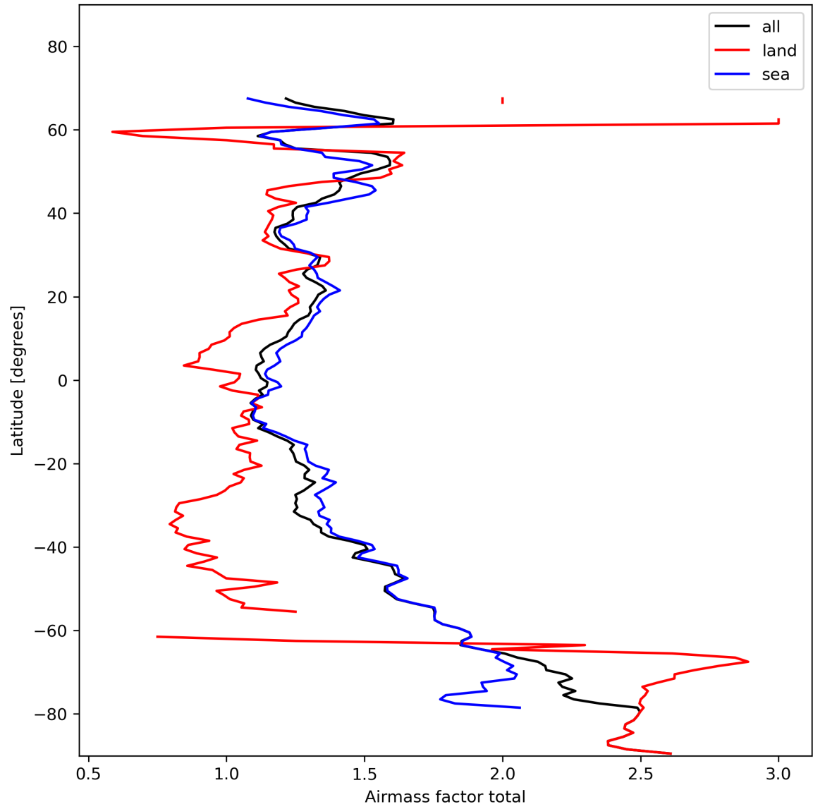
Figure 26: Zonal average of “Airmass factor total” for 2024-01-31 to 2024-02-02.
