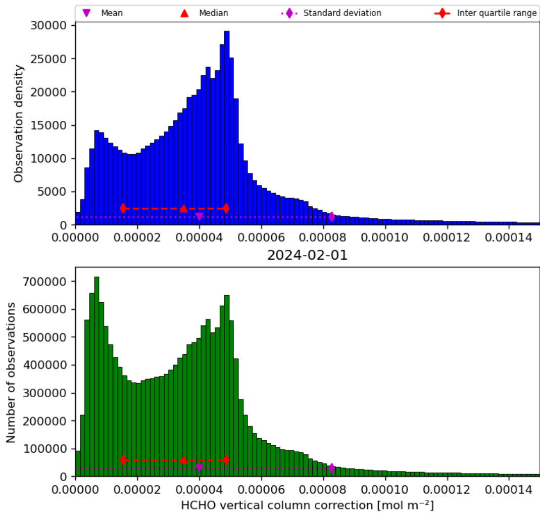
Figure 37: Histogram of “HCHO vertical column correction” for 2024-01-31 to 2024-02-02
