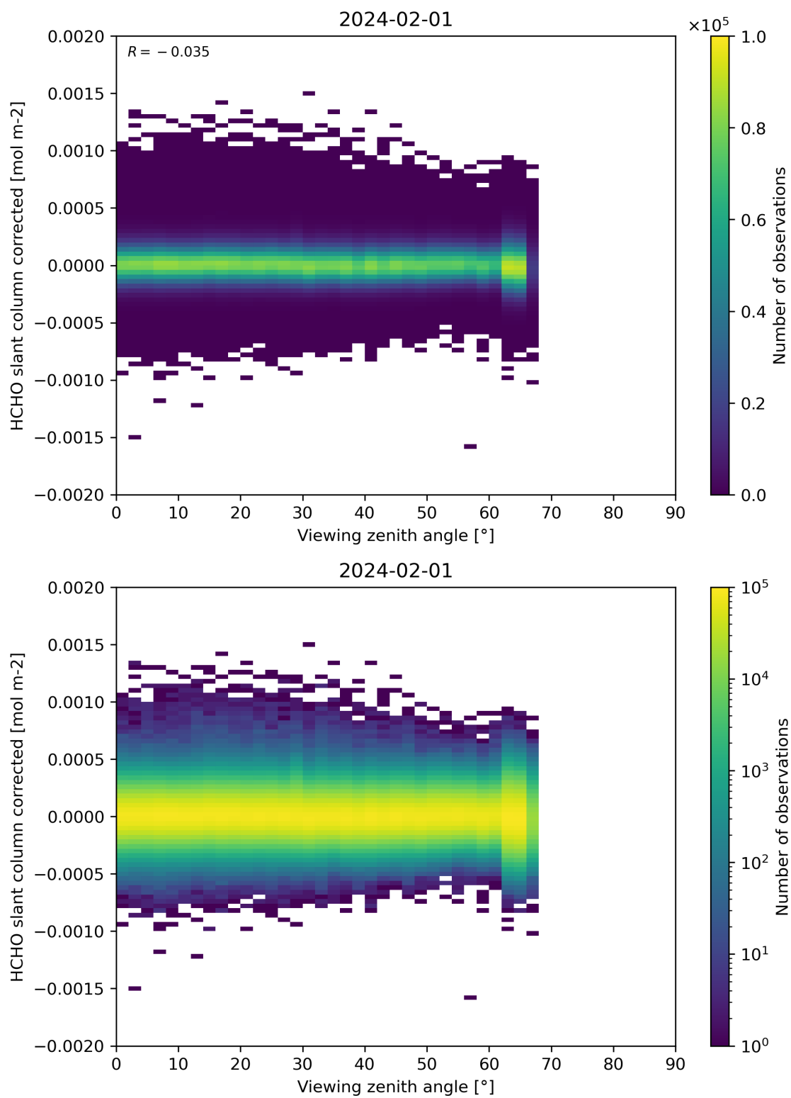
Figure 186: Scatter density plot of “Viewing zenith angle” against “HCHO slant column corrected” for 2024-01-31 to 2024-02-02.
