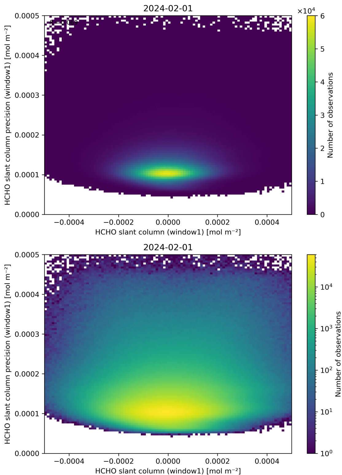
Figure 84: Scatter density plot of “HCHO slant column (window1)” against “HCHO slant column precision (window1)” for 2024-01-31 to 2024-02-02.
