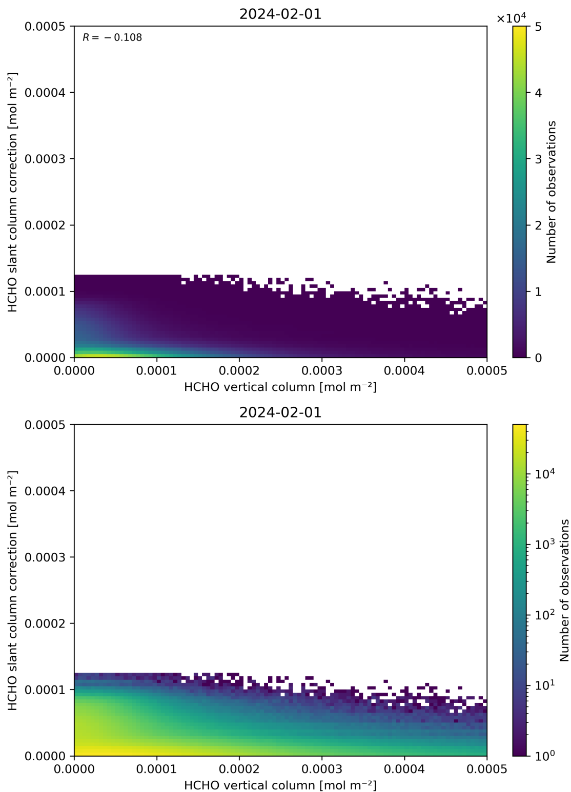
Figure 128: Scatter density plot of “HCHO vertical column” against “HCHO slant column correction” for 2024-01-31 to 2024-02-02.
