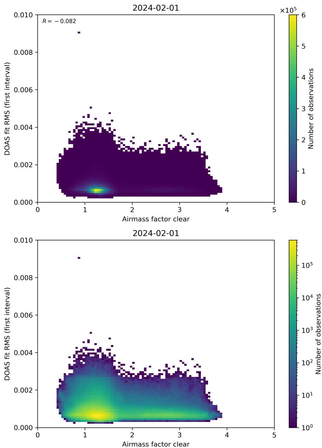
Figure 71: Scatter density plot of “Airmass factor clear” against “DOAS fit RMS (first interval)” for 2024-01-31 to 2024-02-02.
