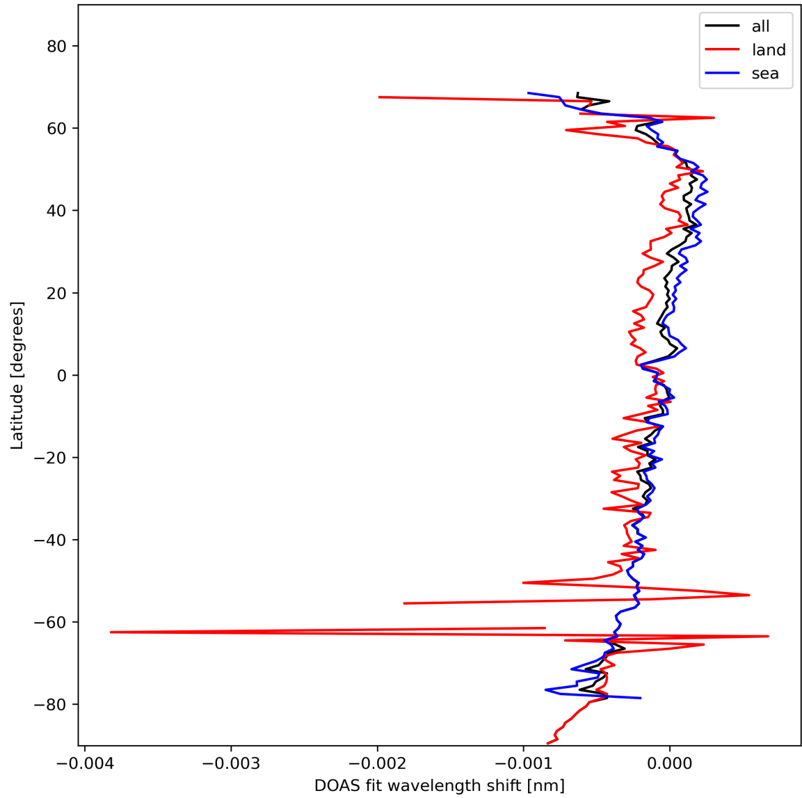
Figure 30: Zonal average of “DOAS fit wavelength shift” for 2024-02-02 to 2024-02-04.
