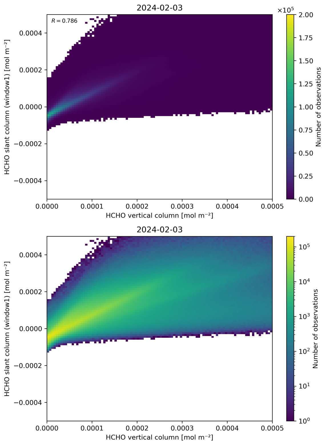
Figure 129: Scatter density plot of “HCHO vertical column” against “HCHO slant column (window1)” for 2024-02-02 to 2024-02-04.
