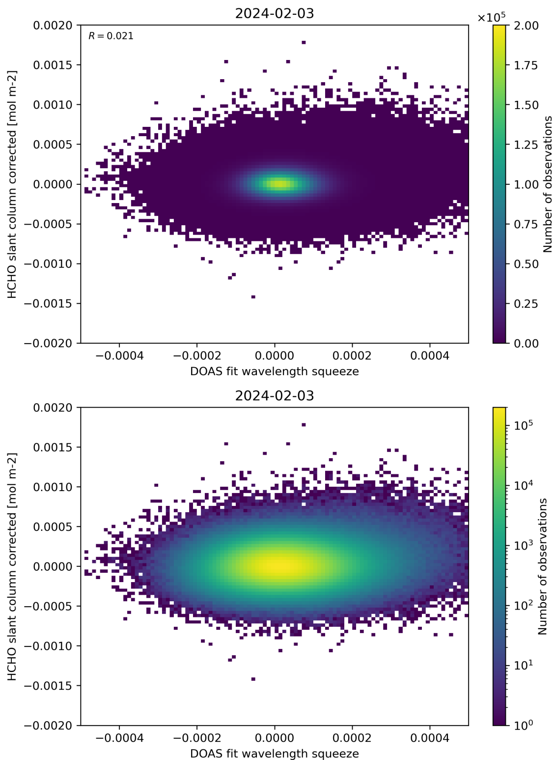
Figure 69: Scatter density plot of “DOAS fit wavelength squeeze” against “HCHO slant column corrected” for 2024-02-02 to 2024-02-04.
