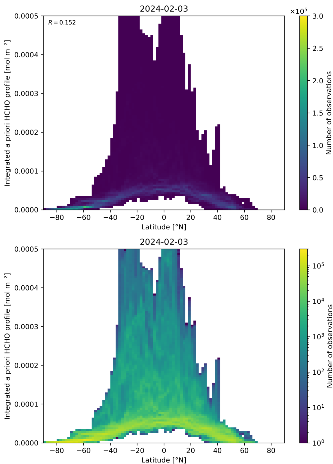
Figure 166: Scatter density plot of “Latitude” against “Integrated a priori HCHO profile” for 2024-02-02 to 2024-02-04.
