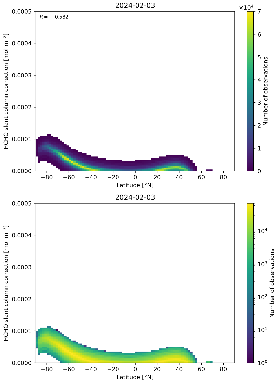
Figure 158: Scatter density plot of “Latitude” against “HCHO slant column correction” for 2024-02-02 to 2024-02-04.
