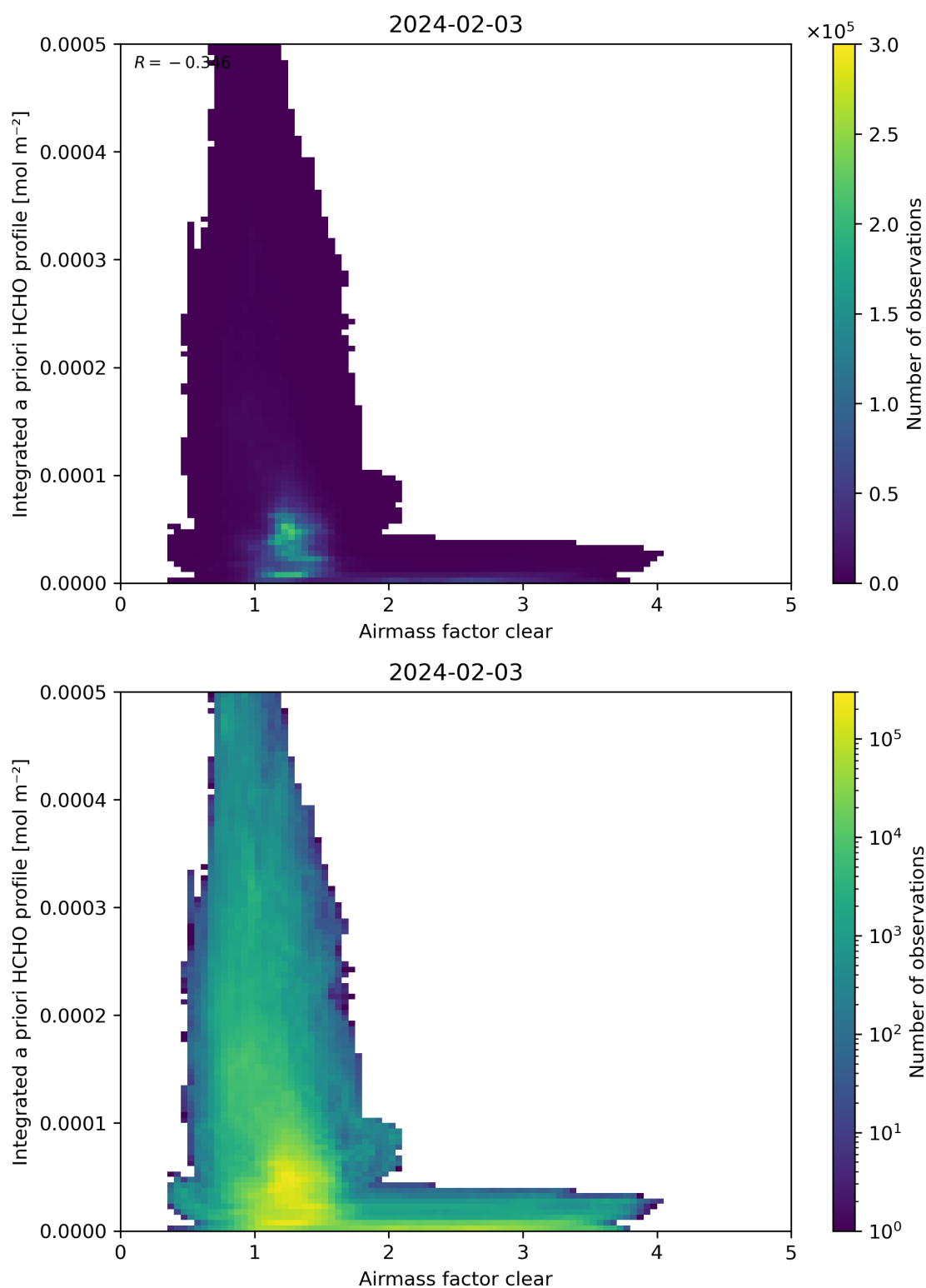
Figure 76: Scatter density plot of “Airmass factor clear” against “Integrated a priori HCHO profile” for 2024-02-02 to 2024-02-04.
