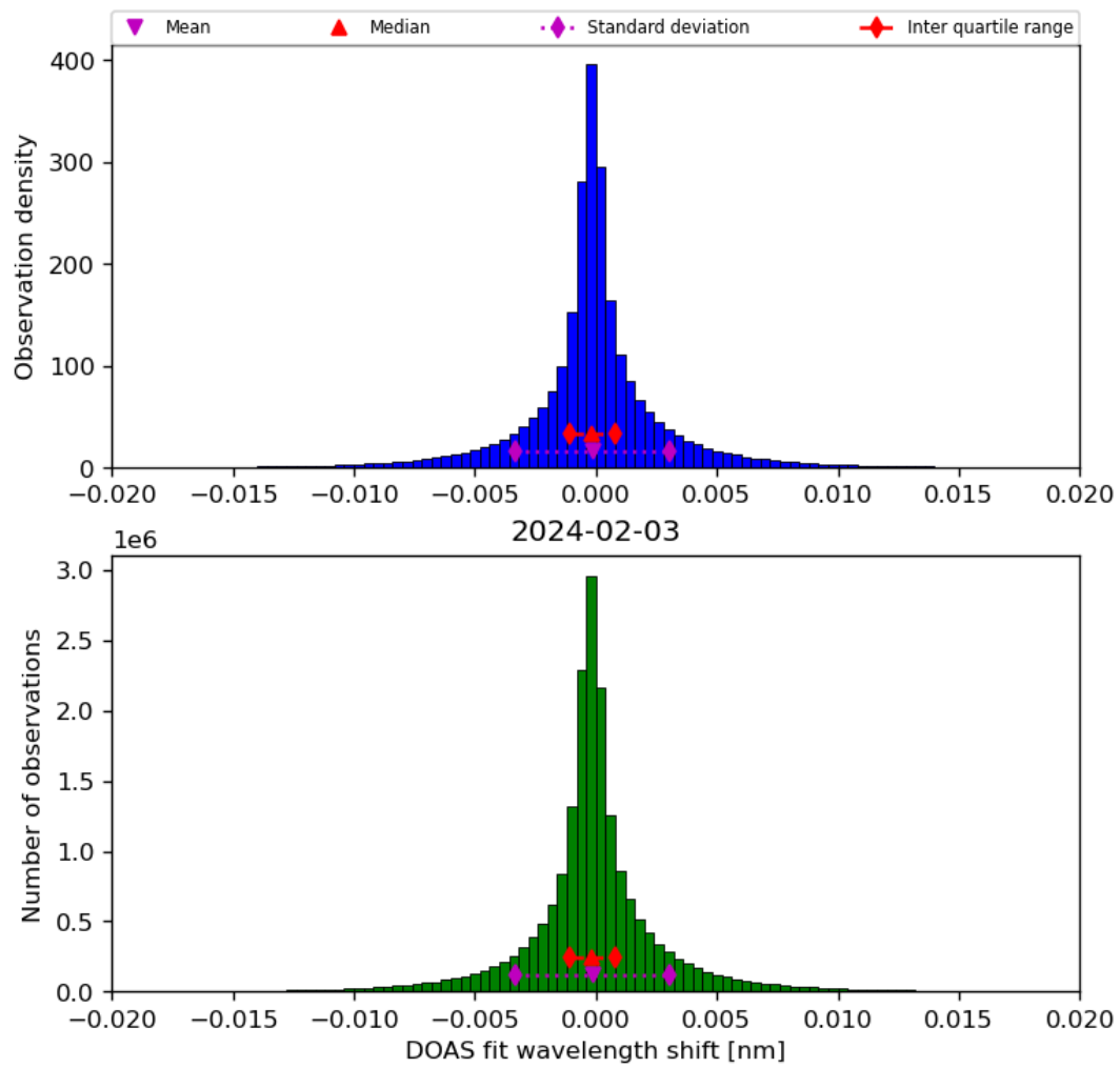
Figure 44: Histogram of “DOAS fit wavelength shift” for 2024-02-02 to 2024-02-04
