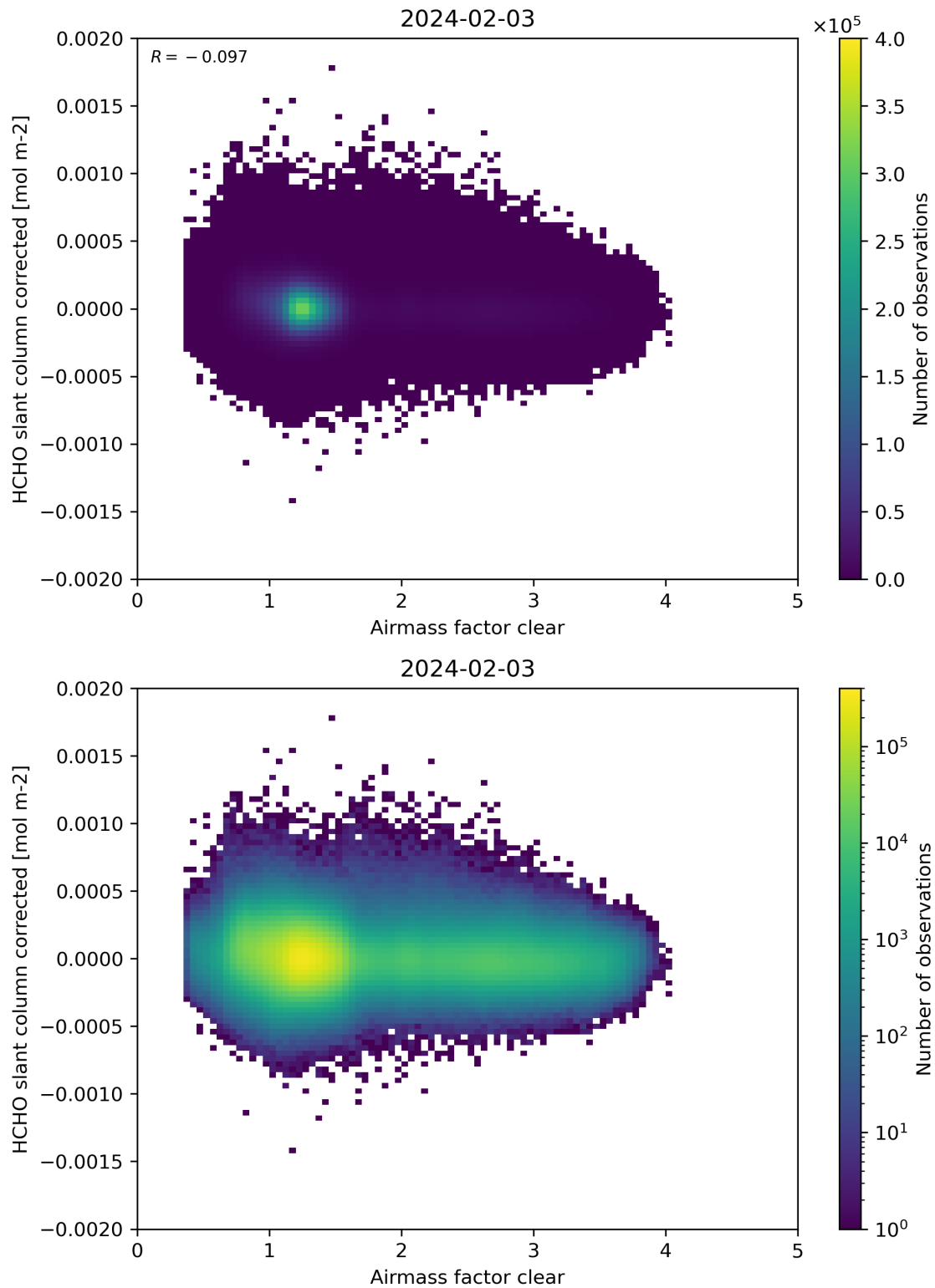
Figure 74: Scatter density plot of “Airmass factor clear” against “HCHO slant column corrected” for 2024-02-02 to 2024-02-04.
