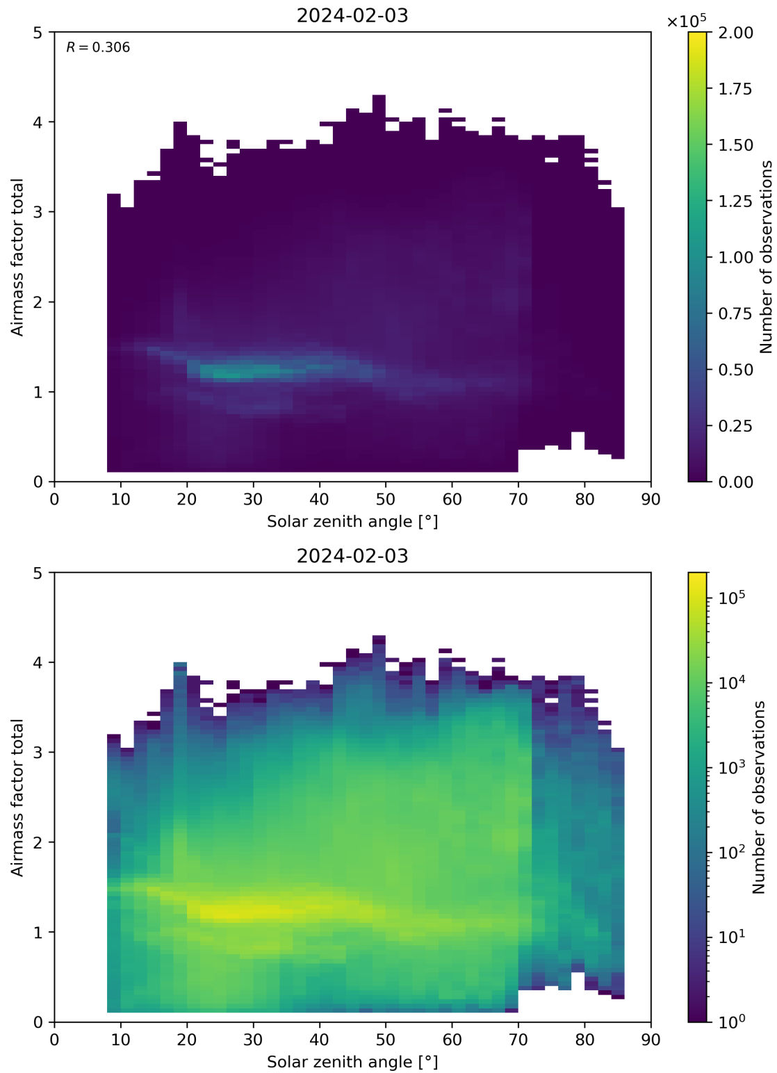
Figure 175: Scatter density plot of “Solar zenith angle” against “Airmass factor total” for 2024-02-02 to 2024-02-04.
