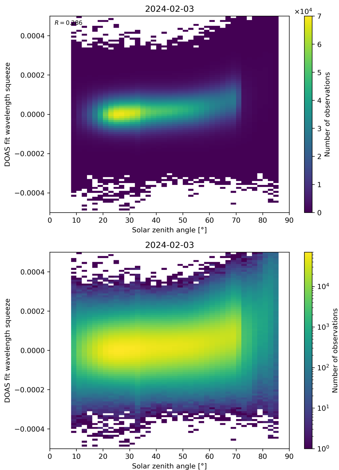
Figure 169: Scatter density plot of “Solar zenith angle” against “DOAS fit wavelength squeeze” for 2024-02-02 to 2024-02-04.
