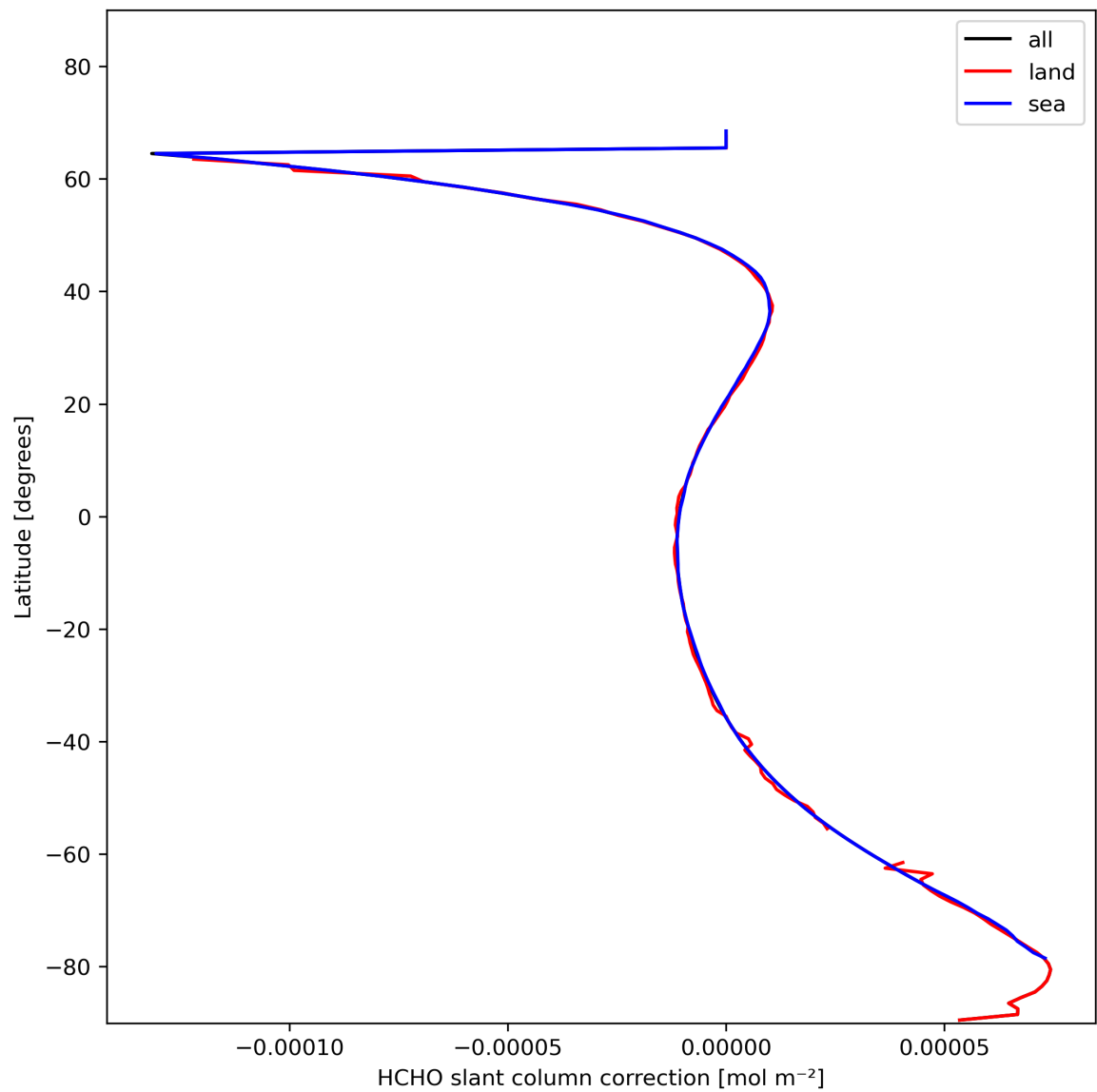
Figure 33: Zonal average of “HCHO slant column correction” for 2024-02-02 to 2024-02-04.
