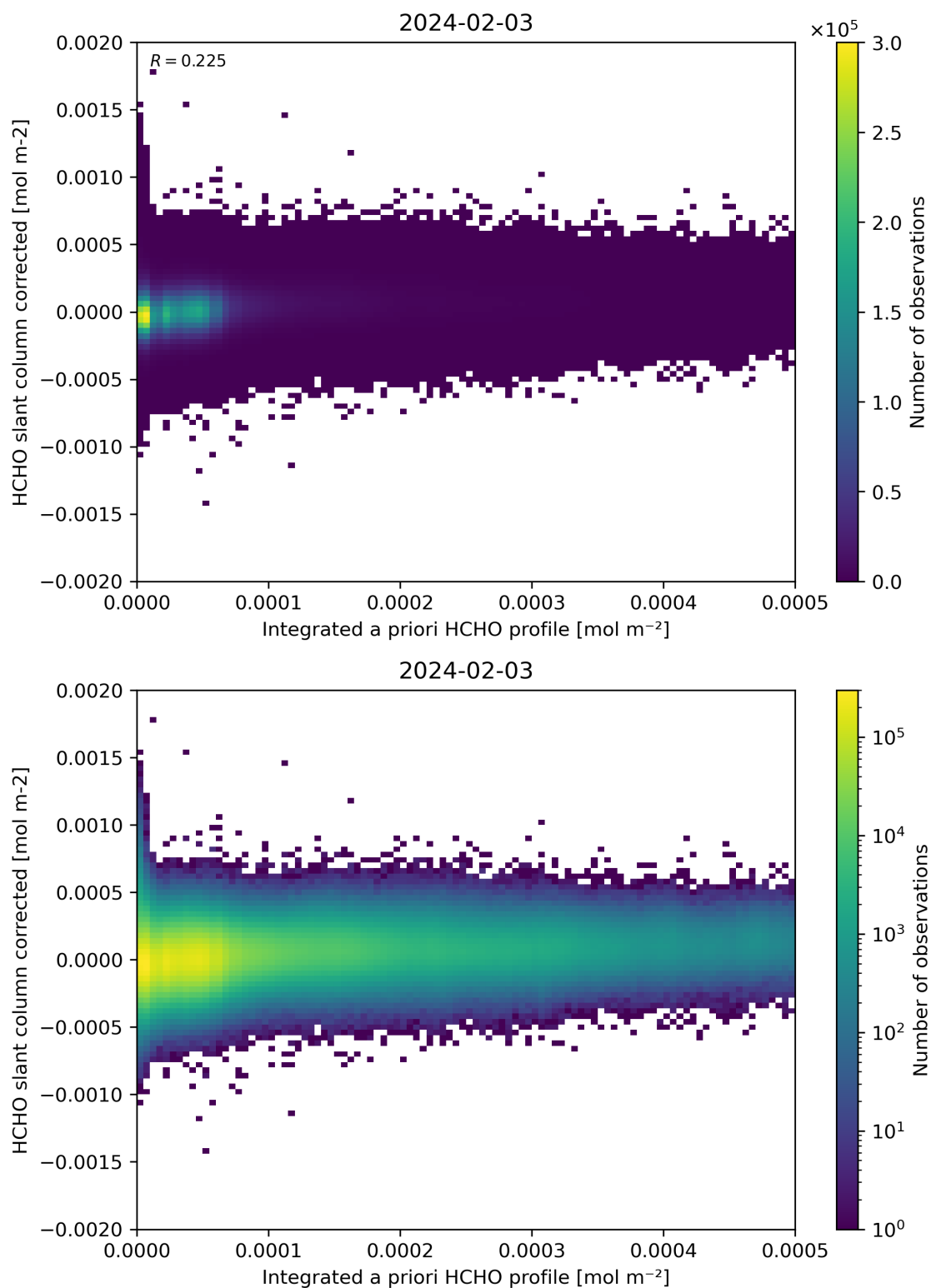
Figure 151: Scatter density plot of “Integrated a priori HCHO profile” against “HCHO slant column corrected” for 2024-02-02 to 2024-02-04.
