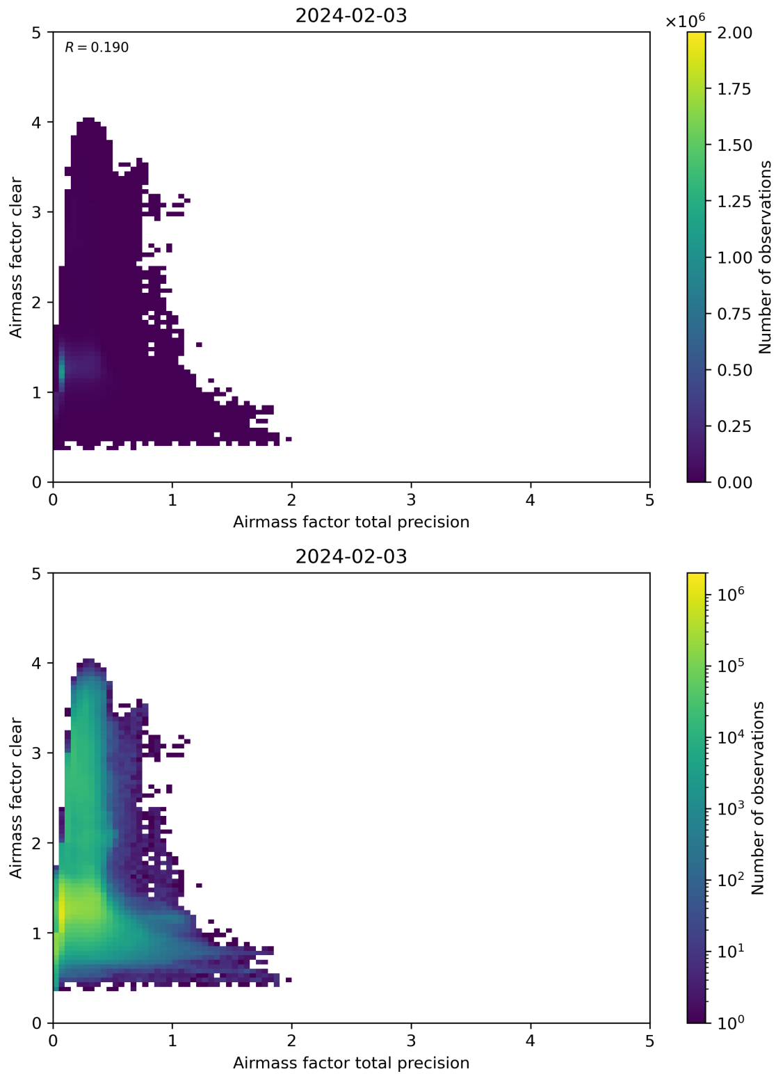
Figure 108: Scatter density plot of “Airmass factor total precision” against “Airmass factor clear” for 2024-02-02 to 2024-02-04.
