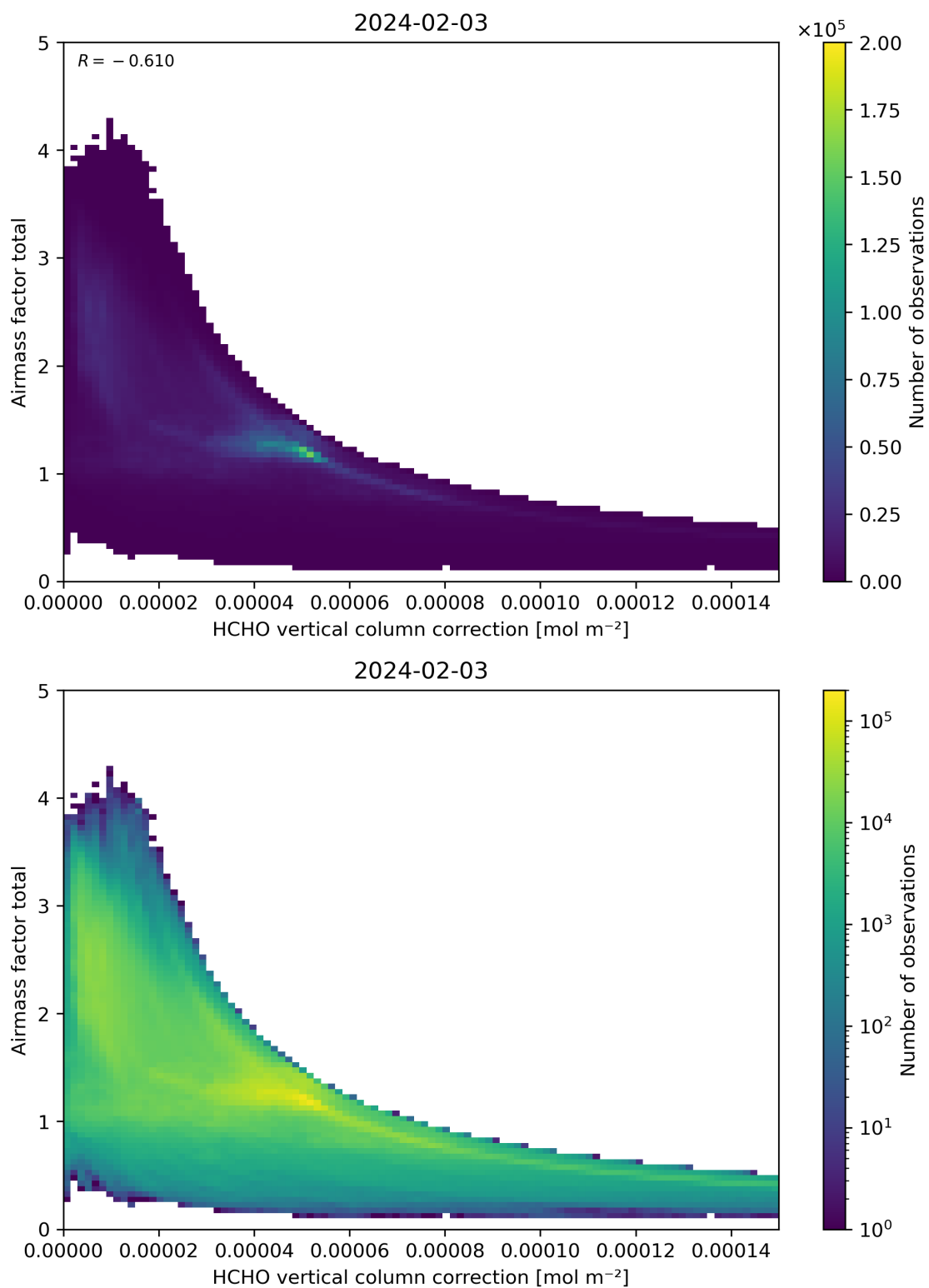
Figure 120: Scatter density plot of “HCHO vertical column correction” against “Airmass factor total” for 2024-02-02 to 2024-02-04.
