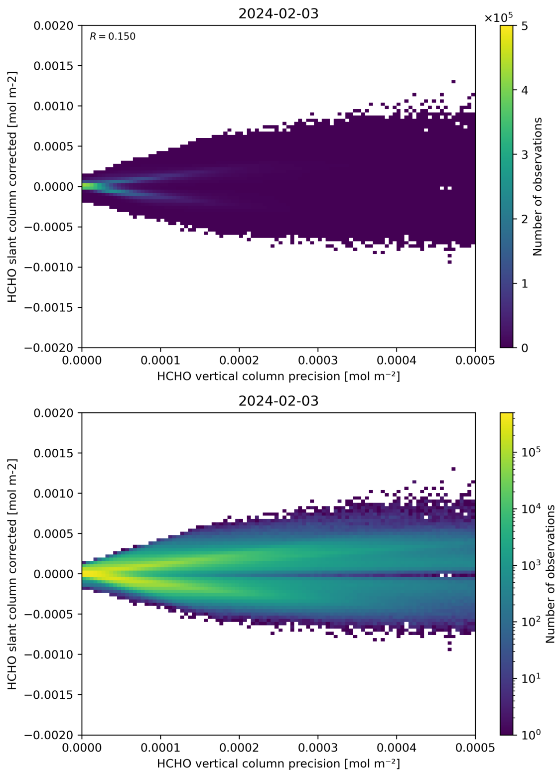
Figure 140: Scatter density plot of “HCHO vertical column precision” against “HCHO slant column corrected” for 2024-02-02 to 2024-02-04.
