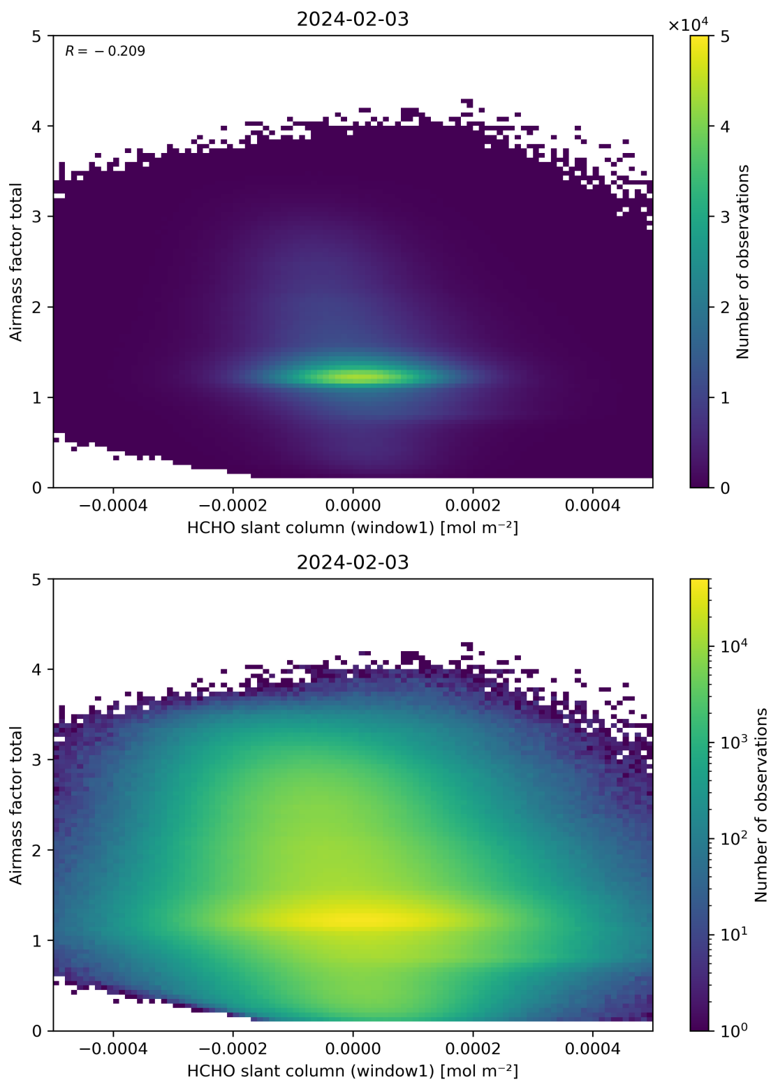
Figure 85: Scatter density plot of “HCHO slant column (window1)” against “Airmass factor total” for 2024-02-02 to 2024-02-04.
