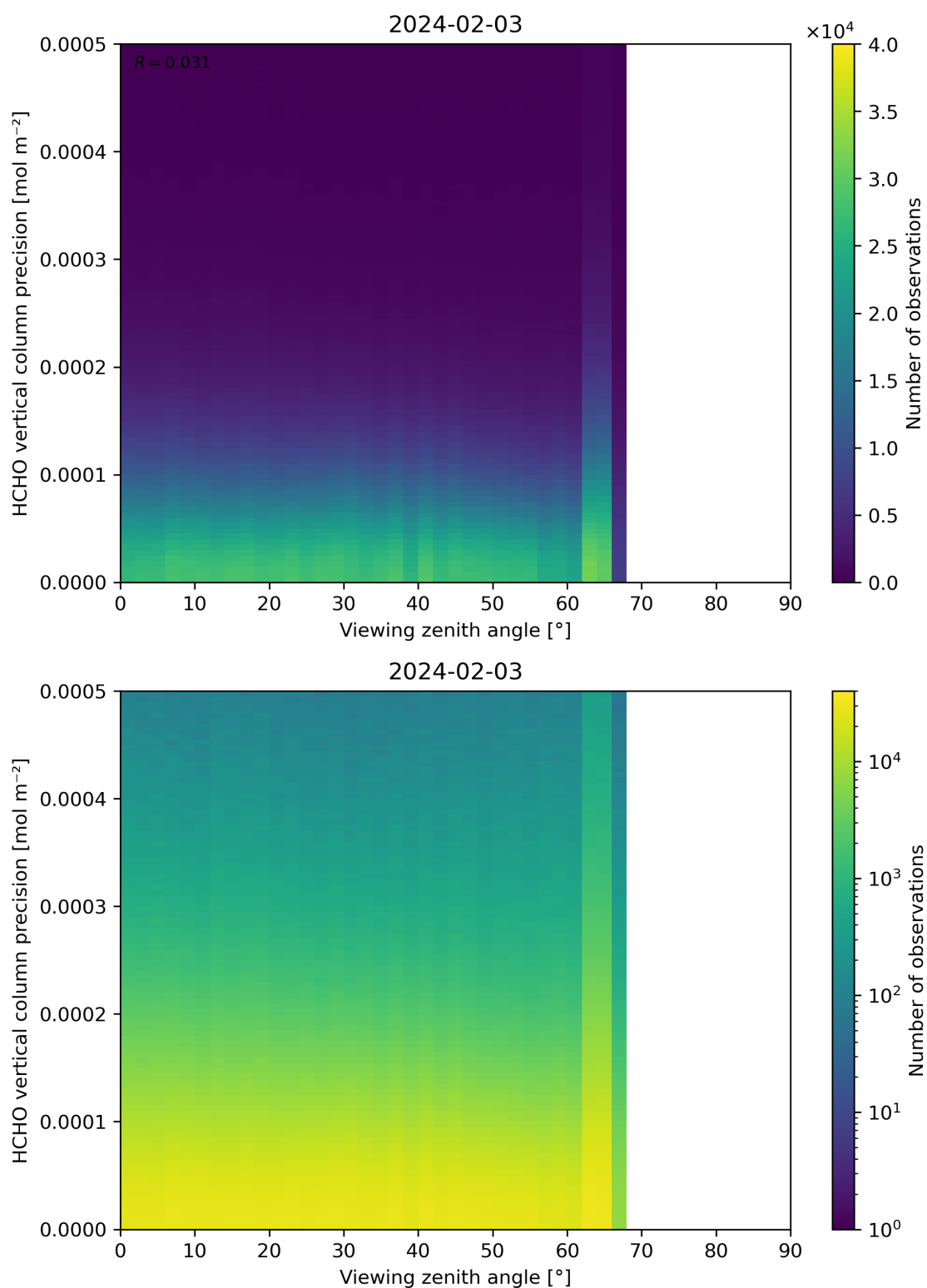
Figure 194: Scatter density plot of “Viewing zenith angle” against “HCHO vertical column precision” for 2024-02-02 to 2024-02-04.
