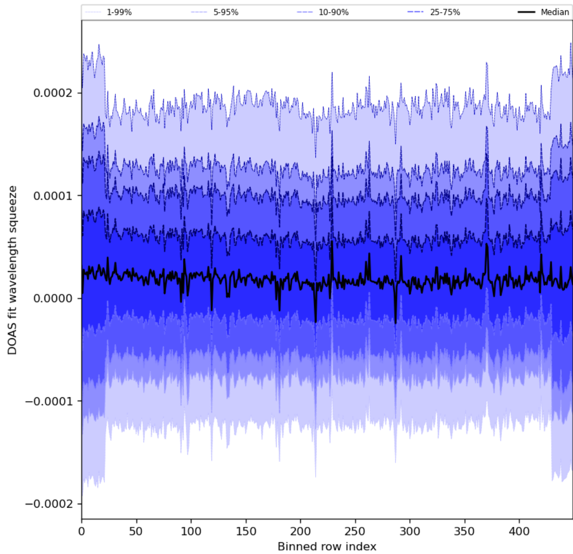
Figure 59: Along track statistics of “DOAS fit wavelength squeeze” for 2024-02-02 to 2024-02-04
