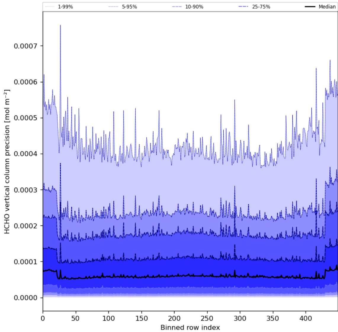
Figure 50: Along track statistics of “HCHO vertical column precision” for 2024-02-02 to 2024-02-04
