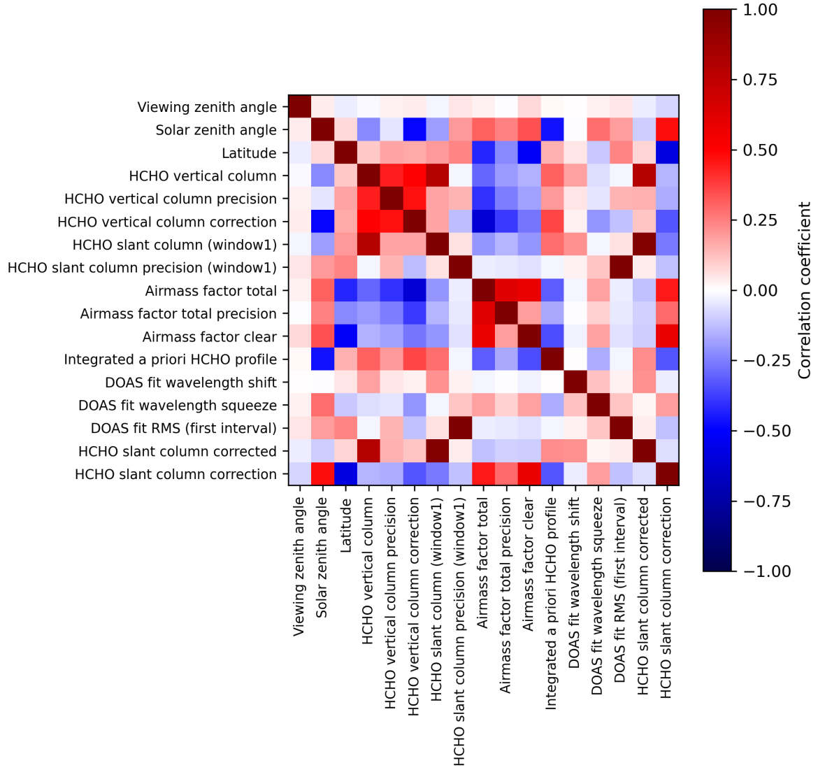
Figure 2: Map of correlation matrix for 2024-02-02 to 2024-02-04.
