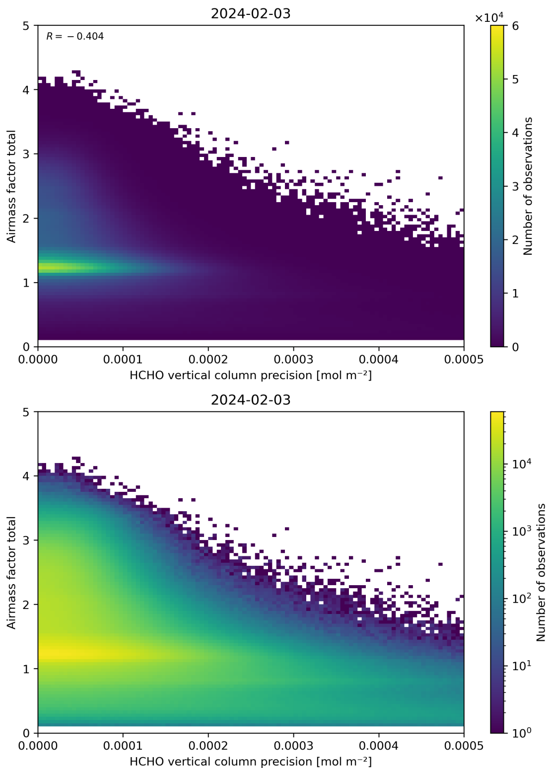
Figure 144: Scatter density plot of “HCHO vertical column precision” against “Airmass factor total” for 2024-02-02 to 2024-02-04.
