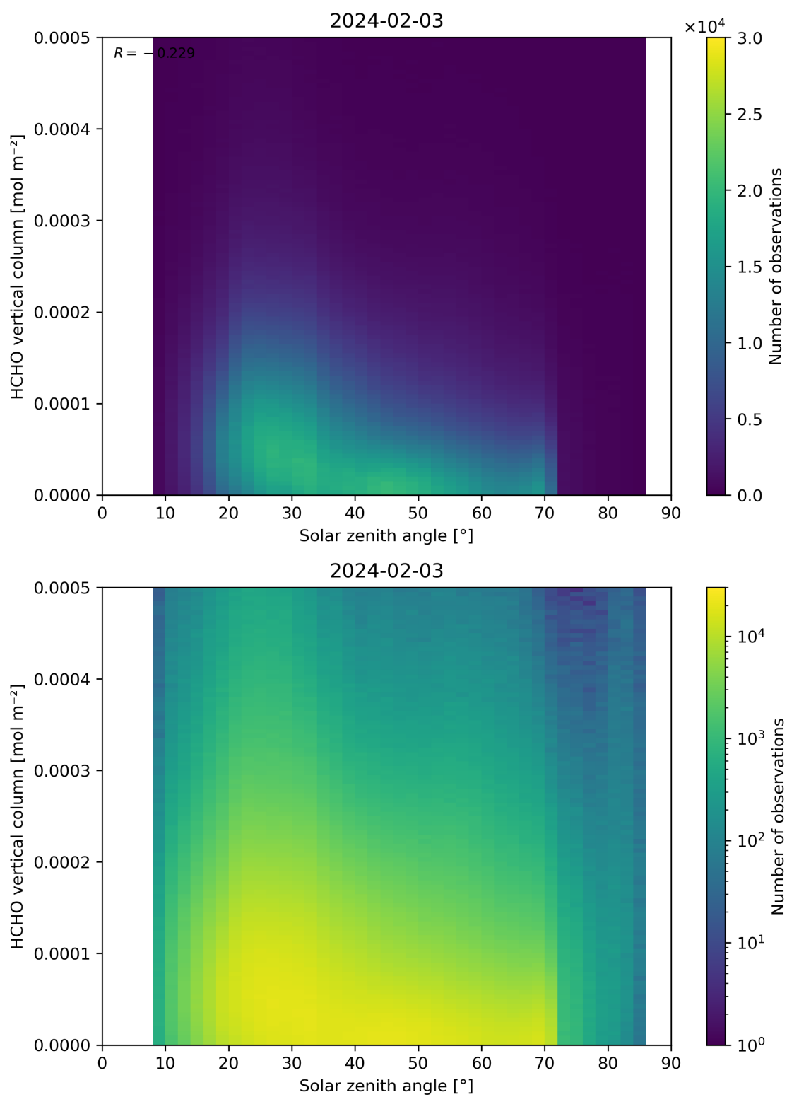
Figure 177: Scatter density plot of “Solar zenith angle” against “HCHO vertical column” for 2024-02-02 to 2024-02-04.
