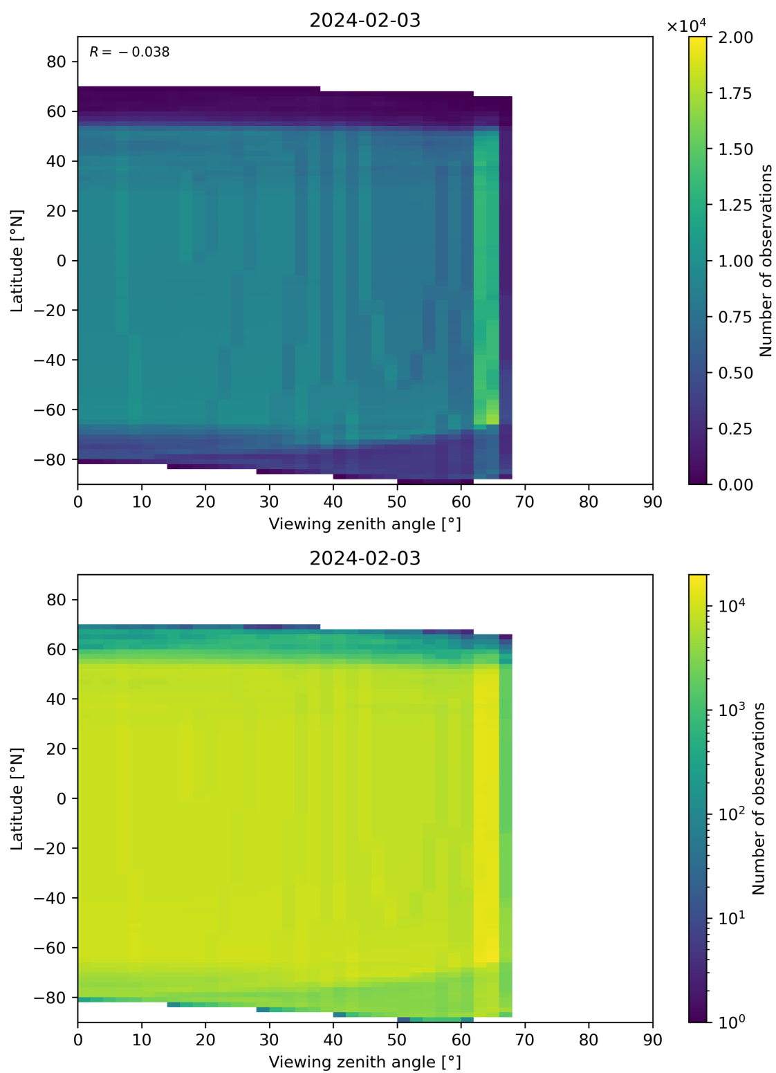
Figure 196: Scatter density plot of “Viewing zenith angle” against “Latitude” for 2024-02-02 to 2024-02-04.
