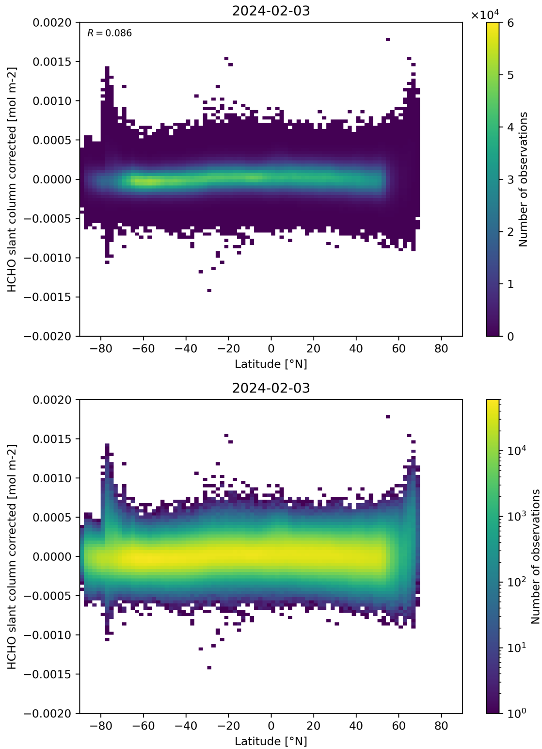
Figure 157: Scatter density plot of “Latitude” against “HCHO slant column corrected” for 2024-02-02 to 2024-02-04.
