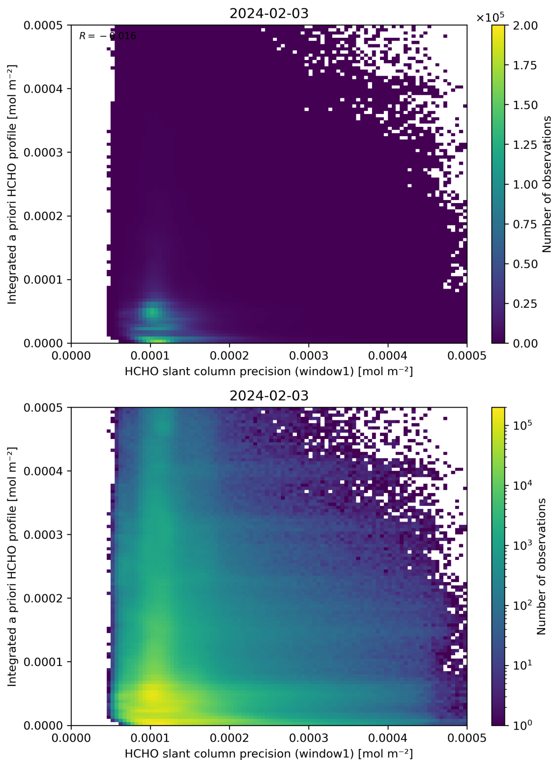
Figure 96: Scatter density plot of “HCHO slant column precision (window1)” against “Integrated a priori HCHO profile” for 2024-02-02 to 2024-02-04.
