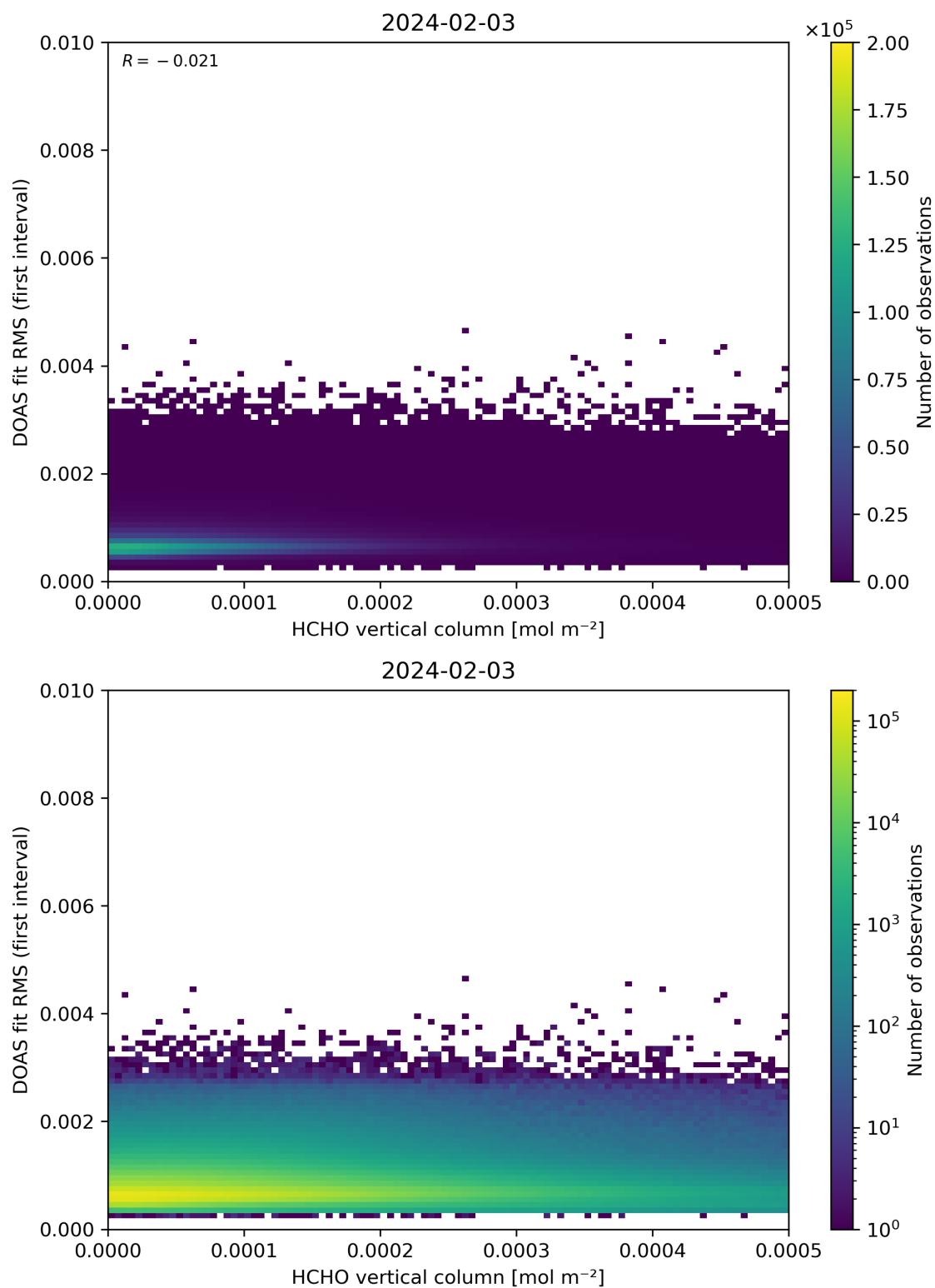
Figure 123: Scatter density plot of “HCHO vertical column” against “DOAS fit RMS (first interval)” for 2024-02-02 to 2024-02-04.
