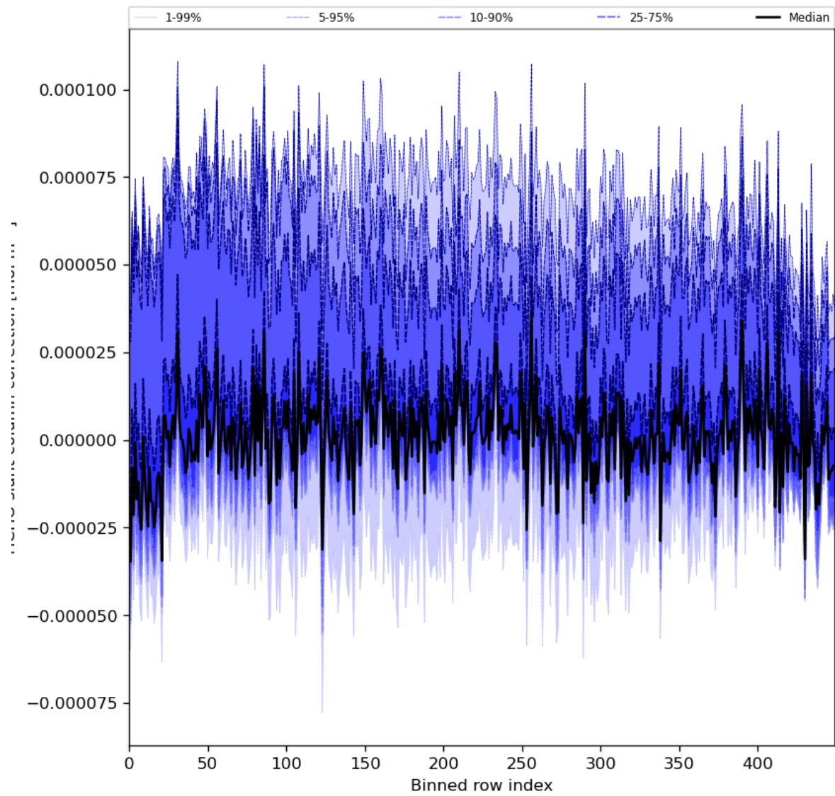
Figure 61: Along track statistics of “HCHO slant column correction” for 2024-02-02 to 2024-02-04
