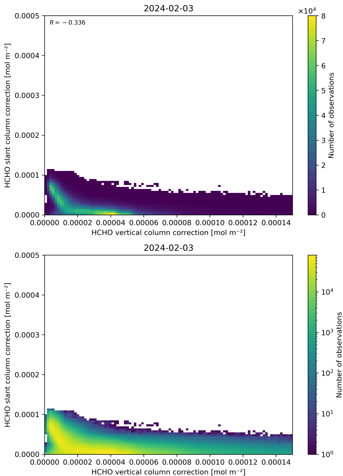
Figure 117: Scatter density plot of “HCHO vertical column correction” against “HCHO slant column correction” for 2024-02-02 to 2024-02-04.
