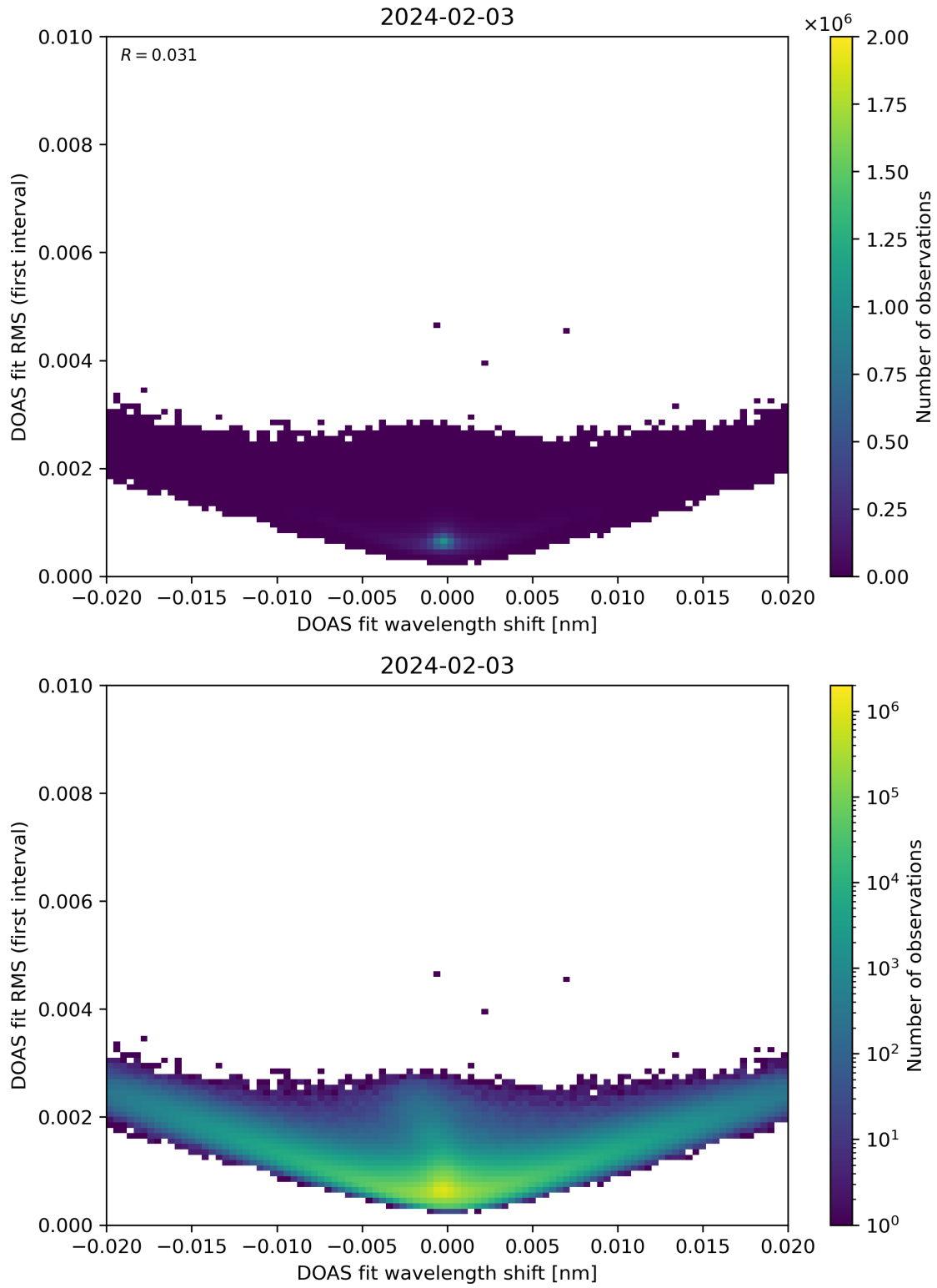
Figure 64: Scatter density plot of “DOAS fit wavelength shift” against “DOAS fit RMS (first interval)” for 2024-02-02 to 2024-02-04.
