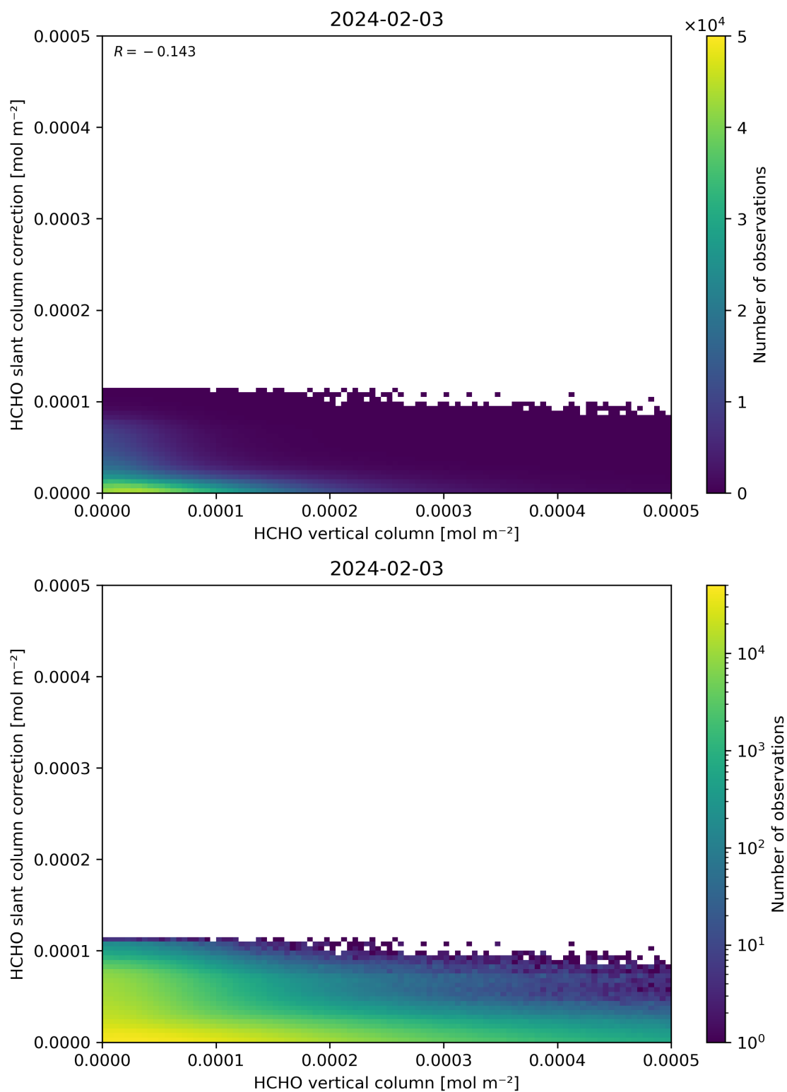
Figure 128: Scatter density plot of “HCHO vertical column” against “HCHO slant column correction” for 2024-02-02 to 2024-02-04.
