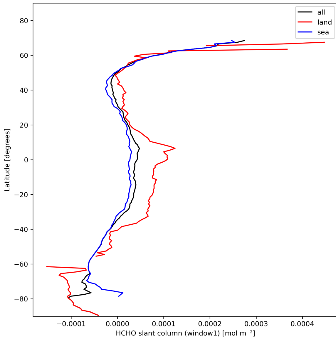
Figure 24: Zonal average of “HCHO slant column (window1)” for 2024-02-02 to 2024-02-04.
