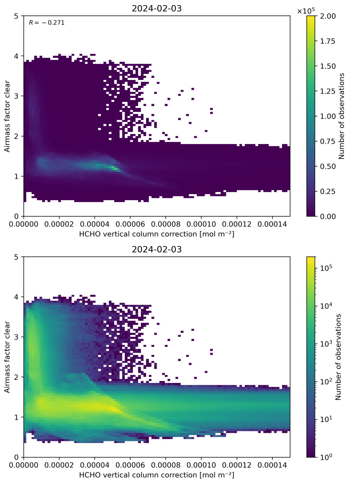
Figure 115: Scatter density plot of “HCHO vertical column correction” against “Airmass factor clear” for 2024-02-02 to 2024-02-04.
