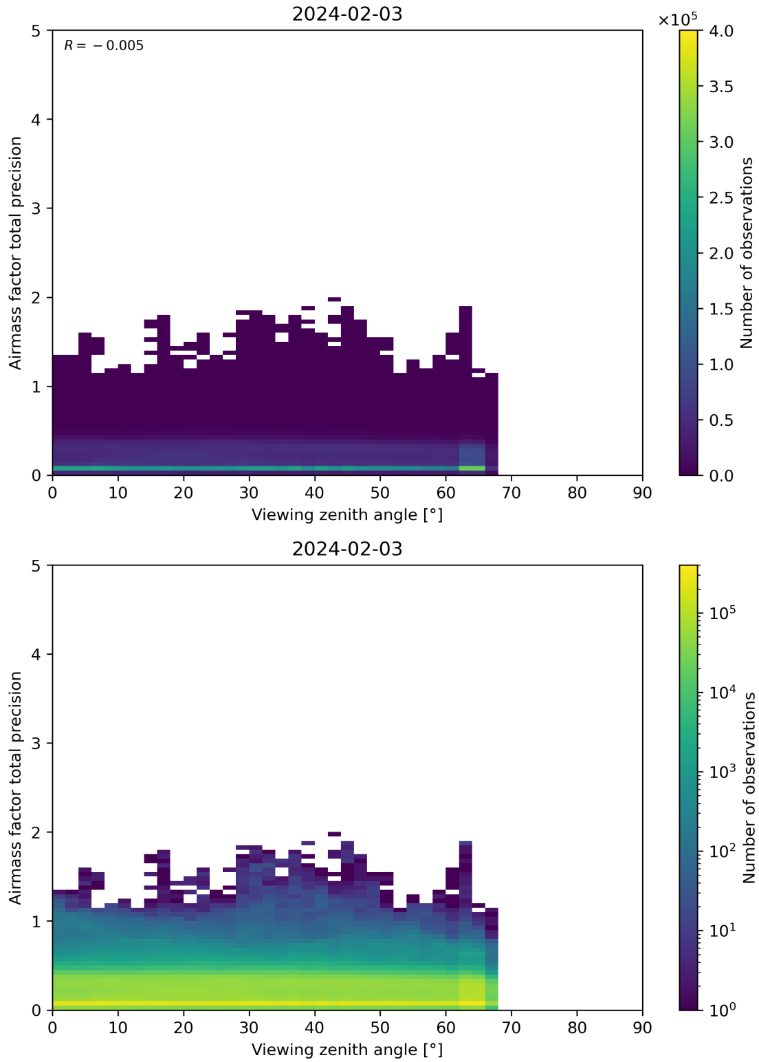
Figure 191: Scatter density plot of “Viewing zenith angle” against “Airmass factor total precision” for 2024-02-02 to 2024-02-04.
