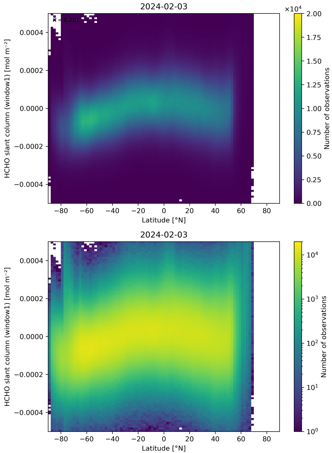
Figure 159: Scatter density plot of “Latitude” against “HCHO slant column (window1)” for 2024-02-02 to 2024-02-04.
