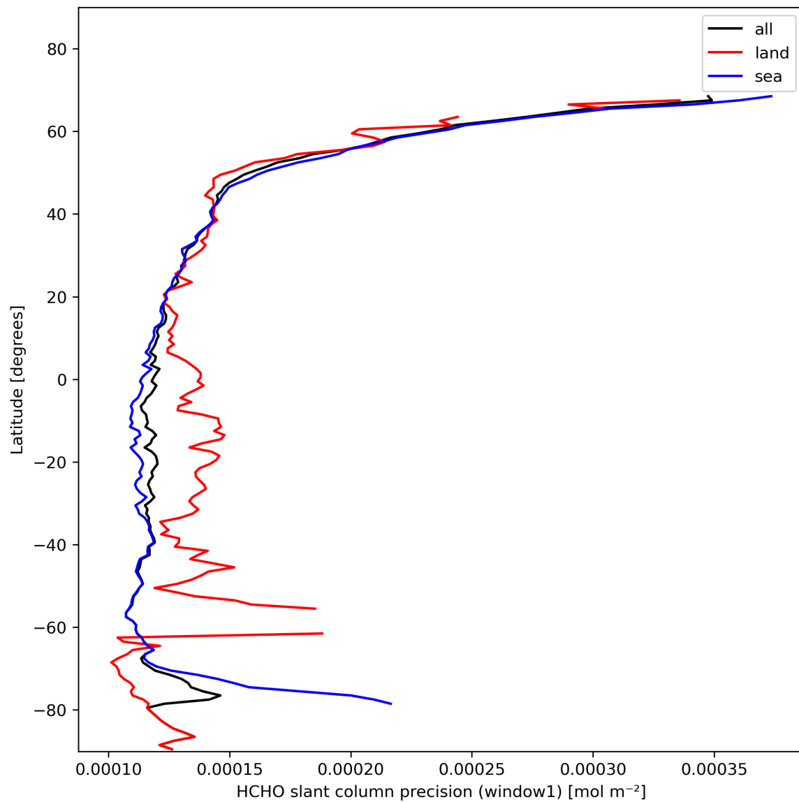
Figure 25: Zonal average of “HCHO slant column precision (window1)” for 2024-02-02 to 2024-02-04.
