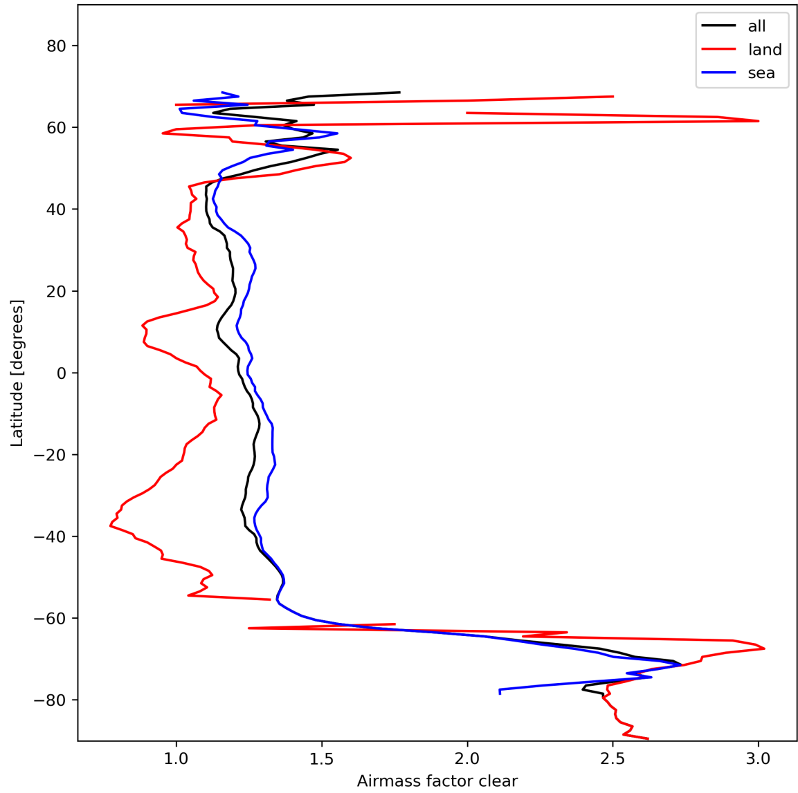
Figure 28: Zonal average of “Airmass factor clear” for 2024-02-02 to 2024-02-04.
