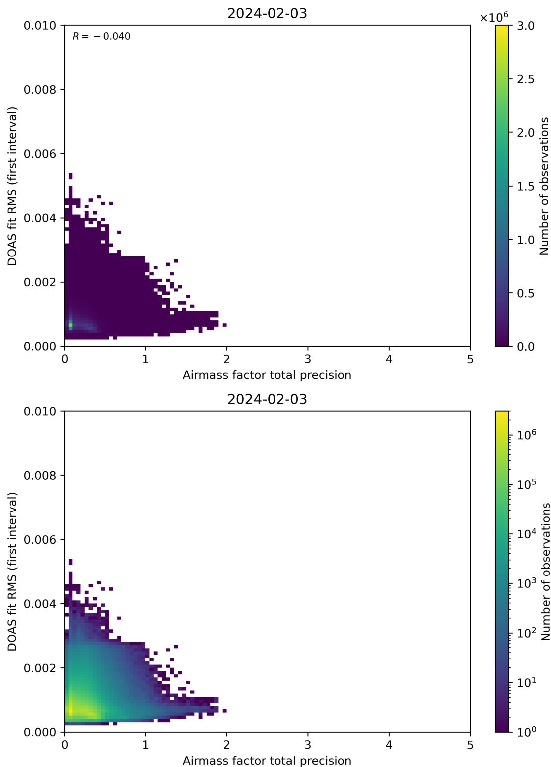
Figure 105: Scatter density plot of “Airmass factor total precision” against “DOAS fit RMS (first interval)” for 2024-02-02 to 2024-02-04.
