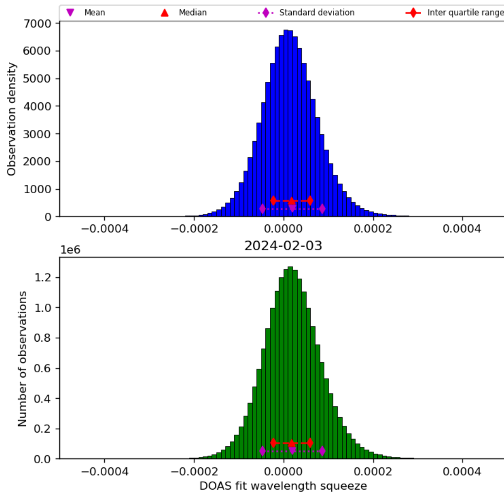
Figure 45: Histogram of “DOAS fit wavelength squeeze” for 2024-02-02 to 2024-02-04
