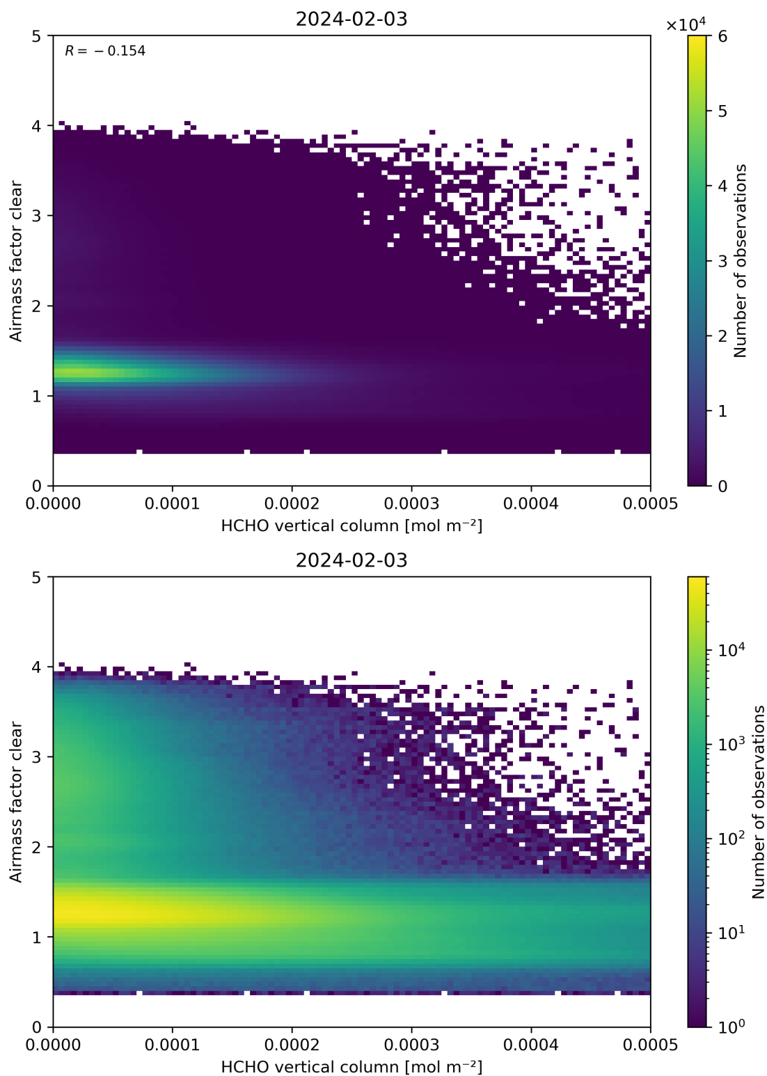
Figure 126: Scatter density plot of “HCHO vertical column” against “Airmass factor clear” for 2024-02-02 to 2024-02-04.
