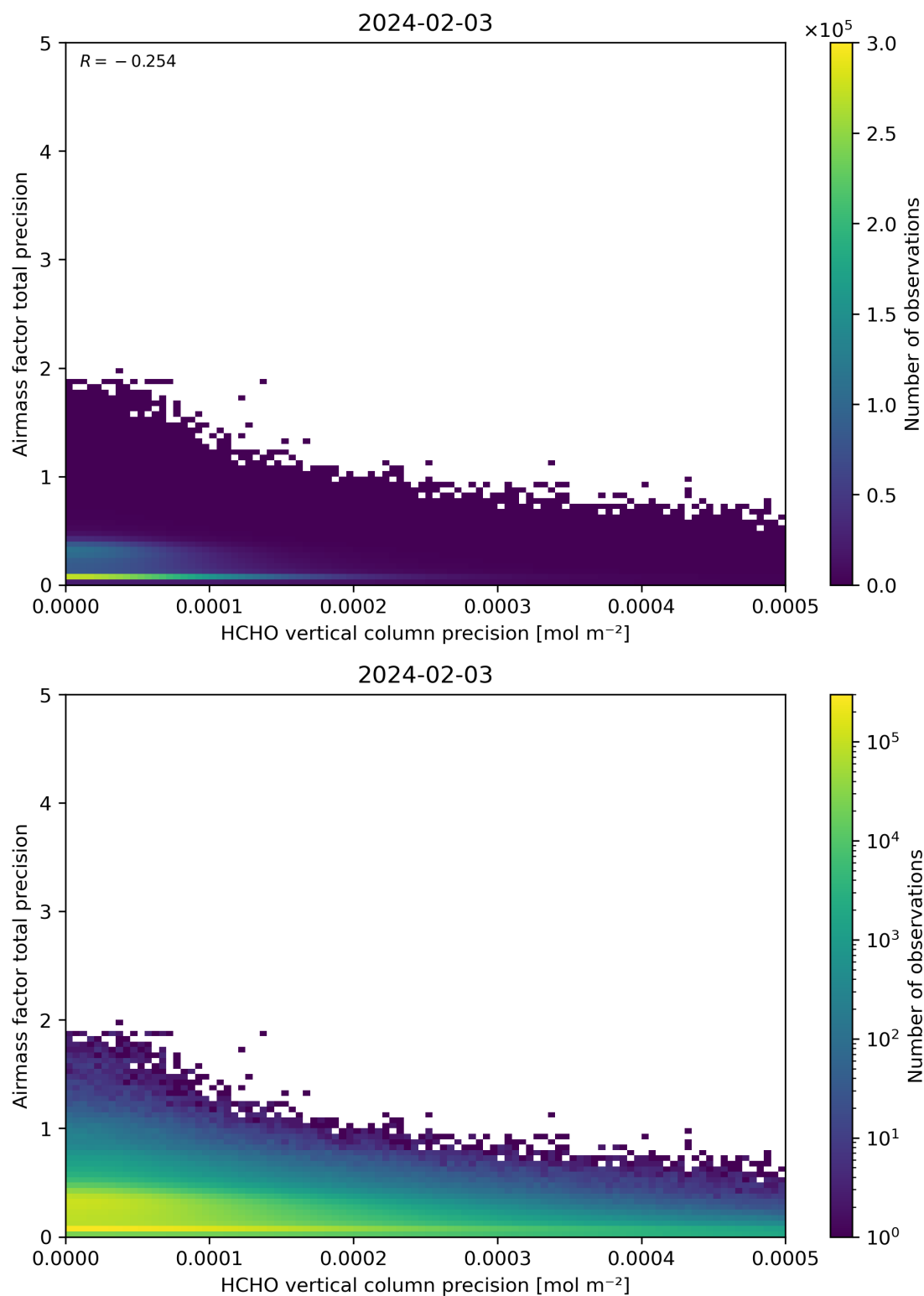
Figure 145: Scatter density plot of “HCHO vertical column precision” against “Airmass factor total precision” for 2024-02-02 to 2024-02-04.
