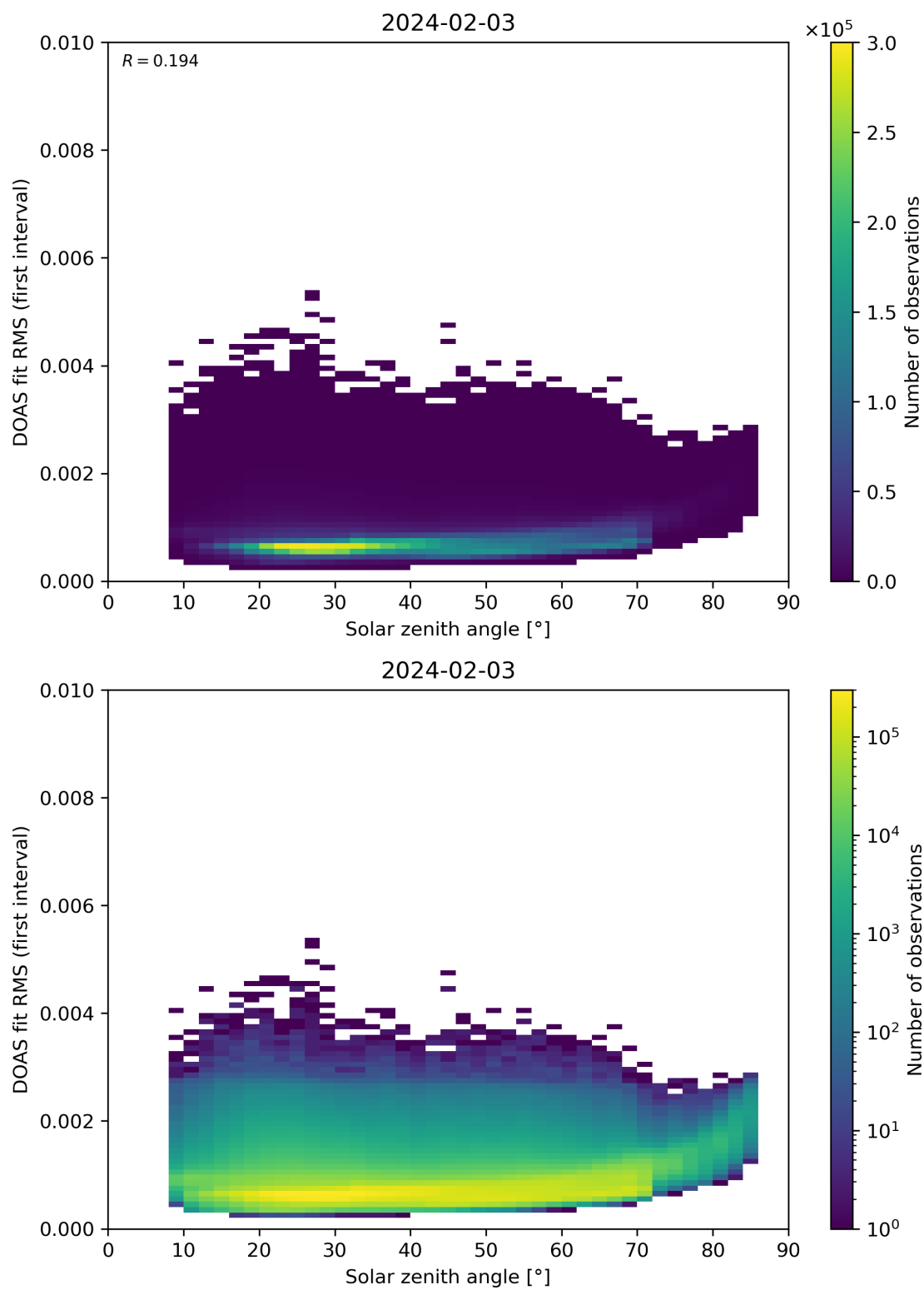
Figure 167: Scatter density plot of “Solar zenith angle” against “DOAS fit RMS (first interval)” for 2024-02-02 to 2024-02-04.
