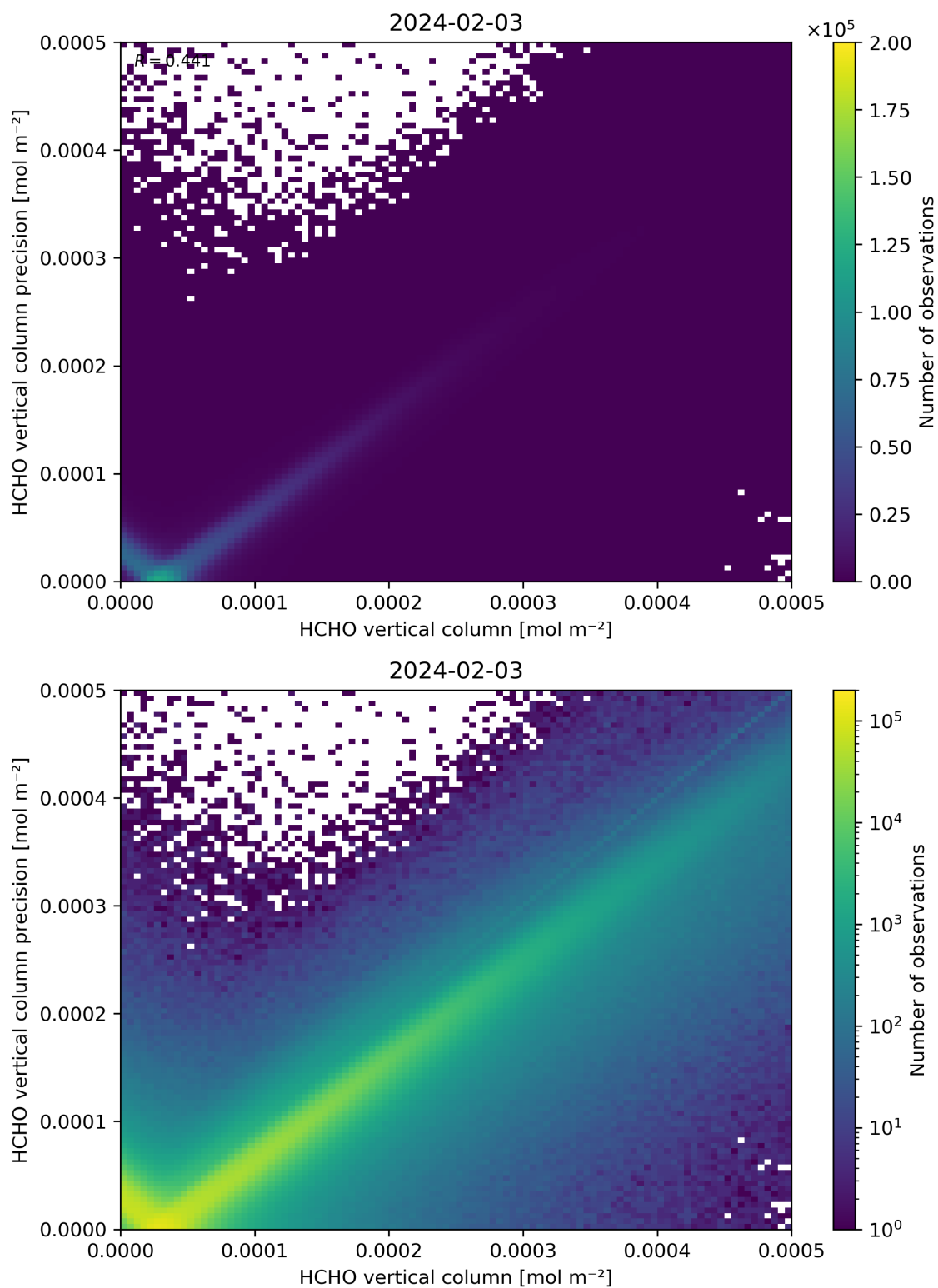
Figure 134: Scatter density plot of “HCHO vertical column” against “HCHO vertical column precision” for 2024-02-02 to 2024-02-04.
