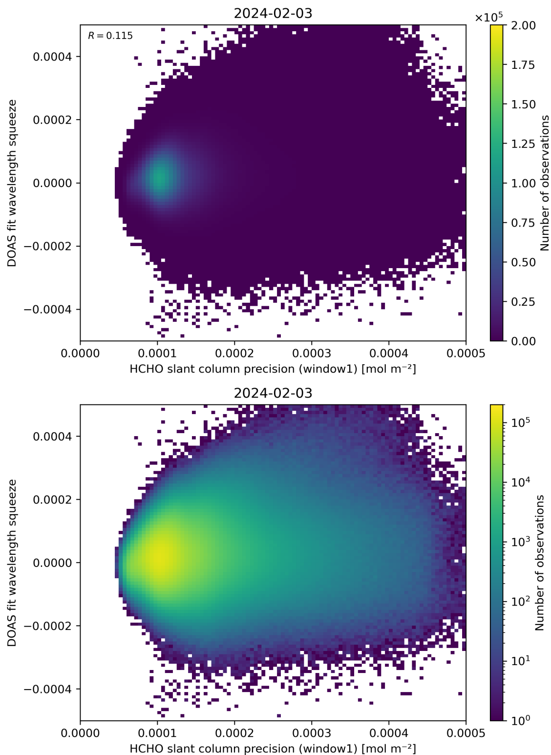
Figure 90: Scatter density plot of “HCHO slant column precision (window1)” against “DOAS fit wavelength squeeze” for 2024-02-02 to 2024-02-04.
