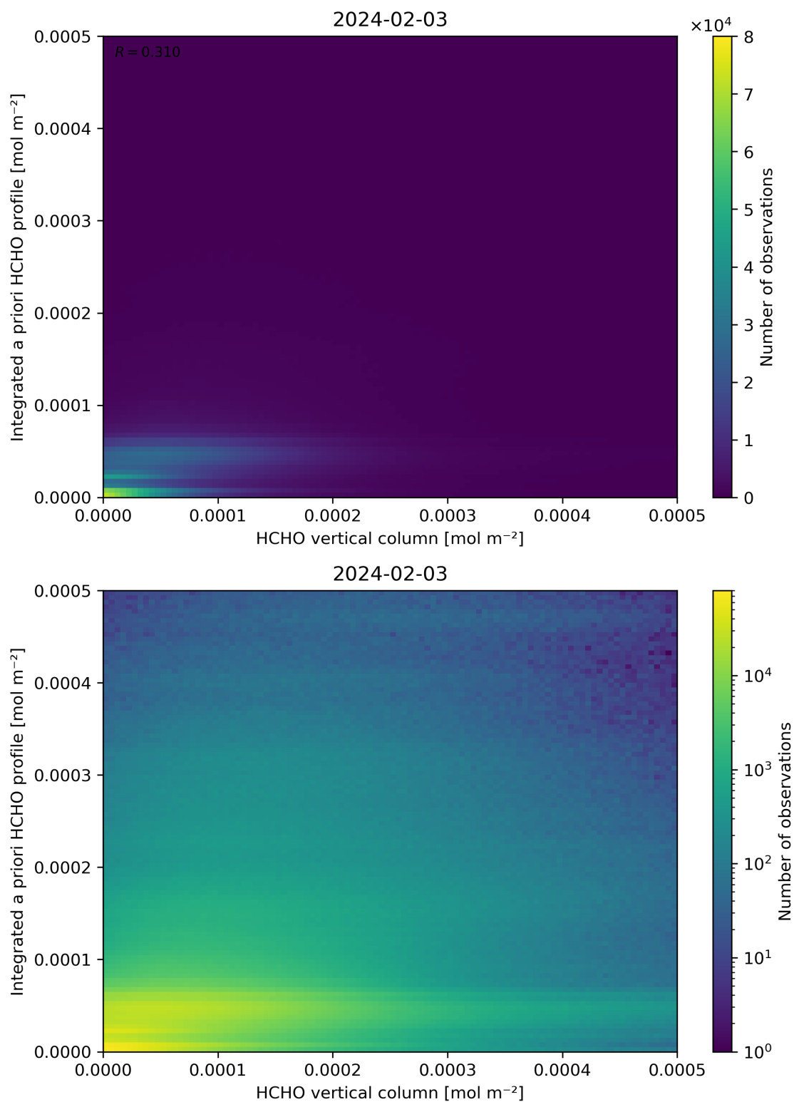
Figure 135: Scatter density plot of “HCHO vertical column” against “Integrated a priori HCHO profile” for 2024-02-02 to 2024-02-04.
