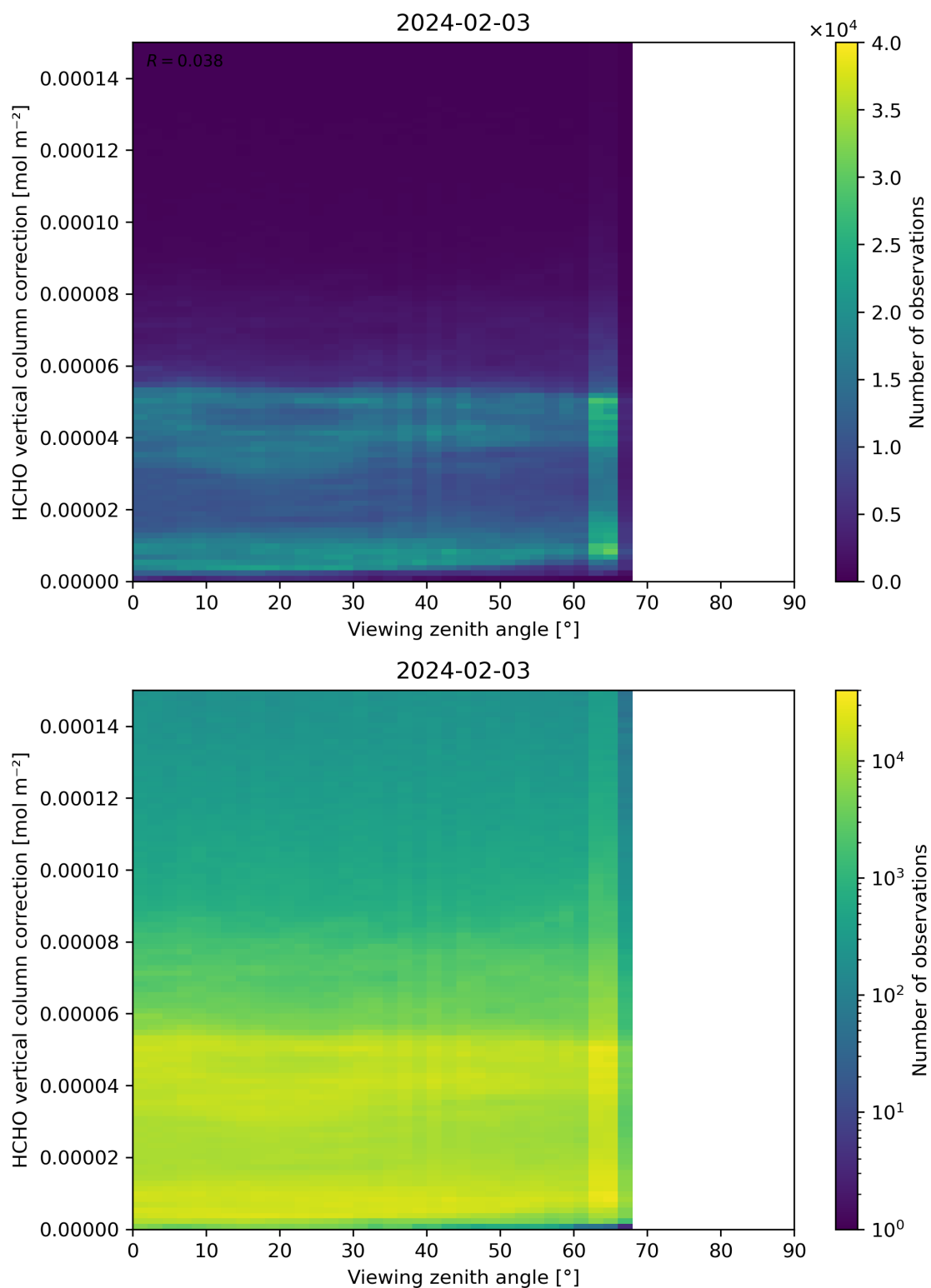
Figure 193: Scatter density plot of “Viewing zenith angle” against “HCHO vertical column correction” for 2024-02-02 to 2024-02-04.
