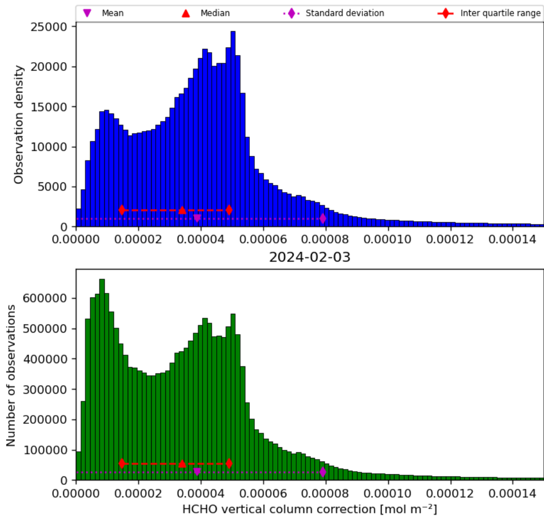
Figure 37: Histogram of “HCHO vertical column correction” for 2024-02-02 to 2024-02-04
