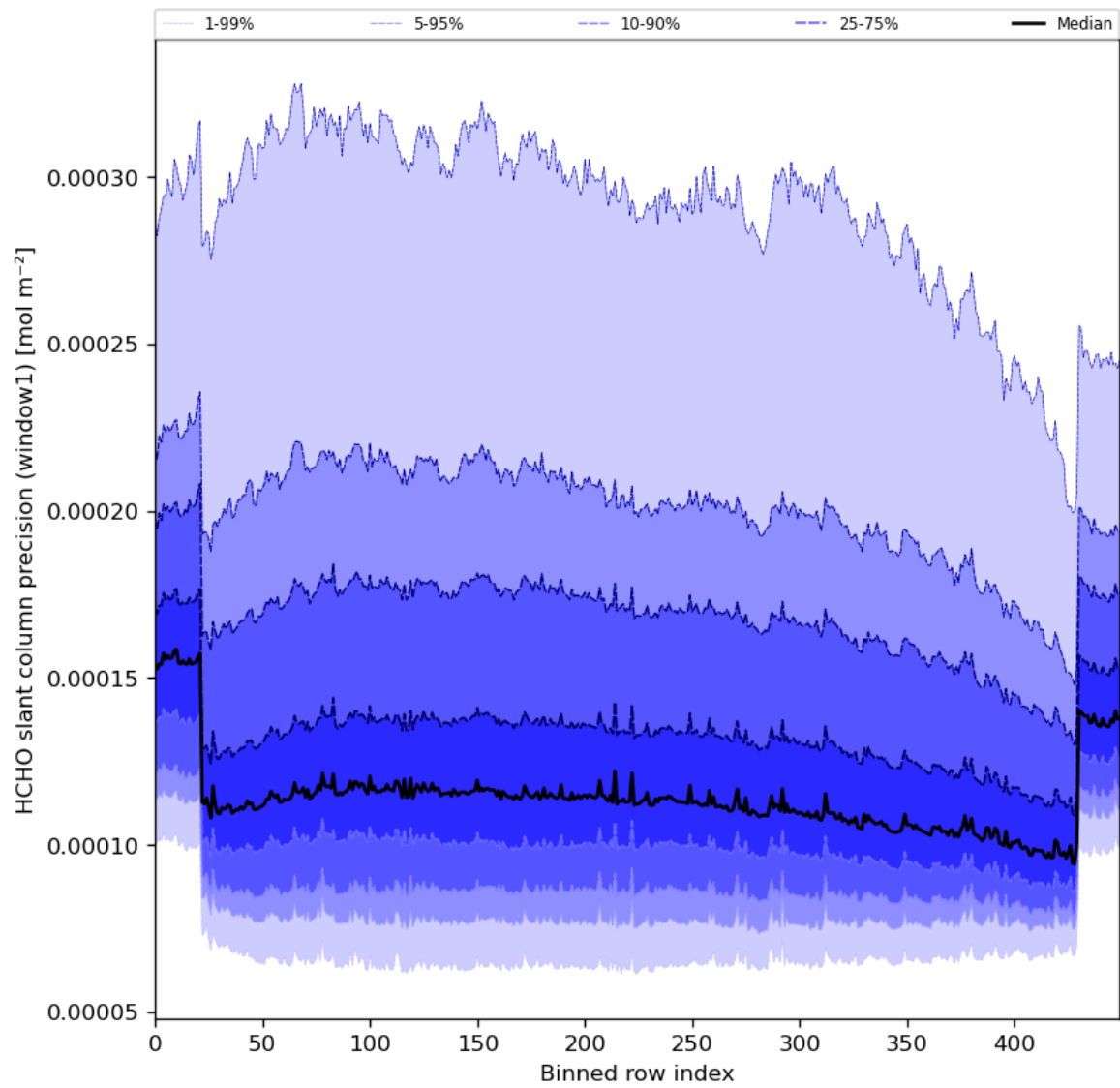
Figure 53: Along track statistics of “HCHO slant column precision (window1)” for 2024-02-02 to 2024-02-04
