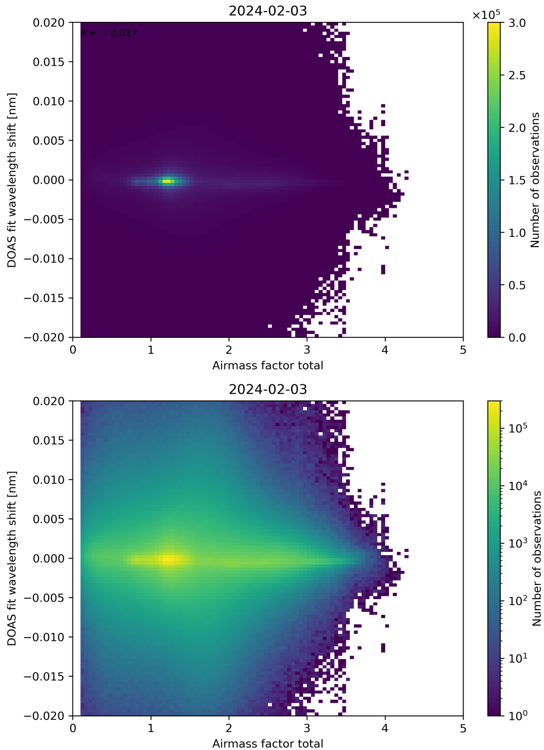
Figure 98: Scatter density plot of “Airmass factor total” against “DOAS fit wavelength shift” for 2024-02-02 to 2024-02-04.
