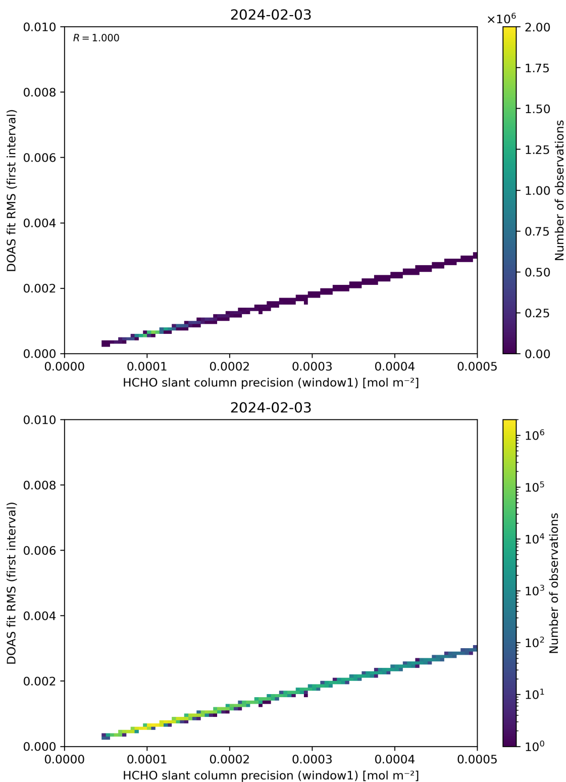
Figure 88: Scatter density plot of “HCHO slant column precision (window1)” against “DOAS fit RMS (first interval)” for 2024-02-02 to 2024-02-04.
