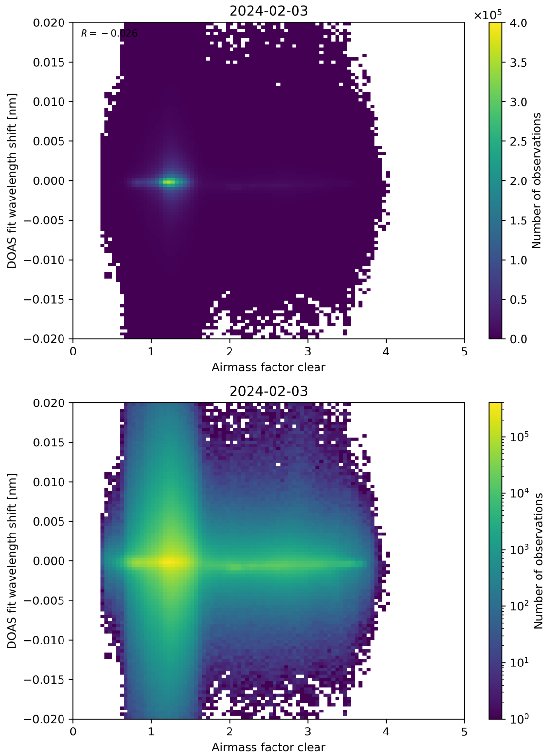
Figure 72: Scatter density plot of “Airmass factor clear” against “DOAS fit wavelength shift” for 2024-02-02 to 2024-02-04.
