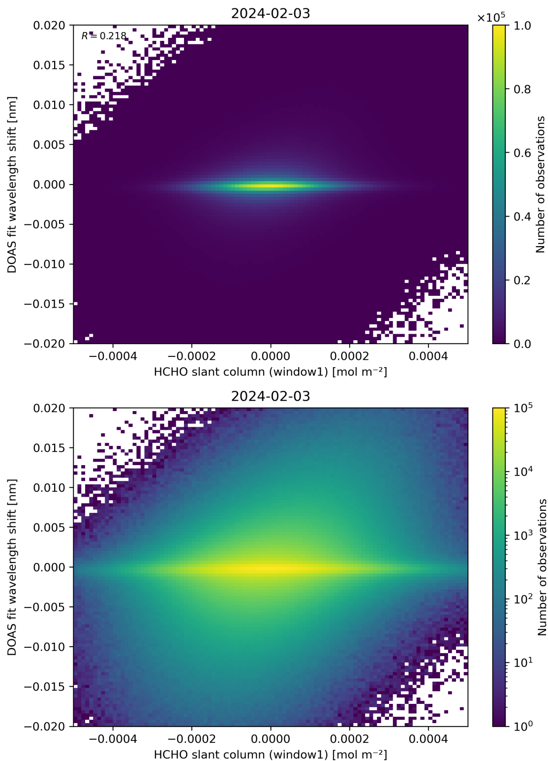
Figure 79: Scatter density plot of “HCHO slant column (window1)” against “DOAS fit wavelength shift” for 2024-02-02 to 2024-02-04.
