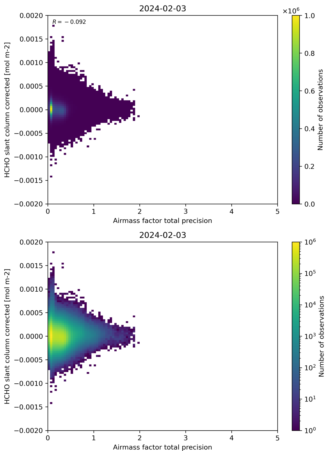
Figure 109: Scatter density plot of “Airmass factor total precision” against “HCHO slant column corrected” for 2024-02-02 to 2024-02-04.
