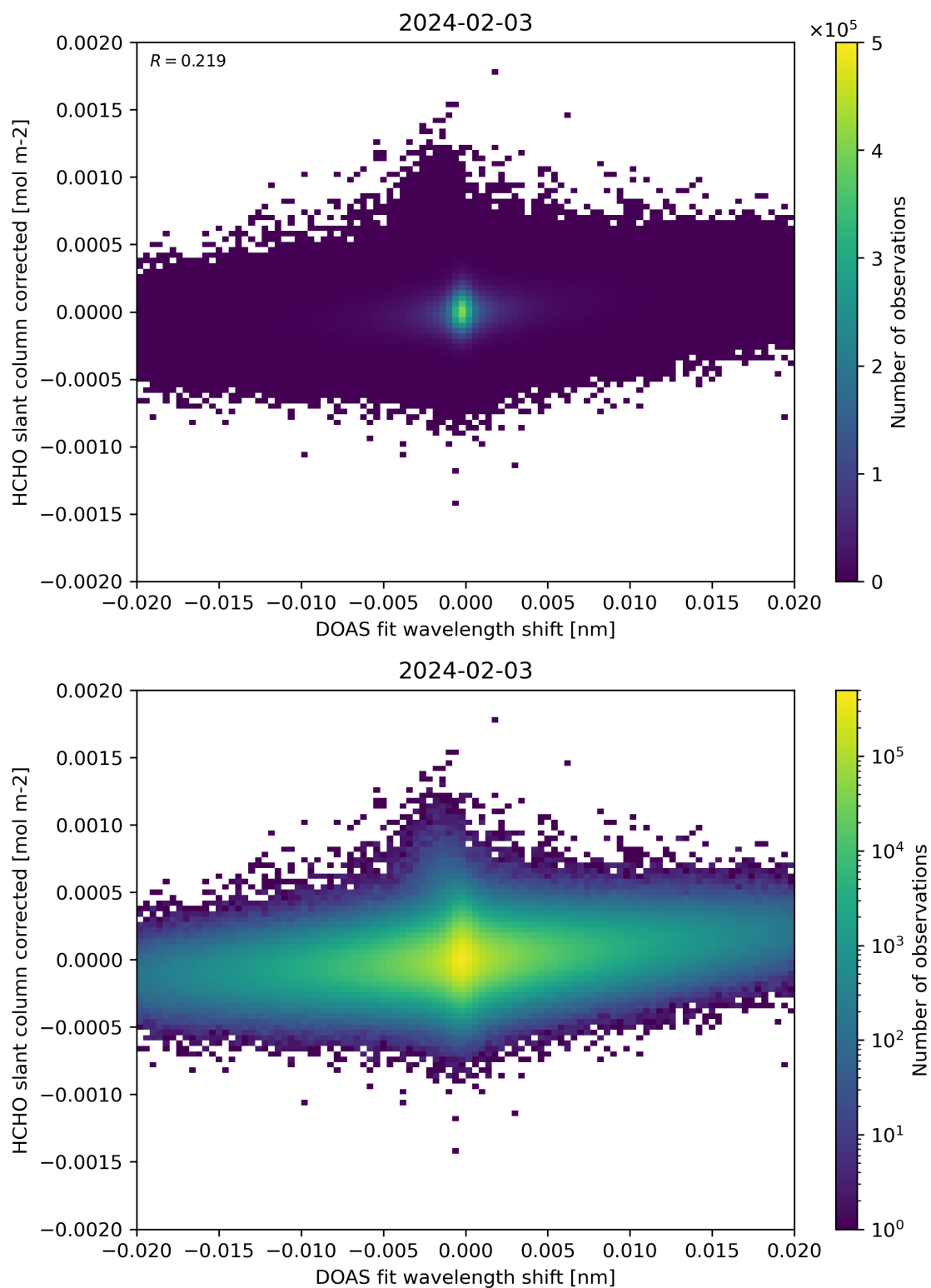
Figure 66: Scatter density plot of “DOAS fit wavelength shift” against “HCHO slant column corrected” for 2024-02-02 to 2024-02-04.
