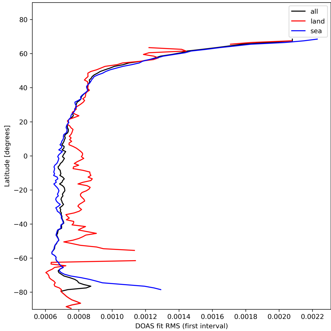
Figure 32: Zonal average of “DOAS fit RMS (first interval)” for 2024-02-02 to 2024-02-04.
