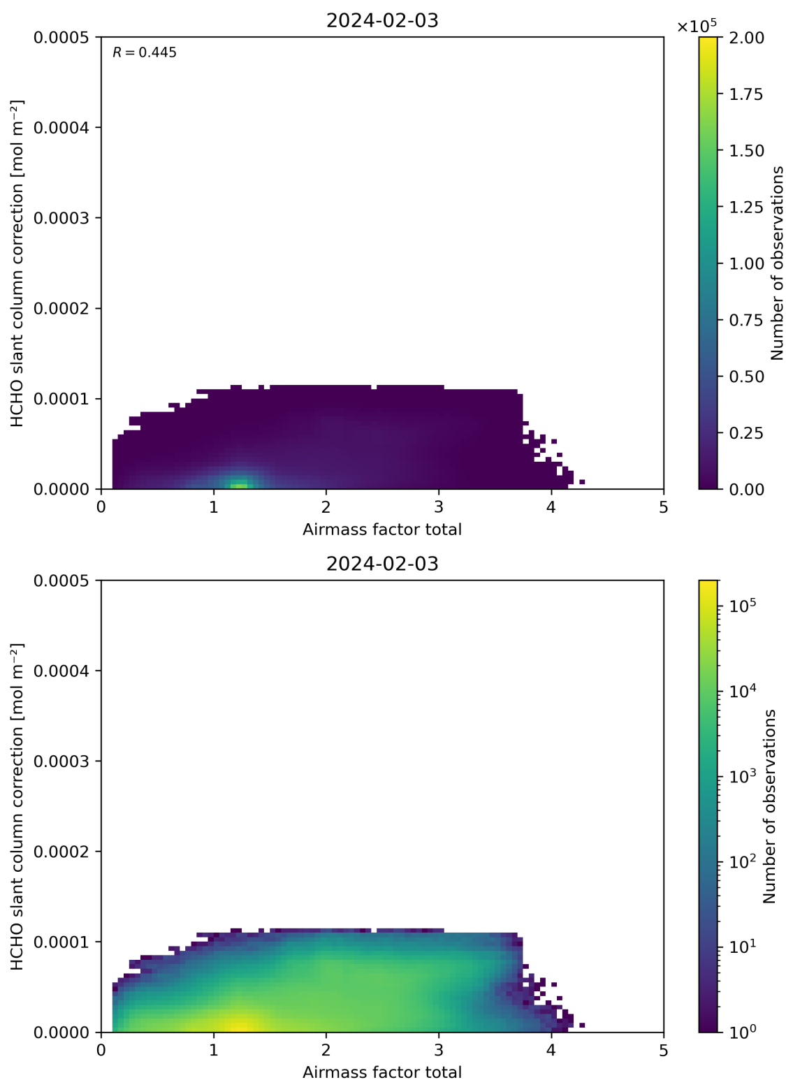
Figure 102: Scatter density plot of “Airmass factor total” against “HCHO slant column correction” for 2024-02-02 to 2024-02-04.
