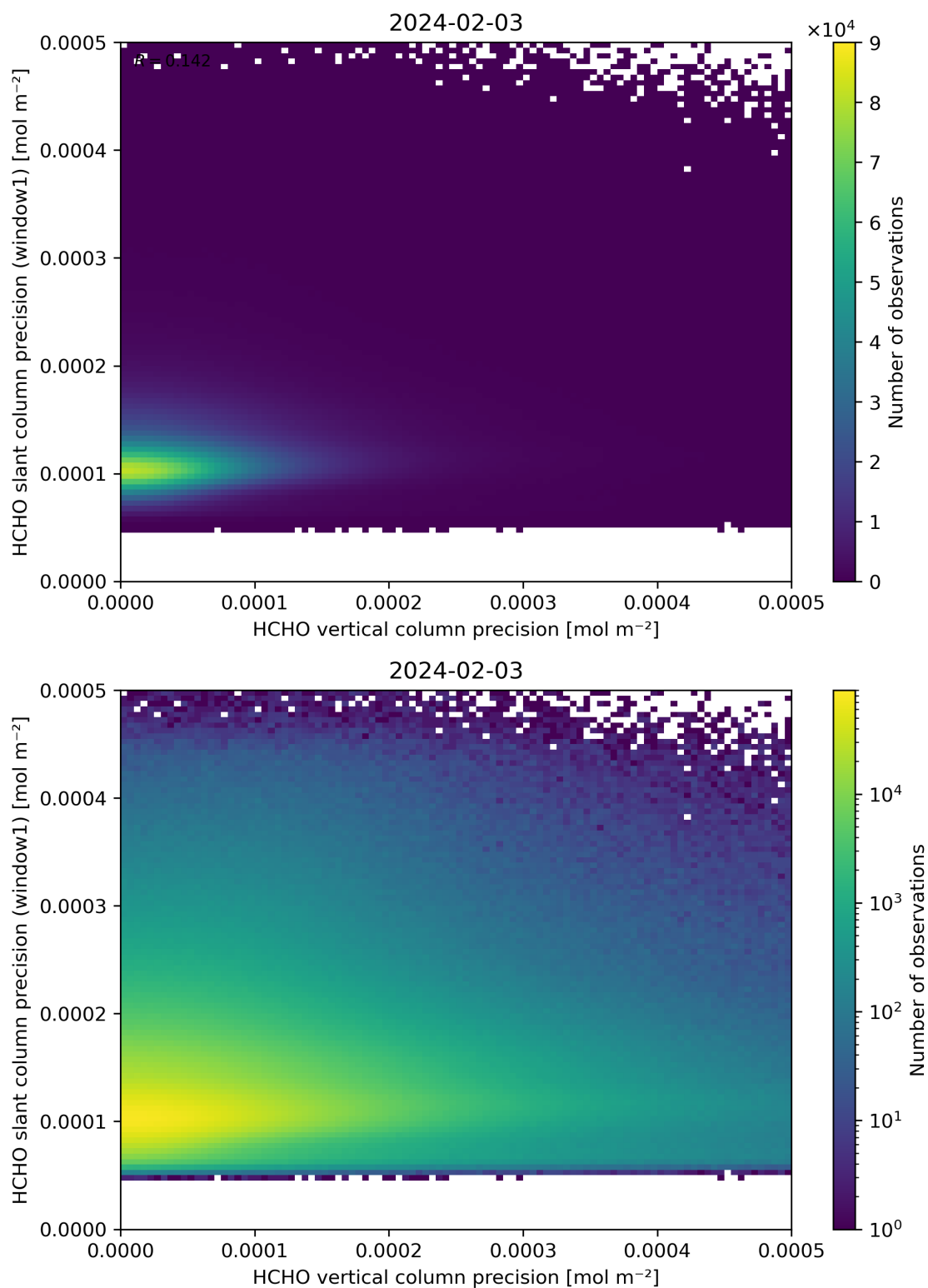
Figure 143: Scatter density plot of “HCHO vertical column precision” against “HCHO slant column precision (window1)” for 2024-02-02 to 2024-02-04.
