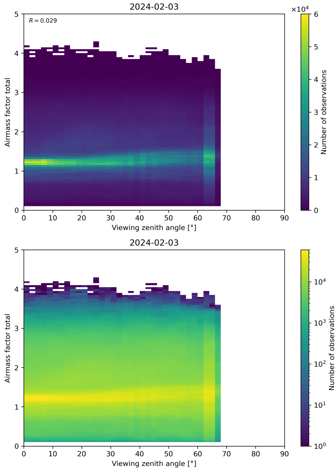
Figure 190: Scatter density plot of “Viewing zenith angle” against “Airmass factor total” for 2024-02-02 to 2024-02-04.
