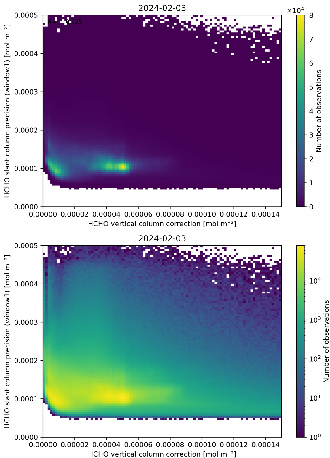
Figure 119: Scatter density plot of “HCHO vertical column correction” against “HCHO slant column precision (window1)” for 2024-02-02 to 2024-02-04.
