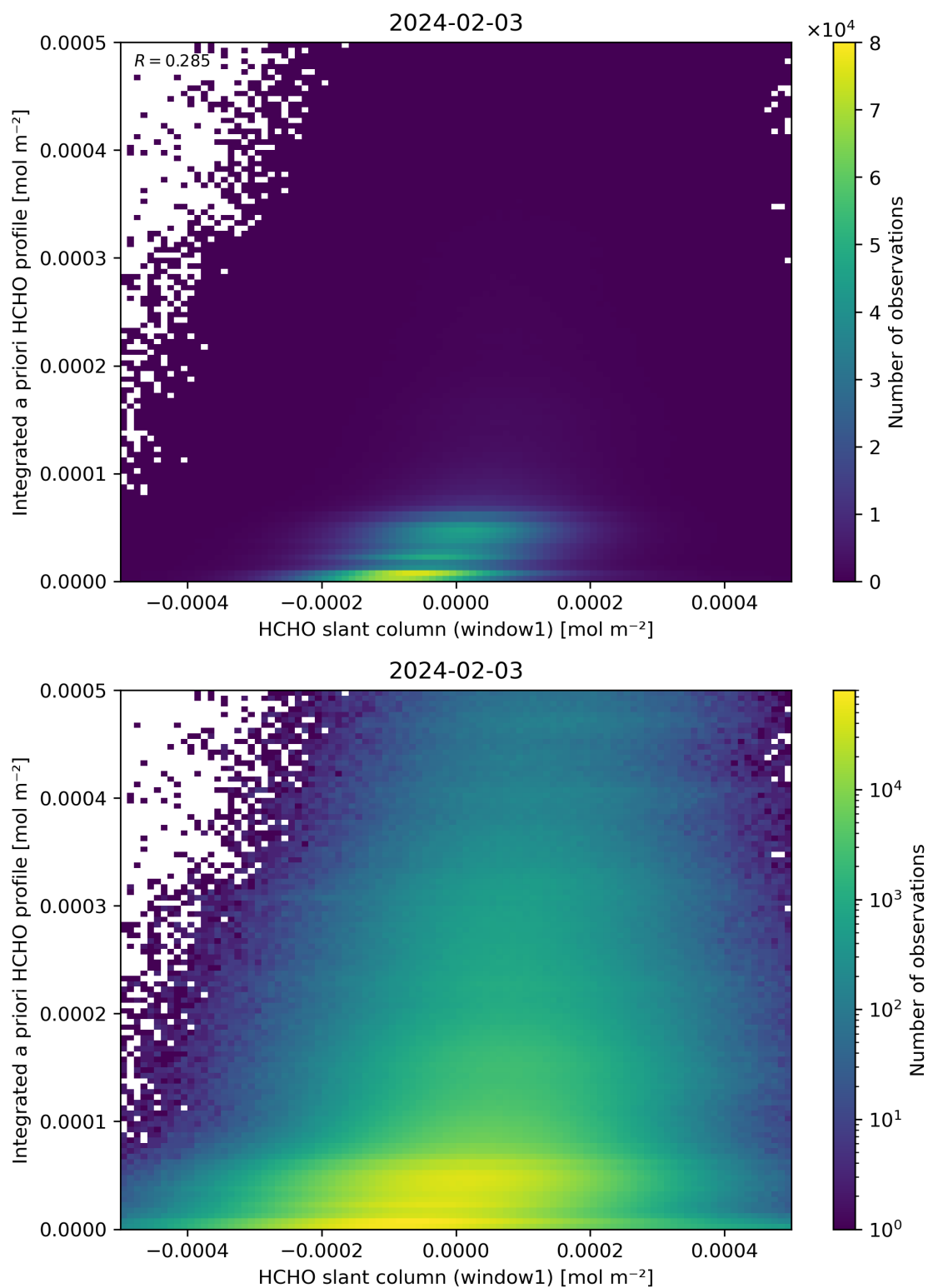
Figure 87: Scatter density plot of “HCHO slant column (window1)” against “Integrated a priori HCHO profile” for 2024-02-02 to 2024-02-04.
