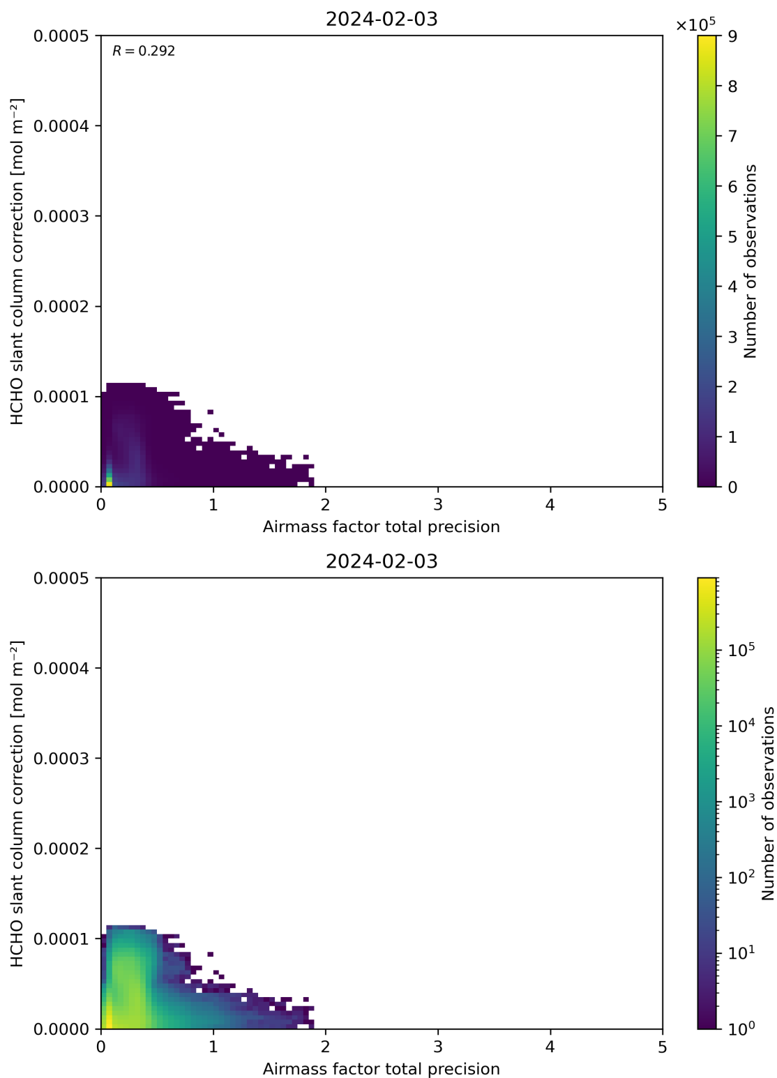
Figure 110: Scatter density plot of “Airmass factor total precision” against “HCHO slant column correction” for 2024-02-02 to 2024-02-04.
