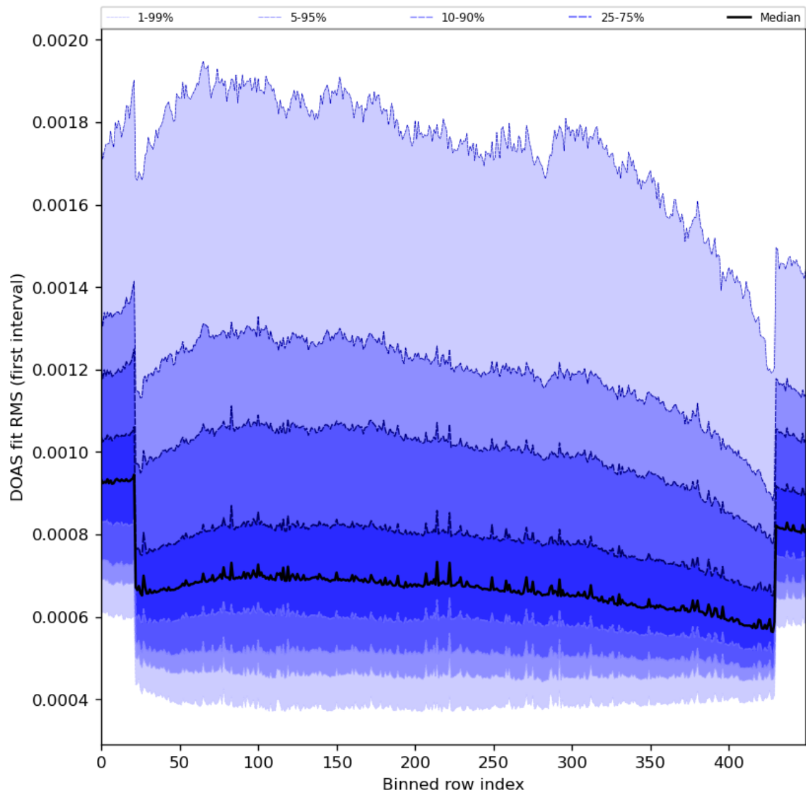
Figure 60: Along track statistics of “DOAS fit RMS (first interval)” for 2024-02-02 to 2024-02-04
