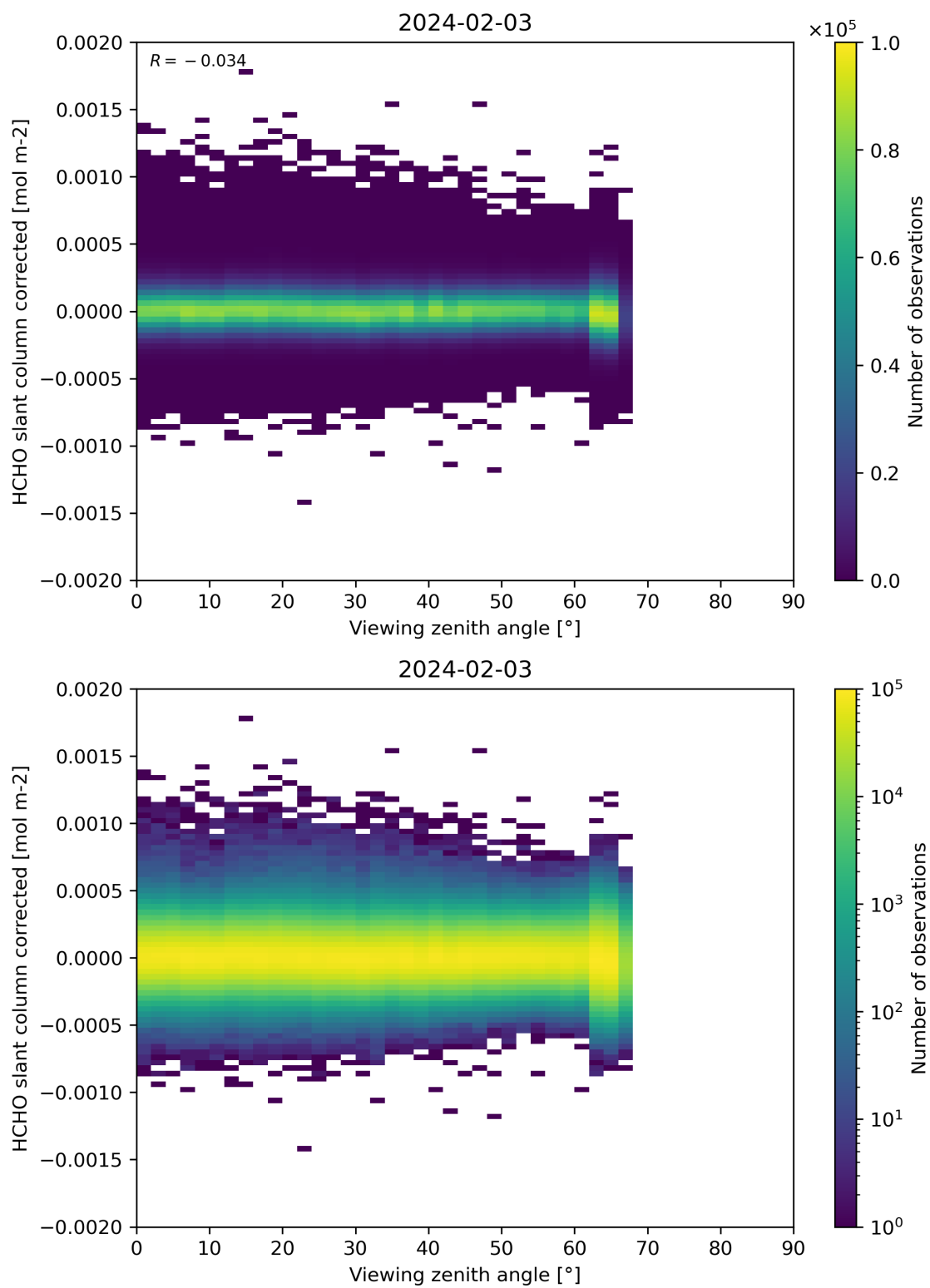
Figure 186: Scatter density plot of “Viewing zenith angle” against “HCHO slant column corrected” for 2024-02-02 to 2024-02-04.
