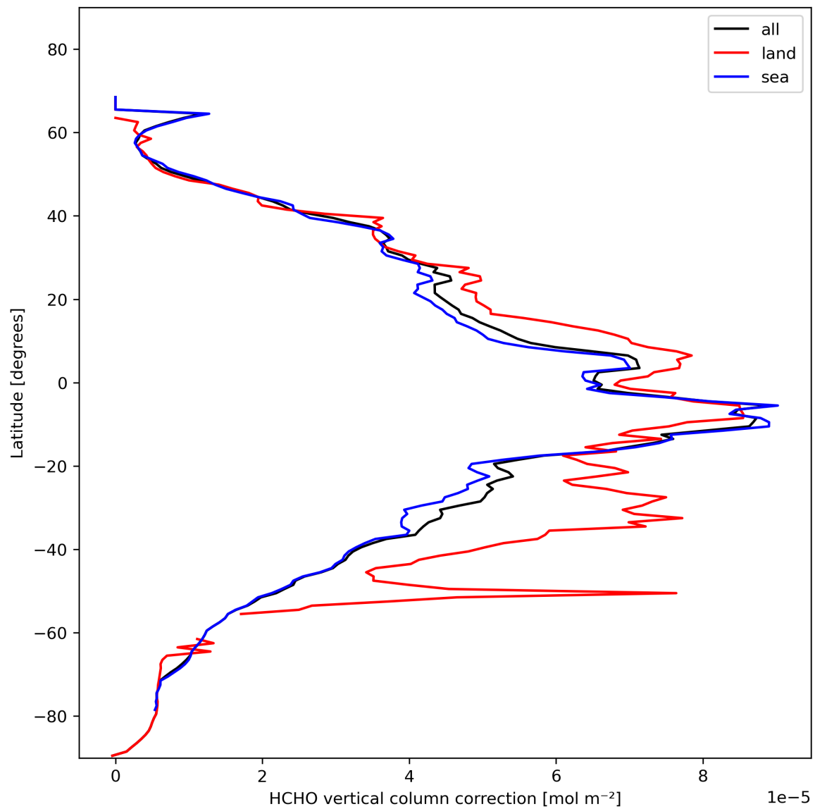
Figure 23: Zonal average of “HCHO vertical column correction” for 2024-02-02 to 2024-02-04.
