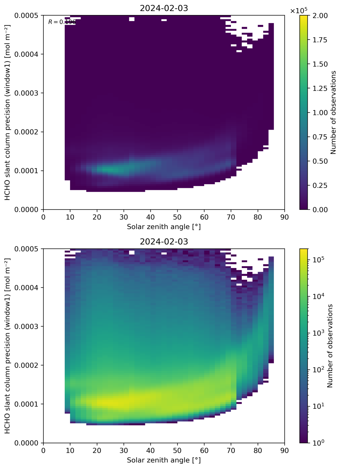
Figure 174: Scatter density plot of “Solar zenith angle” against “HCHO slant column precision (window1)” for 2024-02-02 to 2024-02-04.
