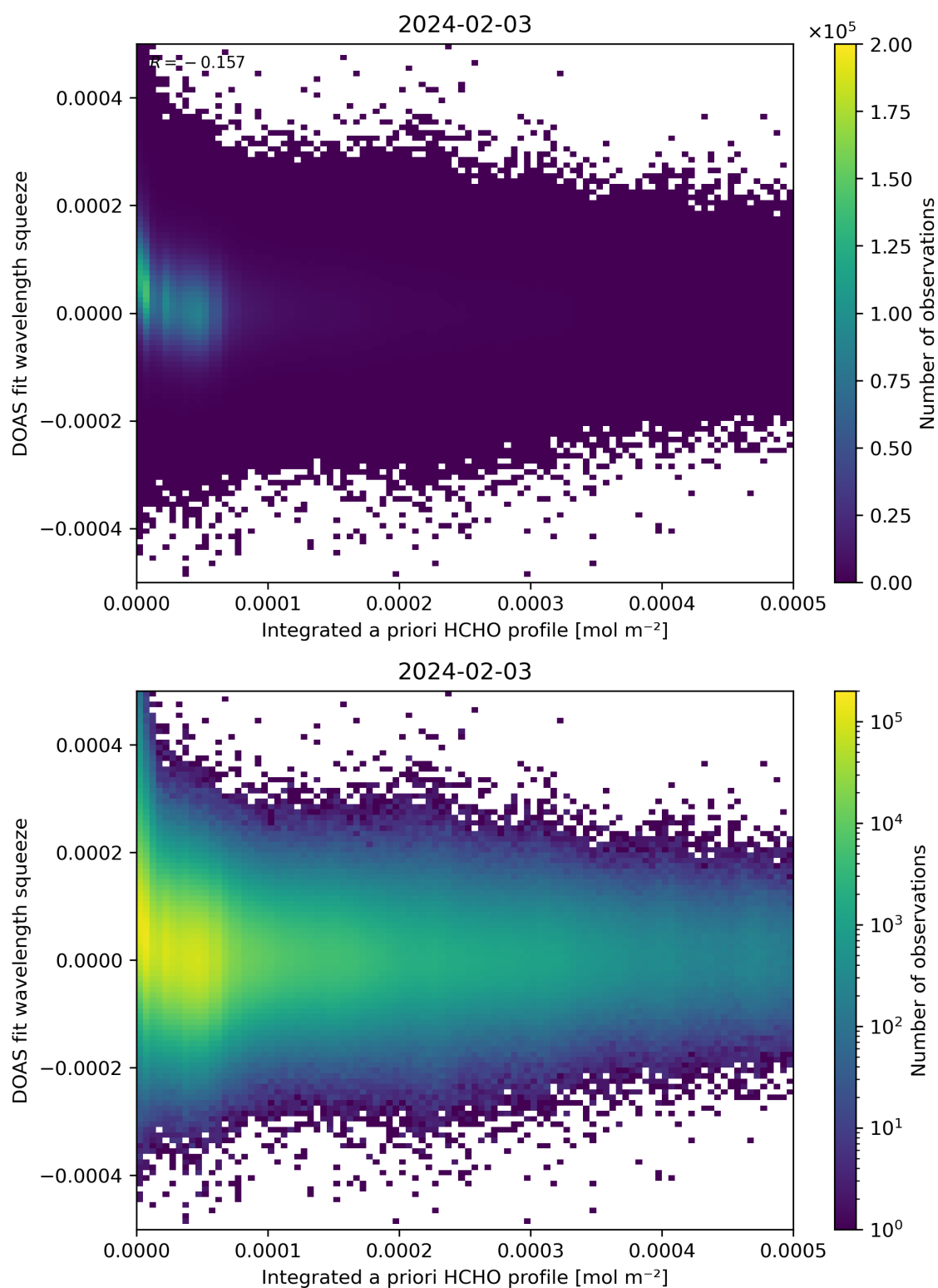
Figure 150: Scatter density plot of “Integrated a priori HCHO profile” against “DOAS fit wavelength squeeze” for 2024-02-02 to 2024-02-04.
