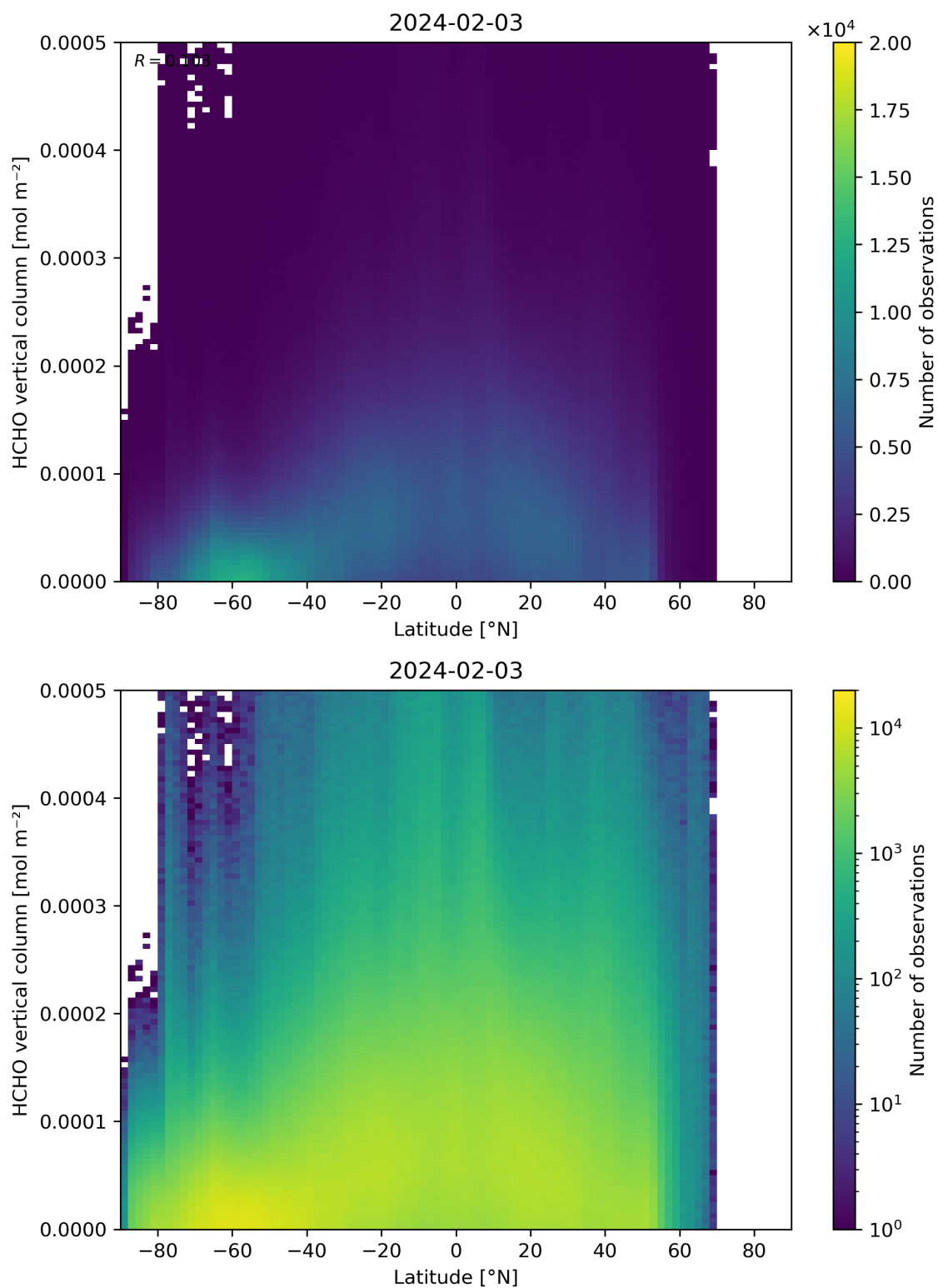
Figure 163: Scatter density plot of “Latitude” against “HCHO vertical column” for 2024-02-02 to 2024-02-04.
