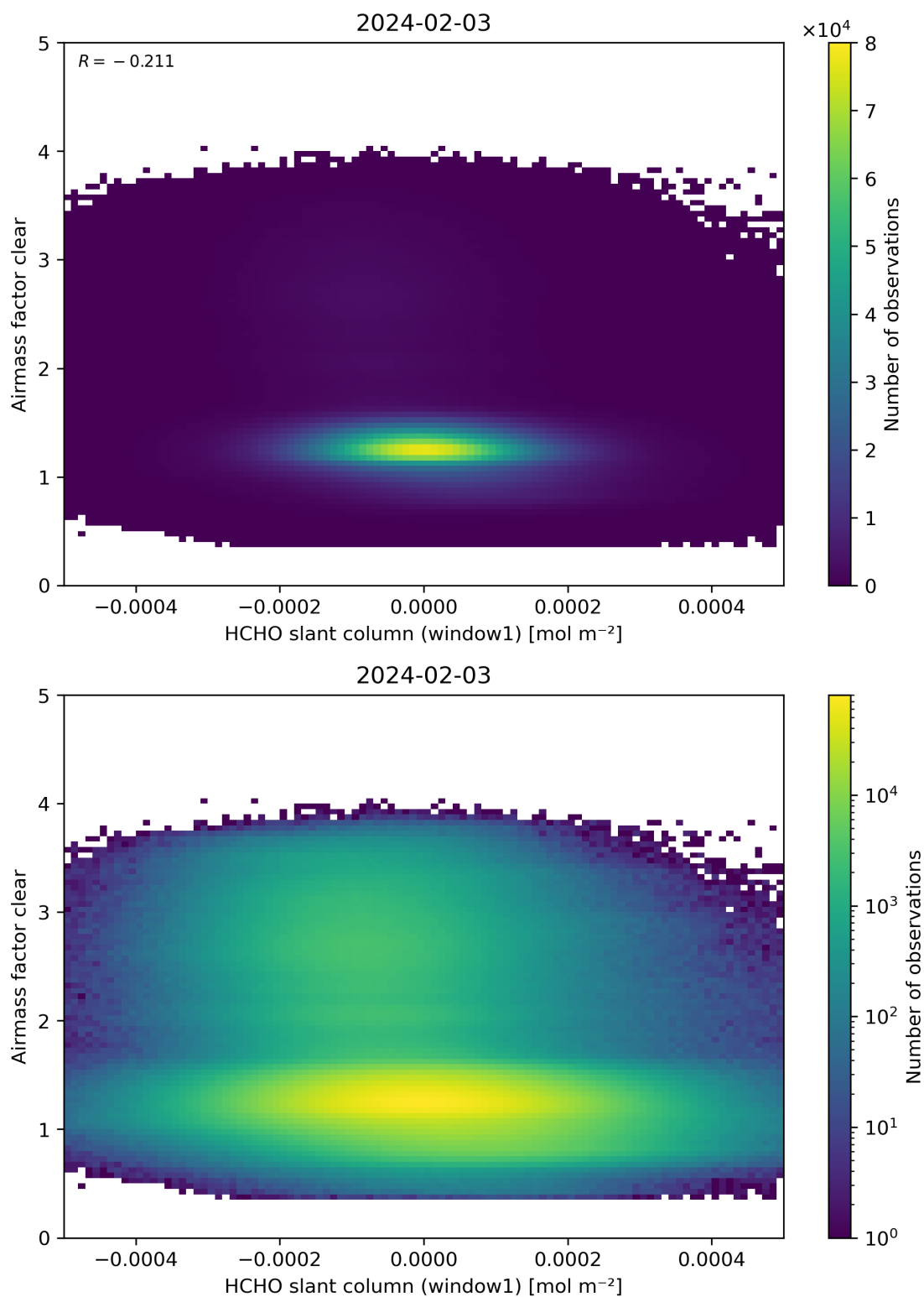
Figure 81: Scatter density plot of “HCHO slant column (window1)” against “Airmass factor clear” for 2024-02-02 to 2024-02-04.
