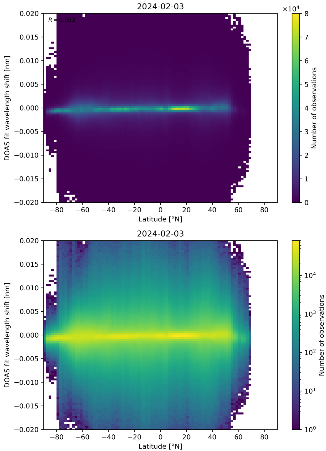
Figure 154: Scatter density plot of “Latitude” against “DOAS fit wavelength shift” for 2024-02-02 to 2024-02-04.
