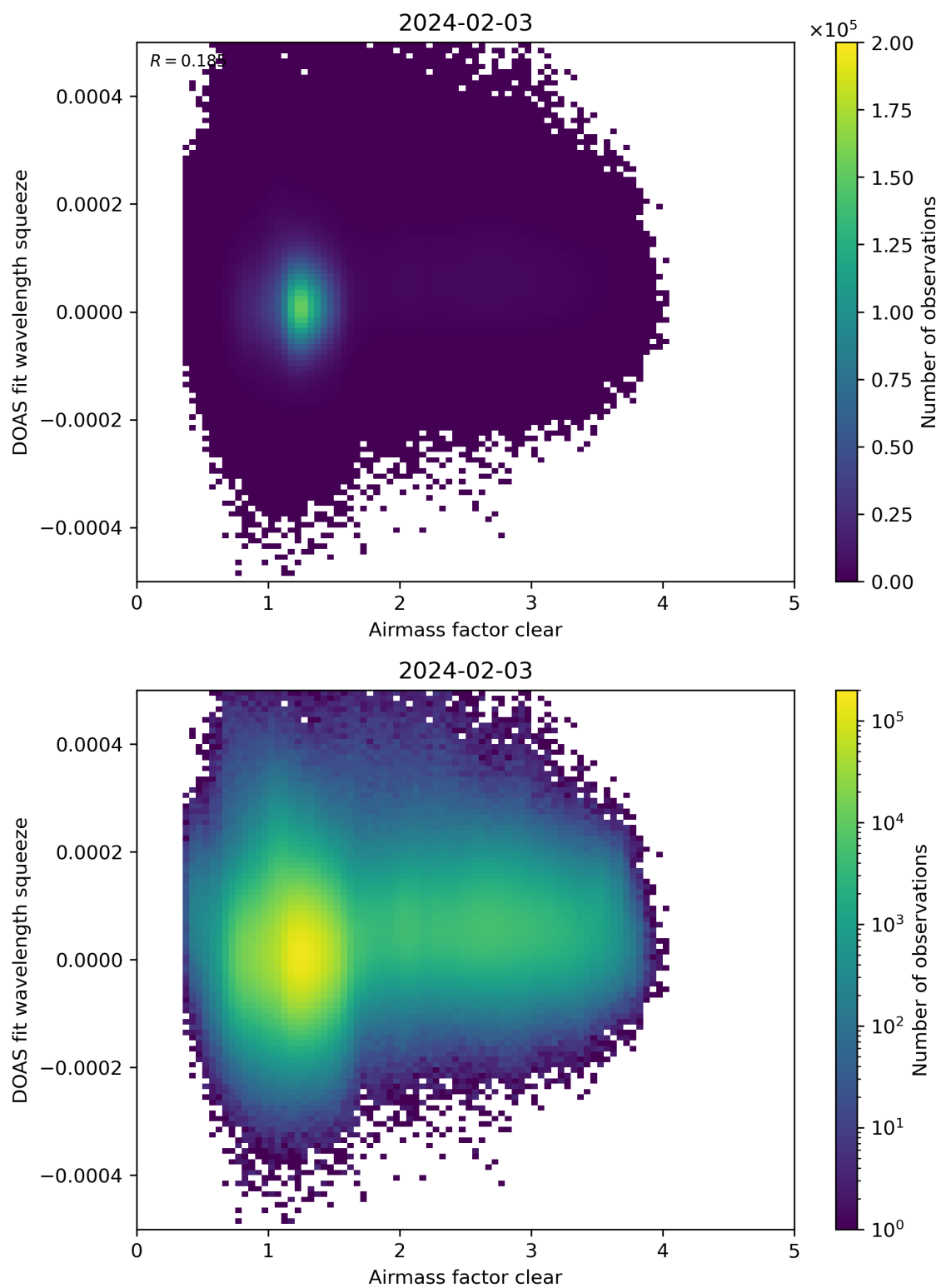
Figure 73: Scatter density plot of “Airmass factor clear” against “DOAS fit wavelength squeeze” for 2024-02-02 to 2024-02-04.
