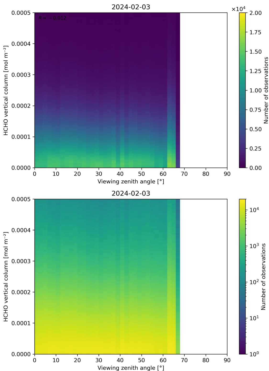
Figure 192: Scatter density plot of “Viewing zenith angle” against “HCHO vertical column” for 2024-02-02 to 2024-02-04.
