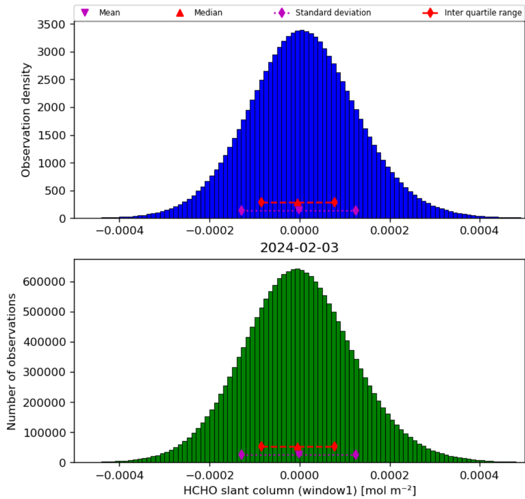
Figure 38: Histogram of “HCHO slant column (window1)” for 2024-02-02 to 2024-02-04
