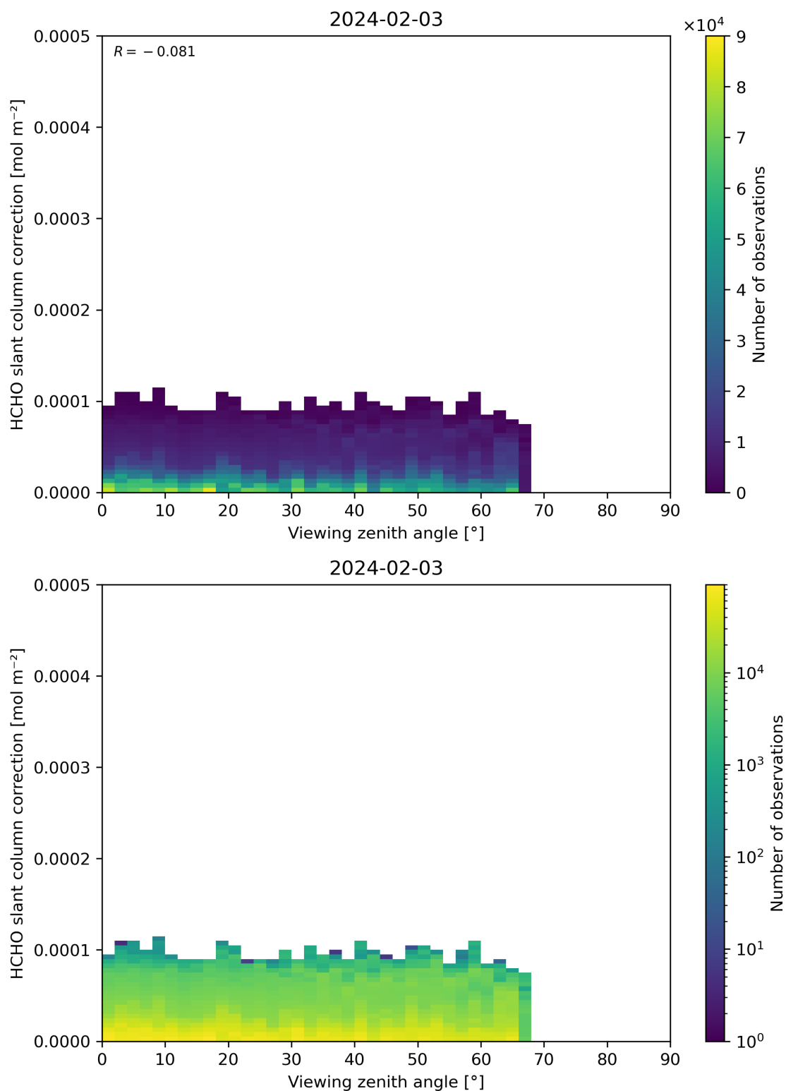
Figure 187: Scatter density plot of “Viewing zenith angle” against “HCHO slant column correction” for 2024-02-02 to 2024-02-04.
