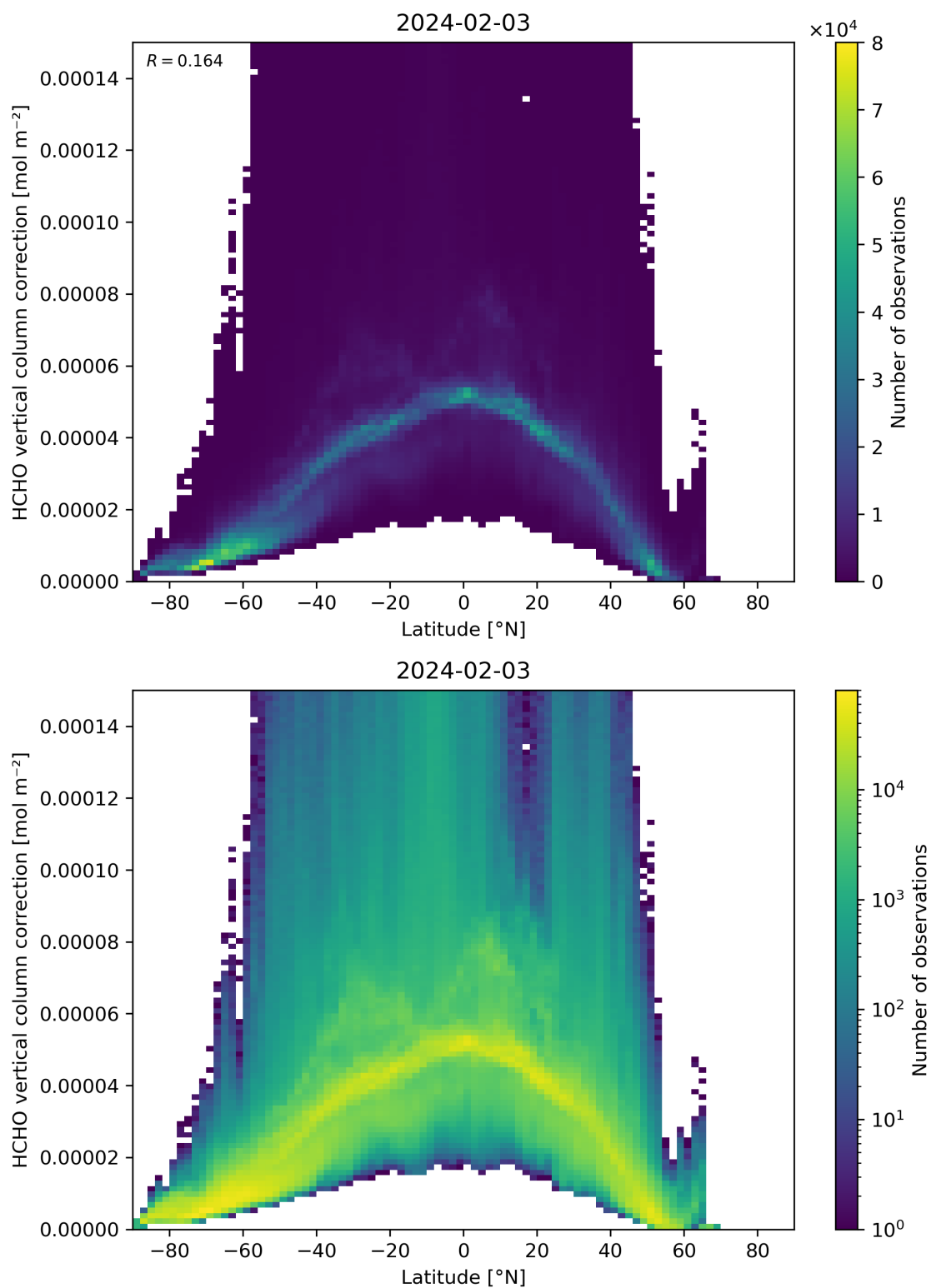
Figure 164: Scatter density plot of “Latitude” against “HCHO vertical column correction” for 2024-02-02 to 2024-02-04.
