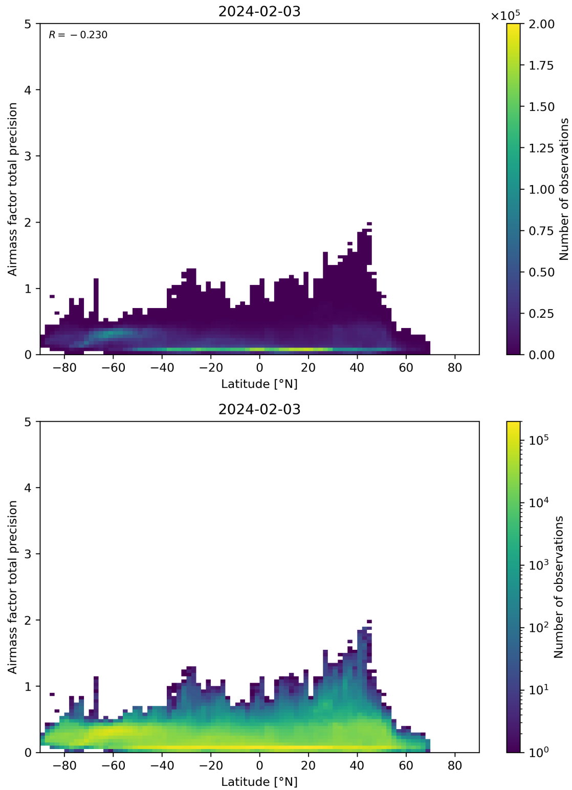
Figure 162: Scatter density plot of “Latitude” against “Airmass factor total precision” for 2024-02-02 to 2024-02-04.
