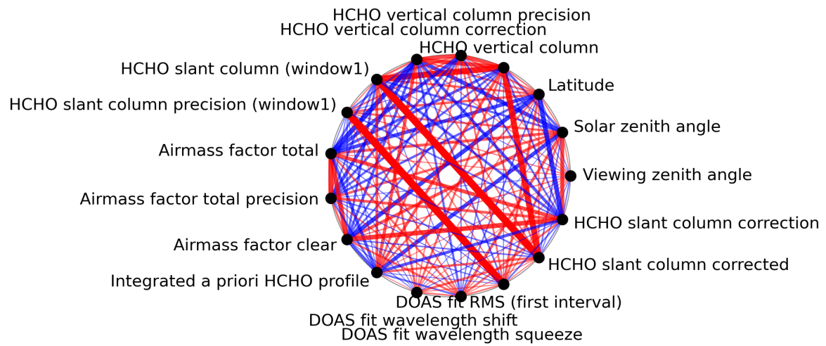
Figure 1: Map of correlation graph for 2024-02-02 to 2024-02-04.
