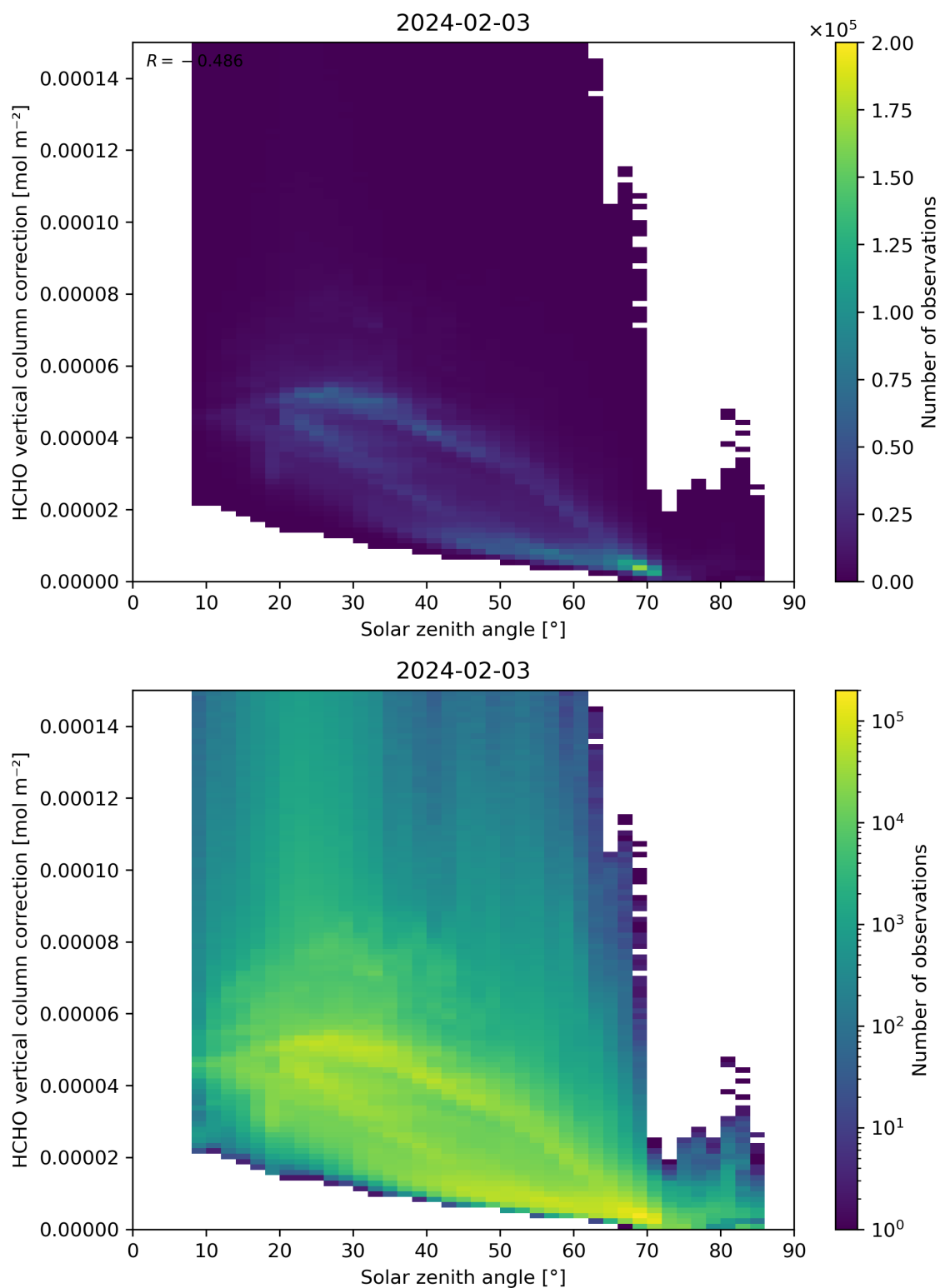
Figure 178: Scatter density plot of “Solar zenith angle” against “HCHO vertical column correction” for 2024-02-02 to 2024-02-04.
