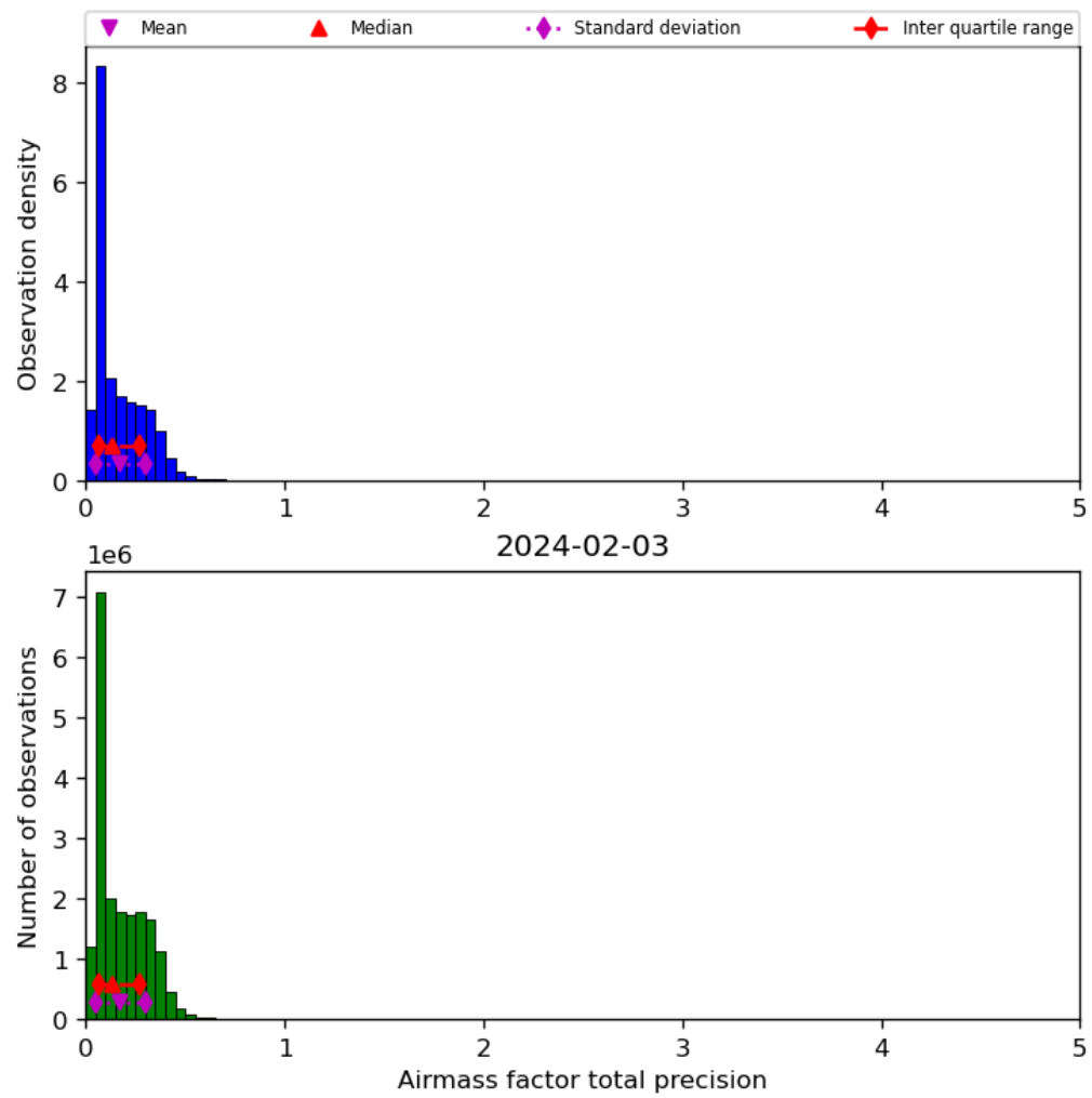
Figure 41: Histogram of “Airmass factor total precision” for 2024-02-02 to 2024-02-04
