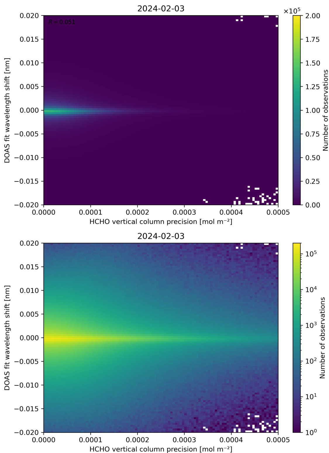
Figure 137: Scatter density plot of “HCHO vertical column precision” against “DOAS fit wavelength shift” for 2024-02-02 to 2024-02-04.
