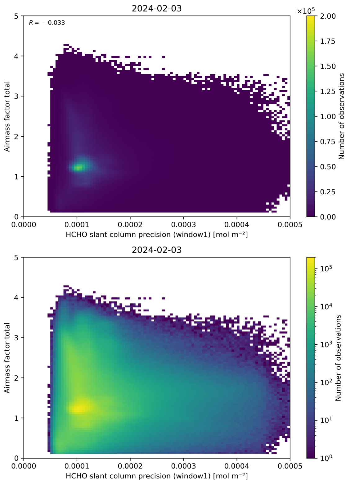
Figure 94: Scatter density plot of “HCHO slant column precision (window1)” against “Airmass factor total” for 2024-02-02 to 2024-02-04.
