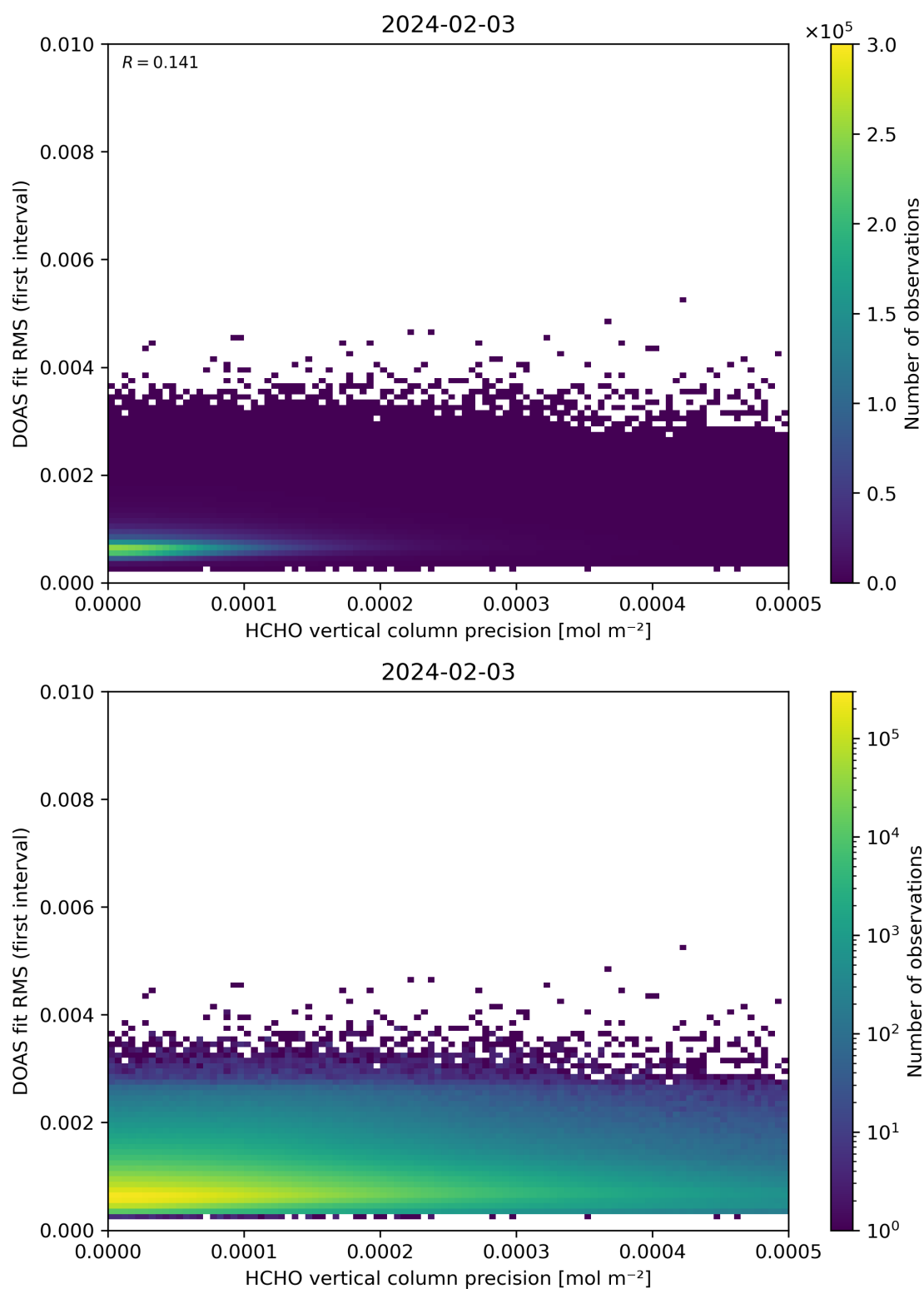
Figure 136: Scatter density plot of “HCHO vertical column precision” against “DOAS fit RMS (first interval)” for 2024-02-02 to 2024-02-04.
