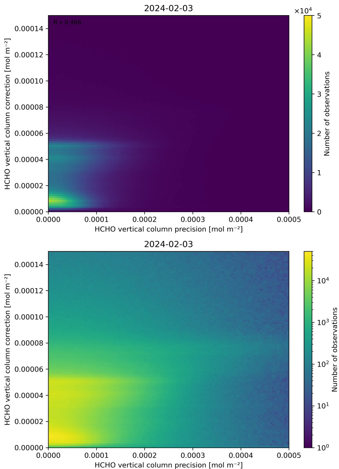
Figure 146: Scatter density plot of “HCHO vertical column precision” against “HCHO vertical column correction” for 2024-02-02 to 2024-02-04.
