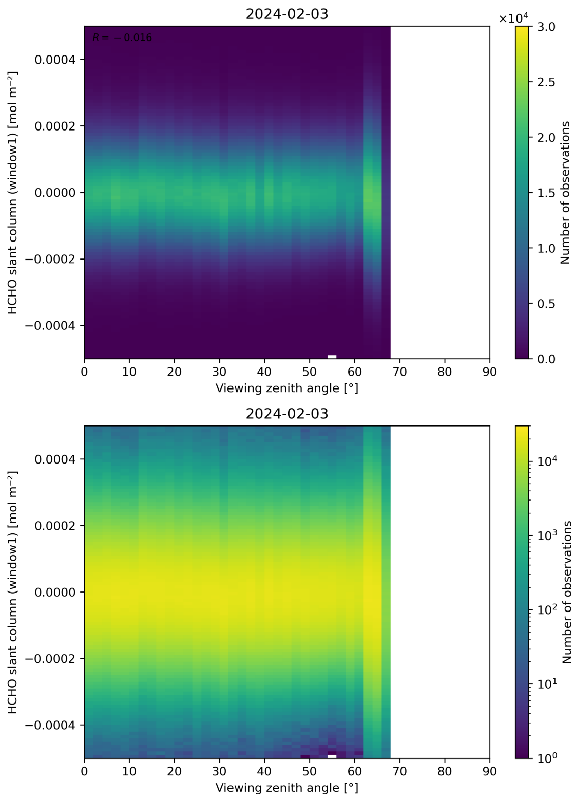
Figure 188: Scatter density plot of “Viewing zenith angle” against “HCHO slant column (window1)” for 2024-02-02 to 2024-02-04.
