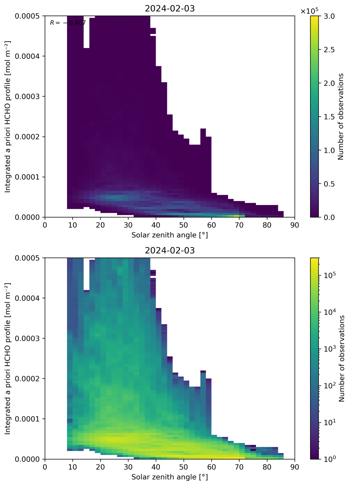
Figure 180: Scatter density plot of “Solar zenith angle” against “Integrated a priori HCHO profile” for 2024-02-02 to 2024-02-04.
