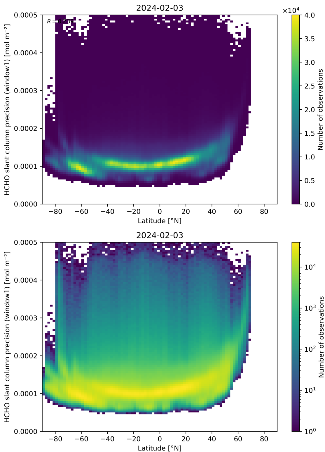
Figure 160: Scatter density plot of “Latitude” against “HCHO slant column precision (window1)” for 2024-02-02 to 2024-02-04.
