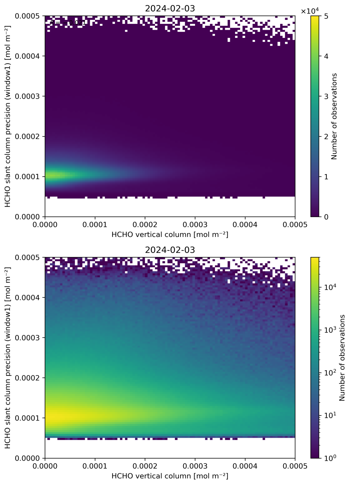
Figure 130: Scatter density plot of “HCHO vertical column” against “HCHO slant column precision (window1)” for 2024-02-02 to 2024-02-04.
