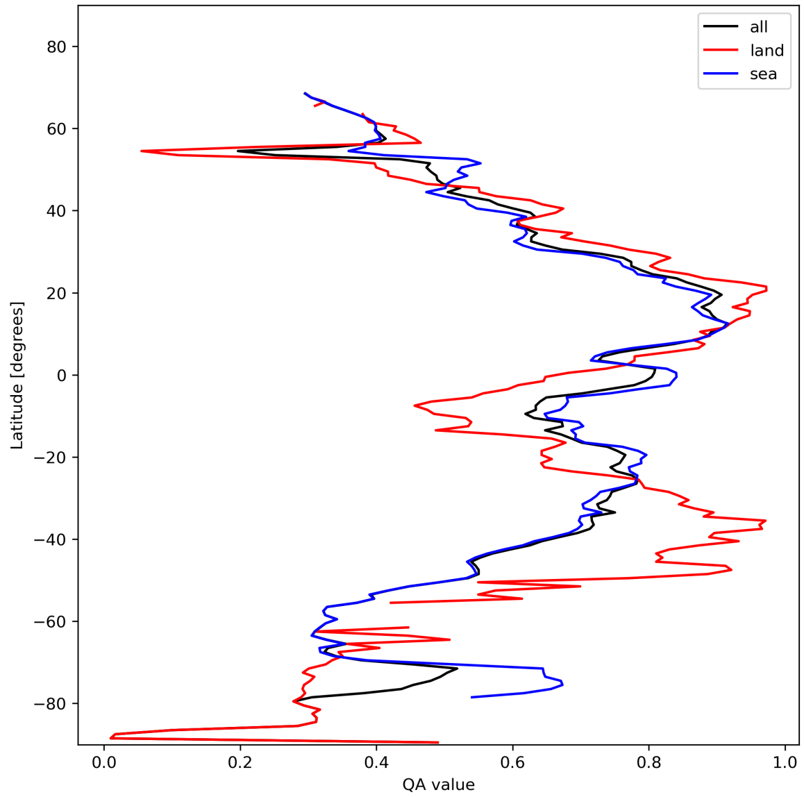
Figure 20: Zonal average of “QA value” for 2024-02-02 to 2024-02-04.
