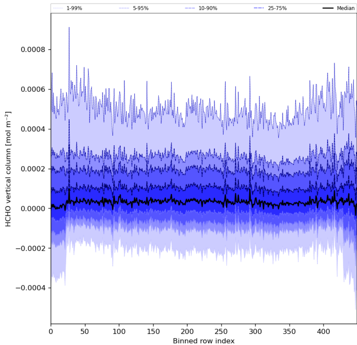
Figure 49: Along track statistics of “HCHO vertical column” for 2024-02-02 to 2024-02-04
