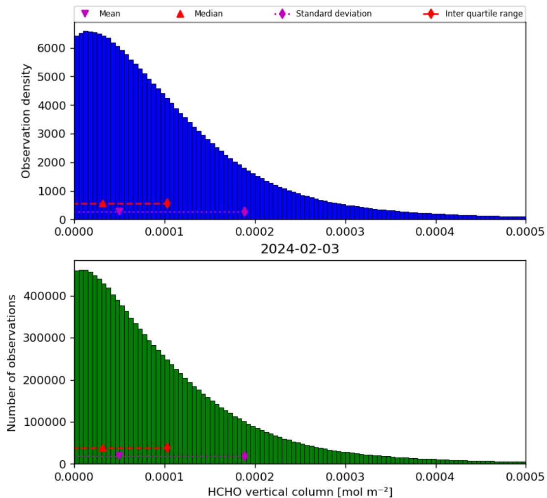
Figure 35: Histogram of “HCHO vertical column” for 2024-02-02 to 2024-02-04
