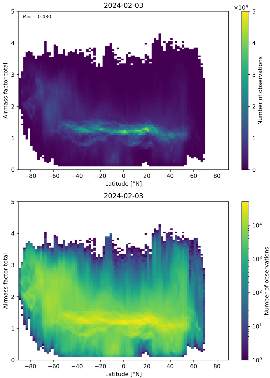
Figure 161: Scatter density plot of “Latitude” against “Airmass factor total” for 2024-02-02 to 2024-02-04.
