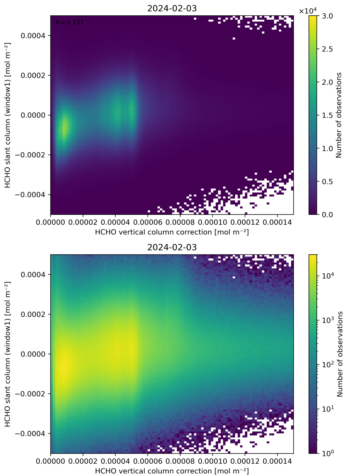
Figure 118: Scatter density plot of “HCHO vertical column correction” against “HCHO slant column (window1)” for 2024-02-02 to 2024-02-04.
