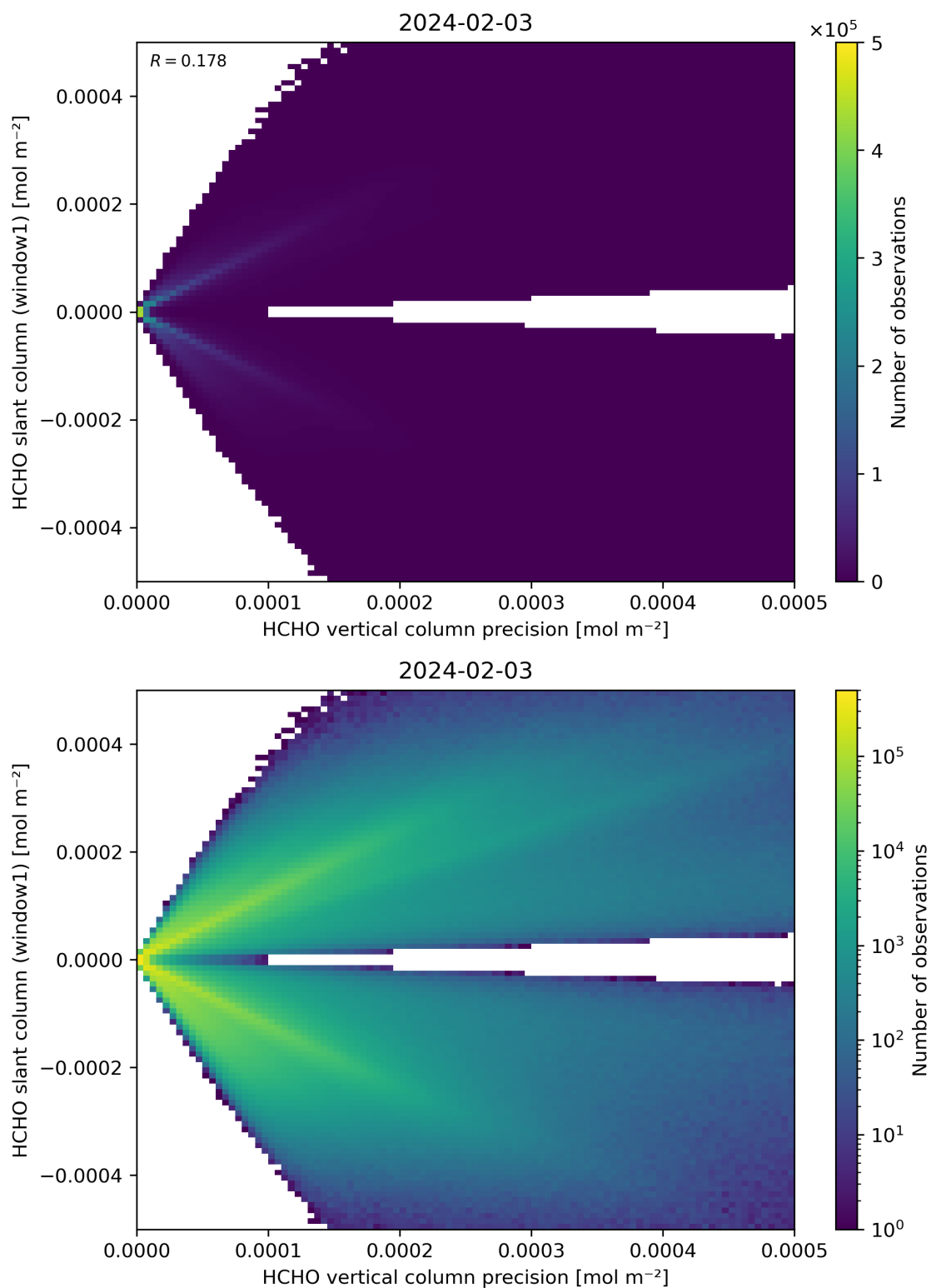
Figure 142: Scatter density plot of “HCHO vertical column precision” against “HCHO slant column (window1)” for 2024-02-02 to 2024-02-04.
