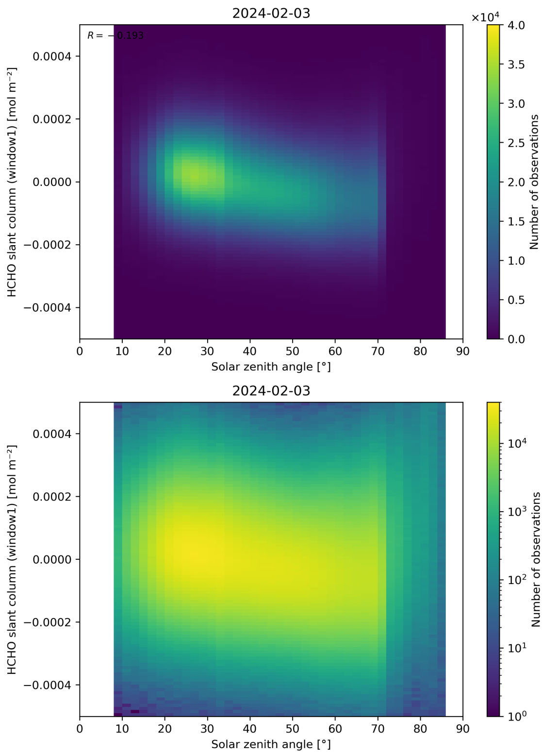
Figure 173: Scatter density plot of “Solar zenith angle” against “HCHO slant column (window1)” for 2024-02-02 to 2024-02-04.
