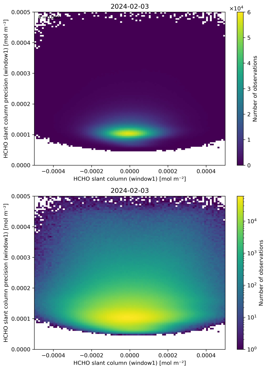
Figure 84: Scatter density plot of “HCHO slant column (window1)” against “HCHO slant column precision (window1)” for 2024-02-02 to 2024-02-04.
