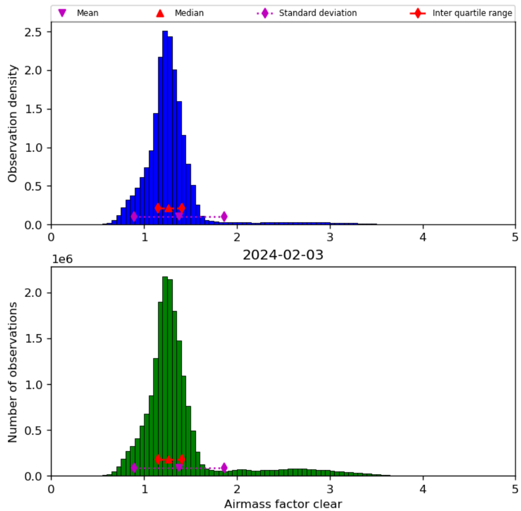
Figure 42: Histogram of “Airmass factor clear” for 2024-02-02 to 2024-02-04
