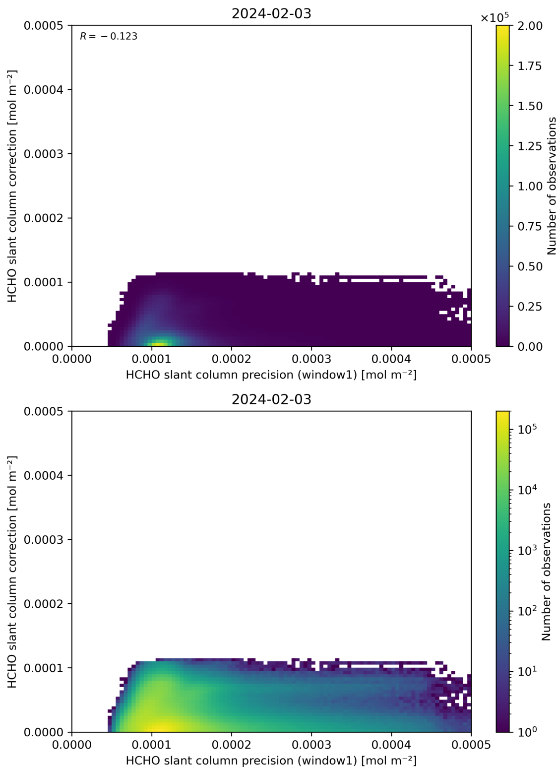
Figure 93: Scatter density plot of “HCHO slant column precision (window1)” against “HCHO slant column correction” for 2024-02-02 to 2024-02-04.
