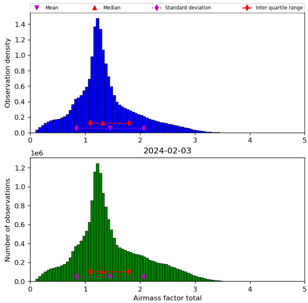
Figure 40: Histogram of “Airmass factor total” for 2024-02-02 to 2024-02-04
