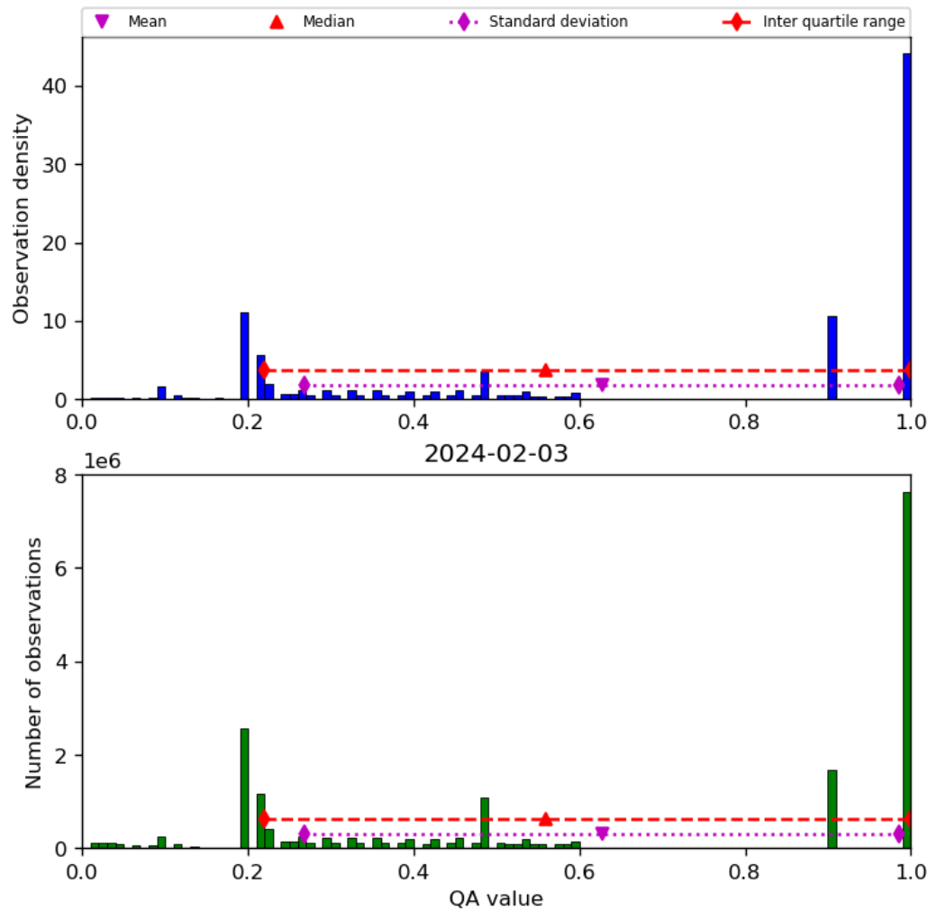
Figure 34: Histogram of “QA value” for 2024-02-02 to 2024-02-04
