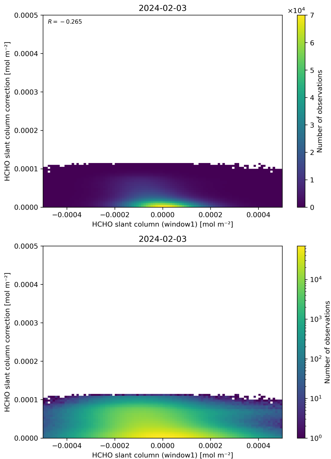
Figure 83: Scatter density plot of “HCHO slant column (window1)” against “HCHO slant column correction” for 2024-02-02 to 2024-02-04.
