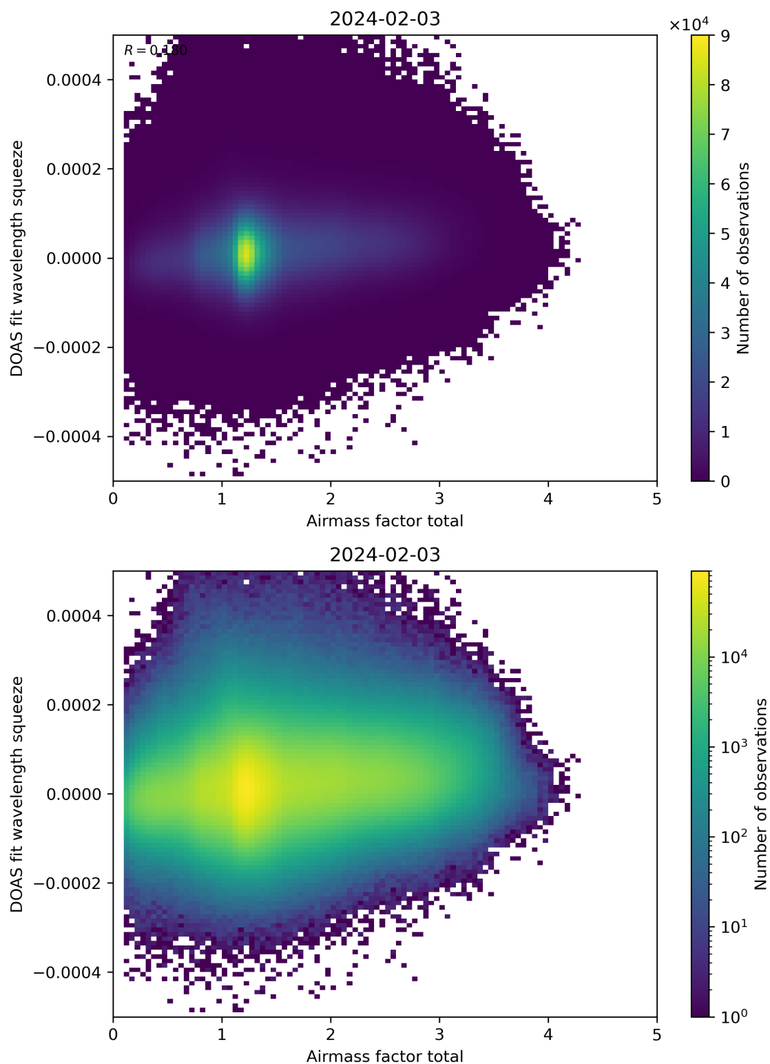
Figure 99: Scatter density plot of “Airmass factor total” against “DOAS fit wavelength squeeze” for 2024-02-02 to 2024-02-04.
