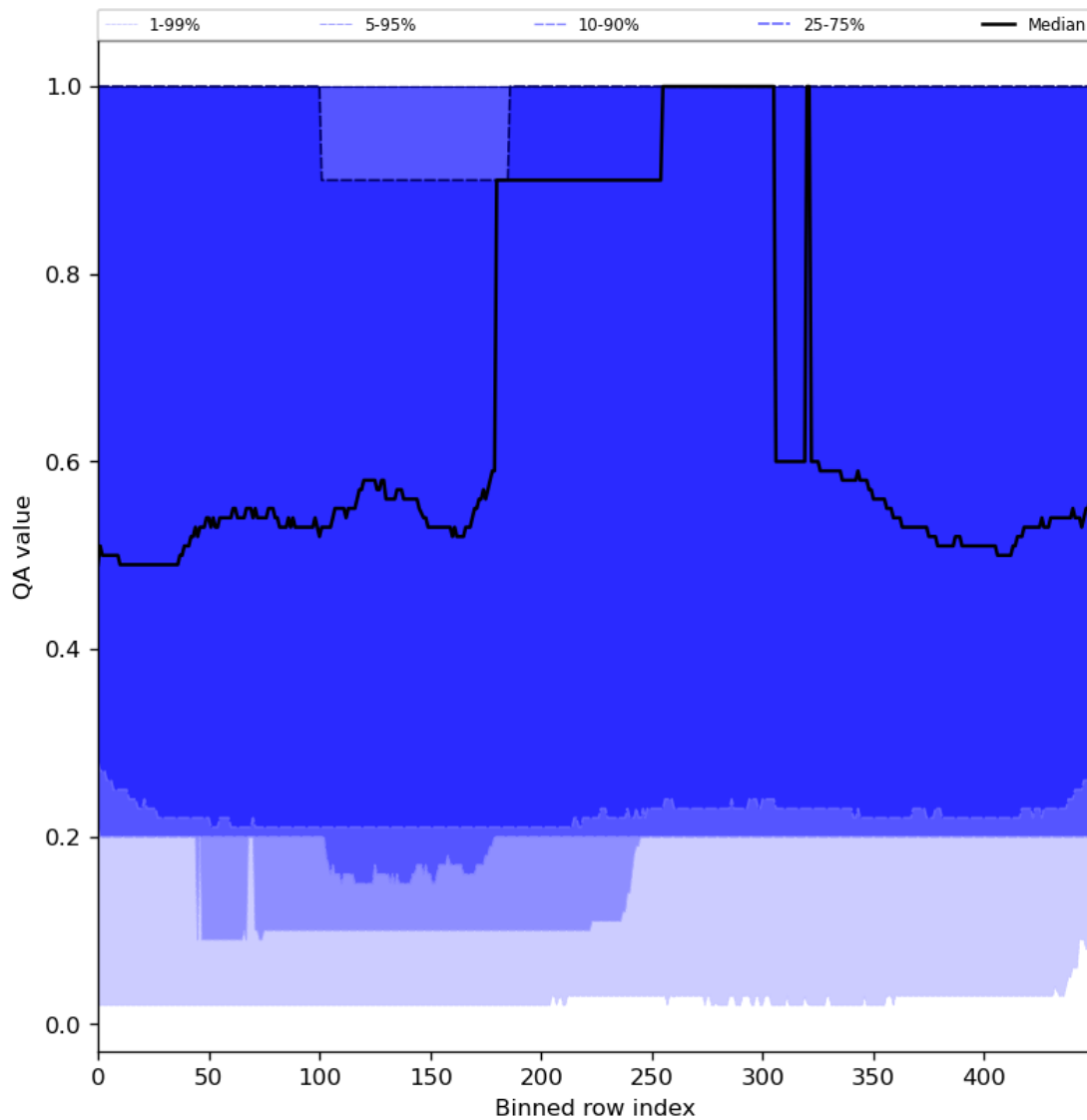
Figure 48: Along track statistics of “QA value” for 2024-02-02 to 2024-02-04
