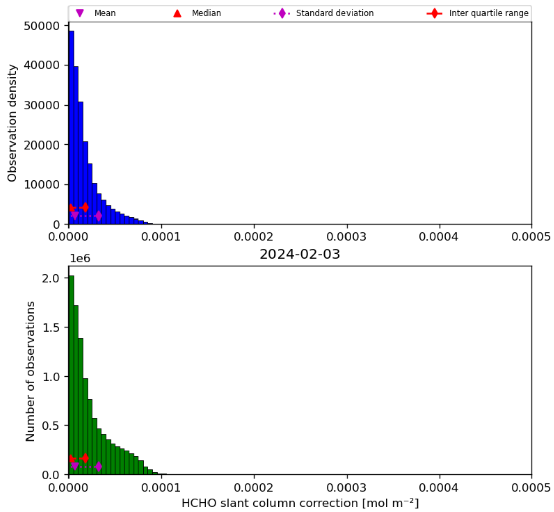
Figure 47: Histogram of “HCHO slant column correction” for 2024-02-02 to 2024-02-04
