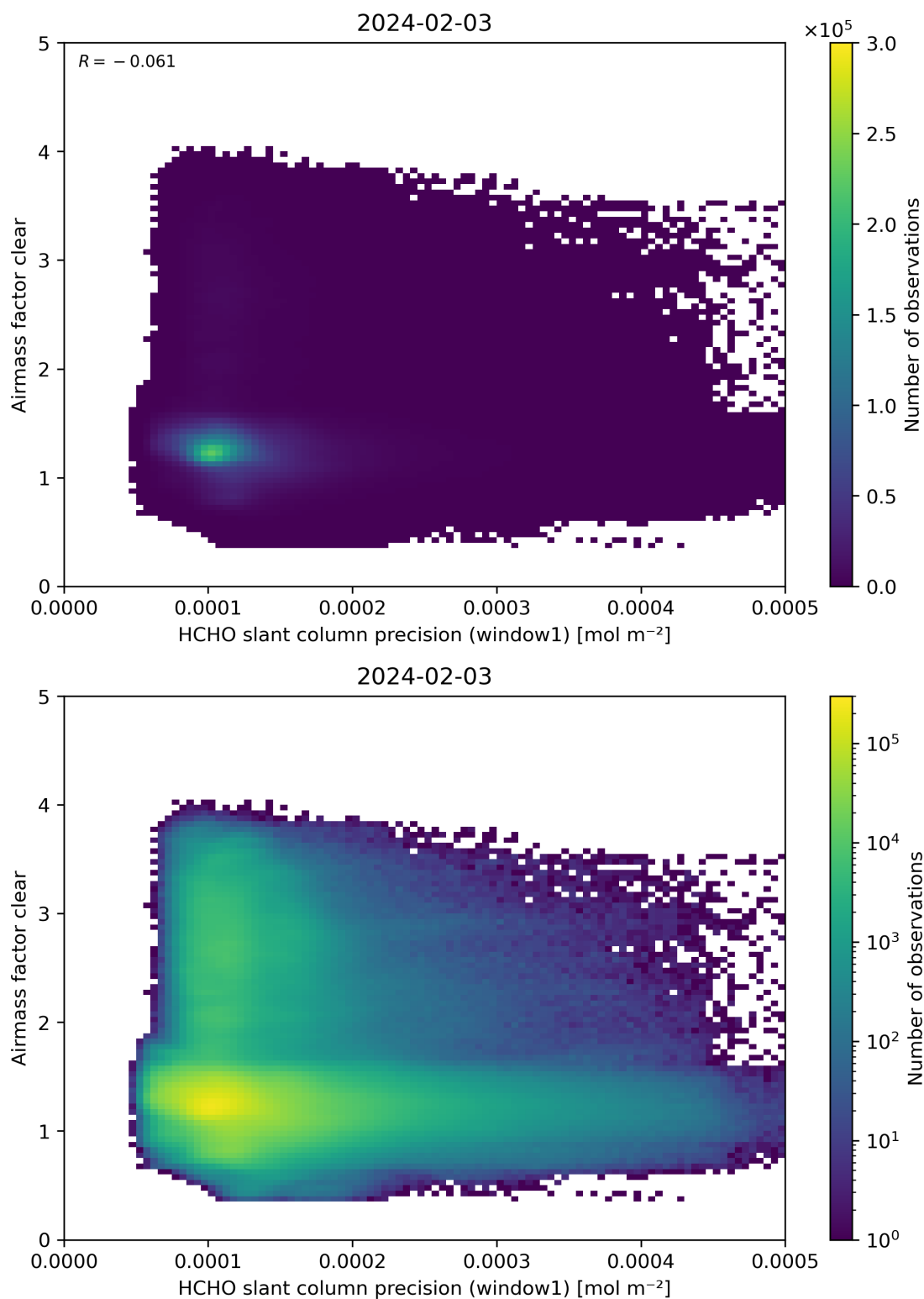
Figure 91: Scatter density plot of “HCHO slant column precision (window1)” against “Airmass factor clear” for 2024-02-02 to 2024-02-04.
