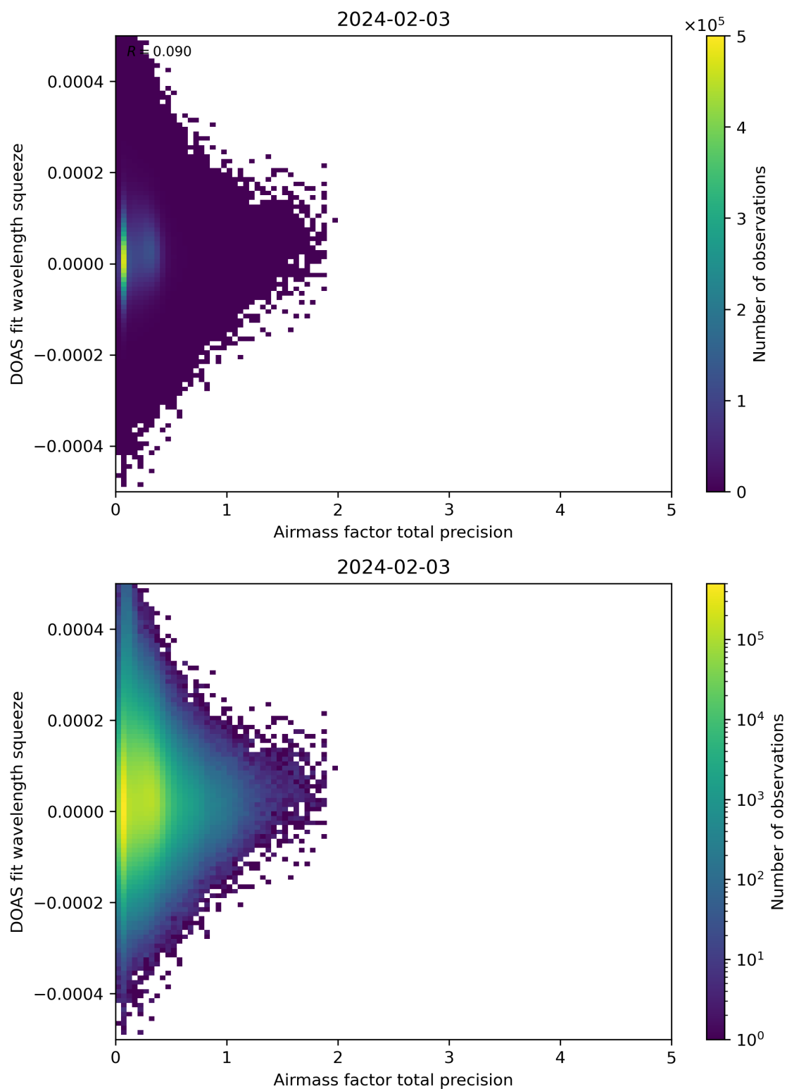
Figure 107: Scatter density plot of “Airmass factor total precision” against “DOAS fit wavelength squeeze” for 2024-02-02 to 2024-02-04.
