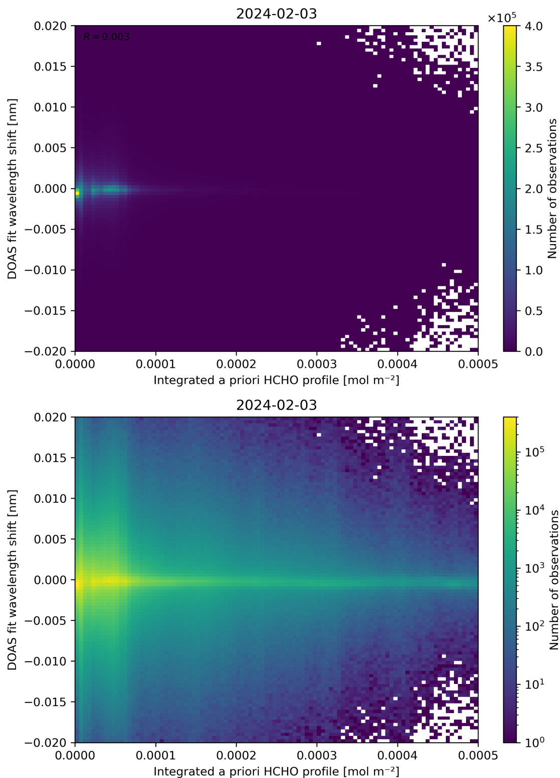
Figure 149: Scatter density plot of “Integrated a priori HCHO profile” against “DOAS fit wavelength shift” for 2024-02-02 to 2024-02-04.
