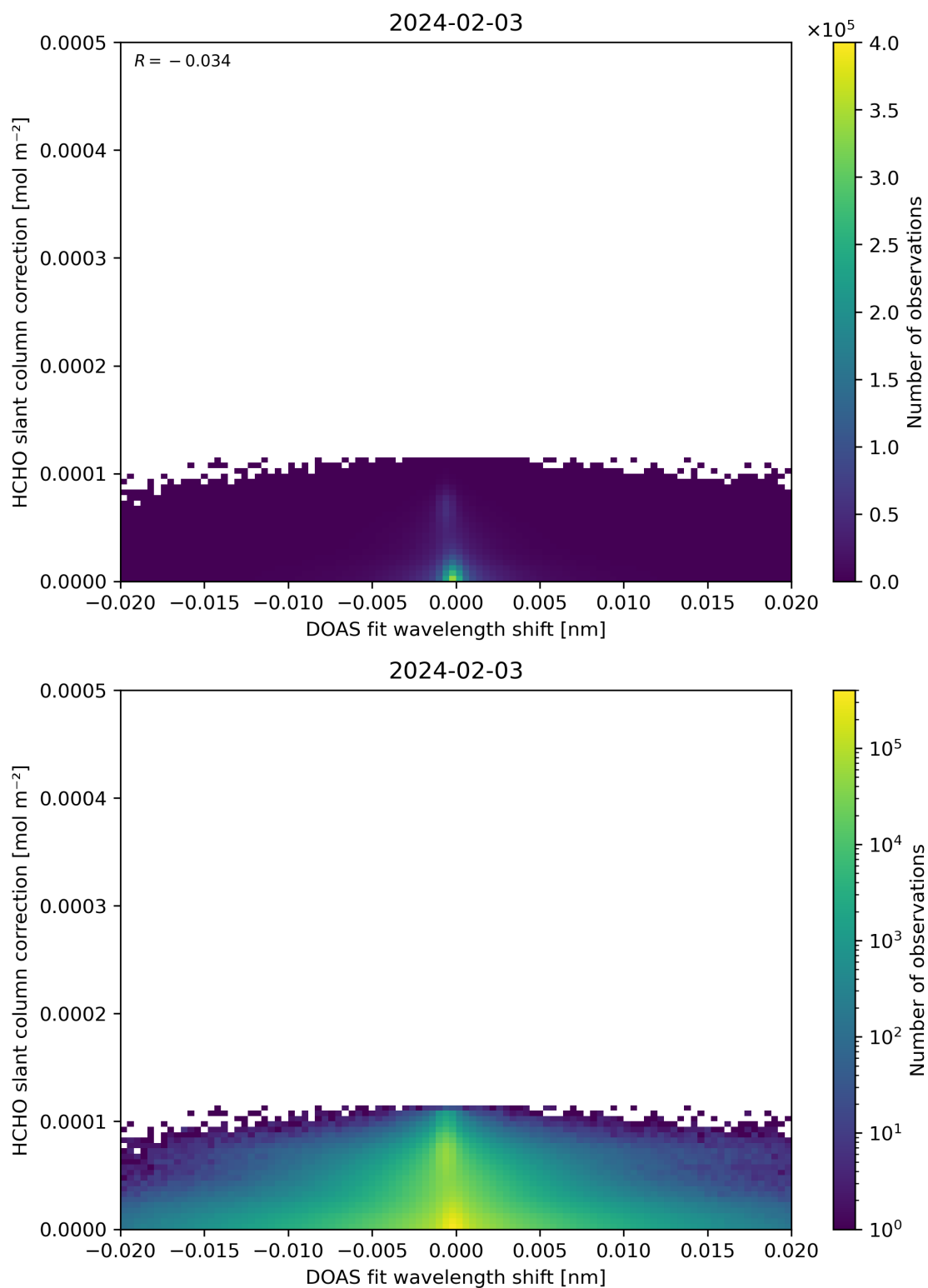
Figure 67: Scatter density plot of “DOAS fit wavelength shift” against “HCHO slant column correction” for 2024-02-02 to 2024-02-04.
