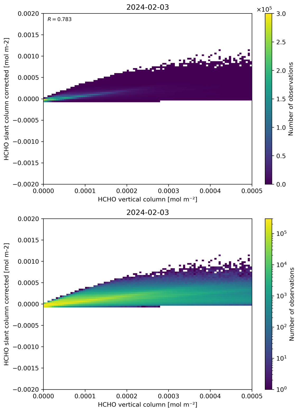
Figure 127: Scatter density plot of “HCHO vertical column” against “HCHO slant column corrected” for 2024-02-02 to 2024-02-04.
