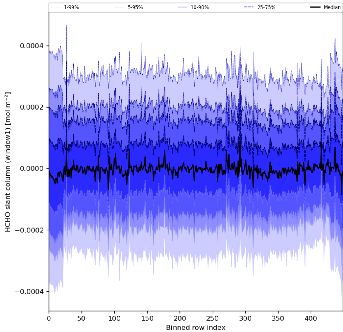
Figure 52: Along track statistics of “HCHO slant column (window1)” for 2024-02-02 to 2024-02-04
