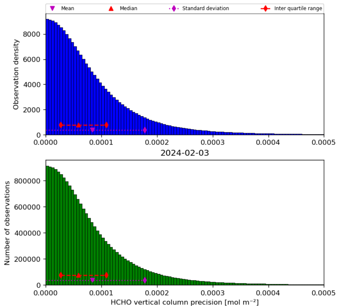
Figure 36: Histogram of “HCHO vertical column precision” for 2024-02-02 to 2024-02-04
