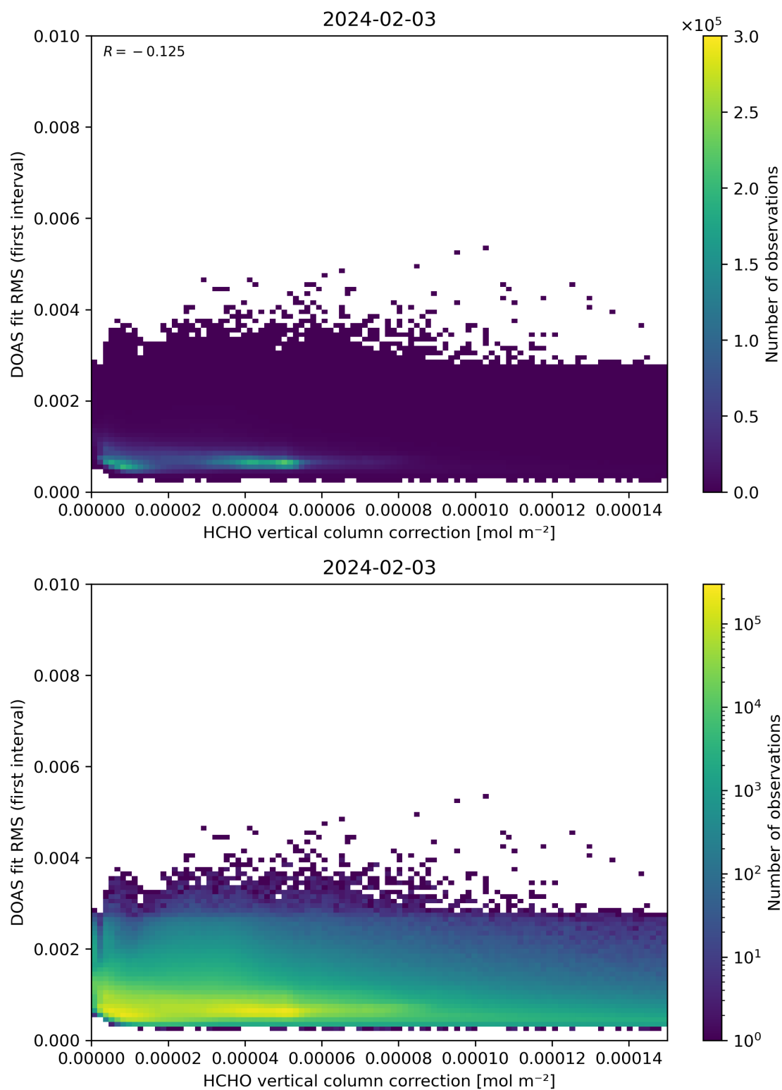
Figure 112: Scatter density plot of “HCHO vertical column correction” against “DOAS fit RMS (first interval)” for 2024-02-02 to 2024-02-04.
