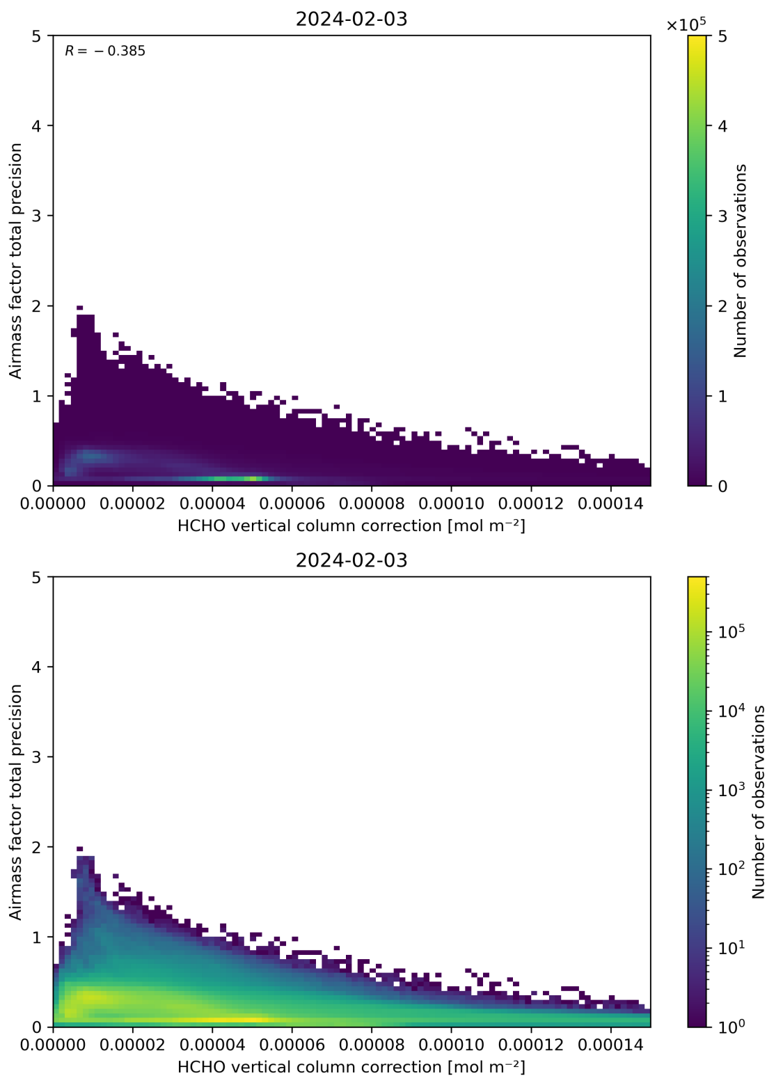
Figure 121: Scatter density plot of “HCHO vertical column correction” against “Airmass factor total precision” for 2024-02-02 to 2024-02-04.
