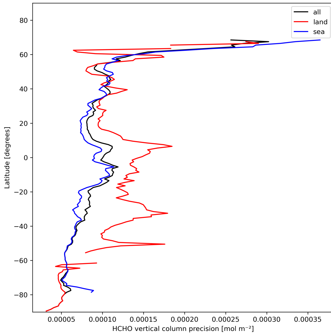
Figure 22: Zonal average of “HCHO vertical column precision” for 2024-02-02 to 2024-02-04.
