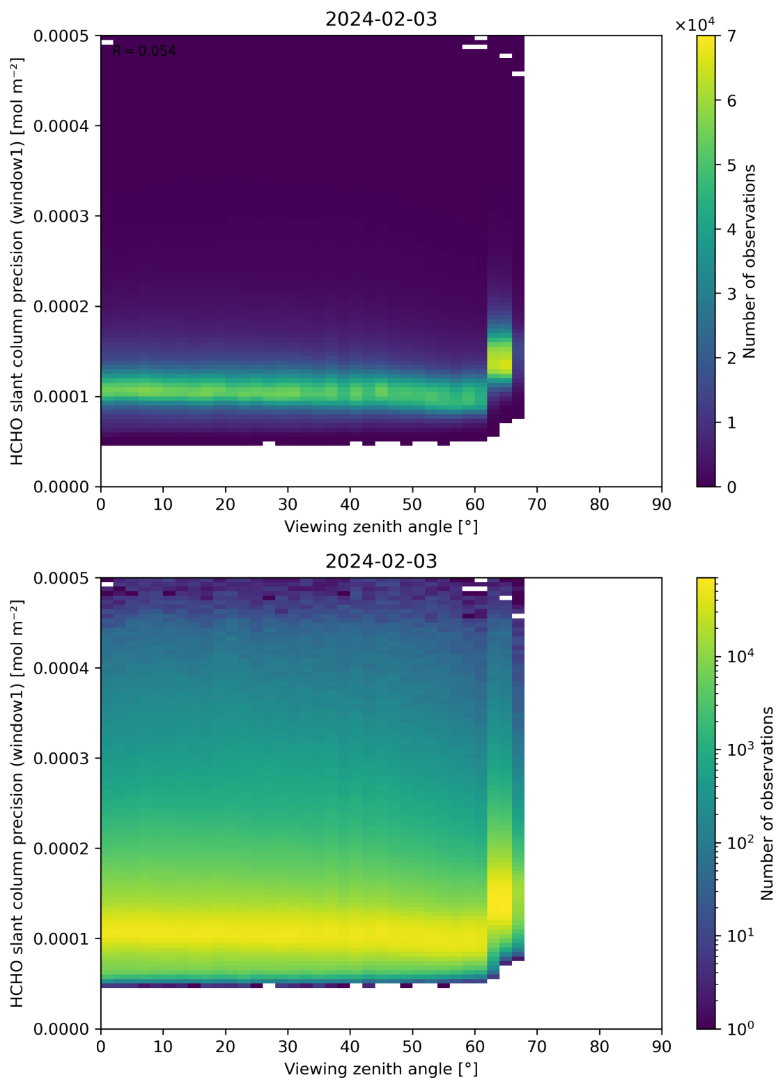
Figure 189: Scatter density plot of “Viewing zenith angle” against “HCHO slant column precision (window1)” for 2024-02-02 to 2024-02-04.
