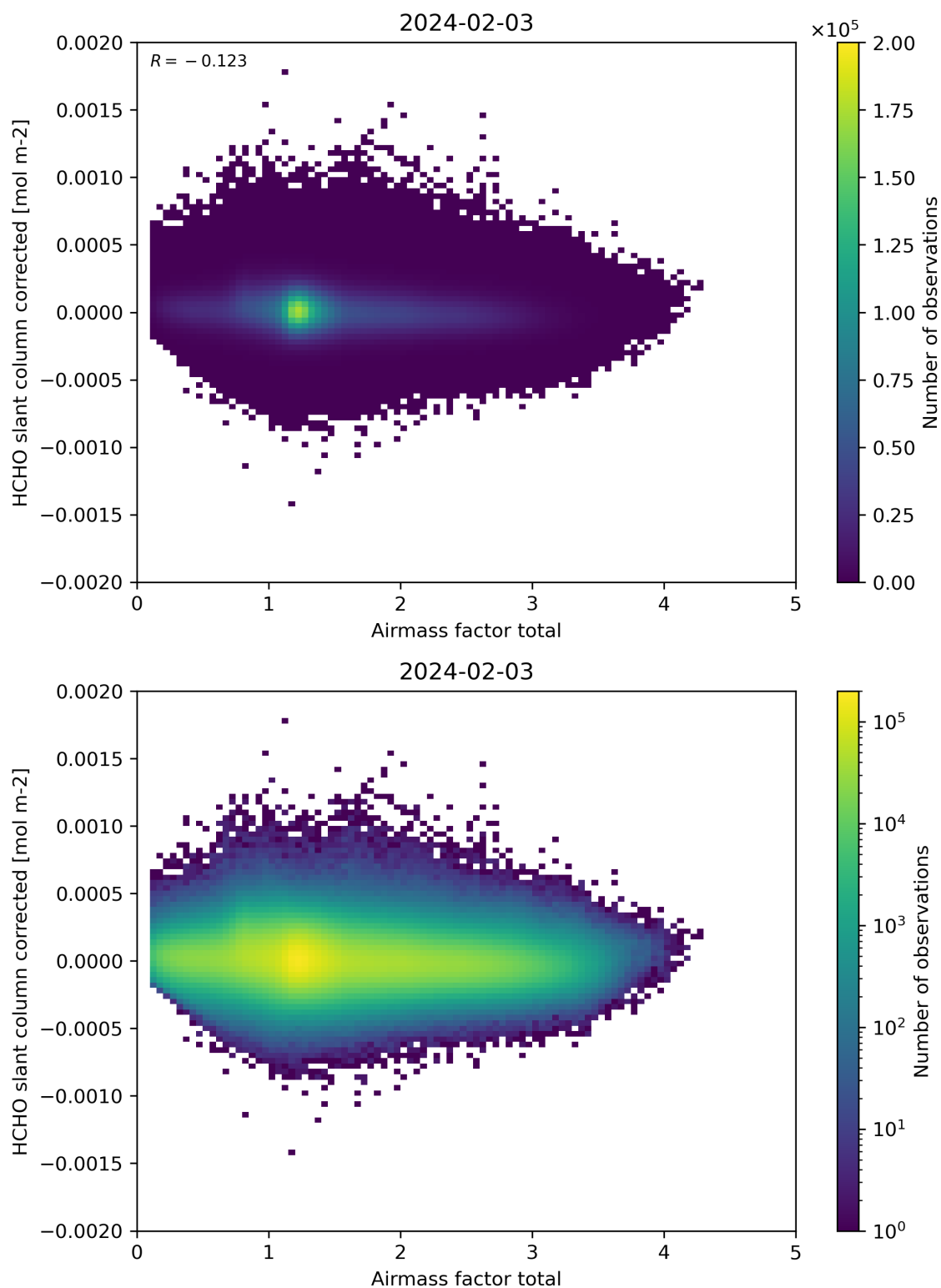
Figure 101: Scatter density plot of “Airmass factor total” against “HCHO slant column corrected” for 2024-02-02 to 2024-02-04.
