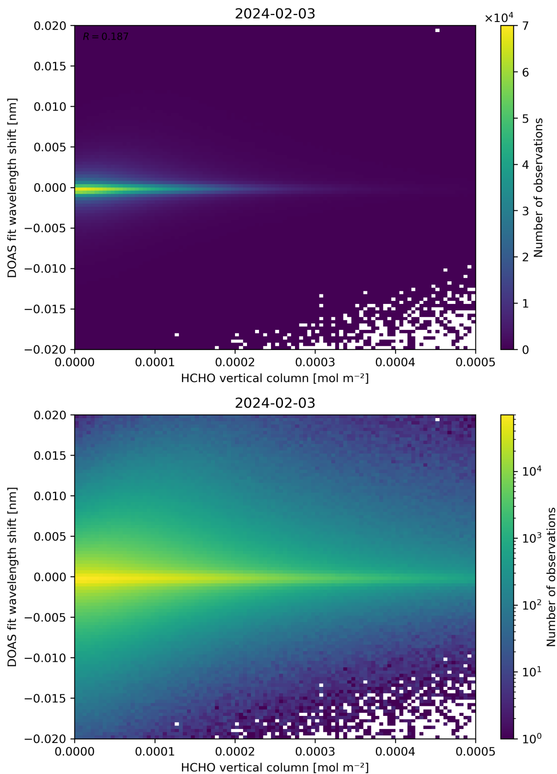
Figure 124: Scatter density plot of “HCHO vertical column” against “DOAS fit wavelength shift” for 2024-02-02 to 2024-02-04.
