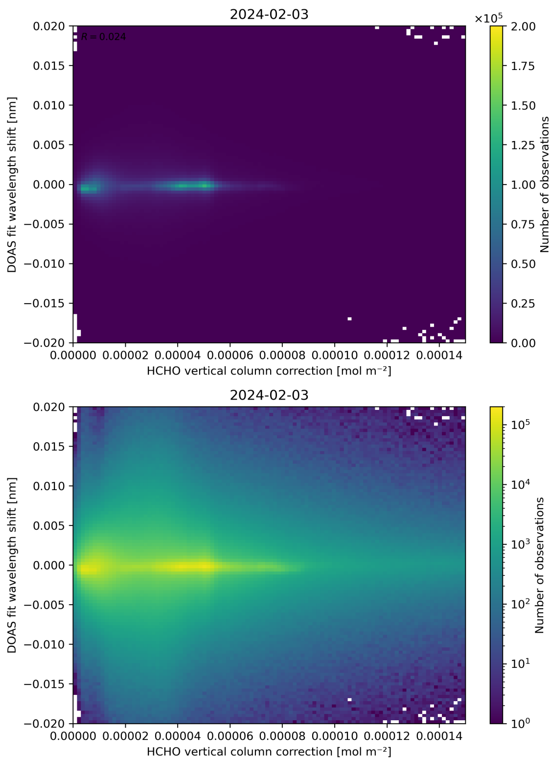
Figure 113: Scatter density plot of “HCHO vertical column correction” against “DOAS fit wavelength shift” for 2024-02-02 to 2024-02-04.
