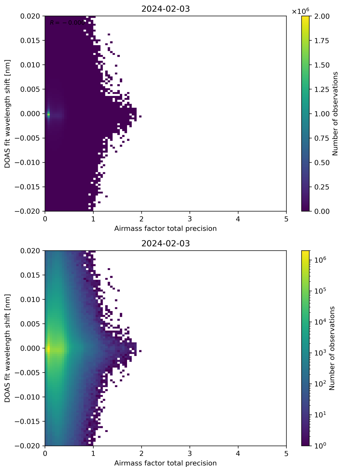
Figure 106: Scatter density plot of “Airmass factor total precision” against “DOAS fit wavelength shift” for 2024-02-02 to 2024-02-04.
