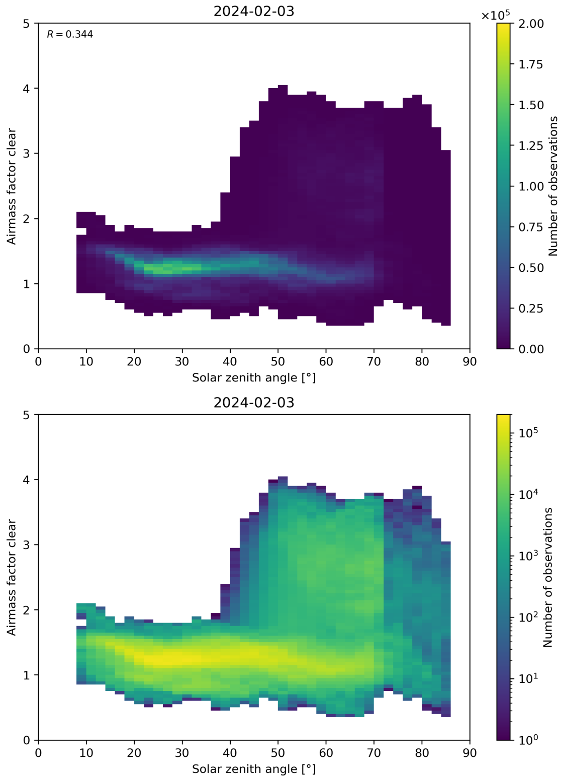
Figure 170: Scatter density plot of “Solar zenith angle” against “Airmass factor clear” for 2024-02-02 to 2024-02-04.
