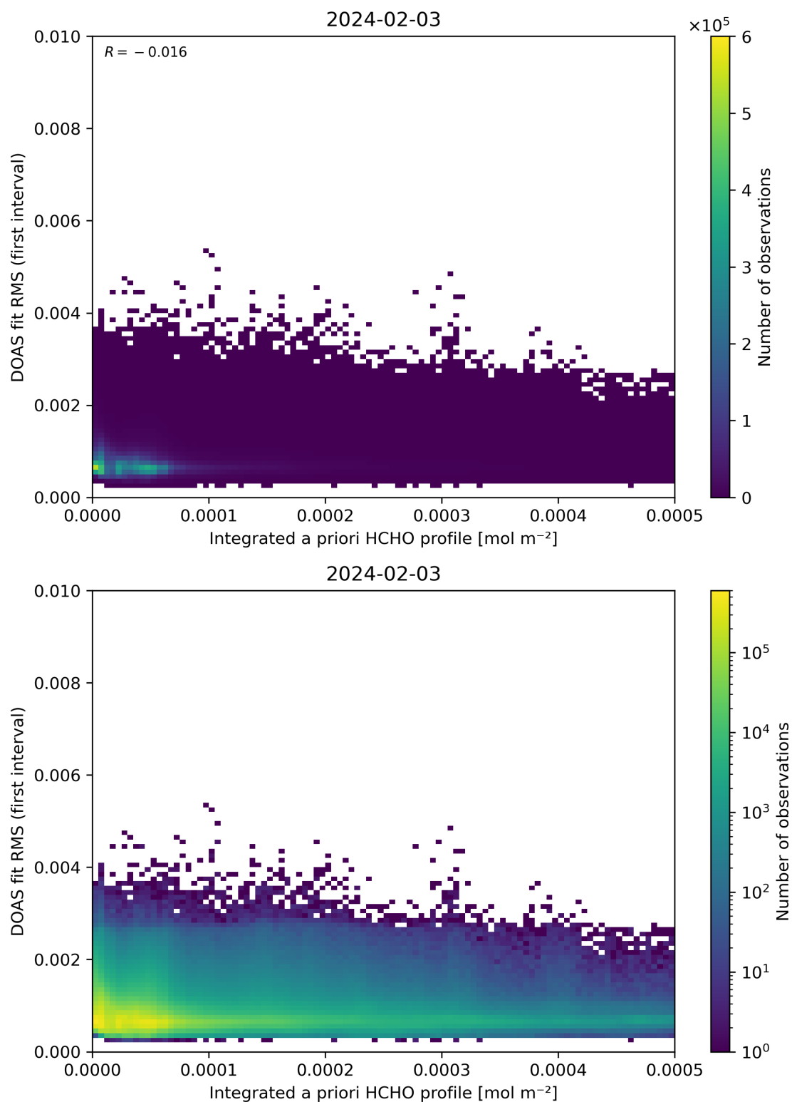
Figure 148: Scatter density plot of “Integrated a priori HCHO profile” against “DOAS fit RMS (first interval)” for 2024-02-02 to 2024-02-04.
