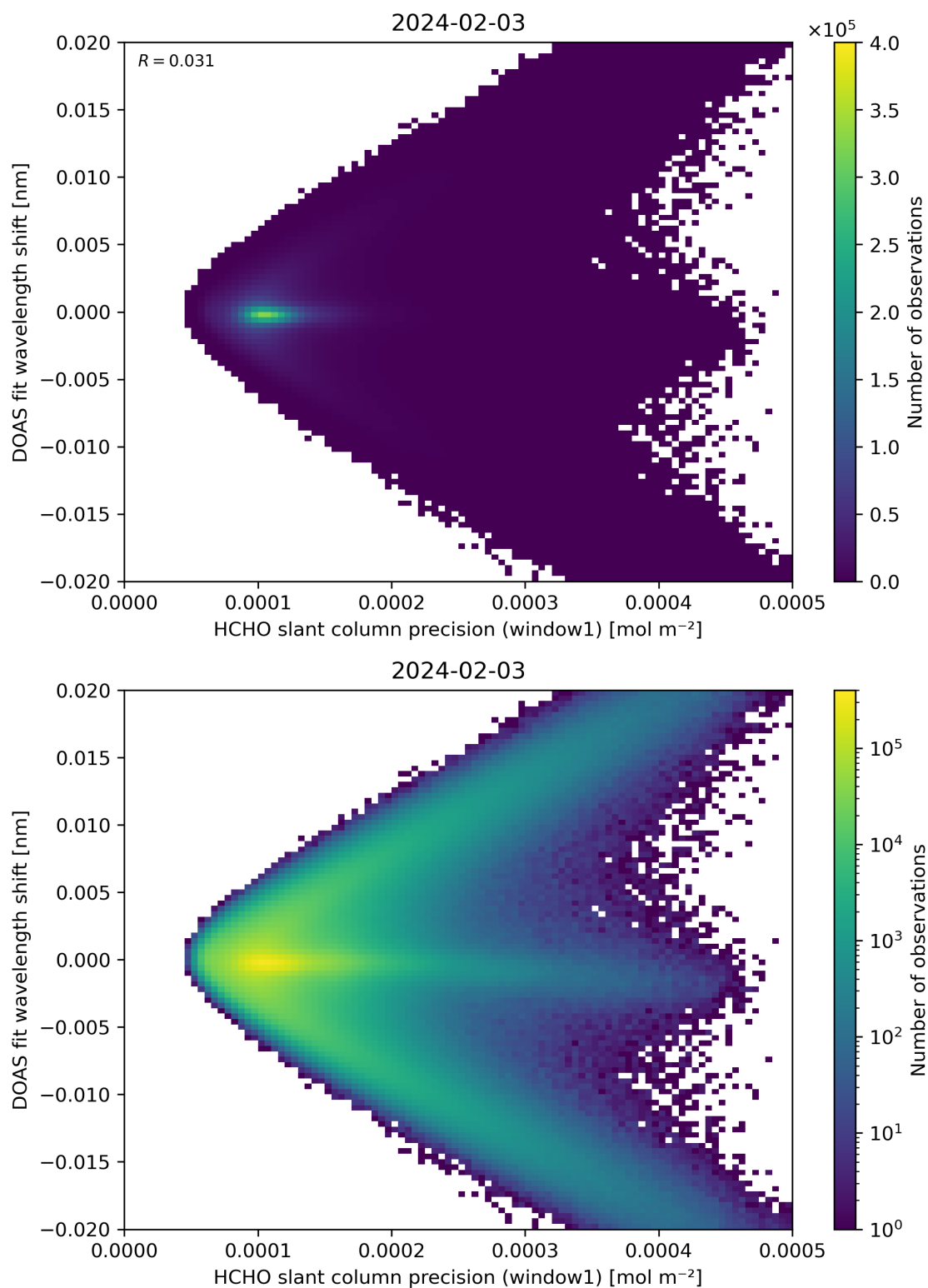
Figure 89: Scatter density plot of “HCHO slant column precision (window1)” against “DOAS fit wavelength shift” for 2024-02-02 to 2024-02-04.
