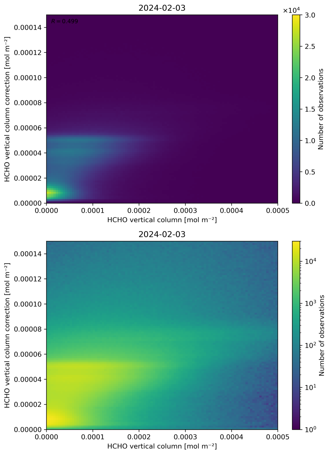
Figure 133: Scatter density plot of “HCHO vertical column” against “HCHO vertical column correction” for 2024-02-02 to 2024-02-04.
