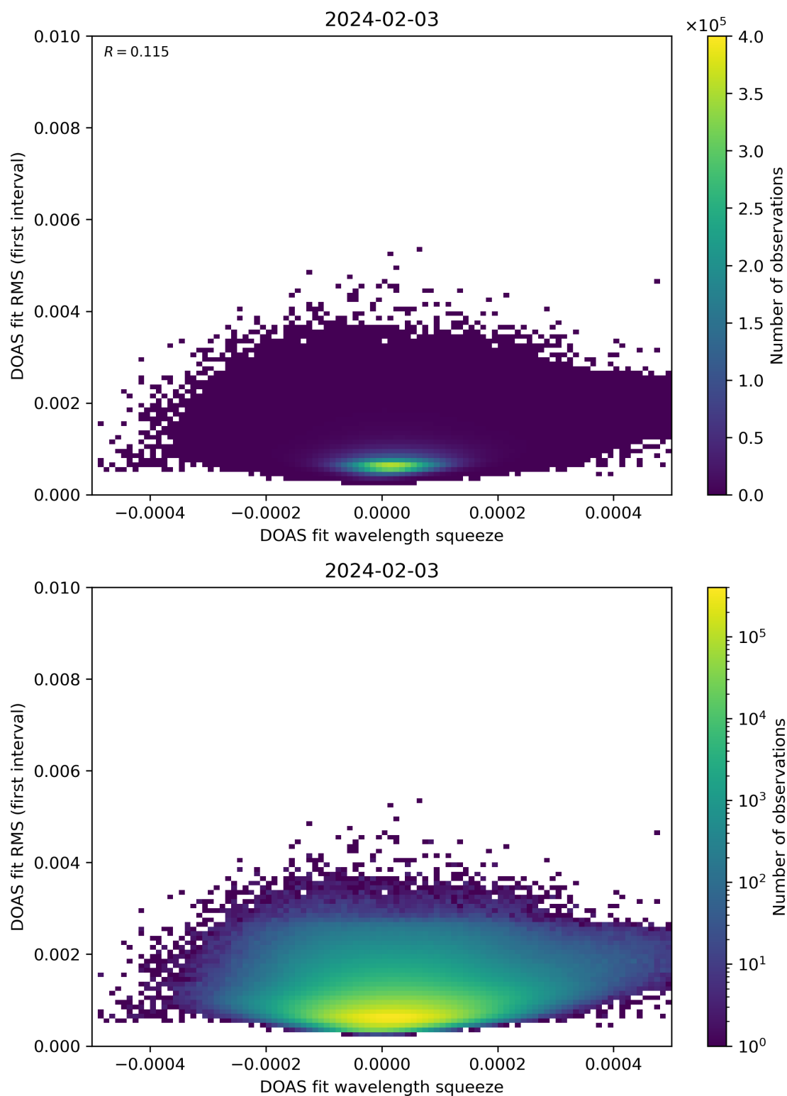
Figure 68: Scatter density plot of “DOAS fit wavelength squeeze” against “DOAS fit RMS (first interval)” for 2024-02-02 to 2024-02-04.
