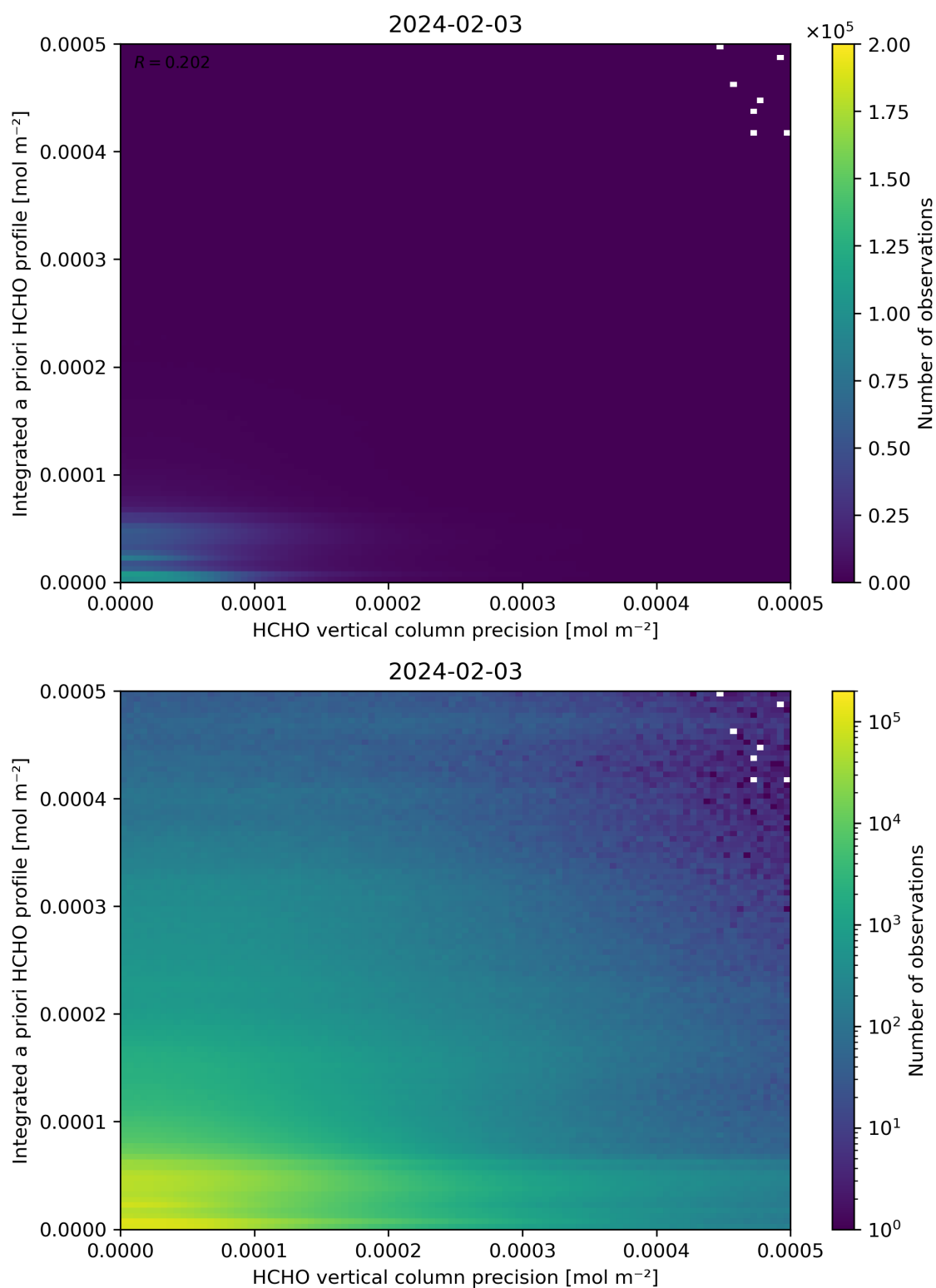
Figure 147: Scatter density plot of “HCHO vertical column precision” against “Integrated a priori HCHO profile” for 2024-02-02 to 2024-02-04.
