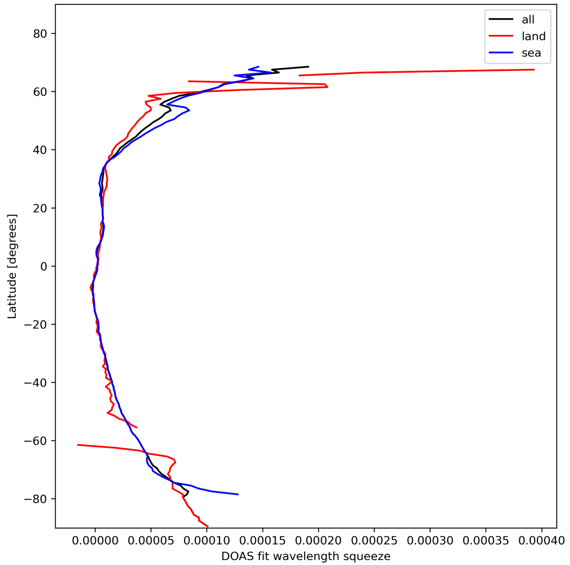
Figure 31: Zonal average of “DOAS fit wavelength squeeze” for 2024-02-02 to 2024-02-04.
