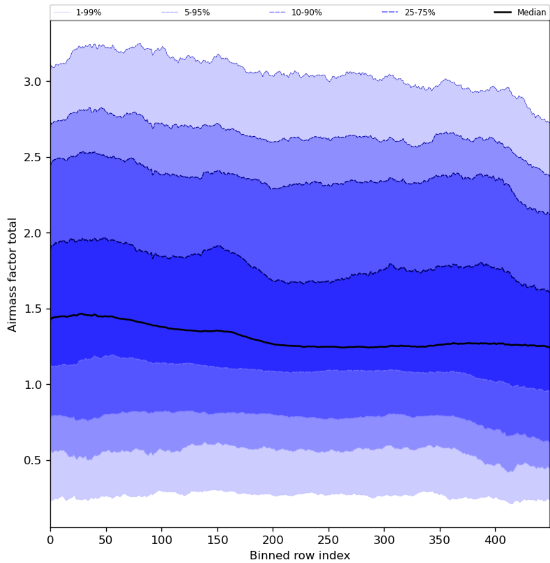
Figure 54: Along track statistics of “Airmass factor total” for 2024-02-02 to 2024-02-04
