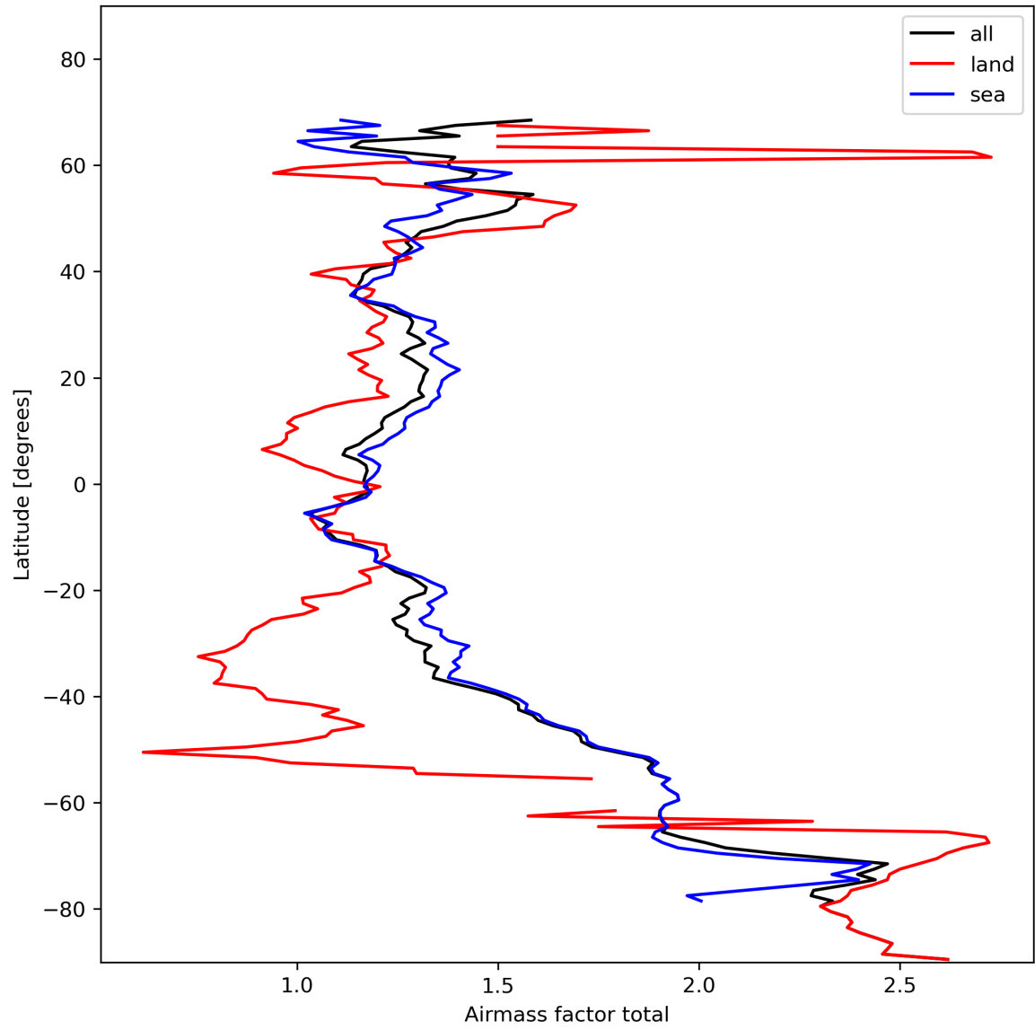
Figure 26: Zonal average of “Airmass factor total” for 2024-02-02 to 2024-02-04.
