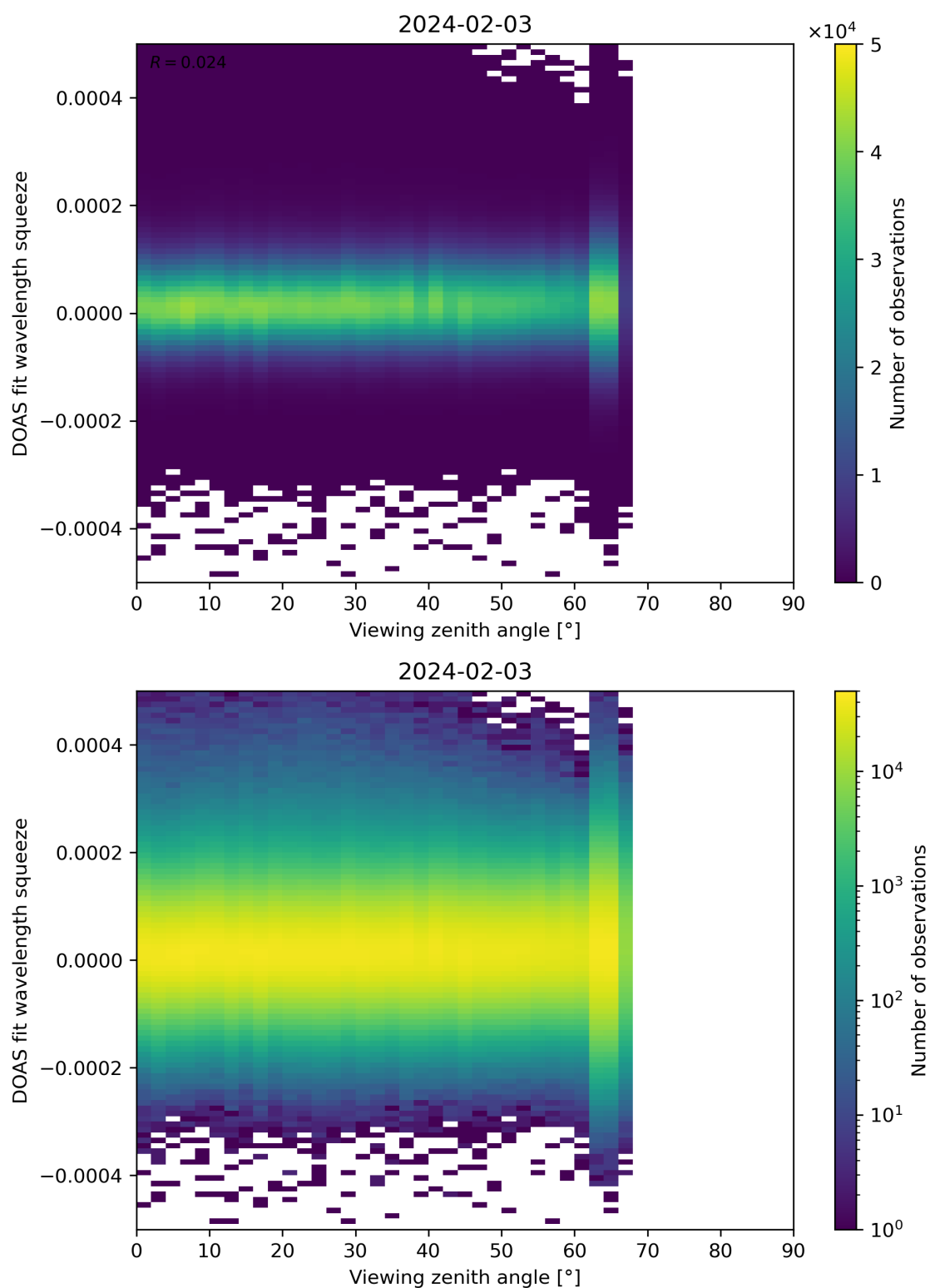
Figure 184: Scatter density plot of “Viewing zenith angle” against “DOAS fit wavelength squeeze” for 2024-02-02 to 2024-02-04.
