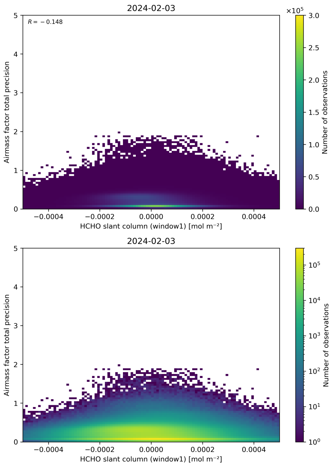
Figure 86: Scatter density plot of “HCHO slant column (window1)” against “Airmass factor total precision” for 2024-02-02 to 2024-02-04.
