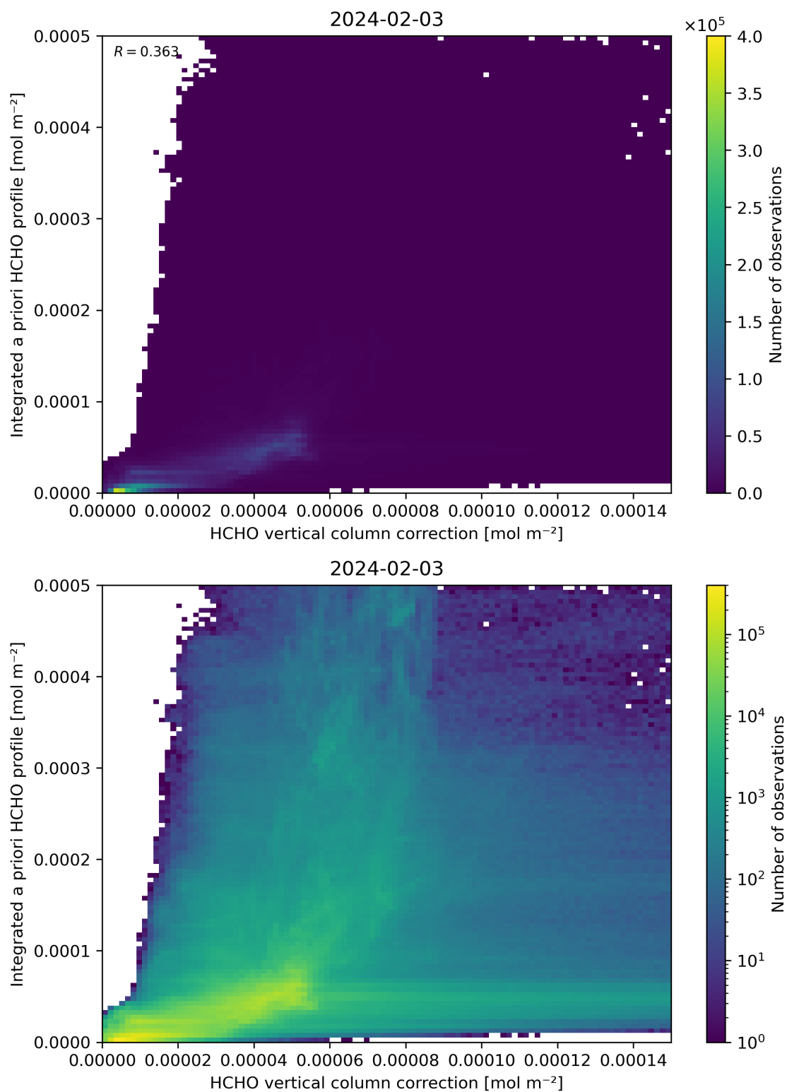
Figure 122: Scatter density plot of “HCHO vertical column correction” against “Integrated a priori HCHO profile” for 2024-02-02 to 2024-02-04.
