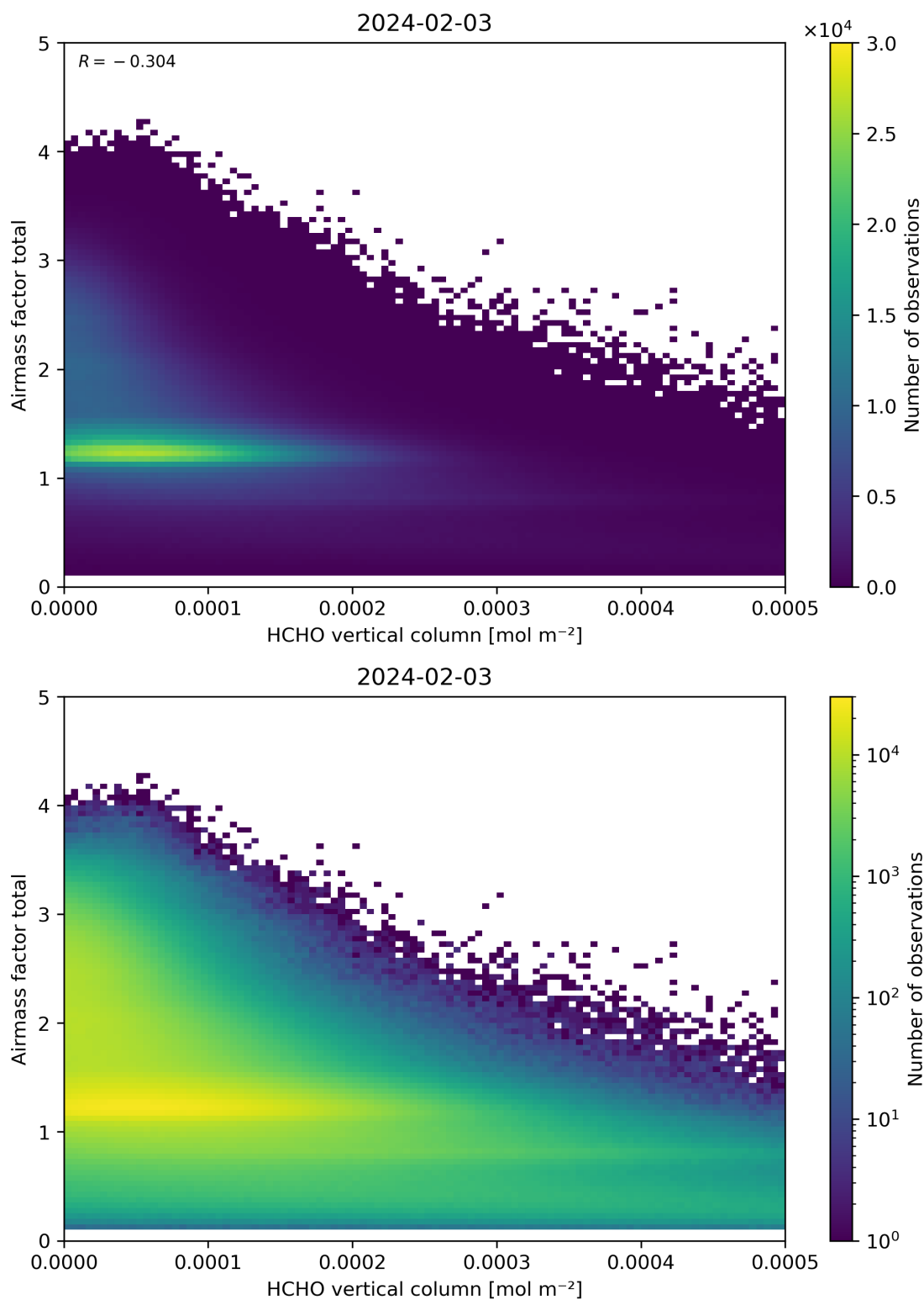
Figure 131: Scatter density plot of “HCHO vertical column” against “Airmass factor total” for 2024-02-02 to 2024-02-04.
