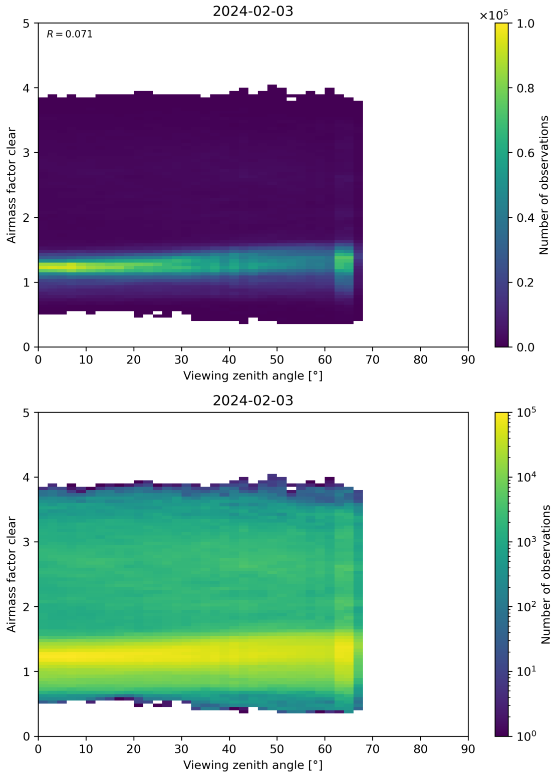
Figure 185: Scatter density plot of “Viewing zenith angle” against “Airmass factor clear” for 2024-02-02 to 2024-02-04.
