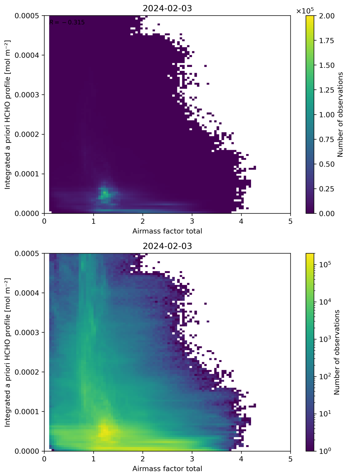
Figure 104: Scatter density plot of “Air mass factor total” against “Integrated a priori HCHO profile” for 2024-02-02 to 2024-02-04.
