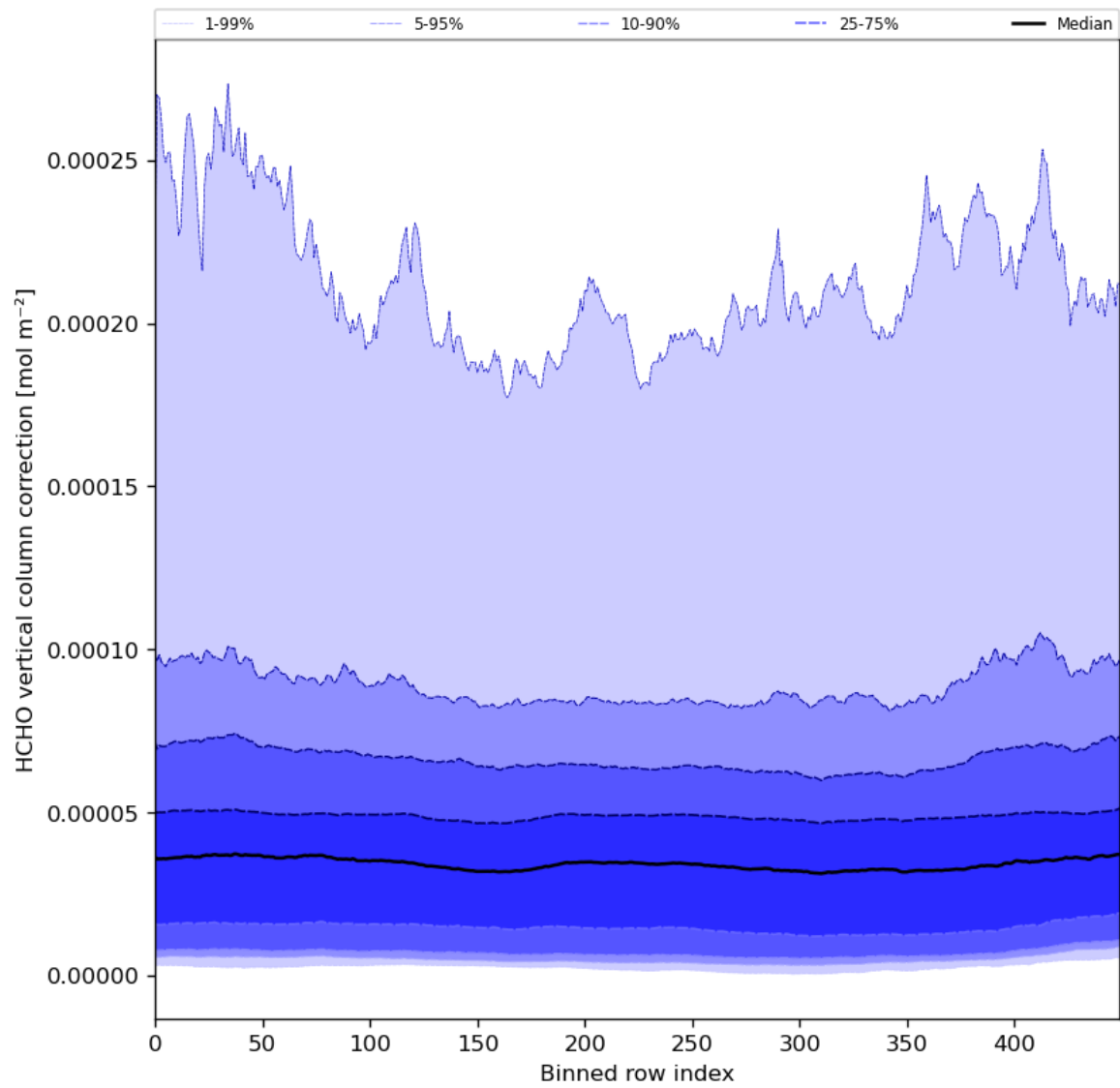
Figure 51: Along track statistics of “HCHO vertical column correction” for 2024-02-02 to 2024-02-04
