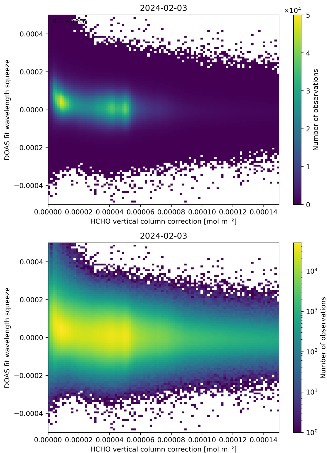
Figure 114: Scatter density plot of “HCHO vertical column correction” against “DOAS fit wavelength squeeze” for 2024-02-02 to 2024-02-04.
