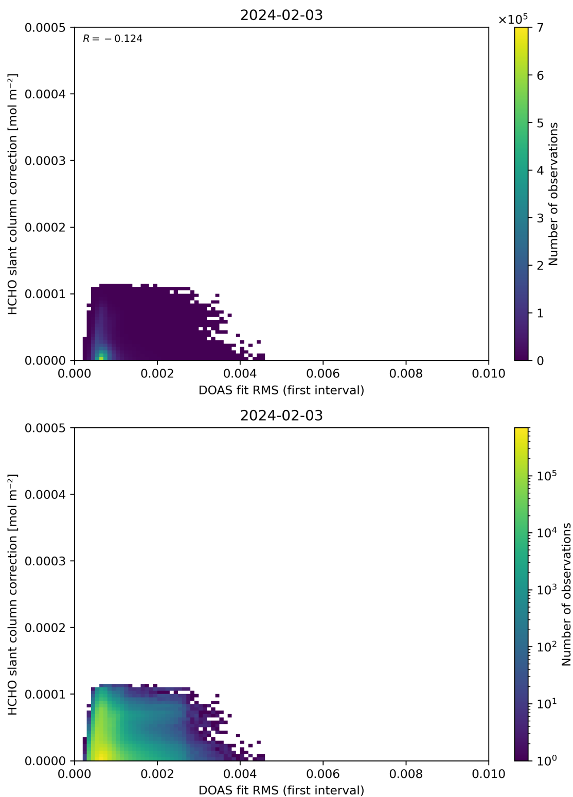
Figure 63: Scatter density plot of “DOAS fit RMS (first interval)” against “HCHO slant column correction” for 2024-02-02 to 2024-02-04.
