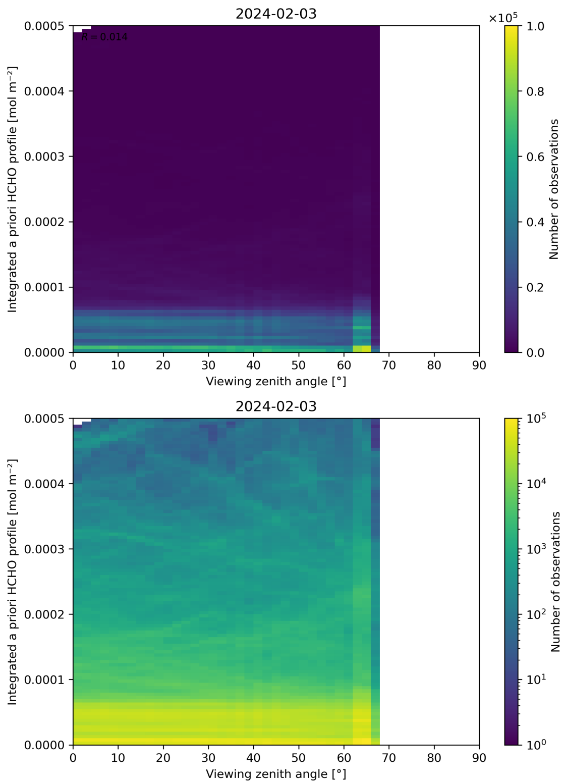
Figure 195: Scatter density plot of “Viewing zenith angle” against “Integrated a priori HCHO profile” for 2024-02-02 to 2024-02-04.
