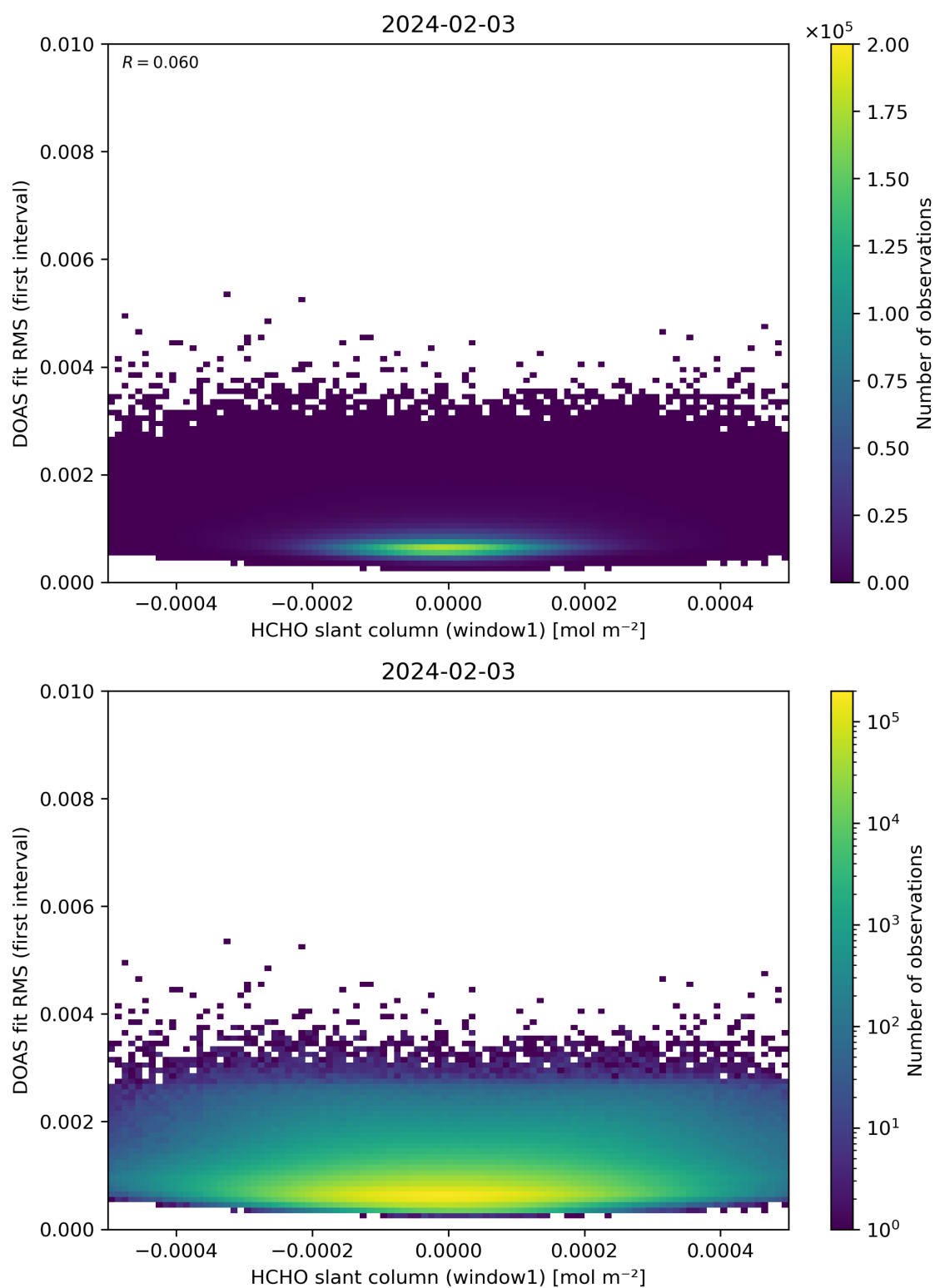
Figure 78: Scatter density plot of “HCHO slant column (window1)” against “DOAS fit RMS (first interval)” for 2024-02-02 to 2024-02-04.
