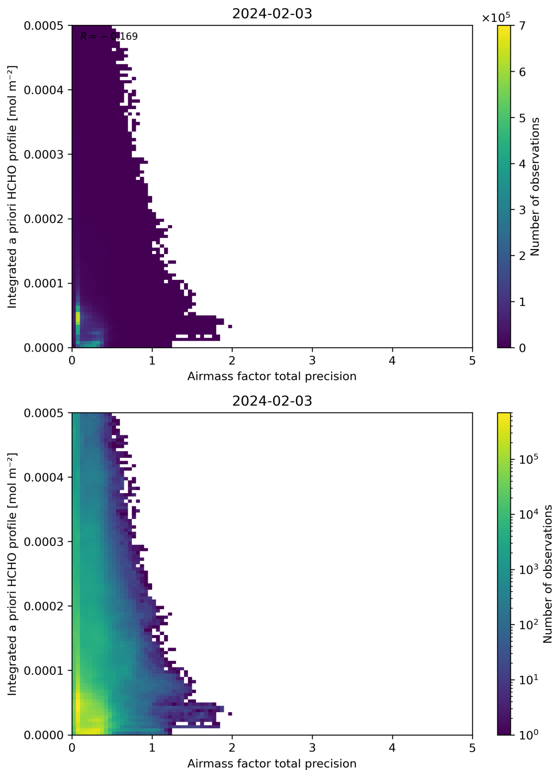
Figure 111: Scatter density plot of “Airmass factor total precision” against “Integrated a priori HCHO profile” for 2024-02-02 to 2024-02-04.
