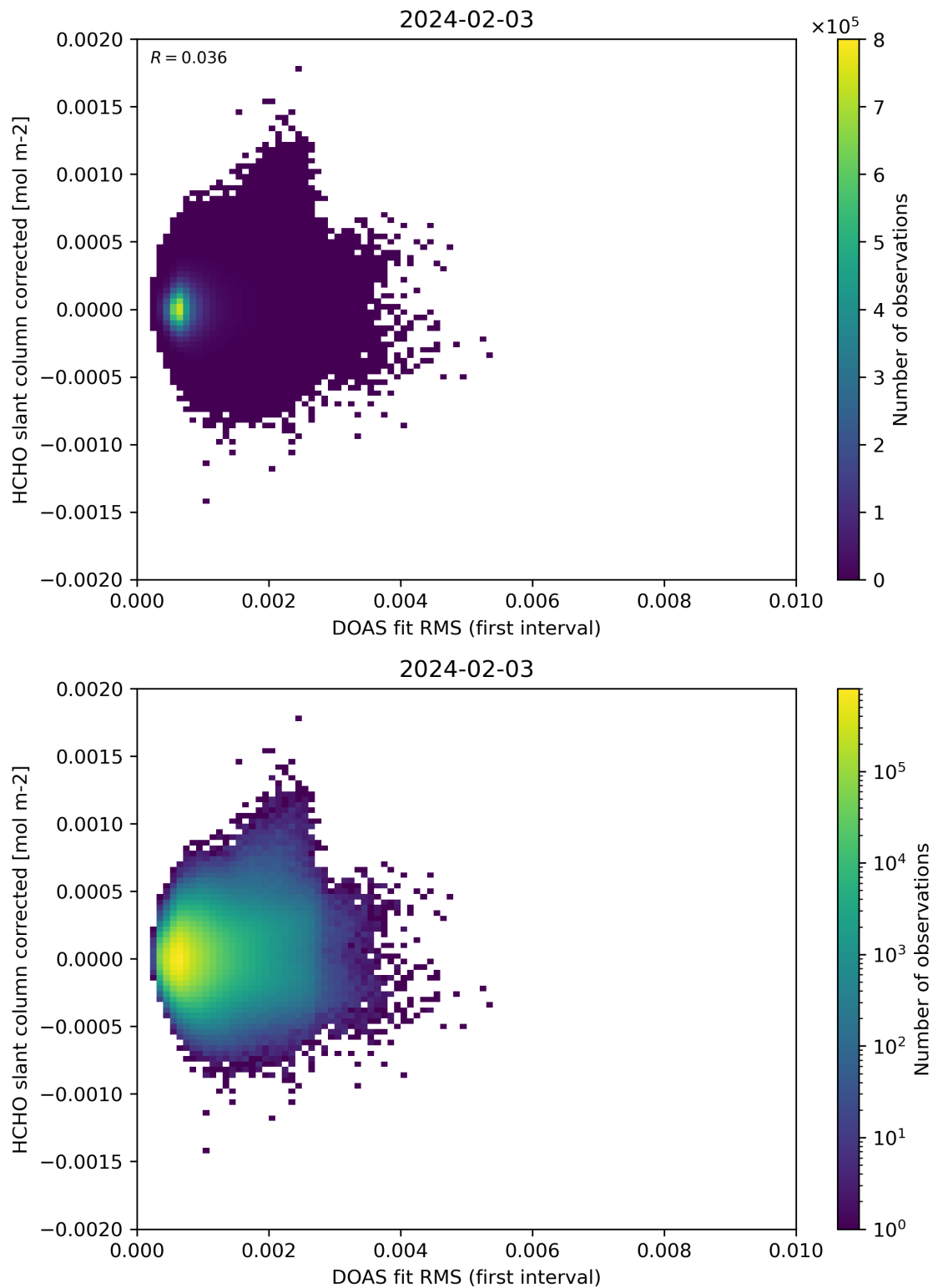
Figure 62: Scatter density plot of “DOAS fit RMS (first interval)” against “HCHO slant column corrected” for 2024-02-02 to 2024-02-04.
