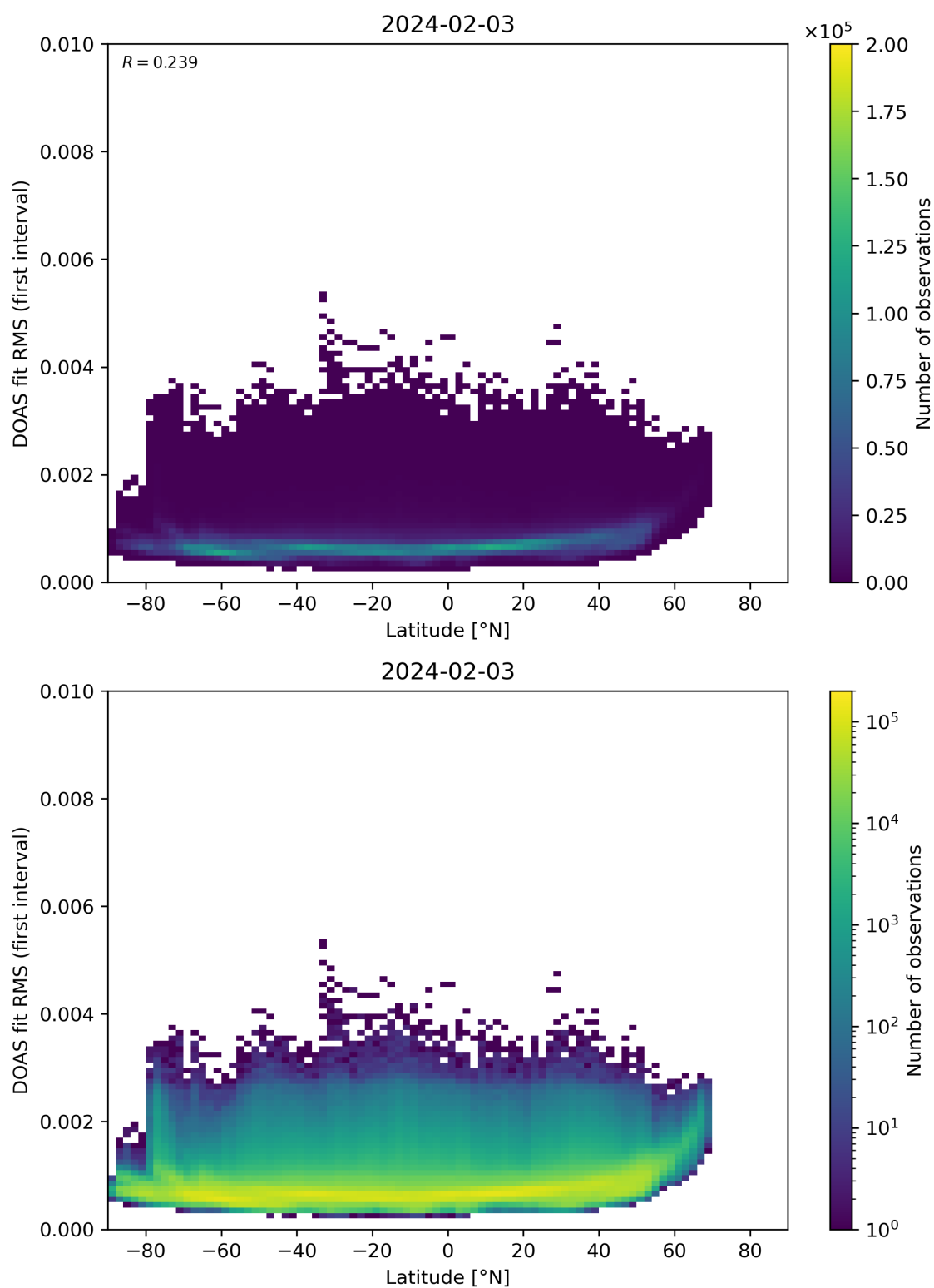
Figure 153: Scatter density plot of “Latitude” against “DOAS fit RMS (first interval)” for 2024-02-02 to 2024-02-04.
