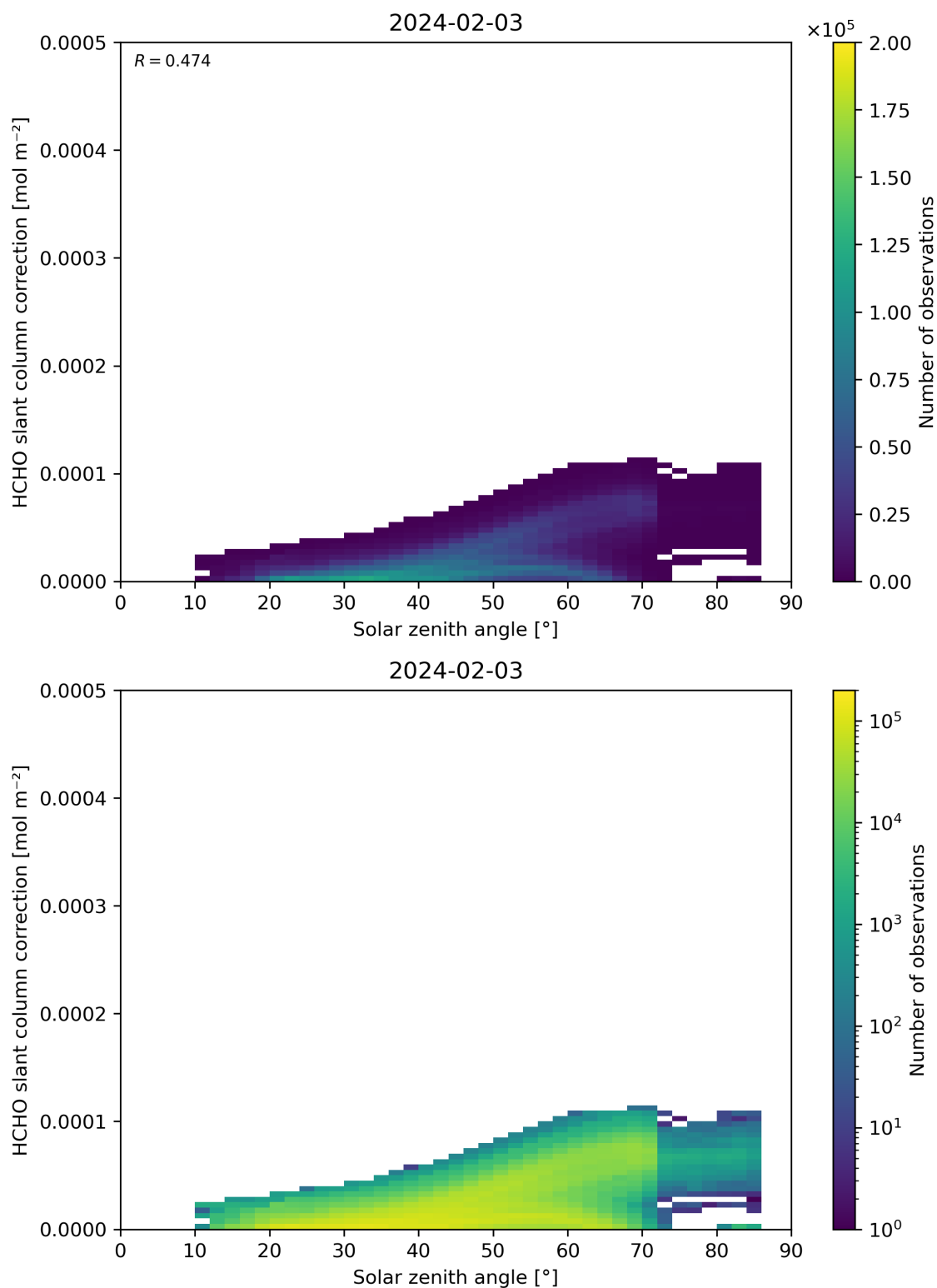
Figure 172: Scatter density plot of “Solar zenith angle” against “HCHO slant column correction” for 2024-02-02 to 2024-02-04.
