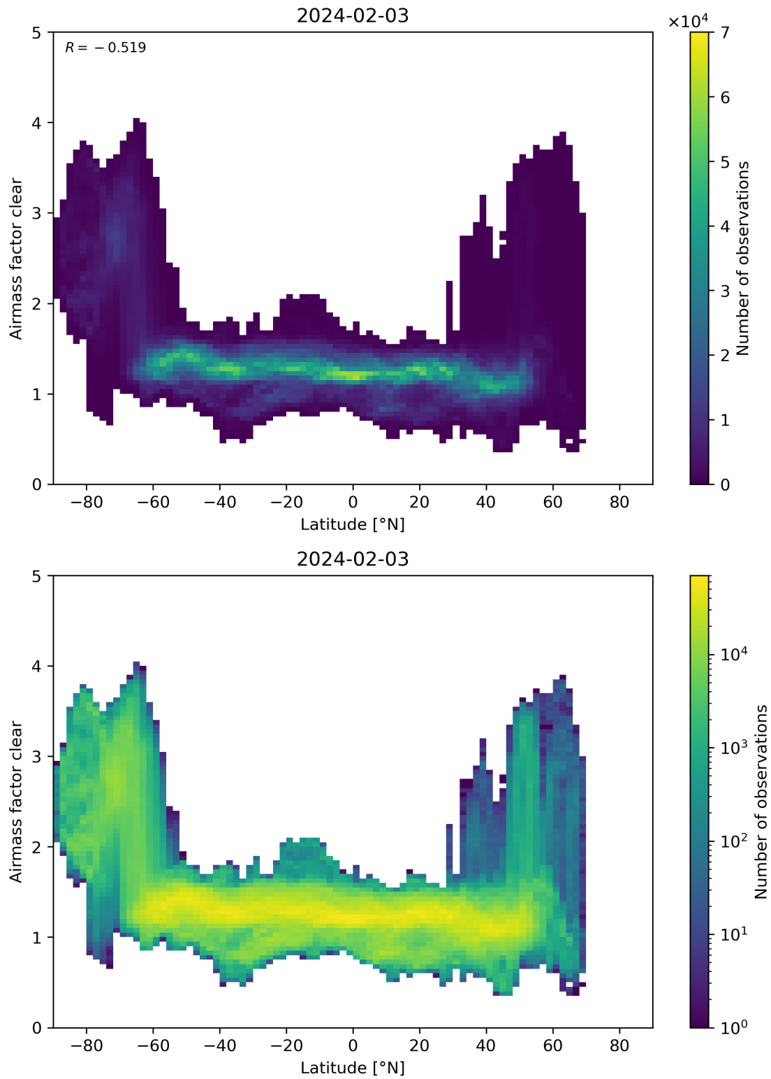
Figure 156: Scatter density plot of “Latitude” against “Airmass factor clear” for 2024-02-02 to 2024-02-04.
