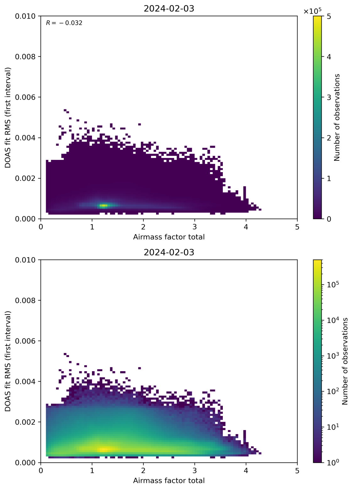
Figure 97: Scatter density plot of “Airmass factor total” against “DOAS fit RMS (first interval)” for 2024-02-02 to 2024-02-04.
