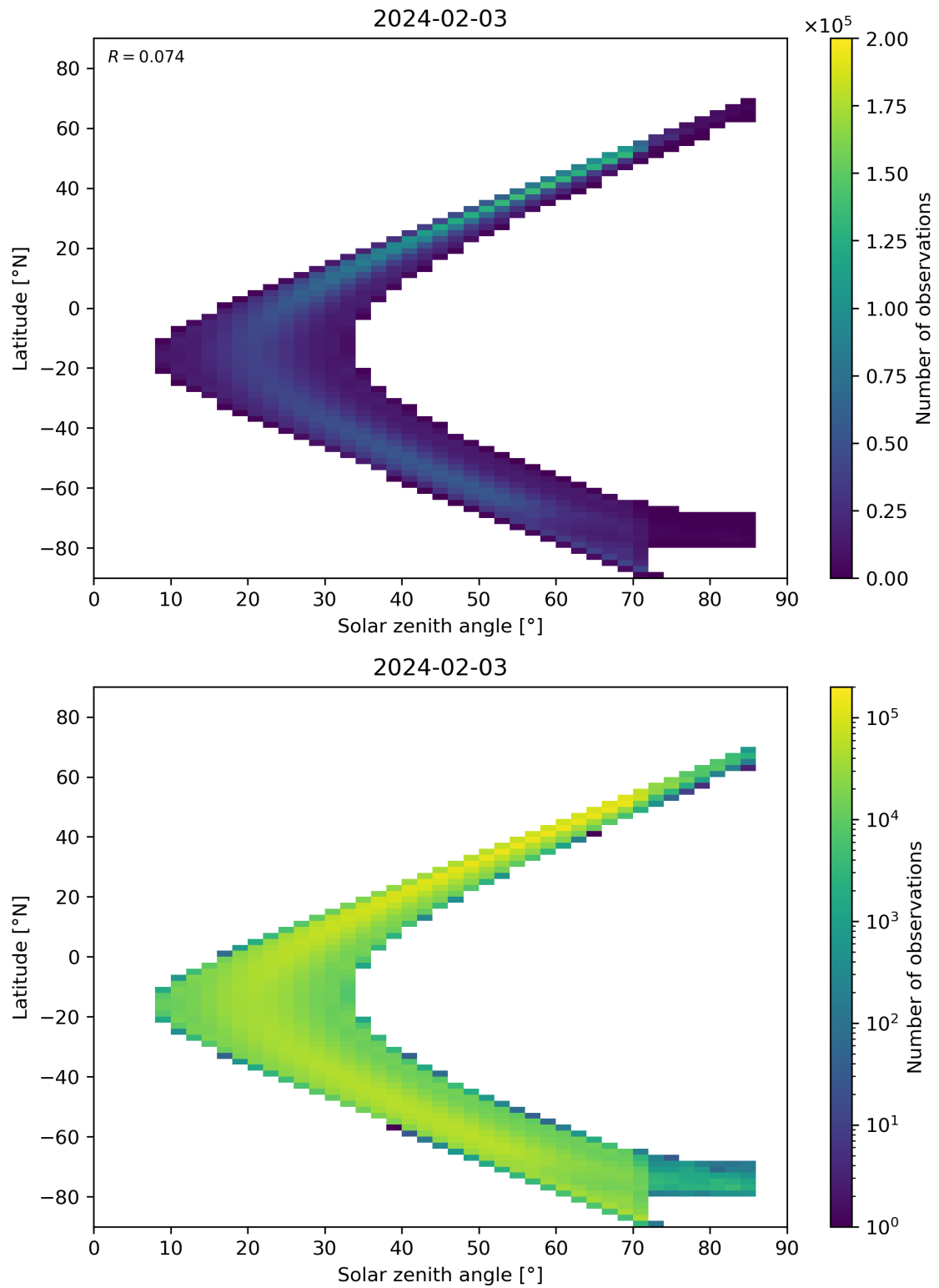
Figure 181: Scatter density plot of “Solar zenith angle” against “Latitude” for 2024-02-02 to 2024-02-04.
