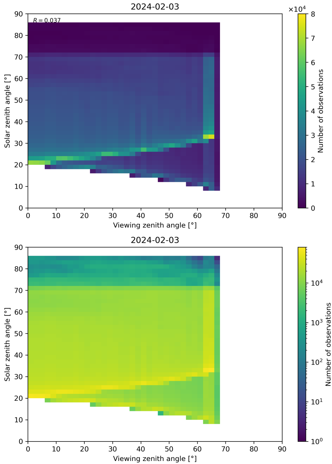
Figure 197: Scatter density plot of “Viewing zenith angle” against “Solar zenith angle” for 2024-02-02 to 2024-02-04.
