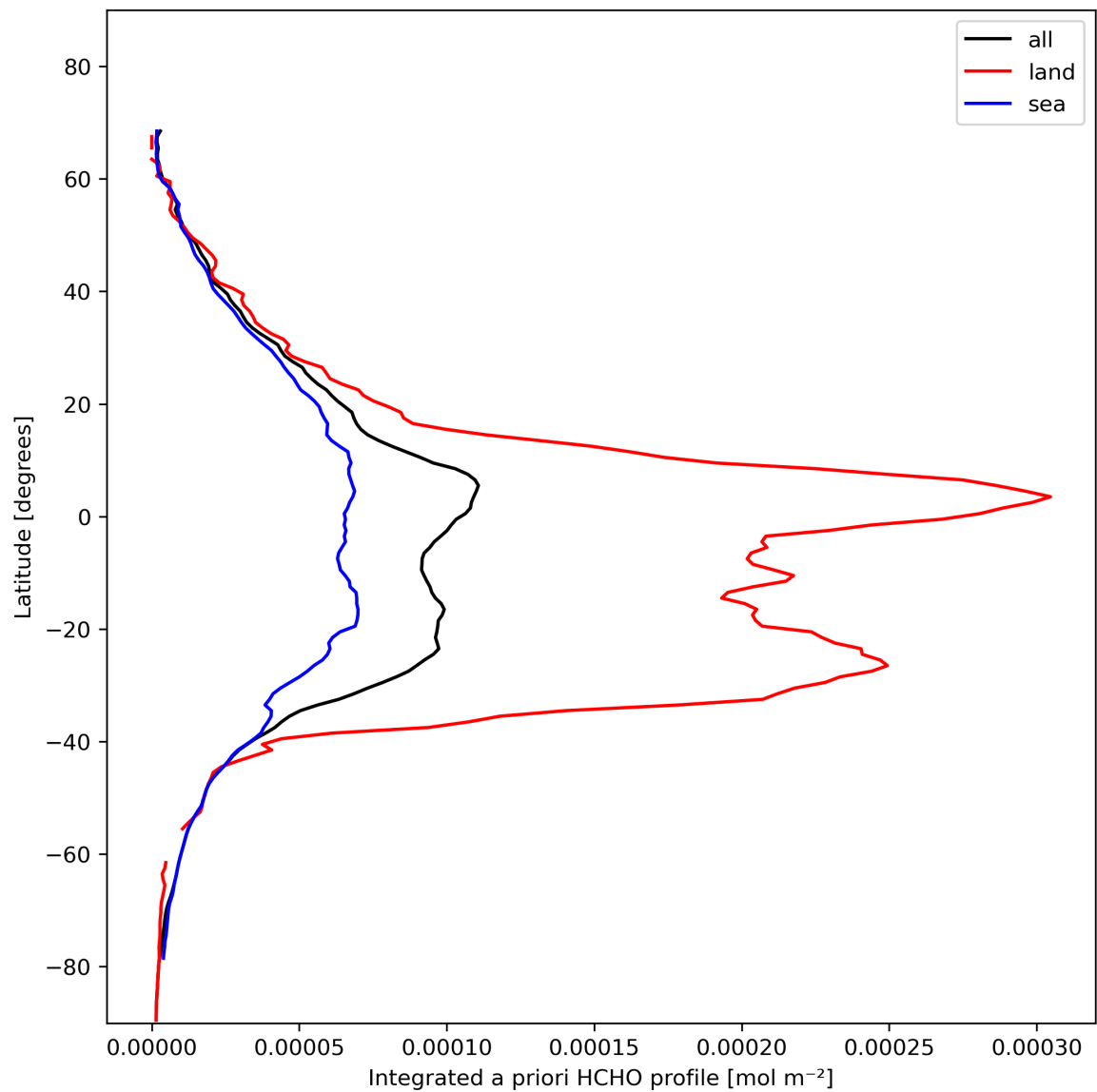
Figure 29: Zonal average of “Integrated a priori HCHO profile” for 2024-02-02 to 2024-02-04.
