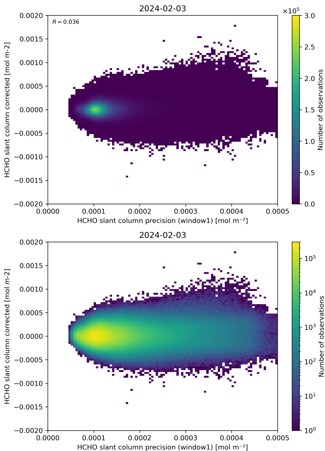
Figure 92: Scatter density plot of “HCHO slant column precision (window1)” against “HCHO slant column corrected” for 2024-02-02 to 2024-02-04.
