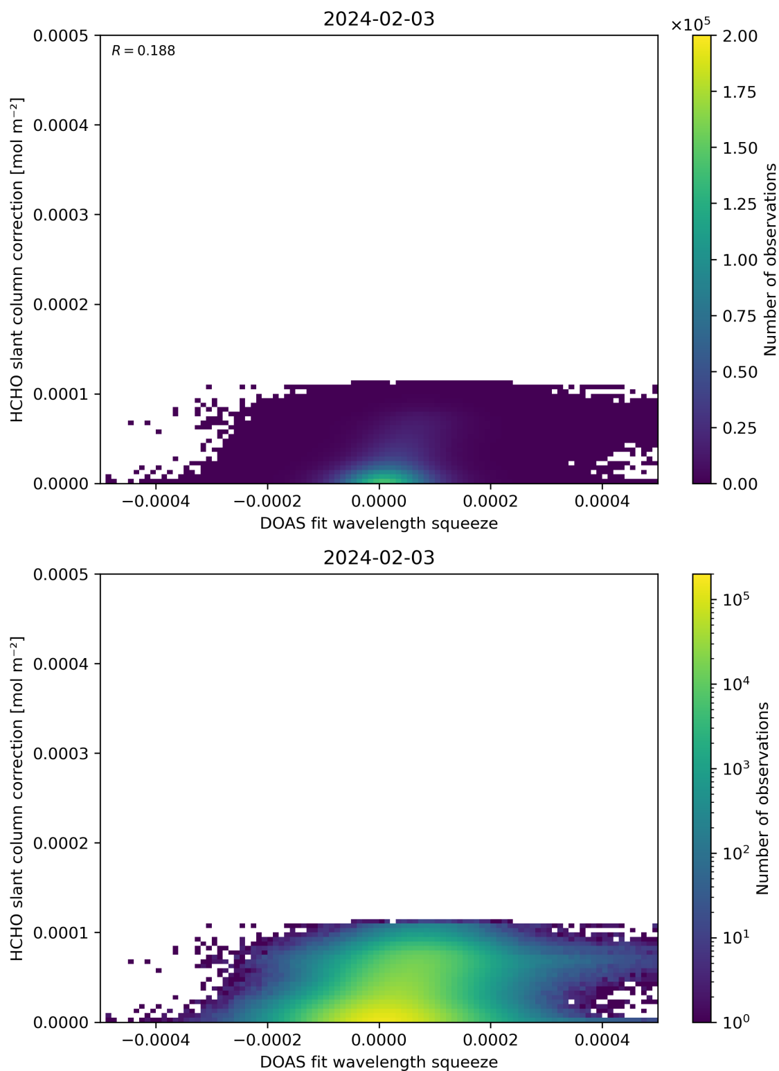
Figure 70: Scatter density plot of “DOAS fit wavelength squeeze” against “HCHO slant column correction” for 2024-02-02 to 2024-02-04.
