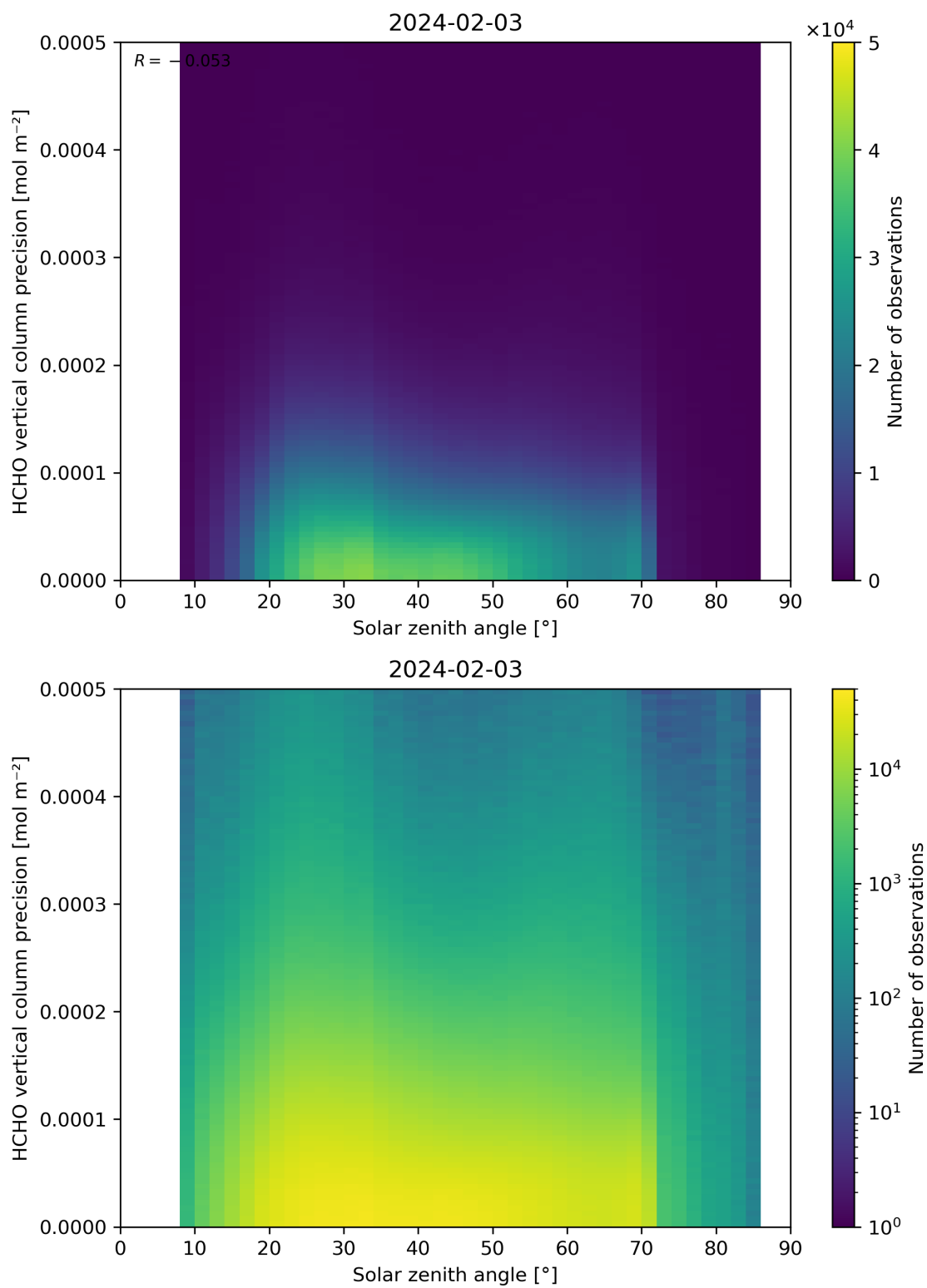
Figure 179: Scatter density plot of “Solar zenith angle” against “HCHO vertical column precision” for 2024-02-02 to 2024-02-04.
