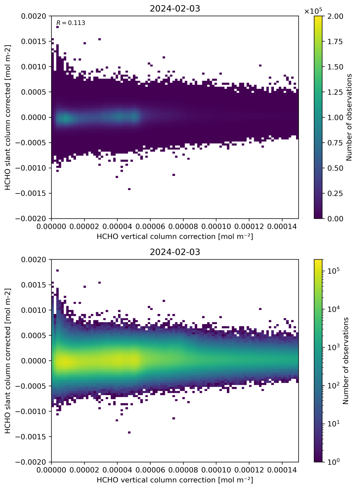
Figure 116: Scatter density plot of “HCHO vertical column correction” against “HCHO slant column corrected” for 2024-02-02 to 2024-02-04.
