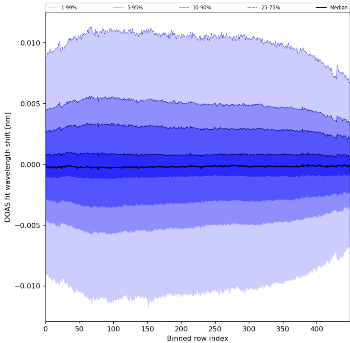
Figure 58: Along track statistics of “DOAS fit wavelength shift” for 2024-02-02 to 2024-02-04
