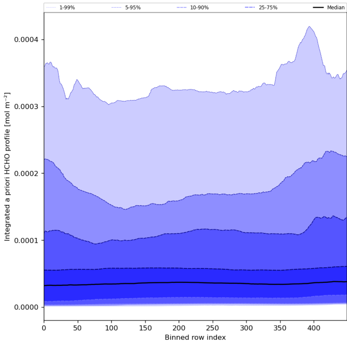
Figure 57: Along track statistics of “Integrated a priori HCHO profile” for 2024-02-02 to 2024-02-04
