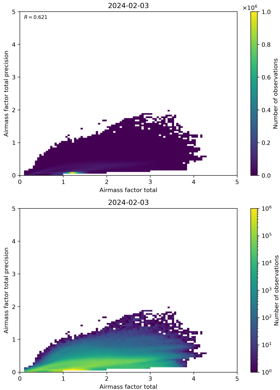
Figure 103: Scatter density plot of “Airmass factor total” against “Airmass factor total precision” for 2024-02-02 to 2024-02-04.
