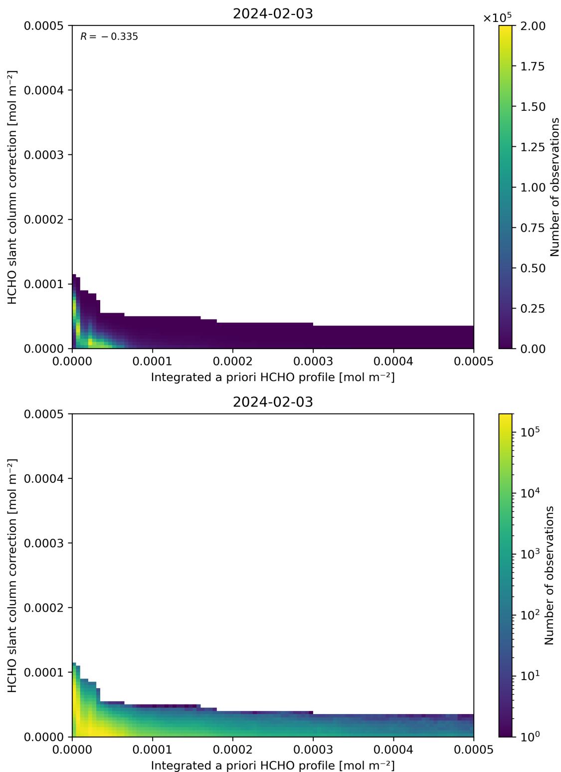
Figure 152: Scatter density plot of “Integrated a priori HCHO profile” against “HCHO slant column correction” for 2024-02-02 to 2024-02-04.
