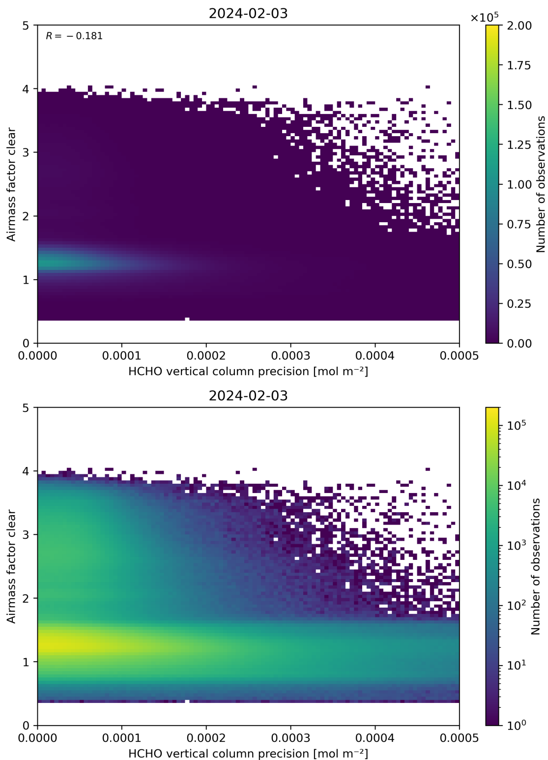
Figure 139: Scatter density plot of “HCHO vertical column precision” against “Airmass factor clear” for 2024-02-02 to 2024-02-04.
