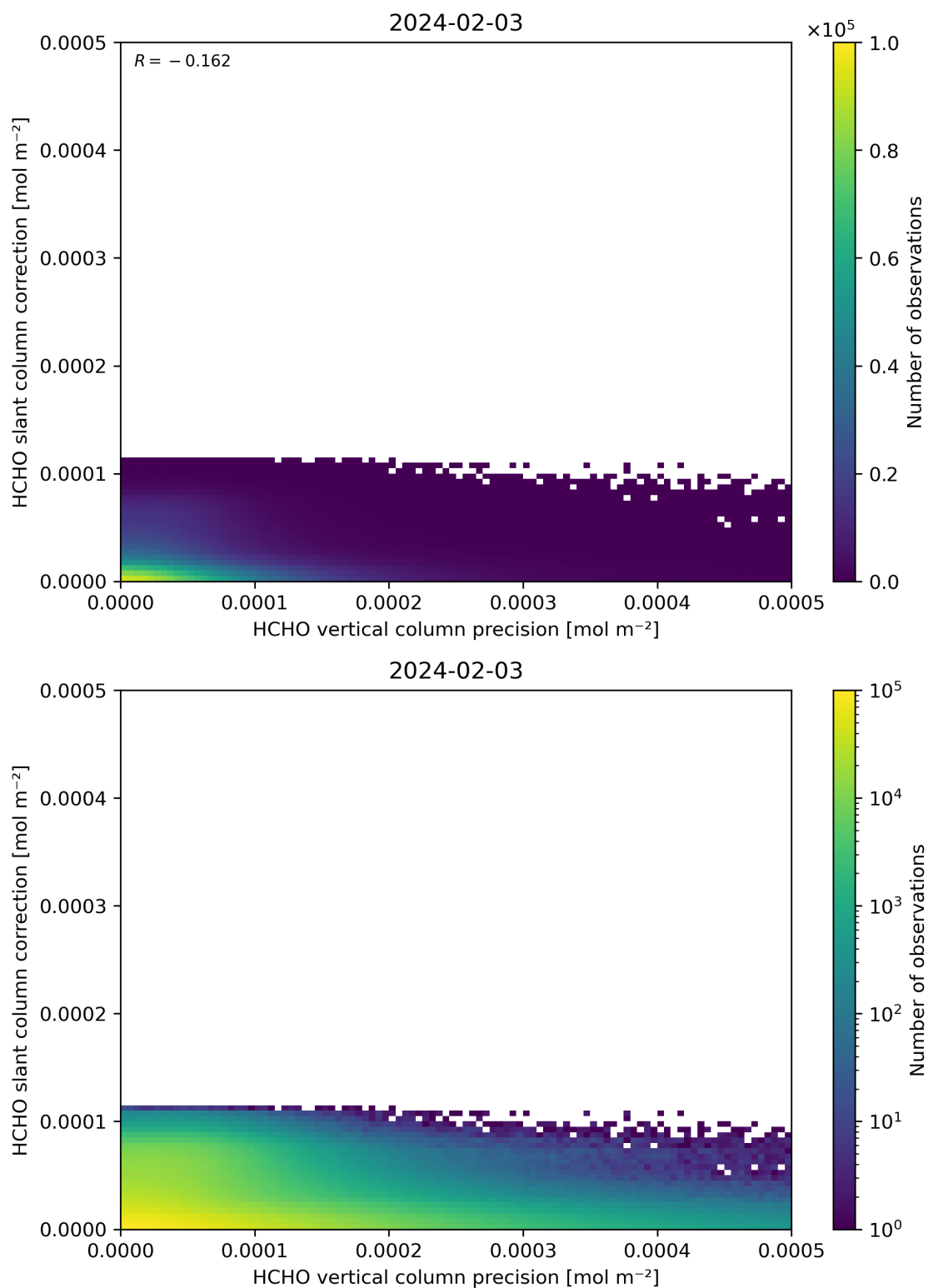
Figure 141: Scatter density plot of “HCHO vertical column precision” against “HCHO slant column correction” for 2024-02-02 to 2024-02-04.
