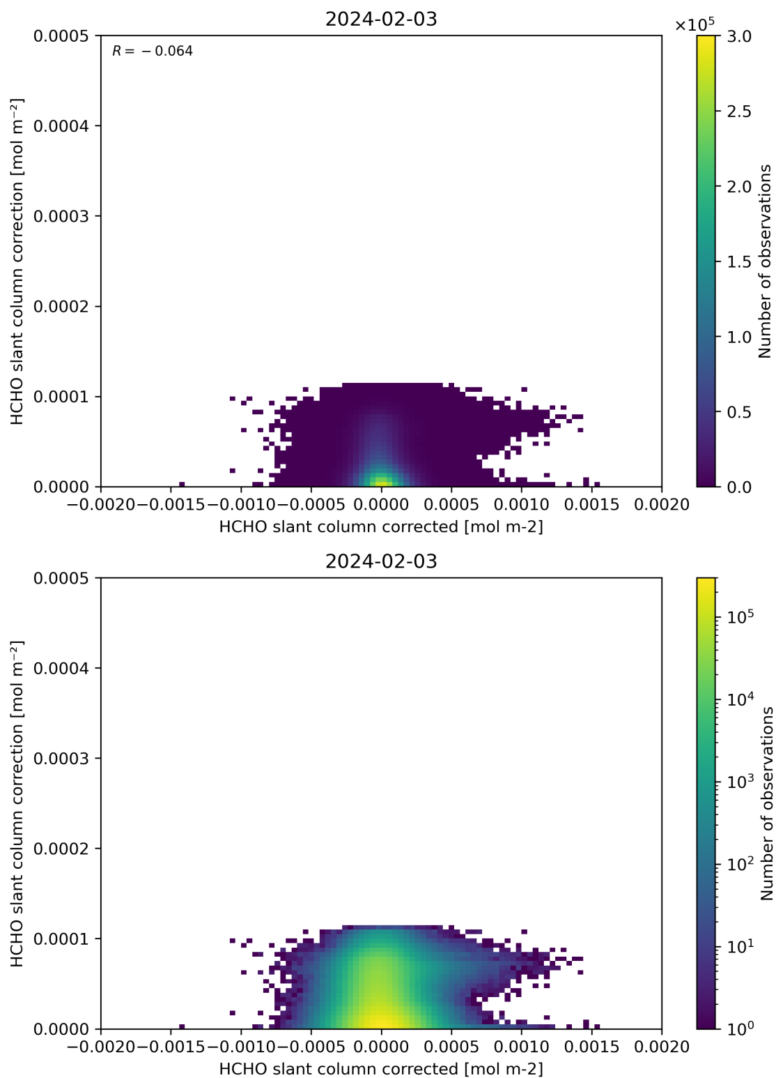
Figure 77: Scatter density plot of “HCHO slant column corrected” against “HCHO slant column correction” for 2024-02-02 to 2024-02-04.
