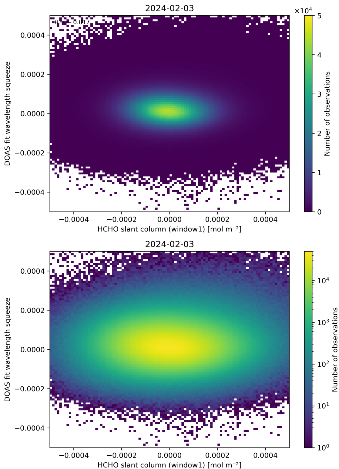
Figure 80: Scatter density plot of “HCHO slant column (window1)” against “DOAS fit wavelength squeeze” for 2024-02-02 to 2024-02-04.
