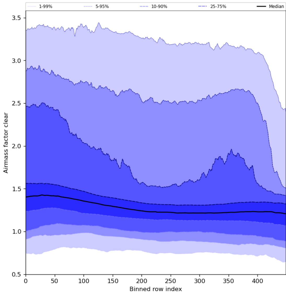
Figure 56: Along track statistics of “Airmass factor clear” for 2024-02-02 to 2024-02-04
