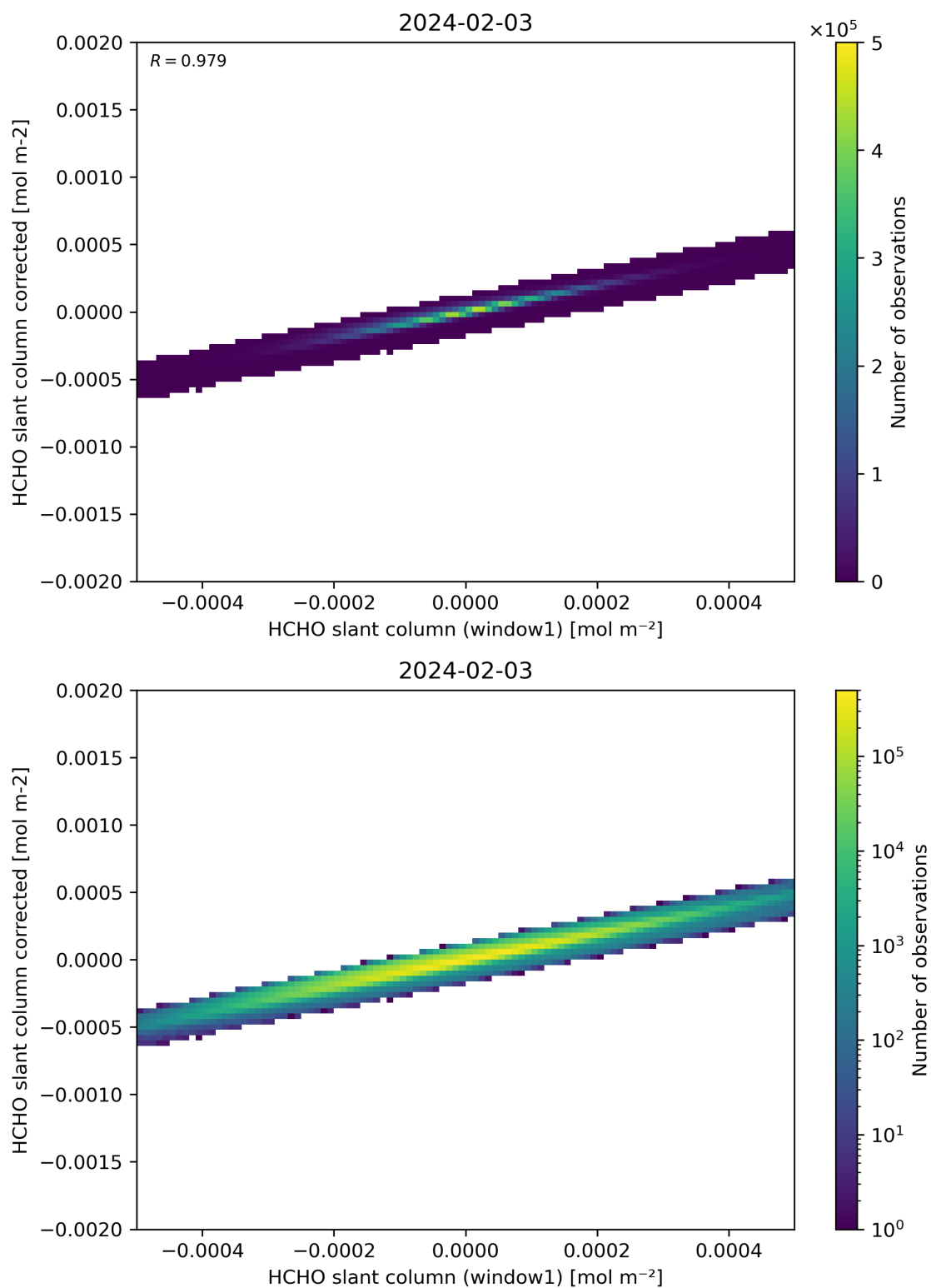
Figure 82: Scatter density plot of “HCHO slant column (window1)” against “HCHO slant column corrected” for 2024-02-02 to 2024-02-04.
