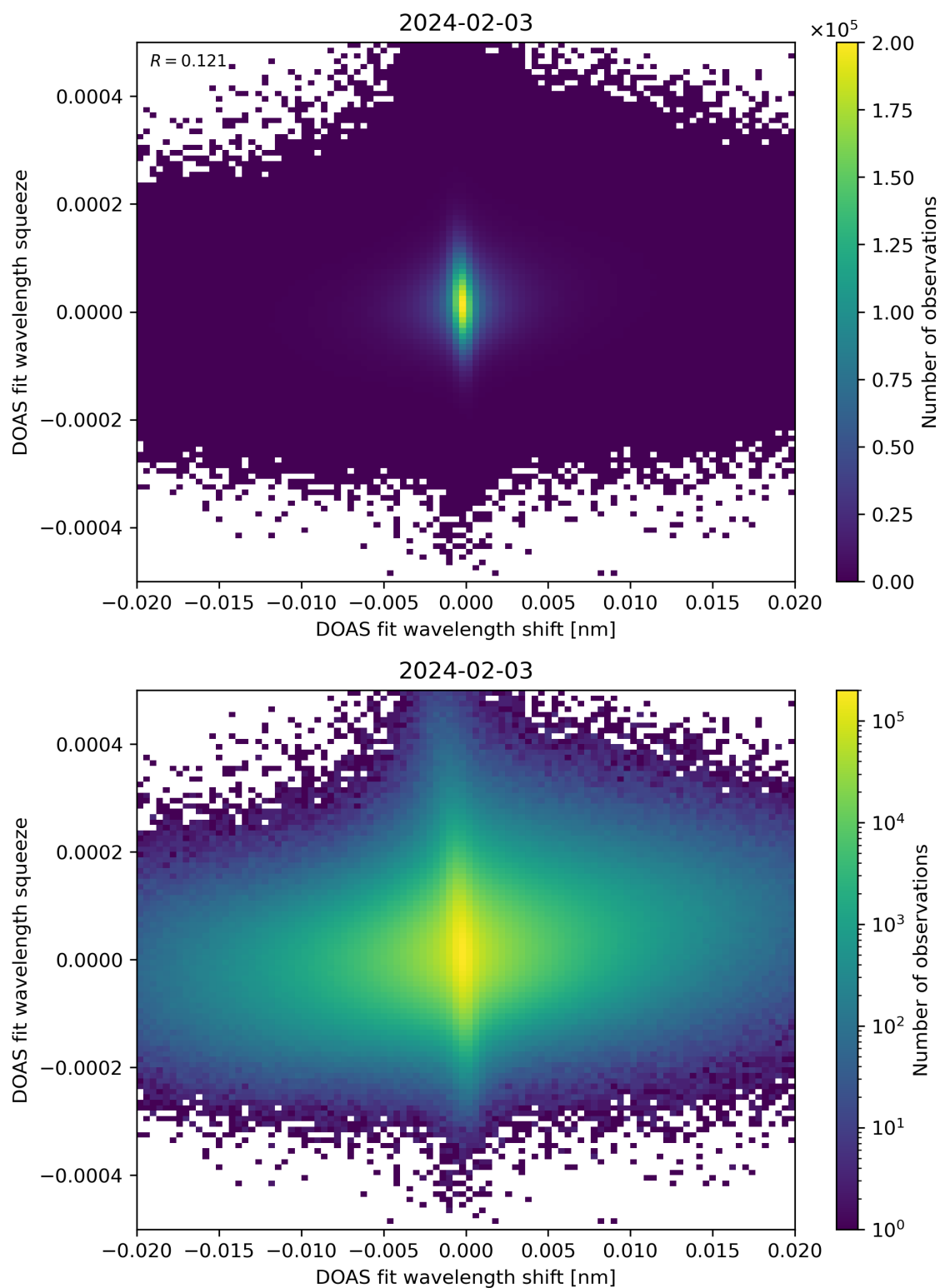
Figure 65: Scatter density plot of “DOAS fit wavelength shift” against “DOAS fit wavelength squeeze” for 2024-02-02 to 2024-02-04.
