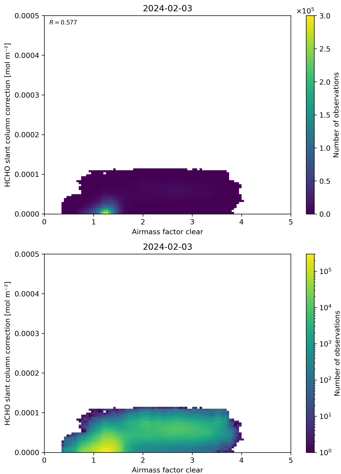
Figure 75: Scatter density plot of “Airmass factor clear” against “HCHO slant column correction” for 2024-02-02 to 2024-02-04.
