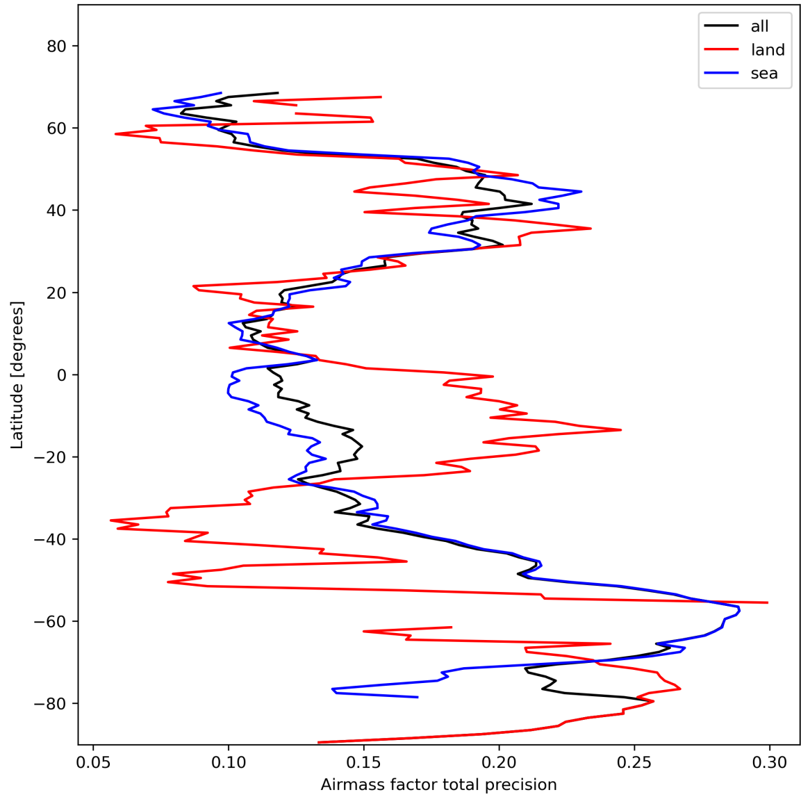
Figure 27: Zonal average of “Airmass factor total precision” for 2024-02-02 to 2024-02-04.
