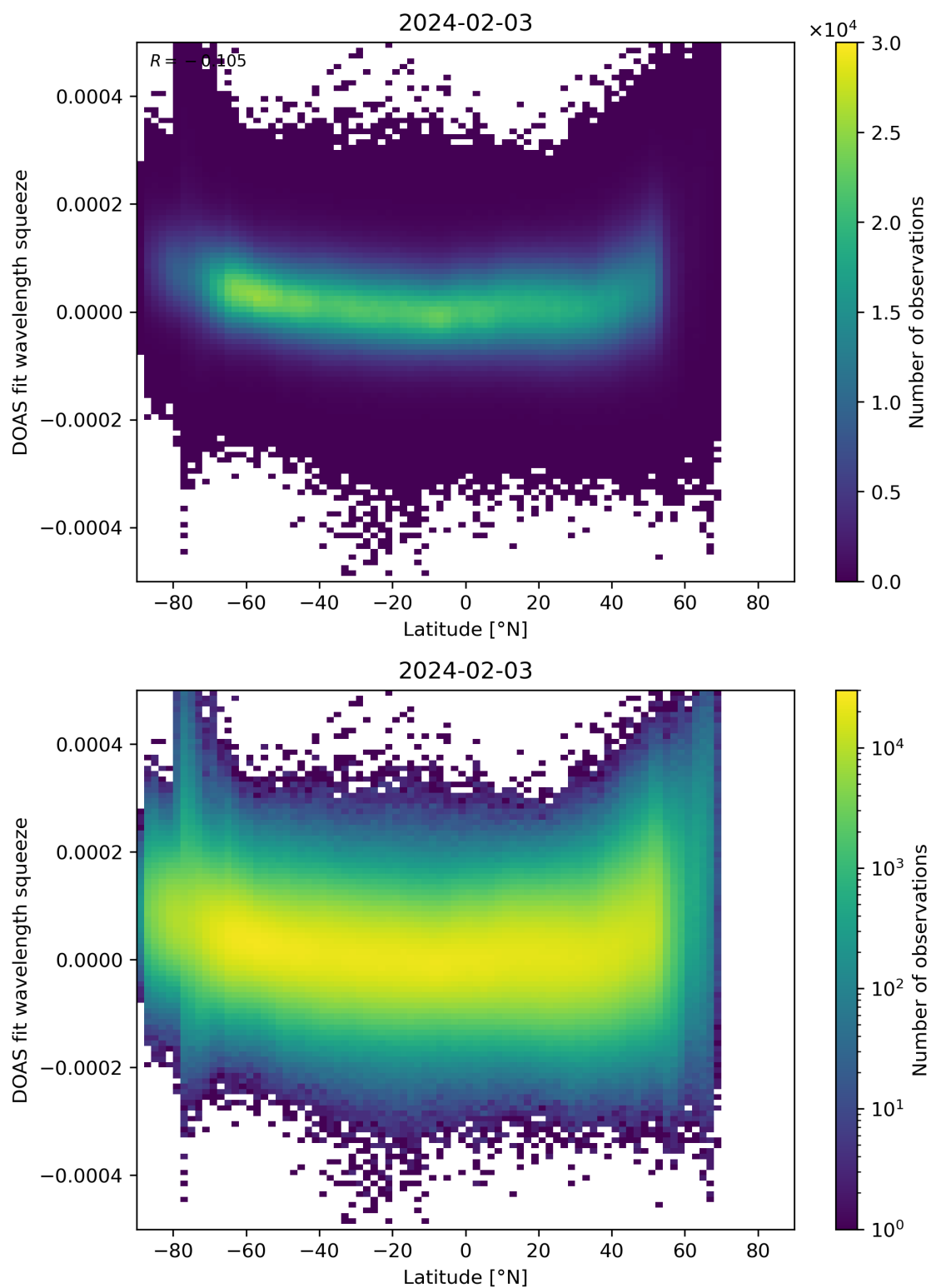
Figure 155: Scatter density plot of “Latitude” against “DOAS fit wavelength squeeze” for 2024-02-02 to 2024-02-04.
