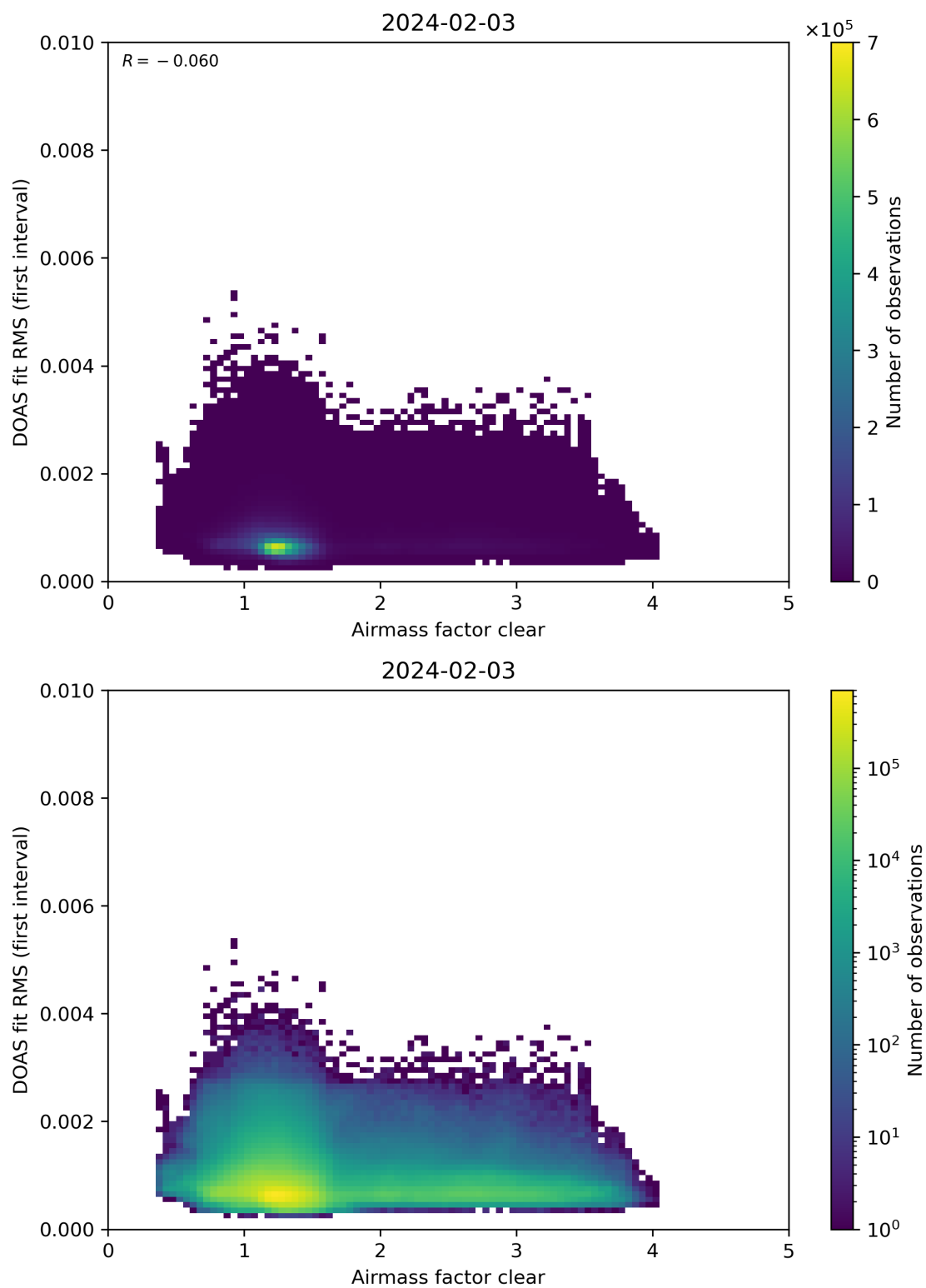
Figure 71: Scatter density plot of “Airmass factor clear” against “DOAS fit RMS (first interval)” for 2024-02-02 to 2024-02-04.
