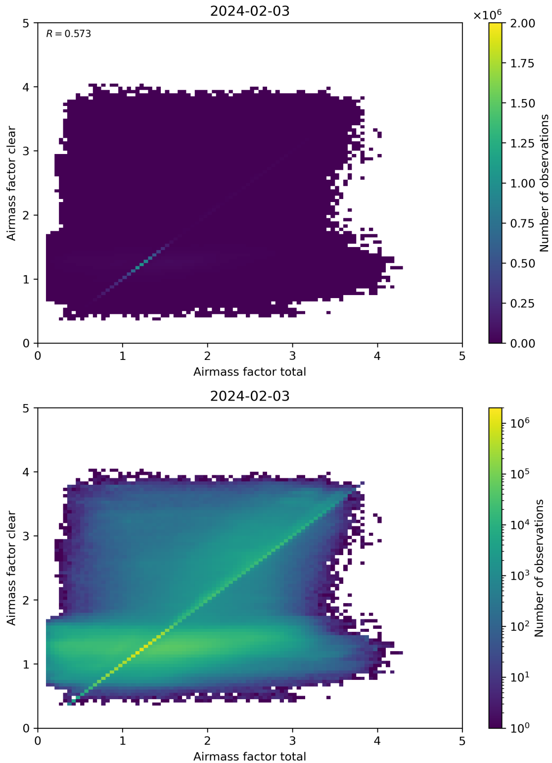
Figure 100: Scatter density plot of “Airmass factor total” against “Airmass factor clear” for 2024-02-02 to 2024-02-04.
