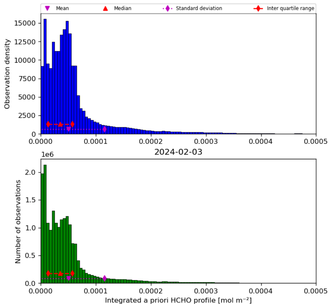
Figure 43: Histogram of “Integrated a priori HCHO profile” for 2024-02-02 to 2024-02-04
