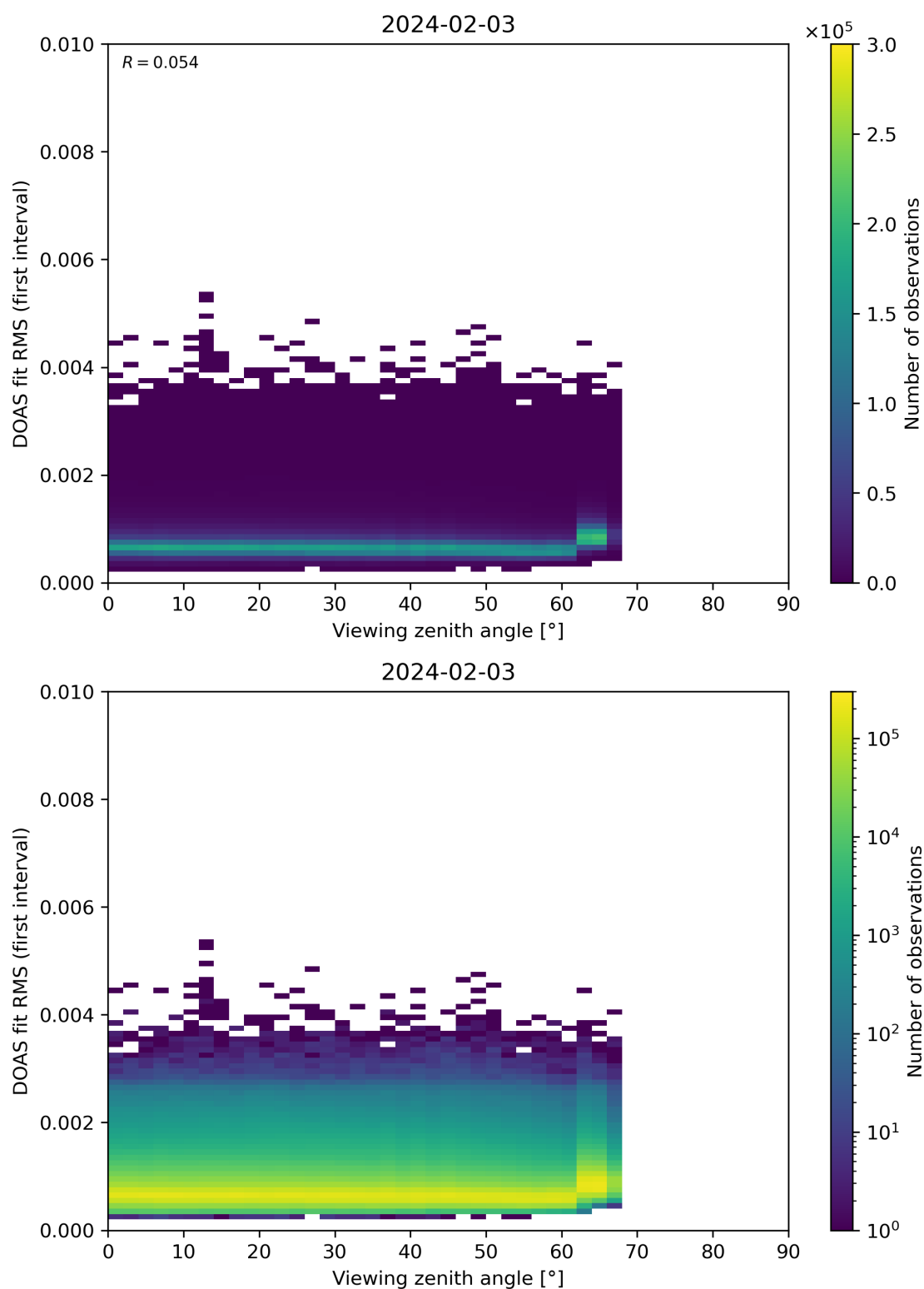
Figure 182: Scatter density plot of “Viewing zenith angle” against “DOAS fit RMS (first interval)” for 2024-02-02 to 2024-02-04.
