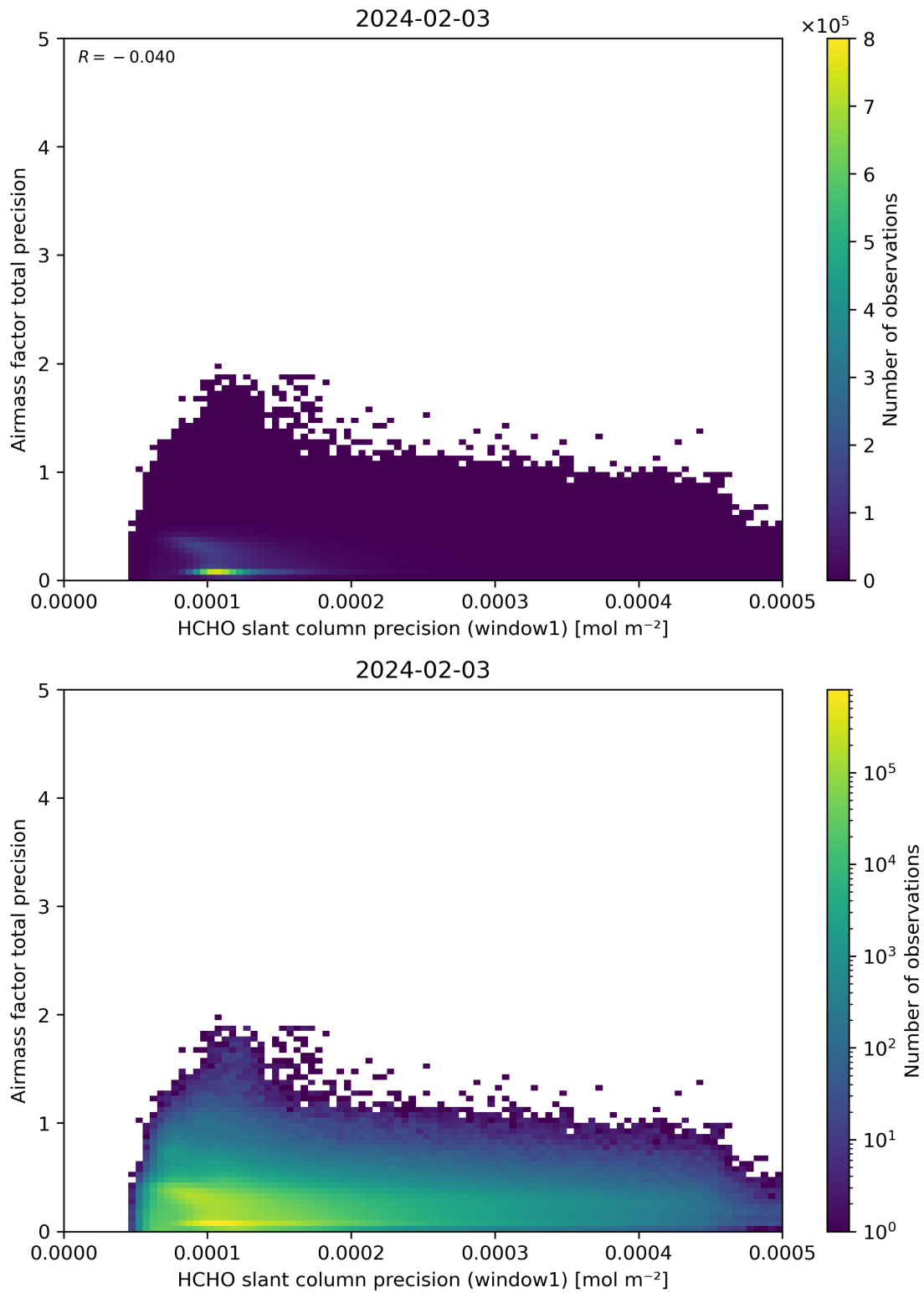
Figure 95: Scatter density plot of “HCHO slant column precision (window1)” against “Airmass factor total precision” for 2024-02-02 to 2024-02-04.
