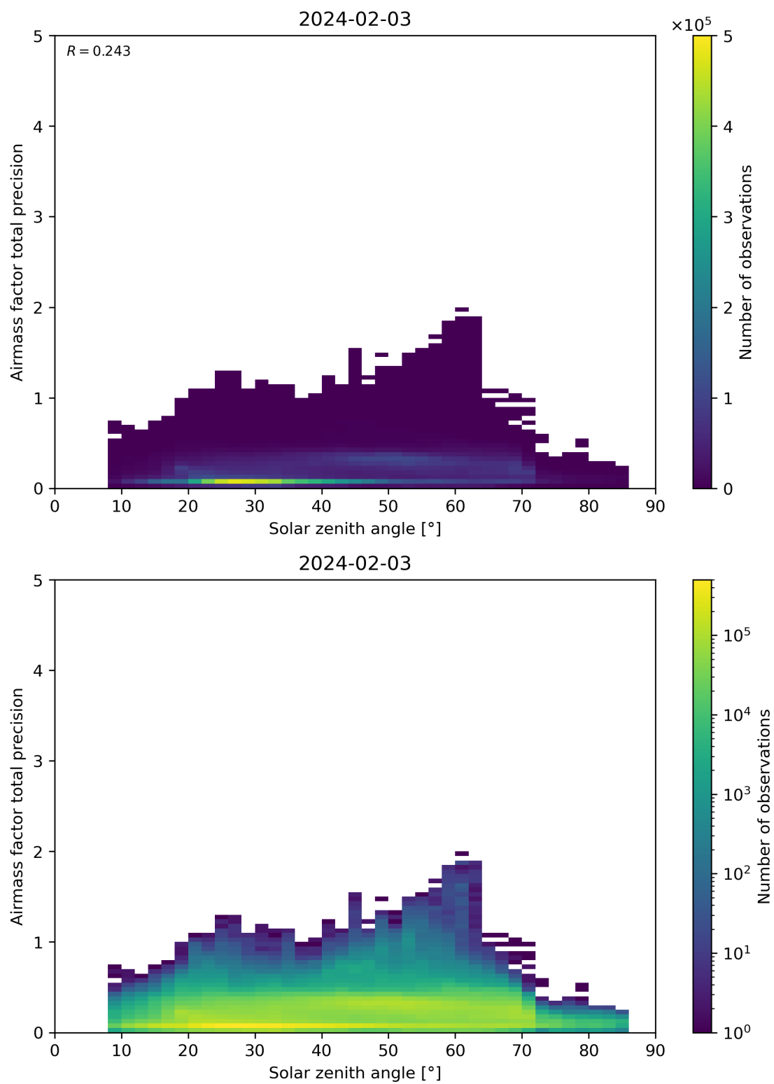
Figure 176: Scatter density plot of “Solar zenith angle” against “Airmass factor total precision” for 2024-02-02 to 2024-02-04.
