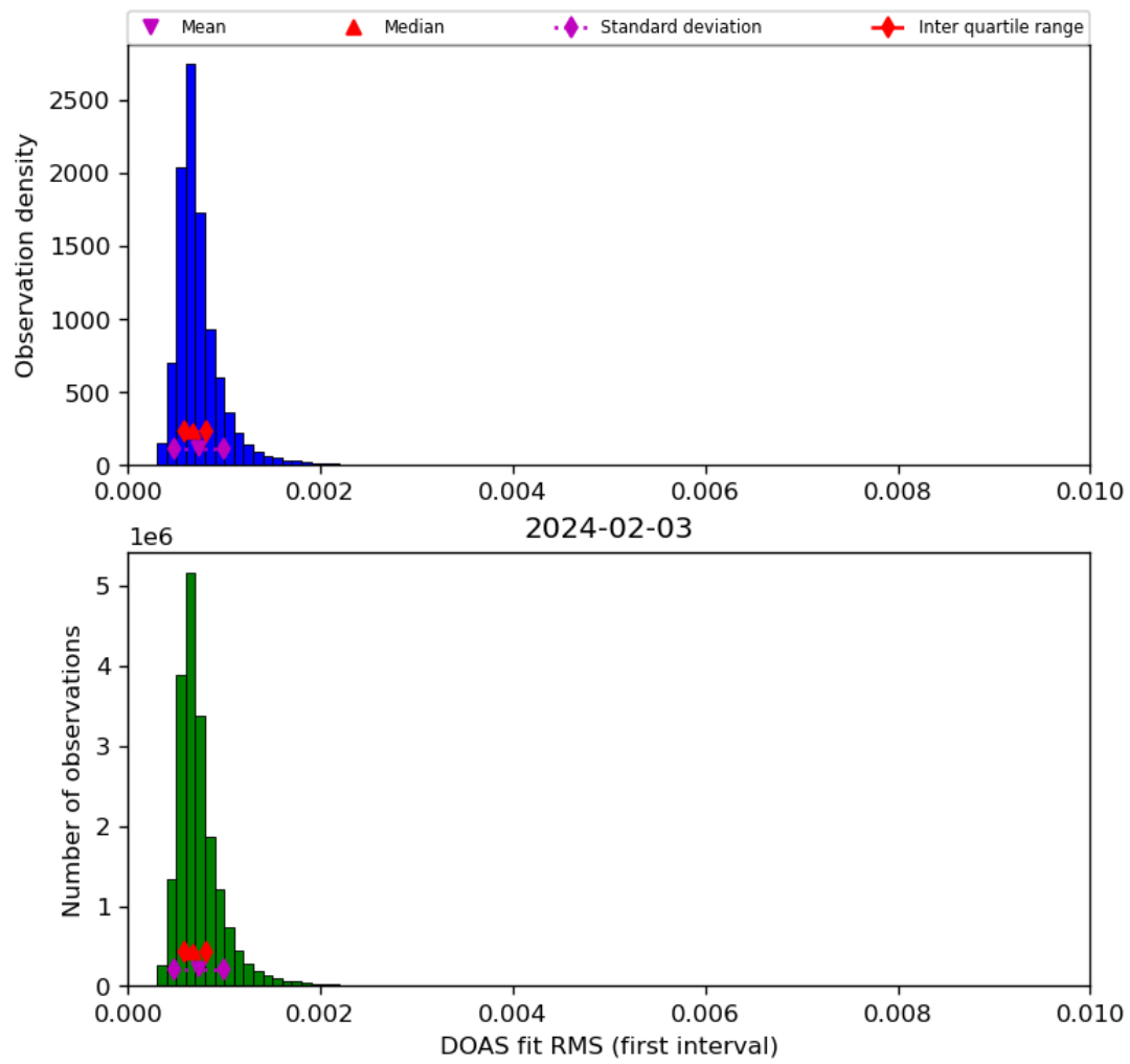
Figure 46: Histogram of “DOAS fit RMS (first interval)” for 2024-02-02 to 2024-02-04
