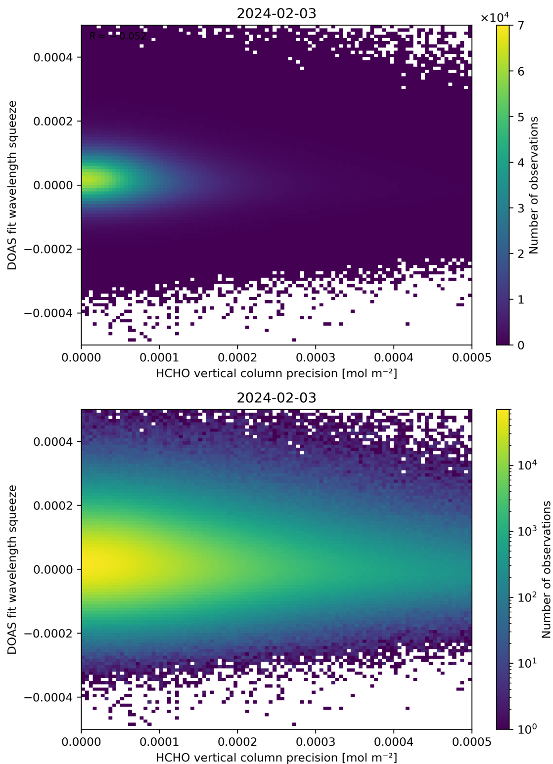
Figure 138: Scatter density plot of “HCHO vertical column precision” against “DOAS fit wavelength squeeze” for 2024-02-02 to 2024-02-04.
