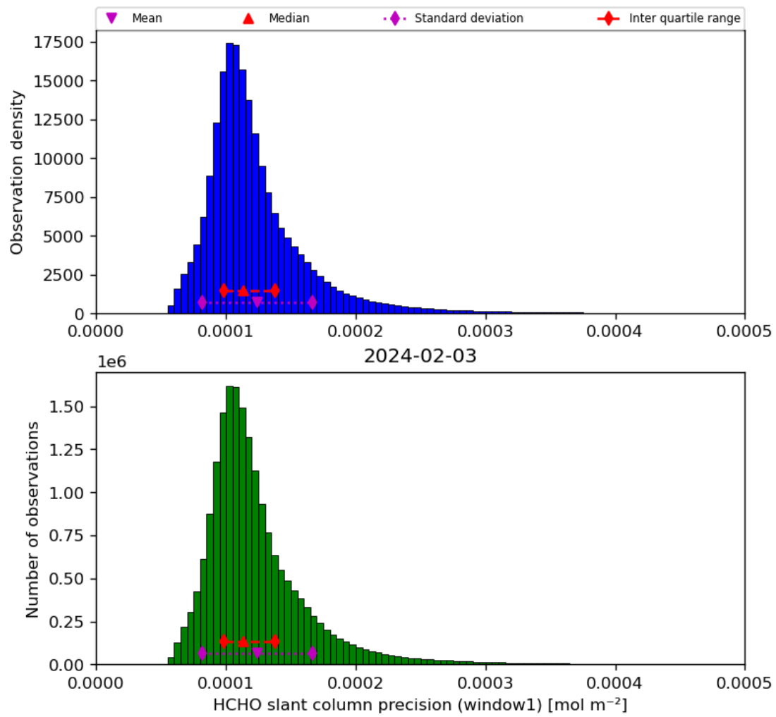
Figure 39: Histogram of “HCHO slant column precision (window1)” for 2024-02-02 to 2024-02-04
