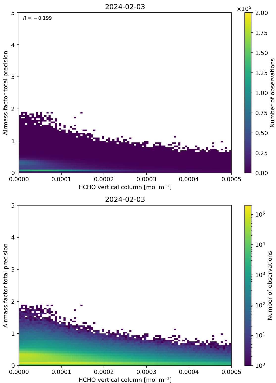
Figure 132: Scatter density plot of “HCHO vertical column” against “Airmass factor total precision” for 2024-02-02 to 2024-02-04.
