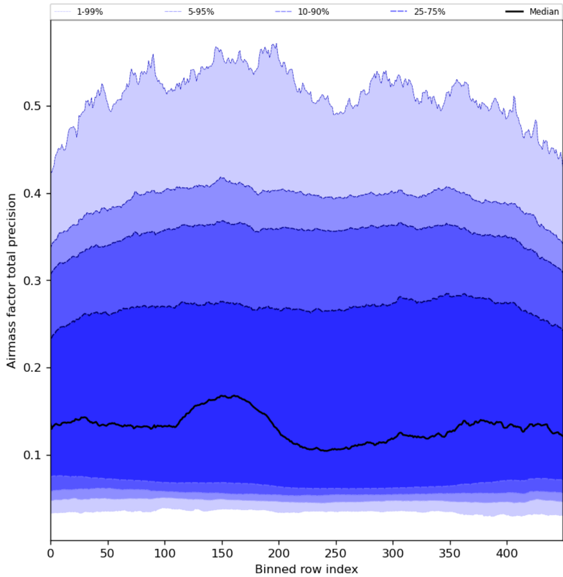
Figure 55: Along track statistics of “Airmass factor total precision” for 2024-02-02 to 2024-02-04
