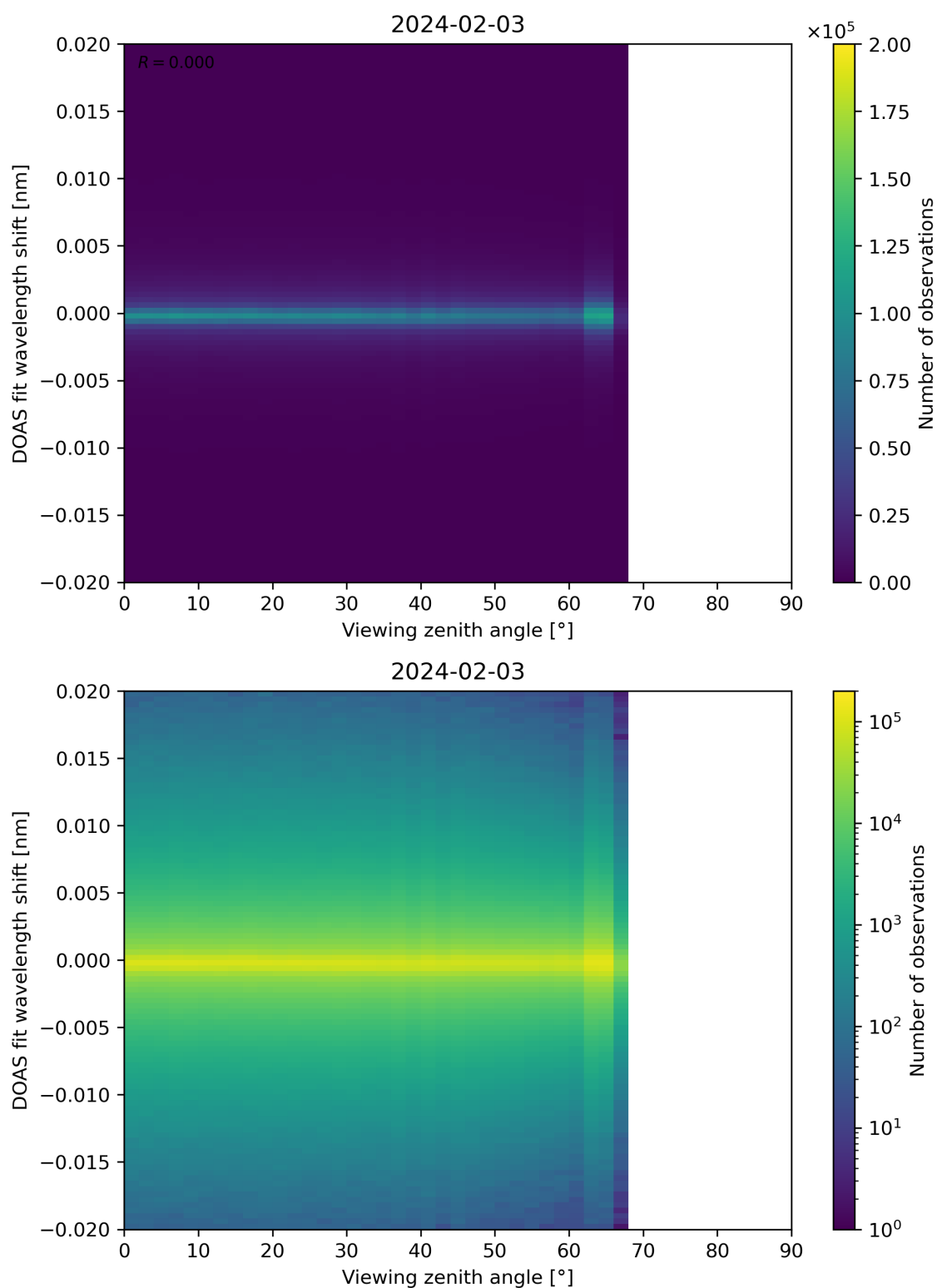
Figure 183: Scatter density plot of “Viewing zenith angle” against “DOAS fit wavelength shift” for 2024-02-02 to 2024-02-04.
