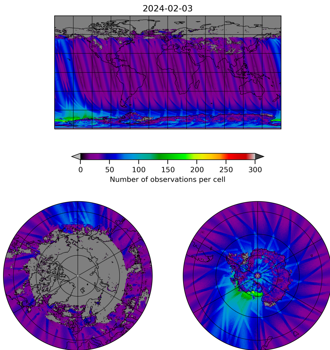
Figure 19: Map of the number of observations for 2024-02-02 to 2024-02-04
