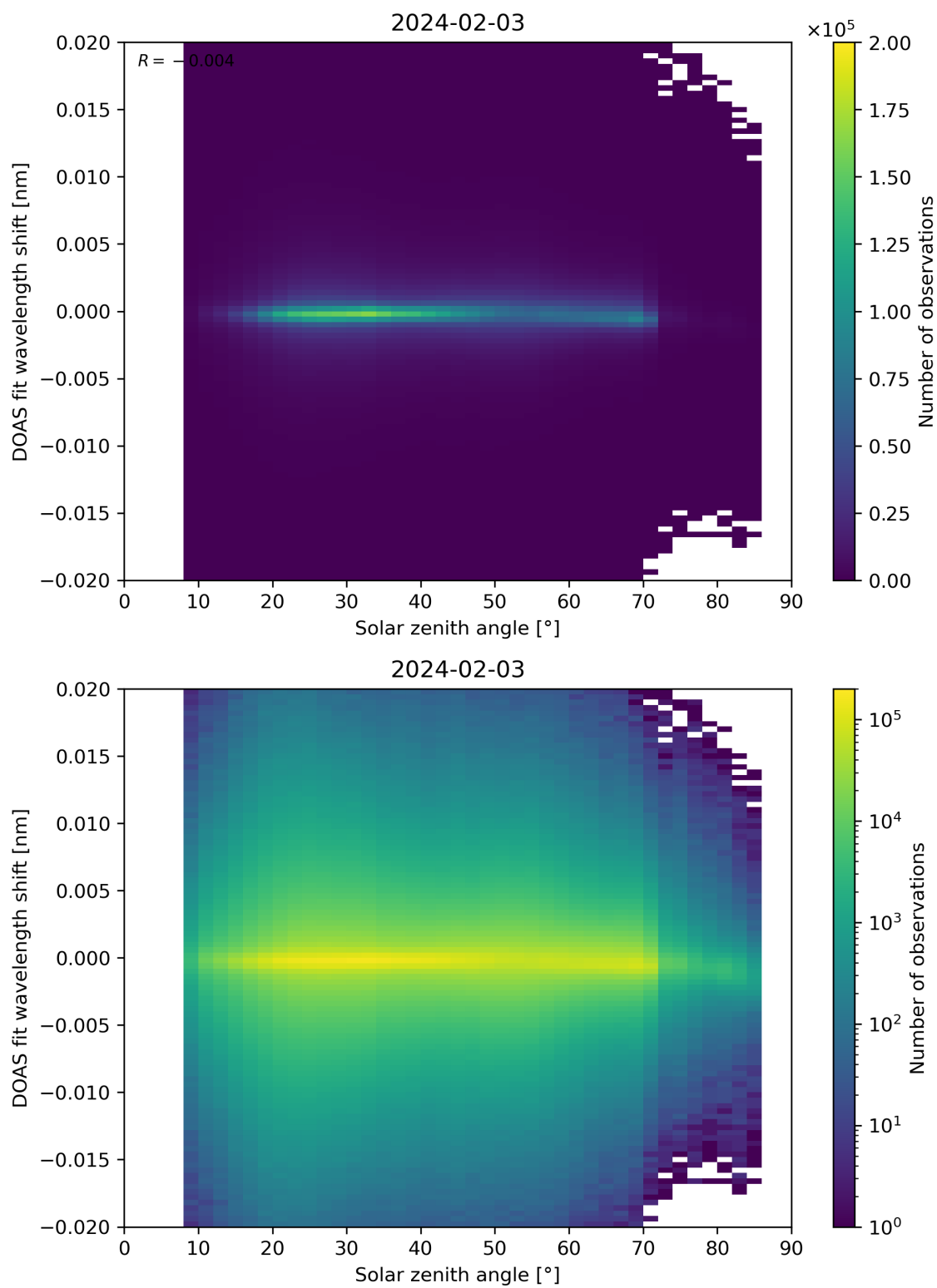
Figure 168: Scatter density plot of “Solar zenith angle” against “DOAS fit wavelength shift” for 2024-02-02 to 2024-02-04.
