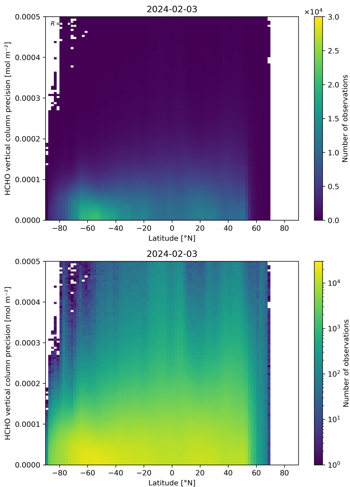
Figure 165: Scatter density plot of “Latitude” against “HCHO vertical column precision” for 2024-02-02 to 2024-02-04.
