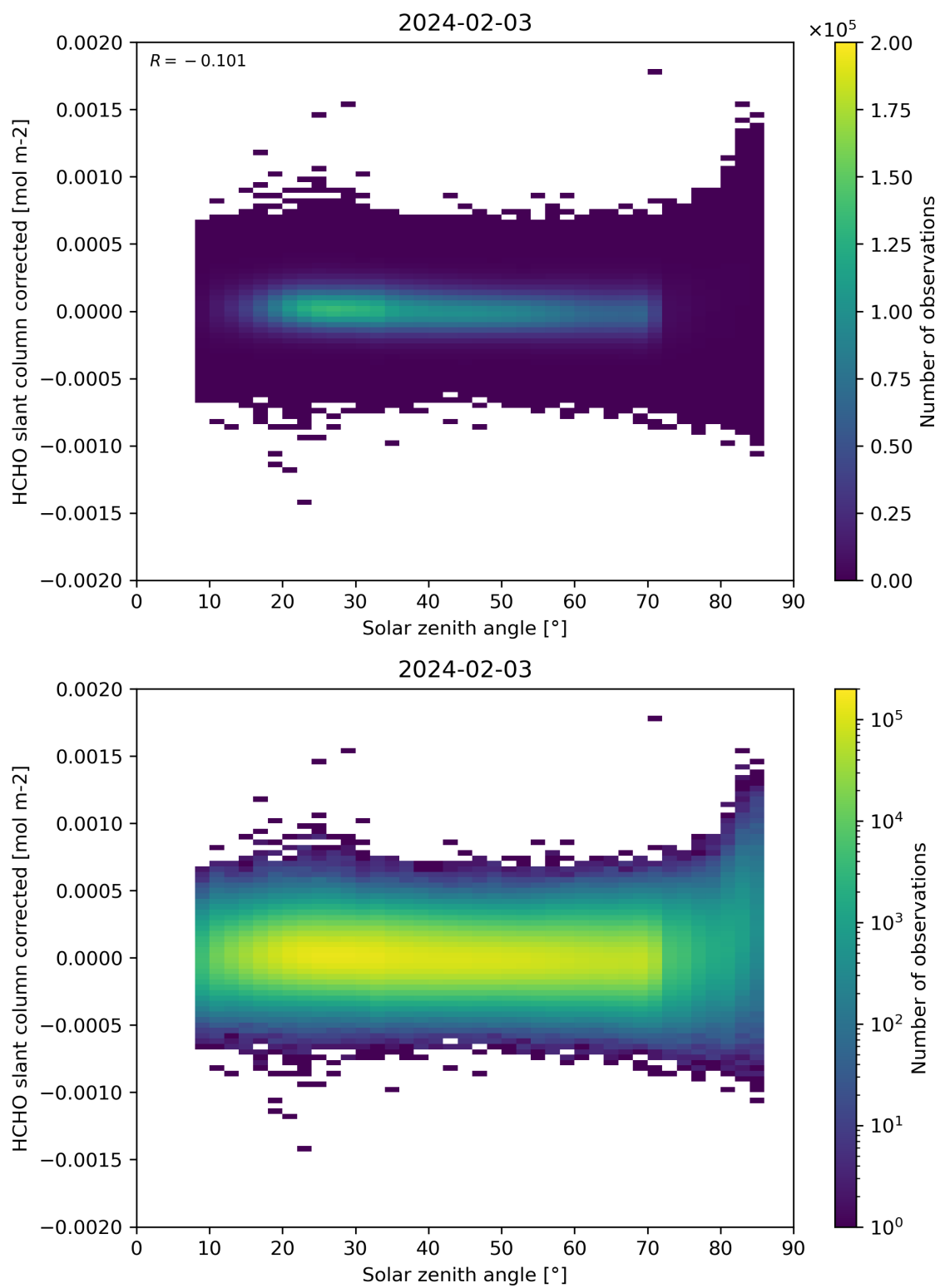
Figure 171: Scatter density plot of “Solar zenith angle” against “HCHO slant column corrected” for 2024-02-02 to 2024-02-04.
