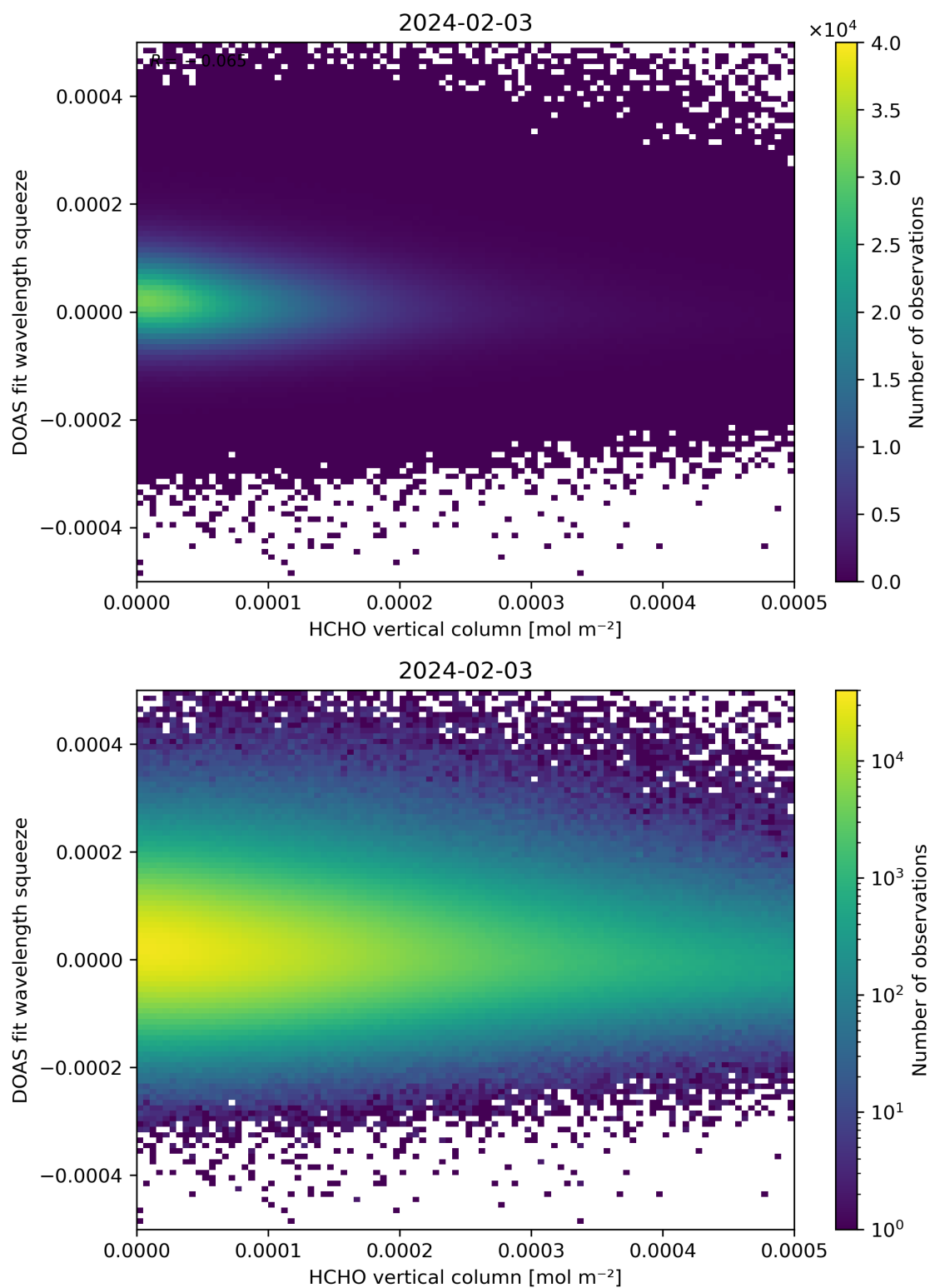
Figure 125: Scatter density plot of “HCHO vertical column” against “DOAS fit wavelength squeeze” for 2024-02-02 to 2024-02-04.
