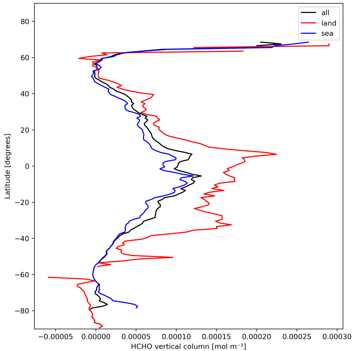
Figure 21: Zonal average of “HCHO vertical column” for 2024-02-02 to 2024-02-04.
