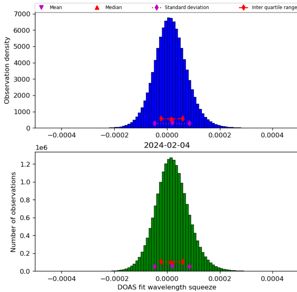
Figure 45: Histogram of “DOAS fit wavelength squeeze” for 2024-02-03 to 2024-02-05
