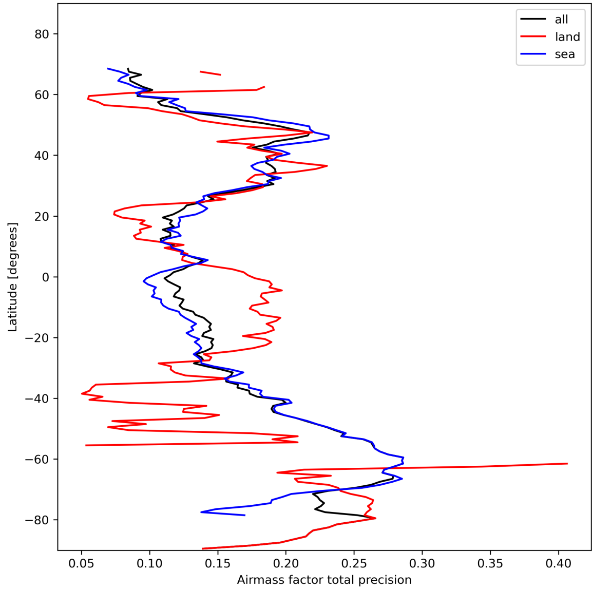
Figure 27: Zonal average of “Airmass factor total precision” for 2024-02-03 to 2024-02-05.
