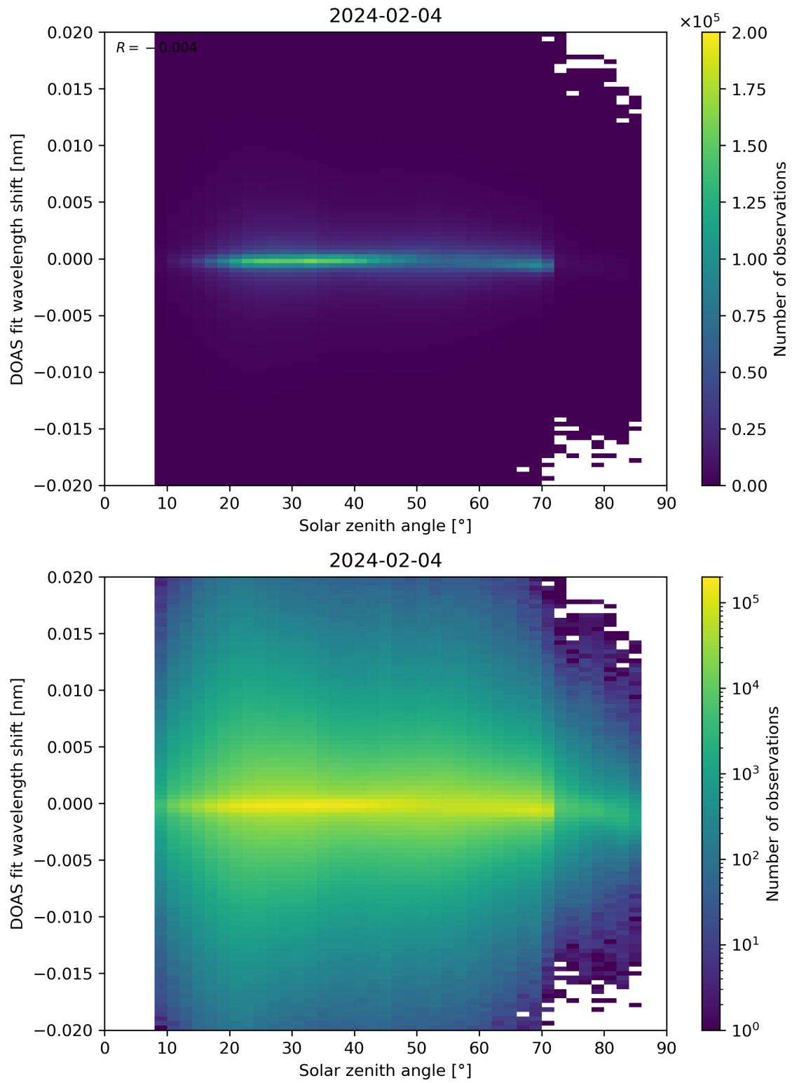
Figure 168: Scatter density plot of “Solar zenith angle” against “DOAS fit wavelength shift” for 2024-02-03 to 2024-02-05.
