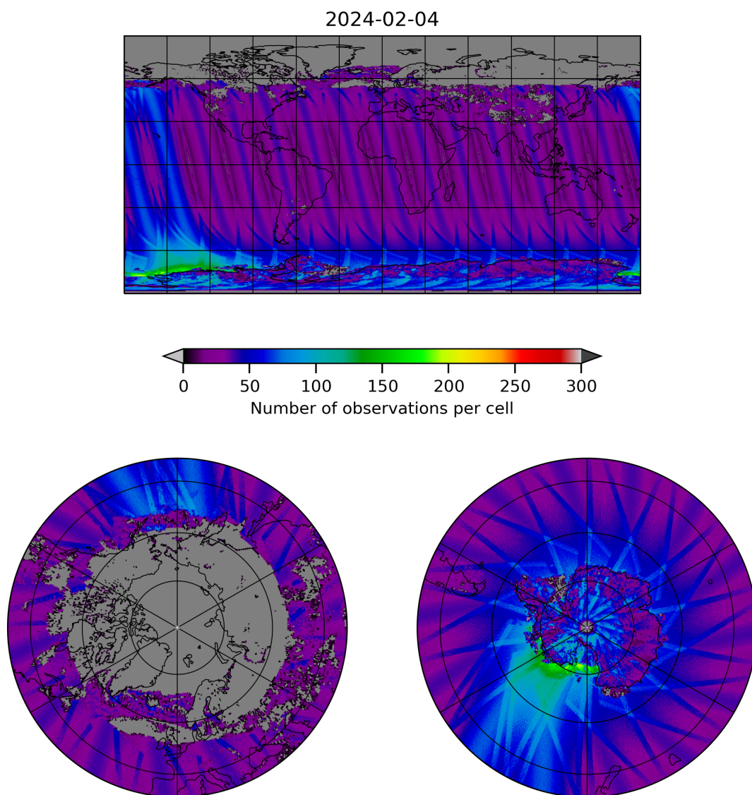
Figure 19: Map of the number of observations for 2024-02-03 to 2024-02-05
