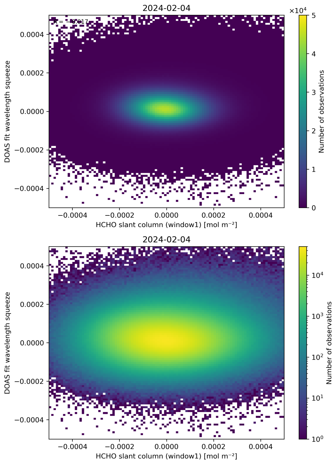
Figure 80: Scatter density plot of “HCHO slant column (window1)” against “DOAS fit wavelength squeeze” for 2024-02-03 to 2024-02-05.
