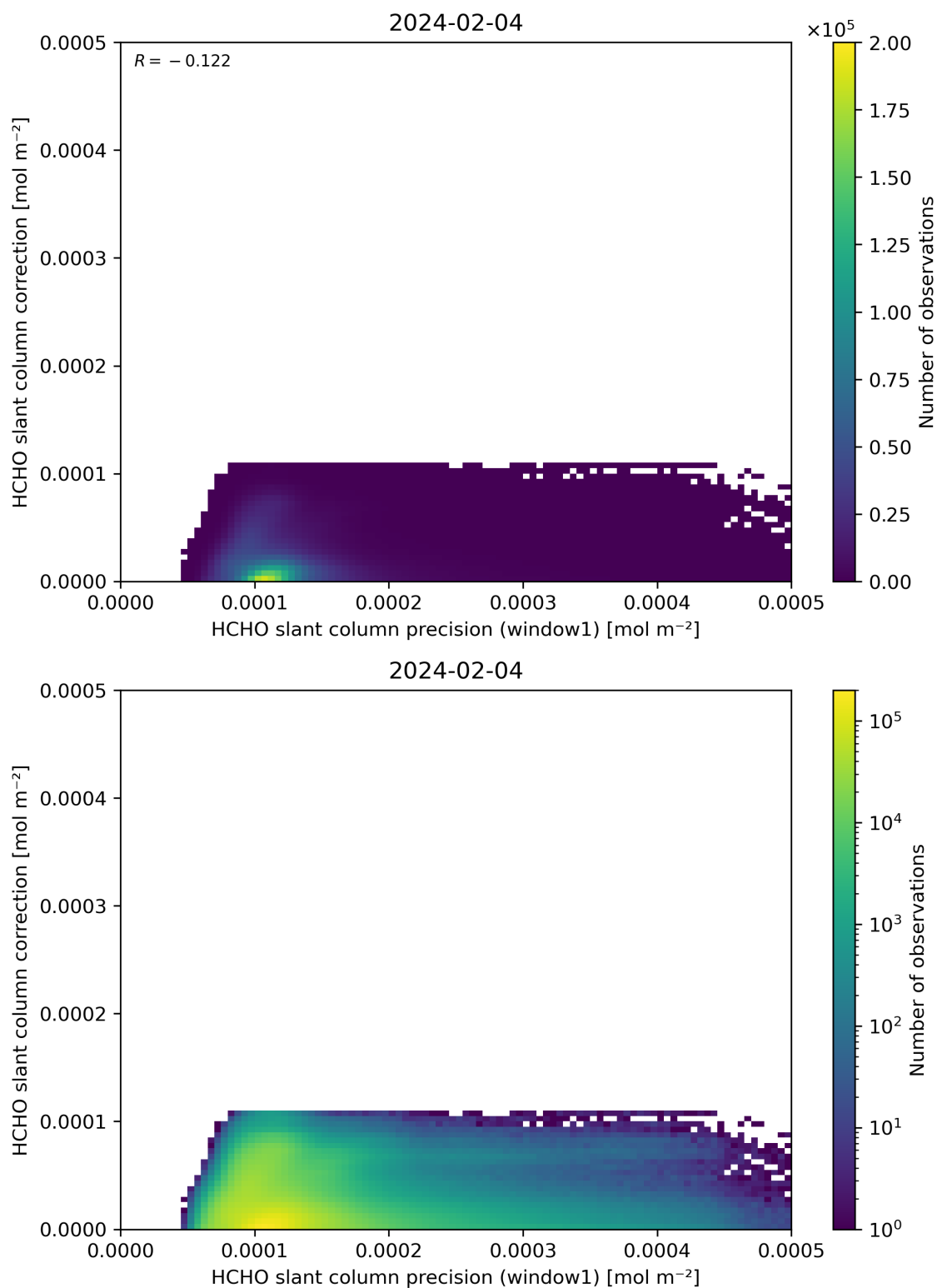
Figure 93: Scatter density plot of “HCHO slant column precision (window1)” against “HCHO slant column correction” for 2024-02-03 to 2024-02-05.
