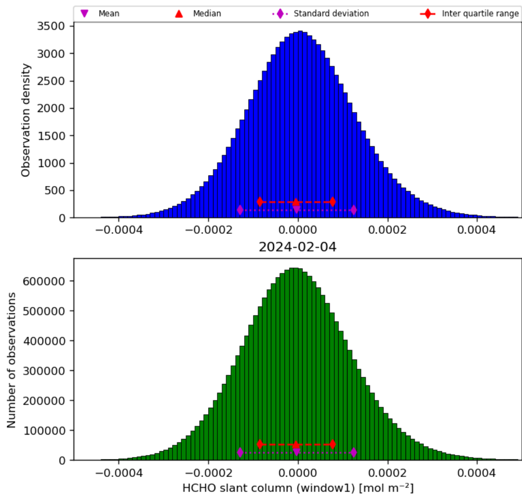
Figure 38: Histogram of “HCHO slant column (window1)” for 2024-02-03 to 2024-02-05
