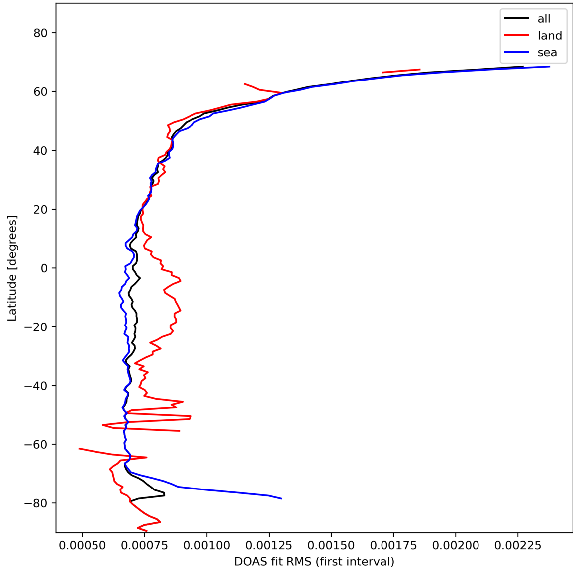
Figure 32: Zonal average of “DOAS fit RMS (first interval)” for 2024-02-03 to 2024-02-05.
