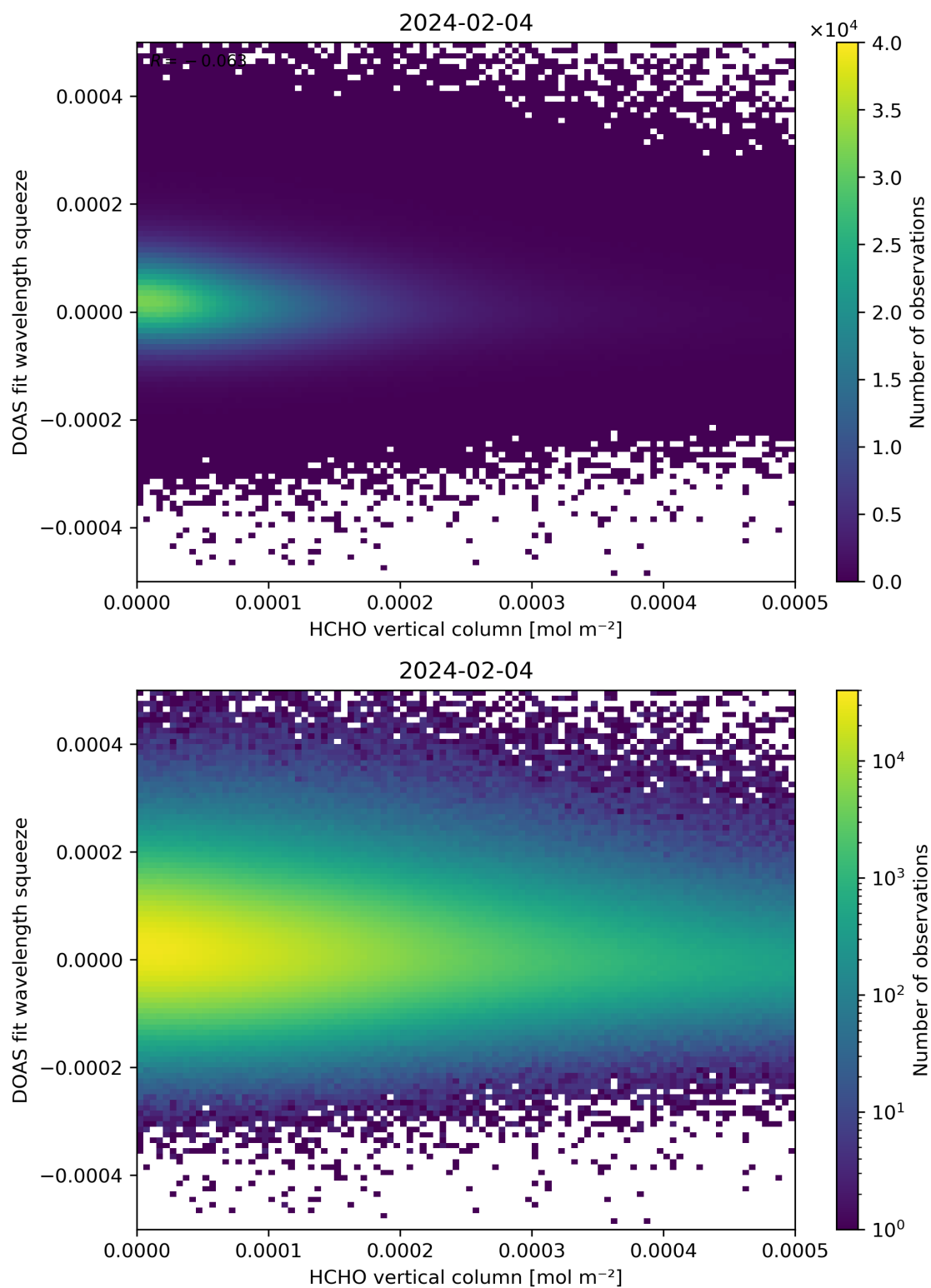
Figure 125: Scatter density plot of “HCHO vertical column” against “DOAS fit wavelength squeeze” for 2024-02-03 to 2024-02-05.
