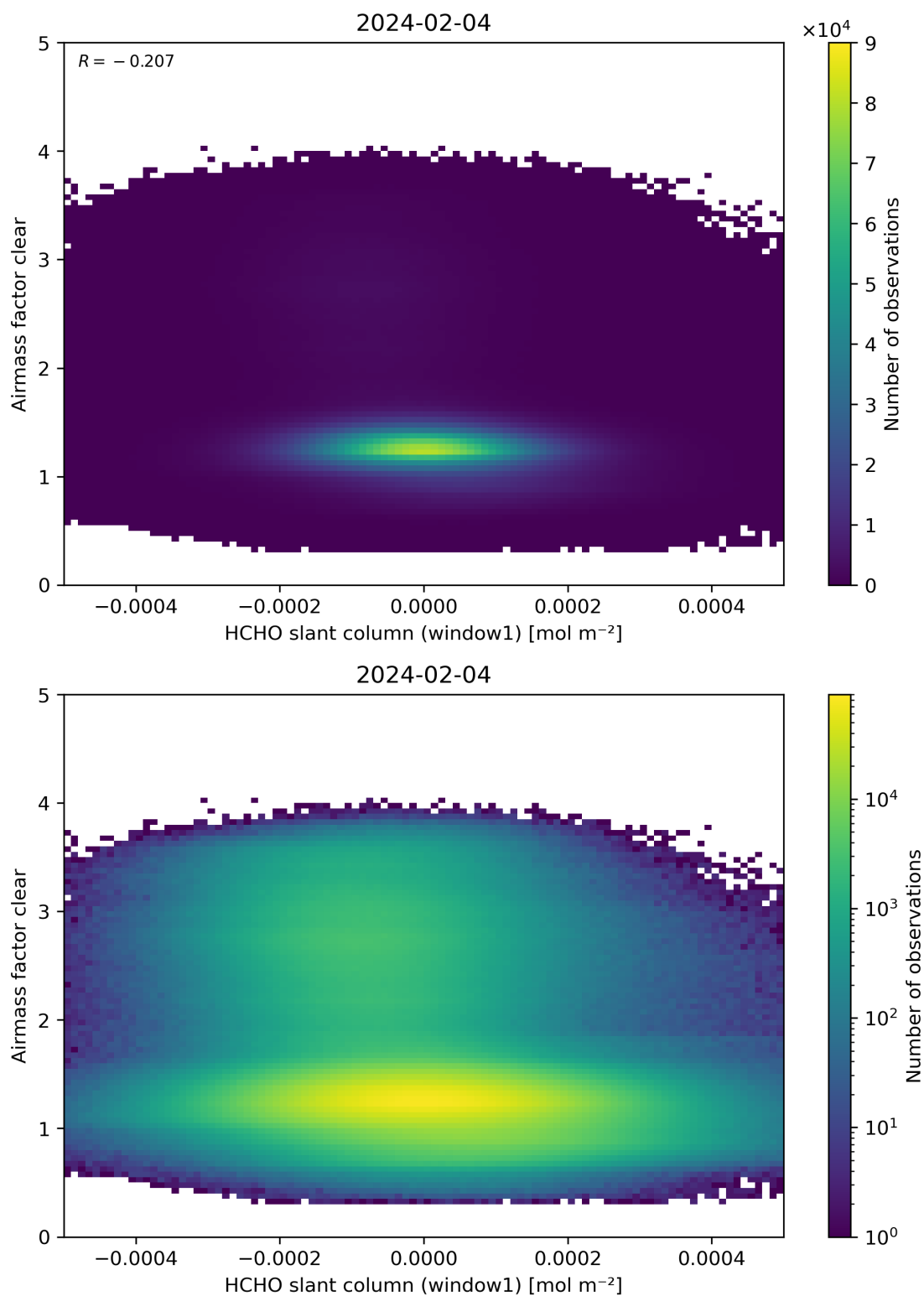
Figure 81: Scatter density plot of “HCHO slant column (window1)” against “Airmass factor clear” for 2024-02-03 to 2024-02-05.
