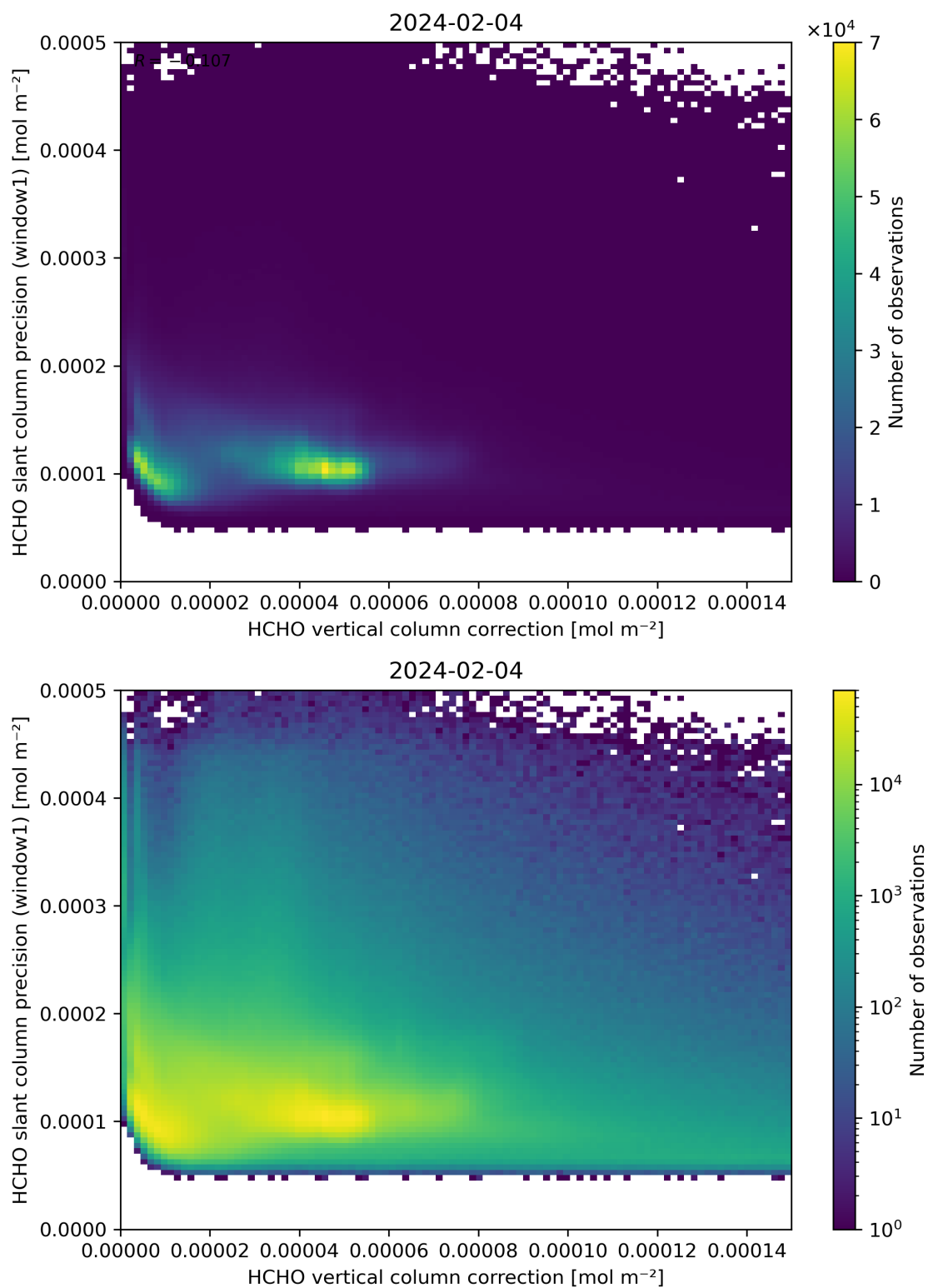
Figure 119: Scatter density plot of “HCHO vertical column correction” against “HCHO slant column precision (window1)” for 2024-02-03 to 2024-02-05.
