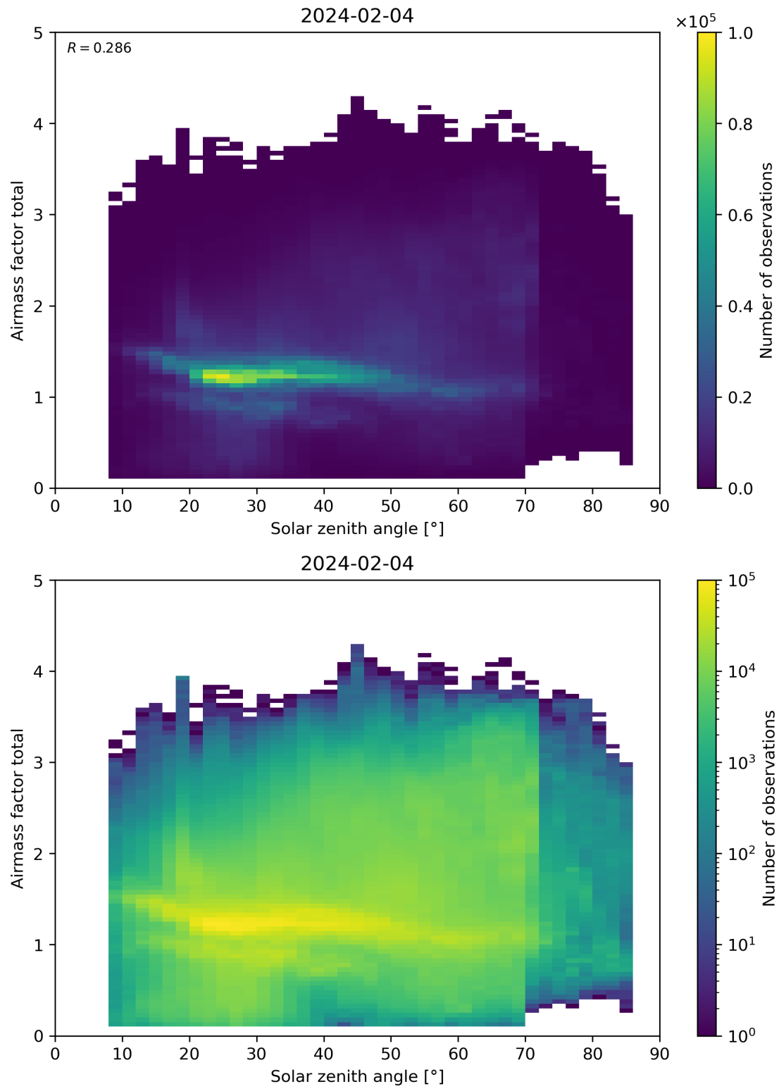
Figure 175: Scatter density plot of “Solar zenith angle” against “Airmass factor total” for 2024-02-03 to 2024-02-05.
