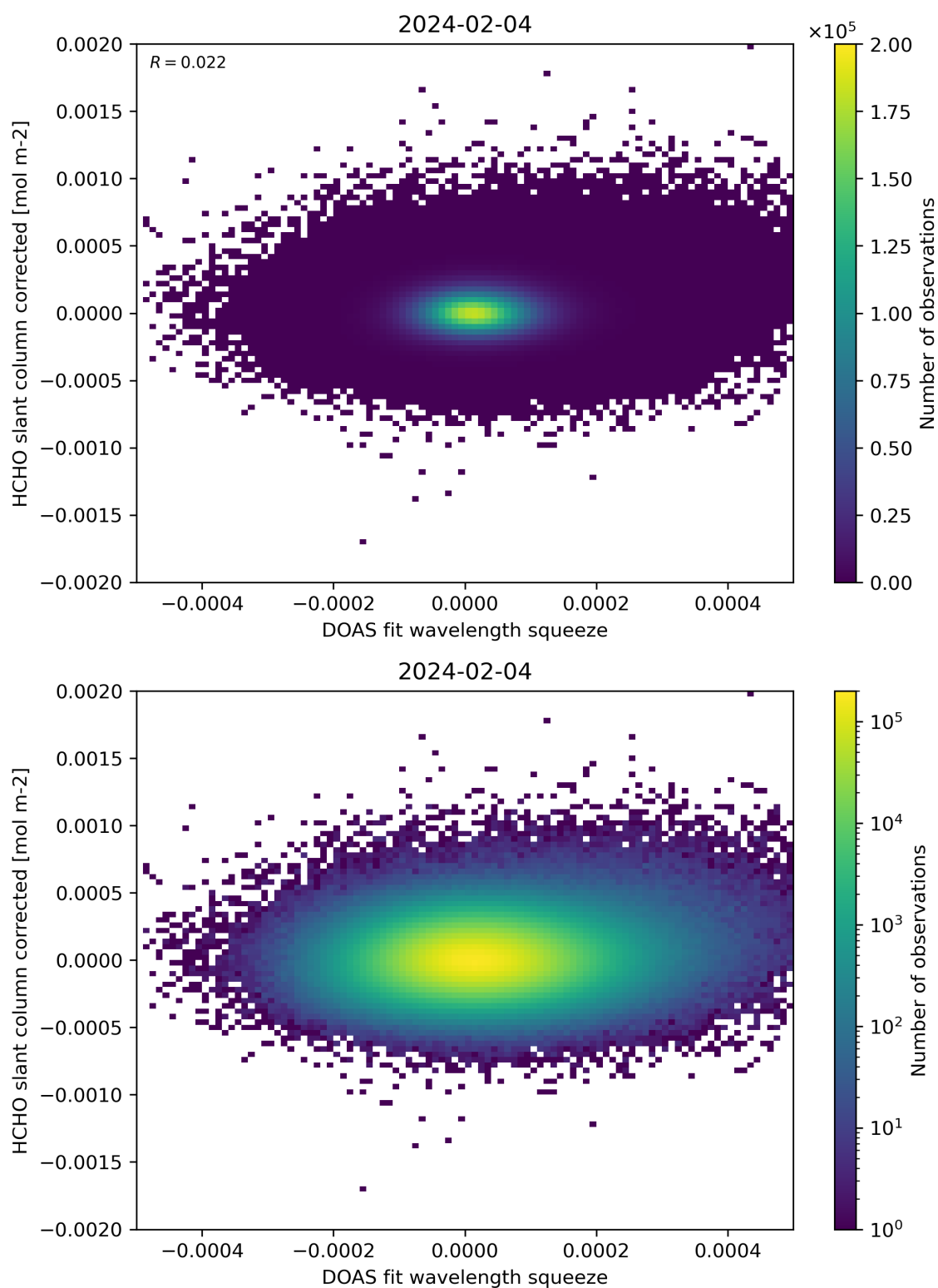
Figure 69: Scatter density plot of “DOAS fit wavelength squeeze” against “HCHO slant column corrected” for 2024-02-03 to 2024-02-05.
