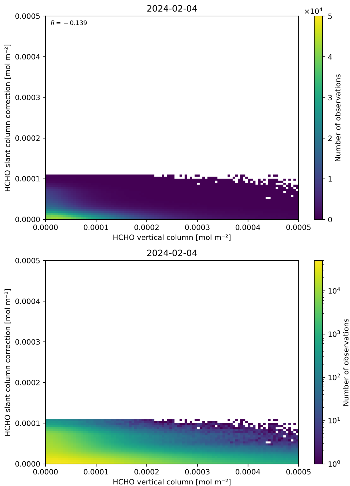
Figure 128: Scatter density plot of “HCHO vertical column” against “HCHO slant column correction” for 2024-02-03 to 2024-02-05.
