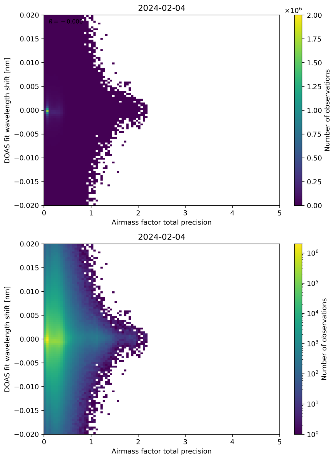
Figure 106: Scatter density plot of “Airmass factor total precision” against “DOAS fit wavelength shift” for 2024-02-03 to 2024-02-05.
