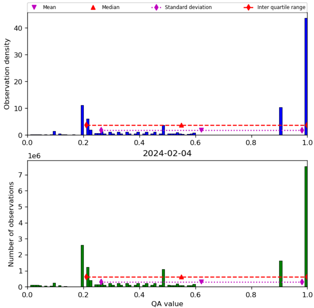
Figure 34: Histogram of “QA value” for 2024-02-03 to 2024-02-05
