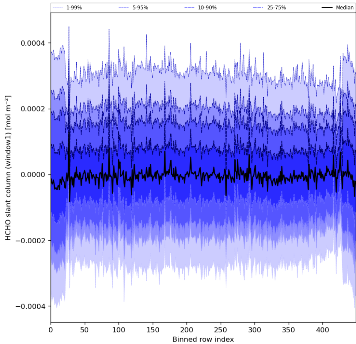
Figure 52: Along track statistics of “HCHO slant column (window1)” for 2024-02-03 to 2024-02-05
