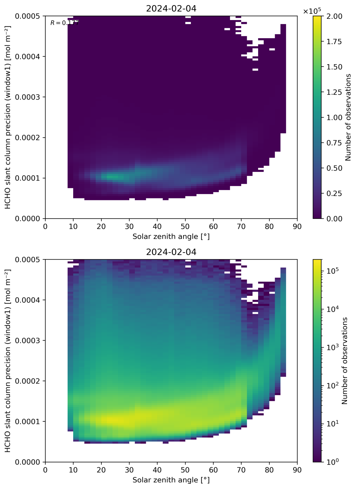
Figure 174: Scatter density plot of “Solar zenith angle” against “HCHO slant column precision (window1)” for 2024-02-03 to 2024-02-05.
