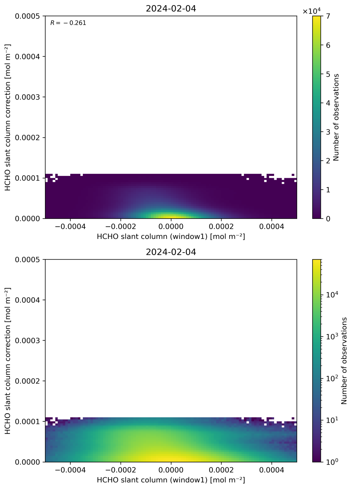
Figure 83: Scatter density plot of “HCHO slant column (window1)” against “HCHO slant column correction” for 2024-02-03 to 2024-02-05.
