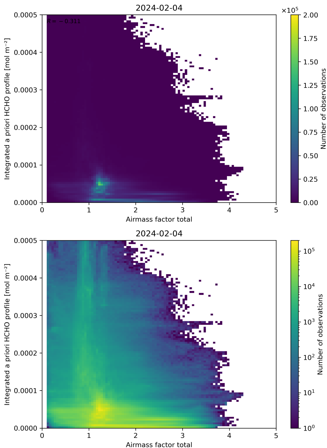
Figure 104: Scatter density plot of “Air mass factor total” against “Integrated a priori HCHO profile” for 2024-02-03 to 2024-02-05.
