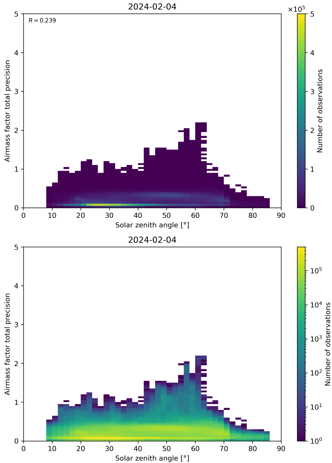
Figure 176: Scatter density plot of “Solar zenith angle” against “Airmass factor total precision” for 2024-02-03 to 2024-02-05.
