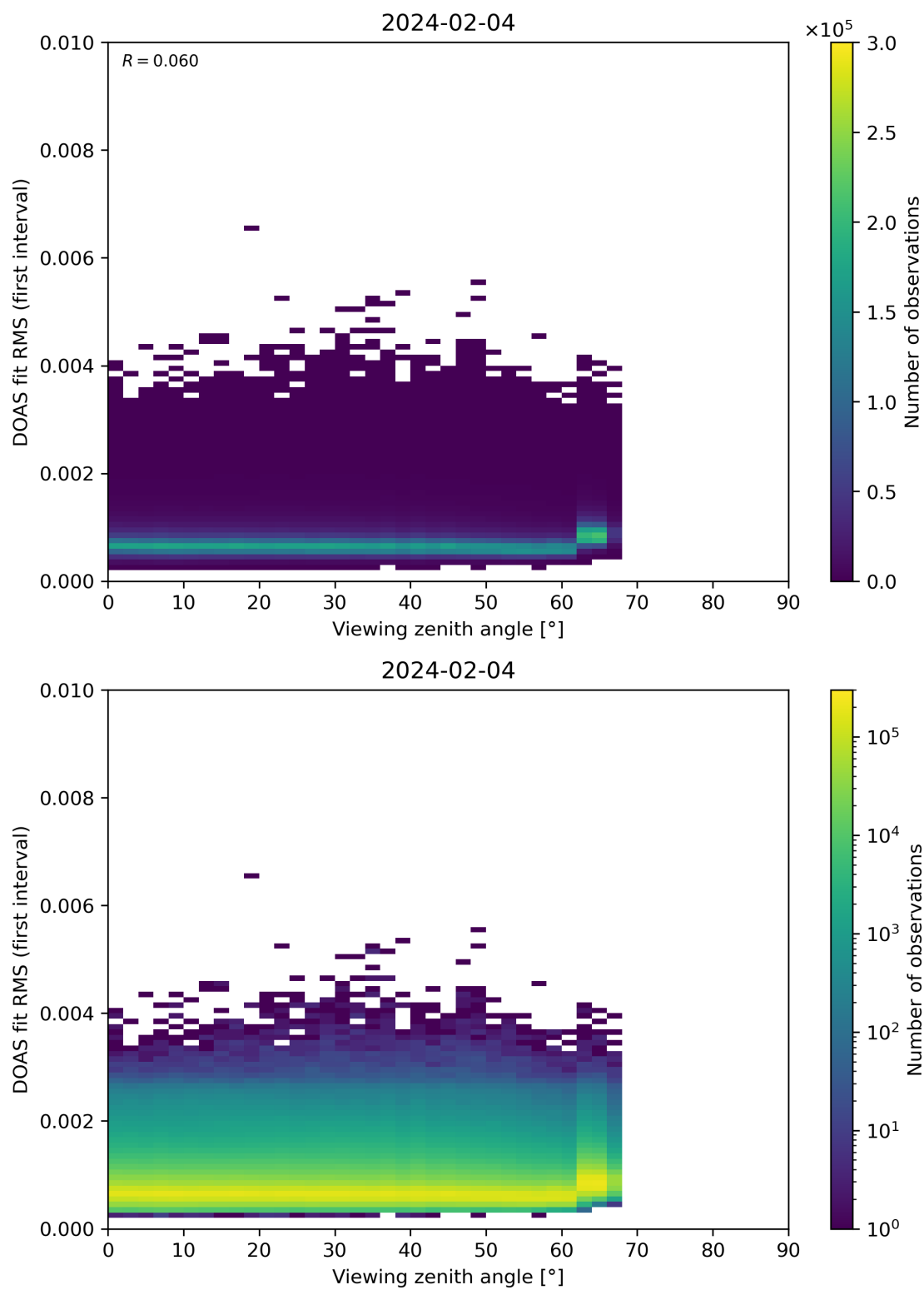
Figure 182: Scatter density plot of “Viewing zenith angle” against “DOAS fit RMS (first interval)” for 2024-02-03 to 2024-02-05.
