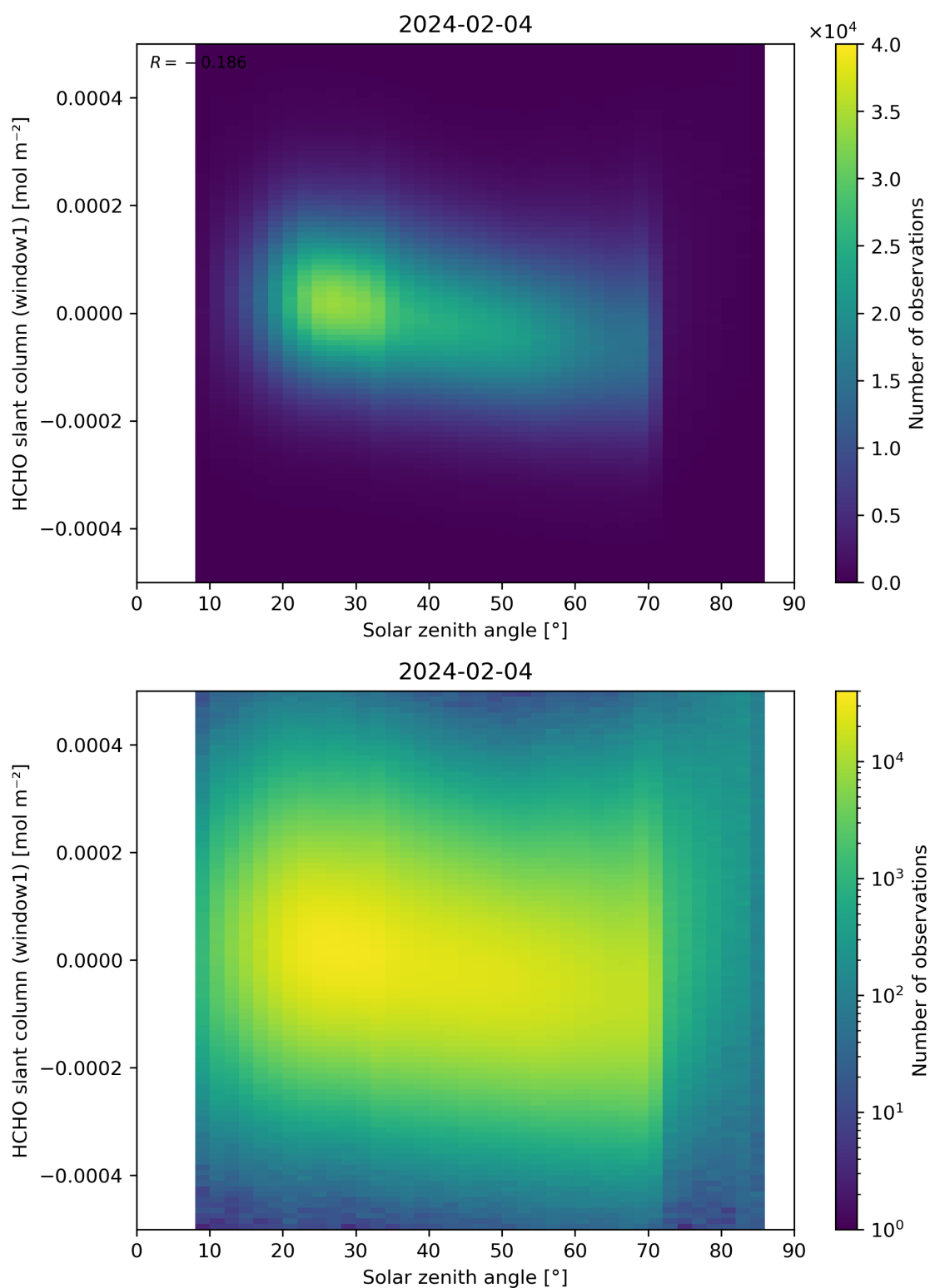
Figure 173: Scatter density plot of “Solar zenith angle” against “HCHO slant column (window1)” for 2024-02-03 to 2024-02-05.
