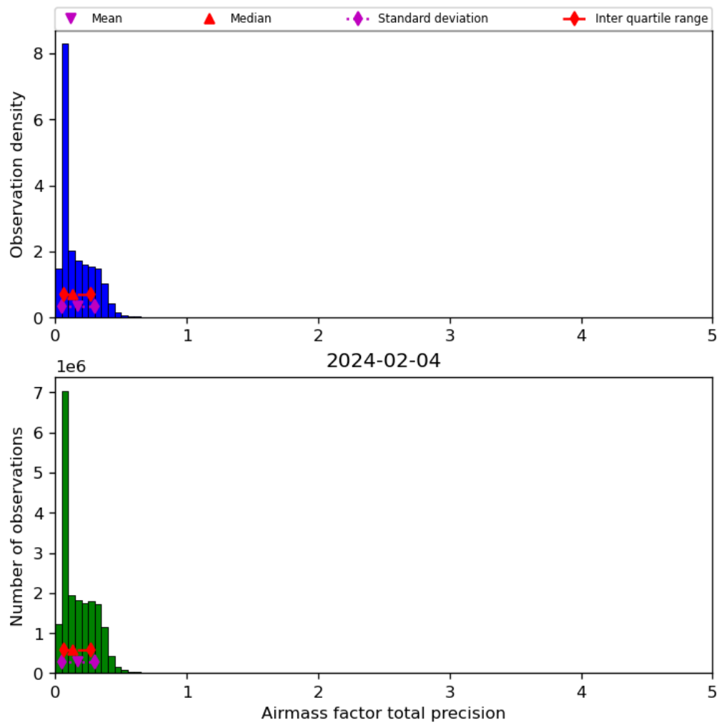
Figure 41: Histogram of “Airmass factor total precision” for 2024-02-03 to 2024-02-05
