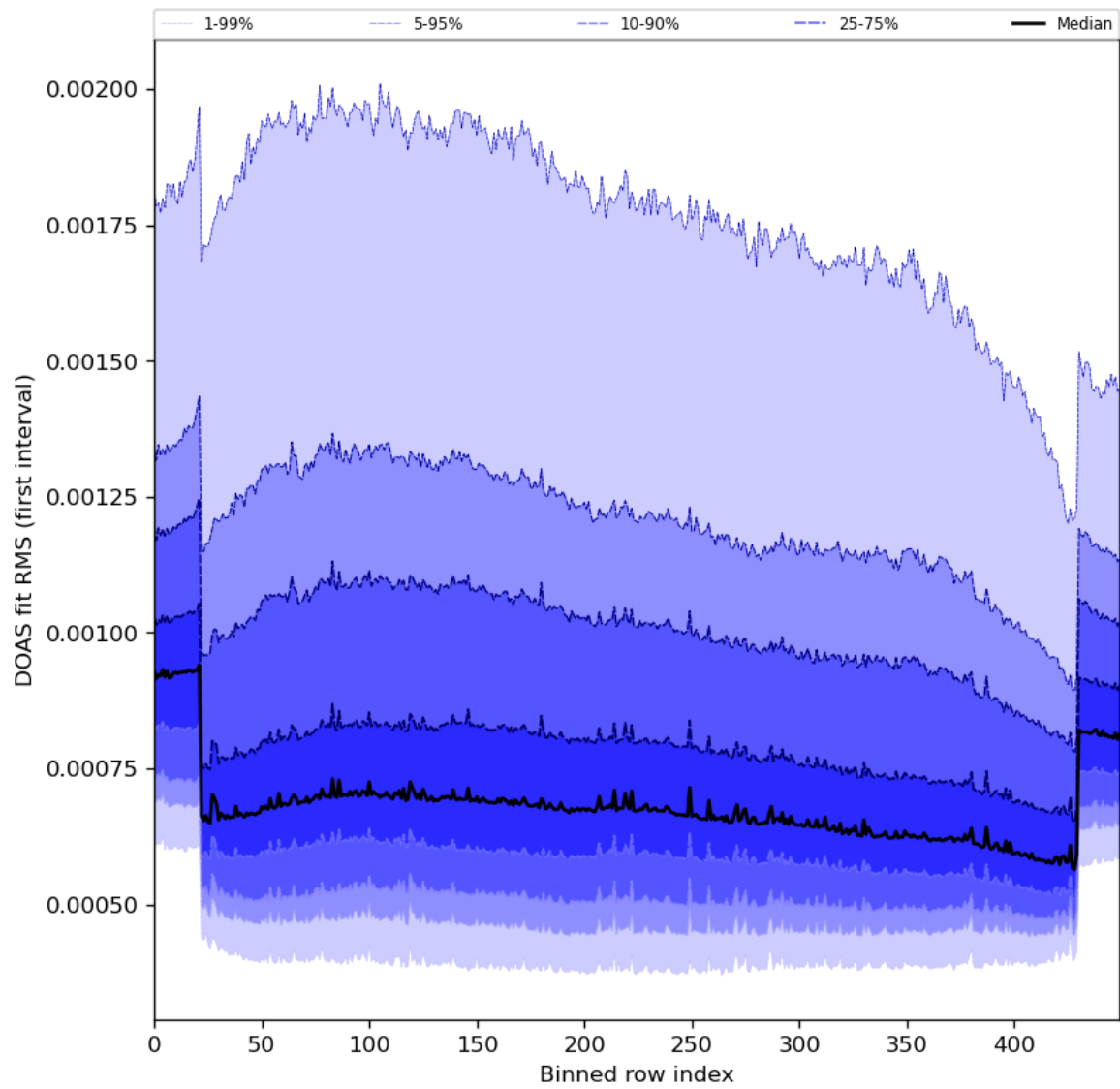
Figure 60: Along track statistics of “DOAS fit RMS (first interval)” for 2024-02-03 to 2024-02-05
