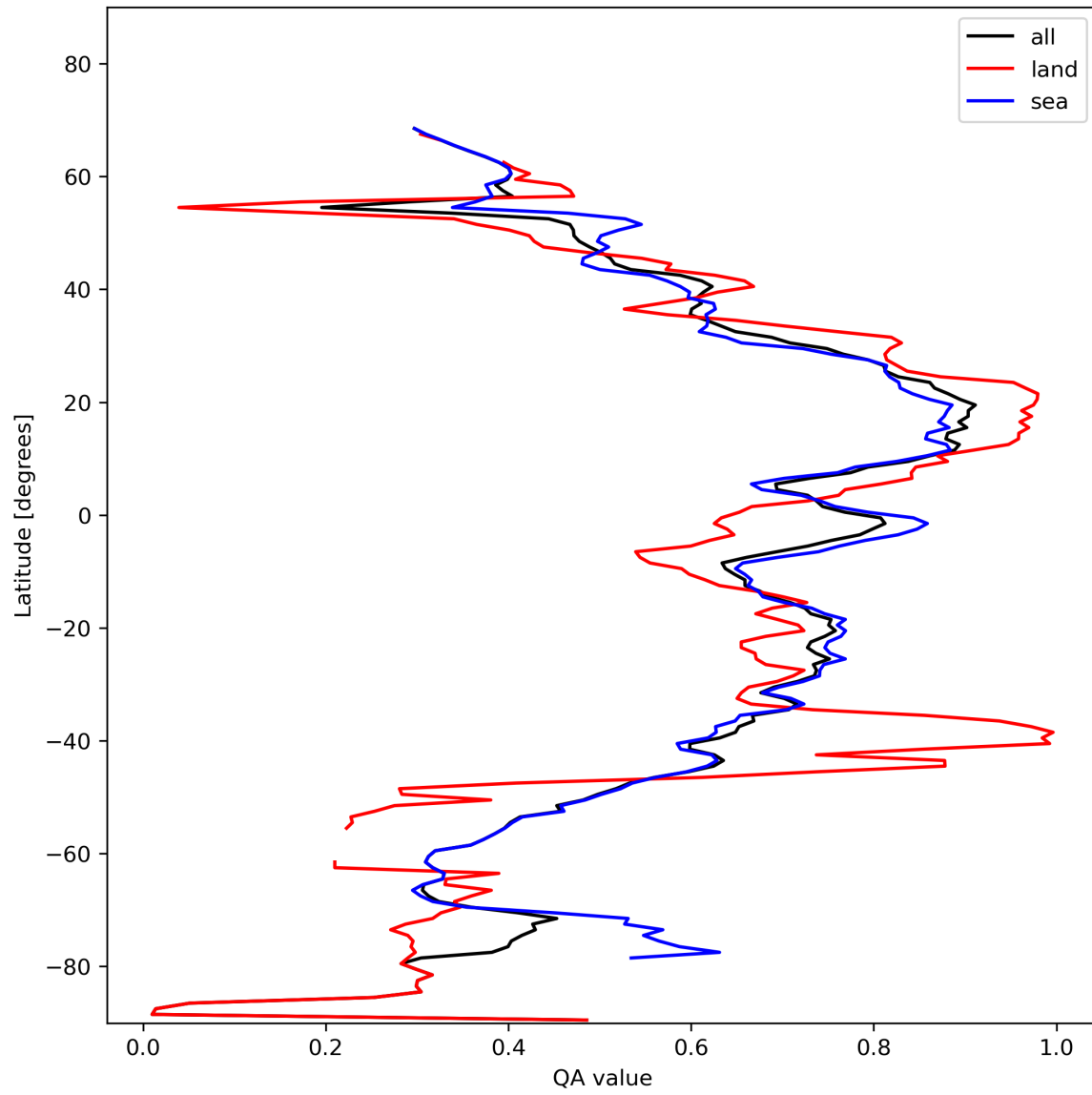
Figure 20: Zonal average of “QA value” for 2024-02-03 to 2024-02-05.
