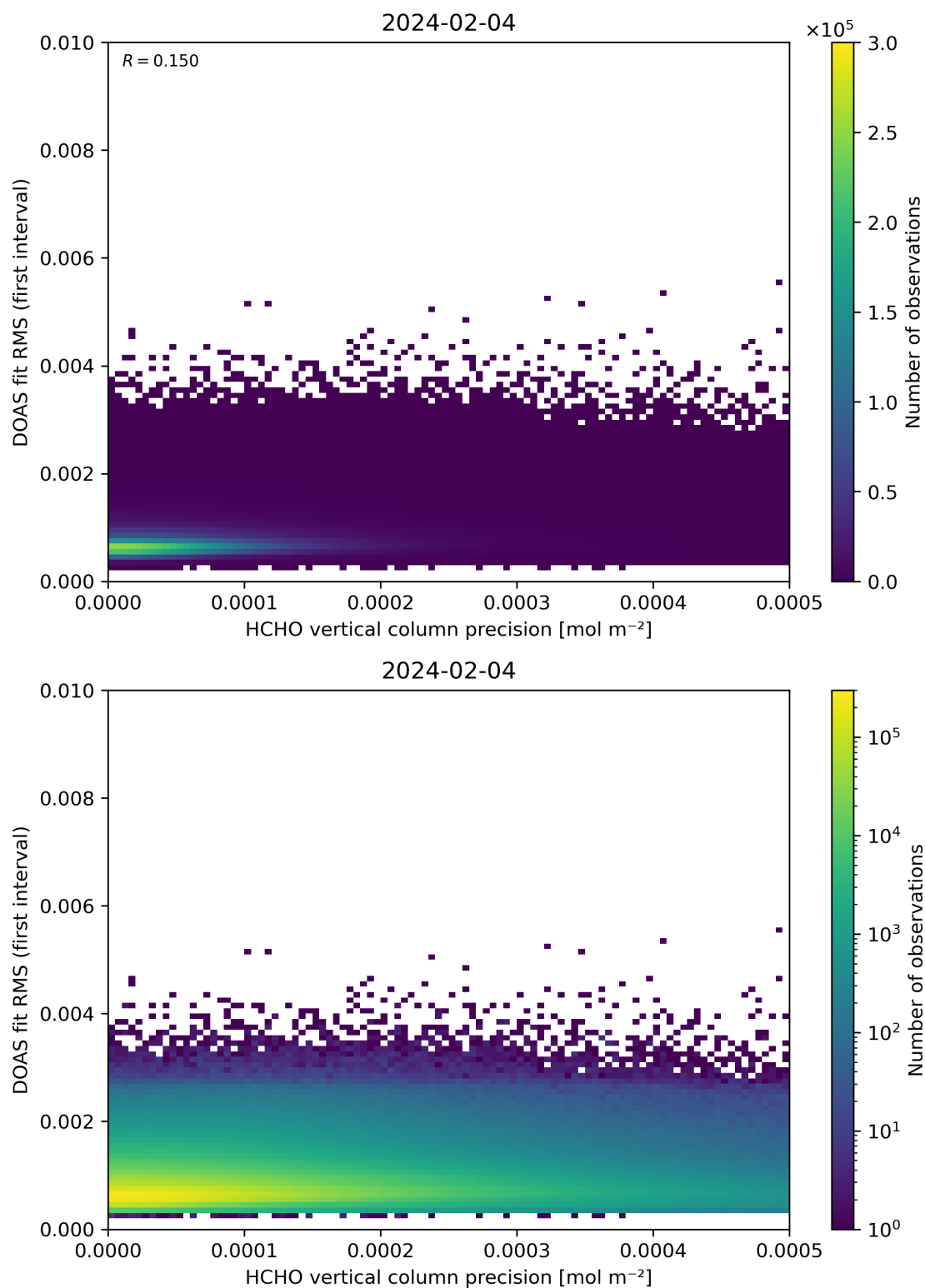
Figure 136: Scatter density plot of “HCHO vertical column precision” against “DOAS fit RMS (first interval)” for 2024-02-03 to 2024-02-05.
