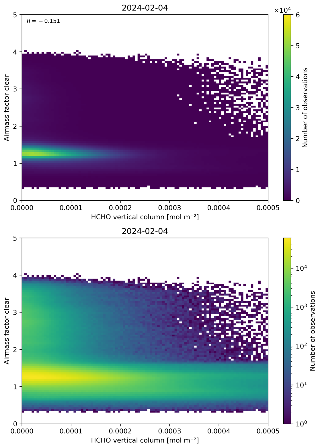
Figure 126: Scatter density plot of “HCHO vertical column” against “Airmass factor clear” for 2024-02-03 to 2024-02-05.
