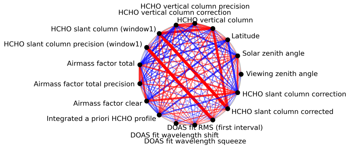
Figure 1: Map of correlation graph for 2024-02-03 to 2024-02-05.
