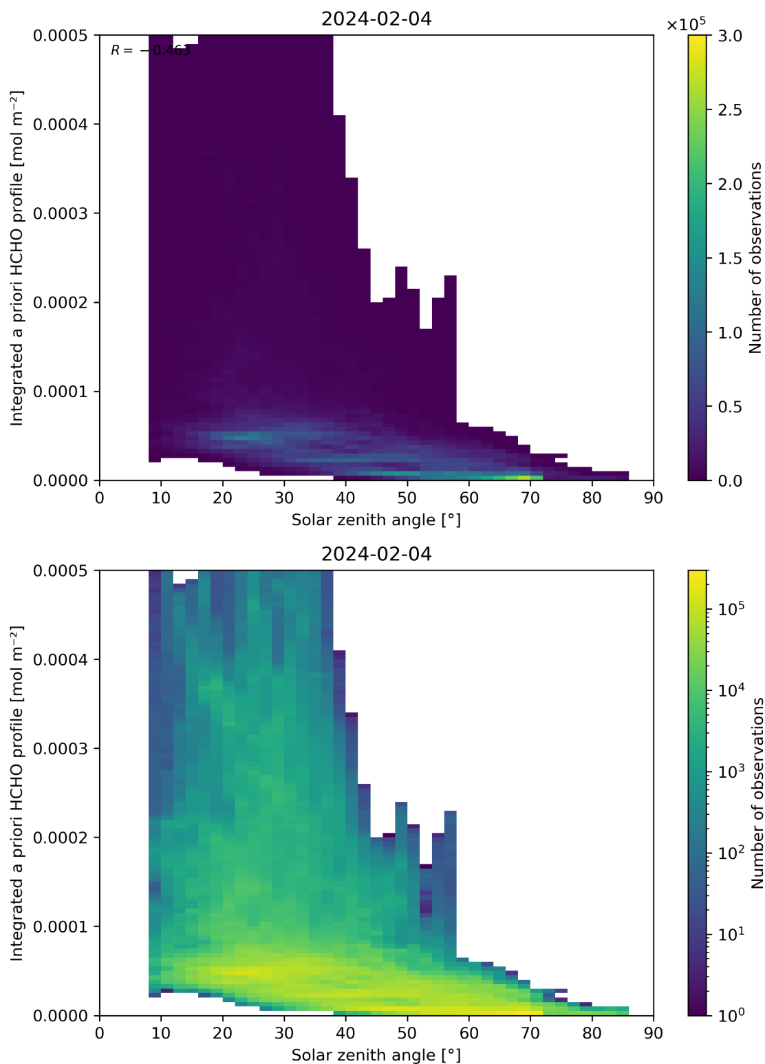
Figure 180: Scatter density plot of “Solar zenith angle” against “Integrated a priori HCHO profile” for 2024-02-03 to 2024-02-05.
