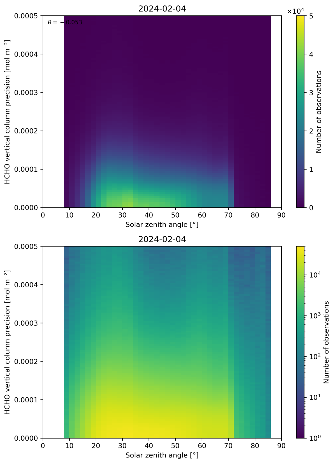
Figure 179: Scatter density plot of “Solar zenith angle” against “HCHO vertical column precision” for 2024-02-03 to 2024-02-05.
