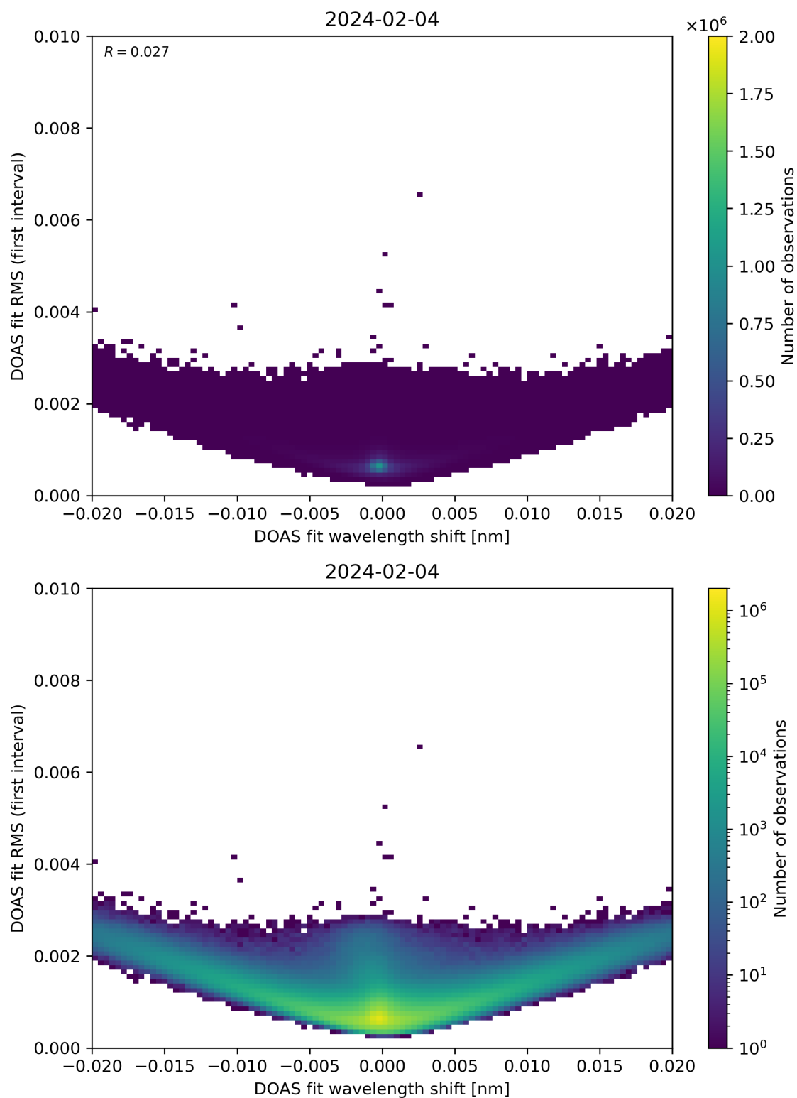
Figure 64: Scatter density plot of “DOAS fit wavelength shift” against “DOAS fit RMS (first interval)” for 2024-02-03 to 2024-02-05.
