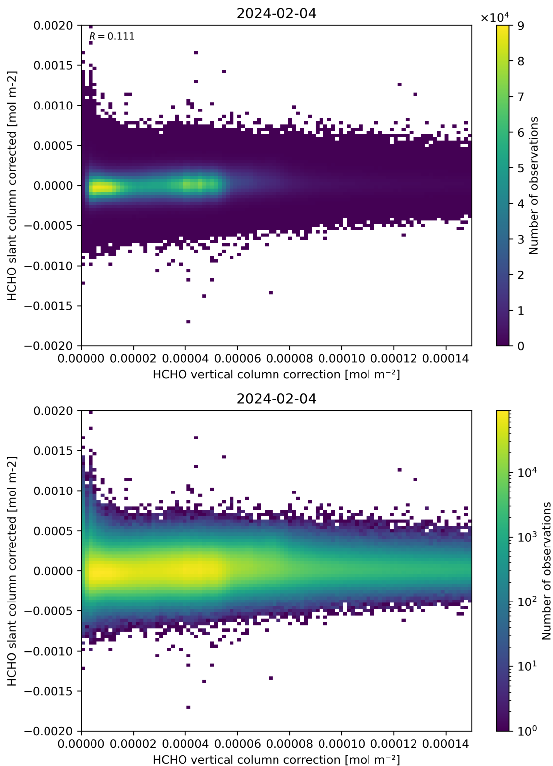
Figure 116: Scatter density plot of “HCHO vertical column correction” against “HCHO slant column corrected” for 2024-02-03 to 2024-02-05.
