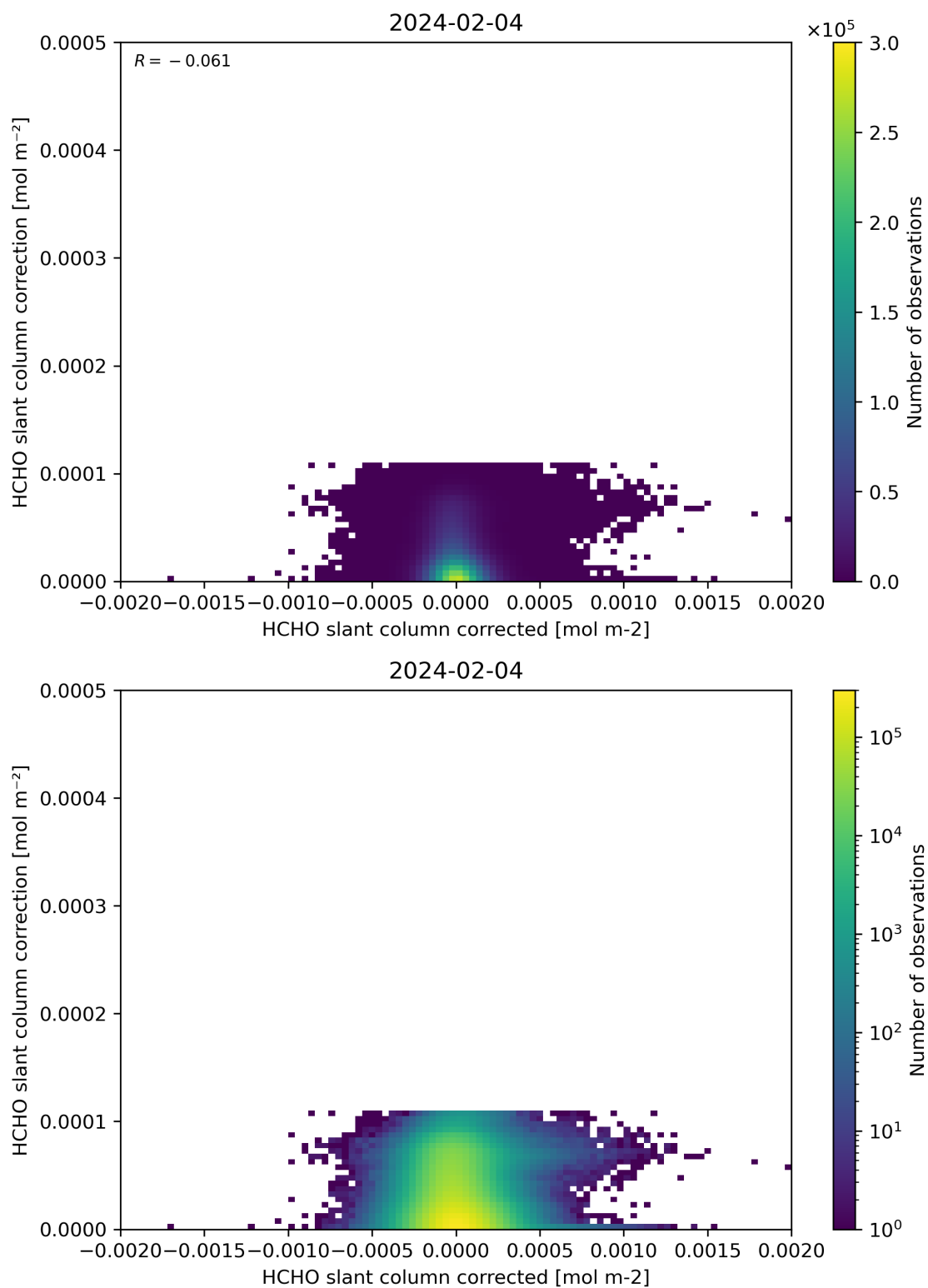
Figure 77: Scatter density plot of “HCHO slant column corrected” against “HCHO slant column correction” for 2024-02-03 to 2024-02-05.
