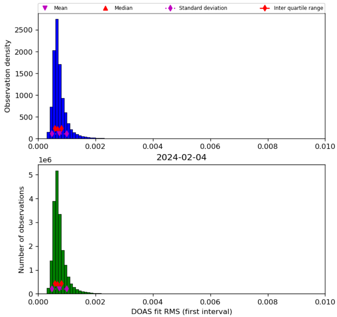
Figure 46: Histogram of “DOAS fit RMS (first interval)” for 2024-02-03 to 2024-02-05
