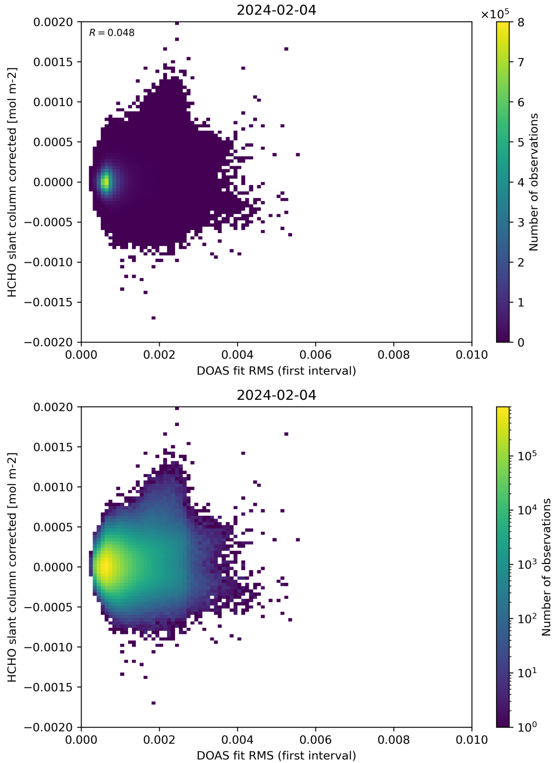
Figure 62: Scatter density plot of “DOAS fit RMS (first interval)” against “HCHO slant column corrected” for 2024-02-03 to 2024-02-05.
