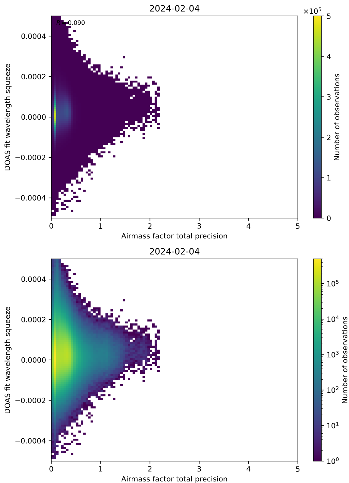
Figure 107: Scatter density plot of “Airmass factor total precision” against “DOAS fit wavelength squeeze” for 2024-02-03 to 2024-02-05.
