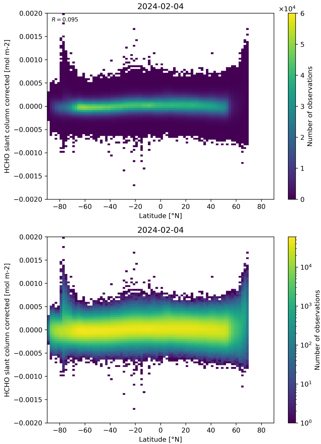
Figure 157: Scatter density plot of “Latitude” against “HCHO slant column corrected” for 2024-02-03 to 2024-02-05.
