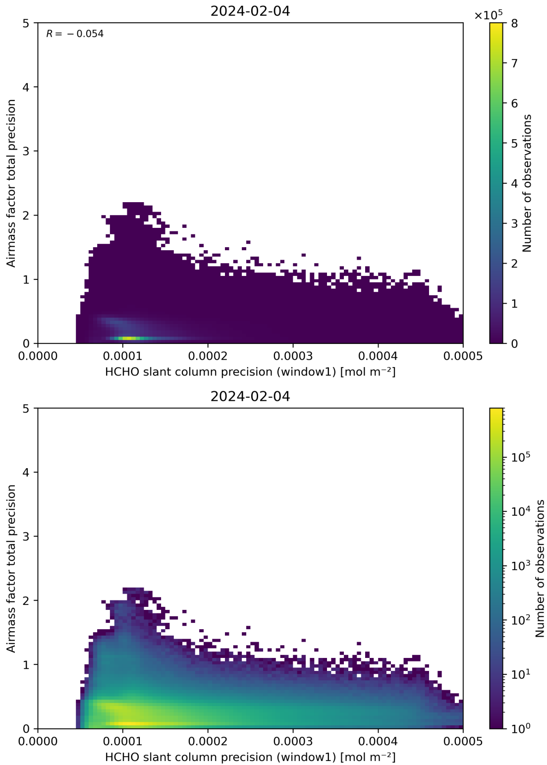
Figure 95: Scatter density plot of “HCHO slant column precision (window1)” against “Airmass factor total precision” for 2024-02-03 to 2024-02-05.
