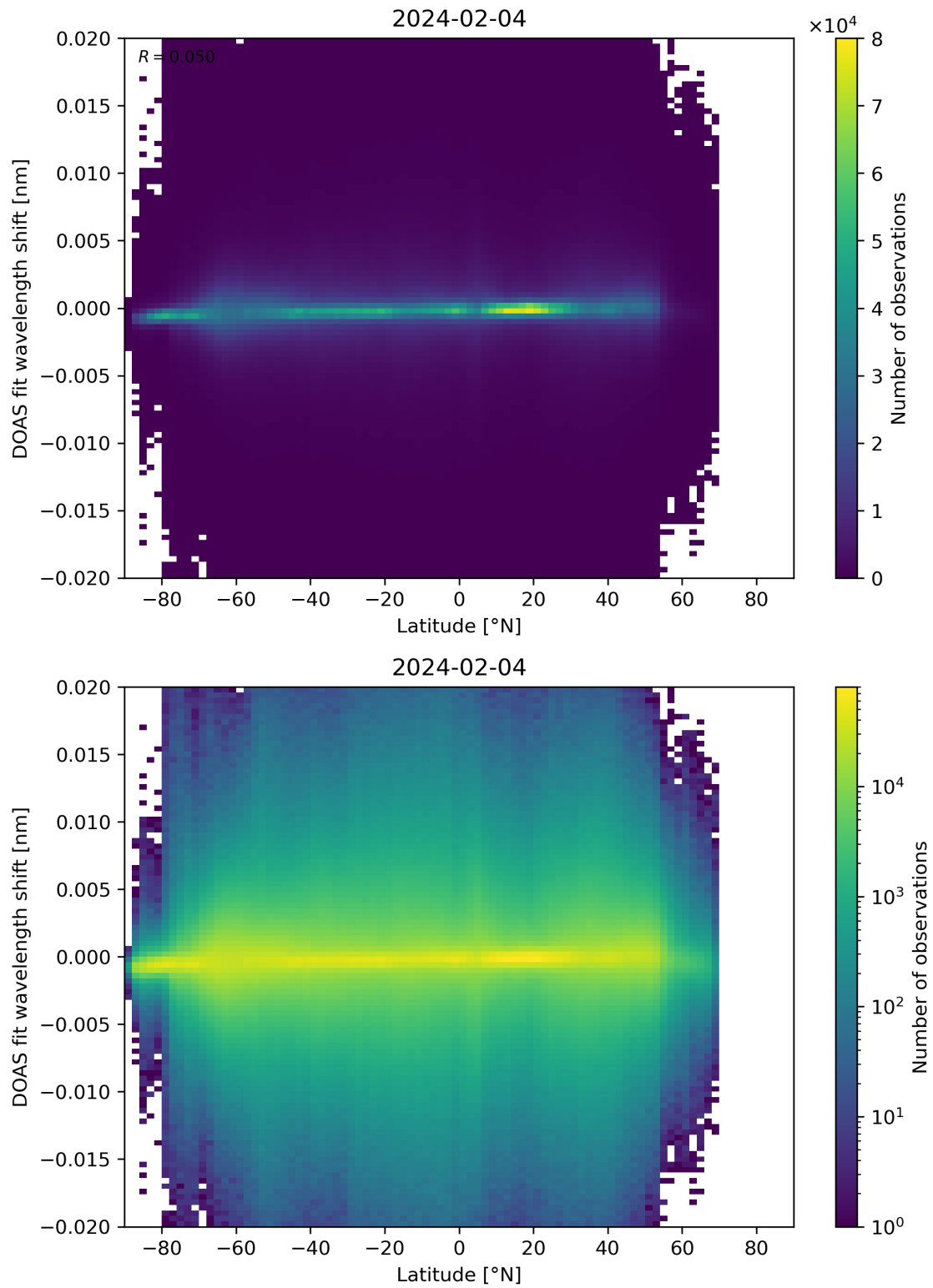
Figure 154: Scatter density plot of “Latitude” against “DOAS fit wavelength shift” for 2024-02-03 to 2024-02-05.
