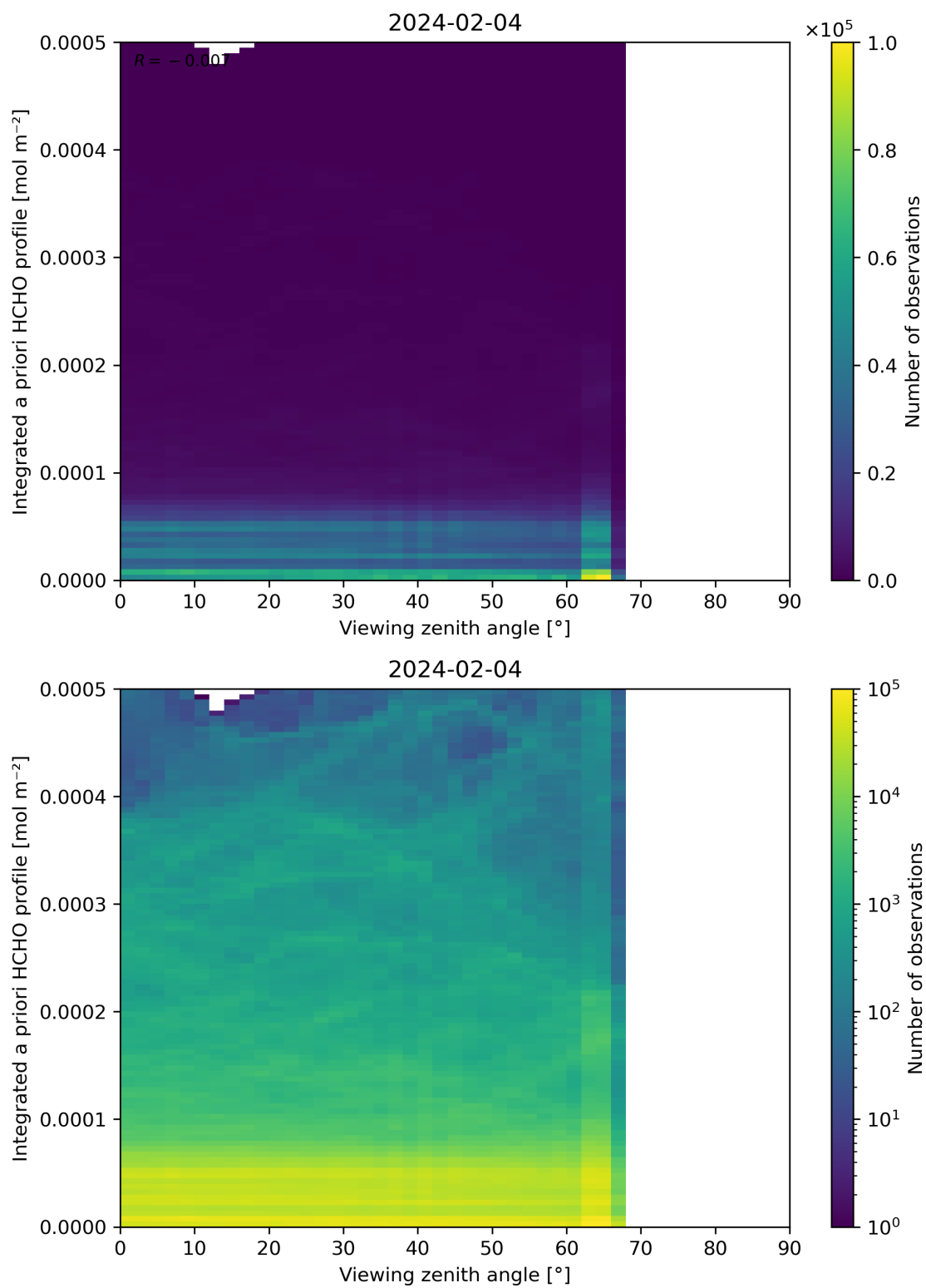
Figure 195: Scatter density plot of “Viewing zenith angle” against “Integrated a priori HCHO profile” for 2024-02-03 to 2024-02-05.
