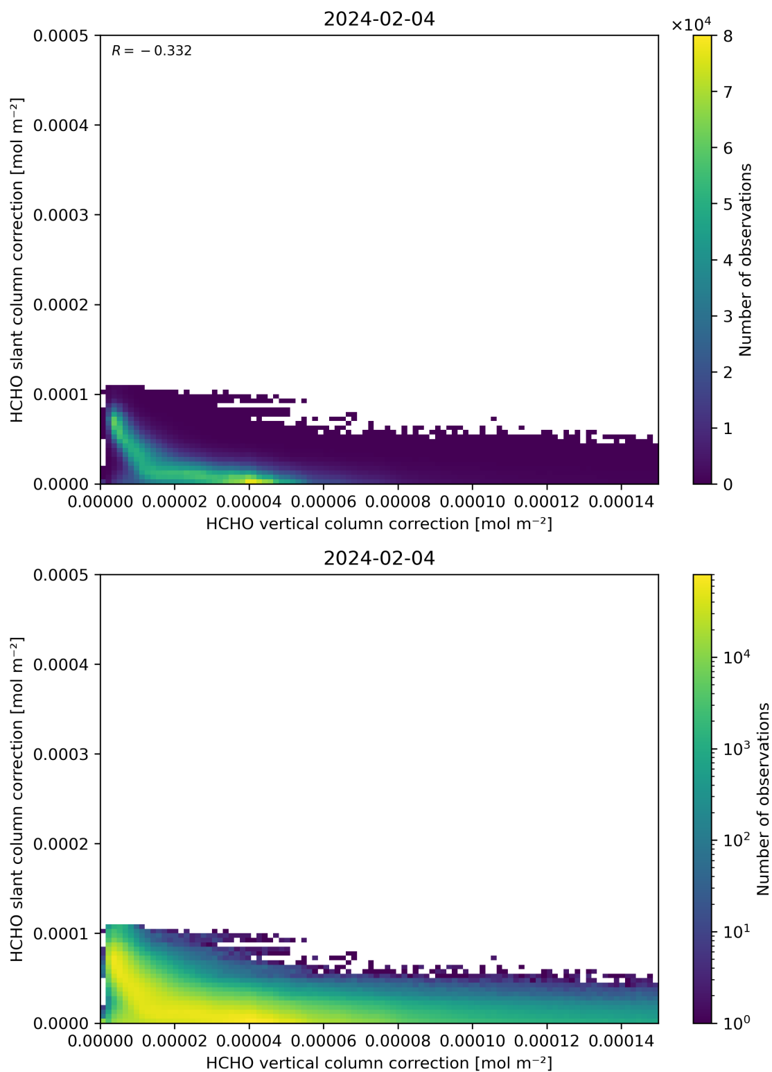
Figure 117: Scatter density plot of “HCHO vertical column correction” against “HCHO slant column correction” for 2024-02-03 to 2024-02-05.
