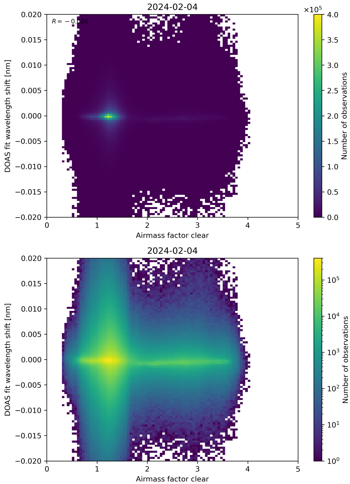
Figure 72: Scatter density plot of “Airmass factor clear” against “DOAS fit wavelength shift” for 2024-02-03 to 2024-02-05.
