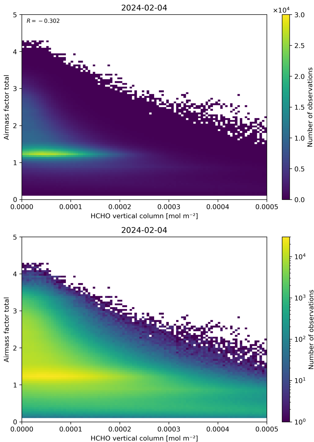
Figure 131: Scatter density plot of “HCHO vertical column” against “Airmass factor total” for 2024-02-03 to 2024-02-05.
