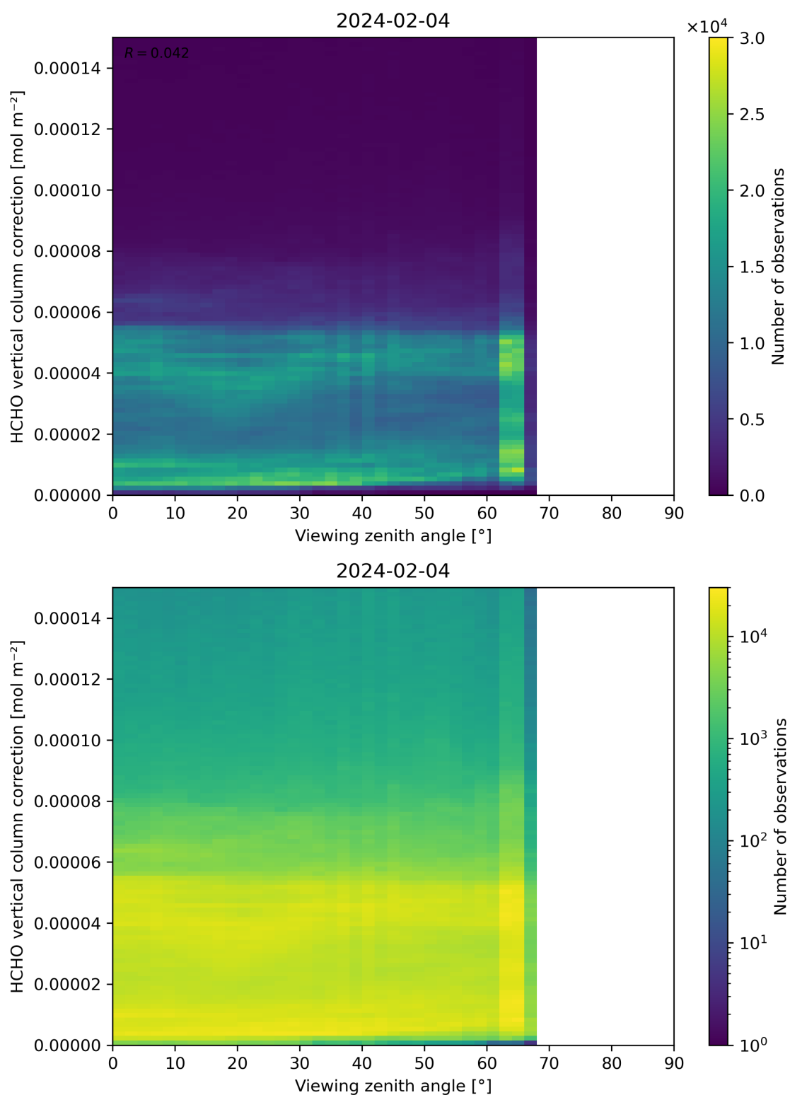
Figure 193: Scatter density plot of “Viewing zenith angle” against “HCHO vertical column correction” for 2024-02-03 to 2024-02-05.
