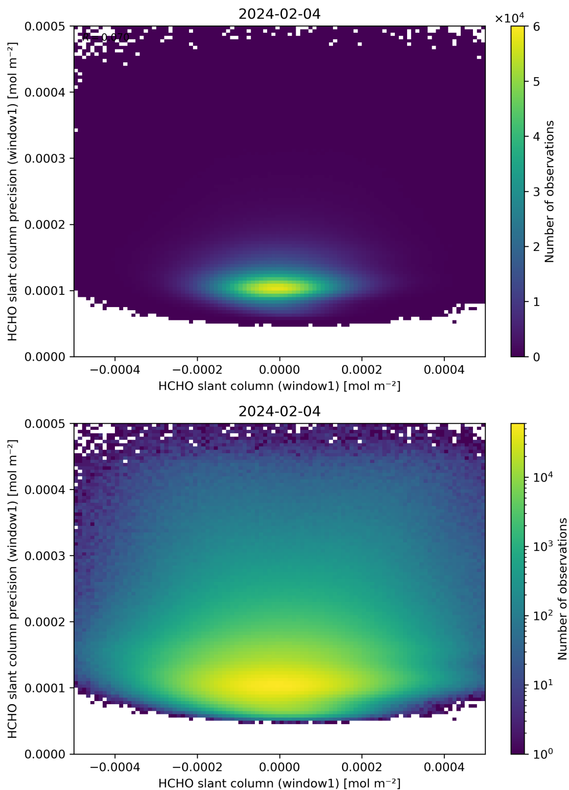
Figure 84: Scatter density plot of “HCHO slant column (window1)” against “HCHO slant column precision (window1)” for 2024-02-03 to 2024-02-05.
