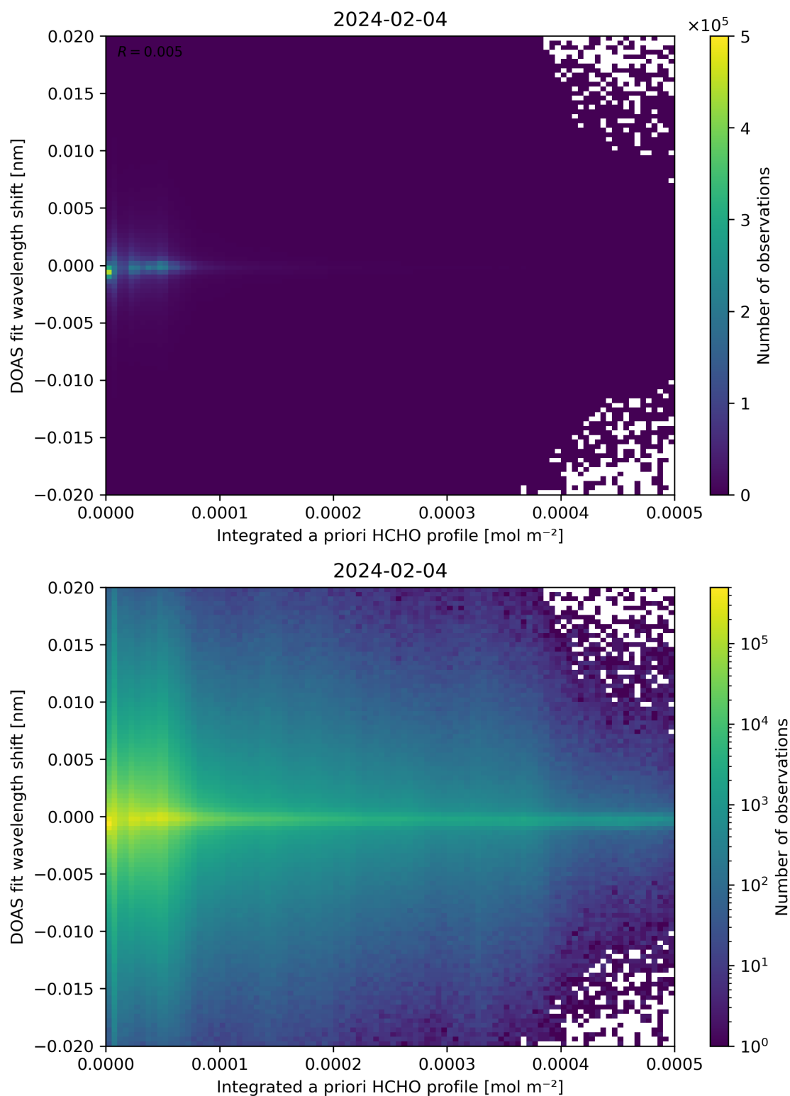
Figure 149: Scatter density plot of “Integrated a priori HCHO profile” against “DOAS fit wavelength shift” for 2024-02-03 to 2024-02-05.
