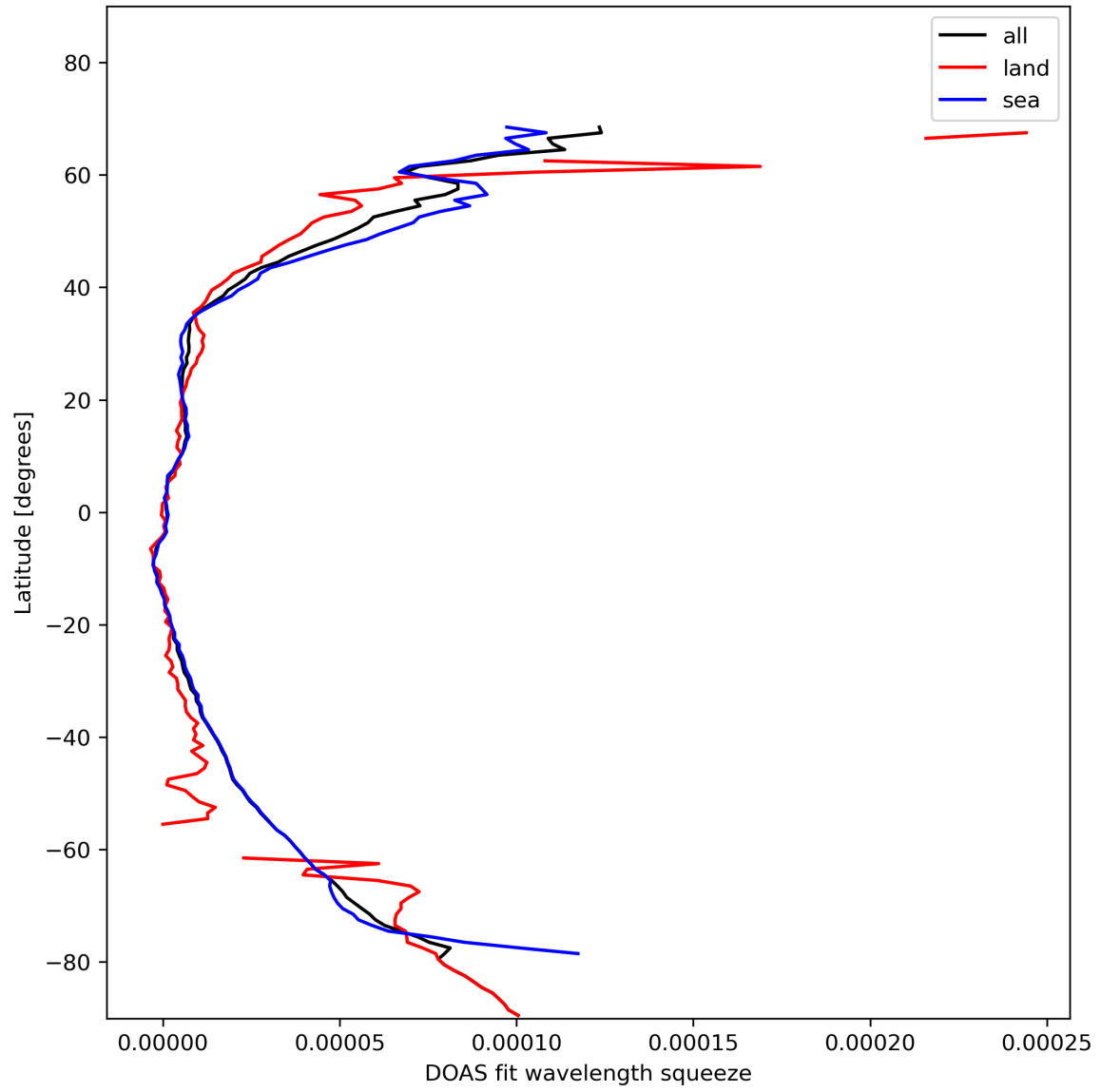
Figure 31: Zonal average of “DOAS fit wavelength squeeze” for 2024-02-03 to 2024-02-05.
