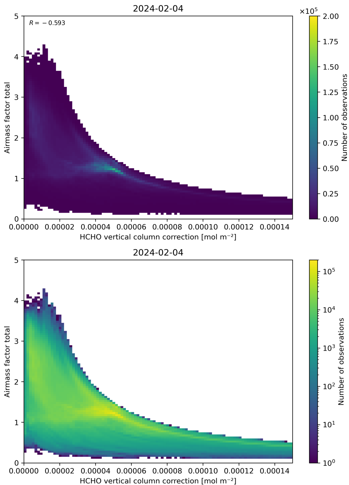
Figure 120: Scatter density plot of “HCHO vertical column correction” against “Airmass factor total” for 2024-02-03 to 2024-02-05.
