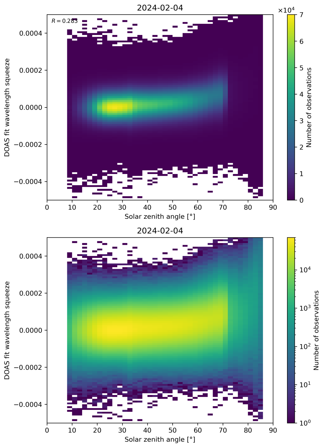
Figure 169: Scatter density plot of “Solar zenith angle” against “DOAS fit wavelength squeeze” for 2024-02-03 to 2024-02-05.
