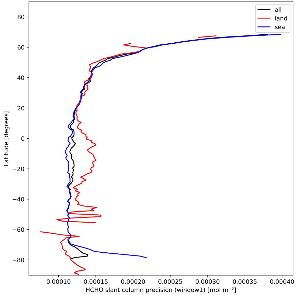
Figure 25: Zonal average of “HCHO slant column precision (window1)” for 2024-02-03 to 2024-02-05.
