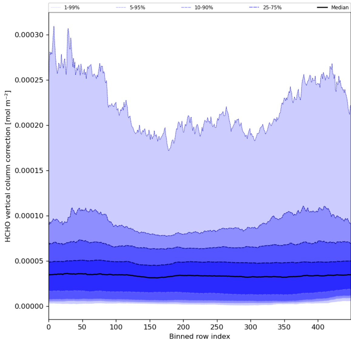
Figure 51: Along track statistics of “HCHO vertical column correction” for 2024-02-03 to 2024-02-05
