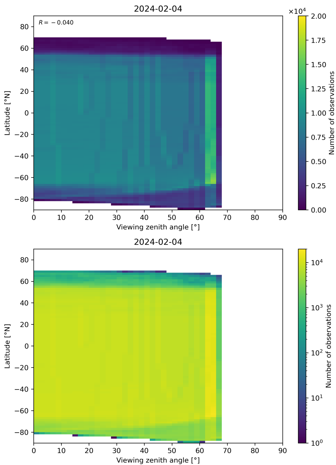
Figure 196: Scatter density plot of “Viewing zenith angle” against “Latitude” for 2024-02-03 to 2024-02-05.
