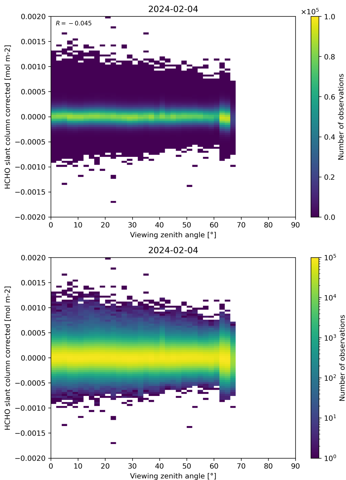
Figure 186: Scatter density plot of “Viewing zenith angle” against “HCHO slant column corrected” for 2024-02-03 to 2024-02-05.
