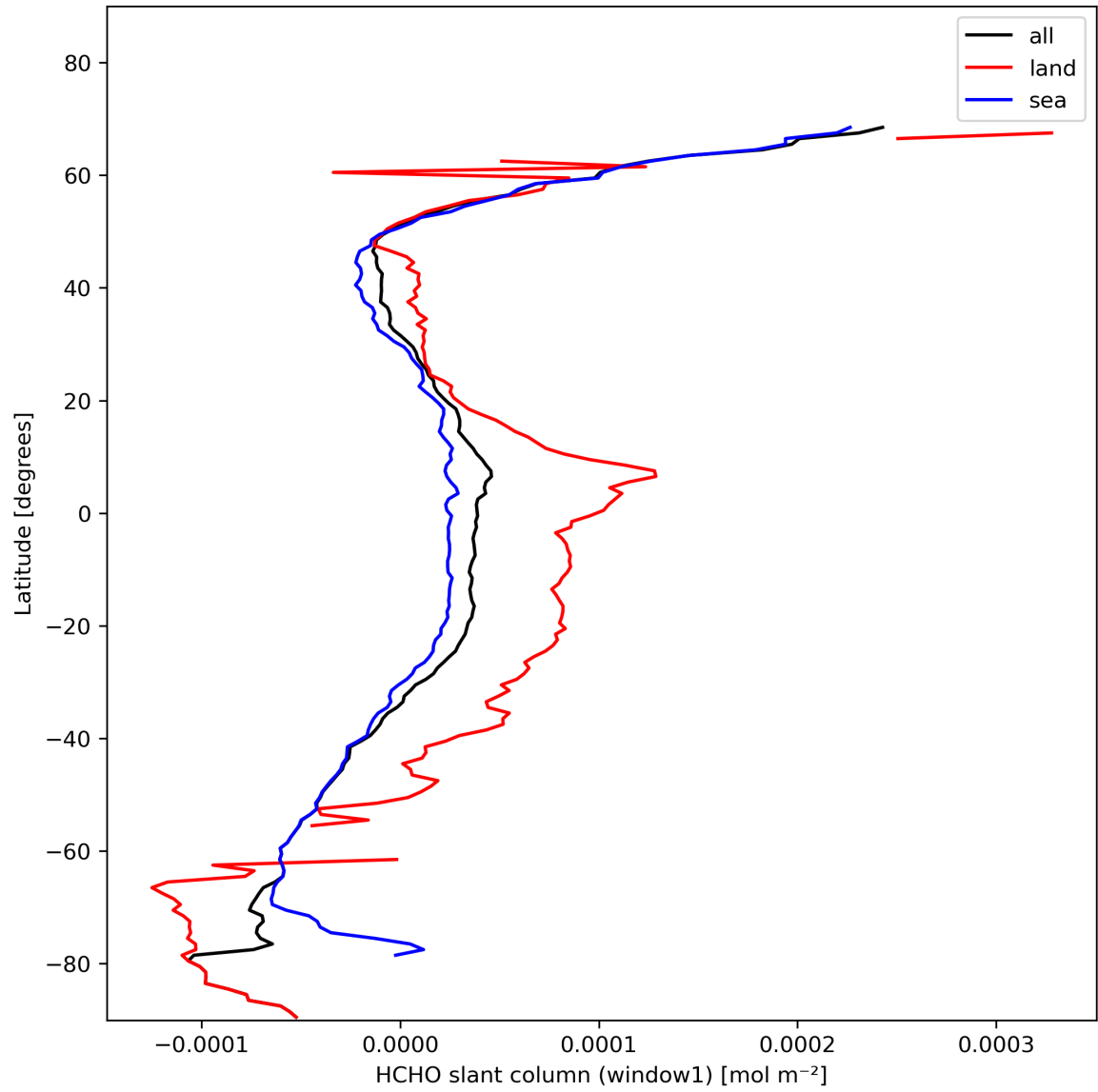
Figure 24: Zonal average of “HCHO slant column (window1)” for 2024-02-03 to 2024-02-05.
