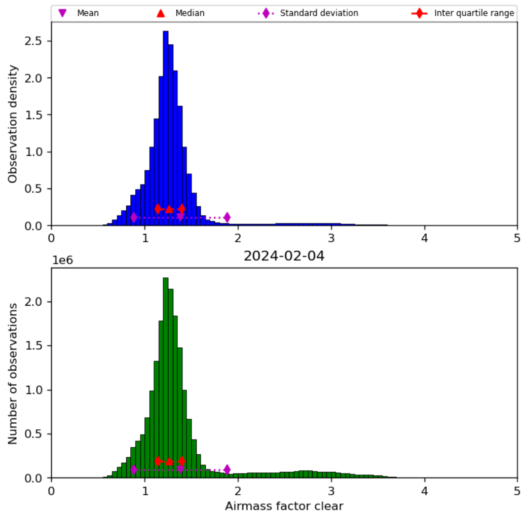
Figure 42: Histogram of “Airmass factor clear” for 2024-02-03 to 2024-02-05
