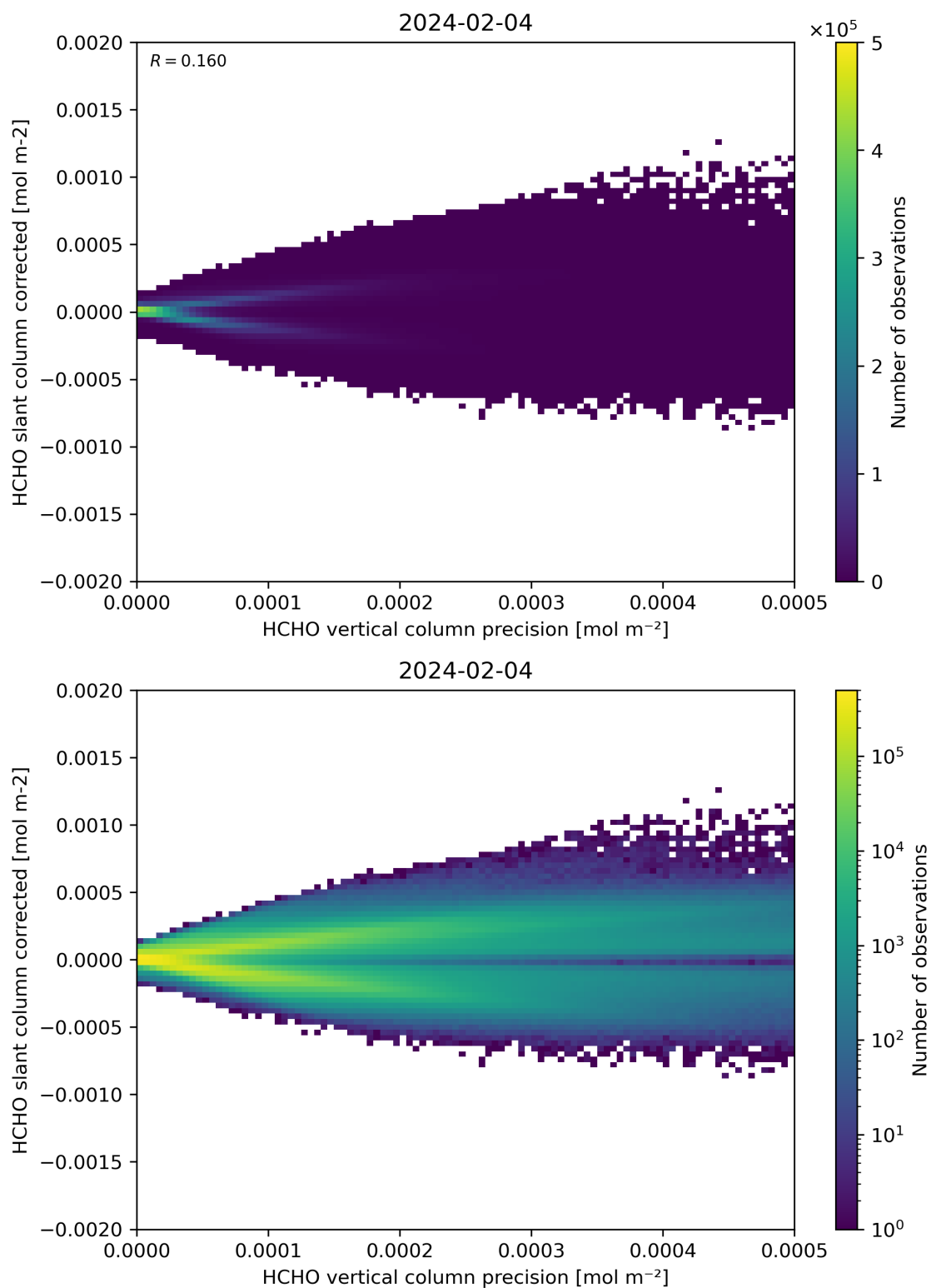
Figure 140: Scatter density plot of “HCHO vertical column precision” against “HCHO slant column corrected” for 2024-02-03 to 2024-02-05.
