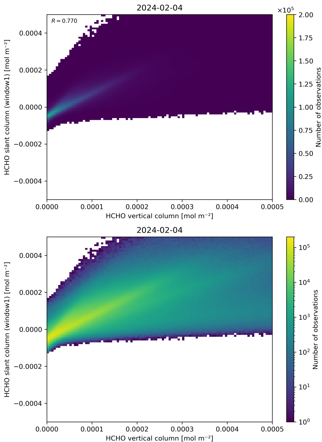
Figure 129: Scatter density plot of “HCHO vertical column” against “HCHO slant column (window1)” for 2024-02-03 to 2024-02-05.
