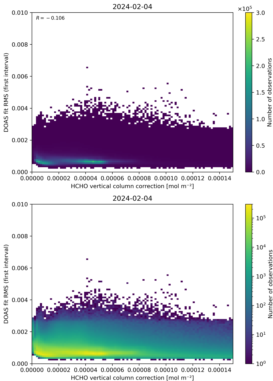
Figure 112: Scatter density plot of “HCHO vertical column correction” against “DOAS fit RMS (first interval)” for 2024-02-03 to 2024-02-05.
