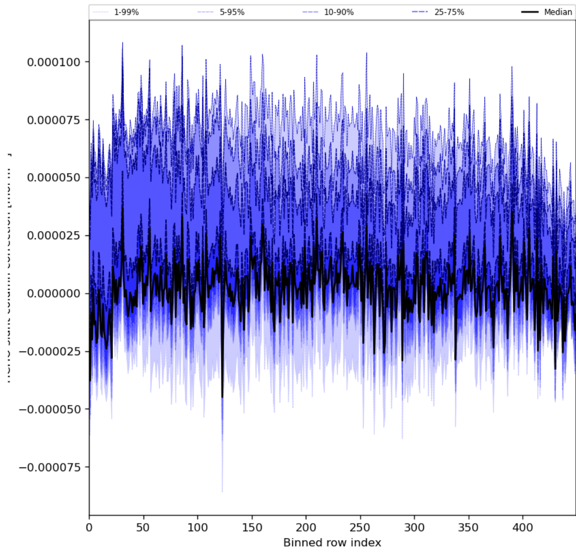
Figure 61: Along track statistics of “HCHO slant column correction” for 2024-02-03 to 2024-02-05
