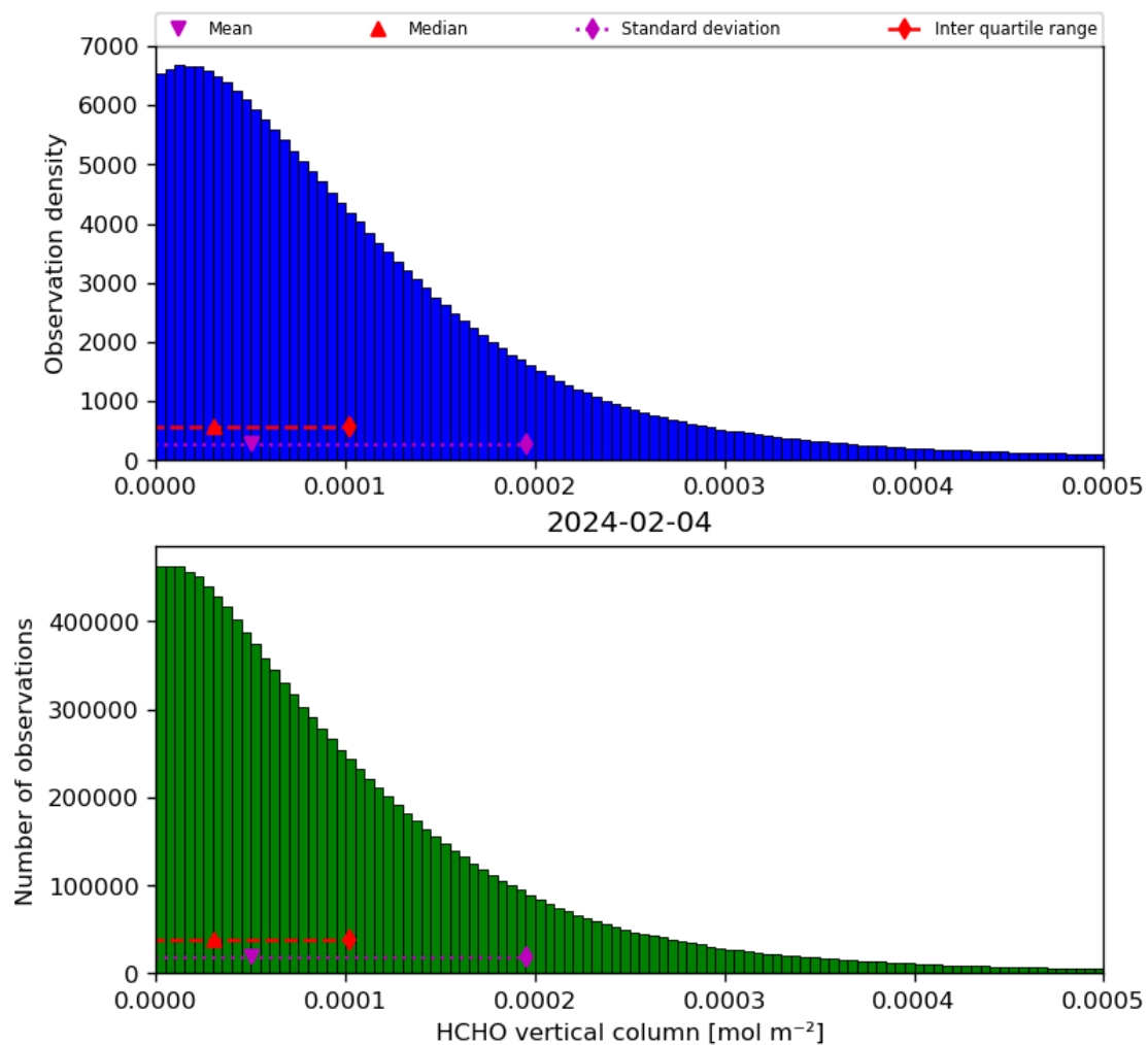
Figure 35: Histogram of “HCHO vertical column” for 2024-02-03 to 2024-02-05
