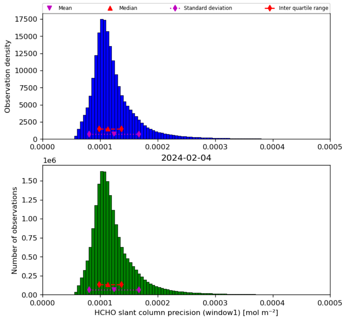
Figure 39: Histogram of “HCHO slant column precision (window1)” for 2024-02-03 to 2024-02-05
