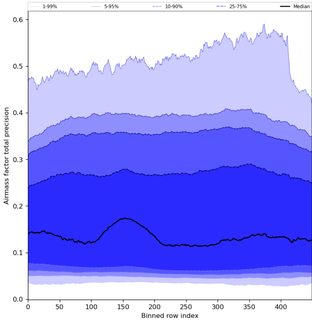
Figure 55: Along track statistics of “Airmass factor total precision” for 2024-02-03 to 2024-02-05
