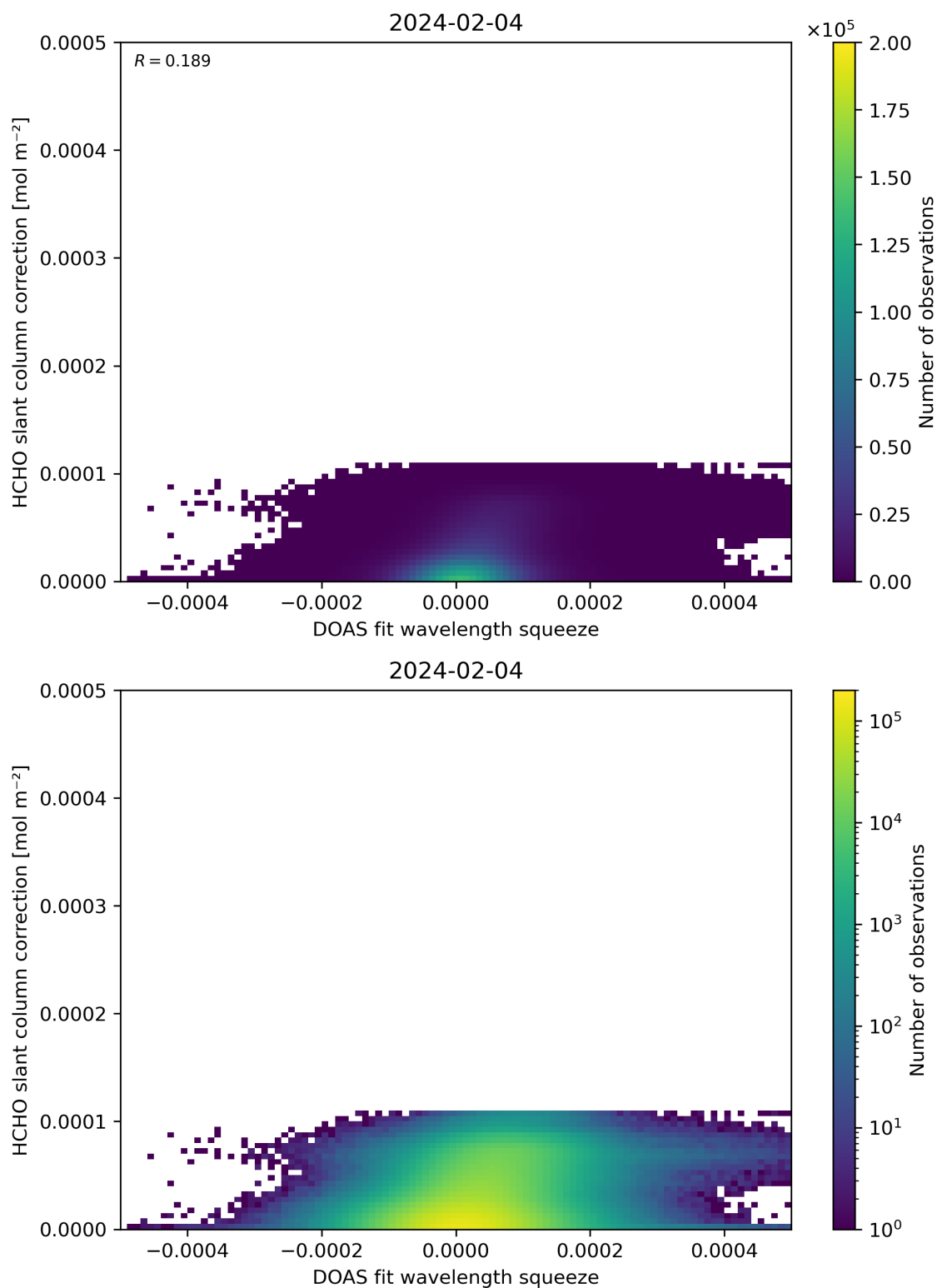
Figure 70: Scatter density plot of “DOAS fit wavelength squeeze” against “HCHO slant column correction” for 2024-02-03 to 2024-02-05.
