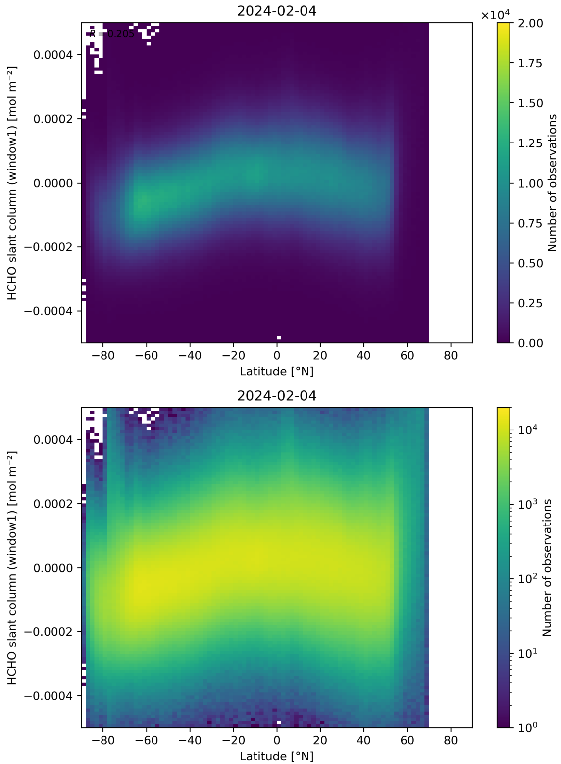
Figure 159: Scatter density plot of “Latitude” against “HCHO slant column (window1)” for 2024-02-03 to 2024-02-05.
