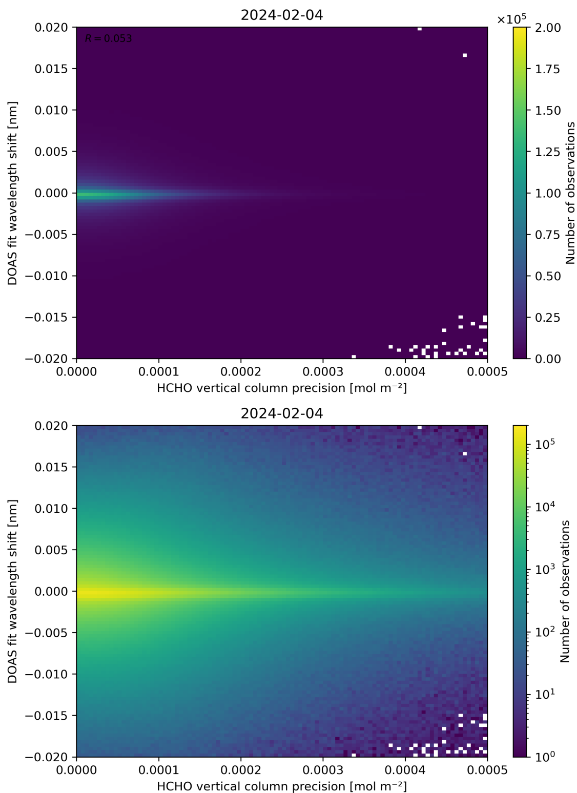
Figure 137: Scatter density plot of “HCHO vertical column precision” against “DOAS fit wavelength shift” for 2024-02-03 to 2024-02-05.
