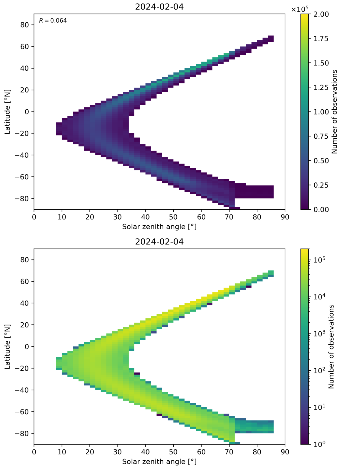
Figure 181: Scatter density plot of “Solar zenith angle” against “Latitude” for 2024-02-03 to 2024-02-05.
