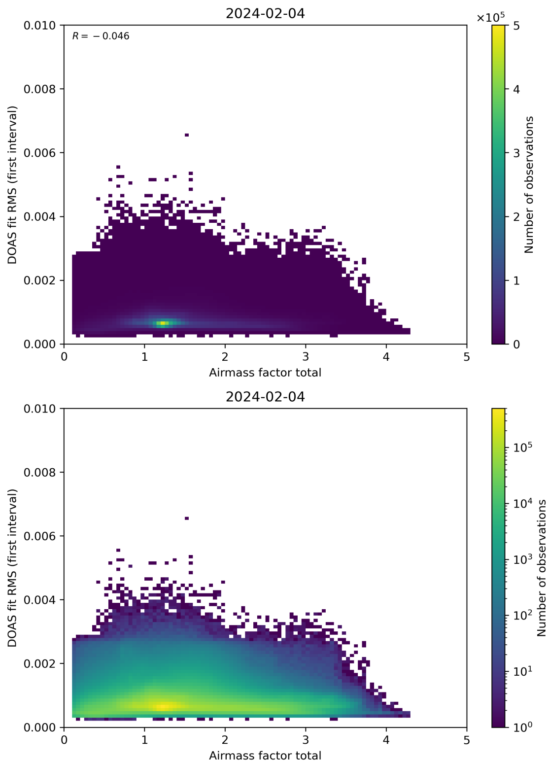
Figure 97: Scatter density plot of “Airmass factor total” against “DOAS fit RMS (first interval)” for 2024-02-03 to 2024-02-05.
