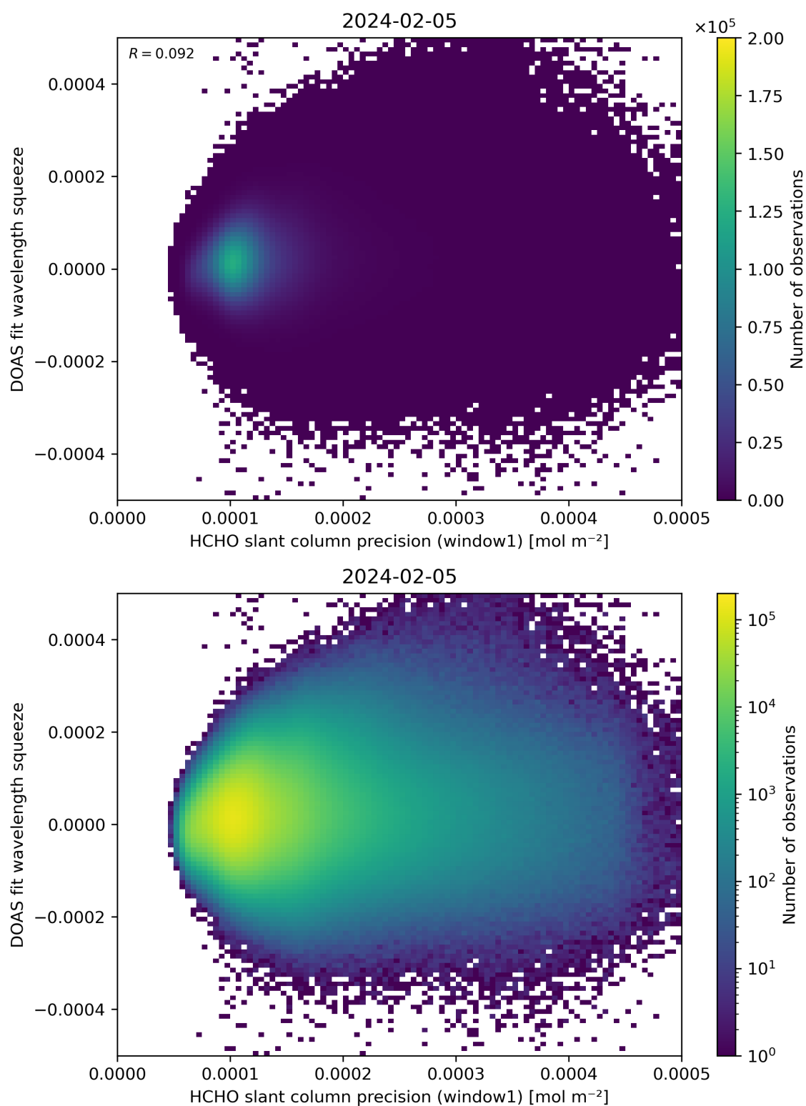
Figure 90: Scatter density plot of “HCHO slant column precision (window1)” against “DOAS fit wavelength squeeze” for 2024-02-04 to 2024-02-06.
