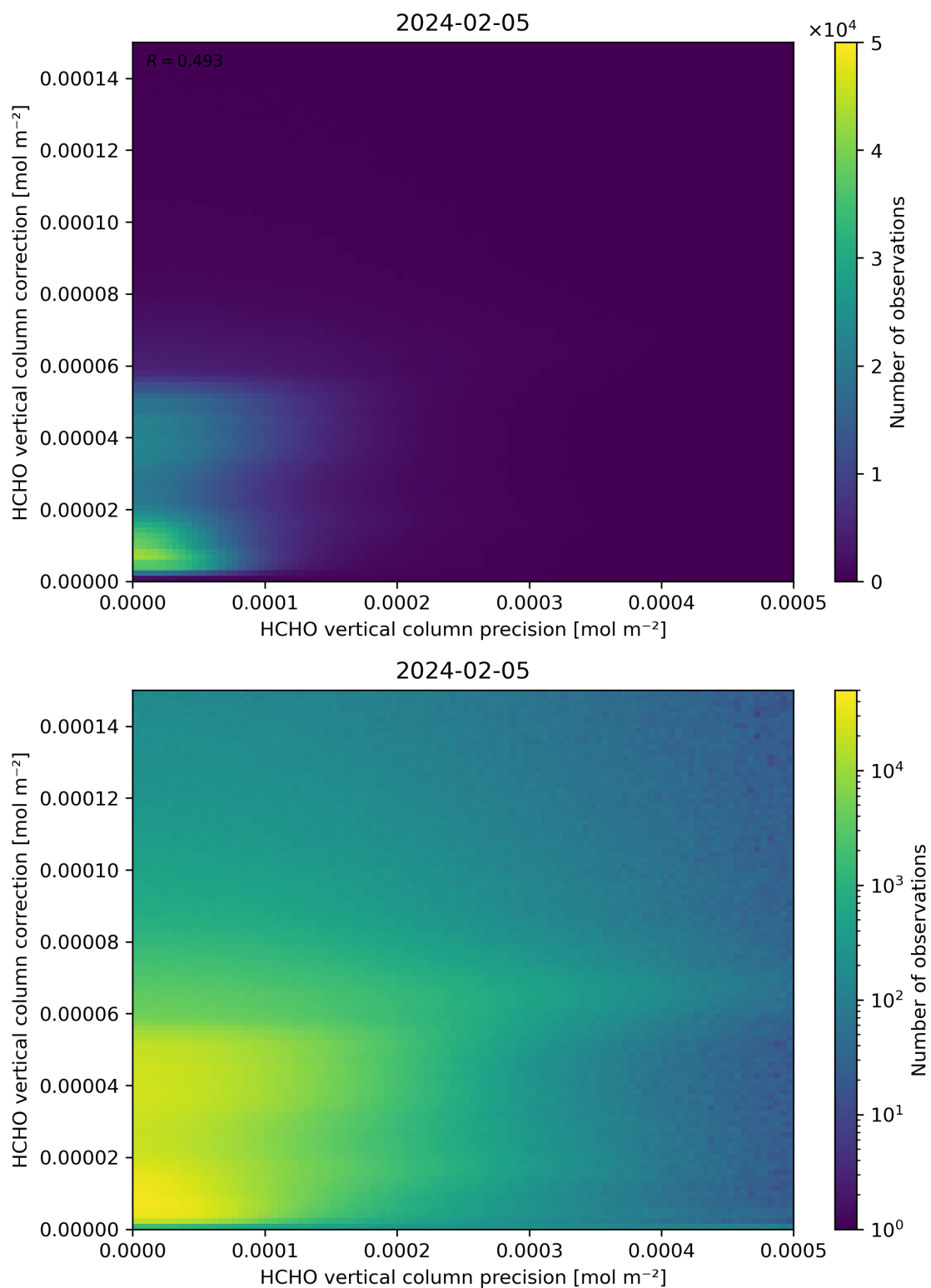
Figure 146: Scatter density plot of “HCHO vertical column precision” against “HCHO vertical column correction” for 2024-02-04 to 2024-02-06.
