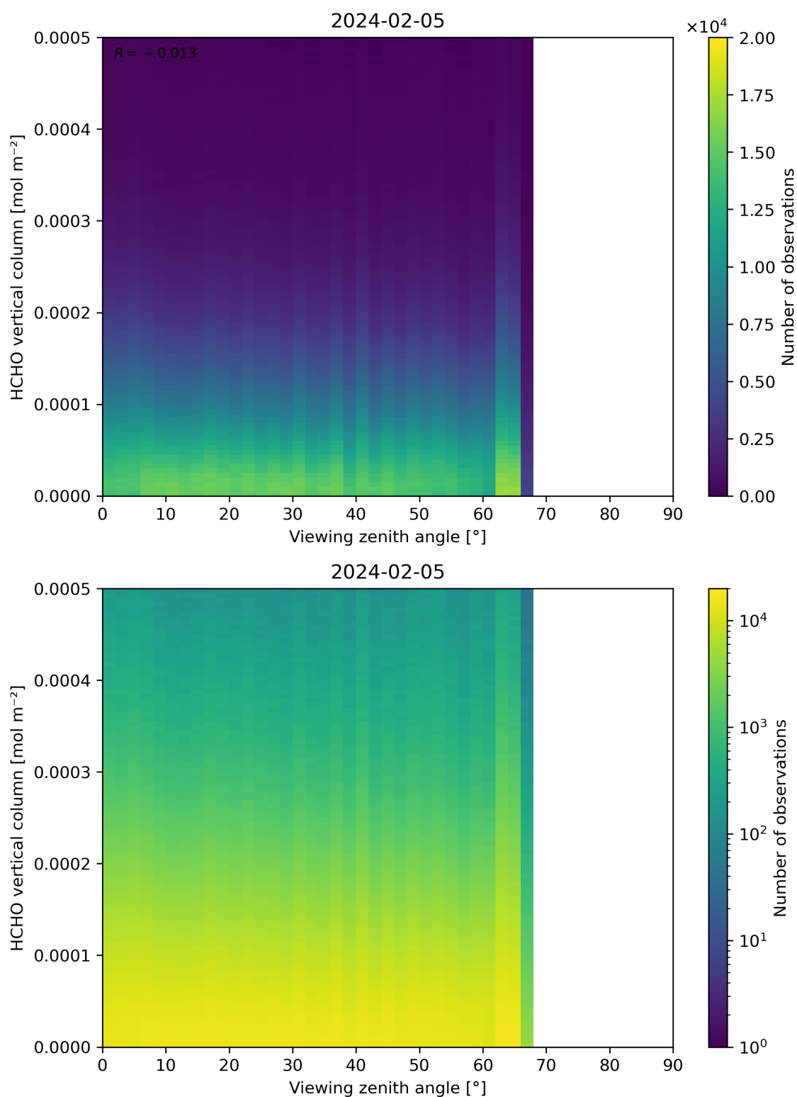
Figure 192: Scatter density plot of “Viewing zenith angle” against “HCHO vertical column” for 2024-02-04 to 2024-02-06.
