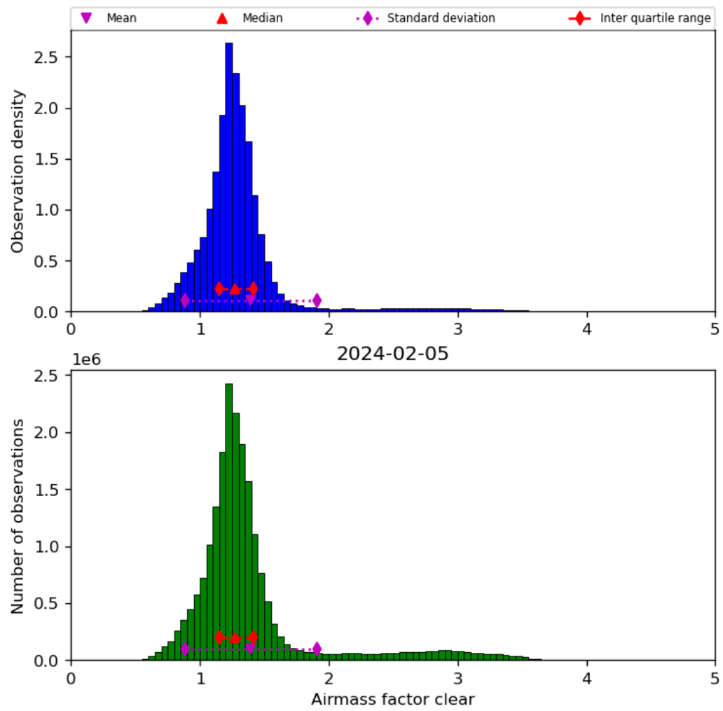
Figure 42: Histogram of “Airmass factor clear” for 2024-02-04 to 2024-02-06
