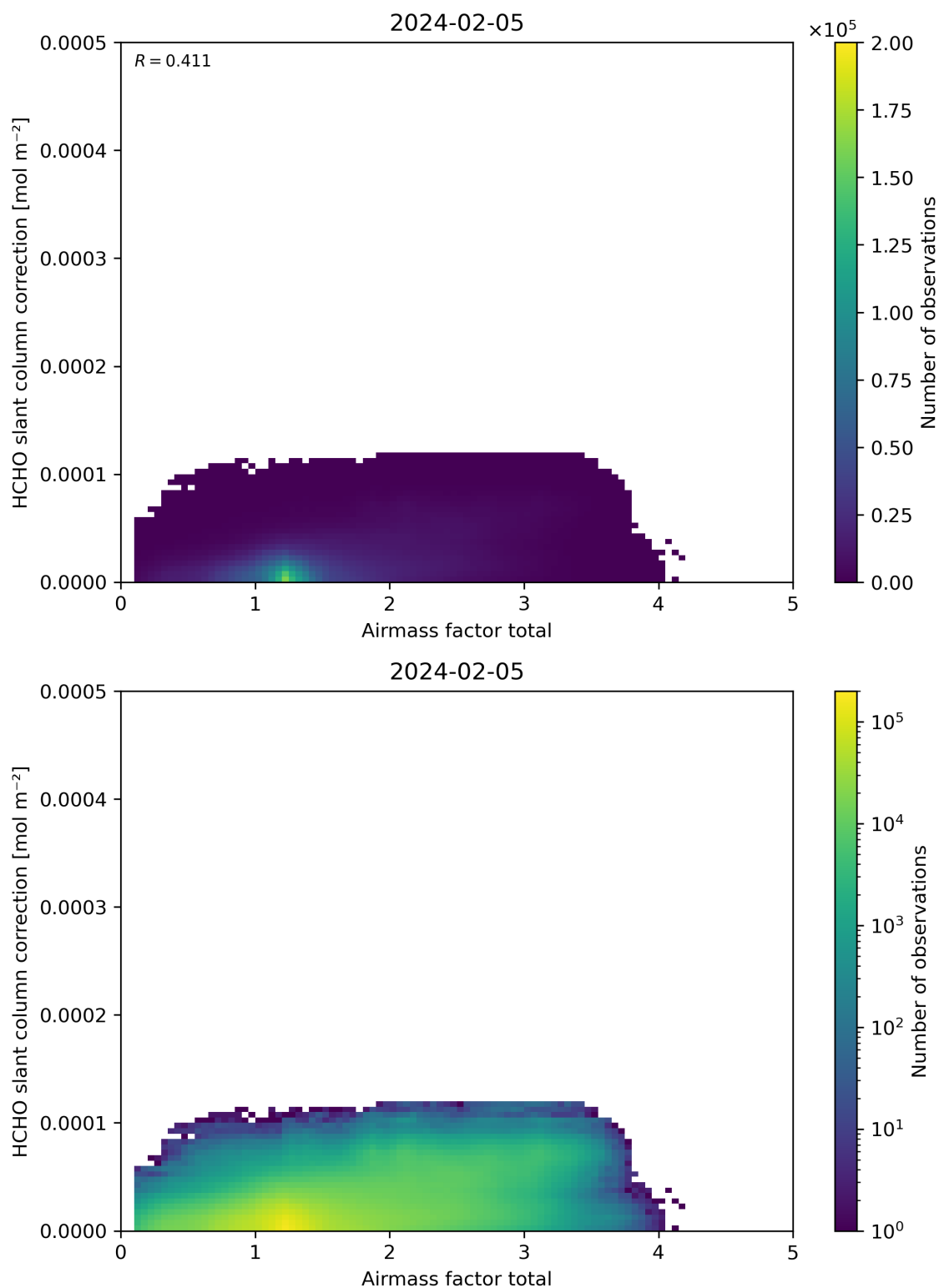
Figure 102: Scatter density plot of “Airmass factor total” against “HCHO slant column correction” for 2024-02-04 to 2024-02-06.
