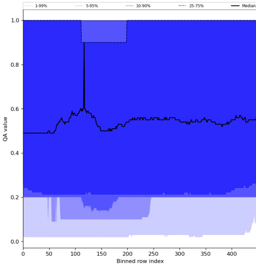
Figure 48: Along track statistics of “QA value” for 2024-02-04 to 2024-02-06
