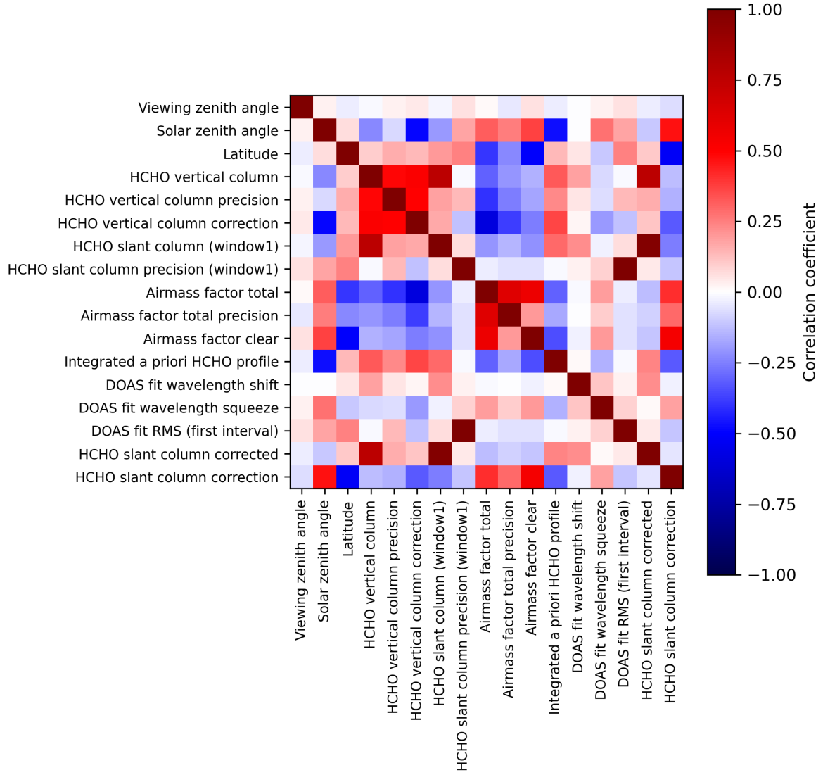
Figure 2: Map of correlation matrix for 2024-02-04 to 2024-02-06.
