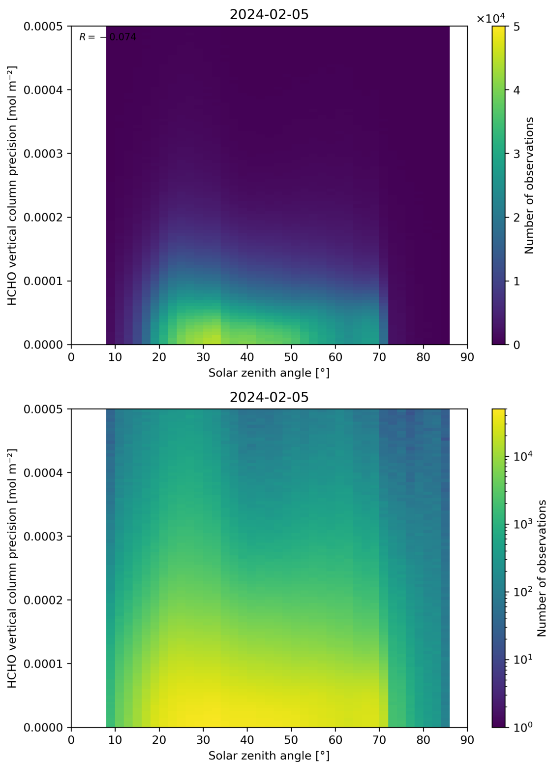
Figure 179: Scatter density plot of “Solar zenith angle” against “HCHO vertical column precision” for 2024-02-04 to 2024-02-06.
