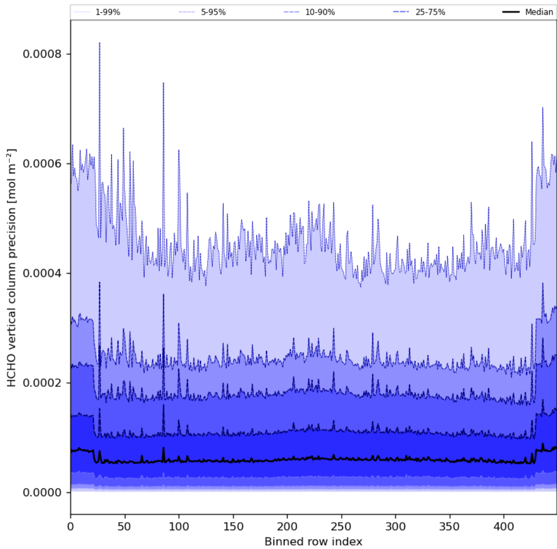
Figure 50: Along track statistics of “HCHO vertical column precision” for 2024-02-04 to 2024-02-06
