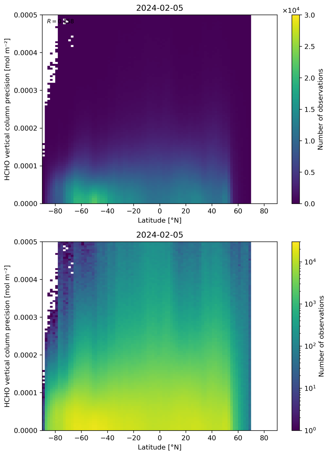
Figure 165: Scatter density plot of “Latitude” against “HCHO vertical column precision” for 2024-02-04 to 2024-02-06.
