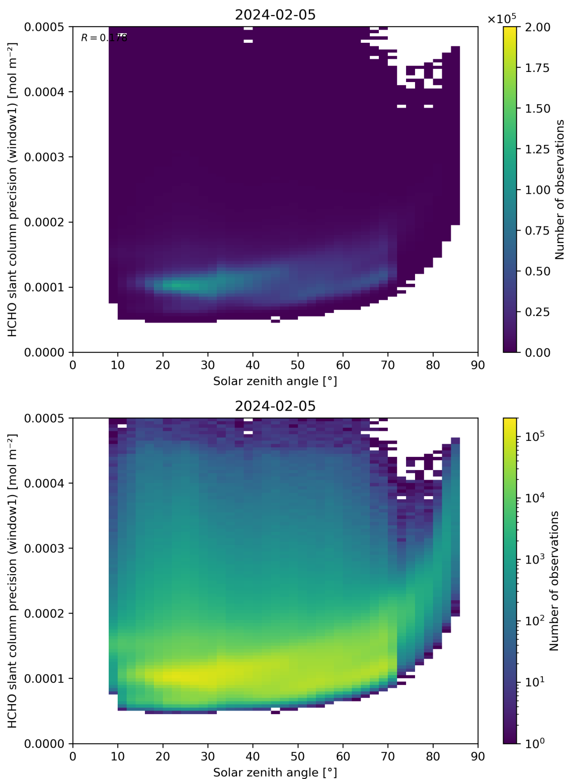
Figure 174: Scatter density plot of “Solar zenith angle” against “HCHO slant column precision (window1)” for 2024-02-04 to 2024-02-06.
