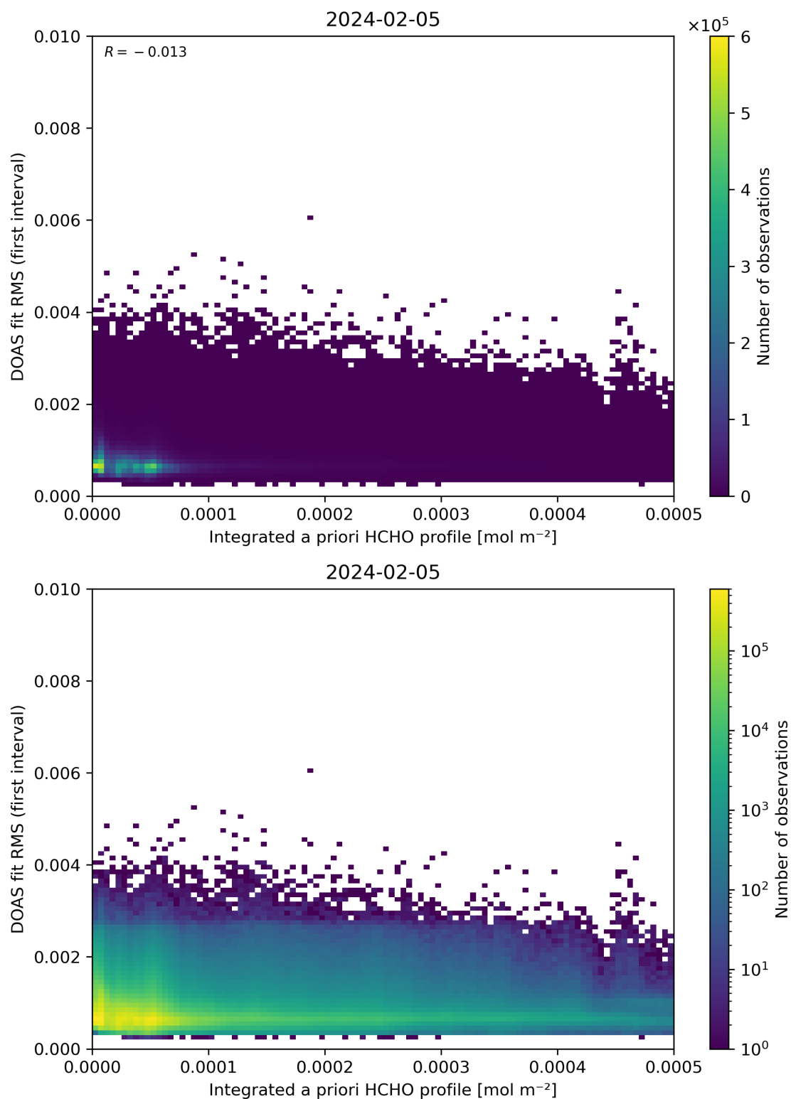
Figure 148: Scatter density plot of “Integrated a priori HCHO profile” against “DOAS fit RMS (first interval)” for 2024-02-04 to 2024-02-06.
