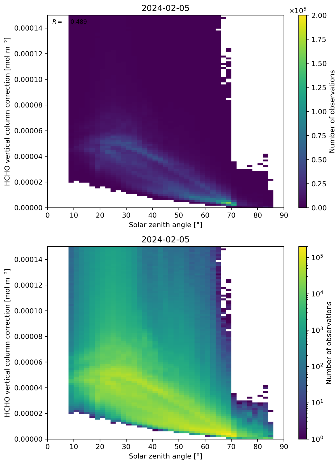
Figure 178: Scatter density plot of “Solar zenith angle” against “HCHO vertical column correction” for 2024-02-04 to 2024-02-06.
