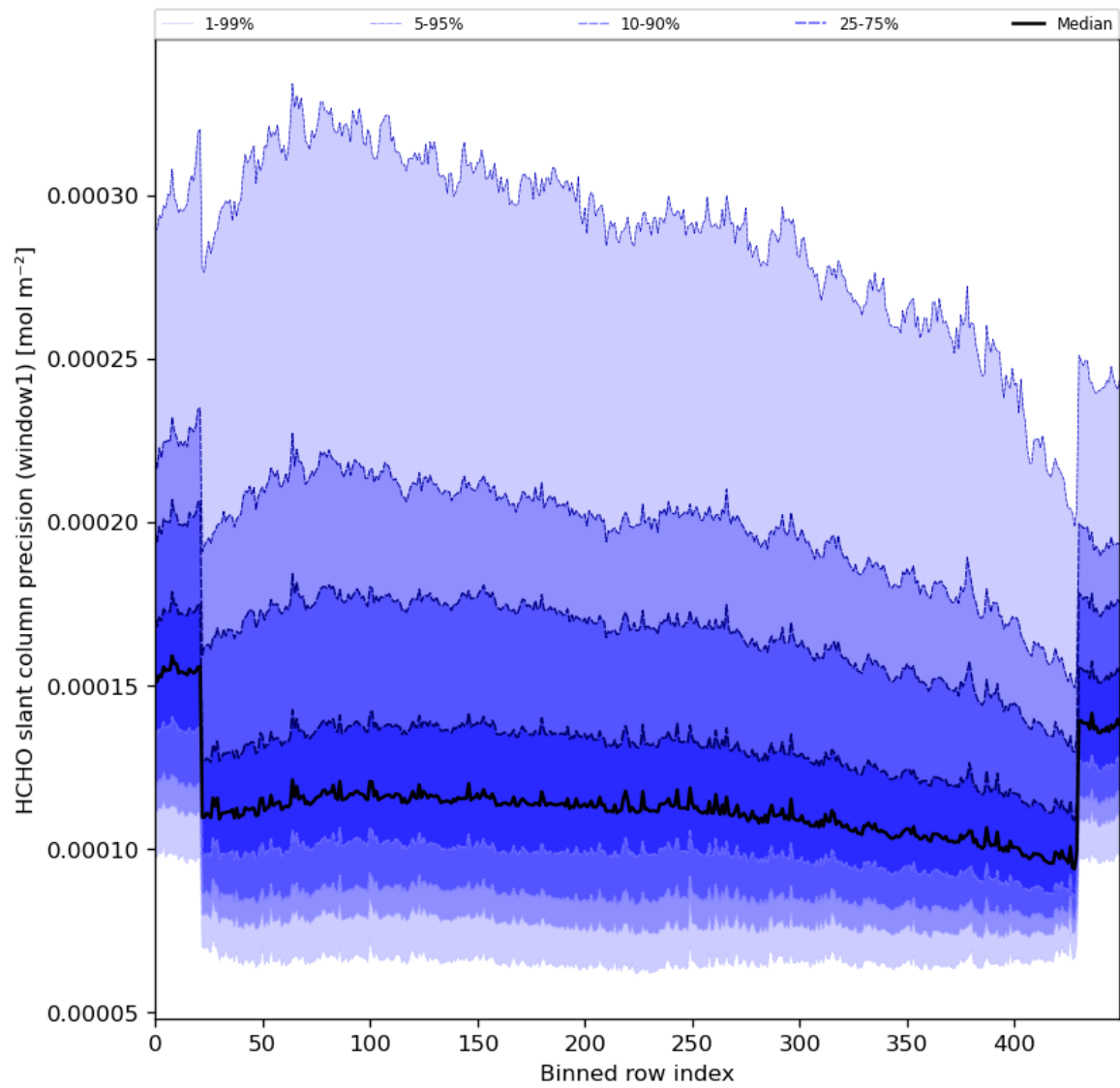
Figure 53: Along track statistics of “HCHO slant column precision (window1)” for 2024-02-04 to 2024-02-06
