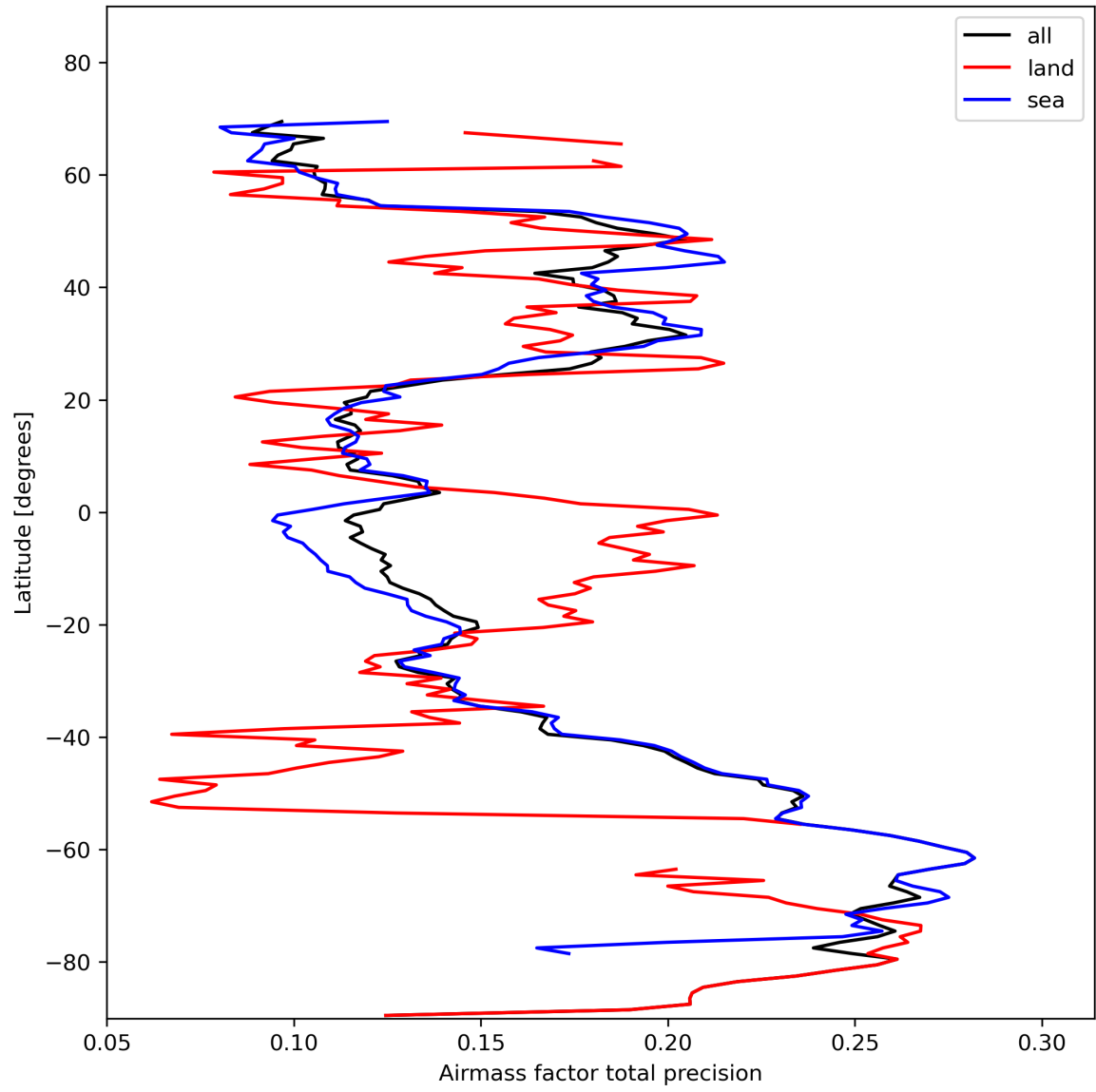
Figure 27: Zonal average of “Airmass factor total precision” for 2024-02-04 to 2024-02-06.
