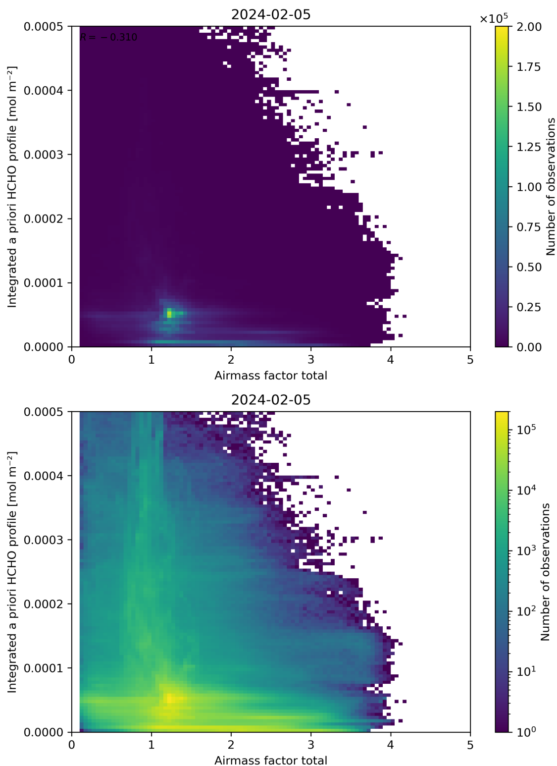
Figure 104: Scatter density plot of “Airmass factor total” against “Integrated a priori HCHO profile” for 2024-02-04 to 2024-02-06.
