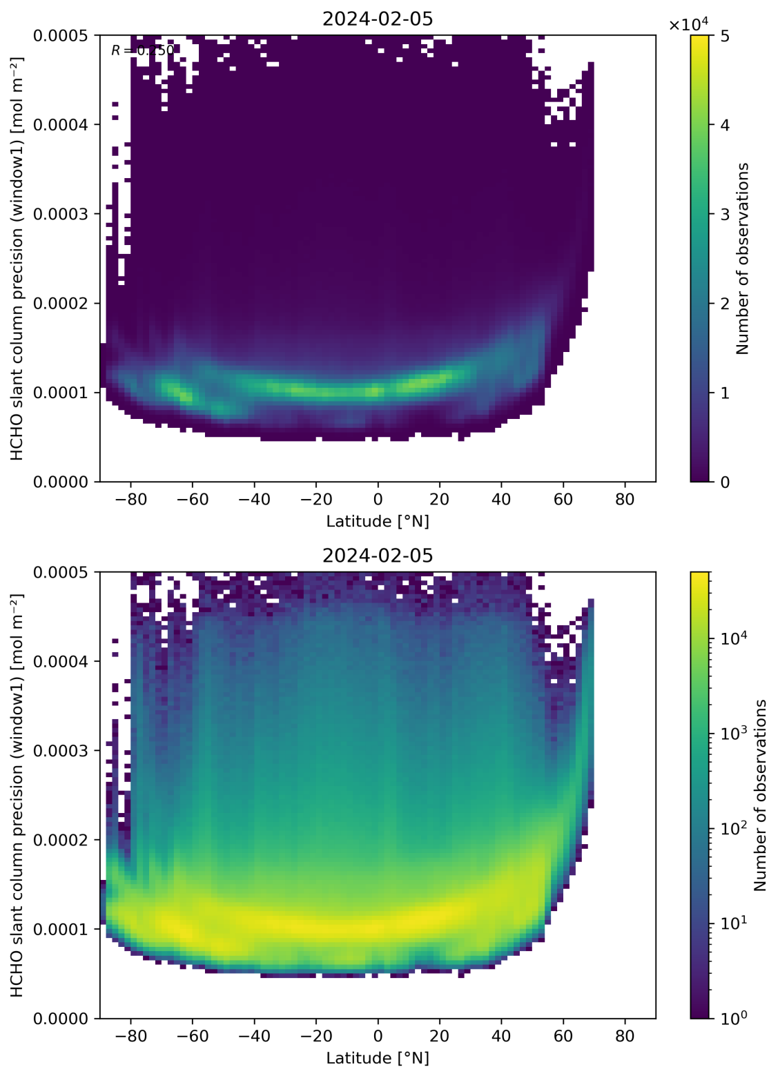
Figure 160: Scatter density plot of “Latitude” against “HCHO slant column precision (window1)” for 2024-02-04 to 2024-02-06.
