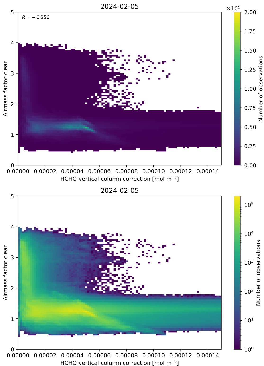
Figure 115: Scatter density plot of “HCHO vertical column correction” against “Airmass factor clear” for 2024-02-04 to 2024-02-06.
