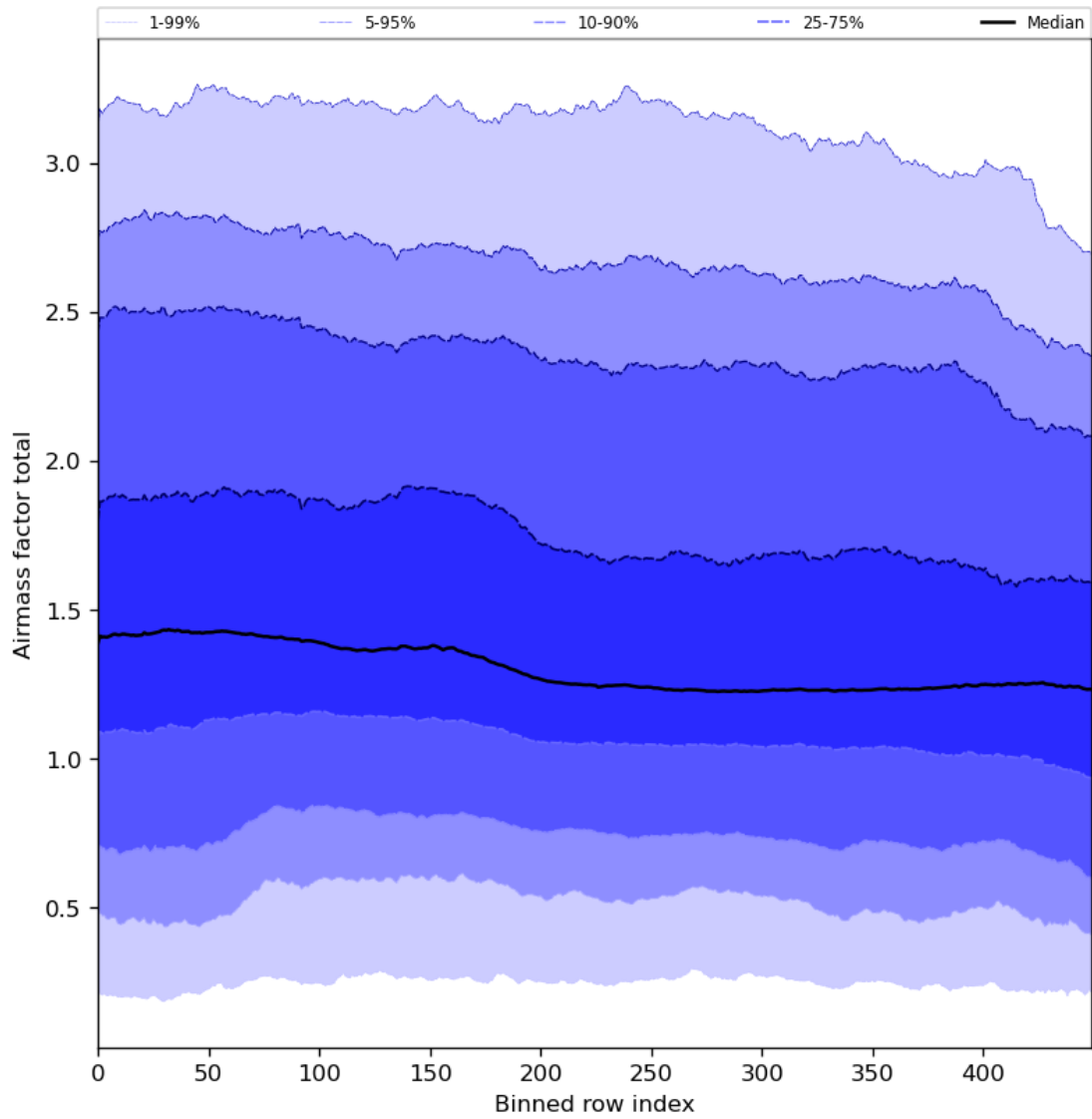
Figure 54: Along track statistics of “Airmass factor total” for 2024-02-04 to 2024-02-06
