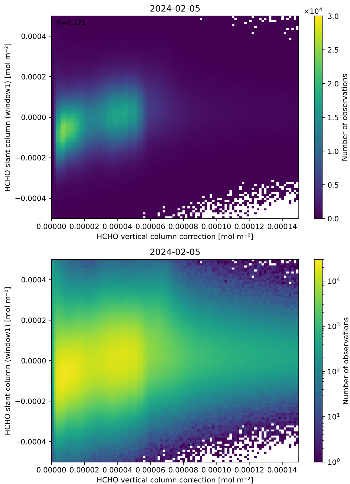
Figure 118: Scatter density plot of “HCHO vertical column correction” against “HCHO slant column (window1)” for 2024-02-04 to 2024-02-06.
