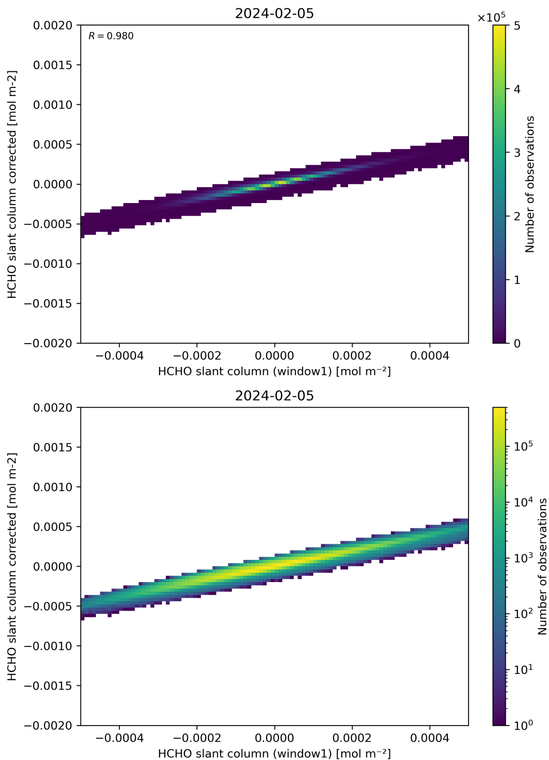
Figure 82: Scatter density plot of “HCHO slant column (window1)” against “HCHO slant column corrected” for 2024-02-04 to 2024-02-06.
