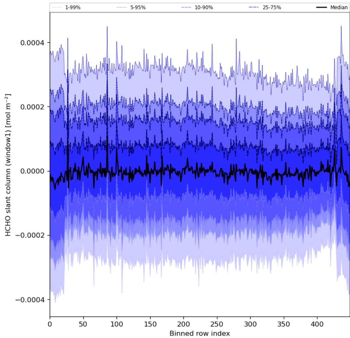
Figure 52: Along track statistics of “HCHO slant column (window1)” for 2024-02-04 to 2024-02-06
