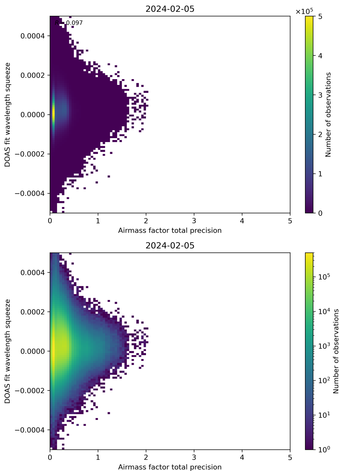
Figure 107: Scatter density plot of “Airmass factor total precision” against “DOAS fit wavelength squeeze” for 2024-02-04 to 2024-02-06.
