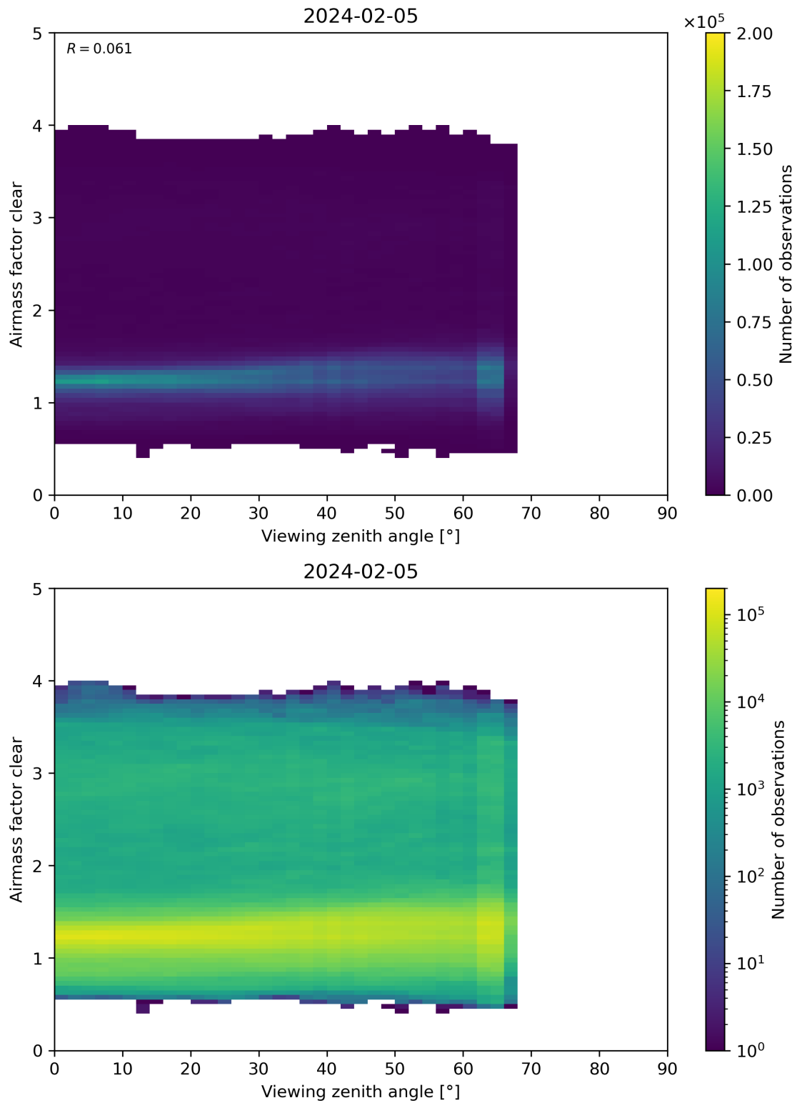
Figure 185: Scatter density plot of “Viewing zenith angle” against “Airmass factor clear” for 2024-02-04 to 2024-02-06.
