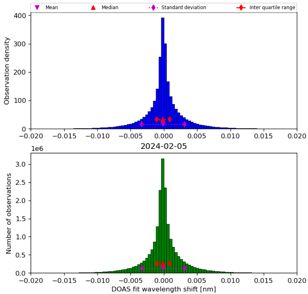
Figure 44: Histogram of “DOAS fit wavelength shift” for 2024-02-04 to 2024-02-06
