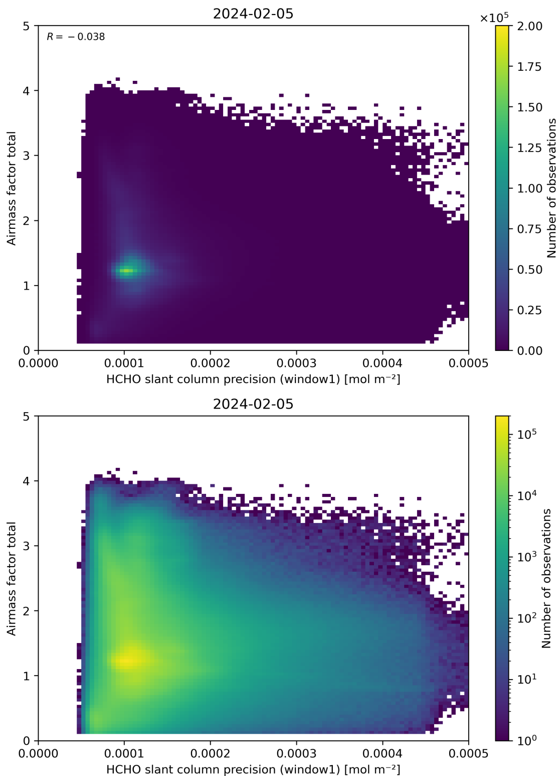
Figure 94: Scatter density plot of “HCHO slant column precision (window1)” against “Airmass factor total” for 2024-02-04 to 2024-02-06.
