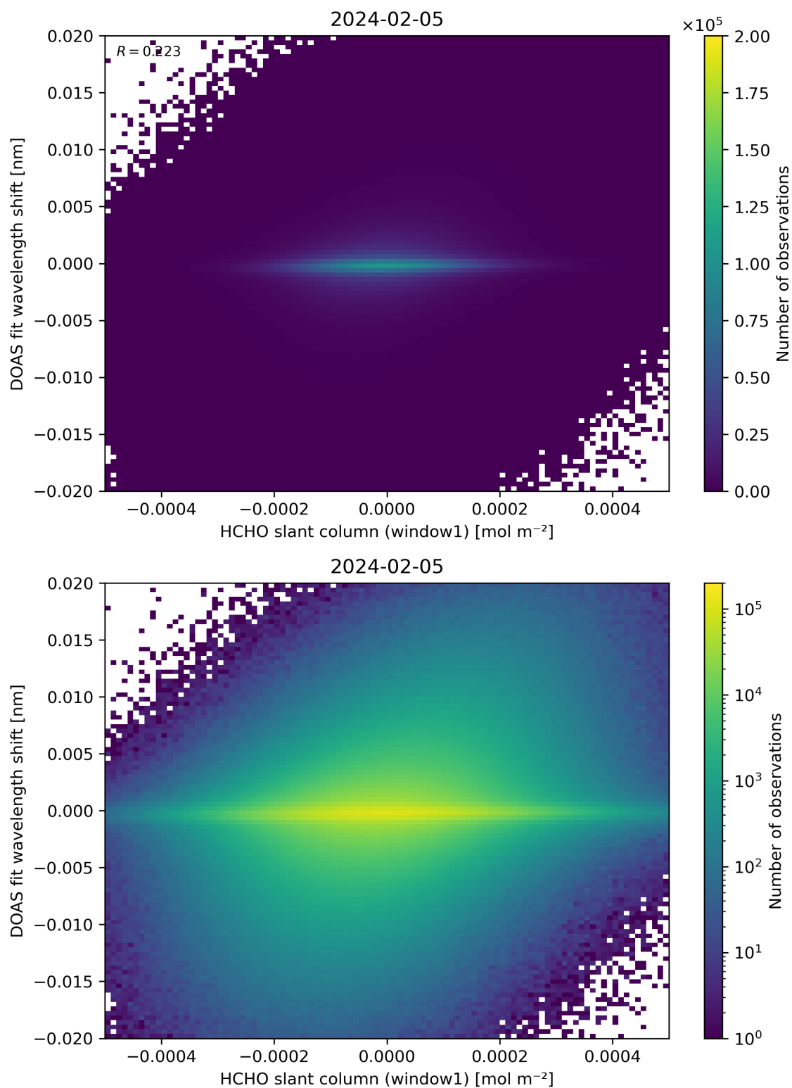
Figure 79: Scatter density plot of “HCHO slant column (window1)” against “DOAS fit wavelength shift” for 2024-02-04 to 2024-02-06.
