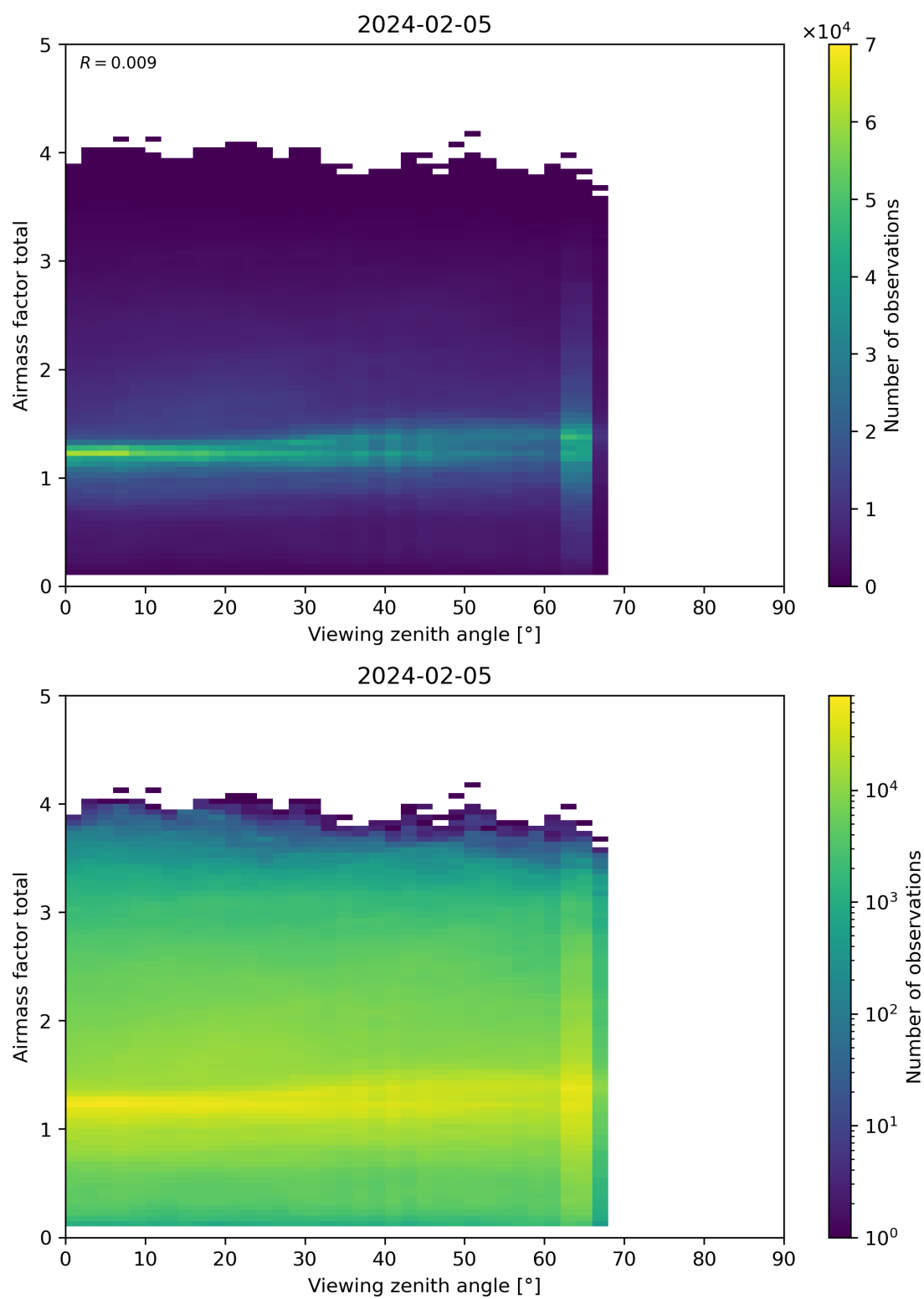
Figure 190: Scatter density plot of “Viewing zenith angle” against “Airmass factor total” for 2024-02-04 to 2024-02-06.
