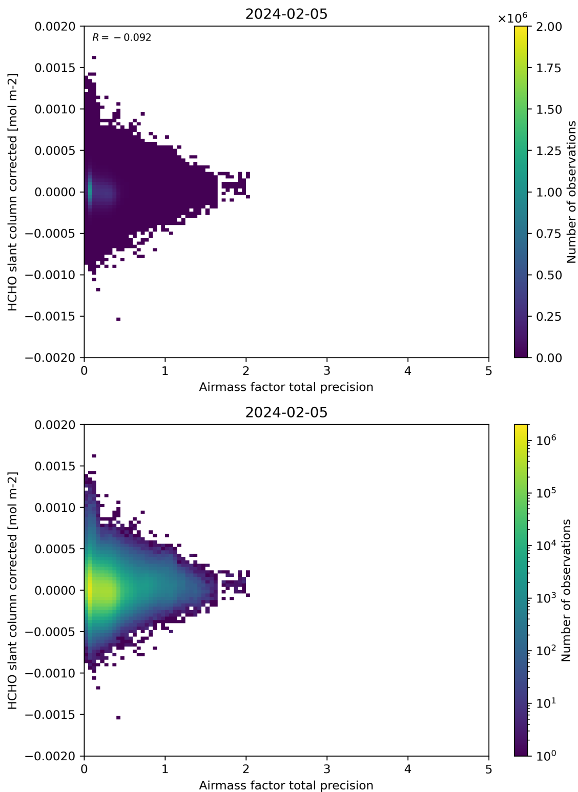
Figure 109: Scatter density plot of “Airmass factor total precision” against “HCHO slant column corrected” for 2024-02-04 to 2024-02-06.
