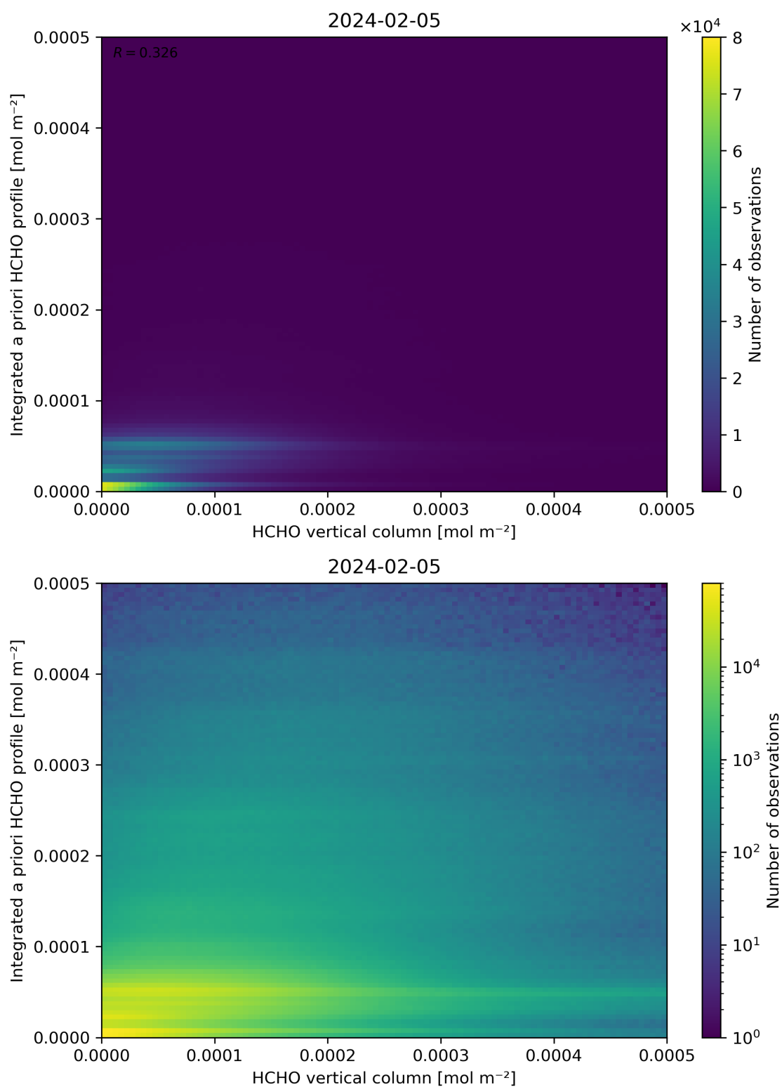
Figure 135: Scatter density plot of “HCHO vertical column” against “Integrated a priori HCHO profile” for 2024-02-04 to 2024-02-06.
