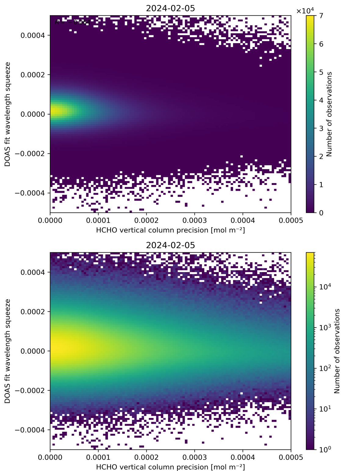
Figure 138: Scatter density plot of “HCHO vertical column precision” against “DOAS fit wavelength squeeze” for 2024-02-04 to 2024-02-06.
