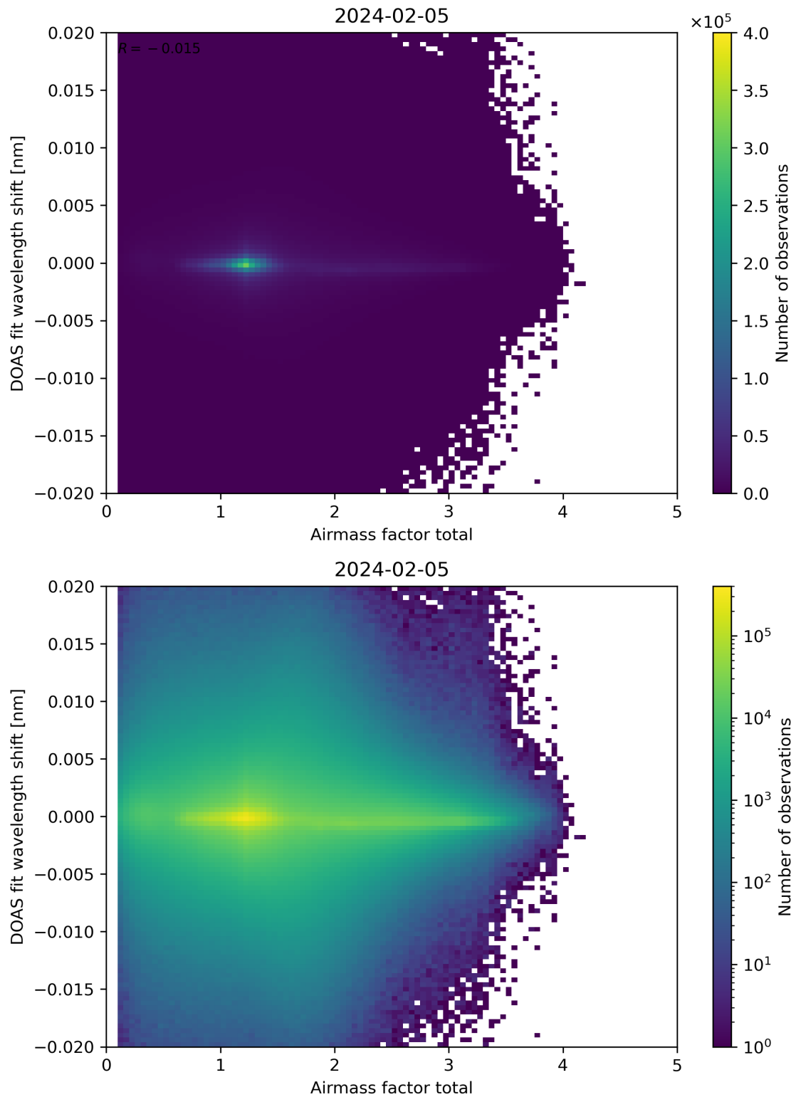
Figure 98: Scatter density plot of “Airmass factor total” against “DOAS fit wavelength shift” for 2024-02-04 to 2024-02-06.
