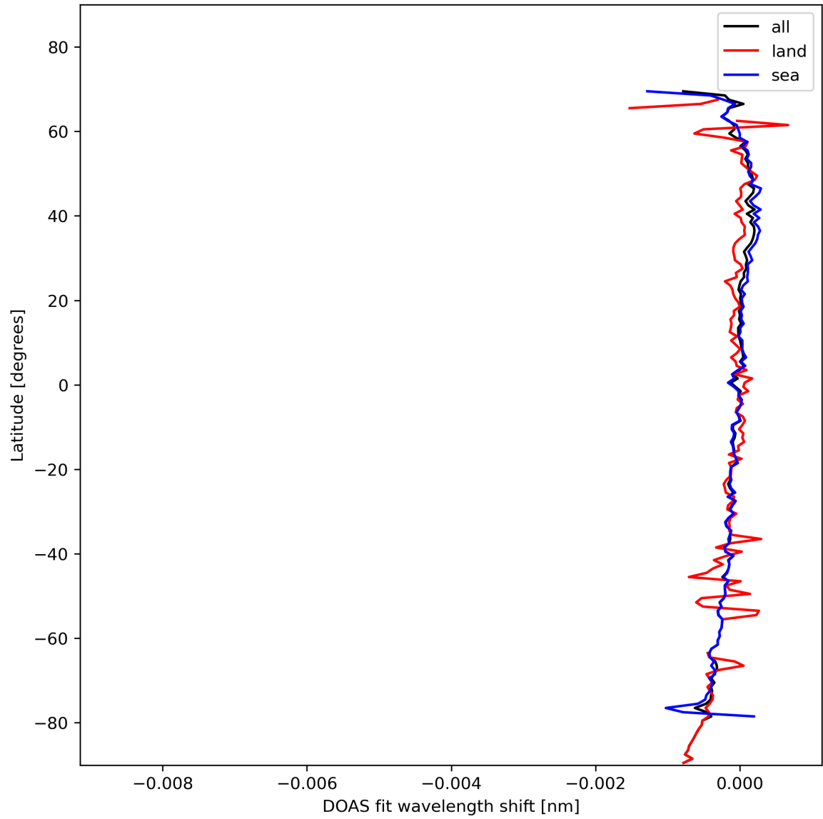
Figure 30: Zonal average of “DOAS fit wavelength shift” for 2024-02-04 to 2024-02-06.
