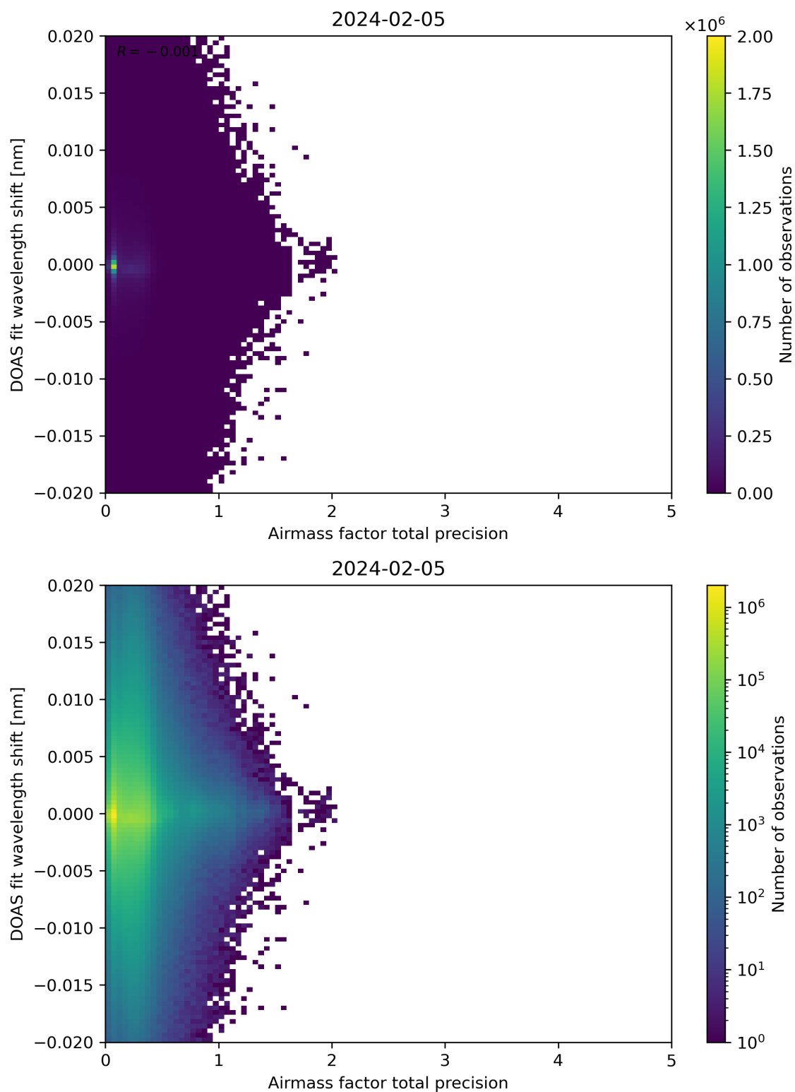
Figure 106: Scatter density plot of “Airmass factor total precision” against “DOAS fit wavelength shift” for 2024-02-04 to 2024-02-06.
