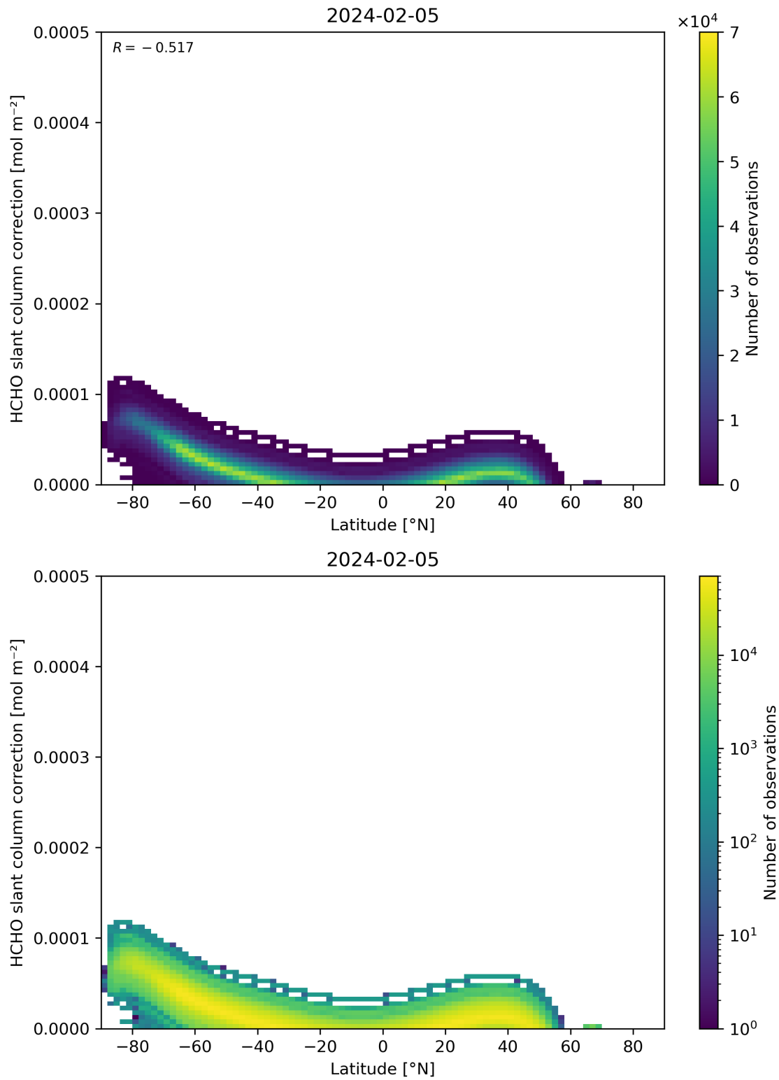
Figure 158: Scatter density plot of “Latitude” against “HCHO slant column correction” for 2024-02-04 to 2024-02-06.
