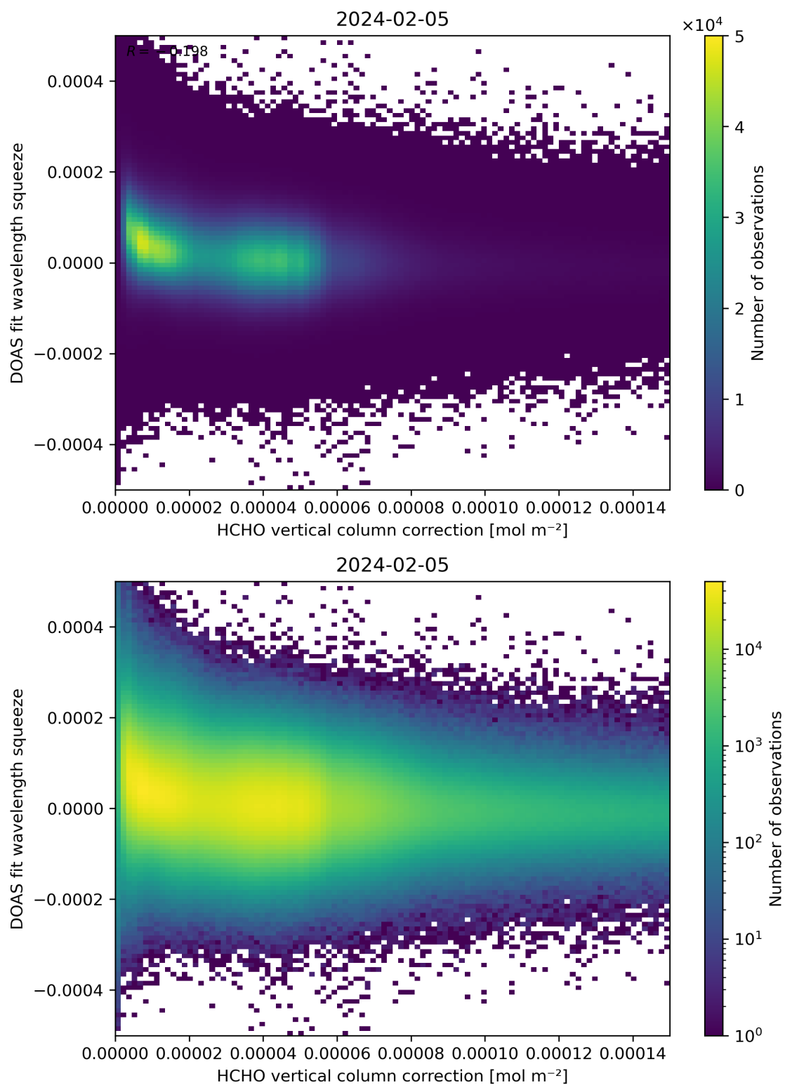
Figure 114: Scatter density plot of “HCHO vertical column correction” against “DOAS fit wavelength squeeze” for 2024-02-04 to 2024-02-06.
