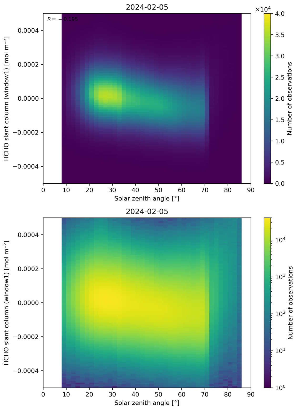
Figure 173: Scatter density plot of “Solar zenith angle” against “HCHO slant column (window1)” for 2024-02-04 to 2024-02-06.
