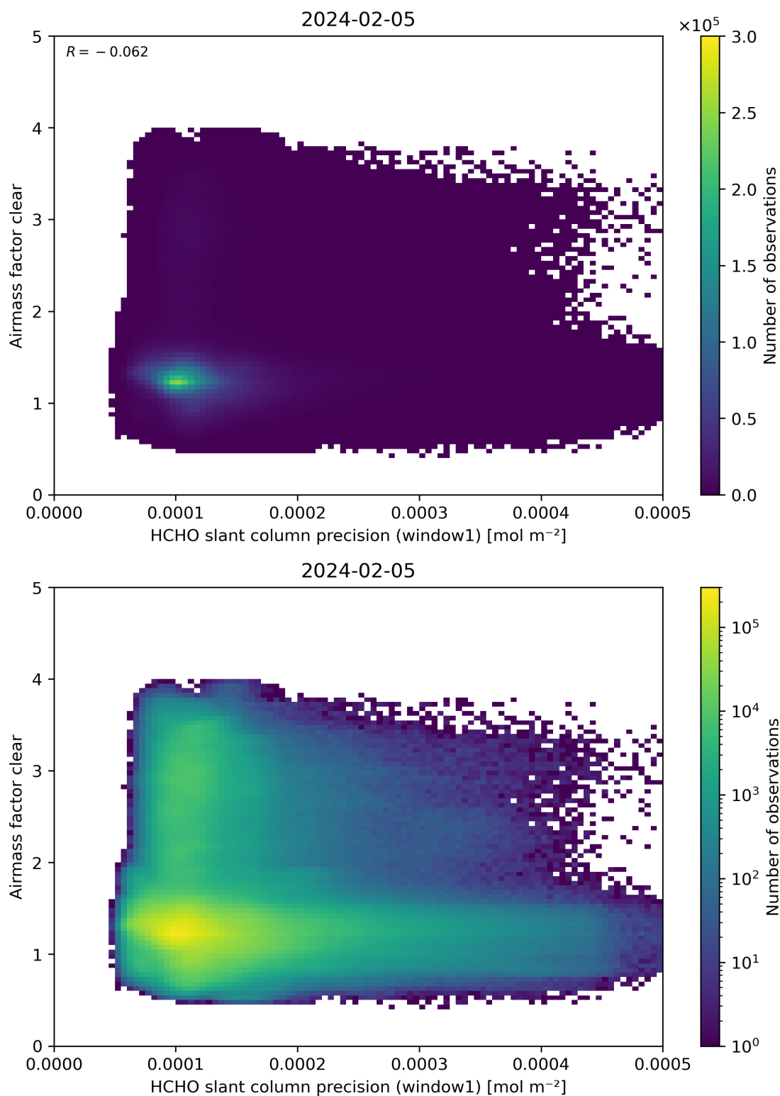
Figure 91: Scatter density plot of “HCHO slant column precision (window1)” against “Airmass factor clear” for 2024-02-04 to 2024-02-06.
