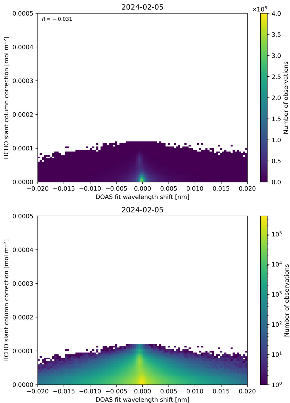
Figure 67: Scatter density plot of “DOAS fit wavelength shift” against “HCHO slant column correction” for 2024-02-04 to 2024-02-06.
