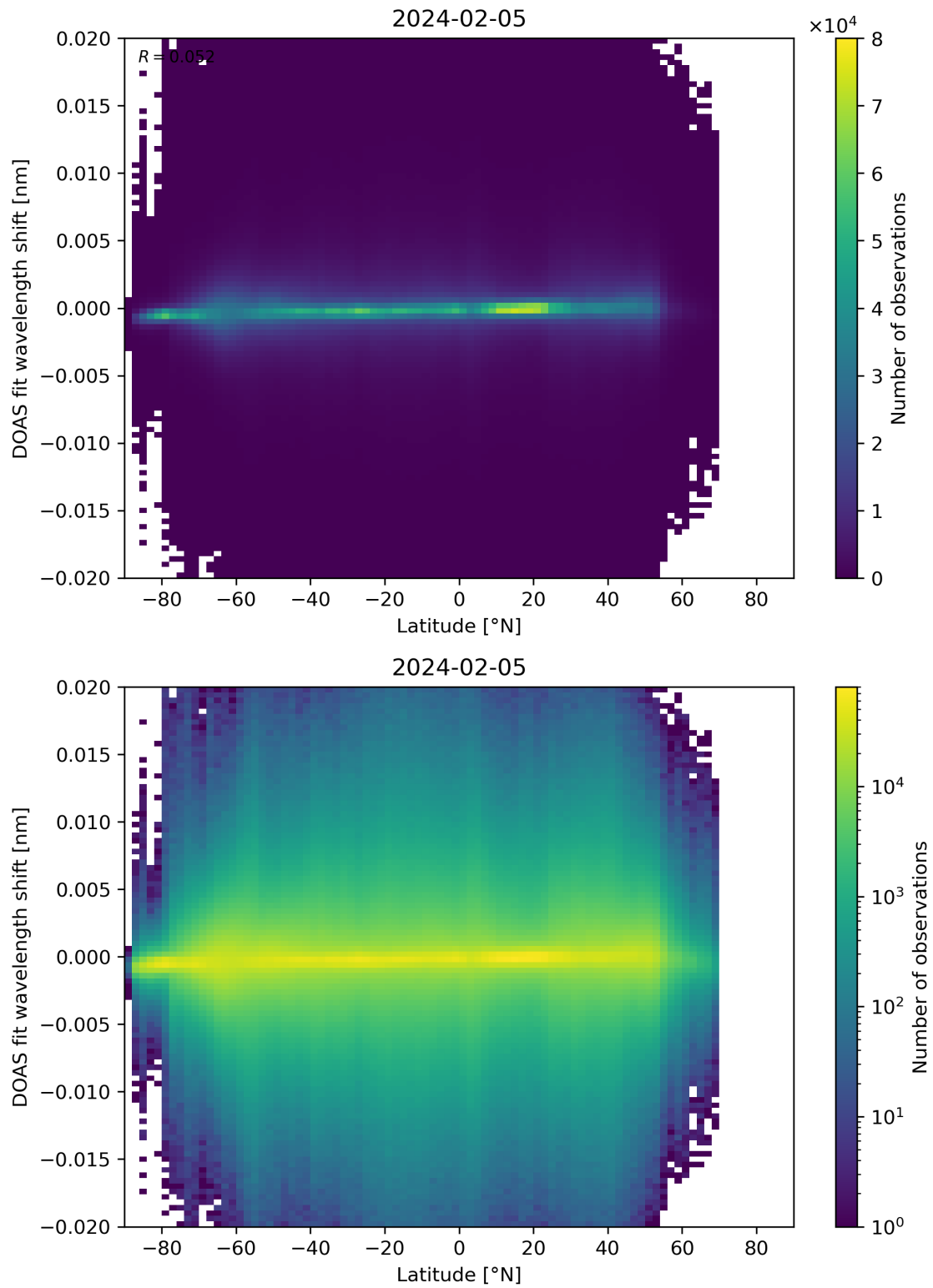
Figure 154: Scatter density plot of “Latitude” against “DOAS fit wavelength shift” for 2024-02-04 to 2024-02-06.
