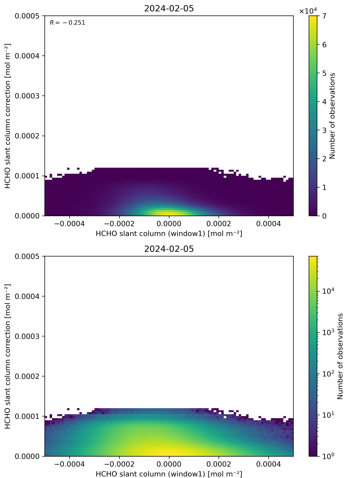
Figure 83: Scatter density plot of “HCHO slant column (window1)” against “HCHO slant column correction” for 2024-02-04 to 2024-02-06.
