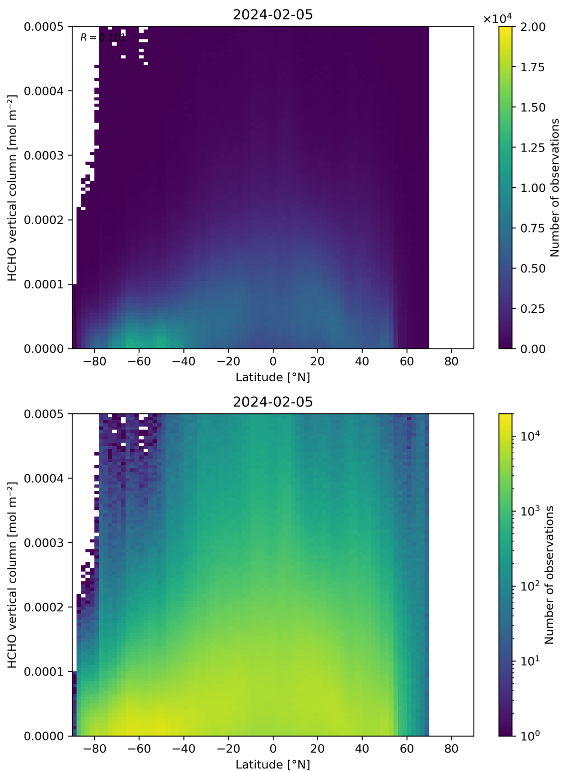
Figure 163: Scatter density plot of “Latitude” against “HCHO vertical column” for 2024-02-04 to 2024-02-06.
