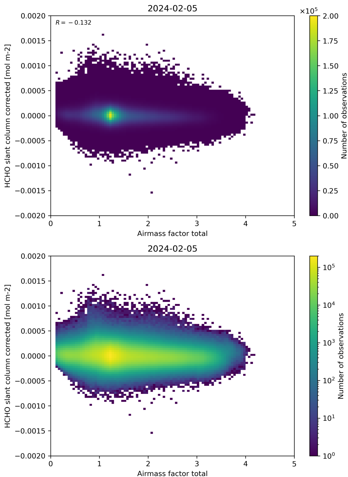
Figure 101: Scatter density plot of “Airmass factor total” against “HCHO slant column corrected” for 2024-02-04 to 2024-02-06.
