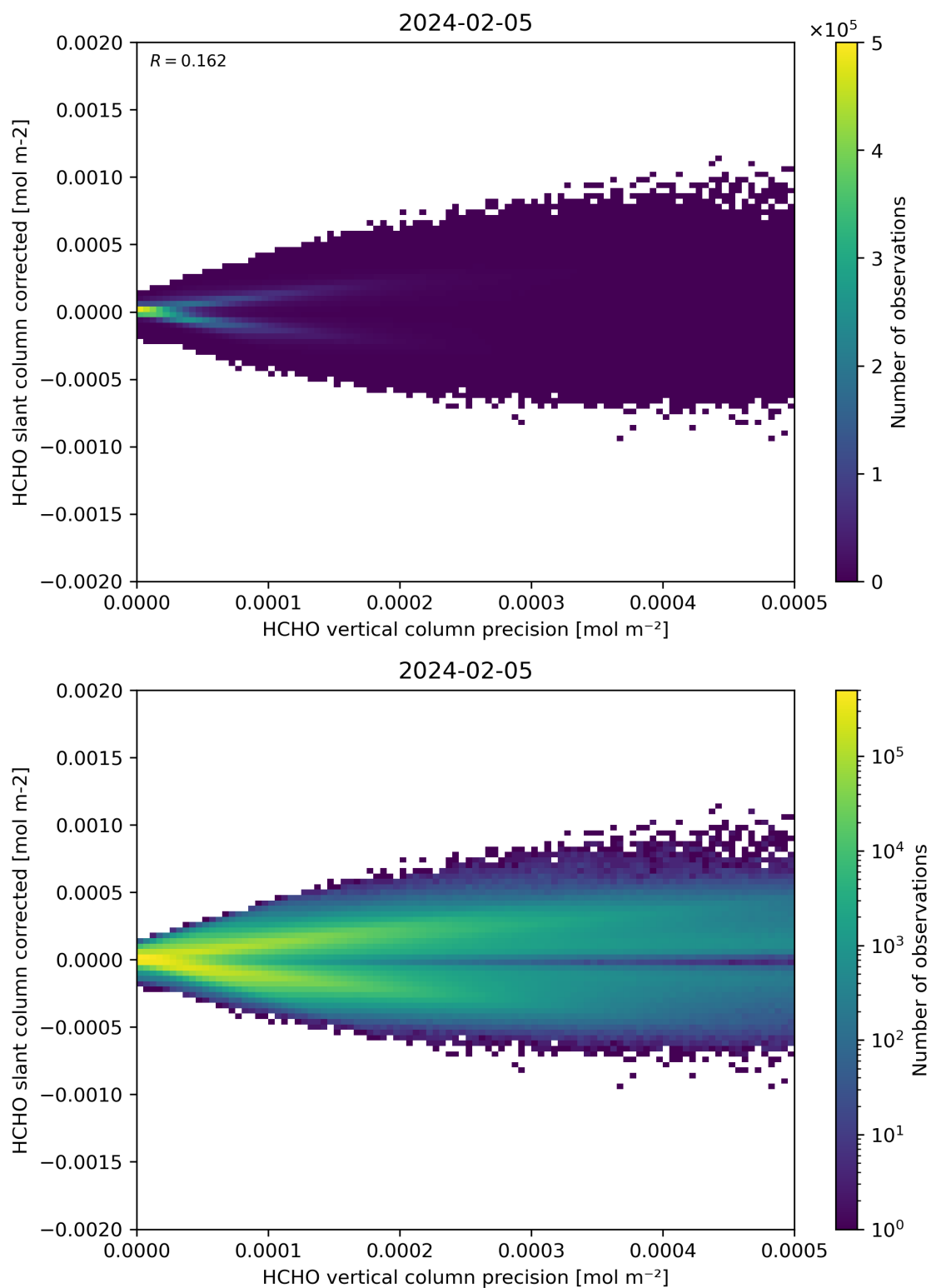
Figure 140: Scatter density plot of “HCHO vertical column precision” against “HCHO slant column corrected” for 2024-02-04 to 2024-02-06.
