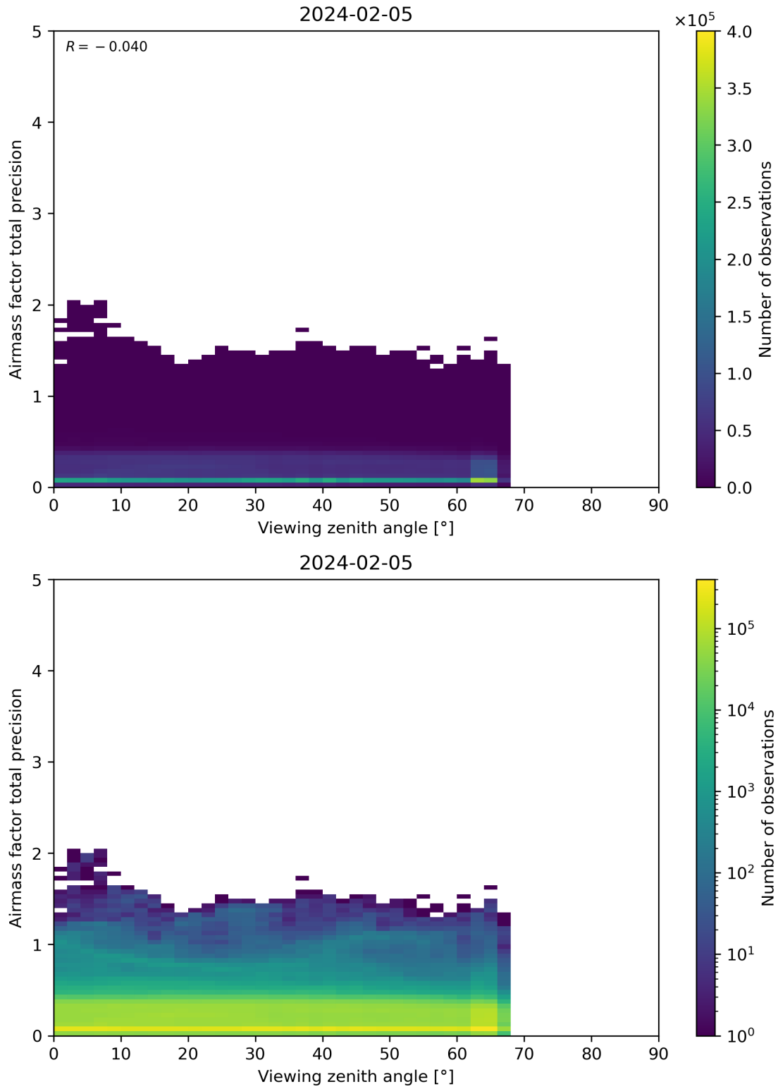
Figure 191: Scatter density plot of “Viewing zenith angle” against “Airmass factor total precision” for 2024-02-04 to 2024-02-06.
