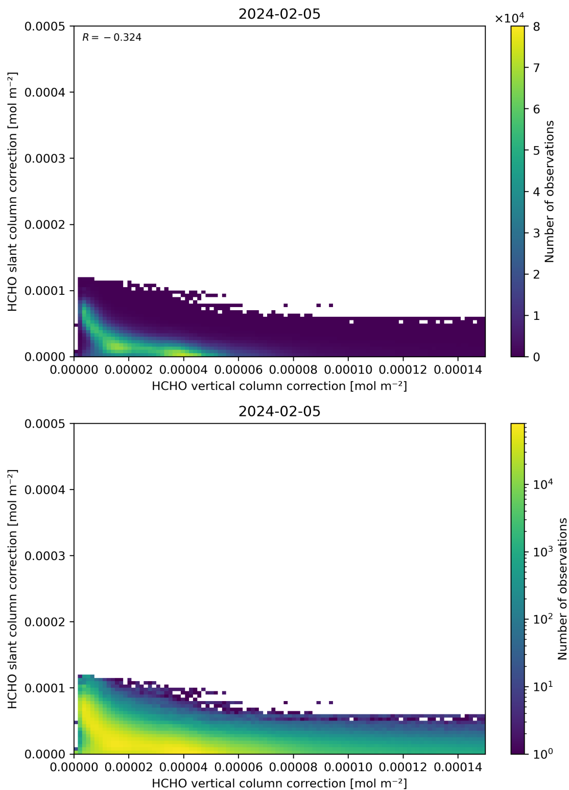
Figure 117: Scatter density plot of “HCHO vertical column correction” against “HCHO slant column correction” for 2024-02-04 to 2024-02-06.
