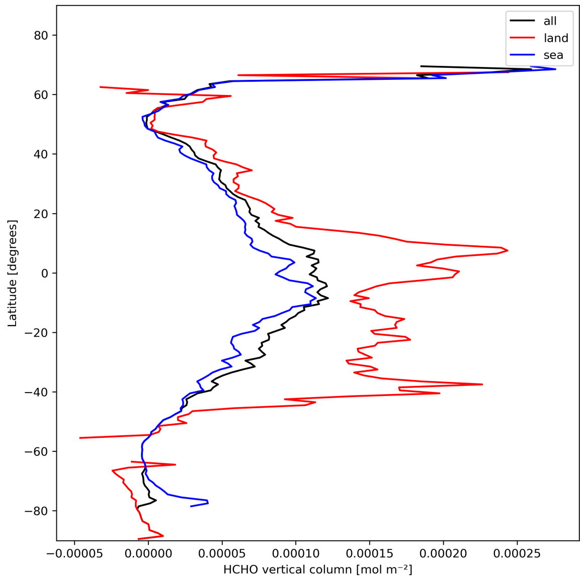
Figure 21: Zonal average of “HCHO vertical column” for 2024-02-04 to 2024-02-06.
