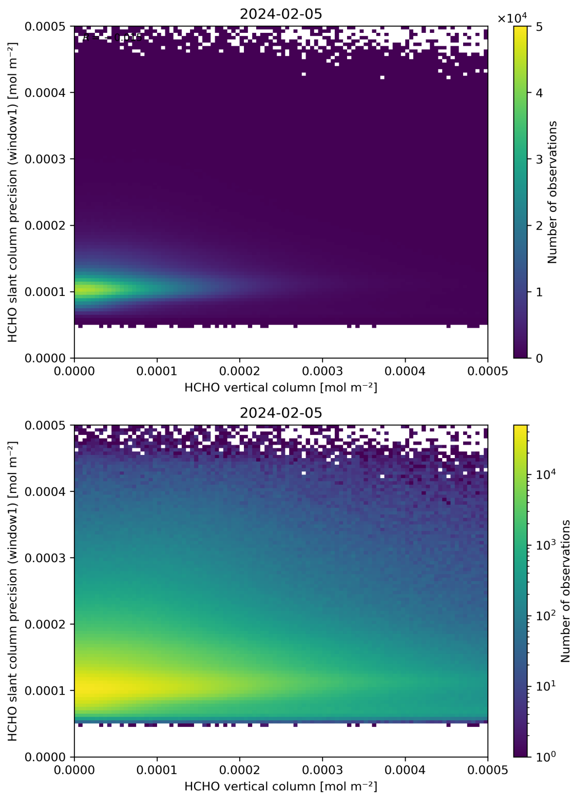
Figure 130: Scatter density plot of “HCHO vertical column” against “HCHO slant column precision (window1)” for 2024-02-04 to 2024-02-06.
