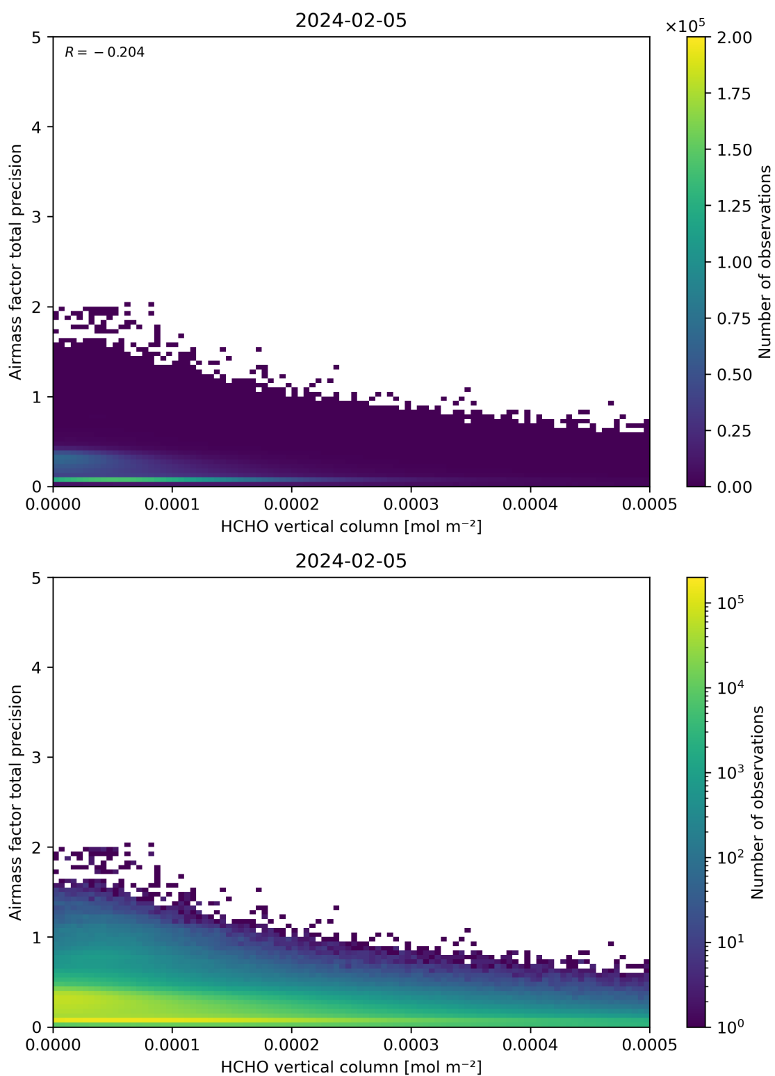
Figure 132: Scatter density plot of “HCHO vertical column” against “Airmass factor total precision” for 2024-02-04 to 2024-02-06.
