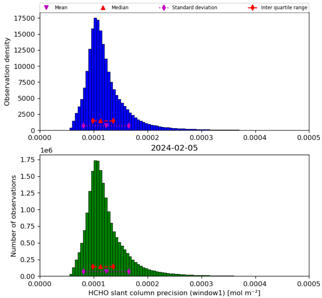
Figure 39: Histogram of “HCHO slant column precision (window1)” for 2024-02-04 to 2024-02-06
