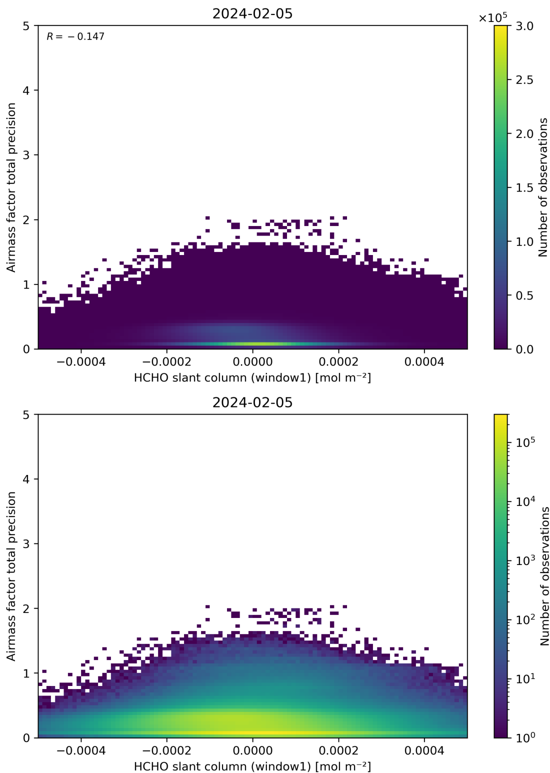
Figure 86: Scatter density plot of “HCHO slant column (window1)” against “Airmass factor total precision” for 2024-02-04 to 2024-02-06.
