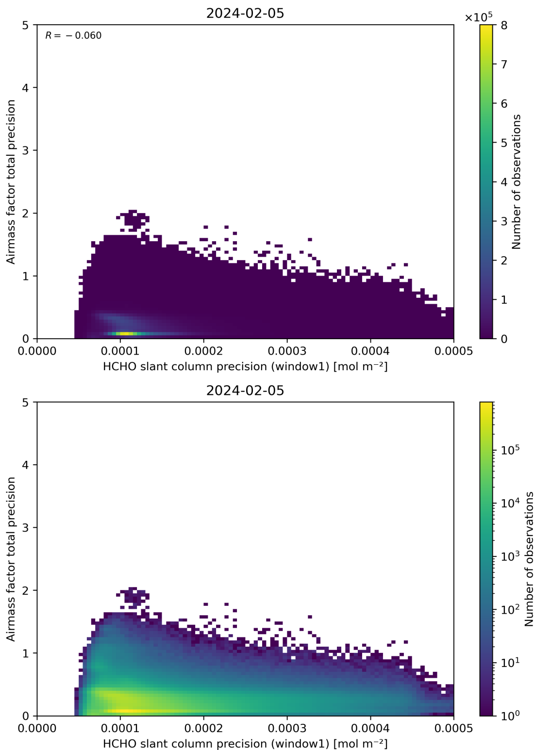
Figure 95: Scatter density plot of “HCHO slant column precision (window1)” against “Airmass factor total precision” for 2024-02-04 to 2024-02-06.
