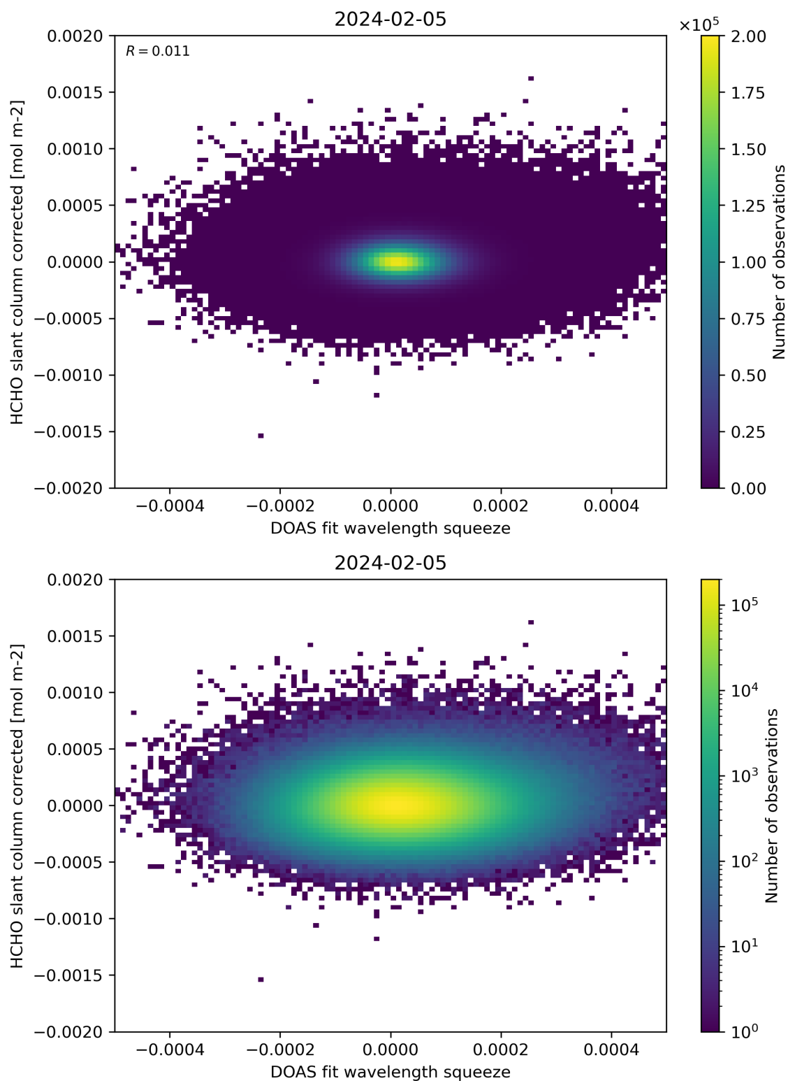
Figure 69: Scatter density plot of “DOAS fit wavelength squeeze” against “HCHO slant column corrected” for 2024-02-04 to 2024-02-06.
