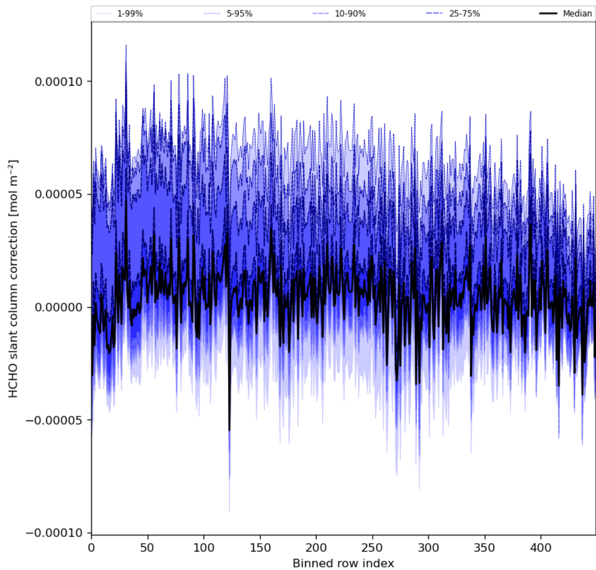
Figure 61: Along track statistics of “HCHO slant column correction” for 2024-02-04 to 2024-02-06
