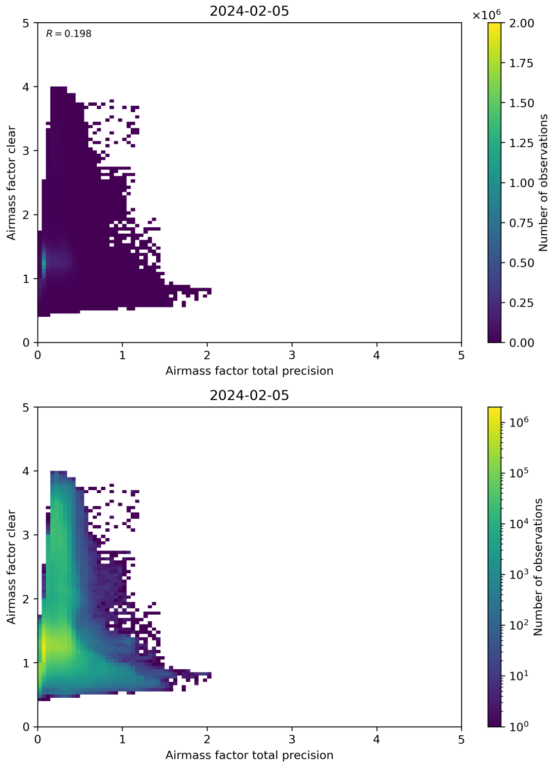
Figure 108: Scatter density plot of “Airmass factor total precision” against “Airmass factor clear” for 2024-02-04 to 2024-02-06.
