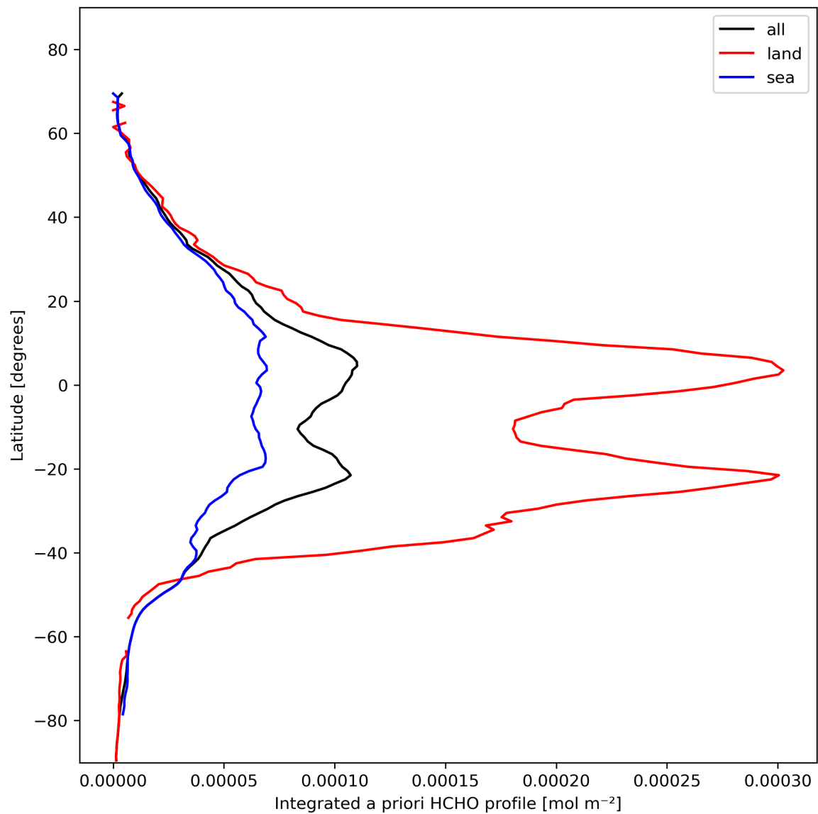
Figure 29: Zonal average of “Integrated a priori HCHO profile” for 2024-02-04 to 2024-02-06.
