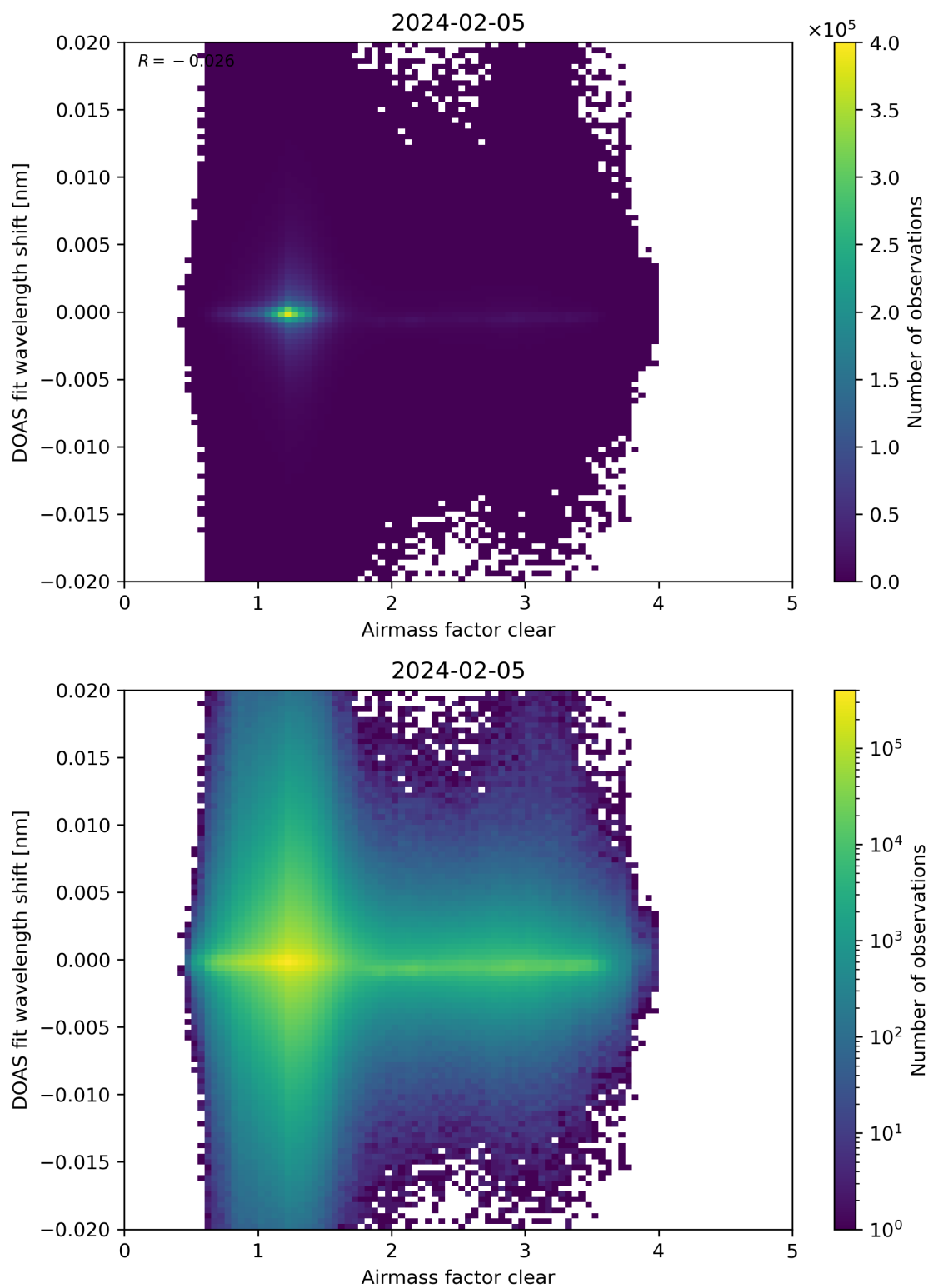
Figure 72: Scatter density plot of “Airmass factor clear” against “DOAS fit wavelength shift” for 2024-02-04 to 2024-02-06.
