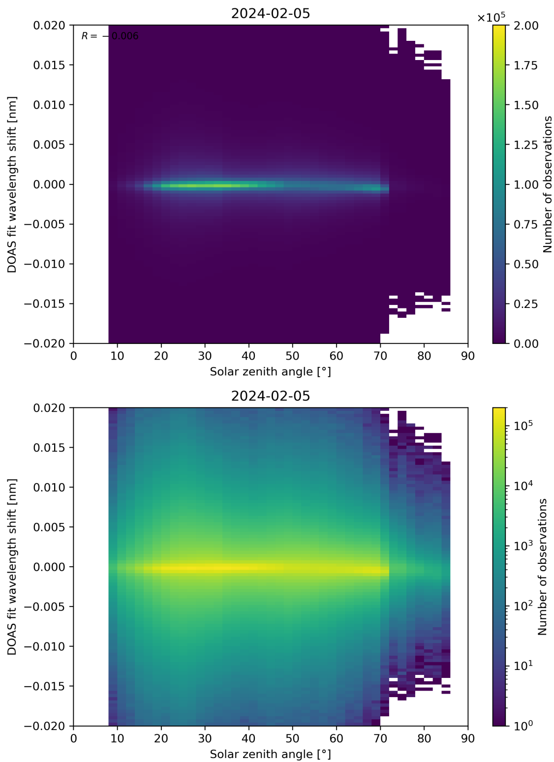
Figure 168: Scatter density plot of “Solar zenith angle” against “DOAS fit wavelength shift” for 2024-02-04 to 2024-02-06.
