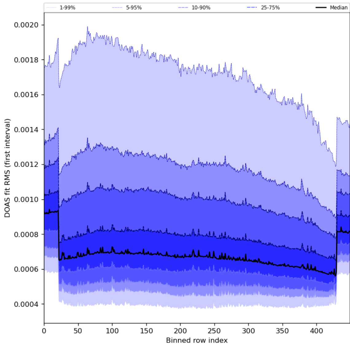
Figure 60: Along track statistics of “DOAS fit RMS (first interval)” for 2024-02-04 to 2024-02-06
