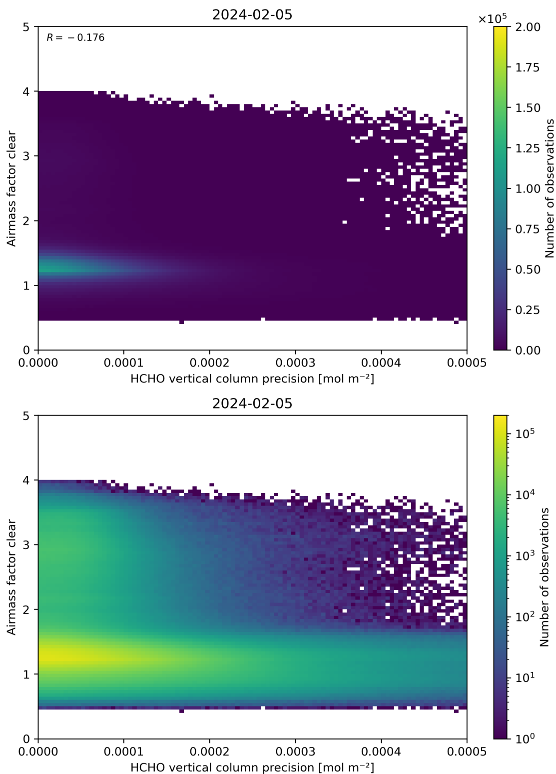
Figure 139: Scatter density plot of “HCHO vertical column precision” against “Airmass factor clear” for 2024-02-04 to 2024-02-06.
