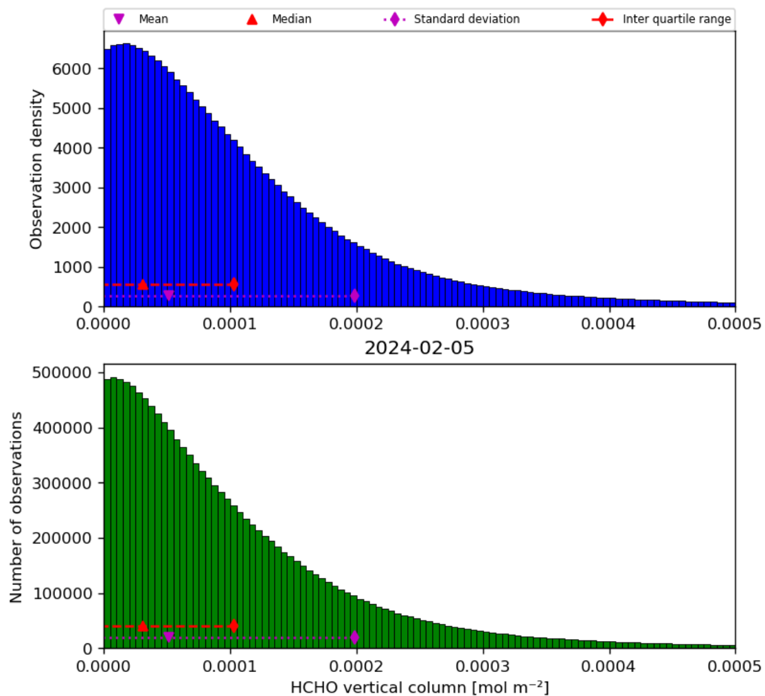
Figure 35: Histogram of “HCHO vertical column” for 2024-02-04 to 2024-02-06
