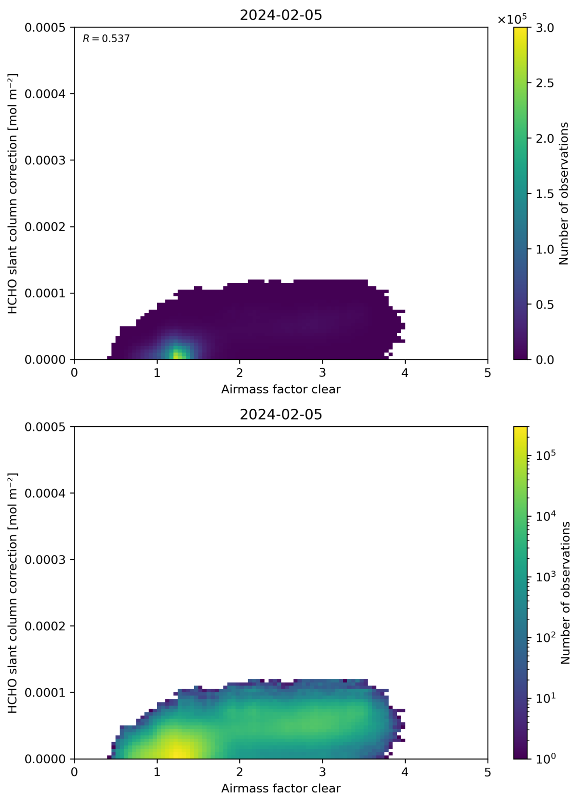
Figure 75: Scatter density plot of “Airmass factor clear” against “HCHO slant column correction” for 2024-02-04 to 2024-02-06.
