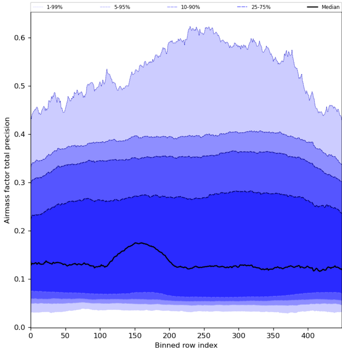
Figure 55: Along track statistics of “Airmass factor total precision” for 2024-02-04 to 2024-02-06
