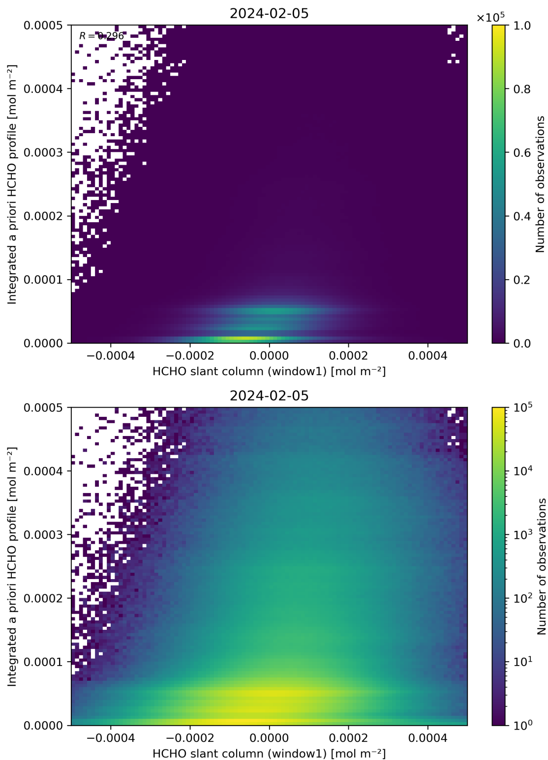
Figure 87: Scatter density plot of “HCHO slant column (window1)” against “Integrated a priori HCHO profile” for 2024-02-04 to 2024-02-06.
