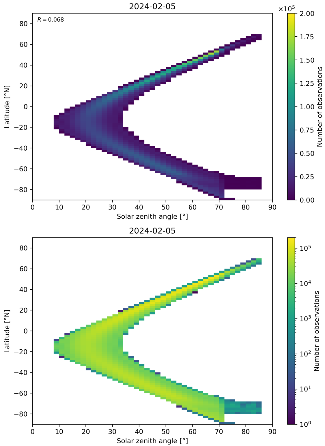
Figure 181: Scatter density plot of “Solar zenith angle” against “Latitude” for 2024-02-04 to 2024-02-06.
