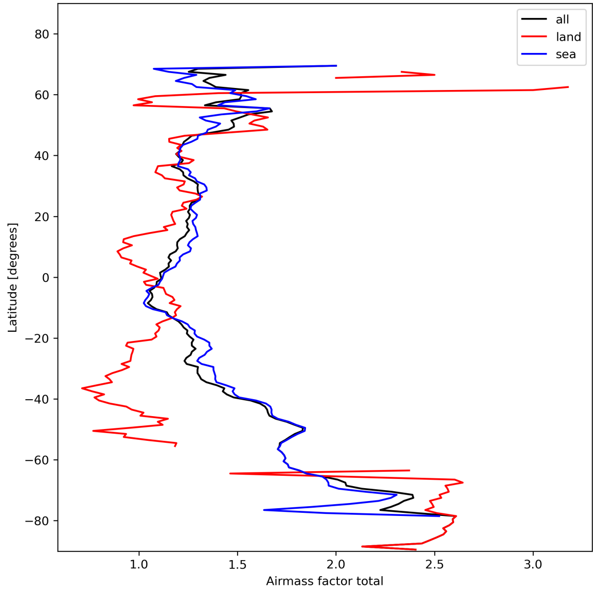
Figure 26: Zonal average of “Airmass factor total” for 2024-02-04 to 2024-02-06.
