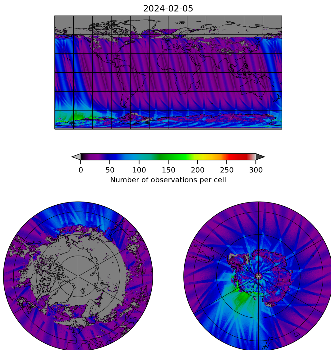
Figure 19: Map of the number of observations for 2024-02-04 to 2024-02-06
