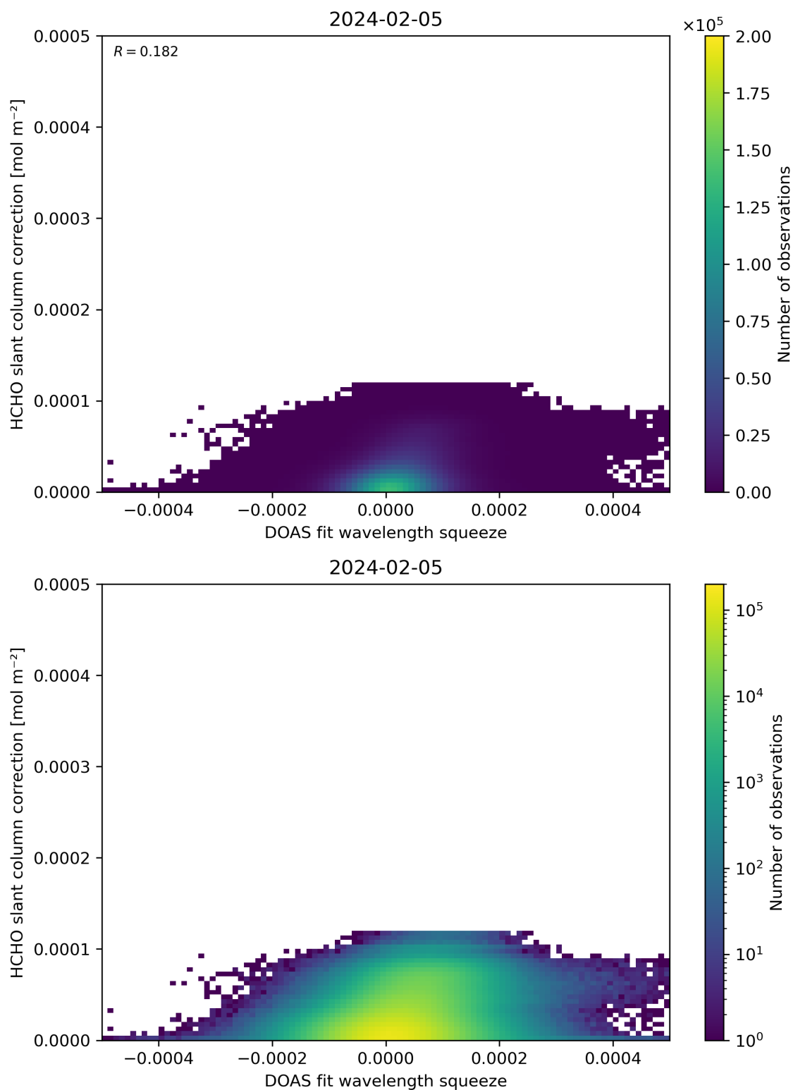
Figure 70: Scatter density plot of “DOAS fit wavelength squeeze” against “HCHO slant column correction” for 2024-02-04 to 2024-02-06.
