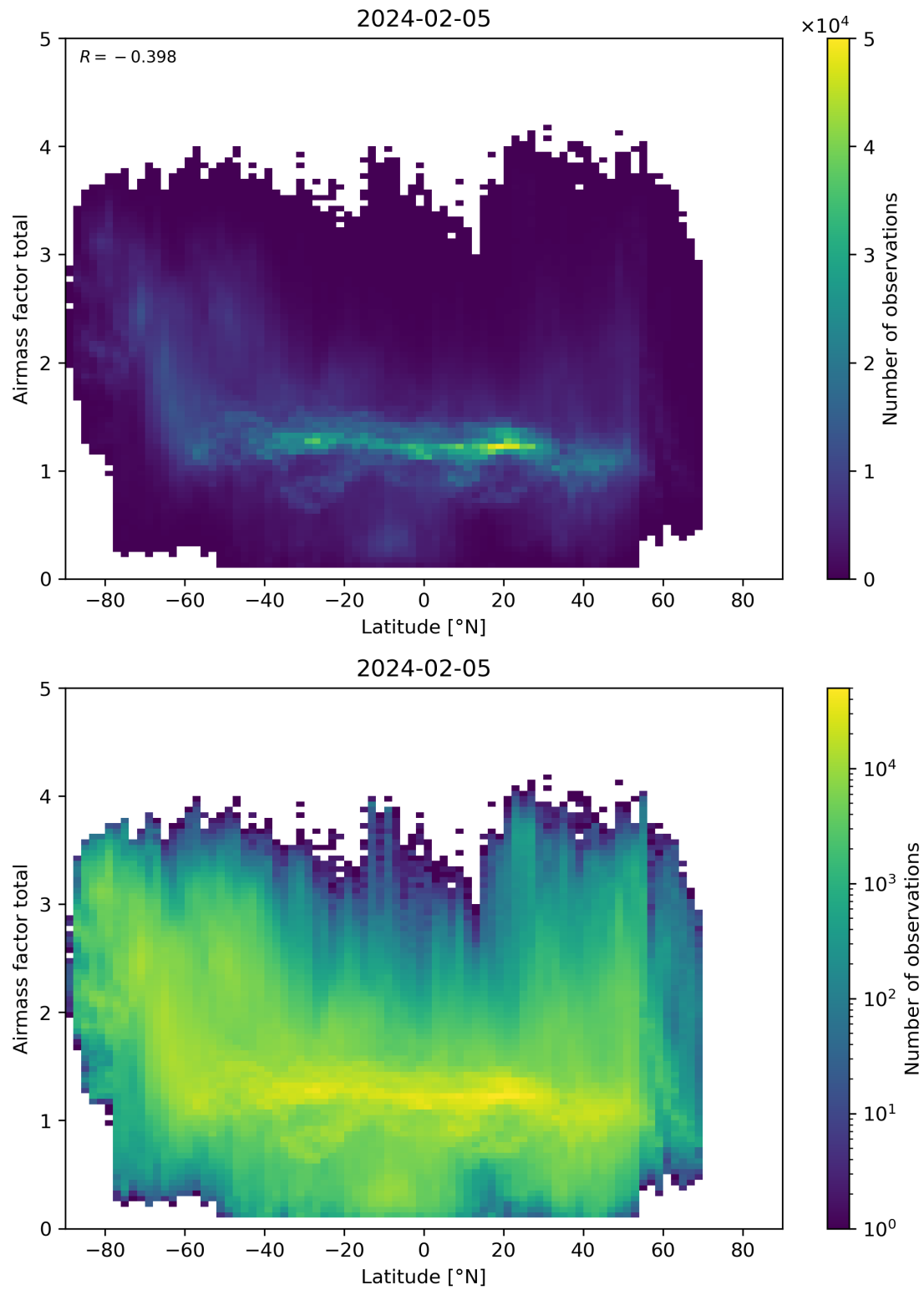
Figure 161: Scatter density plot of “Latitude” against “Airmass factor total” for 2024-02-04 to 2024-02-06.
