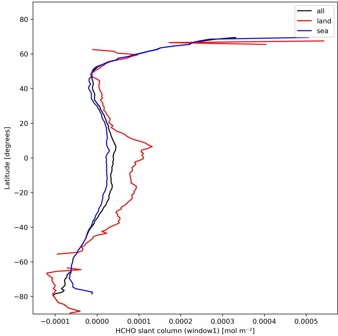
Figure 24: Zonal average of “HCHO slant column (window1)” for 2024-02-04 to 2024-02-06.
