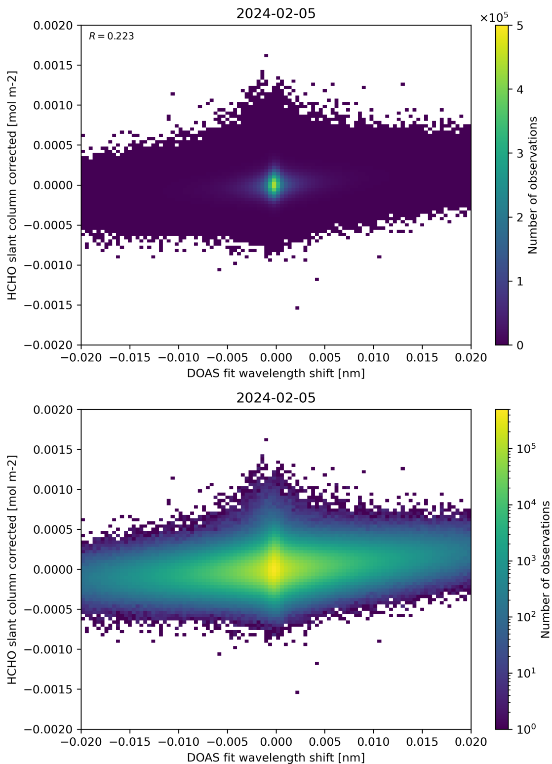
Figure 66: Scatter density plot of “DOAS fit wavelength shift” against “HCHO slant column corrected” for 2024-02-04 to 2024-02-06.
