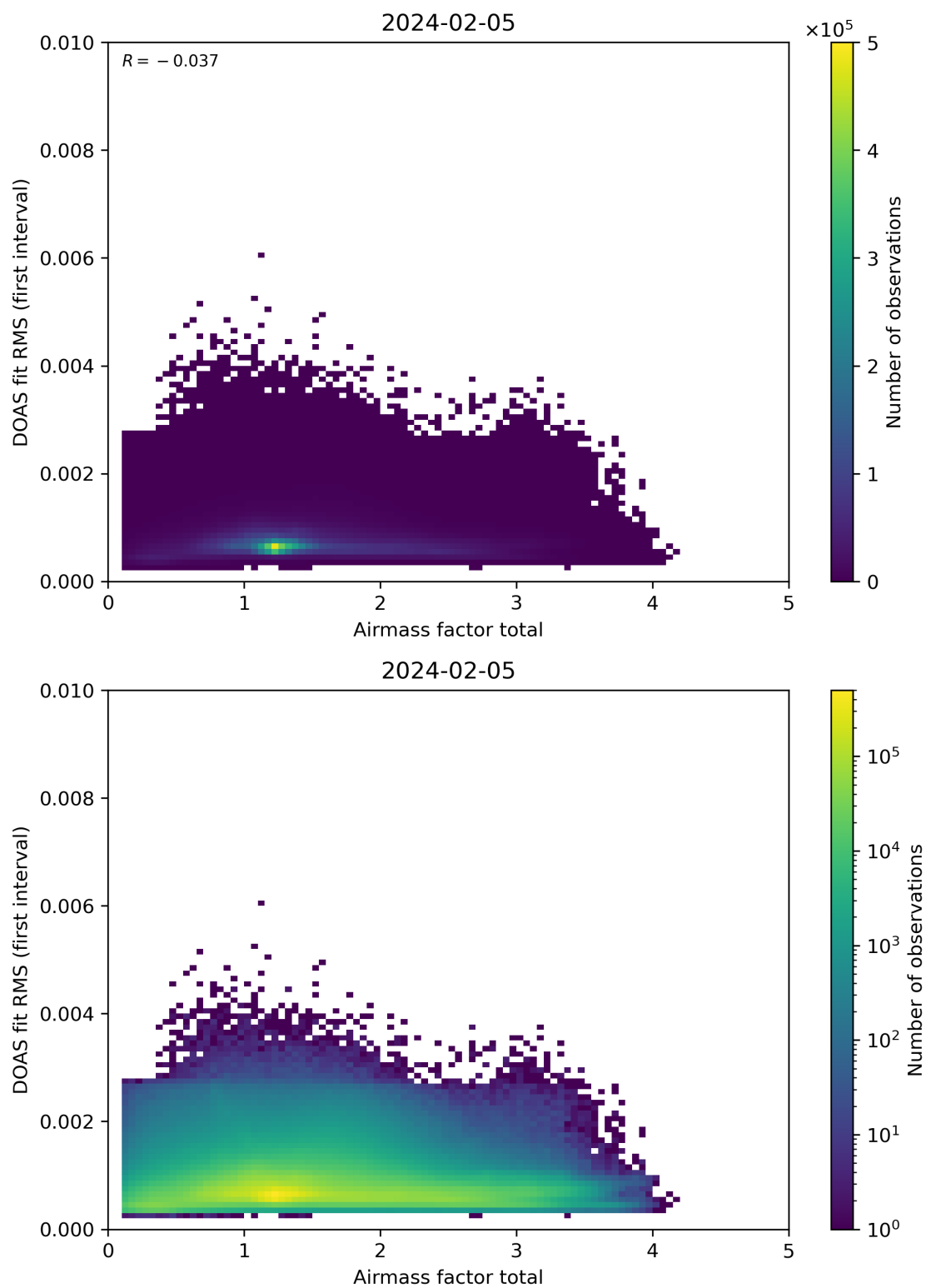
Figure 97: Scatter density plot of “Airmass factor total” against “DOAS fit RMS (first interval)” for 2024-02-04 to 2024-02-06.
