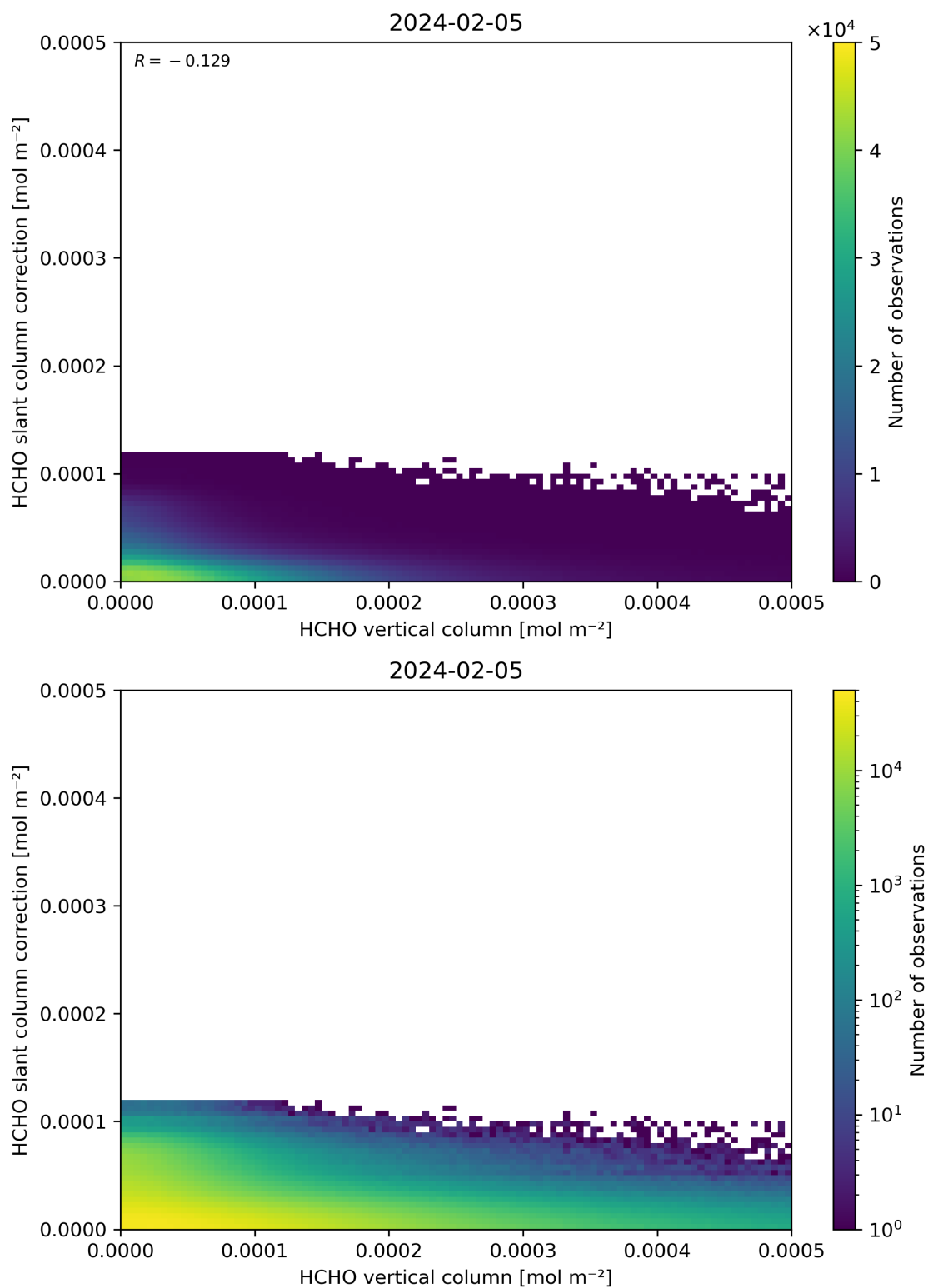
Figure 128: Scatter density plot of “HCHO vertical column” against “HCHO slant column correction” for 2024-02-04 to 2024-02-06.
