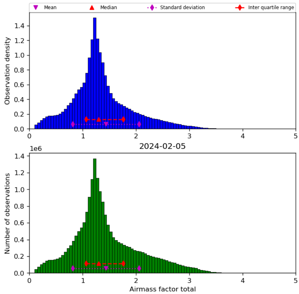
Figure 40: Histogram of “Airmass factor total” for 2024-02-04 to 2024-02-06
