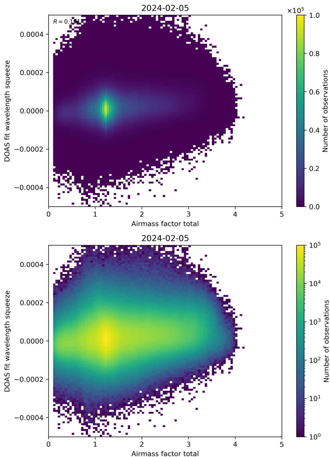
Figure 99: Scatter density plot of “Airmass factor total” against “DOAS fit wavelength squeeze” for 2024-02-04 to 2024-02-06.
