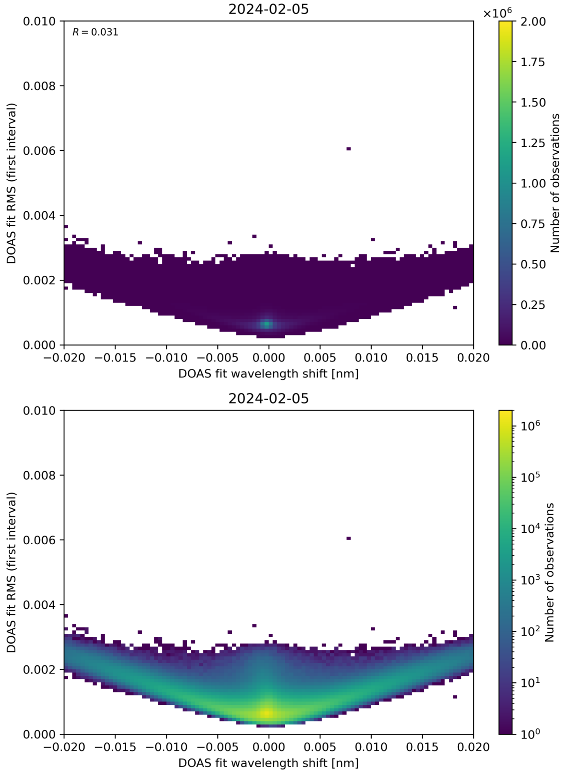
Figure 64: Scatter density plot of “DOAS fit wavelength shift” against “DOAS fit RMS (first interval)” for 2024-02-04 to 2024-02-06.
