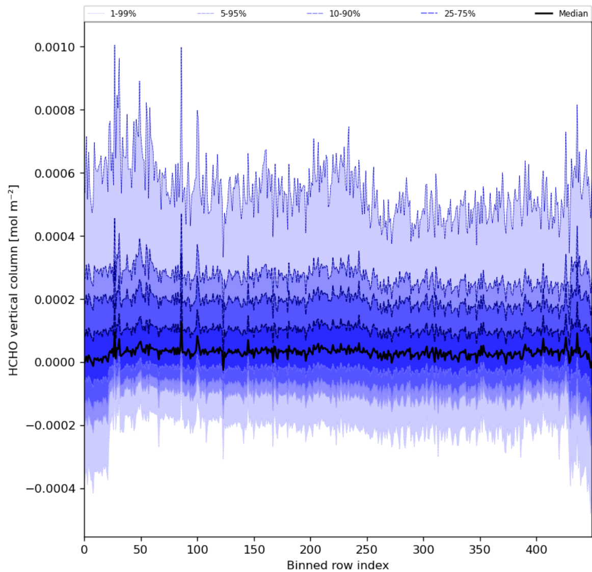
Figure 49: Along track statistics of “HCHO vertical column” for 2024-02-04 to 2024-02-06
