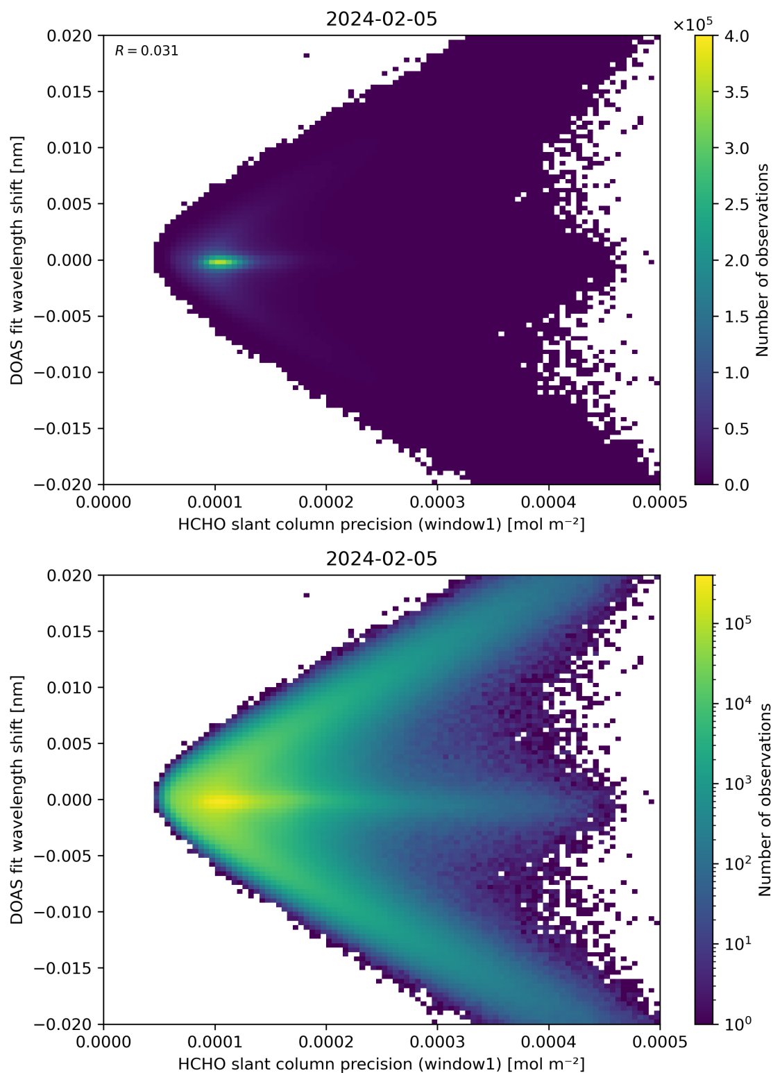
Figure 89: Scatter density plot of “HCHO slant column precision (window1)” against “DOAS fit wavelength shift” for 2024-02-04 to 2024-02-06.
