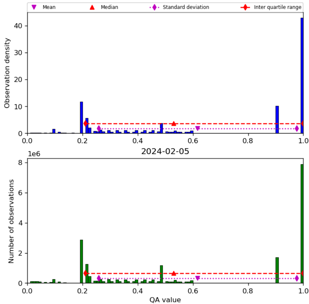
Figure 34: Histogram of “QA value” for 2024-02-04 to 2024-02-06
