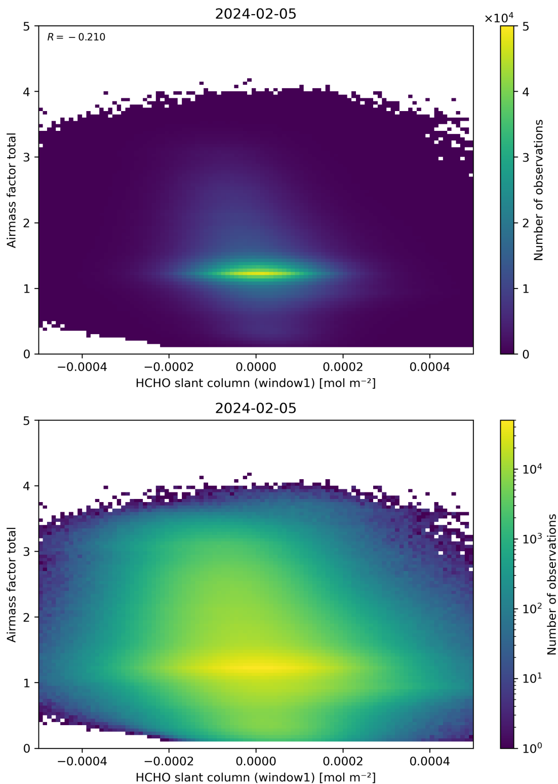
Figure 85: Scatter density plot of “HCHO slant column (window1)” against “Airmass factor total” for 2024-02-04 to 2024-02-06.
