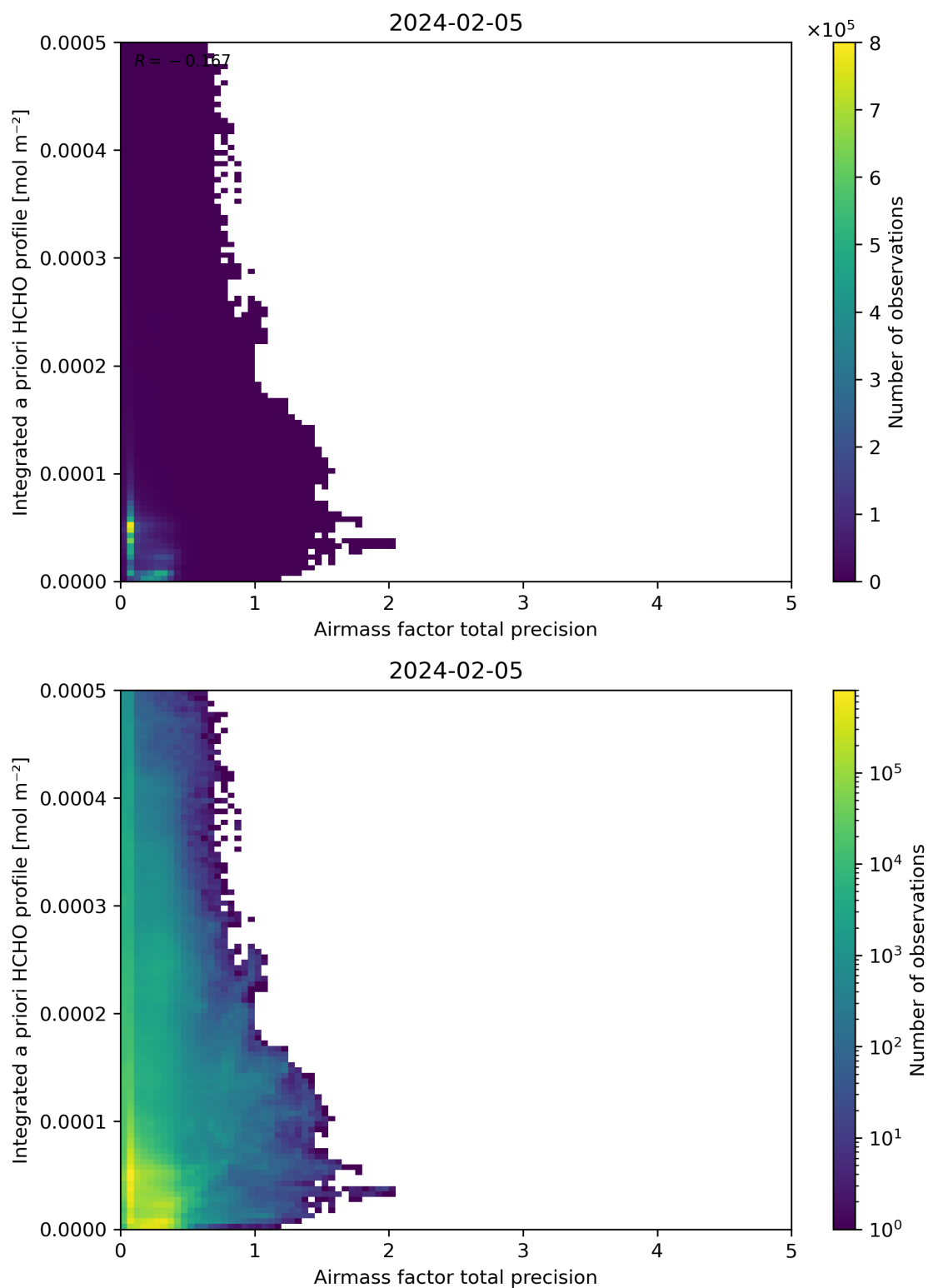
Figure 111: Scatter density plot of “Airmass factor total precision” against “Integrated a priori HCHO profile” for 2024-02-04 to 2024-02-06.
