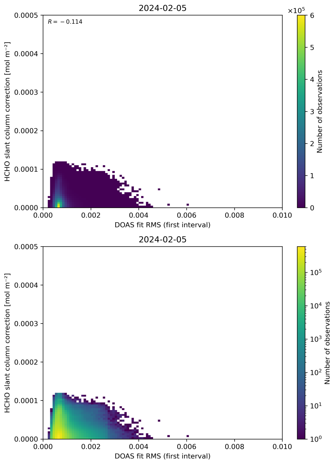
Figure 63: Scatter density plot of “DOAS fit RMS (first interval)” against “HCHO slant column correction” for 2024-02-04 to 2024-02-06.
