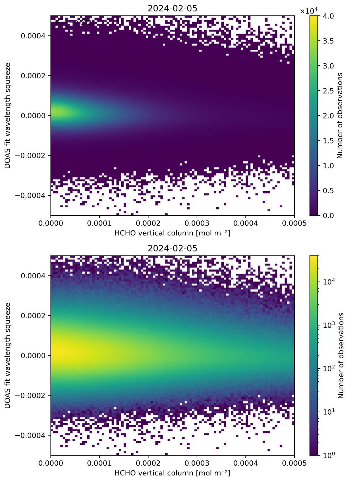
Figure 125: Scatter density plot of “HCHO vertical column” against “DOAS fit wavelength squeeze” for 2024-02-04 to 2024-02-06.
