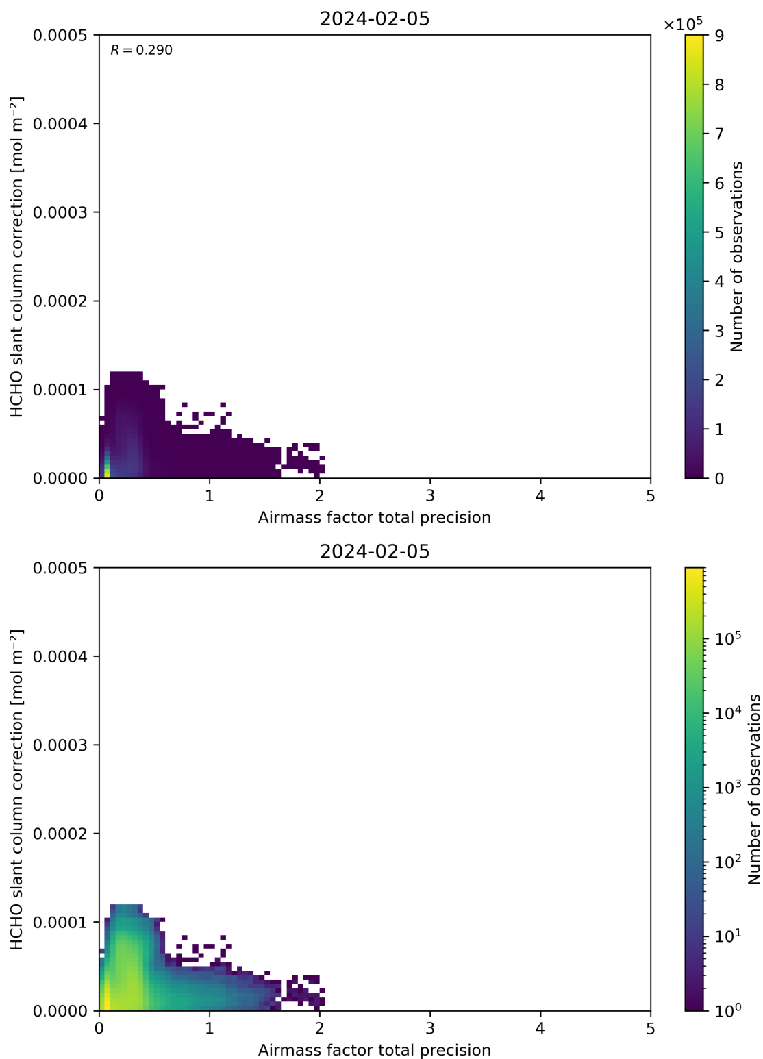
Figure 110: Scatter density plot of “Airmass factor total precision” against “HCHO slant column correction” for 2024-02-04 to 2024-02-06.
