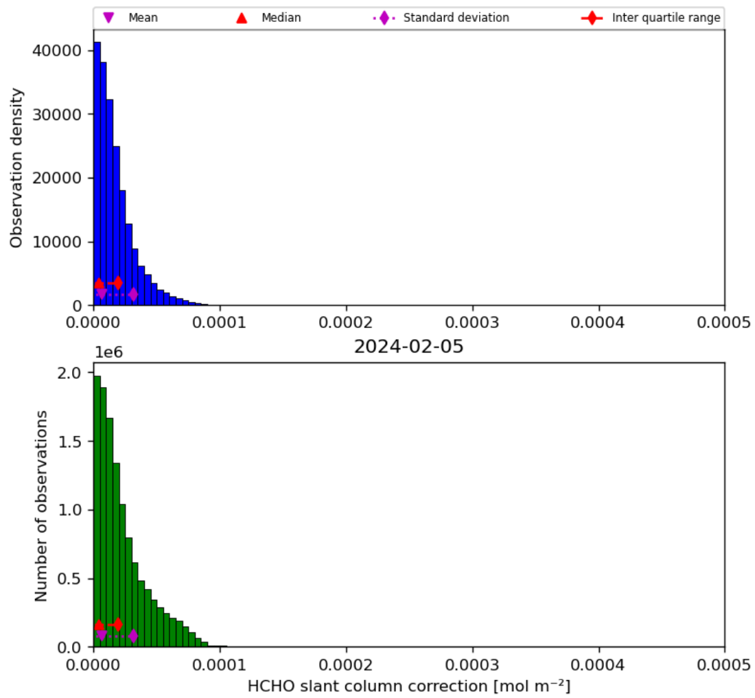
Figure 47: Histogram of “HCHO slant column correction” for 2024-02-04 to 2024-02-06
