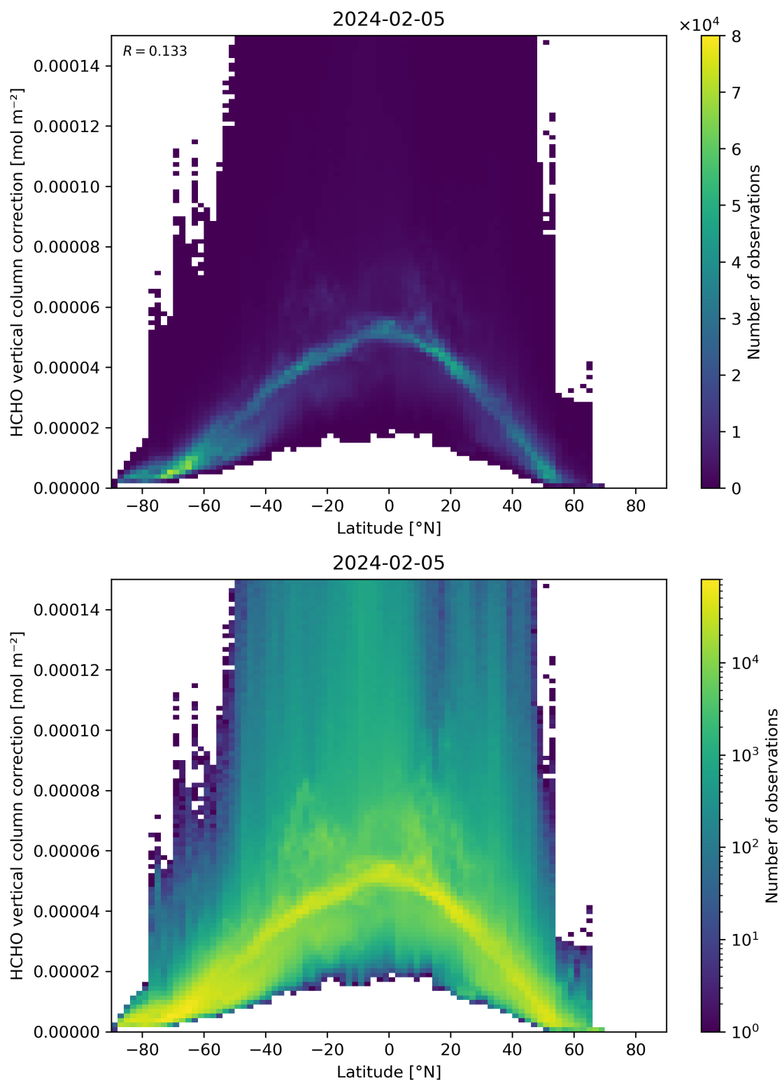
Figure 164: Scatter density plot of “Latitude” against “HCHO vertical column correction” for 2024-02-04 to 2024-02-06.
