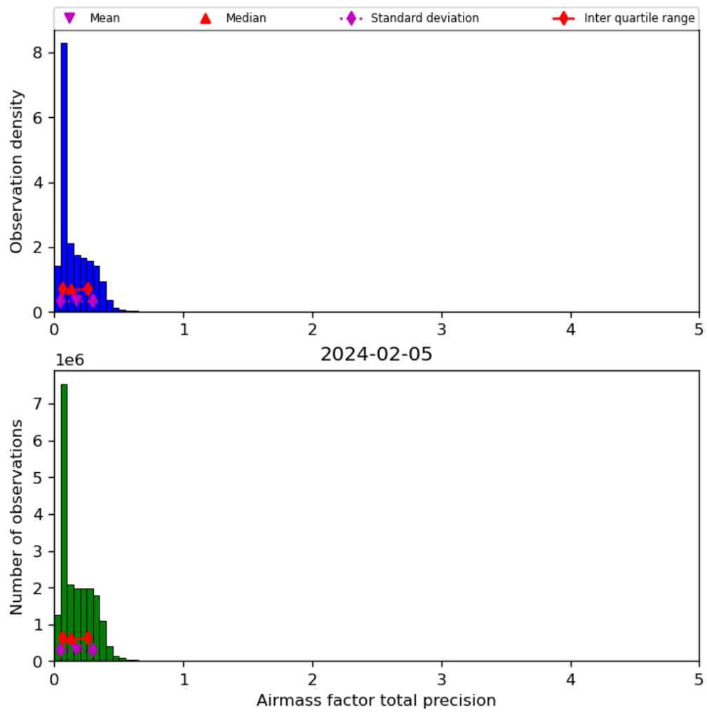
Figure 41: Histogram of “Airmass factor total precision” for 2024-02-04 to 2024-02-06
