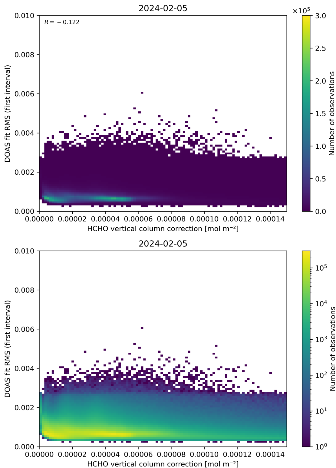
Figure 112: Scatter density plot of “HCHO vertical column correction” against “DOAS fit RMS (first interval)” for 2024-02-04 to 2024-02-06.
