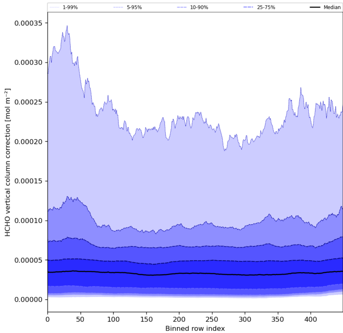
Figure 51: Along track statistics of “HCHO vertical column correction” for 2024-02-04 to 2024-02-06
