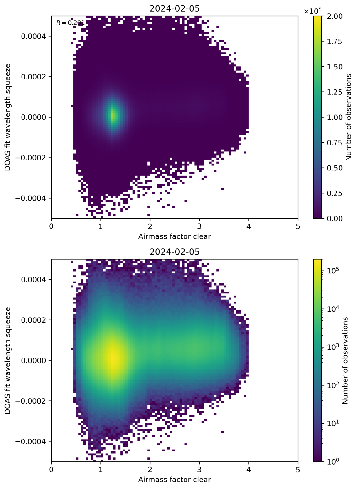
Figure 73: Scatter density plot of “Airmass factor clear” against “DOAS fit wavelength squeeze” for 2024-02-04 to 2024-02-06.
