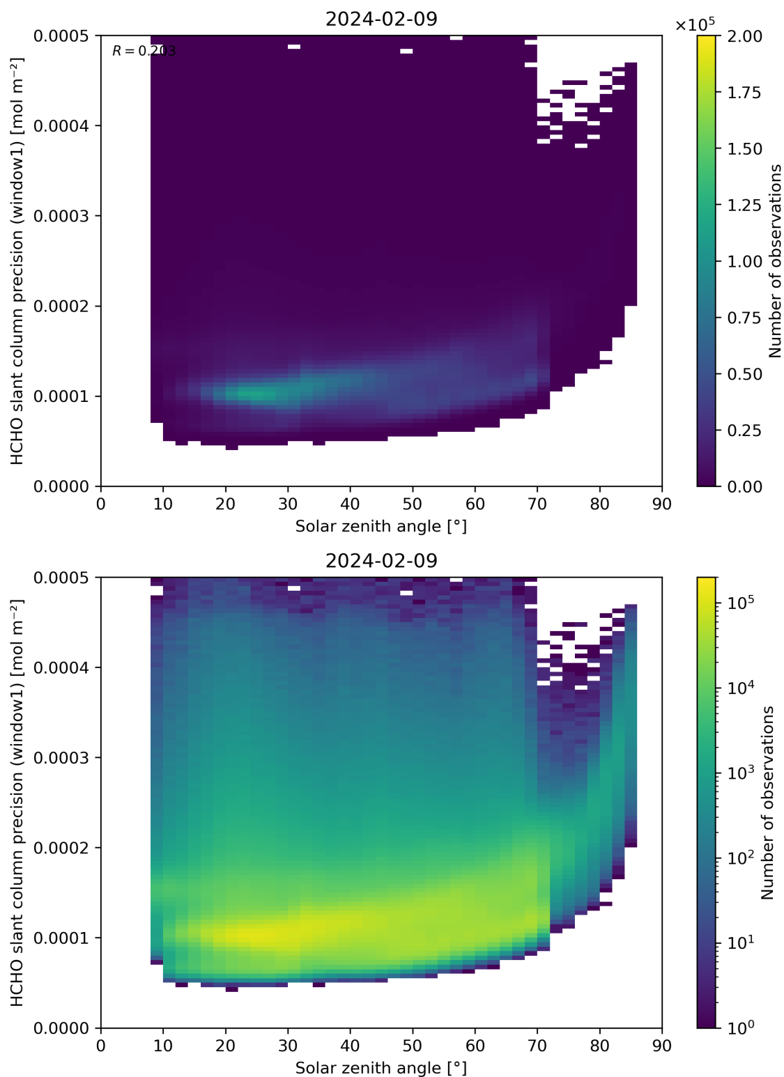
Figure 174: Scatter density plot of “Solar zenith angle” against “HCHO slant column precision (window1)” for 2024-02-08 to 2024-02-10.
