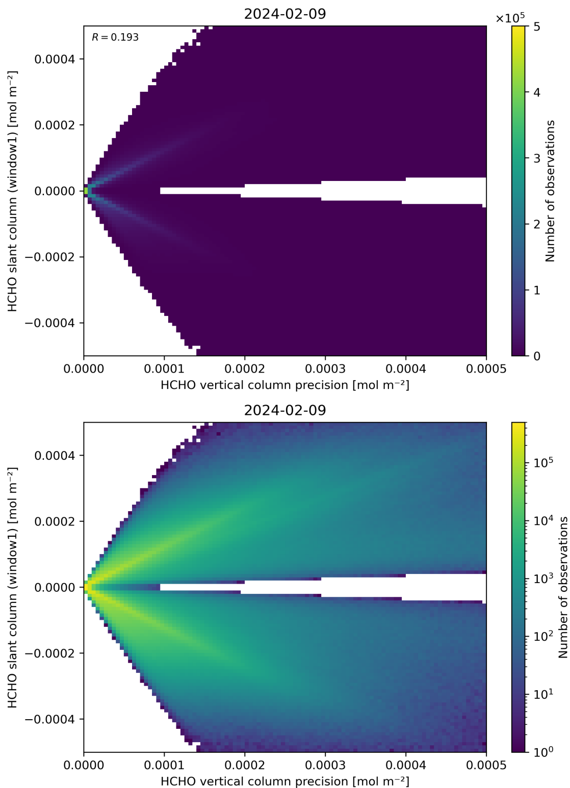
Figure 142: Scatter density plot of “HCHO vertical column precision” against “HCHO slant column (window1)” for 2024-02-08 to 2024-02-10.
