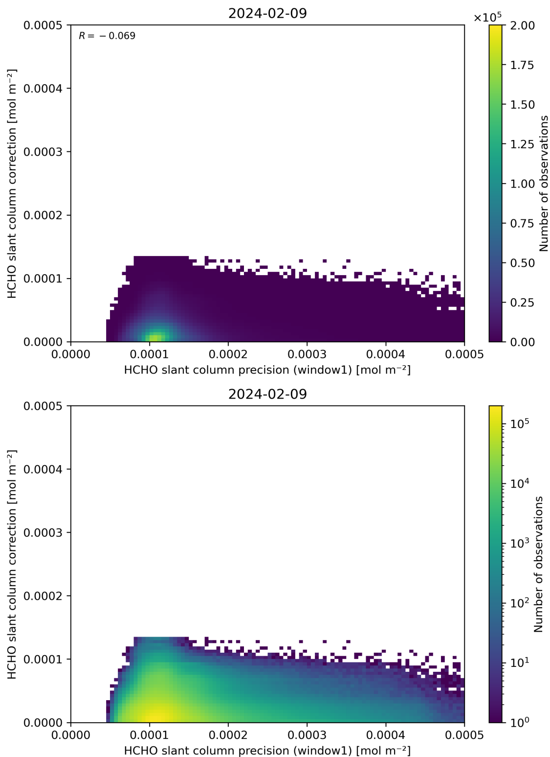
Figure 93: Scatter density plot of “HCHO slant column precision (window1)” against “HCHO slant column correction” for 2024-02-08 to 2024-02-10.
