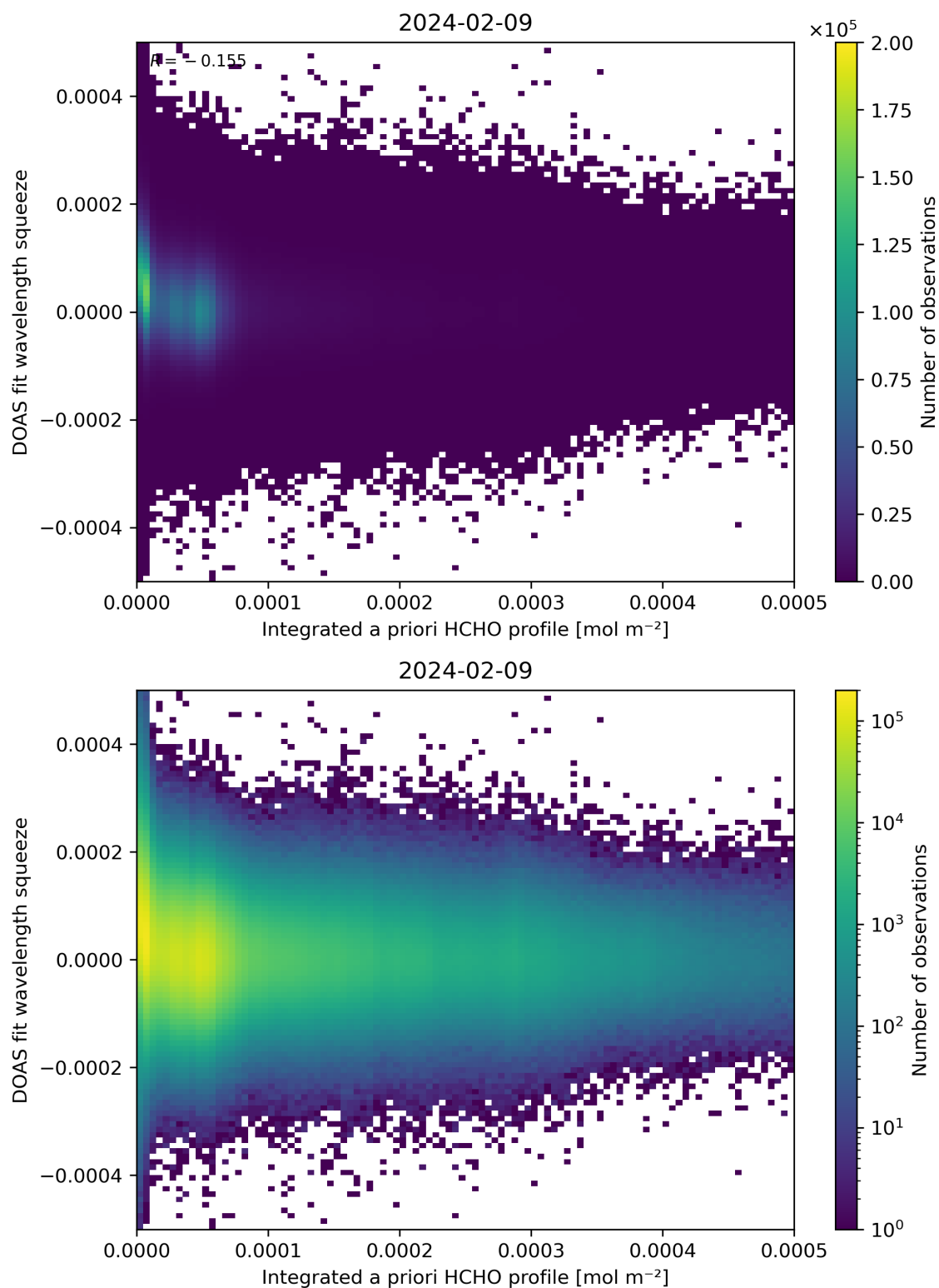
Figure 150: Scatter density plot of “Integrated a priori HCHO profile” against “DOAS fit wavelength squeeze” for 2024-02-08 to 2024-02-10.
