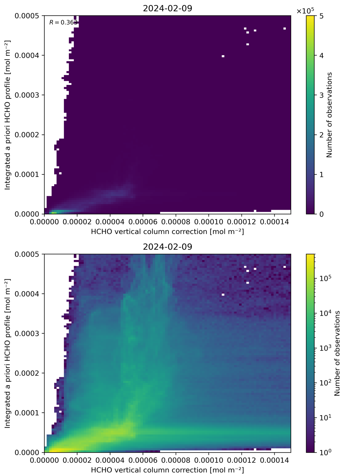
Figure 122: Scatter density plot of “HCHO vertical column correction” against “Integrated a priori HCHO profile” for 2024-02-08 to 2024-02-10.
