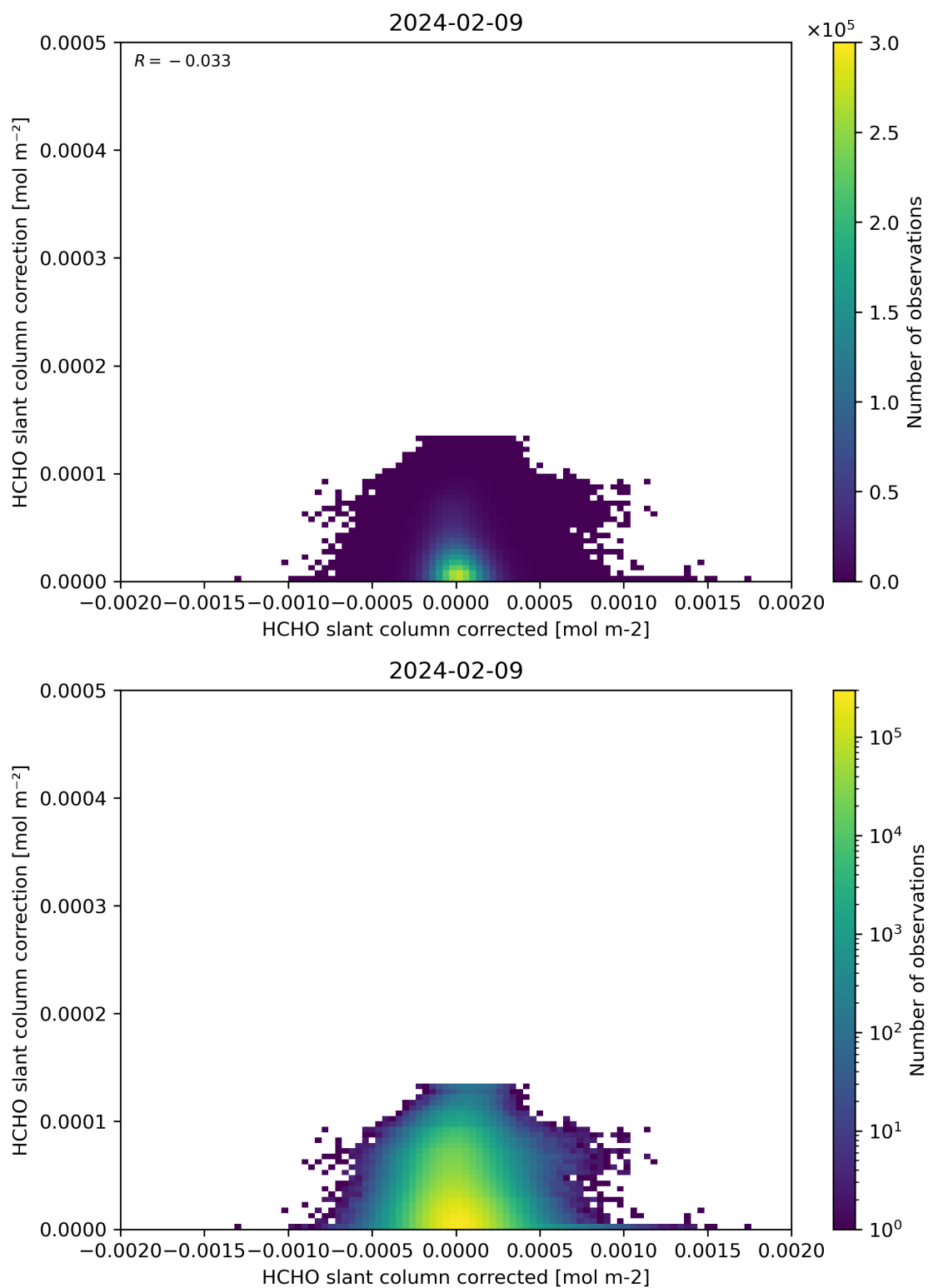
Figure 77: Scatter density plot of “HCHO slant column corrected” against “HCHO slant column correction” for 2024-02-08 to 2024-02-10.
