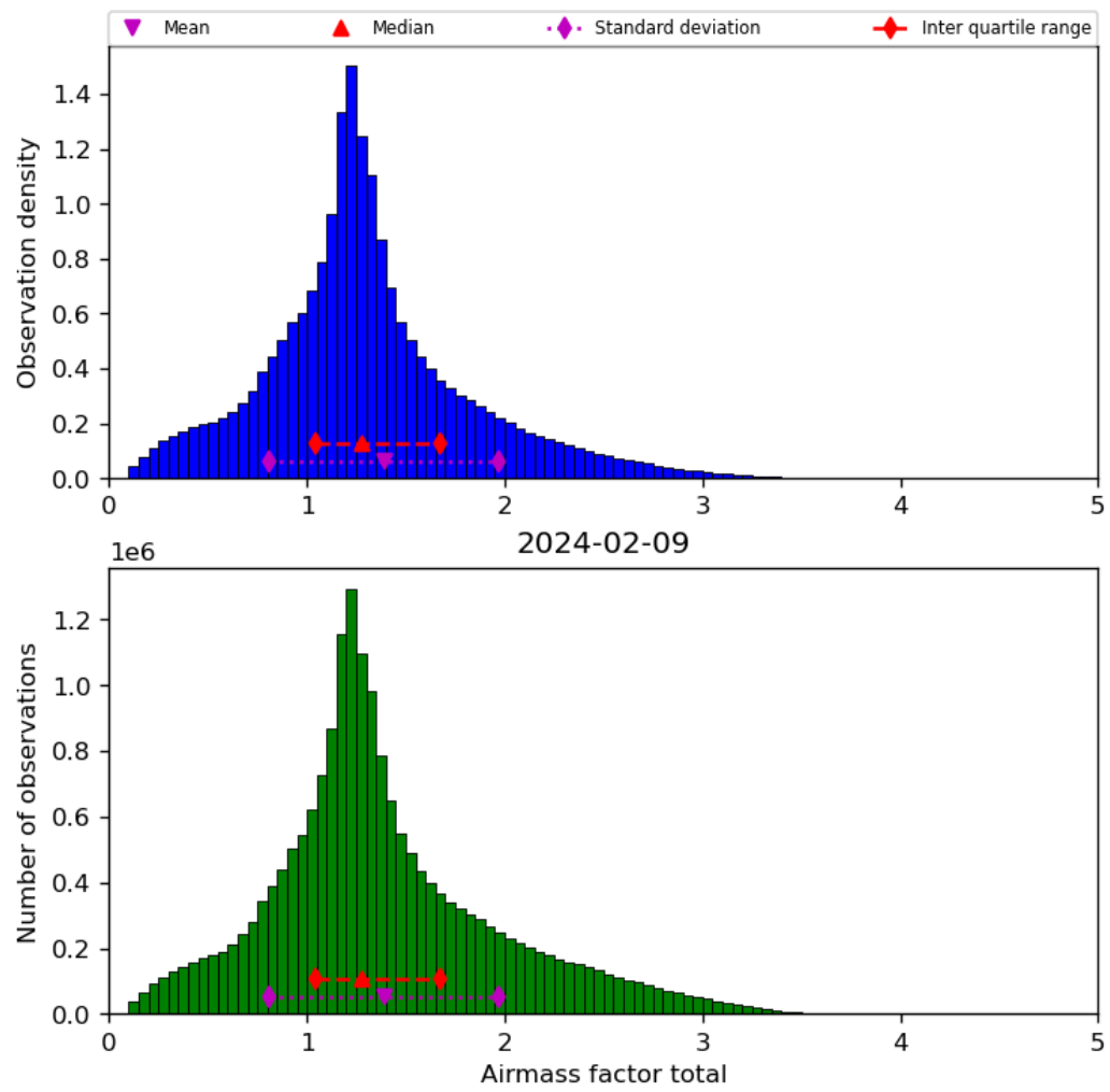
Figure 40: Histogram of “Airmass factor total” for 2024-02-08 to 2024-02-10
