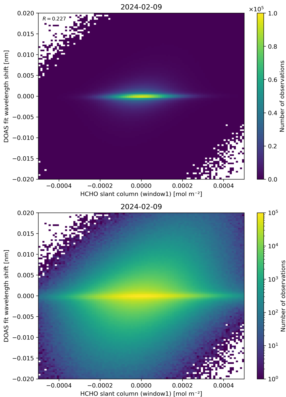
Figure 79: Scatter density plot of “HCHO slant column (window1)” against “DOAS fit wavelength shift” for 2024-02-08 to 2024-02-10.
