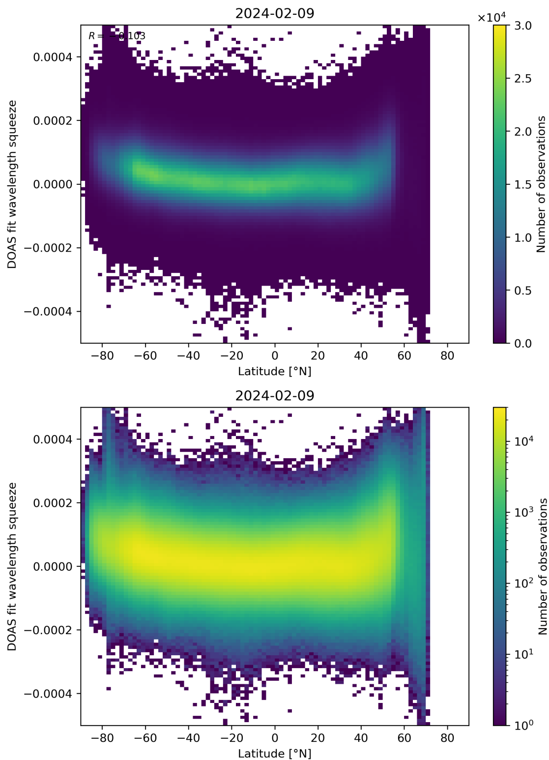
Figure 155: Scatter density plot of “Latitude” against “DOAS fit wavelength squeeze” for 2024-02-08 to 2024-02-10.
