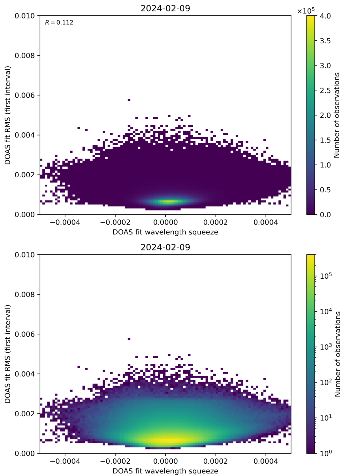
Figure 68: Scatter density plot of “DOAS fit wavelength squeeze” against “DOAS fit RMS (first interval)” for 2024-02-08 to 2024-02-10.
