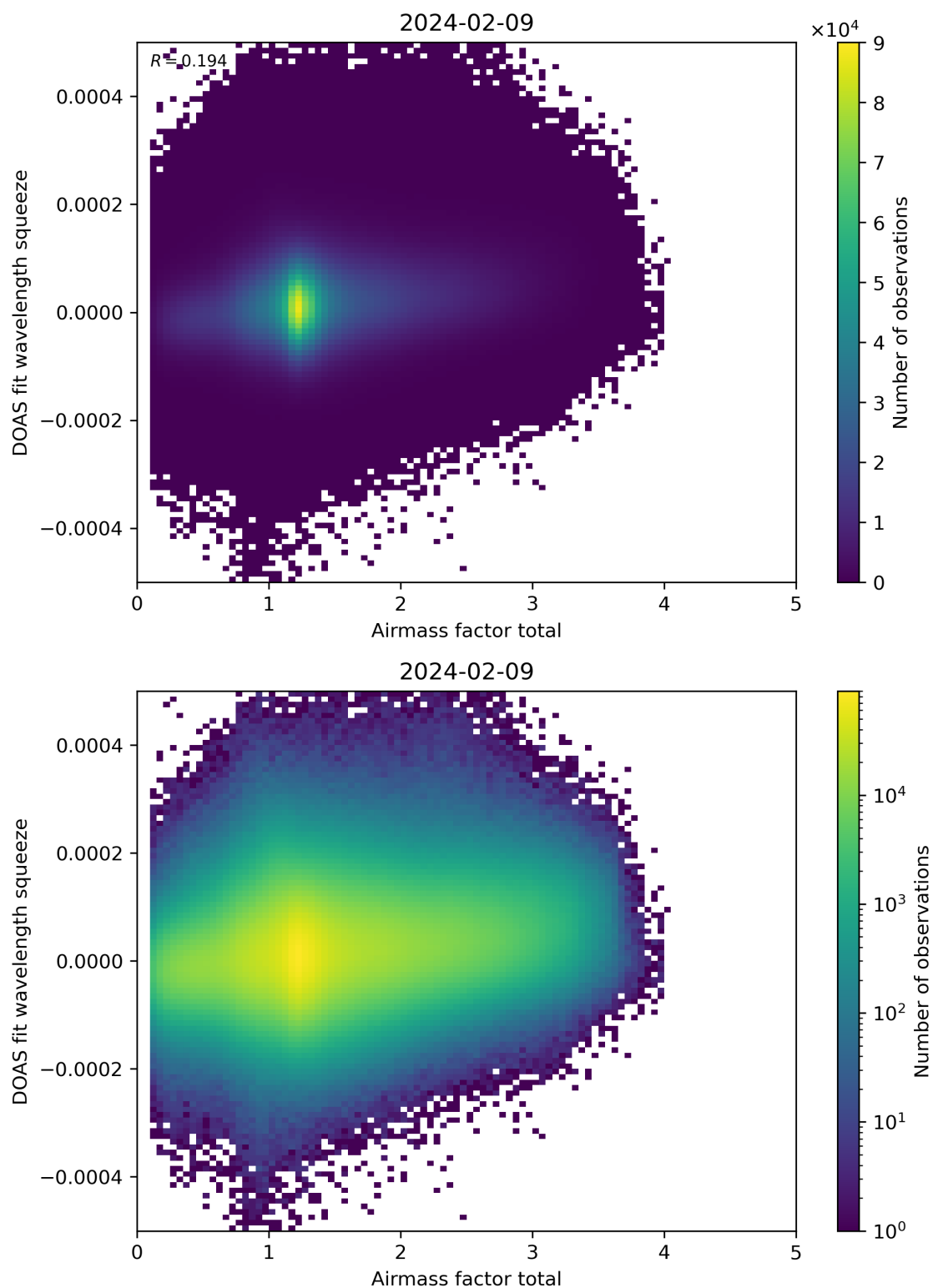
Figure 99: Scatter density plot of “Airmass factor total” against “DOAS fit wavelength squeeze” for 2024-02-08 to 2024-02-10.
