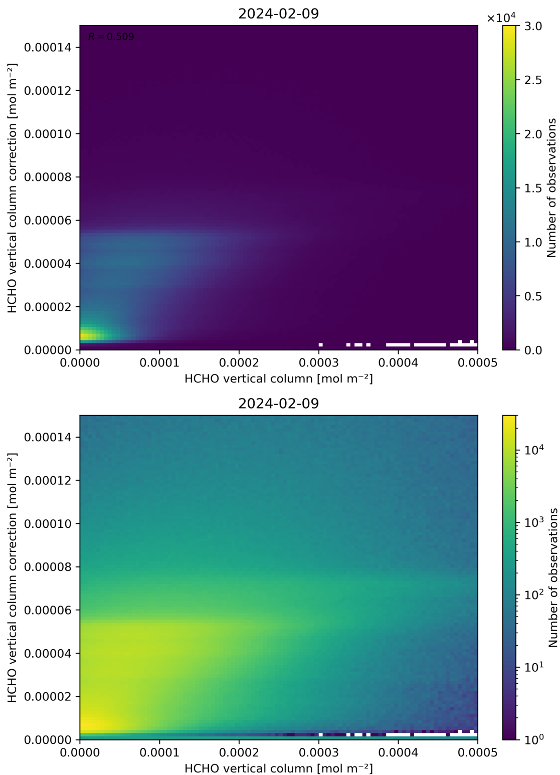
Figure 133: Scatter density plot of “HCHO vertical column” against “HCHO vertical column correction” for 2024-02-08 to 2024-02-10.
