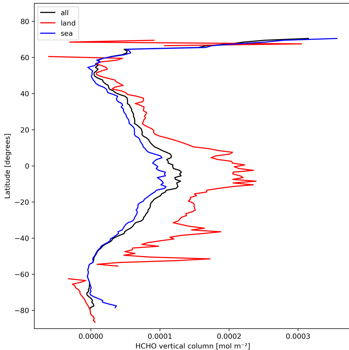
Figure 21: Zonal average of “HCHO vertical column” for 2024-02-08 to 2024-02-10.
