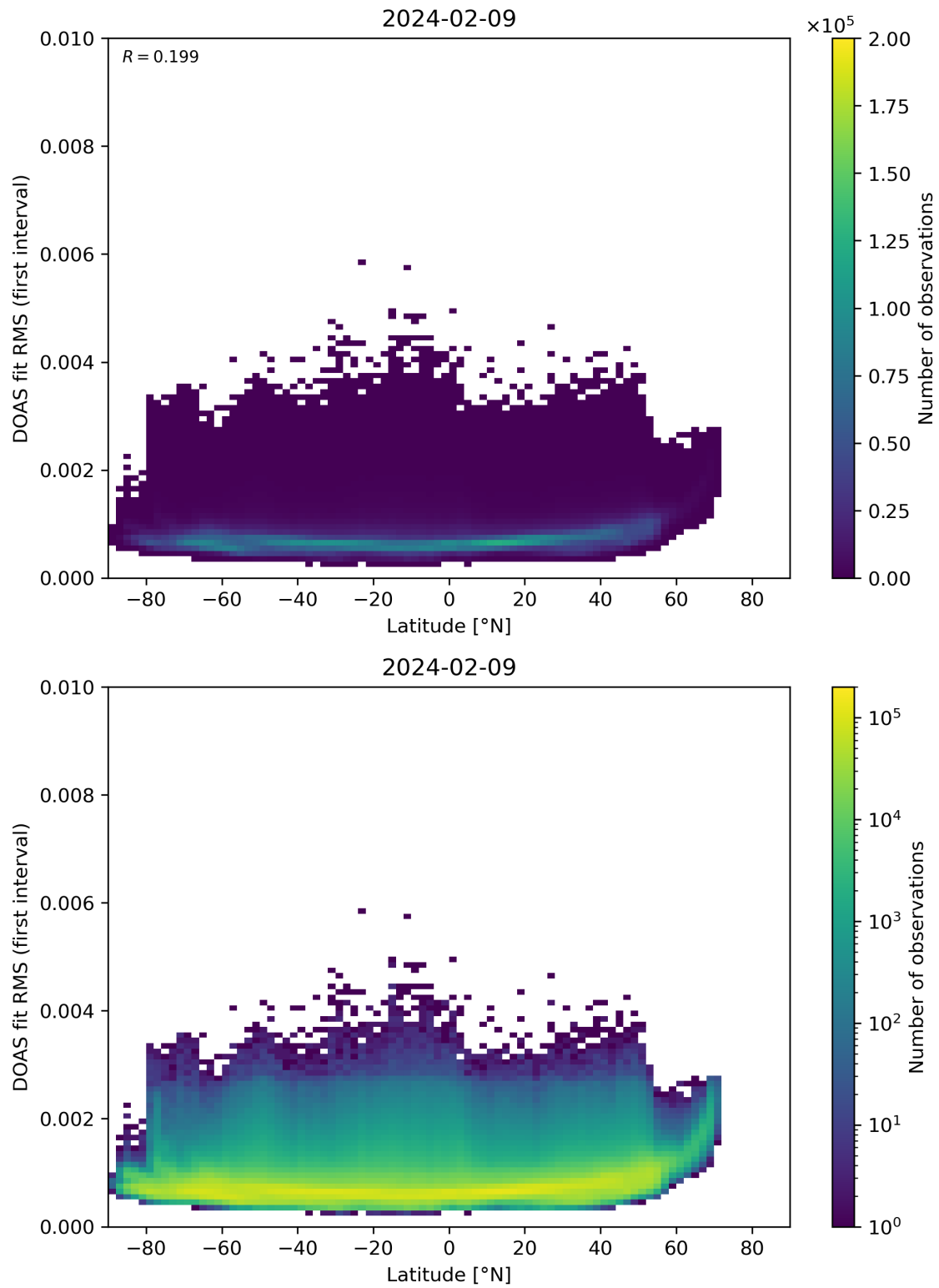
Figure 153: Scatter density plot of “Latitude” against “DOAS fit RMS (first interval)” for 2024-02-08 to 2024-02-10.
