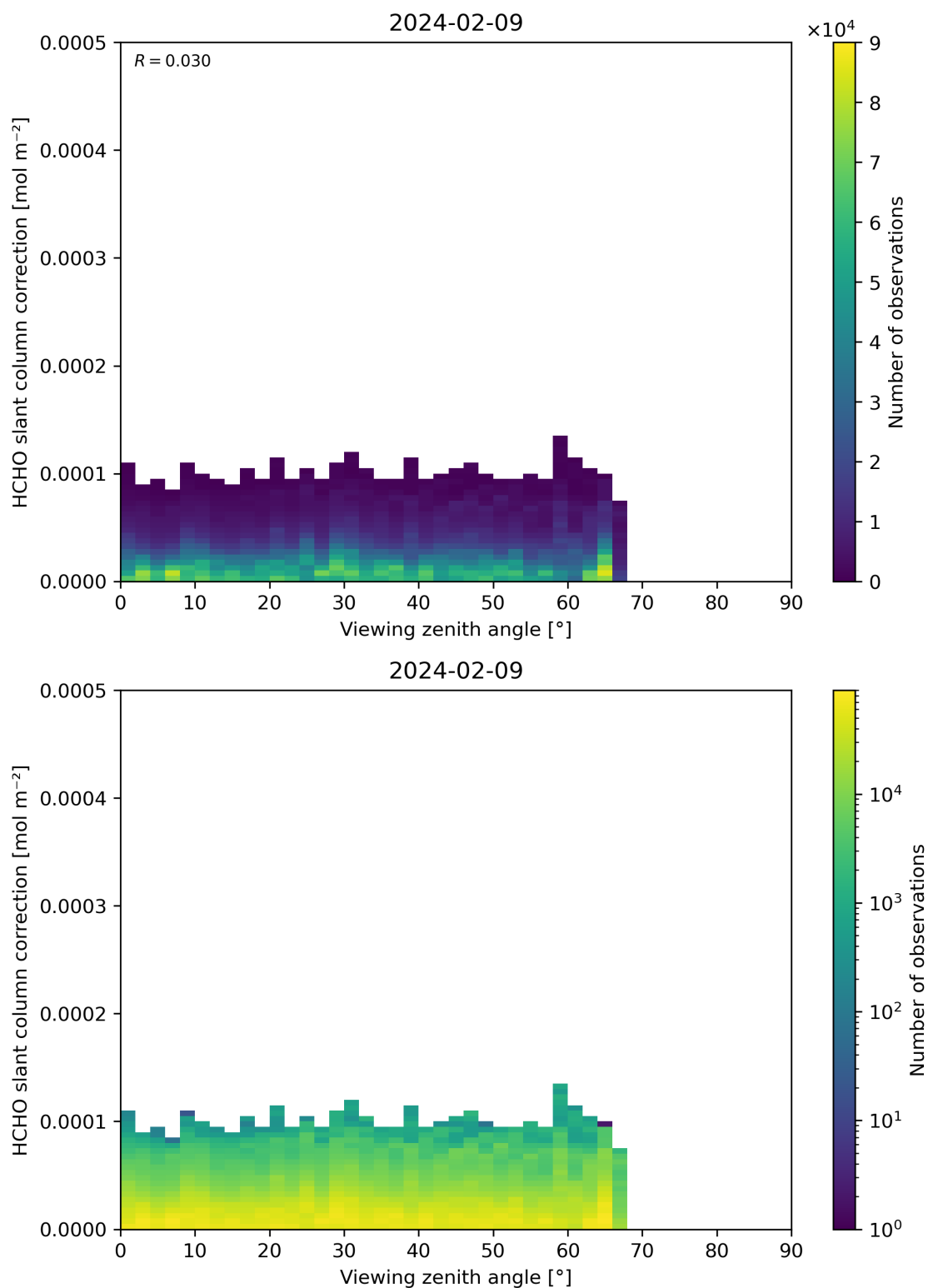
Figure 187: Scatter density plot of “Viewing zenith angle” against “HCHO slant column correction” for 2024-02-08 to 2024-02-10.
