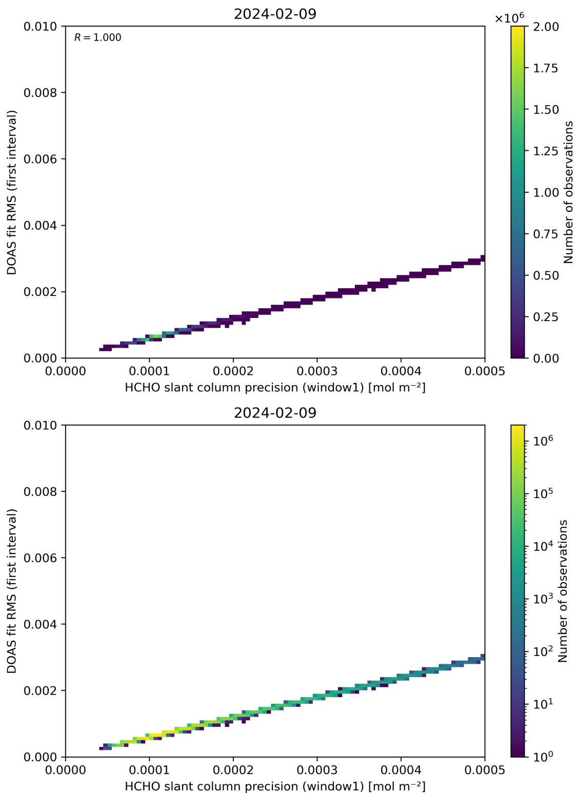
Figure 88: Scatter density plot of “HCHO slant column precision (window1)” against “DOAS fit RMS (first interval)” for 2024-02-08 to 2024-02-10.
