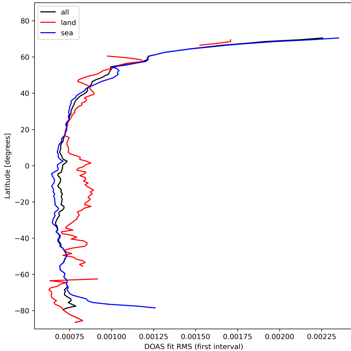
Figure 32: Zonal average of “DOAS fit RMS (first interval)” for 2024-02-08 to 2024-02-10.
