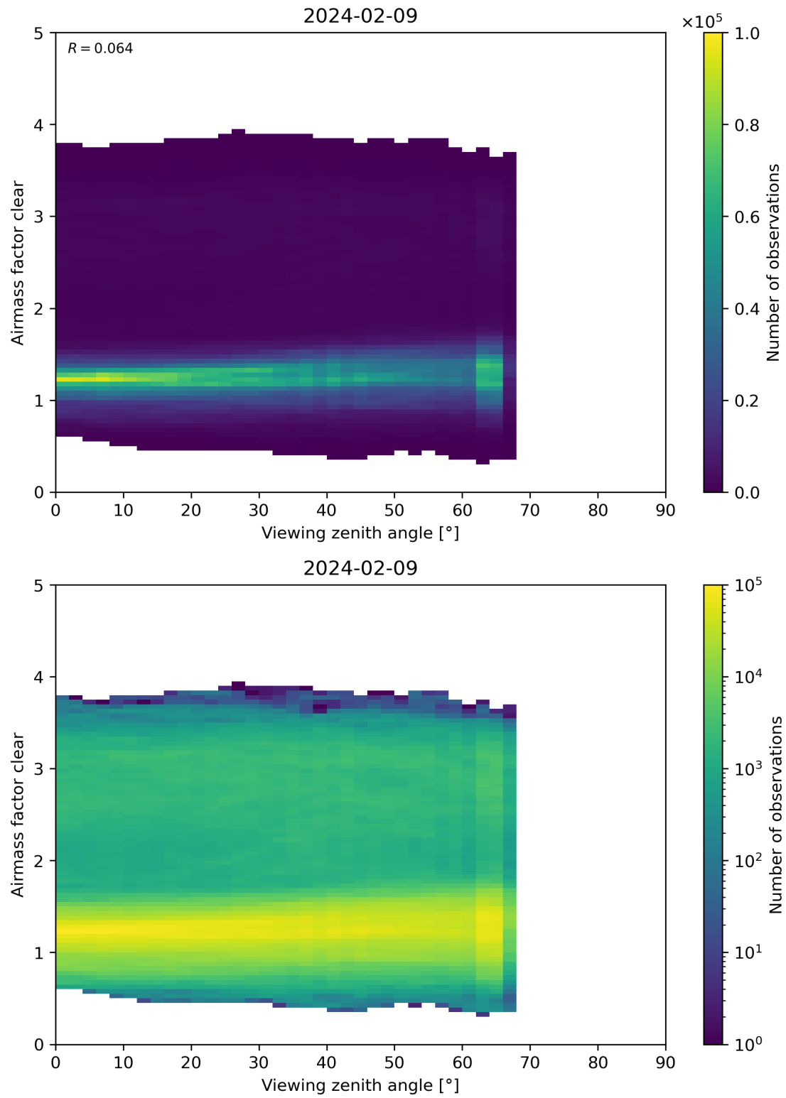
Figure 185: Scatter density plot of “Viewing zenith angle” against “Airmass factor clear” for 2024-02-08 to 2024-02-10.
