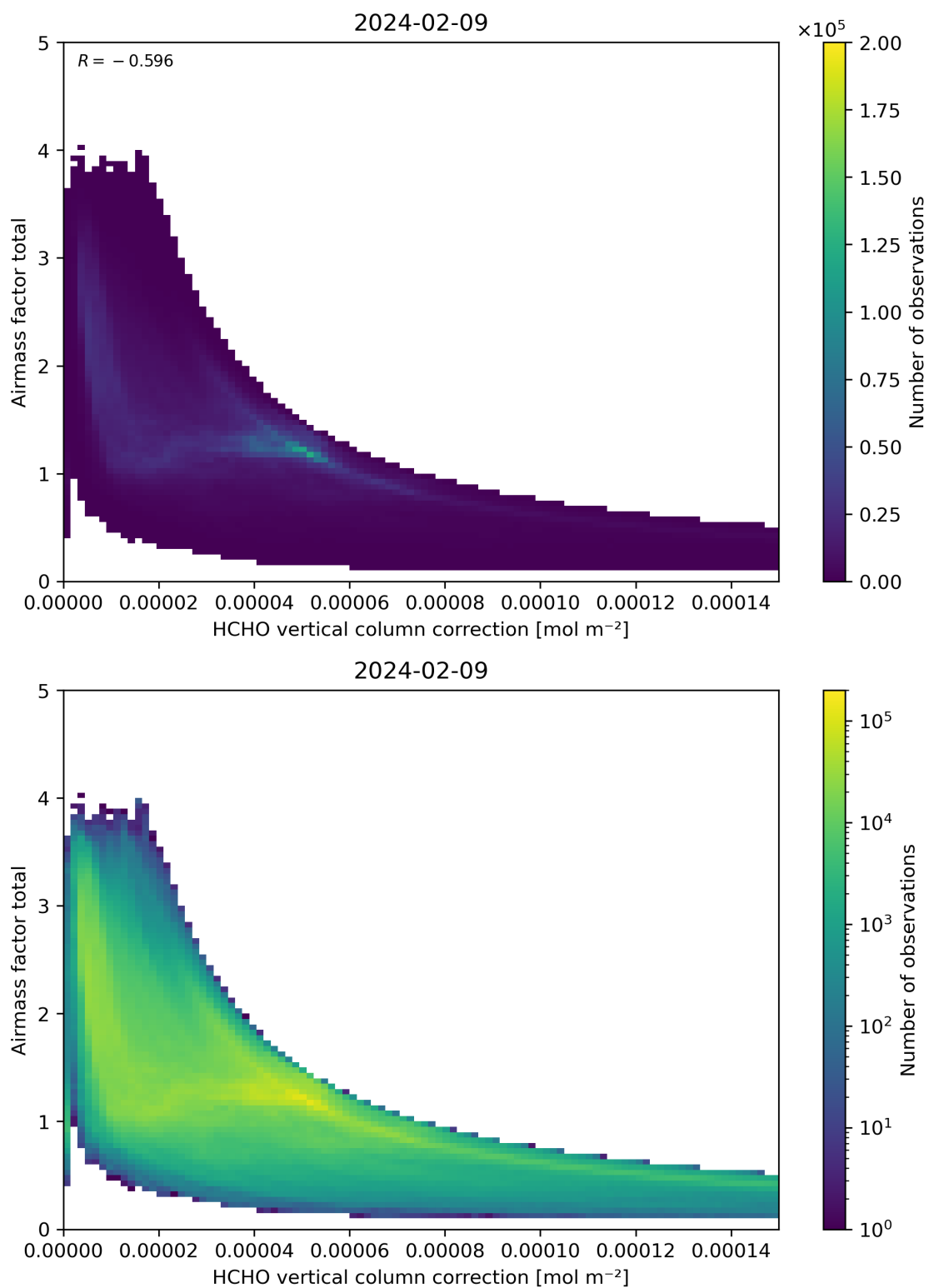
Figure 120: Scatter density plot of “HCHO vertical column correction” against “Airmass factor total” for 2024-02-08 to 2024-02-10.
