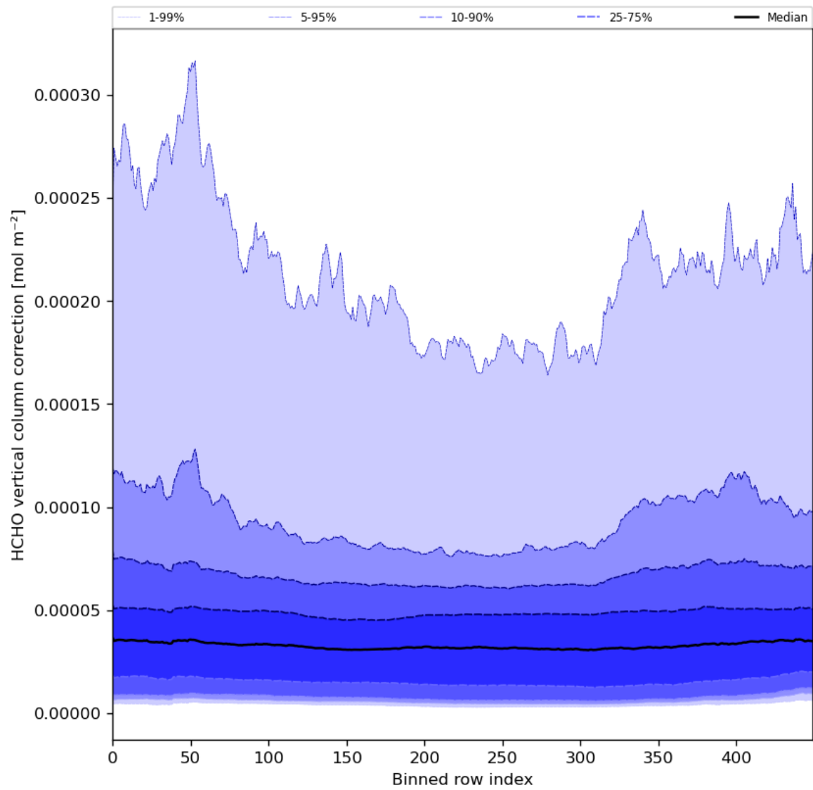
Figure 51: Along track statistics of "HCHO vertical column correction" for 2024-02-08 to 2024-02-10
