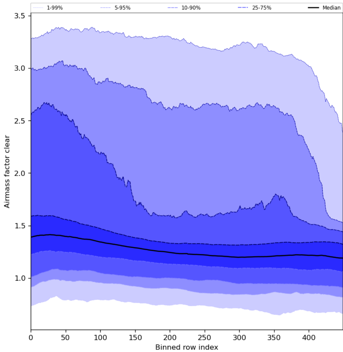
Figure 56: Along track statistics of “Airmass factor clear” for 2024-02-08 to 2024-02-10
