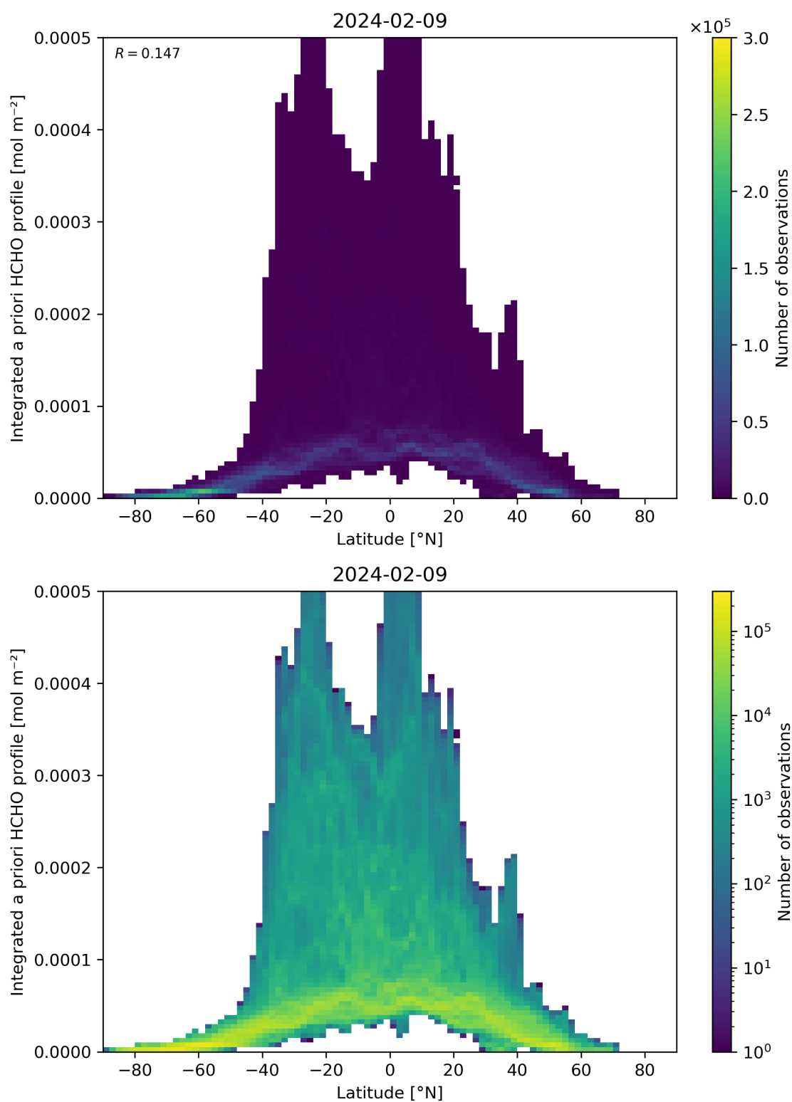
Figure 166: Scatter density plot of “Latitude” against “Integrated a priori HCHO profile” for 2024-02-08 to 2024-02-10.
