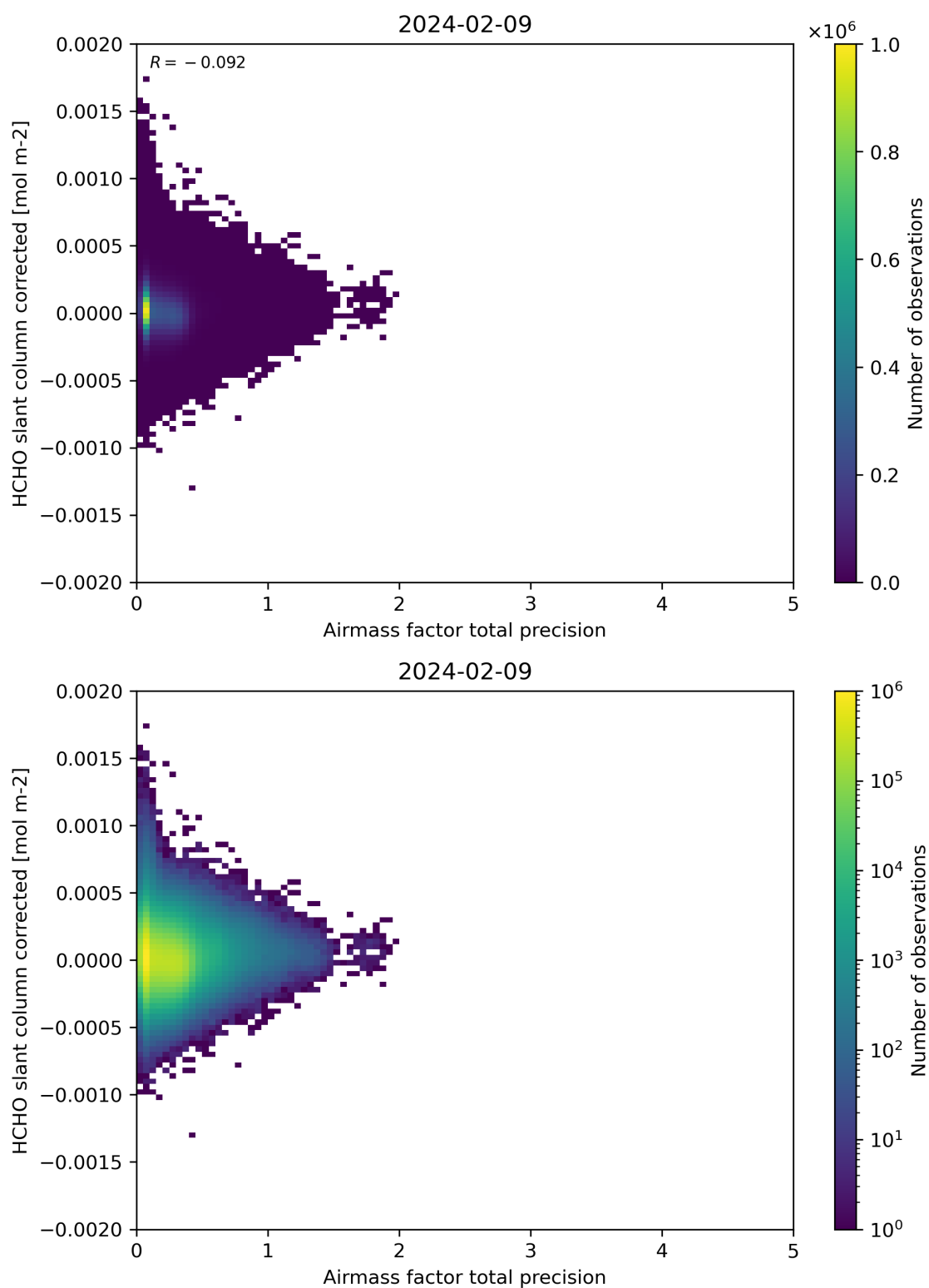
Figure 109: Scatter density plot of “Airmass factor total precision” against “HCHO slant column corrected” for 2024-02-08 to 2024-02-10.
