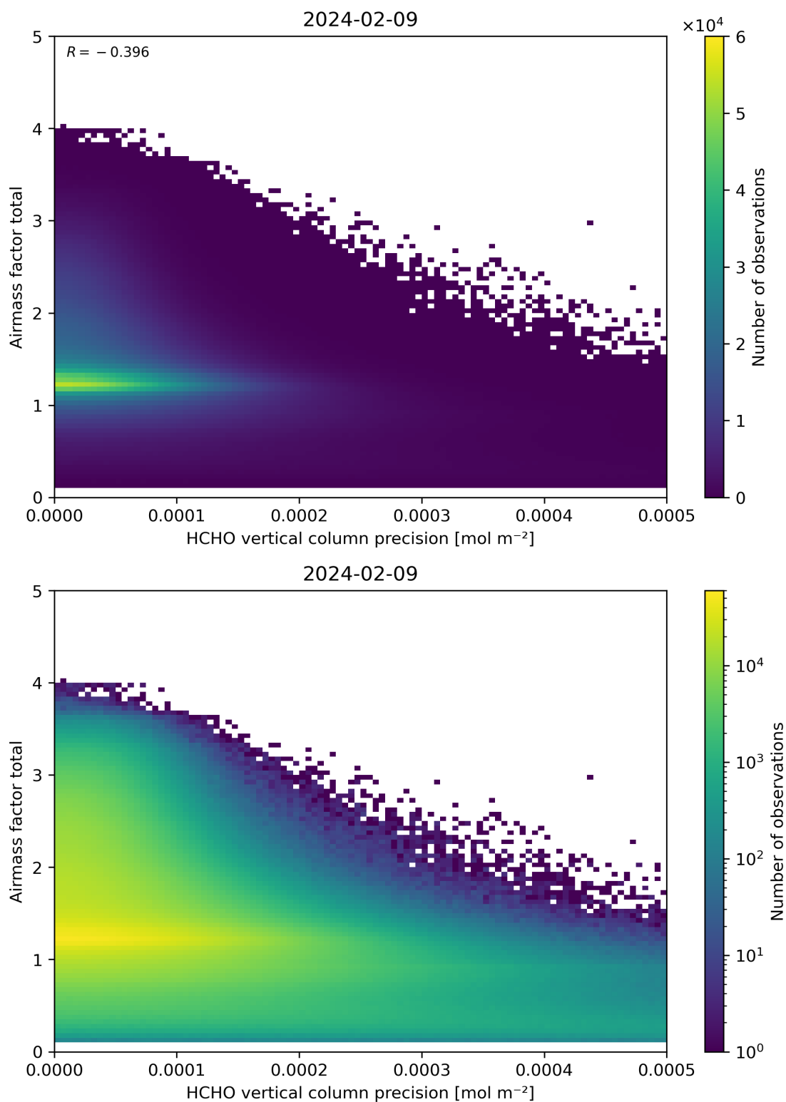
Figure 144: Scatter density plot of “HCHO vertical column precision” against “Airmass factor total” for 2024-02-08 to 2024-02-10.
