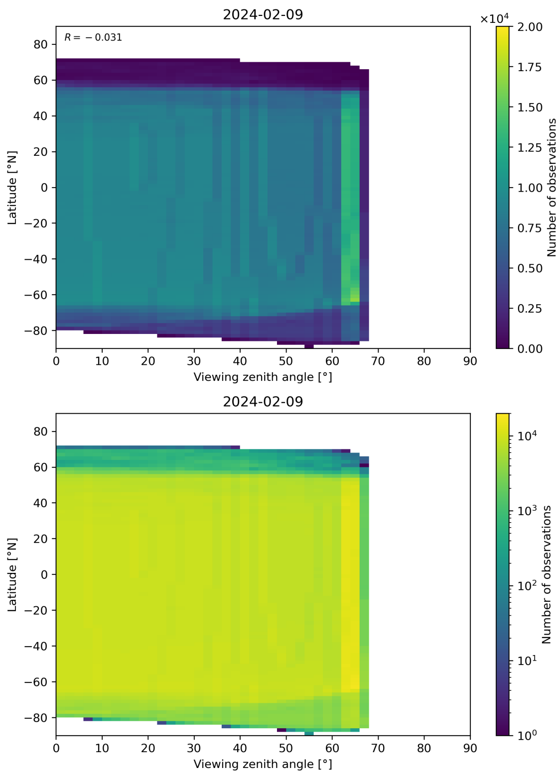
Figure 196: Scatter density plot of “Viewing zenith angle” against “Latitude” for 2024-02-08 to 2024-02-10.
