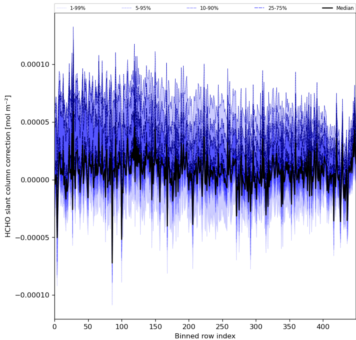
Figure 61: Along track statistics of “HCHO slant column correction” for 2024-02-08 to 2024-02-10
