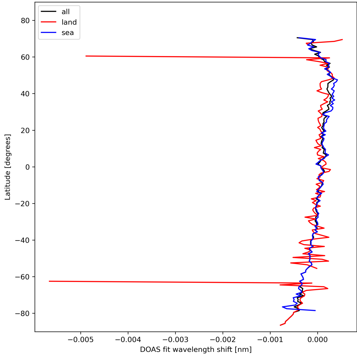
Figure 30: Zonal average of "DOAS fit wavelength shift" for 2024-02-08 to 2024-02-10.
