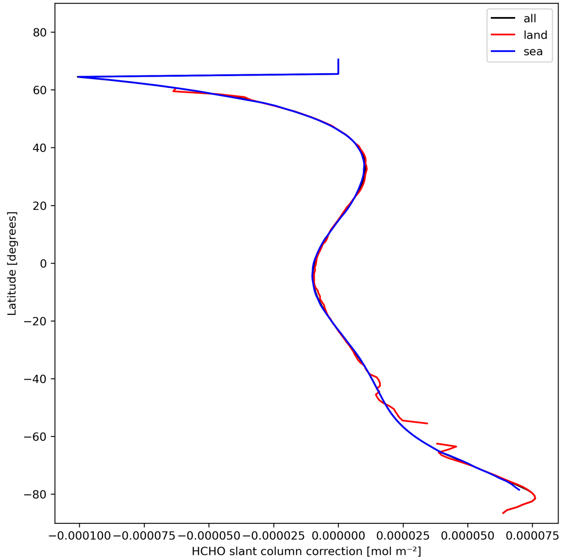
Figure 33: Zonal average of “HCHO slant column correction” for 2024-02-08 to 2024-02-10.
