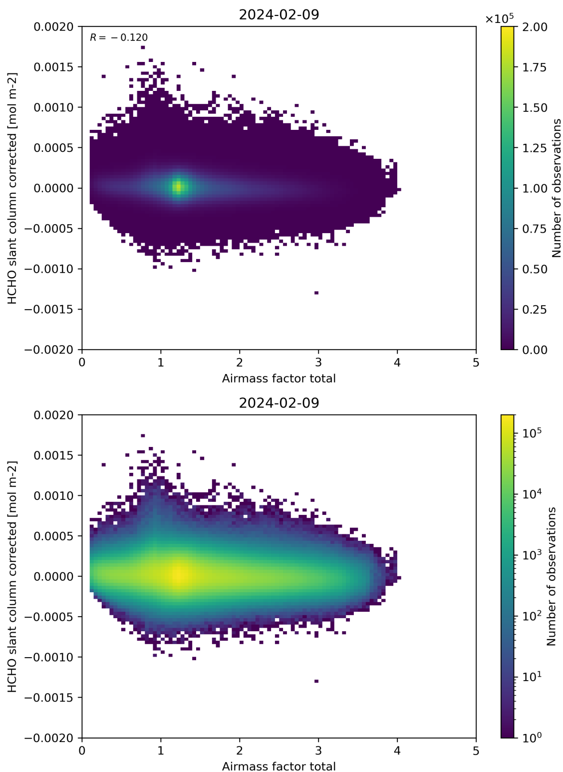
Figure 101: Scatter density plot of “Airmass factor total” against “HCHO slant column corrected” for 2024-02-08 to 2024-02-10.
