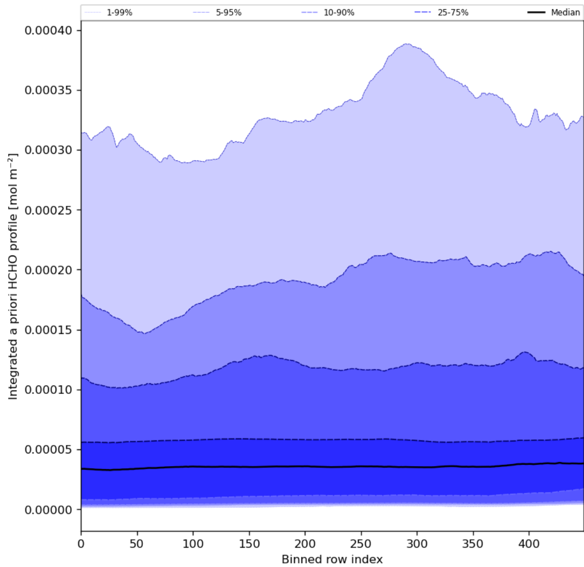
Figure 57: Along track statistics of “Integrated a priori HCHO profile” for 2024-02-08 to 2024-02-10
