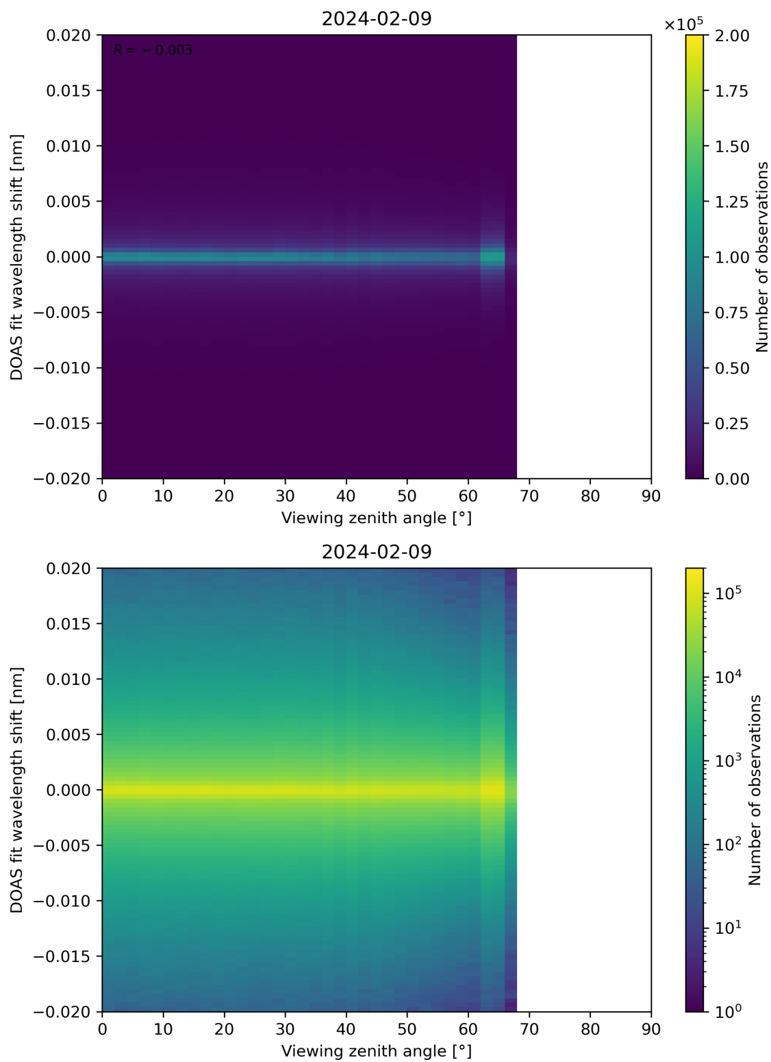
Figure 183: Scatter density plot of “Viewing zenith angle” against “DOAS fit wavelength shift” for 2024-02-08 to 2024-02-10.
