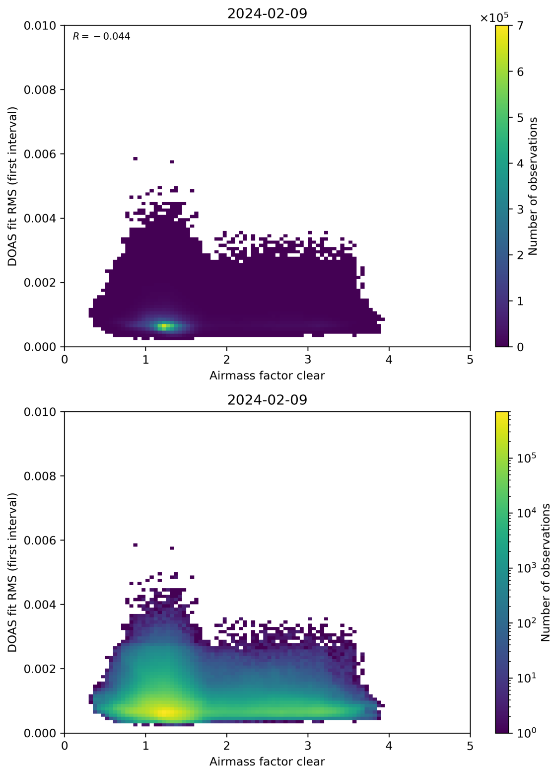
Figure 71: Scatter density plot of “Airmass factor clear” against “DOAS fit RMS (first interval)” for 2024-02-08 to 2024-02-10.
