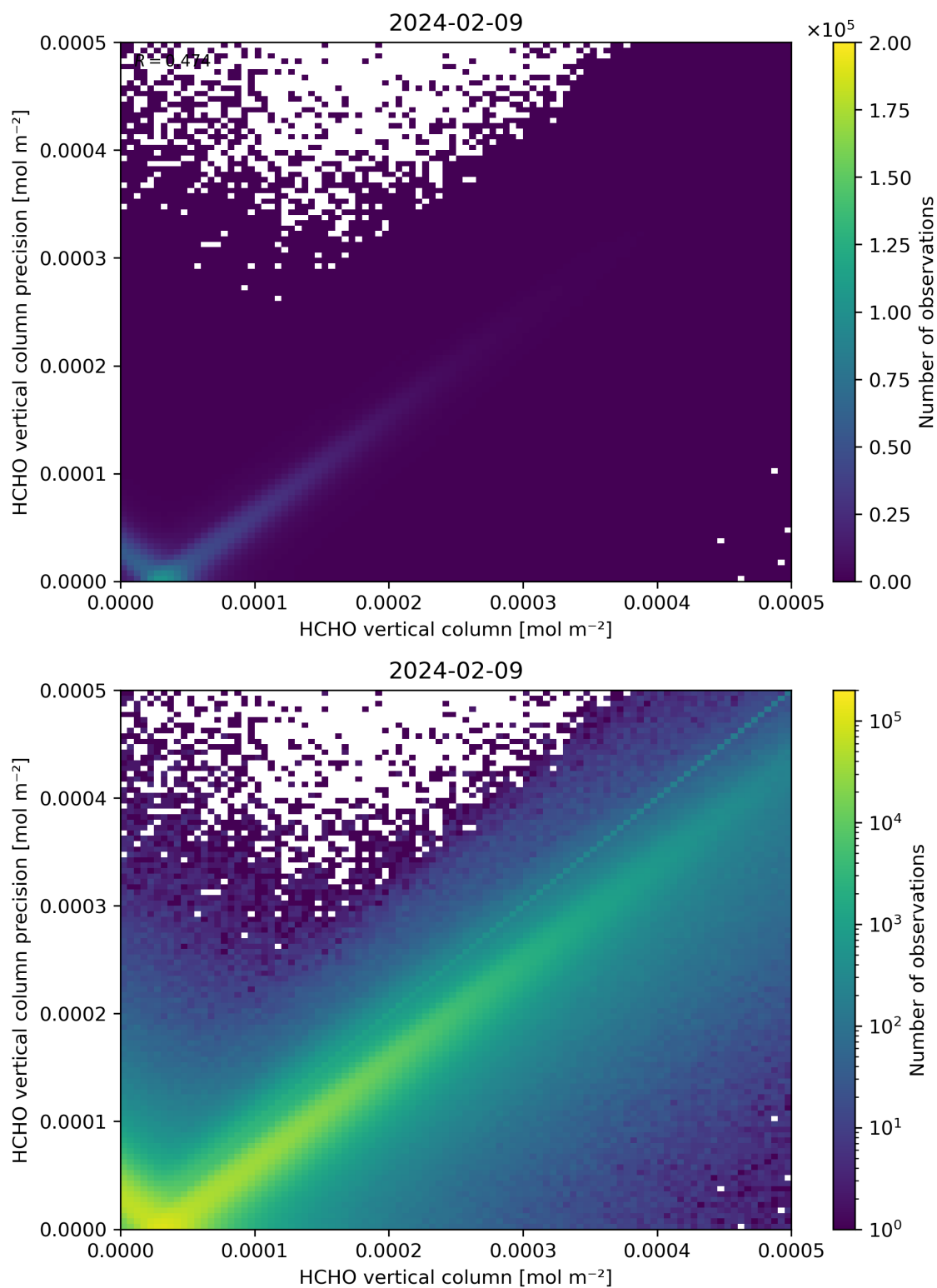
Figure 134: Scatter density plot of “HCHO vertical column” against “HCHO vertical column precision” for 2024-02-08 to 2024-02-10.
