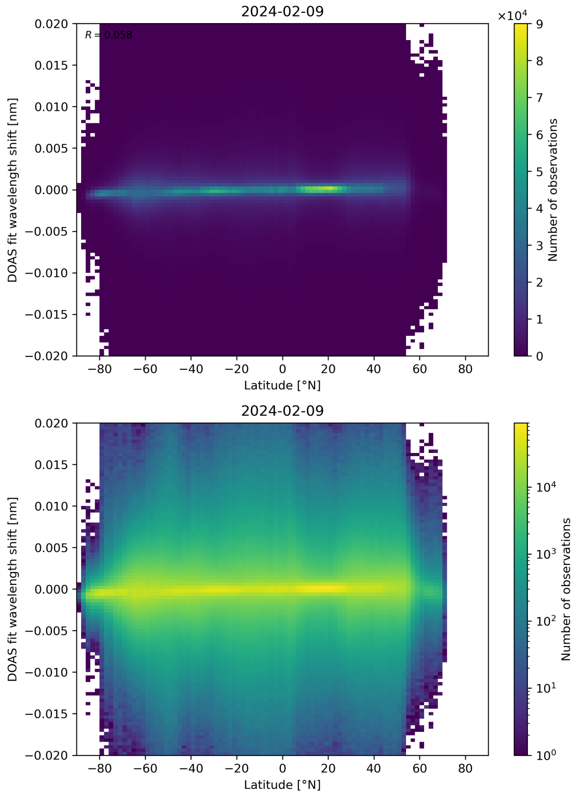
Figure 154: Scatter density plot of “Latitude” against “DOAS fit wavelength shift” for 2024-02-08 to 2024-02-10.
