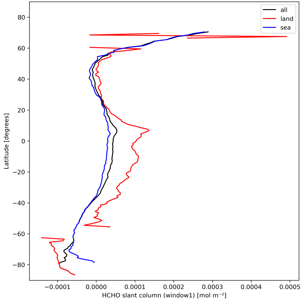
Figure 24: Zonal average of “HCHO slant column (window1)” for 2024-02-08 to 2024-02-10.
