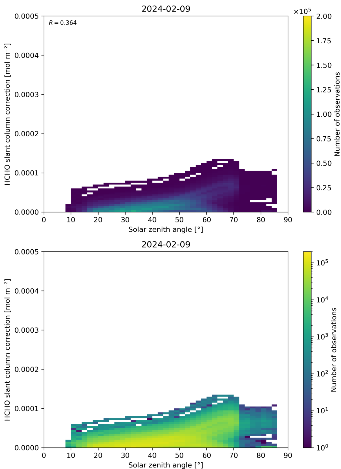
Figure 172: Scatter density plot of “Solar zenith angle” against “HCHO slant column correction” for 2024-02-08 to 2024-02-10.
