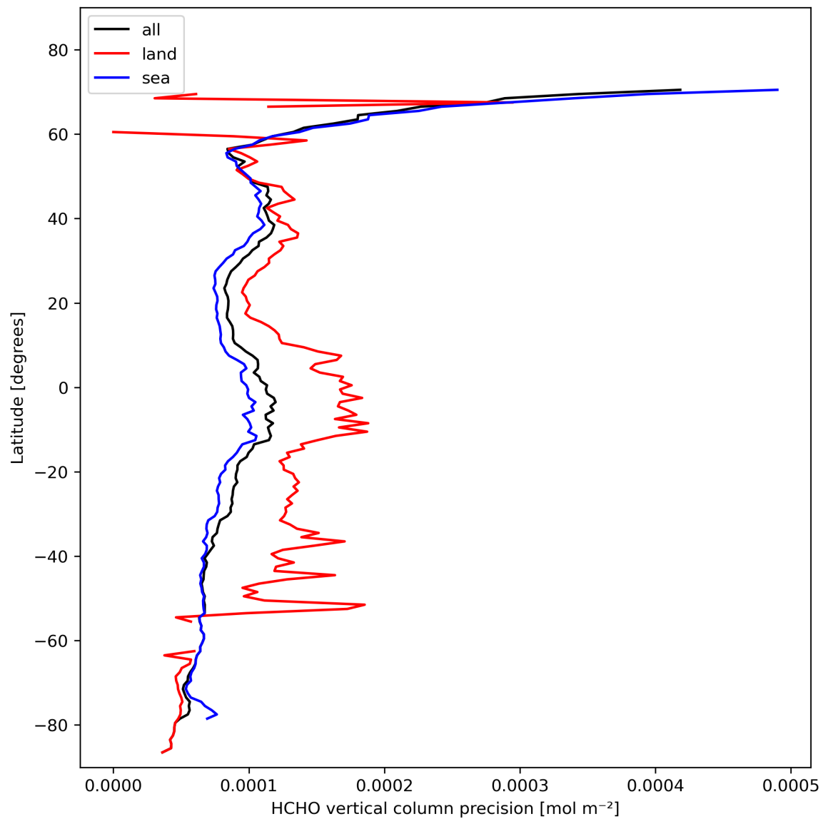
Figure 22: Zonal average of “HCHO vertical column precision” for 2024-02-08 to 2024-02-10.
