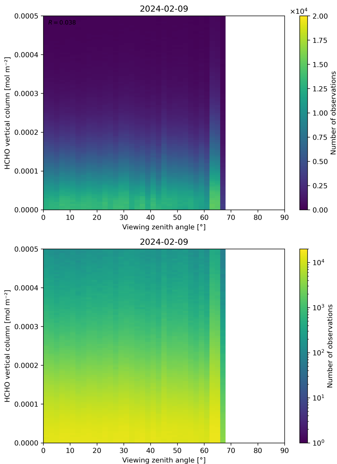
Figure 192: Scatter density plot of “Viewing zenith angle” against “HCHO vertical column” for 2024-02-08 to 2024-02-10.
