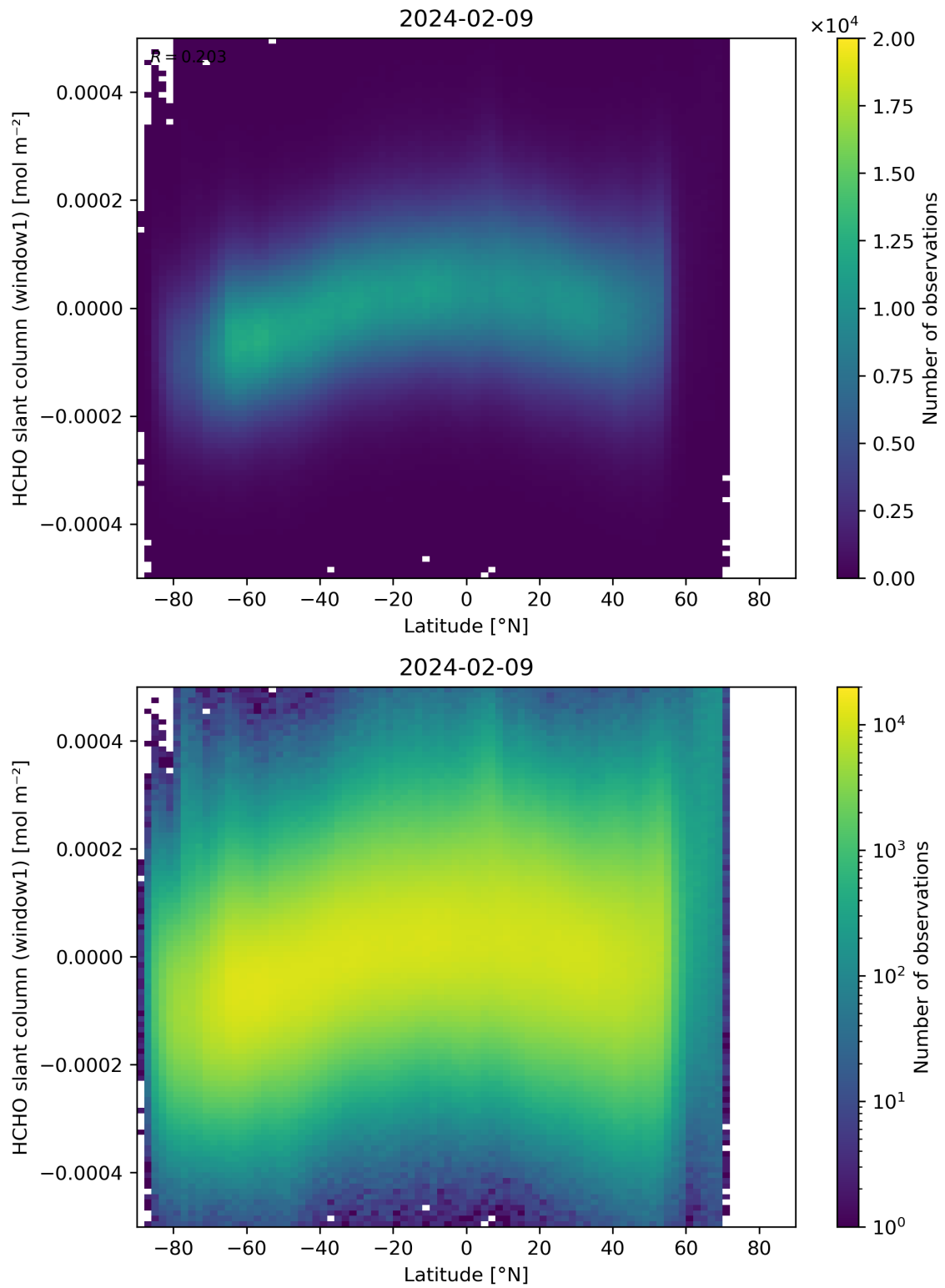
Figure 159: Scatter density plot of “Latitude” against “HCHO slant column (window1)” for 2024-02-08 to 2024-02-10.
