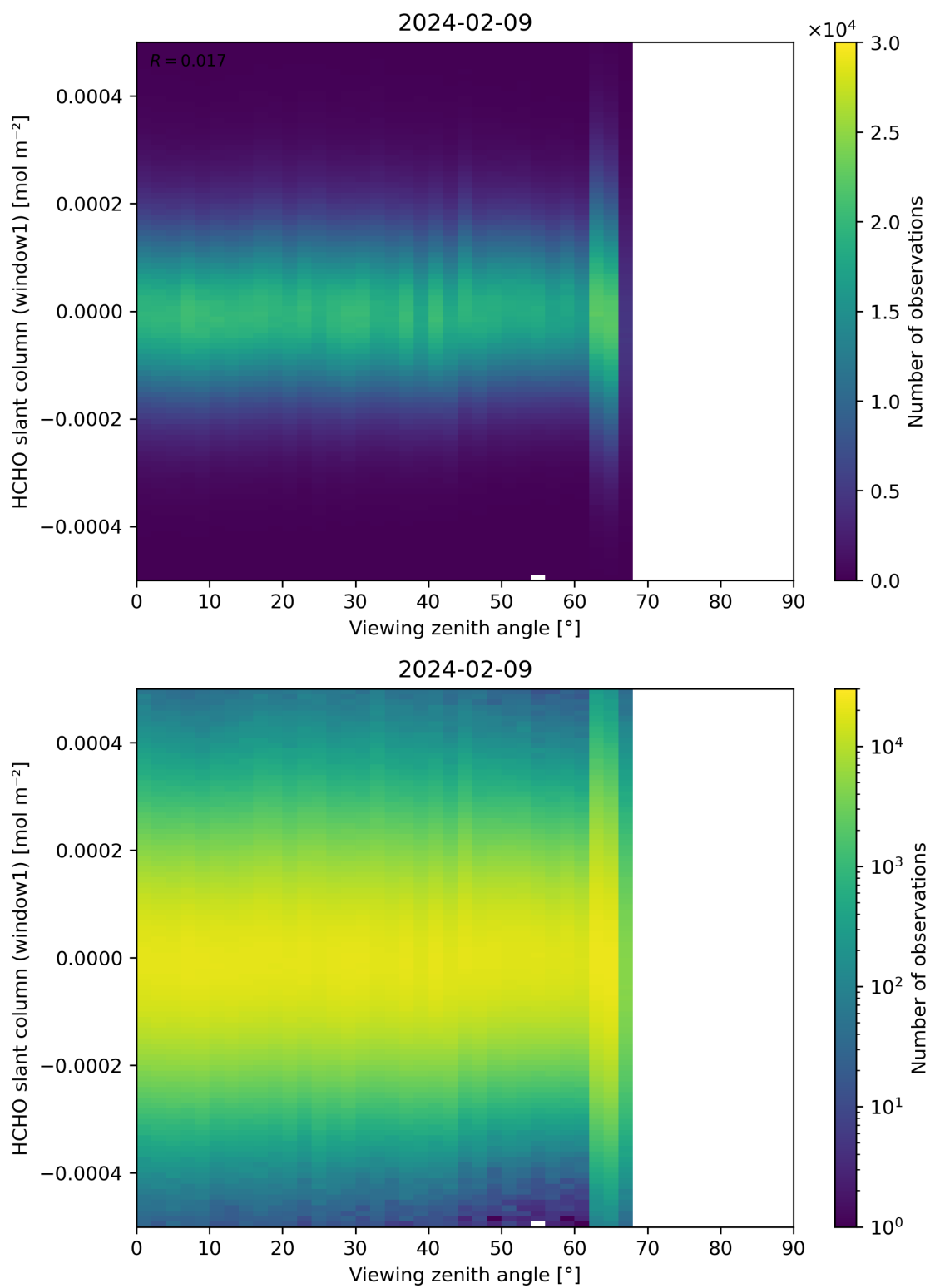
Figure 188: Scatter density plot of “Viewing zenith angle” against “HCHO slant column (window1)” for 2024-02-08 to 2024-02-10.
