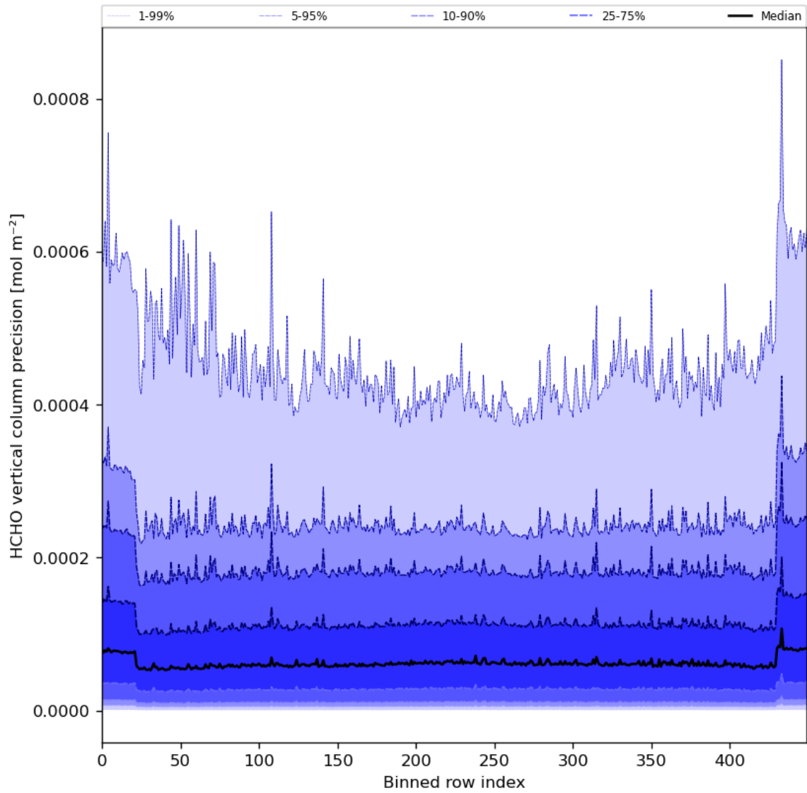
Figure 50: Along track statistics of “HCHO vertical column precision” for 2024-02-08 to 2024-02-10
