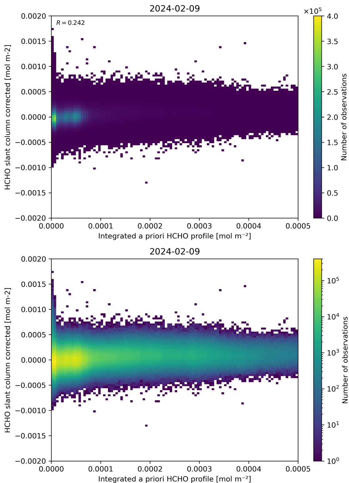
Figure 151: Scatter density plot of “Integrated a priori HCHO profile” against “HCHO slant column corrected” for 2024-02-08 to 2024-02-10.
