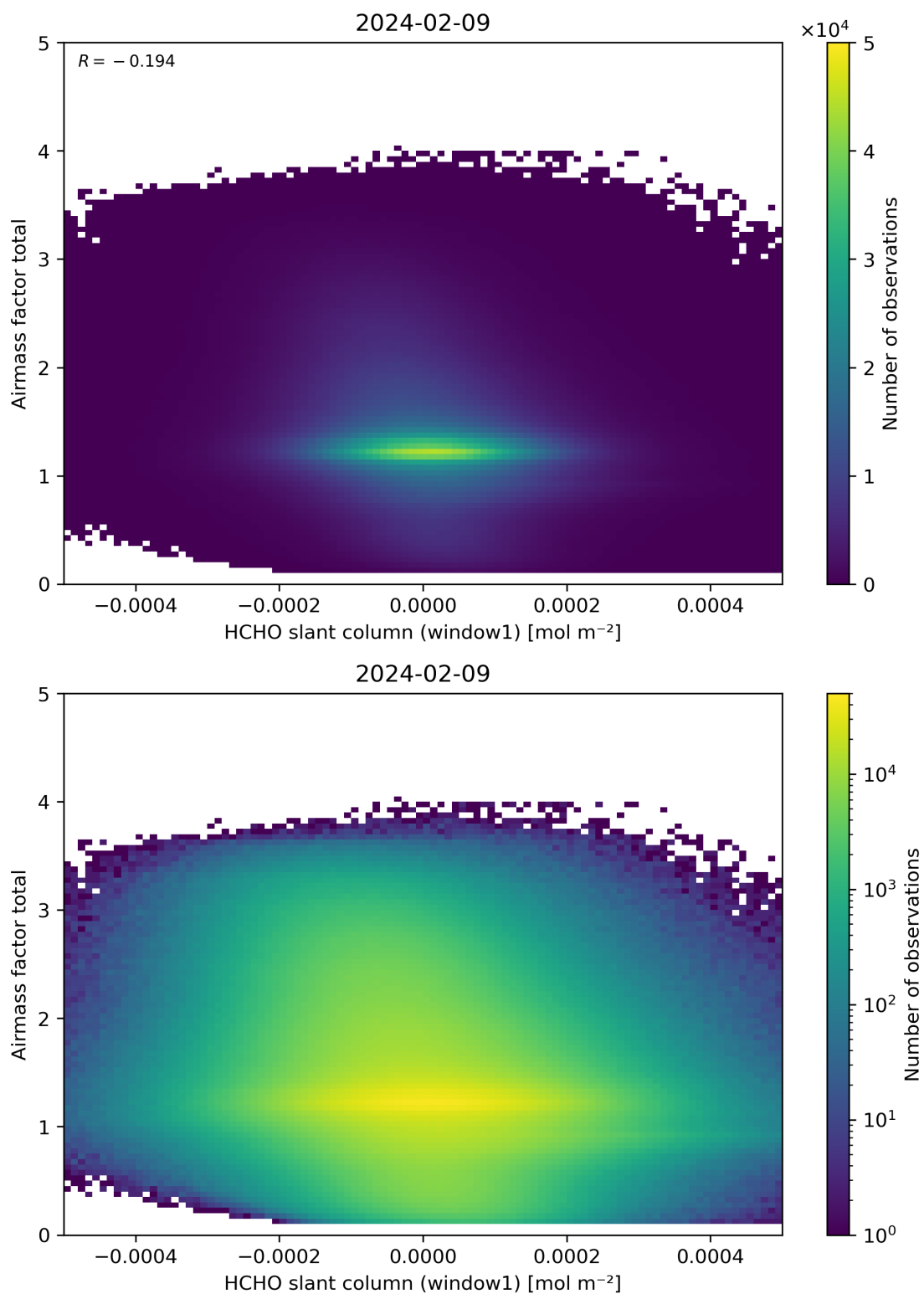
Figure 85: Scatter density plot of “HCHO slant column (window1)” against “Airmass factor total” for 2024-02-08 to 2024-02-10.
