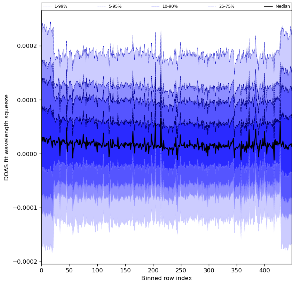
Figure 59: Along track statistics of “DOAS fit wavelength squeeze” for 2024-02-08 to 2024-02-10
