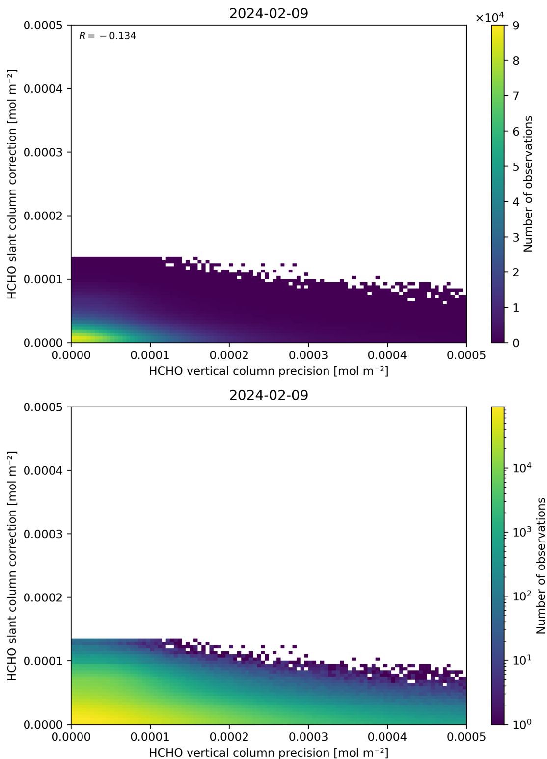
Figure 141: Scatter density plot of “HCHO vertical column precision” against “HCHO slant column correction” for 2024-02-08 to 2024-02-10.
