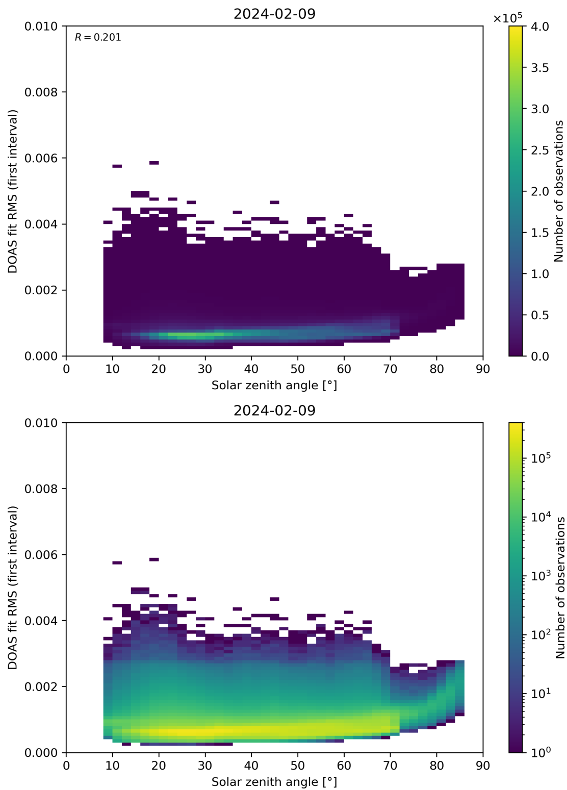
Figure 167: Scatter density plot of “Solar zenith angle” against “DOAS fit RMS (first interval)” for 2024-02-08 to 2024-02-10.
