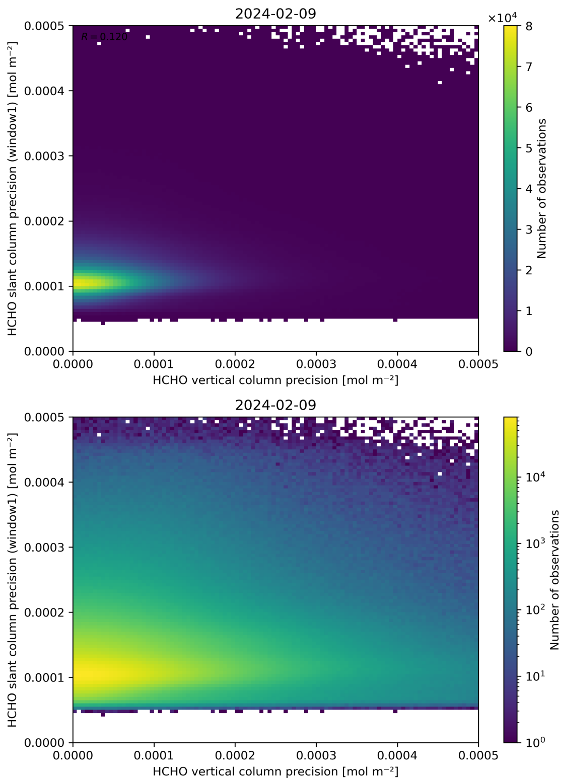
Figure 143: Scatter density plot of “HCHO vertical column precision” against “HCHO slant column precision (window1)” for 2024-02-08 to 2024-02-10.
