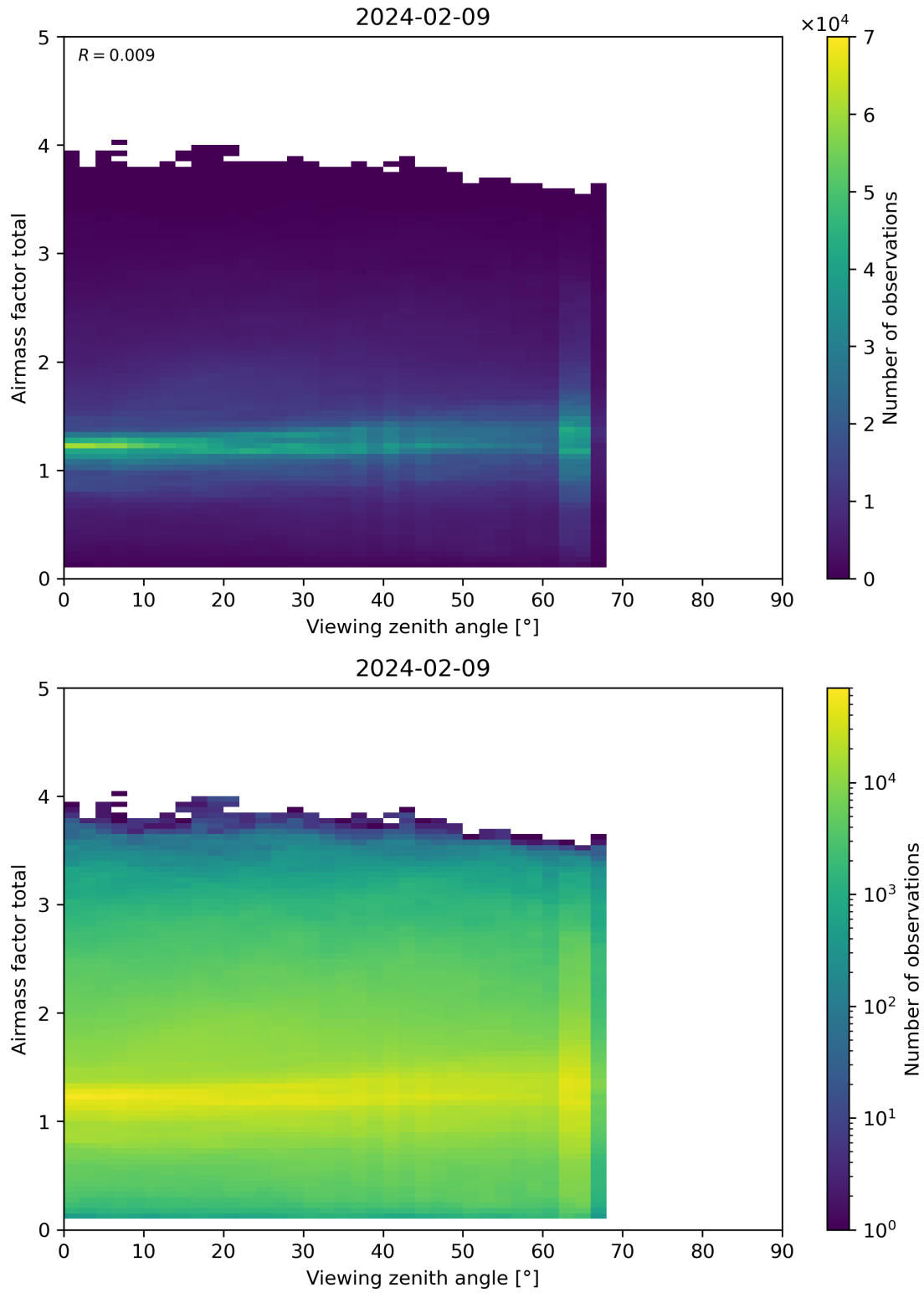
Figure 190: Scatter density plot of “Viewing zenith angle” against “Airmass factor total” for 2024-02-08 to 2024-02-10.
