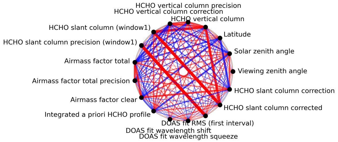
Figure 1: Map of correlation graph for 2024-02-08 to 2024-02-10.
