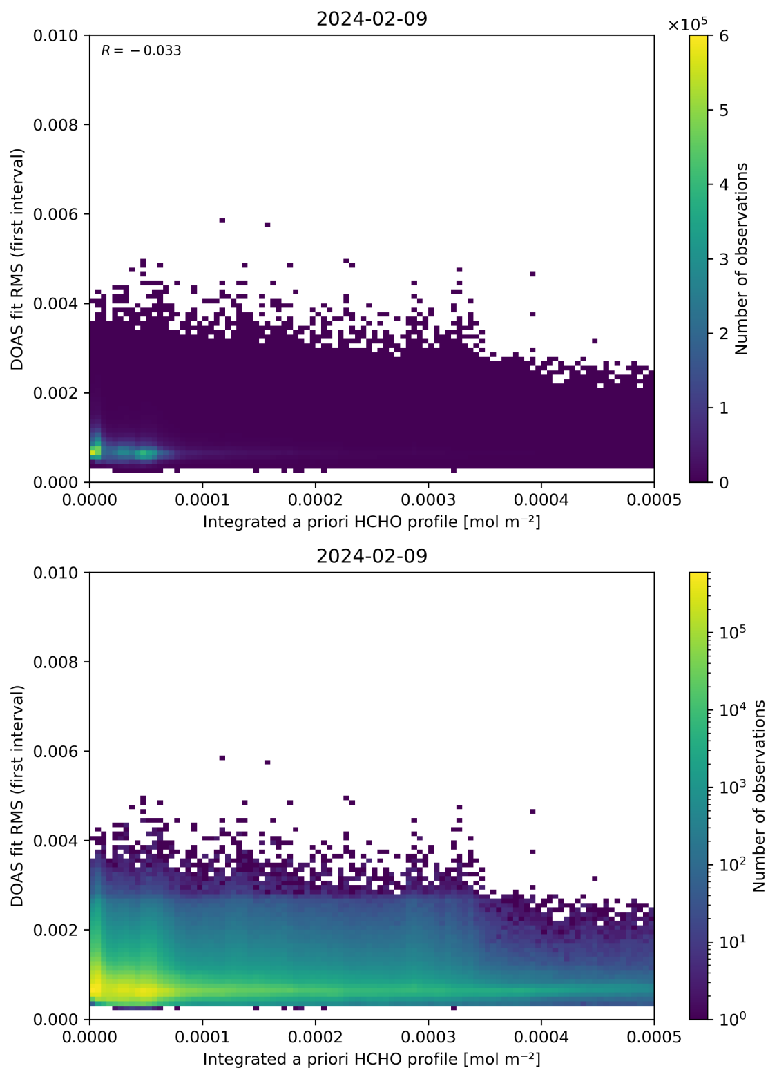
Figure 148: Scatter density plot of “Integrated a priori HCHO profile” against “DOAS fit RMS (first interval)” for 2024-02-08 to 2024-02-10.
