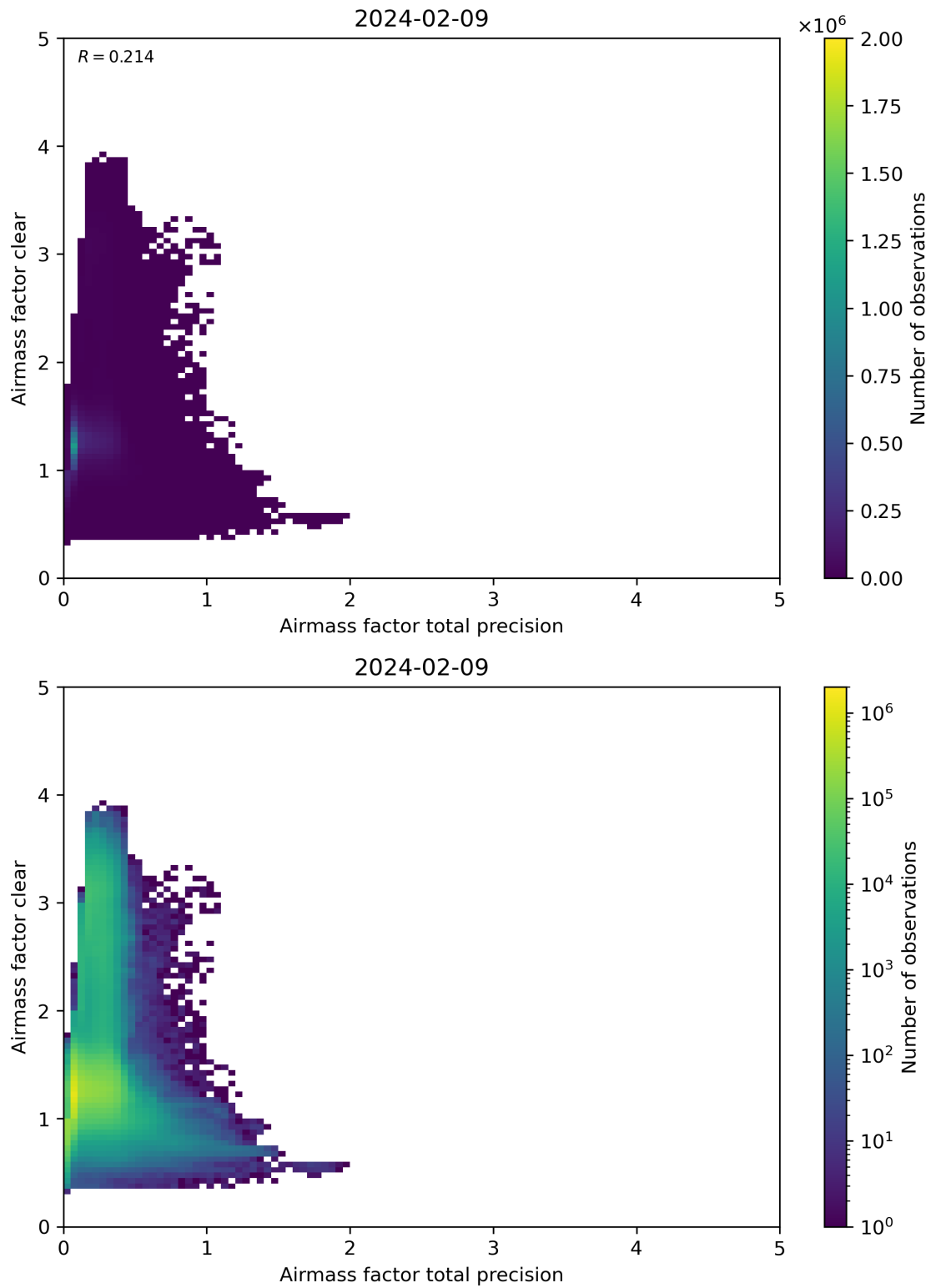
Figure 108: Scatter density plot of “Airmass factor total precision” against “Airmass factor clear” for 2024-02-08 to 2024-02-10.
