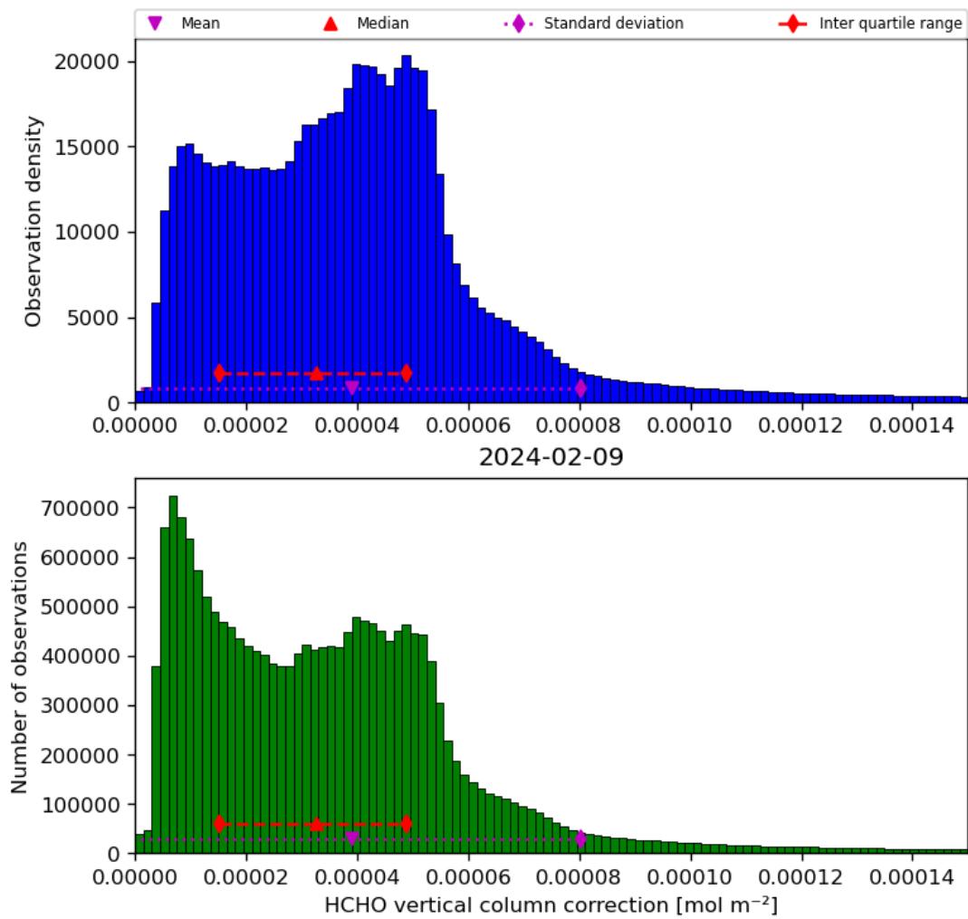
Figure 37: Histogram of “HCHO vertical column correction” for 2024-02-08 to 2024-02-10
