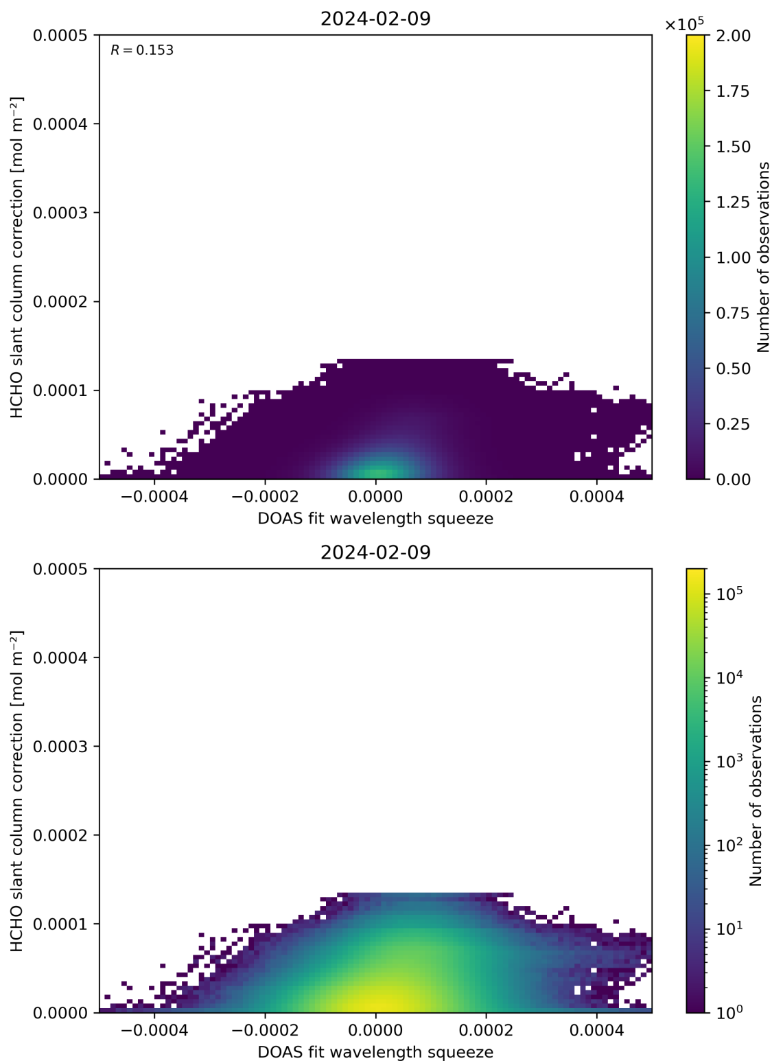
Figure 70: Scatter density plot of “DOAS fit wavelength squeeze” against “HCHO slant column correction” for 2024-02-08 to 2024-02-10.
