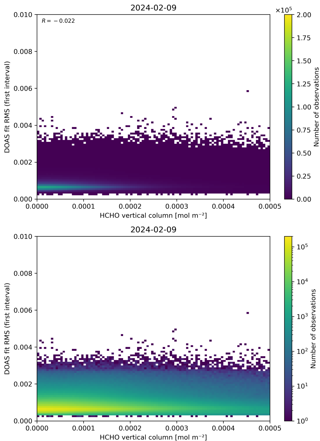
Figure 123: Scatter density plot of “HCHO vertical column” against “DOAS fit RMS (first interval)” for 2024-02-08 to 2024-02-10.
