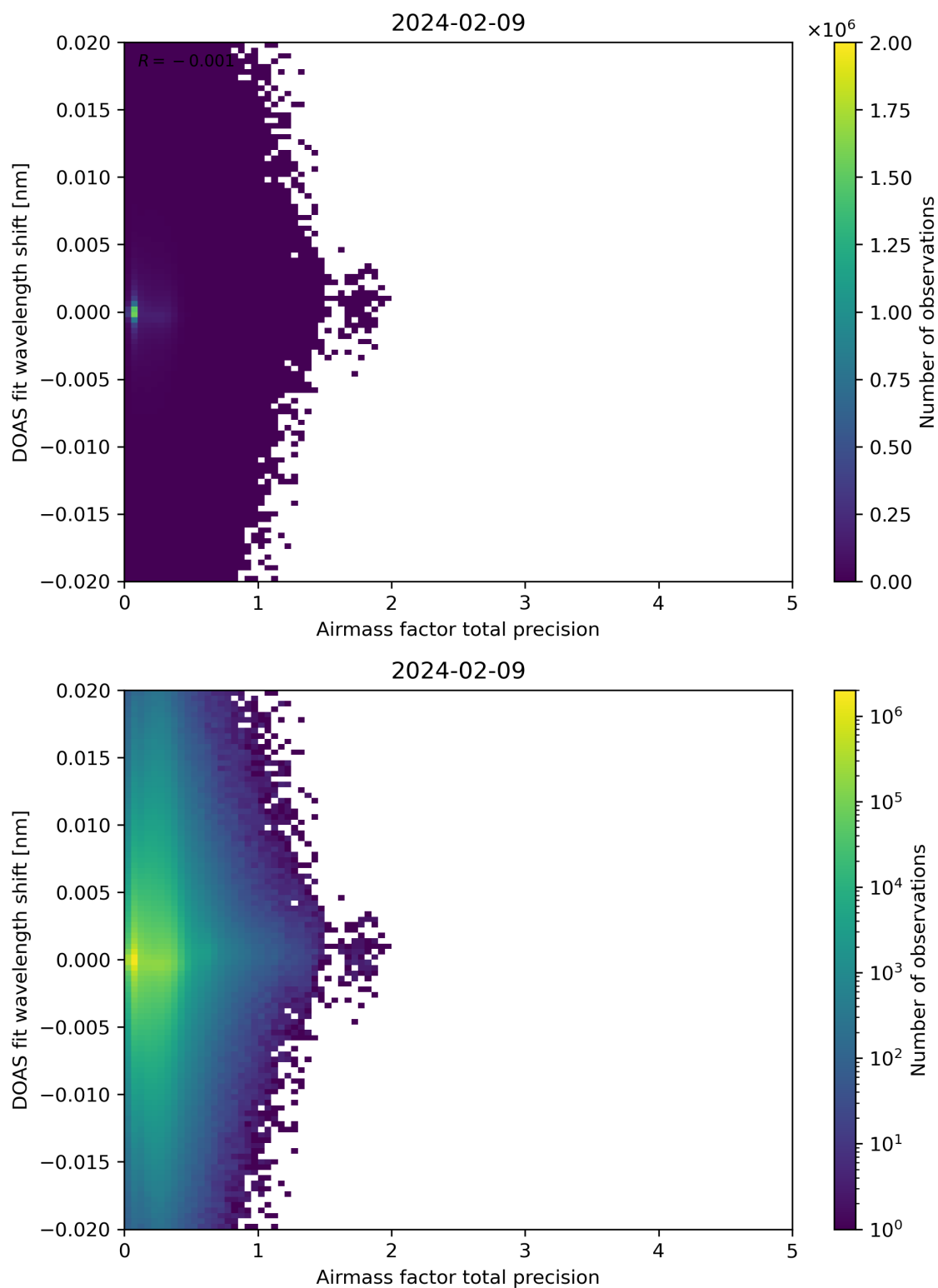
Figure 106: Scatter density plot of “Airmass factor total precision” against “DOAS fit wavelength shift” for 2024-02-08 to 2024-02-10.
