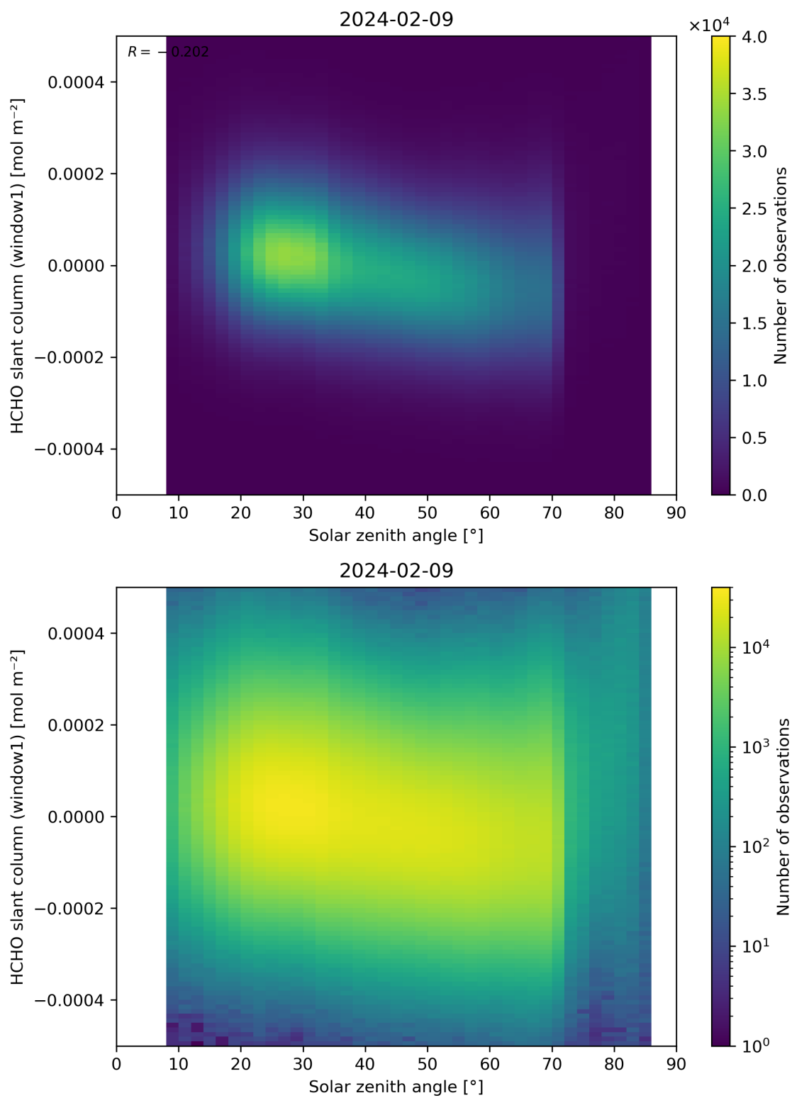
Figure 173: Scatter density plot of “Solar zenith angle” against “HCHO slant column (window1)” for 2024-02-08 to 2024-02-10.
