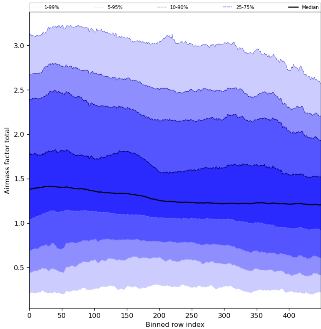
Figure 54: Along track statistics of “Airmass factor total” for 2024-02-08 to 2024-02-10
