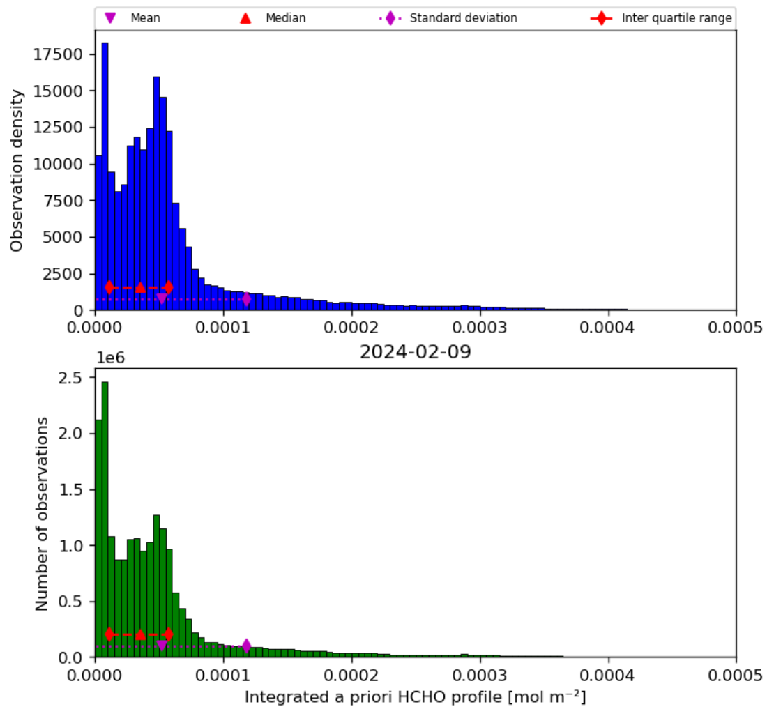
Figure 43: Histogram of “Integrated a priori HCHO profile” for 2024-02-08 to 2024-02-10
