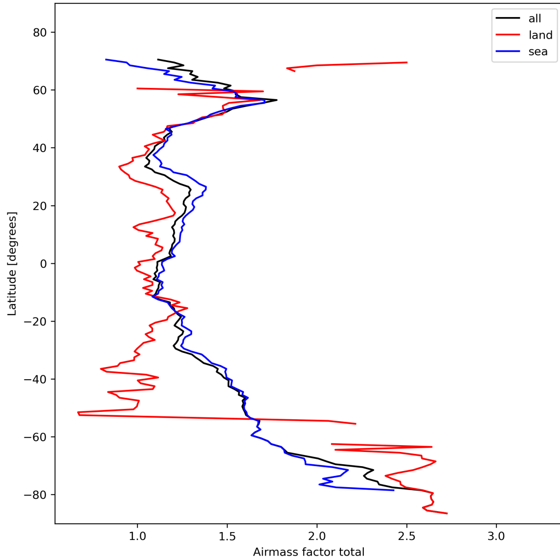
Figure 26: Zonal average of “Airmass factor total” for 2024-02-08 to 2024-02-10.
