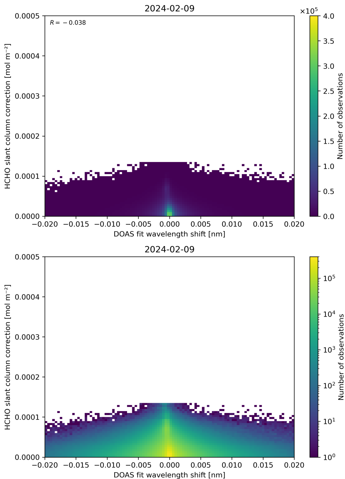
Figure 67: Scatter density plot of “DOAS fit wavelength shift” against “HCHO slant column correction” for 2024-02-08 to 2024-02-10.
