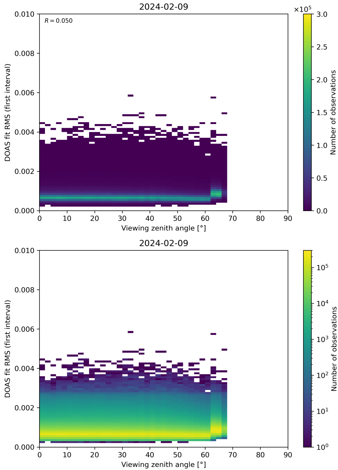
Figure 182: Scatter density plot of “Viewing zenith angle” against “DOAS fit RMS (first interval)” for 2024-02-08 to 2024-02-10.
