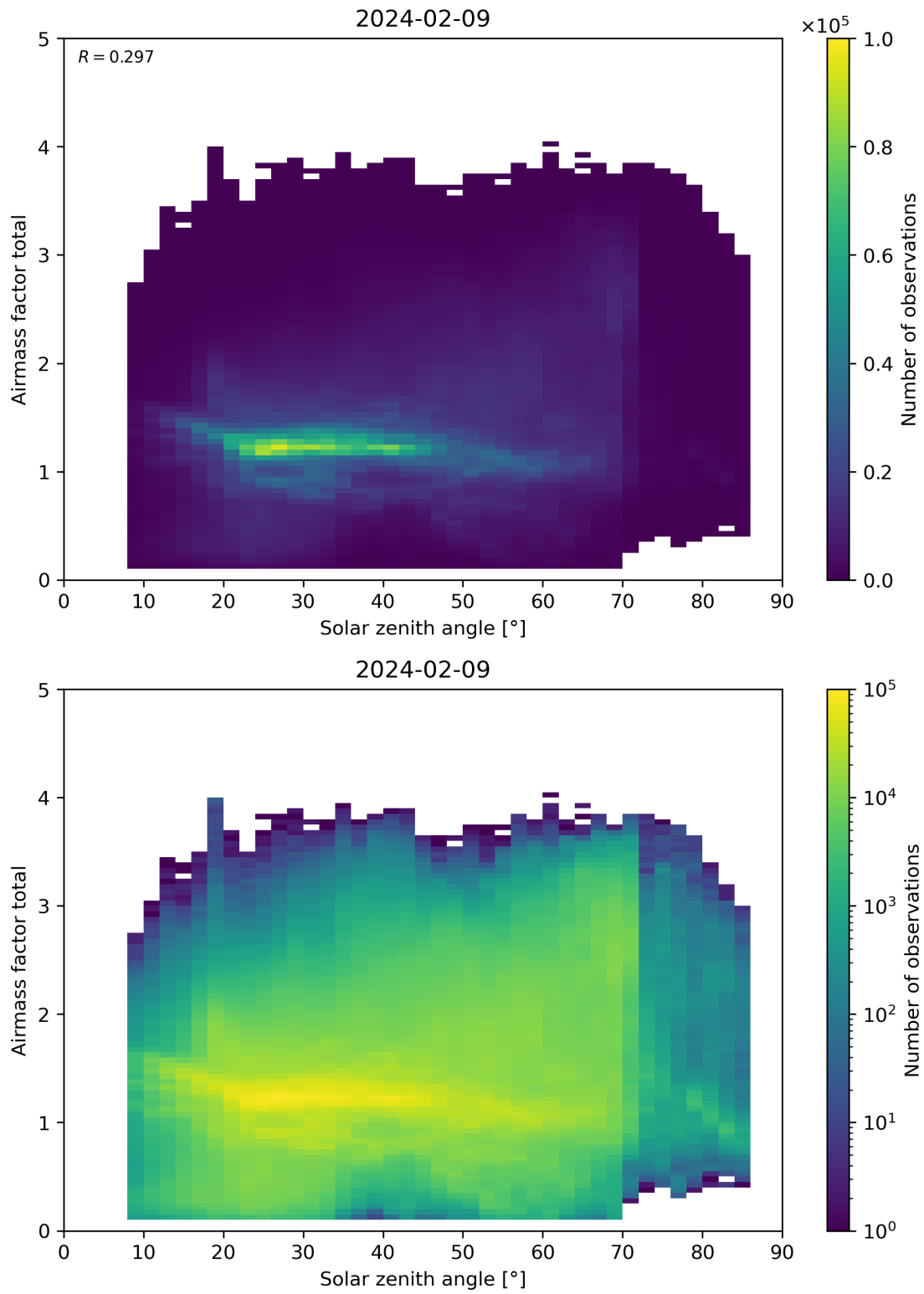
Figure 175: Scatter density plot of “Solar zenith angle” against “Airmass factor total” for 2024-02-08 to 2024-02-10.
