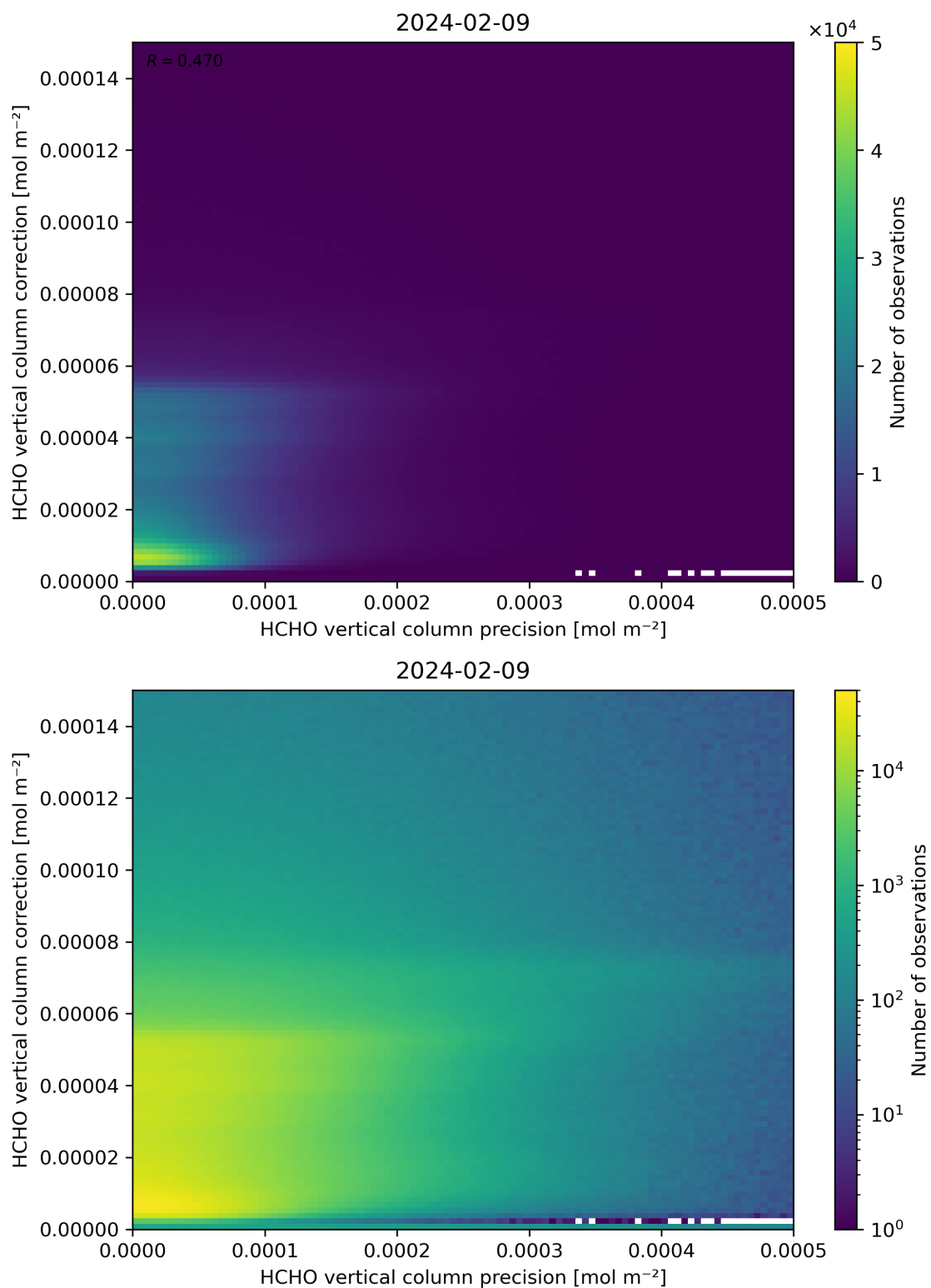
Figure 146: Scatter density plot of “HCHO vertical column precision” against “HCHO vertical column correction” for 2024-02-08 to 2024-02-10.
