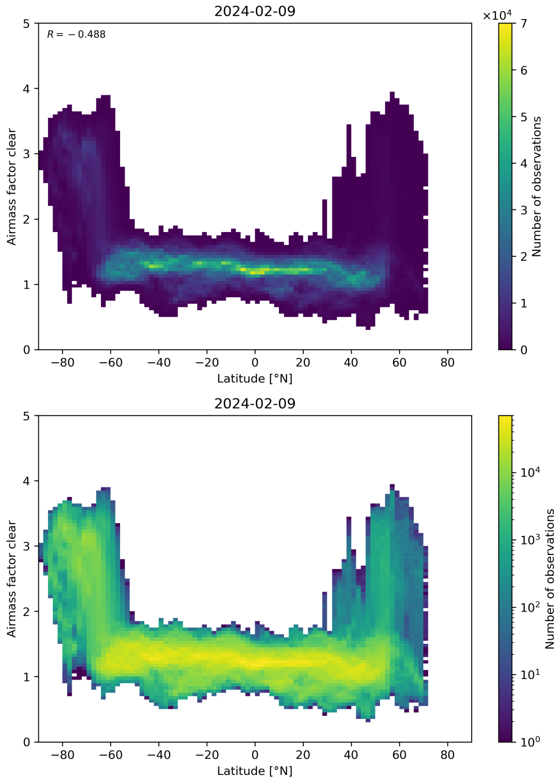
Figure 156: Scatter density plot of “Latitude” against “Airmass factor clear” for 2024-02-08 to 2024-02-10.
