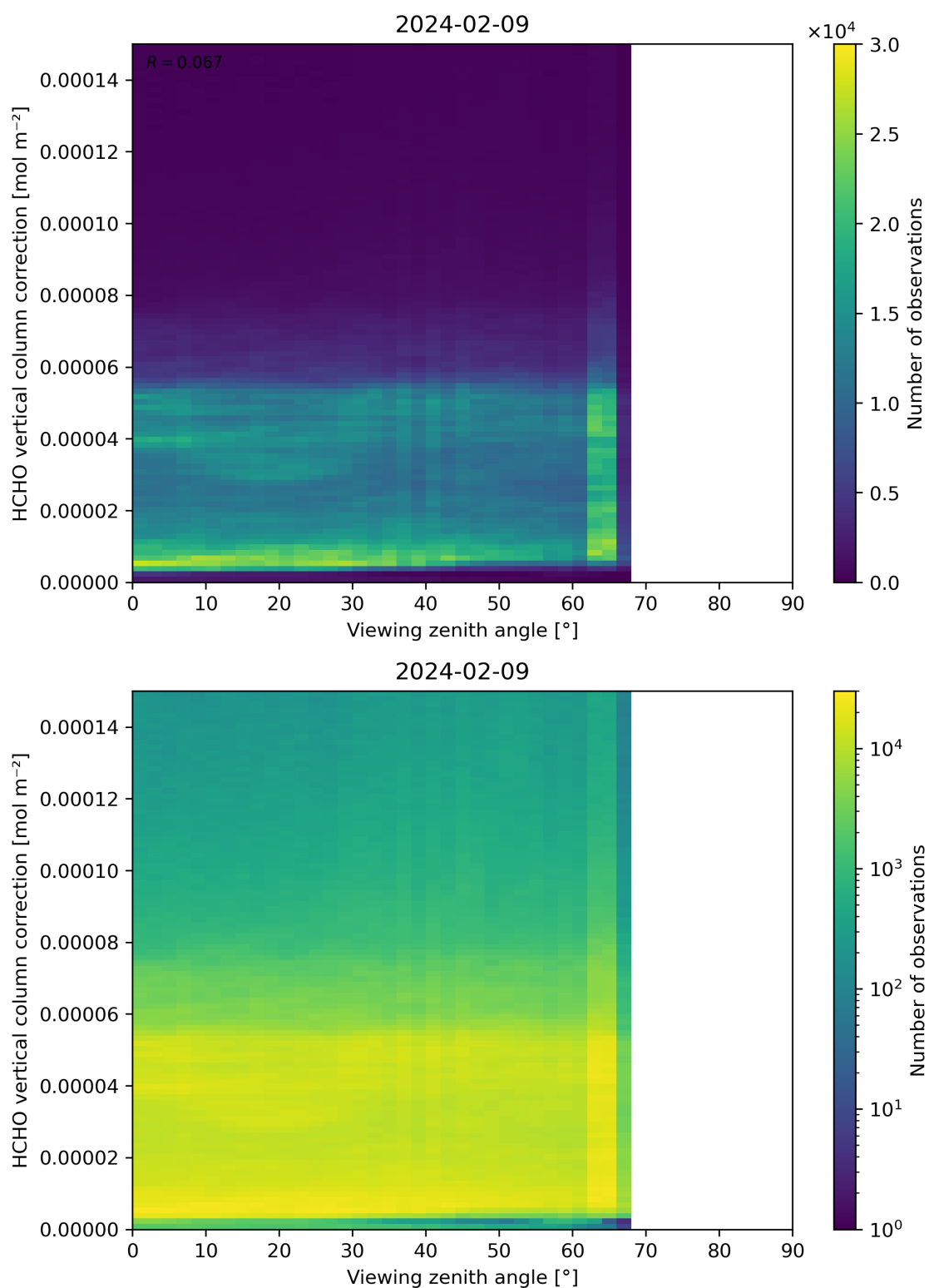
Figure 193: Scatter density plot of “Viewing zenith angle” against “HCHO vertical column correction” for 2024-02-08 to 2024-02-10.
