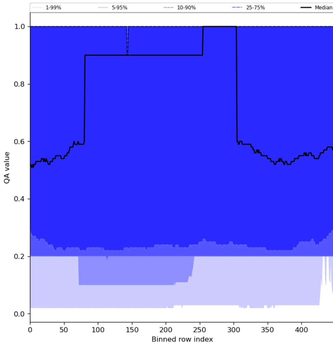
Figure 48: Along track statistics of “QA value” for 2024-02-08 to 2024-02-10
