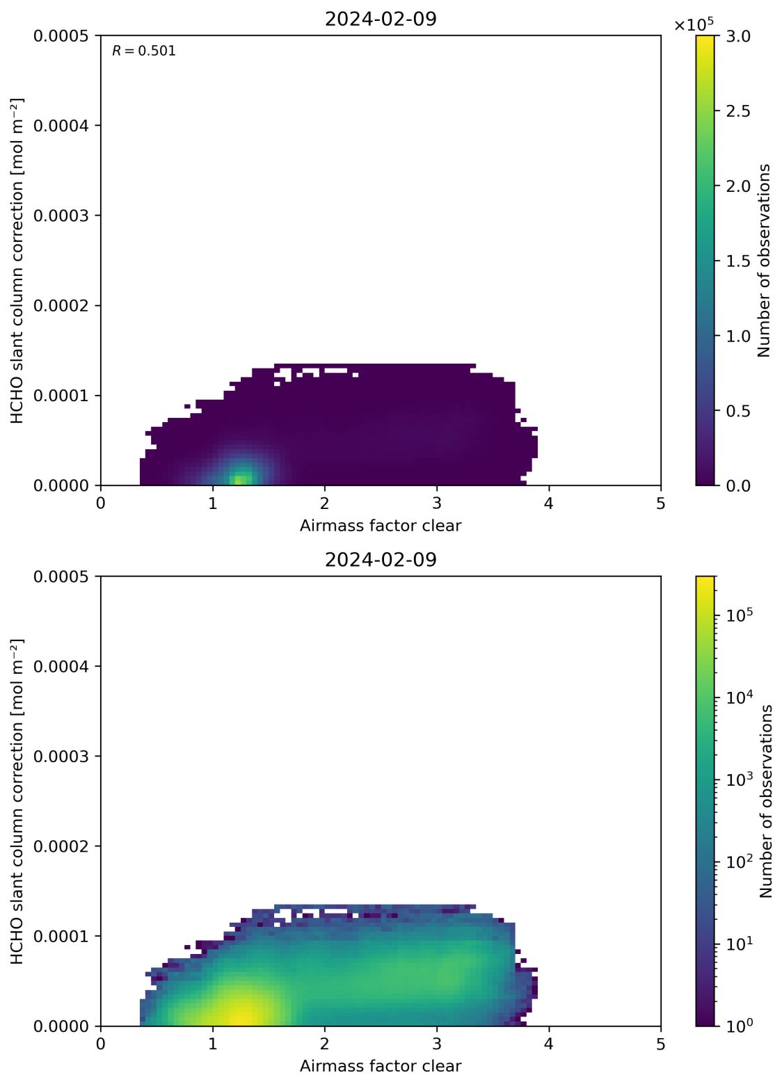
Figure 75: Scatter density plot of “Airmass factor clear” against “HCHO slant column correction” for 2024-02-08 to 2024-02-10.
