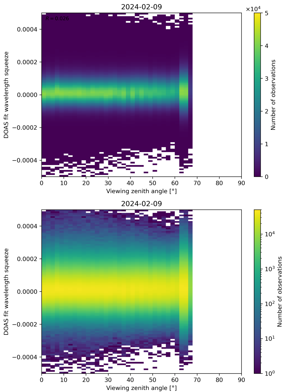
Figure 184: Scatter density plot of “Viewing zenith angle” against “DOAS fit wavelength squeeze” for 2024-02-08 to 2024-02-10.
