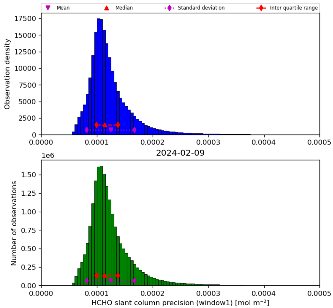
Figure 39: Histogram of “HCHO slant column precision (window1)” for 2024-02-08 to 2024-02-10
