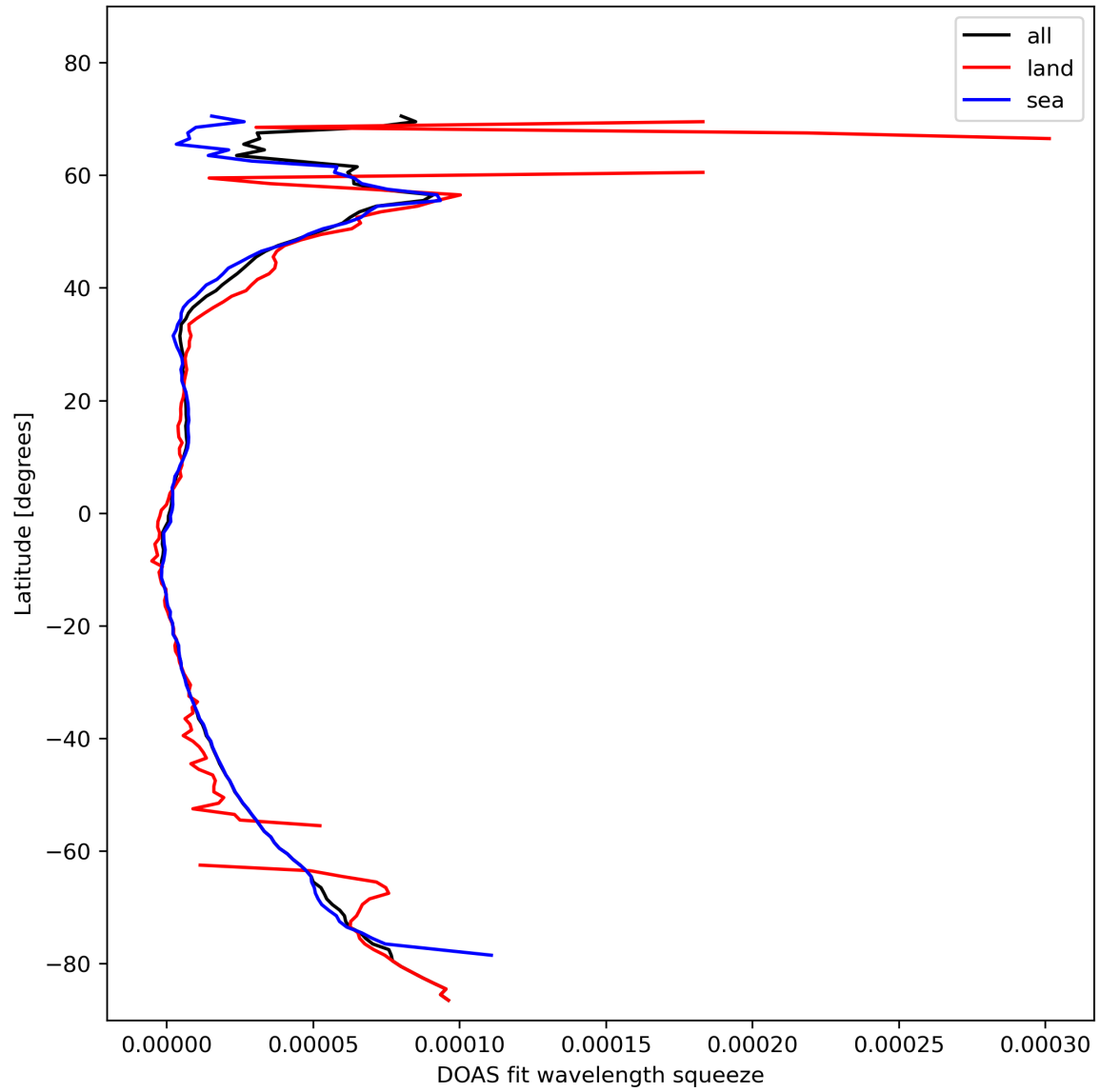
Figure 31: Zonal average of “DOAS fit wavelength squeeze” for 2024-02-08 to 2024-02-10.
