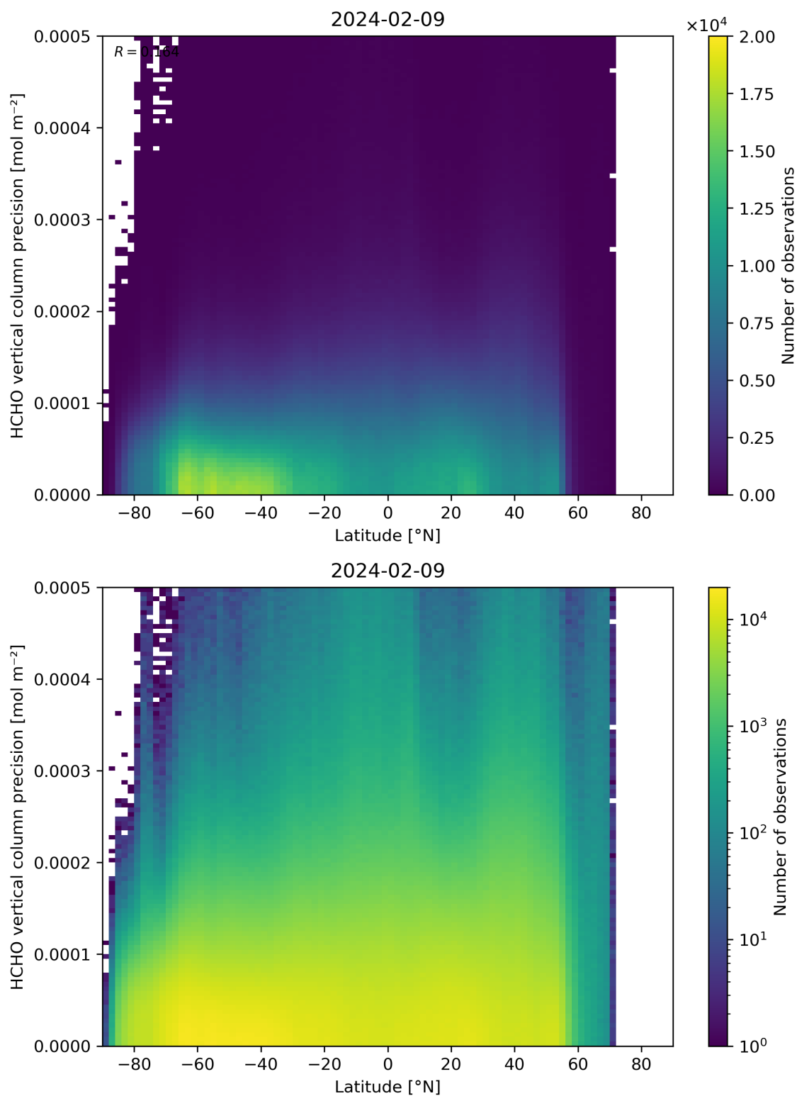
Figure 165: Scatter density plot of “Latitude” against “HCHO vertical column precision” for 2024-02-08 to 2024-02-10.
