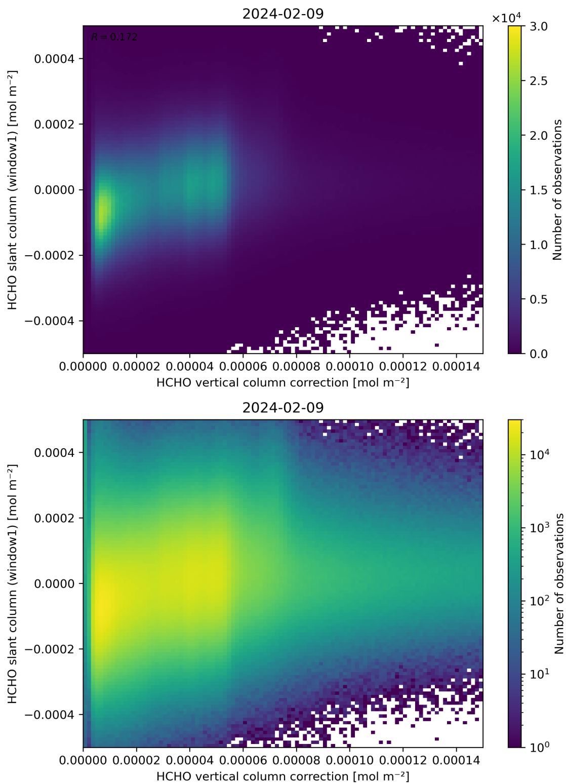
Figure 118: Scatter density plot of “HCHO vertical column correction” against “HCHO slant column (window1)” for 2024-02-08 to 2024-02-10.
