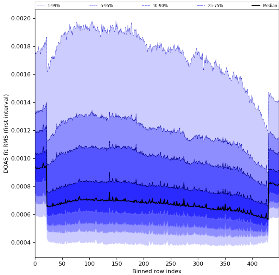
Figure 60: Along track statistics of “DOAS fit RMS (first interval)” for 2024-02-08 to 2024-02-10
