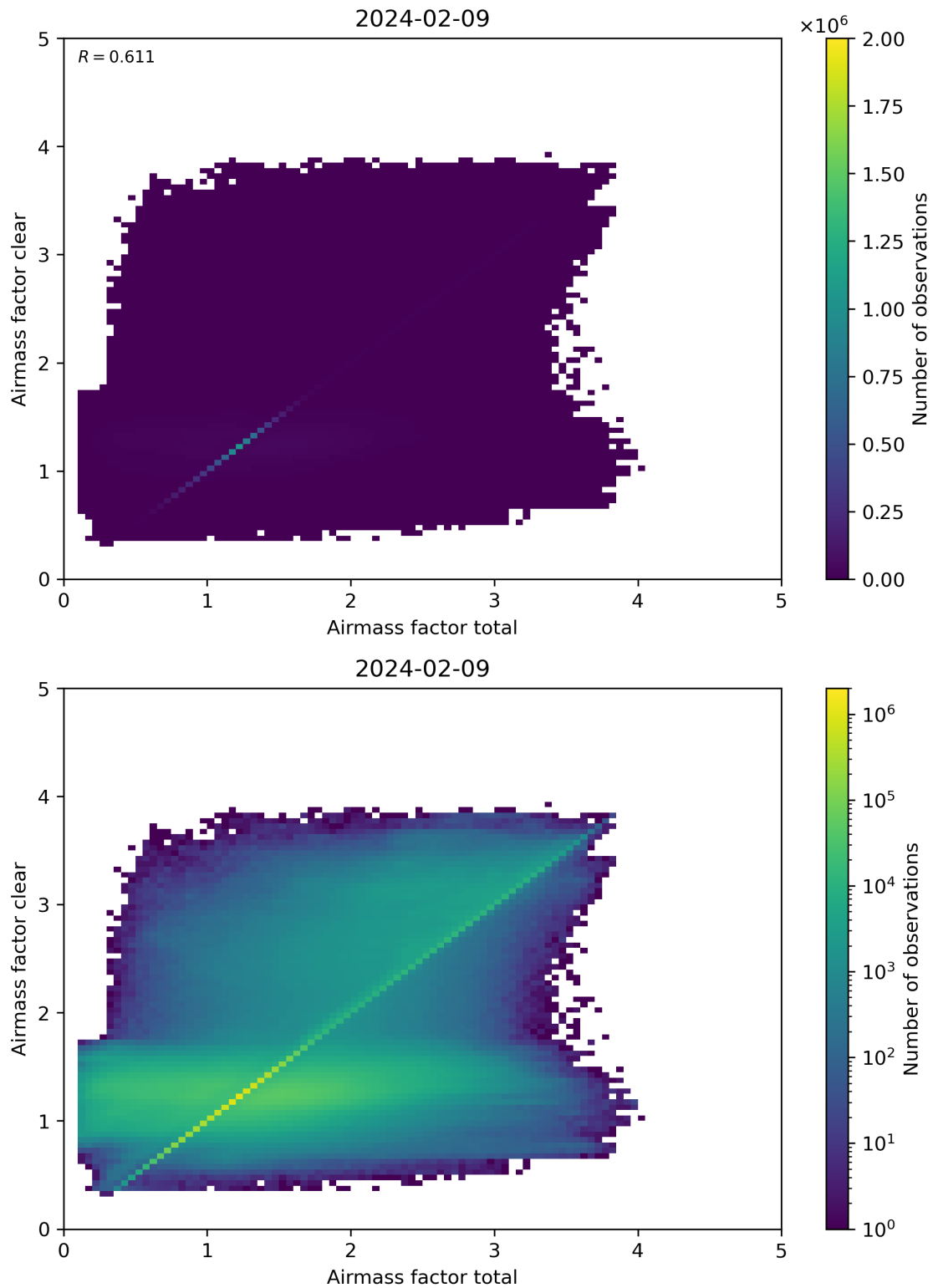
Figure 100: Scatter density plot of “Airmass factor total” against “Airmass factor clear” for 2024-02-08 to 2024-02-10.
