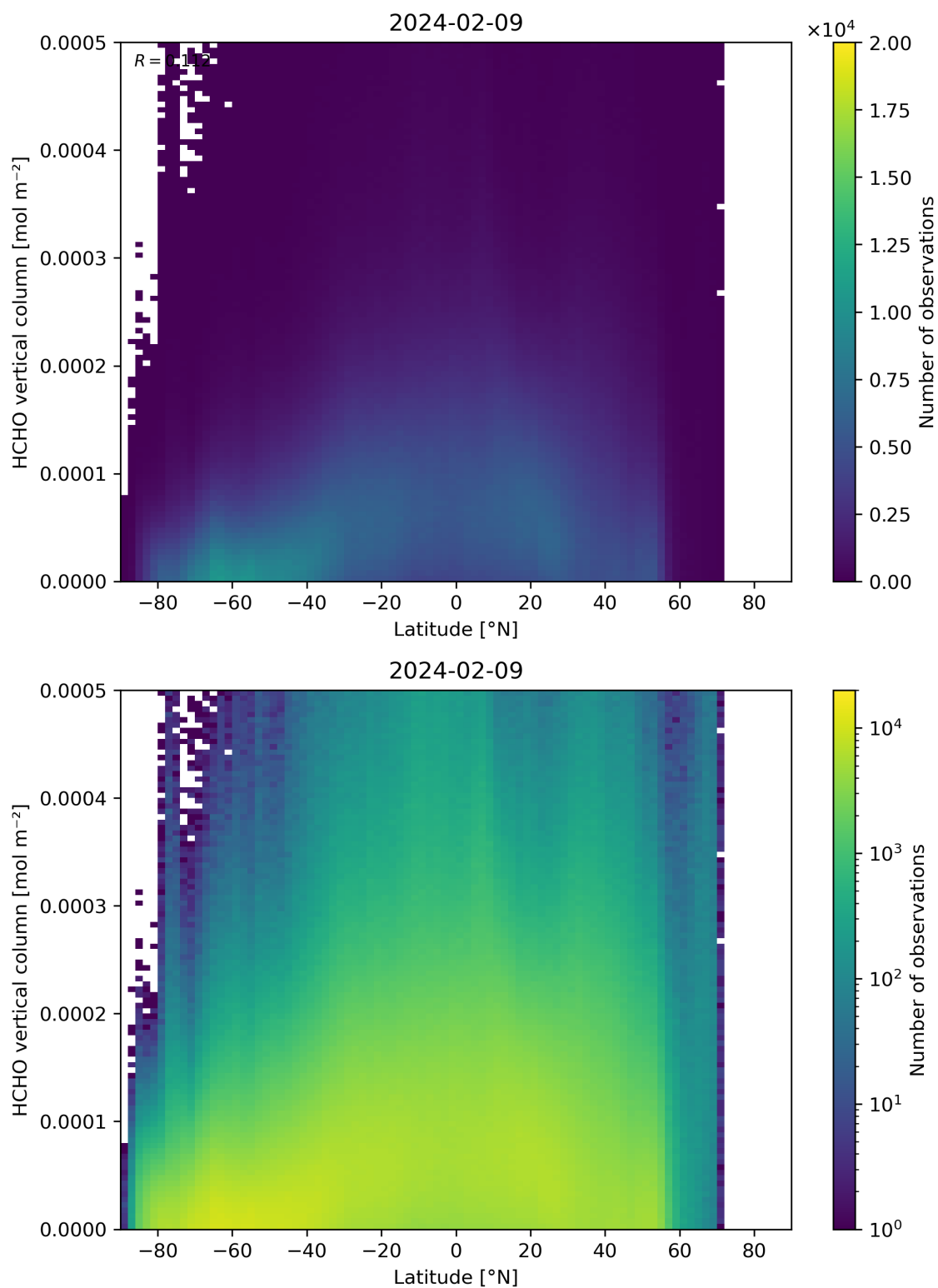
Figure 163: Scatter density plot of “Latitude” against “HCHO vertical column” for 2024-02-08 to 2024-02-10.
