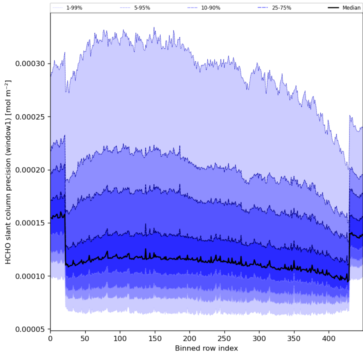
Figure 53: Along track statistics of “HCHO slant column precision (window1)” for 2024-02-08 to 2024-02-10
