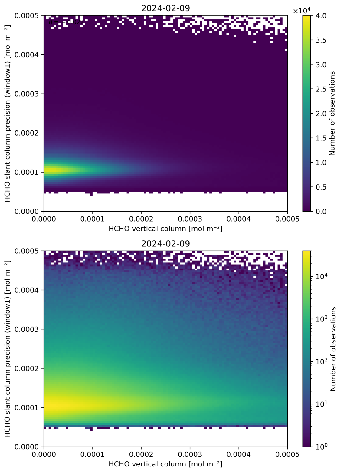
Figure 130: Scatter density plot of “HCHO vertical column” against “HCHO slant column precision (window1)” for 2024-02-08 to 2024-02-10.
