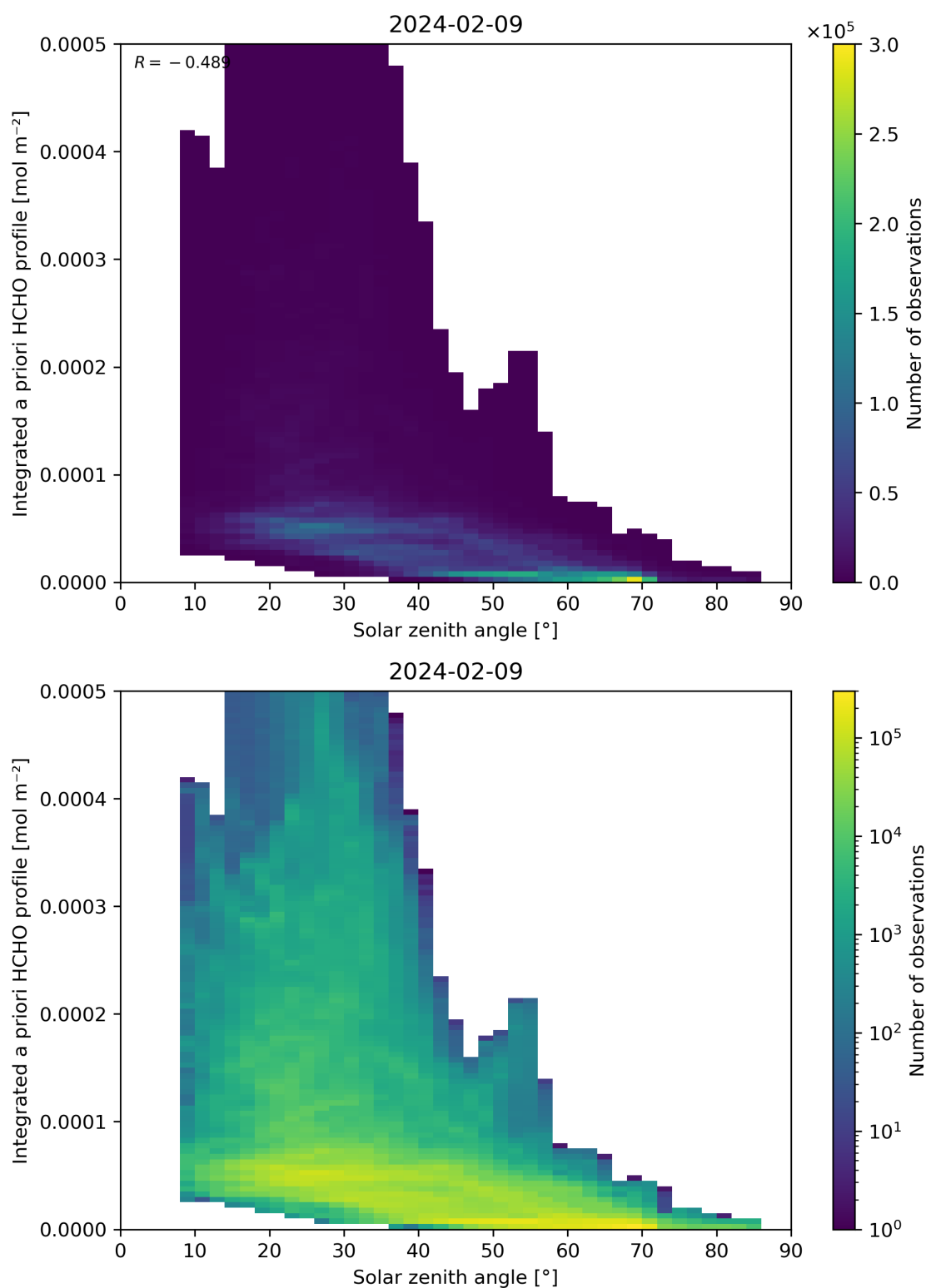
Figure 180: Scatter density plot of “Solar zenith angle” against “Integrated a priori HCHO profile” for 2024-02-08 to 2024-02-10.
