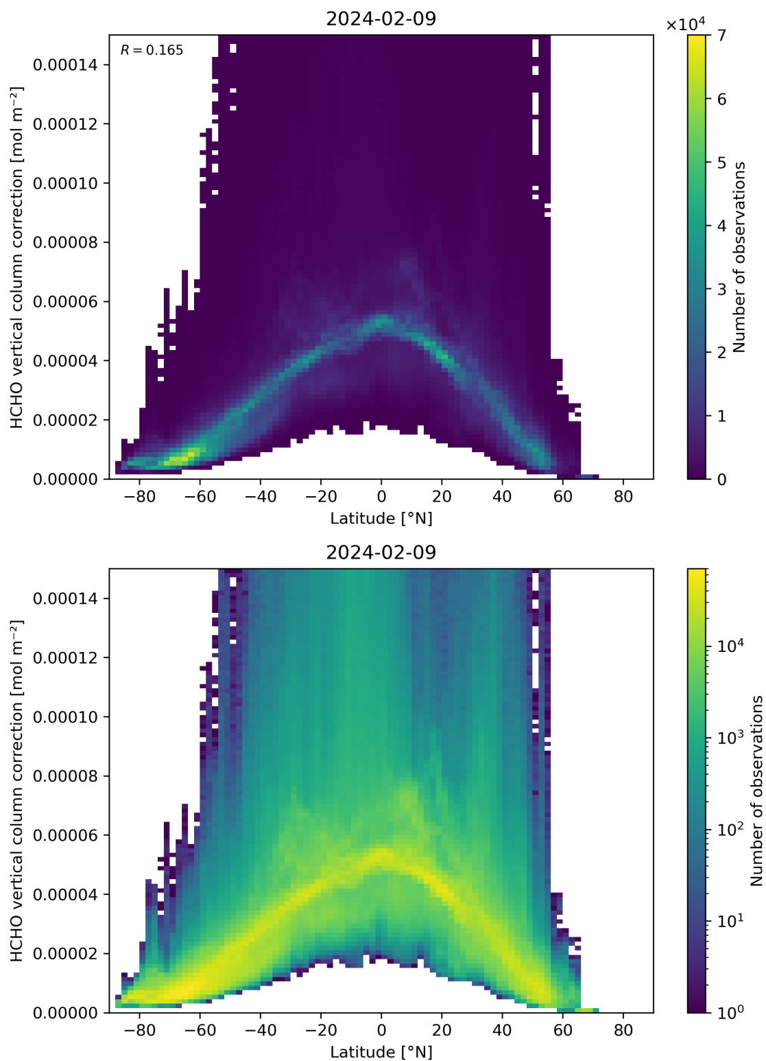
Figure 164: Scatter density plot of “Latitude” against “HCHO vertical column correction” for 2024-02-08 to 2024-02-10.
