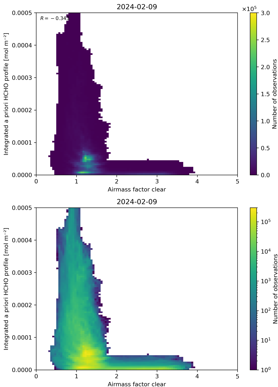
Figure 76: Scatter density plot of “Airmass factor clear” against “Integrated a priori HCHO profile” for 2024-02-08 to 2024-02-10.
