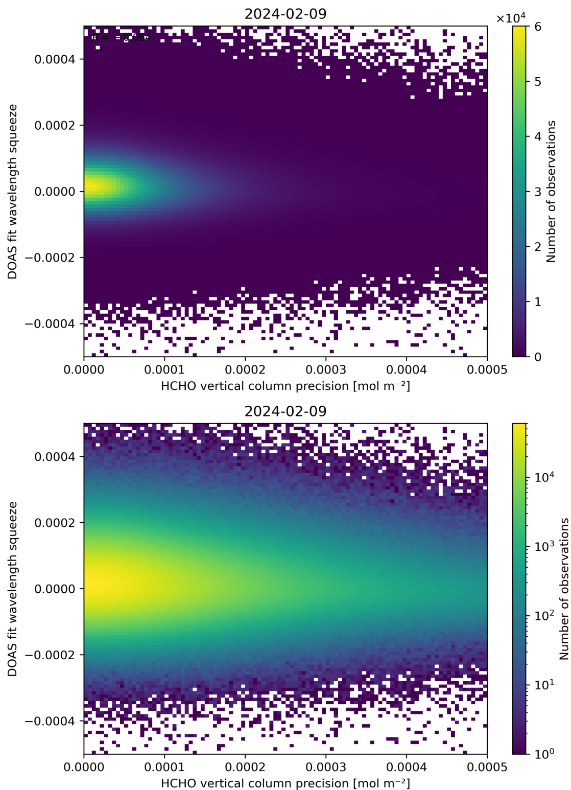
Figure 138: Scatter density plot of “HCHO vertical column precision” against “DOAS fit wavelength squeeze” for 2024-02-08 to 2024-02-10.
