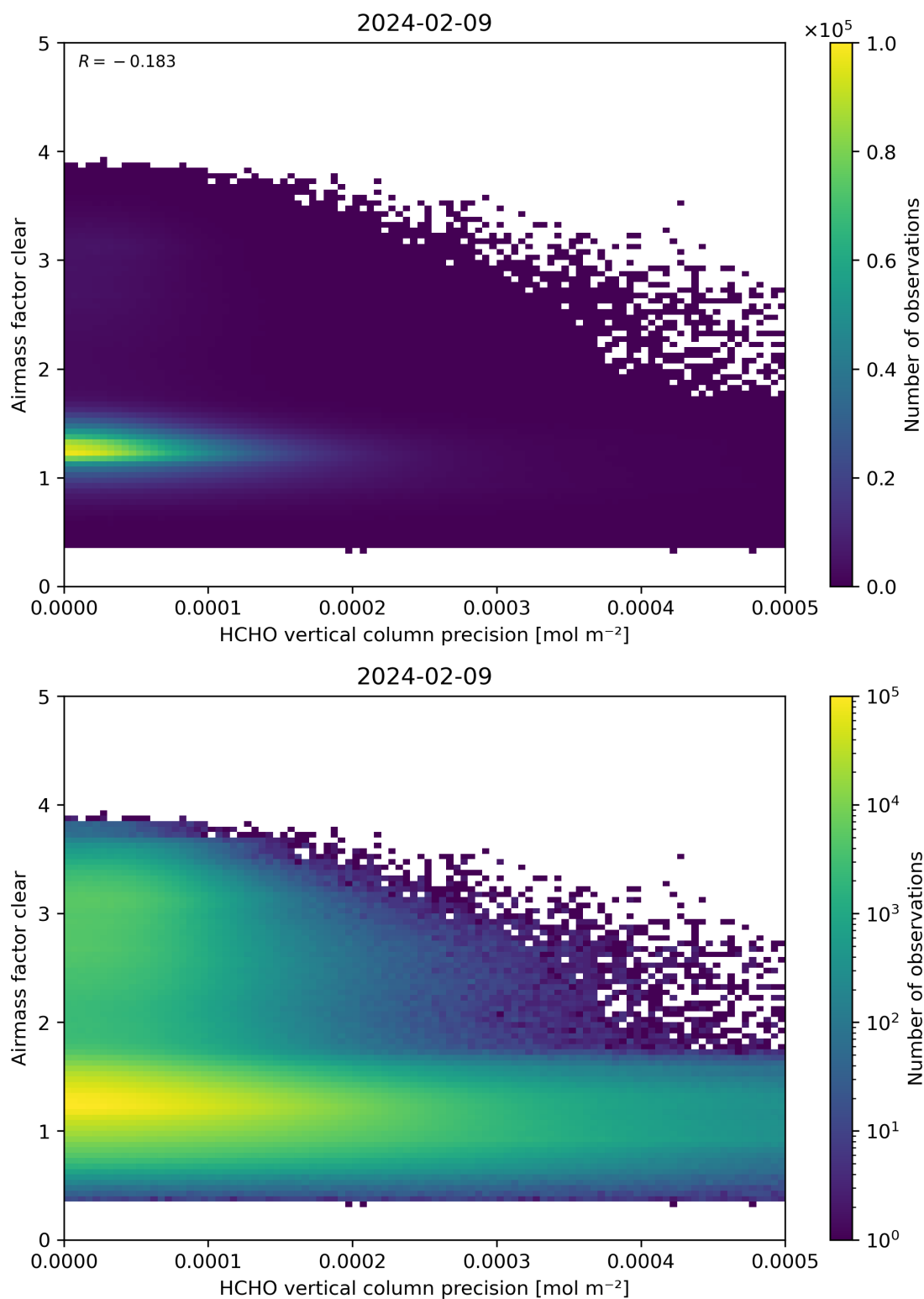
Figure 139: Scatter density plot of “HCHO vertical column precision” against “Airmass factor clear” for 2024-02-08 to 2024-02-10.
