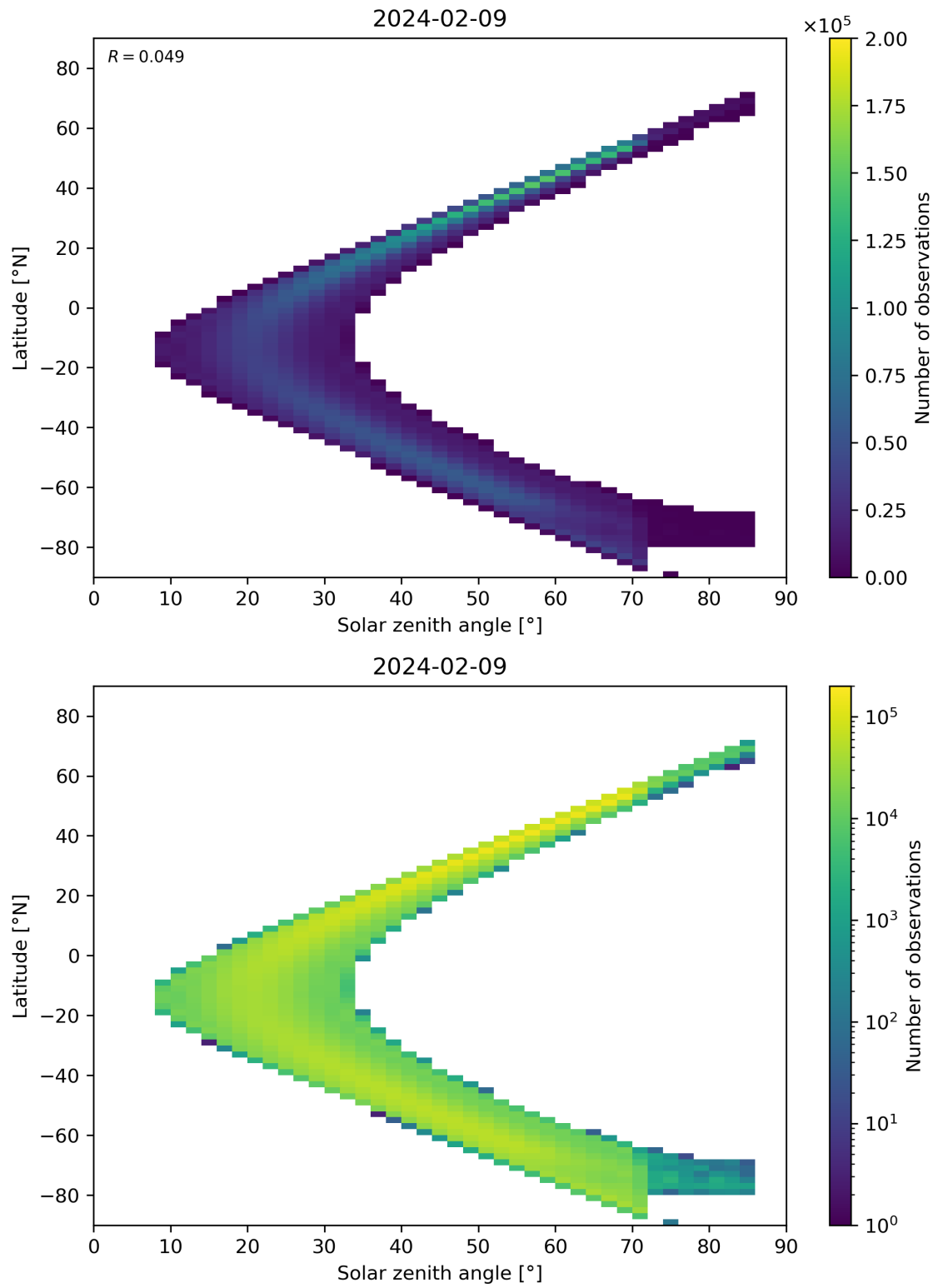
Figure 181: Scatter density plot of “Solar zenith angle” against “Latitude” for 2024-02-08 to 2024-02-10.
