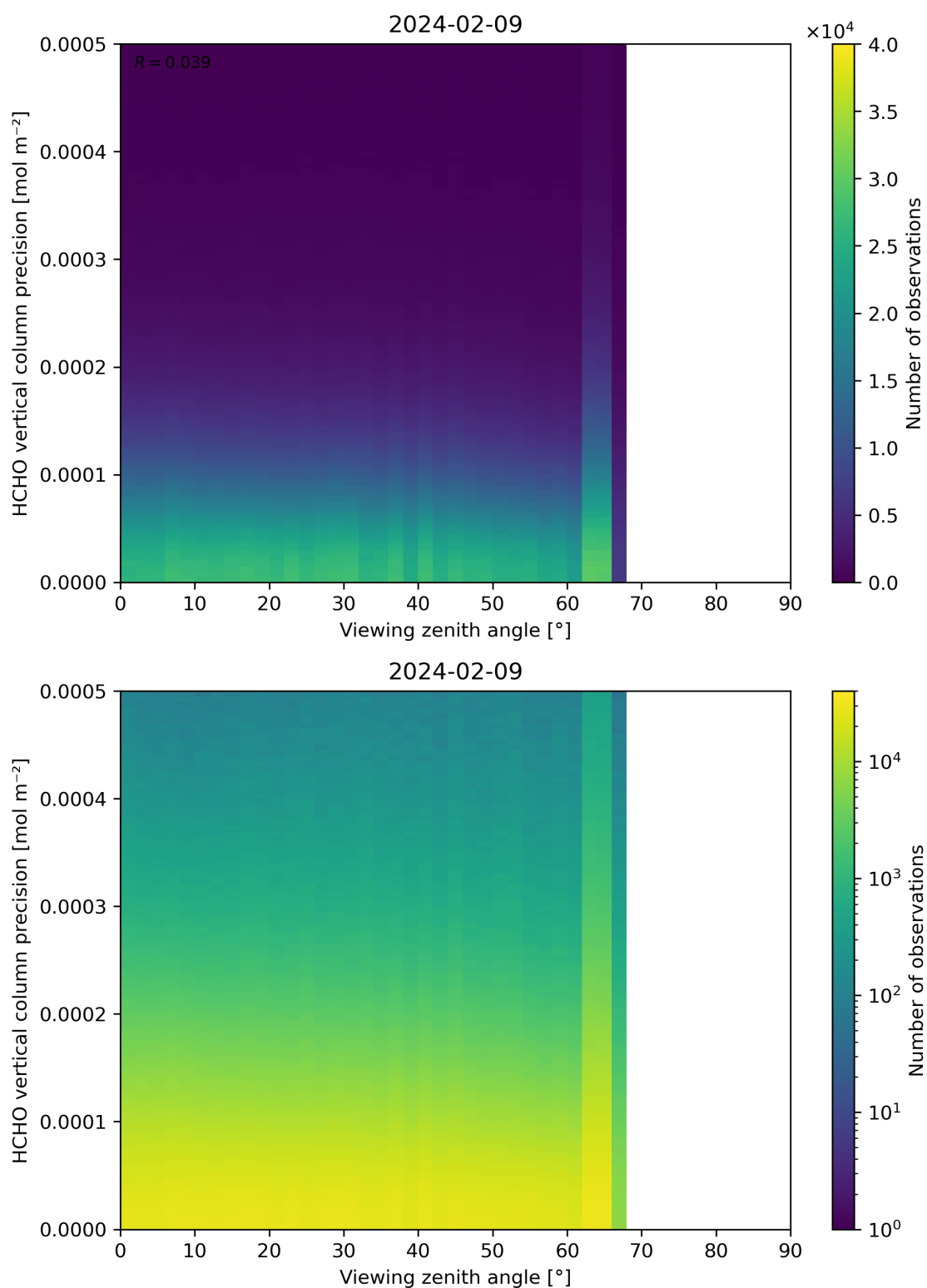
Figure 194: Scatter density plot of “Viewing zenith angle” against “HCHO vertical column precision” for 2024-02-08 to 2024-02-10.
