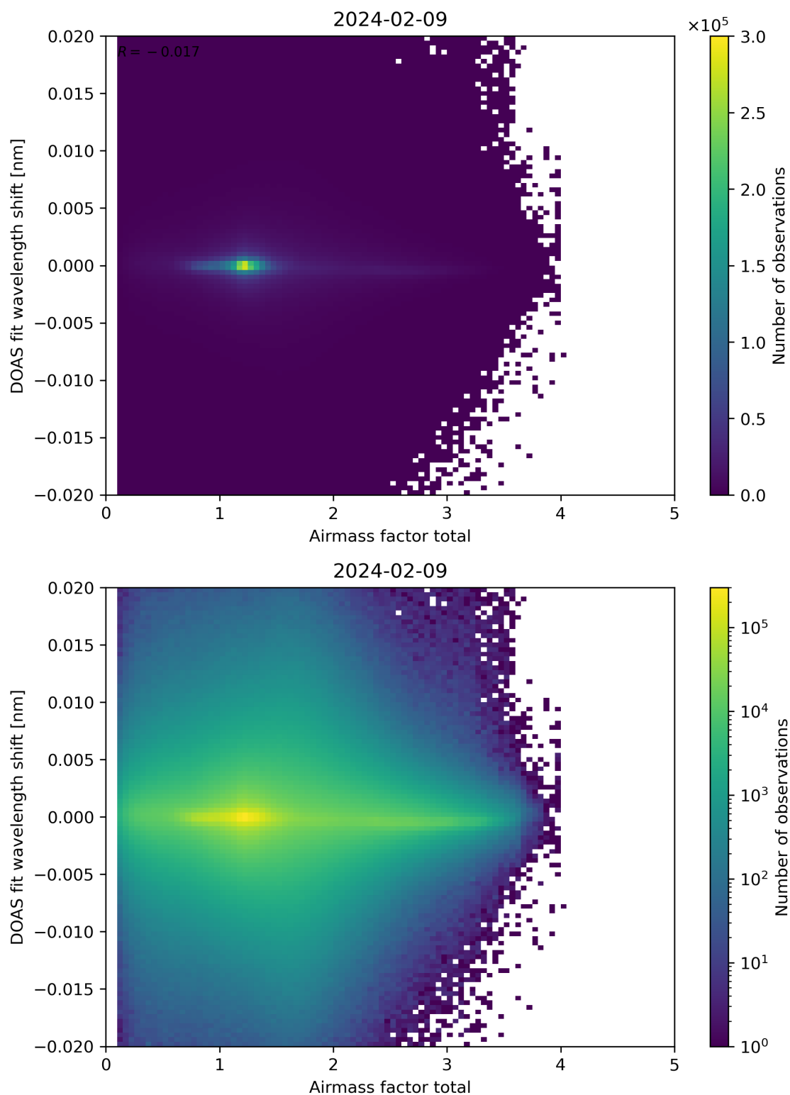
Figure 98: Scatter density plot of “Airmass factor total” against “DOAS fit wavelength shift” for 2024-02-08 to 2024-02-10.
