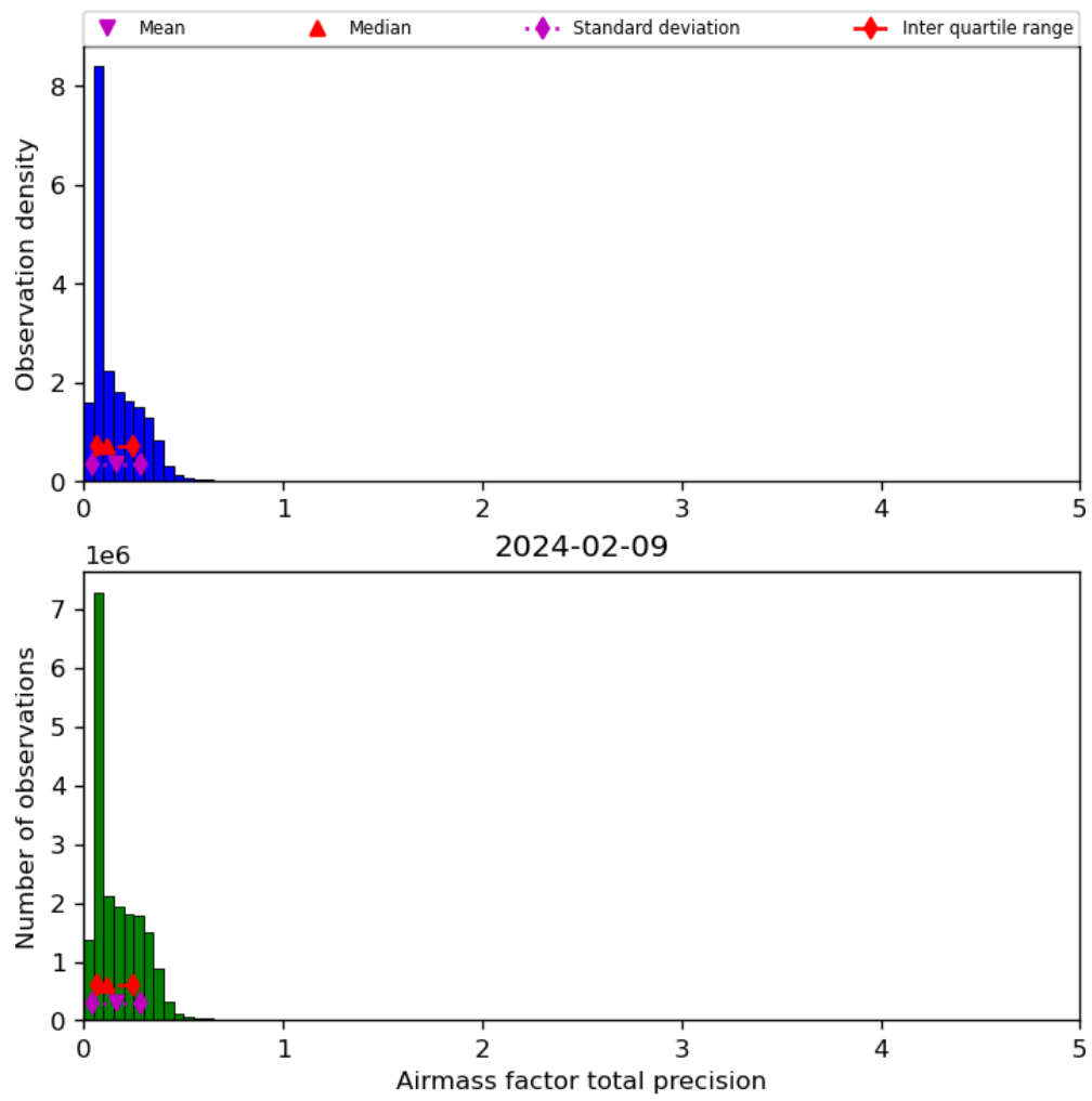
Figure 41: Histogram of “Airmass factor total precision” for 2024-02-08 to 2024-02-10
