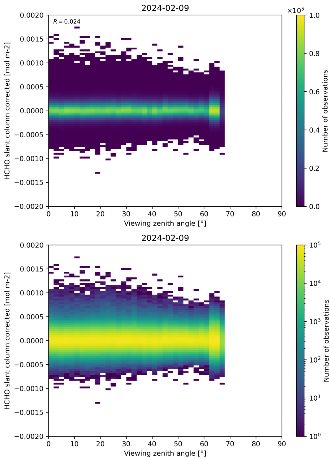
Figure 186: Scatter density plot of “Viewing zenith angle” against “HCHO slant column corrected” for 2024-02-08 to 2024-02-10.
