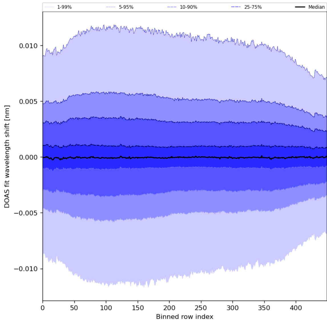
Figure 58: Along track statistics of “DOAS fit wavelength shift” for 2024-02-08 to 2024-02-10
