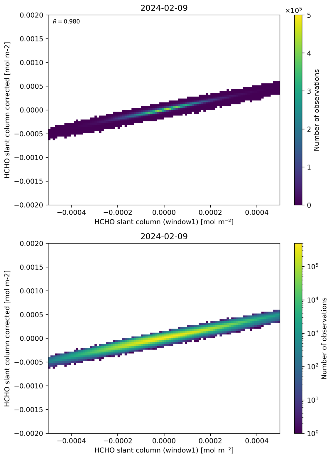
Figure 82: Scatter density plot of “HCHO slant column (window1)” against “HCHO slant column corrected” for 2024-02-08 to 2024-02-10.
