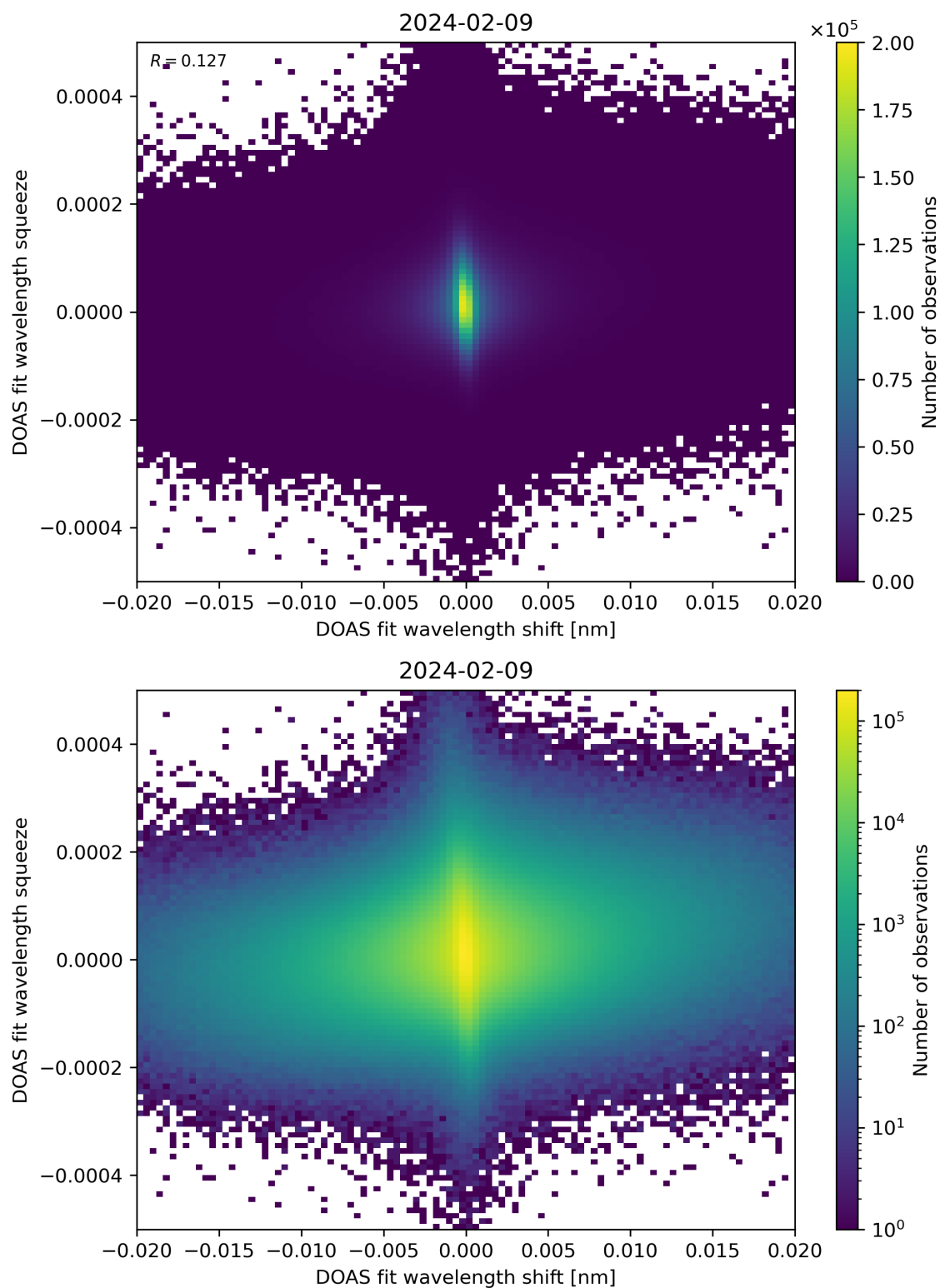
Figure 65: Scatter density plot of “DOAS fit wavelength shift” against “DOAS fit wavelength squeeze” for 2024-02-08 to 2024-02-10.
