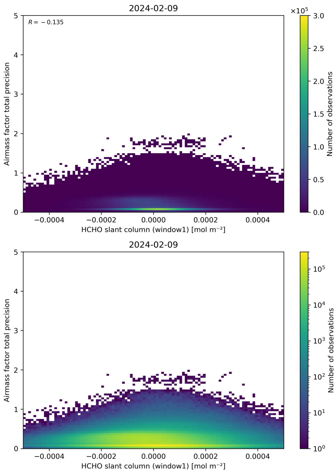
Figure 86: Scatter density plot of “HCHO slant column (window1)” against “Airmass factor total precision” for 2024-02-08 to 2024-02-10.
