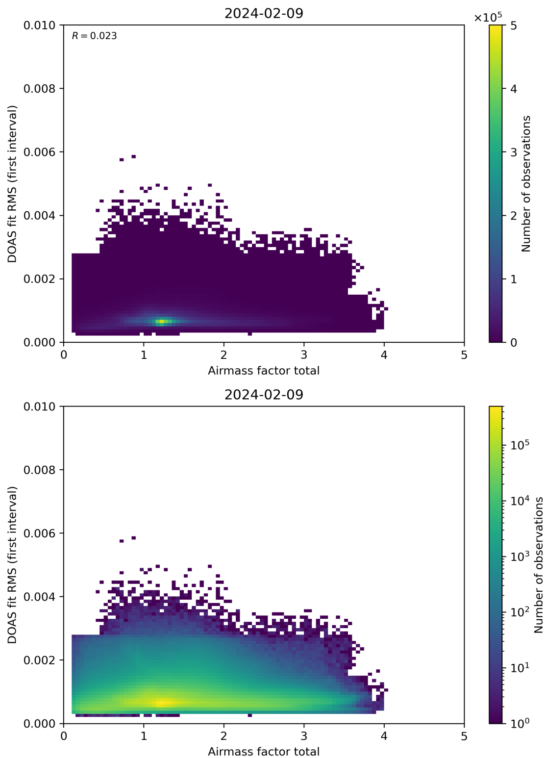
Figure 97: Scatter density plot of “Airmass factor total” against “DOAS fit RMS (first interval)” for 2024-02-08 to 2024-02-10.
