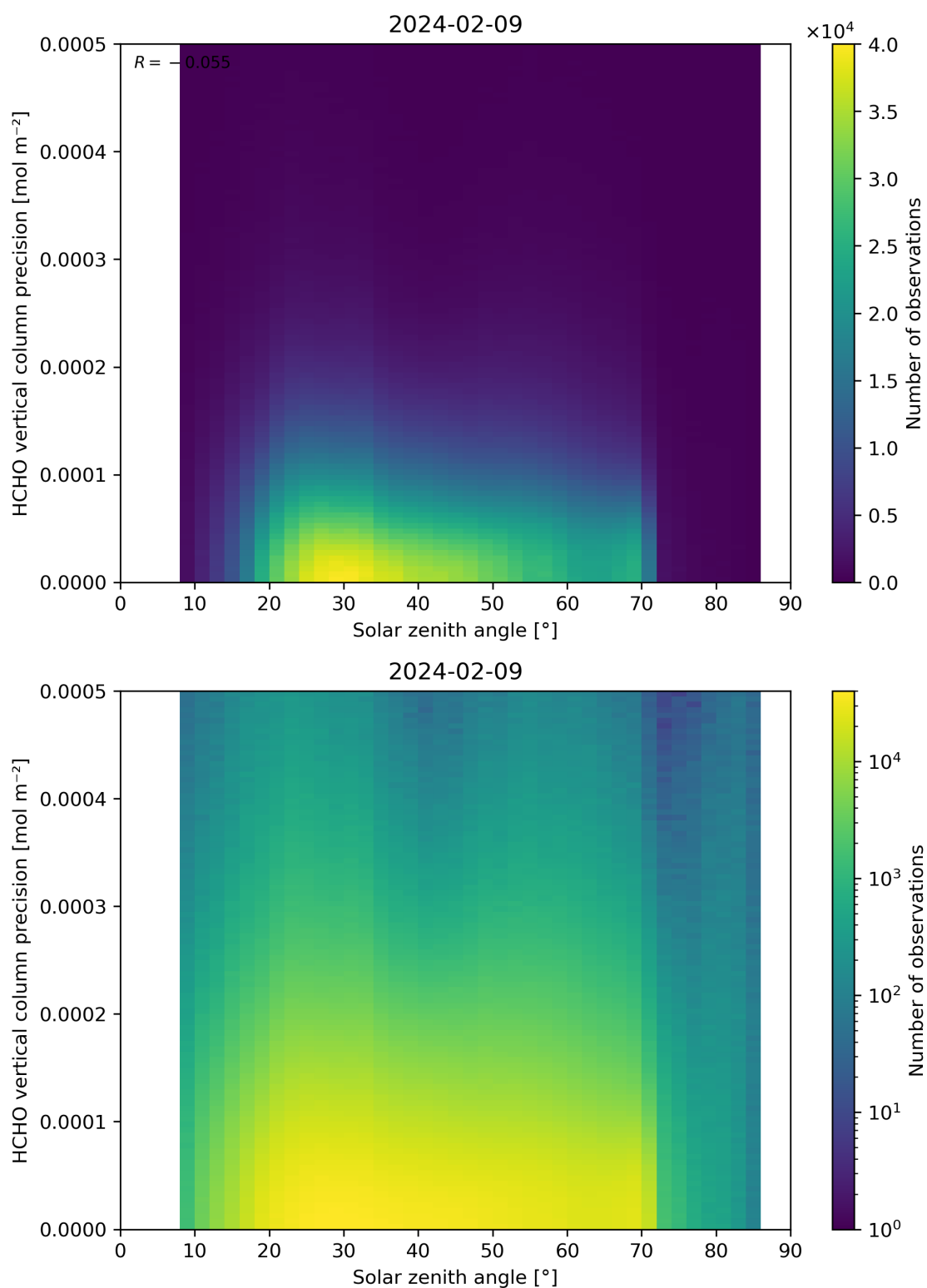
Figure 179: Scatter density plot of “Solar zenith angle” against “HCHO vertical column precision” for 2024-02-08 to 2024-02-10.
