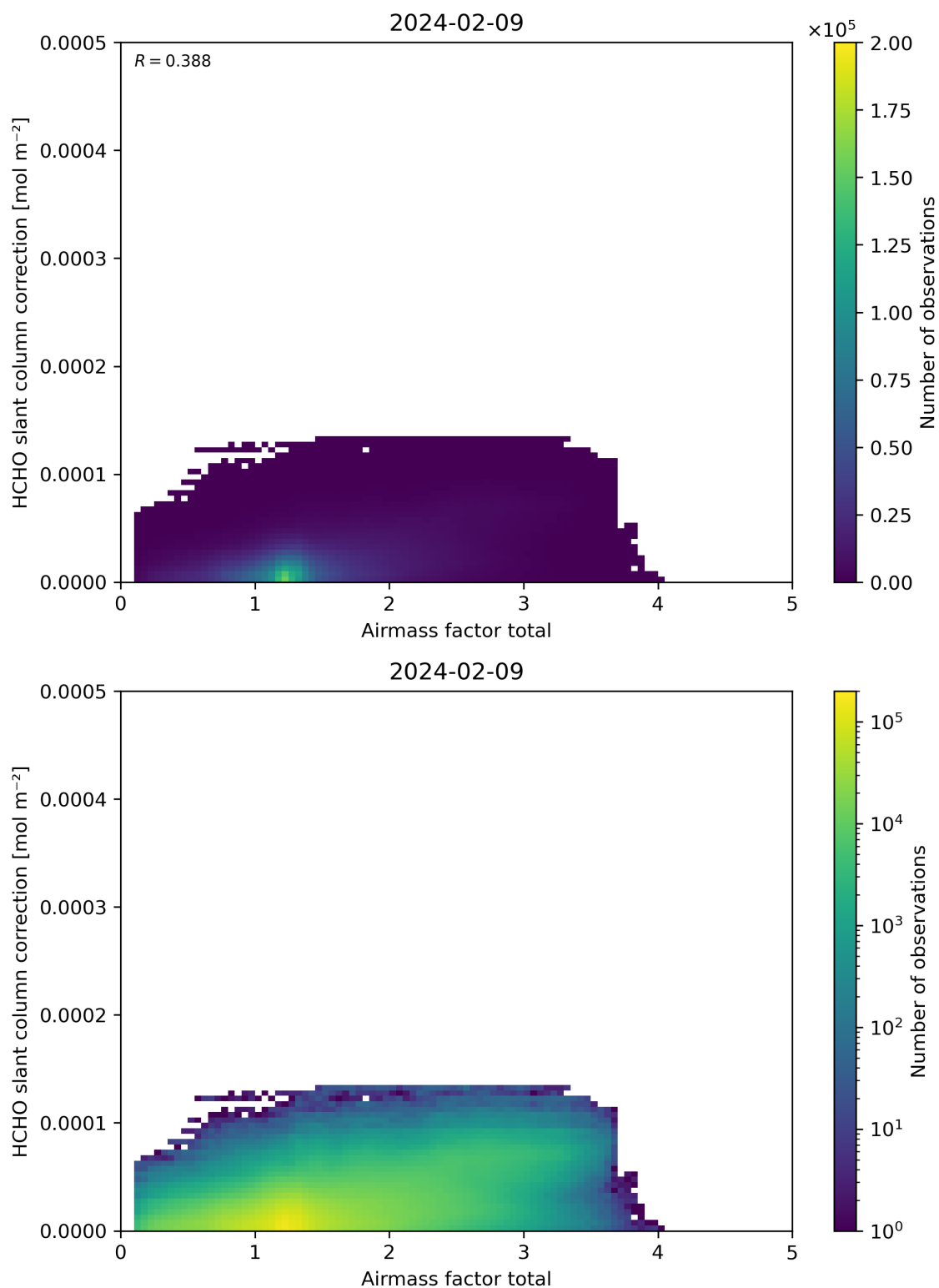
Figure 102: Scatter density plot of “Airmass factor total” against “HCHO slant column correction” for 2024-02-08 to 2024-02-10.
