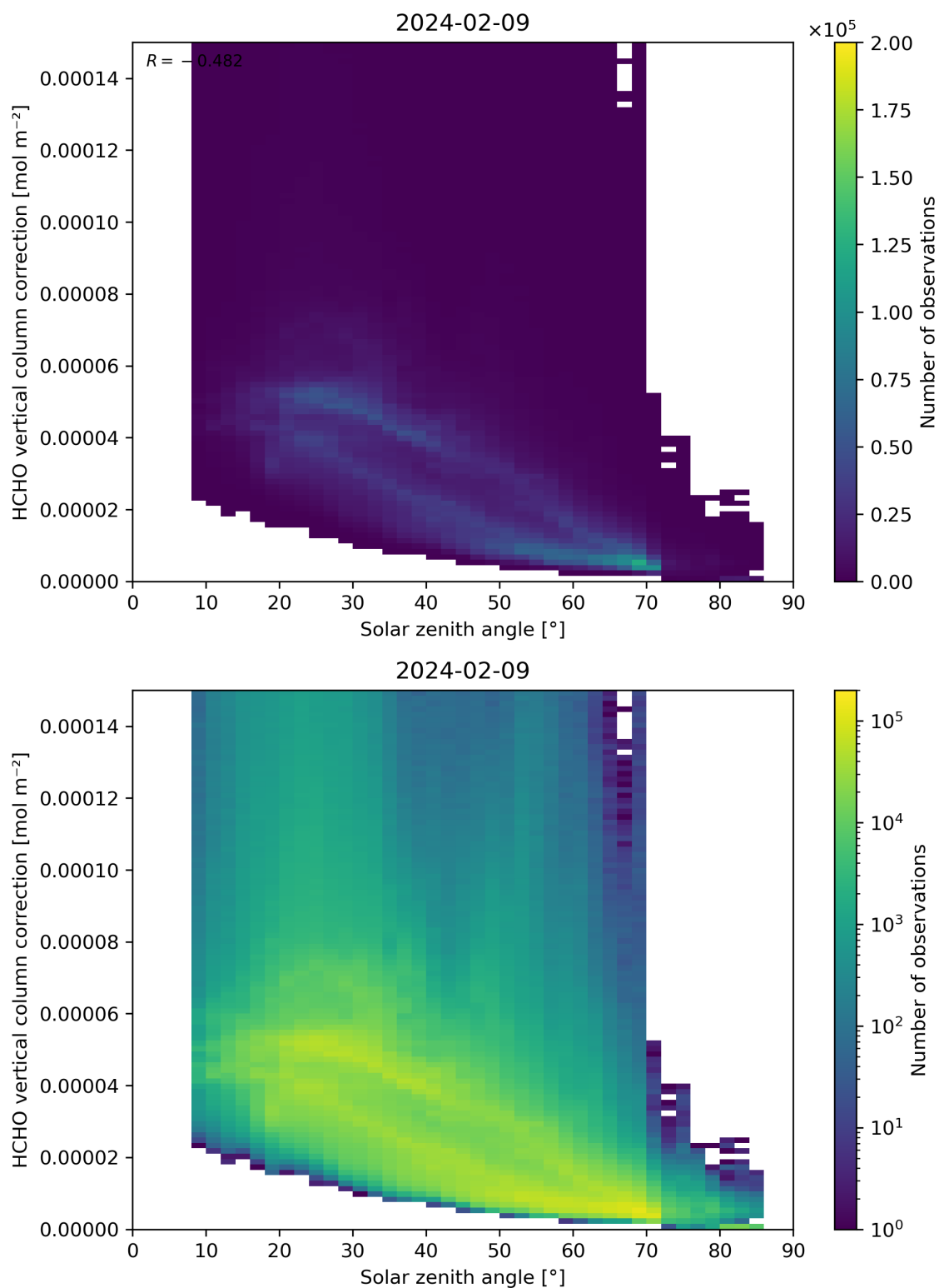
Figure 178: Scatter density plot of “Solar zenith angle” against “HCHO vertical column correction” for 2024-02-08 to 2024-02-10.
