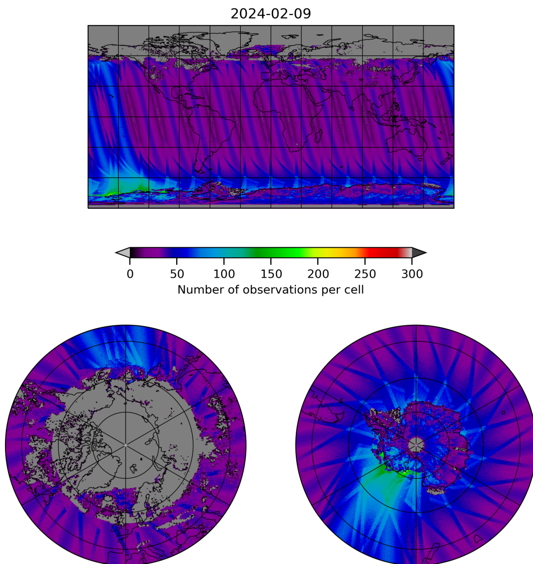
Figure 19: Map of the number of observations for 2024-02-08 to 2024-02-10
