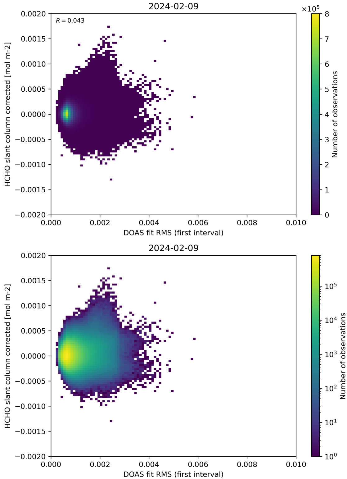
Figure 62: Scatter density plot of “DOAS fit RMS (first interval)” against “HCHO slant column corrected” for 2024-02-08 to 2024-02-10.
