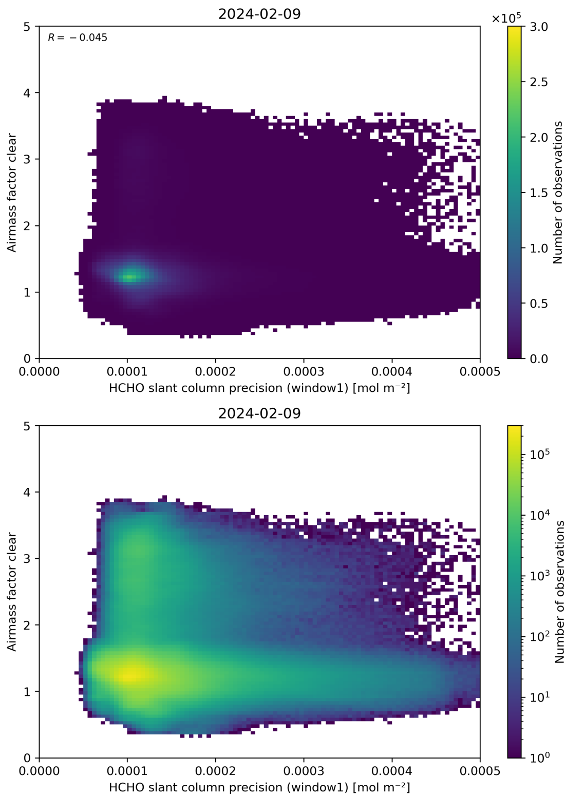
Figure 91: Scatter density plot of “HCHO slant column precision (window1)” against “Airmass factor clear” for 2024-02-08 to 2024-02-10.
