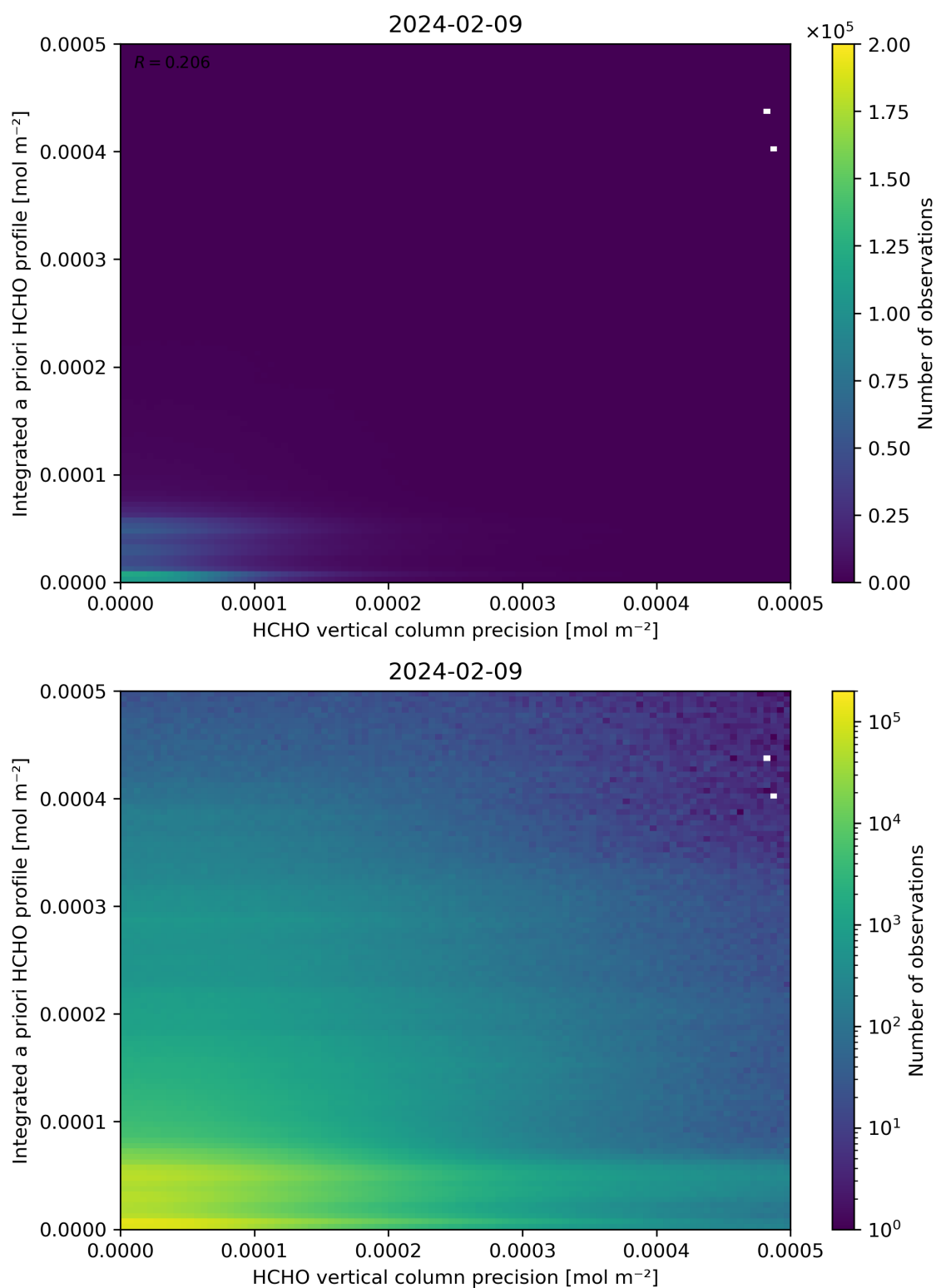
Figure 147: Scatter density plot of “HCHO vertical column precision” against “Integrated a priori HCHO profile” for 2024-02-08 to 2024-02-10.
