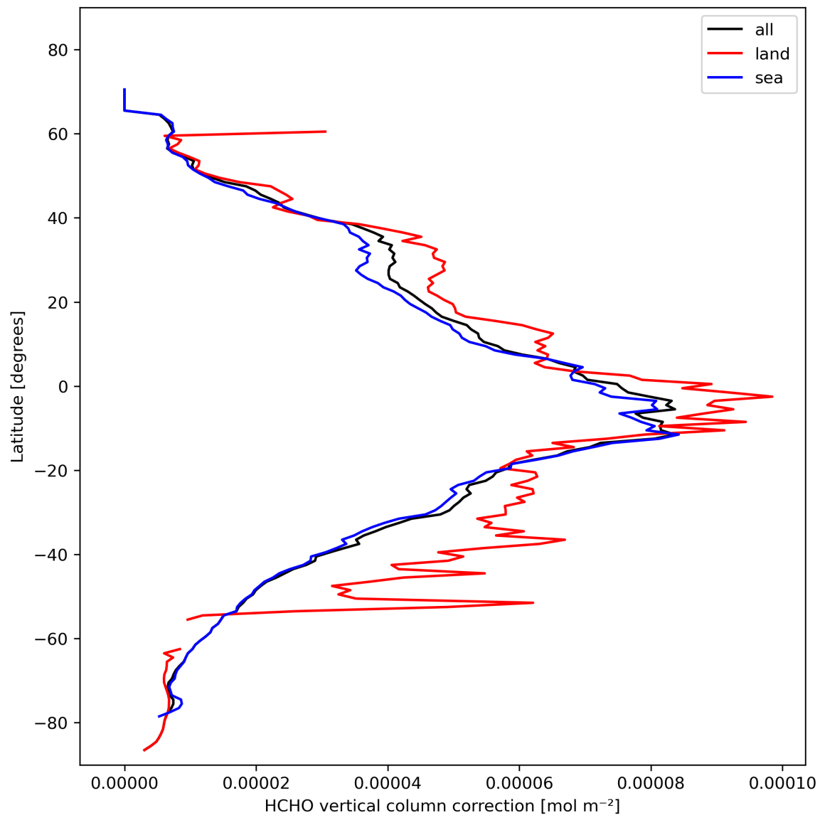
Figure 23: Zonal average of “HCHO vertical column correction” for 2024-02-08 to 2024-02-10.
