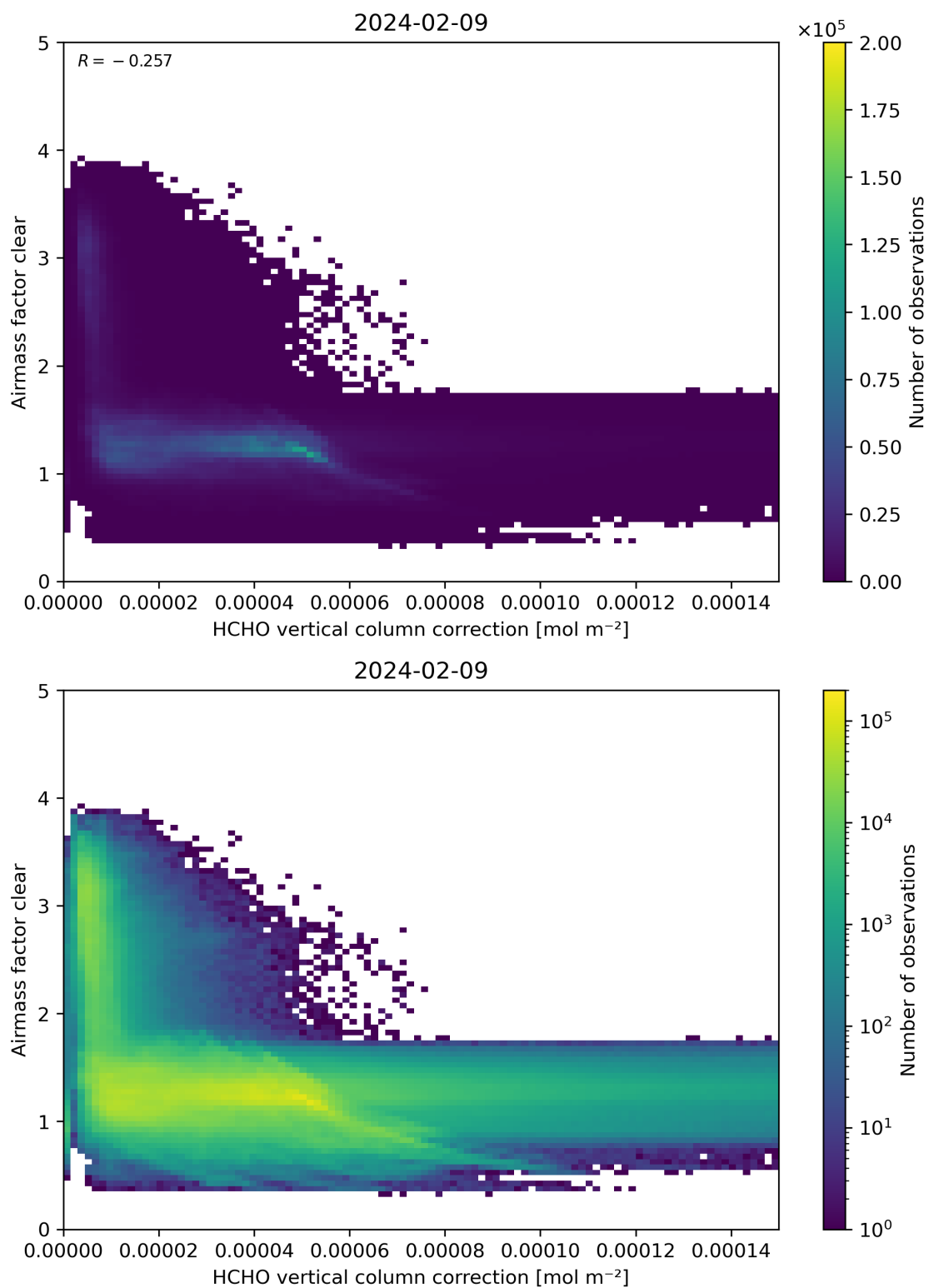
Figure 115: Scatter density plot of “HCHO vertical column correction” against “Airmass factor clear” for 2024-02-08 to 2024-02-10.
