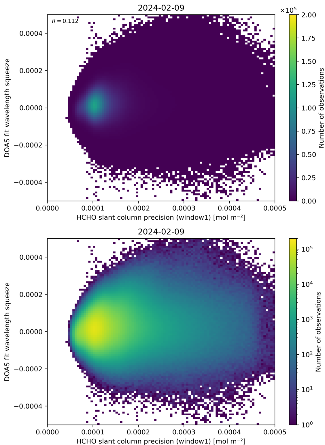
Figure 90: Scatter density plot of “HCHO slant column precision (window1)” against “DOAS fit wavelength squeeze” for 2024-02-08 to 2024-02-10.
