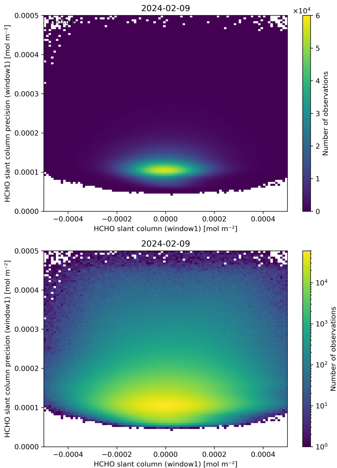
Figure 84: Scatter density plot of “HCHO slant column (window1)” against “HCHO slant column precision (window1)” for 2024-02-08 to 2024-02-10.
