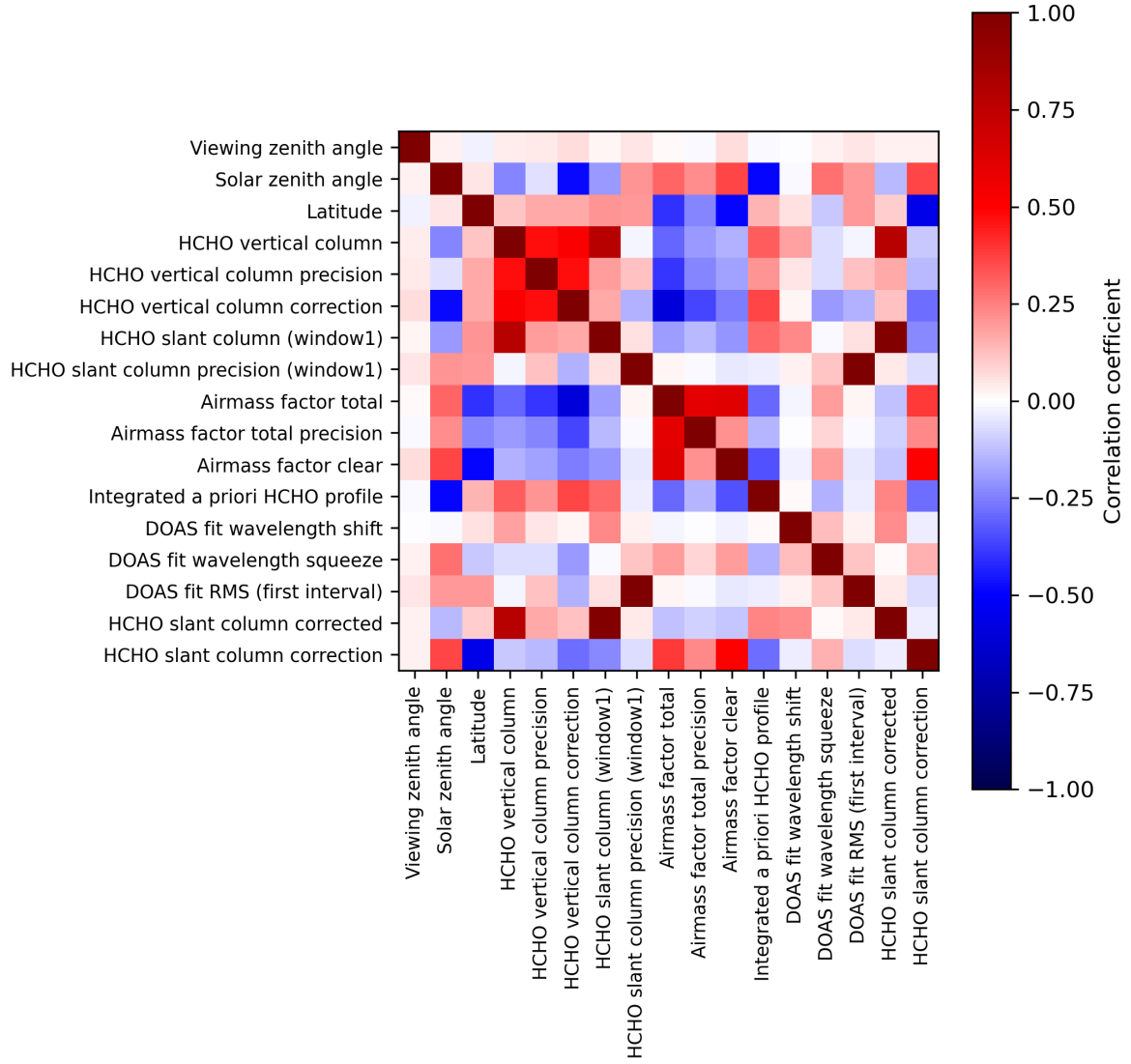
Figure 2: Map of correlation matrix for 2024-02-08 to 2024-02-10.
