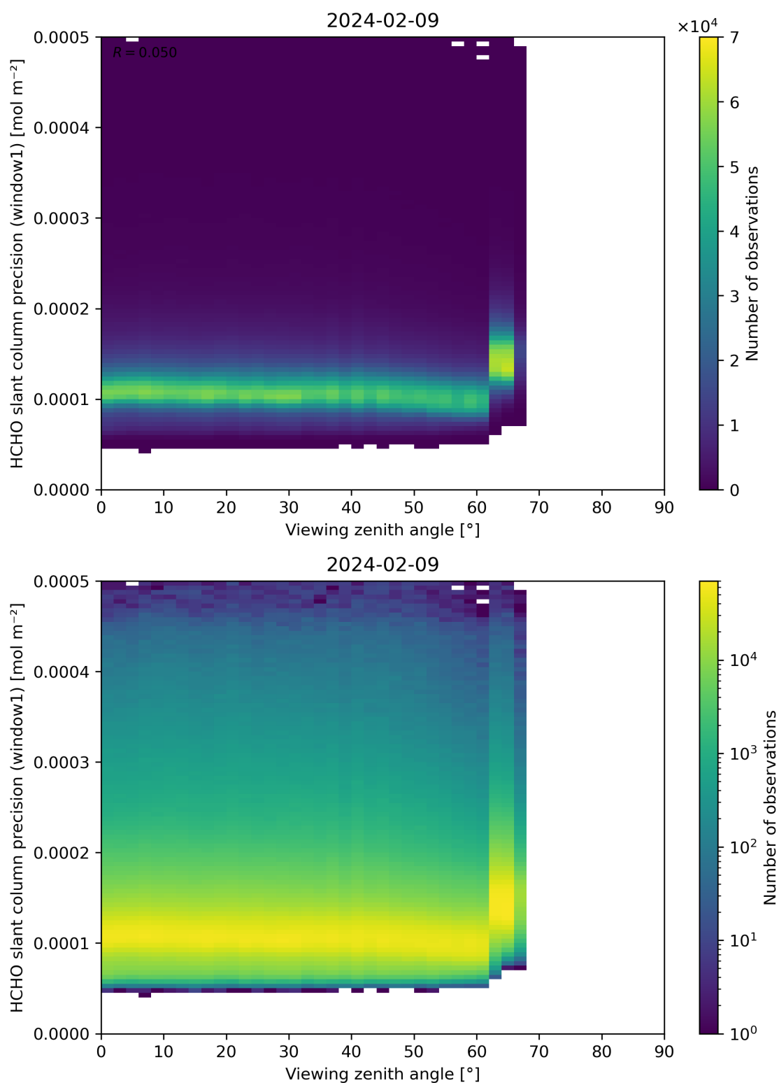
Figure 189: Scatter density plot of “Viewing zenith angle” against “HCHO slant column precision (window1)” for 2024-02-08 to 2024-02-10.
