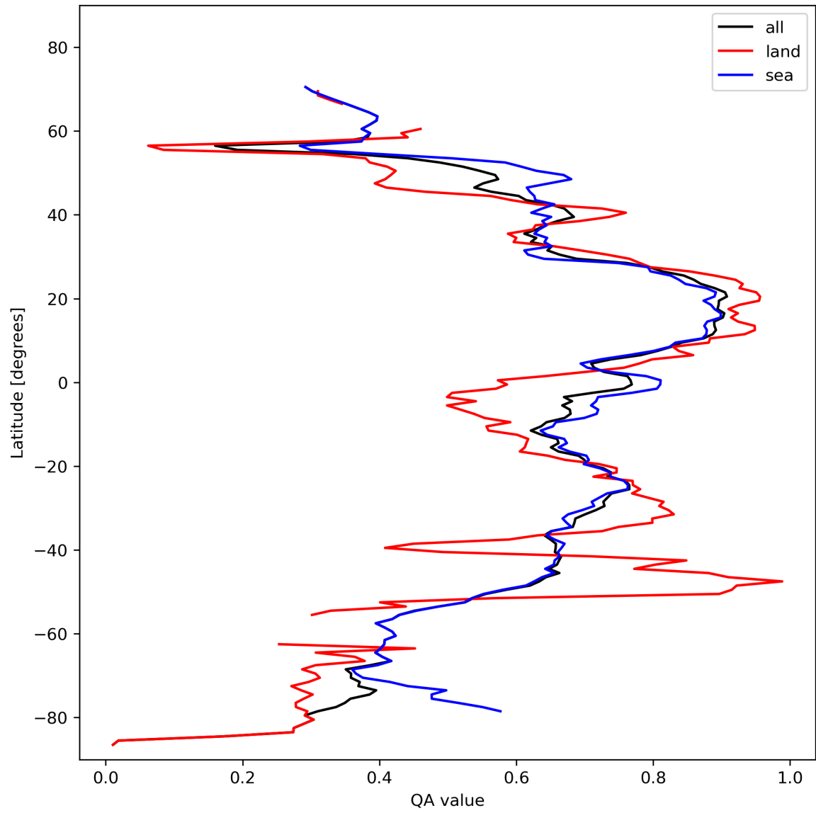
Figure 20: Zonal average of “QA value” for 2024-02-08 to 2024-02-10.
