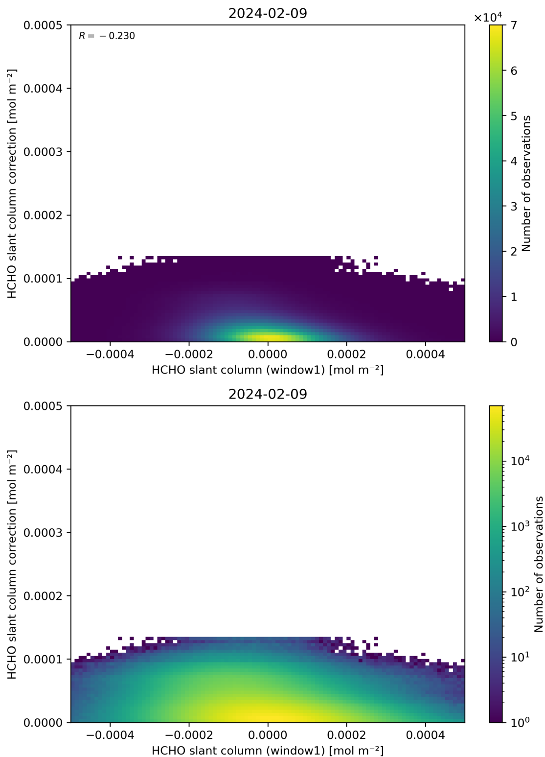
Figure 83: Scatter density plot of “HCHO slant column (window1)” against “HCHO slant column correction” for 2024-02-08 to 2024-02-10.
