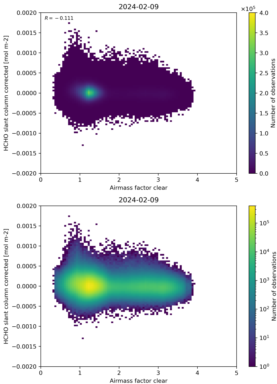
Figure 74: Scatter density plot of “Airmass factor clear” against “HCHO slant column corrected” for 2024-02-08 to 2024-02-10.
