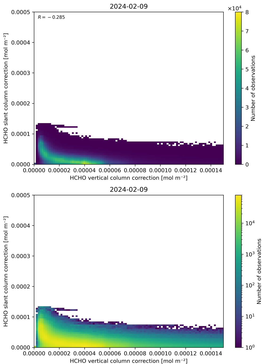
Figure 117: Scatter density plot of “HCHO vertical column correction” against “HCHO slant column correction” for 2024-02-08 to 2024-02-10.
