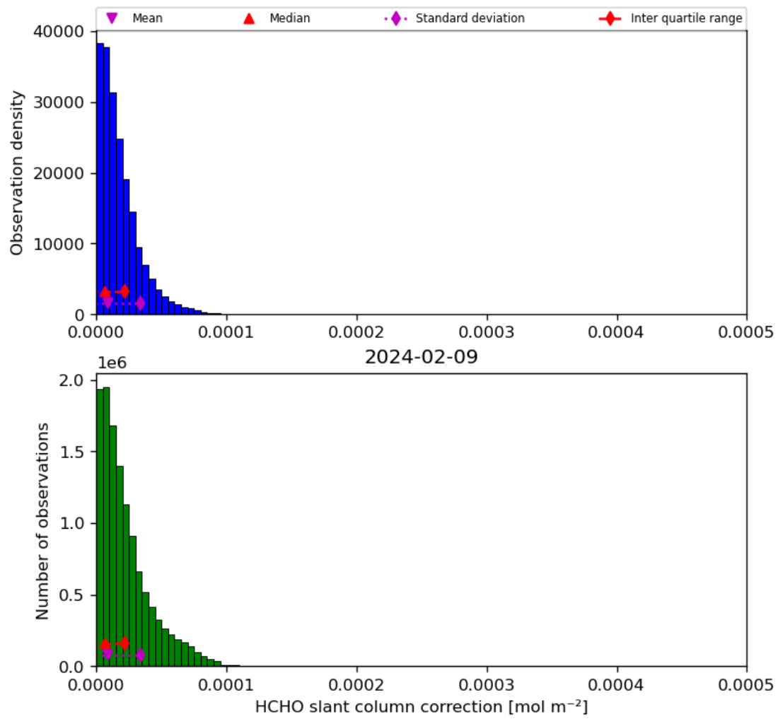
Figure 47: Histogram of “HCHO slant column correction” for 2024-02-08 to 2024-02-10
