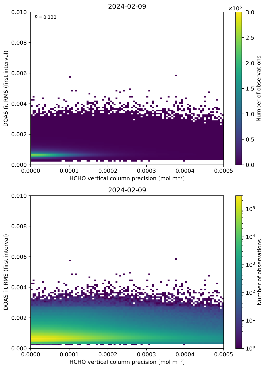
Figure 136: Scatter density plot of “HCHO vertical column precision” against “DOAS fit RMS (first interval)” for 2024-02-08 to 2024-02-10.
