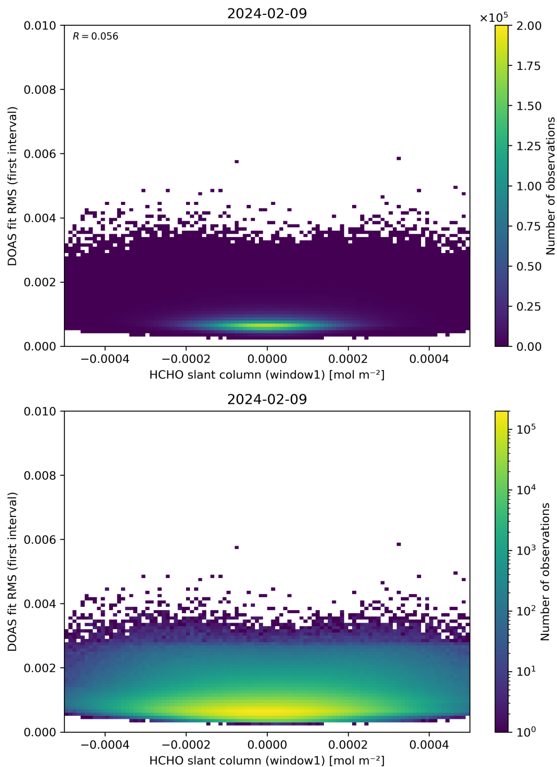
Figure 78: Scatter density plot of “HCHO slant column (window1)” against “DOAS fit RMS (first interval)” for 2024-02-08 to 2024-02-10.
