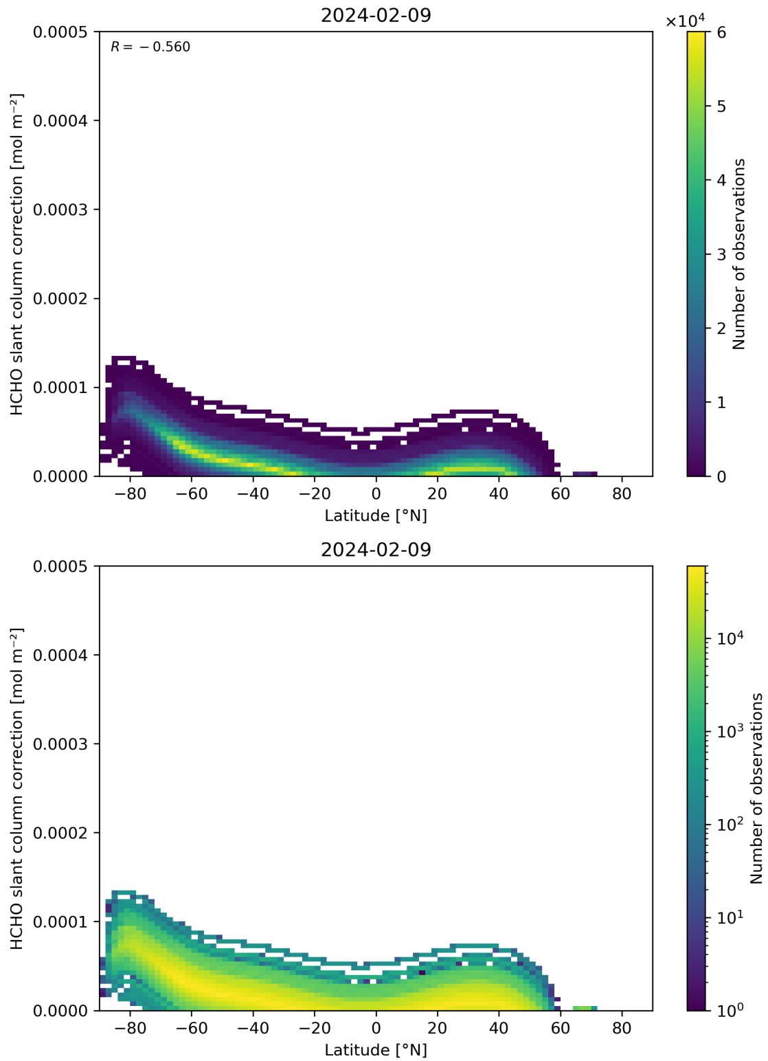
Figure 158: Scatter density plot of “Latitude” against “HCHO slant column correction” for 2024-02-08 to 2024-02-10.
