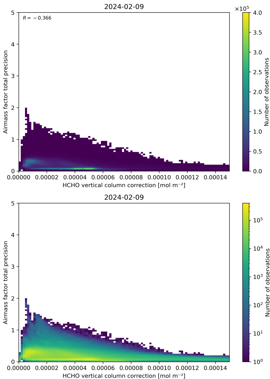
Figure 121: Scatter density plot of “HCHO vertical column correction” against “Airmass factor total precision” for 2024-02-08 to 2024-02-10.
