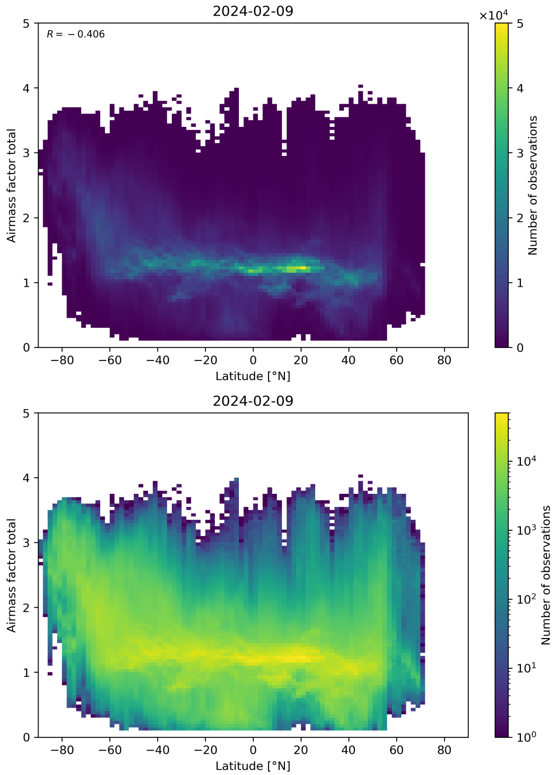
Figure 161: Scatter density plot of “Latitude” against “Airmass factor total” for 2024-02-08 to 2024-02-10.
