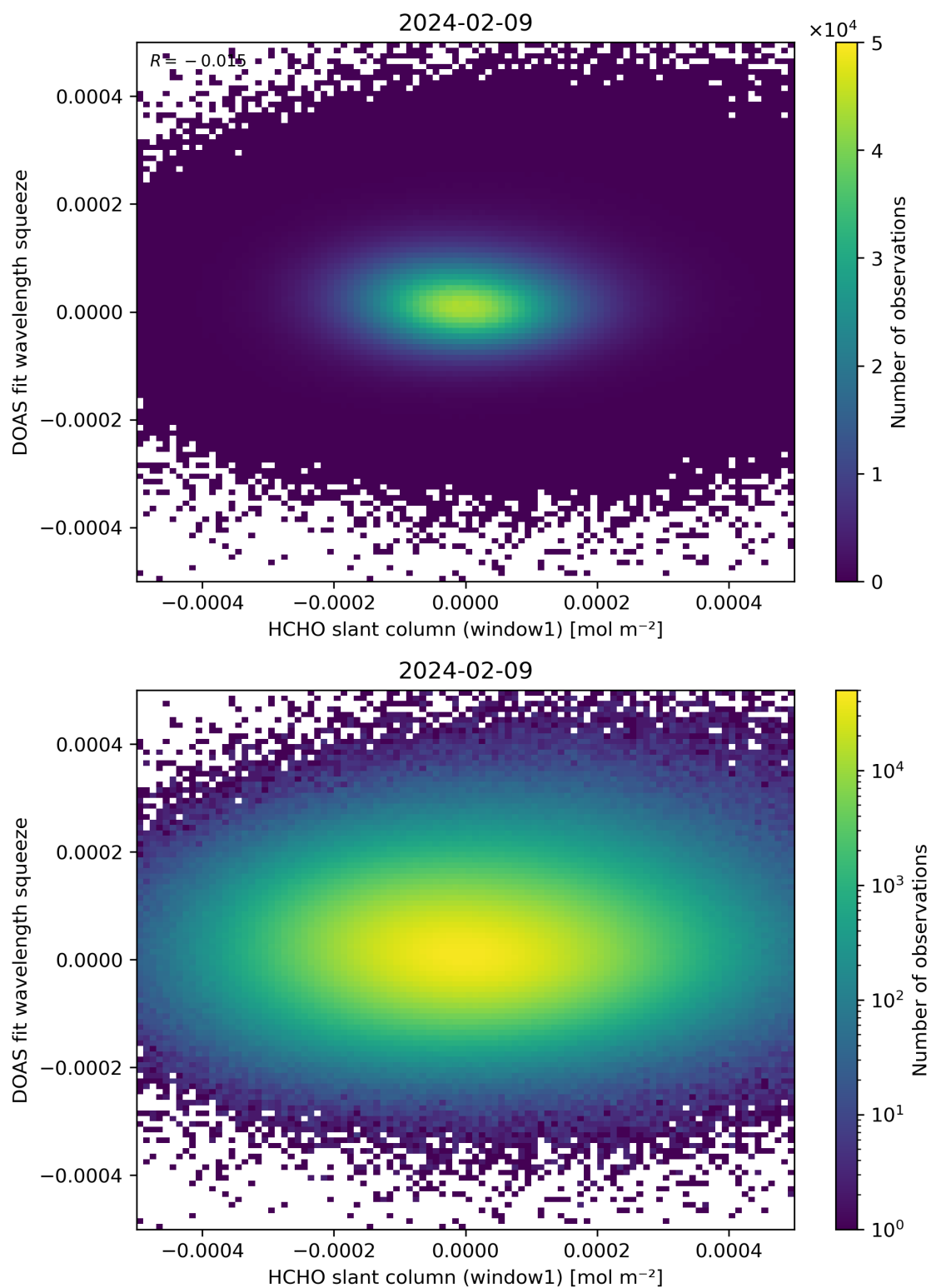
Figure 80: Scatter density plot of “HCHO slant column (window1)” against “DOAS fit wavelength squeeze” for 2024-02-08 to 2024-02-10.
