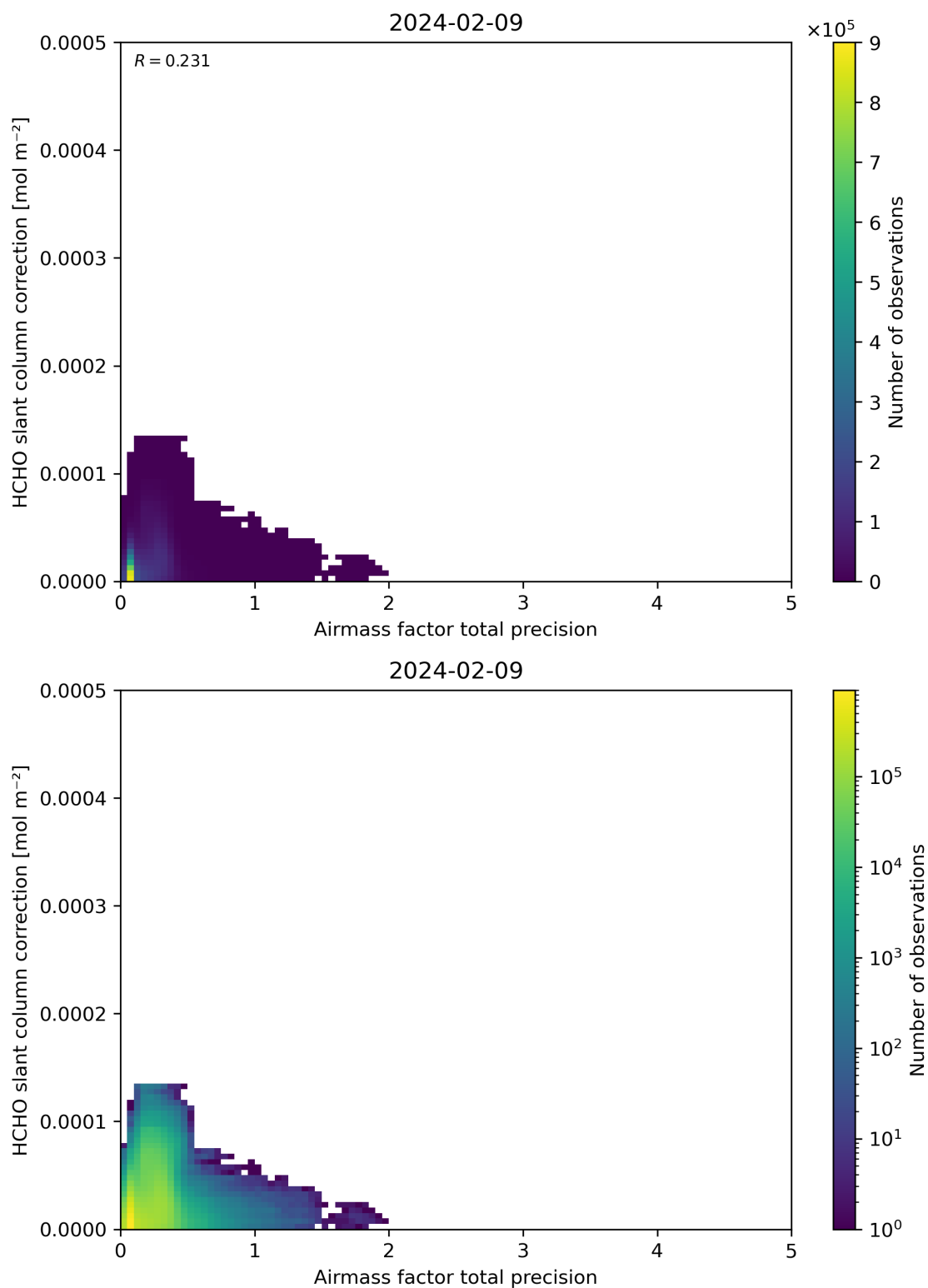
Figure 110: Scatter density plot of “Airmass factor total precision” against “HCHO slant column correction” for 2024-02-08 to 2024-02-10.
