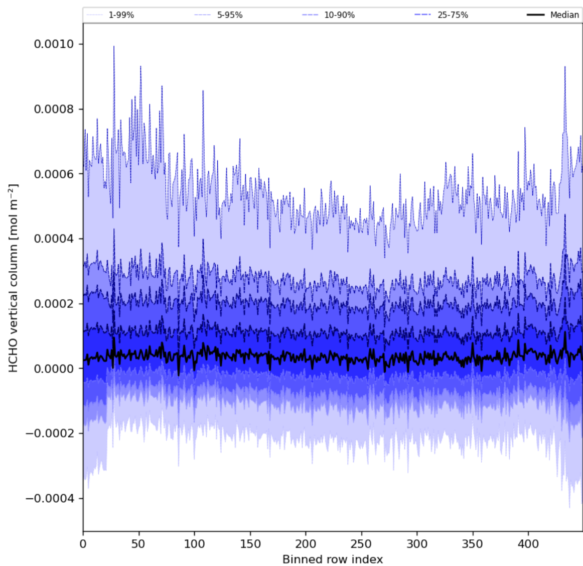
Figure 49: Along track statistics of “HCHO vertical column” for 2024-02-08 to 2024-02-10
