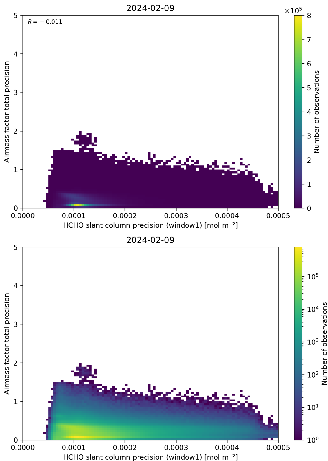
Figure 95: Scatter density plot of “HCHO slant column precision (window1)” against “Airmass factor total precision” for 2024-02-08 to 2024-02-10.
