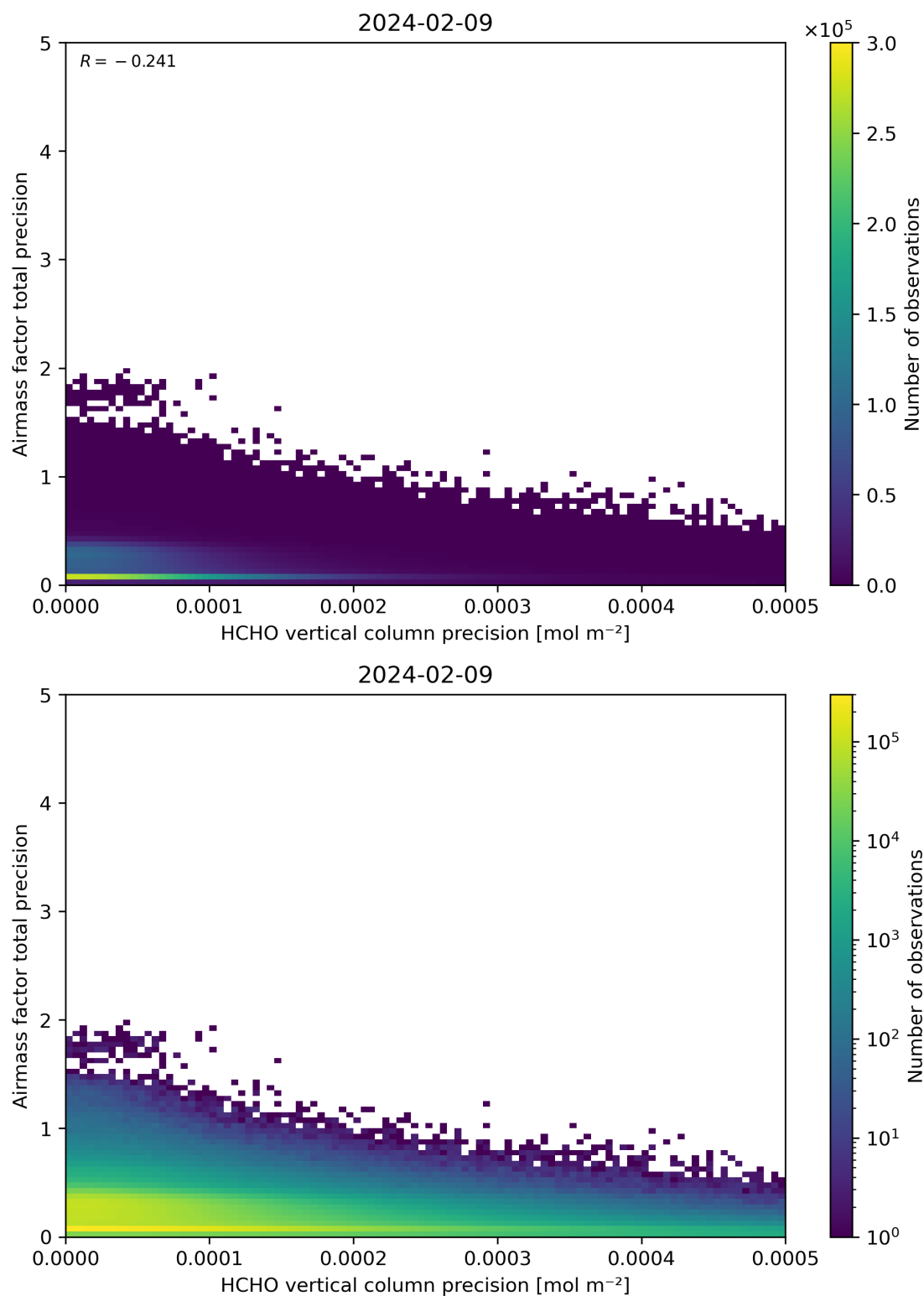
Figure 145: Scatter density plot of “HCHO vertical column precision” against “Airmass factor total precision” for 2024-02-08 to 2024-02-10.
