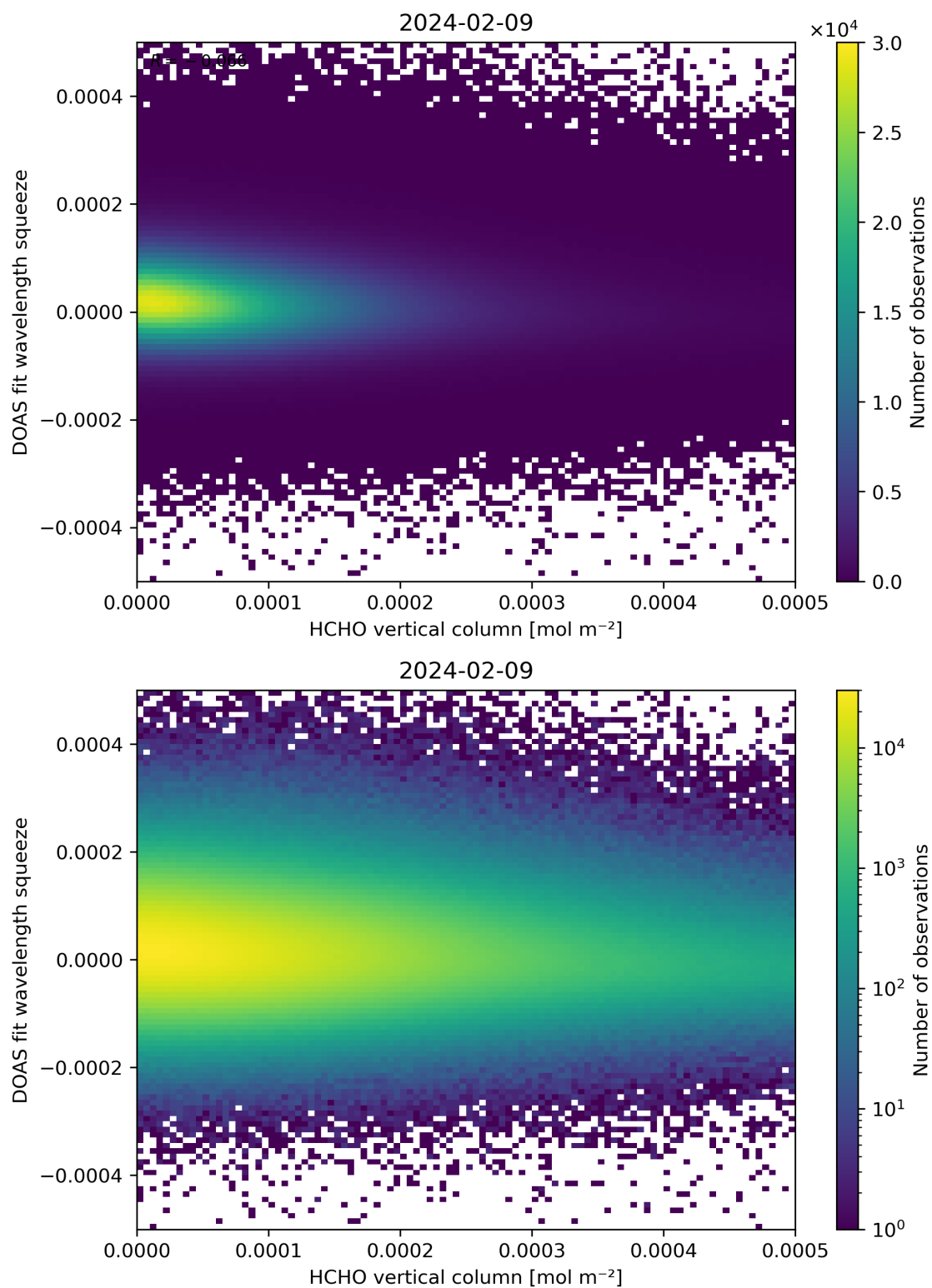
Figure 125: Scatter density plot of “HCHO vertical column” against “DOAS fit wavelength squeeze” for 2024-02-08 to 2024-02-10.
