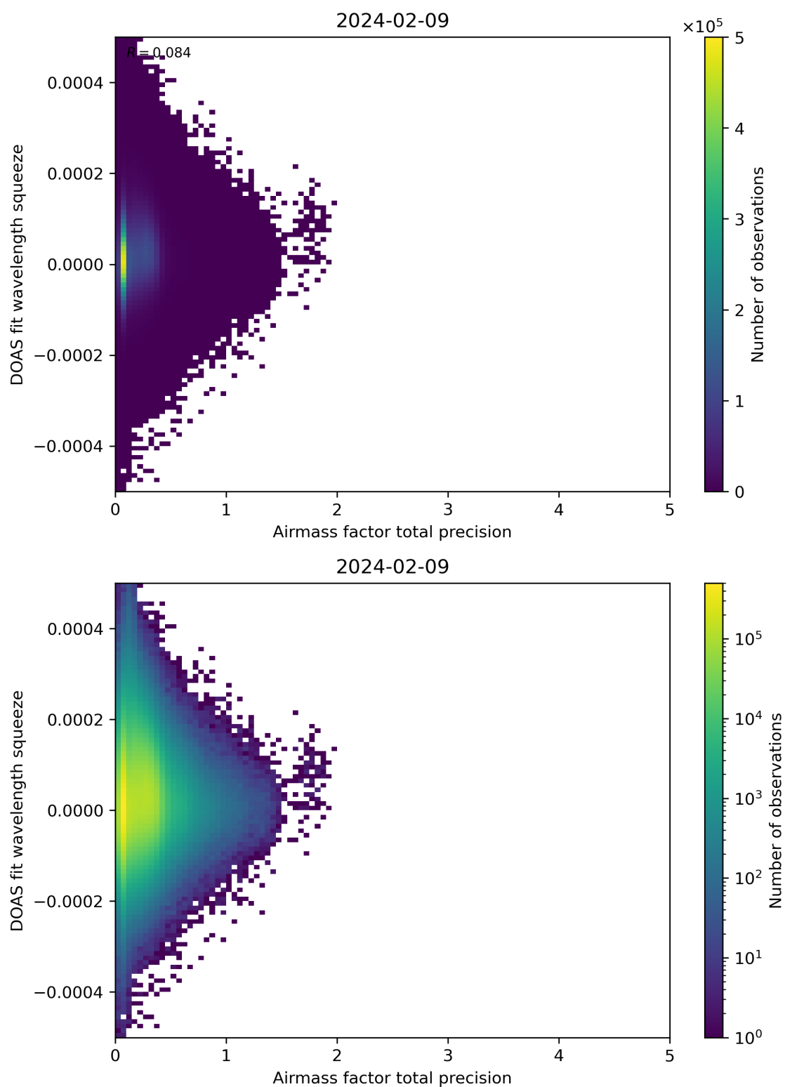
Figure 107: Scatter density plot of “Airmass factor total precision” against “DOAS fit wavelength squeeze” for 2024-02-08 to 2024-02-10.
