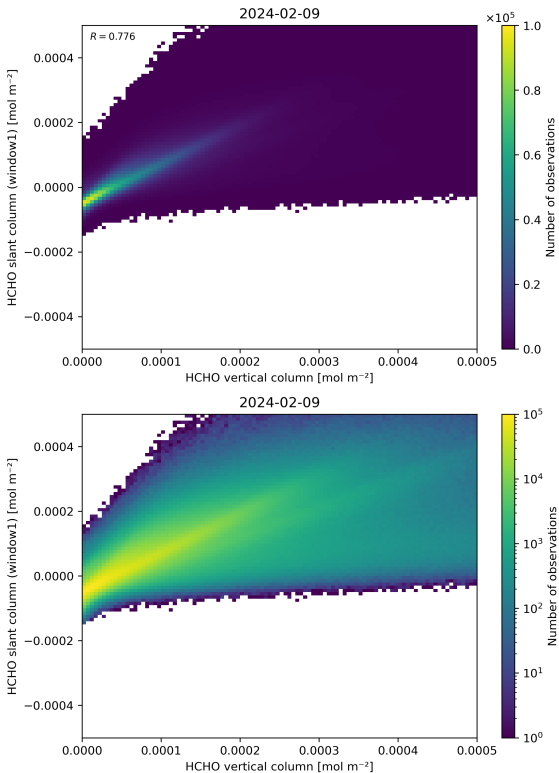
Figure 129: Scatter density plot of “HCHO vertical column” against “HCHO slant column (window1)” for 2024-02-08 to 2024-02-10.
