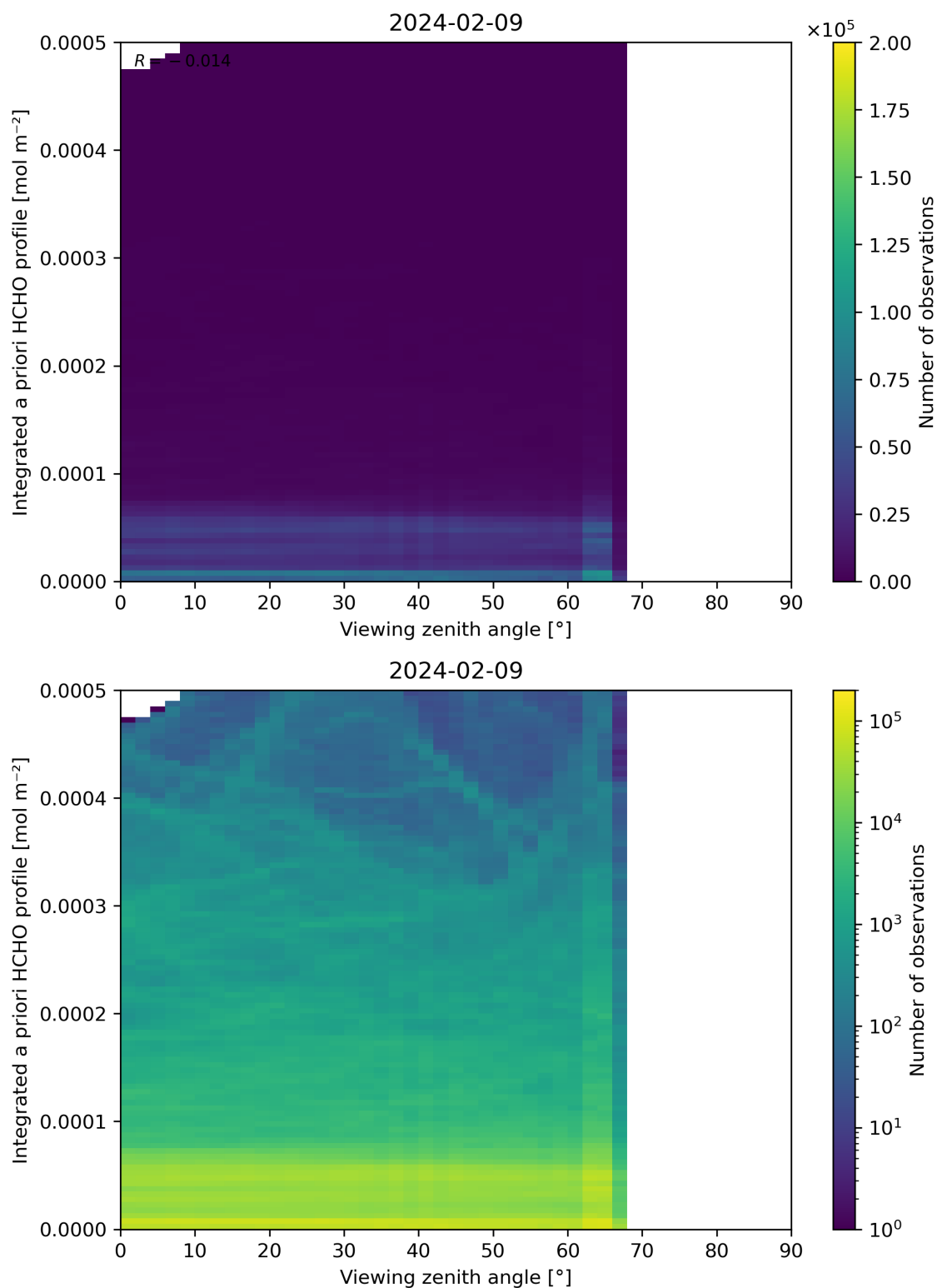
Figure 195: Scatter density plot of “Viewing zenith angle” against “Integrated a priori HCHO profile” for 2024-02-08 to 2024-02-10.
