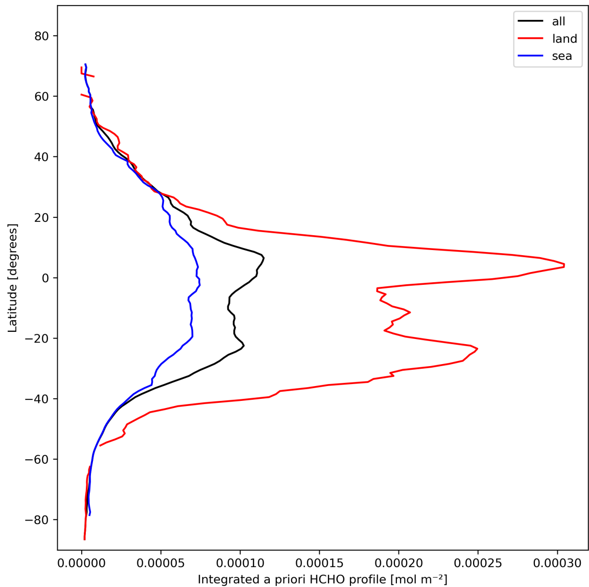
Figure 29: Zonal average of “Integrated a priori HCHO profile” for 2024-02-08 to 2024-02-10.
