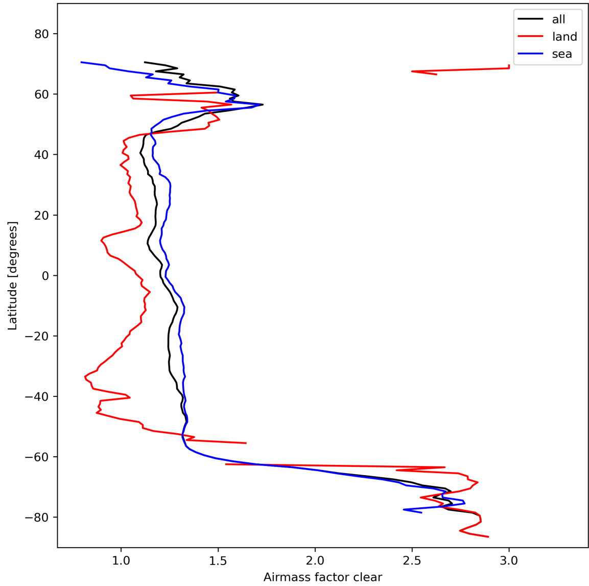
Figure 28: Zonal average of “Airmass factor clear” for 2024-02-08 to 2024-02-10.
