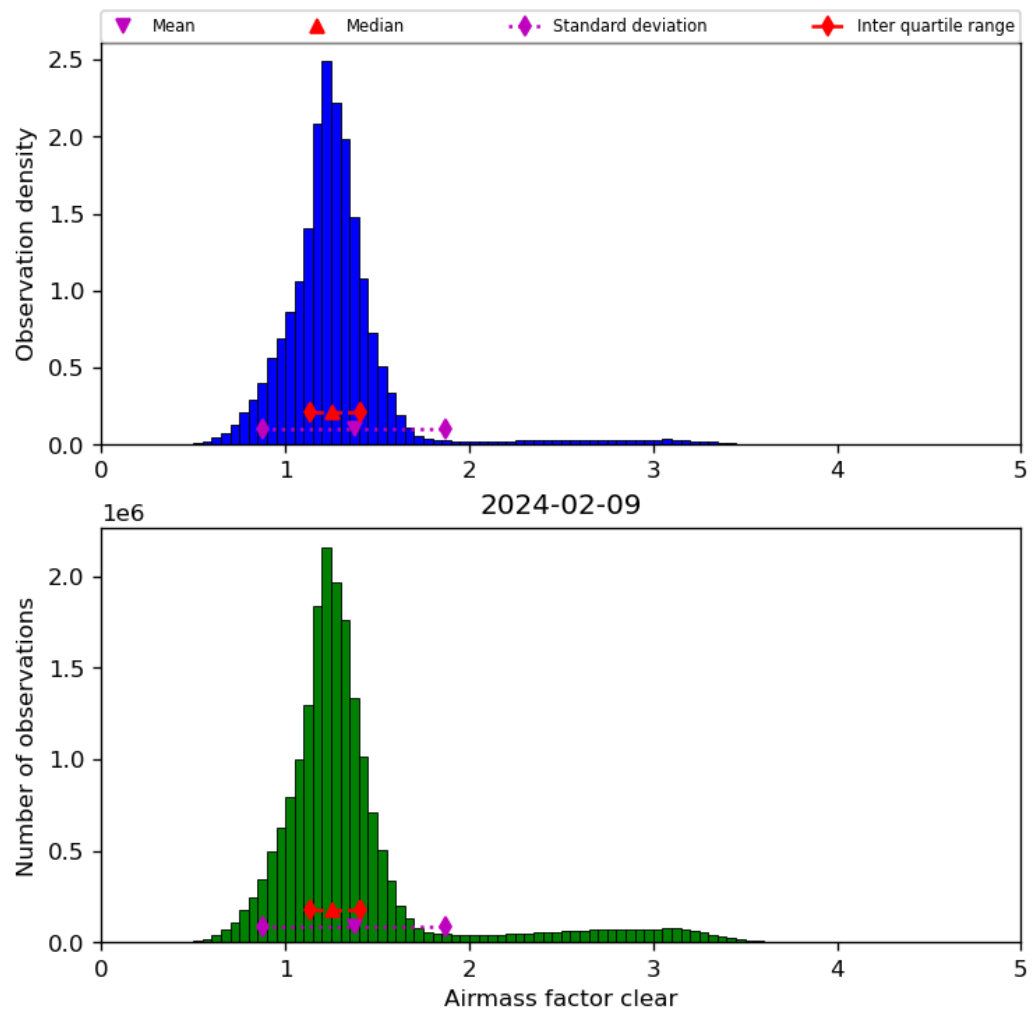
Figure 42: Histogram of “Airmass factor clear” for 2024-02-08 to 2024-02-10
