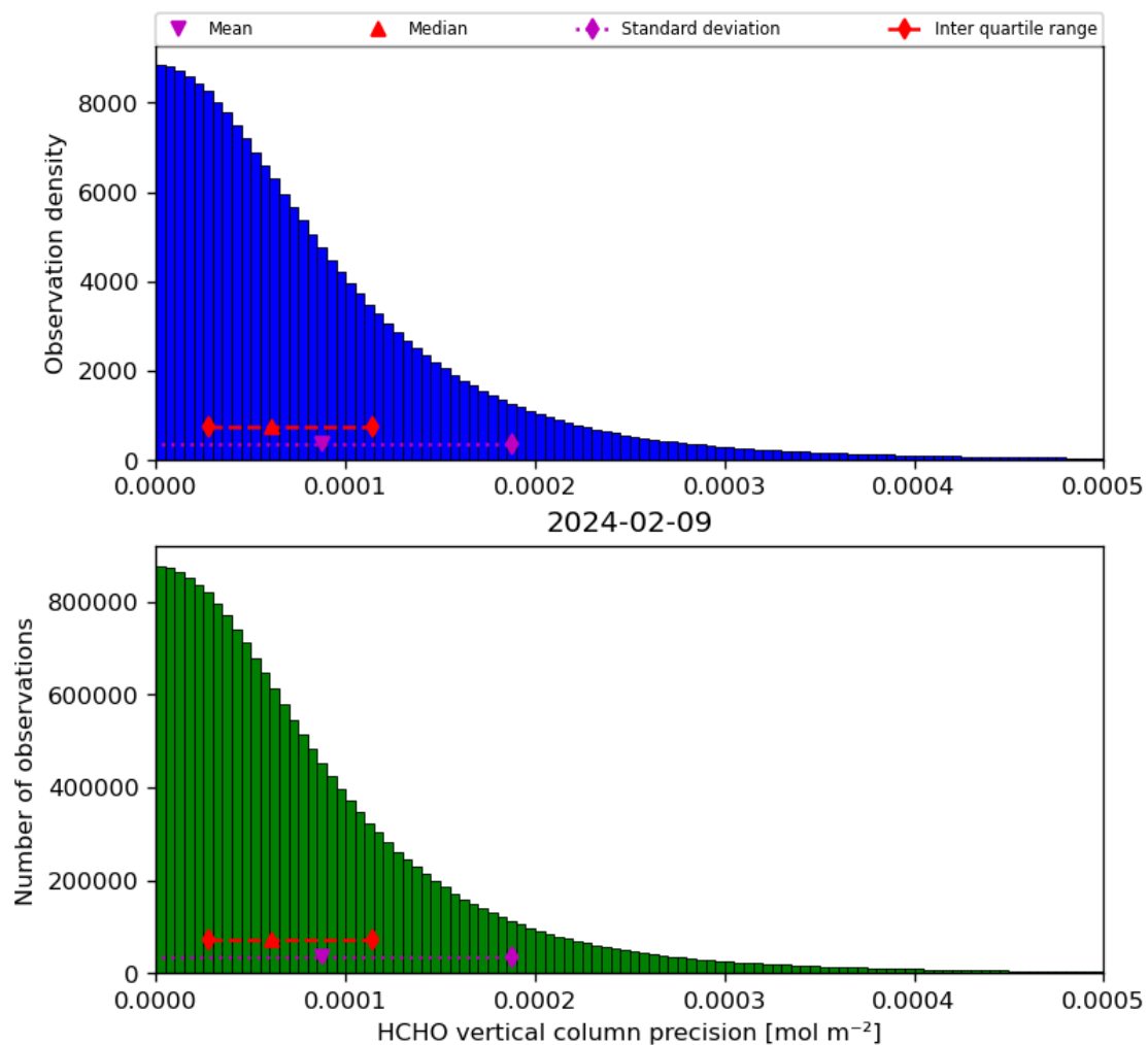
Figure 36: Histogram of “HCHO vertical column precision” for 2024-02-08 to 2024-02-10
