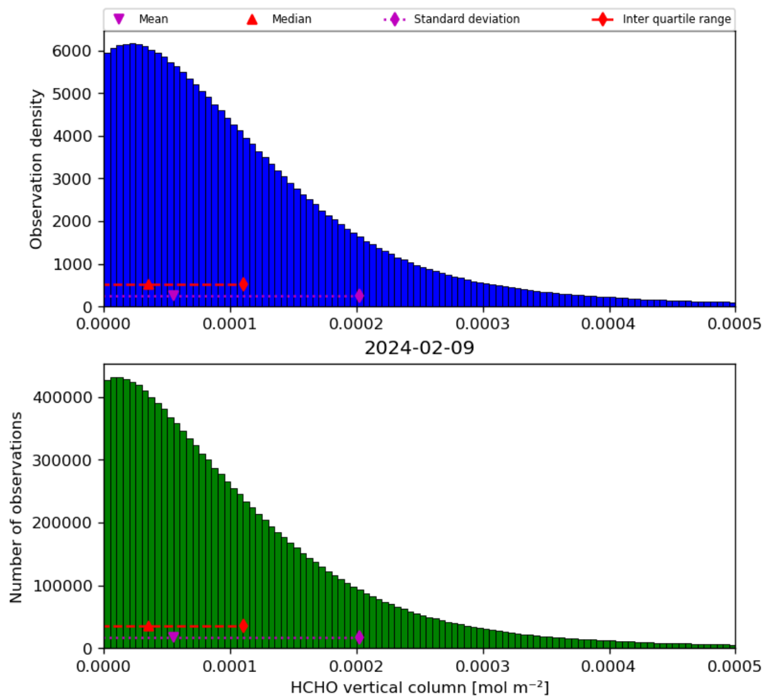
Figure 35: Histogram of “HCHO vertical column” for 2024-02-08 to 2024-02-10
