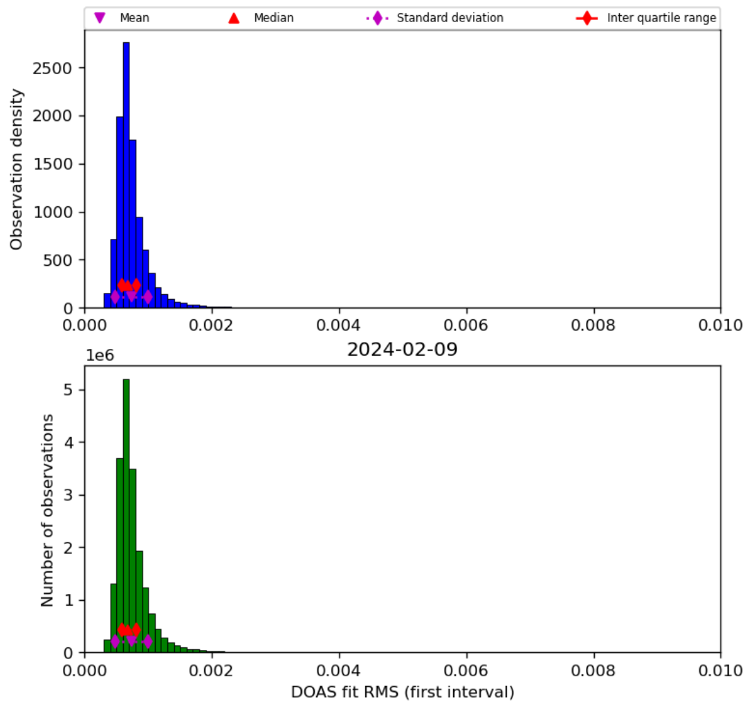
Figure 46: Histogram of “DOAS fit RMS (first interval)” for 2024-02-08 to 2024-02-10
