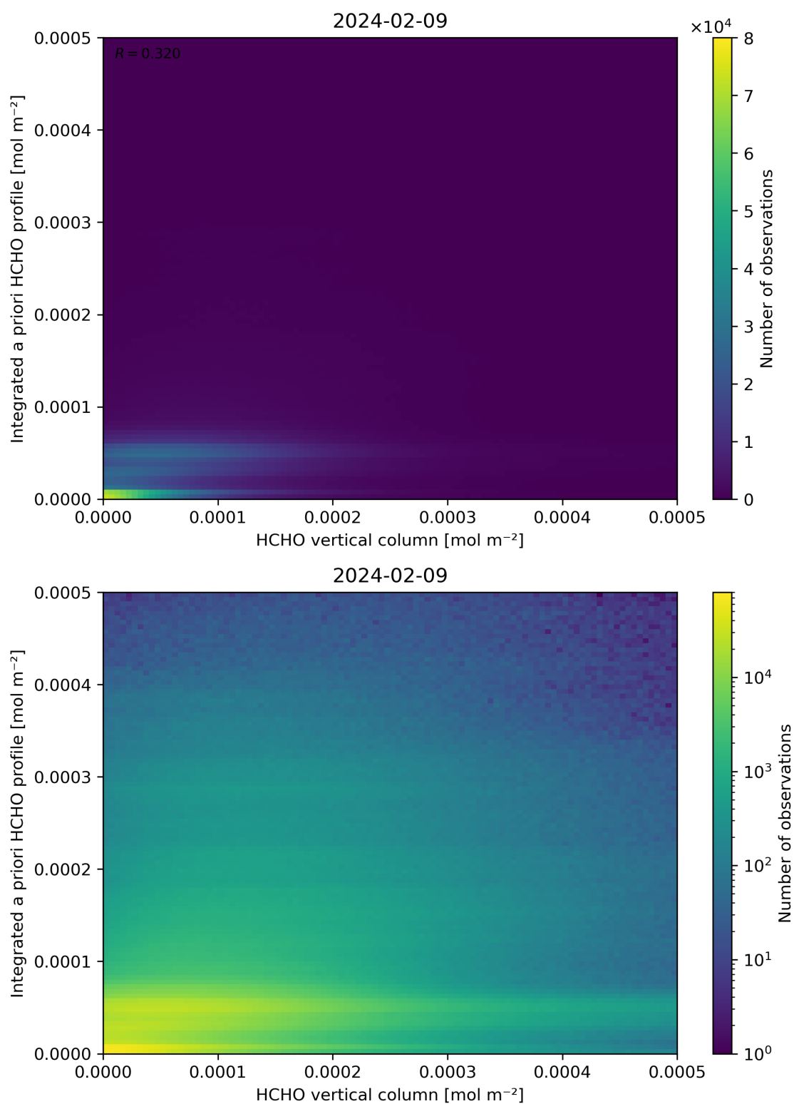
Figure 135: Scatter density plot of “HCHO vertical column” against “Integrated a priori HCHO profile” for 2024-02-08 to 2024-02-10.
