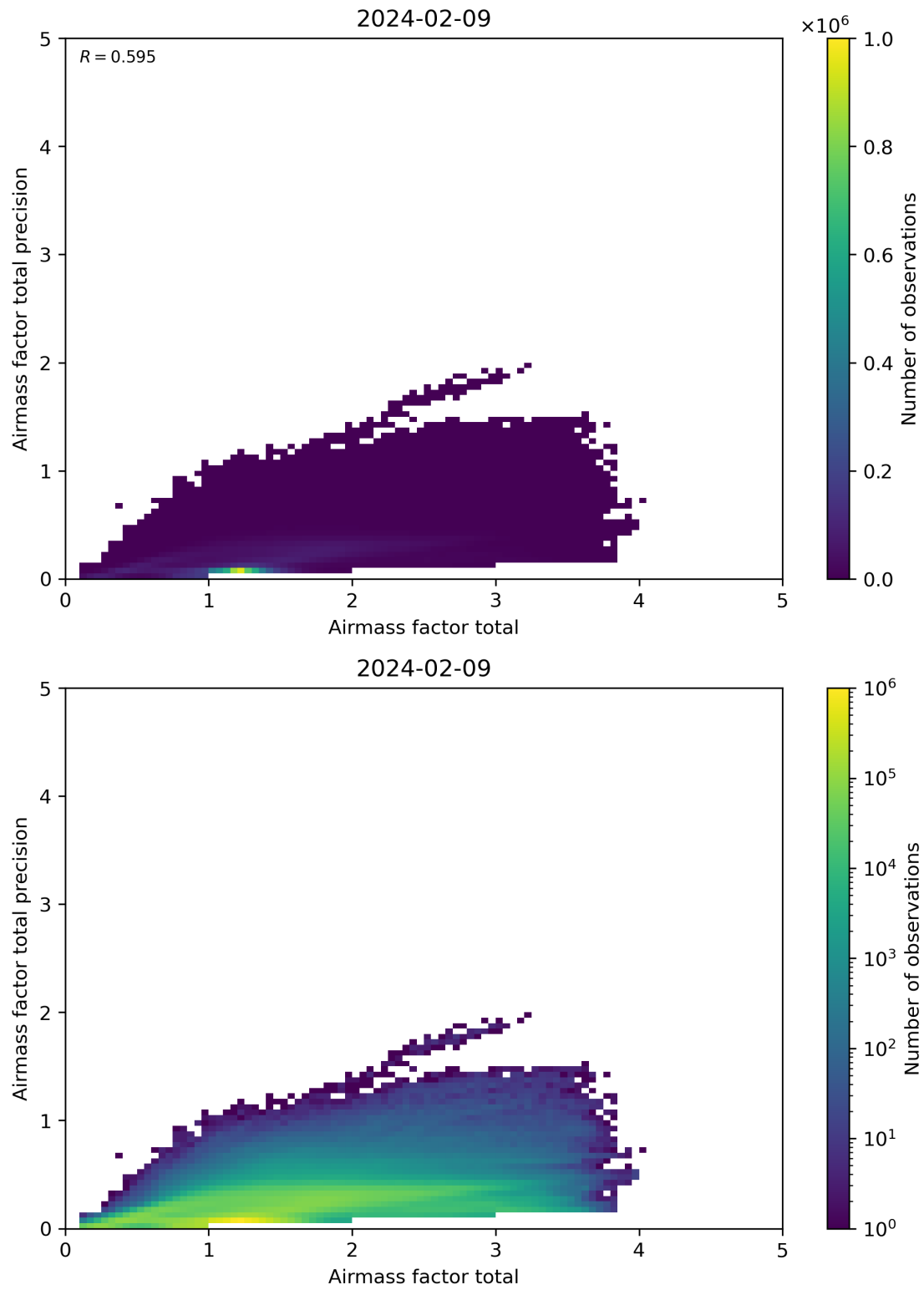
Figure 103: Scatter density plot of “Airmass factor total” against “Airmass factor total precision” for 2024-02-08 to 2024-02-10.
