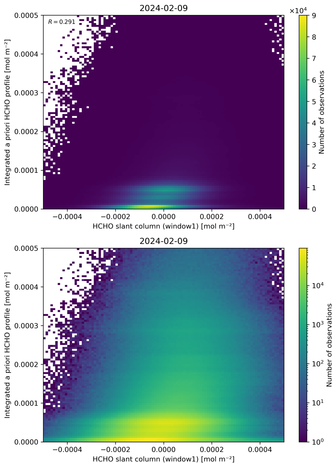
Figure 87: Scatter density plot of “HCHO slant column (window1)” against “Integrated a priori HCHO profile” for 2024-02-08 to 2024-02-10.
