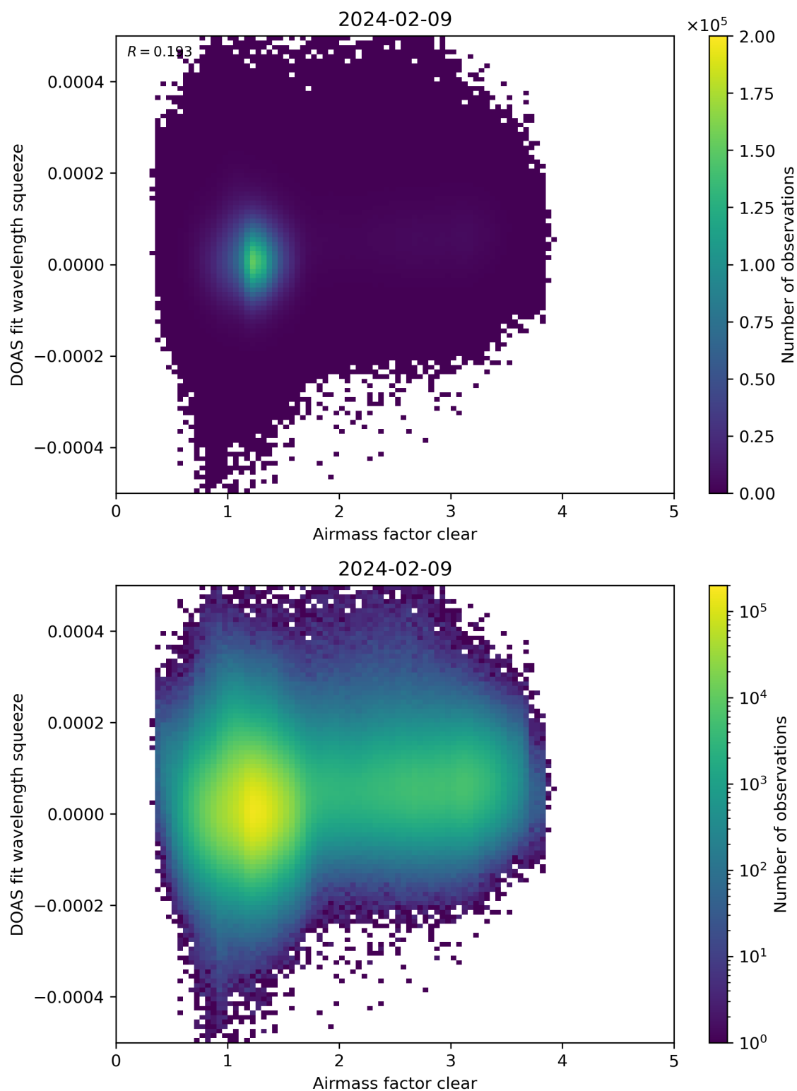
Figure 73: Scatter density plot of “Airmass factor clear” against “DOAS fit wavelength squeeze” for 2024-02-08 to 2024-02-10.
