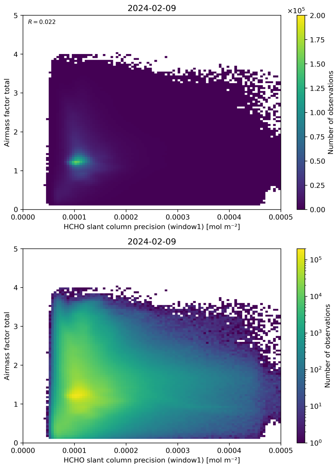
Figure 94: Scatter density plot of “HCHO slant column precision (window1)” against “Airmass factor total” for 2024-02-08 to 2024-02-10.
