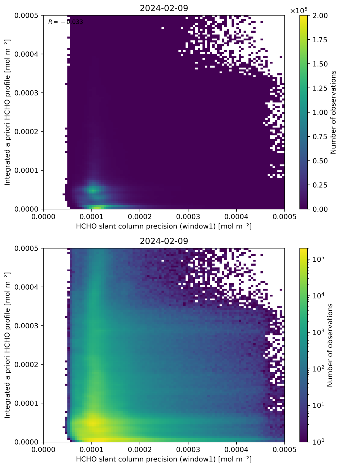
Figure 96: Scatter density plot of “HCHO slant column precision (window1)” against “Integrated a priori HCHO profile” for 2024-02-08 to 2024-02-10.
