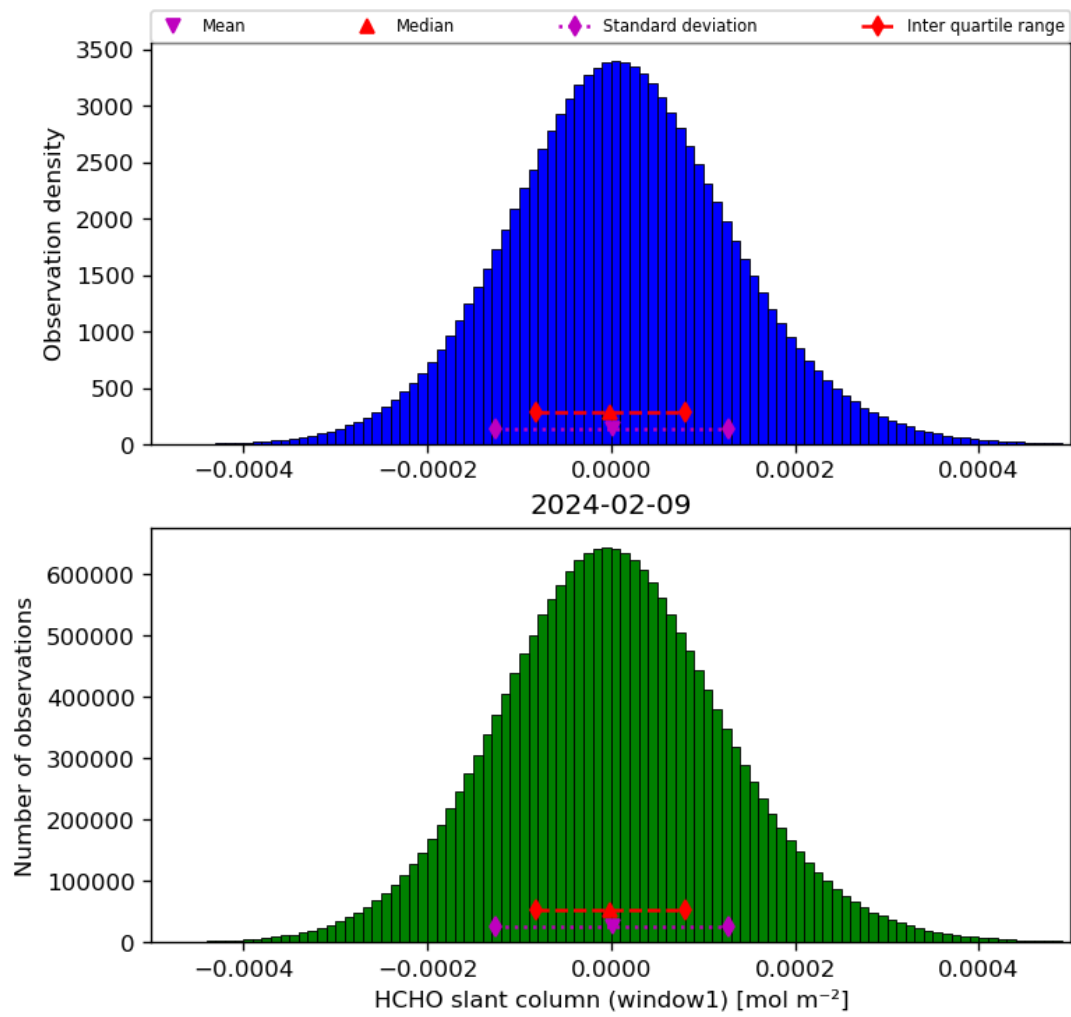
Figure 38: Histogram of “HCHO slant column (window1)” for 2024-02-08 to 2024-02-10
