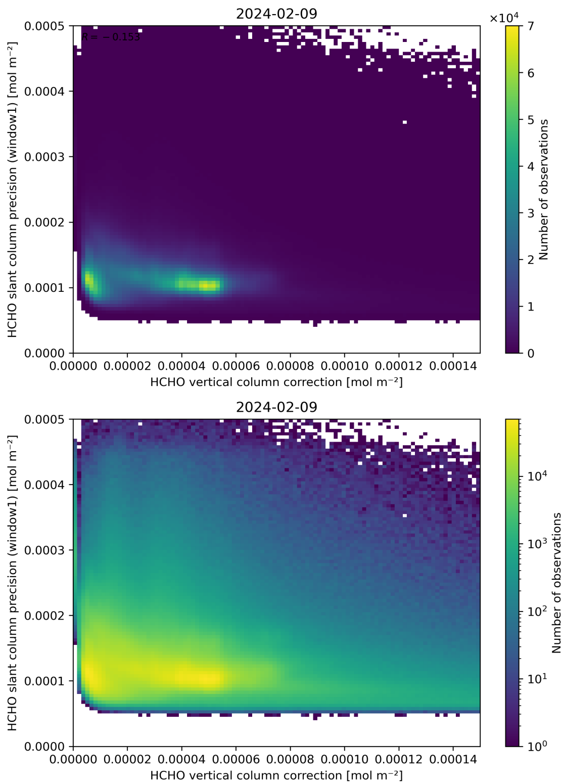
Figure 119: Scatter density plot of “HCHO vertical column correction” against “HCHO slant column precision (window1)” for 2024-02-08 to 2024-02-10.
