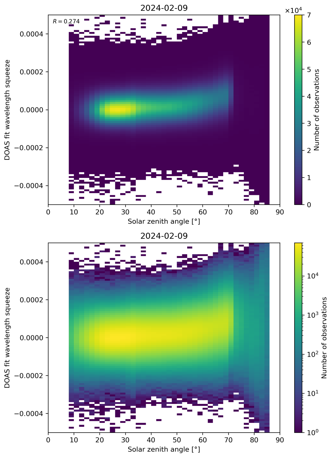
Figure 169: Scatter density plot of “Solar zenith angle” against “DOAS fit wavelength squeeze” for 2024-02-08 to 2024-02-10.
