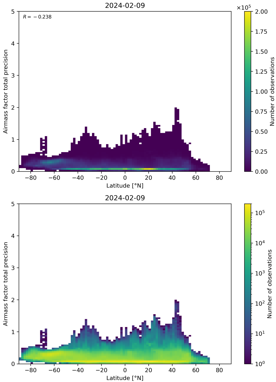
Figure 162: Scatter density plot of “Latitude” against “Airmass factor total precision” for 2024-02-08 to 2024-02-10.
