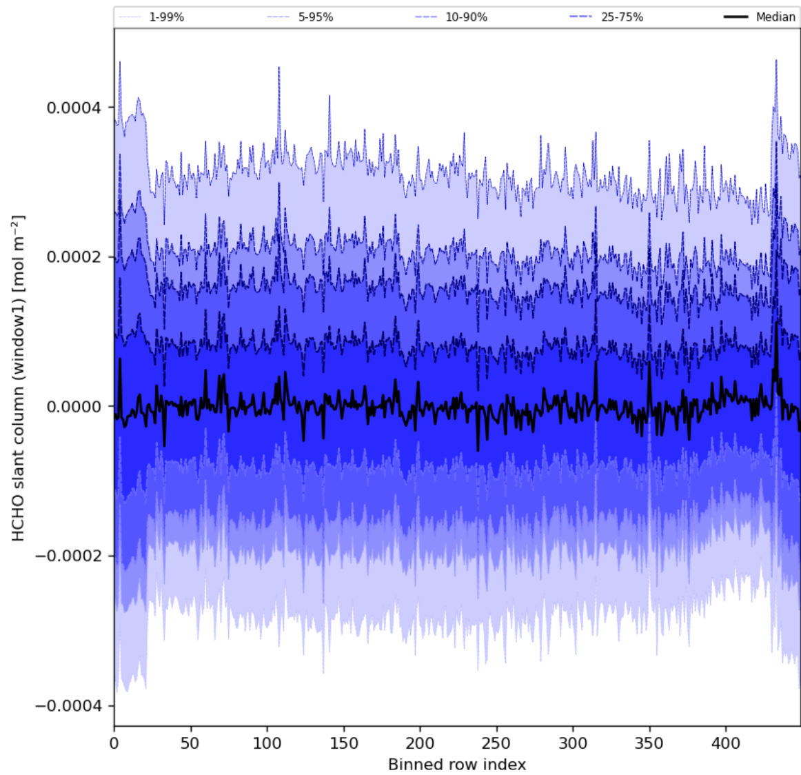
Figure 52: Along track statistics of “HCHO slant column (window1)” for 2024-02-08 to 2024-02-10
