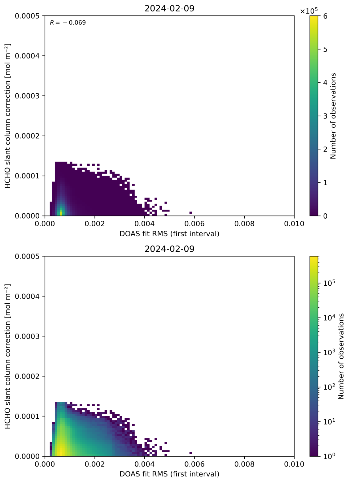
Figure 63: Scatter density plot of “DOAS fit RMS (first interval)” against “HCHO slant column correction” for 2024-02-08 to 2024-02-10.
