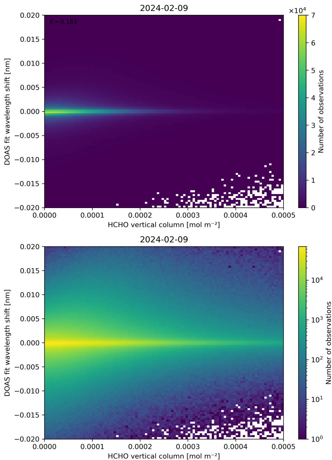
Figure 124: Scatter density plot of “HCHO vertical column” against “DOAS fit wavelength shift” for 2024-02-08 to 2024-02-10.
