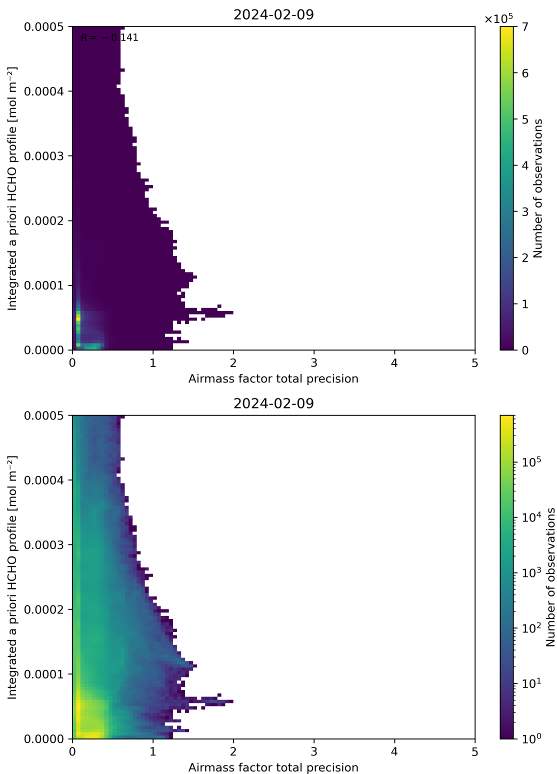
Figure 111: Scatter density plot of “Airmass factor total precision” against “Integrated a priori HCHO profile” for 2024-02-08 to 2024-02-10.
