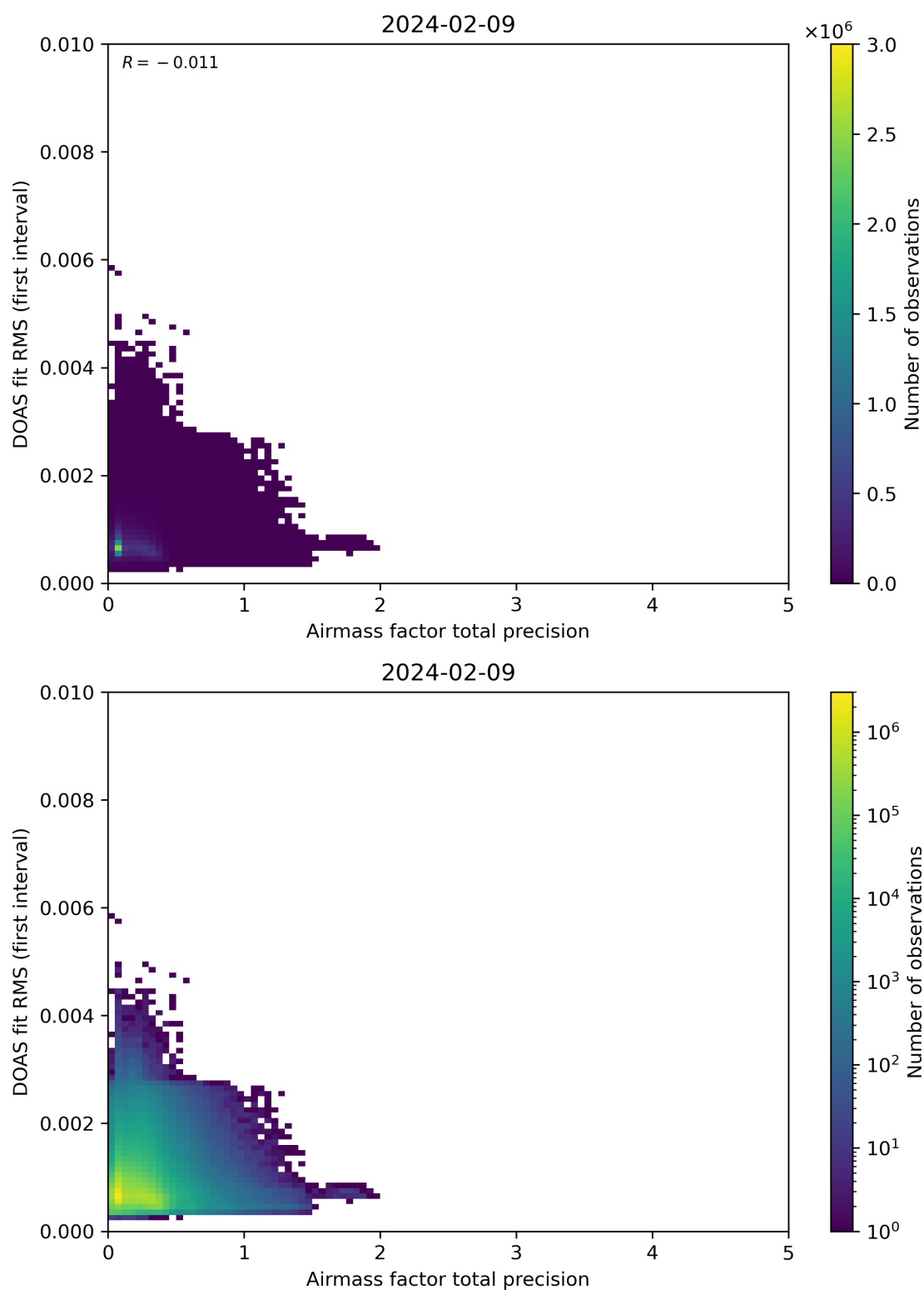
Figure 105: Scatter density plot of “Airmass factor total precision” against “DOAS fit RMS (first interval)” for 2024-02-08 to 2024-02-10.
