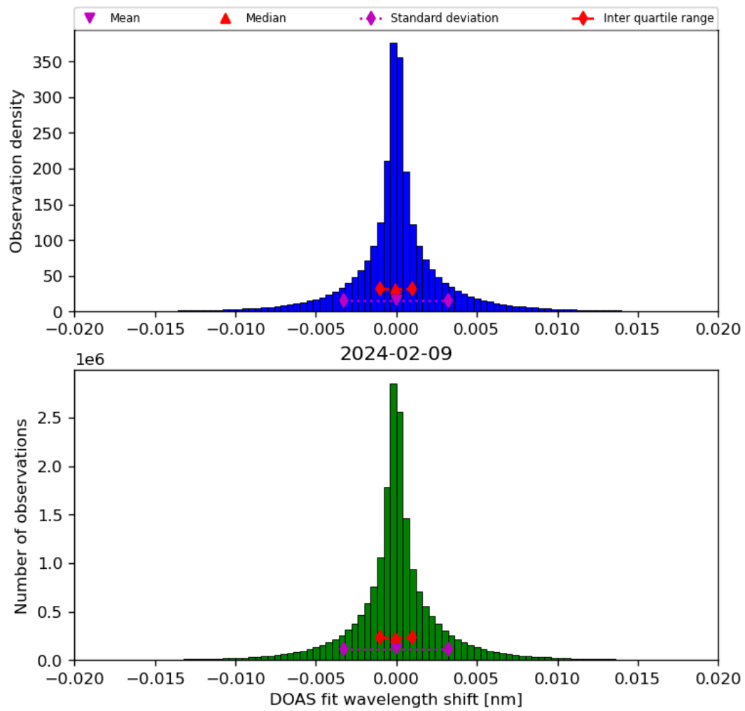
Figure 44: Histogram of “DOAS fit wavelength shift” for 2024-02-08 to 2024-02-10
