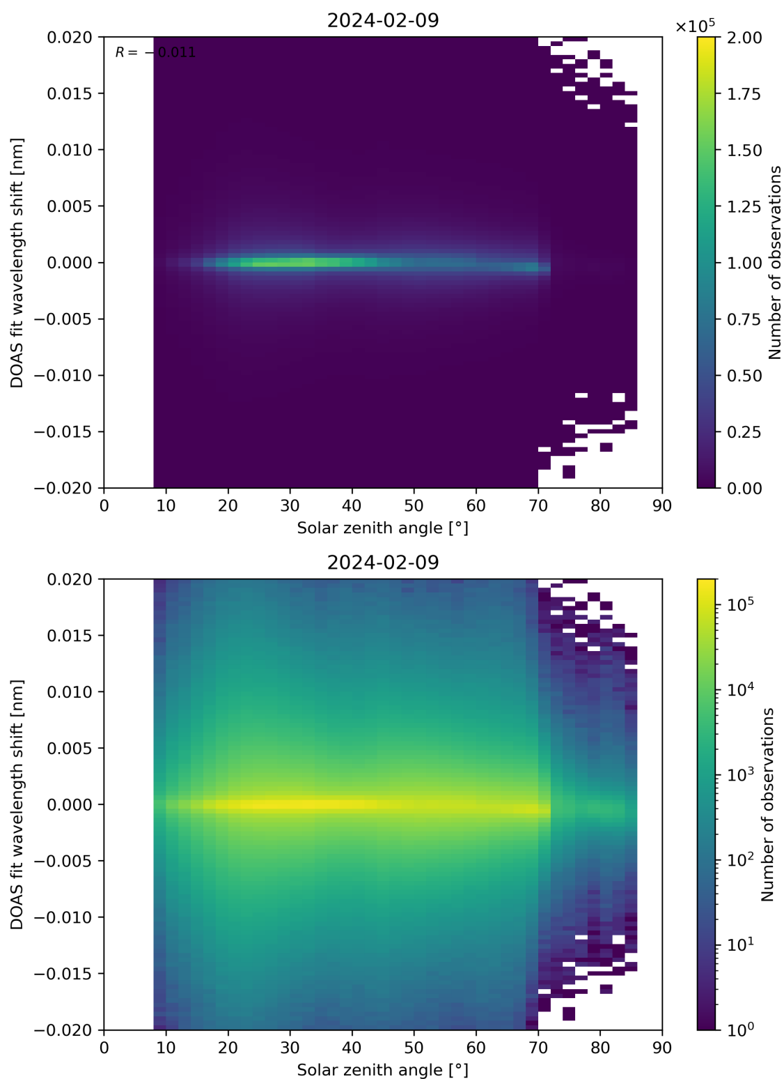
Figure 168: Scatter density plot of “Solar zenith angle” against “DOAS fit wavelength shift” for 2024-02-08 to 2024-02-10.
