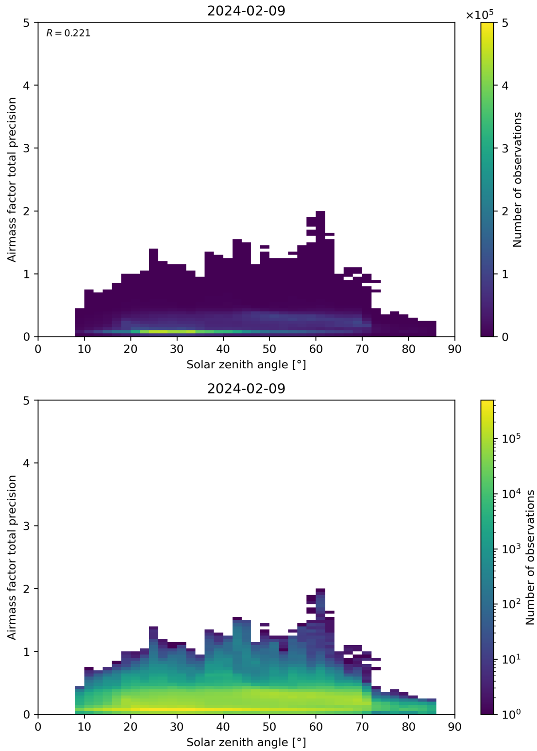
Figure 176: Scatter density plot of “Solar zenith angle” against “Airmass factor total precision” for 2024-02-08 to 2024-02-10.
