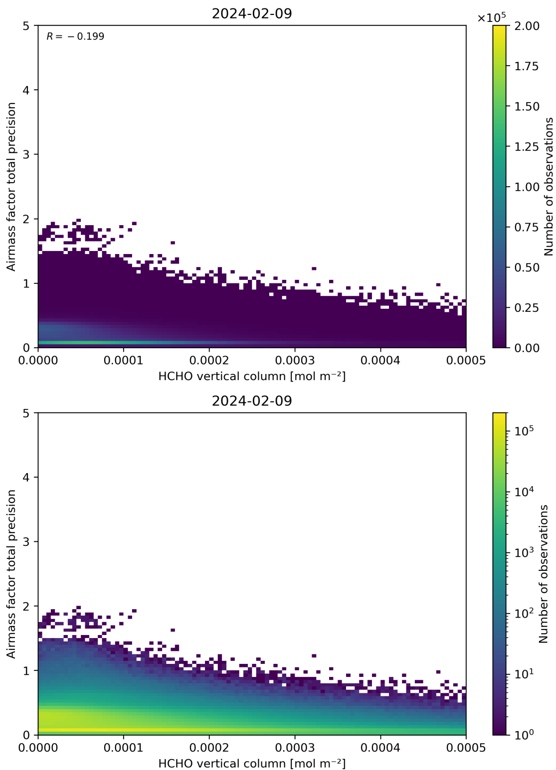
Figure 132: Scatter density plot of “HCHO vertical column” against “Airmass factor total precision” for 2024-02-08 to 2024-02-10.
