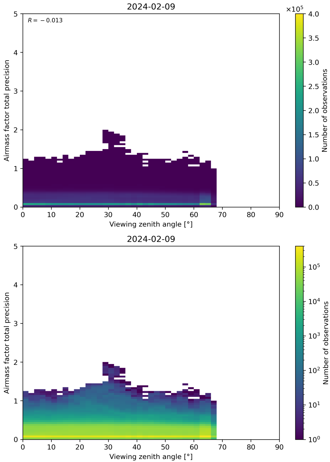
Figure 191: Scatter density plot of “Viewing zenith angle” against “Airmass factor total precision” for 2024-02-08 to 2024-02-10.
