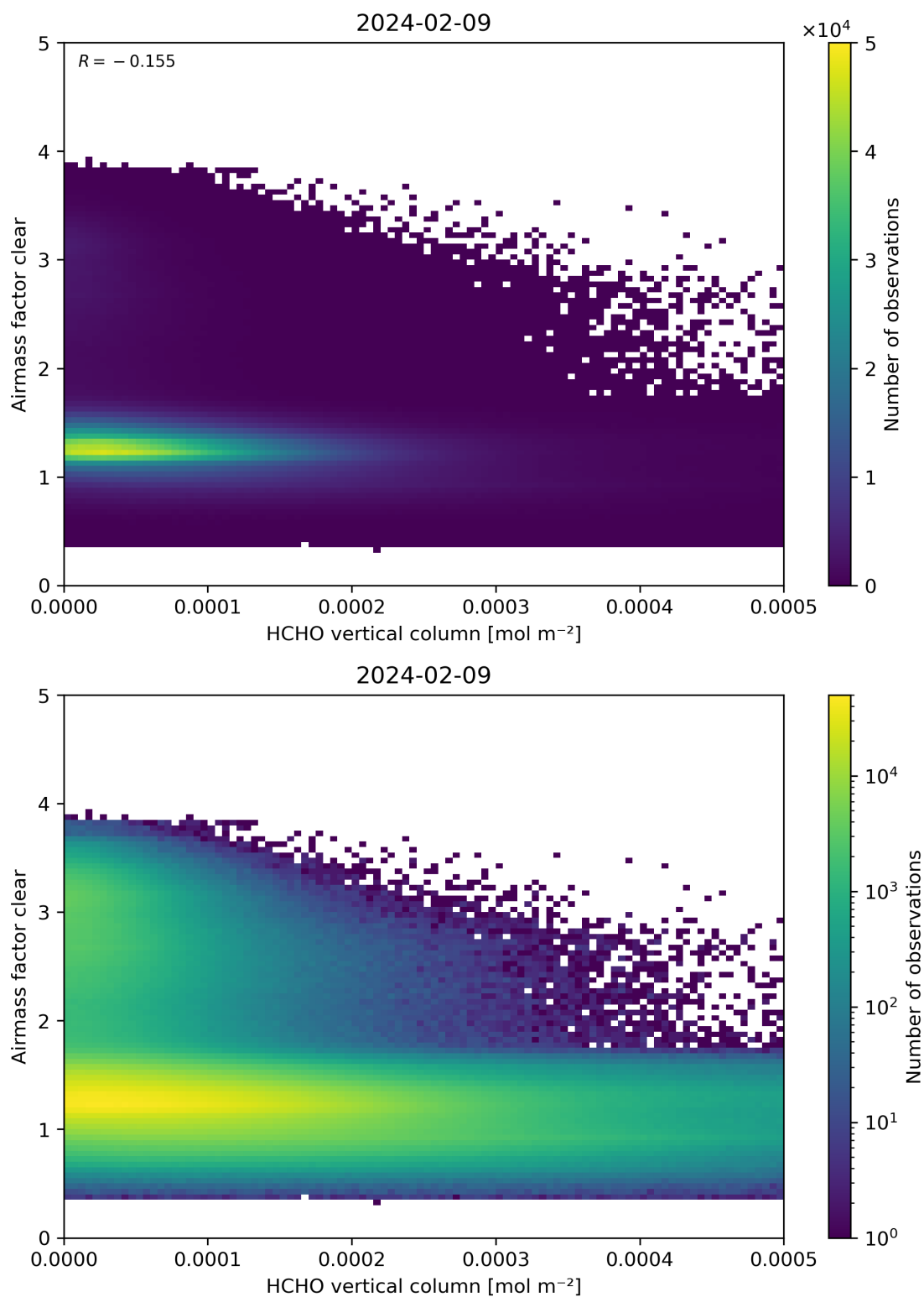
Figure 126: Scatter density plot of “HCHO vertical column” against “Airmass factor clear” for 2024-02-08 to 2024-02-10.
