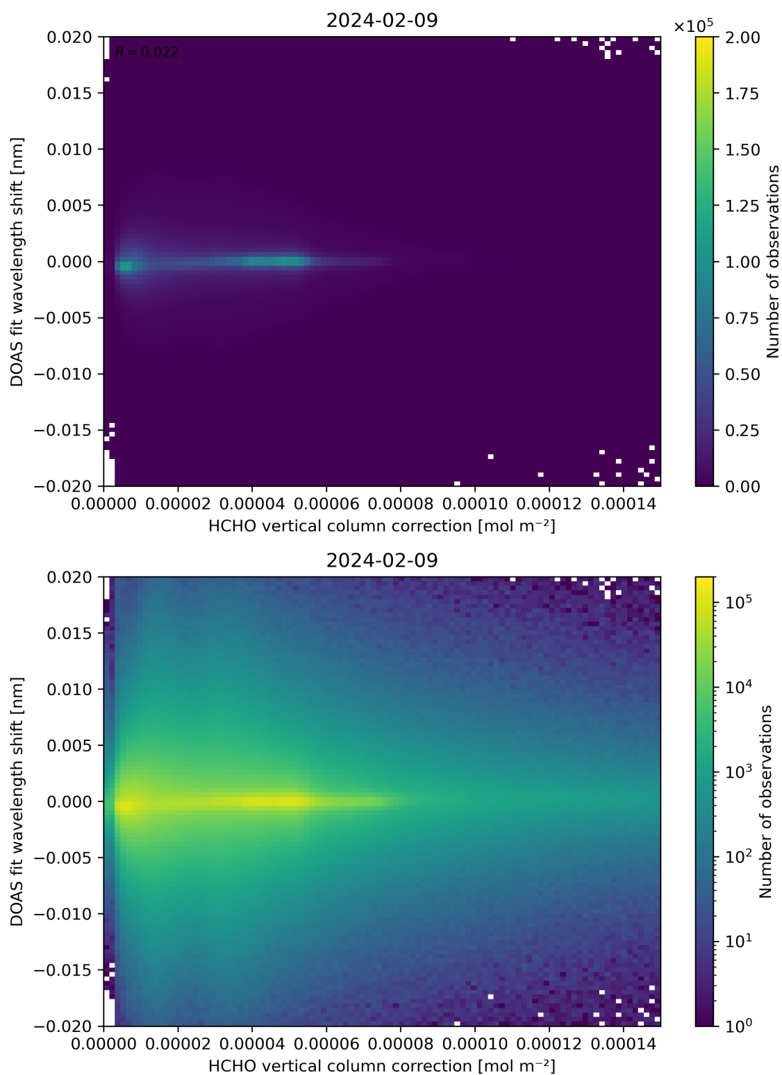
Figure 113: Scatter density plot of “HCHO vertical column correction” against “DOAS fit wavelength shift” for 2024-02-08 to 2024-02-10.
