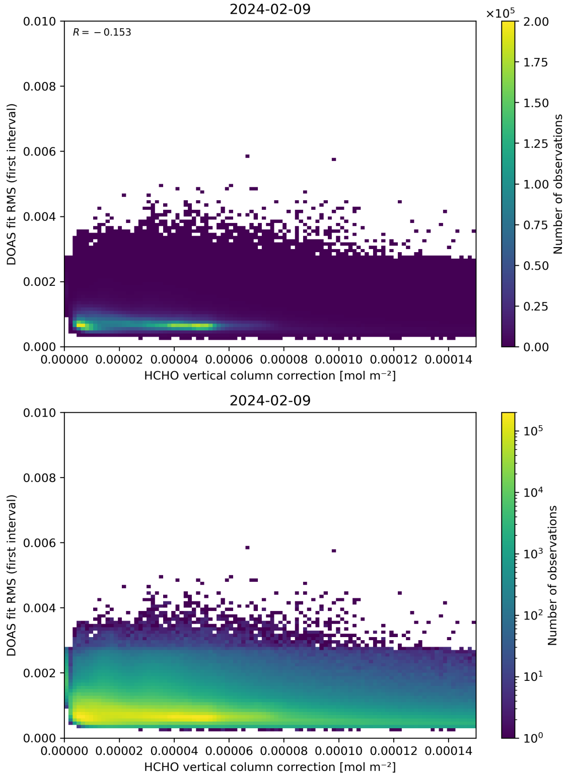
Figure 112: Scatter density plot of “HCHO vertical column correction” against “DOAS fit RMS (first interval)” for 2024-02-08 to 2024-02-10.
