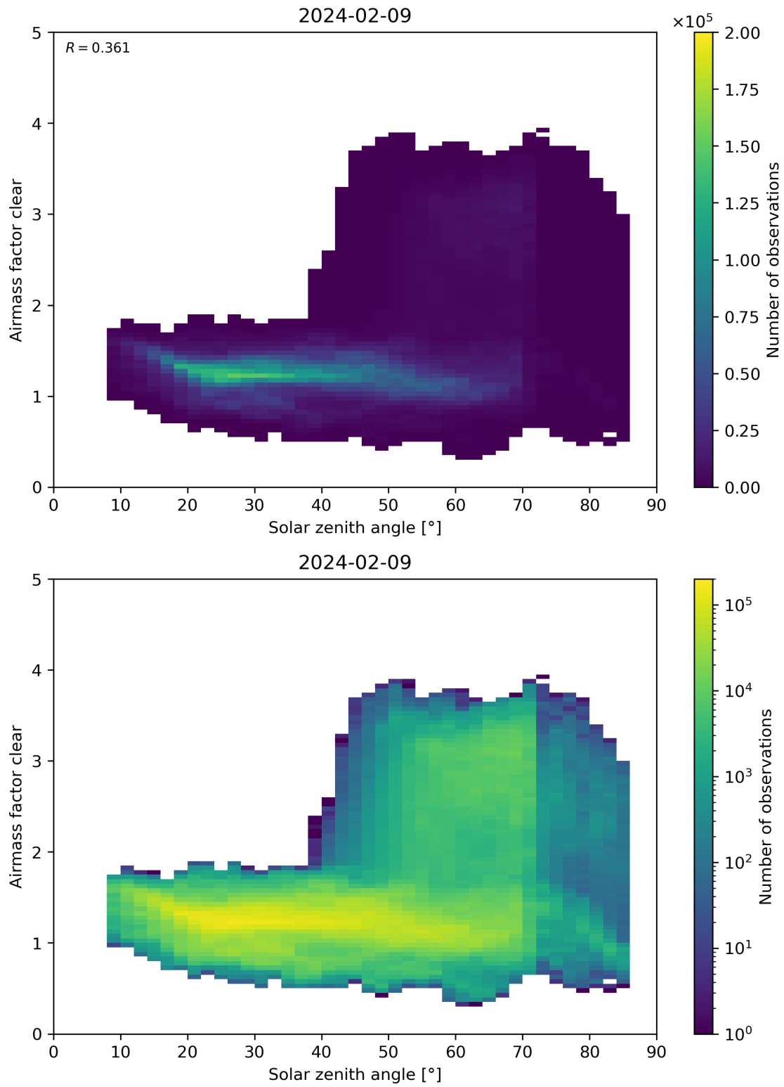
Figure 170: Scatter density plot of “Solar zenith angle” against “Airmass factor clear” for 2024-02-08 to 2024-02-10.
