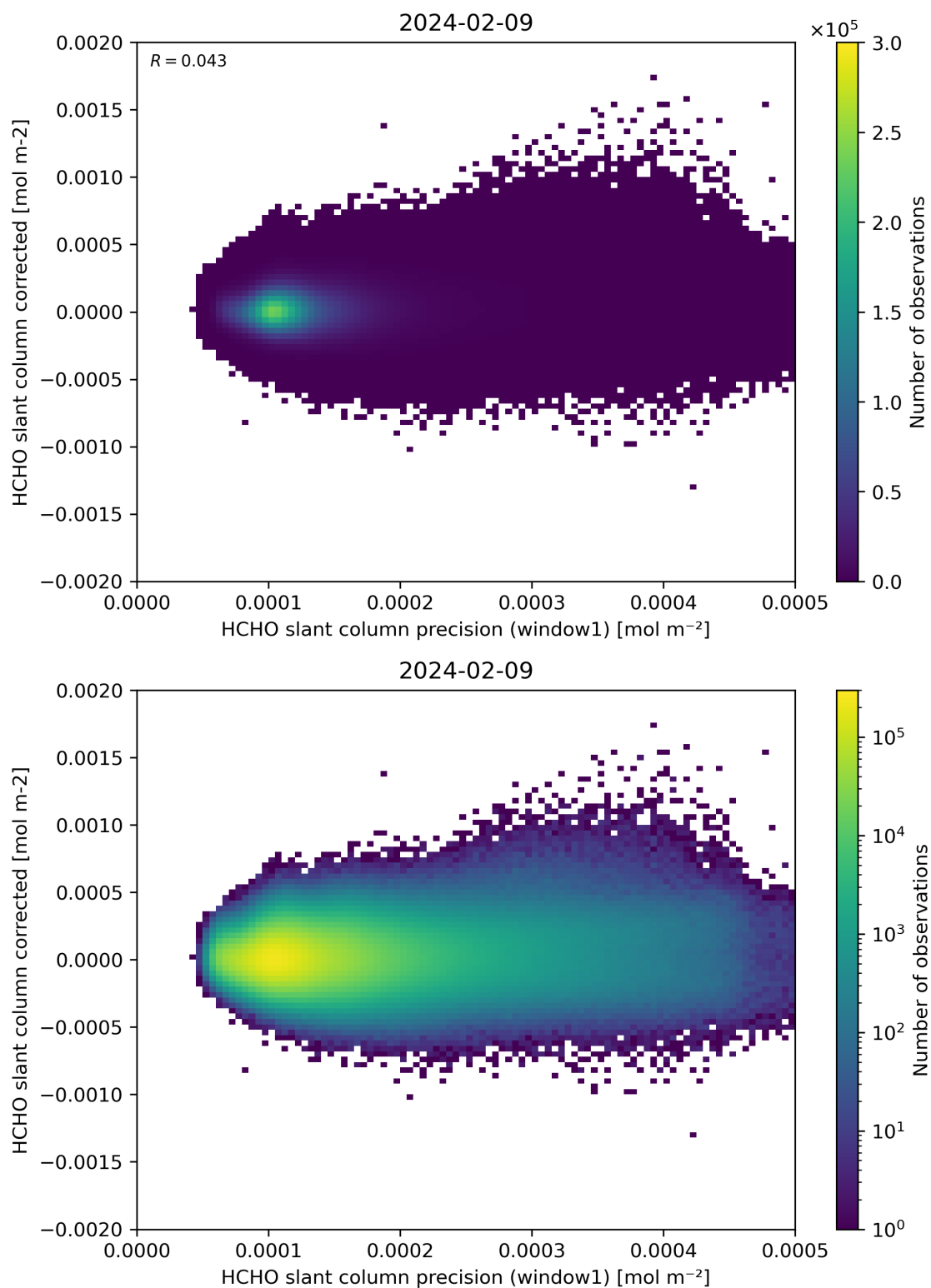
Figure 92: Scatter density plot of “HCHO slant column precision (window1)” against “HCHO slant column corrected” for 2024-02-08 to 2024-02-10.
