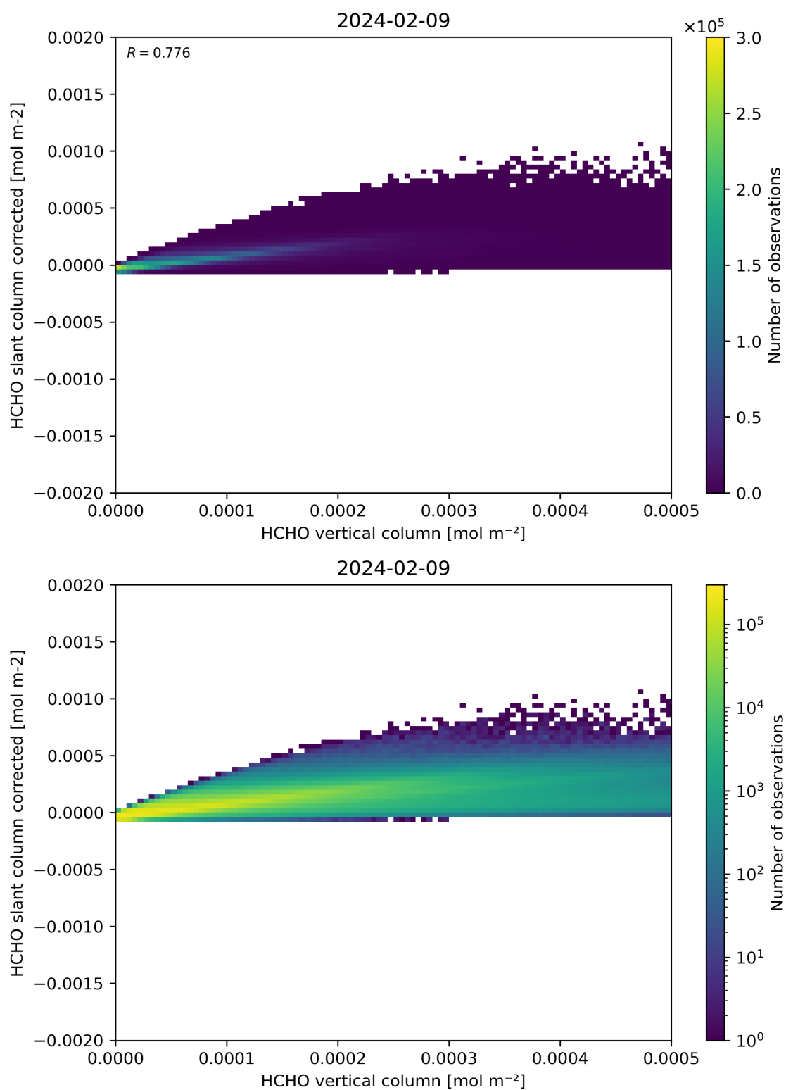
Figure 127: Scatter density plot of “HCHO vertical column” against “HCHO slant column corrected” for 2024-02-08 to 2024-02-10.
