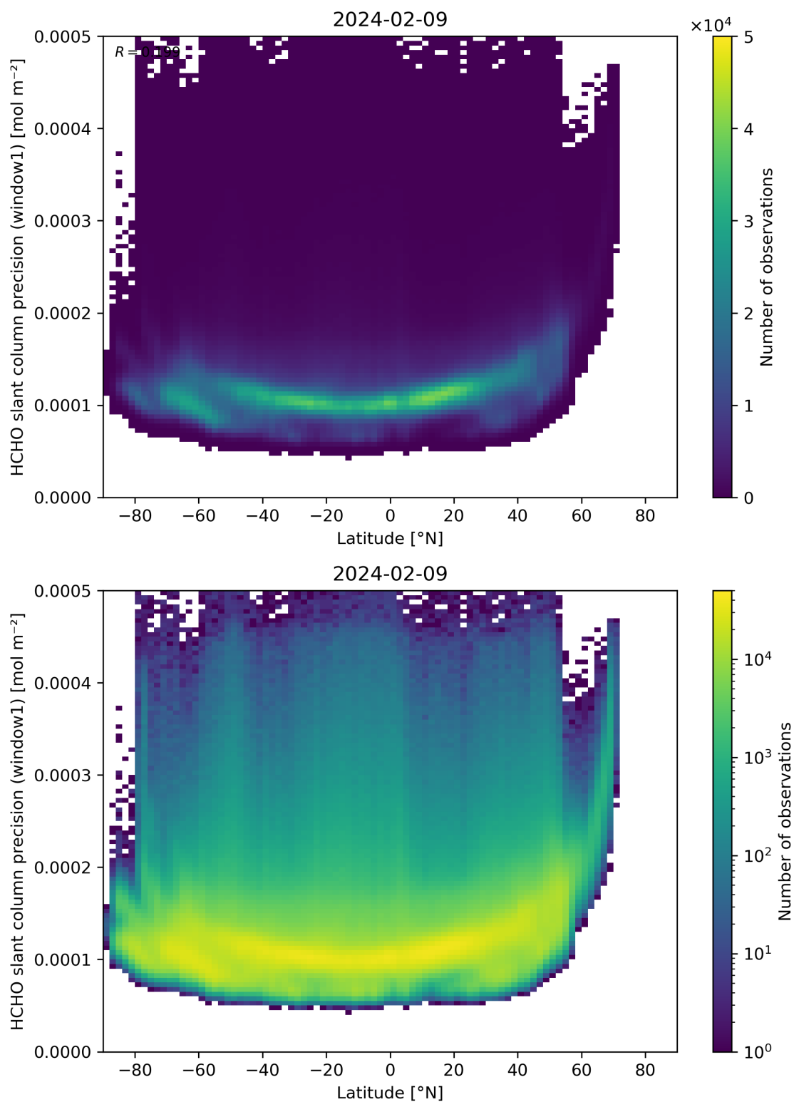
Figure 160: Scatter density plot of “Latitude” against “HCHO slant column precision (window1)” for 2024-02-08 to 2024-02-10.
