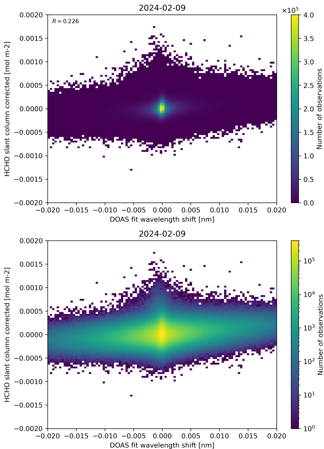
Figure 66: Scatter density plot of “DOAS fit wavelength shift” against “HCHO slant column corrected” for 2024-02-08 to 2024-02-10.
