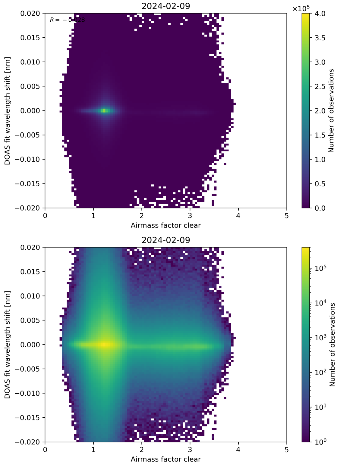
Figure 72: Scatter density plot of “Airmass factor clear” against “DOAS fit wavelength shift” for 2024-02-08 to 2024-02-10.
