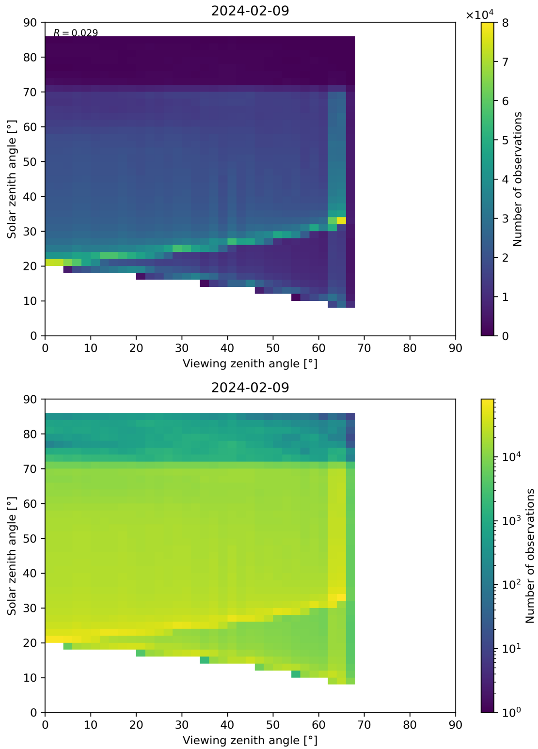
Figure 197: Scatter density plot of “Viewing zenith angle” against “Solar zenith angle” for 2024-02-08 to 2024-02-10.
