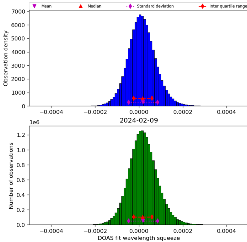
Figure 45: Histogram of “DOAS fit wavelength squeeze” for 2024-02-08 to 2024-02-10
