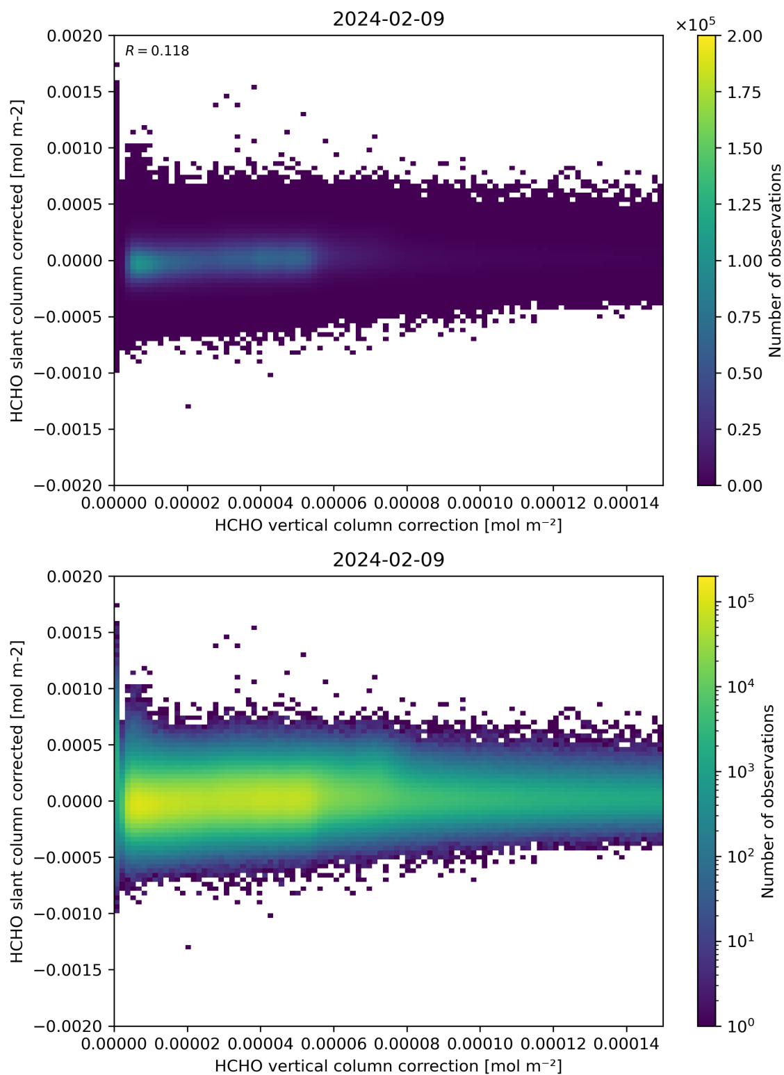
Figure 116: Scatter density plot of “HCHO vertical column correction” against “HCHO slant column corrected” for 2024-02-08 to 2024-02-10.
