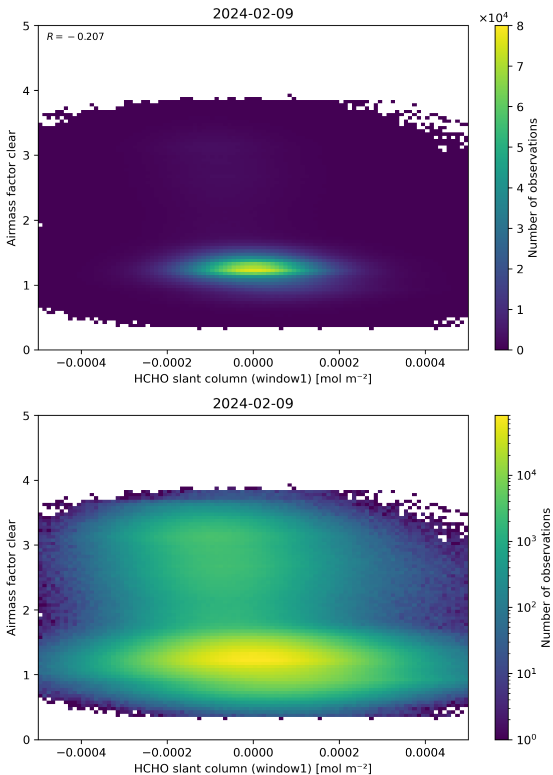
Figure 81: Scatter density plot of “HCHO slant column (window1)” against “Airmass factor clear” for 2024-02-08 to 2024-02-10.
