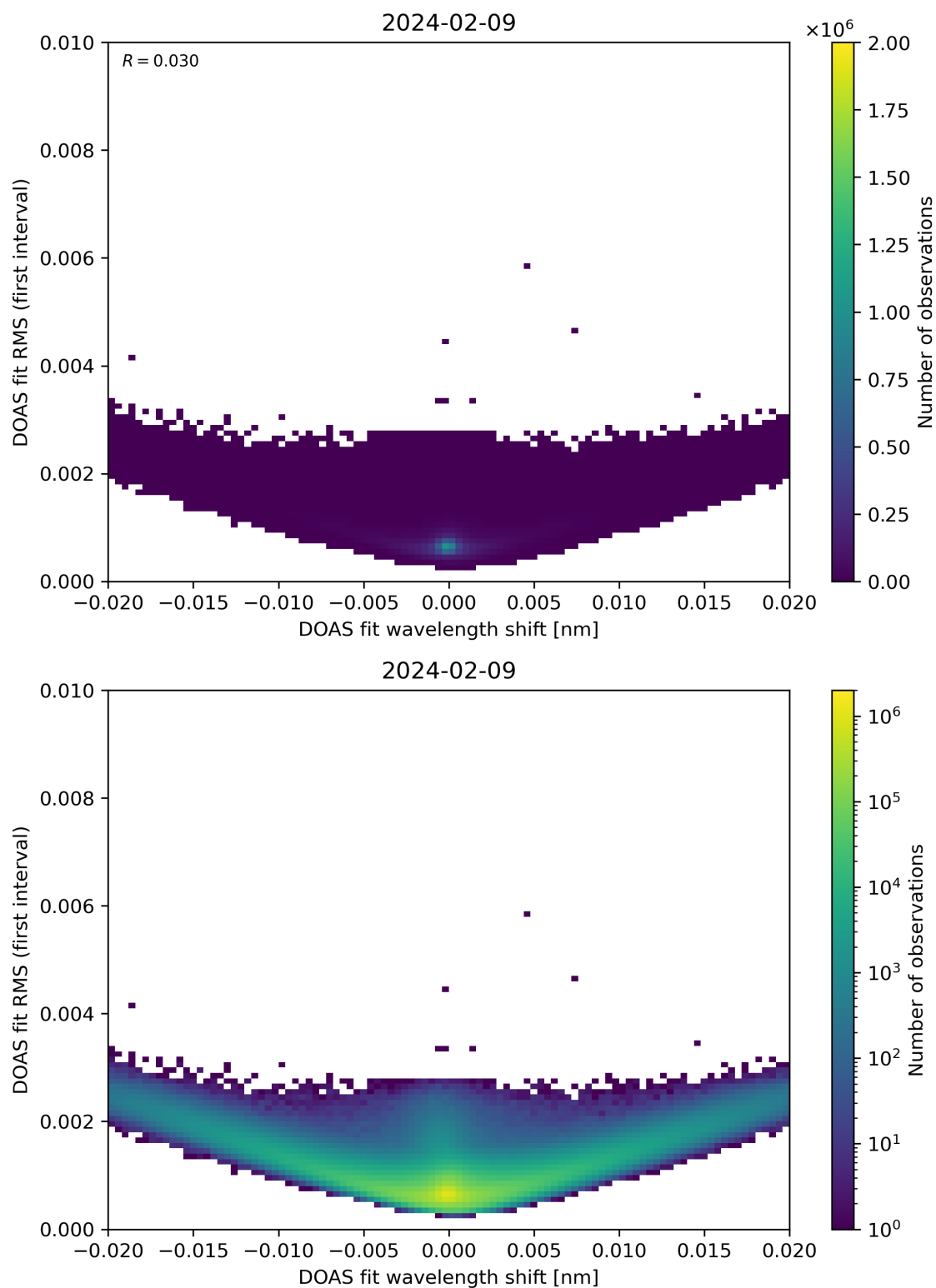
Figure 64: Scatter density plot of “DOAS fit wavelength shift” against “DOAS fit RMS (first interval)” for 2024-02-08 to 2024-02-10.
