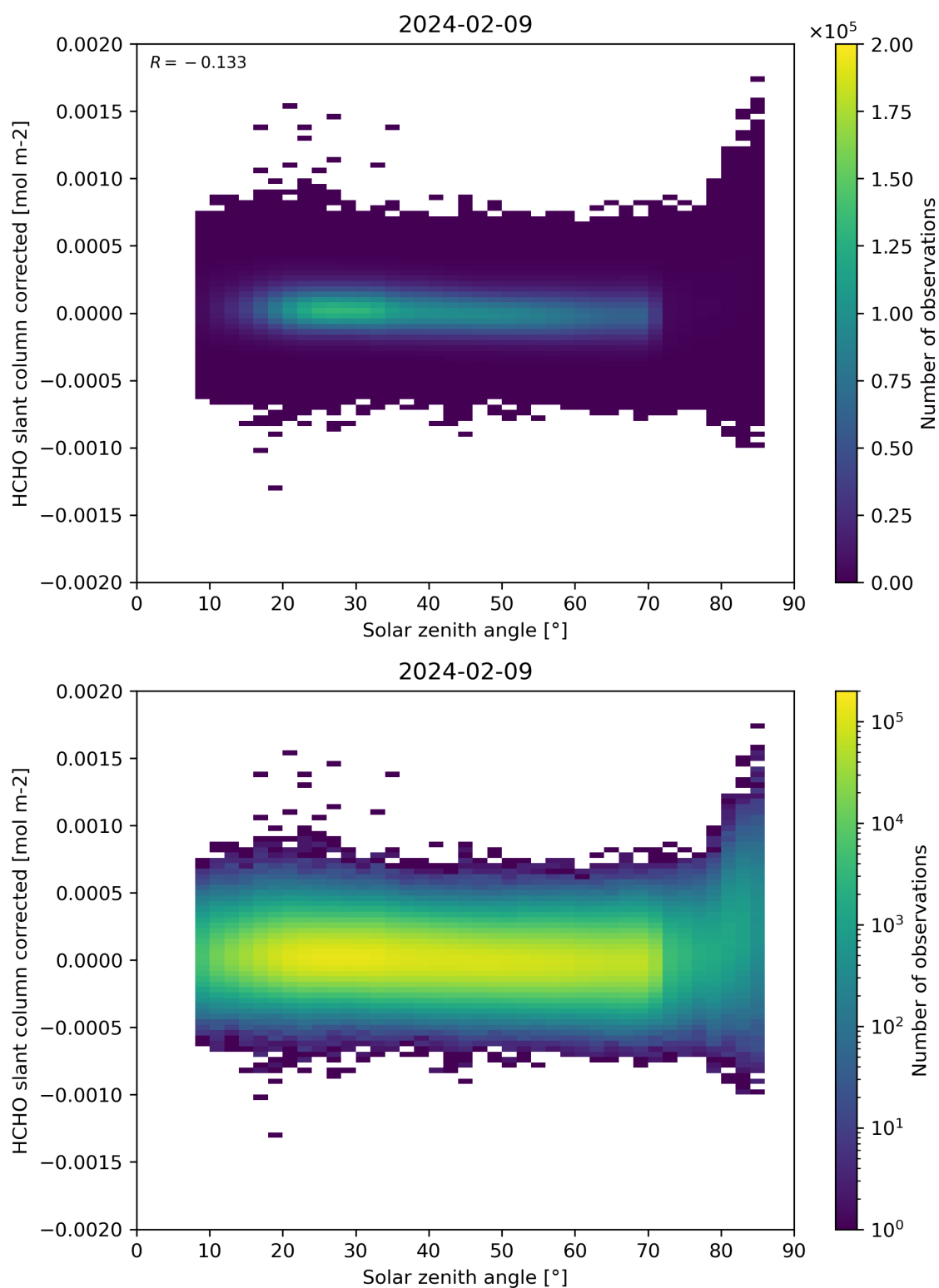
Figure 171: Scatter density plot of “Solar zenith angle” against “HCHO slant column corrected” for 2024-02-08 to 2024-02-10.
