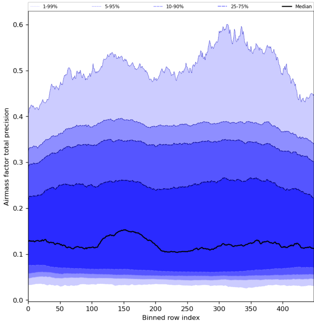
Figure 55: Along track statistics of “Airmass factor total precision” for 2024-02-08 to 2024-02-10
