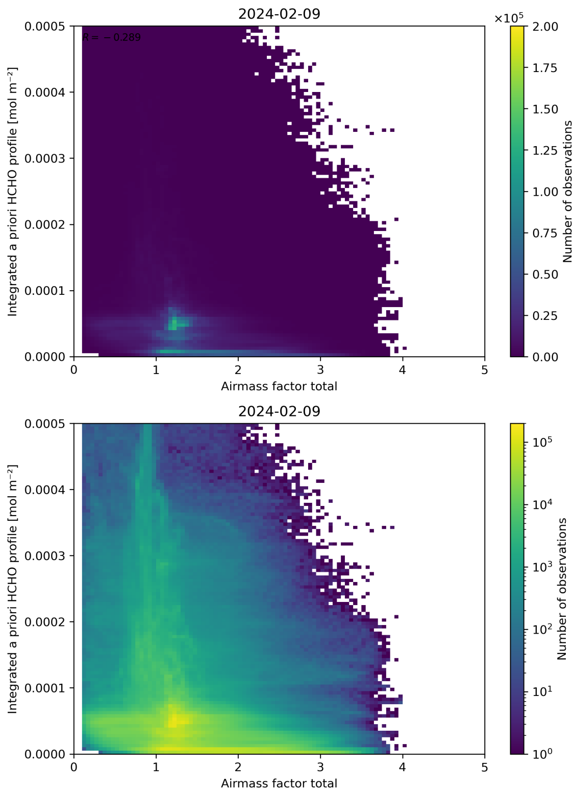
Figure 104: Scatter density plot of “Airmass factor total” against “Integrated a priori HCHO profile” for 2024-02-08 to 2024-02-10.
