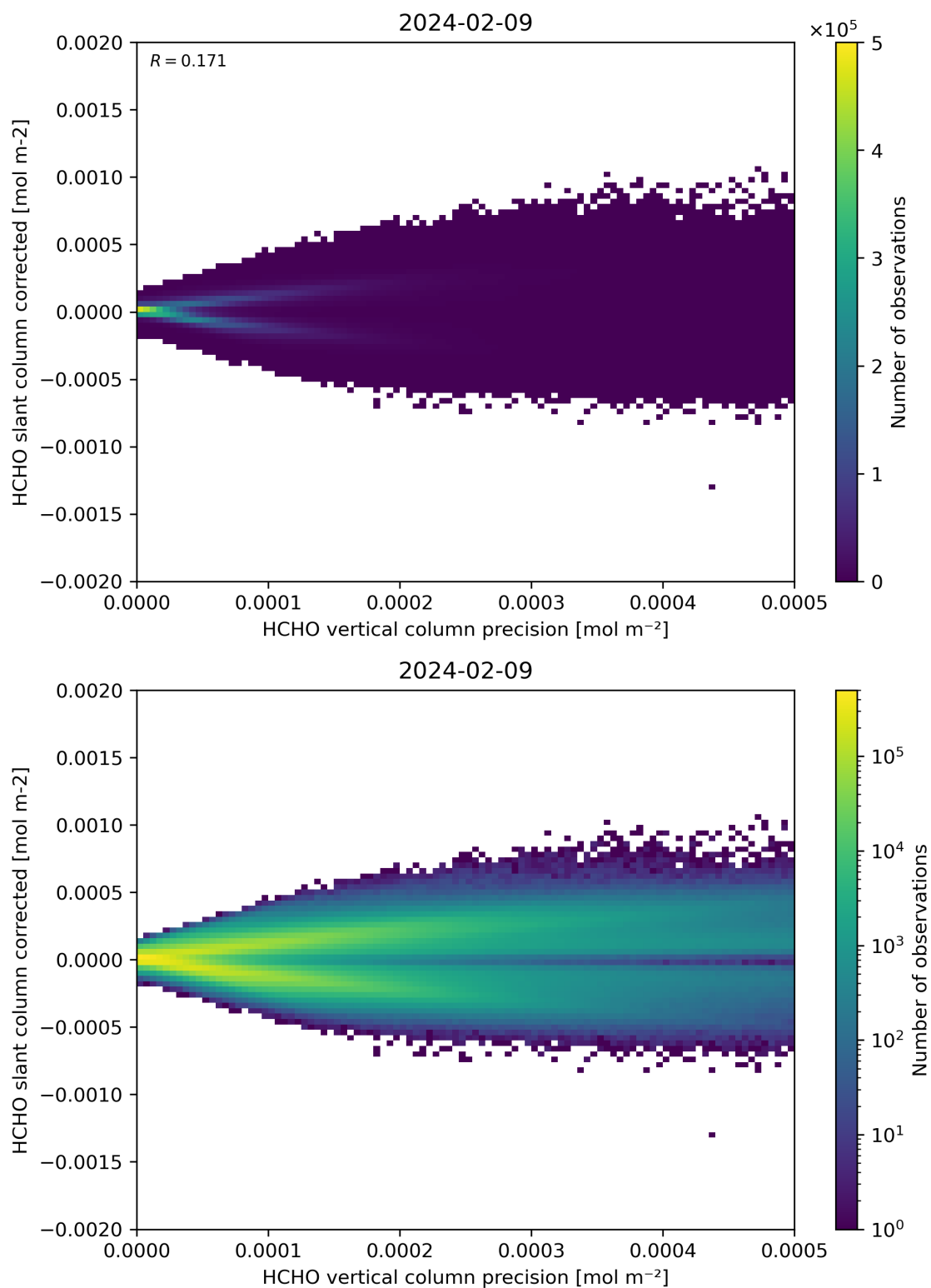
Figure 140: Scatter density plot of “HCHO vertical column precision” against “HCHO slant column corrected” for 2024-02-08 to 2024-02-10.
