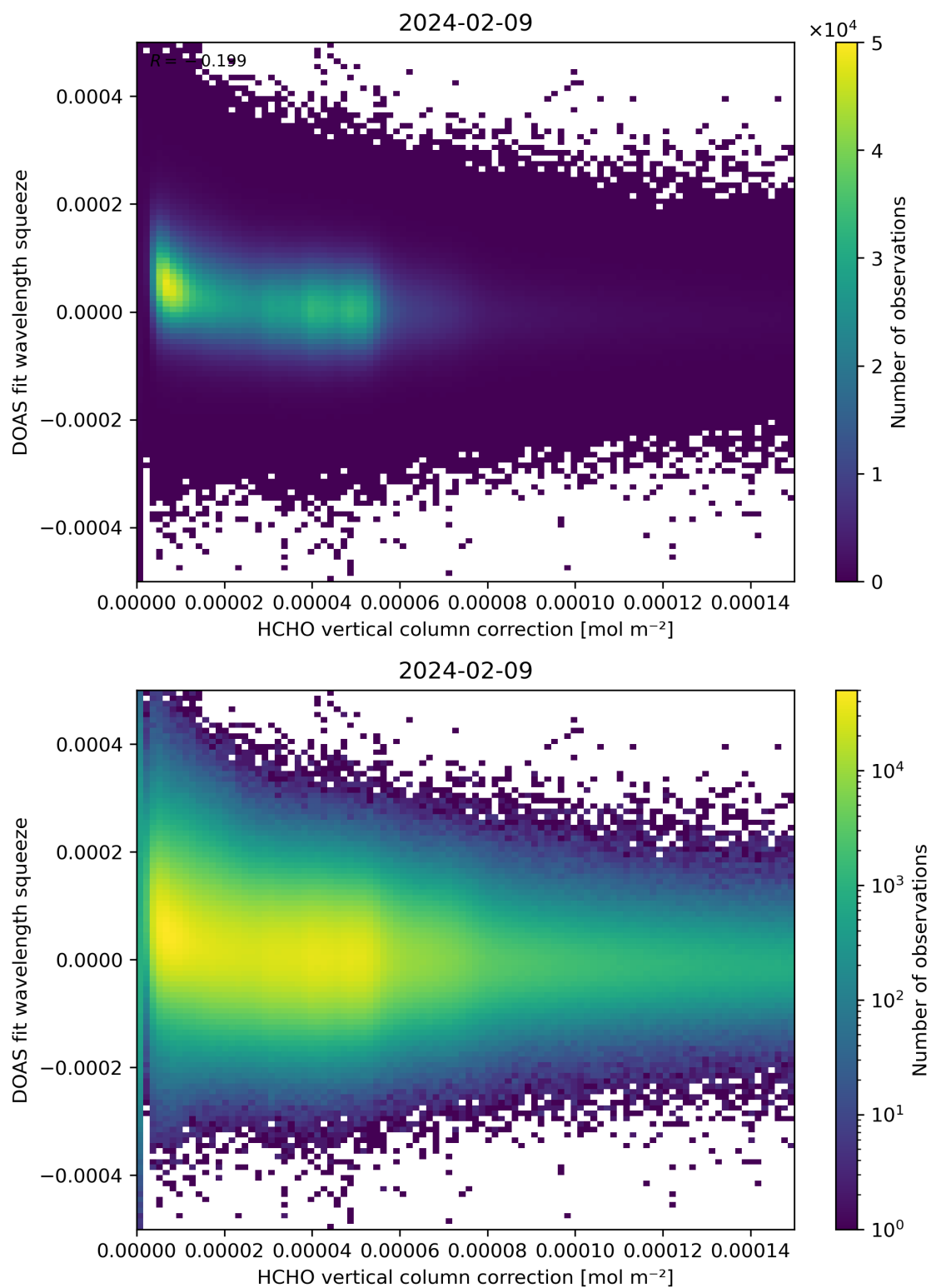
Figure 114: Scatter density plot of “HCHO vertical column correction” against “DOAS fit wavelength squeeze” for 2024-02-08 to 2024-02-10.
