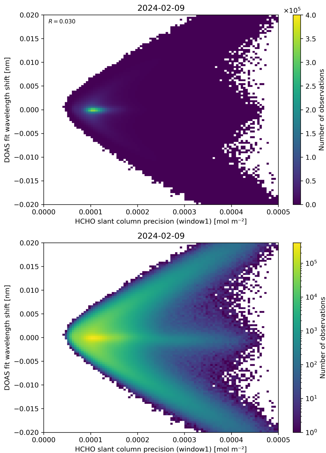
Figure 89: Scatter density plot of “HCHO slant column precision (window1)” against “DOAS fit wavelength shift” for 2024-02-08 to 2024-02-10.
