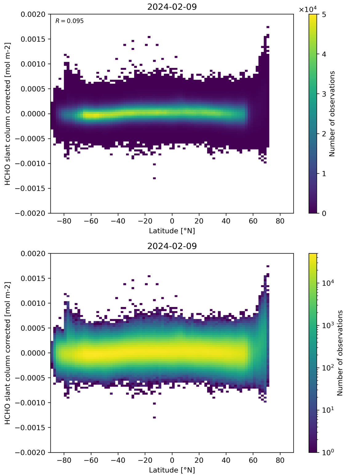
Figure 157: Scatter density plot of “Latitude” against “HCHO slant column corrected” for 2024-02-08 to 2024-02-10.
