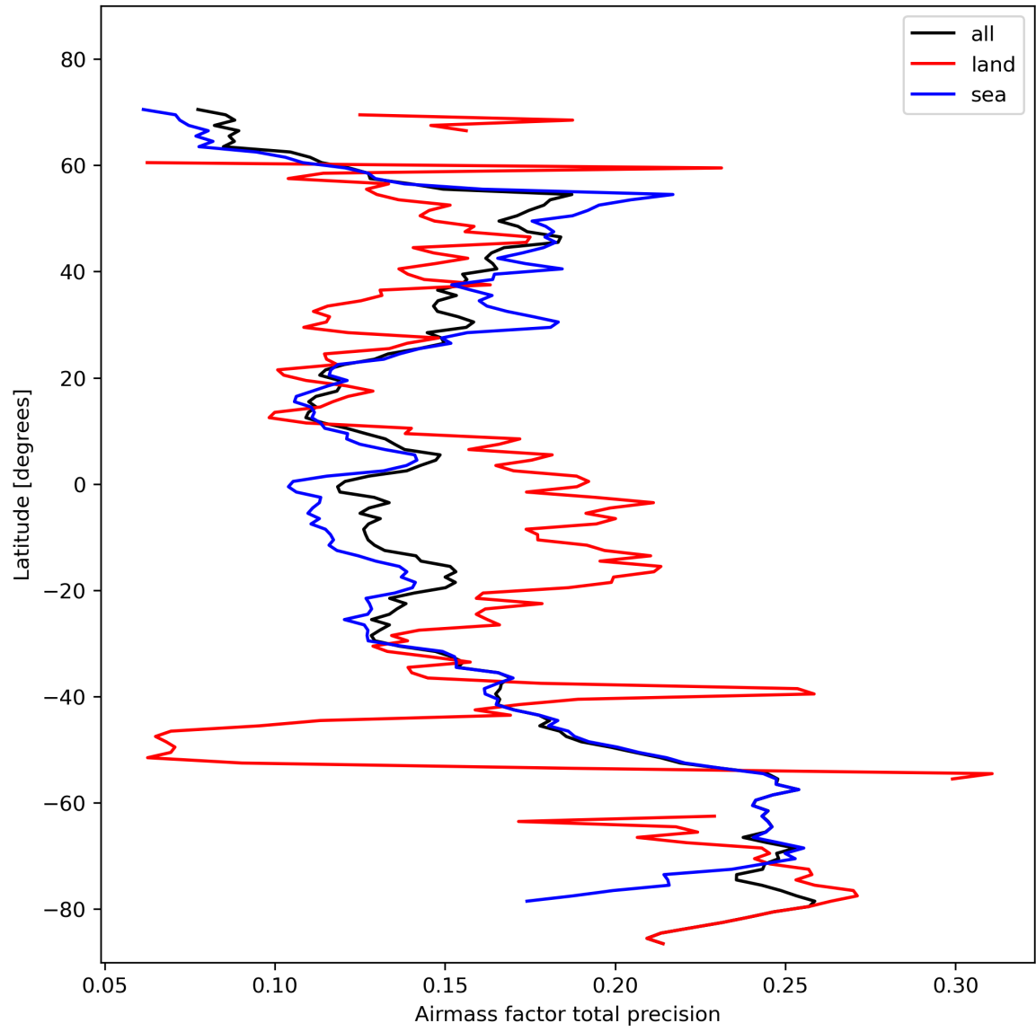
Figure 27: Zonal average of “Airmass factor total precision” for 2024-02-08 to 2024-02-10.
