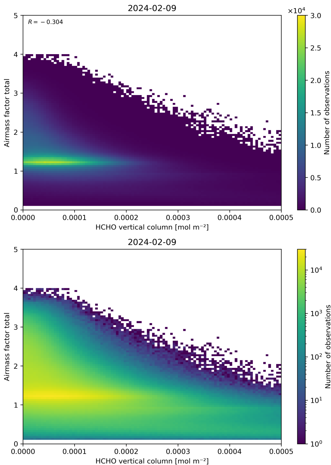
Figure 131: Scatter density plot of “HCHO vertical column” against “Airmass factor total” for 2024-02-08 to 2024-02-10.
