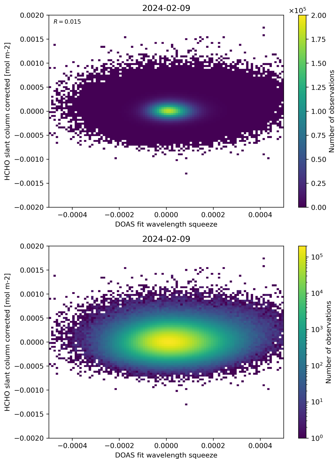
Figure 69: Scatter density plot of “DOAS fit wavelength squeeze” against “HCHO slant column corrected” for 2024-02-08 to 2024-02-10.
