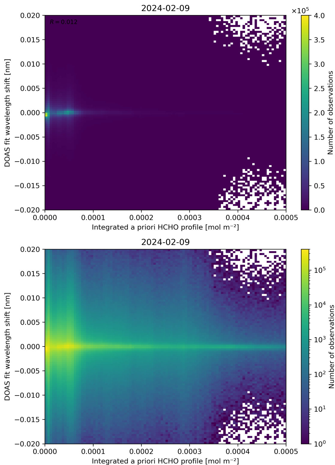
Figure 149: Scatter density plot of “Integrated a priori HCHO profile” against “DOAS fit wavelength shift” for 2024-02-08 to 2024-02-10.
