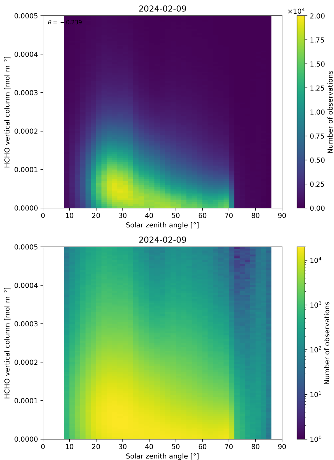
Figure 177: Scatter density plot of “Solar zenith angle” against “HCHO vertical column” for 2024-02-08 to 2024-02-10.
