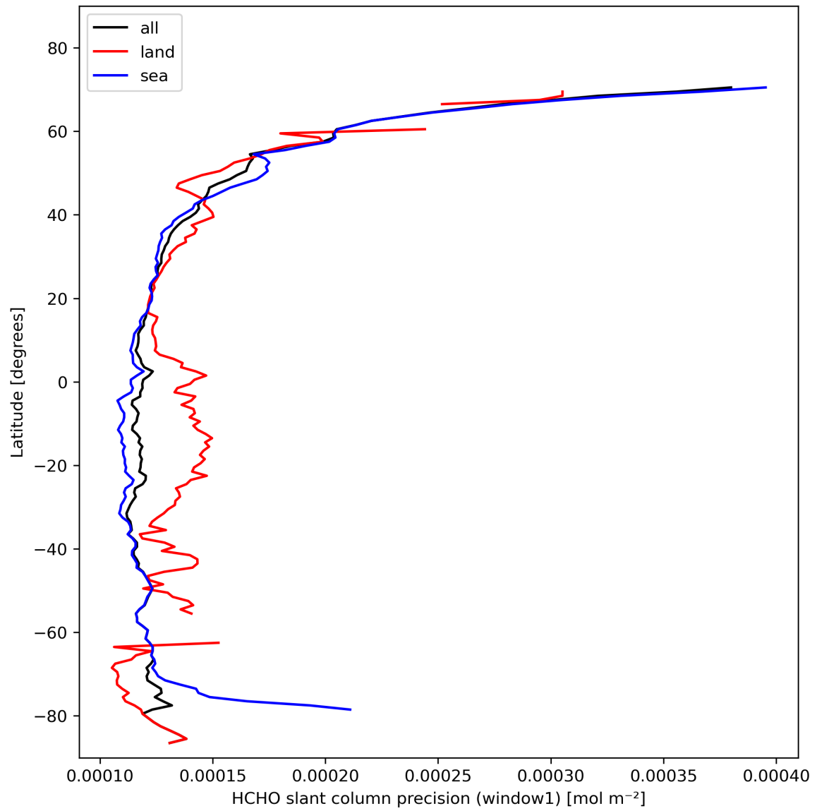
Figure 25: Zonal average of “HCHO slant column precision (window1)” for 2024-02-08 to 2024-02-10.
