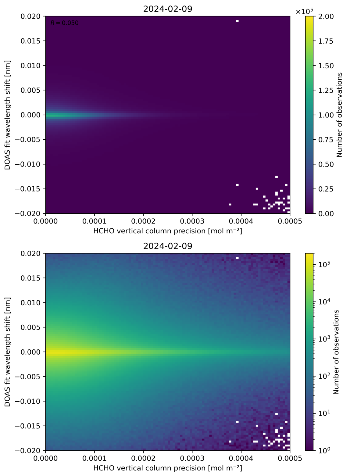
Figure 137: Scatter density plot of “HCHO vertical column precision” against “DOAS fit wavelength shift” for 2024-02-08 to 2024-02-10.
