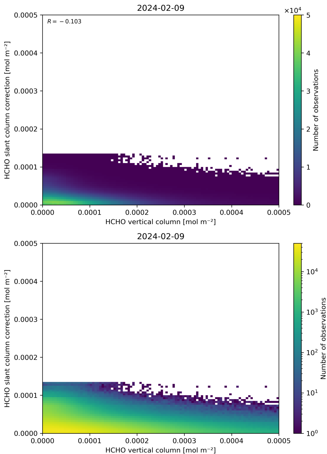
Figure 128: Scatter density plot of “HCHO vertical column” against “HCHO slant column correction” for 2024-02-08 to 2024-02-10.
