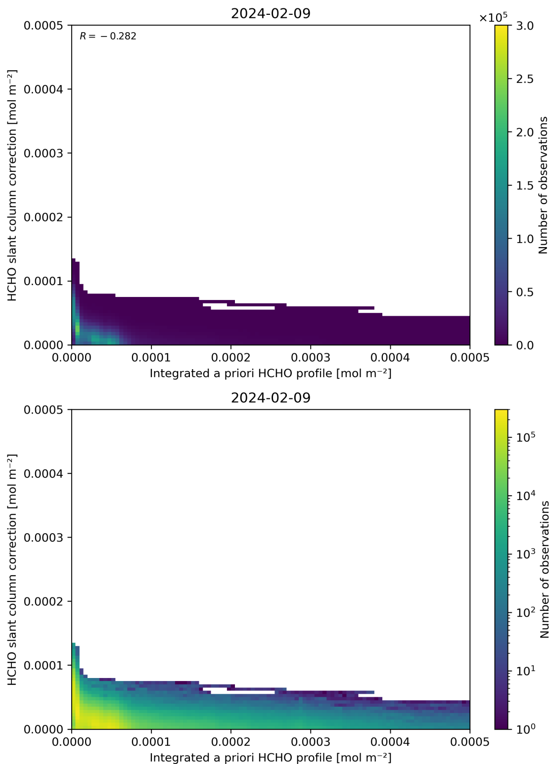
Figure 152: Scatter density plot of “Integrated a priori HCHO profile” against “HCHO slant column correction” for 2024-02-08 to 2024-02-10.
