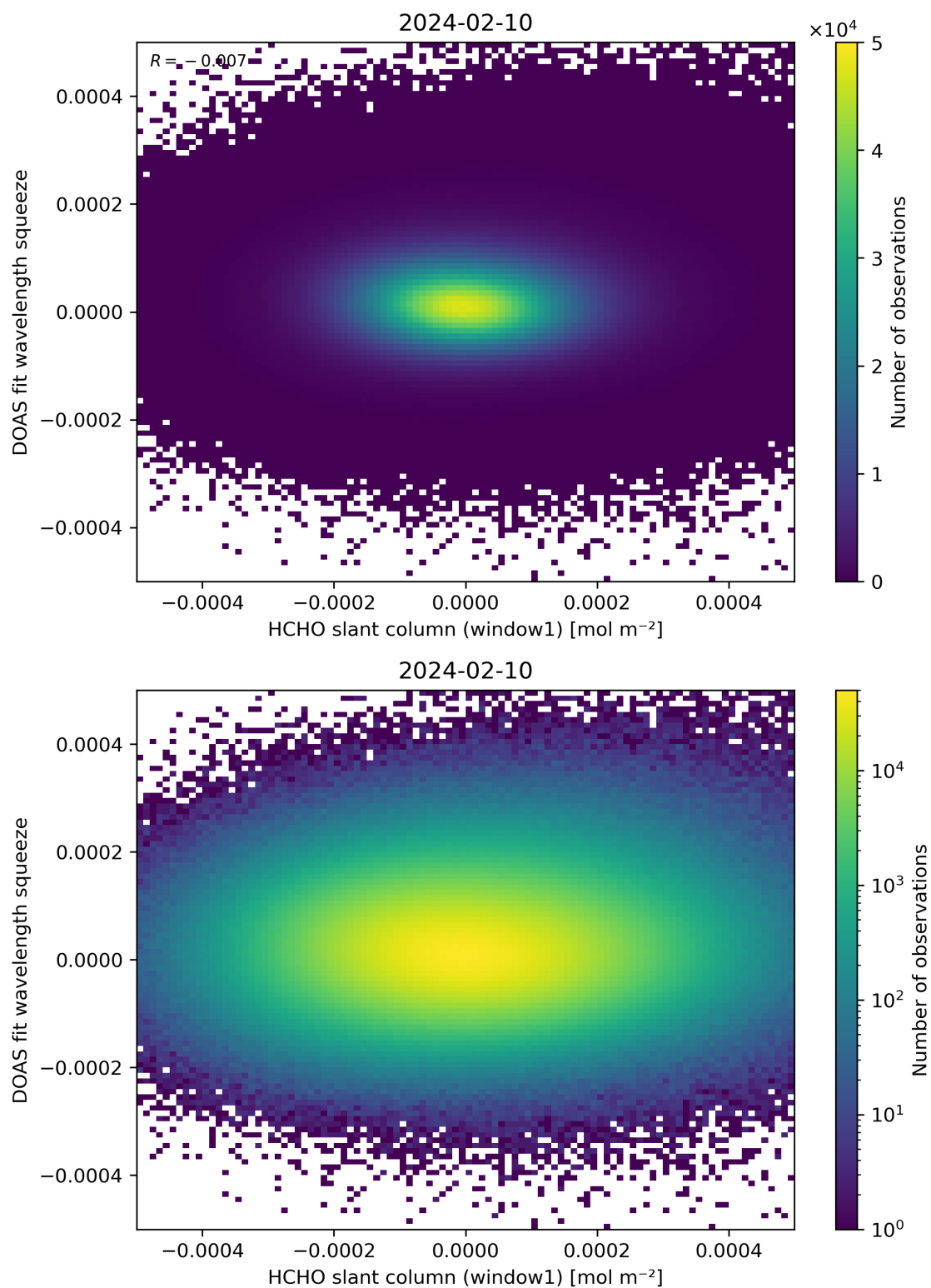
Figure 80: Scatter density plot of “HCHO slant column (window1)” against “DOAS fit wavelength squeeze” for 2024-02-09 to 2024-02-11.
