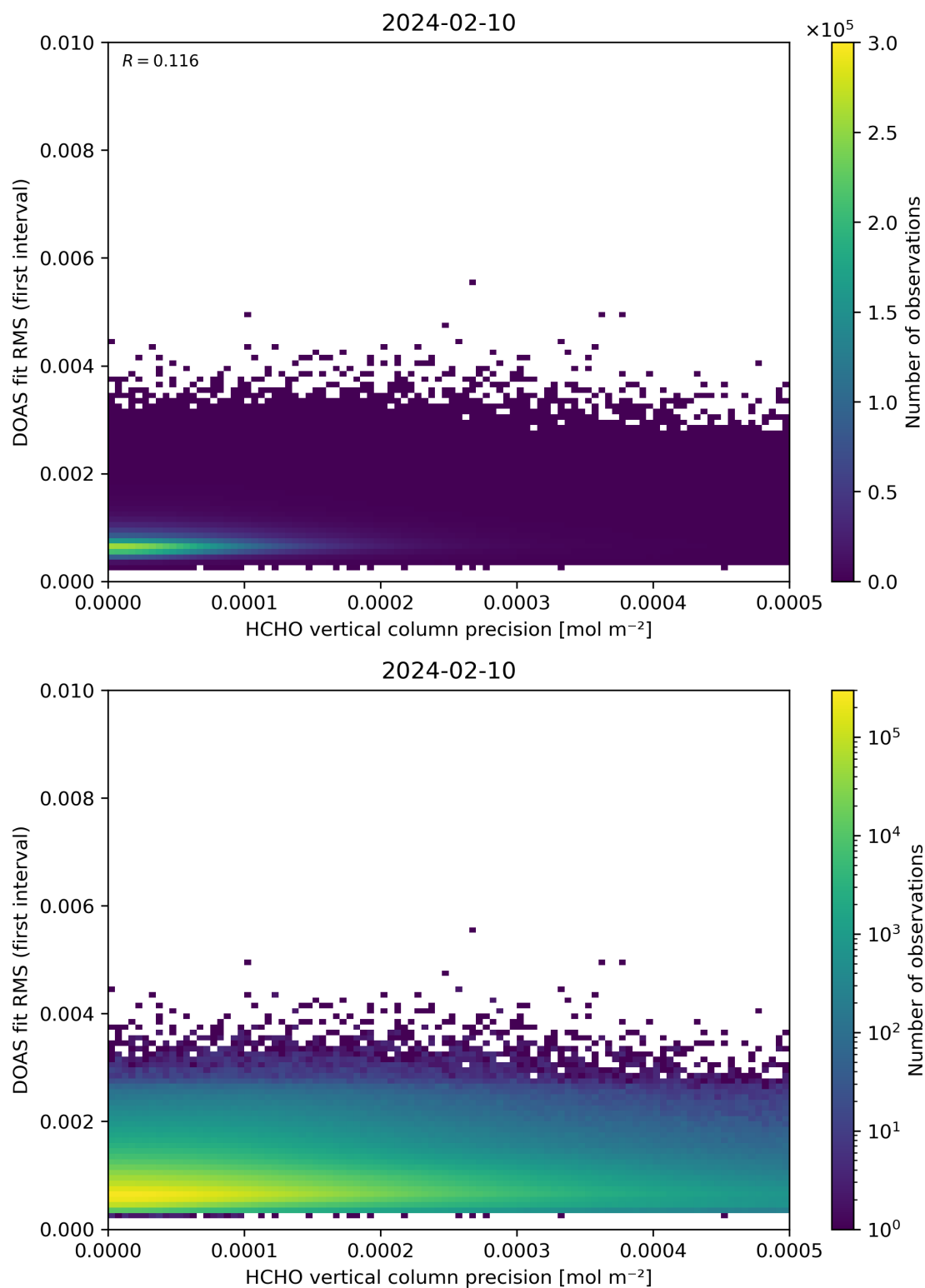
Figure 136: Scatter density plot of “HCHO vertical column precision” against “DOAS fit RMS (first interval)” for 2024-02-09 to 2024-02-11.
