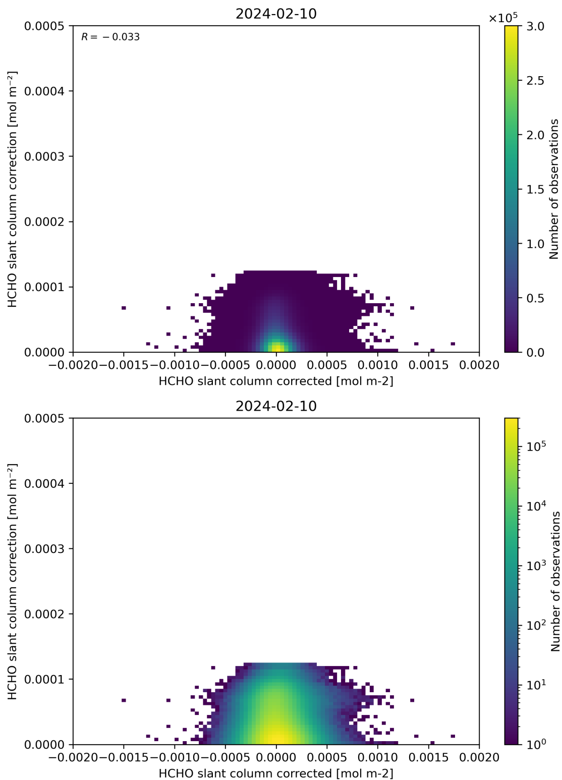
Figure 77: Scatter density plot of “HCHO slant column corrected” against “HCHO slant column correction” for 2024-02-09 to 2024-02-11.
