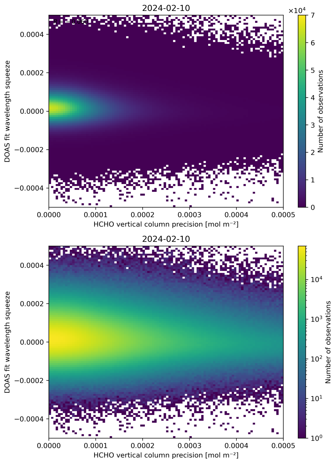
Figure 138: Scatter density plot of “HCHO vertical column precision” against “DOAS fit wavelength squeeze” for 2024-02-09 to 2024-02-11.
