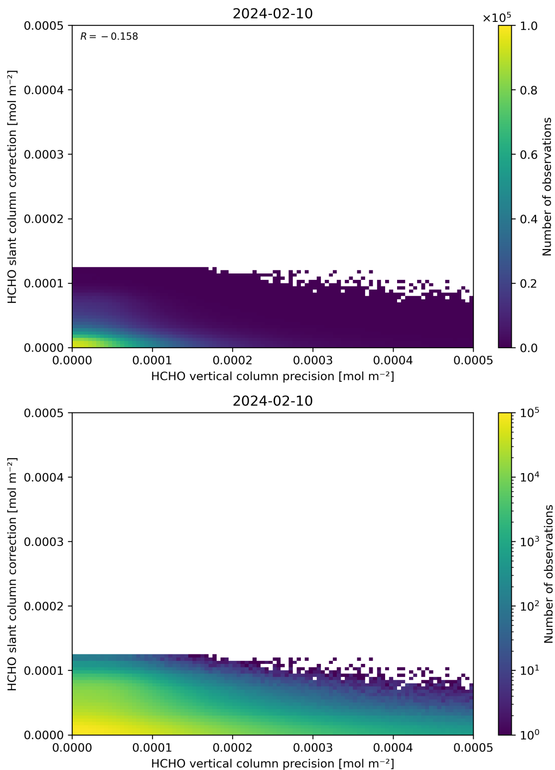
Figure 141: Scatter density plot of “HCHO vertical column precision” against “HCHO slant column correction” for 2024-02-09 to 2024-02-11.
