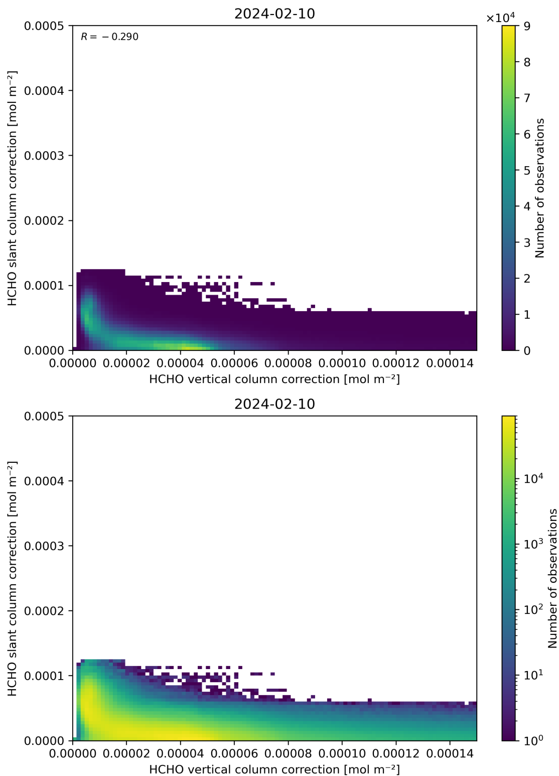
Figure 117: Scatter density plot of “HCHO vertical column correction” against “HCHO slant column correction” for 2024-02-09 to 2024-02-11.
