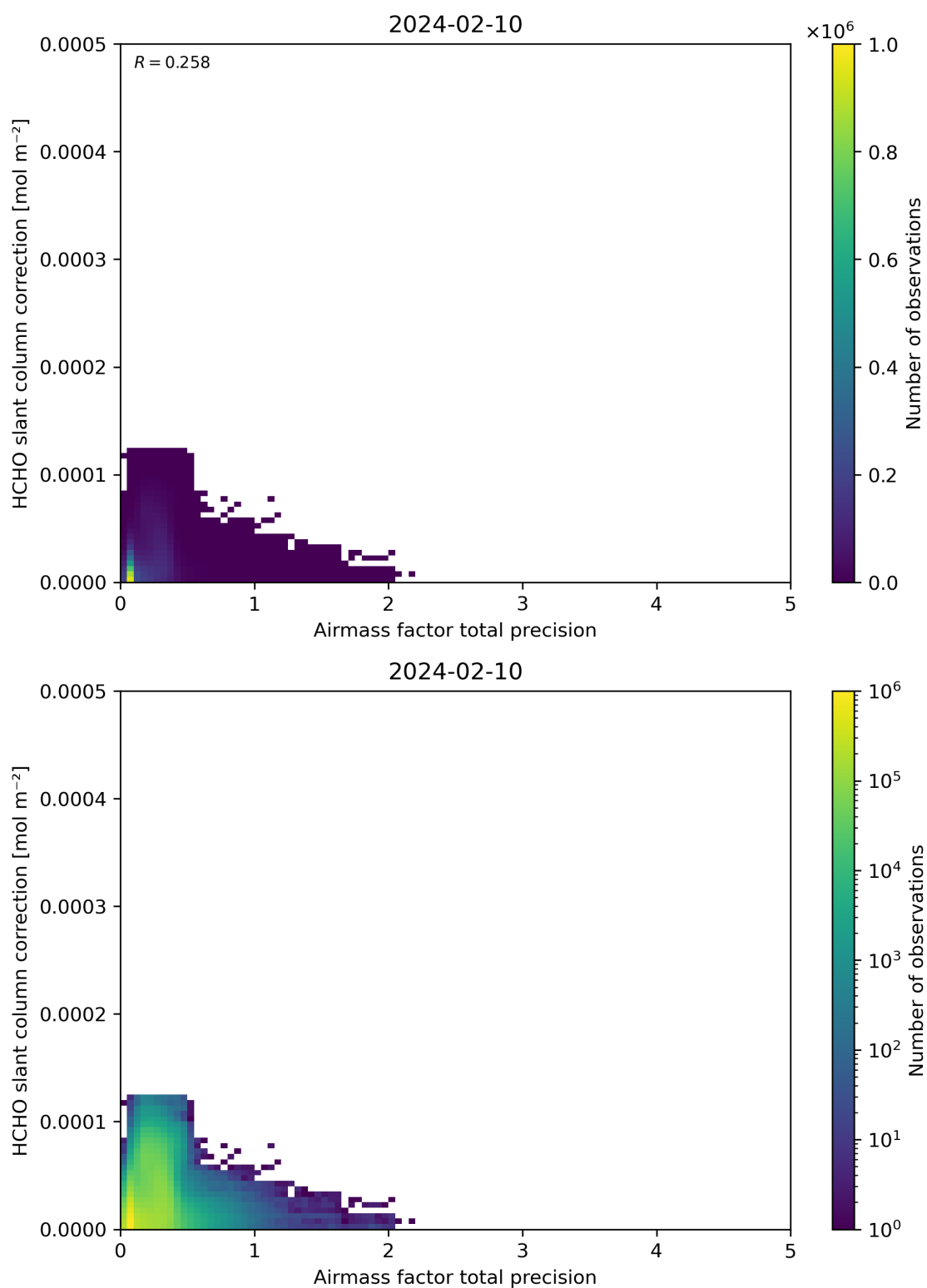
Figure 110: Scatter density plot of “Airmass factor total precision” against “HCHO slant column correction” for 2024-02-09 to 2024-02-11.
