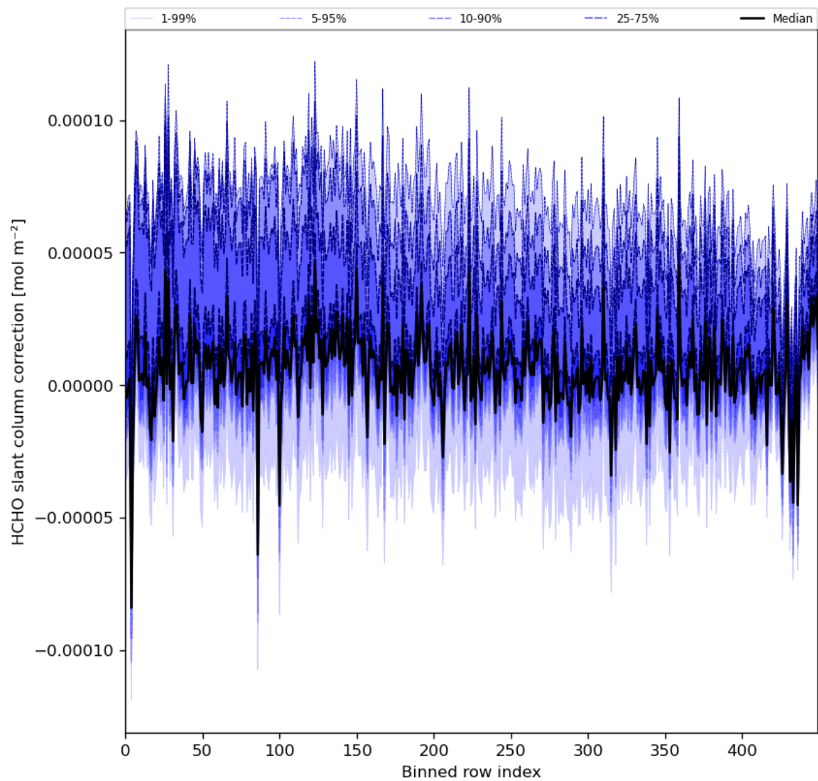
Figure 61: Along track statistics of “HCHO slant column correction” for 2024-02-09 to 2024-02-11
