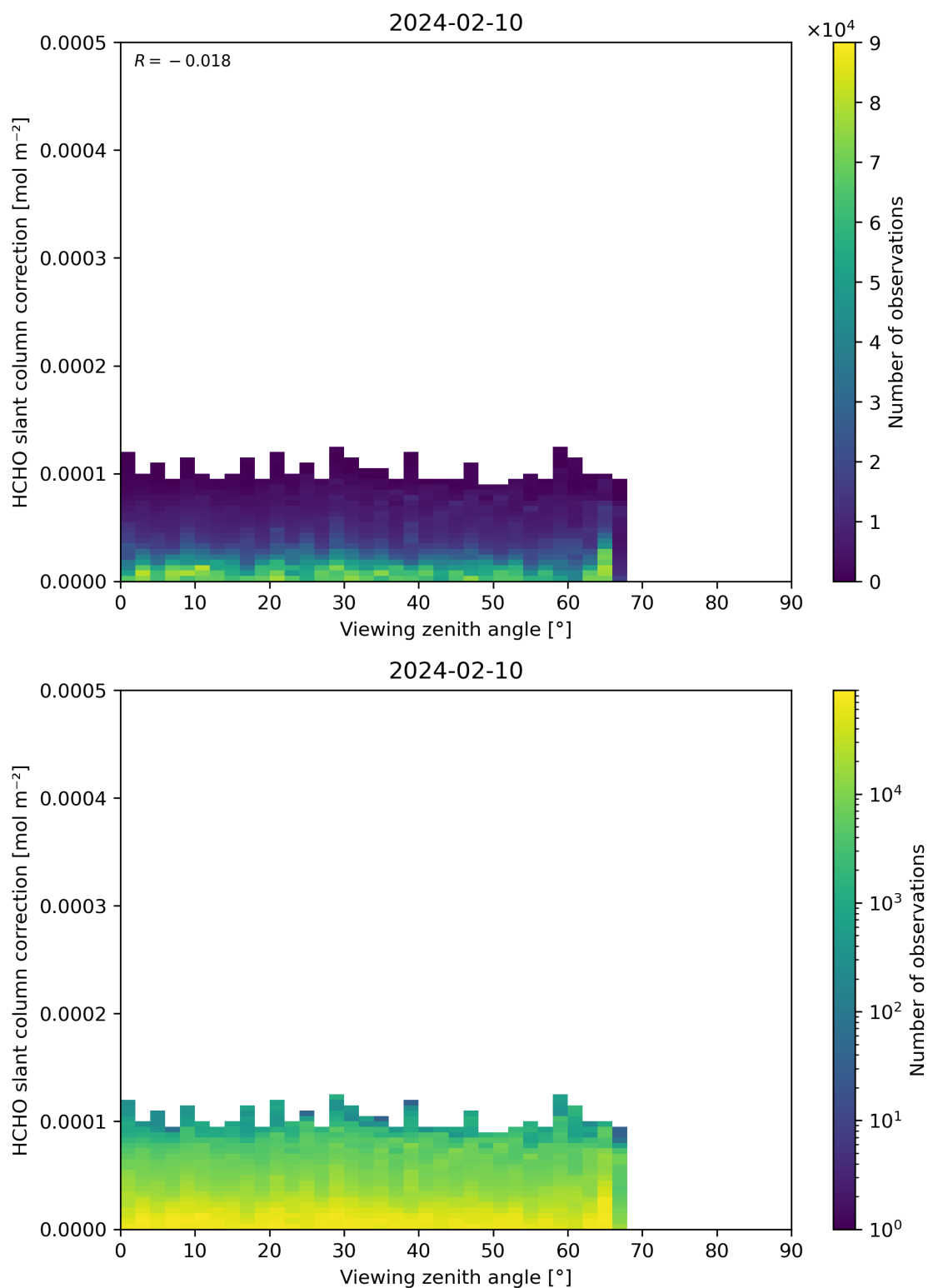
Figure 187: Scatter density plot of “Viewing zenith angle” against “HCHO slant column correction” for 2024-02-09 to 2024-02-11.
