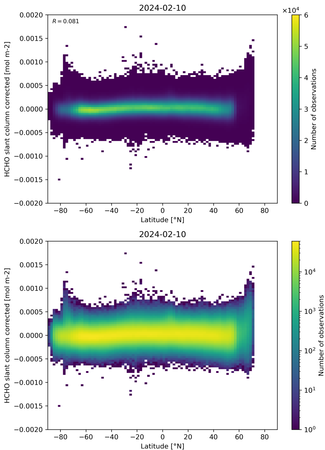
Figure 157: Scatter density plot of “Latitude” against “HCHO slant column corrected” for 2024-02-09 to 2024-02-11.
