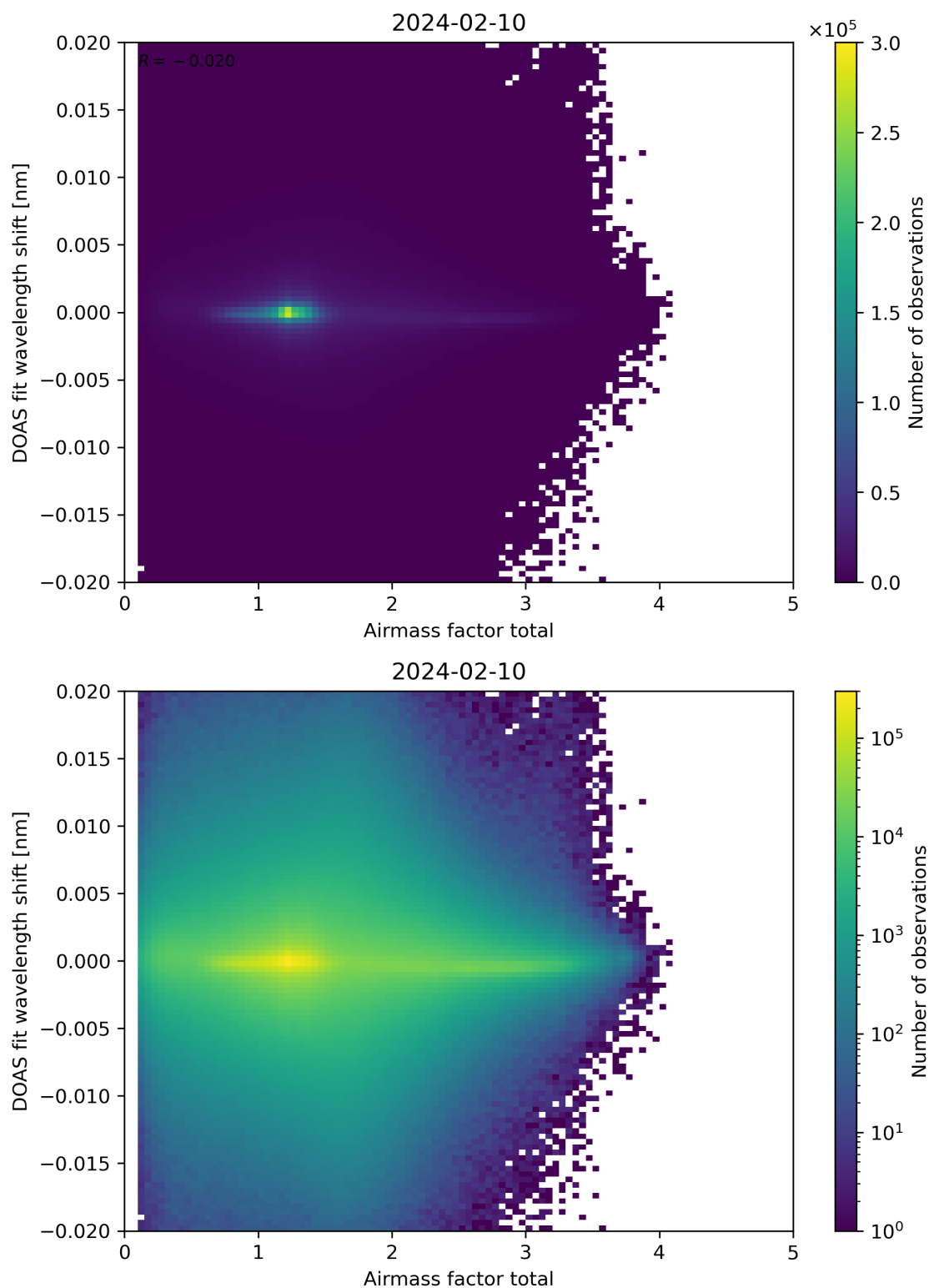
Figure 98: Scatter density plot of “Airmass factor total” against “DOAS fit wavelength shift” for 2024-02-09 to 2024-02-11.
