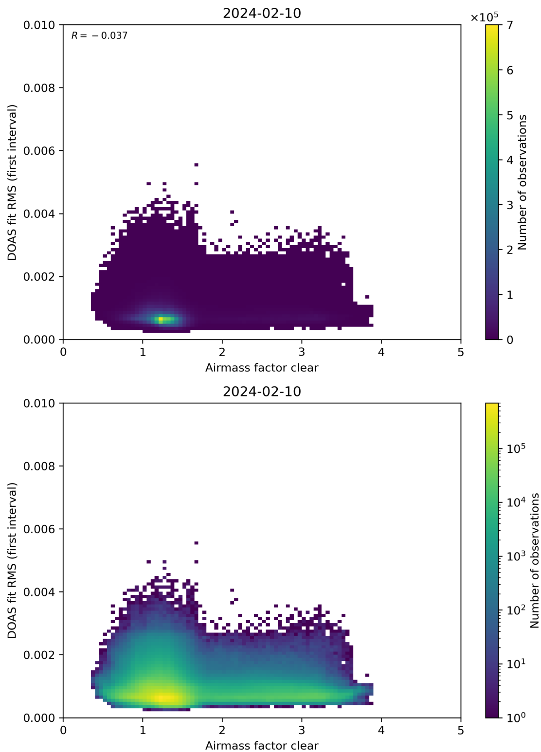
Figure 71: Scatter density plot of “Airmass factor clear” against “DOAS fit RMS (first interval)” for 2024-02-09 to 2024-02-11.
