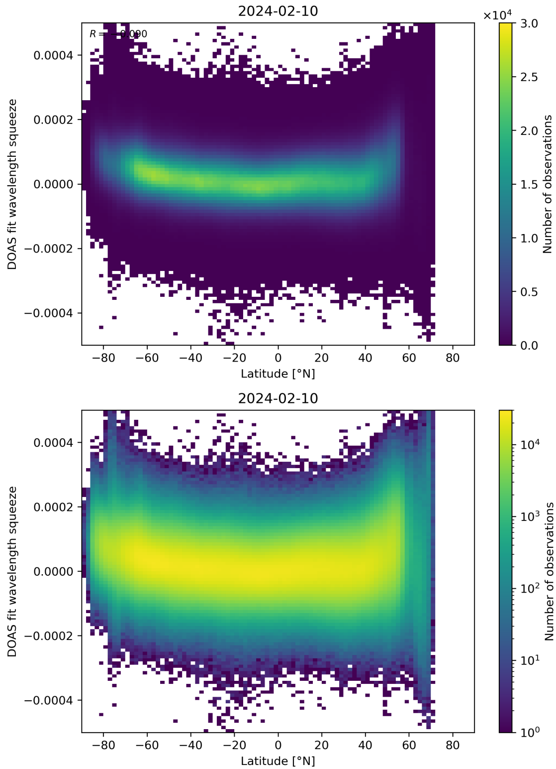
Figure 155: Scatter density plot of “Latitude” against “DOAS fit wavelength squeeze” for 2024-02-09 to 2024-02-11.
