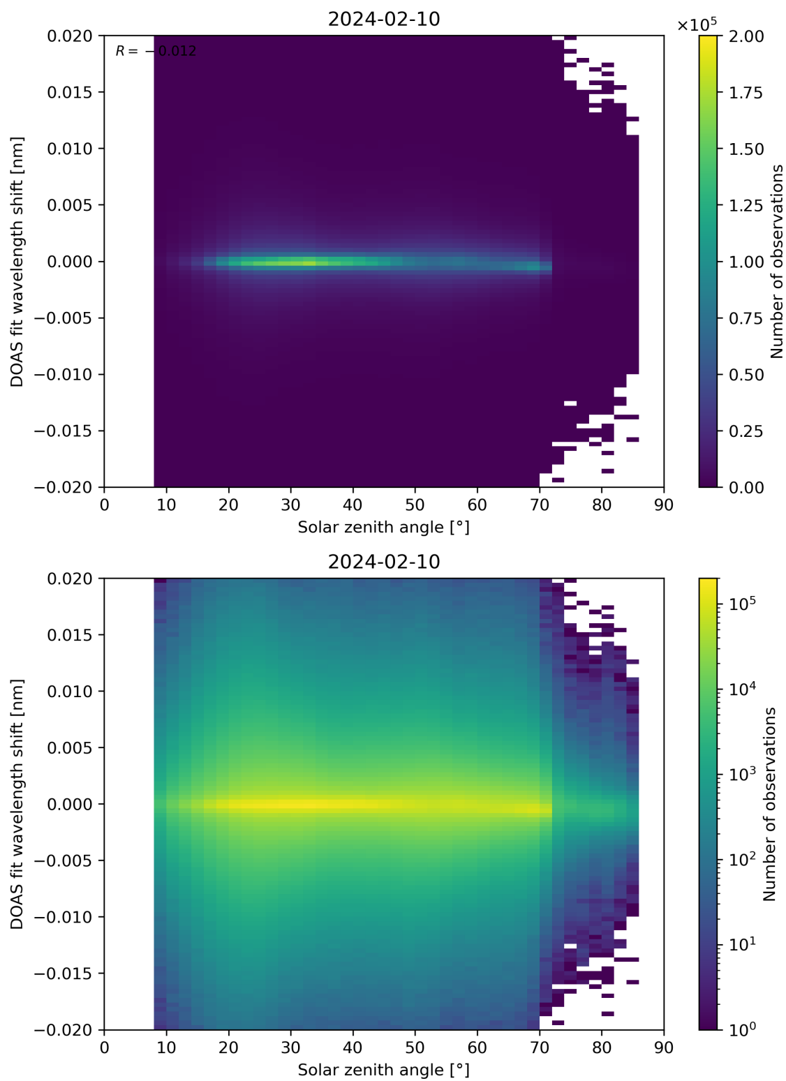
Figure 168: Scatter density plot of “Solar zenith angle” against “DOAS fit wavelength shift” for 2024-02-09 to 2024-02-11.
