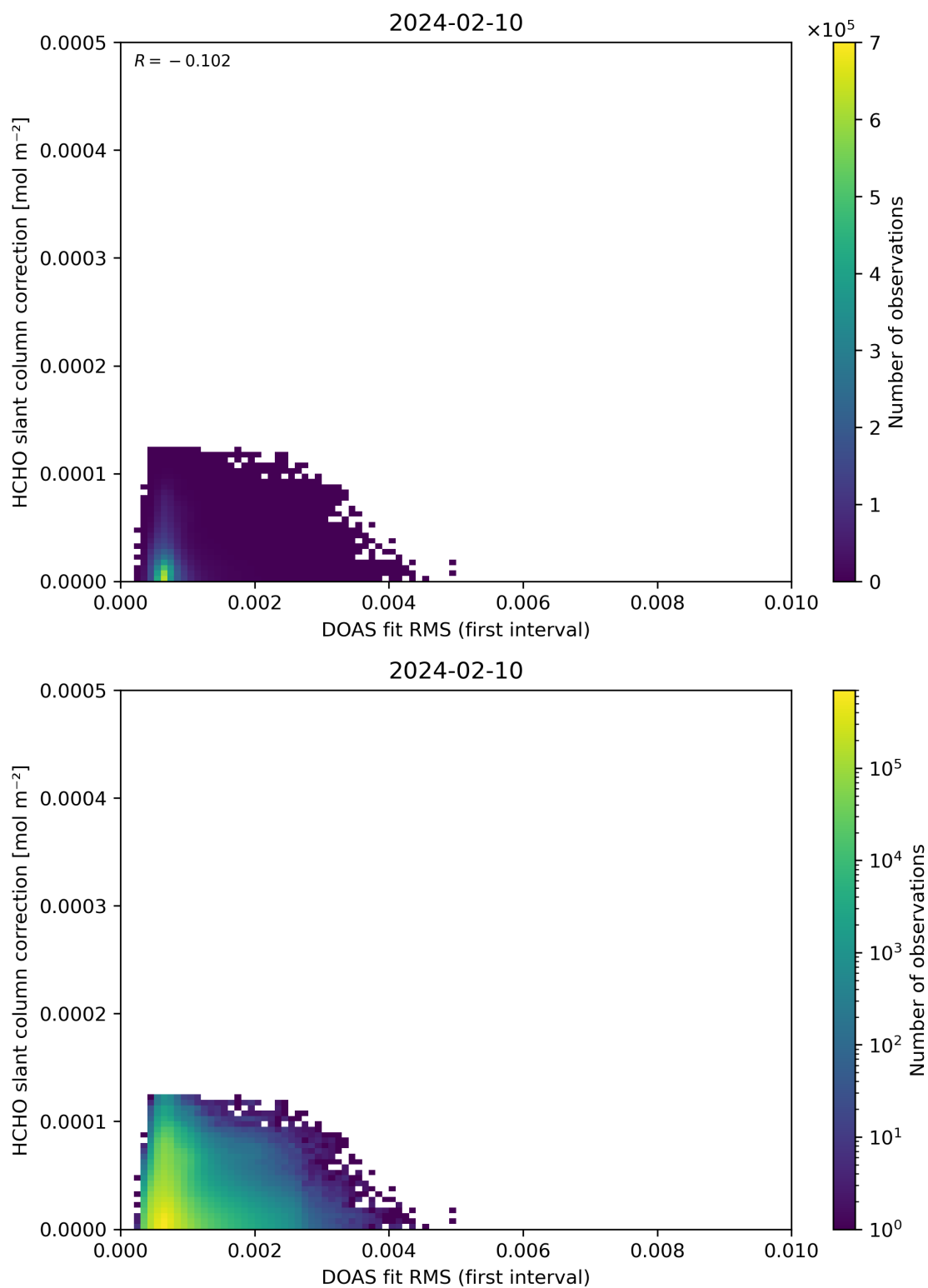
Figure 63: Scatter density plot of “DOAS fit RMS (first interval)” against “HCHO slant column correction” for 2024-02-09 to 2024-02-11.
