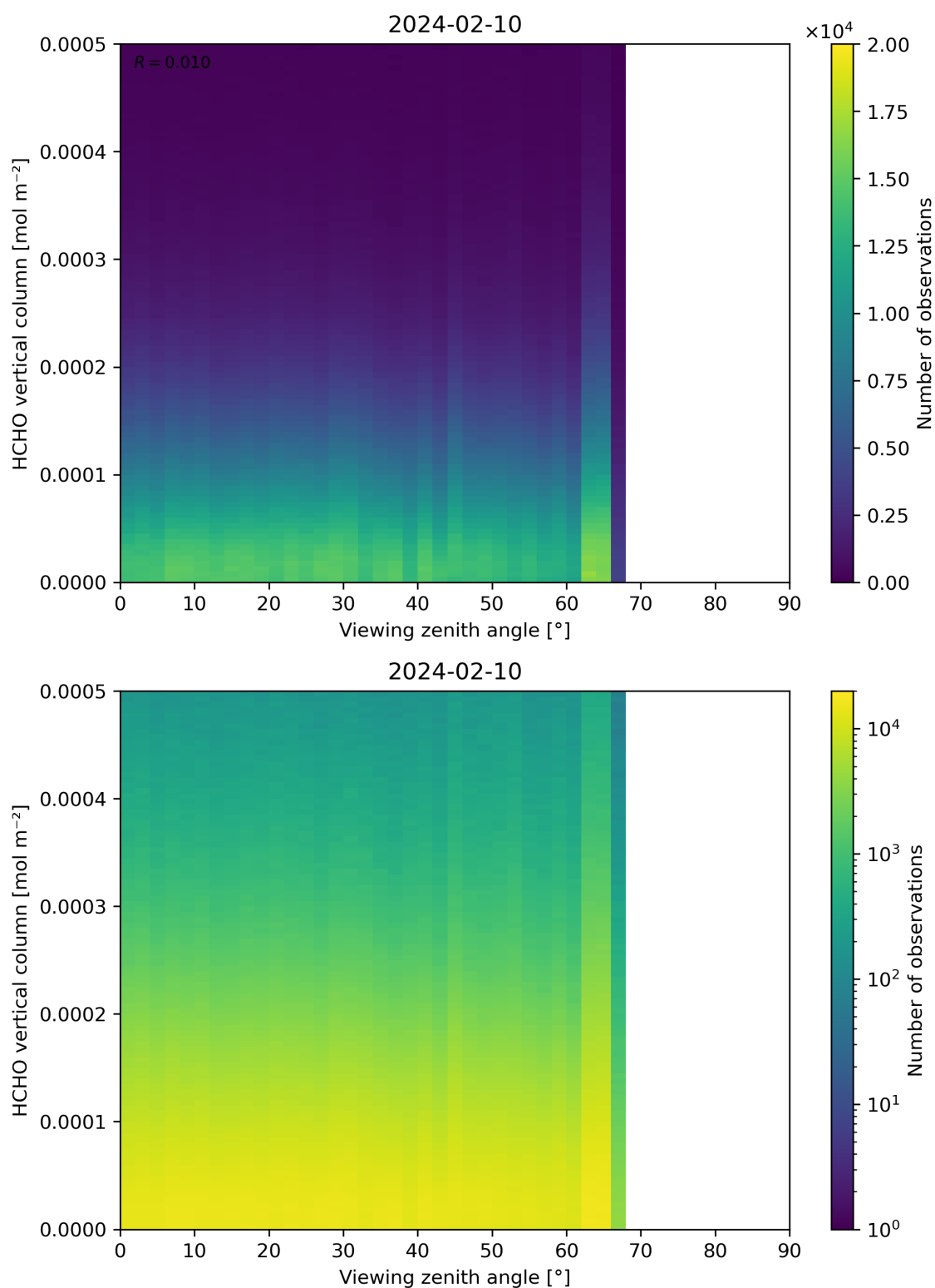
Figure 192: Scatter density plot of “Viewing zenith angle” against “HCHO vertical column” for 2024-02-09 to 2024-02-11.
