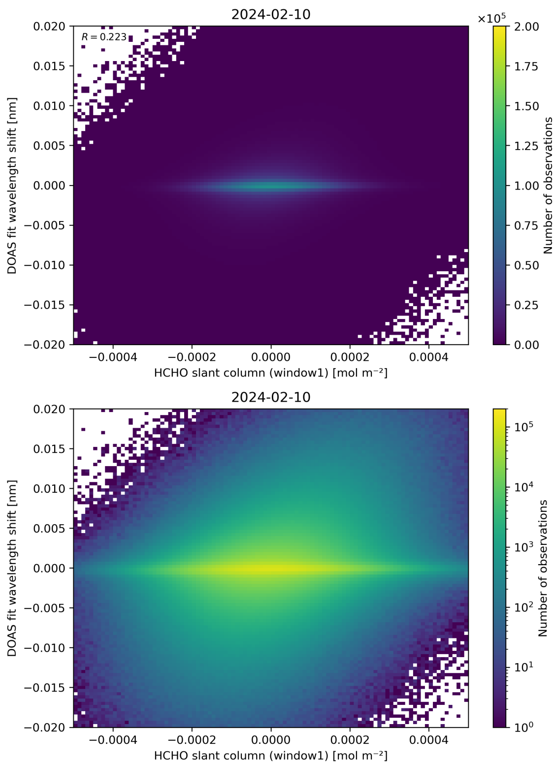
Figure 79: Scatter density plot of “HCHO slant column (window1)” against “DOAS fit wavelength shift” for 2024-02-09 to 2024-02-11.
