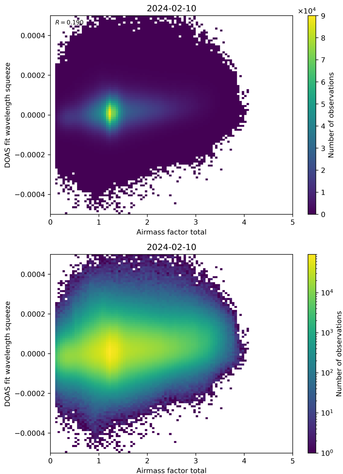
Figure 99: Scatter density plot of “Airmass factor total” against “DOAS fit wavelength squeeze” for 2024-02-09 to 2024-02-11.
