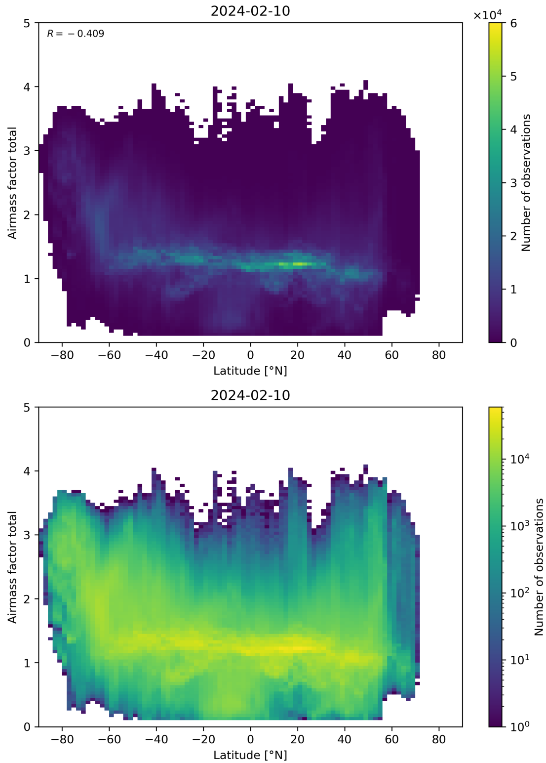
Figure 161: Scatter density plot of “Latitude” against “Airmass factor total” for 2024-02-09 to 2024-02-11.
