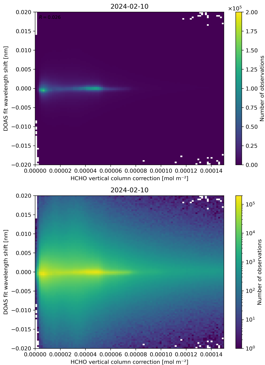
Figure 113: Scatter density plot of “HCHO vertical column correction” against “DOAS fit wavelength shift” for 2024-02-09 to 2024-02-11.
