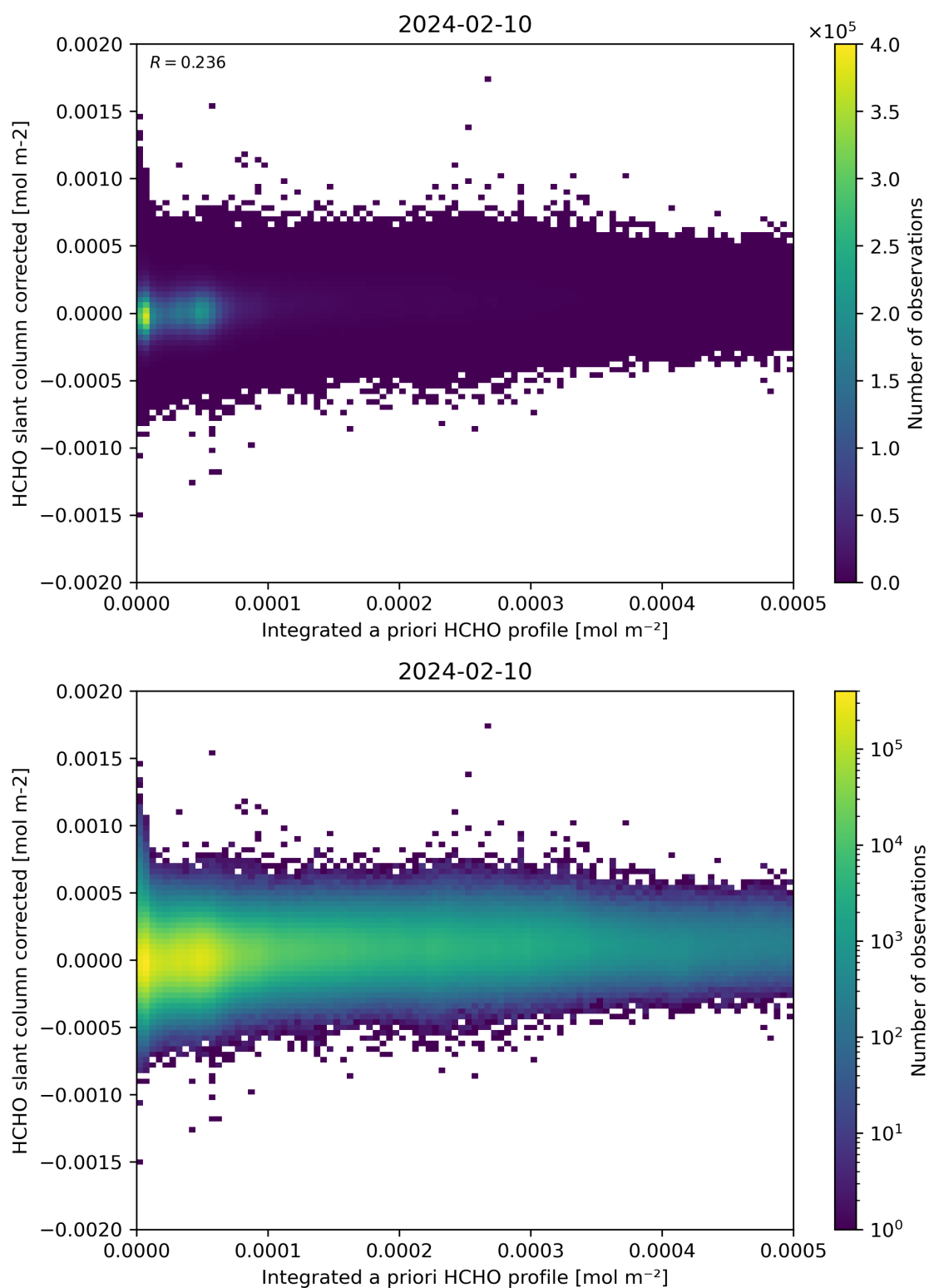
Figure 151: Scatter density plot of “Integrated a priori HCHO profile” against “HCHO slant column corrected” for 2024-02-09 to 2024-02-11.
