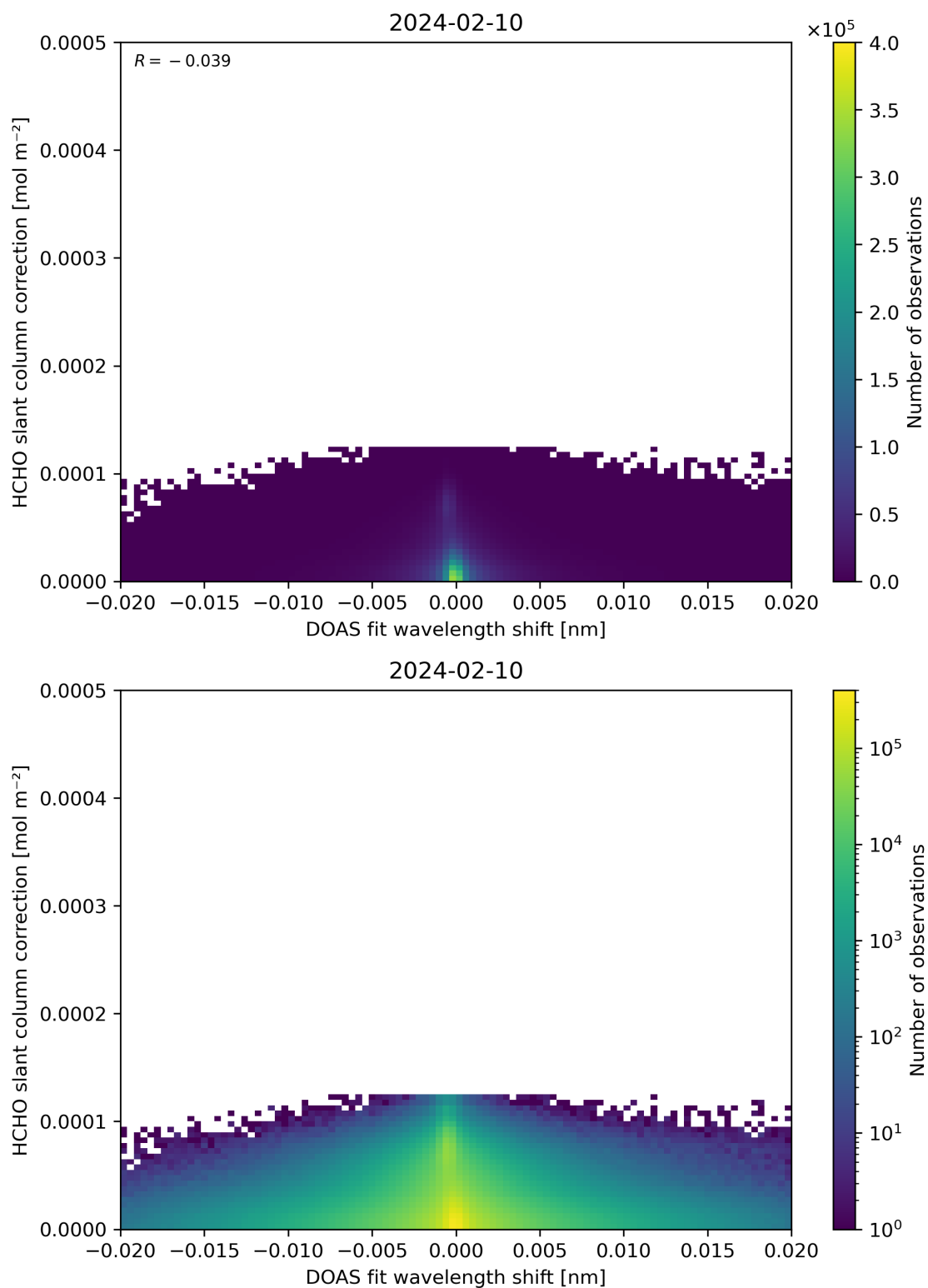
Figure 67: Scatter density plot of “DOAS fit wavelength shift” against “HCHO slant column correction” for 2024-02-09 to 2024-02-11.
