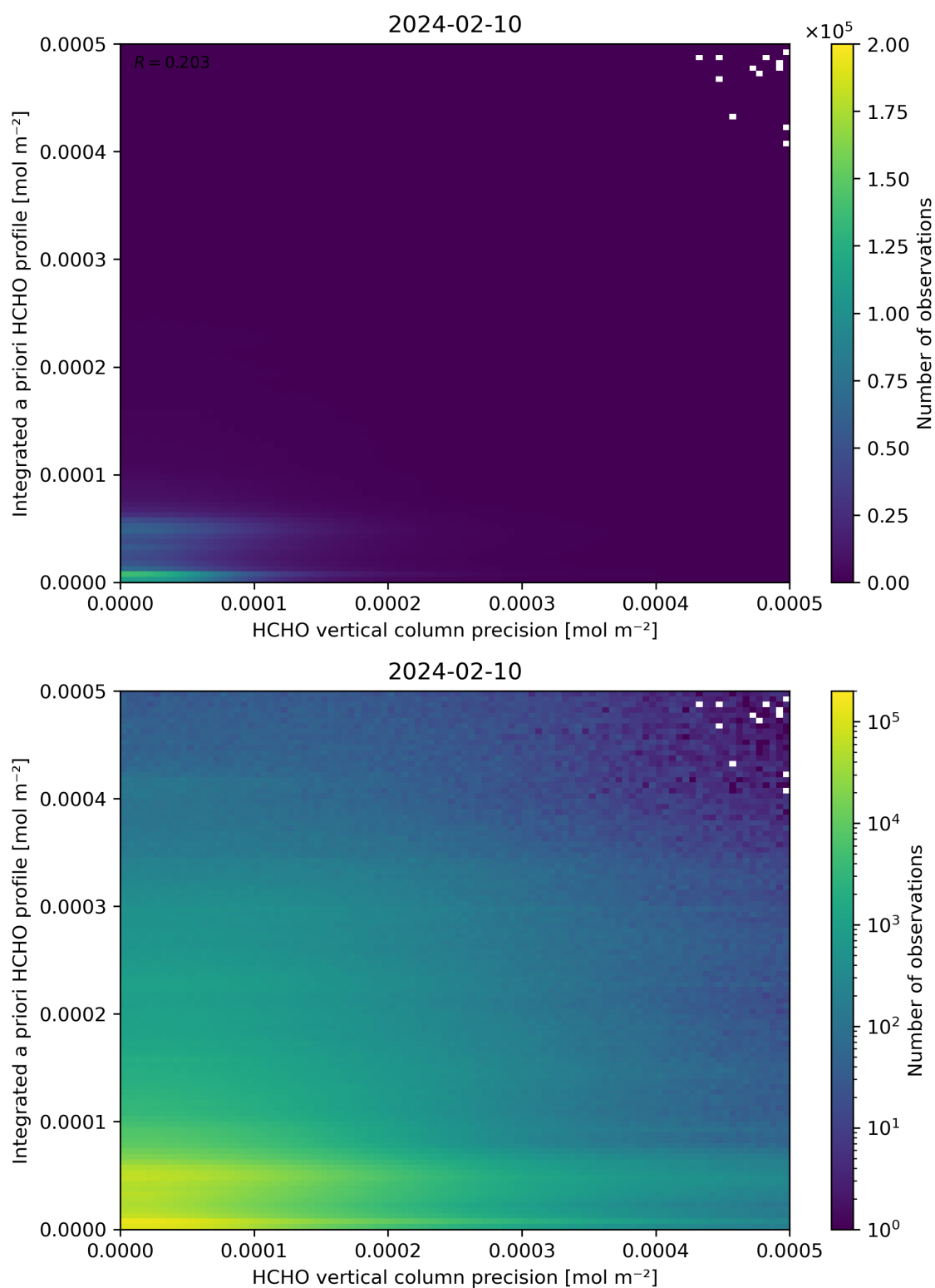
Figure 147: Scatter density plot of “HCHO vertical column precision” against “Integrated a priori HCHO profile” for 2024-02-09 to 2024-02-11.
