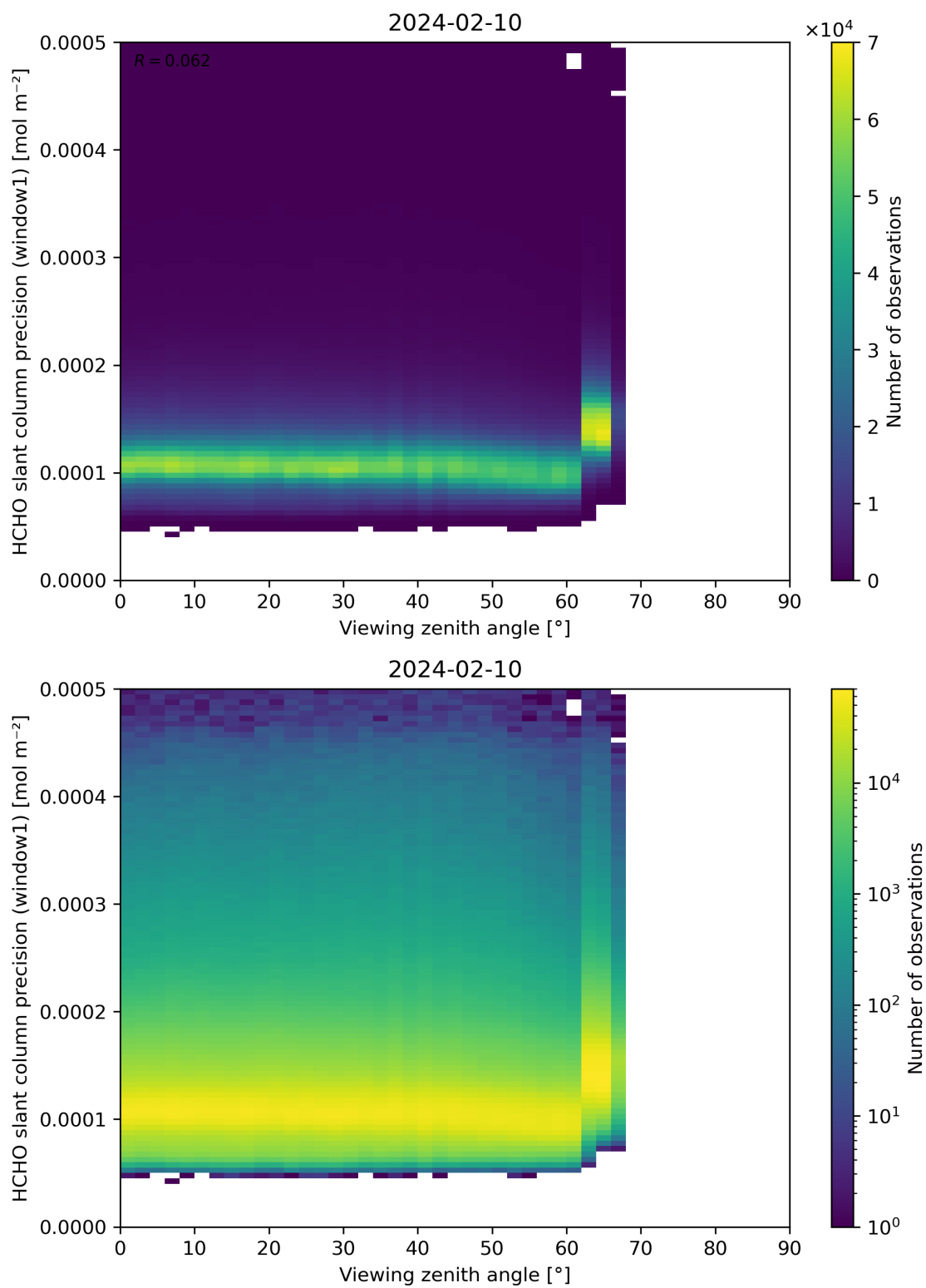
Figure 189: Scatter density plot of “Viewing zenith angle” against “HCHO slant column precision (window1)” for 2024-02-09 to 2024-02-11.
