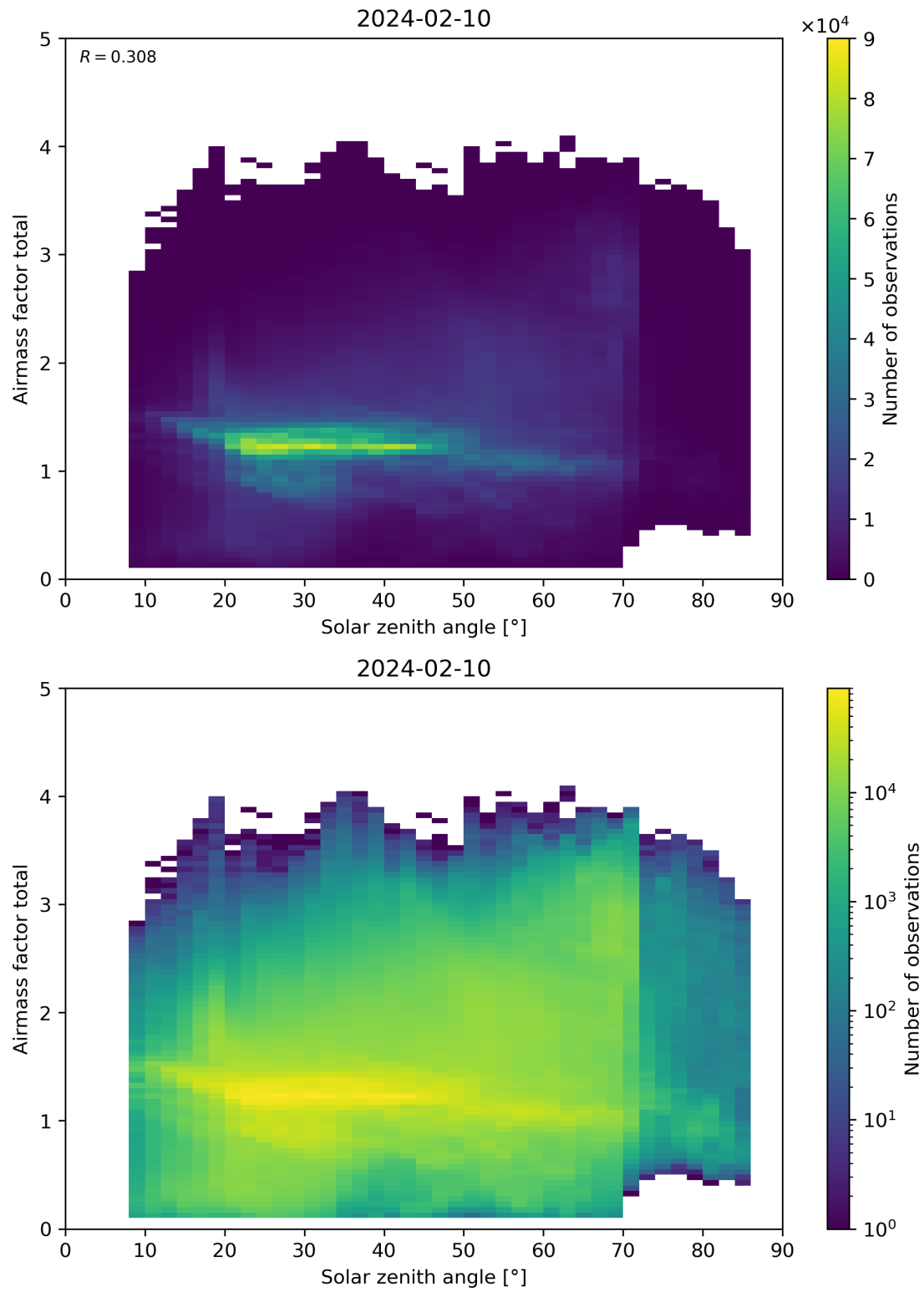
Figure 175: Scatter density plot of “Solar zenith angle” against “Airmass factor total” for 2024-02-09 to 2024-02-11.
