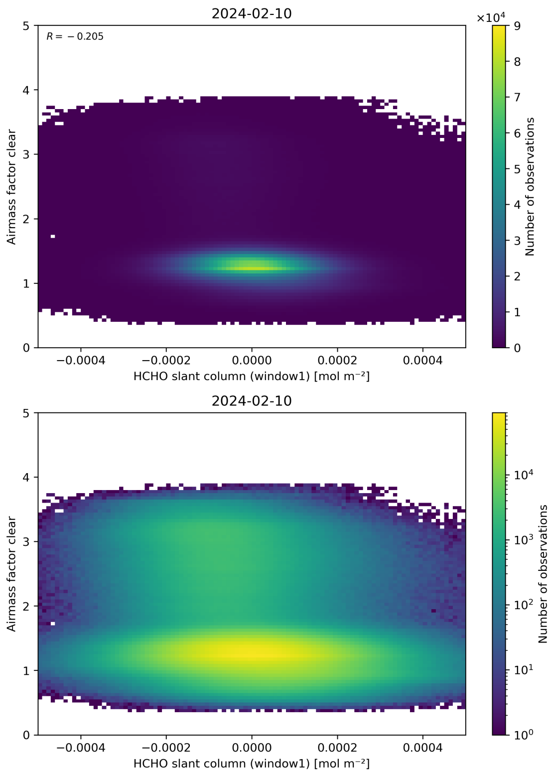
Figure 81: Scatter density plot of “HCHO slant column (window1)” against “Airmass factor clear” for 2024-02-09 to 2024-02-11.
