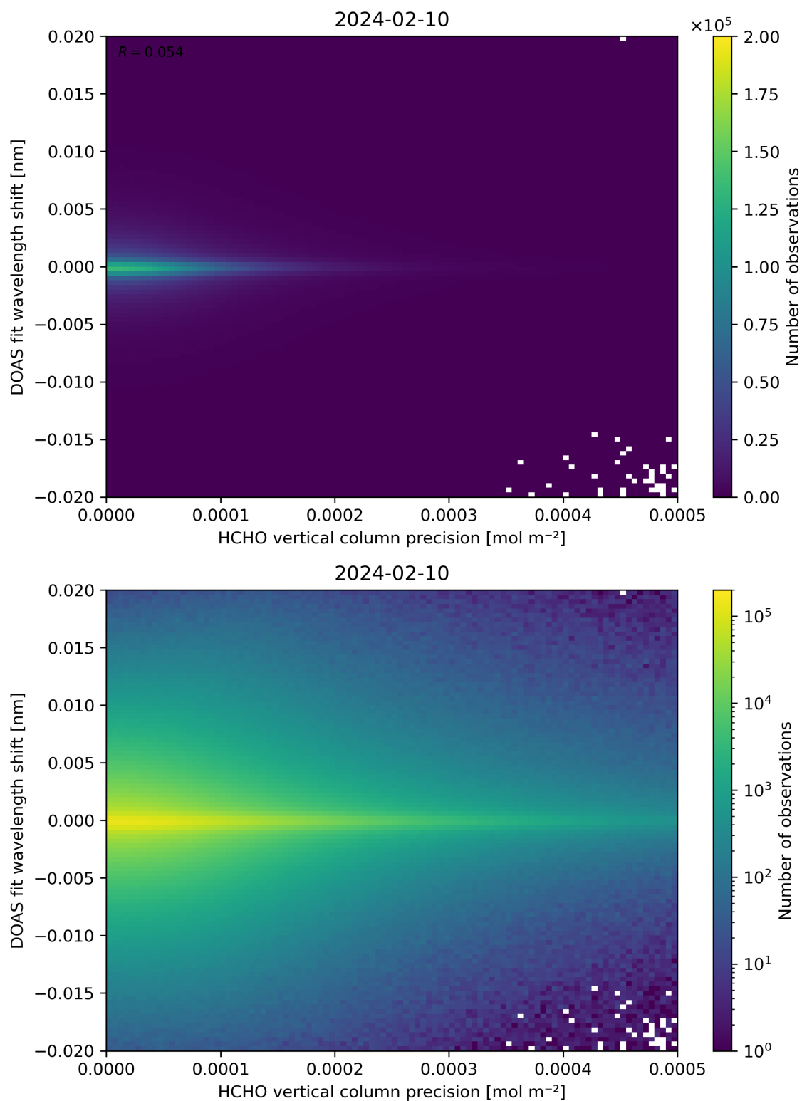
Figure 137: Scatter density plot of “HCHO vertical column precision” against “DOAS fit wavelength shift” for 2024-02-09 to 2024-02-11.
