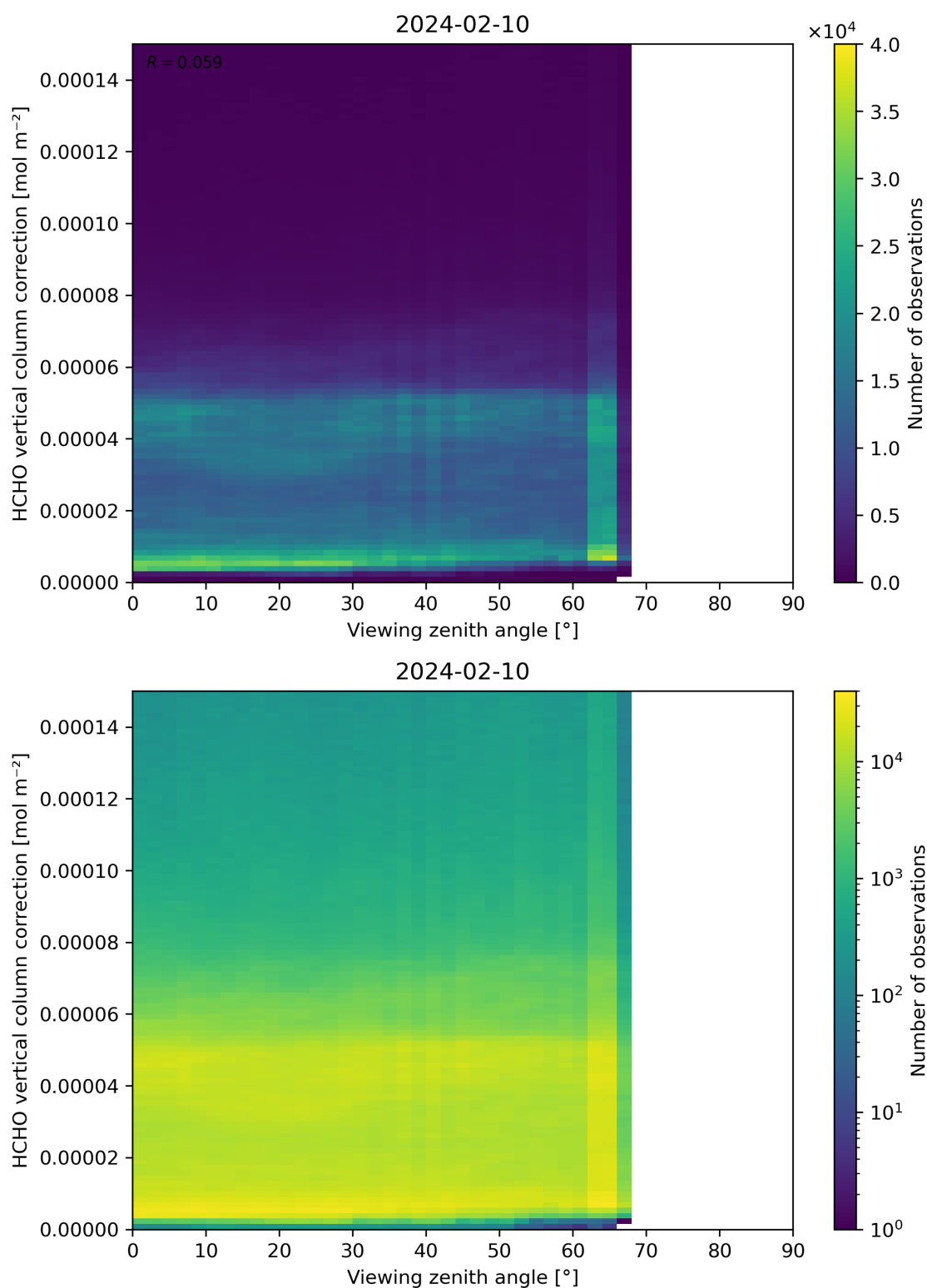
Figure 193: Scatter density plot of “Viewing zenith angle” against “HCHO vertical column correction” for 2024-02-09 to 2024-02-11.
