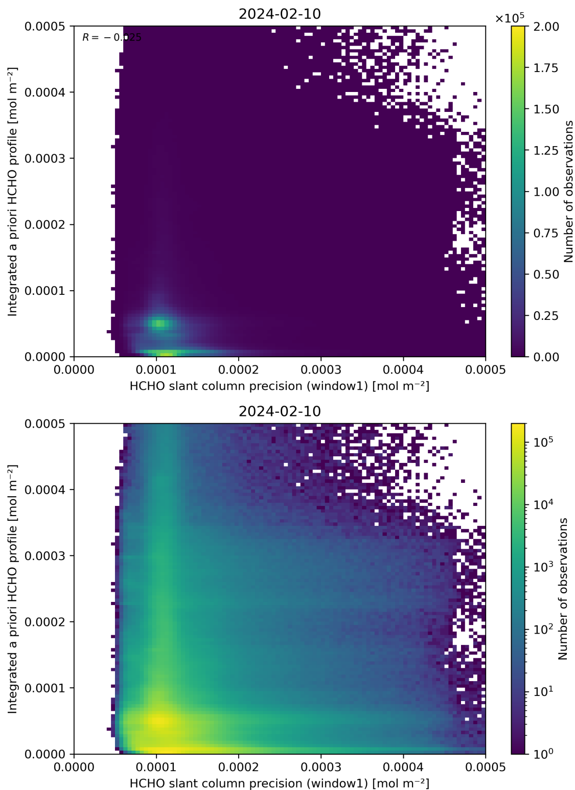
Figure 96: Scatter density plot of “HCHO slant column precision (window1)” against “Integrated a priori HCHO profile” for 2024-02-09 to 2024-02-11.
