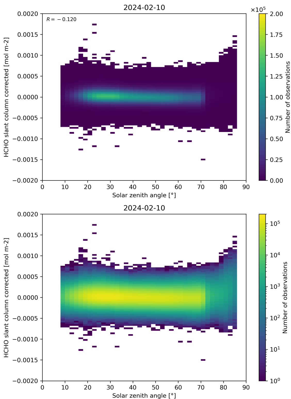
Figure 171: Scatter density plot of “Solar zenith angle” against “HCHO slant column corrected” for 2024-02-09 to 2024-02-11.
