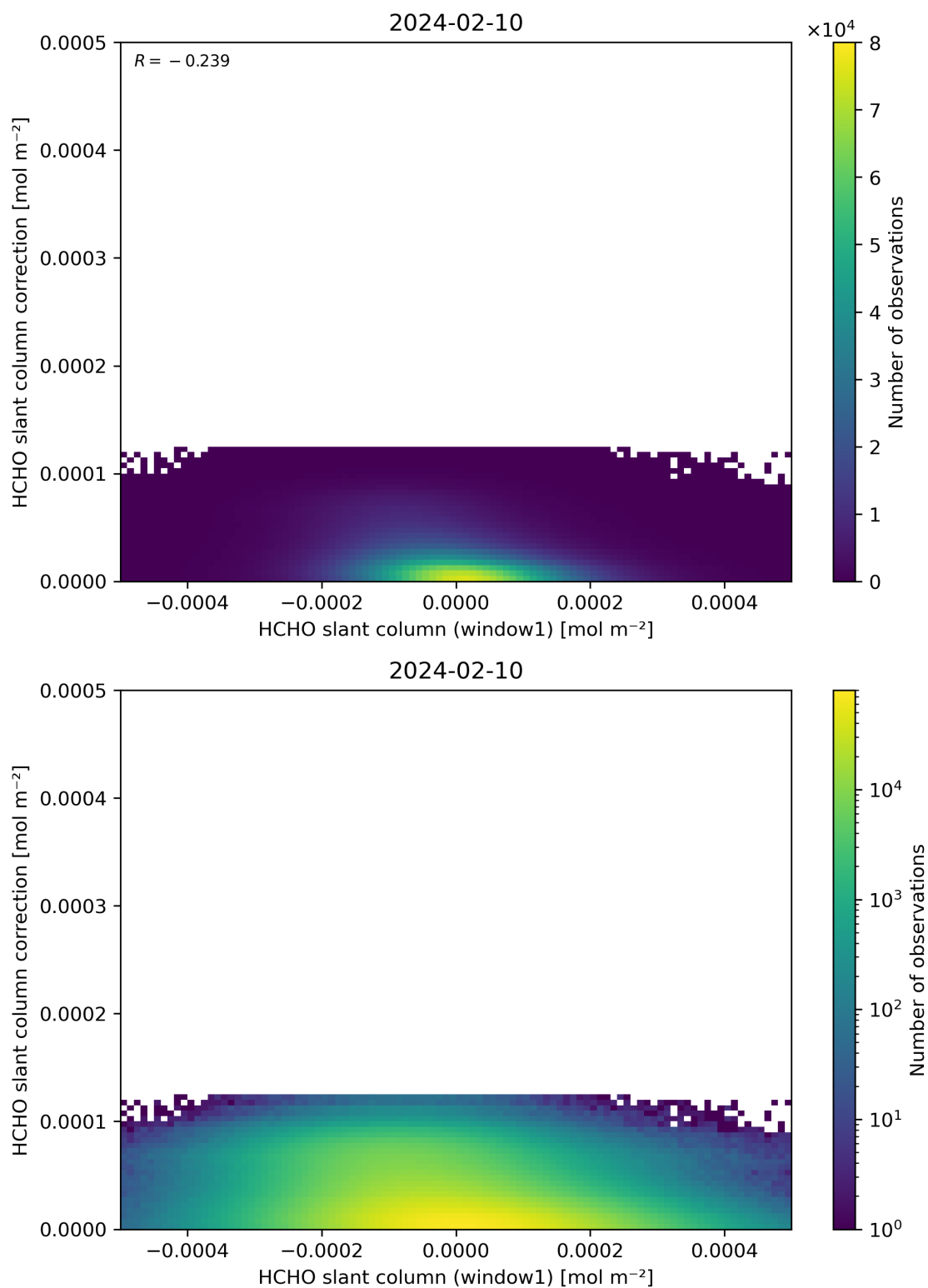
Figure 83: Scatter density plot of “HCHO slant column (window1)” against “HCHO slant column correction” for 2024-02-09 to 2024-02-11.
