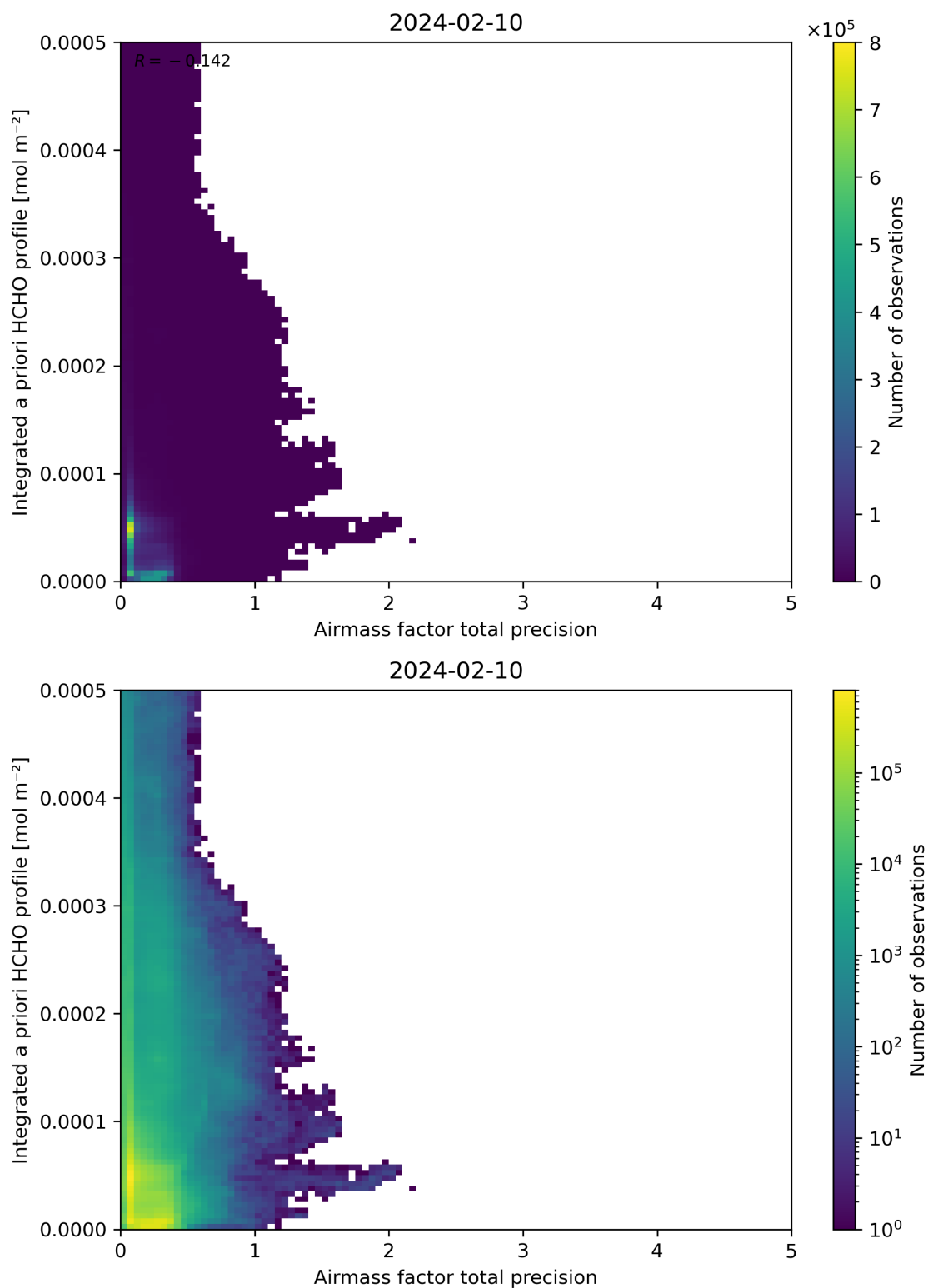
Figure 111: Scatter density plot of “Airmass factor total precision” against “Integrated a priori HCHO profile” for 2024-02-09 to 2024-02-11.
