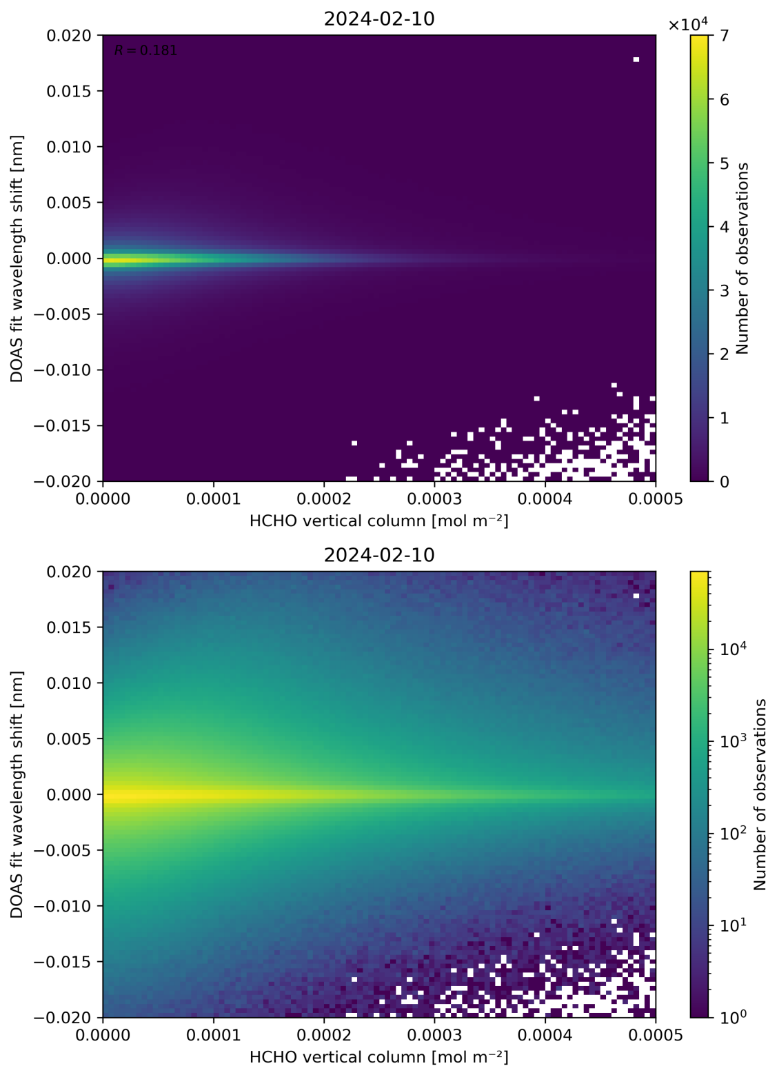
Figure 124: Scatter density plot of “HCHO vertical column” against “DOAS fit wavelength shift” for 2024-02-09 to 2024-02-11.
