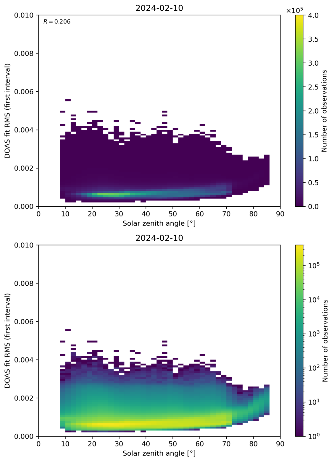
Figure 167: Scatter density plot of “Solar zenith angle” against “DOAS fit RMS (first interval)” for 2024-02-09 to 2024-02-11.
