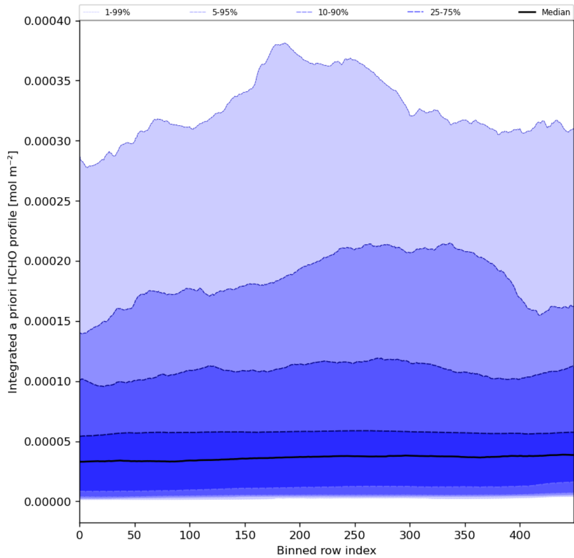
Figure 57: Along track statistics of “Integrated a priori HCHO profile” for 2024-02-09 to 2024-02-11
