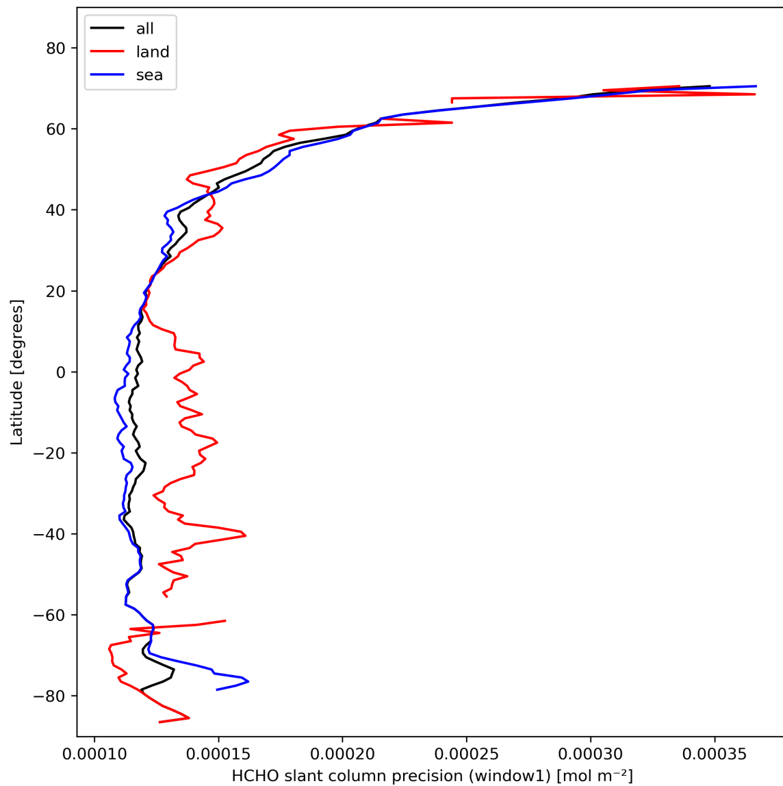
Figure 25: Zonal average of “HCHO slant column precision (window1)” for 2024-02-09 to 2024-02-11.
