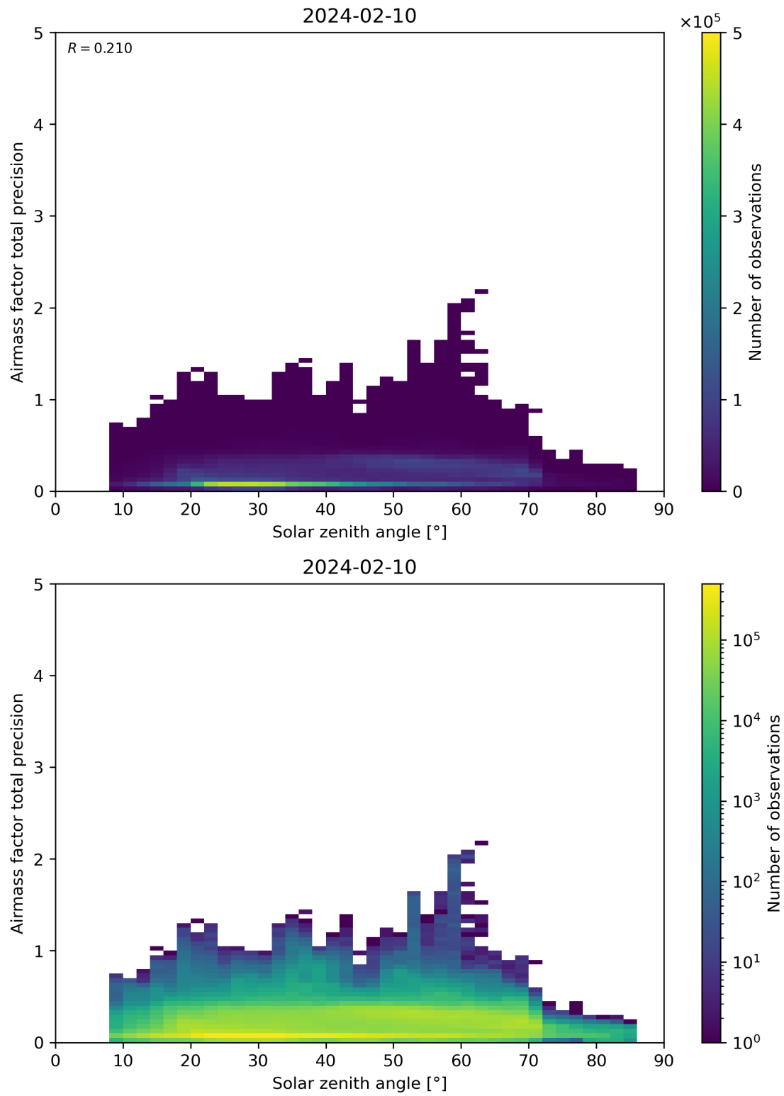
Figure 176: Scatter density plot of “Solar zenith angle” against “Airmass factor total precision” for 2024-02-09 to 2024-02-11.
