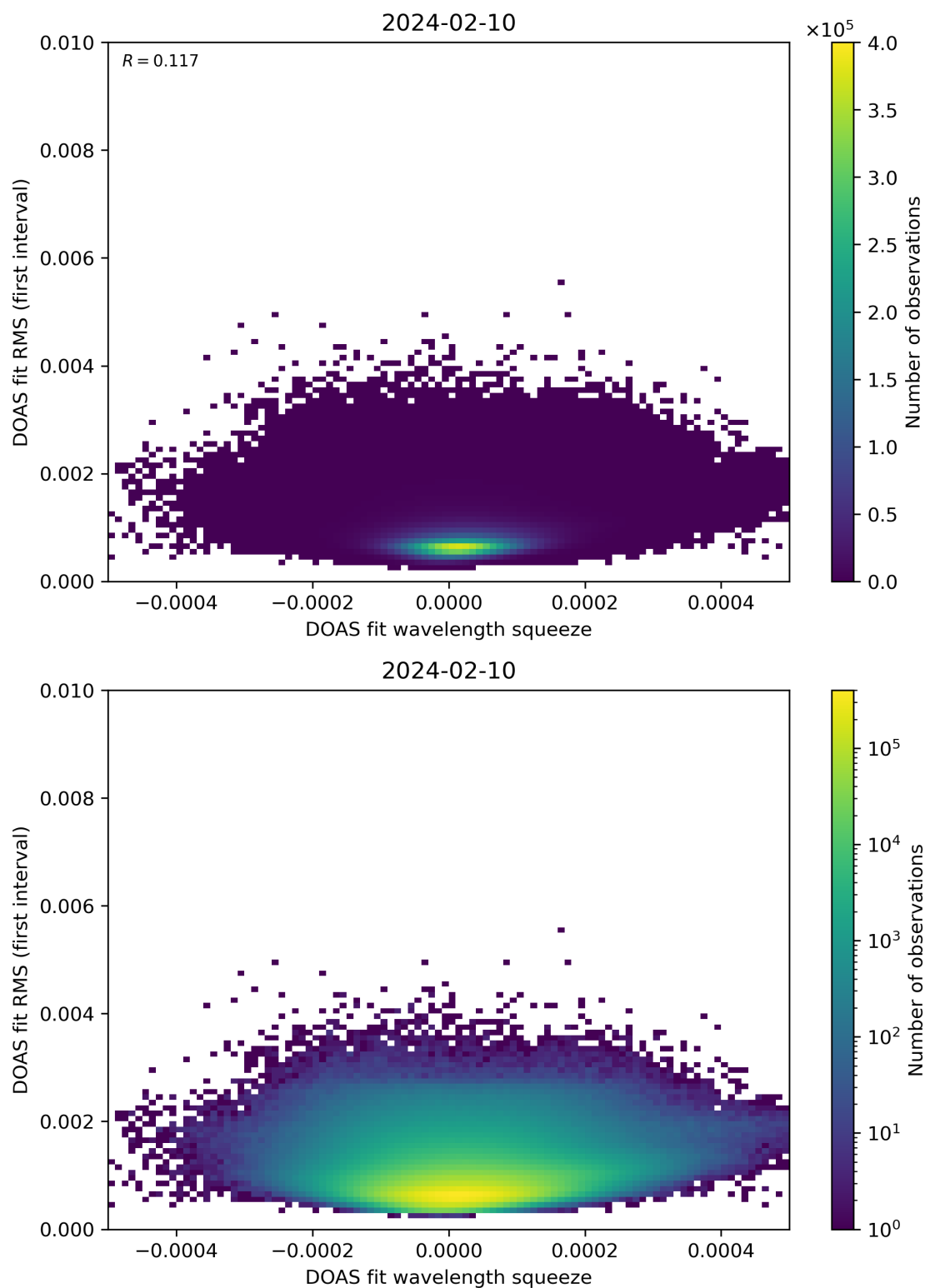
Figure 68: Scatter density plot of “DOAS fit wavelength squeeze” against “DOAS fit RMS (first interval)” for 2024-02-09 to 2024-02-11.
