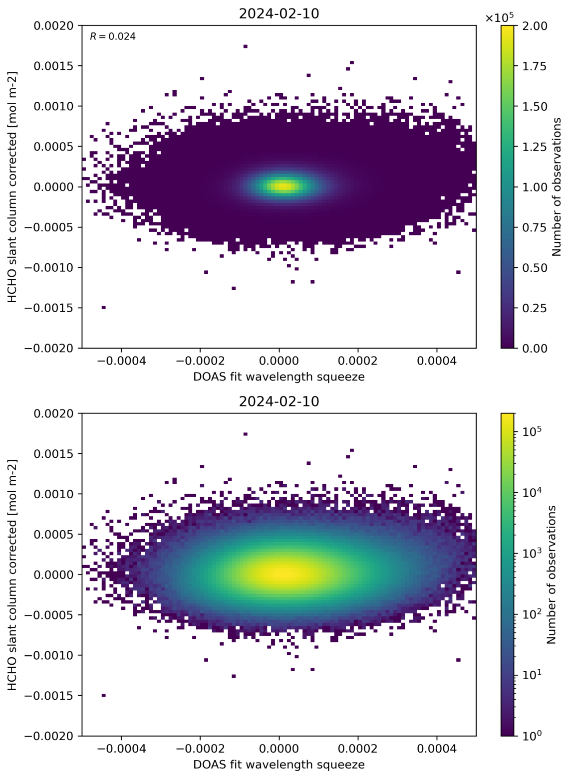
Figure 69: Scatter density plot of “DOAS fit wavelength squeeze” against “HCHO slant column corrected” for 2024-02-09 to 2024-02-11.
