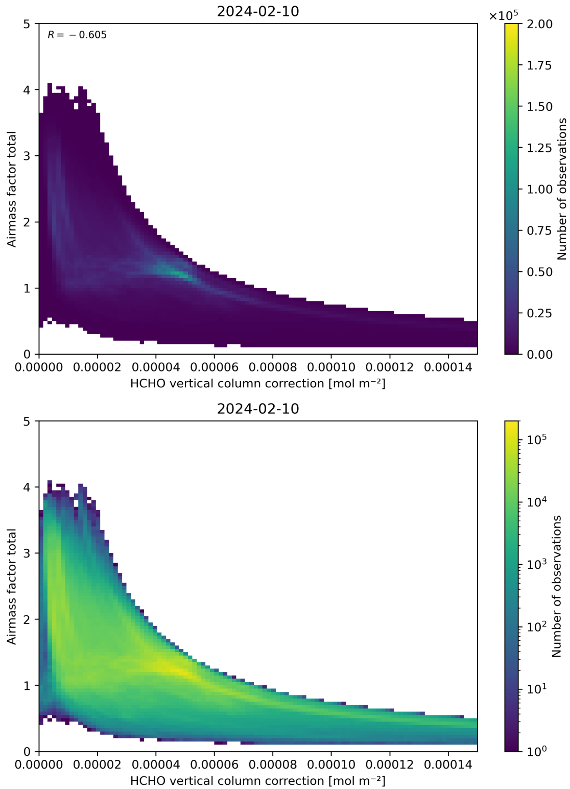
Figure 120: Scatter density plot of “HCHO vertical column correction” against “Airmass factor total” for 2024-02-09 to 2024-02-11.
