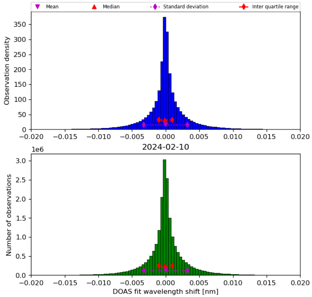
Figure 44: Histogram of “DOAS fit wavelength shift” for 2024-02-09 to 2024-02-11
