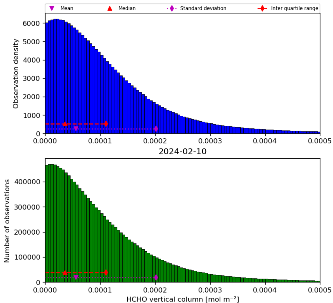
Figure 35: Histogram of “HCHO vertical column” for 2024-02-09 to 2024-02-11
