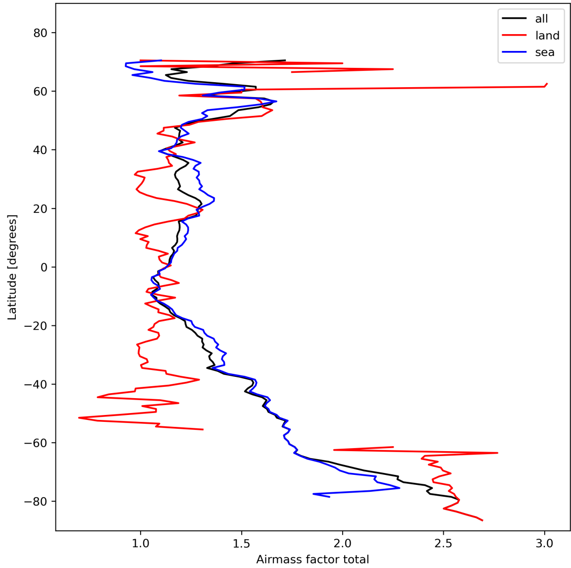
Figure 26: Zonal average of “Airmass factor total” for 2024-02-09 to 2024-02-11.
