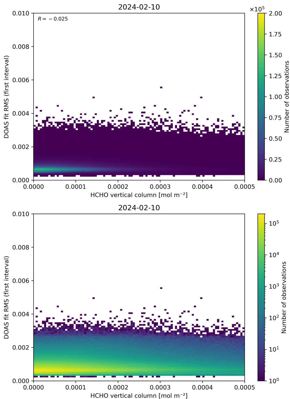
Figure 123: Scatter density plot of “HCHO vertical column” against “DOAS fit RMS (first interval)” for 2024-02-09 to 2024-02-11.
