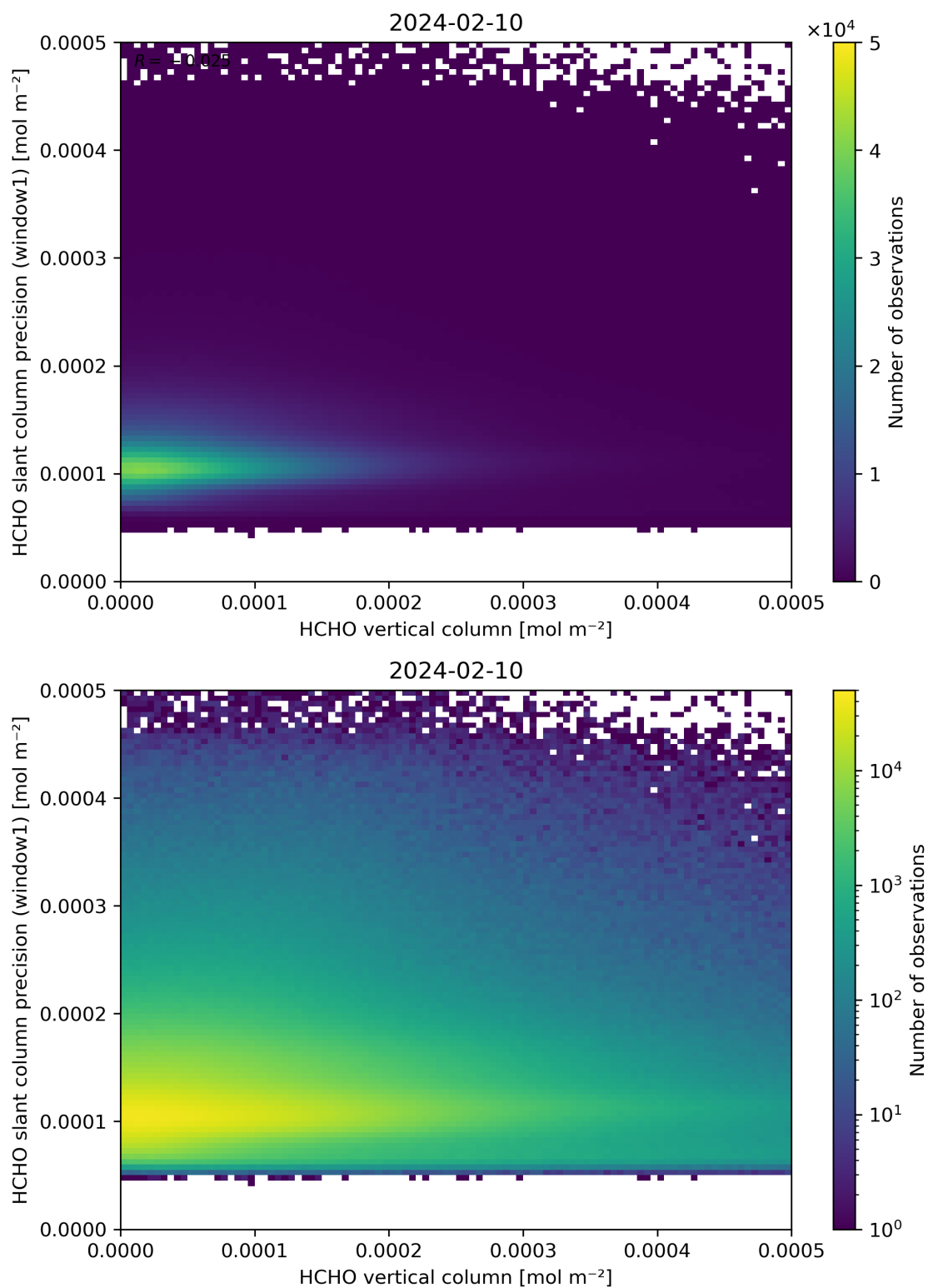
Figure 130: Scatter density plot of “HCHO vertical column” against “HCHO slant column precision (window1)” for 2024-02-09 to 2024-02-11.
