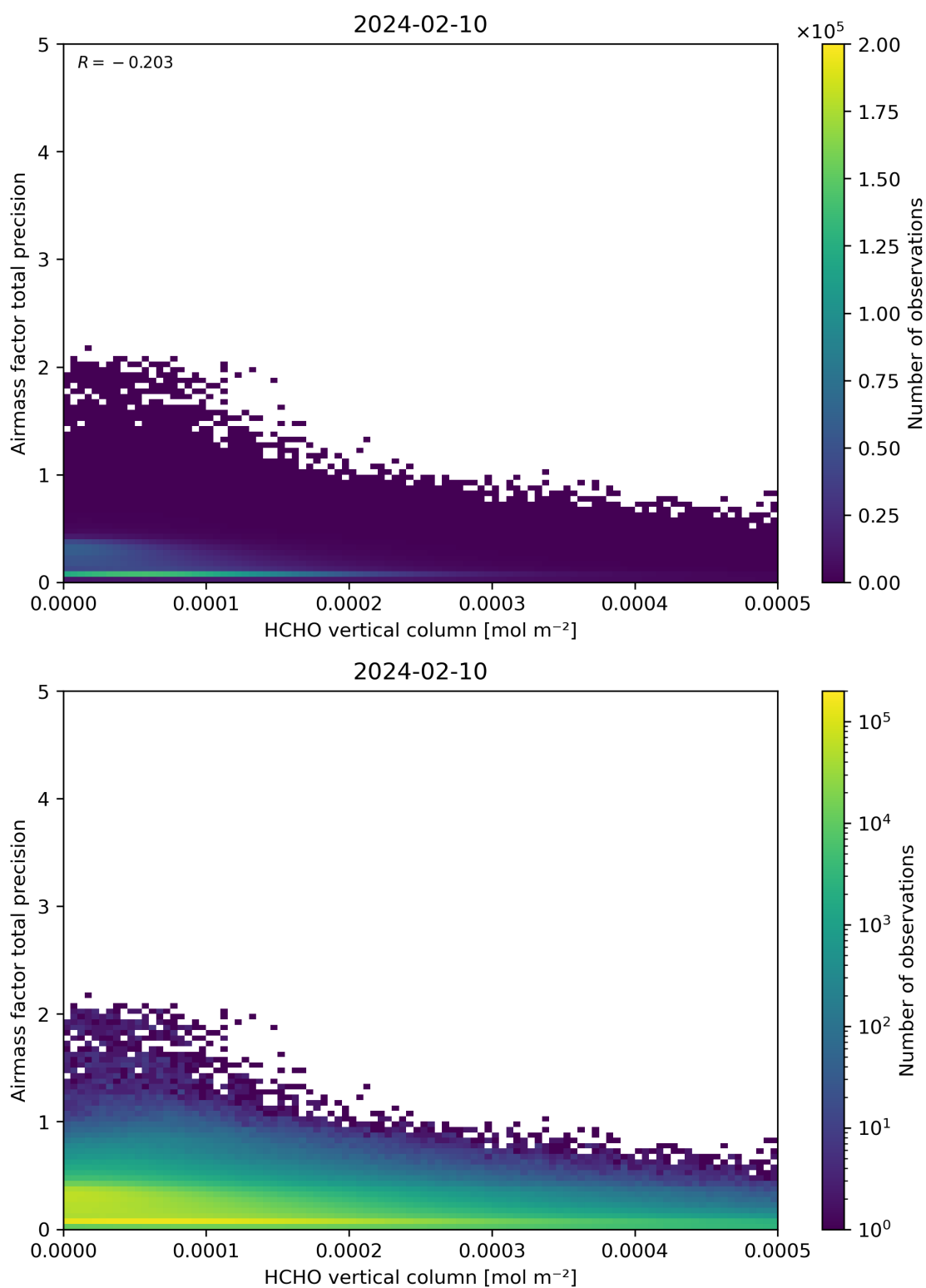
Figure 132: Scatter density plot of “HCHO vertical column” against “Airmass factor total precision” for 2024-02-09 to 2024-02-11.
