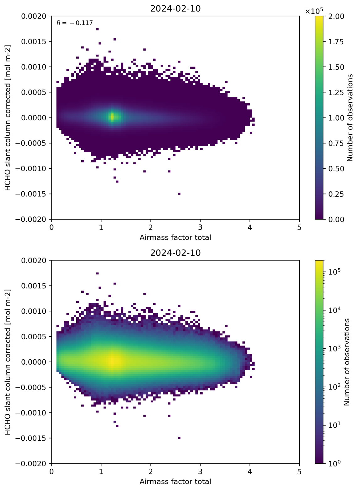
Figure 101: Scatter density plot of “Airmass factor total” against “HCHO slant column corrected” for 2024-02-09 to 2024-02-11.
