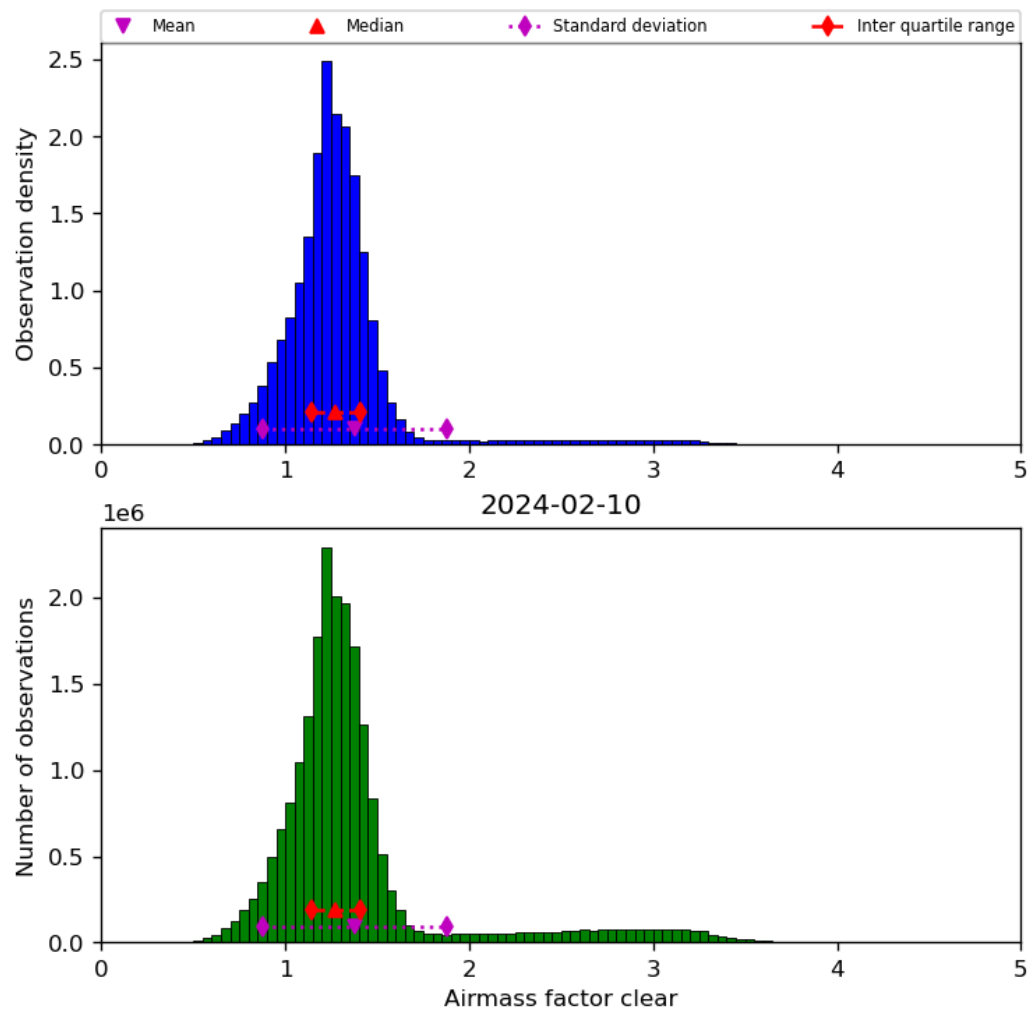
Figure 42: Histogram of “Airmass factor clear” for 2024-02-09 to 2024-02-11
