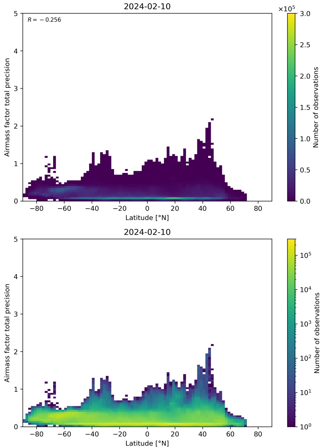
Figure 162: Scatter density plot of “Latitude” against “Airmass factor total precision” for 2024-02-09 to 2024-02-11.
