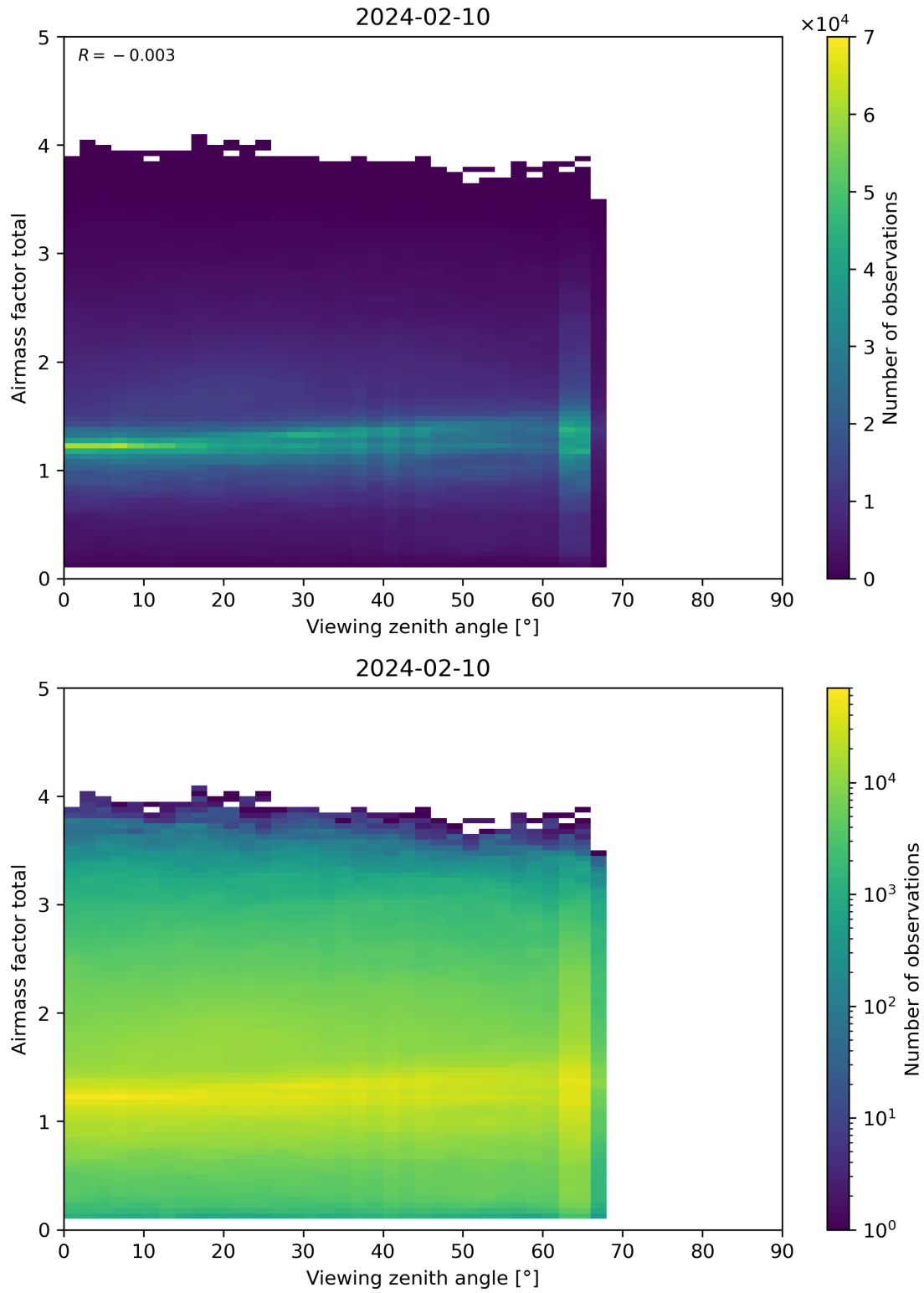
Figure 190: Scatter density plot of “Viewing zenith angle” against “Airmass factor total” for 2024-02-09 to 2024-02-11.
