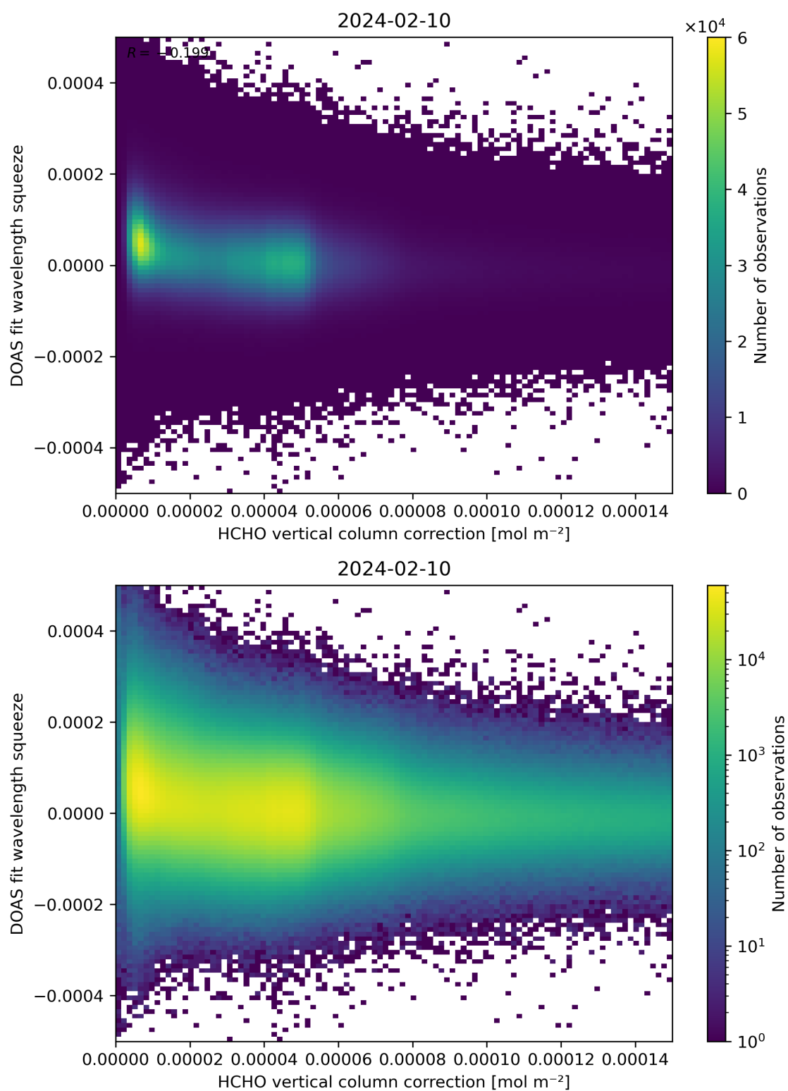
Figure 114: Scatter density plot of “HCHO vertical column correction” against “DOAS fit wavelength squeeze” for 2024-02-09 to 2024-02-11.
