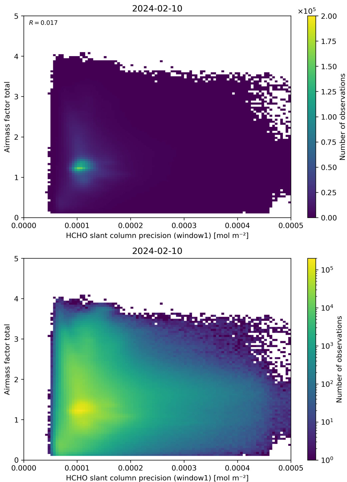
Figure 94: Scatter density plot of “HCHO slant column precision (window1)” against “Airmass factor total” for 2024-02-09 to 2024-02-11.
