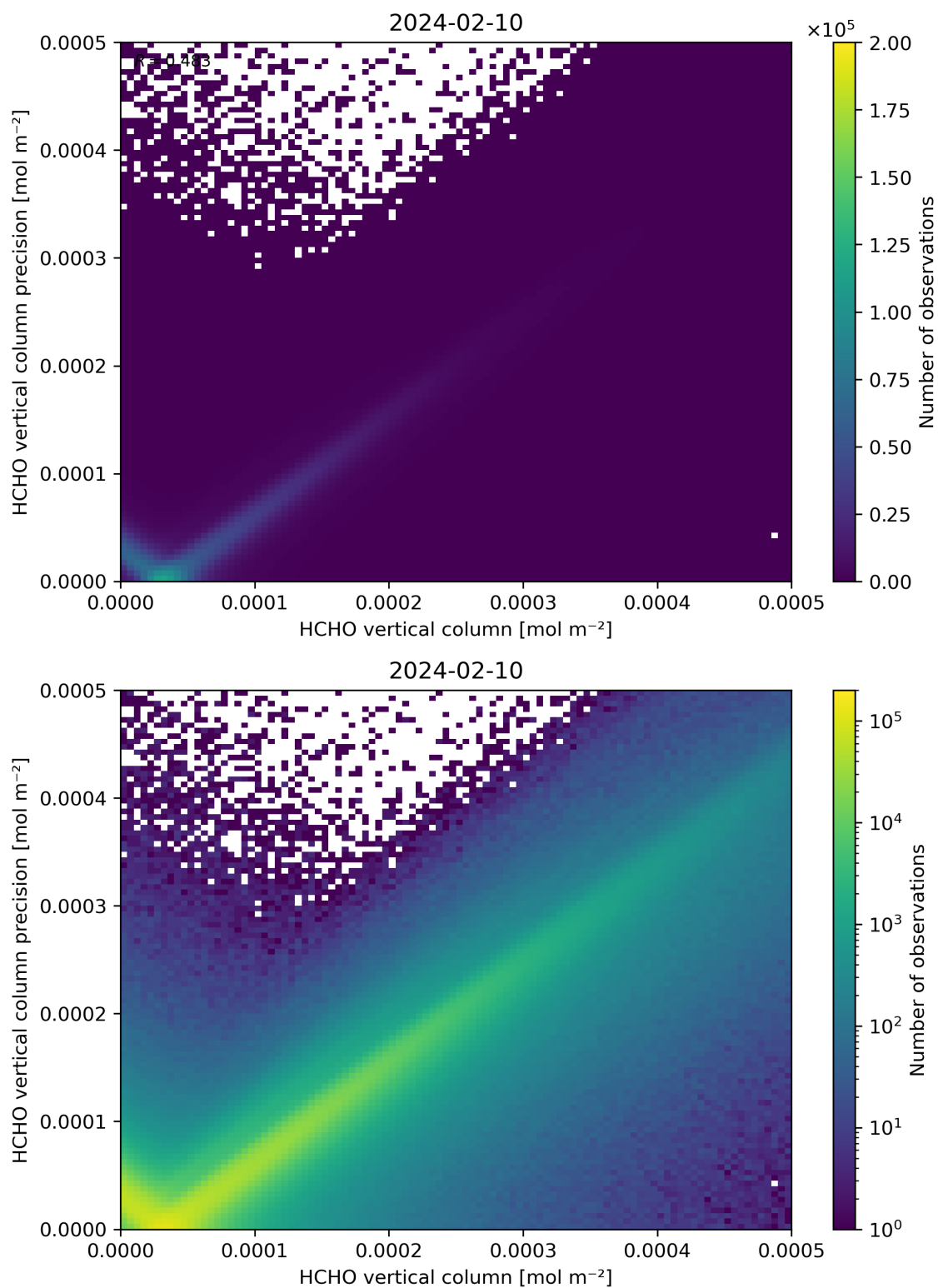
Figure 134: Scatter density plot of “HCHO vertical column” against “HCHO vertical column precision” for 2024-02-09 to 2024-02-11.
