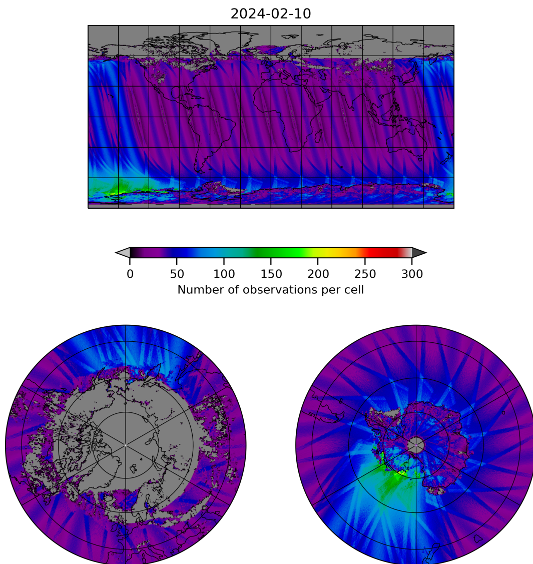
Figure 19: Map of the number of observations for 2024-02-09 to 2024-02-11
