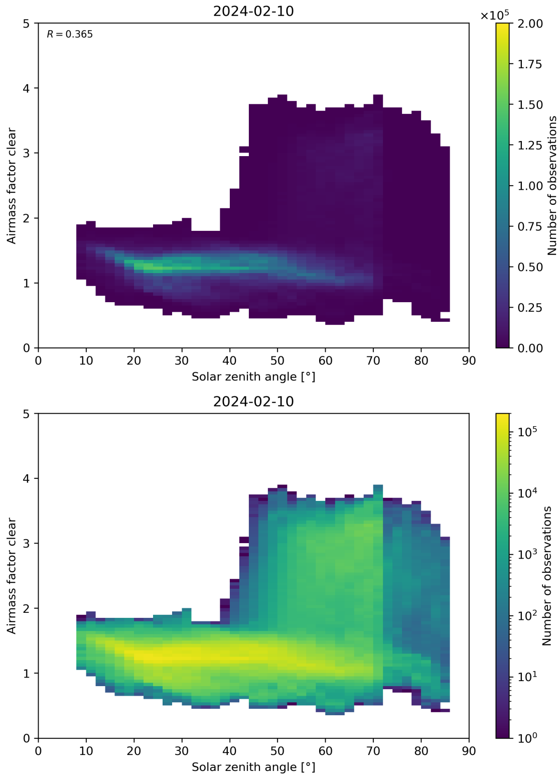
Figure 170: Scatter density plot of “Solar zenith angle” against “Airmass factor clear” for 2024-02-09 to 2024-02-11.
