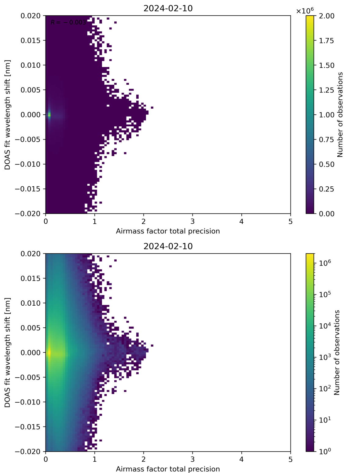
Figure 106: Scatter density plot of “Airmass factor total precision” against “DOAS fit wavelength shift” for 2024-02-09 to 2024-02-11.
