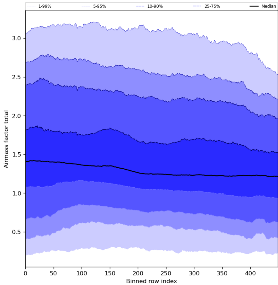
Figure 54: Along track statistics of “Airmass factor total” for 2024-02-09 to 2024-02-11
