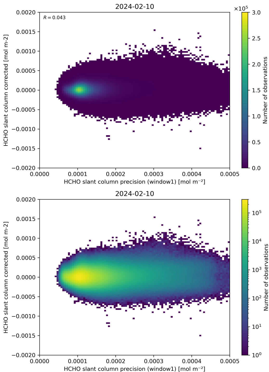
Figure 92: Scatter density plot of “HCHO slant column precision (window1)” against “HCHO slant column corrected” for 2024-02-09 to 2024-02-11.
