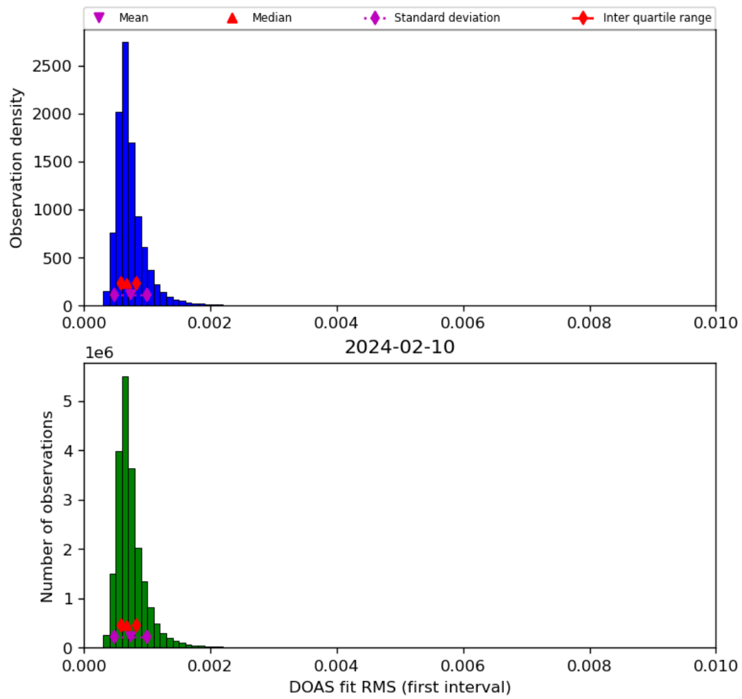
Figure 46: Histogram of “DOAS fit RMS (first interval)” for 2024-02-09 to 2024-02-11
