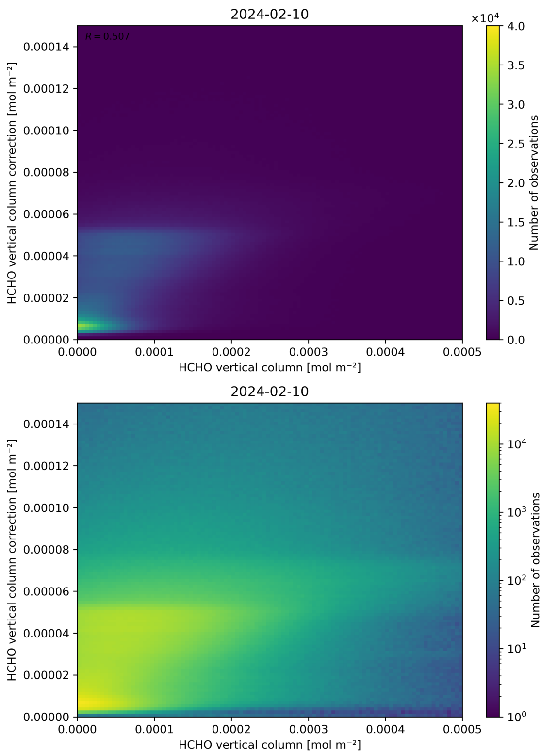
Figure 133: Scatter density plot of “HCHO vertical column” against “HCHO vertical column correction” for 2024-02-09 to 2024-02-11.
