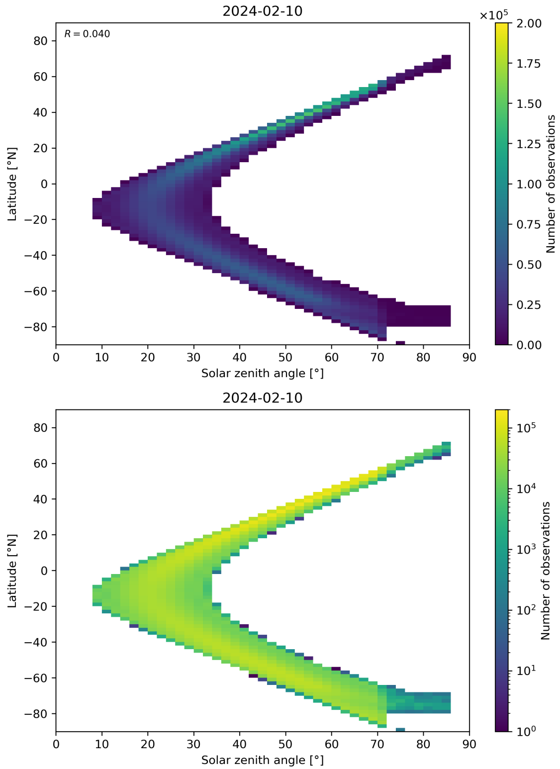
Figure 181: Scatter density plot of “Solar zenith angle” against “Latitude” for 2024-02-09 to 2024-02-11.
