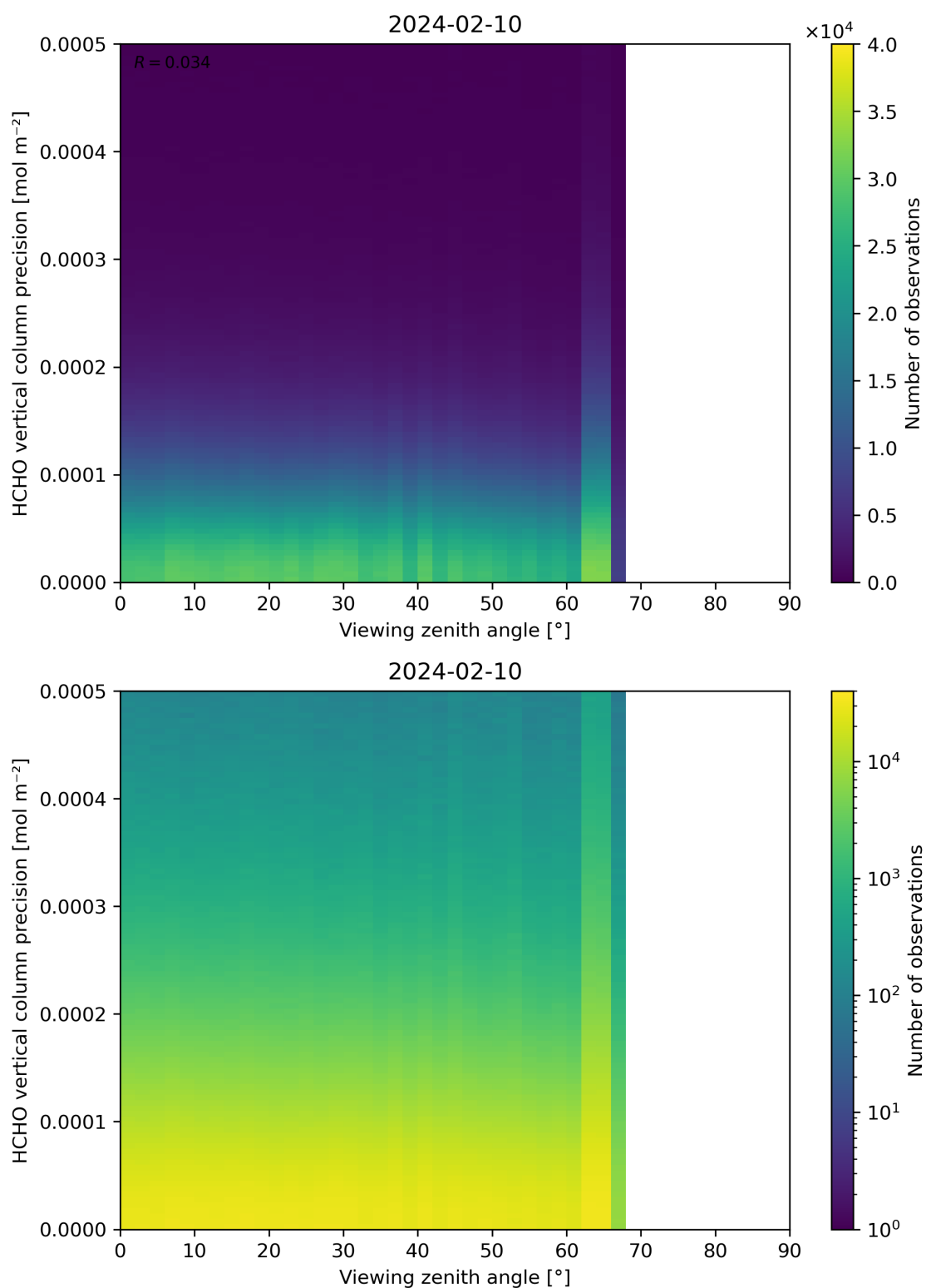
Figure 194: Scatter density plot of “Viewing zenith angle” against “HCHO vertical column precision” for 2024-02-09 to 2024-02-11.
