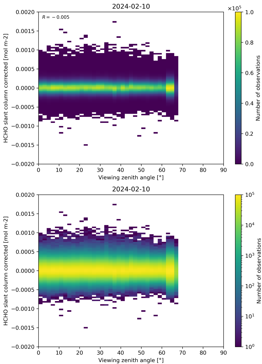
Figure 186: Scatter density plot of “Viewing zenith angle” against “HCHO slant column corrected” for 2024-02-09 to 2024-02-11.
