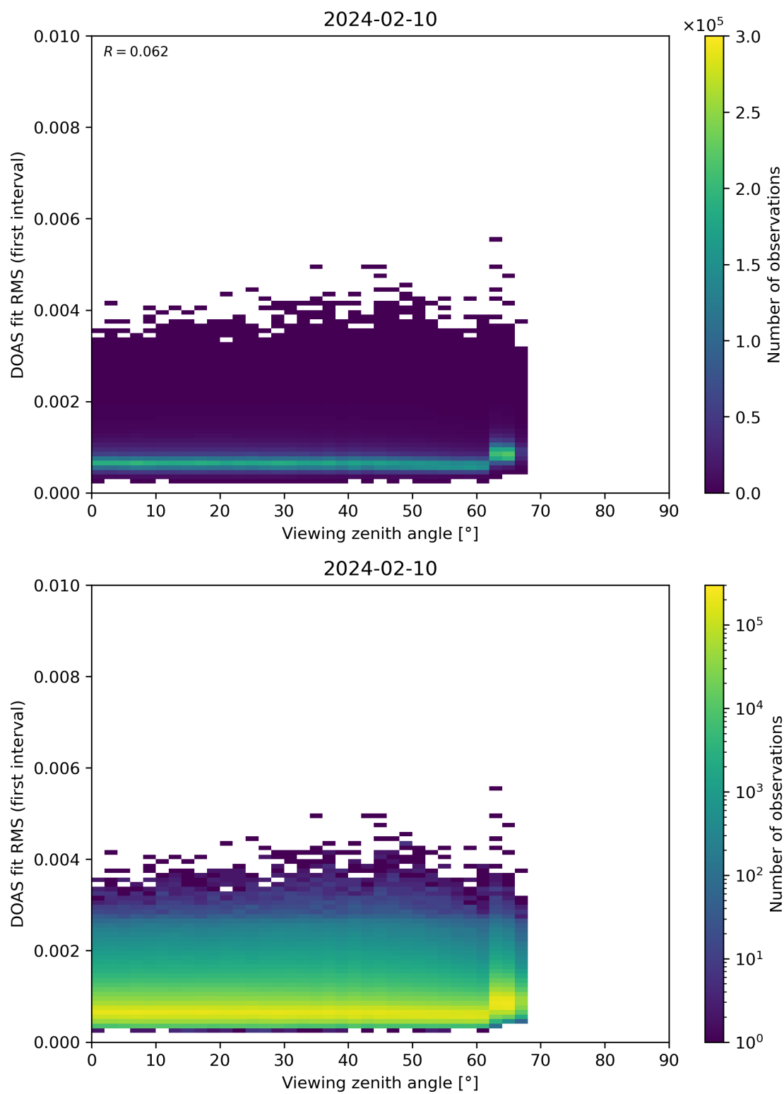
Figure 182: Scatter density plot of “Viewing zenith angle” against “DOAS fit RMS (first interval)” for 2024-02-09 to 2024-02-11.
