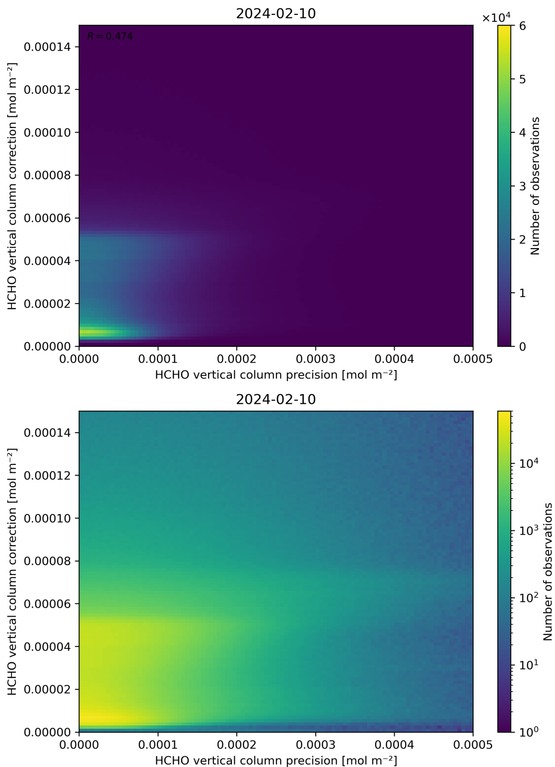
Figure 146: Scatter density plot of “HCHO vertical column precision” against “HCHO vertical column correction” for 2024-02-09 to 2024-02-11.
