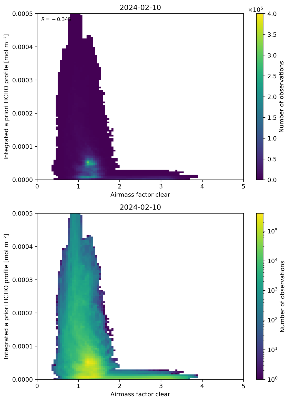
Figure 76: Scatter density plot of “Airmass factor clear” against “Integrated a priori HCHO profile” for 2024-02-09 to 2024-02-11.
