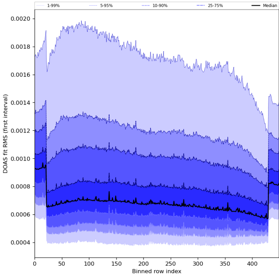
Figure 60: Along track statistics of “DOAS fit RMS (first interval)” for 2024-02-09 to 2024-02-11
