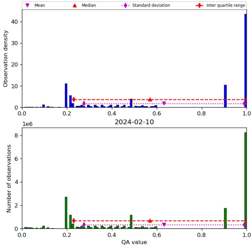
Figure 34: Histogram of “QA value” for 2024-02-09 to 2024-02-11
