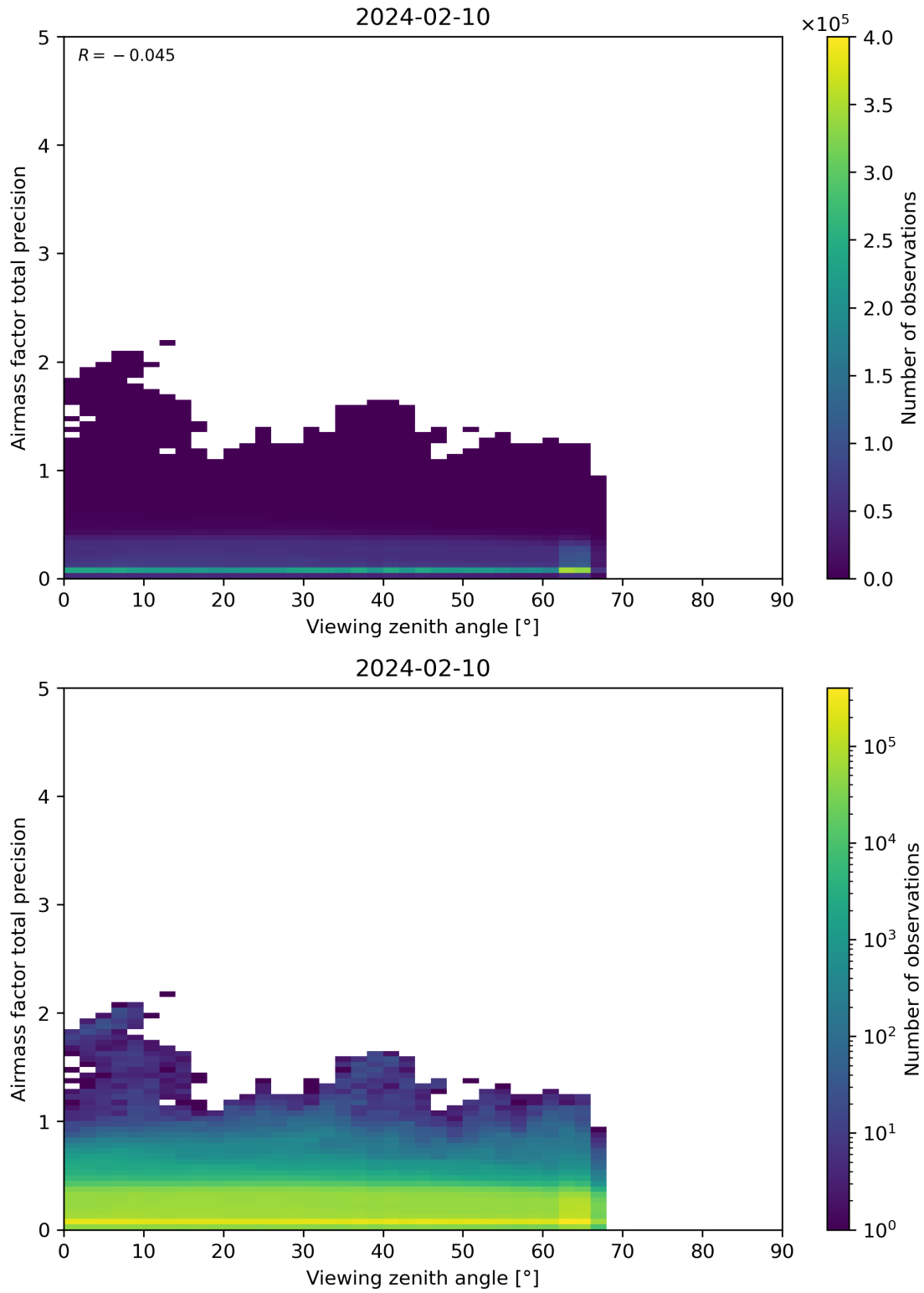
Figure 191: Scatter density plot of “Viewing zenith angle” against “Airmass factor total precision” for 2024-02-09 to 2024-02-11.
