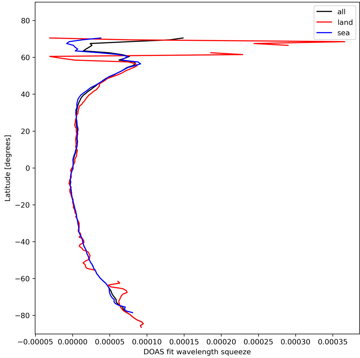
Figure 31: Zonal average of “DOAS fit wavelength squeeze” for 2024-02-09 to 2024-02-11.
