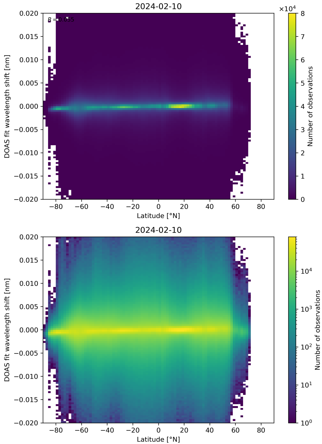
Figure 154: Scatter density plot of “Latitude” against “DOAS fit wavelength shift” for 2024-02-09 to 2024-02-11.
