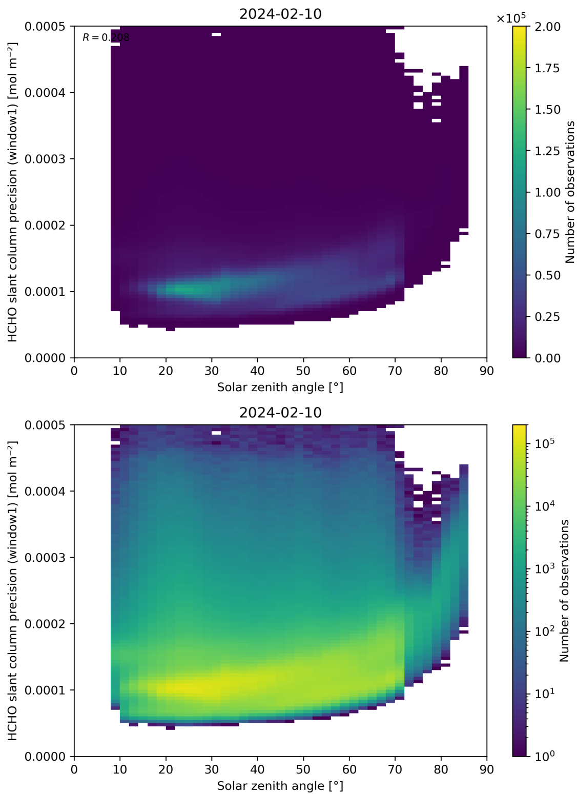
Figure 174: Scatter density plot of “Solar zenith angle” against “HCHO slant column precision (window1)” for 2024-02-09 to 2024-02-11.
