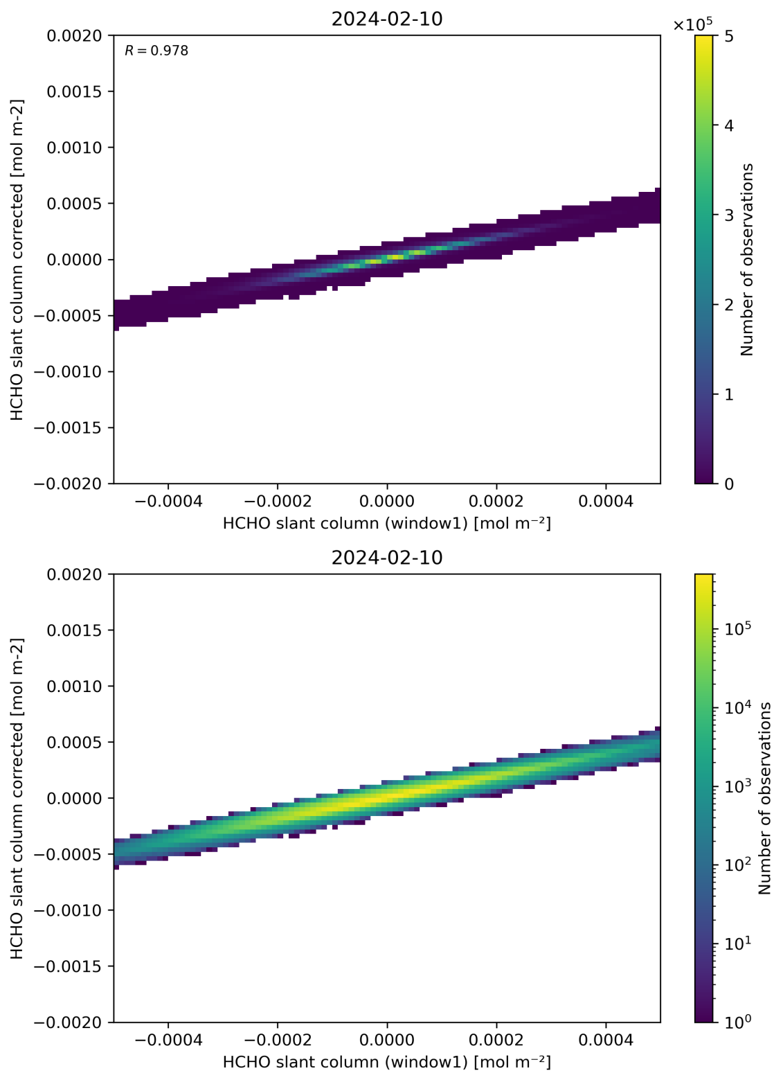
Figure 82: Scatter density plot of “HCHO slant column (window1)” against “HCHO slant column corrected” for 2024-02-09 to 2024-02-11.
