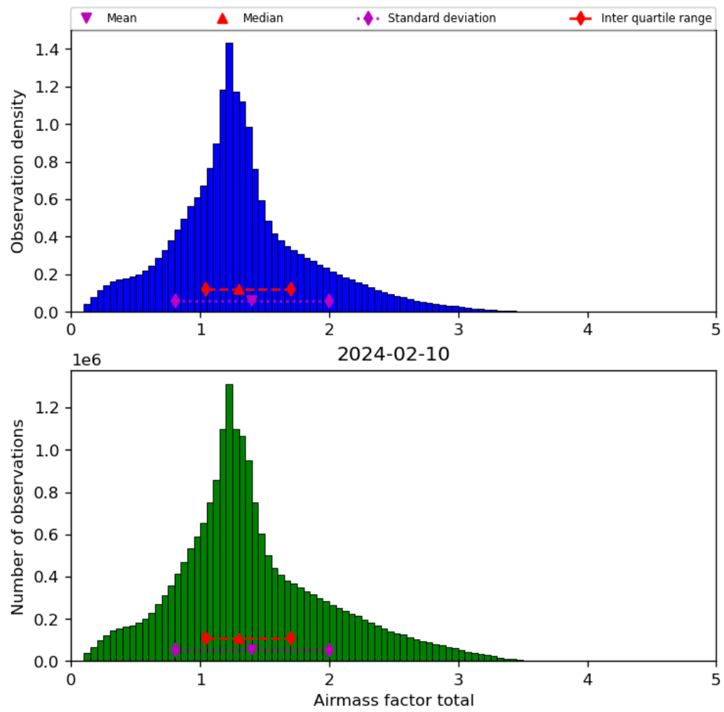
Figure 40: Histogram of “Airmass factor total” for 2024-02-09 to 2024-02-11
