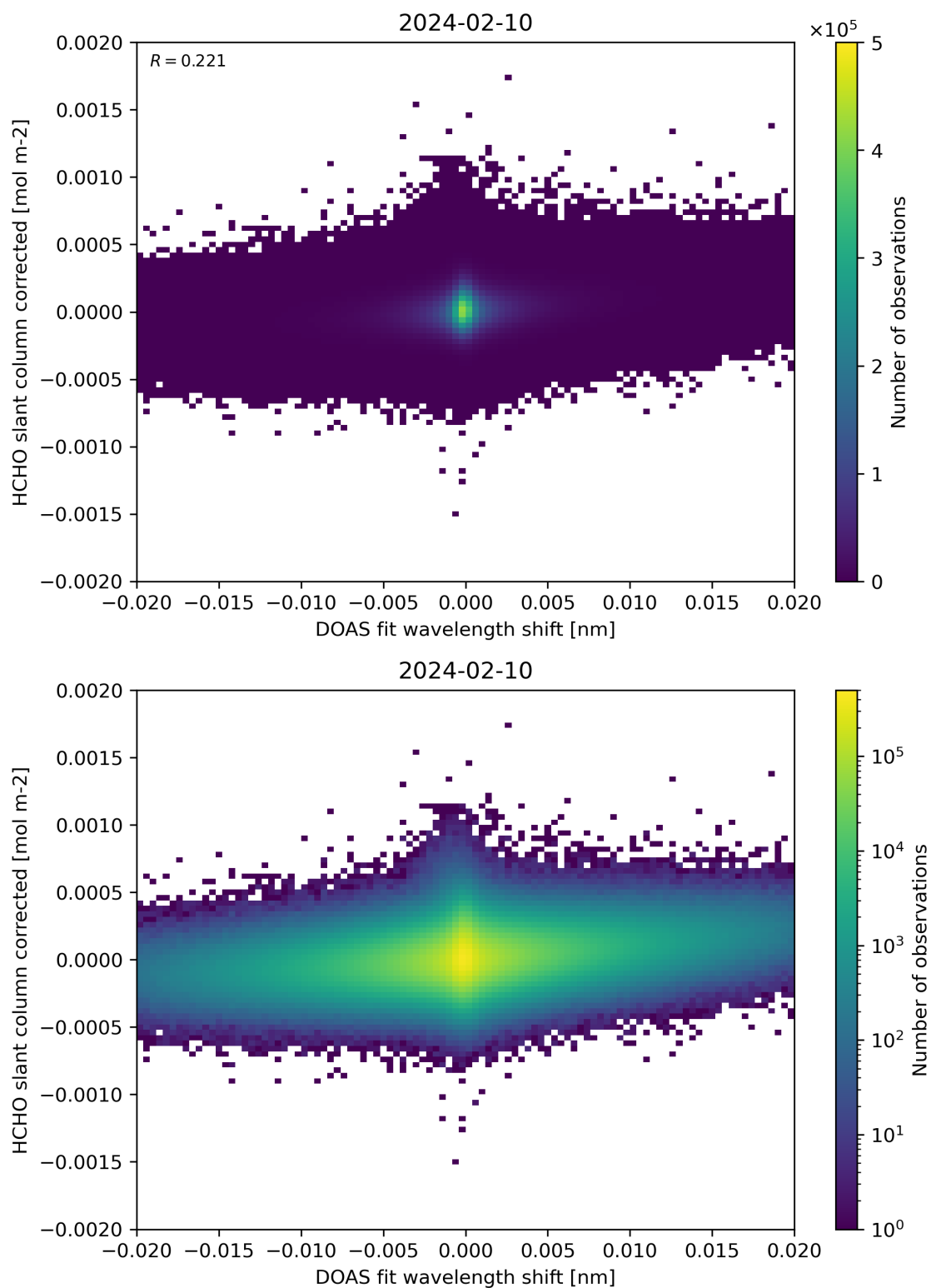
Figure 66: Scatter density plot of “DOAS fit wavelength shift” against “HCHO slant column corrected” for 2024-02-09 to 2024-02-11.
