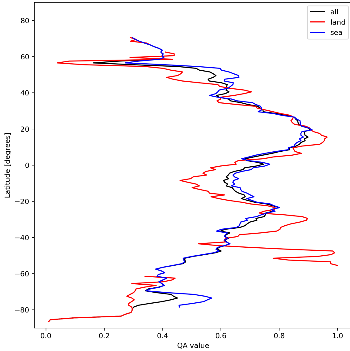
Figure 20: Zonal average of “QA value” for 2024-02-09 to 2024-02-11.
