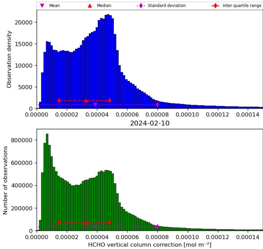
Figure 37: Histogram of “HCHO vertical column correction” for 2024-02-09 to 2024-02-11
