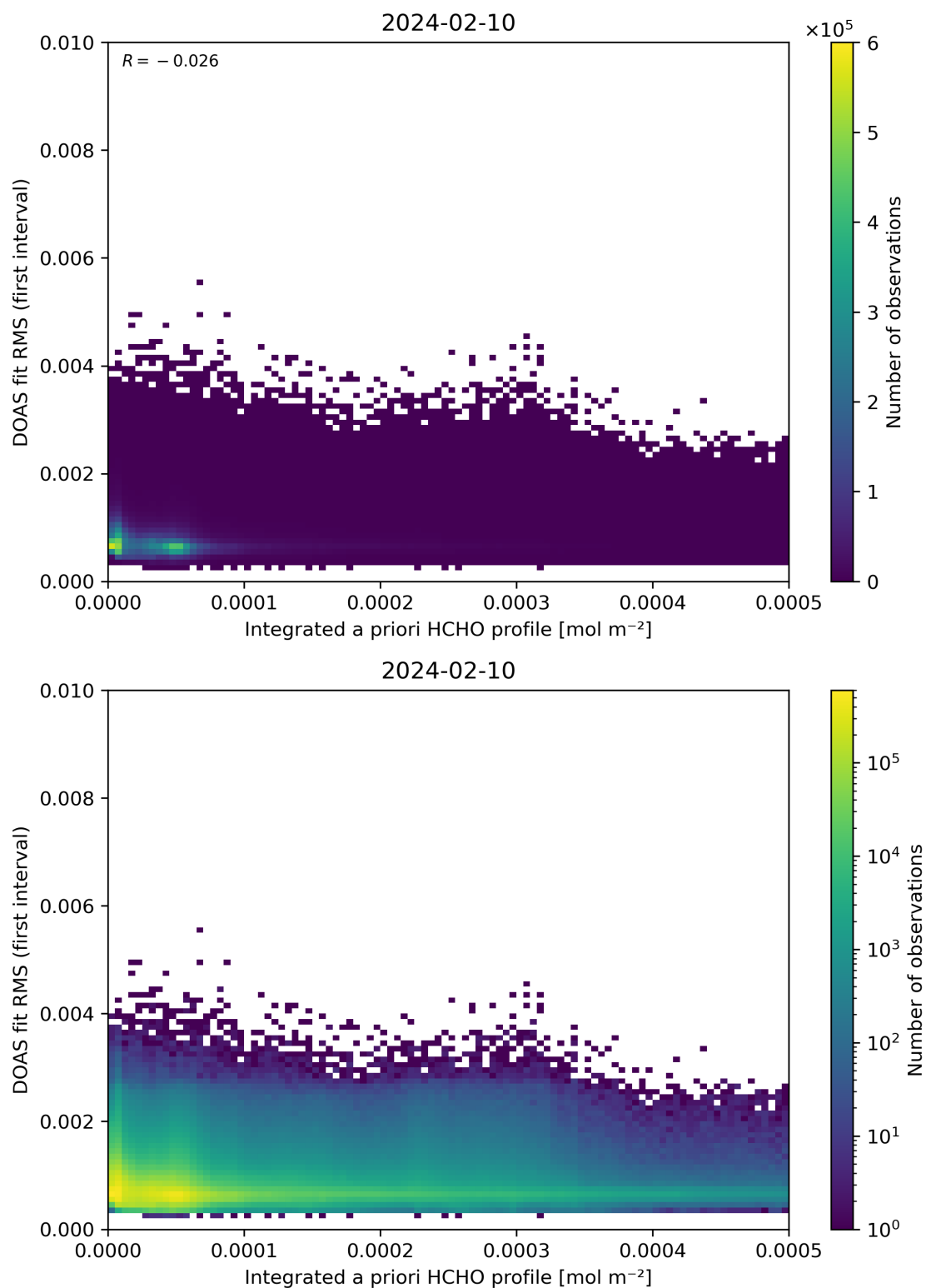
Figure 148: Scatter density plot of “Integrated a priori HCHO profile” against “DOAS fit RMS (first interval)” for 2024-02-09 to 2024-02-11.
