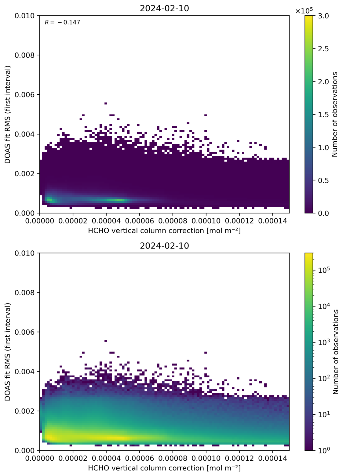
Figure 112: Scatter density plot of “HCHO vertical column correction” against “DOAS fit RMS (first interval)” for 2024-02-09 to 2024-02-11.
