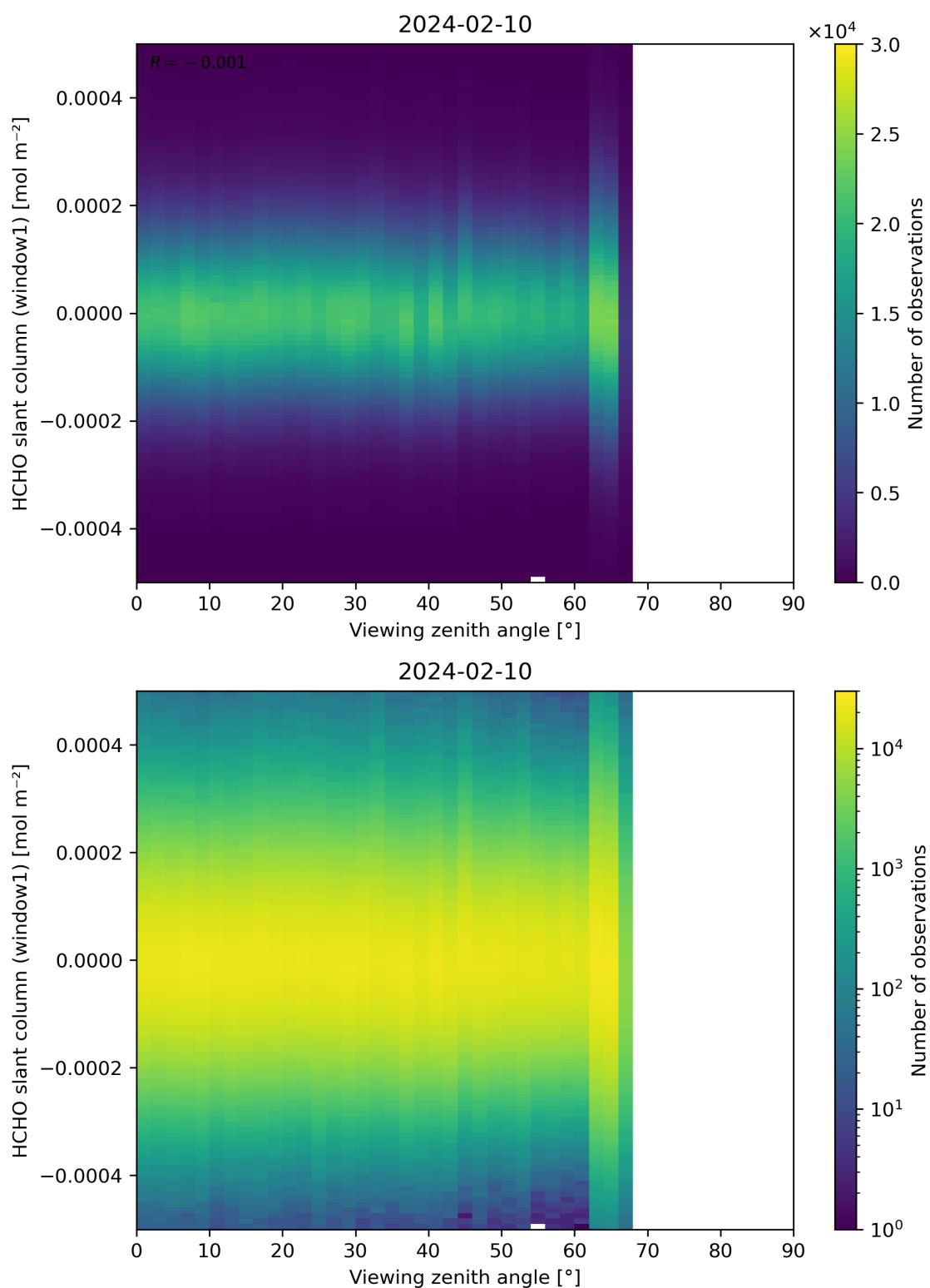
Figure 188: Scatter density plot of “Viewing zenith angle” against “HCHO slant column (window1)” for 2024-02-09 to 2024-02-11.
