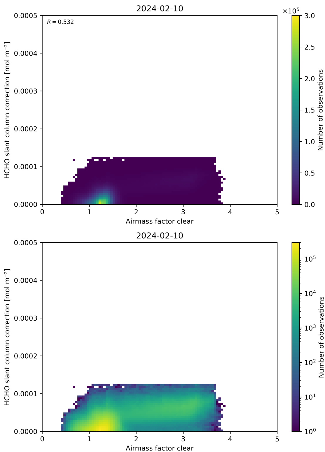
Figure 75: Scatter density plot of “Airmass factor clear” against “HCHO slant column correction” for 2024-02-09 to 2024-02-11.
