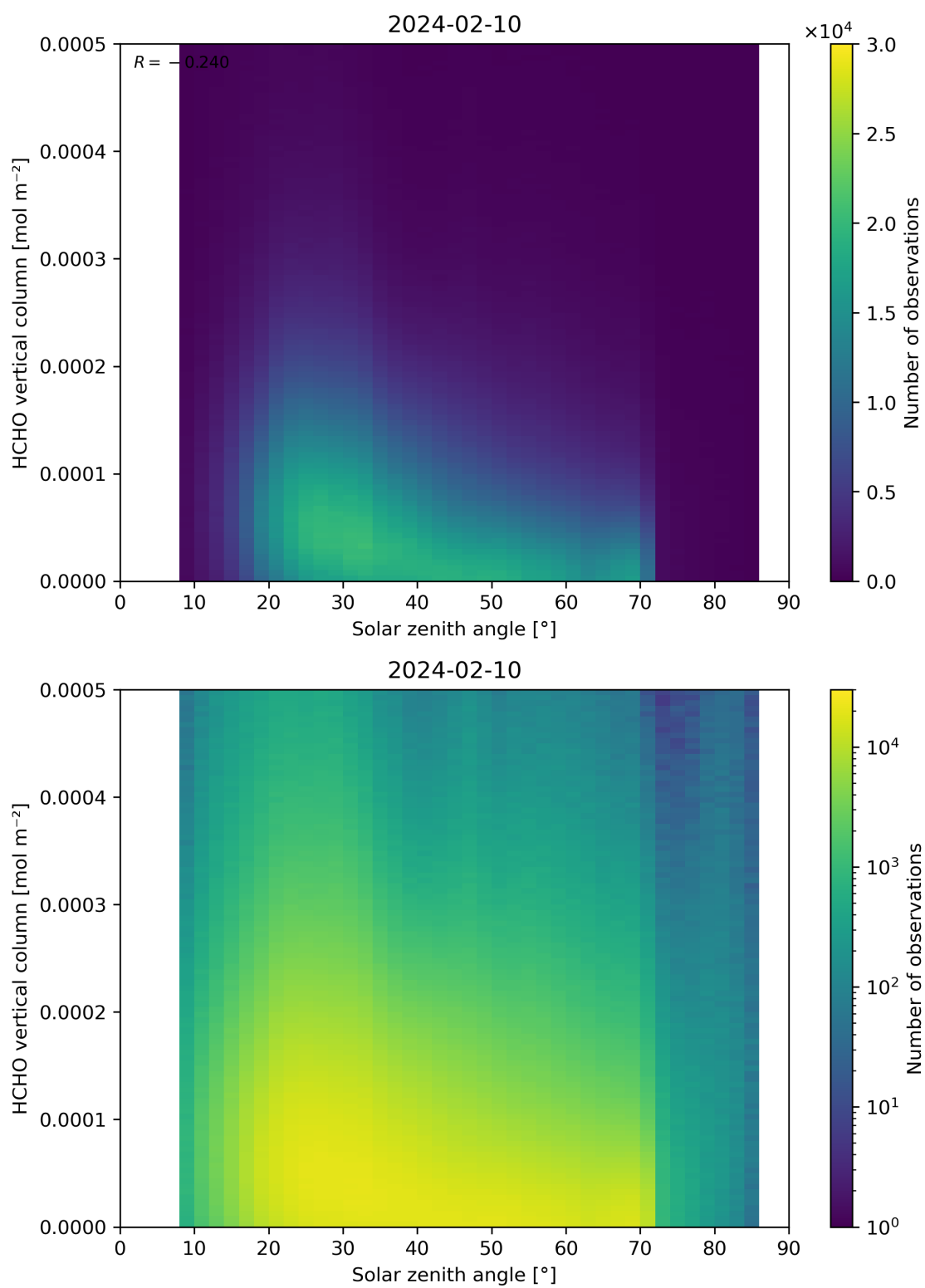
Figure 177: Scatter density plot of “Solar zenith angle” against “HCHO vertical column” for 2024-02-09 to 2024-02-11.
