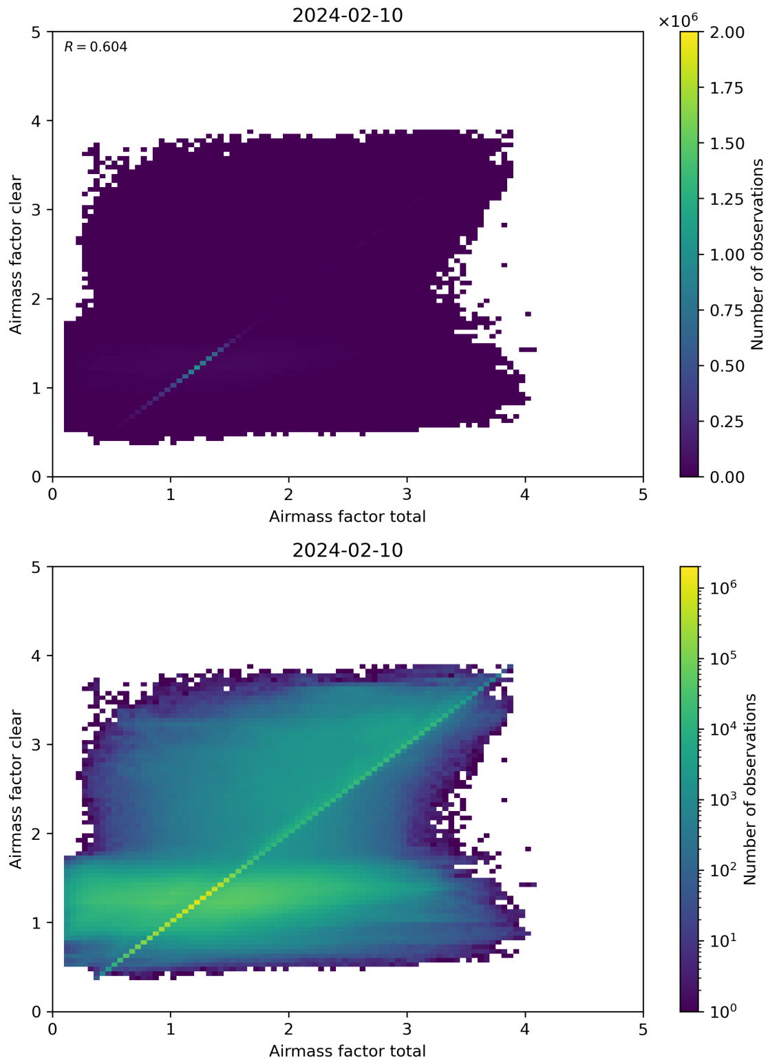
Figure 100: Scatter density plot of “Airmass factor total” against “Airmass factor clear” for 2024-02-09 to 2024-02-11.
