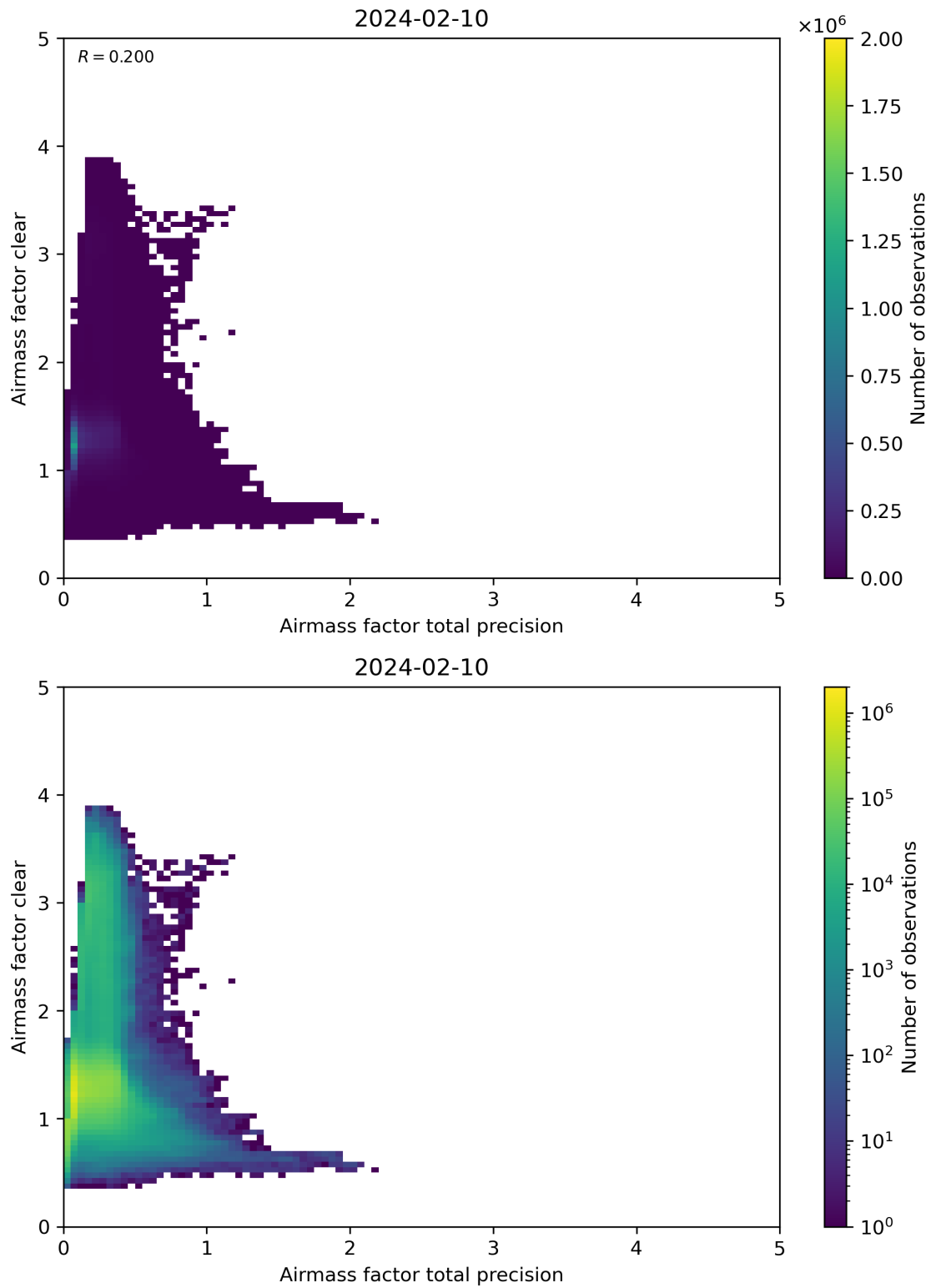
Figure 108: Scatter density plot of “Airmass factor total precision” against “Airmass factor clear” for 2024-02-09 to 2024-02-11.
