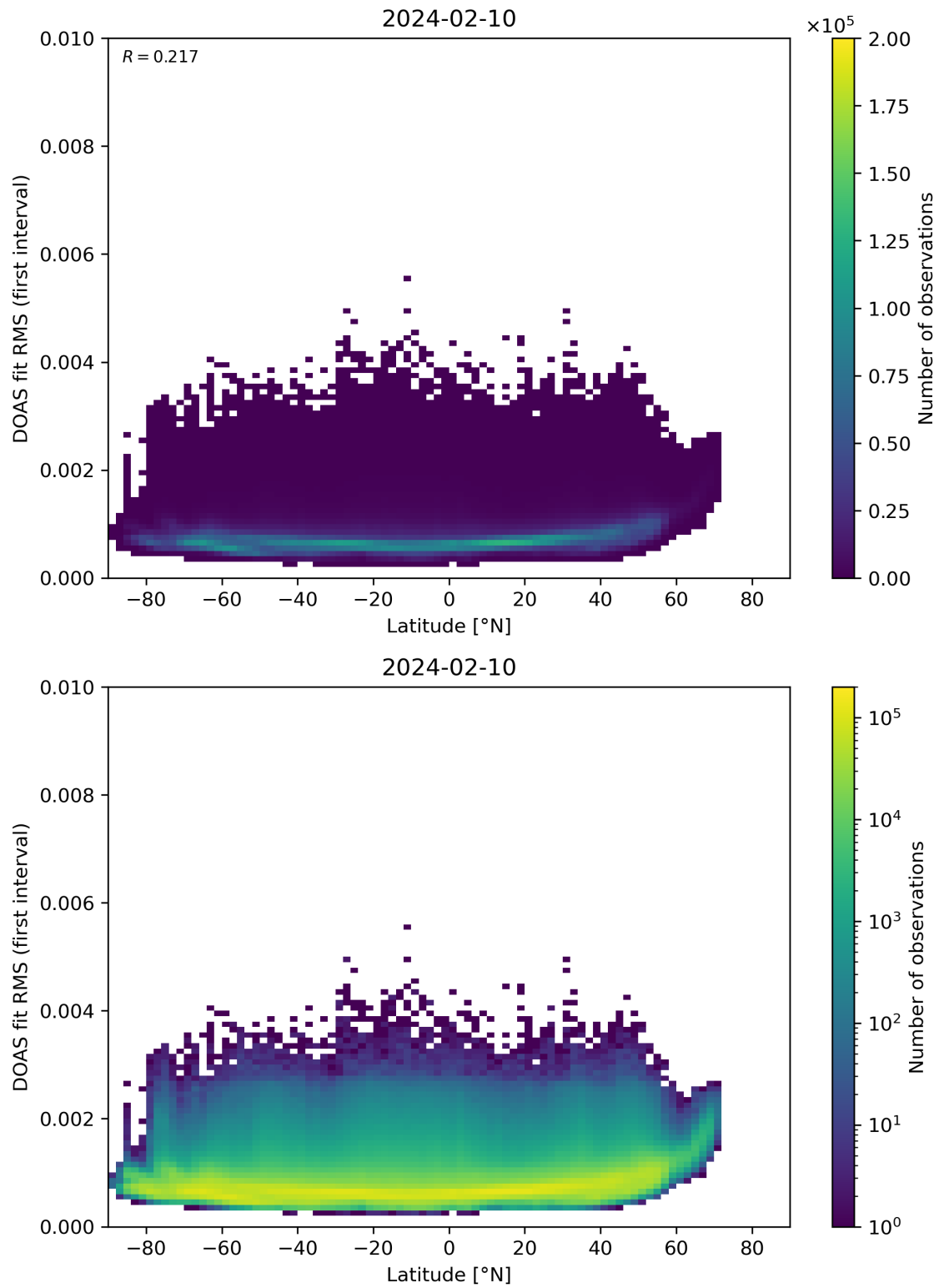
Figure 153: Scatter density plot of “Latitude” against “DOAS fit RMS (first interval)” for 2024-02-09 to 2024-02-11.
