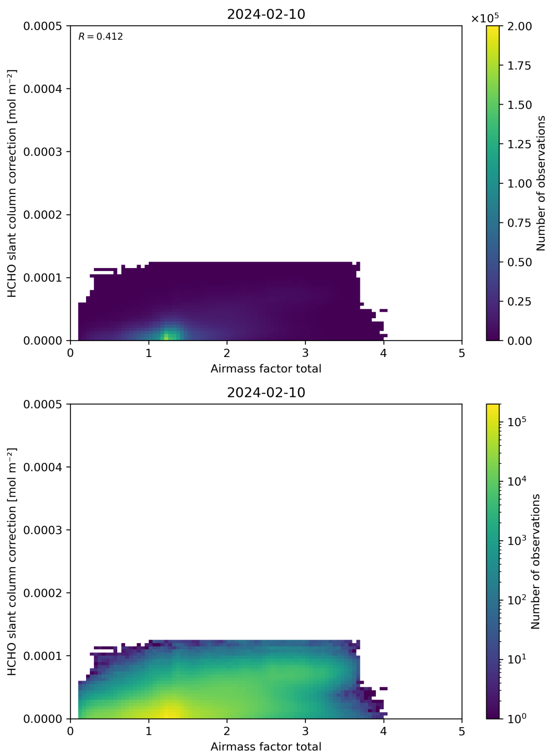
Figure 102: Scatter density plot of “Airmass factor total” against “HCHO slant column correction” for 2024-02-09 to 2024-02-11.
