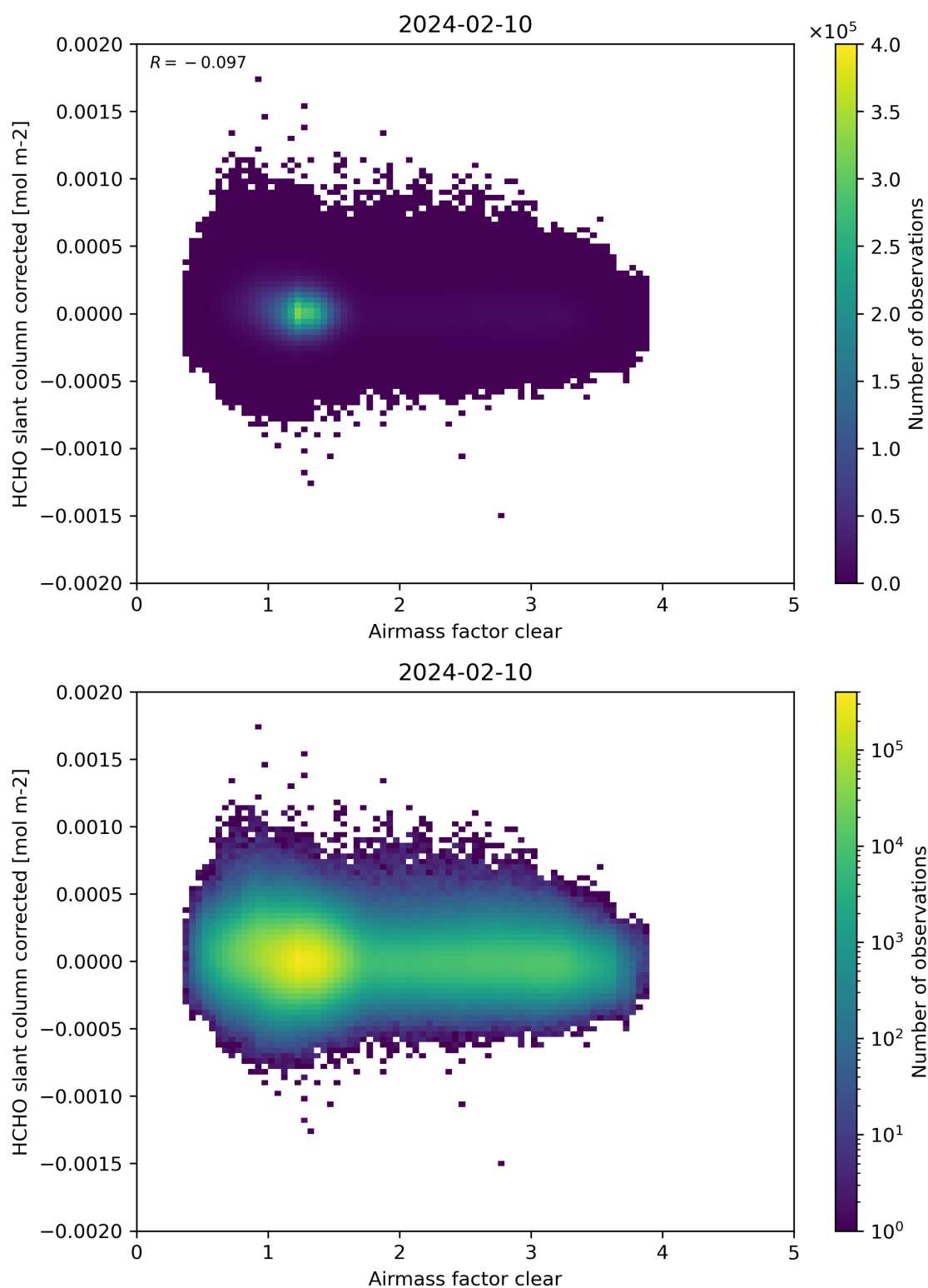
Figure 74: Scatter density plot of “Airmass factor clear” against “HCHO slant column corrected” for 2024-02-09 to 2024-02-11.
