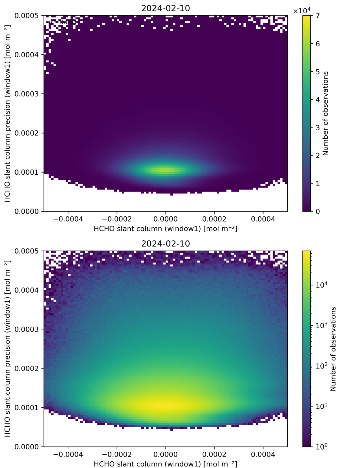
Figure 84: Scatter density plot of “HCHO slant column (window1)” against “HCHO slant column precision (window1)” for 2024-02-09 to 2024-02-11.
