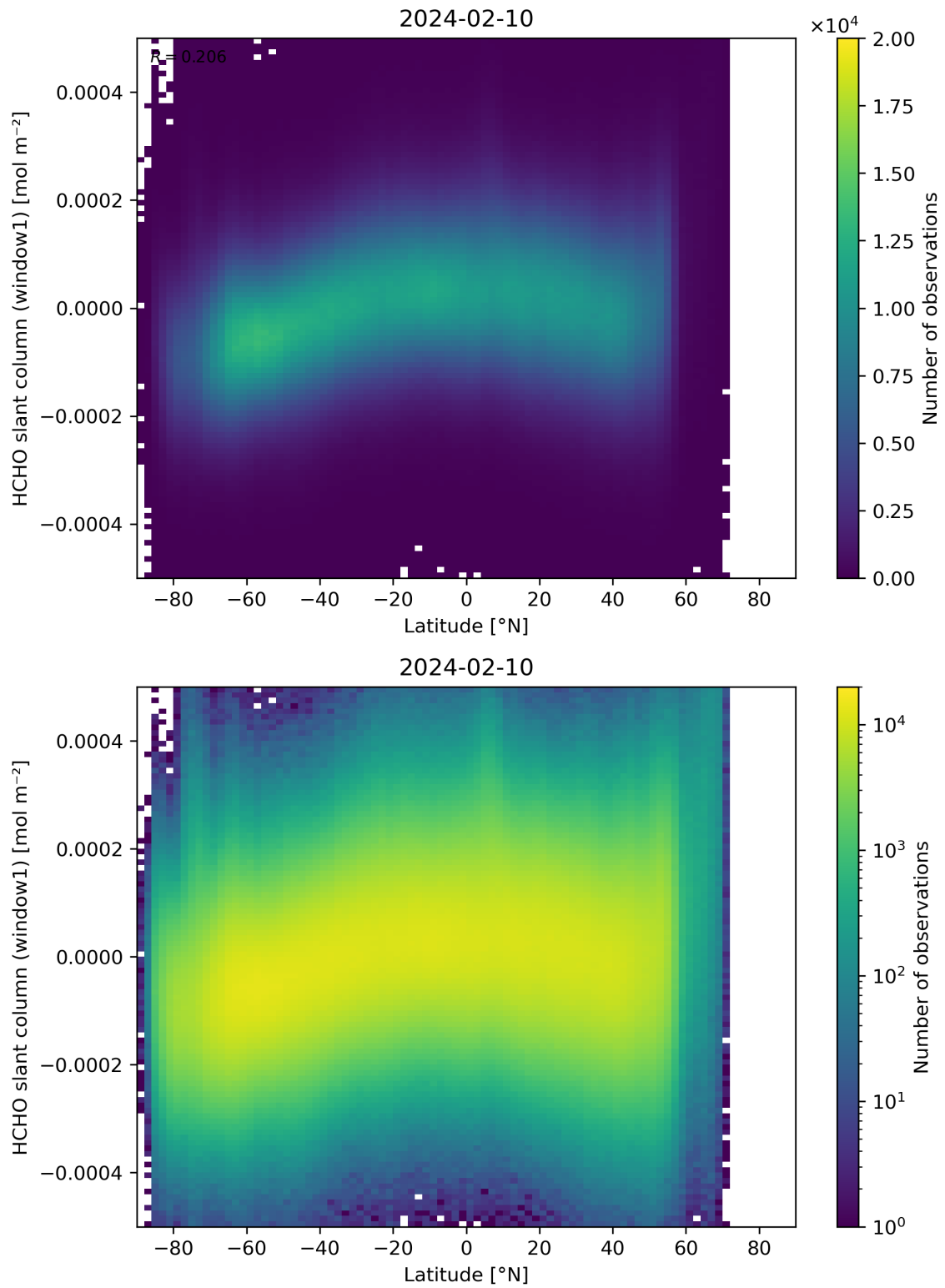
Figure 159: Scatter density plot of “Latitude” against “HCHO slant column (window1)” for 2024-02-09 to 2024-02-11.
