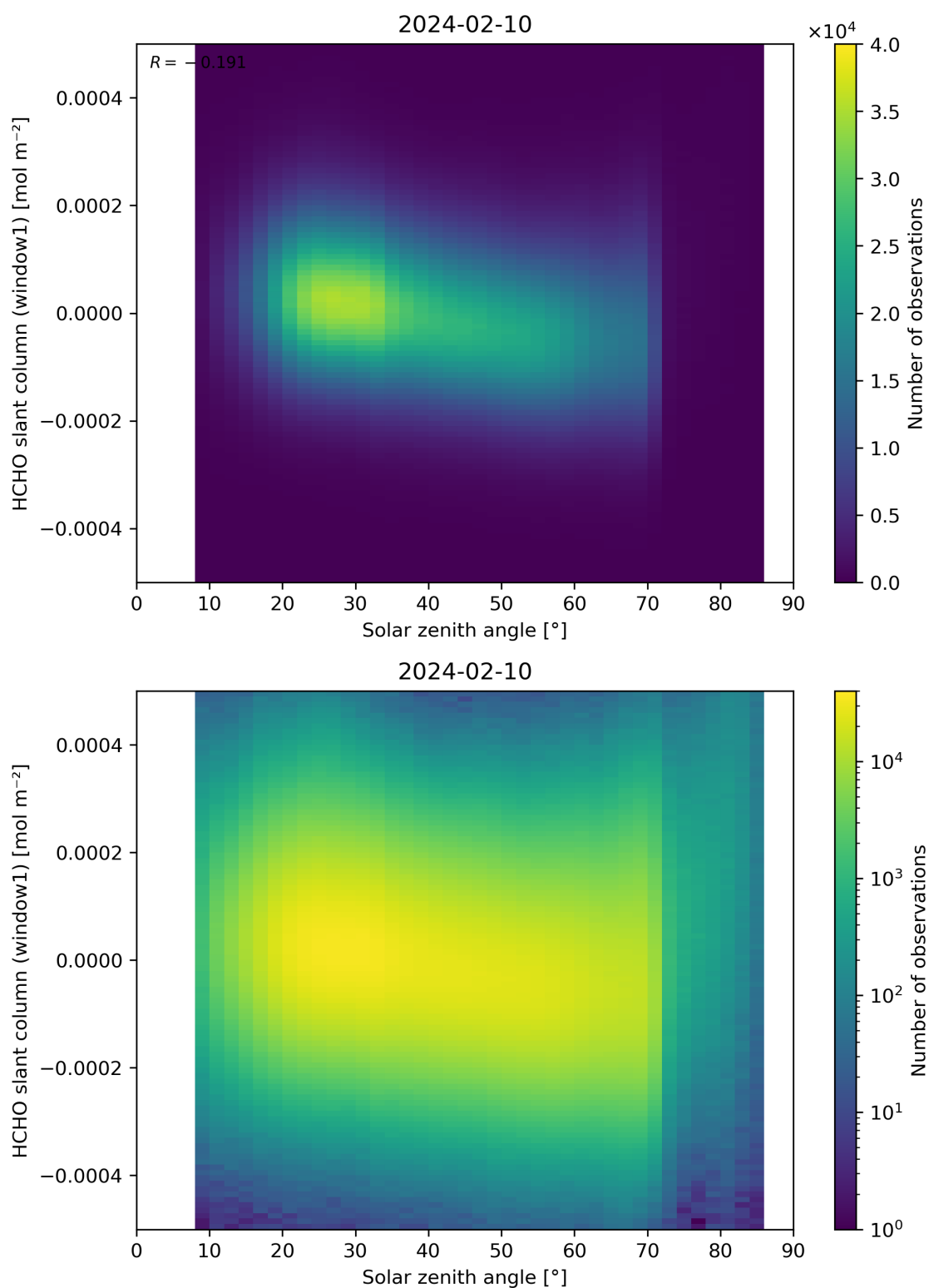
Figure 173: Scatter density plot of “Solar zenith angle” against “HCHO slant column (window1)” for 2024-02-09 to 2024-02-11.
