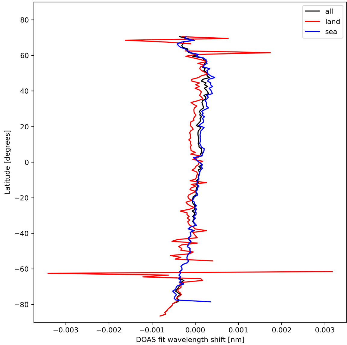
Figure 30: Zonal average of “DOAS fit wavelength shift” for 2024-02-09 to 2024-02-11.
