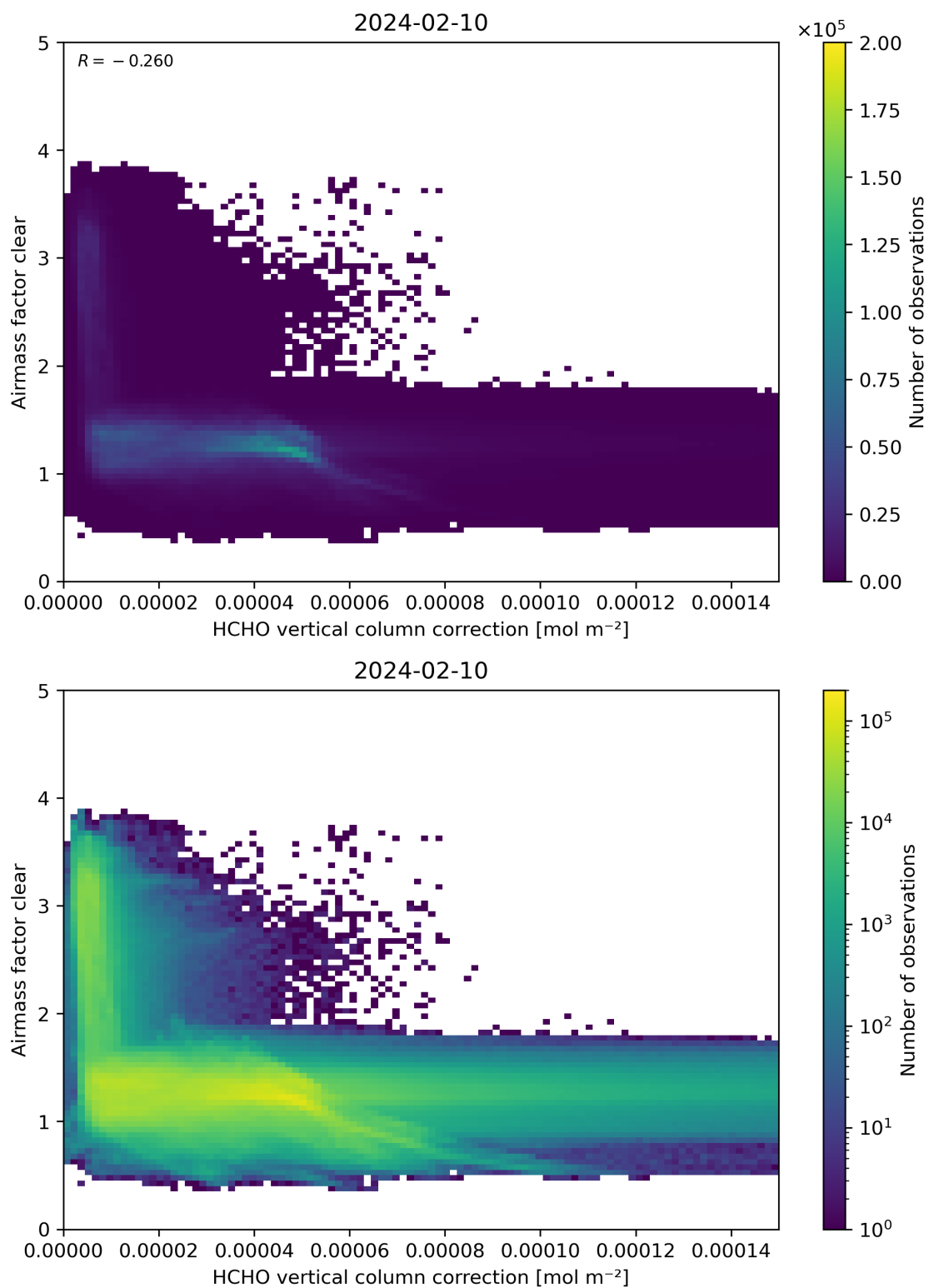
Figure 115: Scatter density plot of “HCHO vertical column correction” against “Airmass factor clear” for 2024-02-09 to 2024-02-11.
