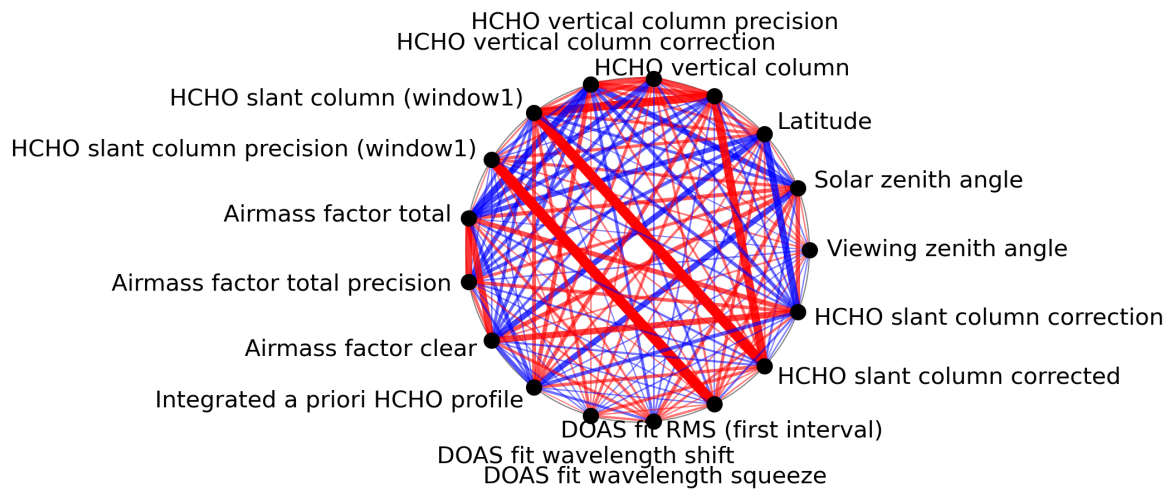
Figure 1: Map of correlation graph for 2024-02-09 to 2024-02-11.
