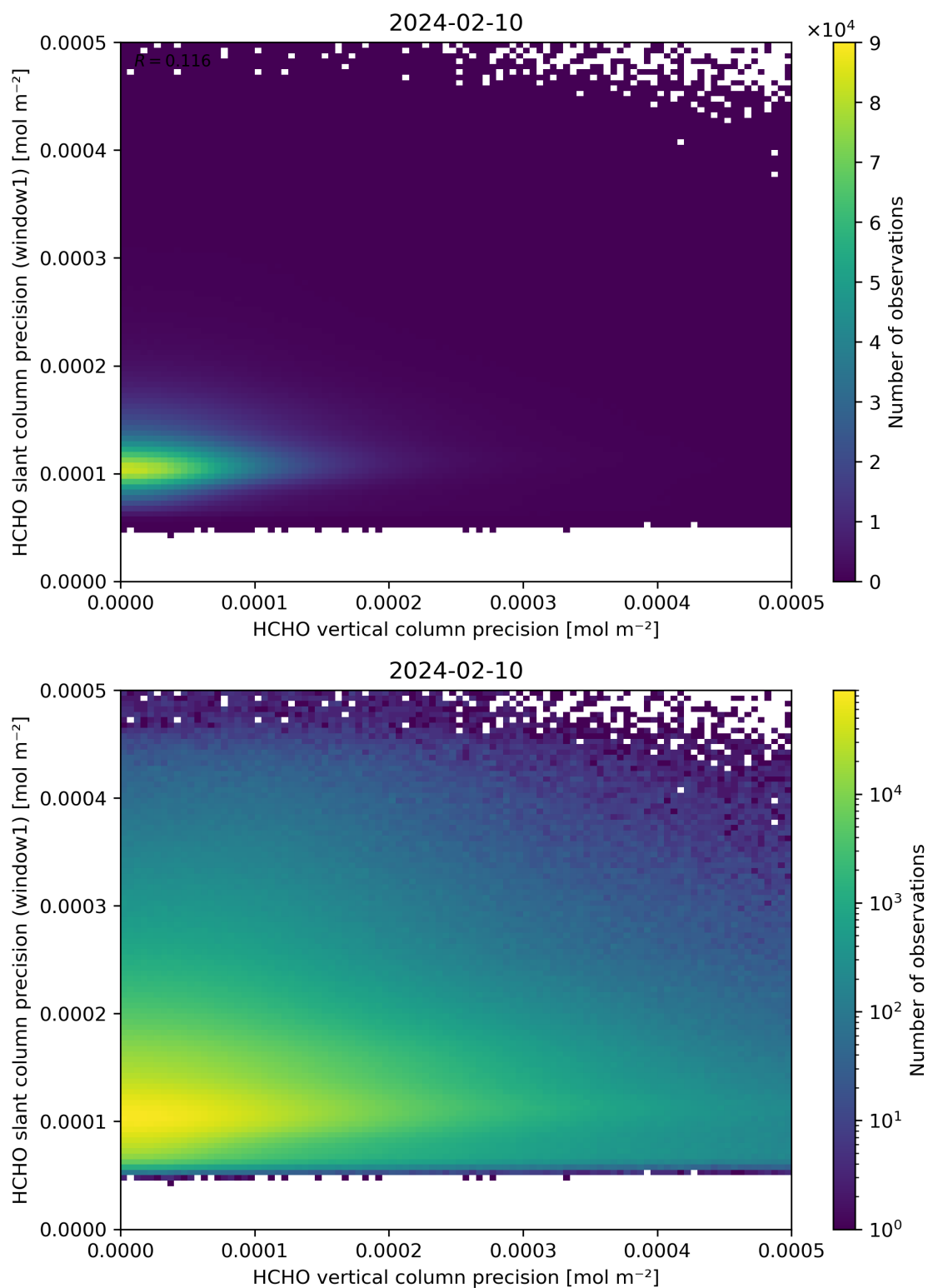
Figure 143: Scatter density plot of “HCHO vertical column precision” against “HCHO slant column precision (window1)” for 2024-02-09 to 2024-02-11.
