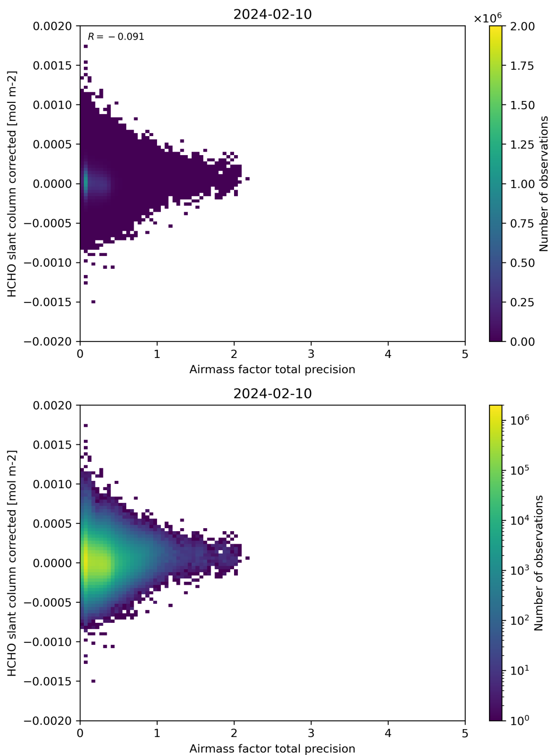
Figure 109: Scatter density plot of “Airmass factor total precision” against “HCHO slant column corrected” for 2024-02-09 to 2024-02-11.
