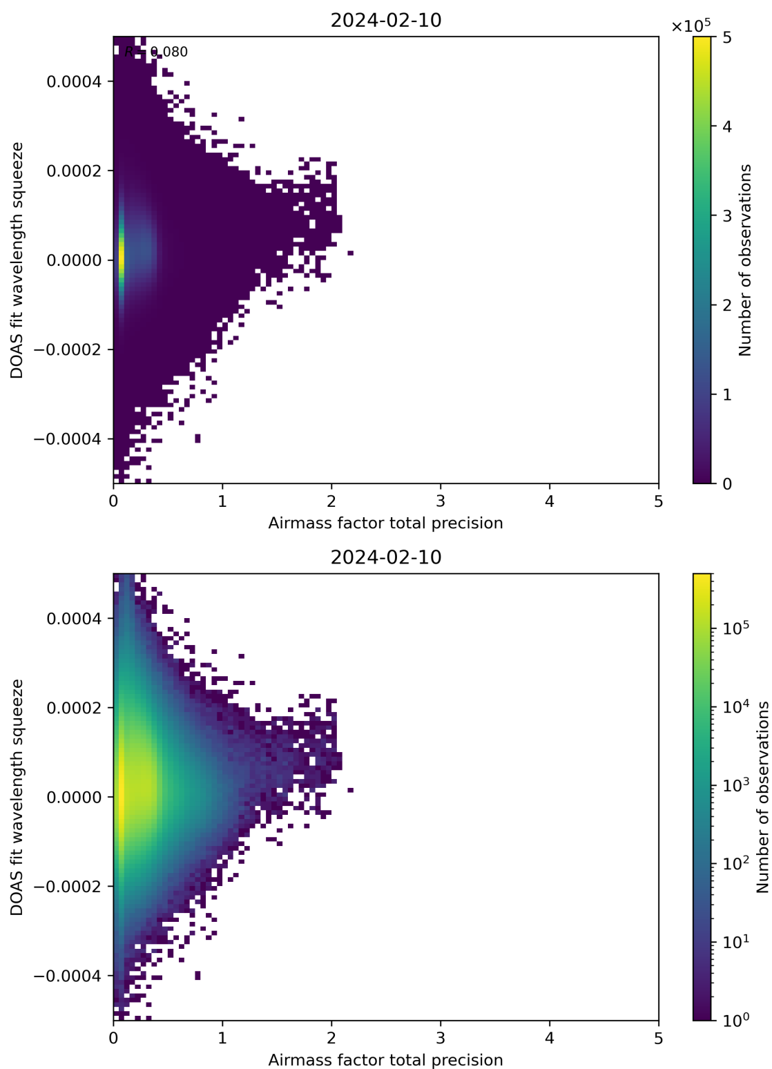
Figure 107: Scatter density plot of “Airmass factor total precision” against “DOAS fit wavelength squeeze” for 2024-02-09 to 2024-02-11.
