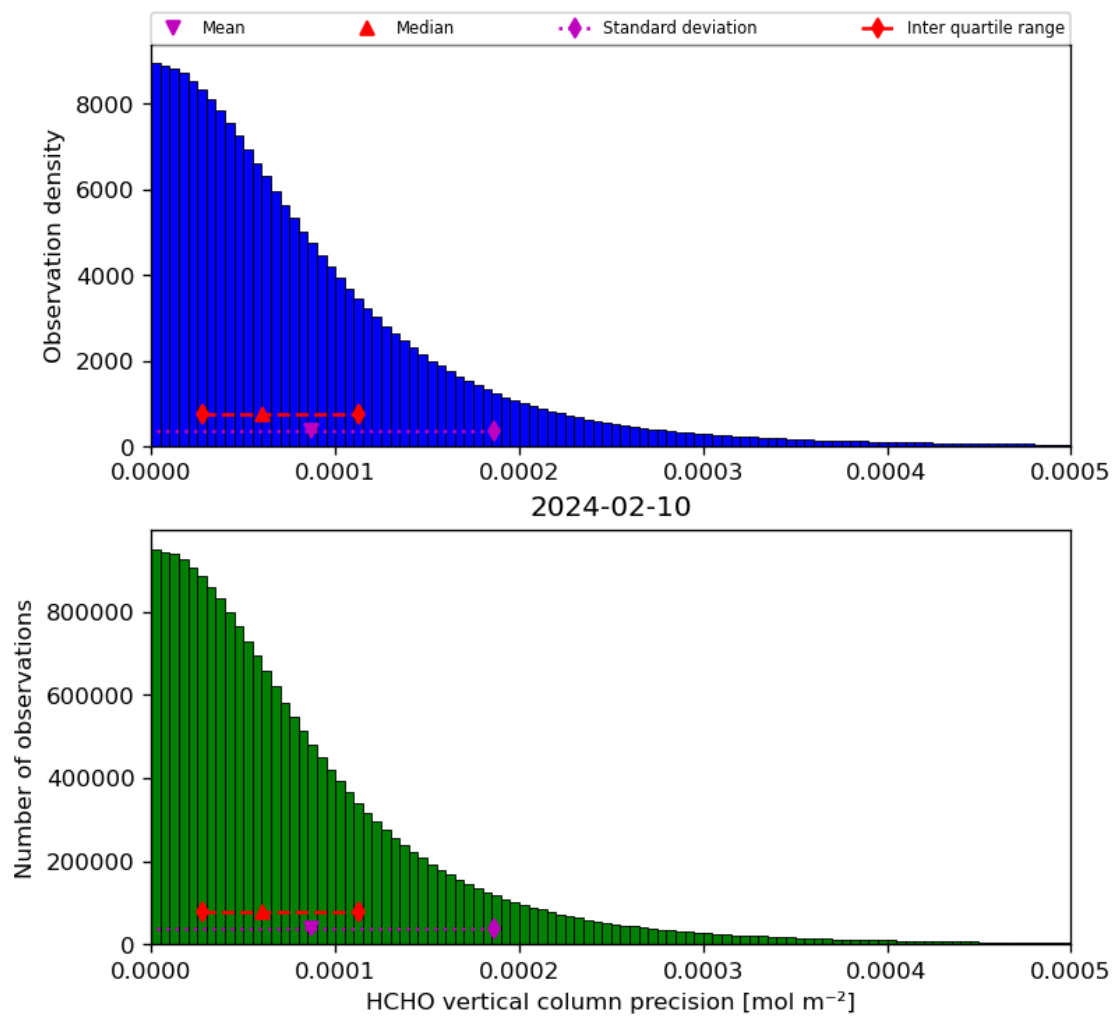
Figure 36: Histogram of “HCHO vertical column precision” for 2024-02-09 to 2024-02-11
