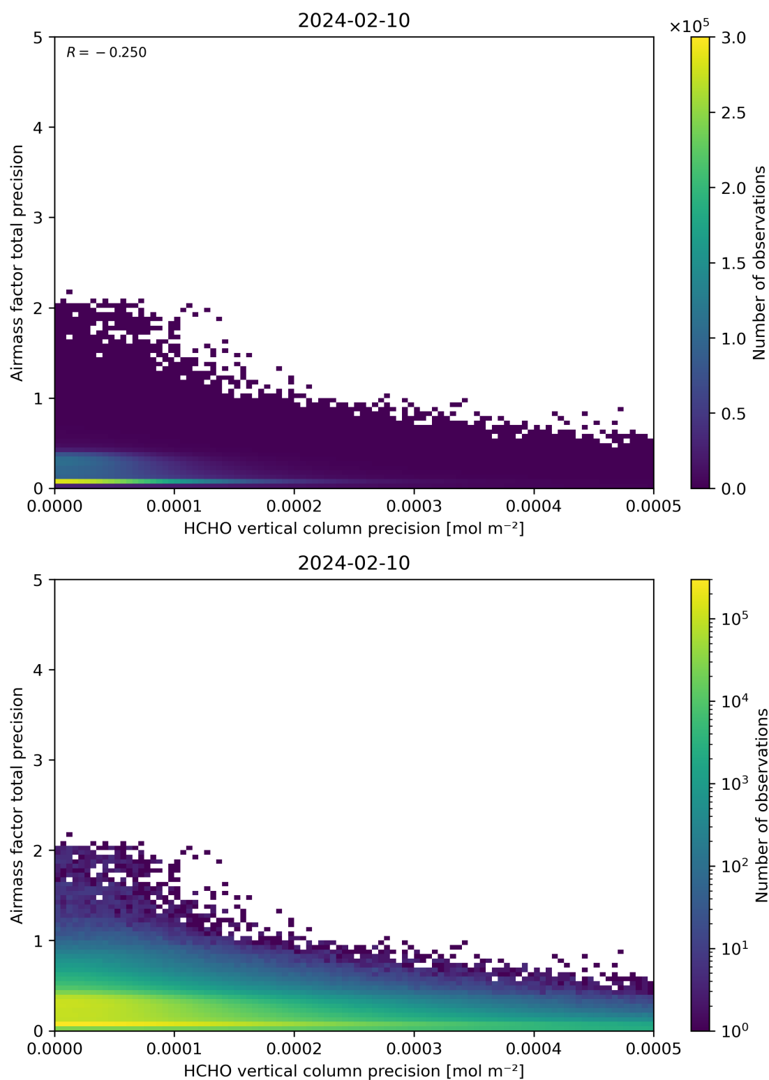
Figure 145: Scatter density plot of “HCHO vertical column precision” against “Airmass factor total precision” for 2024-02-09 to 2024-02-11.
