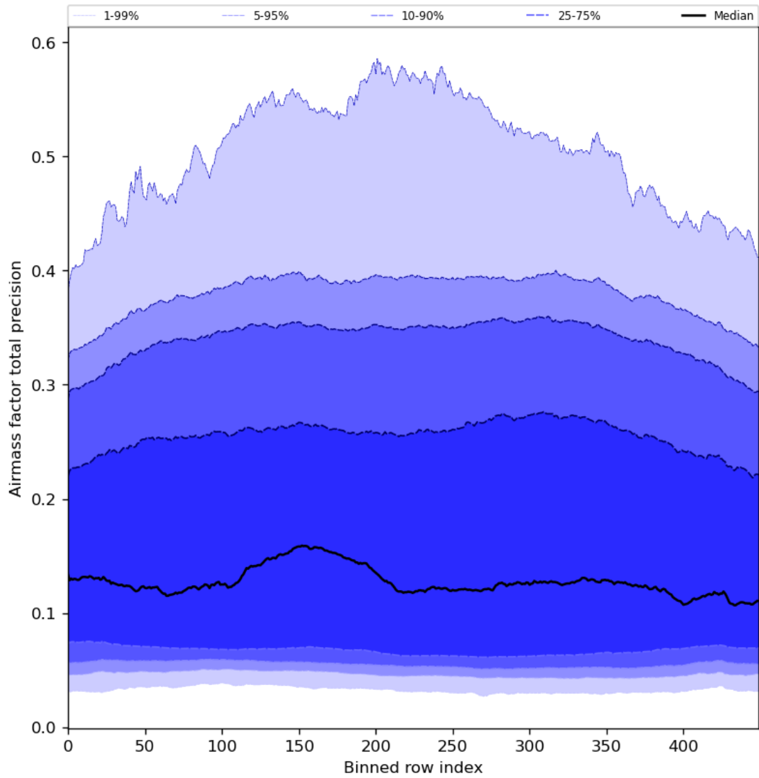
Figure 55: Along track statistics of “Airmass factor total precision” for 2024-02-09 to 2024-02-11
