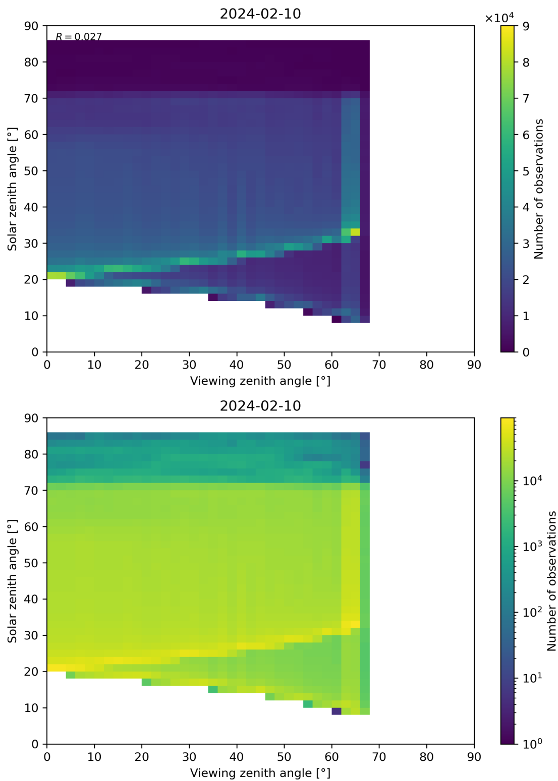
Figure 197: Scatter density plot of “Viewing zenith angle” against “Solar zenith angle” for 2024-02-09 to 2024-02-11.
