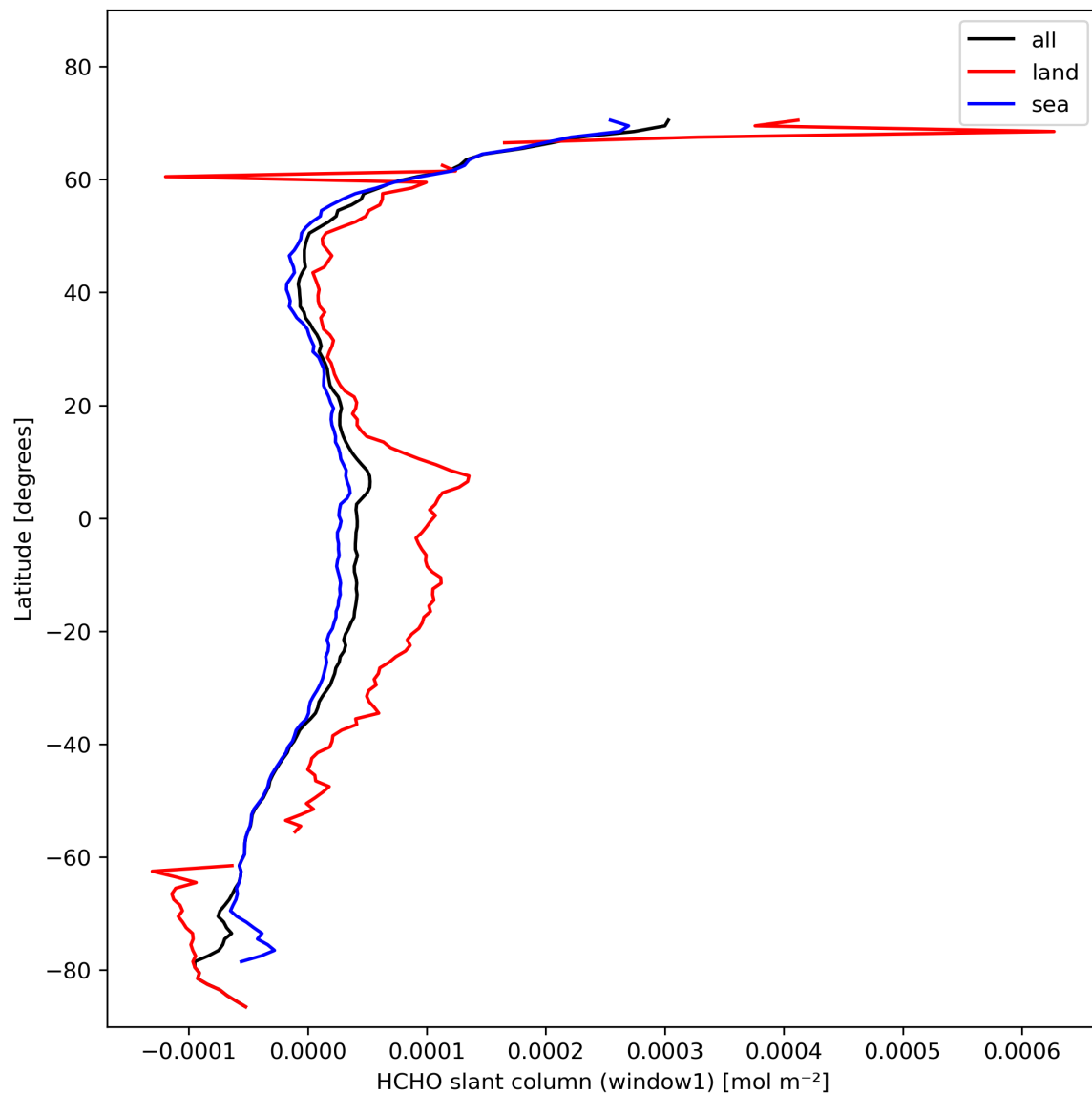
Figure 24: Zonal average of “HCHO slant column (window1)” for 2024-02-09 to 2024-02-11.
