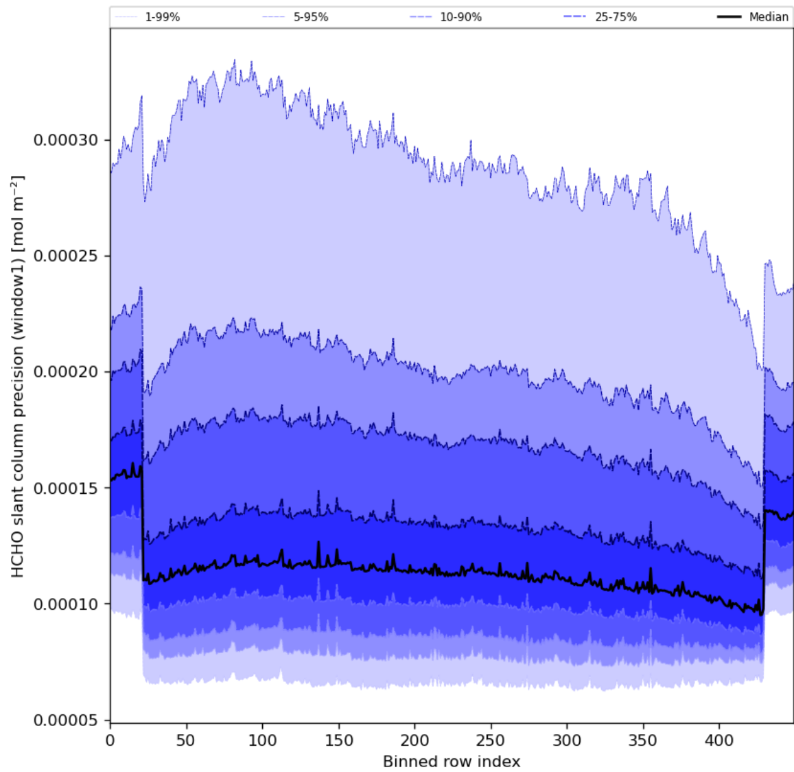
Figure 53: Along track statistics of “HCHO slant column precision (window1)” for 2024-02-09 to 2024-02-11
