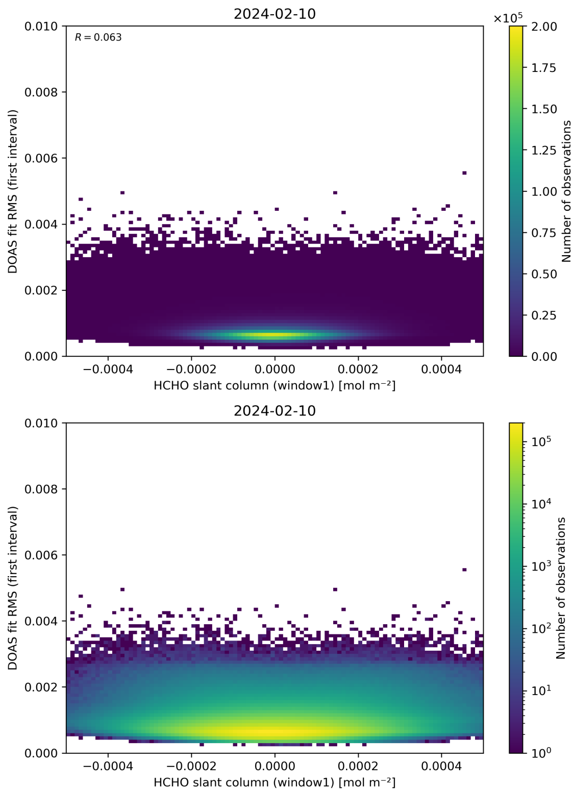
Figure 78: Scatter density plot of “HCHO slant column (window1)” against “DOAS fit RMS (first interval)” for 2024-02-09 to 2024-02-11.
