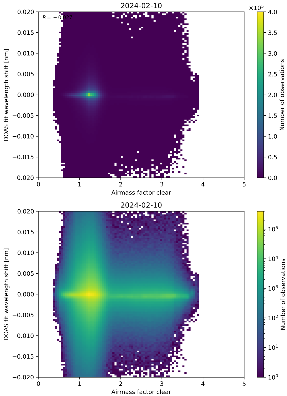
Figure 72: Scatter density plot of “Airmass factor clear” against “DOAS fit wavelength shift” for 2024-02-09 to 2024-02-11.
