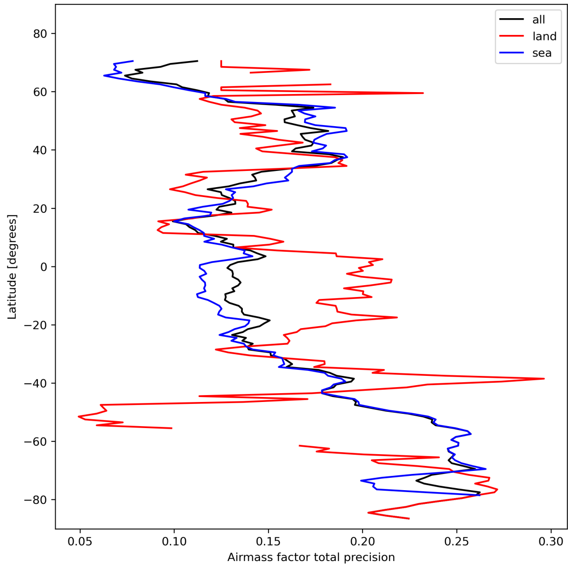
Figure 27: Zonal average of “Airmass factor total precision” for 2024-02-09 to 2024-02-11.
