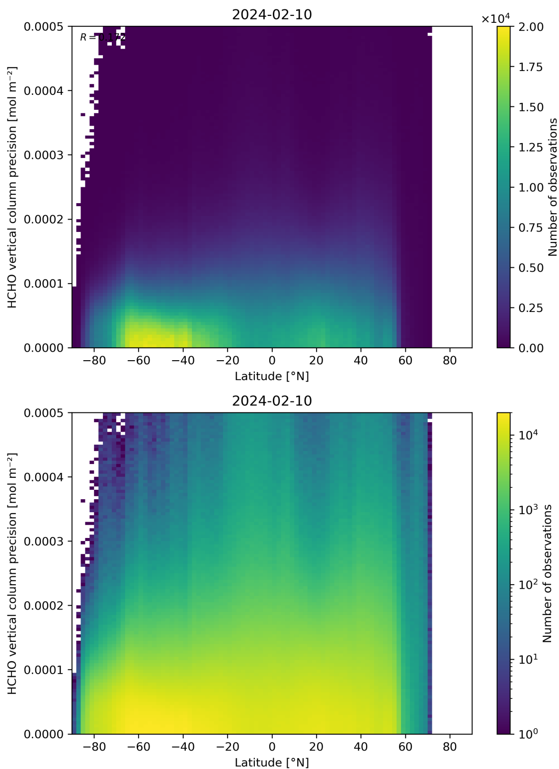
Figure 165: Scatter density plot of “Latitude” against “HCHO vertical column precision” for 2024-02-09 to 2024-02-11.
