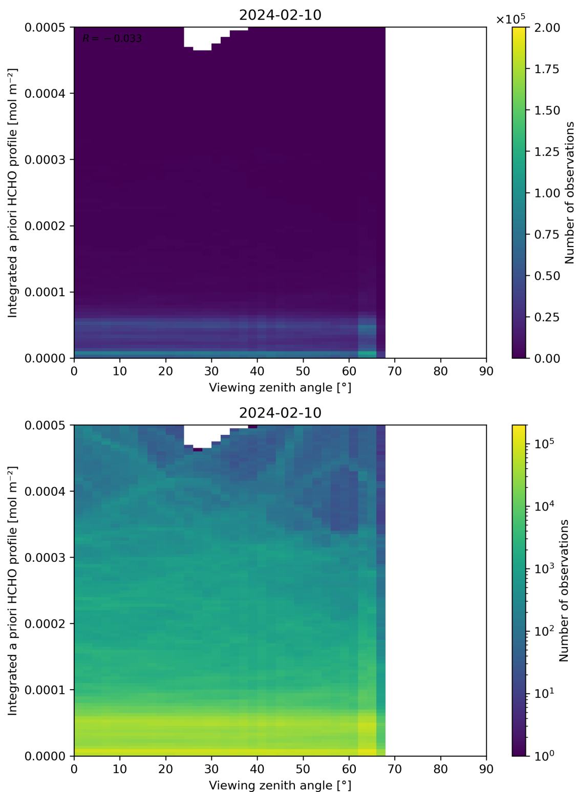
Figure 195: Scatter density plot of “Viewing zenith angle” against “Integrated a priori HCHO profile” for 2024-02-09 to 2024-02-11.
