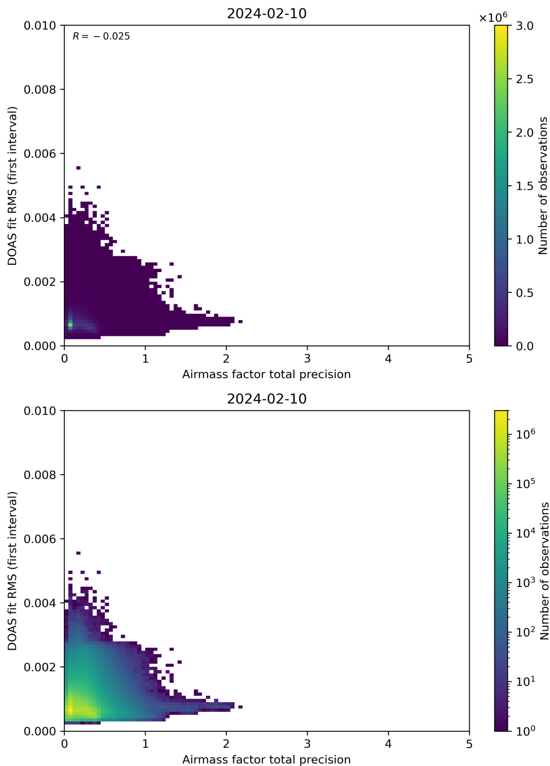
Figure 105: Scatter density plot of “Airmass factor total precision” against “DOAS fit RMS (first interval)” for 2024-02-09 to 2024-02-11.
