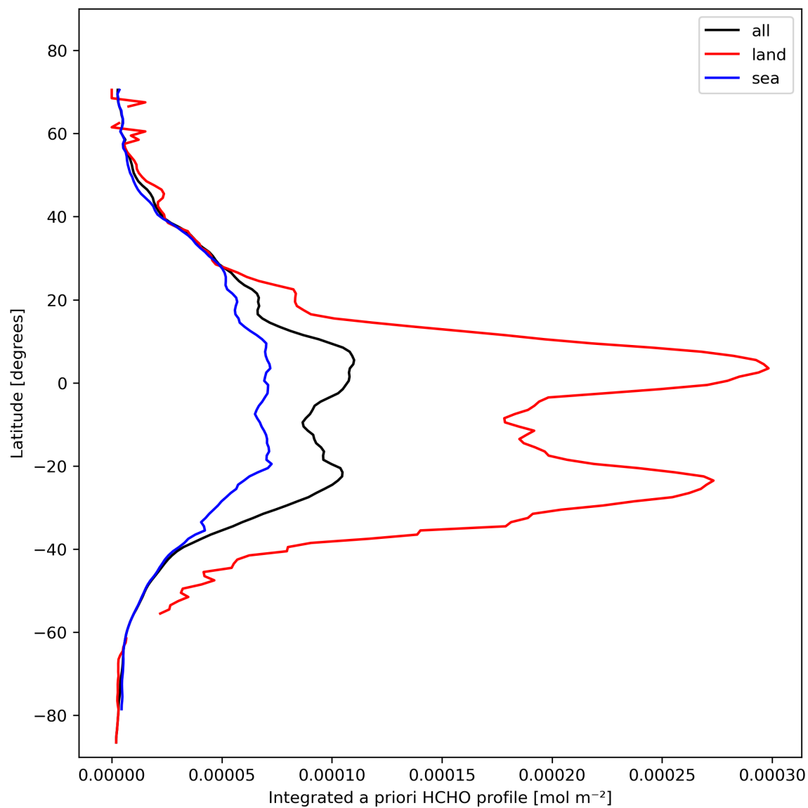
Figure 29: Zonal average of “Integrated a priori HCHO profile” for 2024-02-09 to 2024-02-11.
