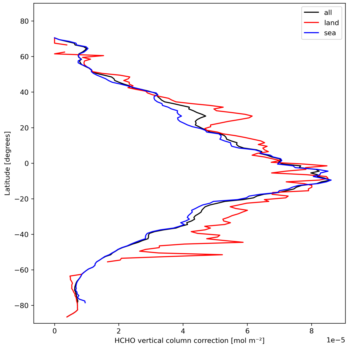
Figure 23: Zonal average of “HCHO vertical column correction” for 2024-02-09 to 2024-02-11.
