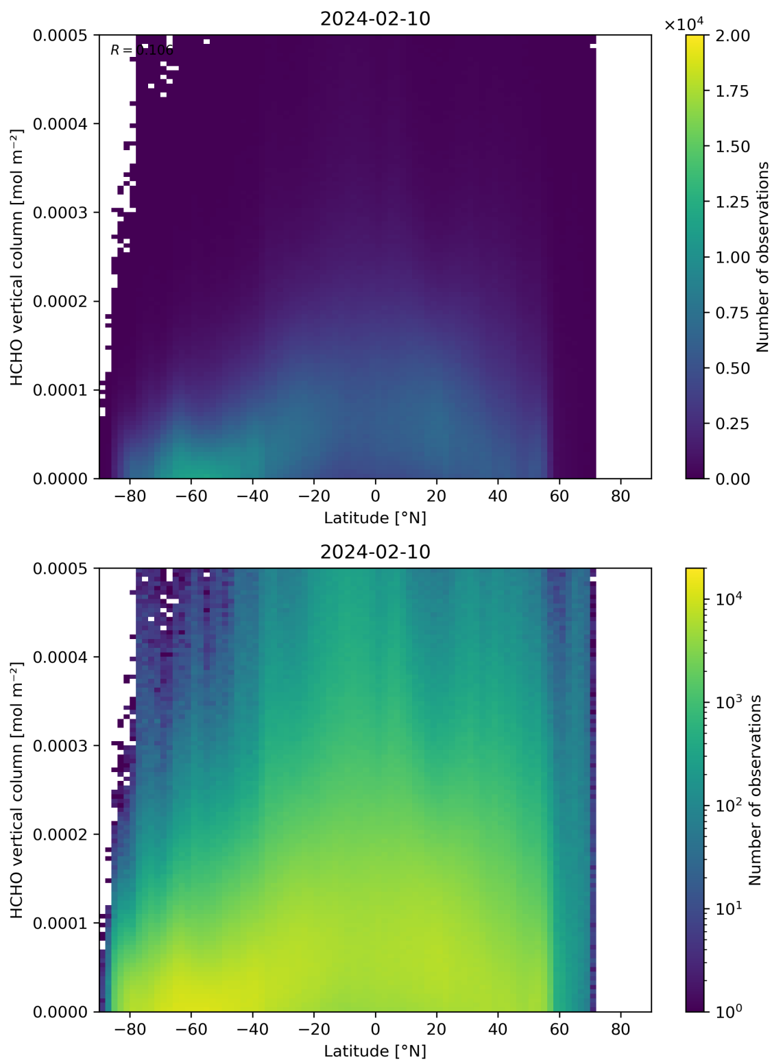
Figure 163: Scatter density plot of “Latitude” against “HCHO vertical column” for 2024-02-09 to 2024-02-11.
