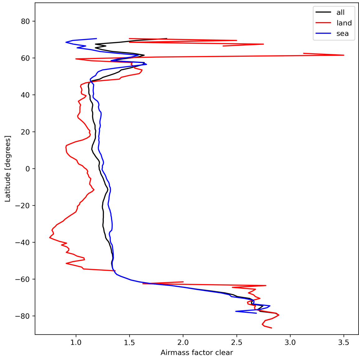
Figure 28: Zonal average of “Airmass factor clear” for 2024-02-09 to 2024-02-11.
