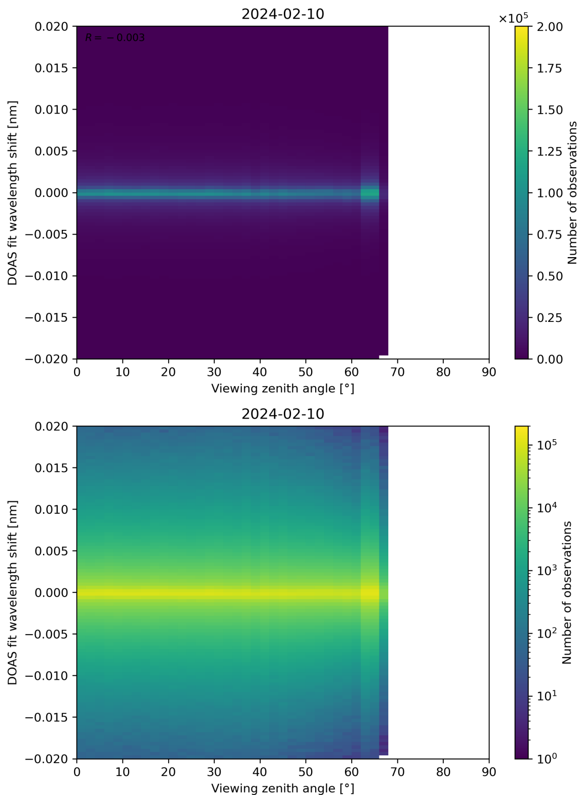
Figure 183: Scatter density plot of “Viewing zenith angle” against “DOAS fit wavelength shift” for 2024-02-09 to 2024-02-11.
