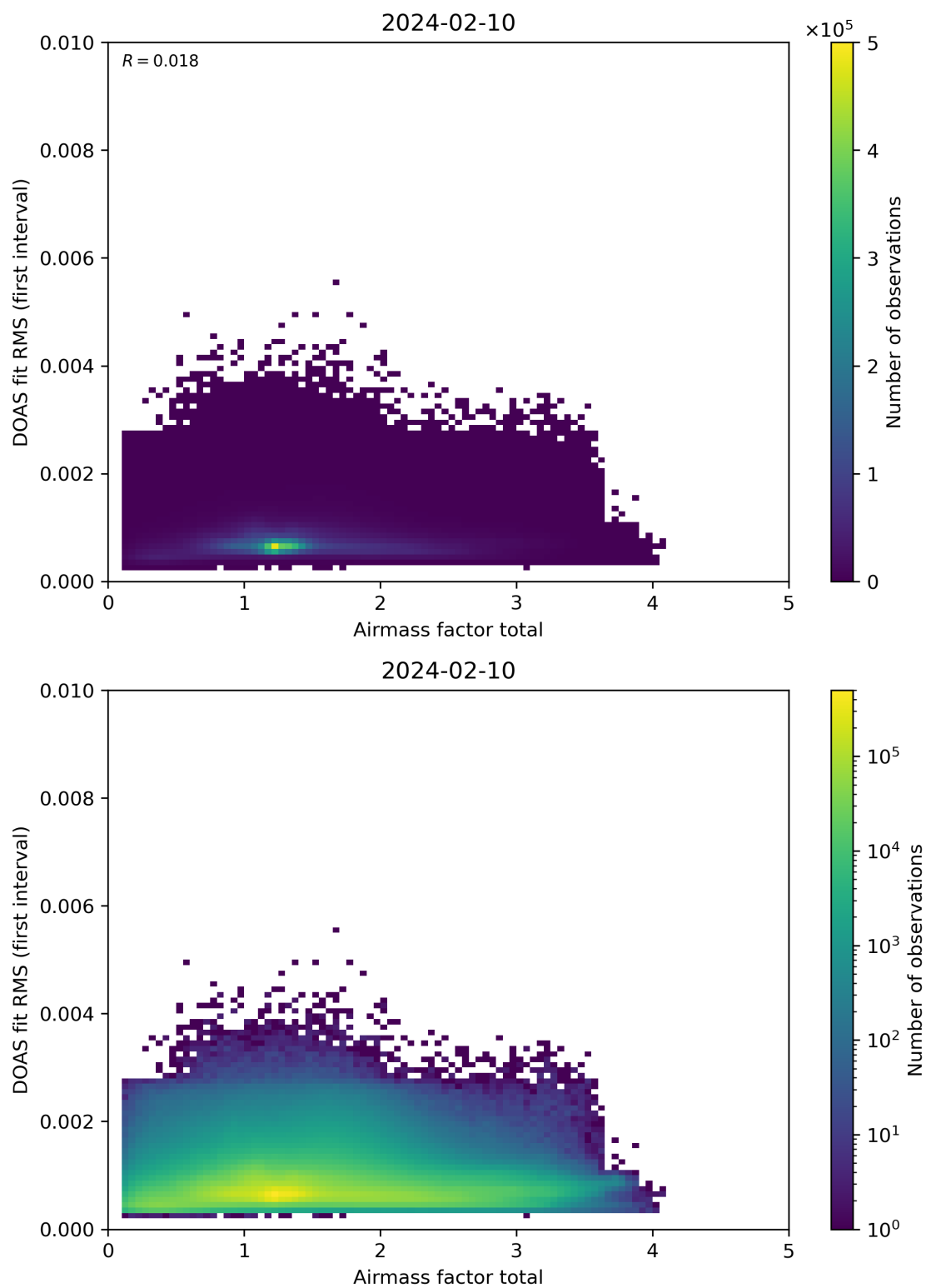
Figure 97: Scatter density plot of “Airmass factor total” against “DOAS fit RMS (first interval)” for 2024-02-09 to 2024-02-11.
