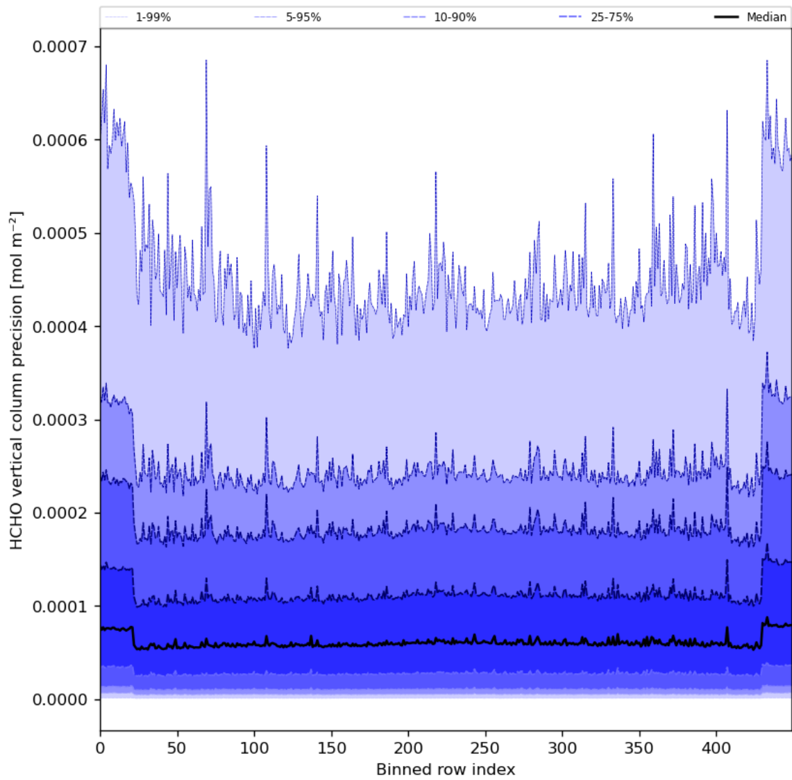
Figure 50: Along track statistics of “HCHO vertical column precision” for 2024-02-09 to 2024-02-11
