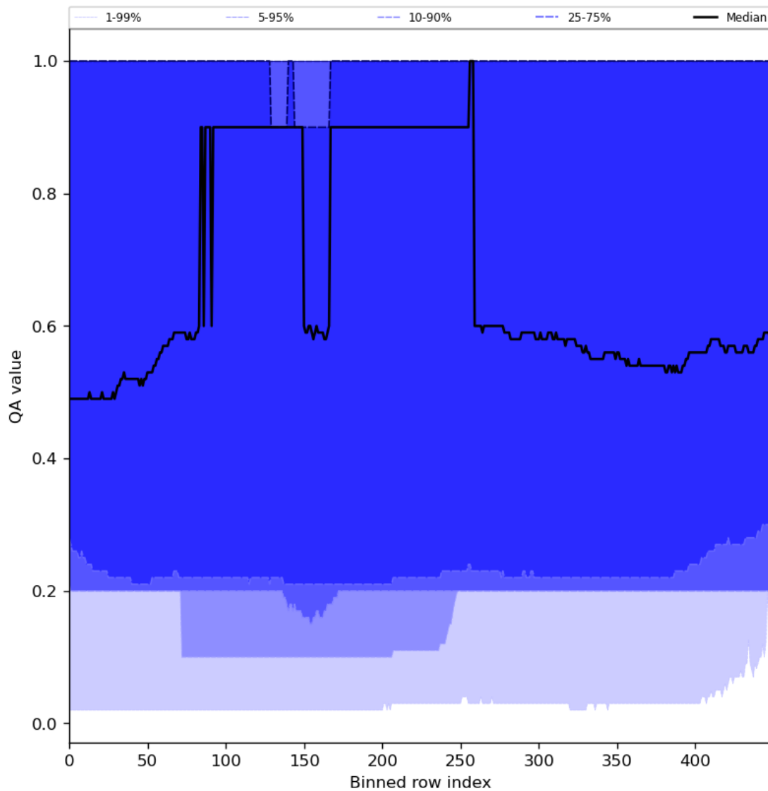
Figure 48: Along track statistics of “QA value” for 2024-02-09 to 2024-02-11
