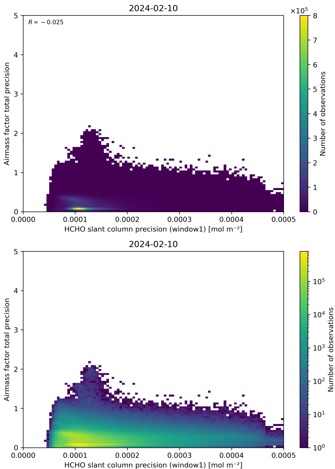
Figure 95: Scatter density plot of “HCHO slant column precision (window1)” against “Airmass factor total precision” for 2024-02-09 to 2024-02-11.
