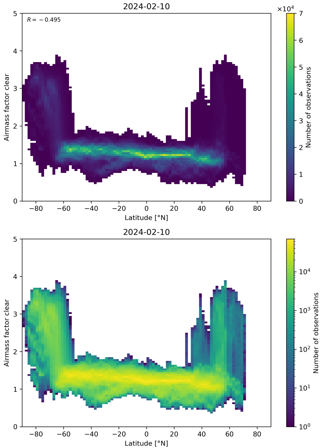
Figure 156: Scatter density plot of “Latitude” against “Airmass factor clear” for 2024-02-09 to 2024-02-11.
