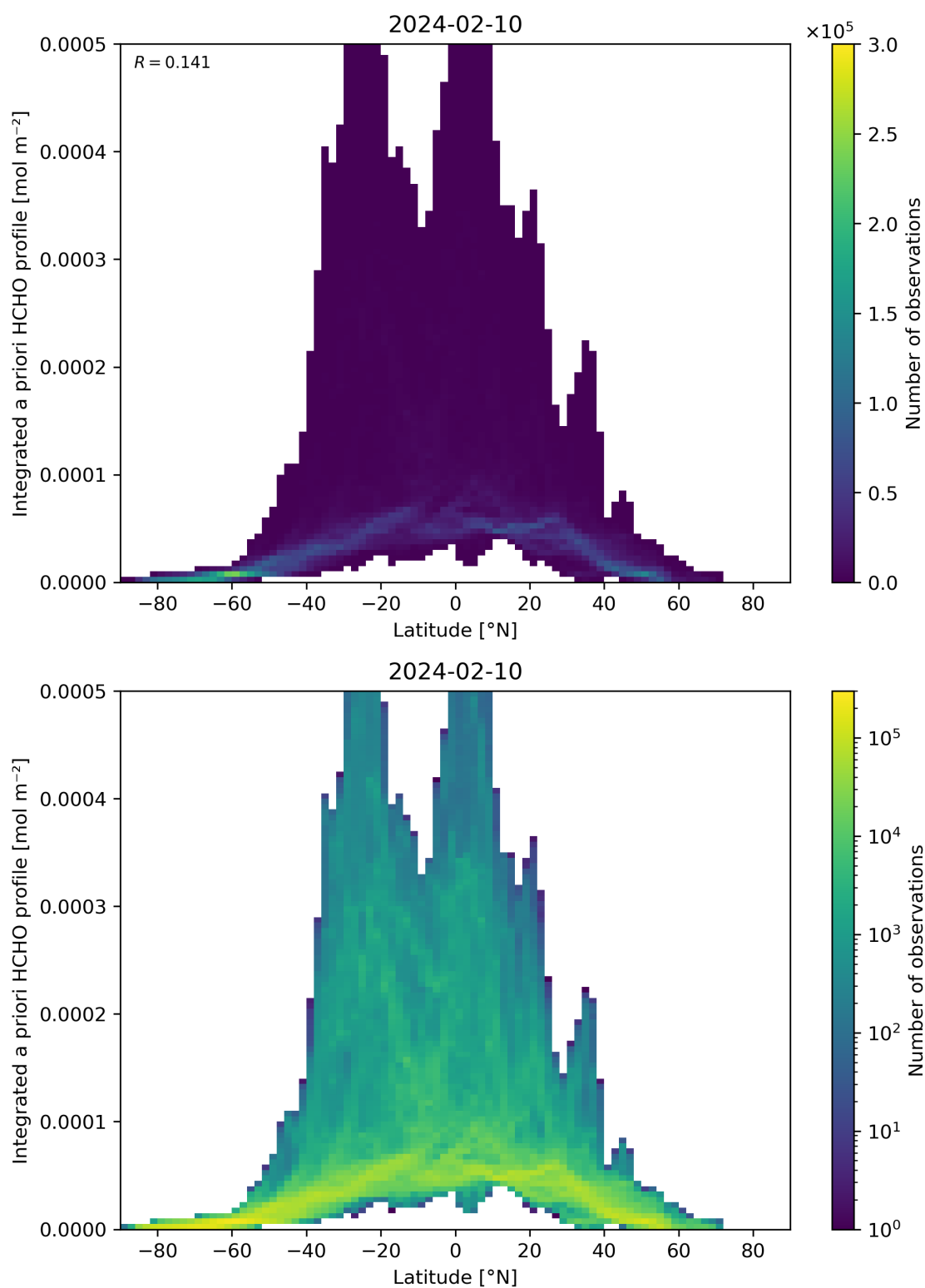
Figure 166: Scatter density plot of “Latitude” against “Integrated a priori HCHO profile” for 2024-02-09 to 2024-02-11.
