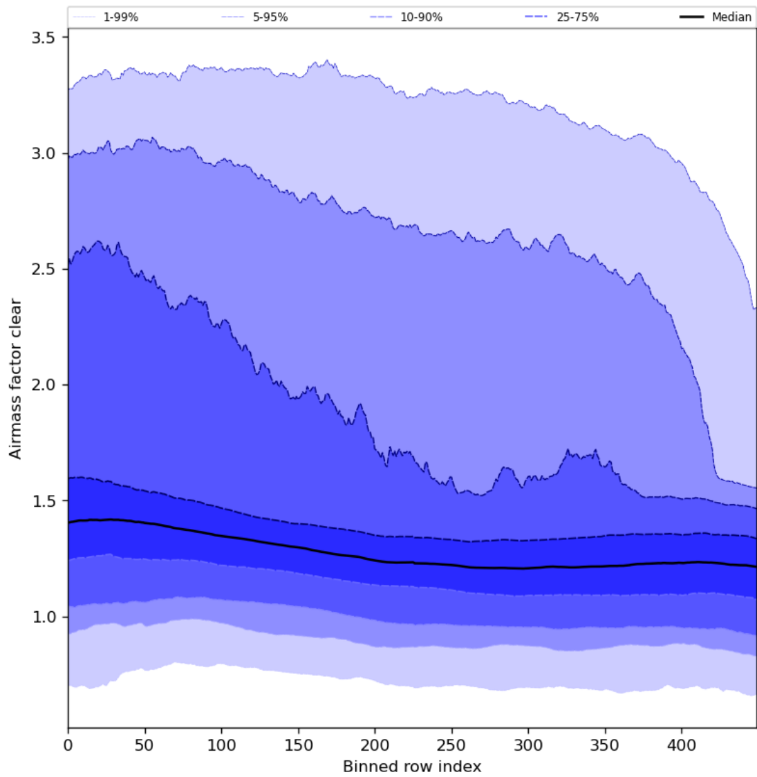
Figure 56: Along track statistics of “Airmass factor clear” for 2024-02-09 to 2024-02-11
