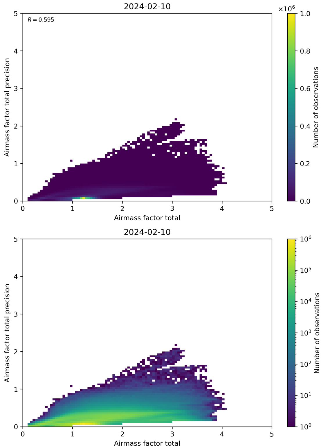
Figure 103: Scatter density plot of “Airmass factor total” against “Airmass factor total precision” for 2024-02-09 to 2024-02-11.
