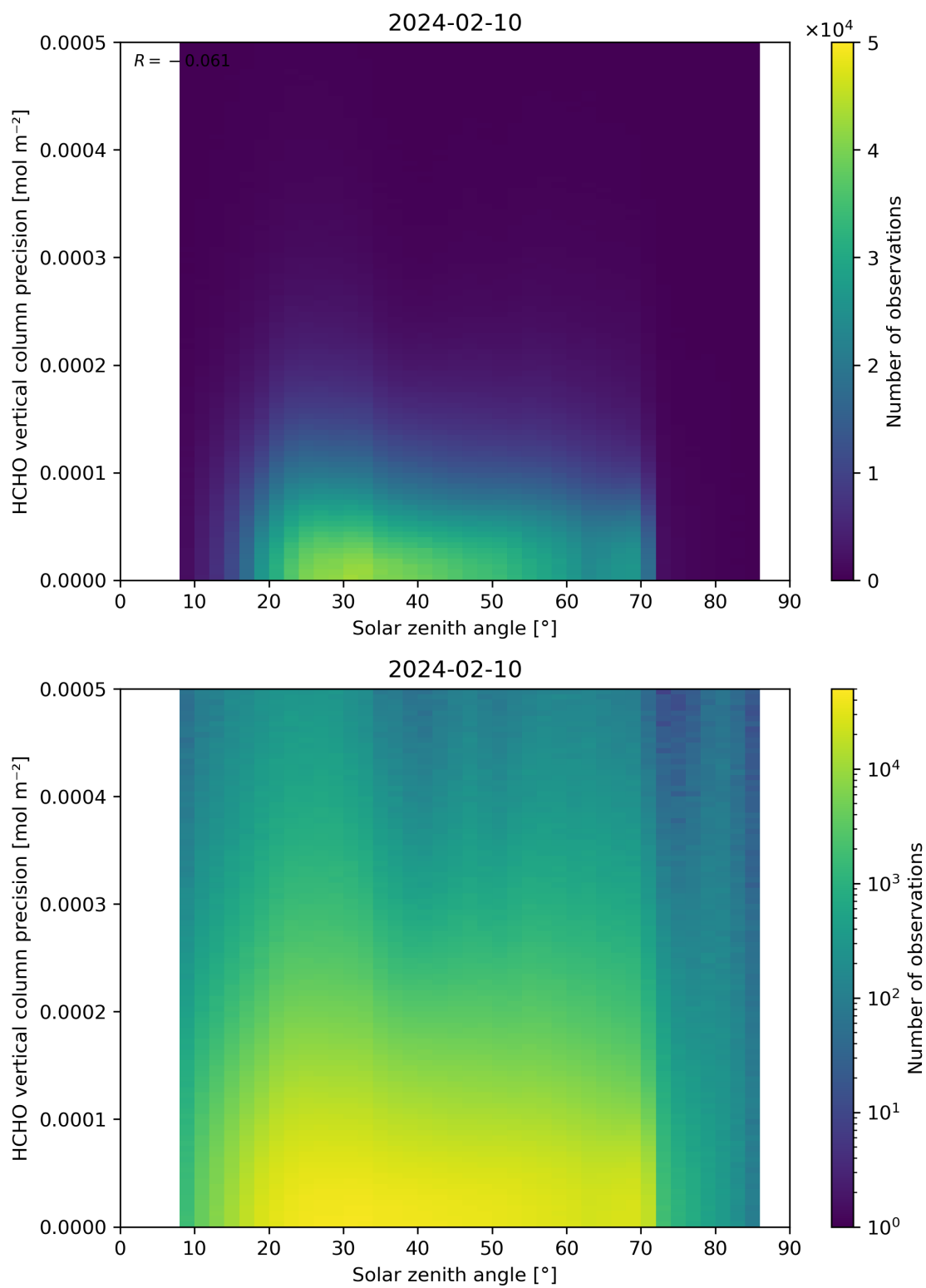
Figure 179: Scatter density plot of “Solar zenith angle” against “HCHO vertical column precision” for 2024-02-09 to 2024-02-11.
