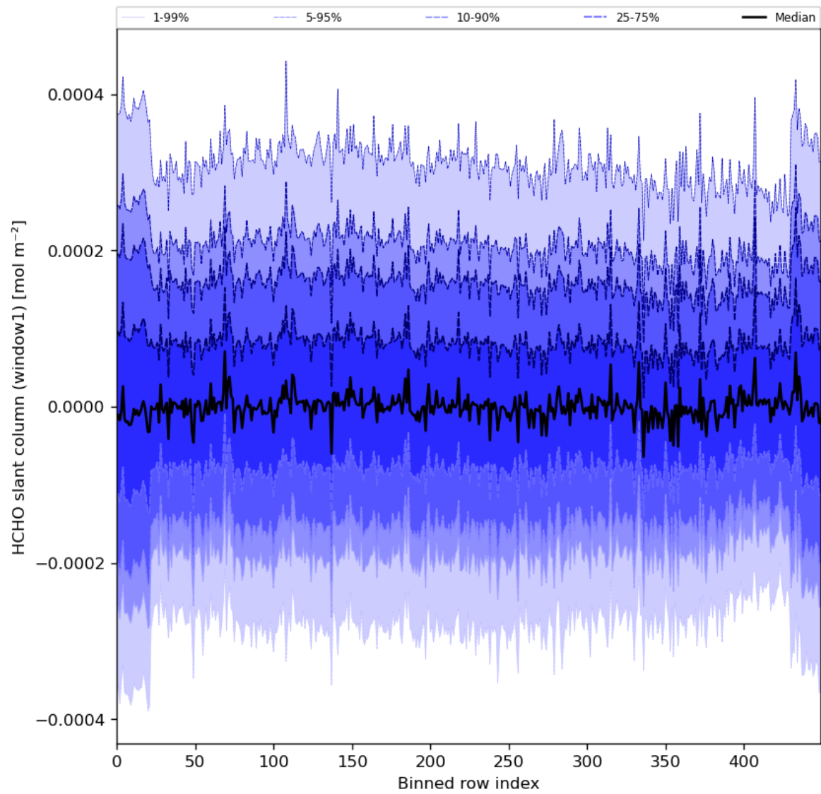
Figure 52: Along track statistics of “HCHO slant column (window1)” for 2024-02-09 to 2024-02-11
