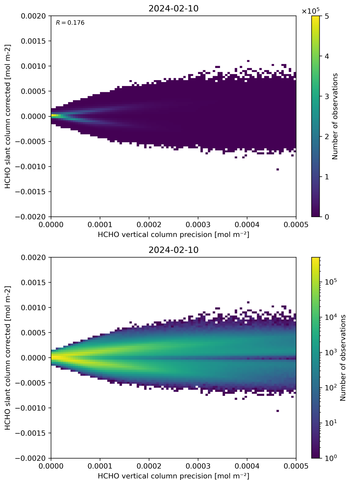
Figure 140: Scatter density plot of “HCHO vertical column precision” against “HCHO slant column corrected” for 2024-02-09 to 2024-02-11.
