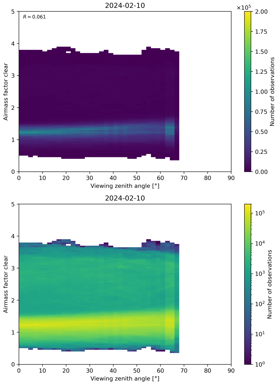
Figure 185: Scatter density plot of “Viewing zenith angle” against “Airmass factor clear” for 2024-02-09 to 2024-02-11.
