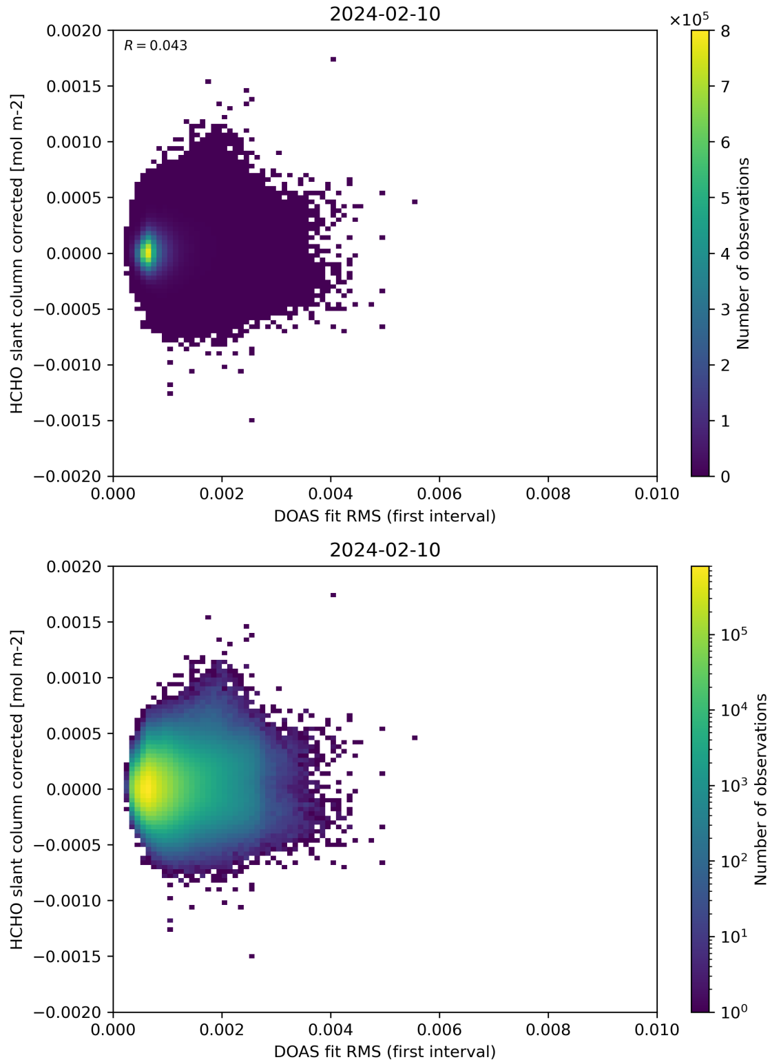
Figure 62: Scatter density plot of “DOAS fit RMS (first interval)” against “HCHO slant column corrected” for 2024-02-09 to 2024-02-11.
