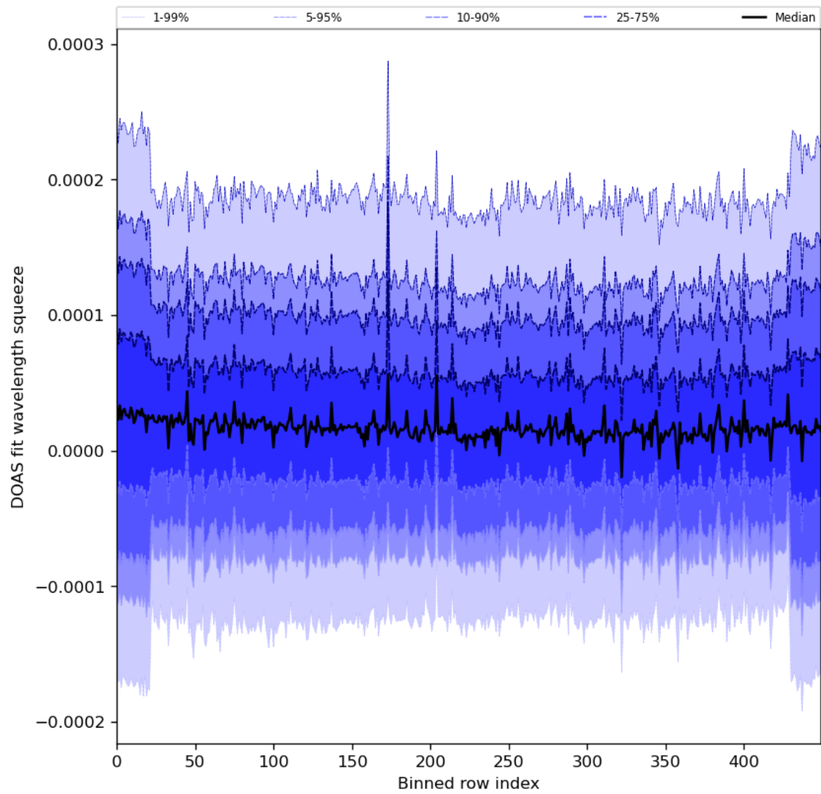
Figure 59: Along track statistics of “DOAS fit wavelength squeeze” for 2024-02-09 to 2024-02-11
