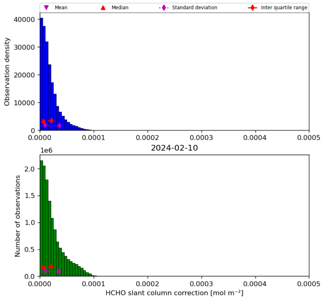
Figure 47: Histogram of “HCHO slant column correction” for 2024-02-09 to 2024-02-11
