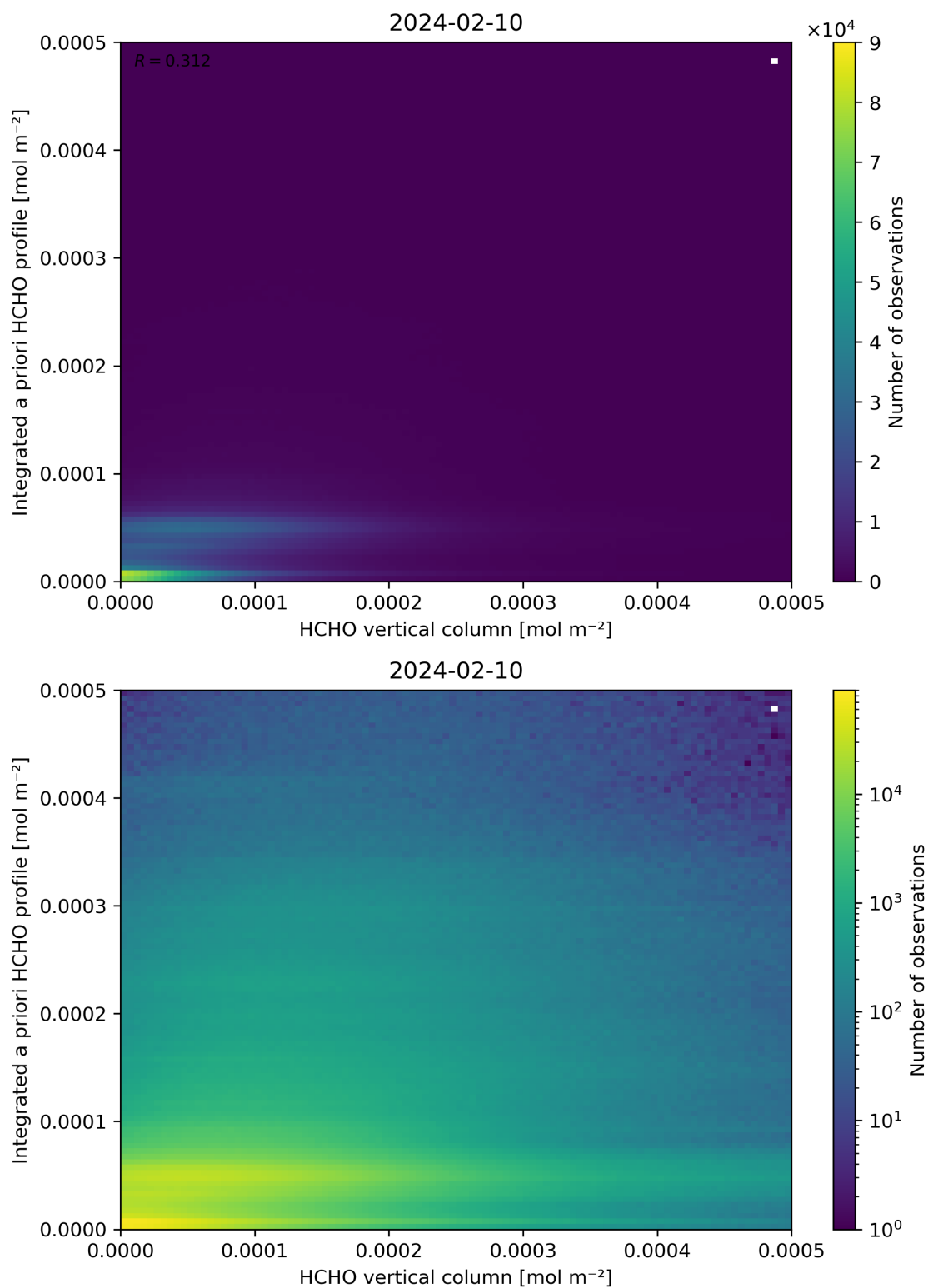
Figure 135: Scatter density plot of “HCHO vertical column” against “Integrated a priori HCHO profile” for 2024-02-09 to 2024-02-11.
