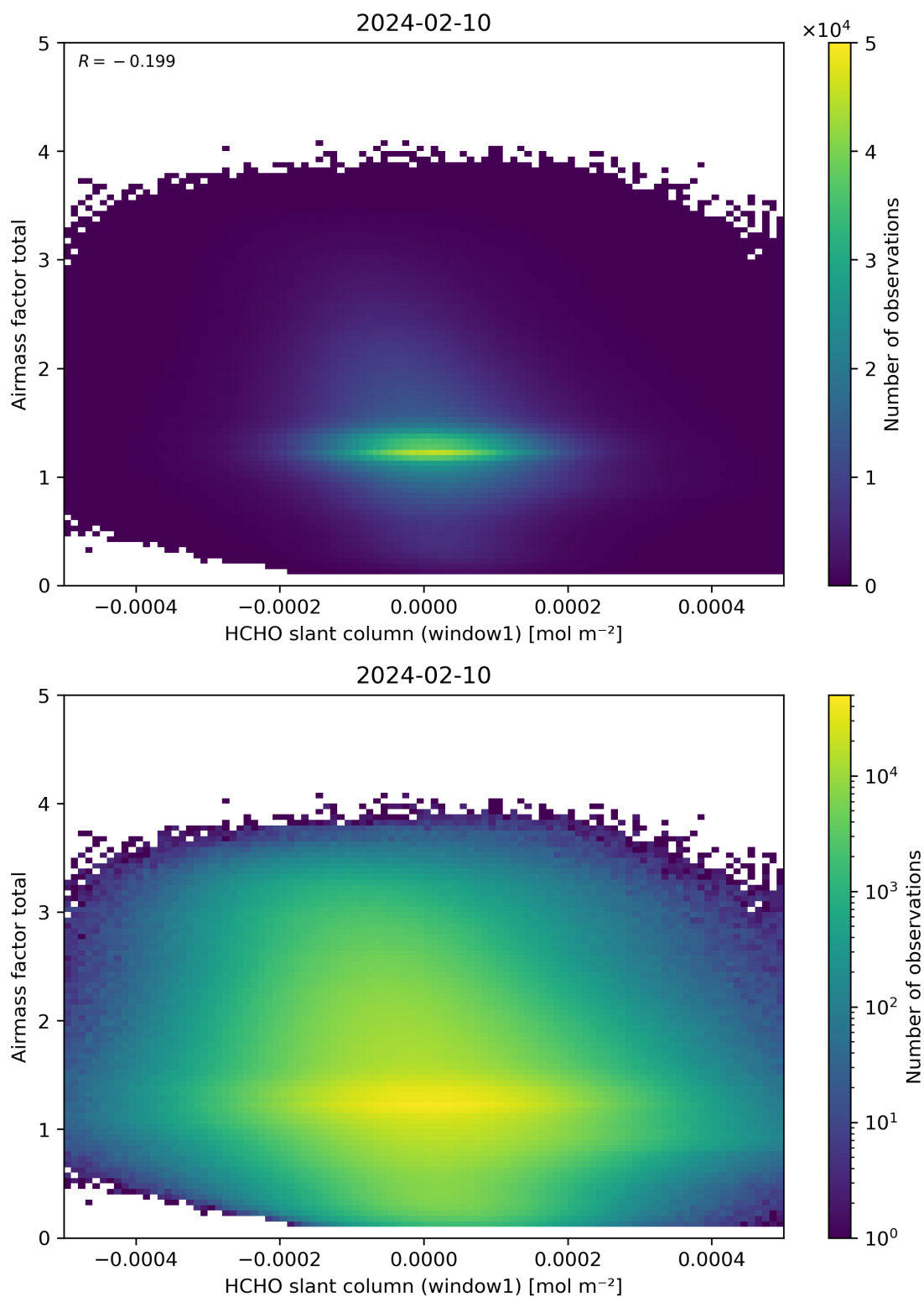
Figure 85: Scatter density plot of “HCHO slant column (window1)” against “Airmass factor total” for 2024-02-09 to 2024-02-11.
