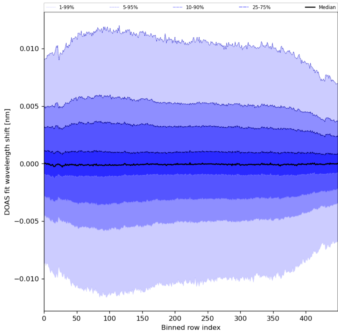
Figure 58: Along track statistics of “DOAS fit wavelength shift” for 2024-02-09 to 2024-02-11
