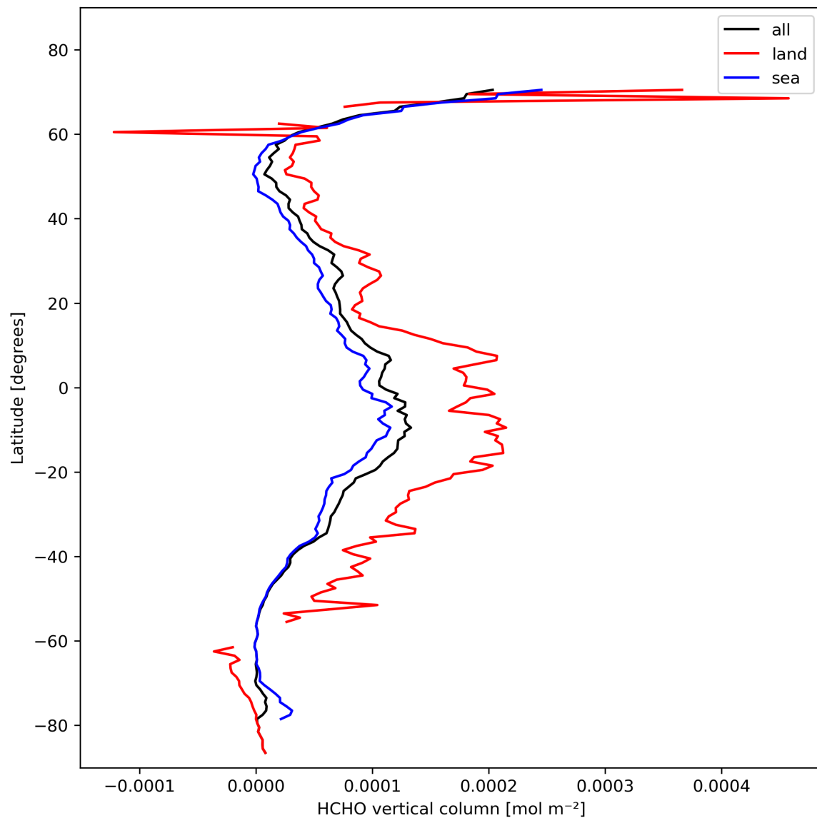
Figure 21: Zonal average of “HCHO vertical column” for 2024-02-09 to 2024-02-11.
