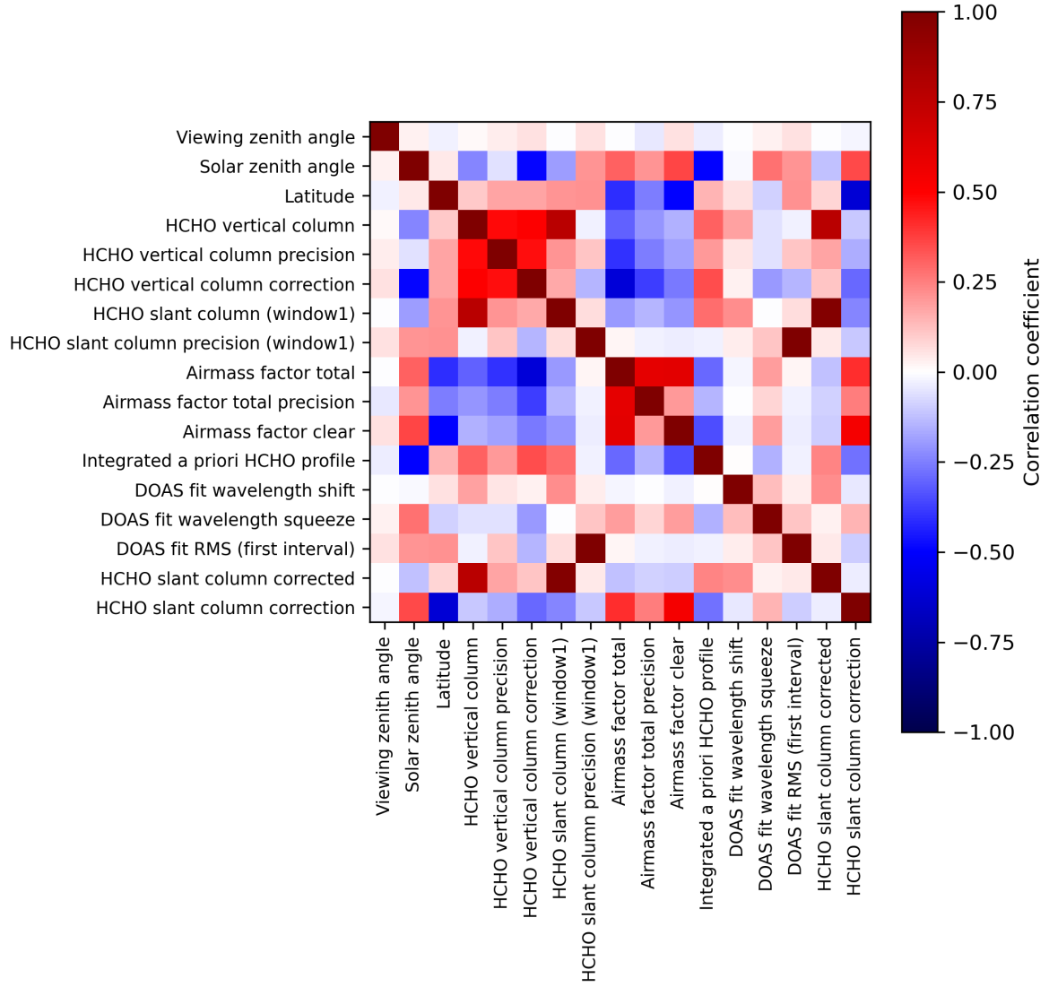
Figure 2: Map of correlation matrix for 2024-02-09 to 2024-02-11.
