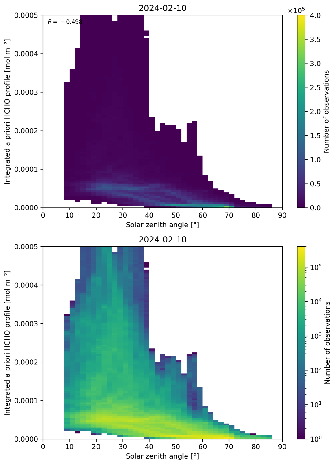
Figure 180: Scatter density plot of “Solar zenith angle” against “Integrated a priori HCHO profile” for 2024-02-09 to 2024-02-11.
