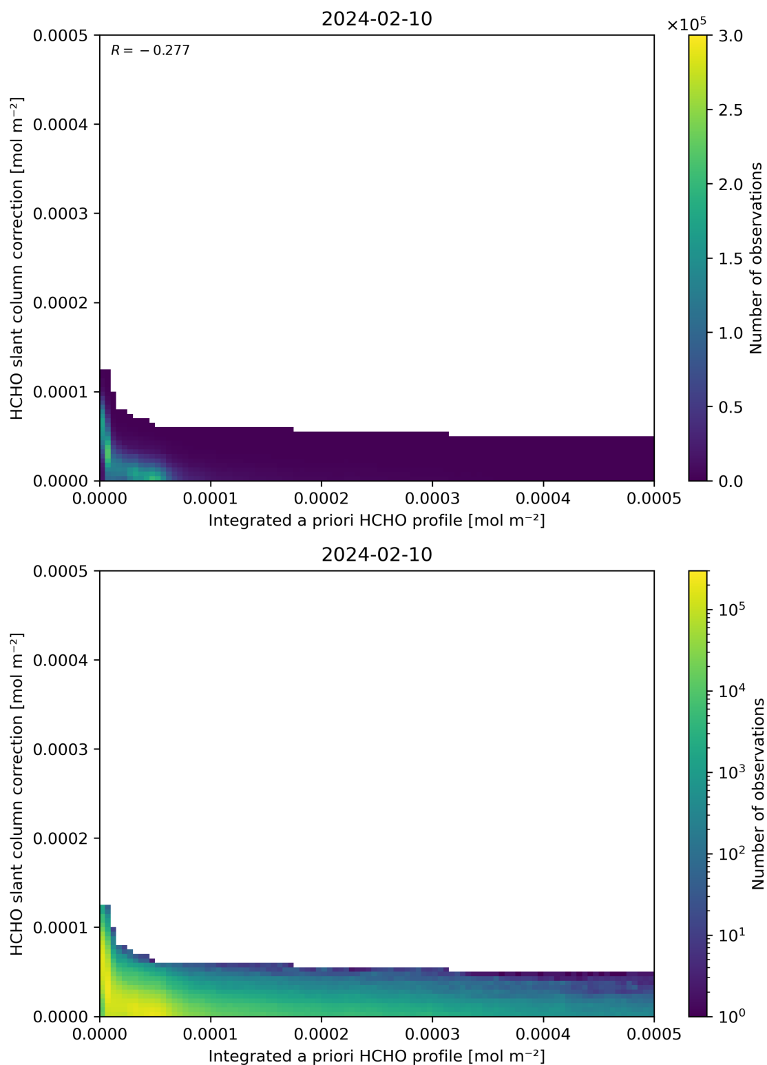
Figure 152: Scatter density plot of “Integrated a priori HCHO profile” against “HCHO slant column correction” for 2024-02-09 to 2024-02-11.
