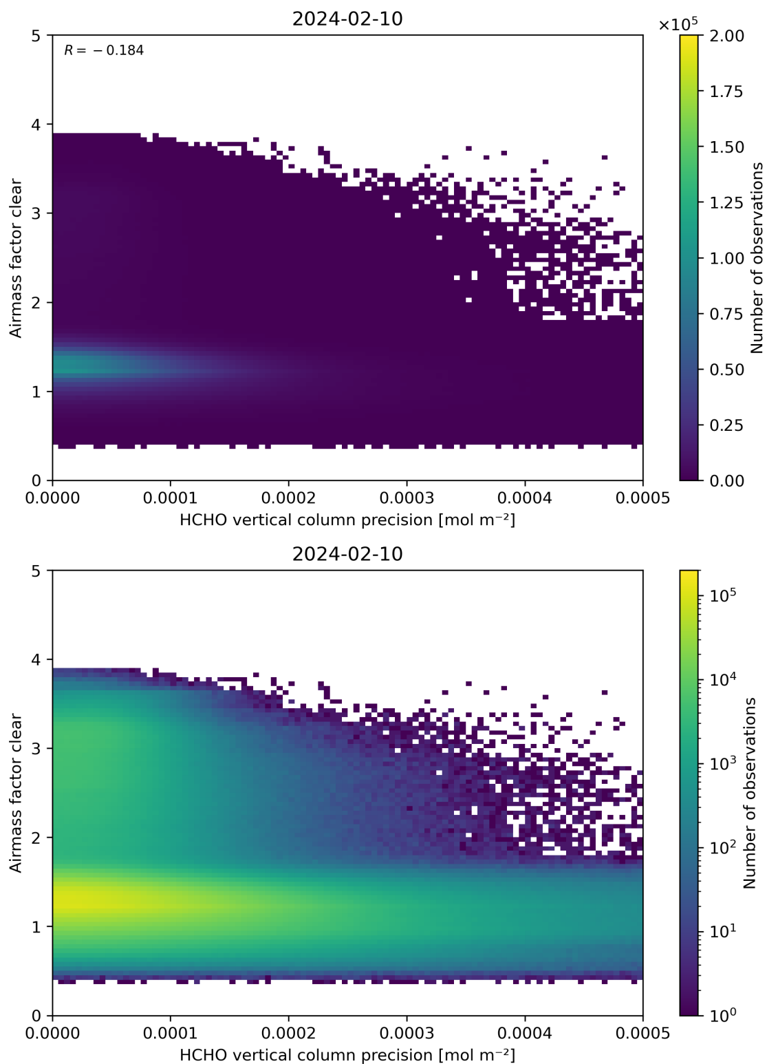
Figure 139: Scatter density plot of “HCHO vertical column precision” against “Airmass factor clear” for 2024-02-09 to 2024-02-11.
