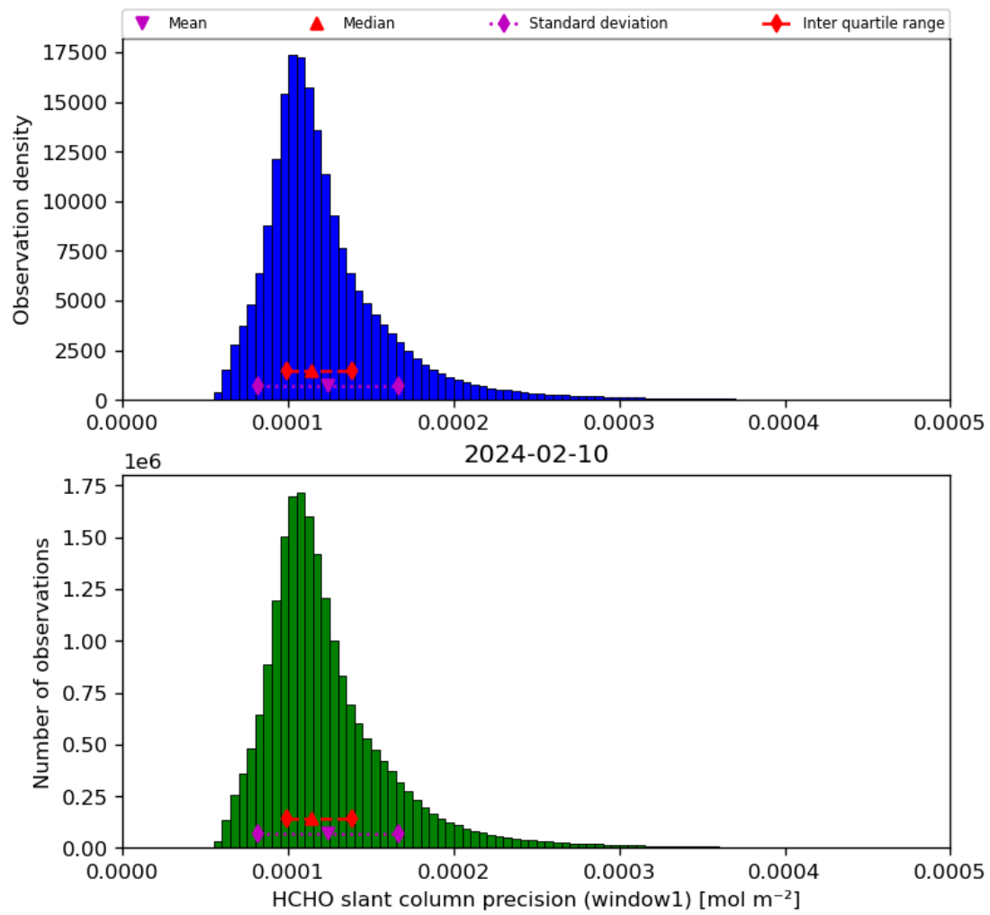
Figure 39: Histogram of “HCHO slant column precision (window1)” for 2024-02-09 to 2024-02-11
