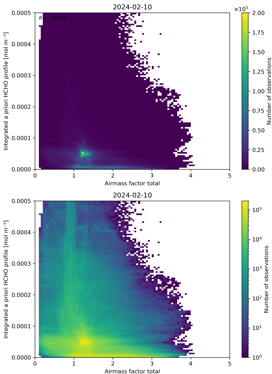
Figure 104: Scatter density plot of “Airmass factor total” against “Integrated a priori HCHO profile” for 2024-02-09 to 2024-02-11.
