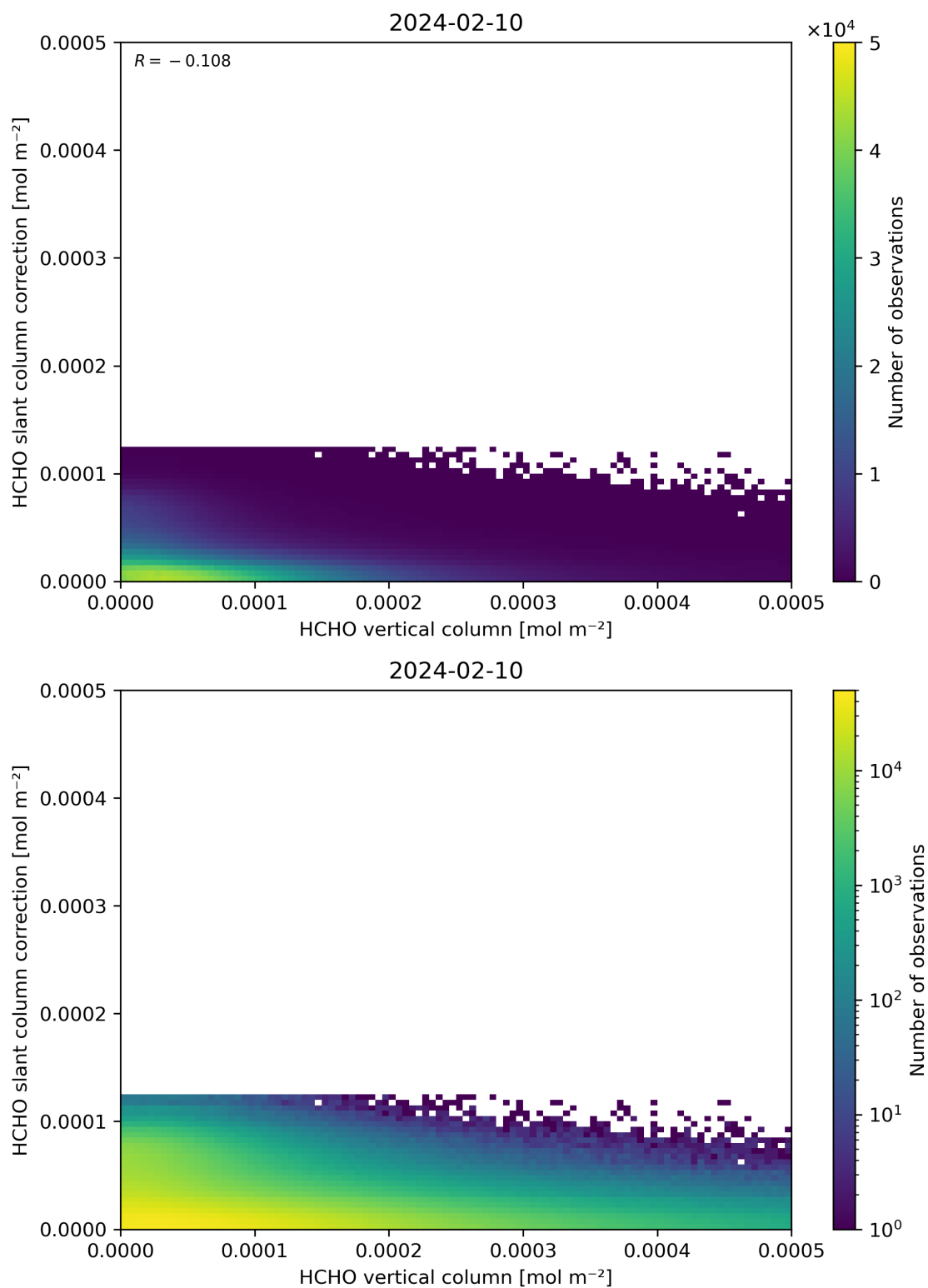
Figure 128: Scatter density plot of “HCHO vertical column” against “HCHO slant column correction” for 2024-02-09 to 2024-02-11.
