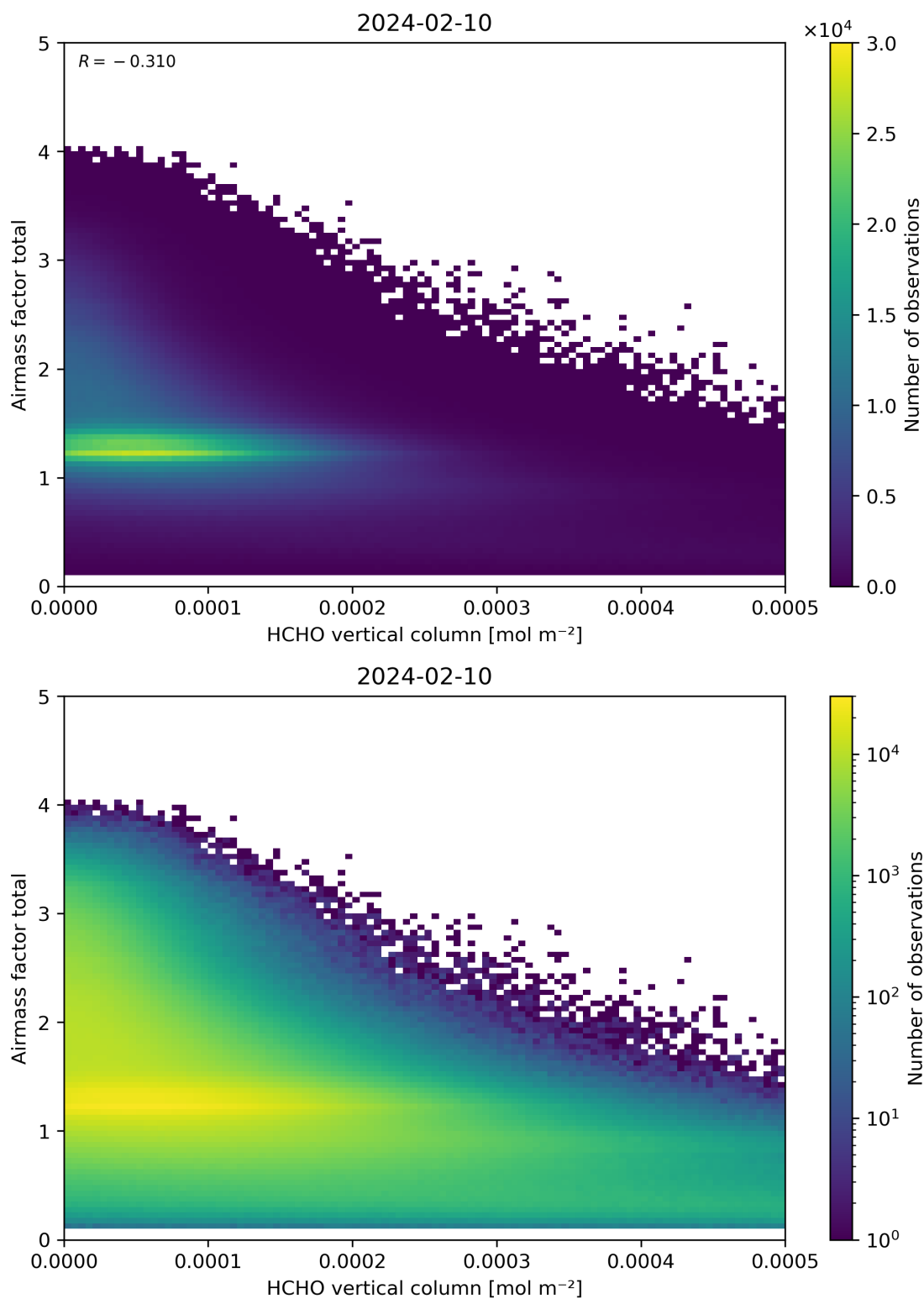
Figure 131: Scatter density plot of “HCHO vertical column” against “Airmass factor total” for 2024-02-09 to 2024-02-11.
