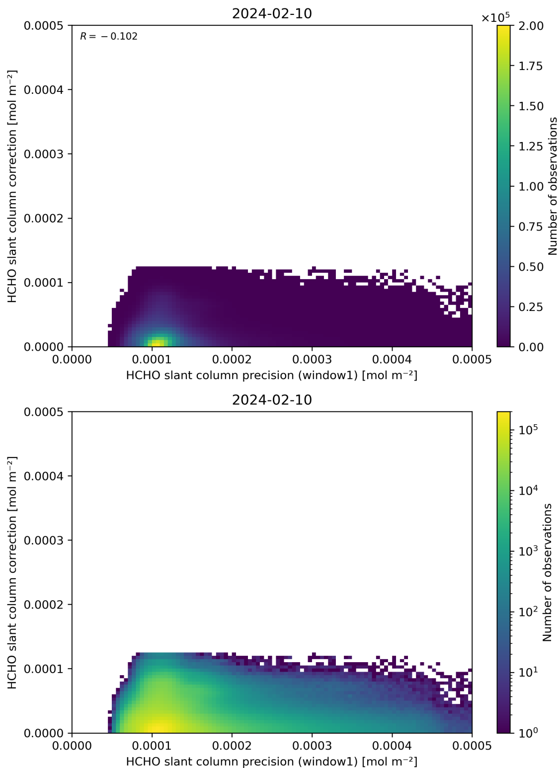
Figure 93: Scatter density plot of “HCHO slant column precision (window1)” against “HCHO slant column correction” for 2024-02-09 to 2024-02-11.
