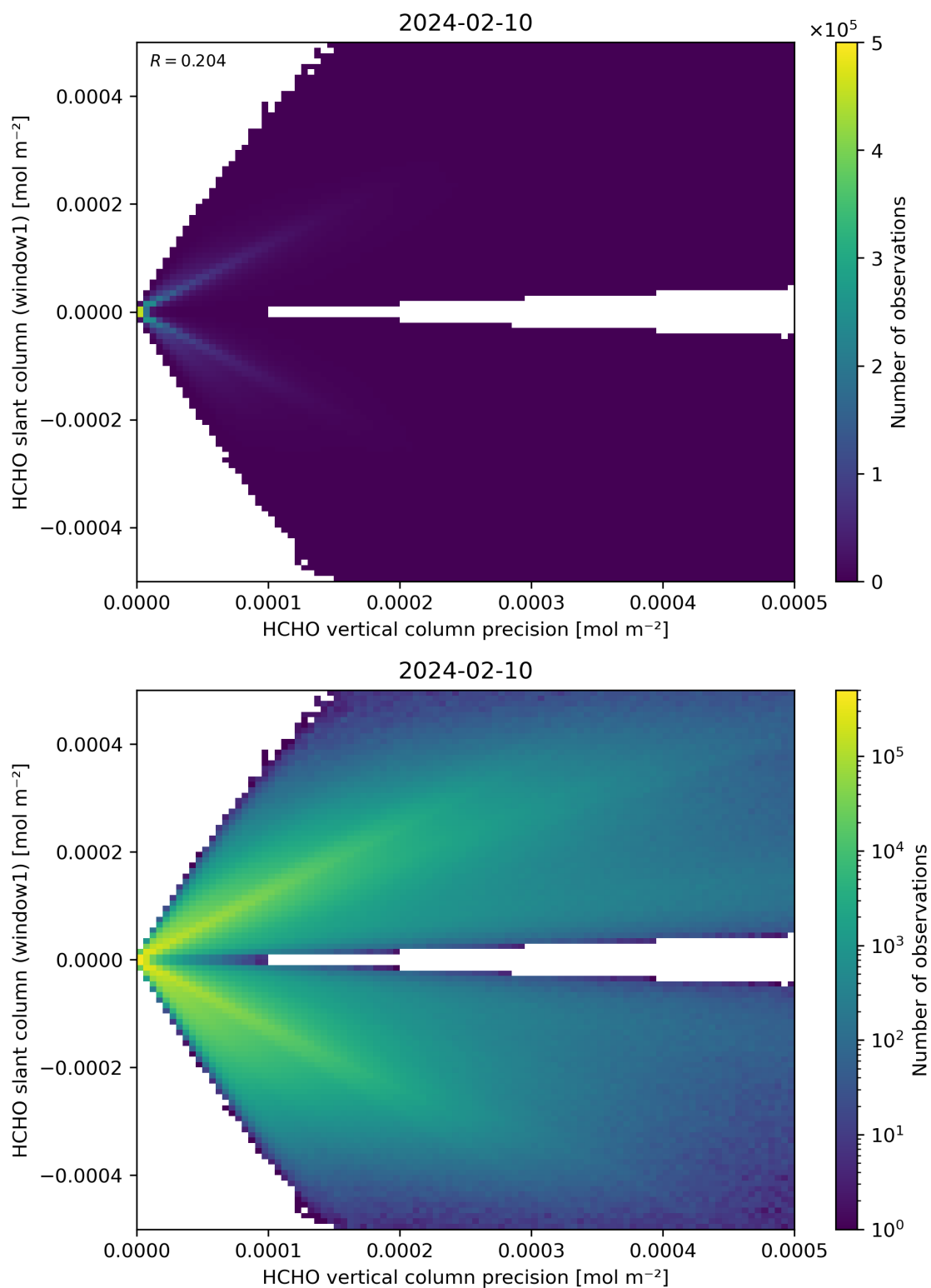
Figure 142: Scatter density plot of “HCHO vertical column precision” against “HCHO slant column (window1)” for 2024-02-09 to 2024-02-11.
