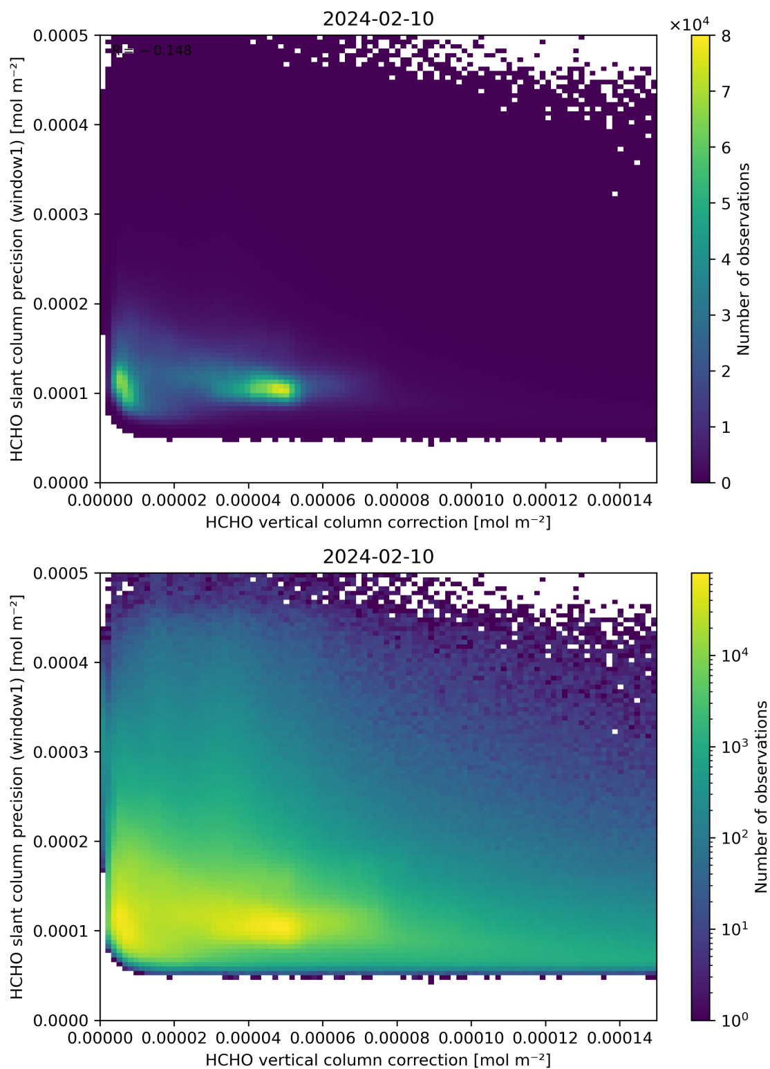
Figure 119: Scatter density plot of “HCHO vertical column correction” against “HCHO slant column precision (window1)” for 2024-02-09 to 2024-02-11.
