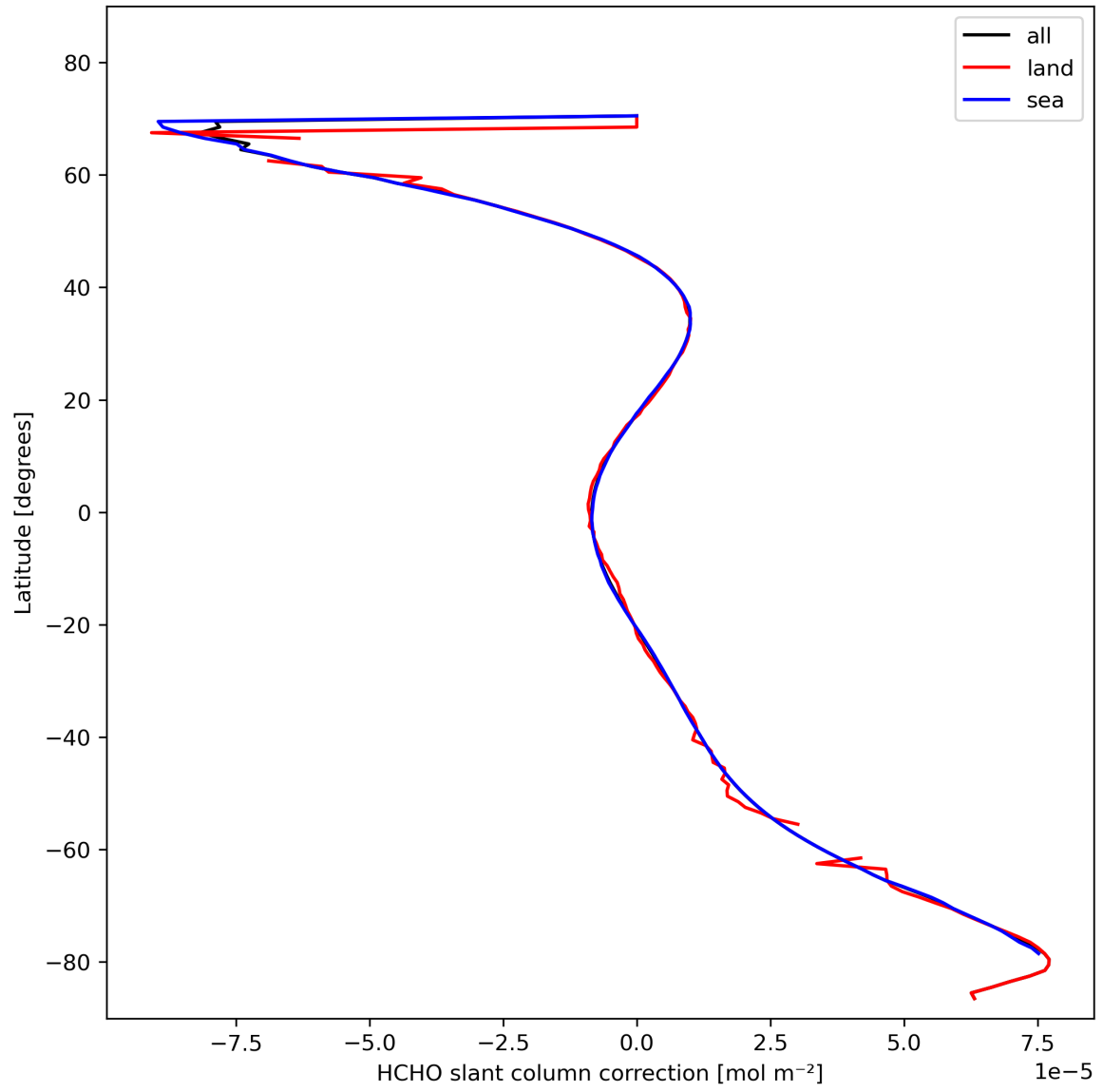
Figure 33: Zonal average of “HCHO slant column correction” for 2024-02-09 to 2024-02-11.
