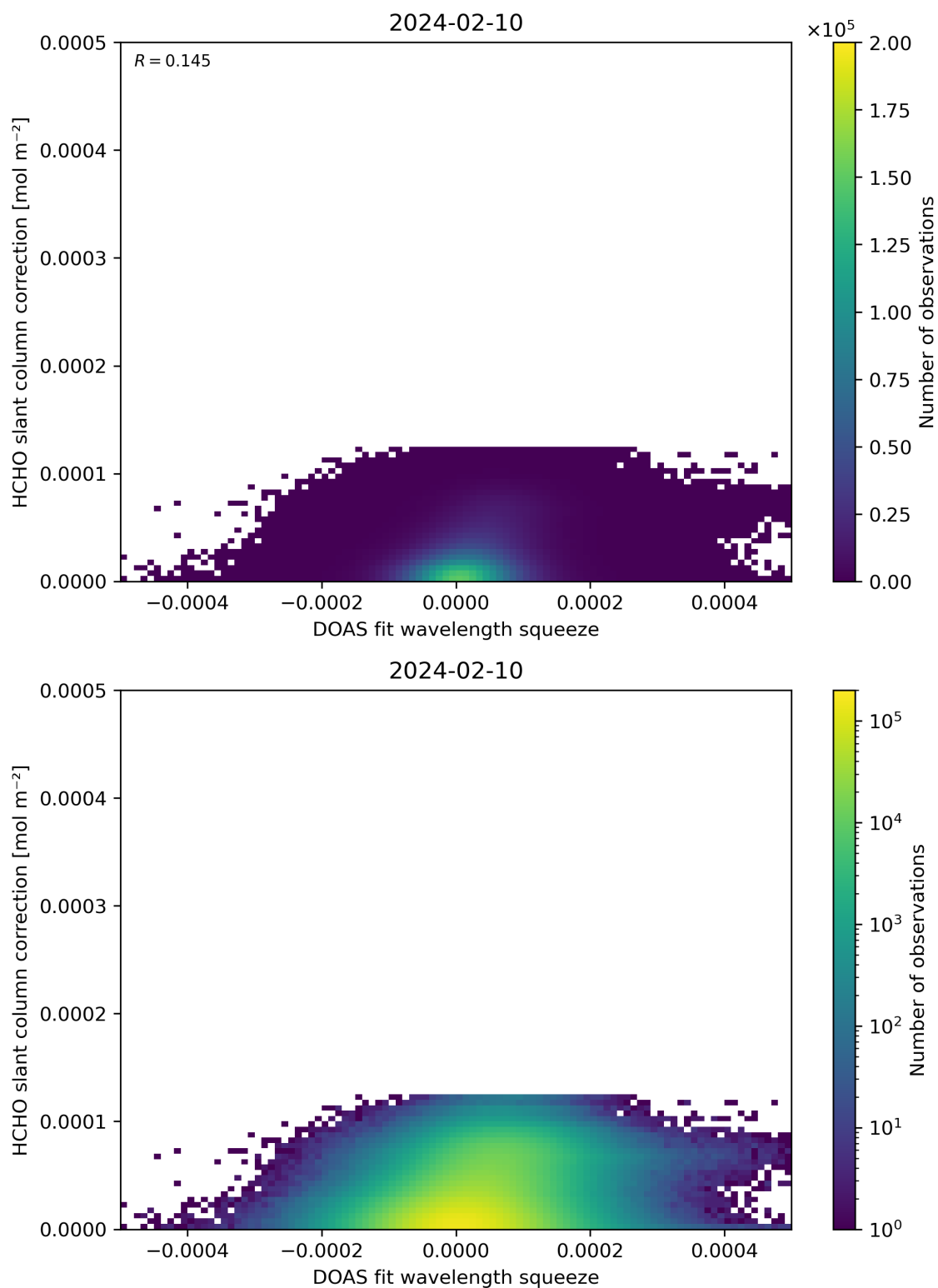
Figure 70: Scatter density plot of “DOAS fit wavelength squeeze” against “HCHO slant column correction” for 2024-02-09 to 2024-02-11.
