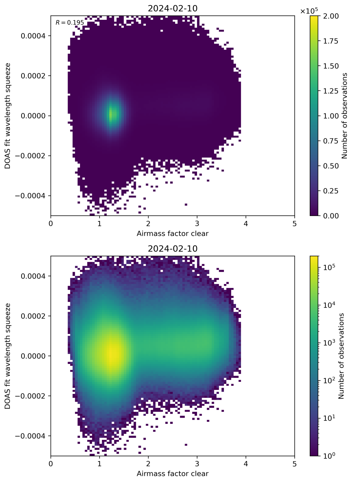
Figure 73: Scatter density plot of “Airmass factor clear” against “DOAS fit wavelength squeeze” for 2024-02-09 to 2024-02-11.
