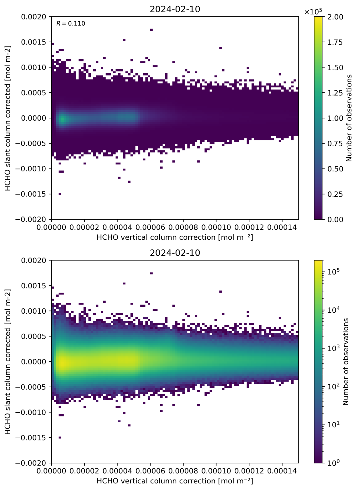
Figure 116: Scatter density plot of “HCHO vertical column correction” against “HCHO slant column corrected” for 2024-02-09 to 2024-02-11.
