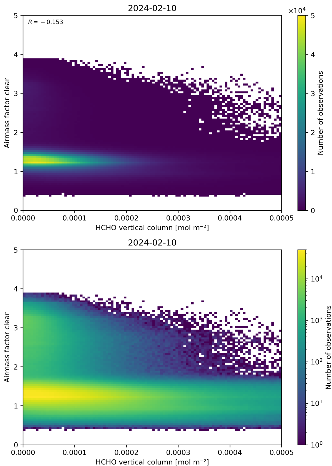
Figure 126: Scatter density plot of “HCHO vertical column” against “Airmass factor clear” for 2024-02-09 to 2024-02-11.
