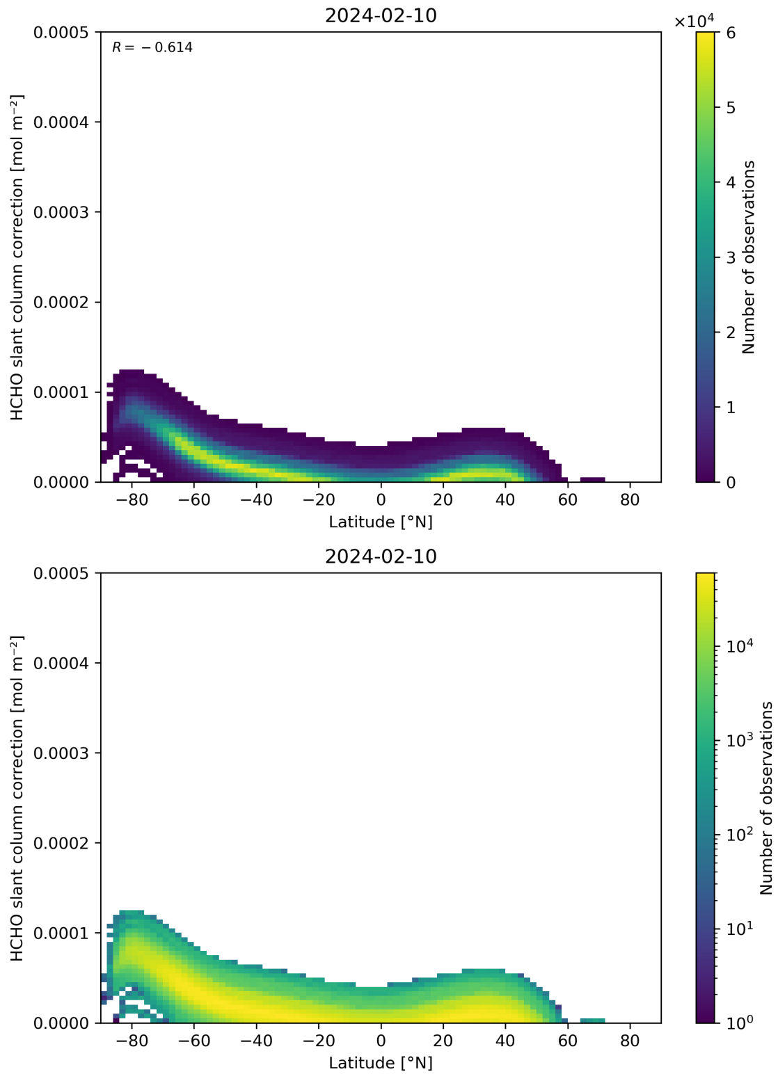
Figure 158: Scatter density plot of “Latitude” against “HCHO slant column correction” for 2024-02-09 to 2024-02-11.
