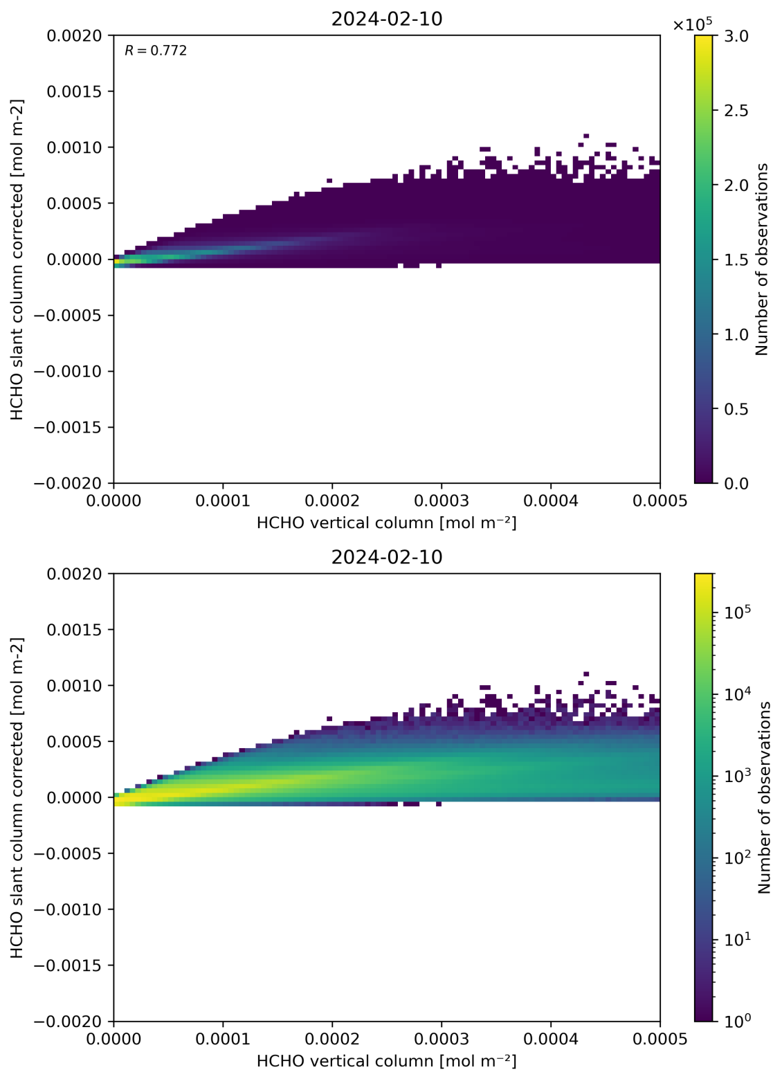
Figure 127: Scatter density plot of “HCHO vertical column” against “HCHO slant column corrected” for 2024-02-09 to 2024-02-11.
