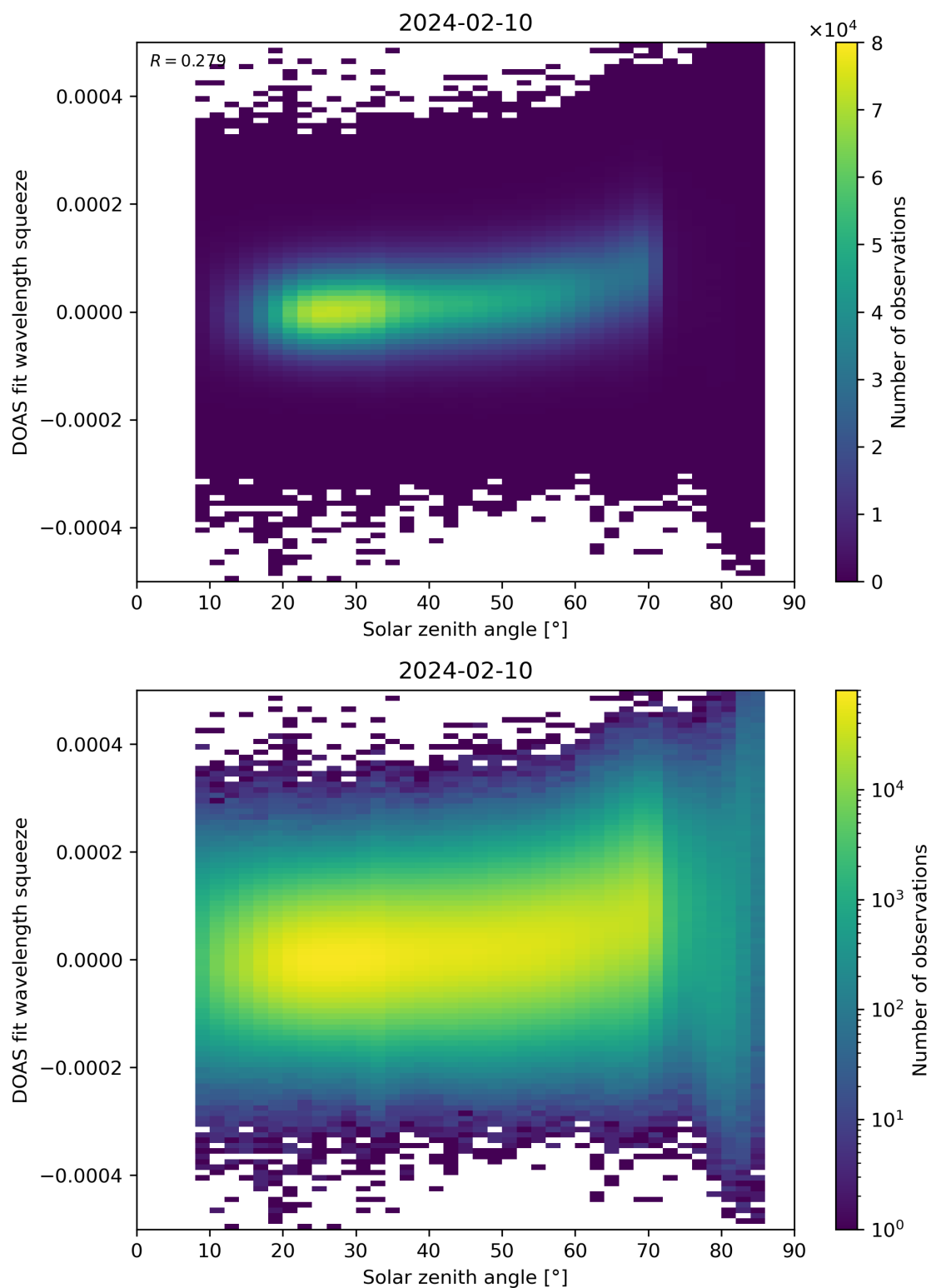
Figure 169: Scatter density plot of “Solar zenith angle” against “DOAS fit wavelength squeeze” for 2024-02-09 to 2024-02-11.
