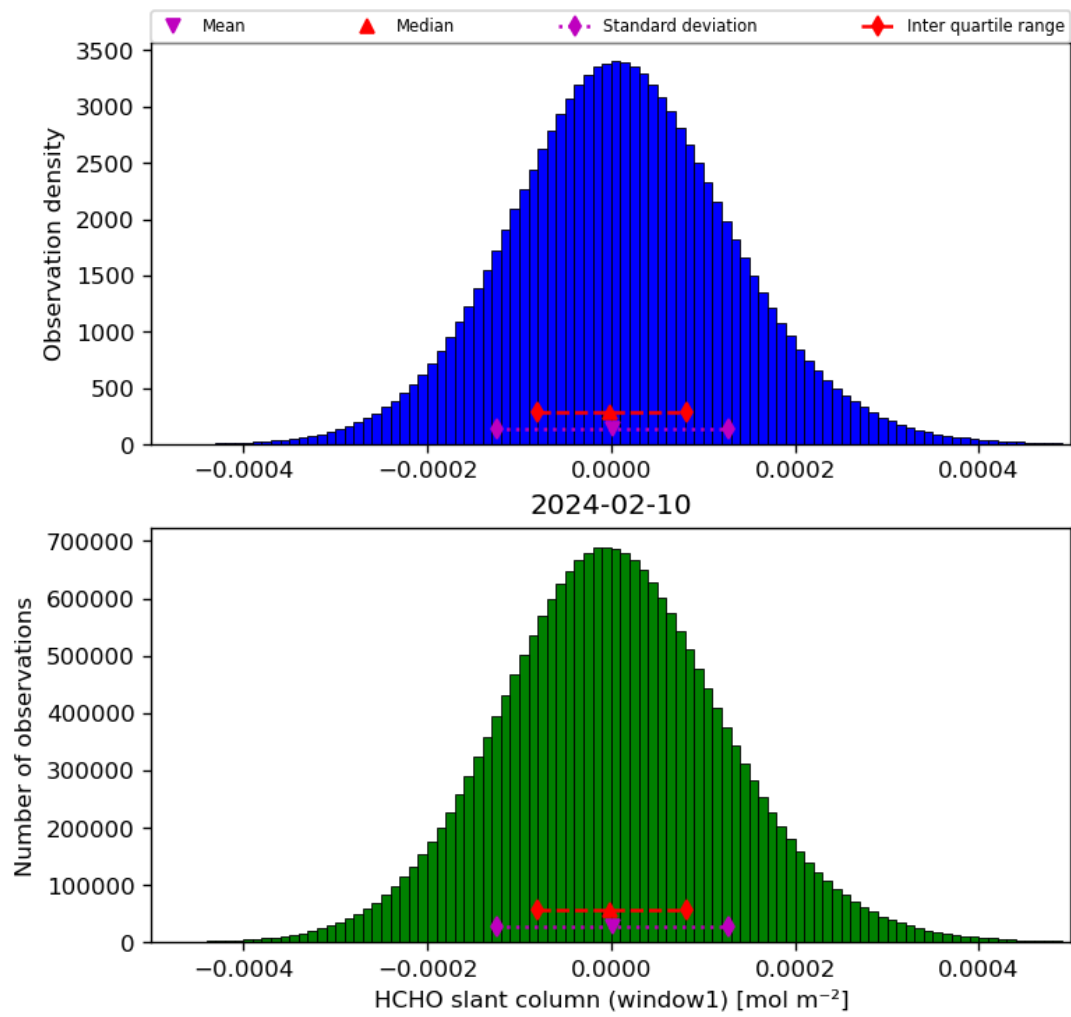
Figure 38: Histogram of “HCHO slant column (window1)” for 2024-02-09 to 2024-02-11
