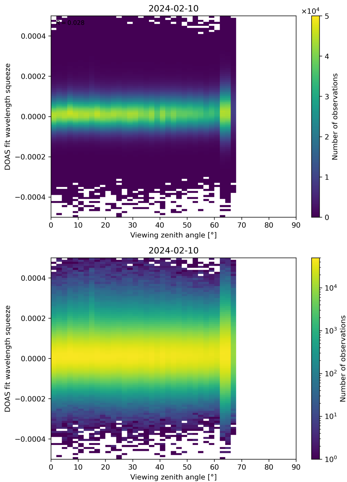
Figure 184: Scatter density plot of “Viewing zenith angle” against “DOAS fit wavelength squeeze” for 2024-02-09 to 2024-02-11.
