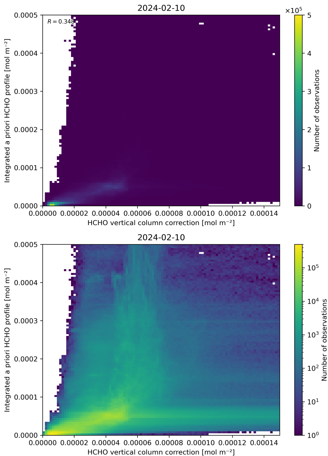
Figure 122: Scatter density plot of “HCHO vertical column correction” against “Integrated a priori HCHO profile” for 2024-02-09 to 2024-02-11.
