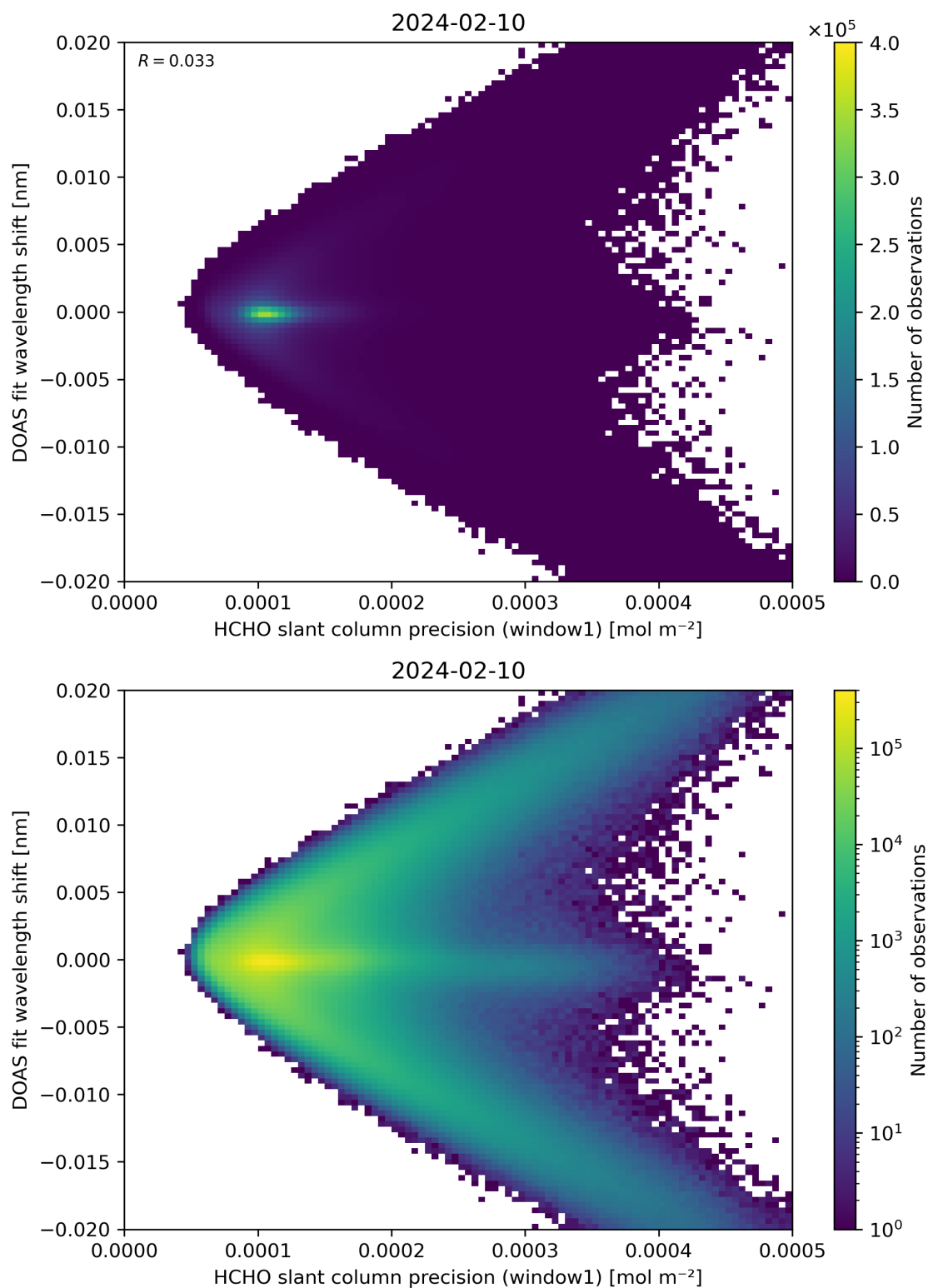
Figure 89: Scatter density plot of “HCHO slant column precision (window1)” against “DOAS fit wavelength shift” for 2024-02-09 to 2024-02-11.
