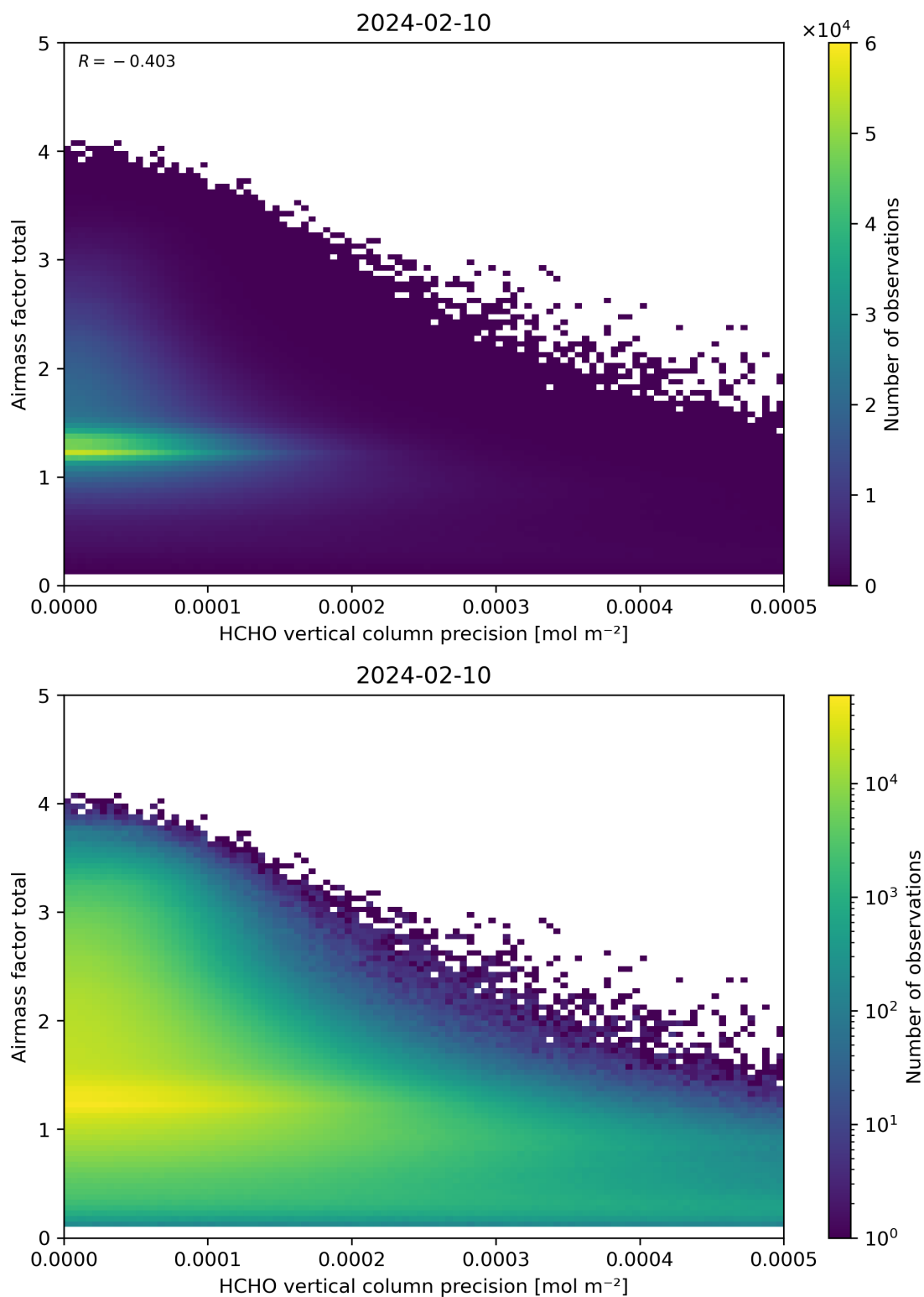
Figure 144: Scatter density plot of “HCHO vertical column precision” against “Airmass factor total” for 2024-02-09 to 2024-02-11.
