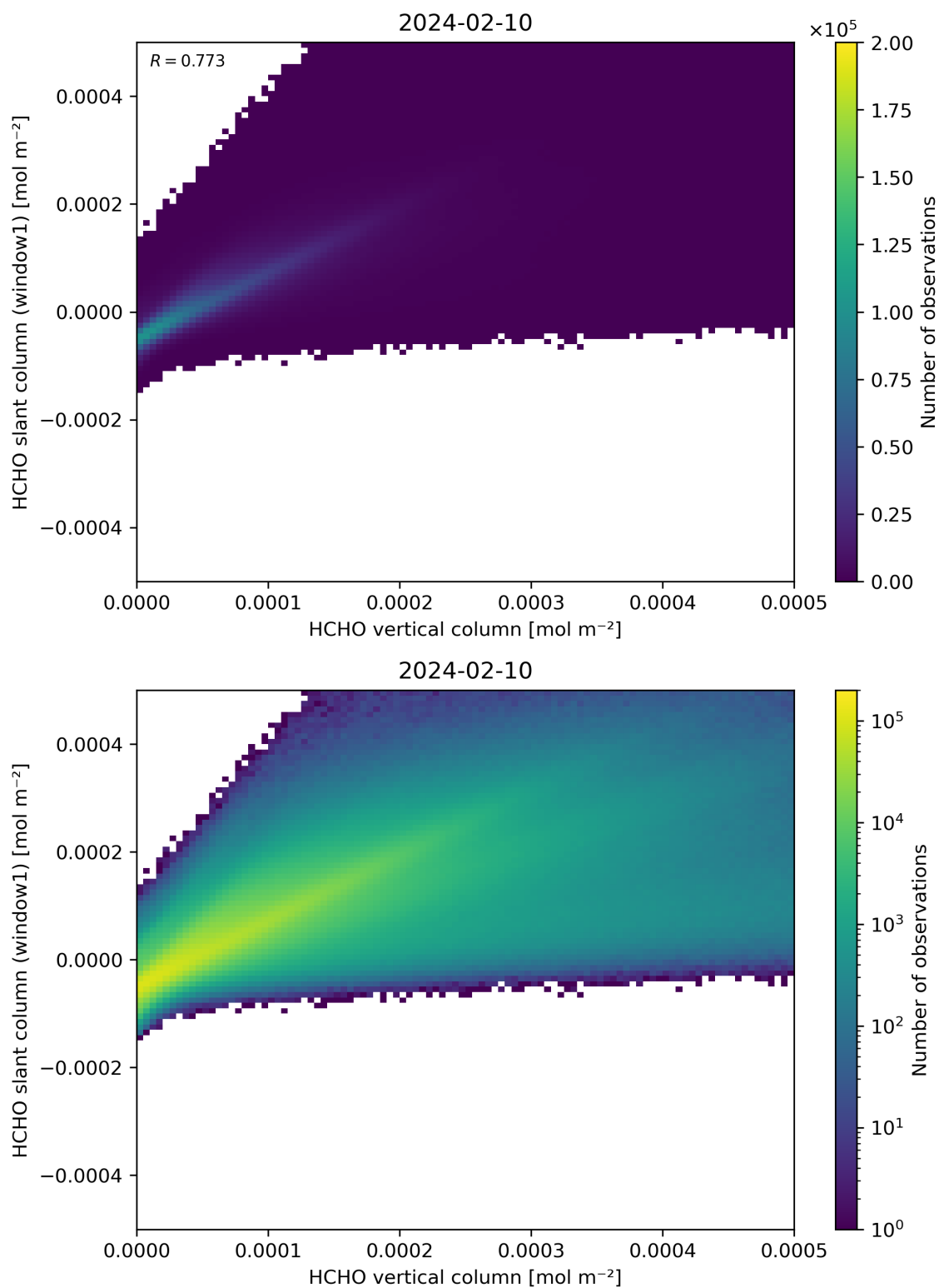
Figure 129: Scatter density plot of “HCHO vertical column” against “HCHO slant column (window1)” for 2024-02-09 to 2024-02-11.
