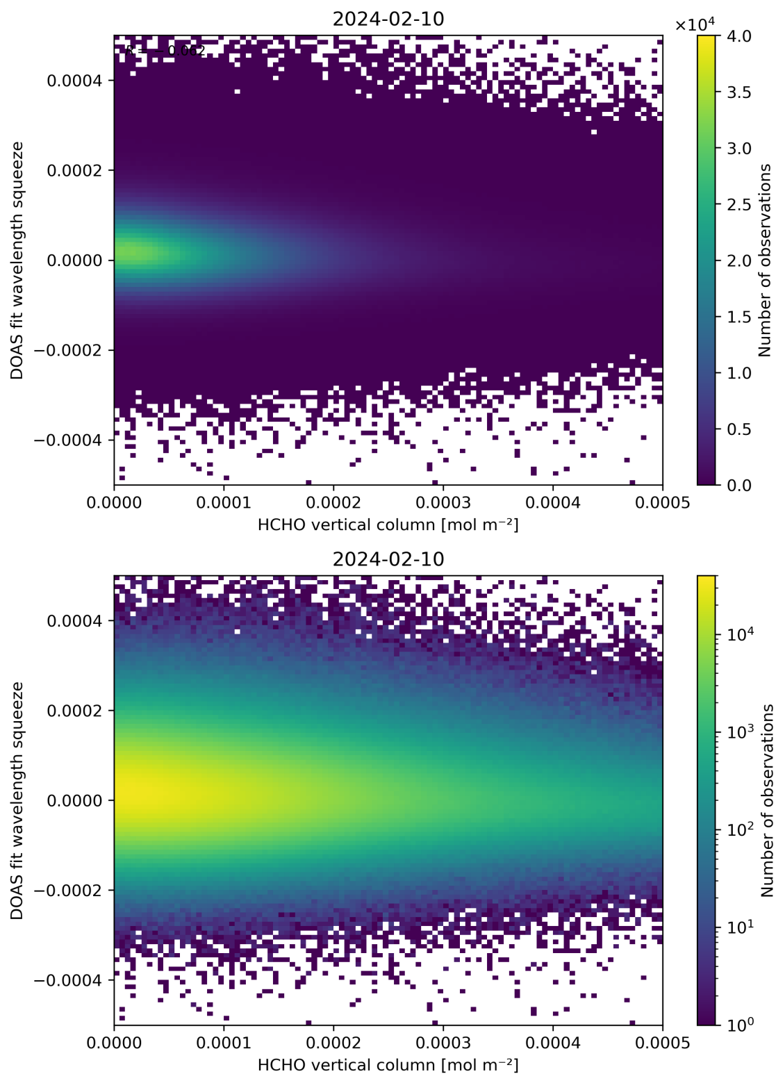
Figure 125: Scatter density plot of “HCHO vertical column” against “DOAS fit wavelength squeeze” for 2024-02-09 to 2024-02-11.
