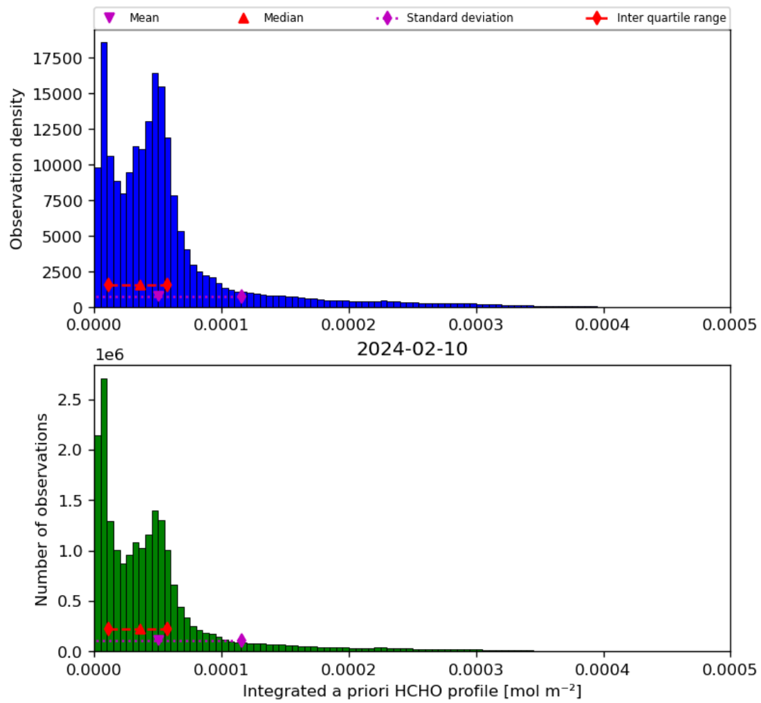
Figure 43: Histogram of “Integrated a priori HCHO profile” for 2024-02-09 to 2024-02-11
