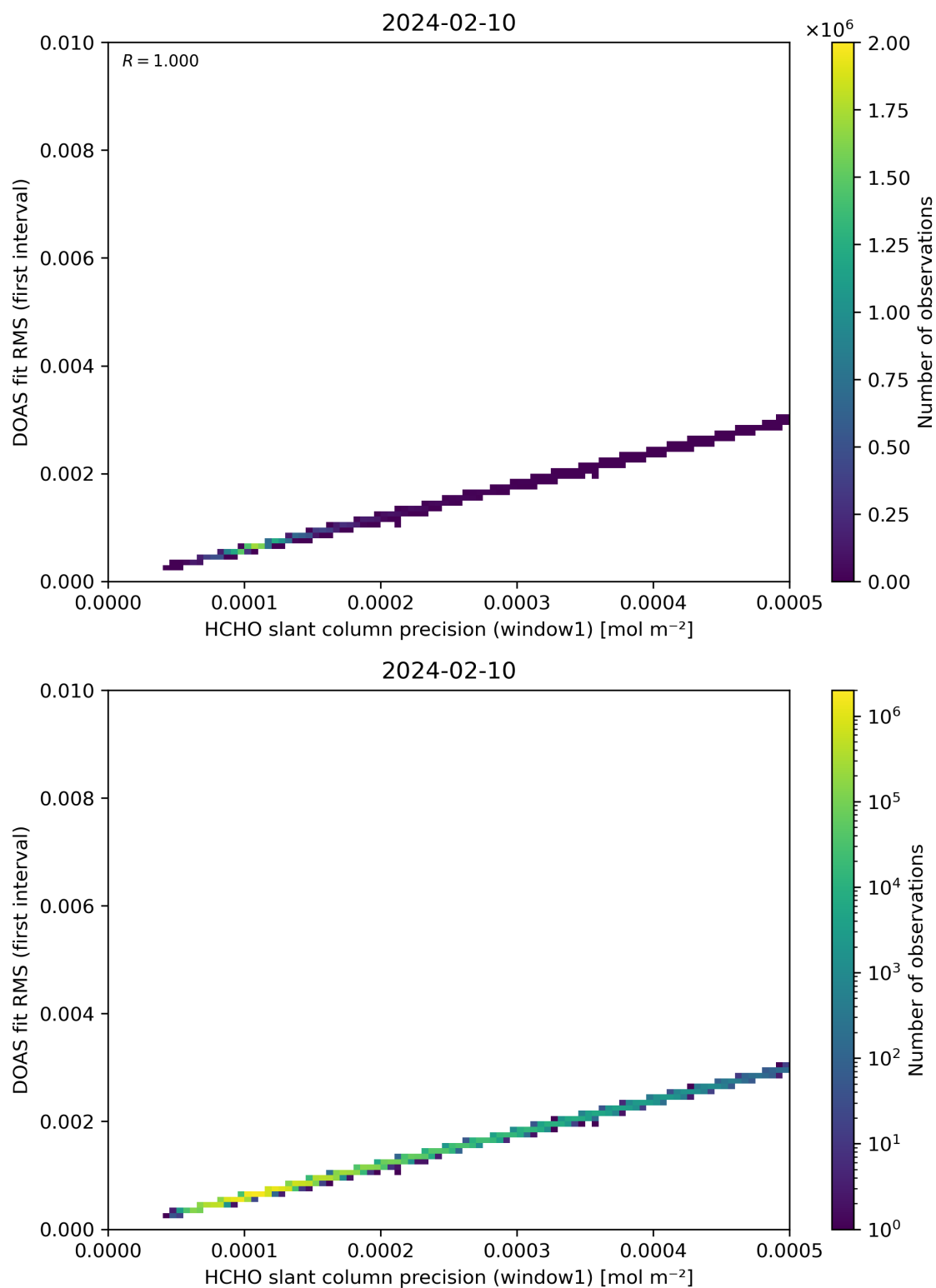
Figure 88: Scatter density plot of “HCHO slant column precision (window1)” against “DOAS fit RMS (first interval)” for 2024-02-09 to 2024-02-11.
