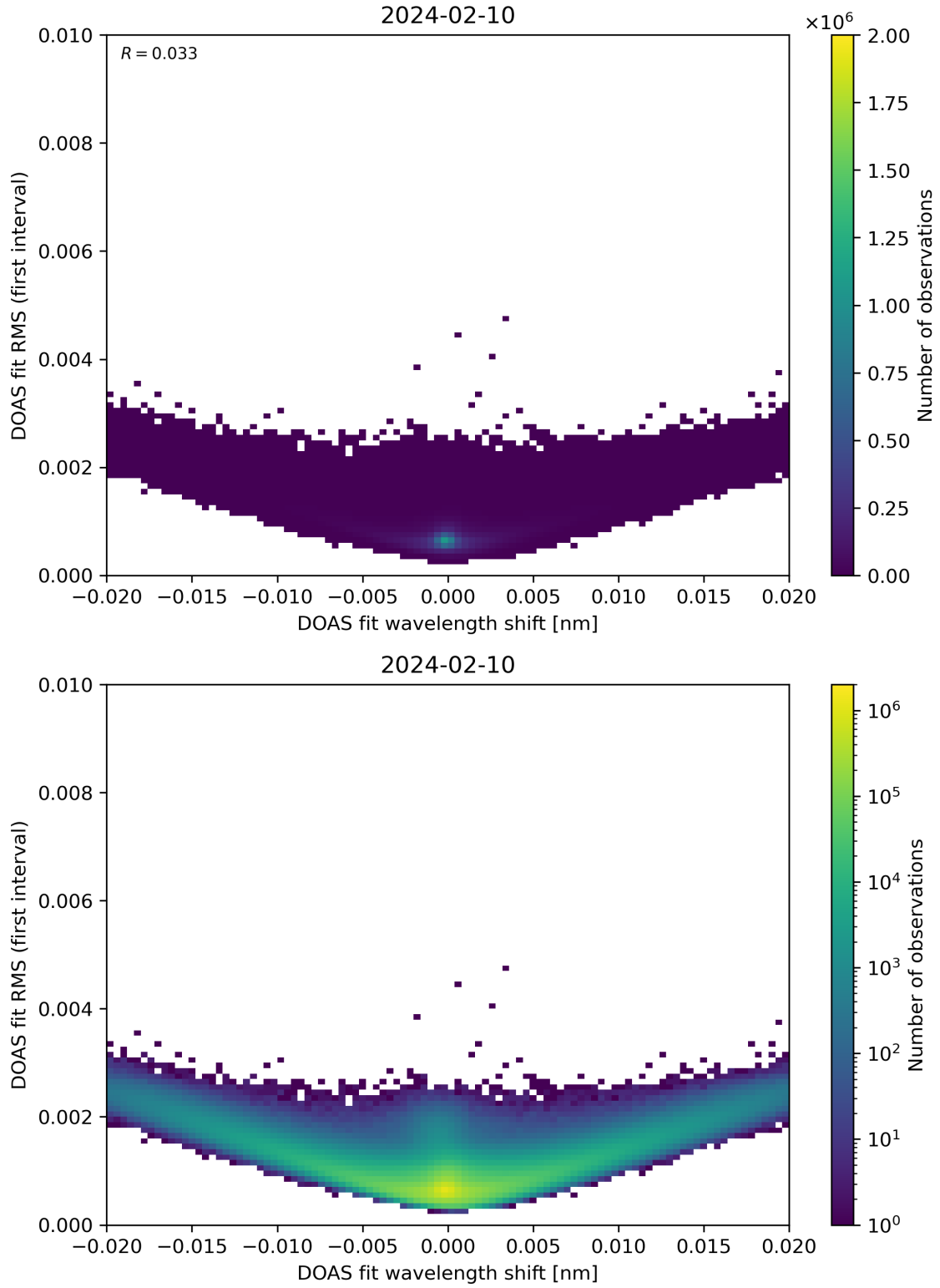
Figure 64: Scatter density plot of “DOAS fit wavelength shift” against “DOAS fit RMS (first interval)” for 2024-02-09 to 2024-02-11.
