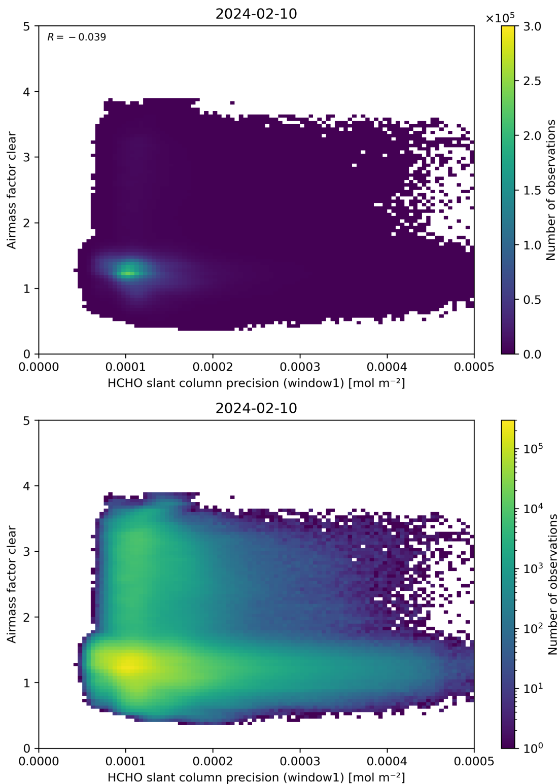
Figure 91: Scatter density plot of “HCHO slant column precision (window1)” against “Airmass factor clear” for 2024-02-09 to 2024-02-11.
