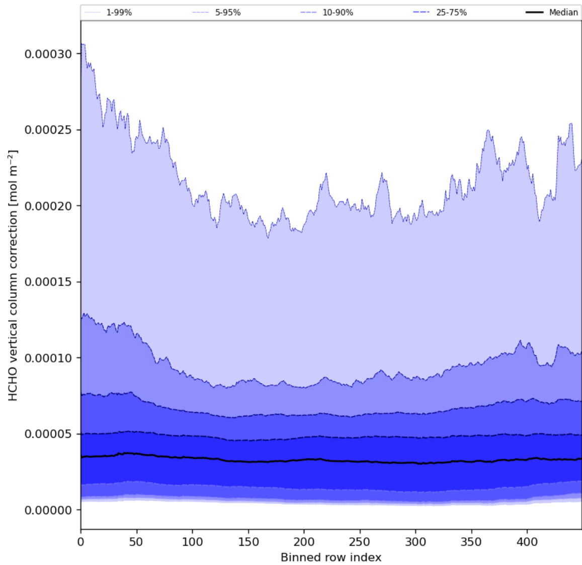
Figure 51: Along track statistics of “HCHO vertical column correction” for 2024-02-09 to 2024-02-11
