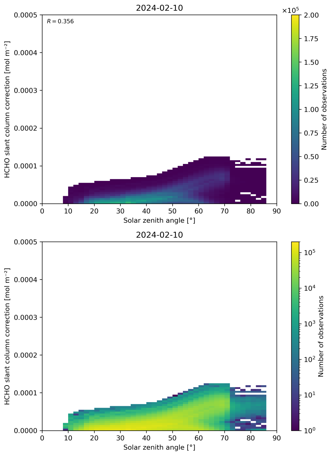
Figure 172: Scatter density plot of “Solar zenith angle” against “HCHO slant column correction” for 2024-02-09 to 2024-02-11.
