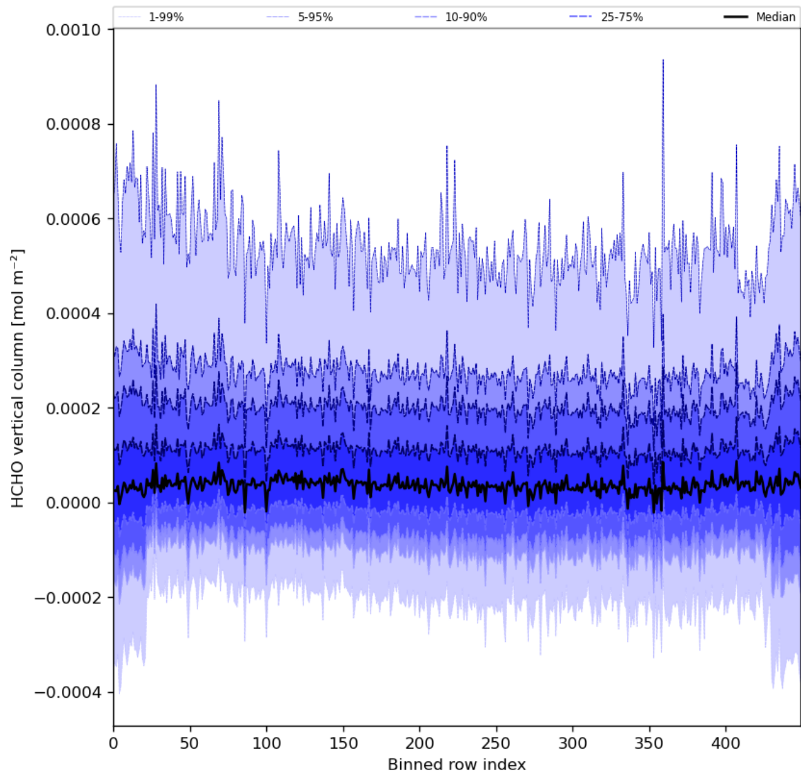
Figure 49: Along track statistics of “HCHO vertical column” for 2024-02-09 to 2024-02-11
