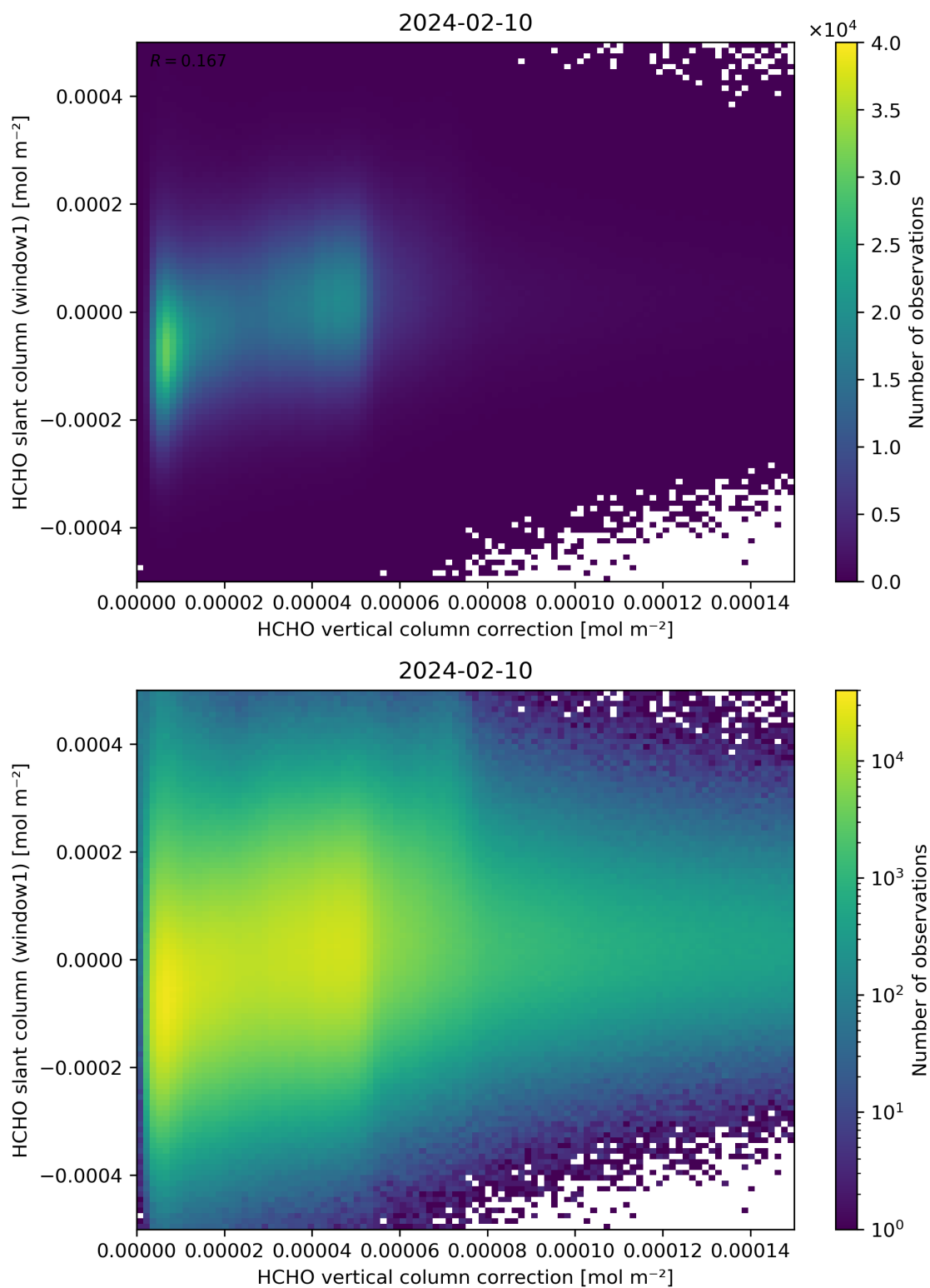
Figure 118: Scatter density plot of “HCHO vertical column correction” against “HCHO slant column (window1)” for 2024-02-09 to 2024-02-11.
