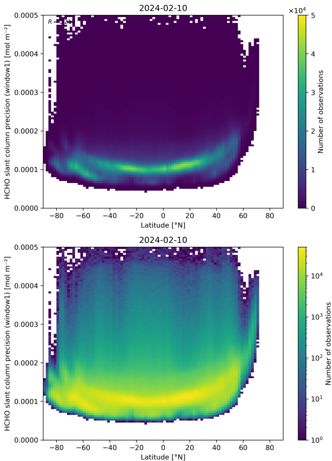
Figure 160: Scatter density plot of “Latitude” against “HCHO slant column precision (window1)” for 2024-02-09 to 2024-02-11.
