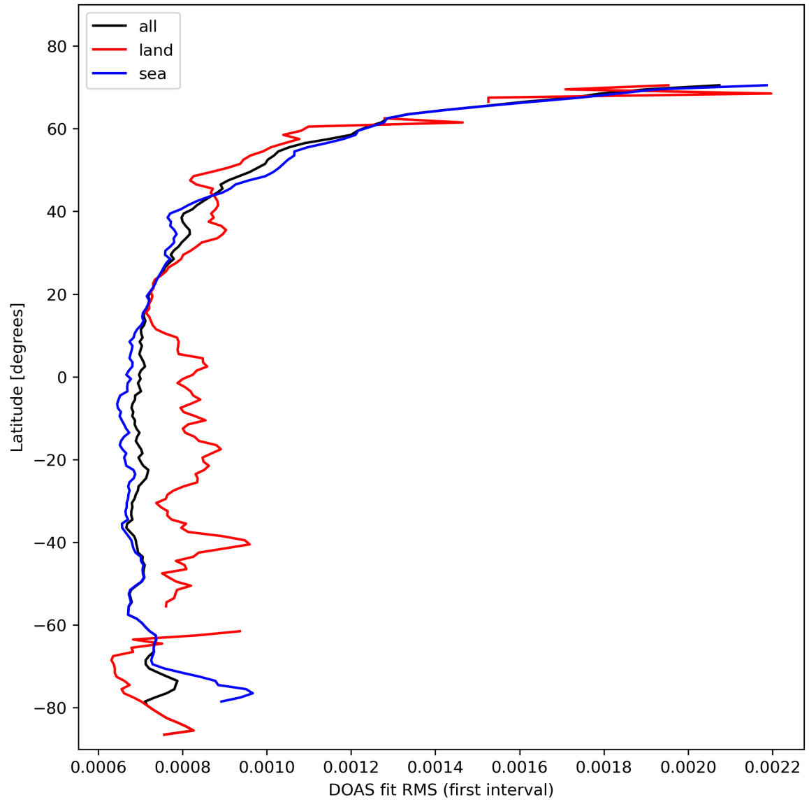
Figure 32: Zonal average of “DOAS fit RMS (first interval)” for 2024-02-09 to 2024-02-11.
