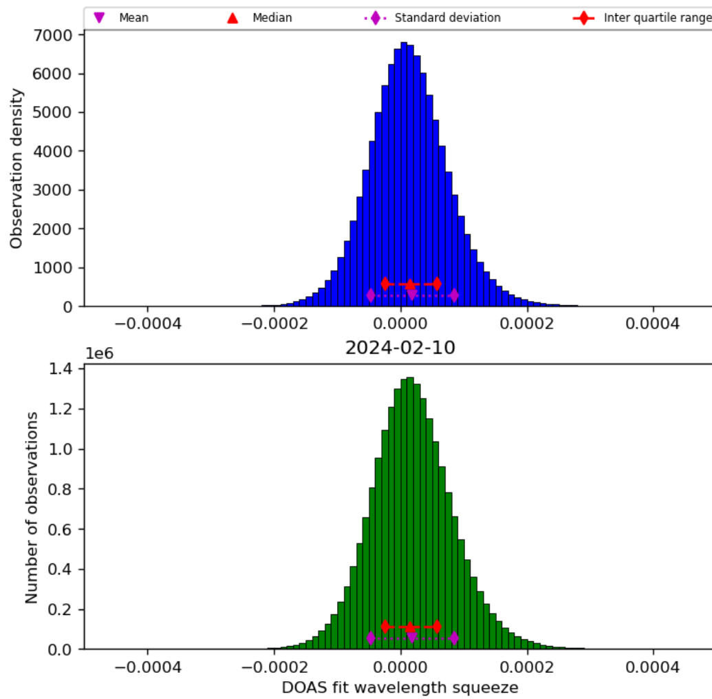
Figure 45: Histogram of “DOAS fit wavelength squeeze” for 2024-02-09 to 2024-02-11
