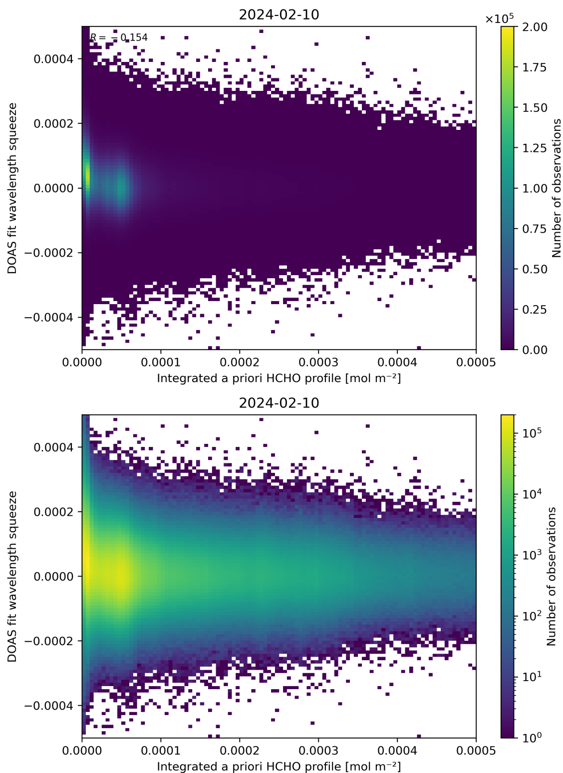
Figure 150: Scatter density plot of “Integrated a priori HCHO profile” against “DOAS fit wavelength squeeze” for 2024-02-09 to 2024-02-11.
