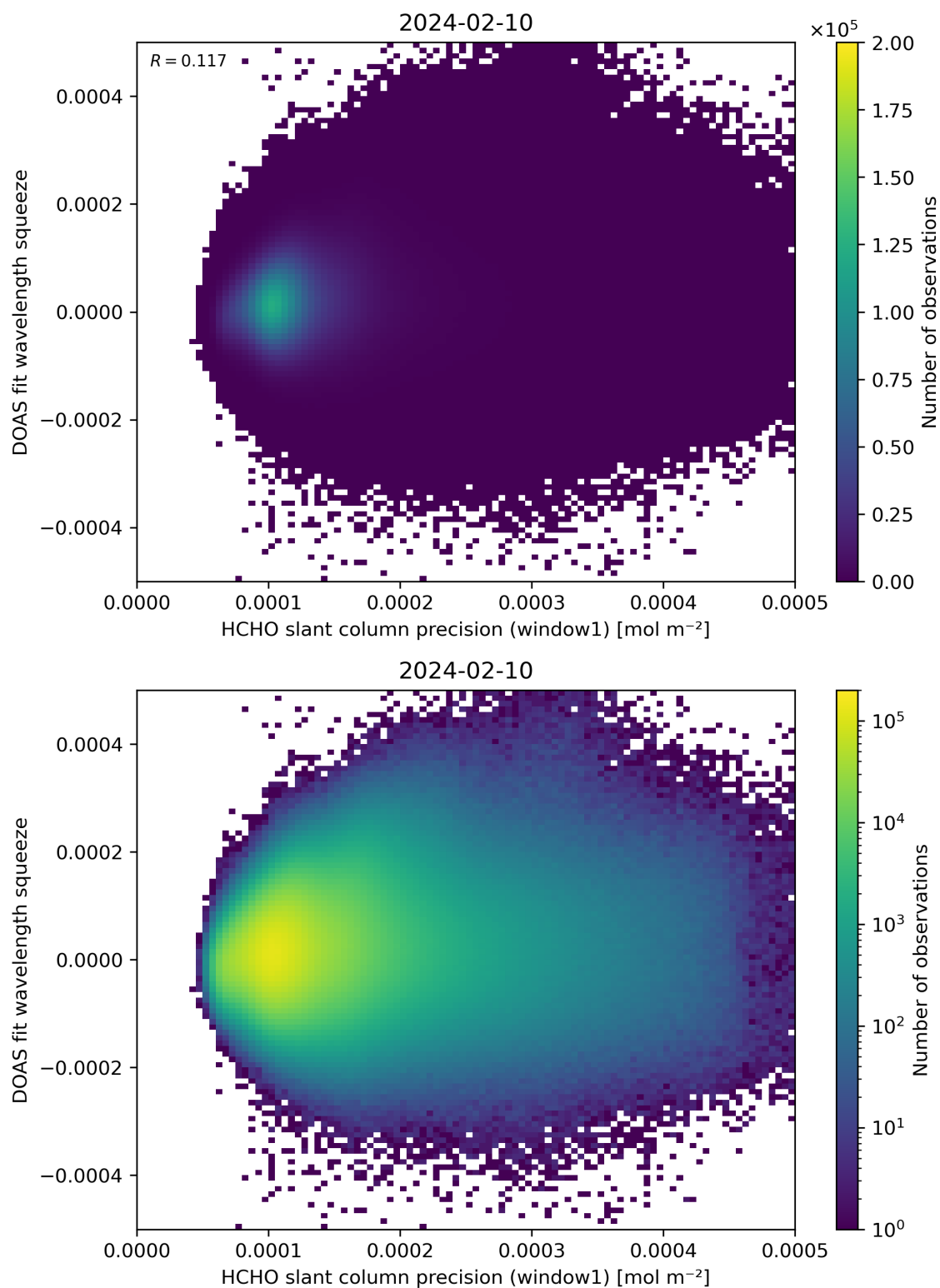
Figure 90: Scatter density plot of “HCHO slant column precision (window1)” against “DOAS fit wavelength squeeze” for 2024-02-09 to 2024-02-11.
