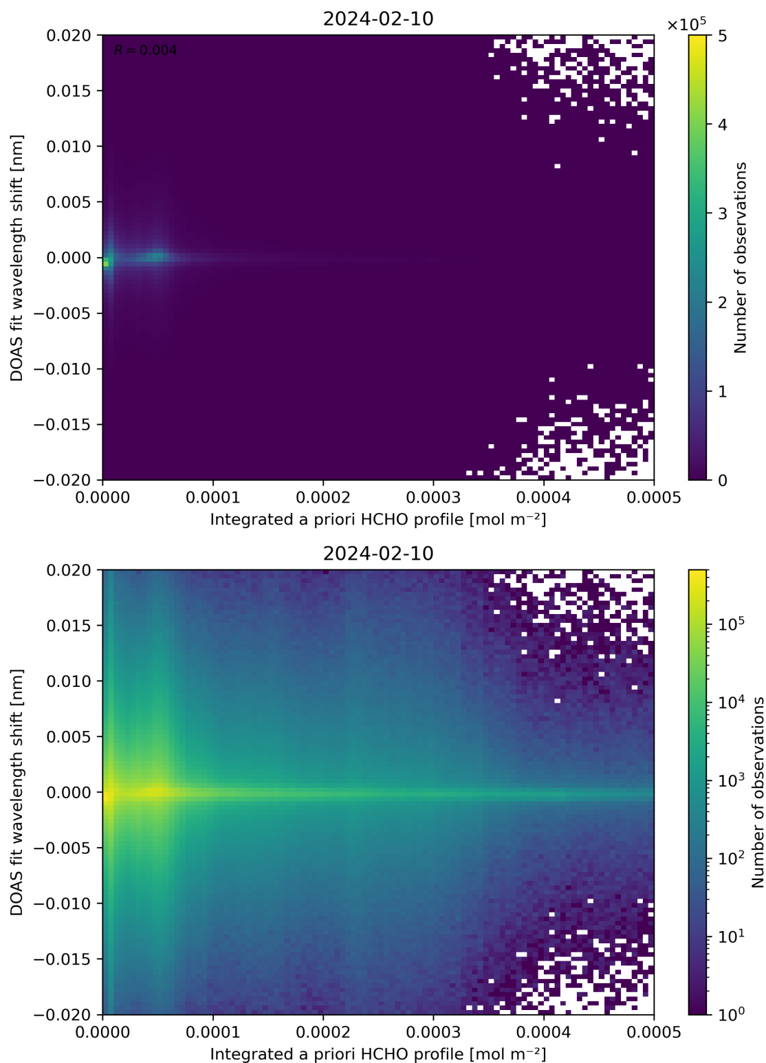
Figure 149: Scatter density plot of “Integrated a priori HCHO profile” against “DOAS fit wavelength shift” for 2024-02-09 to 2024-02-11.
