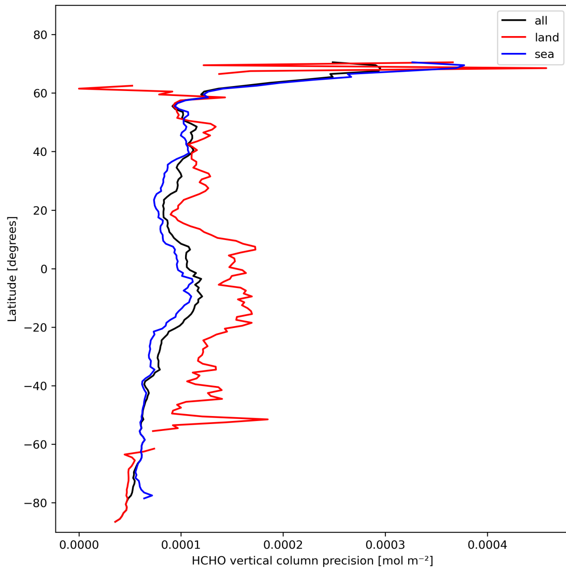
Figure 22: Zonal average of “HCHO vertical column precision” for 2024-02-09 to 2024-02-11.
