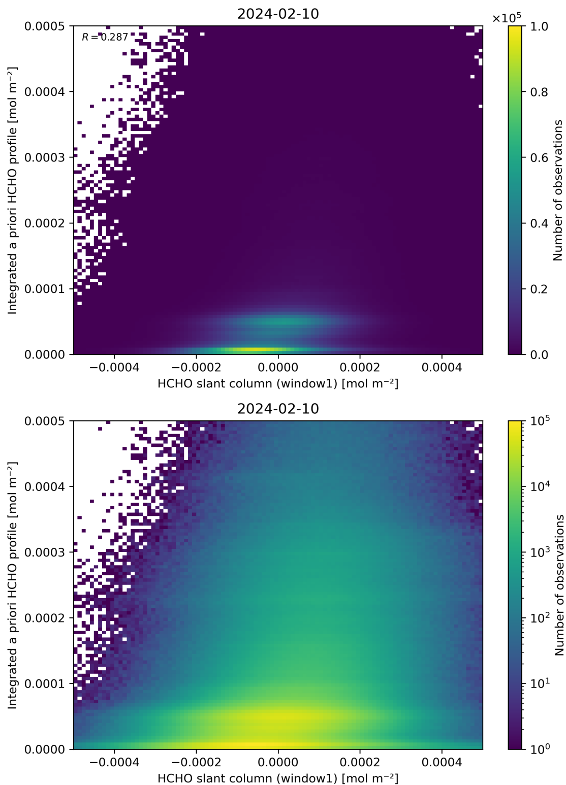
Figure 87: Scatter density plot of “HCHO slant column (window1)” against “Integrated a priori HCHO profile” for 2024-02-09 to 2024-02-11.
