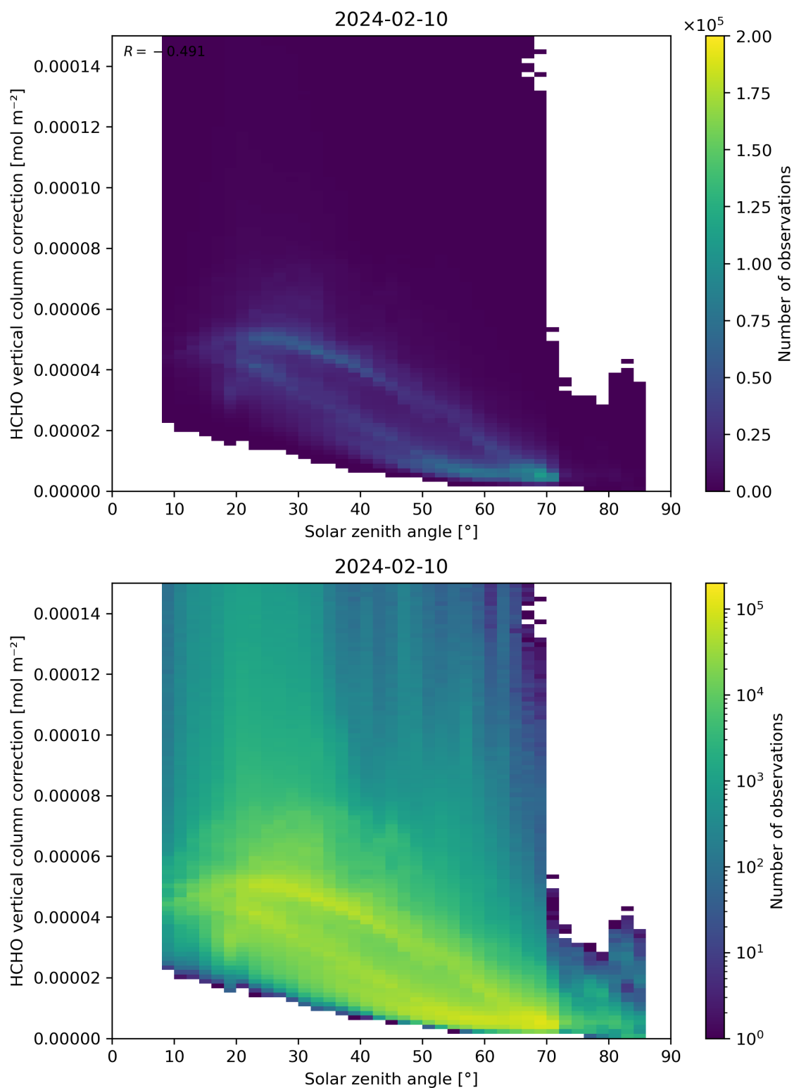
Figure 178: Scatter density plot of “Solar zenith angle” against “HCHO vertical column correction” for 2024-02-09 to 2024-02-11.
