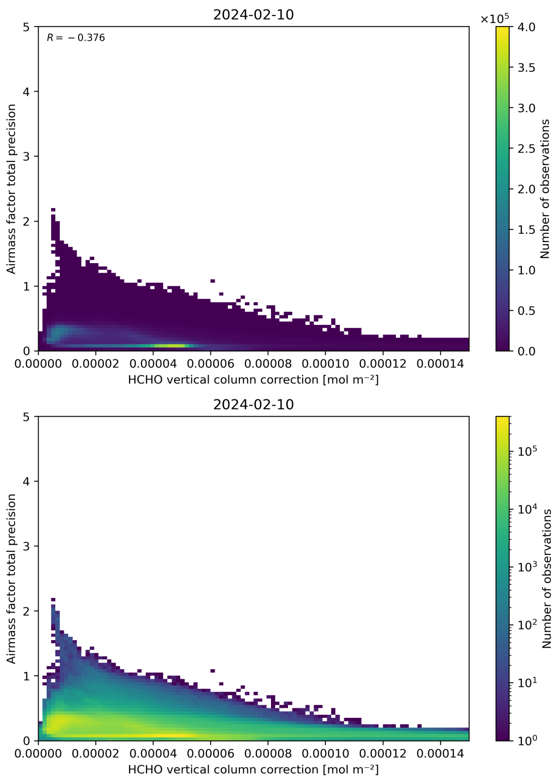
Figure 121: Scatter density plot of “HCHO vertical column correction” against “Airmass factor total precision” for 2024-02-09 to 2024-02-11.
