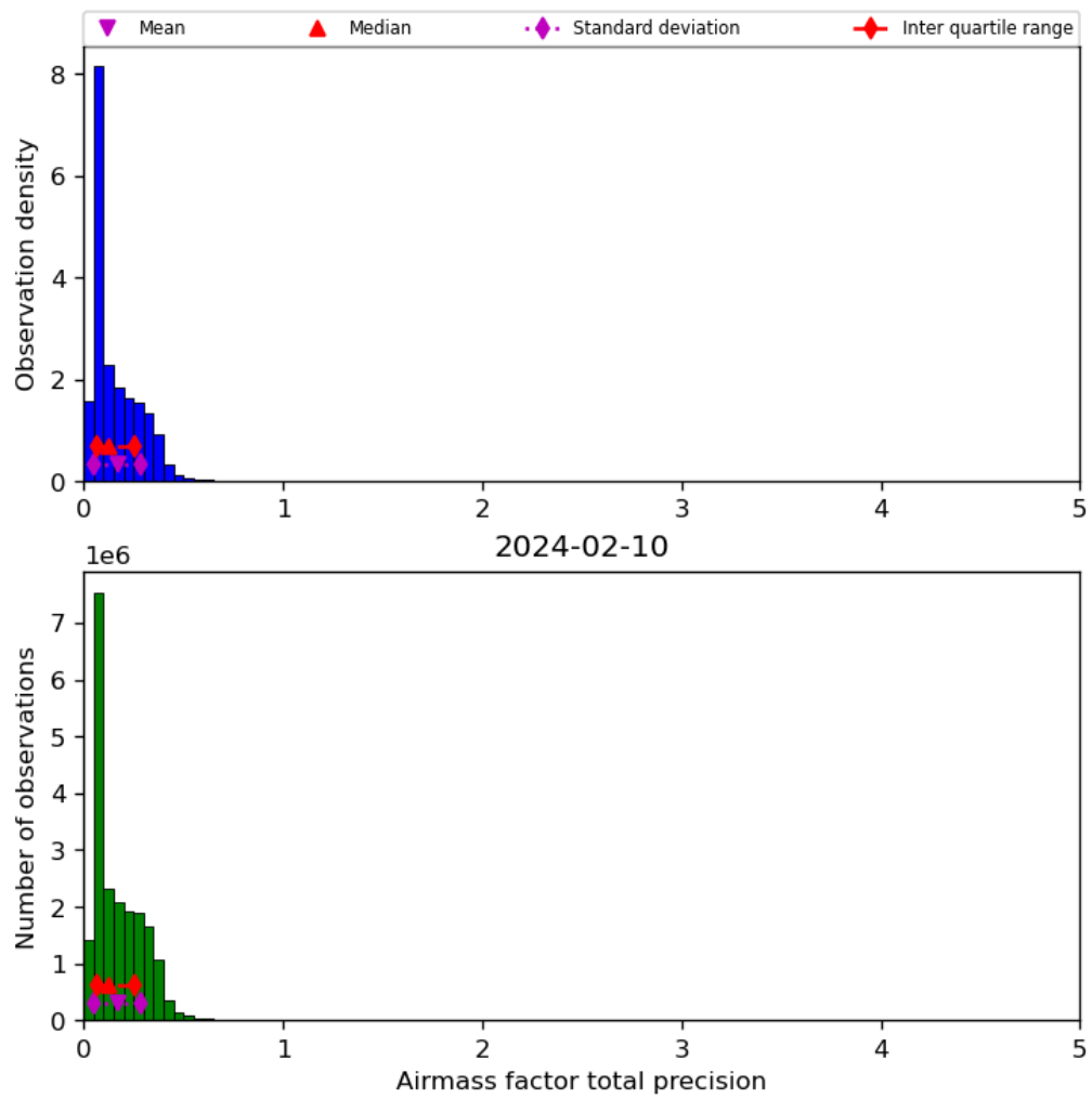
Figure 41: Histogram of “Airmass factor total precision” for 2024-02-09 to 2024-02-11
