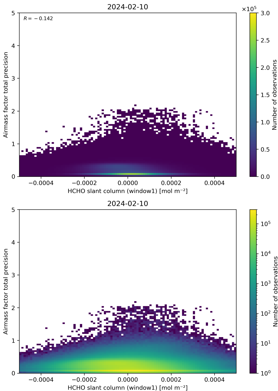
Figure 86: Scatter density plot of “HCHO slant column (window1)” against “Airmass factor total precision” for 2024-02-09 to 2024-02-11.
