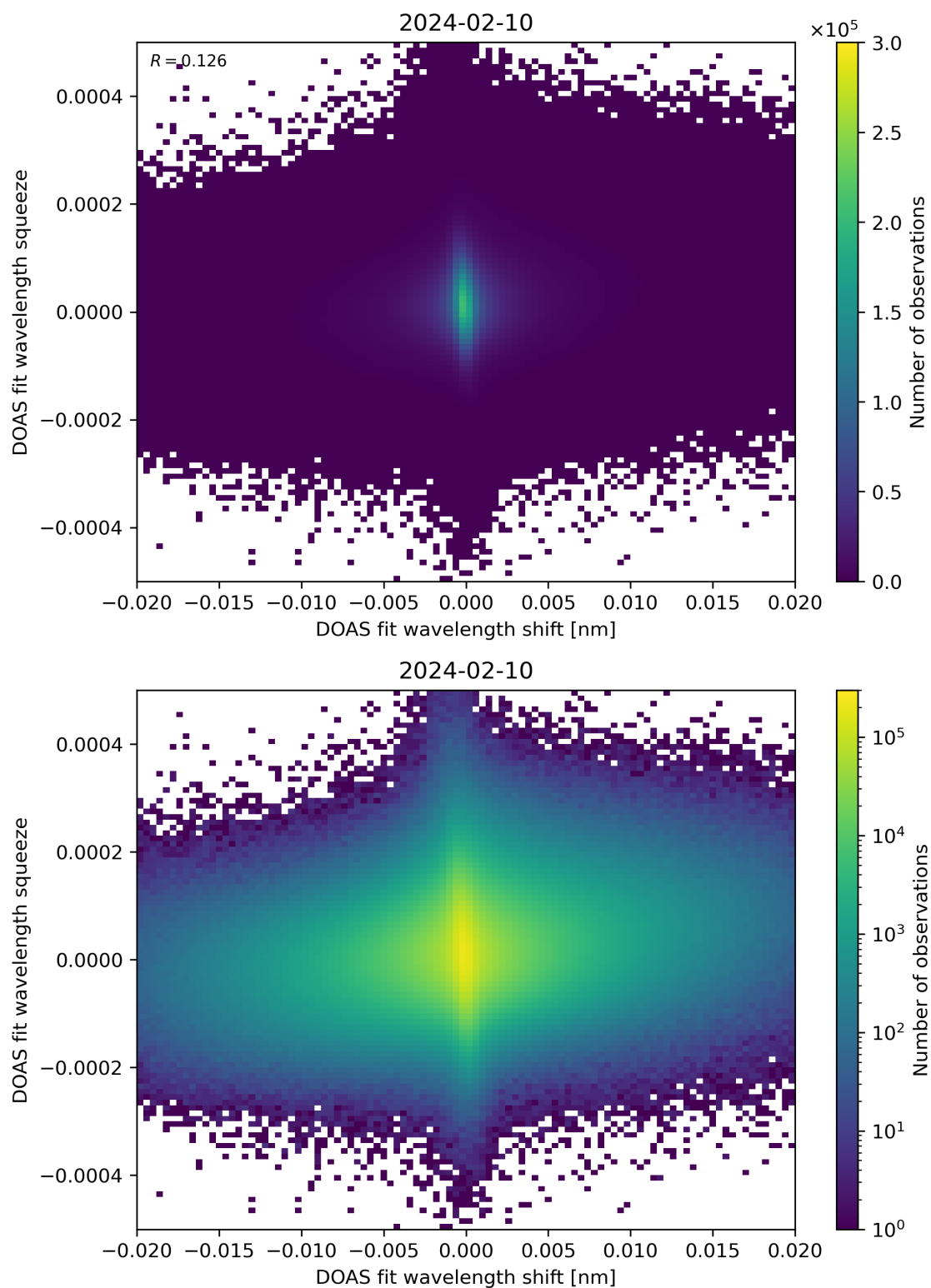
Figure 65: Scatter density plot of “DOAS fit wavelength shift” against “DOAS fit wavelength squeeze” for 2024-02-09 to 2024-02-11.
