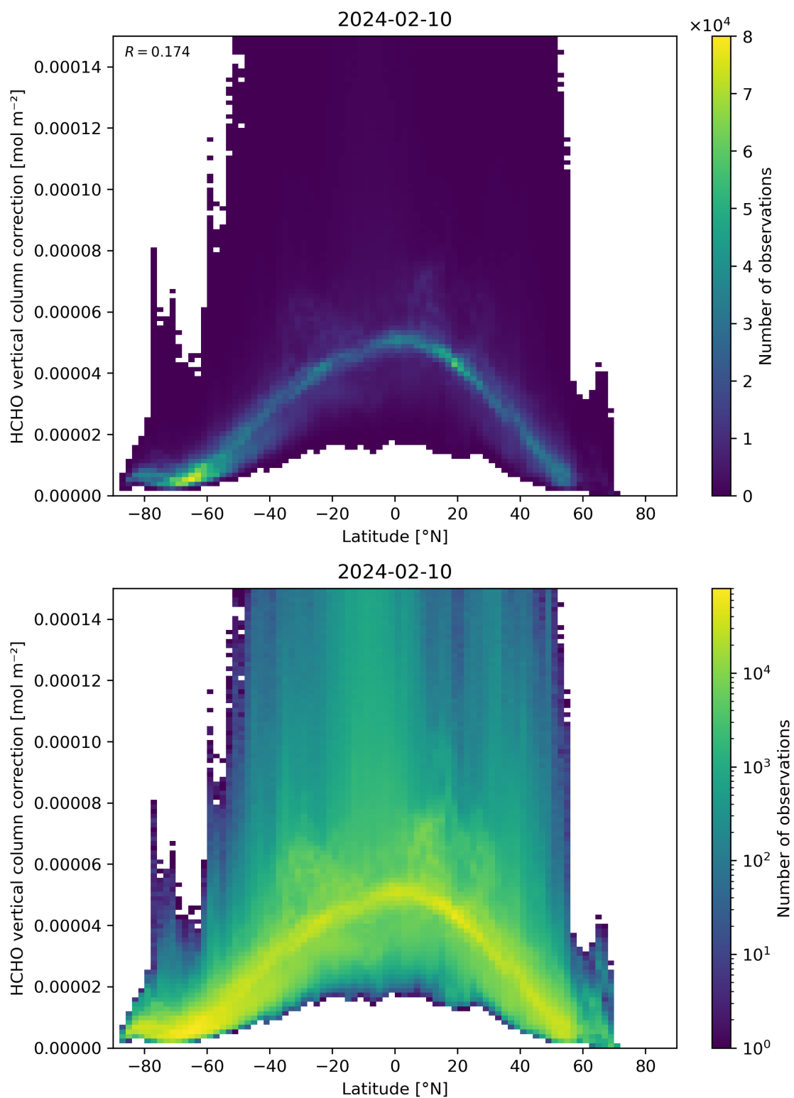
Figure 164: Scatter density plot of “Latitude” against “HCHO vertical column correction” for 2024-02-09 to 2024-02-11.
