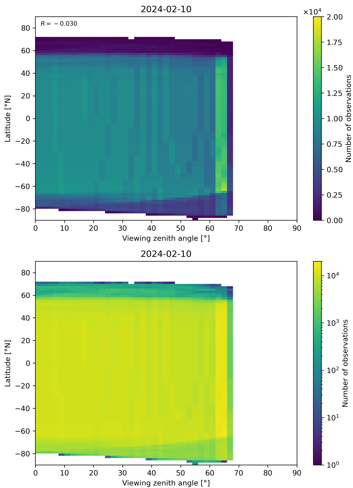
Figure 196: Scatter density plot of “Viewing zenith angle” against “Latitude” for 2024-02-09 to 2024-02-11.
