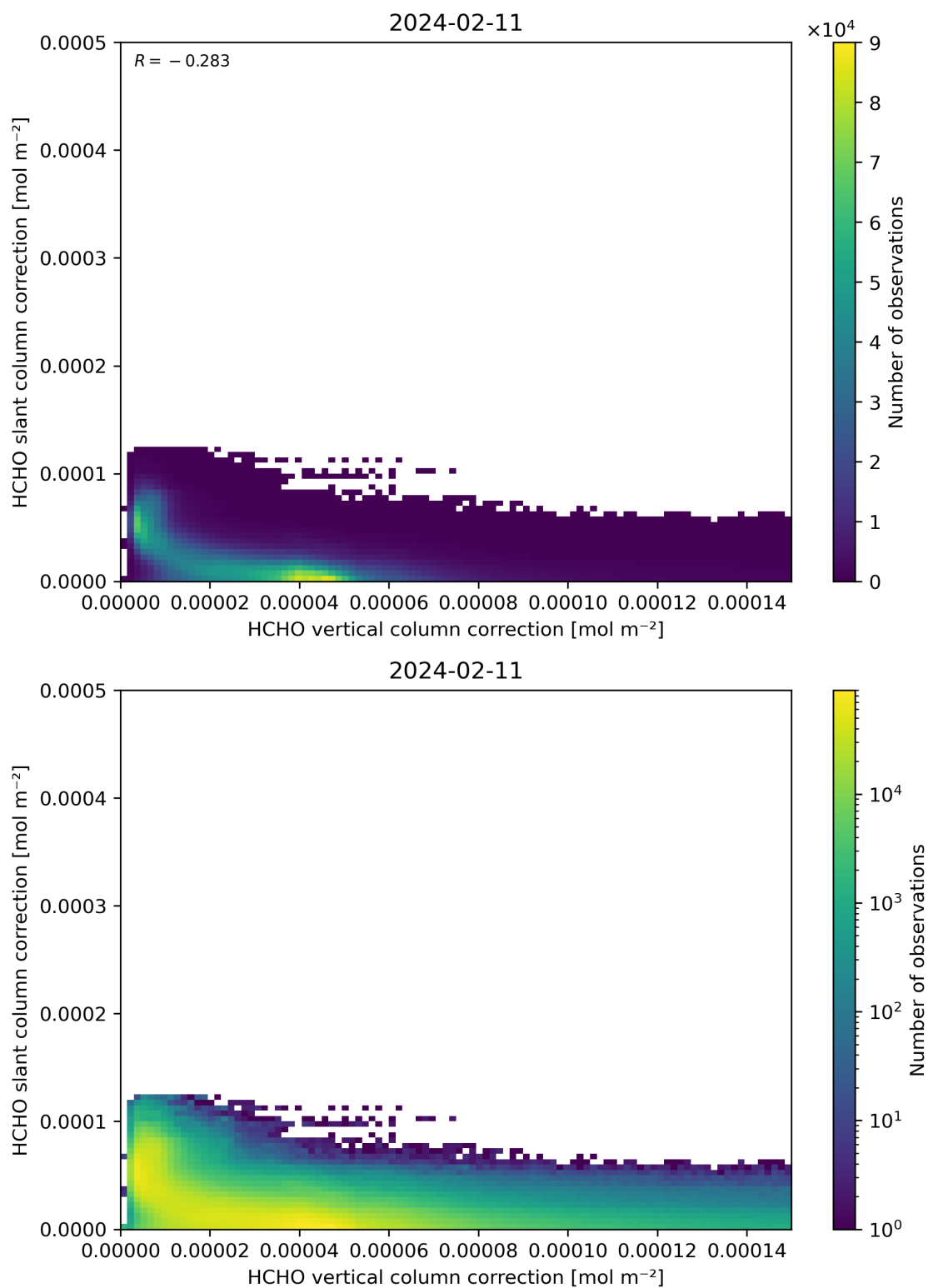
Figure 117: Scatter density plot of “HCHO vertical column correction” against “HCHO slant column correction” for 2024-02-11 to 2024-02-12.
