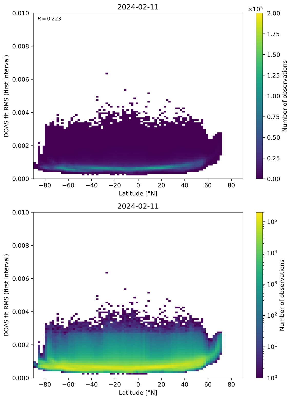
Figure 153: Scatter density plot of “Latitude” against “DOAS fit RMS (first interval)” for 2024-02-11 to 2024-02-12.
