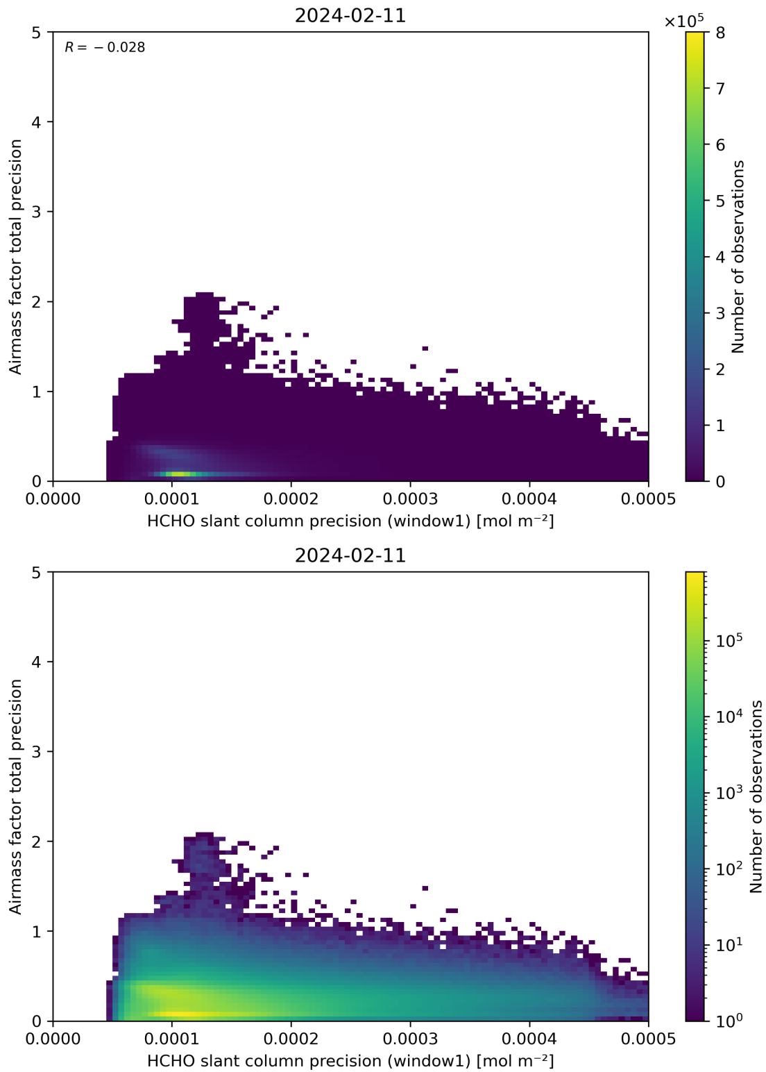
Figure 95: Scatter density plot of “HCHO slant column precision (window1)” against “Airmass factor total precision” for 2024-02-11 to 2024-02-12.
