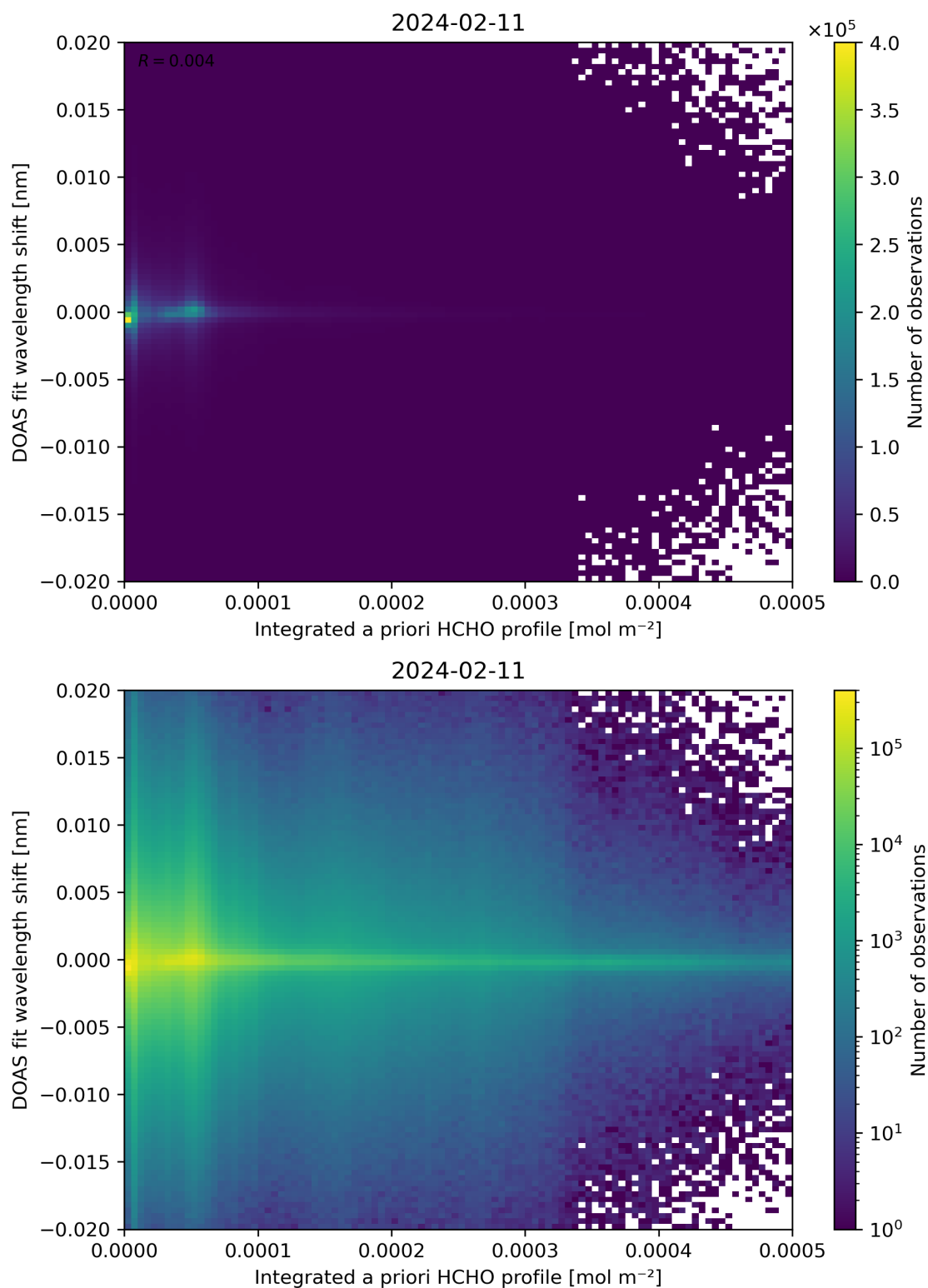
Figure 149: Scatter density plot of “Integrated a priori HCHO profile” against “DOAS fit wavelength shift” for 2024-02-11 to 2024-02-12.
