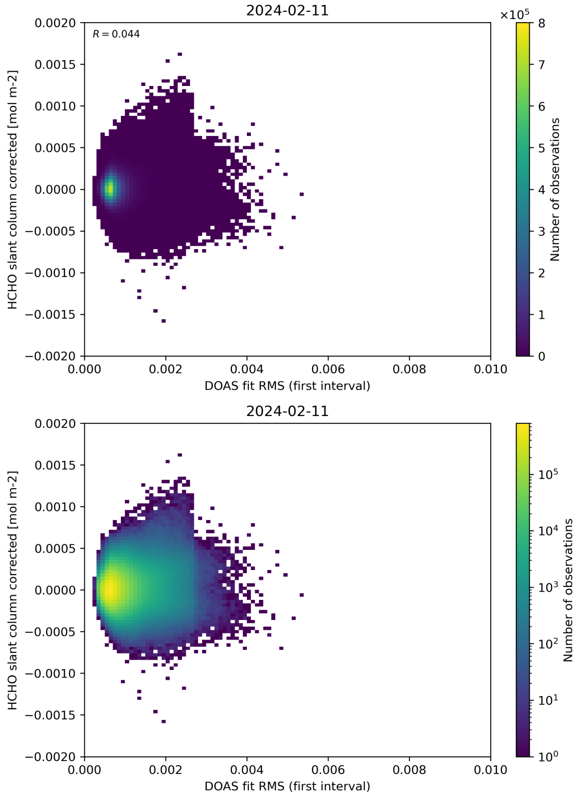
Figure 62: Scatter density plot of “DOAS fit RMS (first interval)” against “HCHO slant column corrected” for 2024-02-11 to 2024-02-12.
