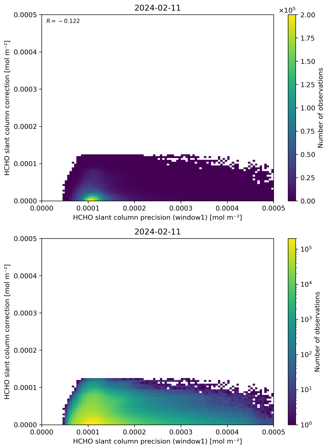
Figure 93: Scatter density plot of “HCHO slant column precision (window1)” against “HCHO slant column correction” for 2024-02-11 to 2024-02-12.
