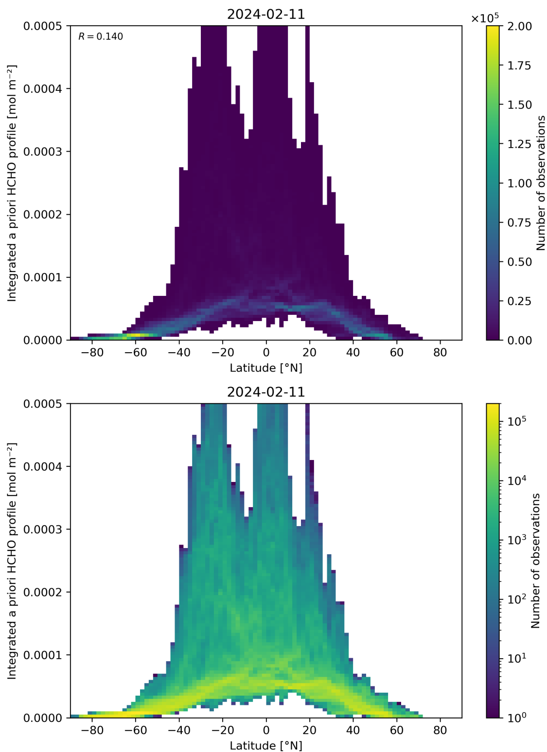
Figure 166: Scatter density plot of “Latitude” against “Integrated a priori HCHO profile” for 2024-02-11 to 2024-02-12.
