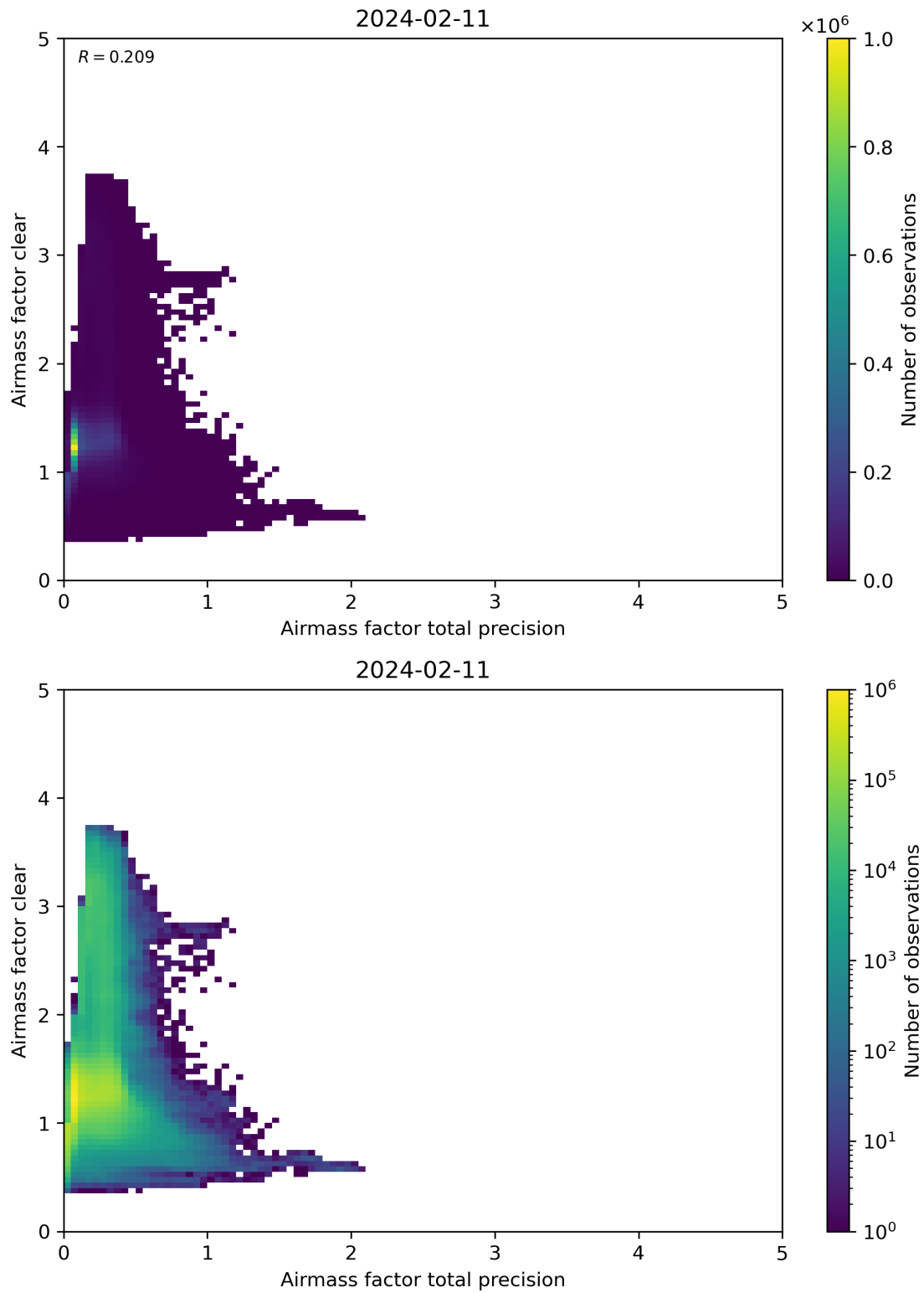
Figure 108: Scatter density plot of “Airmass factor total precision” against “Airmass factor clear” for 2024-02-11 to 2024-02-12.
