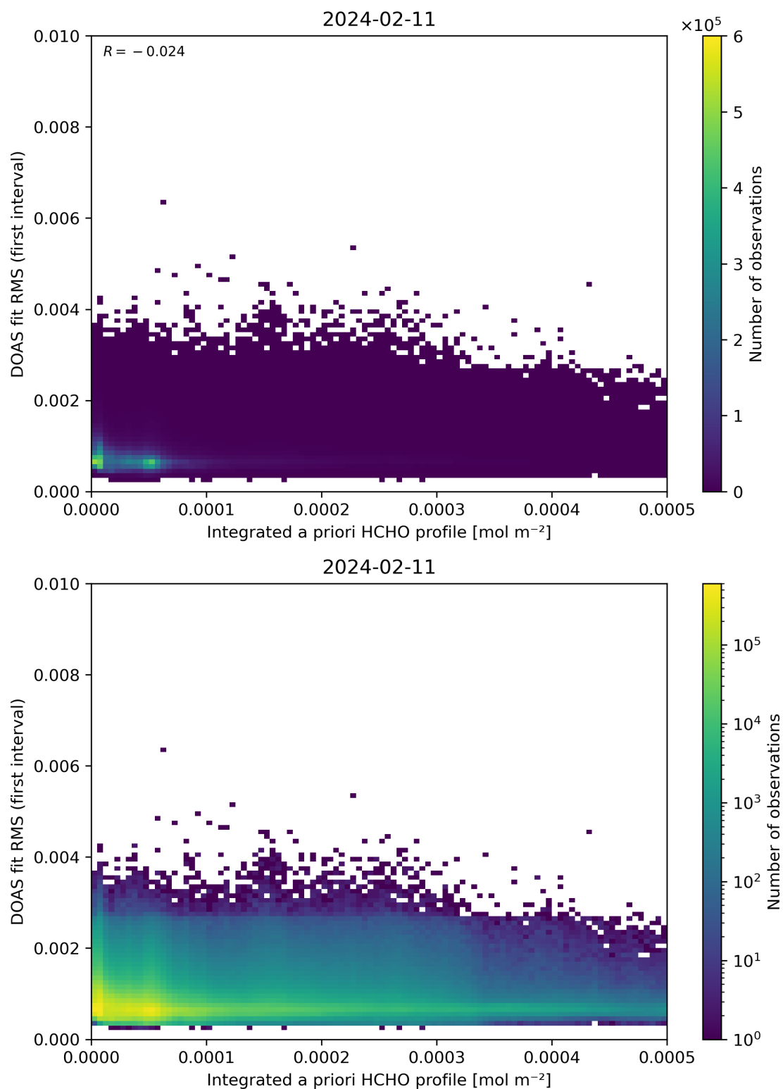
Figure 148: Scatter density plot of “Integrated a priori HCHO profile” against “DOAS fit RMS (first interval)” for 2024-02-11 to 2024-02-12.
