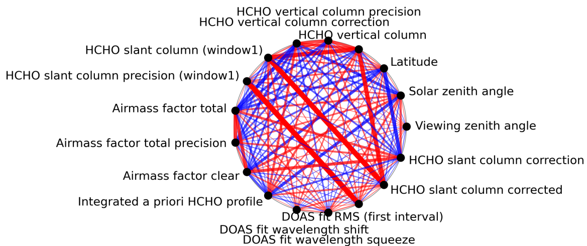
Figure 1: Map of correlation graph for 2024-02-11 to 2024-02-12.
