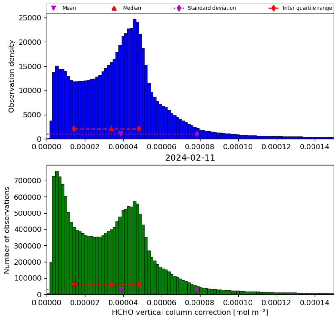
Figure 37: Histogram of “HCHO vertical column correction” for 2024-02-11 to 2024-02-12
