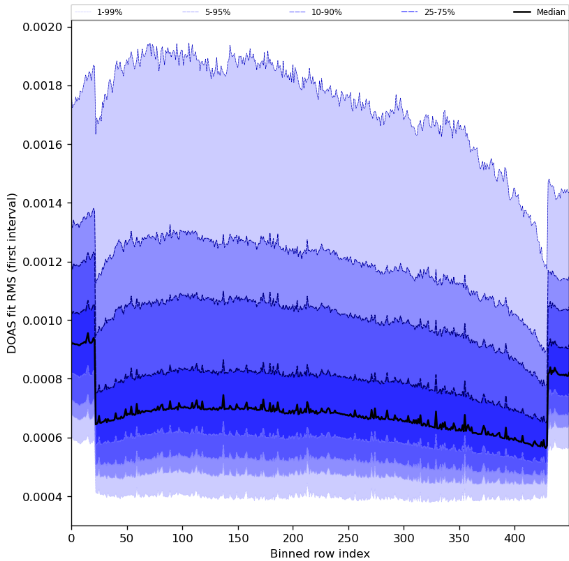
Figure 60: Along track statistics of “DOAS fit RMS (first interval)” for 2024-02-11 to 2024-02-12
