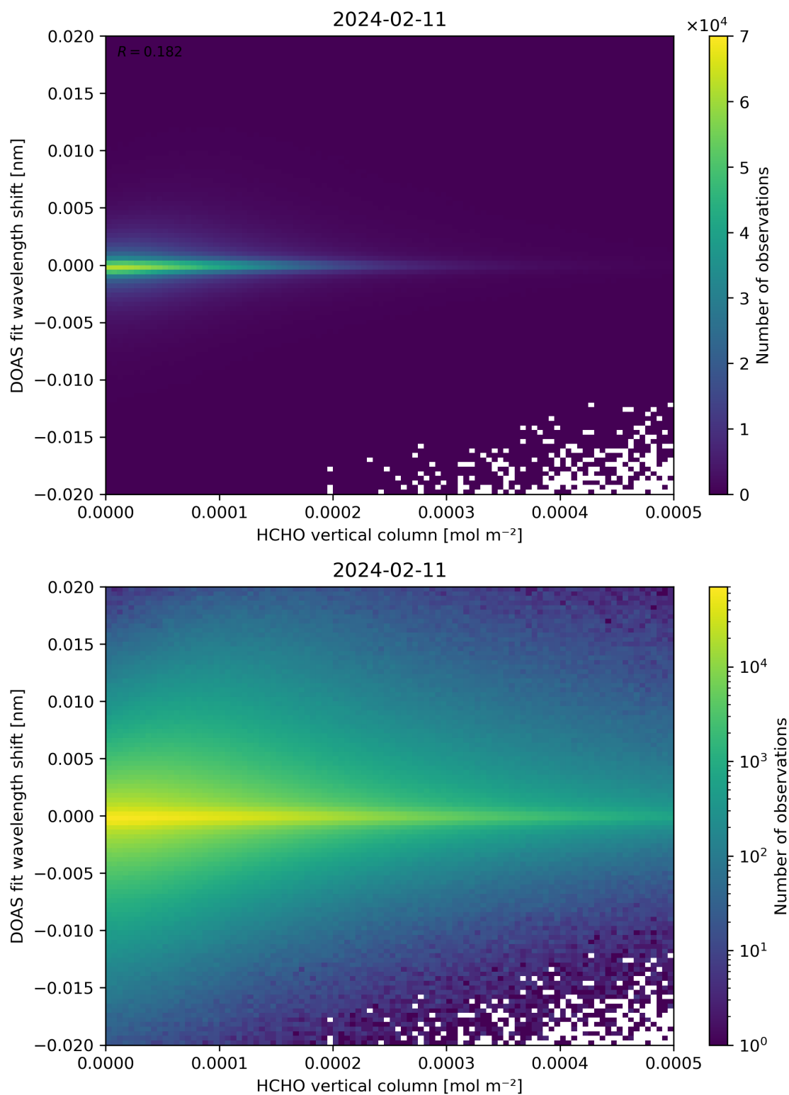
Figure 124: Scatter density plot of “HCHO vertical column” against “DOAS fit wavelength shift” for 2024-02-11 to 2024-02-12.
