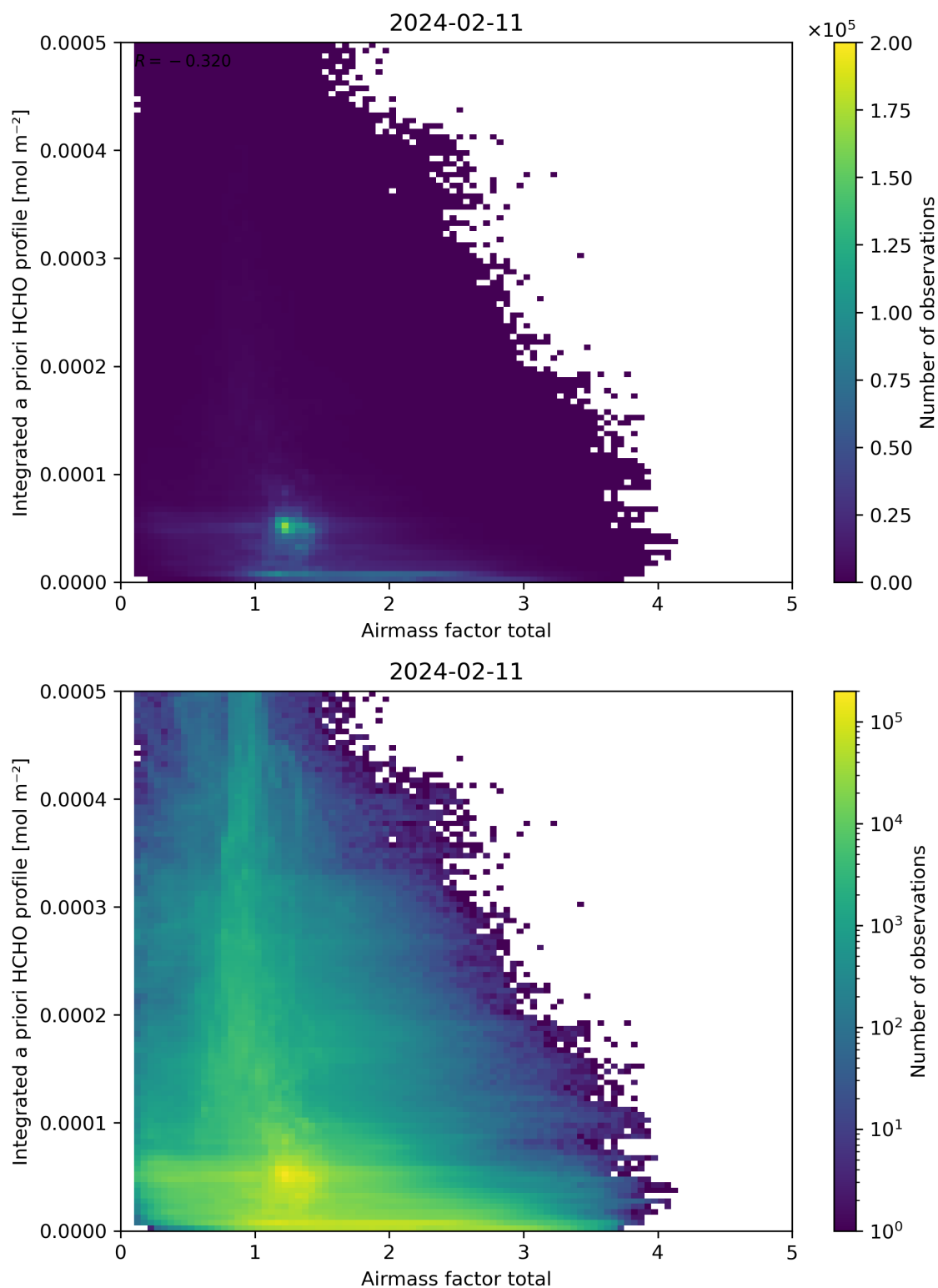
Figure 104: Scatter density plot of “Airmass factor total” against “Integrated a priori HCHO profile” for 2024-02-11 to 2024-02-12.
