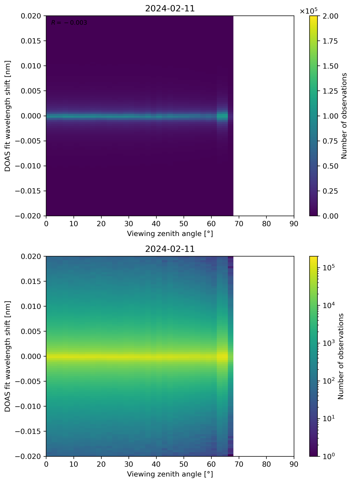
Figure 183: Scatter density plot of “Viewing zenith angle” against “DOAS fit wavelength shift” for 2024-02-11 to 2024-02-12.
