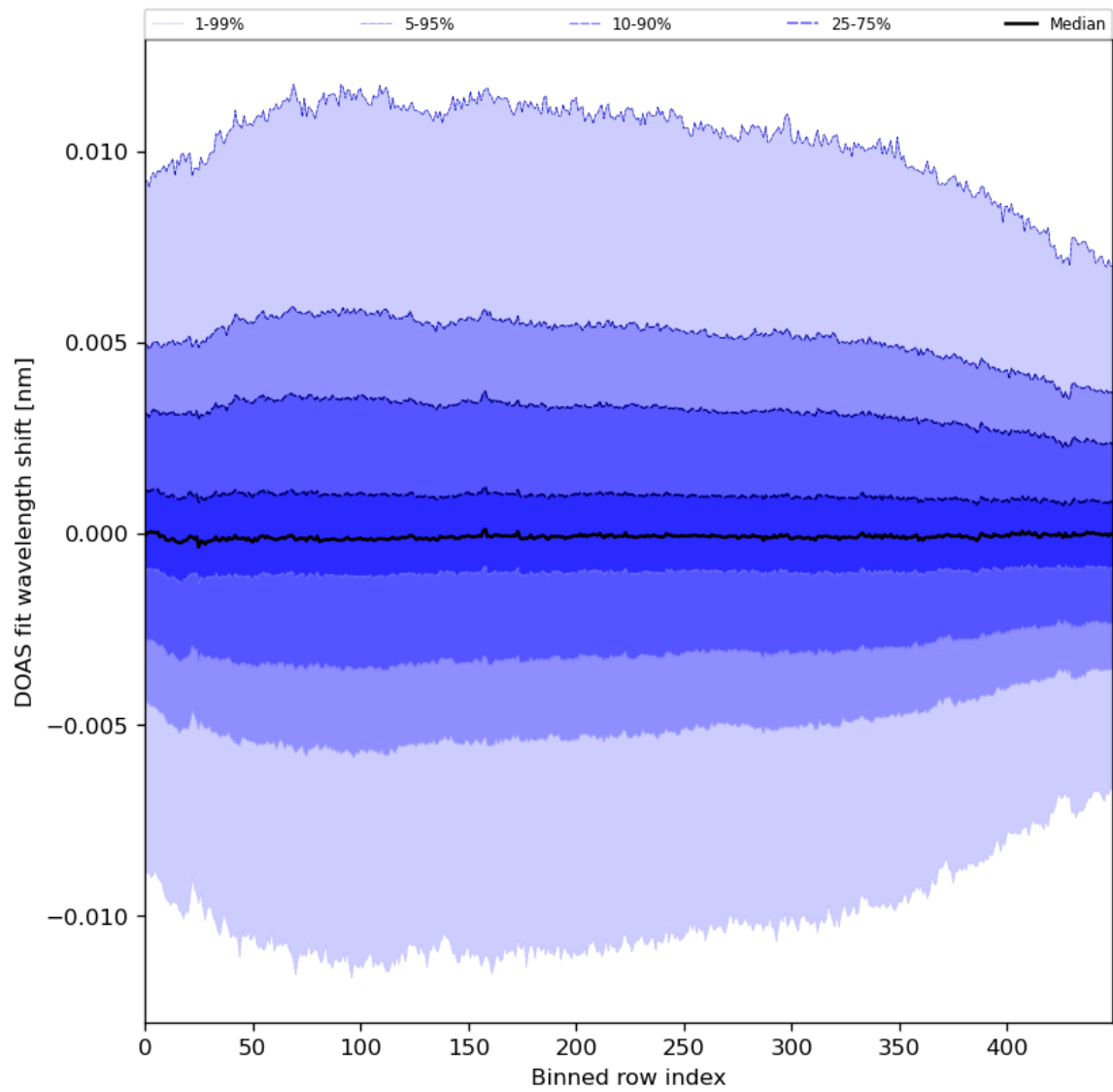
Figure 58: Along track statistics of “DOAS fit wavelength shift” for 2024-02-11 to 2024-02-12
