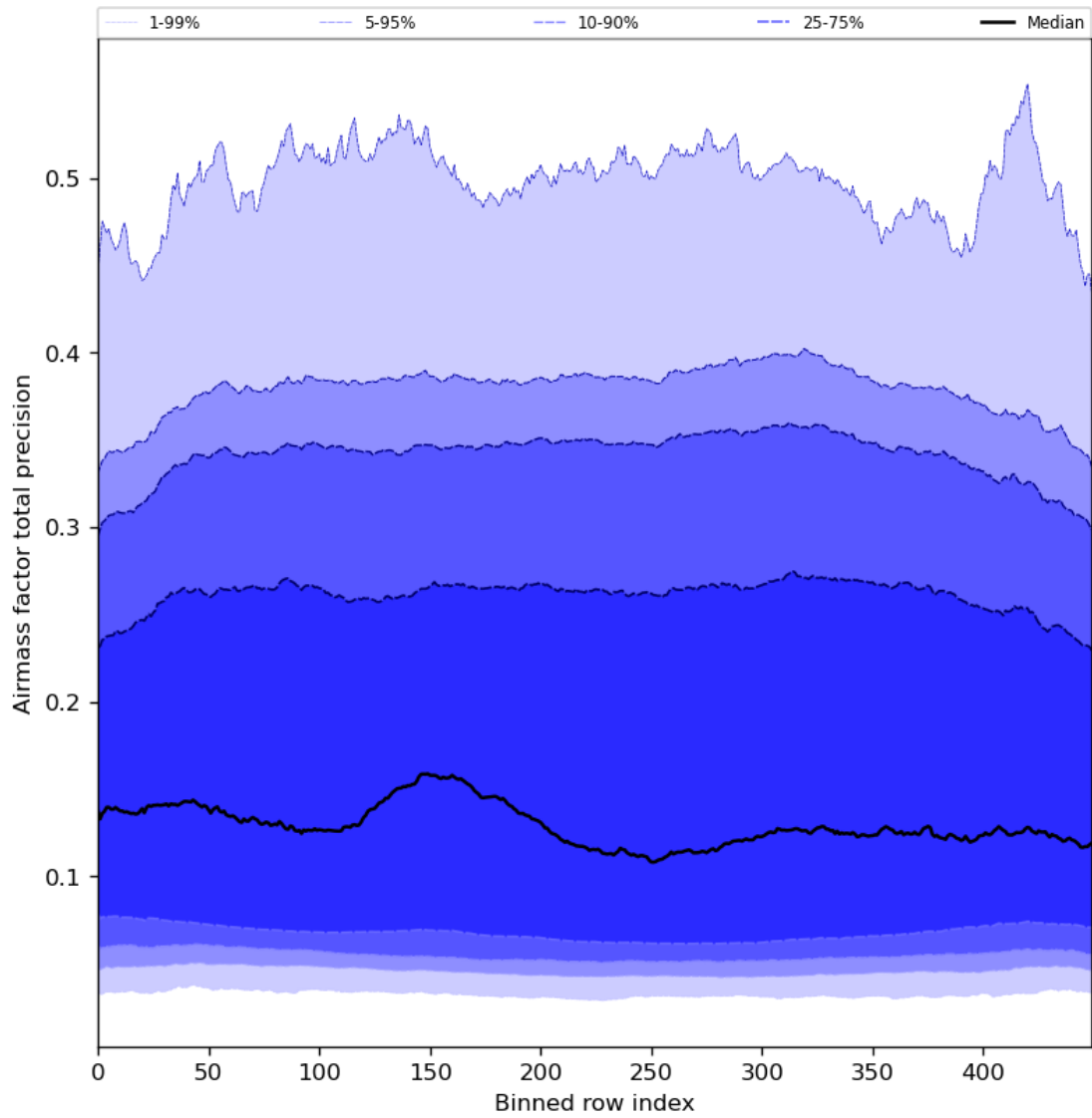
Figure 55: Along track statistics of “Airmass factor total precision” for 2024-02-11 to 2024-02-12
