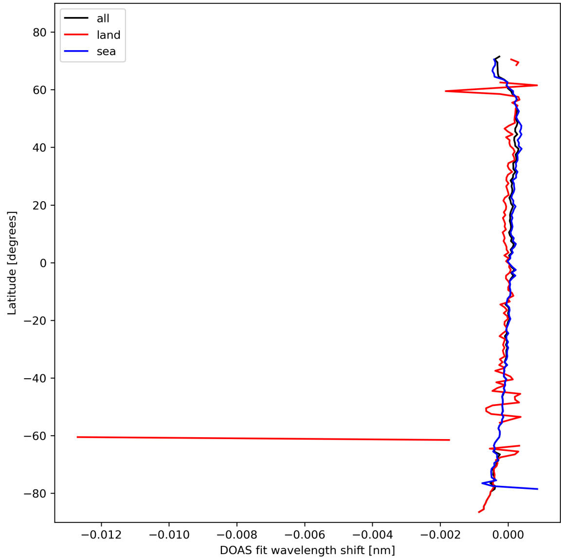
Figure 30: Zonal average of “DOAS fit wavelength shift” for 2024-02-11 to 2024-02-12.
