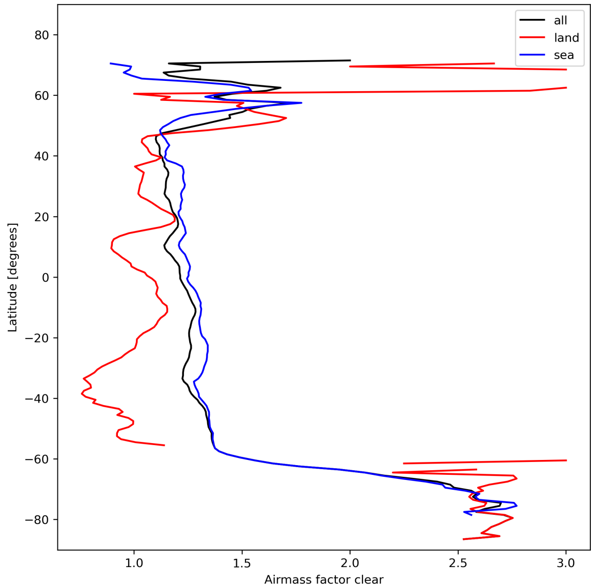
Figure 28: Zonal average of “Airmass factor clear” for 2024-02-11 to 2024-02-12.
