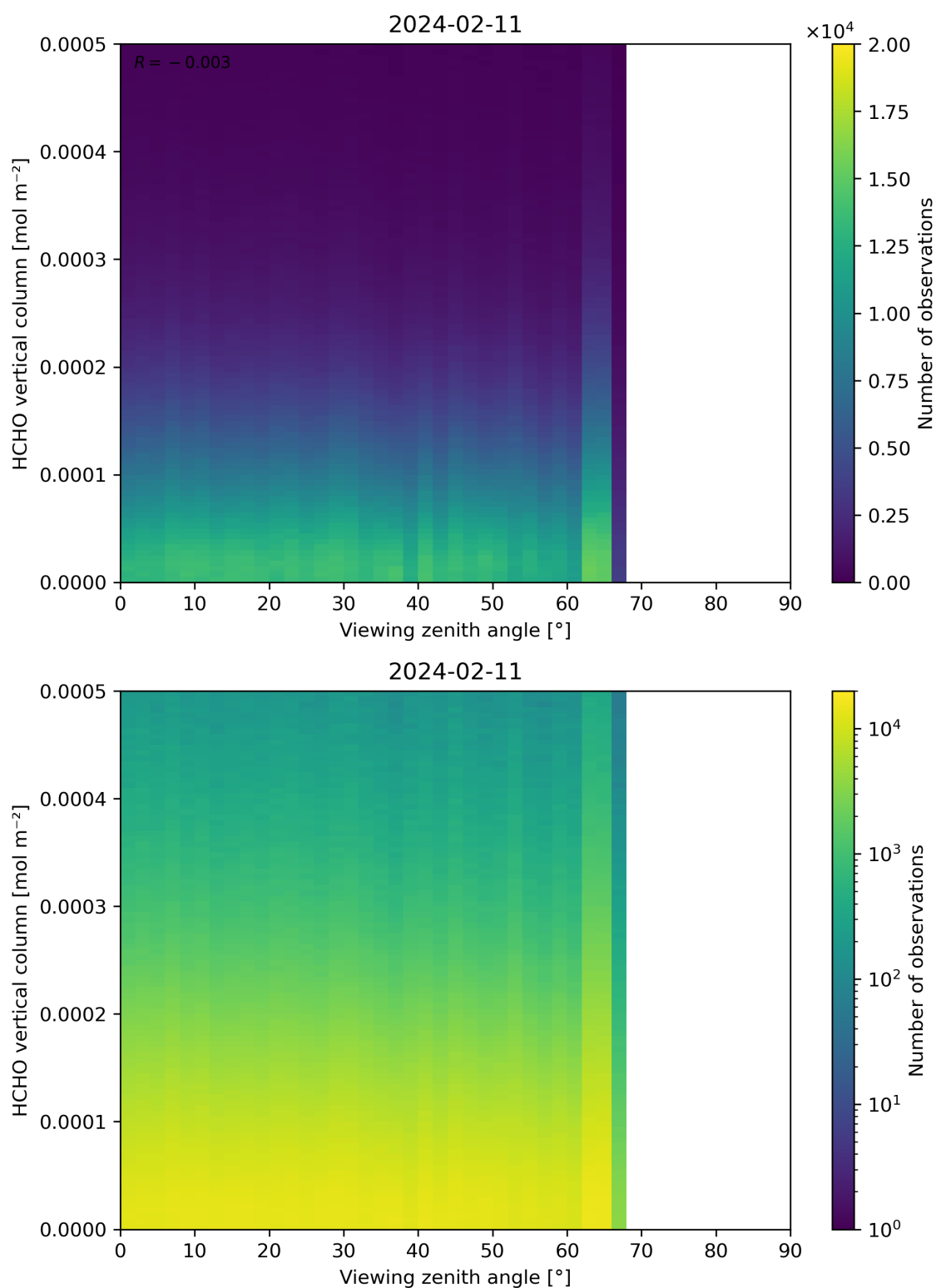
Figure 192: Scatter density plot of “Viewing zenith angle” against “HCHO vertical column” for 2024-02-11 to 2024-02-12.
