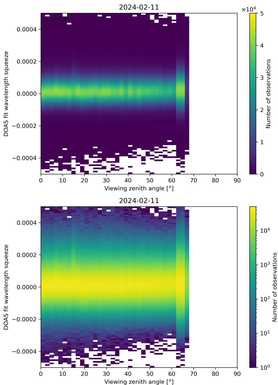
Figure 184: Scatter density plot of “Viewing zenith angle” against “DOAS fit wavelength squeeze” for 2024-02-11 to 2024-02-12.
