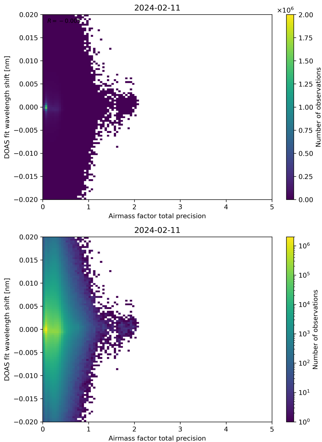
Figure 106: Scatter density plot of “Airmass factor total precision” against “DOAS fit wavelength shift” for 2024-02-11 to 2024-02-12.
