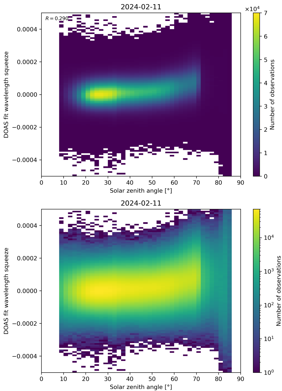
Figure 169: Scatter density plot of “Solar zenith angle” against “DOAS fit wavelength squeeze” for 2024-02-11 to 2024-02-12.
