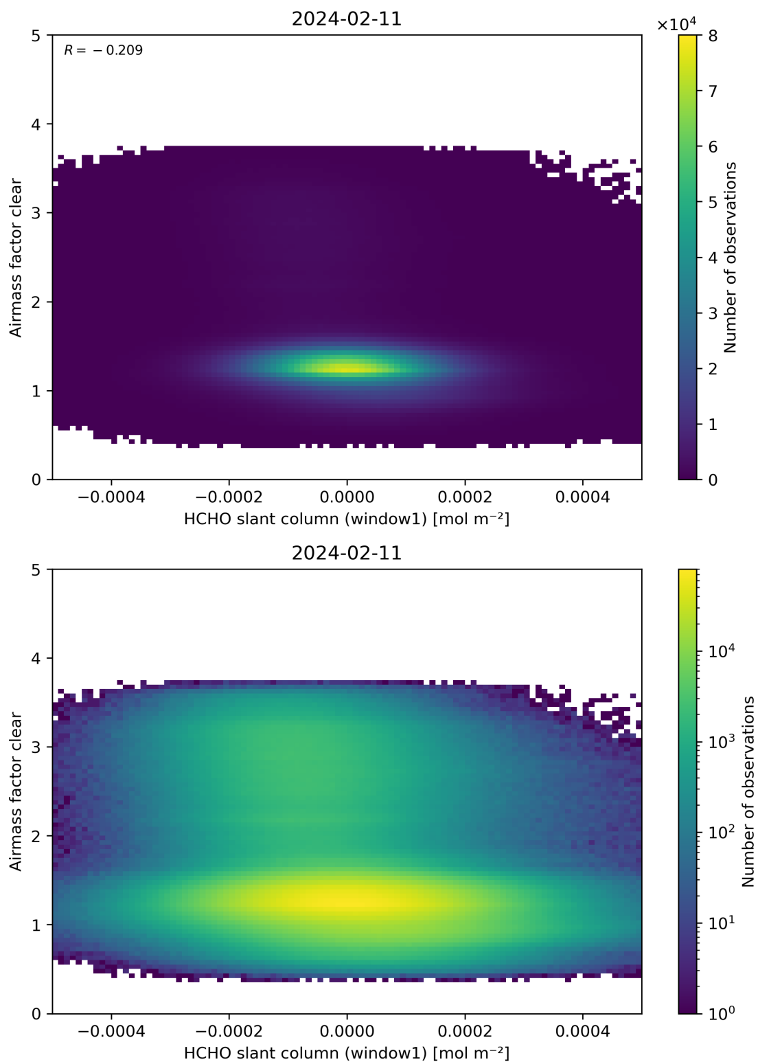
Figure 81: Scatter density plot of “HCHO slant column (window1)” against “Airmass factor clear” for 2024-02-11 to 2024-02-12.
