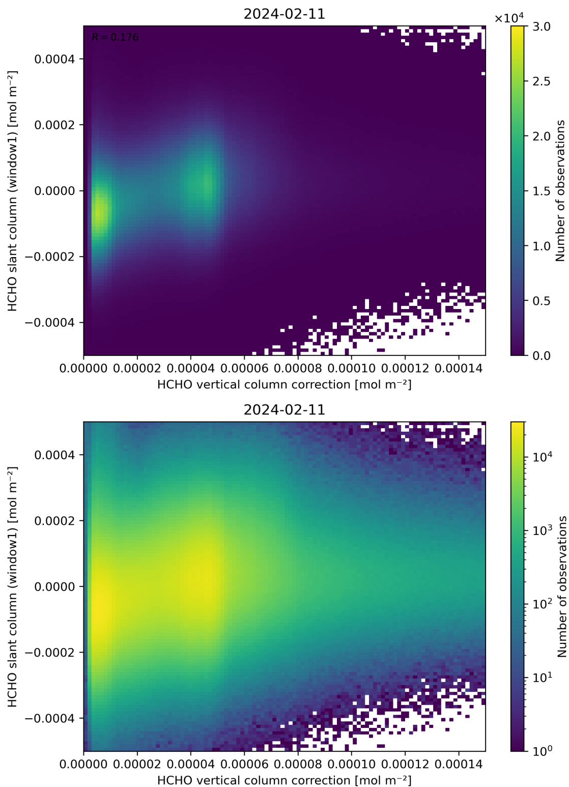
Figure 118: Scatter density plot of “HCHO vertical column correction” against “HCHO slant column (window1)” for 2024-02-11 to 2024-02-12.
