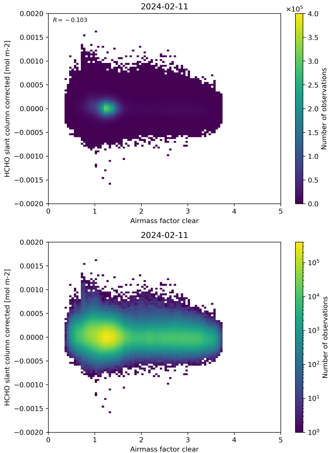
Figure 74: Scatter density plot of “Airmass factor clear” against “HCHO slant column corrected” for 2024-02-11 to 2024-02-12.
