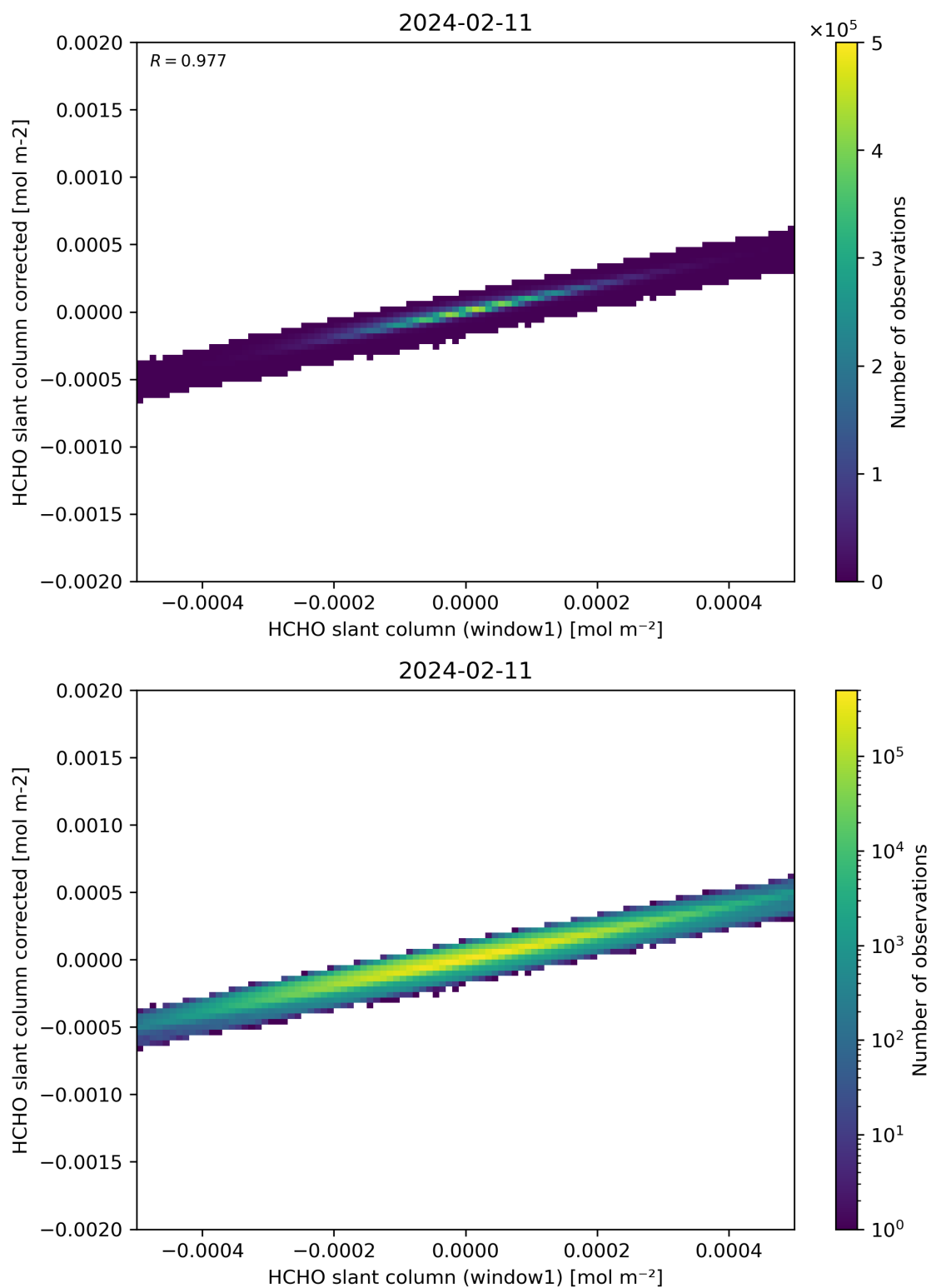
Figure 82: Scatter density plot of “HCHO slant column (window1)” against “HCHO slant column corrected” for 2024-02-11 to 2024-02-12.
