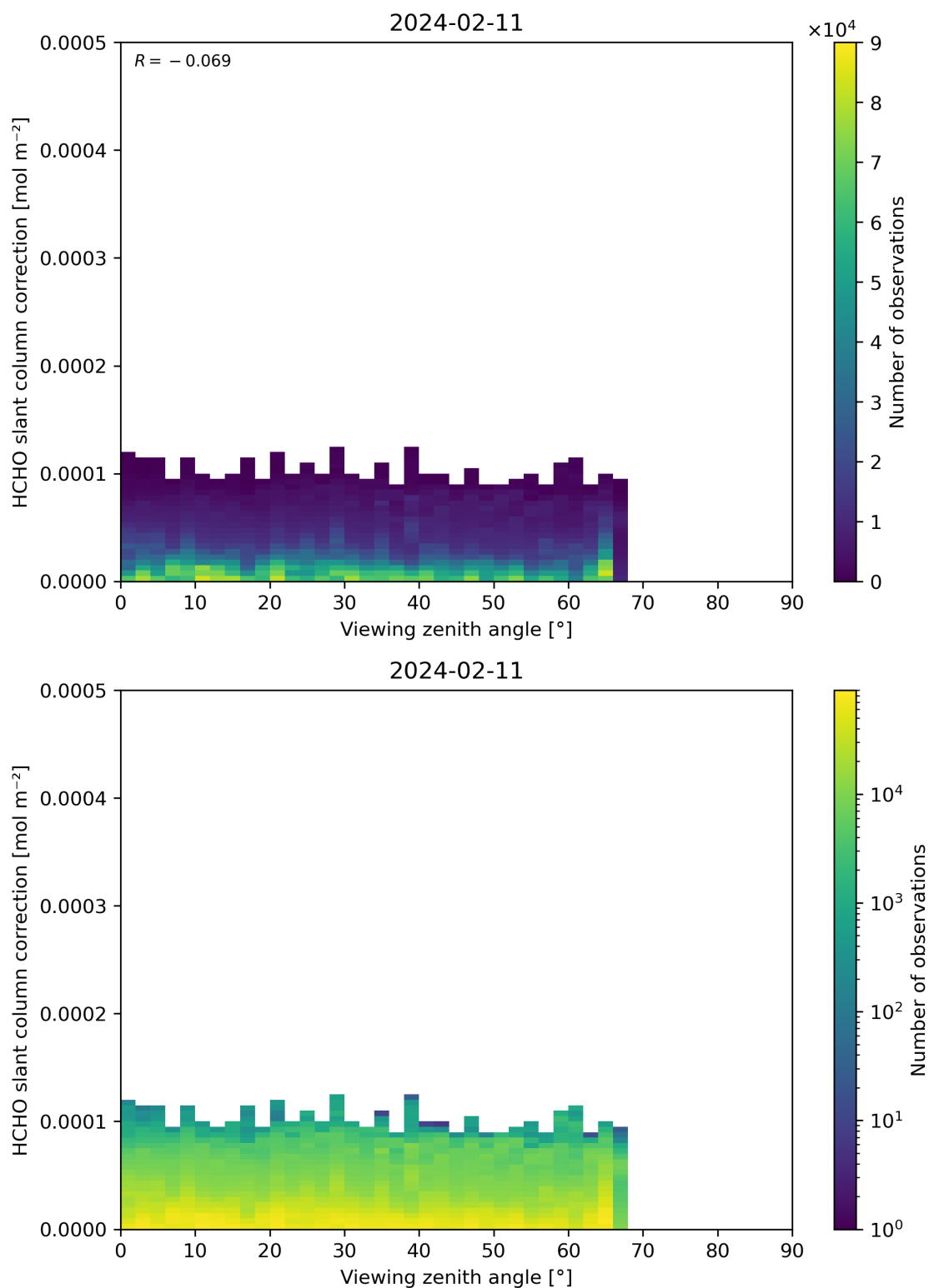
Figure 187: Scatter density plot of “Viewing zenith angle” against “HCHO slant column correction” for 2024-02-11 to 2024-02-12.
