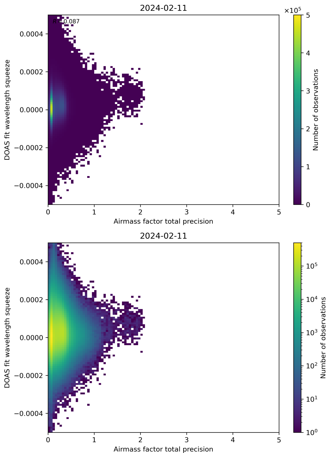
Figure 107: Scatter density plot of “Airmass factor total precision” against “DOAS fit wavelength squeeze” for 2024-02-11 to 2024-02-12.
