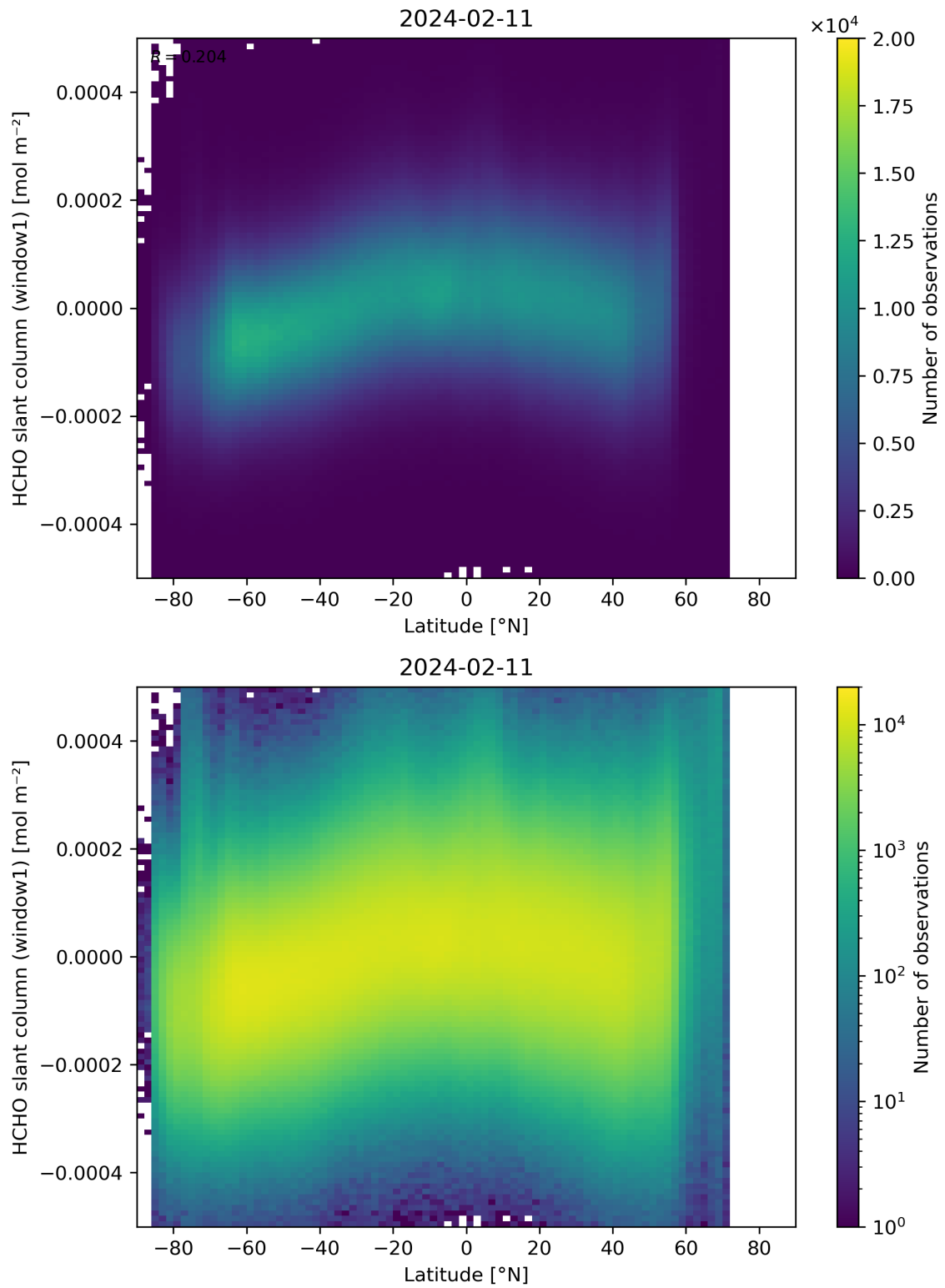
Figure 159: Scatter density plot of “Latitude” against “HCHO slant column (window1)” for 2024-02-11 to 2024-02-12.
