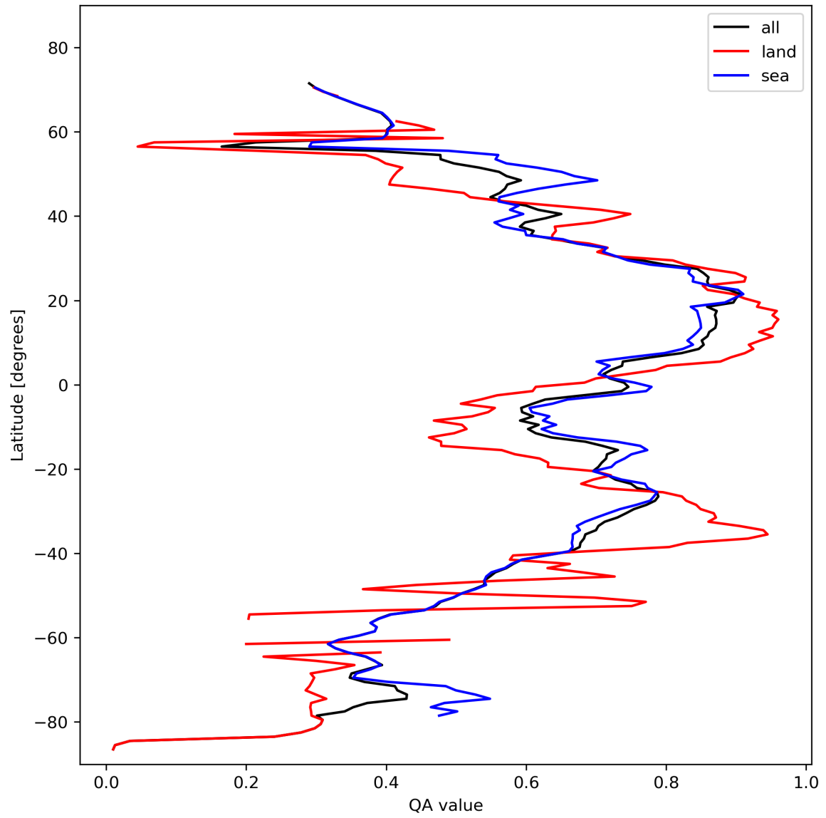
Figure 20: Zonal average of “QA value” for 2024-02-11 to 2024-02-12.
