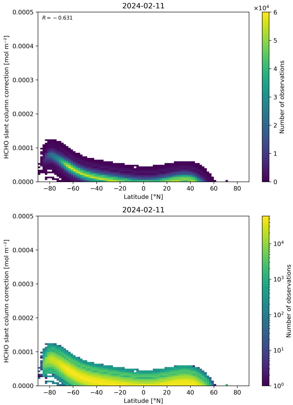
Figure 158: Scatter density plot of “Latitude” against “HCHO slant column correction” for 2024-02-11 to 2024-02-12.
