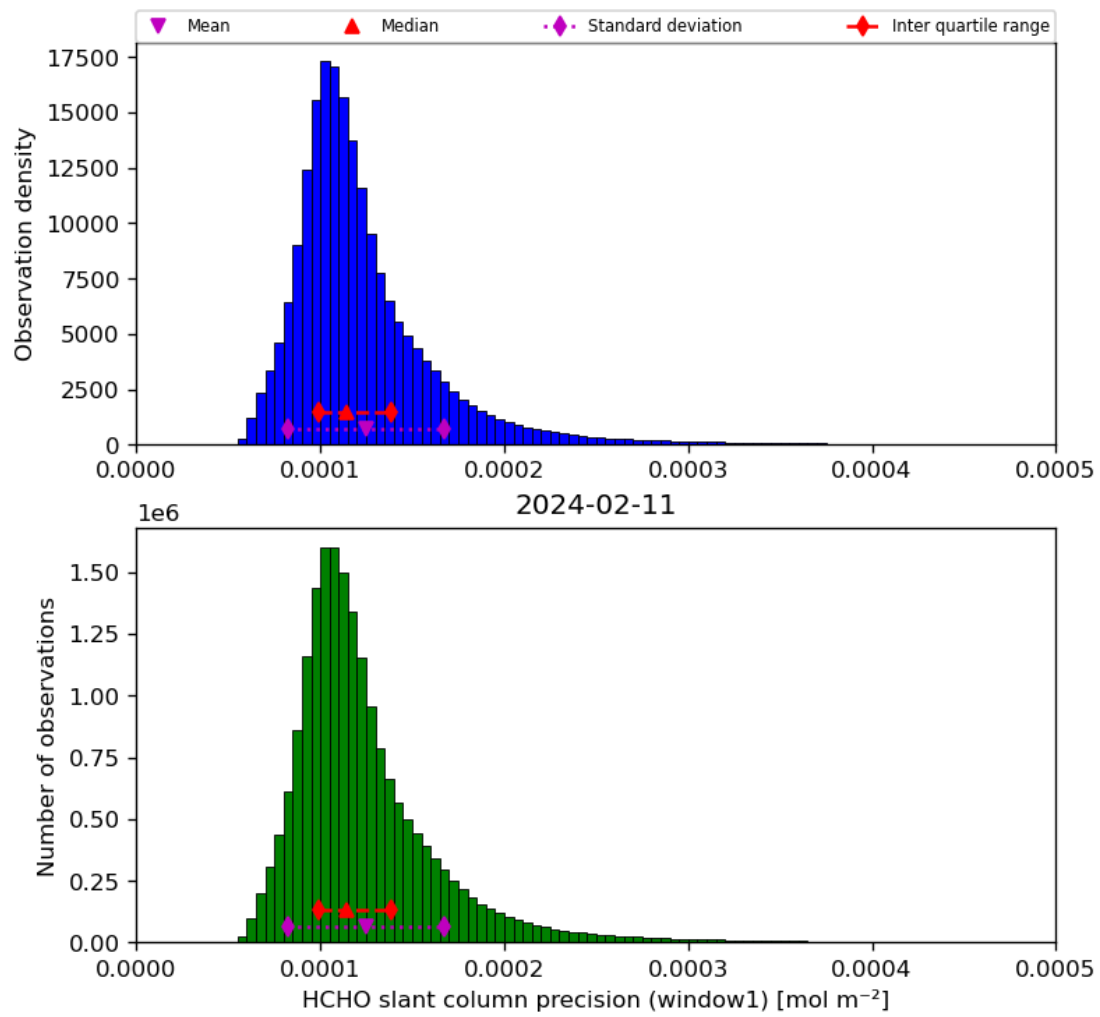
Figure 39: Histogram of “HCHO slant column precision (window1)” for 2024-02-11 to 2024-02-12
