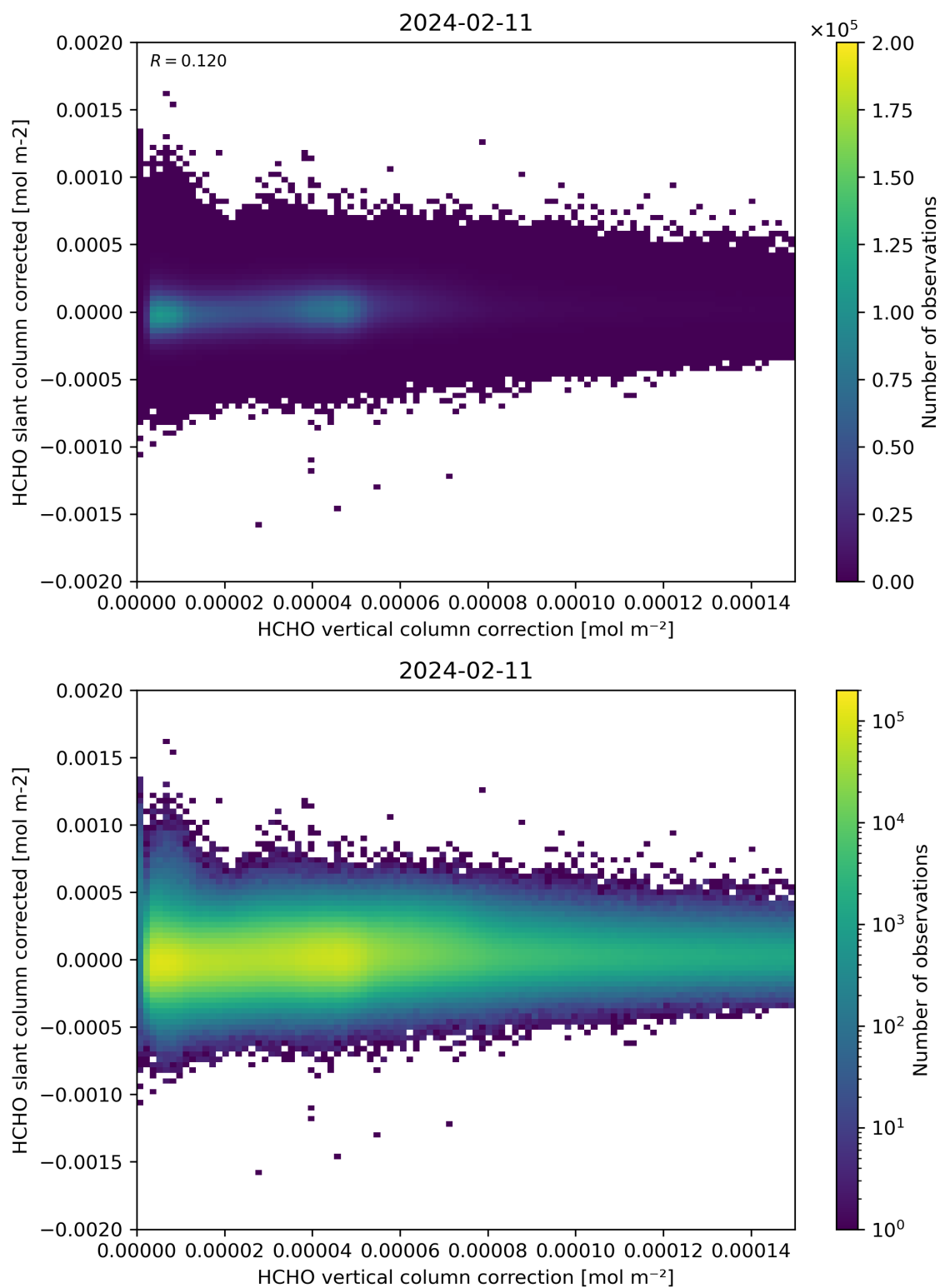
Figure 116: Scatter density plot of “HCHO vertical column correction” against “HCHO slant column corrected” for 2024-02-11 to 2024-02-12.
