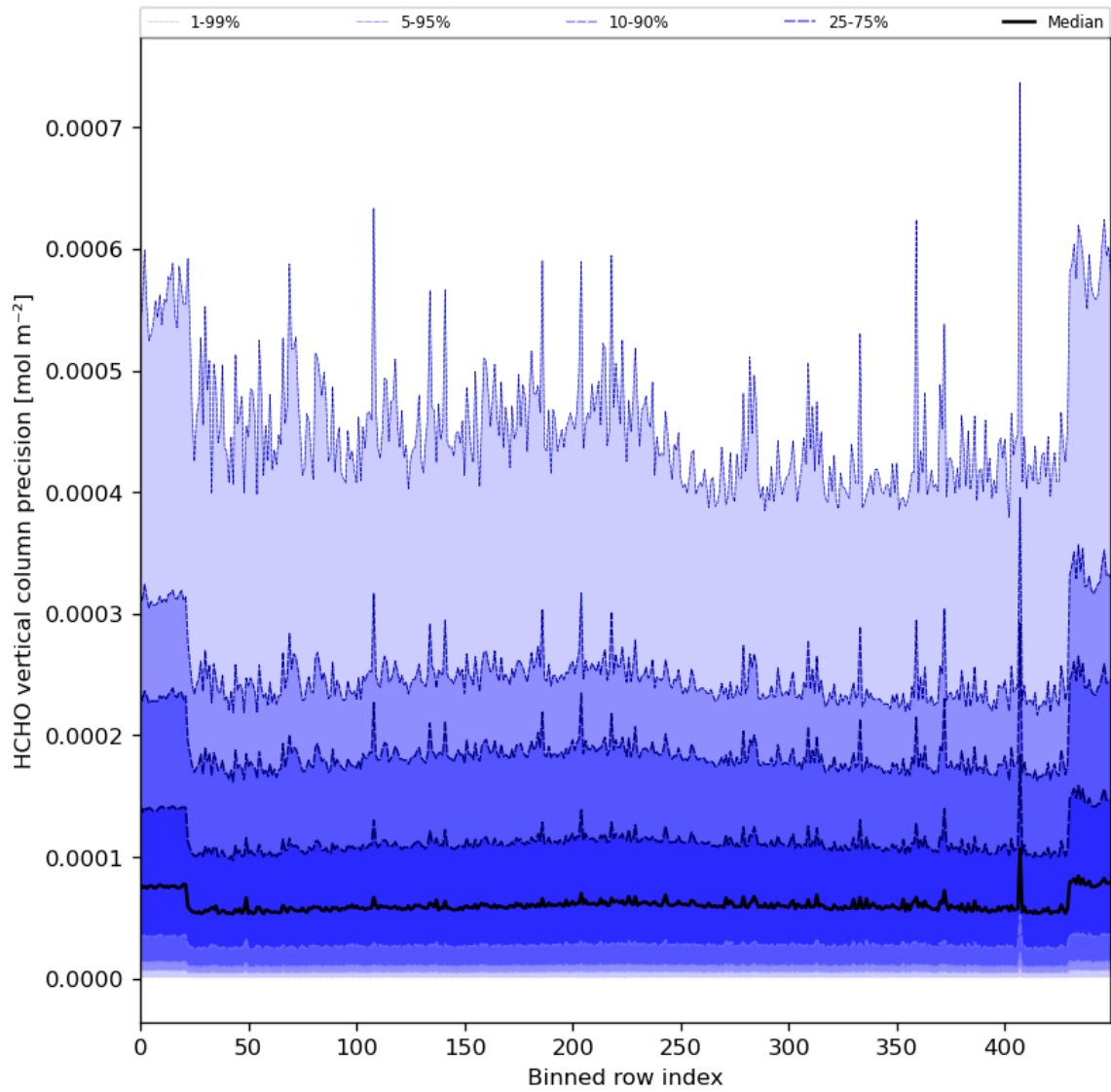
Figure 50: Along track statistics of "HCHO vertical column precision" for 2024-02-11 to 2024-02-12
