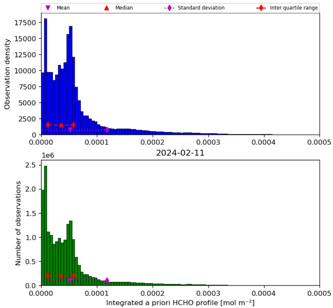
Figure 43: Histogram of “Integrated a priori HCHO profile” for 2024-02-11 to 2024-02-12
