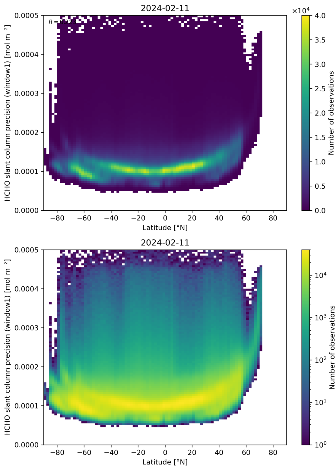
Figure 160: Scatter density plot of “Latitude” against “HCHO slant column precision (window1)” for 2024-02-11 to 2024-02-12.
