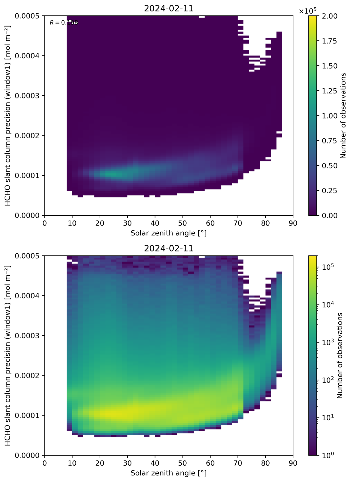
Figure 174: Scatter density plot of “Solar zenith angle” against “HCHO slant column precision (window1)” for 2024-02-11 to 2024-02-12.
