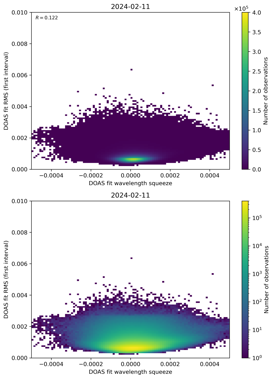
Figure 68: Scatter density plot of “DOAS fit wavelength squeeze” against “DOAS fit RMS (first interval)” for 2024-02-11 to 2024-02-12.
