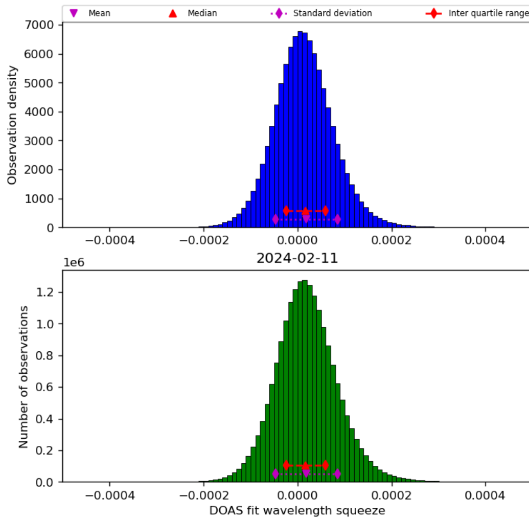
Figure 45: Histogram of “DOAS fit wavelength squeeze” for 2024-02-11 to 2024-02-12
