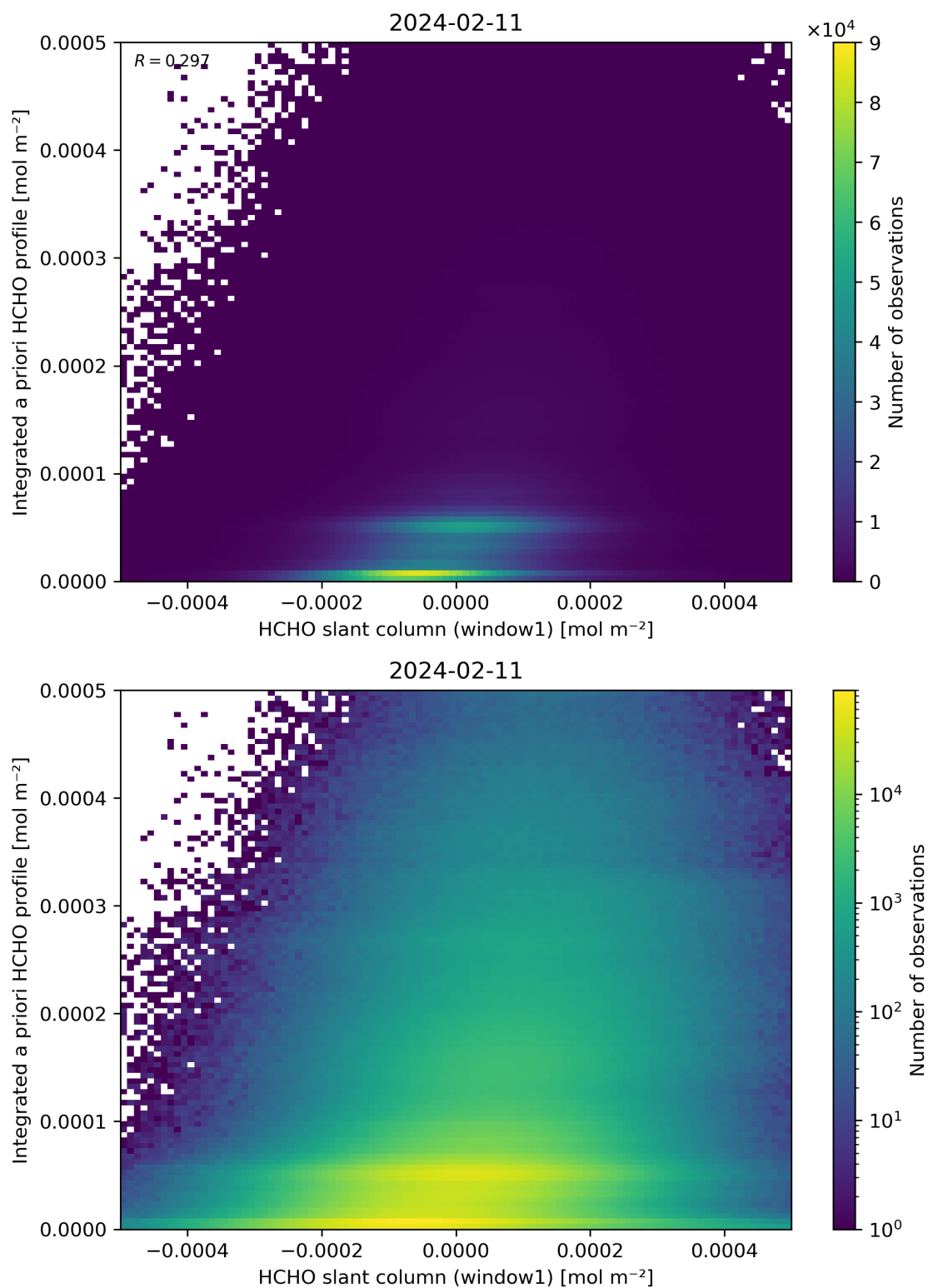
Figure 87: Scatter density plot of “HCHO slant column (window1)” against “Integrated a priori HCHO profile” for 2024-02-11 to 2024-02-12.
