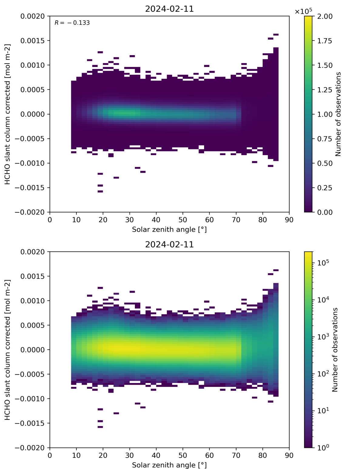
Figure 171: Scatter density plot of “Solar zenith angle” against “HCHO slant column corrected” for 2024-02-11 to 2024-02-12.
