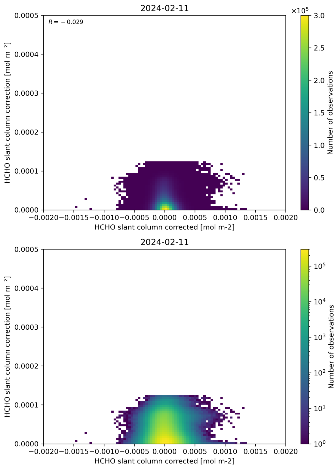
Figure 77: Scatter density plot of “HCHO slant column corrected” against “HCHO slant column correction” for 2024-02-11 to 2024-02-12.
