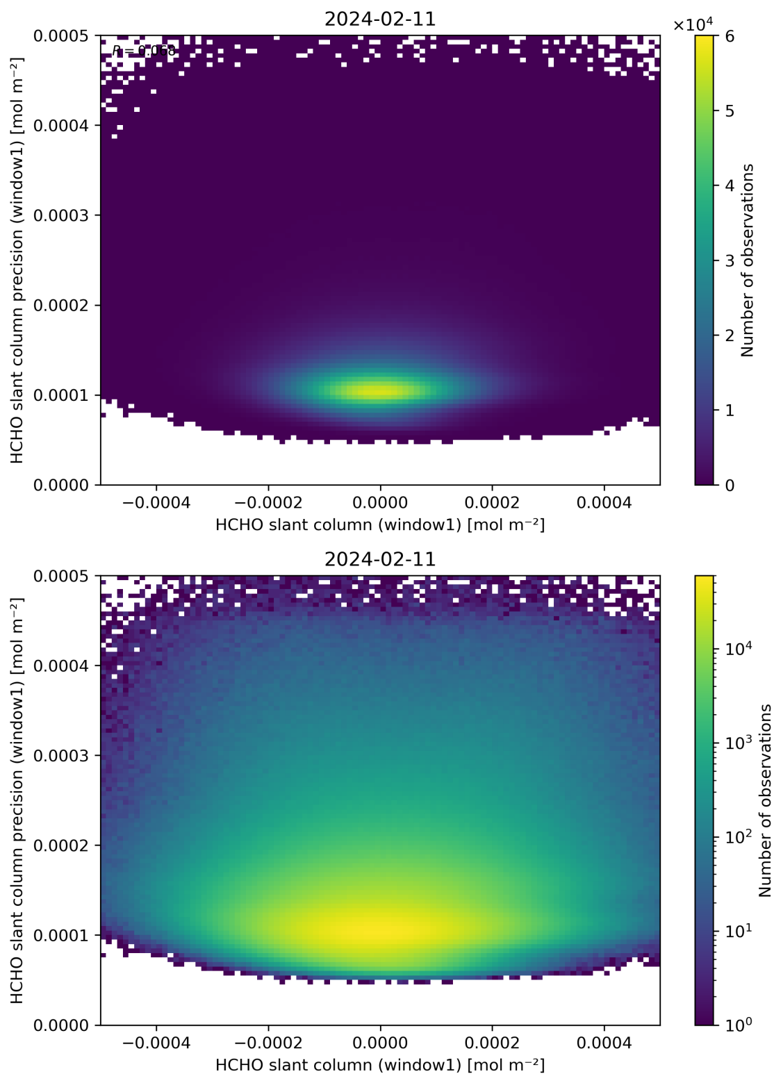
Figure 84: Scatter density plot of “HCHO slant column (window1)” against “HCHO slant column precision (window1)” for 2024-02-11 to 2024-02-12.
