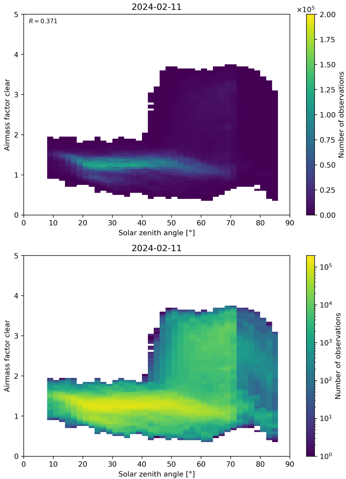
Figure 170: Scatter density plot of “Solar zenith angle” against “Airmass factor clear” for 2024-02-11 to 2024-02-12.
