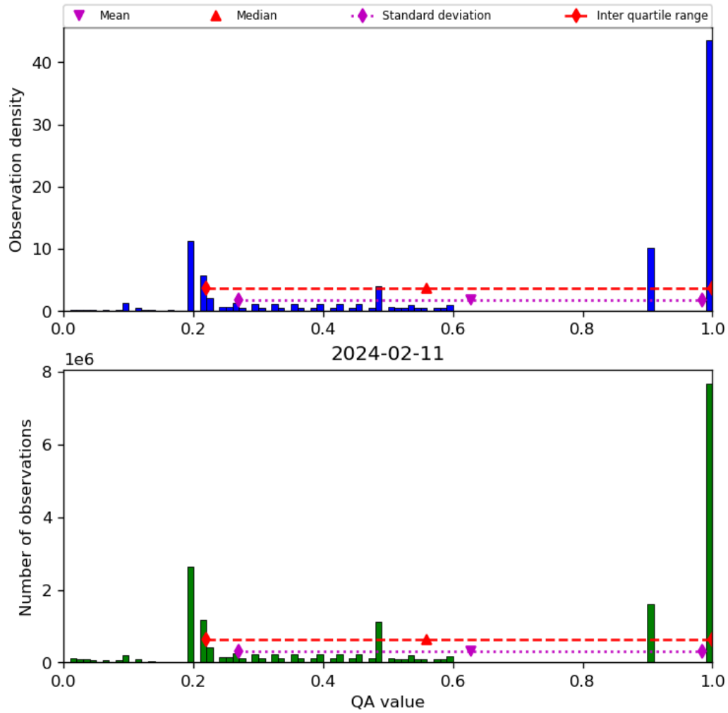
Figure 34: Histogram of “QA value” for 2024-02-11 to 2024-02-12
