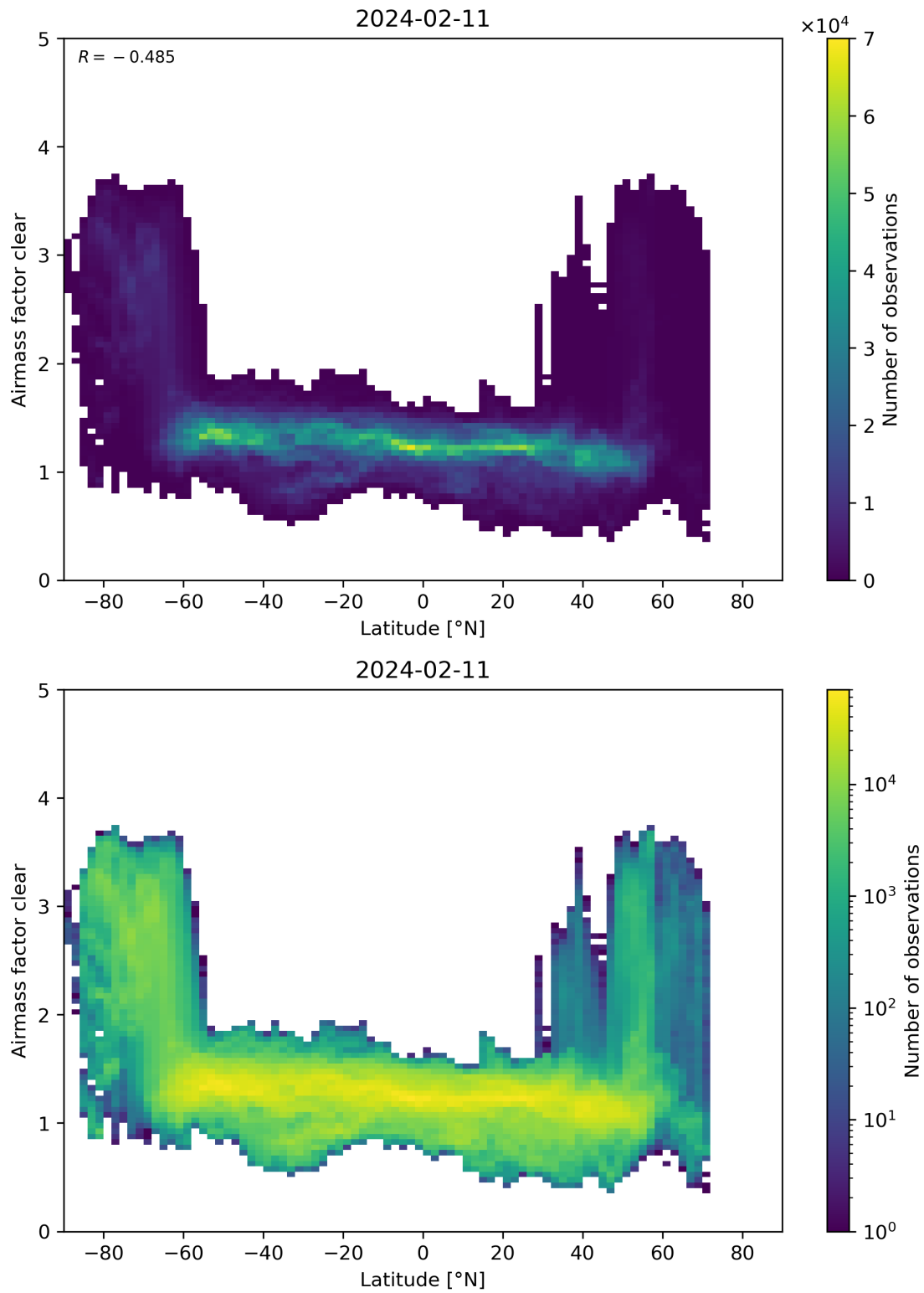
Figure 156: Scatter density plot of “Latitude” against “Airmass factor clear” for 2024-02-11 to 2024-02-12.
