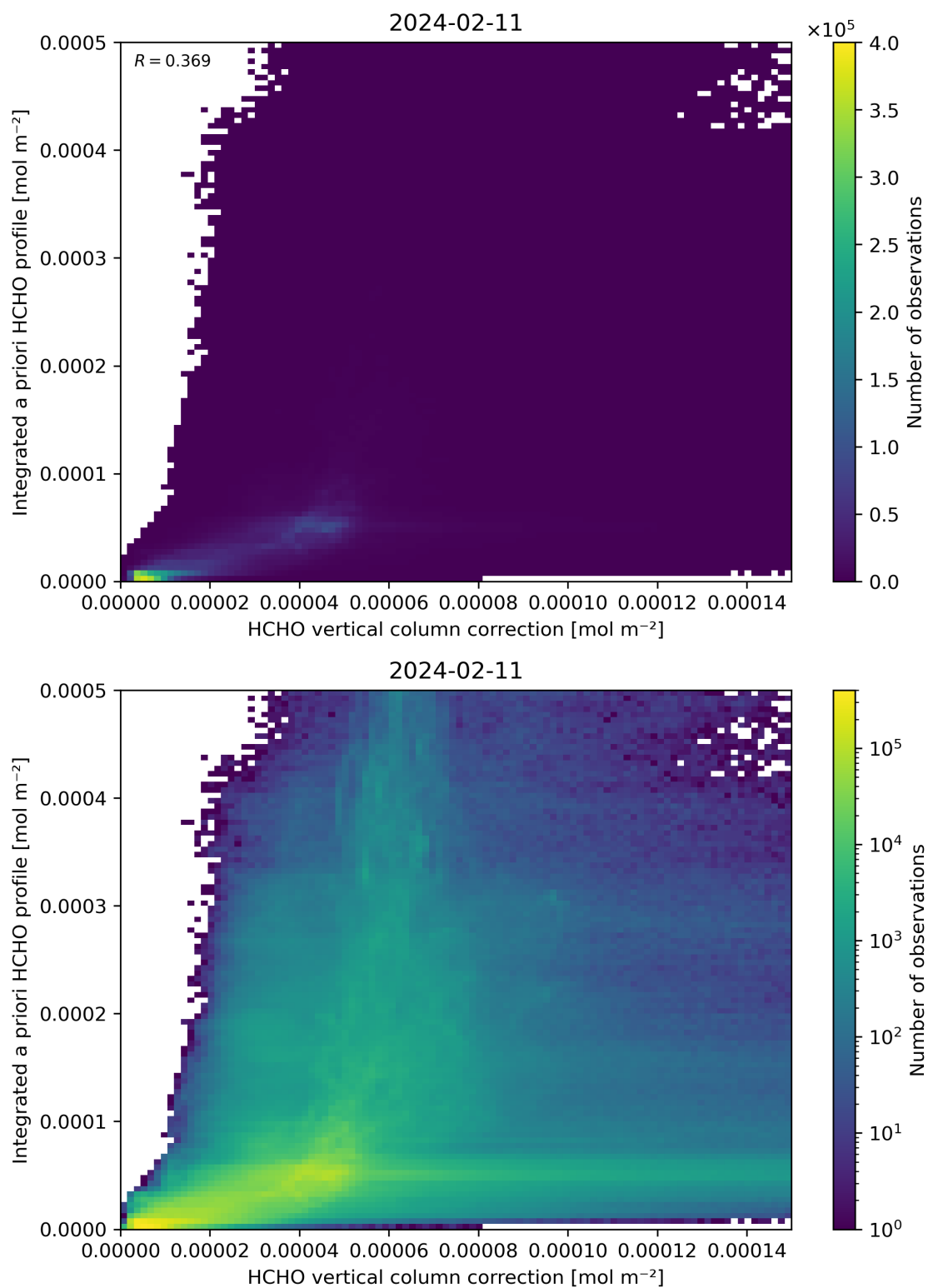
Figure 122: Scatter density plot of “HCHO vertical column correction” against “Integrated a priori HCHO profile” for 2024-02-11 to 2024-02-12.
