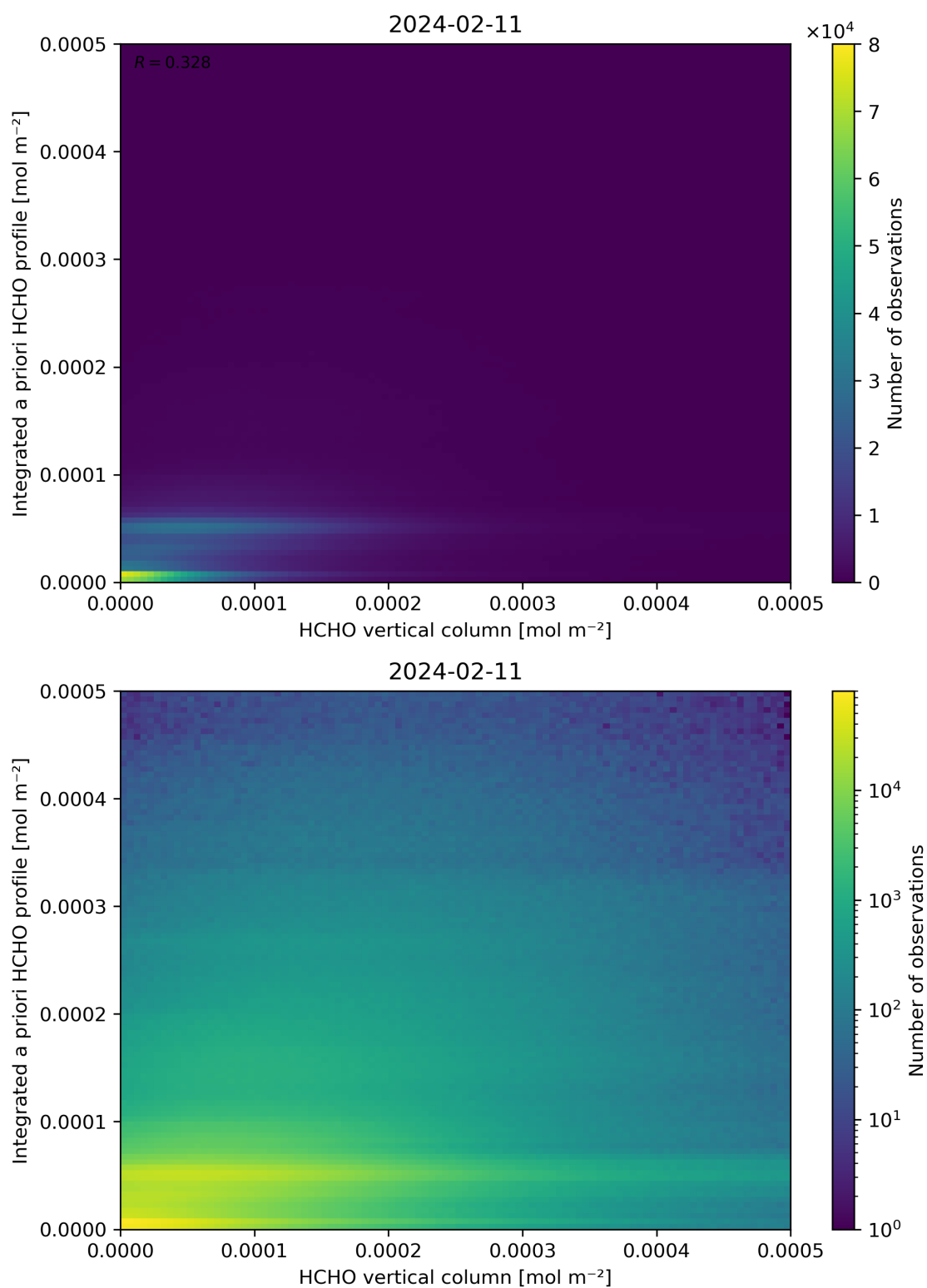
Figure 135: Scatter density plot of “HCHO vertical column” against “Integrated a priori HCHO profile” for 2024-02-11 to 2024-02-12.
