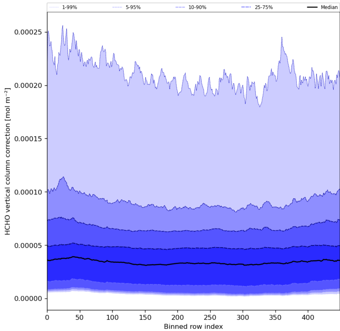
Figure 51: Along track statistics of “HCHO vertical column correction” for 2024-02-11 to 2024-02-12
