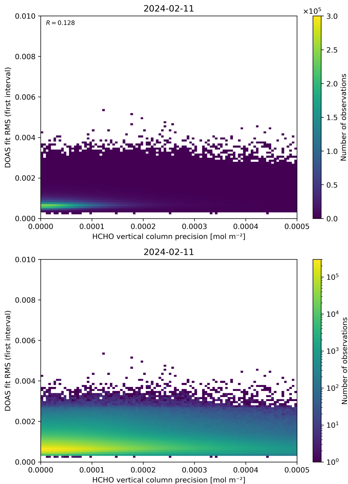
Figure 136: Scatter density plot of “HCHO vertical column precision” against “DOAS fit RMS (first interval)” for 2024-02-11 to 2024-02-12.
