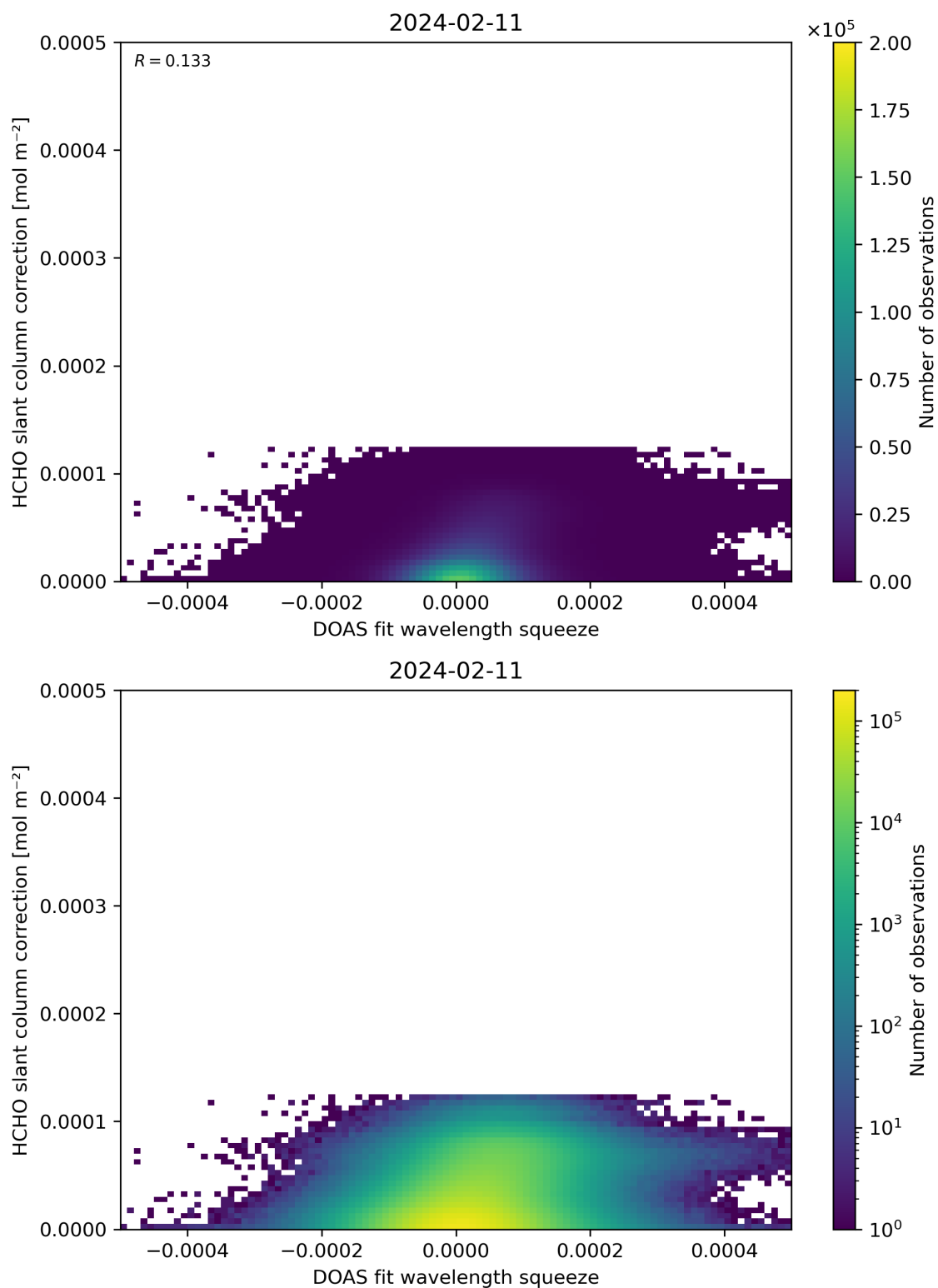
Figure 70: Scatter density plot of “DOAS fit wavelength squeeze” against “HCHO slant column correction” for 2024-02-11 to 2024-02-12.
