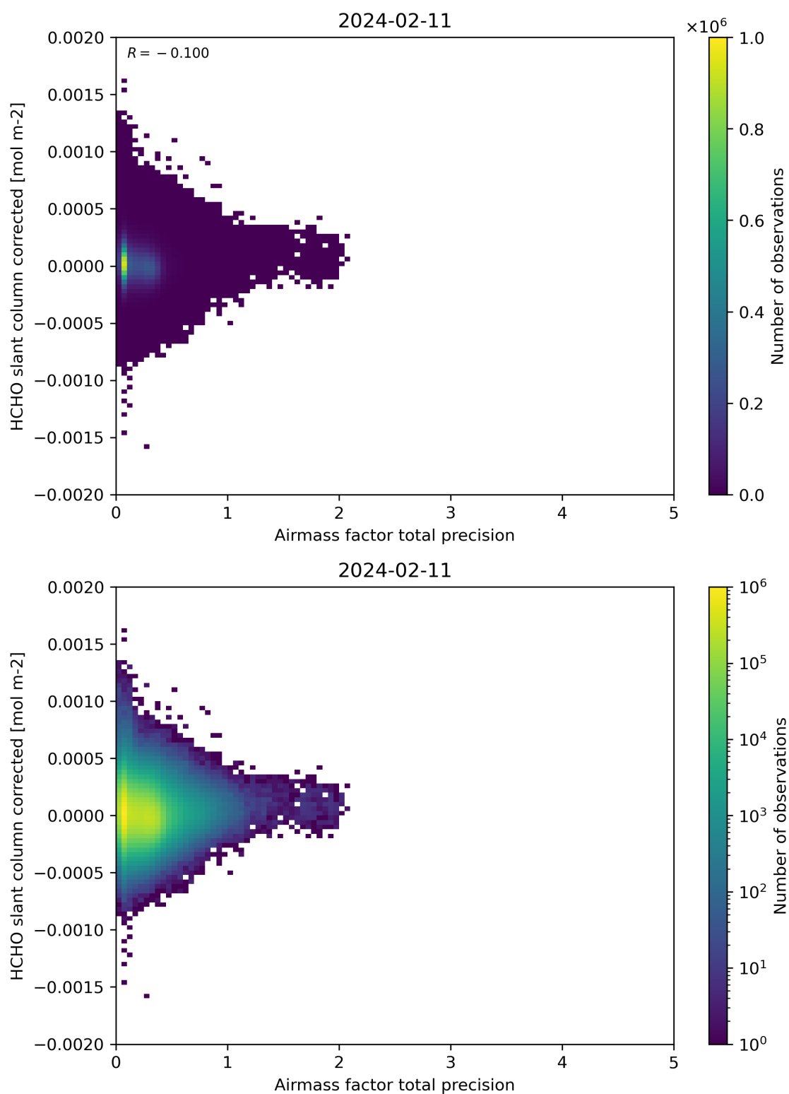
Figure 109: Scatter density plot of “Airmass factor total precision” against “HCHO slant column corrected” for 2024-02-11 to 2024-02-12.
