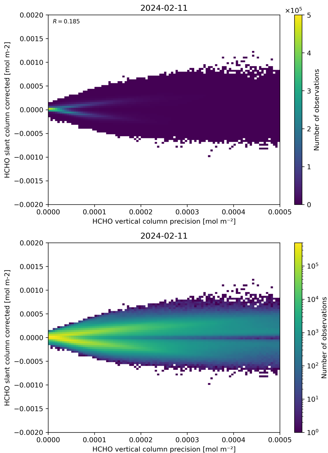
Figure 140: Scatter density plot of “HCHO vertical column precision” against “HCHO slant column corrected” for 2024-02-11 to 2024-02-12.
