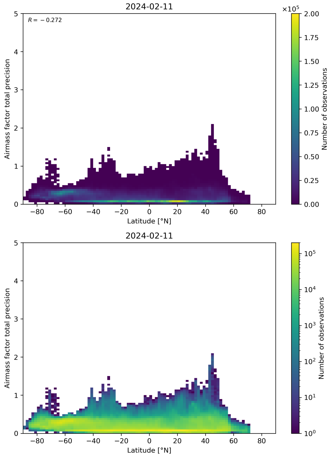
Figure 162: Scatter density plot of “Latitude” against “Airmass factor total precision” for 2024-02-11 to 2024-02-12.
