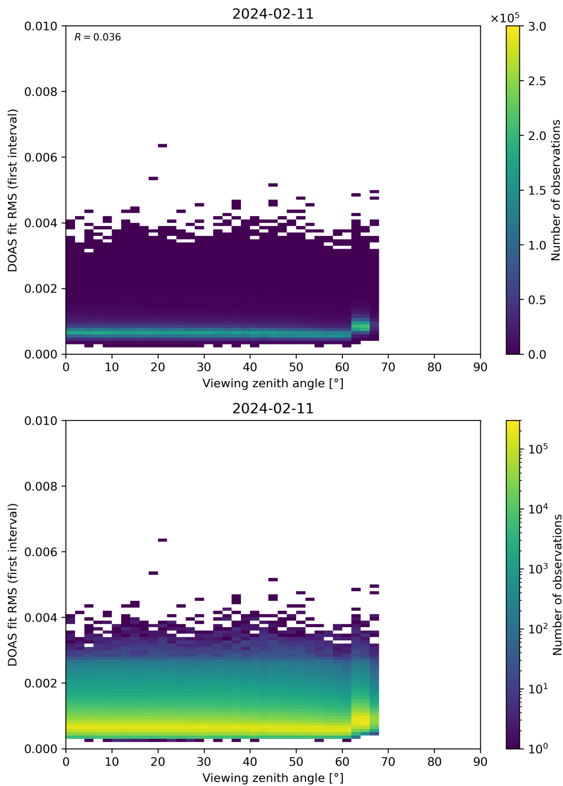
Figure 182: Scatter density plot of “Viewing zenith angle” against “DOAS fit RMS (first interval)” for 2024-02-11 to 2024-02-12.
