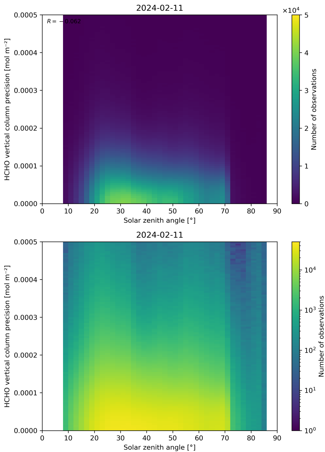
Figure 179: Scatter density plot of “Solar zenith angle” against “HCHO vertical column precision” for 2024-02-11 to 2024-02-12.
