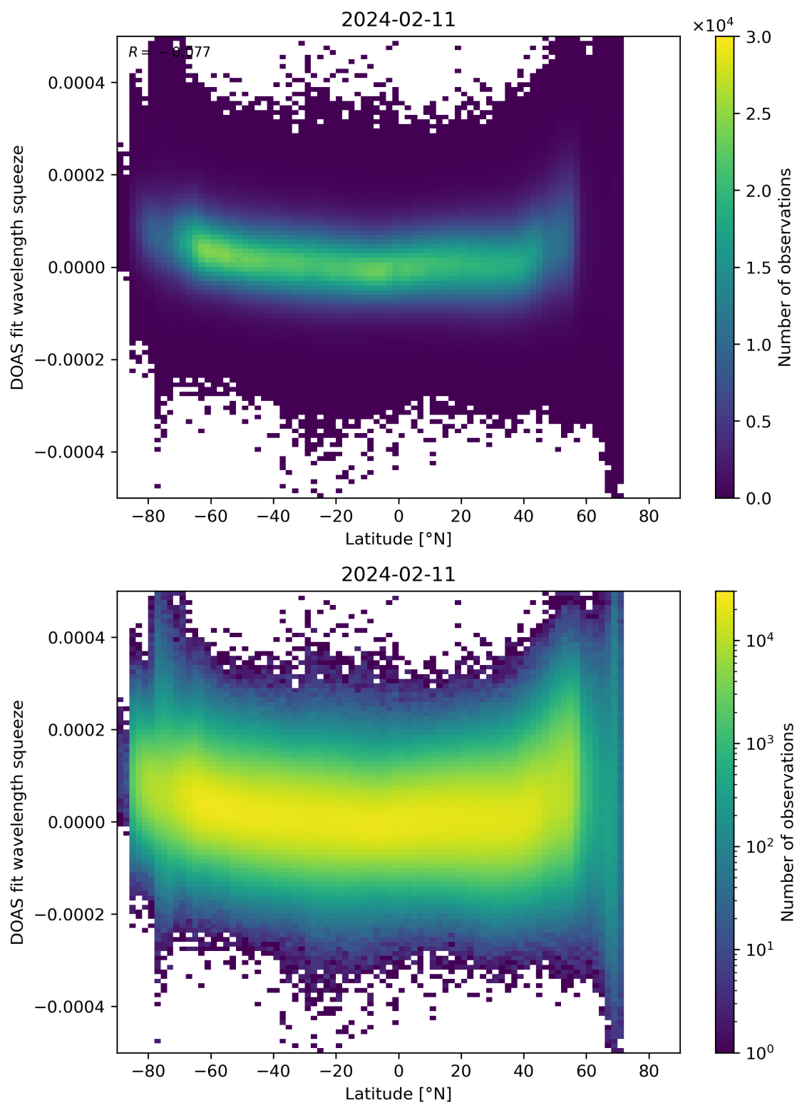
Figure 155: Scatter density plot of “Latitude” against “DOAS fit wavelength squeeze” for 2024-02-11 to 2024-02-12.
