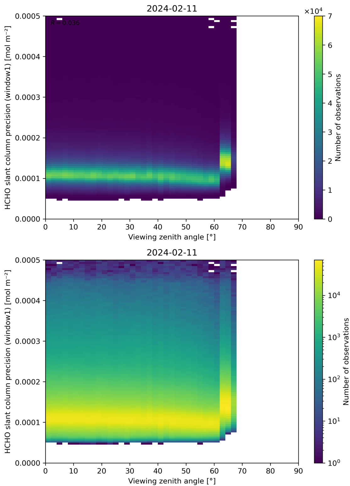
Figure 189: Scatter density plot of “Viewing zenith angle” against “HCHO slant column precision (window1)” for 2024-02-11 to 2024-02-12.
