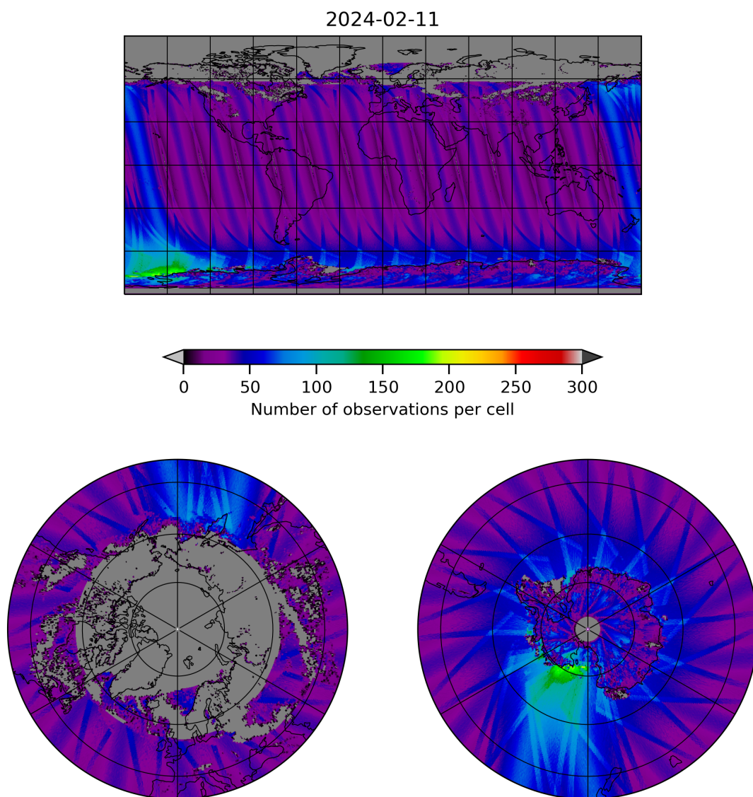
Figure 19: Map of the number of observations for 2024-02-11 to 2024-02-12
