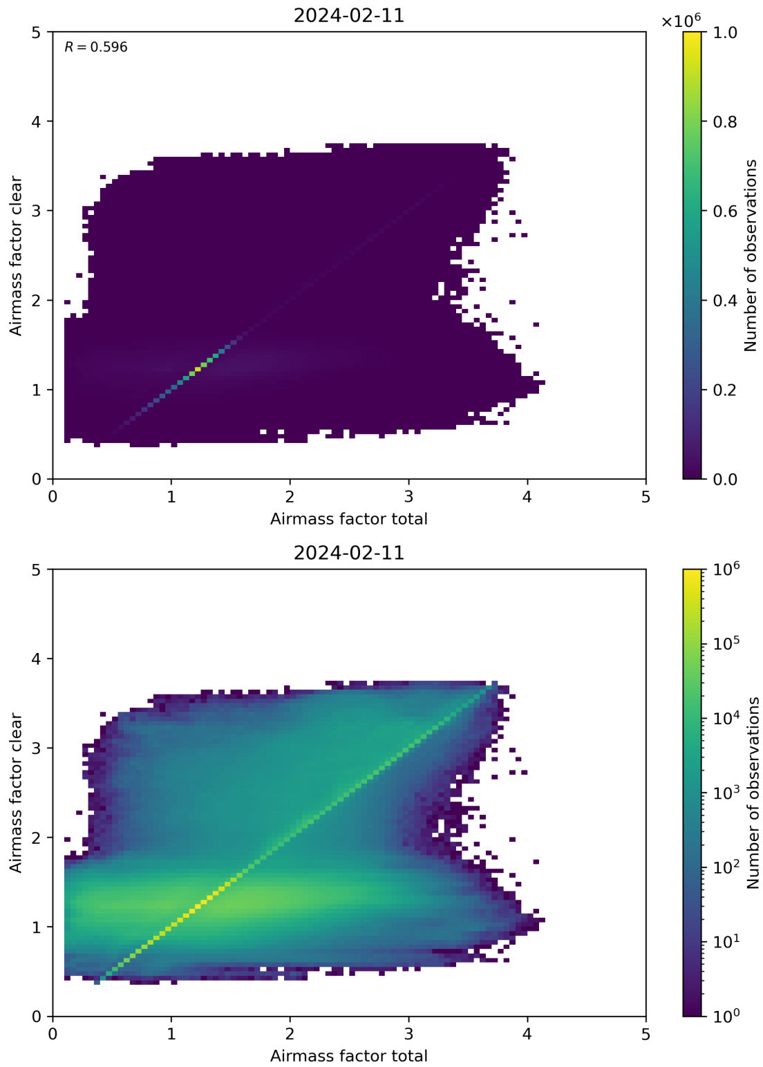
Figure 100: Scatter density plot of “Airmass factor total” against “Airmass factor clear” for 2024-02-11 to 2024-02-12.
