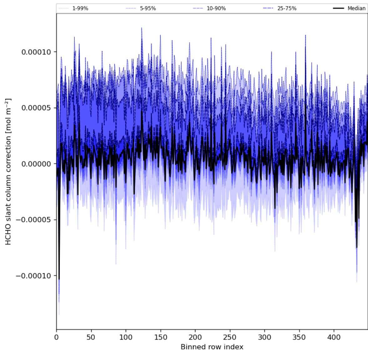
Figure 61: Along track statistics of “HCHO slant column correction” for 2024-02-11 to 2024-02-12
