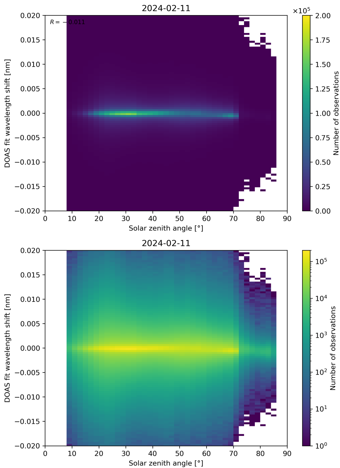
Figure 168: Scatter density plot of “Solar zenith angle” against “DOAS fit wavelength shift” for 2024-02-11 to 2024-02-12.
