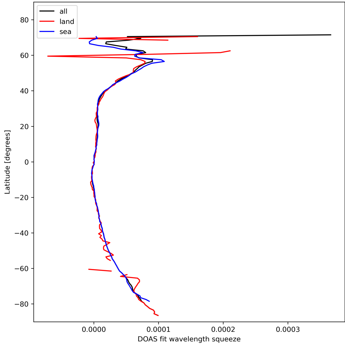
Figure 31: Zonal average of “DOAS fit wavelength squeeze” for 2024-02-11 to 2024-02-12.
