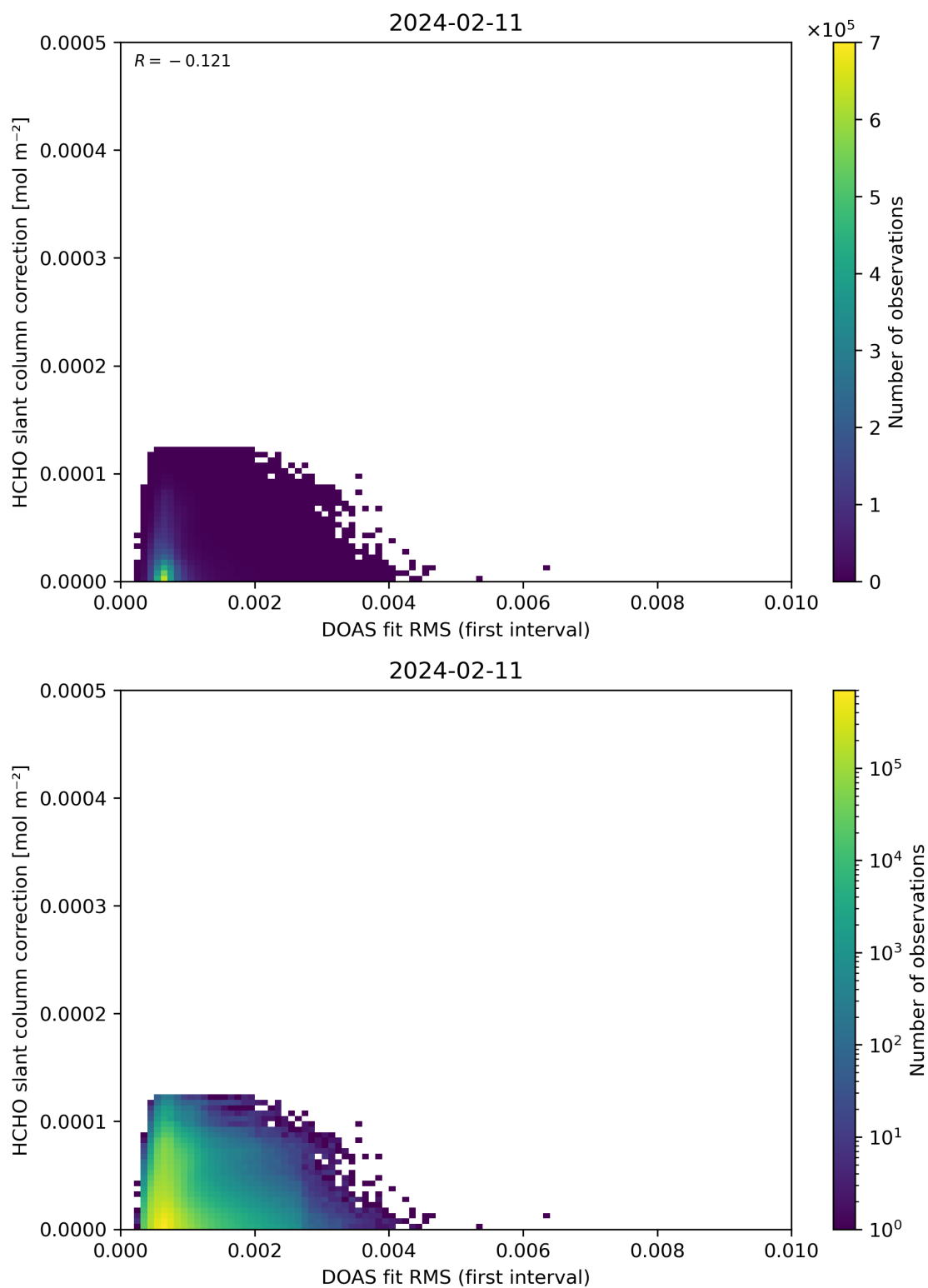
Figure 63: Scatter density plot of “DOAS fit RMS (first interval)” against “HCHO slant column correction” for 2024-02-11 to 2024-02-12.
