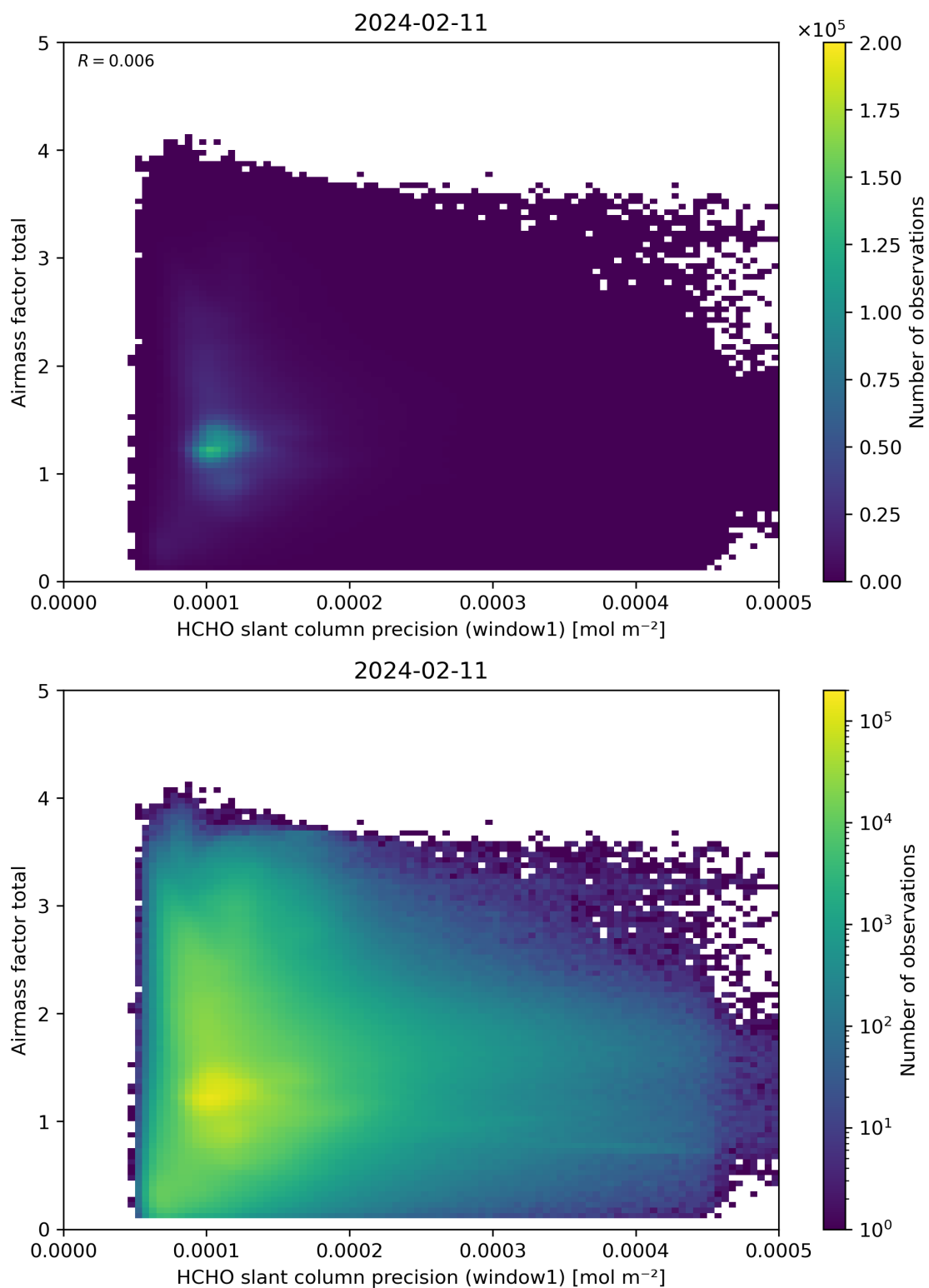
Figure 94: Scatter density plot of “HCHO slant column precision (window1)” against “Airmass factor total” for 2024-02-11 to 2024-02-12.
