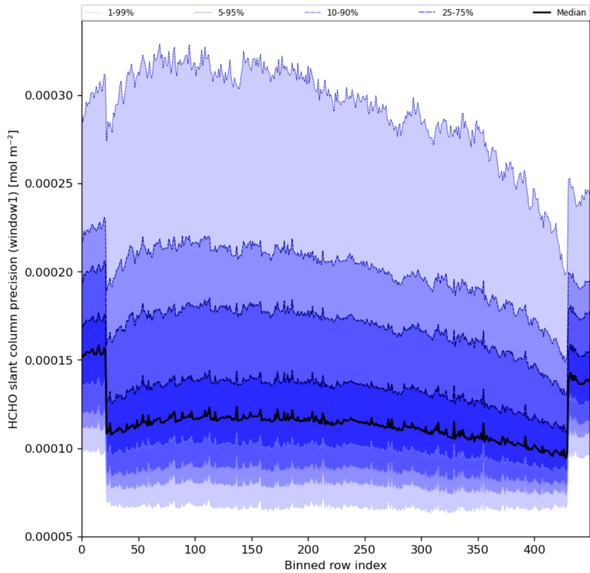
Figure 53: Along track statistics of “HCHO slant column precision (window1)” for 2024-02-11 to 2024-02-12
