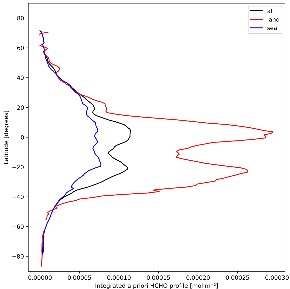
Figure 29: Zonal average of “Integrated a priori HCHO profile” for 2024-02-11 to 2024-02-12.
