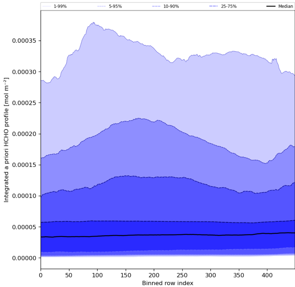
Figure 57: Along track statistics of “Integrated a priori HCHO profile” for 2024-02-11 to 2024-02-12
