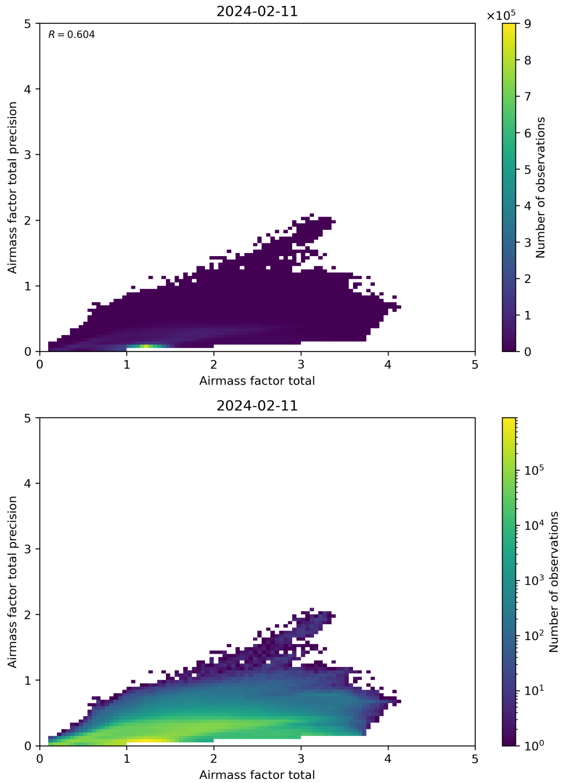
Figure 103: Scatter density plot of “Airmass factor total” against “Airmass factor total precision” for 2024-02-11 to 2024-02-12.
