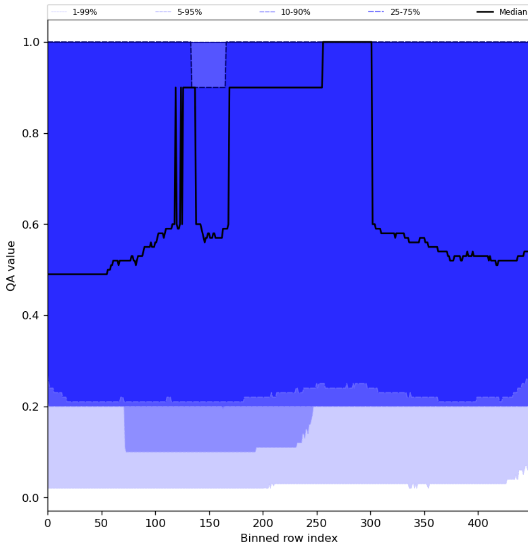
Figure 48: Along track statistics of “QA value” for 2024-02-11 to 2024-02-12
