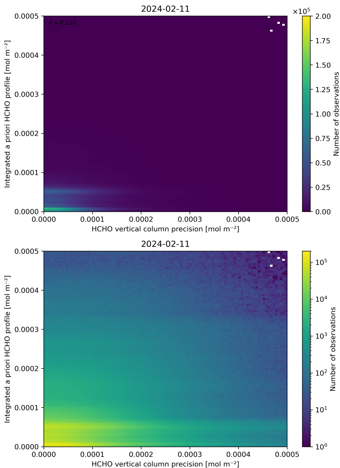
Figure 147: Scatter density plot of “HCHO vertical column precision” against “Integrated a priori HCHO profile” for 2024-02-11 to 2024-02-12.
