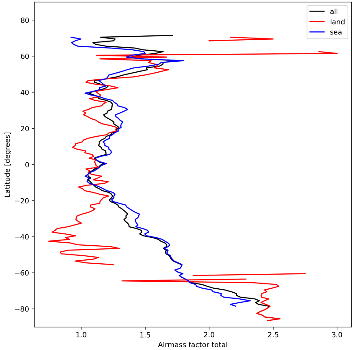
Figure 26: Zonal average of “Airmass factor total” for 2024-02-11 to 2024-02-12.
