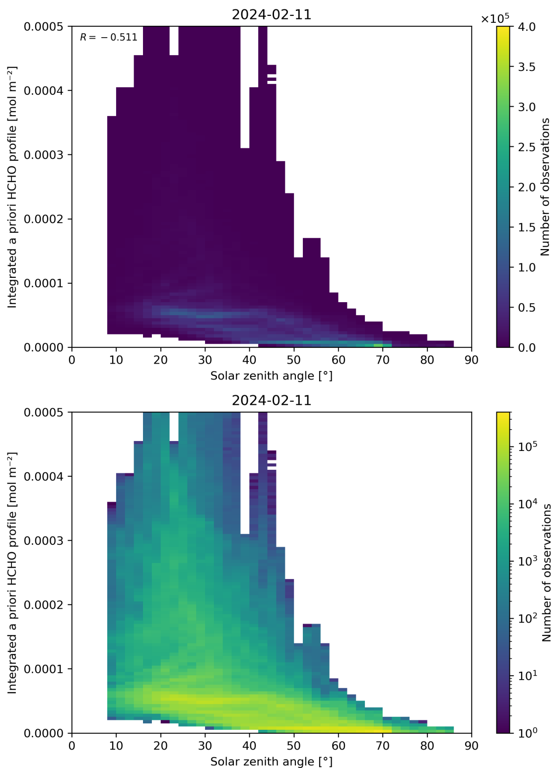
Figure 180: Scatter density plot of “Solar zenith angle” against “Integrated a priori HCHO profile” for 2024-02-11 to 2024-02-12.
