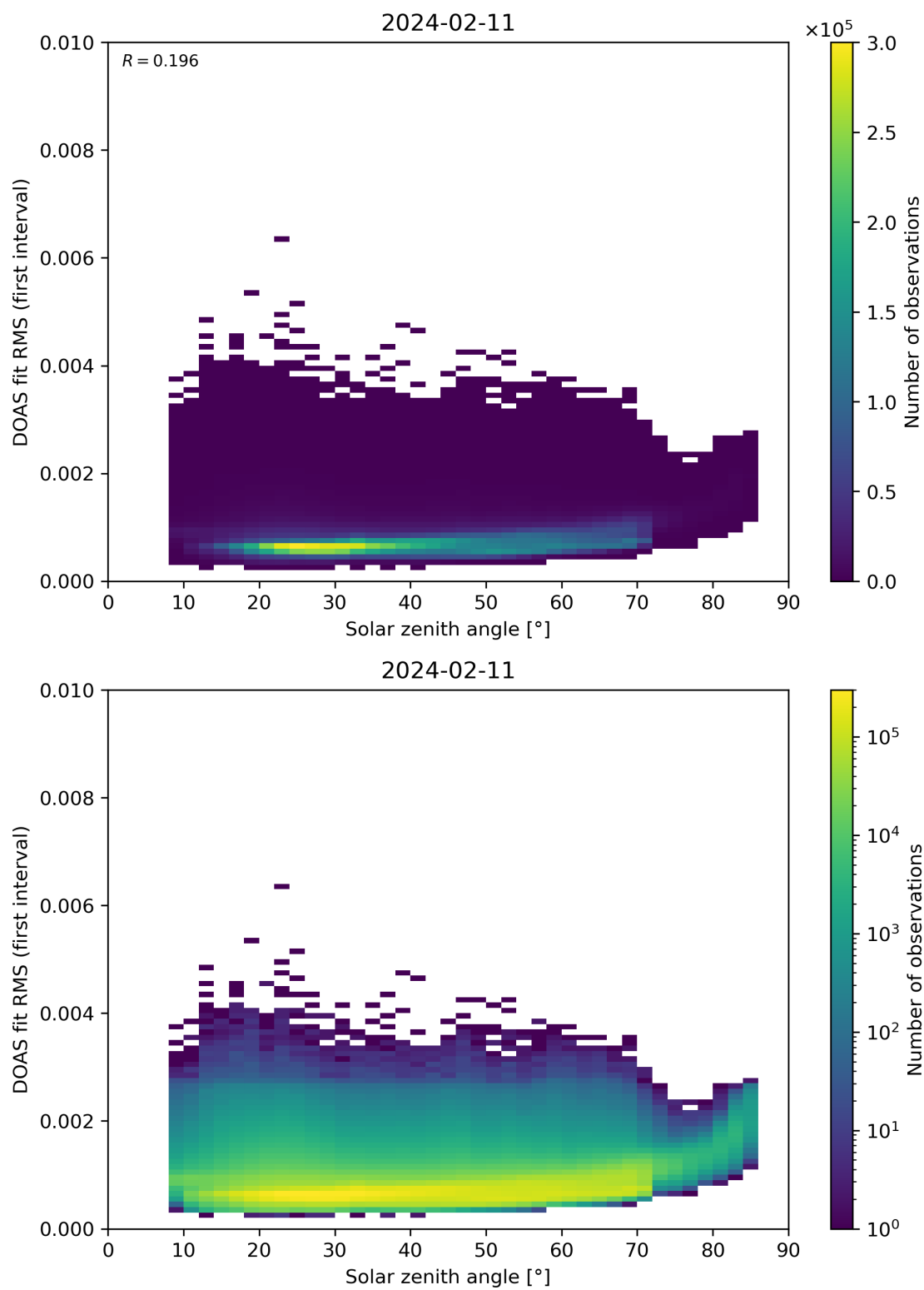
Figure 167: Scatter density plot of “Solar zenith angle” against “DOAS fit RMS (first interval)” for 2024-02-11 to 2024-02-12.
