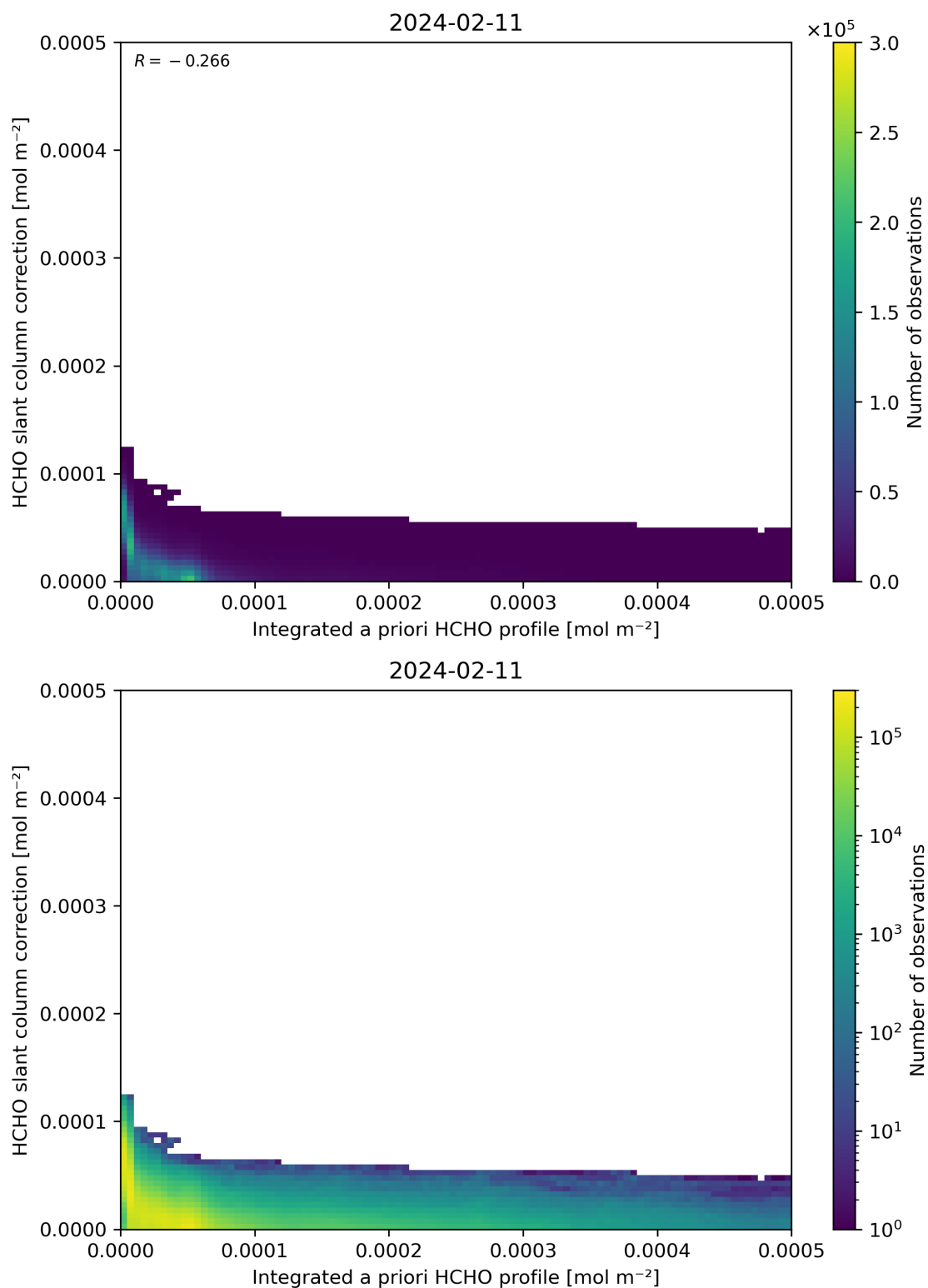
Figure 152: Scatter density plot of “Integrated a priori HCHO profile” against “HCHO slant column correction” for 2024-02-11 to 2024-02-12.
