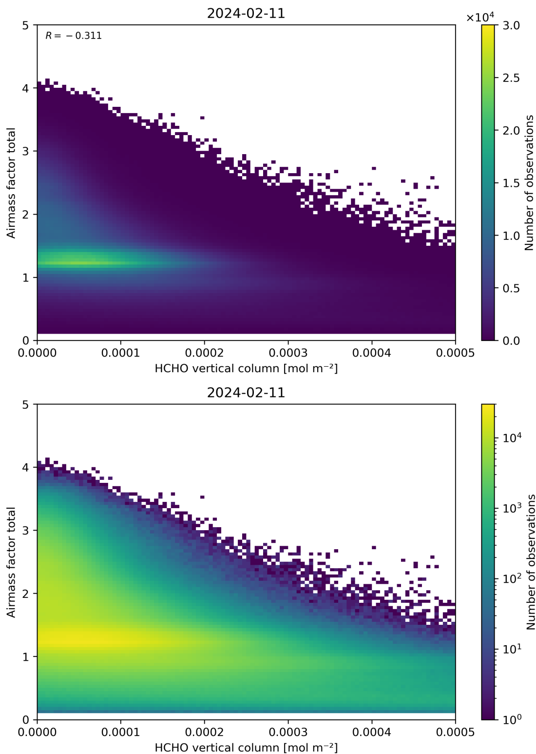
Figure 131: Scatter density plot of “HCHO vertical column” against “Airmass factor total” for 2024-02-11 to 2024-02-12.
