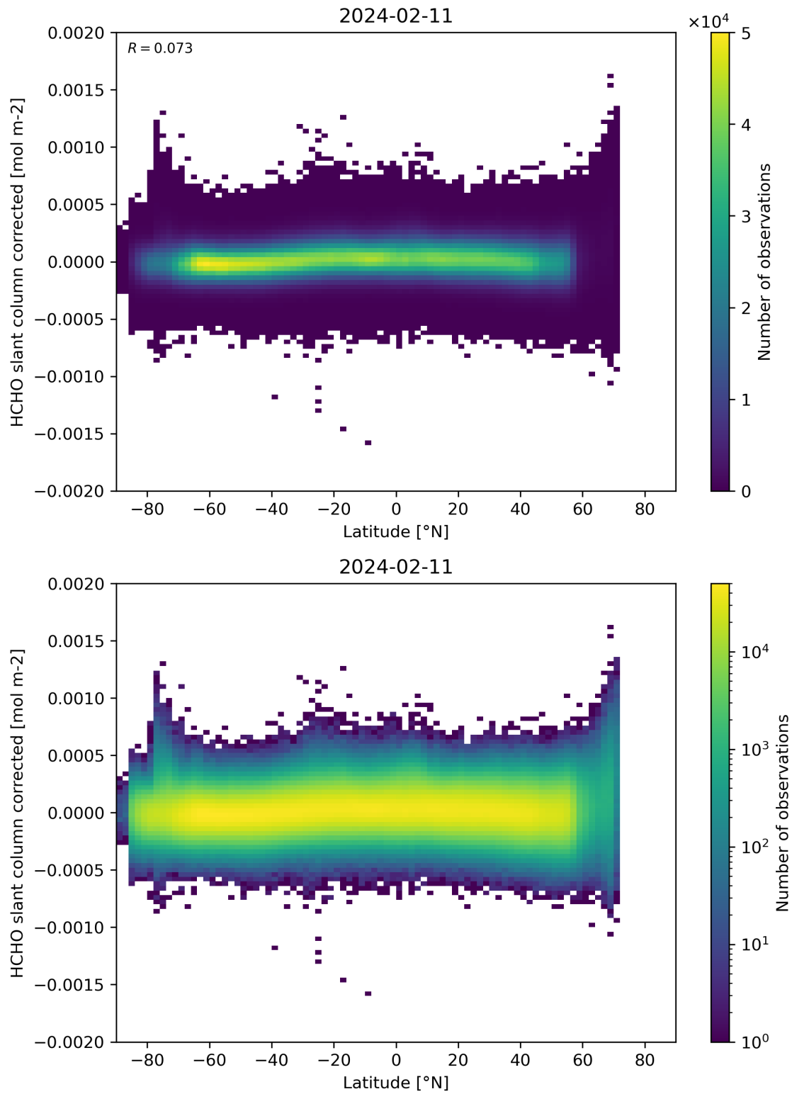
Figure 157: Scatter density plot of “Latitude” against “HCHO slant column corrected” for 2024-02-11 to 2024-02-12.
