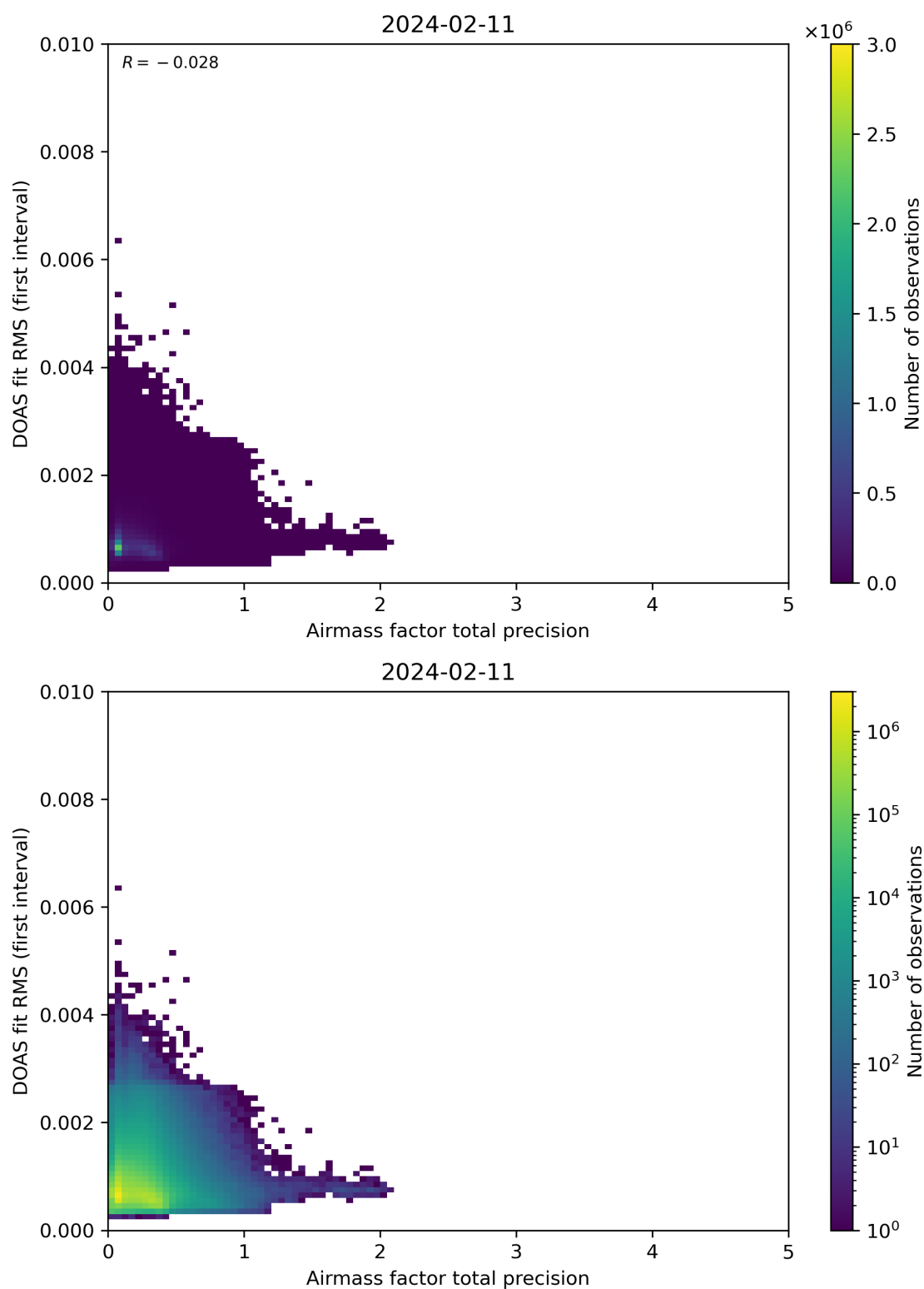
Figure 105: Scatter density plot of “Airmass factor total precision” against “DOAS fit RMS (first interval)” for 2024-02-11 to 2024-02-12.
