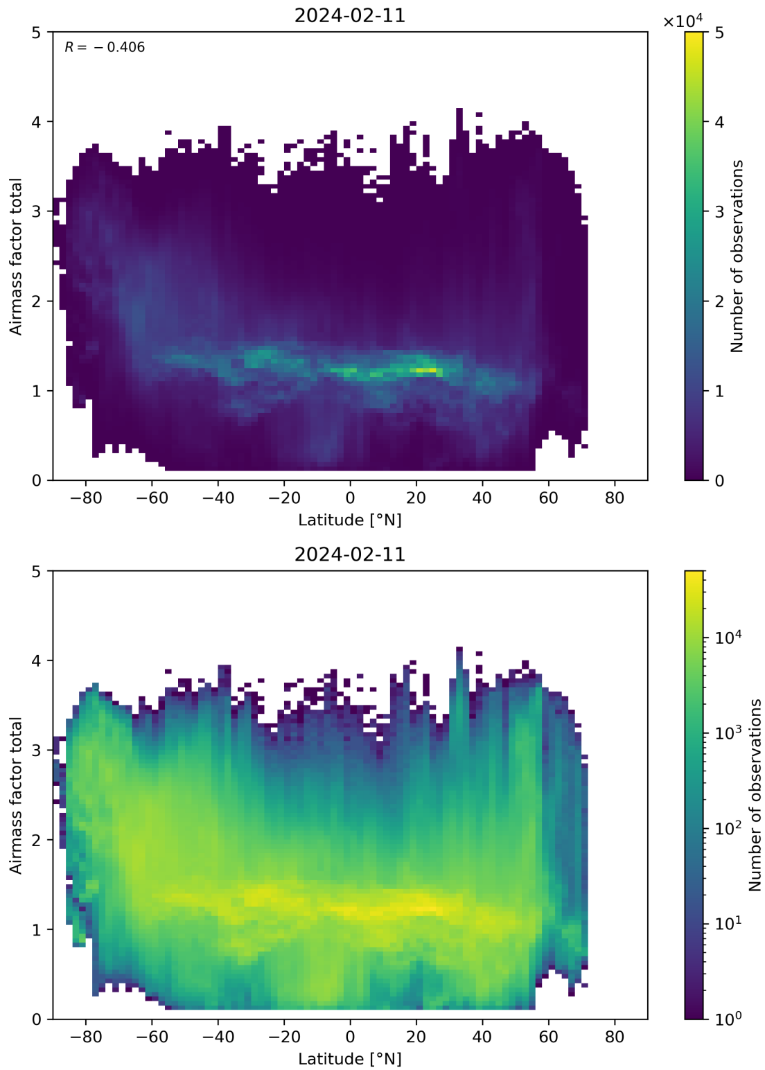
Figure 161: Scatter density plot of “Latitude” against “Airmass factor total” for 2024-02-11 to 2024-02-12.
