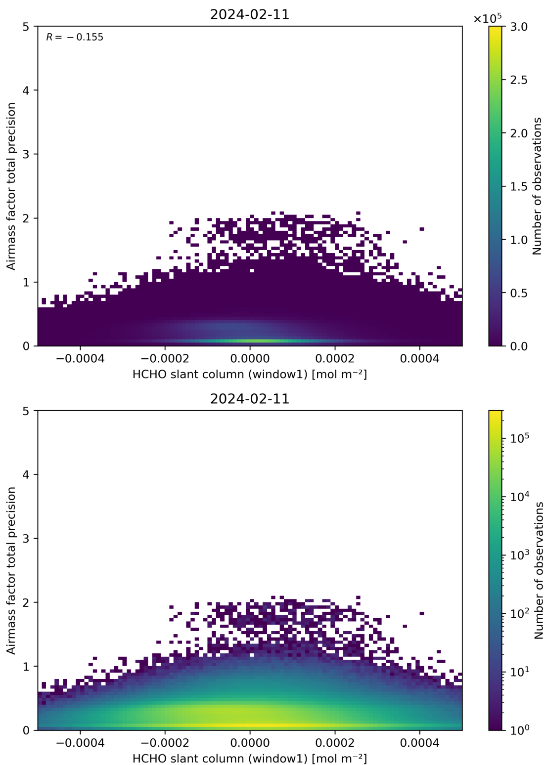
Figure 86: Scatter density plot of “HCHO slant column (window1)” against “Airmass factor total precision” for 2024-02-11 to 2024-02-12.
