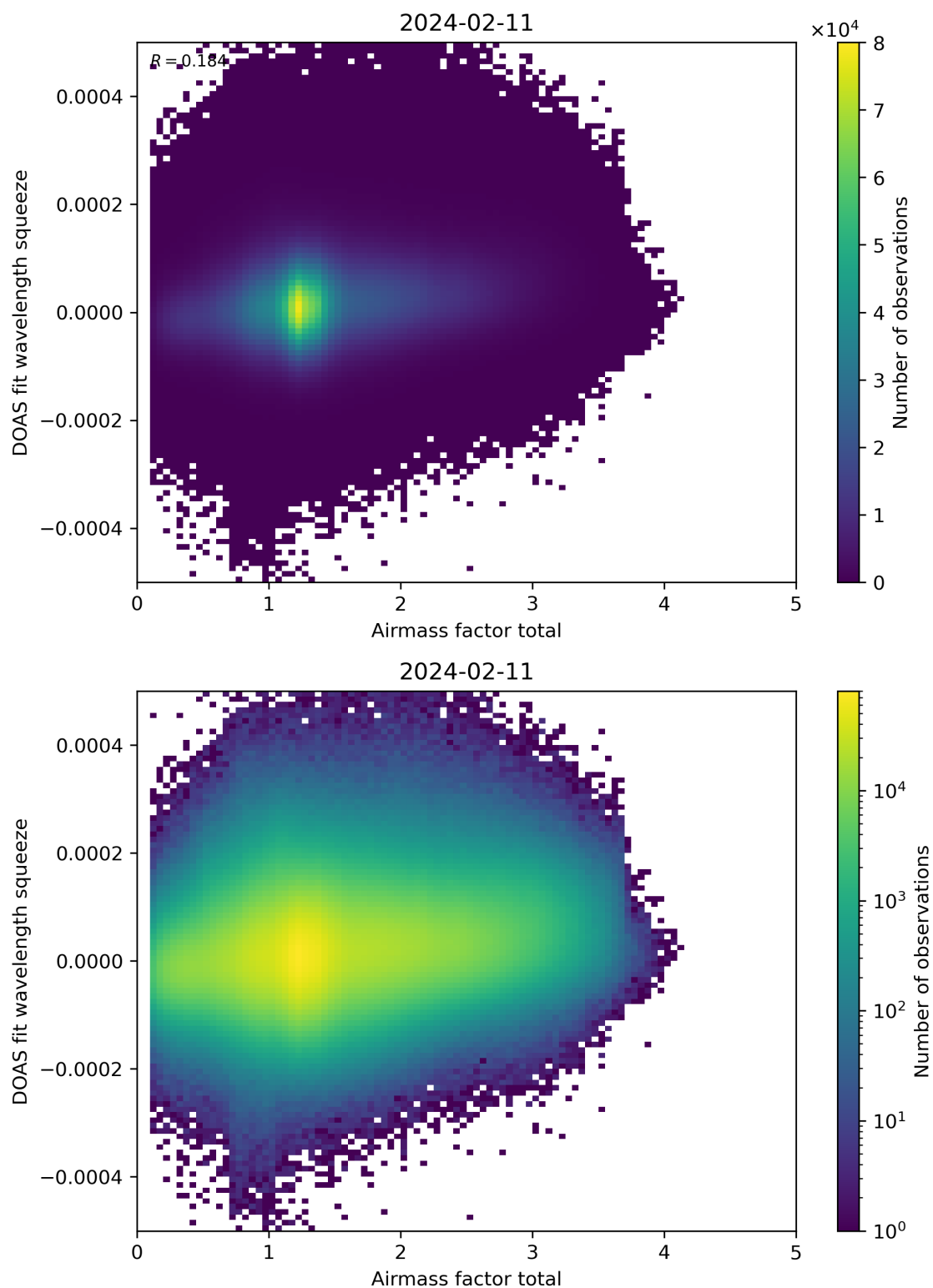
Figure 99: Scatter density plot of “Airmass factor total” against “DOAS fit wavelength squeeze” for 2024-02-11 to 2024-02-12.
