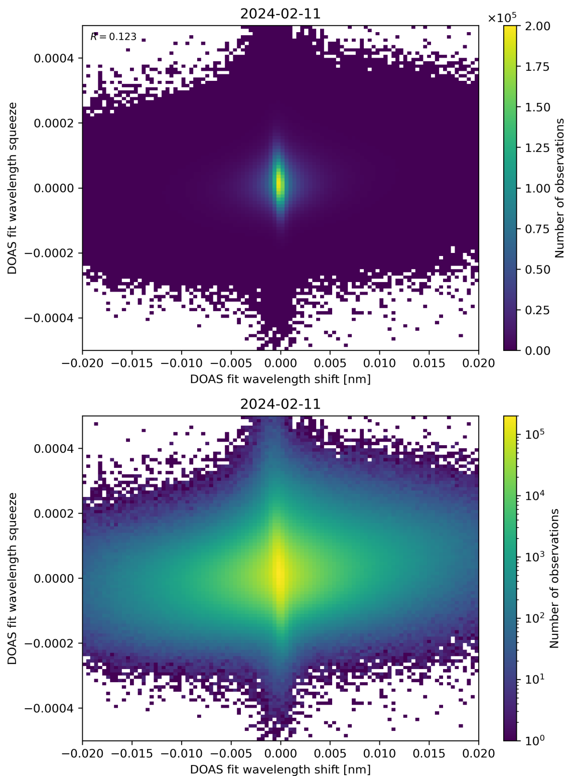
Figure 65: Scatter density plot of “DOAS fit wavelength shift” against “DOAS fit wavelength squeeze” for 2024-02-11 to 2024-02-12.
