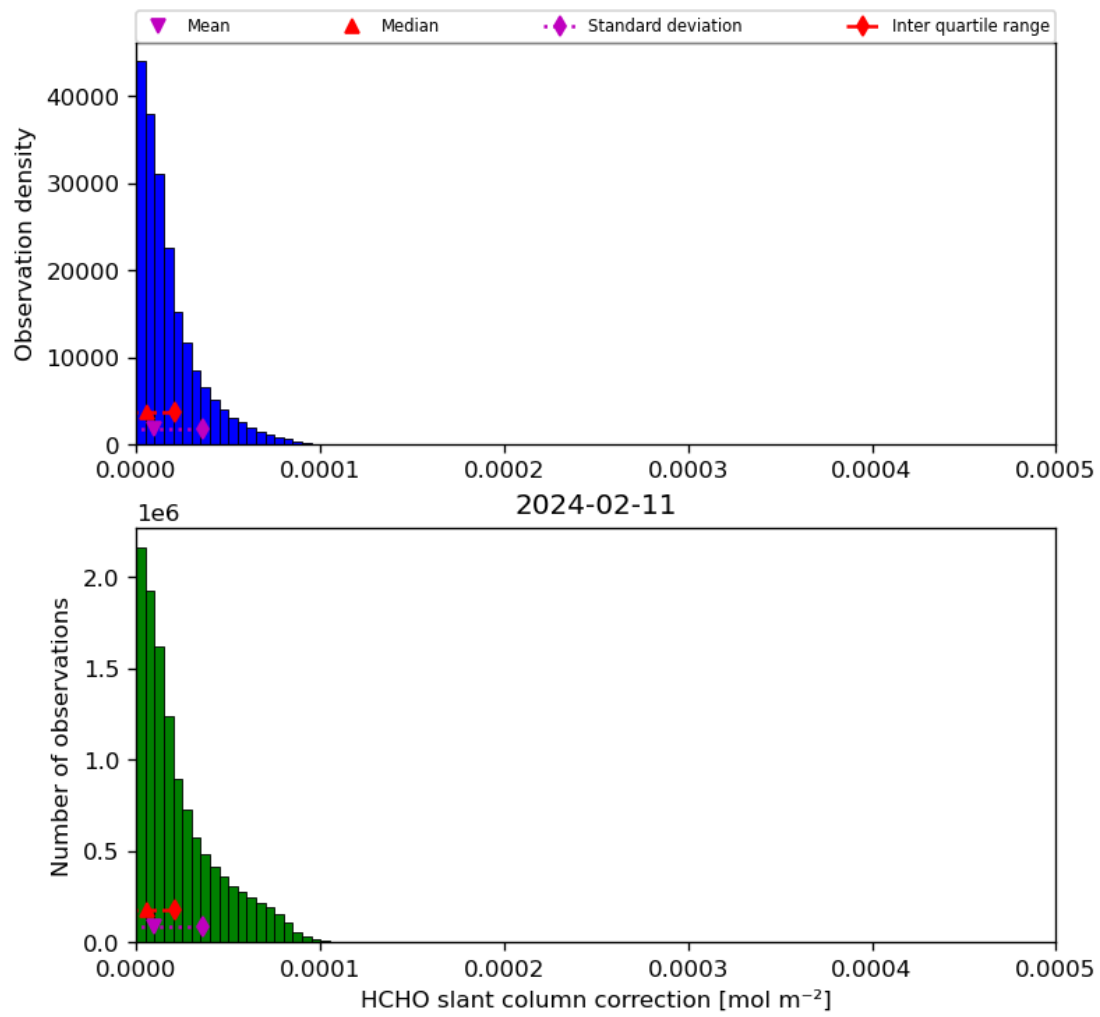
Figure 47: Histogram of “HCHO slant column correction” for 2024-02-11 to 2024-02-12
