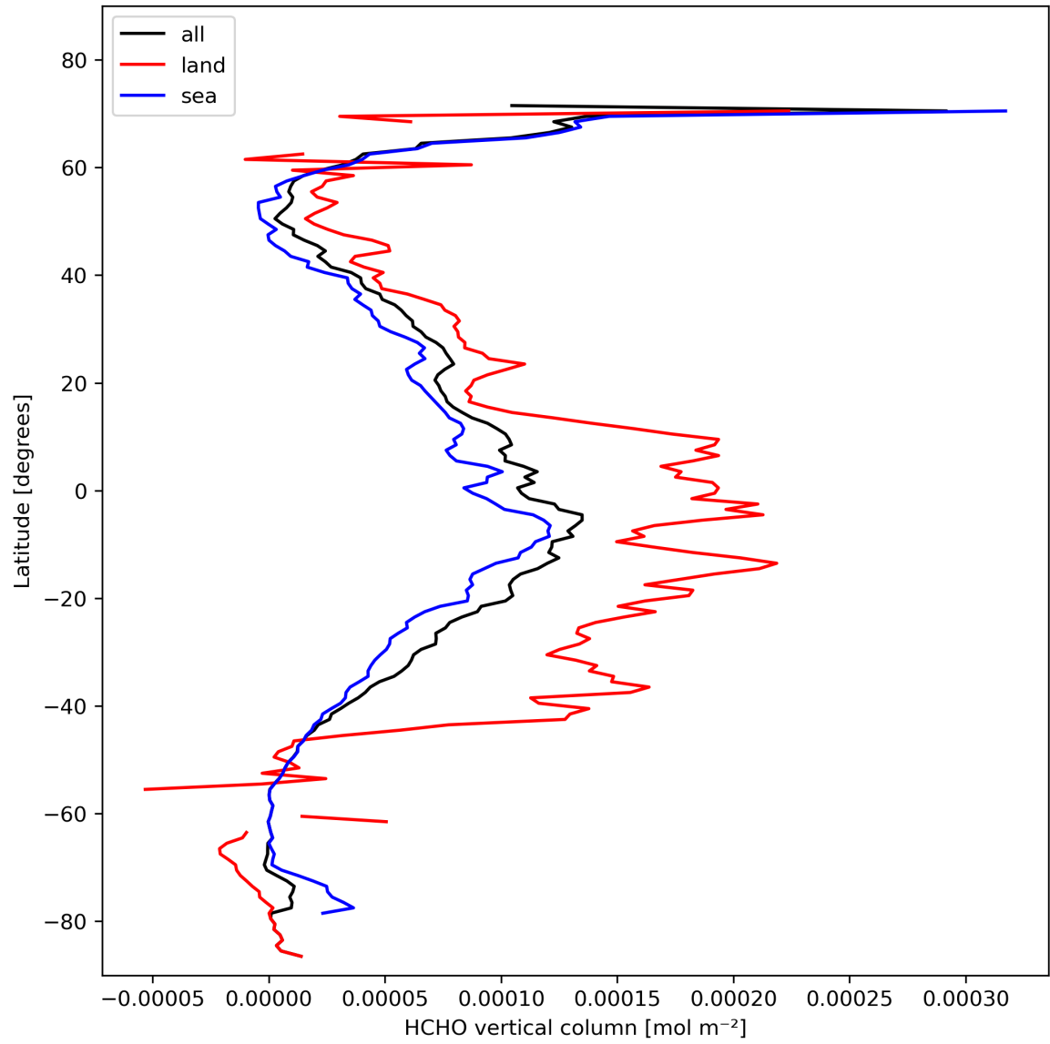
Figure 21: Zonal average of “HCHO vertical column” for 2024-02-11 to 2024-02-12.
