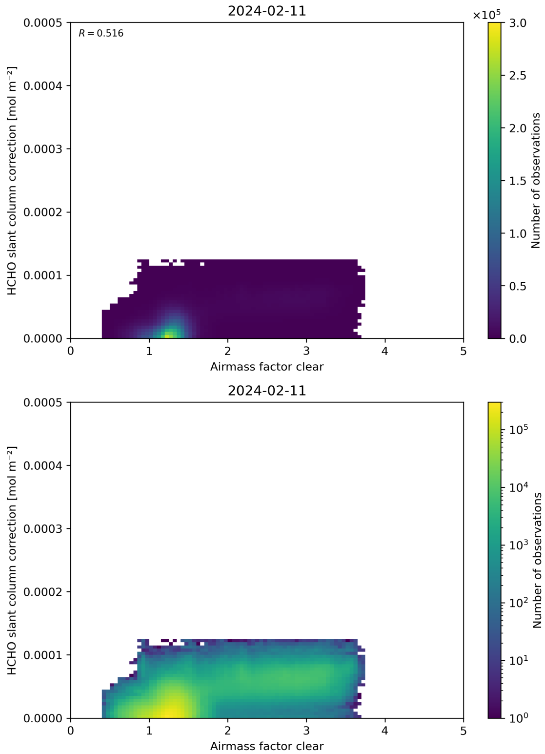
Figure 75: Scatter density plot of “Airmass factor clear” against “HCHO slant column correction” for 2024-02-11 to 2024-02-12.
