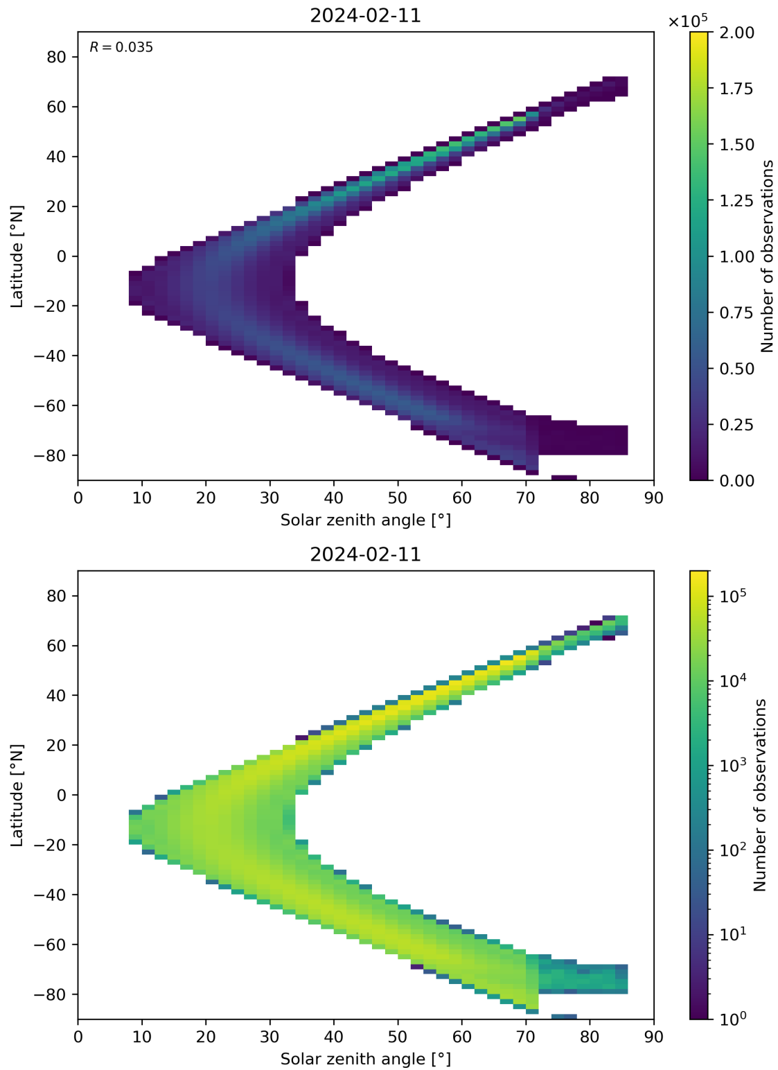
Figure 181: Scatter density plot of “Solar zenith angle” against “Latitude” for 2024-02-11 to 2024-02-12.
