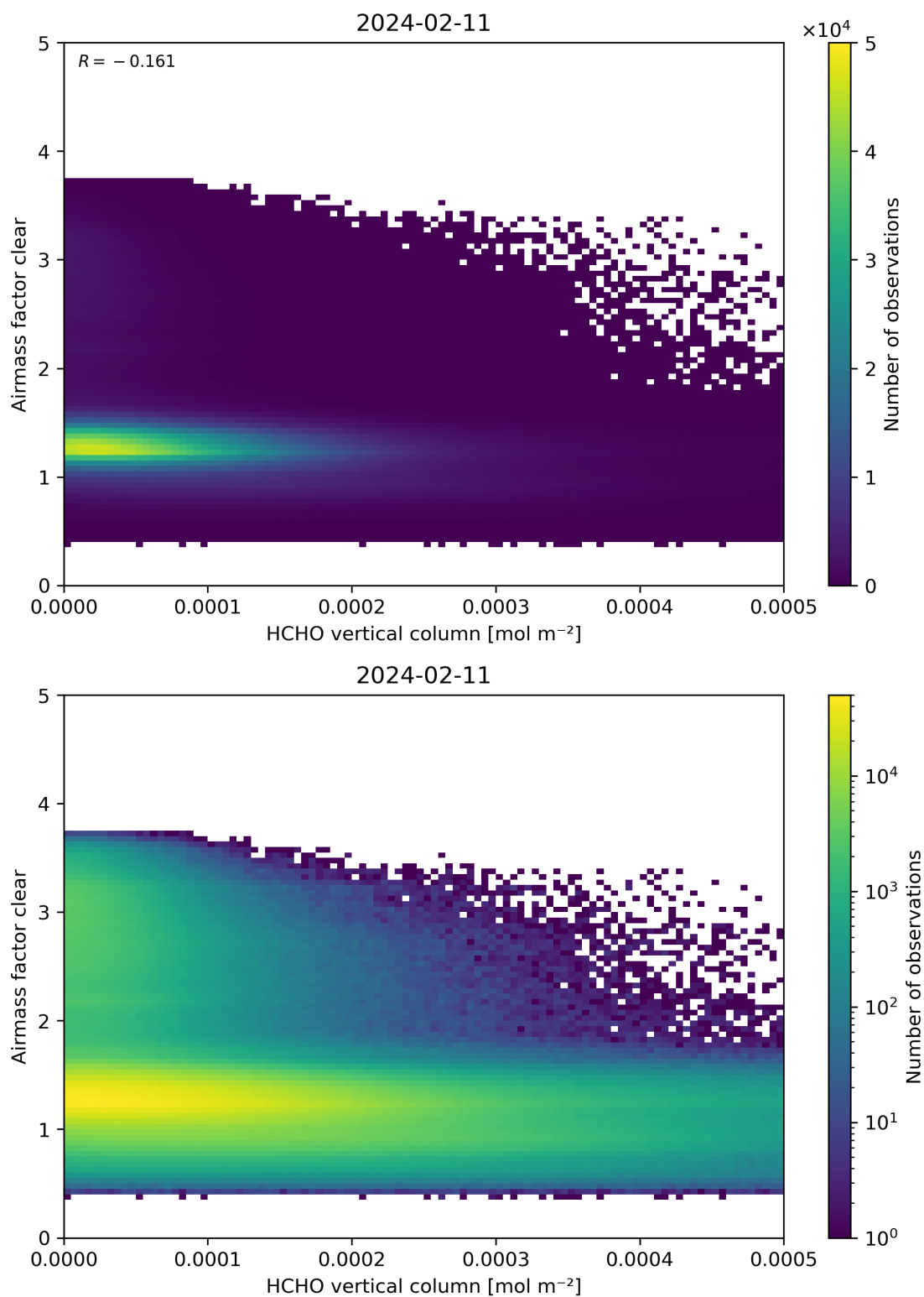
Figure 126: Scatter density plot of “HCHO vertical column” against “Airmass factor clear” for 2024-02-11 to 2024-02-12.
