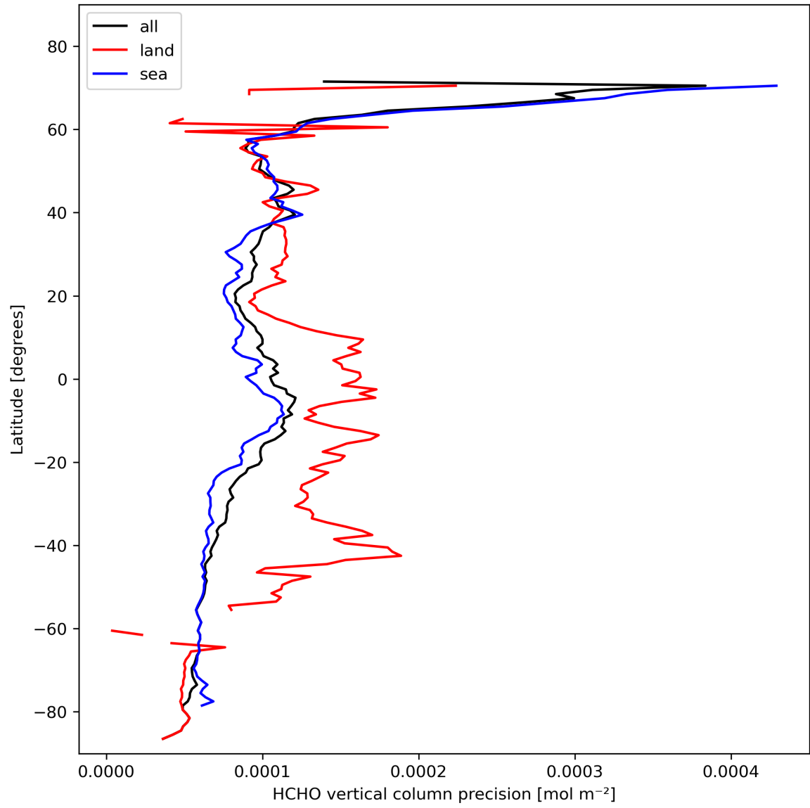
Figure 22: Zonal average of “HCHO vertical column precision” for 2024-02-11 to 2024-02-12.
