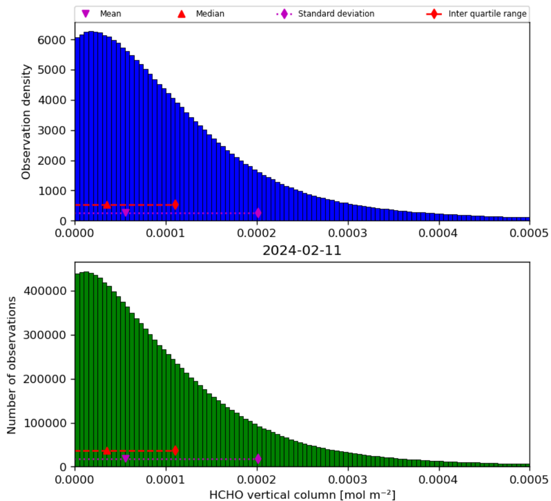
Figure 35: Histogram of “HCHO vertical column” for 2024-02-11 to 2024-02-12
