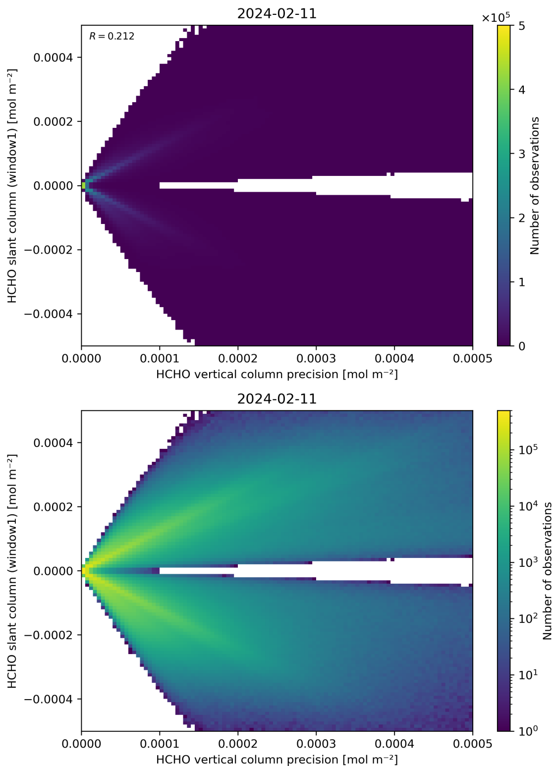
Figure 142: Scatter density plot of “HCHO vertical column precision” against “HCHO slant column (window1)” for 2024-02-11 to 2024-02-12.
