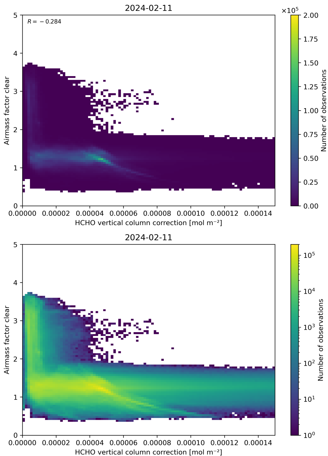
Figure 115: Scatter density plot of “HCHO vertical column correction” against “Airmass factor clear” for 2024-02-11 to 2024-02-12.
