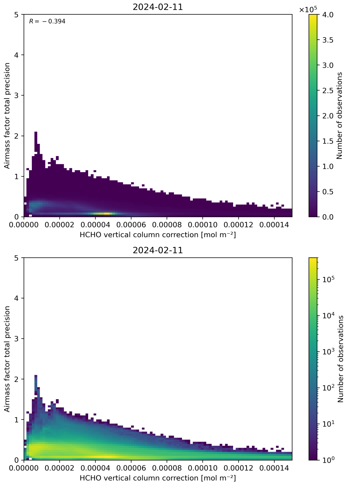
Figure 121: Scatter density plot of “HCHO vertical column correction” against “Airmass factor total precision” for 2024-02-11 to 2024-02-12.
