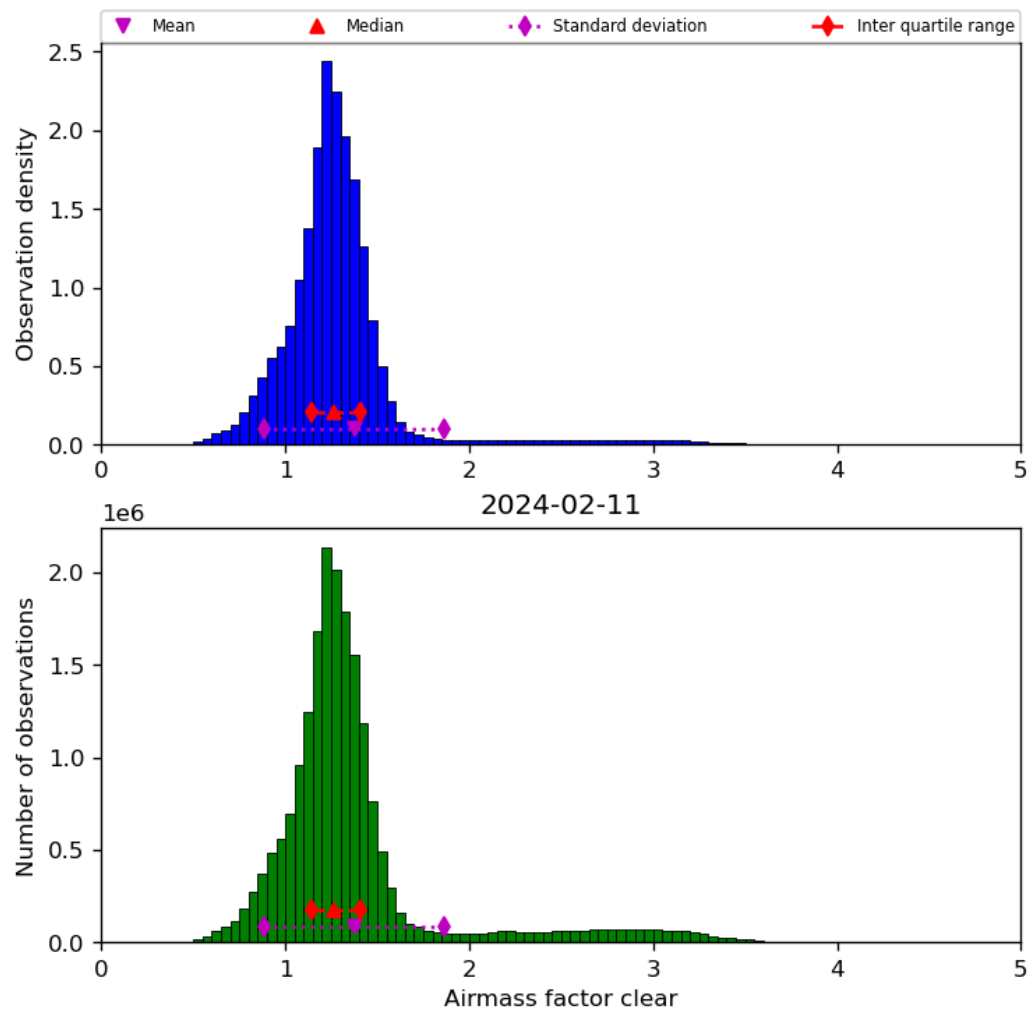
Figure 42: Histogram of “Airmass factor clear” for 2024-02-11 to 2024-02-12
