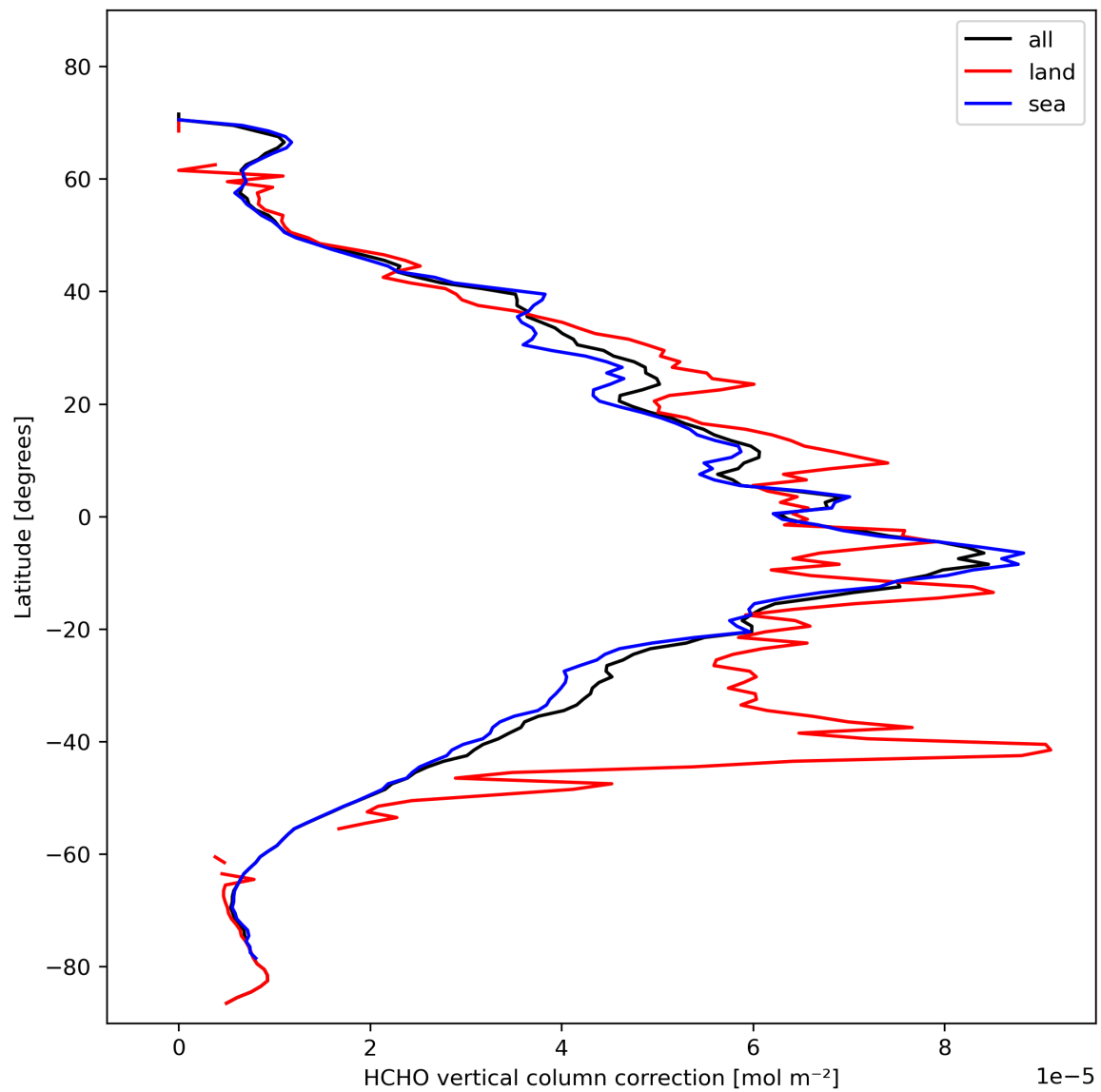
Figure 23: Zonal average of “HCHO vertical column correction” for 2024-02-11 to 2024-02-12.
