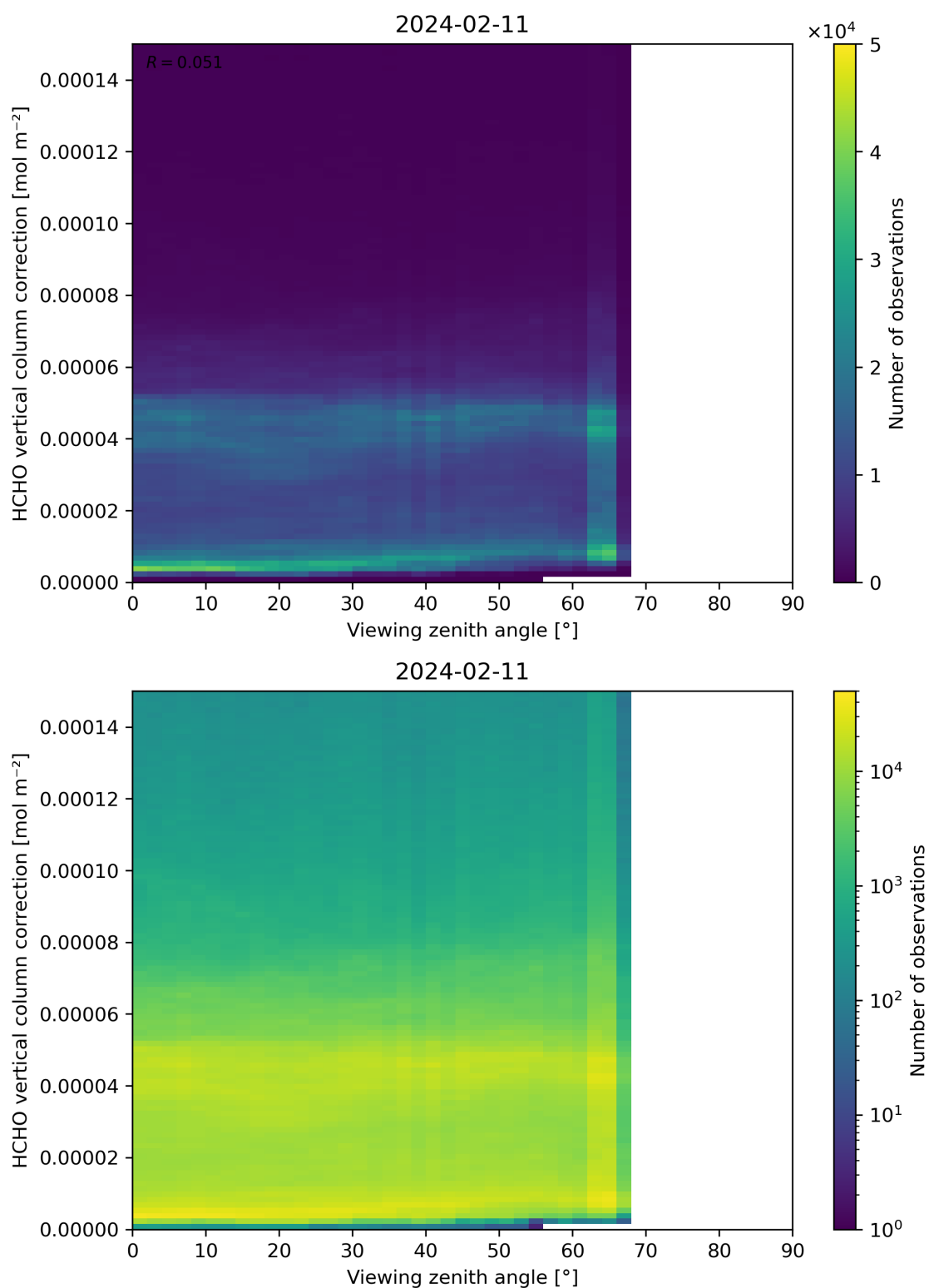
Figure 193: Scatter density plot of “Viewing zenith angle” against “HCHO vertical column correction” for 2024-02-11 to 2024-02-12.
