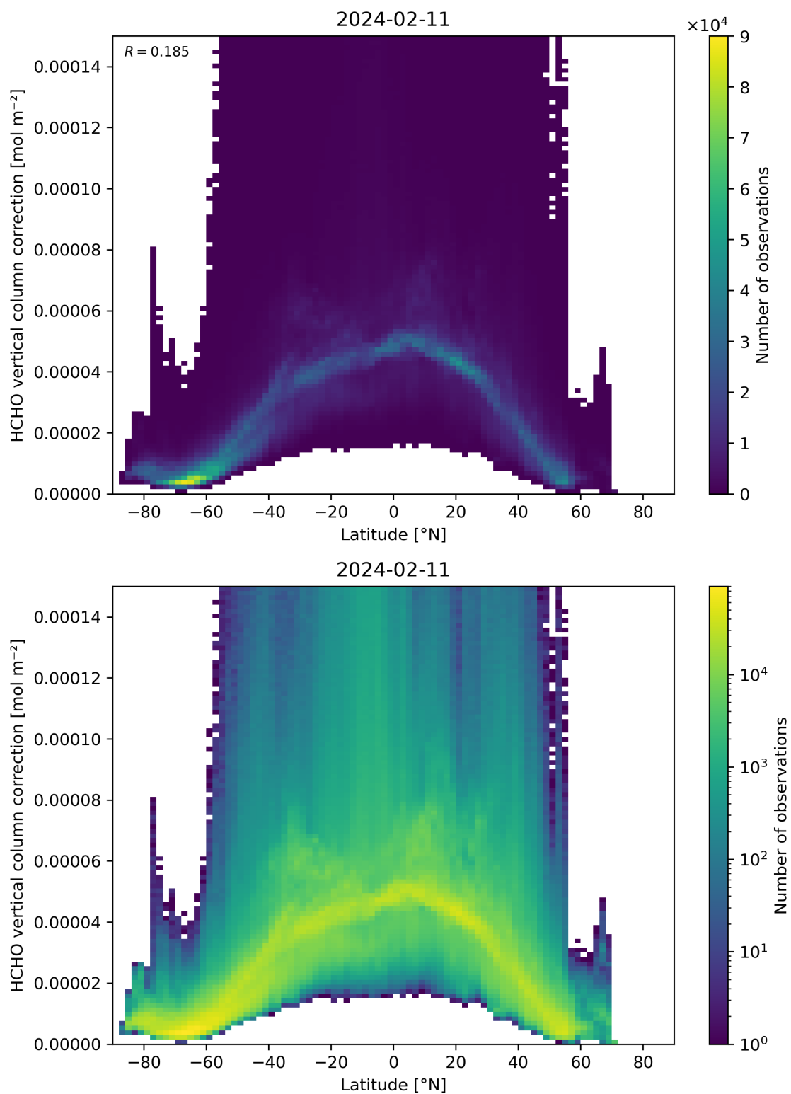
Figure 164: Scatter density plot of “Latitude” against “HCHO vertical column correction” for 2024-02-11 to 2024-02-12.
