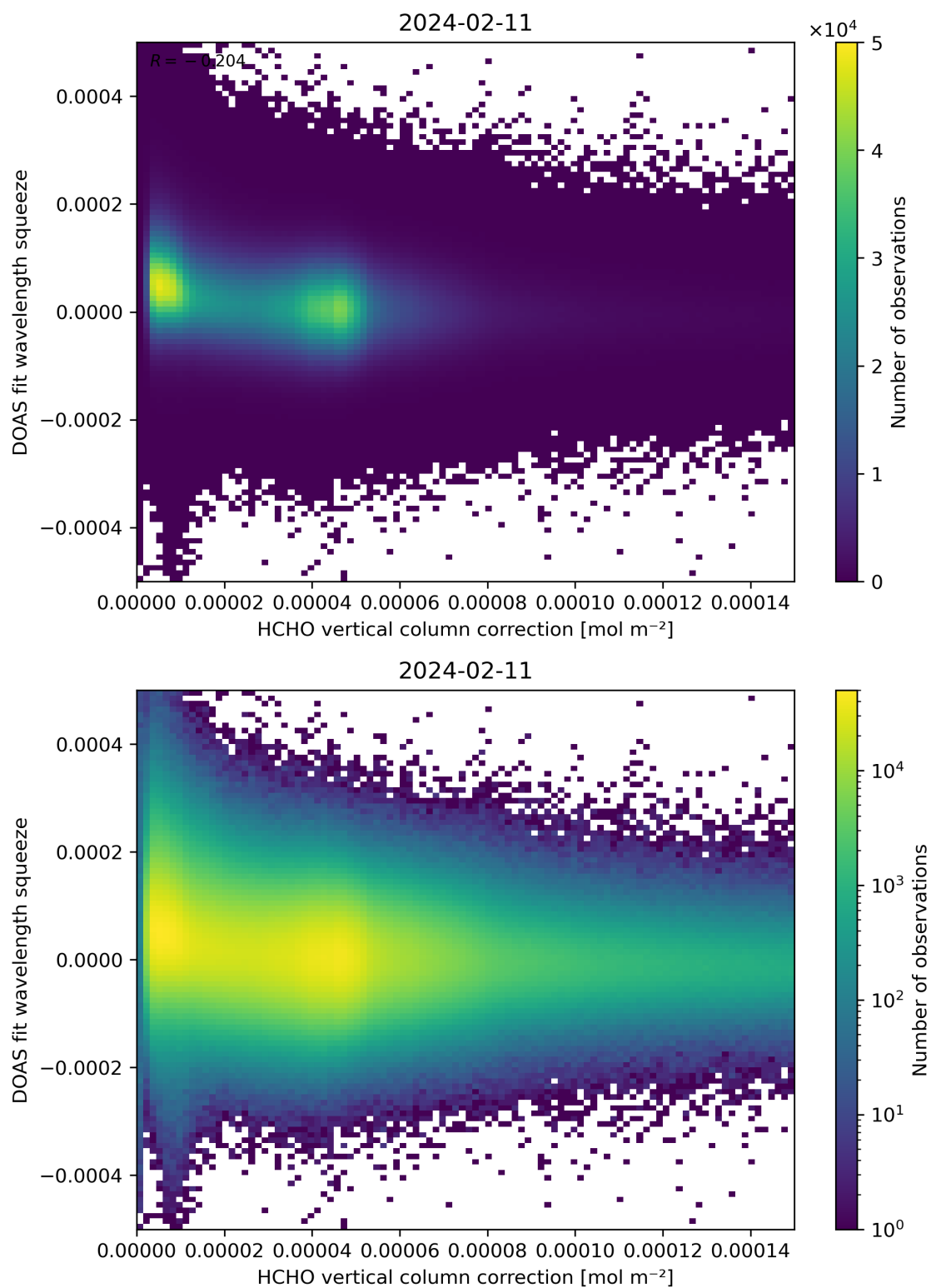
Figure 114: Scatter density plot of “HCHO vertical column correction” against “DOAS fit wavelength squeeze” for 2024-02-11 to 2024-02-12.
