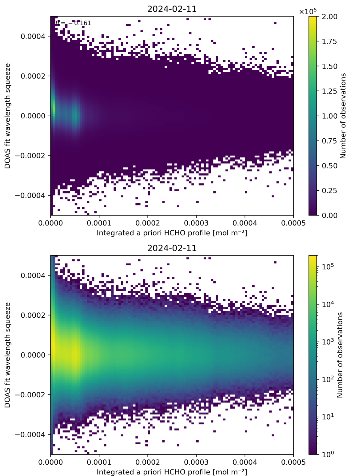
Figure 150: Scatter density plot of “Integrated a priori HCHO profile” against “DOAS fit wavelength squeeze” for 2024-02-11 to 2024-02-12.
