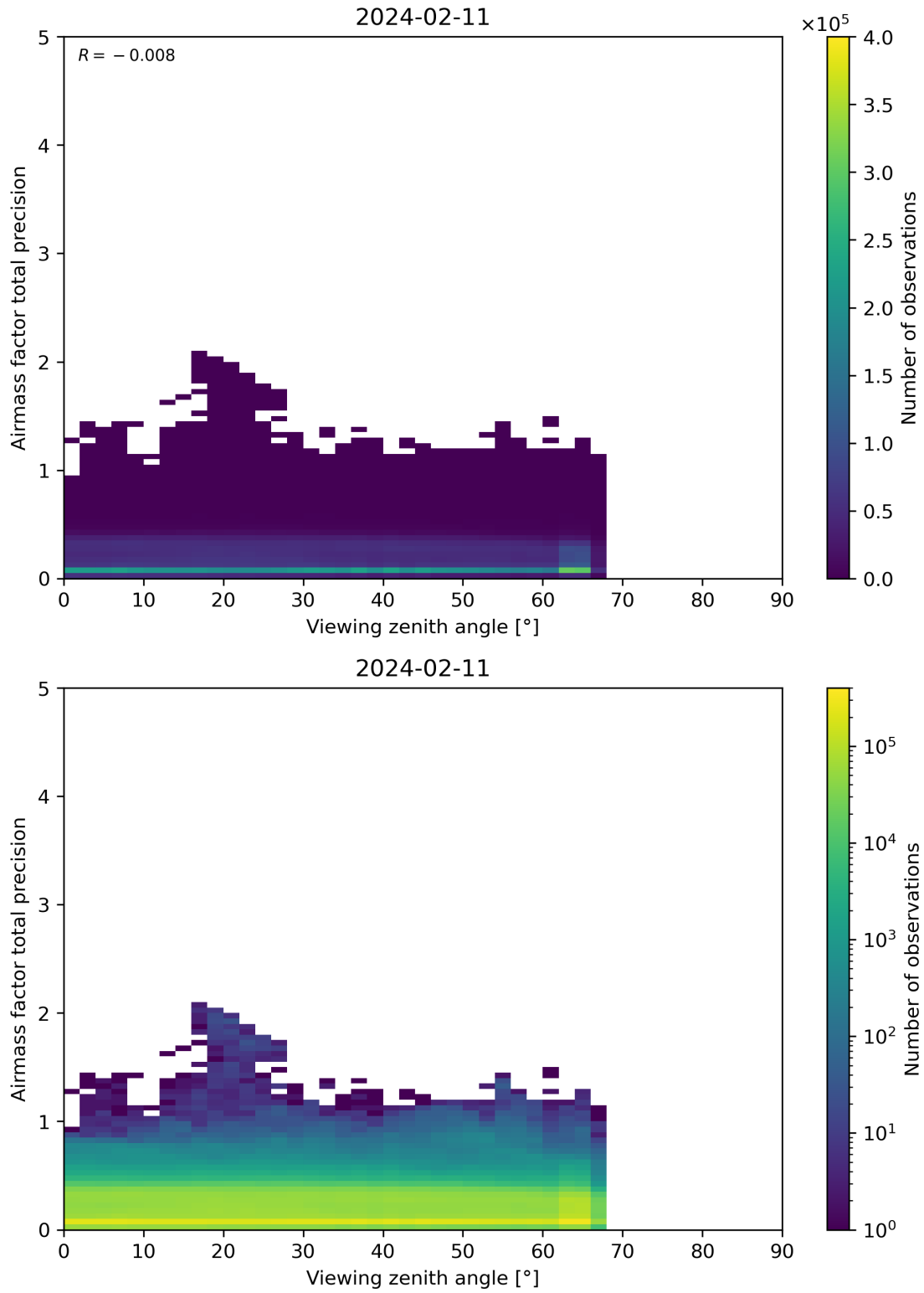
Figure 191: Scatter density plot of “Viewing zenith angle” against “Airmass factor total precision” for 2024-02-11 to 2024-02-12.
