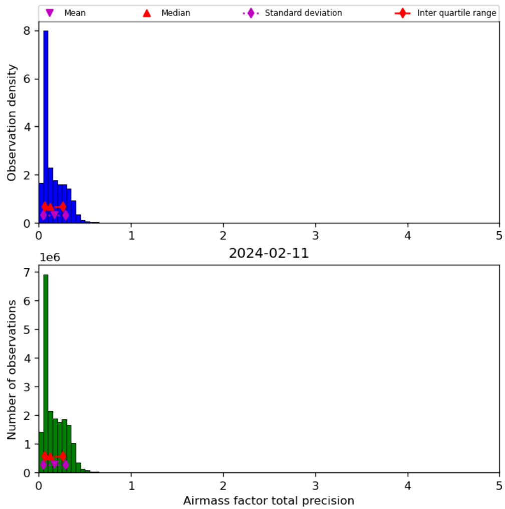
Figure 41: Histogram of “Airmass factor total precision” for 2024-02-11 to 2024-02-12
