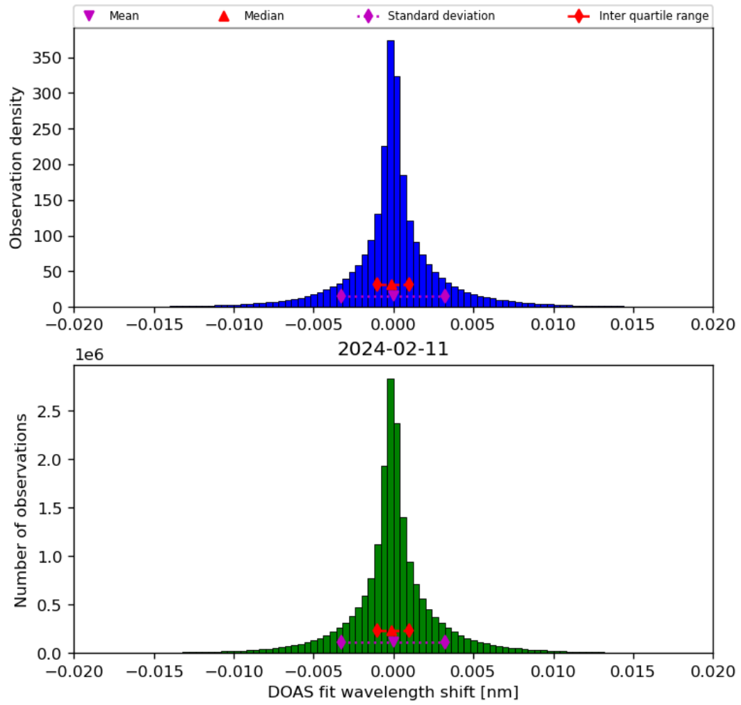
Figure 44: Histogram of “DOAS fit wavelength shift” for 2024-02-11 to 2024-02-12
