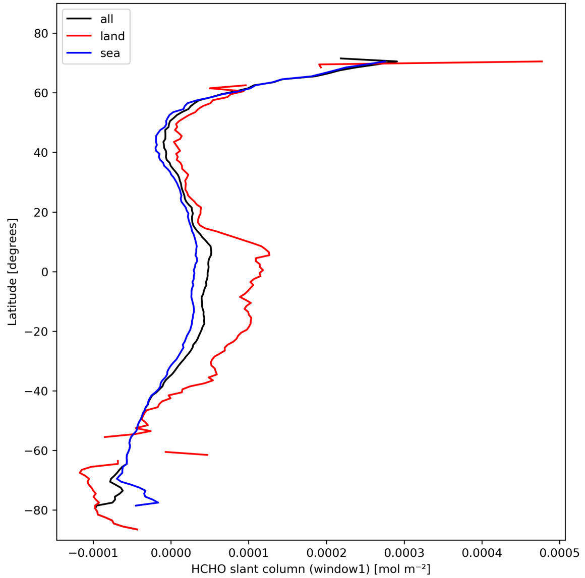
Figure 24: Zonal average of “HCHO slant column (window1)” for 2024-02-11 to 2024-02-12.
