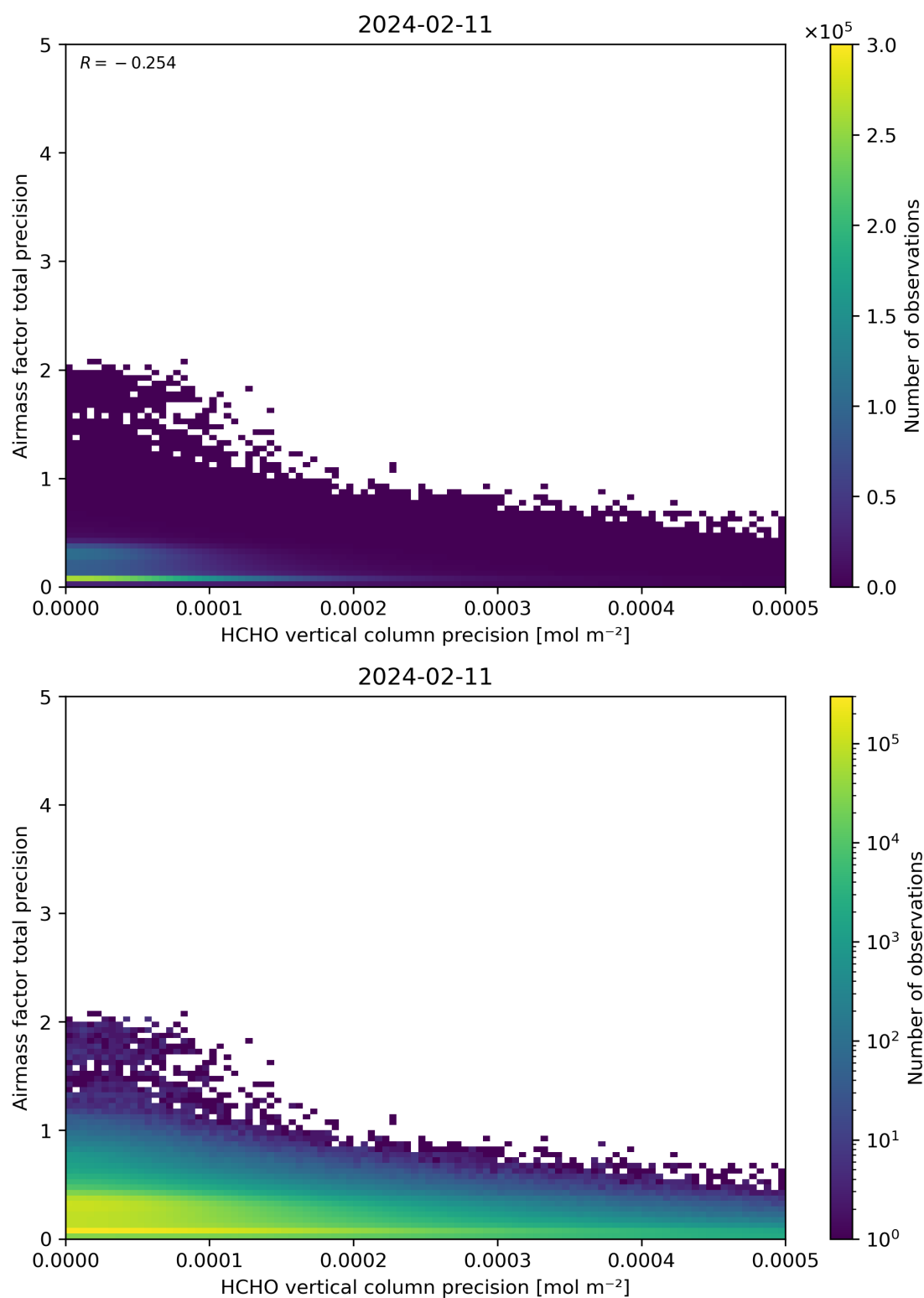
Figure 145: Scatter density plot of “HCHO vertical column precision” against “Airmass factor total precision” for 2024-02-11 to 2024-02-12.
