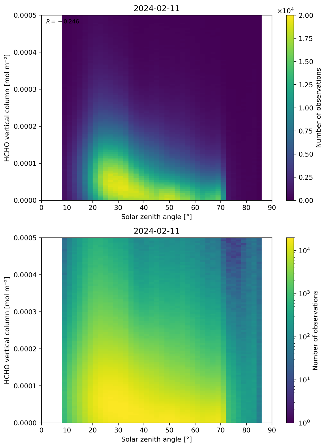
Figure 177: Scatter density plot of “Solar zenith angle” against “HCHO vertical column” for 2024-02-11 to 2024-02-12.
