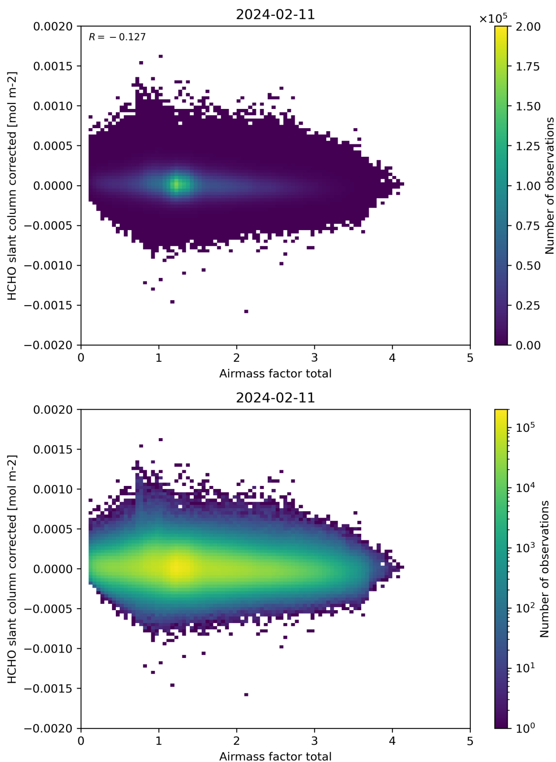
Figure 101: Scatter density plot of “Airmass factor total” against “HCHO slant column corrected” for 2024-02-11 to 2024-02-12.
