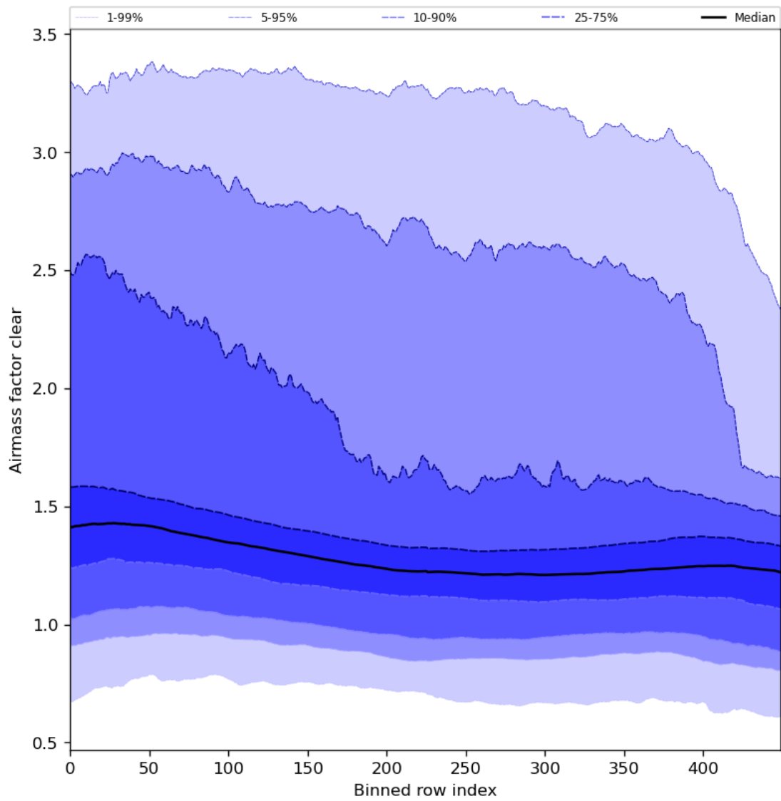
Figure 56: Along track statistics of “Airmass factor clear” for 2024-02-11 to 2024-02-12
