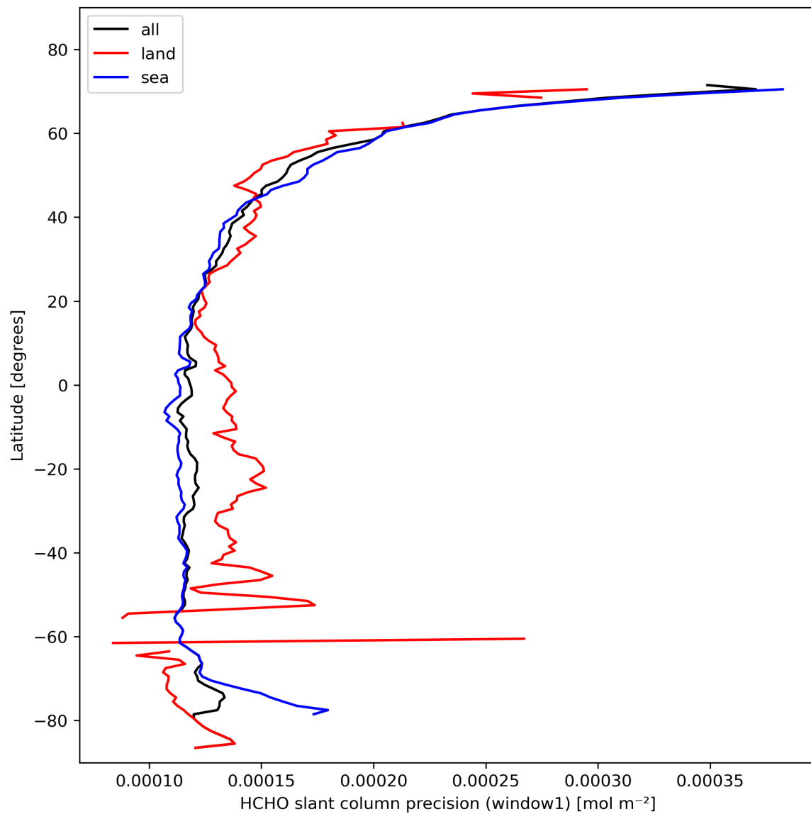
Figure 25: Zonal average of “HCHO slant column precision (window1)” for 2024-02-11 to 2024-02-12.
