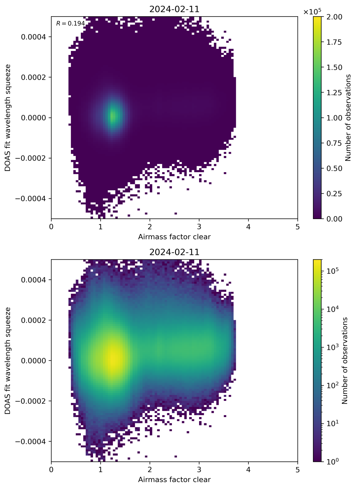
Figure 73: Scatter density plot of “Airmass factor clear” against “DOAS fit wavelength squeeze” for 2024-02-11 to 2024-02-12.
