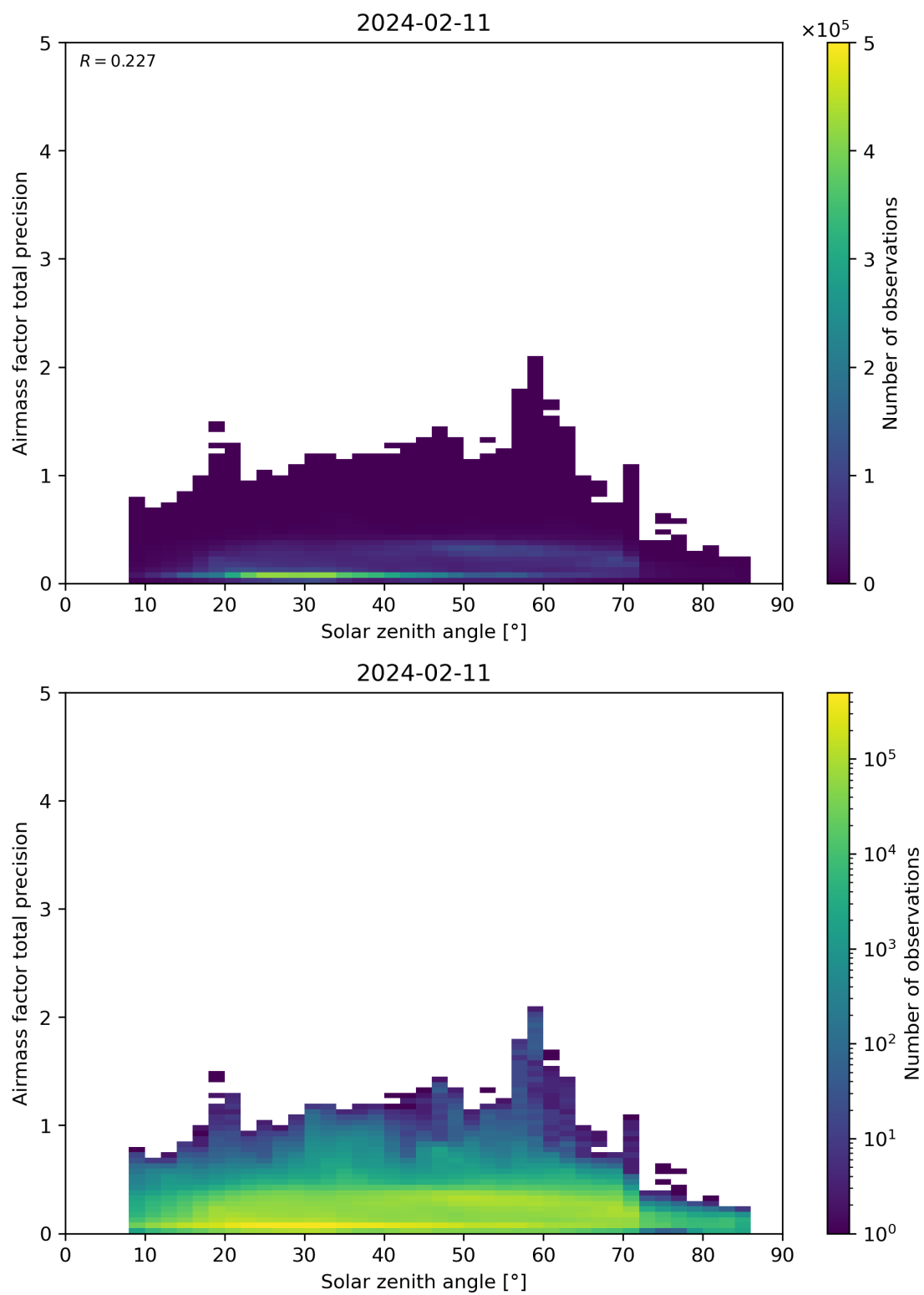
Figure 176: Scatter density plot of “Solar zenith angle” against “Airmass factor total precision” for 2024-02-11 to 2024-02-12.
