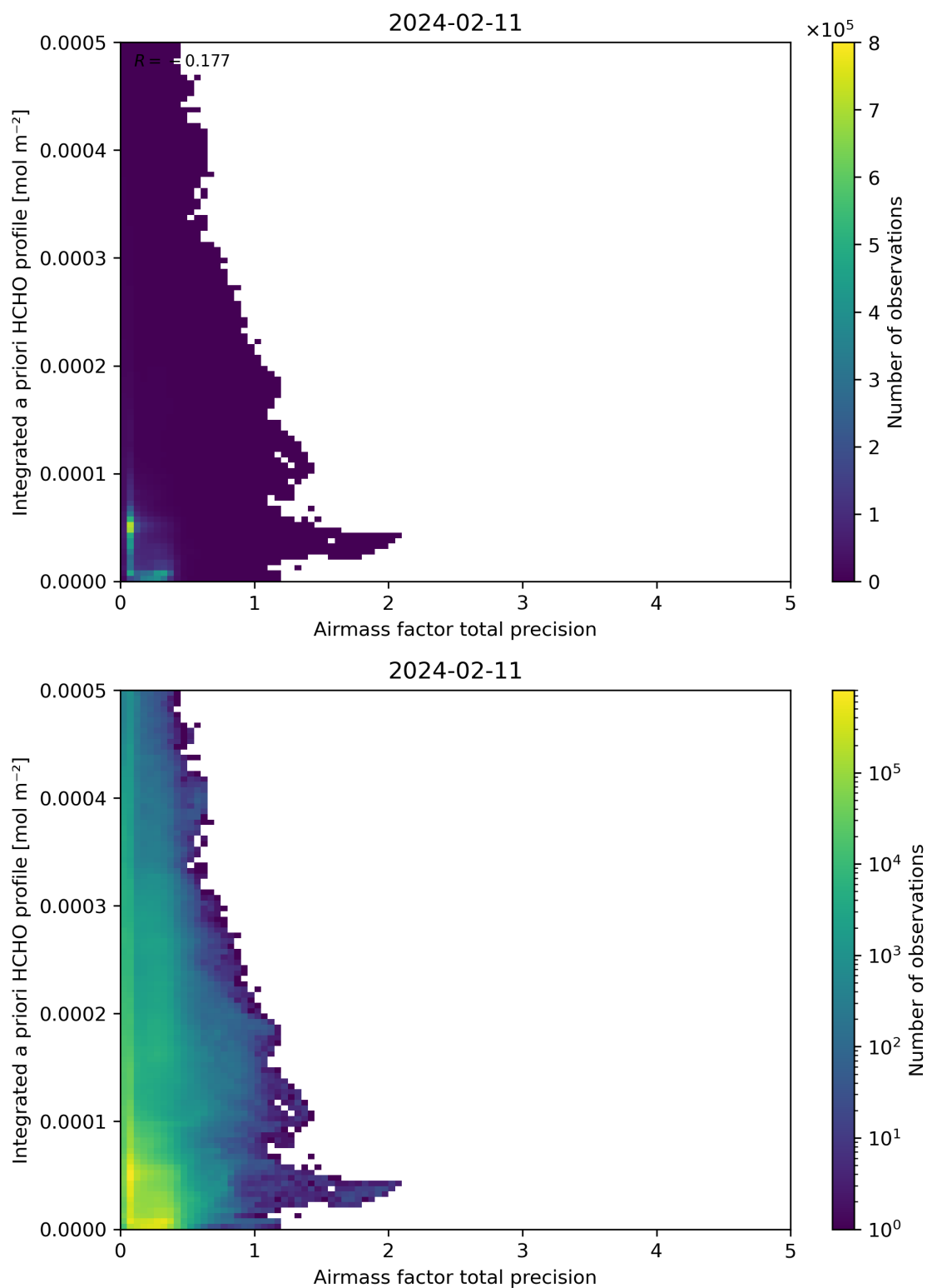
Figure 111: Scatter density plot of “Airmass factor total precision” against “Integrated a priori HCHO profile” for 2024-02-11 to 2024-02-12.
