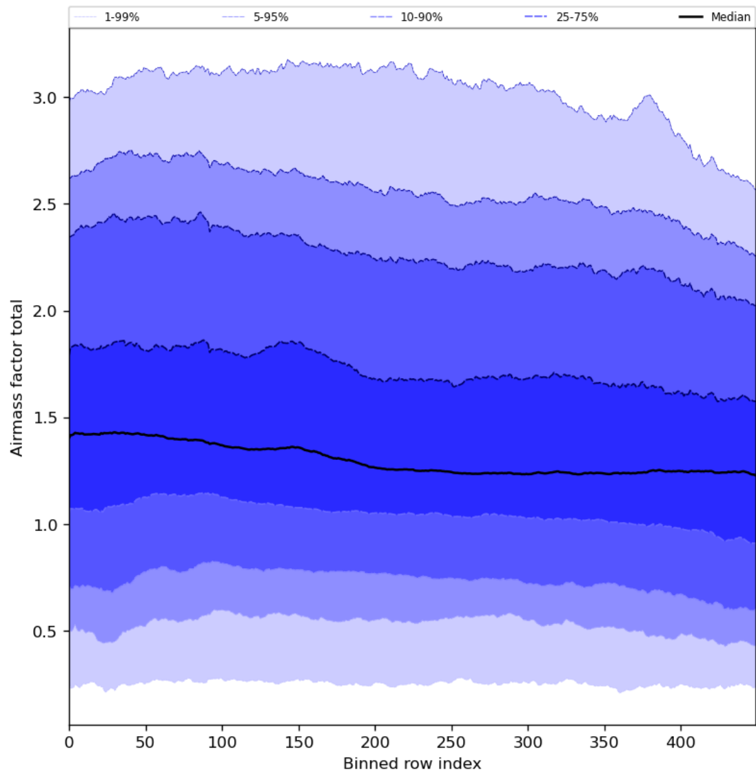
Figure 54: Along track statistics of “Airmass factor total” for 2024-02-11 to 2024-02-12
