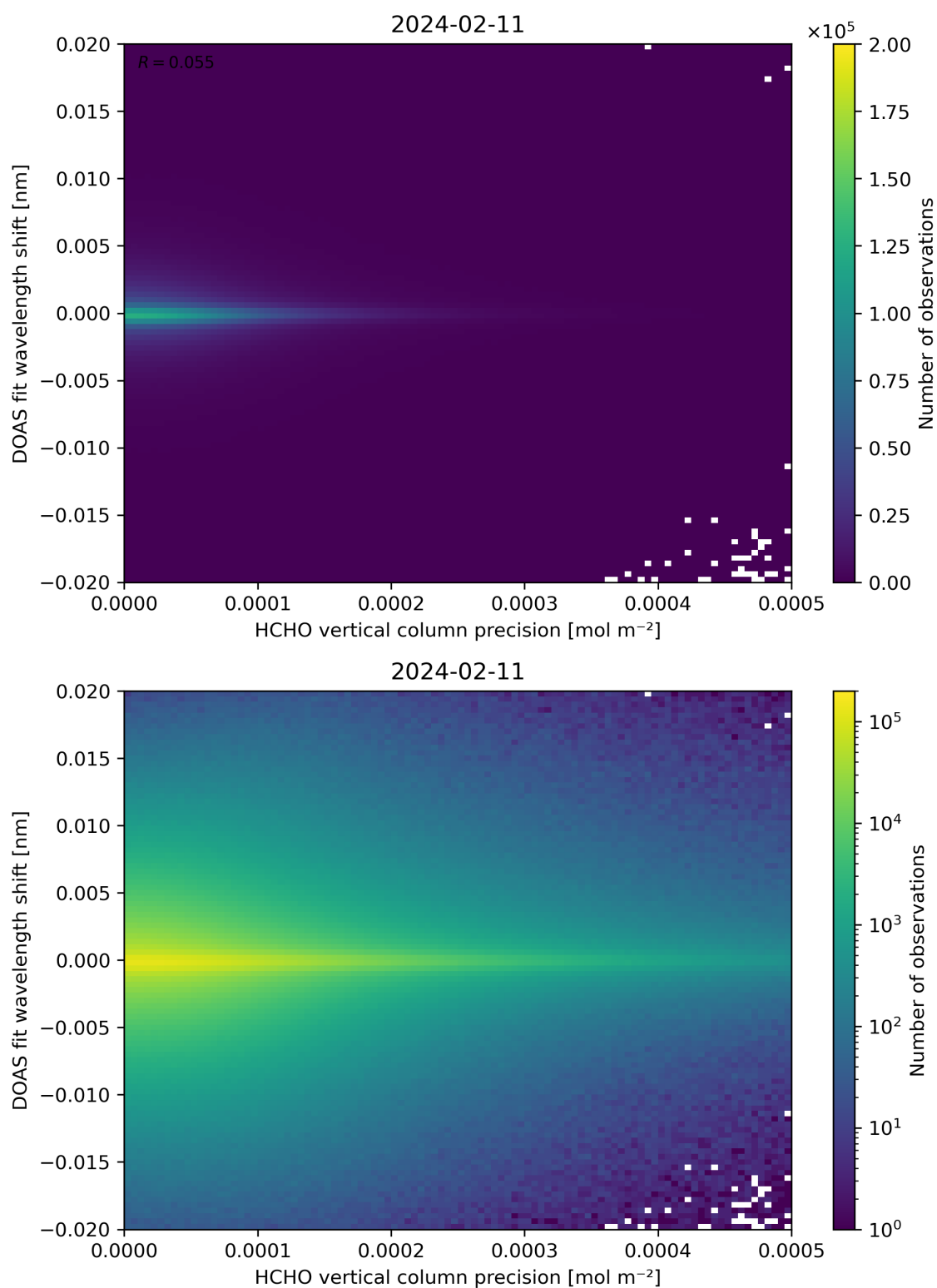
Figure 137: Scatter density plot of “HCHO vertical column precision” against “DOAS fit wavelength shift” for 2024-02-11 to 2024-02-12.
