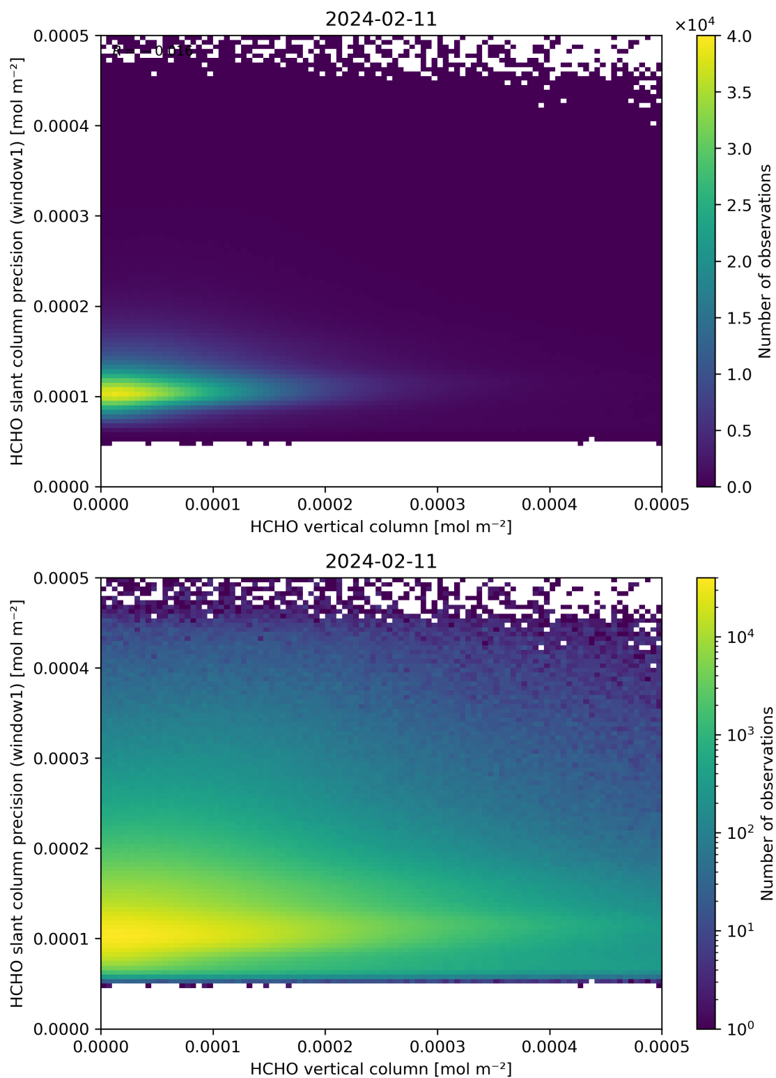
Figure 130: Scatter density plot of “HCHO vertical column” against “HCHO slant column precision (window1)” for 2024-02-11 to 2024-02-12.
