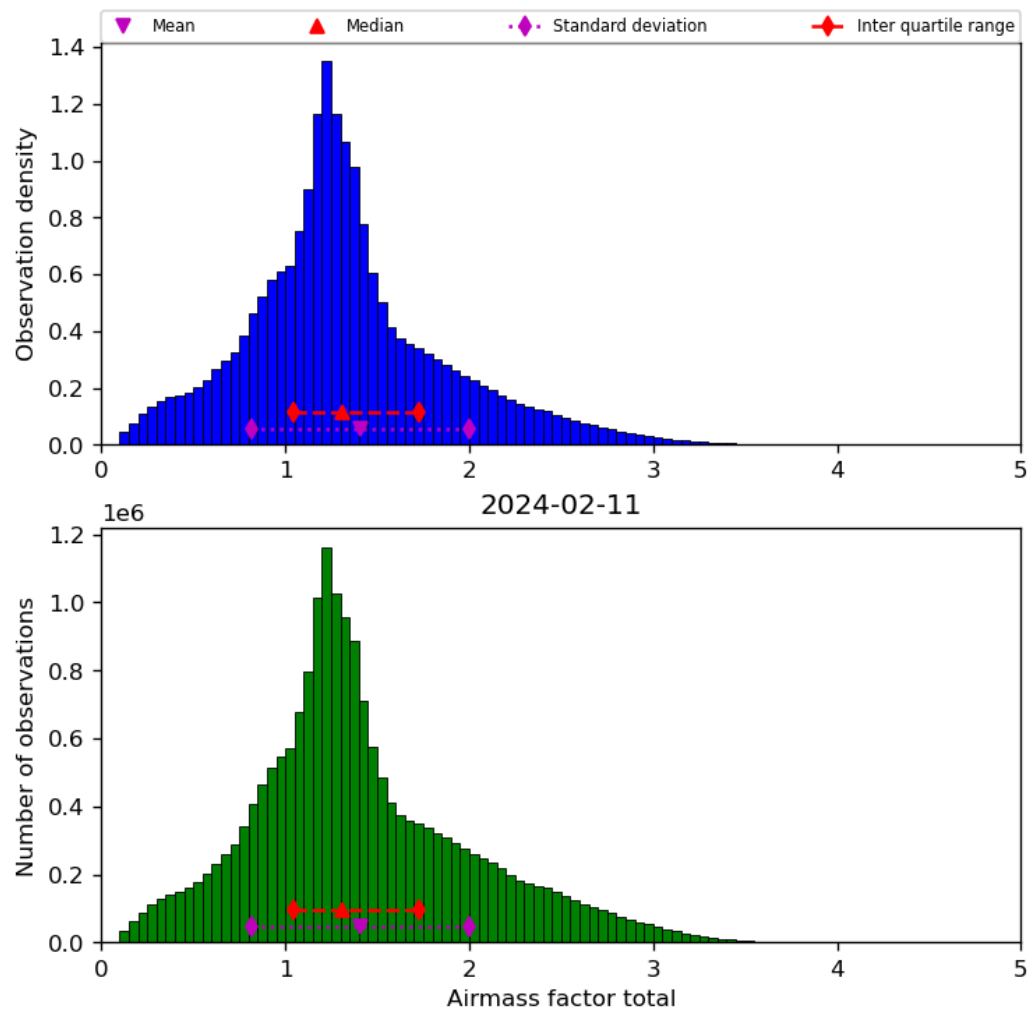
Figure 40: Histogram of “Airmass factor total” for 2024-02-11 to 2024-02-12
