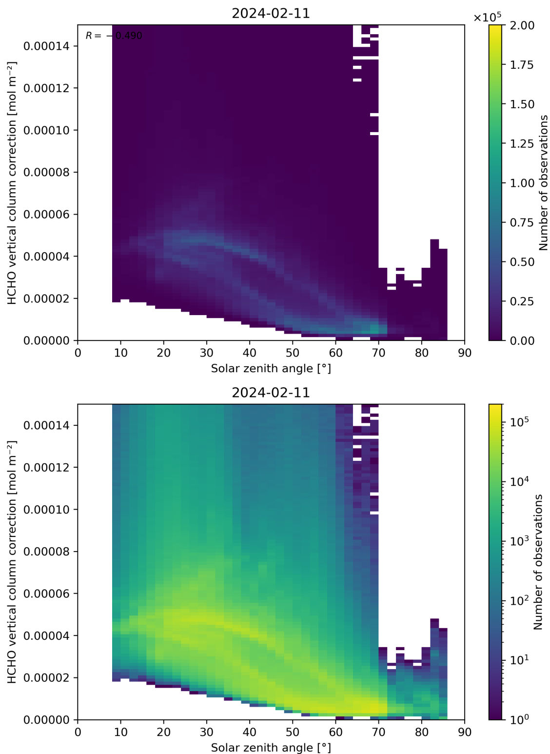
Figure 178: Scatter density plot of “Solar zenith angle” against “HCHO vertical column correction” for 2024-02-11 to 2024-02-12.
