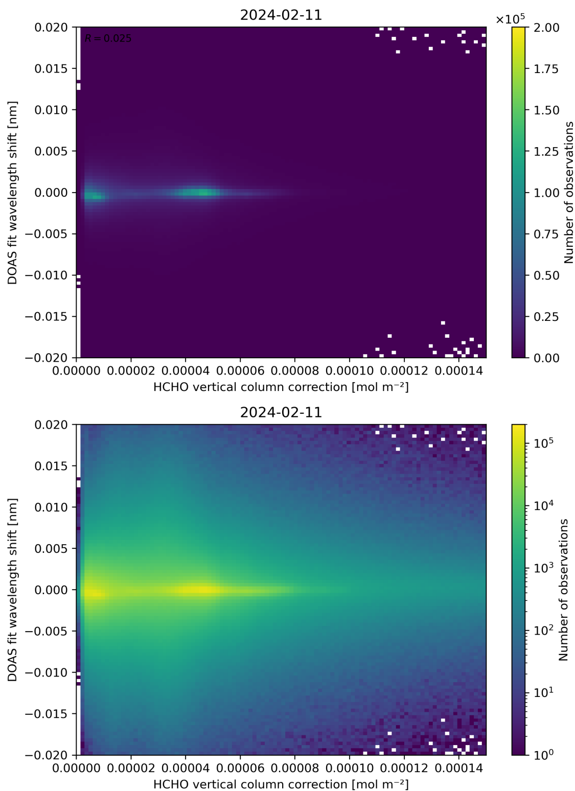
Figure 113: Scatter density plot of “HCHO vertical column correction” against “DOAS fit wavelength shift” for 2024-02-11 to 2024-02-12.
