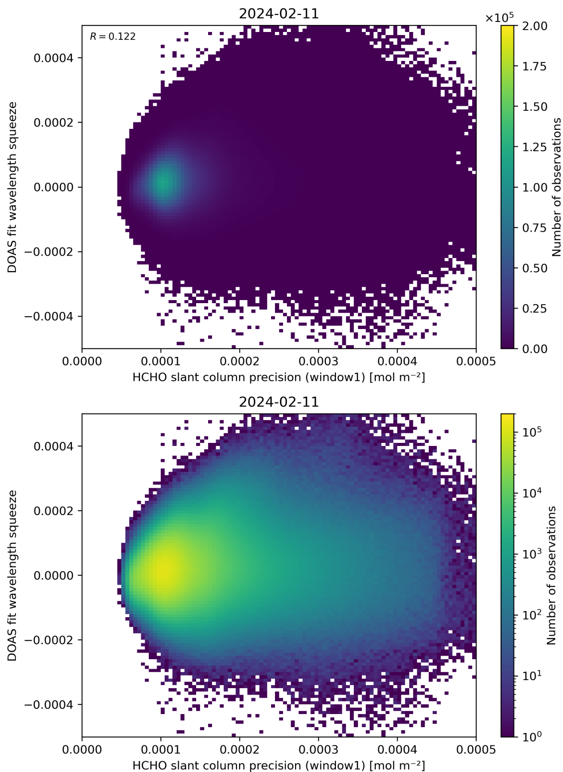
Figure 90: Scatter density plot of “HCHO slant column precision (window1)” against “DOAS fit wavelength squeeze” for 2024-02-11 to 2024-02-12.
