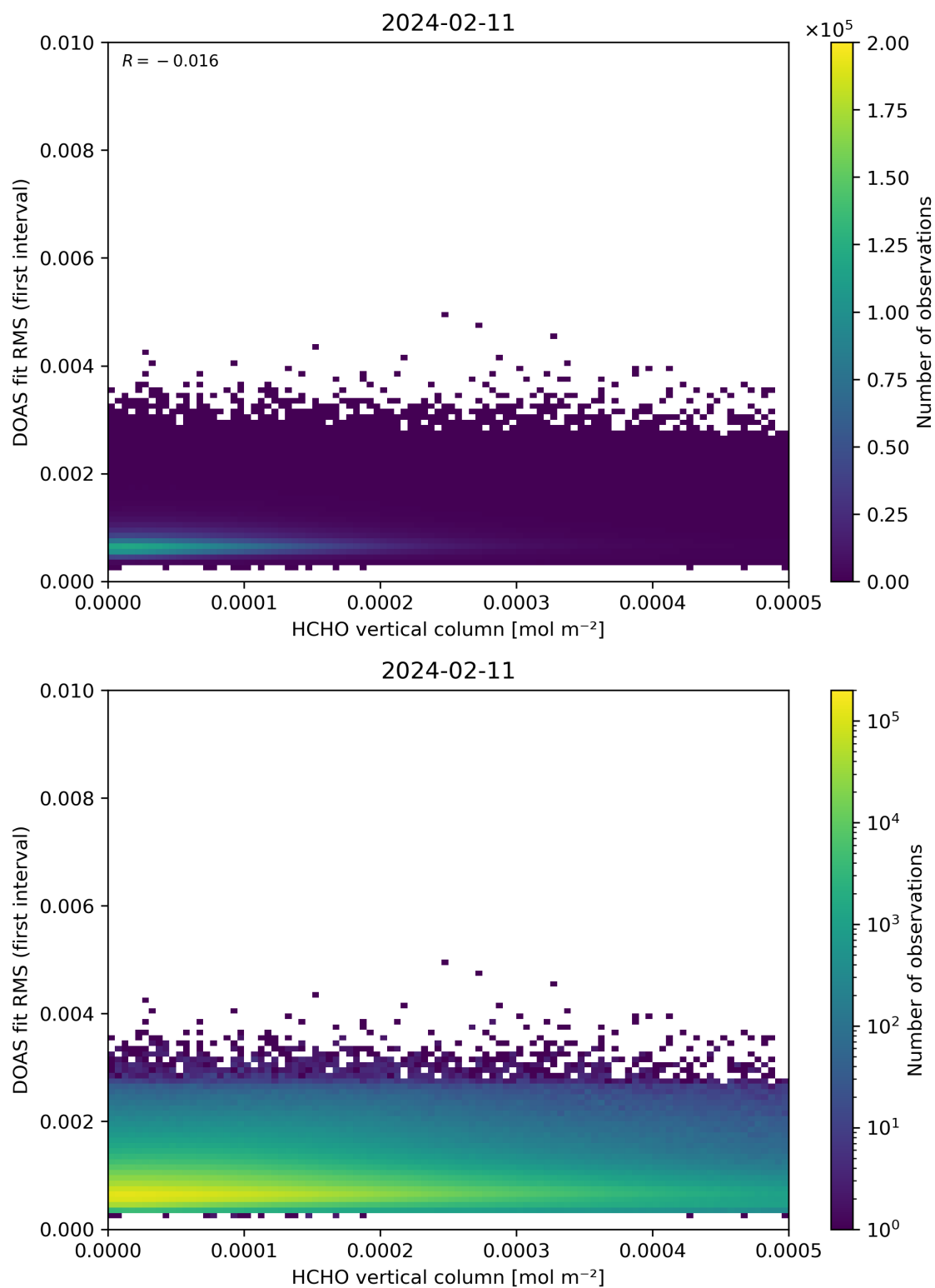
Figure 123: Scatter density plot of “HCHO vertical column” against “DOAS fit RMS (first interval)” for 2024-02-11 to 2024-02-12.
