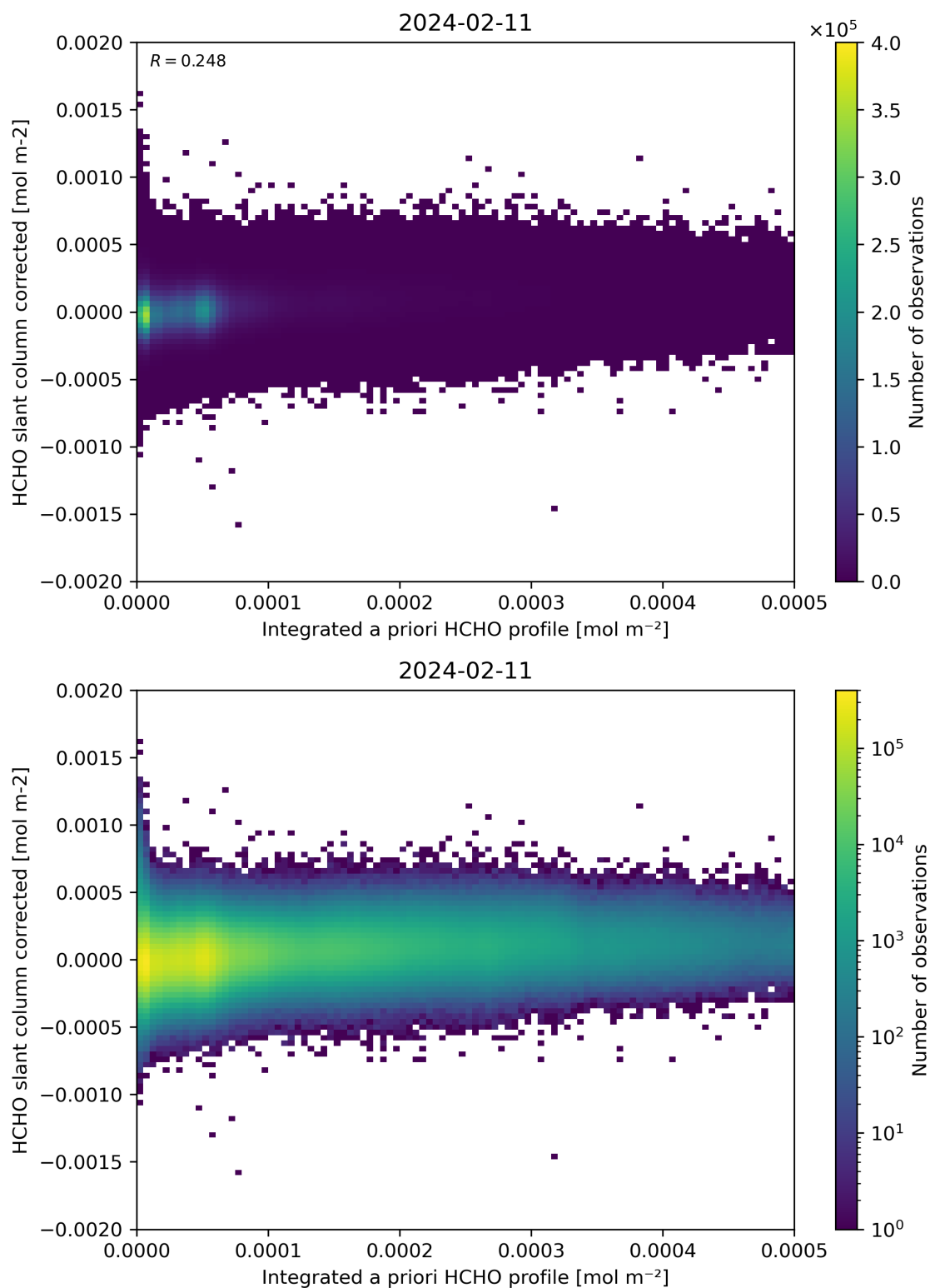
Figure 151: Scatter density plot of “Integrated a priori HCHO profile” against “HCHO slant column corrected” for 2024-02-11 to 2024-02-12.
