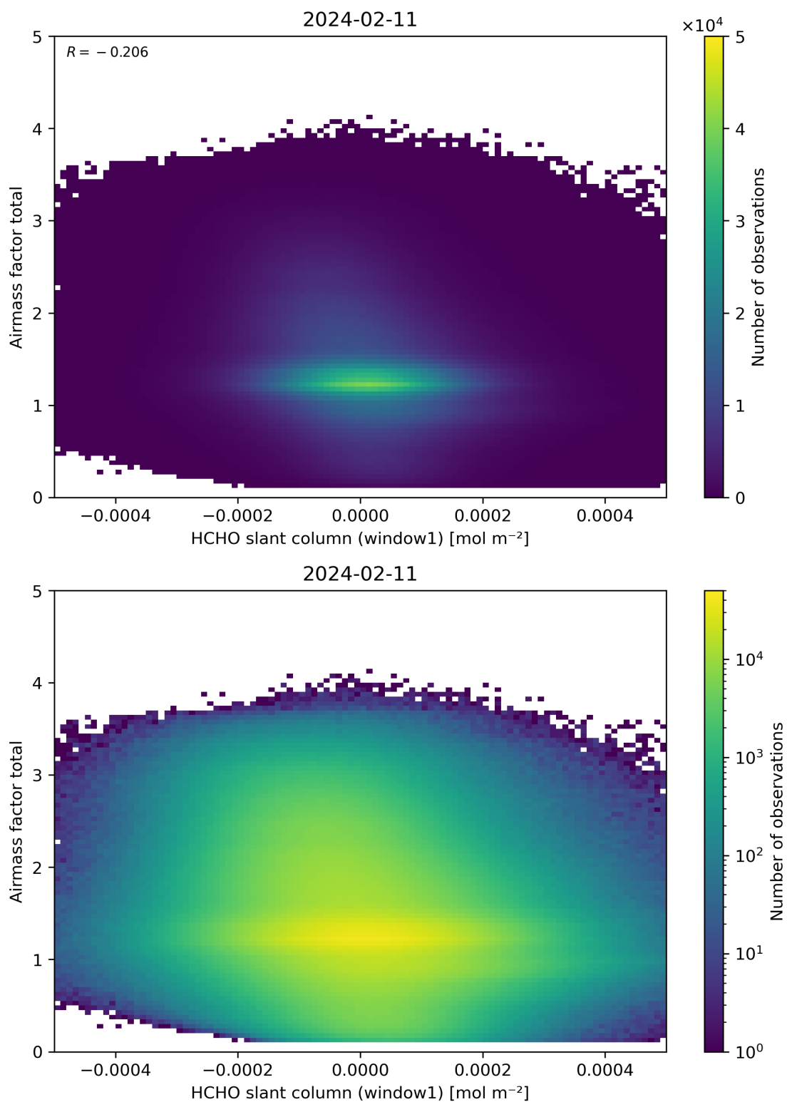
Figure 85: Scatter density plot of “HCHO slant column (window1)” against “Airmass factor total” for 2024-02-11 to 2024-02-12.
