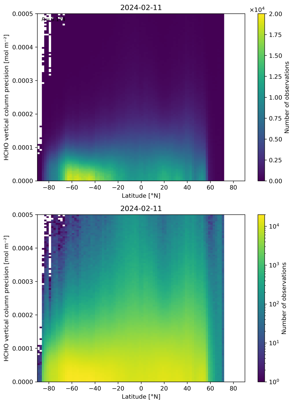
Figure 165: Scatter density plot of “Latitude” against “HCHO vertical column precision” for 2024-02-11 to 2024-02-12.
