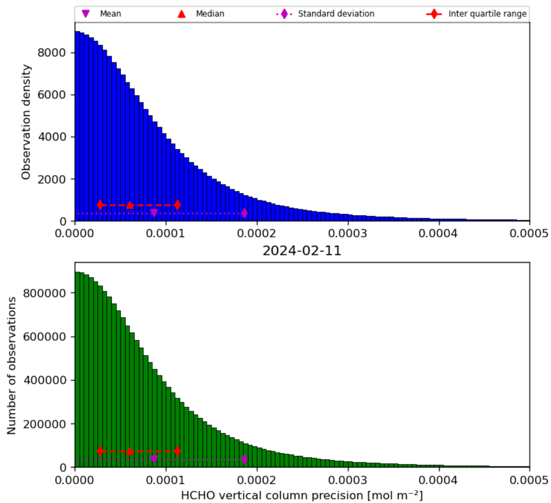
Figure 36: Histogram of “HCHO vertical column precision” for 2024-02-11 to 2024-02-12
