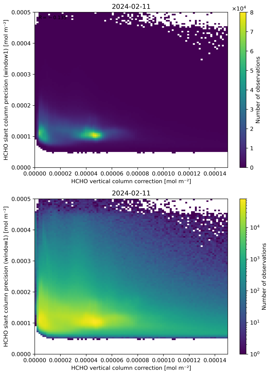
Figure 119: Scatter density plot of “HCHO vertical column correction” against “HCHO slant column precision (window1)” for 2024-02-11 to 2024-02-12.
