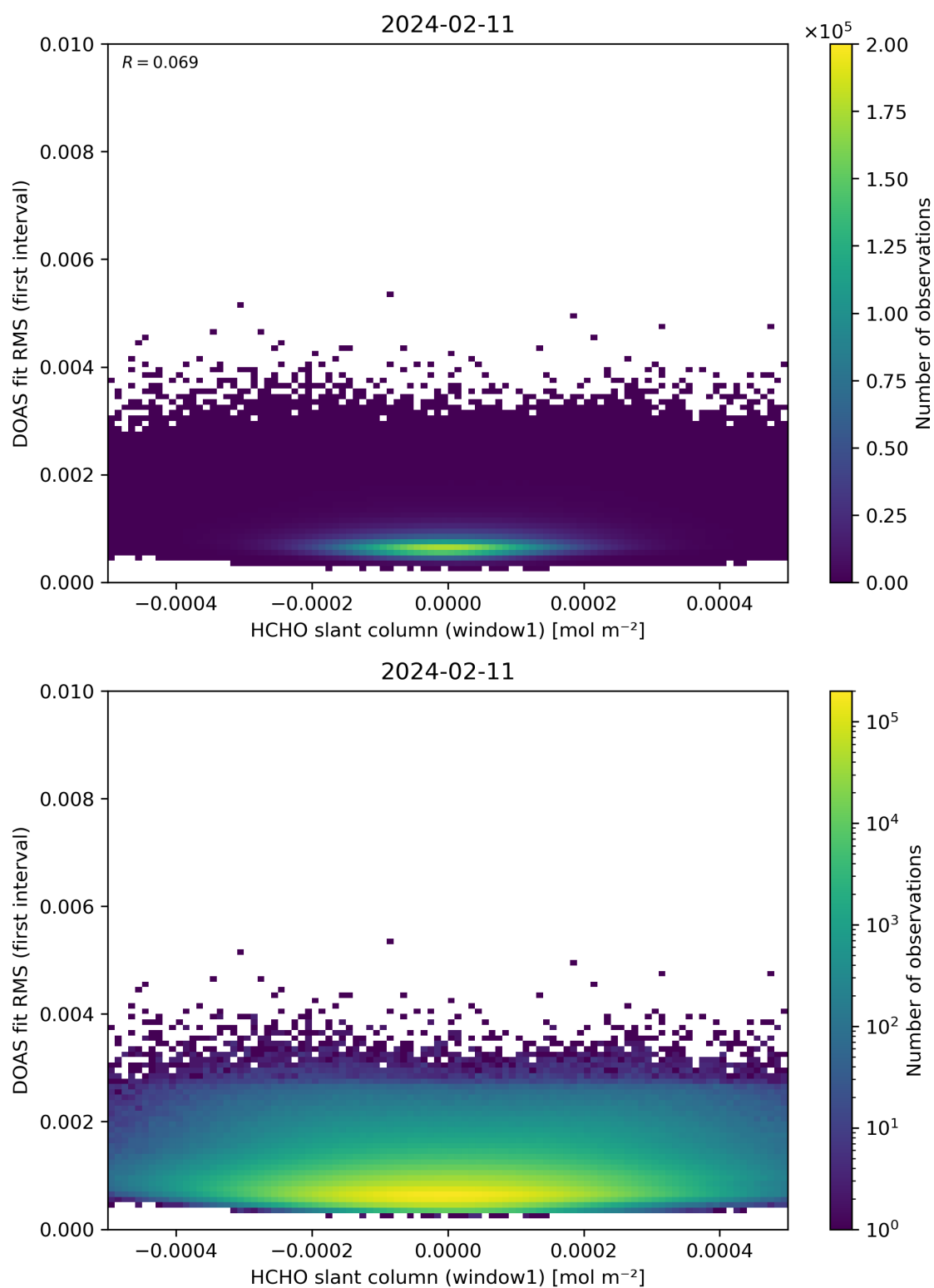
Figure 78: Scatter density plot of “HCHO slant column (window1)” against “DOAS fit RMS (first interval)” for 2024-02-11 to 2024-02-12.
