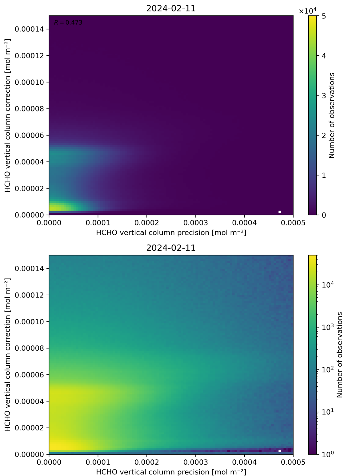
Figure 146: Scatter density plot of “HCHO vertical column precision” against “HCHO vertical column correction” for 2024-02-11 to 2024-02-12.
