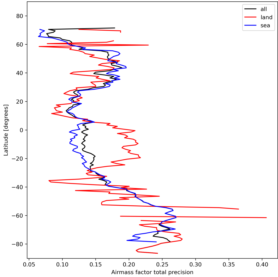
Figure 27: Zonal average of “Airmass factor total precision” for 2024-02-11 to 2024-02-12.
