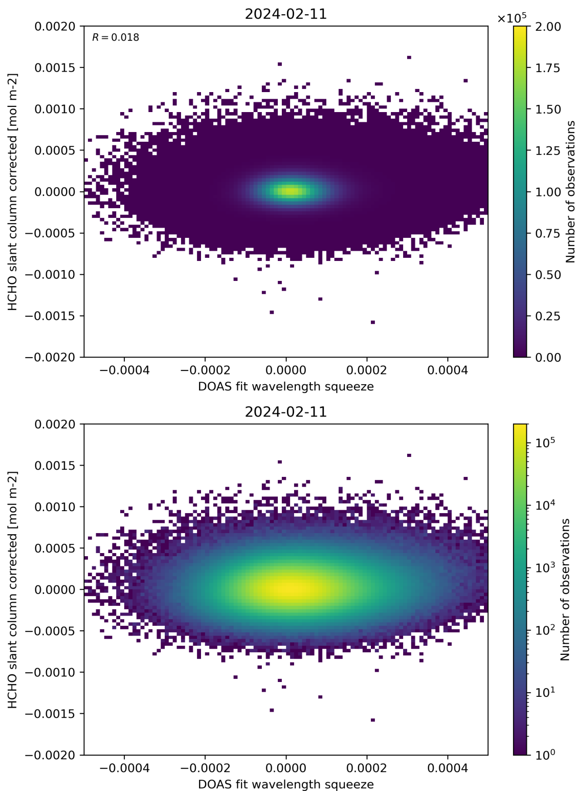
Figure 69: Scatter density plot of “DOAS fit wavelength squeeze” against “HCHO slant column corrected” for 2024-02-11 to 2024-02-12.
