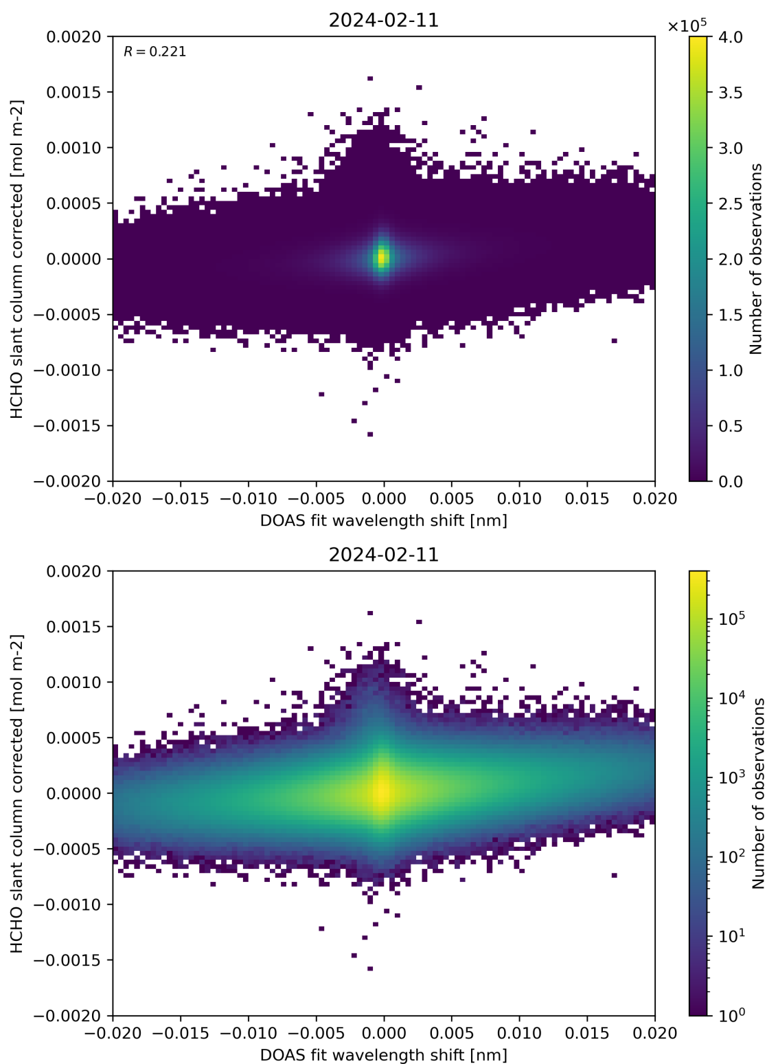
Figure 66: Scatter density plot of “DOAS fit wavelength shift” against “HCHO slant column corrected” for 2024-02-11 to 2024-02-12.
