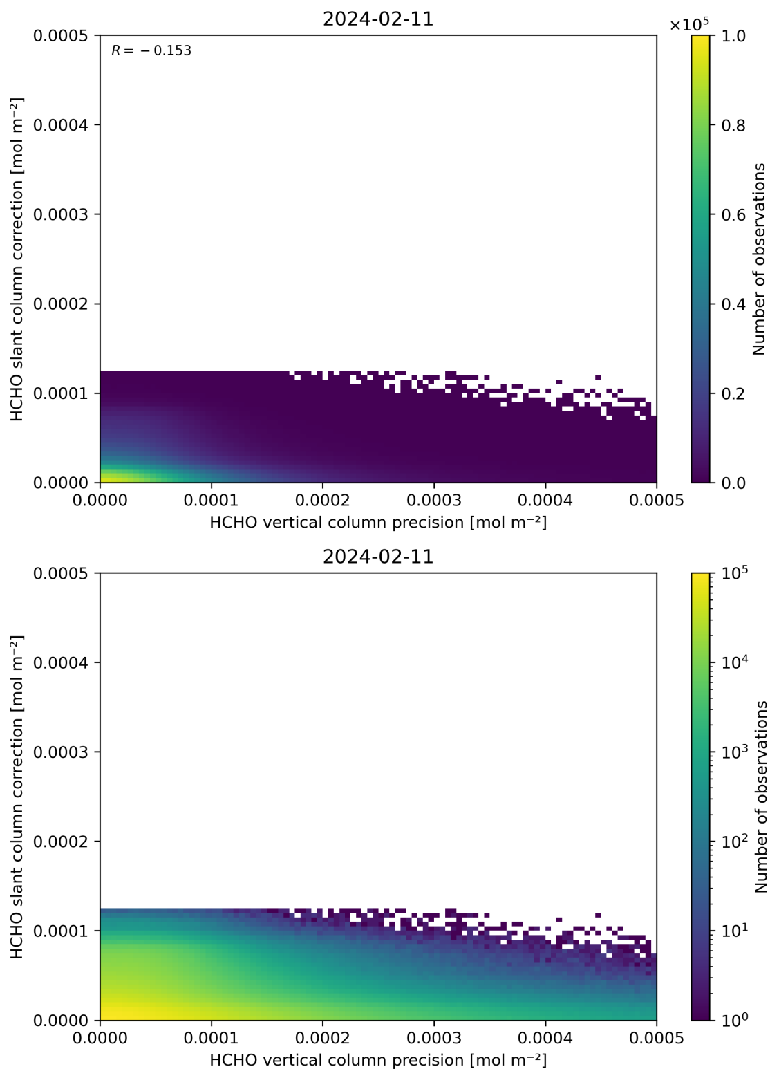
Figure 141: Scatter density plot of “HCHO vertical column precision” against “HCHO slant column correction” for 2024-02-11 to 2024-02-12.
