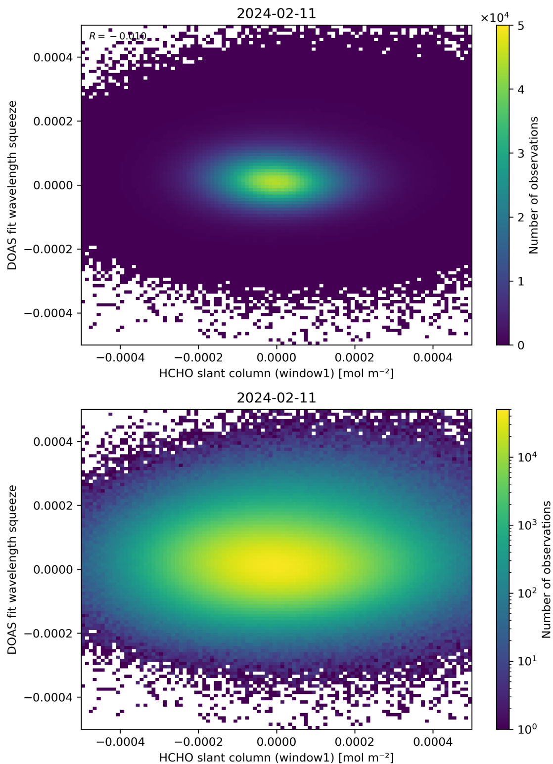
Figure 80: Scatter density plot of “HCHO slant column (window1)” against “DOAS fit wavelength squeeze” for 2024-02-11 to 2024-02-12.
