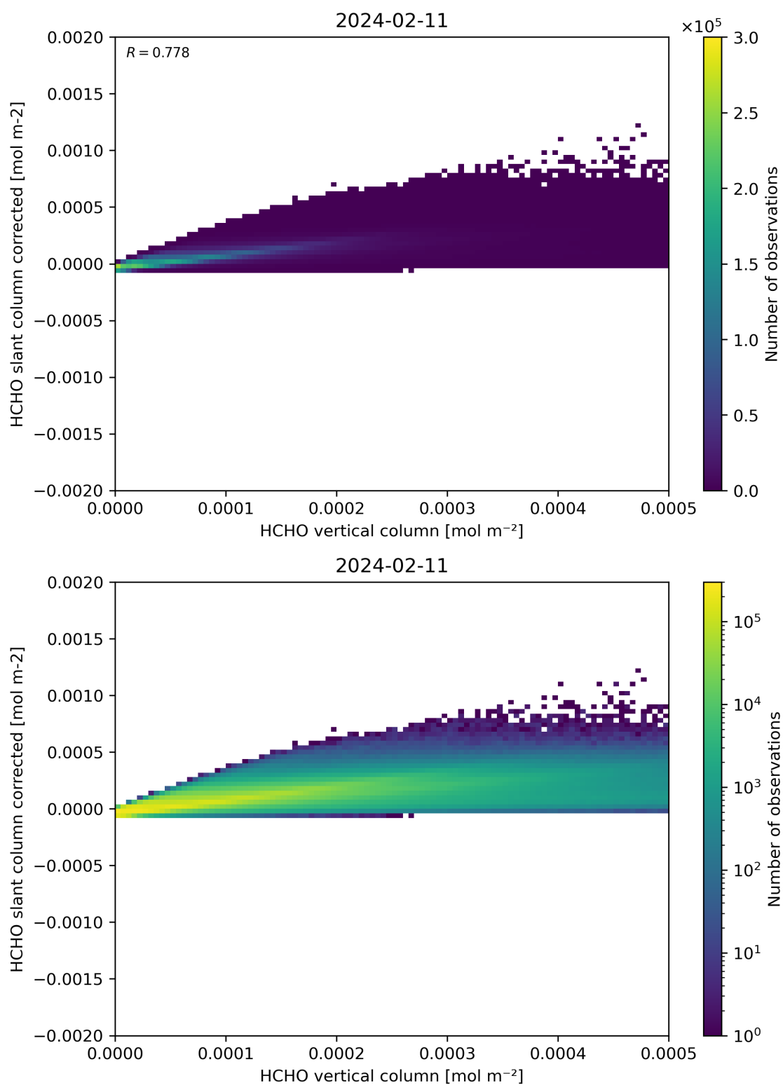
Figure 127: Scatter density plot of “HCHO vertical column” against “HCHO slant column corrected” for 2024-02-11 to 2024-02-12.
