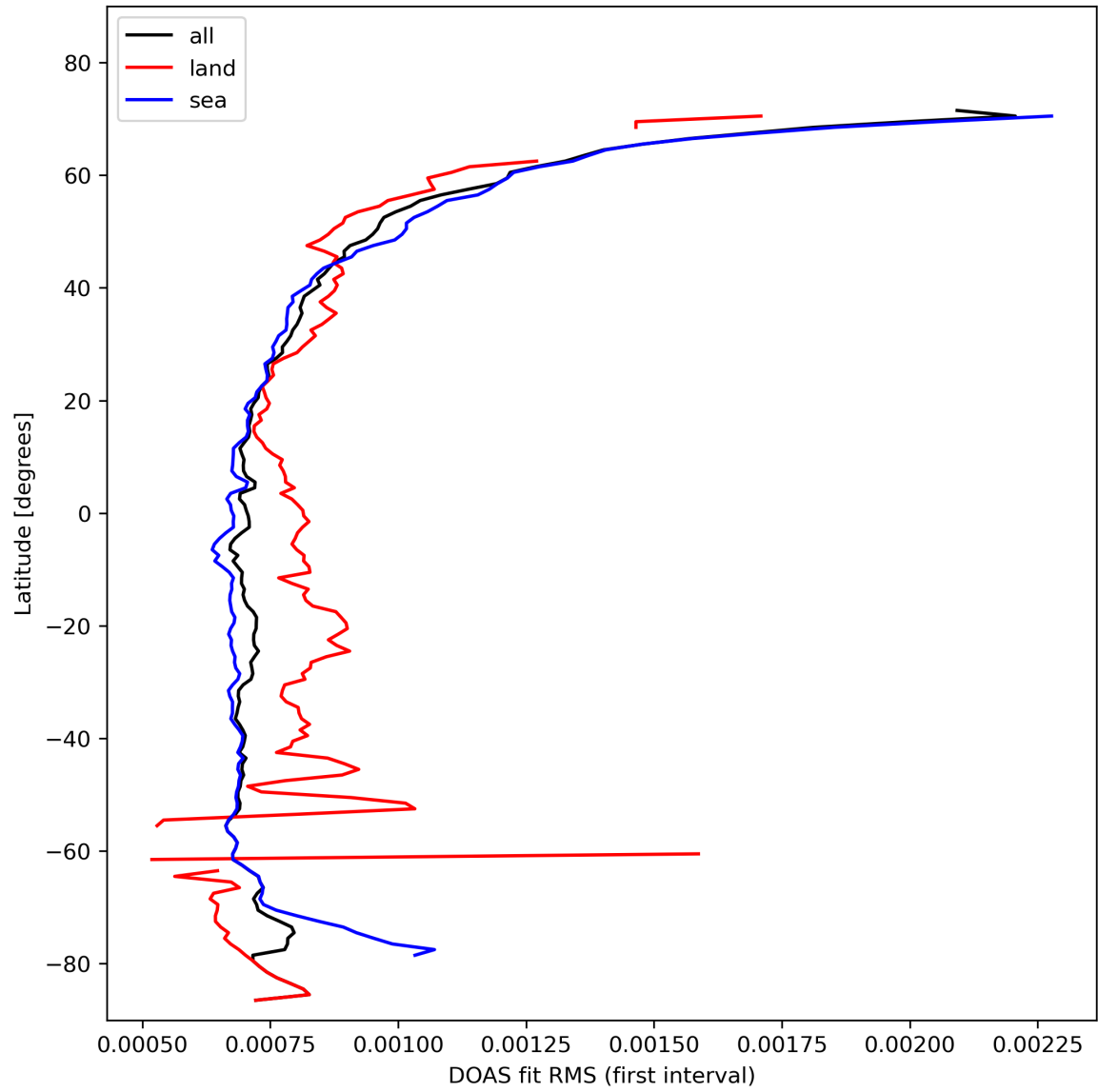
Figure 32: Zonal average of "DOAS fit RMS (first interval)" for 2024-02-11 to 2024-02-12.
