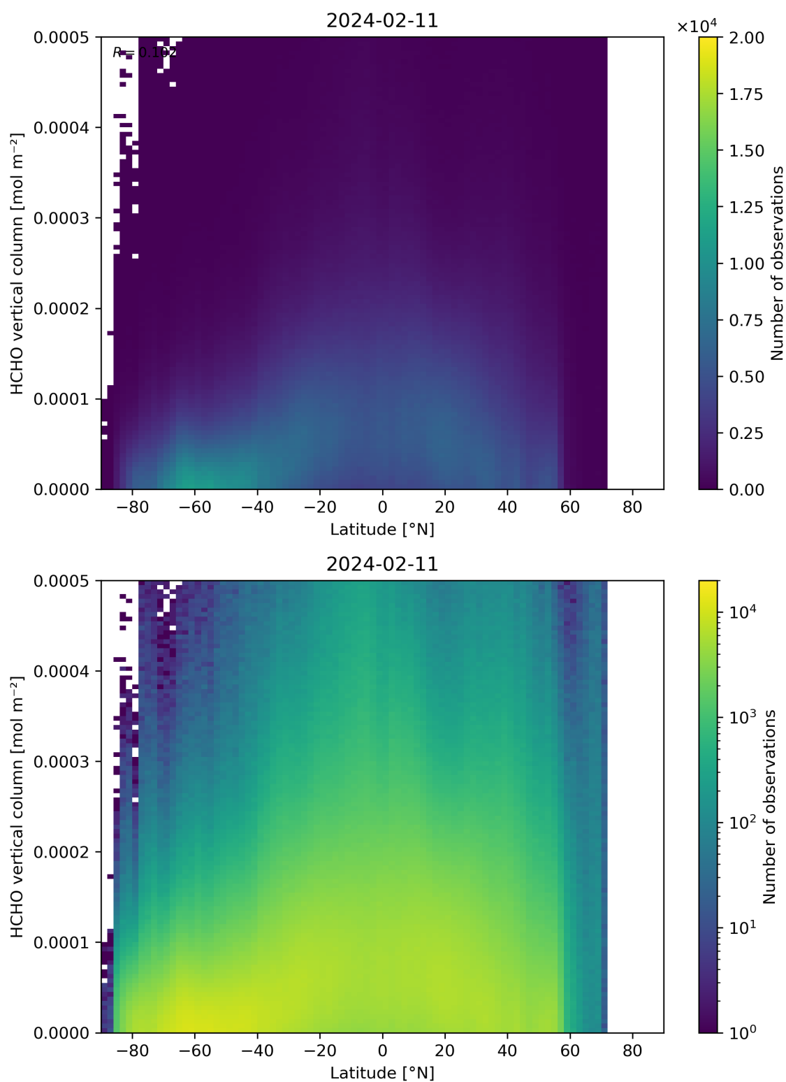
Figure 163: Scatter density plot of “Latitude” against “HCHO vertical column” for 2024-02-11 to 2024-02-12.
