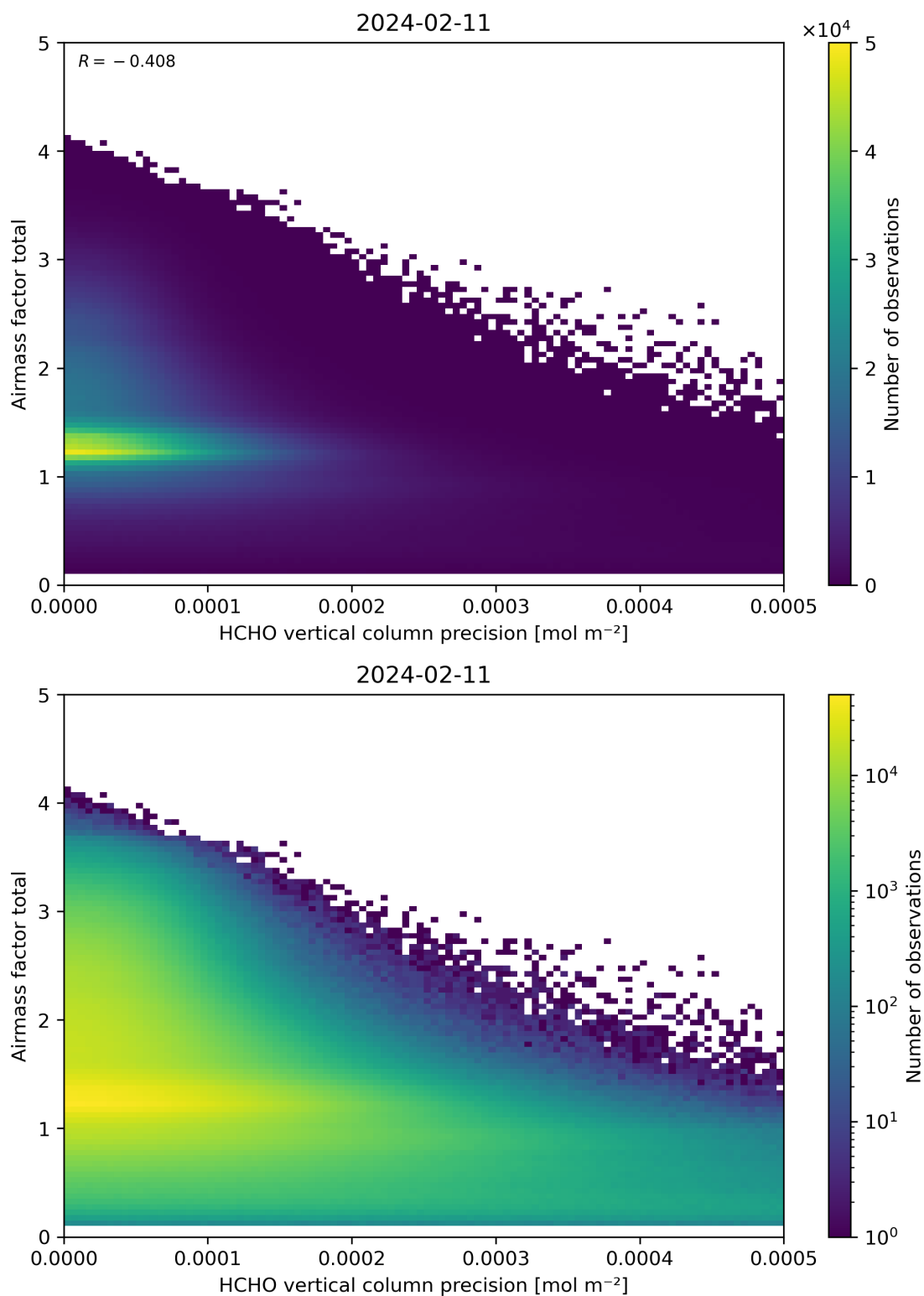
Figure 144: Scatter density plot of “HCHO vertical column precision” against “Airmass factor total” for 2024-02-11 to 2024-02-12.
