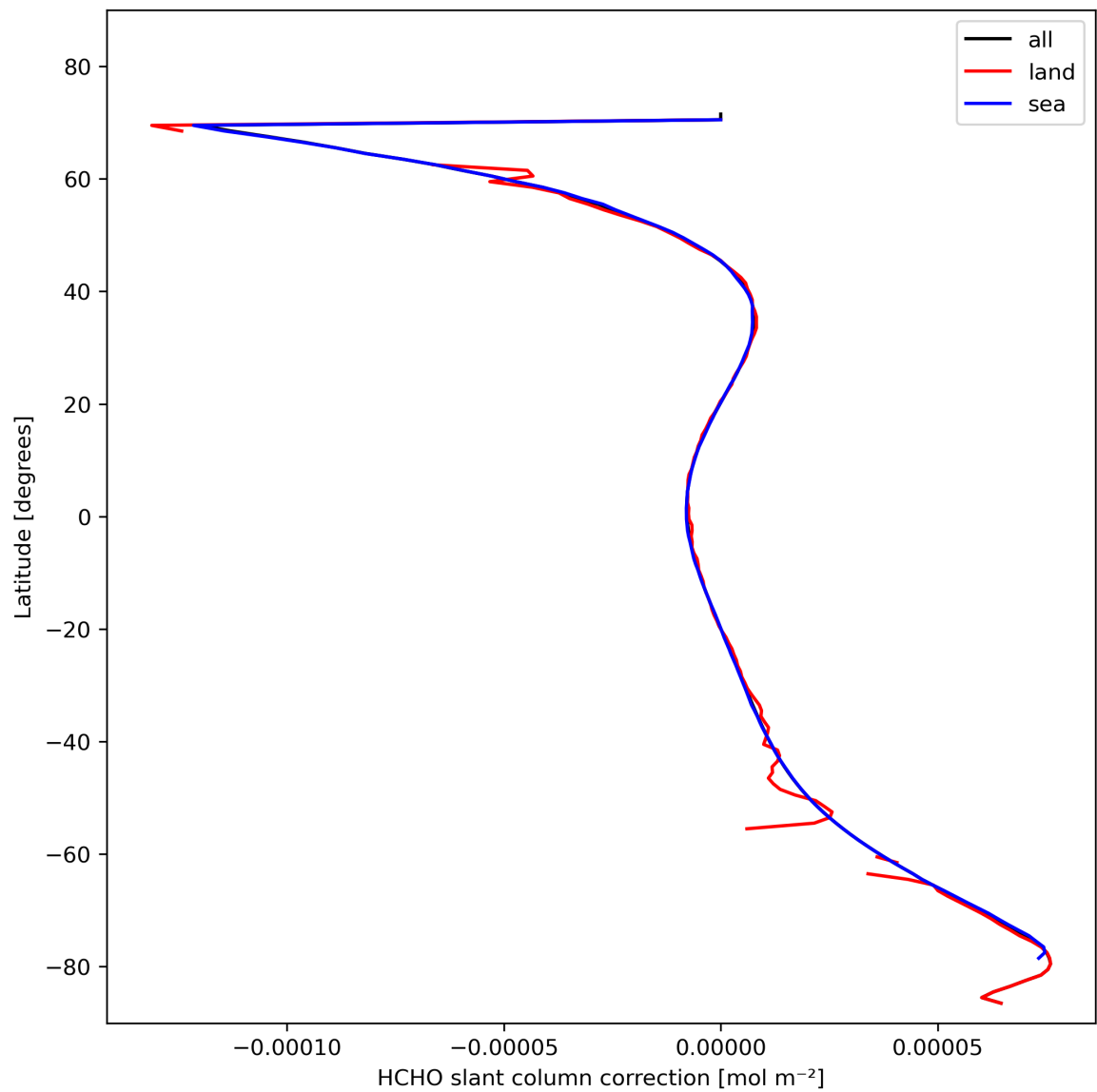
Figure 33: Zonal average of “HCHO slant column correction” for 2024-02-11 to 2024-02-12.
