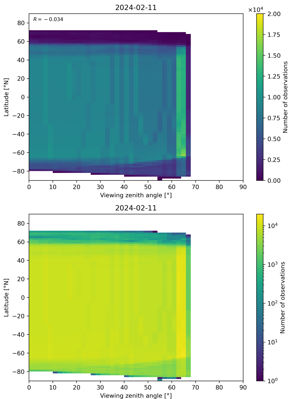
Figure 196: Scatter density plot of “Viewing zenith angle” against “Latitude” for 2024-02-11 to 2024-02-12.
