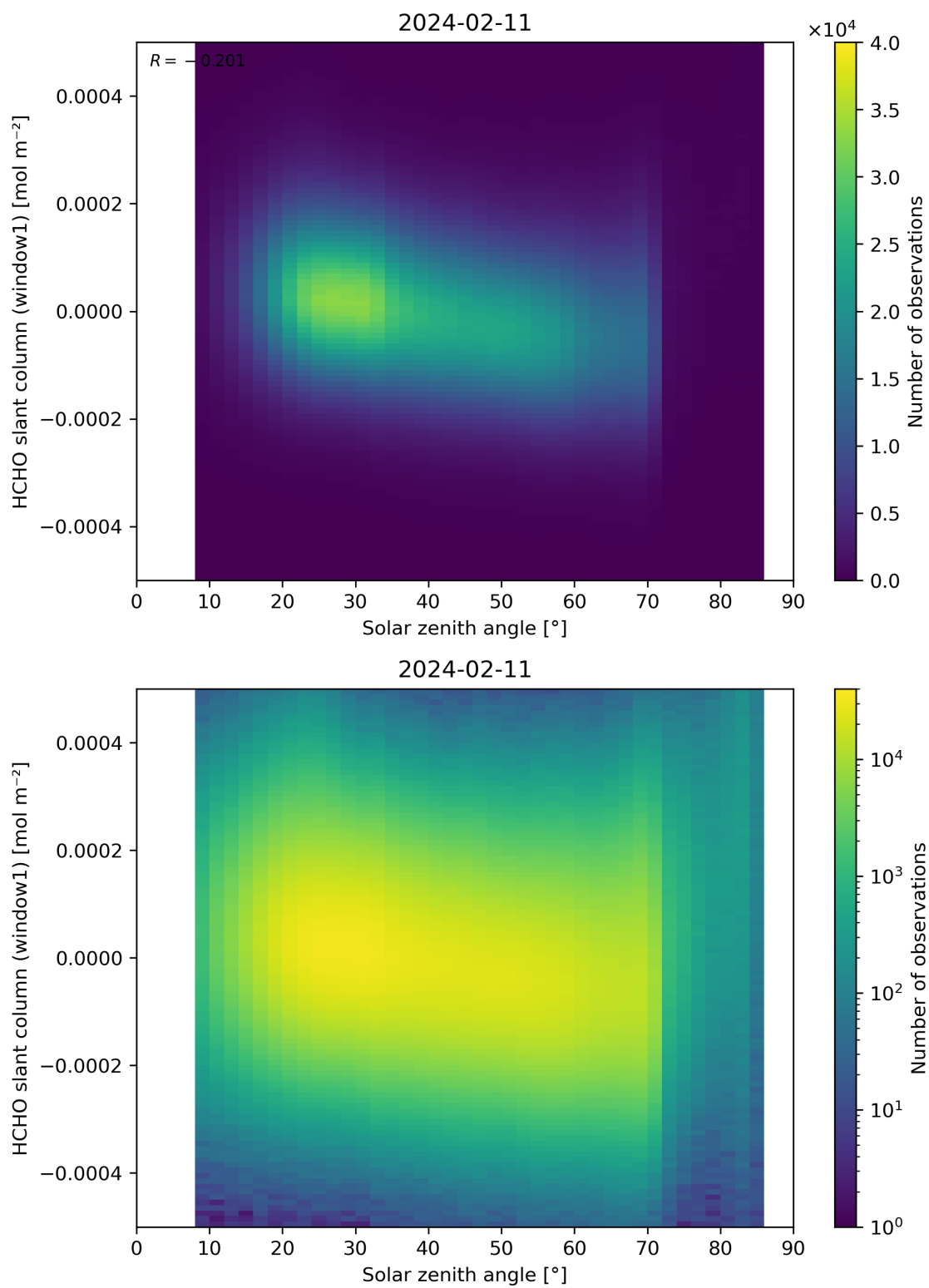
Figure 173: Scatter density plot of “Solar zenith angle” against “HCHO slant column (window1)” for 2024-02-11 to 2024-02-12.
