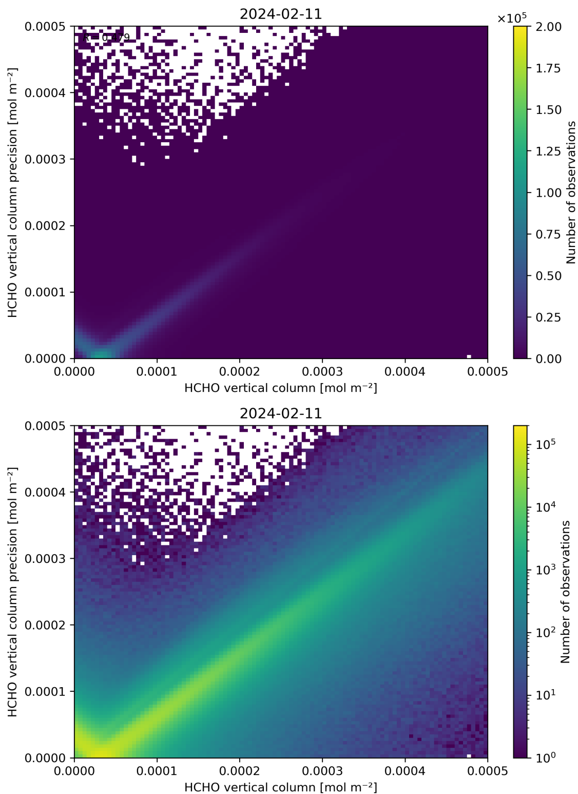
Figure 134: Scatter density plot of “HCHO vertical column” against “HCHO vertical column precision” for 2024-02-11 to 2024-02-12.
