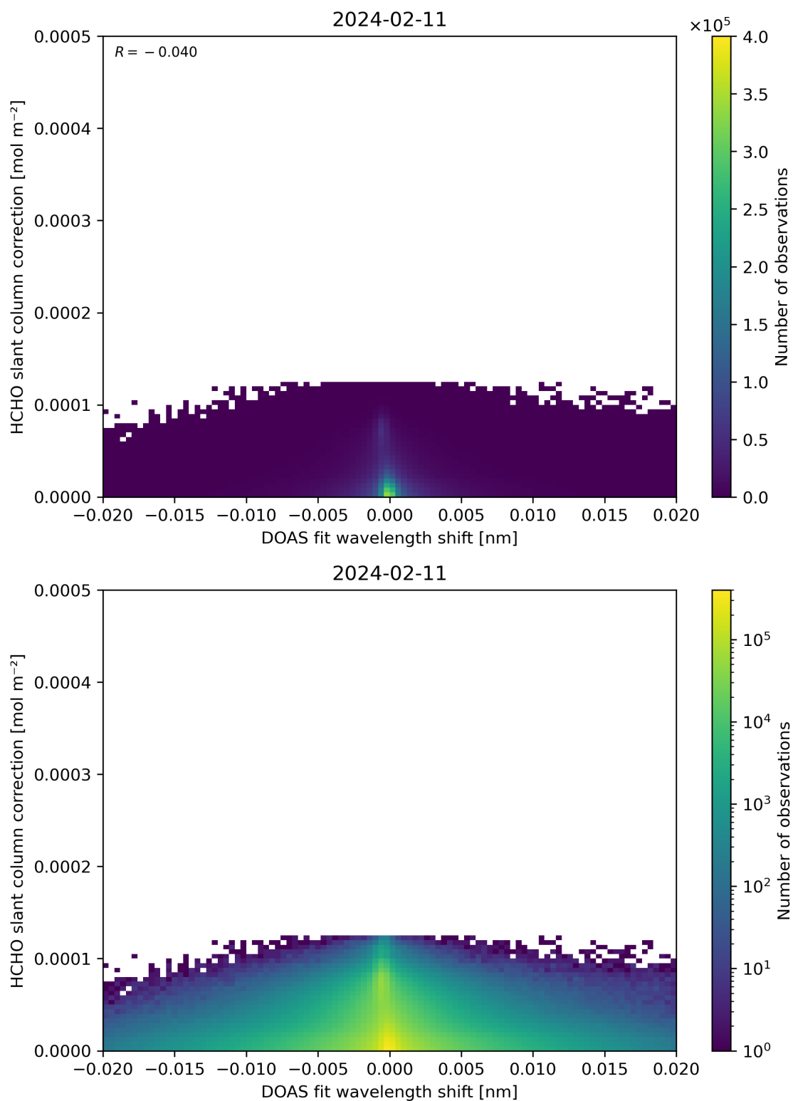
Figure 67: Scatter density plot of “DOAS fit wavelength shift” against “HCHO slant column correction” for 2024-02-11 to 2024-02-12.
