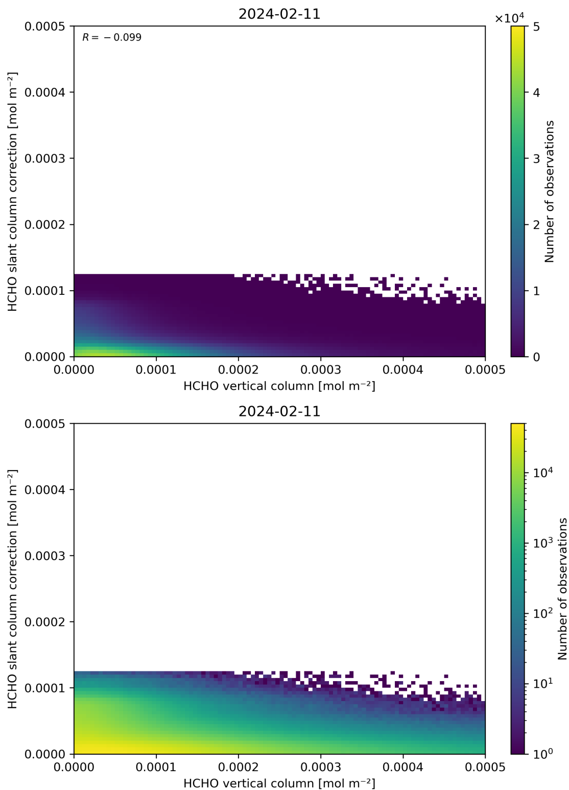
Figure 128: Scatter density plot of “HCHO vertical column” against “HCHO slant column correction” for 2024-02-11 to 2024-02-12.
