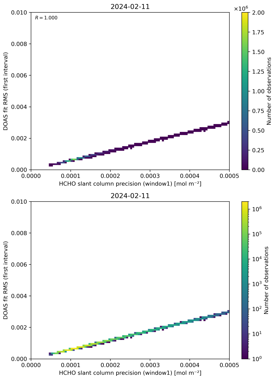
Figure 88: Scatter density plot of “HCHO slant column precision (window1)” against “DOAS fit RMS (first interval)” for 2024-02-11 to 2024-02-12.
