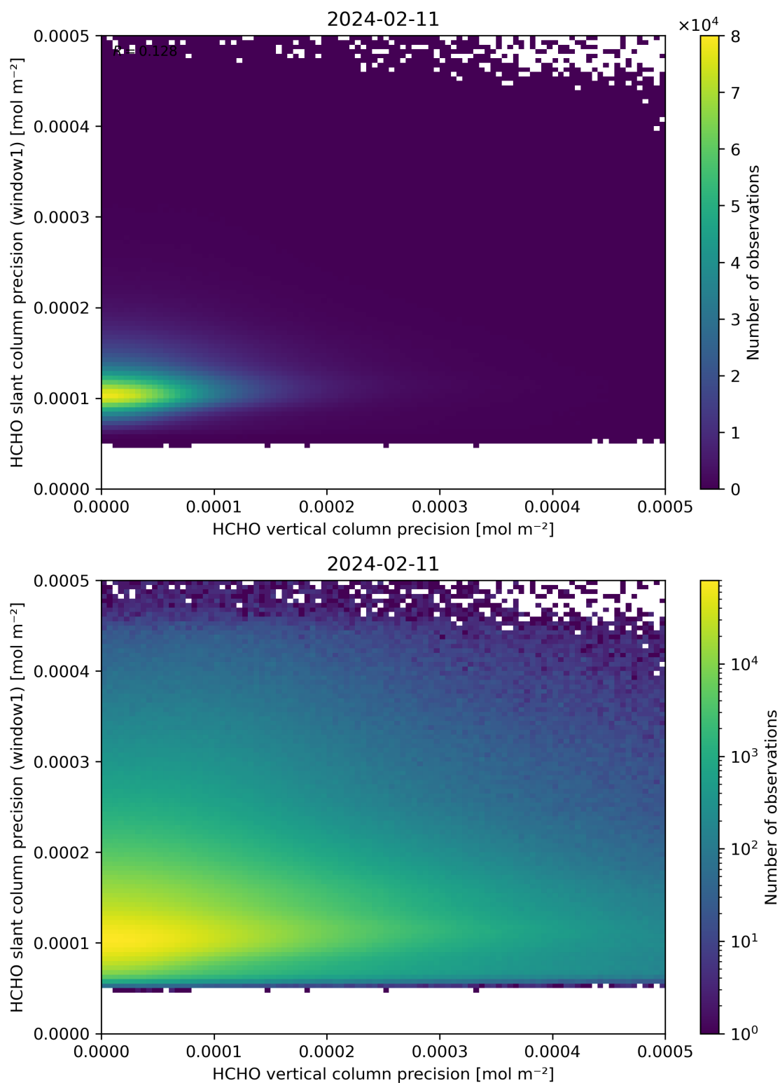
Figure 143: Scatter density plot of “HCHO vertical column precision” against “HCHO slant column precision (window1)” for 2024-02-11 to 2024-02-12.
