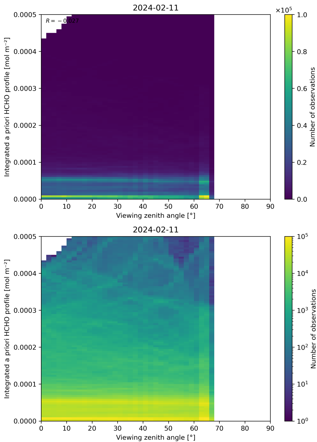
Figure 195: Scatter density plot of “Viewing zenith angle” against “Integrated a priori HCHO profile” for 2024-02-11 to 2024-02-12.
