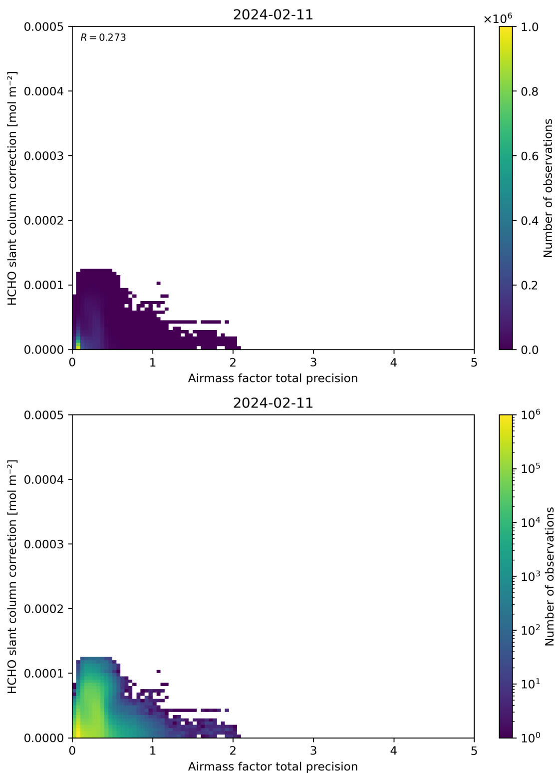
Figure 110: Scatter density plot of “Airmass factor total precision” against “HCHO slant column correction” for 2024-02-11 to 2024-02-12.
