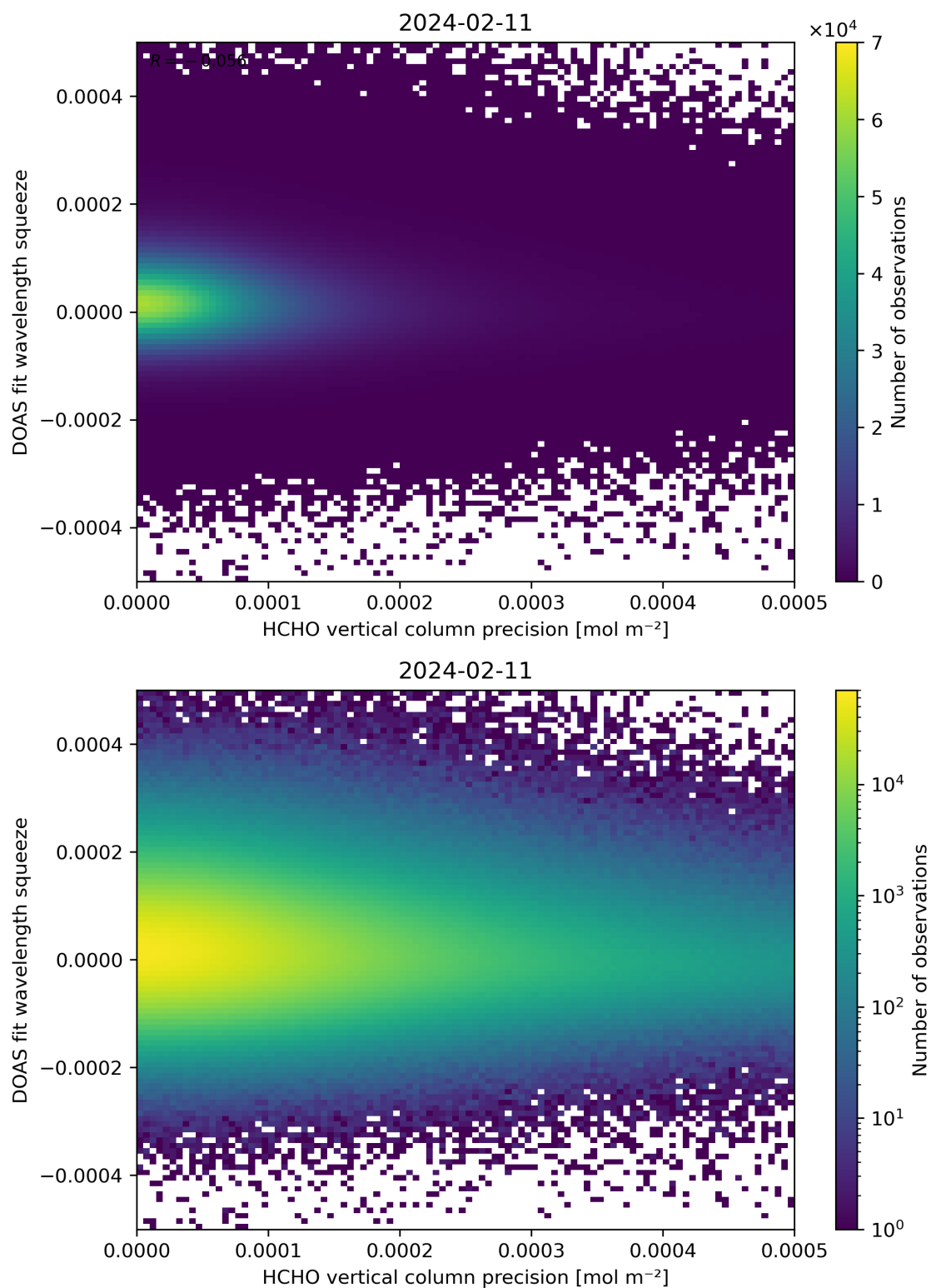
Figure 138: Scatter density plot of “HCHO vertical column precision” against “DOAS fit wavelength squeeze” for 2024-02-11 to 2024-02-12.
