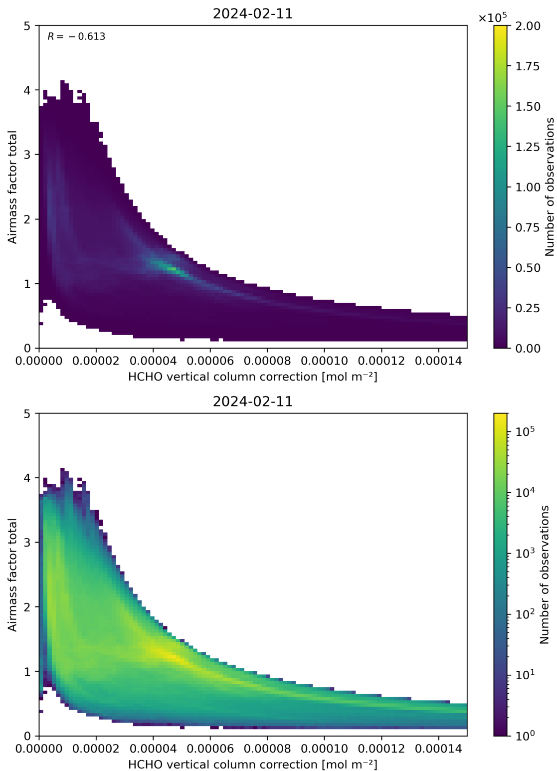
Figure 120: Scatter density plot of “HCHO vertical column correction” against “Airmass factor total” for 2024-02-11 to 2024-02-12.
