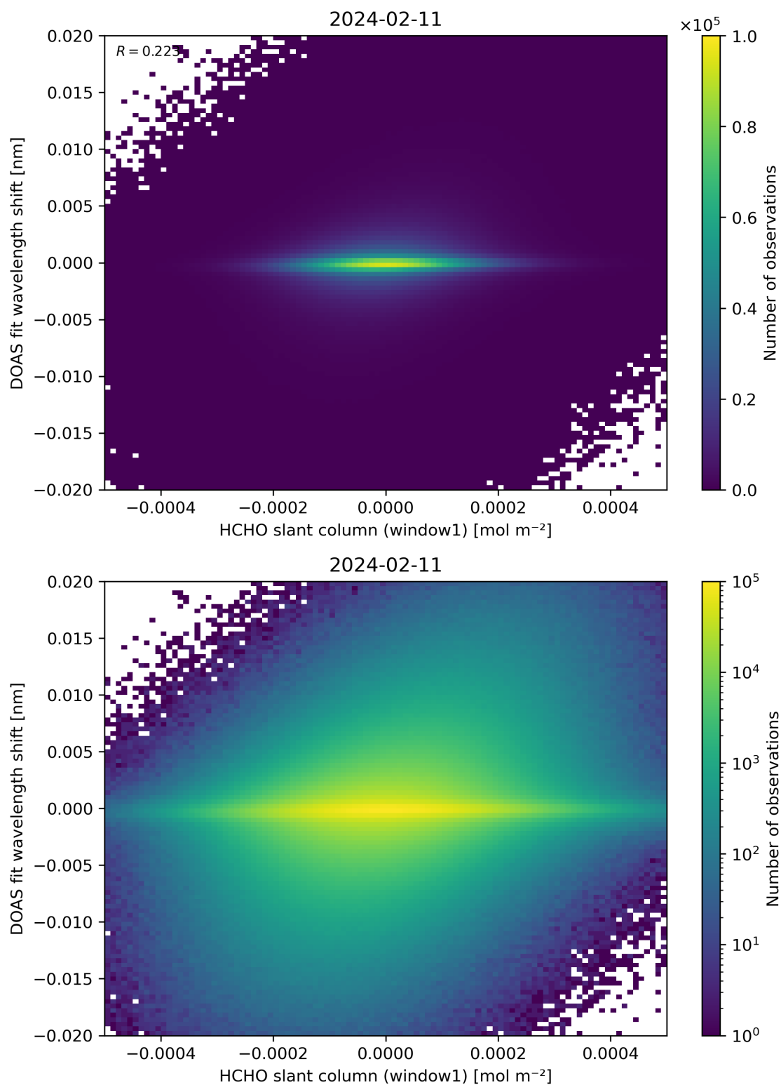
Figure 79: Scatter density plot of “HCHO slant column (window1)” against “DOAS fit wavelength shift” for 2024-02-11 to 2024-02-12.
