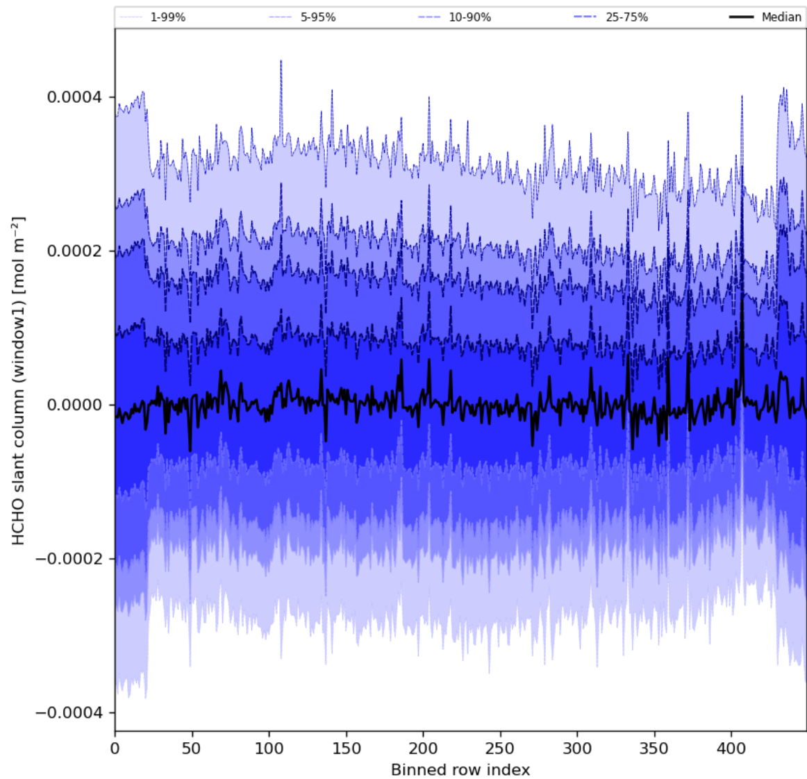
Figure 52: Along track statistics of “HCHO slant column (window1)” for 2024-02-11 to 2024-02-12
