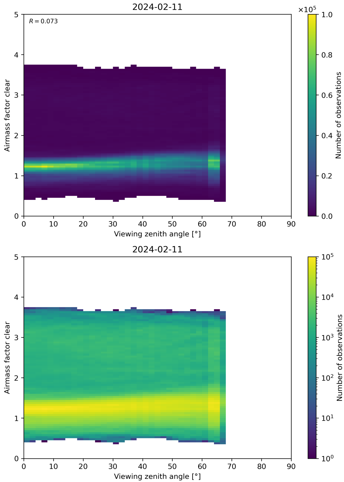
Figure 185: Scatter density plot of “Viewing zenith angle” against “Airmass factor clear” for 2024-02-11 to 2024-02-12.
