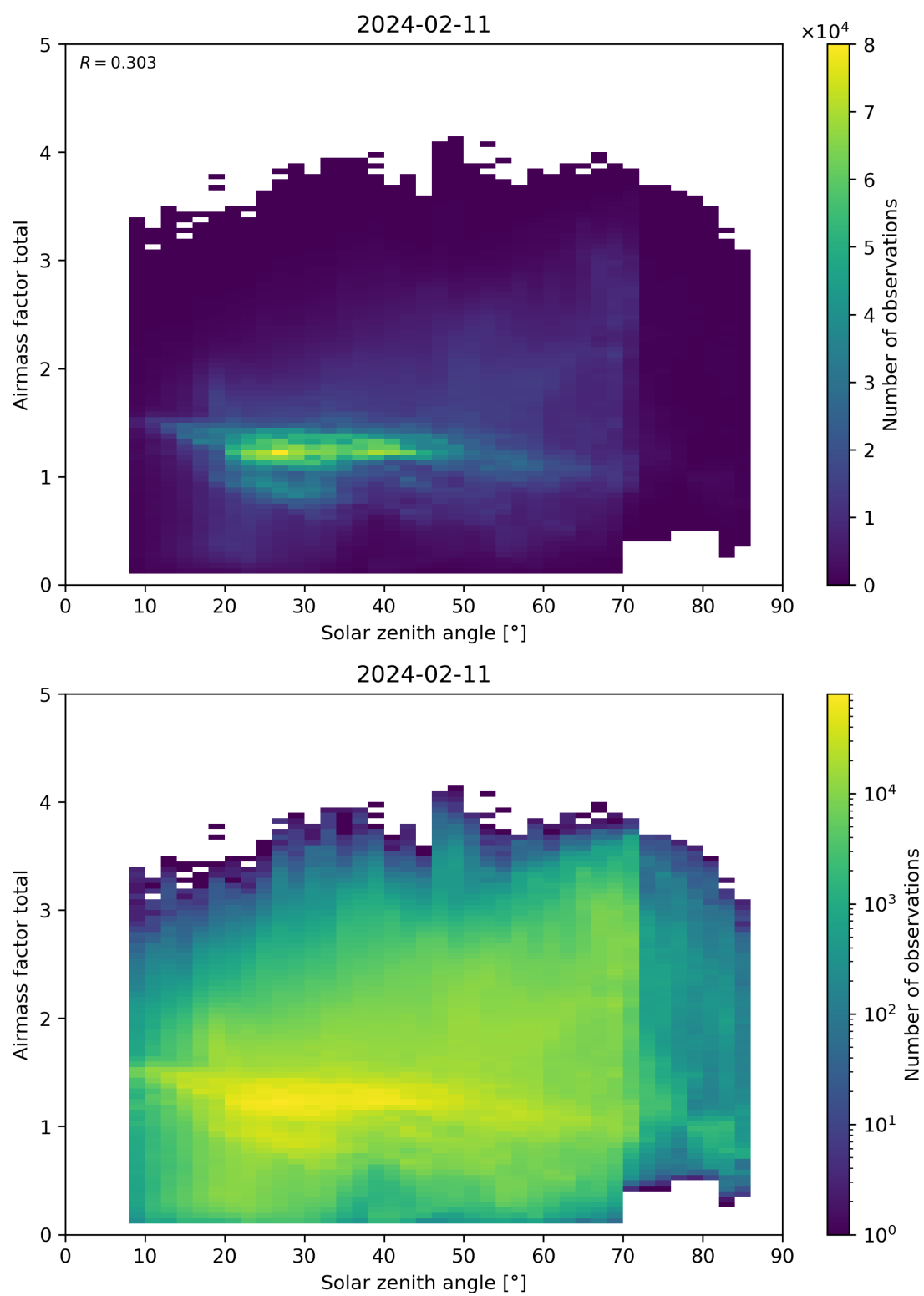
Figure 175: Scatter density plot of “Solar zenith angle” against “Airmass factor total” for 2024-02-11 to 2024-02-12.
