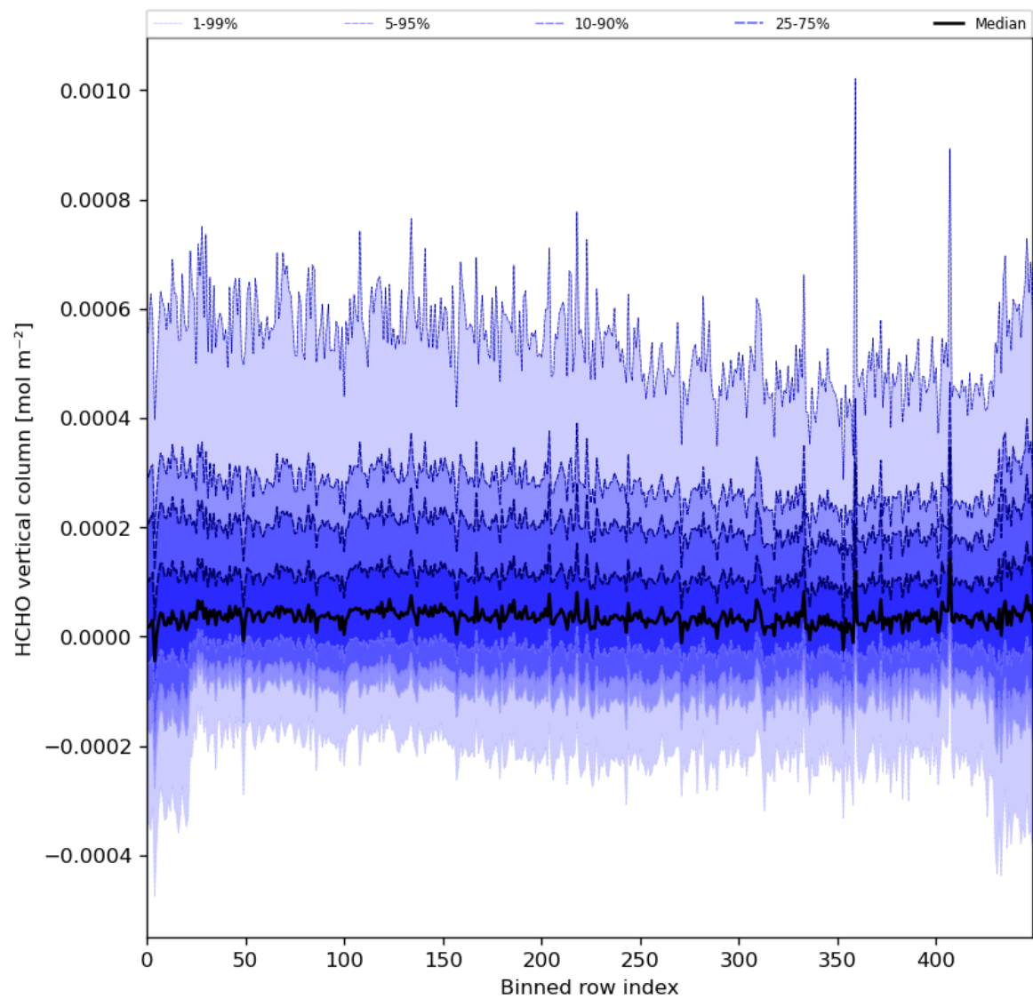
Figure 49: Along track statistics of “HCHO vertical column” for 2024-02-11 to 2024-02-12
