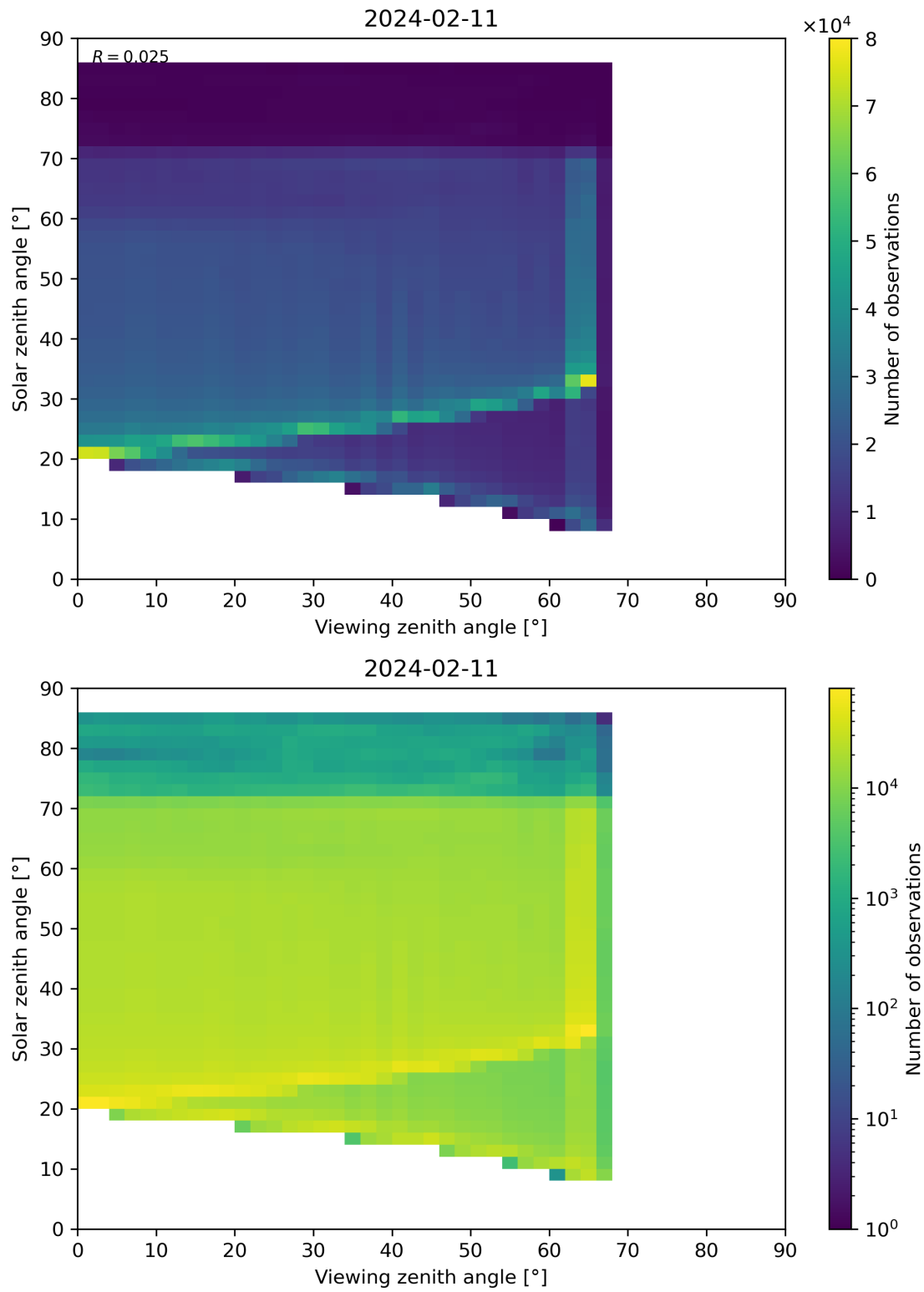
Figure 197: Scatter density plot of “Viewing zenith angle” against “Solar zenith angle” for 2024-02-11 to 2024-02-12.
