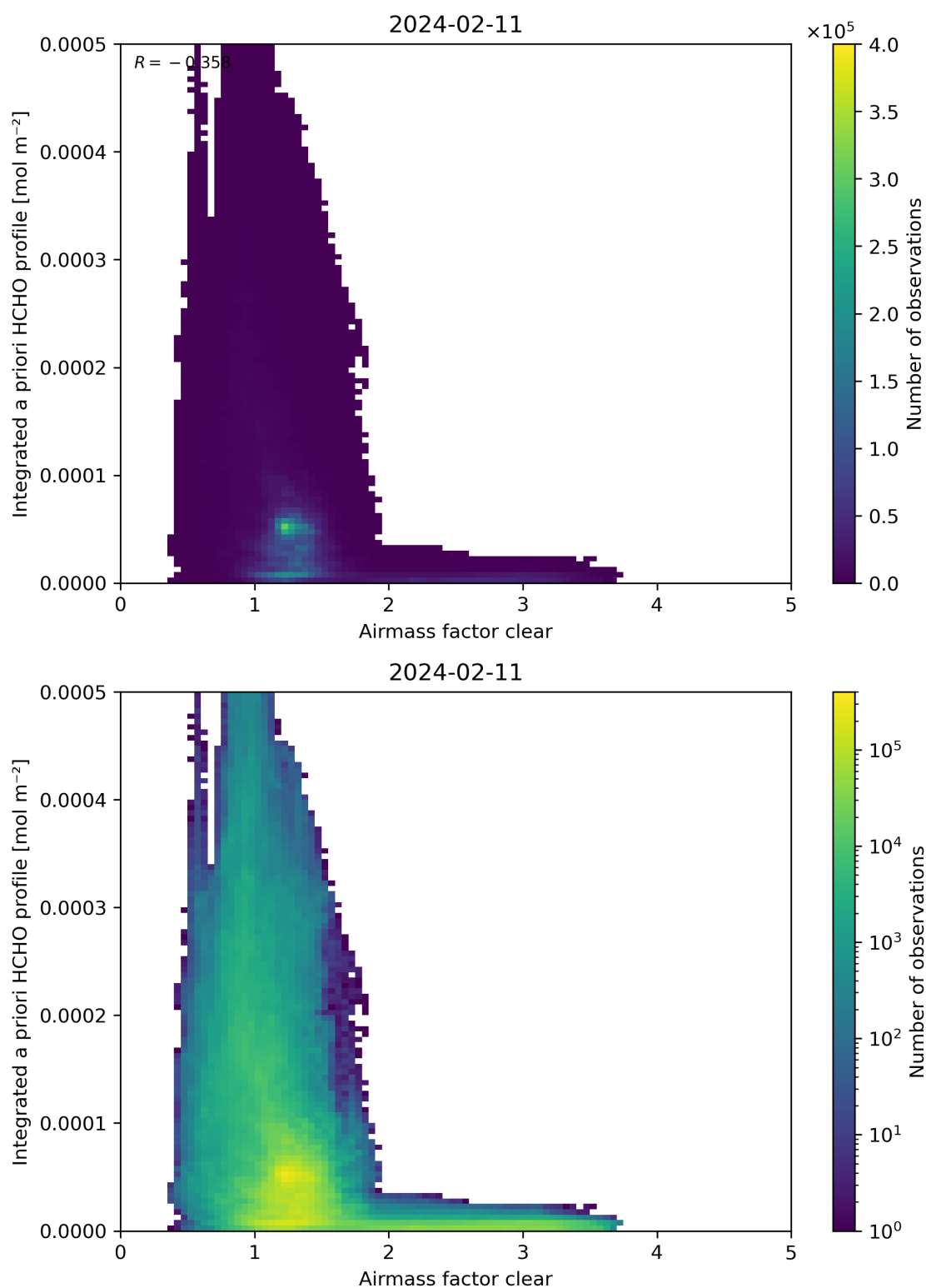
Figure 76: Scatter density plot of “Airmass factor clear” against “Integrated a priori HCHO profile” for 2024-02-11 to 2024-02-12.
