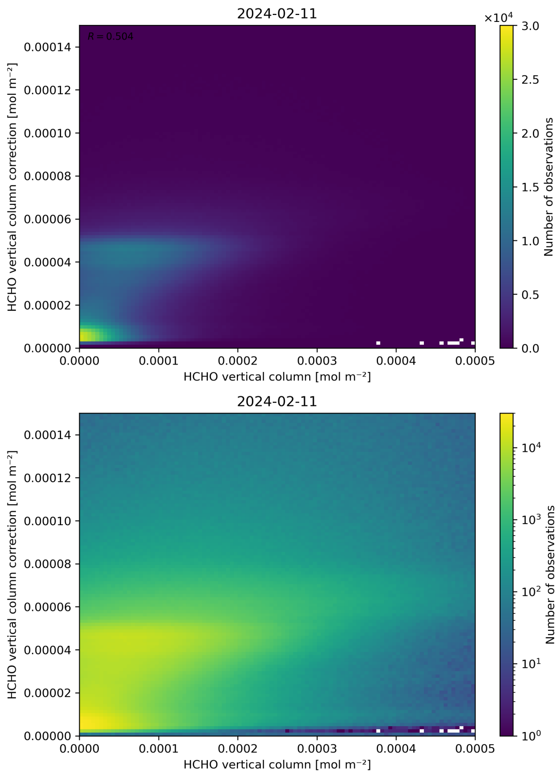
Figure 133: Scatter density plot of “HCHO vertical column” against “HCHO vertical column correction” for 2024-02-11 to 2024-02-12.
