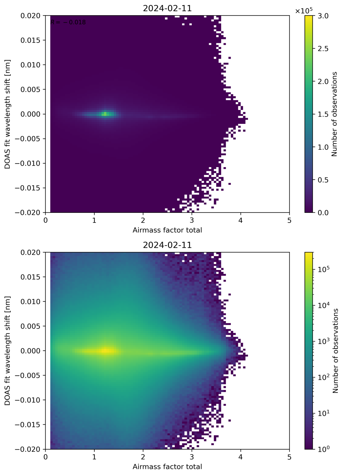
Figure 98: Scatter density plot of “Airmass factor total” against “DOAS fit wavelength shift” for 2024-02-11 to 2024-02-12.
