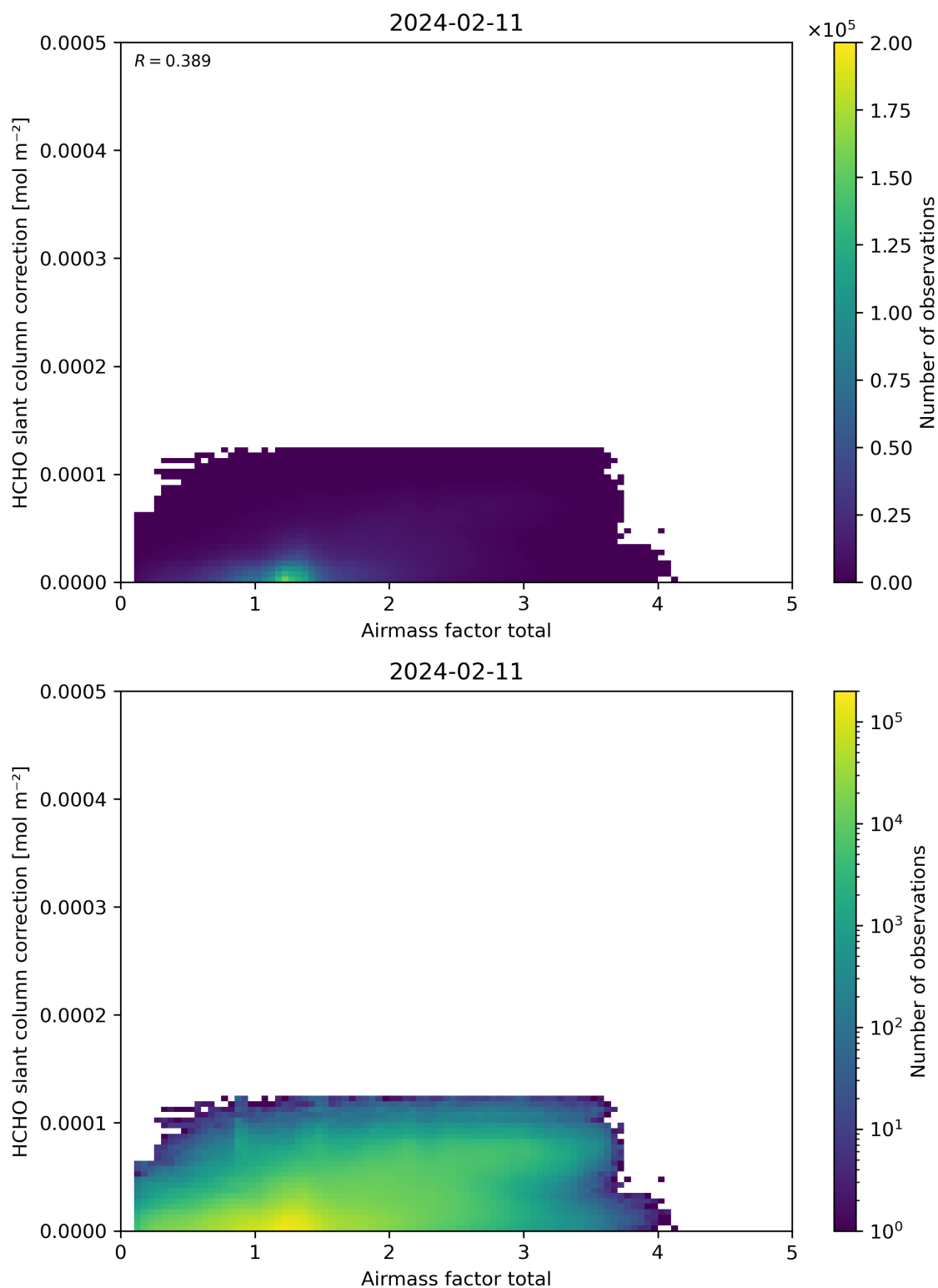
Figure 102: Scatter density plot of “Airmass factor total” against “HCHO slant column correction” for 2024-02-11 to 2024-02-12.
