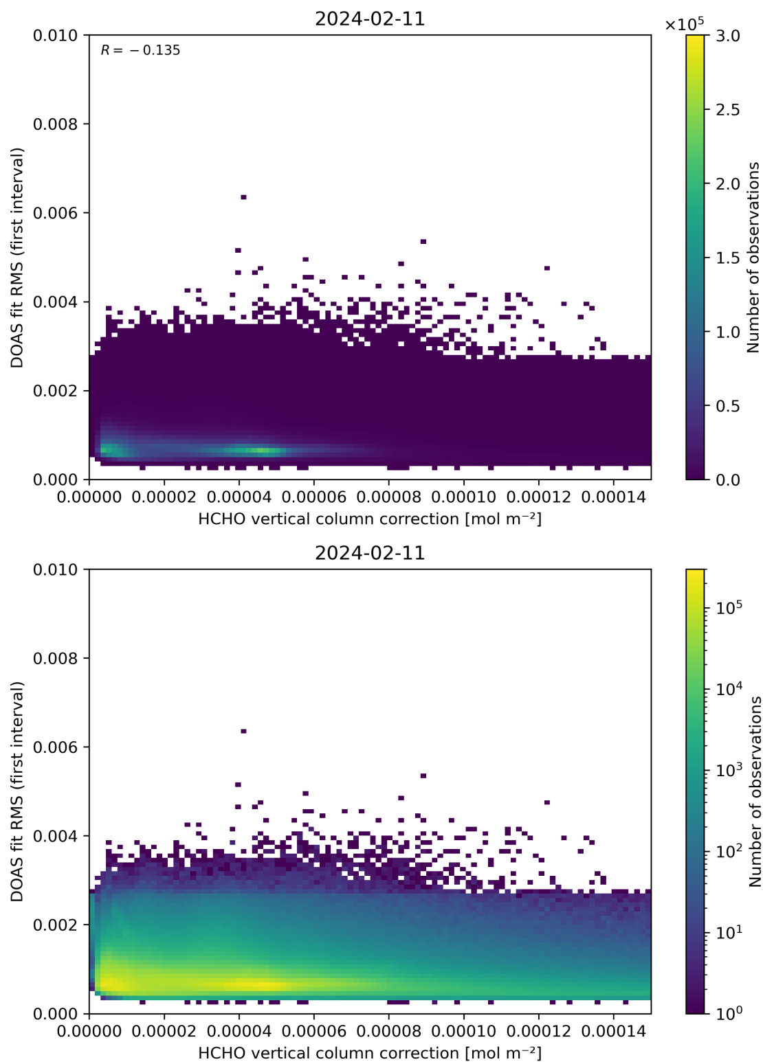
Figure 112: Scatter density plot of “HCHO vertical column correction” against “DOAS fit RMS (first interval)” for 2024-02-11 to 2024-02-12.
