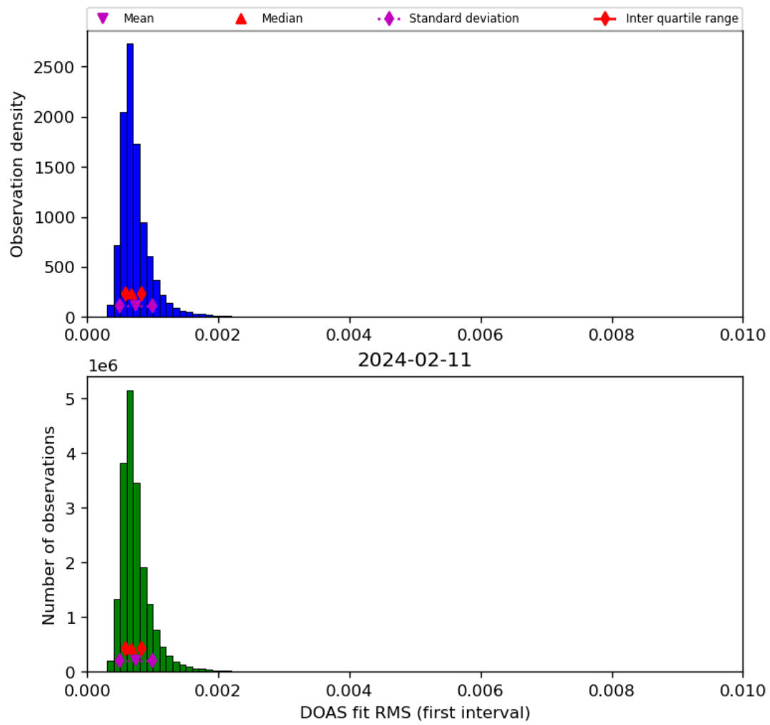
Figure 46: Histogram of “DOAS fit RMS (first interval)” for 2024-02-11 to 2024-02-12
