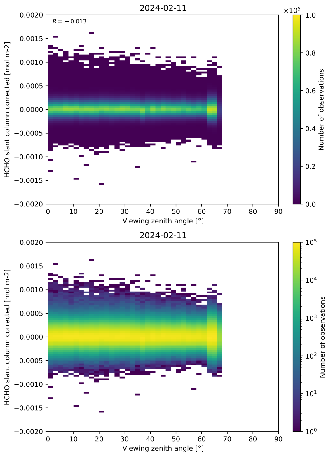
Figure 186: Scatter density plot of “Viewing zenith angle” against “HCHO slant column corrected” for 2024-02-11 to 2024-02-12.
