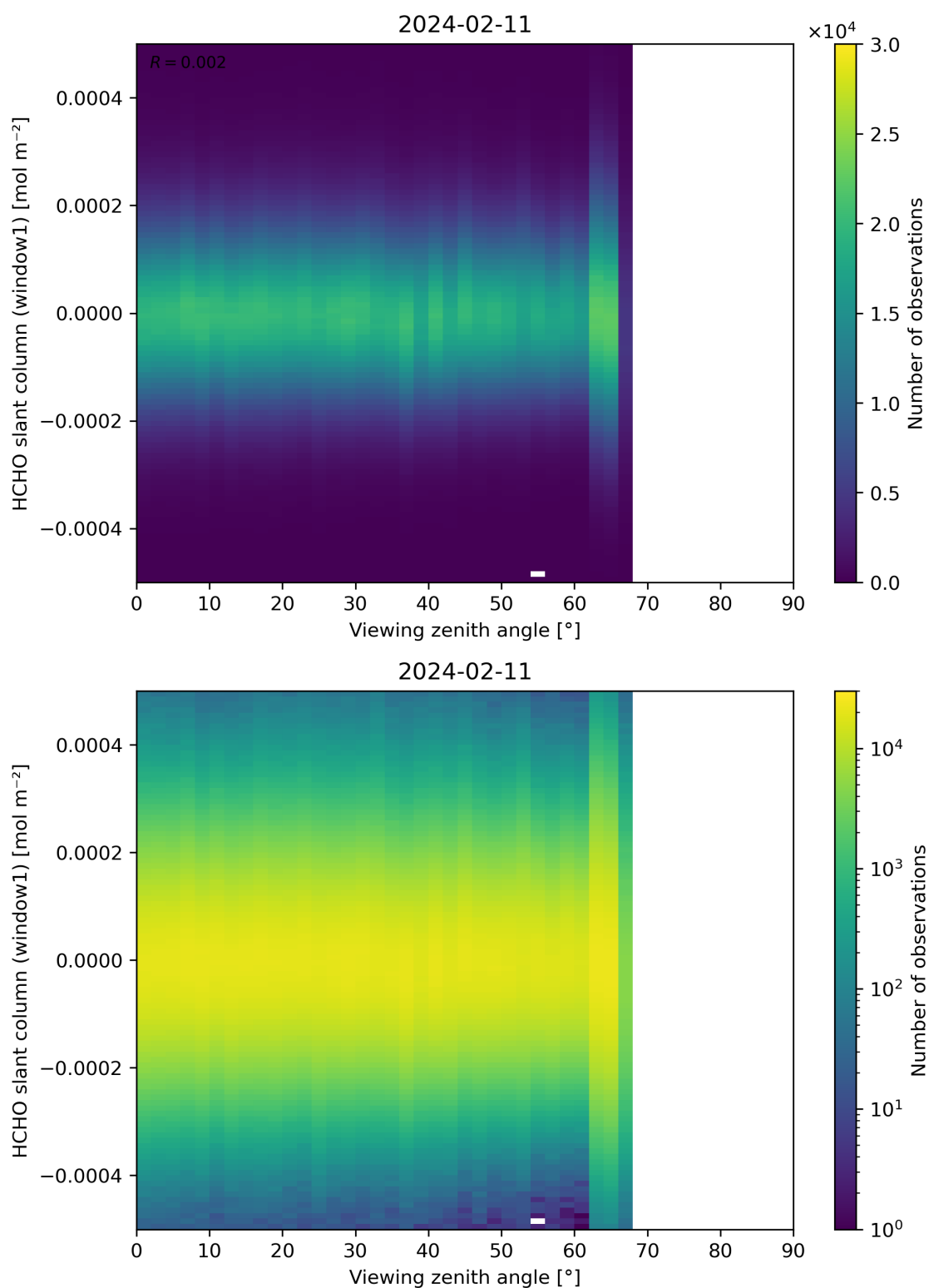
Figure 188: Scatter density plot of “Viewing zenith angle” against “HCHO slant column (window1)” for 2024-02-11 to 2024-02-12.
