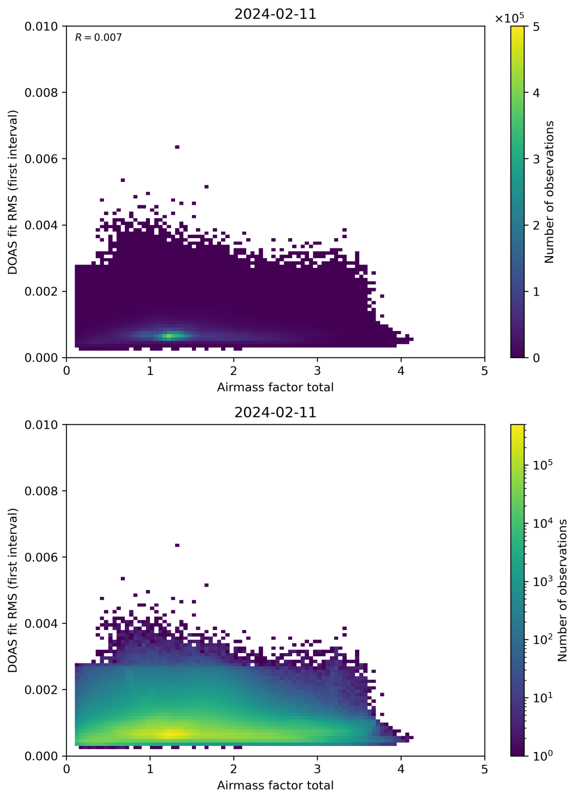
Figure 97: Scatter density plot of “Airmass factor total” against “DOAS fit RMS (first interval)” for 2024-02-11 to 2024-02-12.
