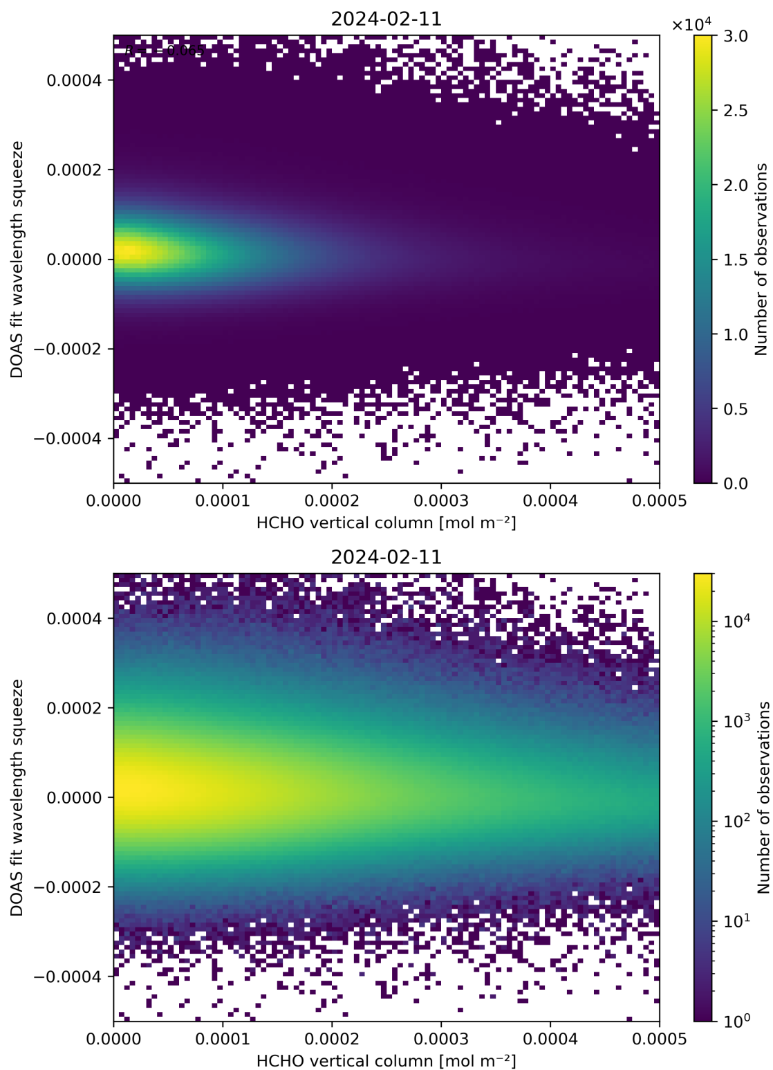
Figure 125: Scatter density plot of “HCHO vertical column” against “DOAS fit wavelength squeeze” for 2024-02-11 to 2024-02-12.
