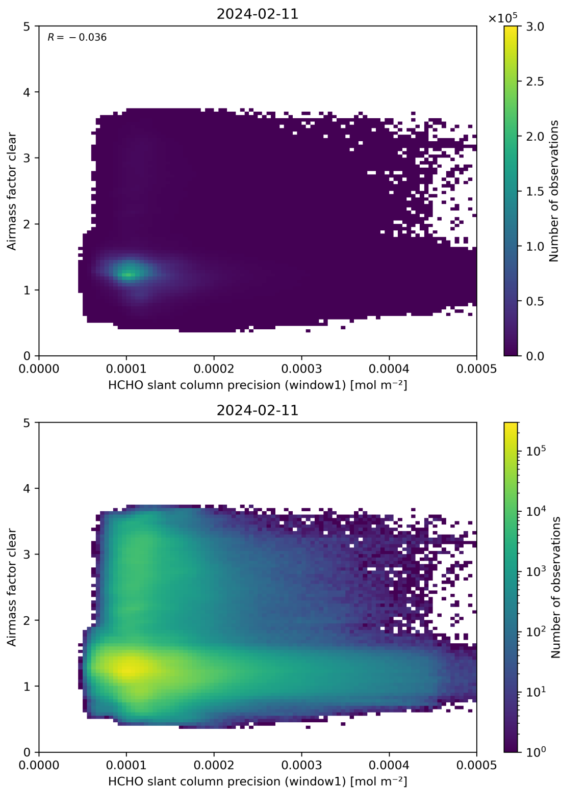
Figure 91: Scatter density plot of “HCHO slant column precision (window1)” against “Airmass factor clear” for 2024-02-11 to 2024-02-12.
