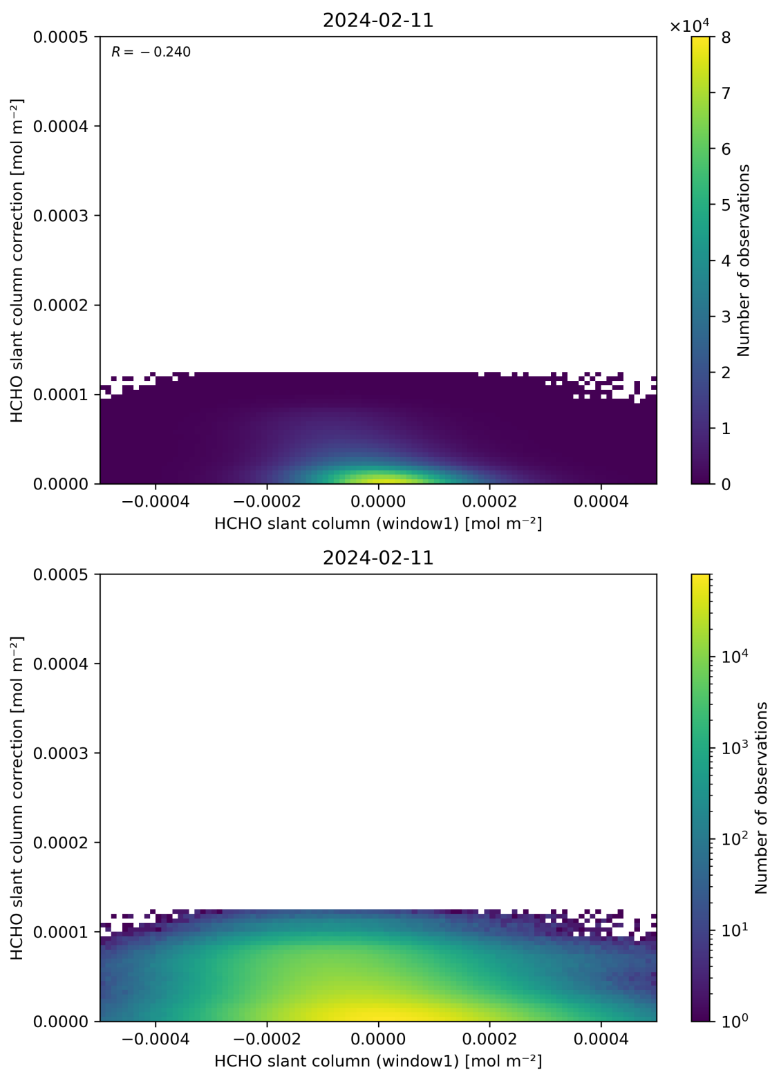
Figure 83: Scatter density plot of “HCHO slant column (window1)” against “HCHO slant column correction” for 2024-02-11 to 2024-02-12.
