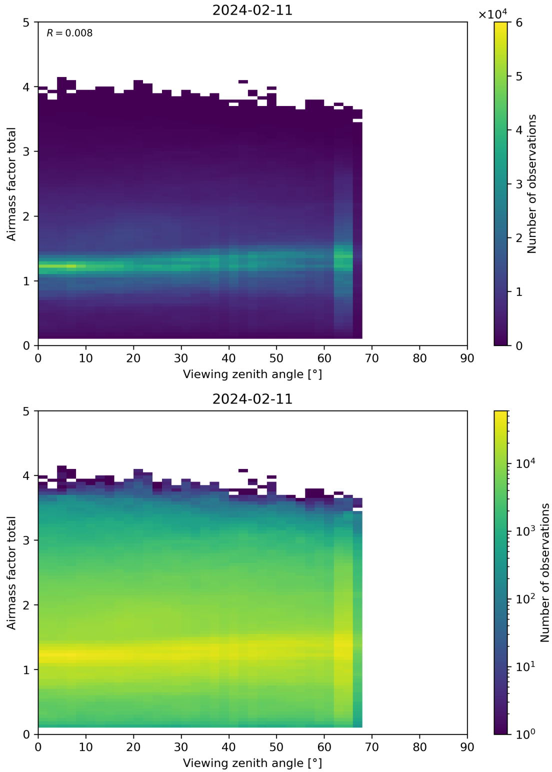
Figure 190: Scatter density plot of “Viewing zenith angle” against “Airmass factor total” for 2024-02-11 to 2024-02-12.
