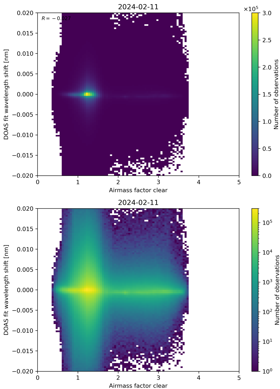
Figure 72: Scatter density plot of “Airmass factor clear” against “DOAS fit wavelength shift” for 2024-02-11 to 2024-02-12.
