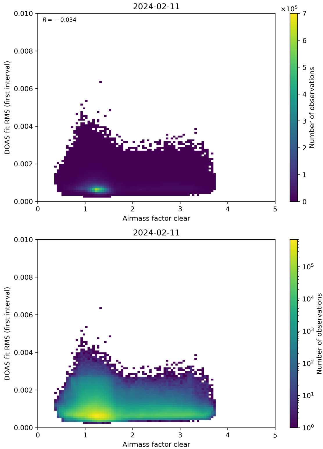
Figure 71: Scatter density plot of “Airmass factor clear” against “DOAS fit RMS (first interval)” for 2024-02-11 to 2024-02-12.
