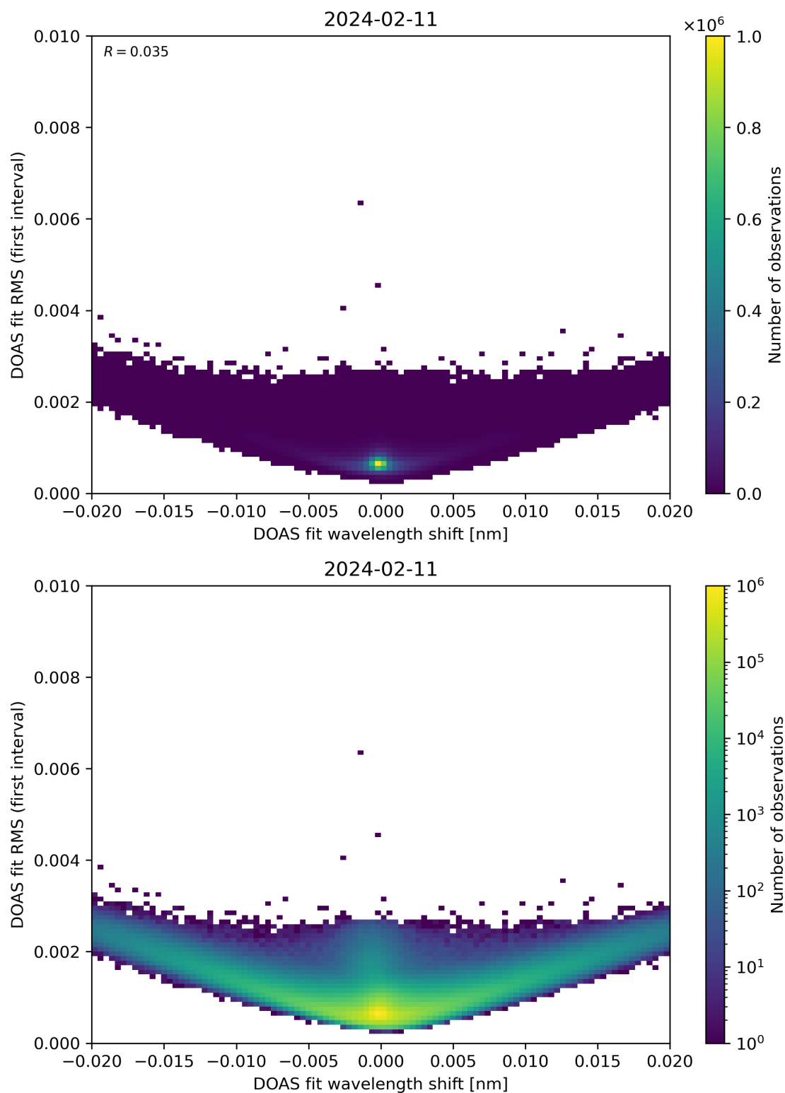
Figure 64: Scatter density plot of “DOAS fit wavelength shift” against “DOAS fit RMS (first interval)” for 2024-02-11 to 2024-02-12.
