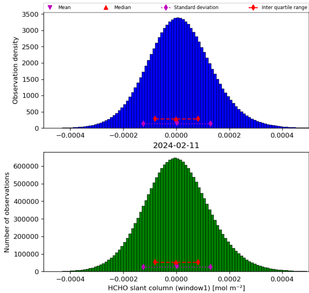
Figure 38: Histogram of “HCHO slant column (window1)” for 2024-02-11 to 2024-02-12
