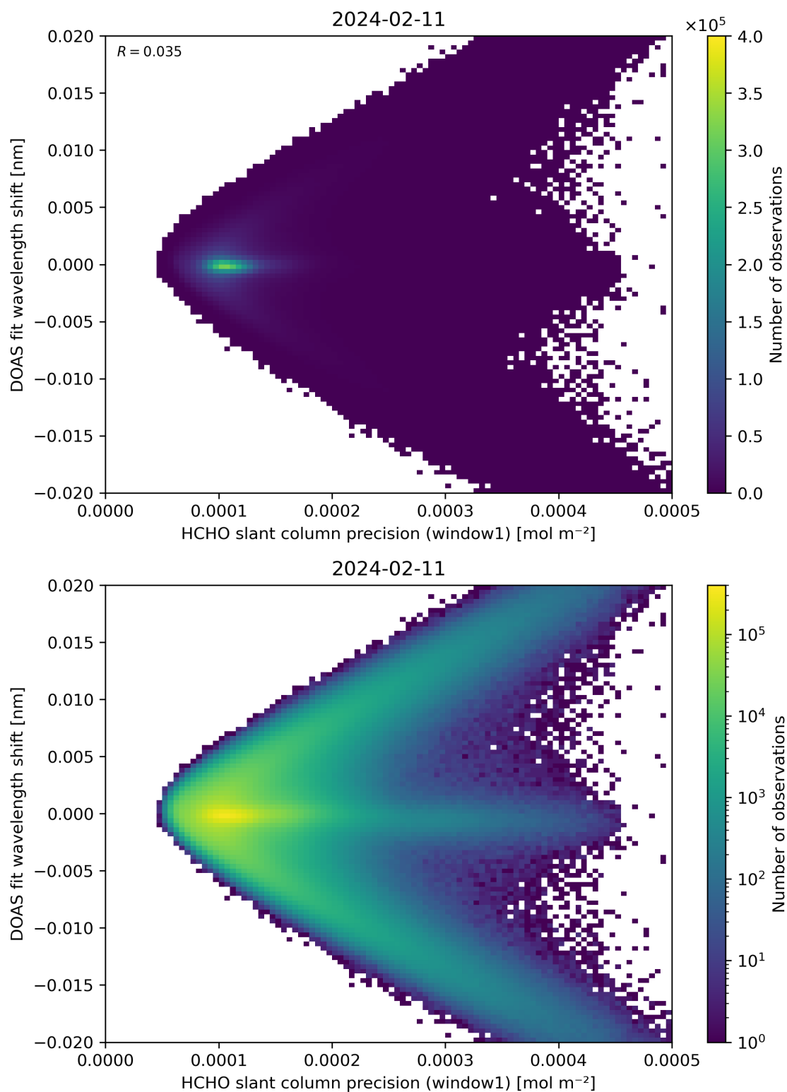
Figure 89: Scatter density plot of “HCHO slant column precision (window1)” against “DOAS fit wavelength shift” for 2024-02-11 to 2024-02-12.
