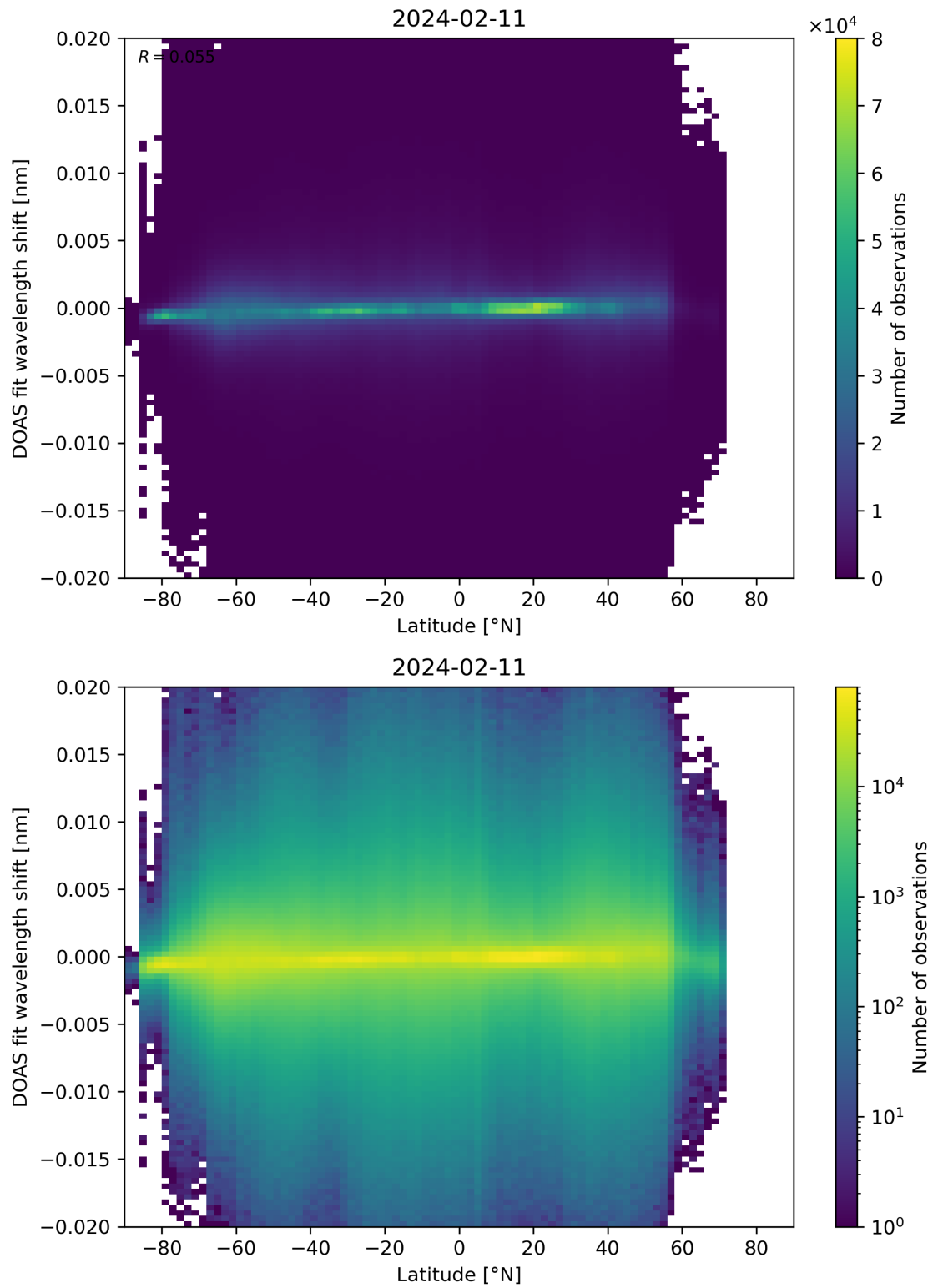
Figure 154: Scatter density plot of “Latitude” against “DOAS fit wavelength shift” for 2024-02-11 to 2024-02-12.
