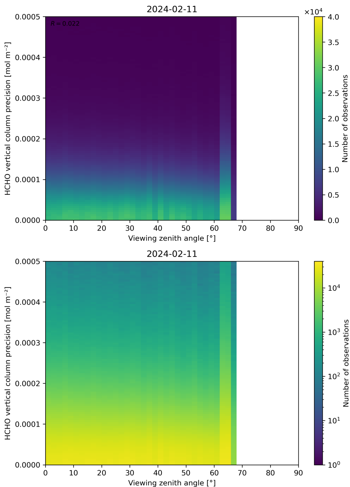
Figure 194: Scatter density plot of “Viewing zenith angle” against “HCHO vertical column precision” for 2024-02-11 to 2024-02-12.
