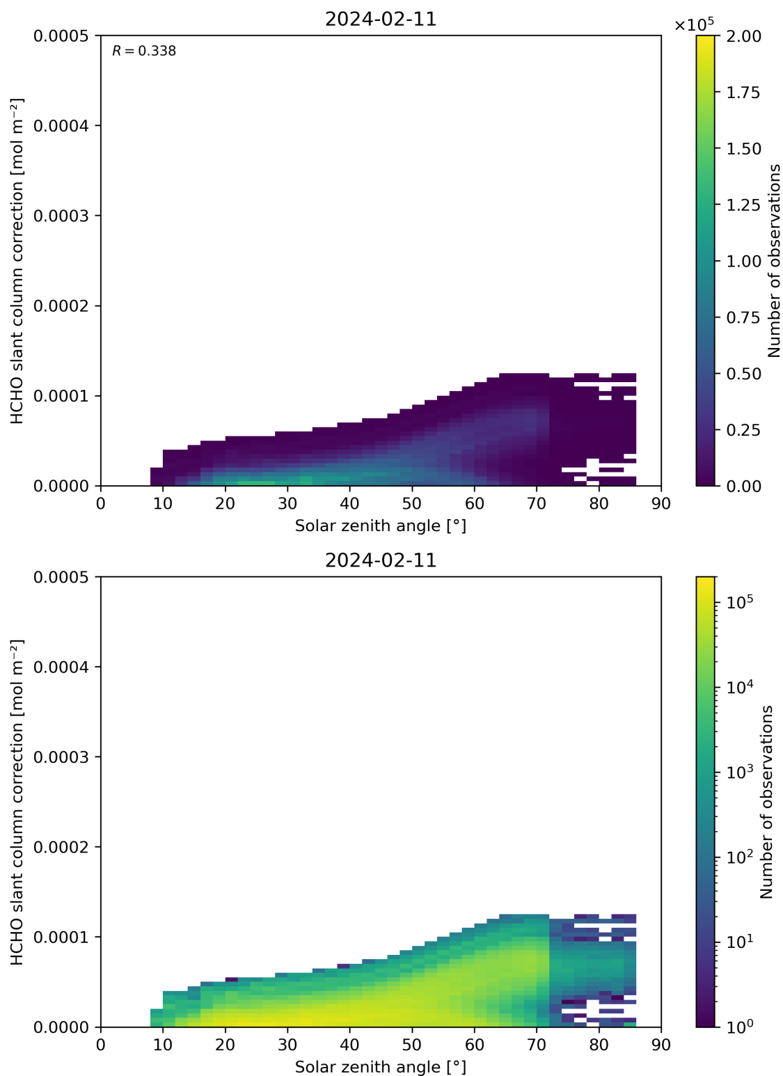
Figure 172: Scatter density plot of “Solar zenith angle” against “HCHO slant column correction” for 2024-02-11 to 2024-02-12.
