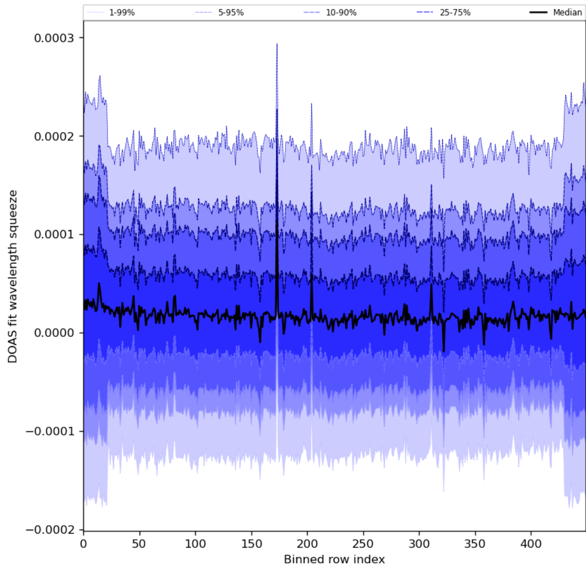
Figure 59: Along track statistics of “DOAS fit wavelength squeeze” for 2024-02-11 to 2024-02-12
