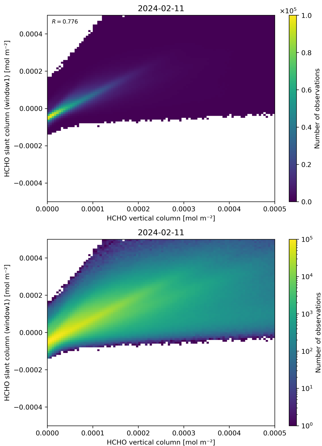
Figure 129: Scatter density plot of “HCHO vertical column” against “HCHO slant column (window1)” for 2024-02-11 to 2024-02-12.
