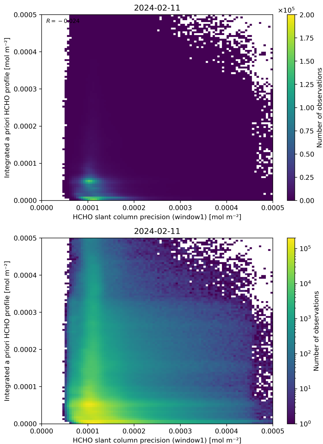
Figure 96: Scatter density plot of “HCHO slant column precision (window1)” against “Integrated a priori HCHO profile” for 2024-02-11 to 2024-02-12.
