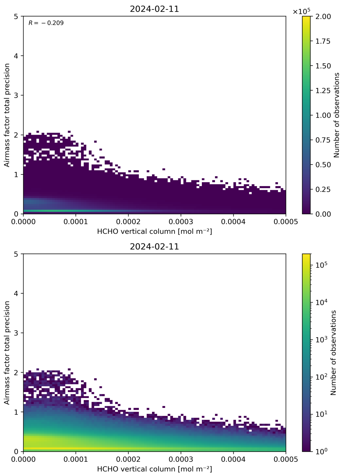
Figure 132: Scatter density plot of “HCHO vertical column” against “Airmass factor total precision” for 2024-02-11 to 2024-02-12.
