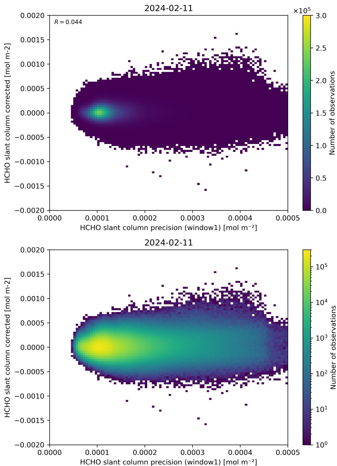
Figure 92: Scatter density plot of “HCHO slant column precision (window1)” against “HCHO slant column corrected” for 2024-02-11 to 2024-02-12.
