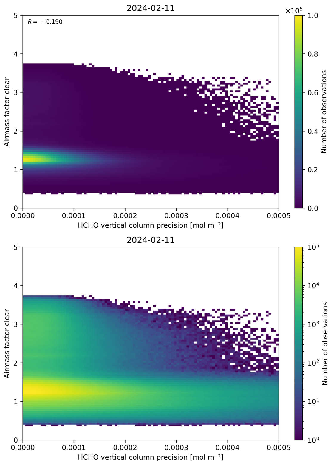
Figure 139: Scatter density plot of “HCHO vertical column precision” against “Airmass factor clear” for 2024-02-11 to 2024-02-12.
