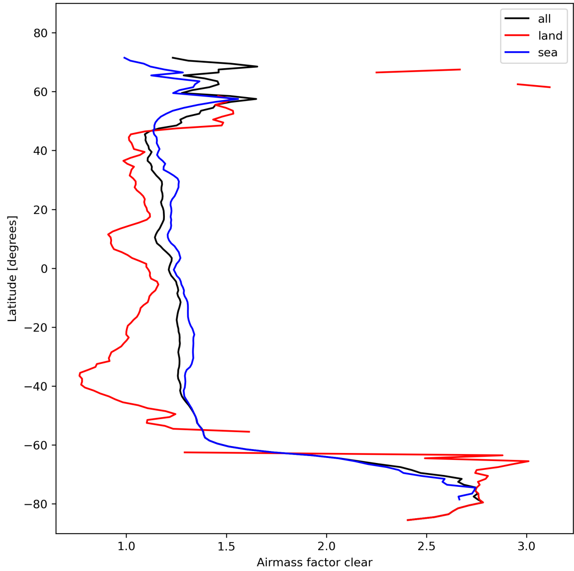
Figure 28: Zonal average of “Airmass factor clear” for 2024-02-12 to 2024-02-14.
