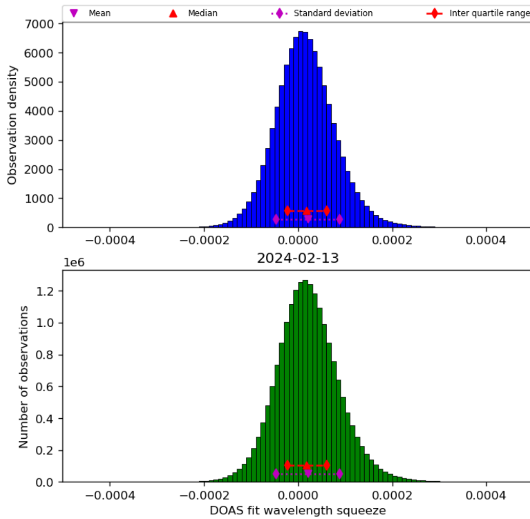
Figure 45: Histogram of “DOAS fit wavelength squeeze” for 2024-02-12 to 2024-02-14
