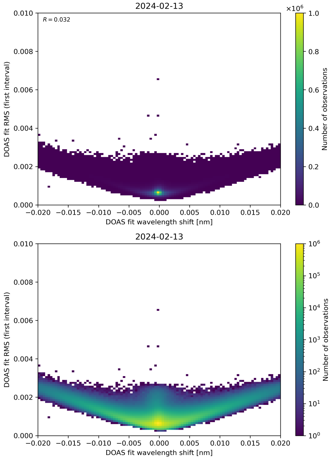
Figure 64: Scatter density plot of “DOAS fit wavelength shift” against “DOAS fit RMS (first interval)” for 2024-02-12 to 2024-02-14.
