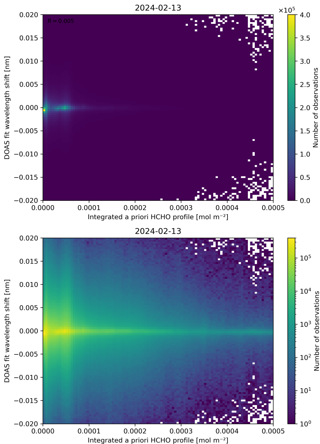
Figure 149: Scatter density plot of “Integrated a priori HCHO profile” against “DOAS fit wavelength shift” for 2024-02-12 to 2024-02-14.
