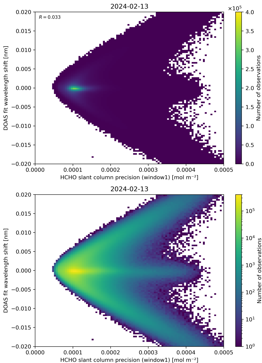
Figure 89: Scatter density plot of “HCHO slant column precision (window1)” against “DOAS fit wavelength shift” for 2024-02-12 to 2024-02-14.
