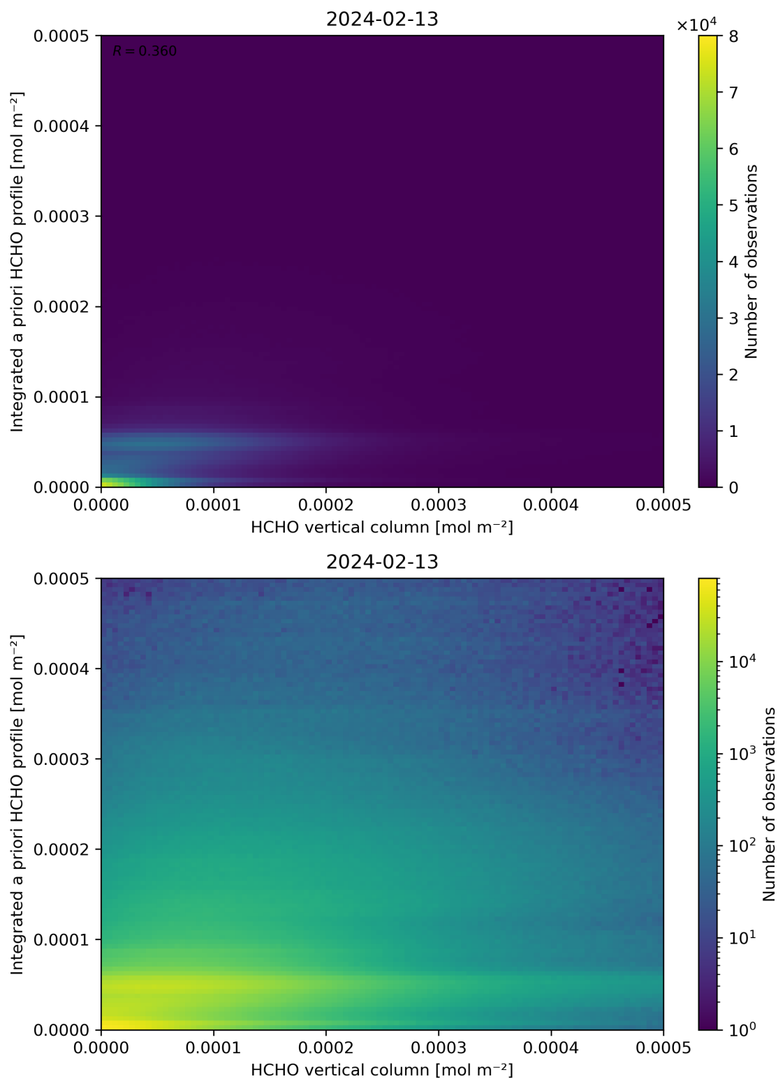
Figure 135: Scatter density plot of “HCHO vertical column” against “Integrated a priori HCHO profile” for 2024-02-12 to 2024-02-14.
