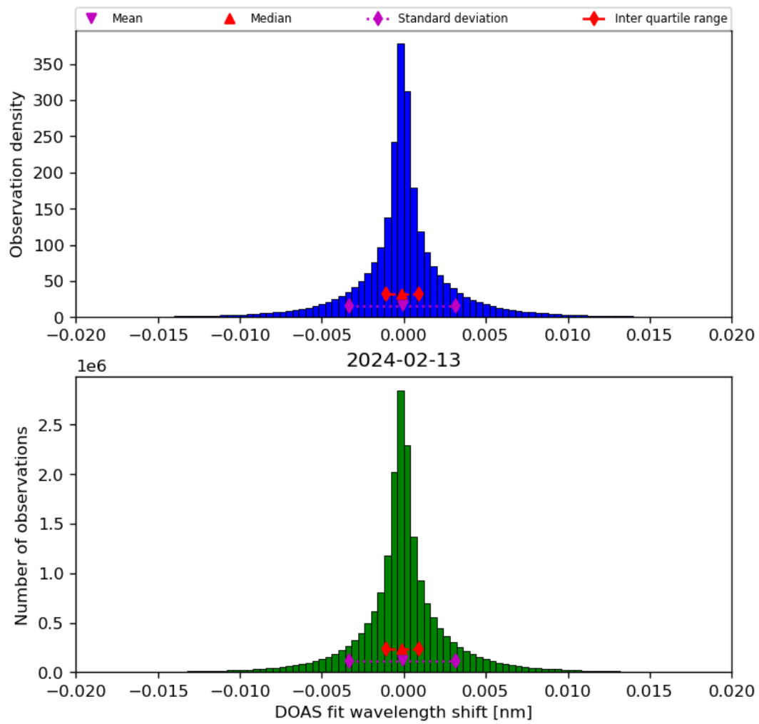
Figure 44: Histogram of “DOAS fit wavelength shift” for 2024-02-12 to 2024-02-14
