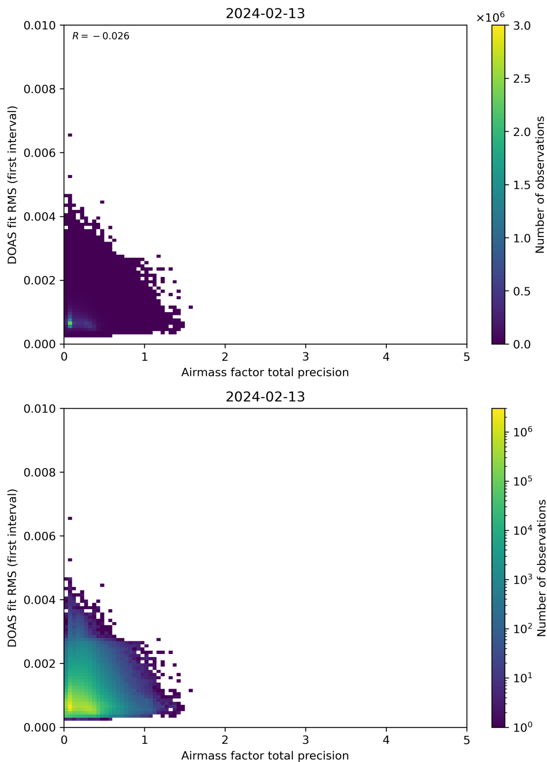
Figure 105: Scatter density plot of “Airmass factor total precision” against “DOAS fit RMS (first interval)” for 2024-02-12 to 2024-02-14.
