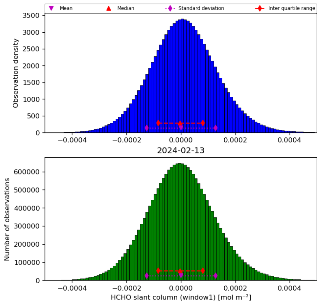
Figure 38: Histogram of “HCHO slant column (window1)” for 2024-02-12 to 2024-02-14
