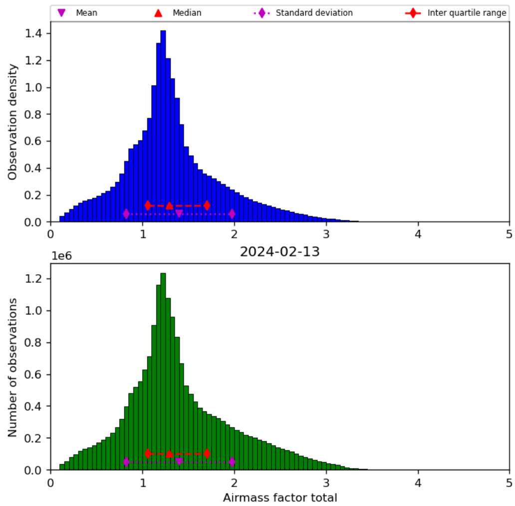
Figure 40: Histogram of “Airmass factor total” for 2024-02-12 to 2024-02-14
