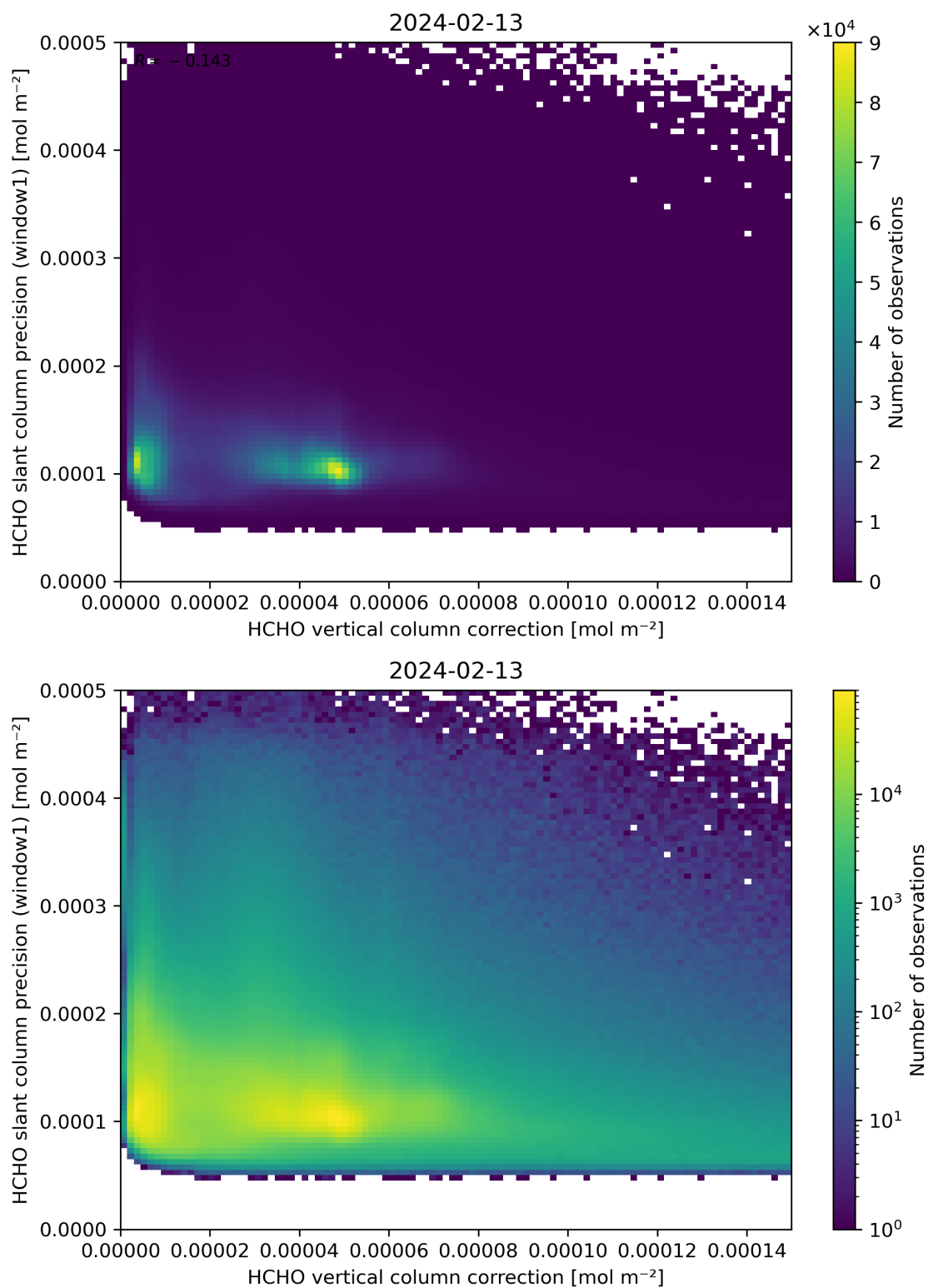
Figure 119: Scatter density plot of “HCHO vertical column correction” against “HCHO slant column precision (window1)” for 2024-02-12 to 2024-02-14.
