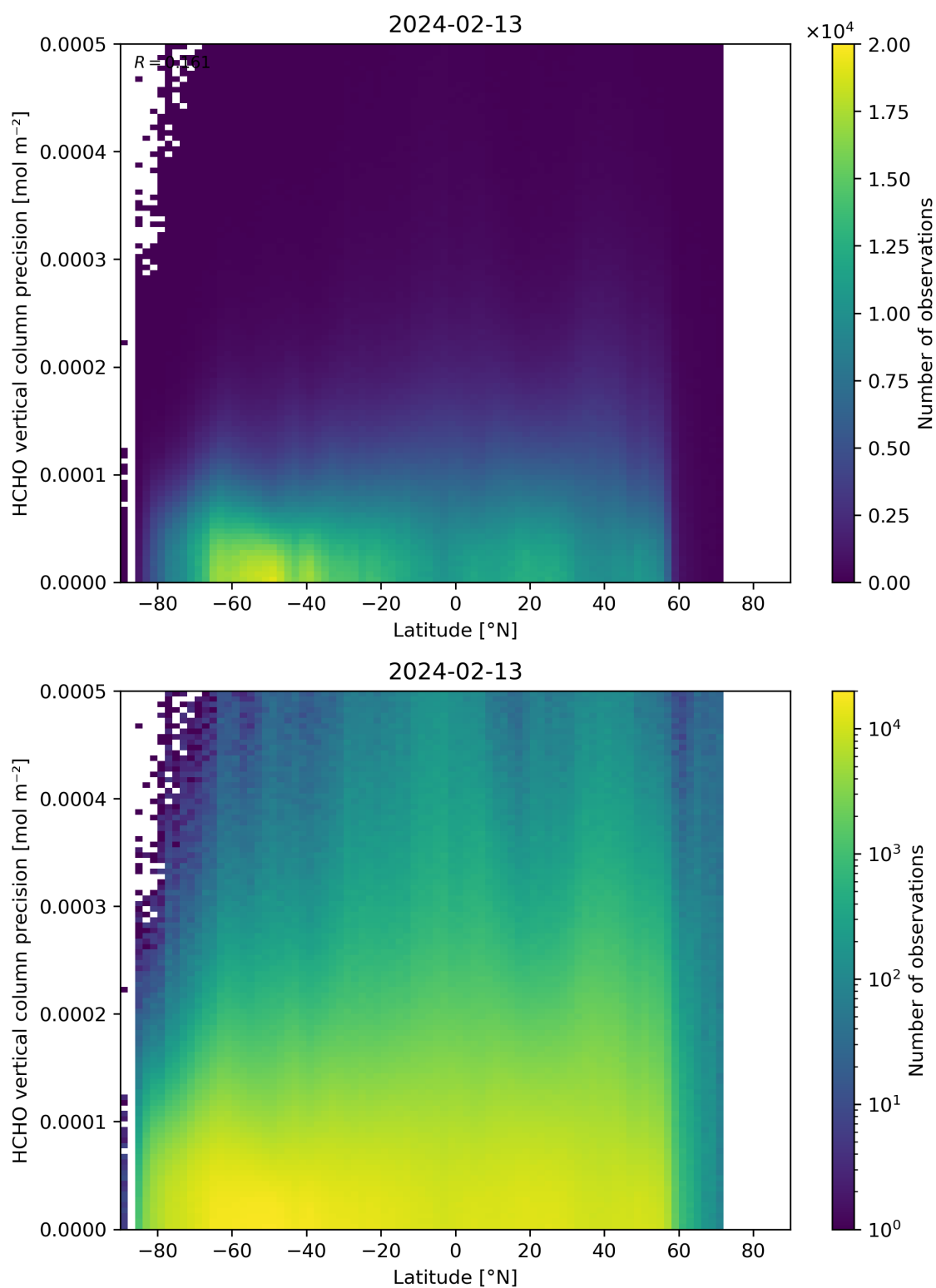
Figure 165: Scatter density plot of “Latitude” against “HCHO vertical column precision” for 2024-02-12 to 2024-02-14.
