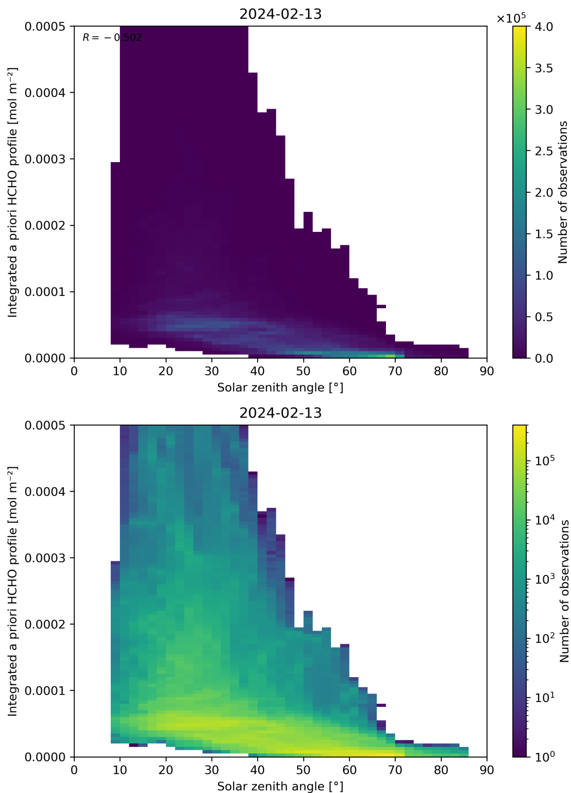
Figure 180: Scatter density plot of “Solar zenith angle” against “Integrated a priori HCHO profile” for 2024-02-12 to 2024-02-14.
