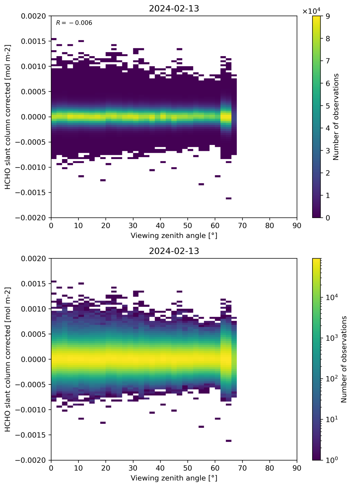
Figure 186: Scatter density plot of “Viewing zenith angle” against “HCHO slant column corrected” for 2024-02-12 to 2024-02-14.
