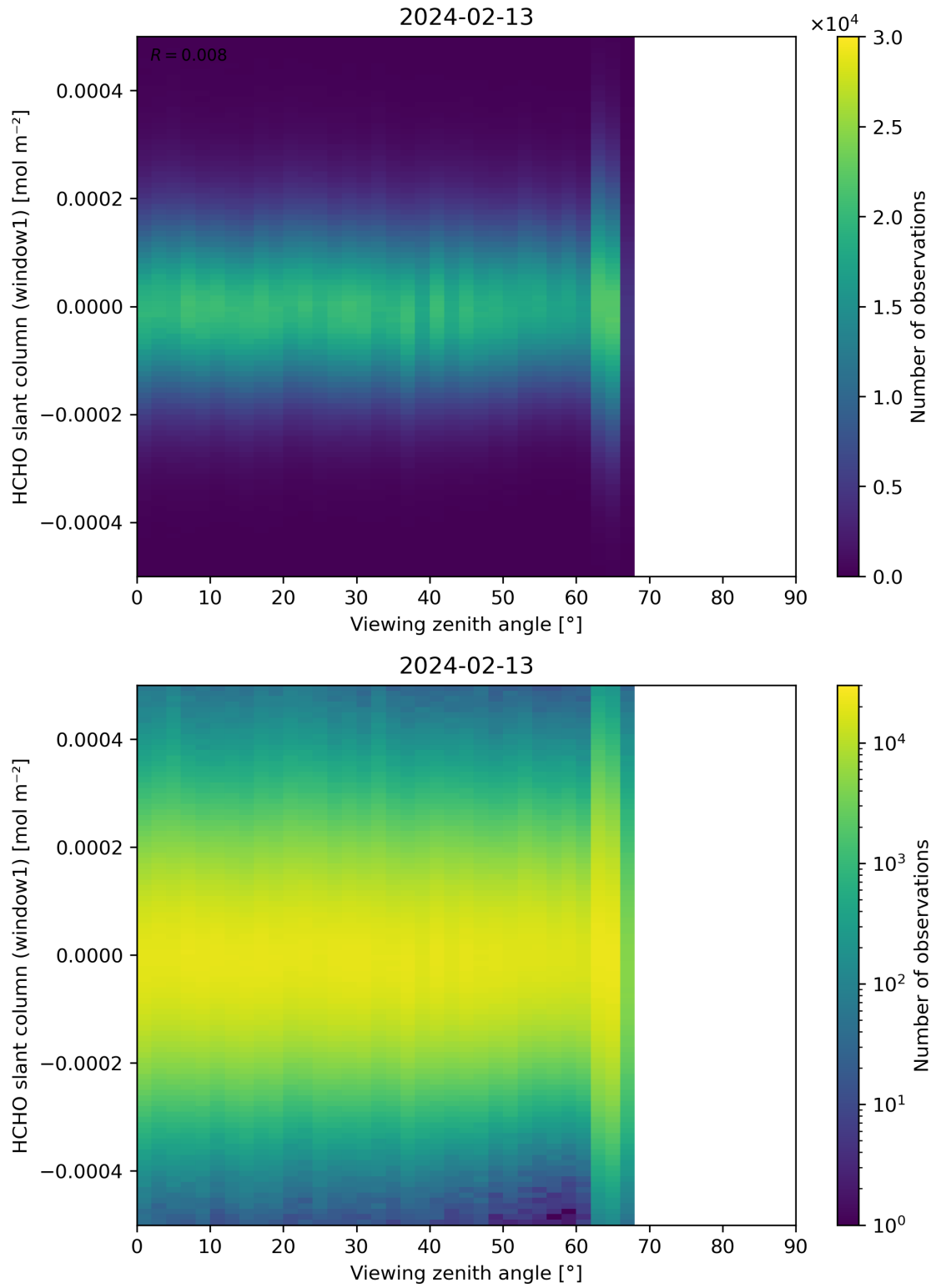
Figure 188: Scatter density plot of “Viewing zenith angle” against “HCHO slant column (window1)” for 2024-02-12 to 2024-02-14.
