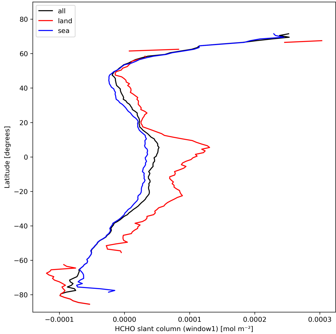
Figure 24: Zonal average of “HCHO slant column (window1)” for 2024-02-12 to 2024-02-14.
