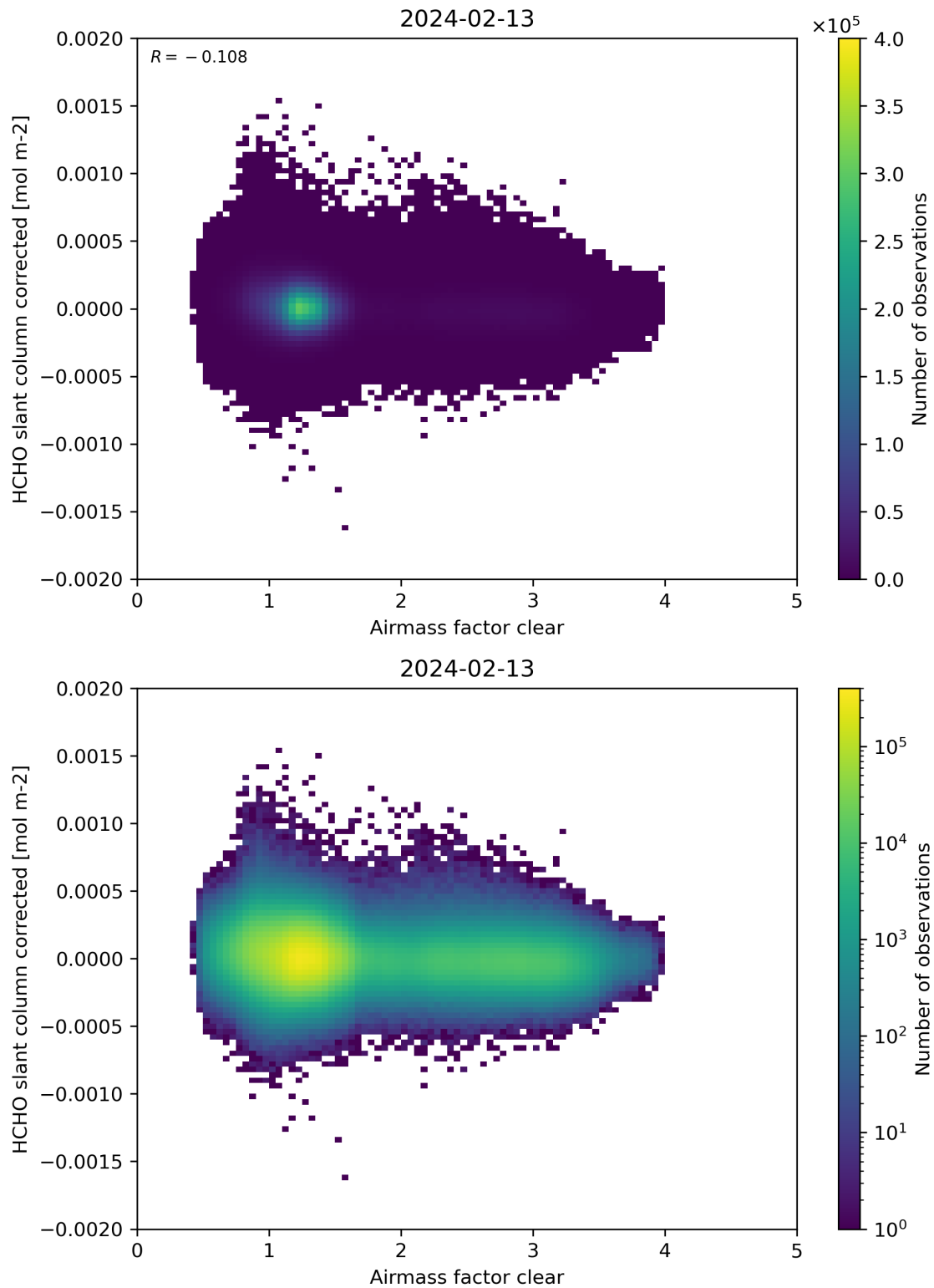
Figure 74: Scatter density plot of “Airmass factor clear” against “HCHO slant column corrected” for 2024-02-12 to 2024-02-14.
