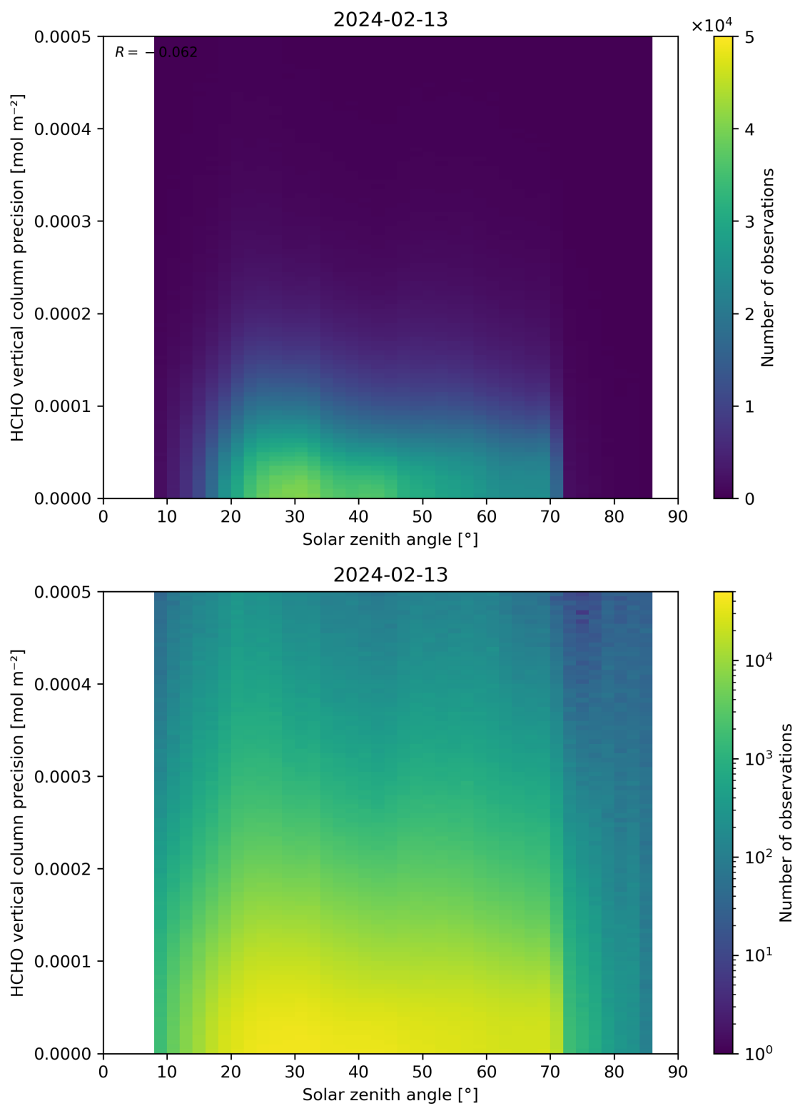
Figure 179: Scatter density plot of “Solar zenith angle” against “HCHO vertical column precision” for 2024-02-12 to 2024-02-14.
