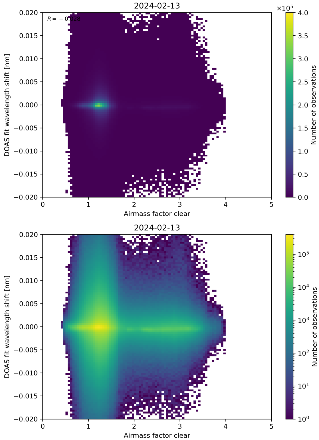
Figure 72: Scatter density plot of “Airmass factor clear” against “DOAS fit wavelength shift” for 2024-02-12 to 2024-02-14.
