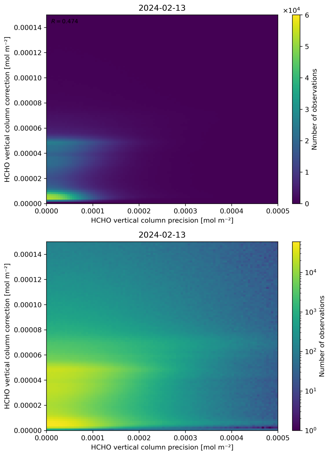
Figure 146: Scatter density plot of “HCHO vertical column precision” against “HCHO vertical column correction” for 2024-02-12 to 2024-02-14.
