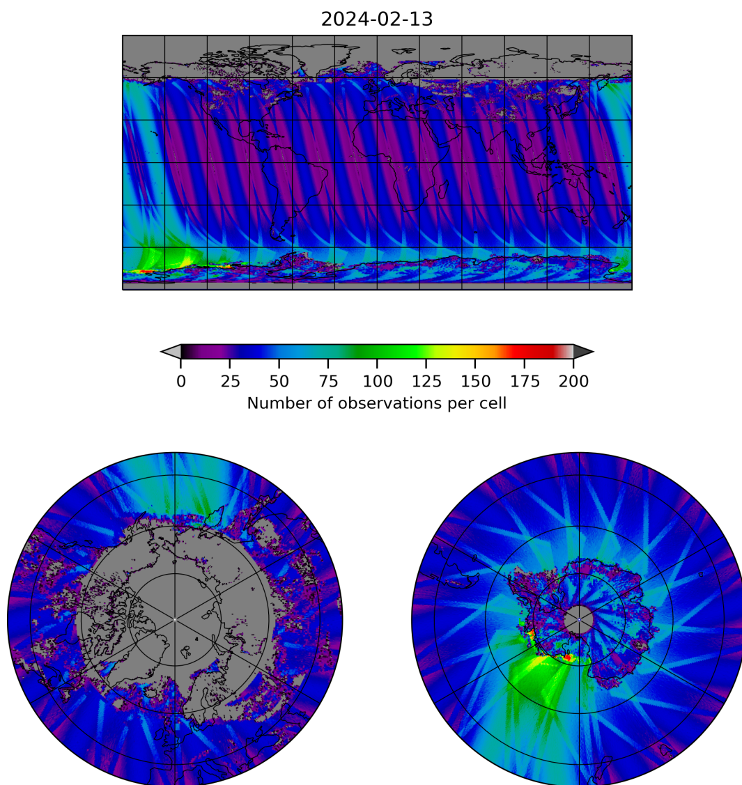
Figure 19: Map of the number of observations for 2024-02-12 to 2024-02-14
