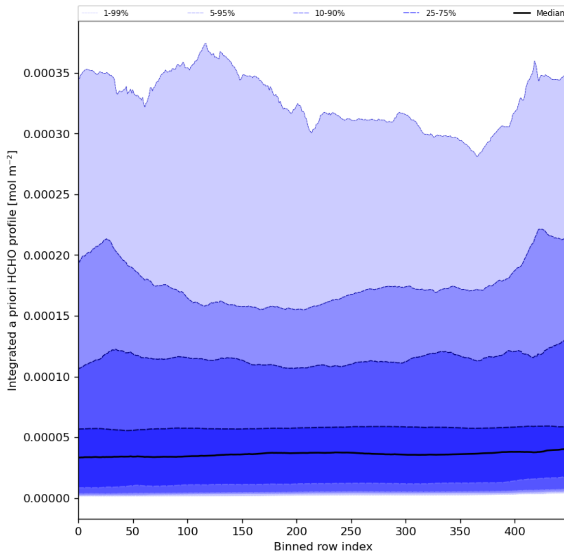
Figure 57: Along track statistics of "Integrated a priori HCHO profile" for 2024-02-12 to 2024-02-14
