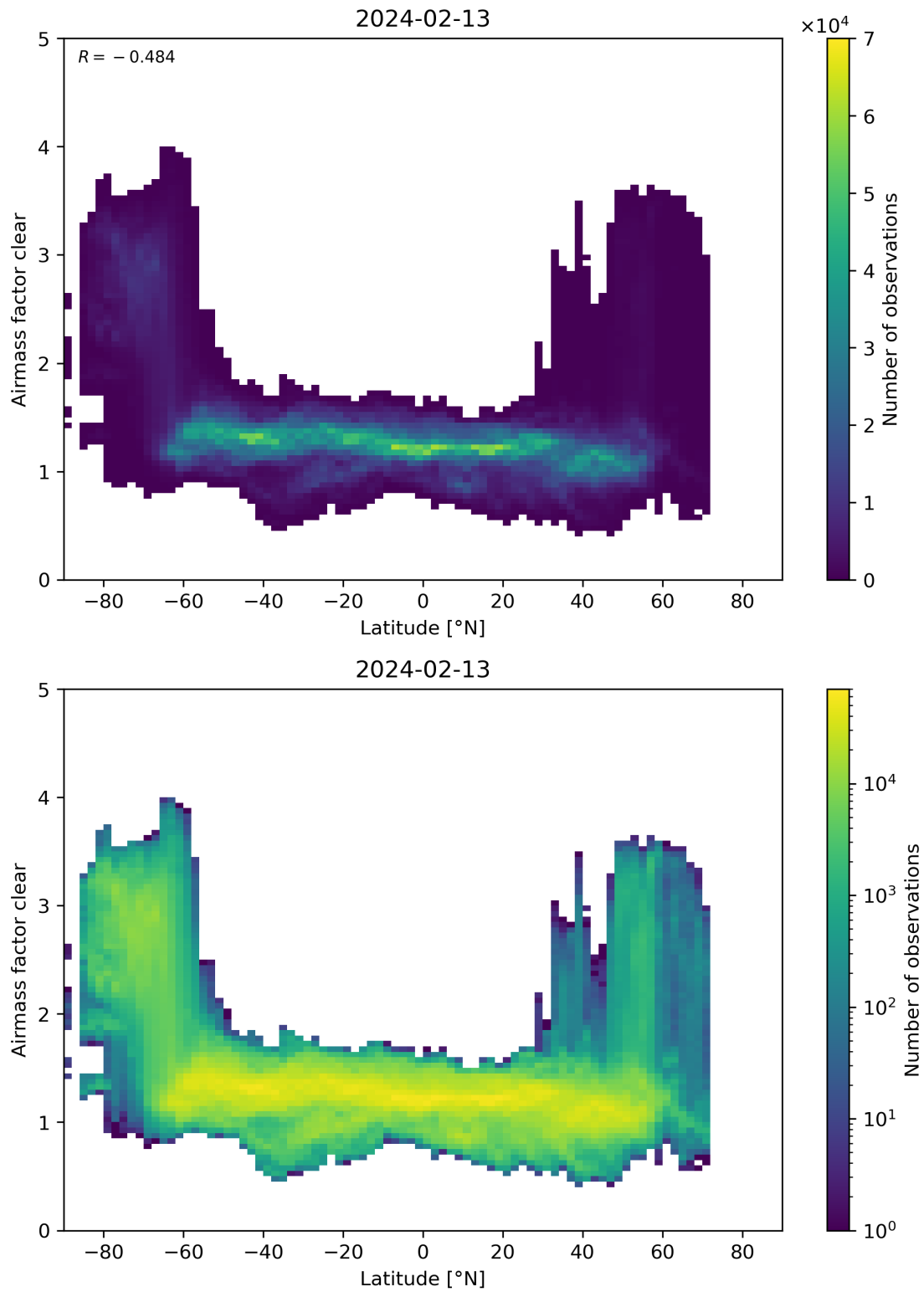
Figure 156: Scatter density plot of “Latitude” against “Airmass factor clear” for 2024-02-12 to 2024-02-14.
