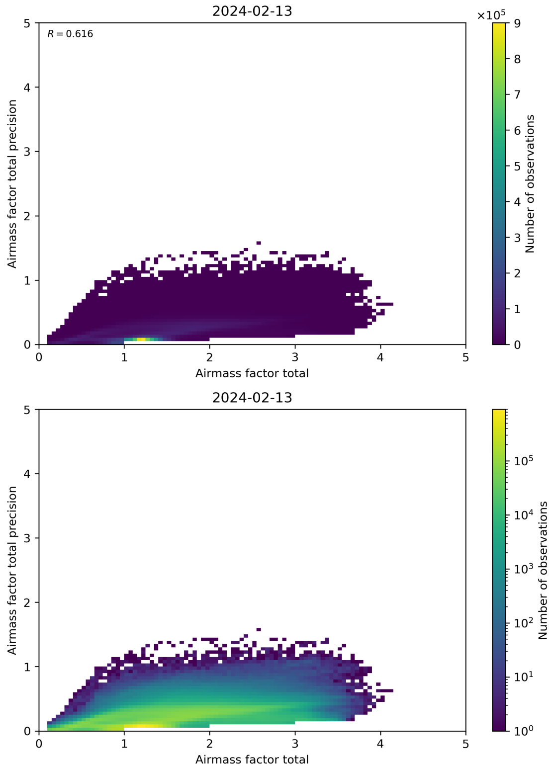
Figure 103: Scatter density plot of “Airmass factor total” against “Airmass factor total precision” for 2024-02-12 to 2024-02-14.
