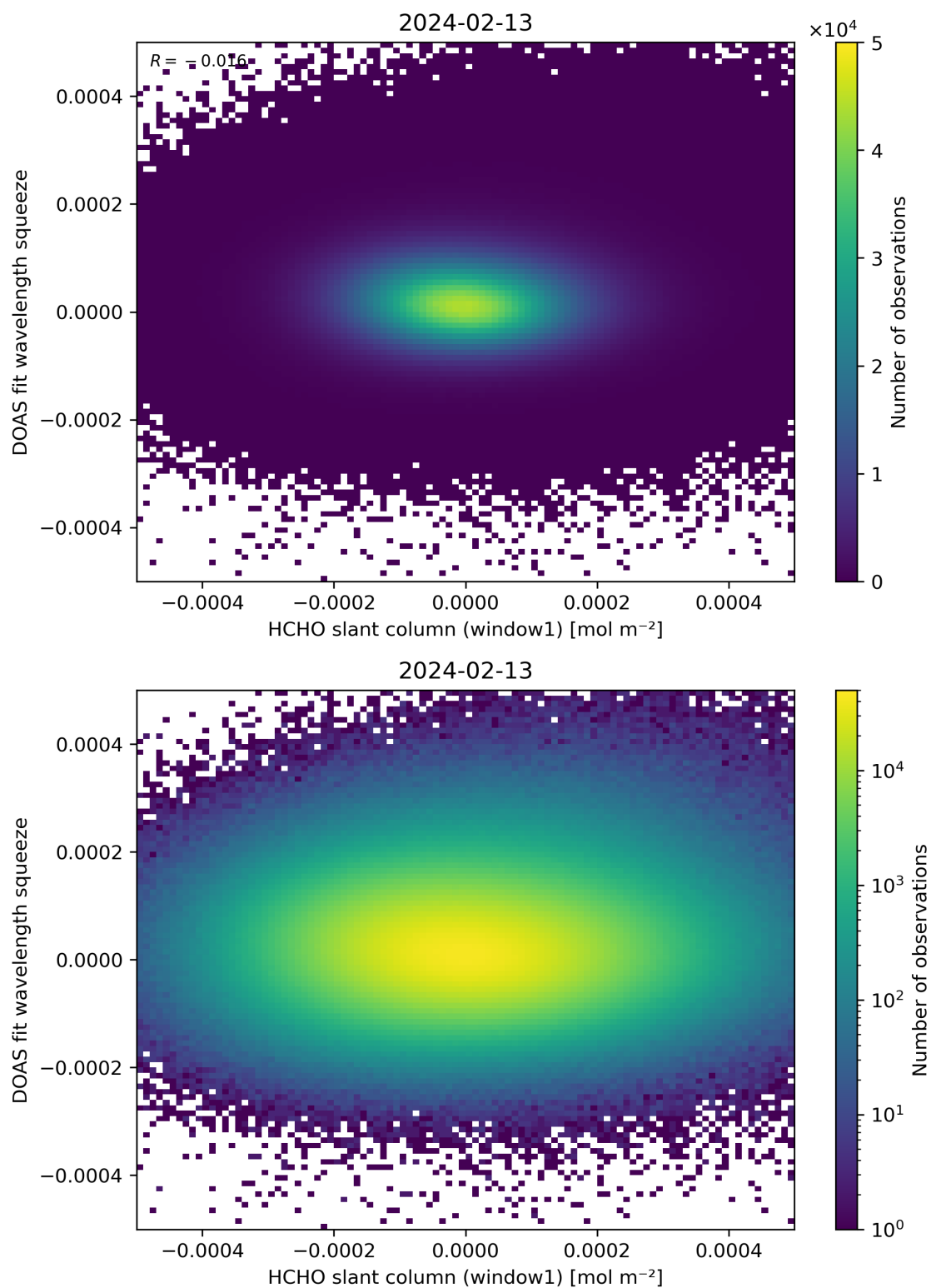
Figure 80: Scatter density plot of “HCHO slant column (window1)” against “DOAS fit wavelength squeeze” for 2024-02-12 to 2024-02-14.
