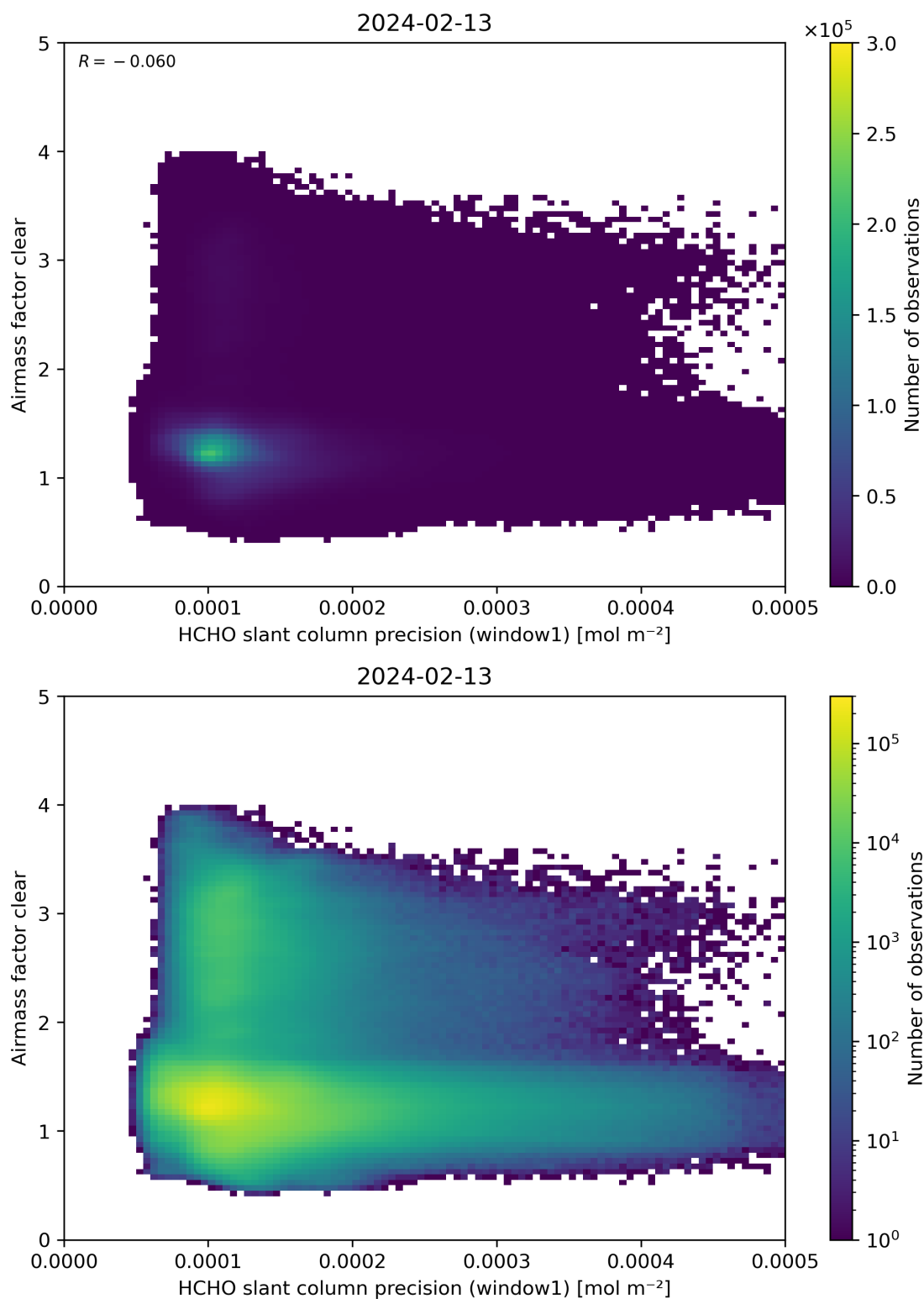
Figure 91: Scatter density plot of “HCHO slant column precision (window1)” against “Airmass factor clear” for 2024-02-12 to 2024-02-14.
