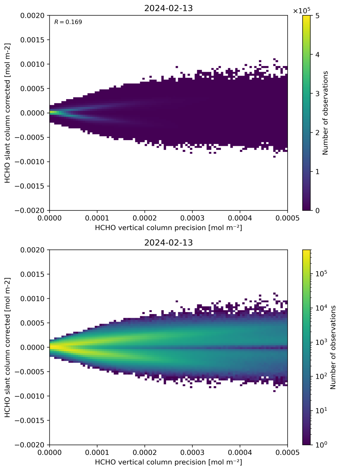
Figure 140: Scatter density plot of “HCHO vertical column precision” against “HCHO slant column corrected” for 2024-02-12 to 2024-02-14.
