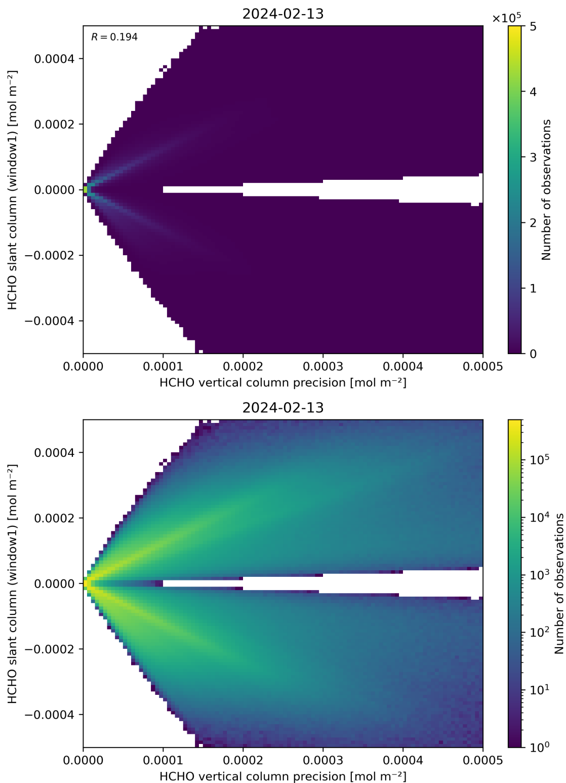
Figure 142: Scatter density plot of “HCHO vertical column precision” against “HCHO slant column (window1)” for 2024-02-12 to 2024-02-14.
