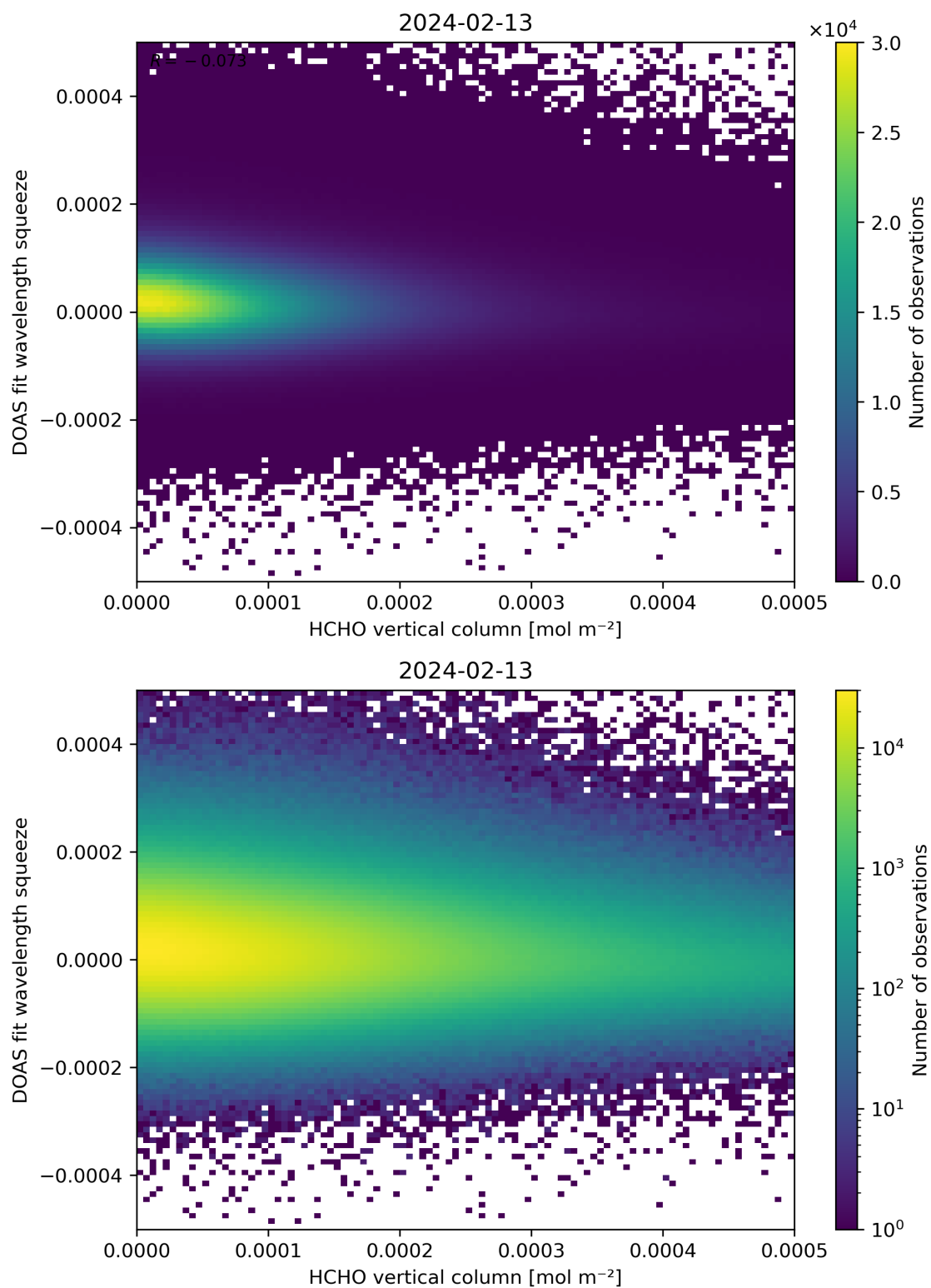
Figure 125: Scatter density plot of “HCHO vertical column” against “DOAS fit wavelength squeeze” for 2024-02-12 to 2024-02-14.
