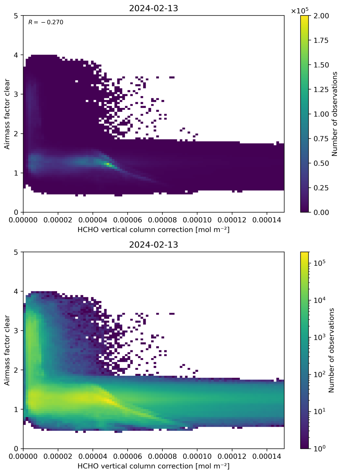
Figure 115: Scatter density plot of “HCHO vertical column correction” against “Airmass factor clear” for 2024-02-12 to 2024-02-14.
