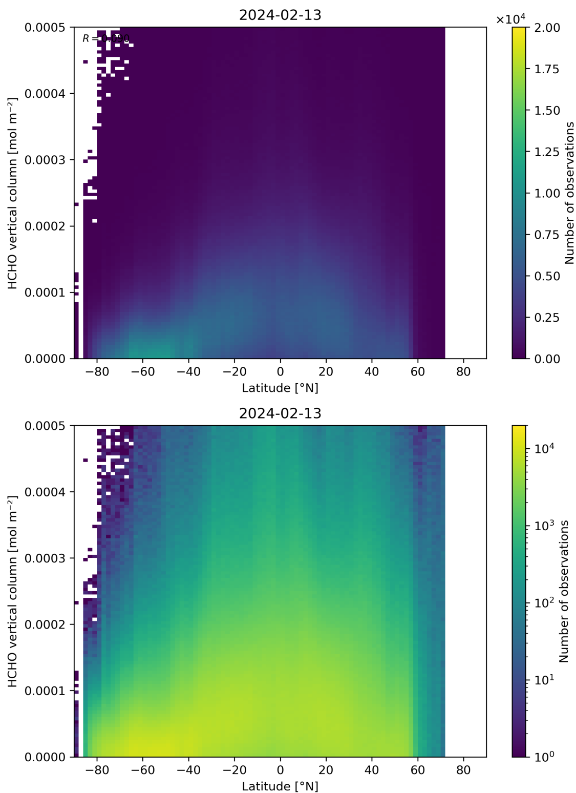
Figure 163: Scatter density plot of “Latitude” against “HCHO vertical column” for 2024-02-12 to 2024-02-14.
