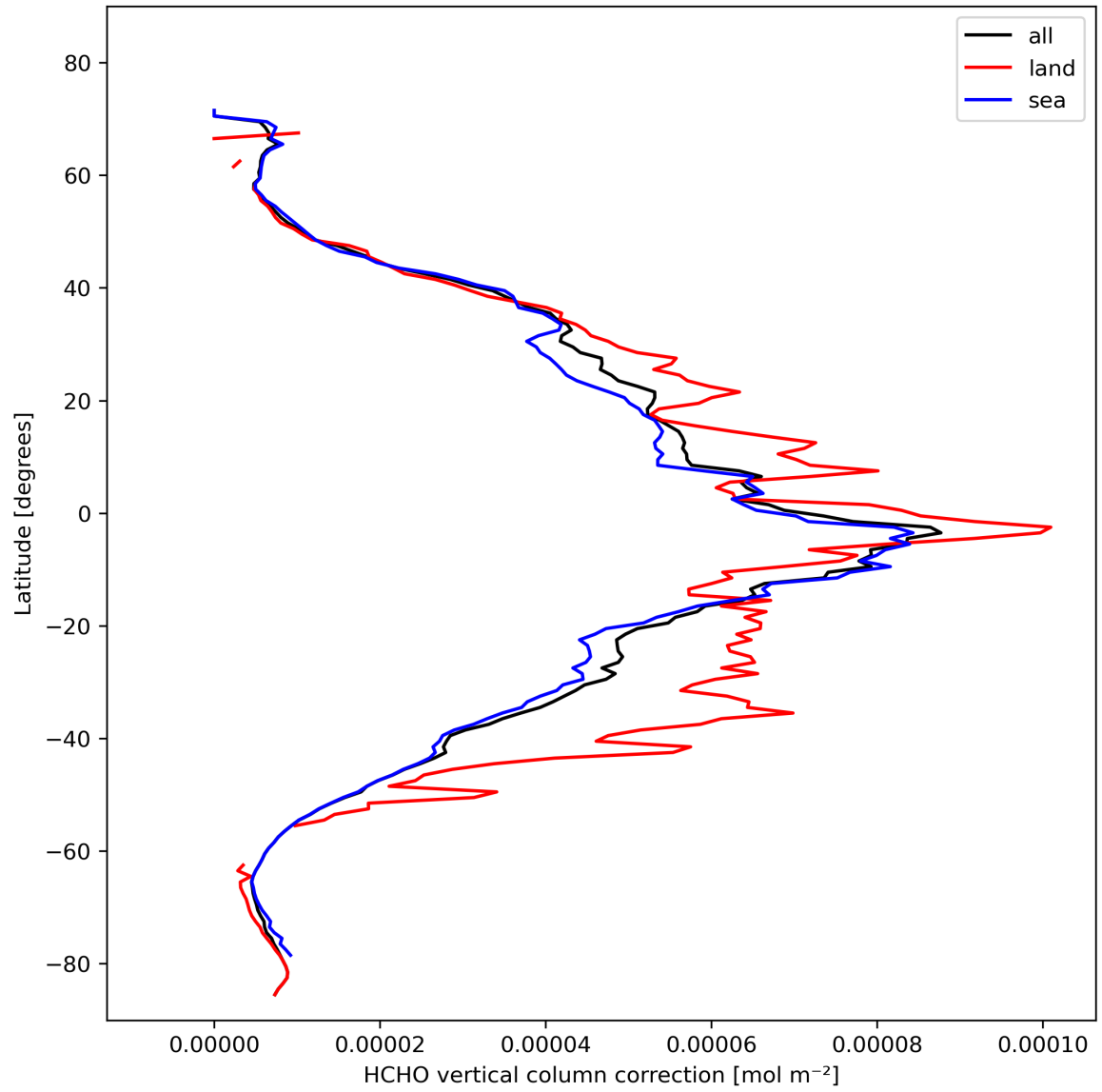
Figure 23: Zonal average of “HCHO vertical column correction” for 2024-02-12 to 2024-02-14.
