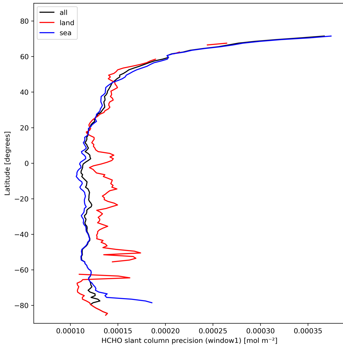
Figure 25: Zonal average of “HCHO slant column precision (window1)” for 2024-02-12 to 2024-02-14.
