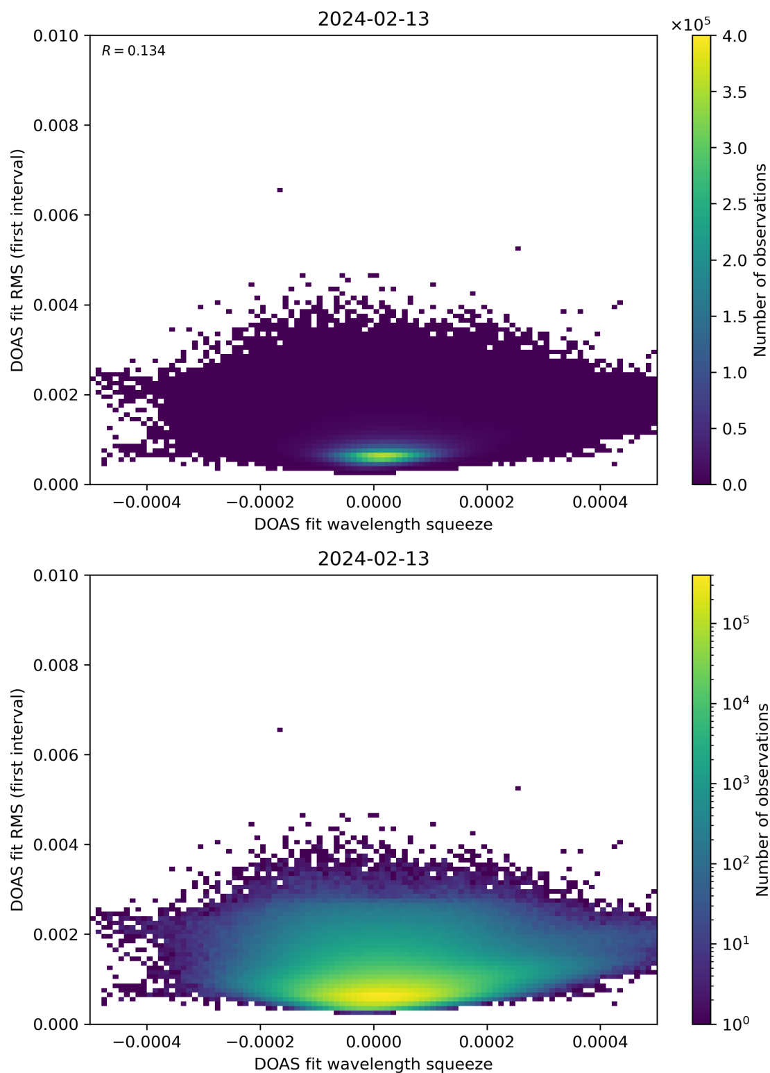
Figure 68: Scatter density plot of “DOAS fit wavelength squeeze” against “DOAS fit RMS (first interval)” for 2024-02-12 to 2024-02-14.
