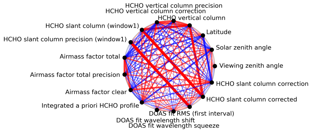
Figure 1: Map of correlation graph for 2024-02-12 to 2024-02-14.
