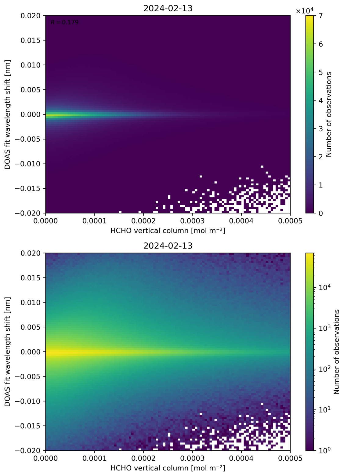
Figure 124: Scatter density plot of “HCHO vertical column” against “DOAS fit wavelength shift” for 2024-02-12 to 2024-02-14.
