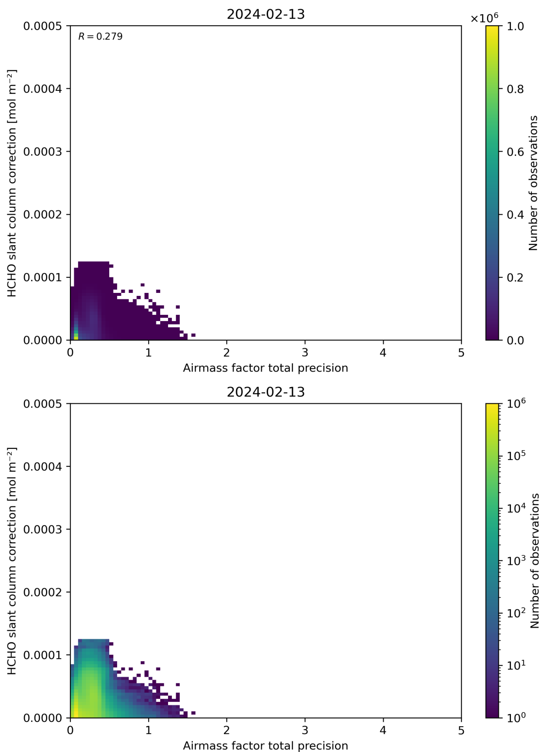
Figure 110: Scatter density plot of “Airmass factor total precision” against “HCHO slant column correction” for 2024-02-12 to 2024-02-14.
