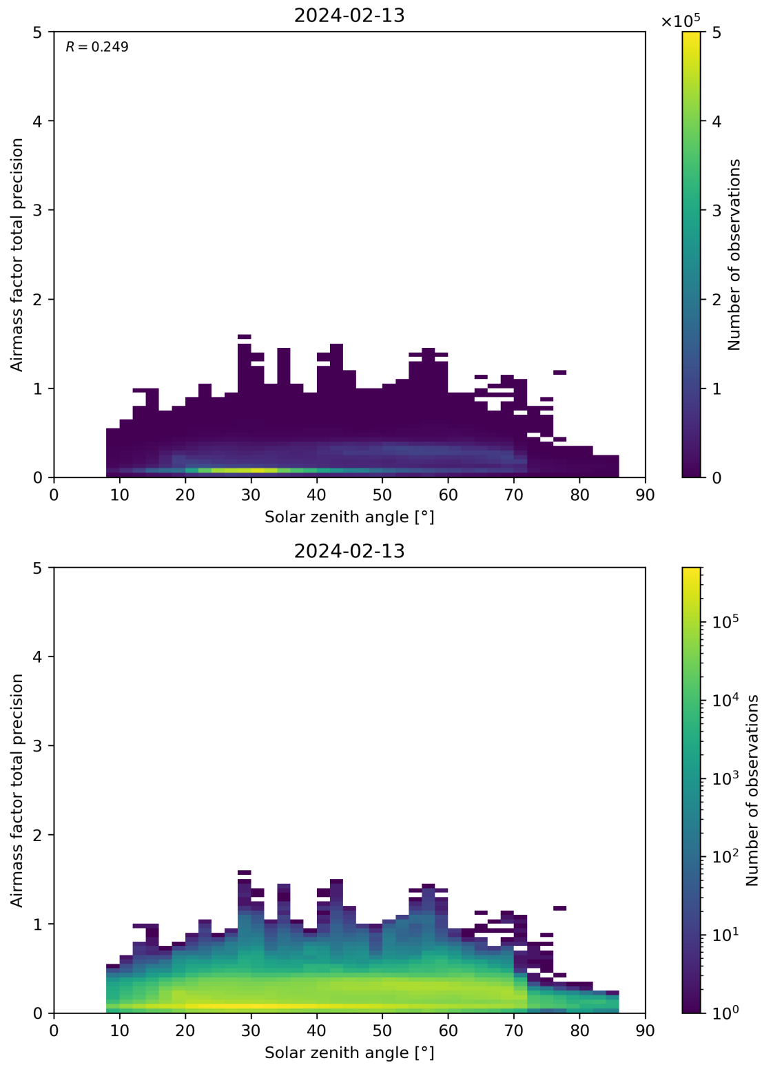
Figure 176: Scatter density plot of “Solar zenith angle” against “Airmass factor total precision” for 2024-02-12 to 2024-02-14.
