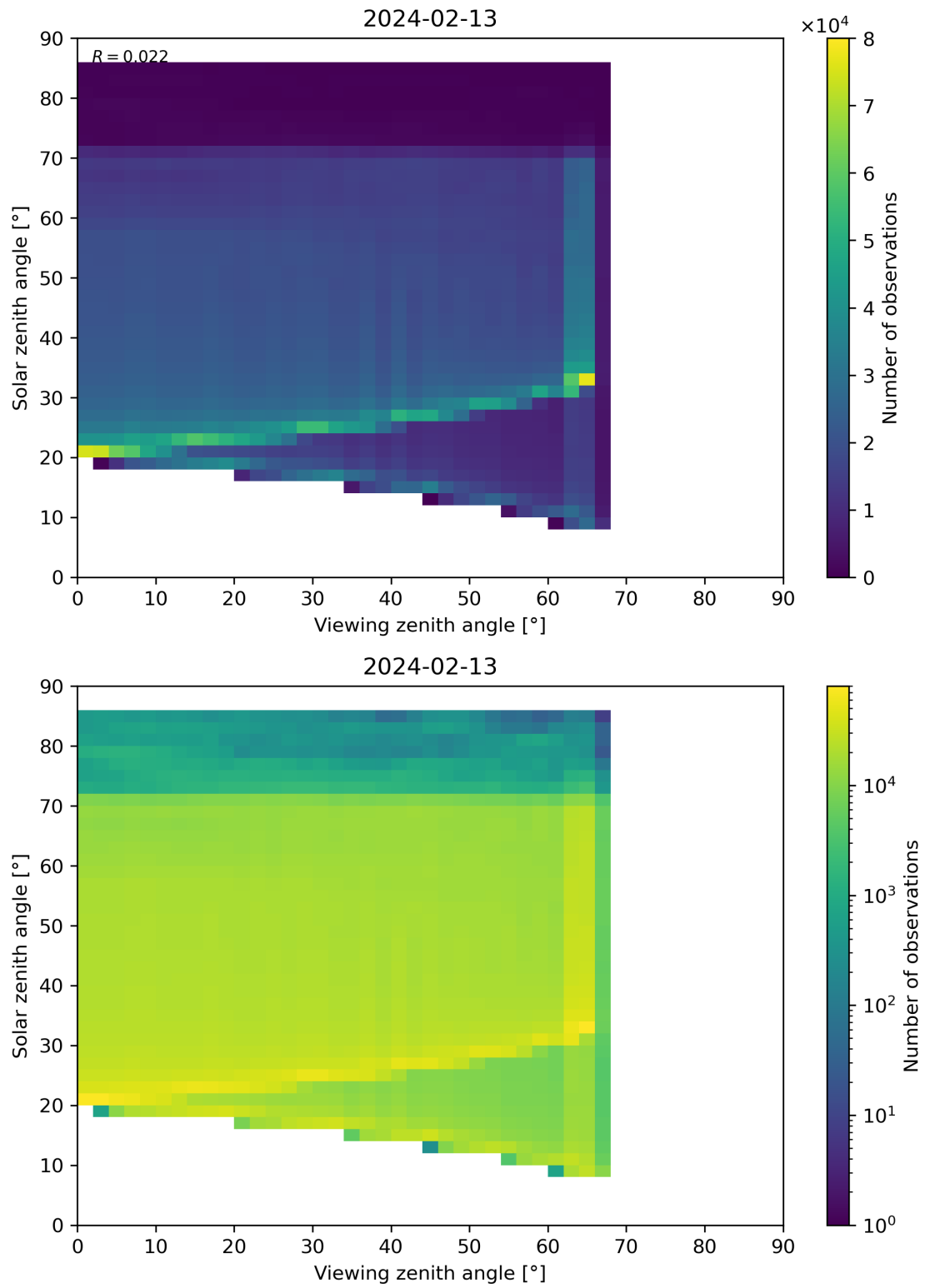
Figure 197: Scatter density plot of “Viewing zenith angle” against “Solar zenith angle” for 2024-02-12 to 2024-02-14.
