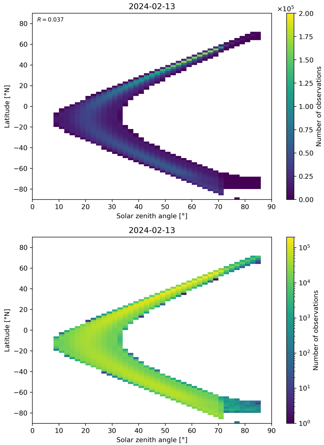
Figure 181: Scatter density plot of “Solar zenith angle” against “Latitude” for 2024-02-12 to 2024-02-14.
