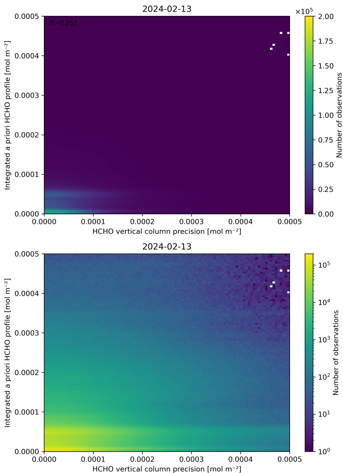
Figure 147: Scatter density plot of “HCHO vertical column precision” against “Integrated a priori HCHO profile” for 2024-02-12 to 2024-02-14.
