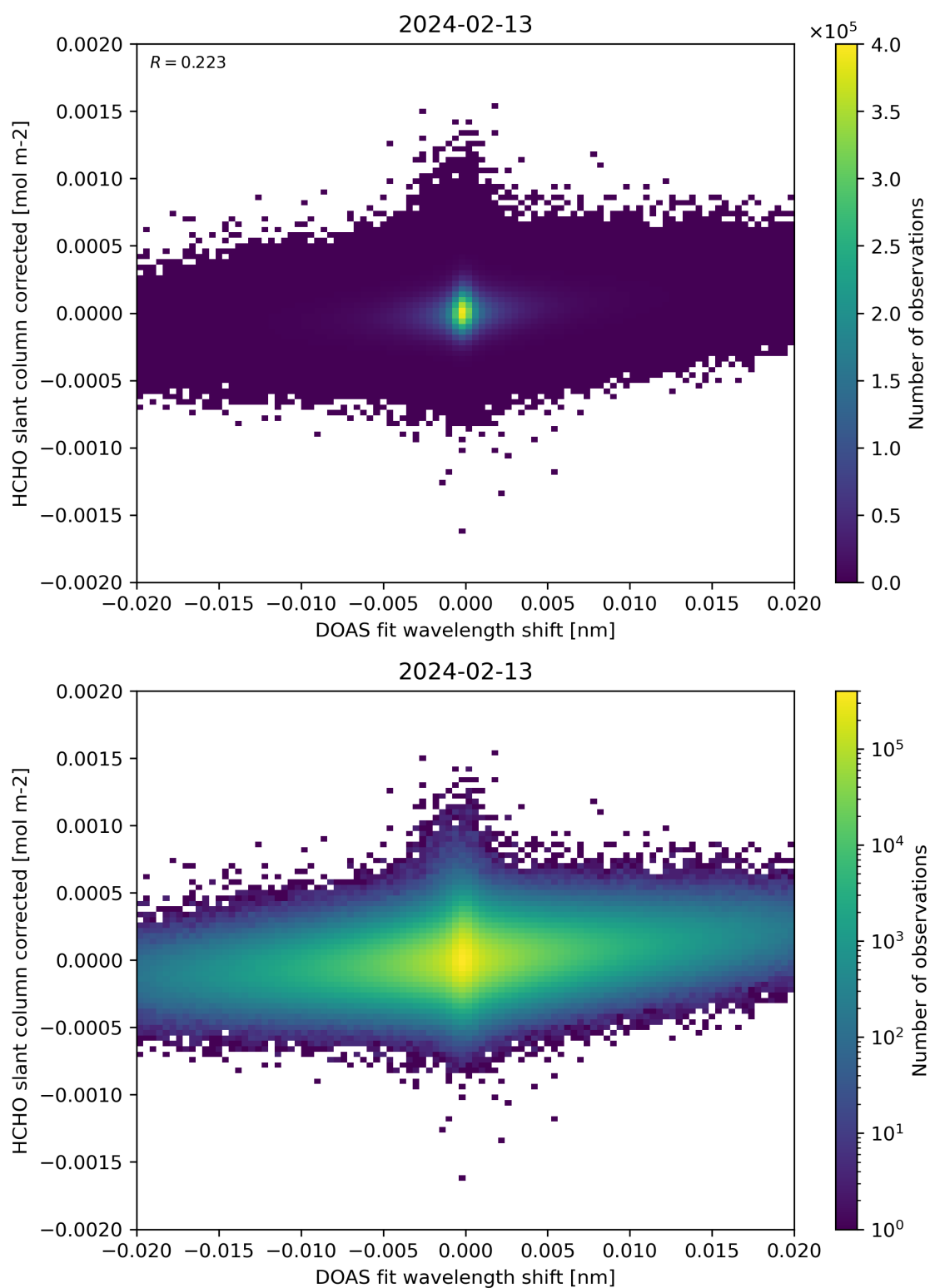
Figure 66: Scatter density plot of “DOAS fit wavelength shift” against “HCHO slant column corrected” for 2024-02-12 to 2024-02-14.
