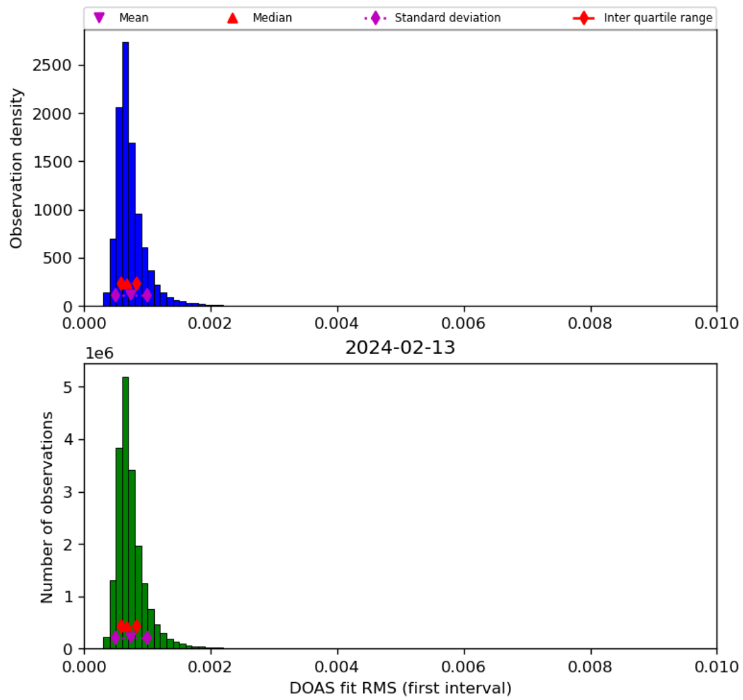
Figure 46: Histogram of “DOAS fit RMS (first interval)” for 2024-02-12 to 2024-02-14
