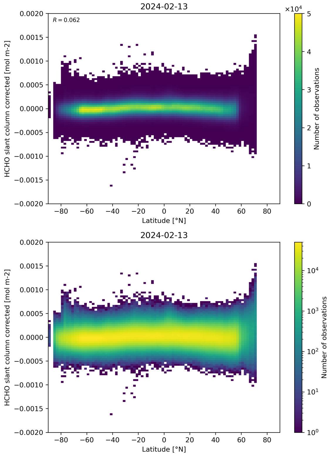
Figure 157: Scatter density plot of “Latitude” against “HCHO slant column corrected” for 2024-02-12 to 2024-02-14.
