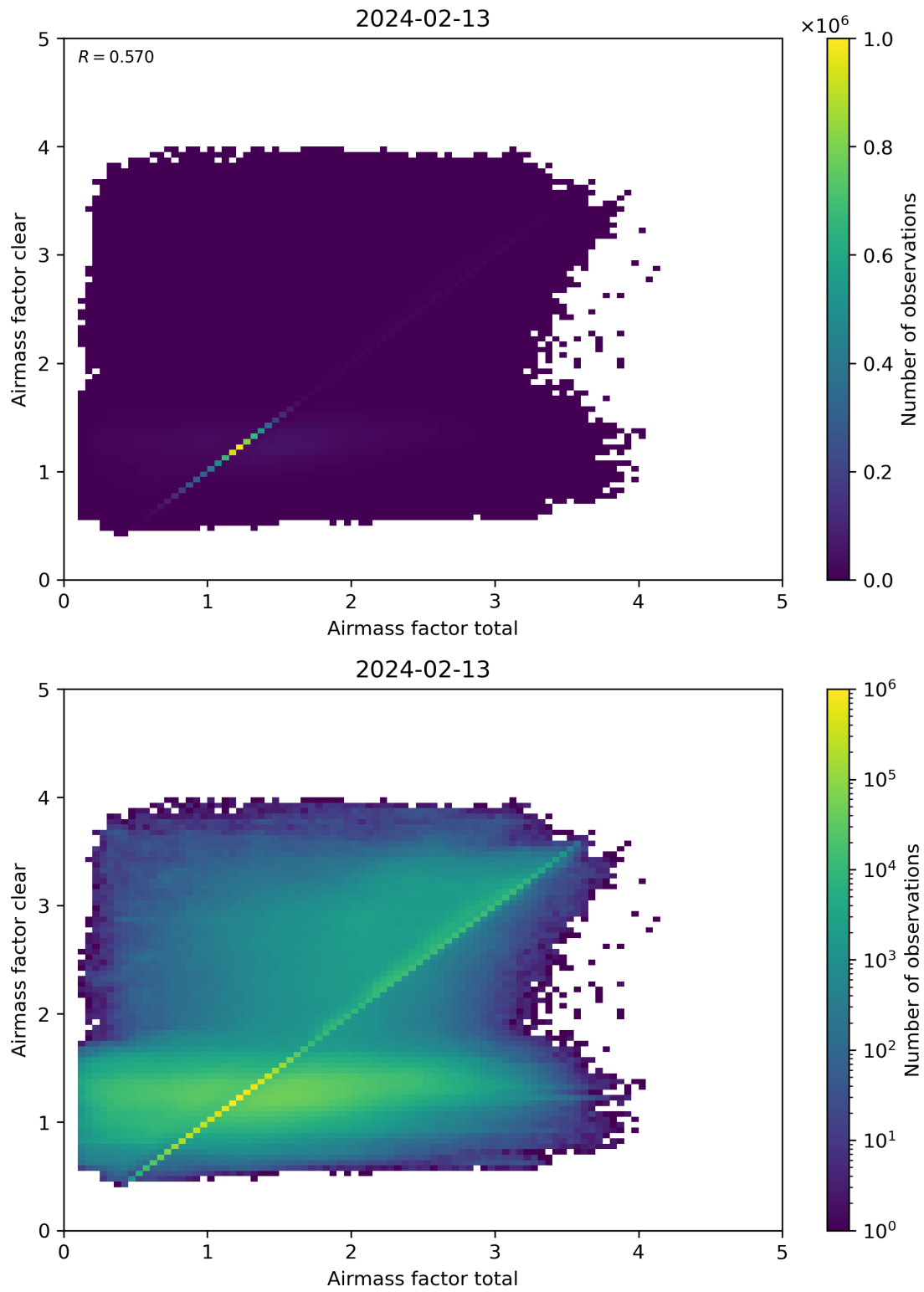
Figure 100: Scatter density plot of “Airmass factor total” against “Airmass factor clear” for 2024-02-12 to 2024-02-14.
