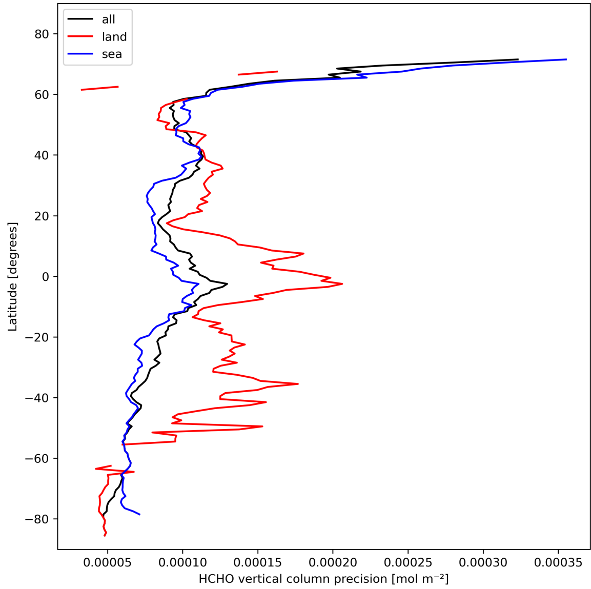
Figure 22: Zonal average of “HCHO vertical column precision” for 2024-02-12 to 2024-02-14.
