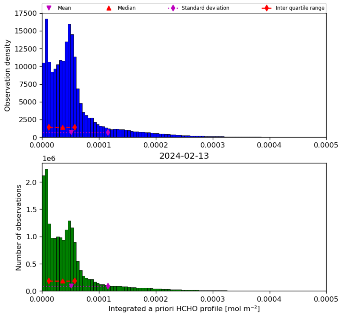
Figure 43: Histogram of “Integrated a priori HCHO profile” for 2024-02-12 to 2024-02-14
