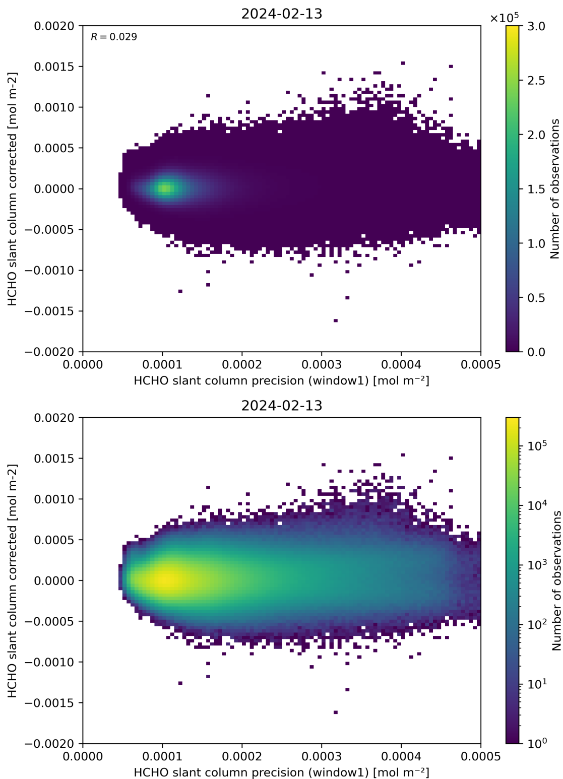
Figure 92: Scatter density plot of “HCHO slant column precision (window1)” against “HCHO slant column corrected” for 2024-02-12 to 2024-02-14.
