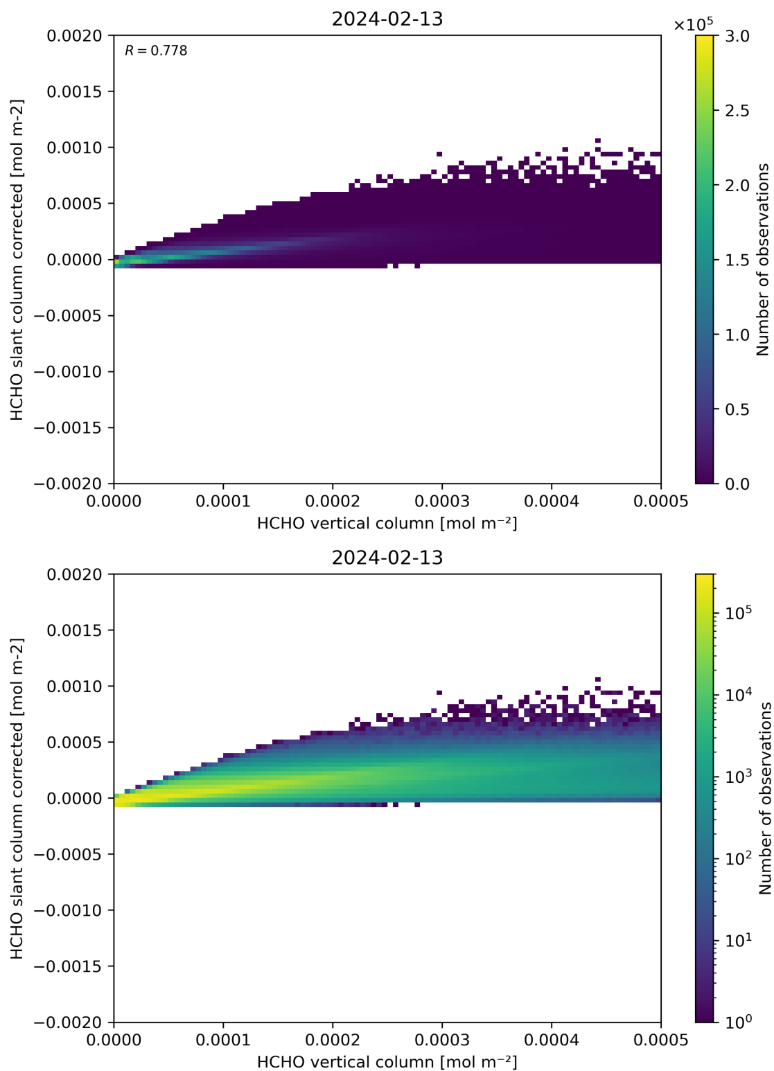
Figure 127: Scatter density plot of “HCHO vertical column” against “HCHO slant column corrected” for 2024-02-12 to 2024-02-14.
