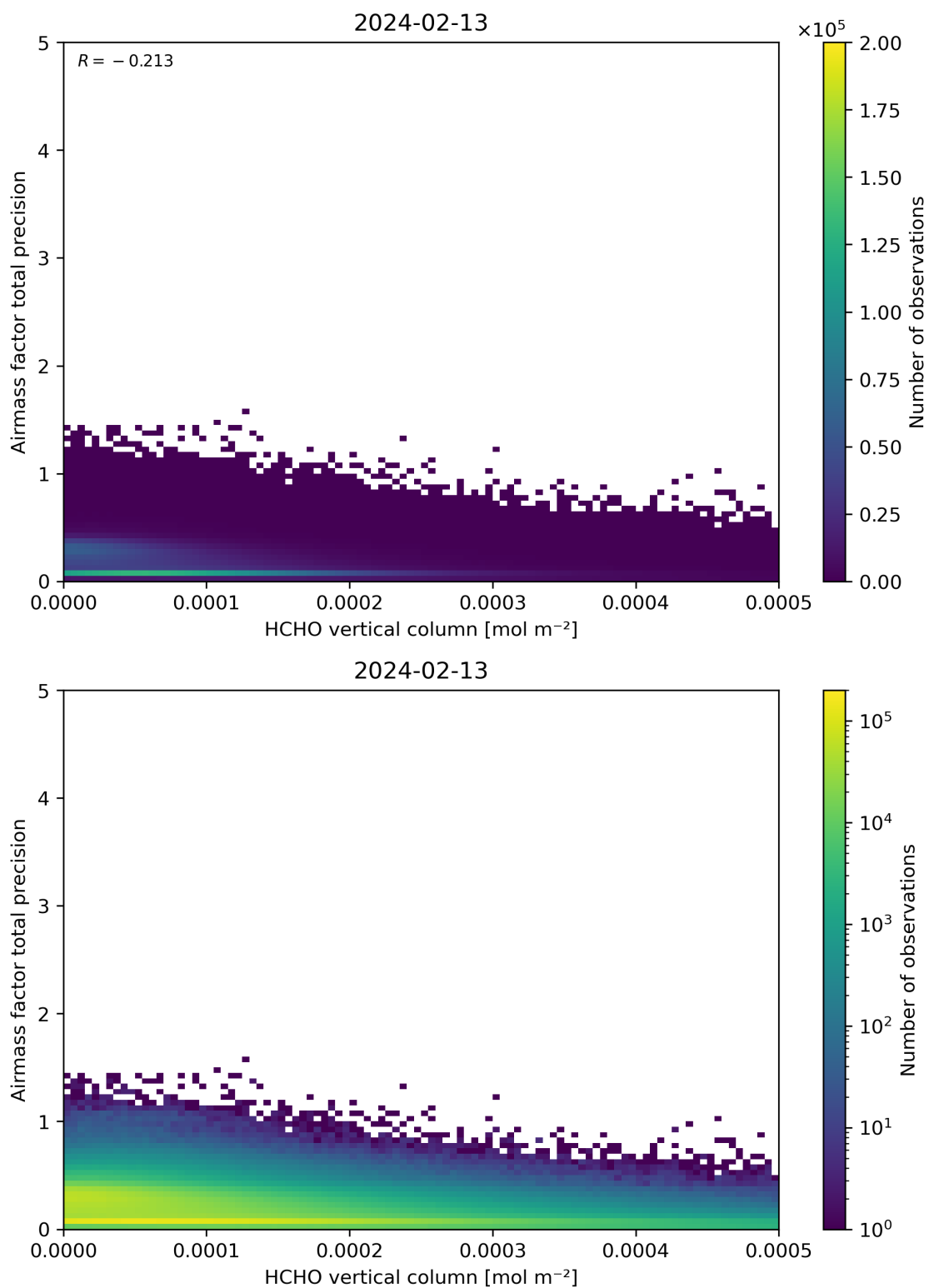
Figure 132: Scatter density plot of “HCHO vertical column” against “Airmass factor total precision” for 2024-02-12 to 2024-02-14.
