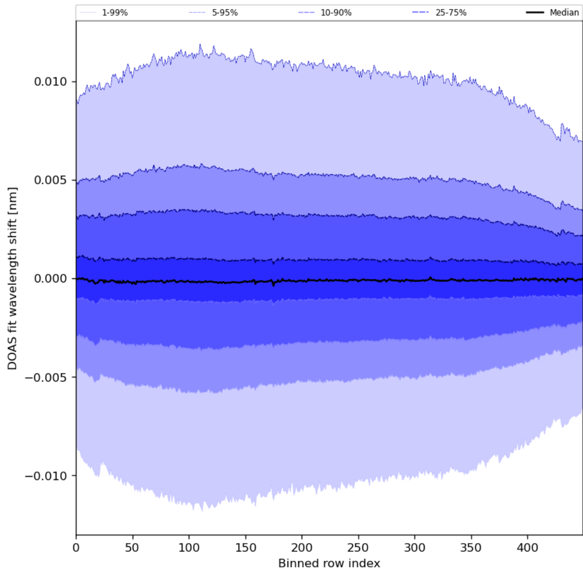
Figure 58: Along track statistics of “DOAS fit wavelength shift” for 2024-02-12 to 2024-02-14
