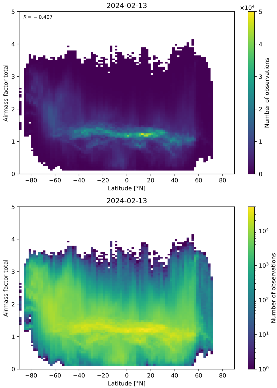
Figure 161: Scatter density plot of “Latitude” against “Airmass factor total” for 2024-02-12 to 2024-02-14.
