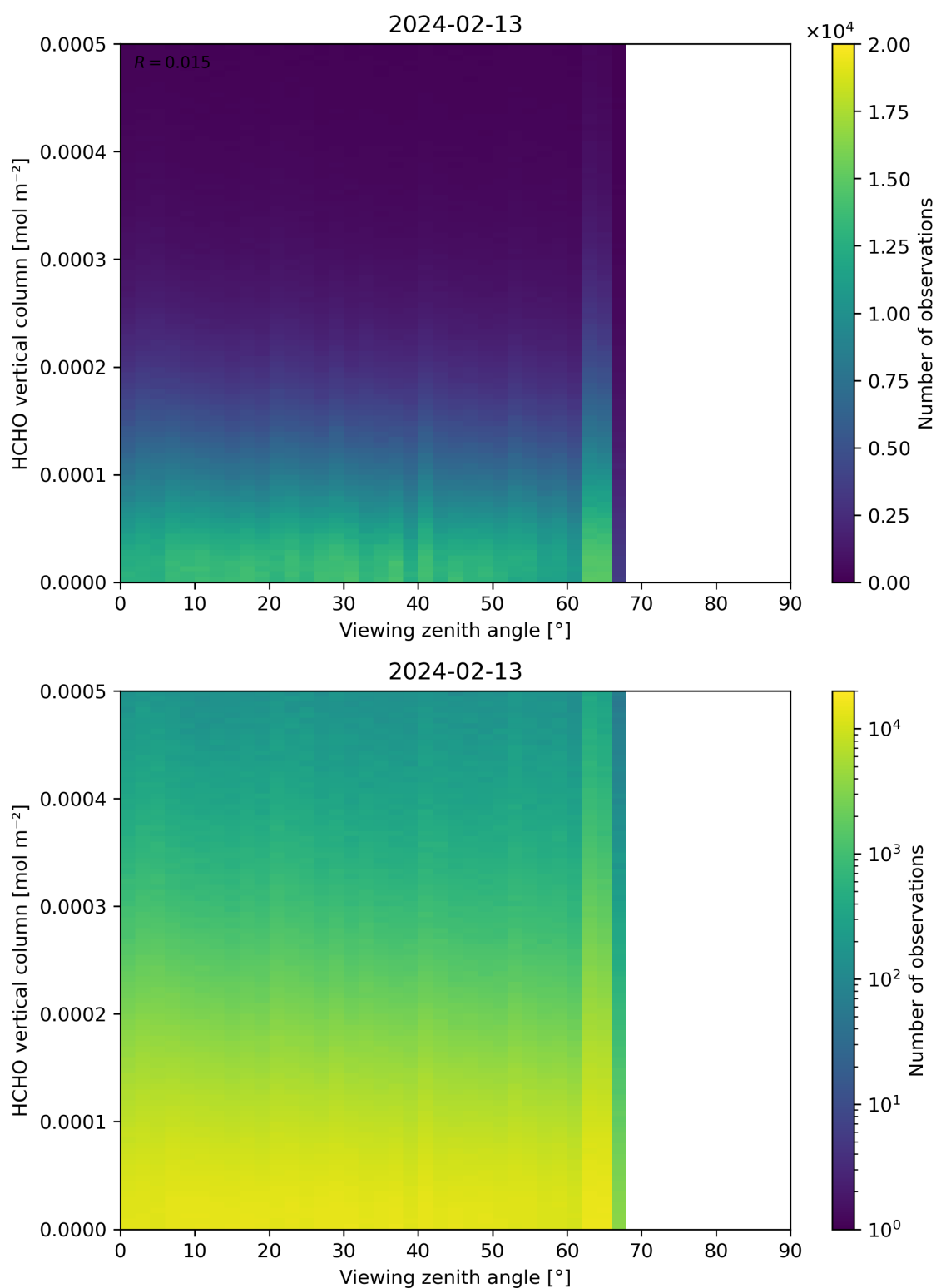
Figure 192: Scatter density plot of “Viewing zenith angle” against “HCHO vertical column” for 2024-02-12 to 2024-02-14.
