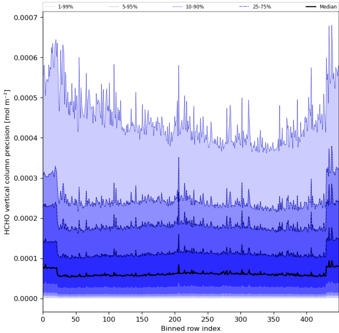
Figure 50: Along track statistics of “HCHO vertical column precision” for 2024-02-12 to 2024-02-14
