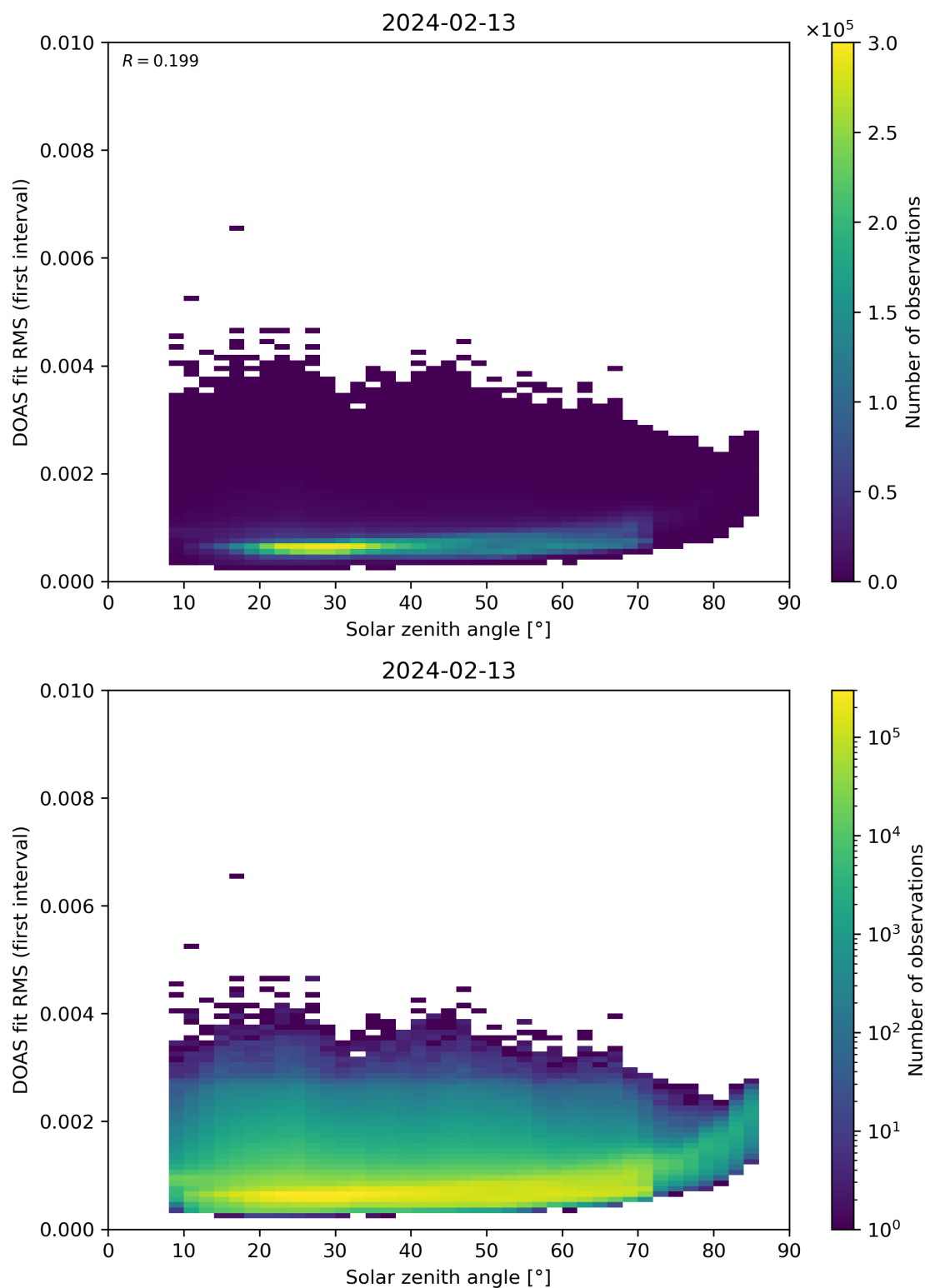
Figure 167: Scatter density plot of “Solar zenith angle” against “DOAS fit RMS (first interval)” for 2024-02-12 to 2024-02-14.
