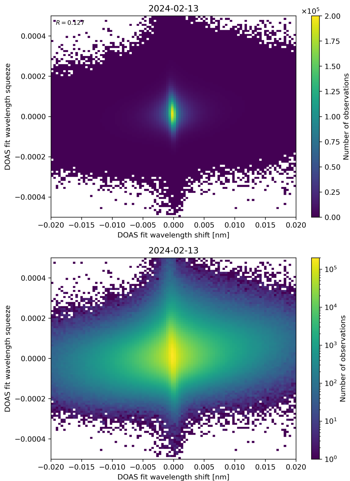
Figure 65: Scatter density plot of “DOAS fit wavelength shift” against “DOAS fit wavelength squeeze” for 2024-02-12 to 2024-02-14.
