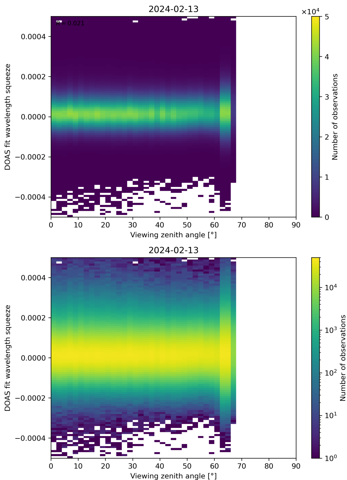
Figure 184: Scatter density plot of “Viewing zenith angle” against “DOAS fit wavelength squeeze” for 2024-02-12 to 2024-02-14.
