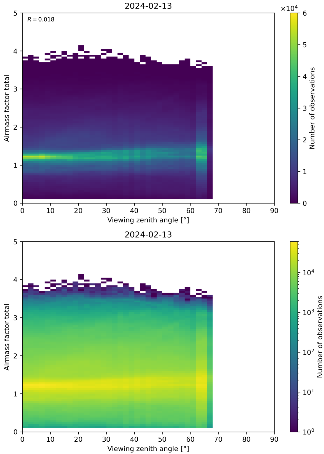
Figure 190: Scatter density plot of “Viewing zenith angle” against “Airmass factor total” for 2024-02-12 to 2024-02-14.
