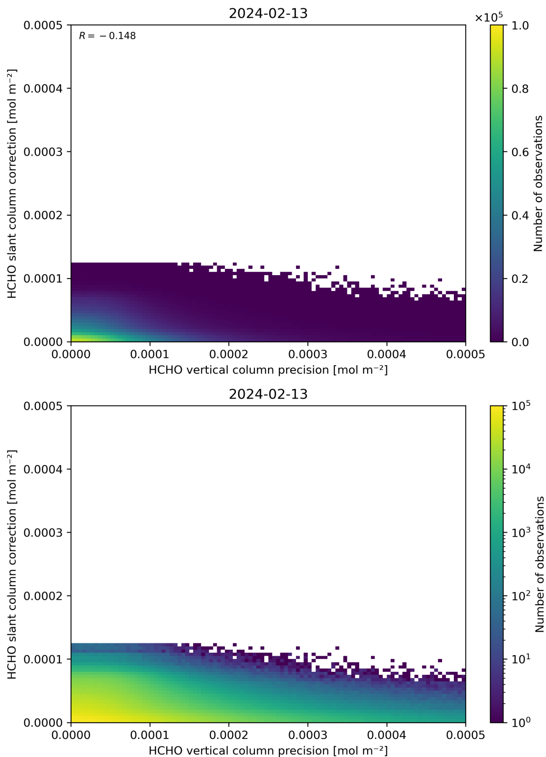
Figure 141: Scatter density plot of “HCHO vertical column precision” against “HCHO slant column correction” for 2024-02-12 to 2024-02-14.
