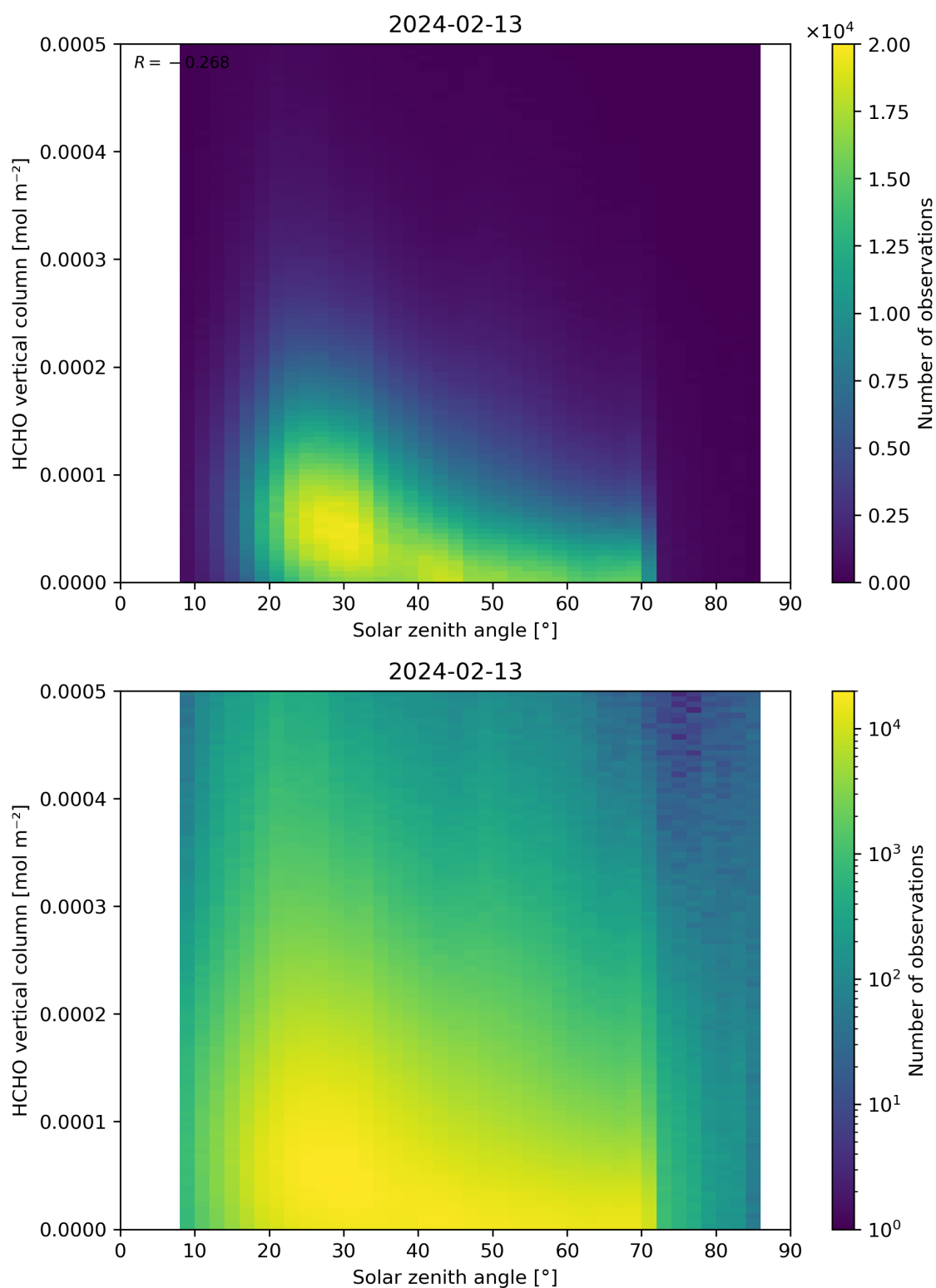
Figure 177: Scatter density plot of “Solar zenith angle” against “HCHO vertical column” for 2024-02-12 to 2024-02-14.
