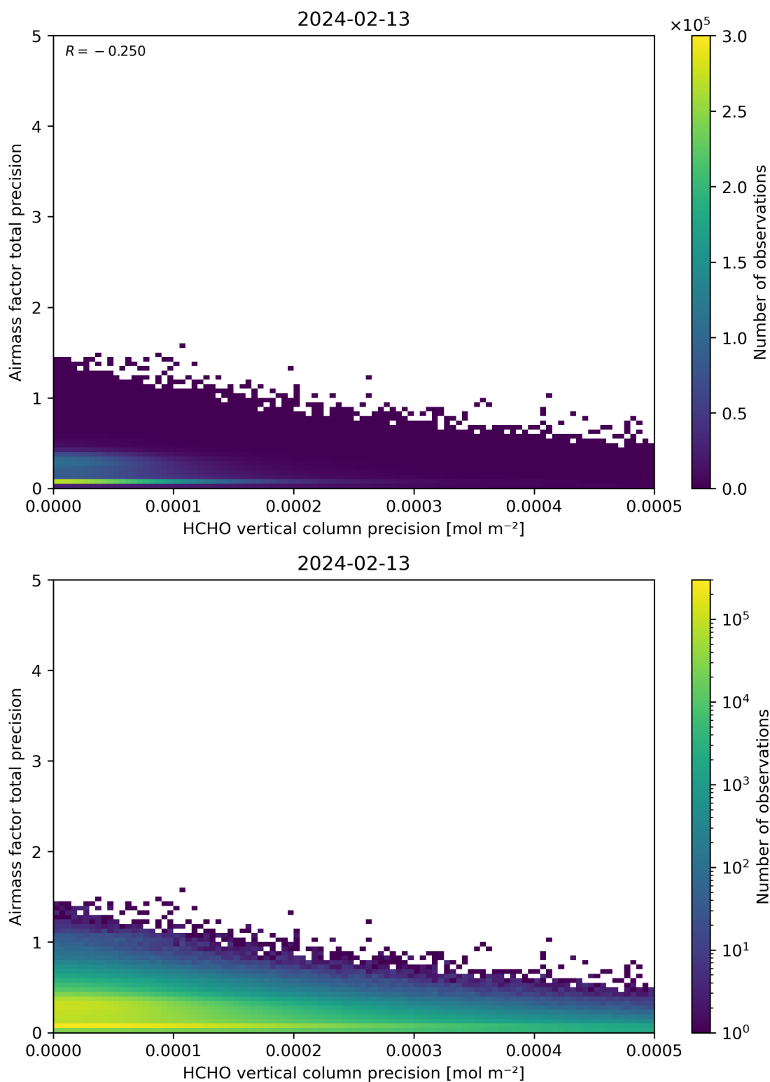
Figure 145: Scatter density plot of “HCHO vertical column precision” against “Airmass factor total precision” for 2024-02-12 to 2024-02-14.
