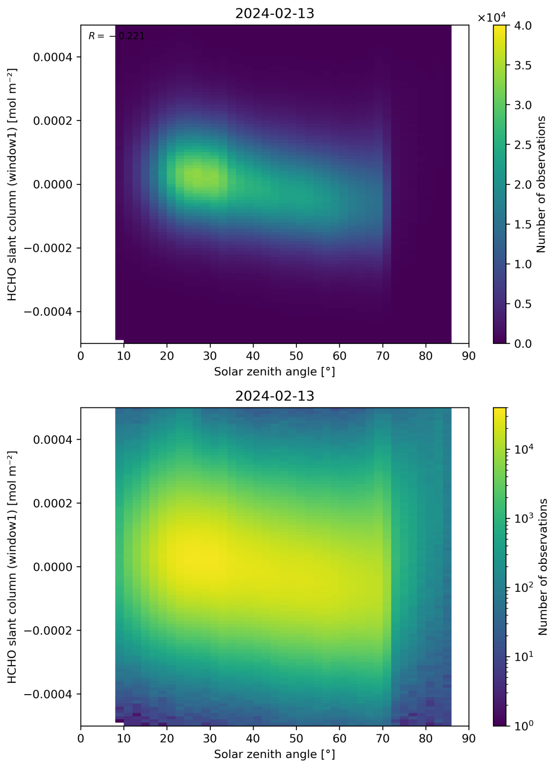
Figure 173: Scatter density plot of “Solar zenith angle” against “HCHO slant column (window1)” for 2024-02-12 to 2024-02-14.
