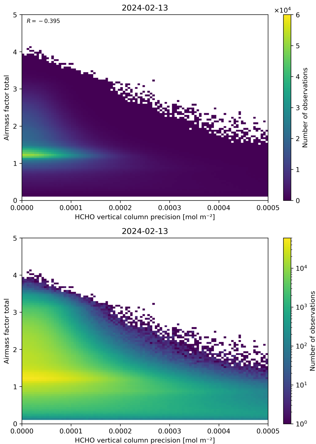
Figure 144: Scatter density plot of “HCHO vertical column precision” against “Airmass factor total” for 2024-02-12 to 2024-02-14.
