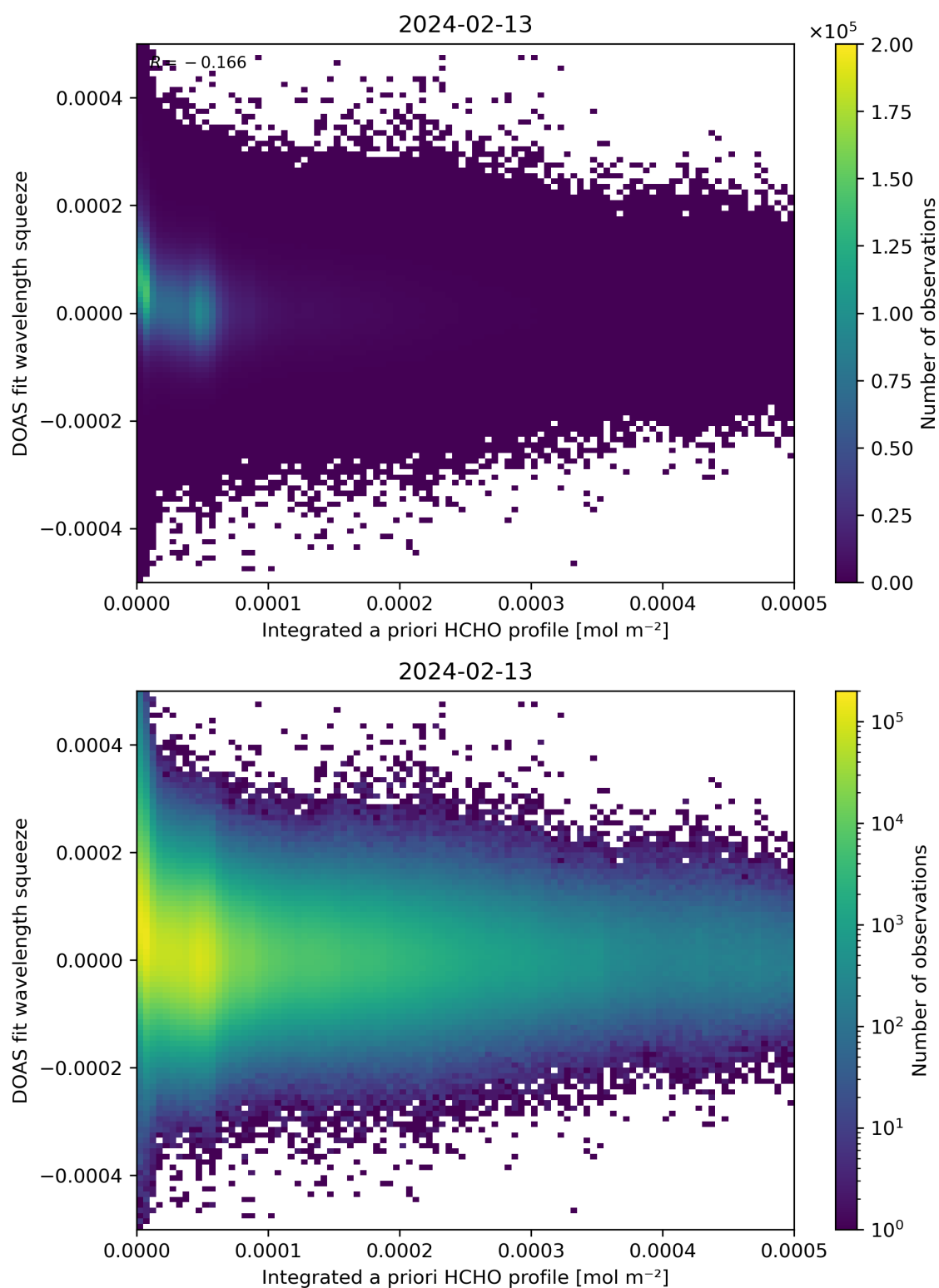
Figure 150: Scatter density plot of “Integrated a priori HCHO profile” against “DOAS fit wavelength squeeze” for 2024-02-12 to 2024-02-14.
