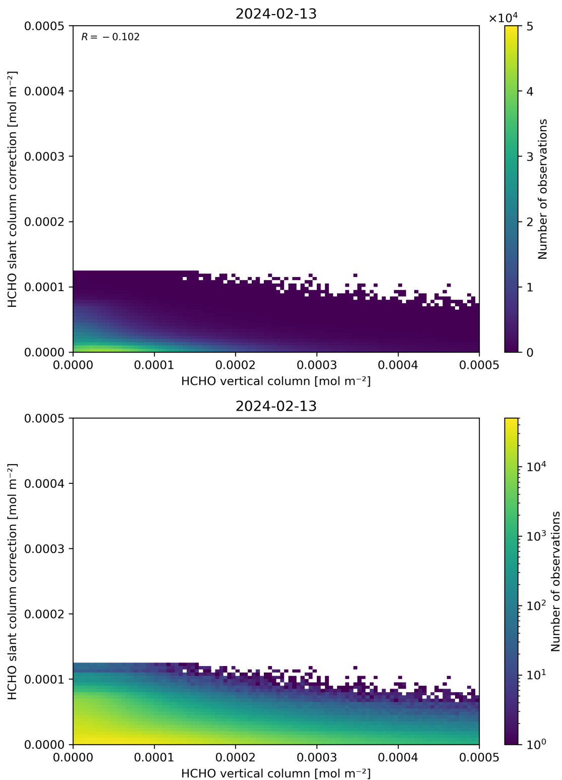
Figure 128: Scatter density plot of “HCHO vertical column” against “HCHO slant column correction” for 2024-02-12 to 2024-02-14.
