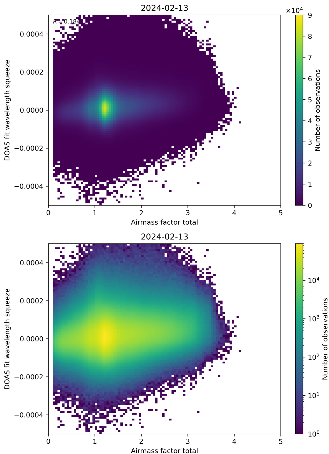
Figure 99: Scatter density plot of “Airmass factor total” against “DOAS fit wavelength squeeze” for 2024-02-12 to 2024-02-14.
