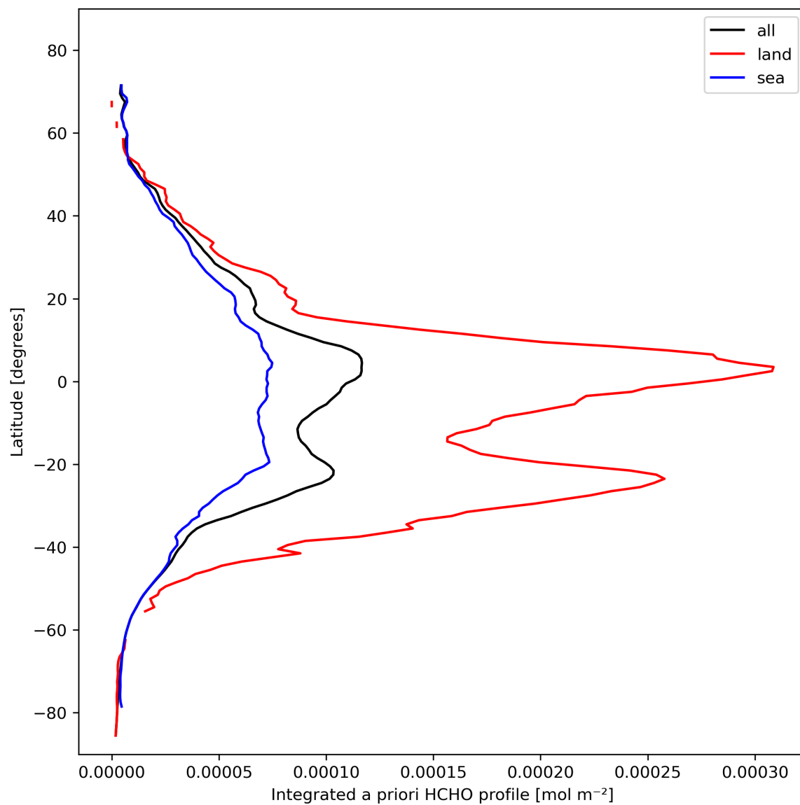
Figure 29: Zonal average of “Integrated a priori HCHO profile” for 2024-02-12 to 2024-02-14.
