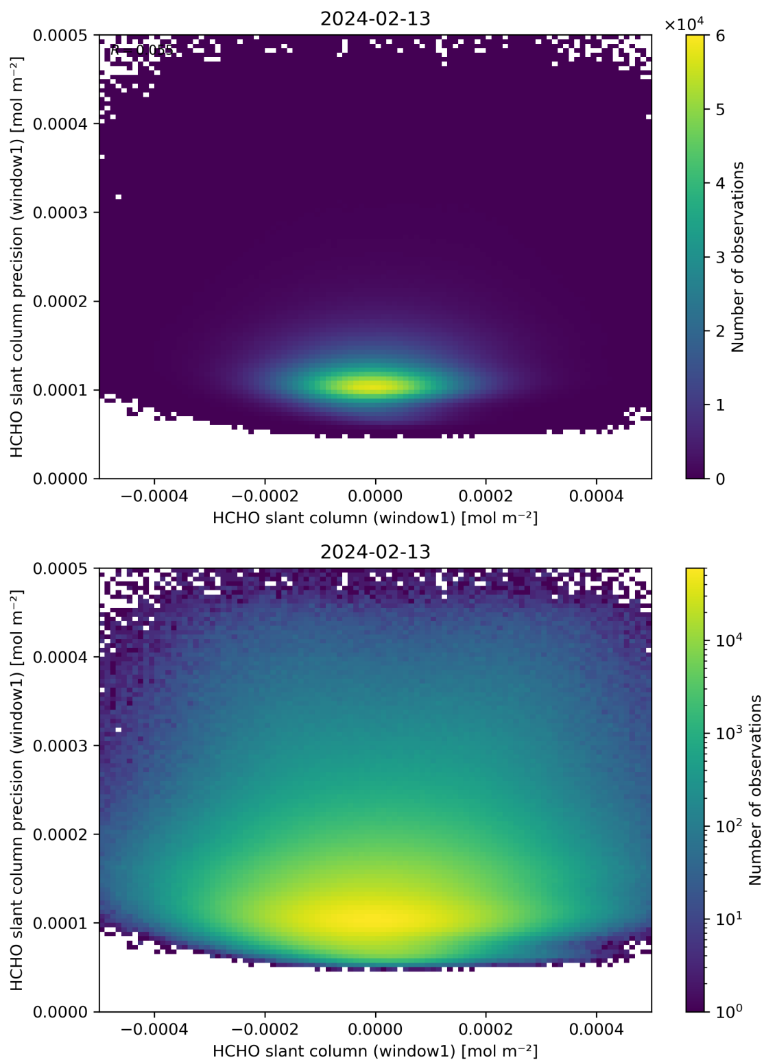
Figure 84: Scatter density plot of “HCHO slant column (window1)” against “HCHO slant column precision (window1)” for 2024-02-12 to 2024-02-14.
