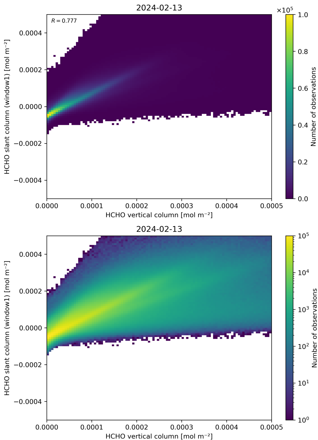
Figure 129: Scatter density plot of “HCHO vertical column” against “HCHO slant column (window1)” for 2024-02-12 to 2024-02-14.
