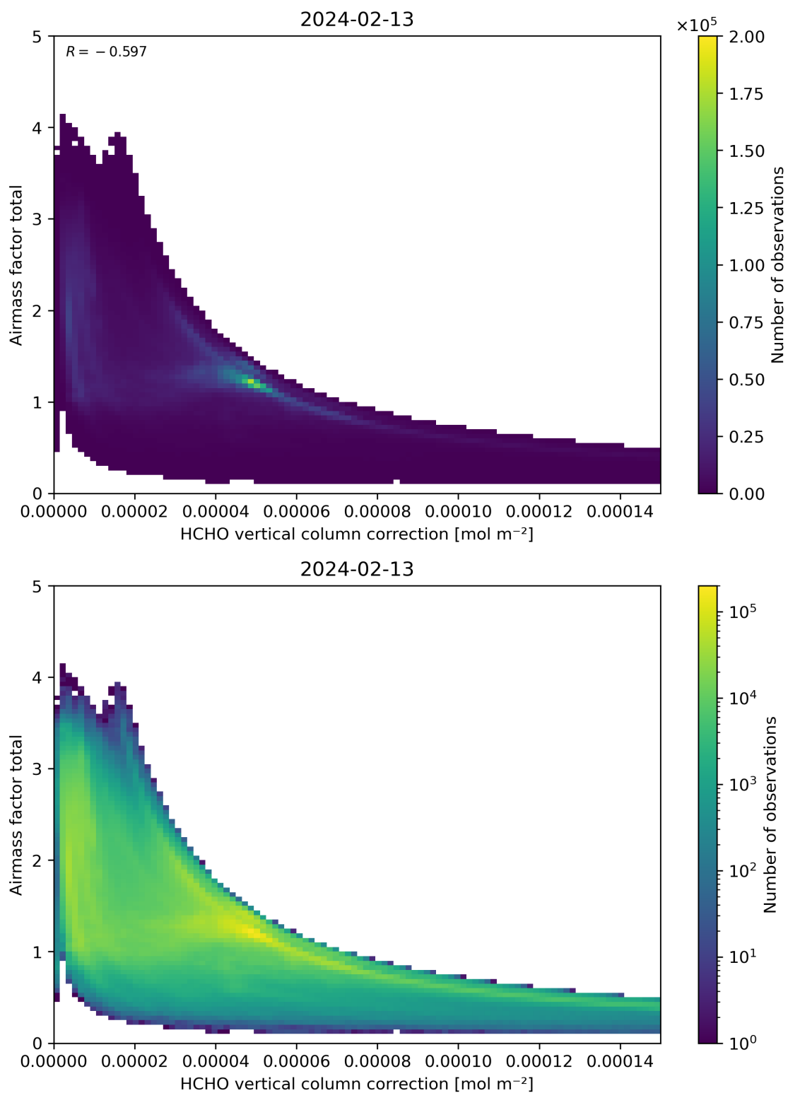
Figure 120: Scatter density plot of “HCHO vertical column correction” against “Airmass factor total” for 2024-02-12 to 2024-02-14.
