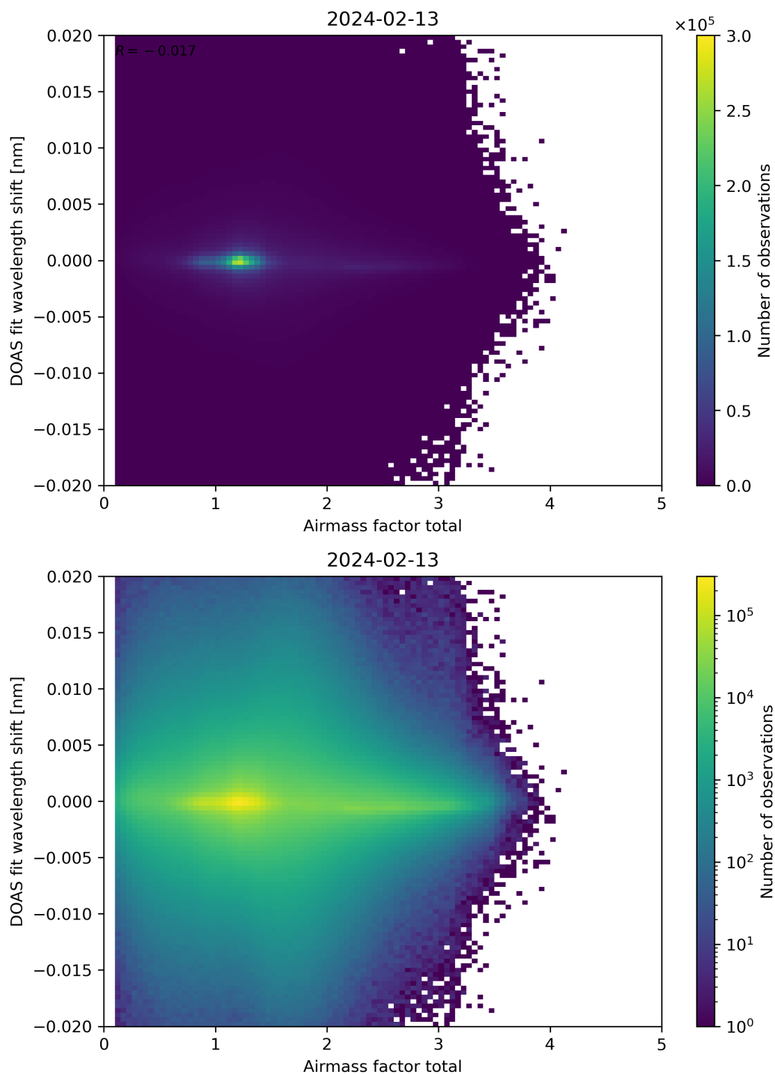
Figure 98: Scatter density plot of “Airmass factor total” against “DOAS fit wavelength shift” for 2024-02-12 to 2024-02-14.
