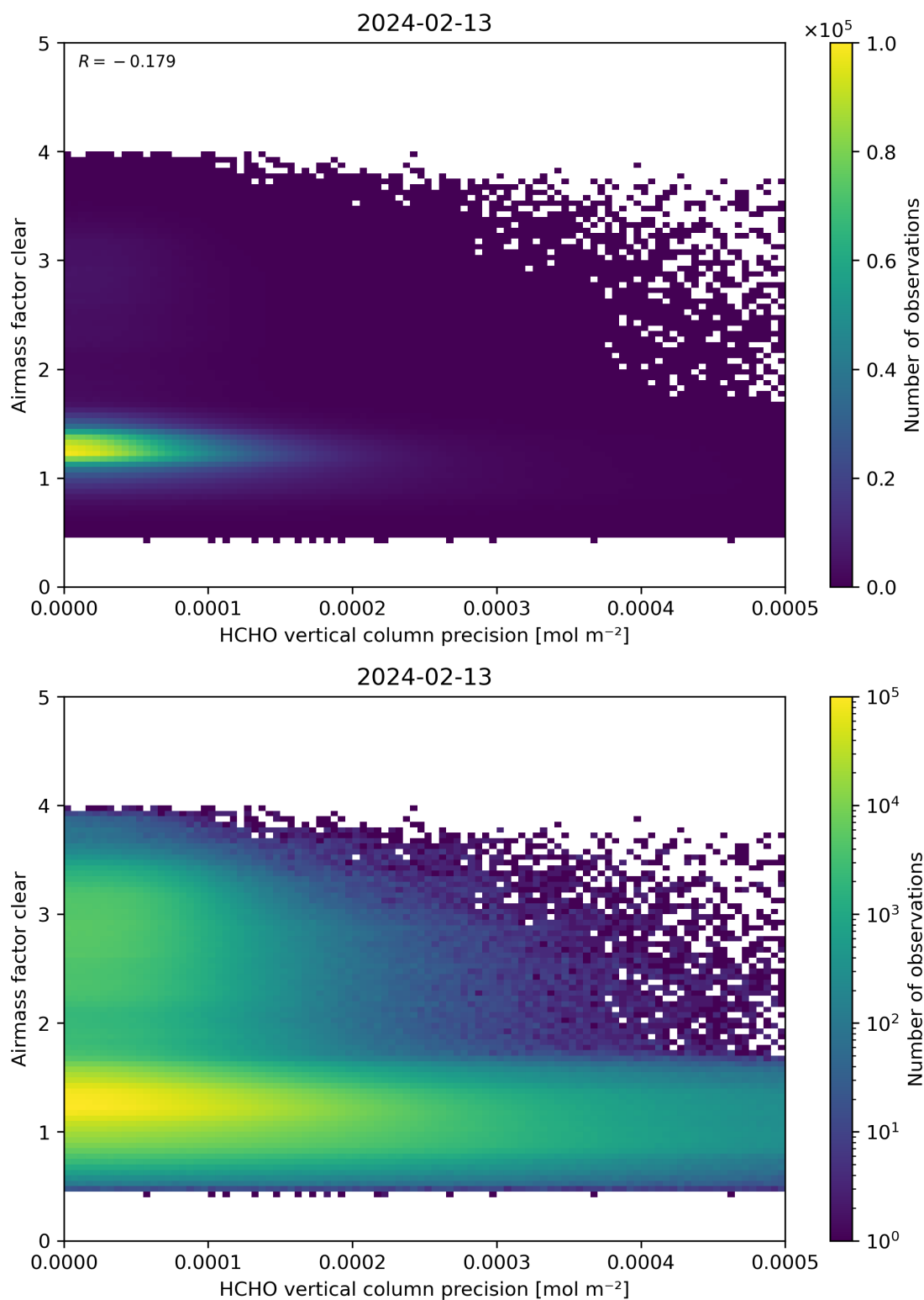
Figure 139: Scatter density plot of “HCHO vertical column precision” against “Airmass factor clear” for 2024-02-12 to 2024-02-14.
