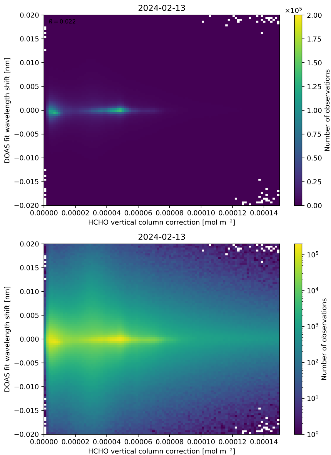
Figure 113: Scatter density plot of “HCHO vertical column correction” against “DOAS fit wavelength shift” for 2024-02-12 to 2024-02-14.
