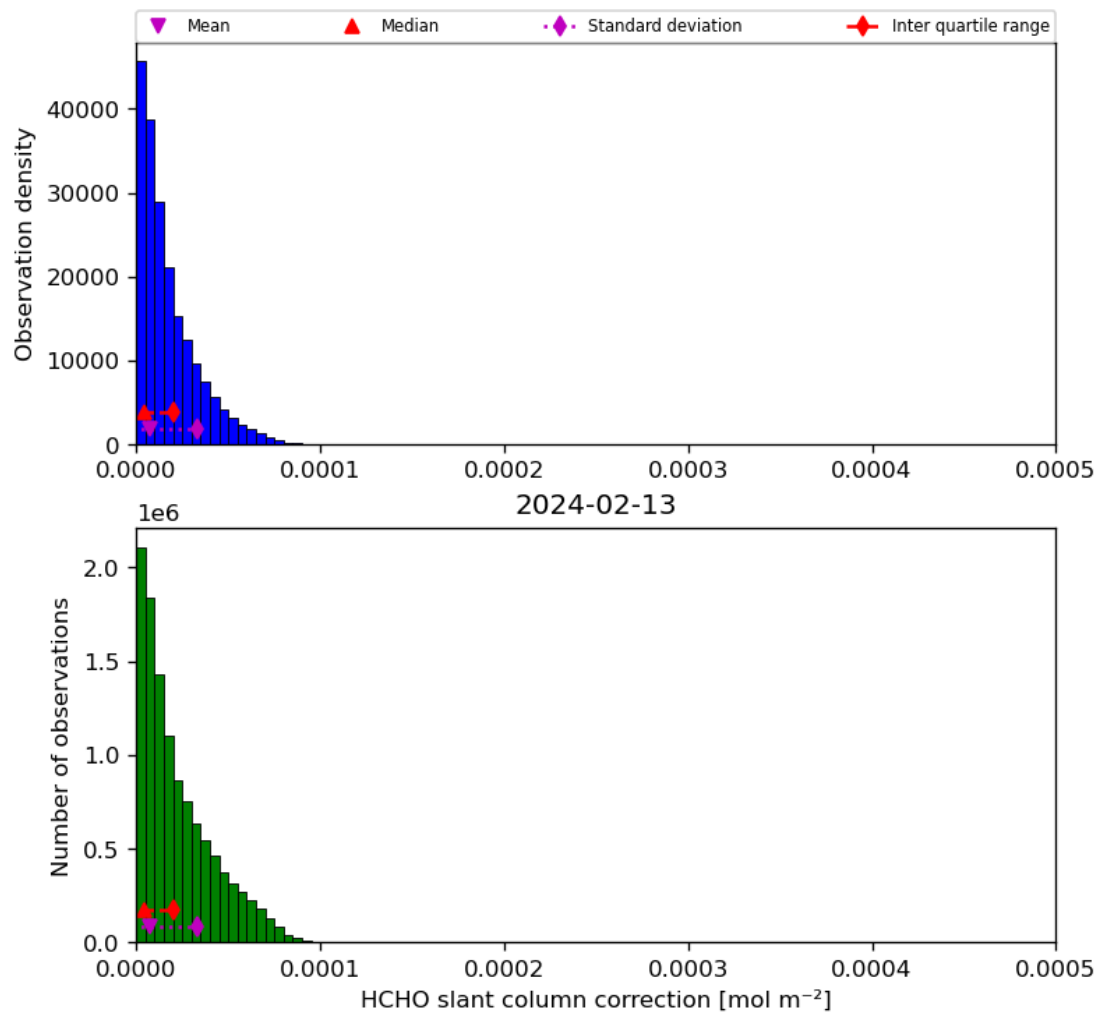
Figure 47: Histogram of “HCHO slant column correction” for 2024-02-12 to 2024-02-14
