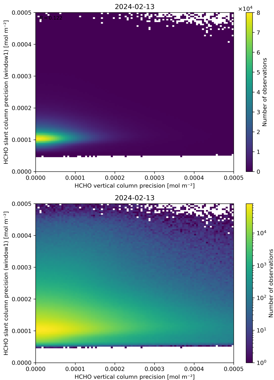
Figure 143: Scatter density plot of “HCHO vertical column precision” against “HCHO slant column precision (window1)” for 2024-02-12 to 2024-02-14.
