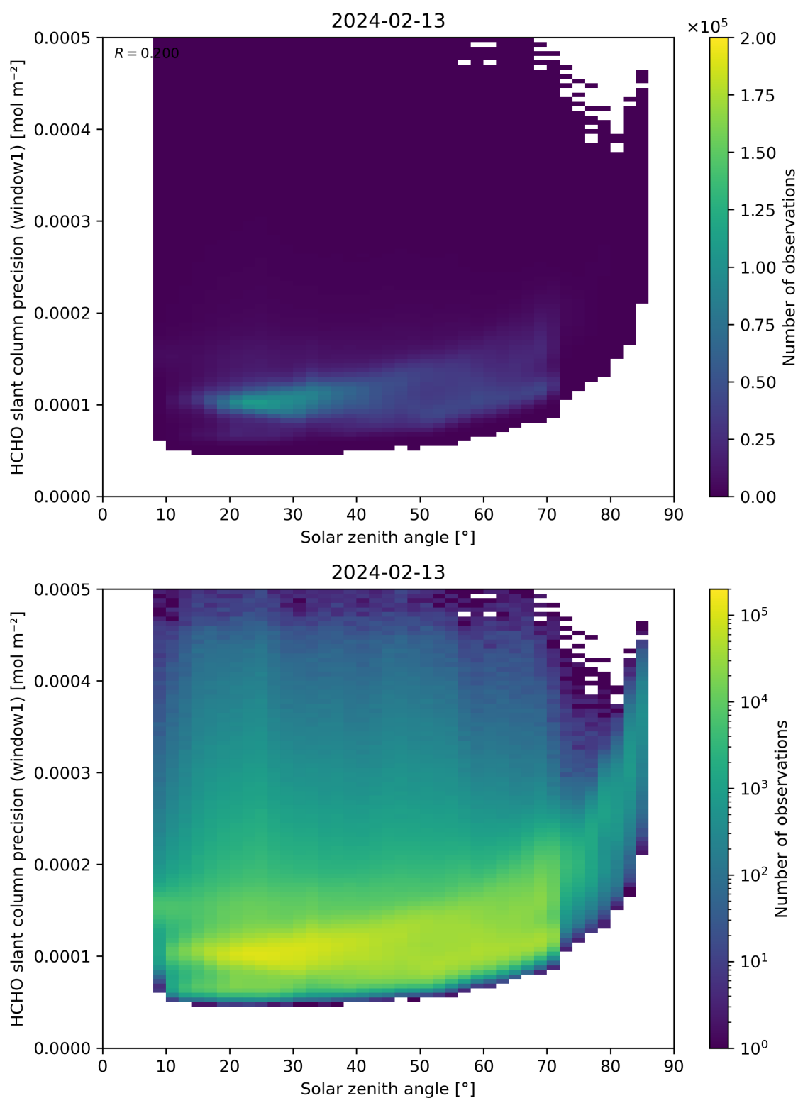
Figure 174: Scatter density plot of “Solar zenith angle” against “HCHO slant column precision (window1)” for 2024-02-12 to 2024-02-14.
