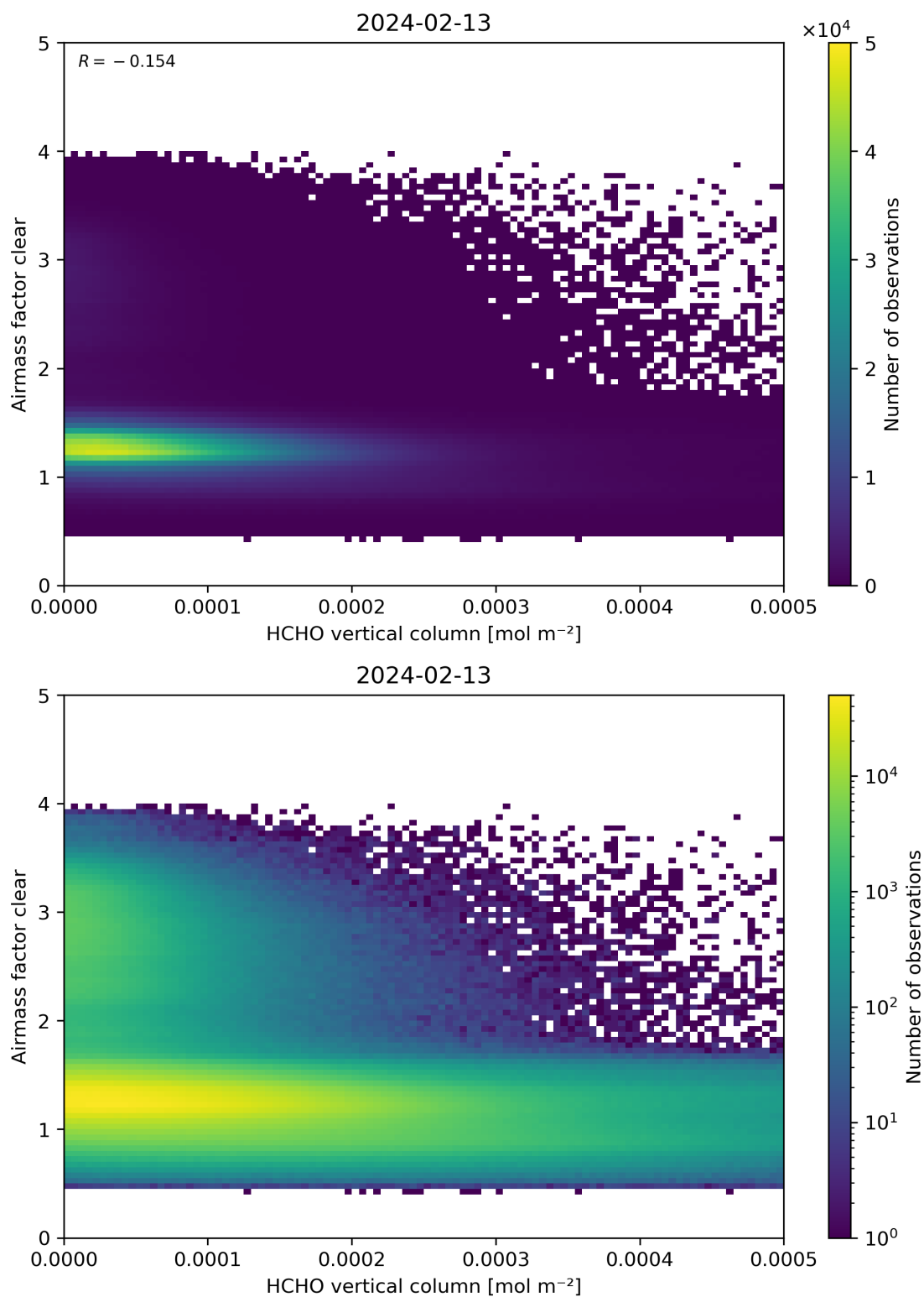
Figure 126: Scatter density plot of “HCHO vertical column” against “Airmass factor clear” for 2024-02-12 to 2024-02-14.
