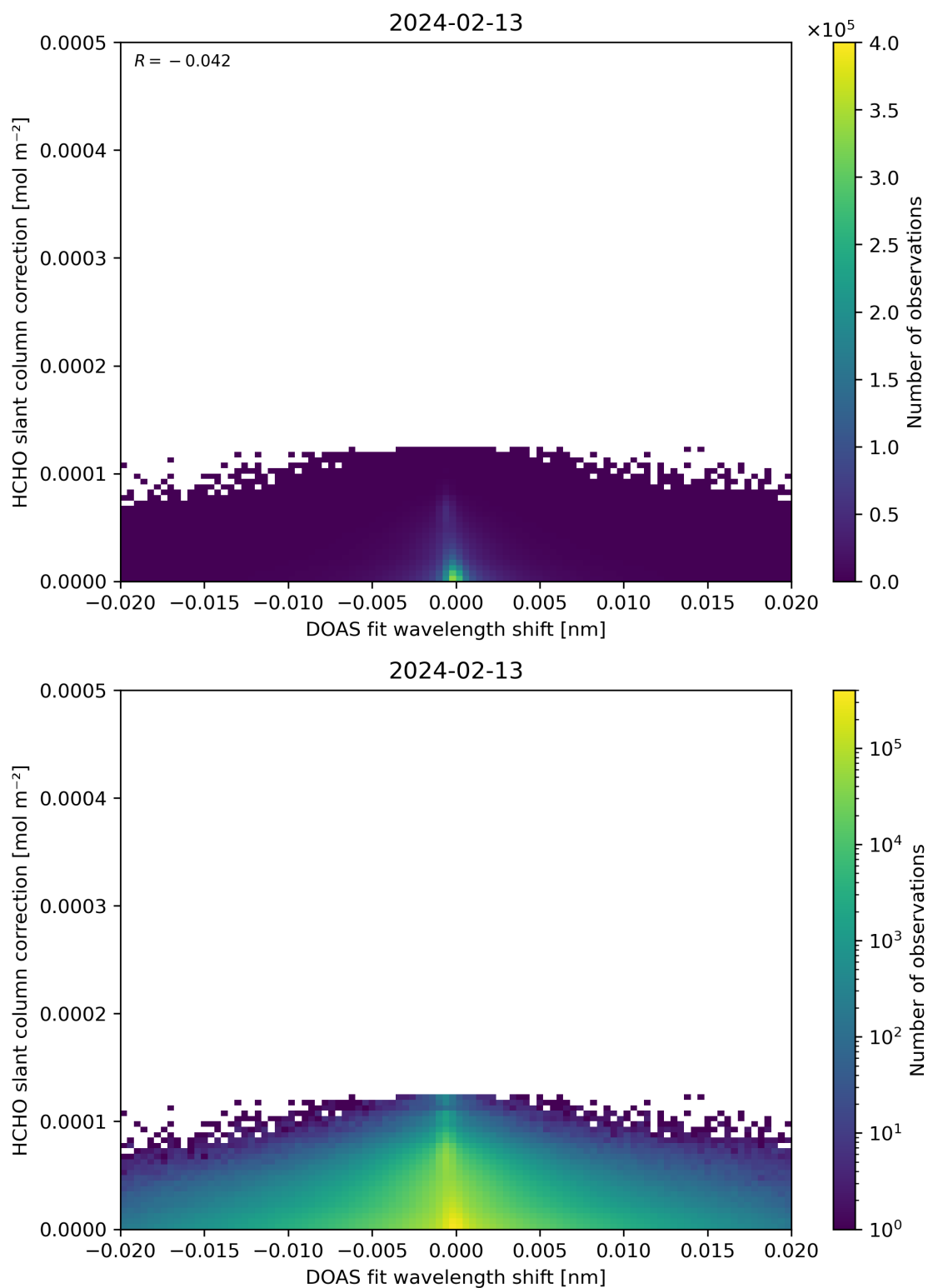
Figure 67: Scatter density plot of “DOAS fit wavelength shift” against “HCHO slant column correction” for 2024-02-12 to 2024-02-14.
