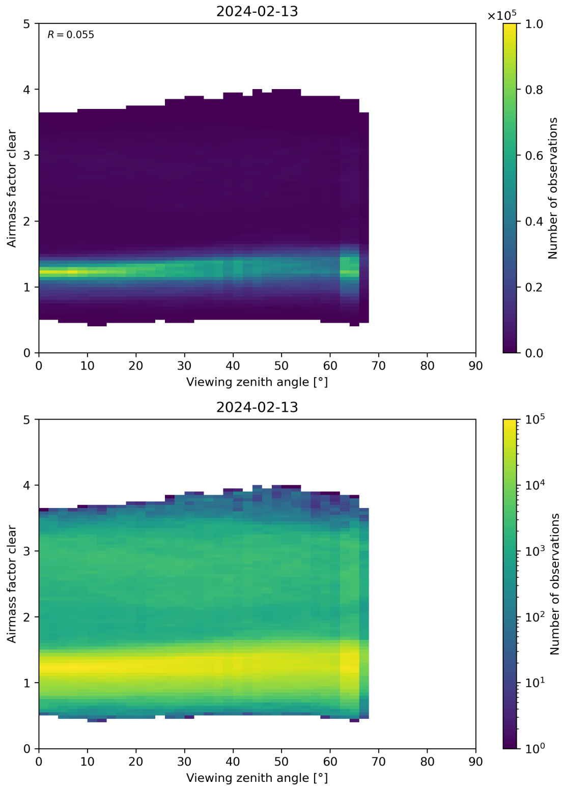
Figure 185: Scatter density plot of “Viewing zenith angle” against “Airmass factor clear” for 2024-02-12 to 2024-02-14.
