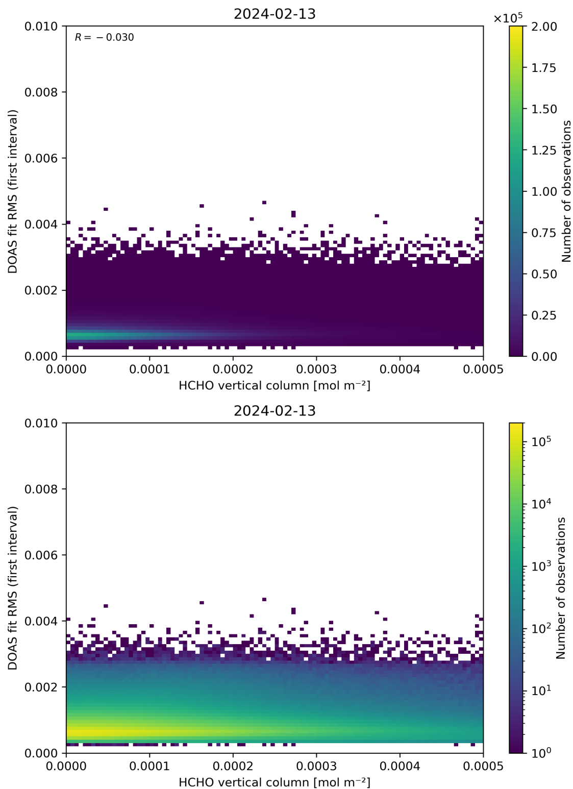
Figure 123: Scatter density plot of “HCHO vertical column” against “DOAS fit RMS (first interval)” for 2024-02-12 to 2024-02-14.
