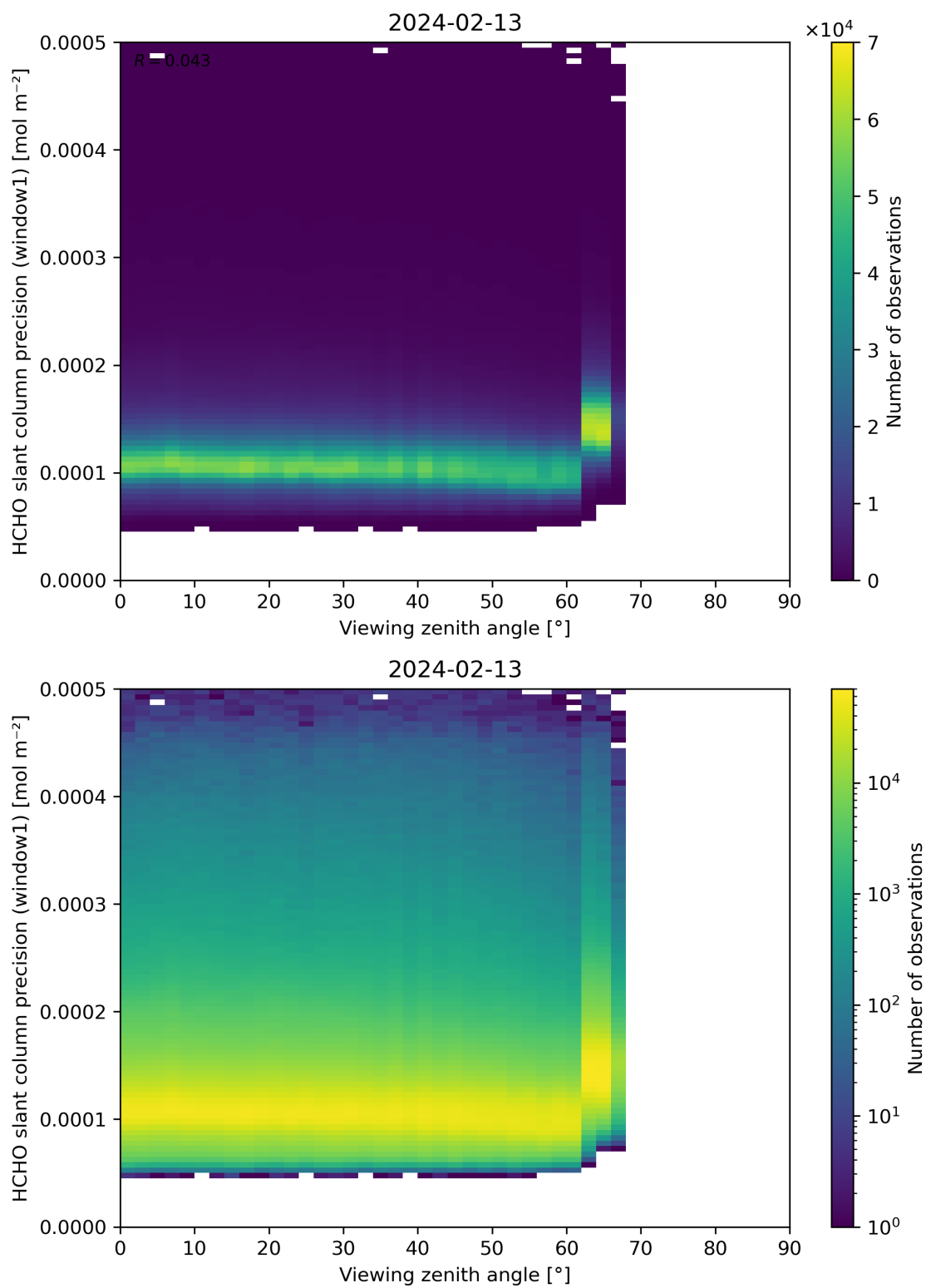
Figure 189: Scatter density plot of “Viewing zenith angle” against “HCHO slant column precision (window1)” for 2024-02-12 to 2024-02-14.
