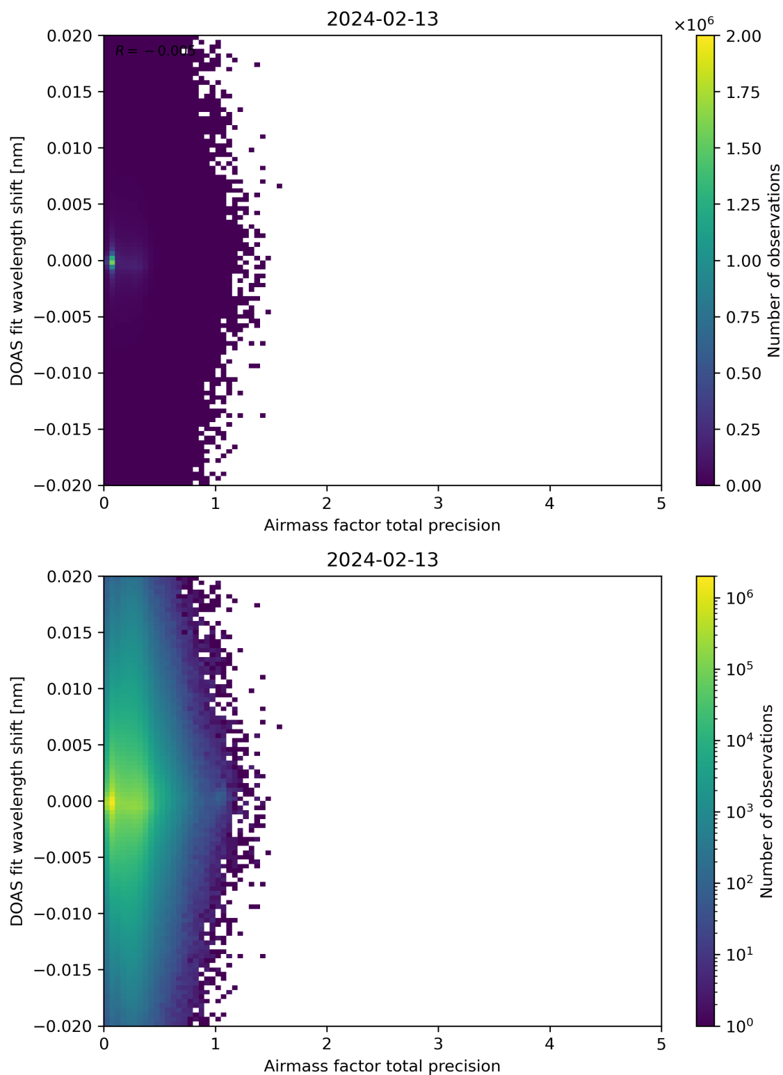
Figure 106: Scatter density plot of “Airmass factor total precision” against “DOAS fit wavelength shift” for 2024-02-12 to 2024-02-14.
