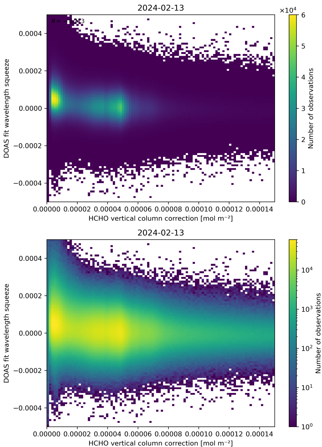
Figure 114: Scatter density plot of “HCHO vertical column correction” against “DOAS fit wavelength squeeze” for 2024-02-12 to 2024-02-14.
