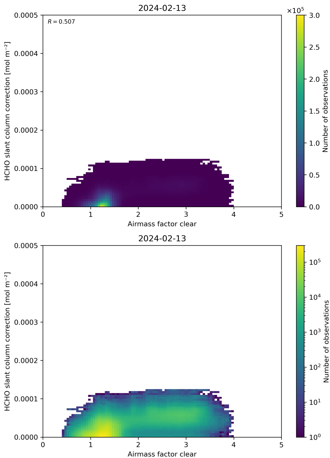
Figure 75: Scatter density plot of “Airmass factor clear” against “HCHO slant column correction” for 2024-02-12 to 2024-02-14.
