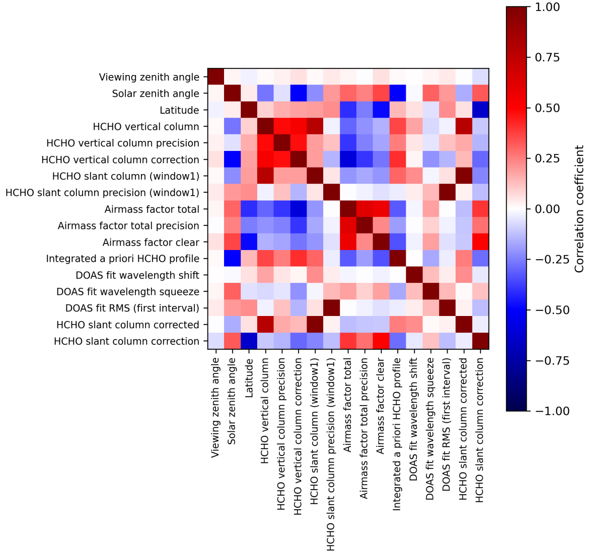
Figure 2: Map of correlation matrix for 2024-02-12 to 2024-02-14.
