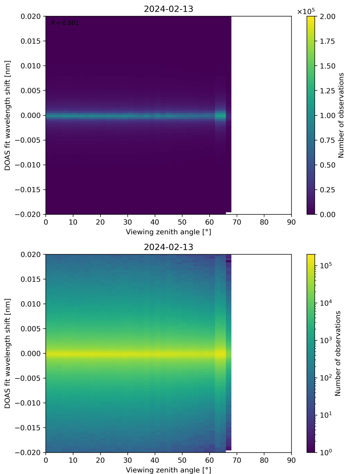
Figure 183: Scatter density plot of “Viewing zenith angle” against “DOAS fit wavelength shift” for 2024-02-12 to 2024-02-14.
