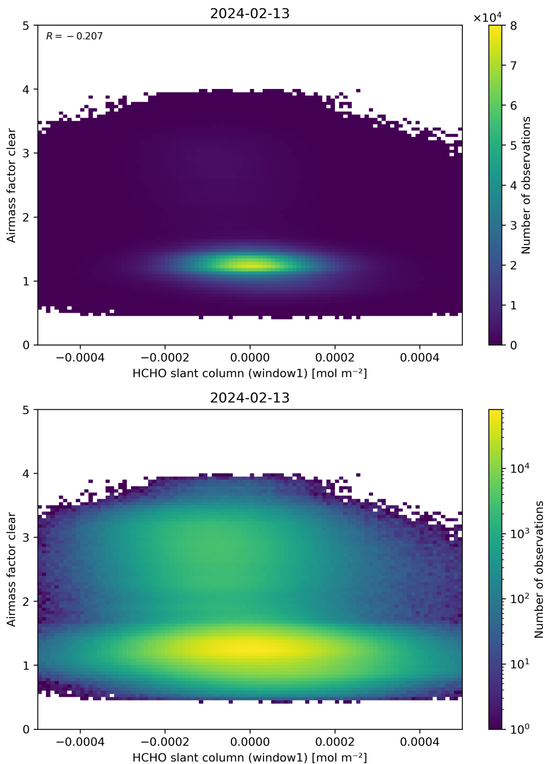
Figure 81: Scatter density plot of “HCHO slant column (window1)” against “Airmass factor clear” for 2024-02-12 to 2024-02-14.
