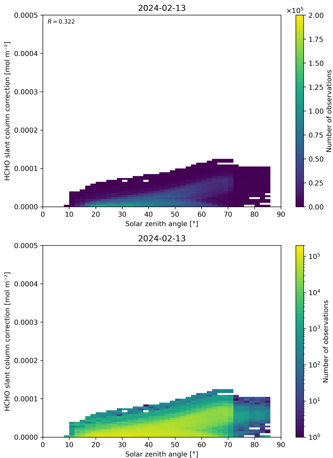
Figure 172: Scatter density plot of “Solar zenith angle” against “HCHO slant column correction” for 2024-02-12 to 2024-02-14.
