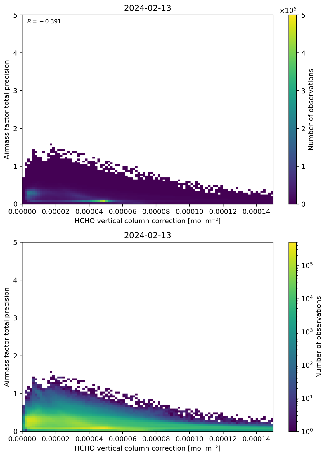
Figure 121: Scatter density plot of “HCHO vertical column correction” against “Airmass factor total precision” for 2024-02-12 to 2024-02-14.
