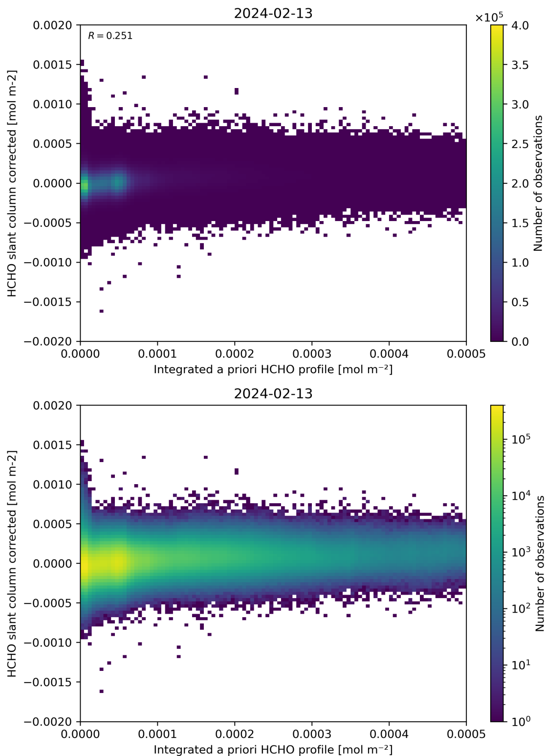
Figure 151: Scatter density plot of “Integrated a priori HCHO profile” against “HCHO slant column corrected” for 2024-02-12 to 2024-02-14.
