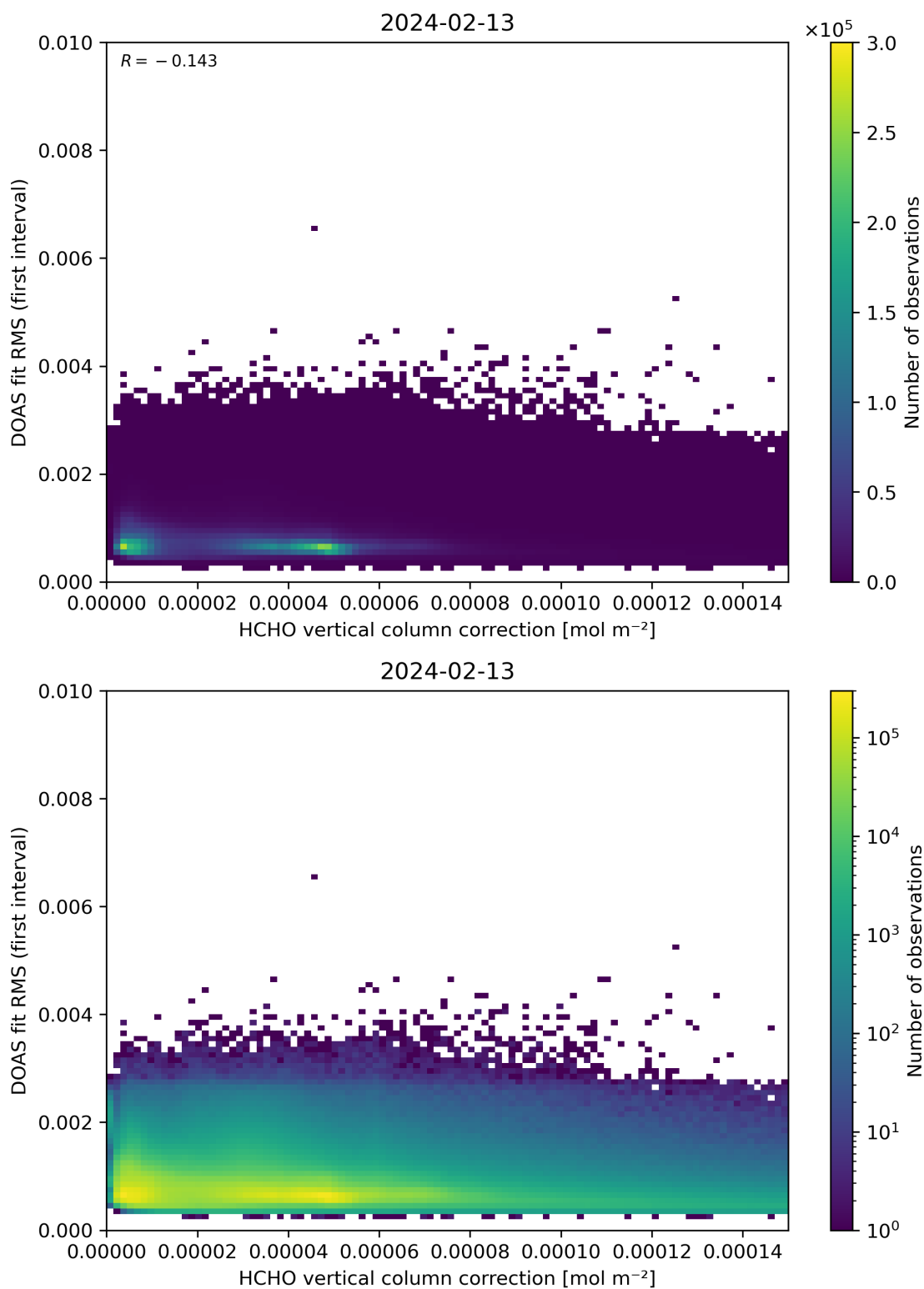
Figure 112: Scatter density plot of “HCHO vertical column correction” against “DOAS fit RMS (first interval)” for 2024-02-12 to 2024-02-14.
