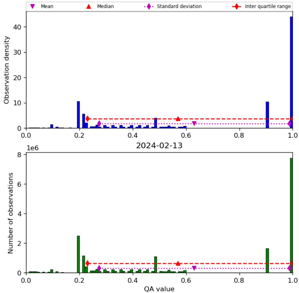
Figure 34: Histogram of “QA value” for 2024-02-12 to 2024-02-14
