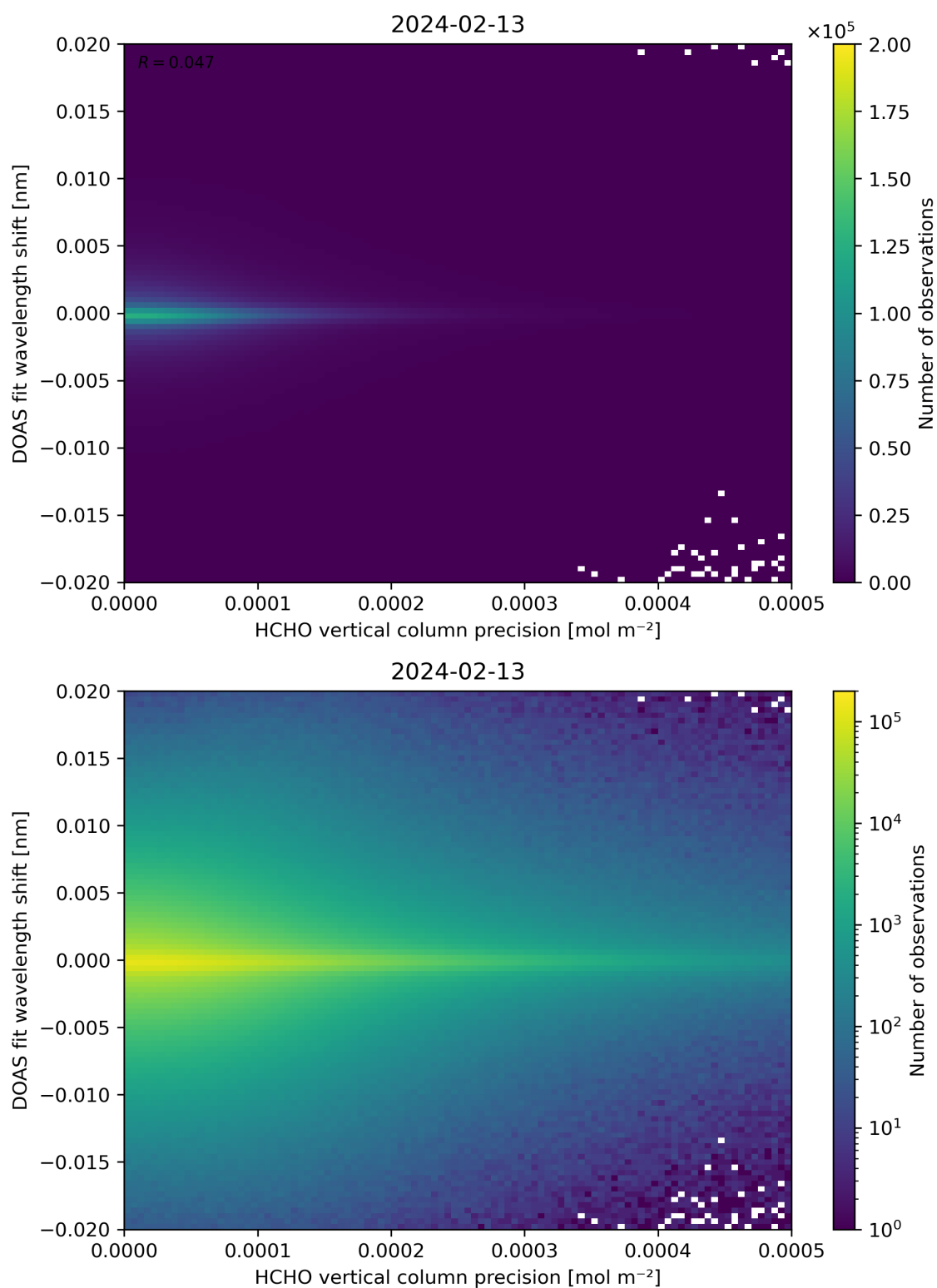
Figure 137: Scatter density plot of “HCHO vertical column precision” against “DOAS fit wavelength shift” for 2024-02-12 to 2024-02-14.
