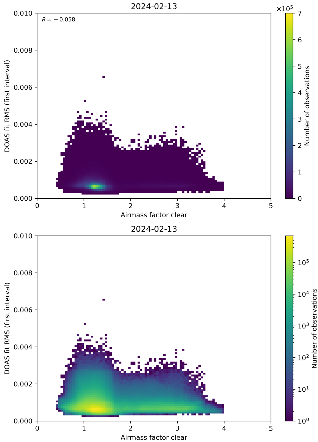
Figure 71: Scatter density plot of “Airmass factor clear” against “DOAS fit RMS (first interval)” for 2024-02-12 to 2024-02-14.
