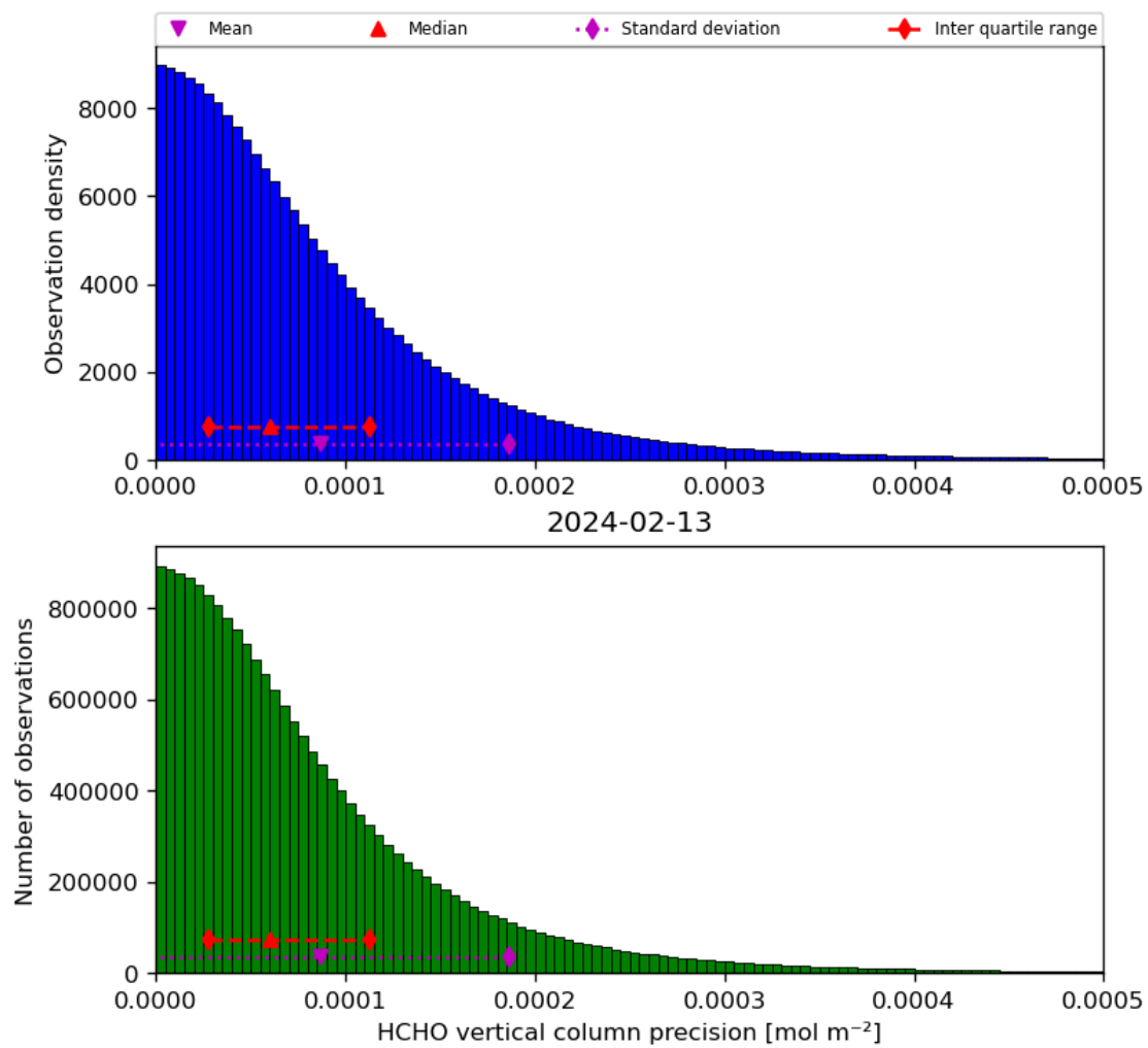
Figure 36: Histogram of “HCHO vertical column precision” for 2024-02-12 to 2024-02-14
