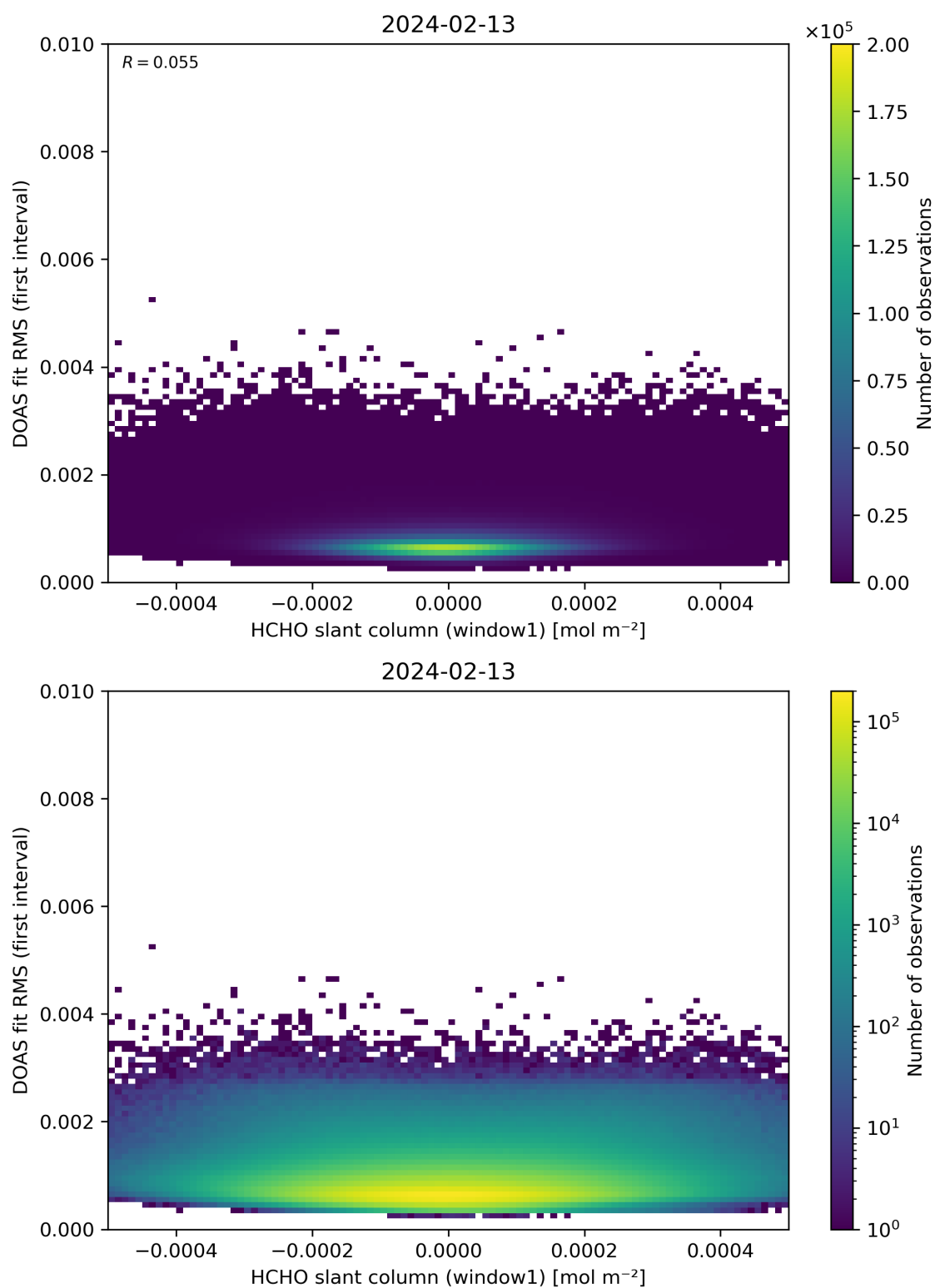
Figure 78: Scatter density plot of “HCHO slant column (window1)” against “DOAS fit RMS (first interval)” for 2024-02-12 to 2024-02-14.
