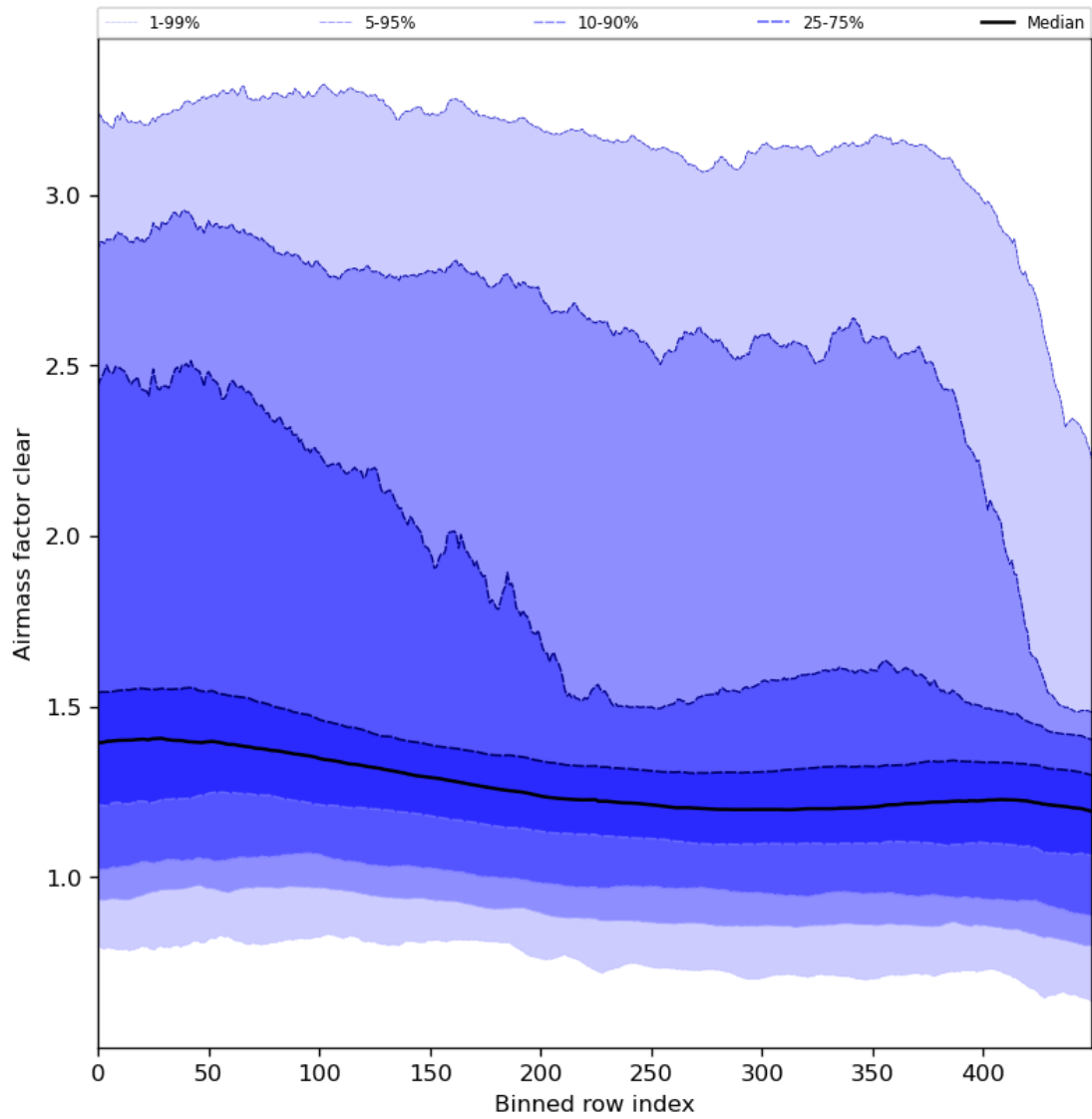
Figure 56: Along track statistics of “Airmass factor clear” for 2024-02-12 to 2024-02-14
