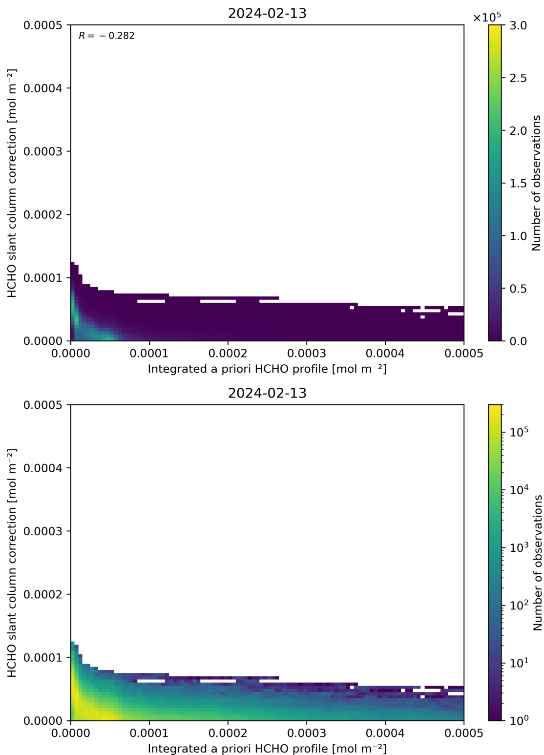
Figure 152: Scatter density plot of “Integrated a priori HCHO profile” against “HCHO slant column correction” for 2024-02-12 to 2024-02-14.
