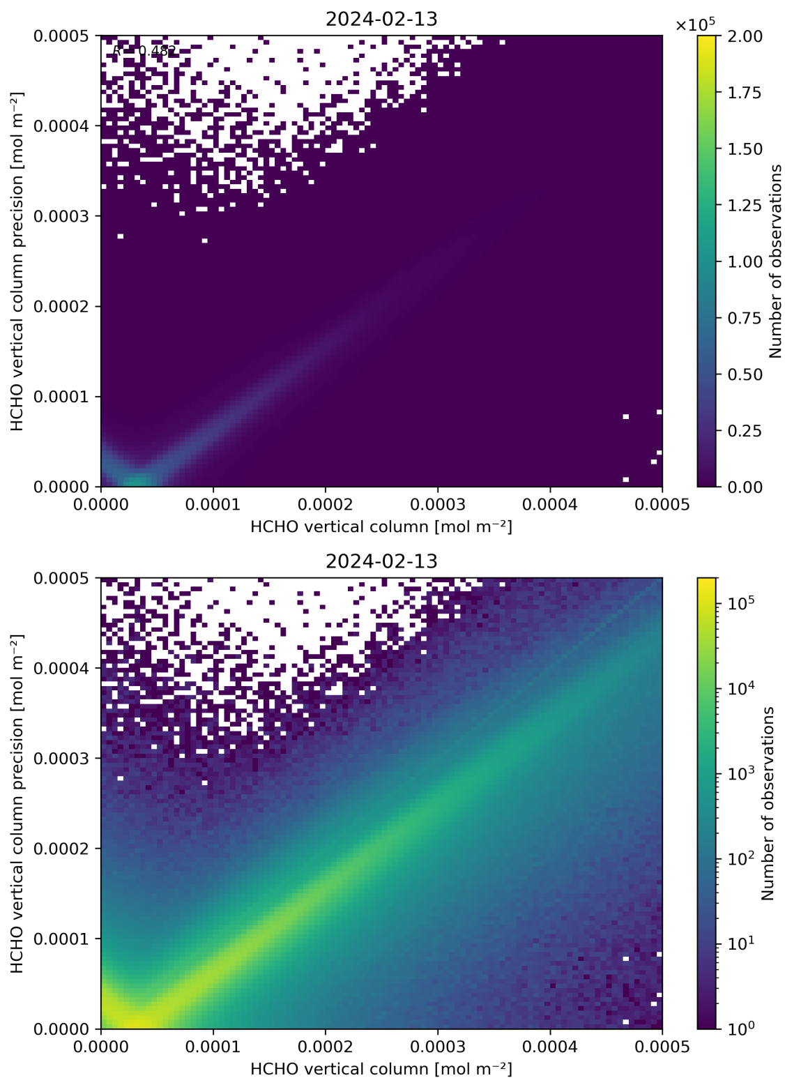
Figure 134: Scatter density plot of “HCHO vertical column” against “HCHO vertical column precision” for 2024-02-12 to 2024-02-14.
