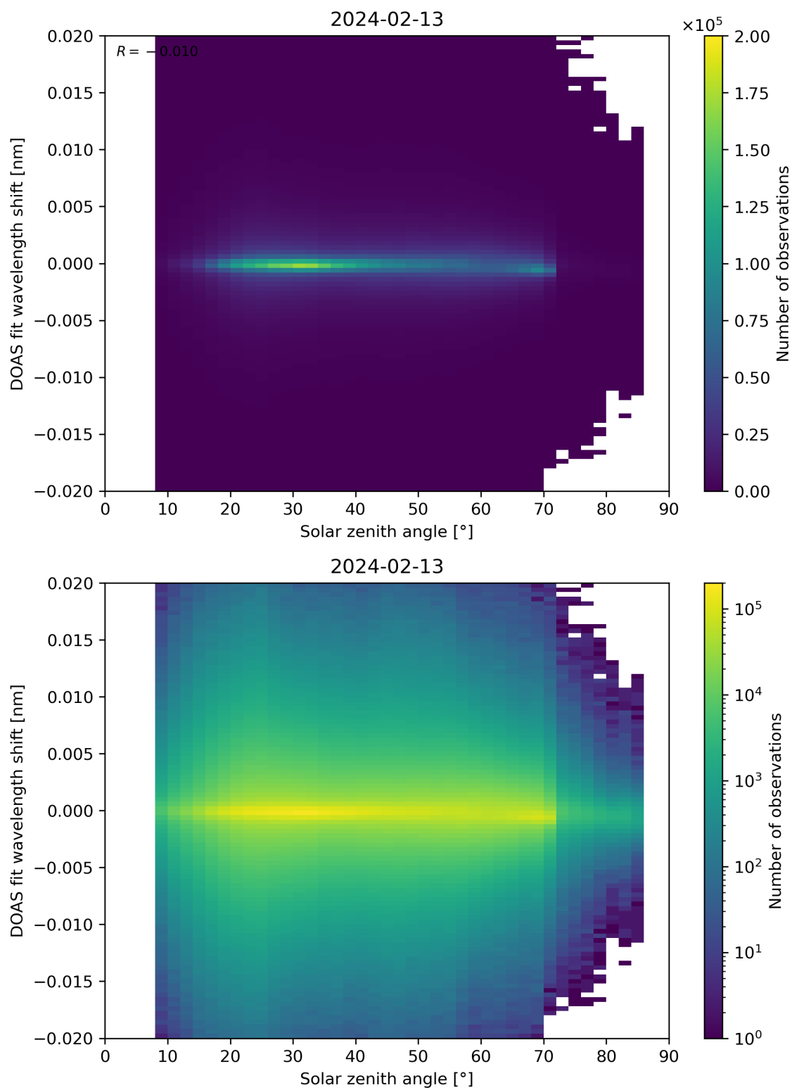
Figure 168: Scatter density plot of “Solar zenith angle” against “DOAS fit wavelength shift” for 2024-02-12 to 2024-02-14.
