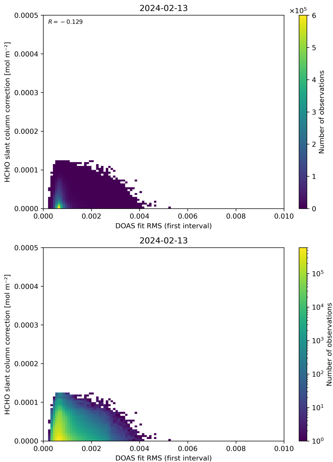
Figure 63: Scatter density plot of “DOAS fit RMS (first interval)” against “HCHO slant column correction” for 2024-02-12 to 2024-02-14.
