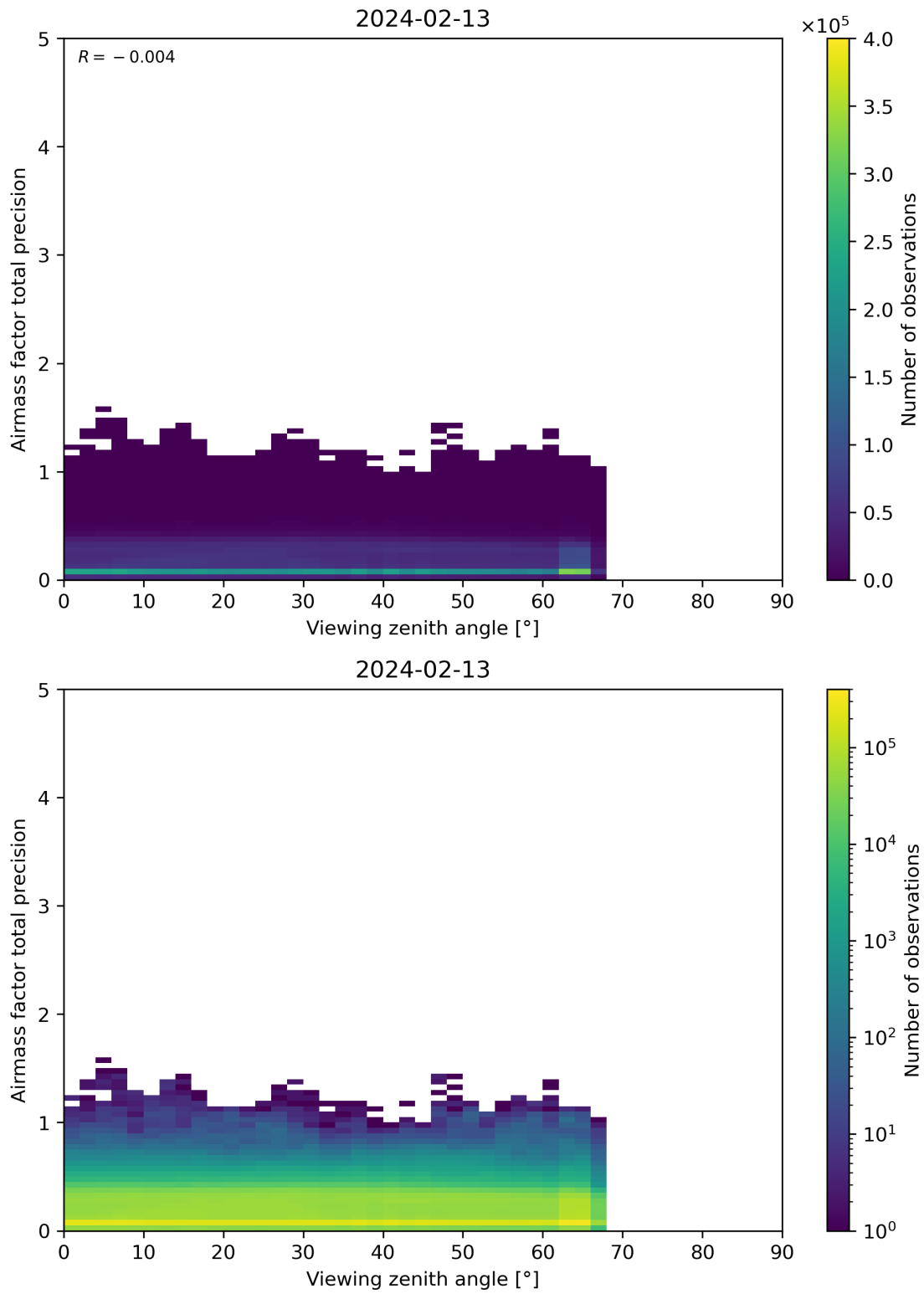
Figure 191: Scatter density plot of “Viewing zenith angle” against “Airmass factor total precision” for 2024-02-12 to 2024-02-14.
