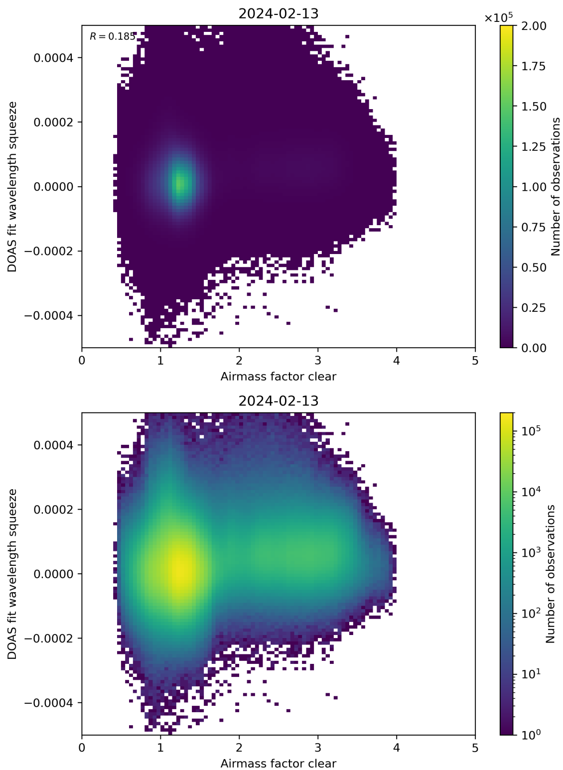
Figure 73: Scatter density plot of “Airmass factor clear” against “DOAS fit wavelength squeeze” for 2024-02-12 to 2024-02-14.
