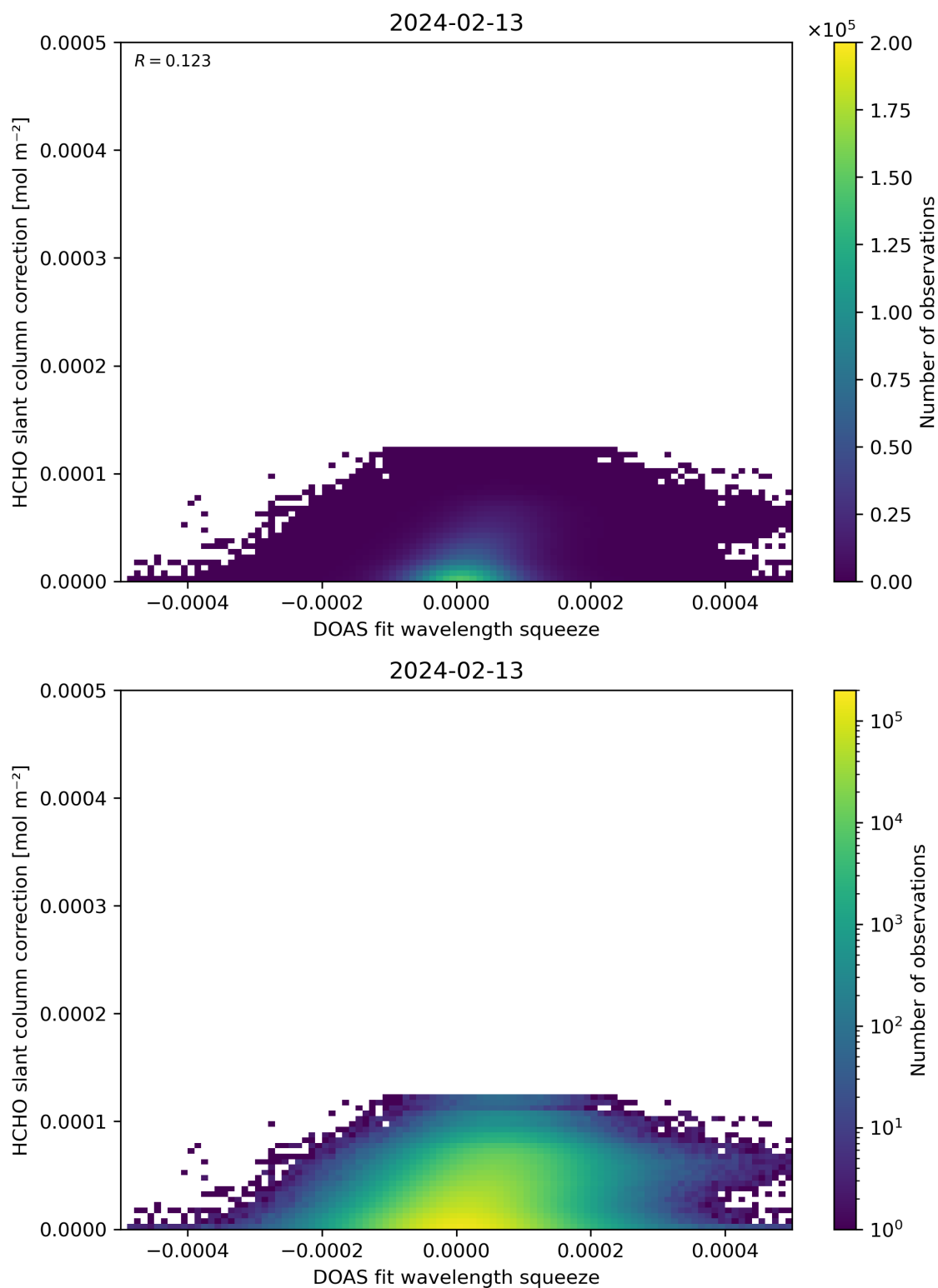
Figure 70: Scatter density plot of “DOAS fit wavelength squeeze” against “HCHO slant column correction” for 2024-02-12 to 2024-02-14.
