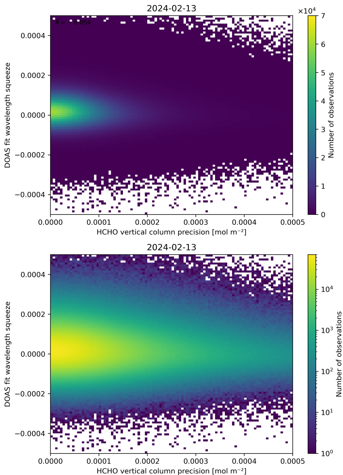
Figure 138: Scatter density plot of “HCHO vertical column precision” against “DOAS fit wavelength squeeze” for 2024-02-12 to 2024-02-14.
