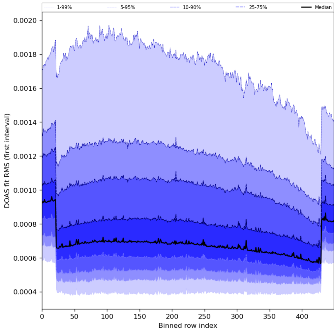
Figure 60: Along track statistics of “DOAS fit RMS (first interval)” for 2024-02-12 to 2024-02-14
