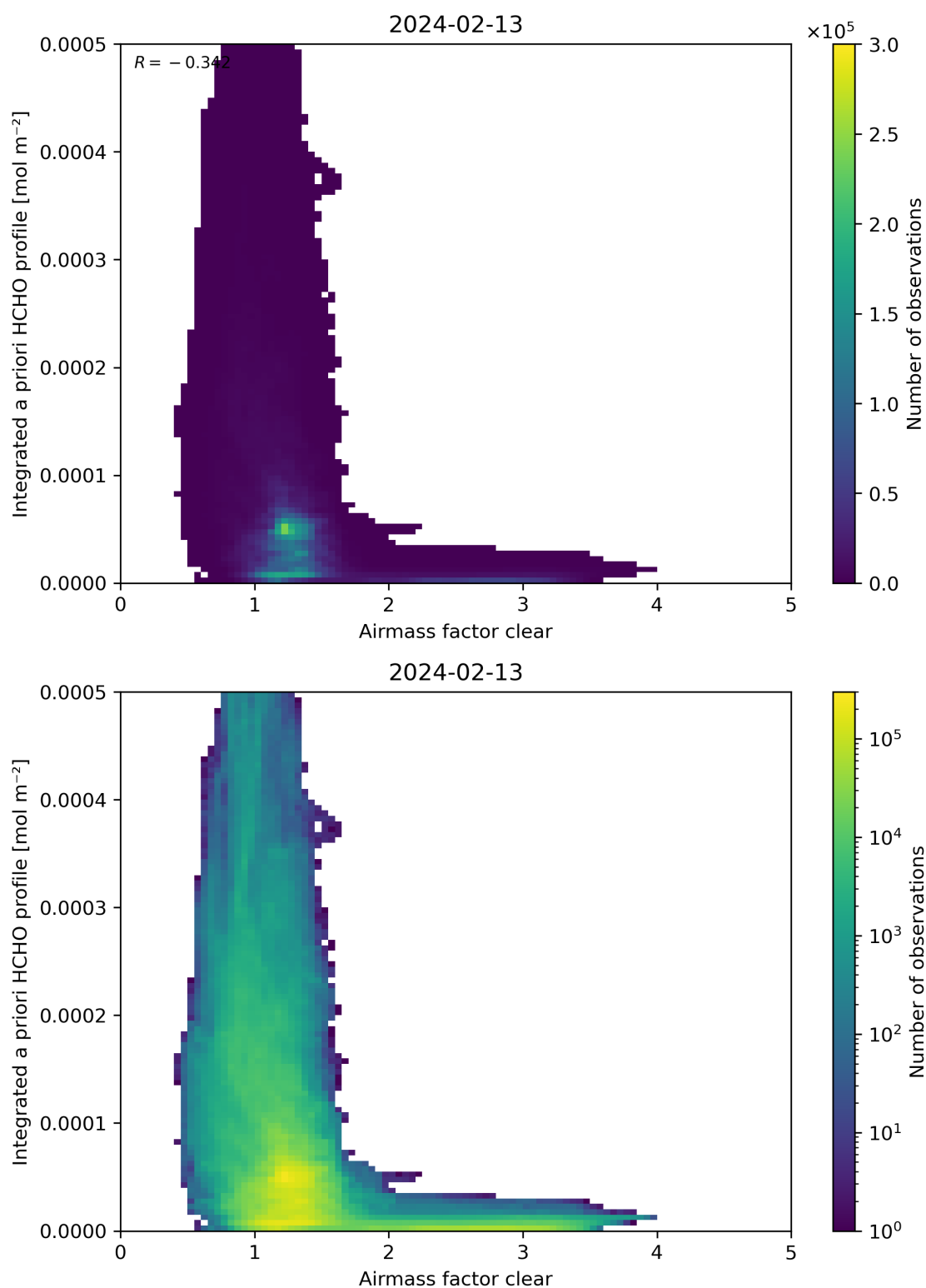
Figure 76: Scatter density plot of “Airmass factor clear” against “Integrated a priori HCHO profile” for 2024-02-12 to 2024-02-14.
