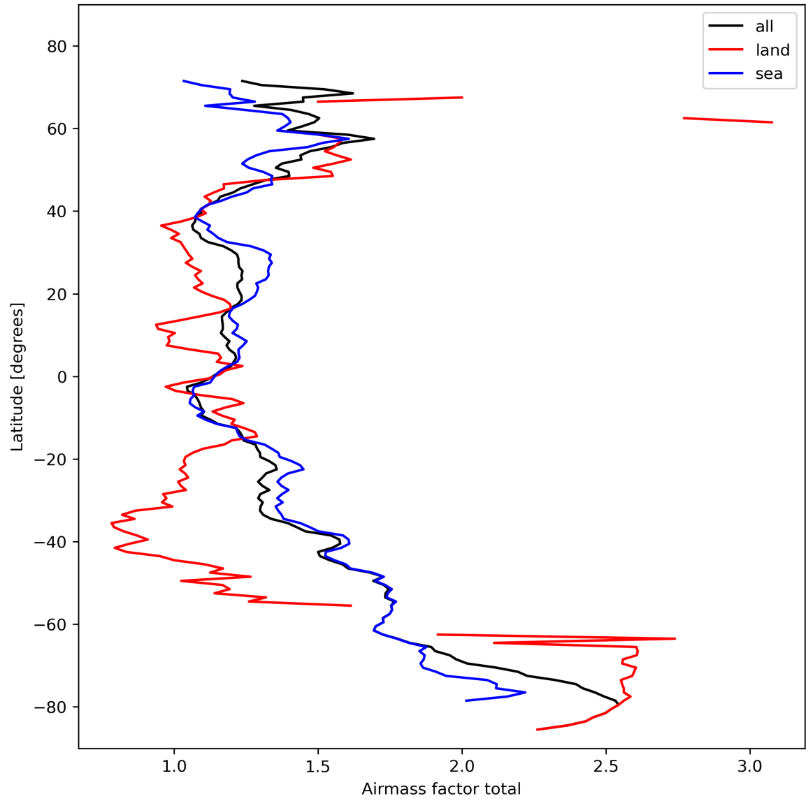
Figure 26: Zonal average of “Airmass factor total” for 2024-02-12 to 2024-02-14.
