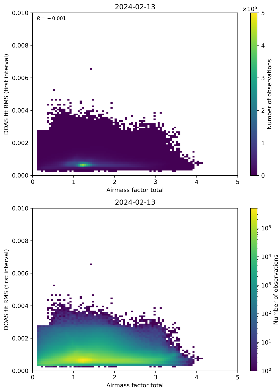
Figure 97: Scatter density plot of “Airmass factor total” against “DOAS fit RMS (first interval)” for 2024-02-12 to 2024-02-14.
