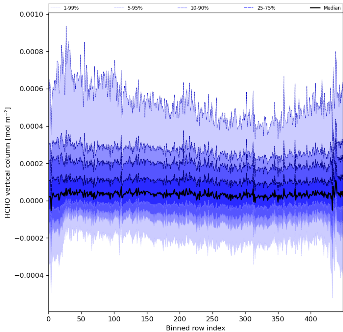
Figure 49: Along track statistics of "HCHO vertical column" for 2024-02-12 to 2024-02-14
