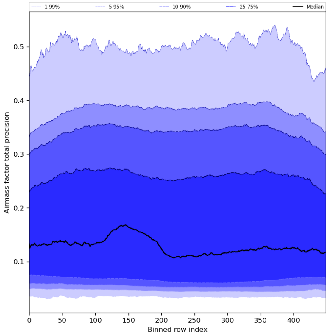
Figure 55: Along track statistics of “Airmass factor total precision” for 2024-02-12 to 2024-02-14
