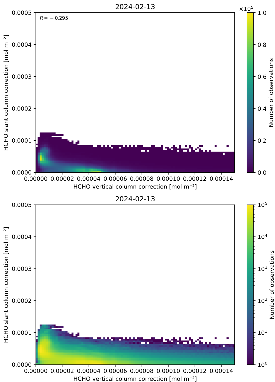
Figure 117: Scatter density plot of “HCHO vertical column correction” against “HCHO slant column correction” for 2024-02-12 to 2024-02-14.
