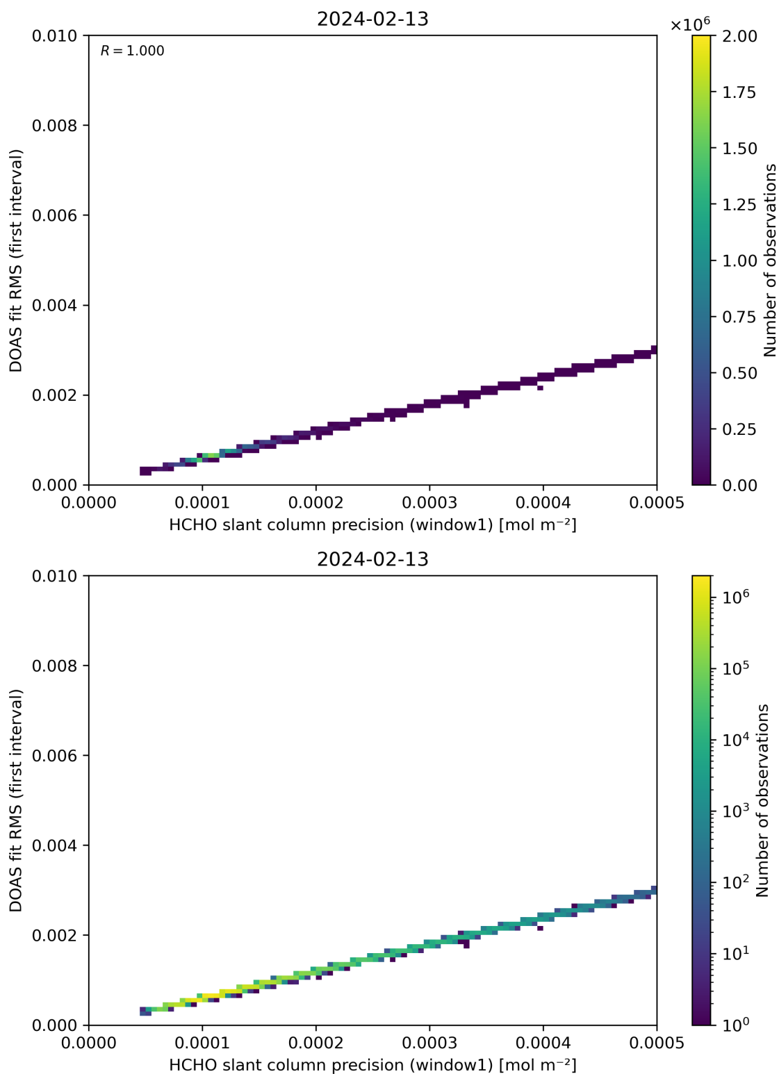
Figure 88: Scatter density plot of “HCHO slant column precision (window1)” against “DOAS fit RMS (first interval)” for 2024-02-12 to 2024-02-14.
