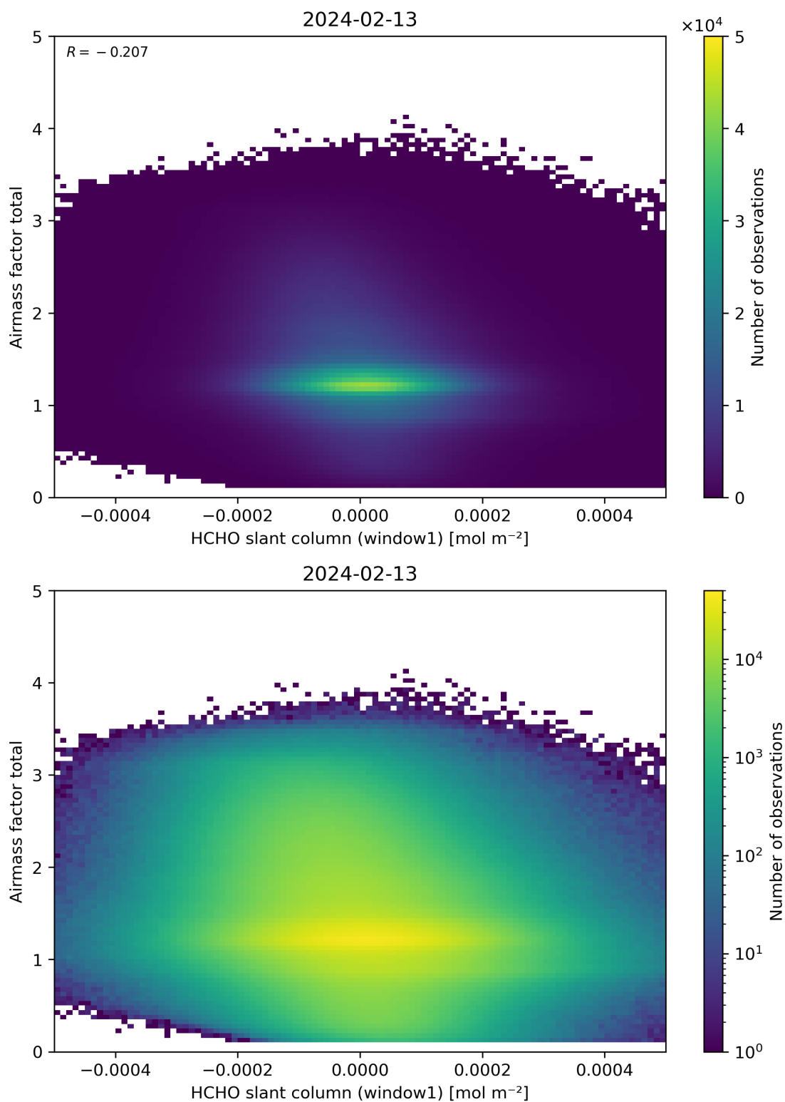
Figure 85: Scatter density plot of “HCHO slant column (window1)” against “Airmass factor total” for 2024-02-12 to 2024-02-14.
