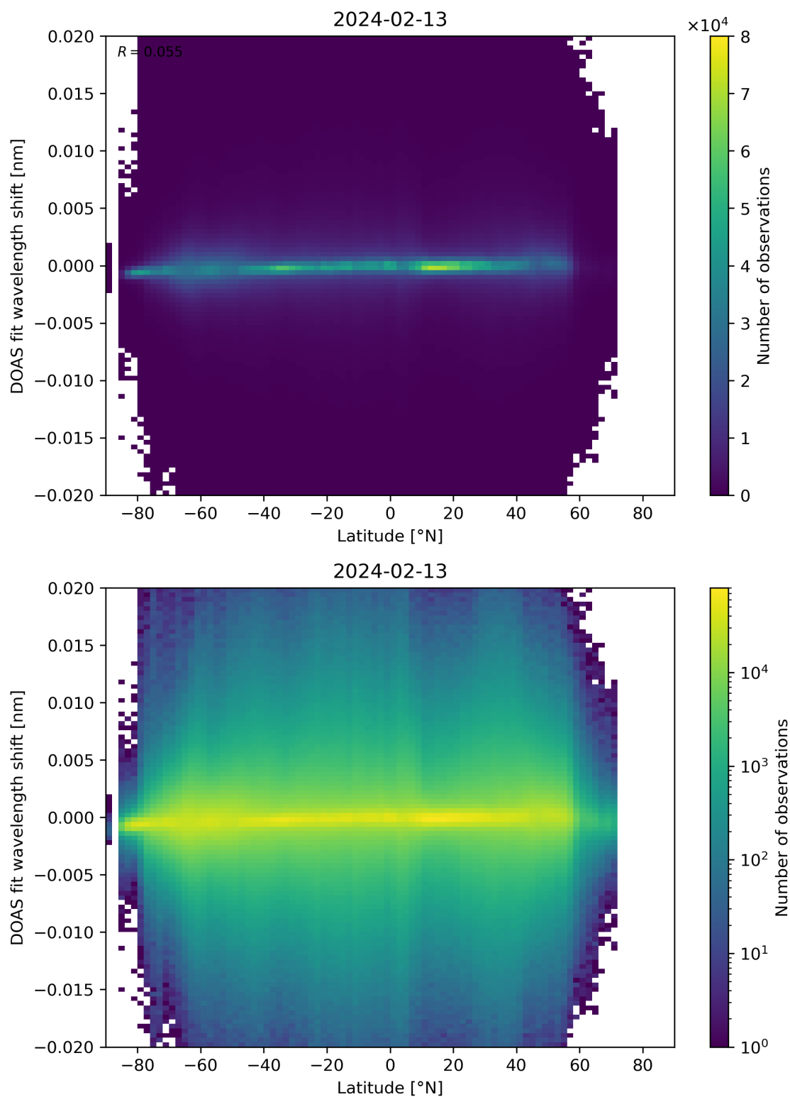
Figure 154: Scatter density plot of “Latitude” against “DOAS fit wavelength shift” for 2024-02-12 to 2024-02-14.
