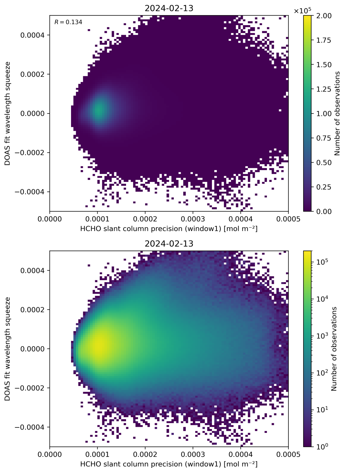
Figure 90: Scatter density plot of “HCHO slant column precision (window1)” against “DOAS fit wavelength squeeze” for 2024-02-12 to 2024-02-14.
