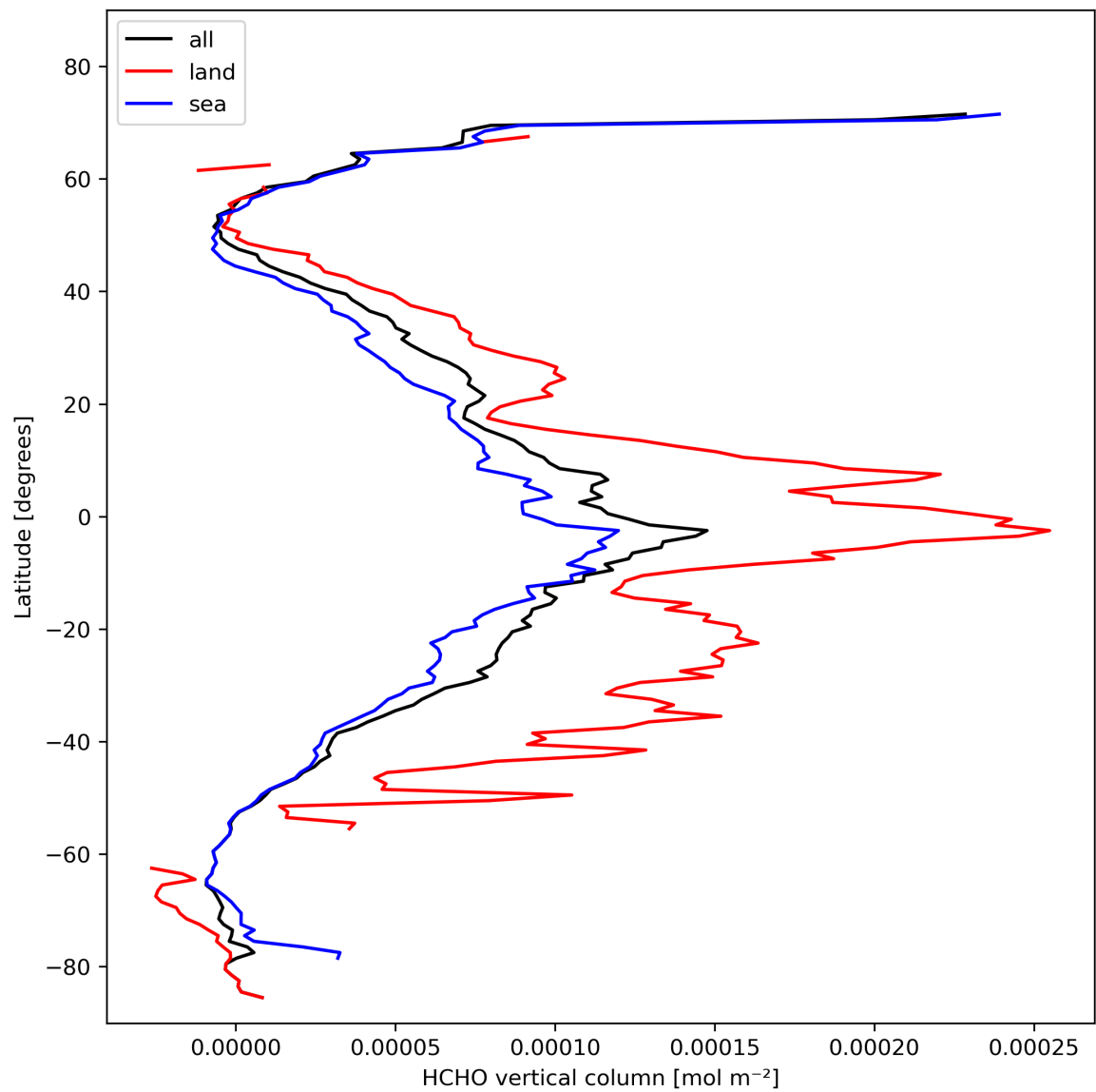
Figure 21: Zonal average of “HCHO vertical column” for 2024-02-12 to 2024-02-14.
