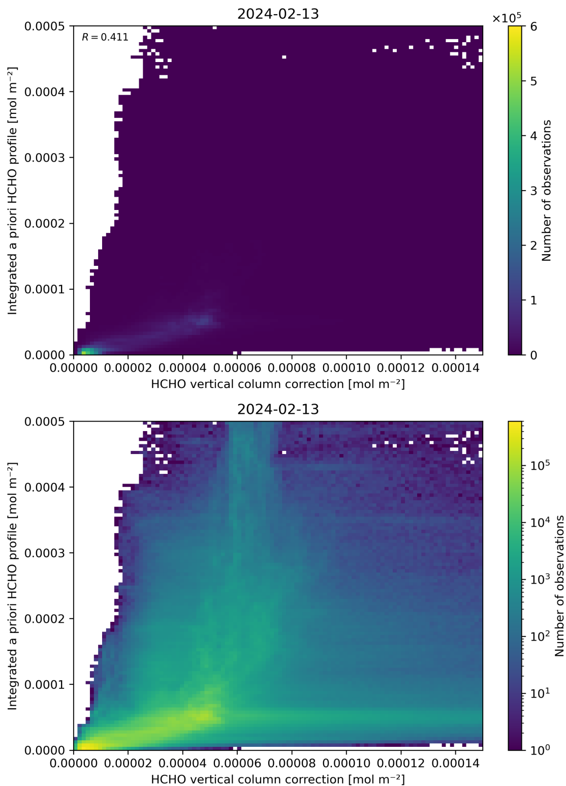
Figure 122: Scatter density plot of “HCHO vertical column correction” against “Integrated a priori HCHO profile” for 2024-02-12 to 2024-02-14.
