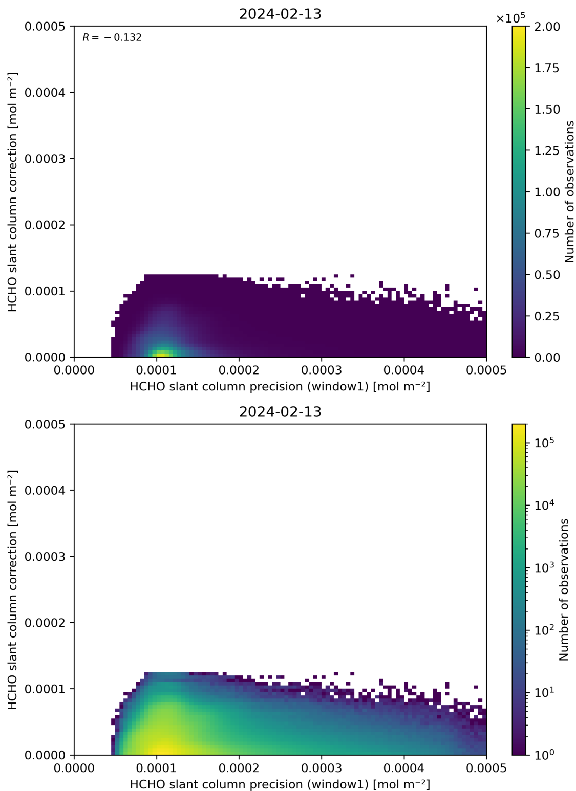
Figure 93: Scatter density plot of “HCHO slant column precision (window1)” against “HCHO slant column correction” for 2024-02-12 to 2024-02-14.
