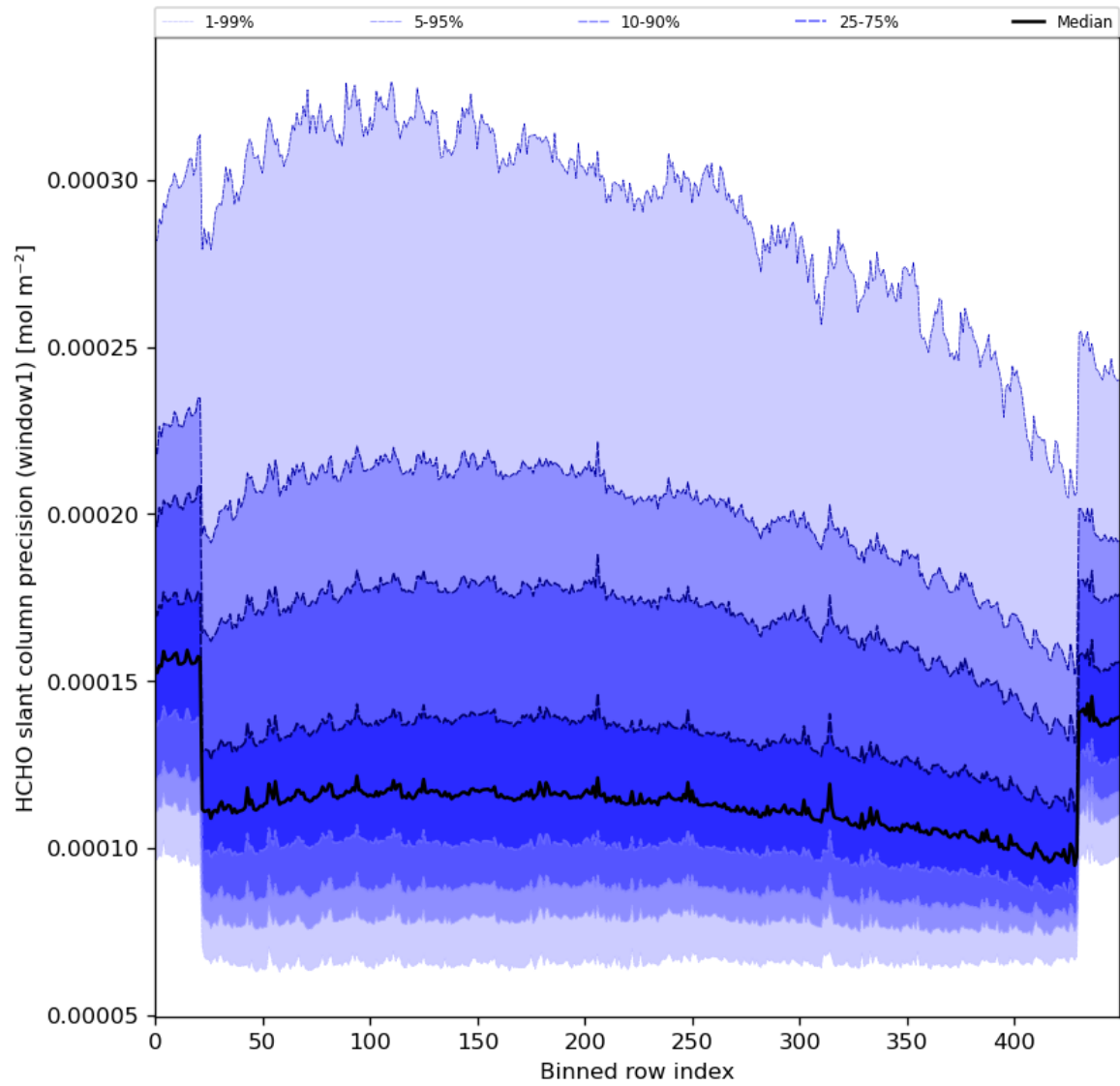
Figure 53: Along track statistics of “HCHO slant column precision (window1)” for 2024-02-12 to 2024-02-14
