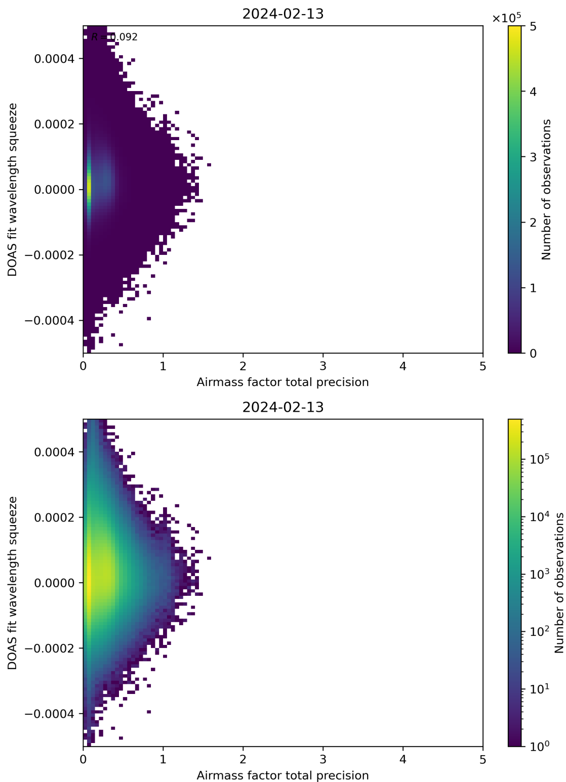
Figure 107: Scatter density plot of “Airmass factor total precision” against “DOAS fit wavelength squeeze” for 2024-02-12 to 2024-02-14.
