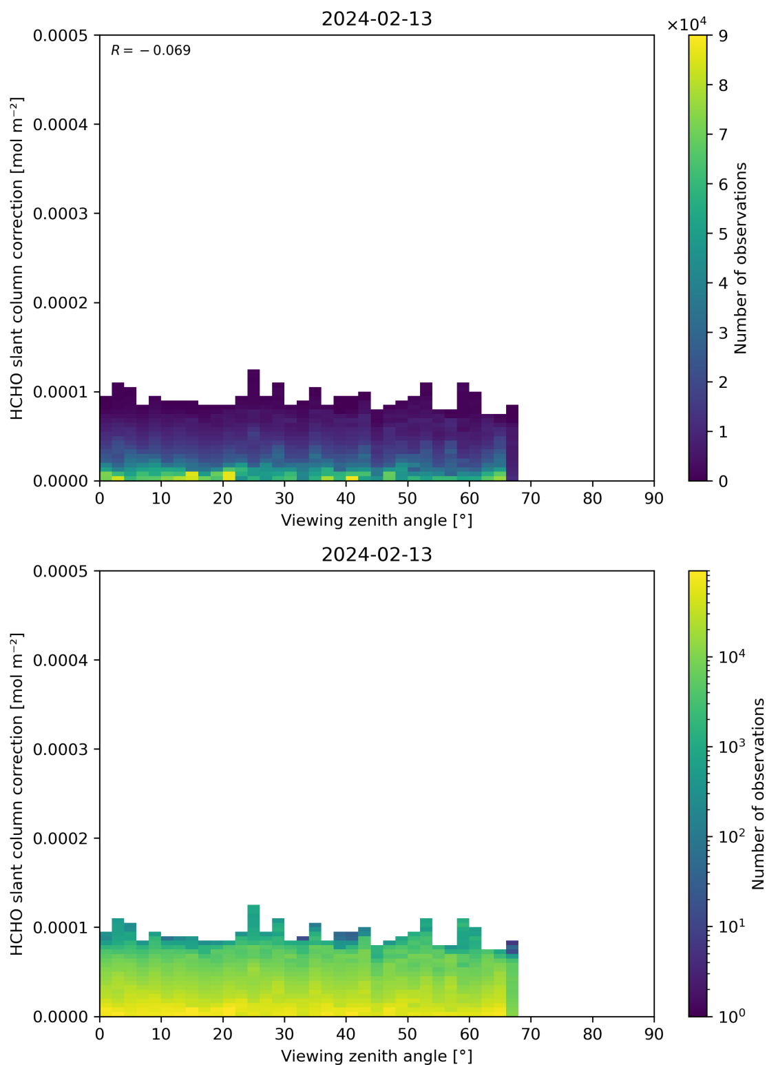
Figure 187: Scatter density plot of “Viewing zenith angle” against “HCHO slant column correction” for 2024-02-12 to 2024-02-14.
