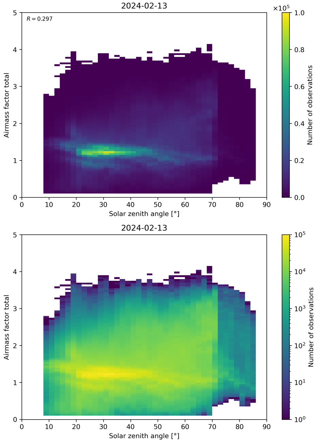
Figure 175: Scatter density plot of “Solar zenith angle” against “Airmass factor total” for 2024-02-12 to 2024-02-14.
