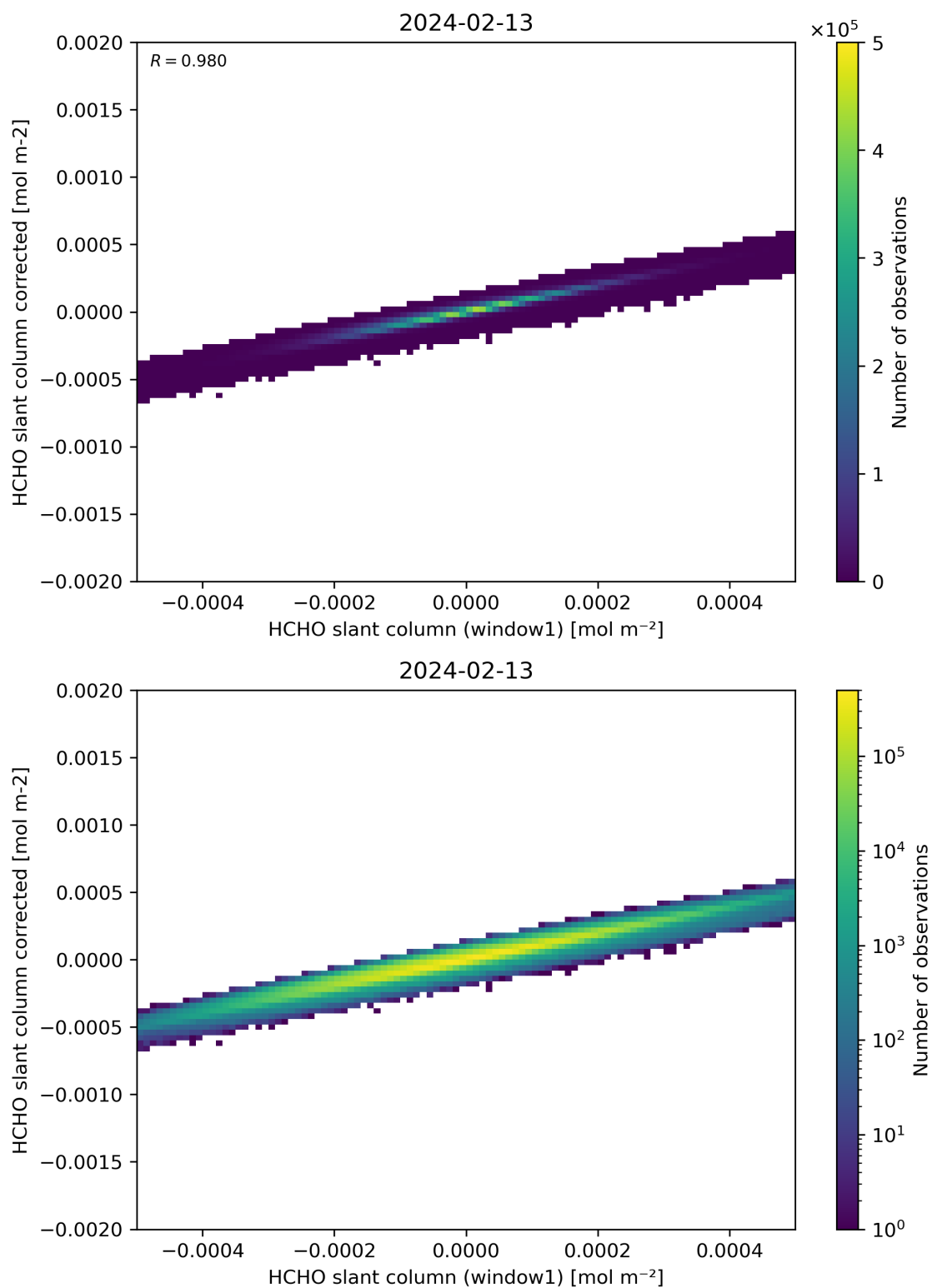
Figure 82: Scatter density plot of “HCHO slant column (window1)” against “HCHO slant column corrected” for 2024-02-12 to 2024-02-14.
