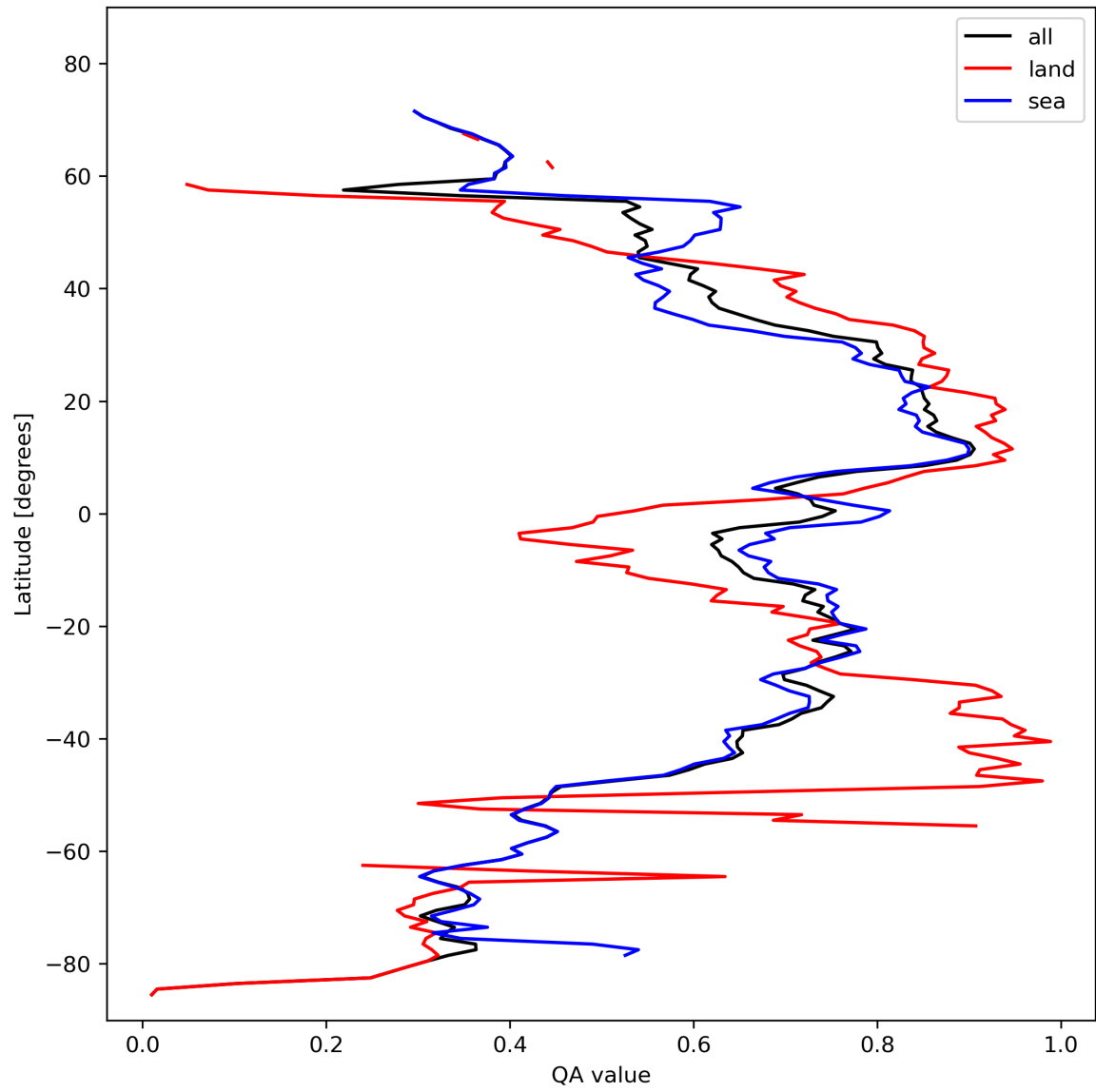
Figure 20: Zonal average of “QA value” for 2024-02-12 to 2024-02-14.
