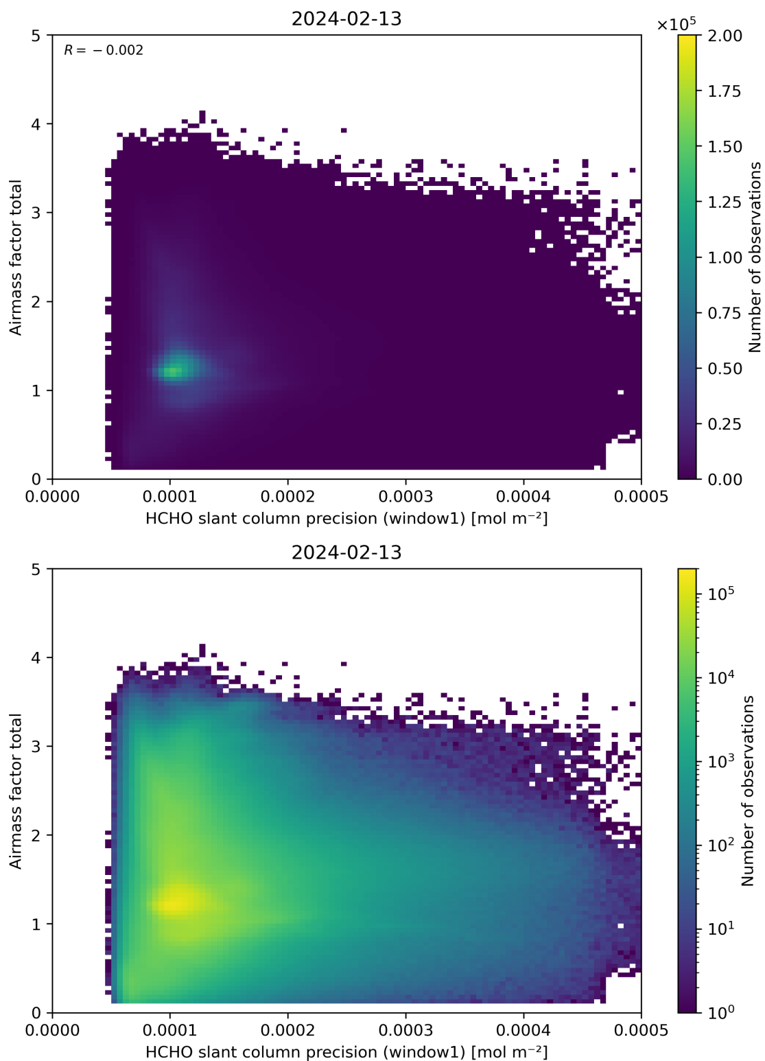
Figure 94: Scatter density plot of “HCHO slant column precision (window1)” against “Airmass factor total” for 2024-02-12 to 2024-02-14.
