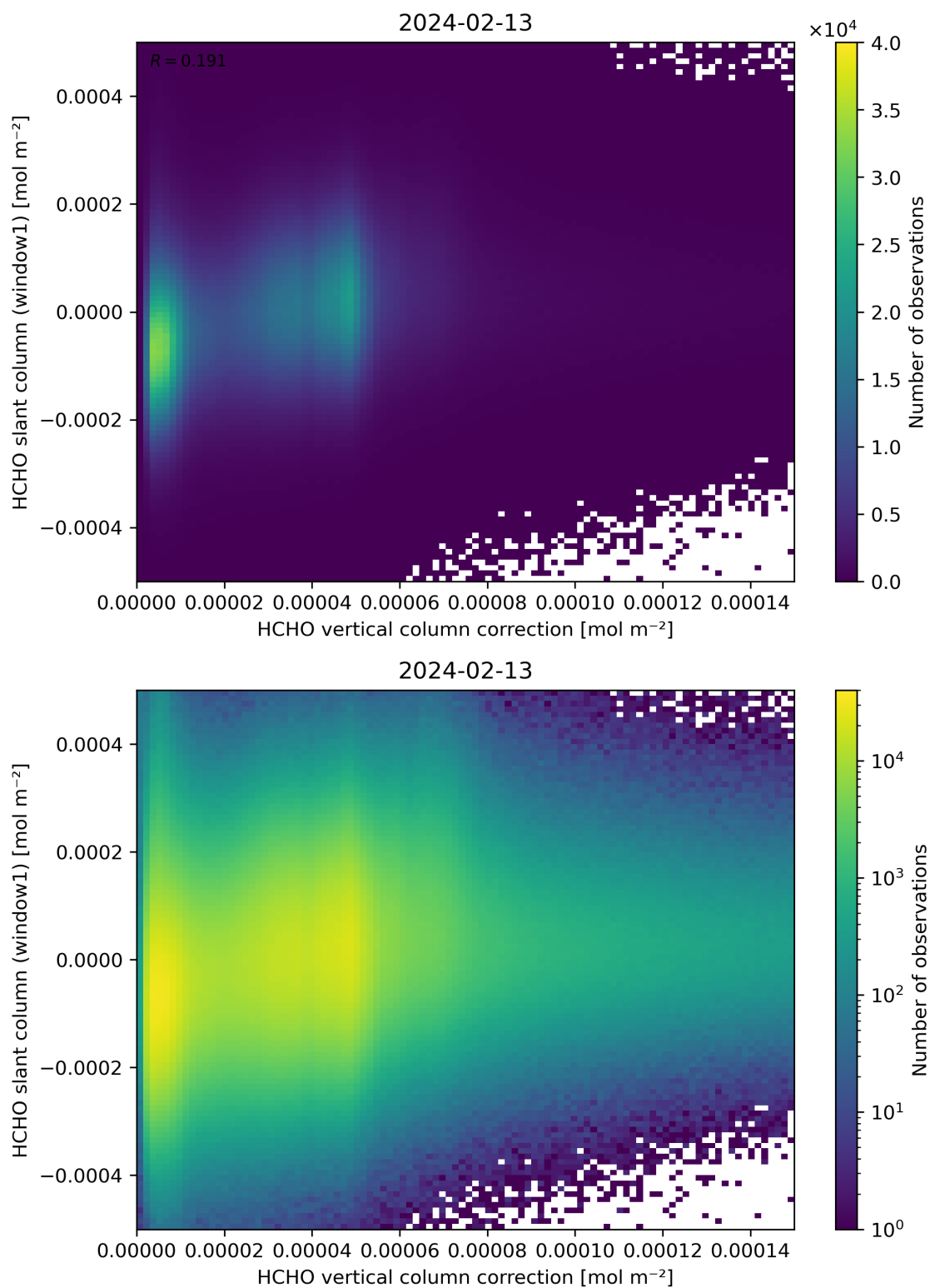
Figure 118: Scatter density plot of “HCHO vertical column correction” against “HCHO slant column (window1)” for 2024-02-12 to 2024-02-14.
