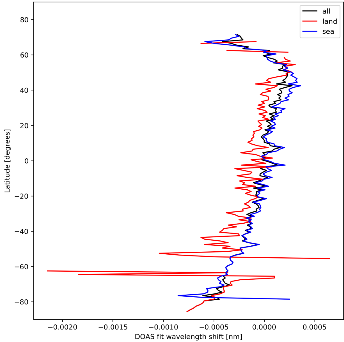
Figure 30: Zonal average of “DOAS fit wavelength shift” for 2024-02-12 to 2024-02-14.
