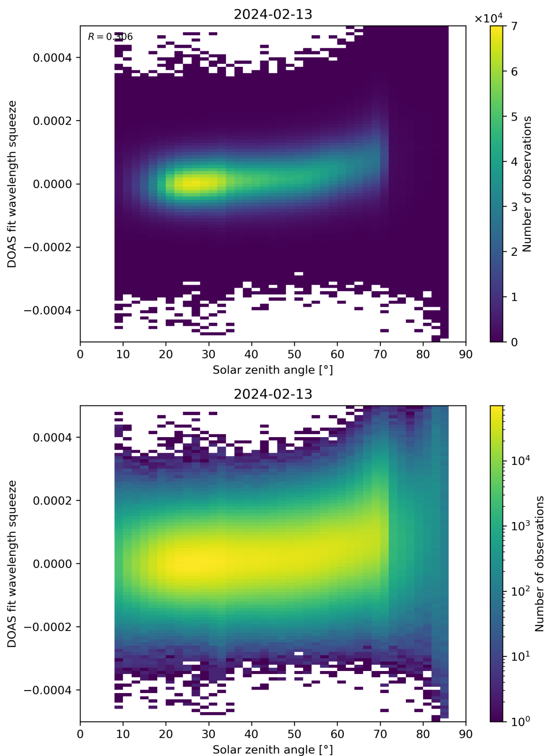
Figure 169: Scatter density plot of “Solar zenith angle” against “DOAS fit wavelength squeeze” for 2024-02-12 to 2024-02-14.
