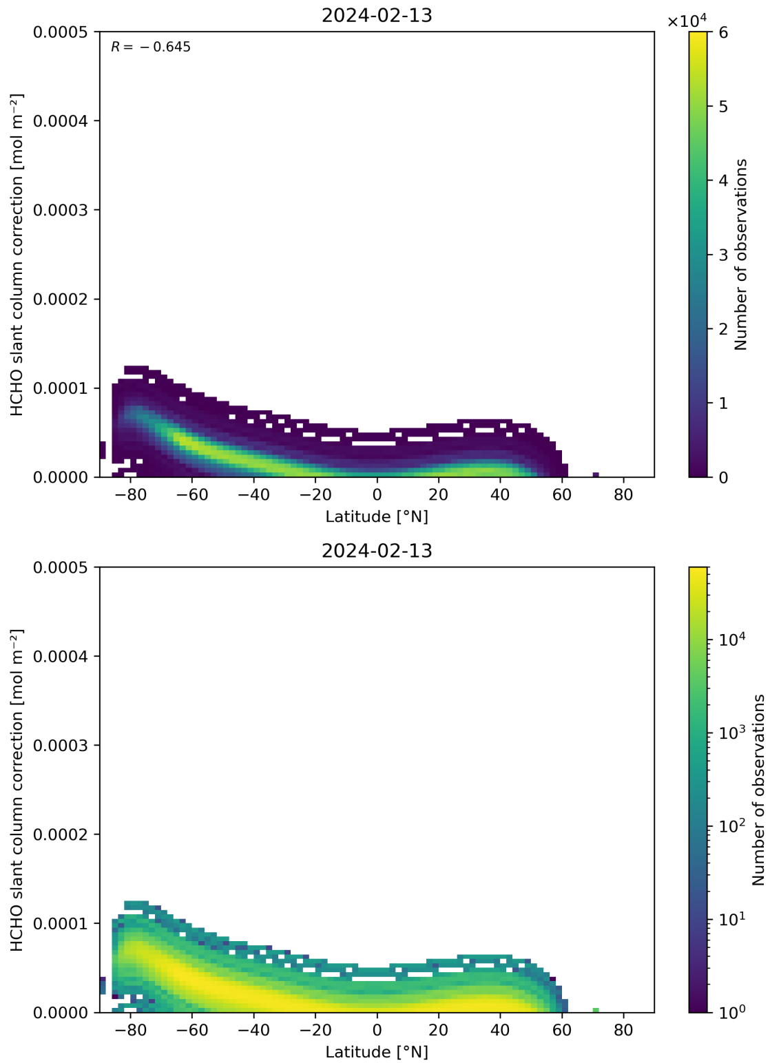
Figure 158: Scatter density plot of “Latitude” against “HCHO slant column correction” for 2024-02-12 to 2024-02-14.
