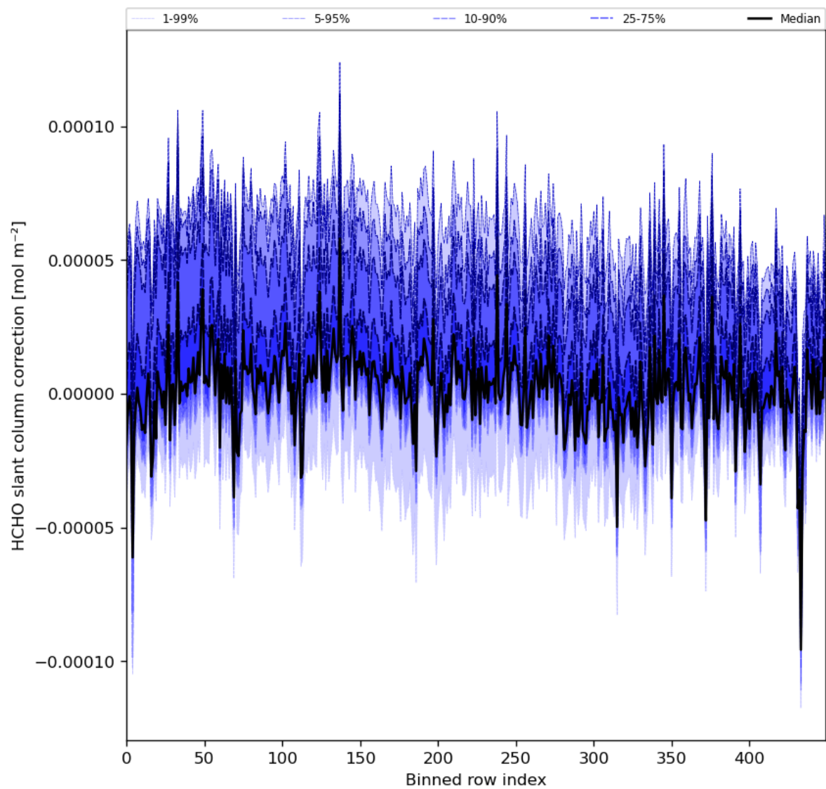
Figure 61: Along track statistics of “HCHO slant column correction” for 2024-02-12 to 2024-02-14
