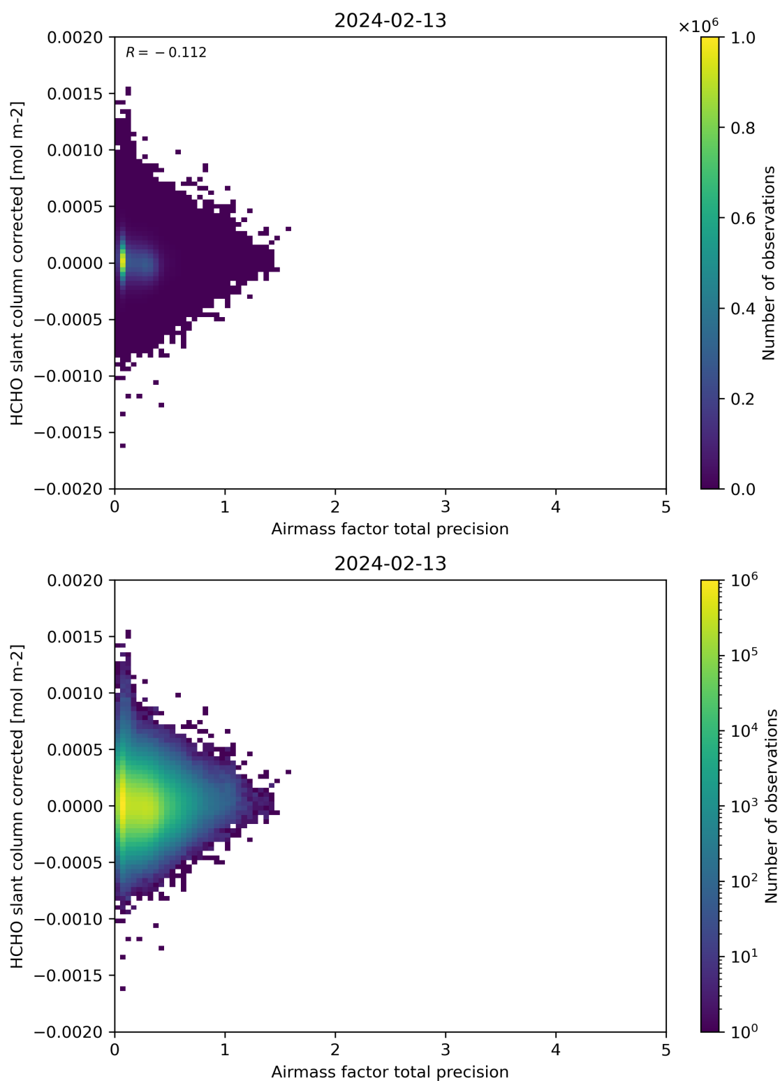
Figure 109: Scatter density plot of “Airmass factor total precision” against “HCHO slant column corrected” for 2024-02-12 to 2024-02-14.
