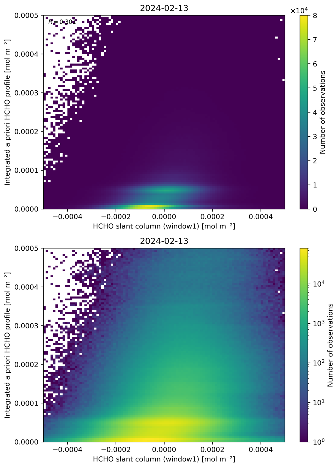
Figure 87: Scatter density plot of “HCHO slant column (window1)” against “Integrated a priori HCHO profile” for 2024-02-12 to 2024-02-14.
