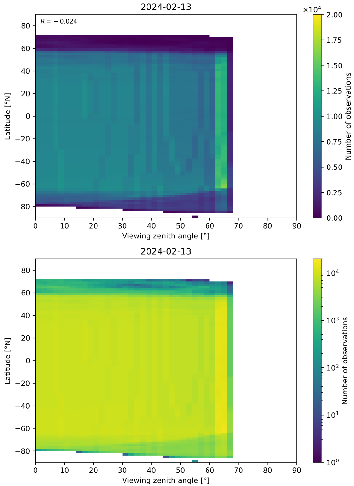
Figure 196: Scatter density plot of “Viewing zenith angle” against “Latitude” for 2024-02-12 to 2024-02-14.
