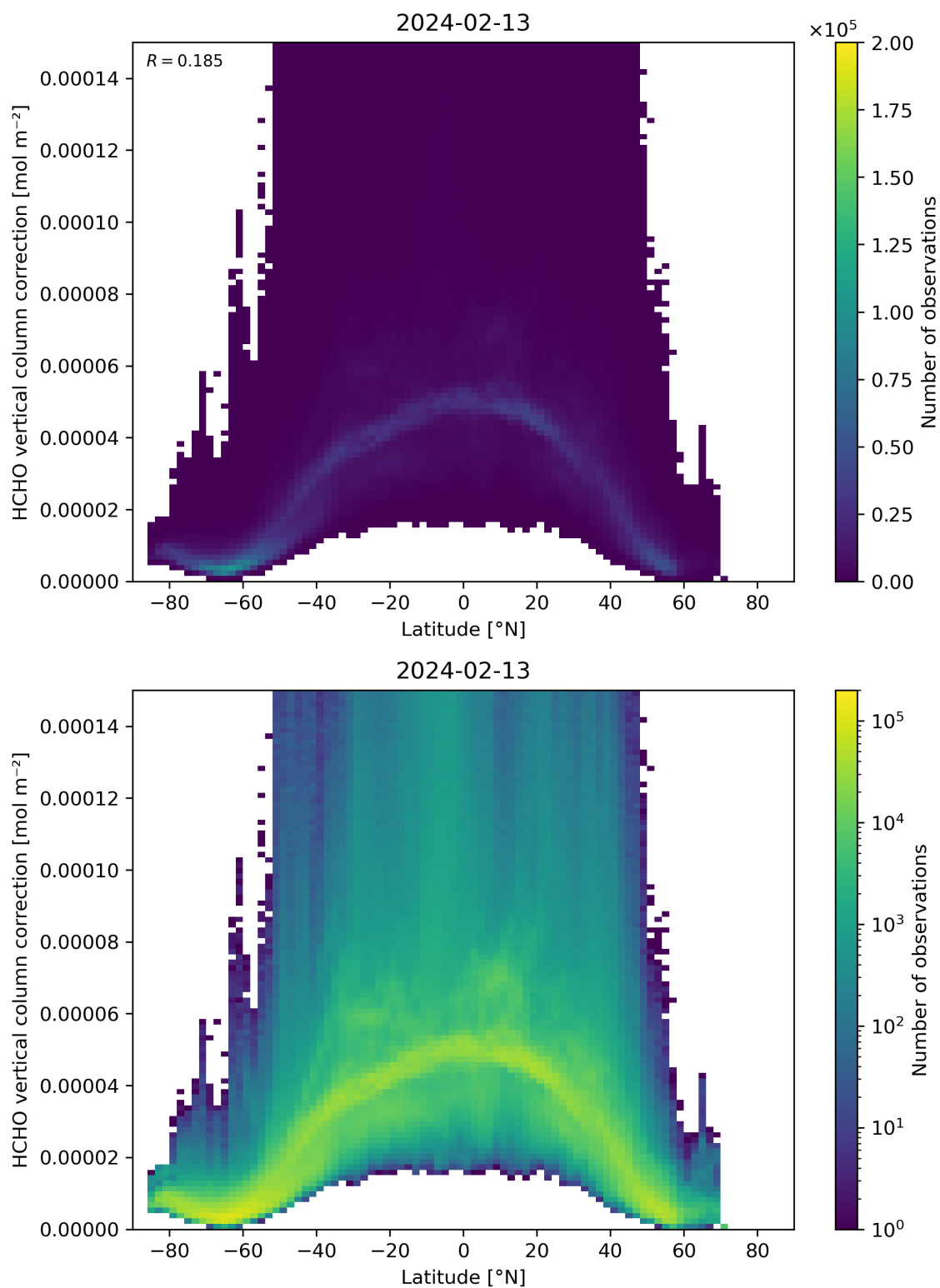
Figure 164: Scatter density plot of “Latitude” against “HCHO vertical column correction” for 2024-02-12 to 2024-02-14.
