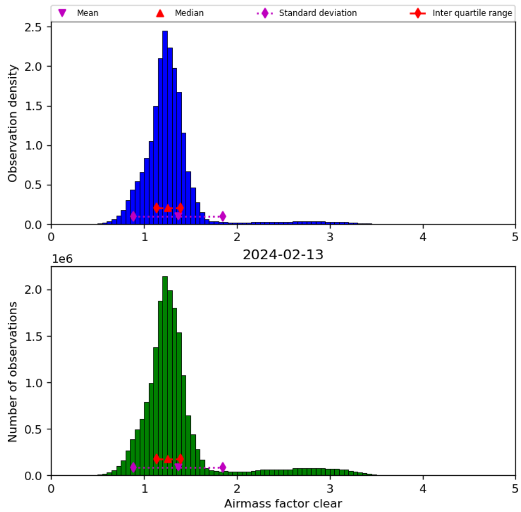
Figure 42: Histogram of “Airmass factor clear” for 2024-02-12 to 2024-02-14
