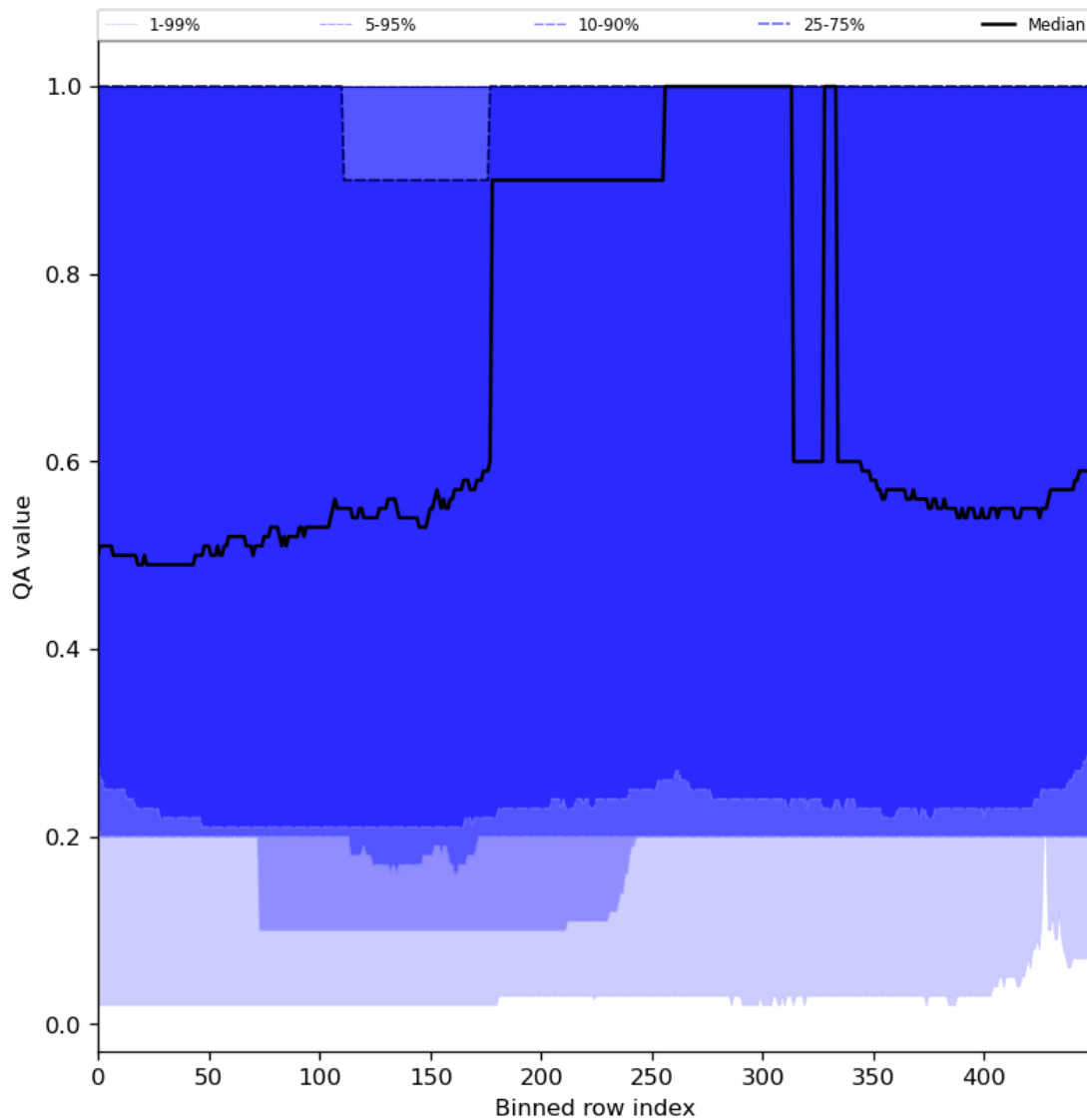
Figure 48: Along track statistics of “QA value” for 2024-02-12 to 2024-02-14
