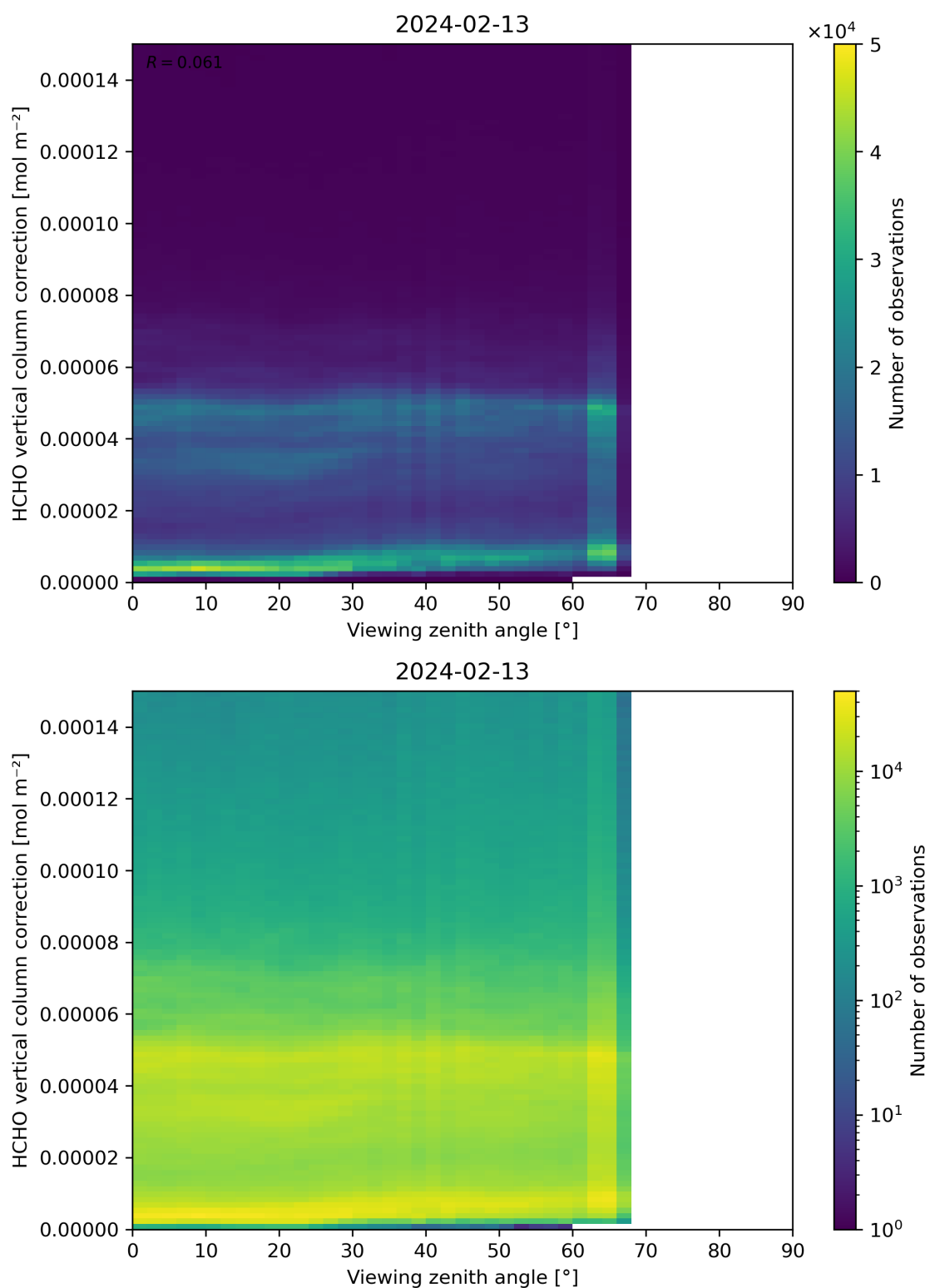
Figure 193: Scatter density plot of “Viewing zenith angle” against “HCHO vertical column correction” for 2024-02-12 to 2024-02-14.
