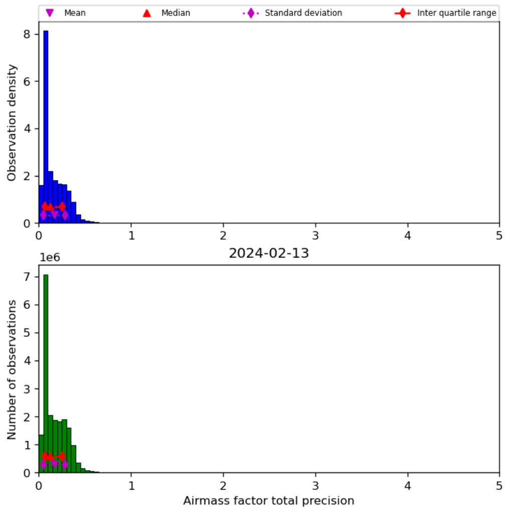
Figure 41: Histogram of “Airmass factor total precision” for 2024-02-12 to 2024-02-14
