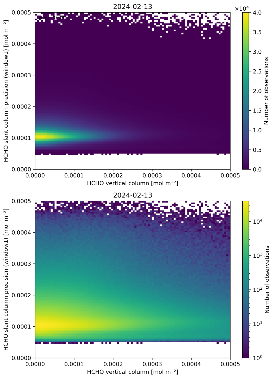
Figure 130: Scatter density plot of “HCHO vertical column” against “HCHO slant column precision (window1)” for 2024-02-12 to 2024-02-14.
