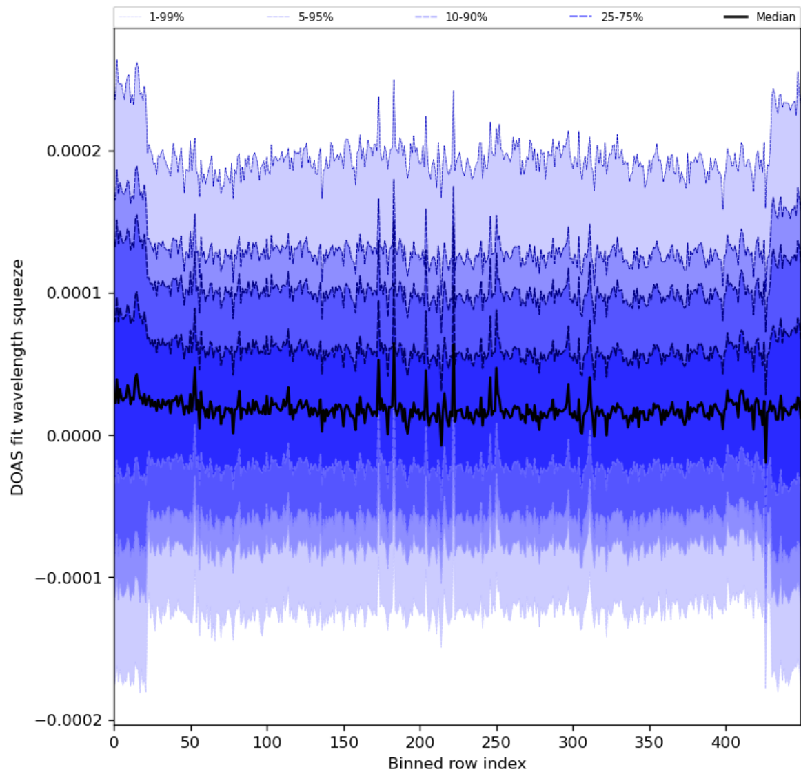
Figure 59: Along track statistics of “DOAS fit wavelength squeeze” for 2024-02-12 to 2024-02-14
