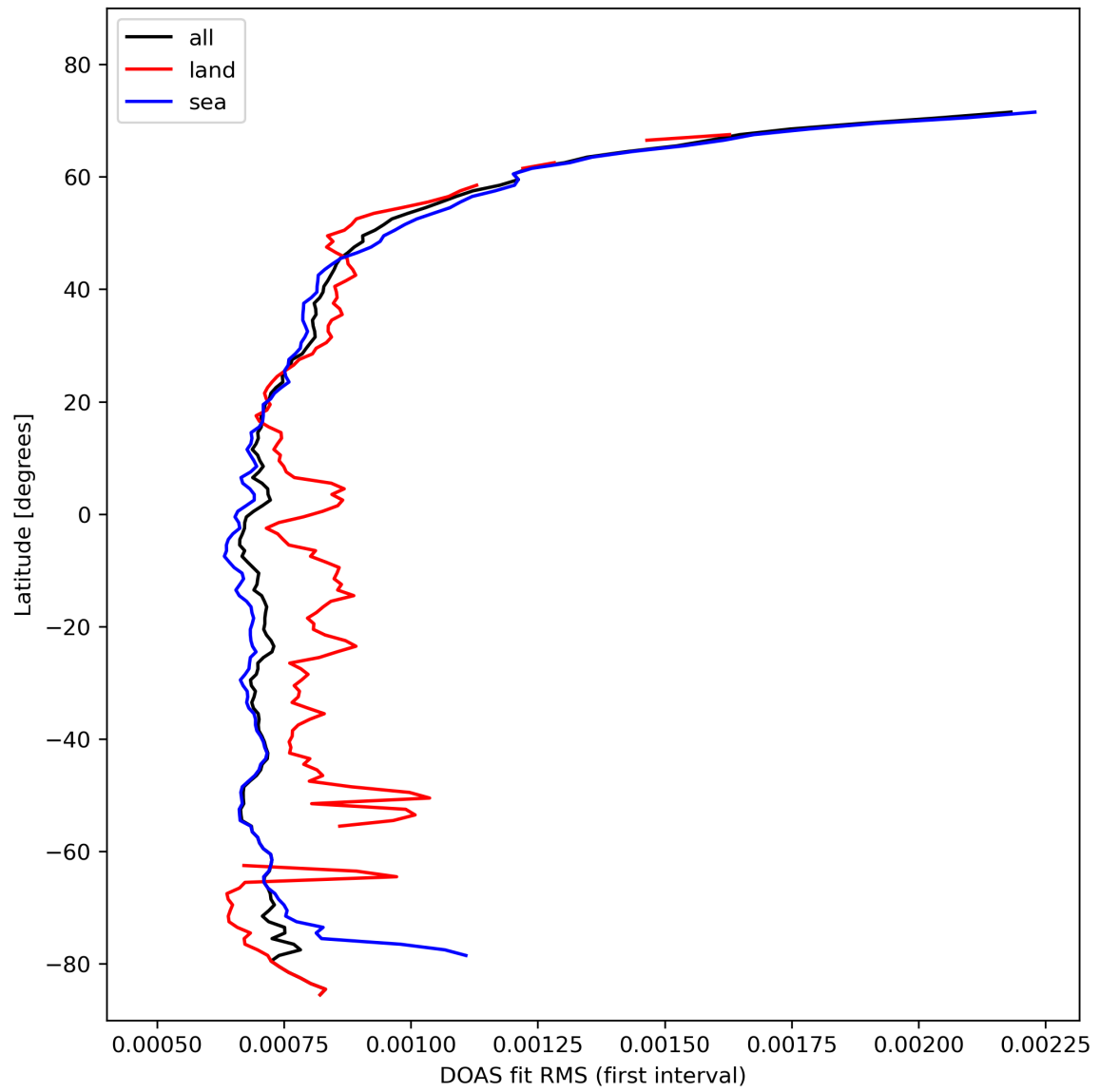
Figure 32: Zonal average of “DOAS fit RMS (first interval)” for 2024-02-12 to 2024-02-14.
