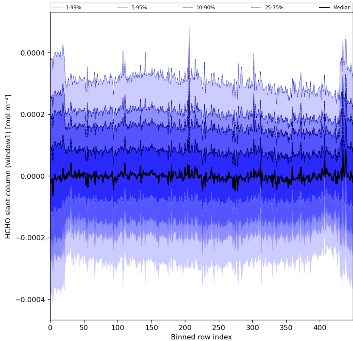
Figure 52: Along track statistics of “HCHO slant column (window1)” for 2024-02-12 to 2024-02-14
