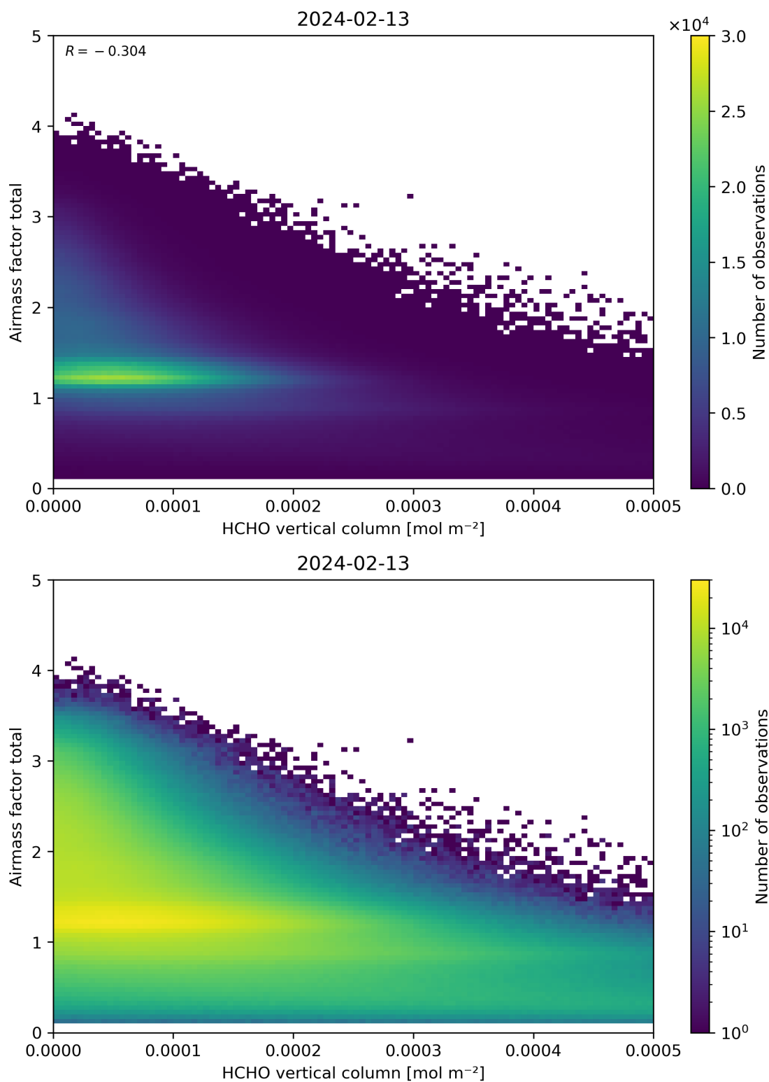
Figure 131: Scatter density plot of “HCHO vertical column” against “Airmass factor total” for 2024-02-12 to 2024-02-14.
