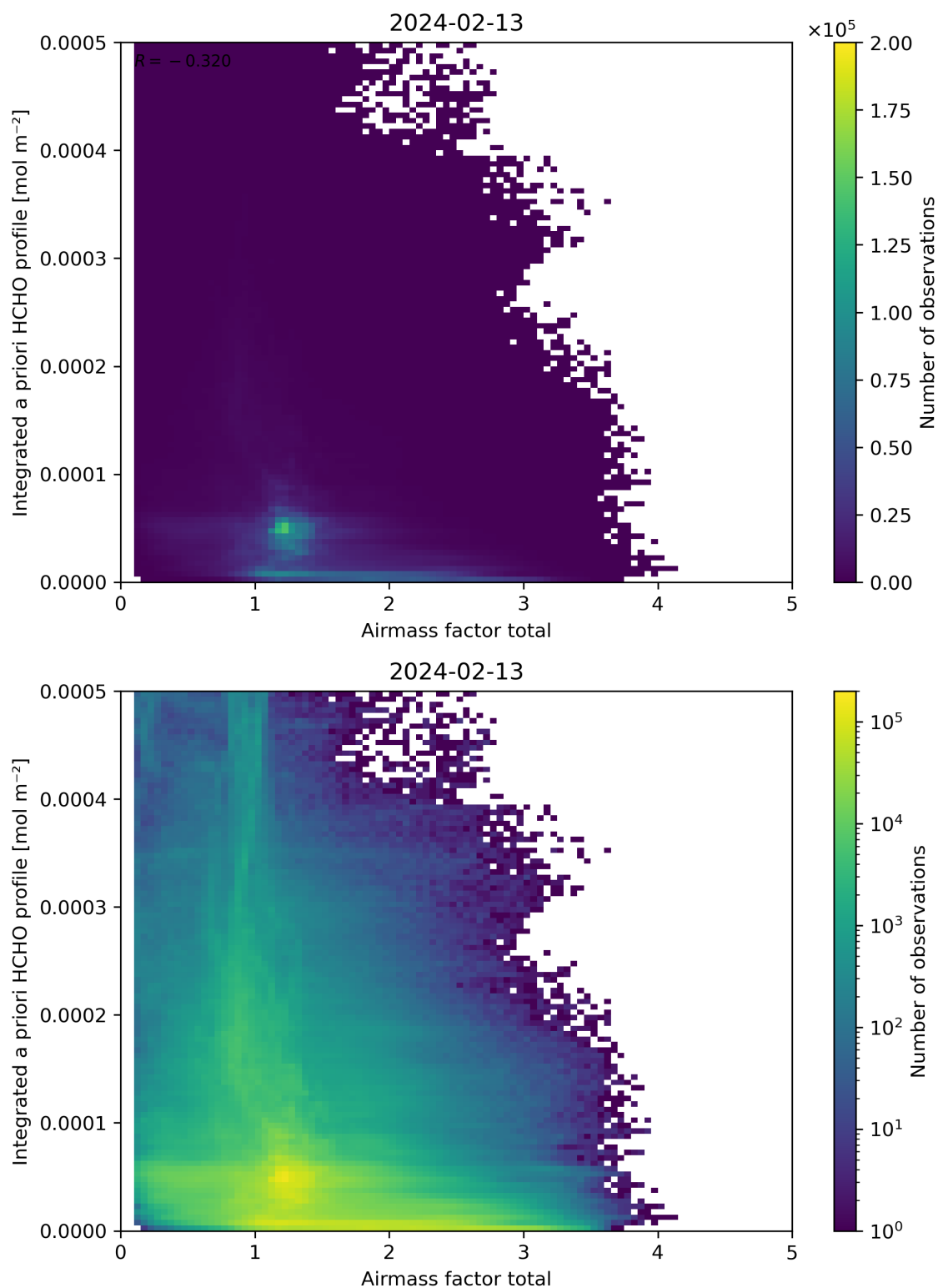
Figure 104: Scatter density plot of “Air mass factor total” against “Integrated a priori HCHO profile” for 2024-02-12 to 2024-02-14.
