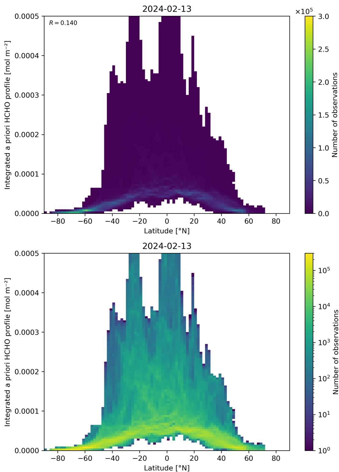
Figure 166: Scatter density plot of “Latitude” against “Integrated a priori HCHO profile” for 2024-02-12 to 2024-02-14.
