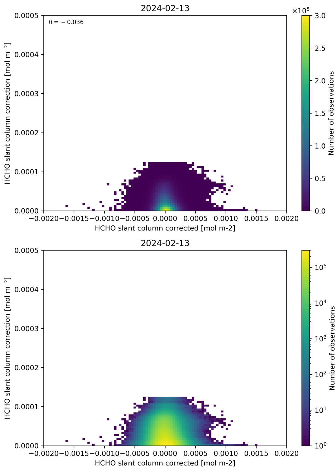
Figure 77: Scatter density plot of “HCHO slant column corrected” against “HCHO slant column correction” for 2024-02-12 to 2024-02-14.
