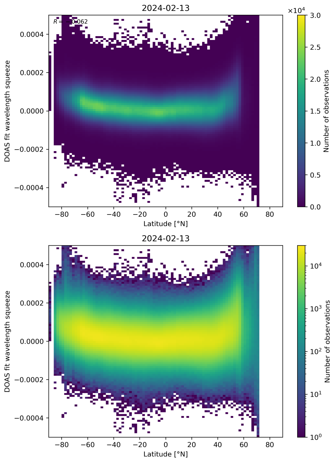
Figure 155: Scatter density plot of “Latitude” against “DOAS fit wavelength squeeze” for 2024-02-12 to 2024-02-14.
