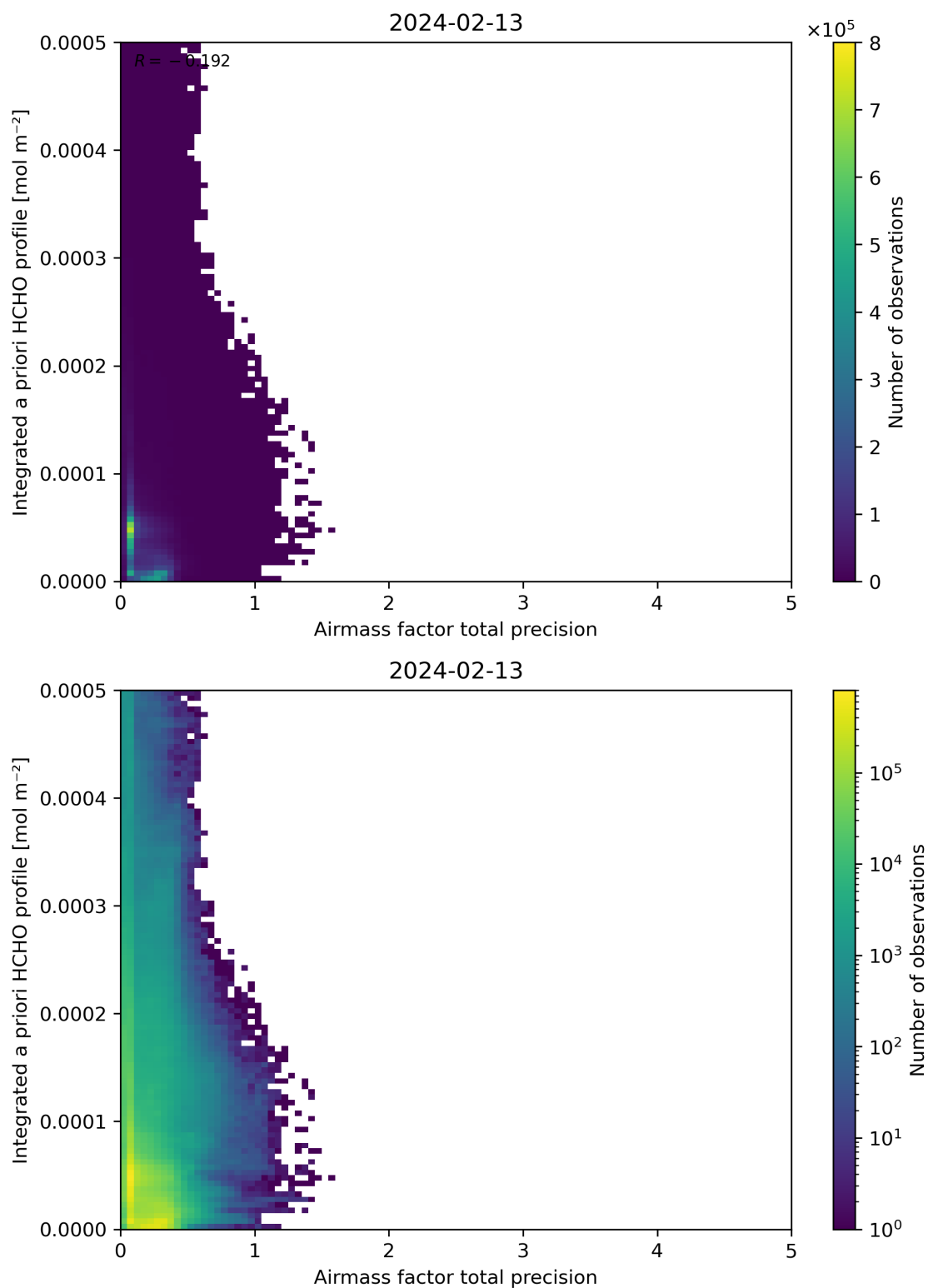
Figure 111: Scatter density plot of “Airmass factor total precision” against “Integrated a priori HCHO profile” for 2024-02-12 to 2024-02-14.
