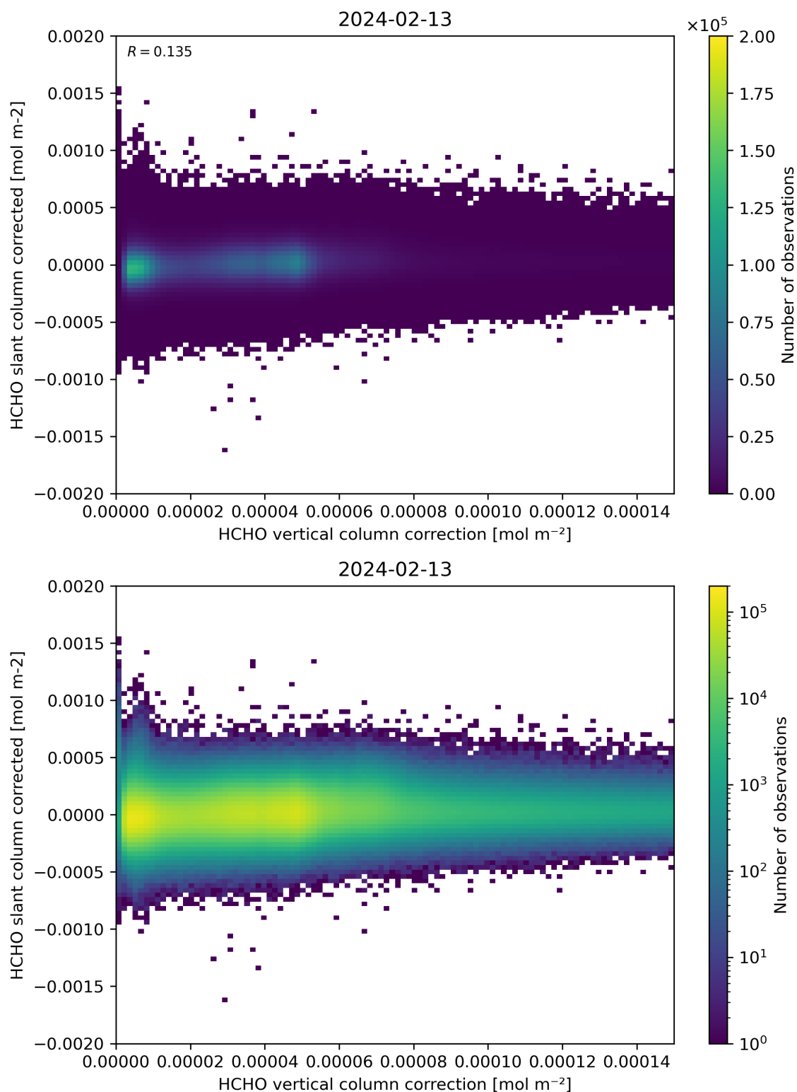
Figure 116: Scatter density plot of “HCHO vertical column correction” against “HCHO slant column corrected” for 2024-02-12 to 2024-02-14.
