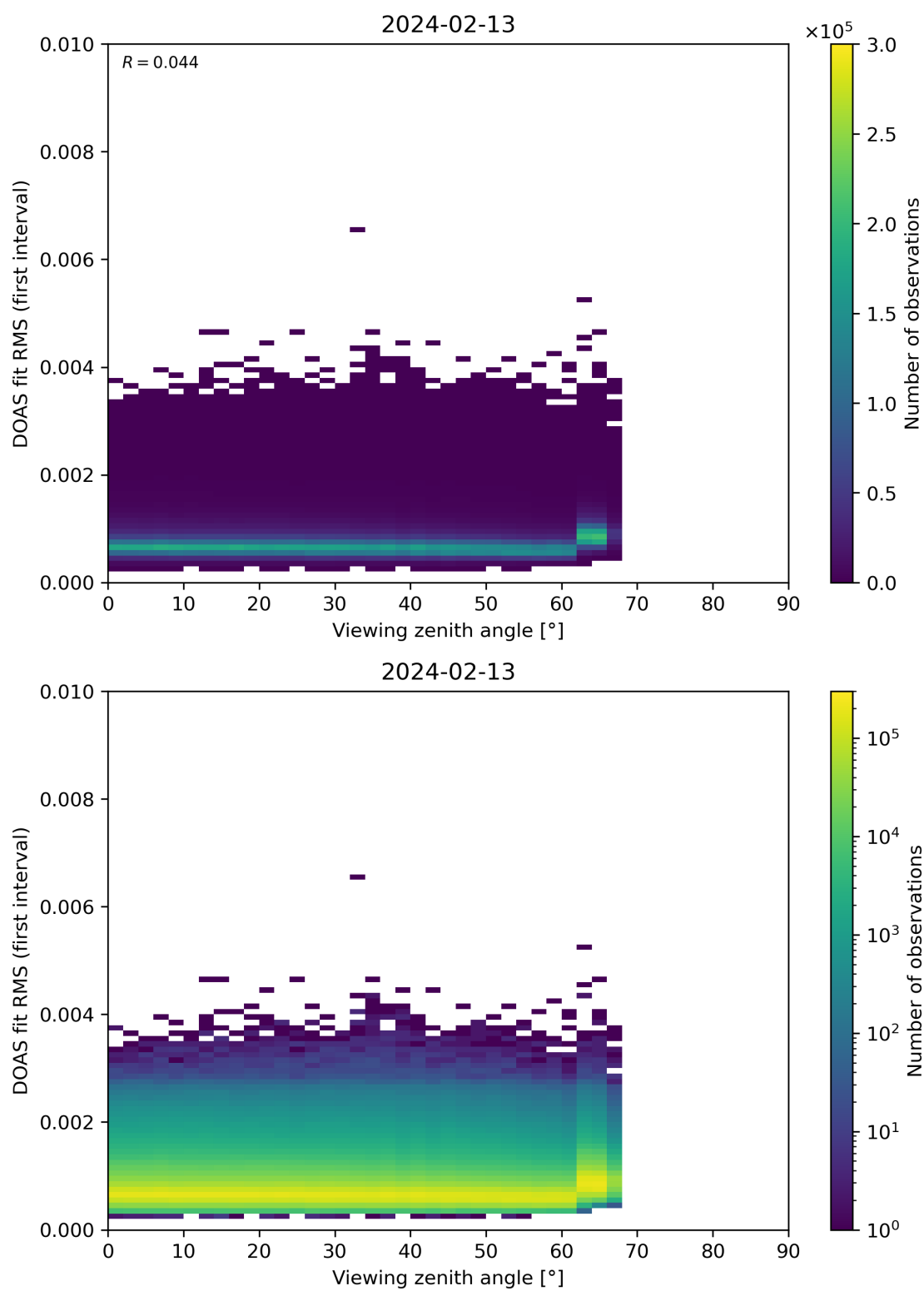
Figure 182: Scatter density plot of “Viewing zenith angle” against “DOAS fit RMS (first interval)” for 2024-02-12 to 2024-02-14.
