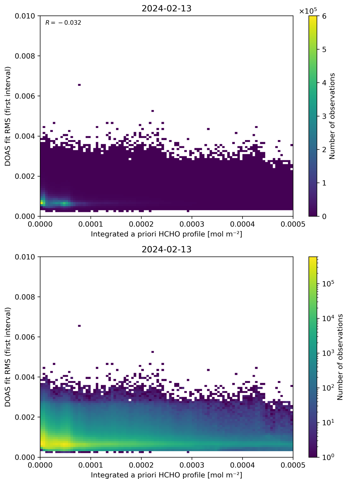
Figure 148: Scatter density plot of “Integrated a priori HCHO profile” against “DOAS fit RMS (first interval)” for 2024-02-12 to 2024-02-14.
