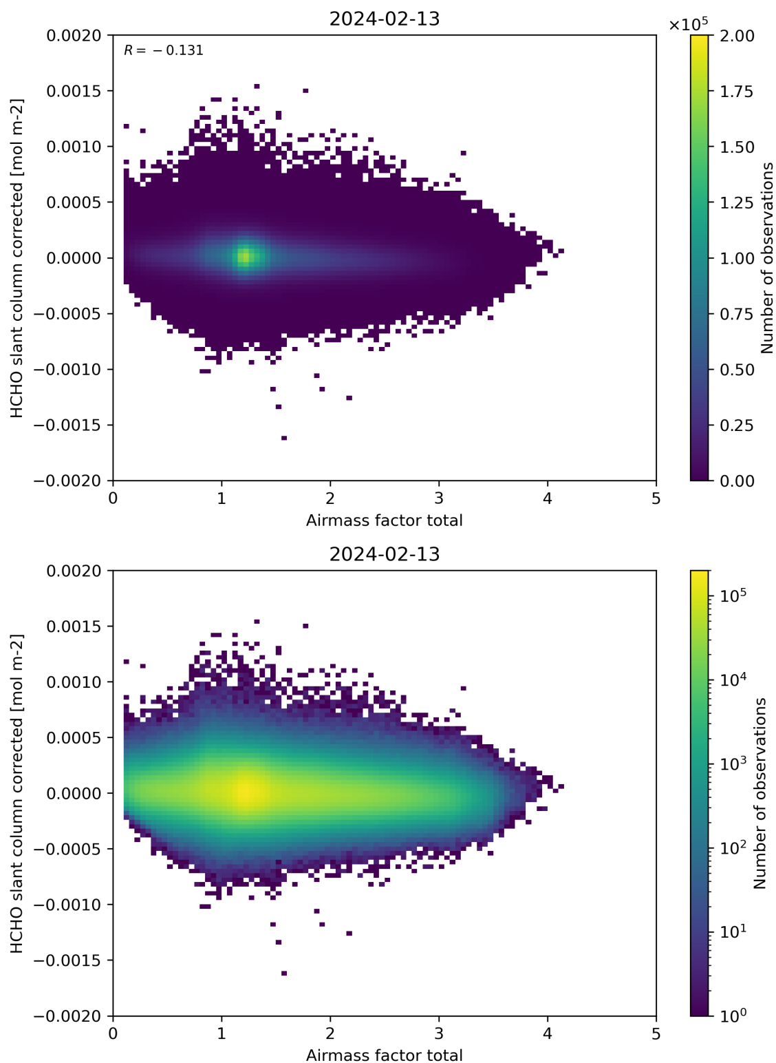
Figure 101: Scatter density plot of “Airmass factor total” against “HCHO slant column corrected” for 2024-02-12 to 2024-02-14.
