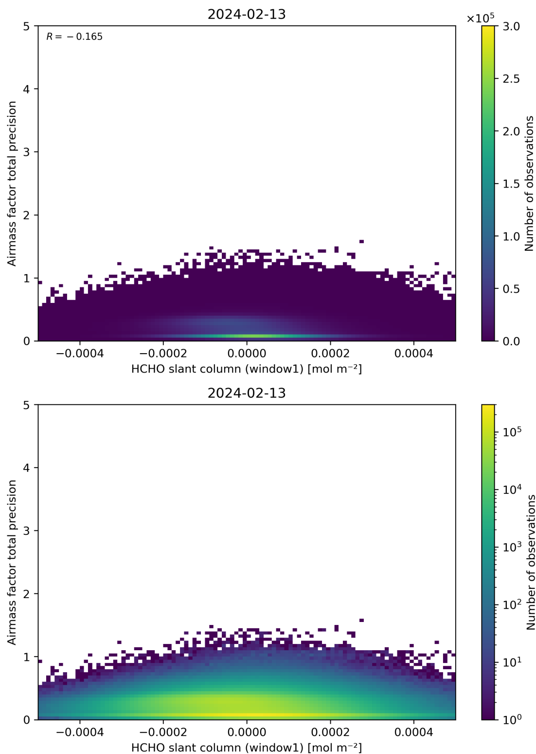
Figure 86: Scatter density plot of “HCHO slant column (window1)” against “Airmass factor total precision” for 2024-02-12 to 2024-02-14.
