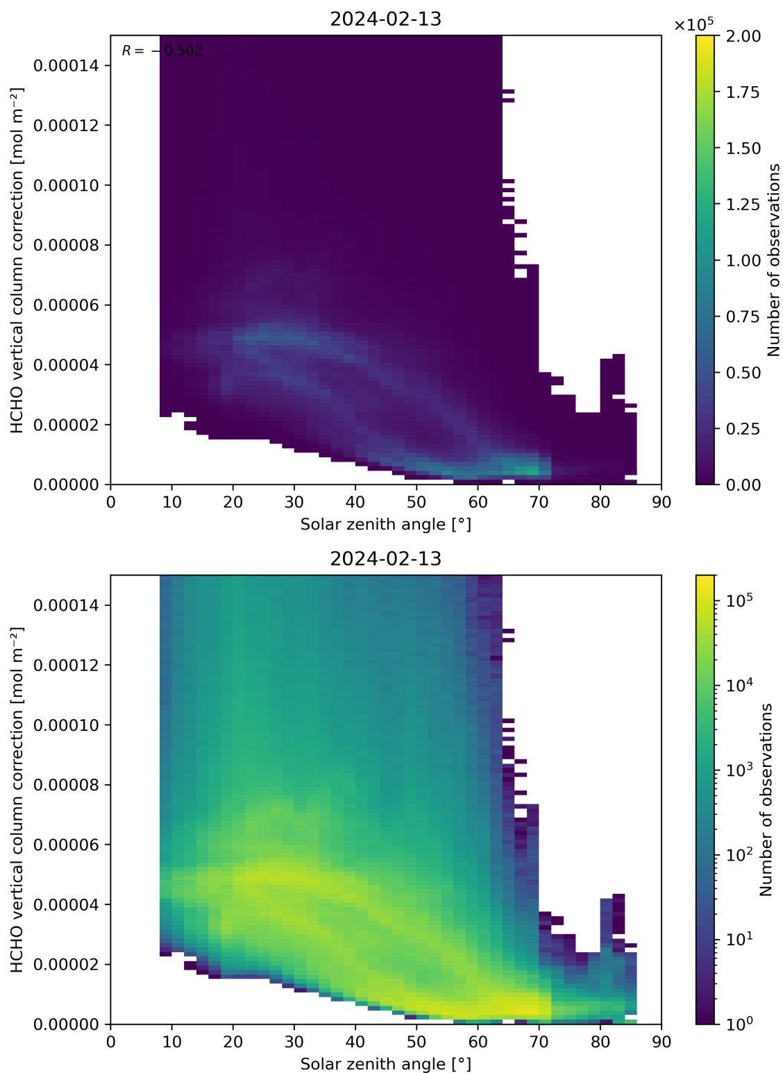
Figure 178: Scatter density plot of “Solar zenith angle” against “HCHO vertical column correction” for 2024-02-12 to 2024-02-14.
