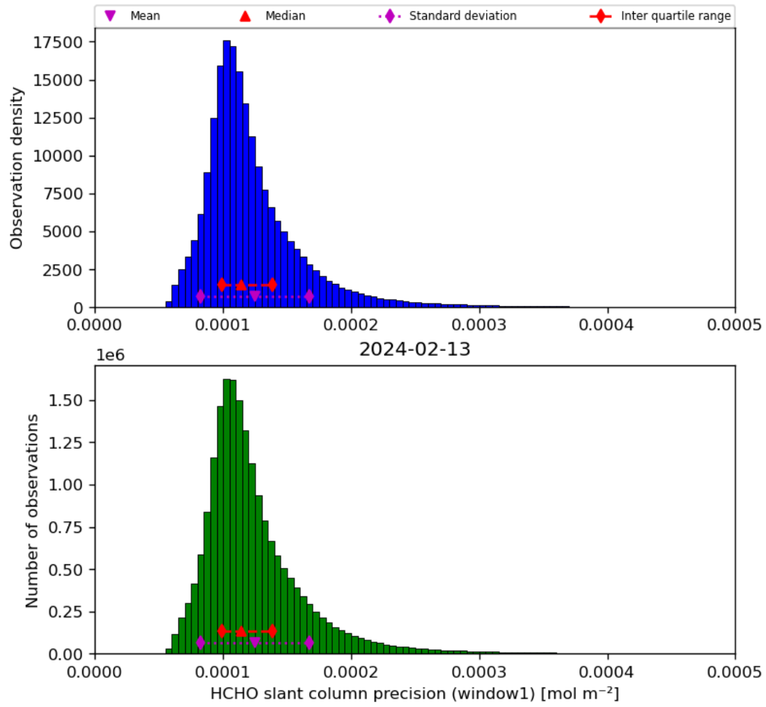
Figure 39: Histogram of “HCHO slant column precision (window1)” for 2024-02-12 to 2024-02-14
