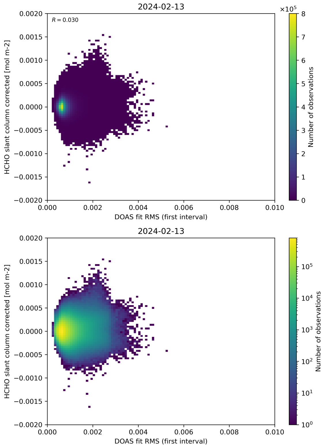
Figure 62: Scatter density plot of “DOAS fit RMS (first interval)” against “HCHO slant column corrected” for 2024-02-12 to 2024-02-14.
