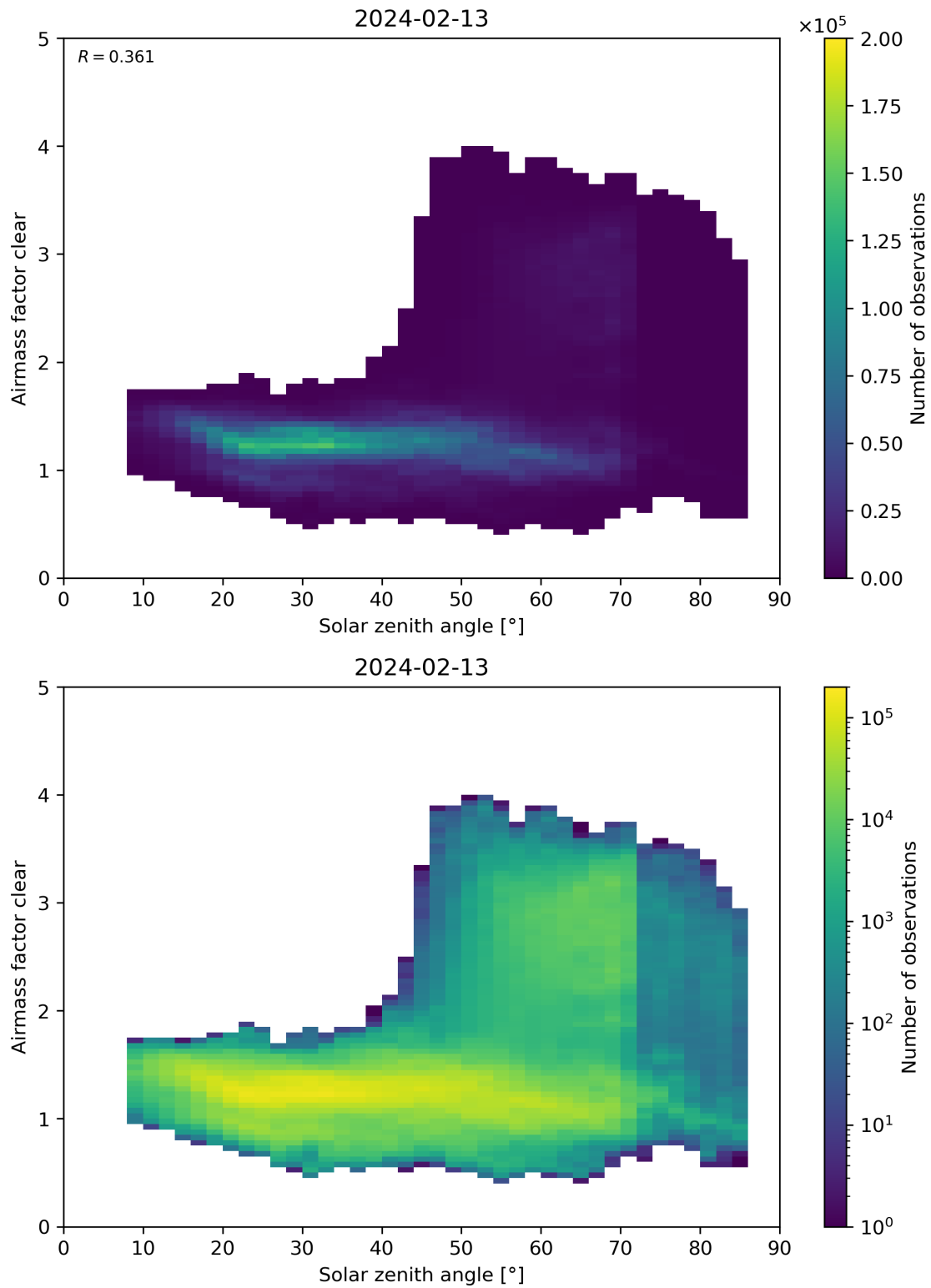
Figure 170: Scatter density plot of “Solar zenith angle” against “Airmass factor clear” for 2024-02-12 to 2024-02-14.
