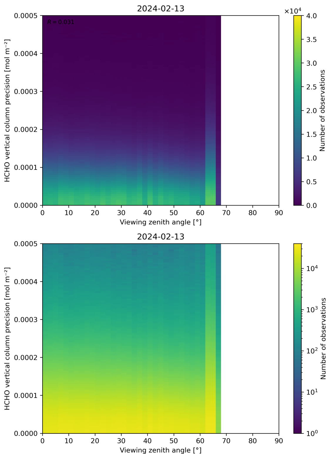
Figure 194: Scatter density plot of “Viewing zenith angle” against “HCHO vertical column precision” for 2024-02-12 to 2024-02-14.
