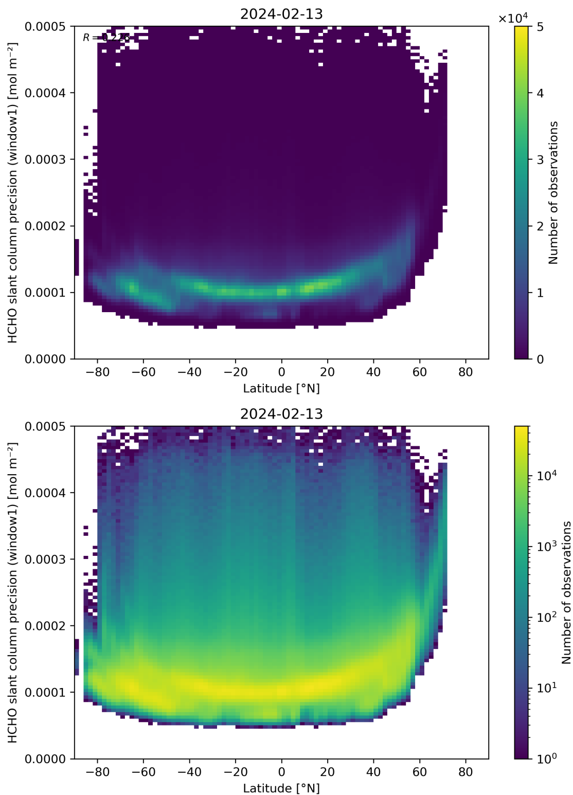
Figure 160: Scatter density plot of “Latitude” against “HCHO slant column precision (window1)” for 2024-02-12 to 2024-02-14.
