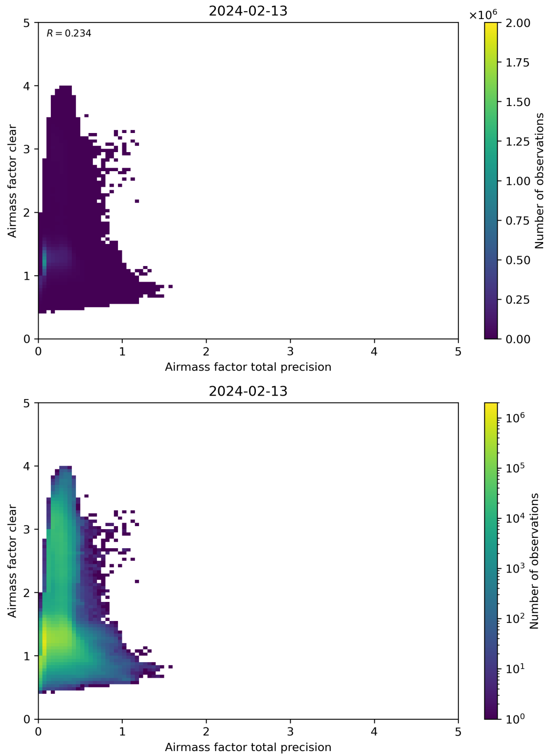
Figure 108: Scatter density plot of “Airmass factor total precision” against “Airmass factor clear” for 2024-02-12 to 2024-02-14.
