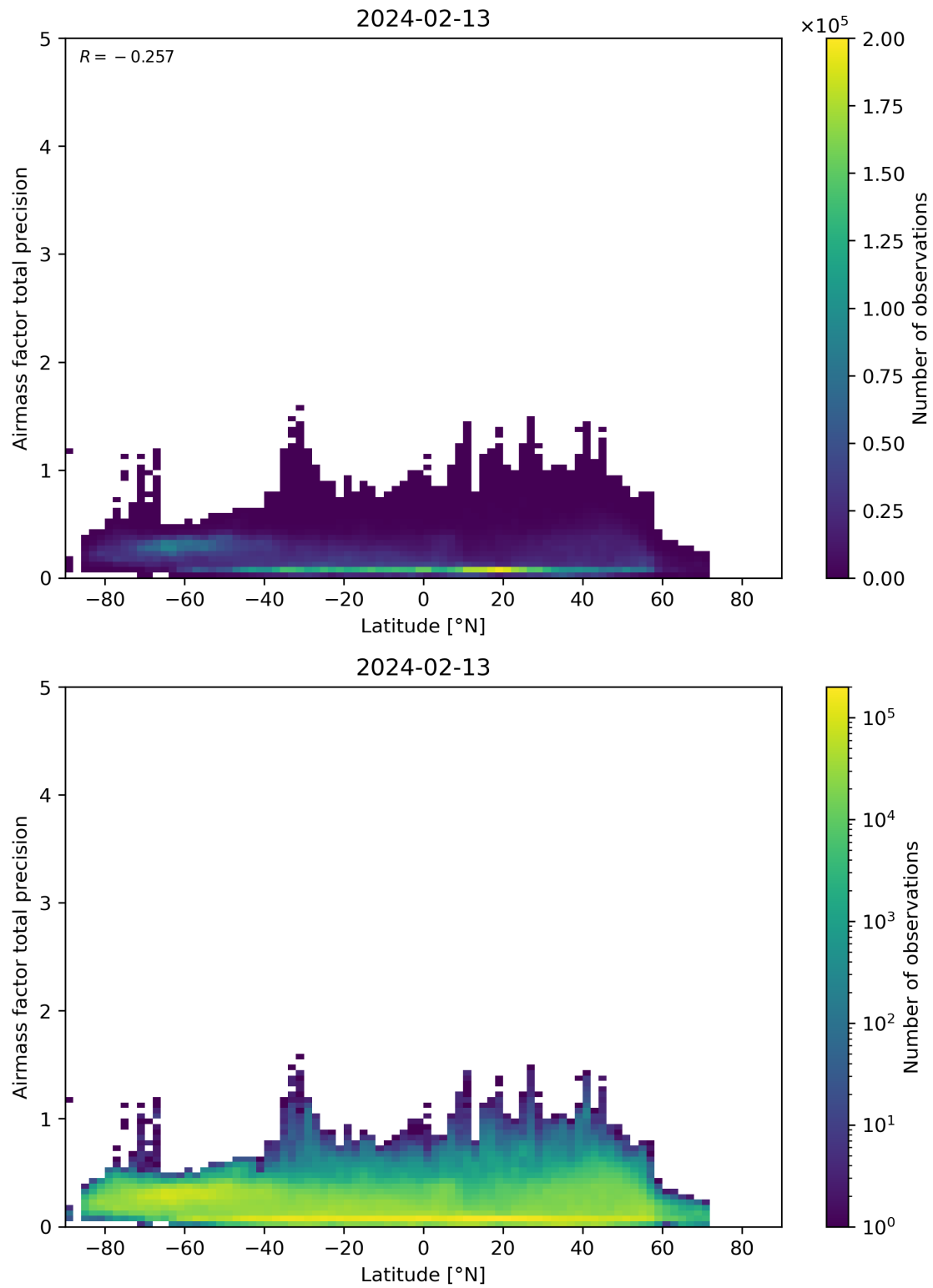
Figure 162: Scatter density plot of “Latitude” against “Airmass factor total precision” for 2024-02-12 to 2024-02-14.
