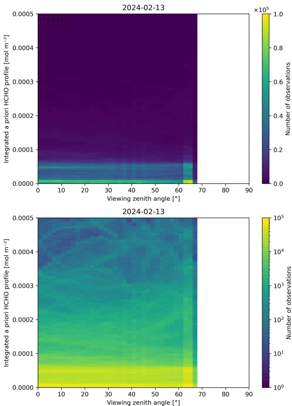
Figure 195: Scatter density plot of “Viewing zenith angle” against “Integrated a priori HCHO profile” for 2024-02-12 to 2024-02-14.
