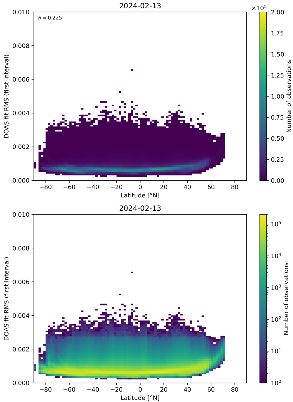
Figure 153: Scatter density plot of “Latitude” against “DOAS fit RMS (first interval)” for 2024-02-12 to 2024-02-14.
