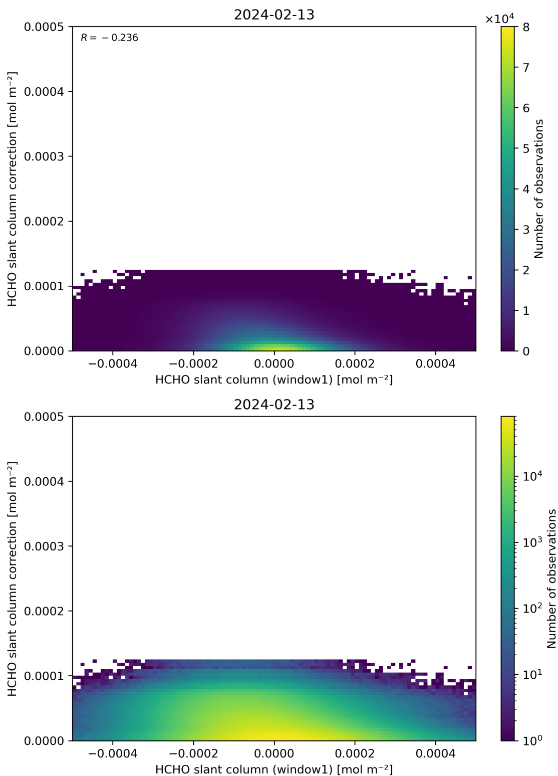
Figure 83: Scatter density plot of “HCHO slant column (window1)” against “HCHO slant column correction” for 2024-02-12 to 2024-02-14.
