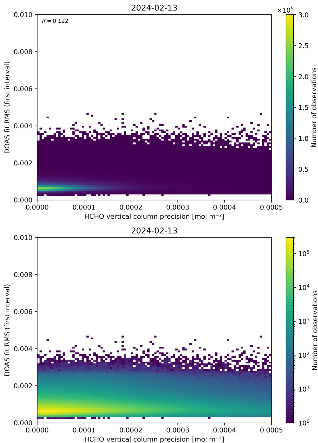
Figure 136: Scatter density plot of “HCHO vertical column precision” against “DOAS fit RMS (first interval)” for 2024-02-12 to 2024-02-14.
