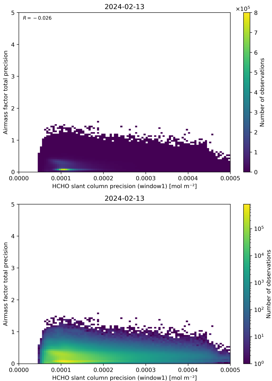
Figure 95: Scatter density plot of “HCHO slant column precision (window1)” against “Airmass factor total precision” for 2024-02-12 to 2024-02-14.
