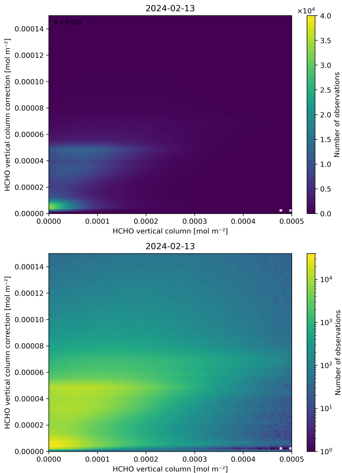
Figure 133: Scatter density plot of “HCHO vertical column” against “HCHO vertical column correction” for 2024-02-12 to 2024-02-14.
