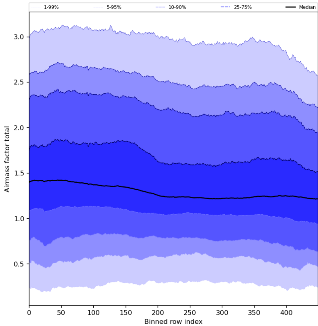
Figure 54: Along track statistics of “Airmass factor total” for 2024-02-12 to 2024-02-14
