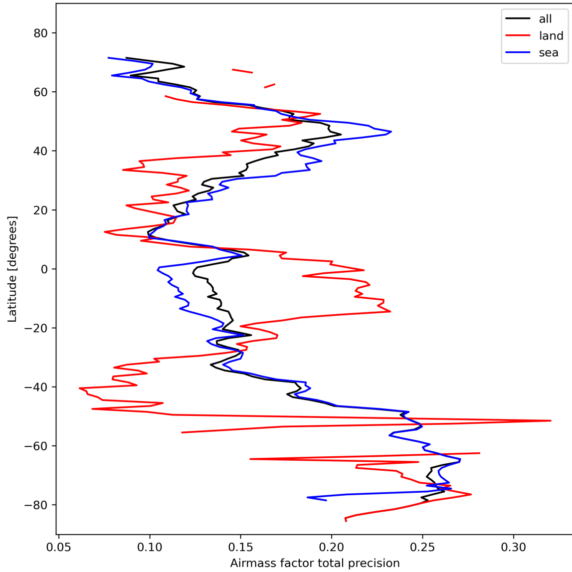
Figure 27: Zonal average of “Airmass factor total precision” for 2024-02-12 to 2024-02-14.
