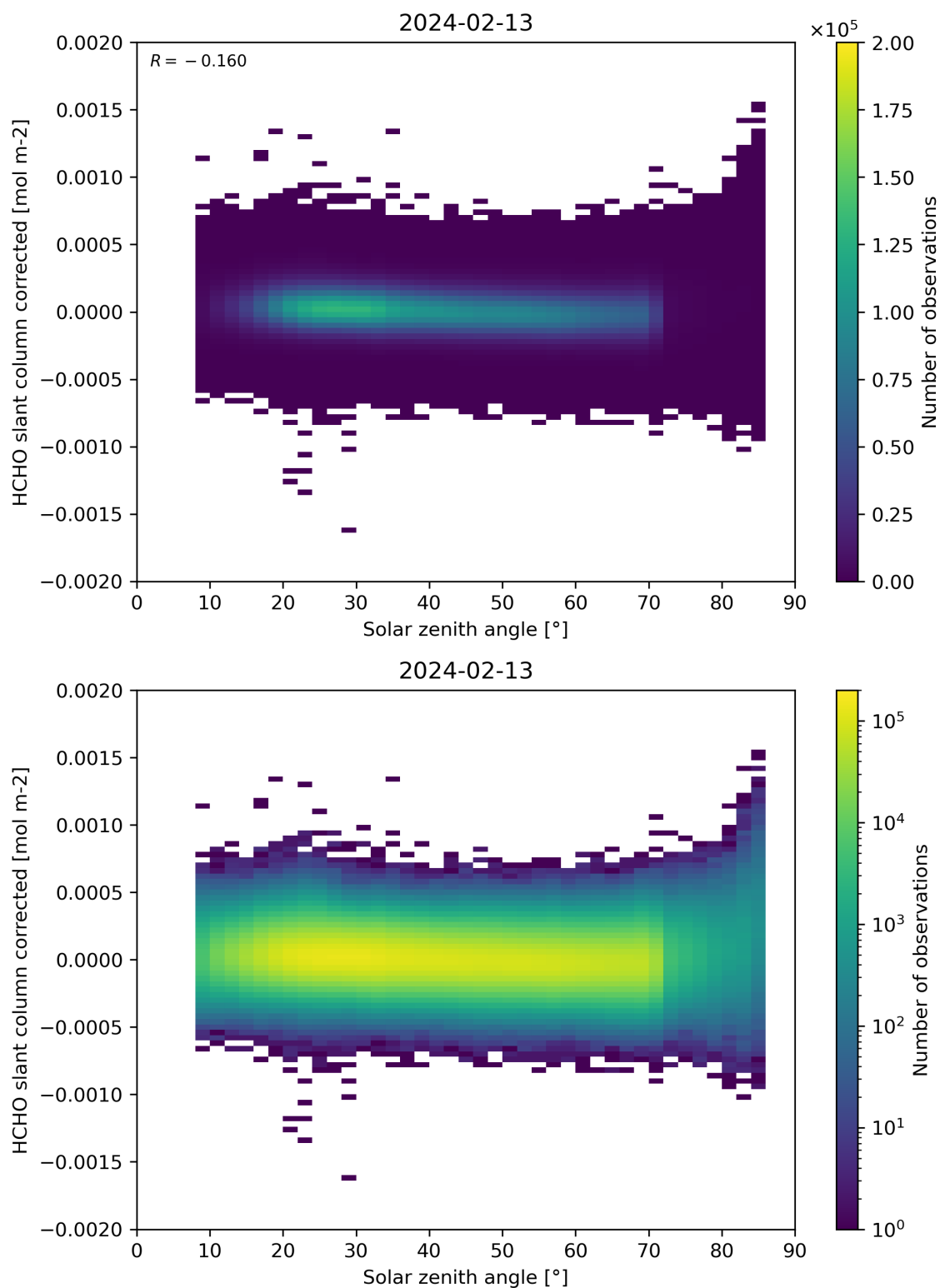
Figure 171: Scatter density plot of “Solar zenith angle” against “HCHO slant column corrected” for 2024-02-12 to 2024-02-14.
