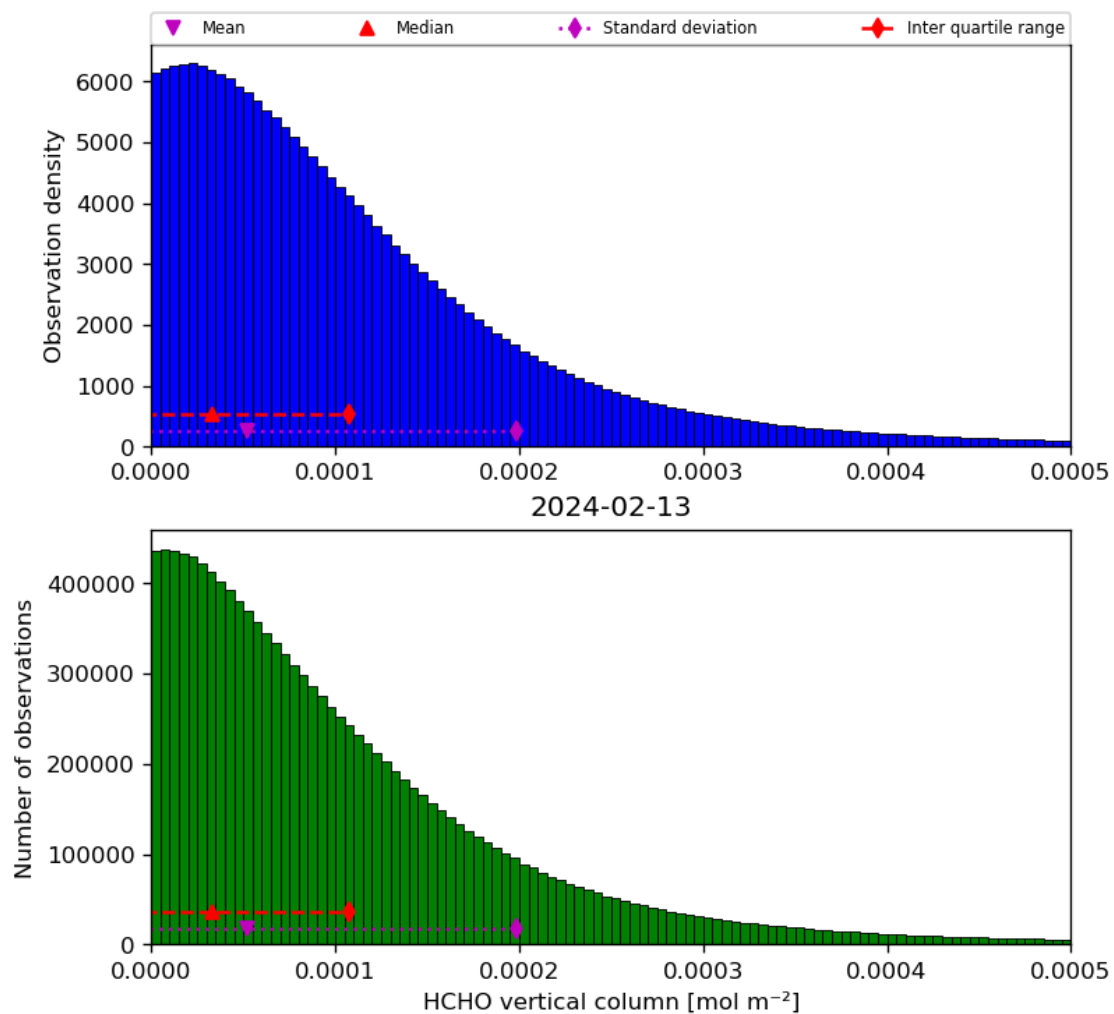
Figure 35: Histogram of “HCHO vertical column” for 2024-02-12 to 2024-02-14
