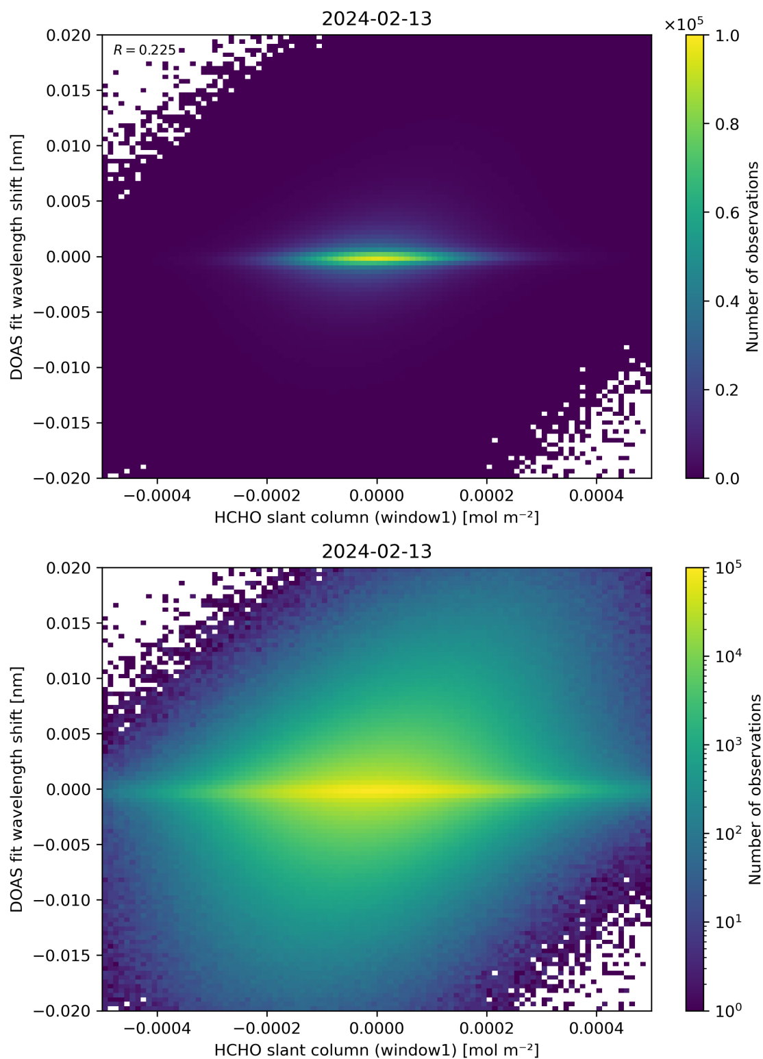
Figure 79: Scatter density plot of “HCHO slant column (window1)” against “DOAS fit wavelength shift” for 2024-02-12 to 2024-02-14.
