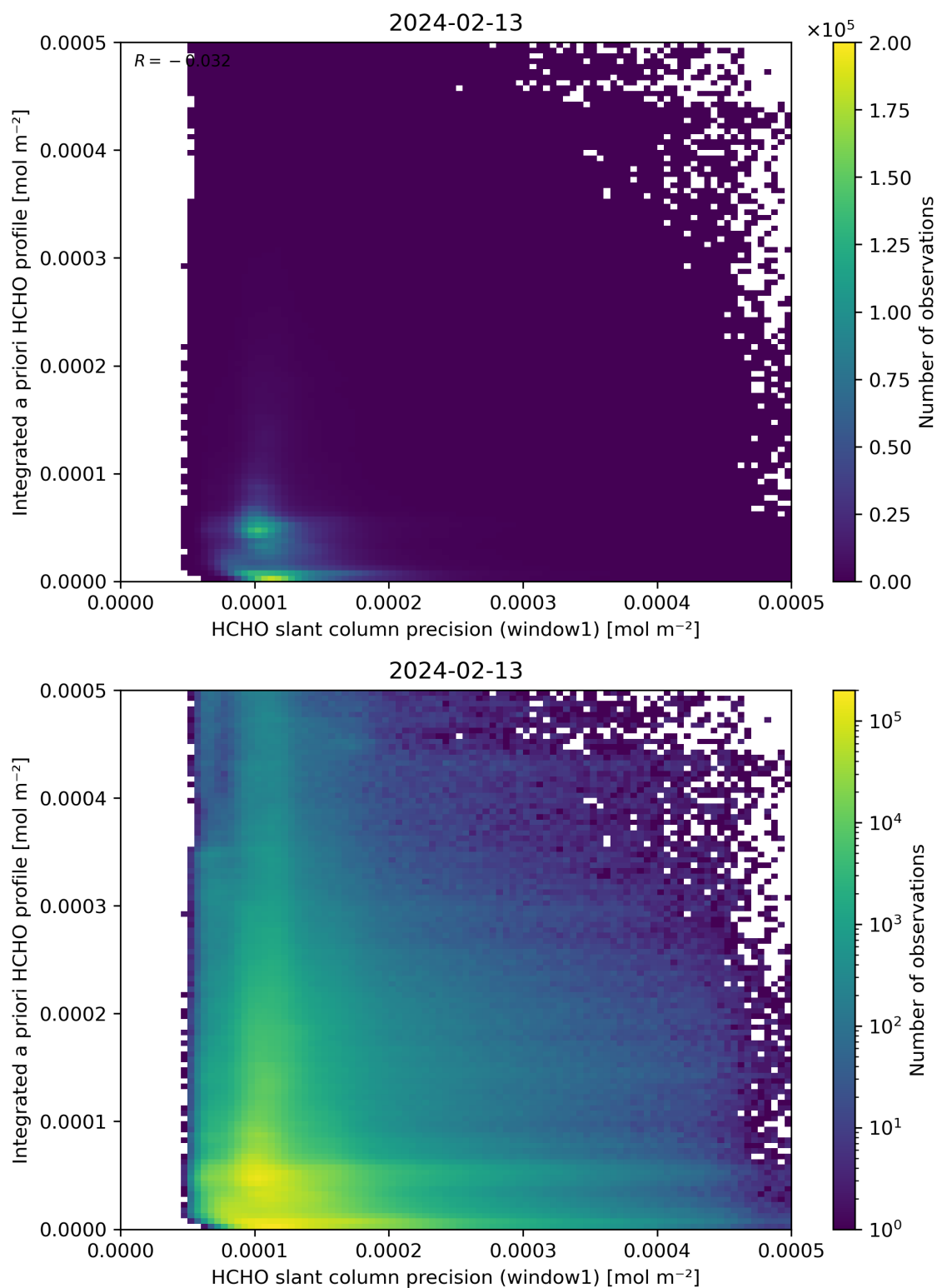
Figure 96: Scatter density plot of “HCHO slant column precision (window1)” against “Integrated a priori HCHO profile” for 2024-02-12 to 2024-02-14.
