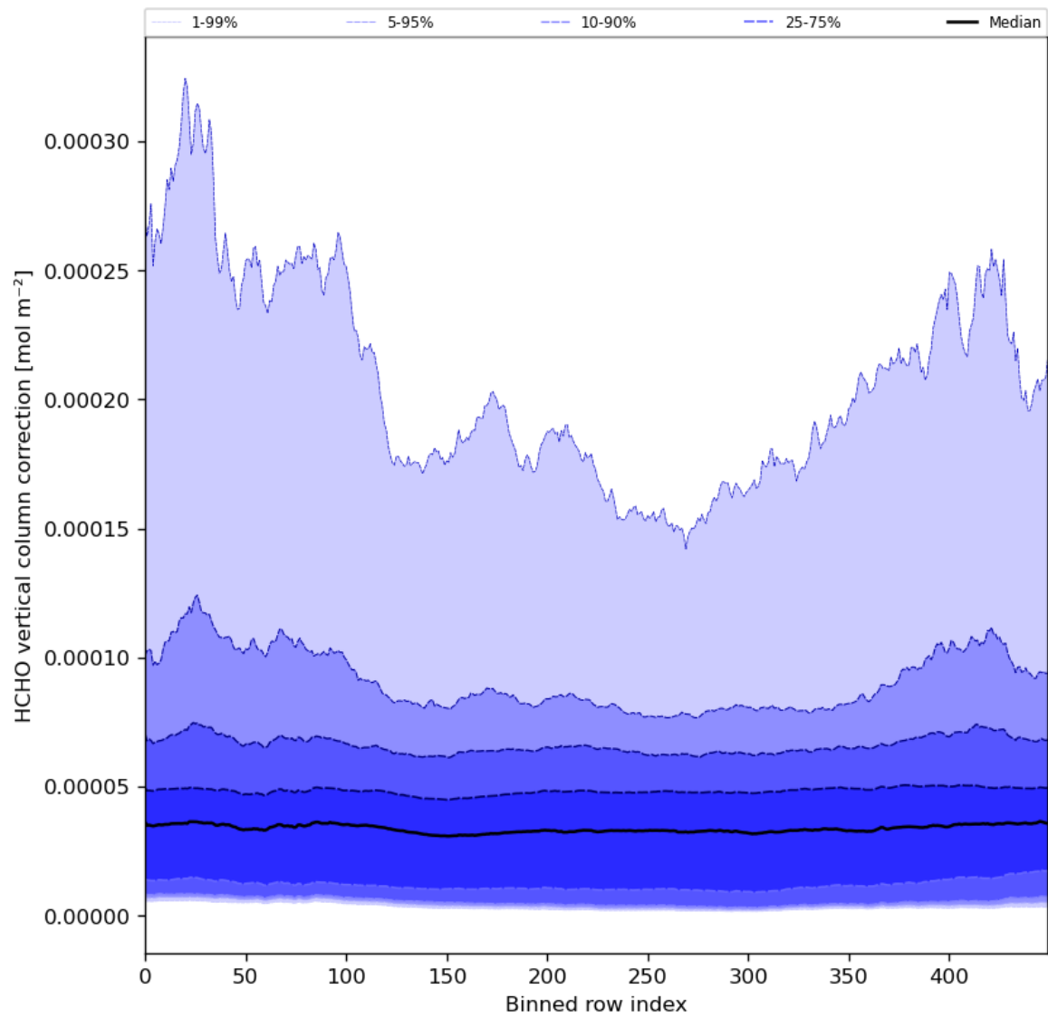
Figure 51: Along track statistics of "HCHO vertical column correction" for 2024-02-12 to 2024-02-14
