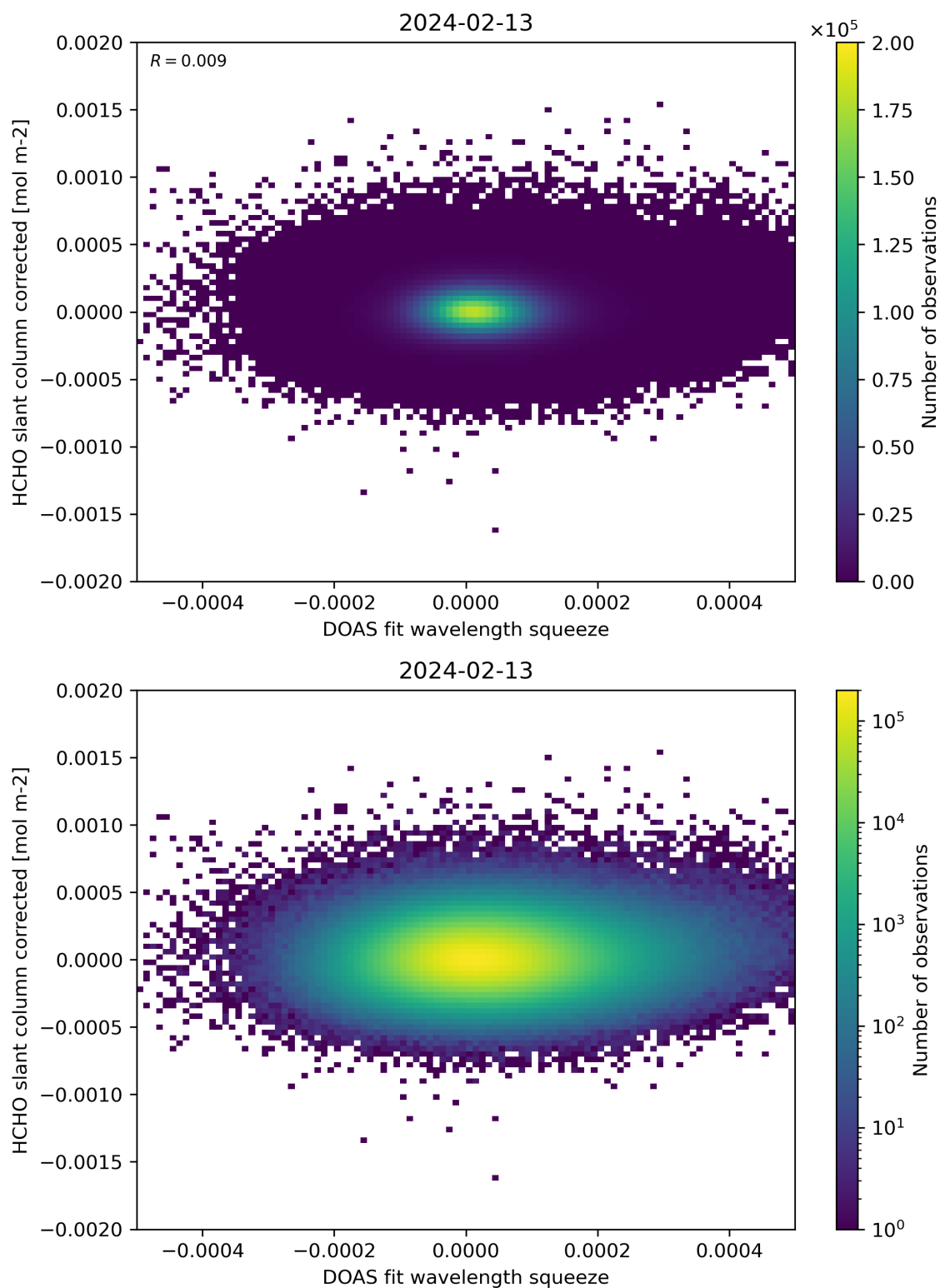
Figure 69: Scatter density plot of “DOAS fit wavelength squeeze” against “HCHO slant column corrected” for 2024-02-12 to 2024-02-14.
