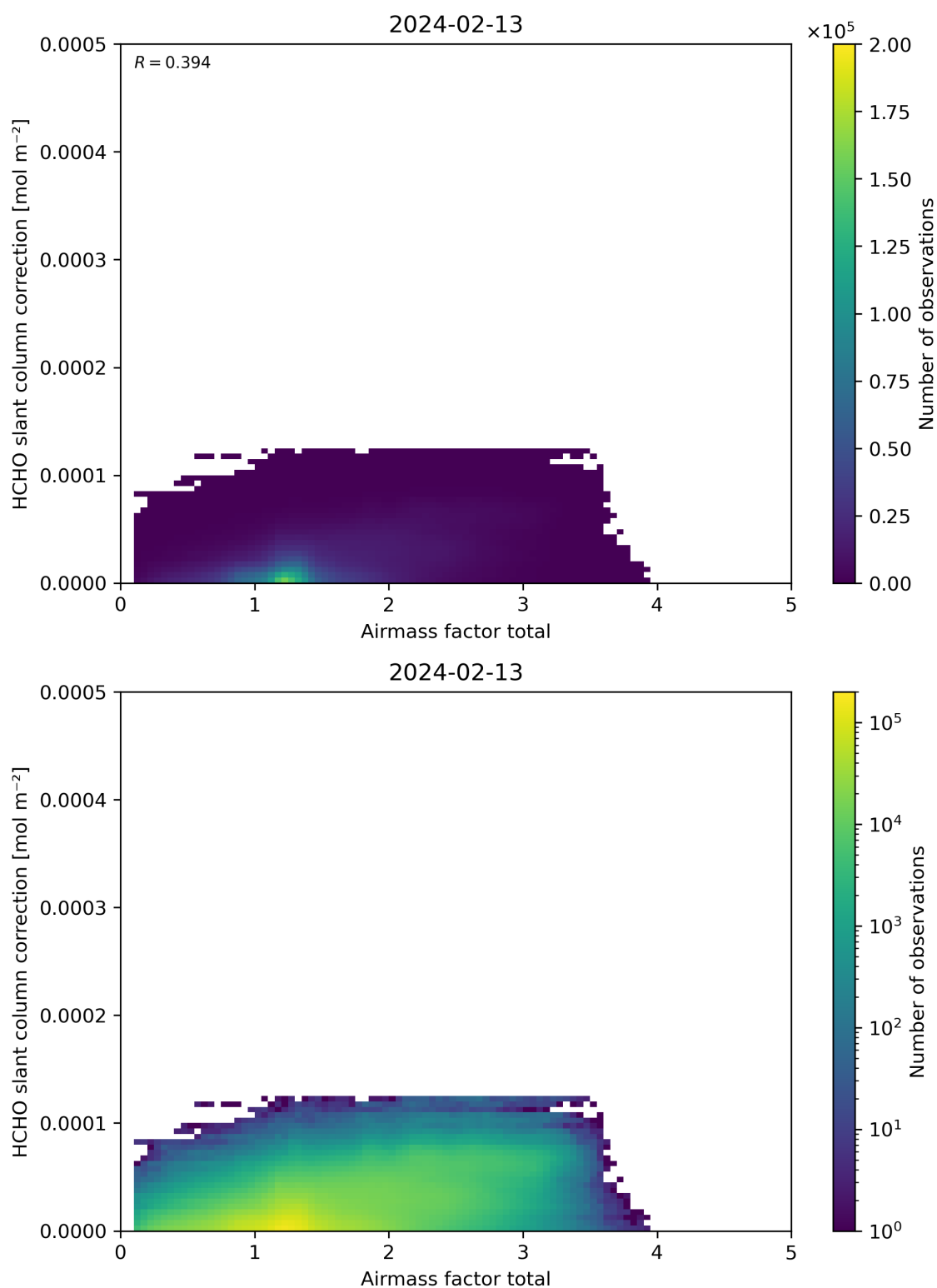
Figure 102: Scatter density plot of “Airmass factor total” against “HCHO slant column correction” for 2024-02-12 to 2024-02-14.
