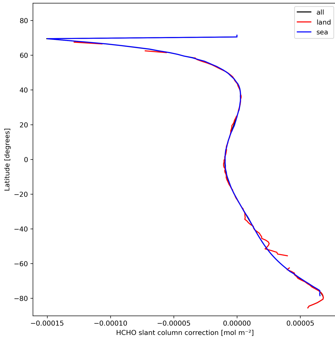
Figure 33: Zonal average of “HCHO slant column correction” for 2024-02-12 to 2024-02-14.
