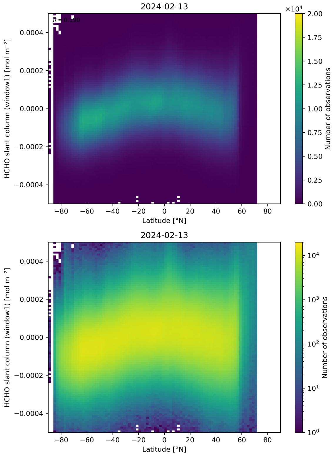
Figure 159: Scatter density plot of “Latitude” against “HCHO slant column (window1)” for 2024-02-12 to 2024-02-14.
