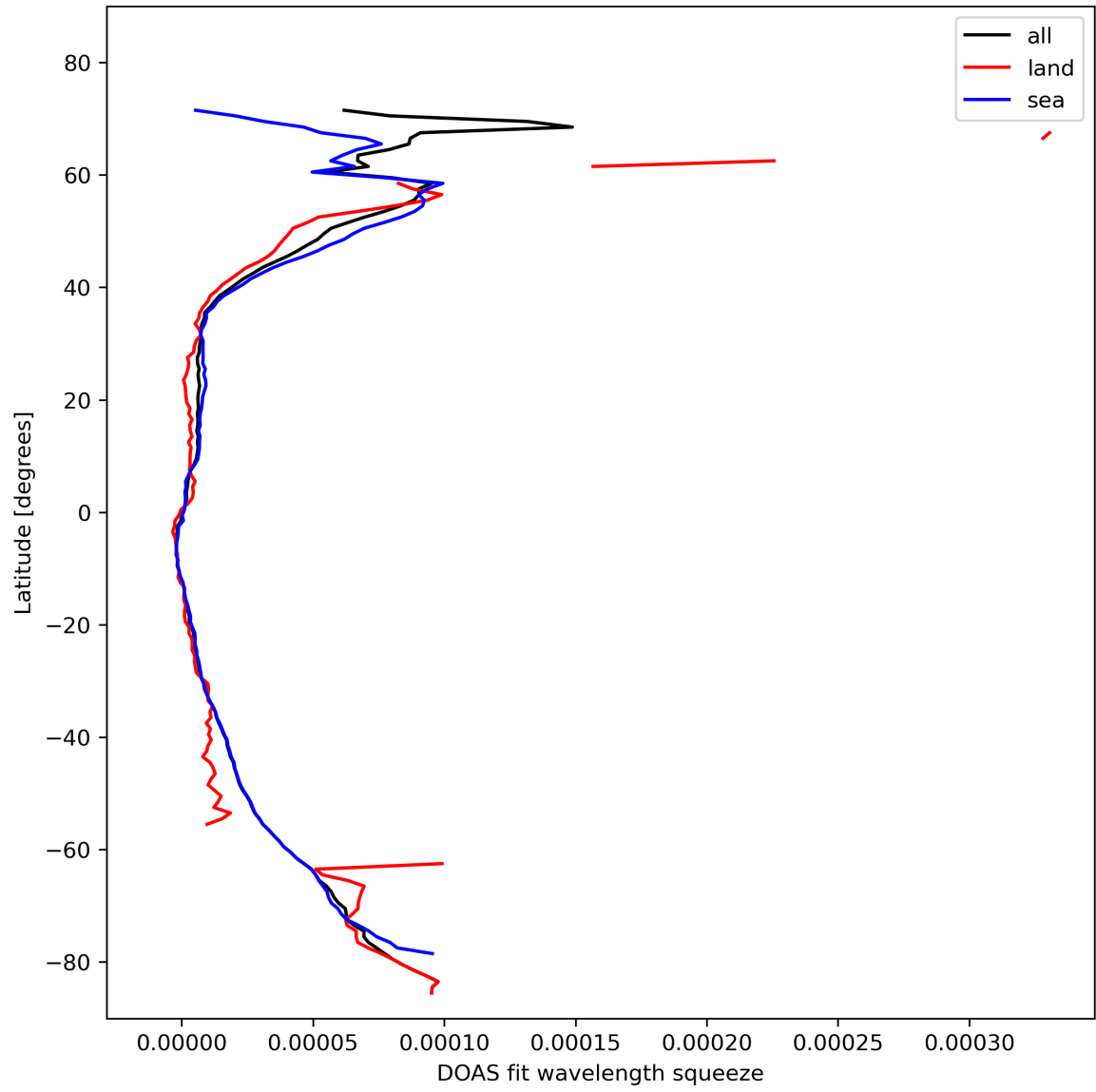
Figure 31: Zonal average of “DOAS fit wavelength squeeze” for 2024-02-12 to 2024-02-14.
