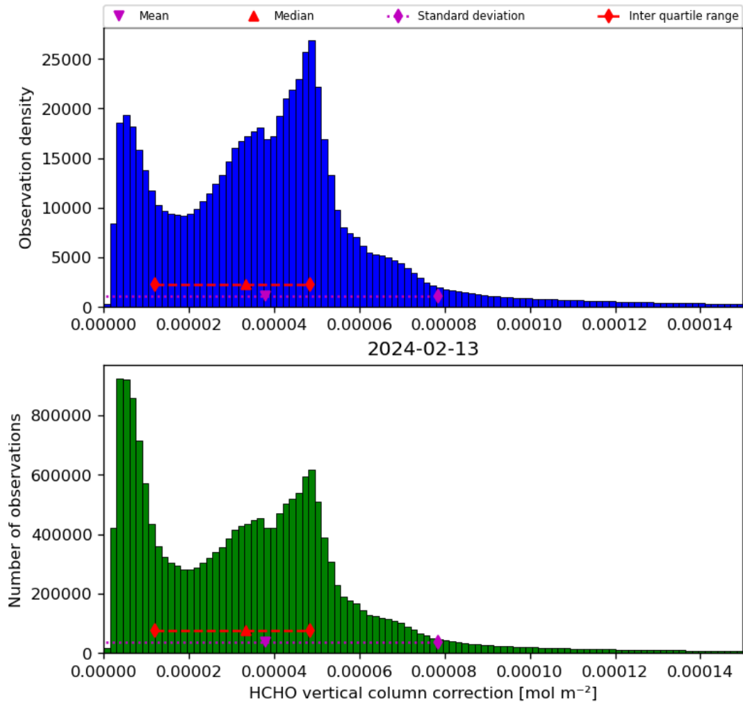
Figure 37: Histogram of “HCHO vertical column correction” for 2024-02-12 to 2024-02-14
