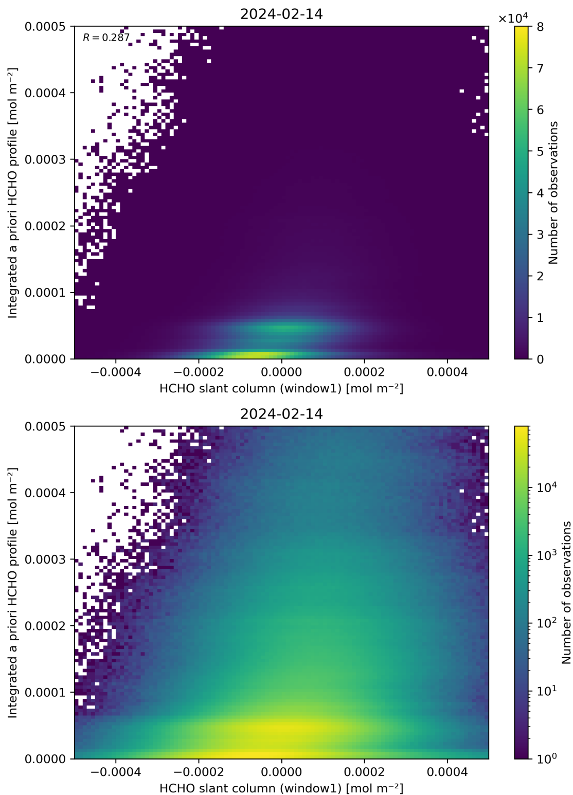
Figure 87: Scatter density plot of “HCHO slant column (window1)” against “Integrated a priori HCHO profile” for 2024-02-13 to 2024-02-15.
