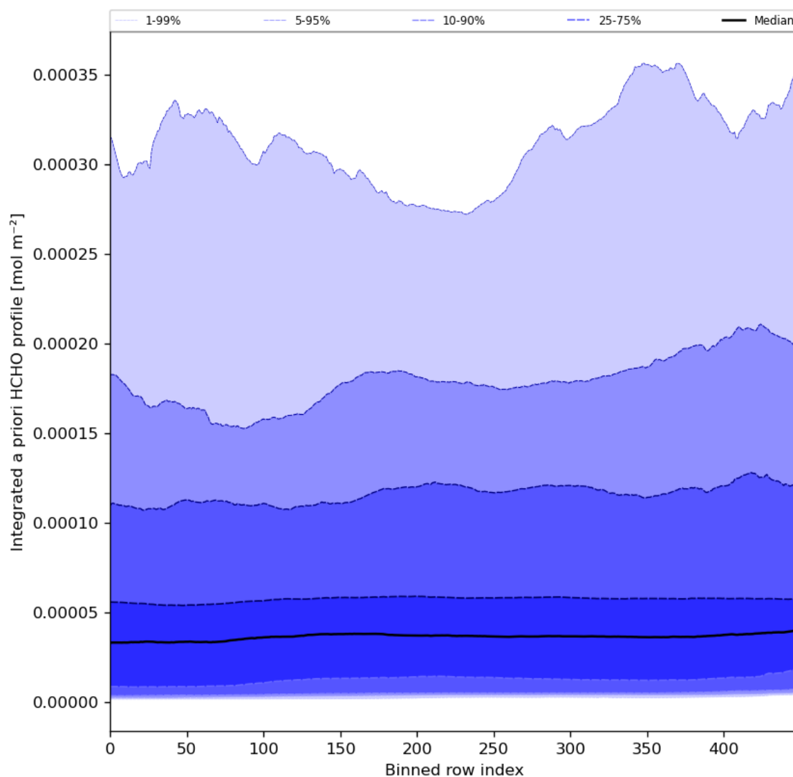
Figure 57: Along track statistics of "Integrated a priori HCHO profile" for 2024-02-13 to 2024-02-15
