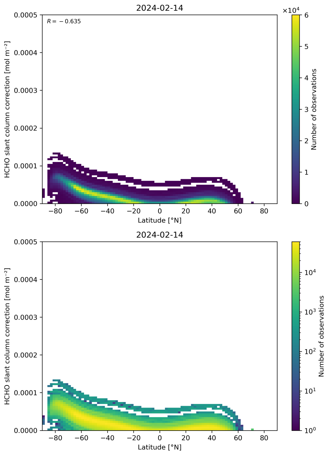
Figure 158: Scatter density plot of “Latitude” against “HCHO slant column correction” for 2024-02-13 to 2024-02-15.
