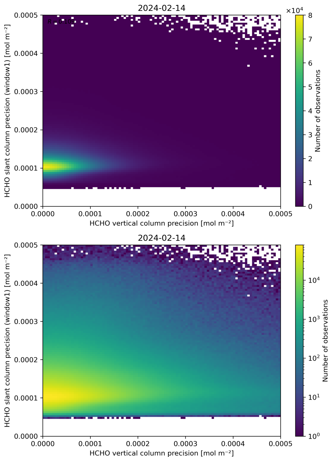
Figure 143: Scatter density plot of “HCHO vertical column precision” against “HCHO slant column precision (window1)” for 2024-02-13 to 2024-02-15.
