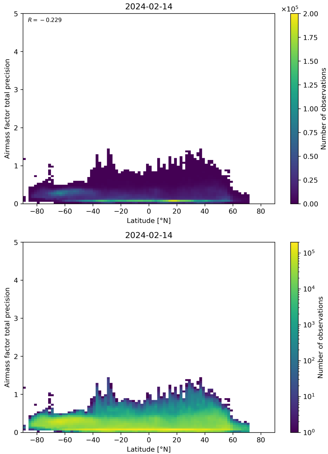
Figure 162: Scatter density plot of “Latitude” against “Airmass factor total precision” for 2024-02-13 to 2024-02-15.
