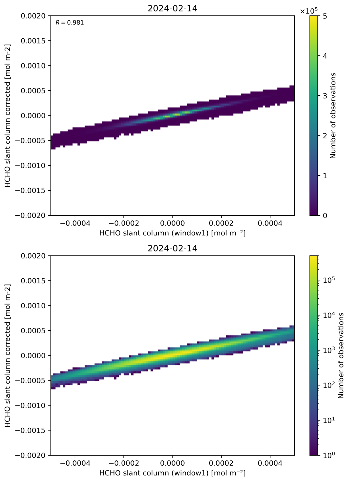
Figure 82: Scatter density plot of “HCHO slant column (window1)” against “HCHO slant column corrected” for 2024-02-13 to 2024-02-15.
