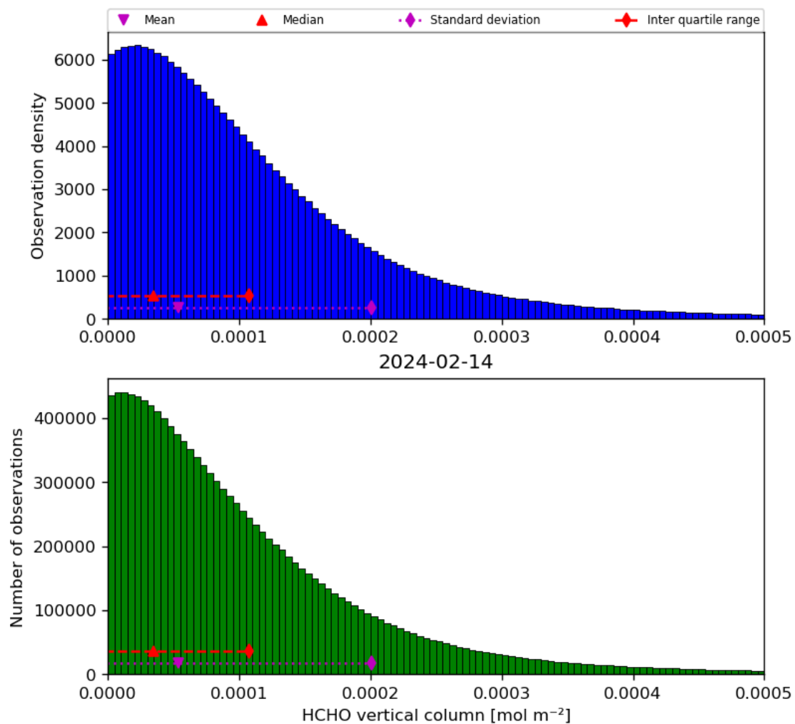
Figure 35: Histogram of “HCHO vertical column” for 2024-02-13 to 2024-02-15
