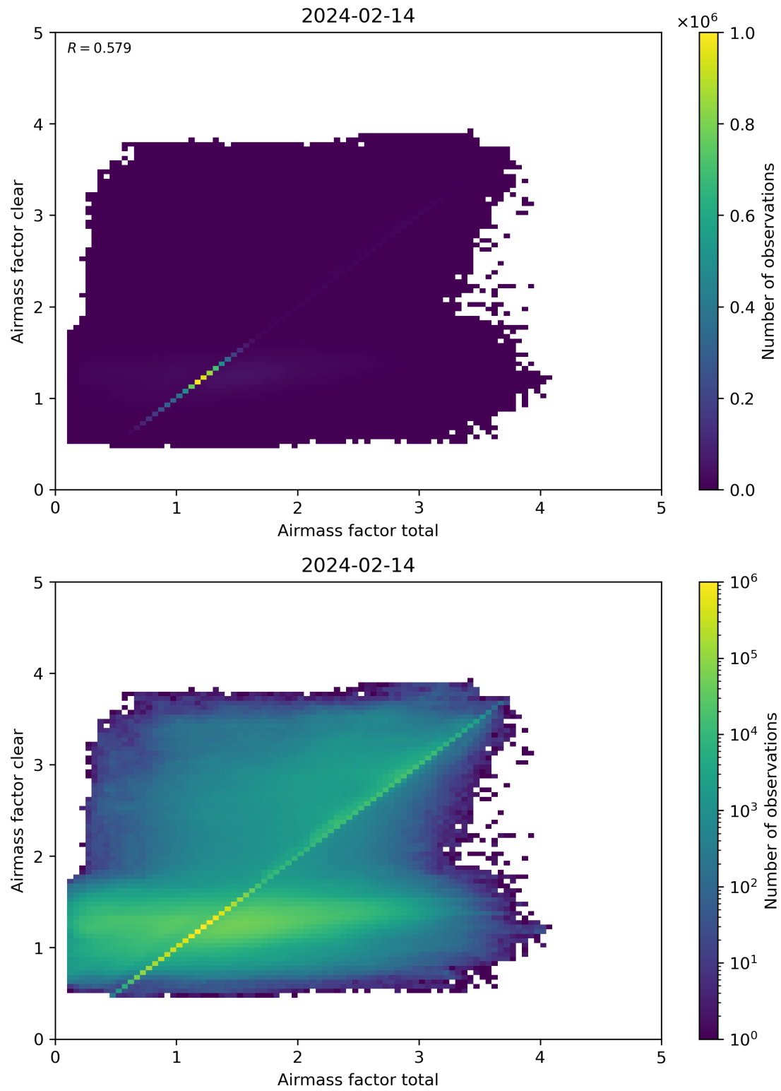
Figure 100: Scatter density plot of “Airmass factor total” against “Airmass factor clear” for 2024-02-13 to 2024-02-15.
