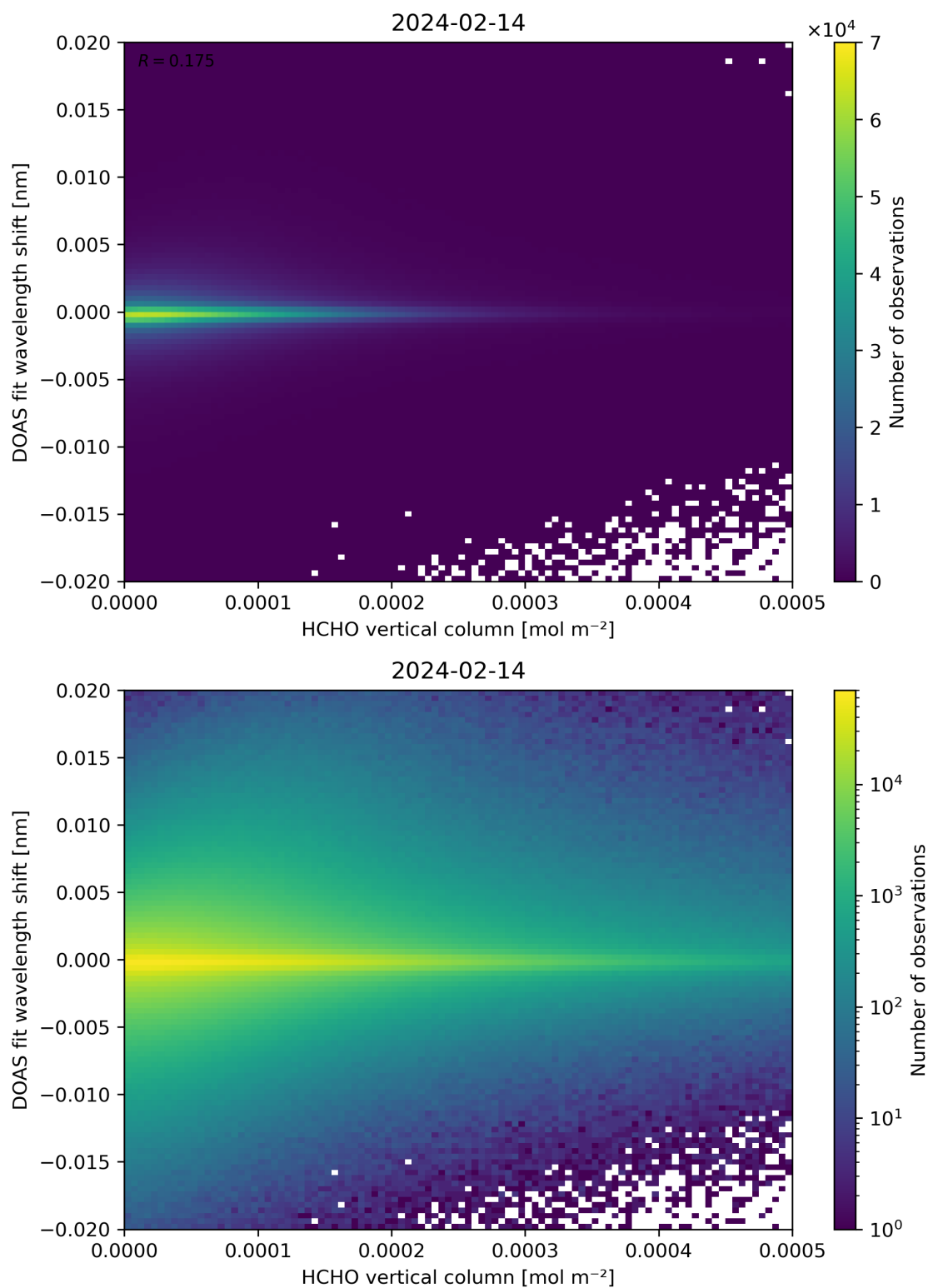
Figure 124: Scatter density plot of “HCHO vertical column” against “DOAS fit wavelength shift” for 2024-02-13 to 2024-02-15.
