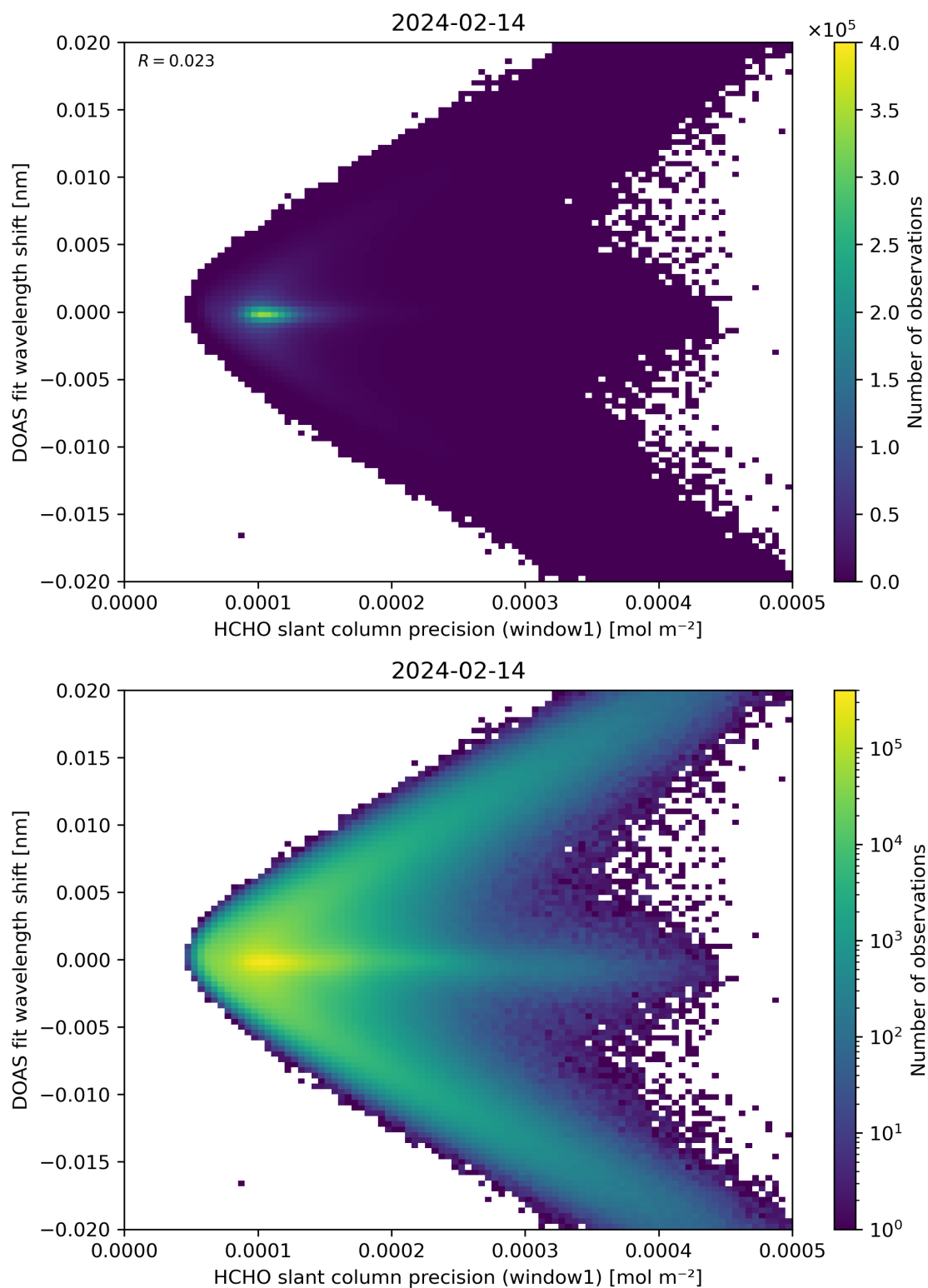
Figure 89: Scatter density plot of “HCHO slant column precision (window1)” against “DOAS fit wavelength shift” for 2024-02-13 to 2024-02-15.
