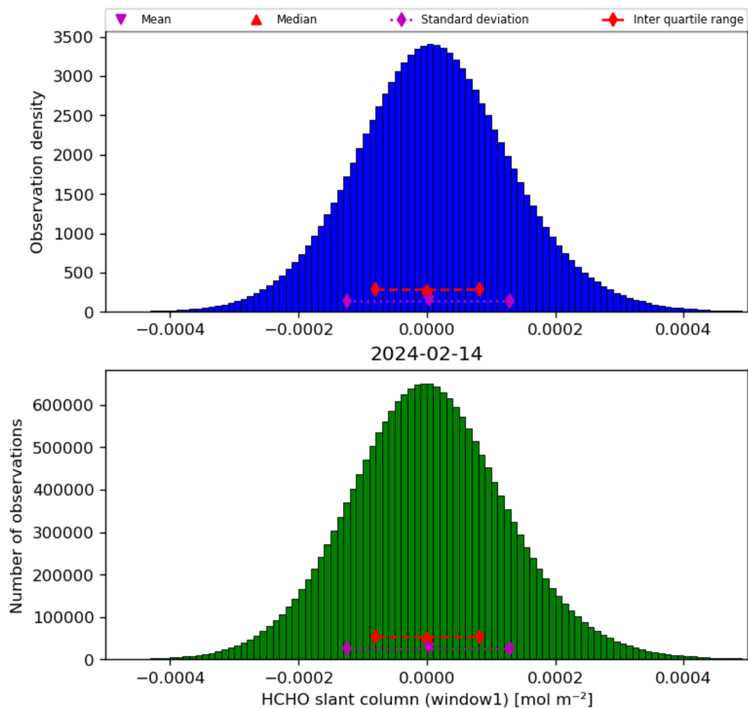
Figure 38: Histogram of “HCHO slant column (window1)” for 2024-02-13 to 2024-02-15
