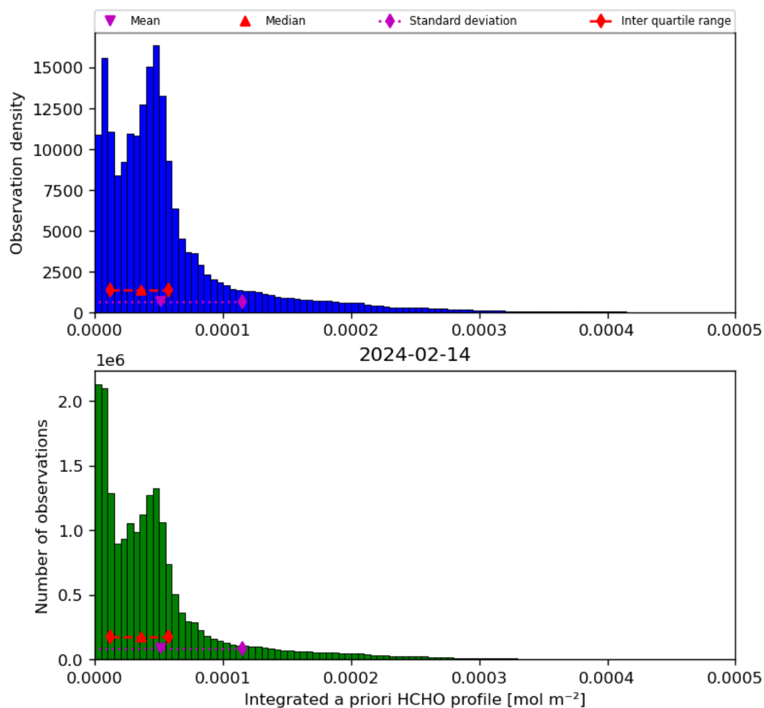
Figure 43: Histogram of “Integrated a priori HCHO profile” for 2024-02-13 to 2024-02-15
