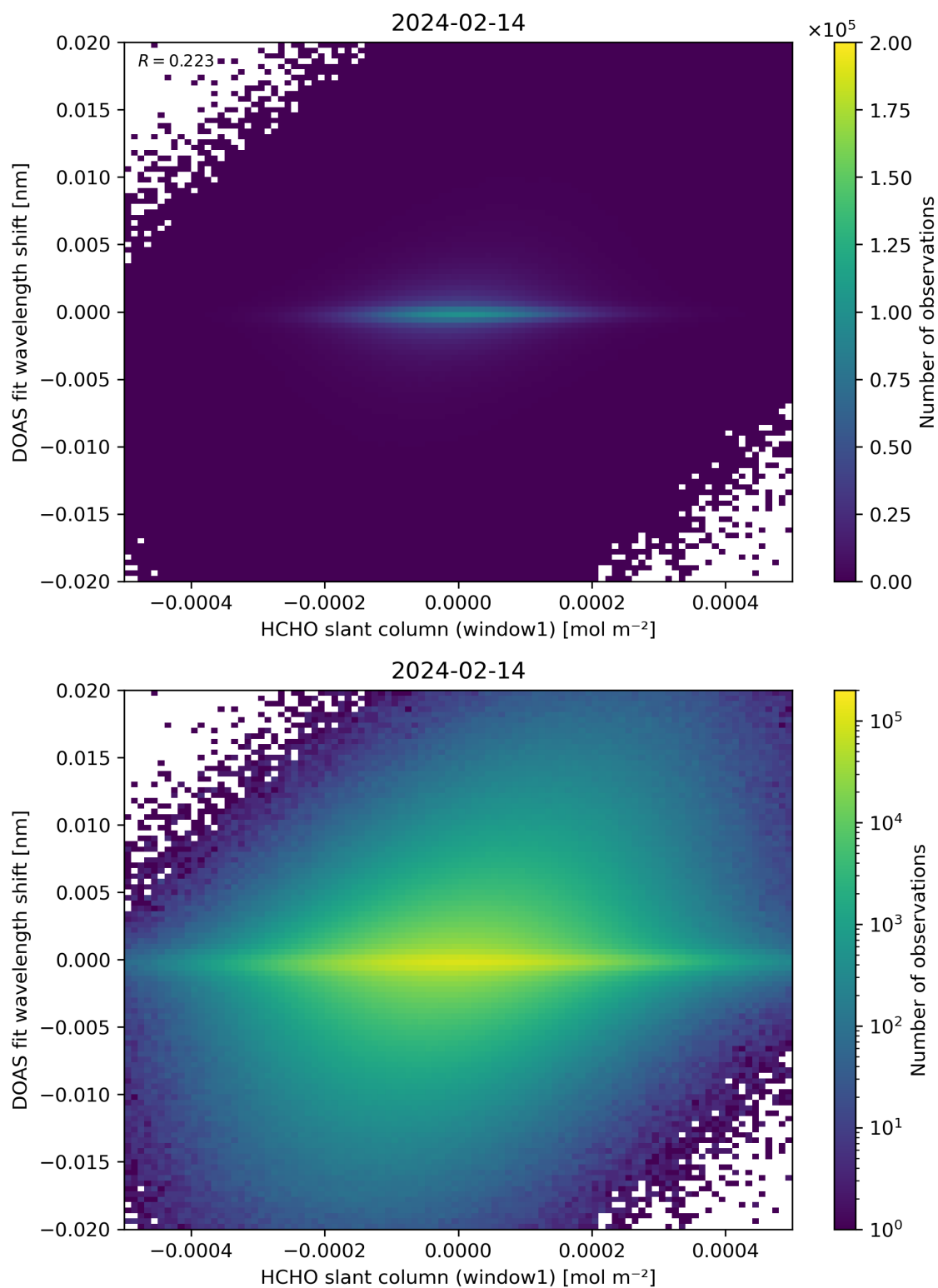
Figure 79: Scatter density plot of “HCHO slant column (window1)” against “DOAS fit wavelength shift” for 2024-02-13 to 2024-02-15.
