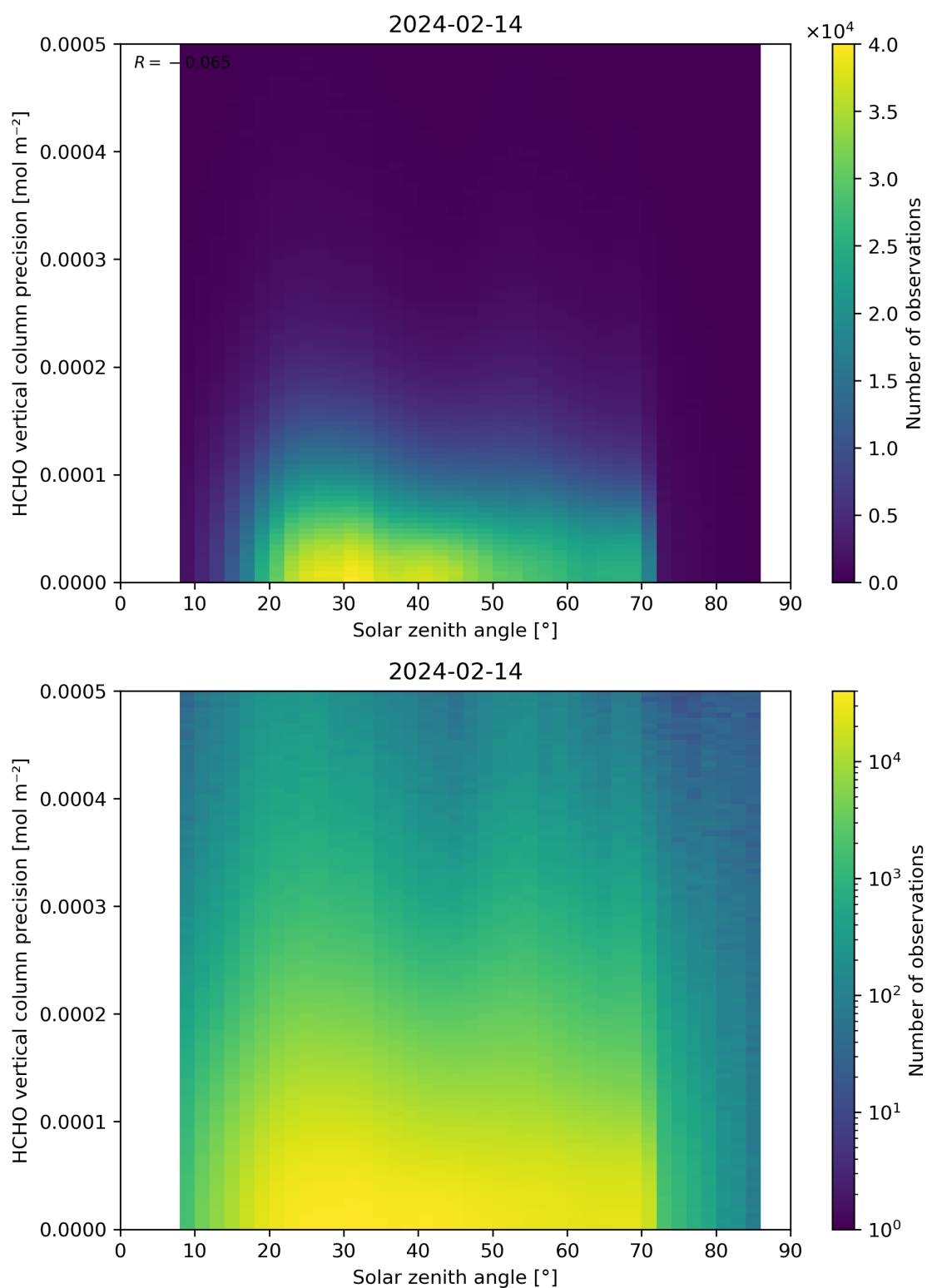
Figure 179: Scatter density plot of “Solar zenith angle” against “HCHO vertical column precision” for 2024-02-13 to 2024-02-15.
