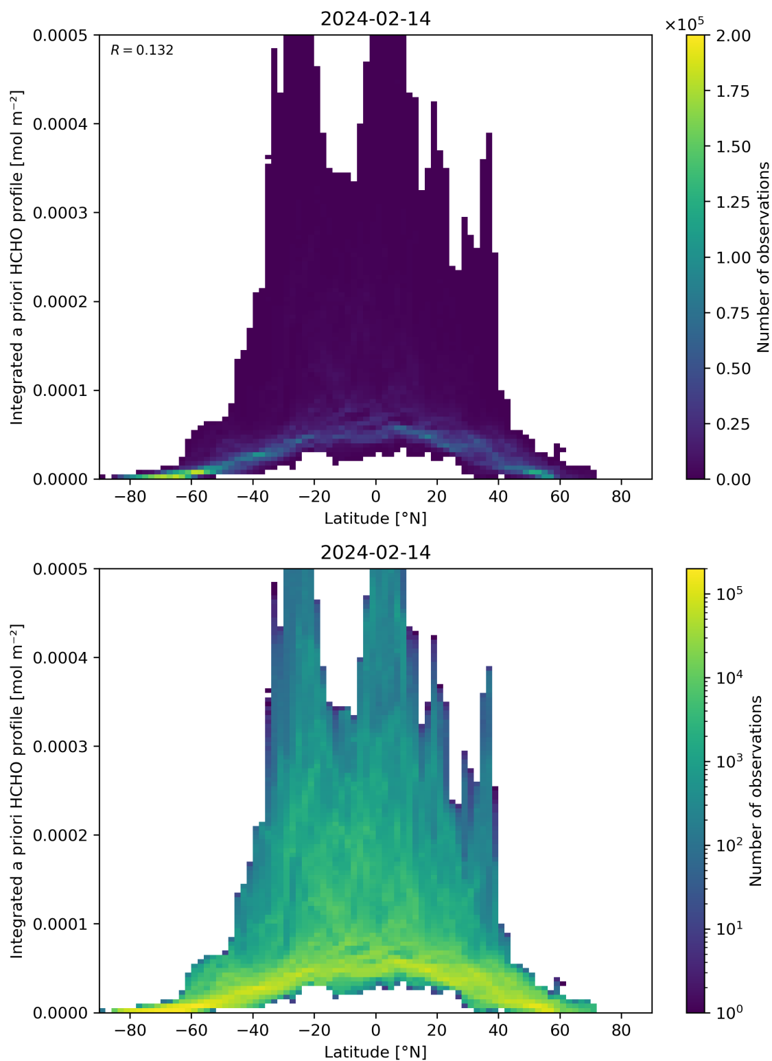
Figure 166: Scatter density plot of “Latitude” against “Integrated a priori HCHO profile” for 2024-02-13 to 2024-02-15.
