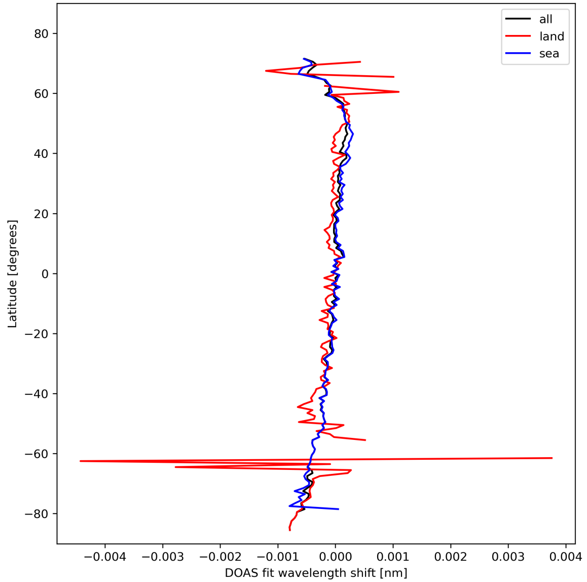
Figure 30: Zonal average of “DOAS fit wavelength shift” for 2024-02-13 to 2024-02-15.
