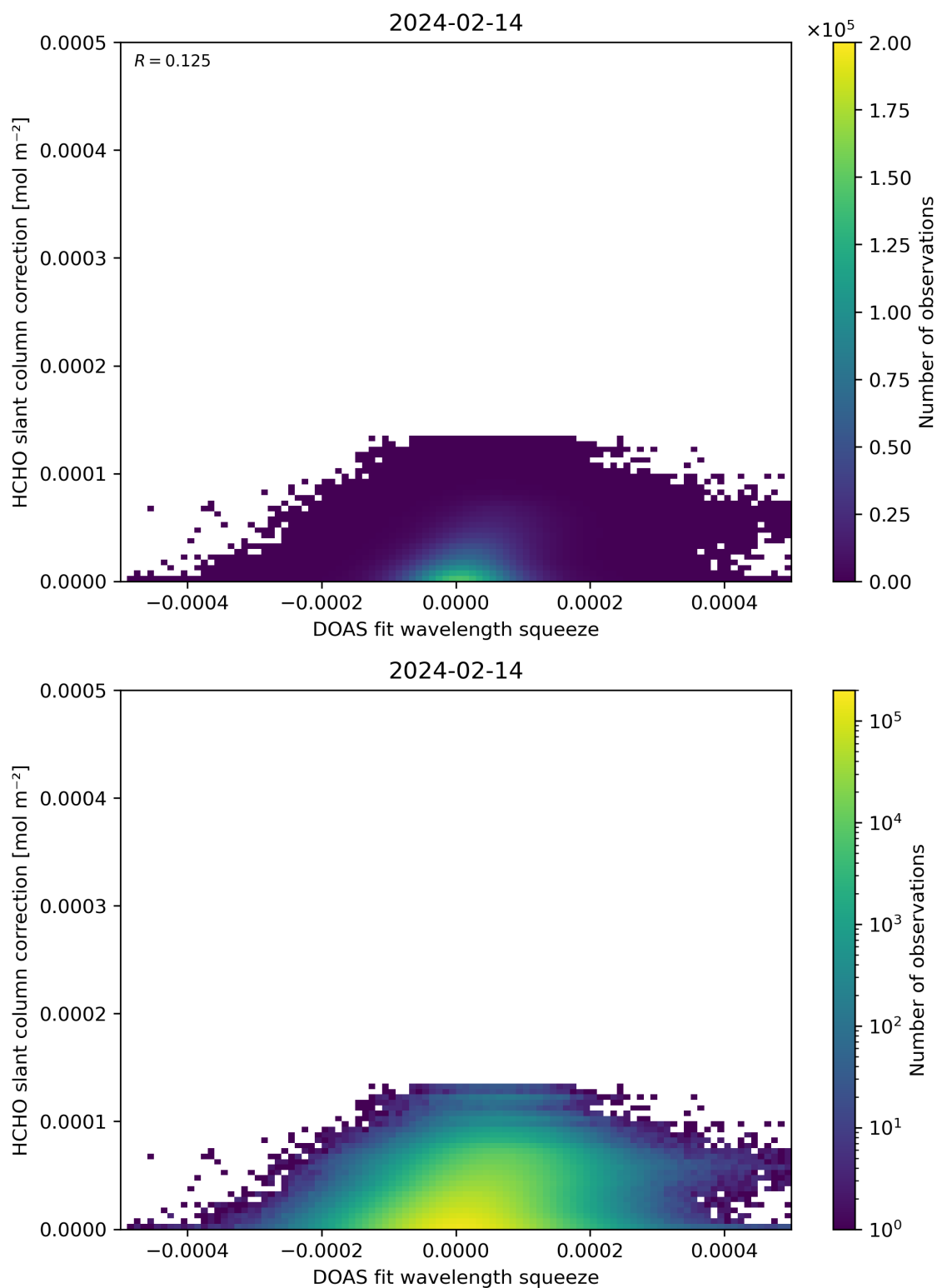
Figure 70: Scatter density plot of “DOAS fit wavelength squeeze” against “HCHO slant column correction” for 2024-02-13 to 2024-02-15.
