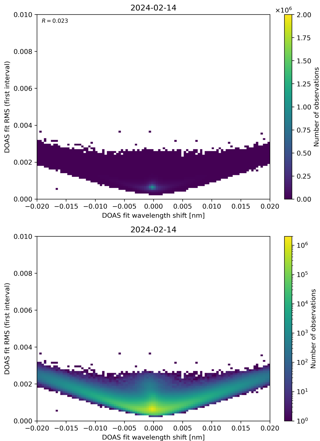
Figure 64: Scatter density plot of “DOAS fit wavelength shift” against “DOAS fit RMS (first interval)” for 2024-02-13 to 2024-02-15.
