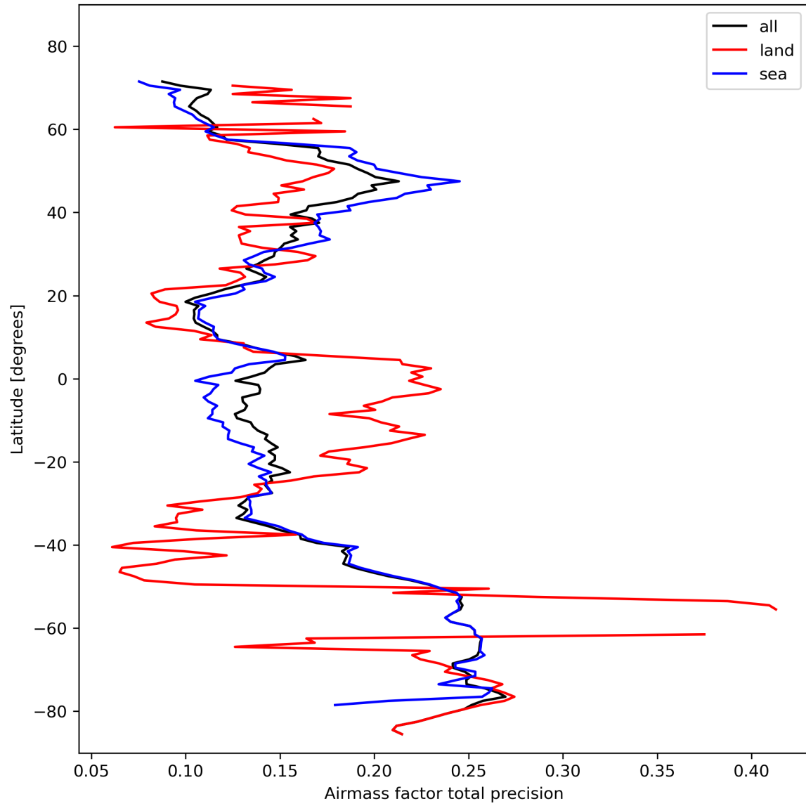
Figure 27: Zonal average of “Airmass factor total precision” for 2024-02-13 to 2024-02-15.
