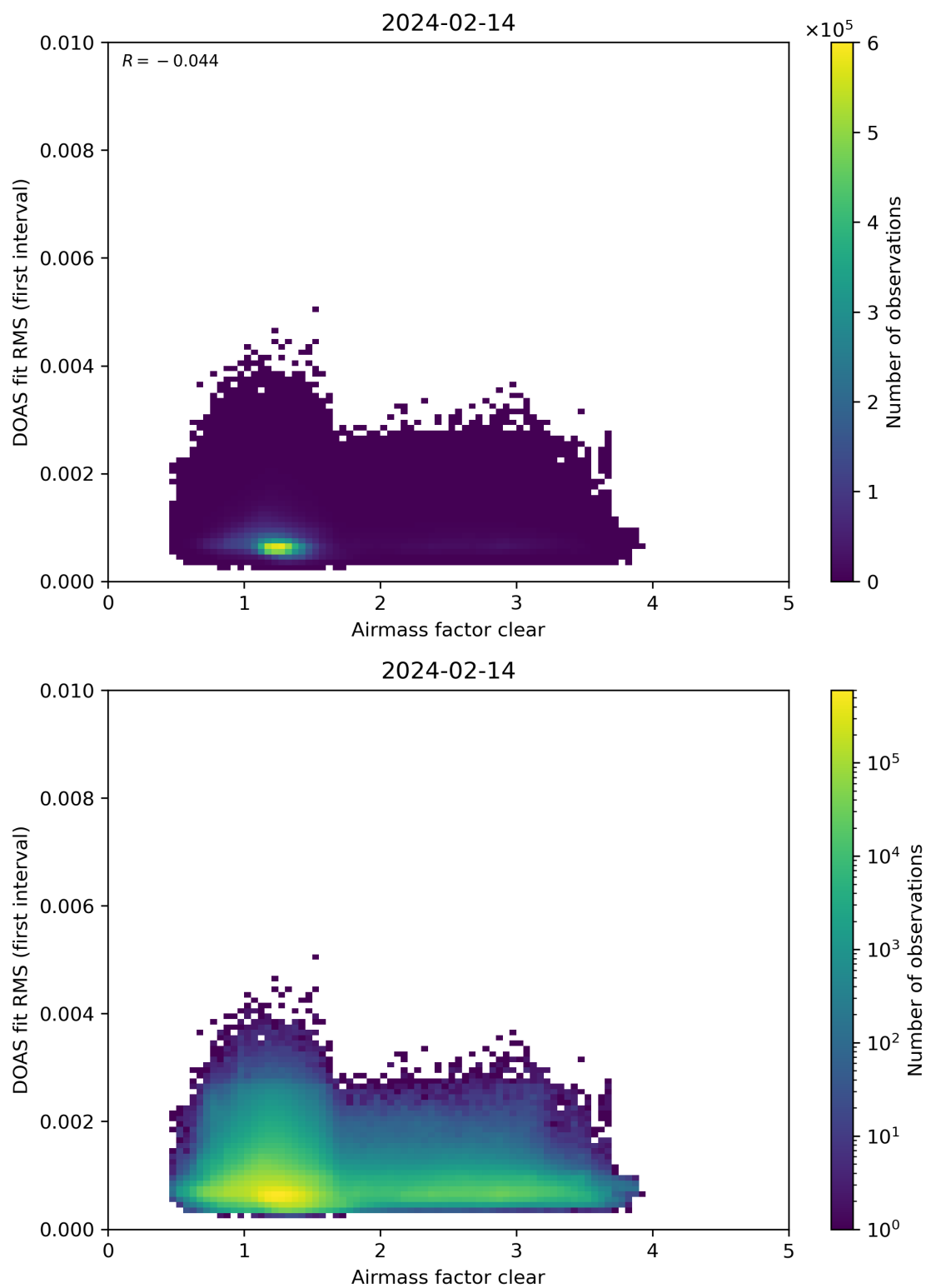
Figure 71: Scatter density plot of “Airmass factor clear” against “DOAS fit RMS (first interval)” for 2024-02-13 to 2024-02-15.
