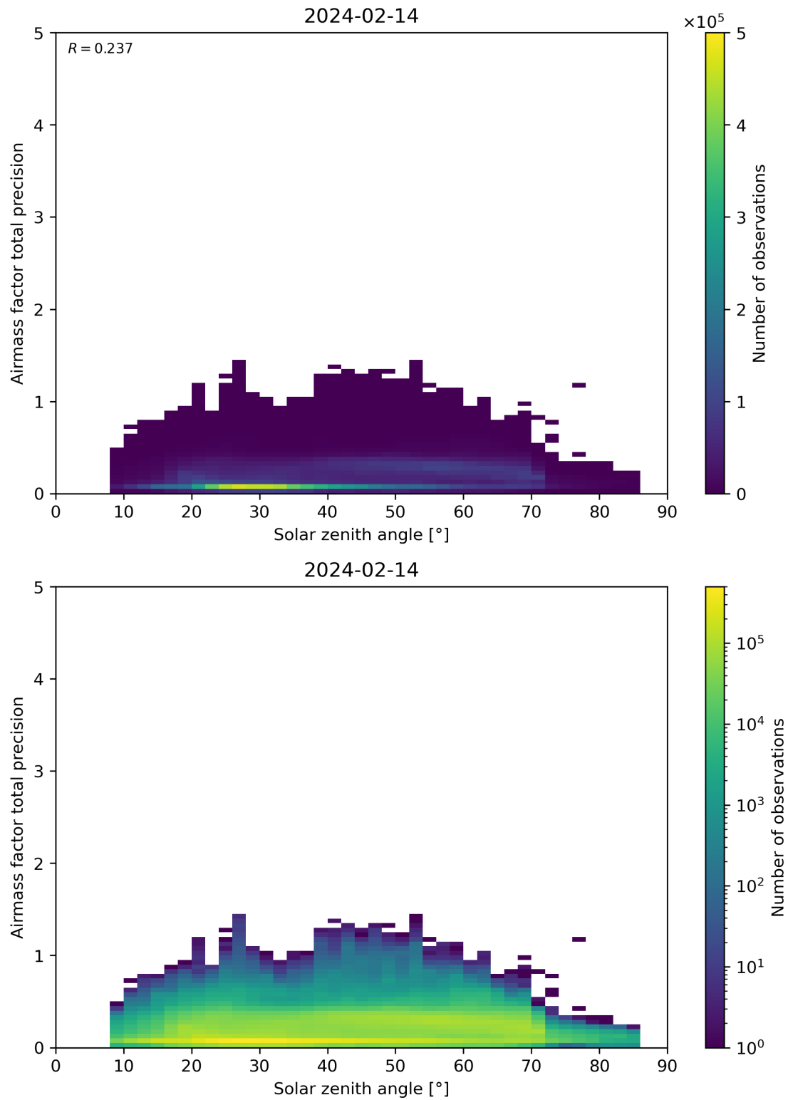
Figure 176: Scatter density plot of “Solar zenith angle” against “Airmass factor total precision” for 2024-02-13 to 2024-02-15.
