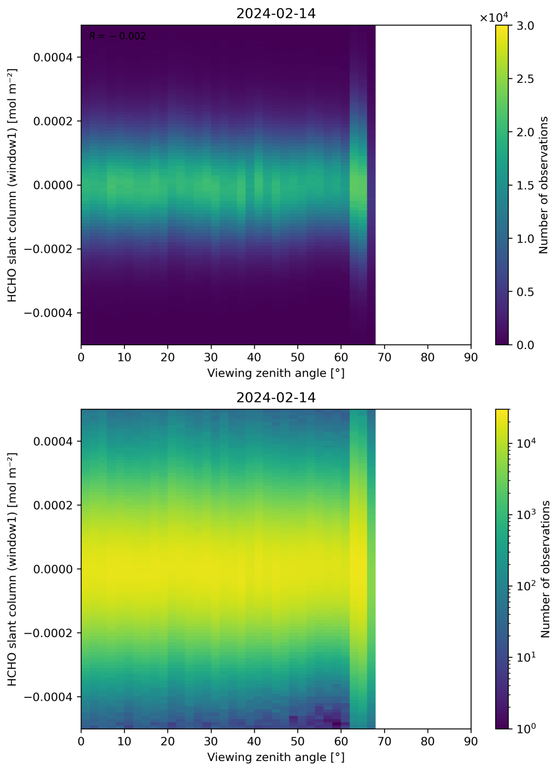
Figure 188: Scatter density plot of “Viewing zenith angle” against “HCHO slant column (window1)” for 2024-02-13 to 2024-02-15.
