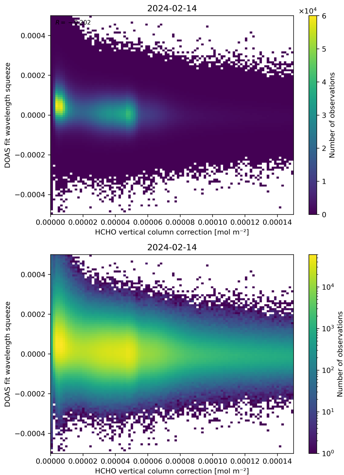
Figure 114: Scatter density plot of “HCHO vertical column correction” against “DOAS fit wavelength squeeze” for 2024-02-13 to 2024-02-15.
