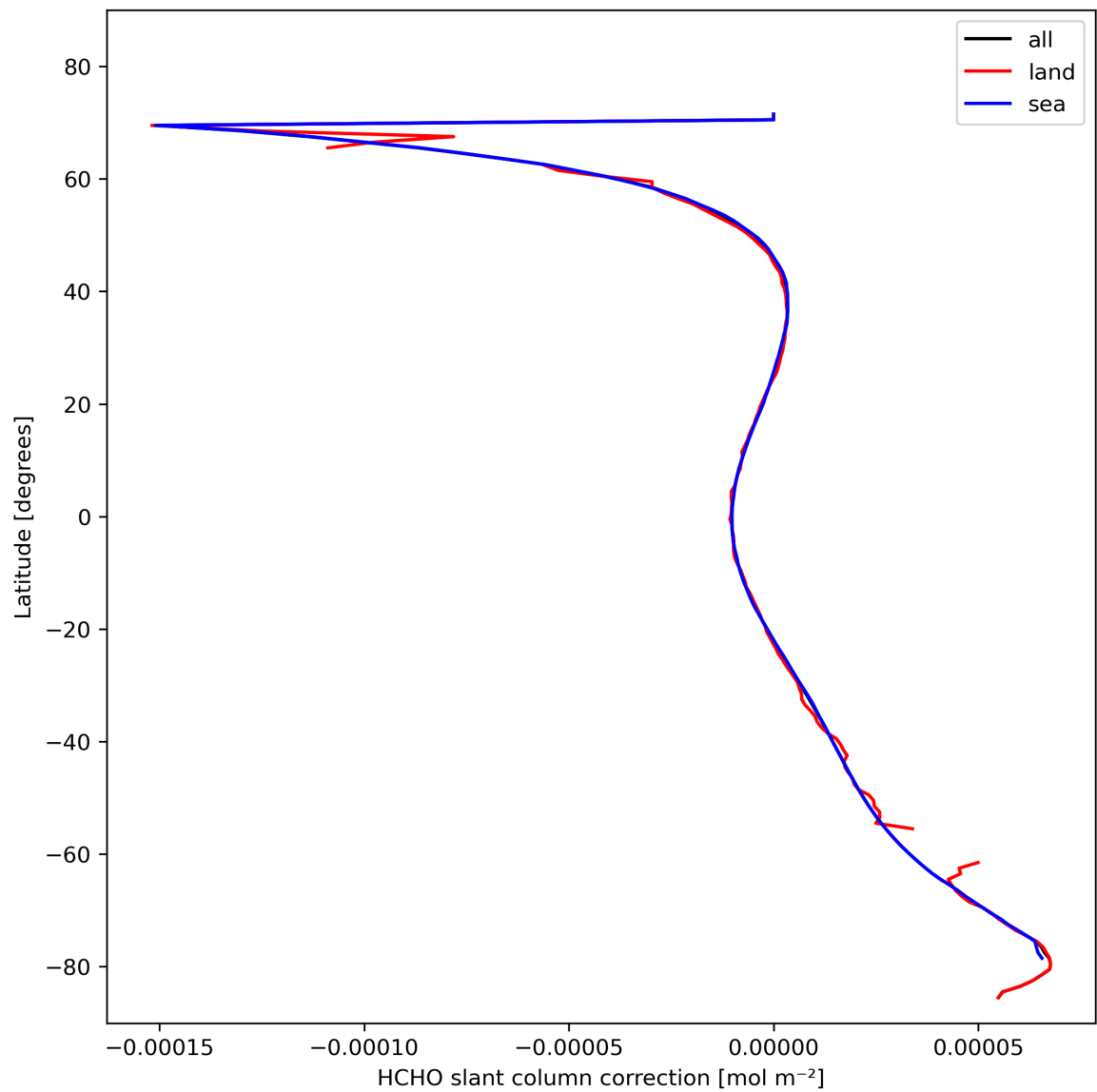
Figure 33: Zonal average of “HCHO slant column correction” for 2024-02-13 to 2024-02-15.
