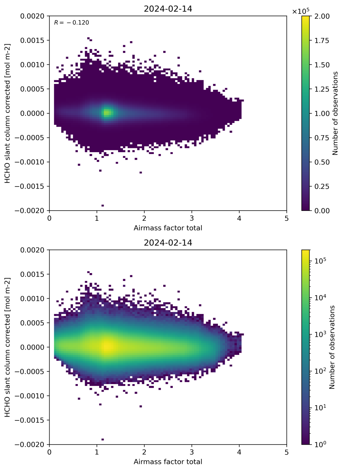
Figure 101: Scatter density plot of “Airmass factor total” against “HCHO slant column corrected” for 2024-02-13 to 2024-02-15.
