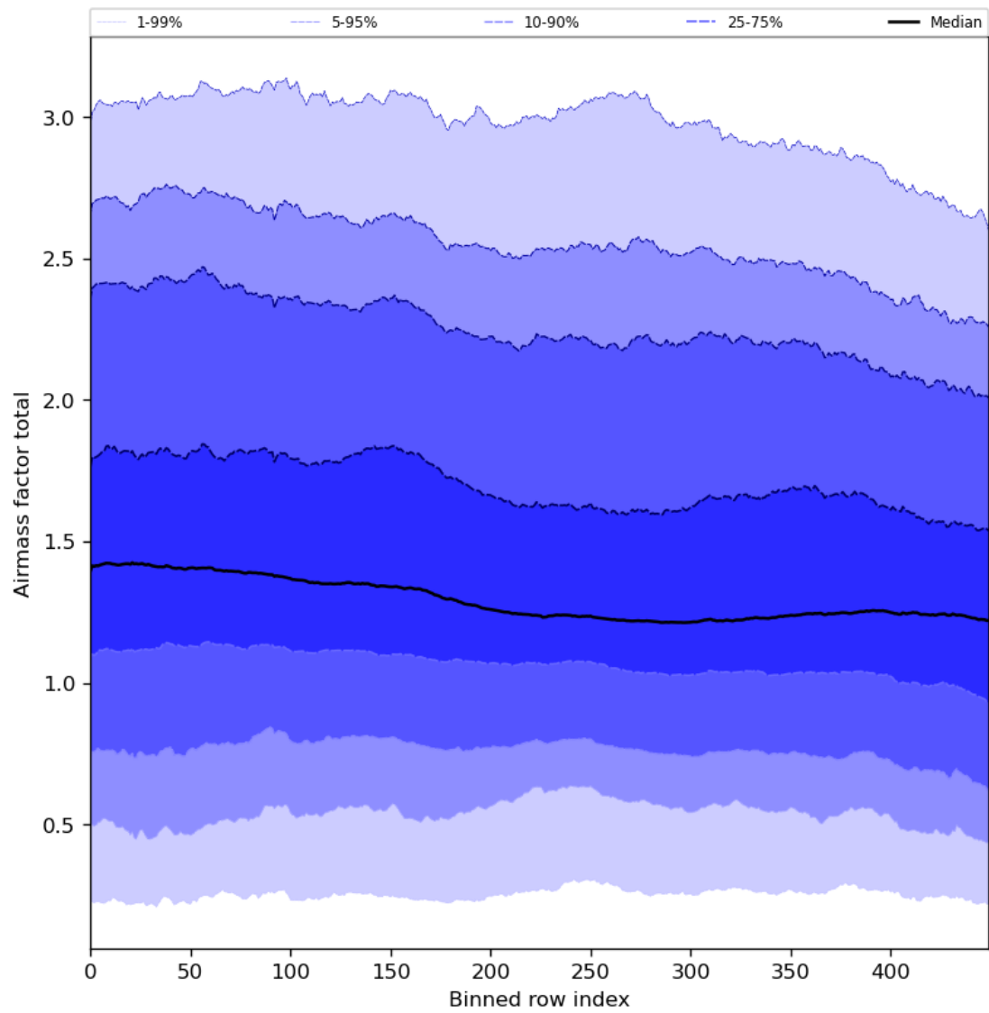
Figure 54: Along track statistics of “Airmass factor total” for 2024-02-13 to 2024-02-15
