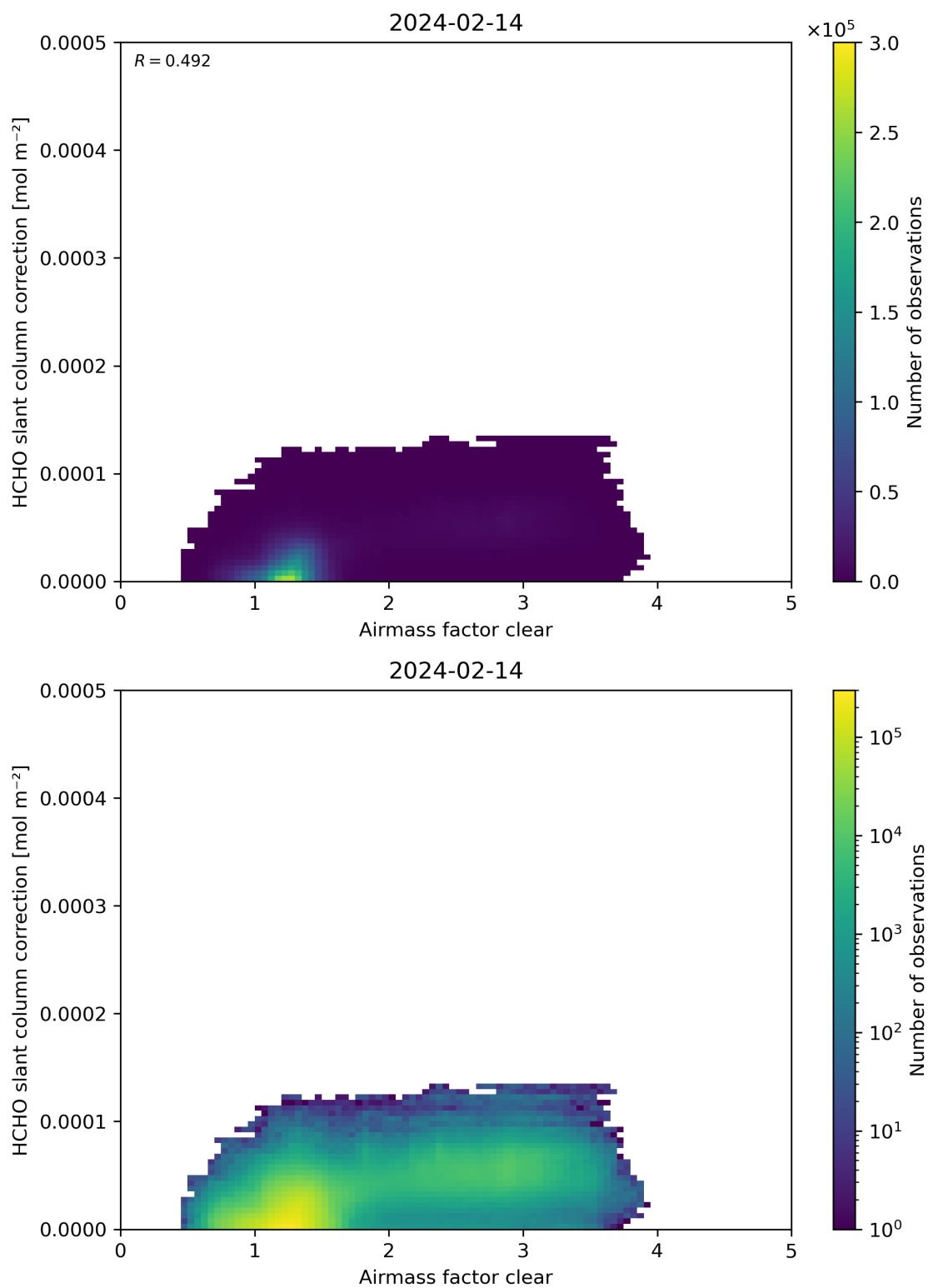
Figure 75: Scatter density plot of “Airmass factor clear” against “HCHO slant column correction” for 2024-02-13 to 2024-02-15.
