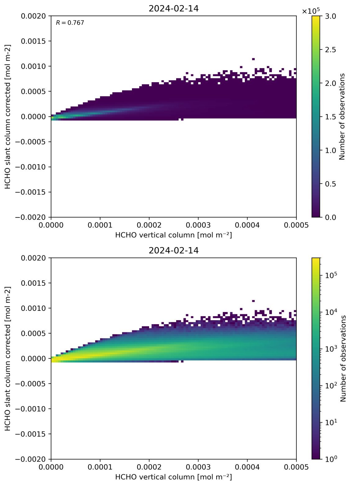
Figure 127: Scatter density plot of “HCHO vertical column” against “HCHO slant column corrected” for 2024-02-13 to 2024-02-15.
