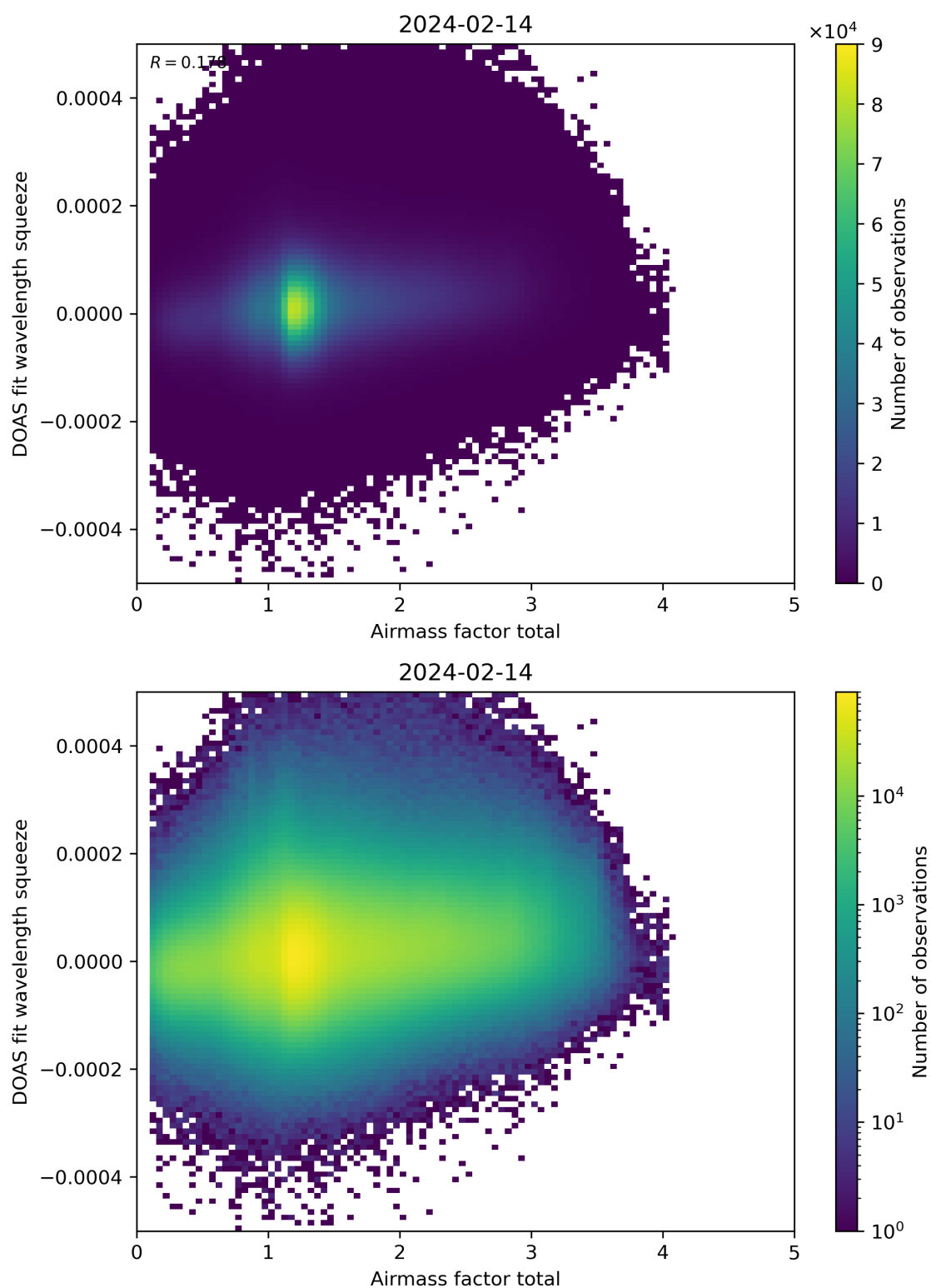
Figure 99: Scatter density plot of “Airmass factor total” against “DOAS fit wavelength squeeze” for 2024-02-13 to 2024-02-15.
