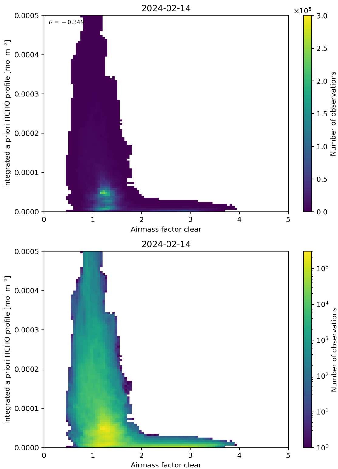
Figure 76: Scatter density plot of “Airmass factor clear” against “Integrated a priori HCHO profile” for 2024-02-13 to 2024-02-15.
