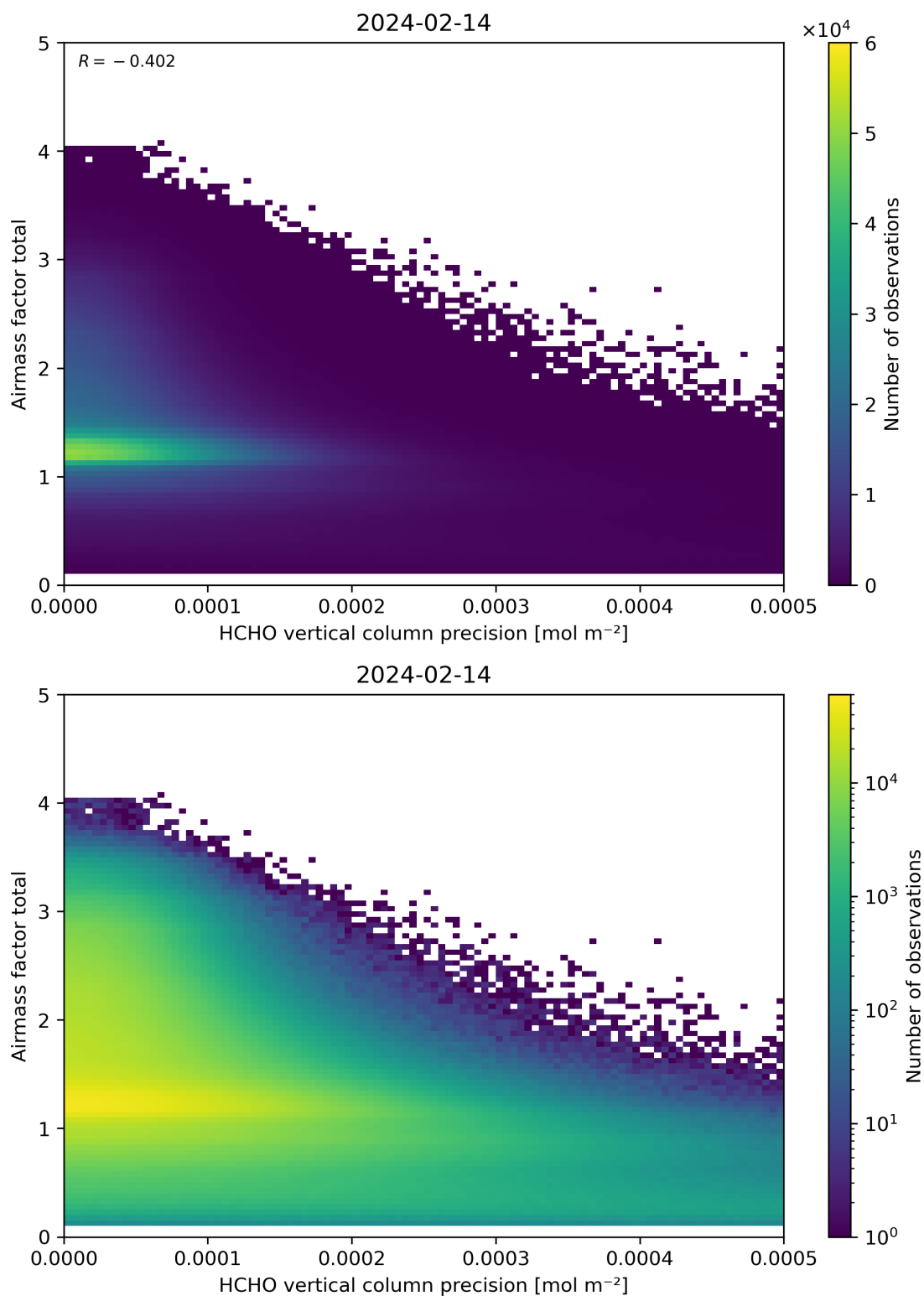
Figure 144: Scatter density plot of “HCHO vertical column precision” against “Airmass factor total” for 2024-02-13 to 2024-02-15.
