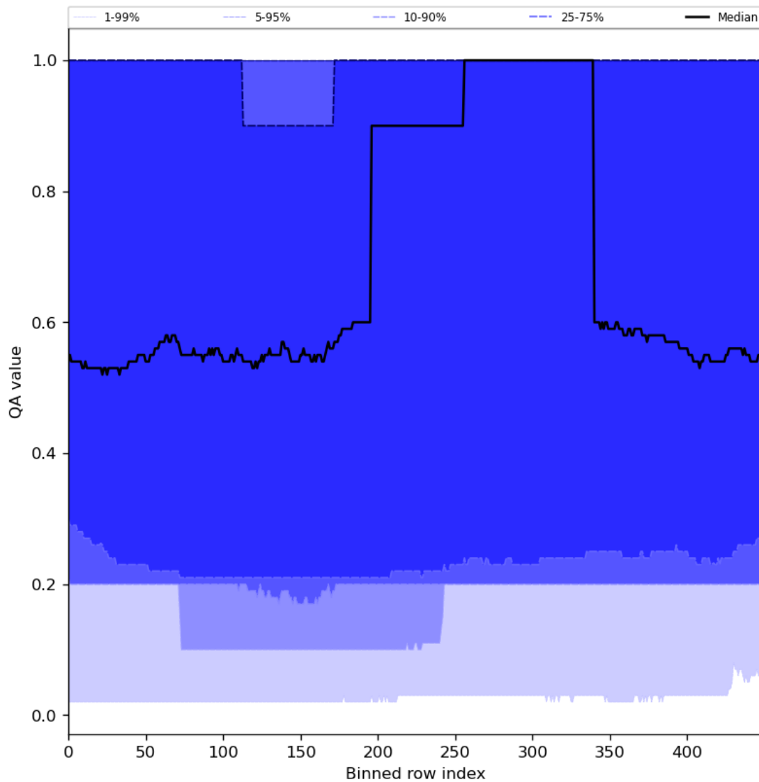
Figure 48: Along track statistics of “QA value” for 2024-02-13 to 2024-02-15
