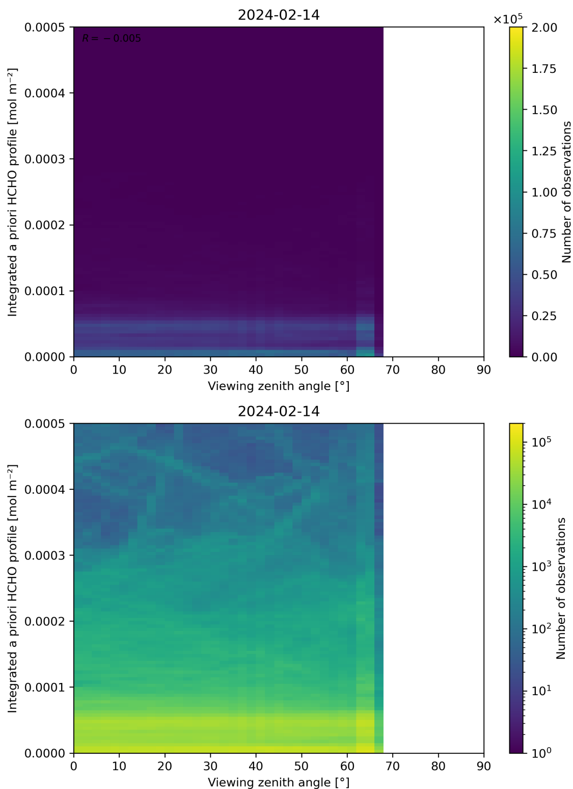
Figure 195: Scatter density plot of “Viewing zenith angle” against “Integrated a priori HCHO profile” for 2024-02-13 to 2024-02-15.
