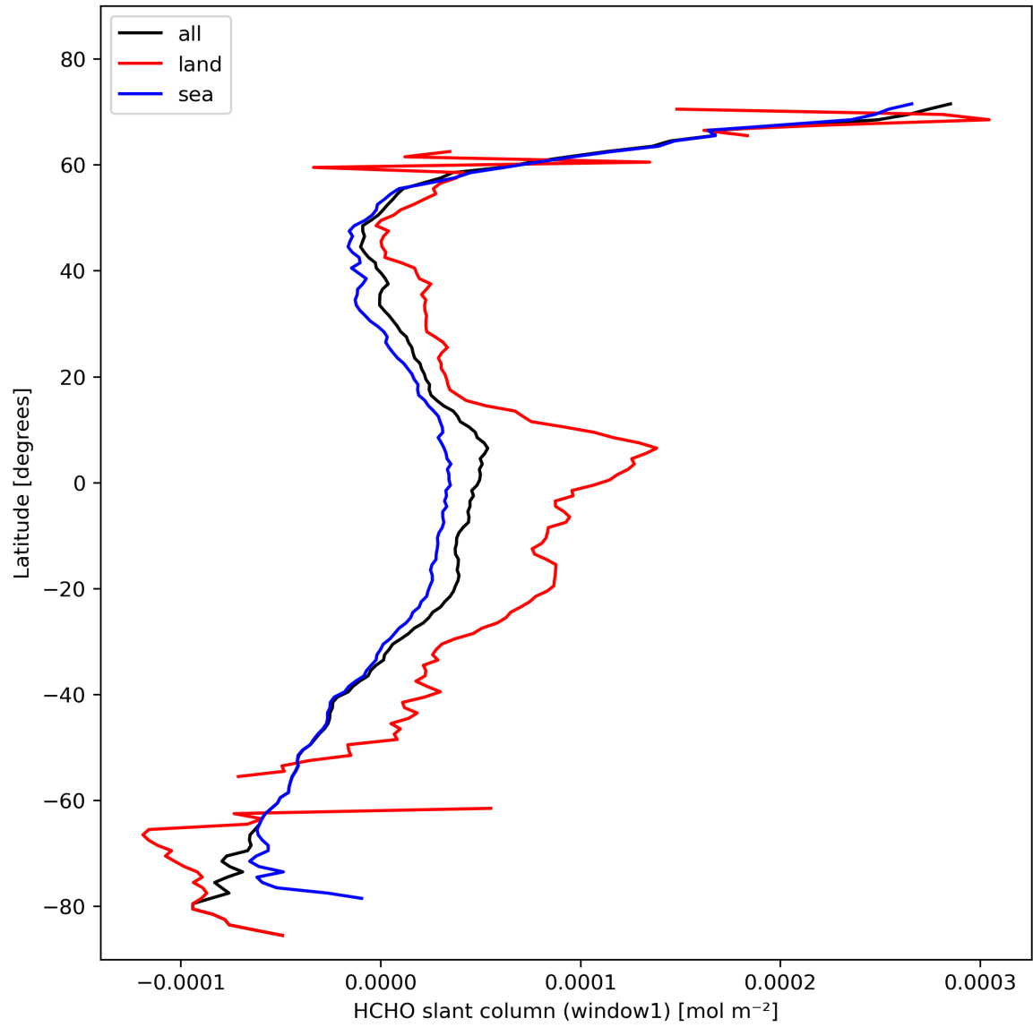
Figure 24: Zonal average of “HCHO slant column (window1)” for 2024-02-13 to 2024-02-15.
