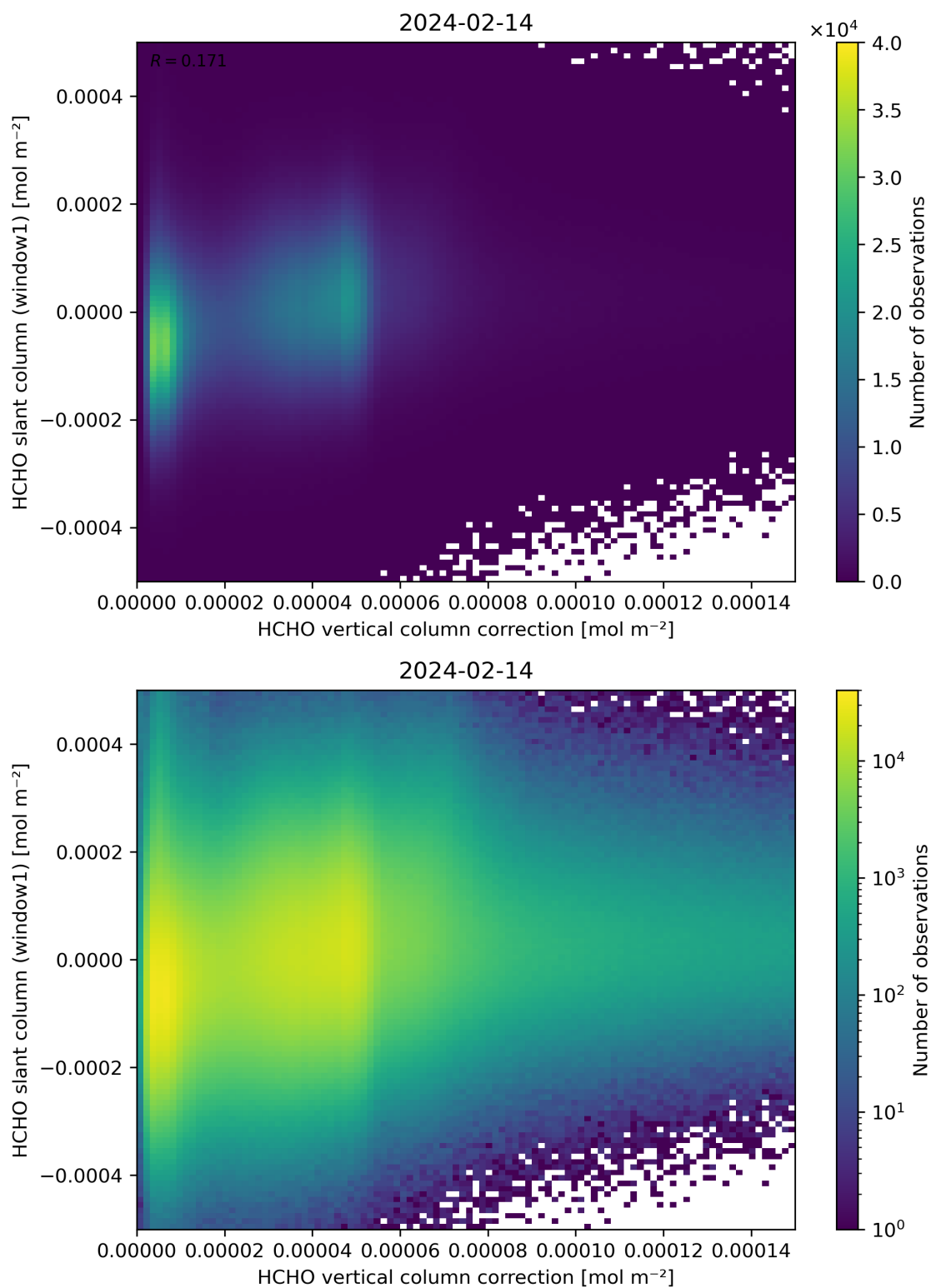
Figure 118: Scatter density plot of “HCHO vertical column correction” against “HCHO slant column (window1)” for 2024-02-13 to 2024-02-15.
