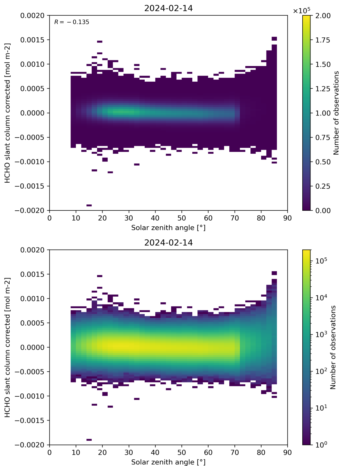
Figure 171: Scatter density plot of “Solar zenith angle” against “HCHO slant column corrected” for 2024-02-13 to 2024-02-15.
