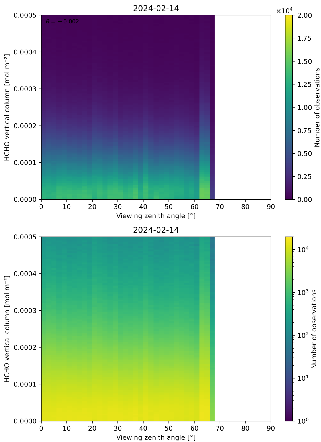
Figure 192: Scatter density plot of “Viewing zenith angle” against “HCHO vertical column” for 2024-02-13 to 2024-02-15.
