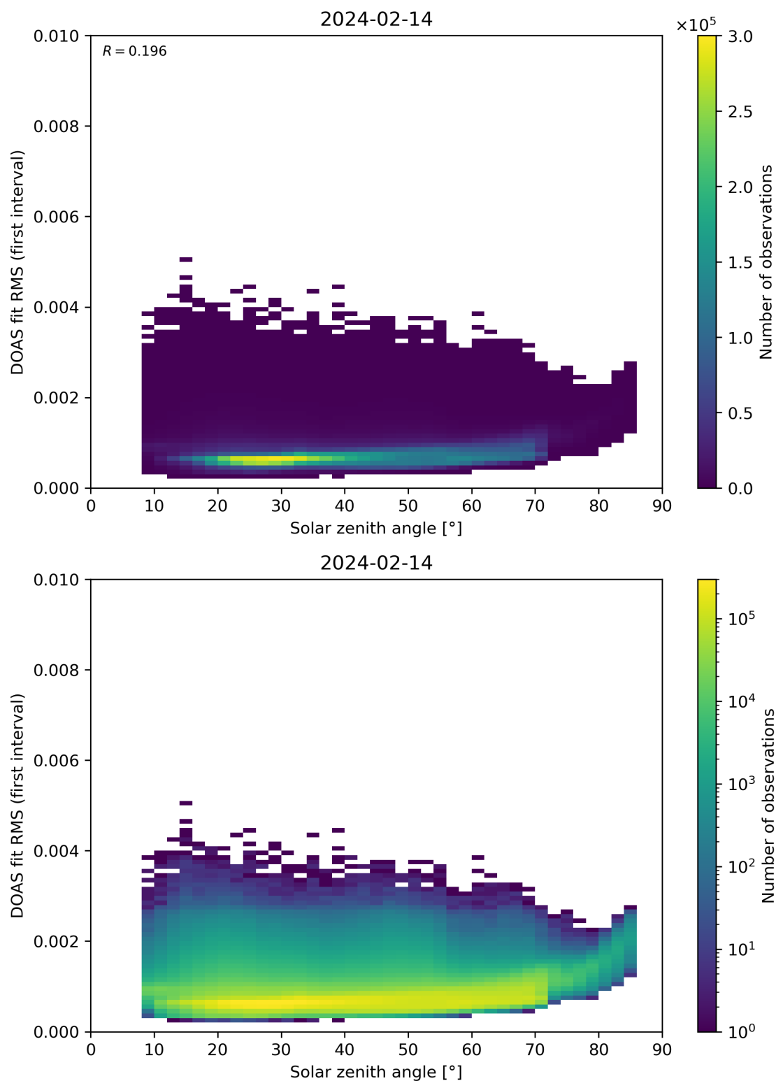
Figure 167: Scatter density plot of “Solar zenith angle” against “DOAS fit RMS (first interval)” for 2024-02-13 to 2024-02-15.
