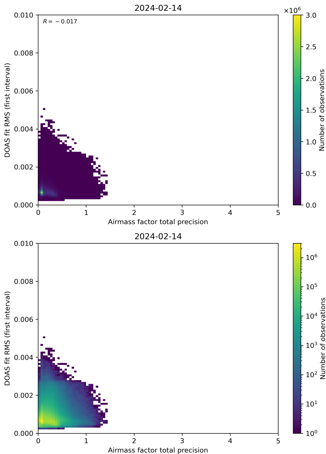
Figure 105: Scatter density plot of “Airmass factor total precision” against “DOAS fit RMS (first interval)” for 2024-02-13 to 2024-02-15.
