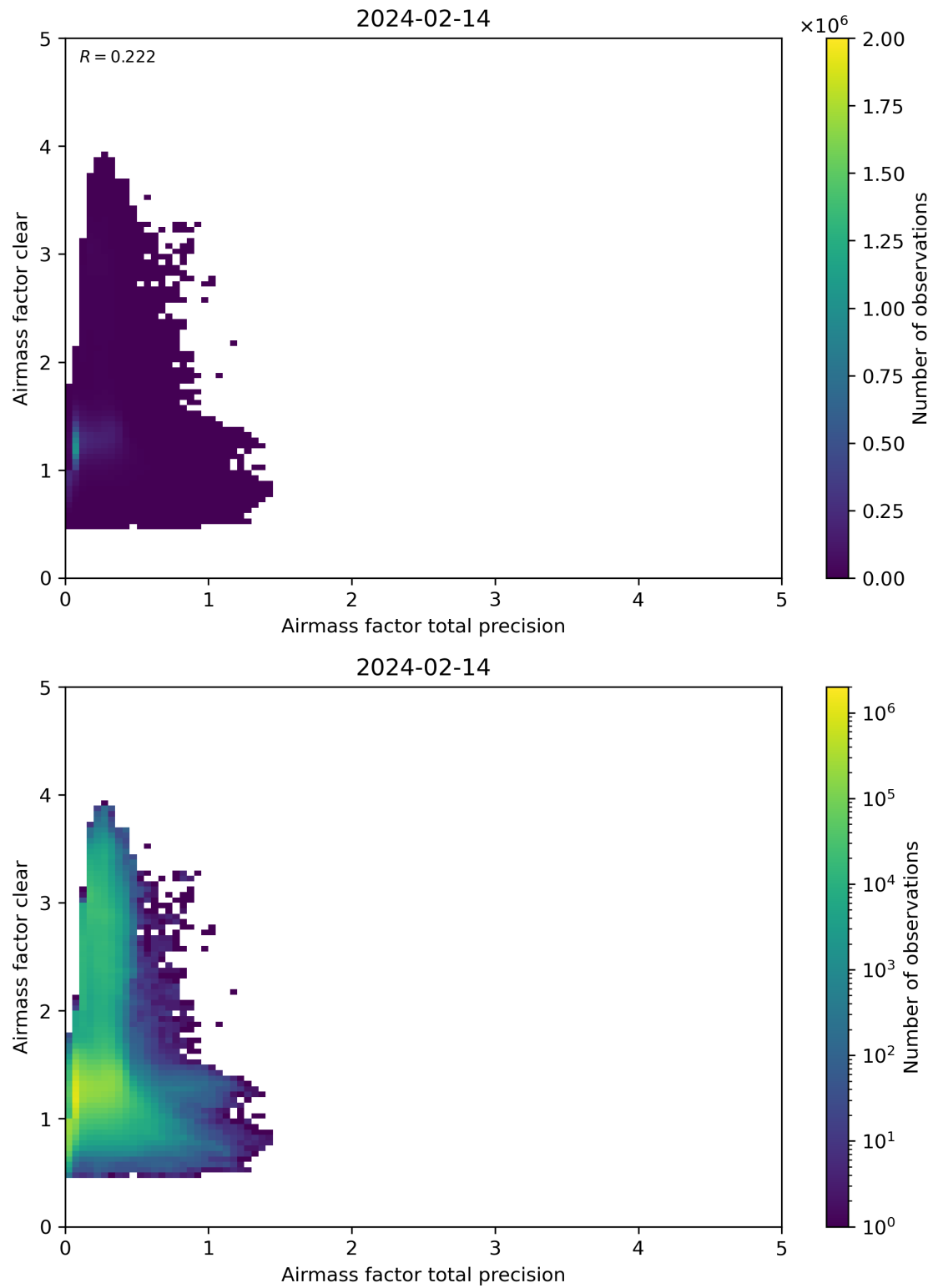
Figure 108: Scatter density plot of “Airmass factor total precision” against “Airmass factor clear” for 2024-02-13 to 2024-02-15.
