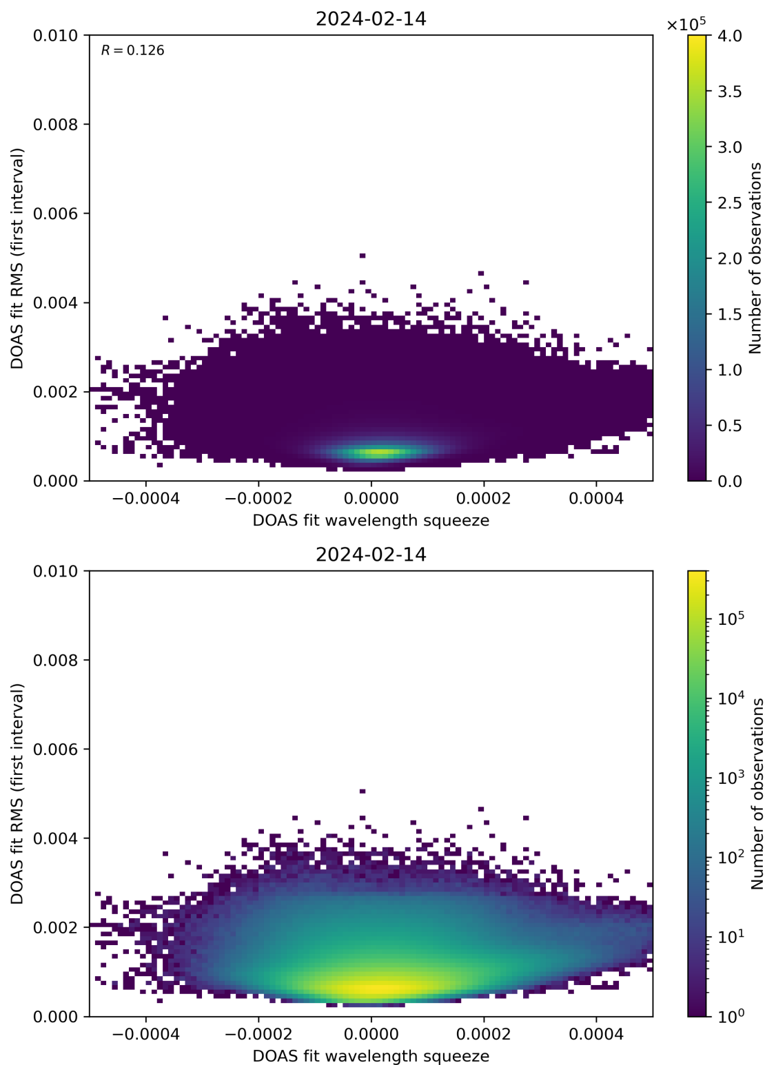
Figure 68: Scatter density plot of “DOAS fit wavelength squeeze” against “DOAS fit RMS (first interval)” for 2024-02-13 to 2024-02-15.
