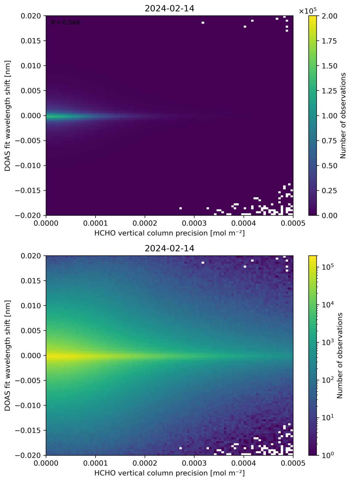
Figure 137: Scatter density plot of “HCHO vertical column precision” against “DOAS fit wavelength shift” for 2024-02-13 to 2024-02-15.
