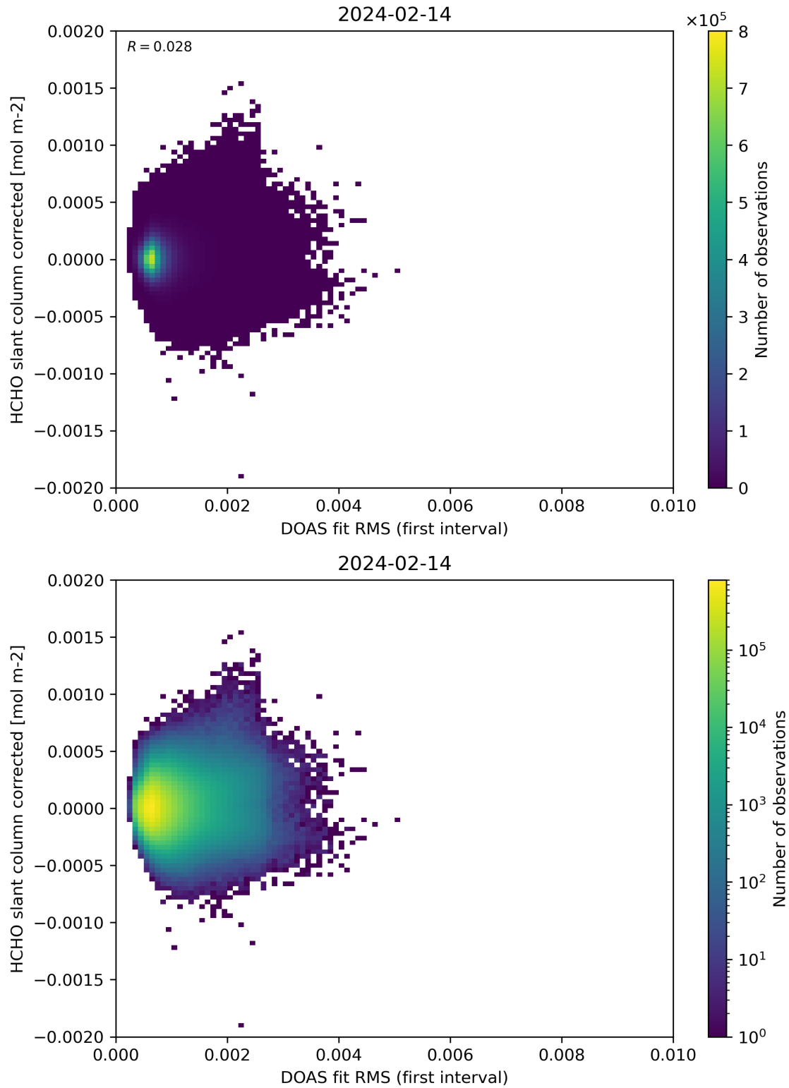
Figure 62: Scatter density plot of “DOAS fit RMS (first interval)” against “HCHO slant column corrected” for 2024-02-13 to 2024-02-15.
