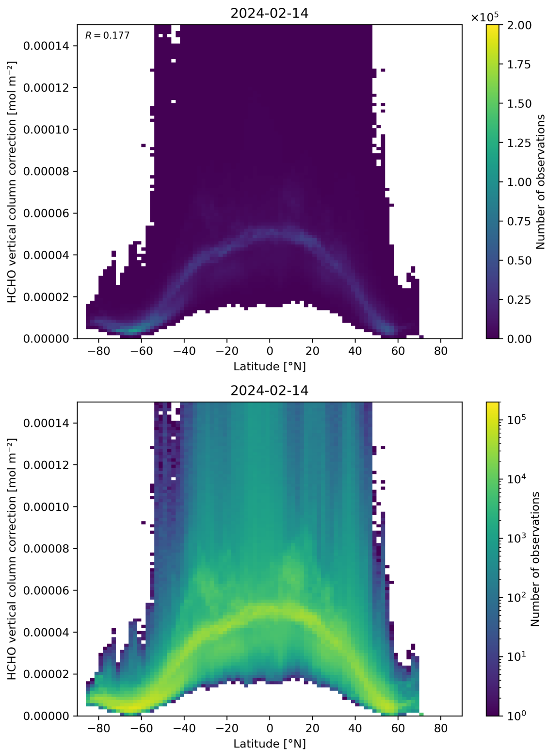
Figure 164: Scatter density plot of “Latitude” against “HCHO vertical column correction” for 2024-02-13 to 2024-02-15.
