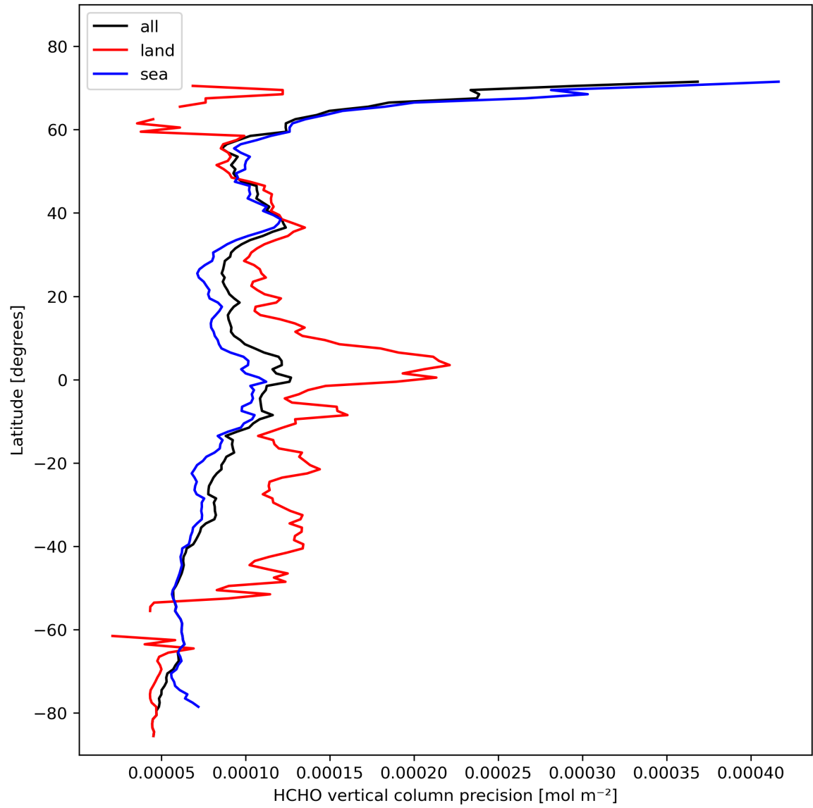
Figure 22: Zonal average of “HCHO vertical column precision” for 2024-02-13 to 2024-02-15.
