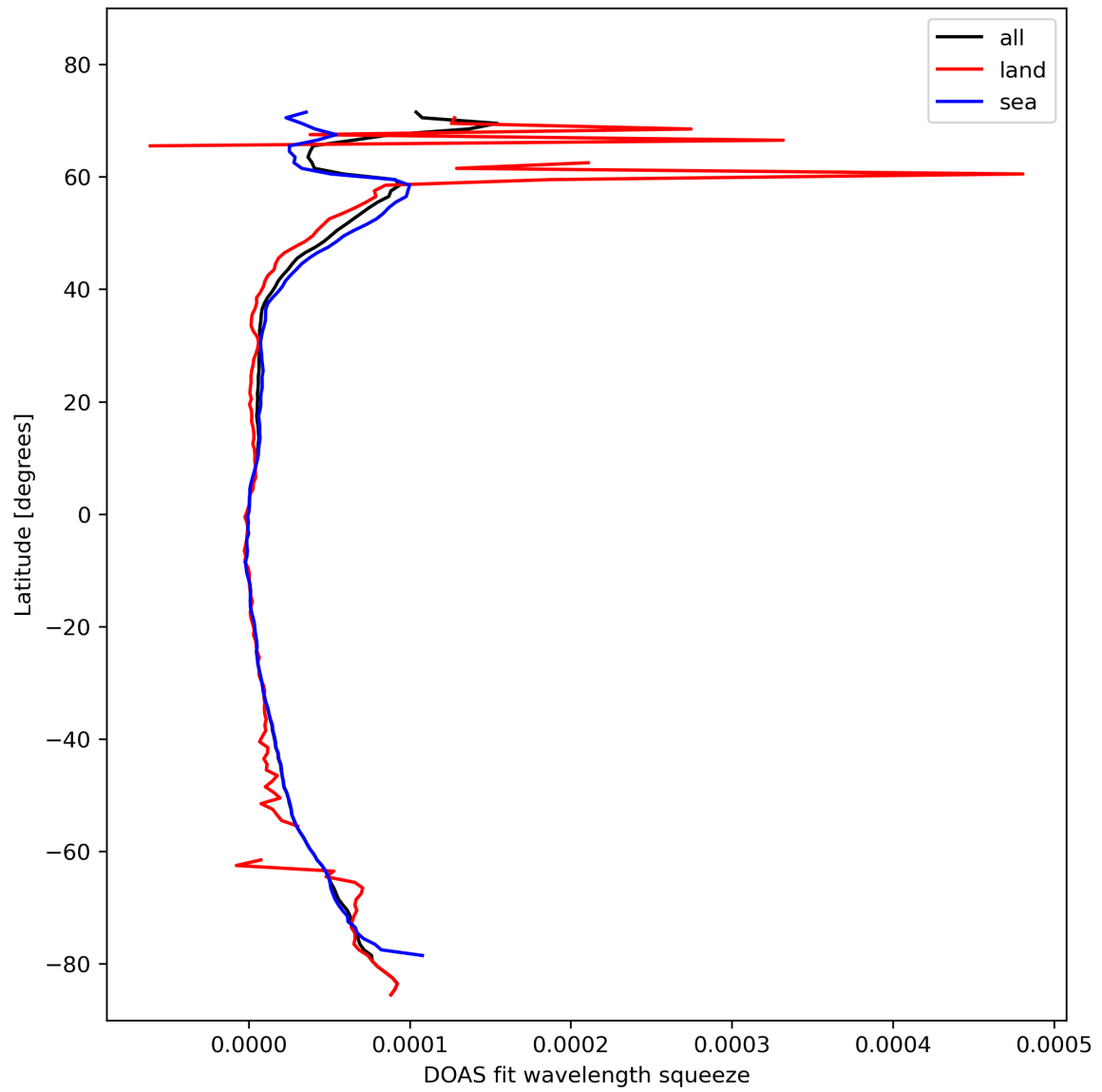
Figure 31: Zonal average of “DOAS fit wavelength squeeze” for 2024-02-13 to 2024-02-15.
