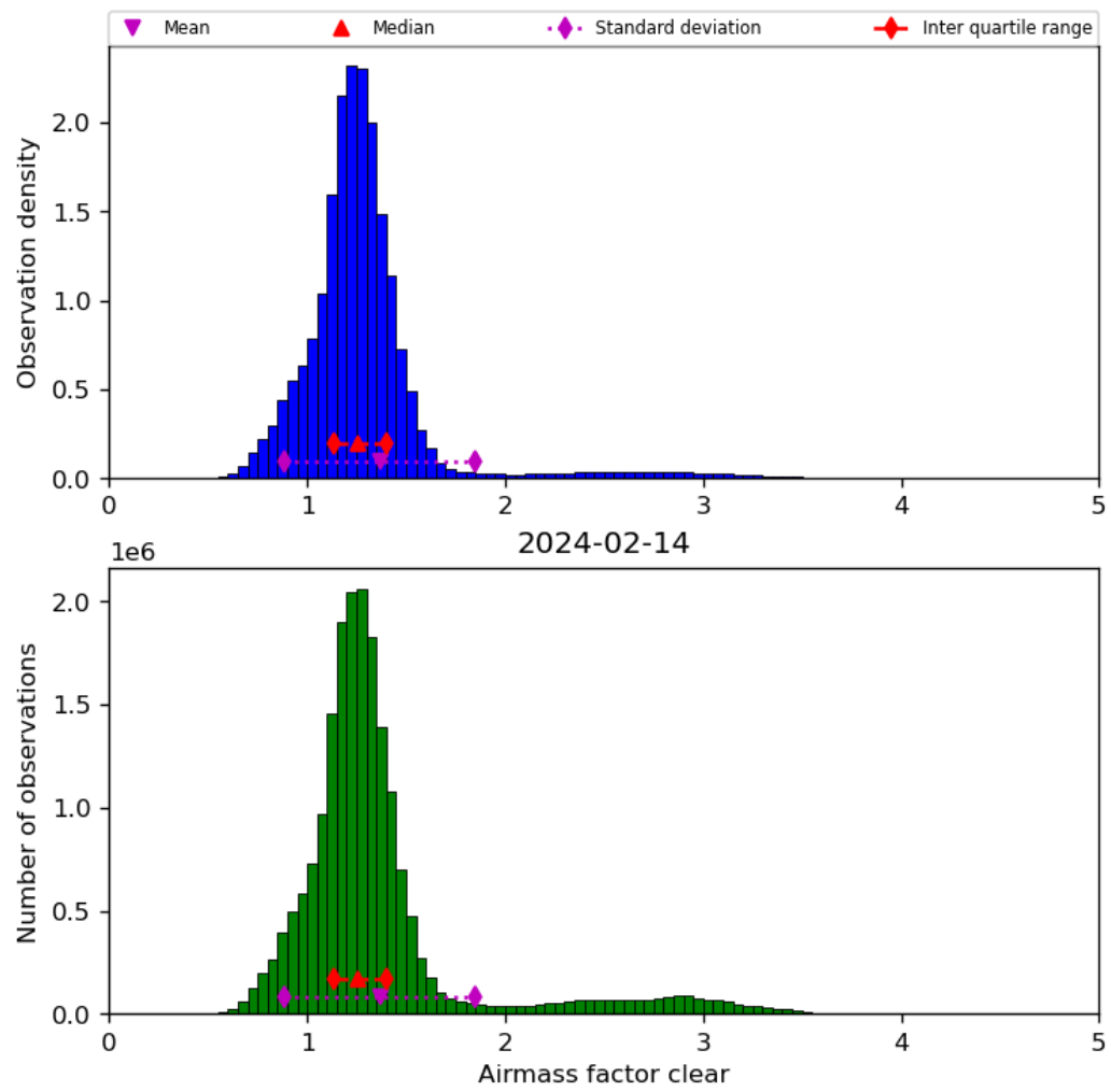
Figure 42: Histogram of “Airmass factor clear” for 2024-02-13 to 2024-02-15
