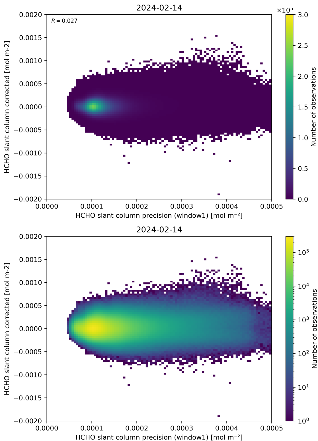
Figure 92: Scatter density plot of “HCHO slant column precision (window1)” against “HCHO slant column corrected” for 2024-02-13 to 2024-02-15.
