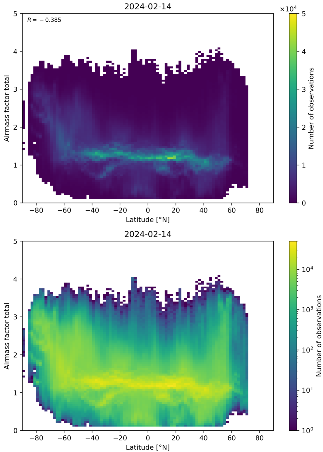
Figure 161: Scatter density plot of “Latitude” against “Airmass factor total” for 2024-02-13 to 2024-02-15.
