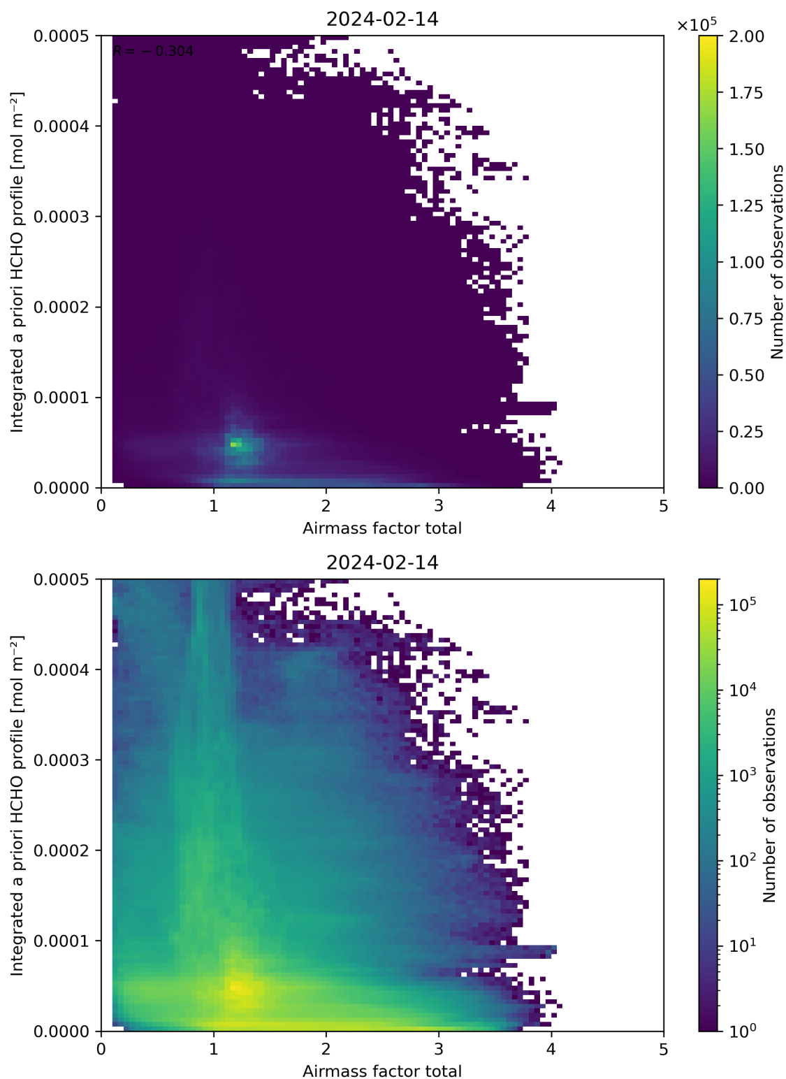
Figure 104: Scatter density plot of “Air mass factor total” against “Integrated a priori HCHO profile” for 2024-02-13 to 2024-02-15.
