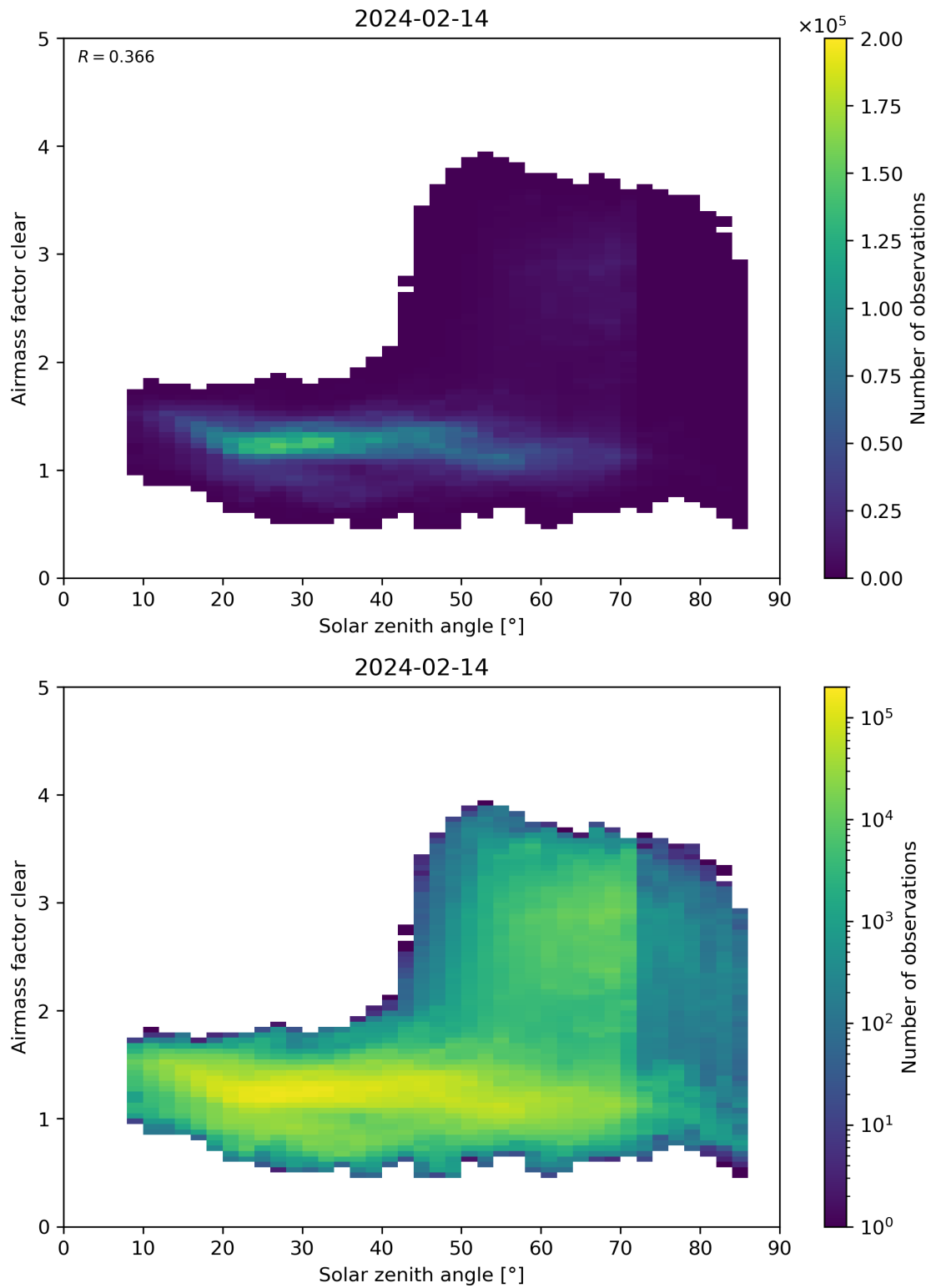
Figure 170: Scatter density plot of “Solar zenith angle” against “Airmass factor clear” for 2024-02-13 to 2024-02-15.
