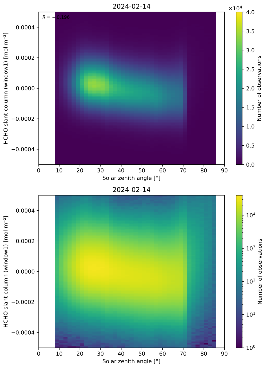
Figure 173: Scatter density plot of “Solar zenith angle” against “HCHO slant column (window1)” for 2024-02-13 to 2024-02-15.
