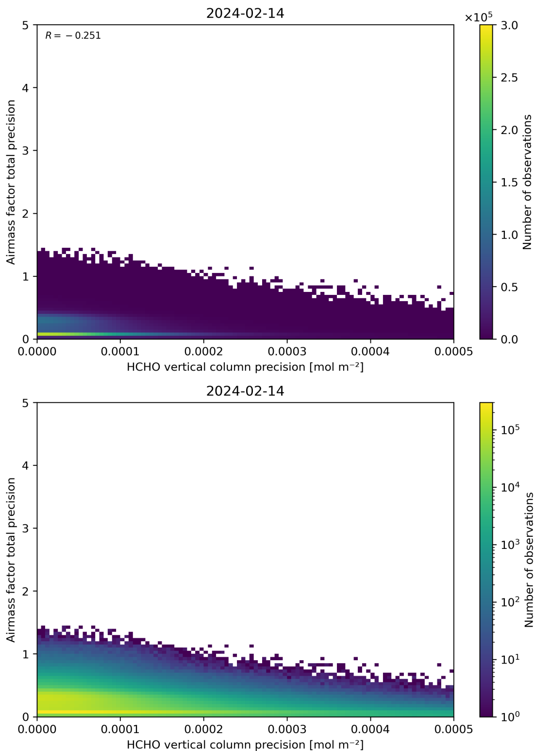
Figure 145: Scatter density plot of “HCHO vertical column precision” against “Airmass factor total precision” for 2024-02-13 to 2024-02-15.
