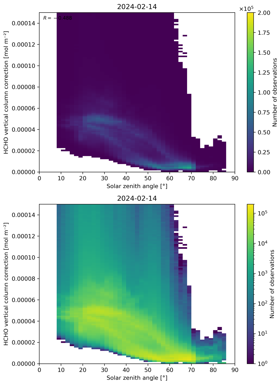
Figure 178: Scatter density plot of “Solar zenith angle” against “HCHO vertical column correction” for 2024-02-13 to 2024-02-15.
