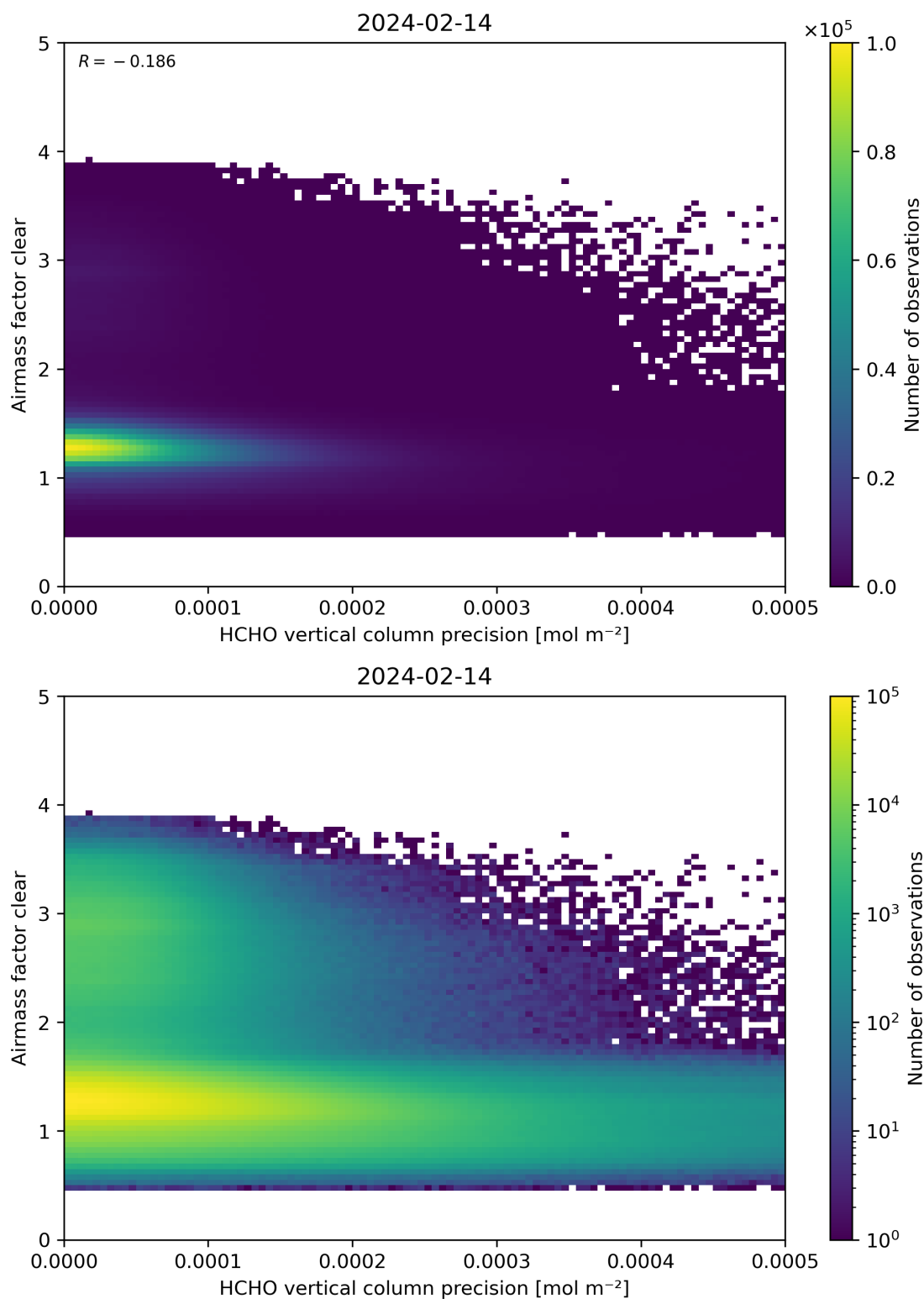
Figure 139: Scatter density plot of “HCHO vertical column precision” against “Airmass factor clear” for 2024-02-13 to 2024-02-15.
