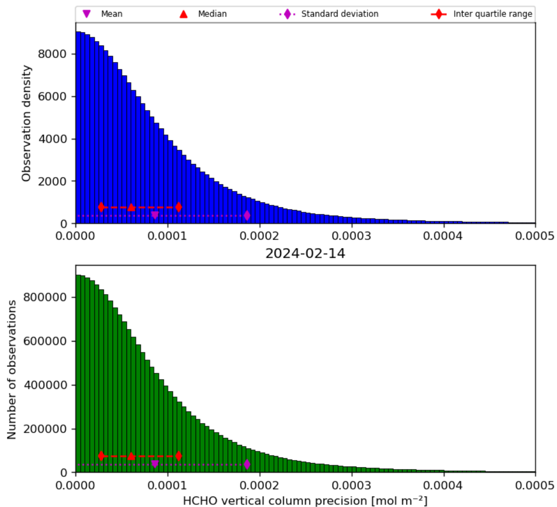
Figure 36: Histogram of “HCHO vertical column precision” for 2024-02-13 to 2024-02-15
