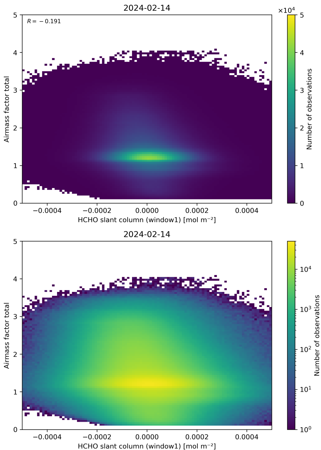
Figure 85: Scatter density plot of “HCHO slant column (window1)” against “Airmass factor total” for 2024-02-13 to 2024-02-15.
