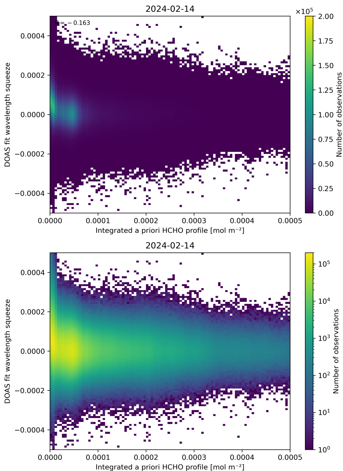
Figure 150: Scatter density plot of “Integrated a priori HCHO profile” against “DOAS fit wavelength squeeze” for 2024-02-13 to 2024-02-15.
