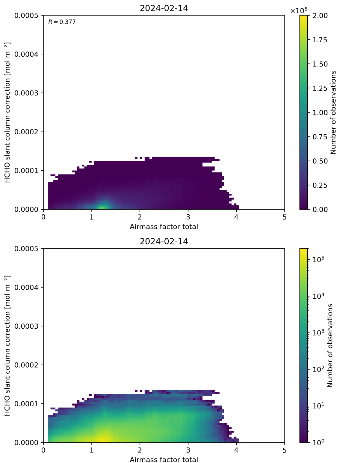
Figure 102: Scatter density plot of “Airmass factor total” against “HCHO slant column correction” for 2024-02-13 to 2024-02-15.
