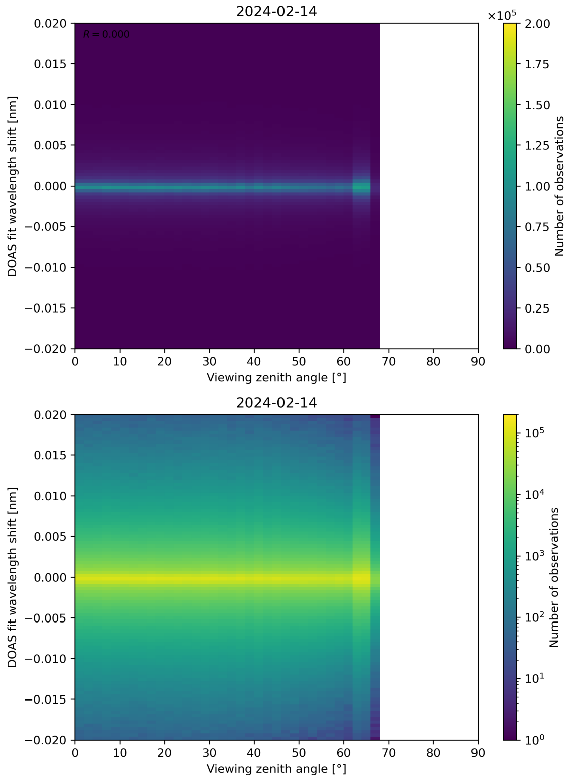
Figure 183: Scatter density plot of “Viewing zenith angle” against “DOAS fit wavelength shift” for 2024-02-13 to 2024-02-15.
