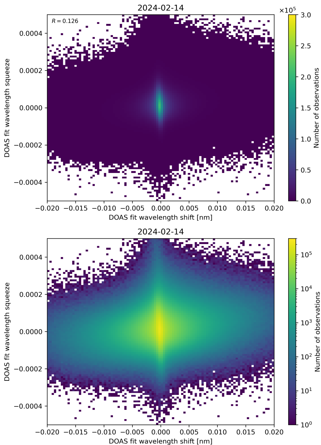
Figure 65: Scatter density plot of “DOAS fit wavelength shift” against “DOAS fit wavelength squeeze” for 2024-02-13 to 2024-02-15.
