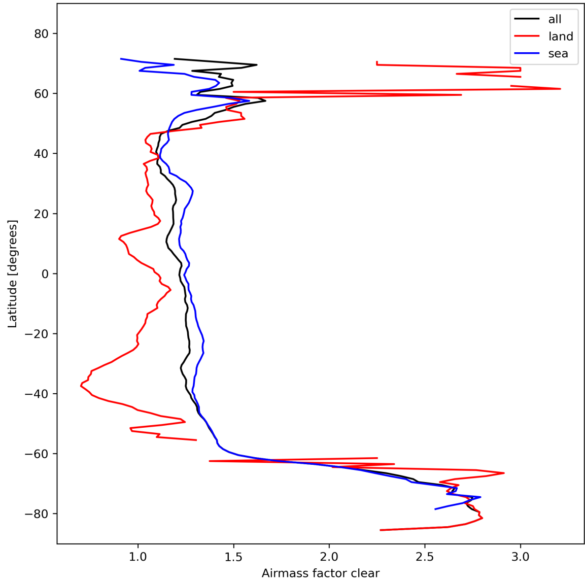
Figure 28: Zonal average of “Airmass factor clear” for 2024-02-13 to 2024-02-15.
