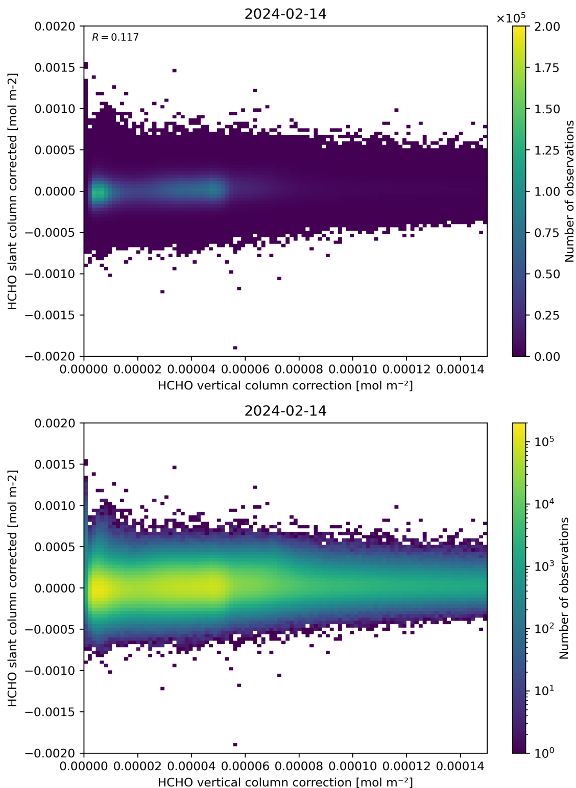
Figure 116: Scatter density plot of “HCHO vertical column correction” against “HCHO slant column corrected” for 2024-02-13 to 2024-02-15.
