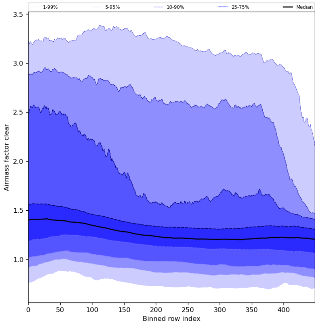
Figure 56: Along track statistics of “Airmass factor clear” for 2024-02-13 to 2024-02-15
