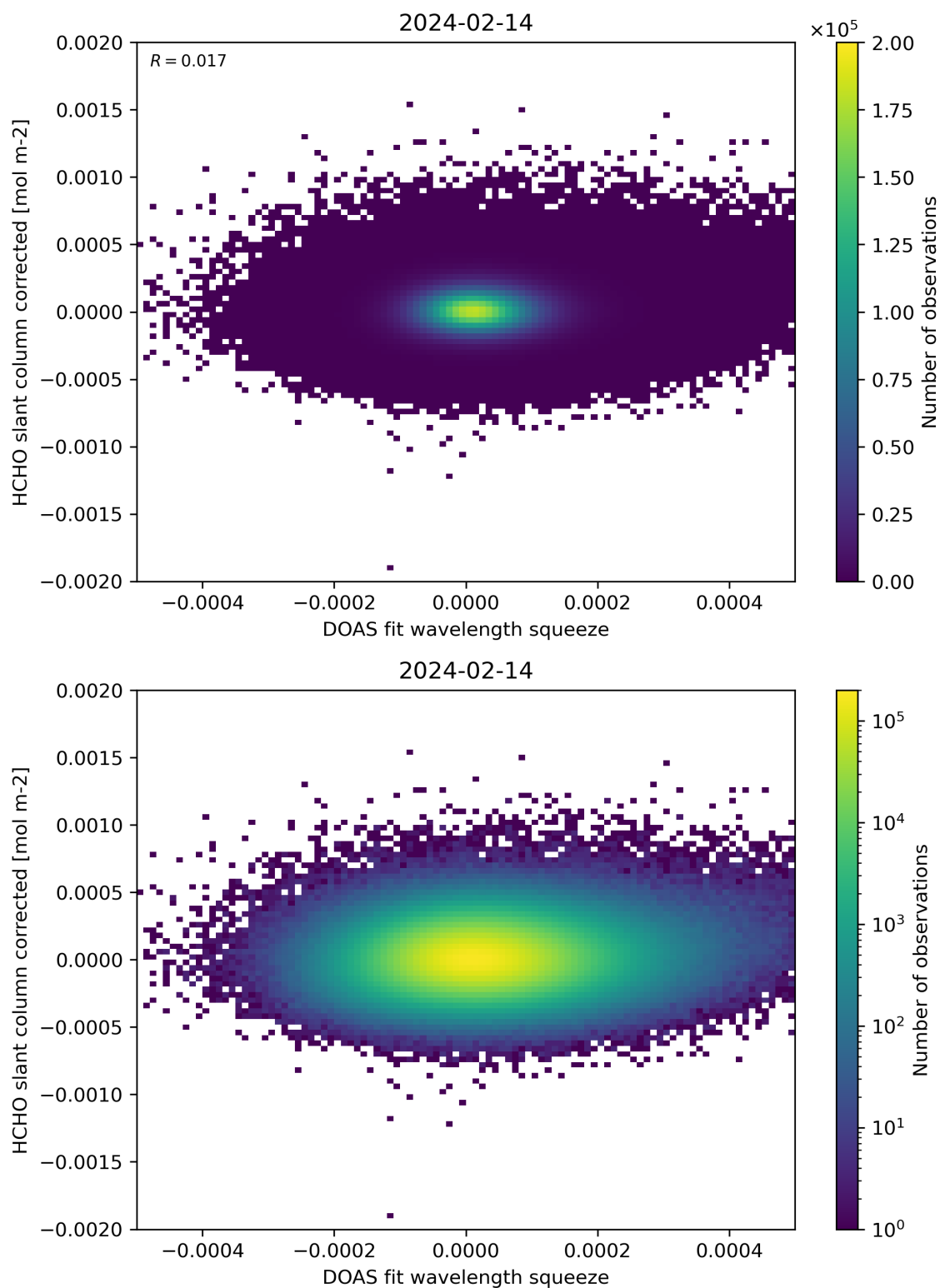
Figure 69: Scatter density plot of “DOAS fit wavelength squeeze” against “HCHO slant column corrected” for 2024-02-13 to 2024-02-15.
