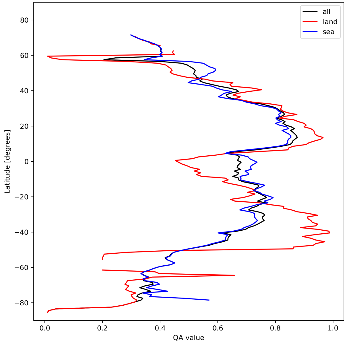
Figure 20: Zonal average of “QA value” for 2024-02-13 to 2024-02-15.
