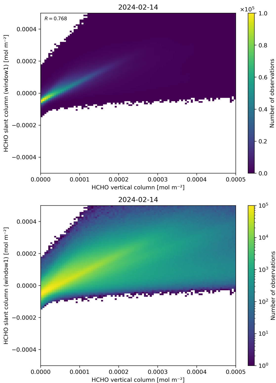
Figure 129: Scatter density plot of “HCHO vertical column” against “HCHO slant column (window1)” for 2024-02-13 to 2024-02-15.
