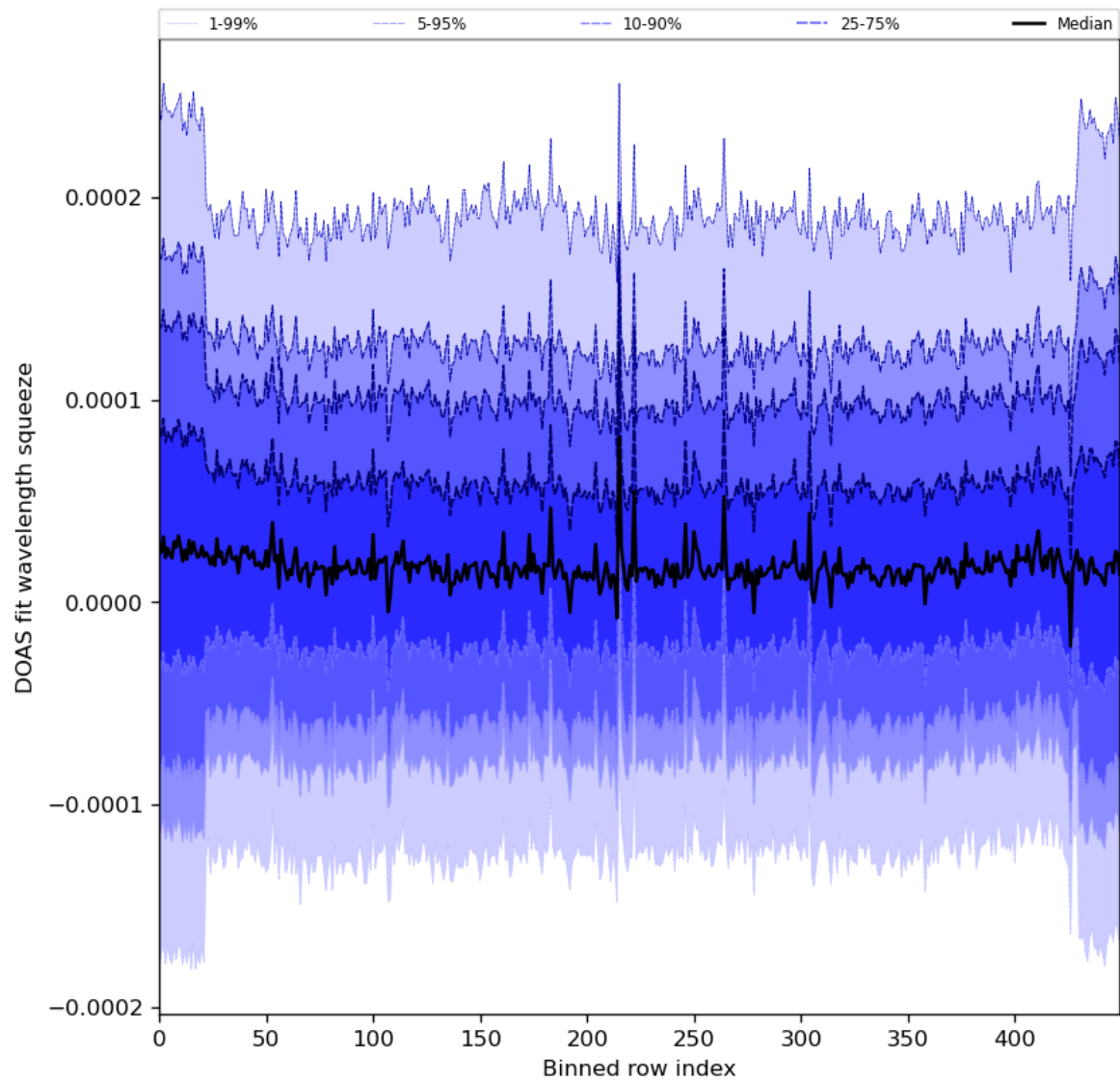
Figure 59: Along track statistics of “DOAS fit wavelength squeeze” for 2024-02-13 to 2024-02-15
