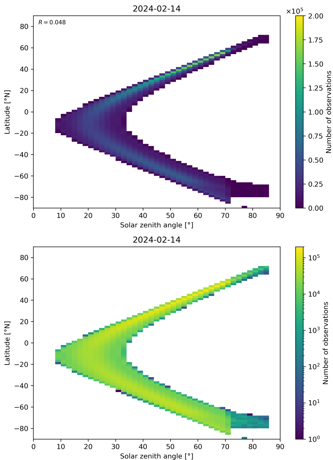
Figure 181: Scatter density plot of “Solar zenith angle” against “Latitude” for 2024-02-13 to 2024-02-15.
