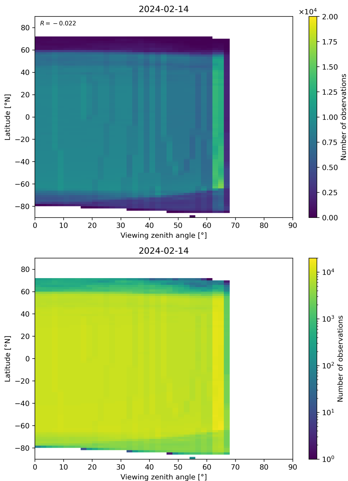
Figure 196: Scatter density plot of “Viewing zenith angle” against “Latitude” for 2024-02-13 to 2024-02-15.
