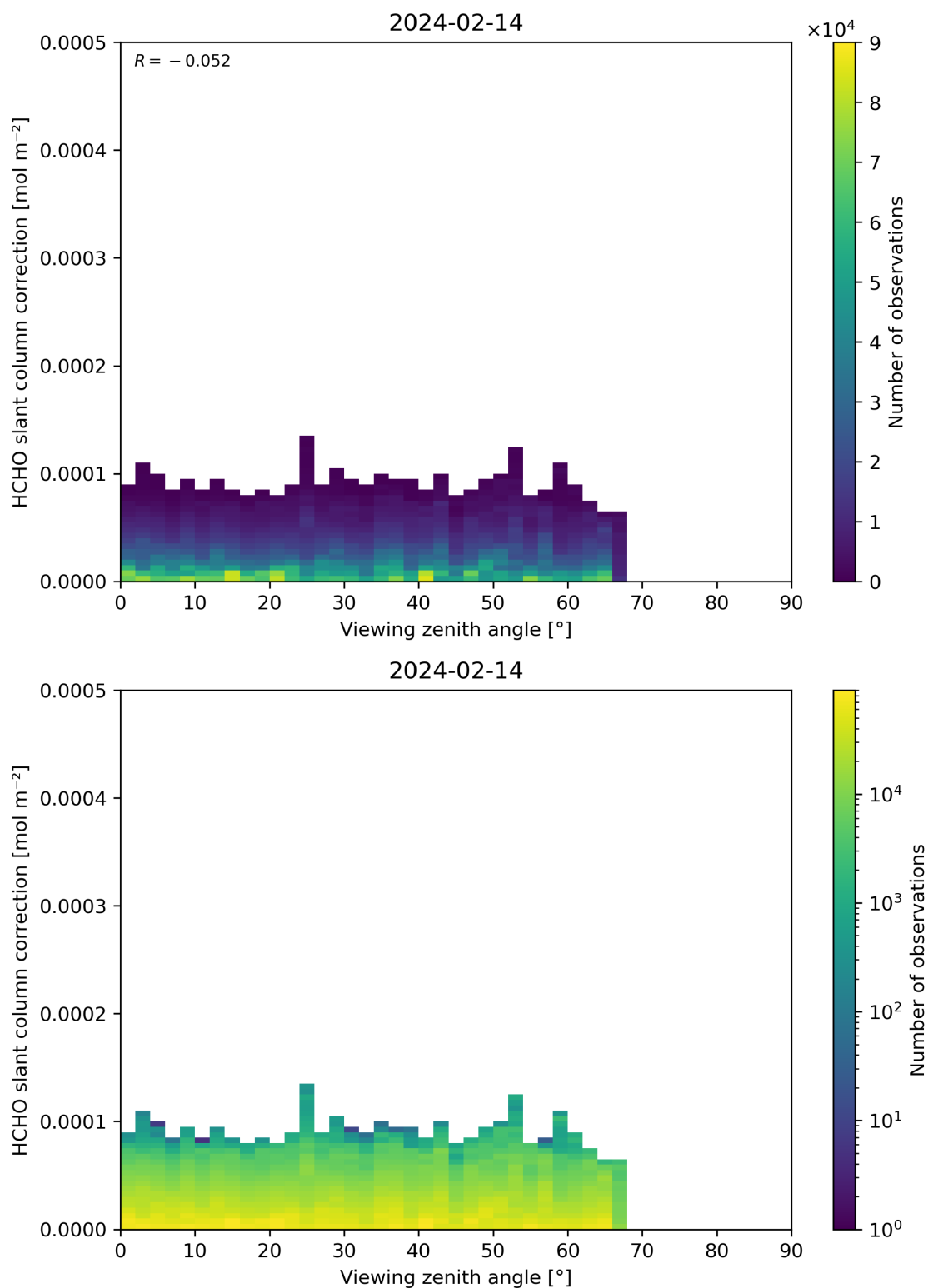
Figure 187: Scatter density plot of “Viewing zenith angle” against “HCHO slant column correction” for 2024-02-13 to 2024-02-15.
