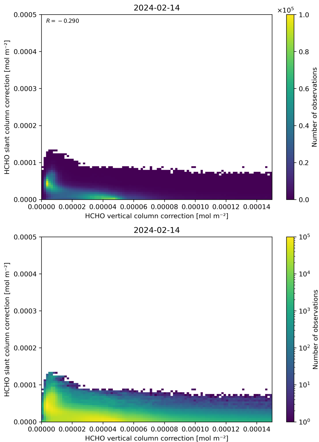
Figure 117: Scatter density plot of “HCHO vertical column correction” against “HCHO slant column correction” for 2024-02-13 to 2024-02-15.
