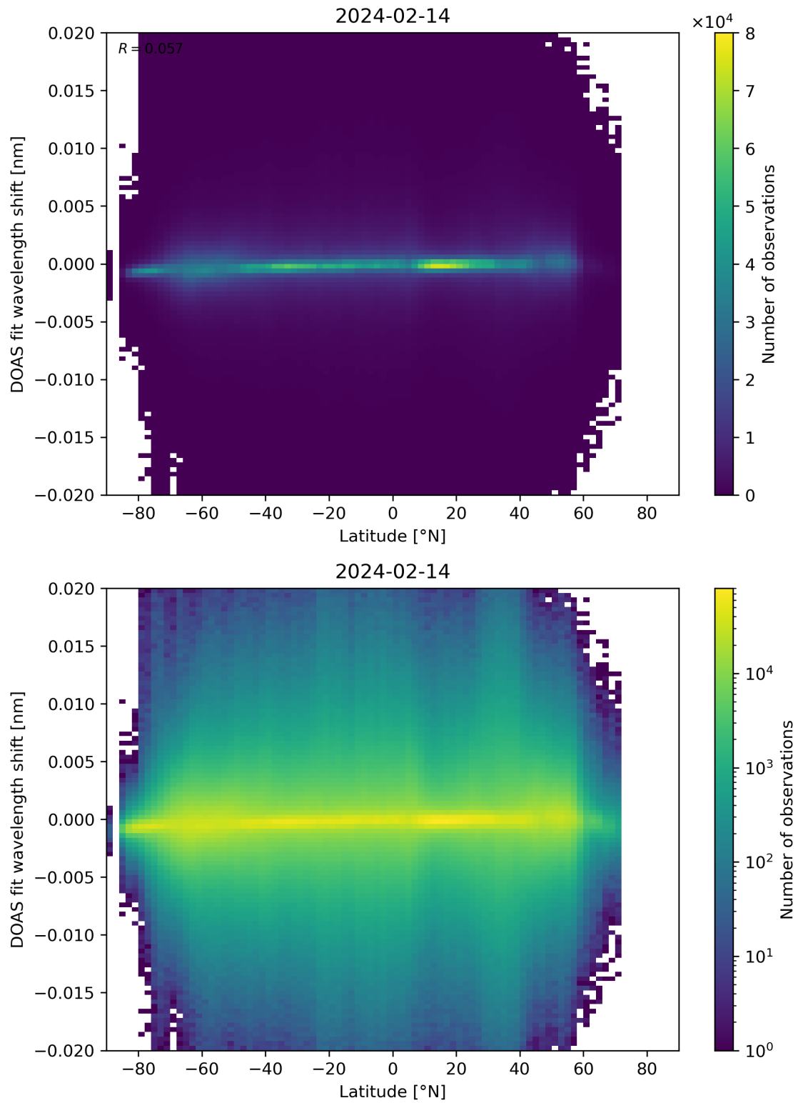
Figure 154: Scatter density plot of “Latitude” against “DOAS fit wavelength shift” for 2024-02-13 to 2024-02-15.
