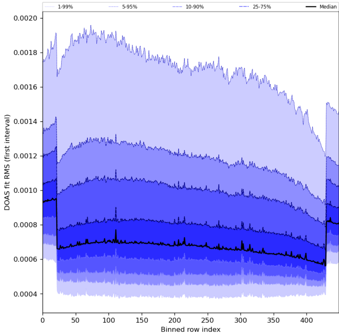
Figure 60: Along track statistics of “DOAS fit RMS (first interval)” for 2024-02-13 to 2024-02-15
