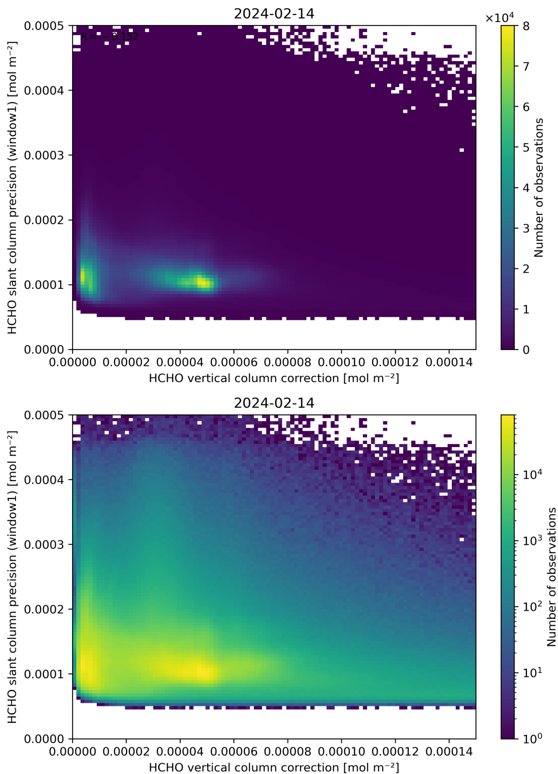
Figure 119: Scatter density plot of “HCHO vertical column correction” against “HCHO slant column precision (window1)” for 2024-02-13 to 2024-02-15.
