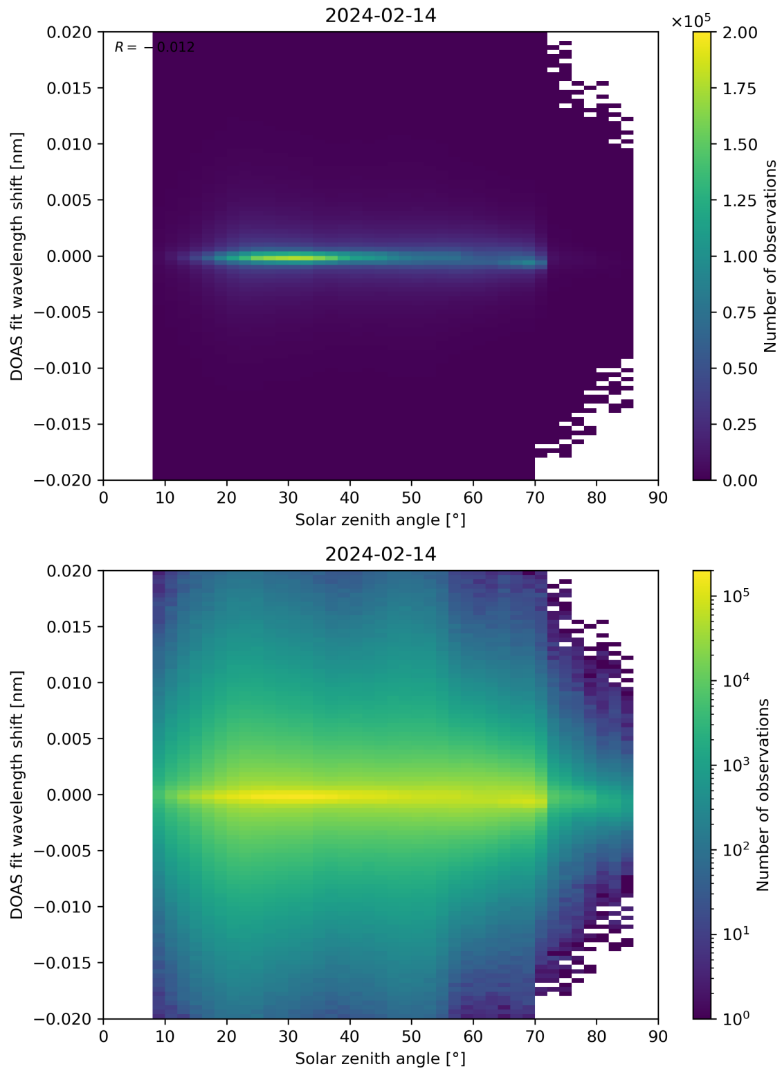
Figure 168: Scatter density plot of “Solar zenith angle” against “DOAS fit wavelength shift” for 2024-02-13 to 2024-02-15.
