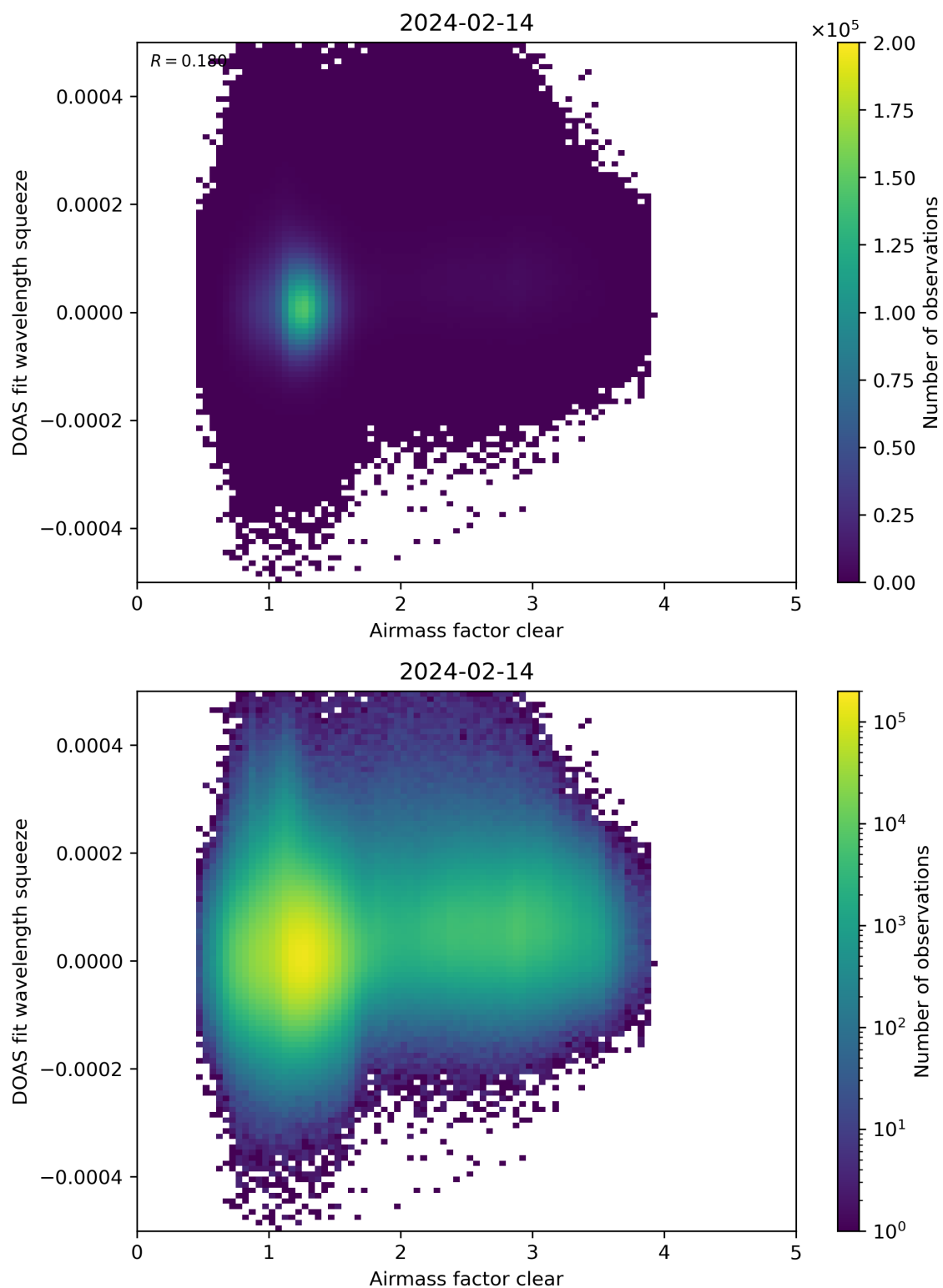
Figure 73: Scatter density plot of “Airmass factor clear” against “DOAS fit wavelength squeeze” for 2024-02-13 to 2024-02-15.
