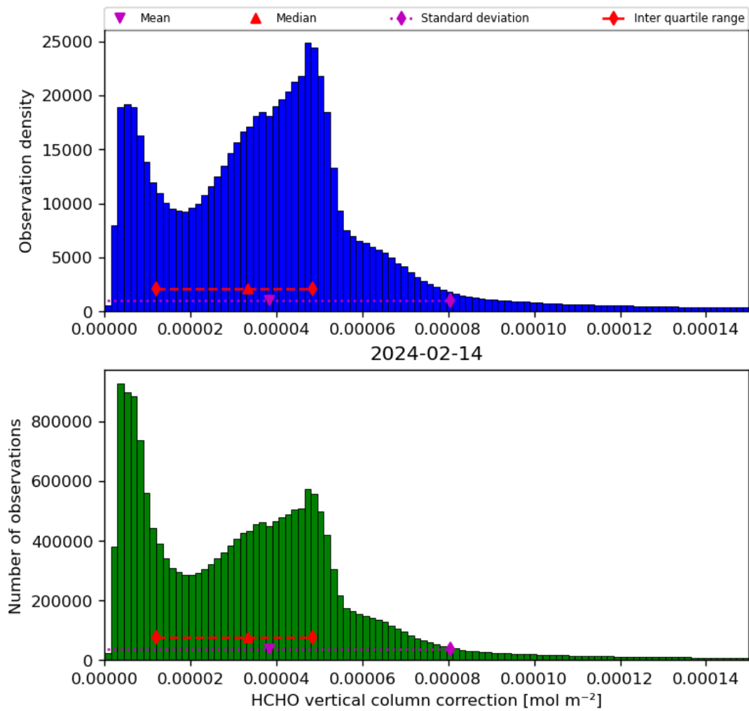
Figure 37: Histogram of “HCHO vertical column correction” for 2024-02-13 to 2024-02-15
