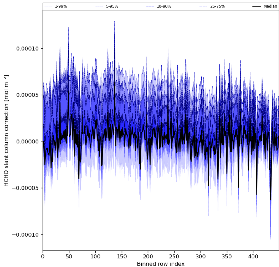
Figure 61: Along track statistics of “HCHO slant column correction” for 2024-02-13 to 2024-02-15
