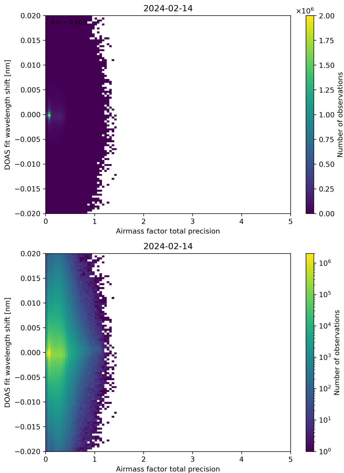
Figure 106: Scatter density plot of “Airmass factor total precision” against “DOAS fit wavelength shift” for 2024-02-13 to 2024-02-15.
