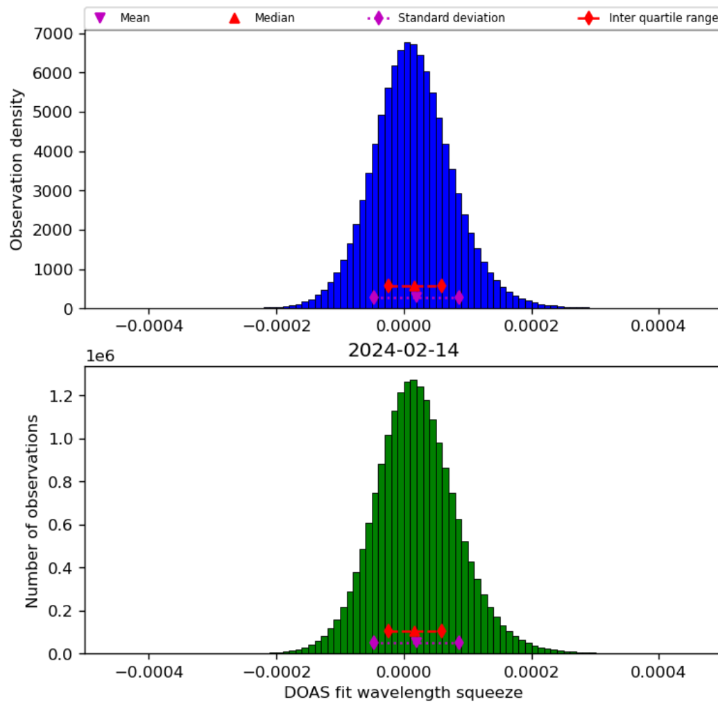
Figure 45: Histogram of “DOAS fit wavelength squeeze” for 2024-02-13 to 2024-02-15
