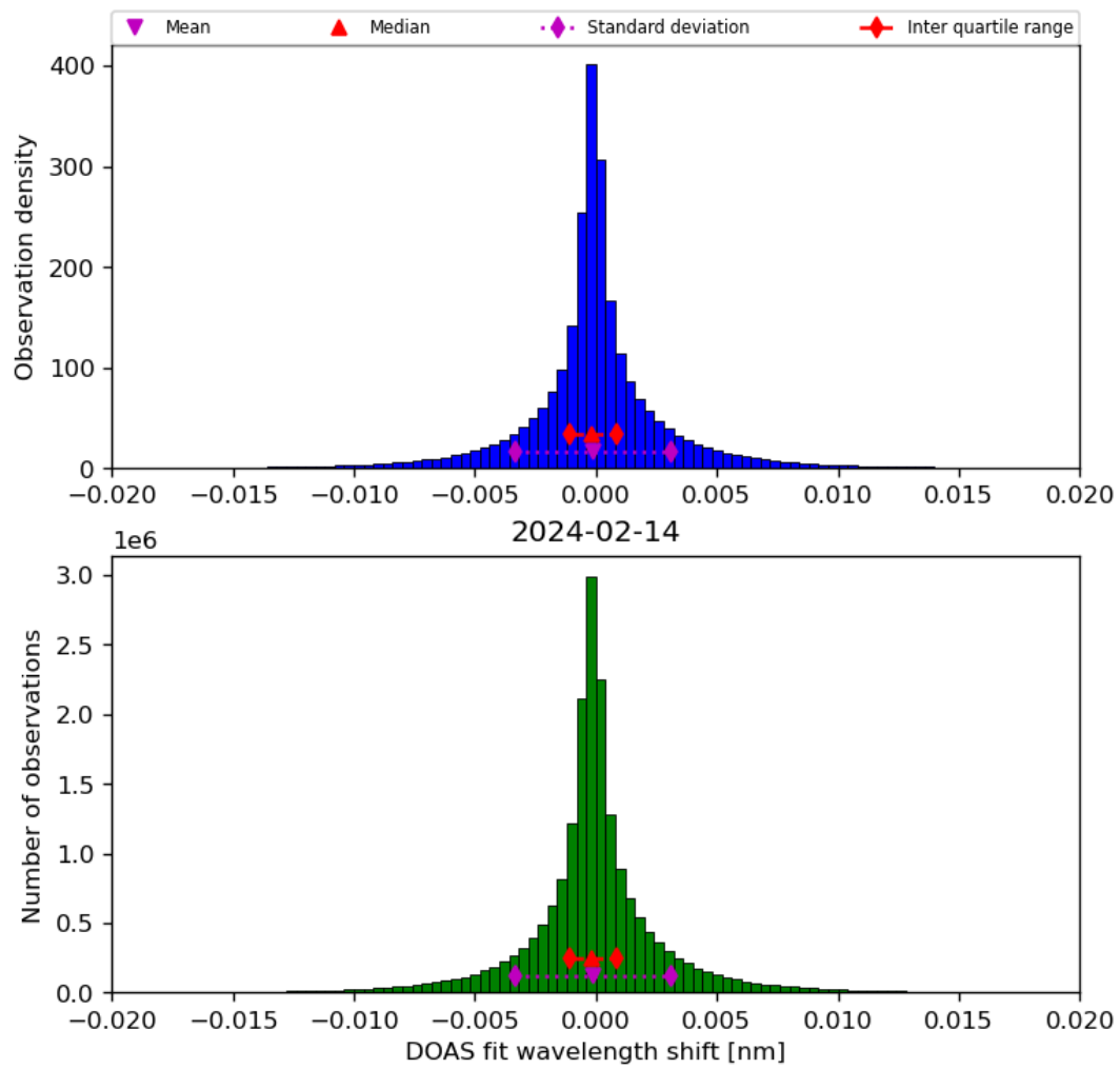
Figure 44: Histogram of “DOAS fit wavelength shift” for 2024-02-13 to 2024-02-15
