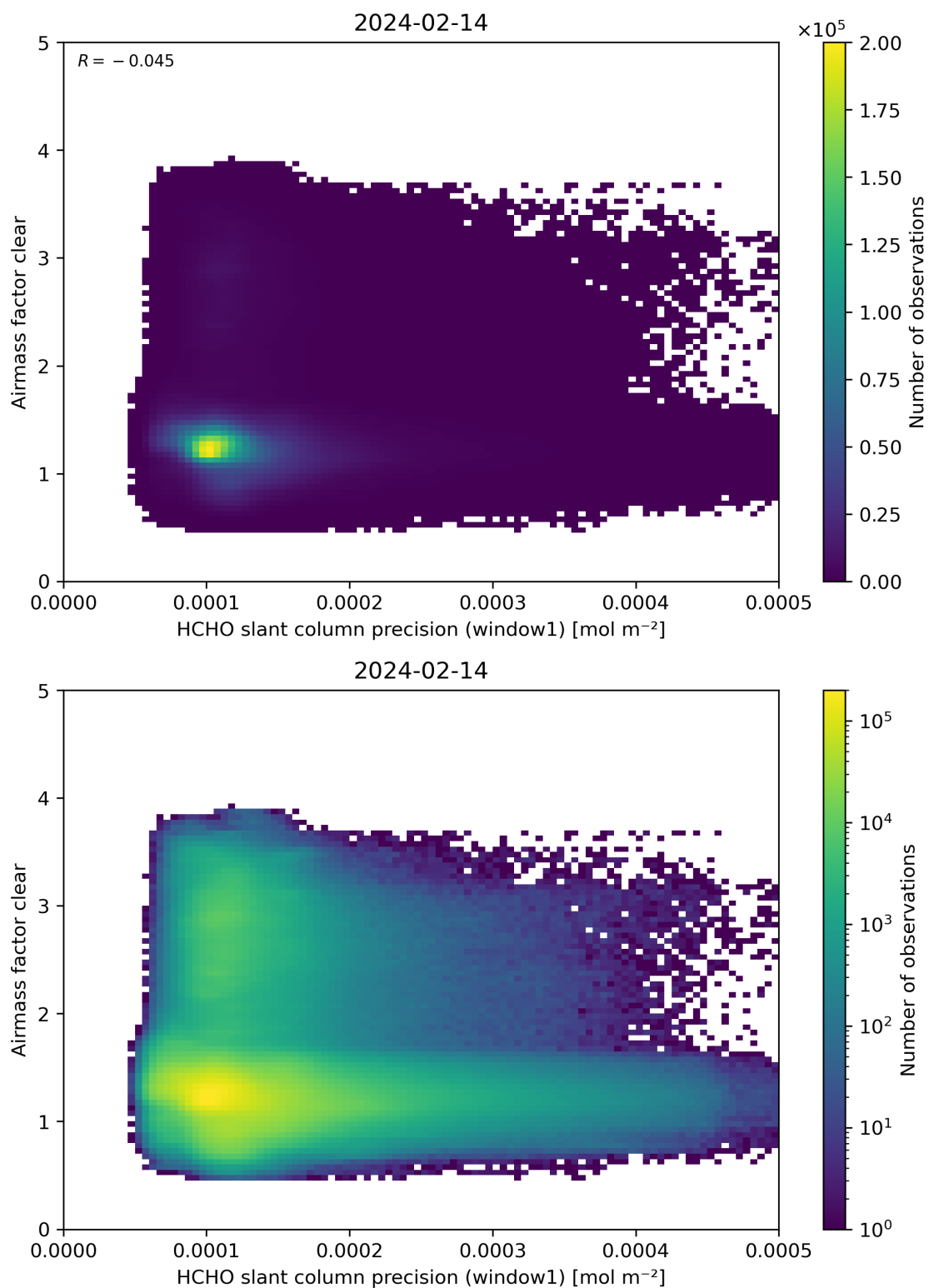
Figure 91: Scatter density plot of “HCHO slant column precision (window1)” against “Airmass factor clear” for 2024-02-13 to 2024-02-15.
