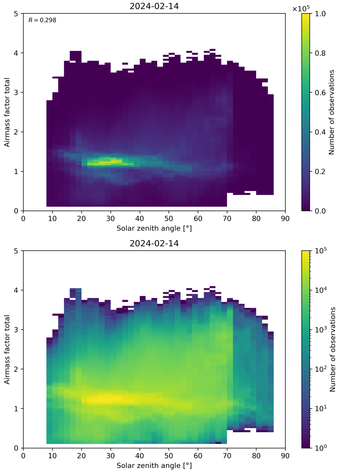
Figure 175: Scatter density plot of “Solar zenith angle” against “Airmass factor total” for 2024-02-13 to 2024-02-15.
