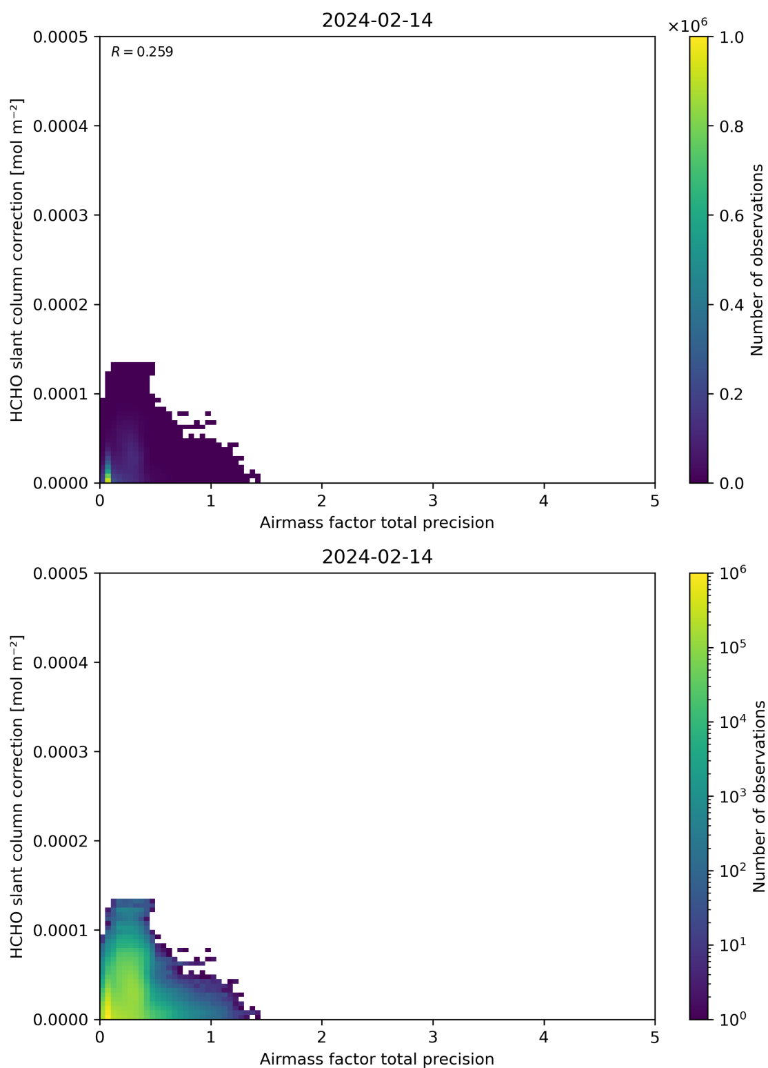
Figure 110: Scatter density plot of “Airmass factor total precision” against “HCHO slant column correction” for 2024-02-13 to 2024-02-15.
