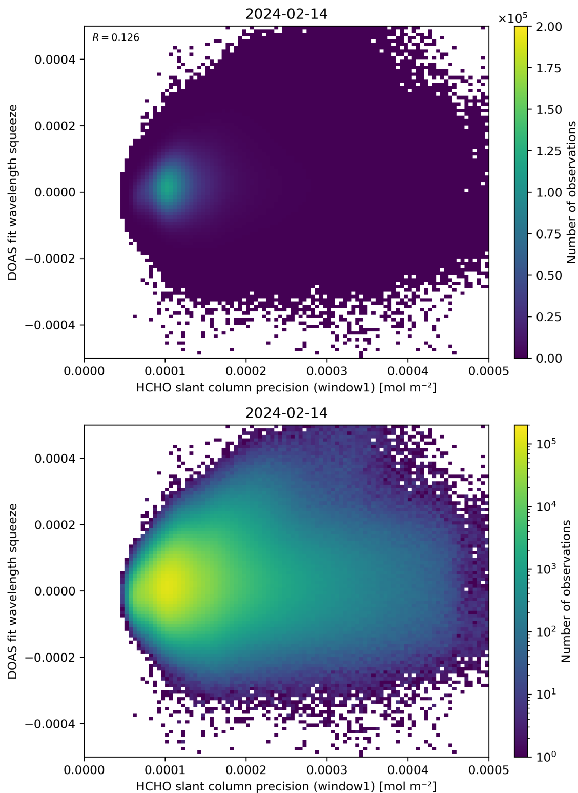
Figure 90: Scatter density plot of “HCHO slant column precision (window1)” against “DOAS fit wavelength squeeze” for 2024-02-13 to 2024-02-15.
