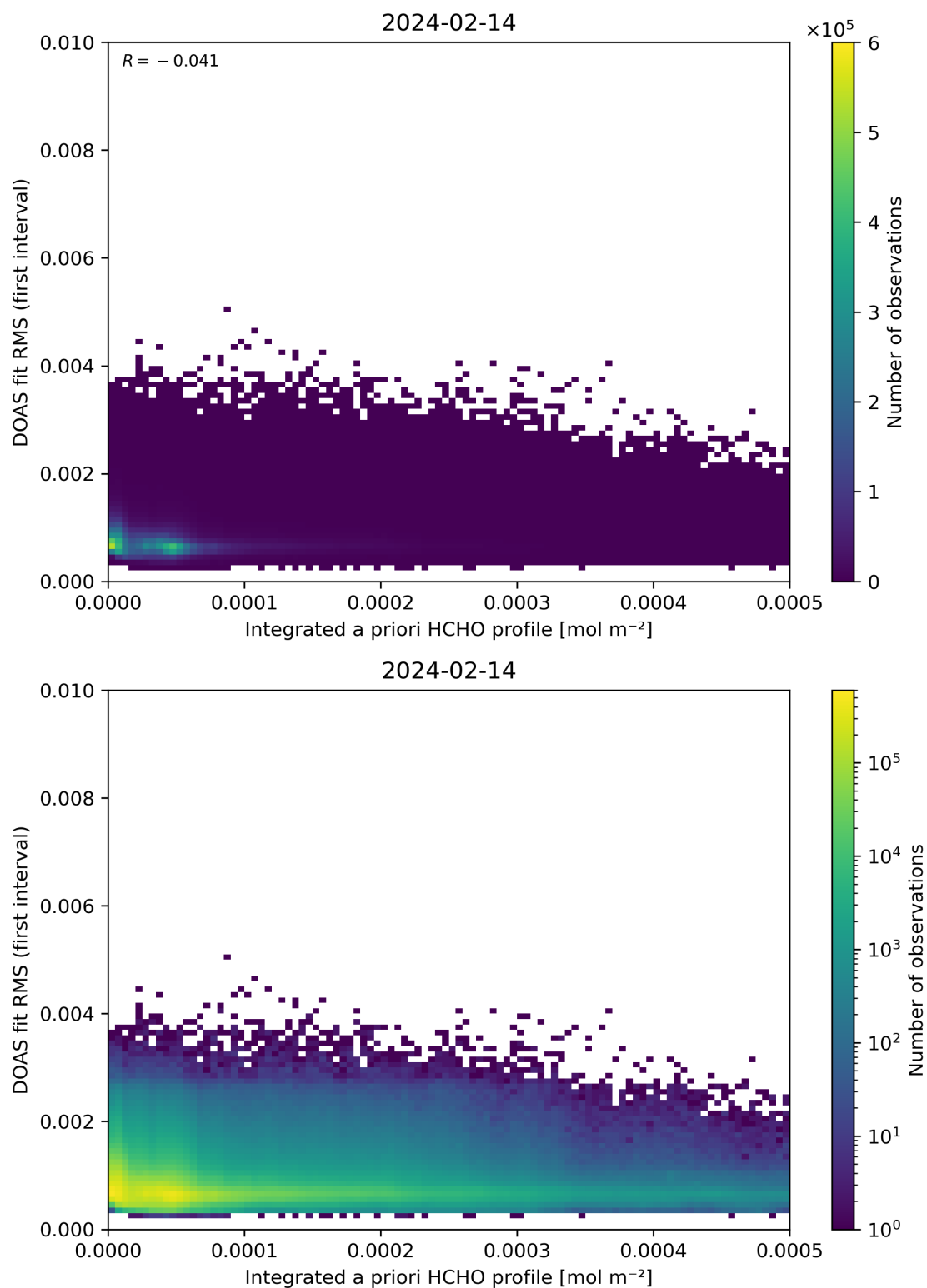
Figure 148: Scatter density plot of “Integrated a priori HCHO profile” against “DOAS fit RMS (first interval)” for 2024-02-13 to 2024-02-15.
