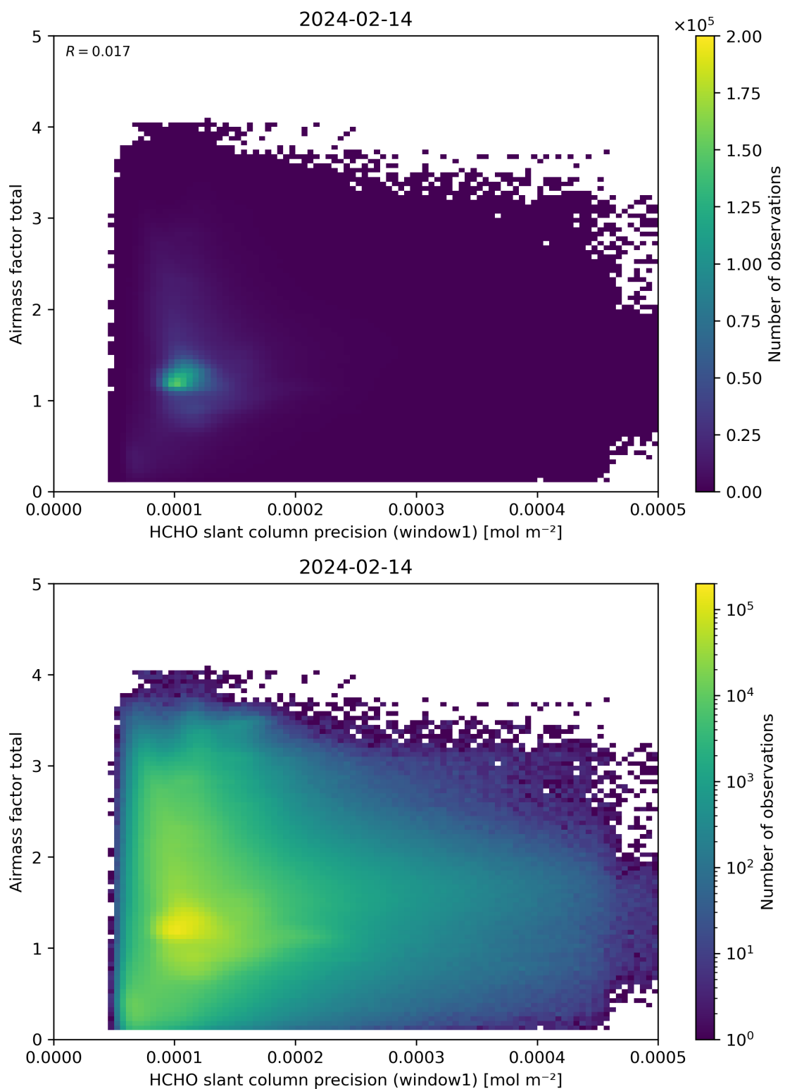
Figure 94: Scatter density plot of “HCHO slant column precision (window1)” against “Airmass factor total” for 2024-02-13 to 2024-02-15.
