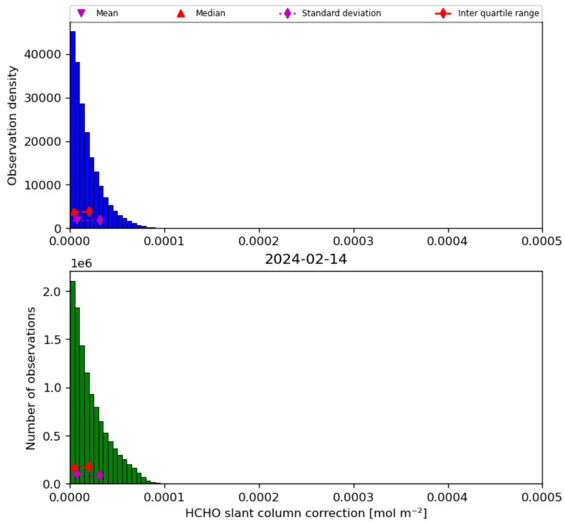
Figure 47: Histogram of “HCHO slant column correction” for 2024-02-13 to 2024-02-15
