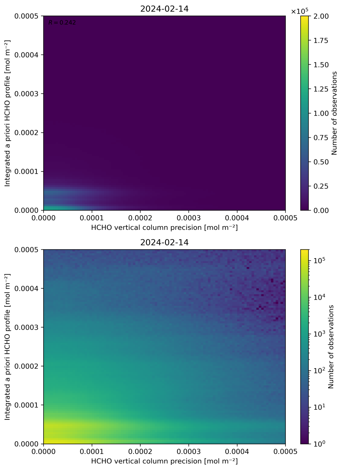
Figure 147: Scatter density plot of “HCHO vertical column precision” against “Integrated a priori HCHO profile” for 2024-02-13 to 2024-02-15.
