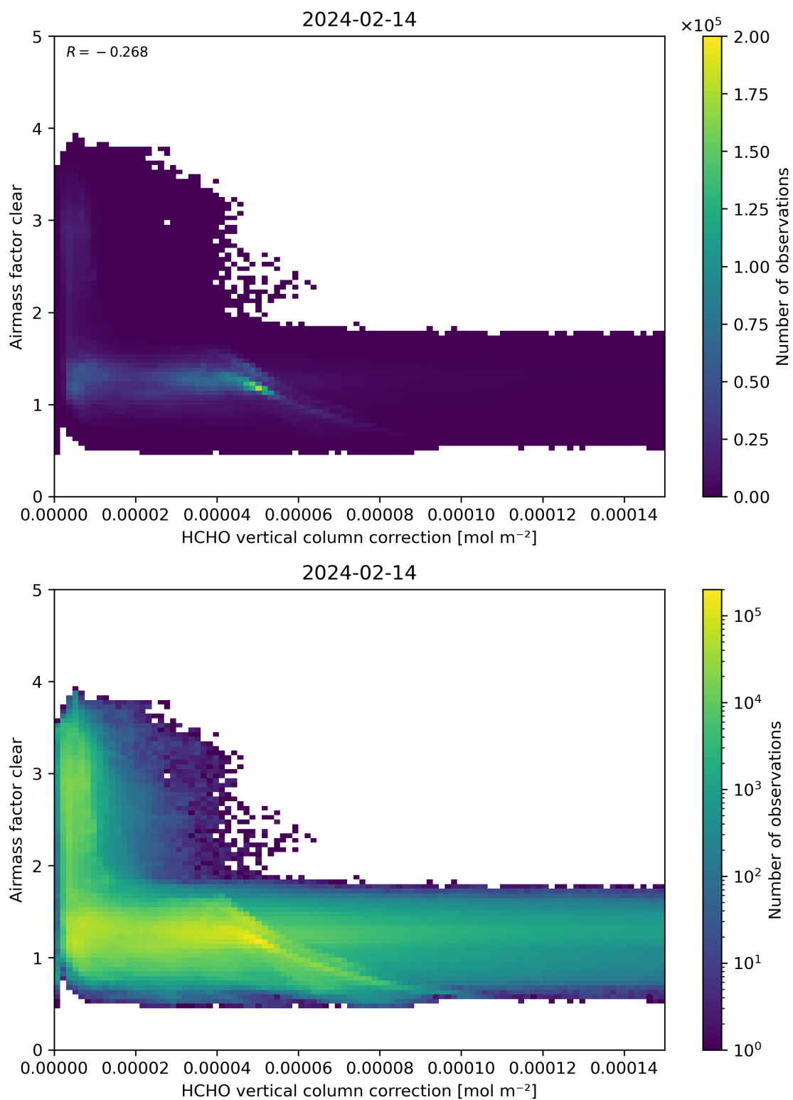
Figure 115: Scatter density plot of “HCHO vertical column correction” against “Airmass factor clear” for 2024-02-13 to 2024-02-15.
