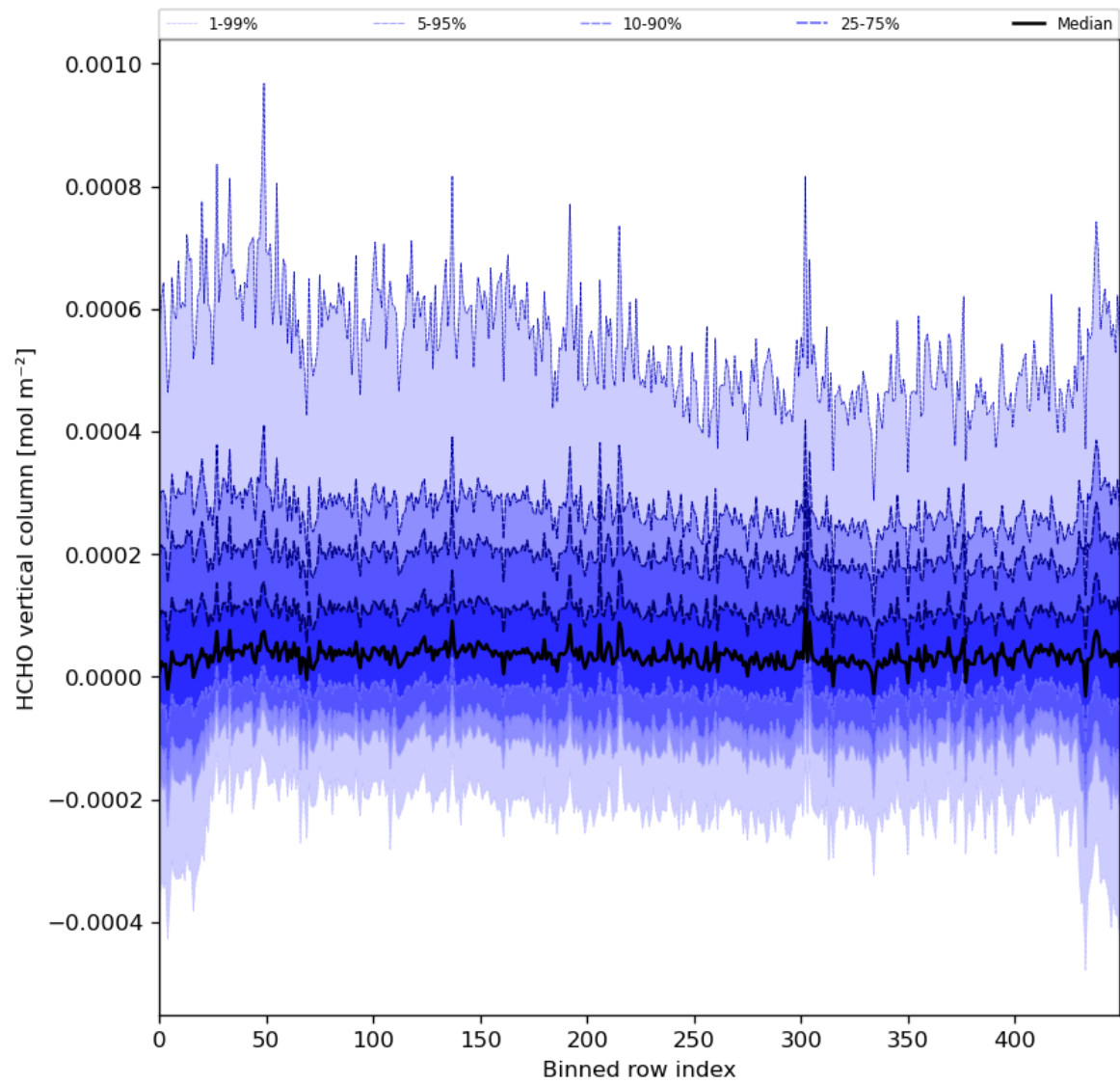
Figure 49: Along track statistics of “HCHO vertical column” for 2024-02-13 to 2024-02-15
