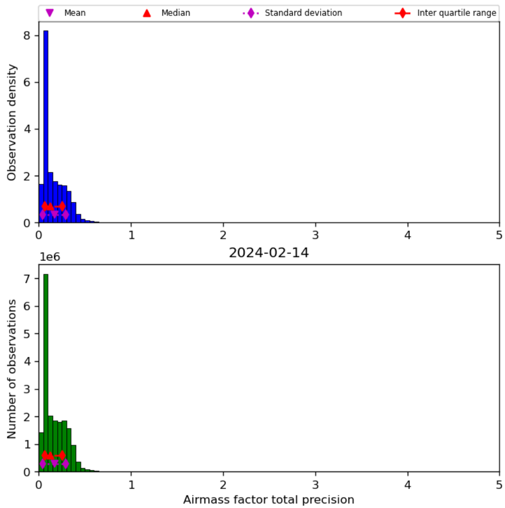
Figure 41: Histogram of “Airmass factor total precision” for 2024-02-13 to 2024-02-15
