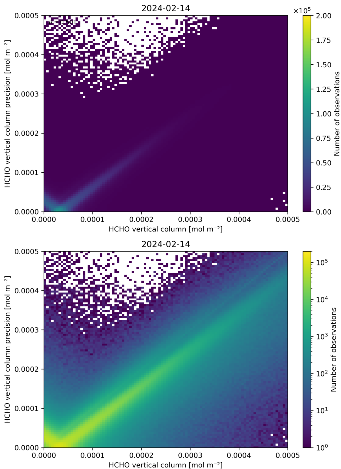
Figure 134: Scatter density plot of “HCHO vertical column” against “HCHO vertical column precision” for 2024-02-13 to 2024-02-15.
