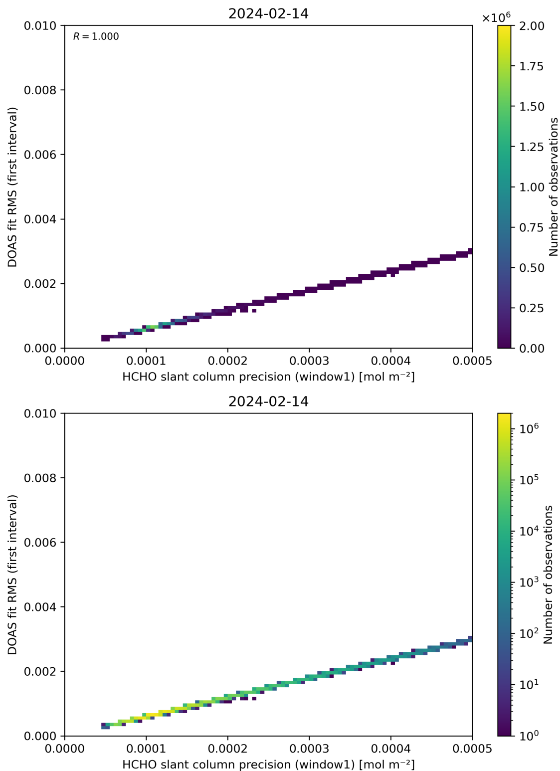
Figure 88: Scatter density plot of “HCHO slant column precision (window1)” against “DOAS fit RMS (first interval)” for 2024-02-13 to 2024-02-15.
