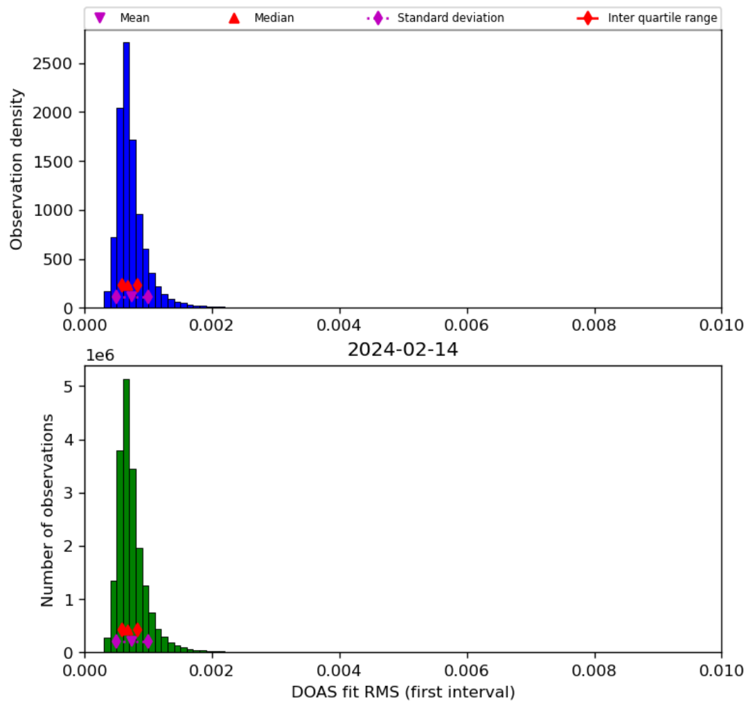
Figure 46: Histogram of “DOAS fit RMS (first interval)” for 2024-02-13 to 2024-02-15
