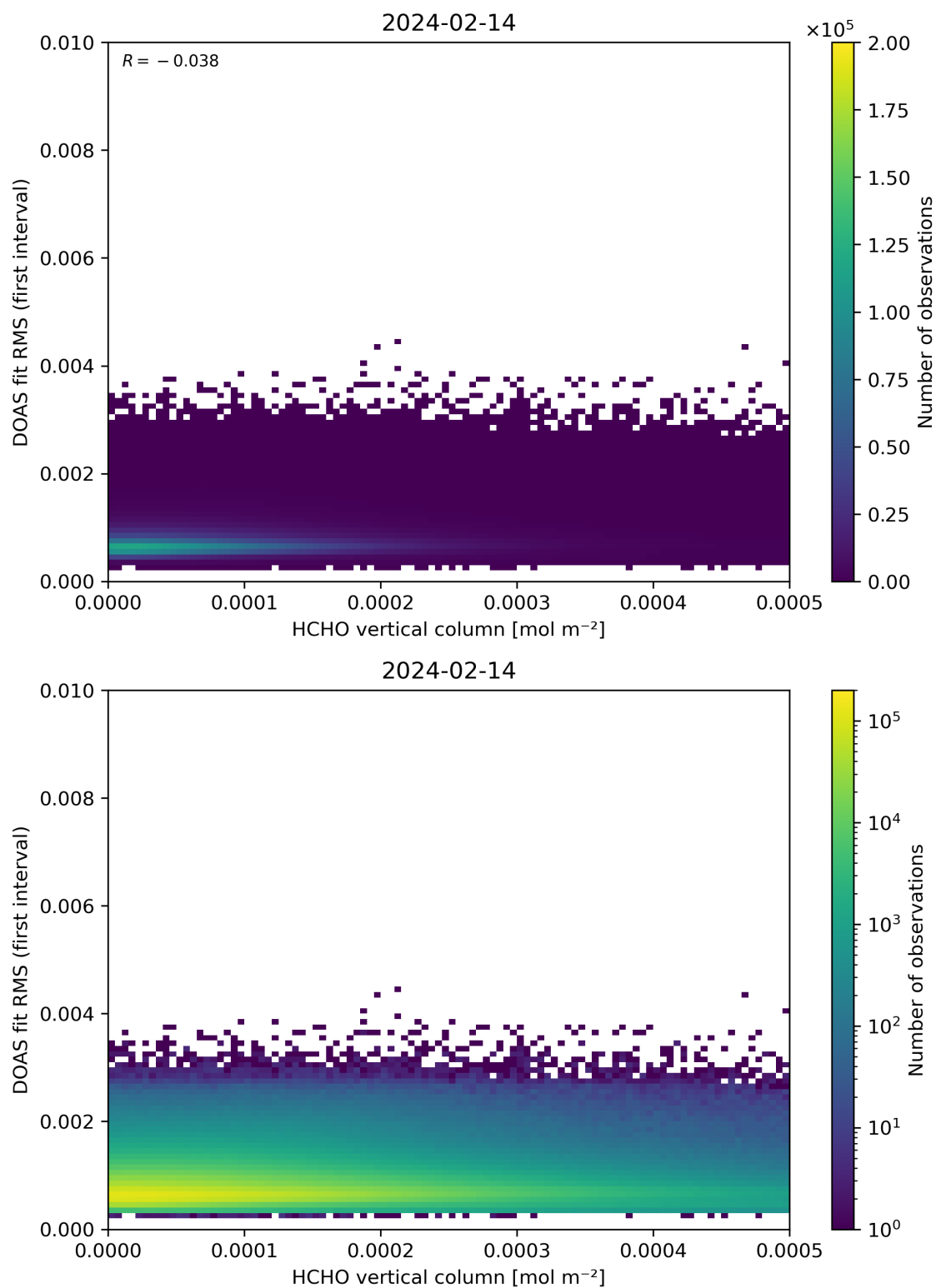
Figure 123: Scatter density plot of “HCHO vertical column” against “DOAS fit RMS (first interval)” for 2024-02-13 to 2024-02-15.
