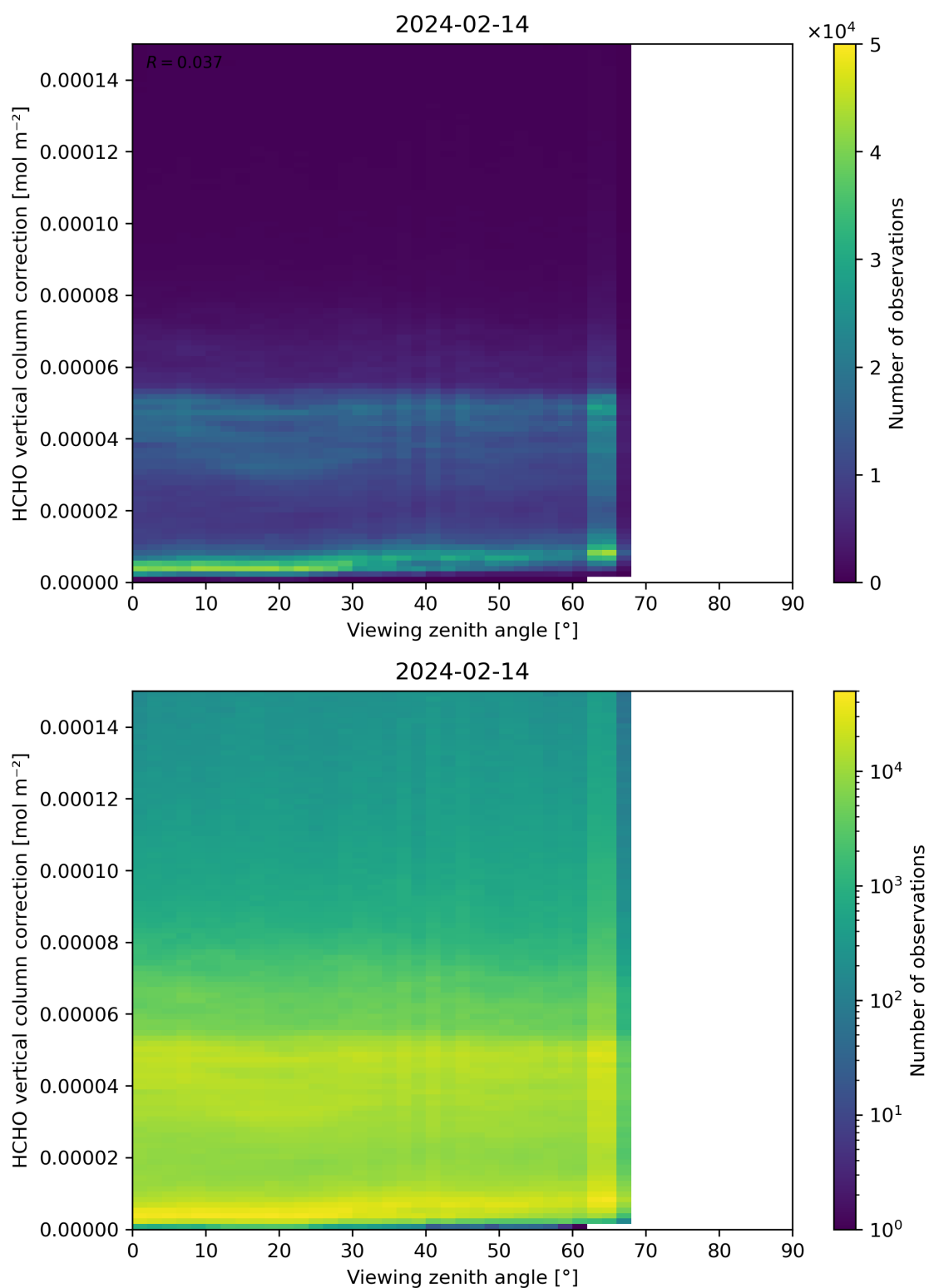
Figure 193: Scatter density plot of “Viewing zenith angle” against “HCHO vertical column correction” for 2024-02-13 to 2024-02-15.
