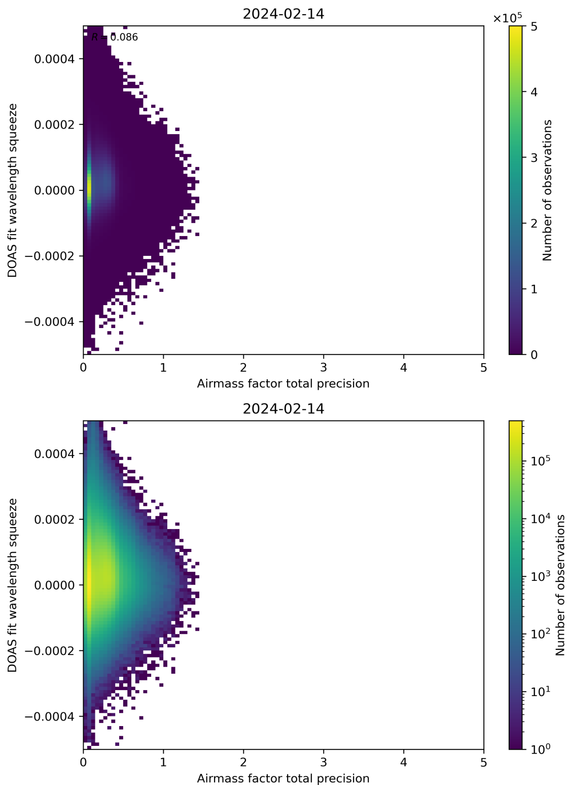
Figure 107: Scatter density plot of “Airmass factor total precision” against “DOAS fit wavelength squeeze” for 2024-02-13 to 2024-02-15.
