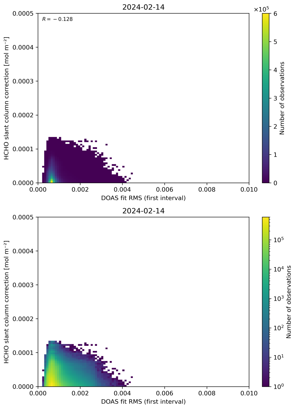
Figure 63: Scatter density plot of “DOAS fit RMS (first interval)” against “HCHO slant column correction” for 2024-02-13 to 2024-02-15.
