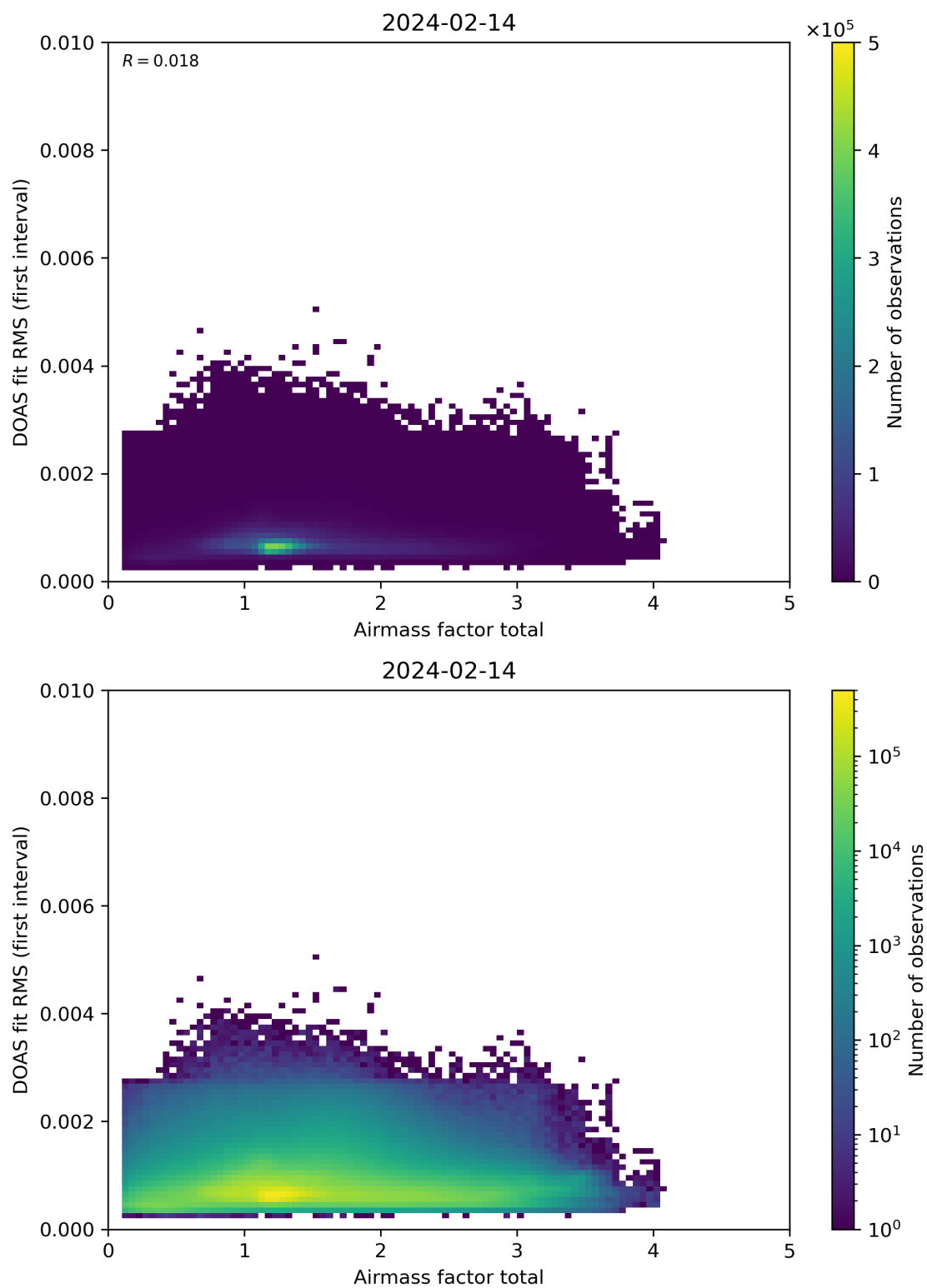
Figure 97: Scatter density plot of “Airmass factor total” against “DOAS fit RMS (first interval)” for 2024-02-13 to 2024-02-15.
