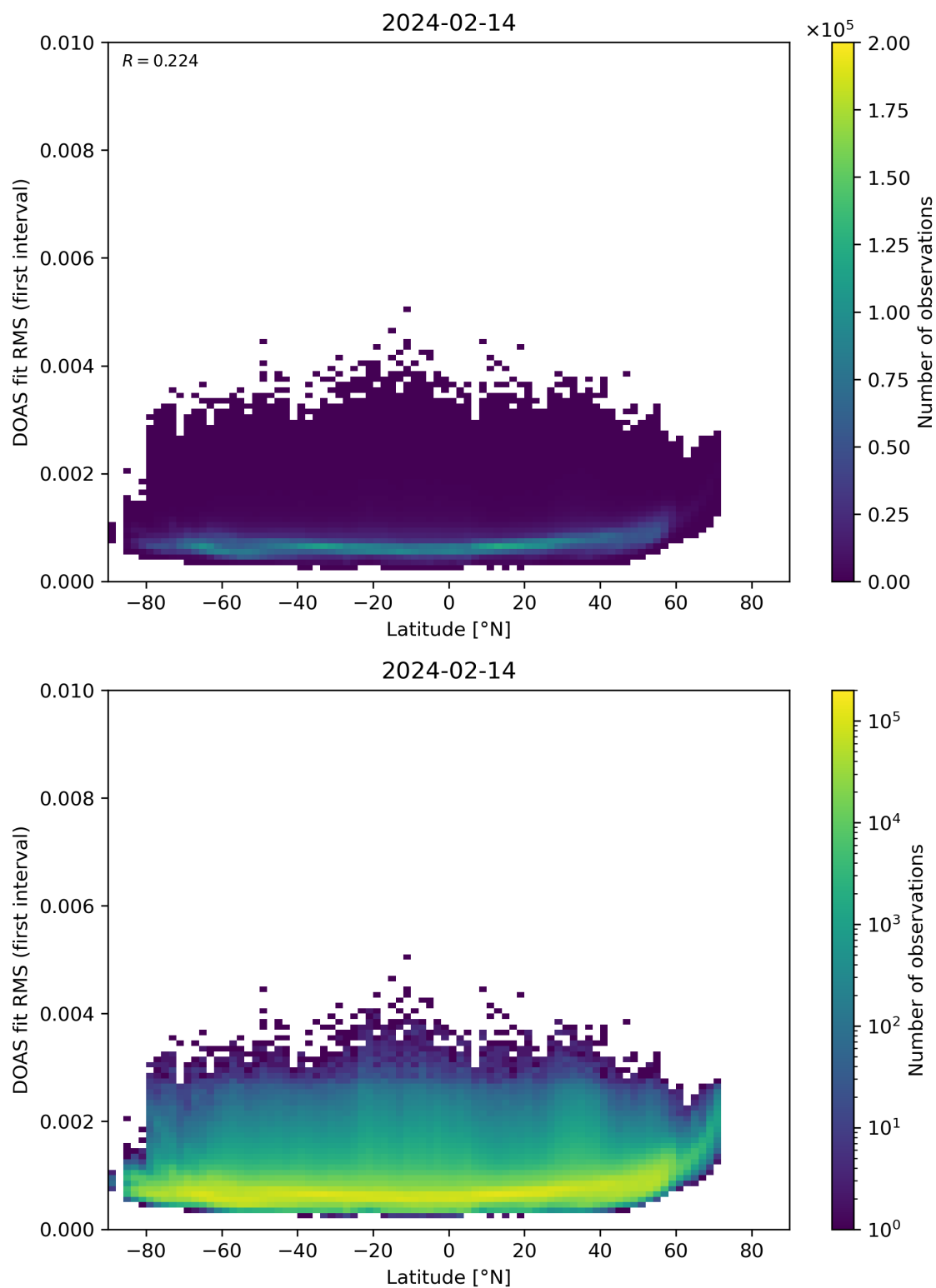
Figure 153: Scatter density plot of “Latitude” against “DOAS fit RMS (first interval)” for 2024-02-13 to 2024-02-15.
