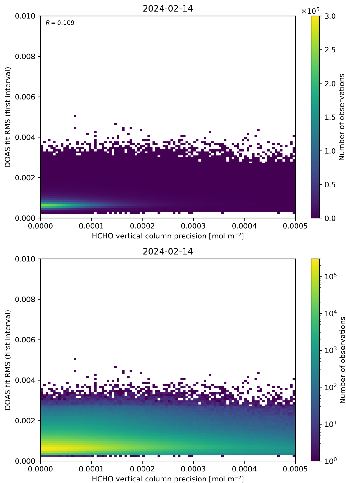
Figure 136: Scatter density plot of “HCHO vertical column precision” against “DOAS fit RMS (first interval)” for 2024-02-13 to 2024-02-15.
