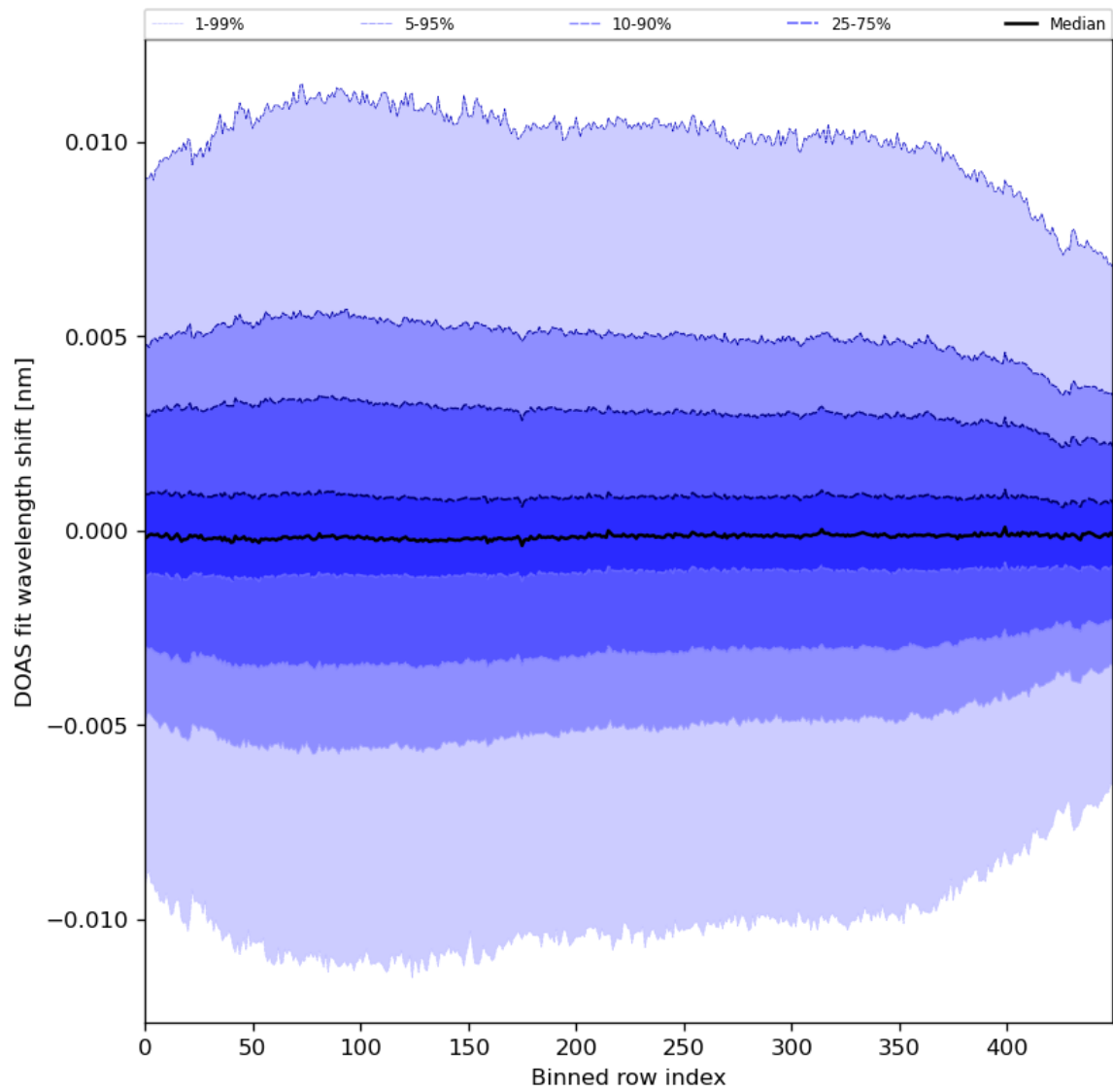
Figure 58: Along track statistics of “DOAS fit wavelength shift” for 2024-02-13 to 2024-02-15
