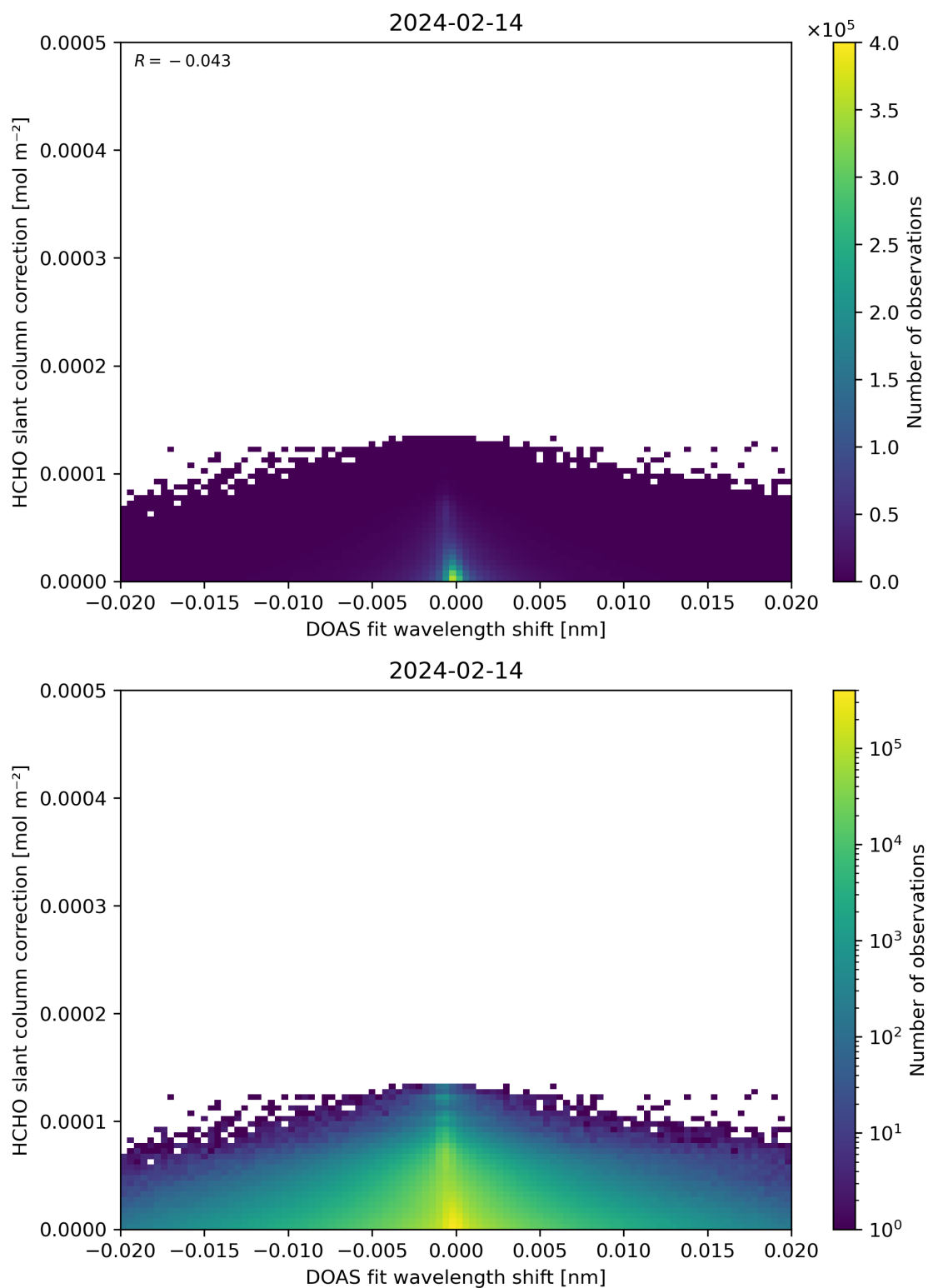
Figure 67: Scatter density plot of “DOAS fit wavelength shift” against “HCHO slant column correction” for 2024-02-13 to 2024-02-15.
