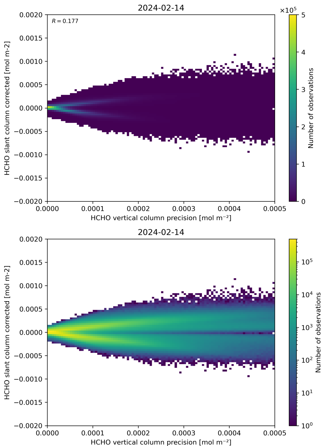
Figure 140: Scatter density plot of “HCHO vertical column precision” against “HCHO slant column corrected” for 2024-02-13 to 2024-02-15.
