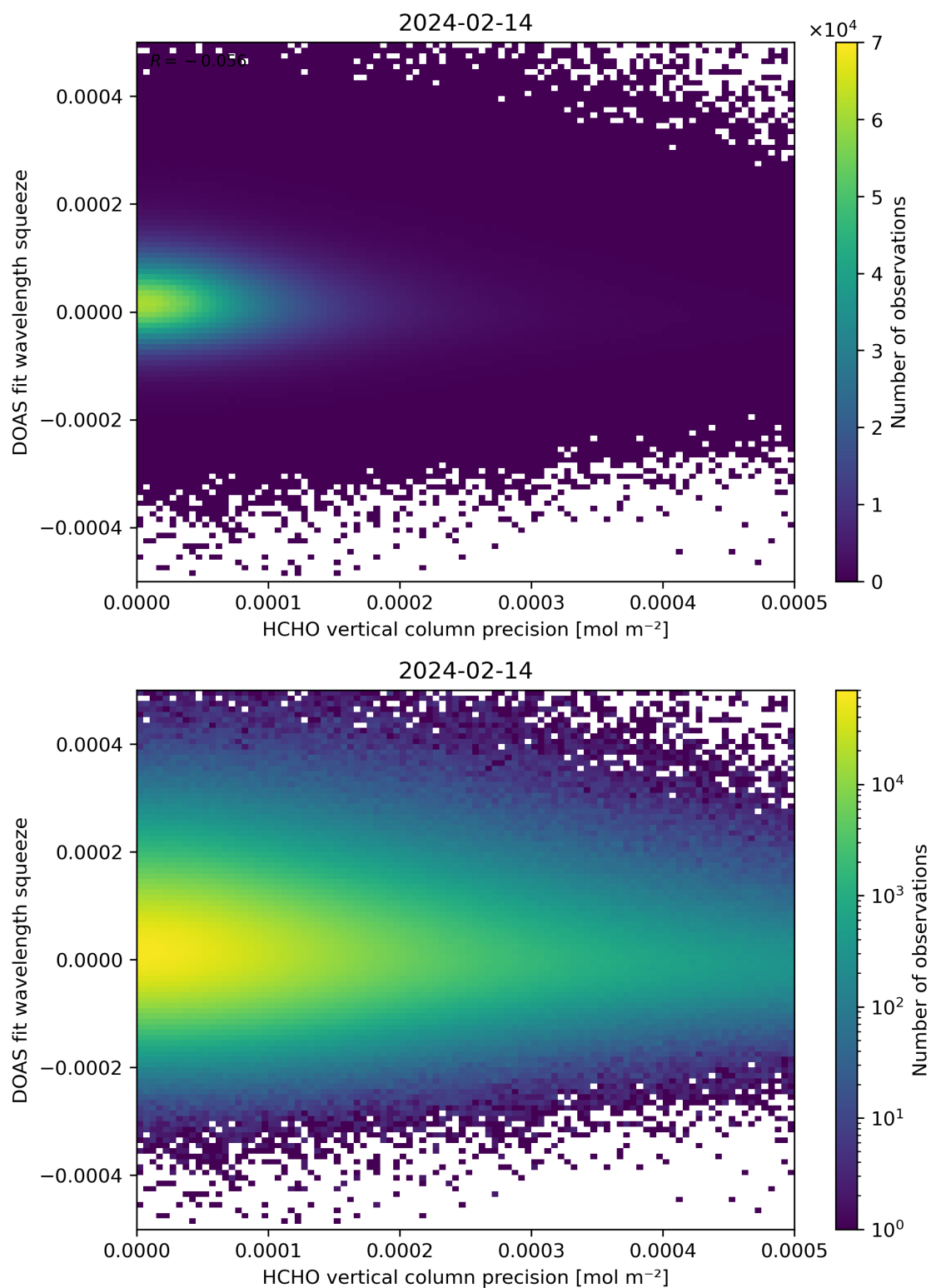
Figure 138: Scatter density plot of “HCHO vertical column precision” against “DOAS fit wavelength squeeze” for 2024-02-13 to 2024-02-15.
