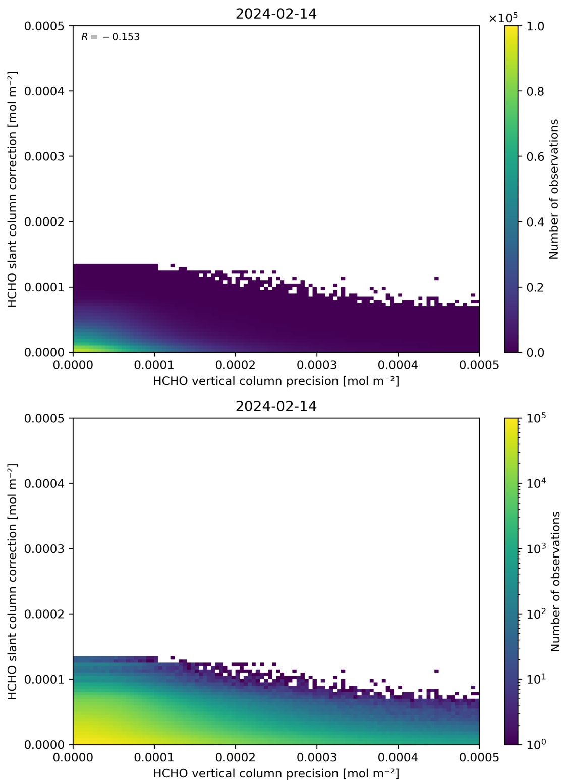
Figure 141: Scatter density plot of “HCHO vertical column precision” against “HCHO slant column correction” for 2024-02-13 to 2024-02-15.
