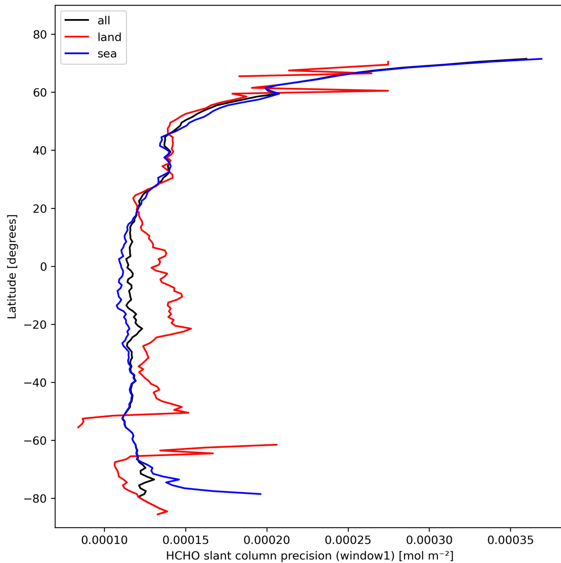
Figure 25: Zonal average of “HCHO slant column precision (window1)” for 2024-02-13 to 2024-02-15.
