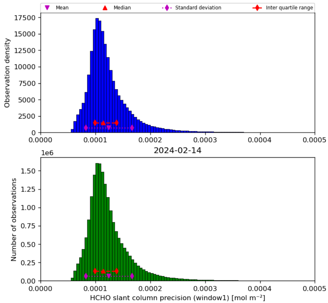
Figure 39: Histogram of “HCHO slant column precision (window1)” for 2024-02-13 to 2024-02-15
