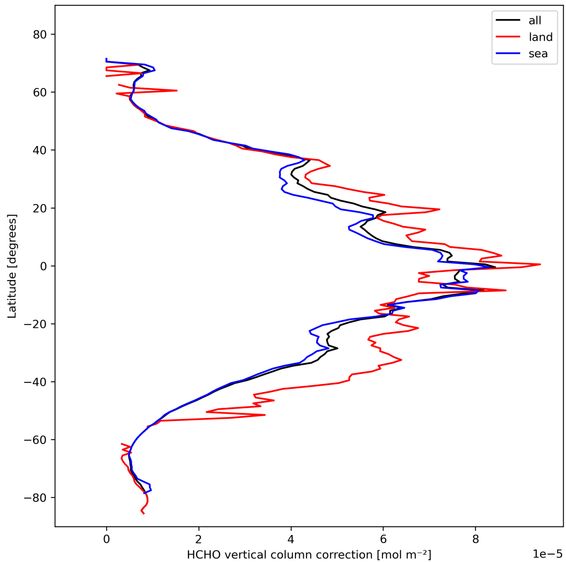
Figure 23: Zonal average of “HCHO vertical column correction” for 2024-02-13 to 2024-02-15.
