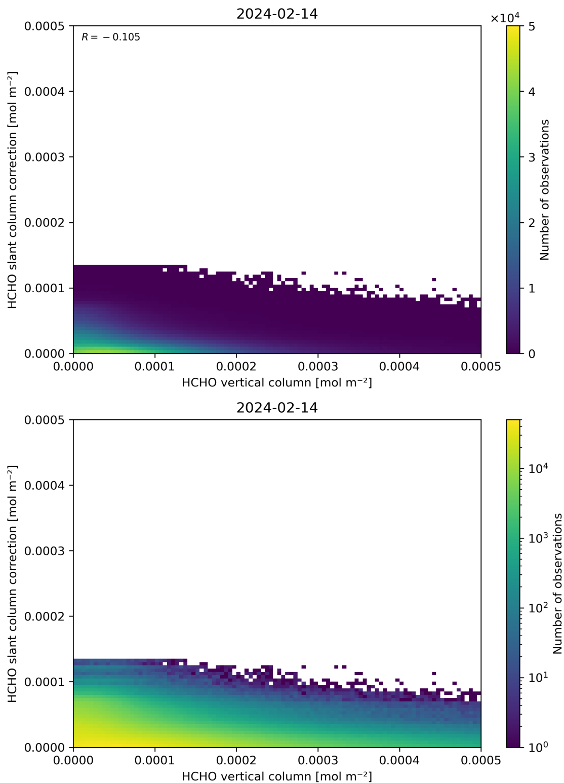
Figure 128: Scatter density plot of “HCHO vertical column” against “HCHO slant column correction” for 2024-02-13 to 2024-02-15.
