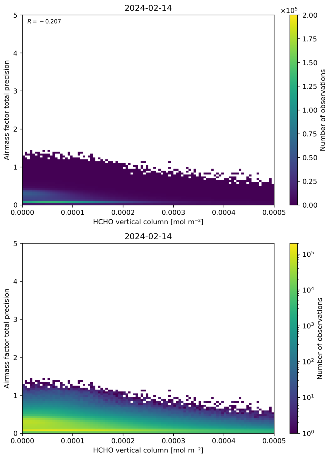
Figure 132: Scatter density plot of “HCHO vertical column” against “Airmass factor total precision” for 2024-02-13 to 2024-02-15.
