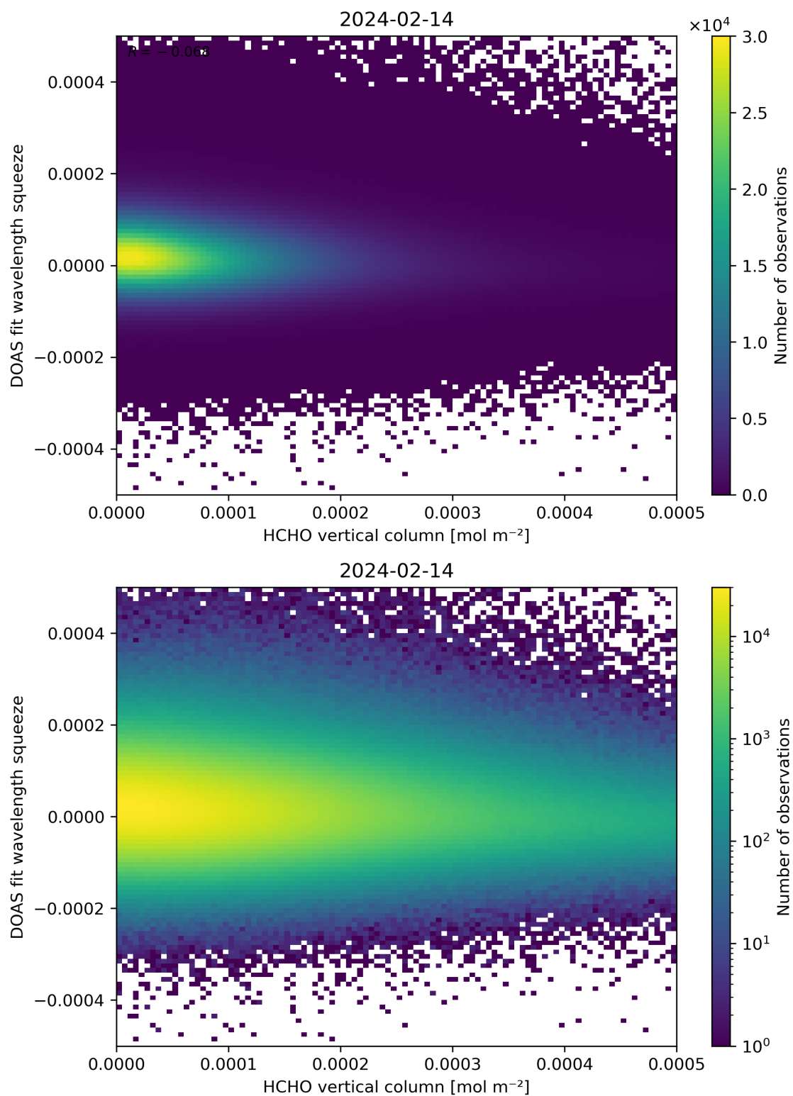
Figure 125: Scatter density plot of “HCHO vertical column” against “DOAS fit wavelength squeeze” for 2024-02-13 to 2024-02-15.
