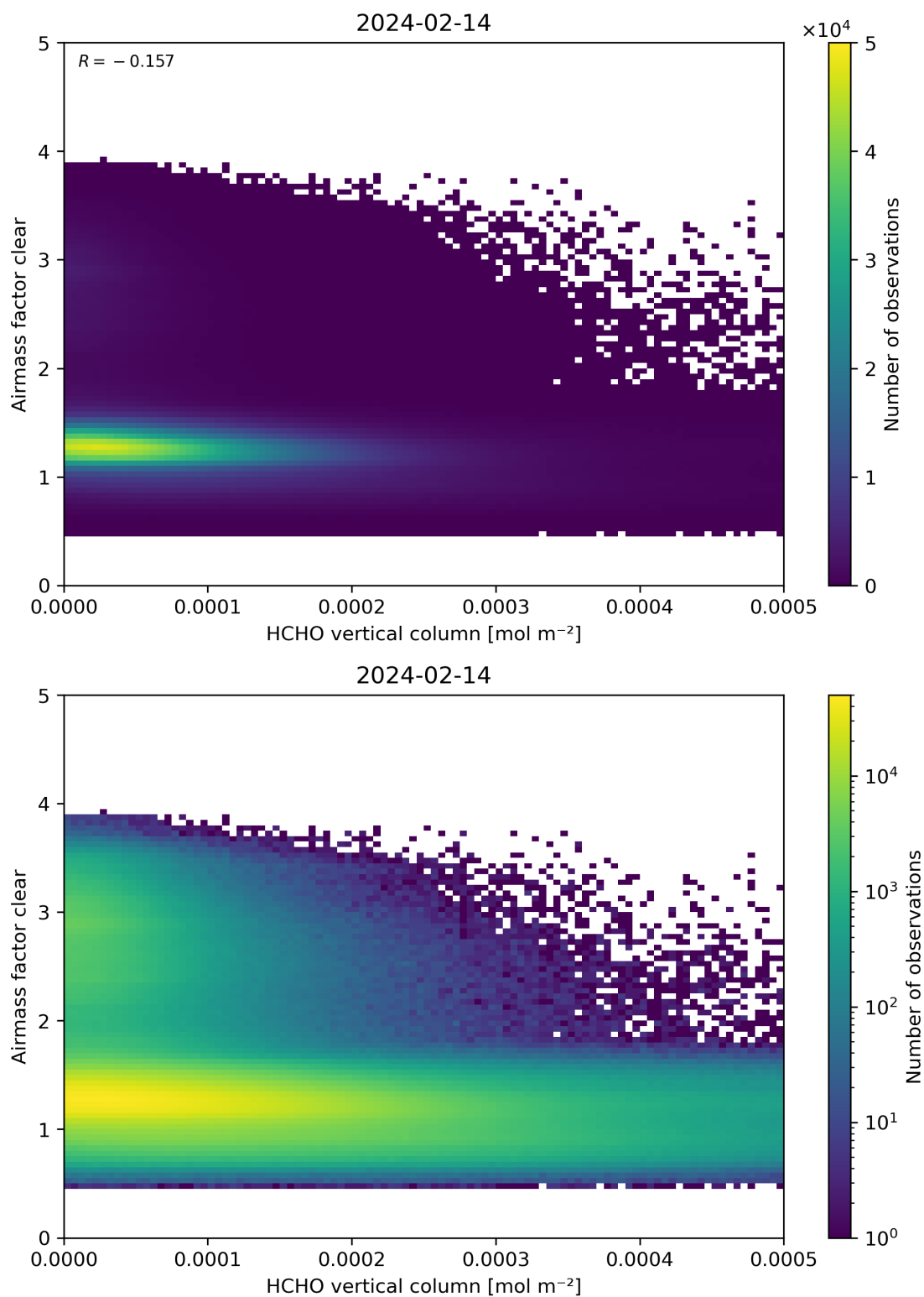
Figure 126: Scatter density plot of “HCHO vertical column” against “Airmass factor clear” for 2024-02-13 to 2024-02-15.
