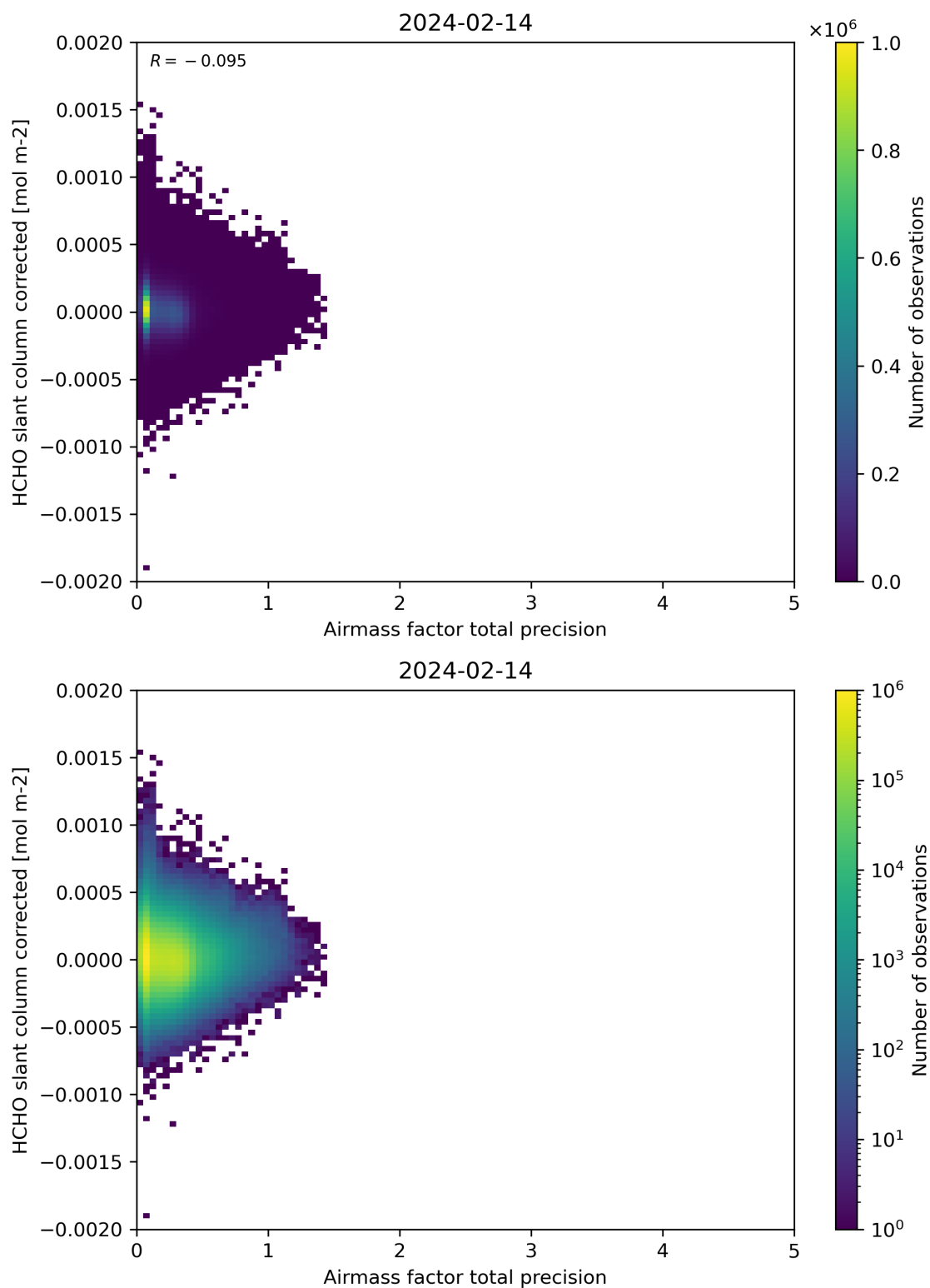
Figure 109: Scatter density plot of “Airmass factor total precision” against “HCHO slant column corrected” for 2024-02-13 to 2024-02-15.
