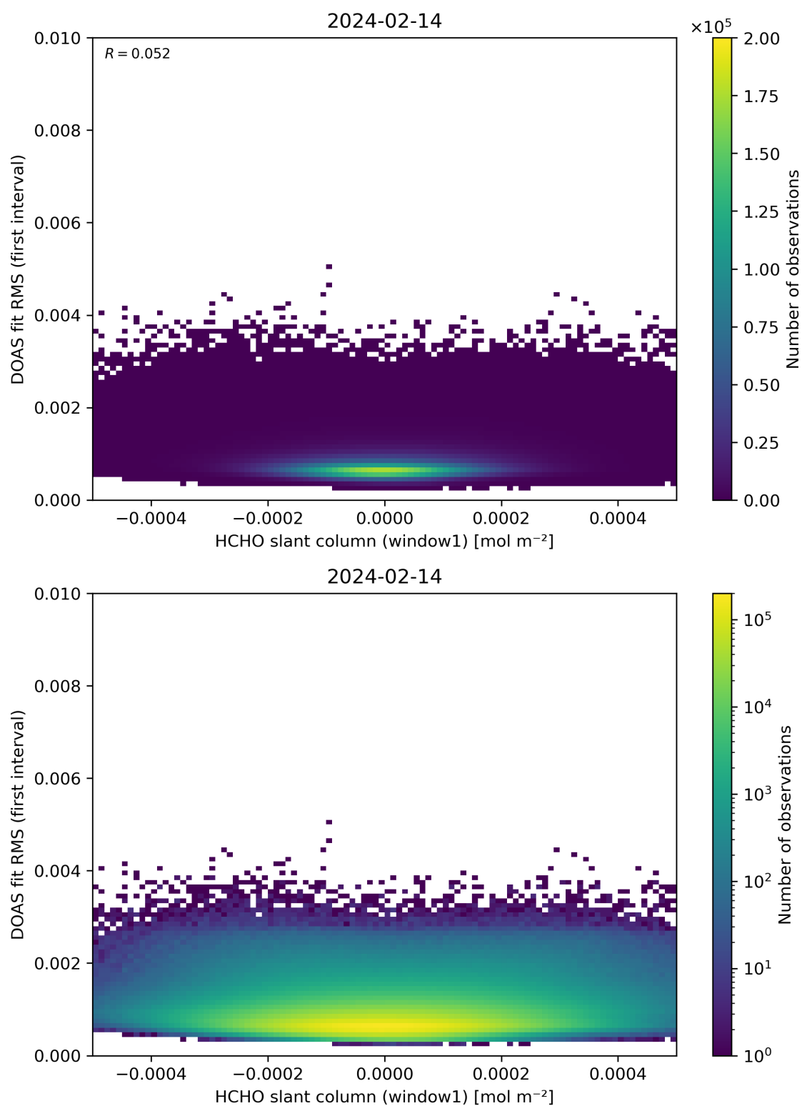
Figure 78: Scatter density plot of “HCHO slant column (window1)” against “DOAS fit RMS (first interval)” for 2024-02-13 to 2024-02-15.
