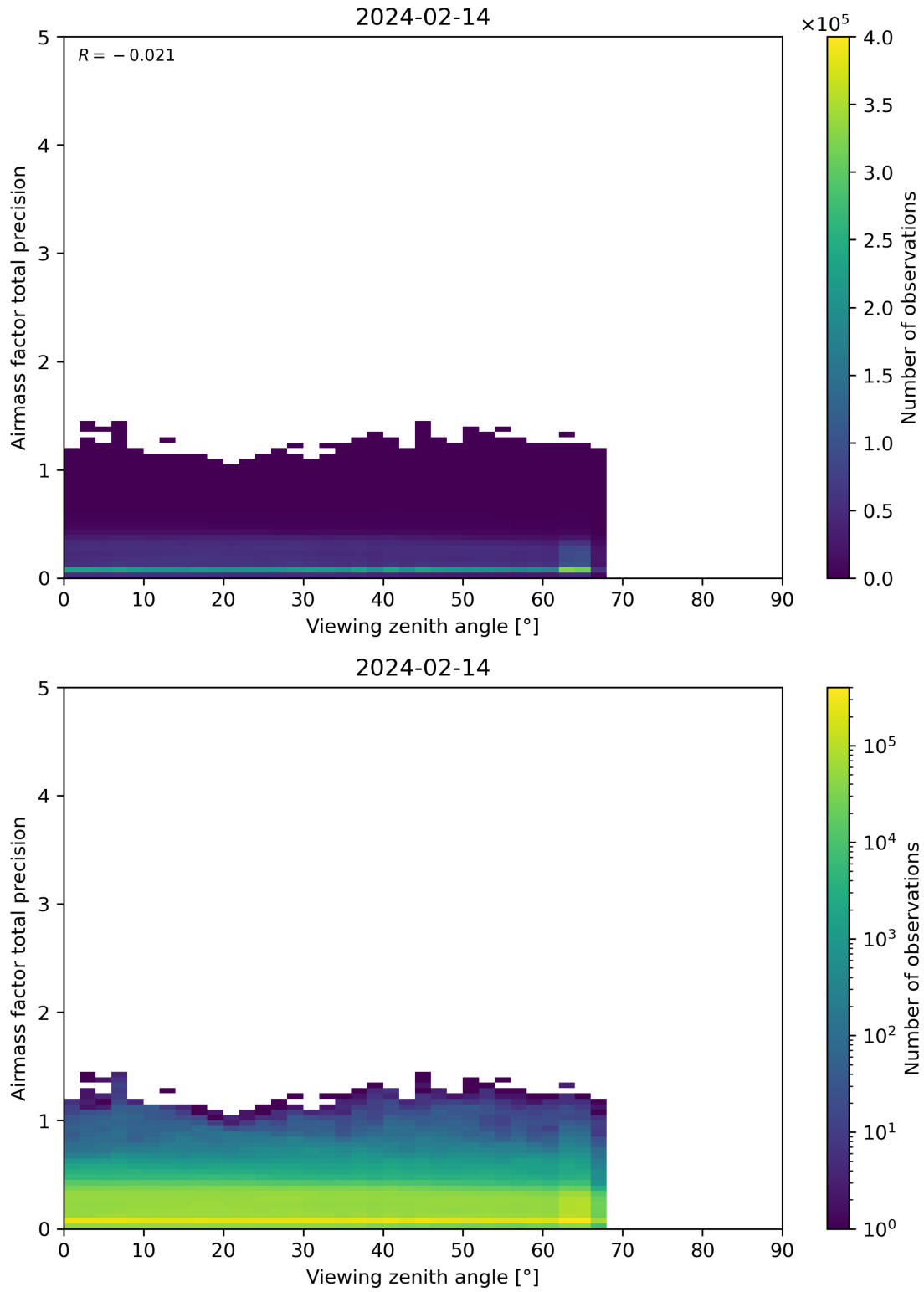
Figure 191: Scatter density plot of “Viewing zenith angle” against “Airmass factor total precision” for 2024-02-13 to 2024-02-15.
