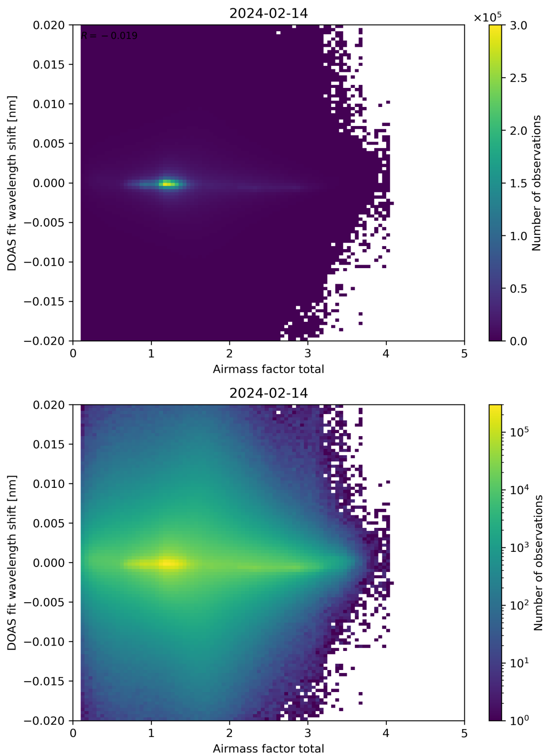
Figure 98: Scatter density plot of “Airmass factor total” against “DOAS fit wavelength shift” for 2024-02-13 to 2024-02-15.
