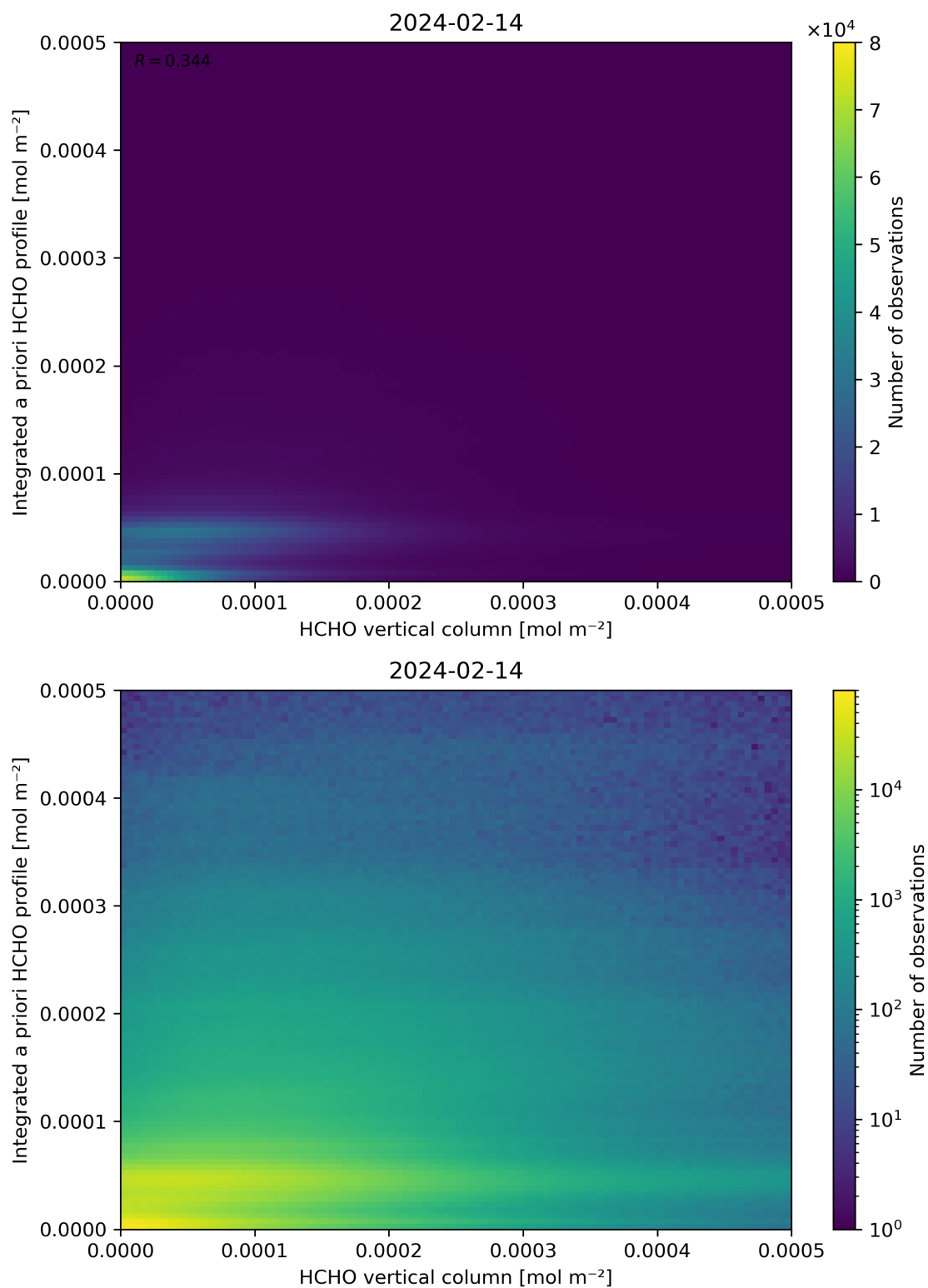
Figure 135: Scatter density plot of “HCHO vertical column” against “Integrated a priori HCHO profile” for 2024-02-13 to 2024-02-15.
