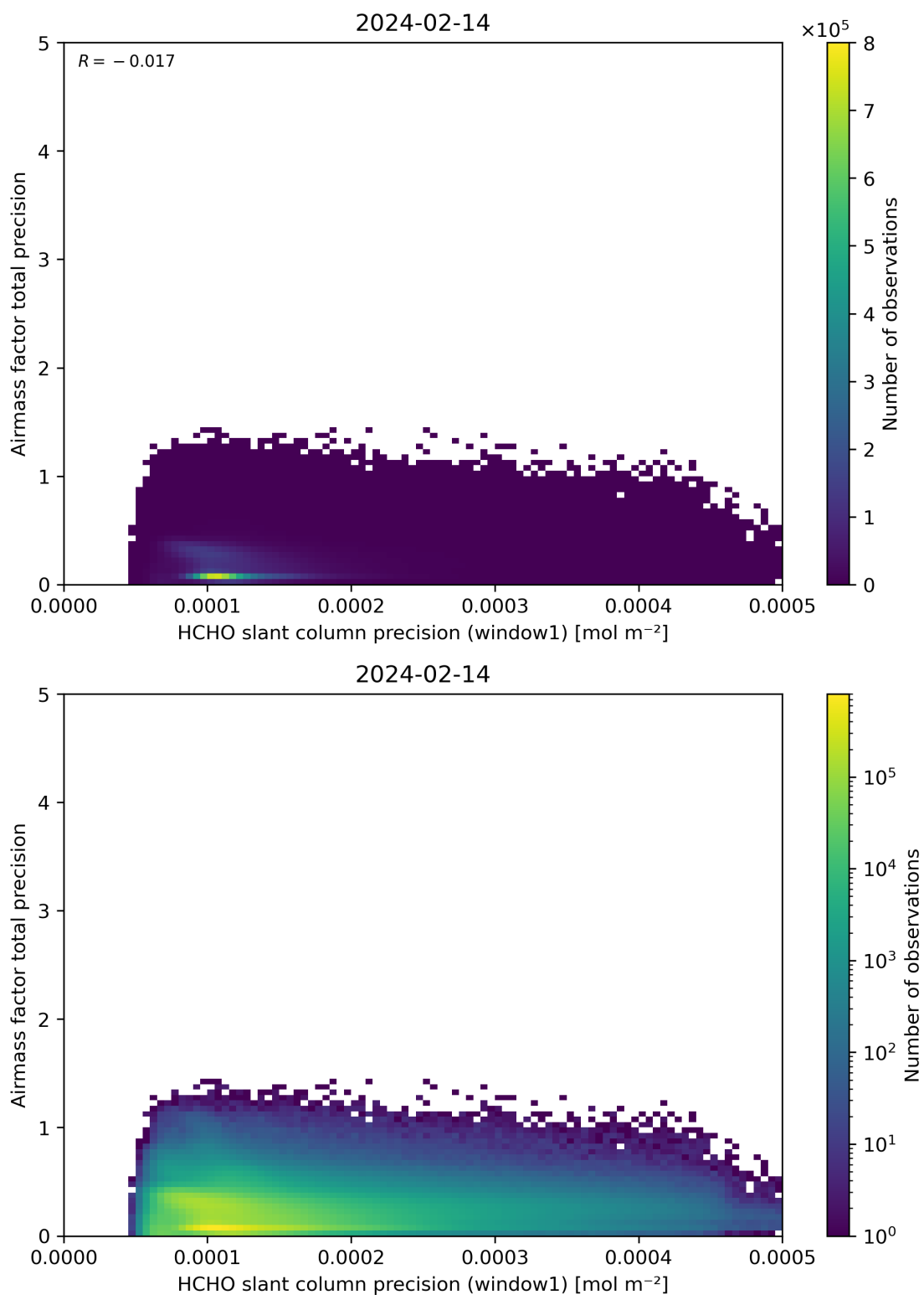
Figure 95: Scatter density plot of “HCHO slant column precision (window1)” against “Airmass factor total precision” for 2024-02-13 to 2024-02-15.
