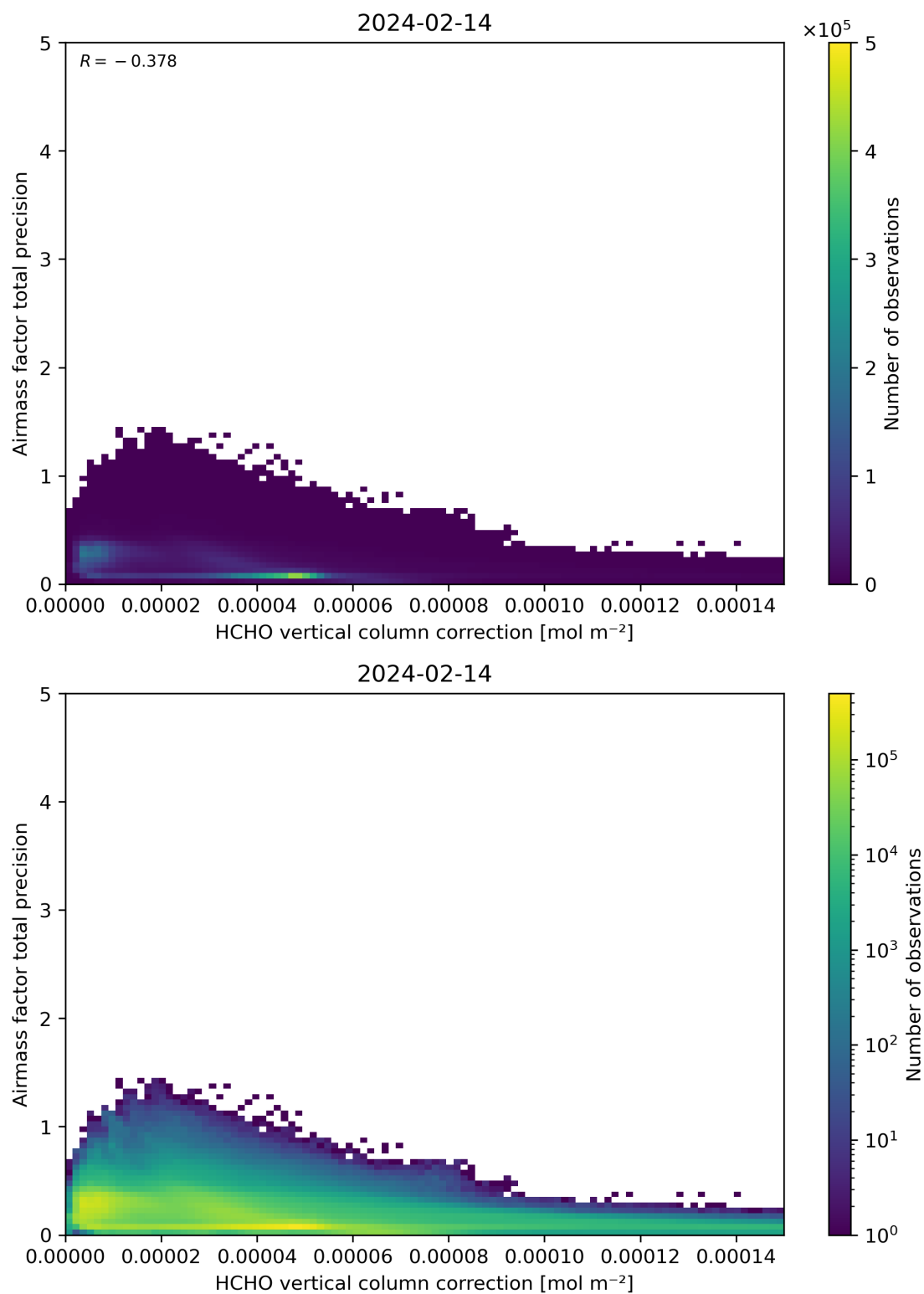
Figure 121: Scatter density plot of “HCHO vertical column correction” against “Airmass factor total precision” for 2024-02-13 to 2024-02-15.
