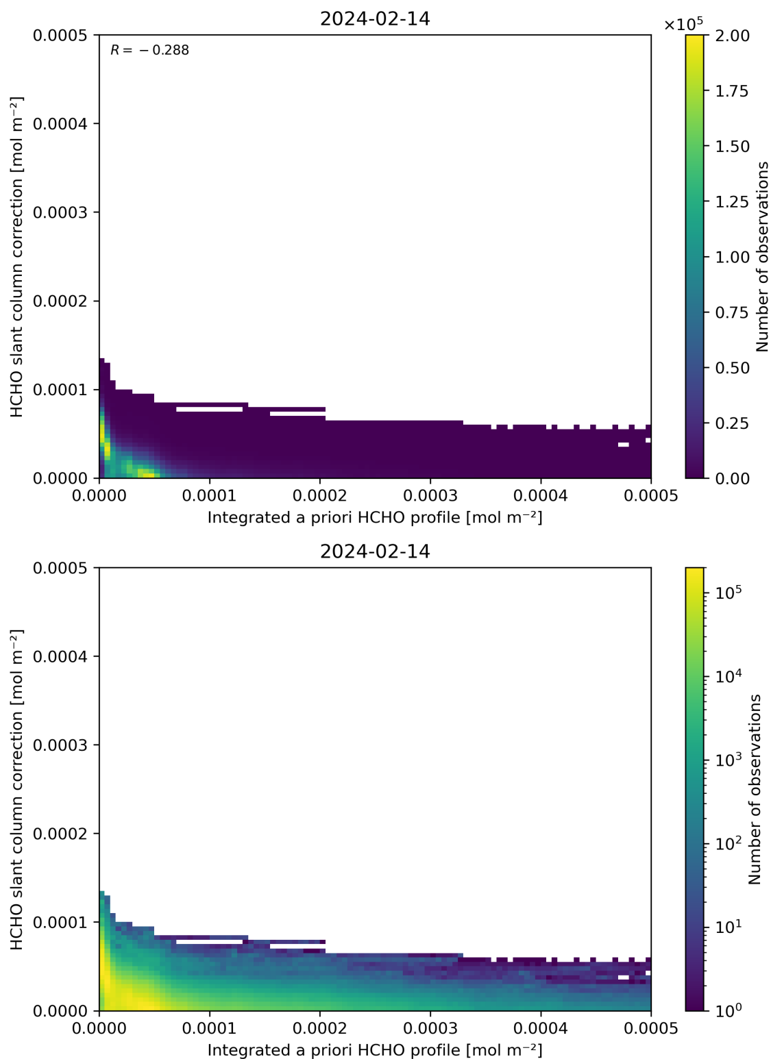
Figure 152: Scatter density plot of “Integrated a priori HCHO profile” against “HCHO slant column correction” for 2024-02-13 to 2024-02-15.
