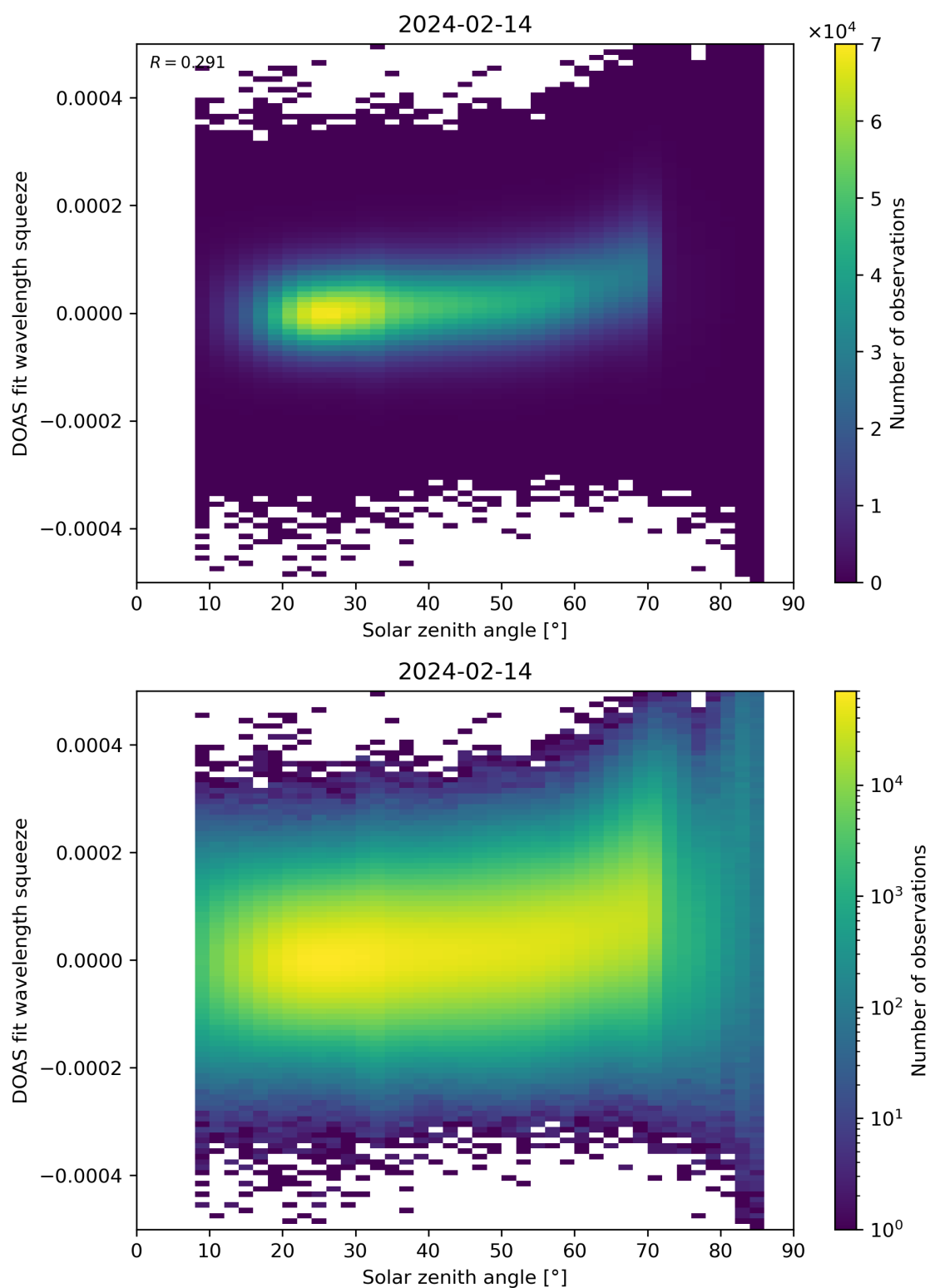
Figure 169: Scatter density plot of “Solar zenith angle” against “DOAS fit wavelength squeeze” for 2024-02-13 to 2024-02-15.
