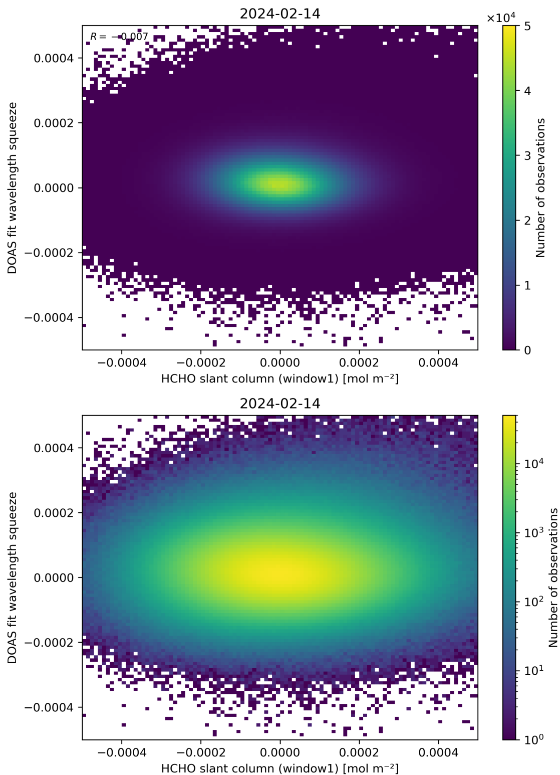
Figure 80: Scatter density plot of “HCHO slant column (window1)” against “DOAS fit wavelength squeeze” for 2024-02-13 to 2024-02-15.
