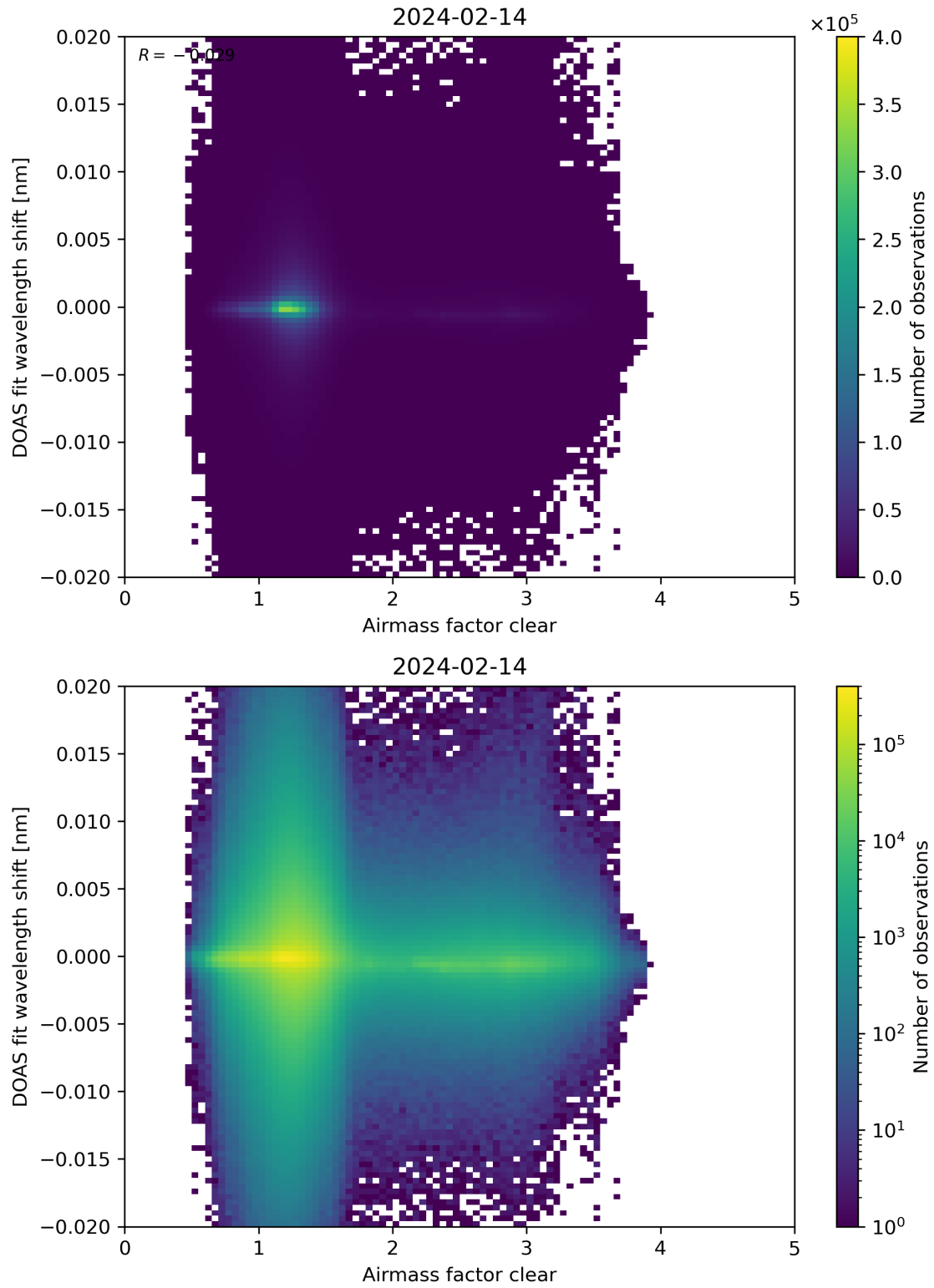
Figure 72: Scatter density plot of “Airmass factor clear” against “DOAS fit wavelength shift” for 2024-02-13 to 2024-02-15.
