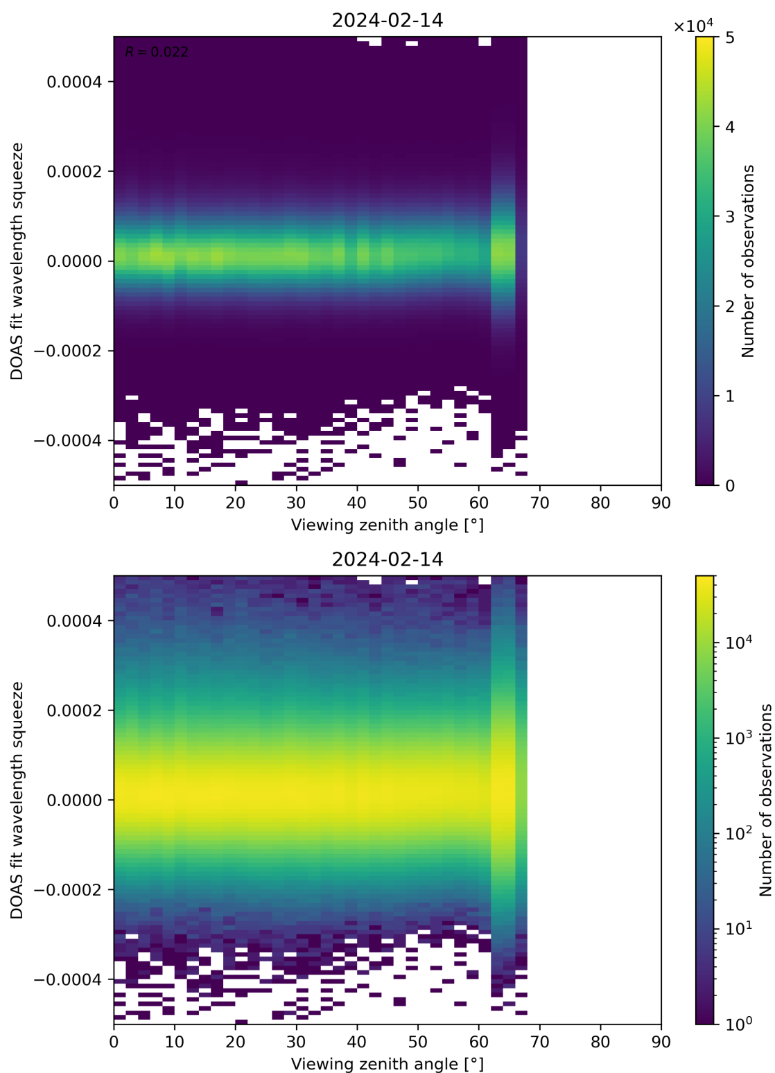
Figure 184: Scatter density plot of “Viewing zenith angle” against “DOAS fit wavelength squeeze” for 2024-02-13 to 2024-02-15.
