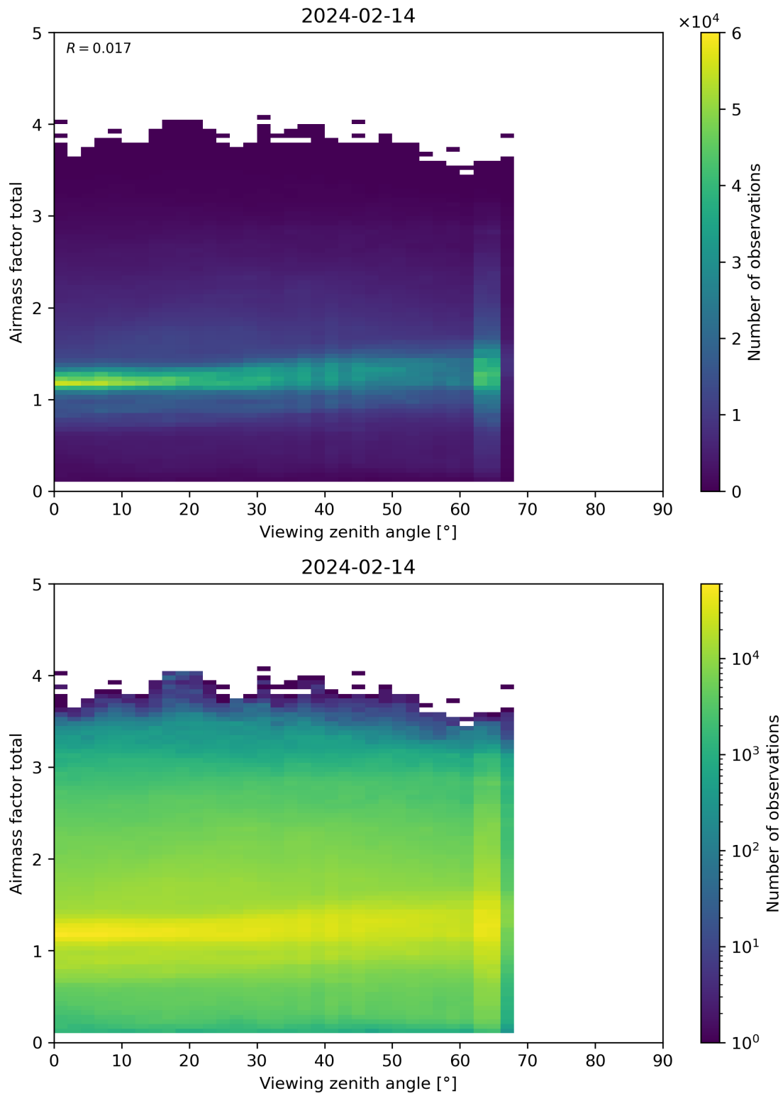
Figure 190: Scatter density plot of “Viewing zenith angle” against “Airmass factor total” for 2024-02-13 to 2024-02-15.
