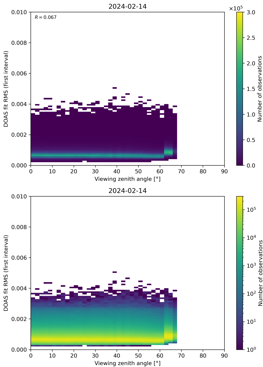
Figure 182: Scatter density plot of “Viewing zenith angle” against “DOAS fit RMS (first interval)” for 2024-02-13 to 2024-02-15.
