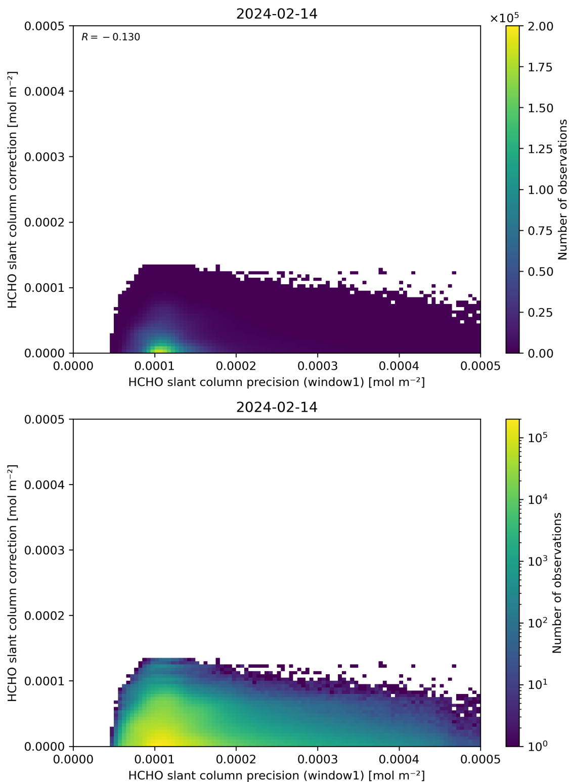
Figure 93: Scatter density plot of “HCHO slant column precision (window1)” against “HCHO slant column correction” for 2024-02-13 to 2024-02-15.
