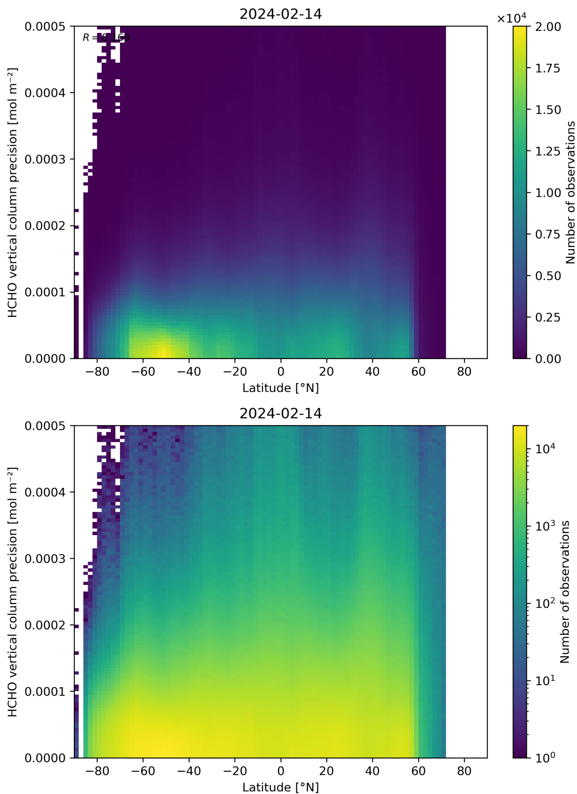
Figure 165: Scatter density plot of “Latitude” against “HCHO vertical column precision” for 2024-02-13 to 2024-02-15.
