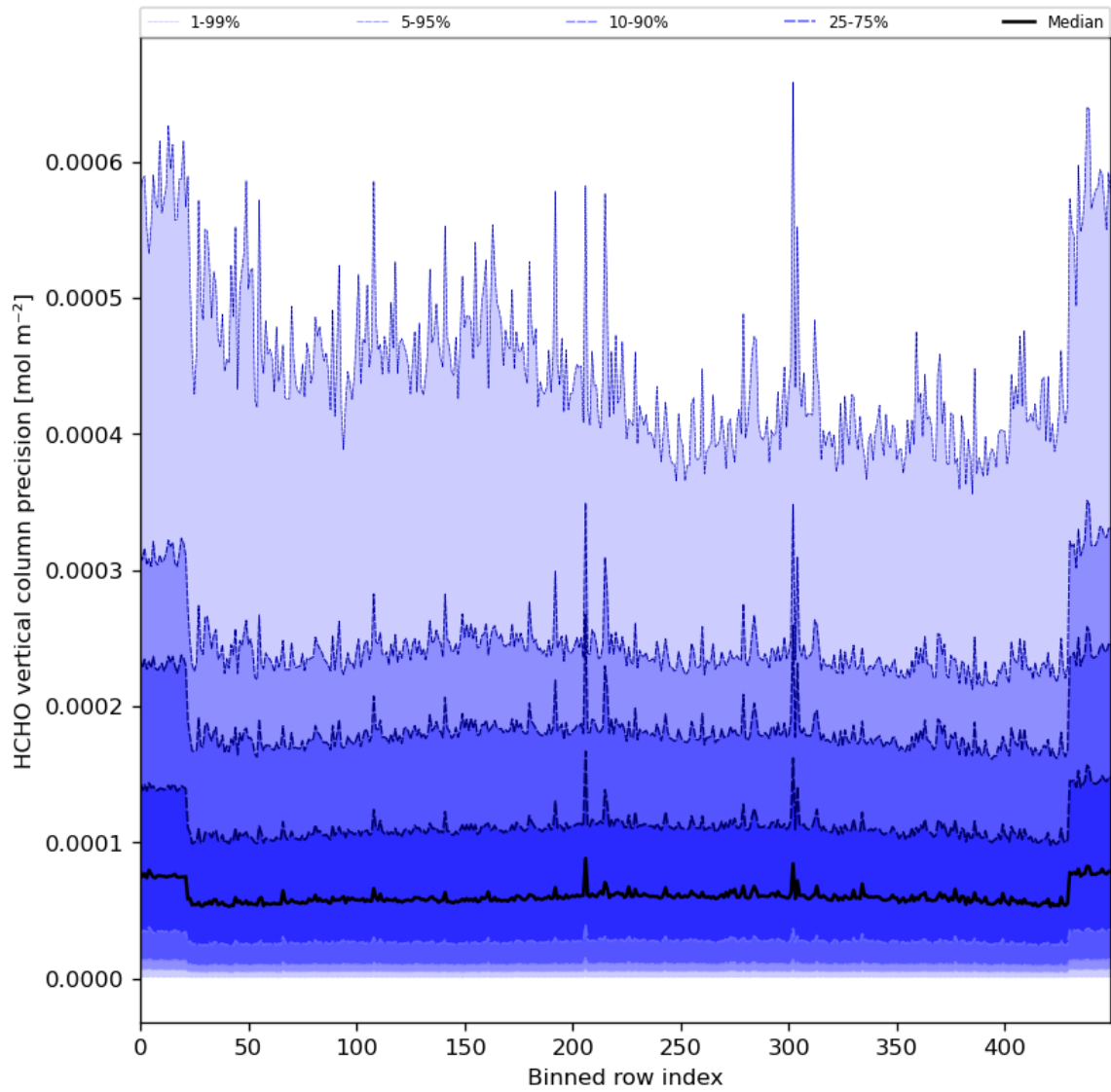
Figure 50: Along track statistics of “HCHO vertical column precision” for 2024-02-13 to 2024-02-15
