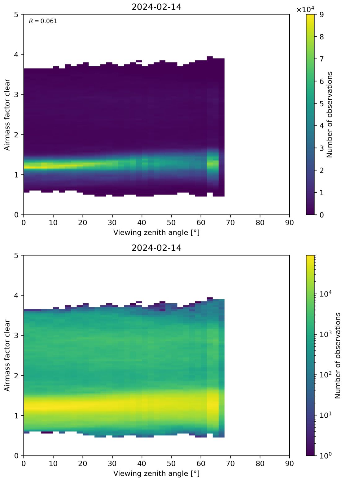
Figure 185: Scatter density plot of “Viewing zenith angle” against “Airmass factor clear” for 2024-02-13 to 2024-02-15.
