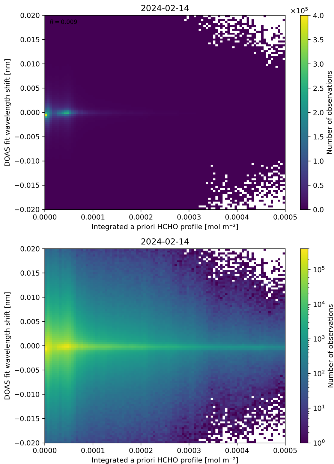
Figure 149: Scatter density plot of “Integrated a priori HCHO profile” against “DOAS fit wavelength shift” for 2024-02-13 to 2024-02-15.
