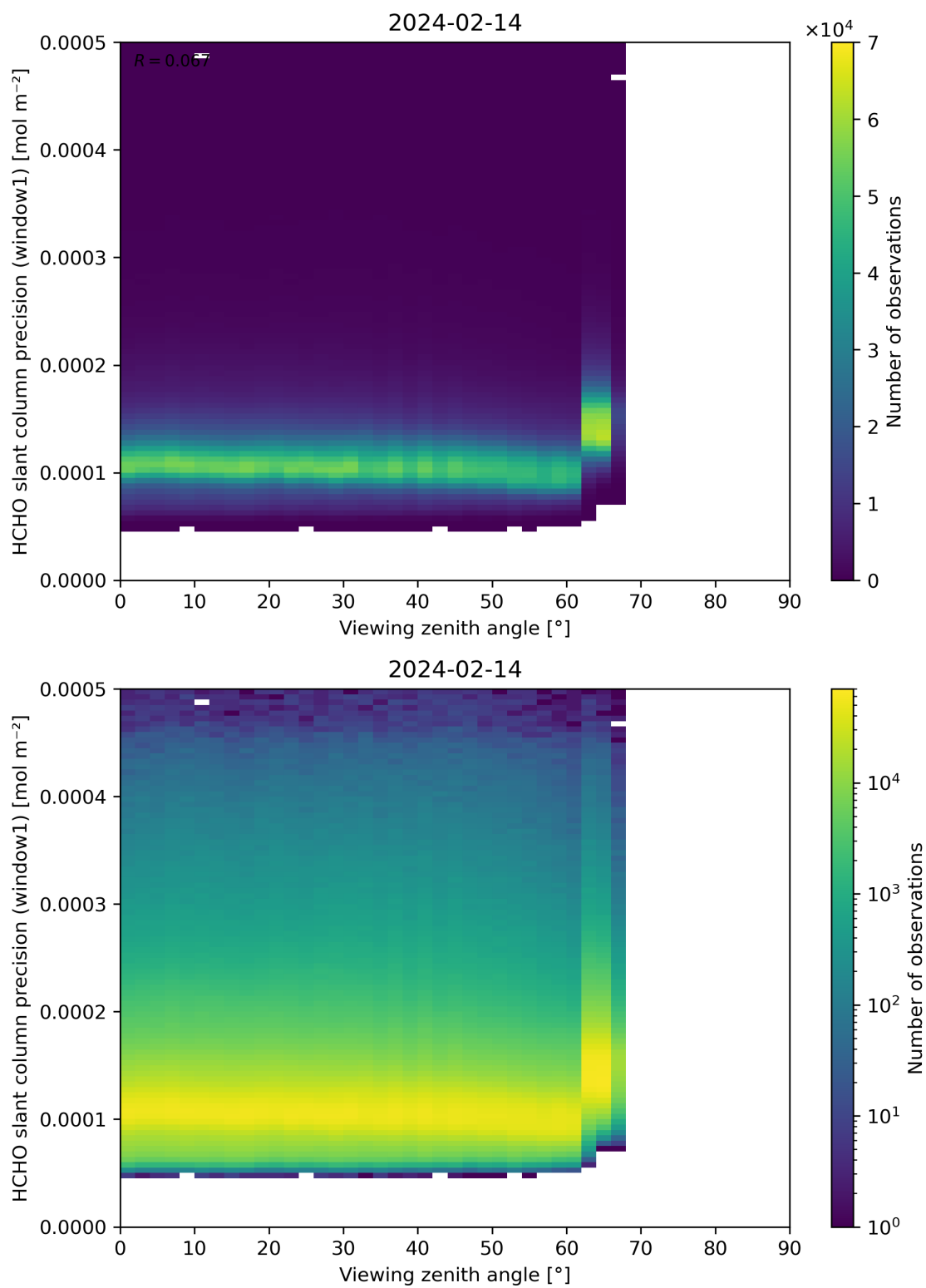
Figure 189: Scatter density plot of “Viewing zenith angle” against “HCHO slant column precision (window1)” for 2024-02-13 to 2024-02-15.
