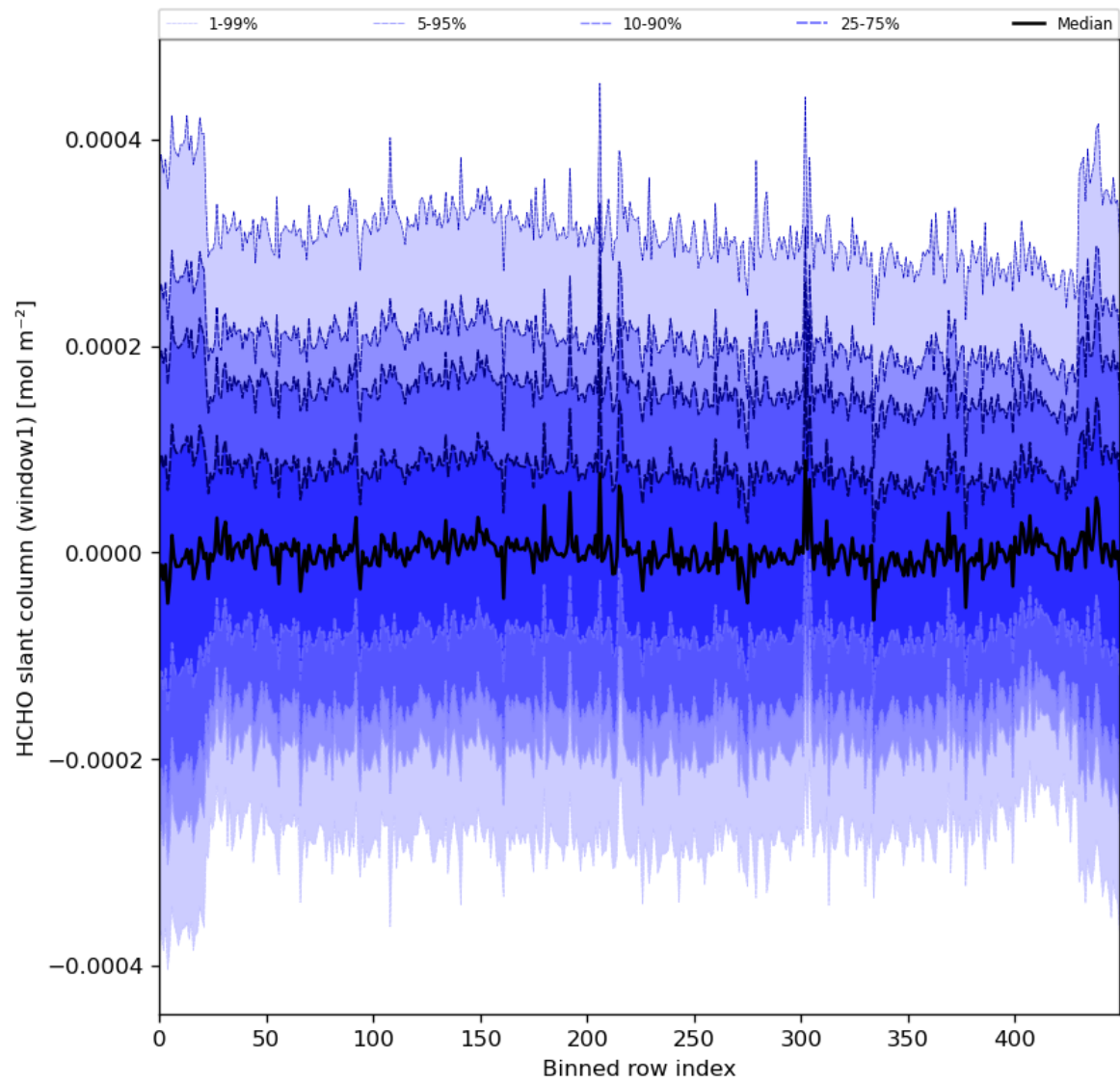
Figure 52: Along track statistics of “HCHO slant column (window1)” for 2024-02-13 to 2024-02-15
