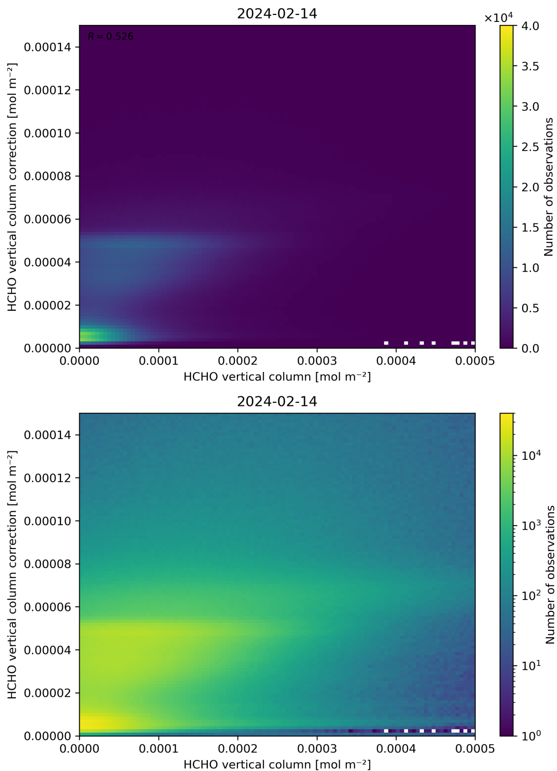
Figure 133: Scatter density plot of “HCHO vertical column” against “HCHO vertical column correction” for 2024-02-13 to 2024-02-15.
