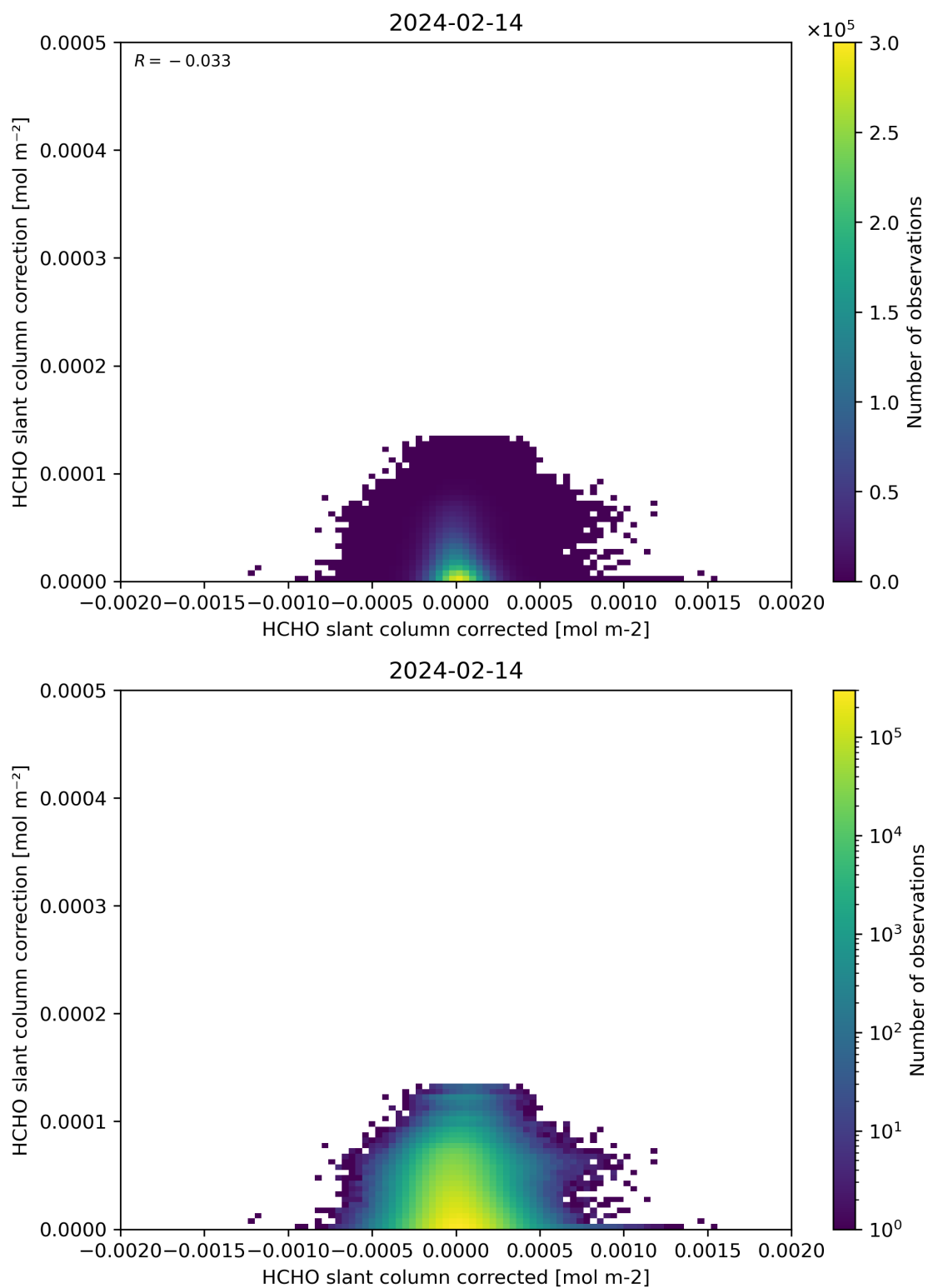
Figure 77: Scatter density plot of “HCHO slant column corrected” against “HCHO slant column correction” for 2024-02-13 to 2024-02-15.
