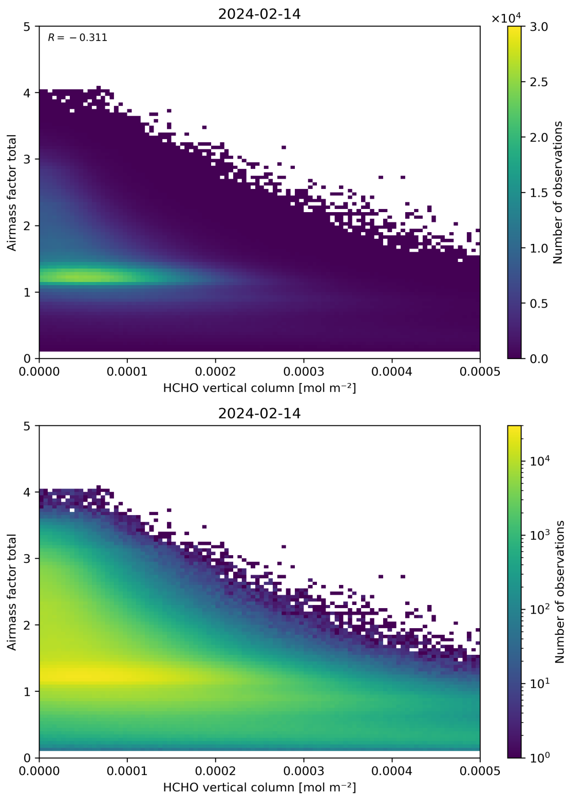
Figure 131: Scatter density plot of “HCHO vertical column” against “Airmass factor total” for 2024-02-13 to 2024-02-15.
