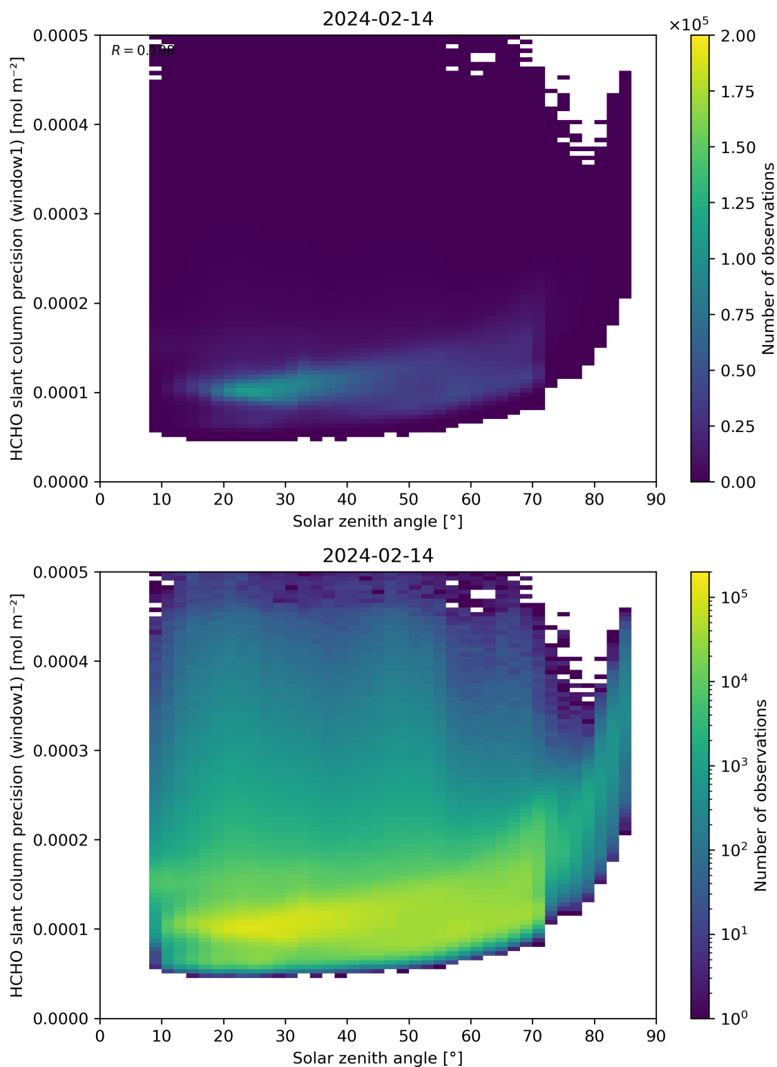
Figure 174: Scatter density plot of “Solar zenith angle” against “HCHO slant column precision (window1)” for 2024-02-13 to 2024-02-15.
