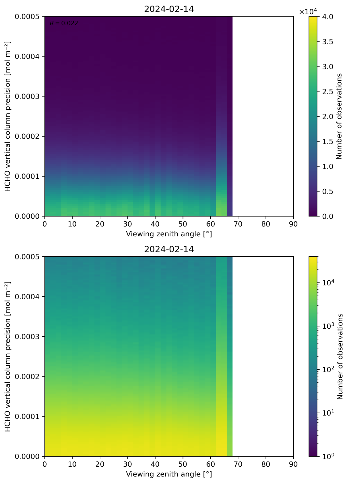
Figure 194: Scatter density plot of “Viewing zenith angle” against “HCHO vertical column precision” for 2024-02-13 to 2024-02-15.
