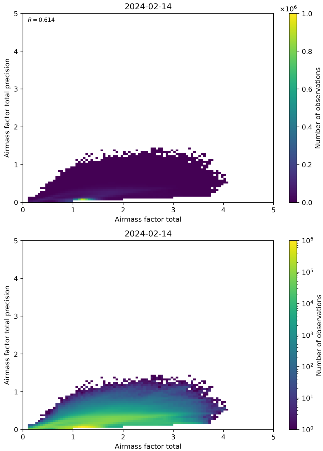
Figure 103: Scatter density plot of “Airmass factor total” against “Airmass factor total precision” for 2024-02-13 to 2024-02-15.
