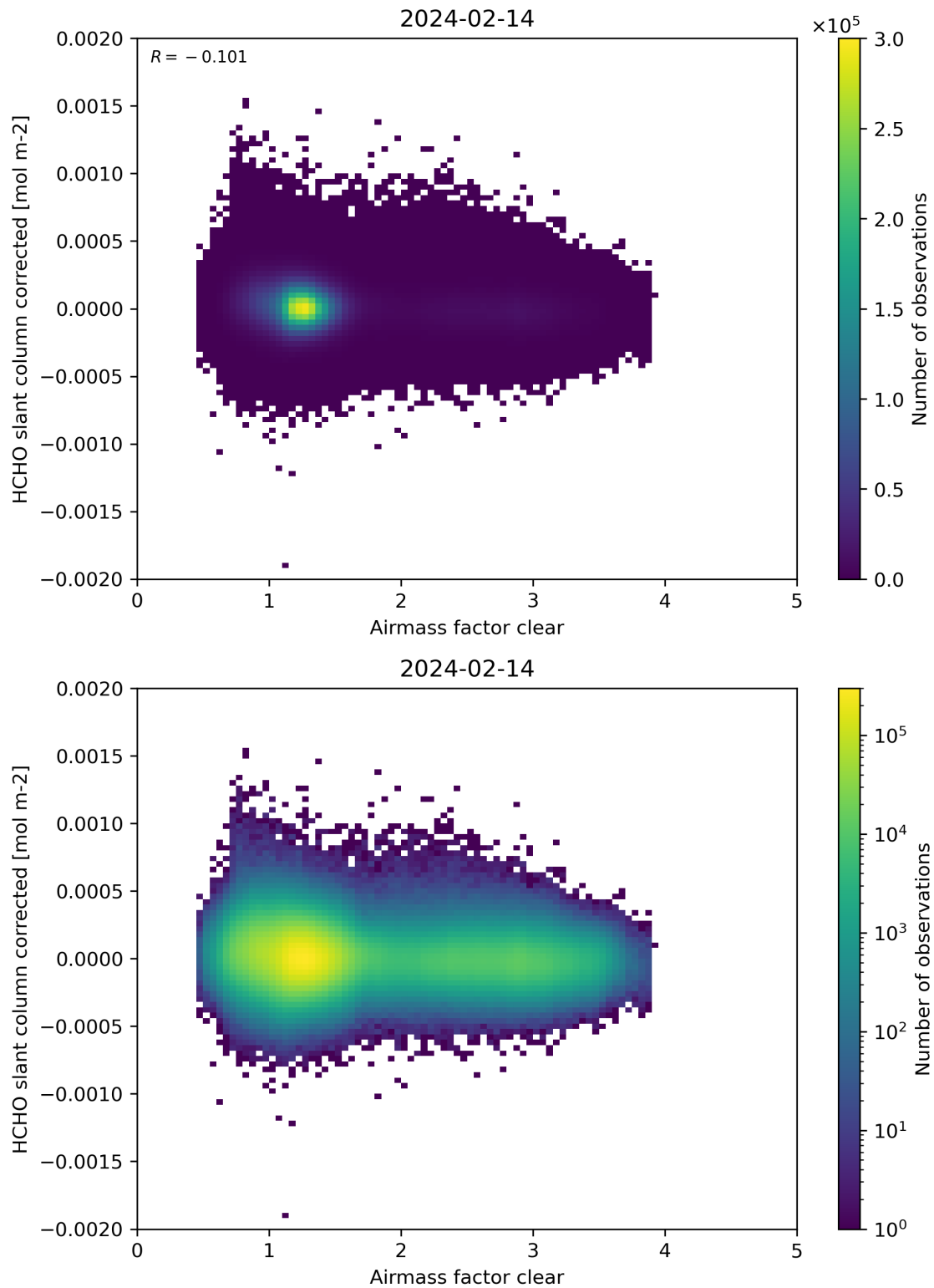
Figure 74: Scatter density plot of “Airmass factor clear” against “HCHO slant column corrected” for 2024-02-13 to 2024-02-15.
