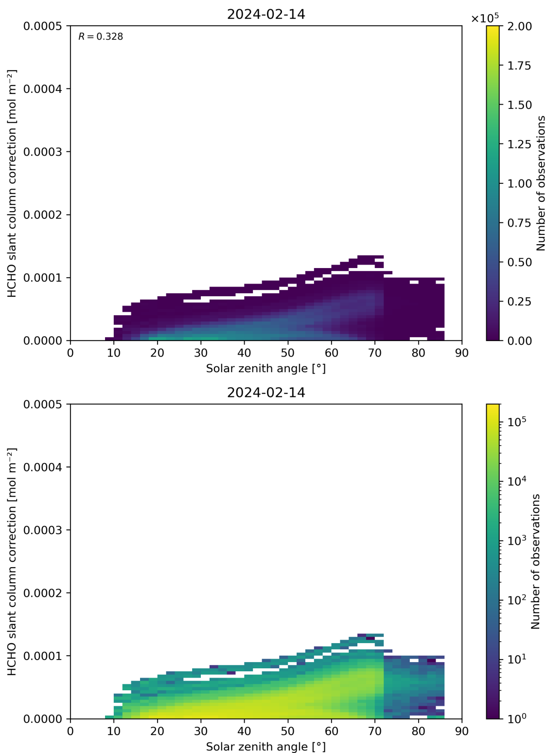
Figure 172: Scatter density plot of “Solar zenith angle” against “HCHO slant column correction” for 2024-02-13 to 2024-02-15.
