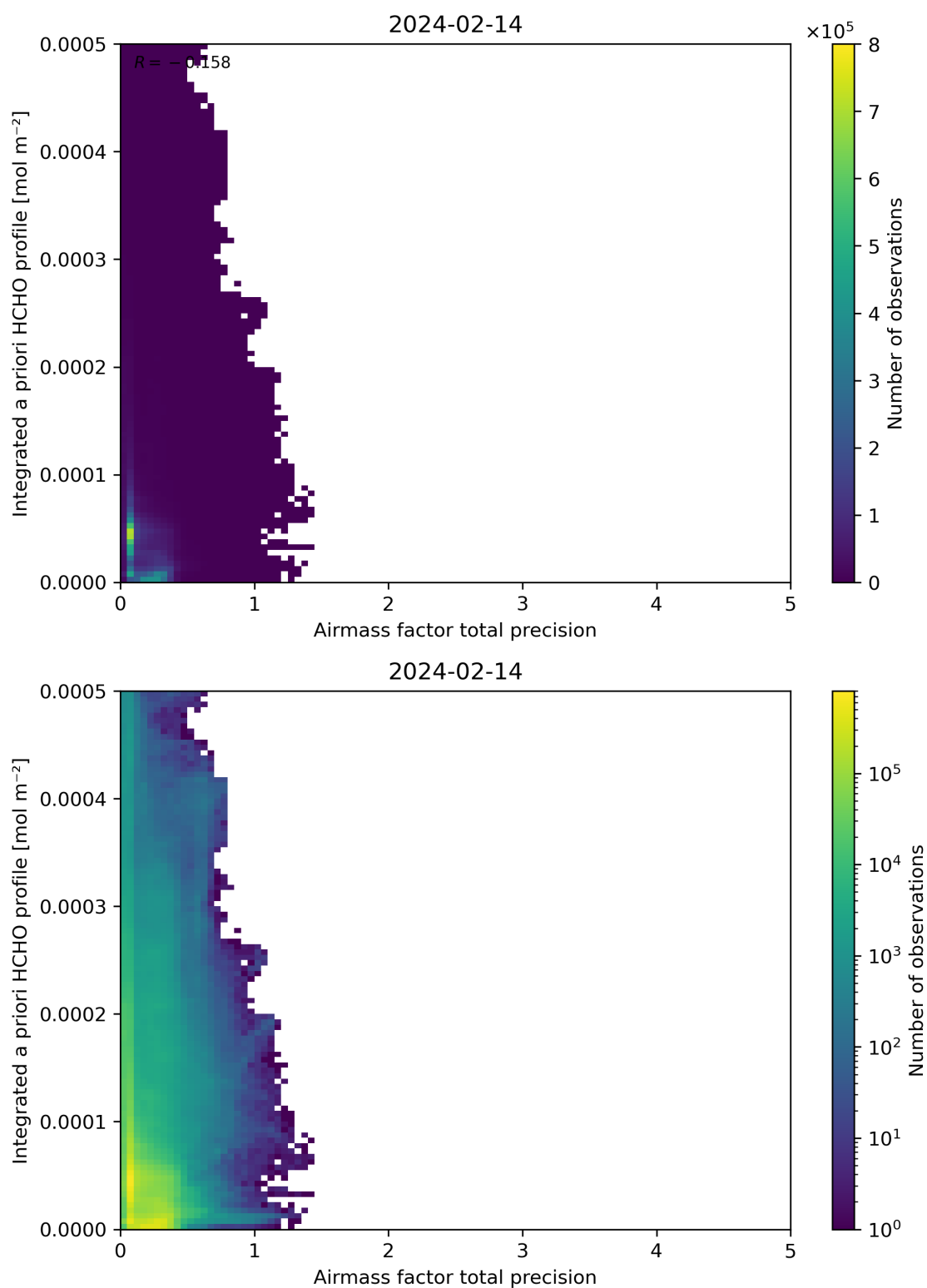
Figure 111: Scatter density plot of “Airmass factor total precision” against “Integrated a priori HCHO profile” for 2024-02-13 to 2024-02-15.
