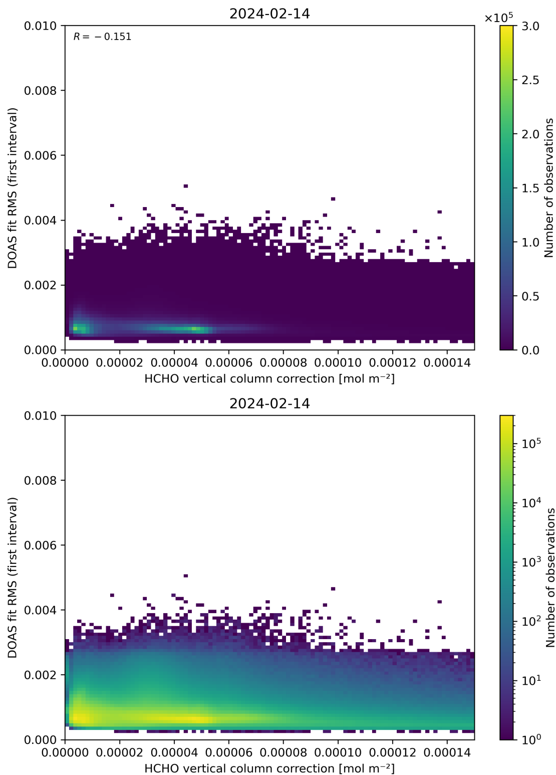
Figure 112: Scatter density plot of “HCHO vertical column correction” against “DOAS fit RMS (first interval)” for 2024-02-13 to 2024-02-15.
