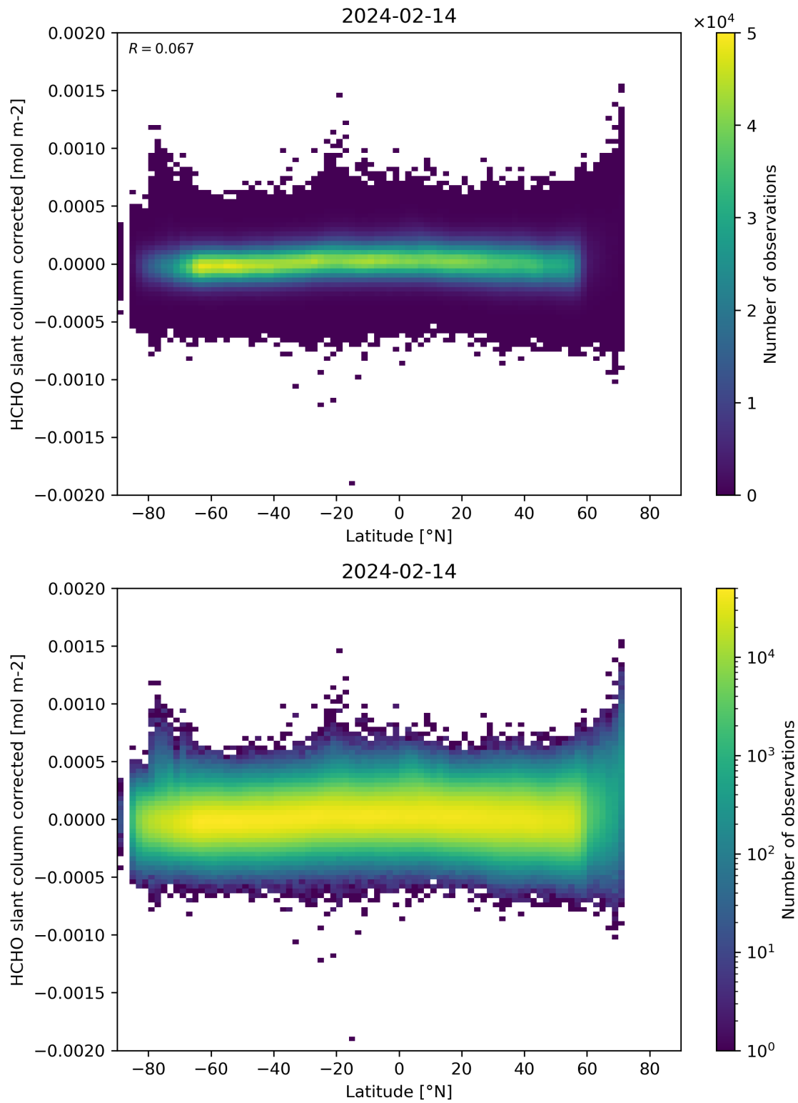
Figure 157: Scatter density plot of “Latitude” against “HCHO slant column corrected” for 2024-02-13 to 2024-02-15.
