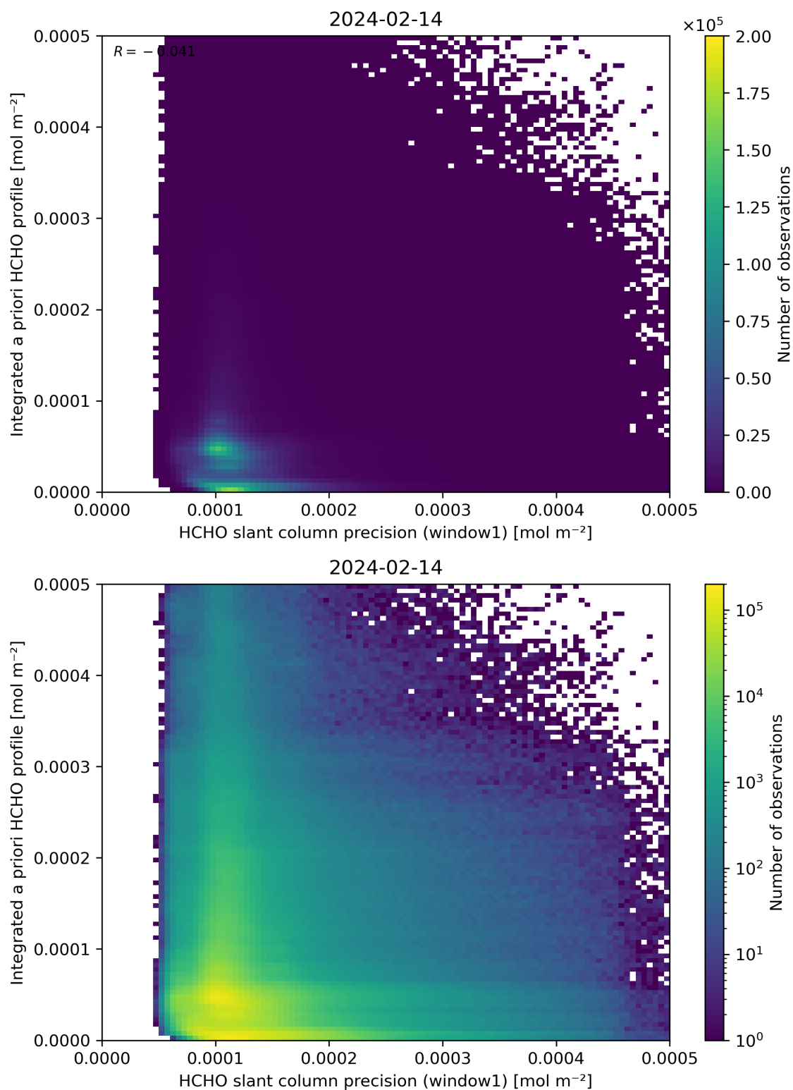
Figure 96: Scatter density plot of “HCHO slant column precision (window1)” against “Integrated a priori HCHO profile” for 2024-02-13 to 2024-02-15.
