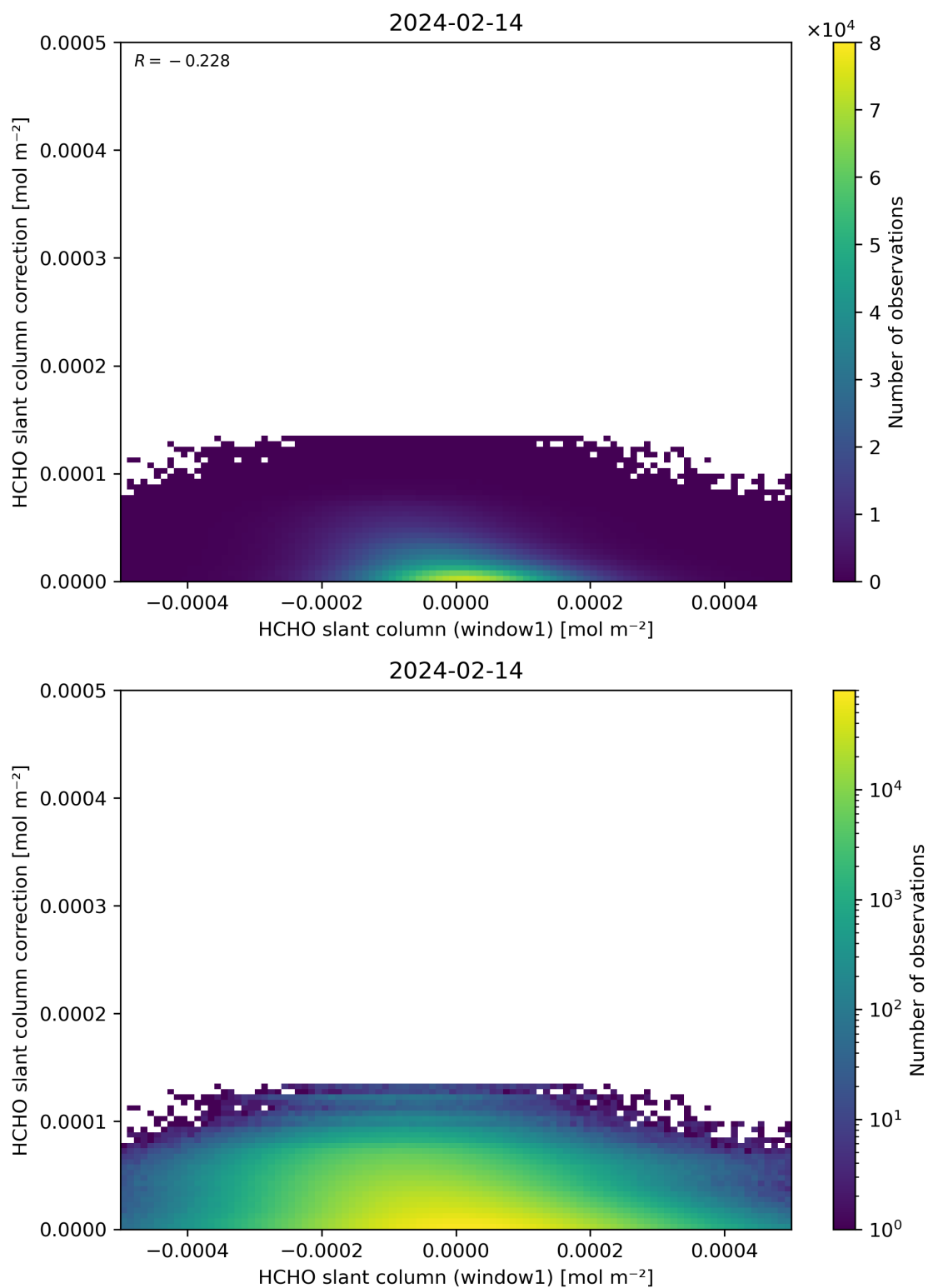
Figure 83: Scatter density plot of “HCHO slant column (window1)” against “HCHO slant column correction” for 2024-02-13 to 2024-02-15.
