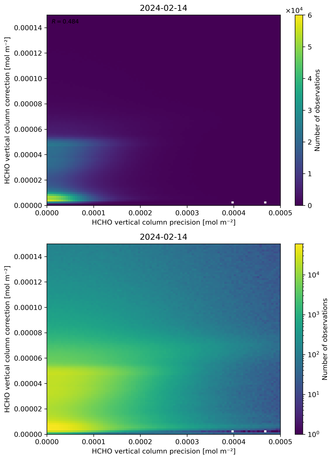
Figure 146: Scatter density plot of “HCHO vertical column precision” against “HCHO vertical column correction” for 2024-02-13 to 2024-02-15.
