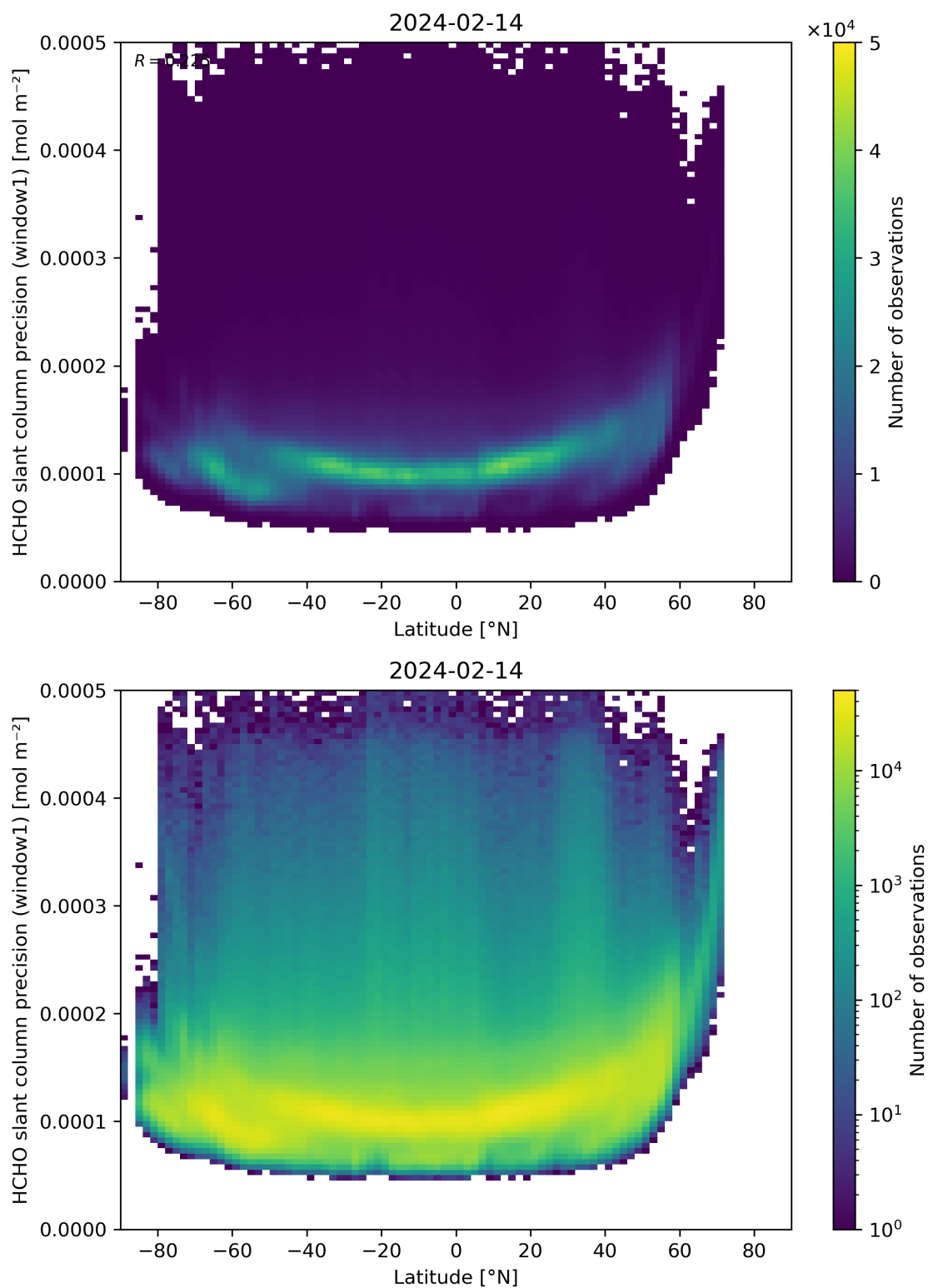
Figure 160: Scatter density plot of “Latitude” against “HCHO slant column precision (window1)” for 2024-02-13 to 2024-02-15.
