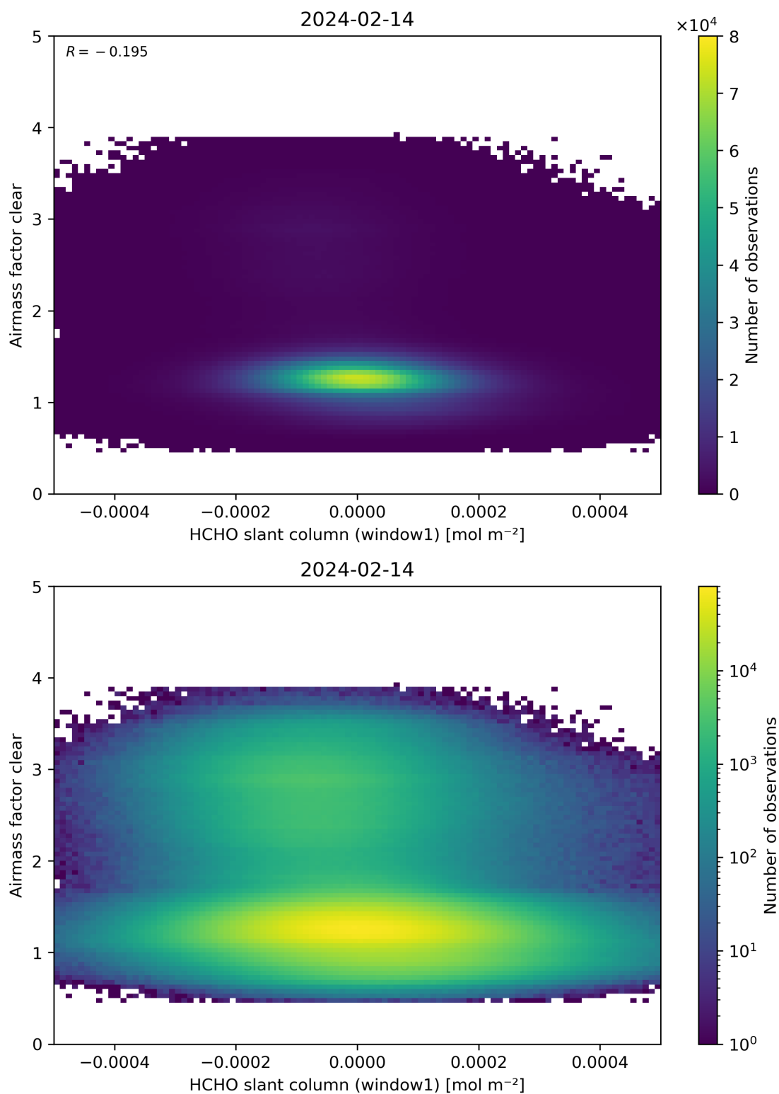
Figure 81: Scatter density plot of “HCHO slant column (window1)” against “Airmass factor clear” for 2024-02-13 to 2024-02-15.
