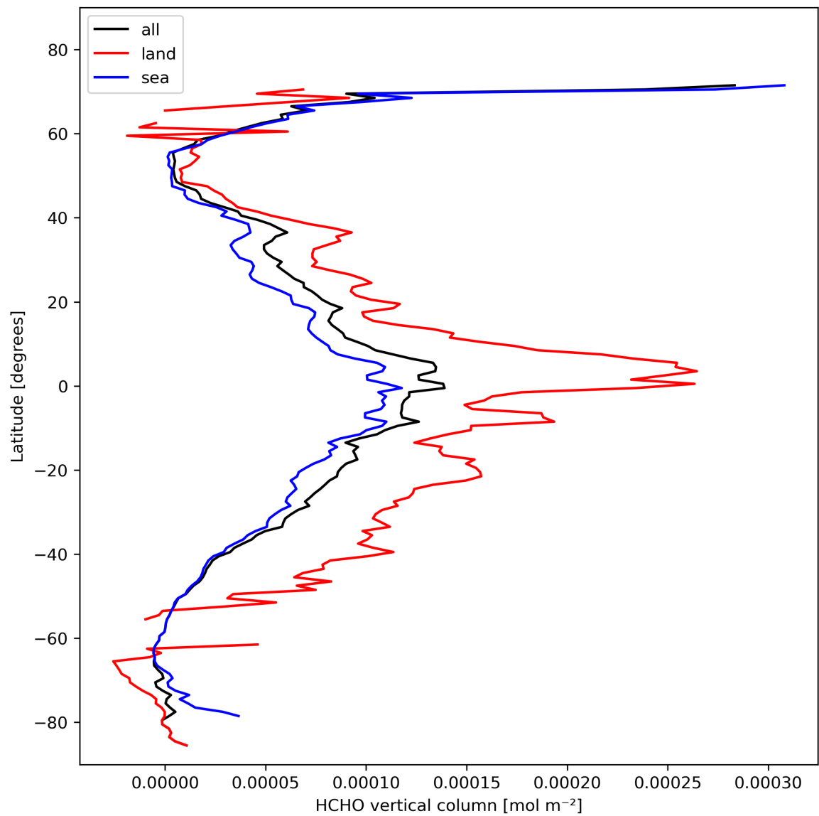
Figure 21: Zonal average of “HCHO vertical column” for 2024-02-13 to 2024-02-15.
