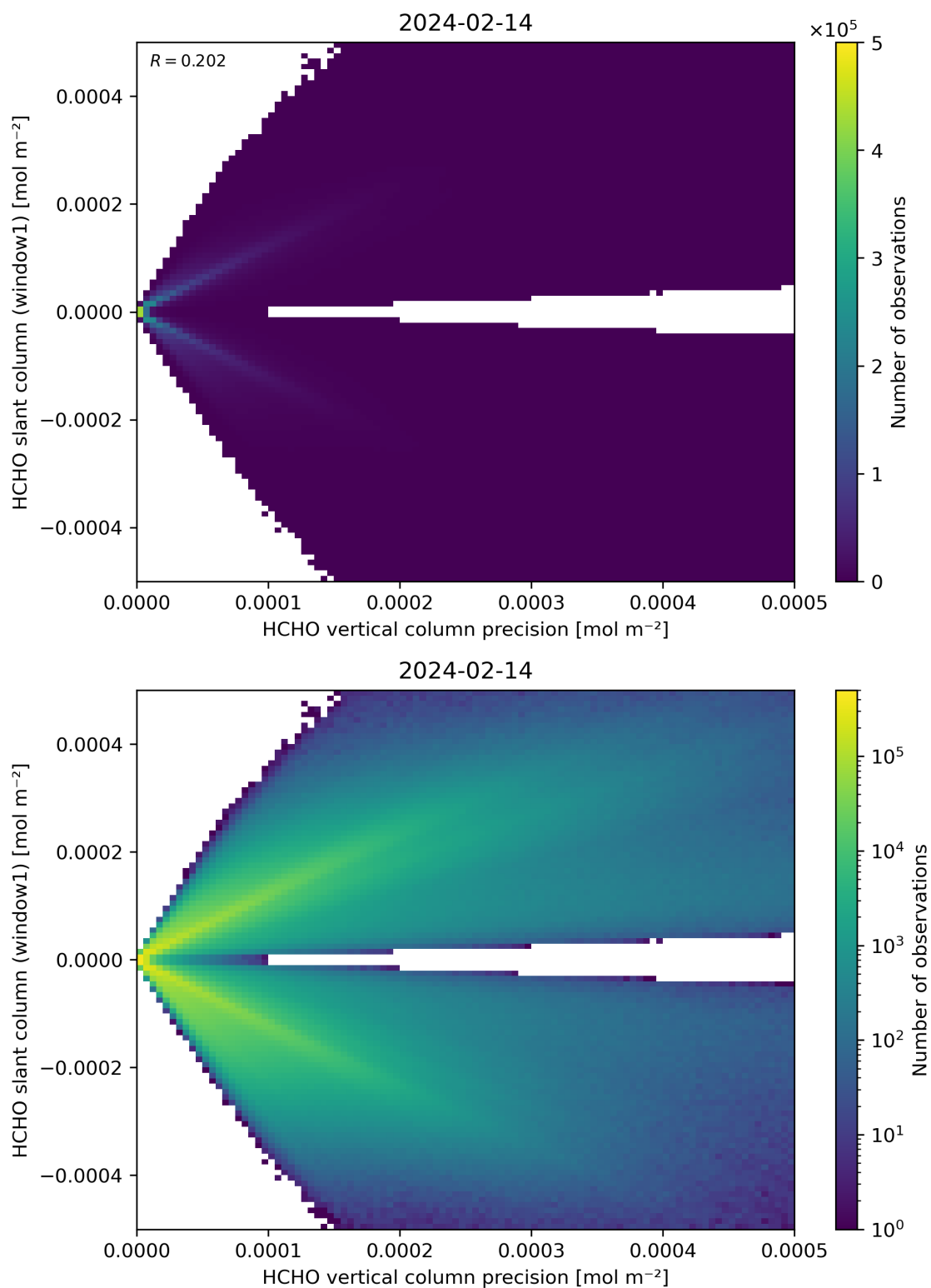
Figure 142: Scatter density plot of “HCHO vertical column precision” against “HCHO slant column (window1)” for 2024-02-13 to 2024-02-15.
