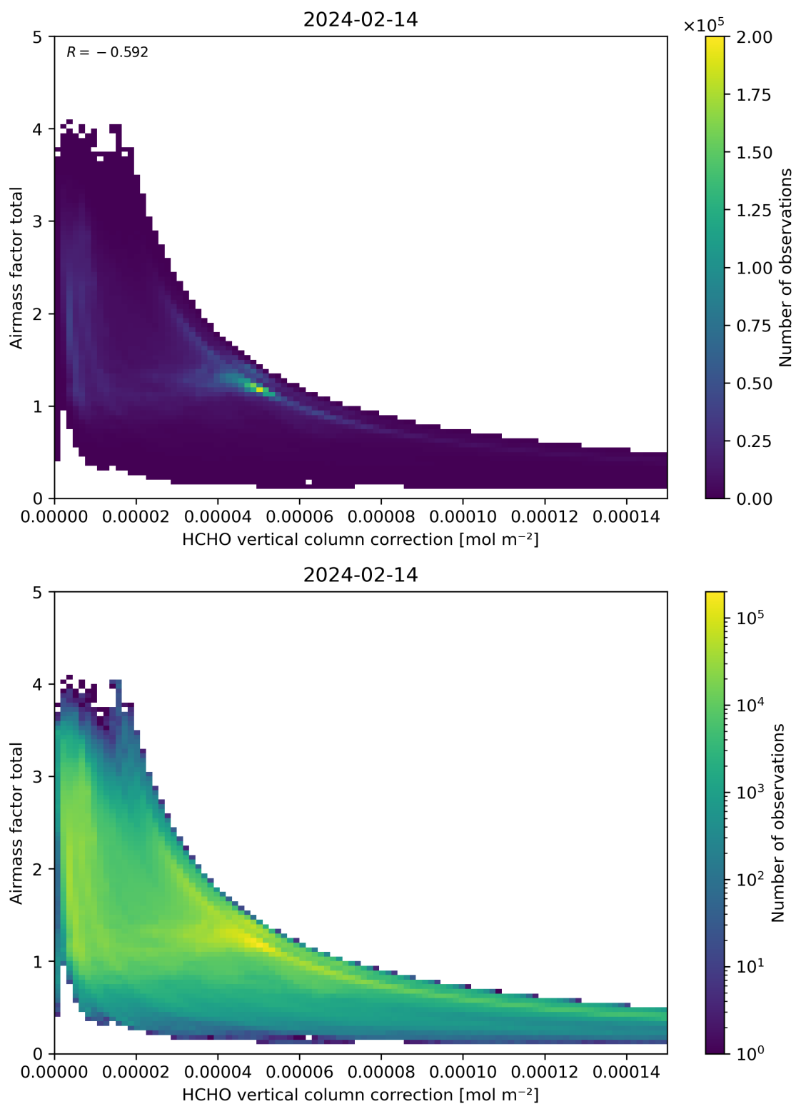
Figure 120: Scatter density plot of “HCHO vertical column correction” against “Airmass factor total” for 2024-02-13 to 2024-02-15.
