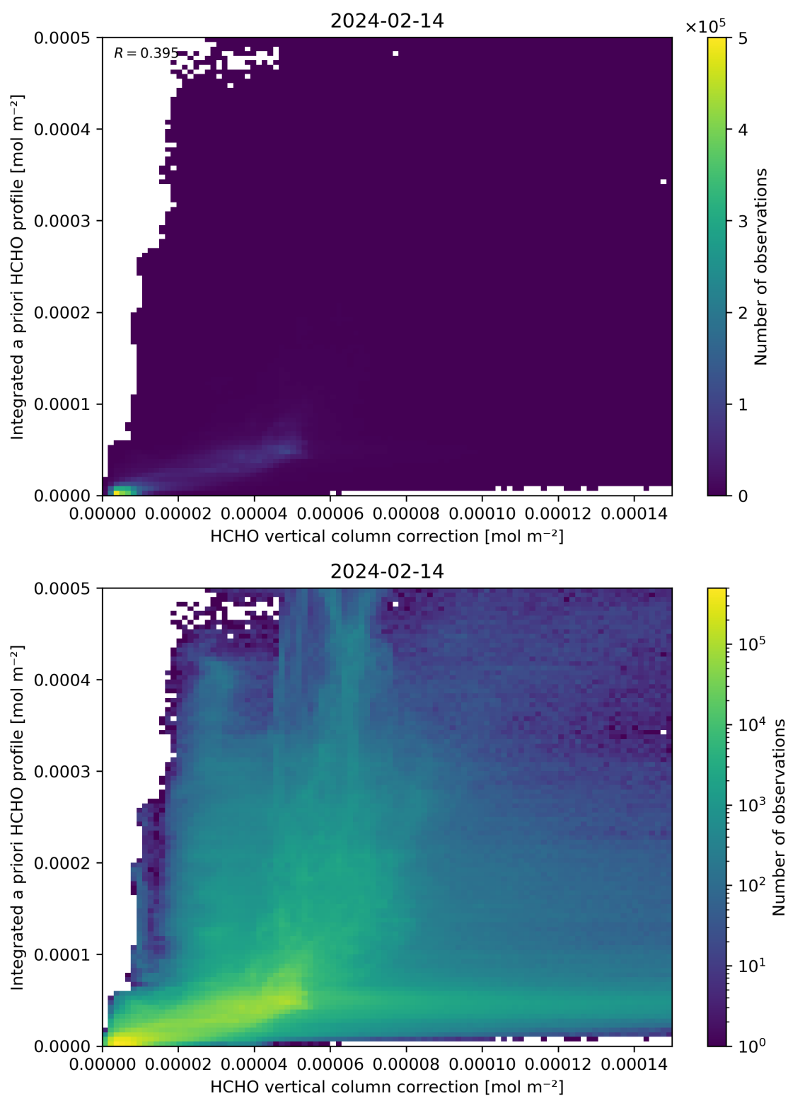
Figure 122: Scatter density plot of “HCHO vertical column correction” against “Integrated a priori HCHO profile” for 2024-02-13 to 2024-02-15.
