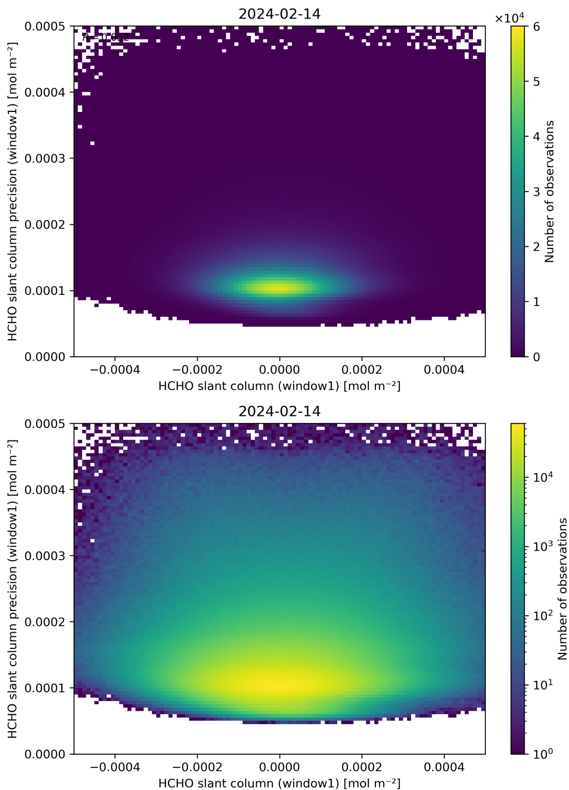
Figure 84: Scatter density plot of “HCHO slant column (window1)” against “HCHO slant column precision (window1)” for 2024-02-13 to 2024-02-15.
