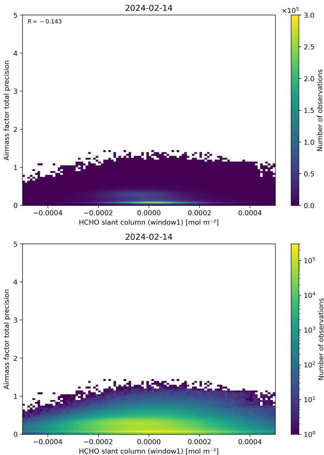
Figure 86: Scatter density plot of “HCHO slant column (window1)” against “Airmass factor total precision” for 2024-02-13 to 2024-02-15.
