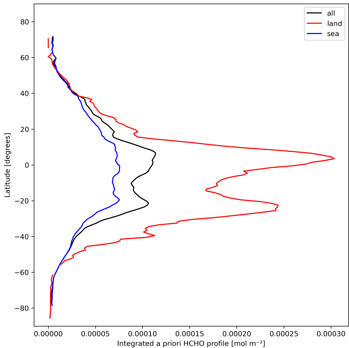
Figure 29: Zonal average of “Integrated a priori HCHO profile” for 2024-02-13 to 2024-02-15.
