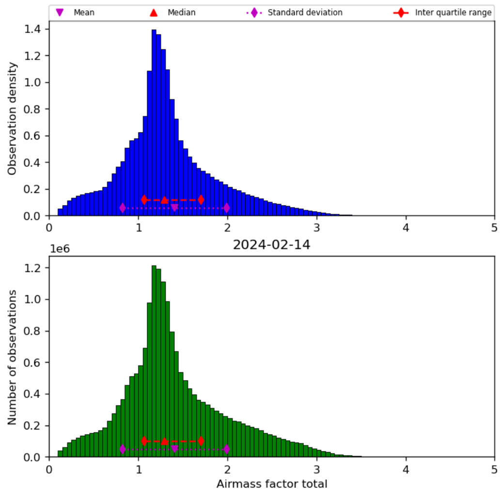
Figure 40: Histogram of “Airmass factor total” for 2024-02-13 to 2024-02-15
