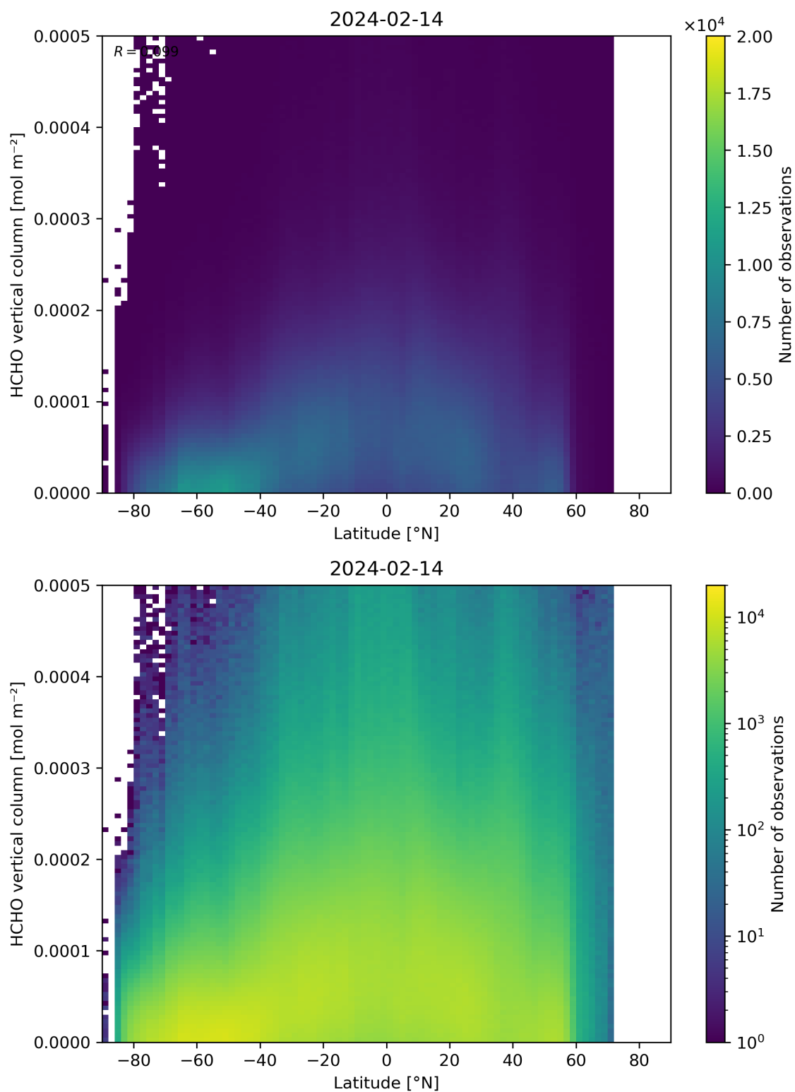
Figure 163: Scatter density plot of “Latitude” against “HCHO vertical column” for 2024-02-13 to 2024-02-15.
