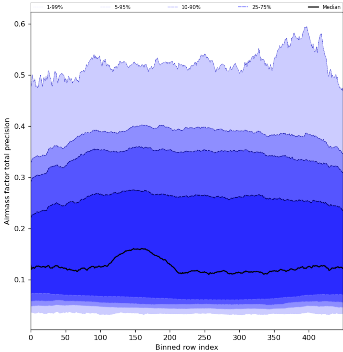
Figure 55: Along track statistics of “Airmass factor total precision” for 2024-02-13 to 2024-02-15
