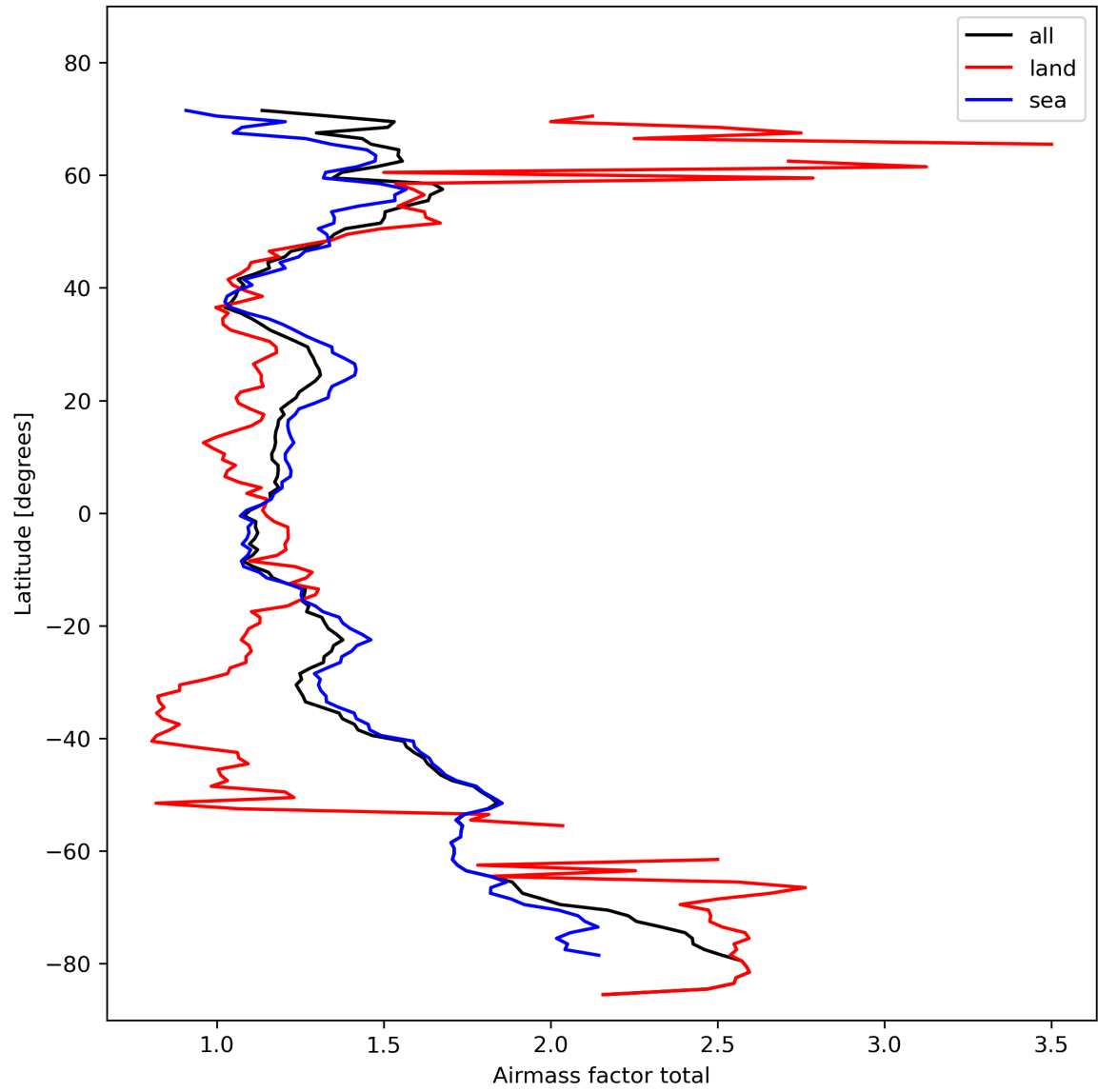
Figure 26: Zonal average of “Airmass factor total” for 2024-02-13 to 2024-02-15.
