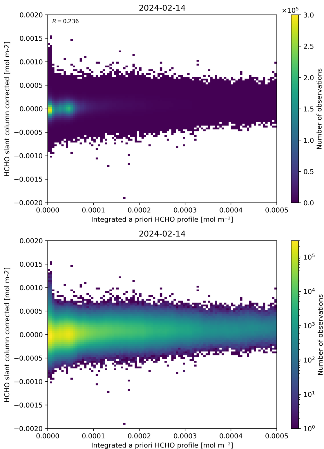
Figure 151: Scatter density plot of “Integrated a priori HCHO profile” against “HCHO slant column corrected” for 2024-02-13 to 2024-02-15.
