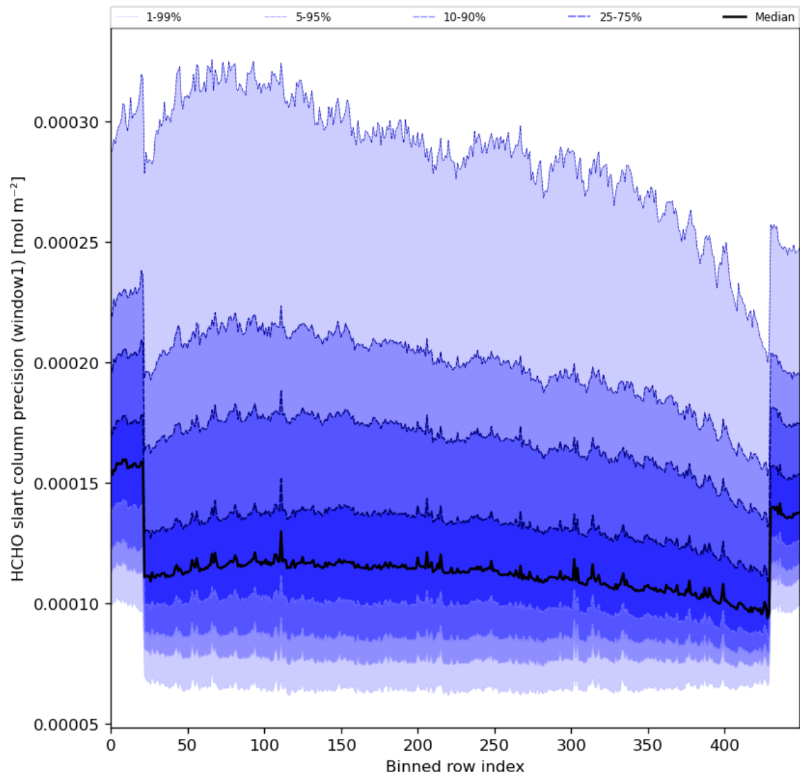
Figure 53: Along track statistics of “HCHO slant column precision (window1)” for 2024-02-13 to 2024-02-15
