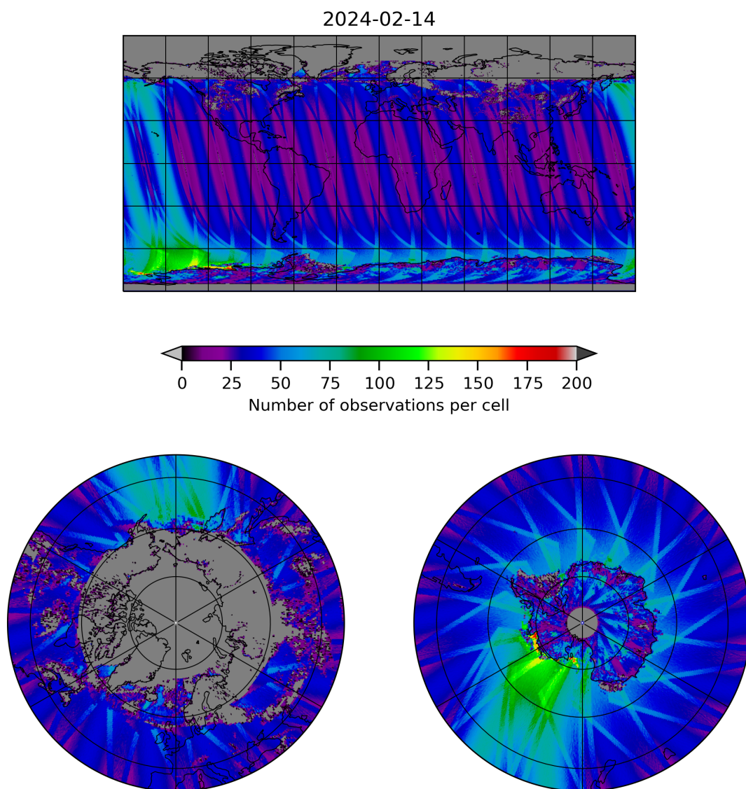
Figure 19: Map of the number of observations for 2024-02-13 to 2024-02-15
