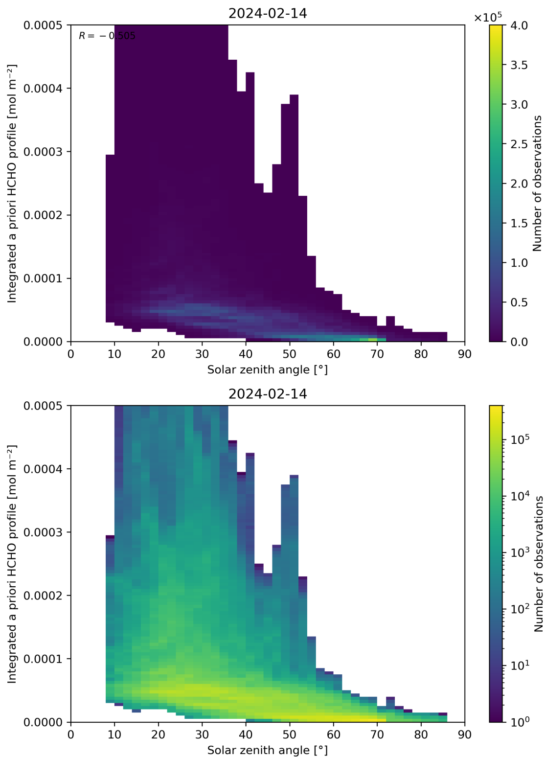
Figure 180: Scatter density plot of “Solar zenith angle” against “Integrated a priori HCHO profile” for 2024-02-13 to 2024-02-15.
