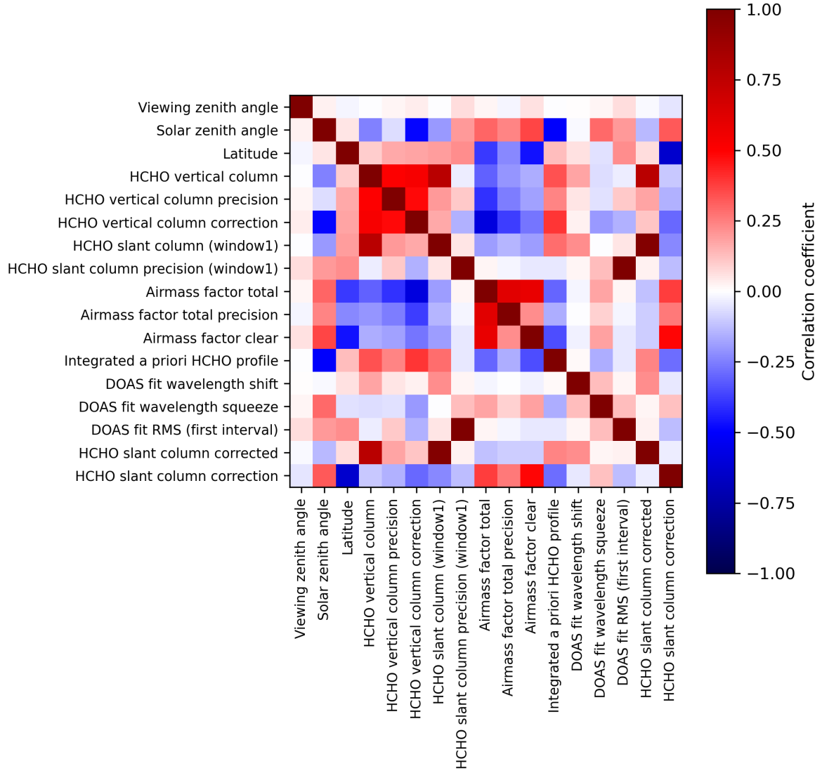
Figure 2: Map of correlation matrix for 2024-02-13 to 2024-02-15.
