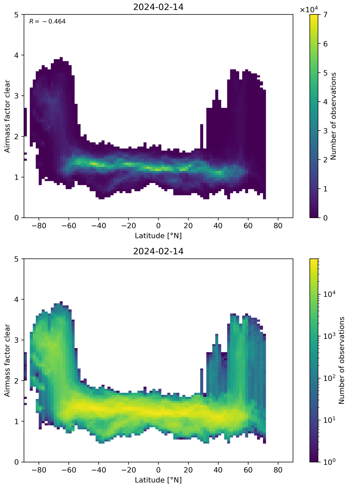
Figure 156: Scatter density plot of “Latitude” against “Airmass factor clear” for 2024-02-13 to 2024-02-15.
