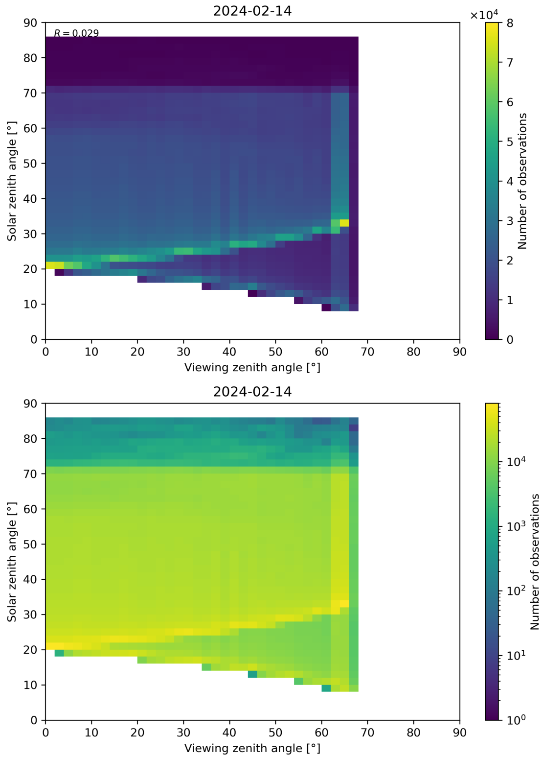
Figure 197: Scatter density plot of “Viewing zenith angle” against “Solar zenith angle” for 2024-02-13 to 2024-02-15.
