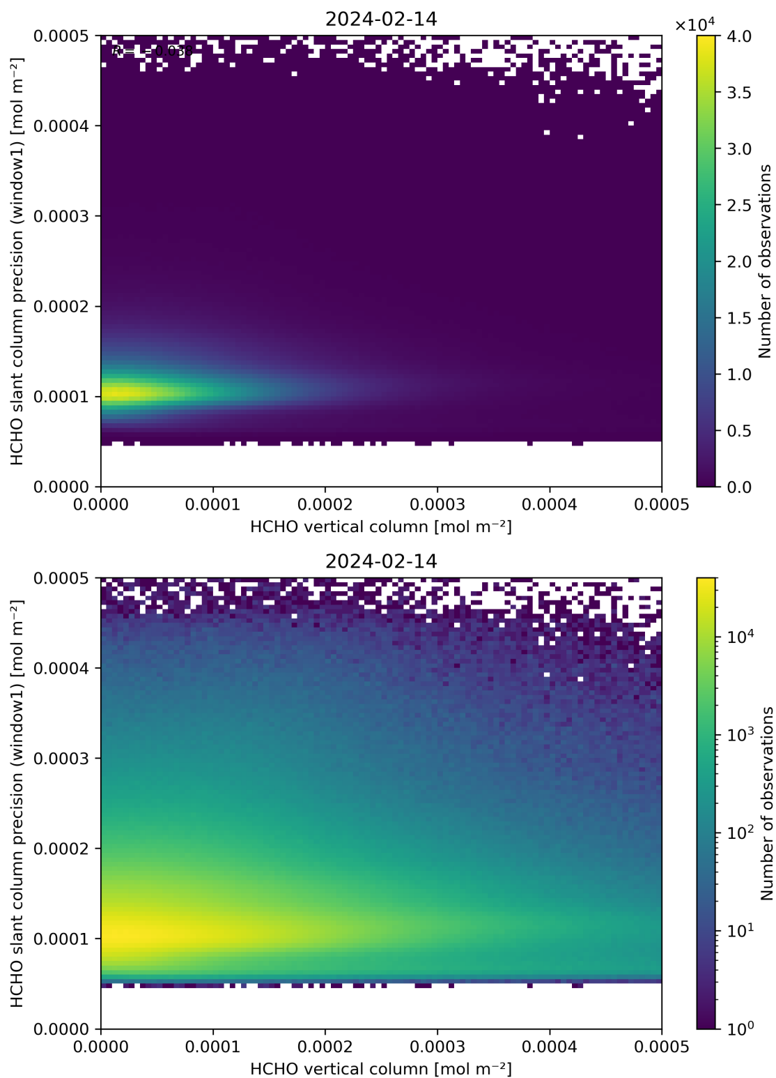
Figure 130: Scatter density plot of “HCHO vertical column” against “HCHO slant column precision (window1)” for 2024-02-13 to 2024-02-15.
