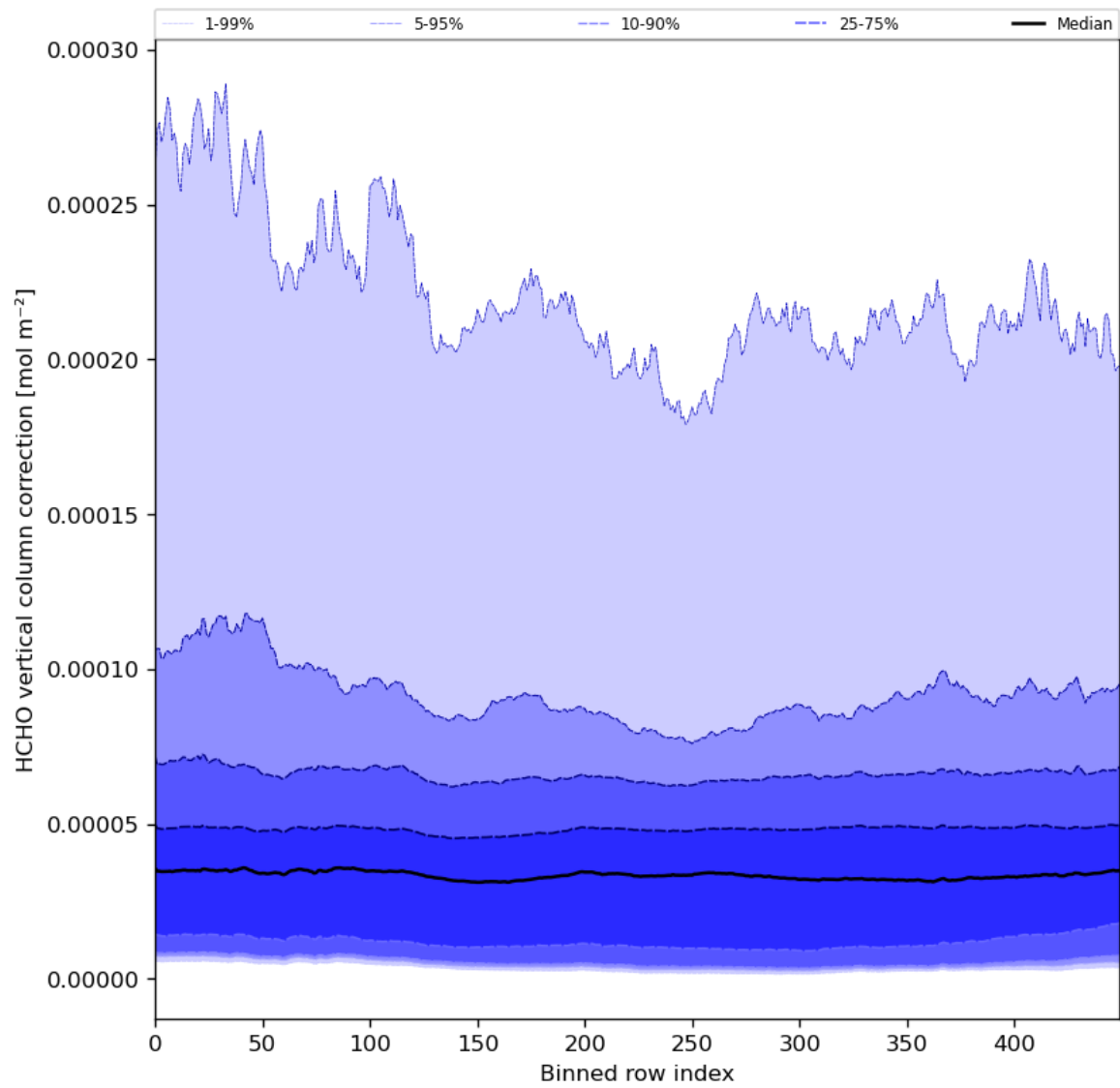
Figure 51: Along track statistics of “HCHO vertical column correction” for 2024-02-13 to 2024-02-15
