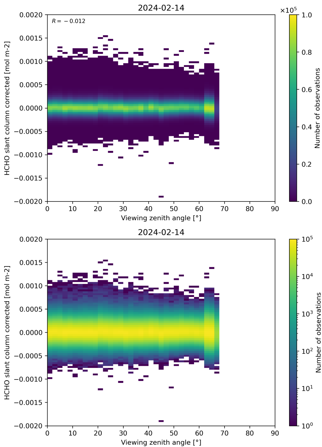
Figure 186: Scatter density plot of “Viewing zenith angle” against “HCHO slant column corrected” for 2024-02-13 to 2024-02-15.
