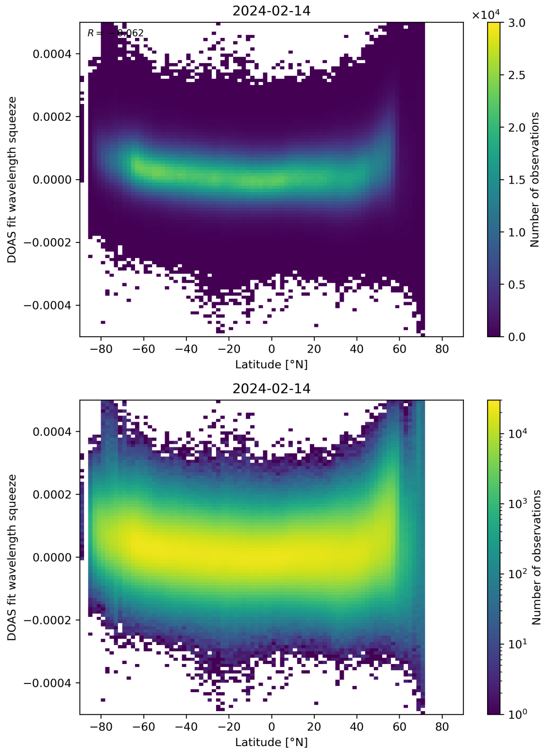
Figure 155: Scatter density plot of “Latitude” against “DOAS fit wavelength squeeze” for 2024-02-13 to 2024-02-15.
