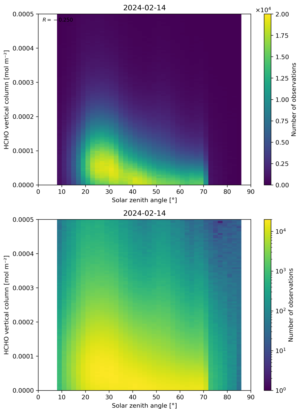
Figure 177: Scatter density plot of “Solar zenith angle” against “HCHO vertical column” for 2024-02-13 to 2024-02-15.
