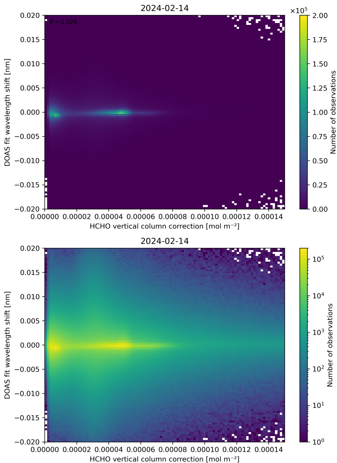
Figure 113: Scatter density plot of “HCHO vertical column correction” against “DOAS fit wavelength shift” for 2024-02-13 to 2024-02-15.
