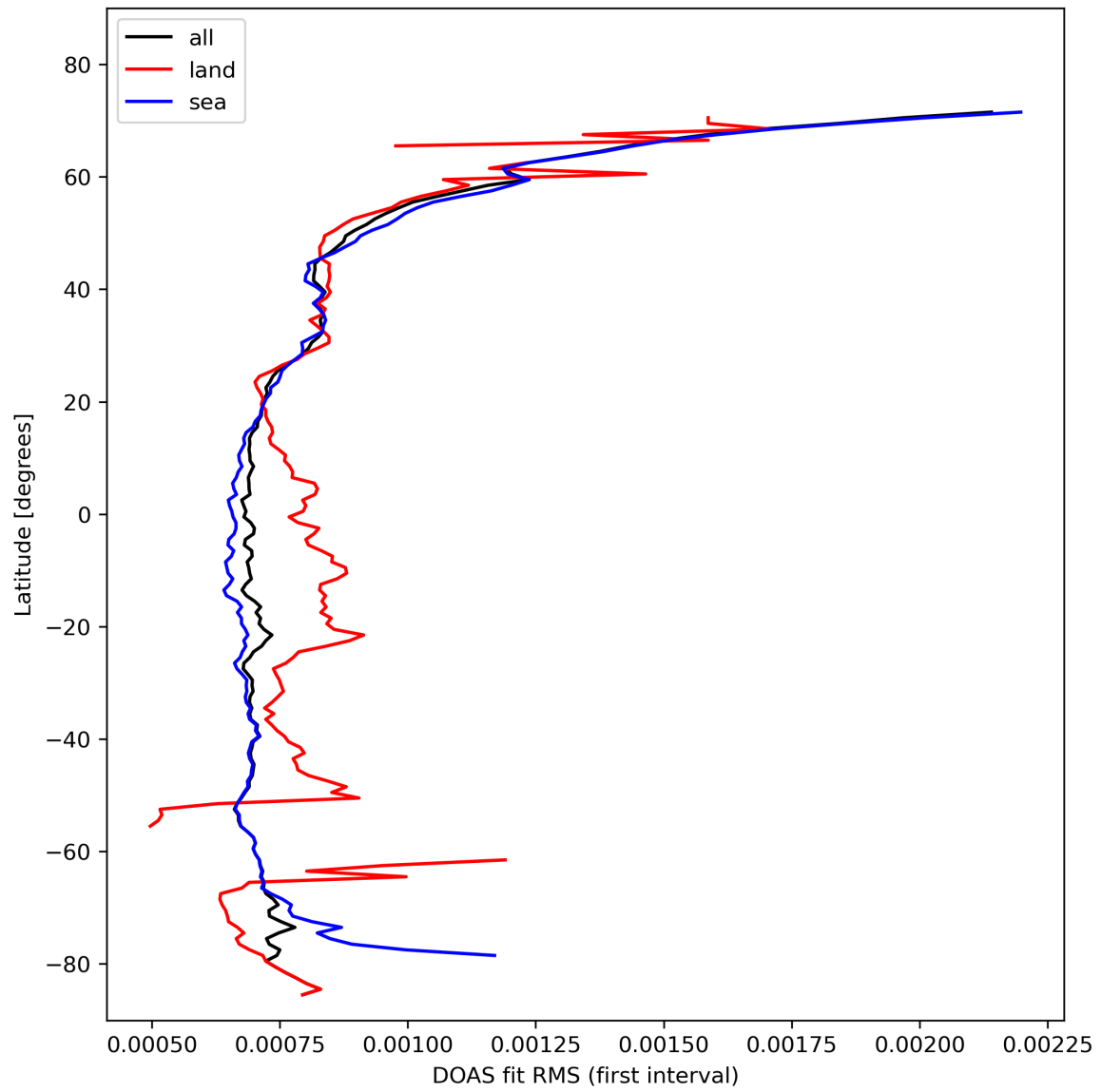
Figure 32: Zonal average of “DOAS fit RMS (first interval)” for 2024-02-13 to 2024-02-15.
