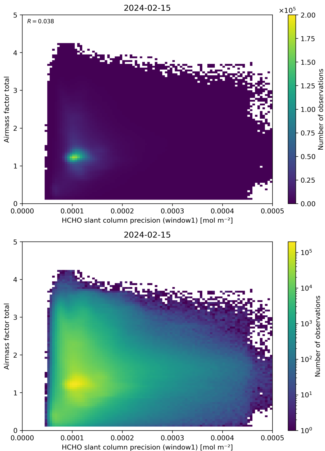
Figure 94: Scatter density plot of “HCHO slant column precision (window1)” against “Airmass factor total” for 2024-02-14 to 2024-02-16.
