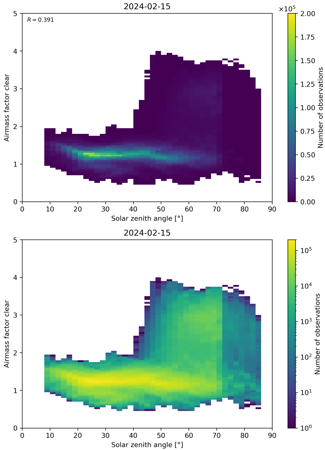
Figure 170: Scatter density plot of “Solar zenith angle” against “Airmass factor clear” for 2024-02-14 to 2024-02-16.
