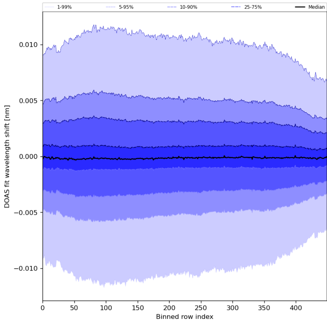
Figure 58: Along track statistics of “DOAS fit wavelength shift” for 2024-02-14 to 2024-02-16
