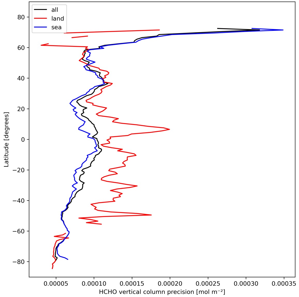
Figure 22: Zonal average of “HCHO vertical column precision” for 2024-02-14 to 2024-02-16.
