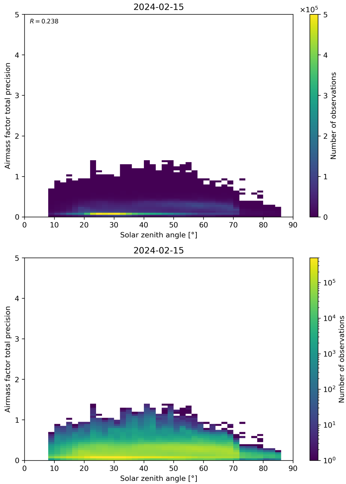
Figure 176: Scatter density plot of “Solar zenith angle” against “Airmass factor total precision” for 2024-02-14 to 2024-02-16.
