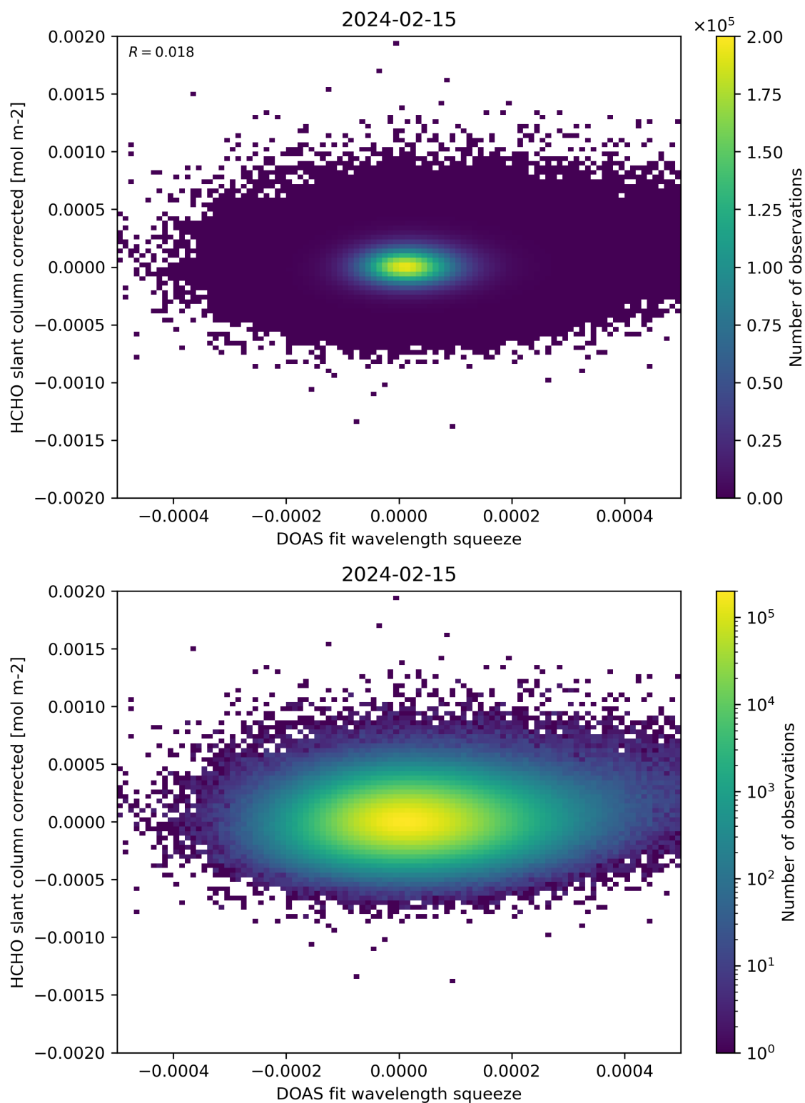
Figure 69: Scatter density plot of “DOAS fit wavelength squeeze” against “HCHO slant column corrected” for 2024-02-14 to 2024-02-16.
