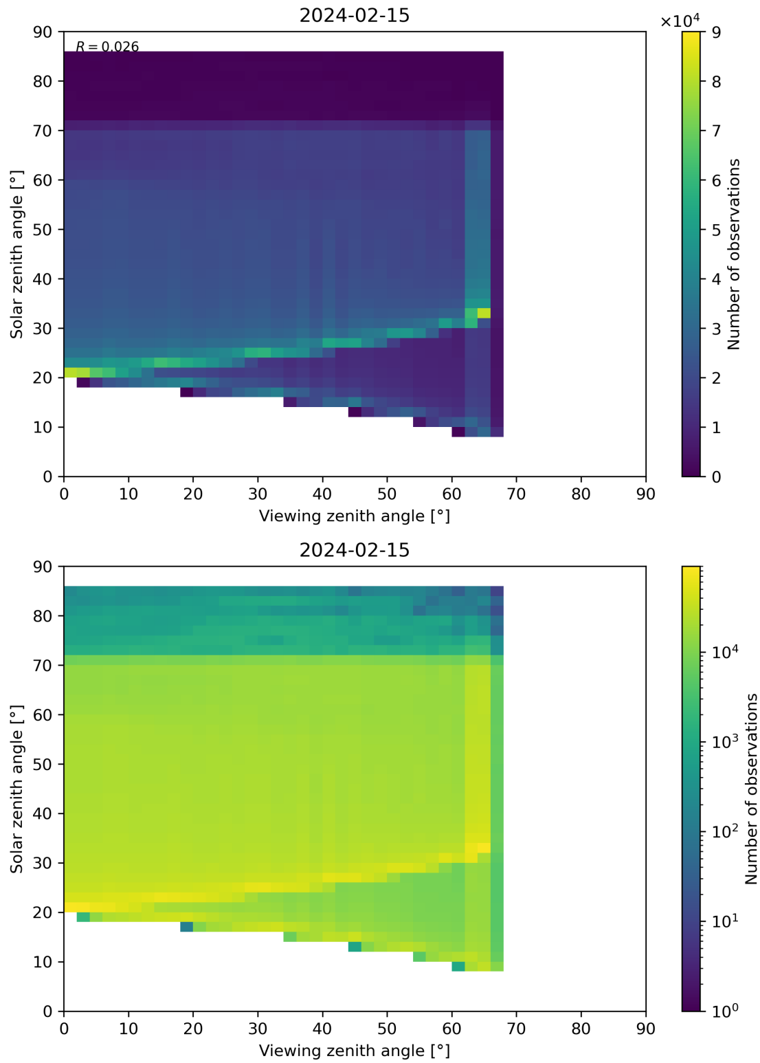
Figure 197: Scatter density plot of “Viewing zenith angle” against “Solar zenith angle” for 2024-02-14 to 2024-02-16.
