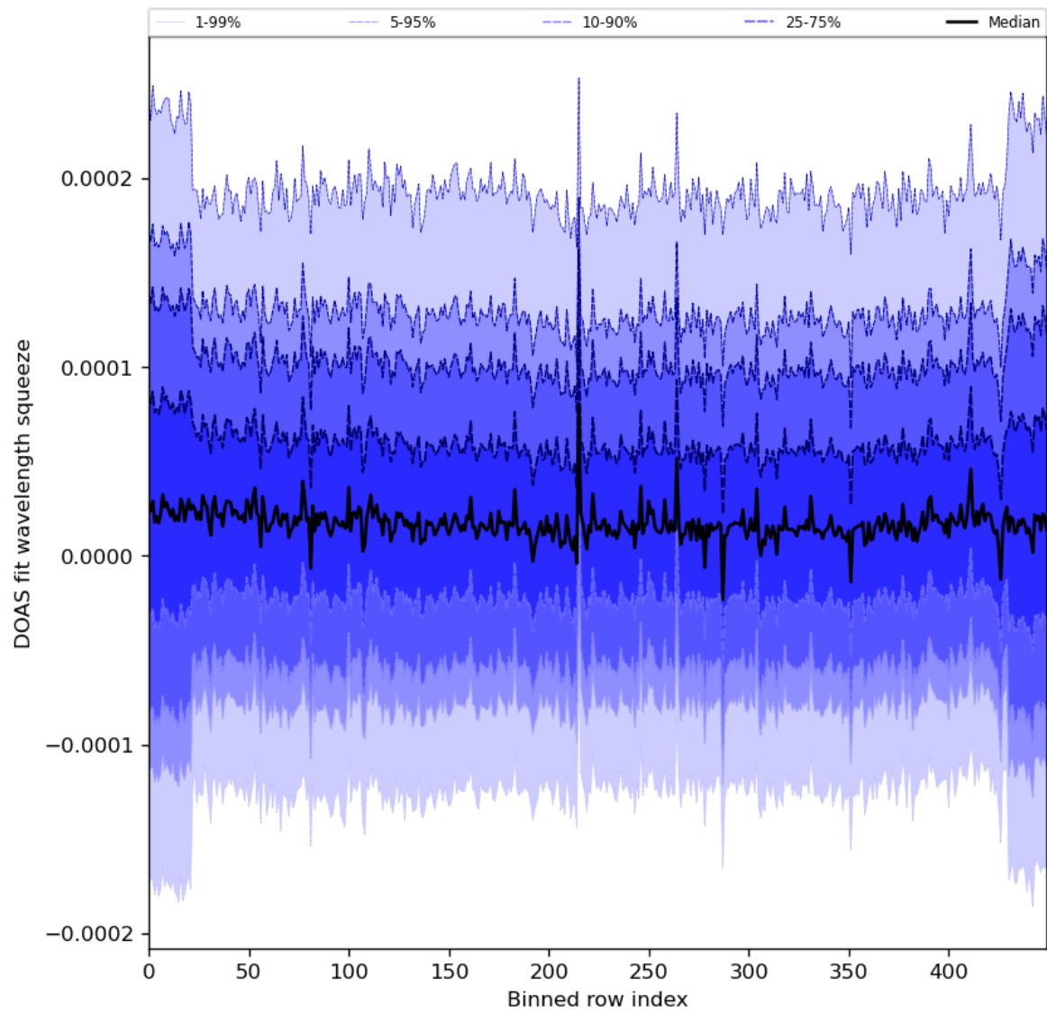
Figure 59: Along track statistics of “DOAS fit wavelength squeeze” for 2024-02-14 to 2024-02-16
