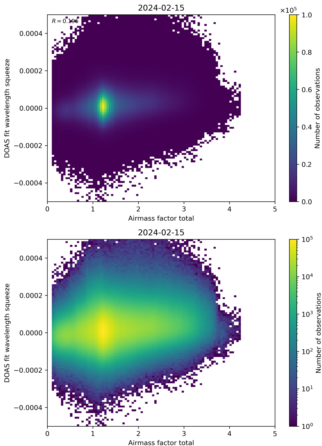
Figure 99: Scatter density plot of “Airmass factor total” against “DOAS fit wavelength squeeze” for 2024-02-14 to 2024-02-16.
