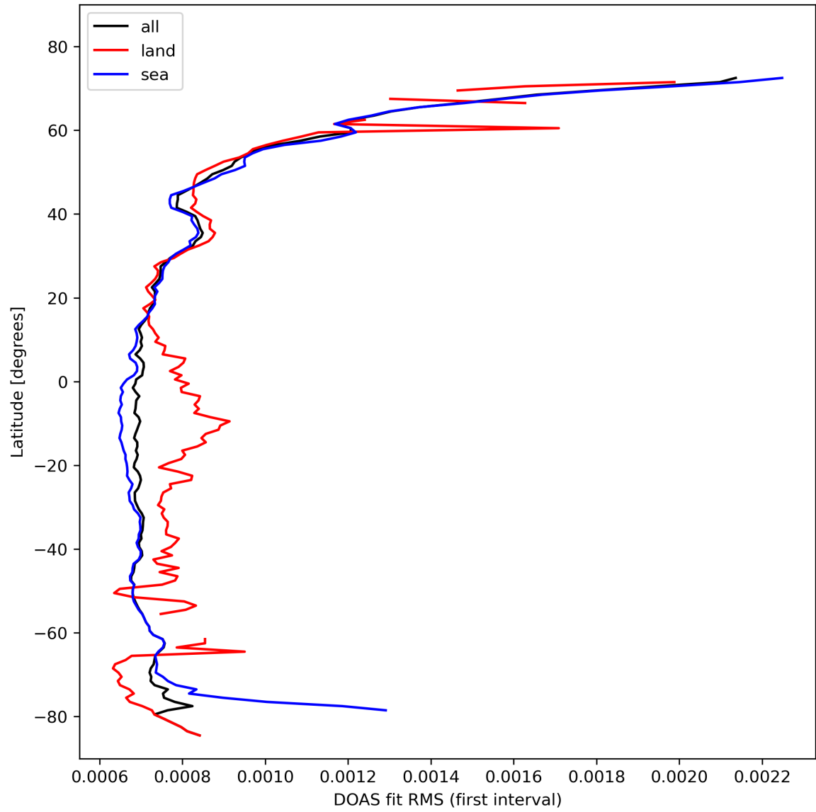
Figure 32: Zonal average of “DOAS fit RMS (first interval)” for 2024-02-14 to 2024-02-16.
