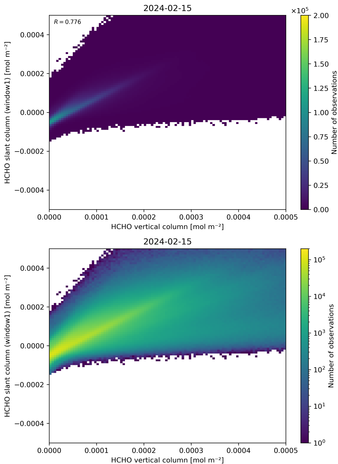
Figure 129: Scatter density plot of “HCHO vertical column” against “HCHO slant column (window1)” for 2024-02-14 to 2024-02-16.
