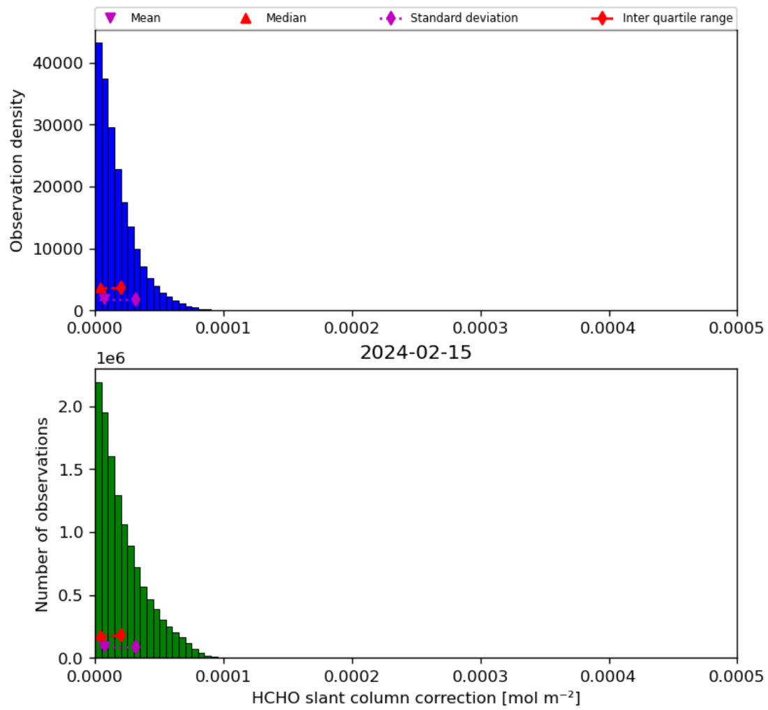
Figure 47: Histogram of “HCHO slant column correction” for 2024-02-14 to 2024-02-16
