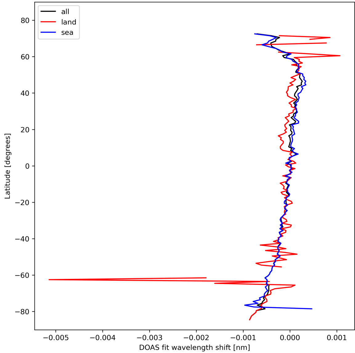
Figure 30: Zonal average of “DOAS fit wavelength shift” for 2024-02-14 to 2024-02-16.
