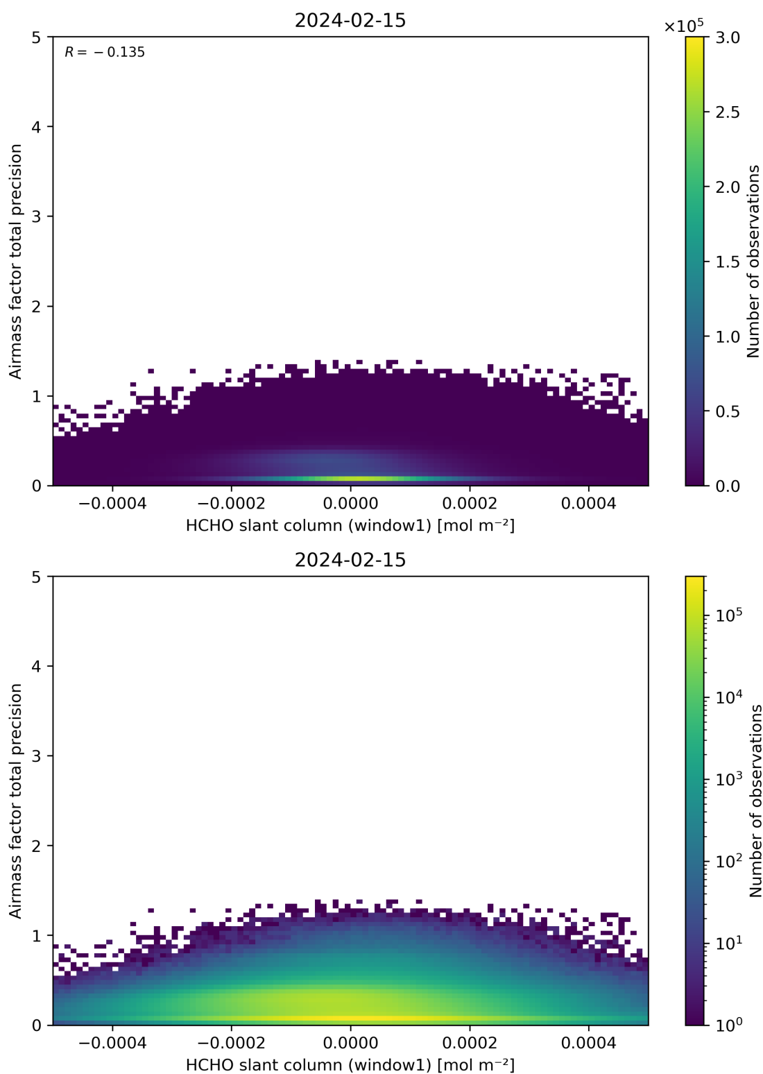
Figure 86: Scatter density plot of “HCHO slant column (window1)” against “Airmass factor total precision” for 2024-02-14 to 2024-02-16.
