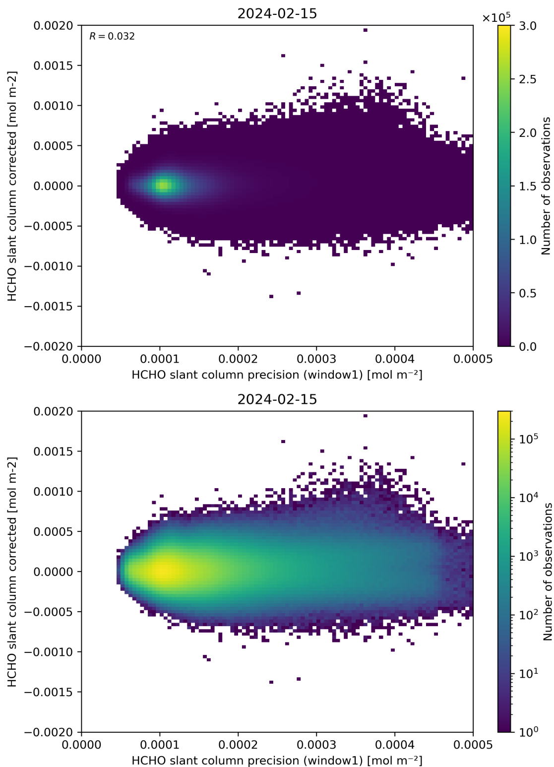
Figure 92: Scatter density plot of “HCHO slant column precision (window1)” against “HCHO slant column corrected” for 2024-02-14 to 2024-02-16.
