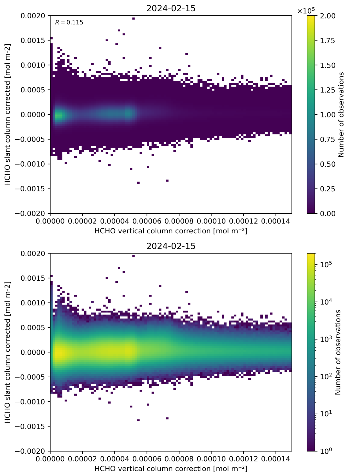
Figure 116: Scatter density plot of “HCHO vertical column correction” against “HCHO slant column corrected” for 2024-02-14 to 2024-02-16.
