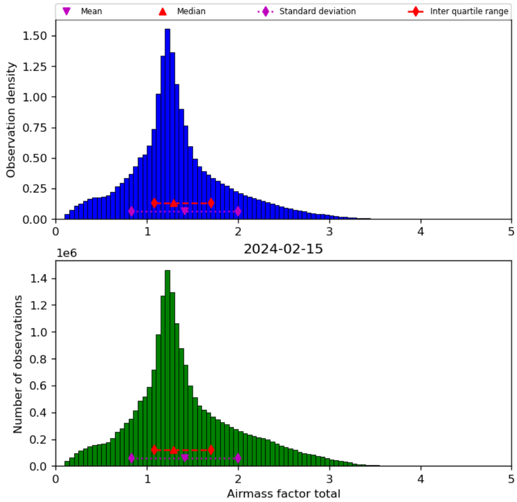
Figure 40: Histogram of “Airmass factor total” for 2024-02-14 to 2024-02-16
