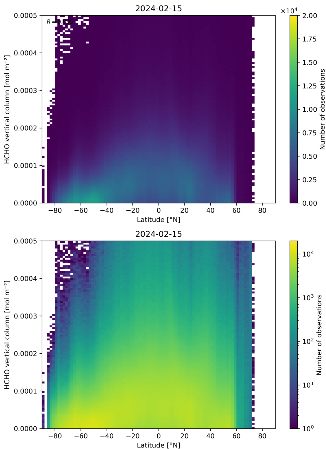
Figure 163: Scatter density plot of “Latitude” against “HCHO vertical column” for 2024-02-14 to 2024-02-16.
