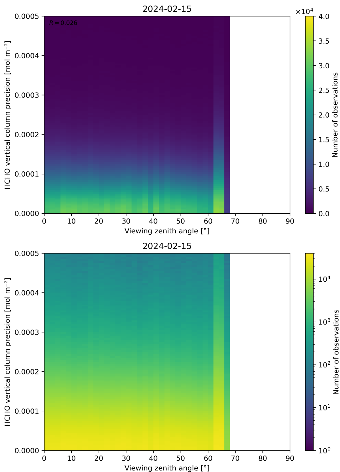
Figure 194: Scatter density plot of “Viewing zenith angle” against “HCHO vertical column precision” for 2024-02-14 to 2024-02-16.
