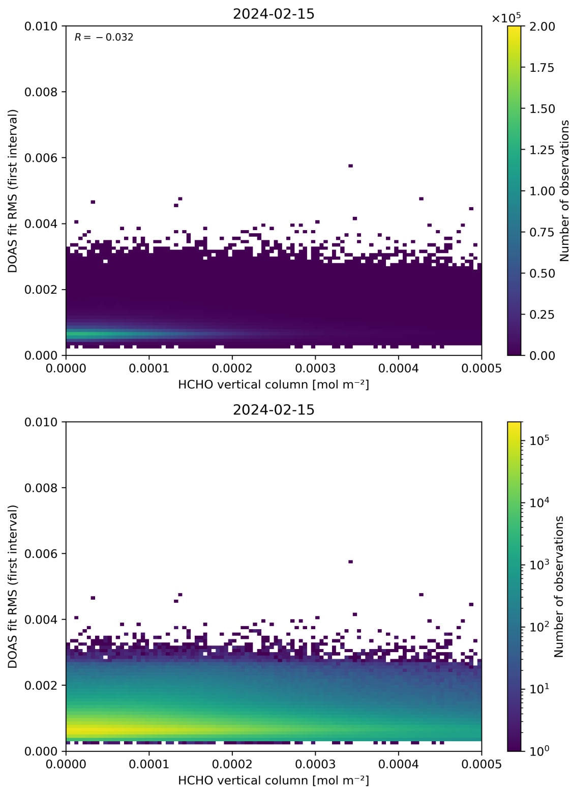
Figure 123: Scatter density plot of “HCHO vertical column” against “DOAS fit RMS (first interval)” for 2024-02-14 to 2024-02-16.
