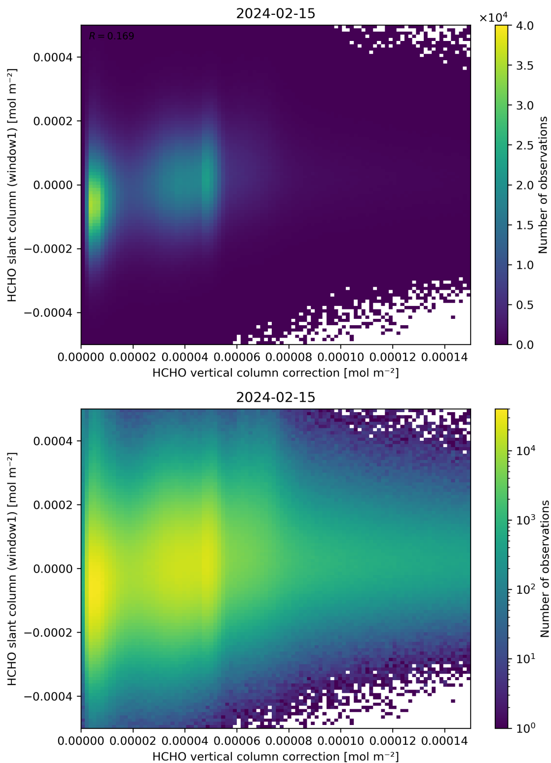
Figure 118: Scatter density plot of “HCHO vertical column correction” against “HCHO slant column (window1)” for 2024-02-14 to 2024-02-16.
