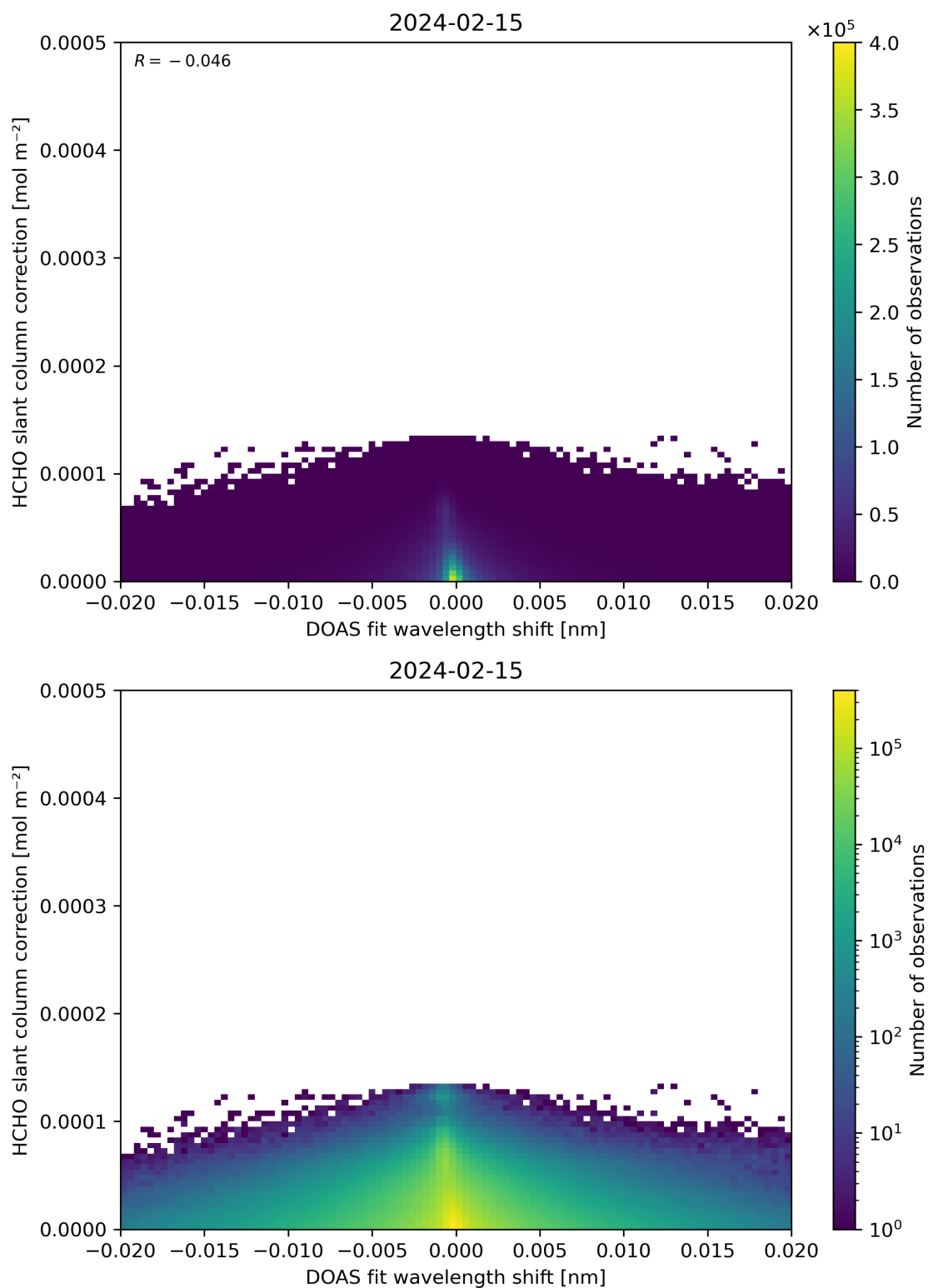
Figure 67: Scatter density plot of “DOAS fit wavelength shift” against “HCHO slant column correction” for 2024-02-14 to 2024-02-16.
