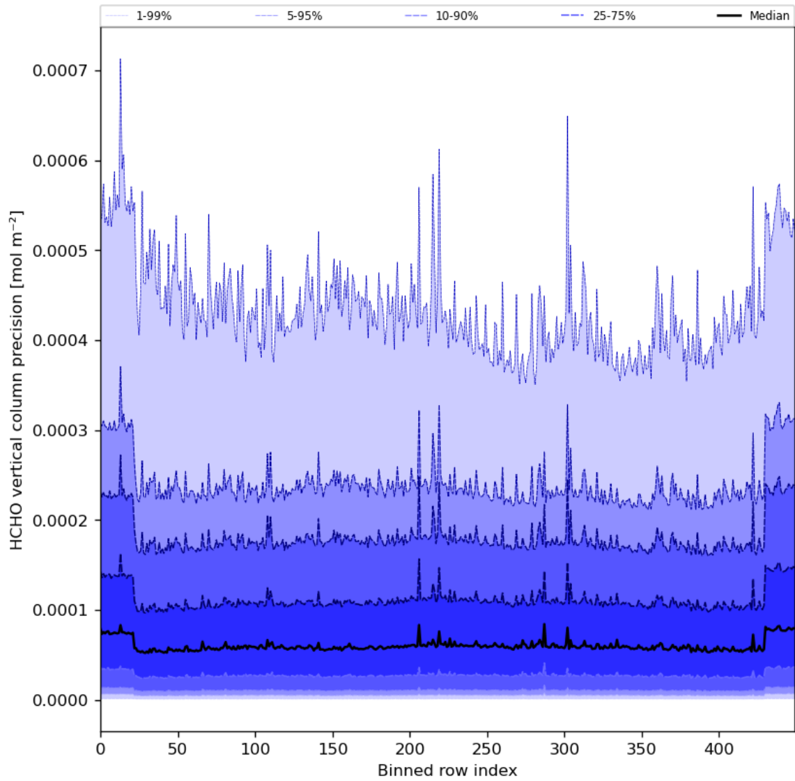
Figure 50: Along track statistics of “HCHO vertical column precision” for 2024-02-14 to 2024-02-16
