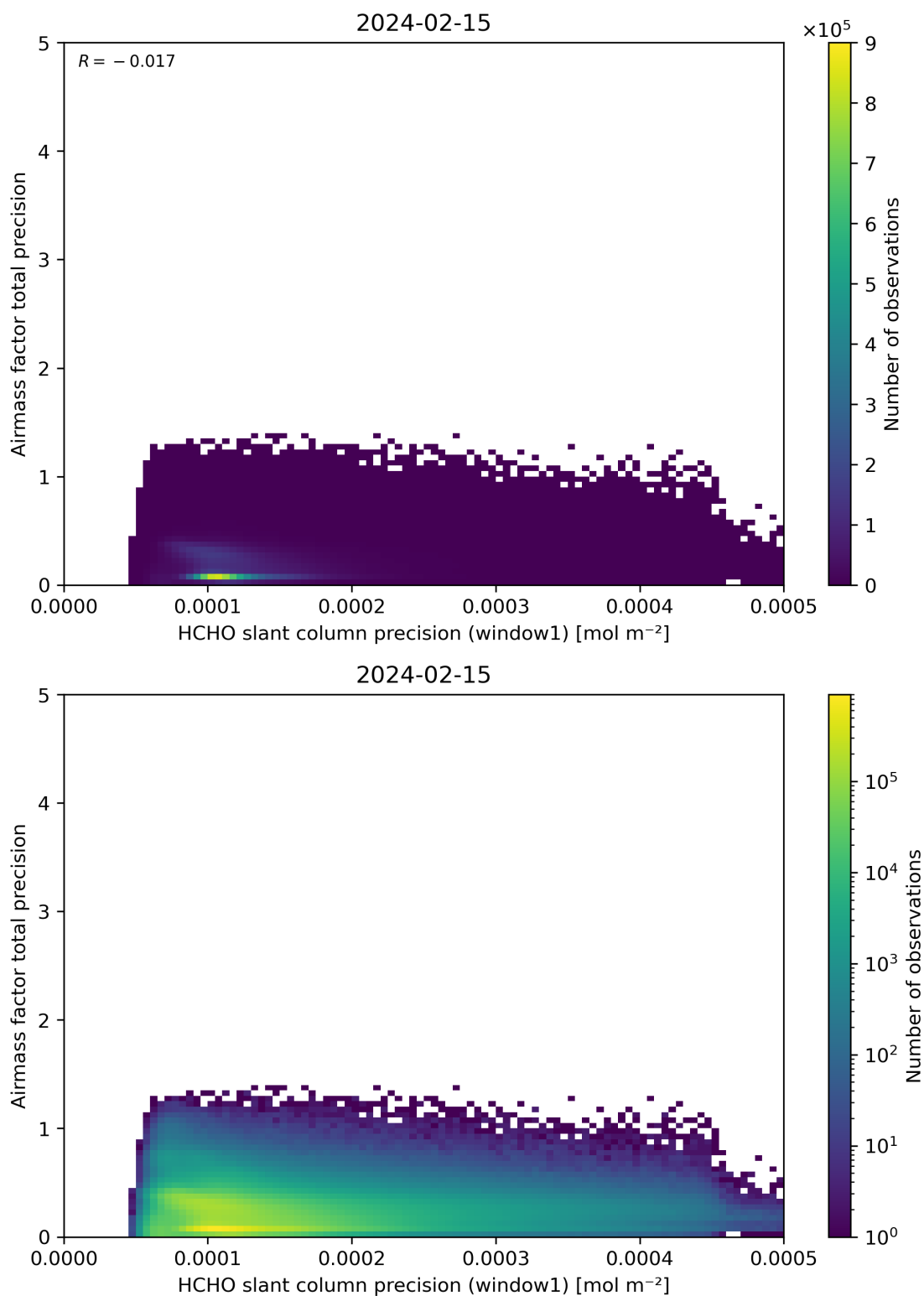
Figure 95: Scatter density plot of “HCHO slant column precision (window1)” against “Airmass factor total precision” for 2024-02-14 to 2024-02-16.
