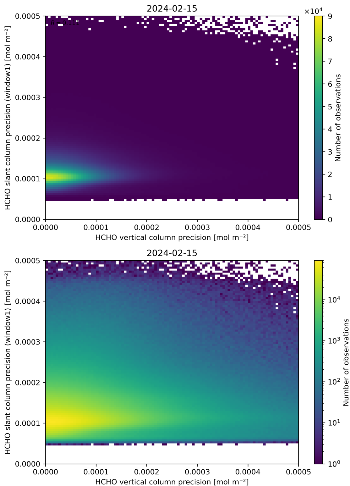
Figure 143: Scatter density plot of “HCHO vertical column precision” against “HCHO slant column precision (window1)” for 2024-02-14 to 2024-02-16.
