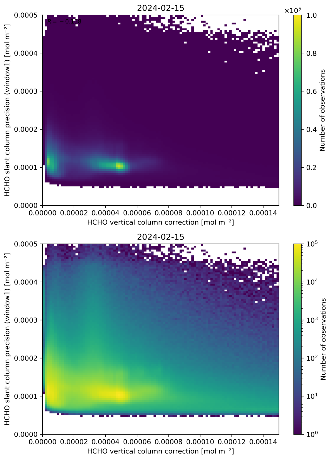
Figure 119: Scatter density plot of “HCHO vertical column correction” against “HCHO slant column precision (window1)” for 2024-02-14 to 2024-02-16.
