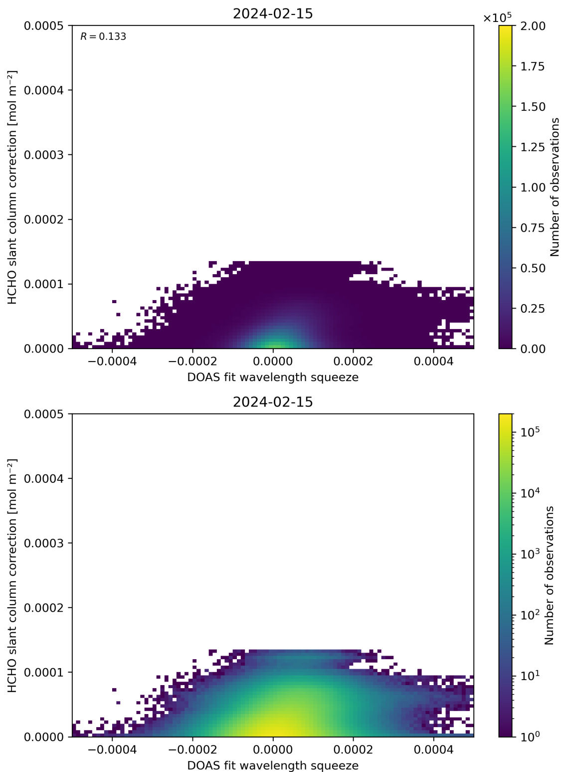
Figure 70: Scatter density plot of “DOAS fit wavelength squeeze” against “HCHO slant column correction” for 2024-02-14 to 2024-02-16.
