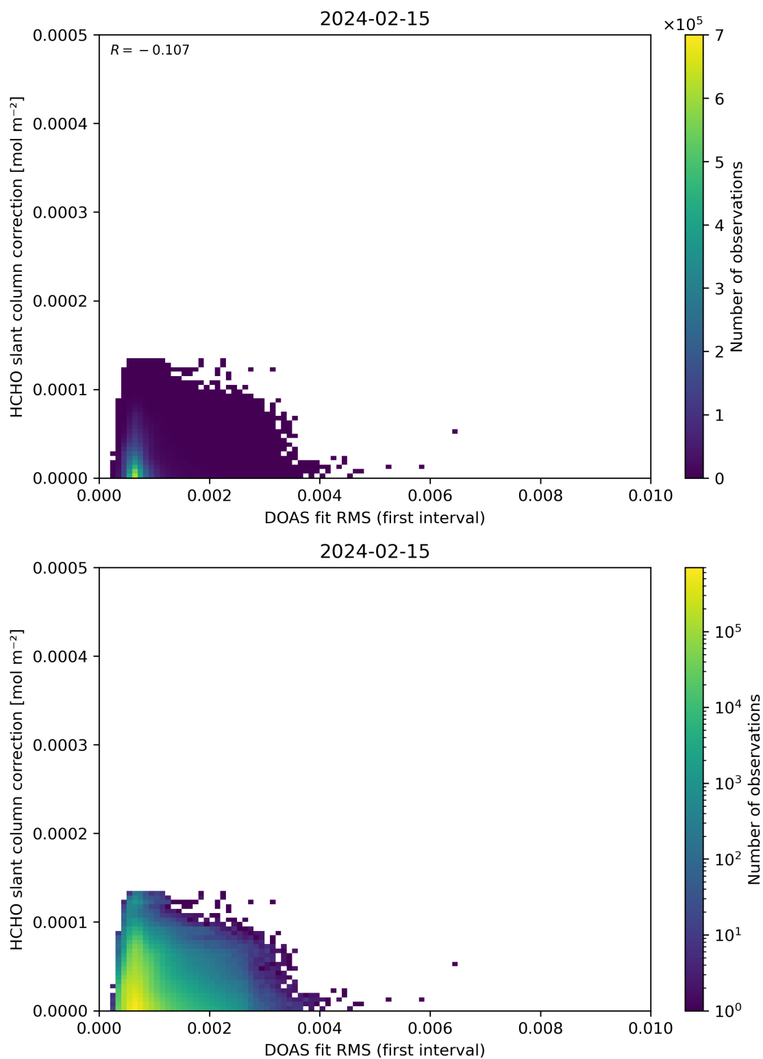
Figure 63: Scatter density plot of “DOAS fit RMS (first interval)” against “HCHO slant column correction” for 2024-02-14 to 2024-02-16.
