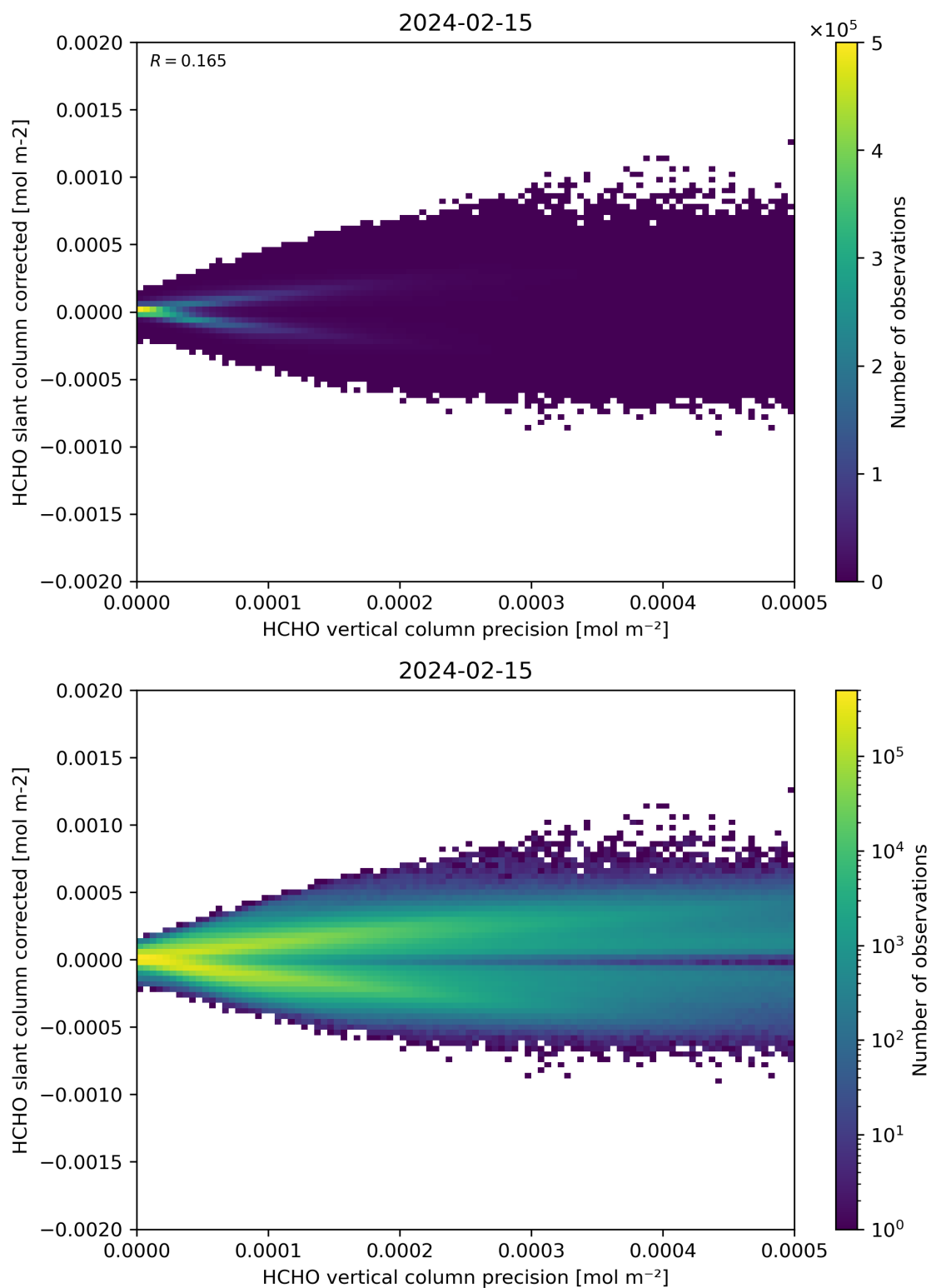
Figure 140: Scatter density plot of “HCHO vertical column precision” against “HCHO slant column corrected” for 2024-02-14 to 2024-02-16.
