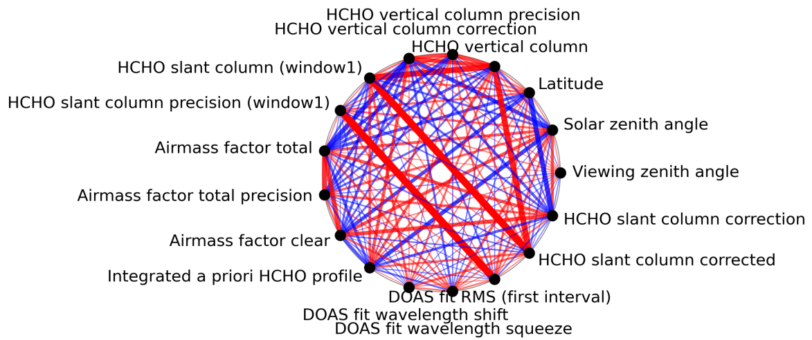
Figure 1: Map of correlation graph for 2024-02-14 to 2024-02-16.
