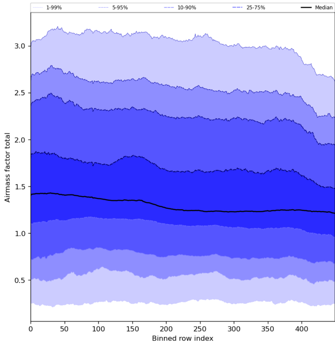
Figure 54: Along track statistics of “Airmass factor total” for 2024-02-14 to 2024-02-16
