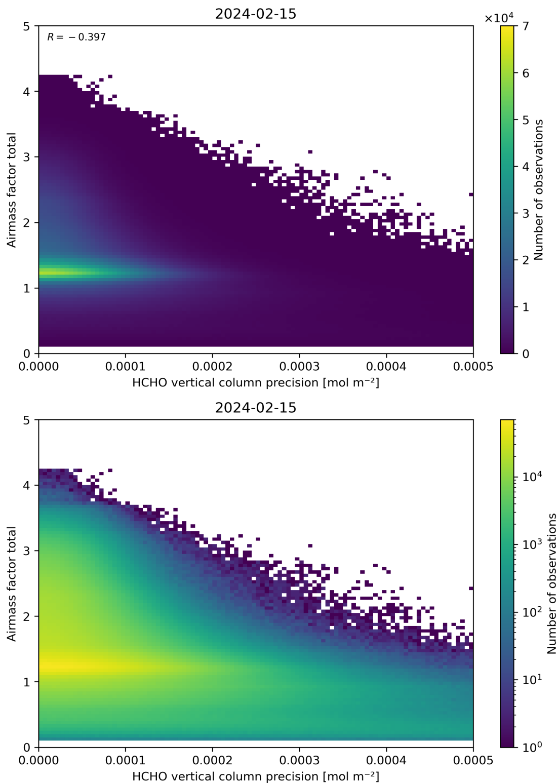
Figure 144: Scatter density plot of “HCHO vertical column precision” against “Airmass factor total” for 2024-02-14 to 2024-02-16.
