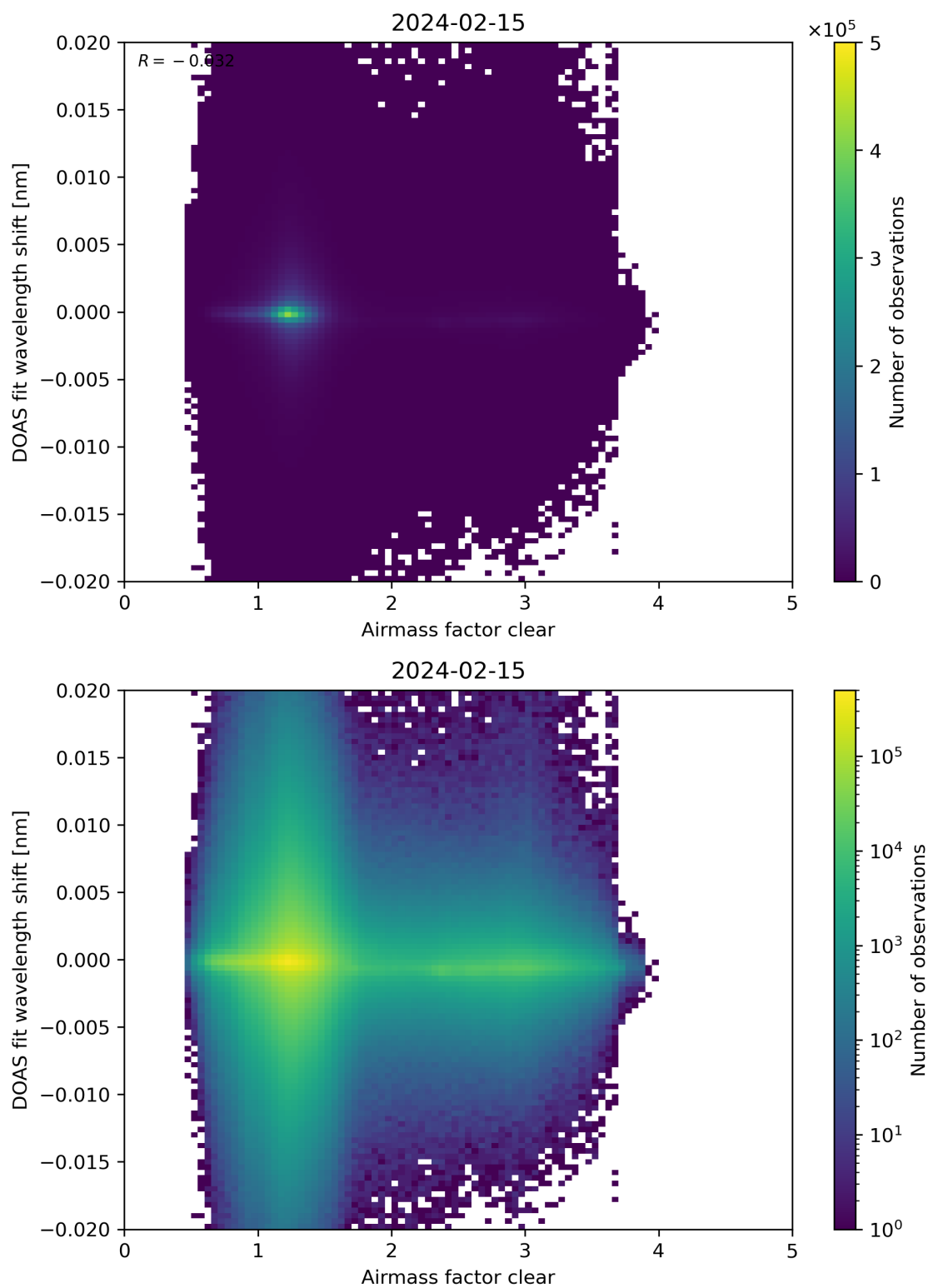
Figure 72: Scatter density plot of “Airmass factor clear” against “DOAS fit wavelength shift” for 2024-02-14 to 2024-02-16.
