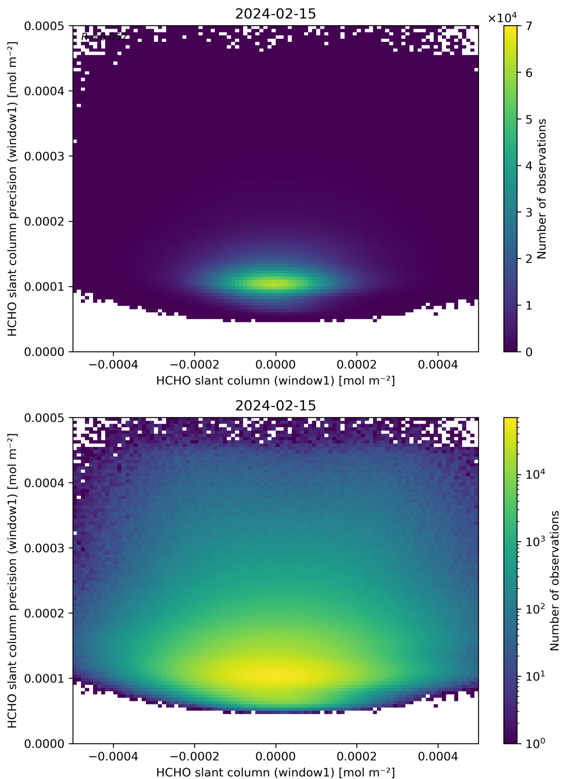
Figure 84: Scatter density plot of “HCHO slant column (window1)” against “HCHO slant column precision (window1)” for 2024-02-14 to 2024-02-16.
