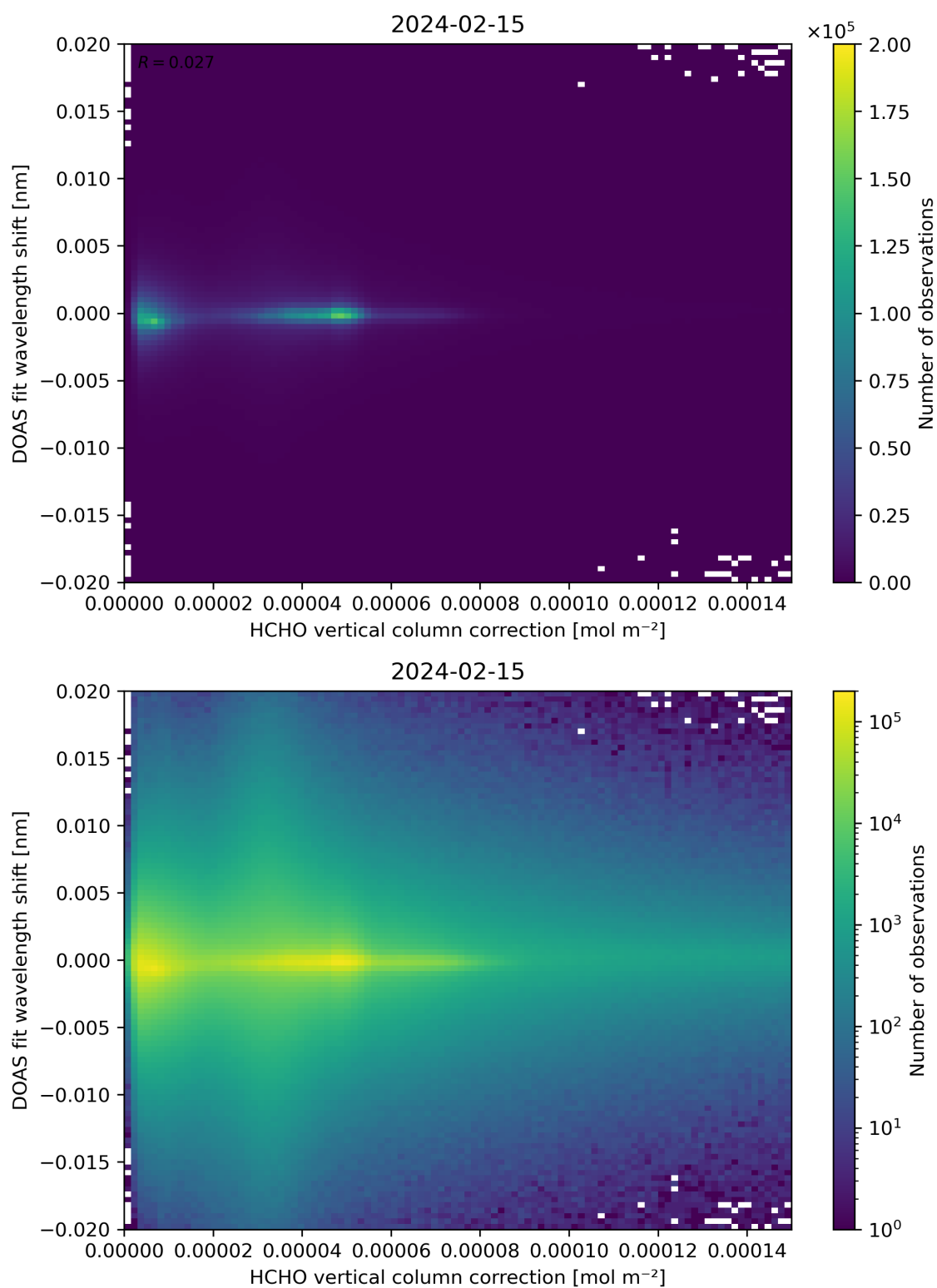
Figure 113: Scatter density plot of “HCHO vertical column correction” against “DOAS fit wavelength shift” for 2024-02-14 to 2024-02-16.
