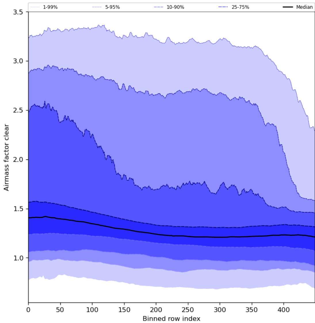
Figure 56: Along track statistics of “Airmass factor clear” for 2024-02-14 to 2024-02-16
