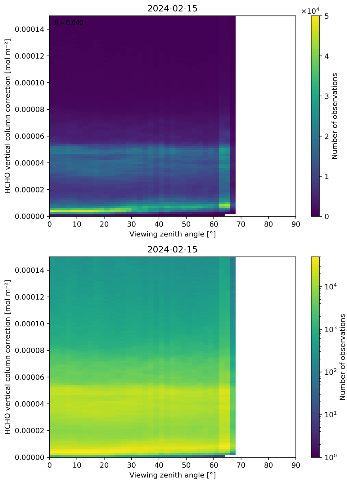
Figure 193: Scatter density plot of “Viewing zenith angle” against “HCHO vertical column correction” for 2024-02-14 to 2024-02-16.
