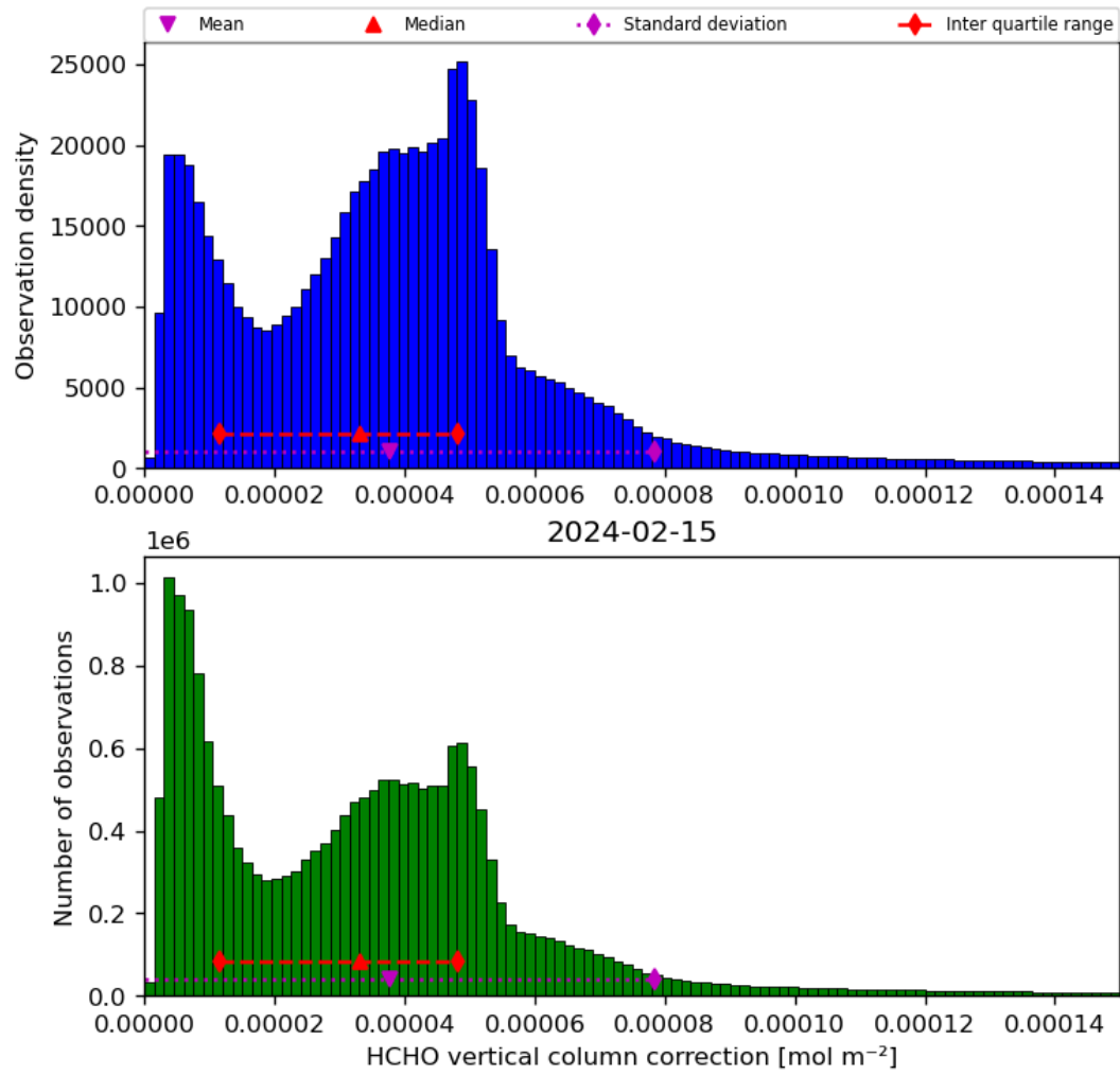
Figure 37: Histogram of “HCHO vertical column correction” for 2024-02-14 to 2024-02-16
