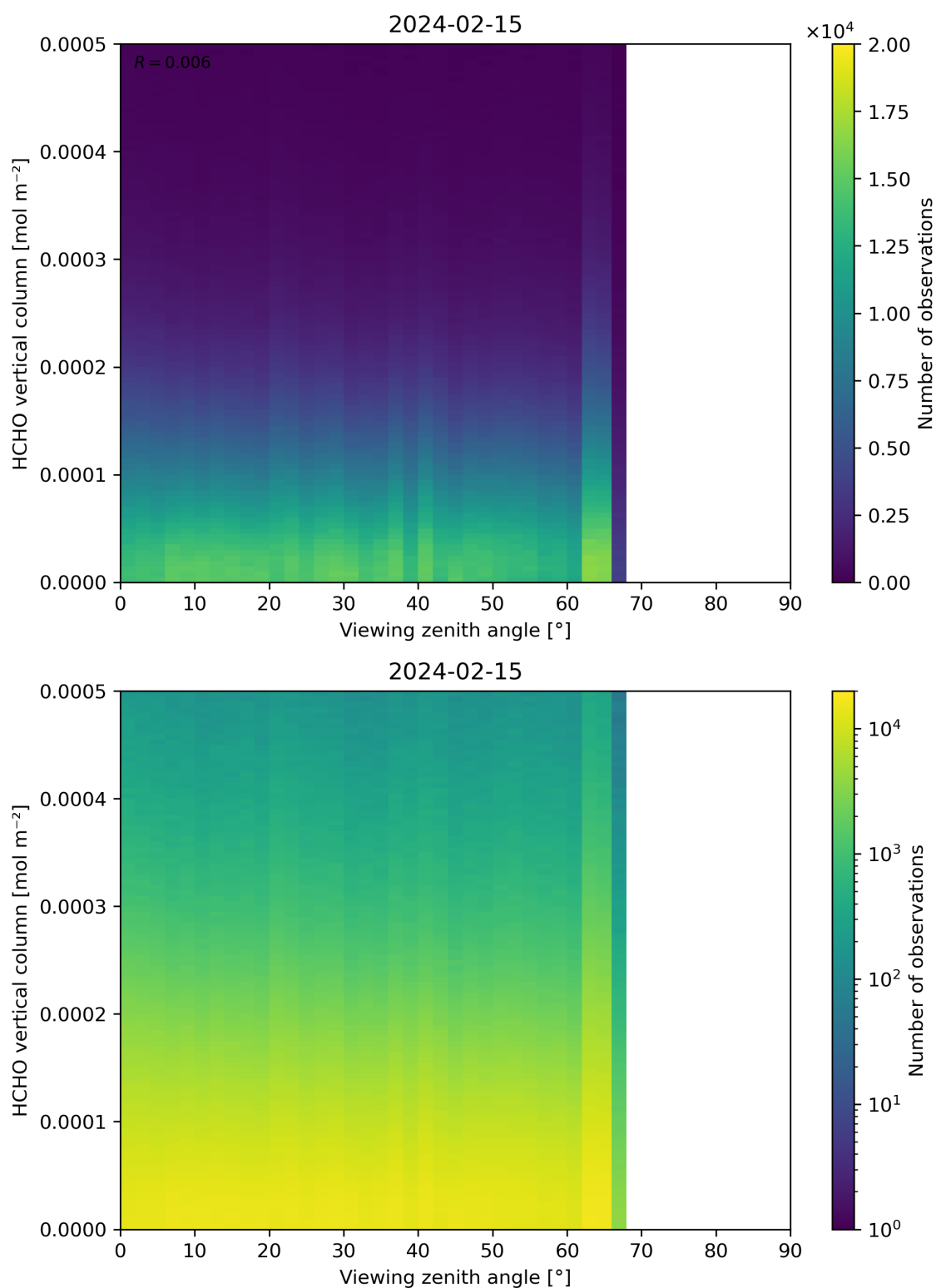
Figure 192: Scatter density plot of “Viewing zenith angle” against “HCHO vertical column” for 2024-02-14 to 2024-02-16.
