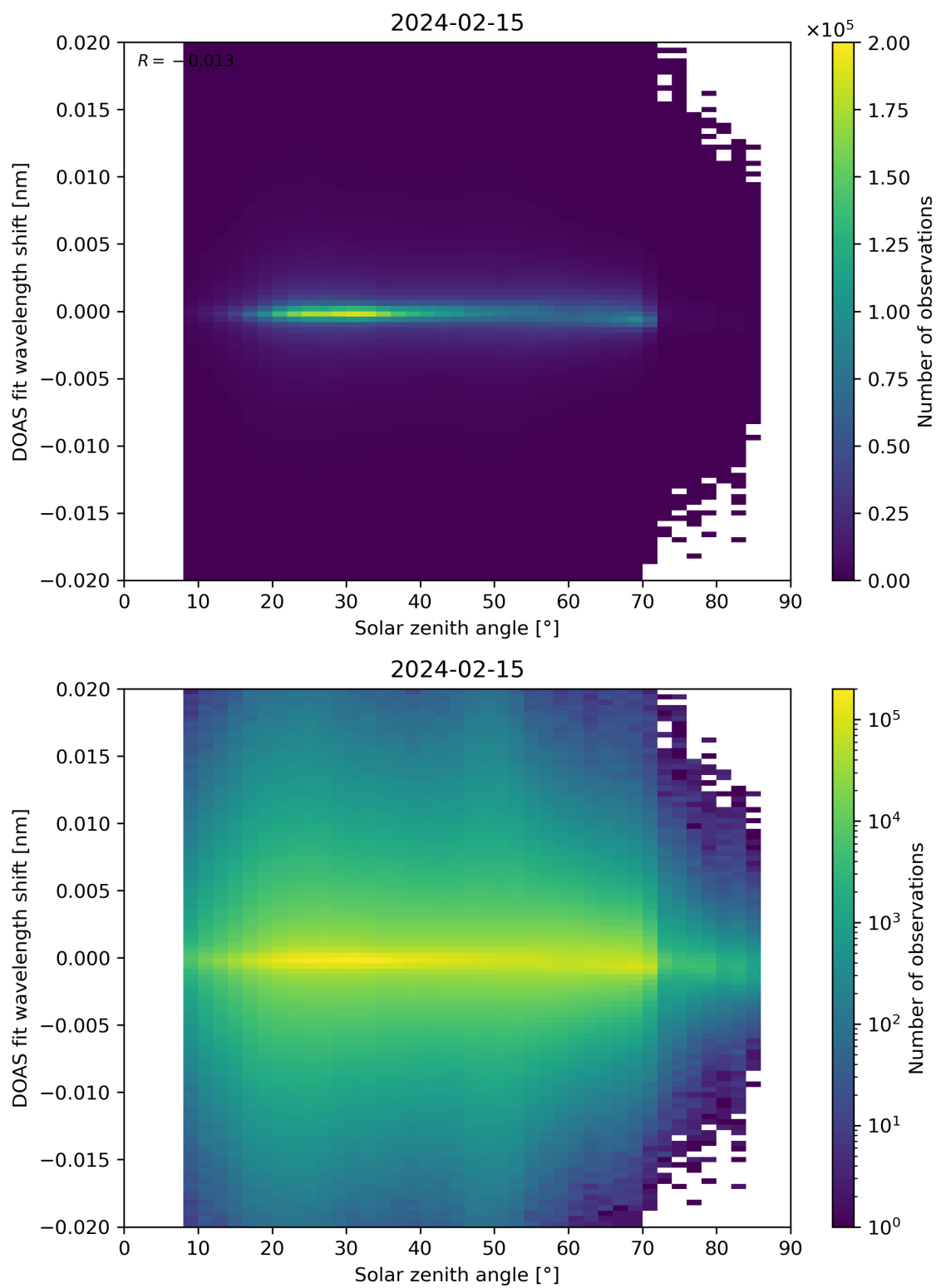
Figure 168: Scatter density plot of “Solar zenith angle” against “DOAS fit wavelength shift” for 2024-02-14 to 2024-02-16.
