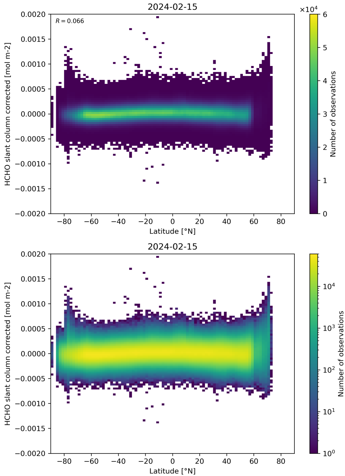
Figure 157: Scatter density plot of “Latitude” against “HCHO slant column corrected” for 2024-02-14 to 2024-02-16.
