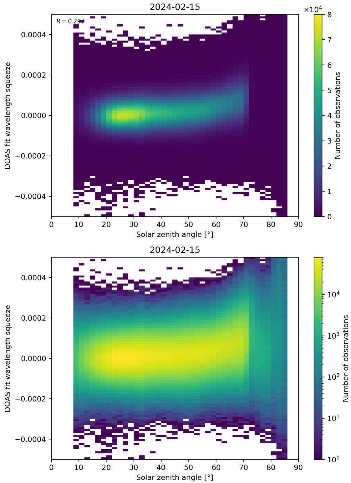
Figure 169: Scatter density plot of “Solar zenith angle” against “DOAS fit wavelength squeeze” for 2024-02-14 to 2024-02-16.
