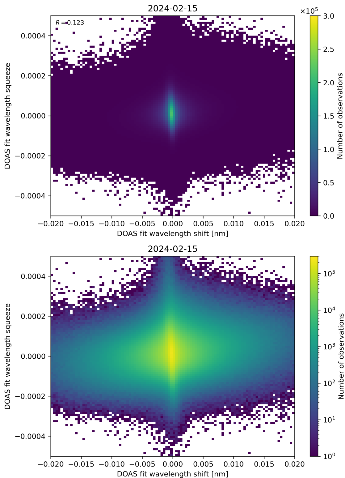
Figure 65: Scatter density plot of “DOAS fit wavelength shift” against “DOAS fit wavelength squeeze” for 2024-02-14 to 2024-02-16.
