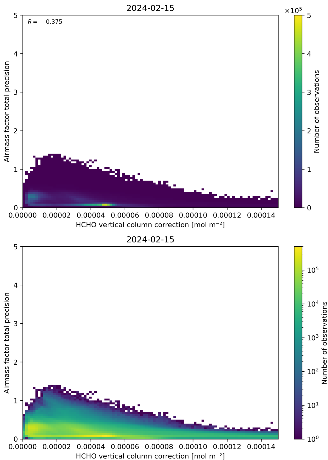
Figure 121: Scatter density plot of “HCHO vertical column correction” against “Airmass factor total precision” for 2024-02-14 to 2024-02-16.
