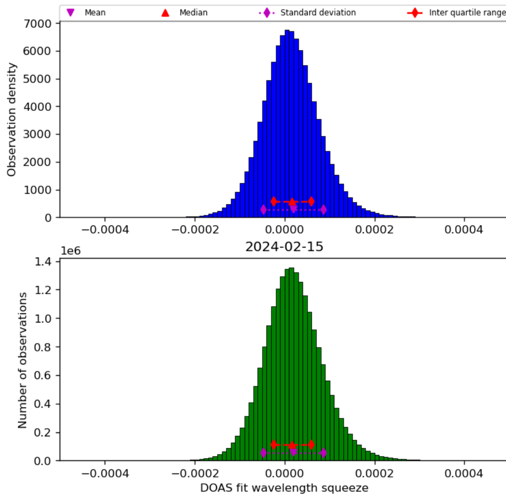
Figure 45: Histogram of “DOAS fit wavelength squeeze” for 2024-02-14 to 2024-02-16
