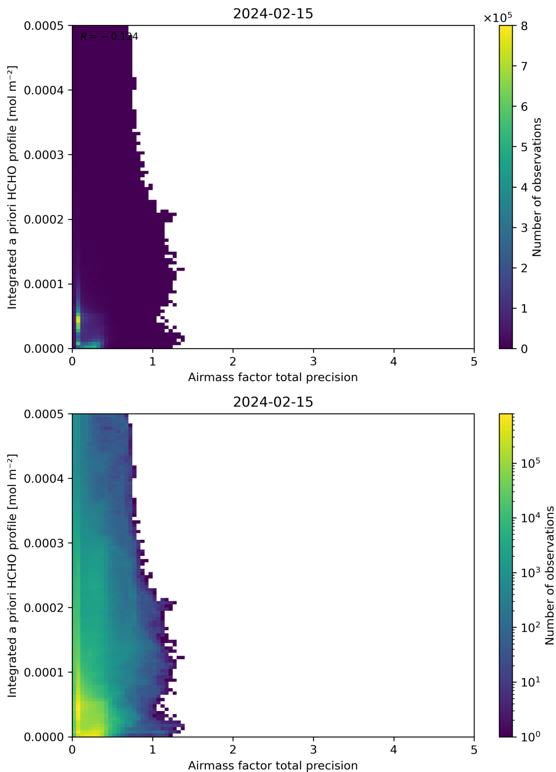
Figure 111: Scatter density plot of “Airmass factor total precision” against “Integrated a priori HCHO profile” for 2024-02-14 to 2024-02-16.
