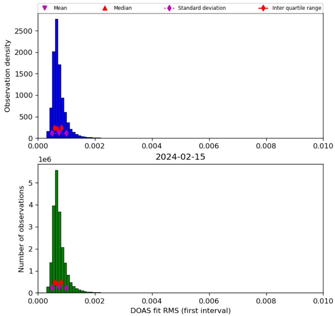
Figure 46: Histogram of “DOAS fit RMS (first interval)” for 2024-02-14 to 2024-02-16
