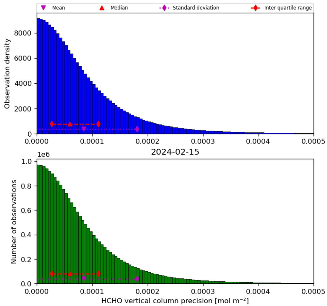
Figure 36: Histogram of “HCHO vertical column precision” for 2024-02-14 to 2024-02-16
