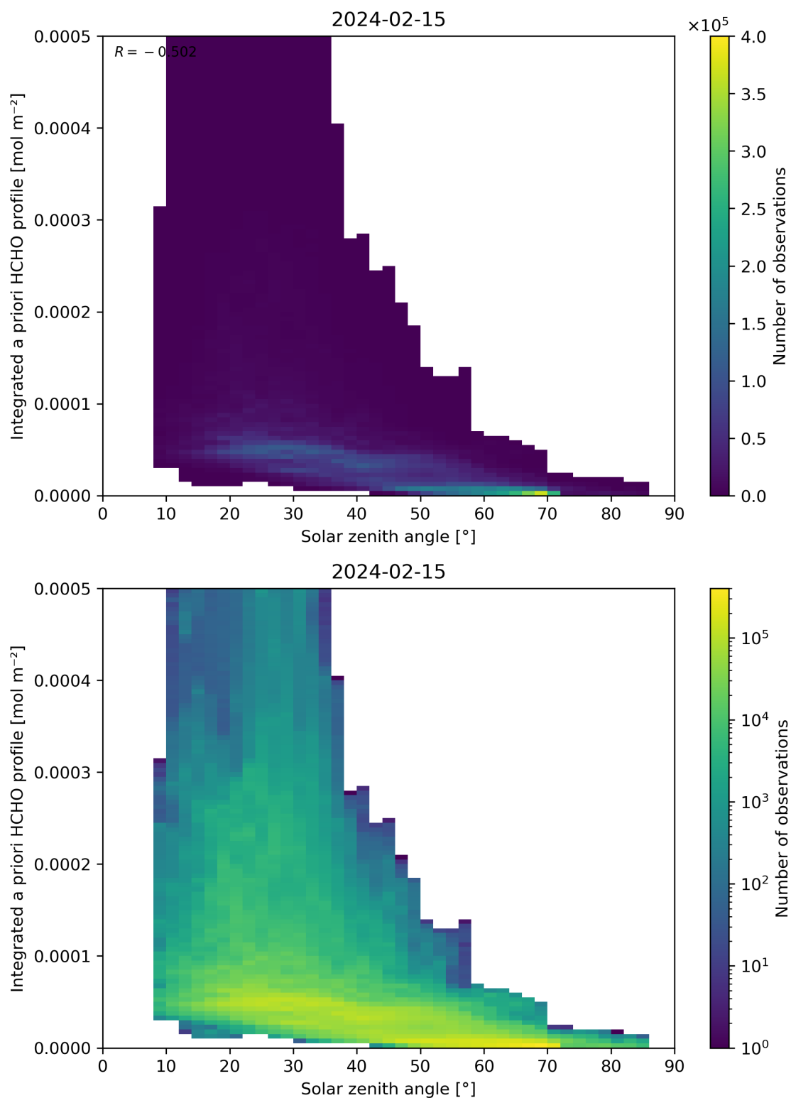
Figure 180: Scatter density plot of “Solar zenith angle” against “Integrated a priori HCHO profile” for 2024-02-14 to 2024-02-16.
