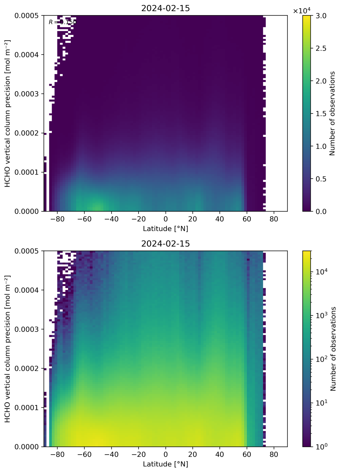
Figure 165: Scatter density plot of “Latitude” against “HCHO vertical column precision” for 2024-02-14 to 2024-02-16.
