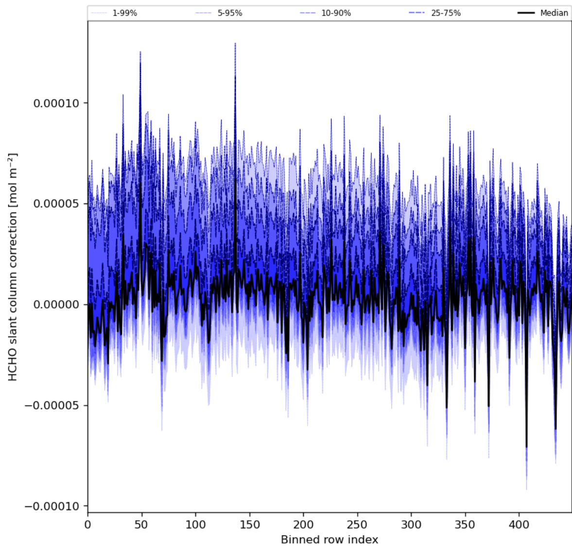
Figure 61: Along track statistics of “HCHO slant column correction” for 2024-02-14 to 2024-02-16
