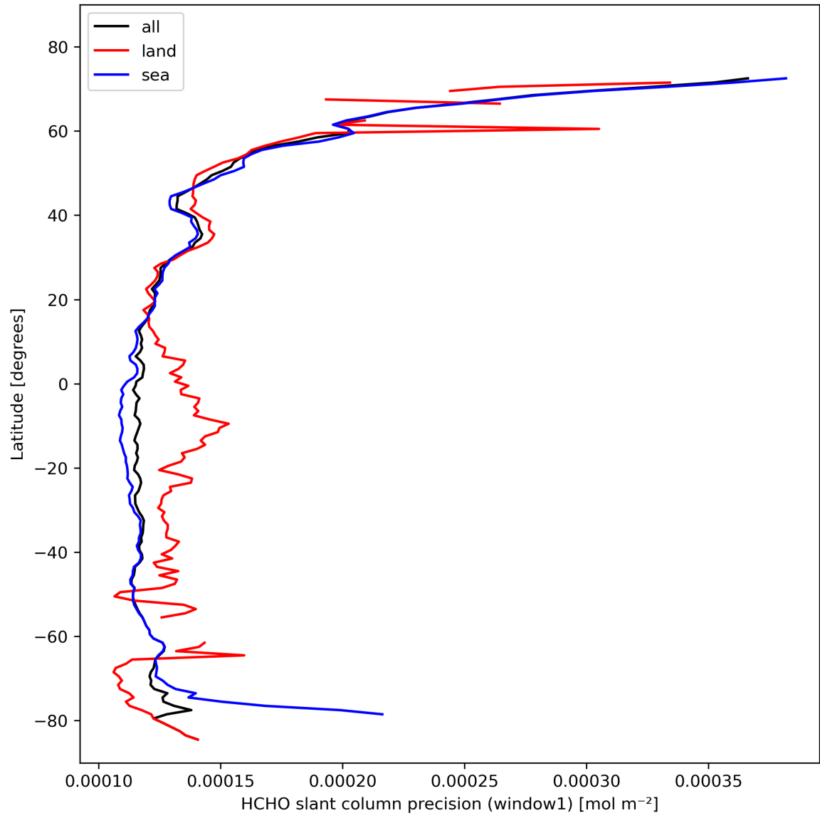
Figure 25: Zonal average of “HCHO slant column precision (window1)” for 2024-02-14 to 2024-02-16.
