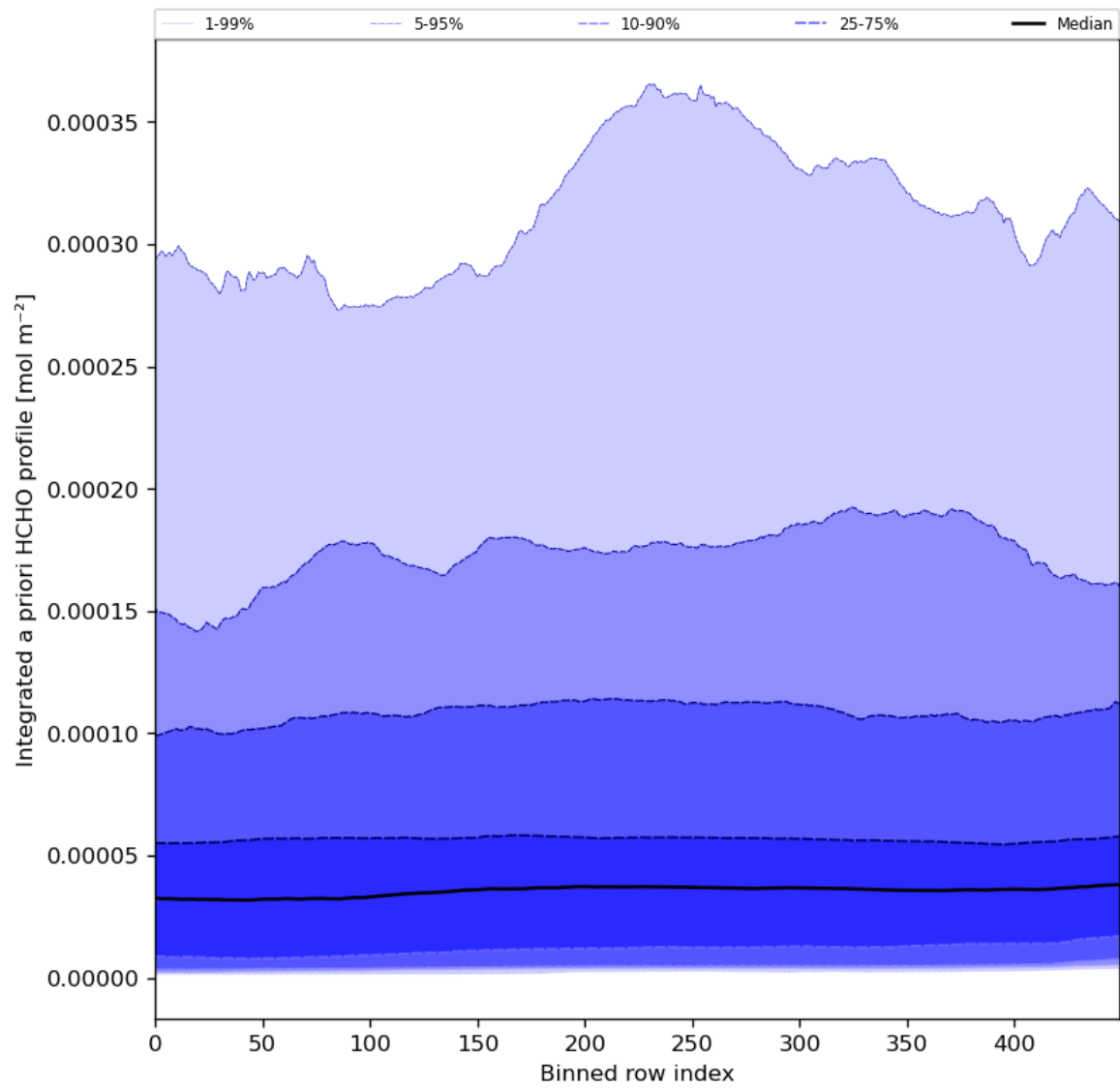
Figure 57: Along track statistics of "Integrated a priori HCHO profile" for 2024-02-14 to 2024-02-16
