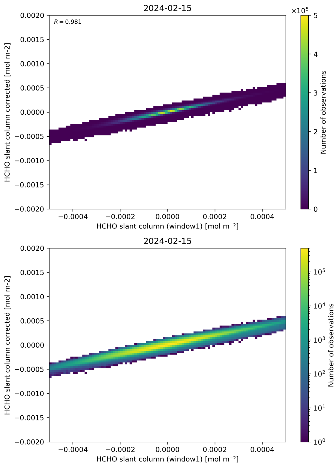
Figure 82: Scatter density plot of “HCHO slant column (window1)” against “HCHO slant column corrected” for 2024-02-14 to 2024-02-16.
