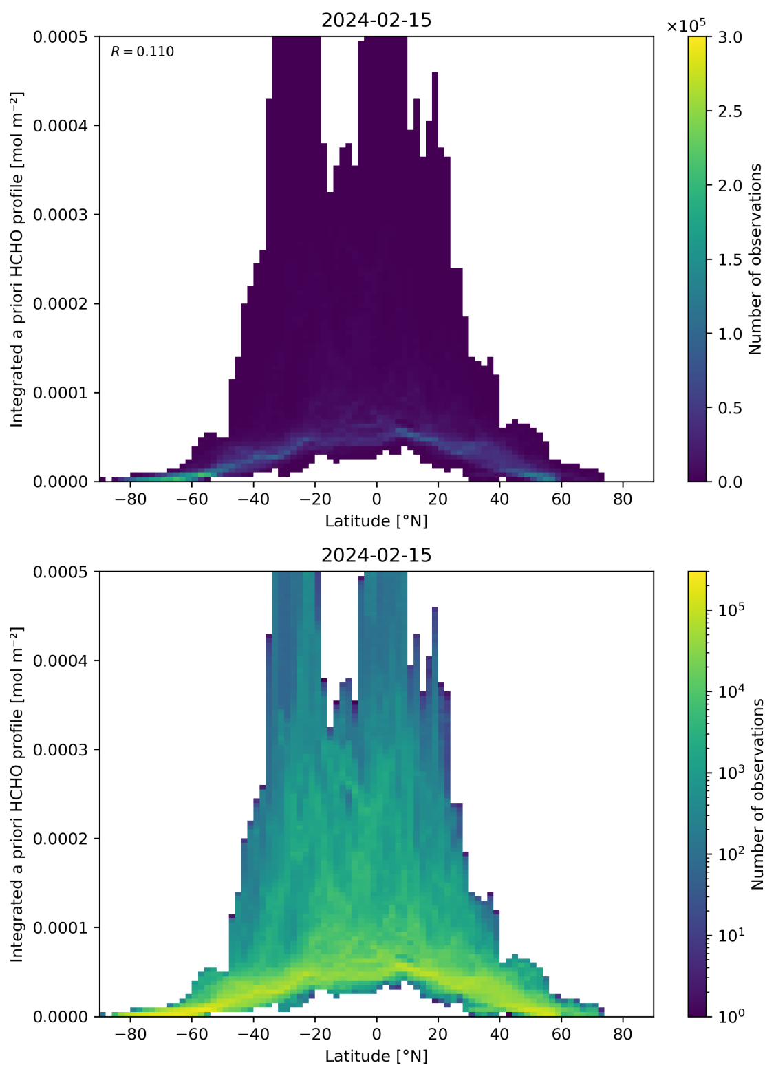
Figure 166: Scatter density plot of “Latitude” against “Integrated a priori HCHO profile” for 2024-02-14 to 2024-02-16.
