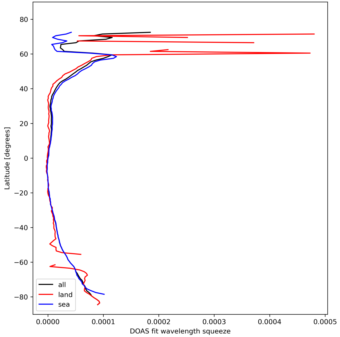
Figure 31: Zonal average of “DOAS fit wavelength squeeze” for 2024-02-14 to 2024-02-16.
