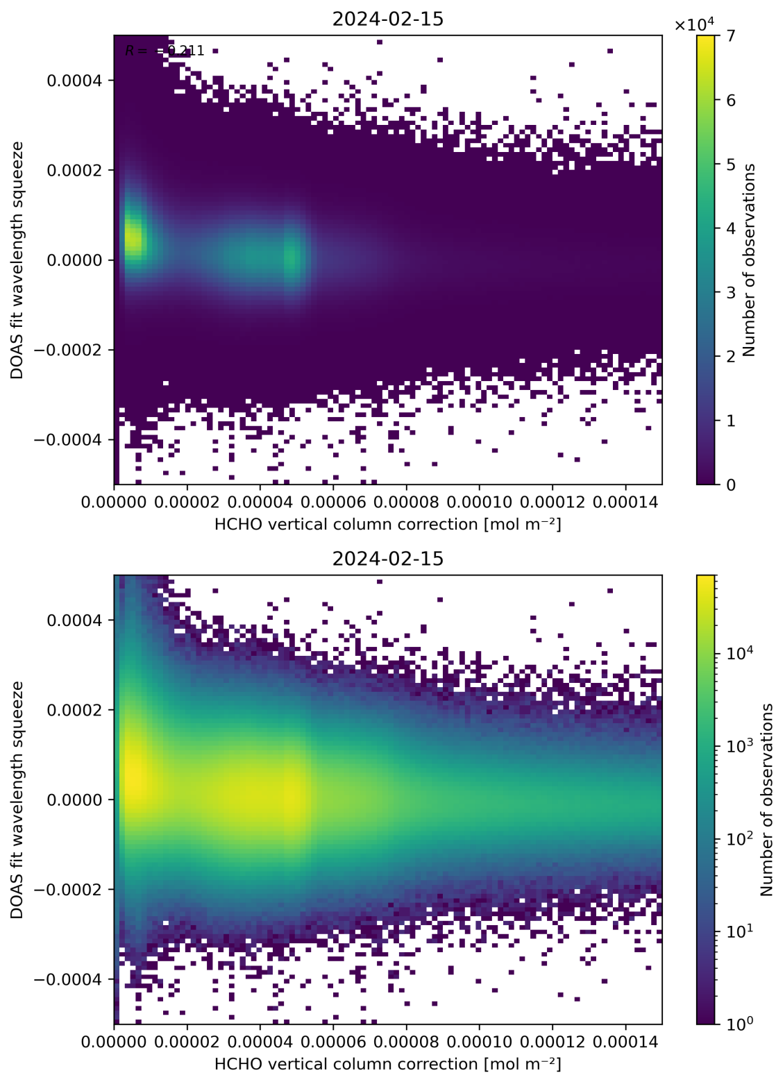
Figure 114: Scatter density plot of “HCHO vertical column correction” against “DOAS fit wavelength squeeze” for 2024-02-14 to 2024-02-16.
