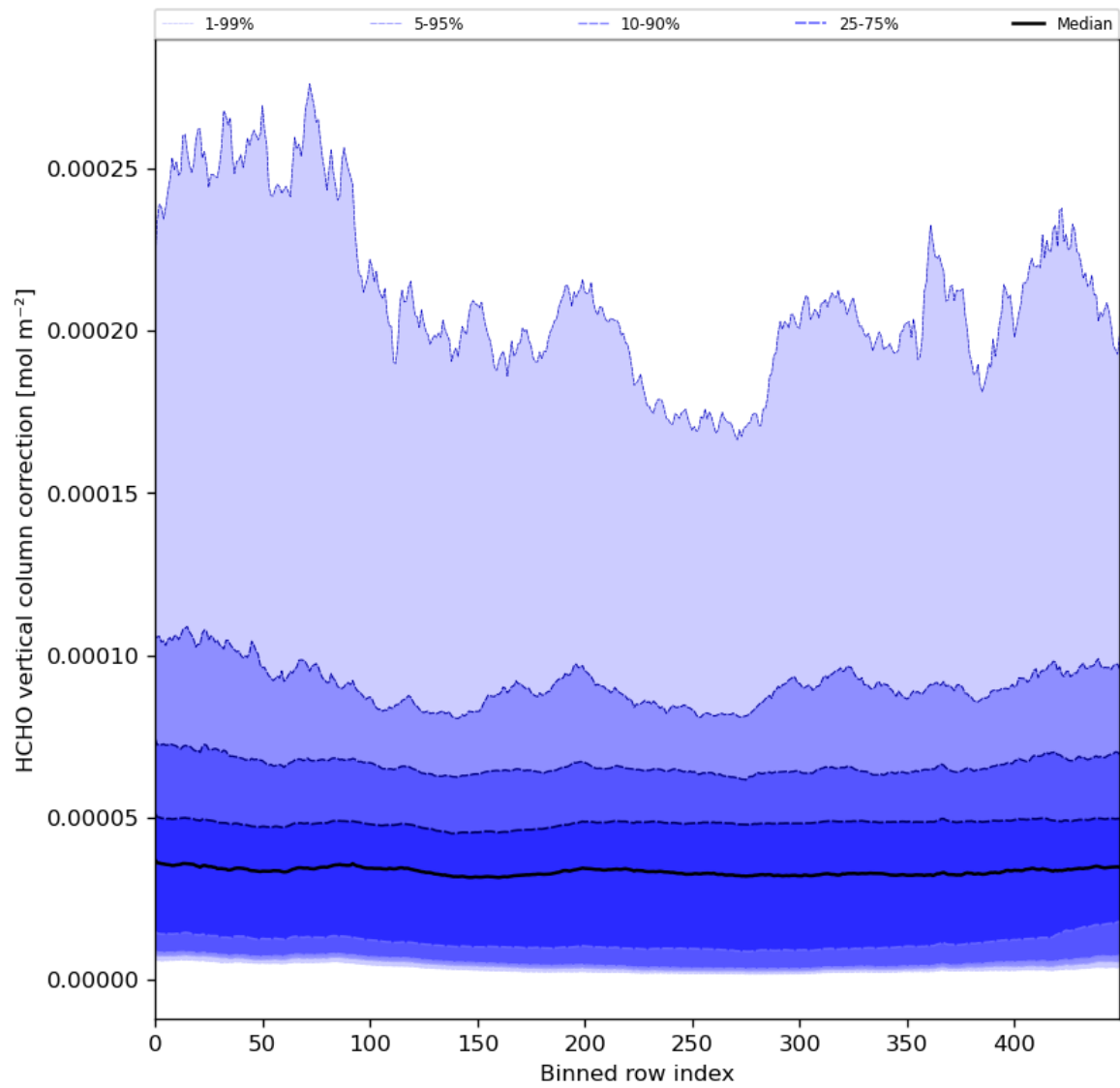
Figure 51: Along track statistics of “HCHO vertical column correction” for 2024-02-14 to 2024-02-16
