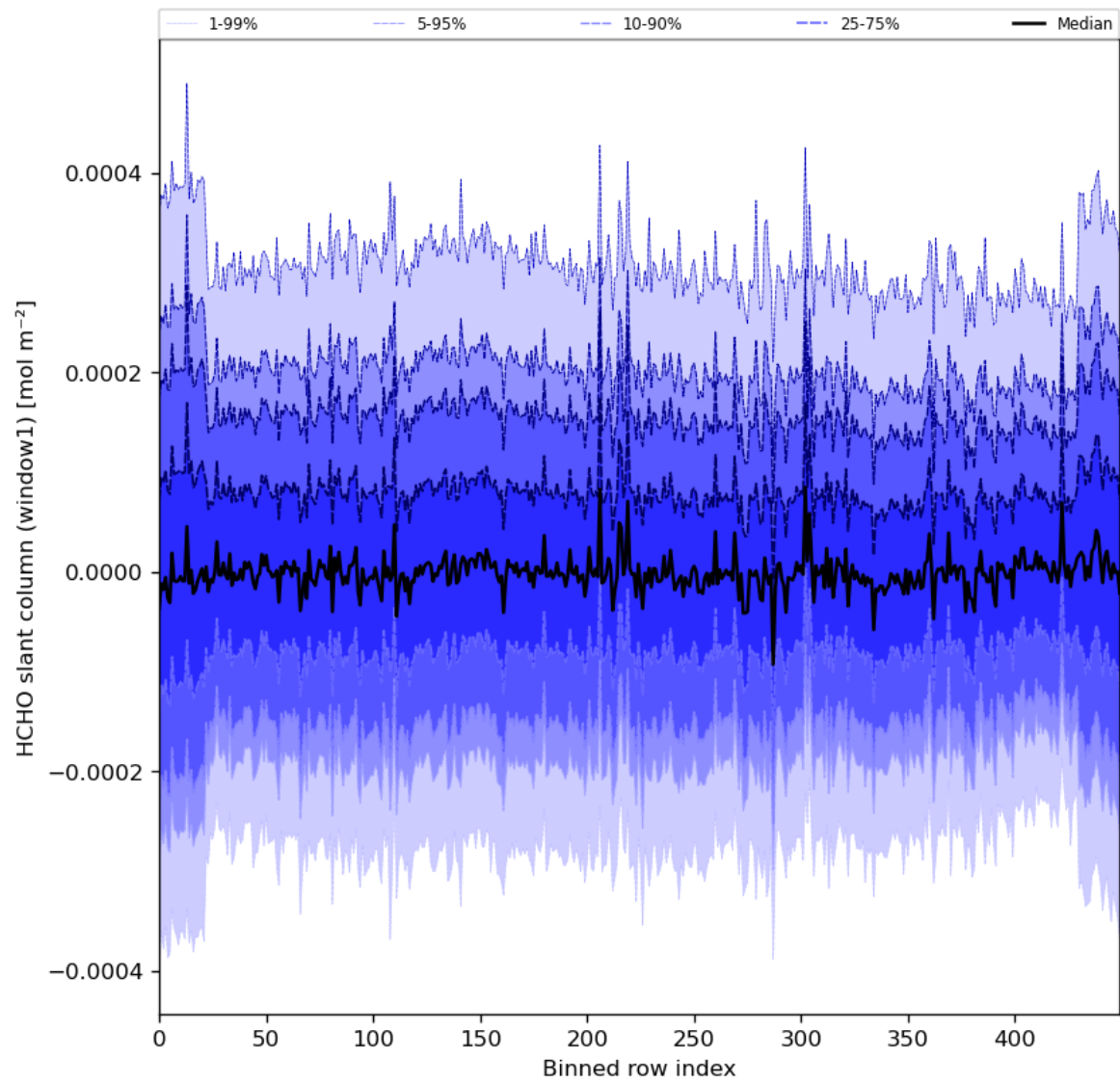
Figure 52: Along track statistics of “HCHO slant column (window1)” for 2024-02-14 to 2024-02-16
