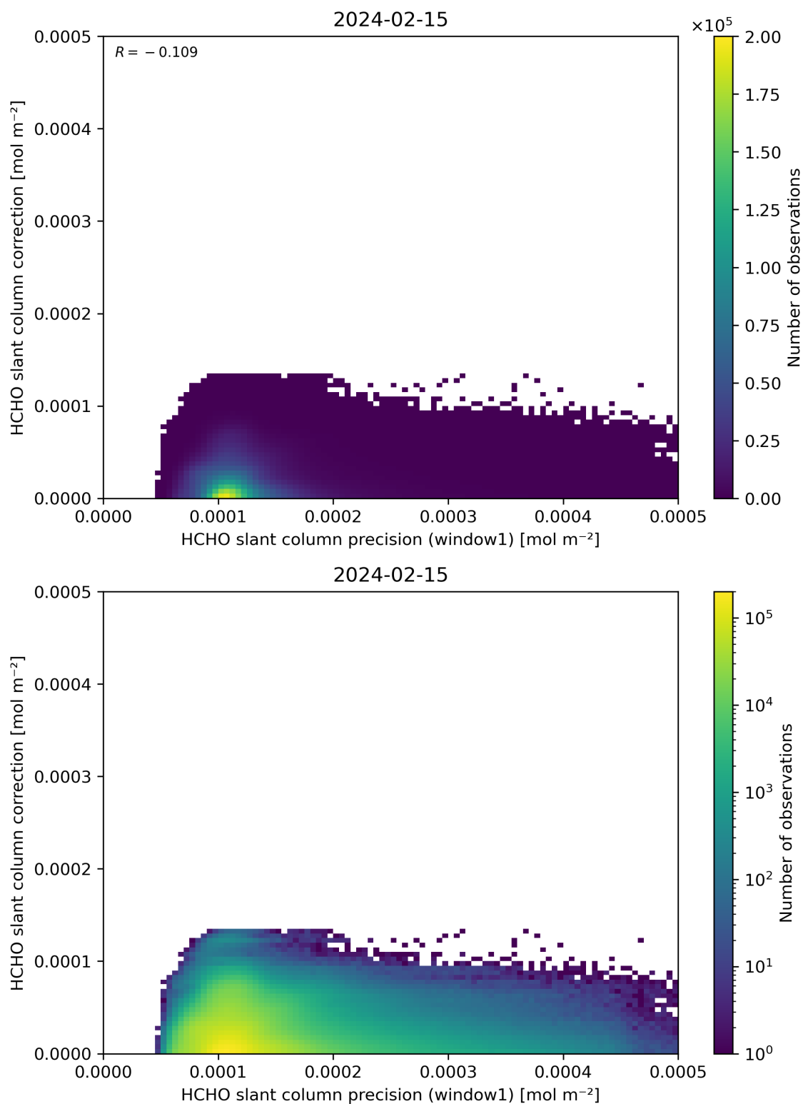
Figure 93: Scatter density plot of “HCHO slant column precision (window1)” against “HCHO slant column correction” for 2024-02-14 to 2024-02-16.
