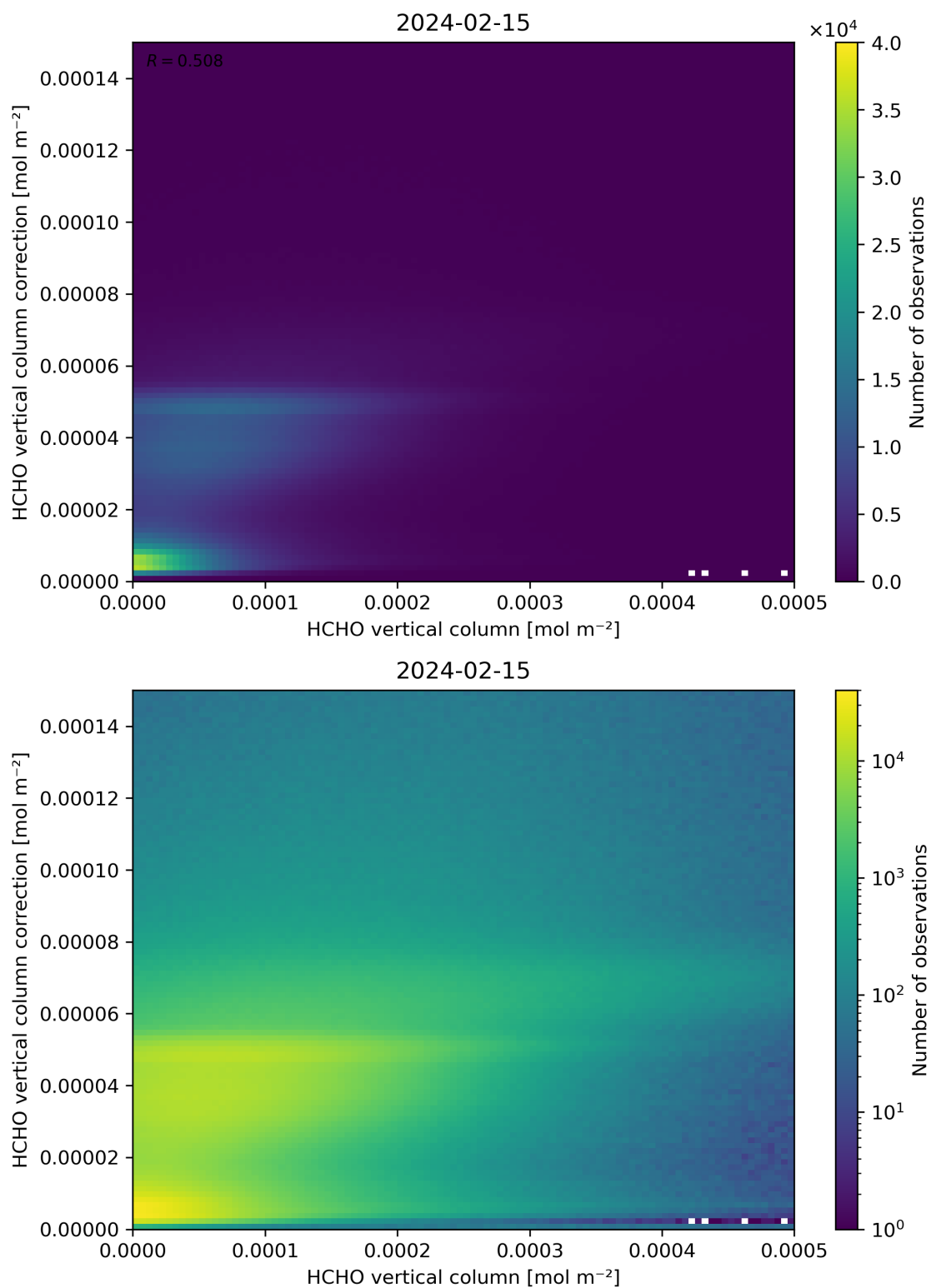
Figure 133: Scatter density plot of “HCHO vertical column” against “HCHO vertical column correction” for 2024-02-14 to 2024-02-16.
