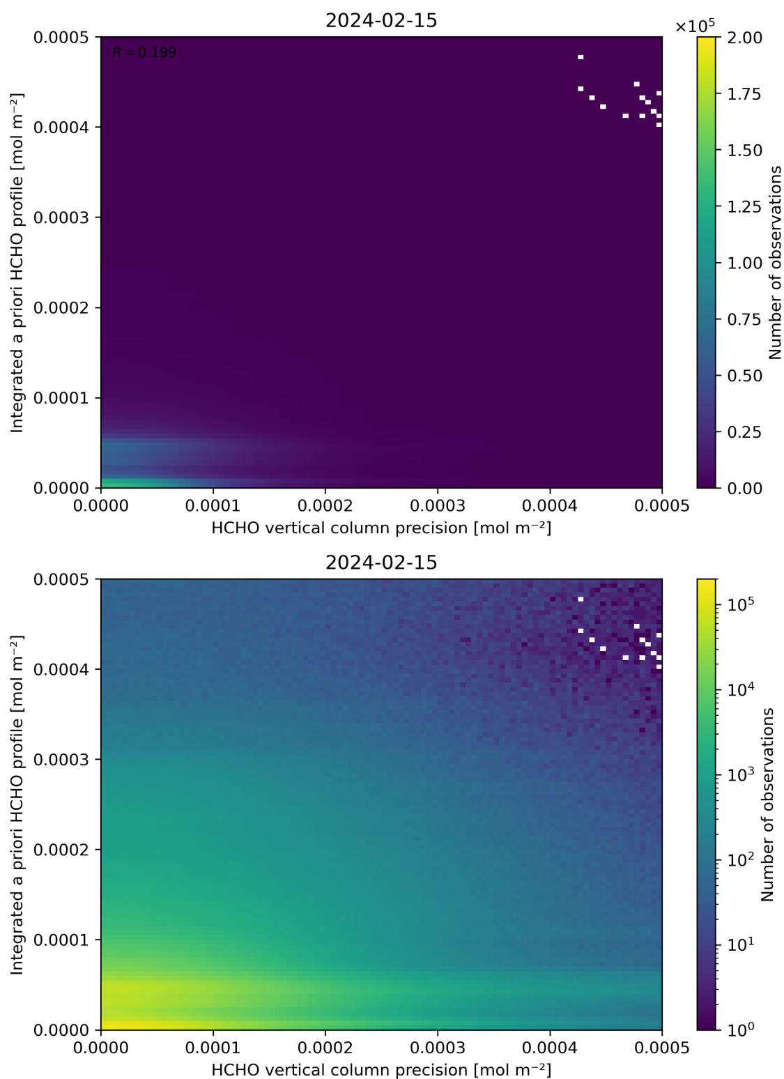
Figure 147: Scatter density plot of “HCHO vertical column precision” against “Integrated a priori HCHO profile” for 2024-02-14 to 2024-02-16.
