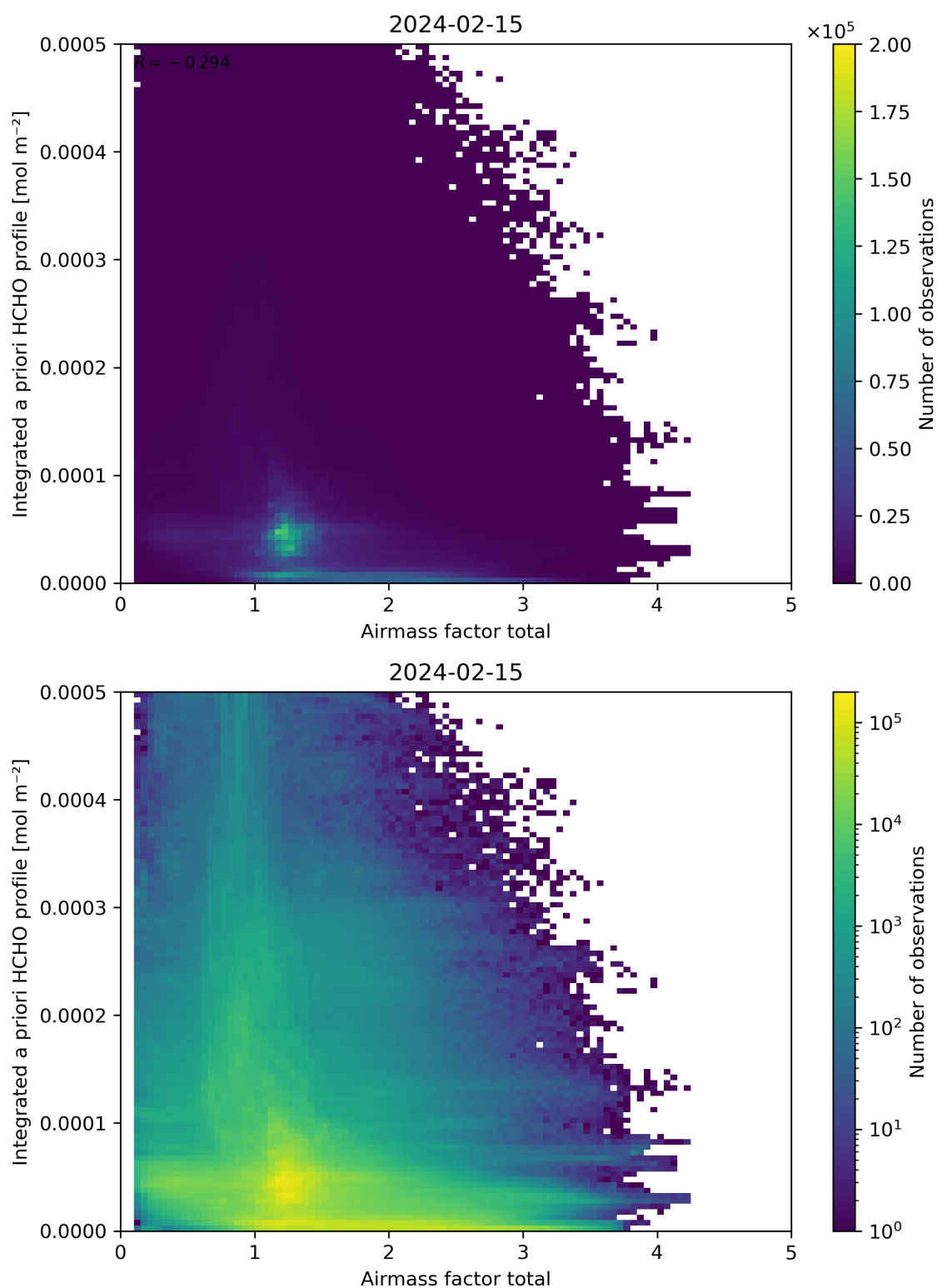
Figure 104: Scatter density plot of “Airmass factor total” against “Integrated a priori HCHO profile” for 2024-02-14 to 2024-02-16.
