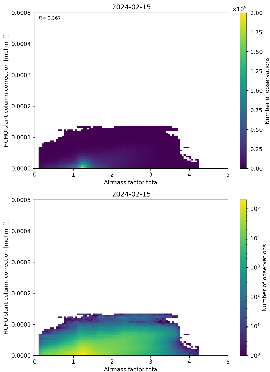
Figure 102: Scatter density plot of “Airmass factor total” against “HCHO slant column correction” for 2024-02-14 to 2024-02-16.
