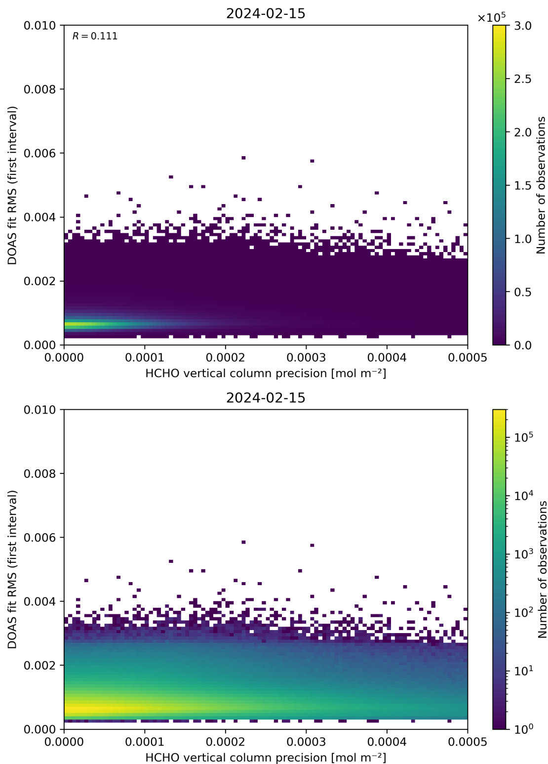
Figure 136: Scatter density plot of “HCHO vertical column precision” against “DOAS fit RMS (first interval)” for 2024-02-14 to 2024-02-16.
