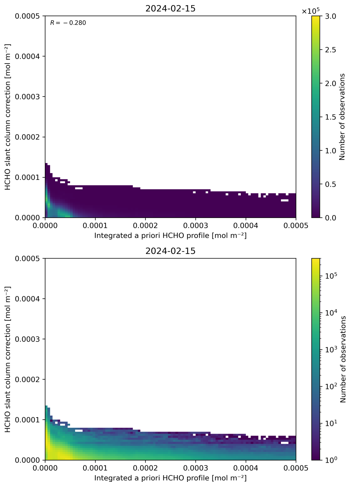
Figure 152: Scatter density plot of “Integrated a priori HCHO profile” against “HCHO slant column correction” for 2024-02-14 to 2024-02-16.
