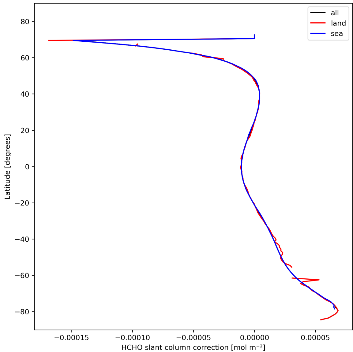
Figure 33: Zonal average of “HCHO slant column correction” for 2024-02-14 to 2024-02-16.
