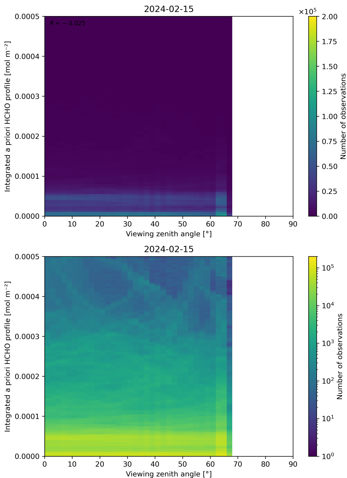
Figure 195: Scatter density plot of “Viewing zenith angle” against “Integrated a priori HCHO profile” for 2024-02-14 to 2024-02-16.
