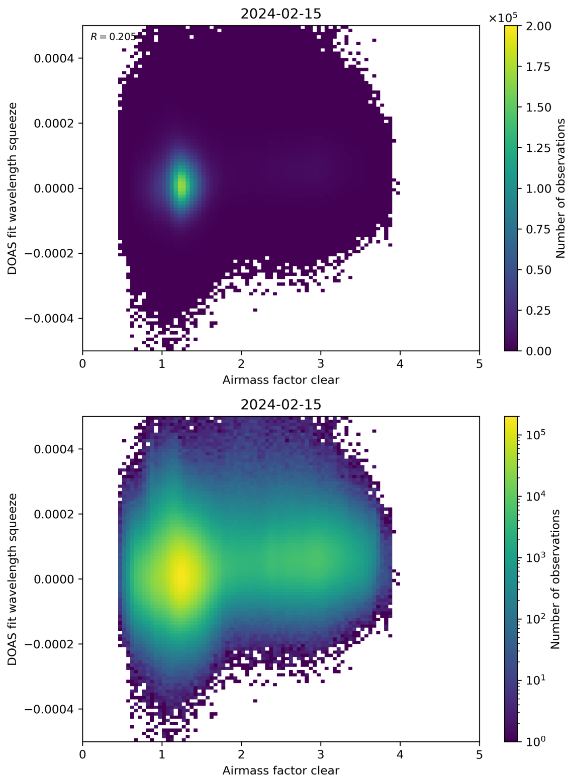
Figure 73: Scatter density plot of “Airmass factor clear” against “DOAS fit wavelength squeeze” for 2024-02-14 to 2024-02-16.
