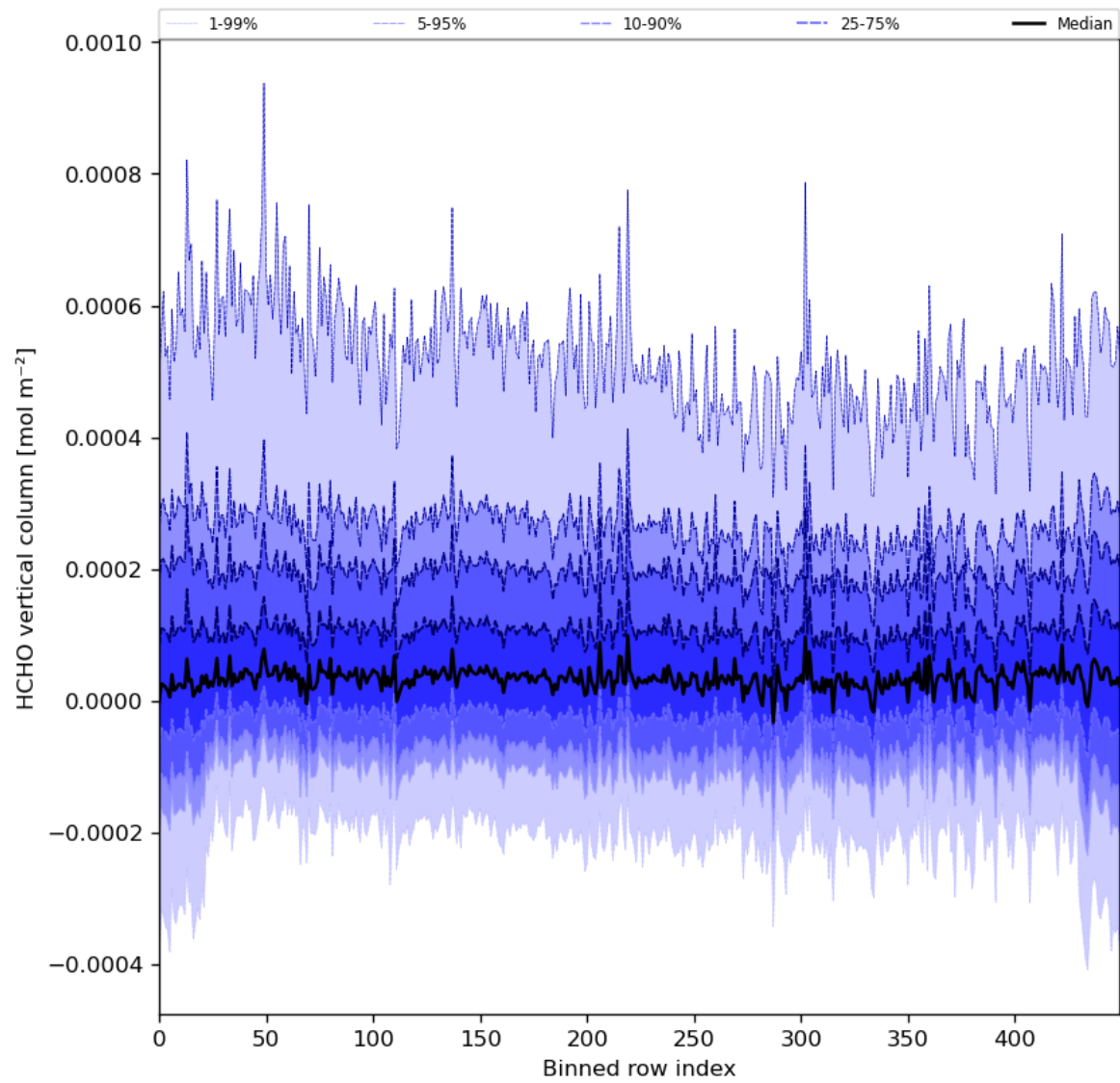
Figure 49: Along track statistics of “HCHO vertical column” for 2024-02-14 to 2024-02-16
