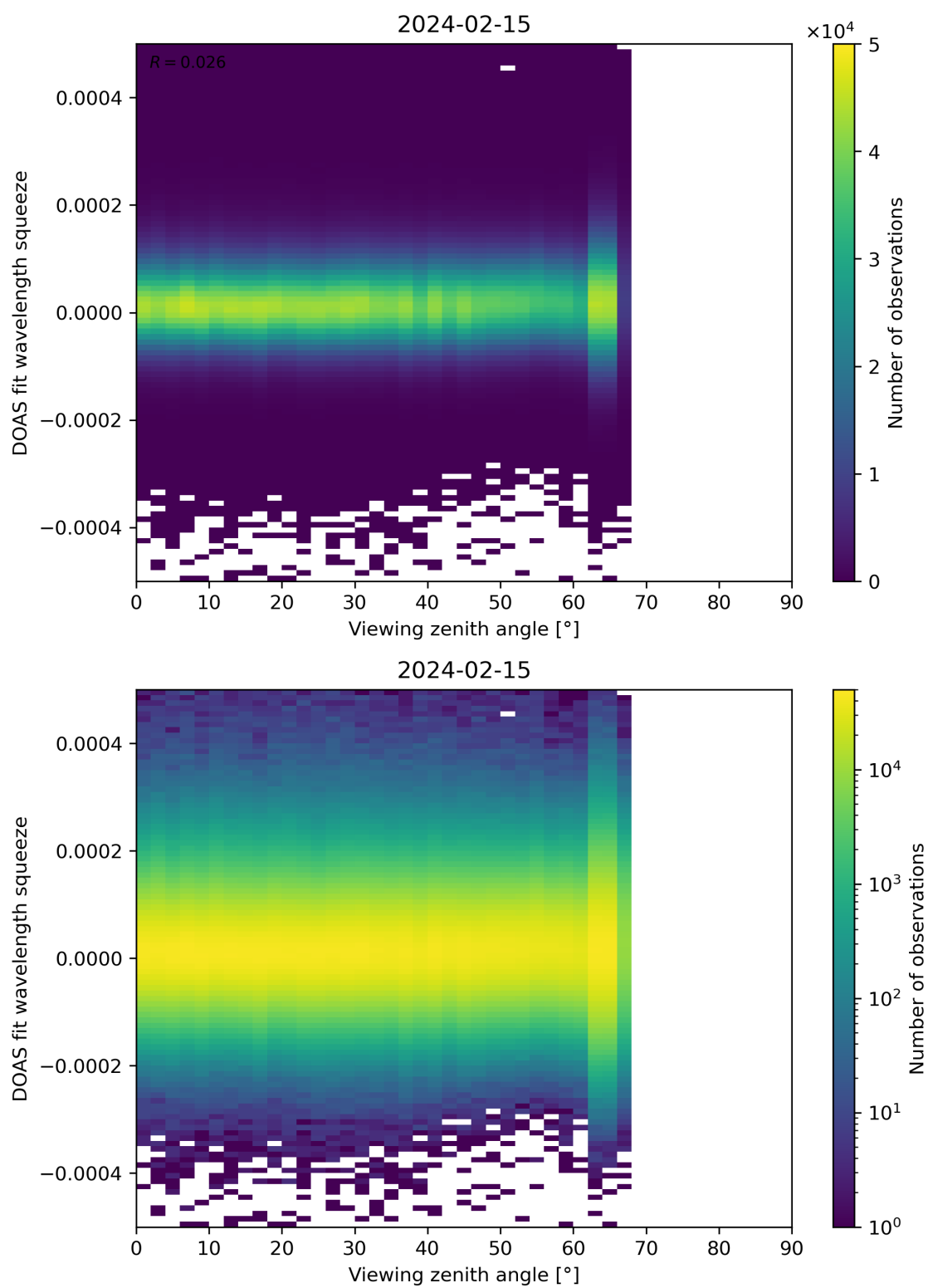
Figure 184: Scatter density plot of “Viewing zenith angle” against “DOAS fit wavelength squeeze” for 2024-02-14 to 2024-02-16.
