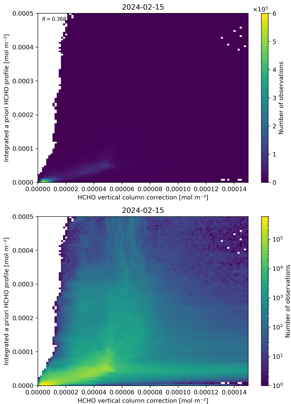
Figure 122: Scatter density plot of “HCHO vertical column correction” against “Integrated a priori HCHO profile” for 2024-02-14 to 2024-02-16.
