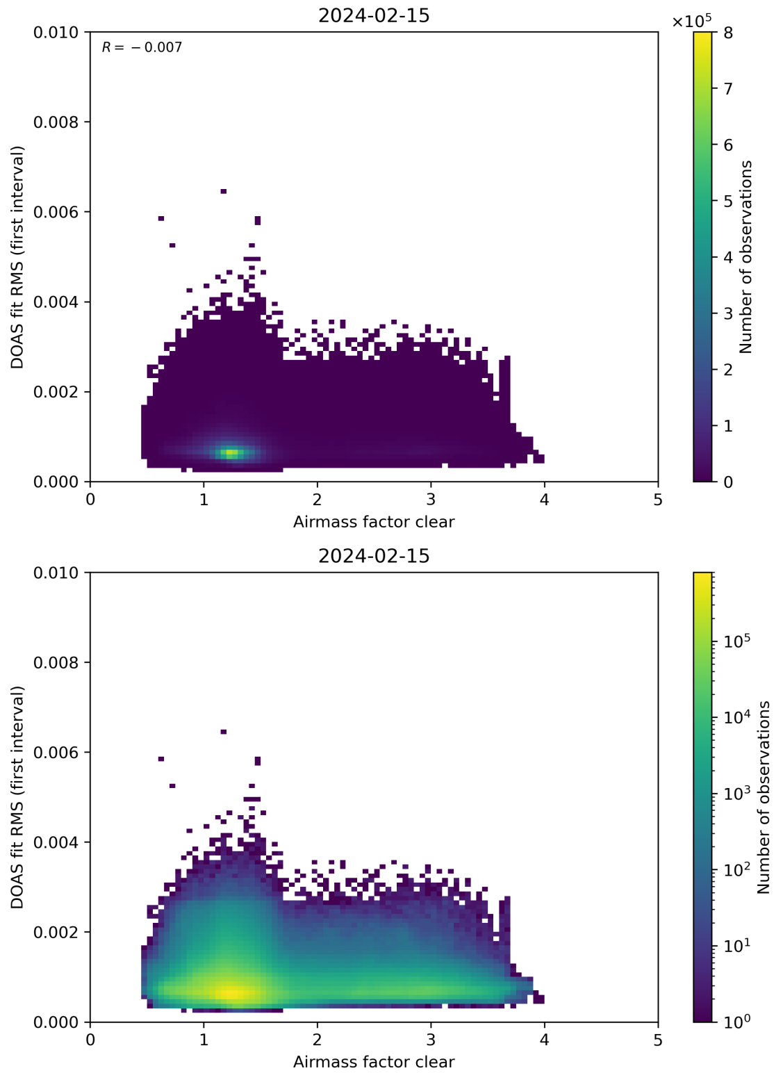
Figure 71: Scatter density plot of “Airmass factor clear” against “DOAS fit RMS (first interval)” for 2024-02-14 to 2024-02-16.
