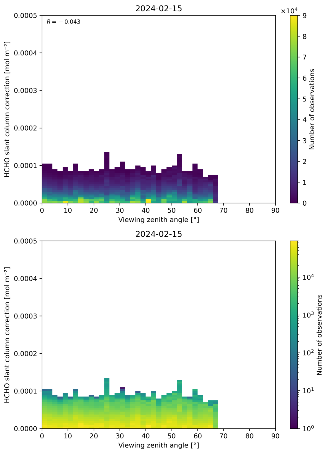
Figure 187: Scatter density plot of “Viewing zenith angle” against “HCHO slant column correction” for 2024-02-14 to 2024-02-16.
