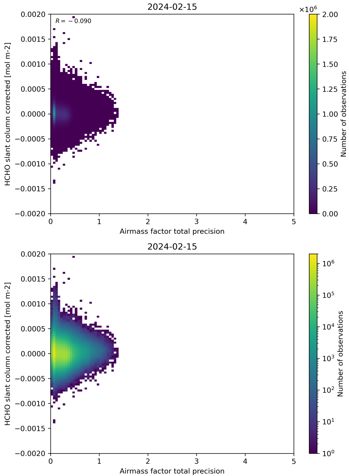
Figure 109: Scatter density plot of “Airmass factor total precision” against “HCHO slant column corrected” for 2024-02-14 to 2024-02-16.
