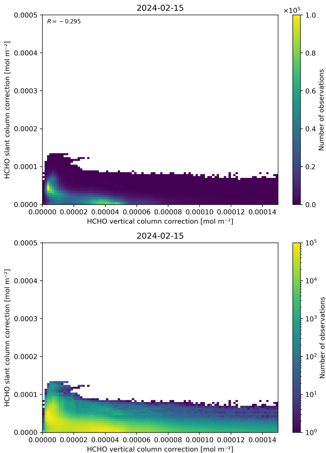
Figure 117: Scatter density plot of “HCHO vertical column correction” against “HCHO slant column correction” for 2024-02-14 to 2024-02-16.
