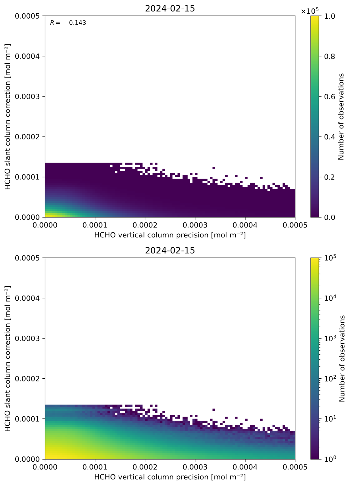
Figure 141: Scatter density plot of “HCHO vertical column precision” against “HCHO slant column correction” for 2024-02-14 to 2024-02-16.
