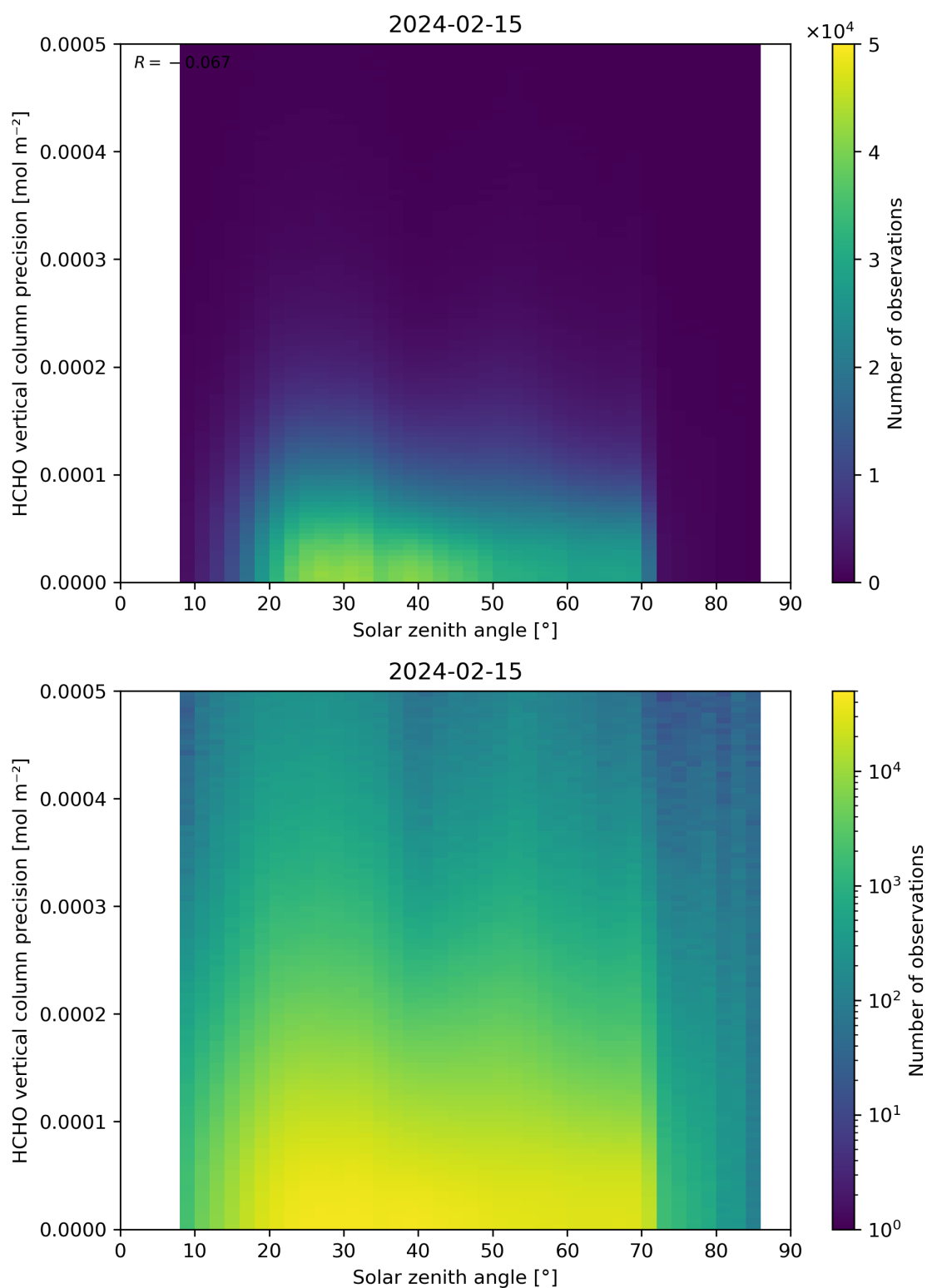
Figure 179: Scatter density plot of “Solar zenith angle” against “HCHO vertical column precision” for 2024-02-14 to 2024-02-16.
