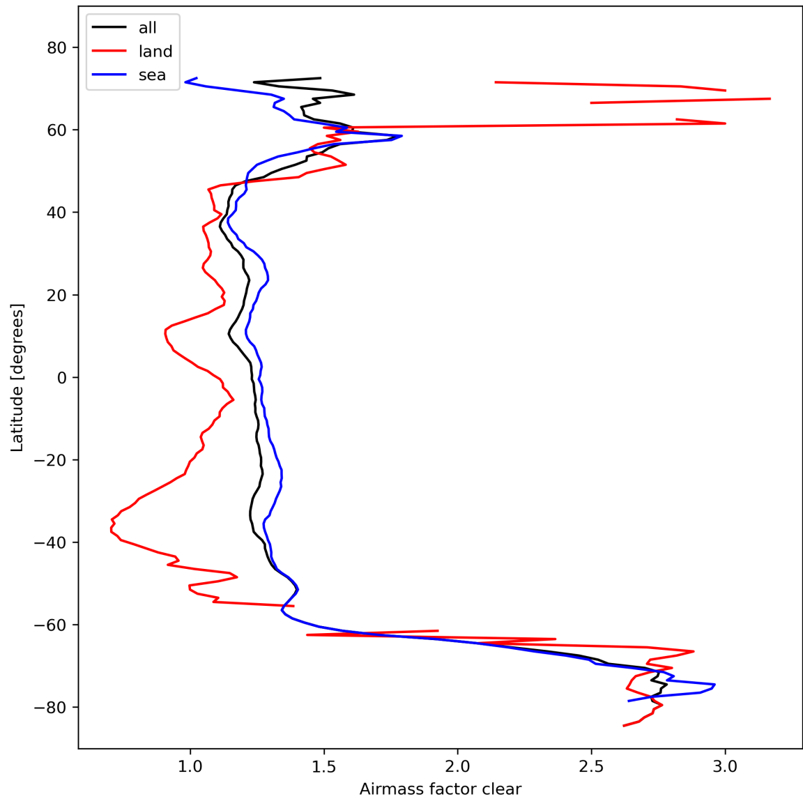
Figure 28: Zonal average of “Airmass factor clear” for 2024-02-14 to 2024-02-16.
