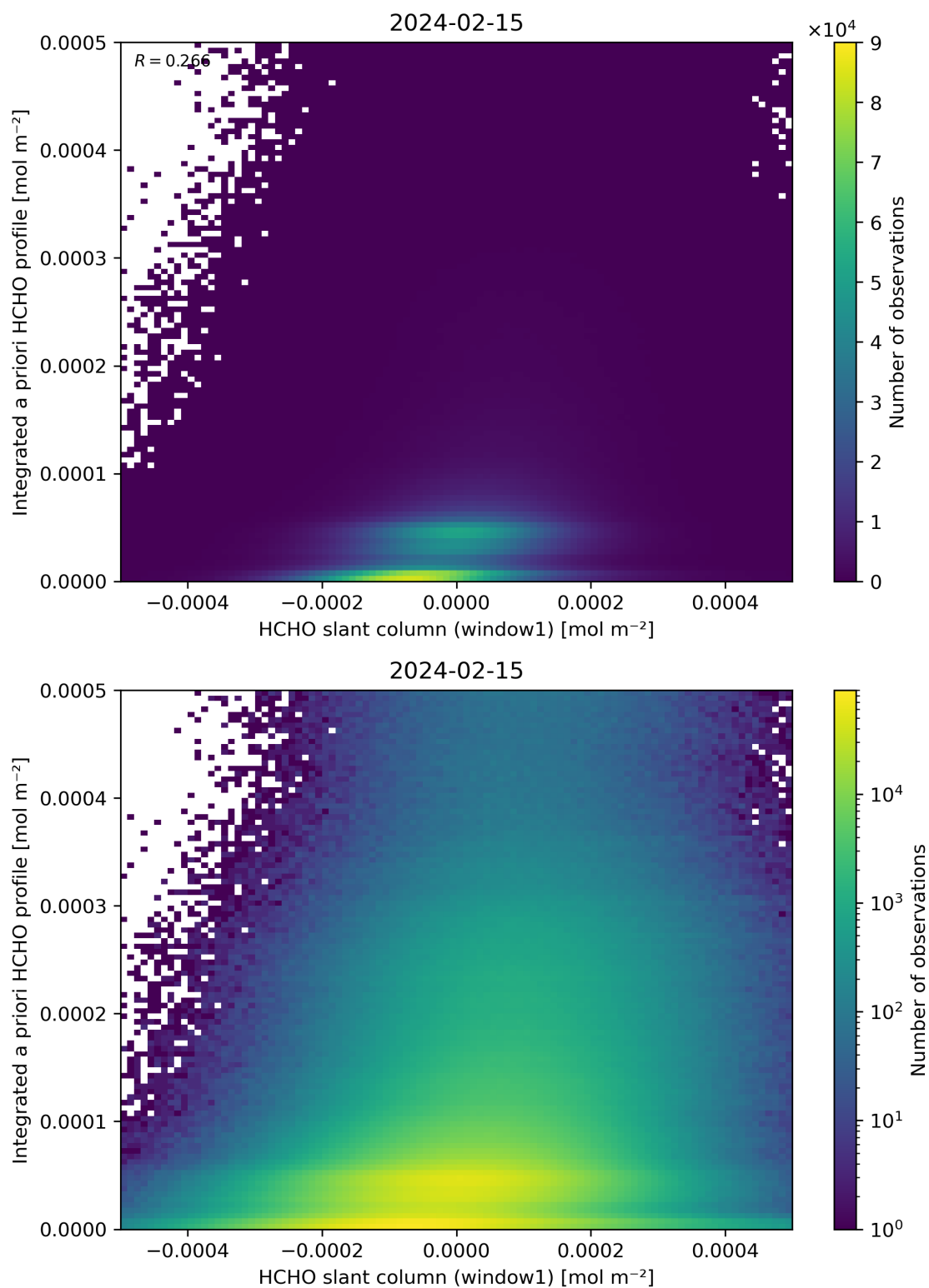
Figure 87: Scatter density plot of “HCHO slant column (window1)” against “Integrated a priori HCHO profile” for 2024-02-14 to 2024-02-16.
