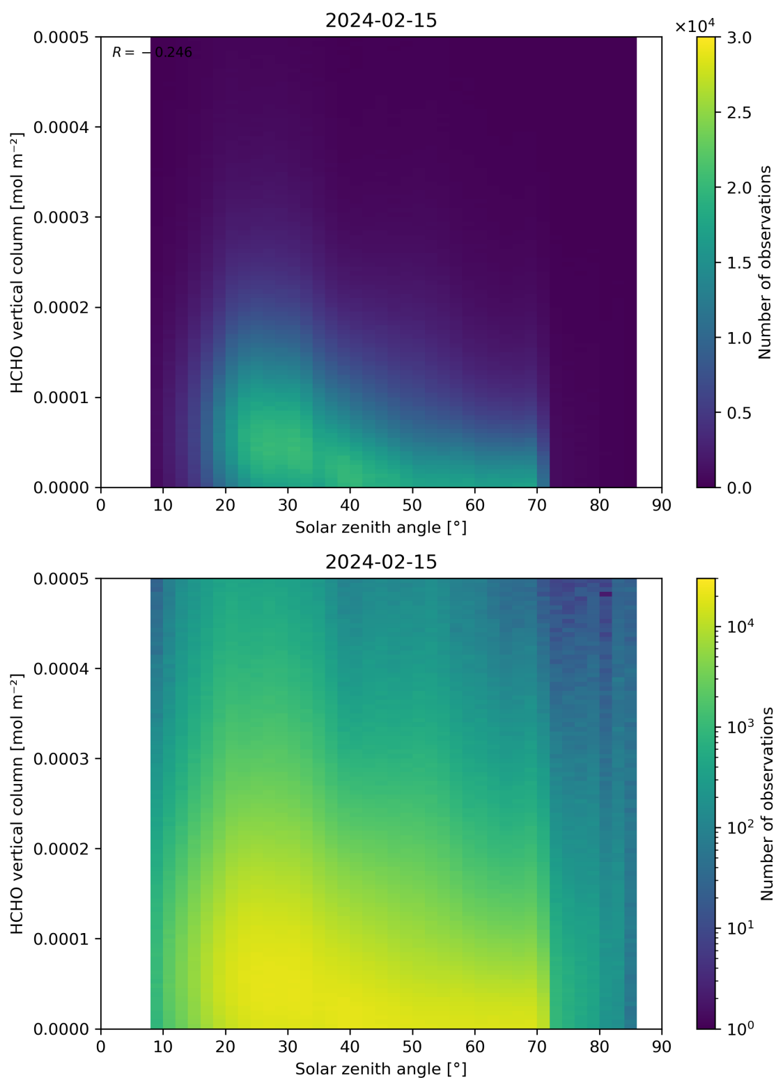
Figure 177: Scatter density plot of “Solar zenith angle” against “HCHO vertical column” for 2024-02-14 to 2024-02-16.
