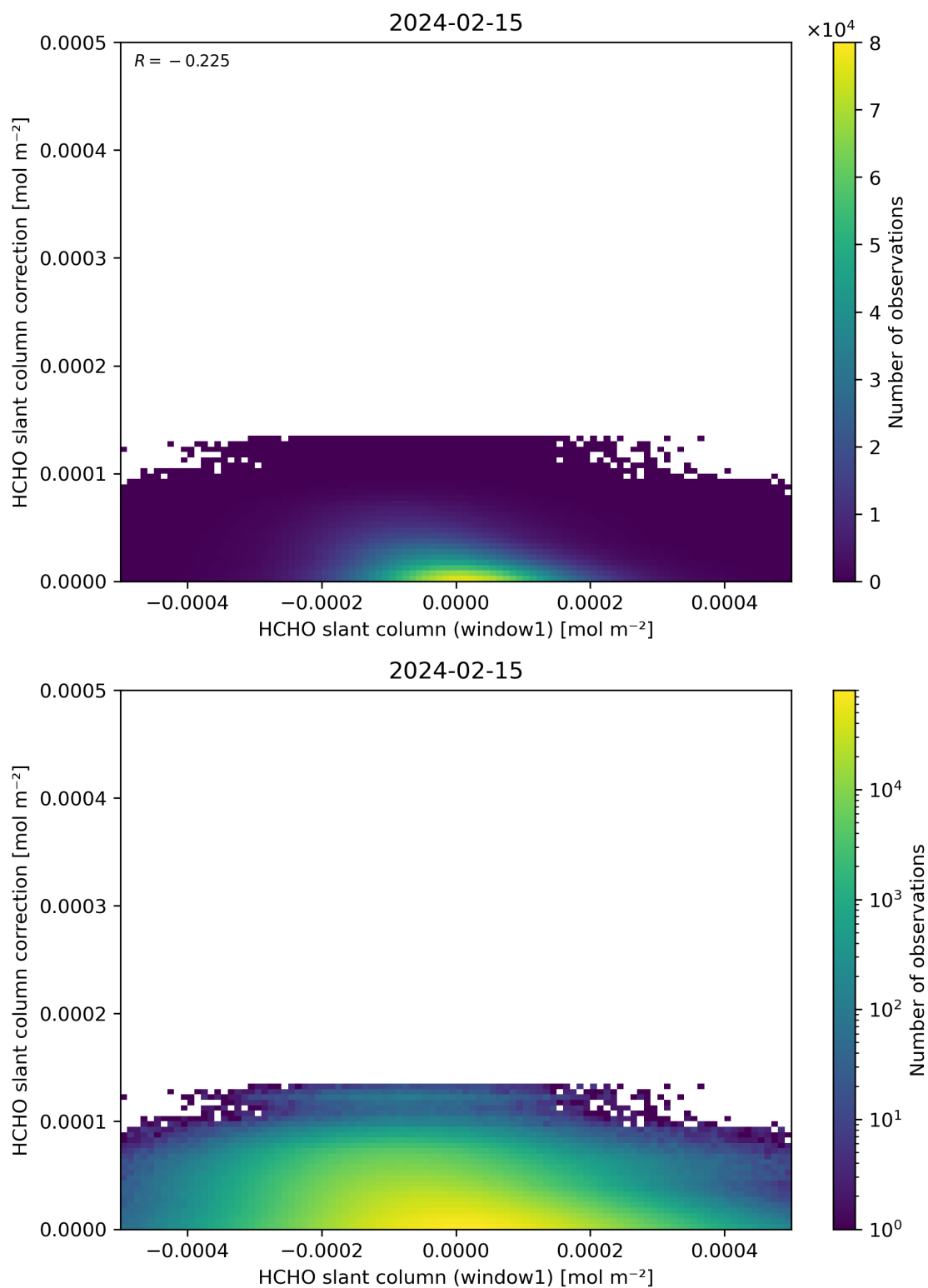
Figure 83: Scatter density plot of “HCHO slant column (window1)” against “HCHO slant column correction” for 2024-02-14 to 2024-02-16.
