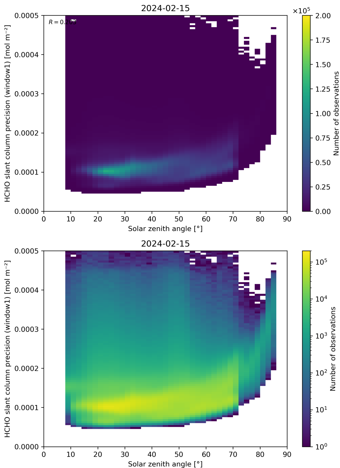
Figure 174: Scatter density plot of “Solar zenith angle” against “HCHO slant column precision (window1)” for 2024-02-14 to 2024-02-16.
