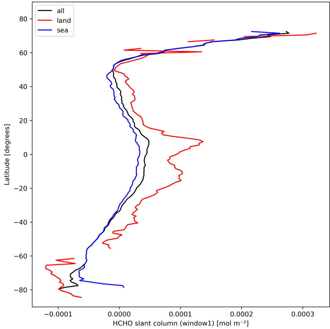
Figure 24: Zonal average of “HCHO slant column (window1)” for 2024-02-14 to 2024-02-16.
