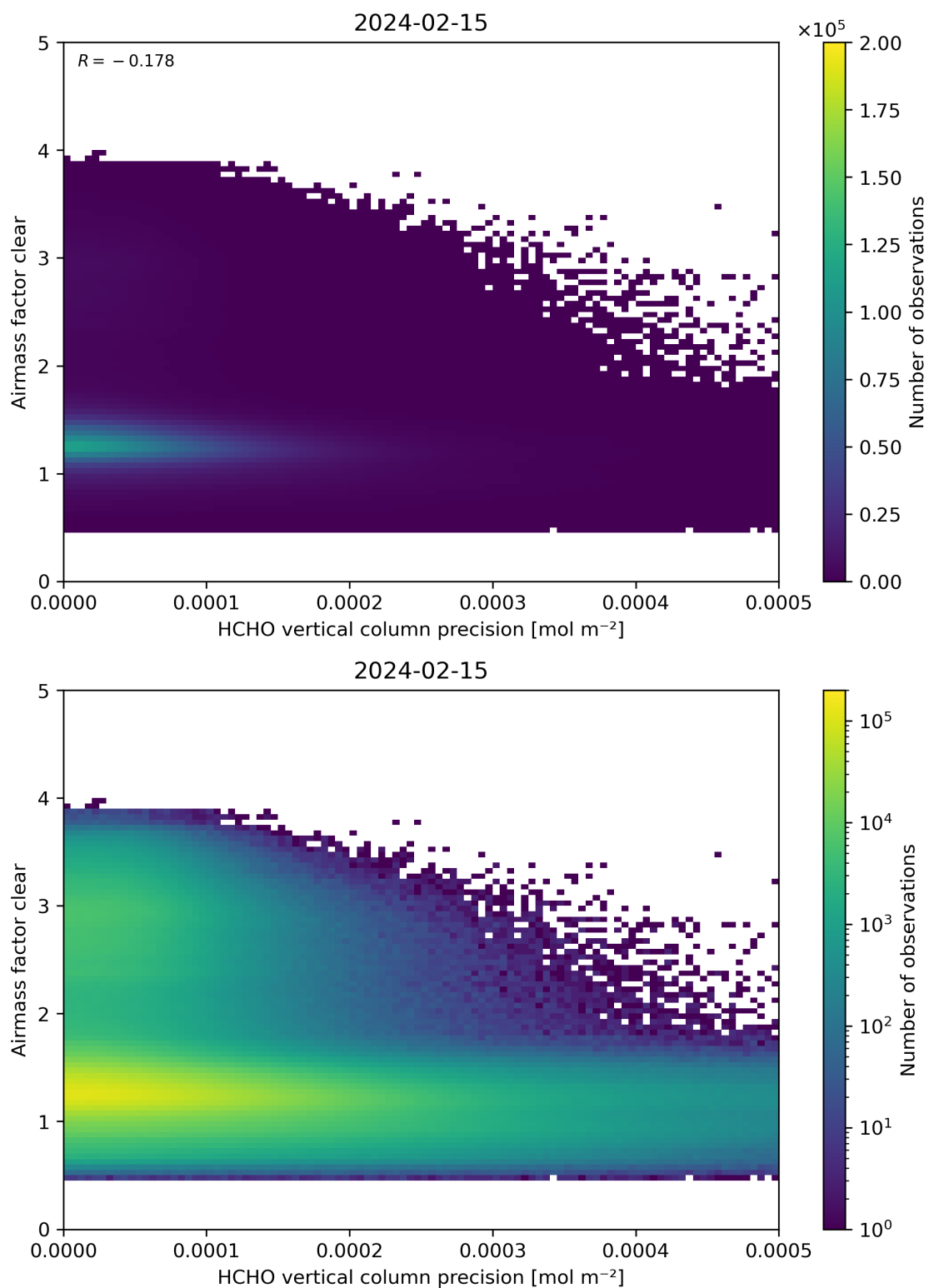
Figure 139: Scatter density plot of “HCHO vertical column precision” against “Airmass factor clear” for 2024-02-14 to 2024-02-16.
