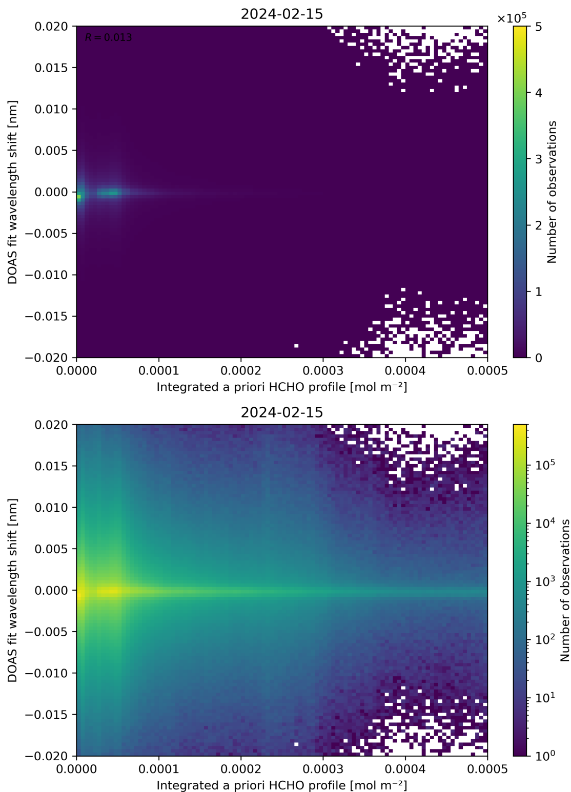
Figure 149: Scatter density plot of “Integrated a priori HCHO profile” against “DOAS fit wavelength shift” for 2024-02-14 to 2024-02-16.
