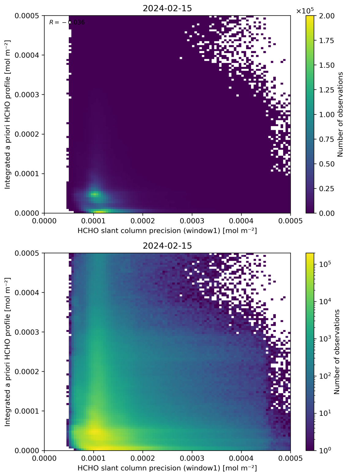
Figure 96: Scatter density plot of “HCHO slant column precision (window1)” against “Integrated a priori HCHO profile” for 2024-02-14 to 2024-02-16.
