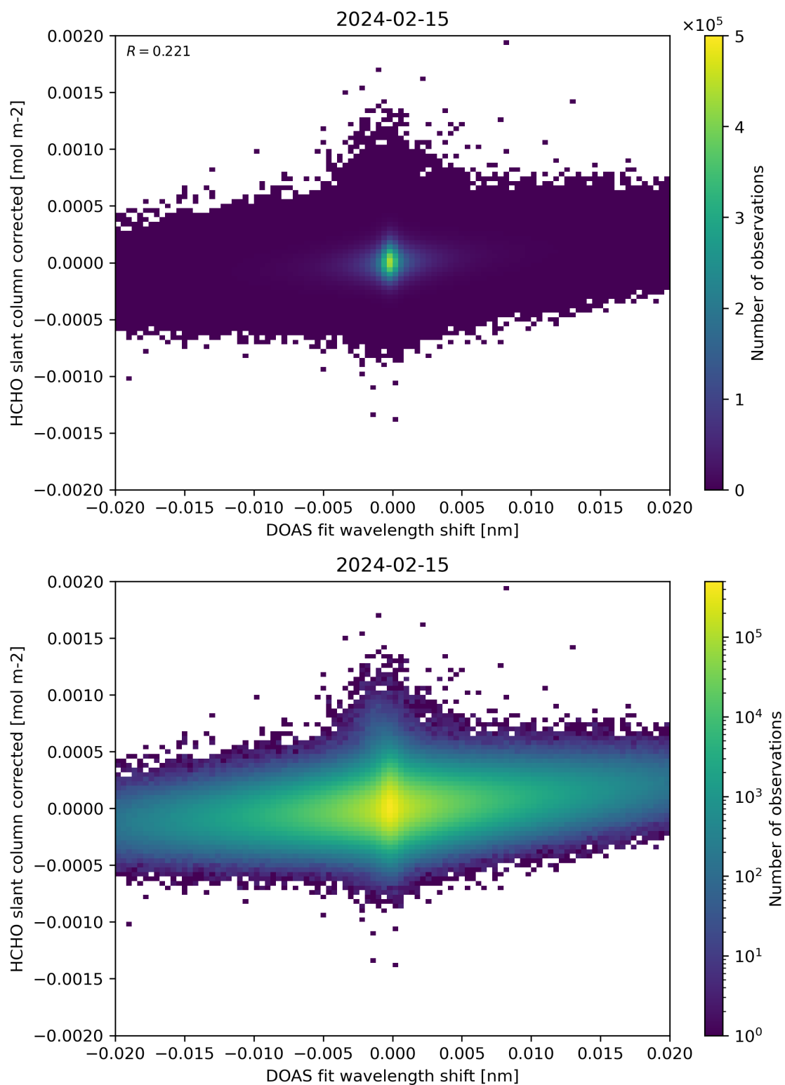
Figure 66: Scatter density plot of “DOAS fit wavelength shift” against “HCHO slant column corrected” for 2024-02-14 to 2024-02-16.
