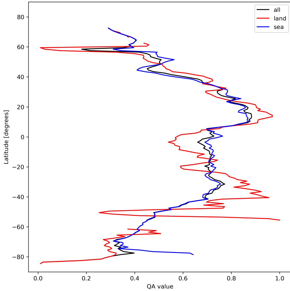
Figure 20: Zonal average of “QA value” for 2024-02-14 to 2024-02-16.
