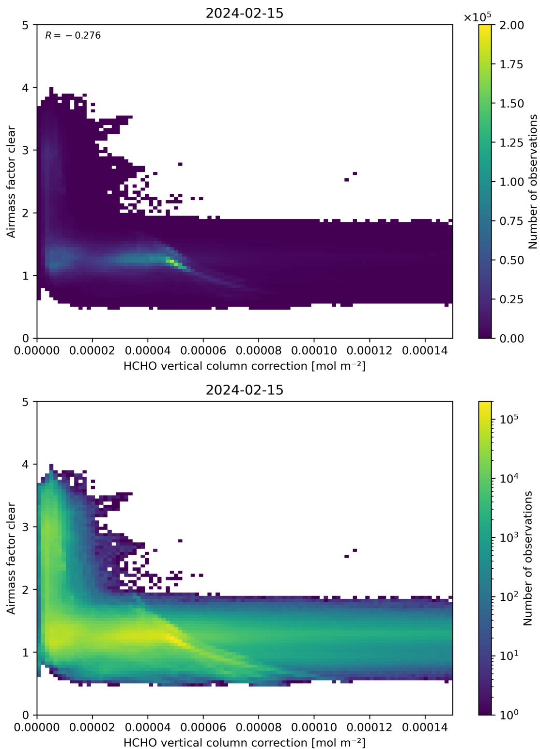
Figure 115: Scatter density plot of “HCHO vertical column correction” against “Airmass factor clear” for 2024-02-14 to 2024-02-16.
