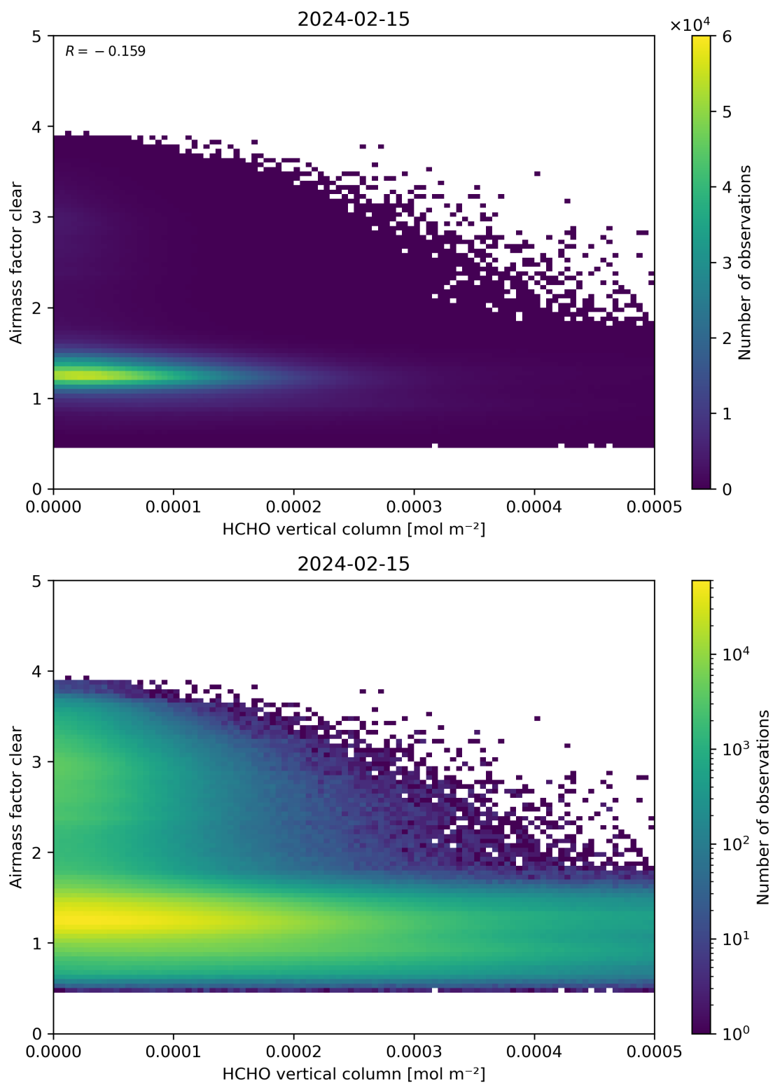
Figure 126: Scatter density plot of “HCHO vertical column” against “Airmass factor clear” for 2024-02-14 to 2024-02-16.
