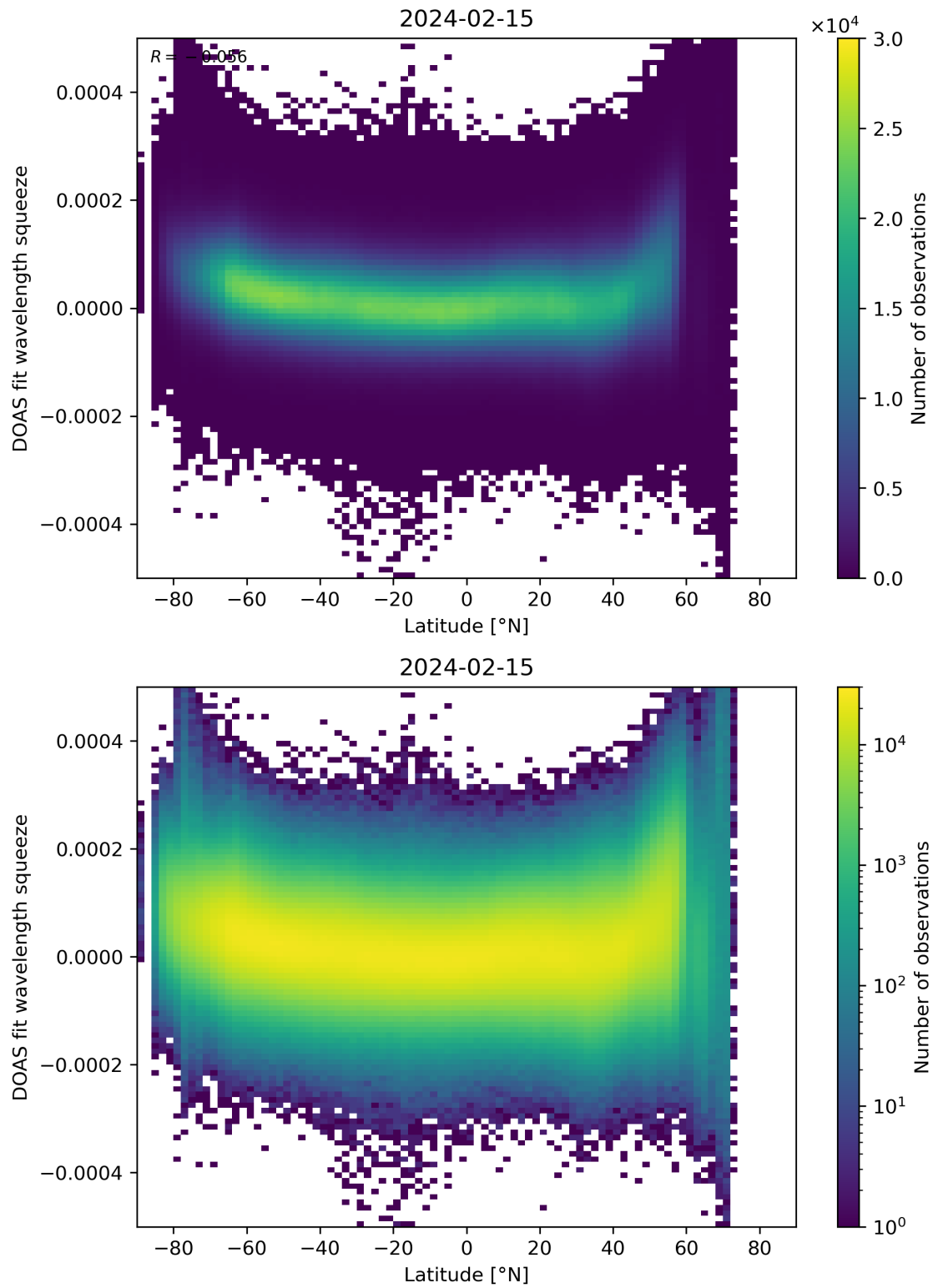
Figure 155: Scatter density plot of “Latitude” against “DOAS fit wavelength squeeze” for 2024-02-14 to 2024-02-16.
