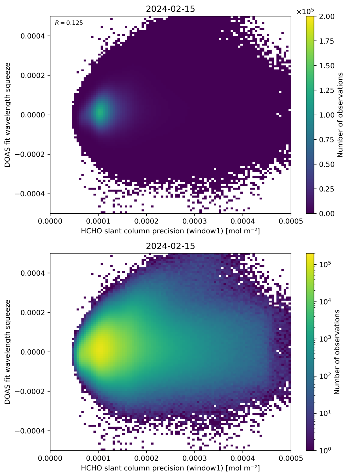
Figure 90: Scatter density plot of “HCHO slant column precision (window1)” against “DOAS fit wavelength squeeze” for 2024-02-14 to 2024-02-16.
