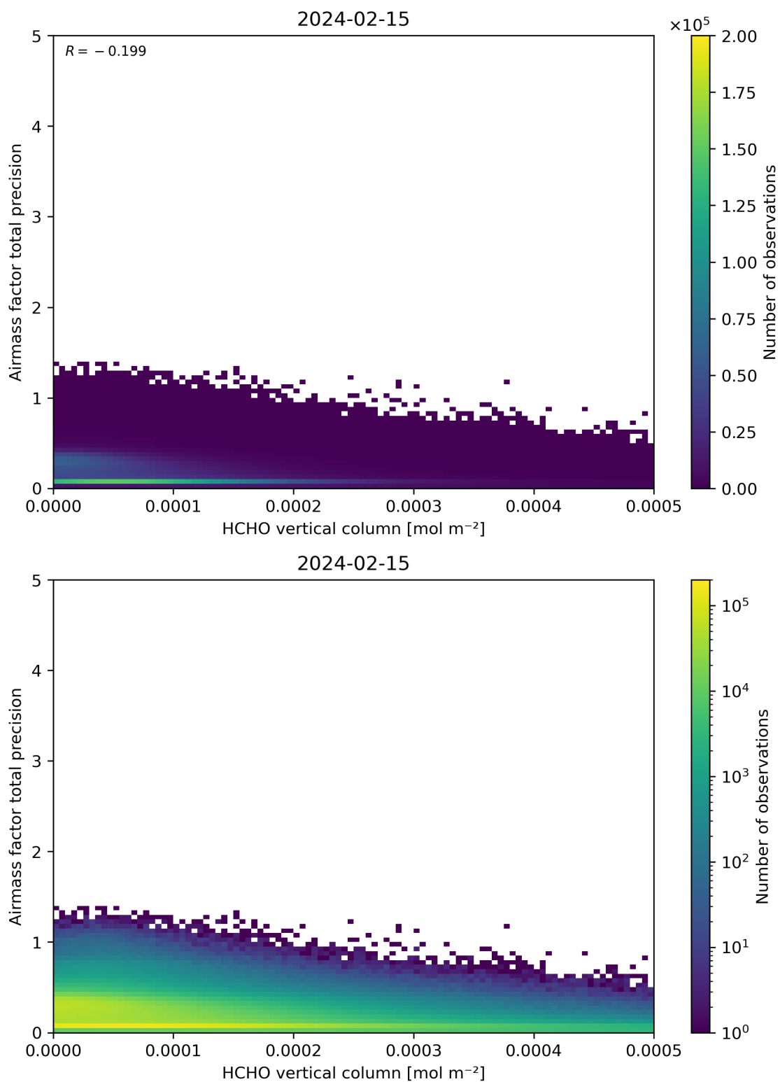
Figure 132: Scatter density plot of “HCHO vertical column” against “Airmass factor total precision” for 2024-02-14 to 2024-02-16.
