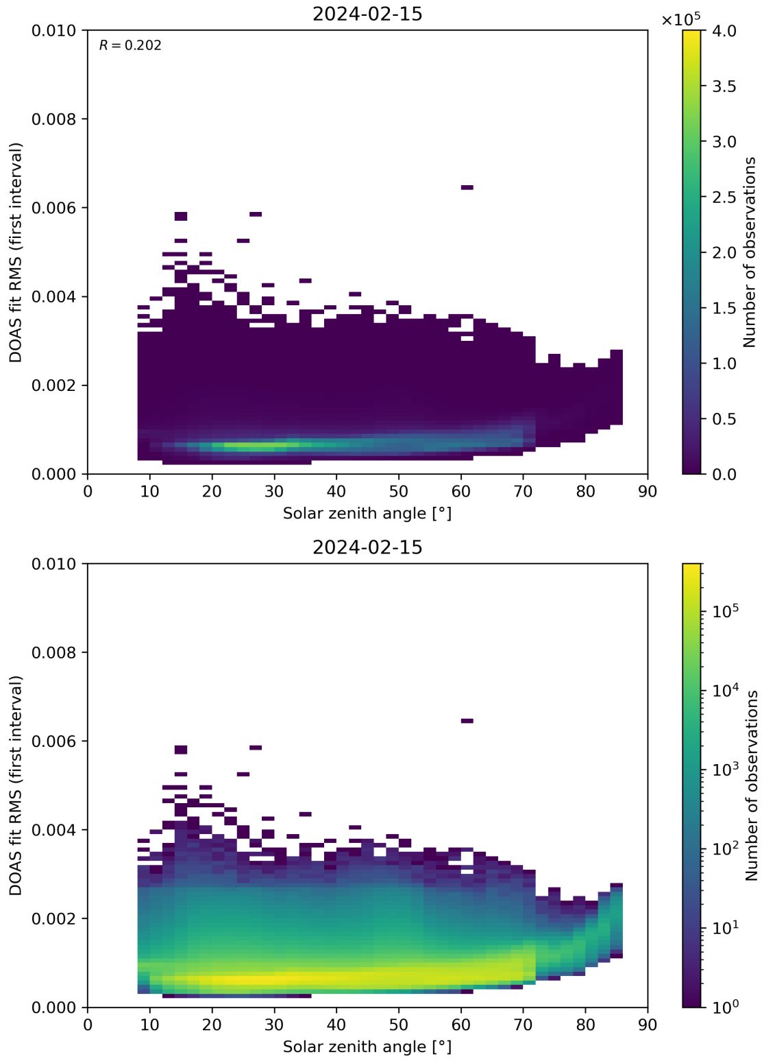
Figure 167: Scatter density plot of “Solar zenith angle” against “DOAS fit RMS (first interval)” for 2024-02-14 to 2024-02-16.
