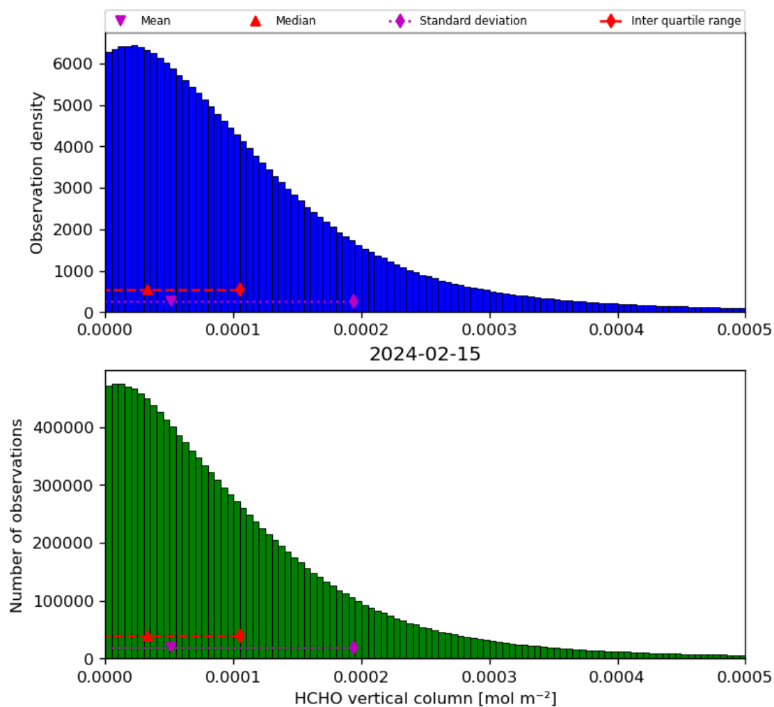
Figure 35: Histogram of “HCHO vertical column” for 2024-02-14 to 2024-02-16
