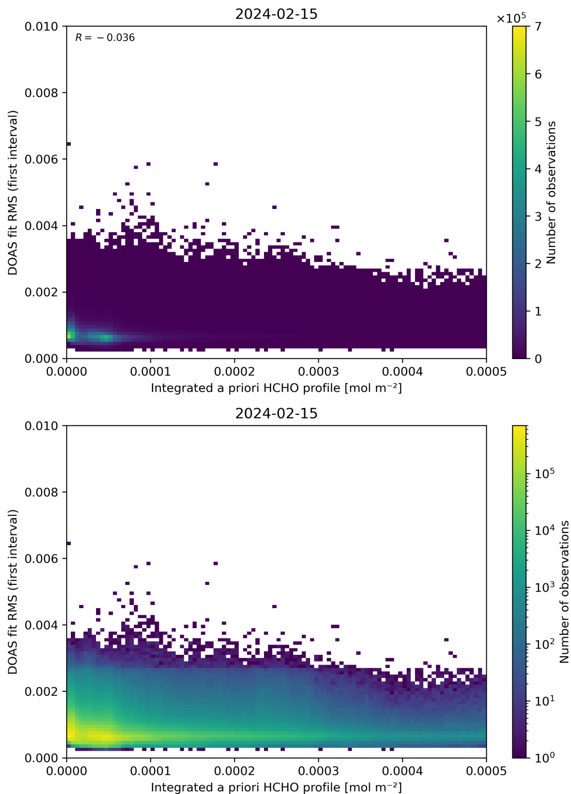
Figure 148: Scatter density plot of “Integrated a priori HCHO profile” against “DOAS fit RMS (first interval)” for 2024-02-14 to 2024-02-16.
