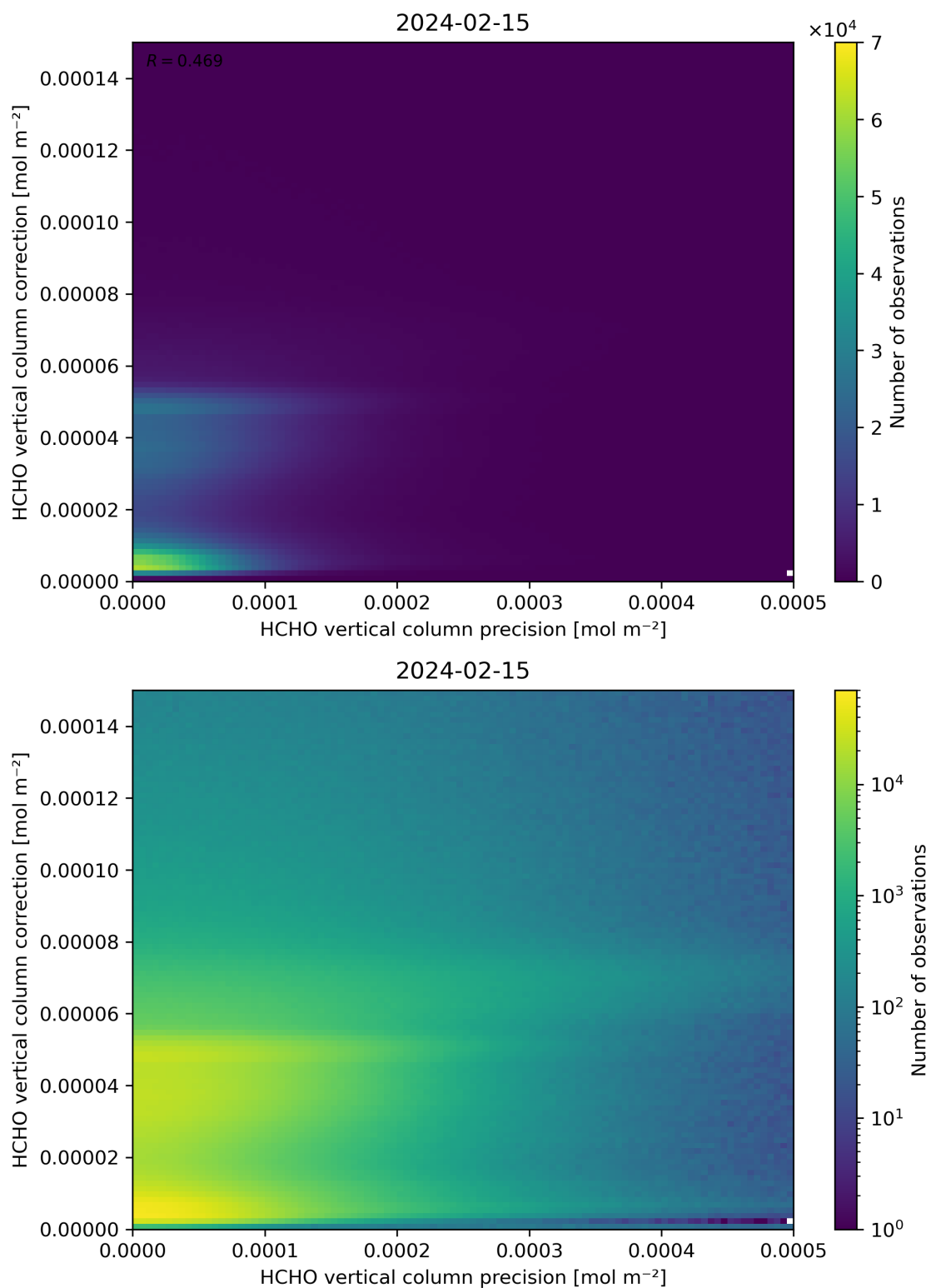
Figure 146: Scatter density plot of “HCHO vertical column precision” against “HCHO vertical column correction” for 2024-02-14 to 2024-02-16.
