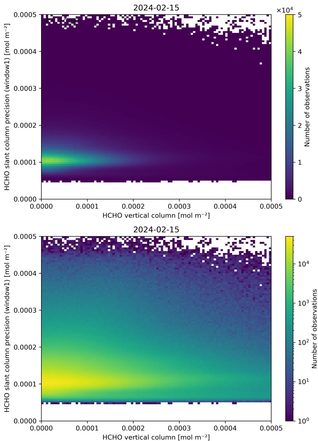
Figure 130: Scatter density plot of “HCHO vertical column” against “HCHO slant column precision (window1)” for 2024-02-14 to 2024-02-16.
