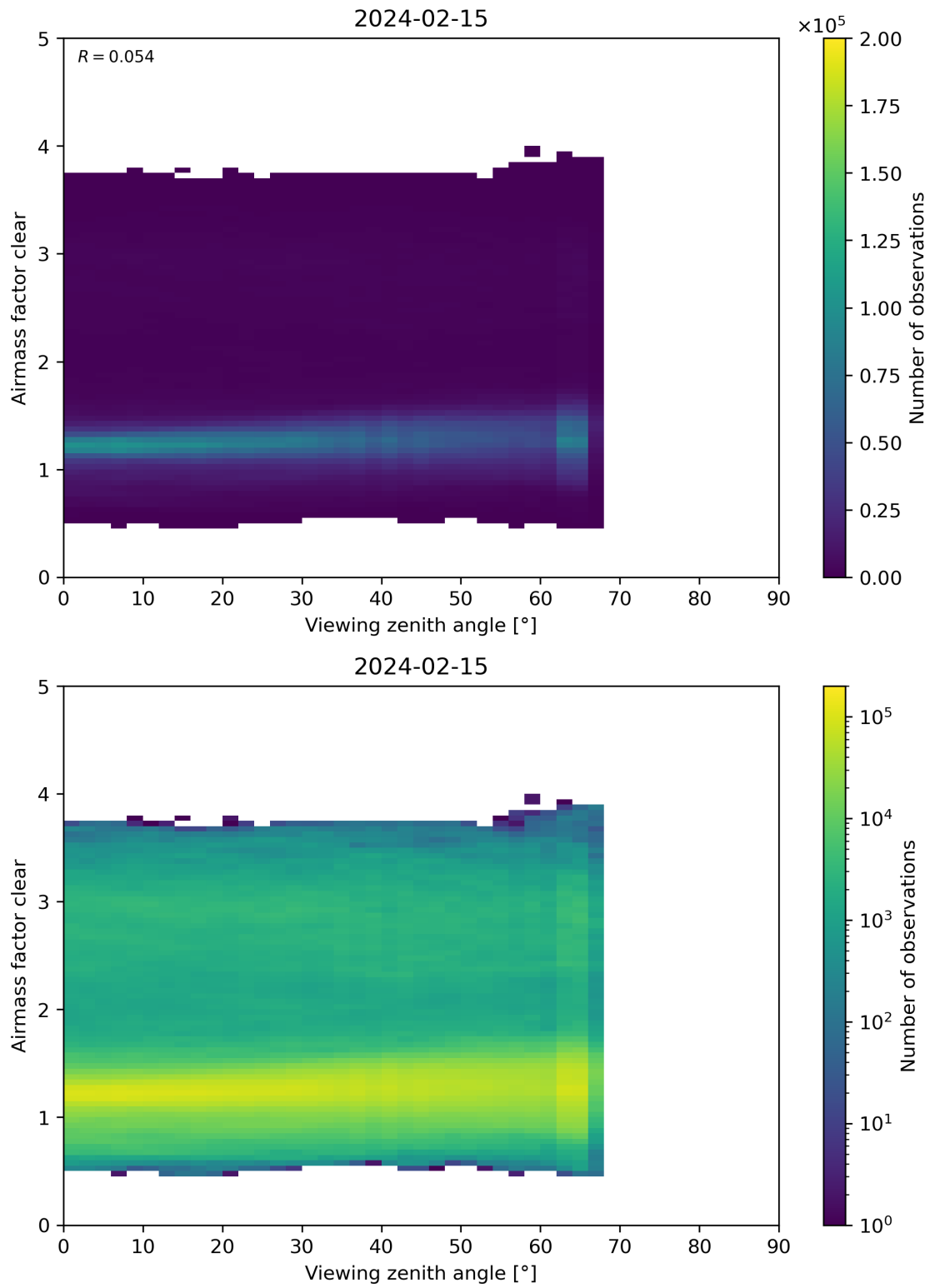
Figure 185: Scatter density plot of “Viewing zenith angle” against “Airmass factor clear” for 2024-02-14 to 2024-02-16.
