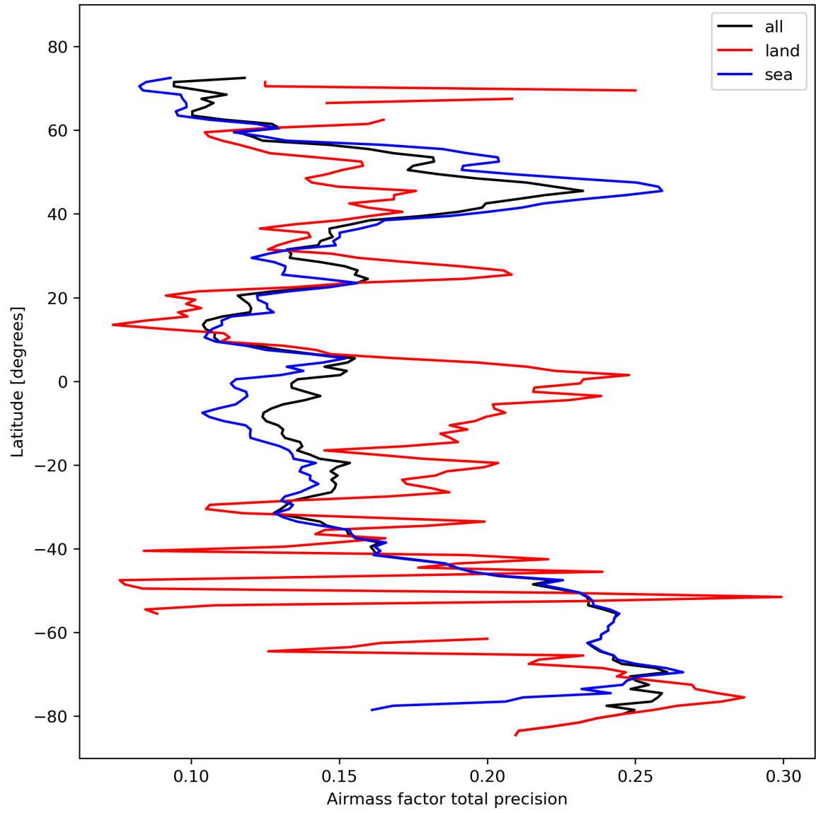
Figure 27: Zonal average of “Airmass factor total precision” for 2024-02-14 to 2024-02-16.
