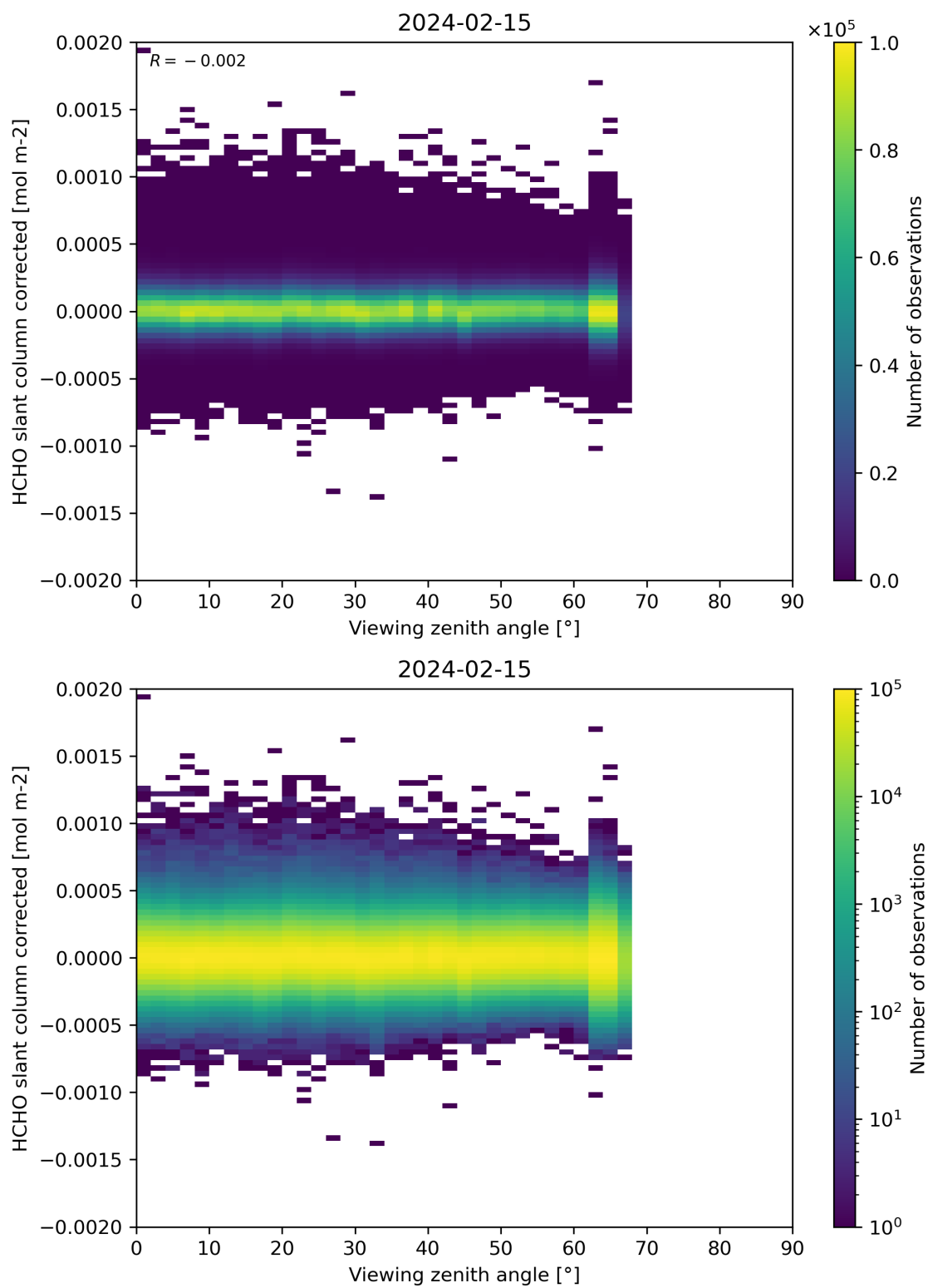
Figure 186: Scatter density plot of “Viewing zenith angle” against “HCHO slant column corrected” for 2024-02-14 to 2024-02-16.
