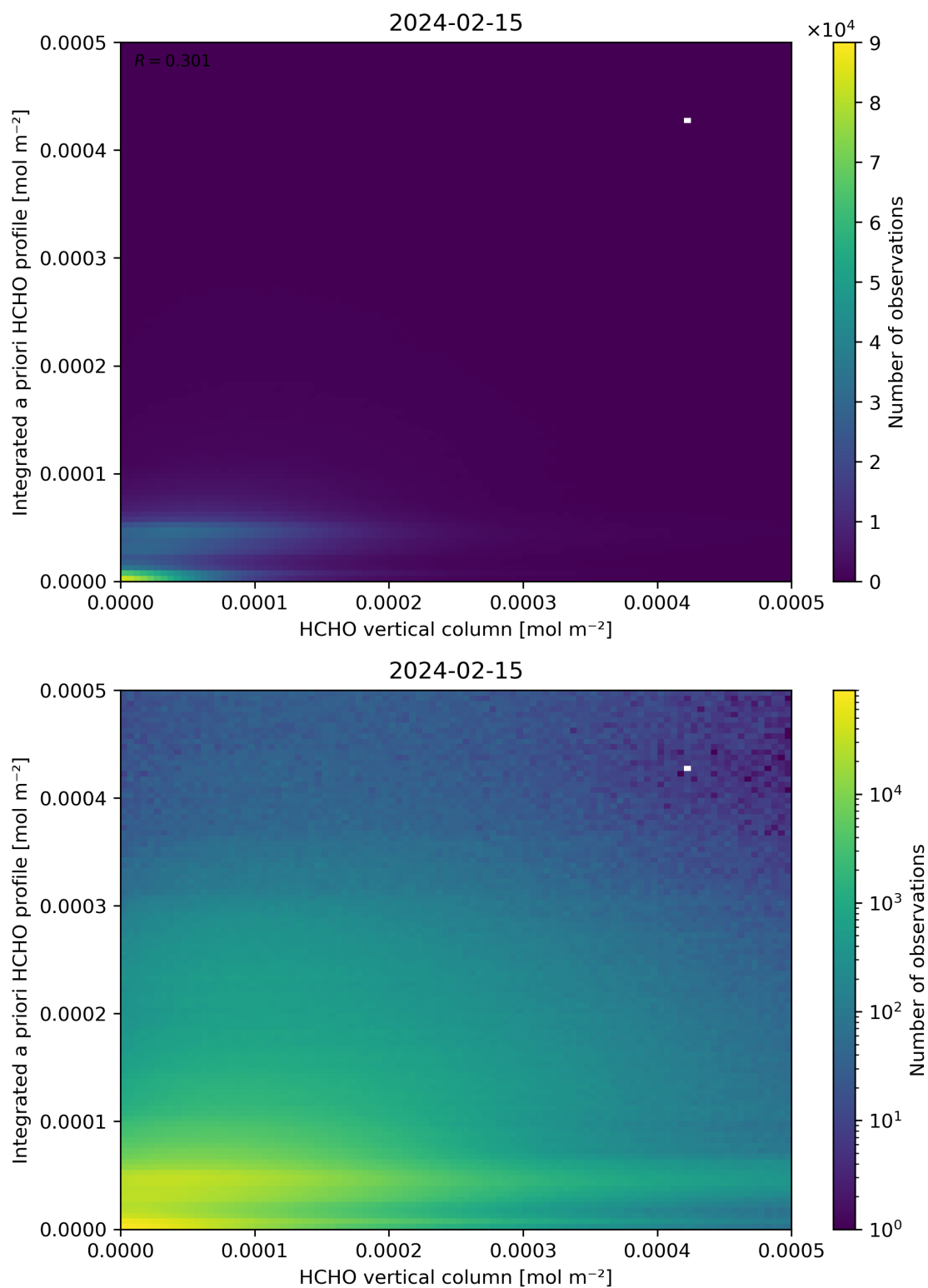
Figure 135: Scatter density plot of “HCHO vertical column” against “Integrated a priori HCHO profile” for 2024-02-14 to 2024-02-16.
