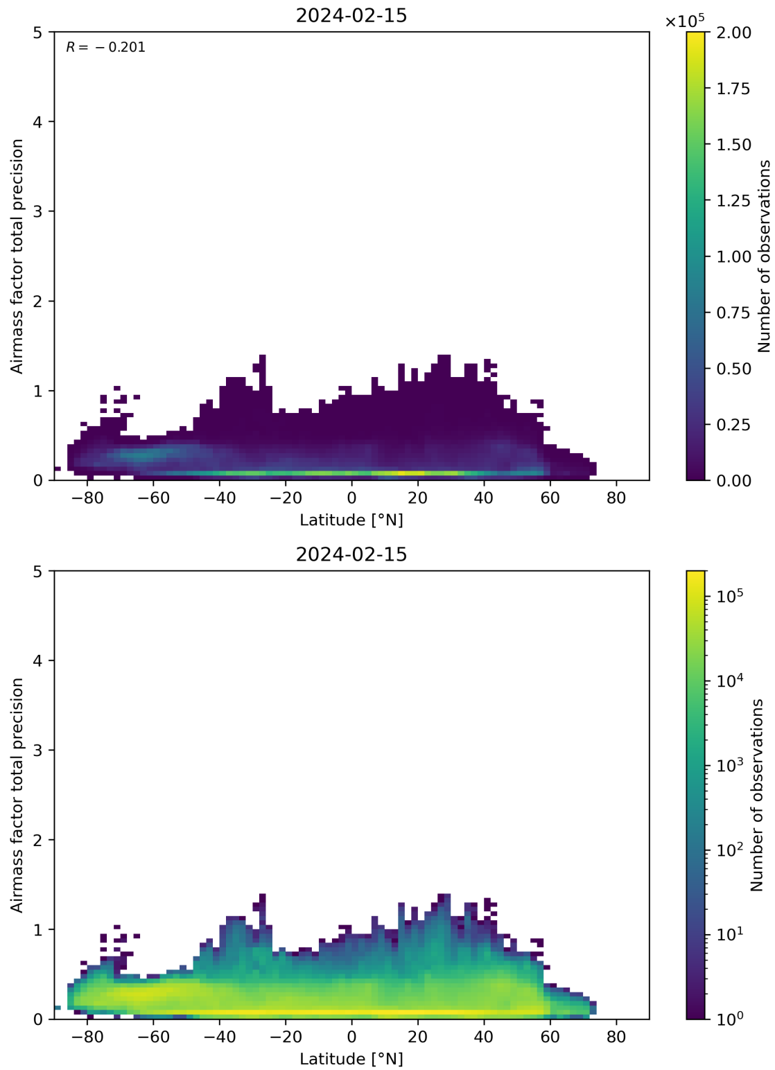
Figure 162: Scatter density plot of “Latitude” against “Airmass factor total precision” for 2024-02-14 to 2024-02-16.
