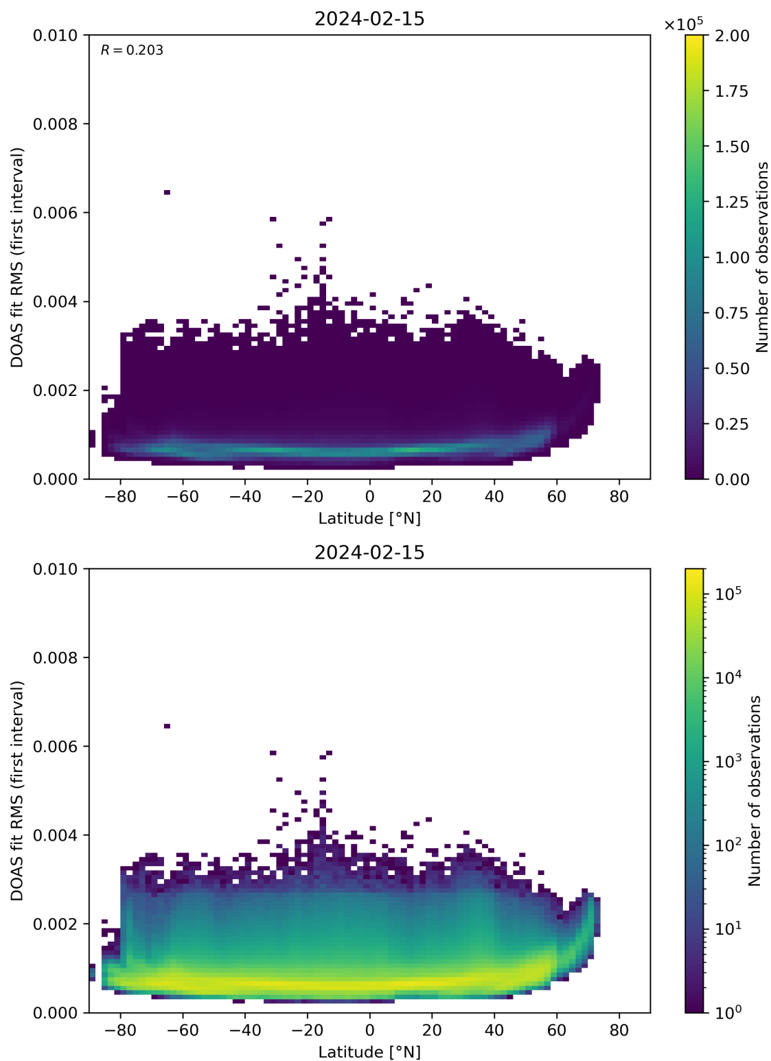
Figure 153: Scatter density plot of “Latitude” against “DOAS fit RMS (first interval)” for 2024-02-14 to 2024-02-16.
