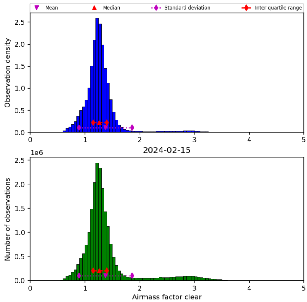
Figure 42: Histogram of “Airmass factor clear” for 2024-02-14 to 2024-02-16
