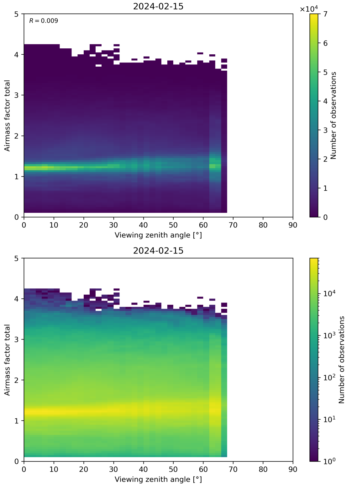
Figure 190: Scatter density plot of “Viewing zenith angle” against “Airmass factor total” for 2024-02-14 to 2024-02-16.
