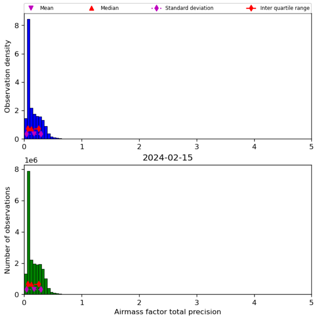
Figure 41: Histogram of “Airmass factor total precision” for 2024-02-14 to 2024-02-16
