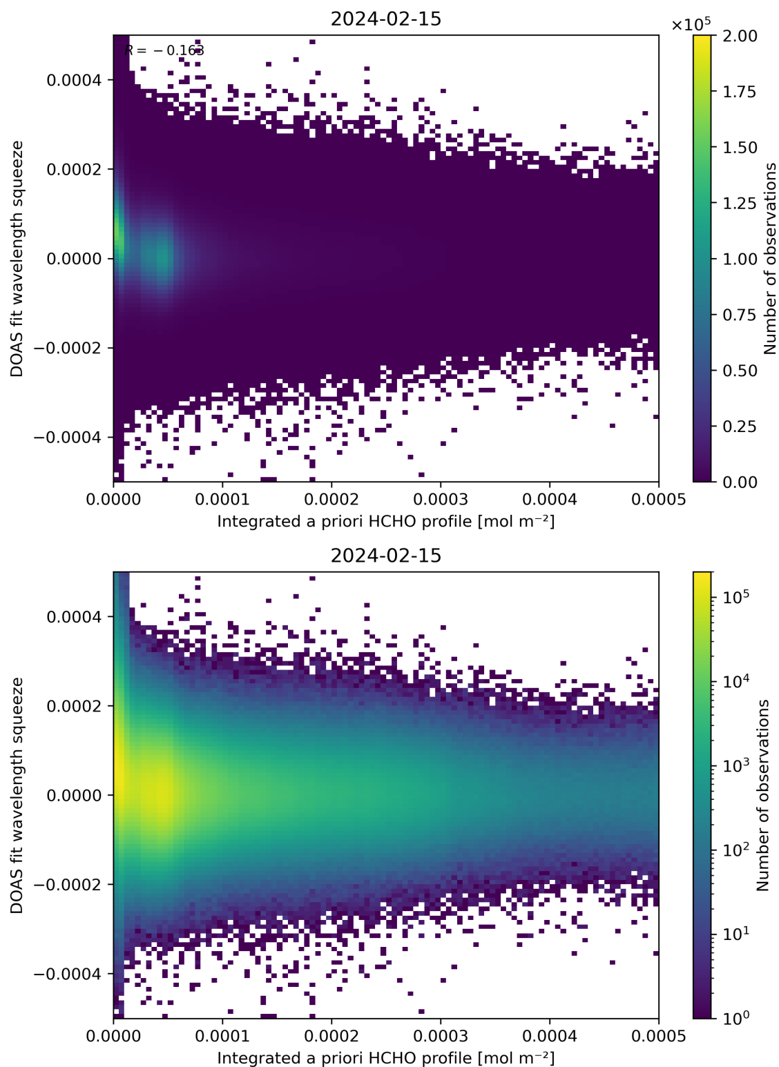
Figure 150: Scatter density plot of “Integrated a priori HCHO profile” against “DOAS fit wavelength squeeze” for 2024-02-14 to 2024-02-16.
