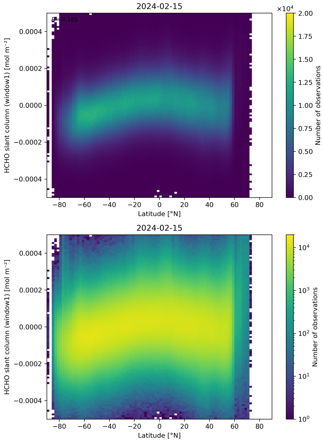
Figure 159: Scatter density plot of “Latitude” against “HCHO slant column (window1)” for 2024-02-14 to 2024-02-16.
