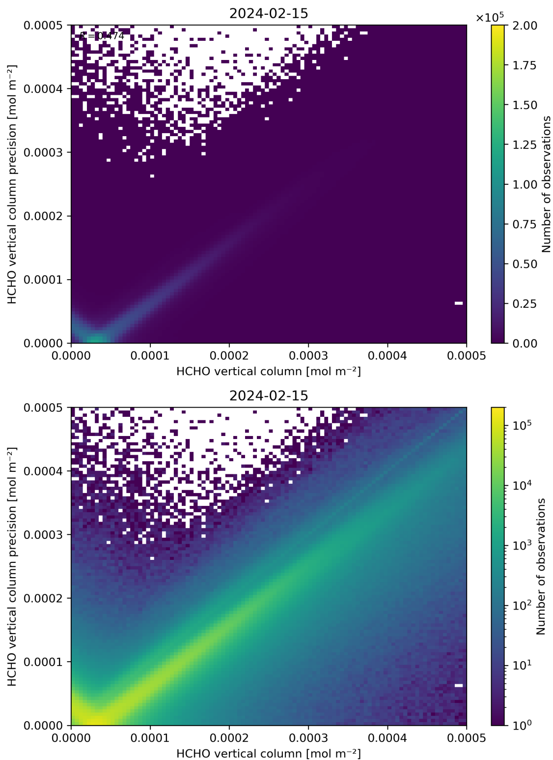
Figure 134: Scatter density plot of “HCHO vertical column” against “HCHO vertical column precision” for 2024-02-14 to 2024-02-16.
