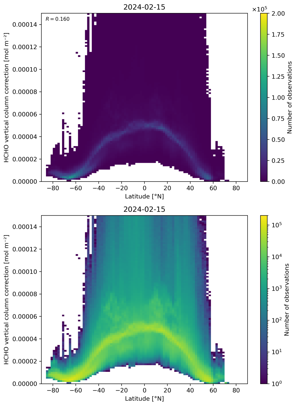
Figure 164: Scatter density plot of “Latitude” against “HCHO vertical column correction” for 2024-02-14 to 2024-02-16.
