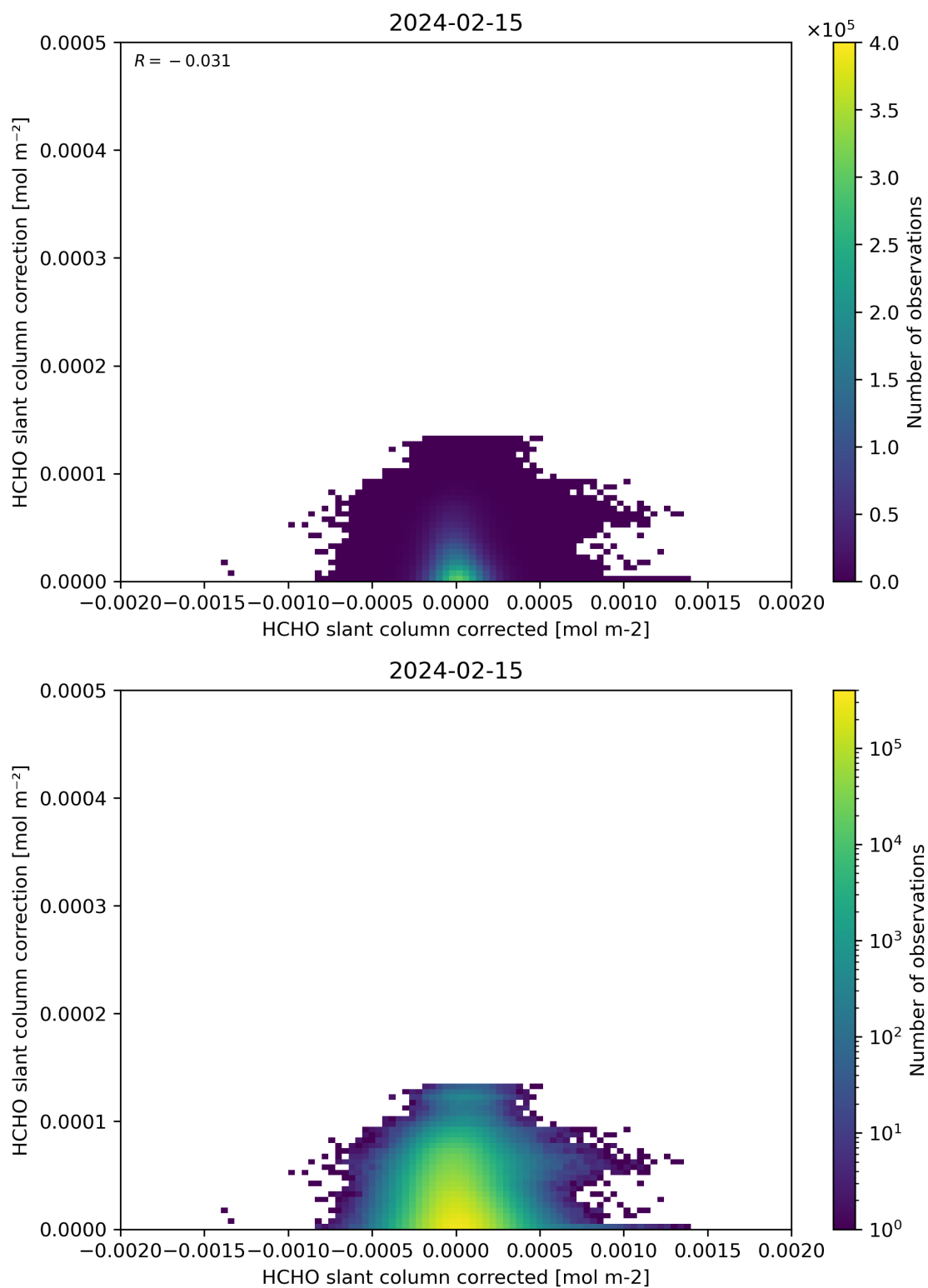
Figure 77: Scatter density plot of “HCHO slant column corrected” against “HCHO slant column correction” for 2024-02-14 to 2024-02-16.
