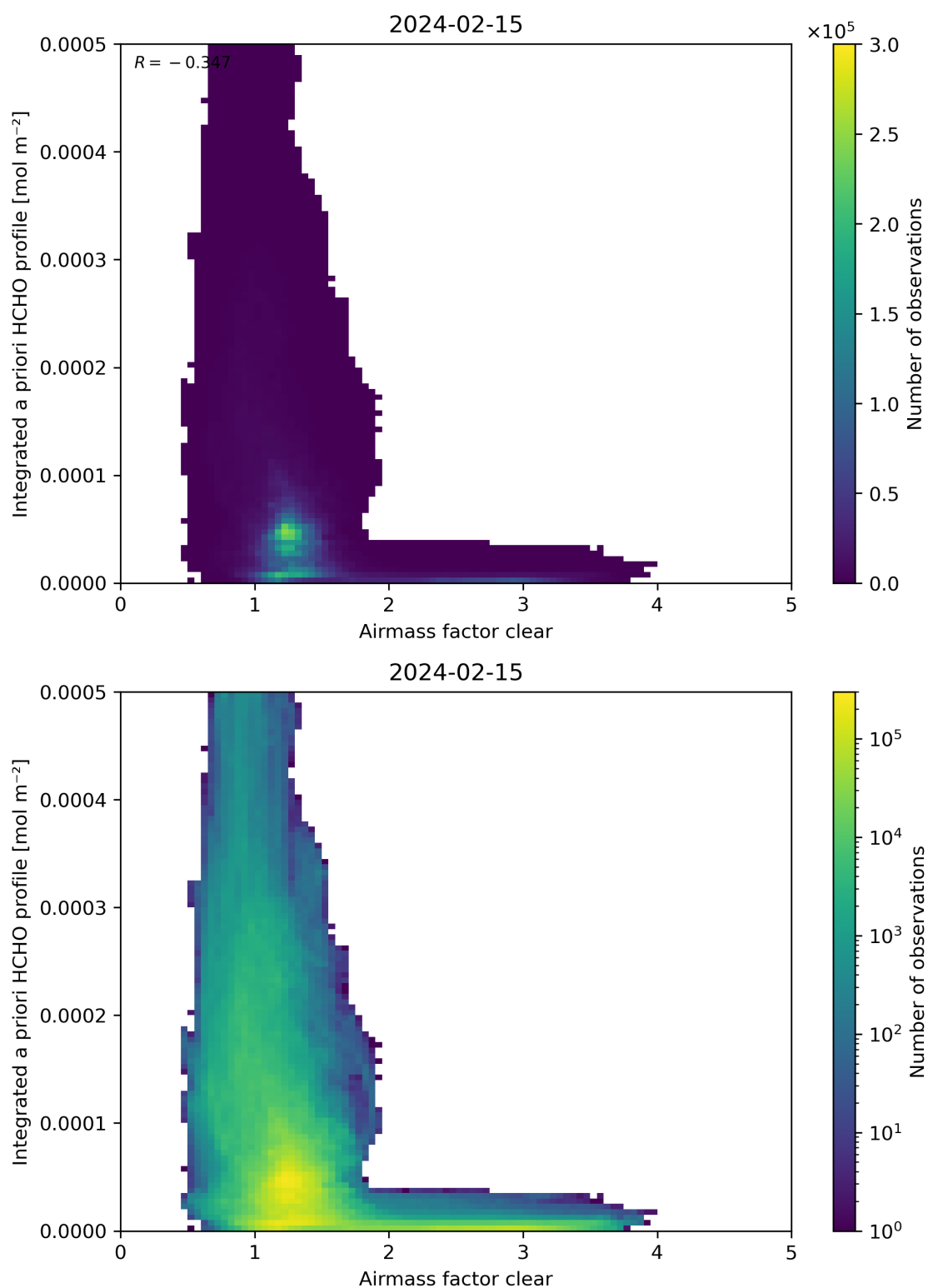
Figure 76: Scatter density plot of “Airmass factor clear” against “Integrated a priori HCHO profile” for 2024-02-14 to 2024-02-16.
