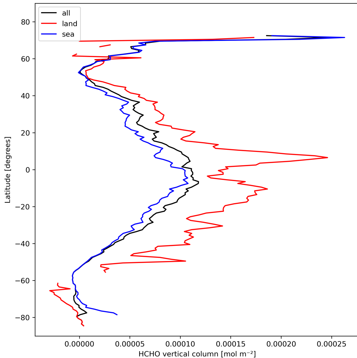
Figure 21: Zonal average of “HCHO vertical column” for 2024-02-14 to 2024-02-16.
