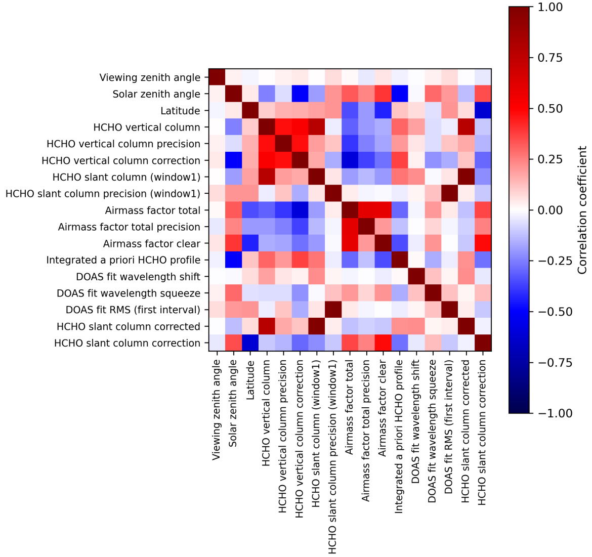
Figure 2: Map of correlation matrix for 2024-02-14 to 2024-02-16.
