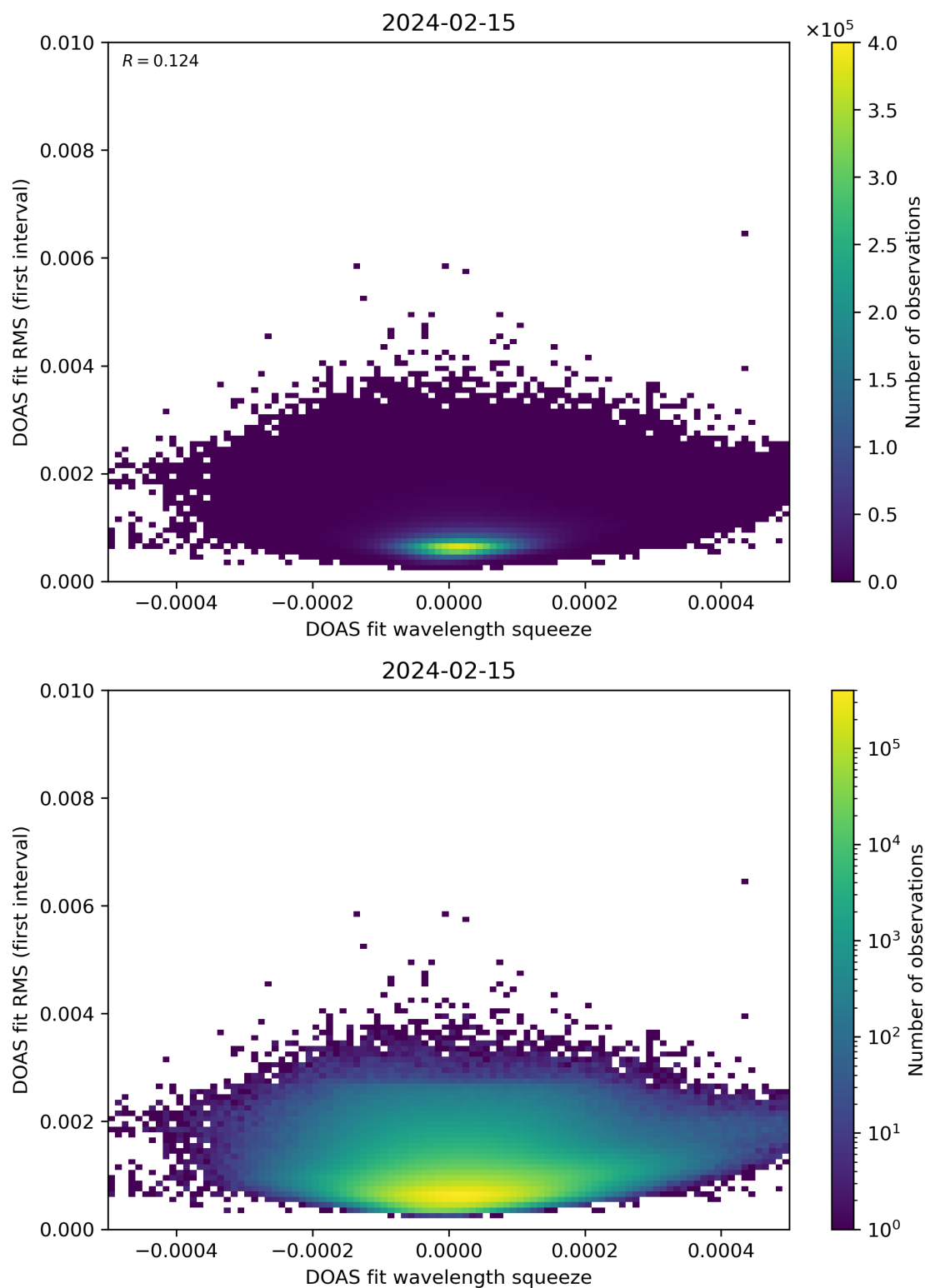
Figure 68: Scatter density plot of “DOAS fit wavelength squeeze” against “DOAS fit RMS (first interval)” for 2024-02-14 to 2024-02-16.
