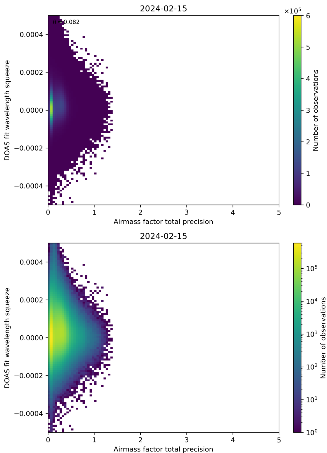
Figure 107: Scatter density plot of “Airmass factor total precision” against “DOAS fit wavelength squeeze” for 2024-02-14 to 2024-02-16.
