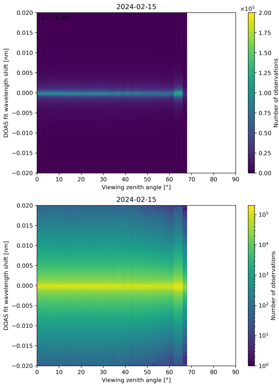
Figure 183: Scatter density plot of “Viewing zenith angle” against “DOAS fit wavelength shift” for 2024-02-14 to 2024-02-16.
