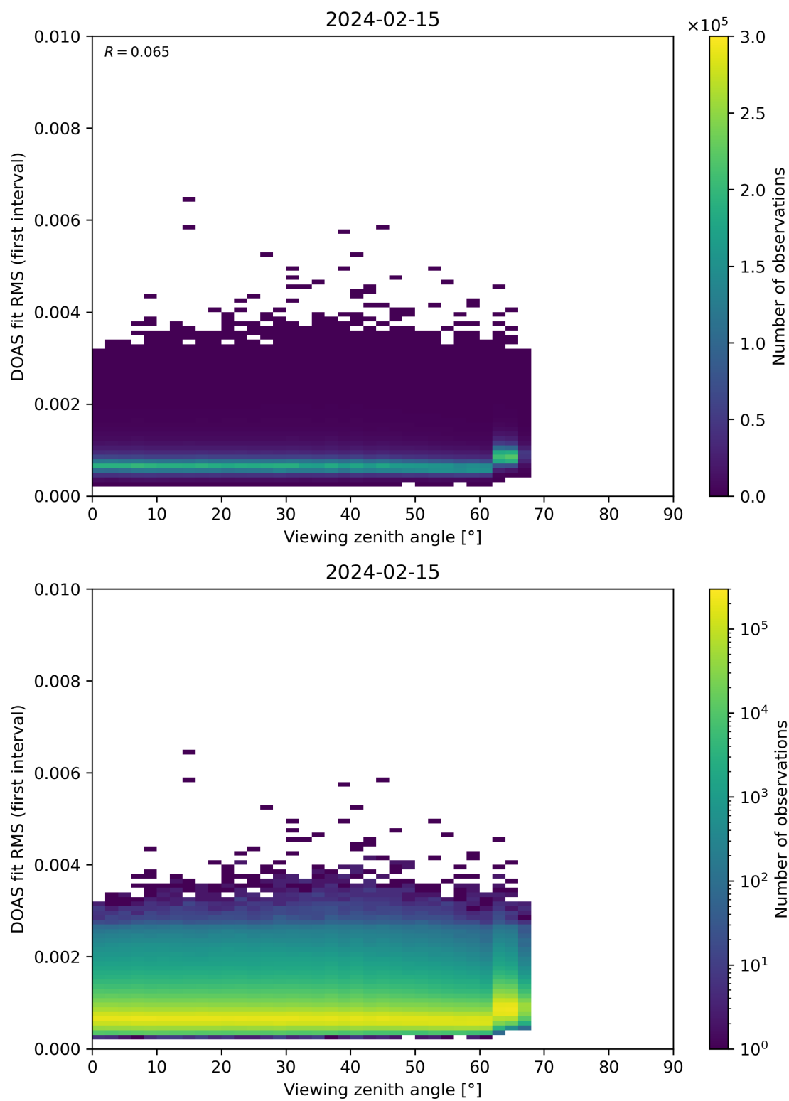
Figure 182: Scatter density plot of “Viewing zenith angle” against “DOAS fit RMS (first interval)” for 2024-02-14 to 2024-02-16.
