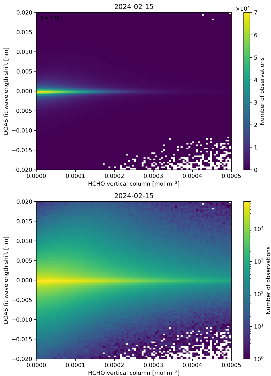
Figure 124: Scatter density plot of “HCHO vertical column” against “DOAS fit wavelength shift” for 2024-02-14 to 2024-02-16.
