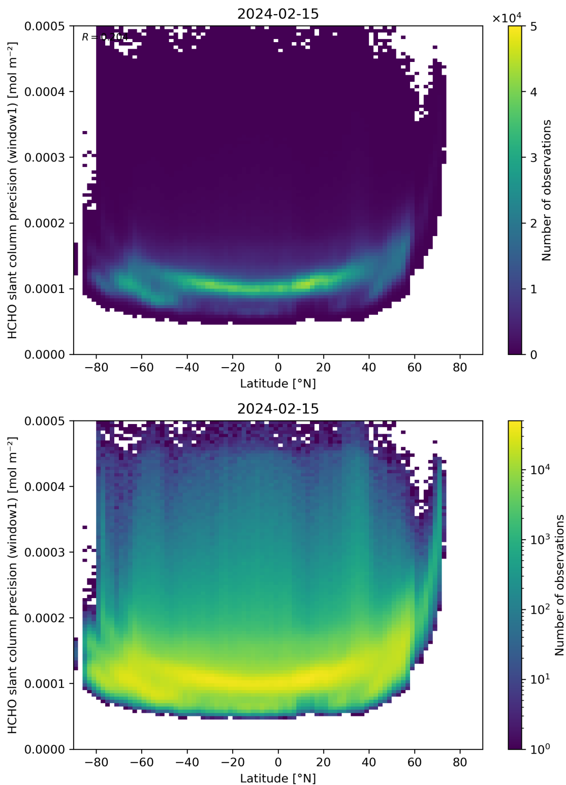
Figure 160: Scatter density plot of “Latitude” against “HCHO slant column precision (window1)” for 2024-02-14 to 2024-02-16.
