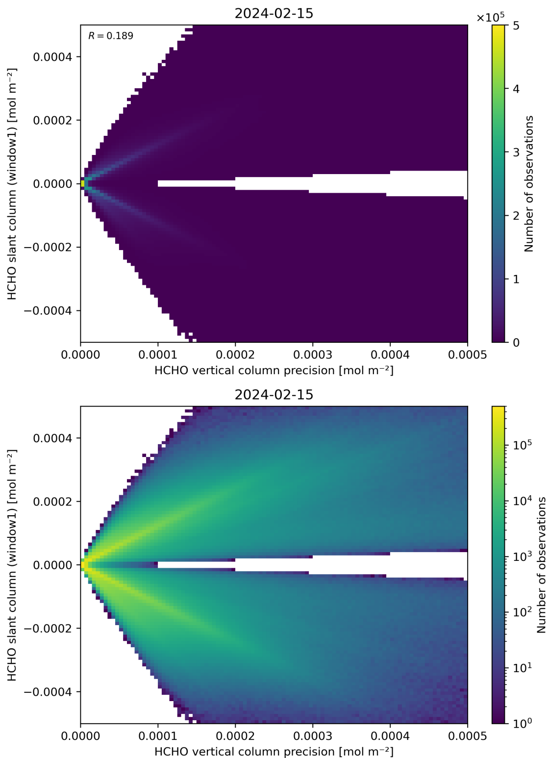
Figure 142: Scatter density plot of “HCHO vertical column precision” against “HCHO slant column (window1)” for 2024-02-14 to 2024-02-16.
