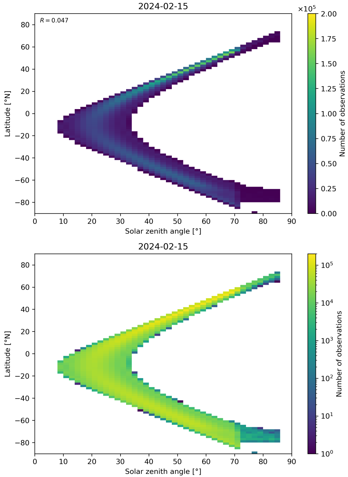
Figure 181: Scatter density plot of “Solar zenith angle” against “Latitude” for 2024-02-14 to 2024-02-16.
