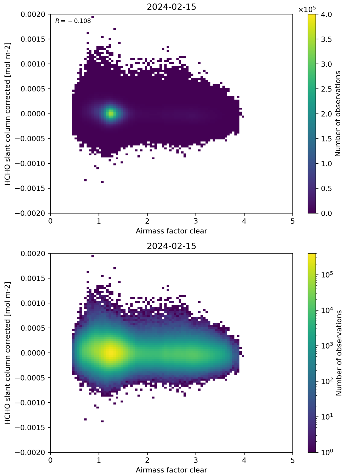
Figure 74: Scatter density plot of “Airmass factor clear” against “HCHO slant column corrected” for 2024-02-14 to 2024-02-16.
