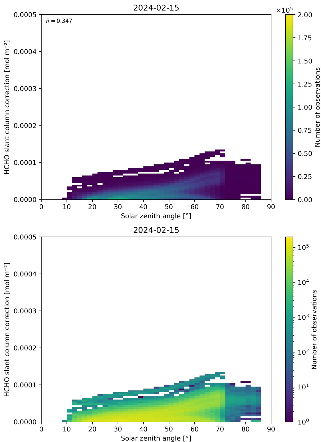
Figure 172: Scatter density plot of “Solar zenith angle” against “HCHO slant column correction” for 2024-02-14 to 2024-02-16.
