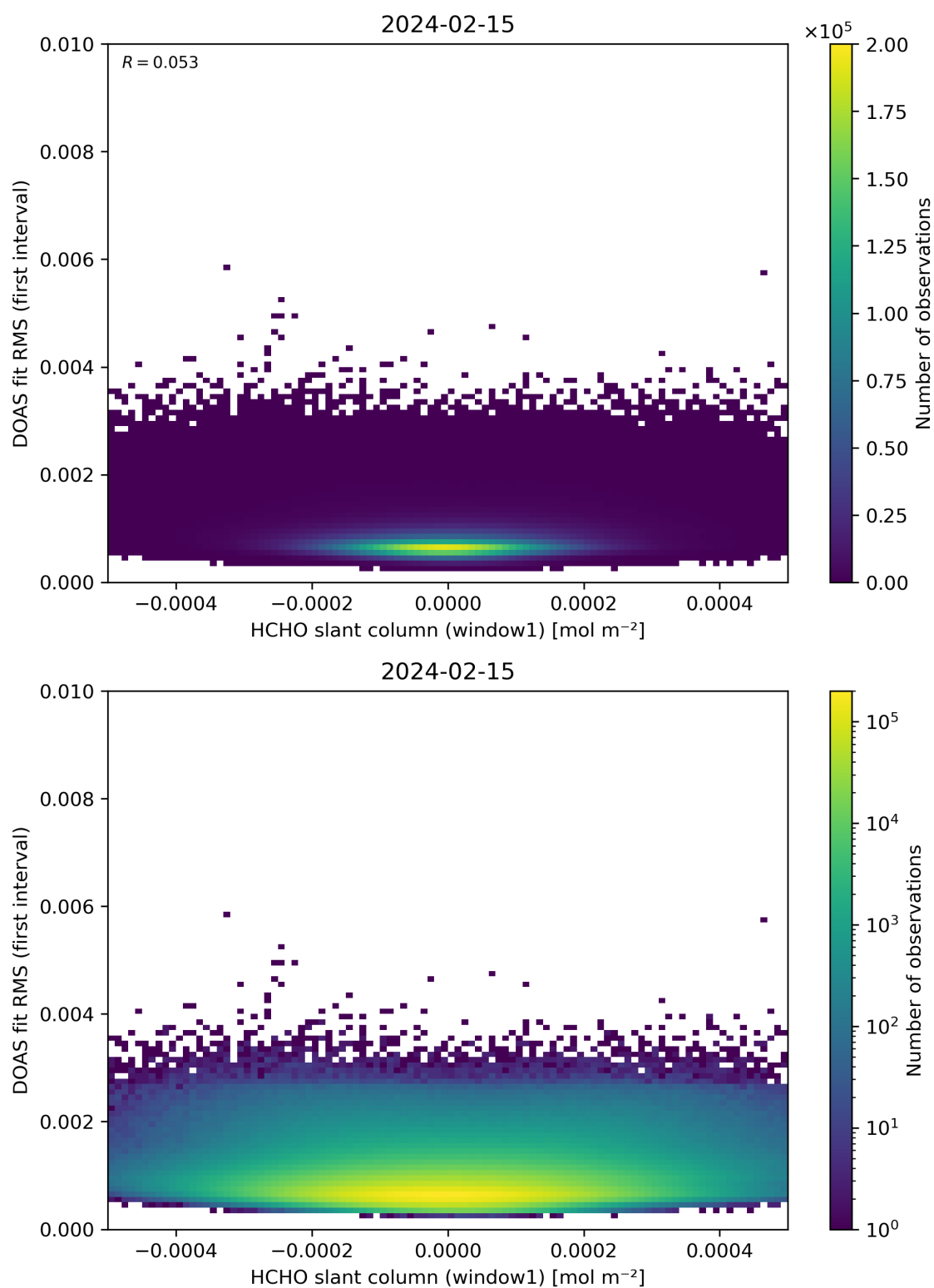
Figure 78: Scatter density plot of “HCHO slant column (window1)” against “DOAS fit RMS (first interval)” for 2024-02-14 to 2024-02-16.
