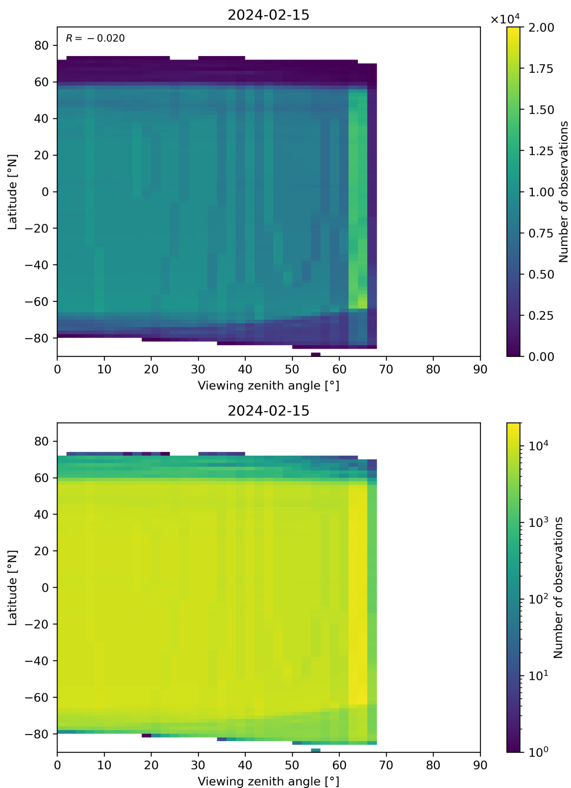
Figure 196: Scatter density plot of “Viewing zenith angle” against “Latitude” for 2024-02-14 to 2024-02-16.
