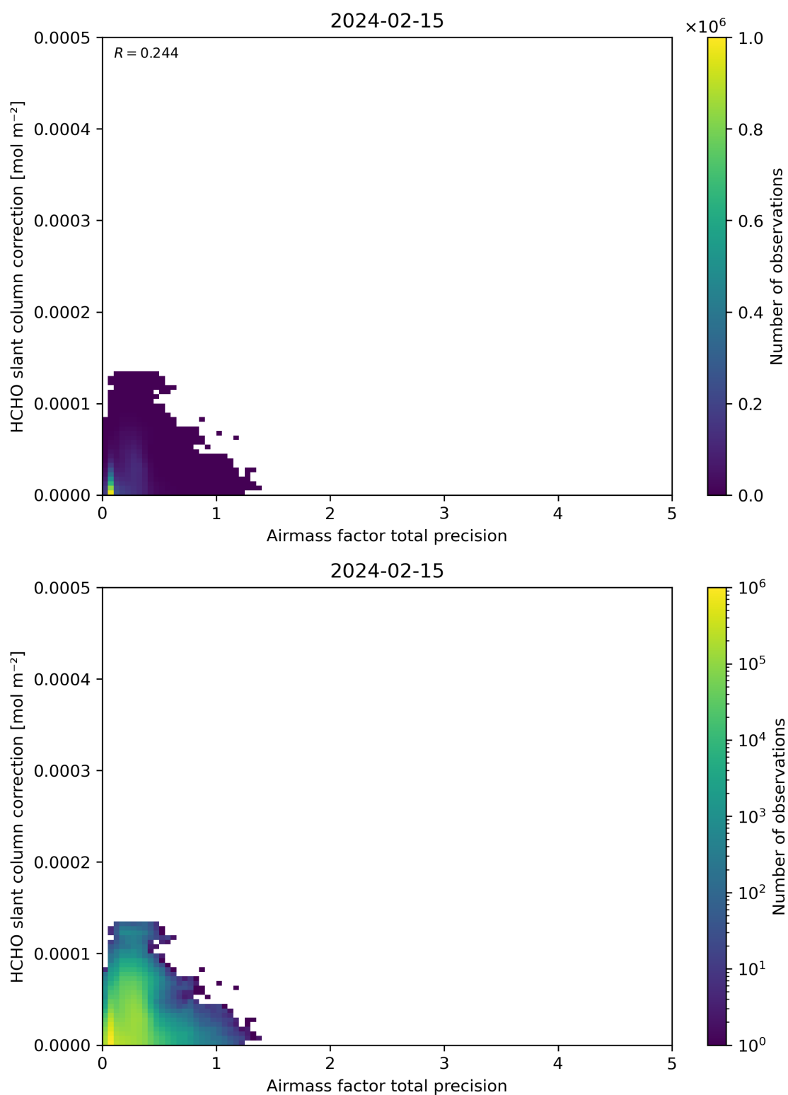
Figure 110: Scatter density plot of “Airmass factor total precision” against “HCHO slant column correction” for 2024-02-14 to 2024-02-16.
