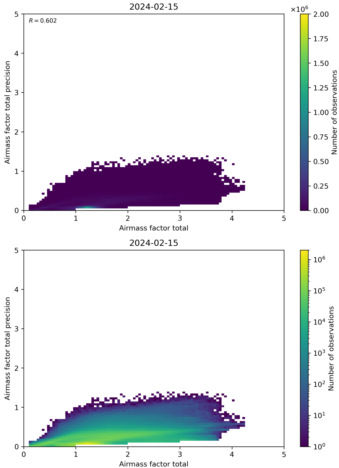
Figure 103: Scatter density plot of “Airmass factor total” against “Airmass factor total precision” for 2024-02-14 to 2024-02-16.
