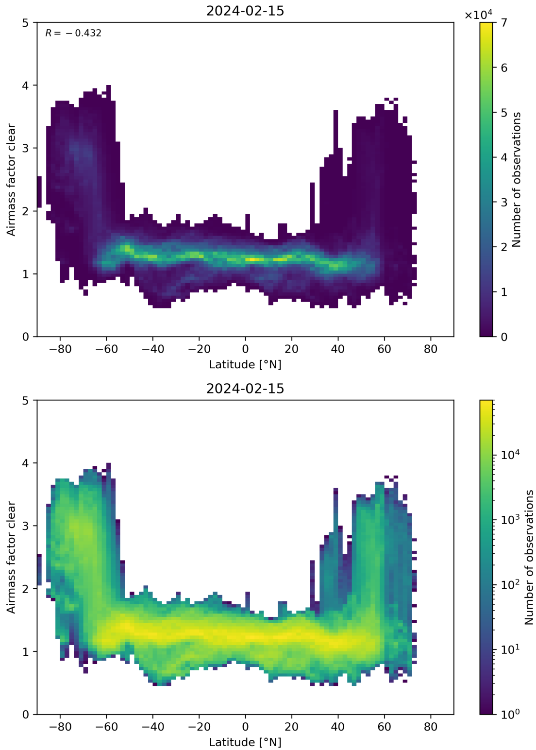
Figure 156: Scatter density plot of “Latitude” against “Airmass factor clear” for 2024-02-14 to 2024-02-16.
