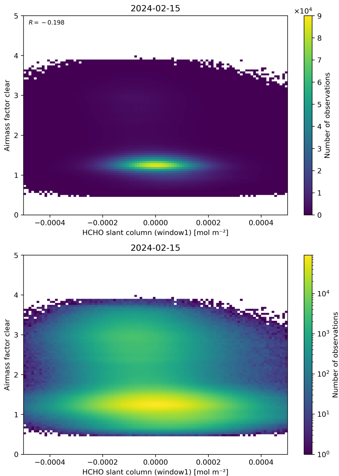
Figure 81: Scatter density plot of “HCHO slant column (window1)” against “Airmass factor clear” for 2024-02-14 to 2024-02-16.
