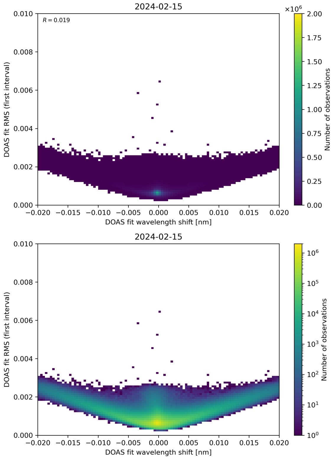
Figure 64: Scatter density plot of “DOAS fit wavelength shift” against “DOAS fit RMS (first interval)” for 2024-02-14 to 2024-02-16.
