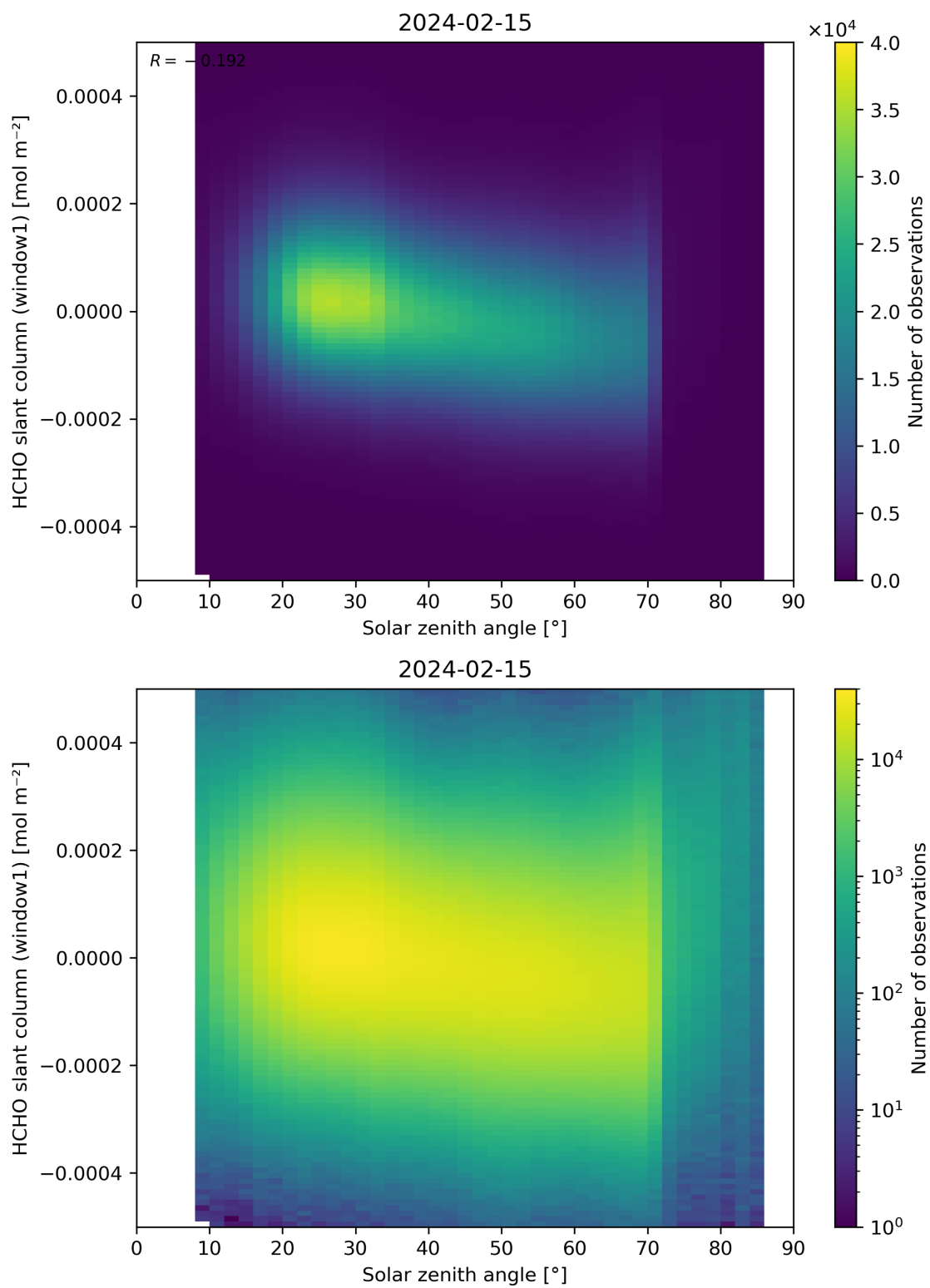
Figure 173: Scatter density plot of “Solar zenith angle” against “HCHO slant column (window1)” for 2024-02-14 to 2024-02-16.
