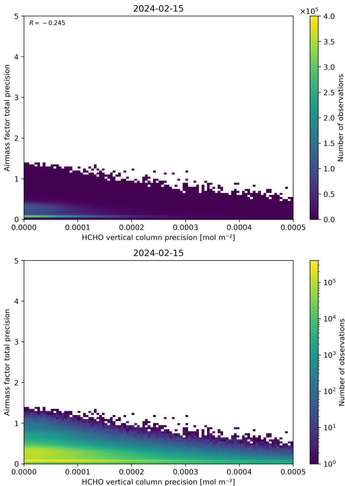
Figure 145: Scatter density plot of “HCHO vertical column precision” against “Airmass factor total precision” for 2024-02-14 to 2024-02-16.
