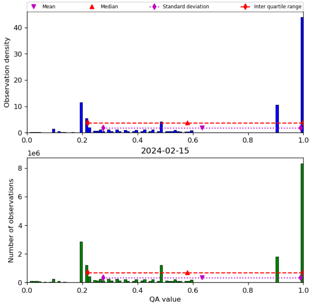
Figure 34: Histogram of “QA value” for 2024-02-14 to 2024-02-16
