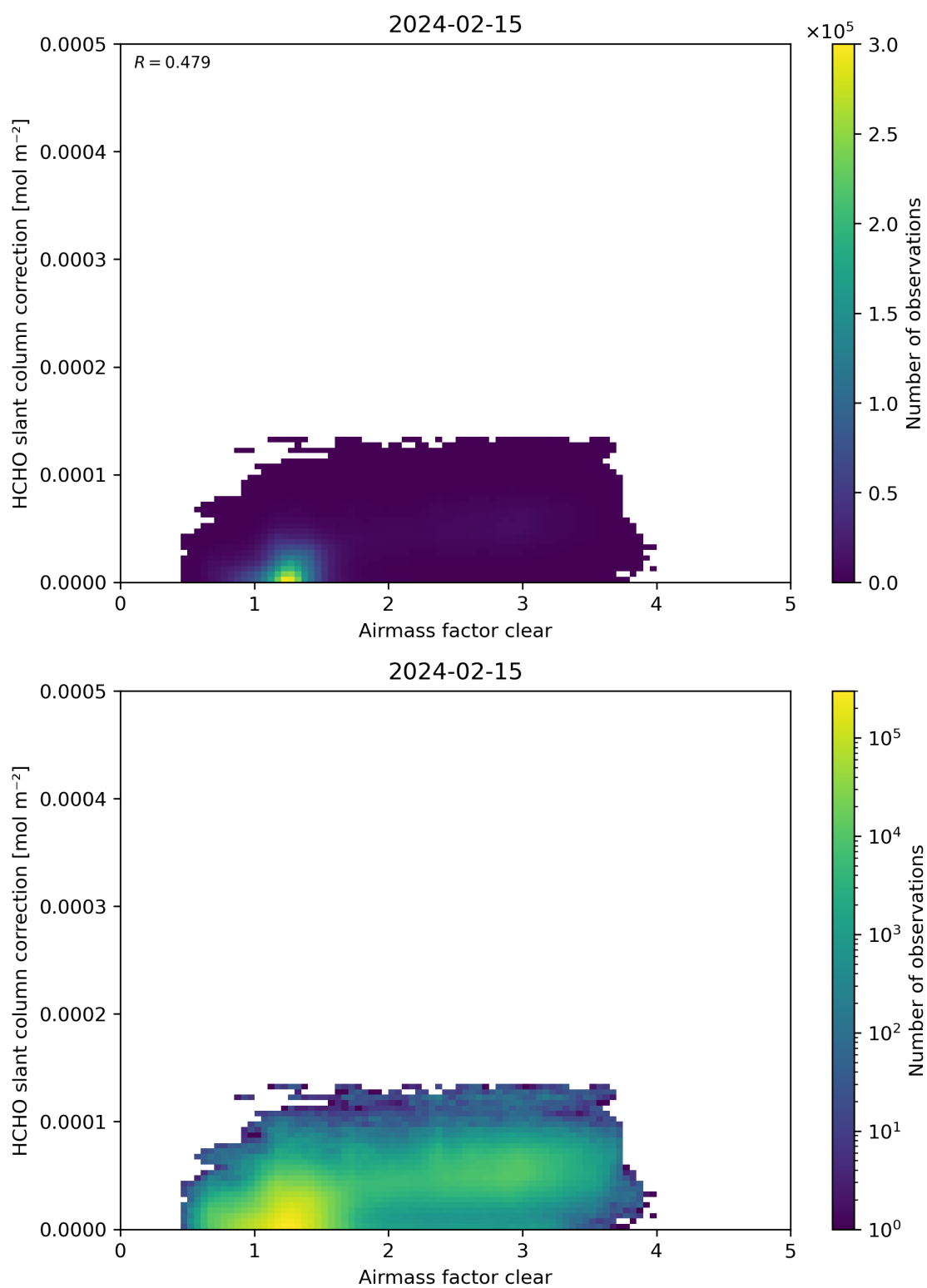
Figure 75: Scatter density plot of “Airmass factor clear” against “HCHO slant column correction” for 2024-02-14 to 2024-02-16.
