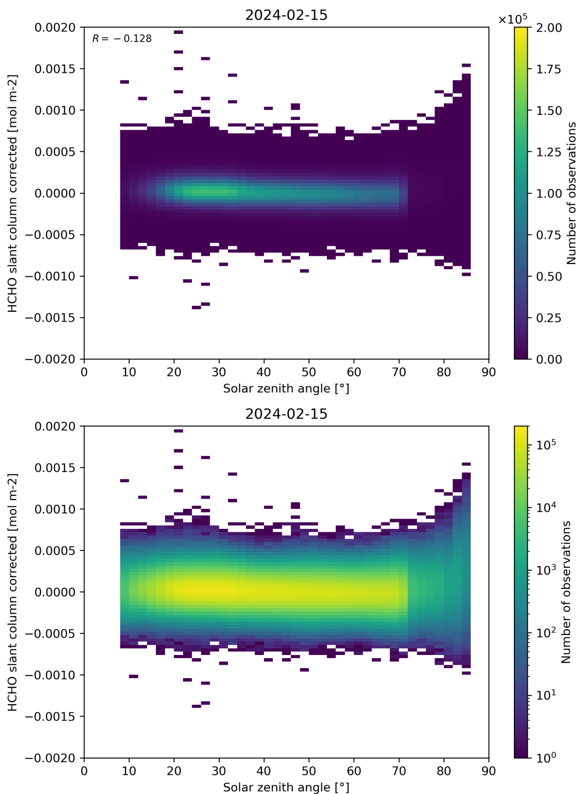
Figure 171: Scatter density plot of “Solar zenith angle” against “HCHO slant column corrected” for 2024-02-14 to 2024-02-16.
