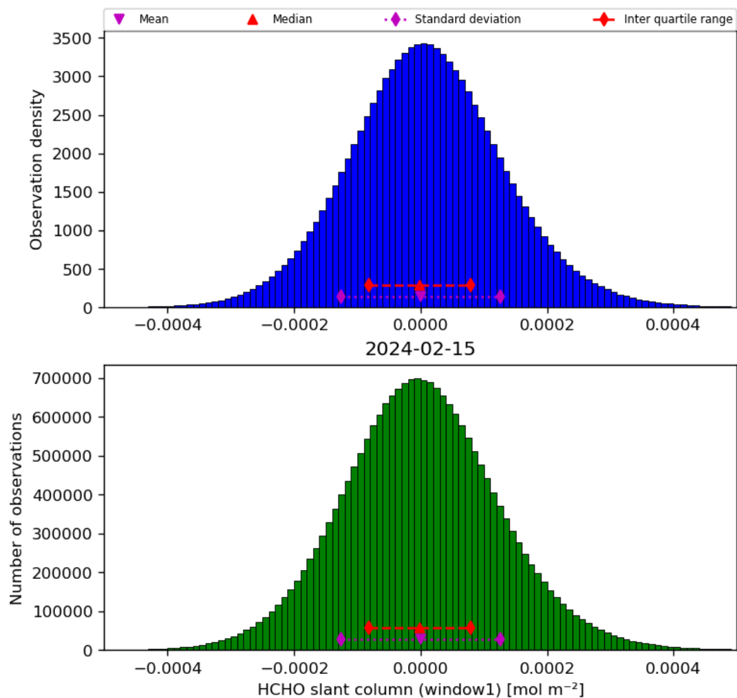
Figure 38: Histogram of “HCHO slant column (window1)” for 2024-02-14 to 2024-02-16
