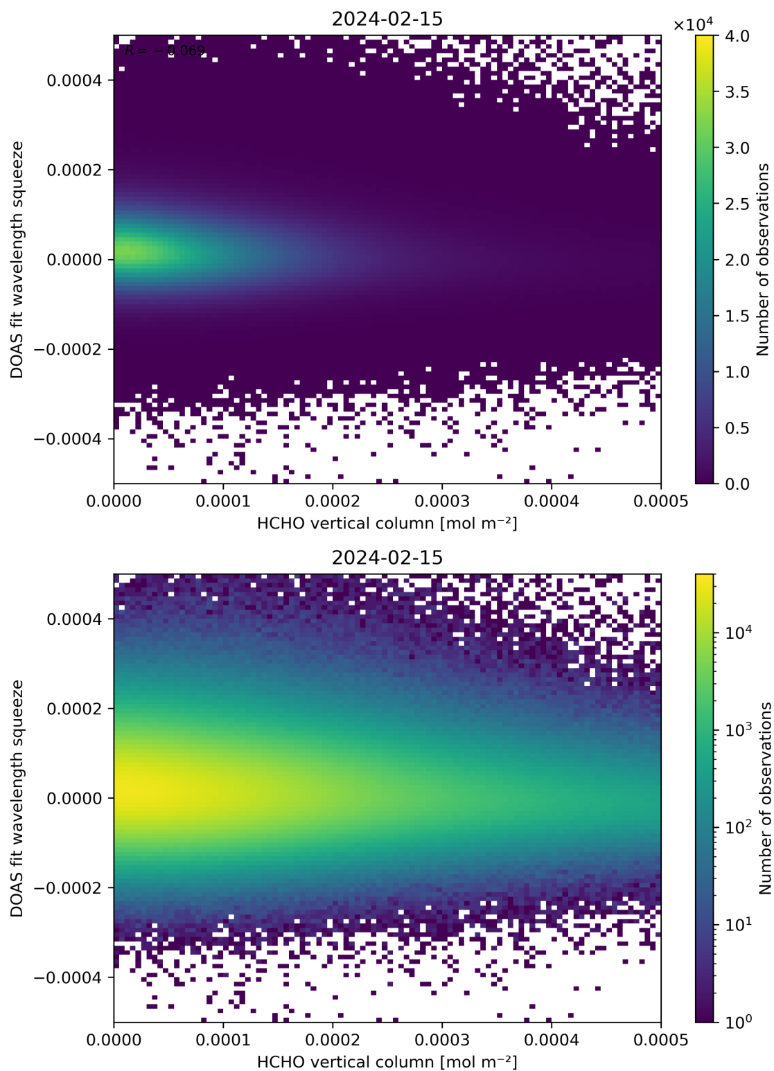
Figure 125: Scatter density plot of “HCHO vertical column” against “DOAS fit wavelength squeeze” for 2024-02-14 to 2024-02-16.
