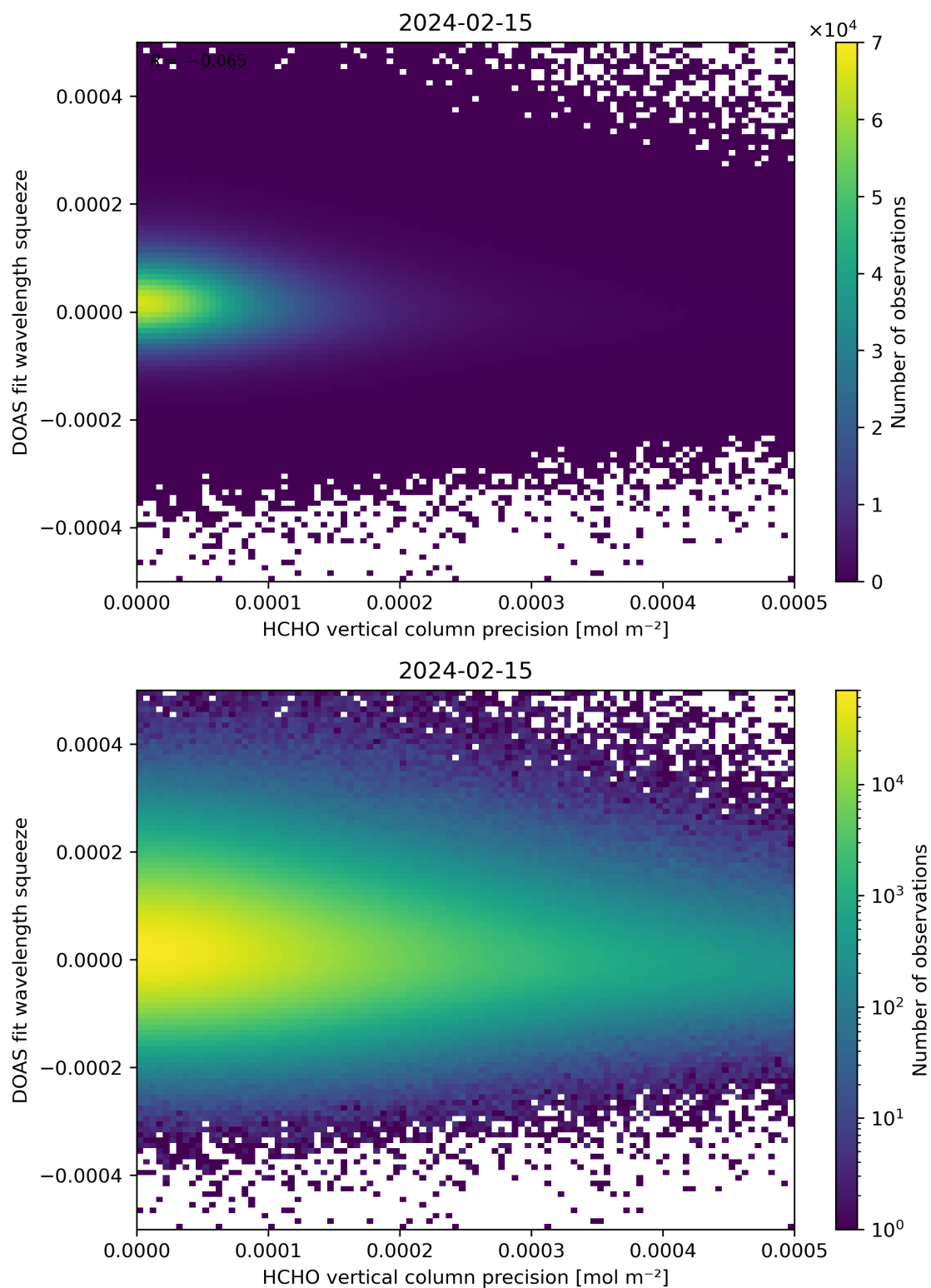
Figure 138: Scatter density plot of “HCHO vertical column precision” against “DOAS fit wavelength squeeze” for 2024-02-14 to 2024-02-16.
