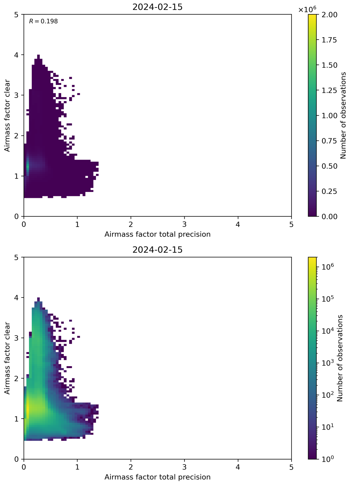
Figure 108: Scatter density plot of “Airmass factor total precision” against “Airmass factor clear” for 2024-02-14 to 2024-02-16.
