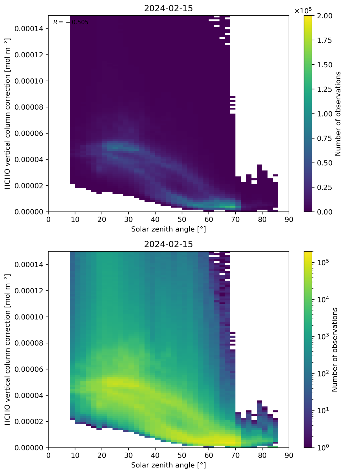
Figure 178: Scatter density plot of “Solar zenith angle” against “HCHO vertical column correction” for 2024-02-14 to 2024-02-16.
