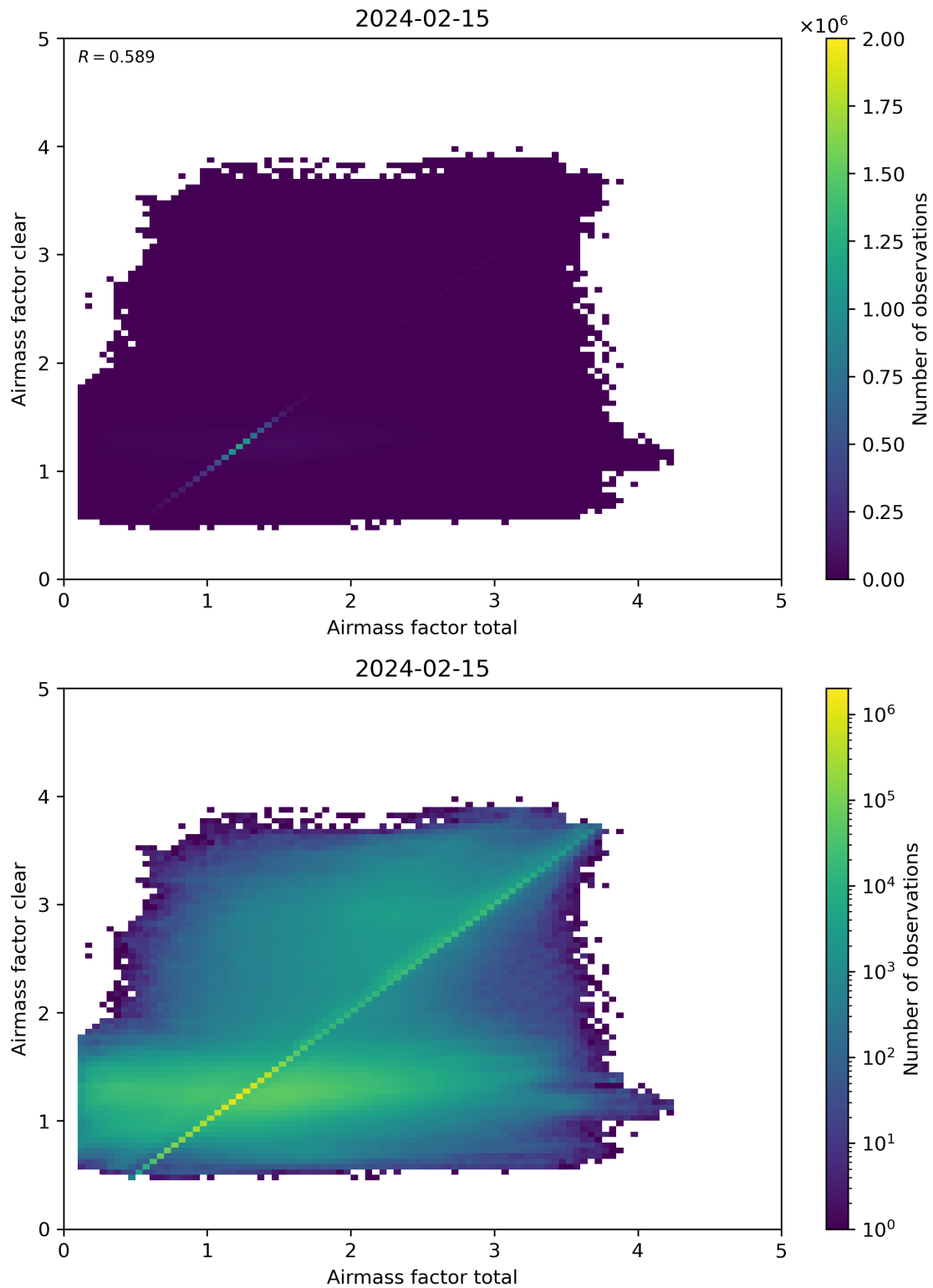
Figure 100: Scatter density plot of “Airmass factor total” against “Airmass factor clear” for 2024-02-14 to 2024-02-16.
