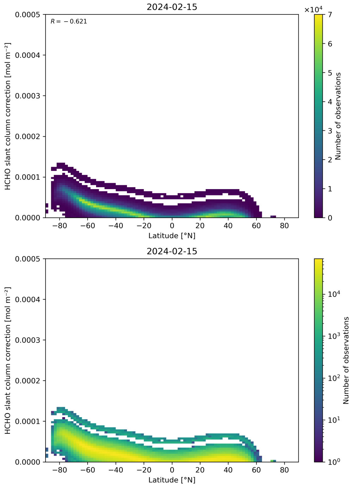
Figure 158: Scatter density plot of “Latitude” against “HCHO slant column correction” for 2024-02-14 to 2024-02-16.
