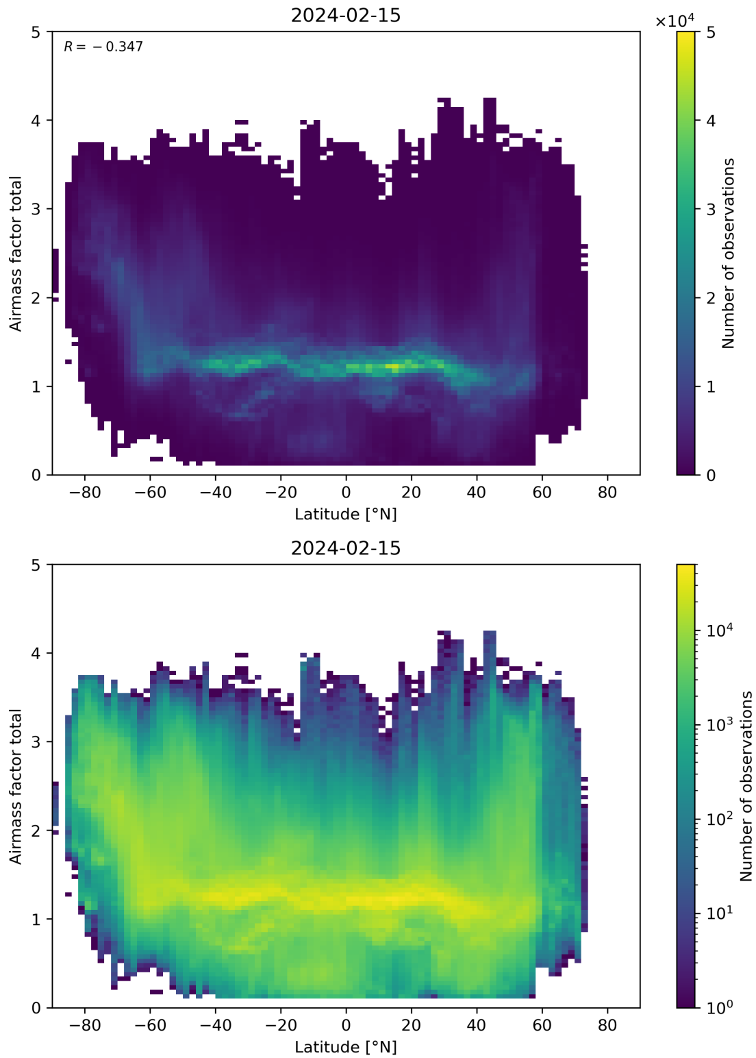
Figure 161: Scatter density plot of “Latitude” against “Airmass factor total” for 2024-02-14 to 2024-02-16.
