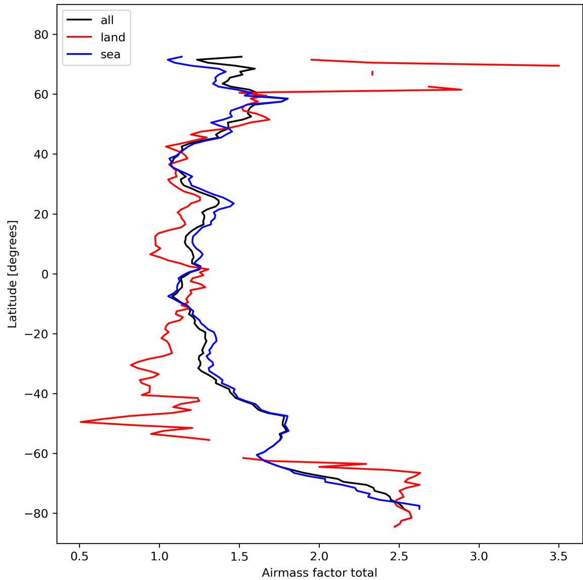
Figure 26: Zonal average of “Airmass factor total” for 2024-02-14 to 2024-02-16.
