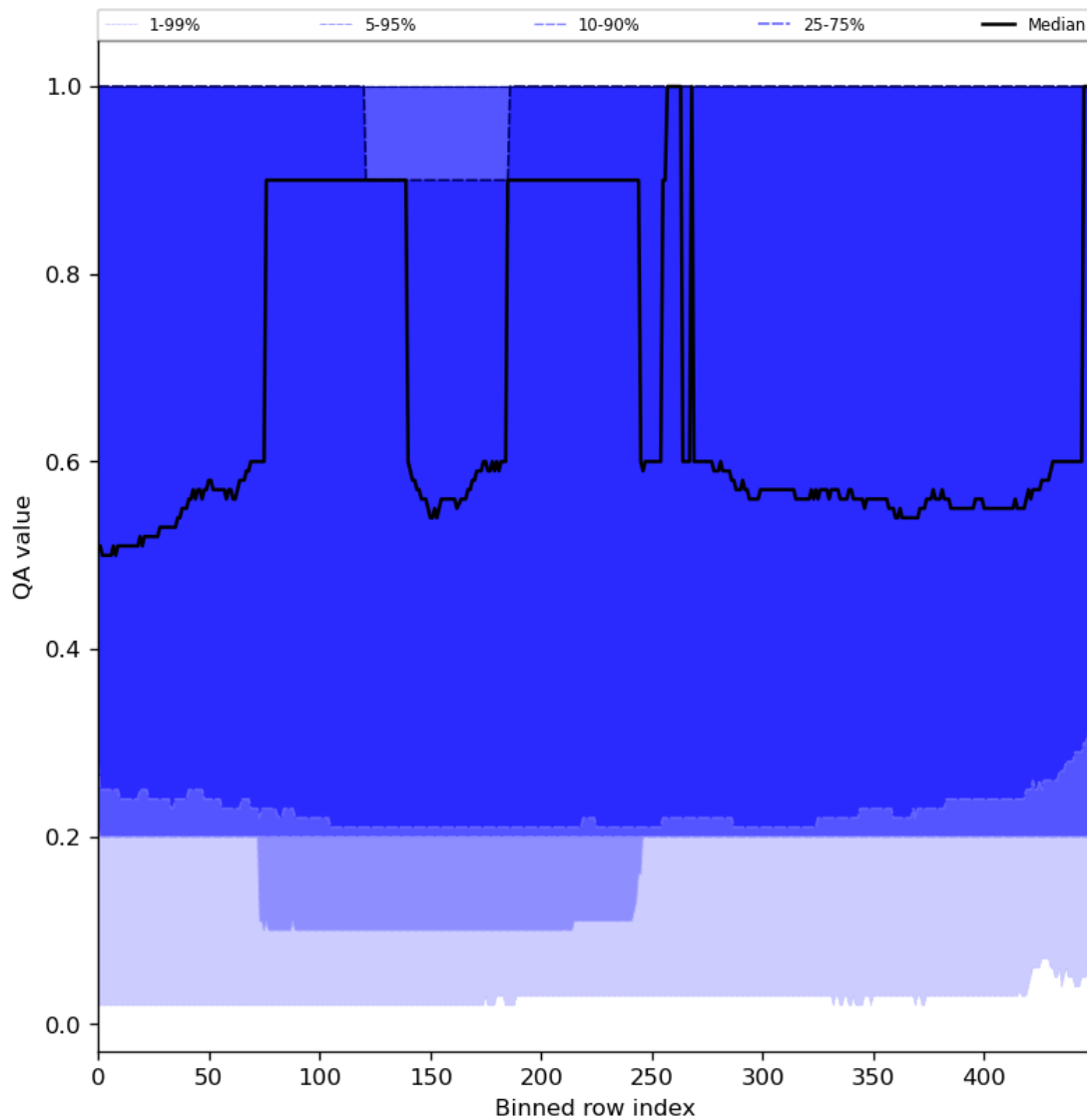
Figure 48: Along track statistics of “QA value” for 2024-02-14 to 2024-02-16
