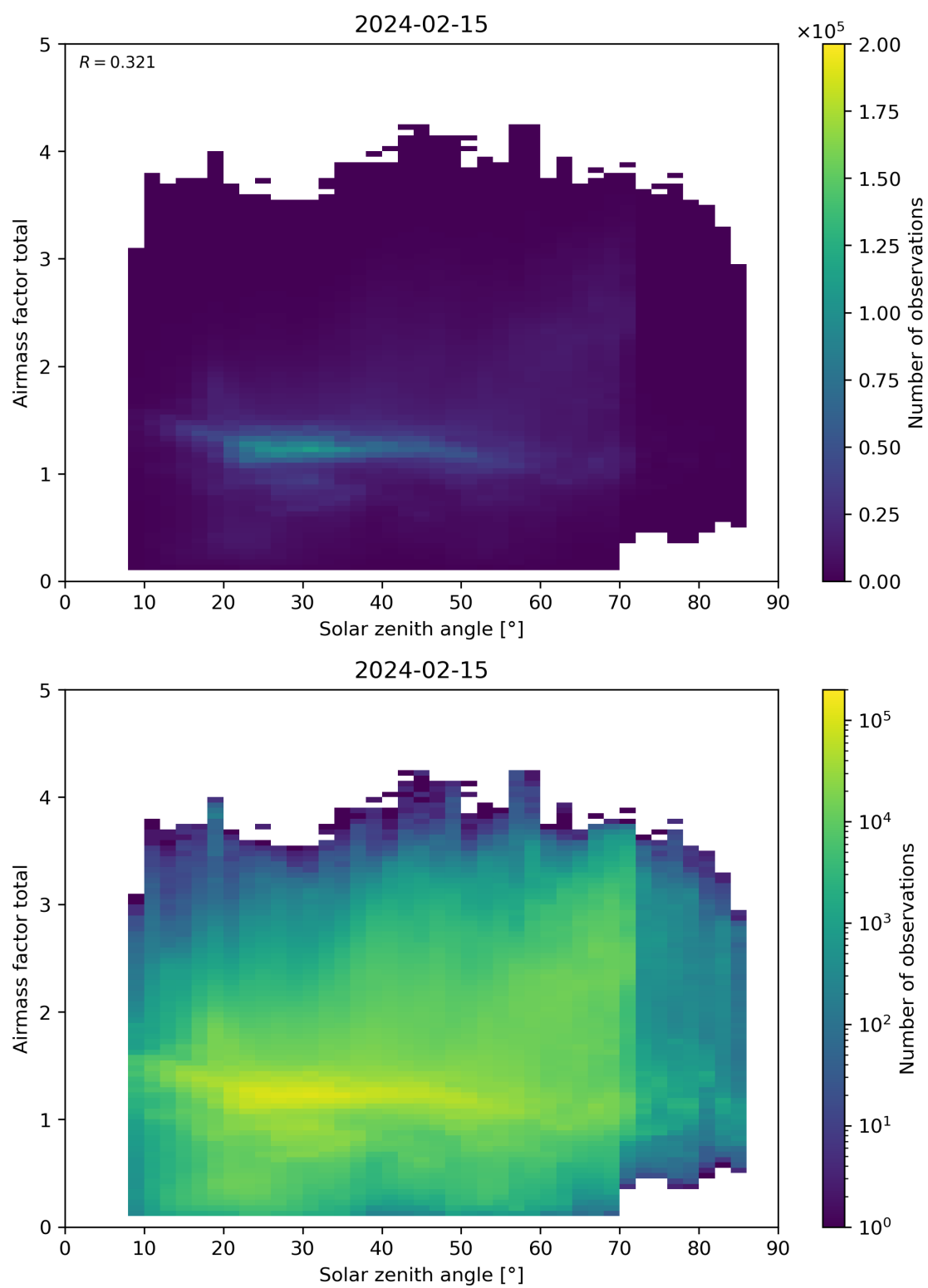
Figure 175: Scatter density plot of “Solar zenith angle” against “Airmass factor total” for 2024-02-14 to 2024-02-16.
