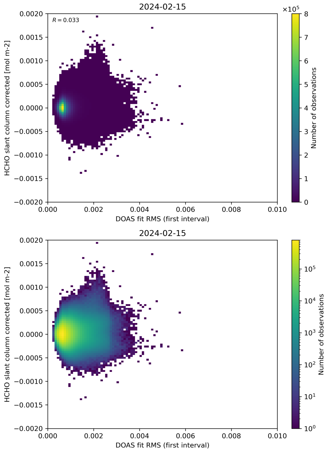
Figure 62: Scatter density plot of “DOAS fit RMS (first interval)” against “HCHO slant column corrected” for 2024-02-14 to 2024-02-16.
