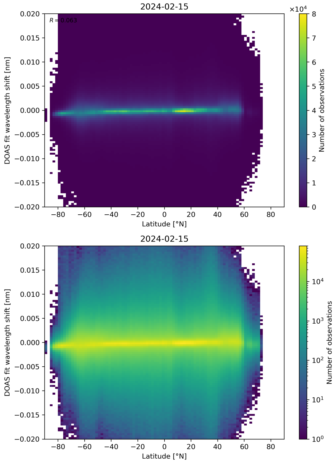
Figure 154: Scatter density plot of “Latitude” against “DOAS fit wavelength shift” for 2024-02-14 to 2024-02-16.
