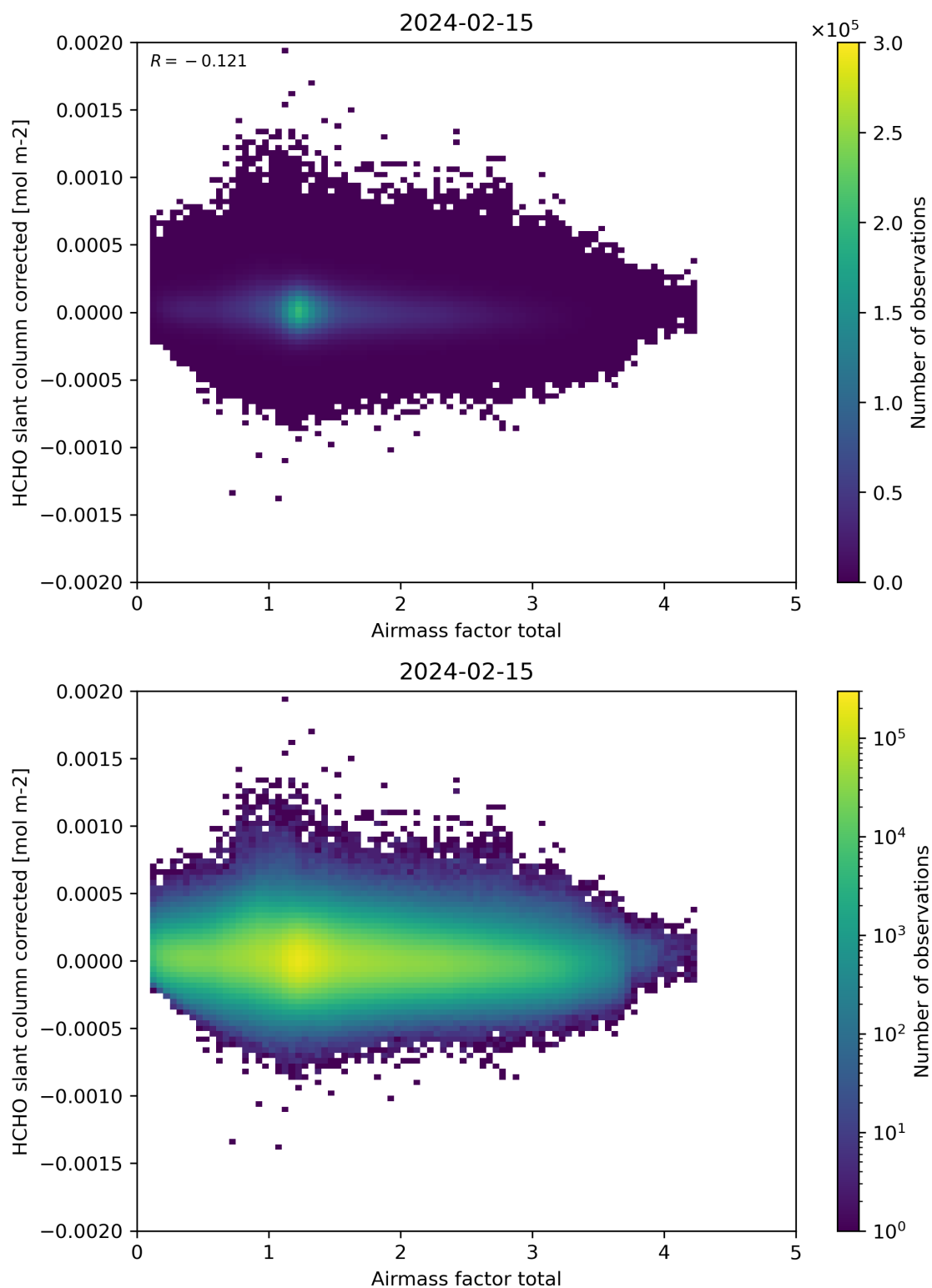
Figure 101: Scatter density plot of “Airmass factor total” against “HCHO slant column corrected” for 2024-02-14 to 2024-02-16.
