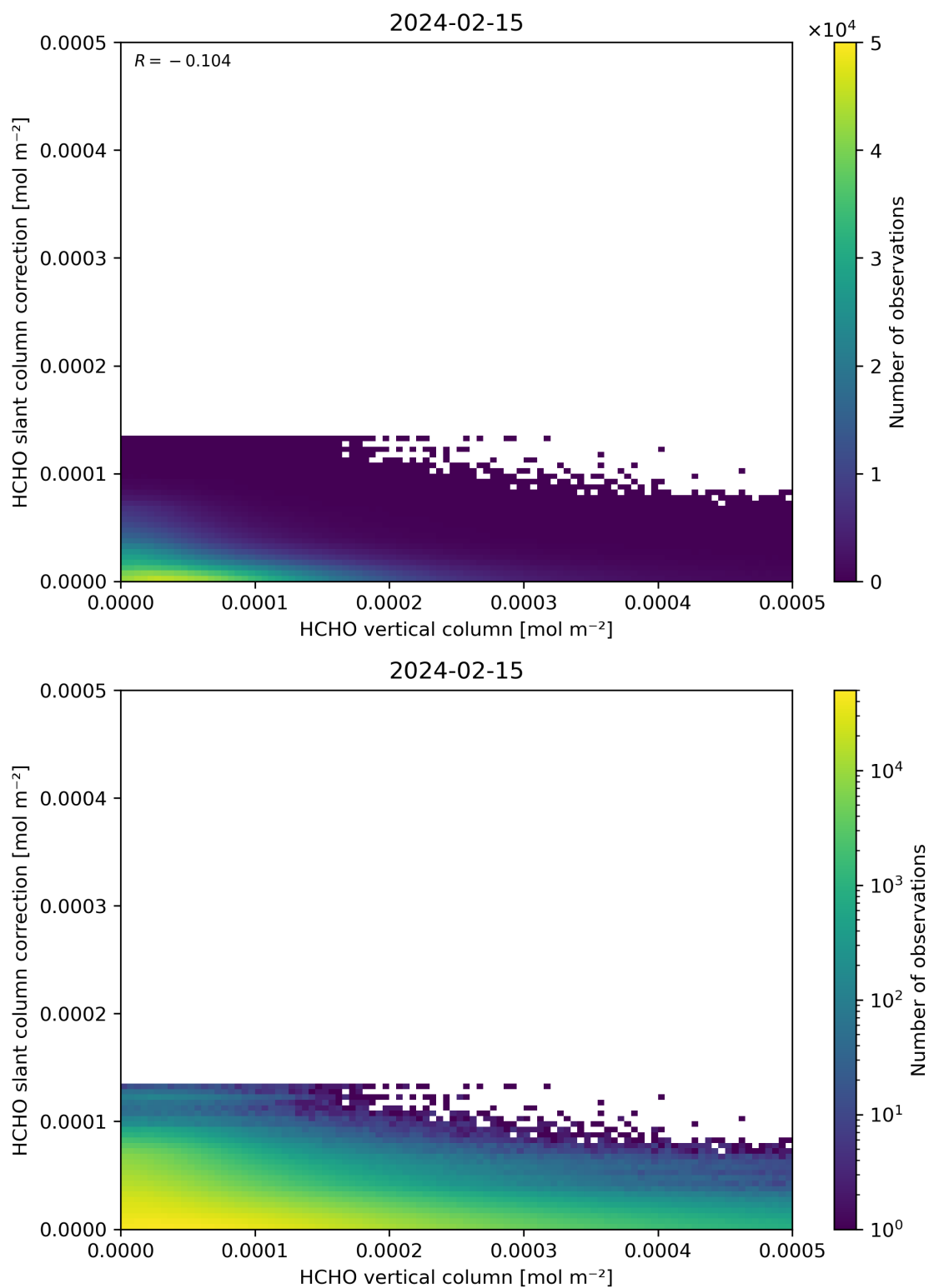
Figure 128: Scatter density plot of “HCHO vertical column” against “HCHO slant column correction” for 2024-02-14 to 2024-02-16.
