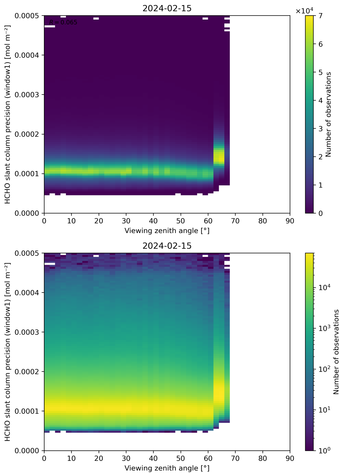
Figure 189: Scatter density plot of “Viewing zenith angle” against “HCHO slant column precision (window1)” for 2024-02-14 to 2024-02-16.
