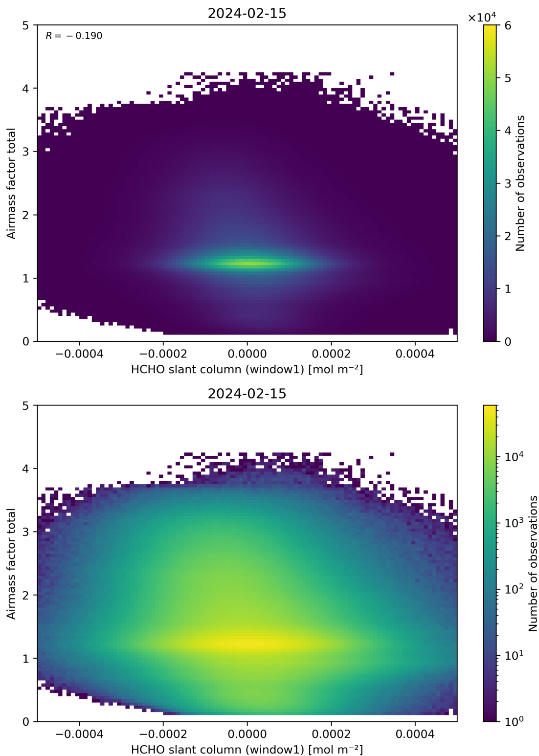
Figure 85: Scatter density plot of “HCHO slant column (window1)” against “Airmass factor total” for 2024-02-14 to 2024-02-16.
