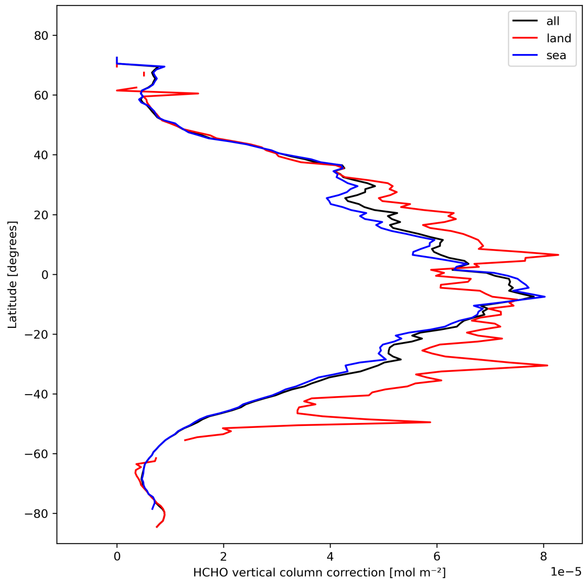
Figure 23: Zonal average of “HCHO vertical column correction” for 2024-02-14 to 2024-02-16.
