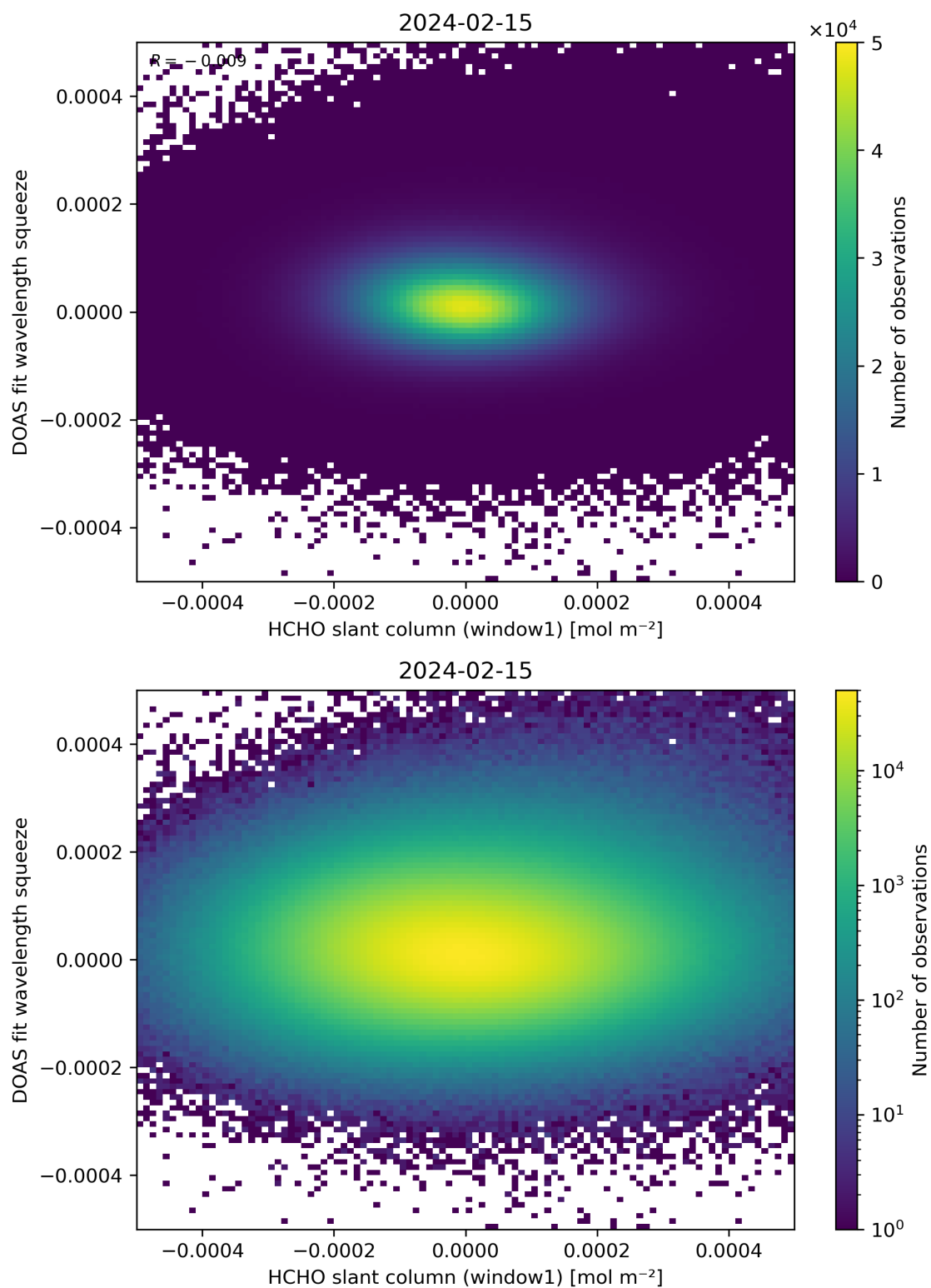
Figure 80: Scatter density plot of “HCHO slant column (window1)” against “DOAS fit wavelength squeeze” for 2024-02-14 to 2024-02-16.
