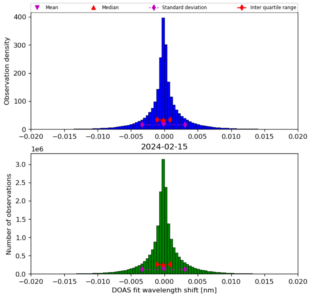
Figure 44: Histogram of “DOAS fit wavelength shift” for 2024-02-14 to 2024-02-16
