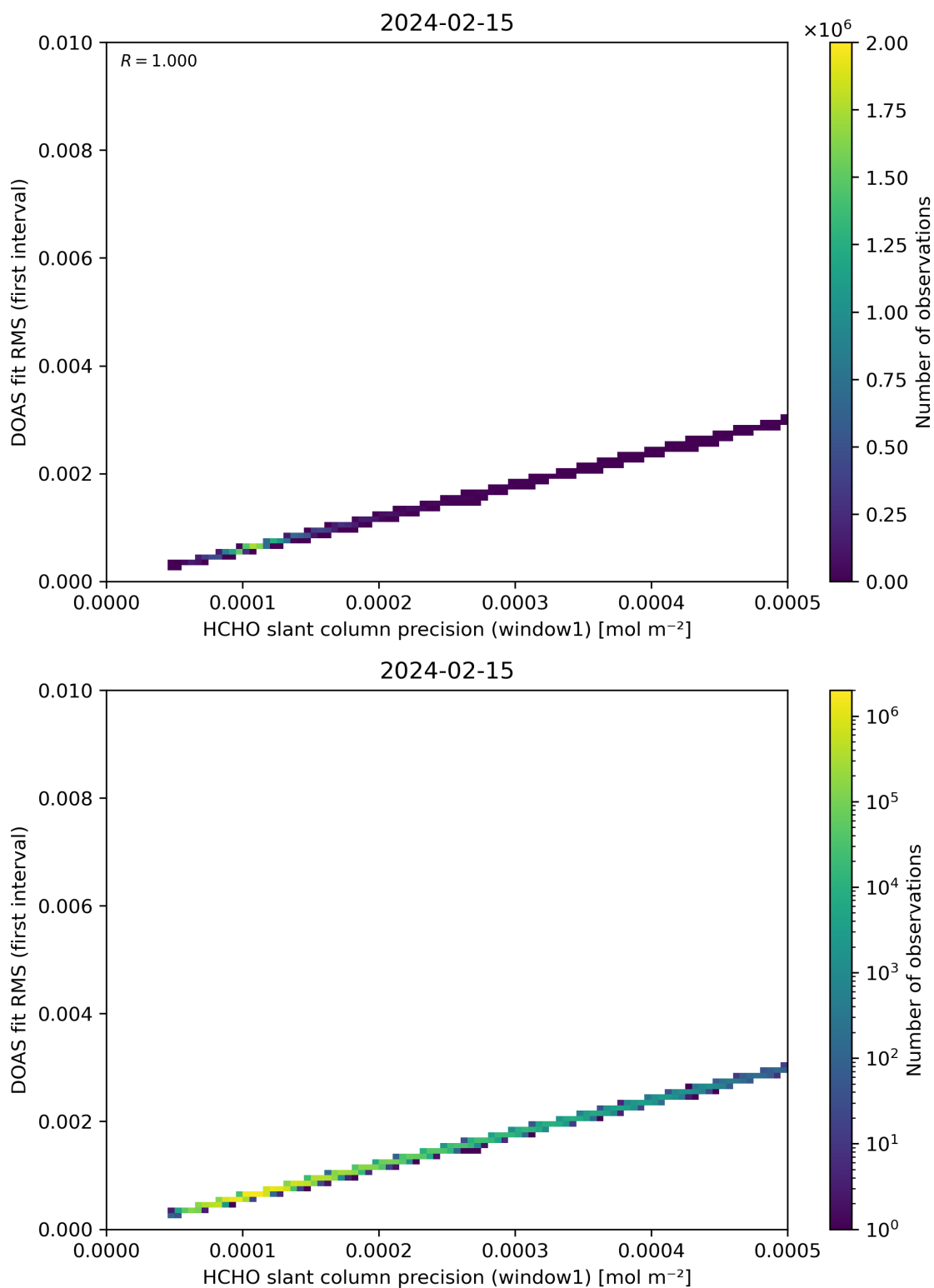
Figure 88: Scatter density plot of “HCHO slant column precision (window1)” against “DOAS fit RMS (first interval)” for 2024-02-14 to 2024-02-16.
