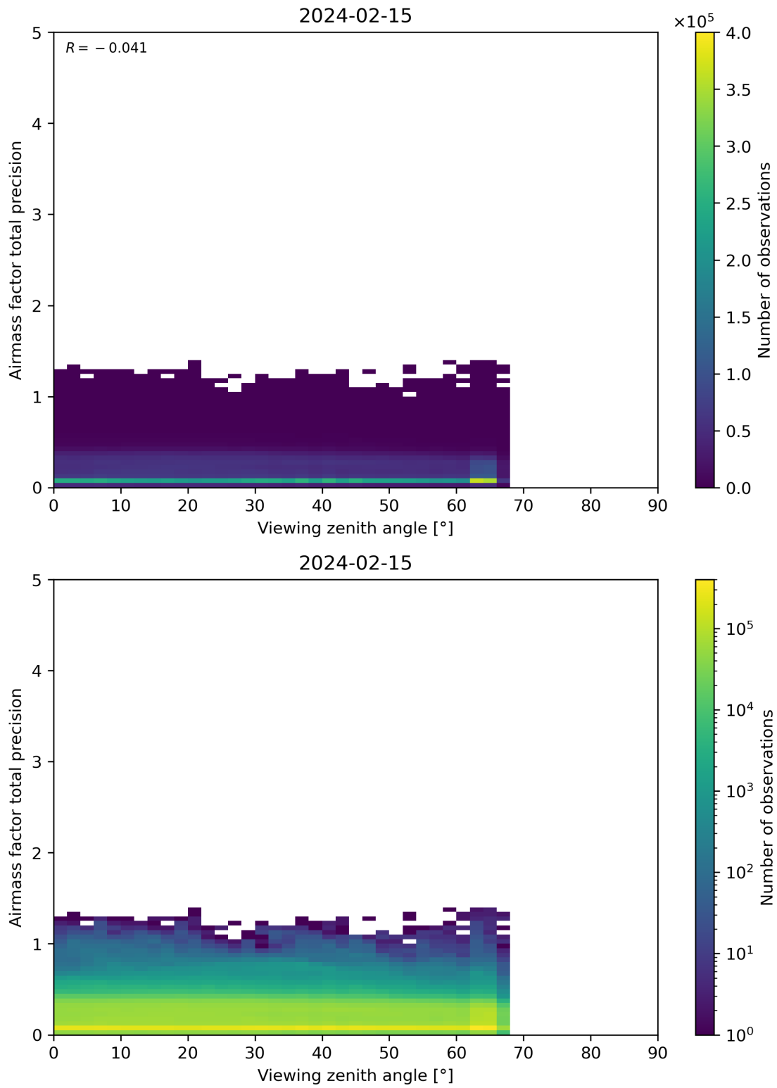
Figure 191: Scatter density plot of “Viewing zenith angle” against “Airmass factor total precision” for 2024-02-14 to 2024-02-16.
