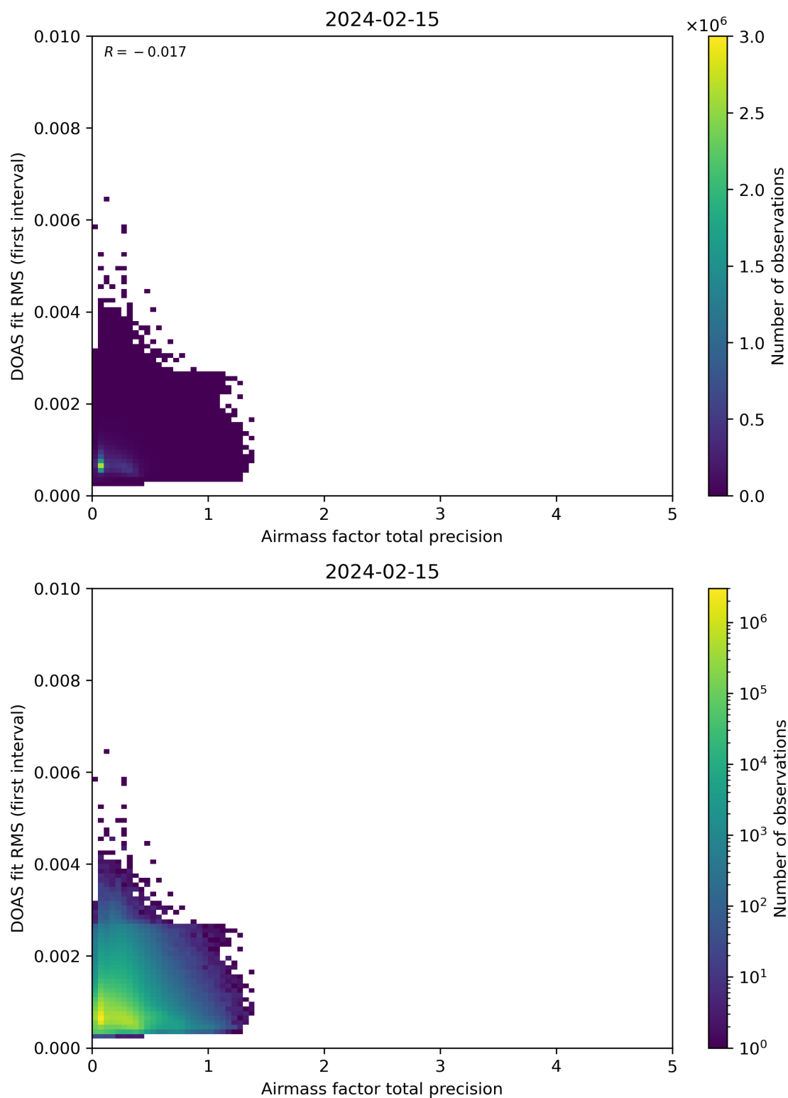
Figure 105: Scatter density plot of “Airmass factor total precision” against “DOAS fit RMS (first interval)” for 2024-02-14 to 2024-02-16.
