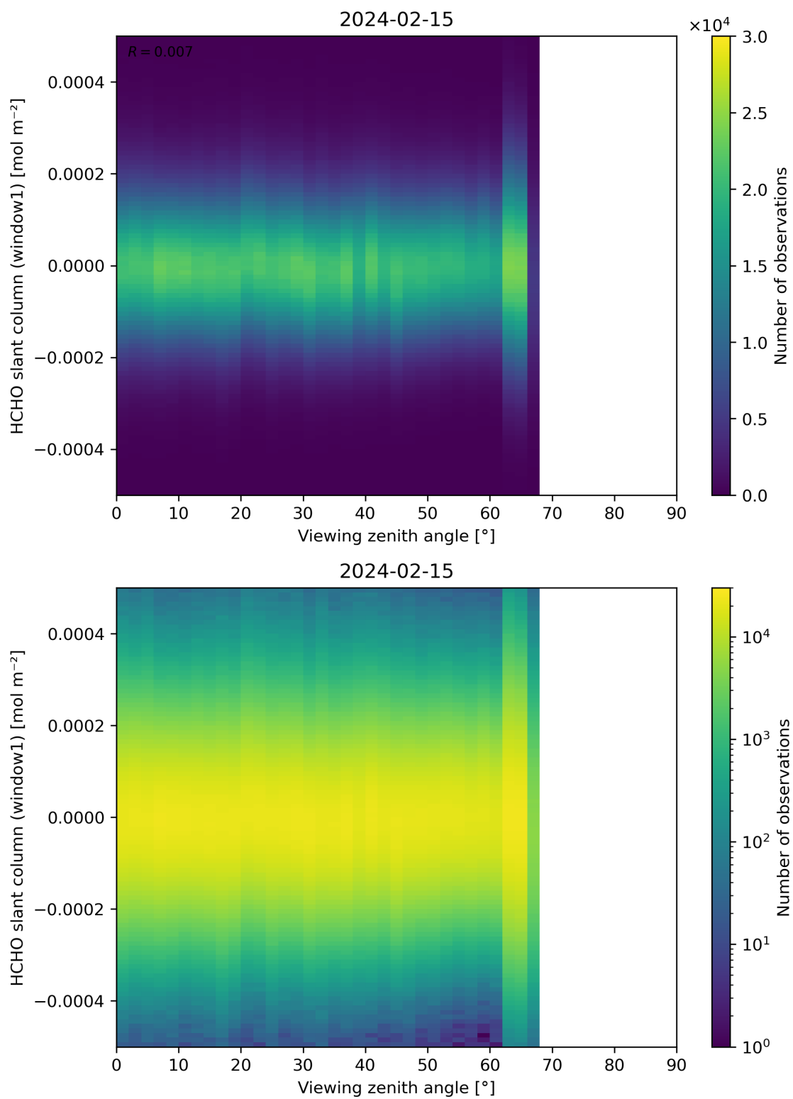
Figure 188: Scatter density plot of “Viewing zenith angle” against “HCHO slant column (window1)” for 2024-02-14 to 2024-02-16.
