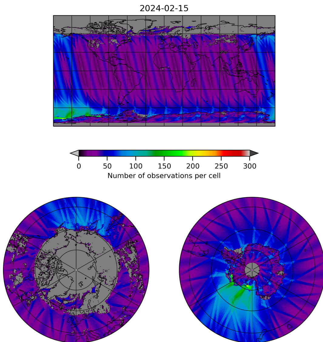
Figure 19: Map of the number of observations for 2024-02-14 to 2024-02-16
