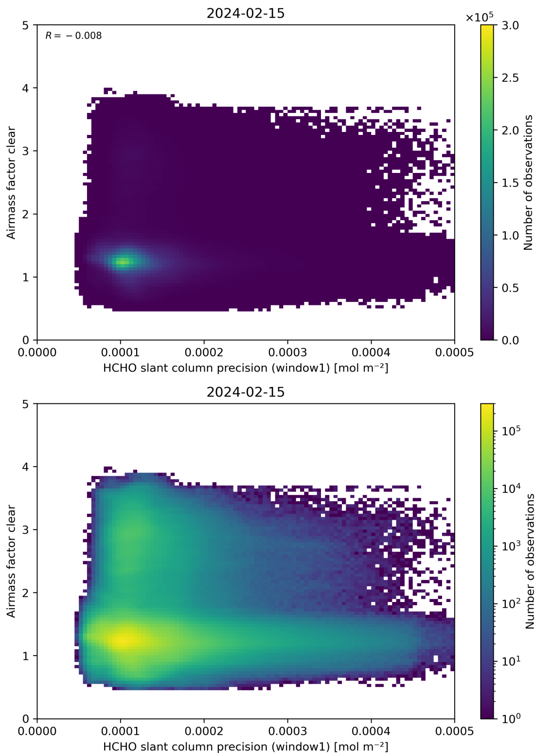
Figure 91: Scatter density plot of “HCHO slant column precision (window1)” against “Airmass factor clear” for 2024-02-14 to 2024-02-16.
