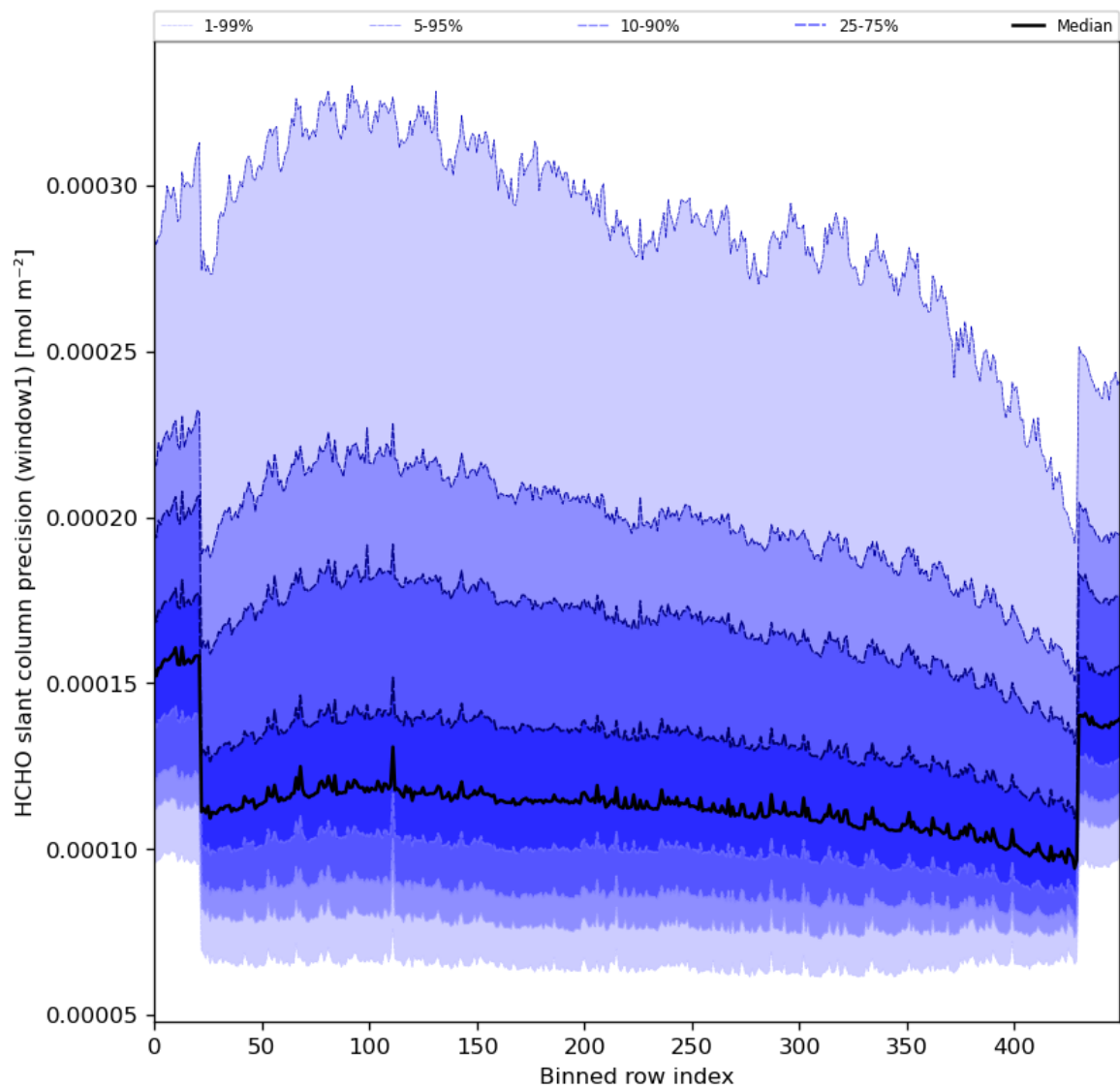
Figure 53: Along track statistics of “HCHO slant column precision (window1)” for 2024-02-14 to 2024-02-16
