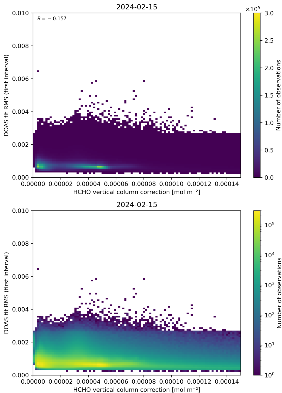
Figure 112: Scatter density plot of “HCHO vertical column correction” against “DOAS fit RMS (first interval)” for 2024-02-14 to 2024-02-16.
