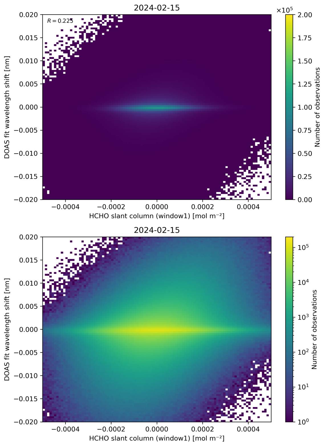
Figure 79: Scatter density plot of “HCHO slant column (window1)” against “DOAS fit wavelength shift” for 2024-02-14 to 2024-02-16.
