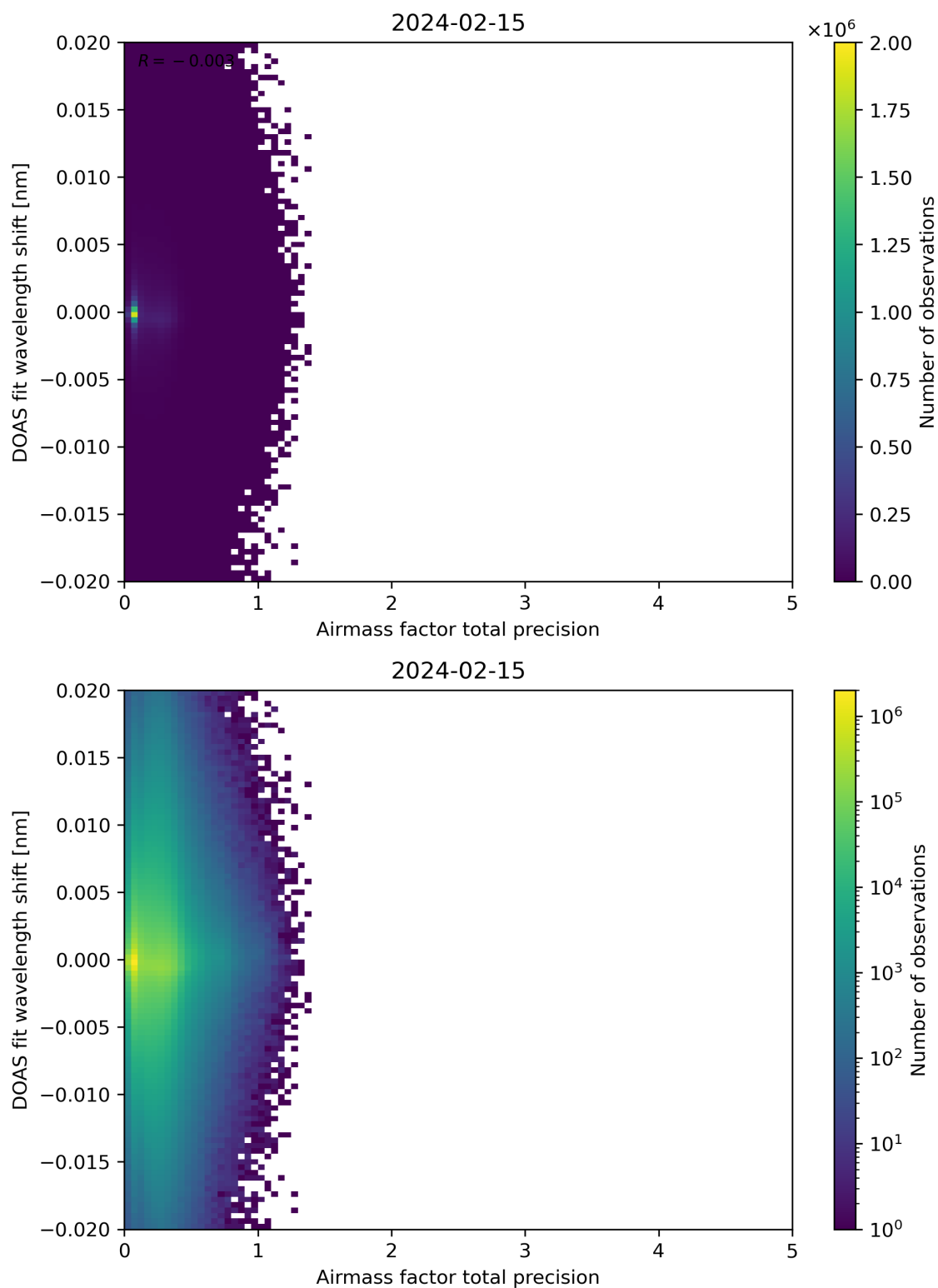
Figure 106: Scatter density plot of “Airmass factor total precision” against “DOAS fit wavelength shift” for 2024-02-14 to 2024-02-16.
