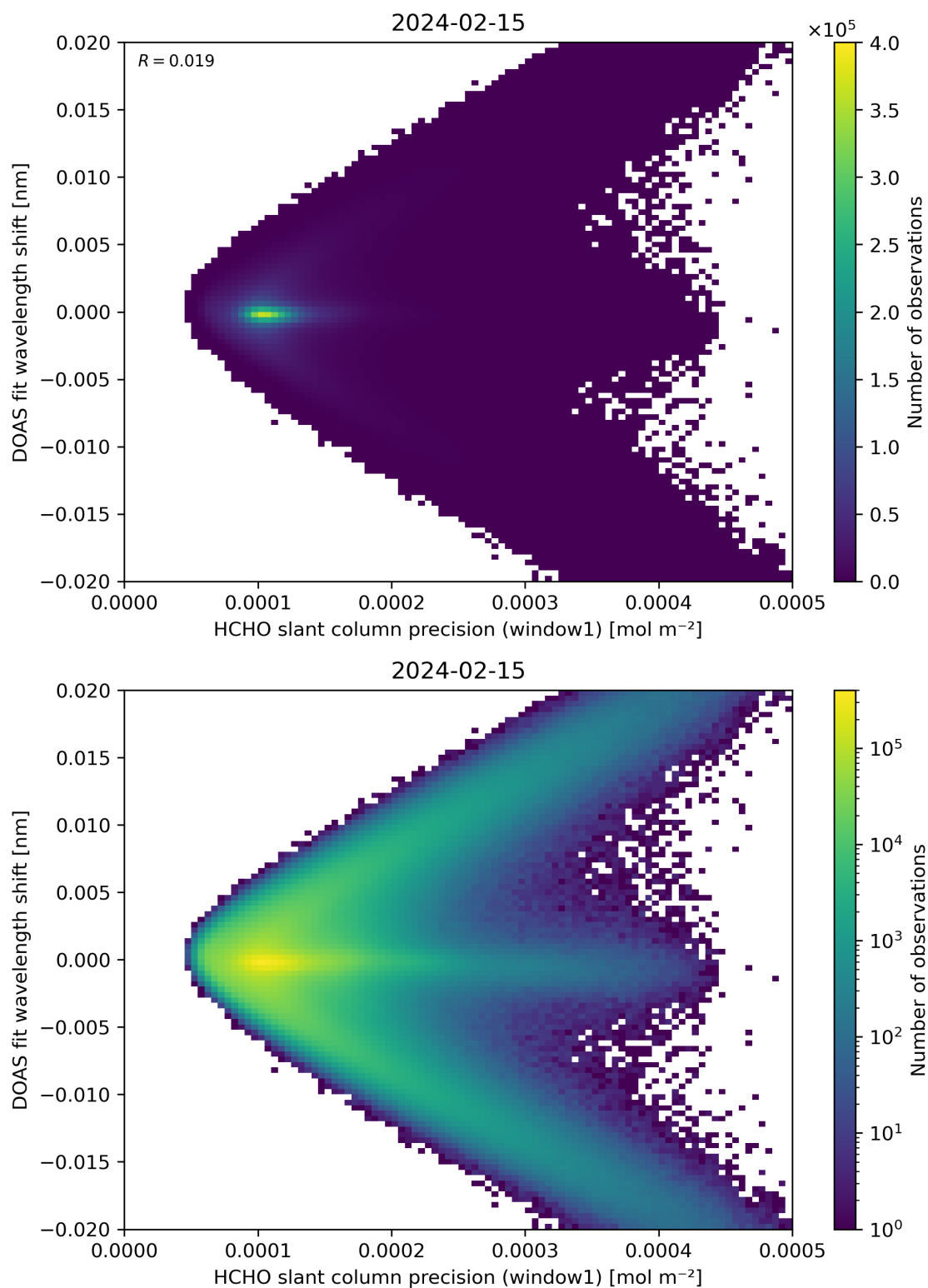
Figure 89: Scatter density plot of “HCHO slant column precision (window1)” against “DOAS fit wavelength shift” for 2024-02-14 to 2024-02-16.
