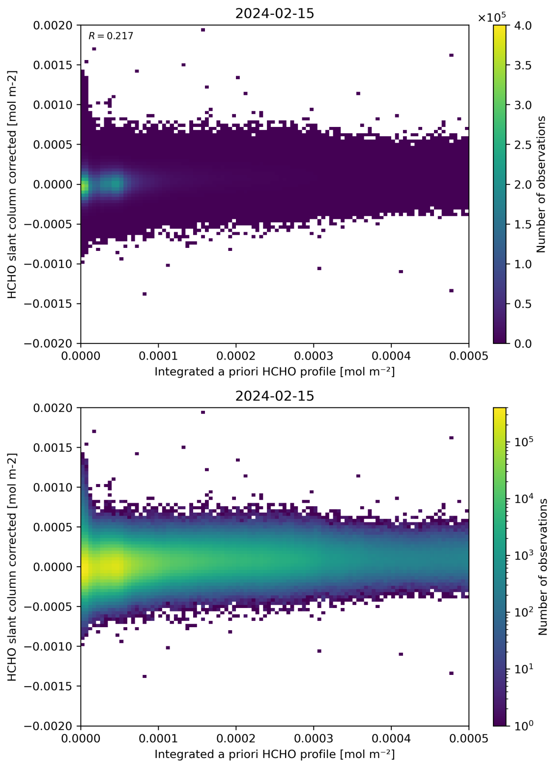
Figure 151: Scatter density plot of “Integrated a priori HCHO profile” against “HCHO slant column corrected” for 2024-02-14 to 2024-02-16.
