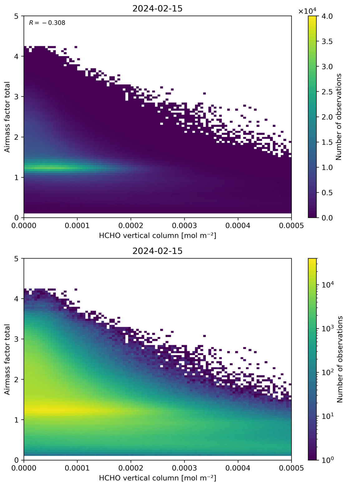
Figure 131: Scatter density plot of “HCHO vertical column” against “Airmass factor total” for 2024-02-14 to 2024-02-16.
