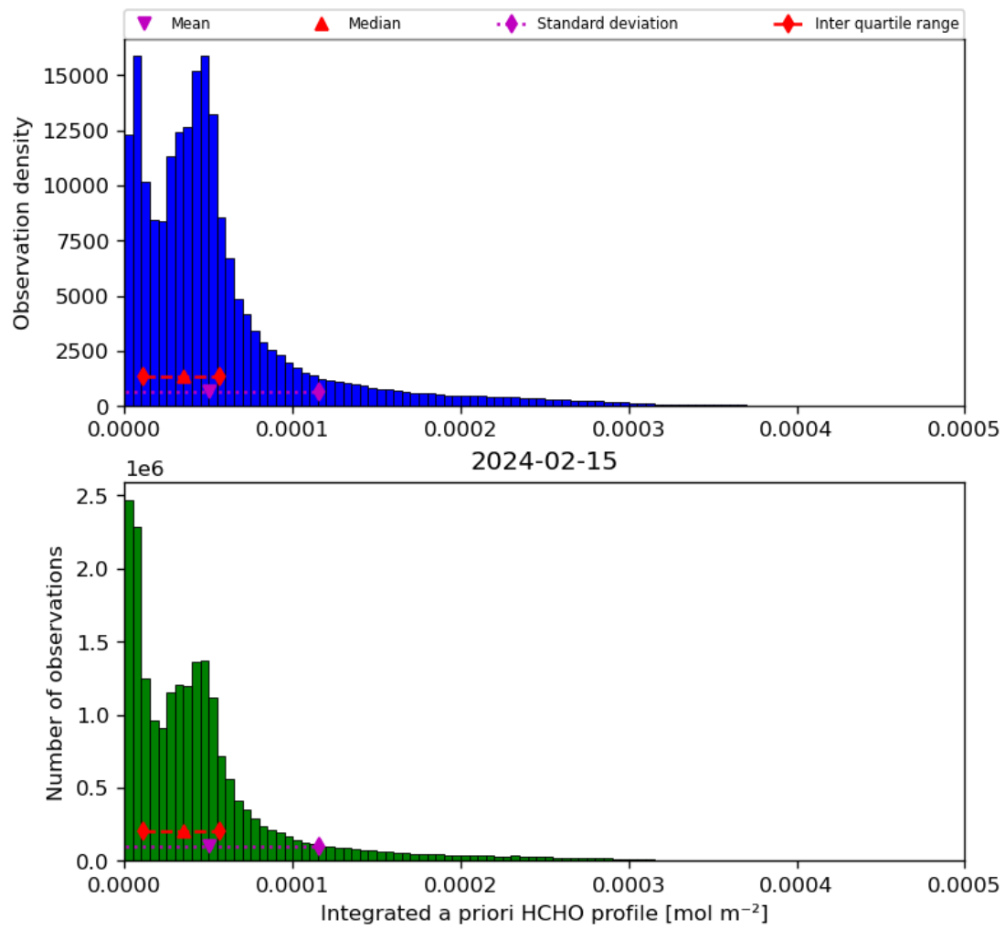
Figure 43: Histogram of “Integrated a priori HCHO profile” for 2024-02-14 to 2024-02-16
