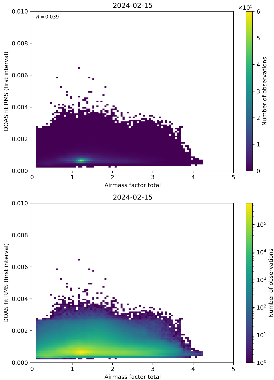
Figure 97: Scatter density plot of “Airmass factor total” against “DOAS fit RMS (first interval)” for 2024-02-14 to 2024-02-16.
