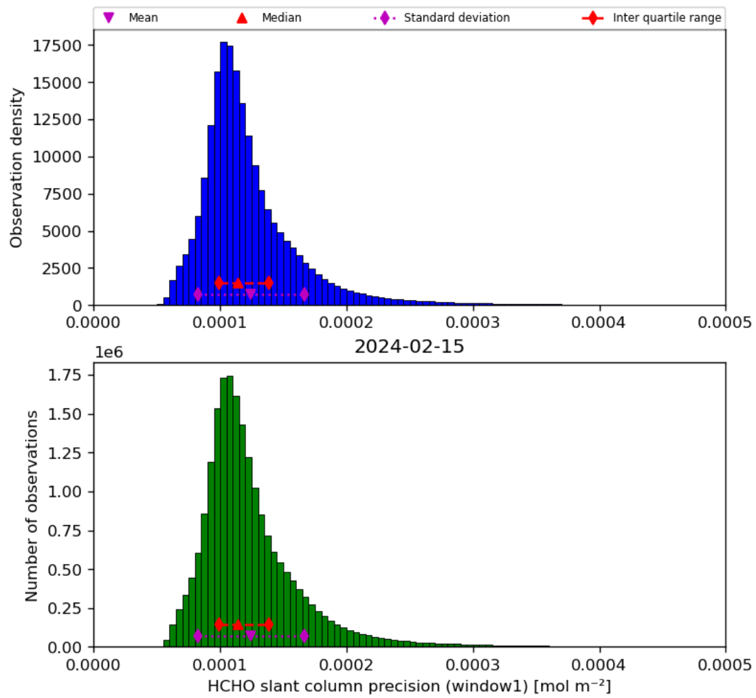
Figure 39: Histogram of “HCHO slant column precision (window1)” for 2024-02-14 to 2024-02-16
