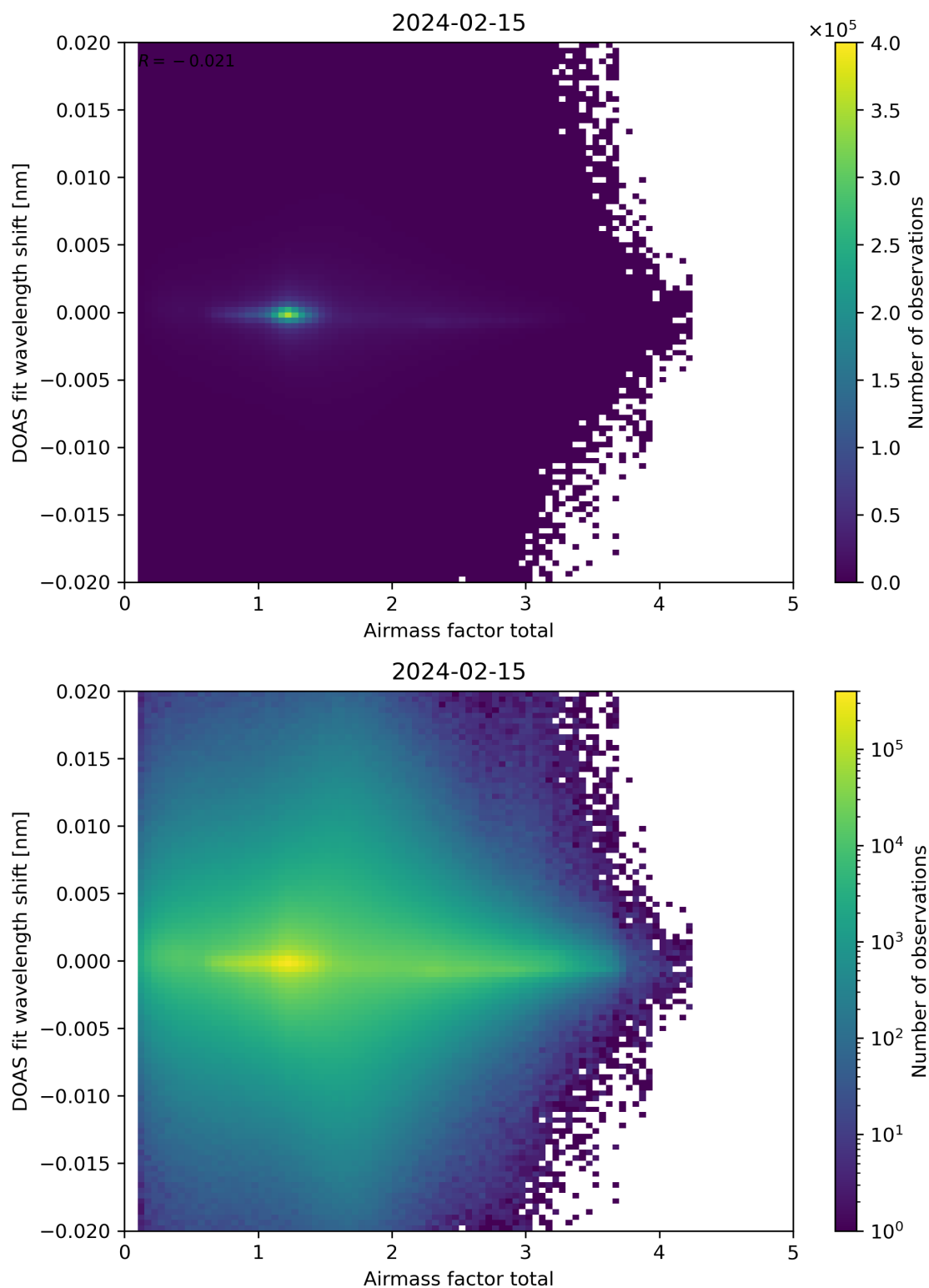
Figure 98: Scatter density plot of “Airmass factor total” against “DOAS fit wavelength shift” for 2024-02-14 to 2024-02-16.
