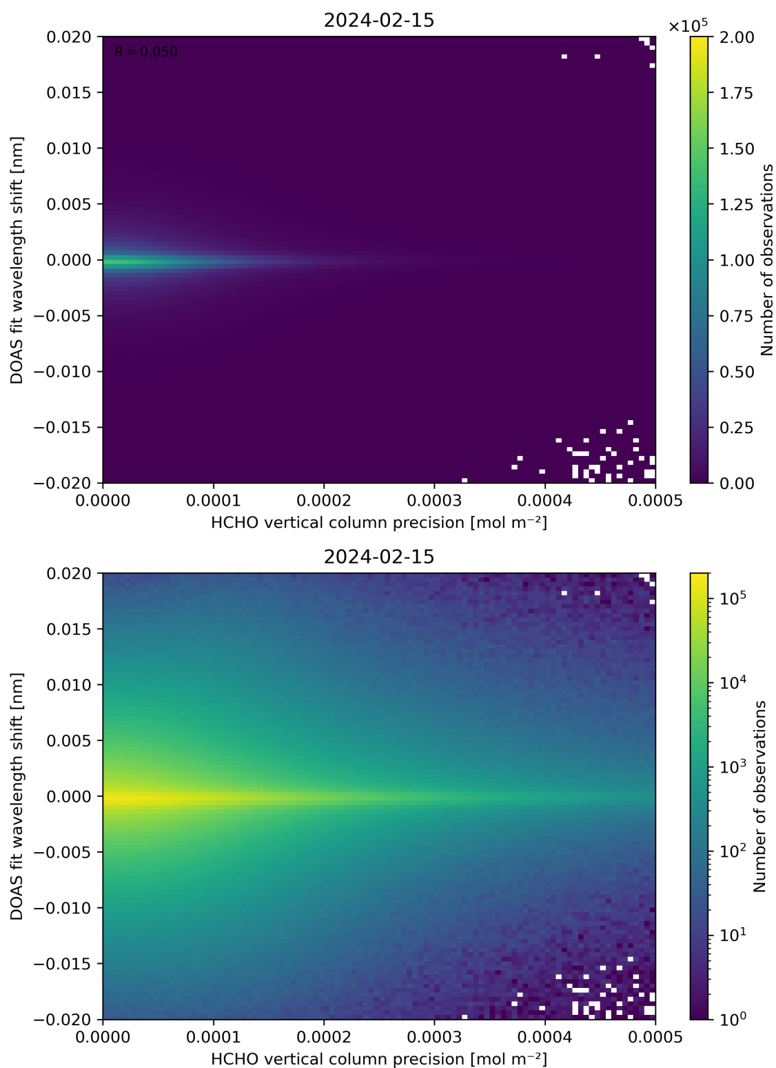
Figure 137: Scatter density plot of “HCHO vertical column precision” against “DOAS fit wavelength shift” for 2024-02-14 to 2024-02-16.
