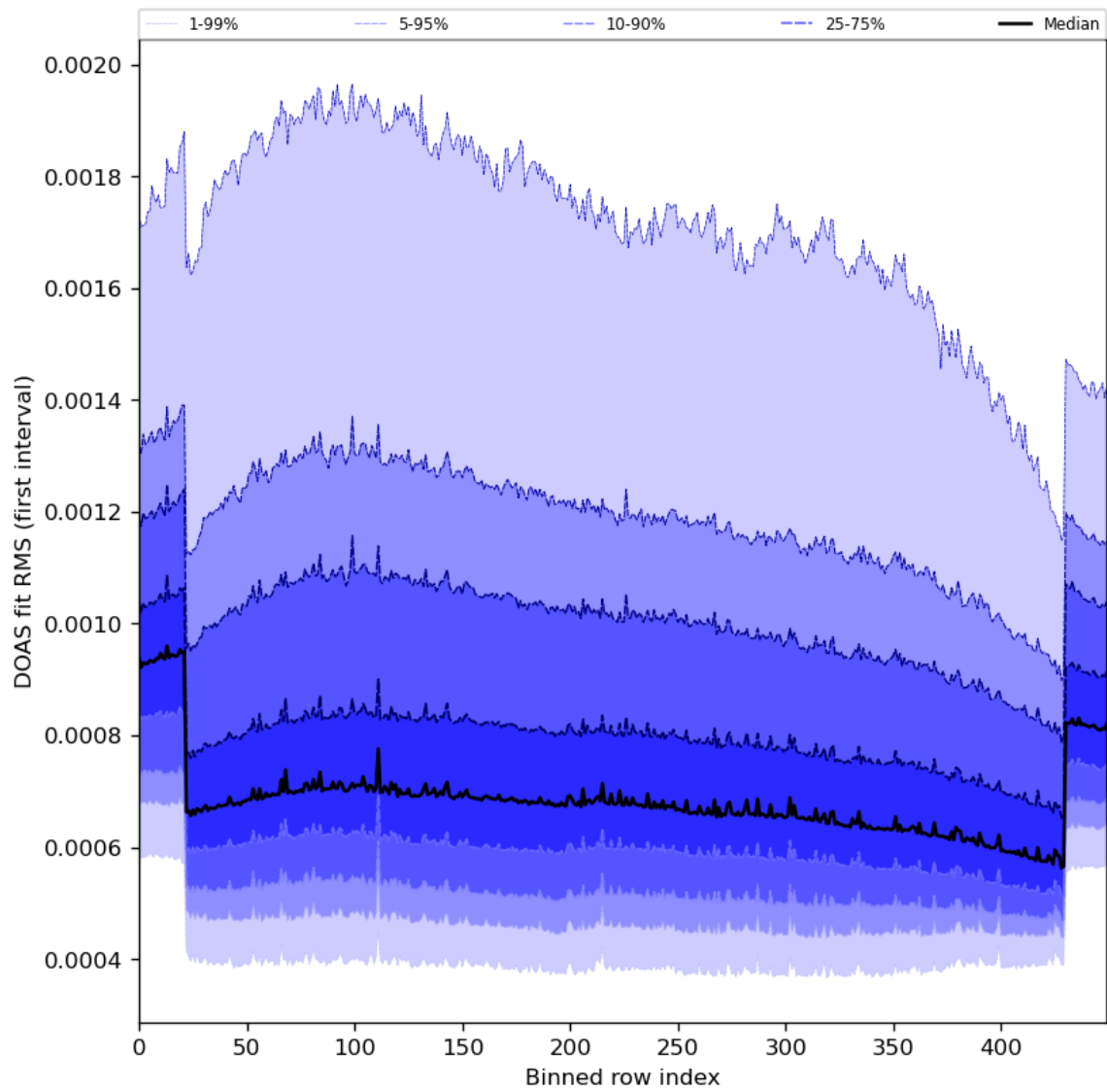
Figure 60: Along track statistics of “DOAS fit RMS (first interval)” for 2024-02-14 to 2024-02-16
