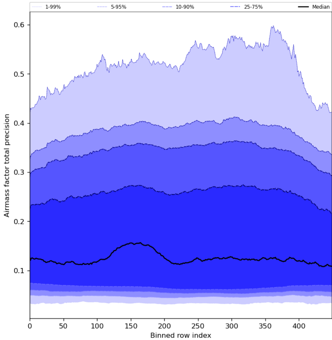
Figure 55: Along track statistics of “Airmass factor total precision” for 2024-02-14 to 2024-02-16
