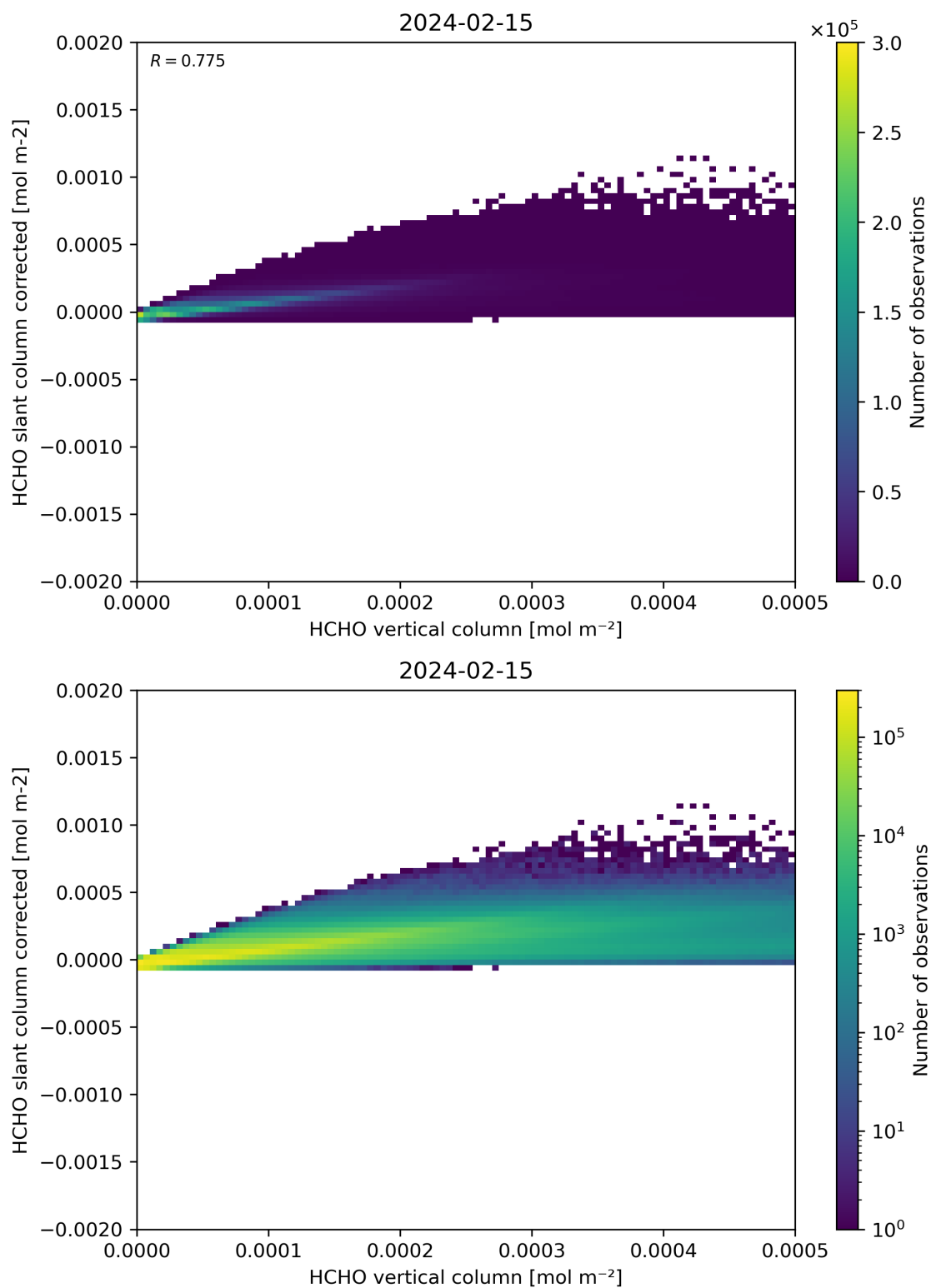
Figure 127: Scatter density plot of “HCHO vertical column” against “HCHO slant column corrected” for 2024-02-14 to 2024-02-16.
