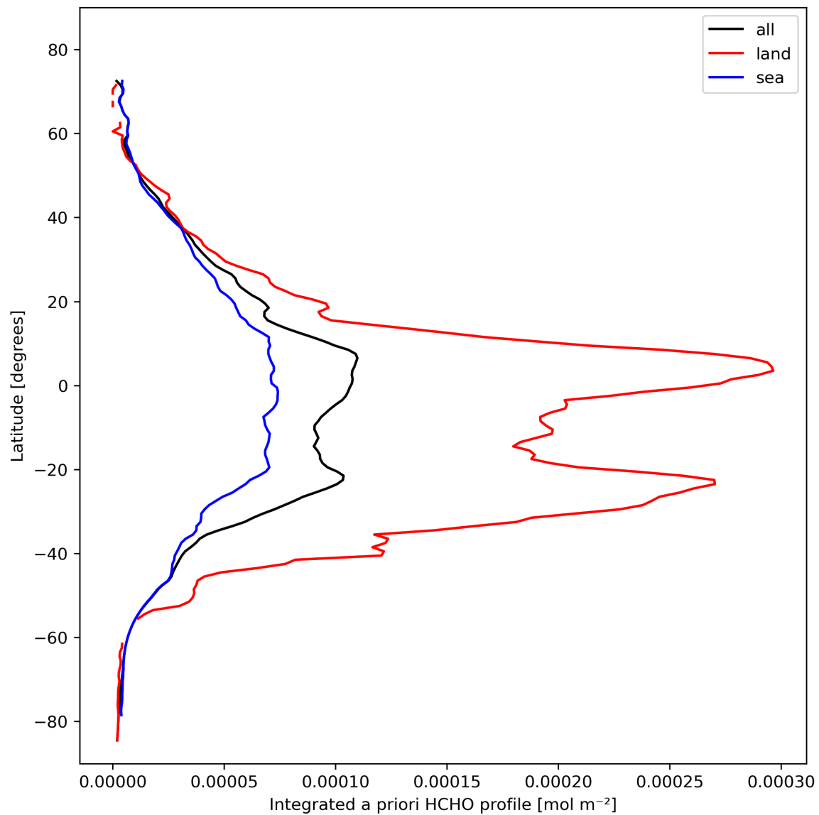
Figure 29: Zonal average of “Integrated a priori HCHO profile” for 2024-02-14 to 2024-02-16.
