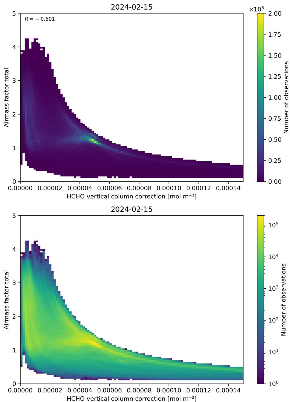
Figure 120: Scatter density plot of “HCHO vertical column correction” against “Airmass factor total” for 2024-02-14 to 2024-02-16.
